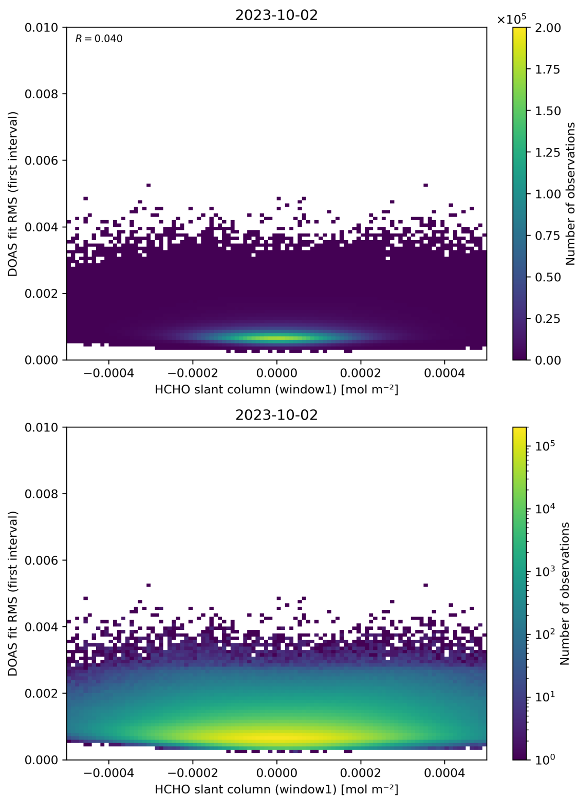
Figure 78: Scatter density plot of “HCHO slant column (window1)” against “DOAS fit RMS (first interval)” for 2023-10-01 to 2023-10-03.
