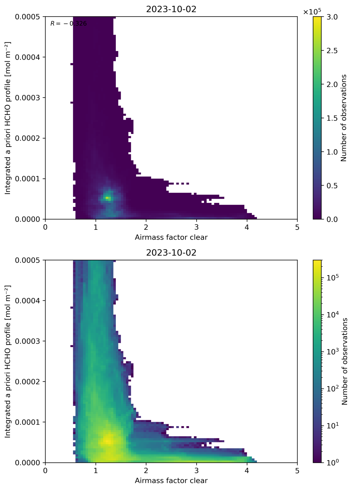
Figure 76: Scatter density plot of “Airmass factor clear” against “Integrated a priori HCHO profile” for 2023-10-01 to 2023-10-03.
