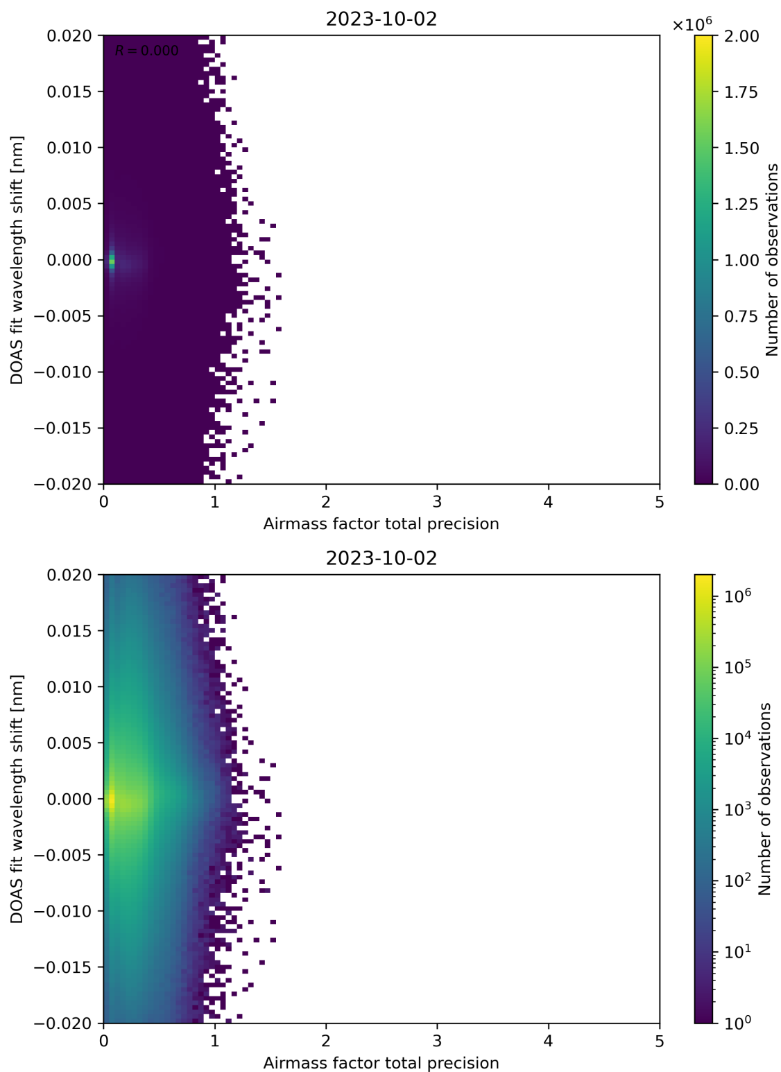
Figure 106: Scatter density plot of “Airmass factor total precision” against “DOAS fit wavelength shift” for 2023-10-01 to 2023-10-03.
