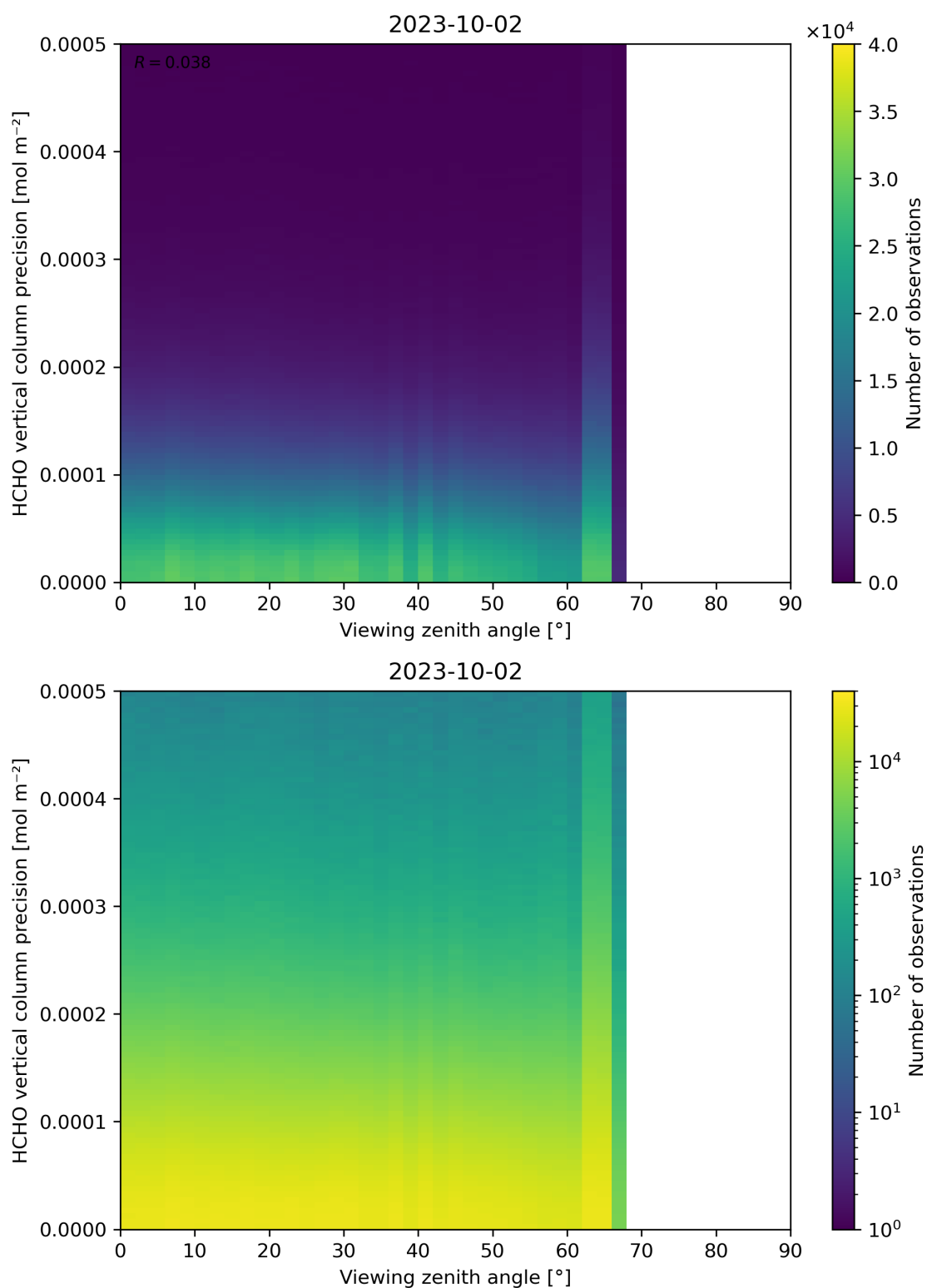
Figure 194: Scatter density plot of “Viewing zenith angle” against “HCHO vertical column precision” for 2023-10-01 to 2023-10-03.
