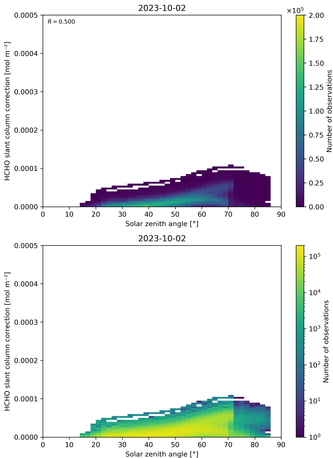
Figure 172: Scatter density plot of “Solar zenith angle” against “HCHO slant column correction” for 2023-10-01 to 2023-10-03.
