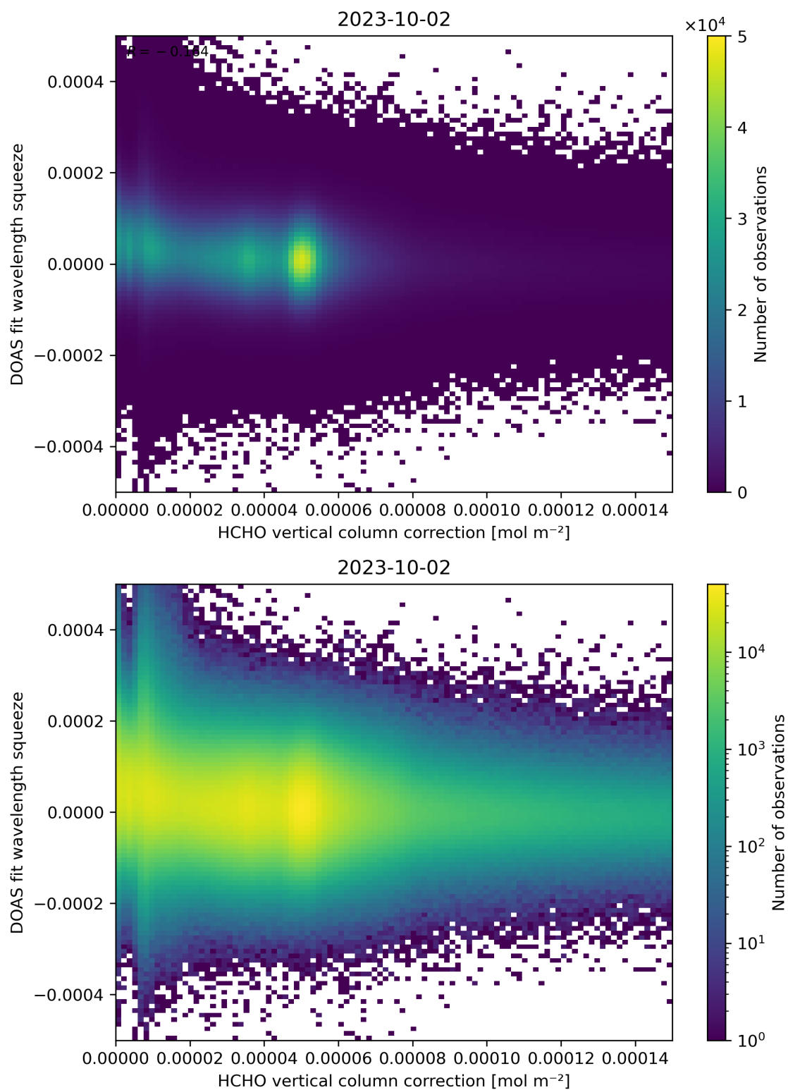
Figure 114: Scatter density plot of “HCHO vertical column correction” against “DOAS fit wavelength squeeze” for 2023-10-01 to 2023-10-03.
