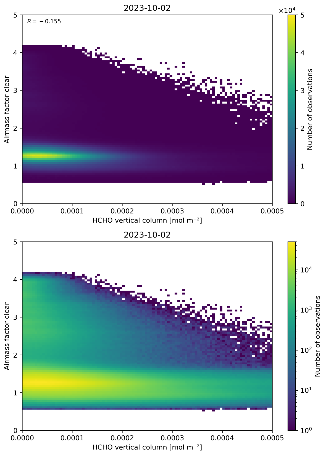
Figure 126: Scatter density plot of “HCHO vertical column” against “Airmass factor clear” for 2023-10-01 to 2023-10-03.
