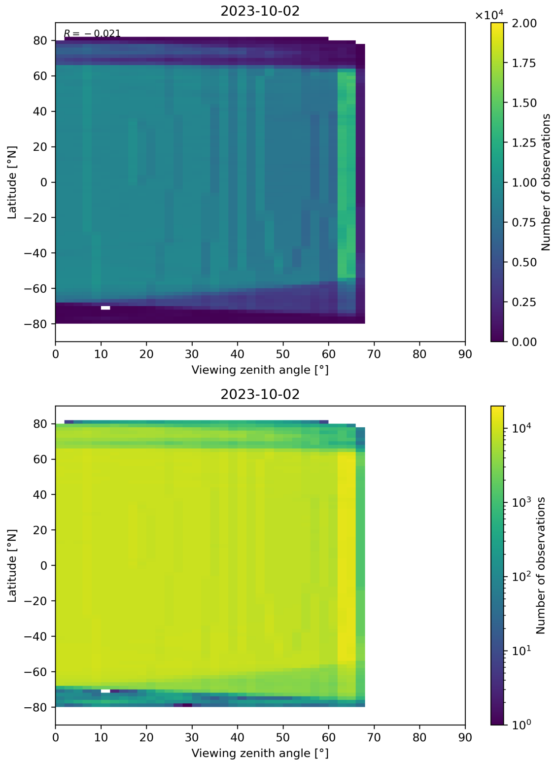
Figure 196: Scatter density plot of “Viewing zenith angle” against “Latitude” for 2023-10-01 to 2023-10-03.
