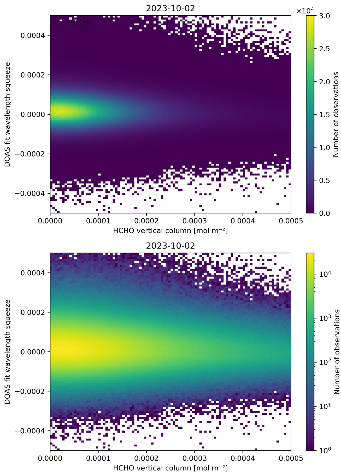
Figure 125: Scatter density plot of “HCHO vertical column” against “DOAS fit wavelength squeeze” for 2023-10-01 to 2023-10-03.
