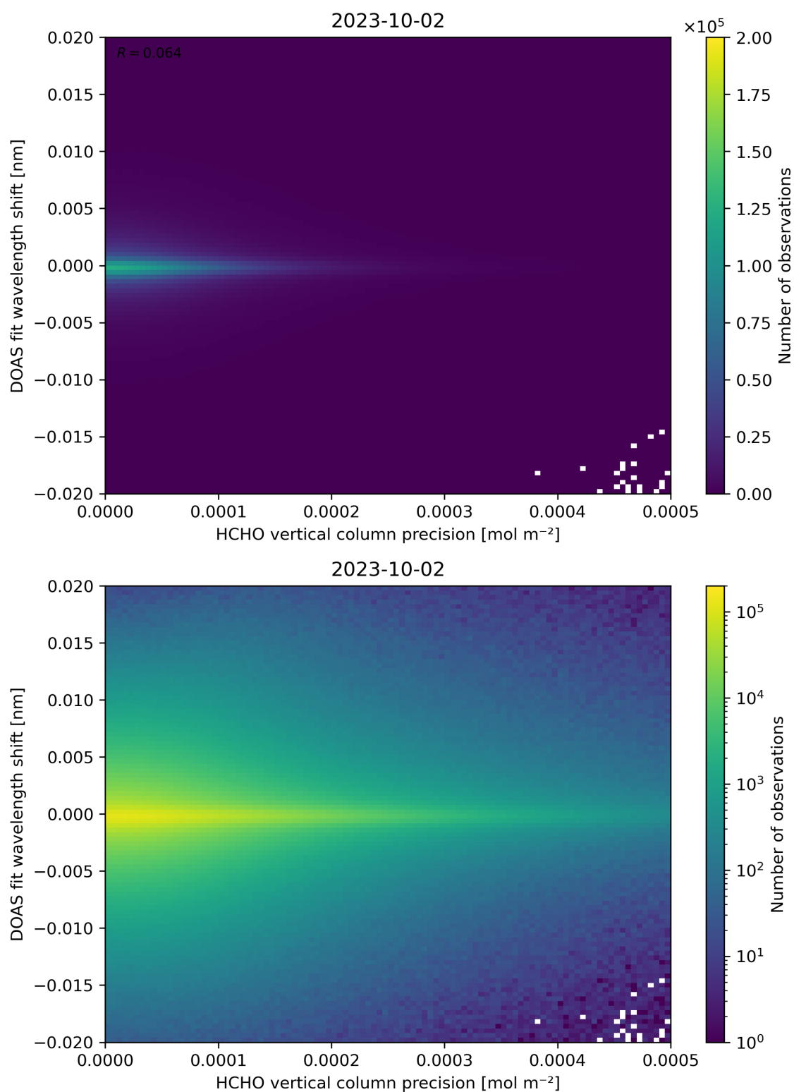
Figure 137: Scatter density plot of “HCHO vertical column precision” against “DOAS fit wavelength shift” for 2023-10-01 to 2023-10-03.
