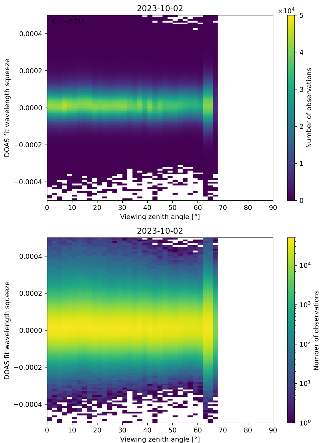
Figure 184: Scatter density plot of “Viewing zenith angle” against “DOAS fit wavelength squeeze” for 2023-10-01 to 2023-10-03.
