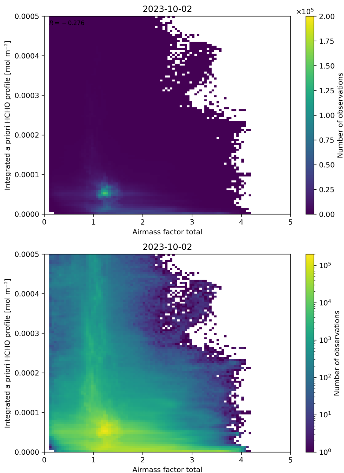
Figure 104: Scatter density plot of “Airmass factor total” against “Integrated a priori HCHO profile” for 2023-10-01 to 2023-10-03.
