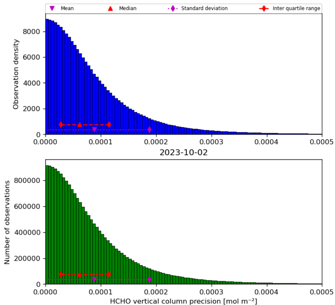
Figure 36: Histogram of “HCHO vertical column precision” for 2023-10-01 to 2023-10-03
