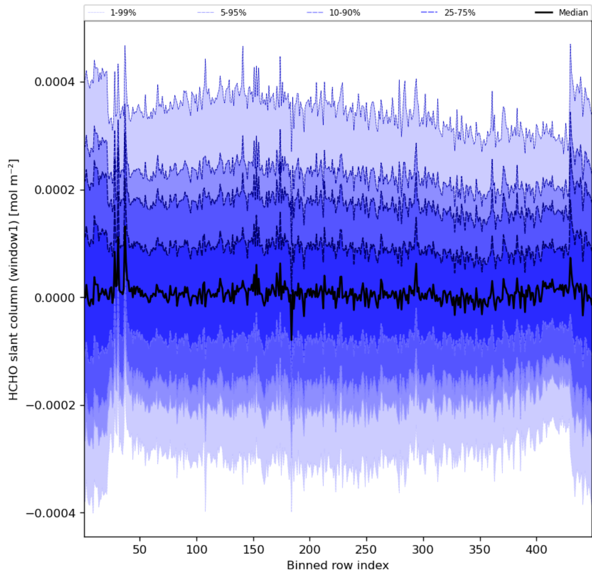
Figure 52: Along track statistics of “HCHO slant column (window1)” for 2023-10-01 to 2023-10-03
