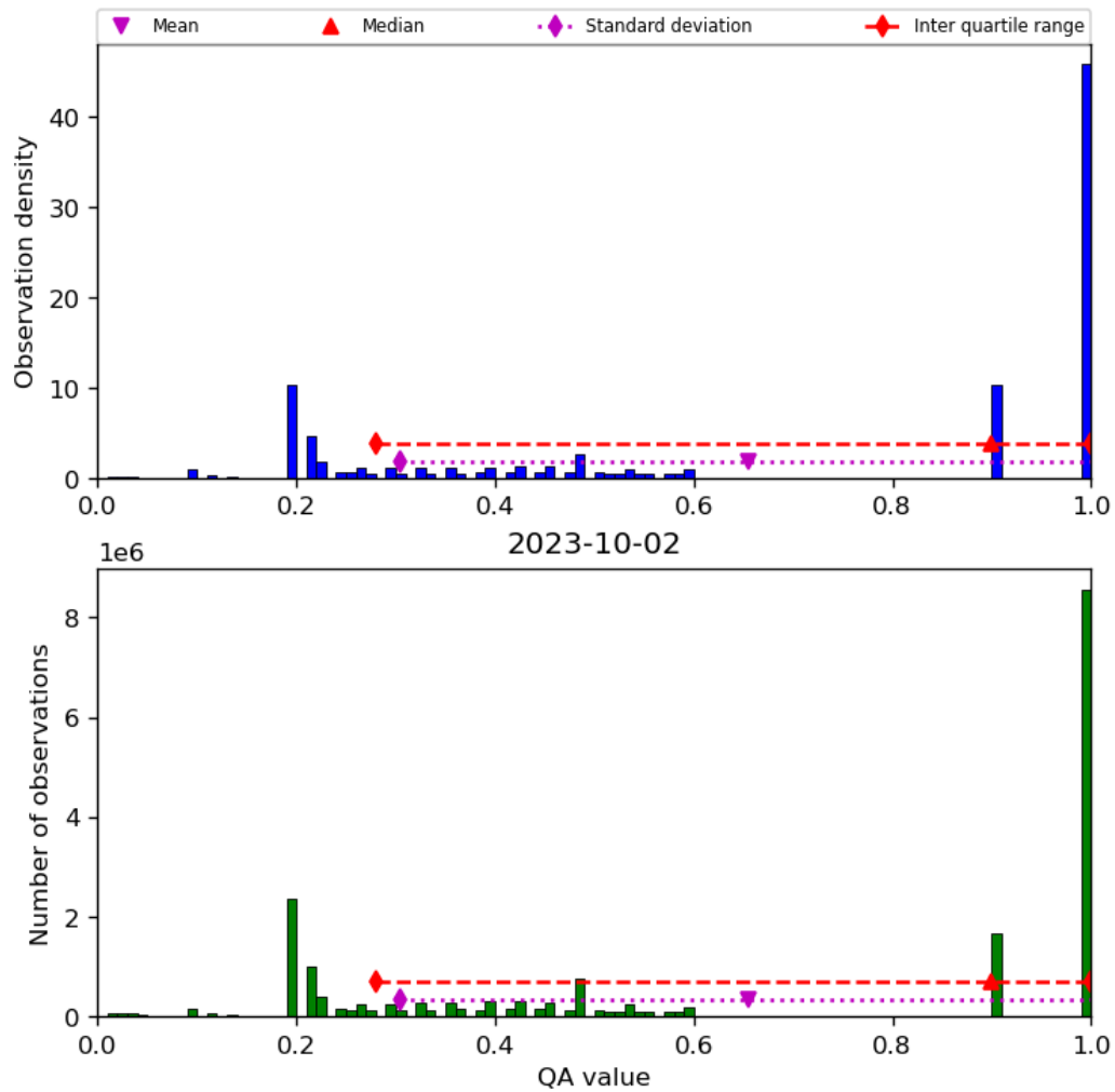
Figure 34: Histogram of “QA value” for 2023-10-01 to 2023-10-03
