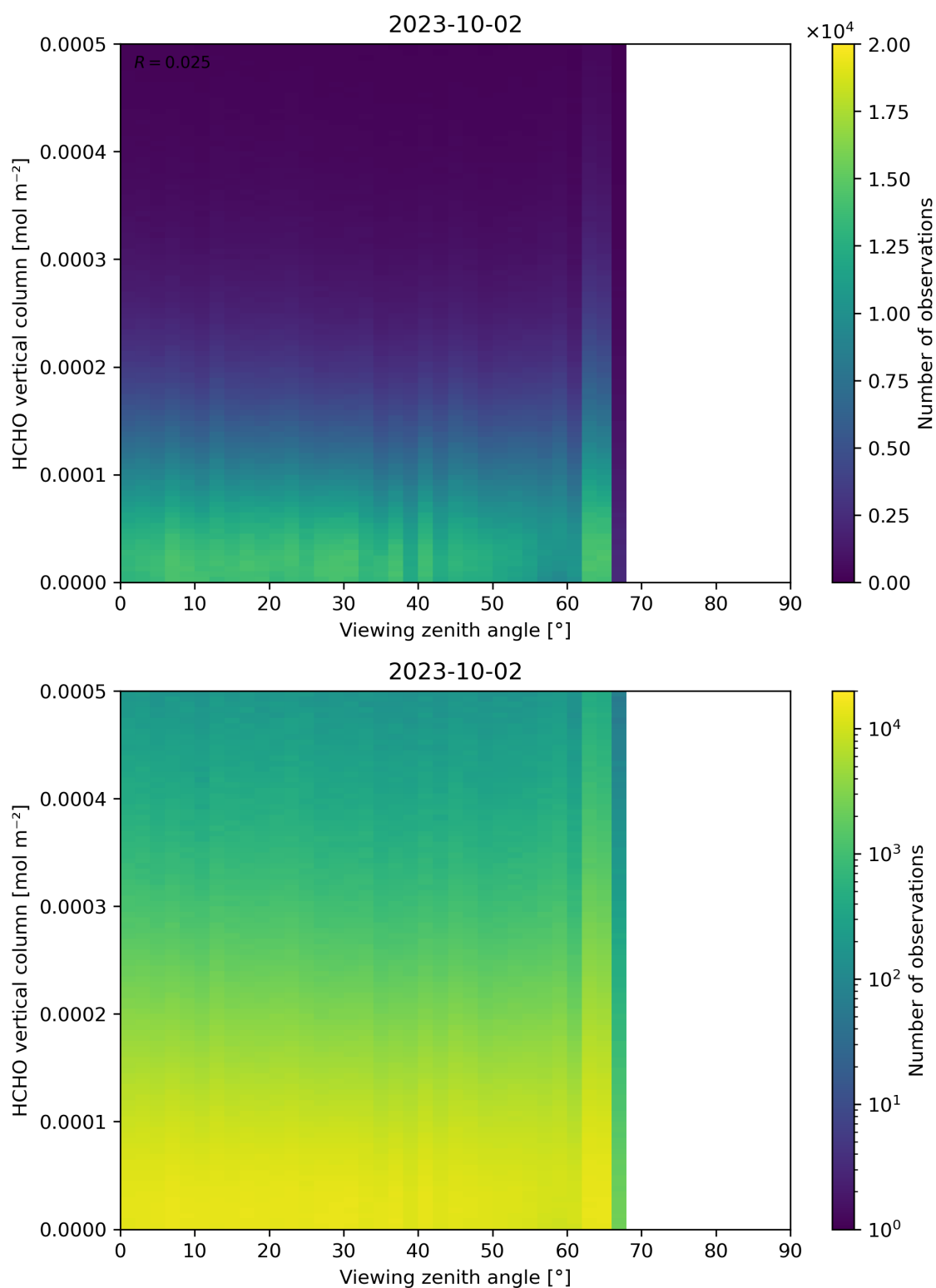
Figure 192: Scatter density plot of “Viewing zenith angle” against “HCHO vertical column” for 2023-10-01 to 2023-10-03.
