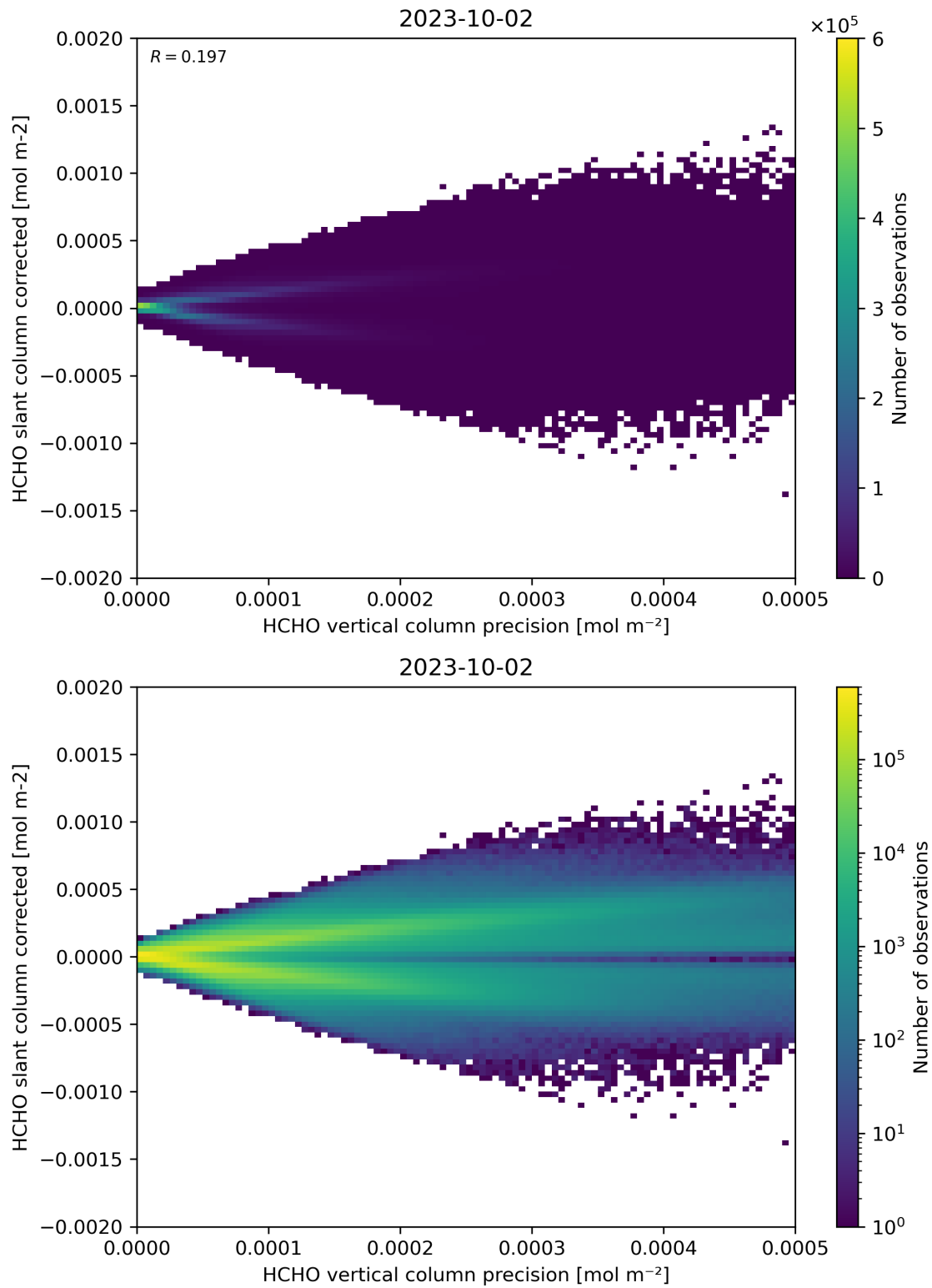
Figure 140: Scatter density plot of “HCHO vertical column precision” against “HCHO slant column corrected” for 2023-10-01 to 2023-10-03.
