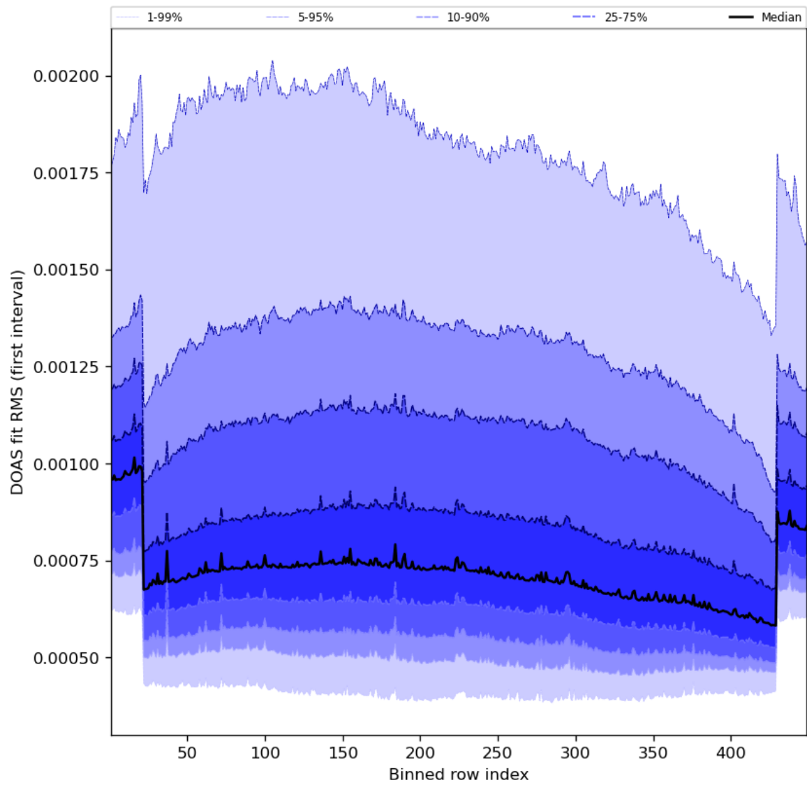
Figure 60: Along track statistics of “DOAS fit RMS (first interval)” for 2023-10-01 to 2023-10-03
