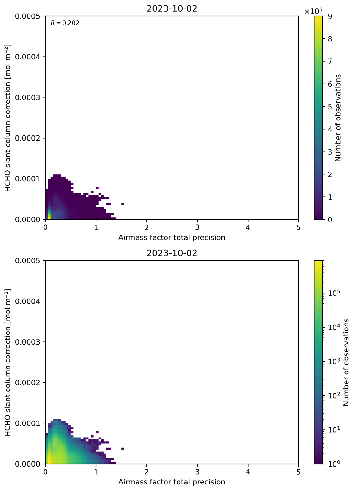
Figure 110: Scatter density plot of “Airmass factor total precision” against “HCHO slant column correction” for 2023-10-01 to 2023-10-03.
