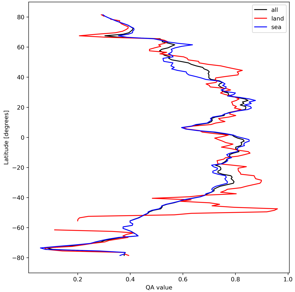
Figure 20: Zonal average of “QA value” for 2023-10-01 to 2023-10-03.
