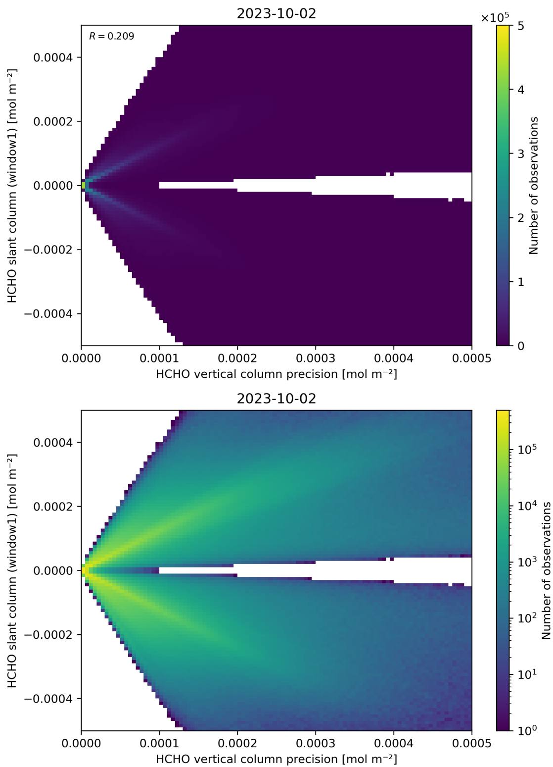
Figure 142: Scatter density plot of “HCHO vertical column precision” against “HCHO slant column (window1)” for 2023-10-01 to 2023-10-03.
