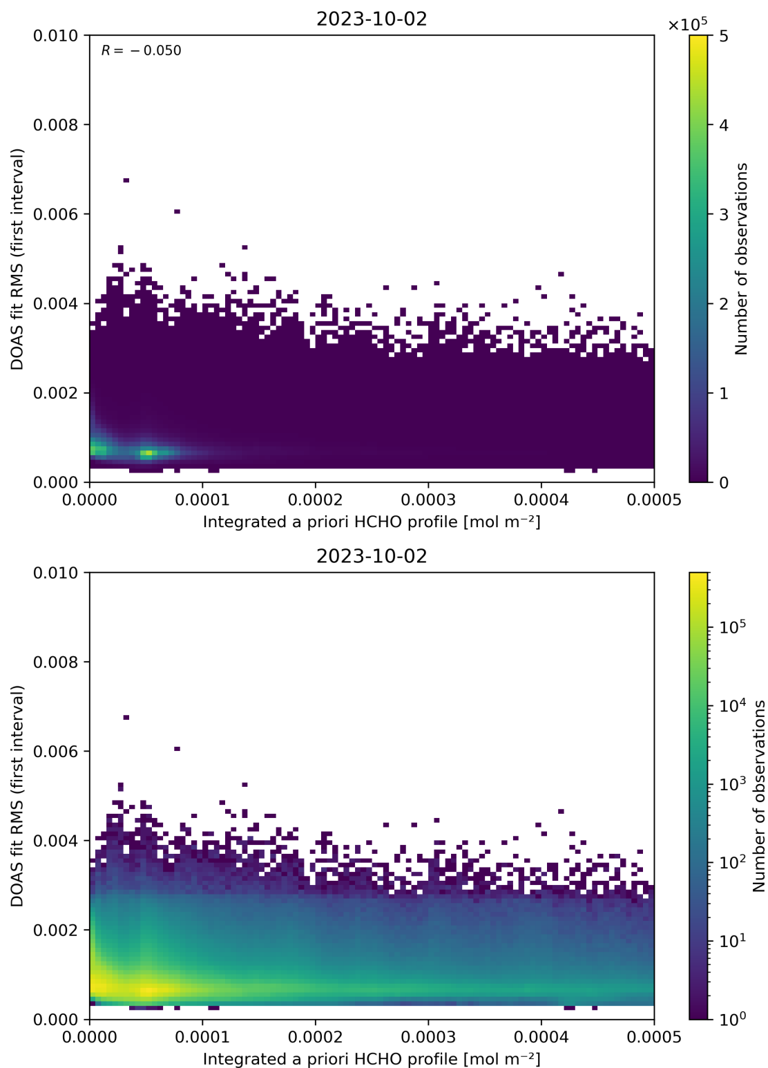
Figure 148: Scatter density plot of “Integrated a priori HCHO profile” against “DOAS fit RMS (first interval)” for 2023-10-01 to 2023-10-03.
