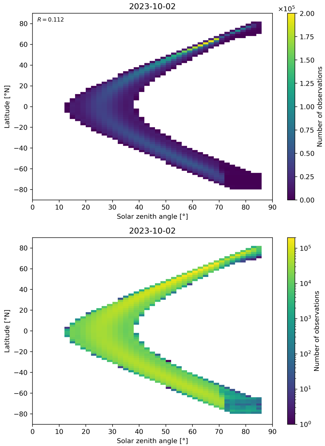
Figure 181: Scatter density plot of “Solar zenith angle” against “Latitude” for 2023-10-01 to 2023-10-03.
