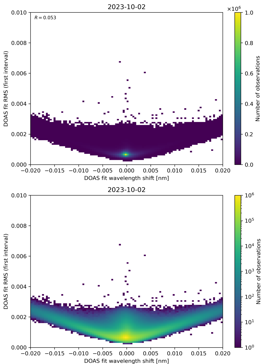
Figure 64: Scatter density plot of “DOAS fit wavelength shift” against “DOAS fit RMS (first interval)” for 2023-10-01 to 2023-10-03.
