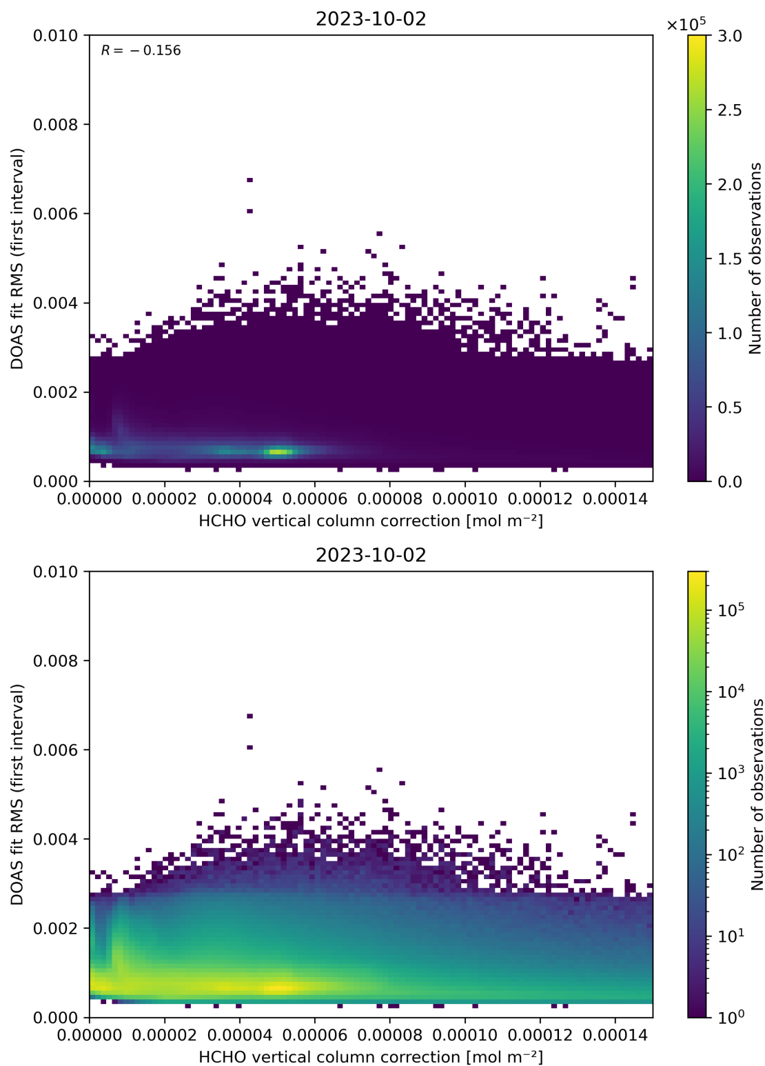
Figure 112: Scatter density plot of “HCHO vertical column correction” against “DOAS fit RMS (first interval)” for 2023-10-01 to 2023-10-03.
