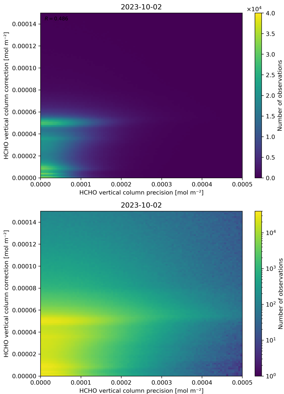
Figure 146: Scatter density plot of “HCHO vertical column precision” against “HCHO vertical column correction” for 2023-10-01 to 2023-10-03.
