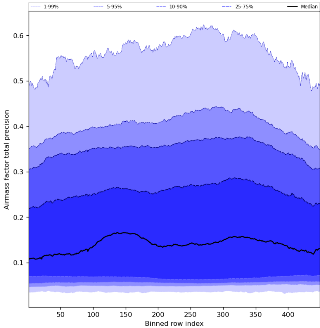
Figure 55: Along track statistics of “Airmass factor total precision” for 2023-10-01 to 2023-10-03
