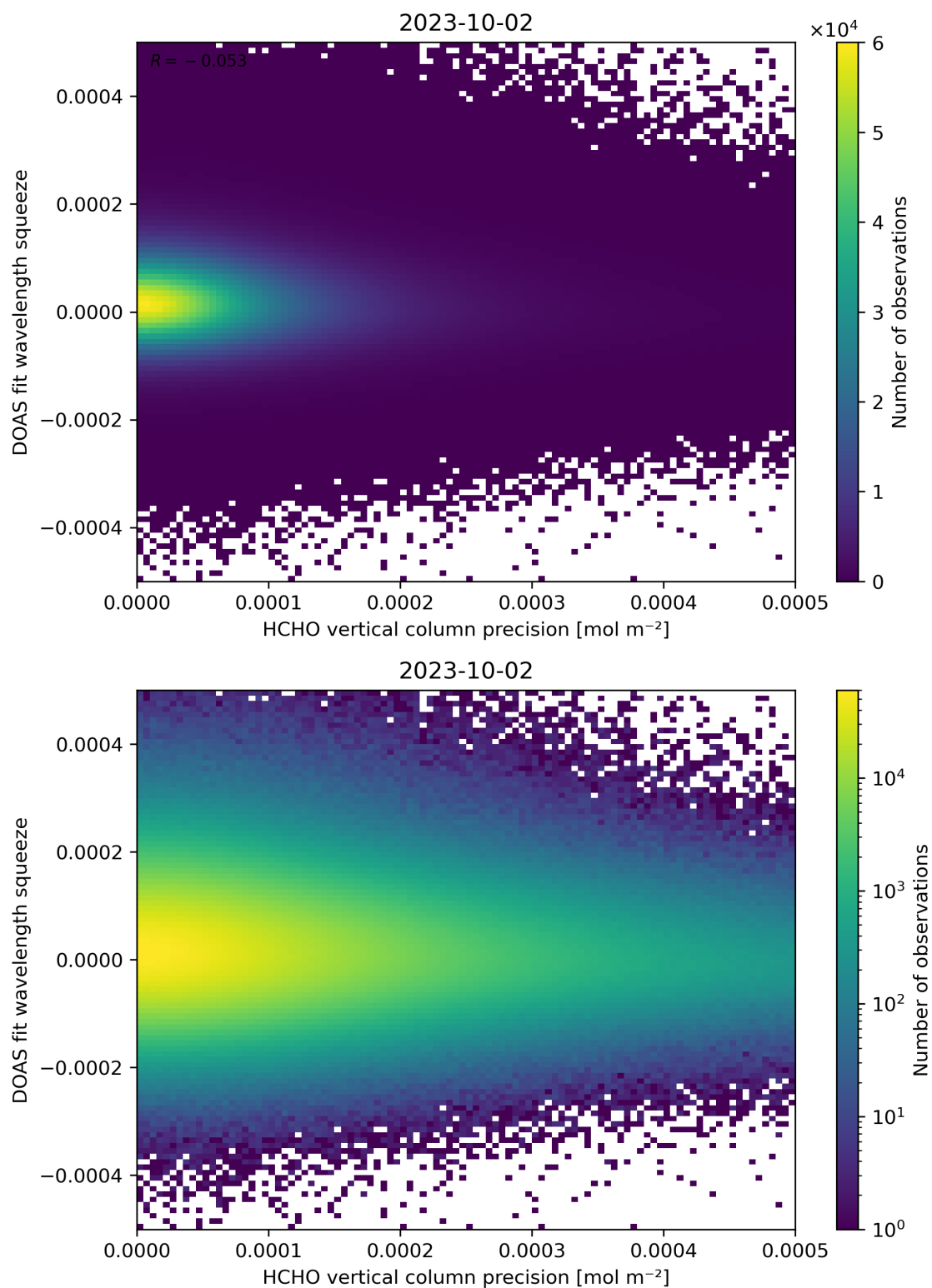
Figure 138: Scatter density plot of “HCHO vertical column precision” against “DOAS fit wavelength squeeze” for 2023-10-01 to 2023-10-03.
