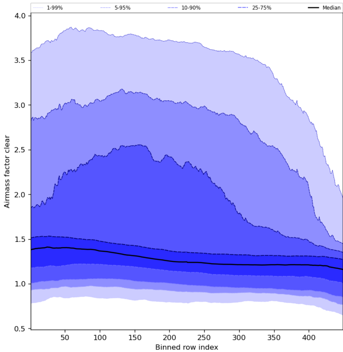
Figure 56: Along track statistics of “Airmass factor clear” for 2023-10-01 to 2023-10-03
