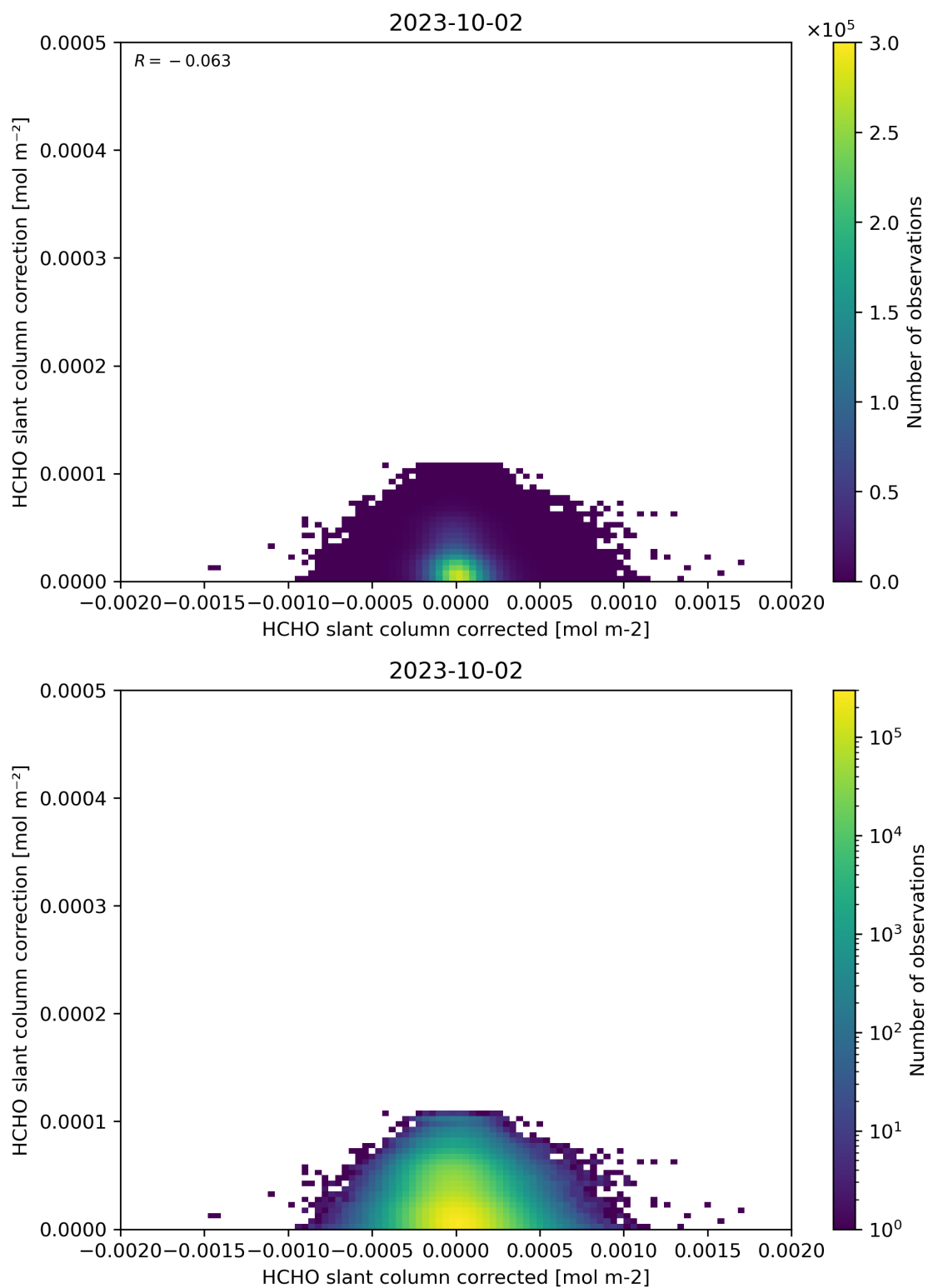
Figure 77: Scatter density plot of “HCHO slant column corrected” against “HCHO slant column correction” for 2023-10-01 to 2023-10-03.
