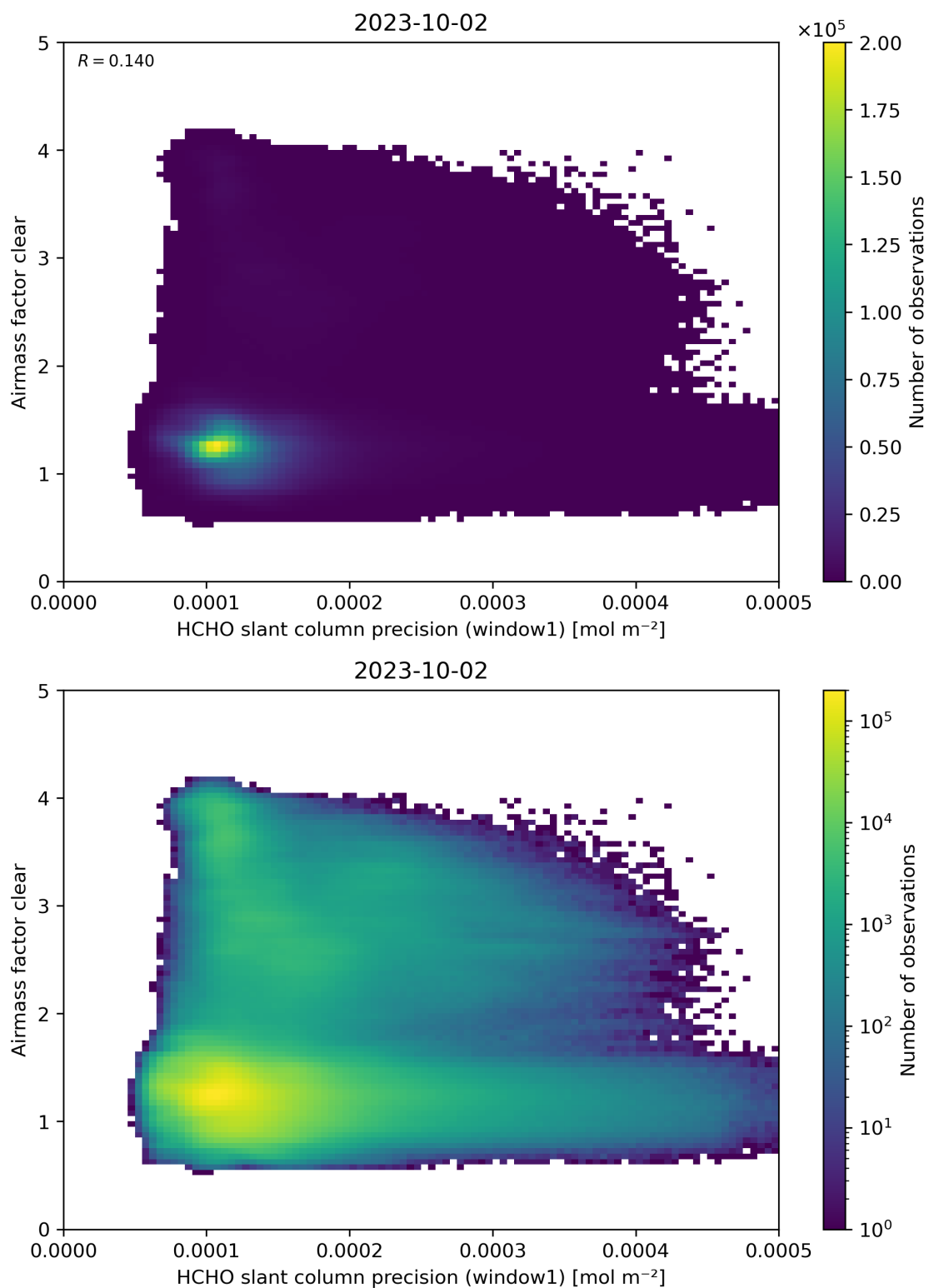
Figure 91: Scatter density plot of “HCHO slant column precision (window1)” against “Airmass factor clear” for 2023-10-01 to 2023-10-03.
