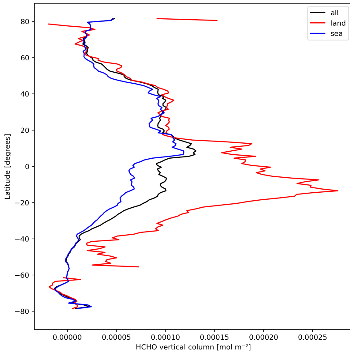
Figure 21: Zonal average of “HCHO vertical column” for 2023-10-01 to 2023-10-03.
