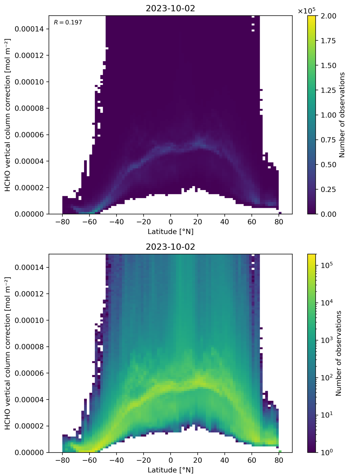
Figure 164: Scatter density plot of “Latitude” against “HCHO vertical column correction” for 2023-10-01 to 2023-10-03.
