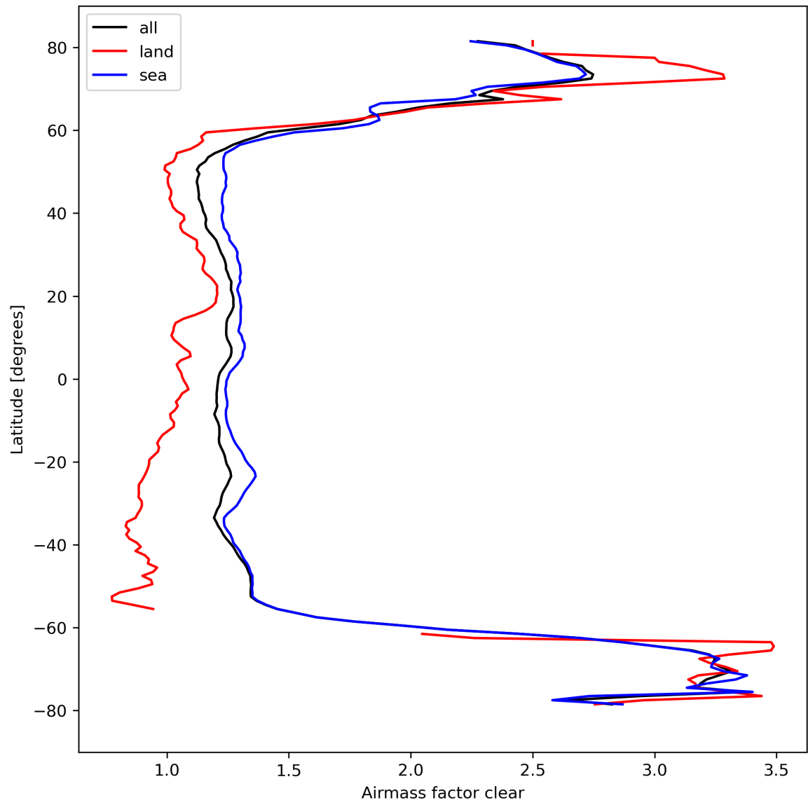
Figure 28: Zonal average of “Airmass factor clear” for 2023-10-01 to 2023-10-03.
