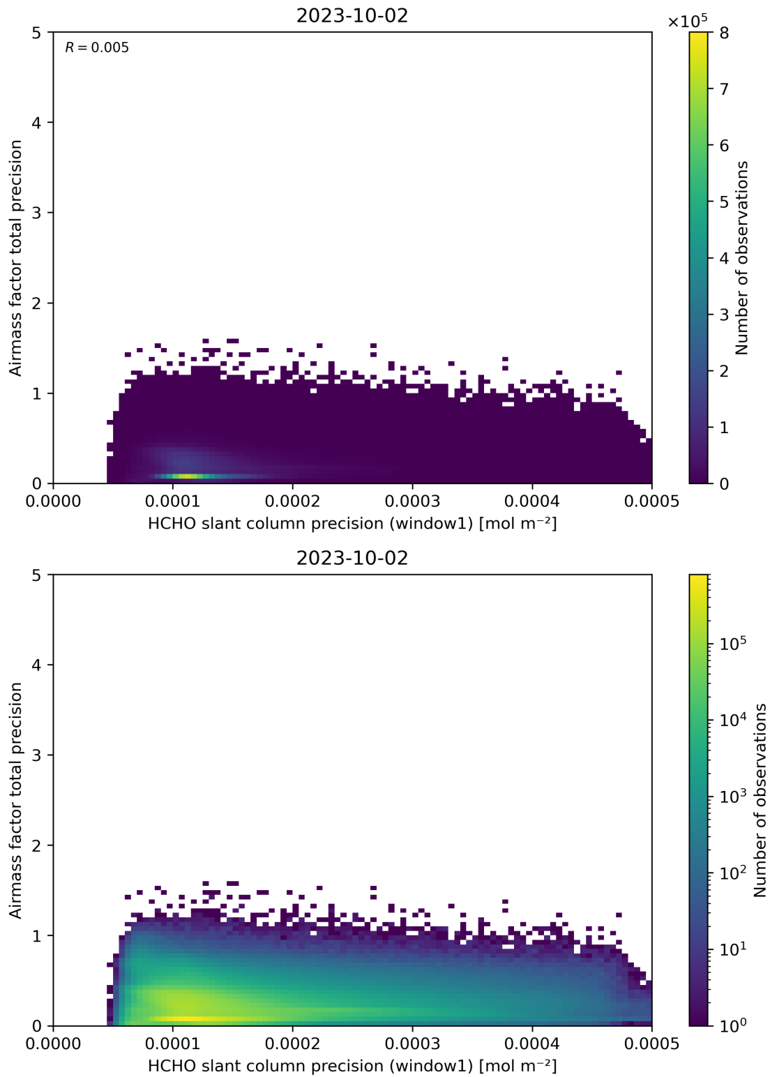
Figure 95: Scatter density plot of “HCHO slant column precision (window1)” against “Airmass factor total precision” for 2023-10-01 to 2023-10-03.
