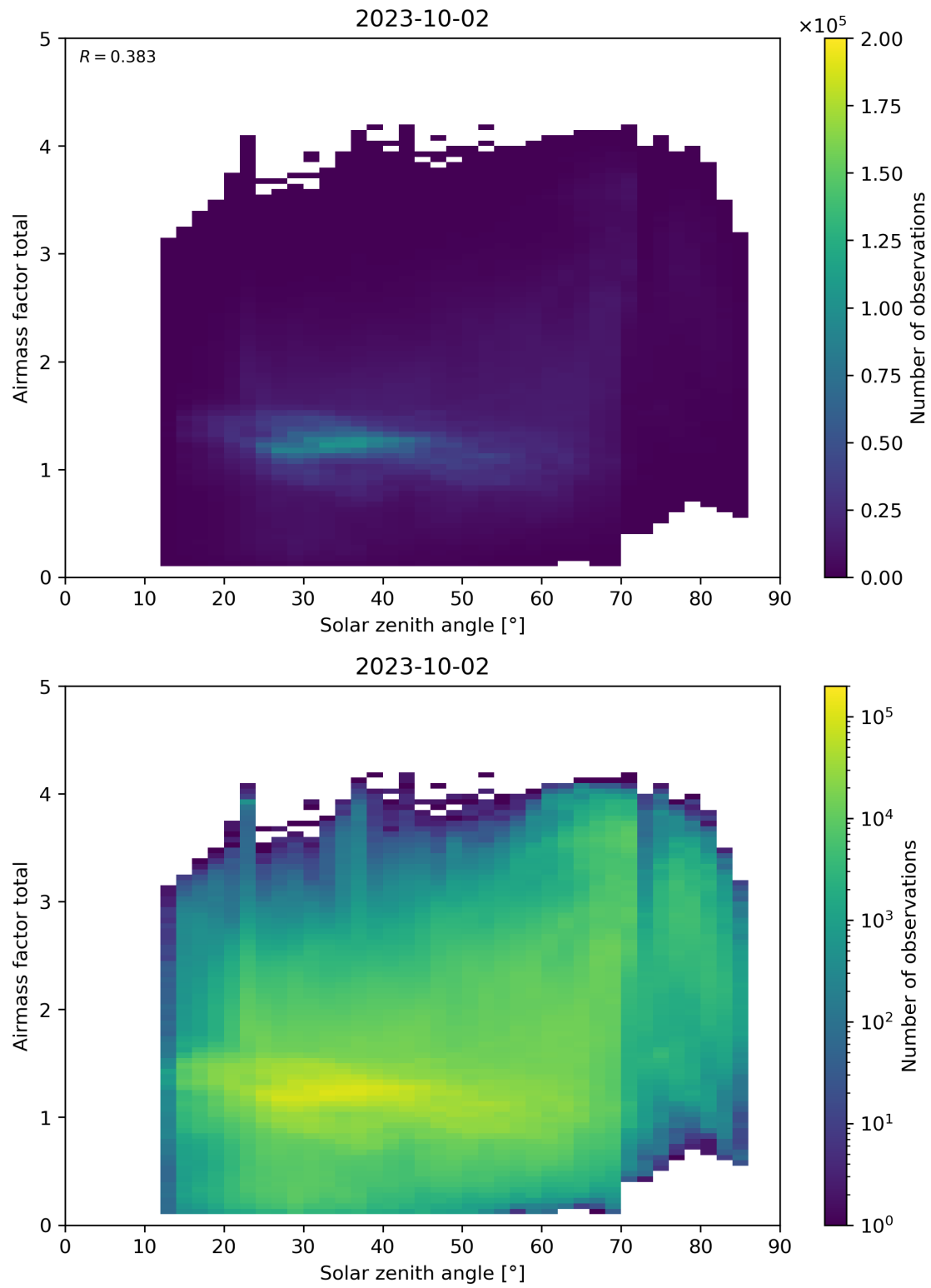
Figure 175: Scatter density plot of “Solar zenith angle” against “Airmass factor total” for 2023-10-01 to 2023-10-03.
