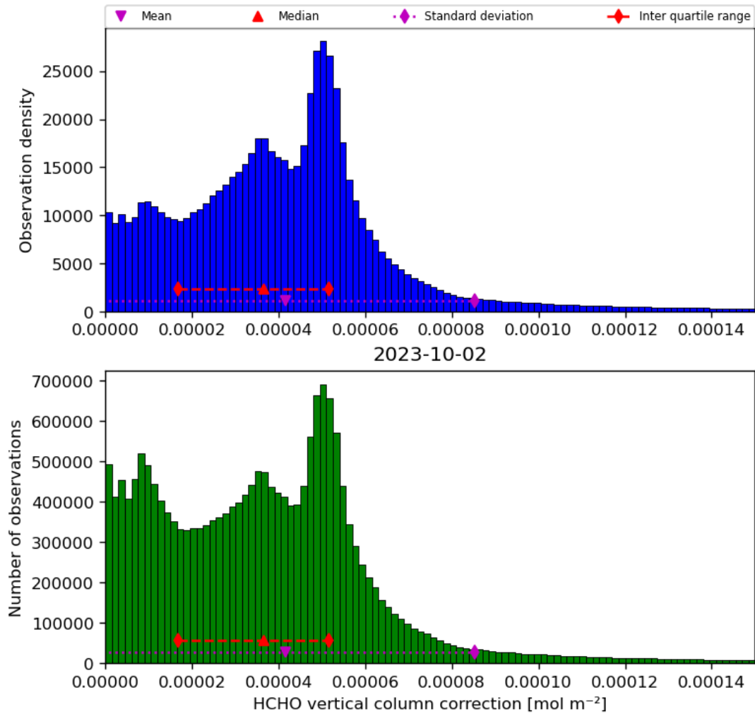
Figure 37: Histogram of “HCHO vertical column correction” for 2023-10-01 to 2023-10-03
