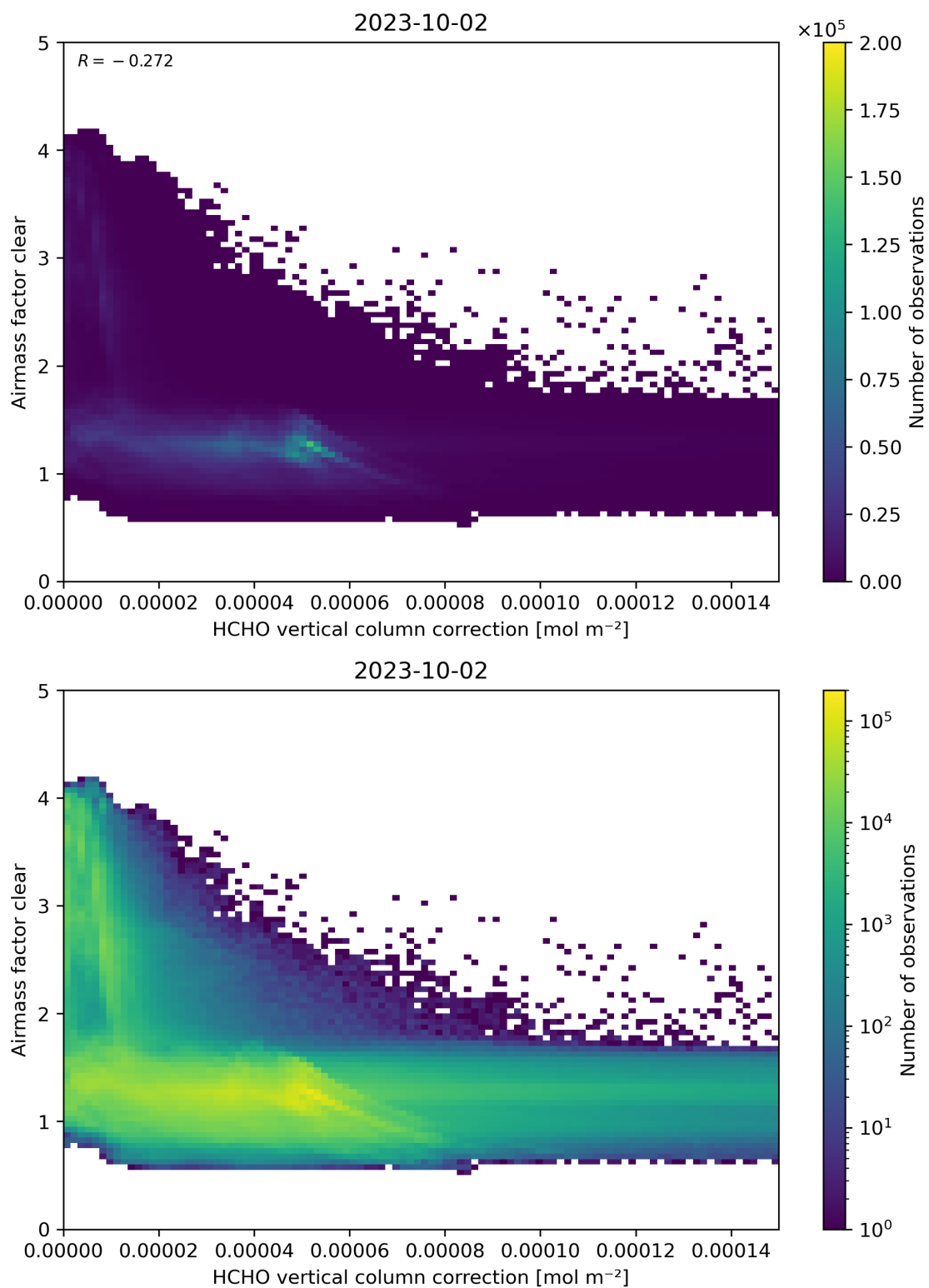
Figure 115: Scatter density plot of “HCHO vertical column correction” against “Airmass factor clear” for 2023-10-01 to 2023-10-03.
