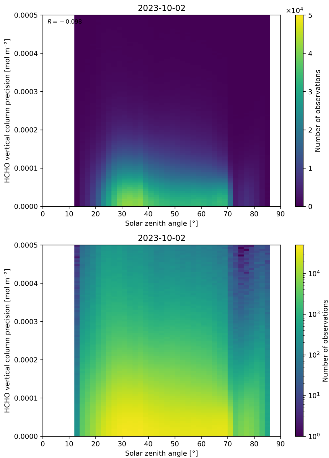
Figure 179: Scatter density plot of “Solar zenith angle” against “HCHO vertical column precision” for 2023-10-01 to 2023-10-03.
