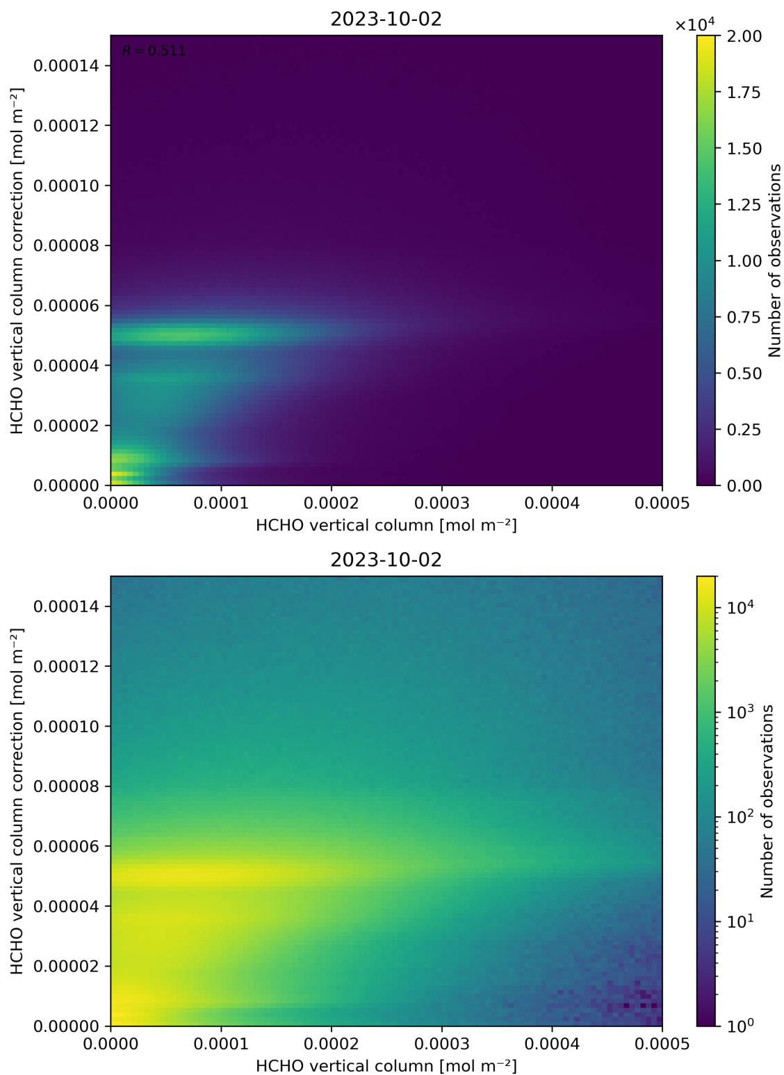
Figure 133: Scatter density plot of “HCHO vertical column” against “HCHO vertical column correction” for 2023-10-01 to 2023-10-03.
