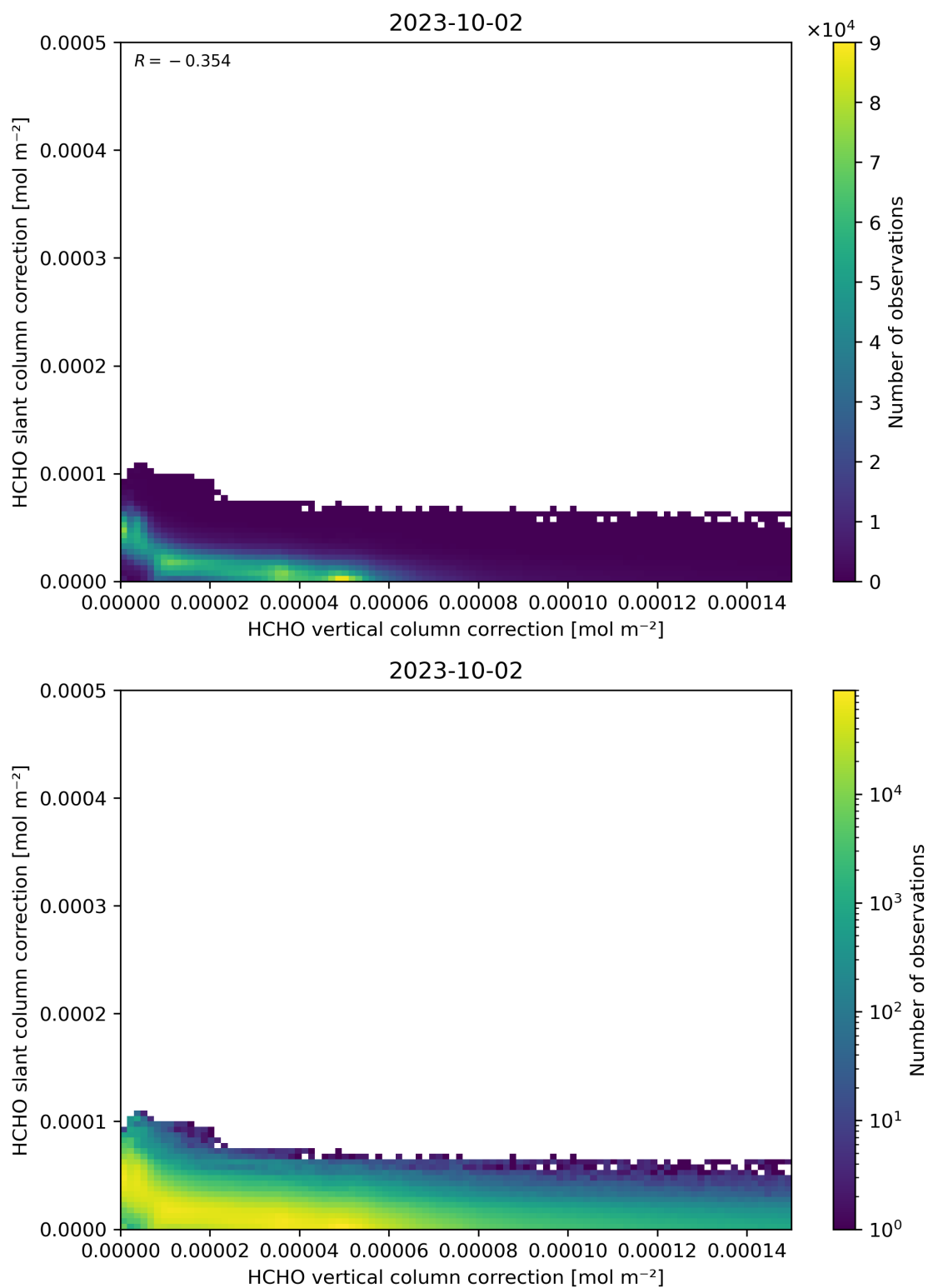
Figure 117: Scatter density plot of “HCHO vertical column correction” against “HCHO slant column correction” for 2023-10-01 to 2023-10-03.
