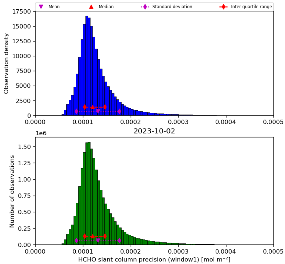
Figure 39: Histogram of “HCHO slant column precision (window1)” for 2023-10-01 to 2023-10-03
