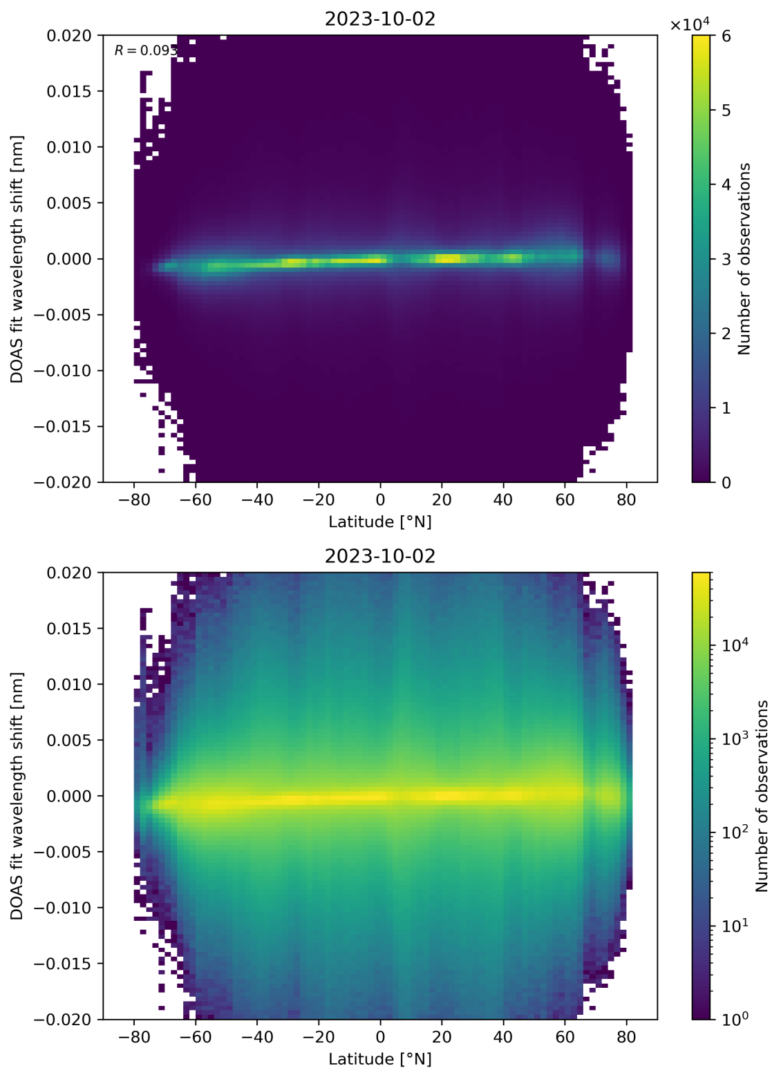
Figure 154: Scatter density plot of “Latitude” against “DOAS fit wavelength shift” for 2023-10-01 to 2023-10-03.
