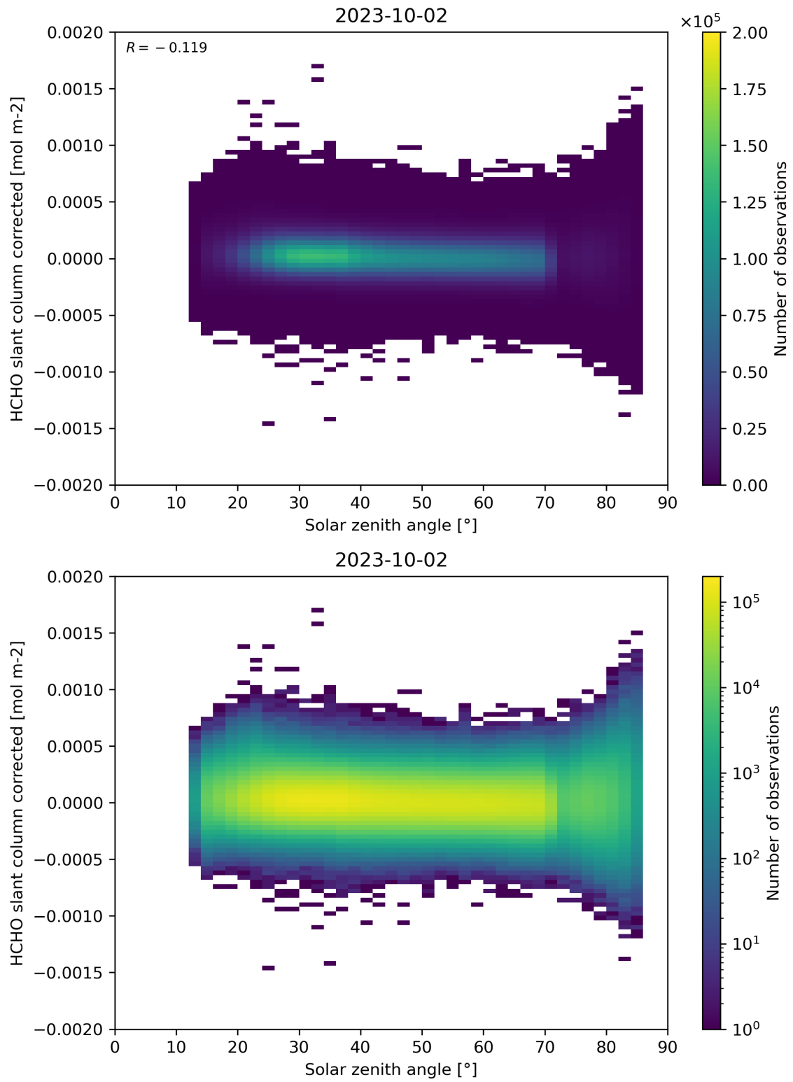
Figure 171: Scatter density plot of “Solar zenith angle” against “HCHO slant column corrected” for 2023-10-01 to 2023-10-03.
