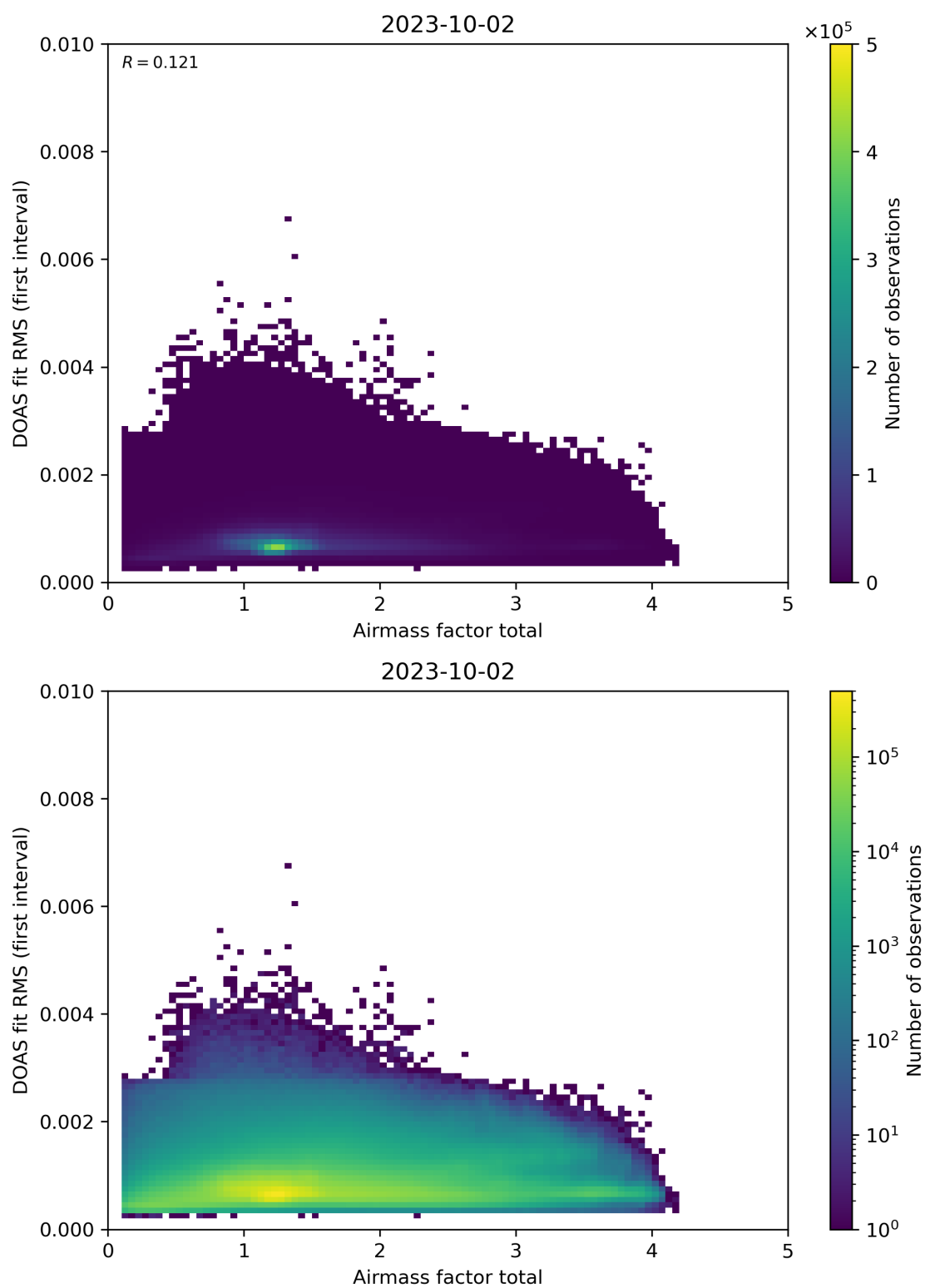
Figure 97: Scatter density plot of “Airmass factor total” against “DOAS fit RMS (first interval)” for 2023-10-01 to 2023-10-03.
