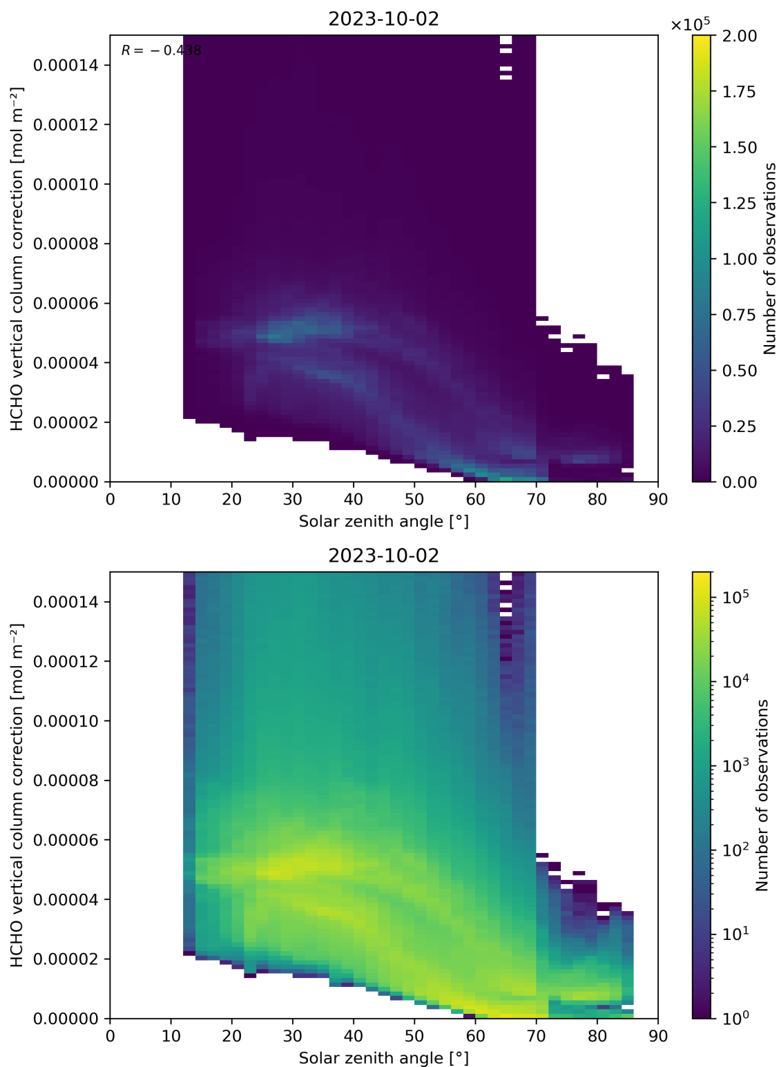
Figure 178: Scatter density plot of “Solar zenith angle” against “HCHO vertical column correction” for 2023-10-01 to 2023-10-03.
