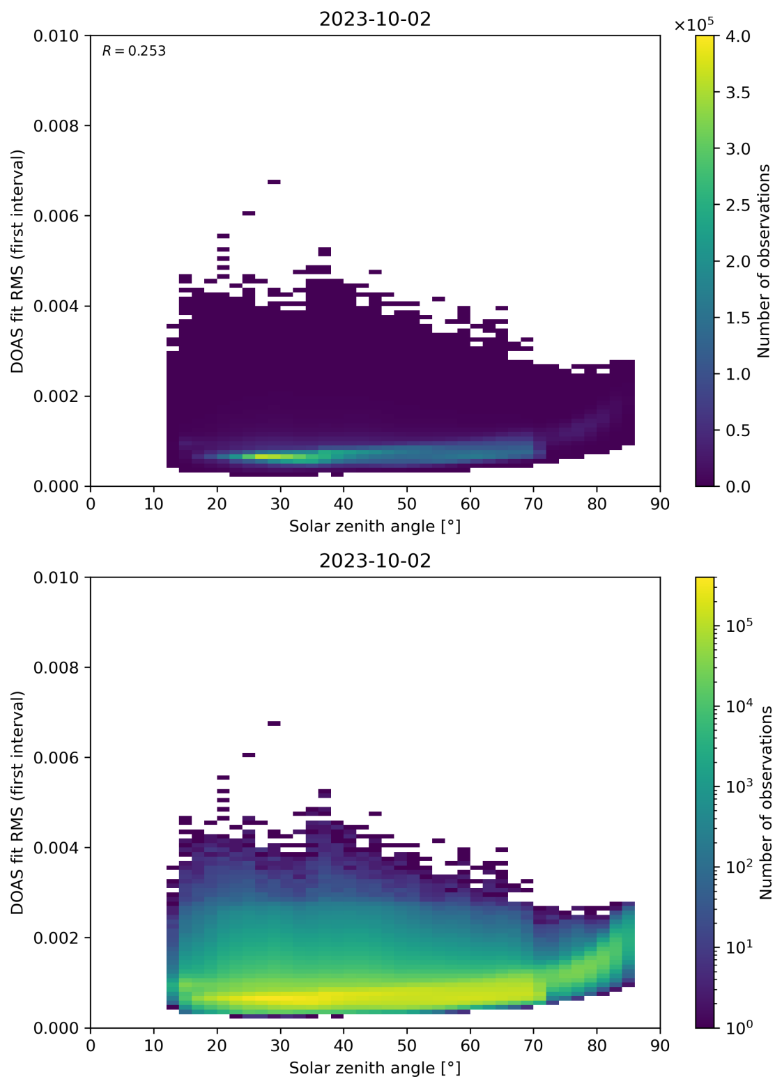
Figure 167: Scatter density plot of “Solar zenith angle” against “DOAS fit RMS (first interval)” for 2023-10-01 to 2023-10-03.
