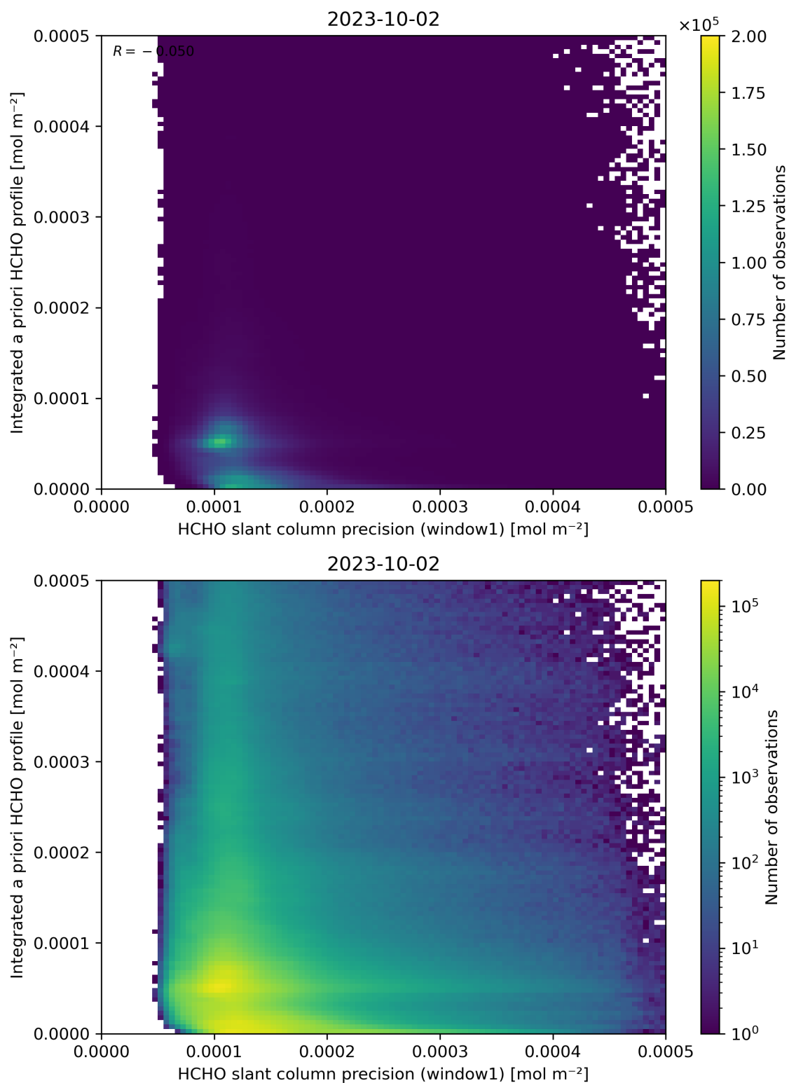
Figure 96: Scatter density plot of “HCHO slant column precision (window1)” against “Integrated a priori HCHO profile” for 2023-10-01 to 2023-10-03.
