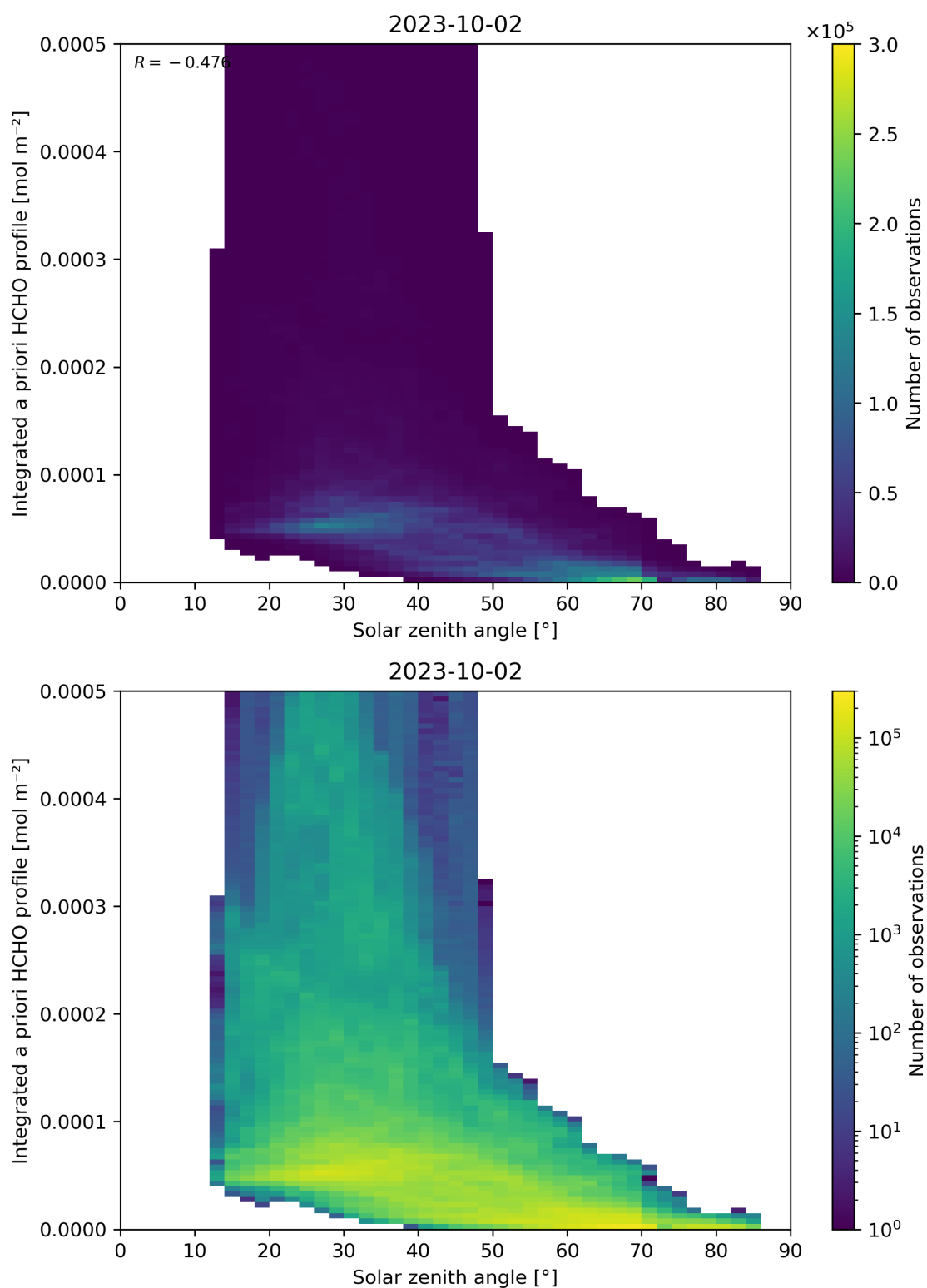
Figure 180: Scatter density plot of “Solar zenith angle” against “Integrated a priori HCHO profile” for 2023-10-01 to 2023-10-03.
