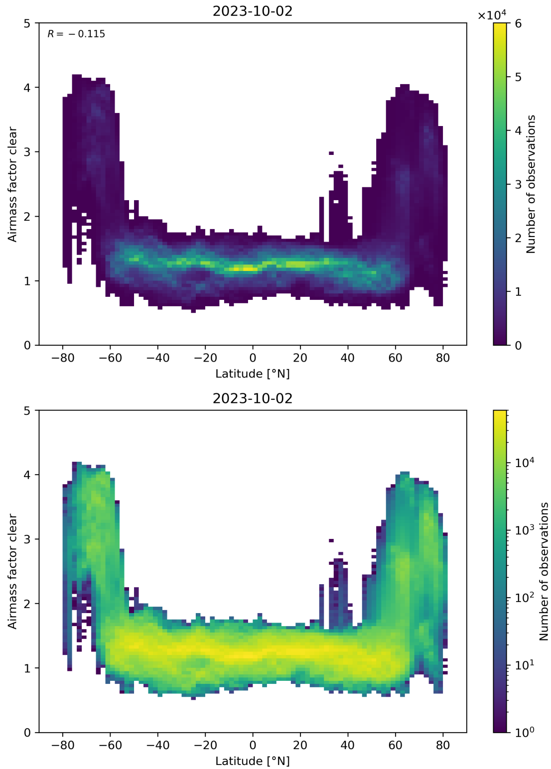
Figure 156: Scatter density plot of “Latitude” against “Airmass factor clear” for 2023-10-01 to 2023-10-03.
