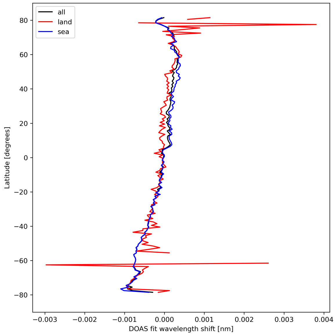
Figure 30: Zonal average of “DOAS fit wavelength shift” for 2023-10-01 to 2023-10-03.
