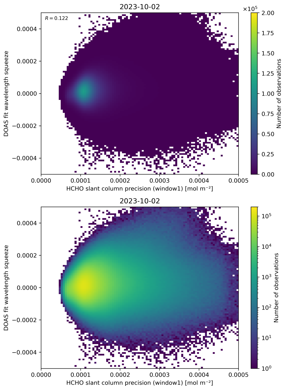
Figure 90: Scatter density plot of “HCHO slant column precision (window1)” against “DOAS fit wavelength squeeze” for 2023-10-01 to 2023-10-03.
