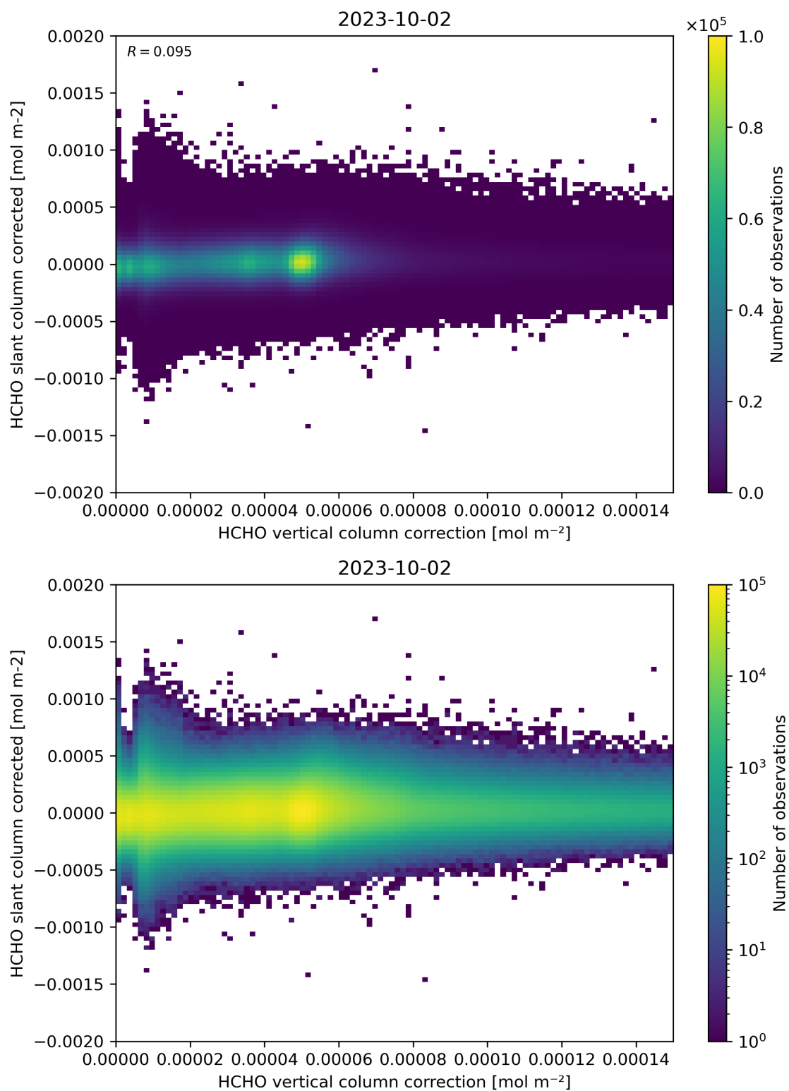
Figure 116: Scatter density plot of “HCHO vertical column correction” against “HCHO slant column corrected” for 2023-10-01 to 2023-10-03.
