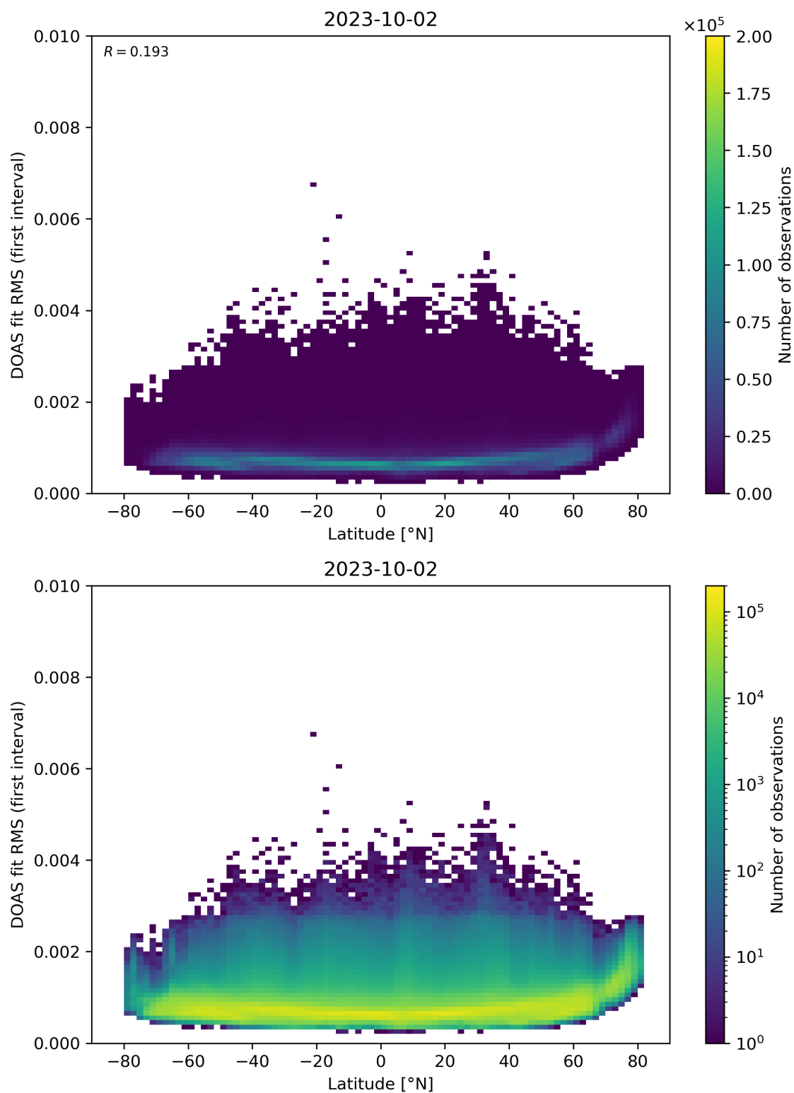
Figure 153: Scatter density plot of “Latitude” against “DOAS fit RMS (first interval)” for 2023-10-01 to 2023-10-03.
