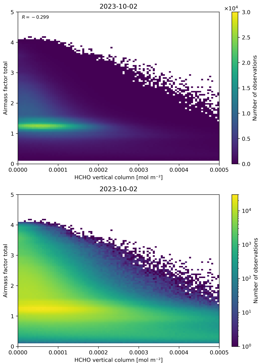
Figure 131: Scatter density plot of “HCHO vertical column” against “Airmass factor total” for 2023-10-01 to 2023-10-03.
