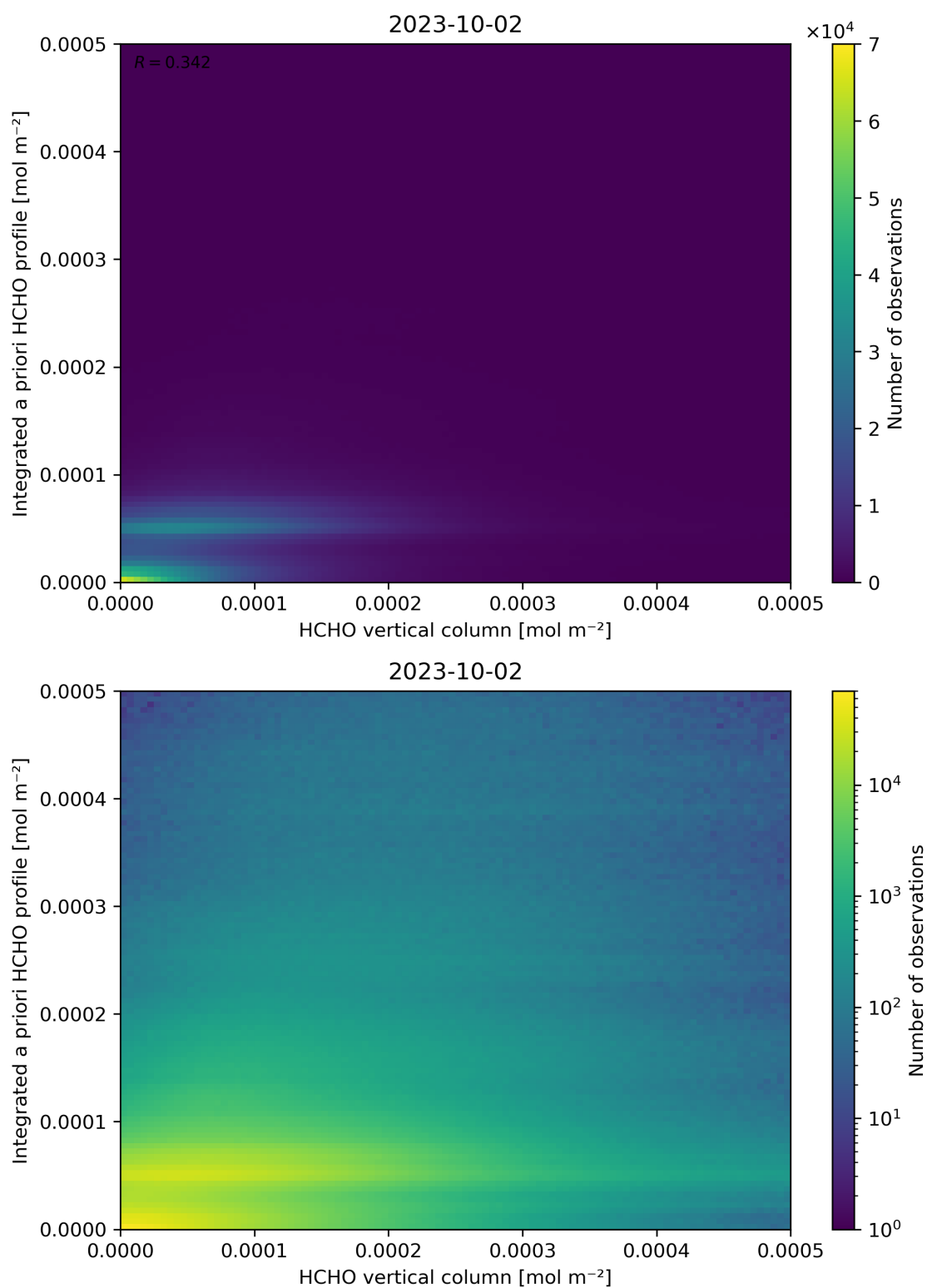
Figure 135: Scatter density plot of “HCHO vertical column” against “Integrated a priori HCHO profile” for 2023-10-01 to 2023-10-03.
