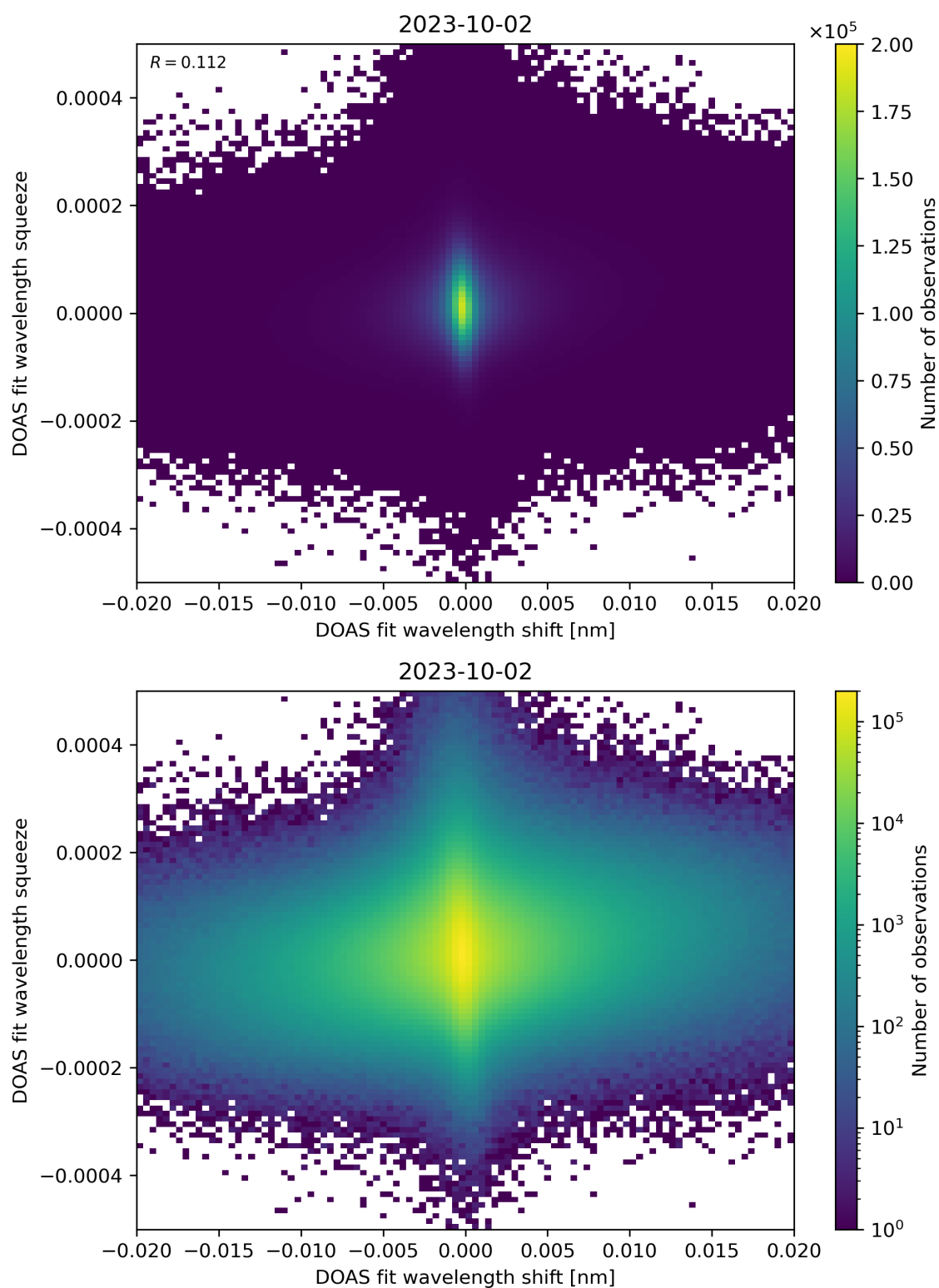
Figure 65: Scatter density plot of “DOAS fit wavelength shift” against “DOAS fit wavelength squeeze” for 2023-10-01 to 2023-10-03.
