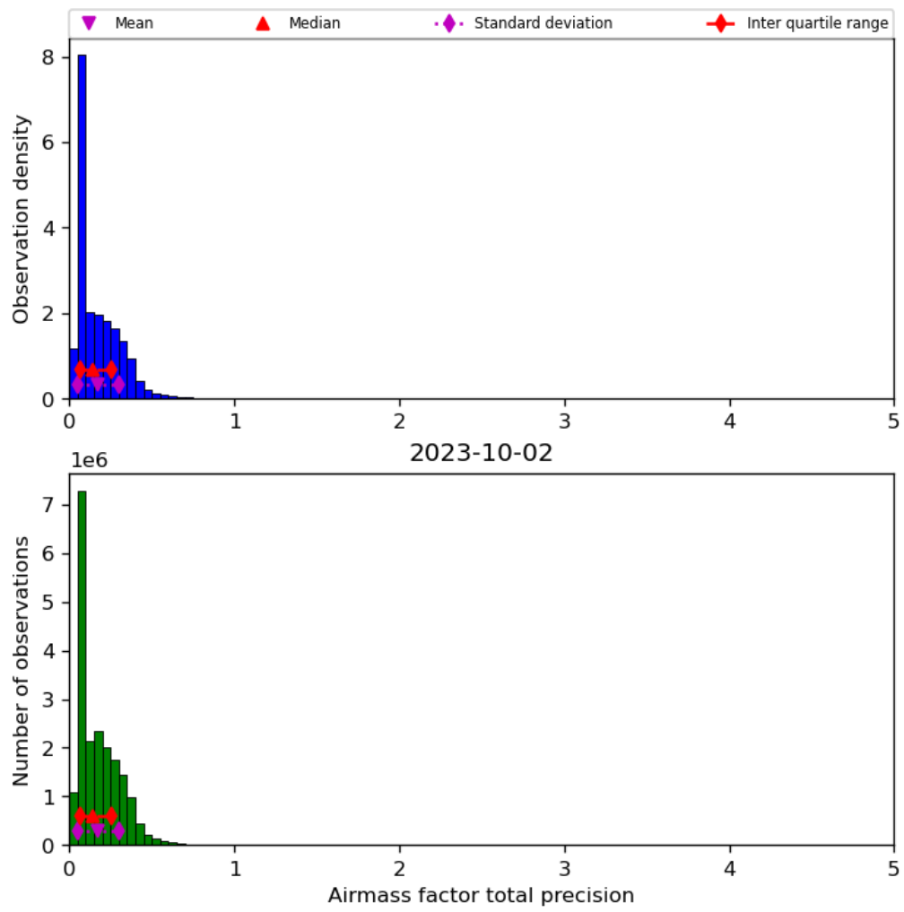
Figure 41: Histogram of “Airmass factor total precision” for 2023-10-01 to 2023-10-03
