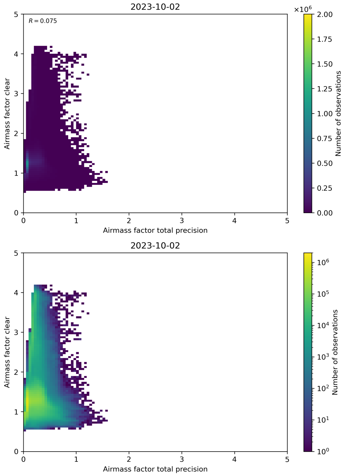
Figure 108: Scatter density plot of “Airmass factor total precision” against “Airmass factor clear” for 2023-10-01 to 2023-10-03.
