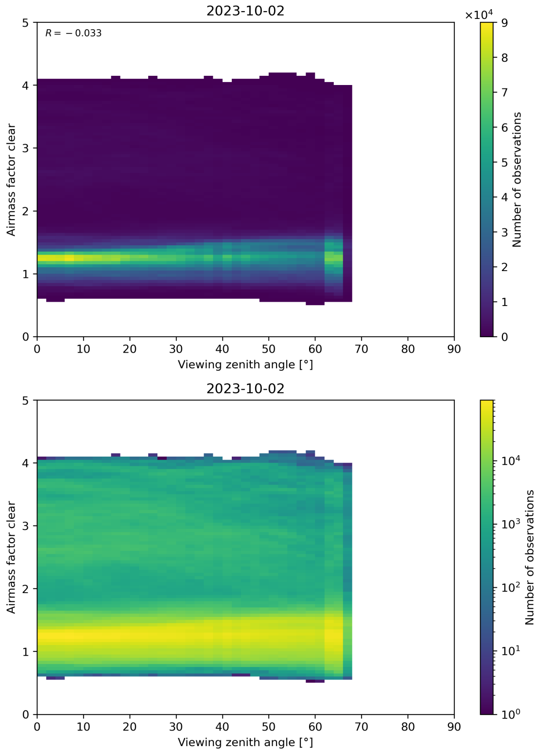
Figure 185: Scatter density plot of “Viewing zenith angle” against “Airmass factor clear” for 2023-10-01 to 2023-10-03.
