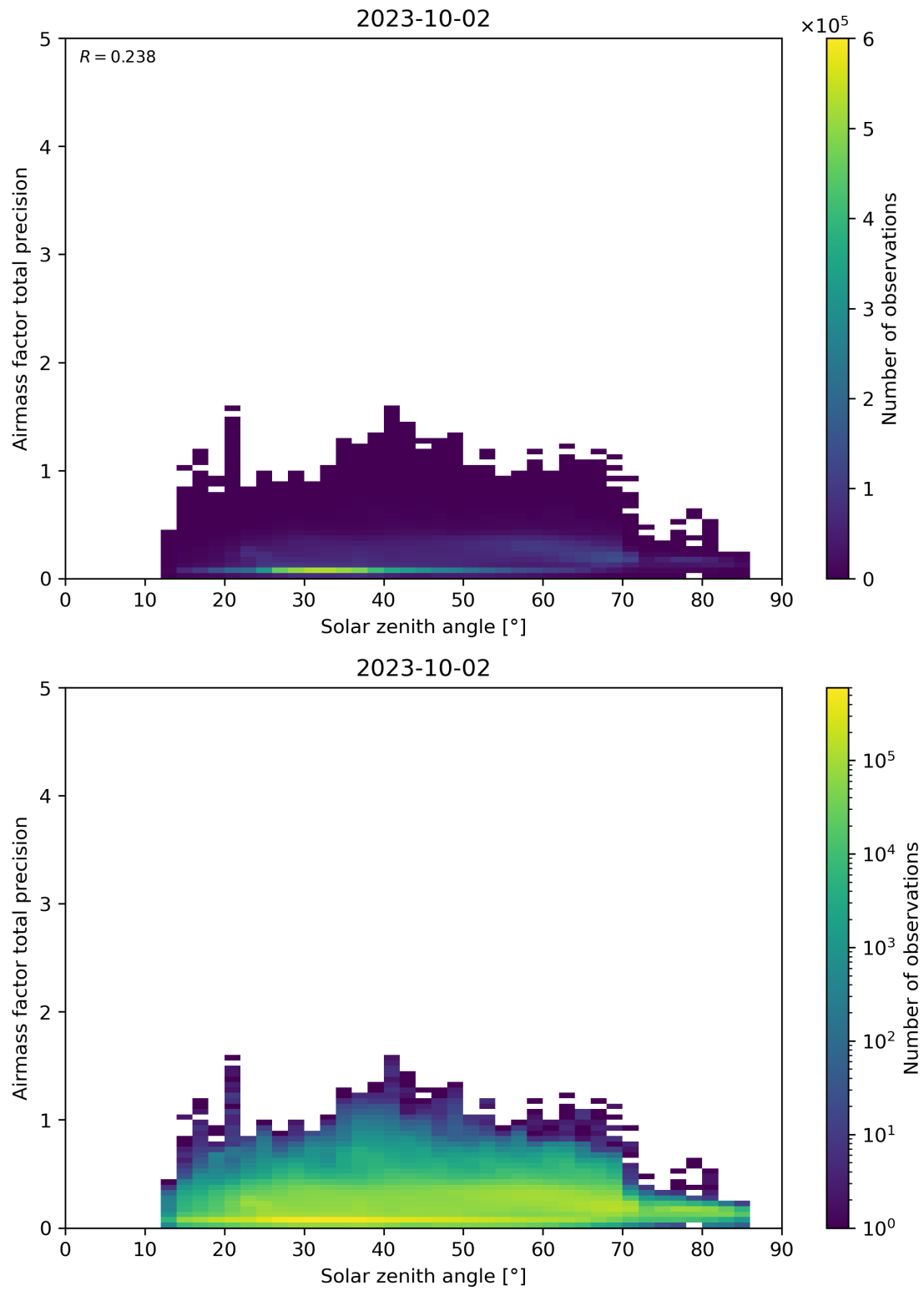
Figure 176: Scatter density plot of “Solar zenith angle” against “Airmass factor total precision” for 2023-10-01 to 2023-10-03.
