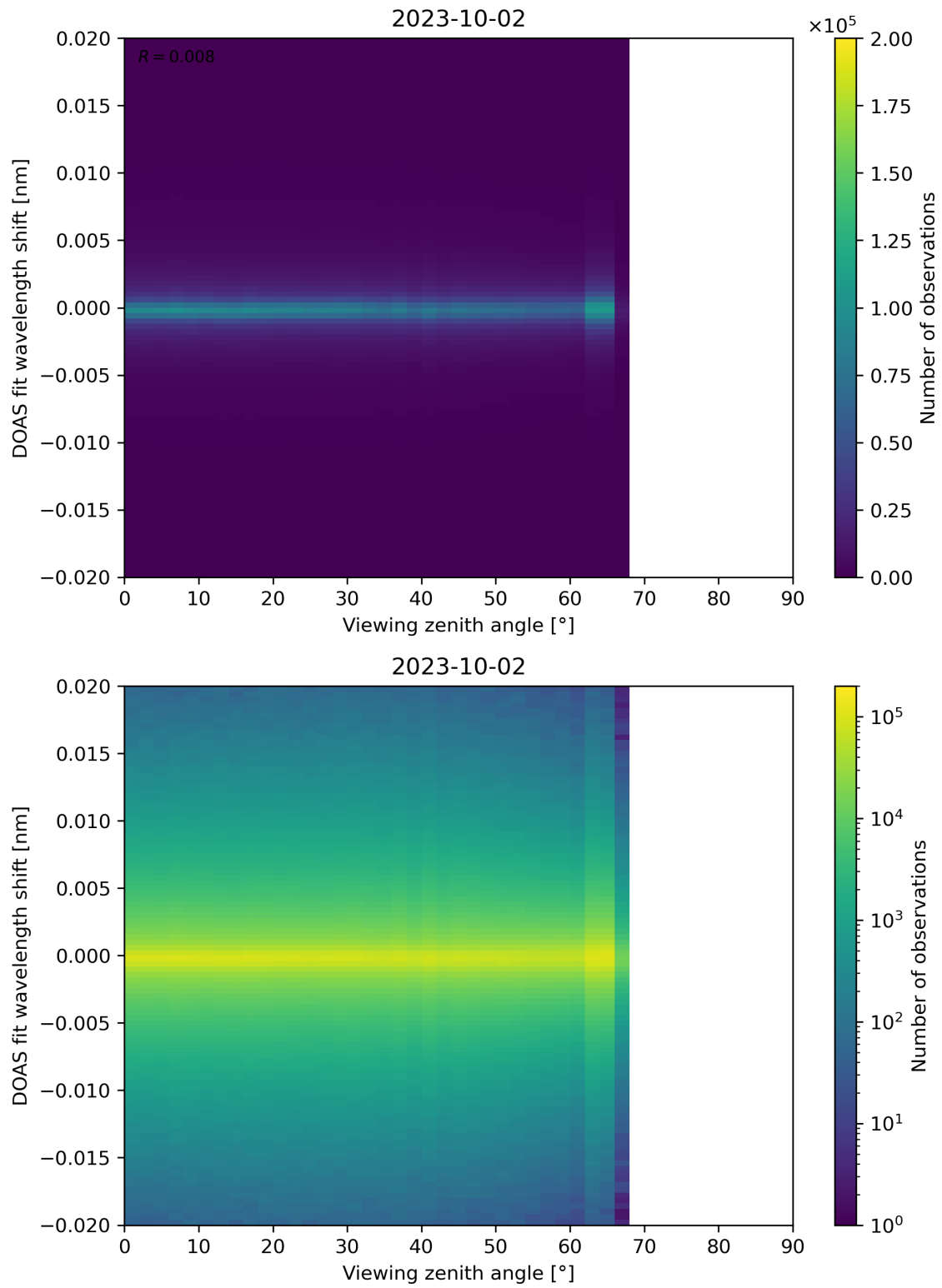
Figure 183: Scatter density plot of “Viewing zenith angle” against “DOAS fit wavelength shift” for 2023-10-01 to 2023-10-03.
