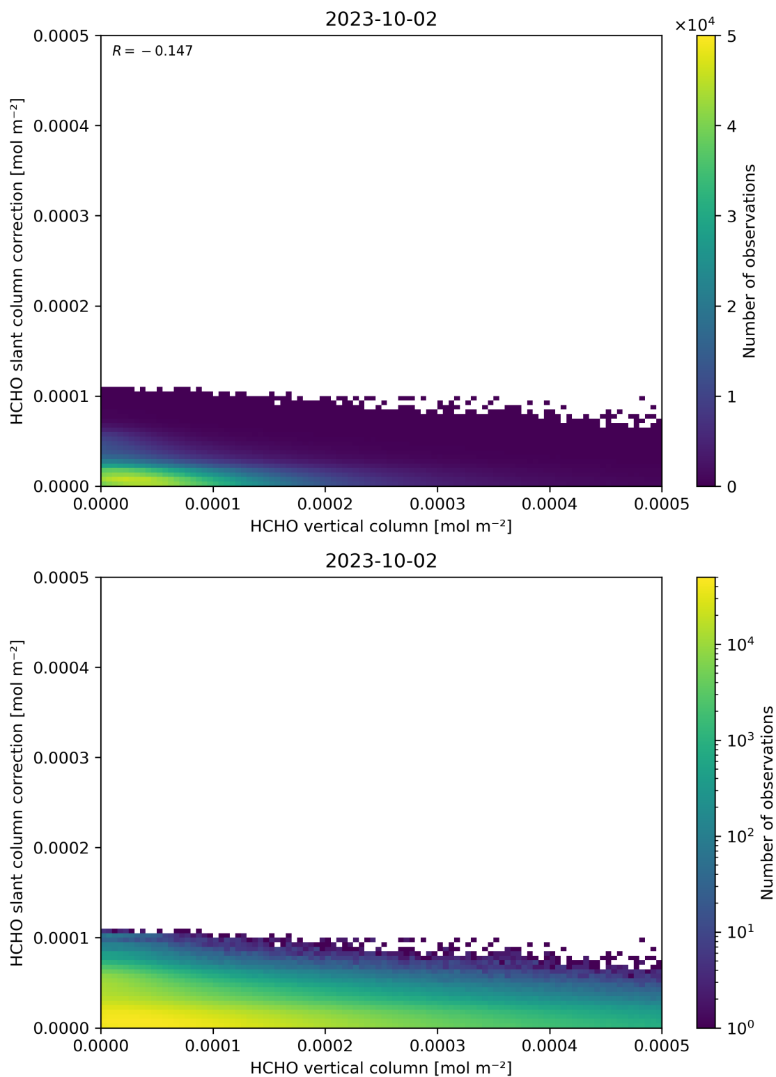
Figure 128: Scatter density plot of “HCHO vertical column” against “HCHO slant column correction” for 2023-10-01 to 2023-10-03.
