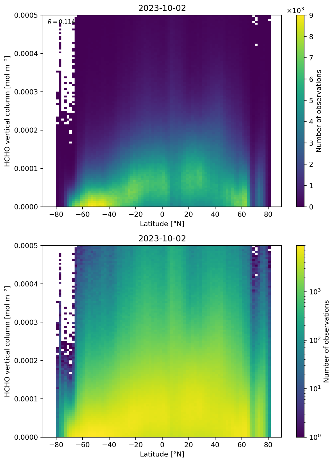
Figure 163: Scatter density plot of “Latitude” against “HCHO vertical column” for 2023-10-01 to 2023-10-03.
