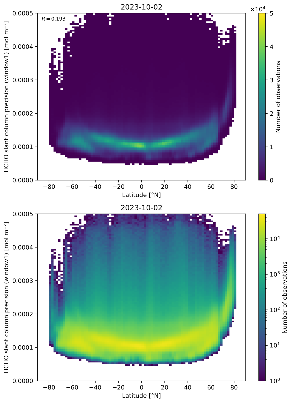
Figure 160: Scatter density plot of “Latitude” against “HCHO slant column precision (window1)” for 2023-10-01 to 2023-10-03.
