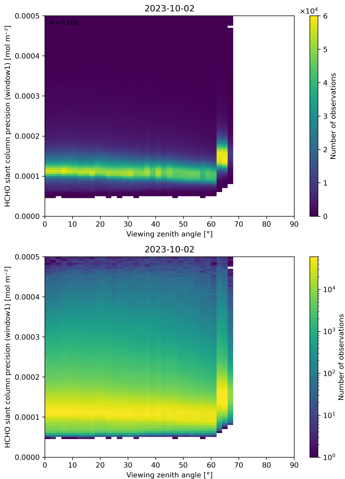
Figure 189: Scatter density plot of “Viewing zenith angle” against “HCHO slant column precision (window1)” for 2023-10-01 to 2023-10-03.
