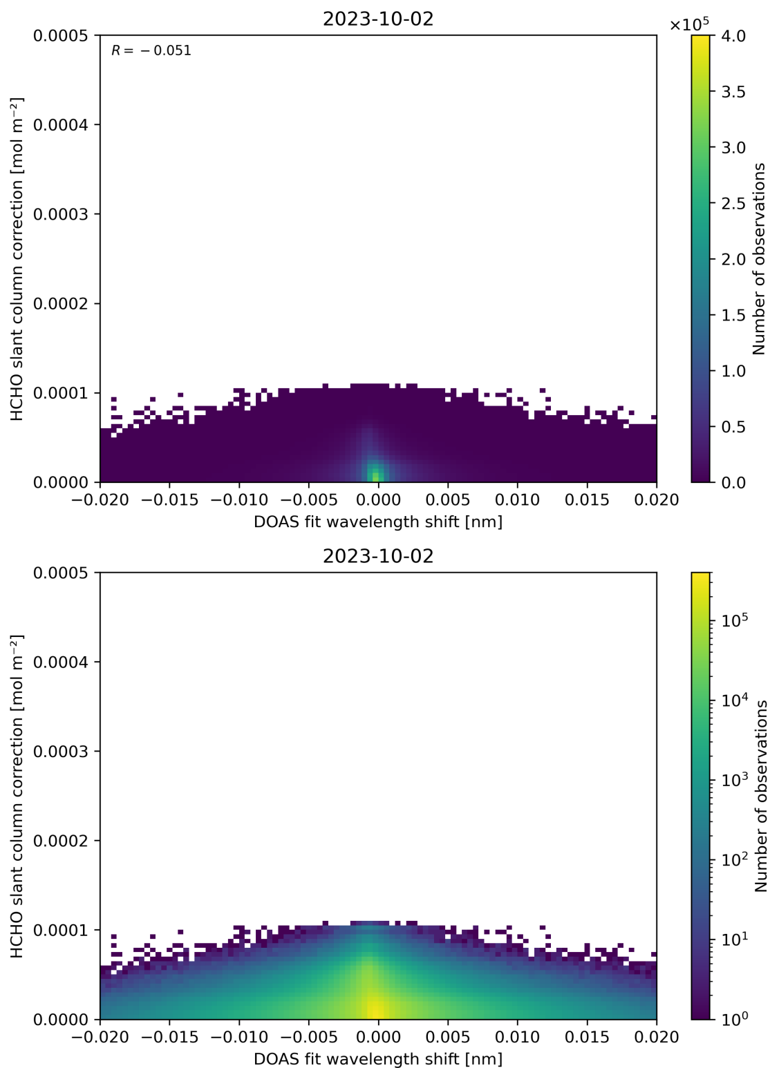
Figure 67: Scatter density plot of “DOAS fit wavelength shift” against “HCHO slant column correction” for 2023-10-01 to 2023-10-03.
