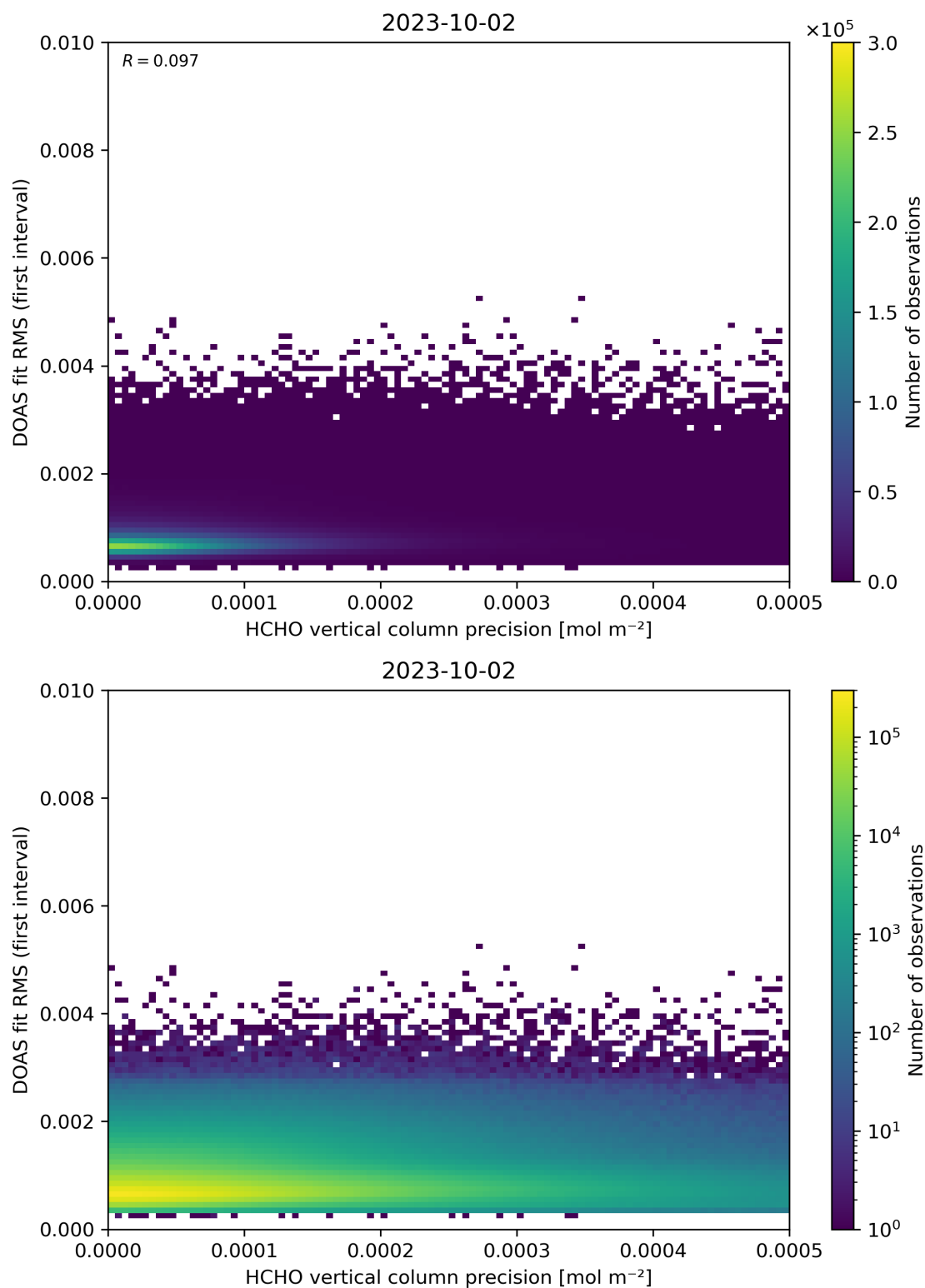
Figure 136: Scatter density plot of “HCHO vertical column precision” against “DOAS fit RMS (first interval)” for 2023-10-01 to 2023-10-03.
