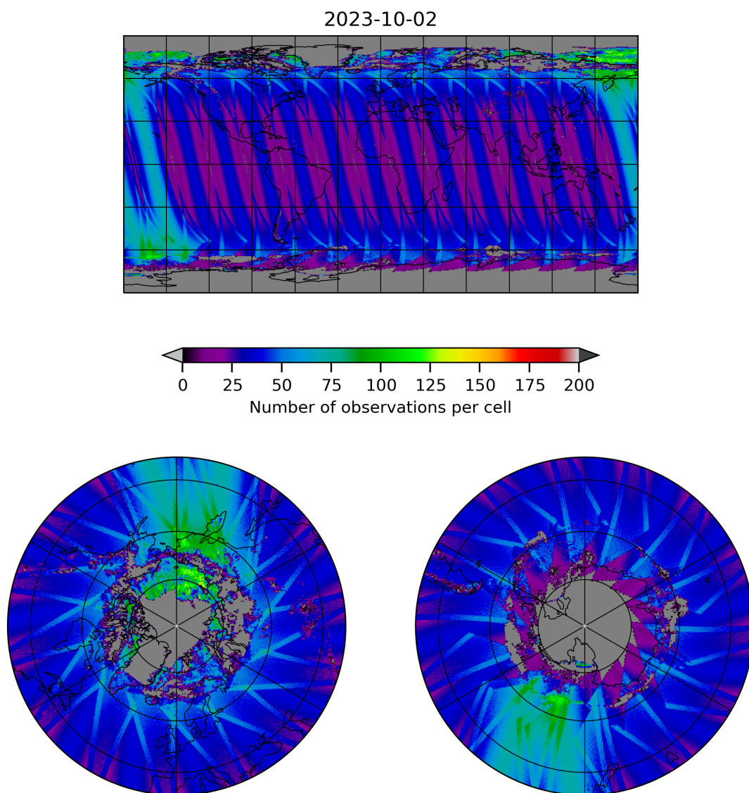
Figure 19: Map of the number of observations for 2023-10-01 to 2023-10-03
