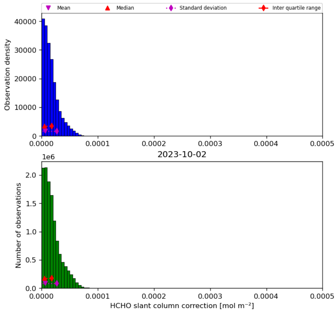
Figure 47: Histogram of “HCHO slant column correction” for 2023-10-01 to 2023-10-03
