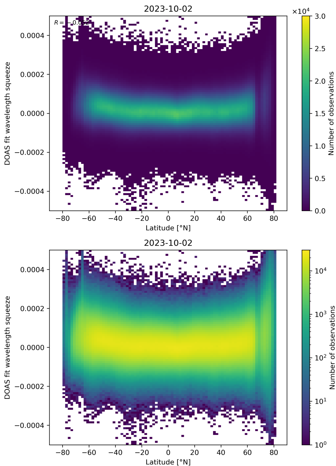
Figure 155: Scatter density plot of “Latitude” against “DOAS fit wavelength squeeze” for 2023-10-01 to 2023-10-03.
