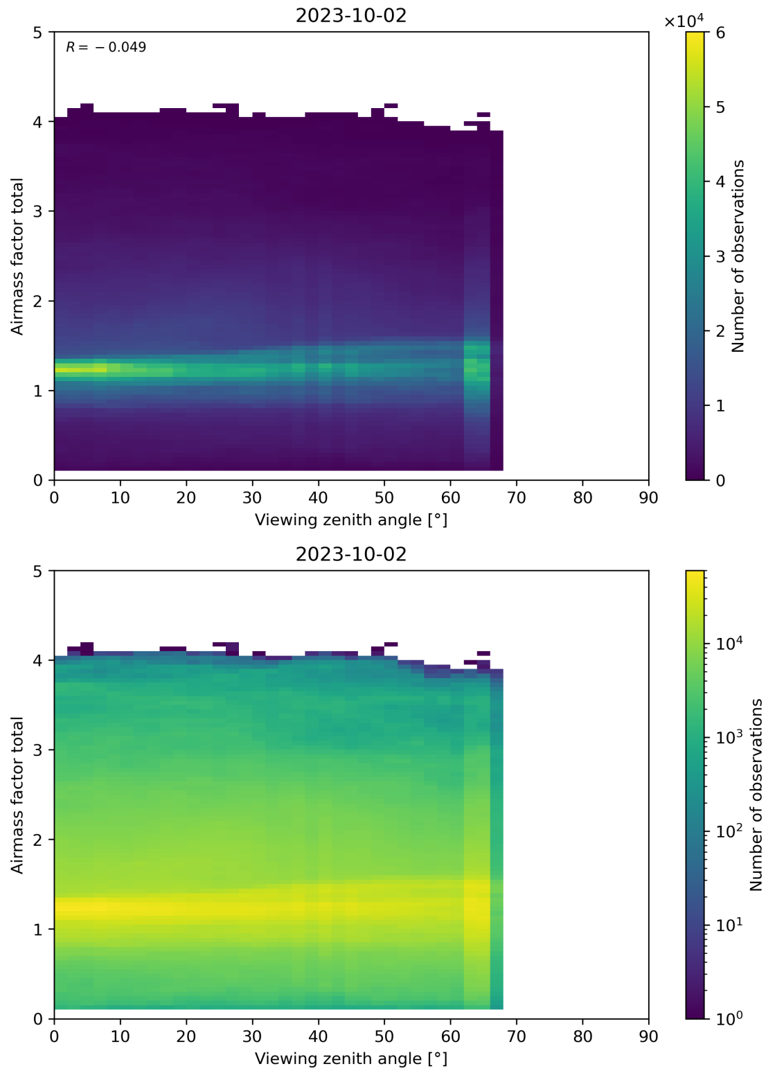
Figure 190: Scatter density plot of “Viewing zenith angle” against “Airmass factor total” for 2023-10-01 to 2023-10-03.
