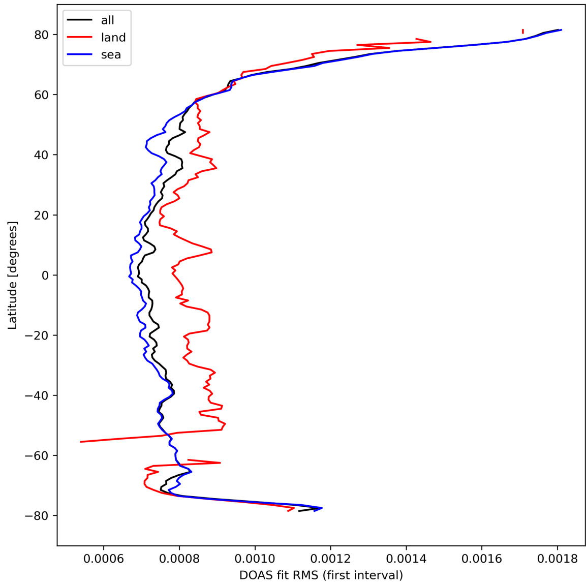
Figure 32: Zonal average of “DOAS fit RMS (first interval)” for 2023-10-01 to 2023-10-03.
