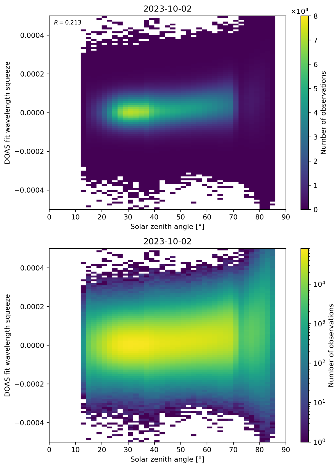
Figure 169: Scatter density plot of “Solar zenith angle” against “DOAS fit wavelength squeeze” for 2023-10-01 to 2023-10-03.
