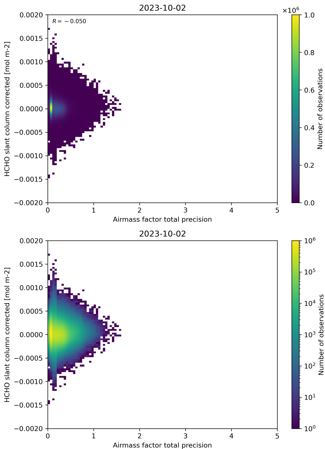
Figure 109: Scatter density plot of “Airmass factor total precision” against “HCHO slant column corrected” for 2023-10-01 to 2023-10-03.
