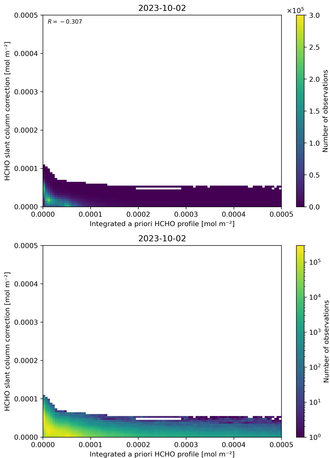
Figure 152: Scatter density plot of “Integrated a priori HCHO profile” against “HCHO slant column correction” for 2023-10-01 to 2023-10-03.
