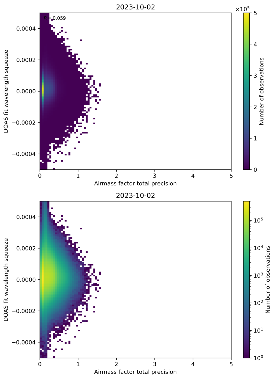
Figure 107: Scatter density plot of “Airmass factor total precision” against “DOAS fit wavelength squeeze” for 2023-10-01 to 2023-10-03.
