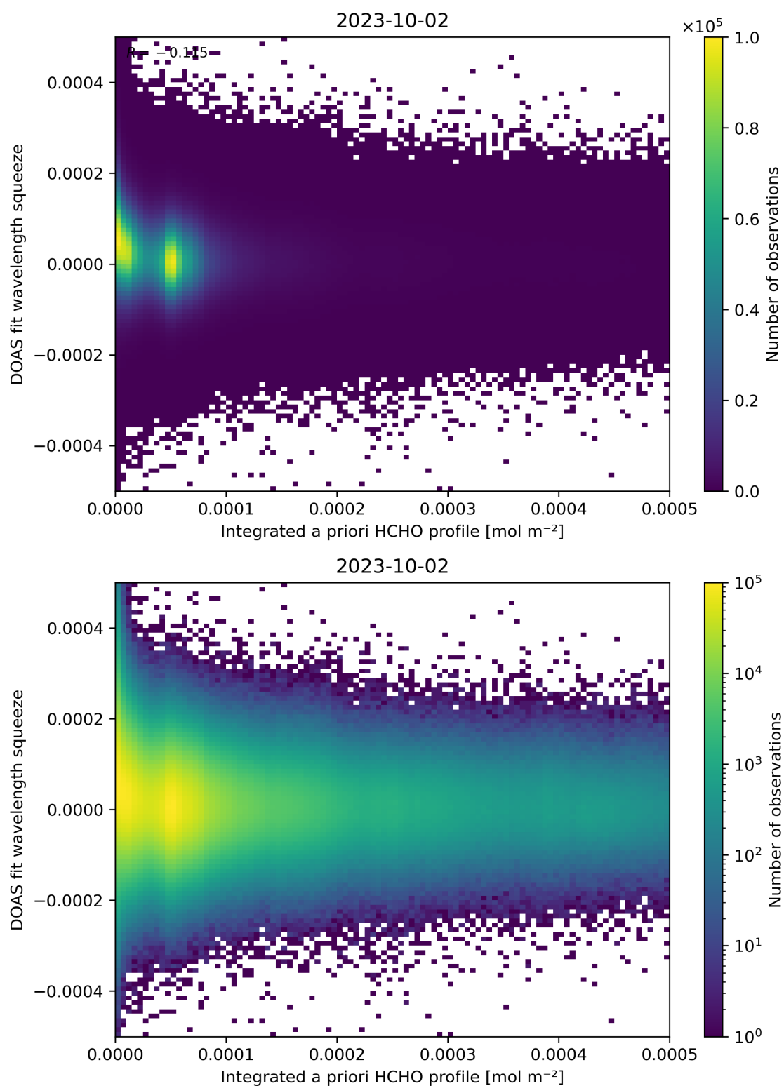
Figure 150: Scatter density plot of “Integrated a priori HCHO profile” against “DOAS fit wavelength squeeze” for 2023-10-01 to 2023-10-03.
