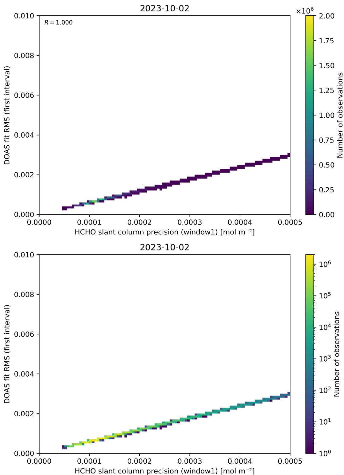
Figure 88: Scatter density plot of “HCHO slant column precision (window1)” against “DOAS fit RMS (first interval)” for 2023-10-01 to 2023-10-03.
