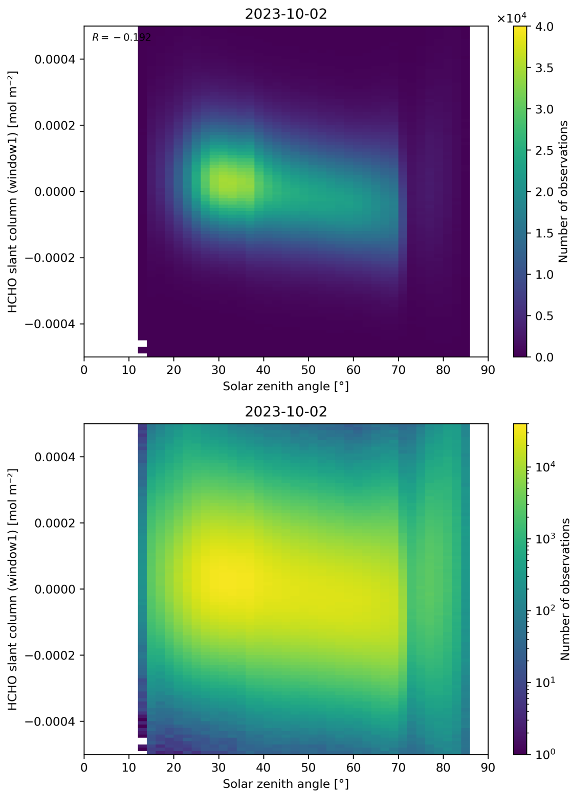
Figure 173: Scatter density plot of “Solar zenith angle” against “HCHO slant column (window1)” for 2023-10-01 to 2023-10-03.
