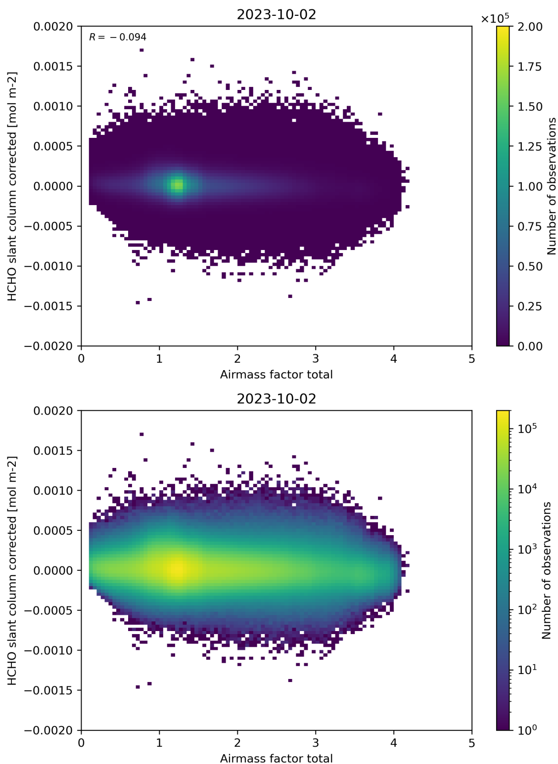
Figure 101: Scatter density plot of “Airmass factor total” against “HCHO slant column corrected” for 2023-10-01 to 2023-10-03.
