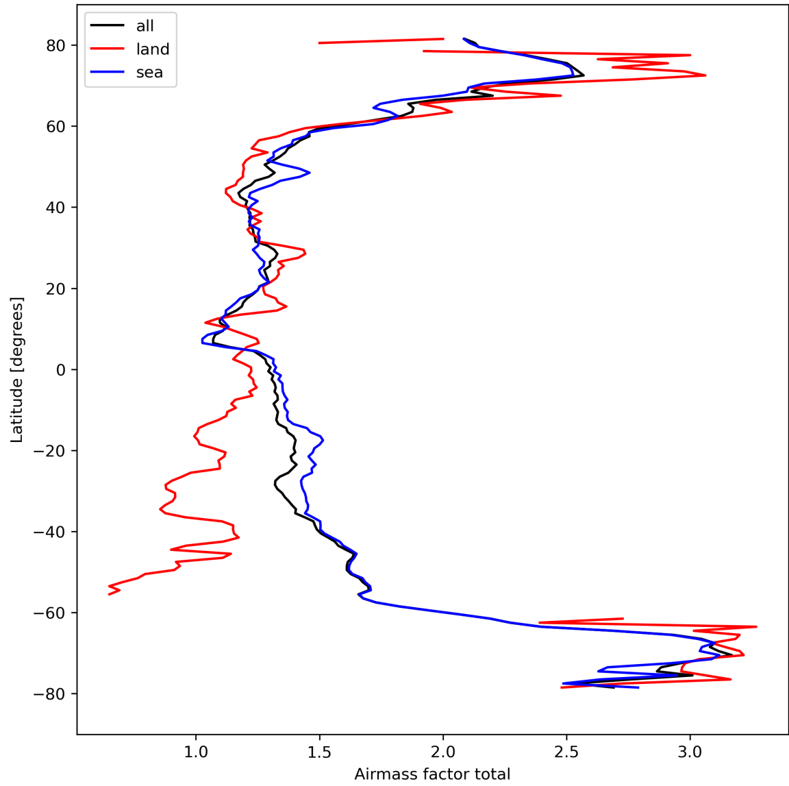
Figure 26: Zonal average of “Airmass factor total” for 2023-10-01 to 2023-10-03.
