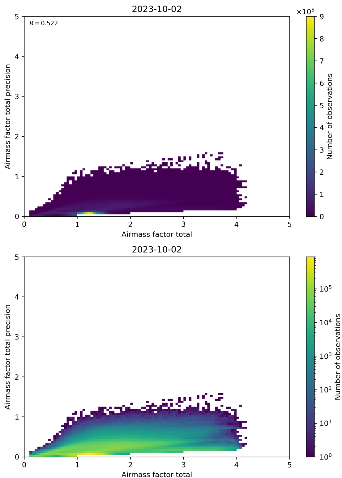
Figure 103: Scatter density plot of “Airmass factor total” against “Airmass factor total precision” for 2023-10-01 to 2023-10-03.
