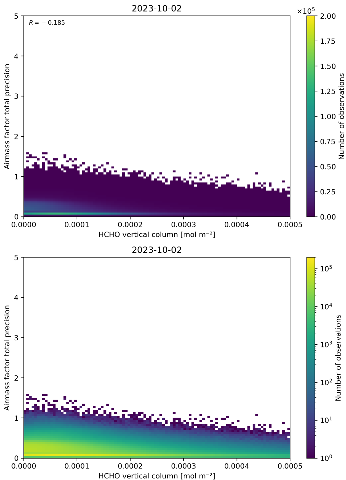
Figure 132: Scatter density plot of “HCHO vertical column” against “Airmass factor total precision” for 2023-10-01 to 2023-10-03.
