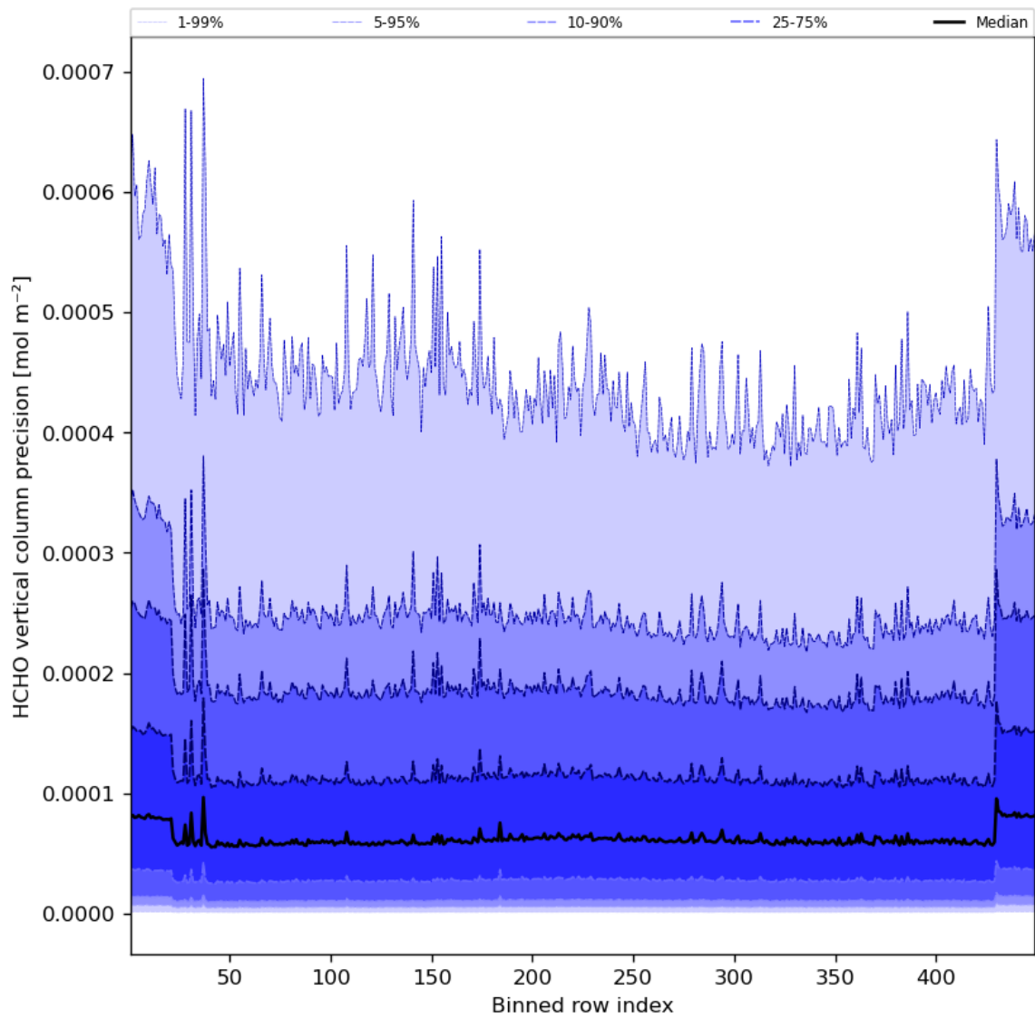
Figure 50: Along track statistics of “HCHO vertical column precision” for 2023-10-01 to 2023-10-03
