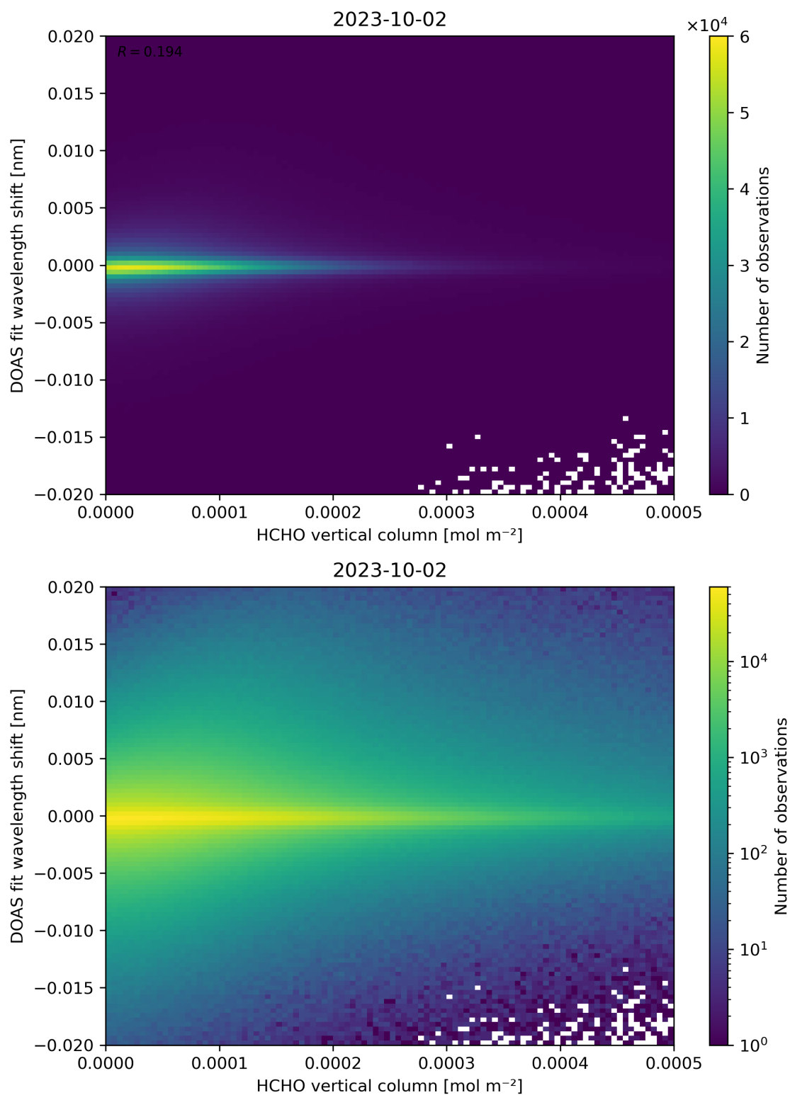
Figure 124: Scatter density plot of “HCHO vertical column” against “DOAS fit wavelength shift” for 2023-10-01 to 2023-10-03.
