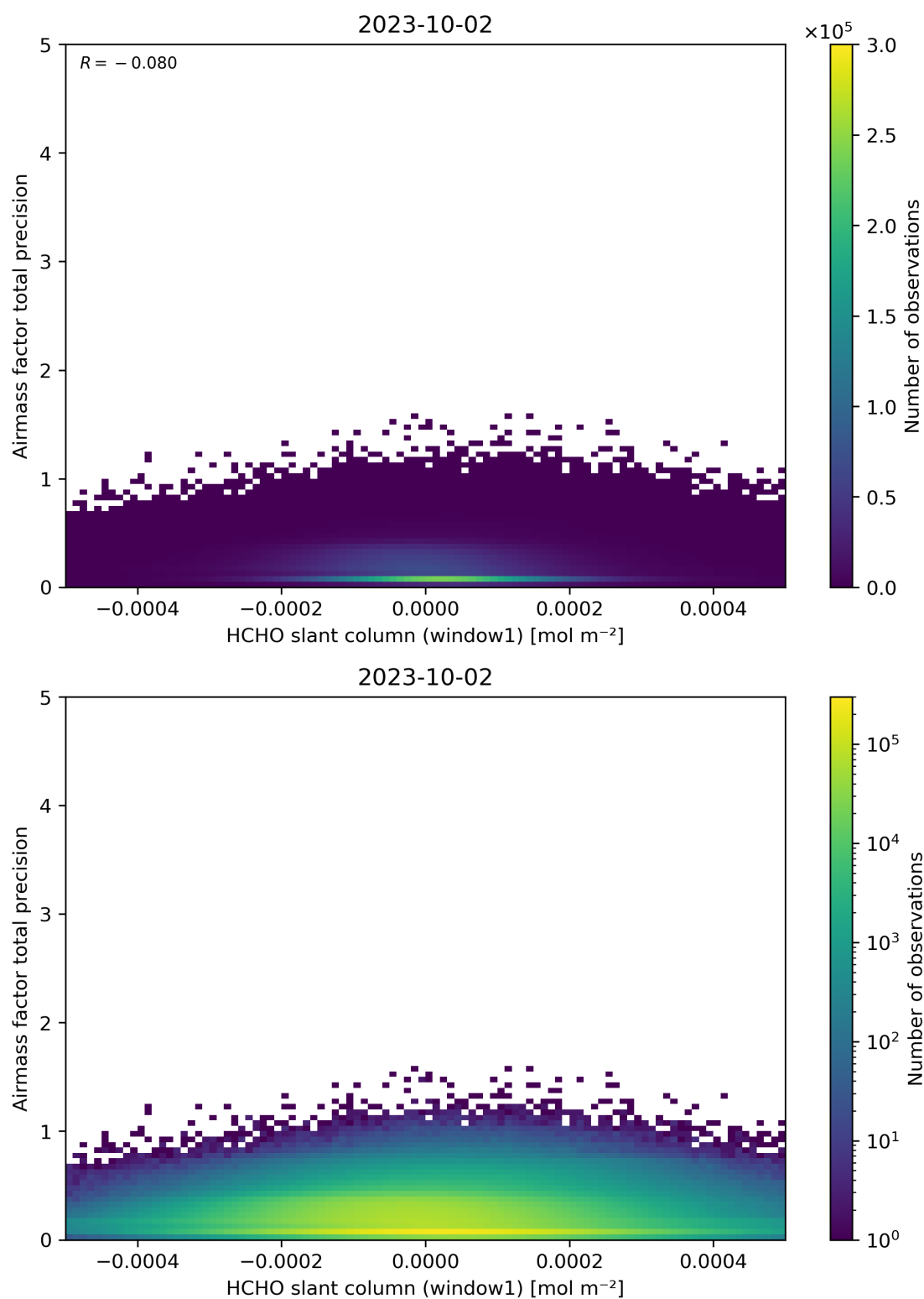
Figure 86: Scatter density plot of “HCHO slant column (window1)” against “Airmass factor total precision” for 2023-10-01 to 2023-10-03.
