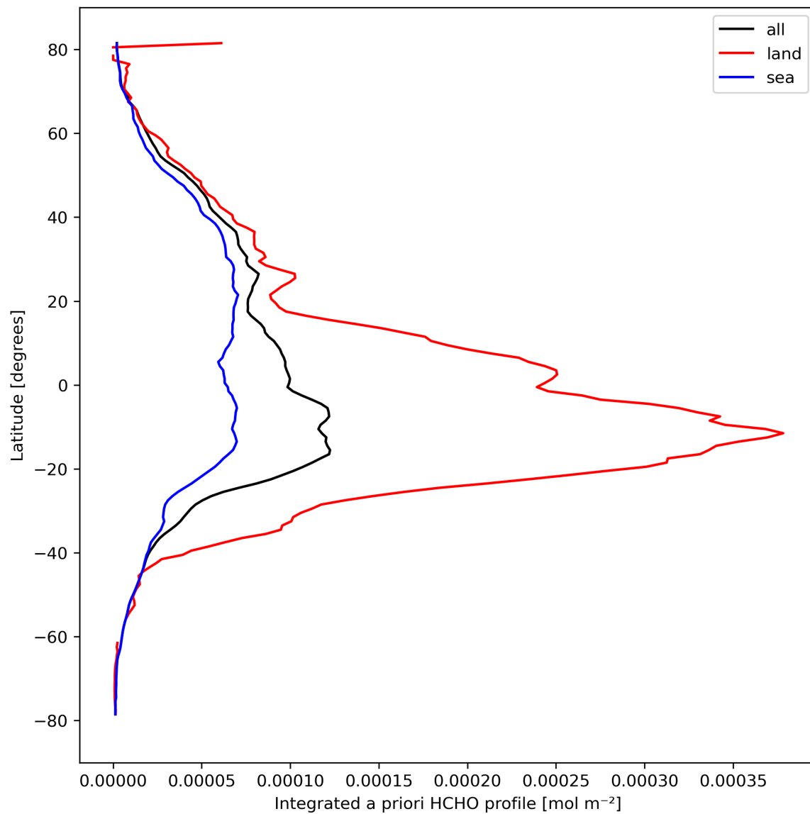
Figure 29: Zonal average of “Integrated a priori HCHO profile” for 2023-10-01 to 2023-10-03.
