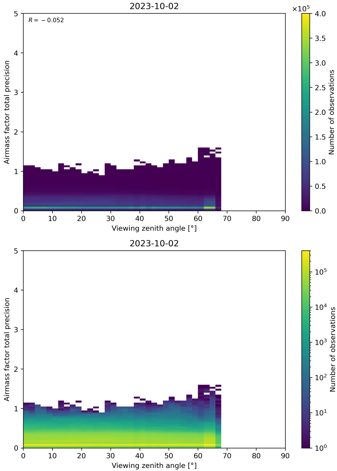
Figure 191: Scatter density plot of “Viewing zenith angle” against “Airmass factor total precision” for 2023-10-01 to 2023-10-03.
