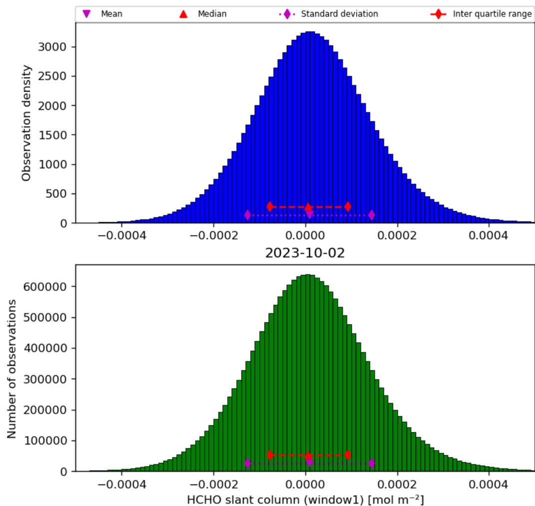
Figure 38: Histogram of “HCHO slant column (window1)” for 2023-10-01 to 2023-10-03
