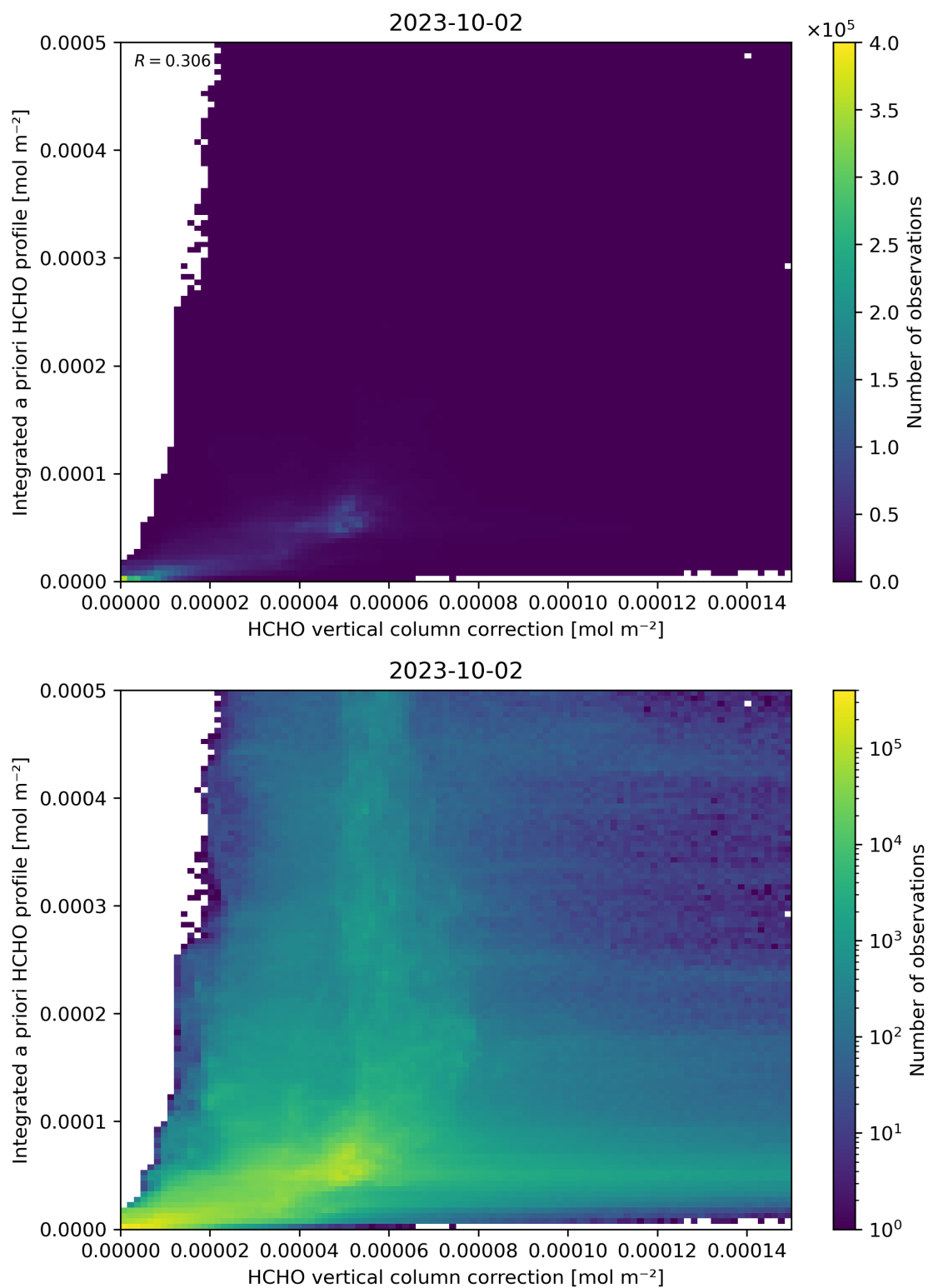
Figure 122: Scatter density plot of “HCHO vertical column correction” against “Integrated a priori HCHO profile” for 2023-10-01 to 2023-10-03.
