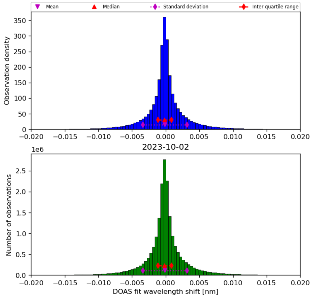
Figure 44: Histogram of “DOAS fit wavelength shift” for 2023-10-01 to 2023-10-03
