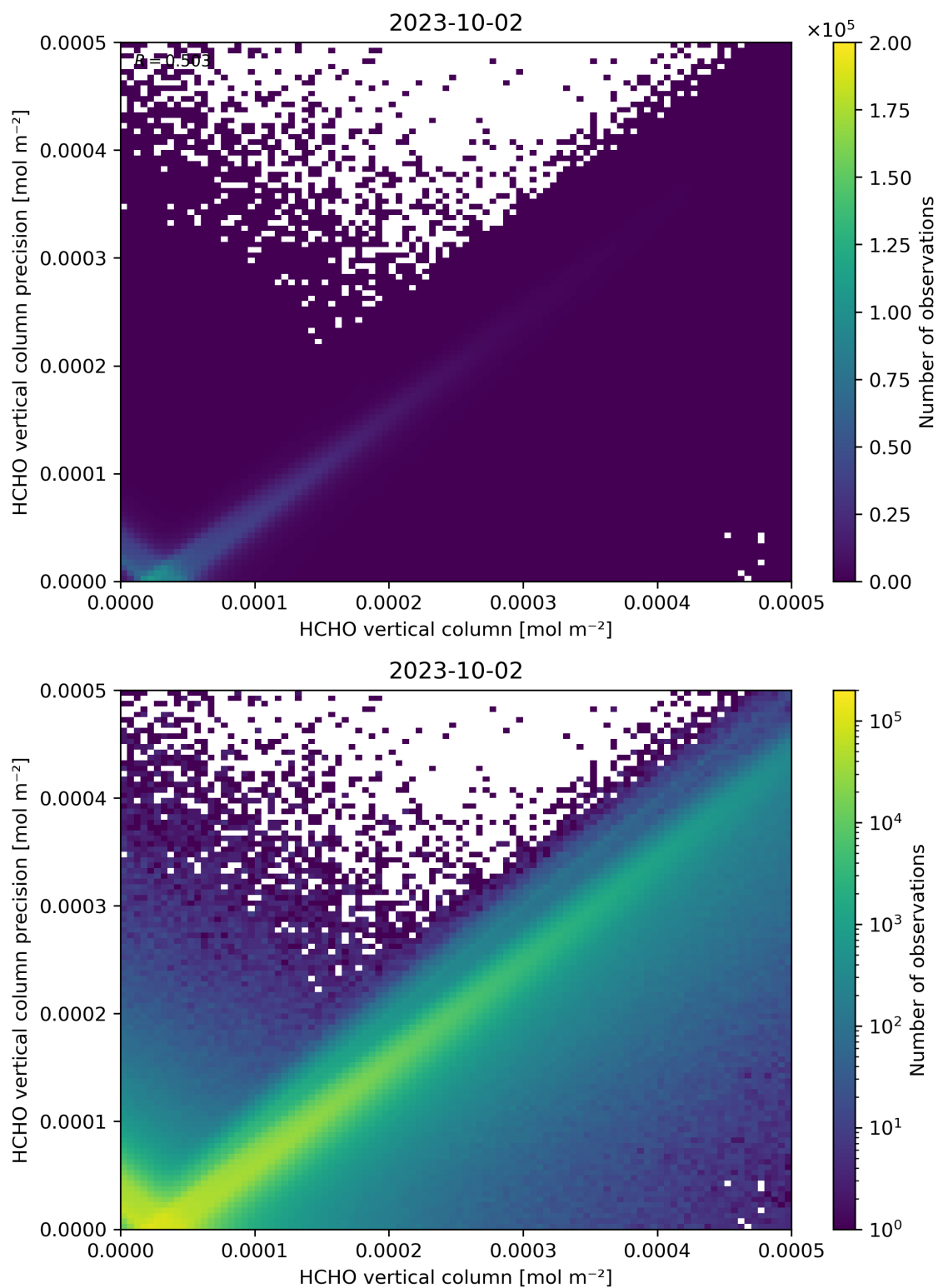
Figure 134: Scatter density plot of “HCHO vertical column” against “HCHO vertical column precision” for 2023-10-01 to 2023-10-03.
