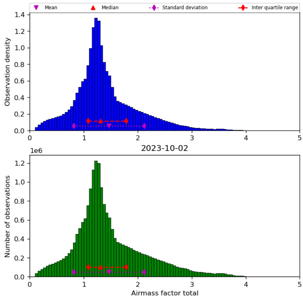
Figure 40: Histogram of “Airmass factor total” for 2023-10-01 to 2023-10-03
