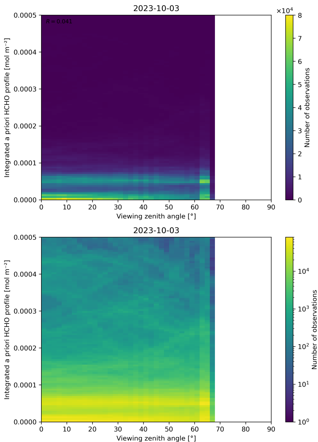
Figure 195: Scatter density plot of “Viewing zenith angle” against “Integrated a priori HCHO profile” for 2023-10-02 to 2023-10-04.
