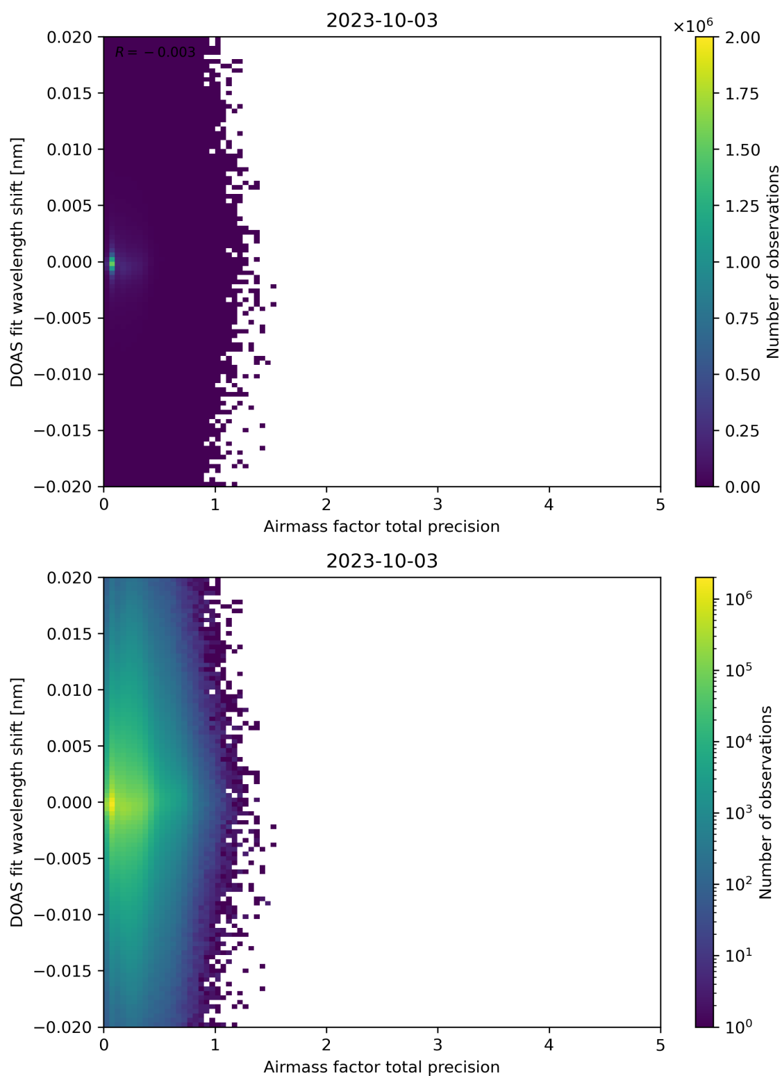
Figure 106: Scatter density plot of “Airmass factor total precision” against “DOAS fit wavelength shift” for 2023-10-02 to 2023-10-04.
