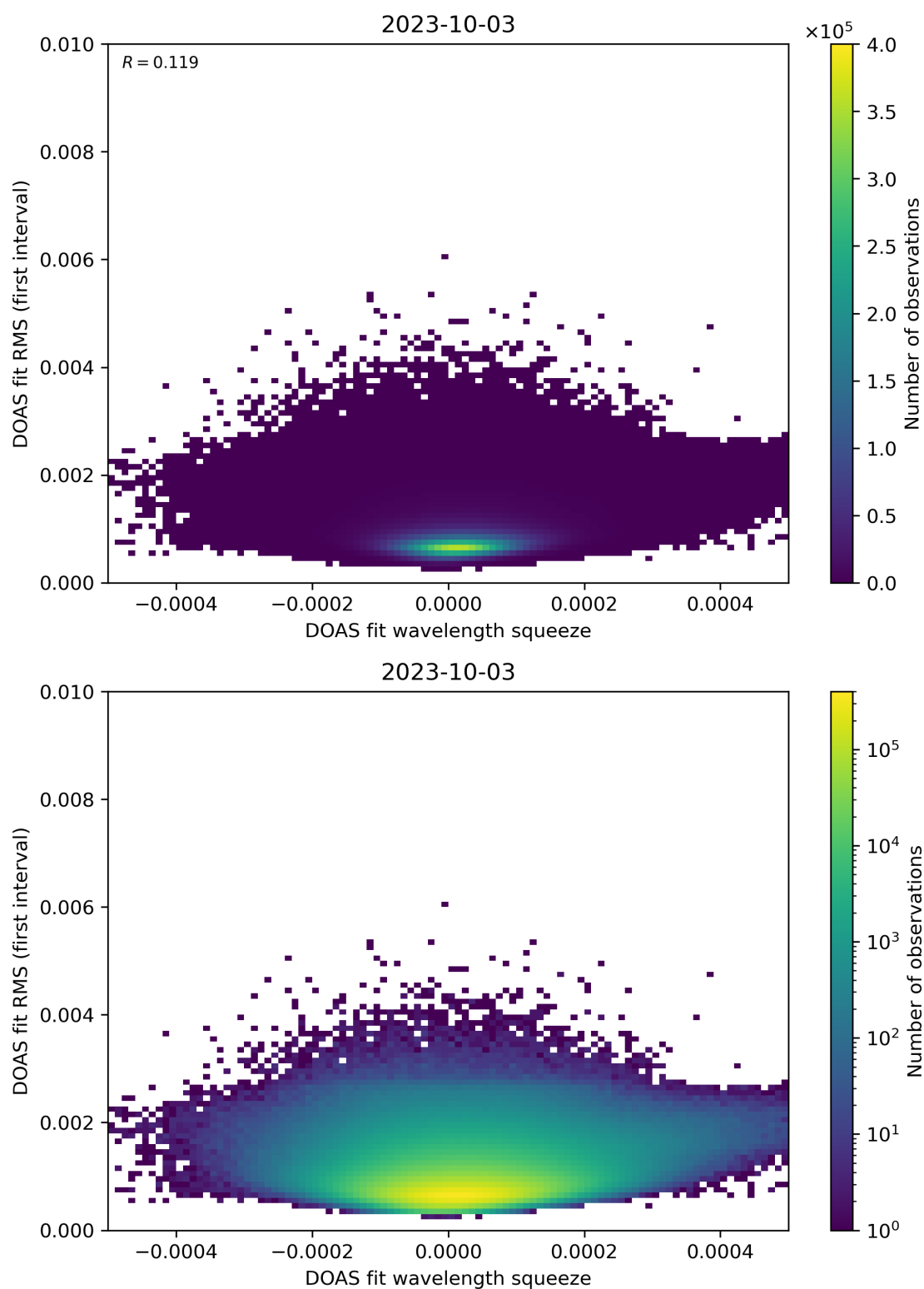
Figure 68: Scatter density plot of “DOAS fit wavelength squeeze” against “DOAS fit RMS (first interval)” for 2023-10-02 to 2023-10-04.
