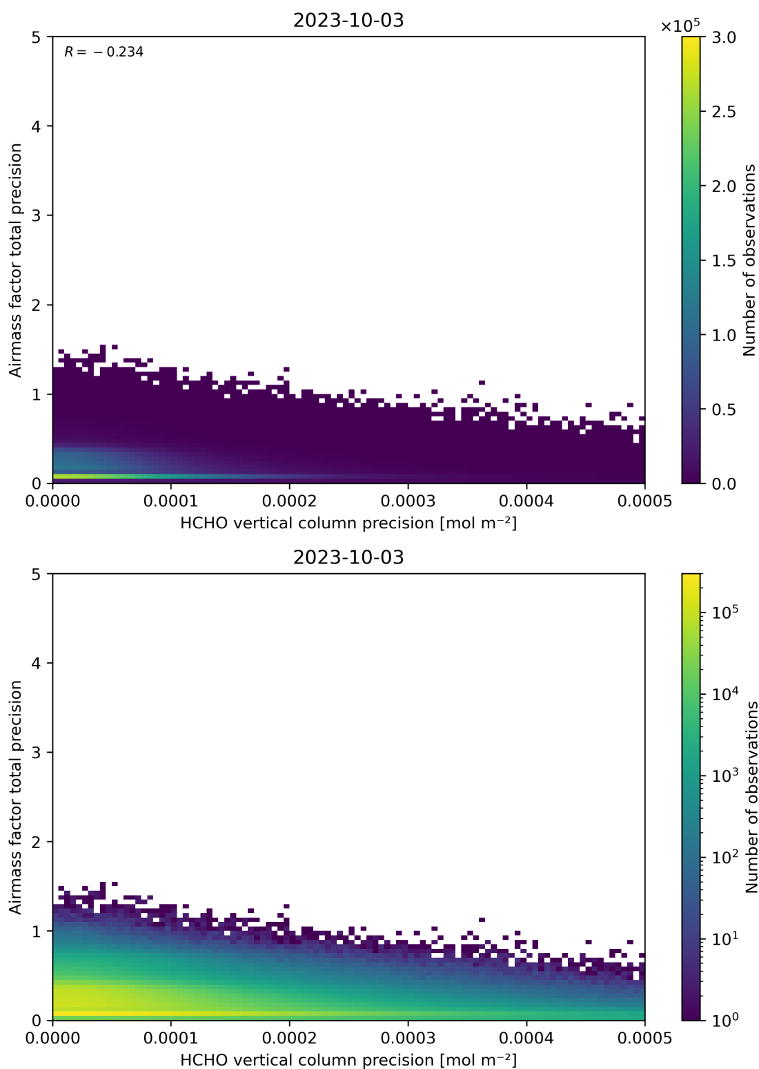
Figure 145: Scatter density plot of “HCHO vertical column precision” against “Airmass factor total precision” for 2023-10-02 to 2023-10-04.
