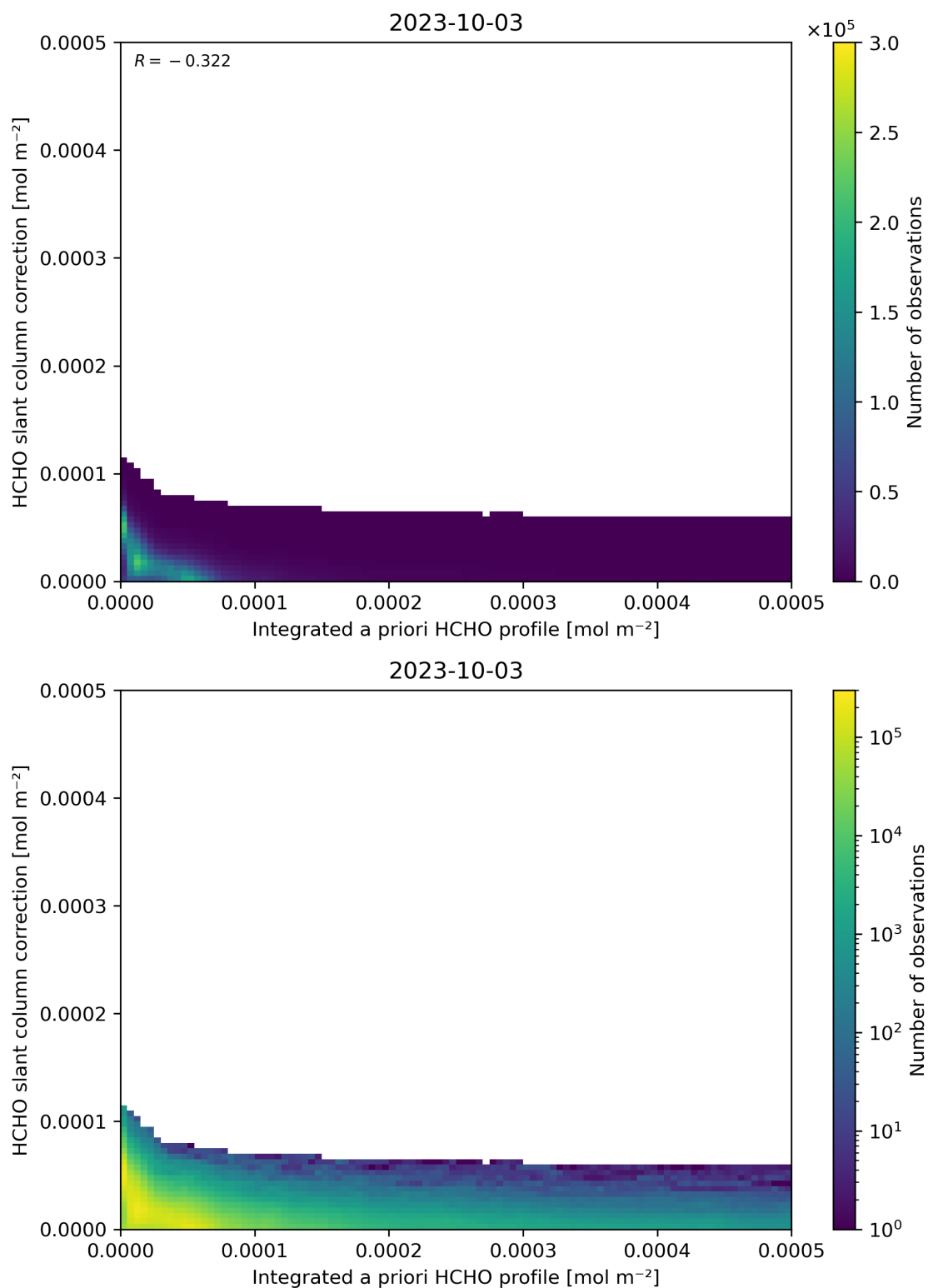
Figure 152: Scatter density plot of “Integrated a priori HCHO profile” against “HCHO slant column correction” for 2023-10-02 to 2023-10-04.
