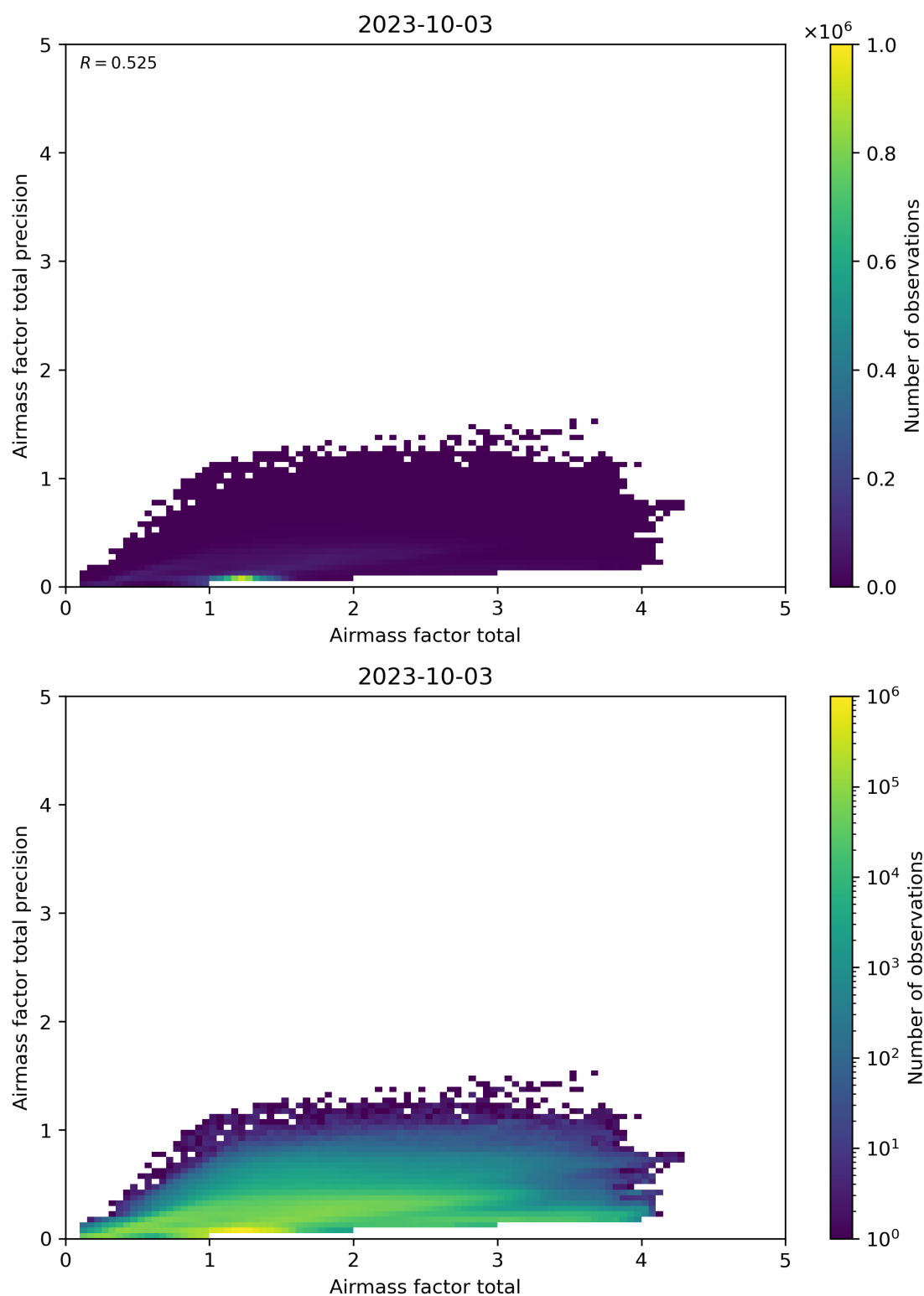
Figure 103: Scatter density plot of “Airmass factor total” against “Airmass factor total precision” for 2023-10-02 to 2023-10-04.
