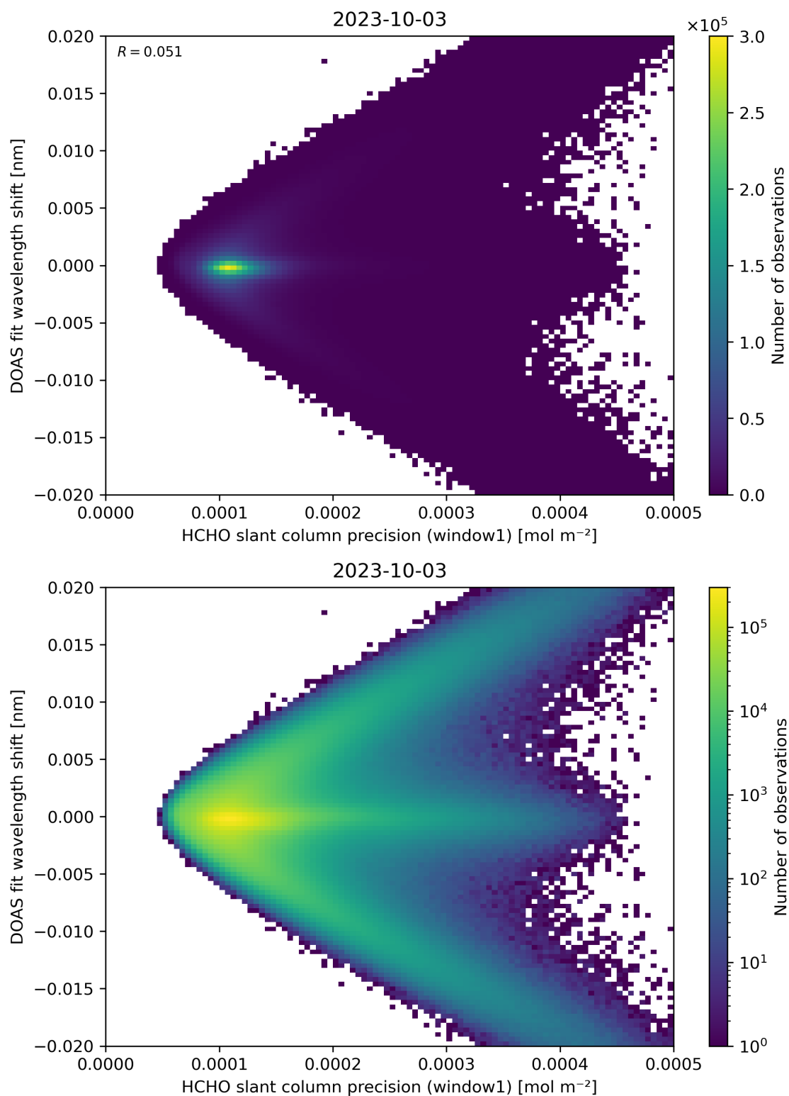
Figure 89: Scatter density plot of “HCHO slant column precision (window1)” against “DOAS fit wavelength shift” for 2023-10-02 to 2023-10-04.
