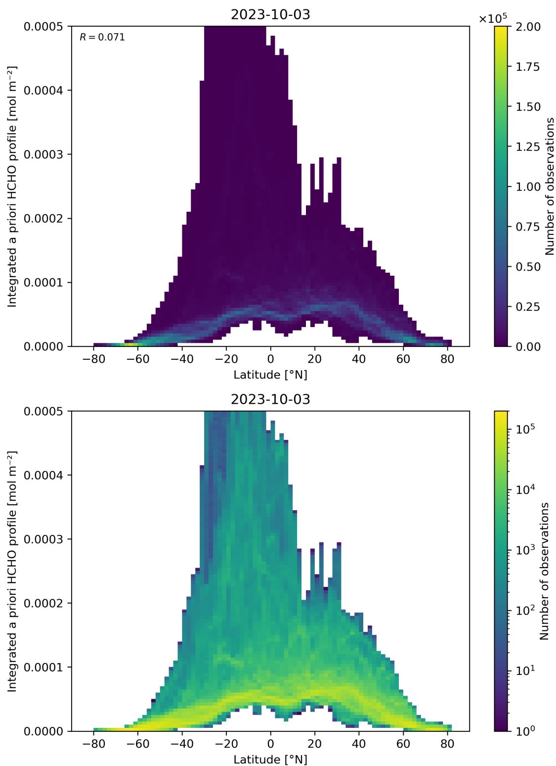
Figure 166: Scatter density plot of “Latitude” against “Integrated a priori HCHO profile” for 2023-10-02 to 2023-10-04.
