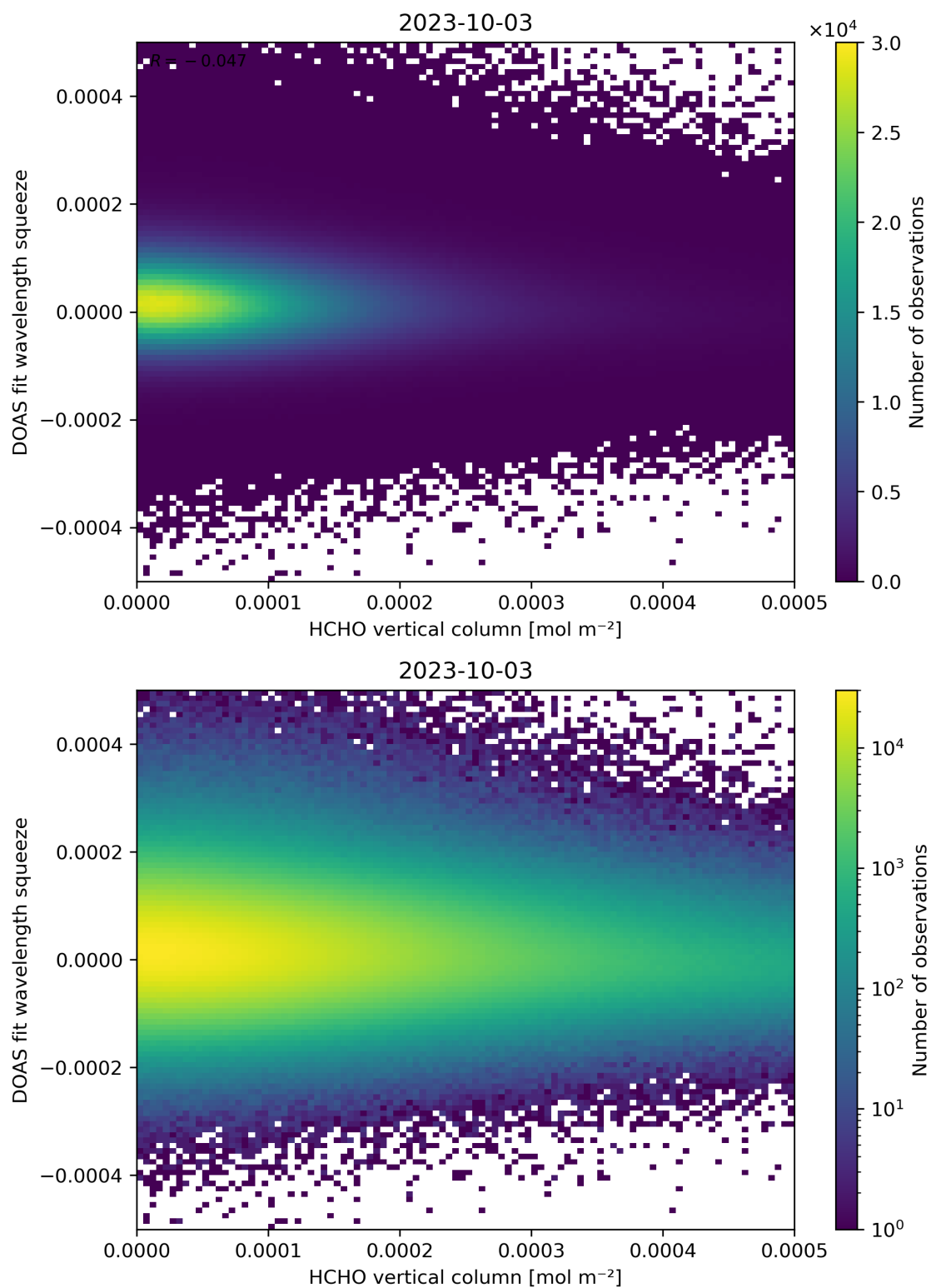
Figure 125: Scatter density plot of “HCHO vertical column” against “DOAS fit wavelength squeeze” for 2023-10-02 to 2023-10-04.
