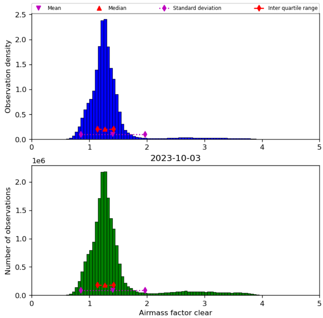
Figure 42: Histogram of “Airmass factor clear” for 2023-10-02 to 2023-10-04
