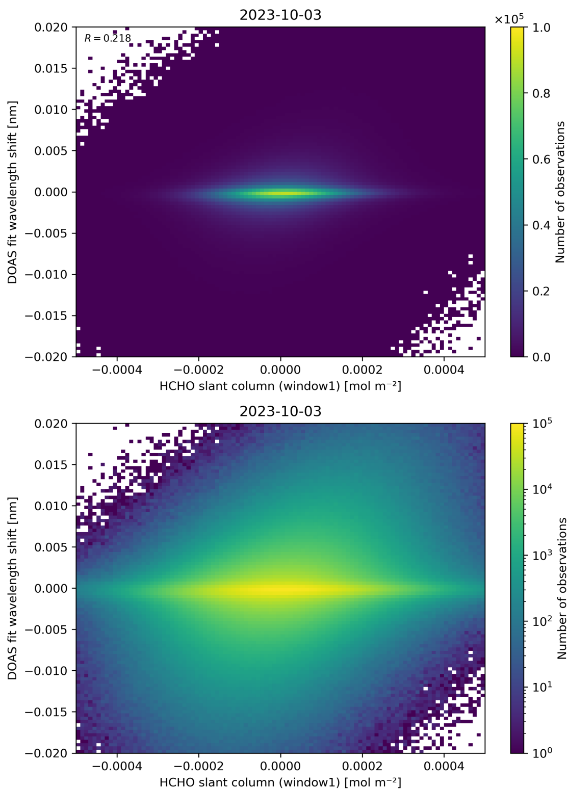
Figure 79: Scatter density plot of “HCHO slant column (window1)” against “DOAS fit wavelength shift” for 2023-10-02 to 2023-10-04.
