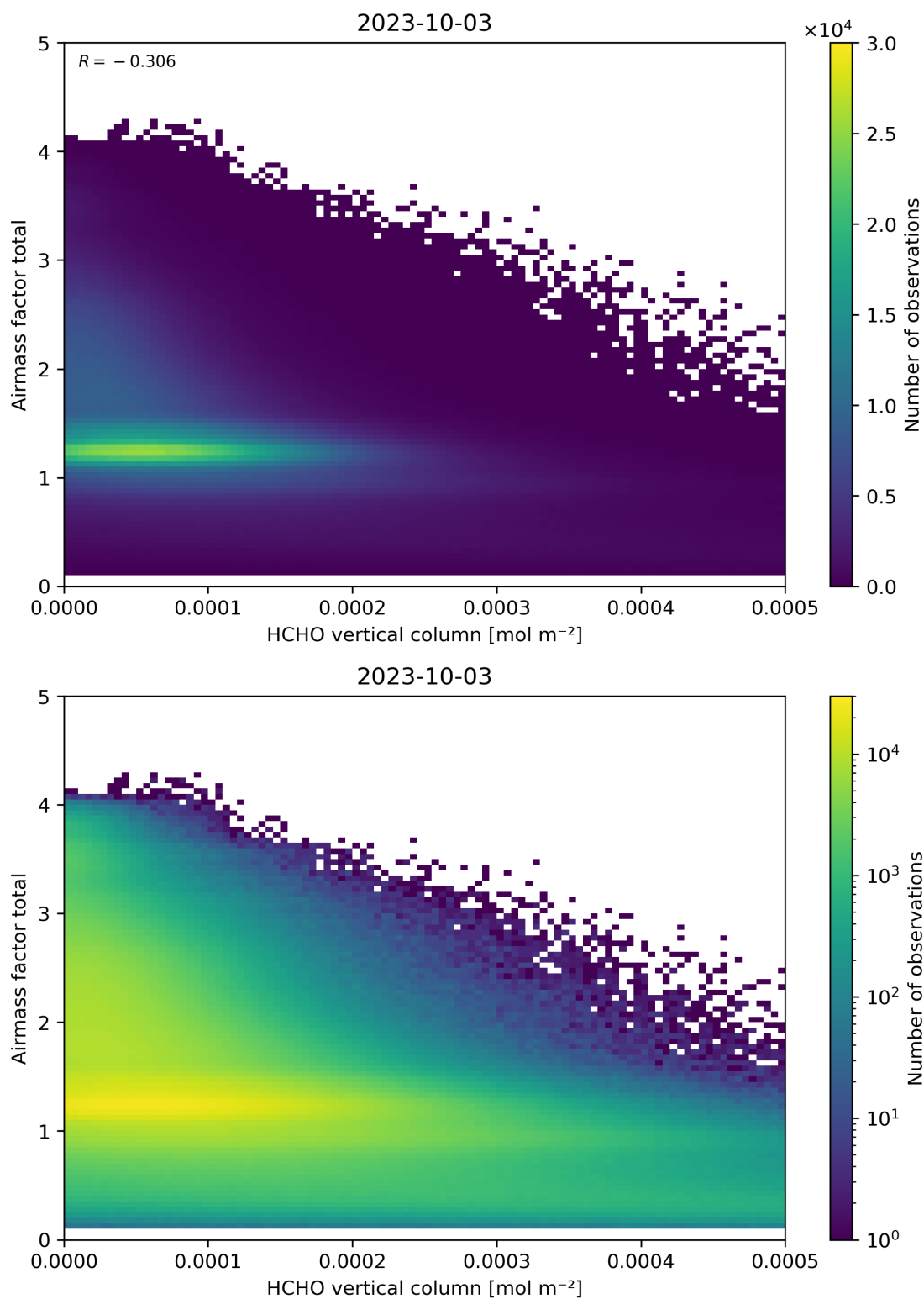
Figure 131: Scatter density plot of “HCHO vertical column” against “Airmass factor total” for 2023-10-02 to 2023-10-04.
