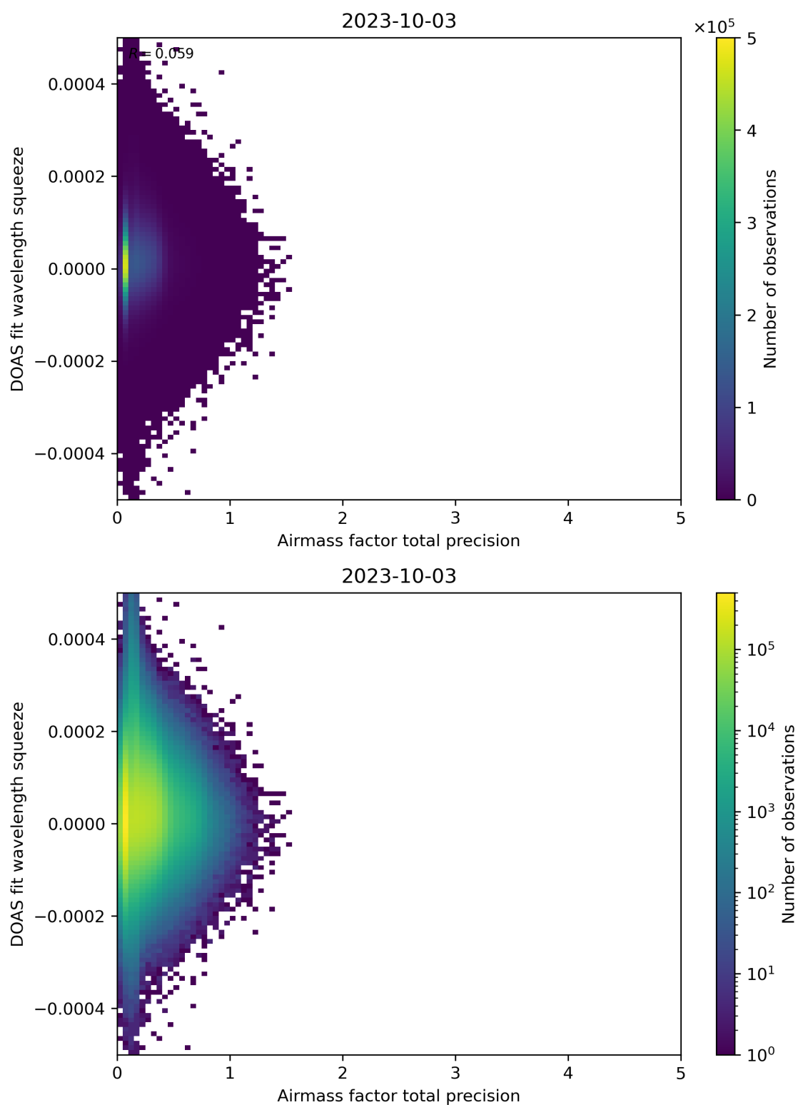
Figure 107: Scatter density plot of “Airmass factor total precision” against “DOAS fit wavelength squeeze” for 2023-10-02 to 2023-10-04.
