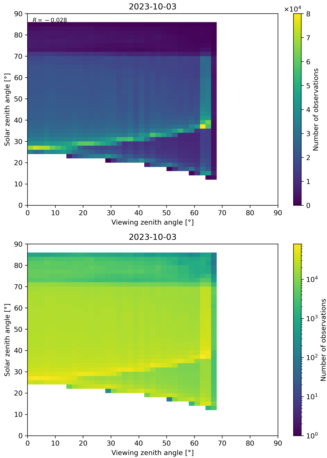
Figure 197: Scatter density plot of “Viewing zenith angle” against “Solar zenith angle” for 2023-10-02 to 2023-10-04.
