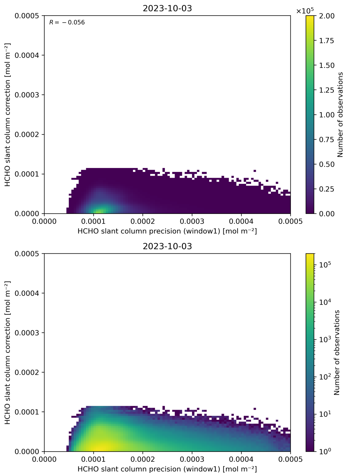
Figure 93: Scatter density plot of “HCHO slant column precision (window1)” against “HCHO slant column correction” for 2023-10-02 to 2023-10-04.
