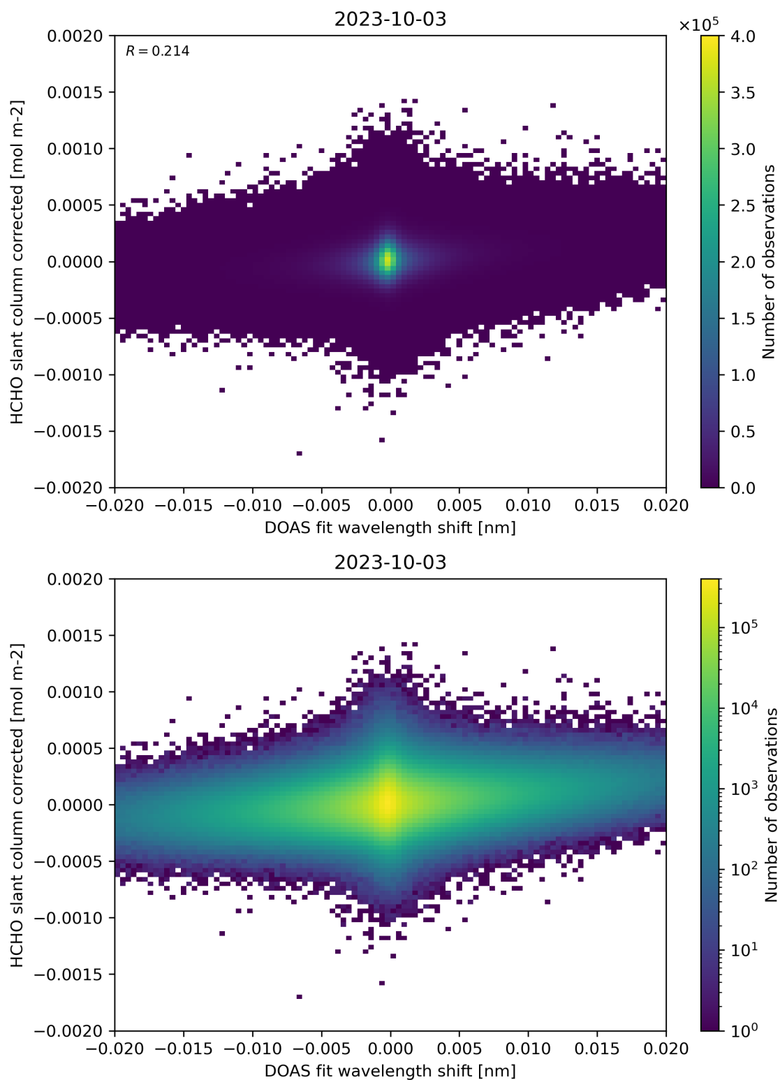
Figure 66: Scatter density plot of “DOAS fit wavelength shift” against “HCHO slant column corrected” for 2023-10-02 to 2023-10-04.
