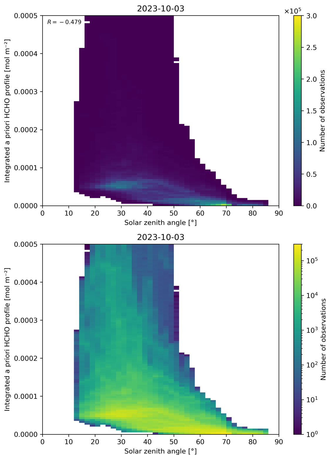
Figure 180: Scatter density plot of “Solar zenith angle” against “Integrated a priori HCHO profile” for 2023-10-02 to 2023-10-04.
