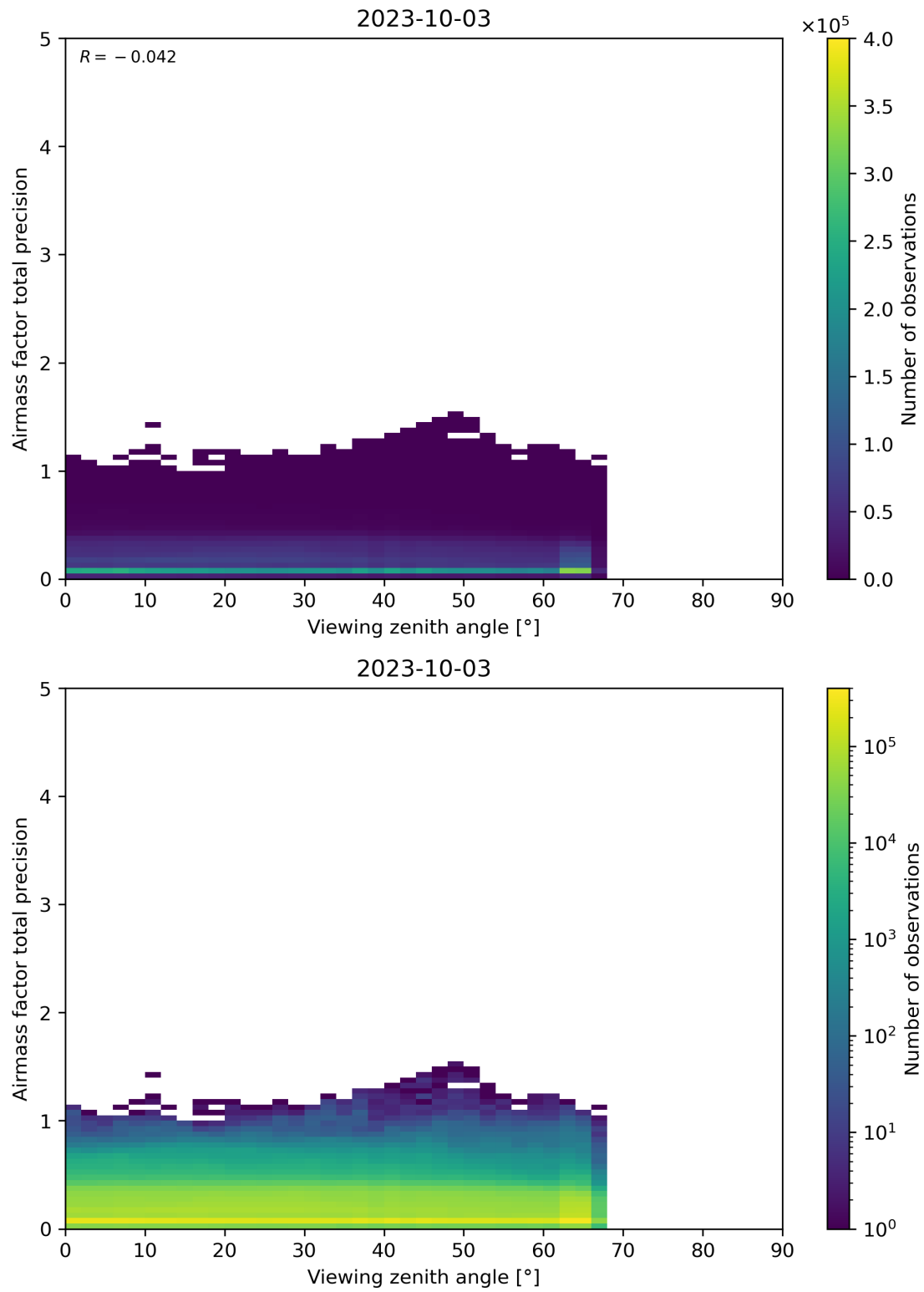
Figure 191: Scatter density plot of “Viewing zenith angle” against “Airmass factor total precision” for 2023-10-02 to 2023-10-04.
