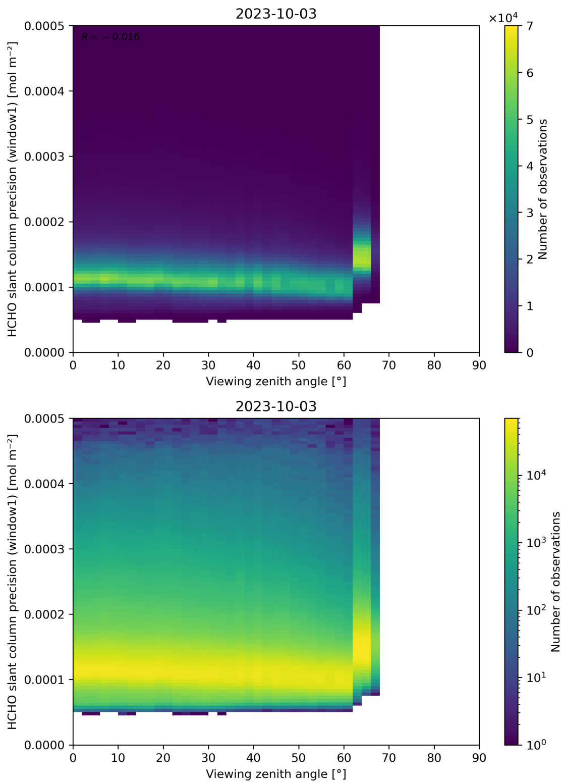
Figure 189: Scatter density plot of “Viewing zenith angle” against “HCHO slant column precision (window1)” for 2023-10-02 to 2023-10-04.
