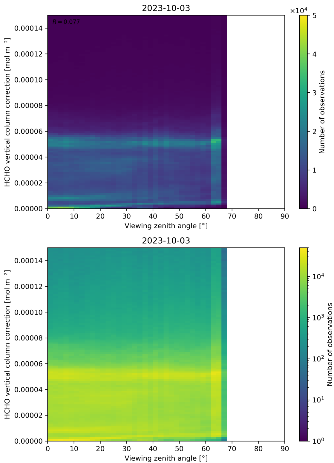
Figure 193: Scatter density plot of “Viewing zenith angle” against “HCHO vertical column correction” for 2023-10-02 to 2023-10-04.
