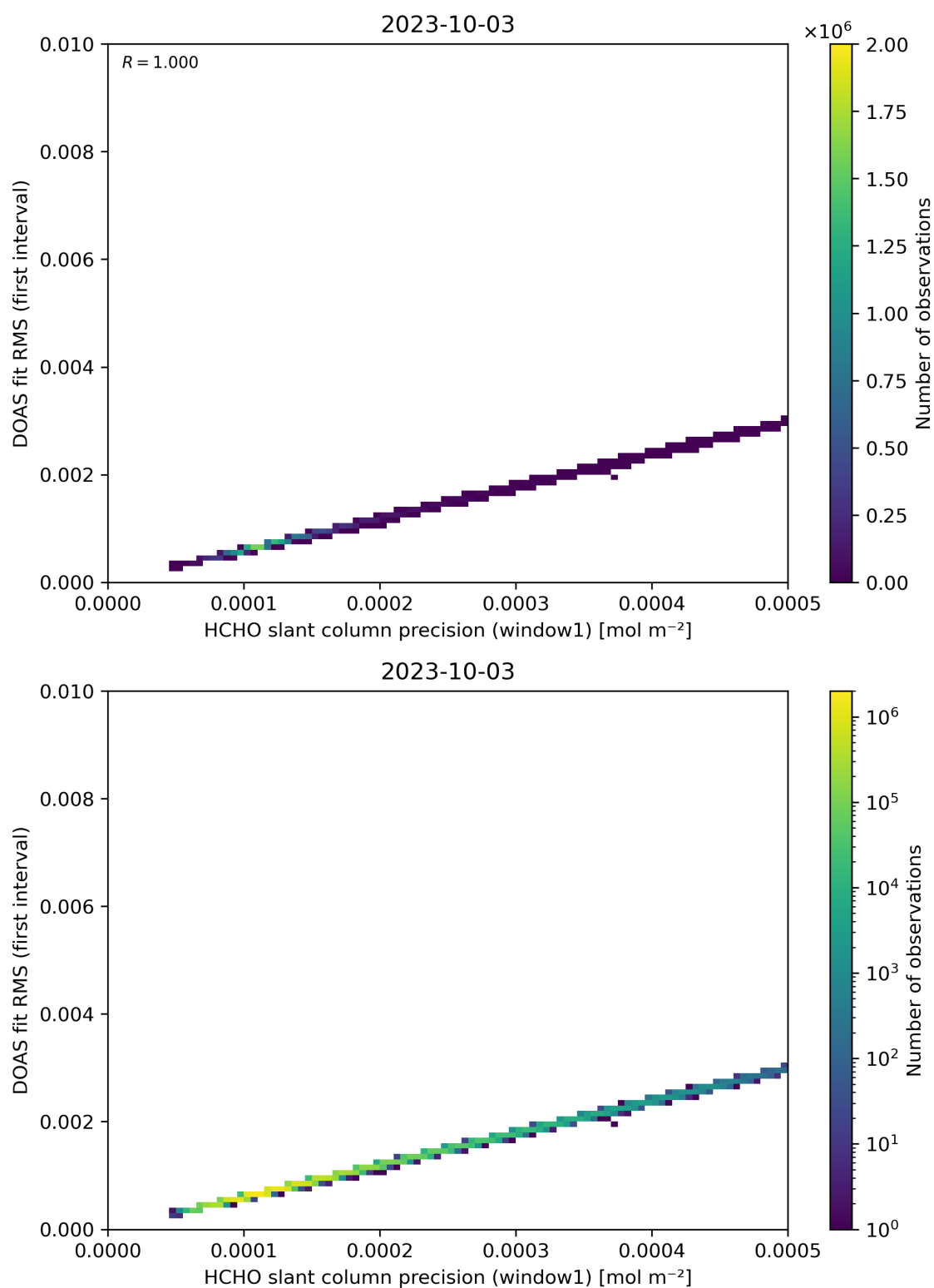
Figure 88: Scatter density plot of “HCHO slant column precision (window1)” against “DOAS fit RMS (first interval)” for 2023-10-02 to 2023-10-04.
