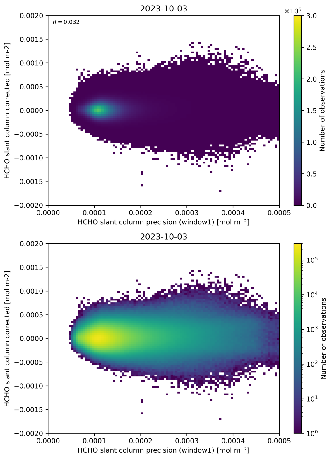
Figure 92: Scatter density plot of “HCHO slant column precision (window1)” against “HCHO slant column corrected” for 2023-10-02 to 2023-10-04.
