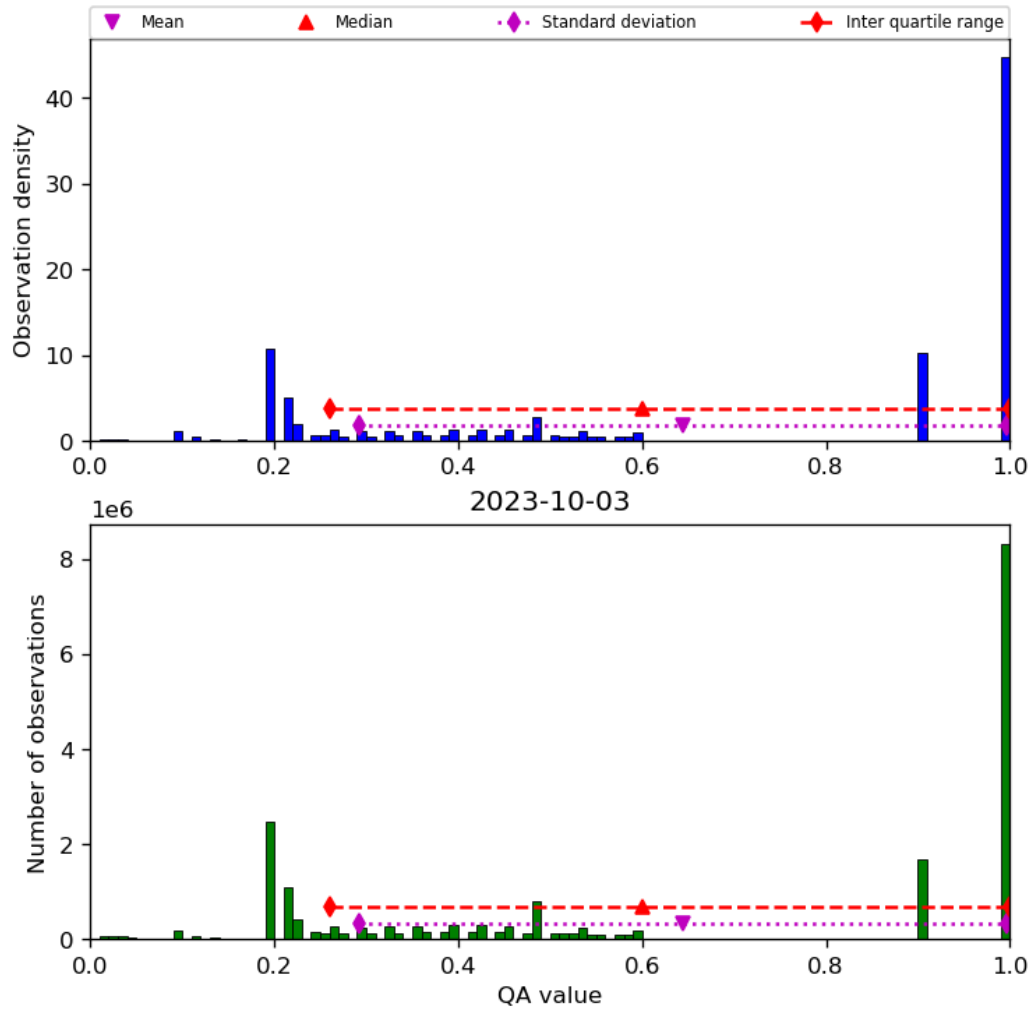
Figure 34: Histogram of “QA value” for 2023-10-02 to 2023-10-04
