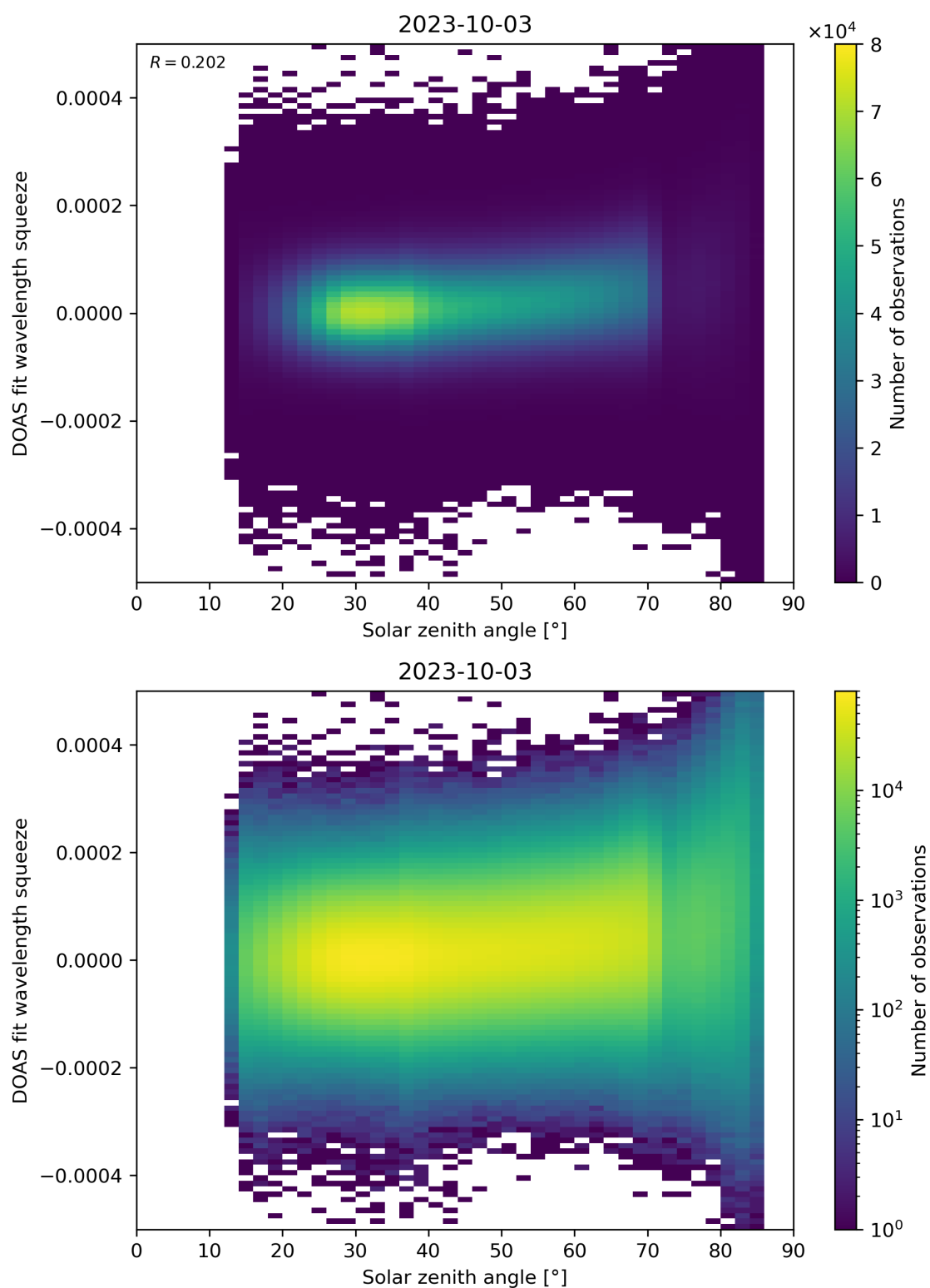
Figure 169: Scatter density plot of “Solar zenith angle” against “DOAS fit wavelength squeeze” for 2023-10-02 to 2023-10-04.
