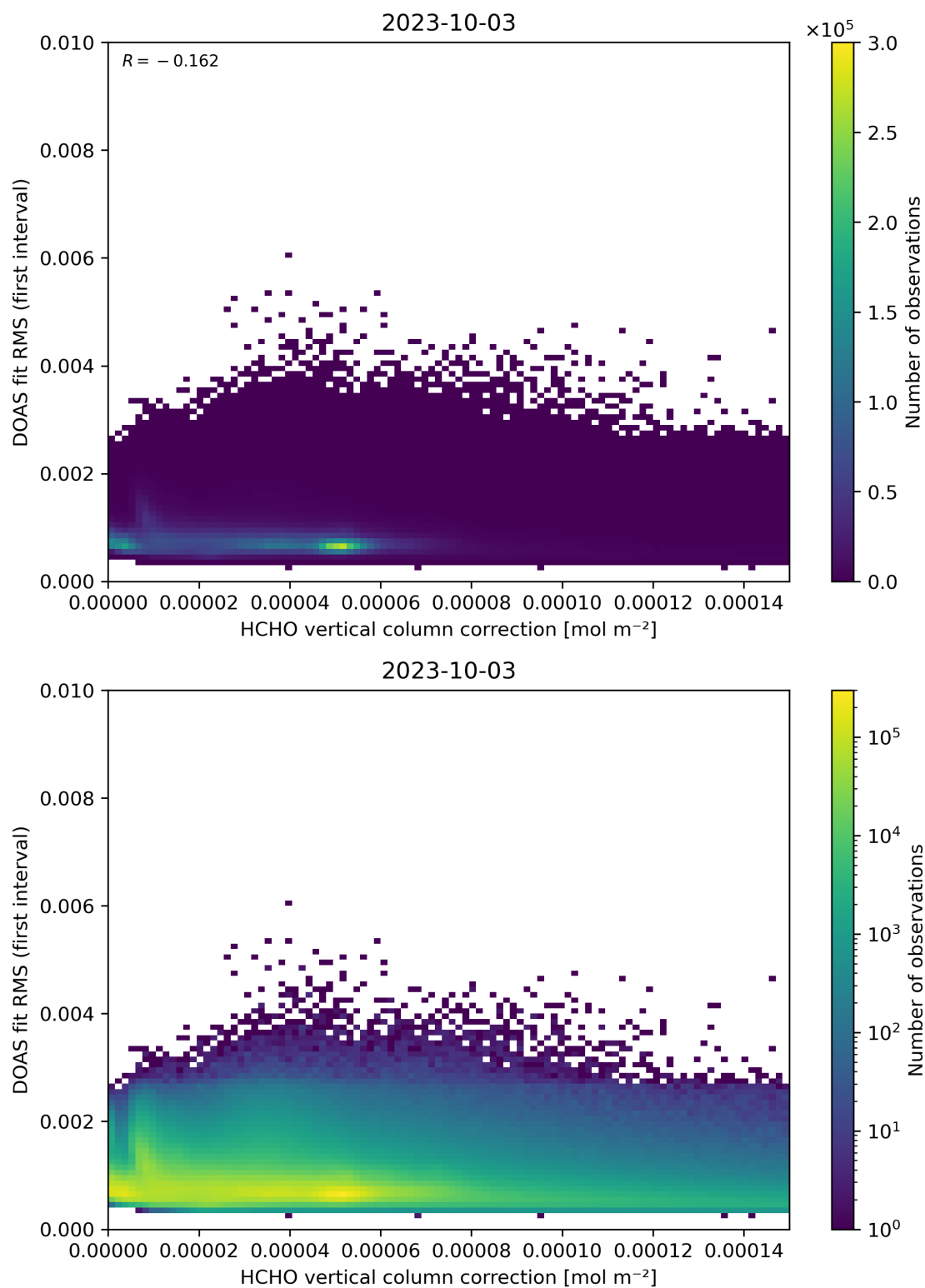
Figure 112: Scatter density plot of “HCHO vertical column correction” against “DOAS fit RMS (first interval)” for 2023-10-02 to 2023-10-04.
