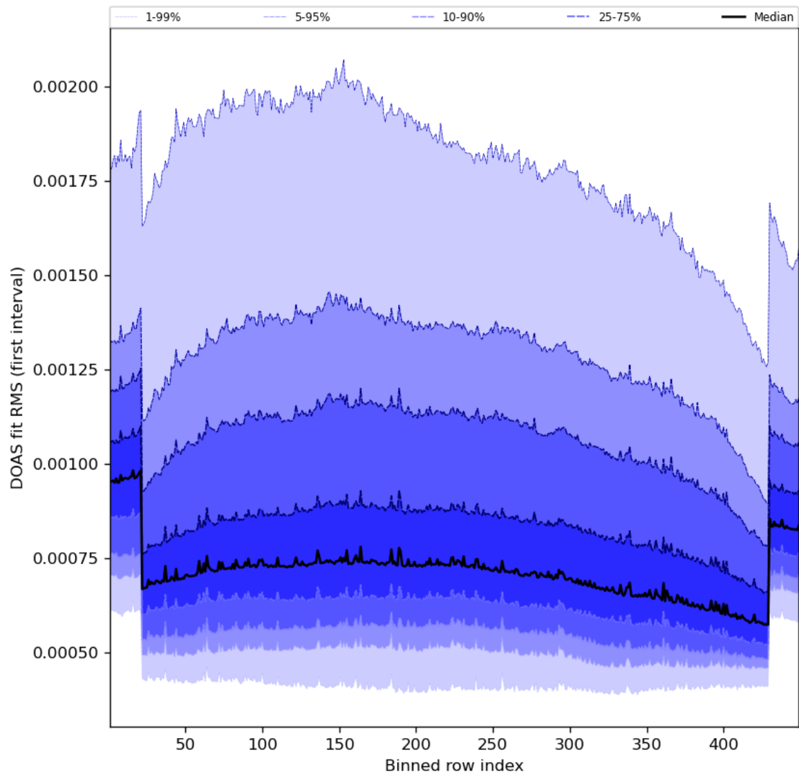
Figure 60: Along track statistics of “DOAS fit RMS (first interval)” for 2023-10-02 to 2023-10-04
