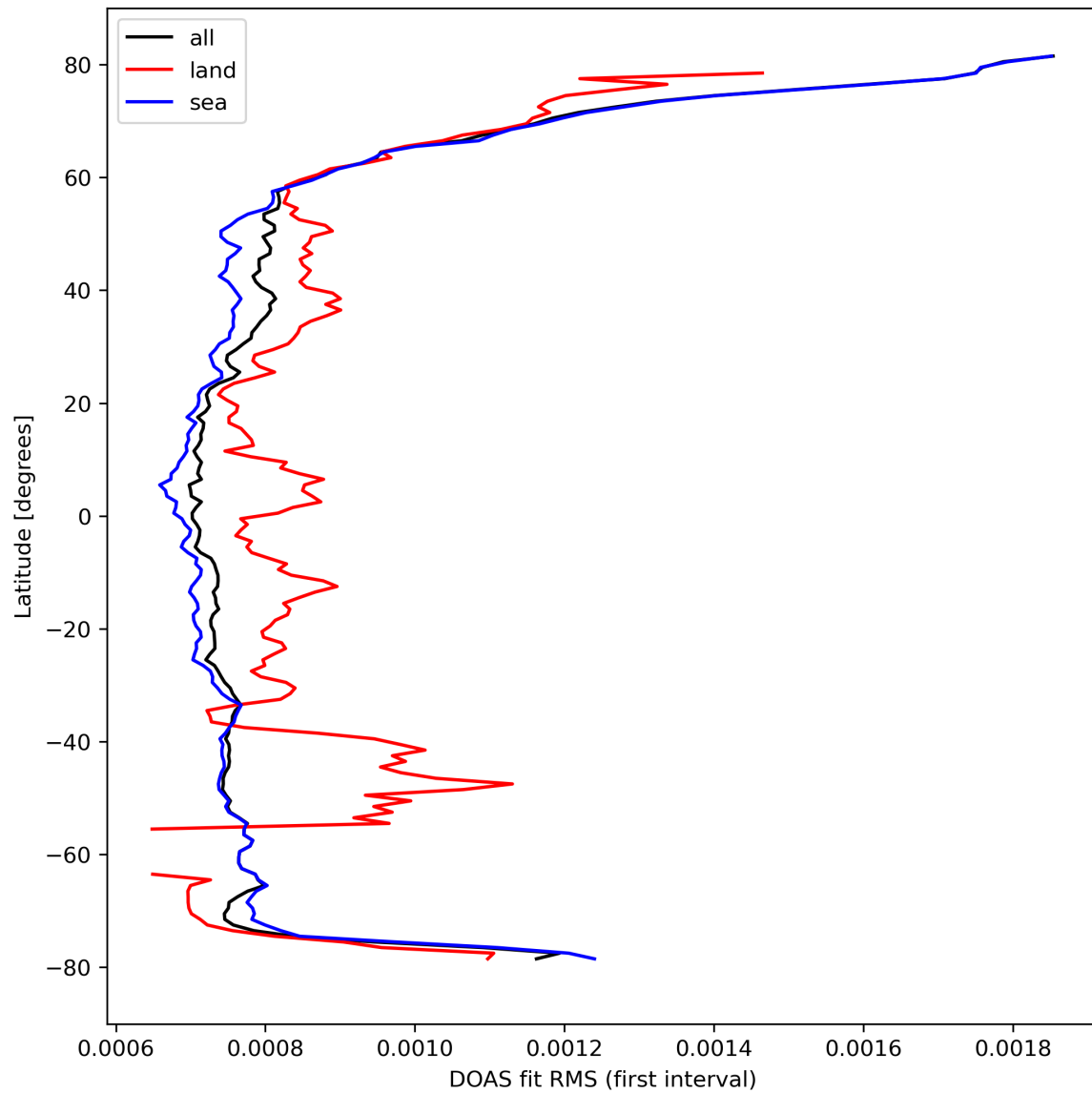
Figure 32: Zonal average of “DOAS fit RMS (first interval)” for 2023-10-02 to 2023-10-04.
