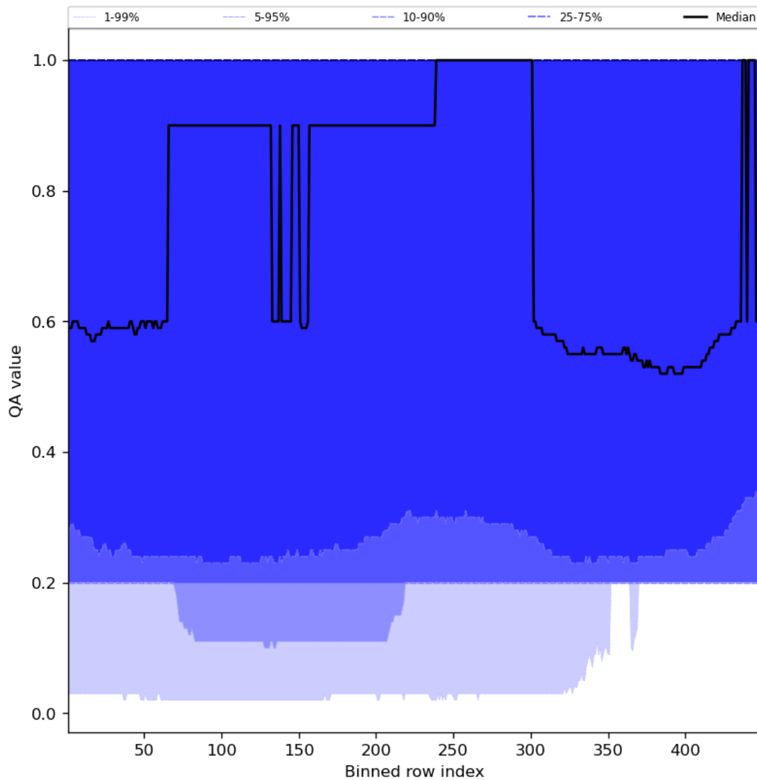
Figure 48: Along track statistics of “QA value” for 2023-10-02 to 2023-10-04
