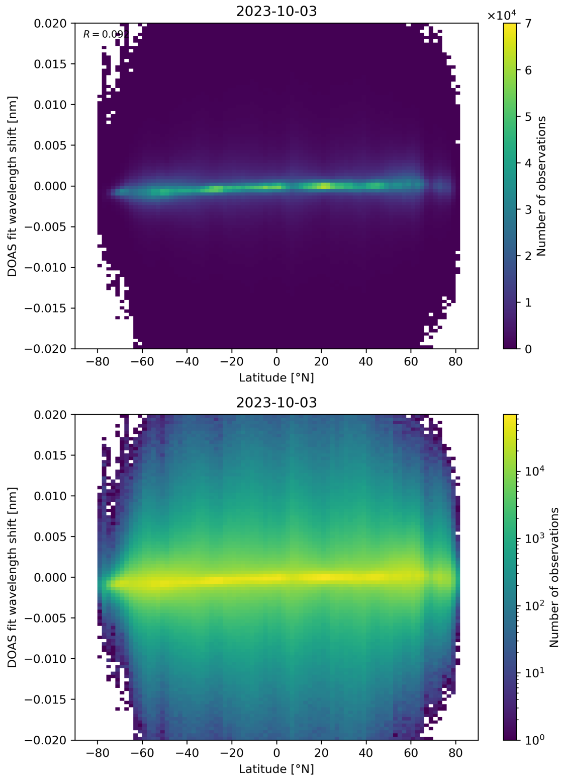
Figure 154: Scatter density plot of “Latitude” against “DOAS fit wavelength shift” for 2023-10-02 to 2023-10-04.
