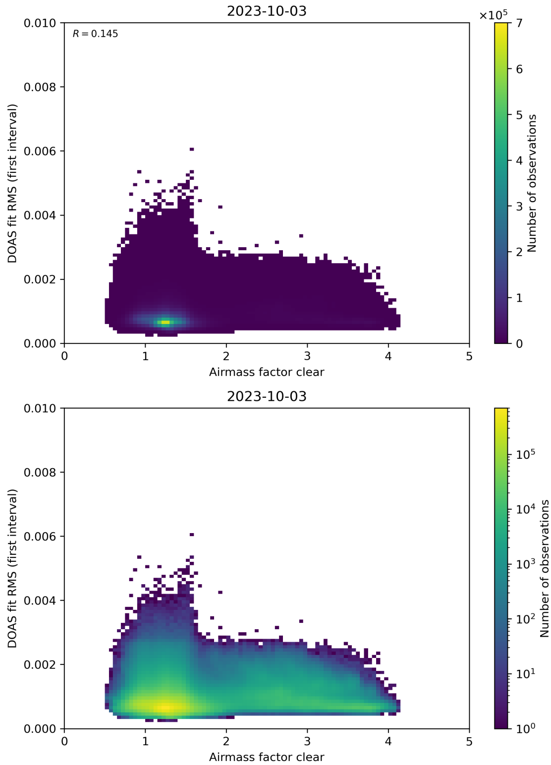
Figure 71: Scatter density plot of “Airmass factor clear” against “DOAS fit RMS (first interval)” for 2023-10-02 to 2023-10-04.
