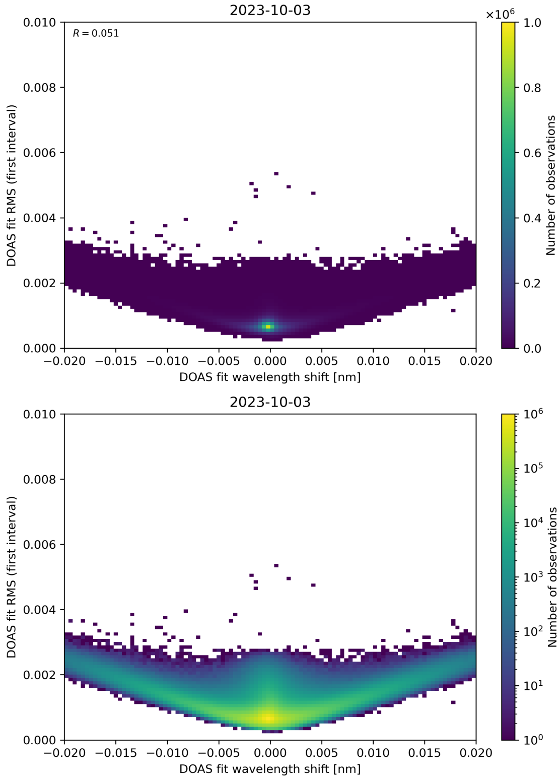
Figure 64: Scatter density plot of “DOAS fit wavelength shift” against “DOAS fit RMS (first interval)” for 2023-10-02 to 2023-10-04.
