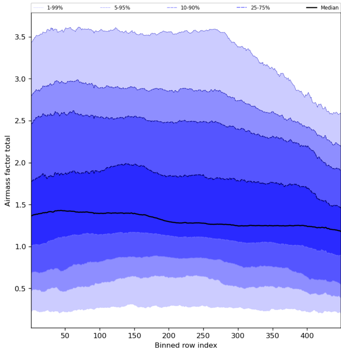
Figure 54: Along track statistics of “Airmass factor total” for 2023-10-02 to 2023-10-04
