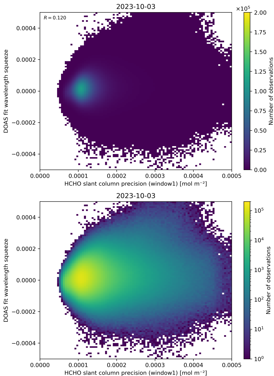
Figure 90: Scatter density plot of “HCHO slant column precision (window1)” against “DOAS fit wavelength squeeze” for 2023-10-02 to 2023-10-04.
