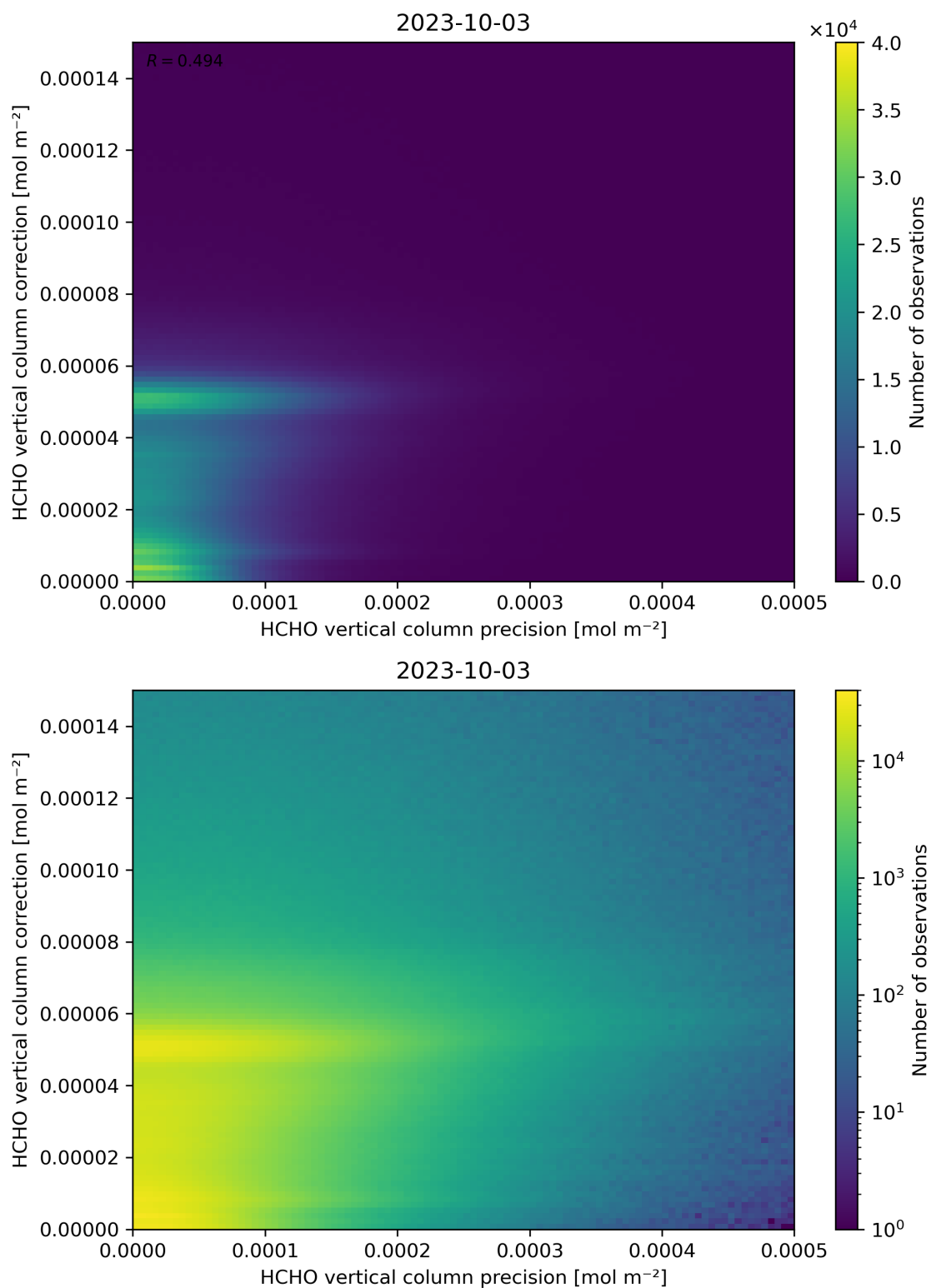
Figure 146: Scatter density plot of “HCHO vertical column precision” against “HCHO vertical column correction” for 2023-10-02 to 2023-10-04.
