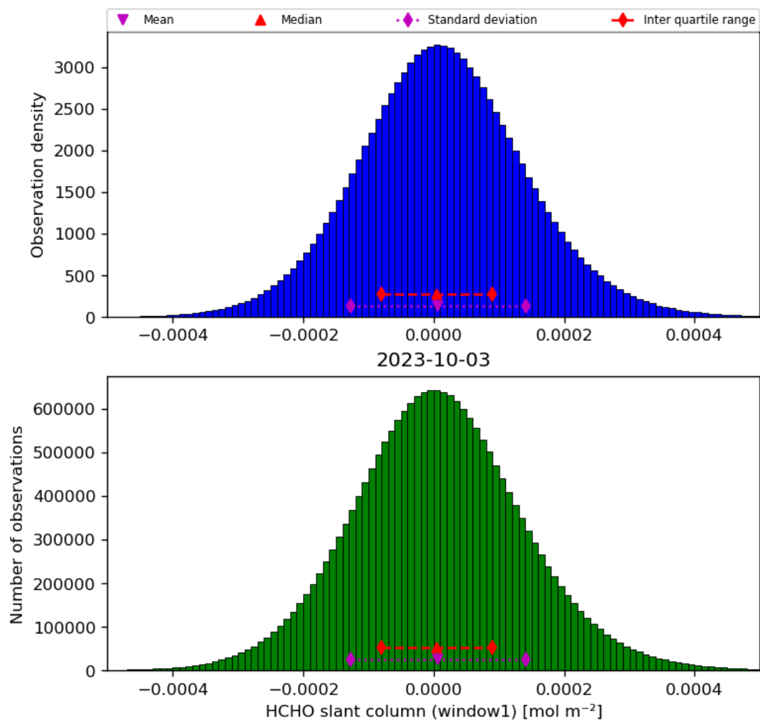
Figure 38: Histogram of “HCHO slant column (window1)” for 2023-10-02 to 2023-10-04
