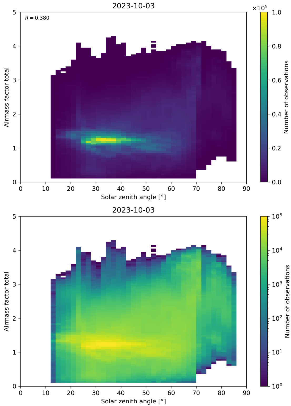
Figure 175: Scatter density plot of “Solar zenith angle” against “Airmass factor total” for 2023-10-02 to 2023-10-04.
