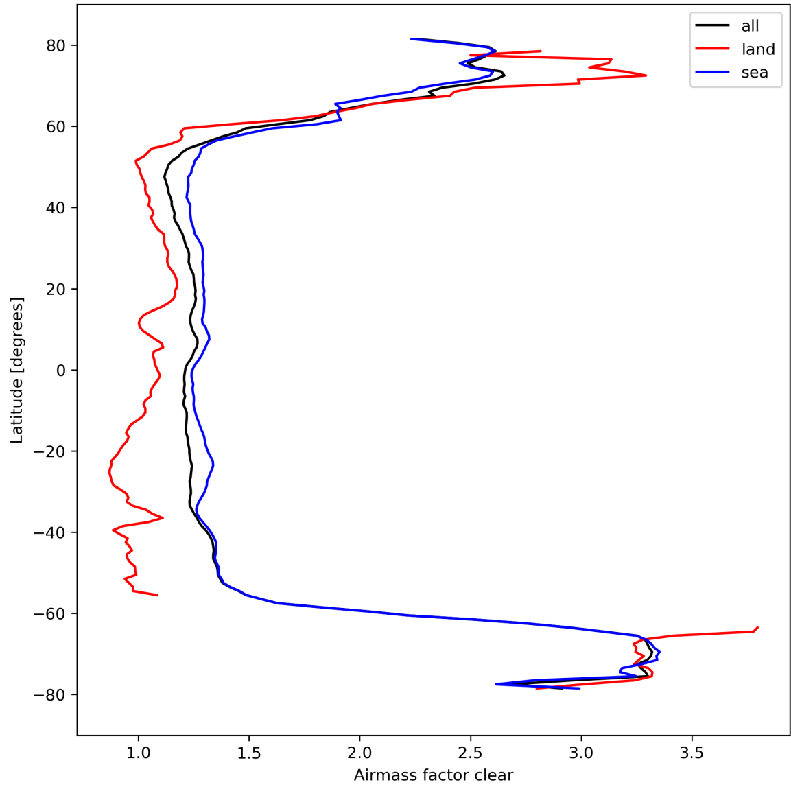
Figure 28: Zonal average of “Airmass factor clear” for 2023-10-02 to 2023-10-04.
