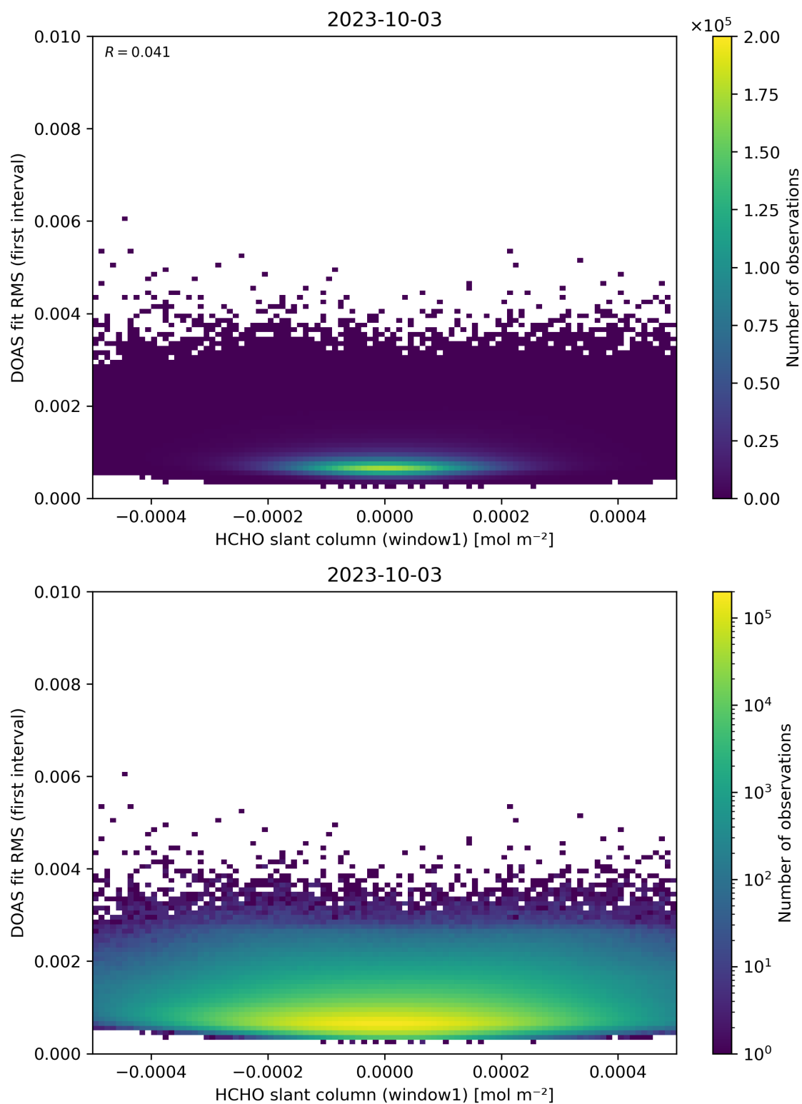
Figure 78: Scatter density plot of “HCHO slant column (window1)” against “DOAS fit RMS (first interval)” for 2023-10-02 to 2023-10-04.
