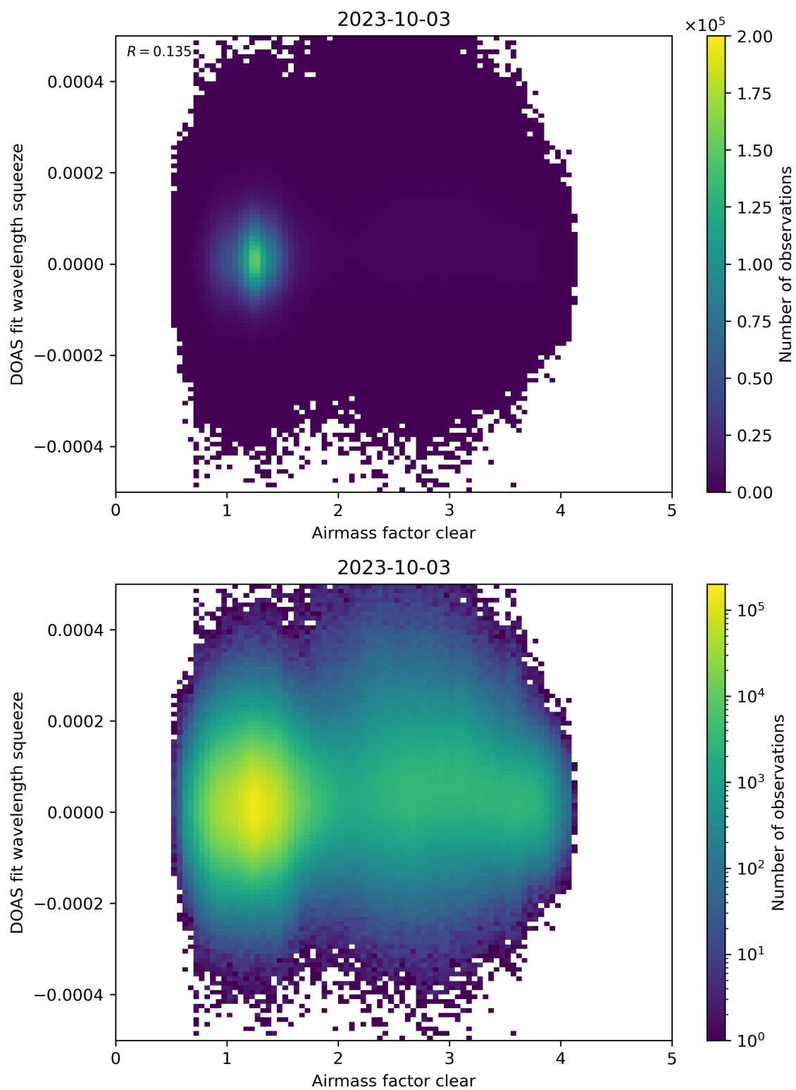
Figure 73: Scatter density plot of “Airmass factor clear” against “DOAS fit wavelength squeeze” for 2023-10-02 to 2023-10-04.
