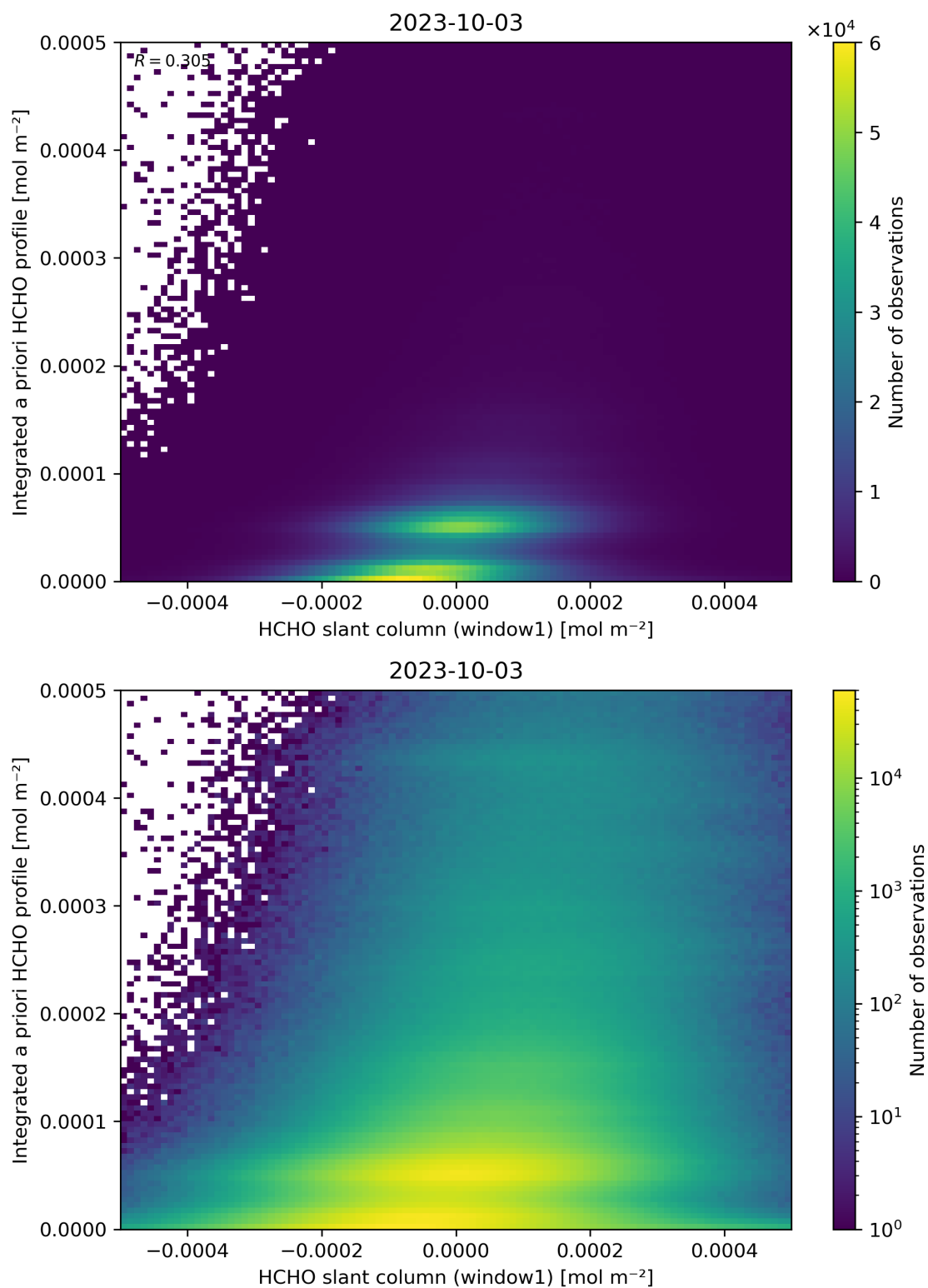
Figure 87: Scatter density plot of “HCHO slant column (window1)” against “Integrated a priori HCHO profile” for 2023-10-02 to 2023-10-04.
