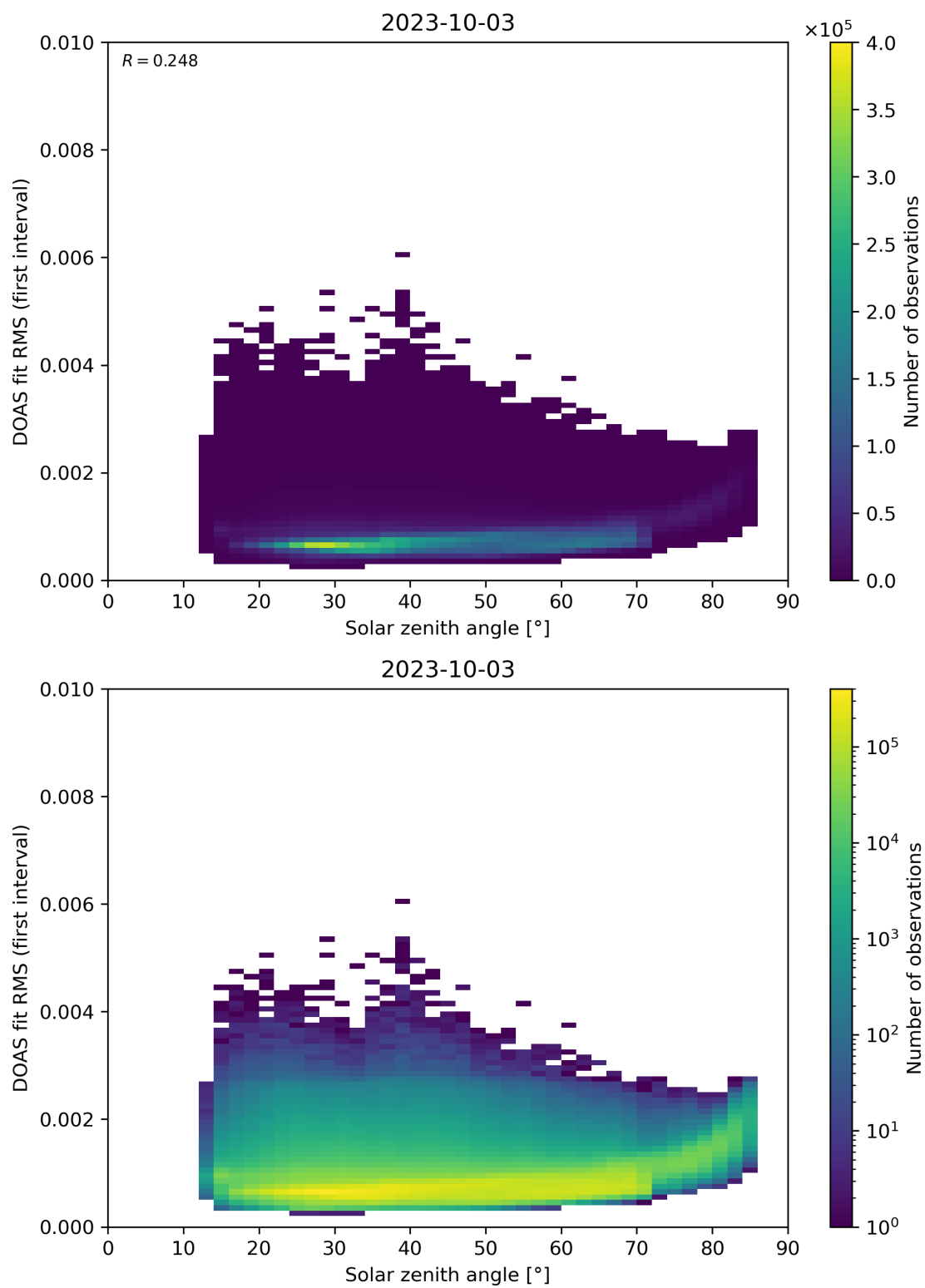
Figure 167: Scatter density plot of “Solar zenith angle” against “DOAS fit RMS (first interval)” for 2023-10-02 to 2023-10-04.
