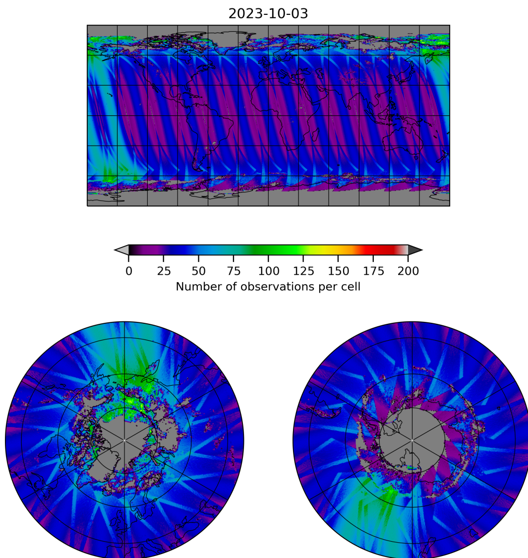
Figure 19: Map of the number of observations for 2023-10-02 to 2023-10-04
