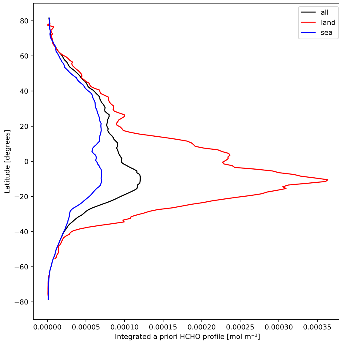
Figure 29: Zonal average of “Integrated a priori HCHO profile” for 2023-10-02 to 2023-10-04.
