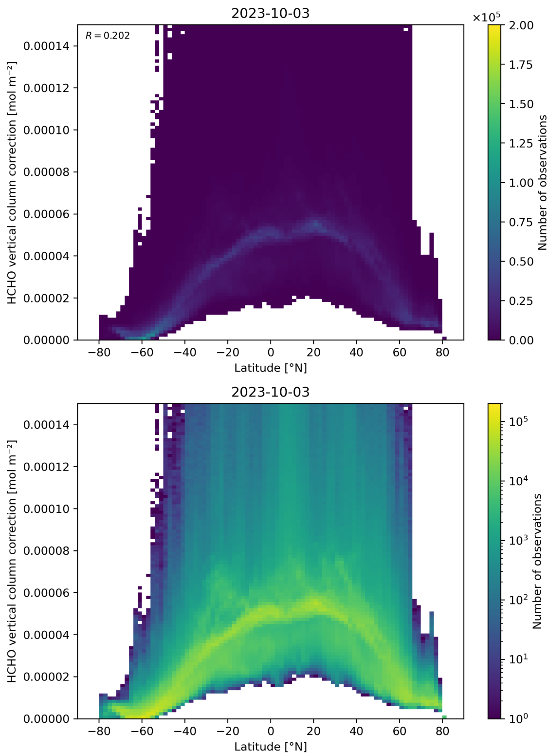
Figure 164: Scatter density plot of “Latitude” against “HCHO vertical column correction” for 2023-10-02 to 2023-10-04.
