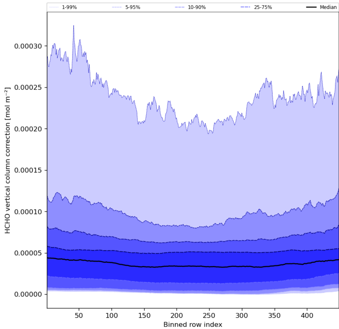
Figure 51: Along track statistics of “HCHO vertical column correction” for 2023-10-02 to 2023-10-04
