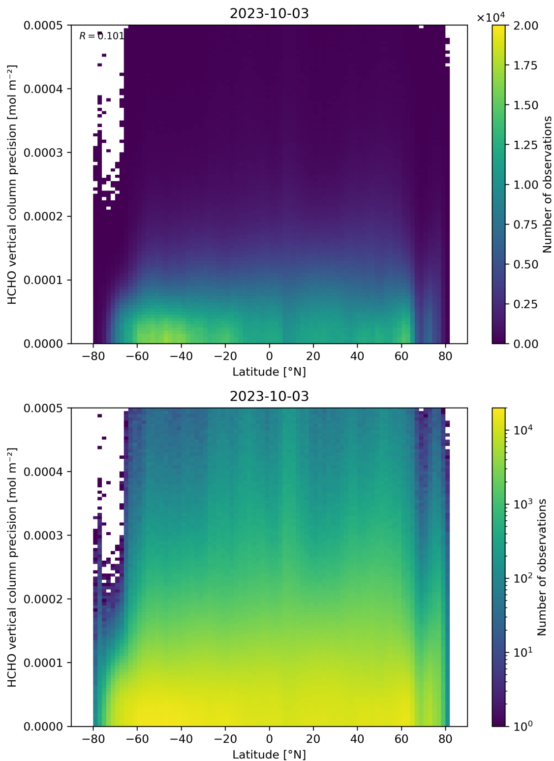
Figure 165: Scatter density plot of “Latitude” against “HCHO vertical column precision” for 2023-10-02 to 2023-10-04.
