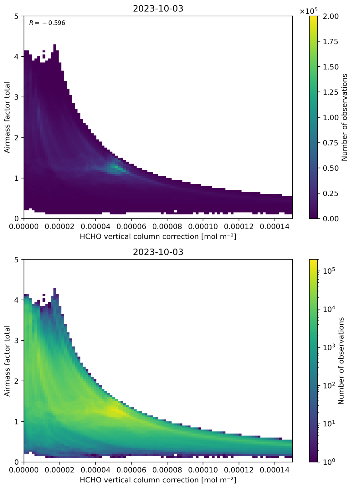
Figure 120: Scatter density plot of “HCHO vertical column correction” against “Airmass factor total” for 2023-10-02 to 2023-10-04.
