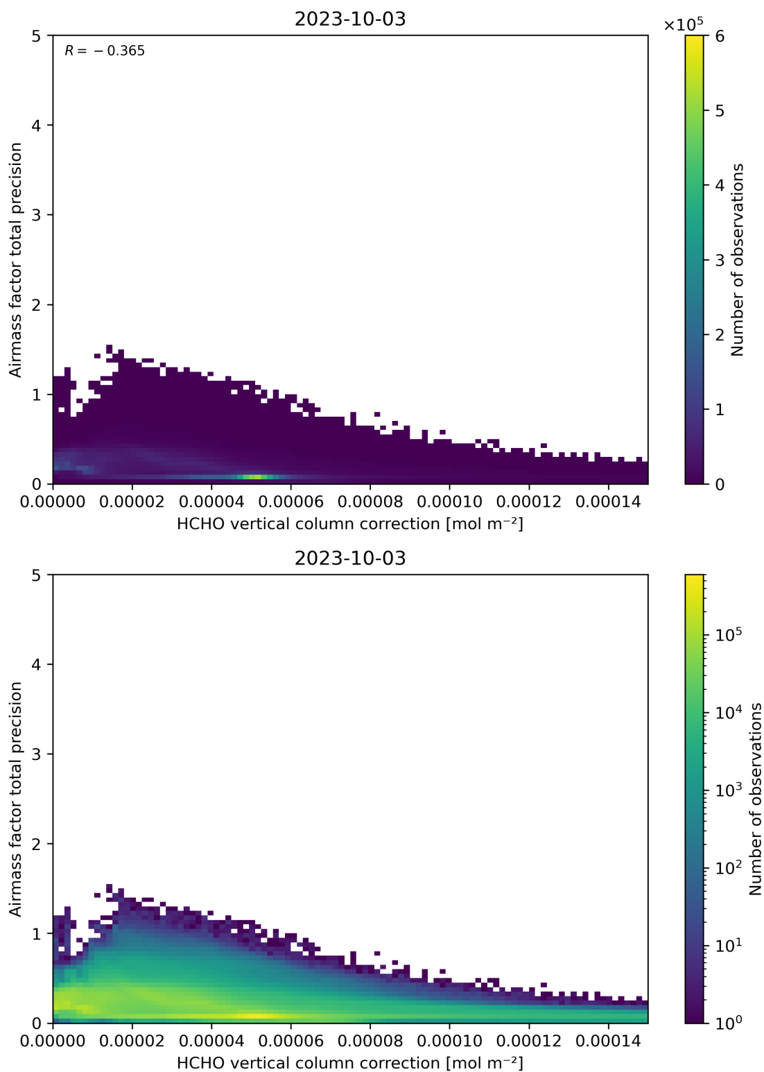
Figure 121: Scatter density plot of “HCHO vertical column correction” against “Airmass factor total precision” for 2023-10-02 to 2023-10-04.
