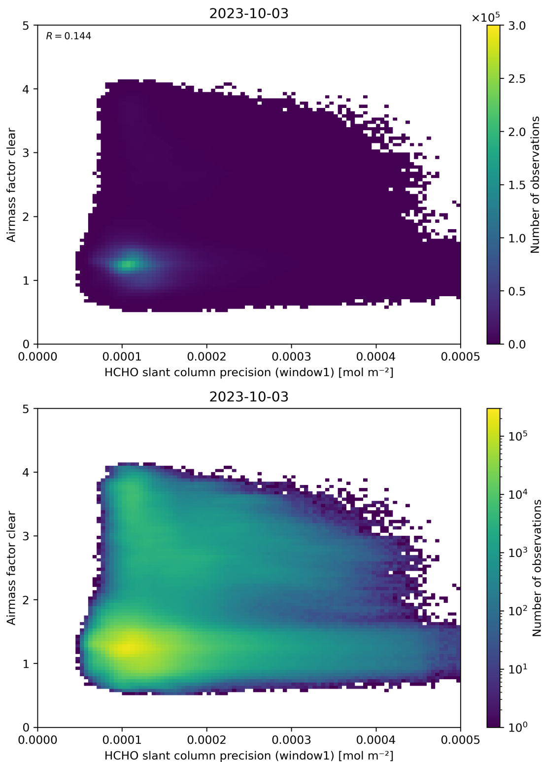
Figure 91: Scatter density plot of “HCHO slant column precision (window1)” against “Airmass factor clear” for 2023-10-02 to 2023-10-04.
