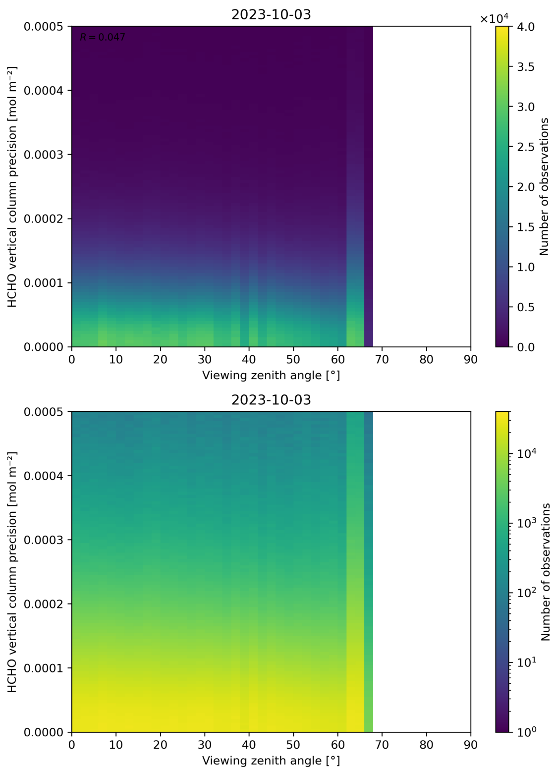
Figure 194: Scatter density plot of “Viewing zenith angle” against “HCHO vertical column precision” for 2023-10-02 to 2023-10-04.
