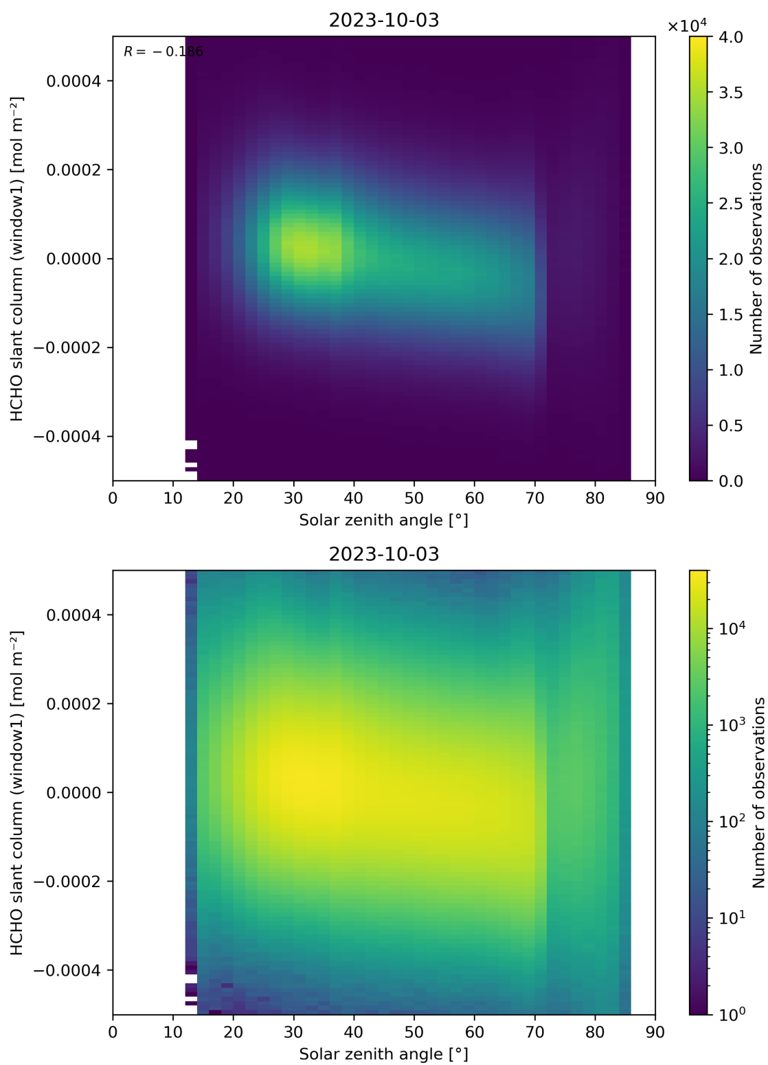
Figure 173: Scatter density plot of “Solar zenith angle” against “HCHO slant column (window1)” for 2023-10-02 to 2023-10-04.
