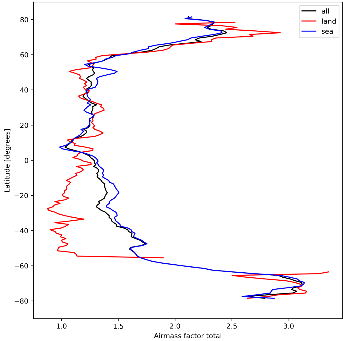
Figure 26: Zonal average of “Airmass factor total” for 2023-10-02 to 2023-10-04.
