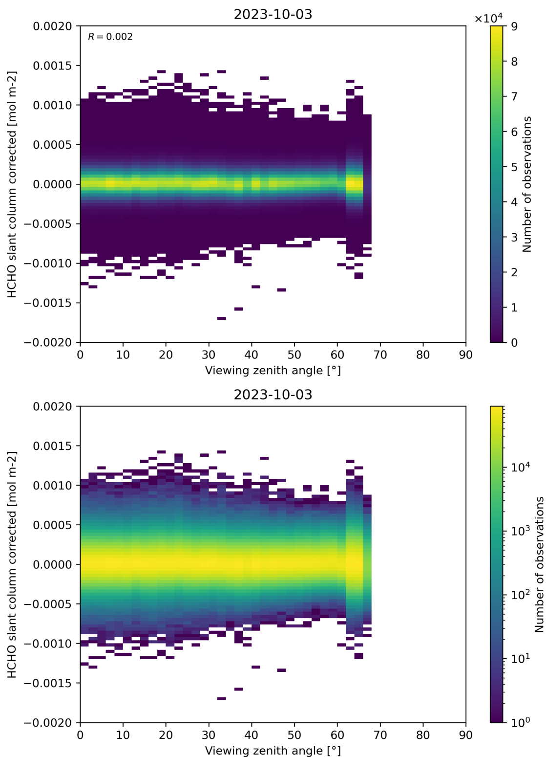
Figure 186: Scatter density plot of “Viewing zenith angle” against “HCHO slant column corrected” for 2023-10-02 to 2023-10-04.
