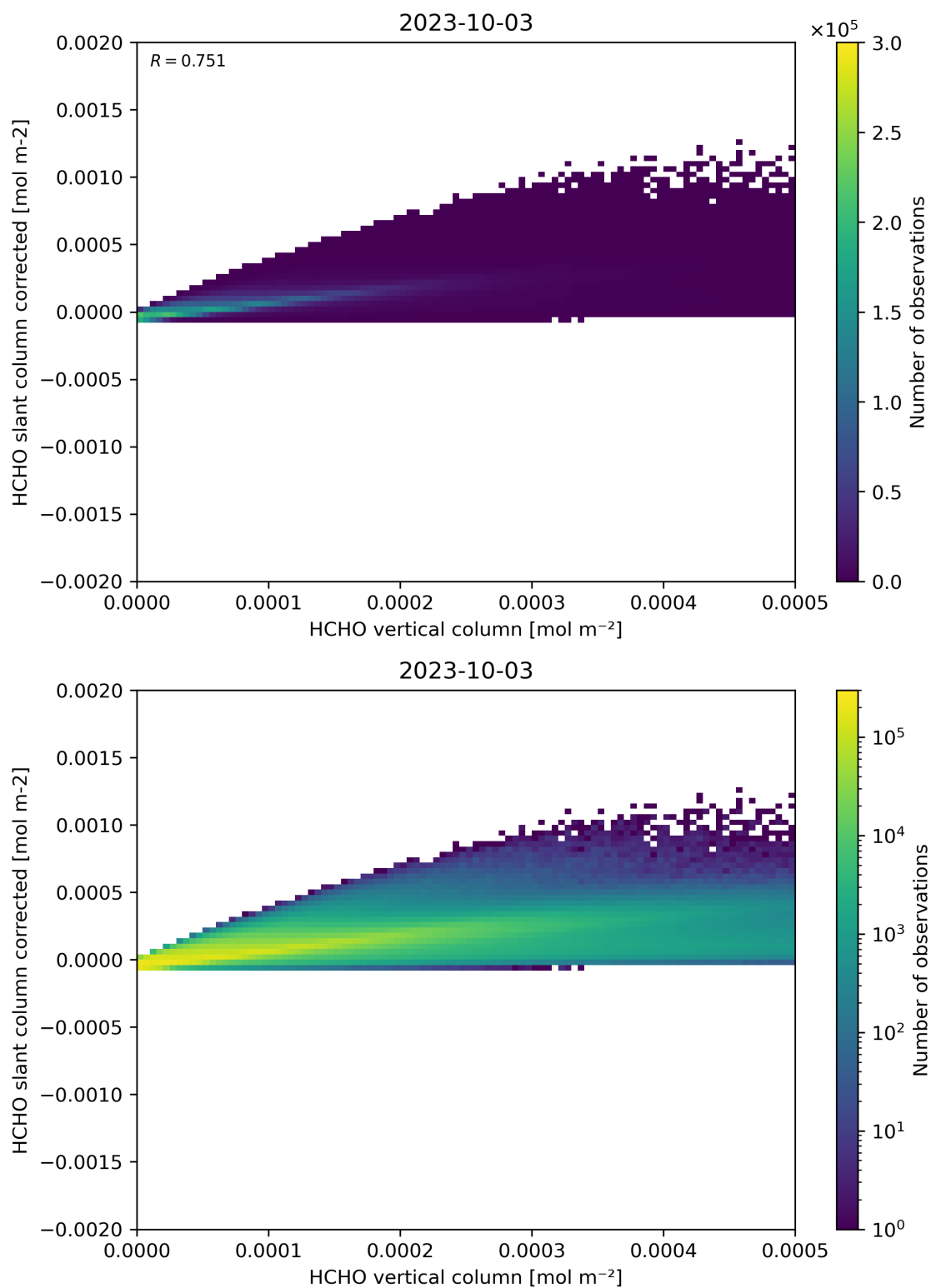
Figure 127: Scatter density plot of “HCHO vertical column” against “HCHO slant column corrected” for 2023-10-02 to 2023-10-04.
