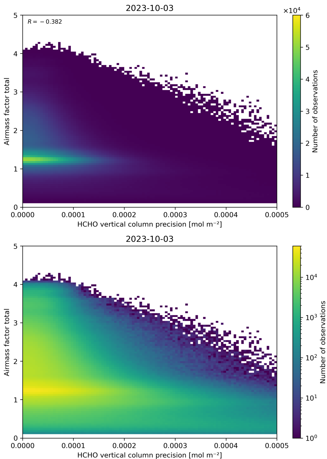
Figure 144: Scatter density plot of “HCHO vertical column precision” against “Airmass factor total” for 2023-10-02 to 2023-10-04.
