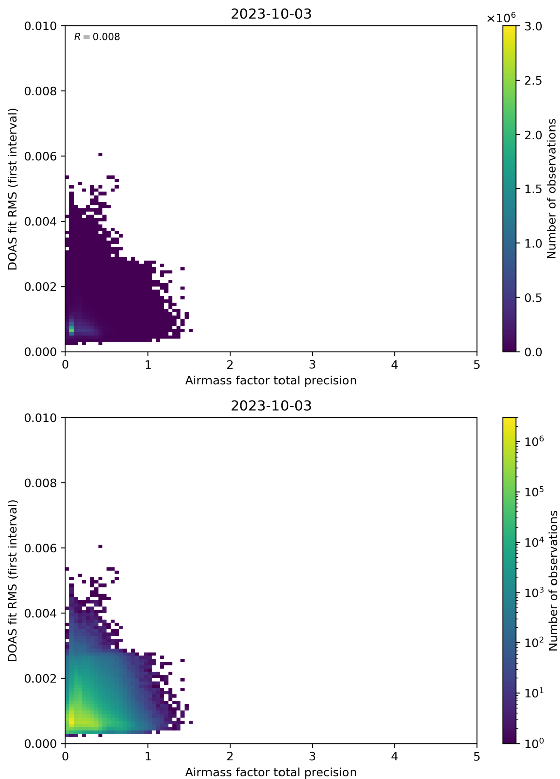
Figure 105: Scatter density plot of “Airmass factor total precision” against “DOAS fit RMS (first interval)” for 2023-10-02 to 2023-10-04.
