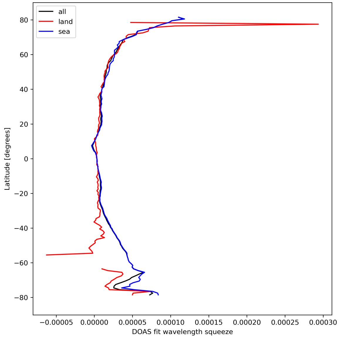
Figure 31: Zonal average of “DOAS fit wavelength squeeze” for 2023-10-02 to 2023-10-04.
