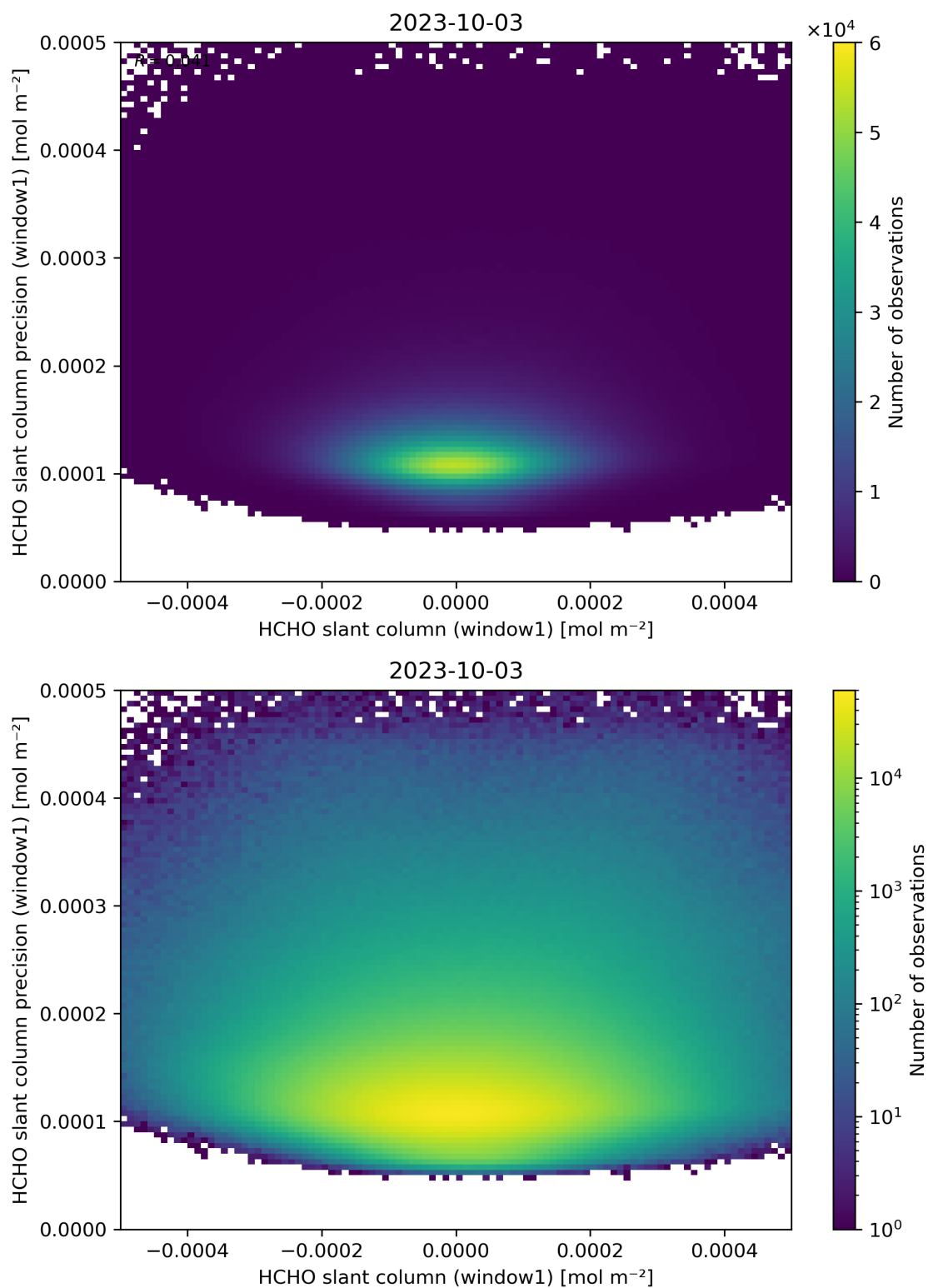
Figure 84: Scatter density plot of “HCHO slant column (window1)” against “HCHO slant column precision (window1)” for 2023-10-02 to 2023-10-04.
