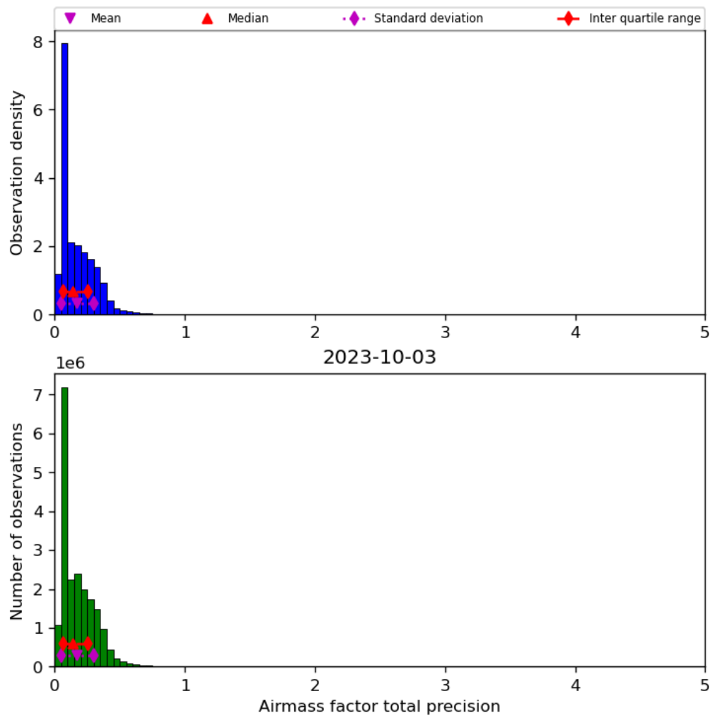
Figure 41: Histogram of “Airmass factor total precision” for 2023-10-02 to 2023-10-04
