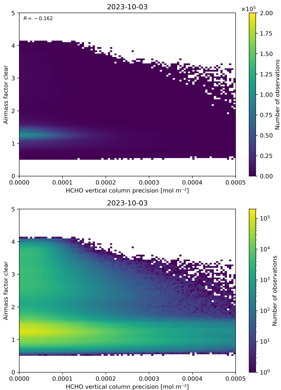
Figure 139: Scatter density plot of “HCHO vertical column precision” against “Airmass factor clear” for 2023-10-02 to 2023-10-04.
