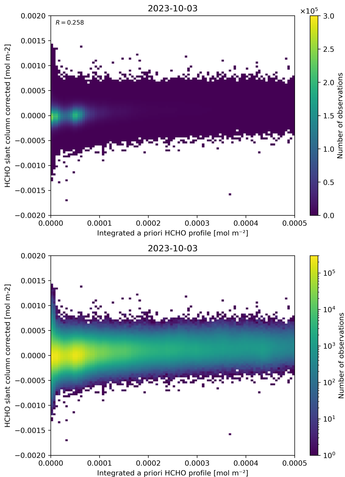
Figure 151: Scatter density plot of “Integrated a priori HCHO profile” against “HCHO slant column corrected” for 2023-10-02 to 2023-10-04.
