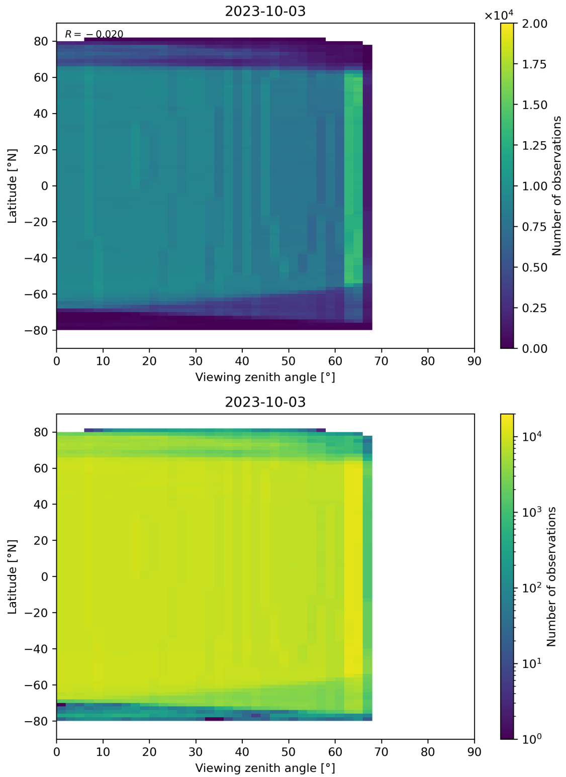
Figure 196: Scatter density plot of “Viewing zenith angle” against “Latitude” for 2023-10-02 to 2023-10-04.
