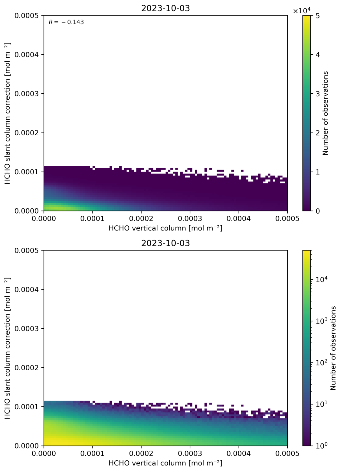
Figure 128: Scatter density plot of “HCHO vertical column” against “HCHO slant column correction” for 2023-10-02 to 2023-10-04.
