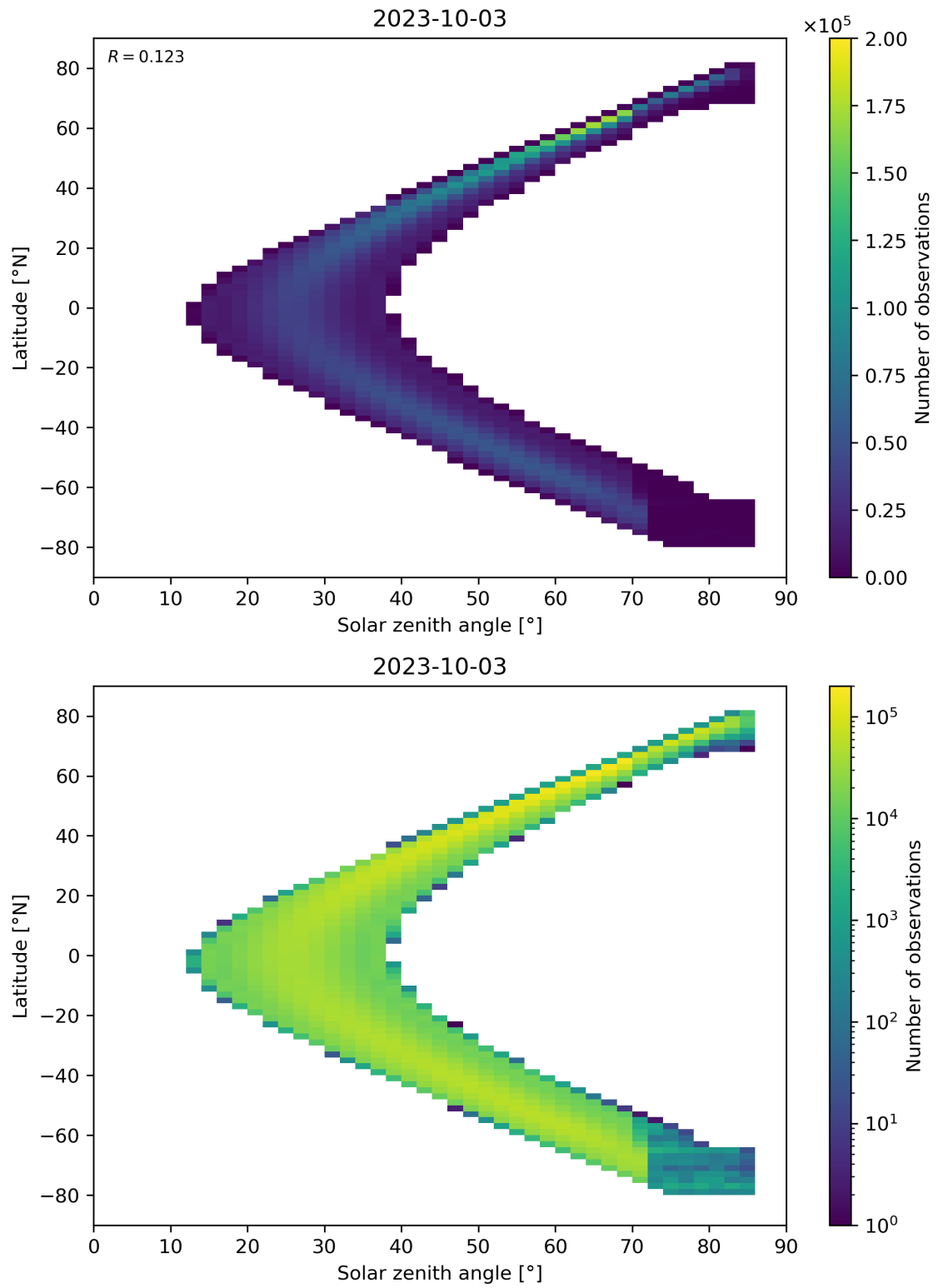
Figure 181: Scatter density plot of “Solar zenith angle” against “Latitude” for 2023-10-02 to 2023-10-04.
