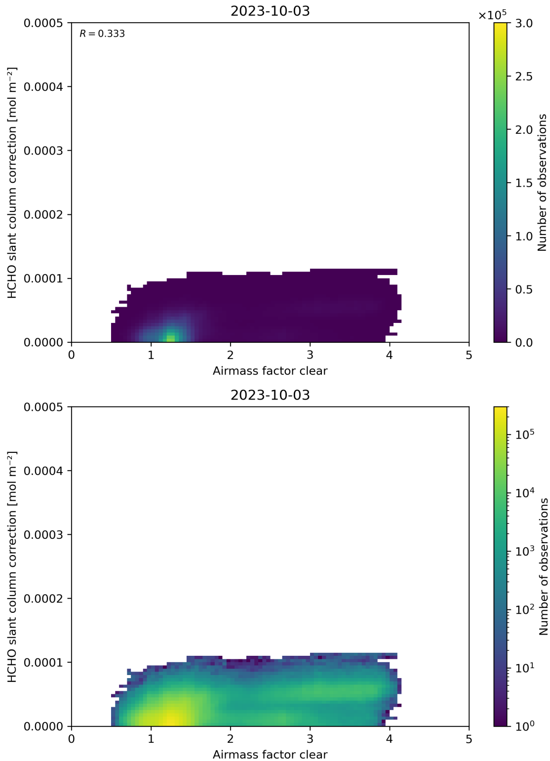
Figure 75: Scatter density plot of “Airmass factor clear” against “HCHO slant column correction” for 2023-10-02 to 2023-10-04.
