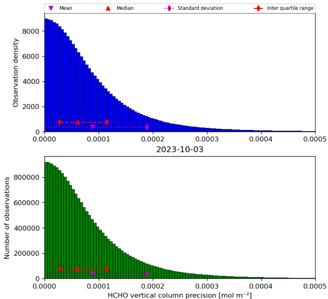
Figure 36: Histogram of “HCHO vertical column precision” for 2023-10-02 to 2023-10-04
