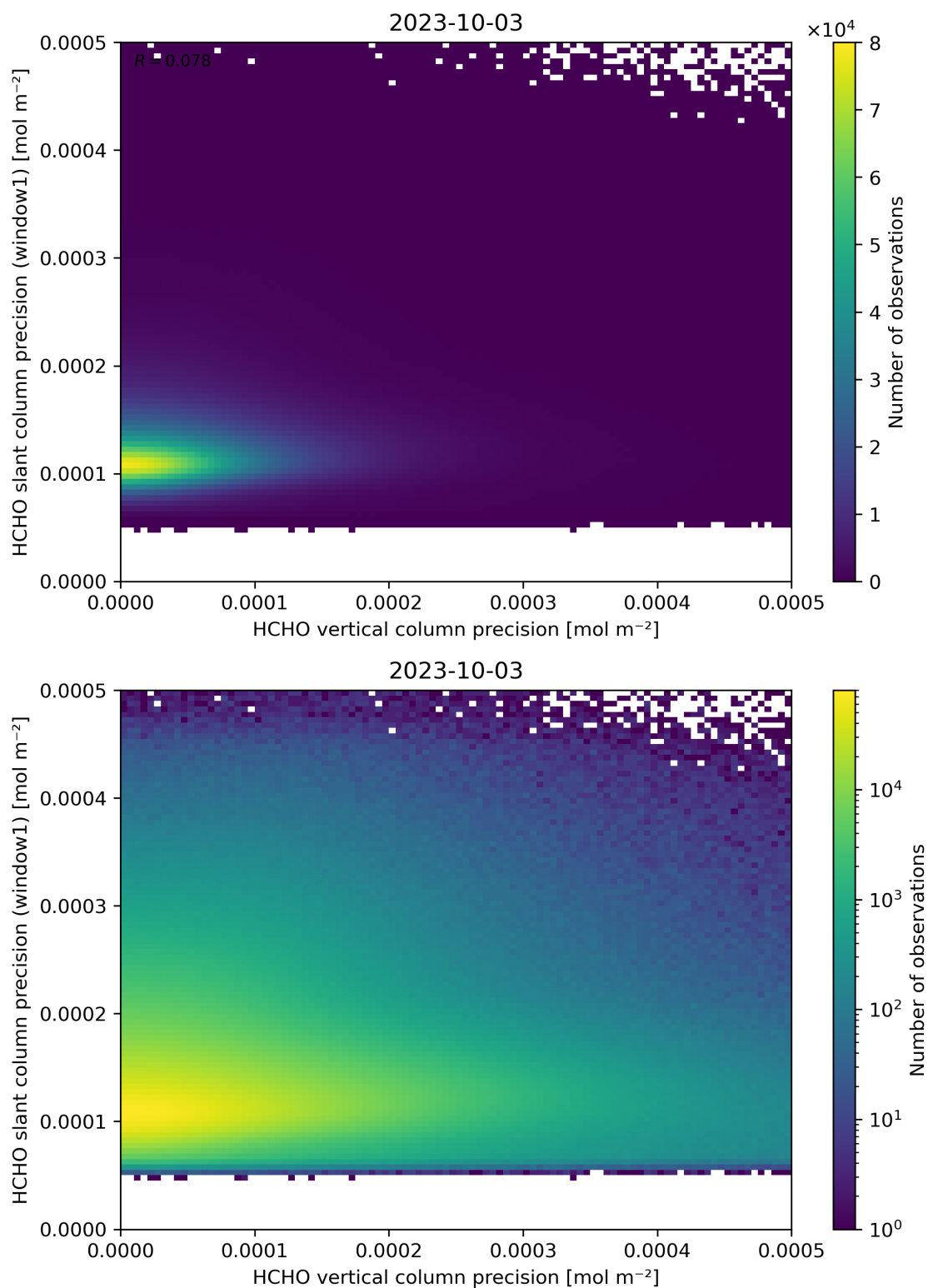
Figure 143: Scatter density plot of “HCHO vertical column precision” against “HCHO slant column precision (window1)” for 2023-10-02 to 2023-10-04.
