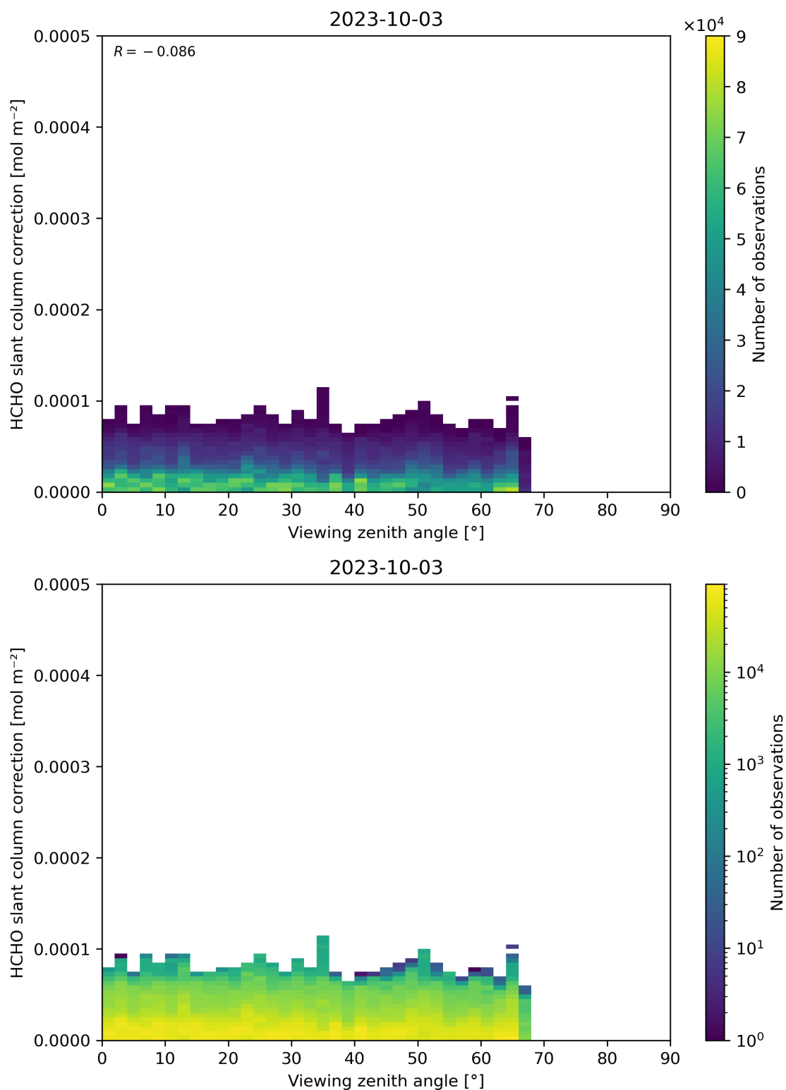
Figure 187: Scatter density plot of “Viewing zenith angle” against “HCHO slant column correction” for 2023-10-02 to 2023-10-04.
