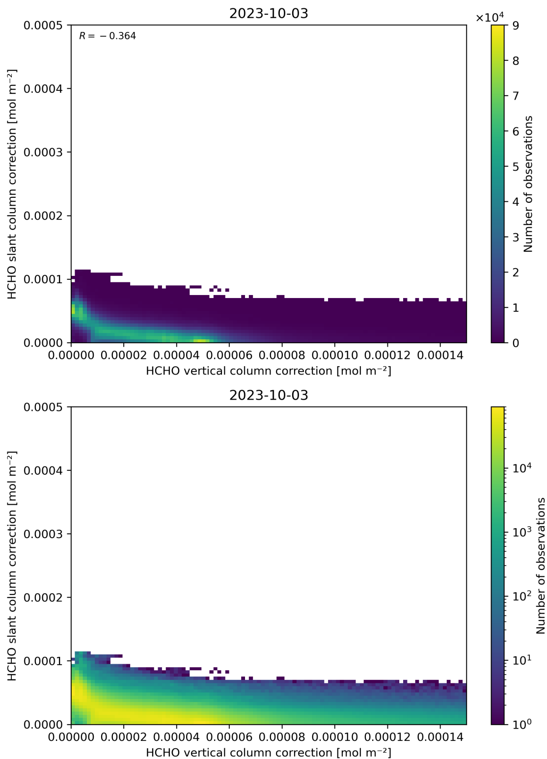
Figure 117: Scatter density plot of “HCHO vertical column correction” against “HCHO slant column correction” for 2023-10-02 to 2023-10-04.
