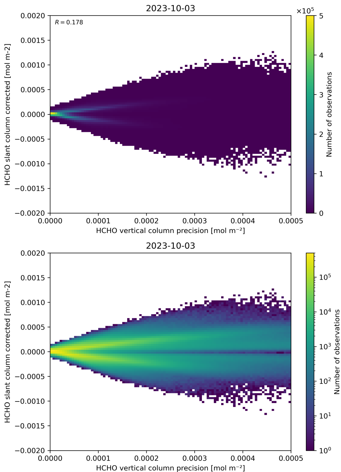
Figure 140: Scatter density plot of “HCHO vertical column precision” against “HCHO slant column corrected” for 2023-10-02 to 2023-10-04.
