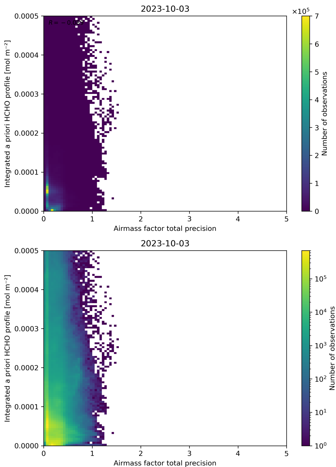
Figure 111: Scatter density plot of “Airmass factor total precision” against “Integrated a priori HCHO profile” for 2023-10-02 to 2023-10-04.
