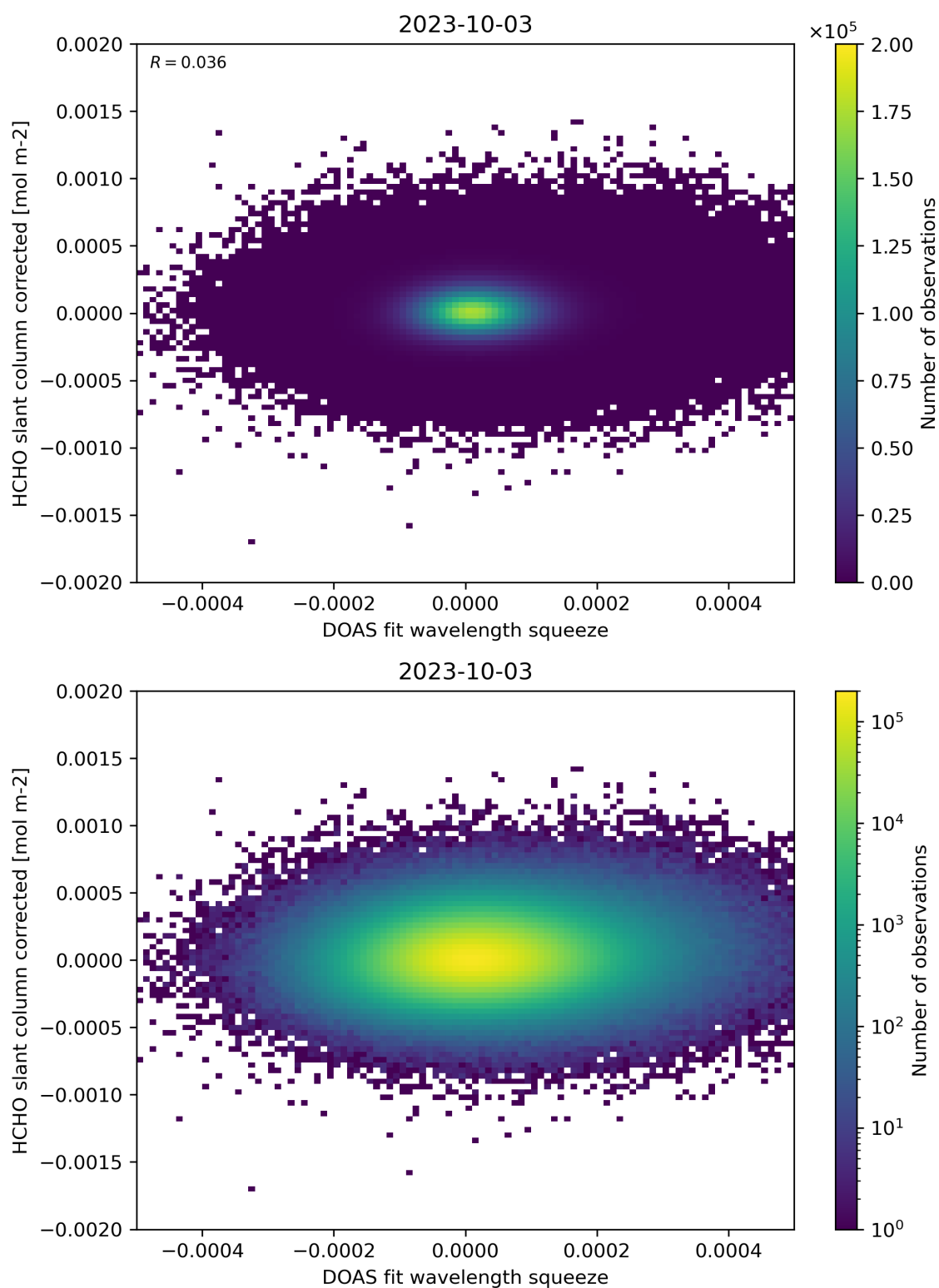
Figure 69: Scatter density plot of “DOAS fit wavelength squeeze” against “HCHO slant column corrected” for 2023-10-02 to 2023-10-04.
