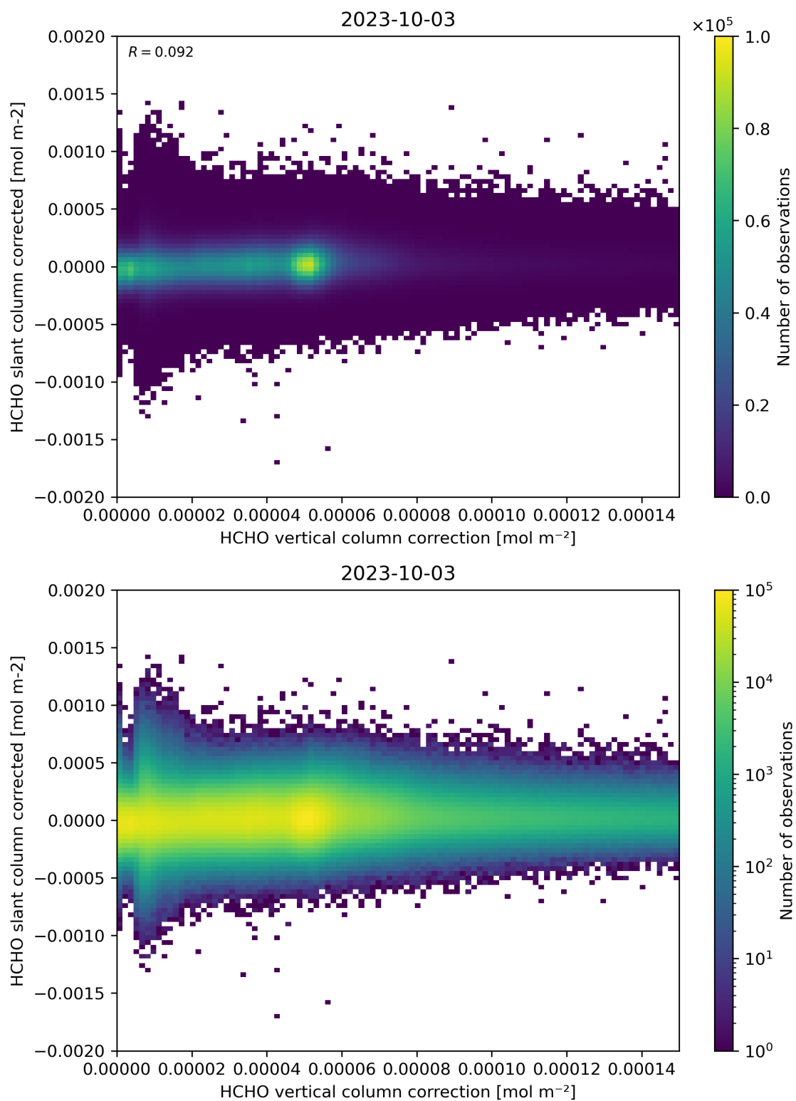
Figure 116: Scatter density plot of “HCHO vertical column correction” against “HCHO slant column corrected” for 2023-10-02 to 2023-10-04.
