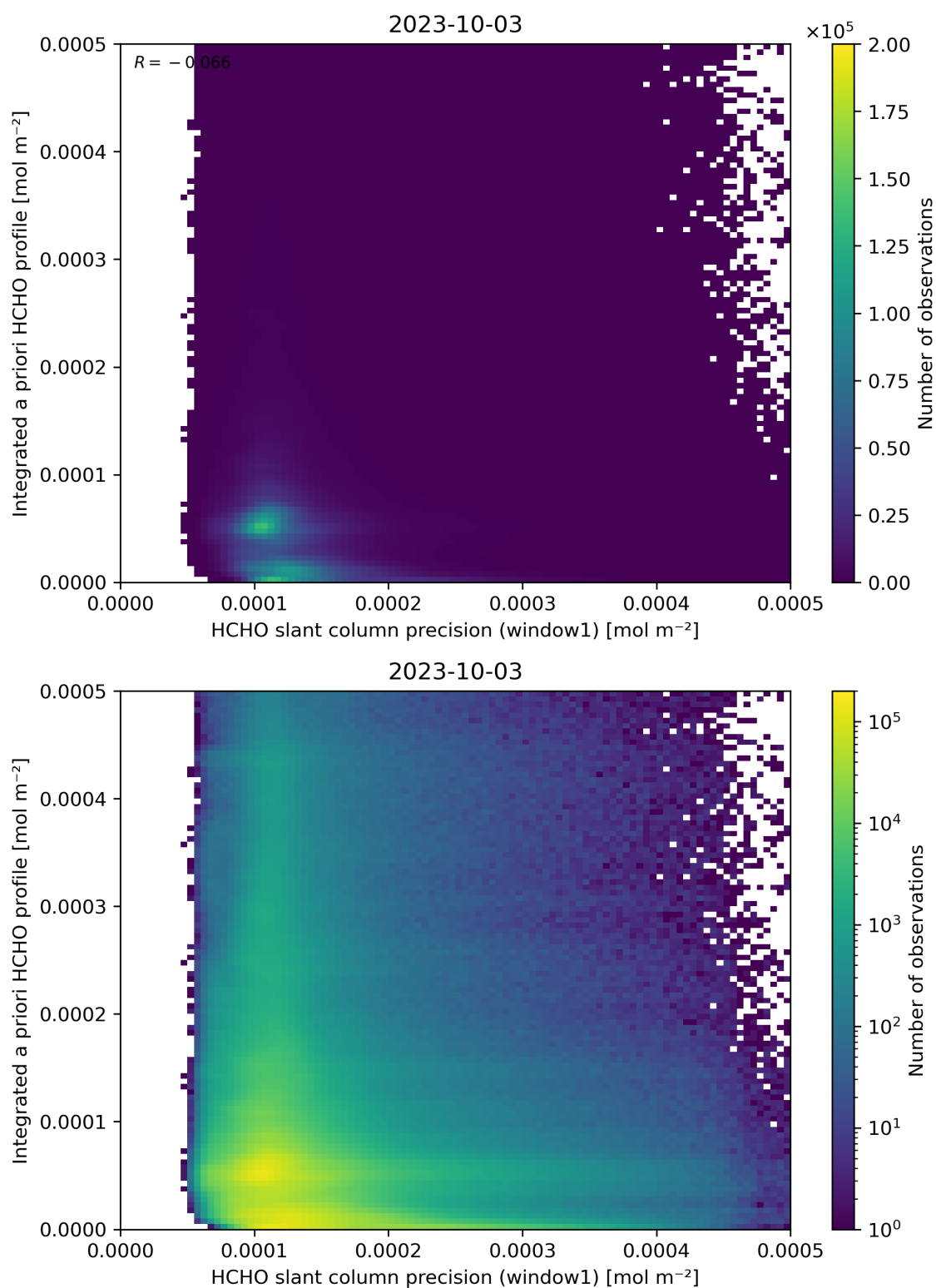
Figure 96: Scatter density plot of “HCHO slant column precision (window1)” against “Integrated a priori HCHO profile” for 2023-10-02 to 2023-10-04.
