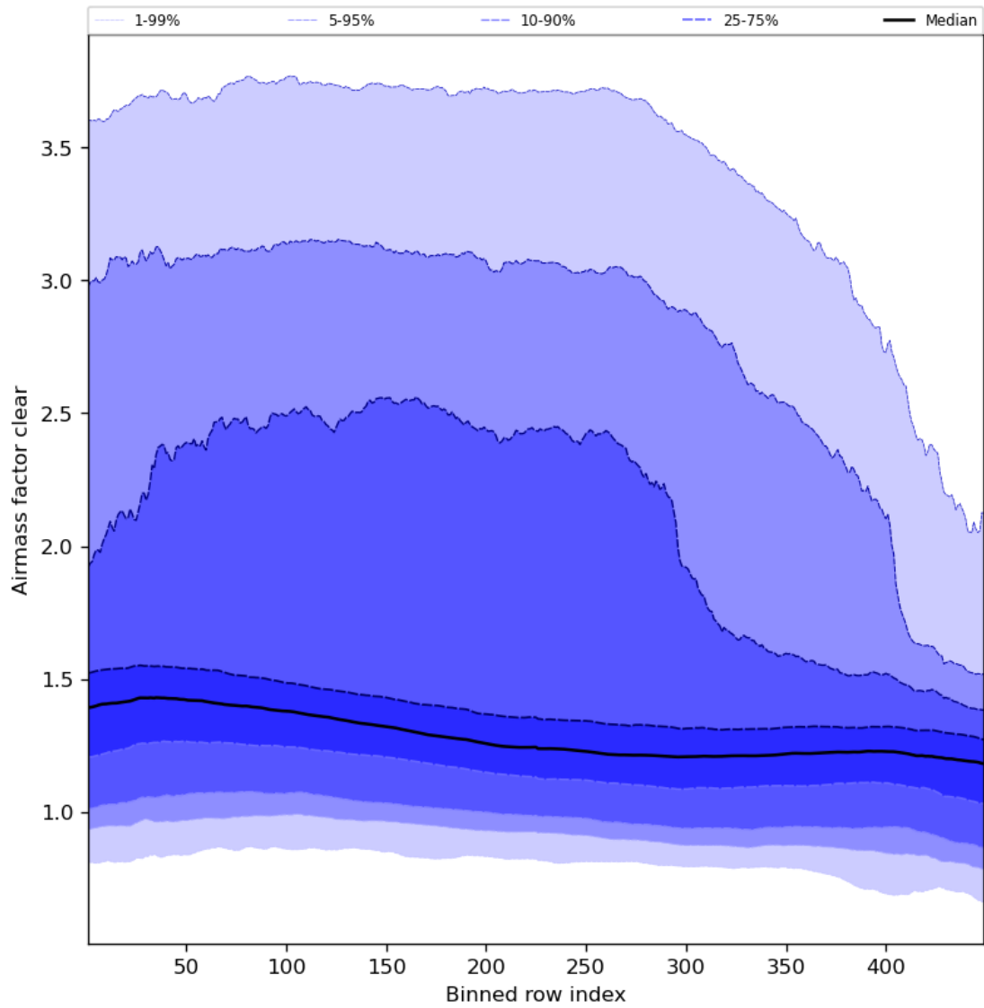
Figure 56: Along track statistics of “Airmass factor clear” for 2023-10-02 to 2023-10-04
