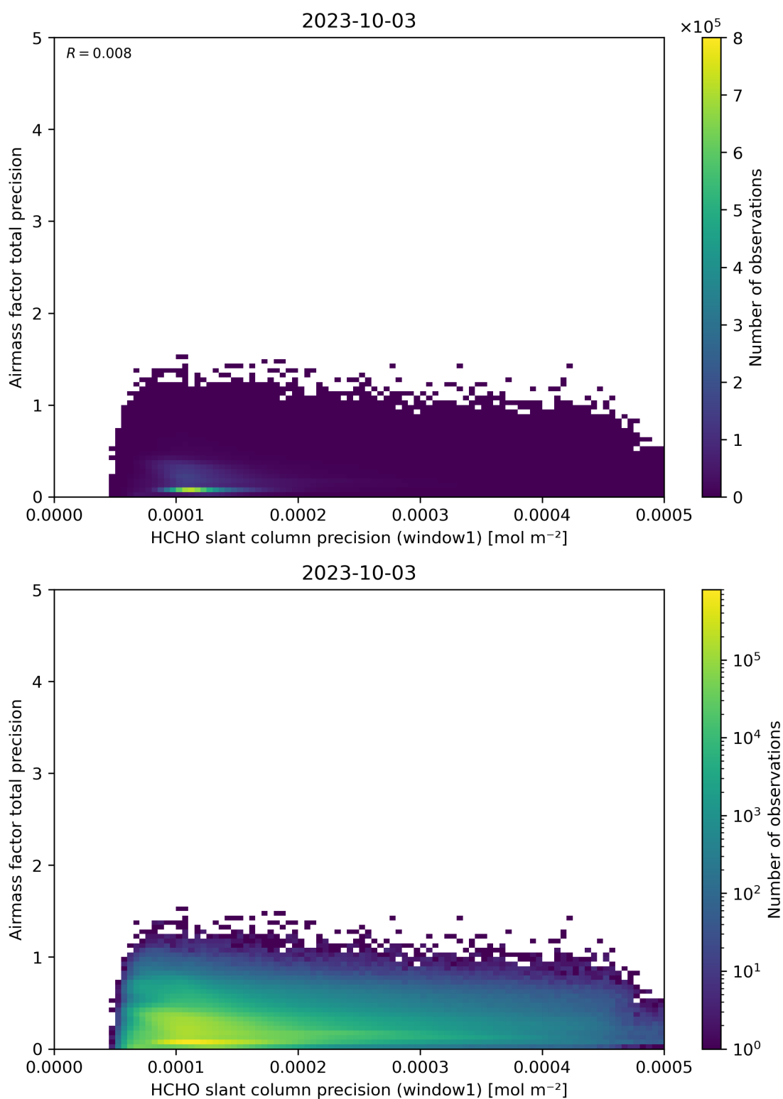
Figure 95: Scatter density plot of “HCHO slant column precision (window1)” against “Airmass factor total precision” for 2023-10-02 to 2023-10-04.
