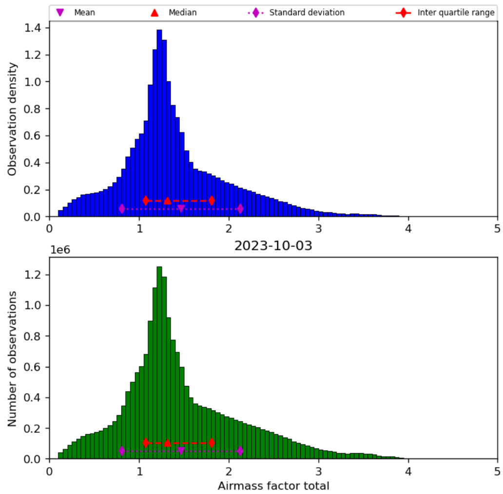
Figure 40: Histogram of “Airmass factor total” for 2023-10-02 to 2023-10-04
