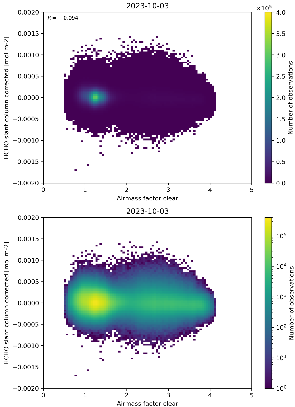
Figure 74: Scatter density plot of “Airmass factor clear” against “HCHO slant column corrected” for 2023-10-02 to 2023-10-04.
