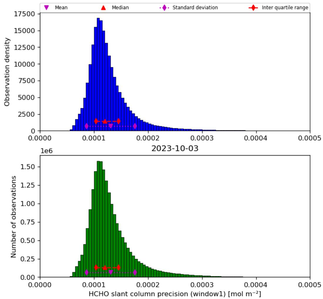
Figure 39: Histogram of “HCHO slant column precision (window1)” for 2023-10-02 to 2023-10-04
