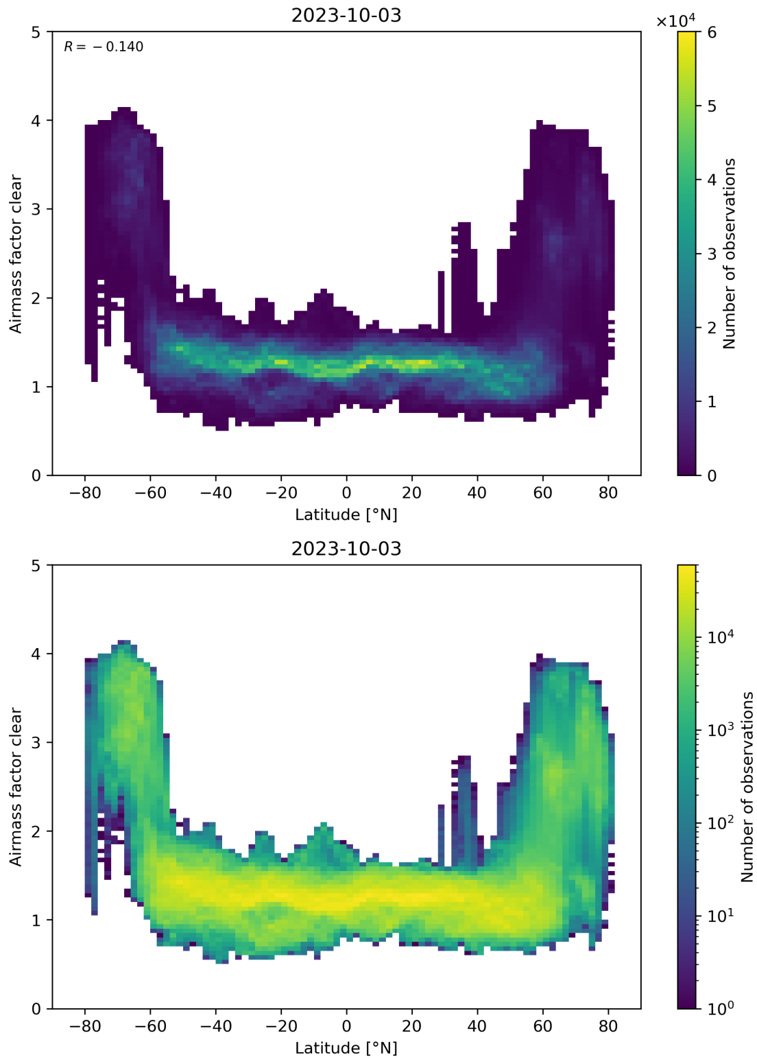
Figure 156: Scatter density plot of “Latitude” against “Airmass factor clear” for 2023-10-02 to 2023-10-04.
