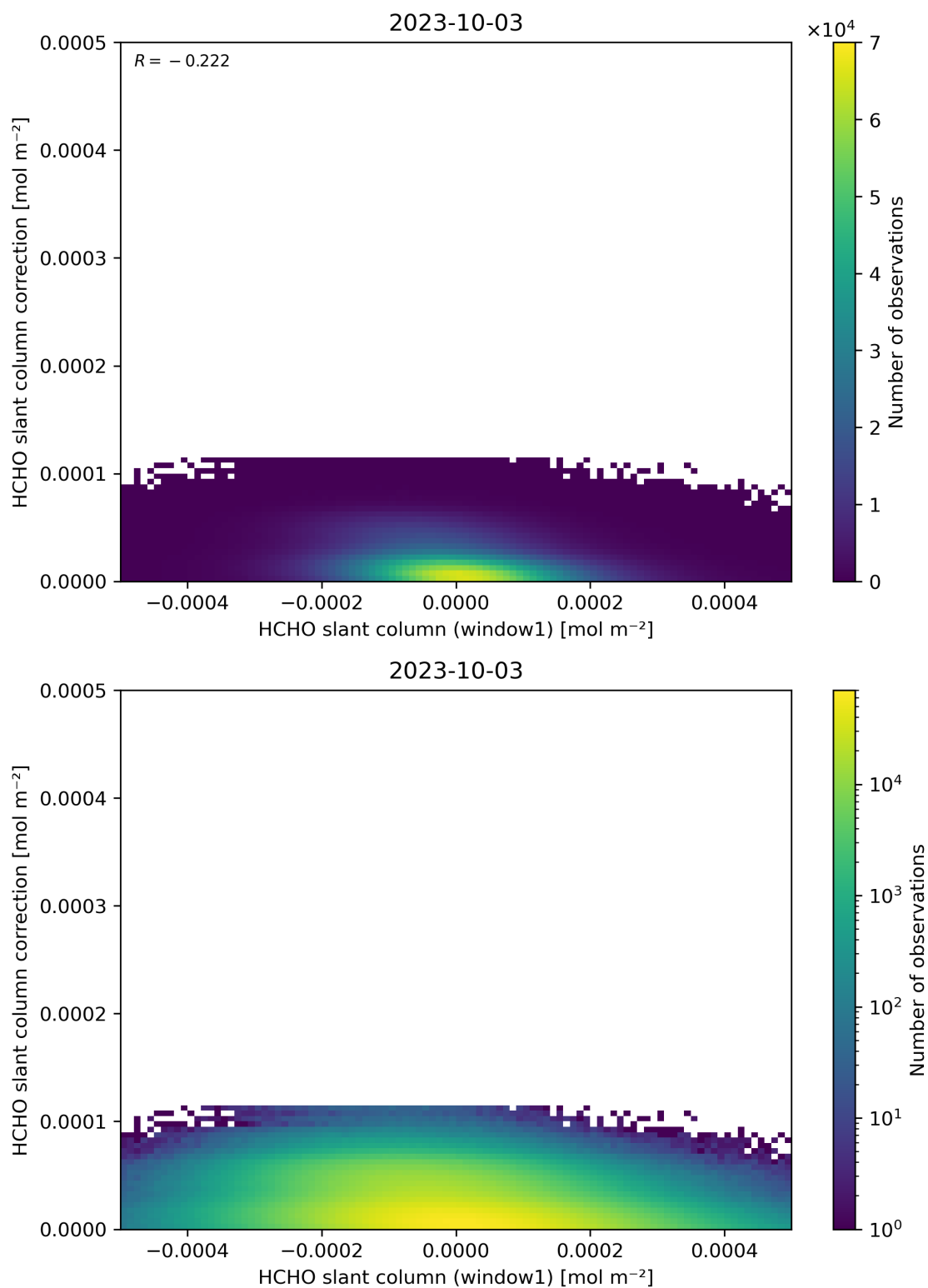
Figure 83: Scatter density plot of “HCHO slant column (window1)” against “HCHO slant column correction” for 2023-10-02 to 2023-10-04.
