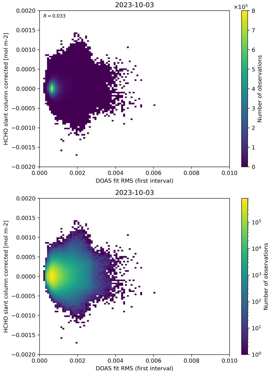
Figure 62: Scatter density plot of “DOAS fit RMS (first interval)” against “HCHO slant column corrected” for 2023-10-02 to 2023-10-04.
