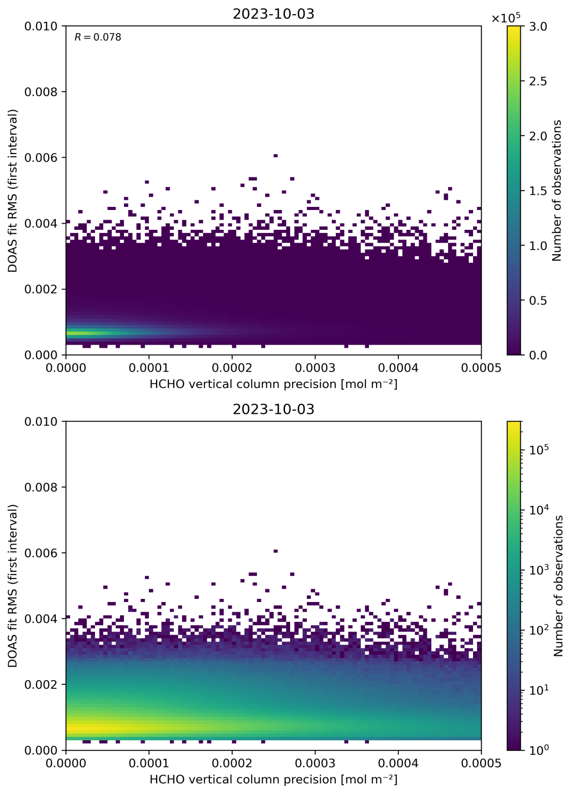
Figure 136: Scatter density plot of “HCHO vertical column precision” against “DOAS fit RMS (first interval)” for 2023-10-02 to 2023-10-04.
