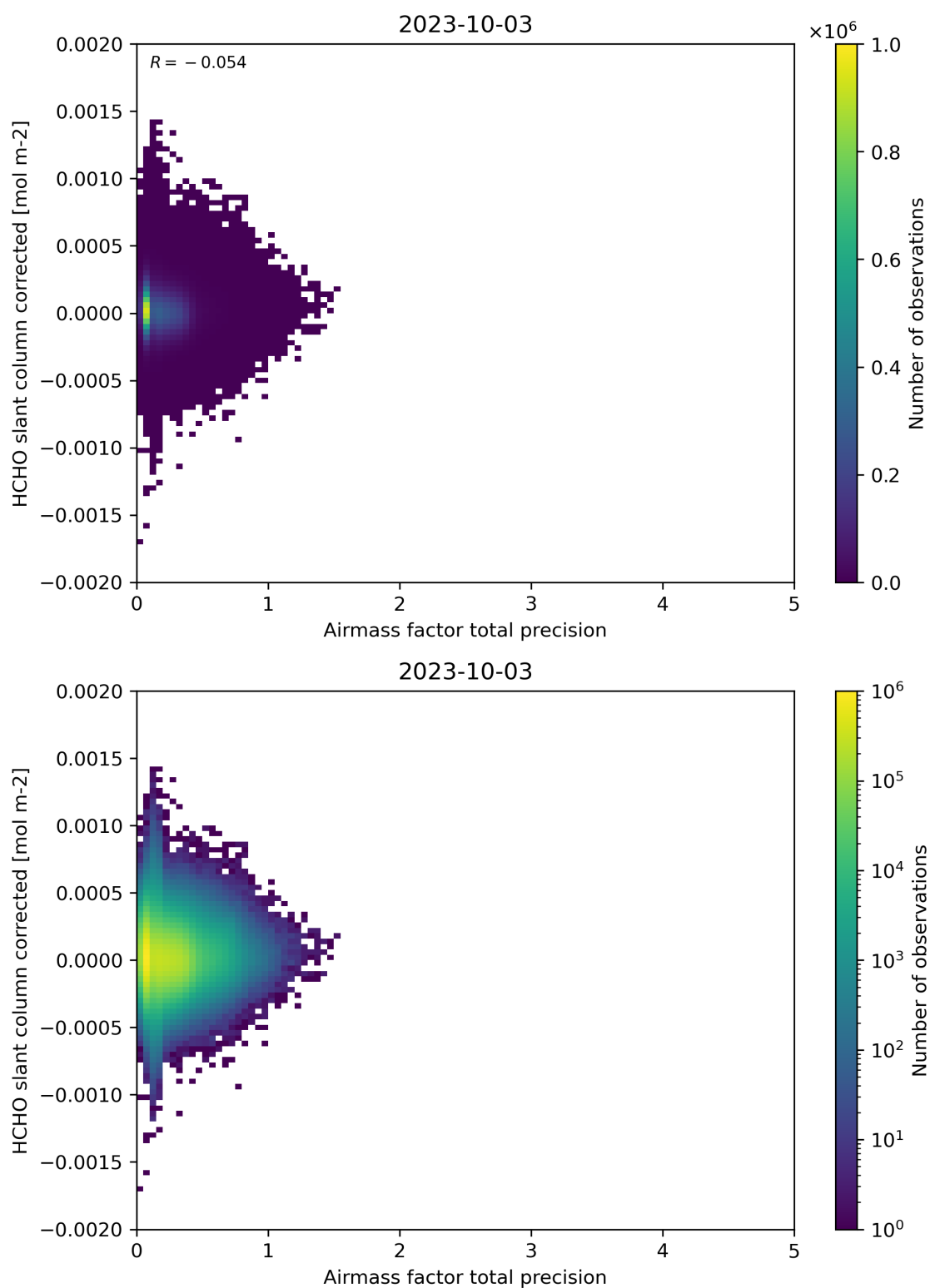
Figure 109: Scatter density plot of “Airmass factor total precision” against “HCHO slant column corrected” for 2023-10-02 to 2023-10-04.
