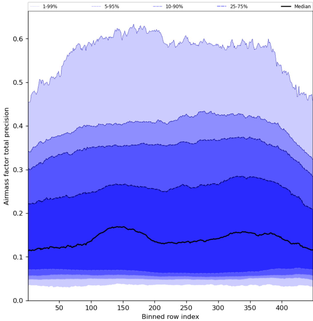
Figure 55: Along track statistics of “Airmass factor total precision” for 2023-10-02 to 2023-10-04
