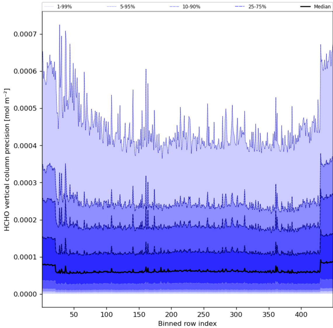
Figure 50: Along track statistics of “HCHO vertical column precision” for 2023-10-02 to 2023-10-04
