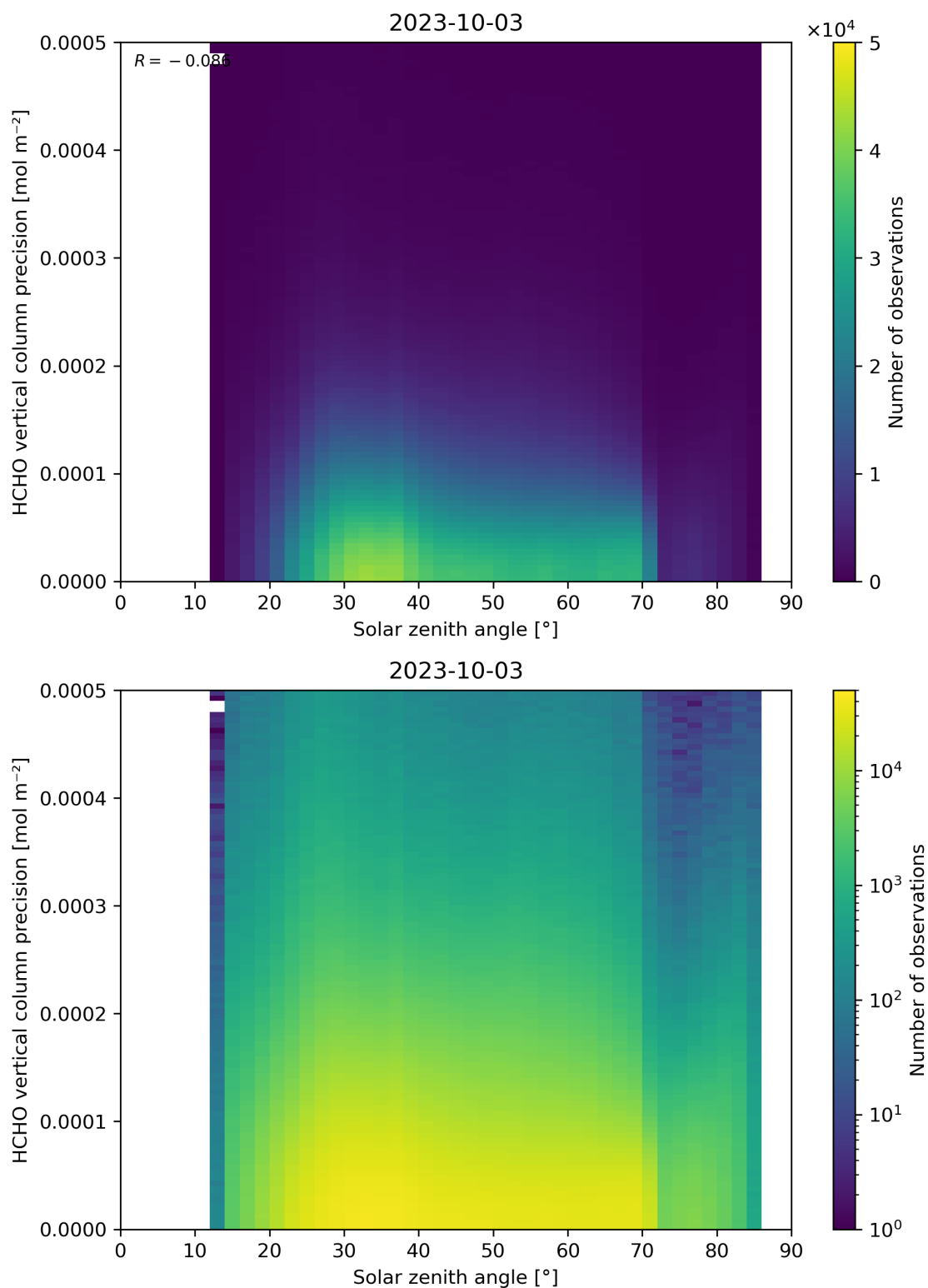
Figure 179: Scatter density plot of “Solar zenith angle” against “HCHO vertical column precision” for 2023-10-02 to 2023-10-04.
