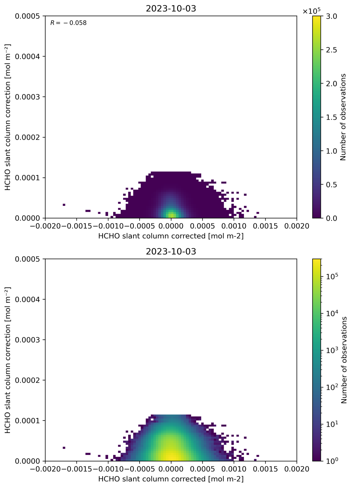
Figure 77: Scatter density plot of “HCHO slant column corrected” against “HCHO slant column correction” for 2023-10-02 to 2023-10-04.
