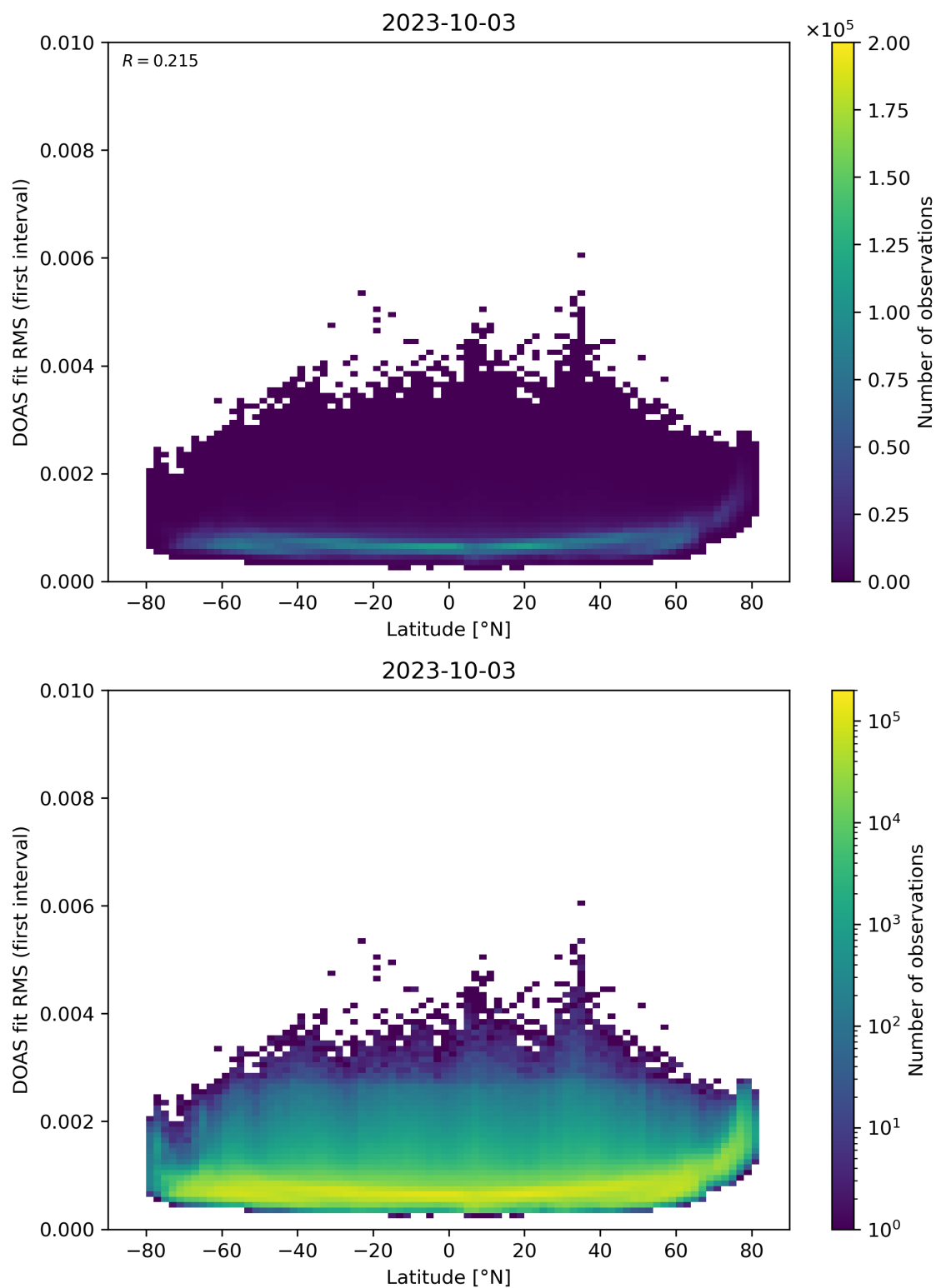
Figure 153: Scatter density plot of “Latitude” against “DOAS fit RMS (first interval)” for 2023-10-02 to 2023-10-04.
