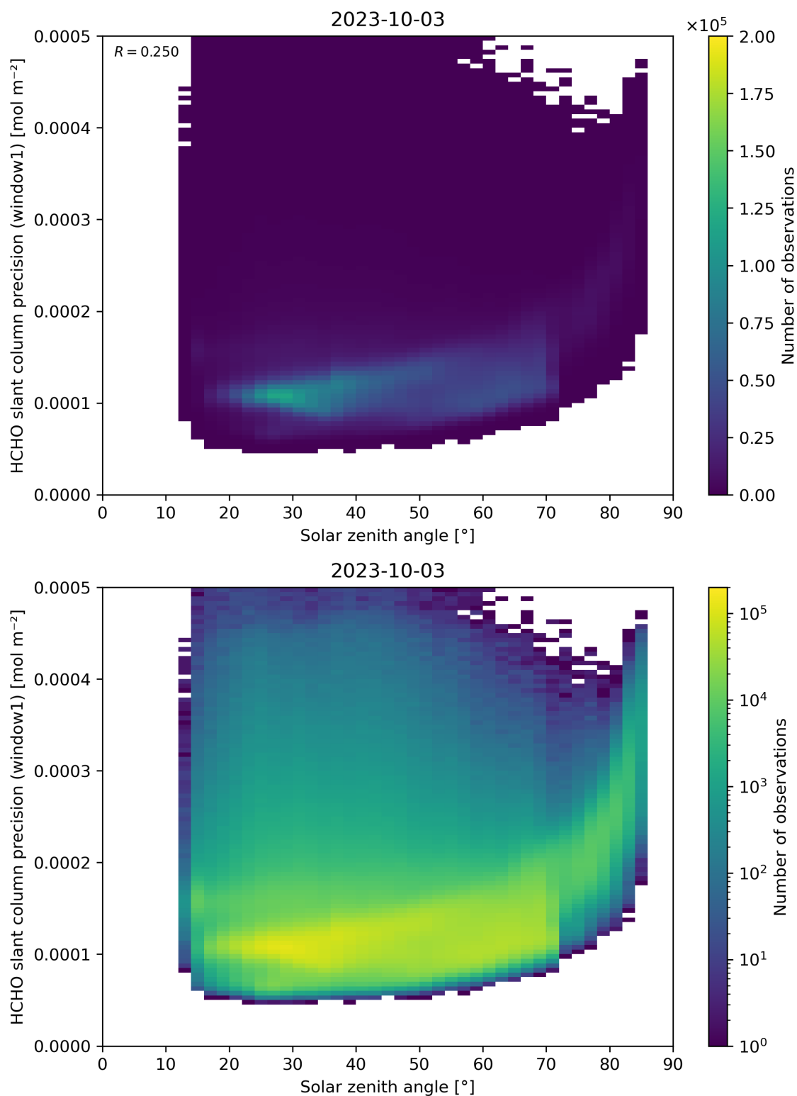
Figure 174: Scatter density plot of “Solar zenith angle” against “HCHO slant column precision (window1)” for 2023-10-02 to 2023-10-04.
