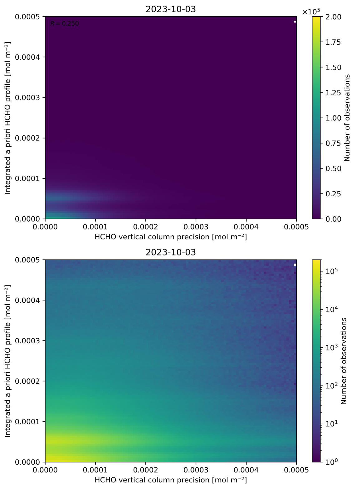
Figure 147: Scatter density plot of “HCHO vertical column precision” against “Integrated a priori HCHO profile” for 2023-10-02 to 2023-10-04.
