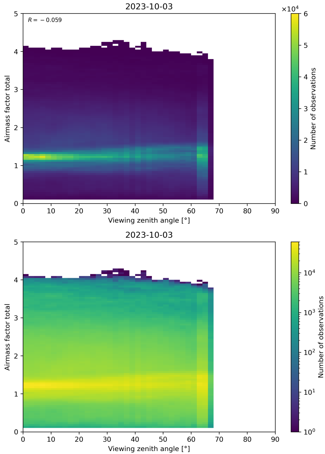
Figure 190: Scatter density plot of “Viewing zenith angle” against “Airmass factor total” for 2023-10-02 to 2023-10-04.
