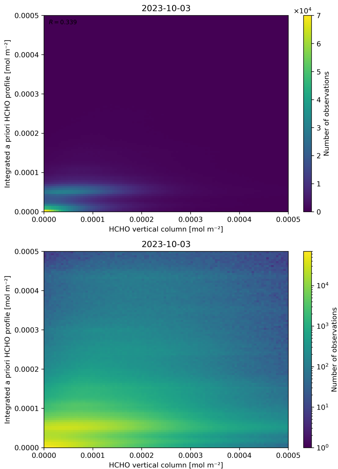
Figure 135: Scatter density plot of “HCHO vertical column” against “Integrated a priori HCHO profile” for 2023-10-02 to 2023-10-04.
