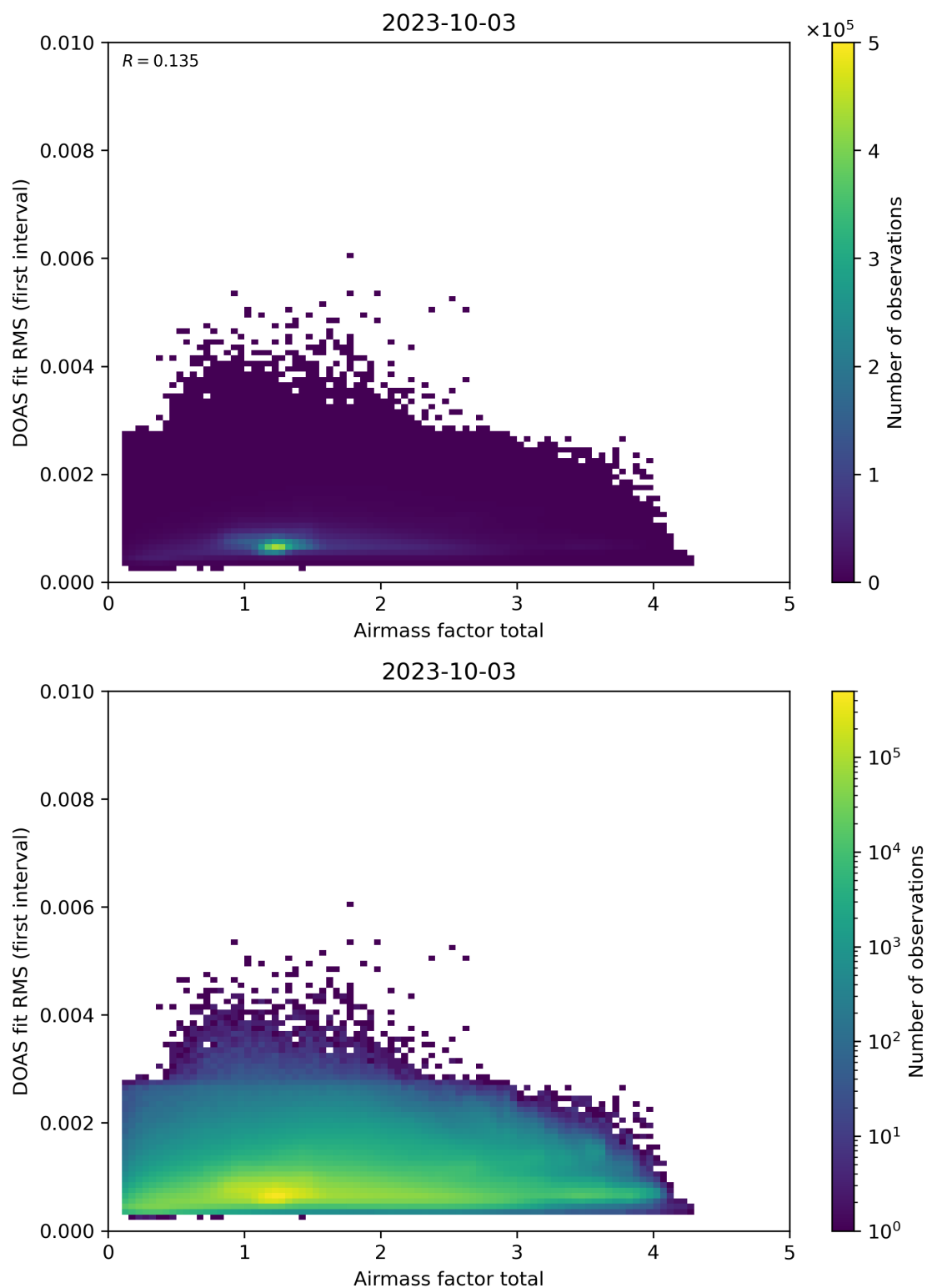
Figure 97: Scatter density plot of “Airmass factor total” against “DOAS fit RMS (first interval)” for 2023-10-02 to 2023-10-04.
