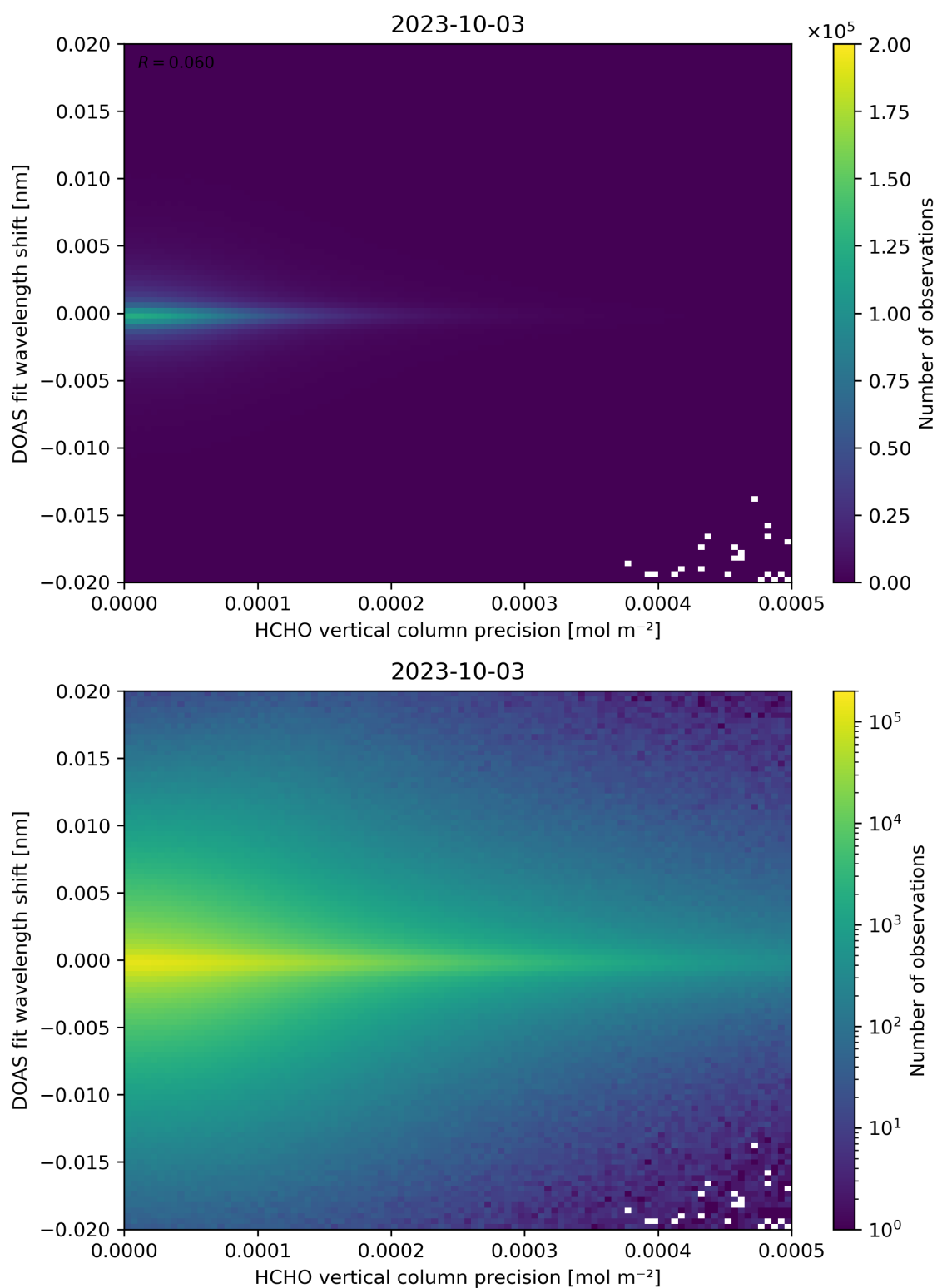
Figure 137: Scatter density plot of “HCHO vertical column precision” against “DOAS fit wavelength shift” for 2023-10-02 to 2023-10-04.
