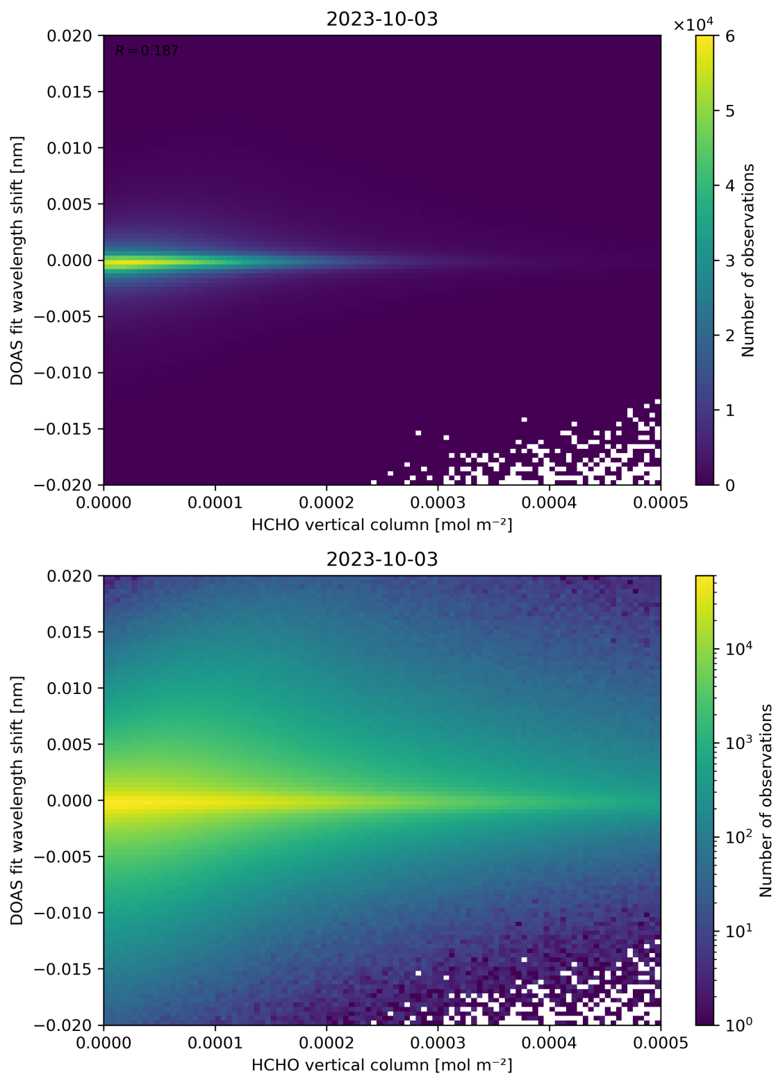
Figure 124: Scatter density plot of “HCHO vertical column” against “DOAS fit wavelength shift” for 2023-10-02 to 2023-10-04.
