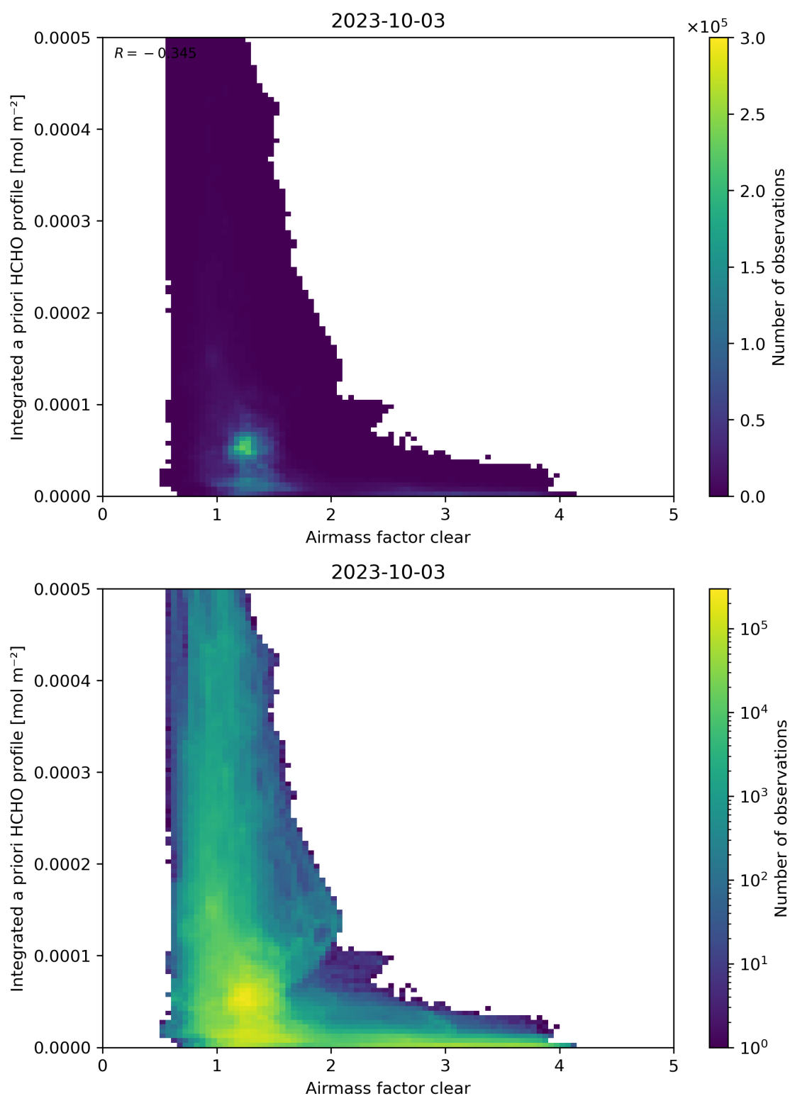
Figure 76: Scatter density plot of “Airmass factor clear” against “Integrated a priori HCHO profile” for 2023-10-02 to 2023-10-04.
