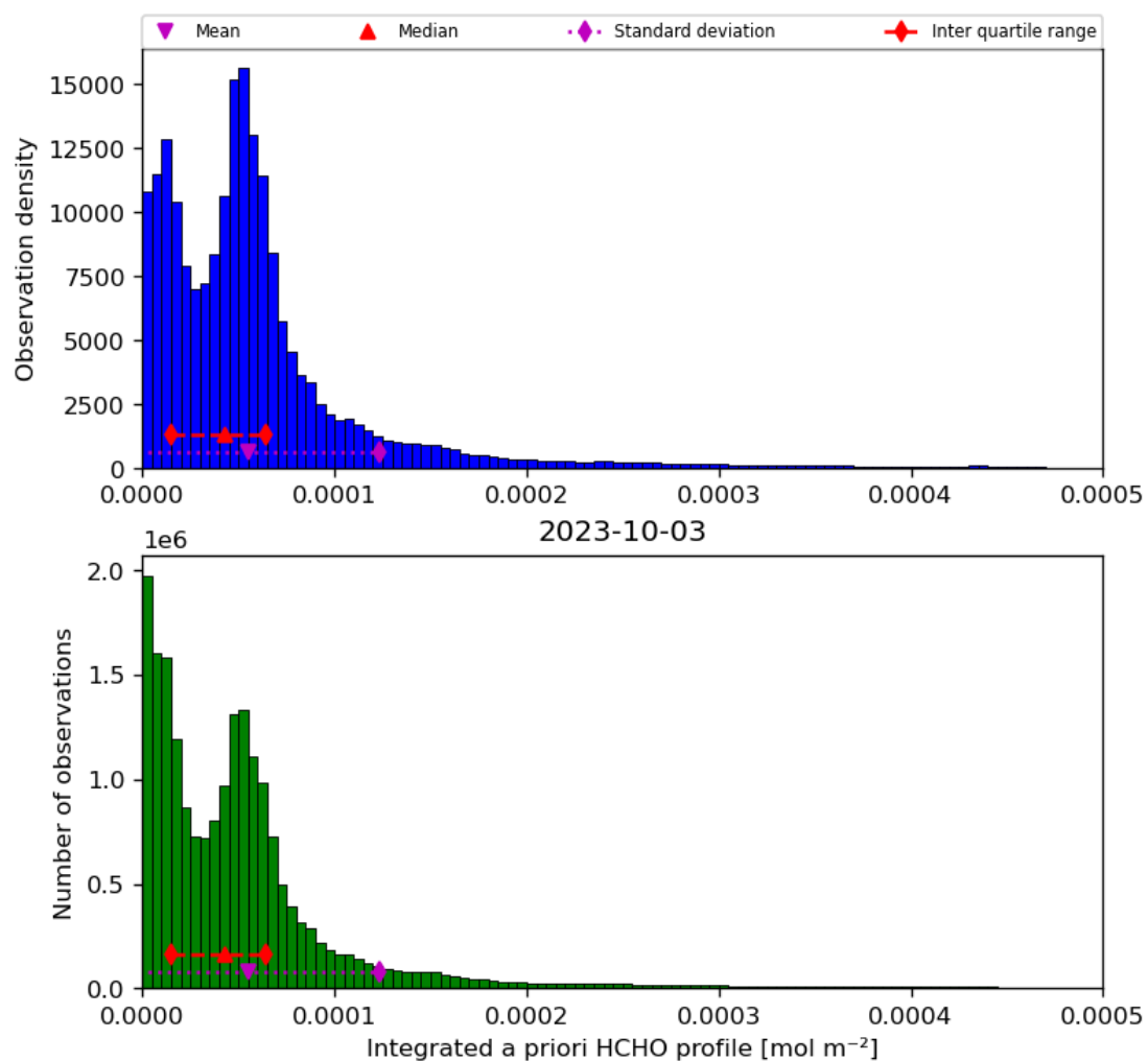
Figure 43: Histogram of “Integrated a priori HCHO profile” for 2023-10-02 to 2023-10-04
