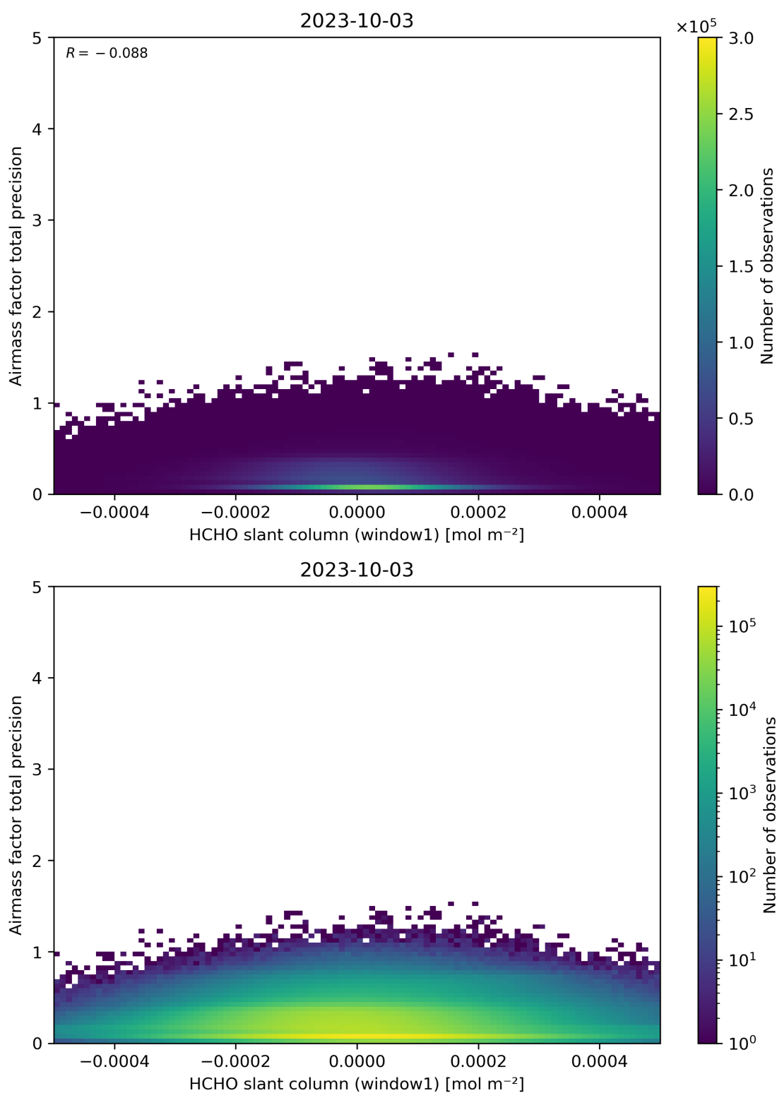
Figure 86: Scatter density plot of “HCHO slant column (window1)” against “Airmass factor total precision” for 2023-10-02 to 2023-10-04.
