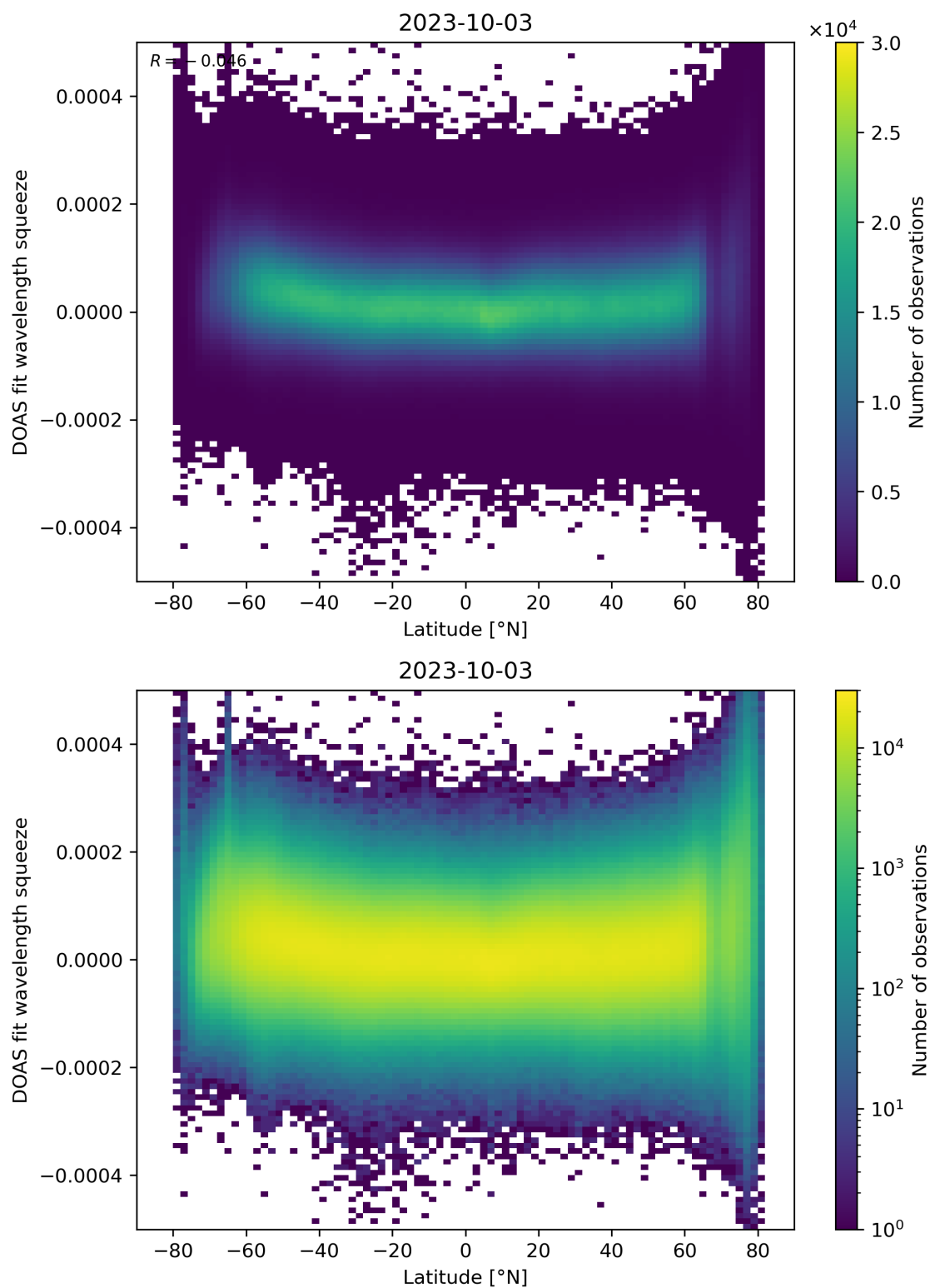
Figure 155: Scatter density plot of “Latitude” against “DOAS fit wavelength squeeze” for 2023-10-02 to 2023-10-04.
