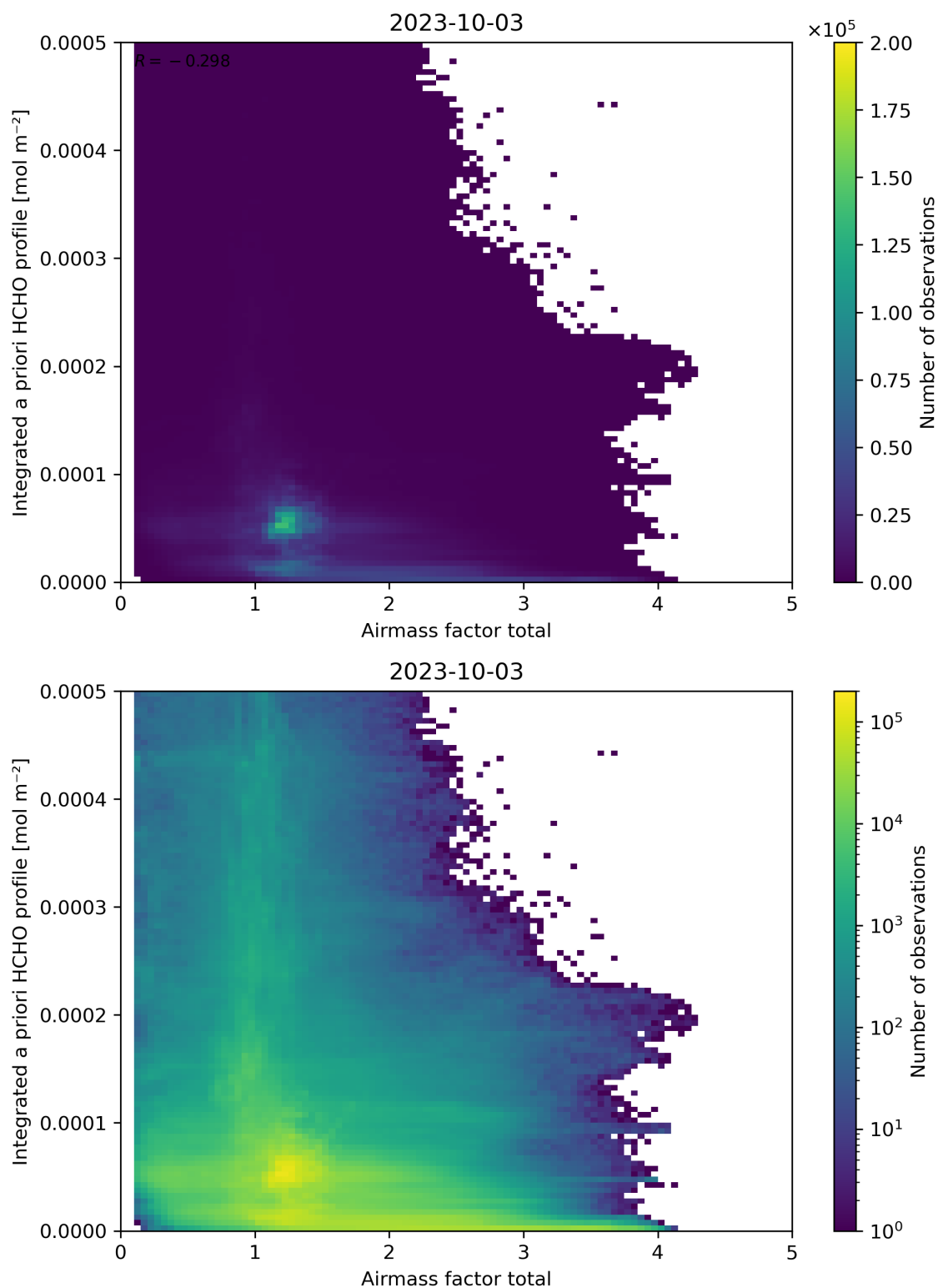
Figure 104: Scatter density plot of “Airmass factor total” against “Integrated a priori HCHO profile” for 2023-10-02 to 2023-10-04.
