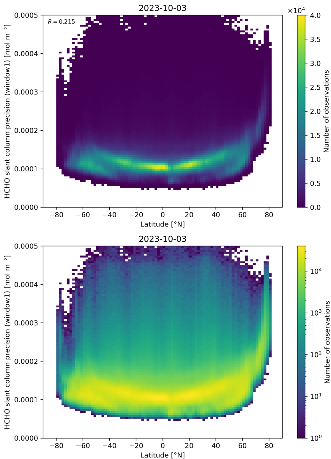
Figure 160: Scatter density plot of “Latitude” against “HCHO slant column precision (window1)” for 2023-10-02 to 2023-10-04.
