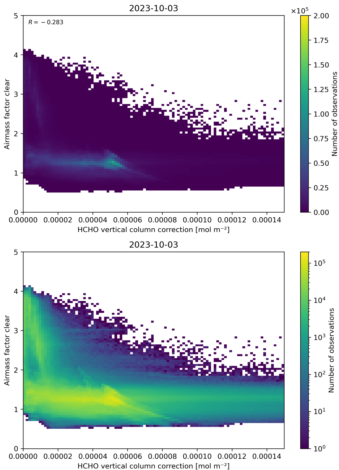
Figure 115: Scatter density plot of “HCHO vertical column correction” against “Airmass factor clear” for 2023-10-02 to 2023-10-04.
