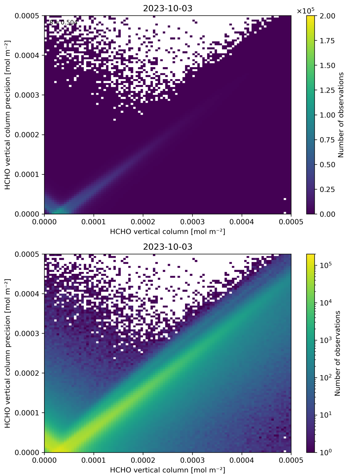
Figure 134: Scatter density plot of “HCHO vertical column” against “HCHO vertical column precision” for 2023-10-02 to 2023-10-04.
