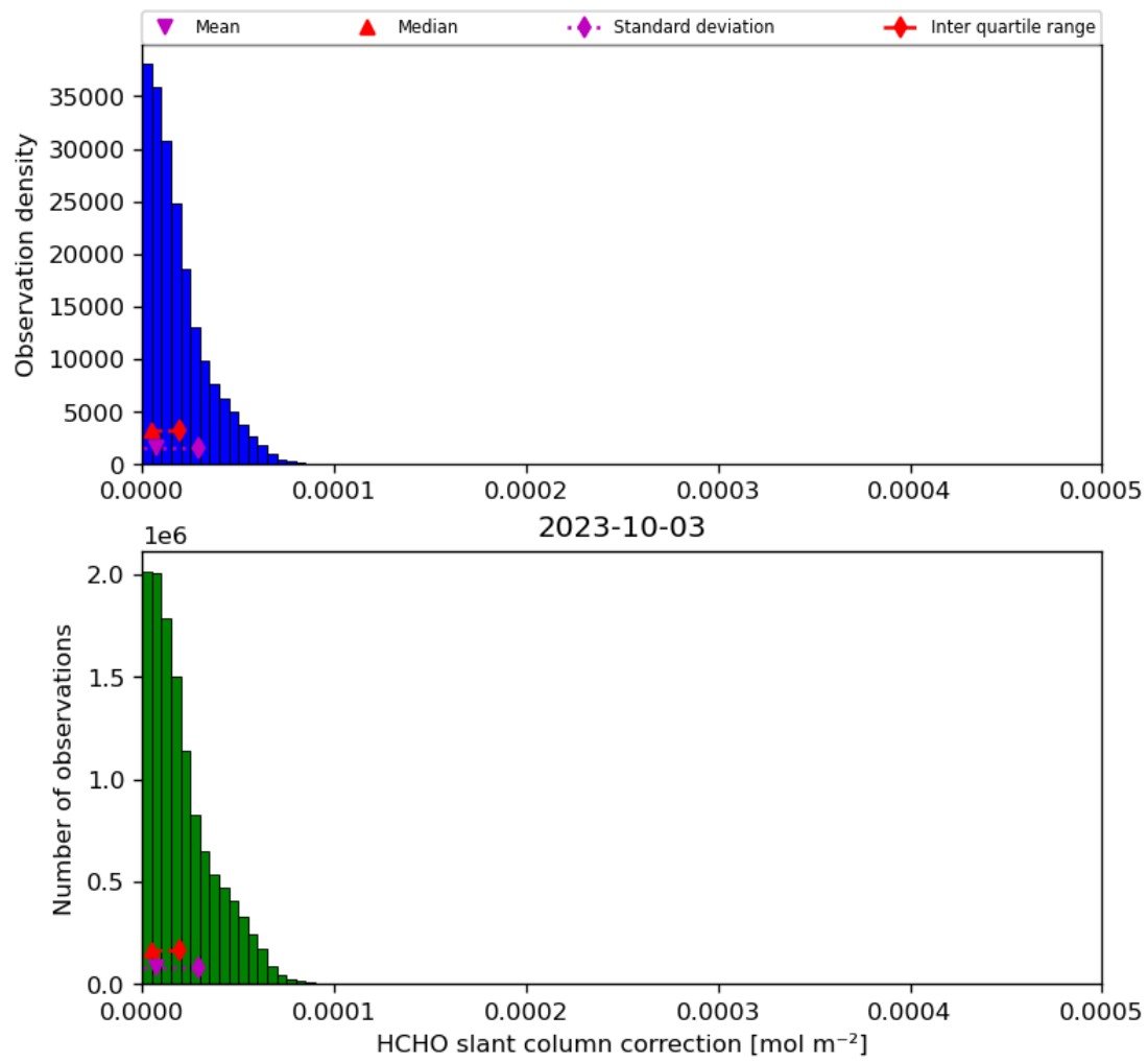
Figure 47: Histogram of “HCHO slant column correction” for 2023-10-02 to 2023-10-04
