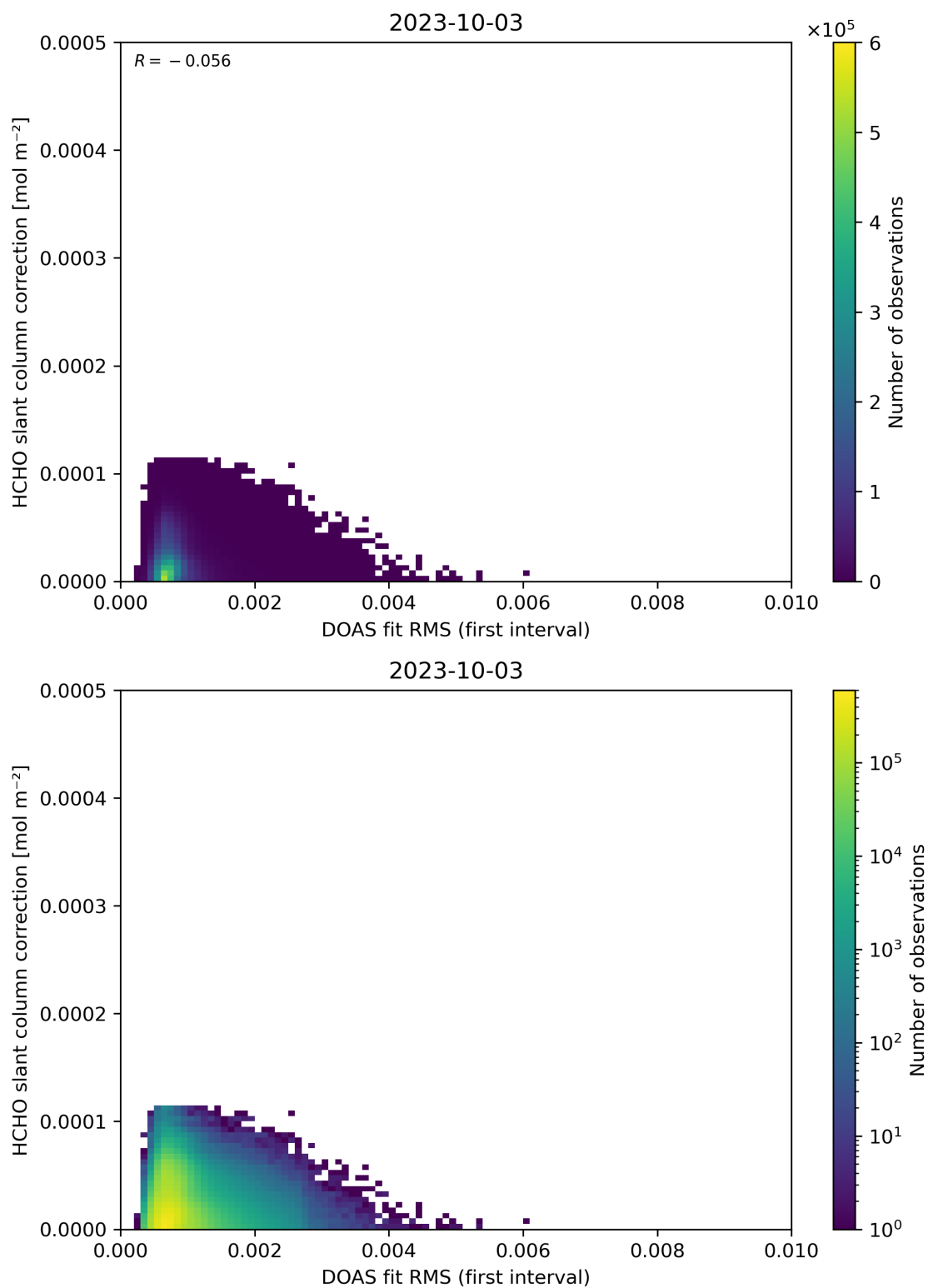
Figure 63: Scatter density plot of “DOAS fit RMS (first interval)” against “HCHO slant column correction” for 2023-10-02 to 2023-10-04.
