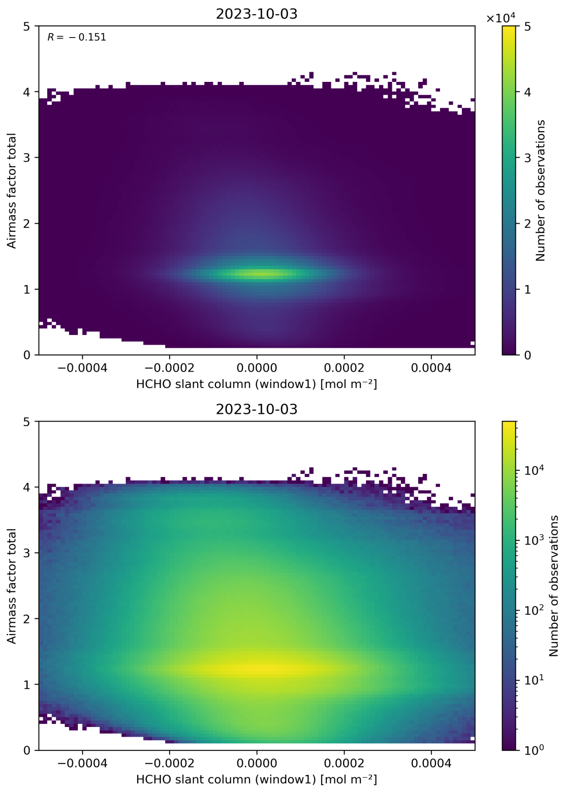
Figure 85: Scatter density plot of “HCHO slant column (window1)” against “Airmass factor total” for 2023-10-02 to 2023-10-04.
