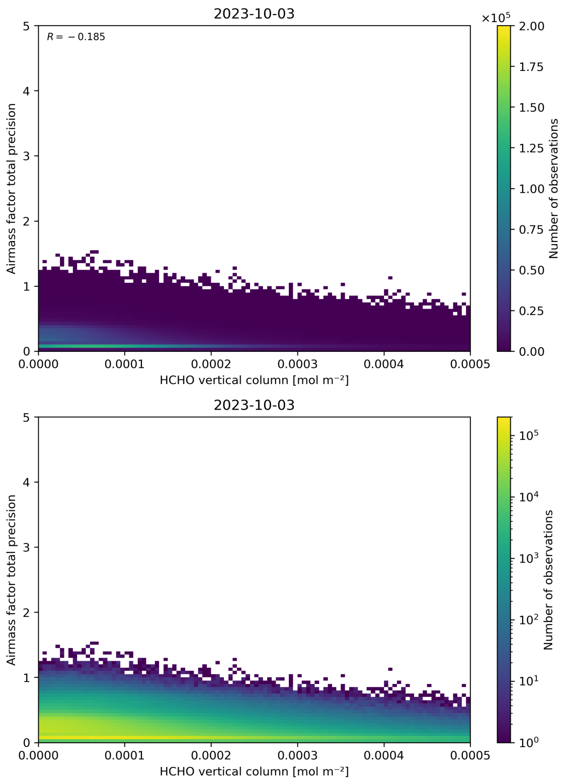
Figure 132: Scatter density plot of “HCHO vertical column” against “Airmass factor total precision” for 2023-10-02 to 2023-10-04.
