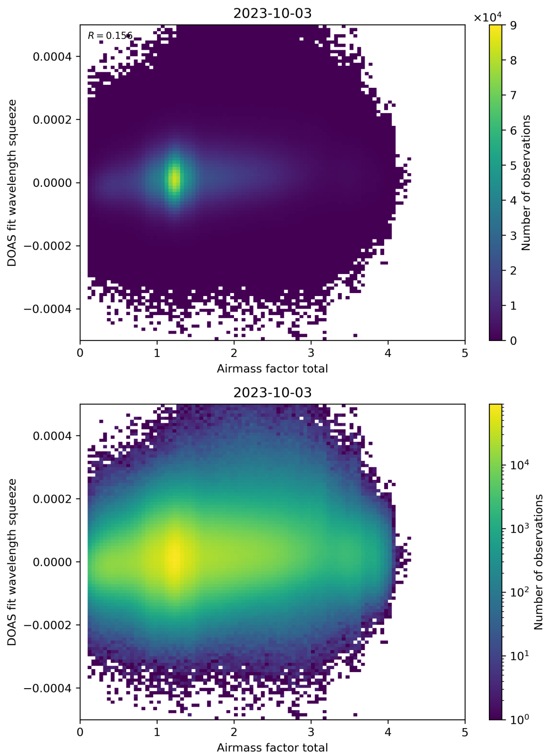
Figure 99: Scatter density plot of “Airmass factor total” against “DOAS fit wavelength squeeze” for 2023-10-02 to 2023-10-04.
