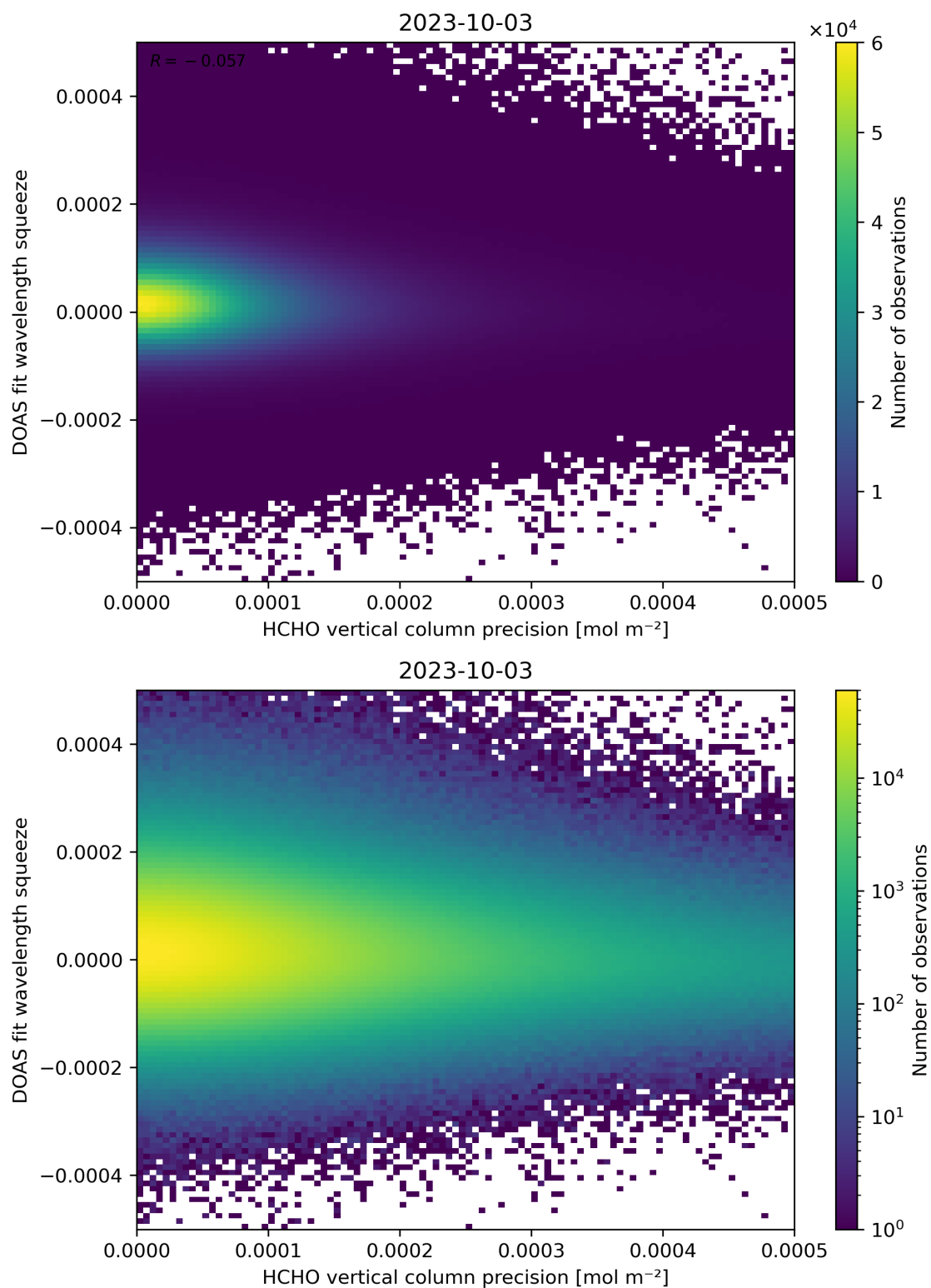
Figure 138: Scatter density plot of “HCHO vertical column precision” against “DOAS fit wavelength squeeze” for 2023-10-02 to 2023-10-04.
