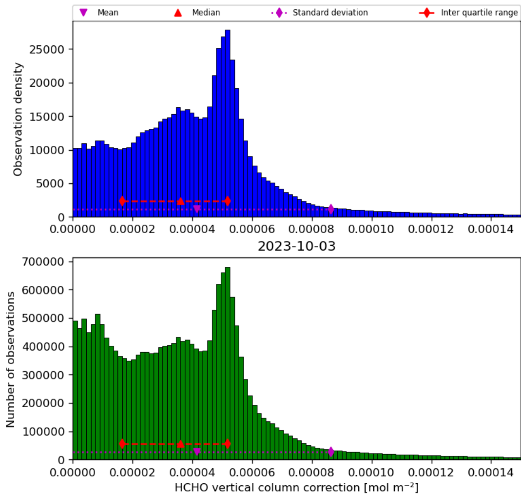
Figure 37: Histogram of “HCHO vertical column correction” for 2023-10-02 to 2023-10-04
