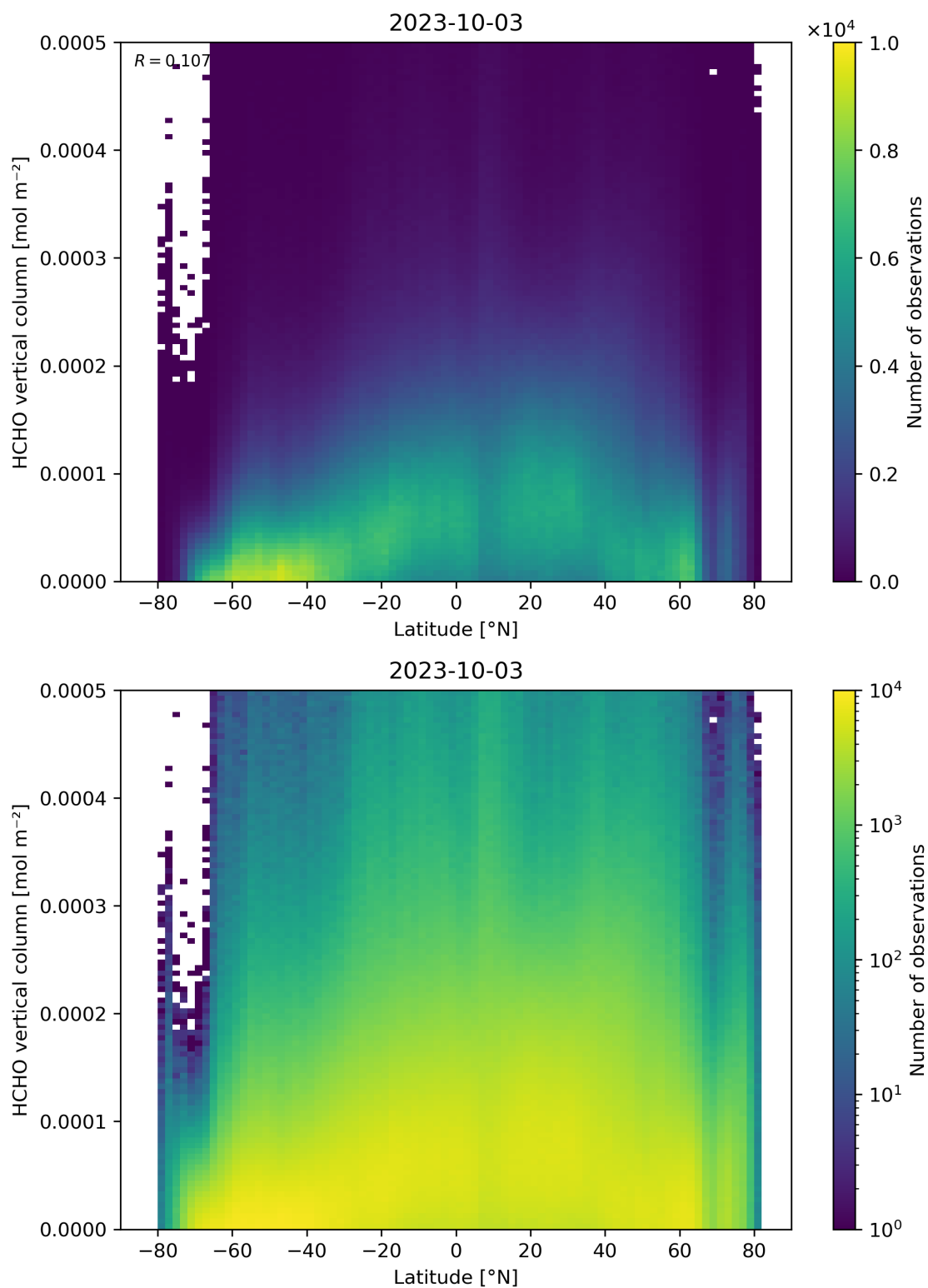
Figure 163: Scatter density plot of “Latitude” against “HCHO vertical column” for 2023-10-02 to 2023-10-04.
