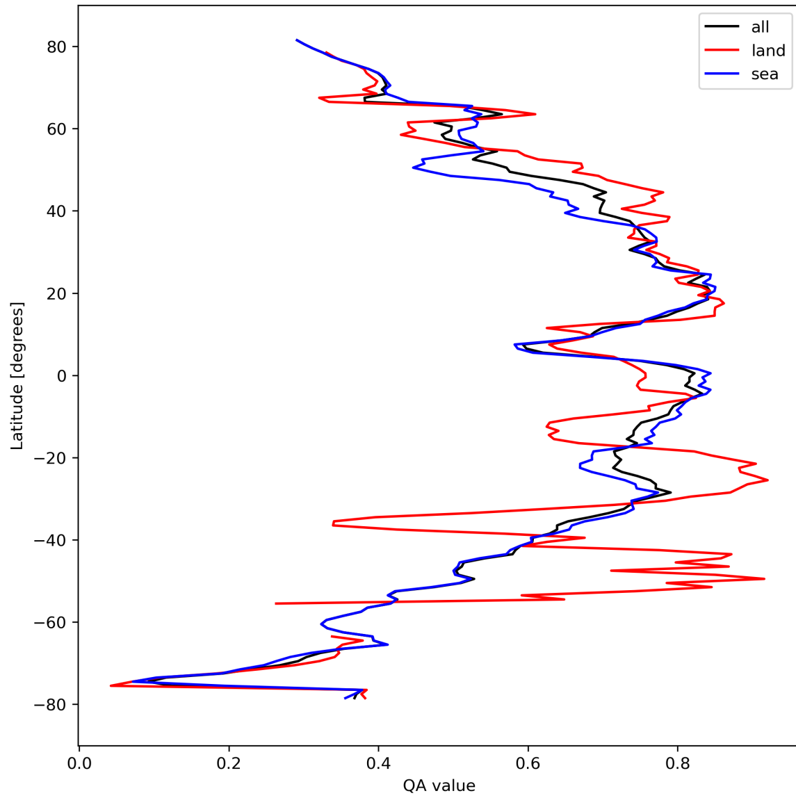
Figure 20: Zonal average of “QA value” for 2023-10-02 to 2023-10-04.
