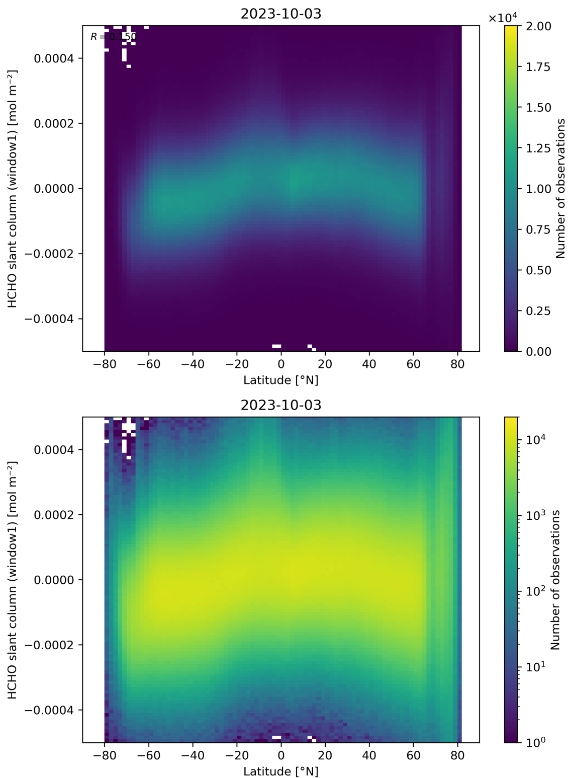
Figure 159: Scatter density plot of “Latitude” against “HCHO slant column (window1)” for 2023-10-02 to 2023-10-04.
