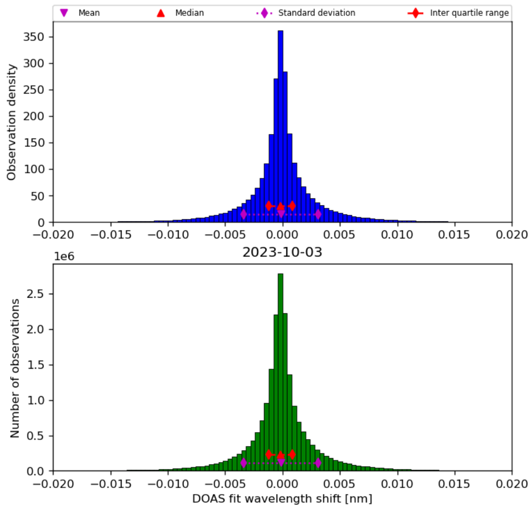
Figure 44: Histogram of “DOAS fit wavelength shift” for 2023-10-02 to 2023-10-04
