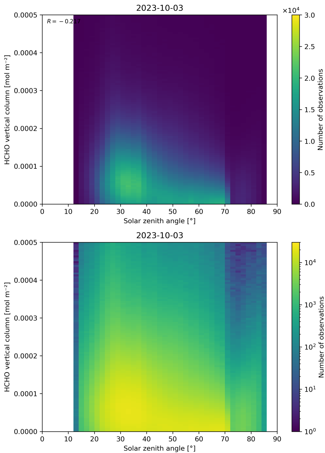
Figure 177: Scatter density plot of “Solar zenith angle” against “HCHO vertical column” for 2023-10-02 to 2023-10-04.
