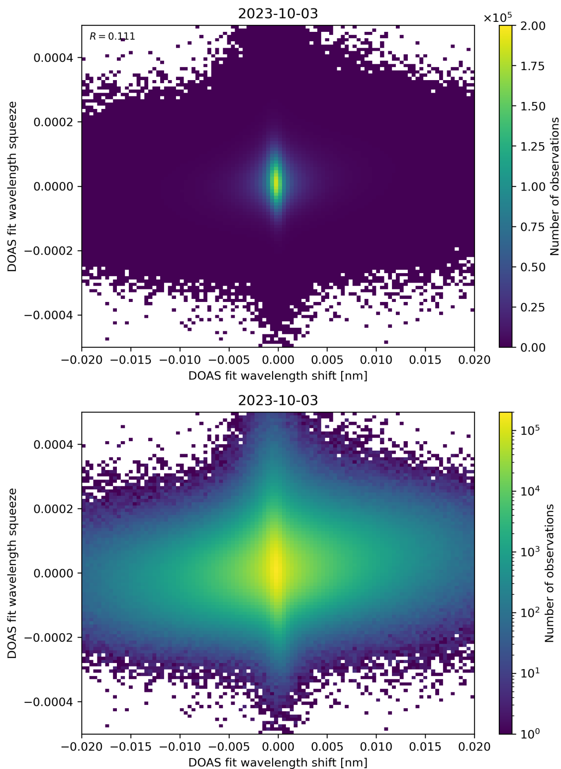
Figure 65: Scatter density plot of “DOAS fit wavelength shift” against “DOAS fit wavelength squeeze” for 2023-10-02 to 2023-10-04.
