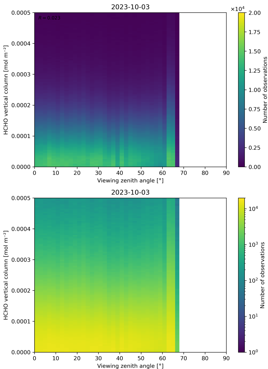
Figure 192: Scatter density plot of “Viewing zenith angle” against “HCHO vertical column” for 2023-10-02 to 2023-10-04.
