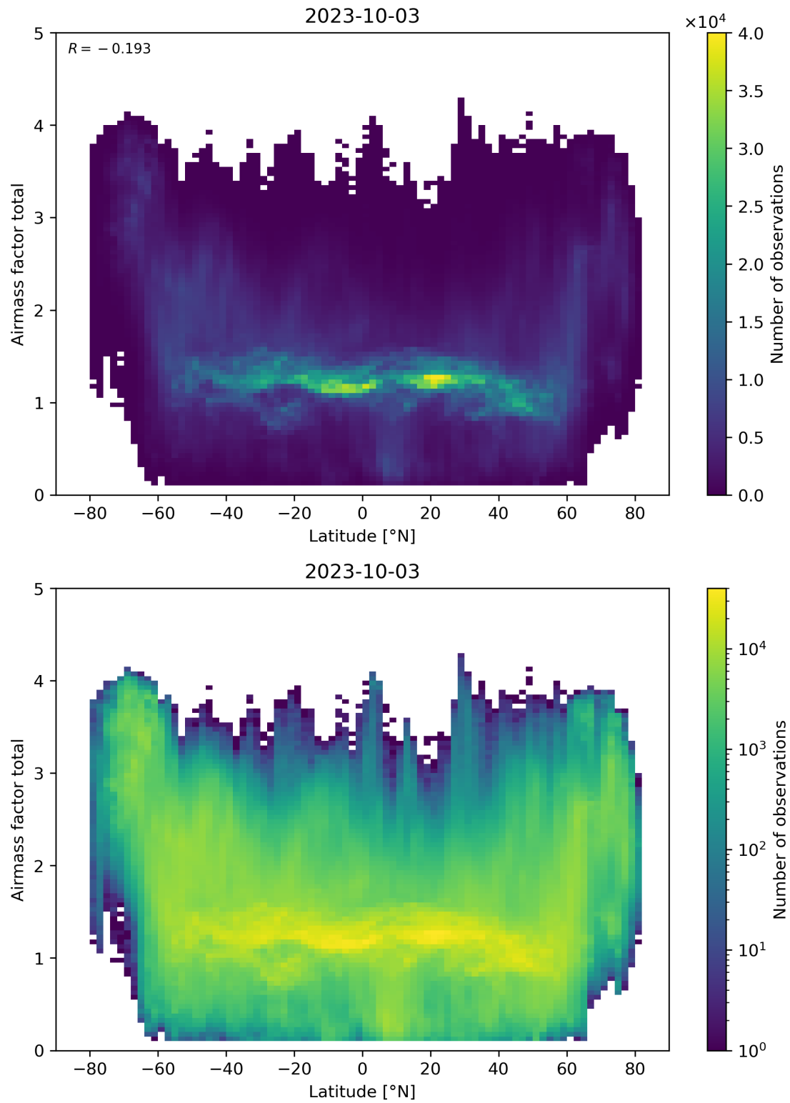
Figure 161: Scatter density plot of “Latitude” against “Airmass factor total” for 2023-10-02 to 2023-10-04.
