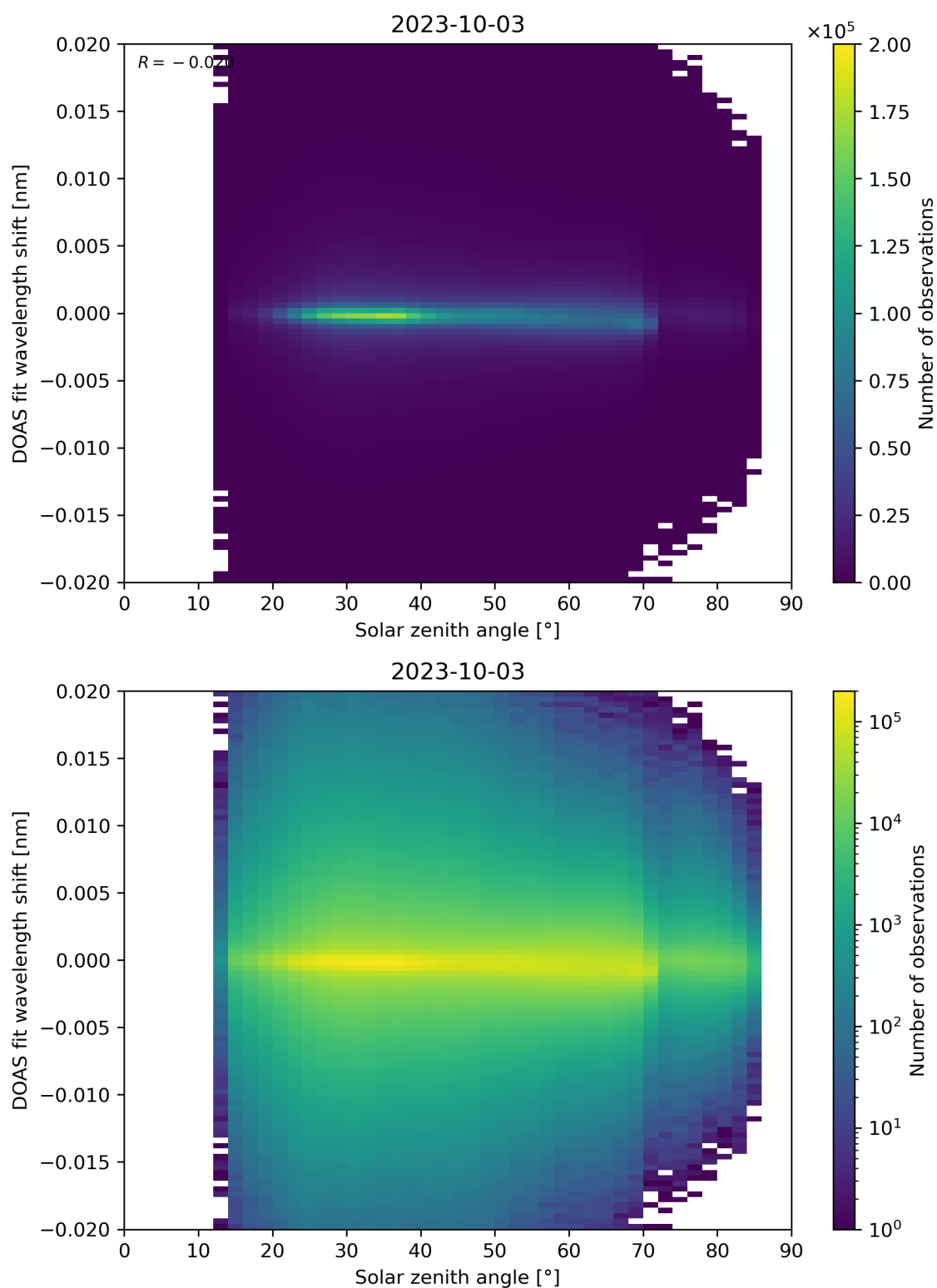
Figure 168: Scatter density plot of “Solar zenith angle” against “DOAS fit wavelength shift” for 2023-10-02 to 2023-10-04.
