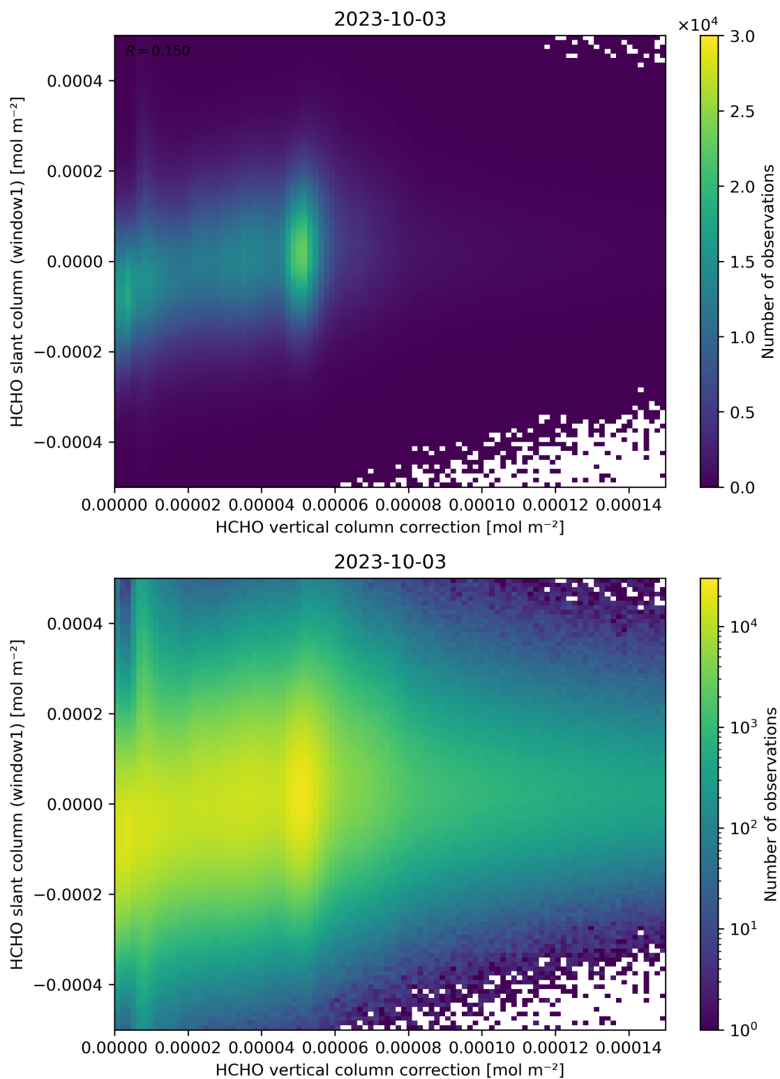
Figure 118: Scatter density plot of “HCHO vertical column correction” against “HCHO slant column (window1)” for 2023-10-02 to 2023-10-04.
