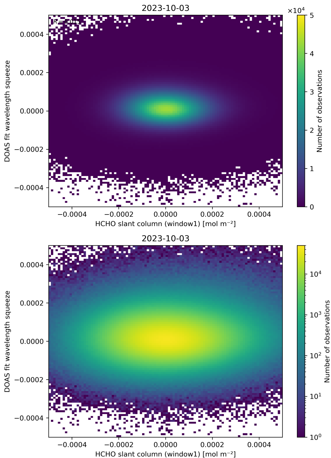
Figure 80: Scatter density plot of “HCHO slant column (window1)” against “DOAS fit wavelength squeeze” for 2023-10-02 to 2023-10-04.
