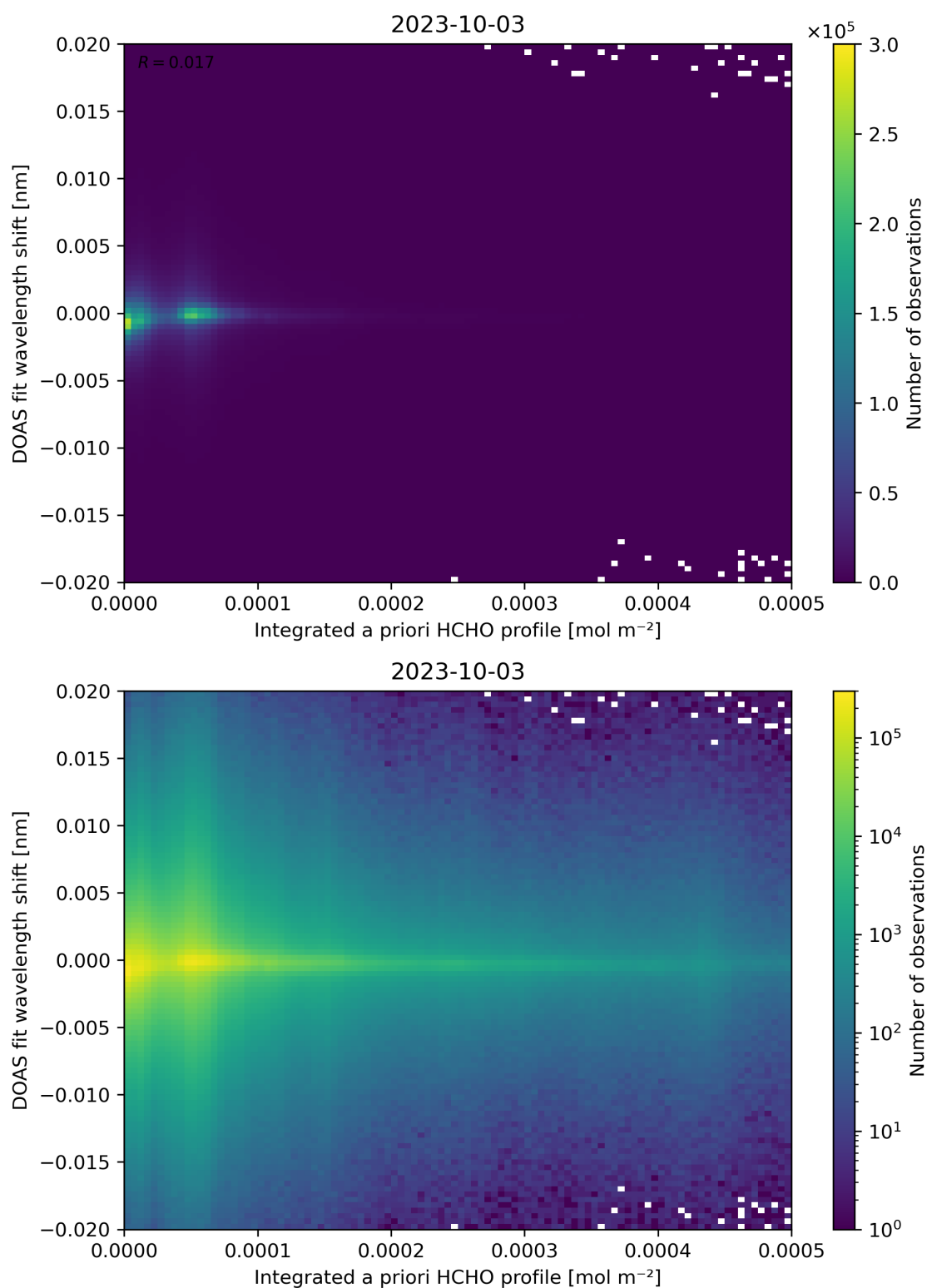
Figure 149: Scatter density plot of “Integrated a priori HCHO profile” against “DOAS fit wavelength shift” for 2023-10-02 to 2023-10-04.
