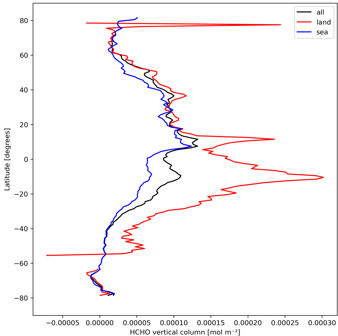
Figure 21: Zonal average of “HCHO vertical column” for 2023-10-02 to 2023-10-04.
