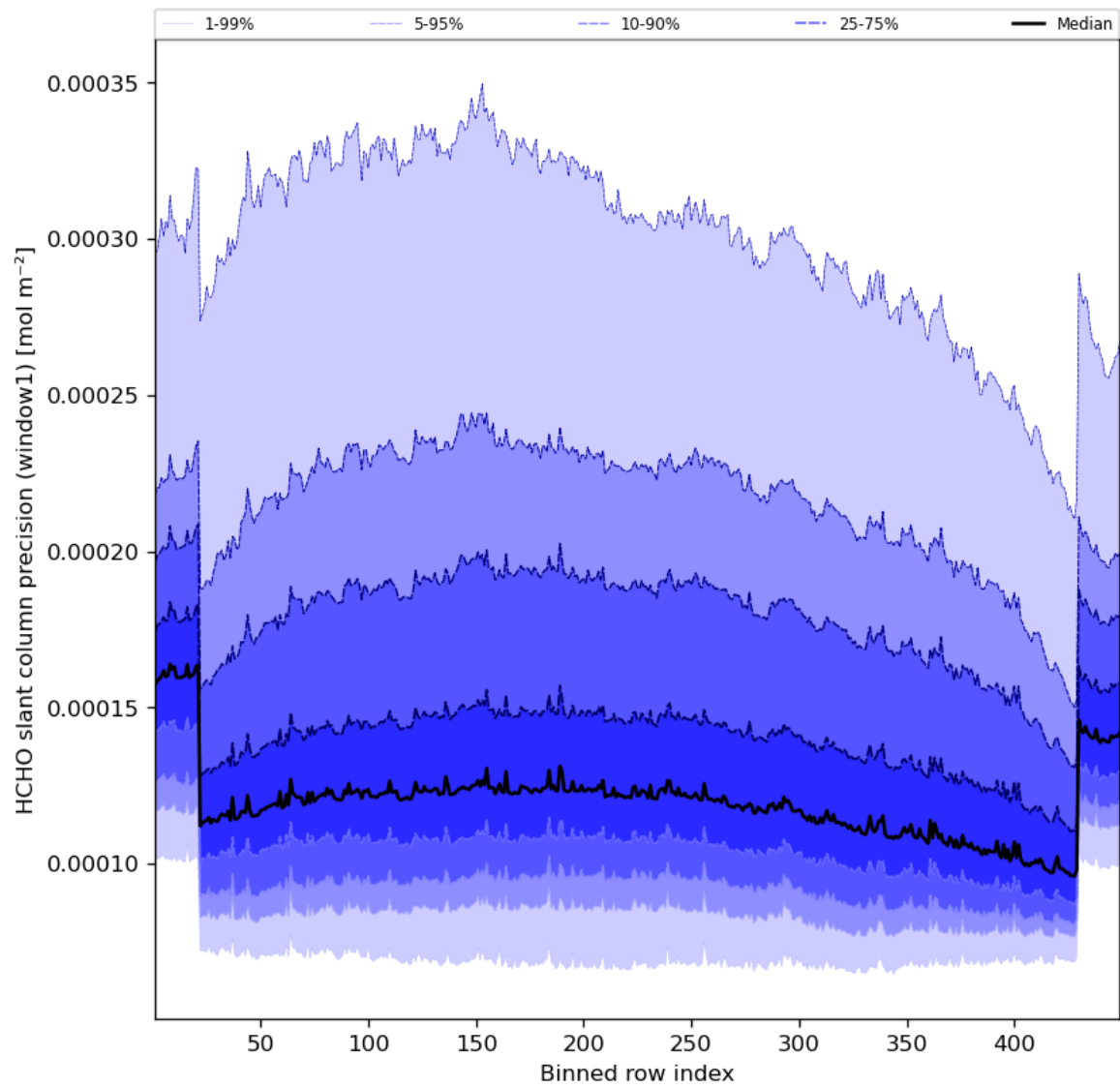
Figure 53: Along track statistics of “HCHO slant column precision (window1)” for 2023-10-02 to 2023-10-04
