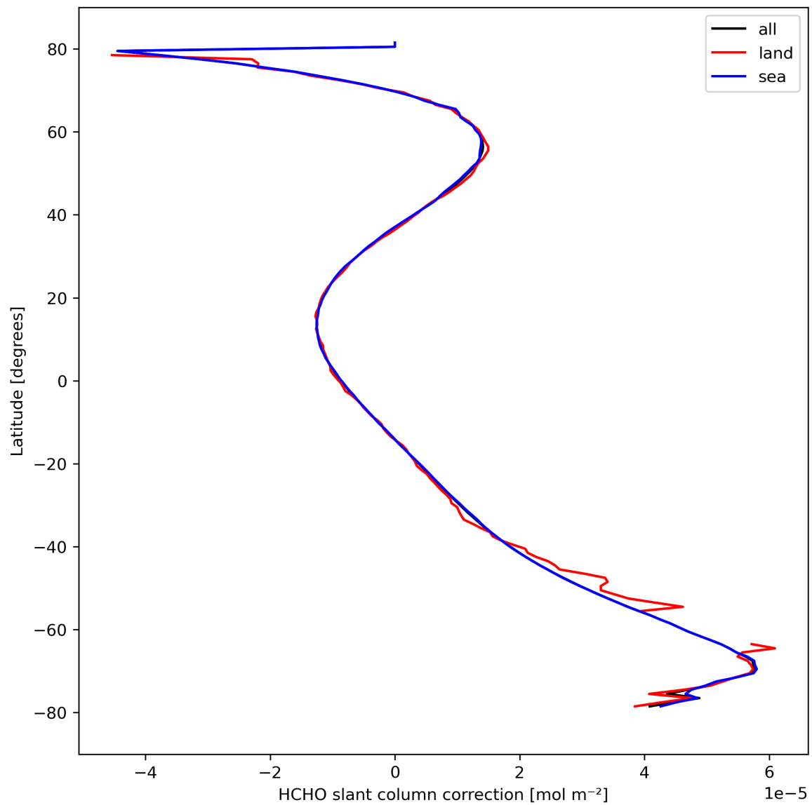
Figure 33: Zonal average of “HCHO slant column correction” for 2023-10-02 to 2023-10-04.
