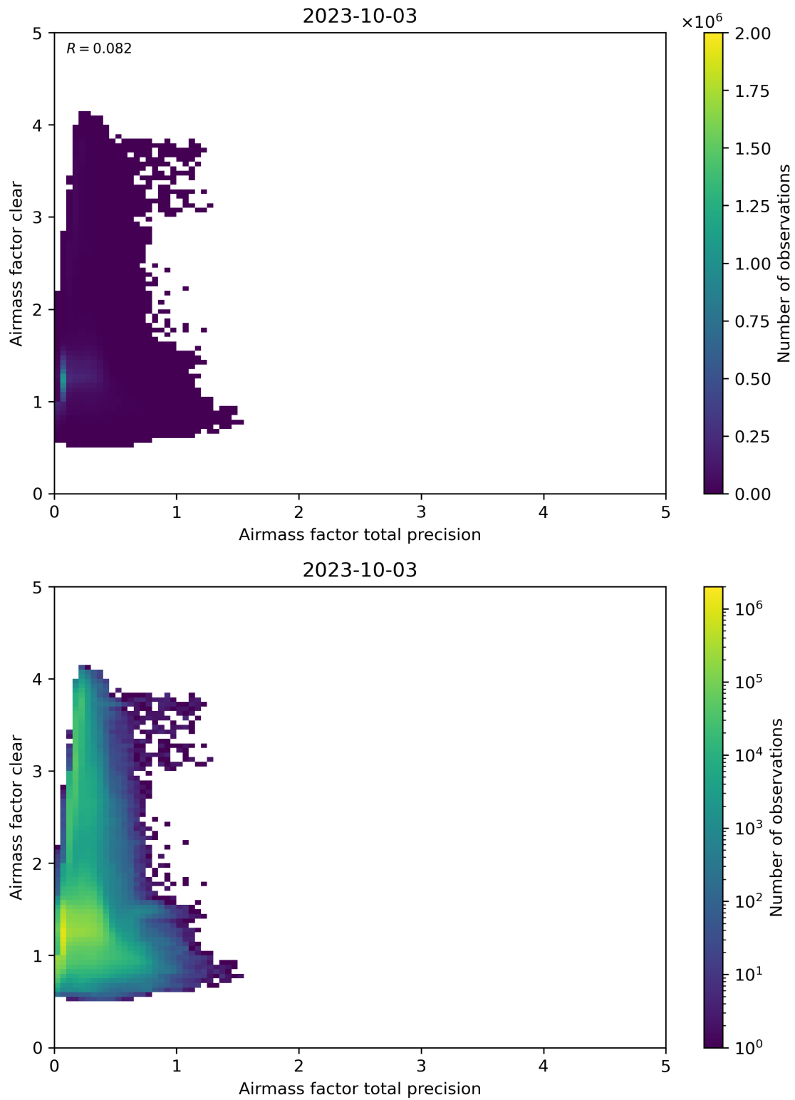
Figure 108: Scatter density plot of “Airmass factor total precision” against “Airmass factor clear” for 2023-10-02 to 2023-10-04.
