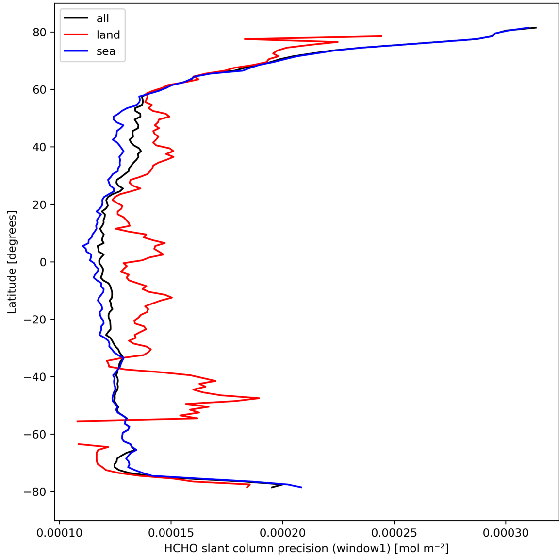
Figure 25: Zonal average of “HCHO slant column precision (window1)” for 2023-10-02 to 2023-10-04.
