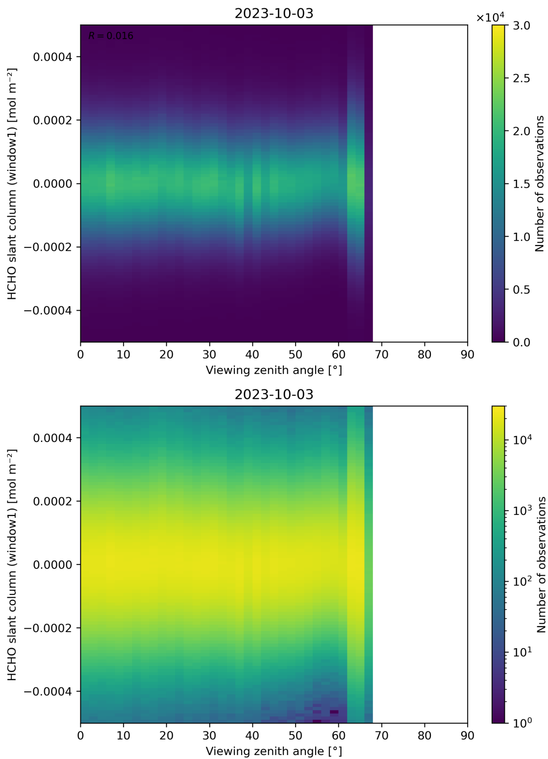
Figure 188: Scatter density plot of “Viewing zenith angle” against “HCHO slant column (window1)” for 2023-10-02 to 2023-10-04.
