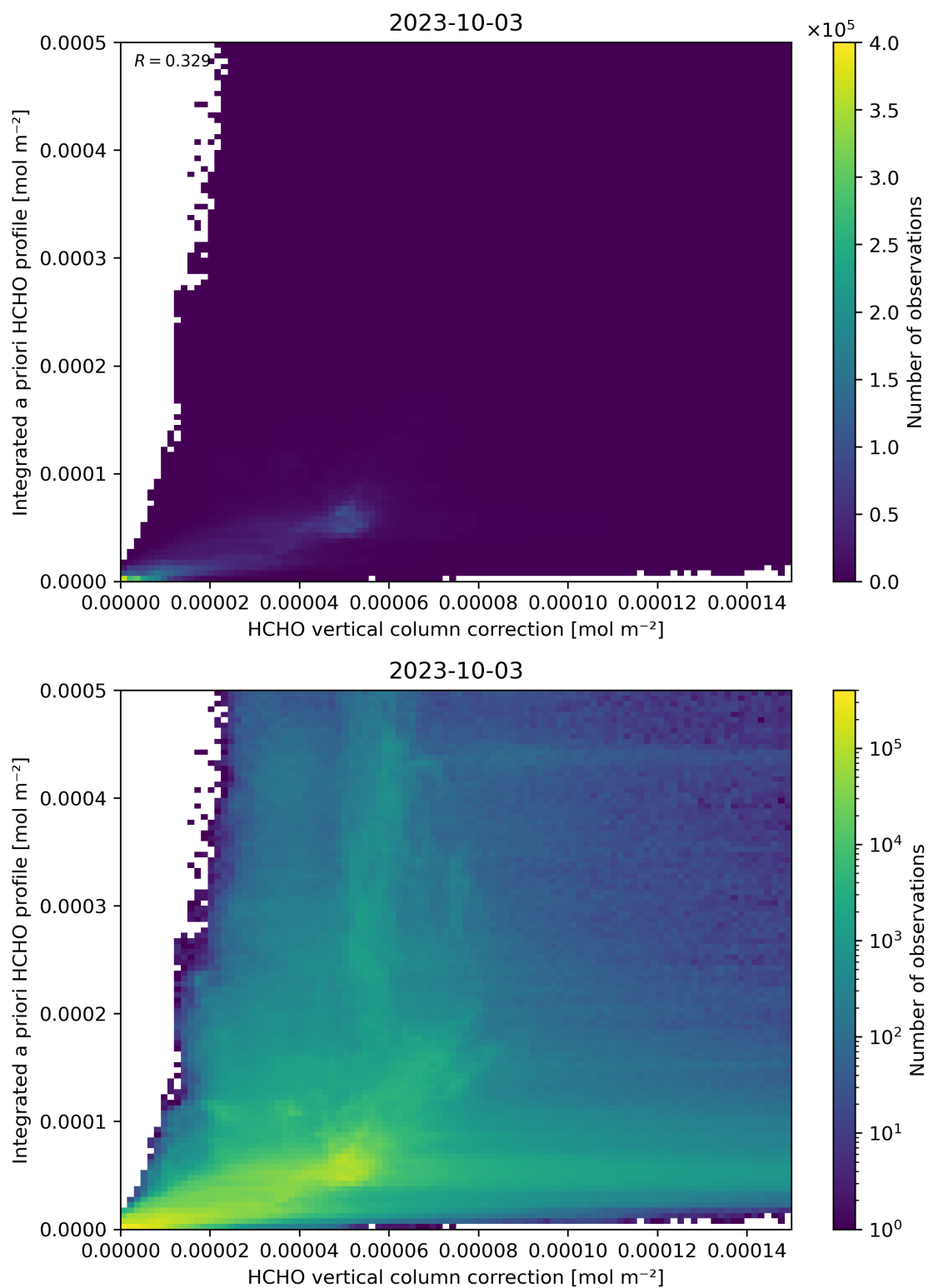
Figure 122: Scatter density plot of “HCHO vertical column correction” against “Integrated a priori HCHO profile” for 2023-10-02 to 2023-10-04.
