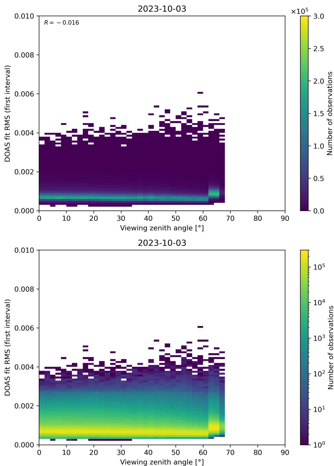
Figure 182: Scatter density plot of “Viewing zenith angle” against “DOAS fit RMS (first interval)” for 2023-10-02 to 2023-10-04.
