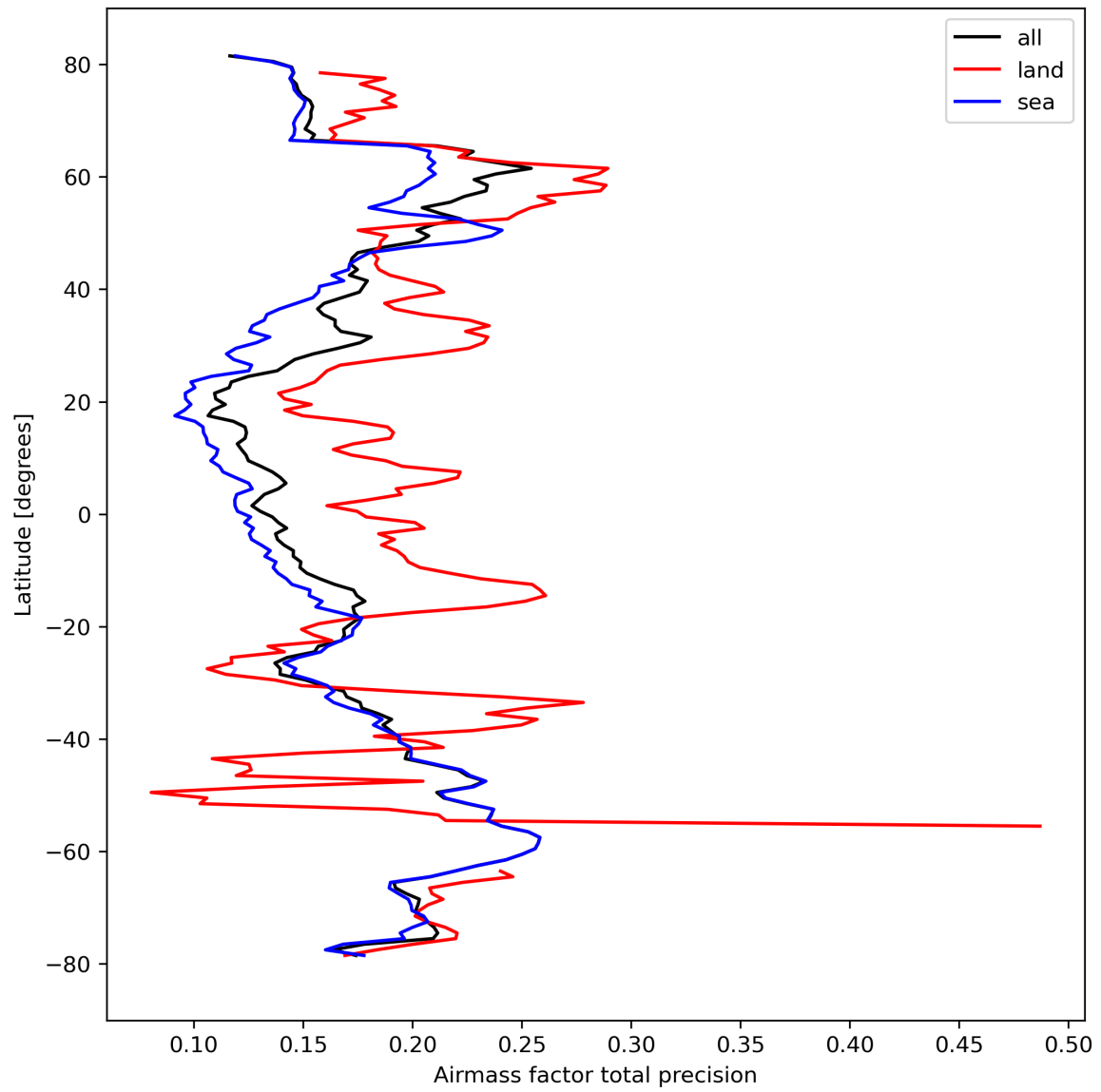
Figure 27: Zonal average of “Airmass factor total precision” for 2023-10-02 to 2023-10-04.
