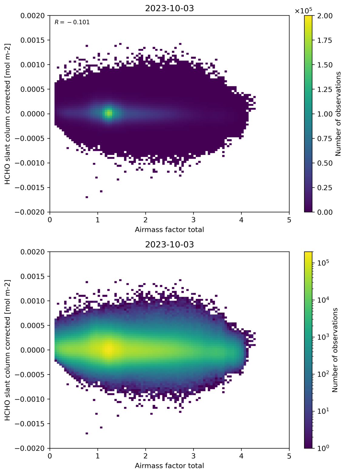
Figure 101: Scatter density plot of “Airmass factor total” against “HCHO slant column corrected” for 2023-10-02 to 2023-10-04.
