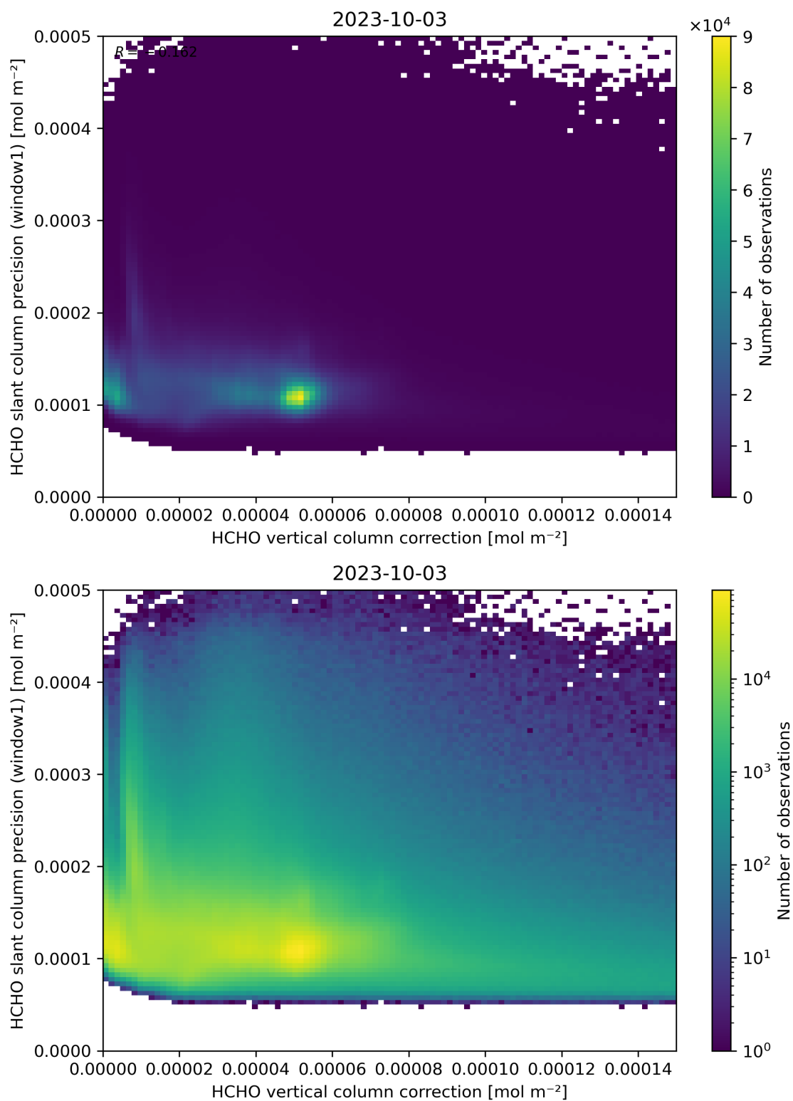
Figure 119: Scatter density plot of “HCHO vertical column correction” against “HCHO slant column precision (window1)” for 2023-10-02 to 2023-10-04.
