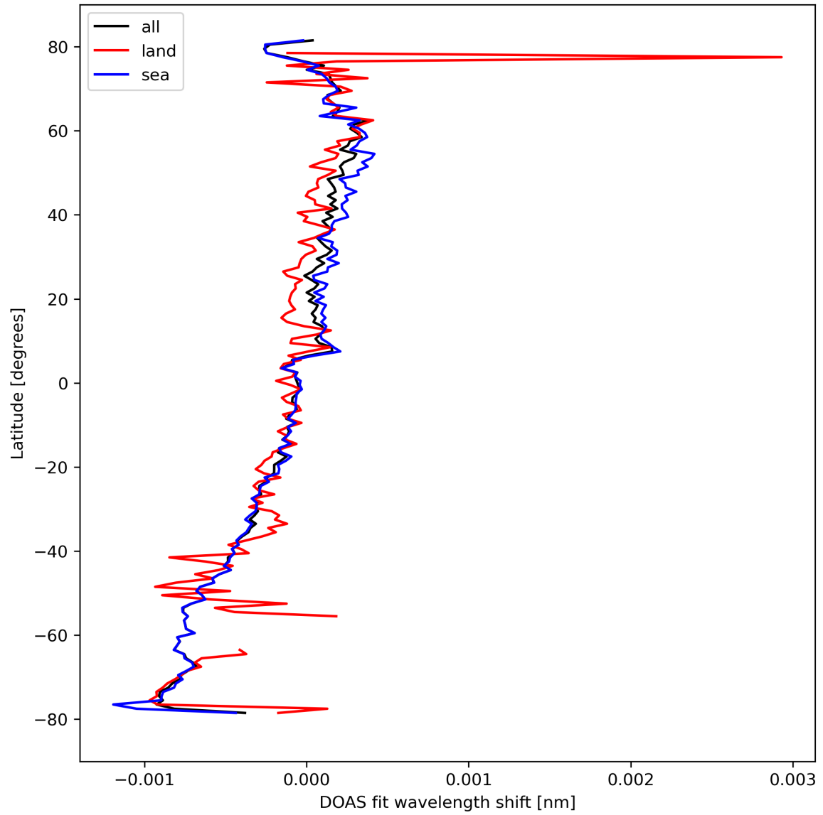
Figure 30: Zonal average of "DOAS fit wavelength shift" for 2023-10-02 to 2023-10-04.
