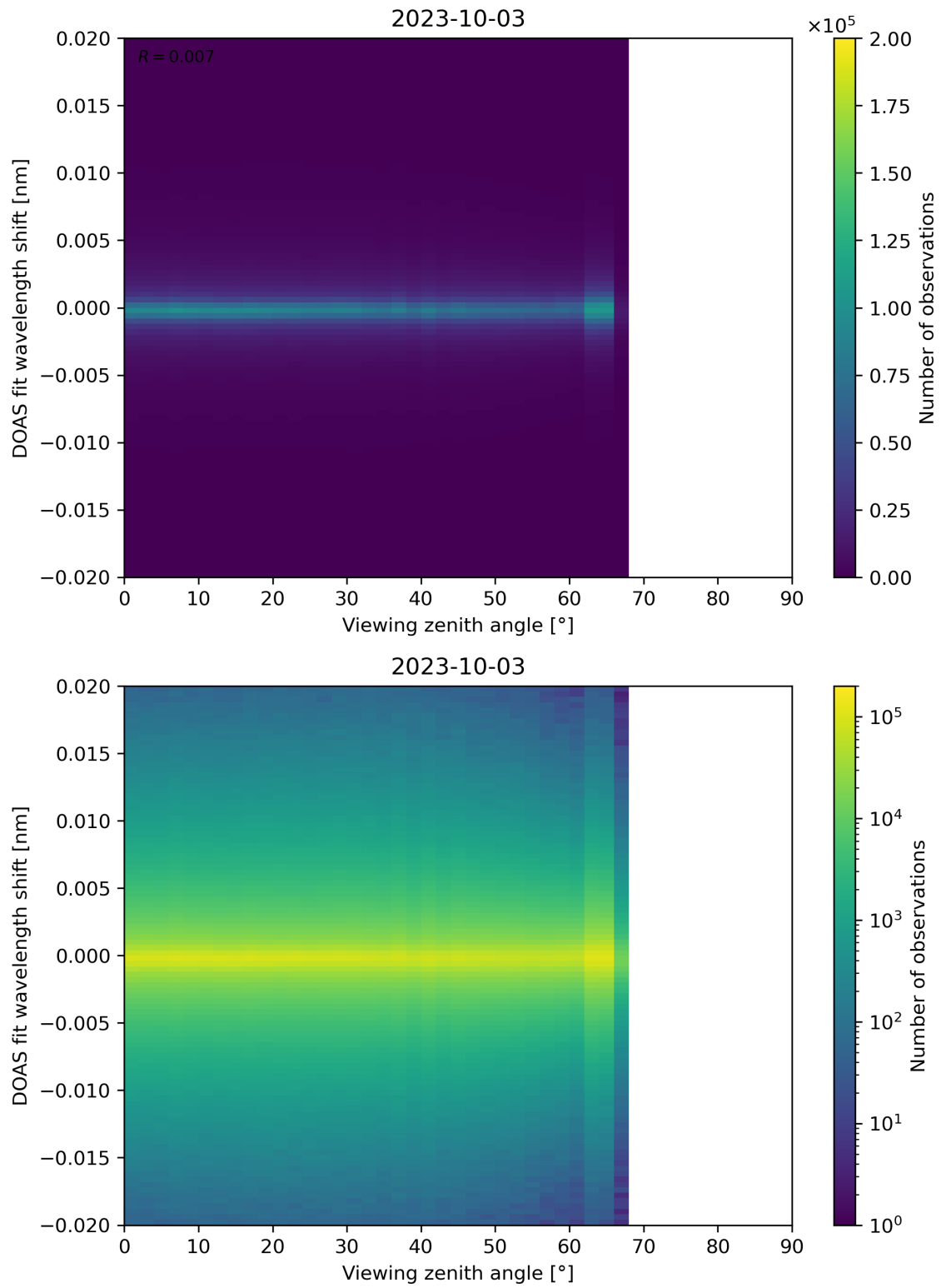
Figure 183: Scatter density plot of “Viewing zenith angle” against “DOAS fit wavelength shift” for 2023-10-02 to 2023-10-04.
