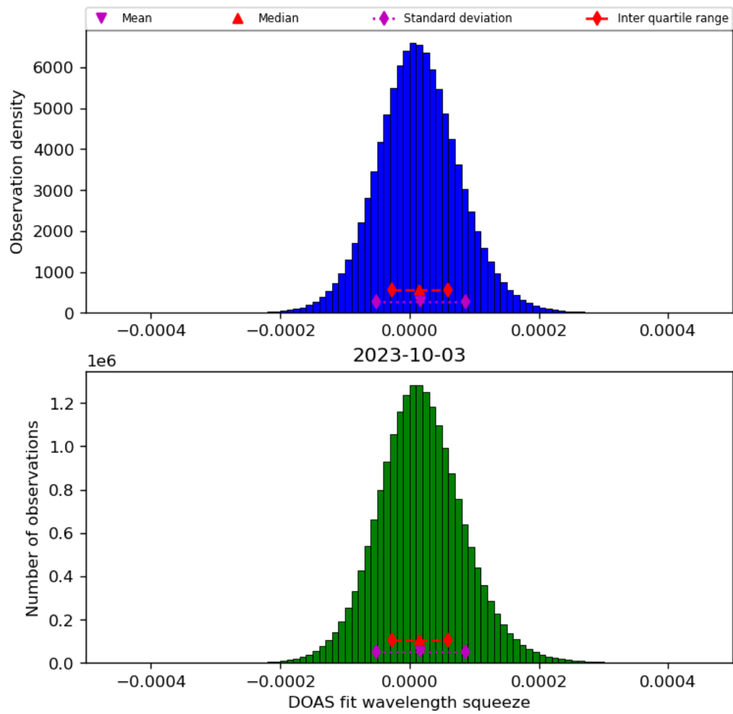
Figure 45: Histogram of “DOAS fit wavelength squeeze” for 2023-10-02 to 2023-10-04
