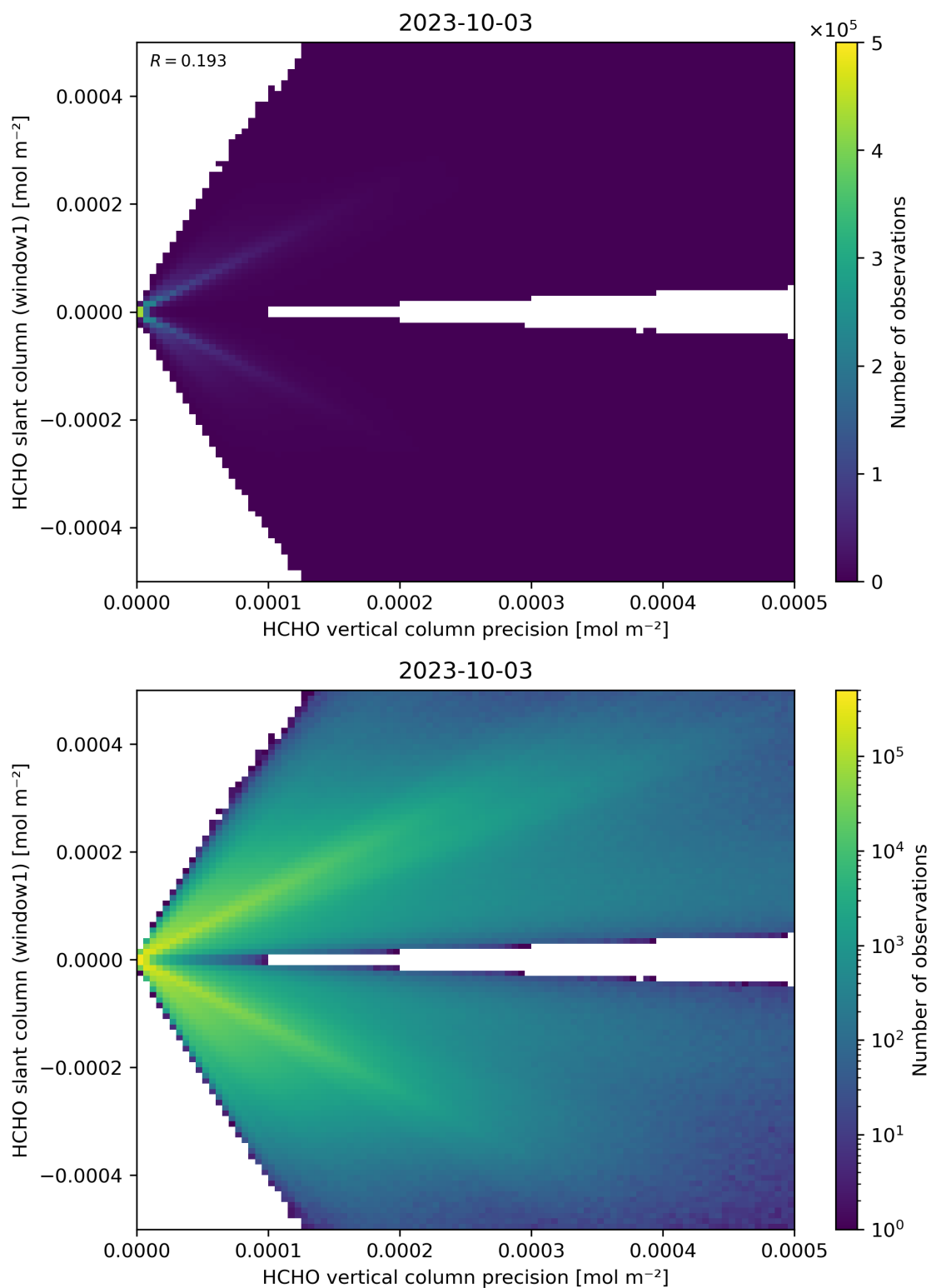
Figure 142: Scatter density plot of “HCHO vertical column precision” against “HCHO slant column (window1)” for 2023-10-02 to 2023-10-04.
