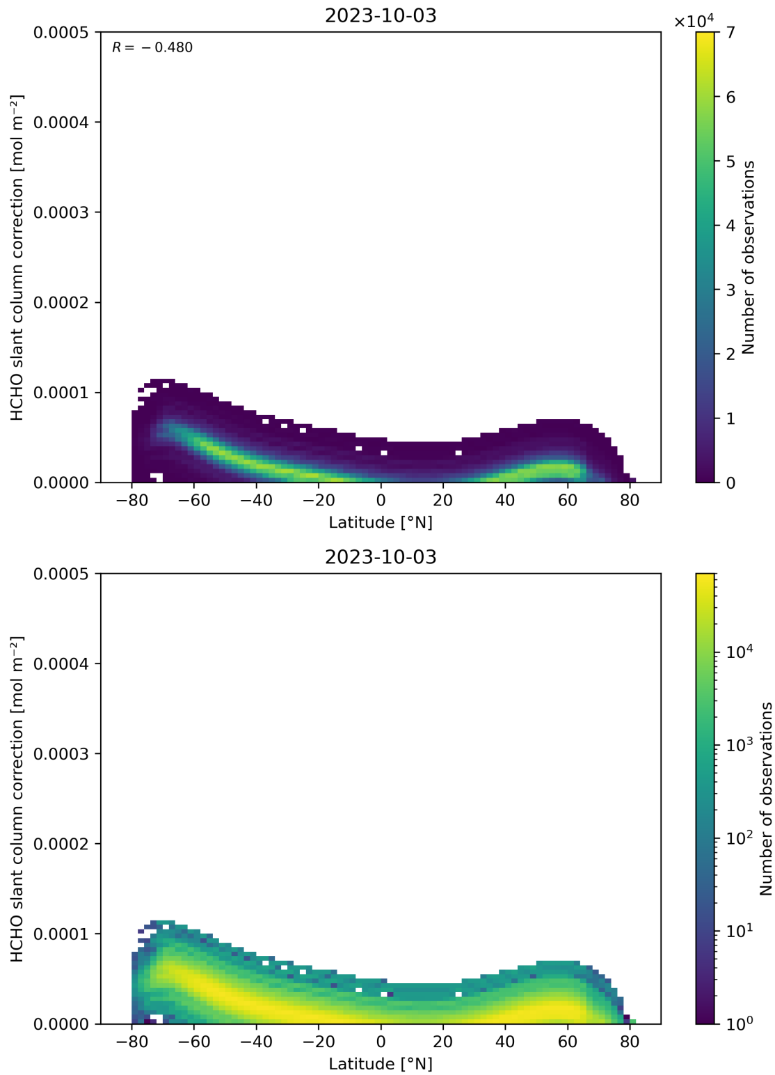
Figure 158: Scatter density plot of “Latitude” against “HCHO slant column correction” for 2023-10-02 to 2023-10-04.
