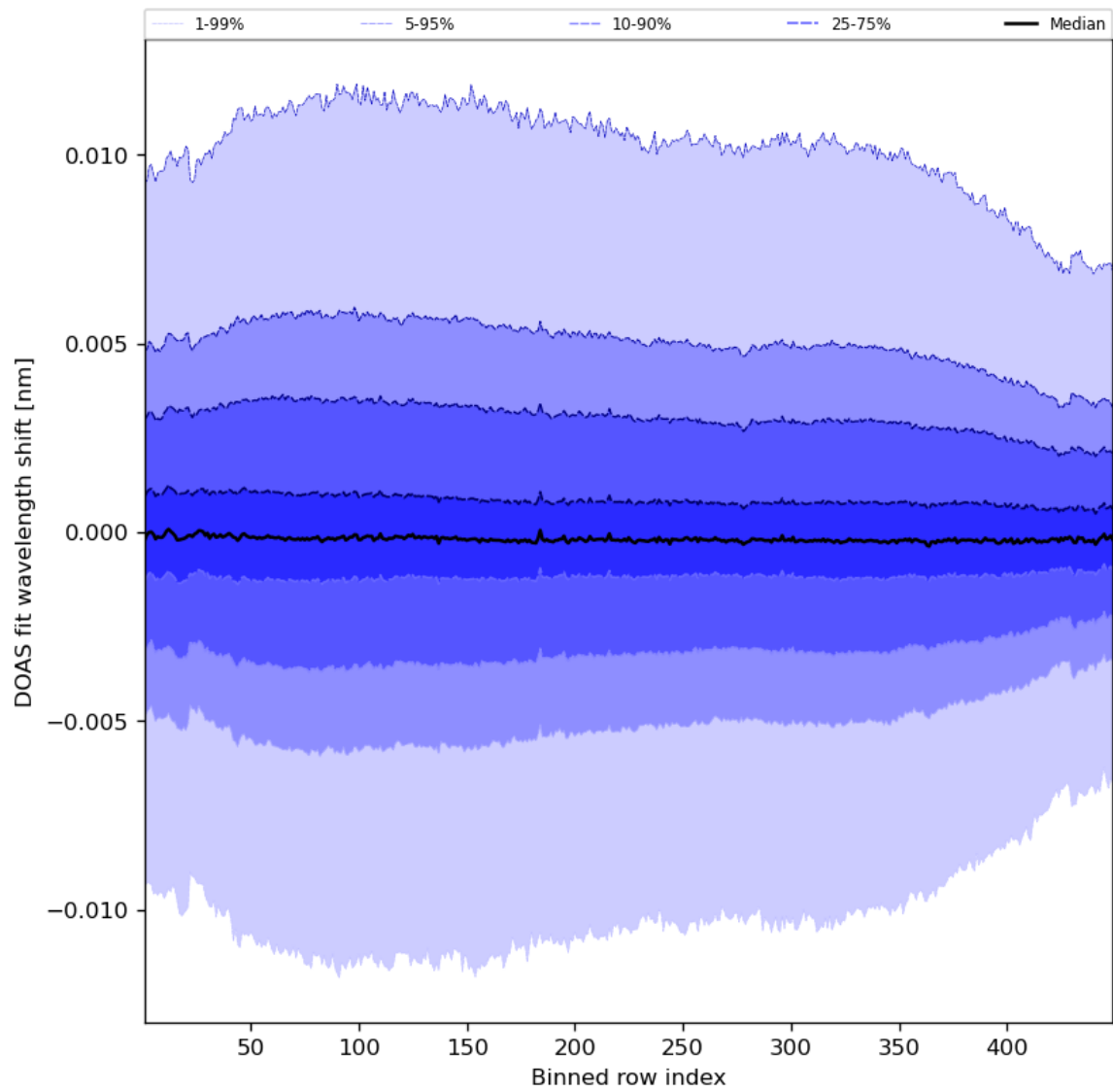
Figure 58: Along track statistics of “DOAS fit wavelength shift” for 2023-10-02 to 2023-10-04
