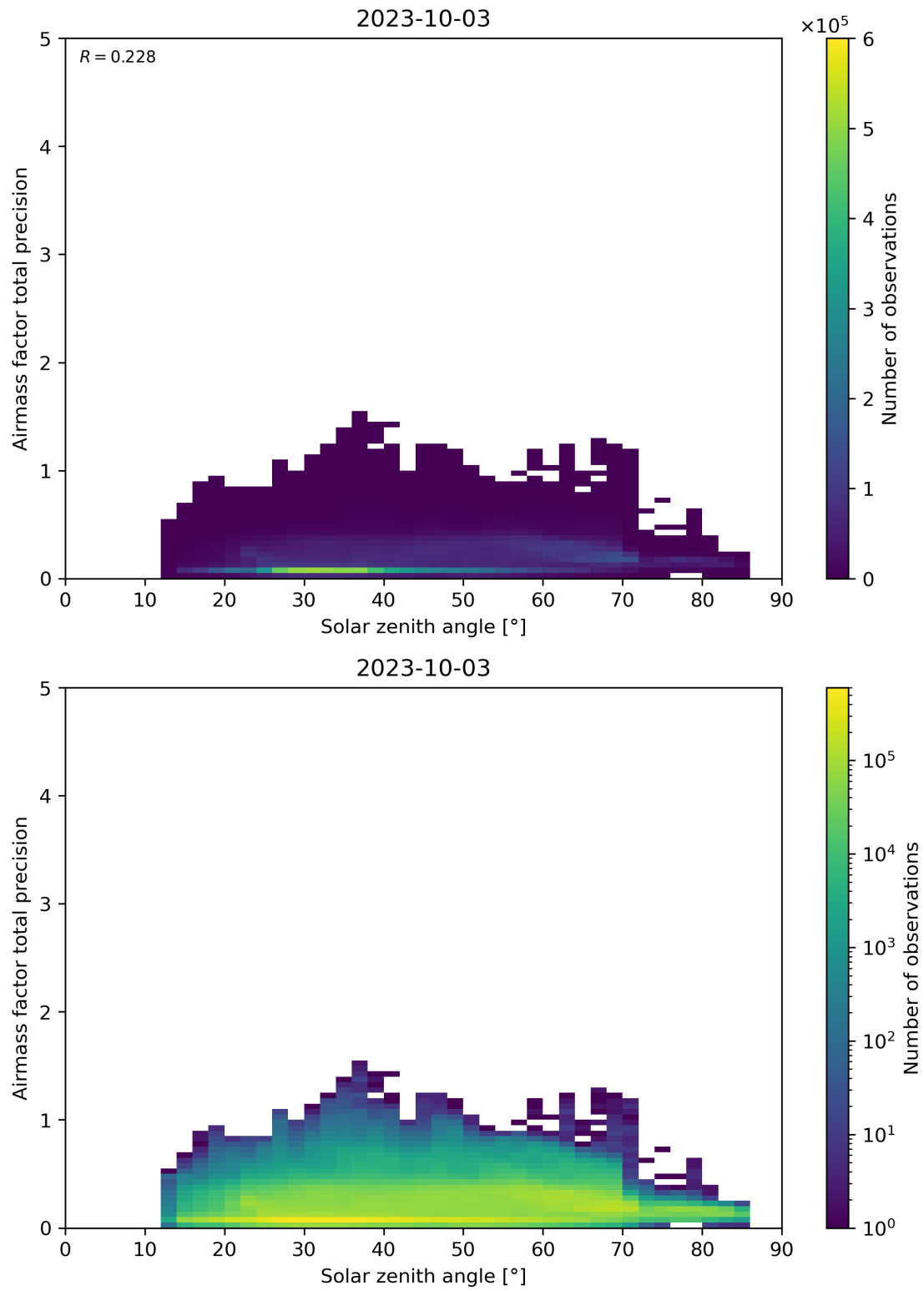
Figure 176: Scatter density plot of “Solar zenith angle” against “Airmass factor total precision” for 2023-10-02 to 2023-10-04.
