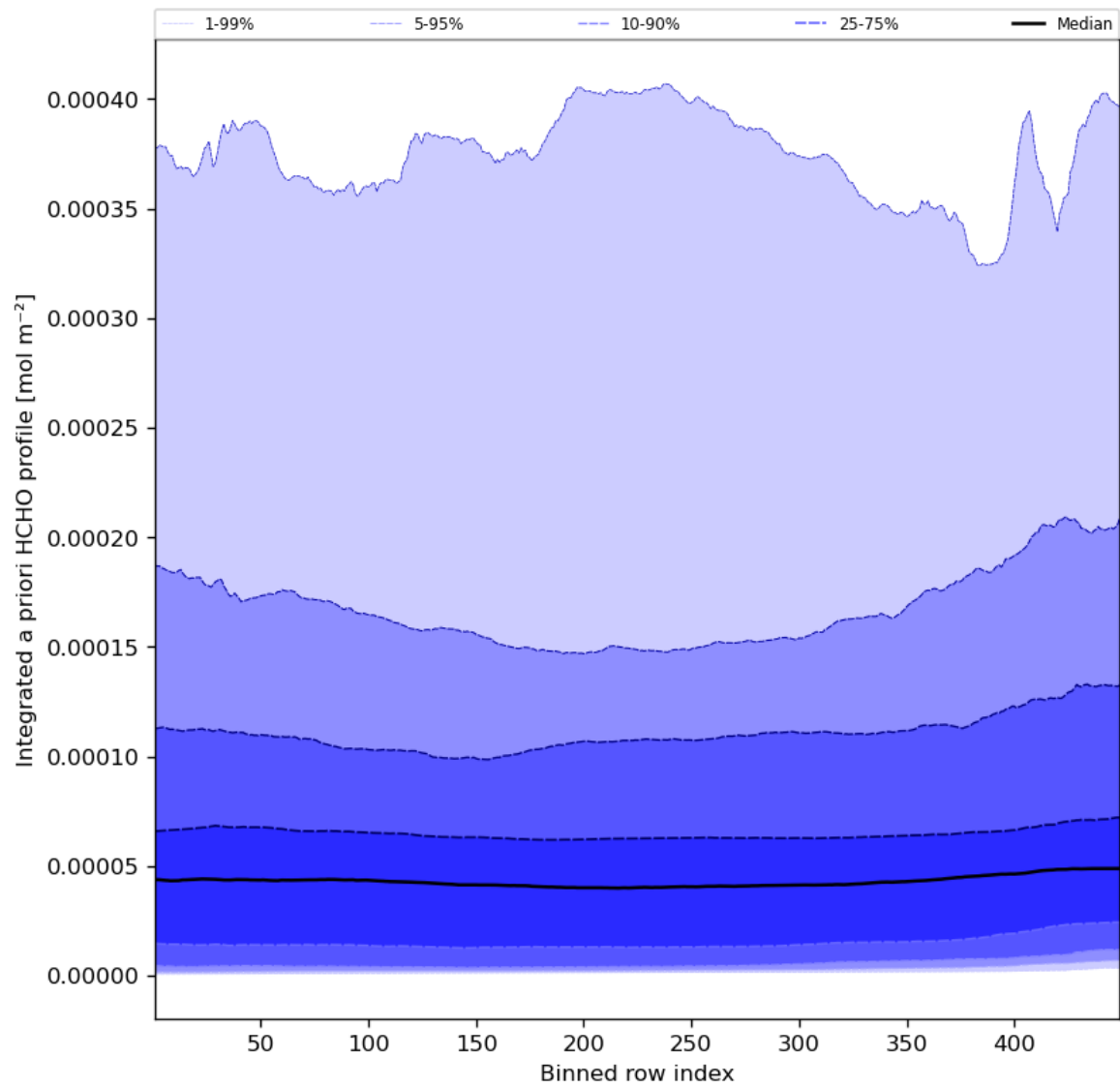
Figure 57: Along track statistics of “Integrated a priori HCHO profile” for 2023-10-02 to 2023-10-04
