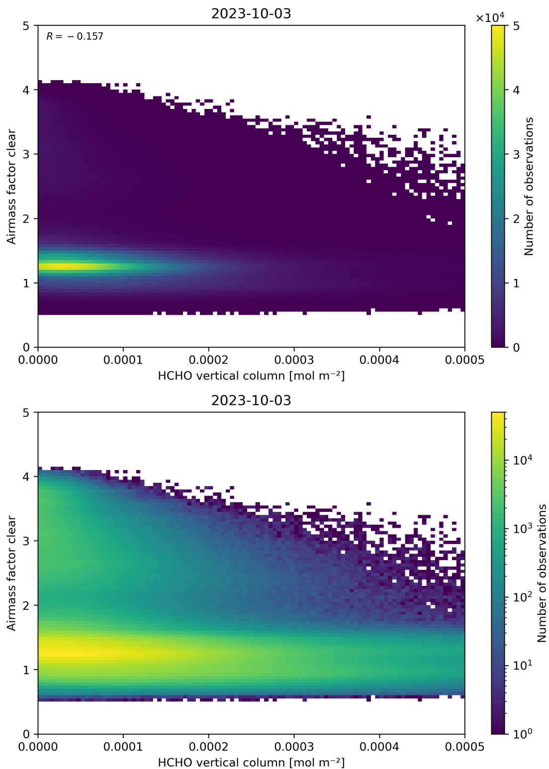
Figure 126: Scatter density plot of “HCHO vertical column” against “Airmass factor clear” for 2023-10-02 to 2023-10-04.
