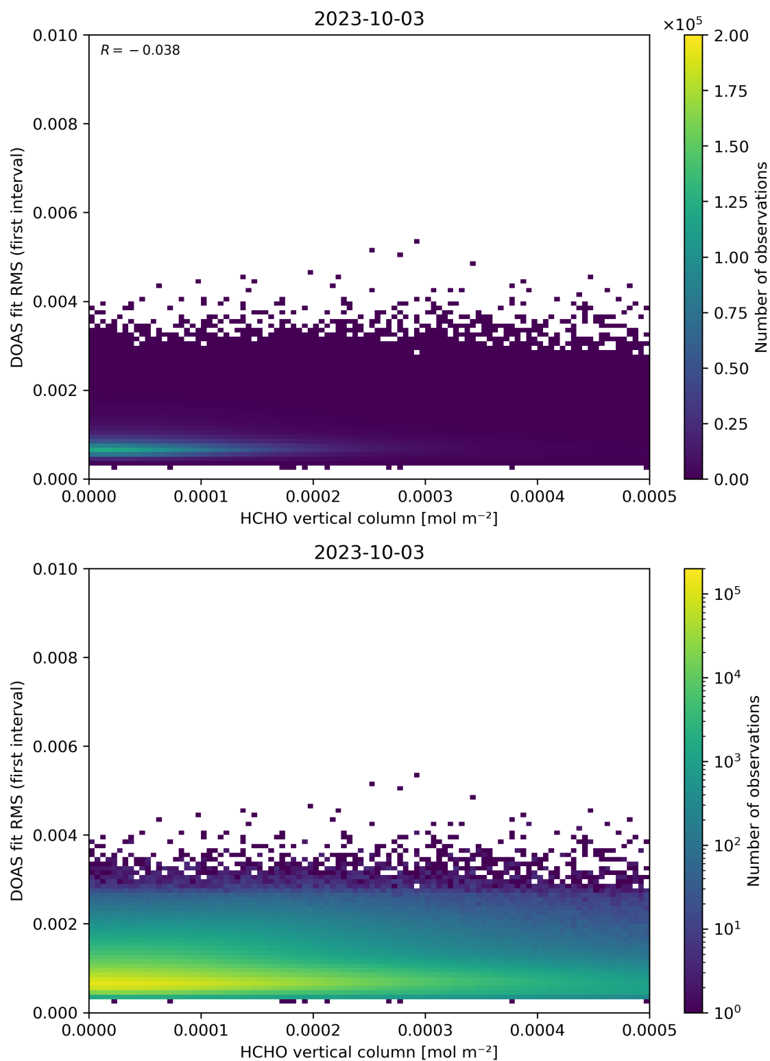
Figure 123: Scatter density plot of “HCHO vertical column” against “DOAS fit RMS (first interval)” for 2023-10-02 to 2023-10-04.
