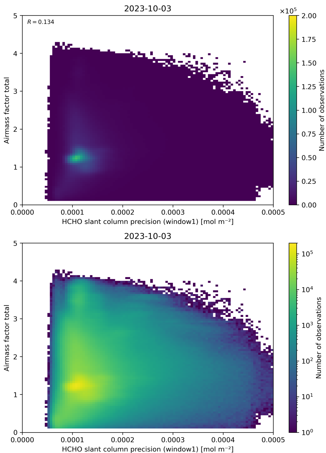
Figure 94: Scatter density plot of “HCHO slant column precision (window1)” against “Airmass factor total” for 2023-10-02 to 2023-10-04.
