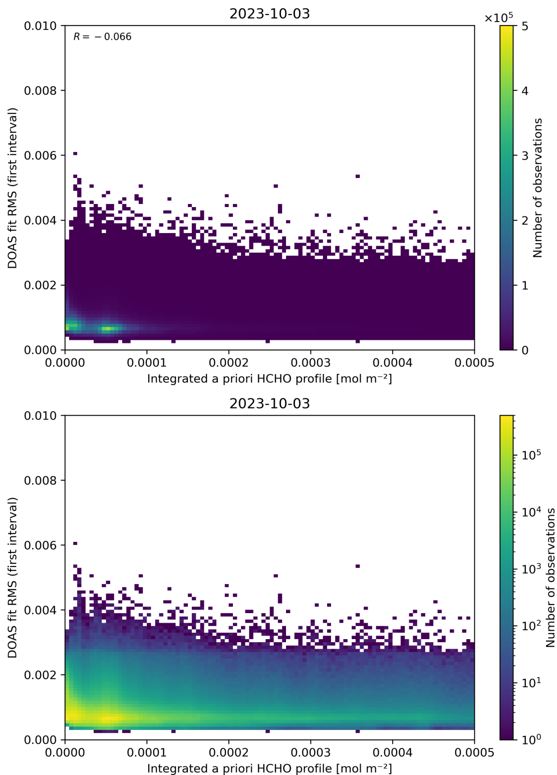
Figure 148: Scatter density plot of “Integrated a priori HCHO profile” against “DOAS fit RMS (first interval)” for 2023-10-02 to 2023-10-04.
