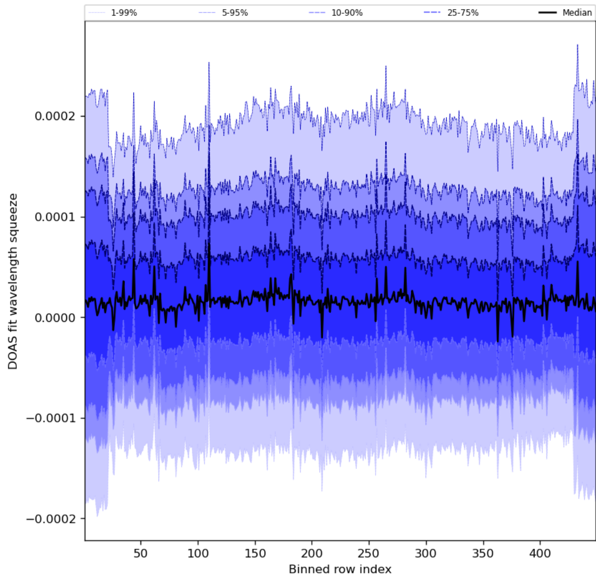
Figure 59: Along track statistics of “DOAS fit wavelength squeeze” for 2023-10-02 to 2023-10-04
