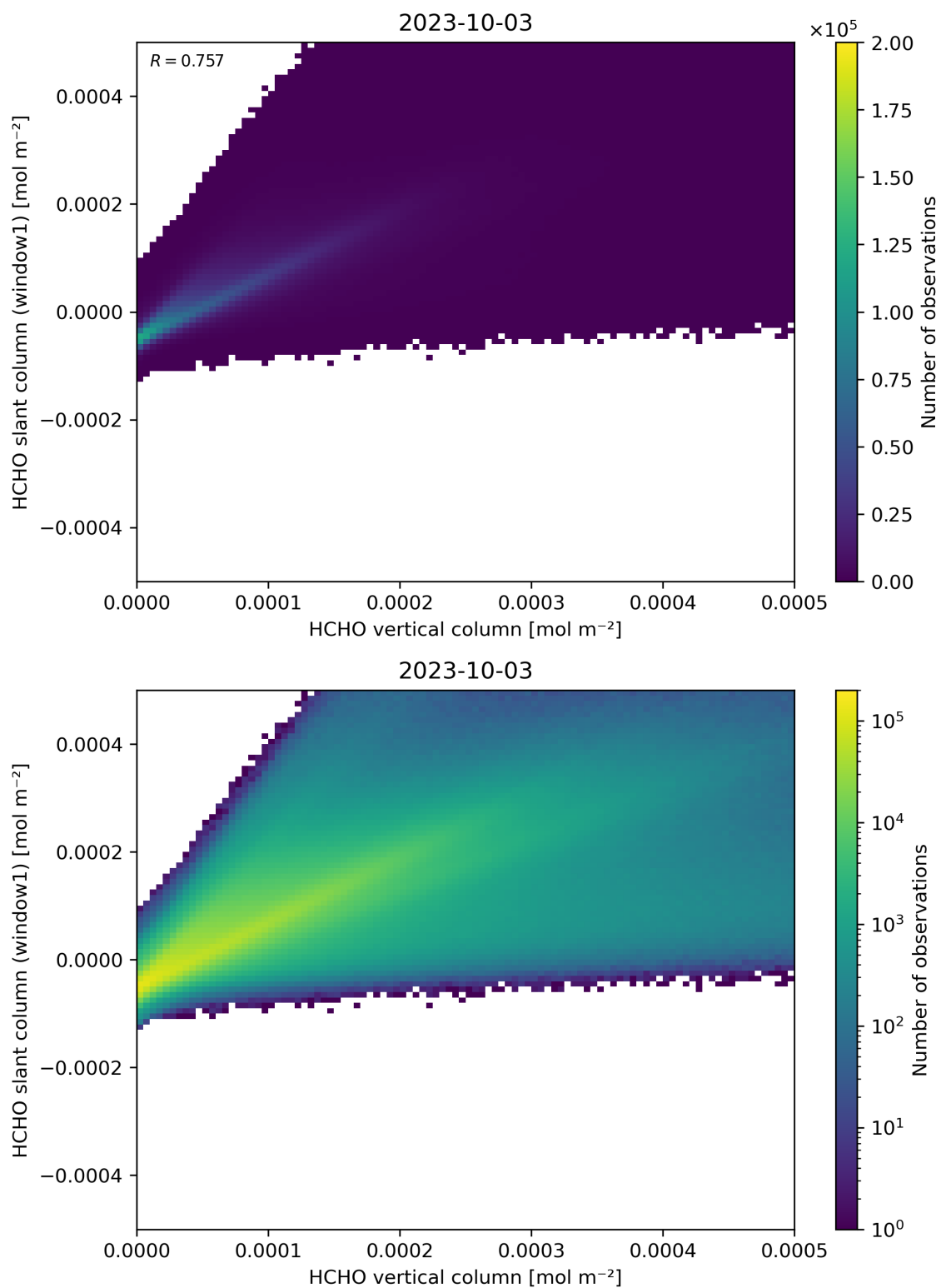
Figure 129: Scatter density plot of “HCHO vertical column” against “HCHO slant column (window1)” for 2023-10-02 to 2023-10-04.
