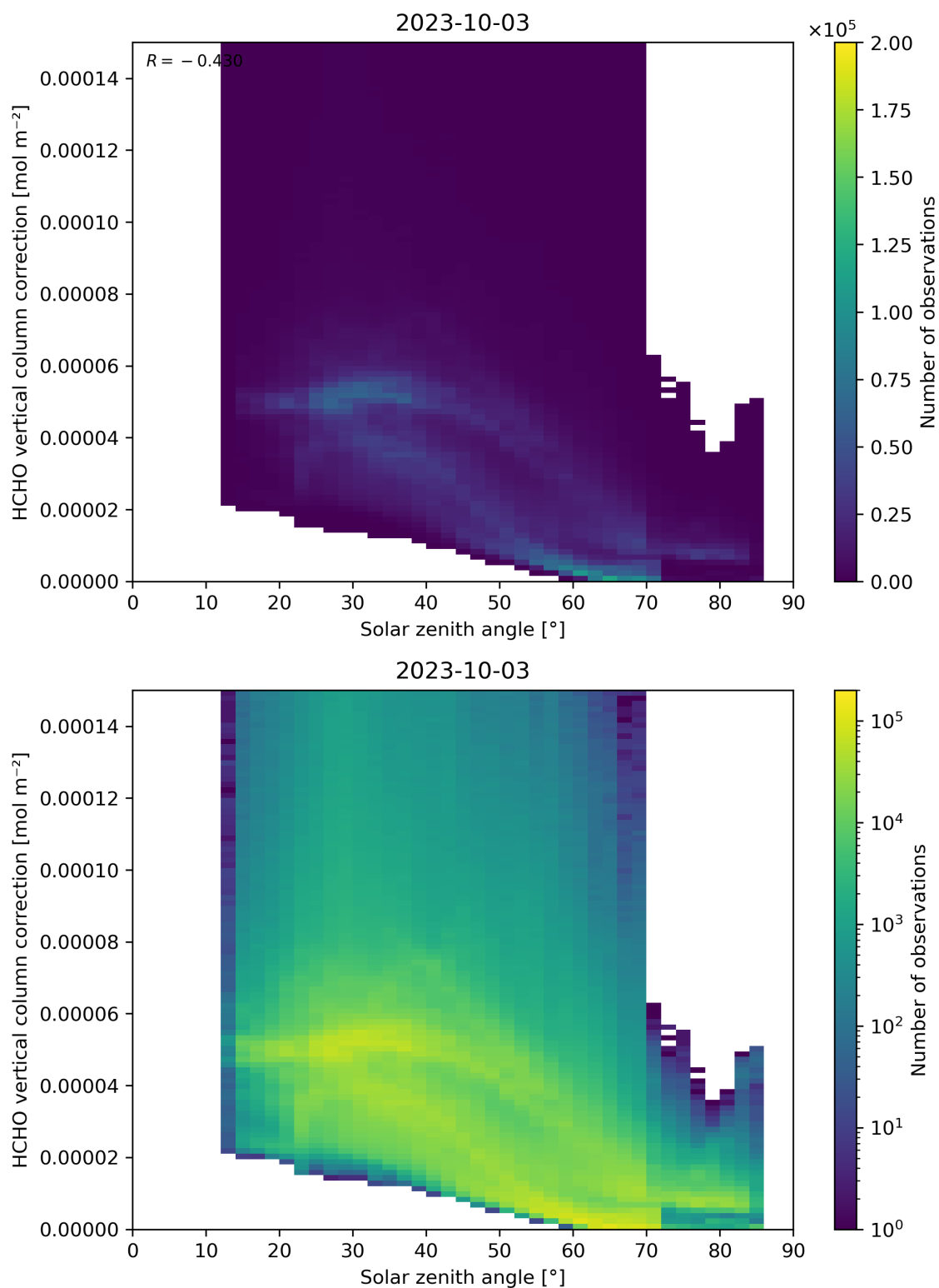
Figure 178: Scatter density plot of “Solar zenith angle” against “HCHO vertical column correction” for 2023-10-02 to 2023-10-04.
