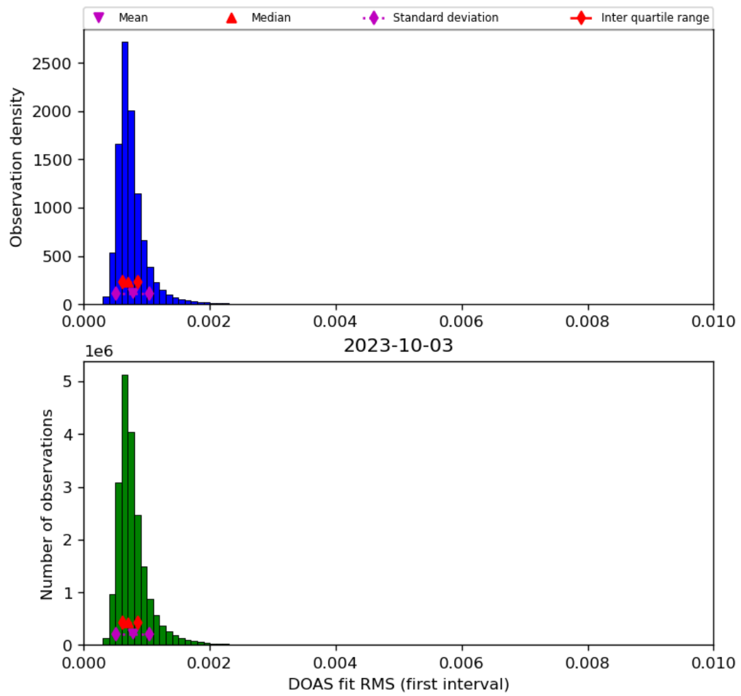
Figure 46: Histogram of “DOAS fit RMS (first interval)” for 2023-10-02 to 2023-10-04
