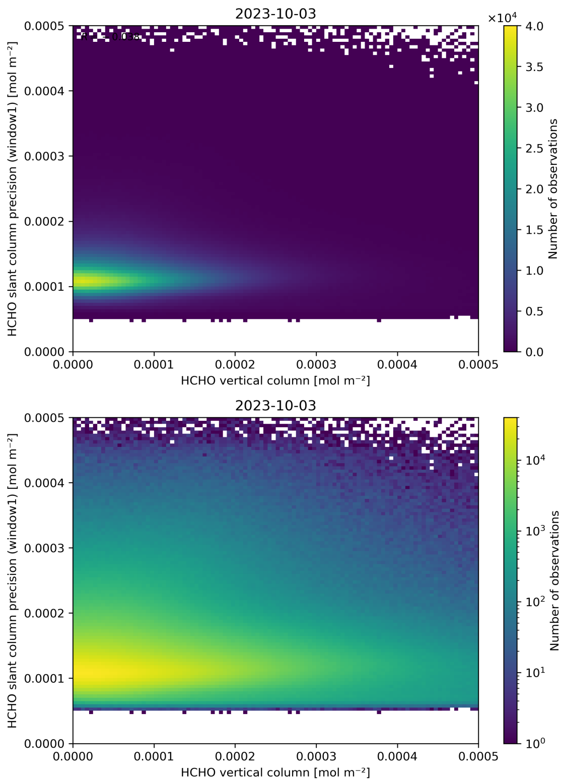
Figure 130: Scatter density plot of “HCHO vertical column” against “HCHO slant column precision (window1)” for 2023-10-02 to 2023-10-04.
