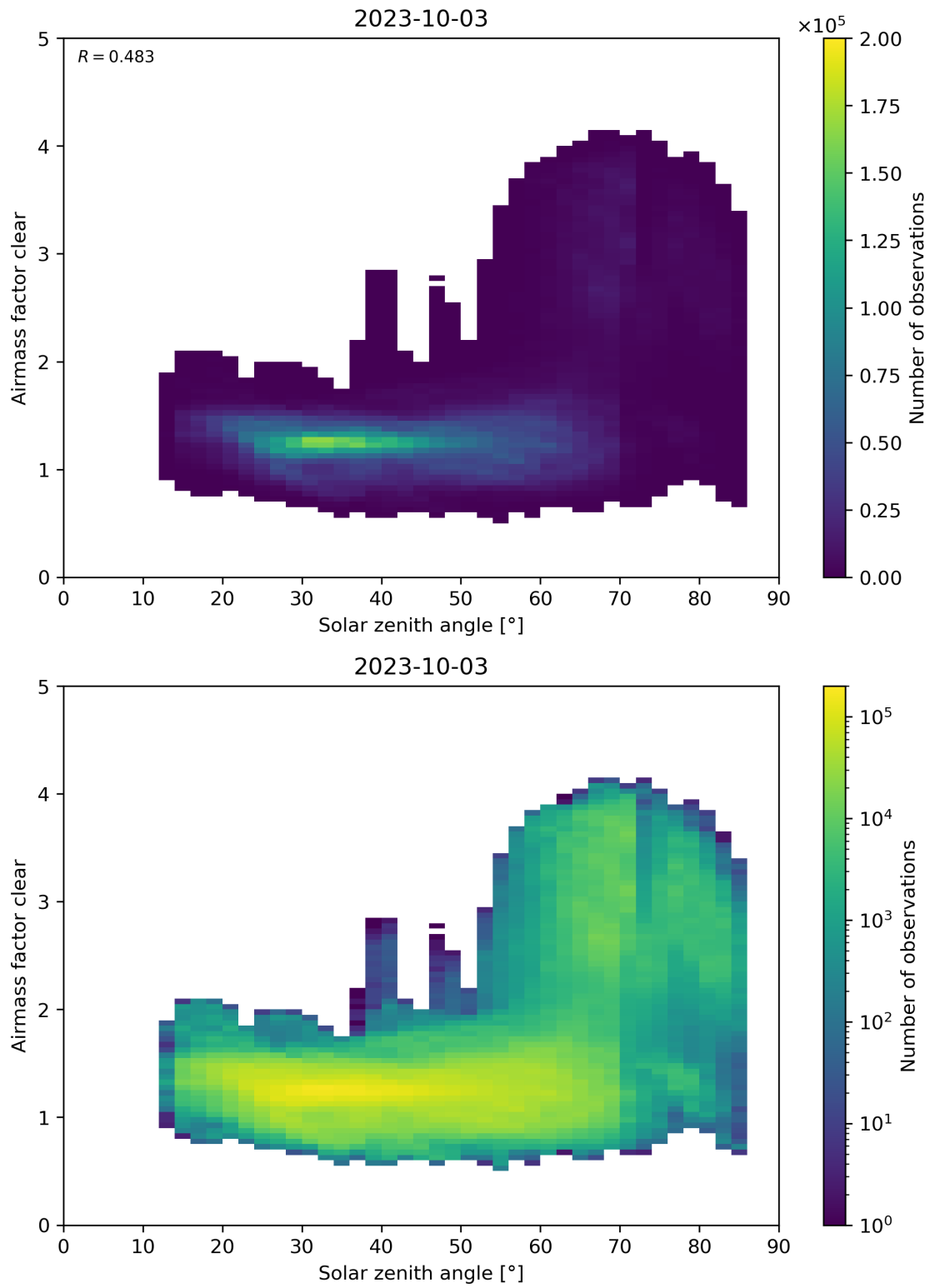
Figure 170: Scatter density plot of “Solar zenith angle” against “Airmass factor clear” for 2023-10-02 to 2023-10-04.
