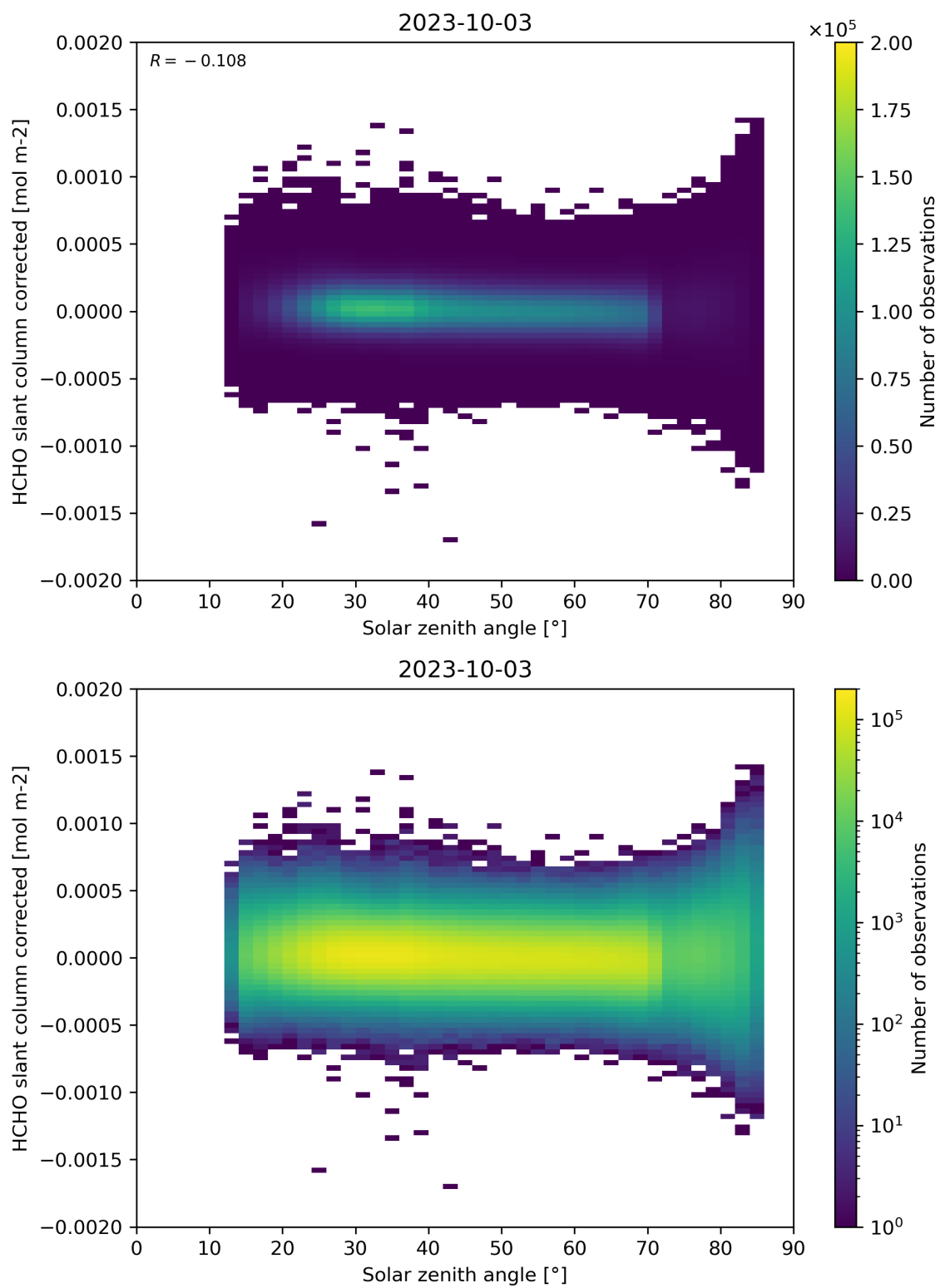
Figure 171: Scatter density plot of “Solar zenith angle” against “HCHO slant column corrected” for 2023-10-02 to 2023-10-04.
