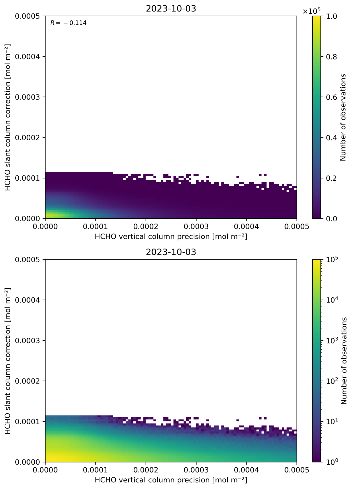
Figure 141: Scatter density plot of “HCHO vertical column precision” against “HCHO slant column correction” for 2023-10-02 to 2023-10-04.
