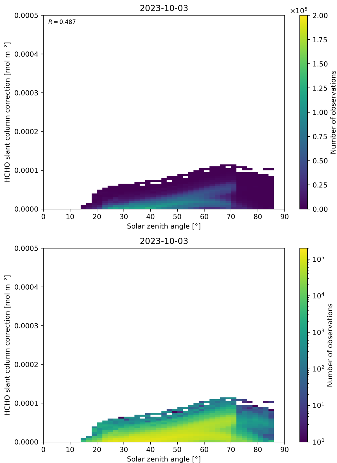
Figure 172: Scatter density plot of “Solar zenith angle” against “HCHO slant column correction” for 2023-10-02 to 2023-10-04.
