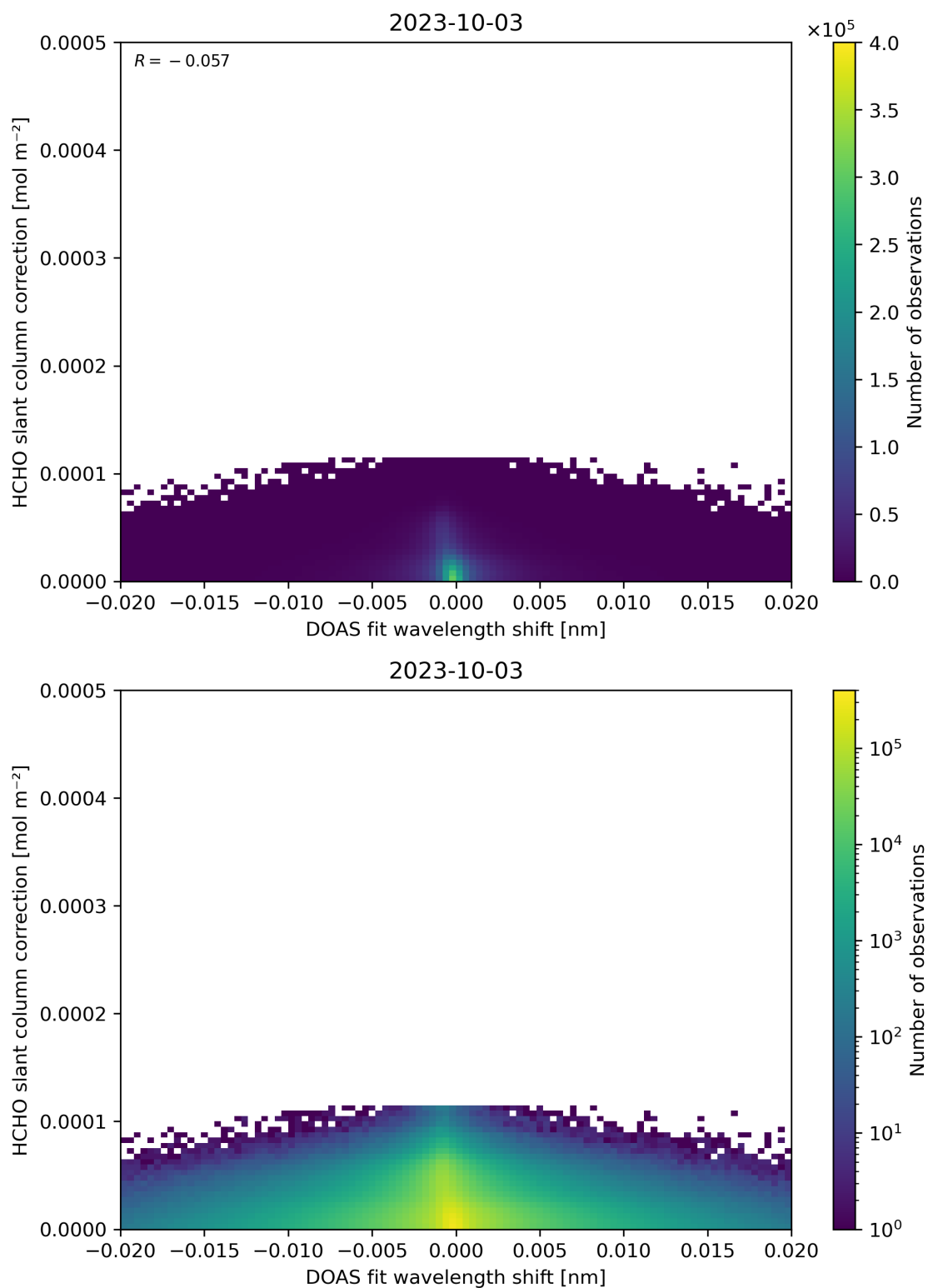
Figure 67: Scatter density plot of “DOAS fit wavelength shift” against “HCHO slant column correction” for 2023-10-02 to 2023-10-04.
