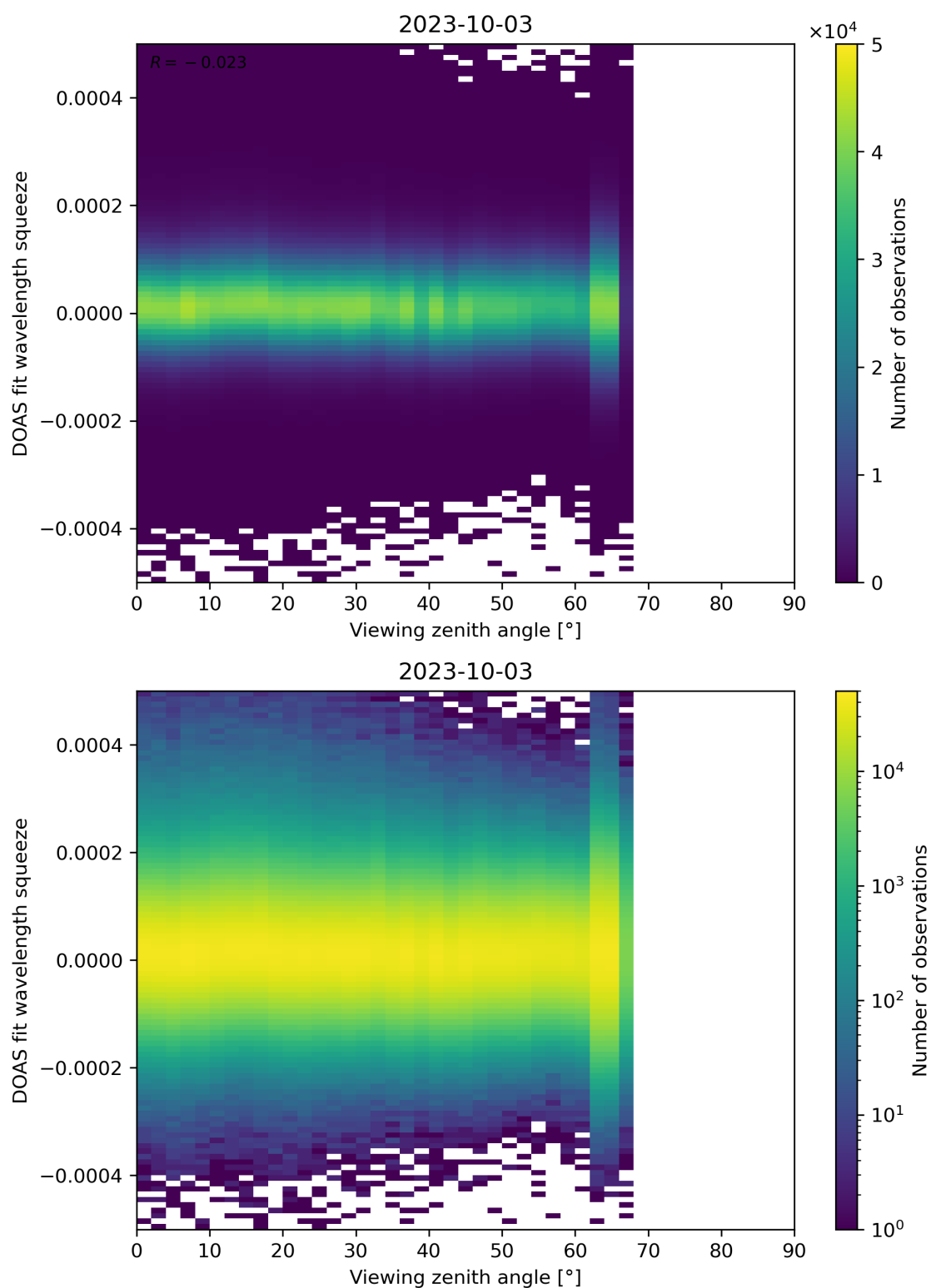
Figure 184: Scatter density plot of “Viewing zenith angle” against “DOAS fit wavelength squeeze” for 2023-10-02 to 2023-10-04.
