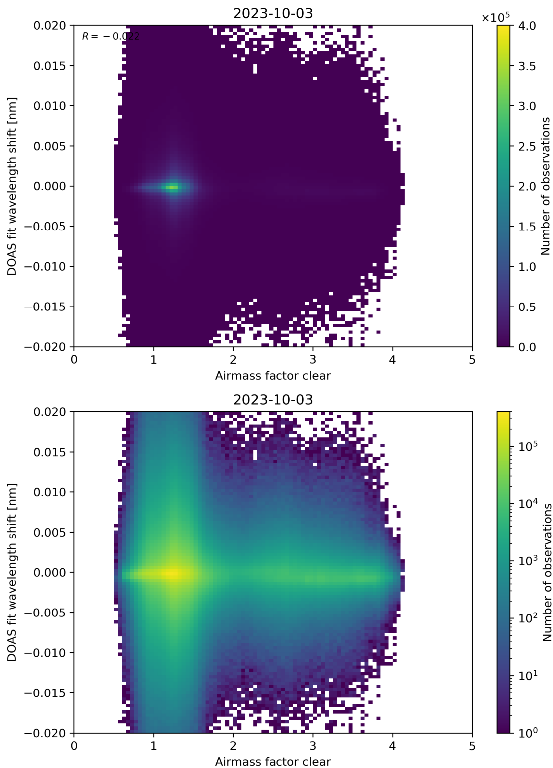
Figure 72: Scatter density plot of “Airmass factor clear” against “DOAS fit wavelength shift” for 2023-10-02 to 2023-10-04.
