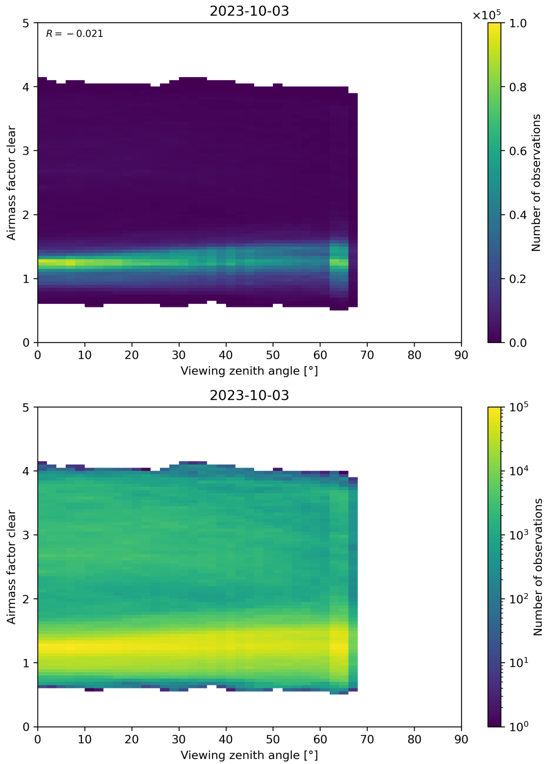
Figure 185: Scatter density plot of “Viewing zenith angle” against “Airmass factor clear” for 2023-10-02 to 2023-10-04.
