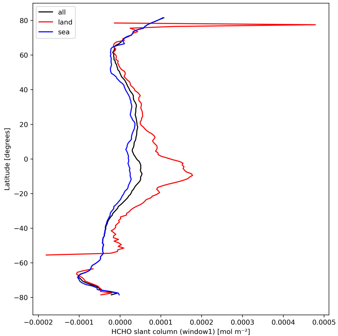
Figure 24: Zonal average of “HCHO slant column (window1)” for 2023-10-02 to 2023-10-04.
