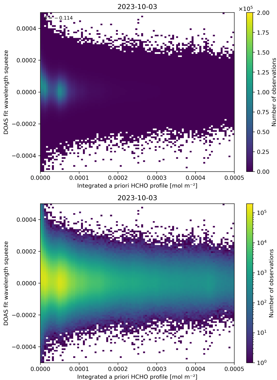
Figure 150: Scatter density plot of “Integrated a priori HCHO profile” against “DOAS fit wavelength squeeze” for 2023-10-02 to 2023-10-04.
