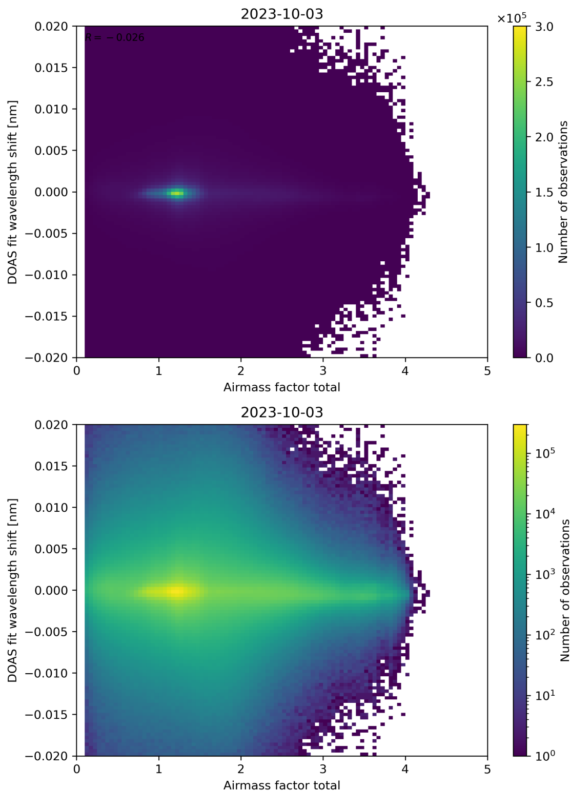
Figure 98: Scatter density plot of “Airmass factor total” against “DOAS fit wavelength shift” for 2023-10-02 to 2023-10-04.
