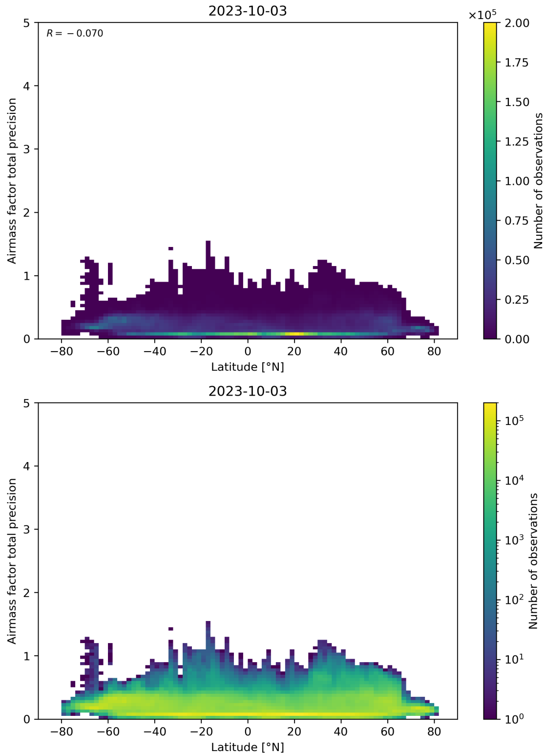
Figure 162: Scatter density plot of “Latitude” against “Airmass factor total precision” for 2023-10-02 to 2023-10-04.
