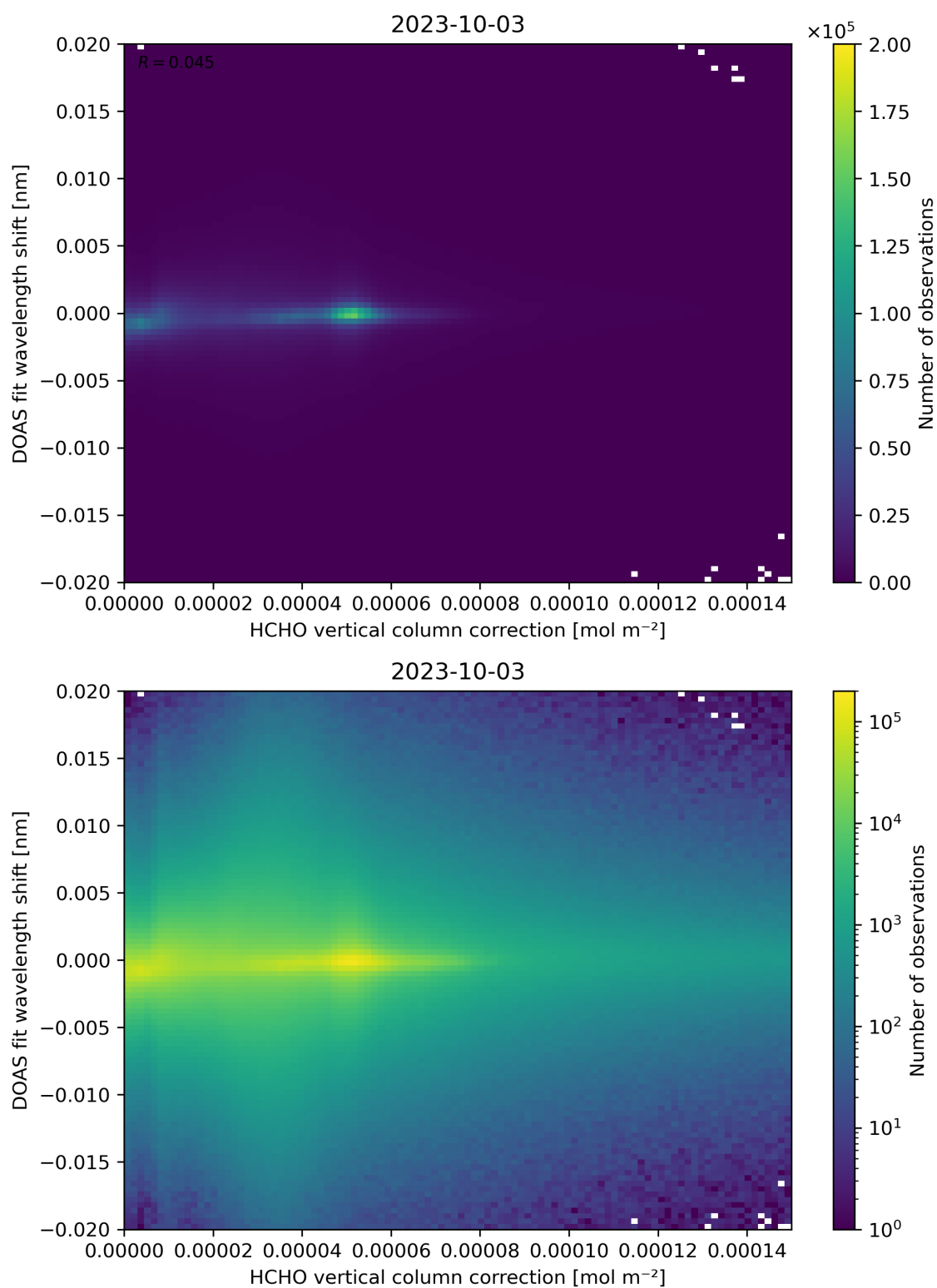
Figure 113: Scatter density plot of “HCHO vertical column correction” against “DOAS fit wavelength shift” for 2023-10-02 to 2023-10-04.
