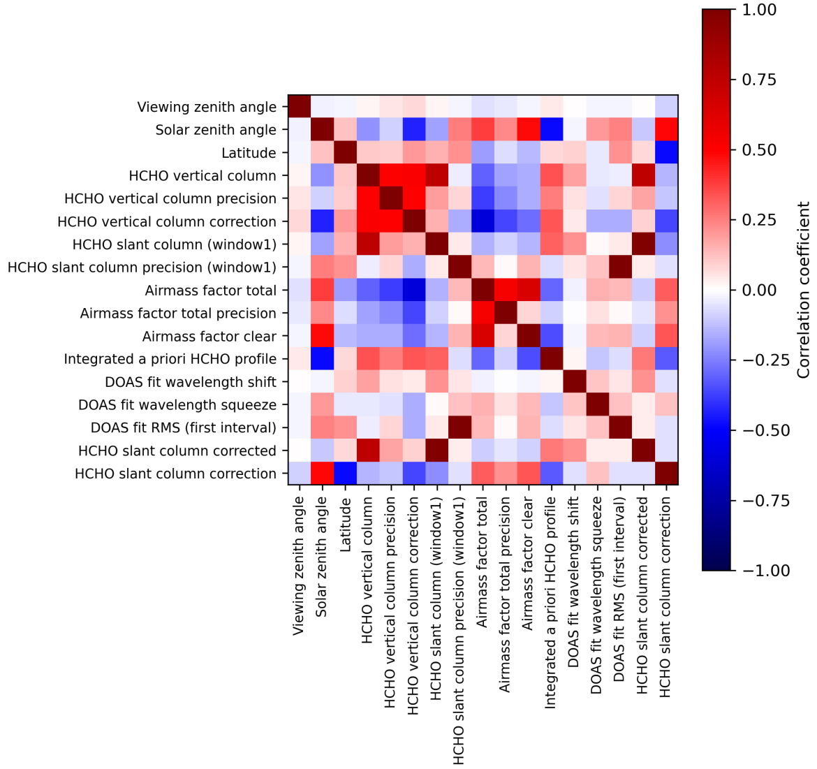
Figure 2: Map of correlation matrix for 2023-10-02 to 2023-10-04.
