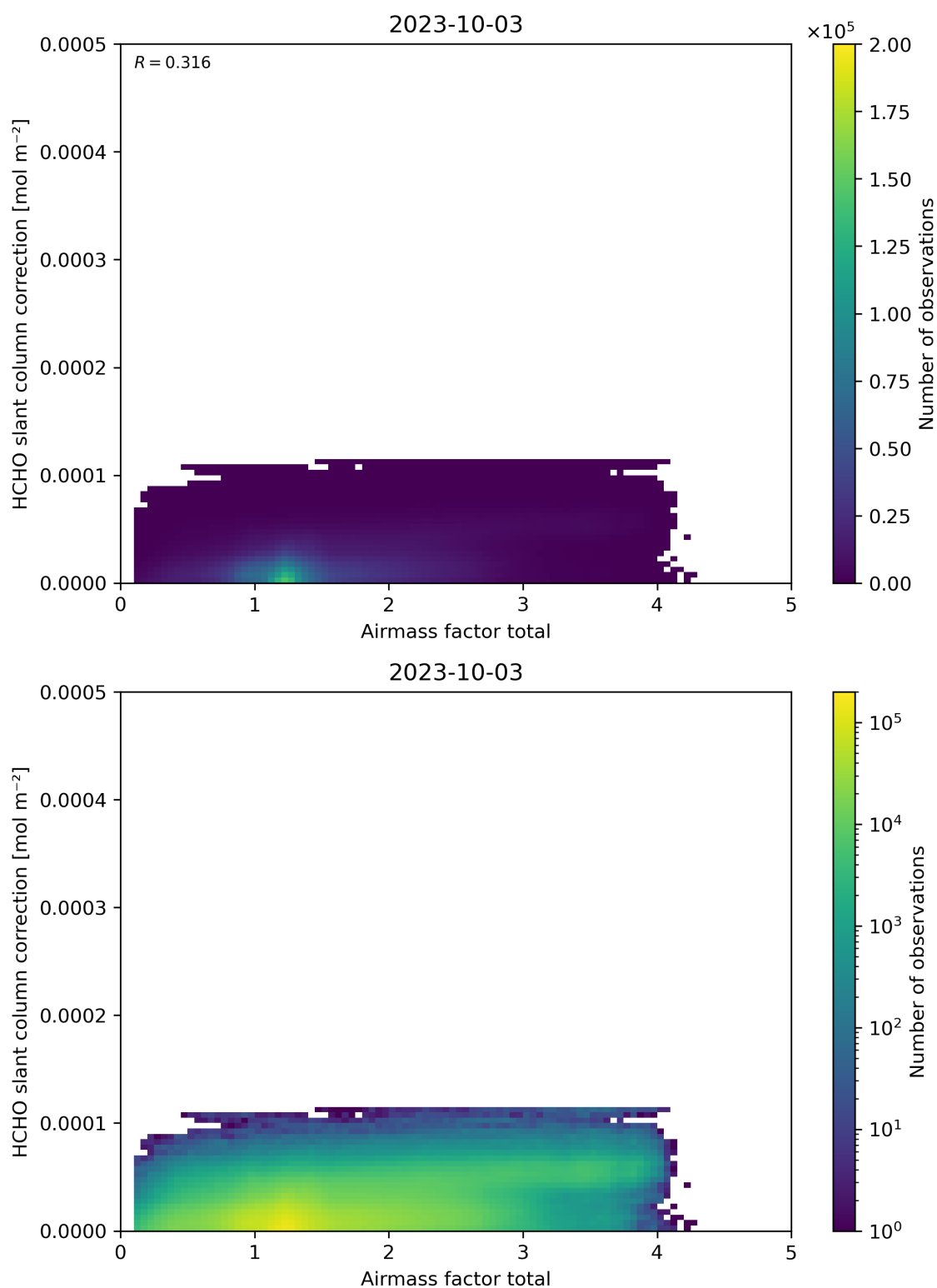
Figure 102: Scatter density plot of “Airmass factor total” against “HCHO slant column correction” for 2023-10-02 to 2023-10-04.
