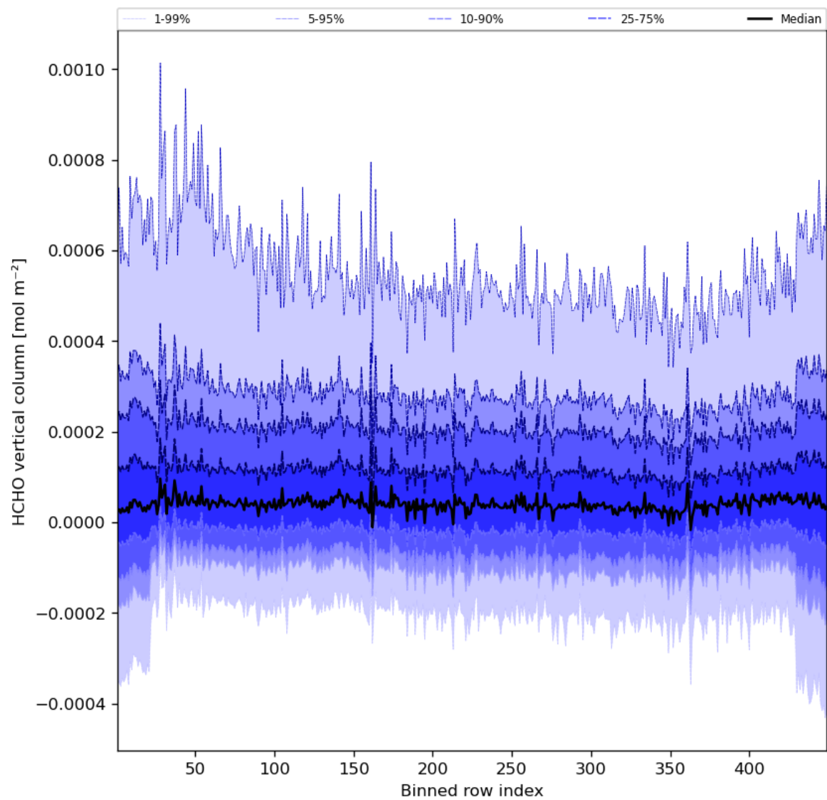
Figure 49: Along track statistics of “HCHO vertical column” for 2023-10-02 to 2023-10-04
