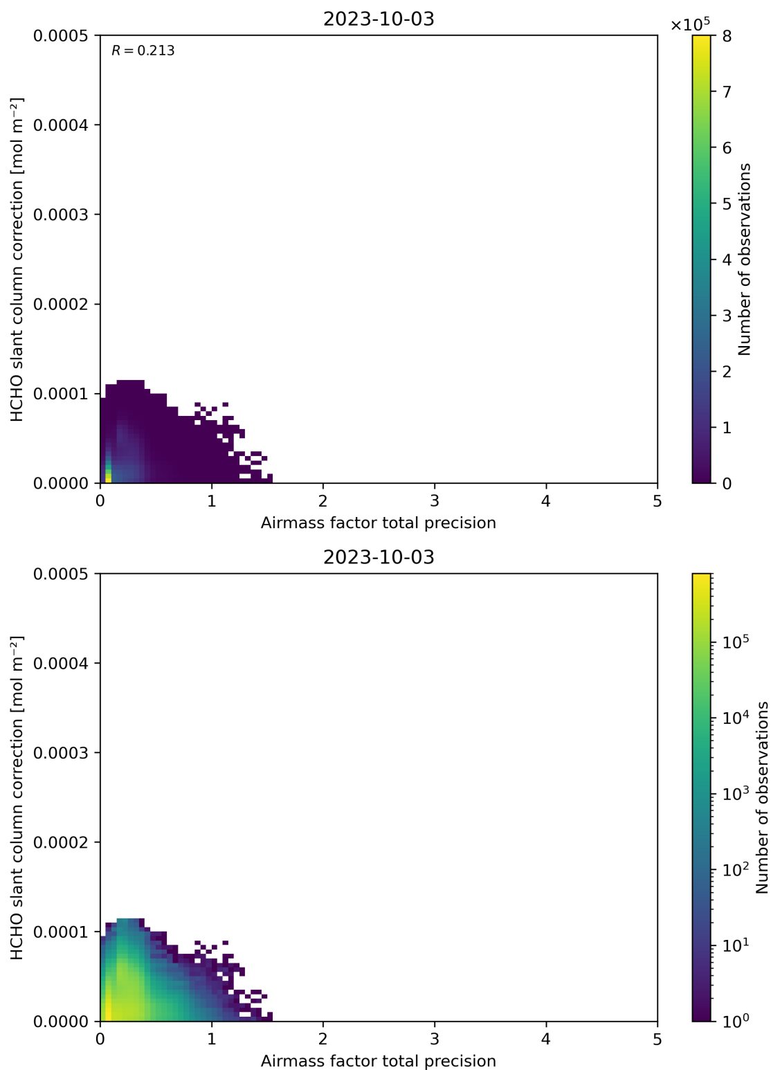
Figure 110: Scatter density plot of “Airmass factor total precision” against “HCHO slant column correction” for 2023-10-02 to 2023-10-04.
