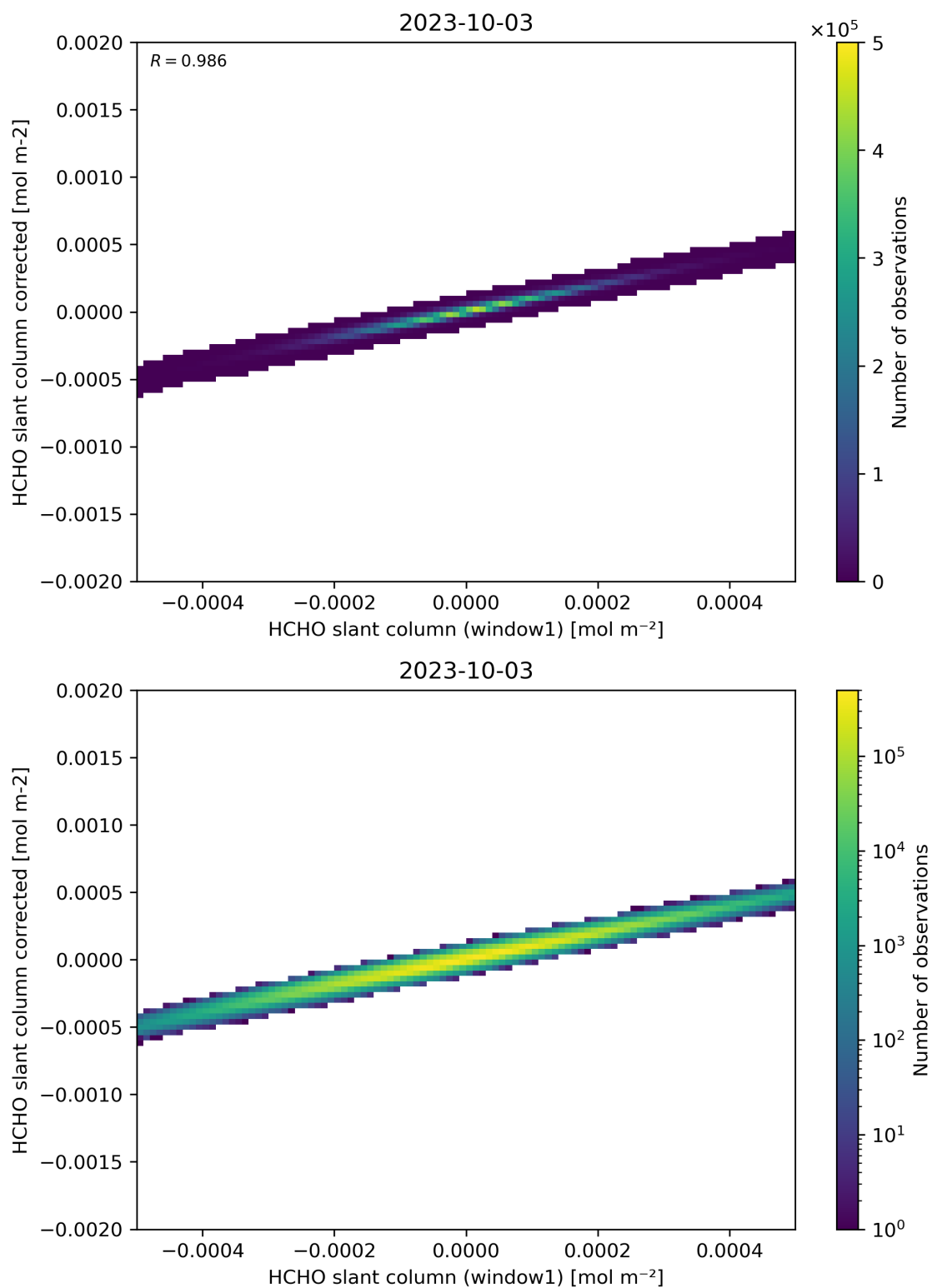
Figure 82: Scatter density plot of “HCHO slant column (window1)” against “HCHO slant column corrected” for 2023-10-02 to 2023-10-04.
