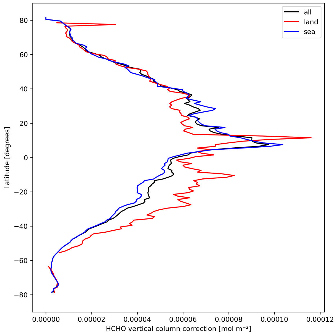
Figure 23: Zonal average of “HCHO vertical column correction” for 2023-10-02 to 2023-10-04.
