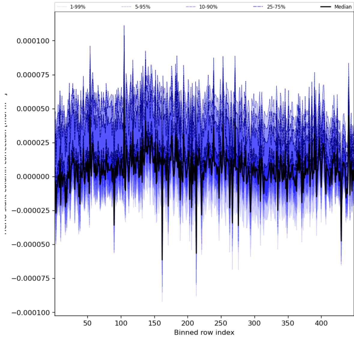
Figure 61: Along track statistics of “HCHO slant column correction” for 2023-10-02 to 2023-10-04
