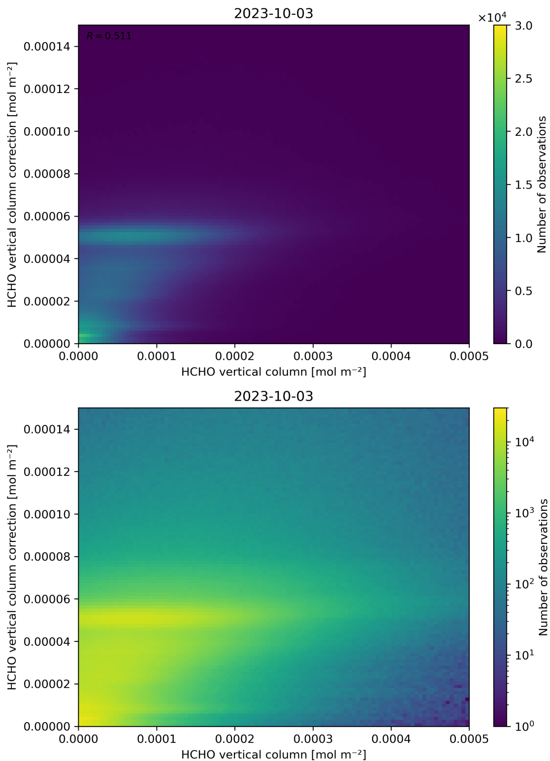
Figure 133: Scatter density plot of “HCHO vertical column” against “HCHO vertical column correction” for 2023-10-02 to 2023-10-04.
