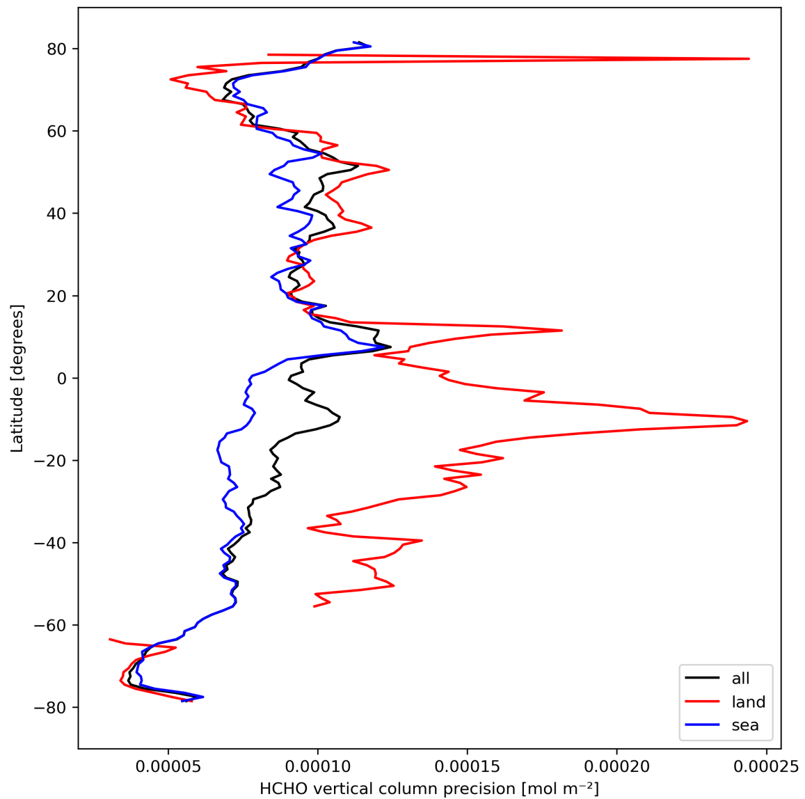
Figure 22: Zonal average of “HCHO vertical column precision” for 2023-10-02 to 2023-10-04.
