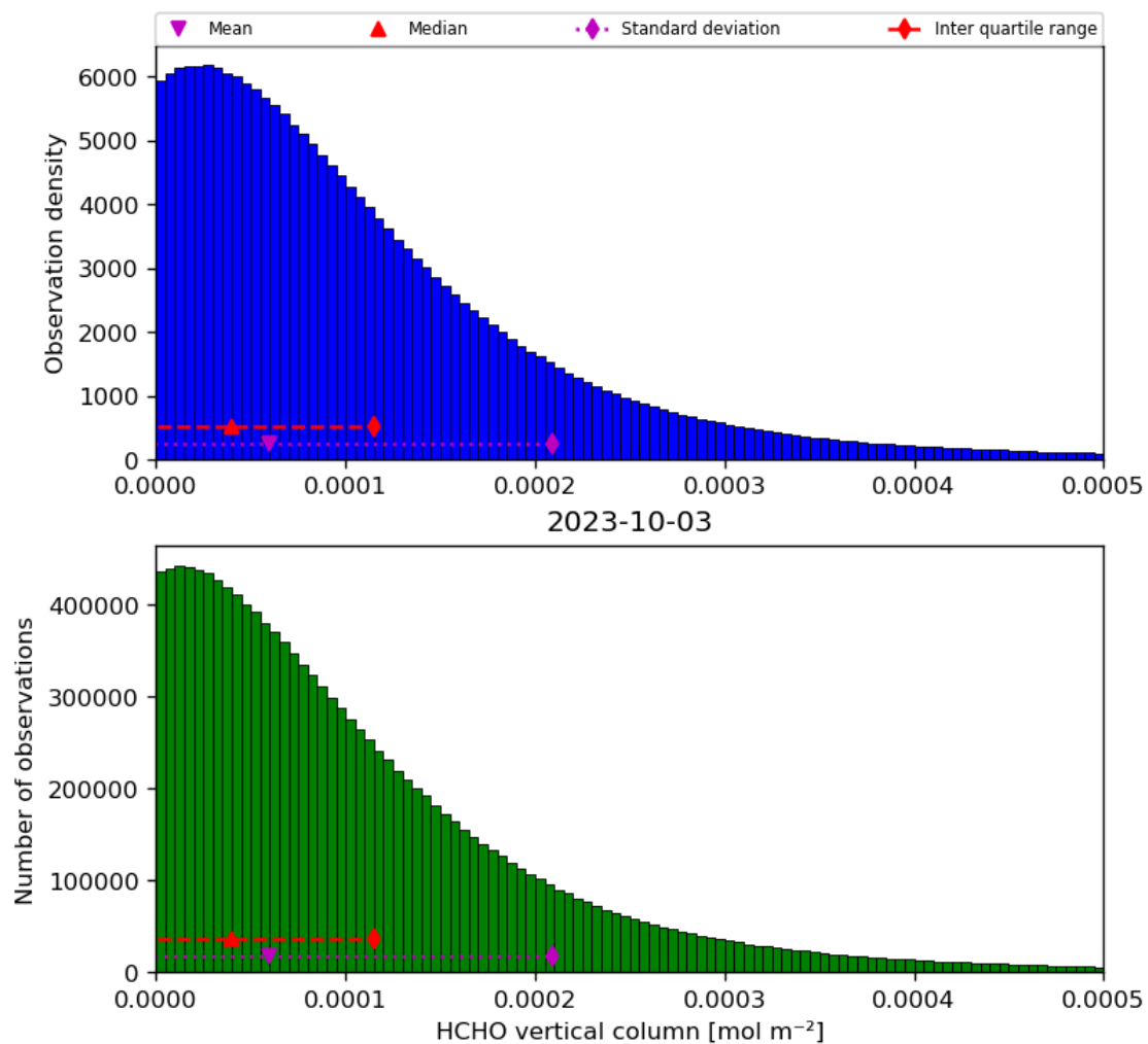
Figure 35: Histogram of “HCHO vertical column” for 2023-10-02 to 2023-10-04
