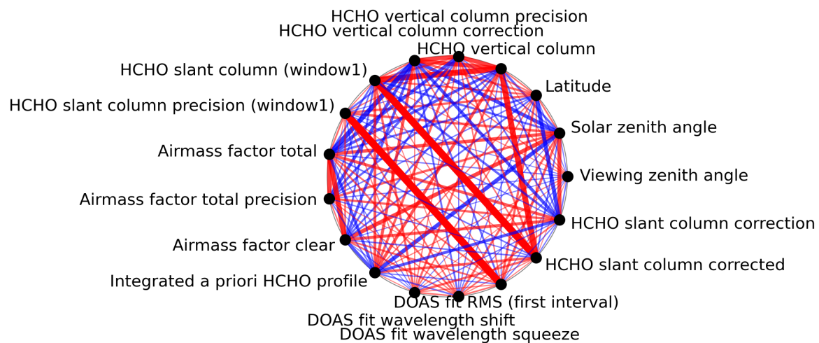
Figure 1: Map of correlation graph for 2023-10-02 to 2023-10-04.
