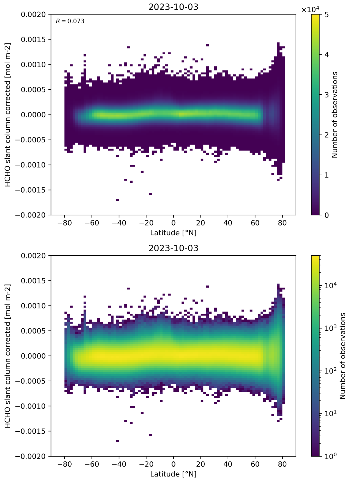
Figure 157: Scatter density plot of “Latitude” against “HCHO slant column corrected” for 2023-10-02 to 2023-10-04.
