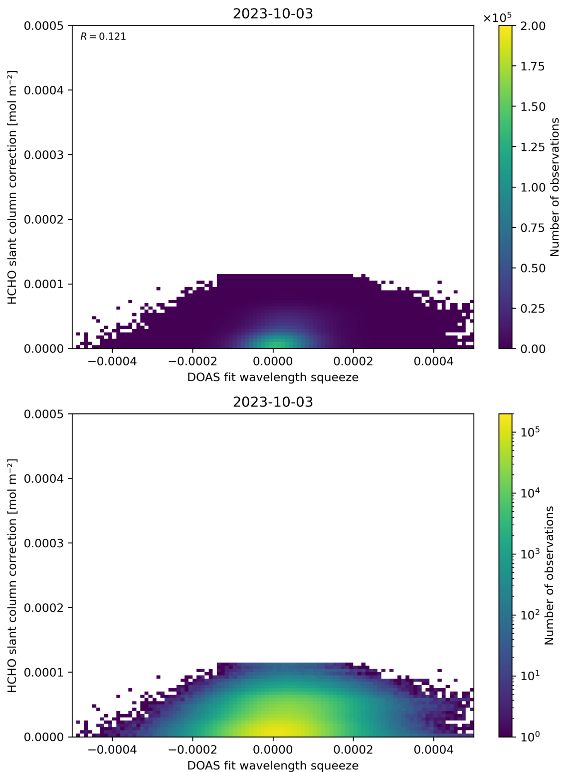
Figure 70: Scatter density plot of “DOAS fit wavelength squeeze” against “HCHO slant column correction” for 2023-10-02 to 2023-10-04.
