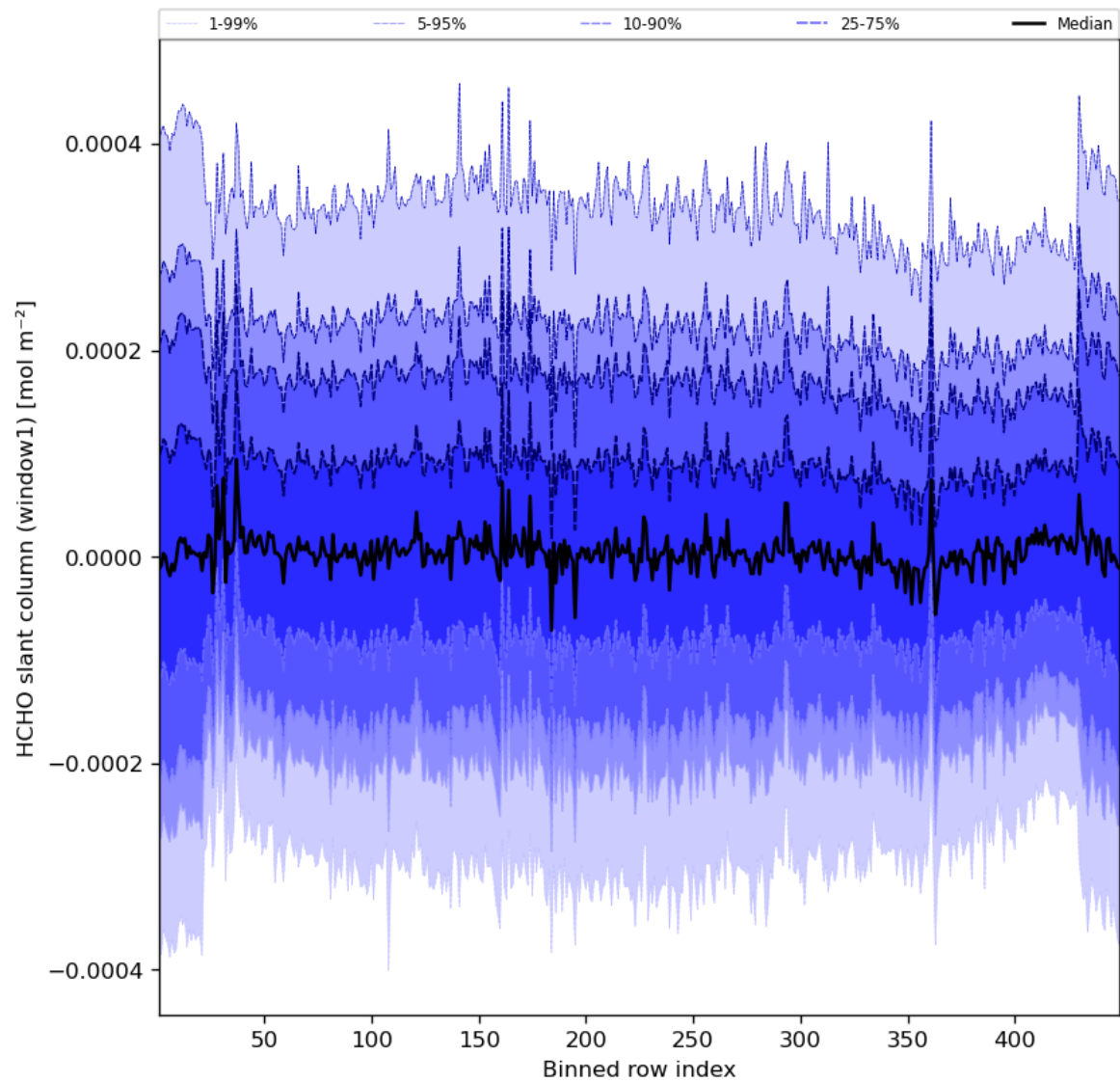
Figure 52: Along track statistics of “HCHO slant column (window1)” for 2023-10-02 to 2023-10-04
