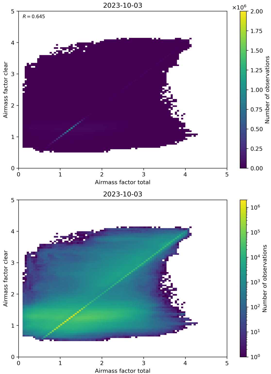
Figure 100: Scatter density plot of “Airmass factor total” against “Airmass factor clear” for 2023-10-02 to 2023-10-04.
