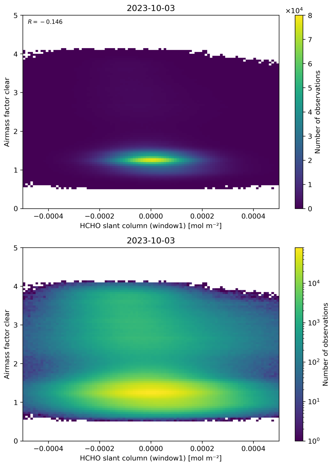
Figure 81: Scatter density plot of “HCHO slant column (window1)” against “Airmass factor clear” for 2023-10-02 to 2023-10-04.
