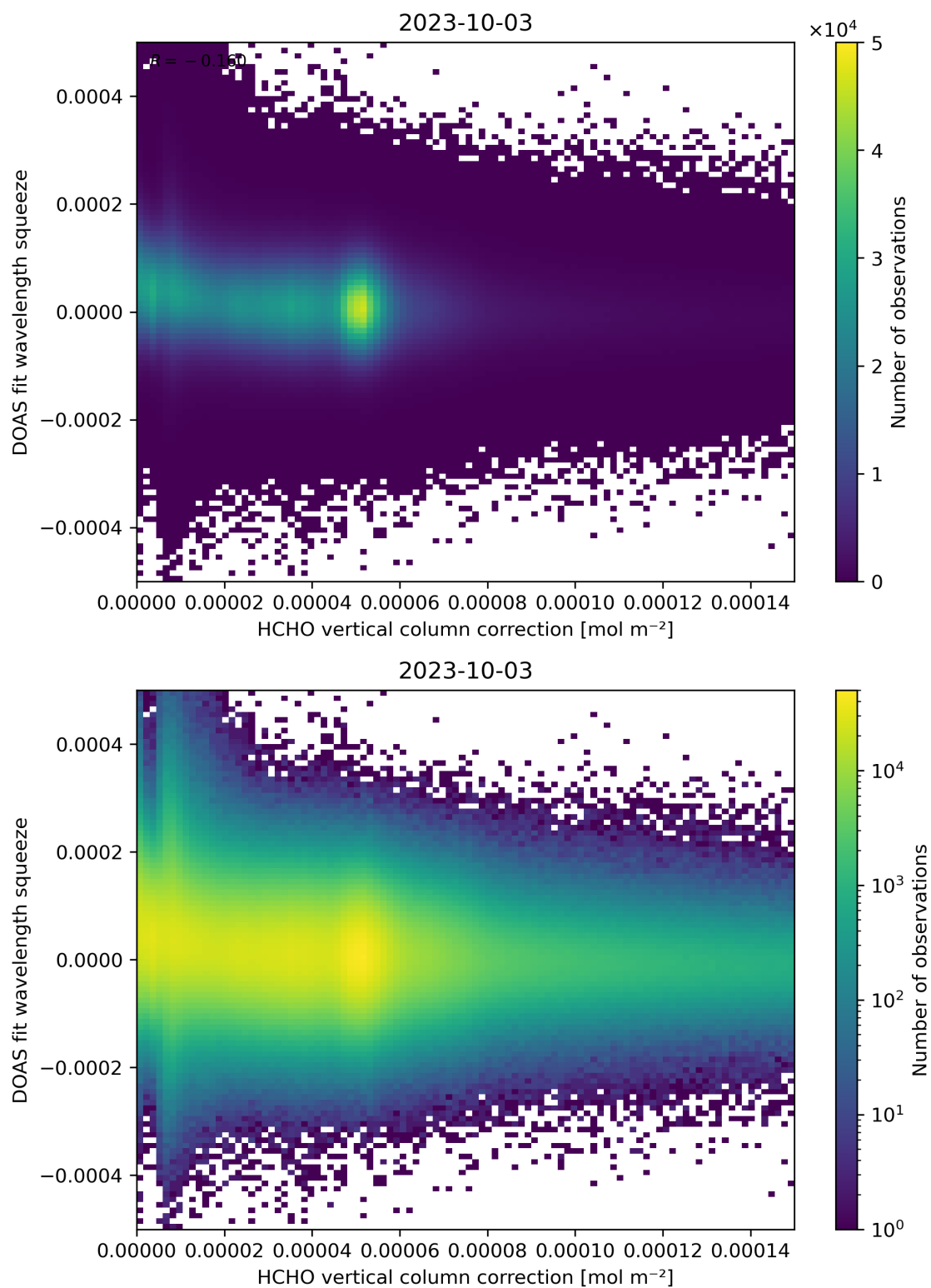
Figure 114: Scatter density plot of “HCHO vertical column correction” against “DOAS fit wavelength squeeze” for 2023-10-02 to 2023-10-04.
