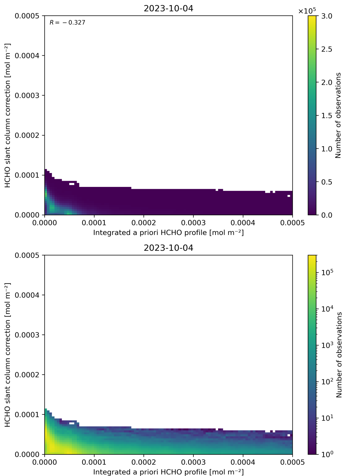
Figure 152: Scatter density plot of “Integrated a priori HCHO profile” against “HCHO slant column correction” for 2023-10-03 to 2023-10-05.
