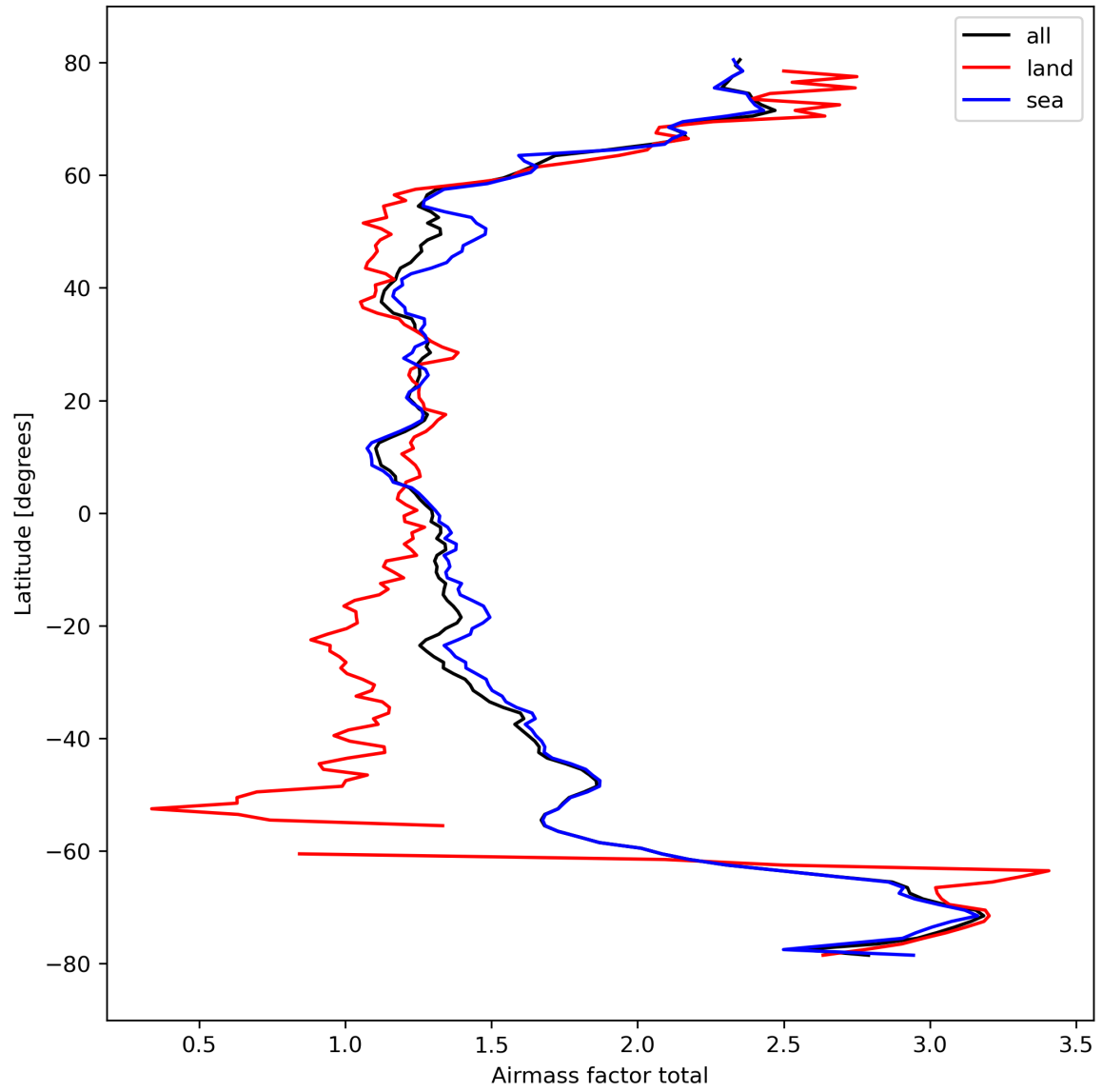
Figure 26: Zonal average of “Airmass factor total” for 2023-10-03 to 2023-10-05.
