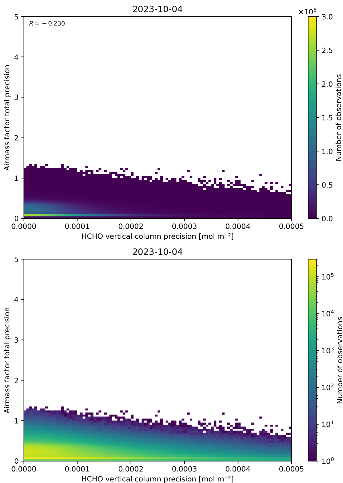
Figure 145: Scatter density plot of “HCHO vertical column precision” against “Airmass factor total precision” for 2023-10-03 to 2023-10-05.
