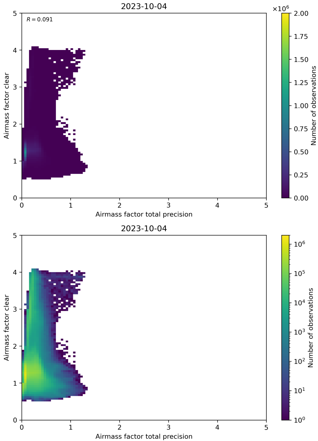
Figure 108: Scatter density plot of “Airmass factor total precision” against “Airmass factor clear” for 2023-10-03 to 2023-10-05.
