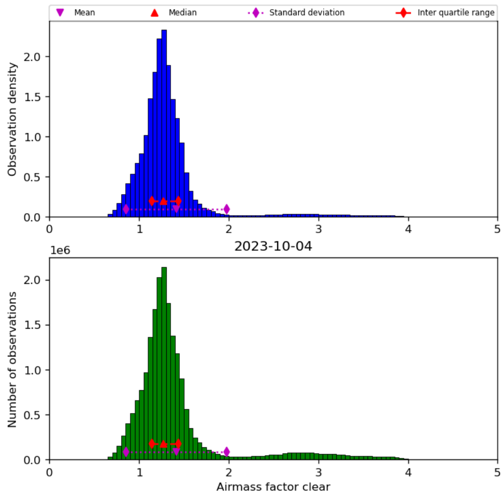
Figure 42: Histogram of “Airmass factor clear” for 2023-10-03 to 2023-10-05
