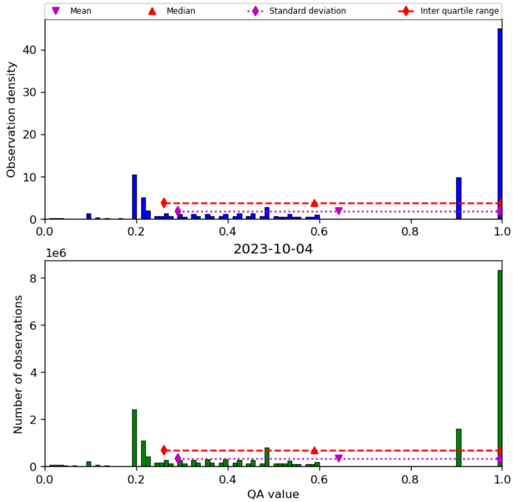
Figure 34: Histogram of “QA value” for 2023-10-03 to 2023-10-05
