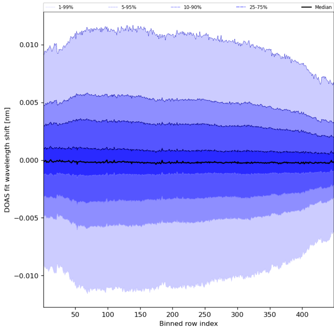
Figure 58: Along track statistics of “DOAS fit wavelength shift” for 2023-10-03 to 2023-10-05
