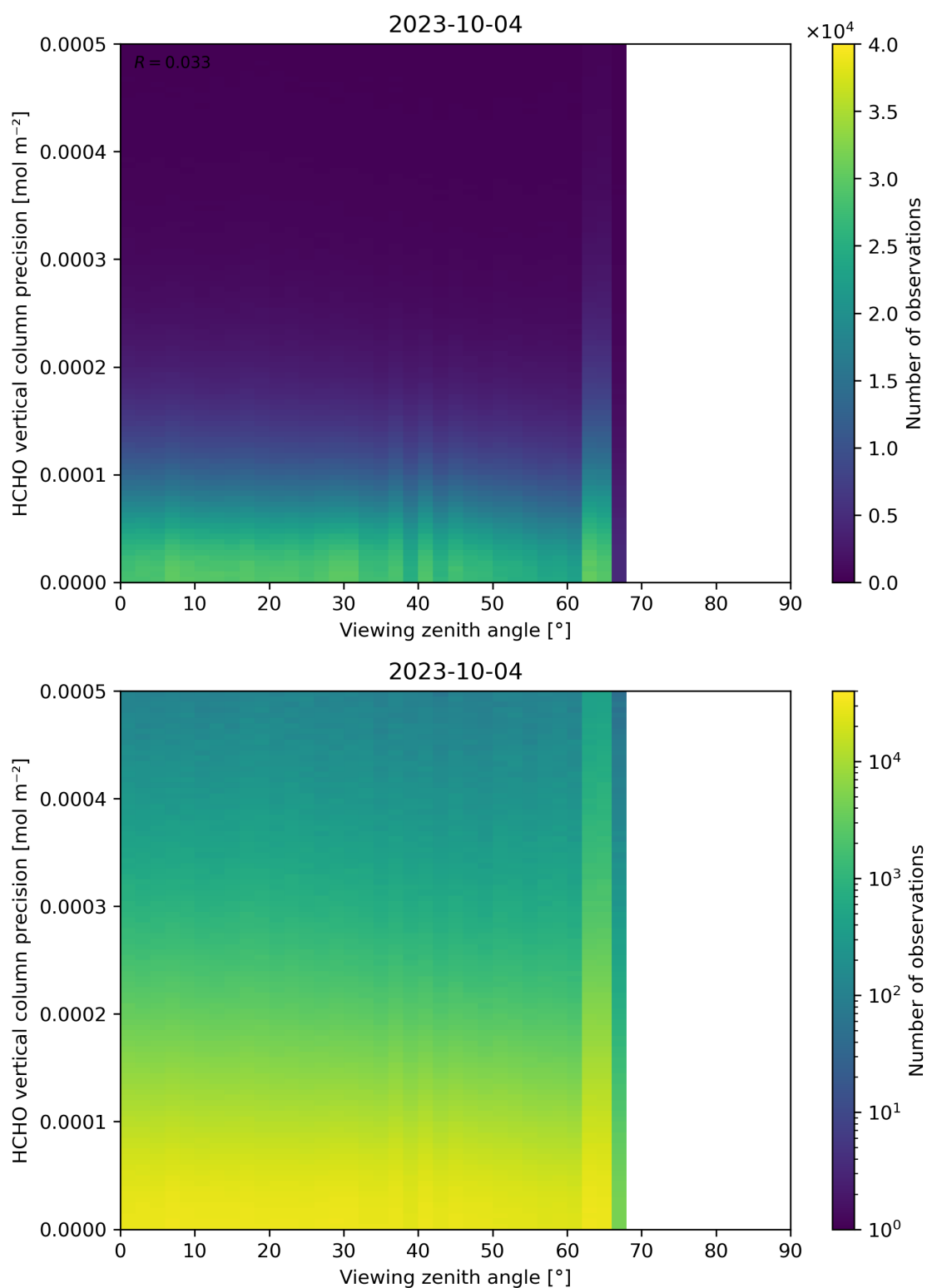
Figure 194: Scatter density plot of “Viewing zenith angle” against “HCHO vertical column precision” for 2023-10-03 to 2023-10-05.
