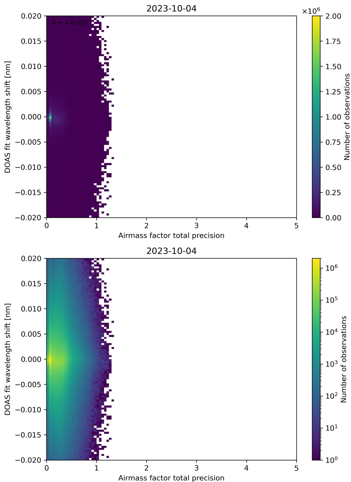
Figure 106: Scatter density plot of “Airmass factor total precision” against “DOAS fit wavelength shift” for 2023-10-03 to 2023-10-05.
