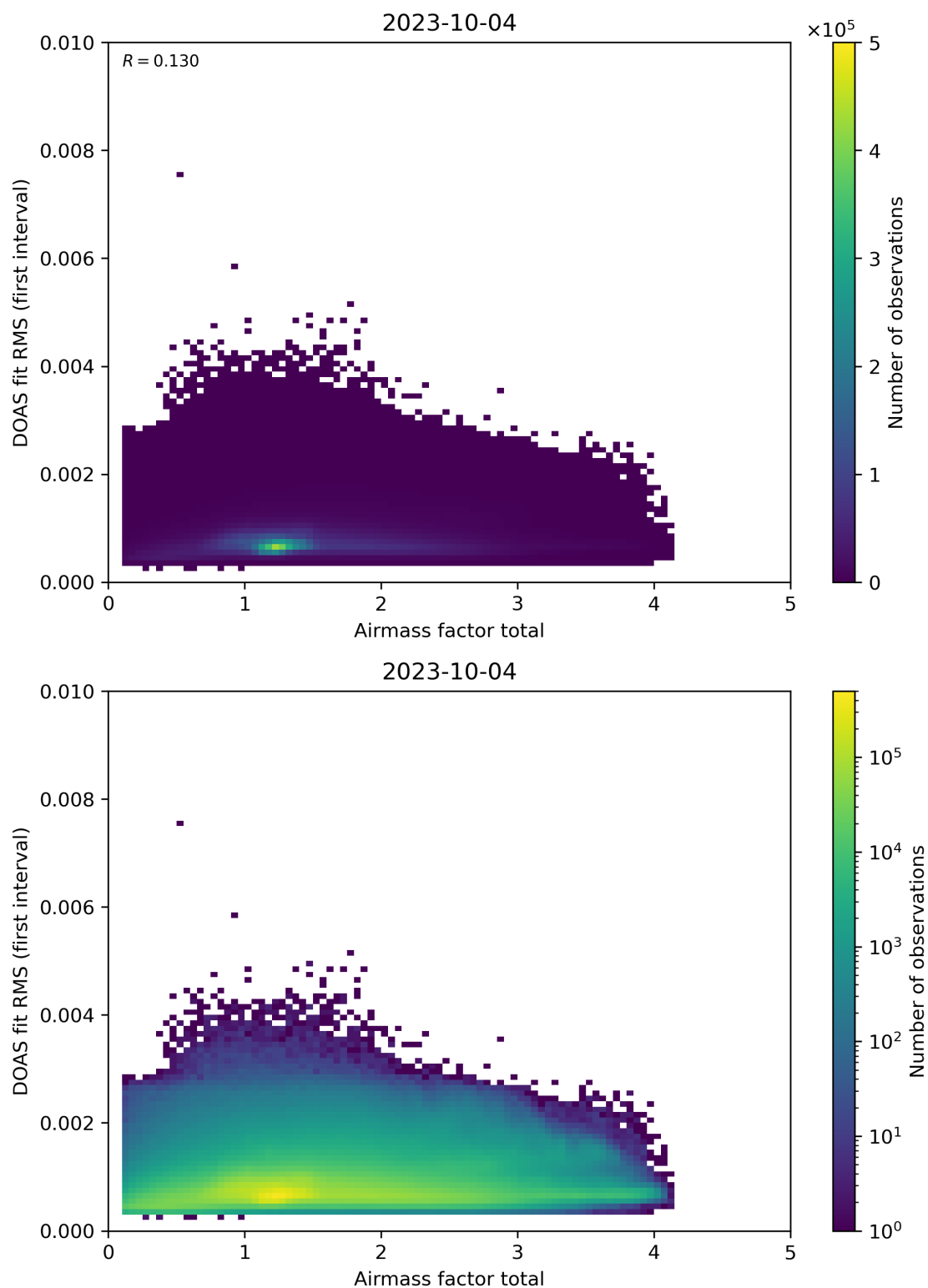
Figure 97: Scatter density plot of “Airmass factor total” against “DOAS fit RMS (first interval)” for 2023-10-03 to 2023-10-05.
