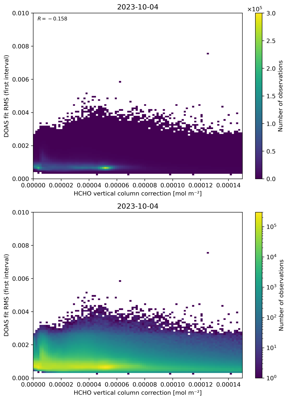
Figure 112: Scatter density plot of “HCHO vertical column correction” against “DOAS fit RMS (first interval)” for 2023-10-03 to 2023-10-05.
