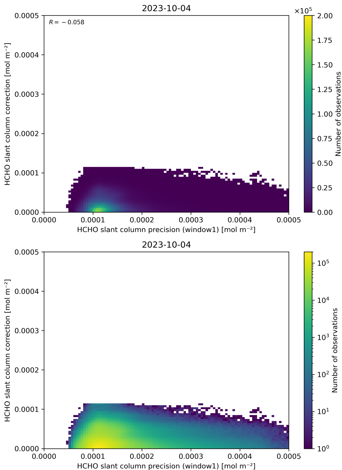
Figure 93: Scatter density plot of “HCHO slant column precision (window1)” against “HCHO slant column correction” for 2023-10-03 to 2023-10-05.
