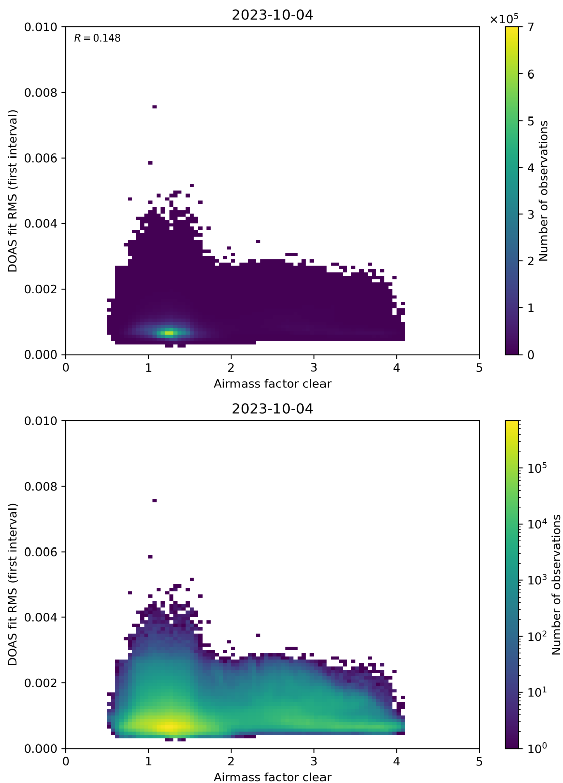
Figure 71: Scatter density plot of “Airmass factor clear” against “DOAS fit RMS (first interval)” for 2023-10-03 to 2023-10-05.
