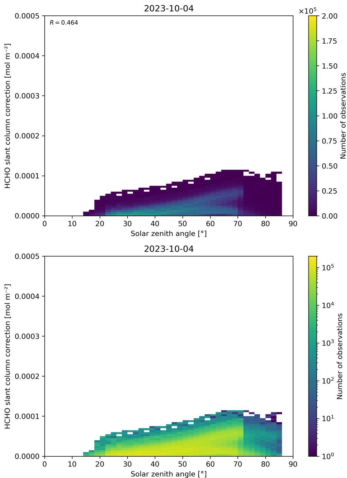
Figure 172: Scatter density plot of “Solar zenith angle” against “HCHO slant column correction” for 2023-10-03 to 2023-10-05.
