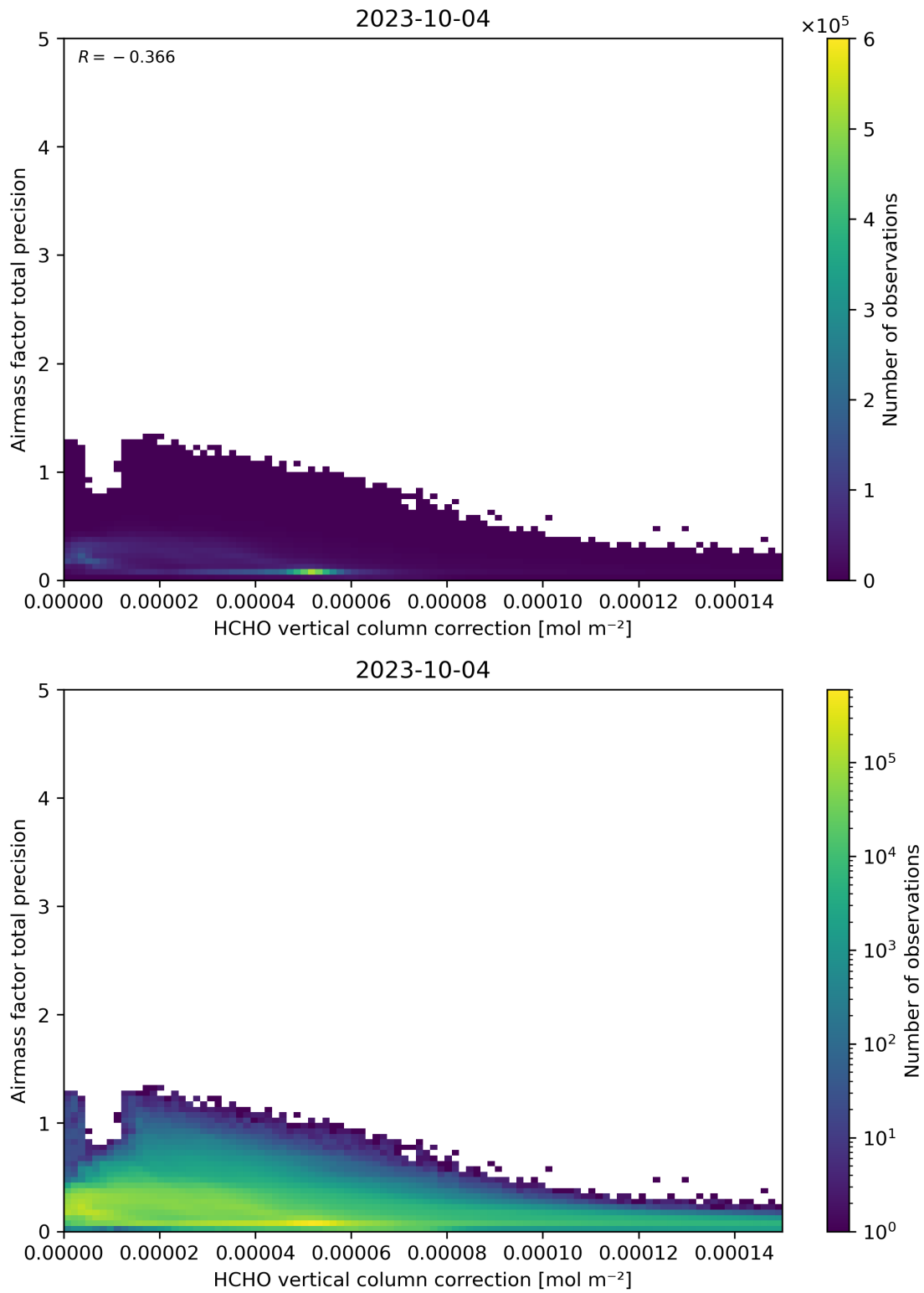
Figure 121: Scatter density plot of “HCHO vertical column correction” against “Airmass factor total precision” for 2023-10-03 to 2023-10-05.
