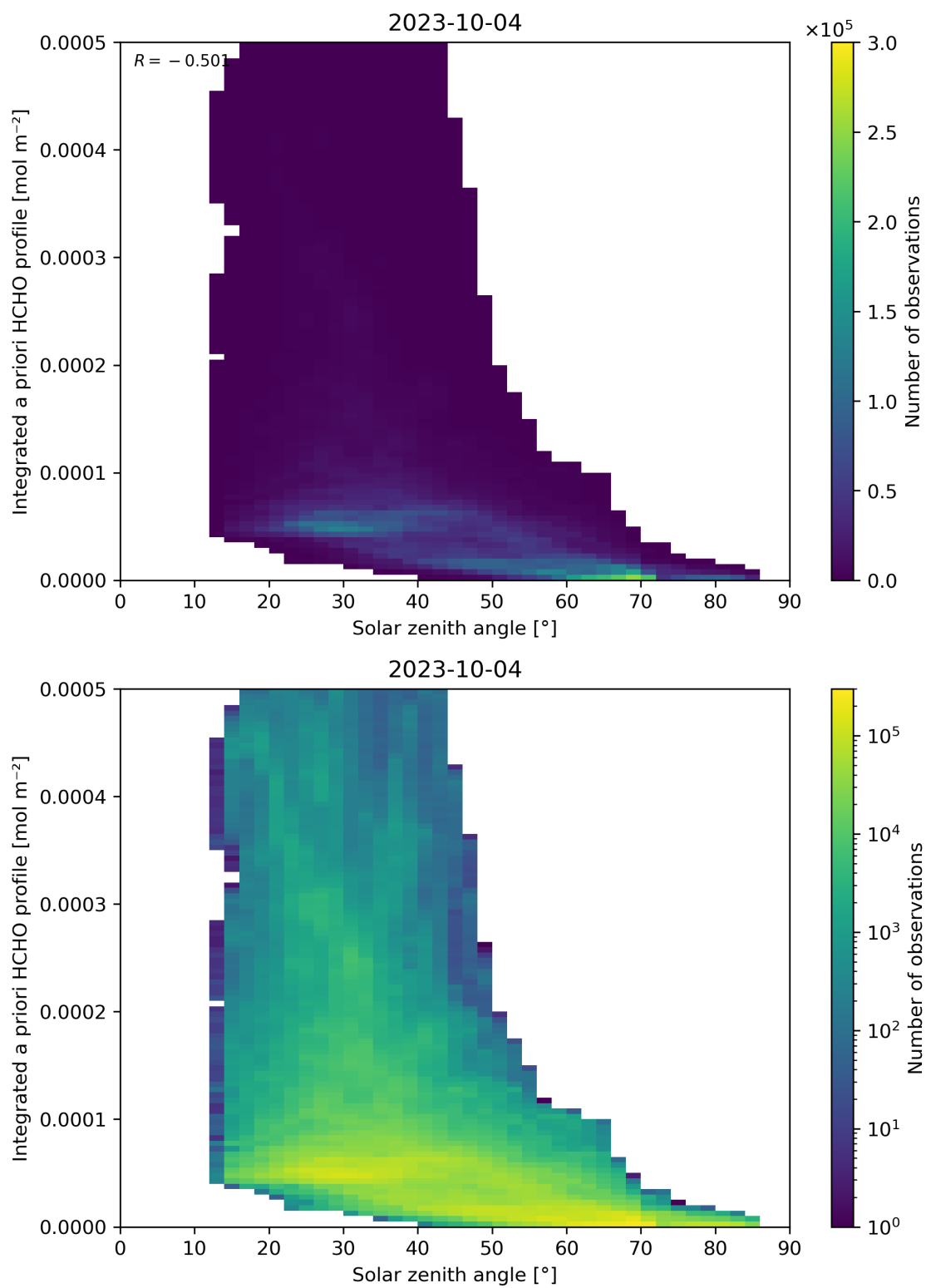
Figure 180: Scatter density plot of “Solar zenith angle” against “Integrated a priori HCHO profile” for 2023-10-03 to 2023-10-05.
