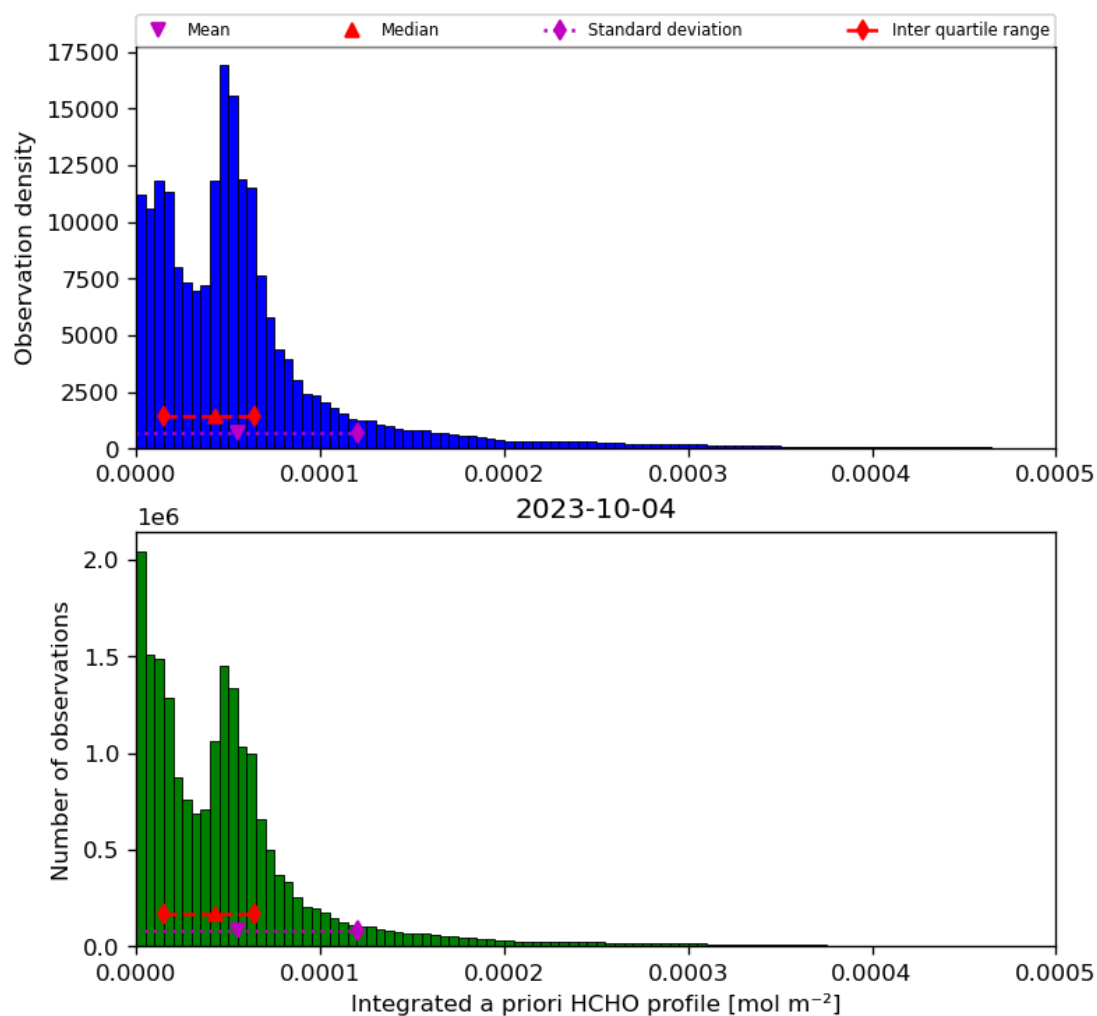
Figure 43: Histogram of “Integrated a priori HCHO profile” for 2023-10-03 to 2023-10-05
