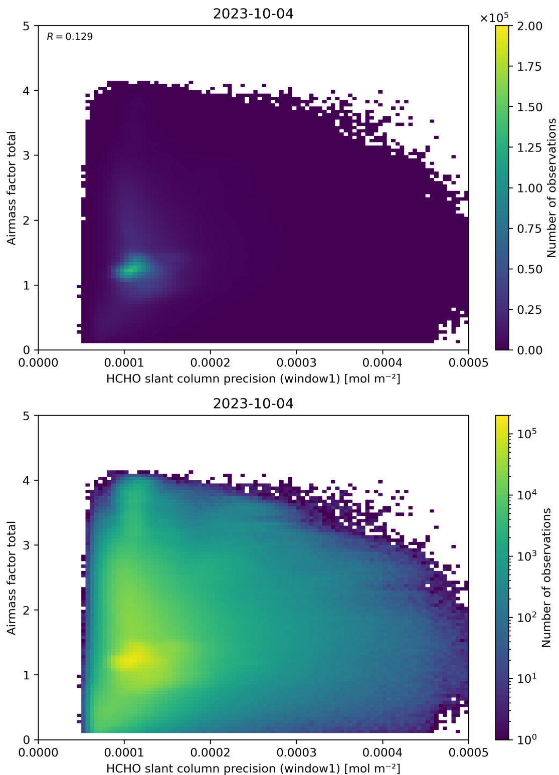
Figure 94: Scatter density plot of “HCHO slant column precision (window1)” against “Airmass factor total” for 2023-10-03 to 2023-10-05.
