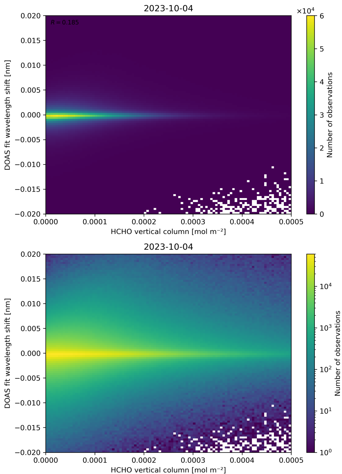
Figure 124: Scatter density plot of “HCHO vertical column” against “DOAS fit wavelength shift” for 2023-10-03 to 2023-10-05.
