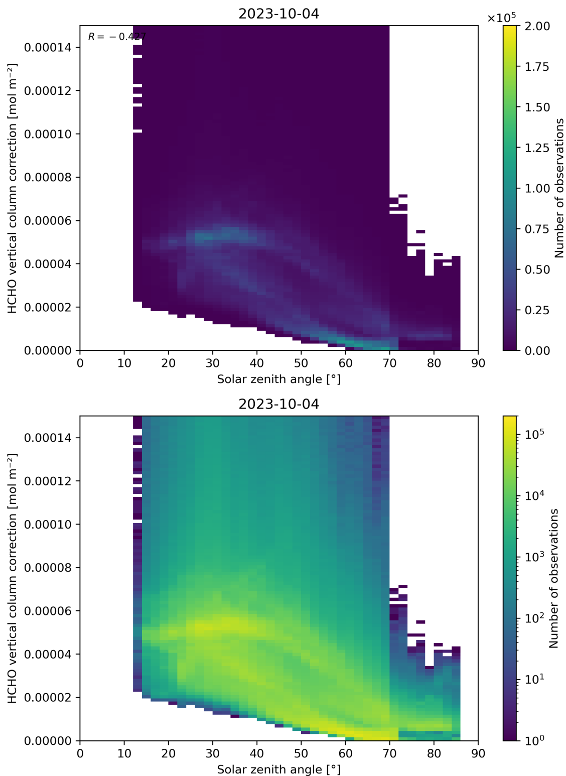
Figure 178: Scatter density plot of “Solar zenith angle” against “HCHO vertical column correction” for 2023-10-03 to 2023-10-05.
