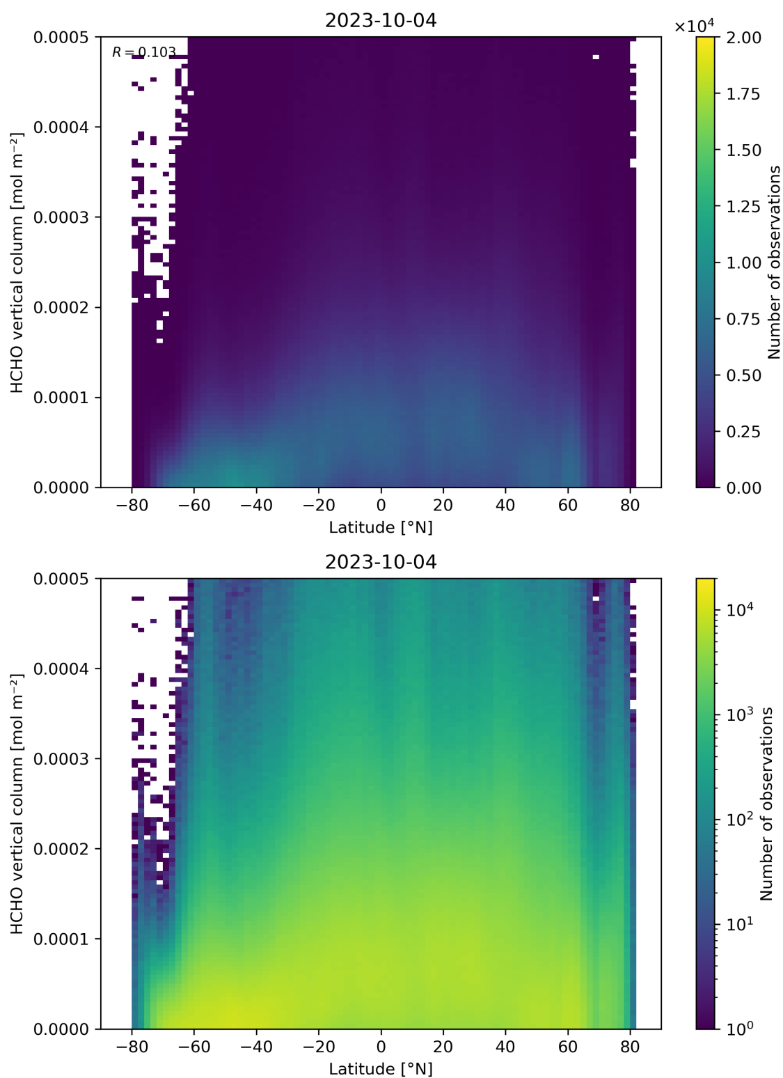
Figure 163: Scatter density plot of “Latitude” against “HCHO vertical column” for 2023-10-03 to 2023-10-05.
