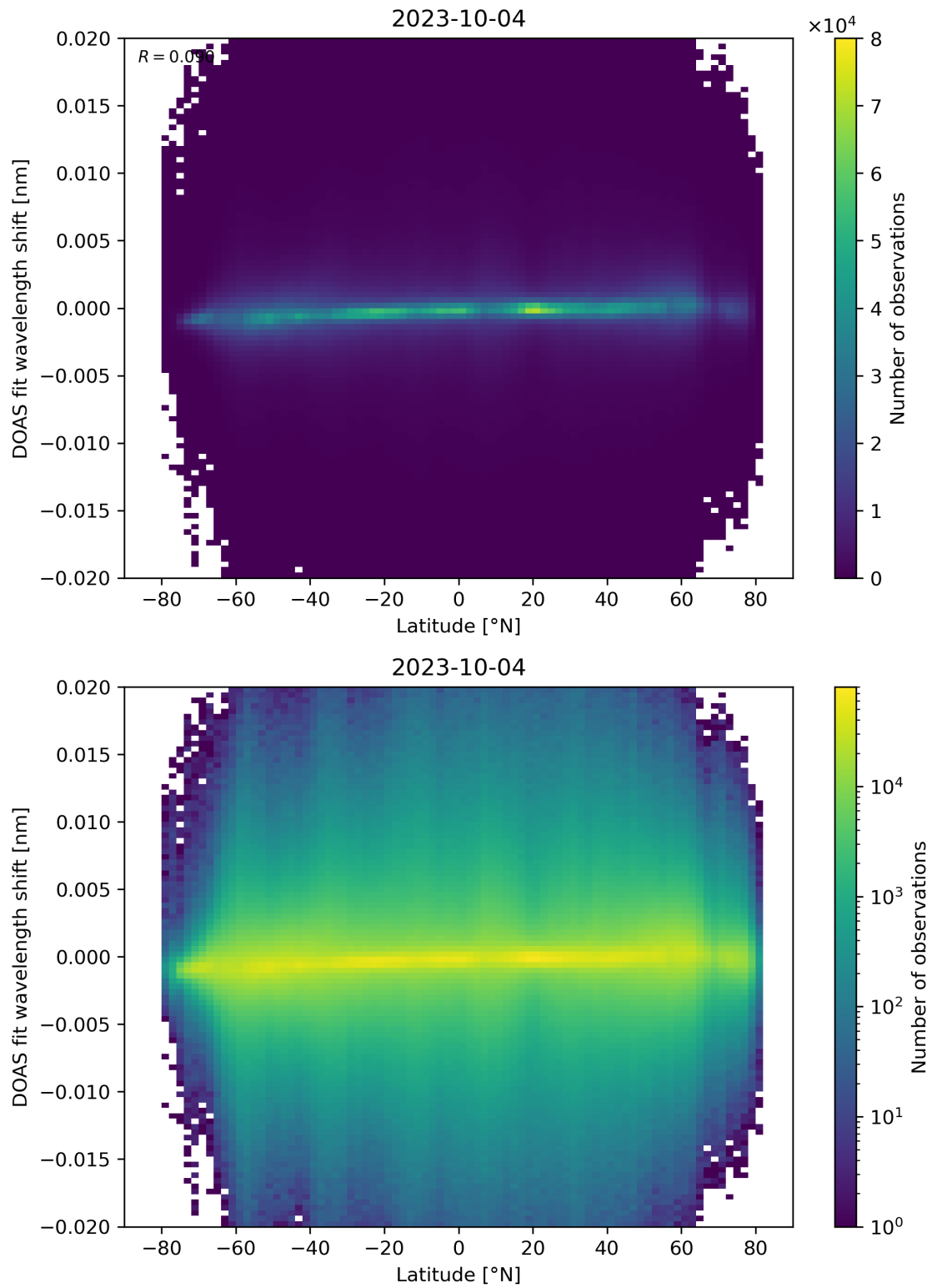
Figure 154: Scatter density plot of “Latitude” against “DOAS fit wavelength shift” for 2023-10-03 to 2023-10-05.
