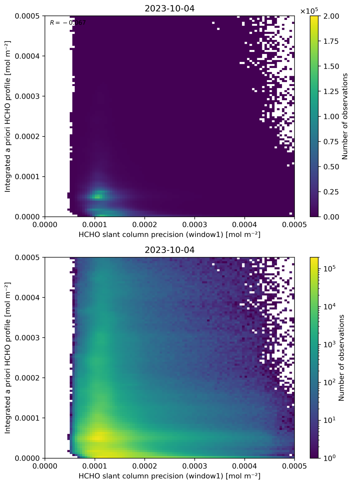
Figure 96: Scatter density plot of “HCHO slant column precision (window1)” against “Integrated a priori HCHO profile” for 2023-10-03 to 2023-10-05.
