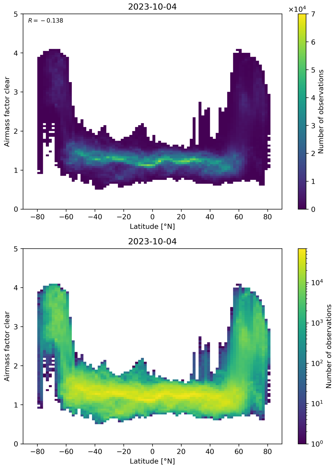
Figure 156: Scatter density plot of “Latitude” against “Airmass factor clear” for 2023-10-03 to 2023-10-05.
