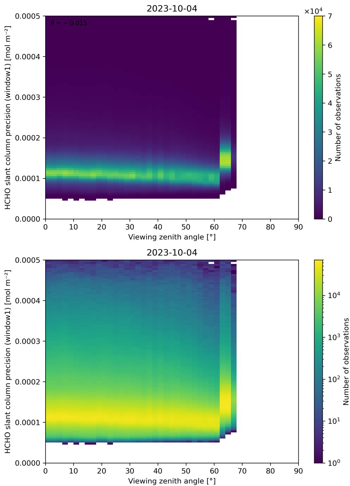
Figure 189: Scatter density plot of “Viewing zenith angle” against “HCHO slant column precision (window1)” for 2023-10-03 to 2023-10-05.
