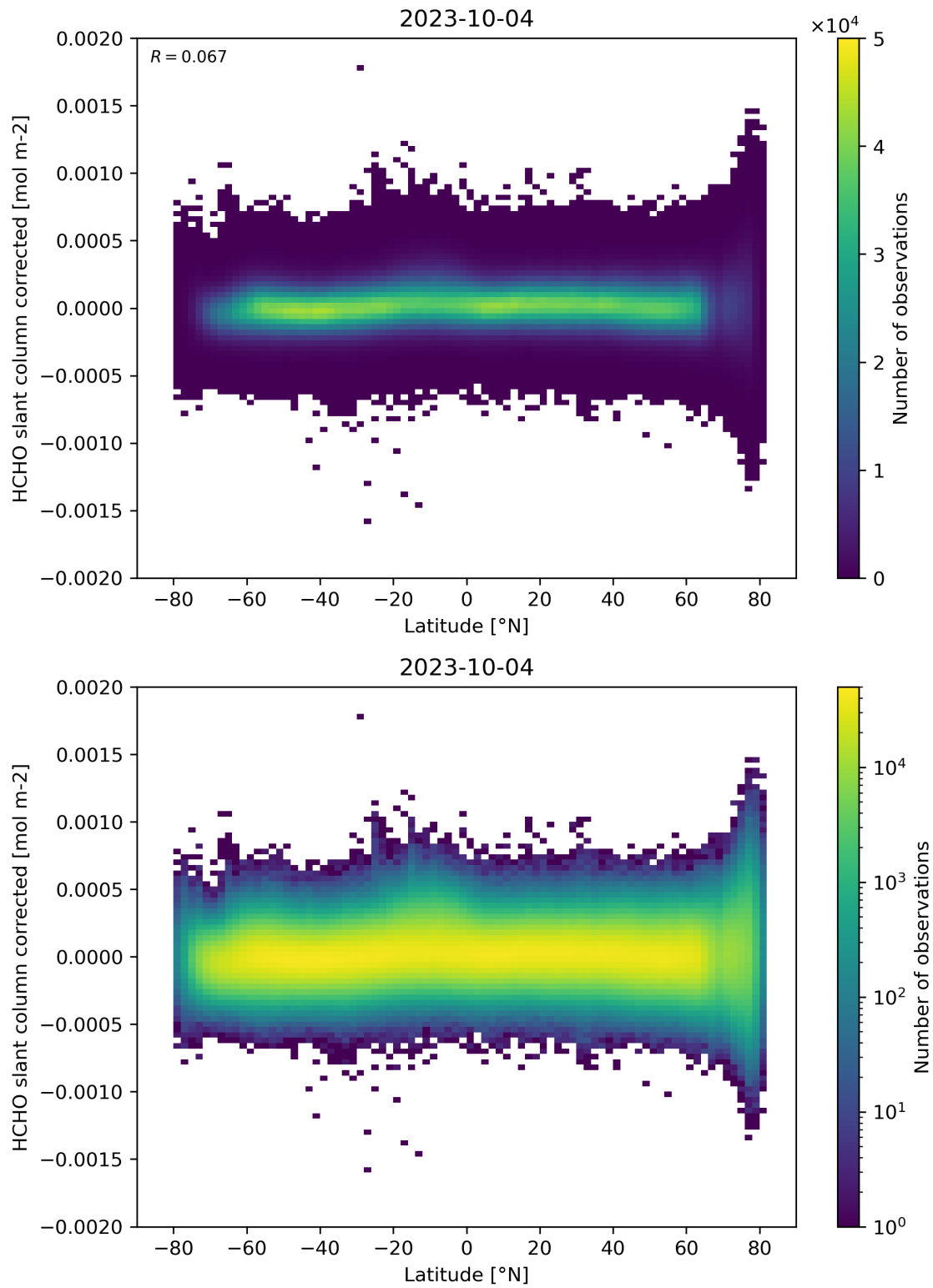
Figure 157: Scatter density plot of “Latitude” against “HCHO slant column corrected” for 2023-10-03 to 2023-10-05.
