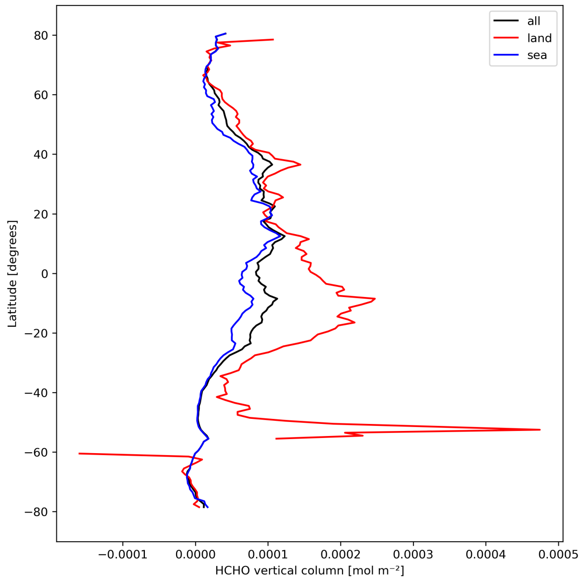
Figure 21: Zonal average of “HCHO vertical column” for 2023-10-03 to 2023-10-05.
