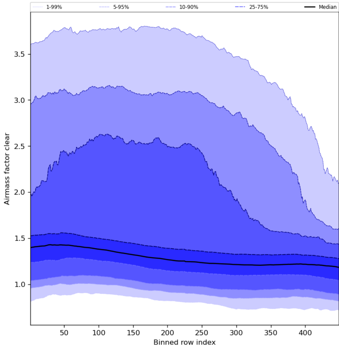
Figure 56: Along track statistics of “Airmass factor clear” for 2023-10-03 to 2023-10-05
