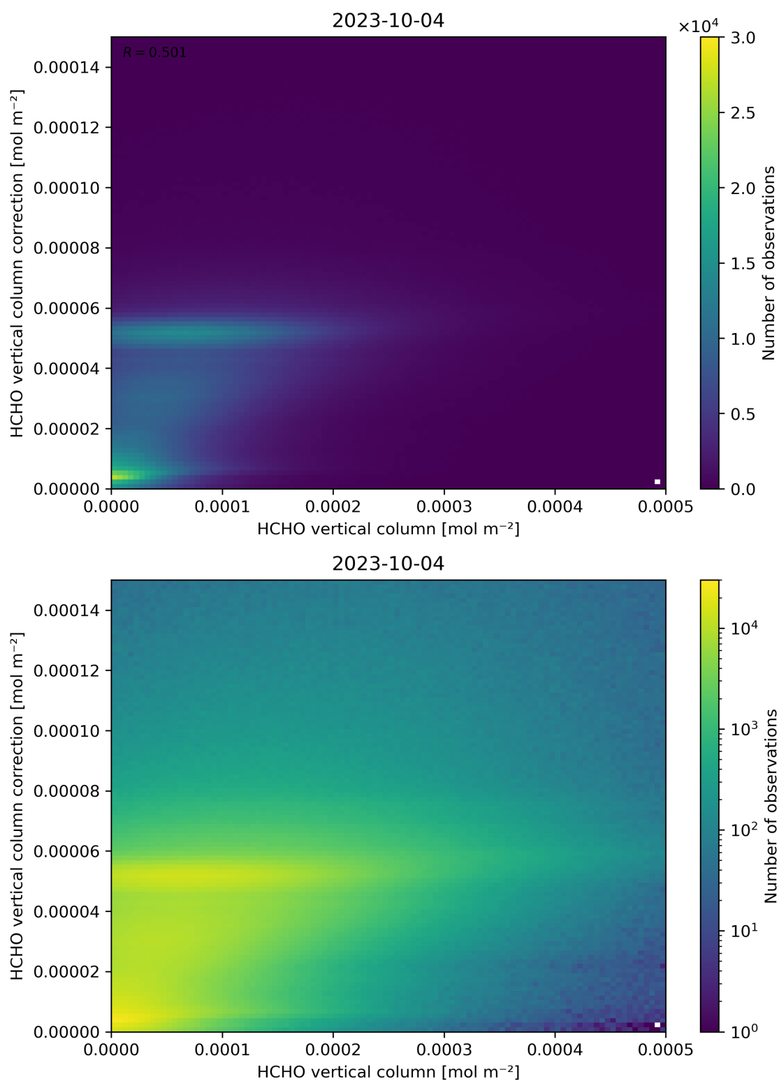
Figure 133: Scatter density plot of “HCHO vertical column” against “HCHO vertical column correction” for 2023-10-03 to 2023-10-05.
