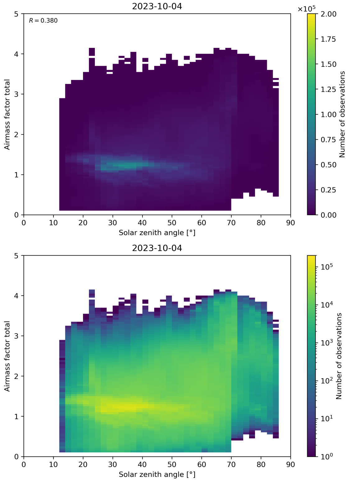
Figure 175: Scatter density plot of “Solar zenith angle” against “Airmass factor total” for 2023-10-03 to 2023-10-05.
