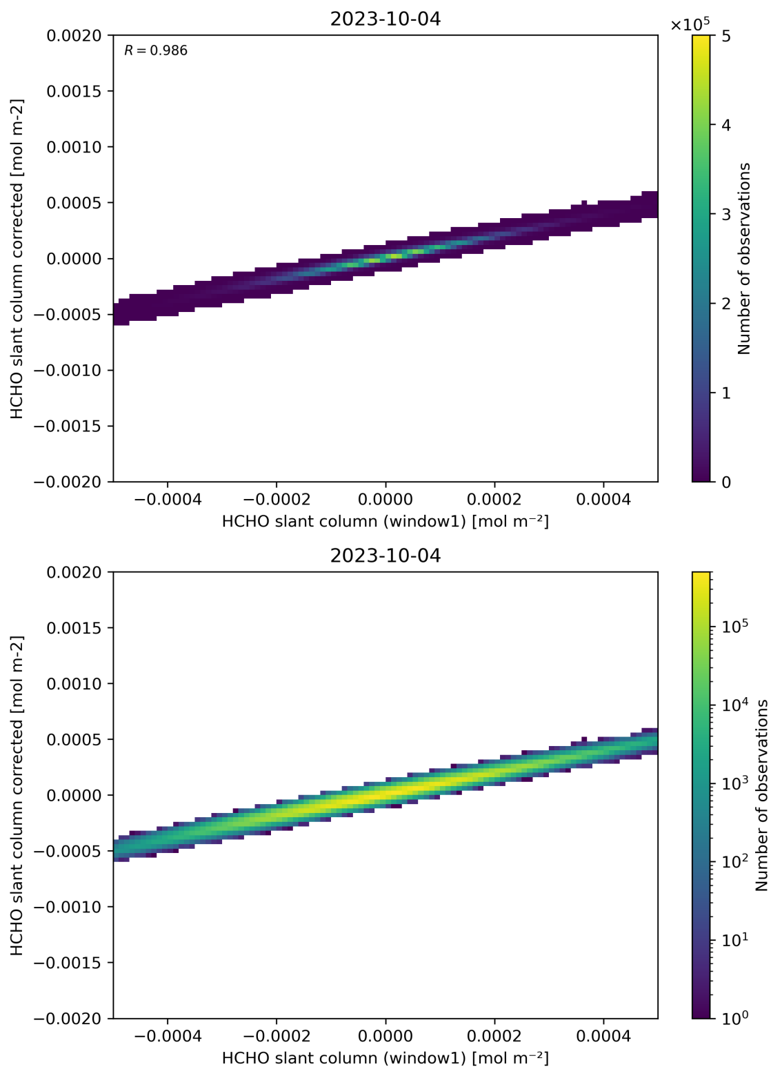
Figure 82: Scatter density plot of “HCHO slant column (window1)” against “HCHO slant column corrected” for 2023-10-03 to 2023-10-05.
