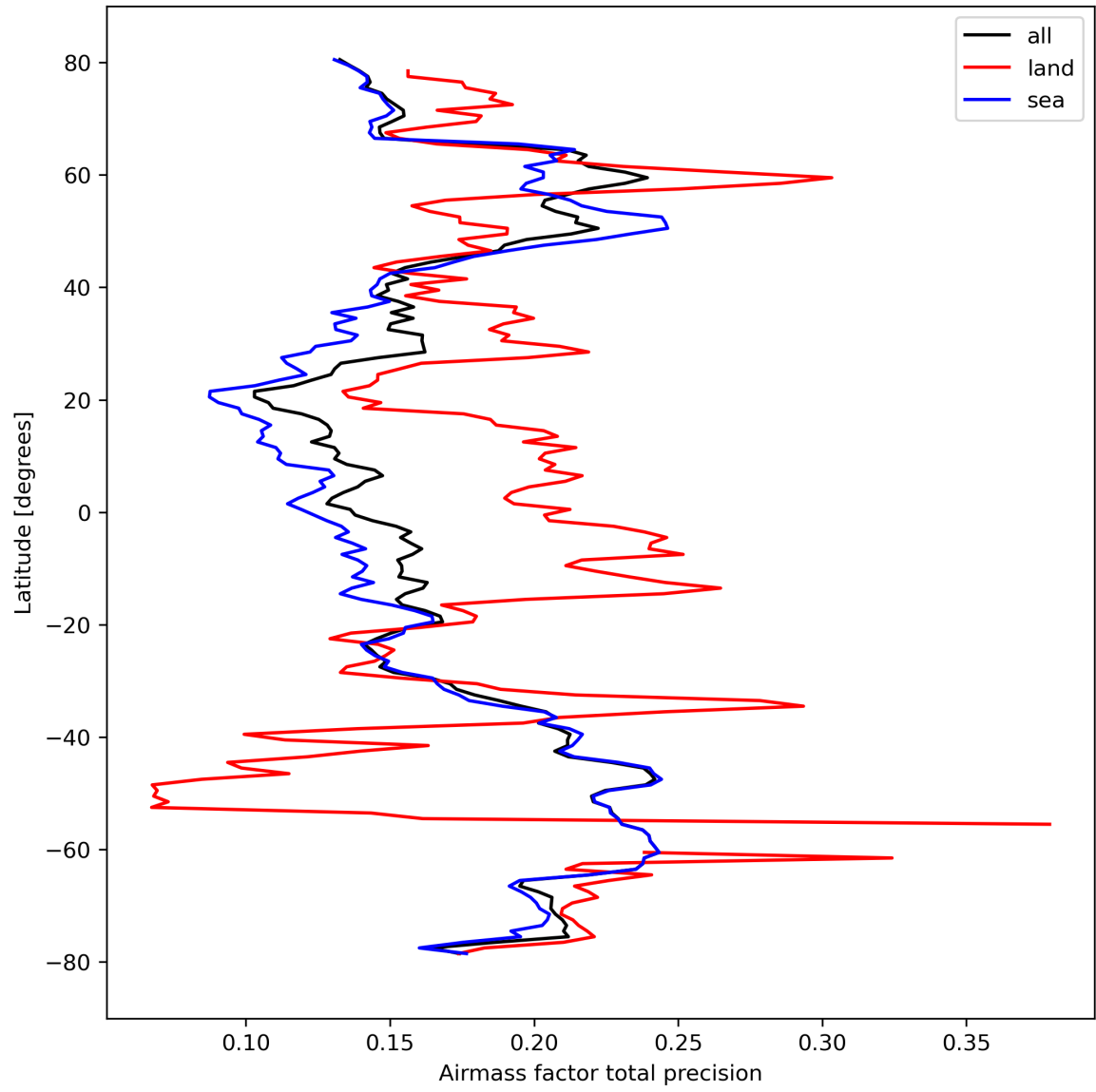
Figure 27: Zonal average of “Airmass factor total precision” for 2023-10-03 to 2023-10-05.
