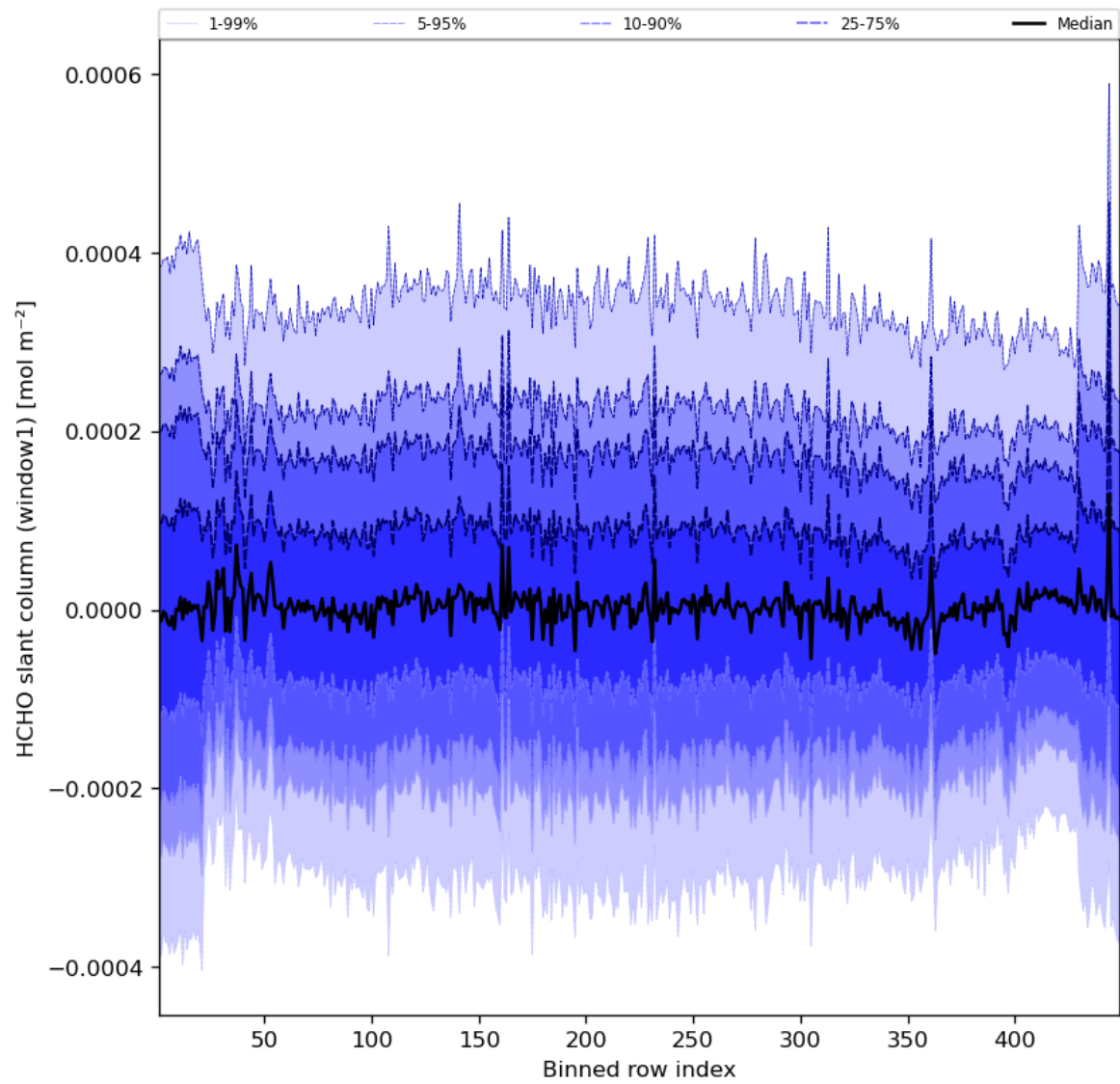
Figure 52: Along track statistics of “HCHO slant column (window1)” for 2023-10-03 to 2023-10-05
