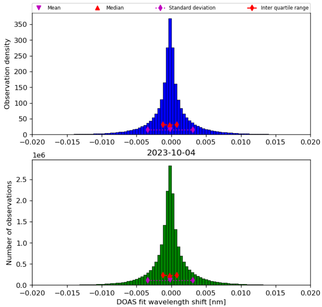
Figure 44: Histogram of “DOAS fit wavelength shift” for 2023-10-03 to 2023-10-05
