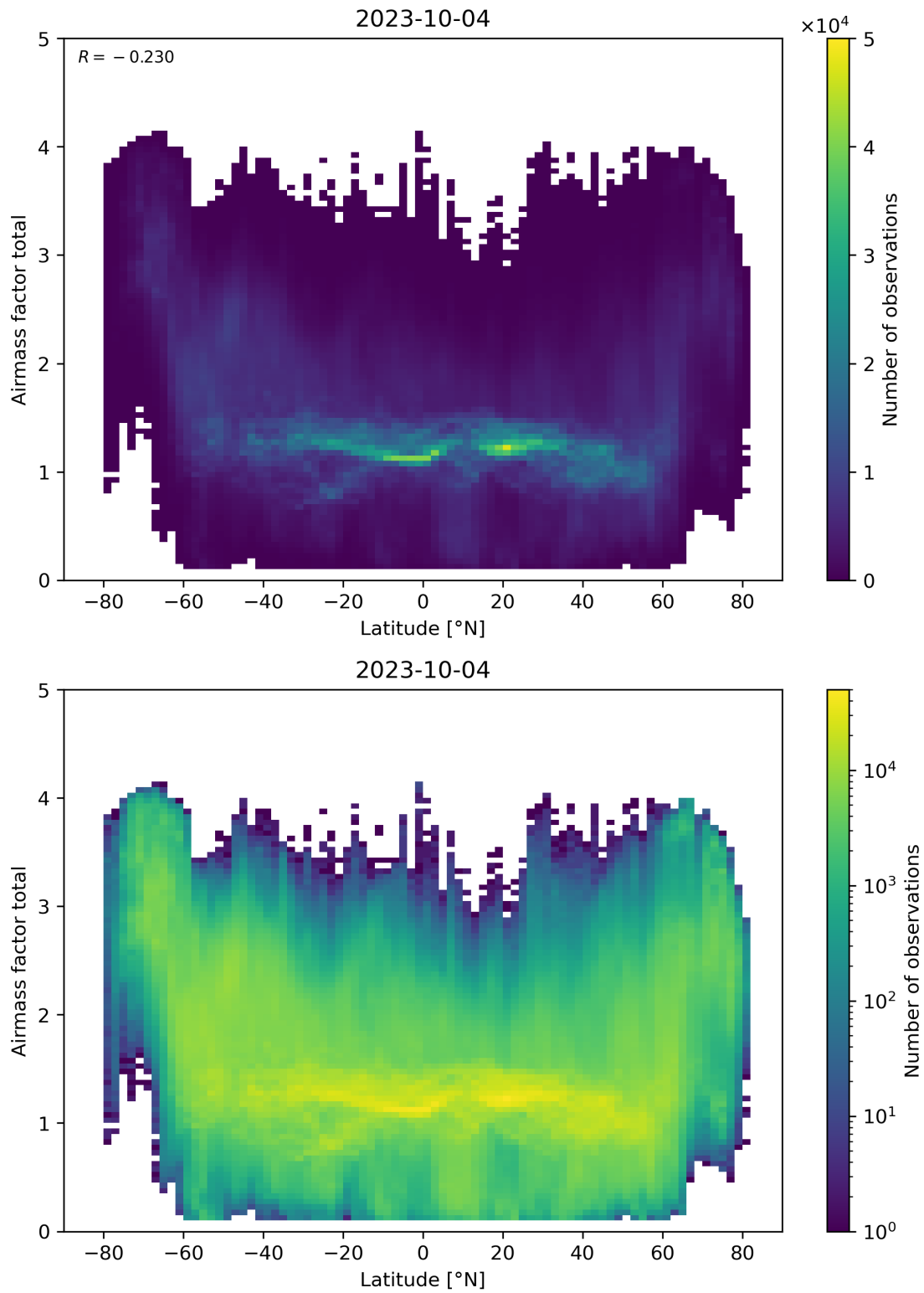
Figure 161: Scatter density plot of “Latitude” against “Airmass factor total” for 2023-10-03 to 2023-10-05.
