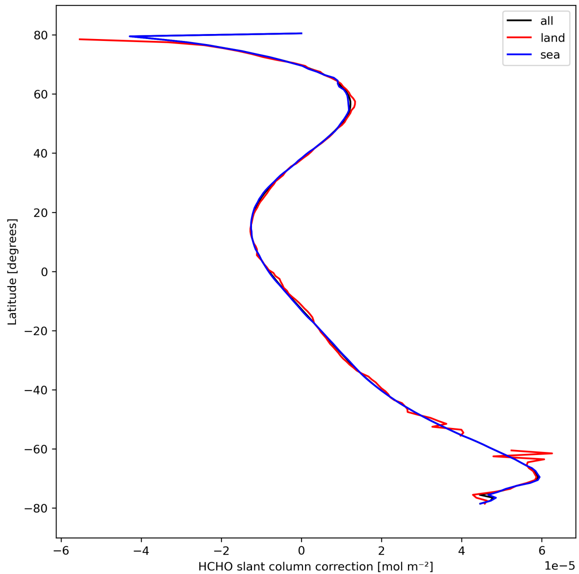
Figure 33: Zonal average of “HCHO slant column correction” for 2023-10-03 to 2023-10-05.
