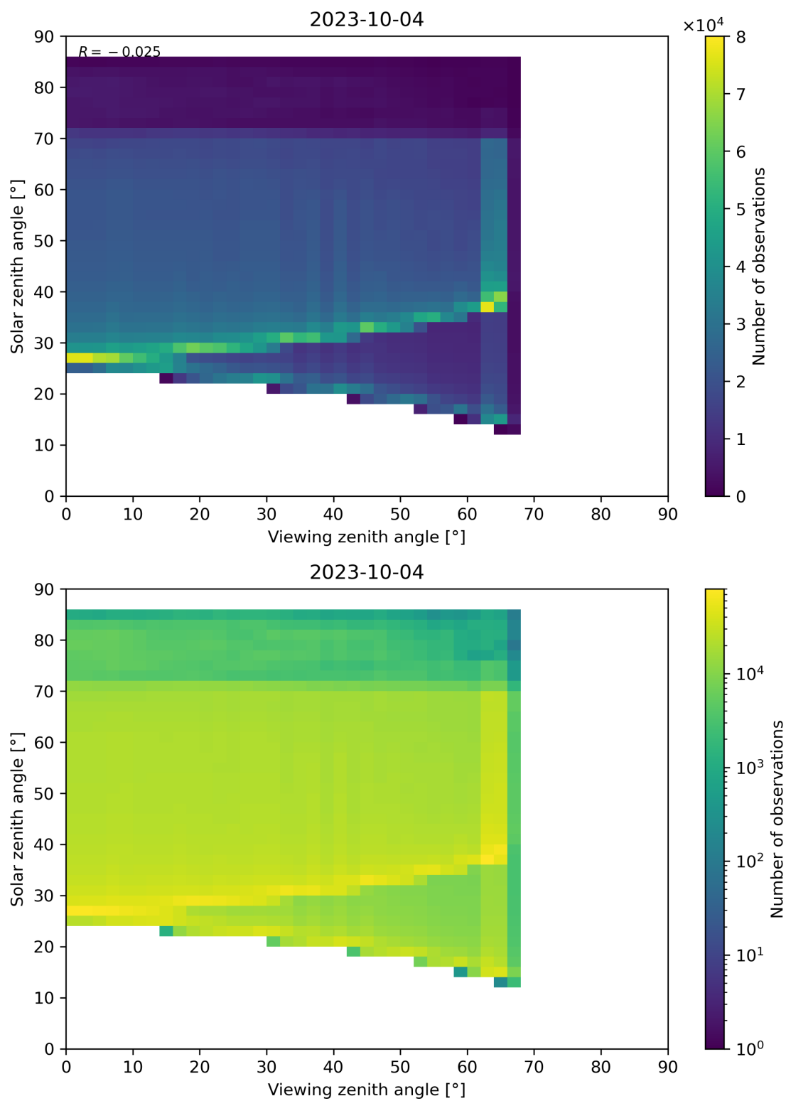
Figure 197: Scatter density plot of “Viewing zenith angle” against “Solar zenith angle” for 2023-10-03 to 2023-10-05.
