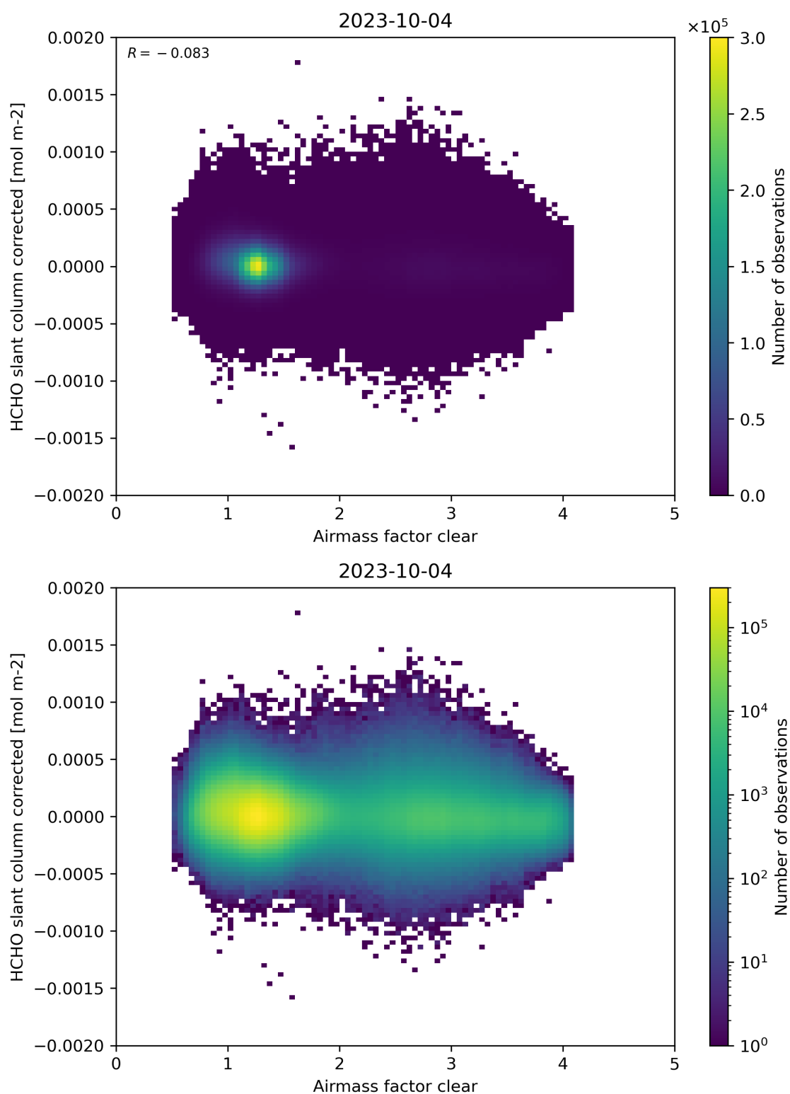
Figure 74: Scatter density plot of “Airmass factor clear” against “HCHO slant column corrected” for 2023-10-03 to 2023-10-05.
