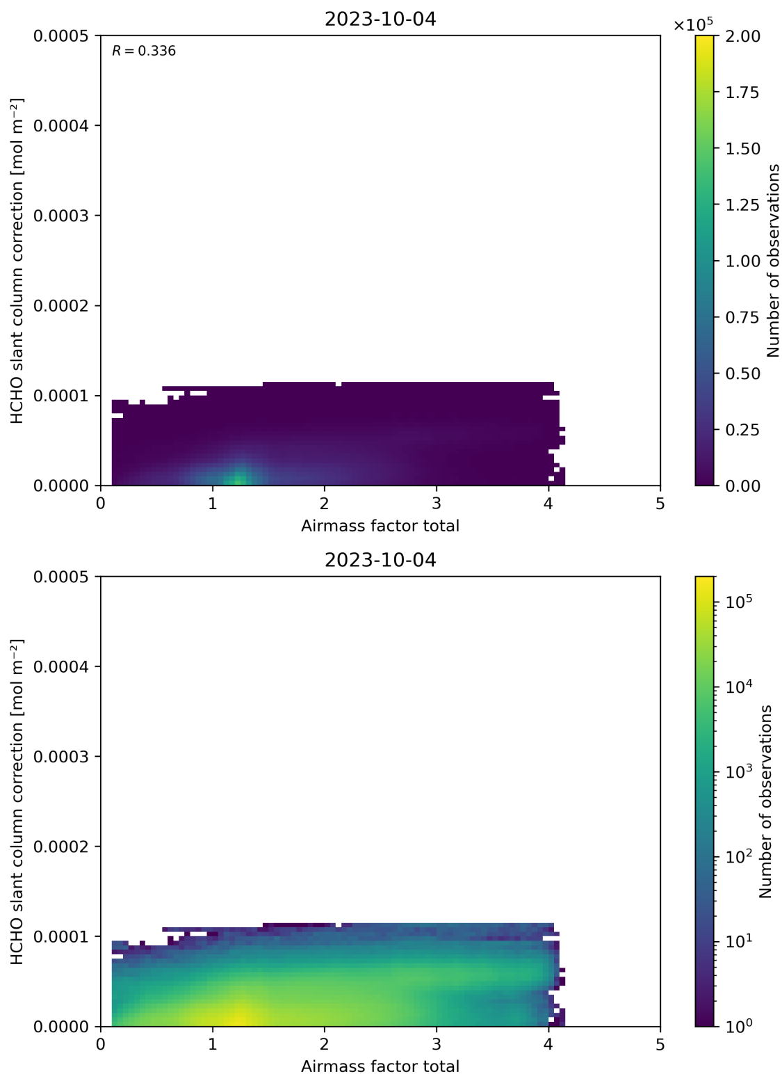
Figure 102: Scatter density plot of “Airmass factor total” against “HCHO slant column correction” for 2023-10-03 to 2023-10-05.
