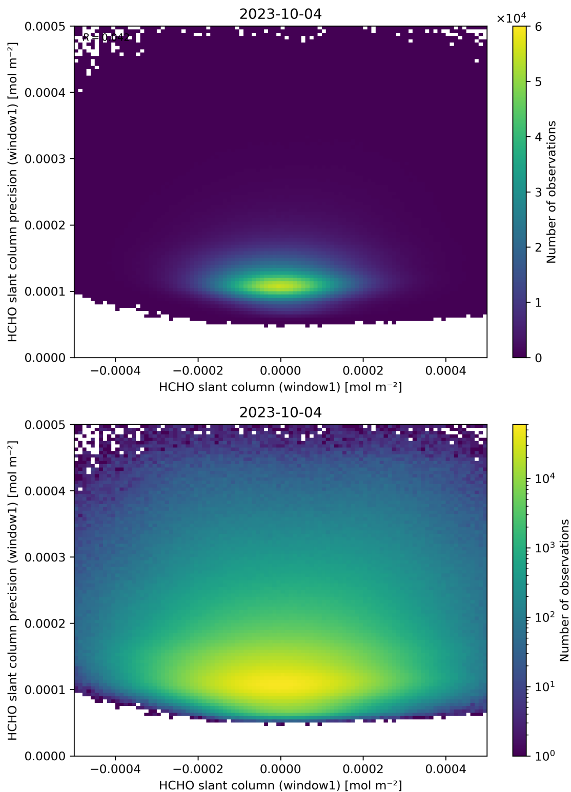
Figure 84: Scatter density plot of “HCHO slant column (window1)” against “HCHO slant column precision (window1)” for 2023-10-03 to 2023-10-05.
