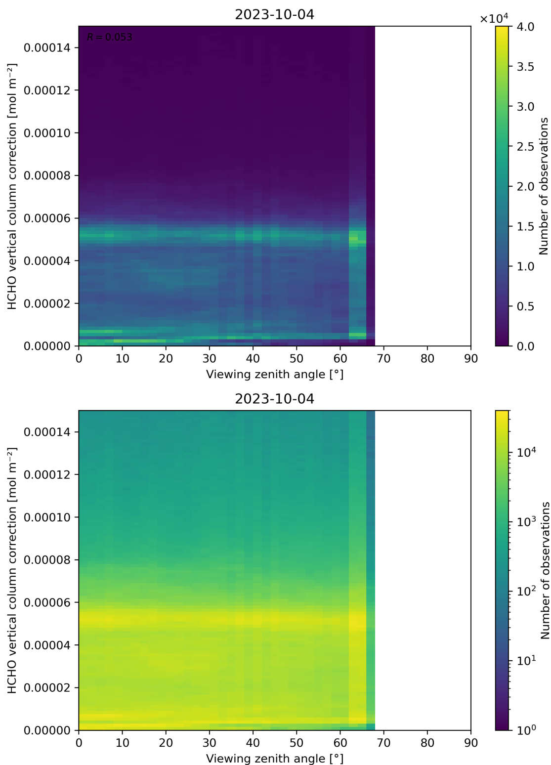
Figure 193: Scatter density plot of “Viewing zenith angle” against “HCHO vertical column correction” for 2023-10-03 to 2023-10-05.
