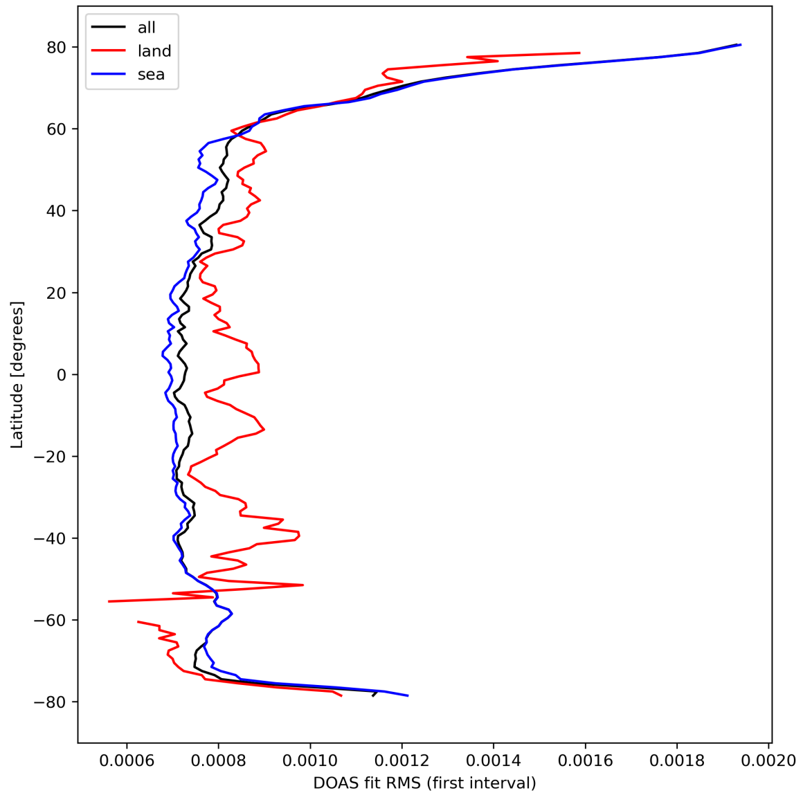
Figure 32: Zonal average of “DOAS fit RMS (first interval)” for 2023-10-03 to 2023-10-05.
