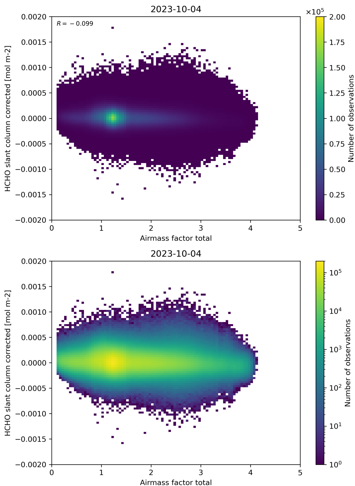
Figure 101: Scatter density plot of “Airmass factor total” against “HCHO slant column corrected” for 2023-10-03 to 2023-10-05.
