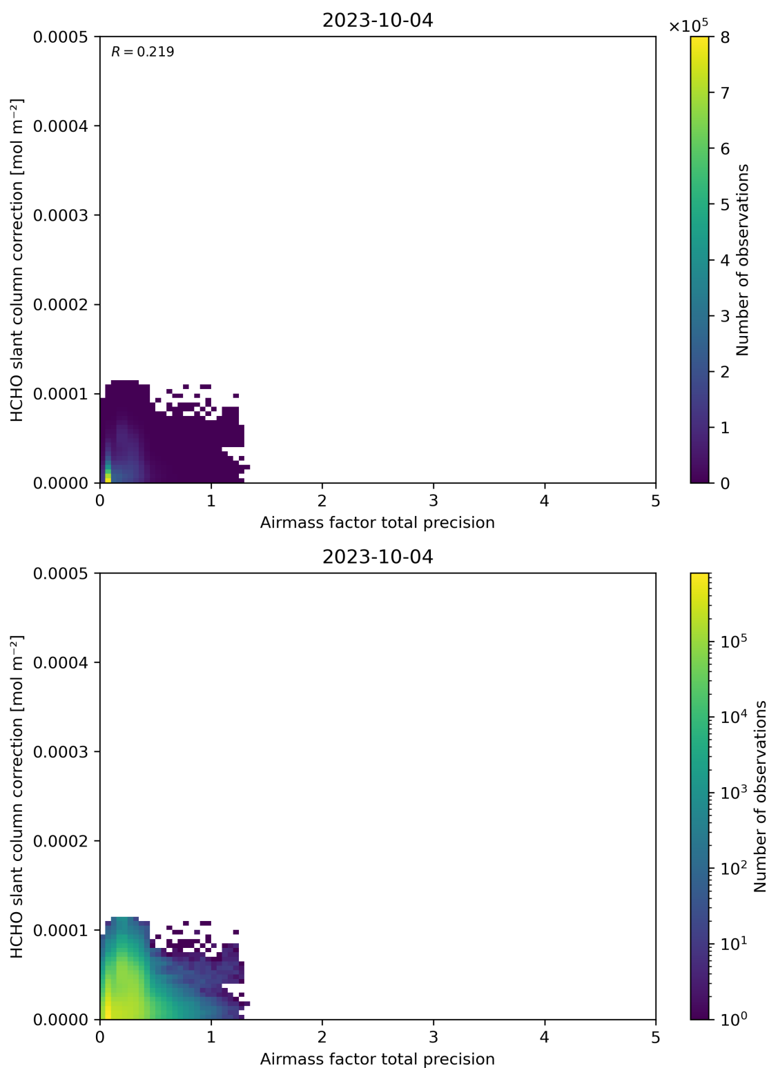
Figure 110: Scatter density plot of “Airmass factor total precision” against “HCHO slant column correction” for 2023-10-03 to 2023-10-05.
