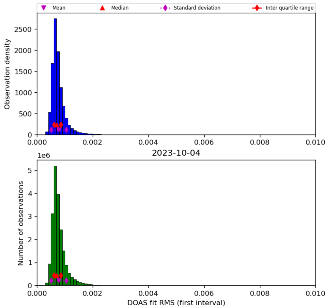
Figure 46: Histogram of “DOAS fit RMS (first interval)” for 2023-10-03 to 2023-10-05
