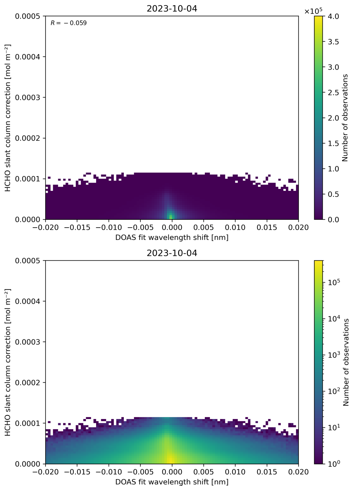
Figure 67: Scatter density plot of “DOAS fit wavelength shift” against “HCHO slant column correction” for 2023-10-03 to 2023-10-05.
