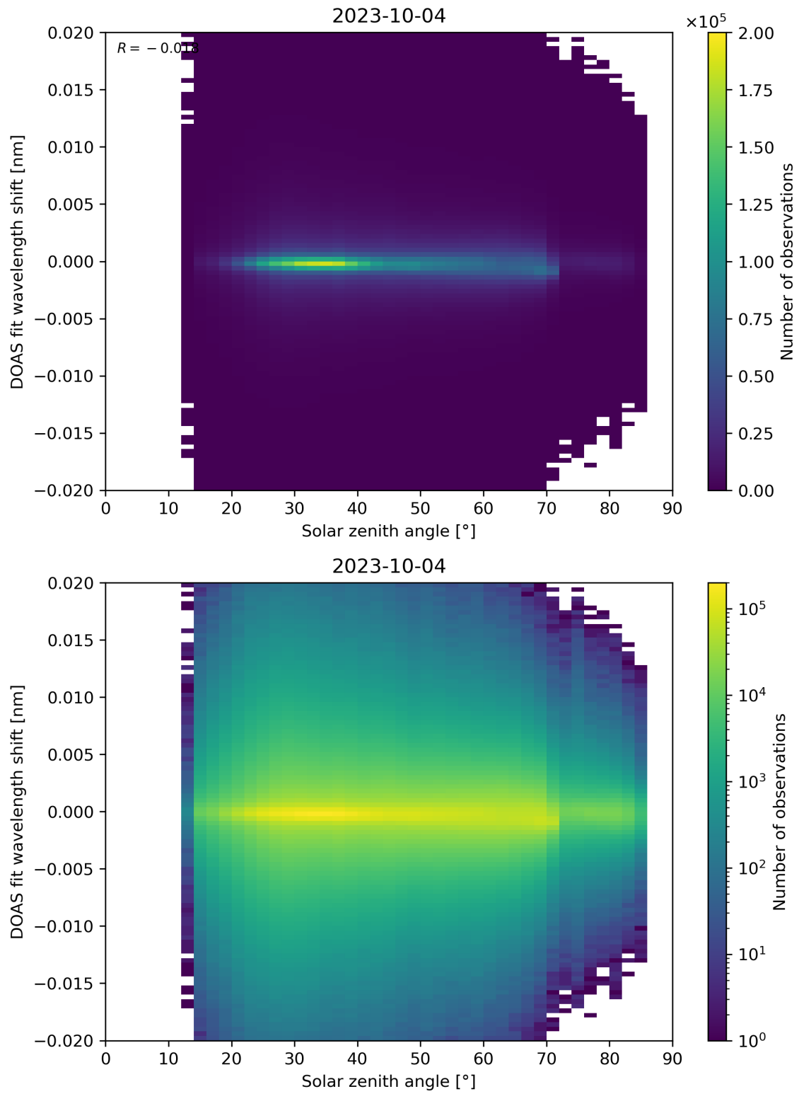
Figure 168: Scatter density plot of “Solar zenith angle” against “DOAS fit wavelength shift” for 2023-10-03 to 2023-10-05.
