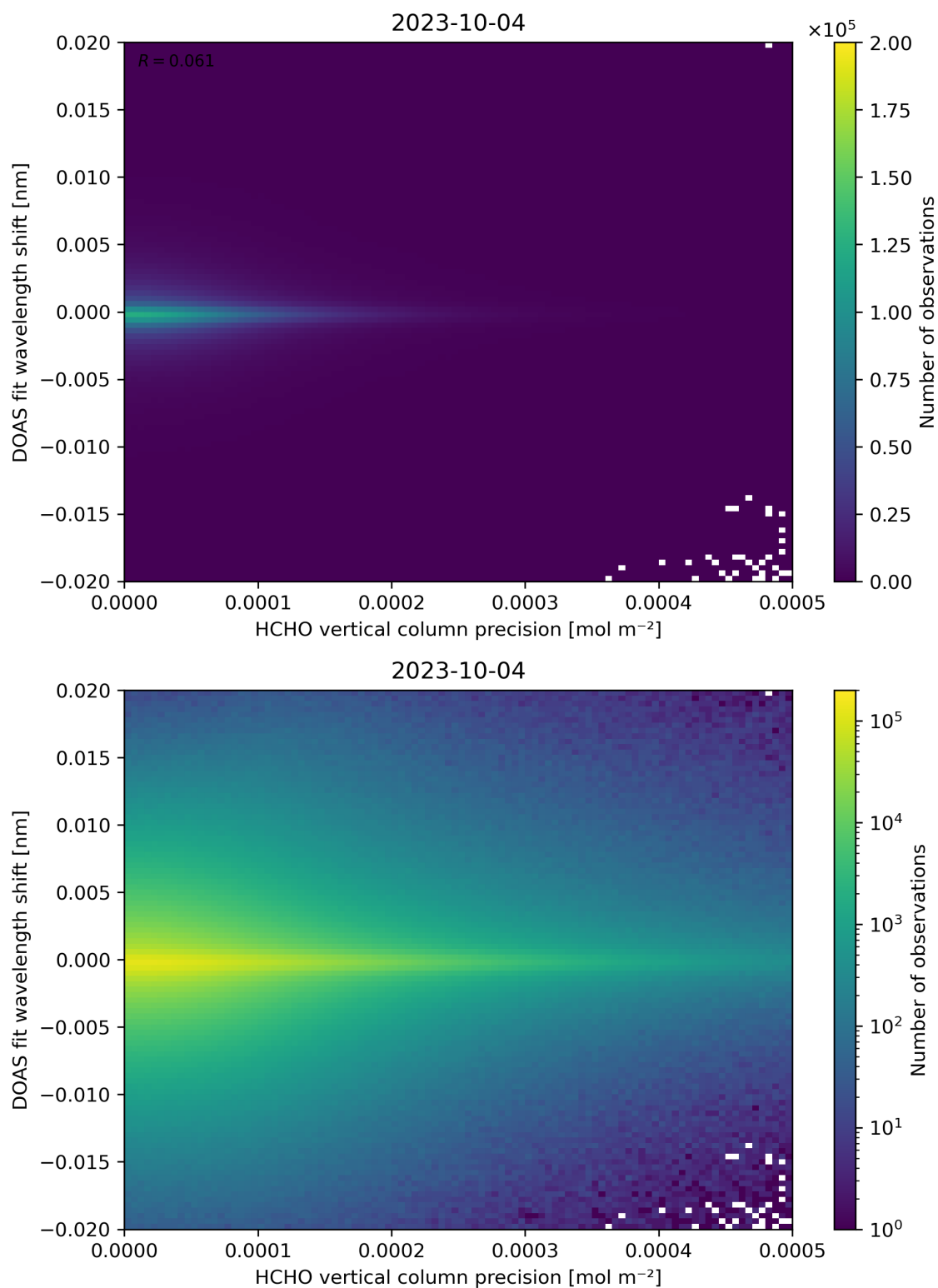
Figure 137: Scatter density plot of “HCHO vertical column precision” against “DOAS fit wavelength shift” for 2023-10-03 to 2023-10-05.
