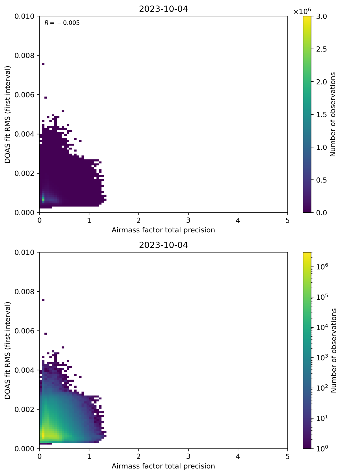
Figure 105: Scatter density plot of “Airmass factor total precision” against “DOAS fit RMS (first interval)” for 2023-10-03 to 2023-10-05.
