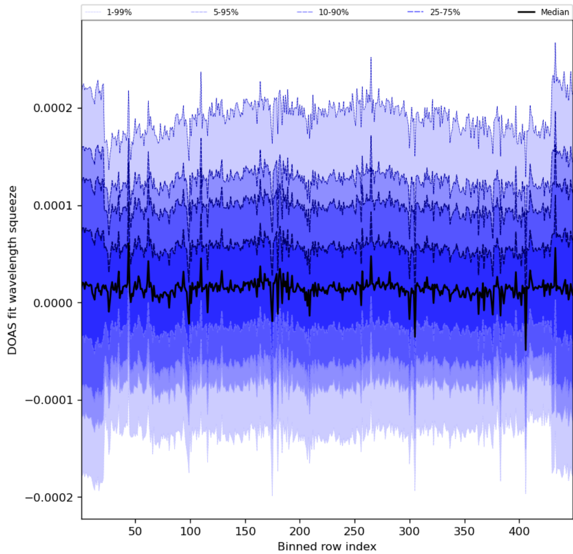
Figure 59: Along track statistics of “DOAS fit wavelength squeeze” for 2023-10-03 to 2023-10-05
