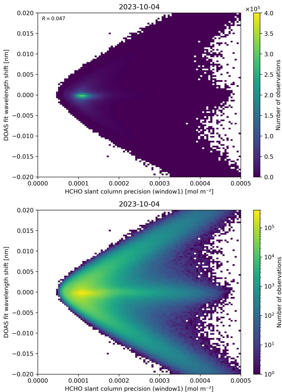
Figure 89: Scatter density plot of “HCHO slant column precision (window1)” against “DOAS fit wavelength shift” for 2023-10-03 to 2023-10-05.
