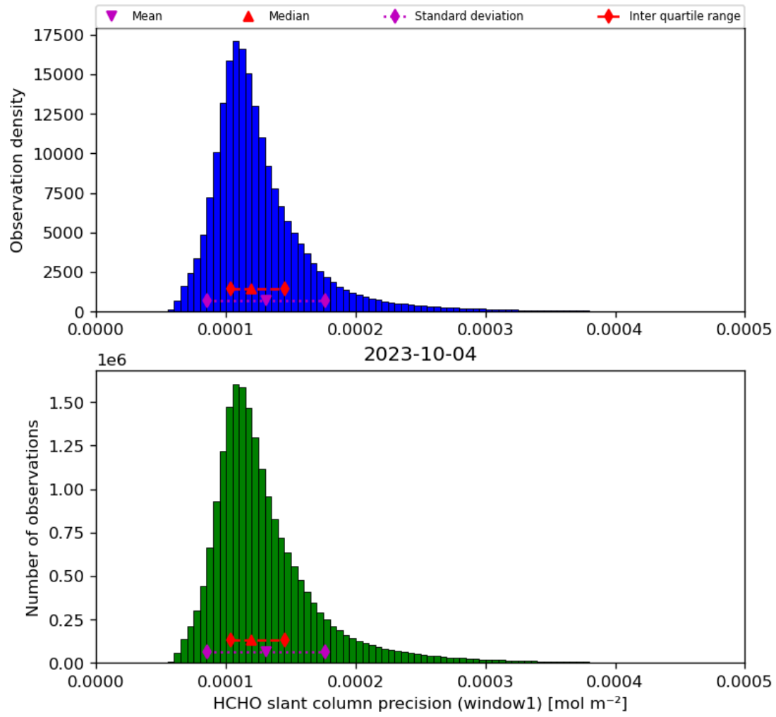
Figure 39: Histogram of “HCHO slant column precision (window1)” for 2023-10-03 to 2023-10-05
