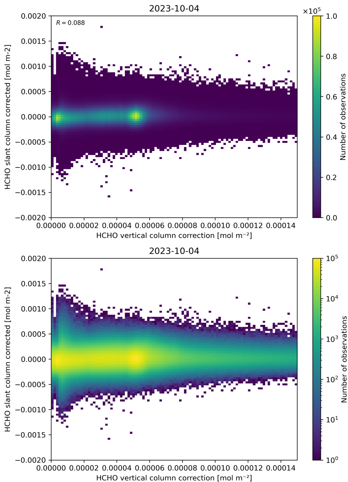
Figure 116: Scatter density plot of “HCHO vertical column correction” against “HCHO slant column corrected” for 2023-10-03 to 2023-10-05.
