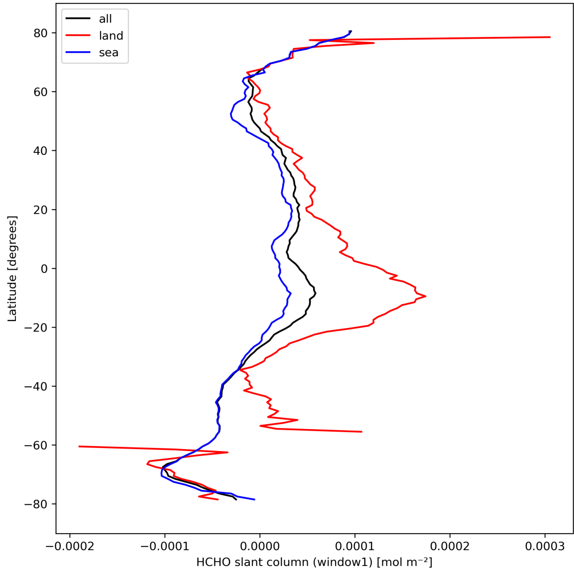
Figure 24: Zonal average of “HCHO slant column (window1)” for 2023-10-03 to 2023-10-05.
