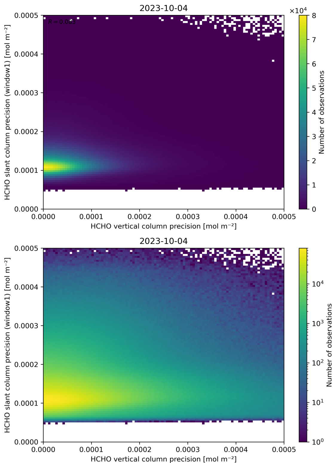
Figure 143: Scatter density plot of “HCHO vertical column precision” against “HCHO slant column precision (window1)” for 2023-10-03 to 2023-10-05.
