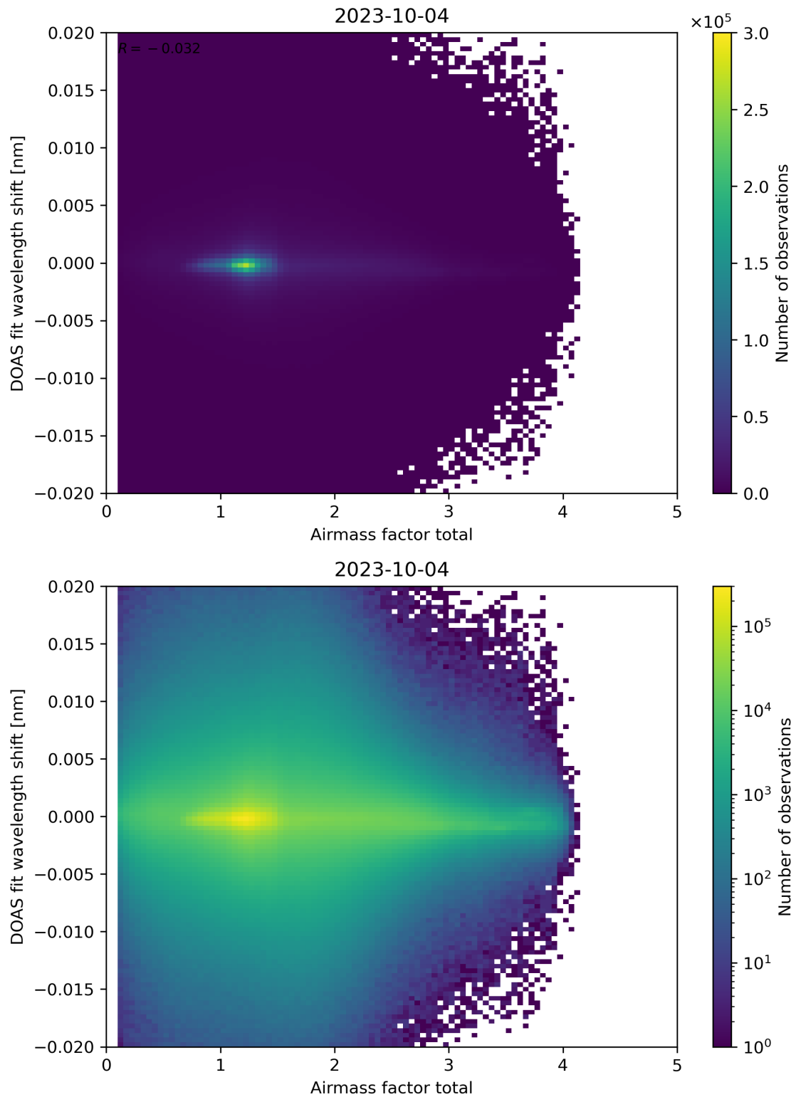
Figure 98: Scatter density plot of “Airmass factor total” against “DOAS fit wavelength shift” for 2023-10-03 to 2023-10-05.
