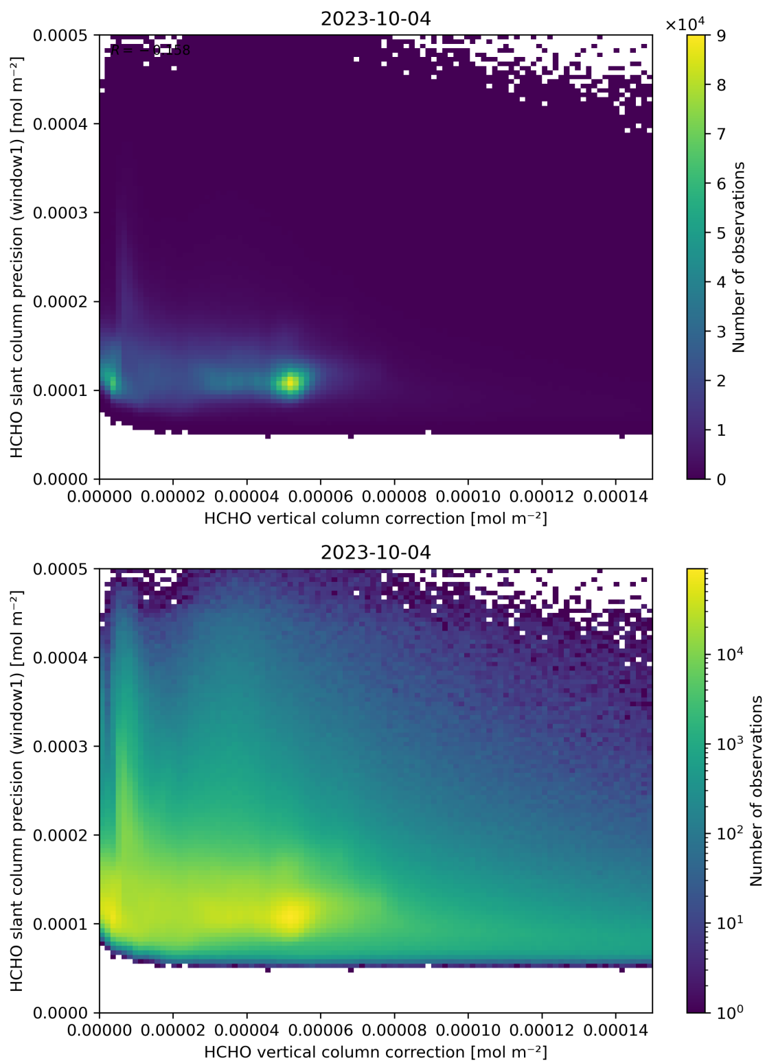
Figure 119: Scatter density plot of “HCHO vertical column correction” against “HCHO slant column precision (window1)” for 2023-10-03 to 2023-10-05.
