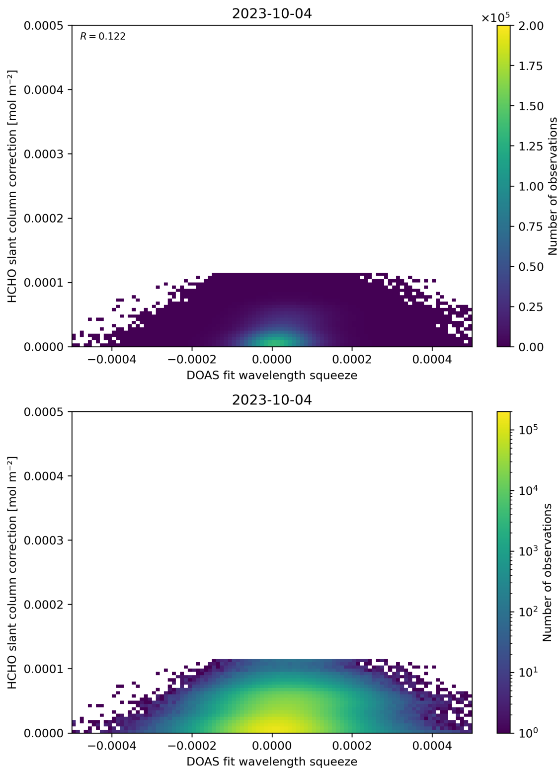
Figure 70: Scatter density plot of “DOAS fit wavelength squeeze” against “HCHO slant column correction” for 2023-10-03 to 2023-10-05.
