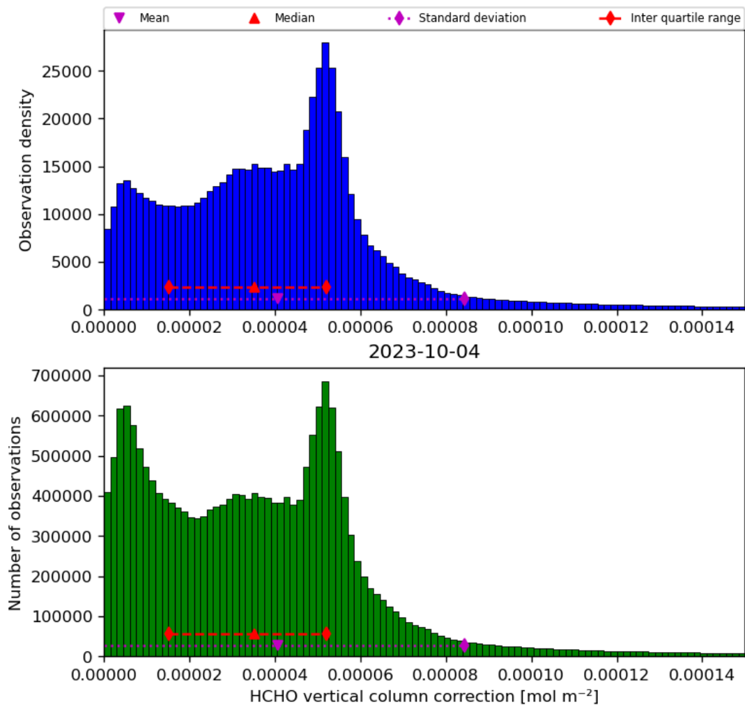
Figure 37: Histogram of “HCHO vertical column correction” for 2023-10-03 to 2023-10-05
