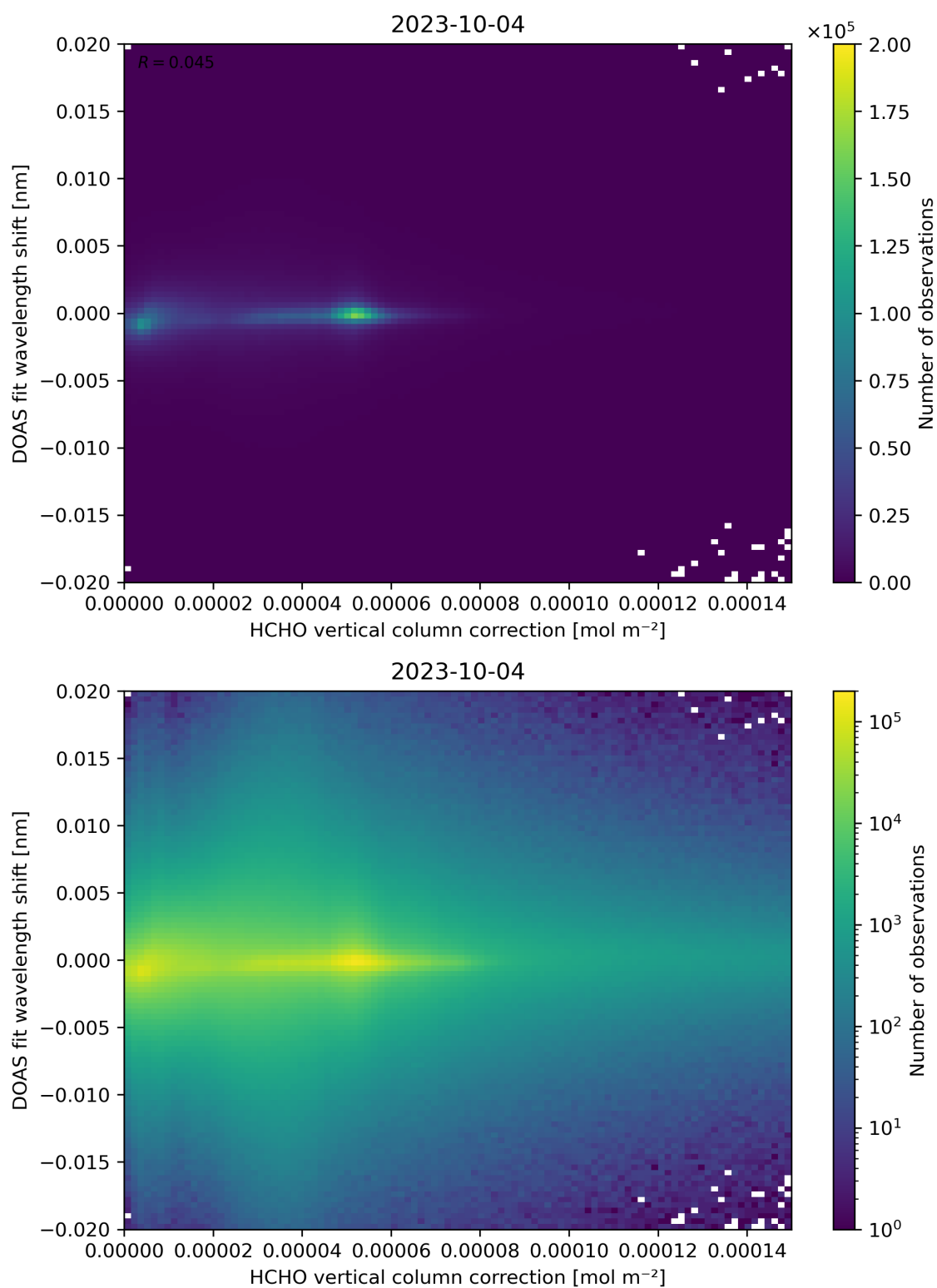
Figure 113: Scatter density plot of “HCHO vertical column correction” against “DOAS fit wavelength shift” for 2023-10-03 to 2023-10-05.
