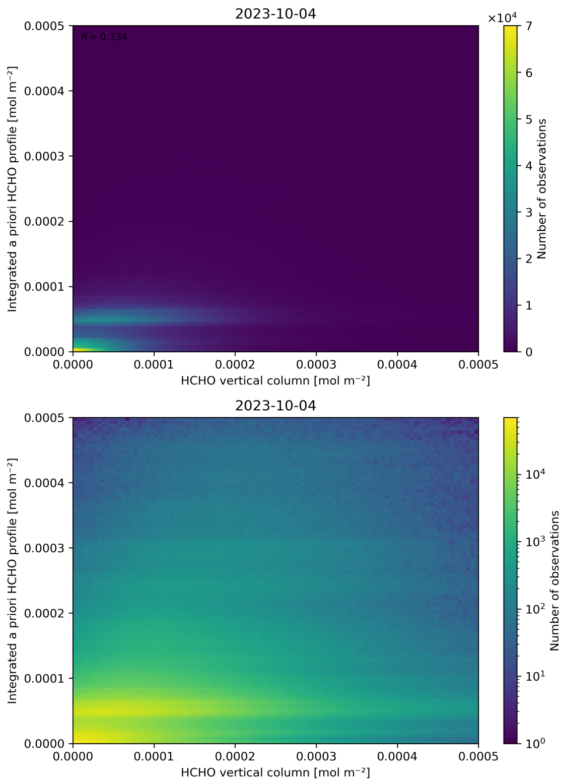
Figure 135: Scatter density plot of “HCHO vertical column” against “Integrated a priori HCHO profile” for 2023-10-03 to 2023-10-05.
