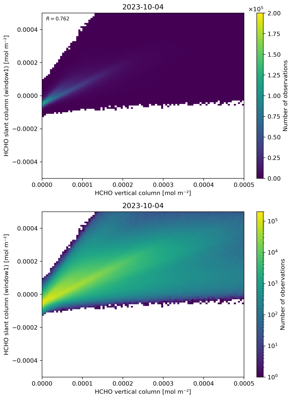
Figure 129: Scatter density plot of “HCHO vertical column” against “HCHO slant column (window1)” for 2023-10-03 to 2023-10-05.
