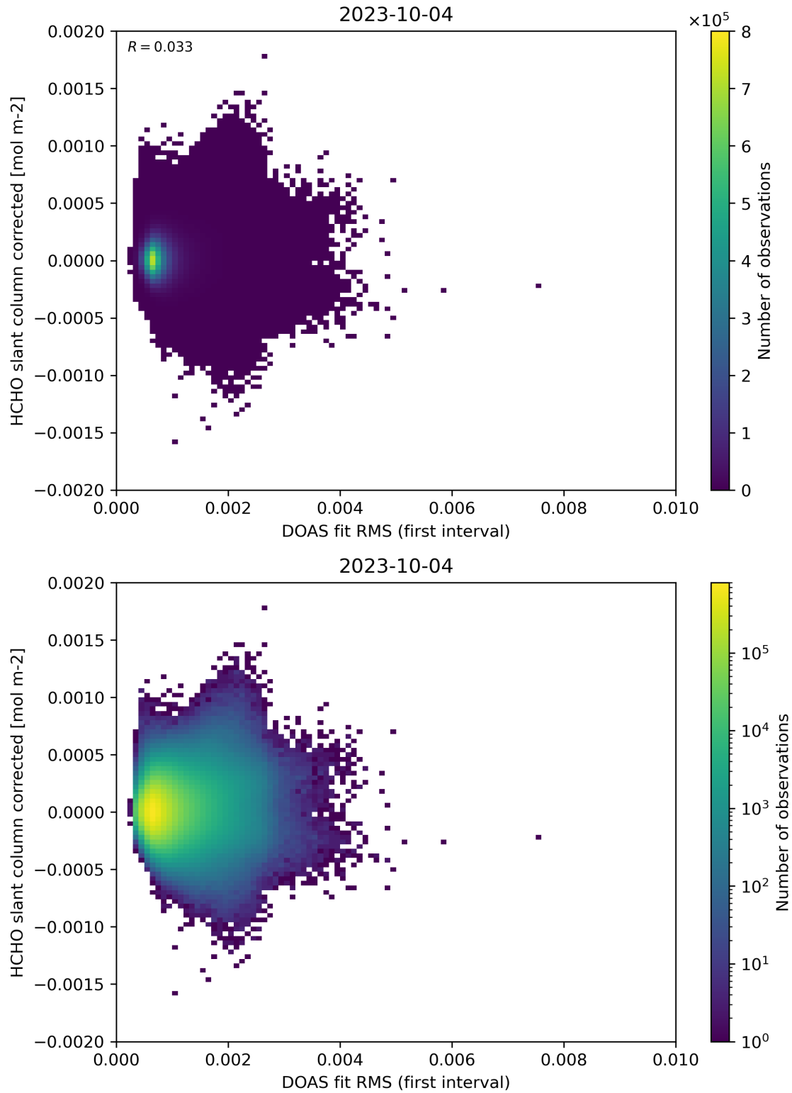
Figure 62: Scatter density plot of “DOAS fit RMS (first interval)” against “HCHO slant column corrected” for 2023-10-03 to 2023-10-05.
