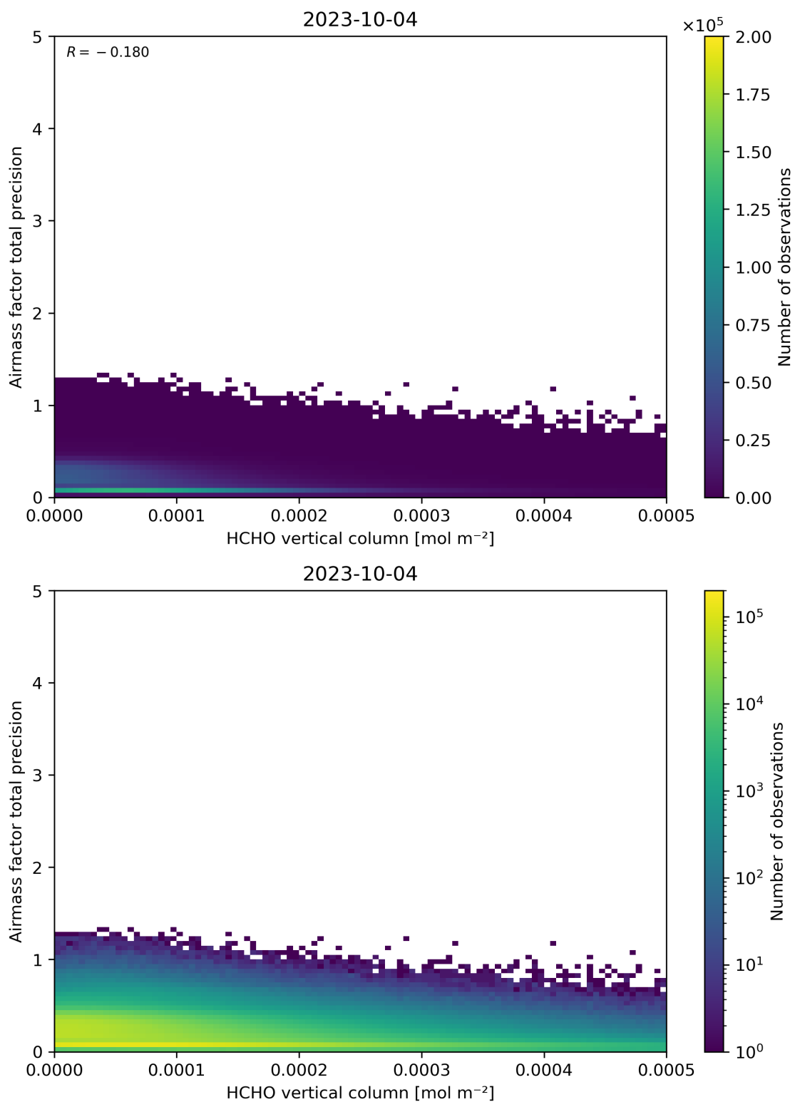
Figure 132: Scatter density plot of “HCHO vertical column” against “Airmass factor total precision” for 2023-10-03 to 2023-10-05.
