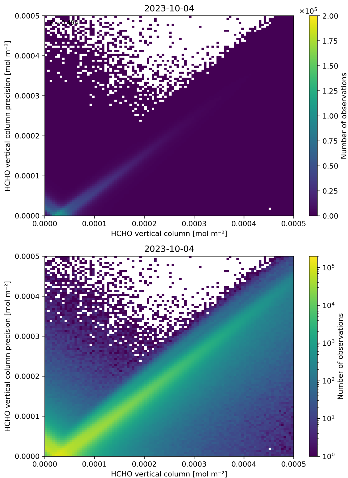
Figure 134: Scatter density plot of “HCHO vertical column” against “HCHO vertical column precision” for 2023-10-03 to 2023-10-05.
