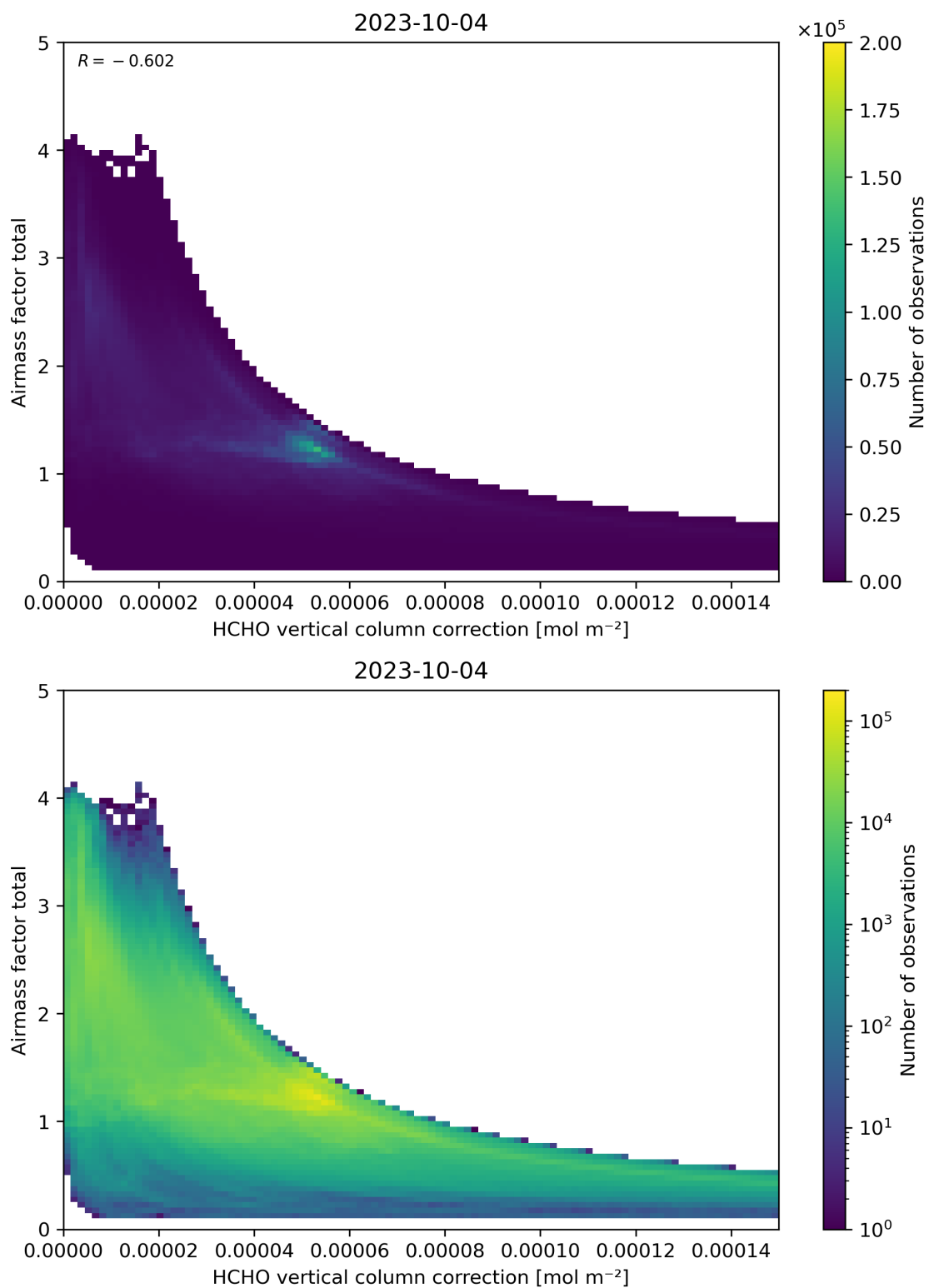
Figure 120: Scatter density plot of “HCHO vertical column correction” against “Airmass factor total” for 2023-10-03 to 2023-10-05.
