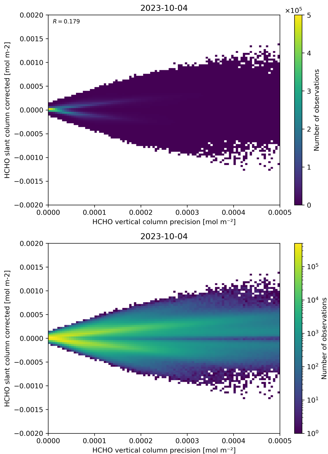
Figure 140: Scatter density plot of “HCHO vertical column precision” against “HCHO slant column corrected” for 2023-10-03 to 2023-10-05.
