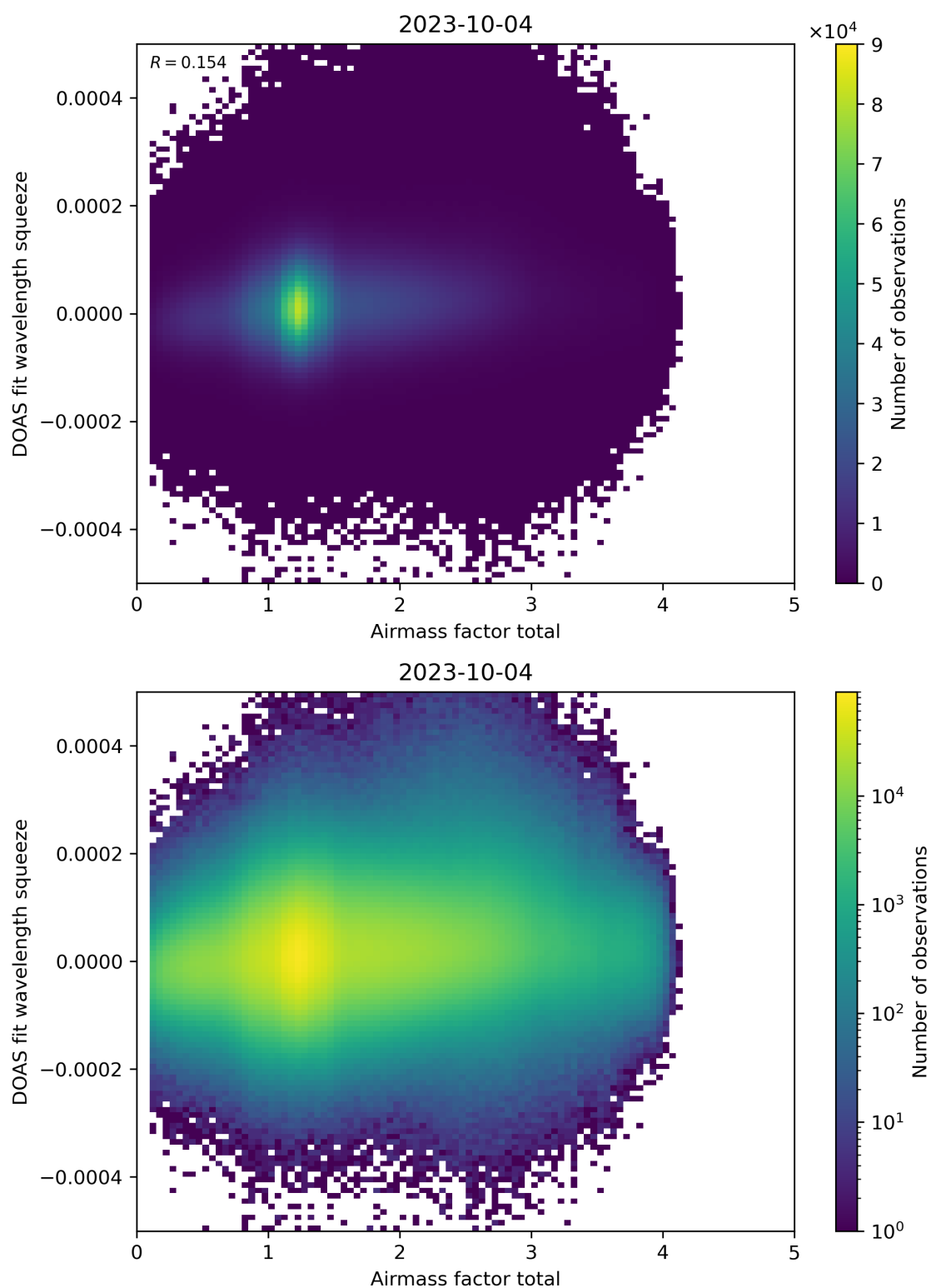
Figure 99: Scatter density plot of “Airmass factor total” against “DOAS fit wavelength squeeze” for 2023-10-03 to 2023-10-05.
