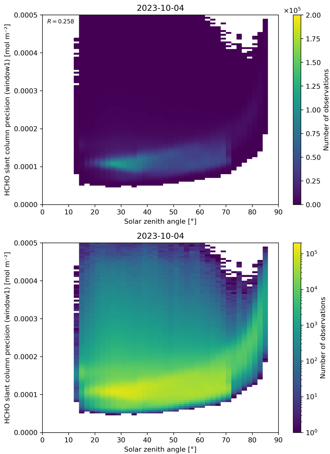
Figure 174: Scatter density plot of “Solar zenith angle” against “HCHO slant column precision (window1)” for 2023-10-03 to 2023-10-05.
