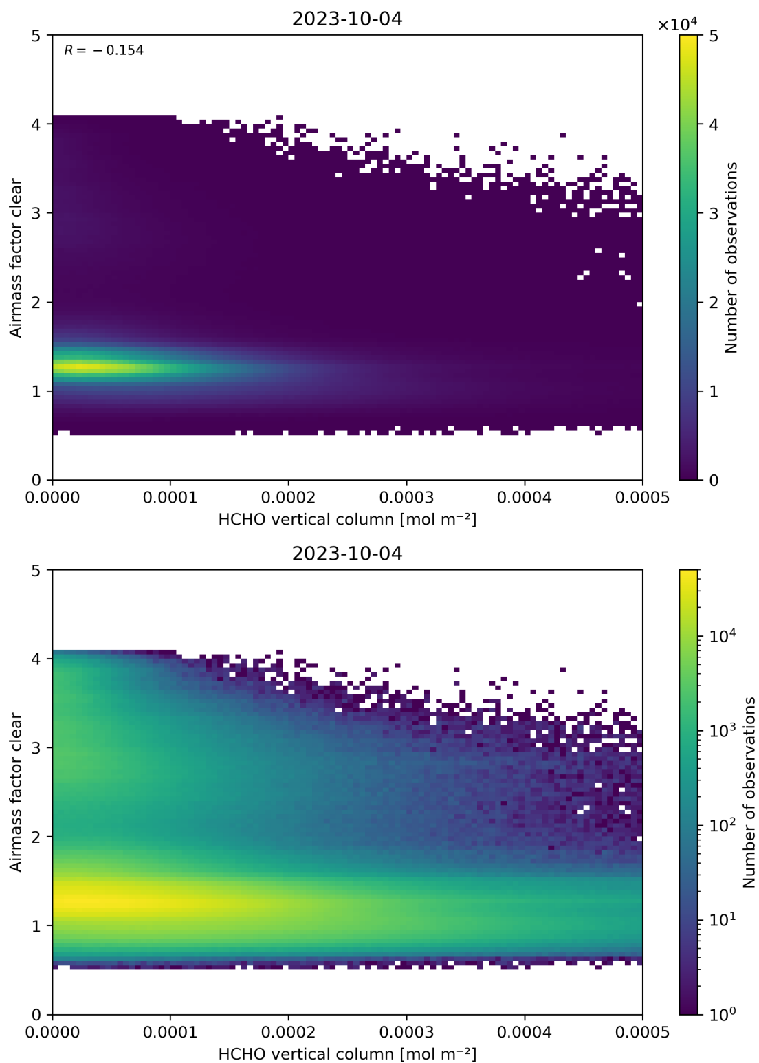
Figure 126: Scatter density plot of “HCHO vertical column” against “Airmass factor clear” for 2023-10-03 to 2023-10-05.
