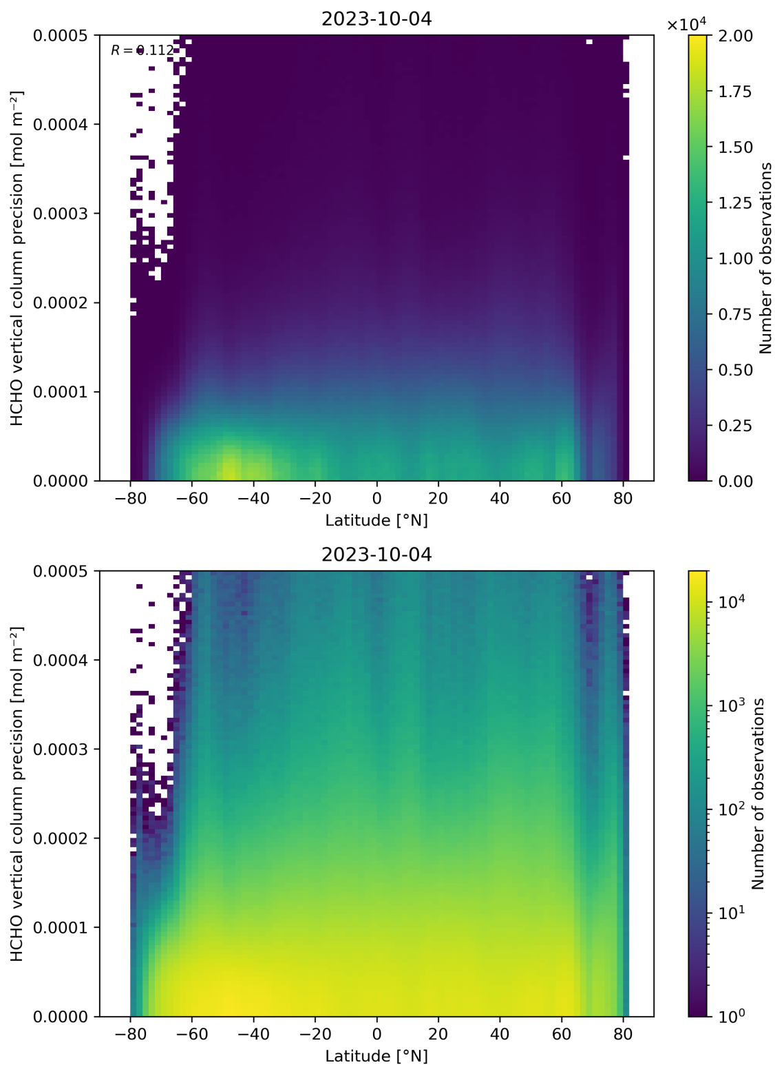
Figure 165: Scatter density plot of “Latitude” against “HCHO vertical column precision” for 2023-10-03 to 2023-10-05.
