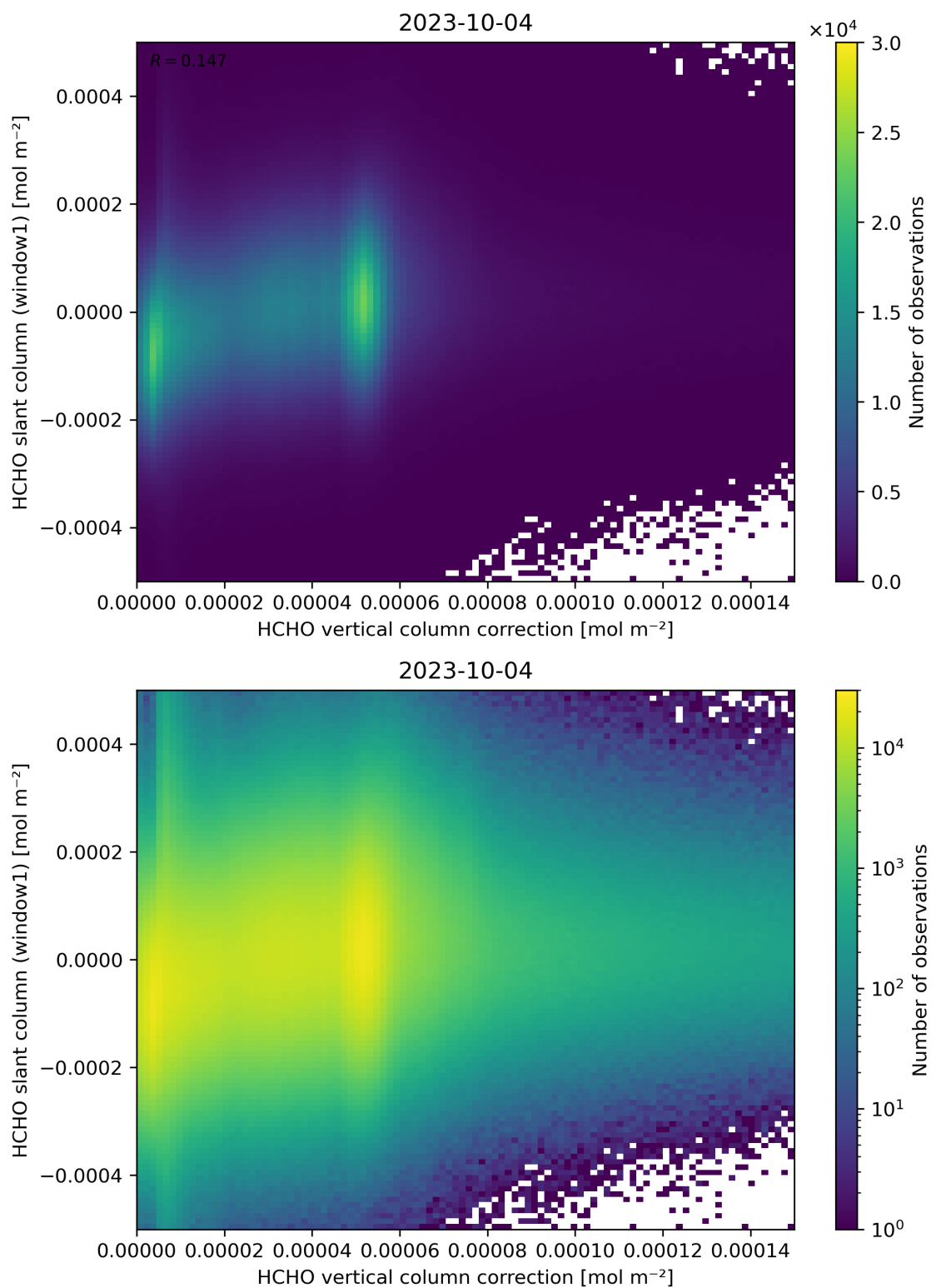
Figure 118: Scatter density plot of “HCHO vertical column correction” against “HCHO slant column (window1)” for 2023-10-03 to 2023-10-05.
