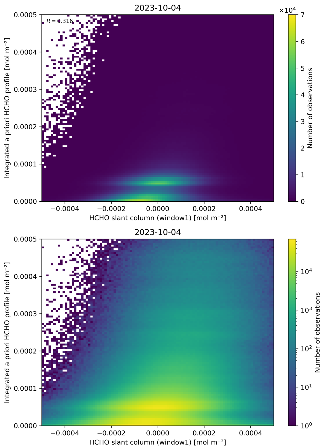
Figure 87: Scatter density plot of “HCHO slant column (window1)” against “Integrated a priori HCHO profile” for 2023-10-03 to 2023-10-05.
