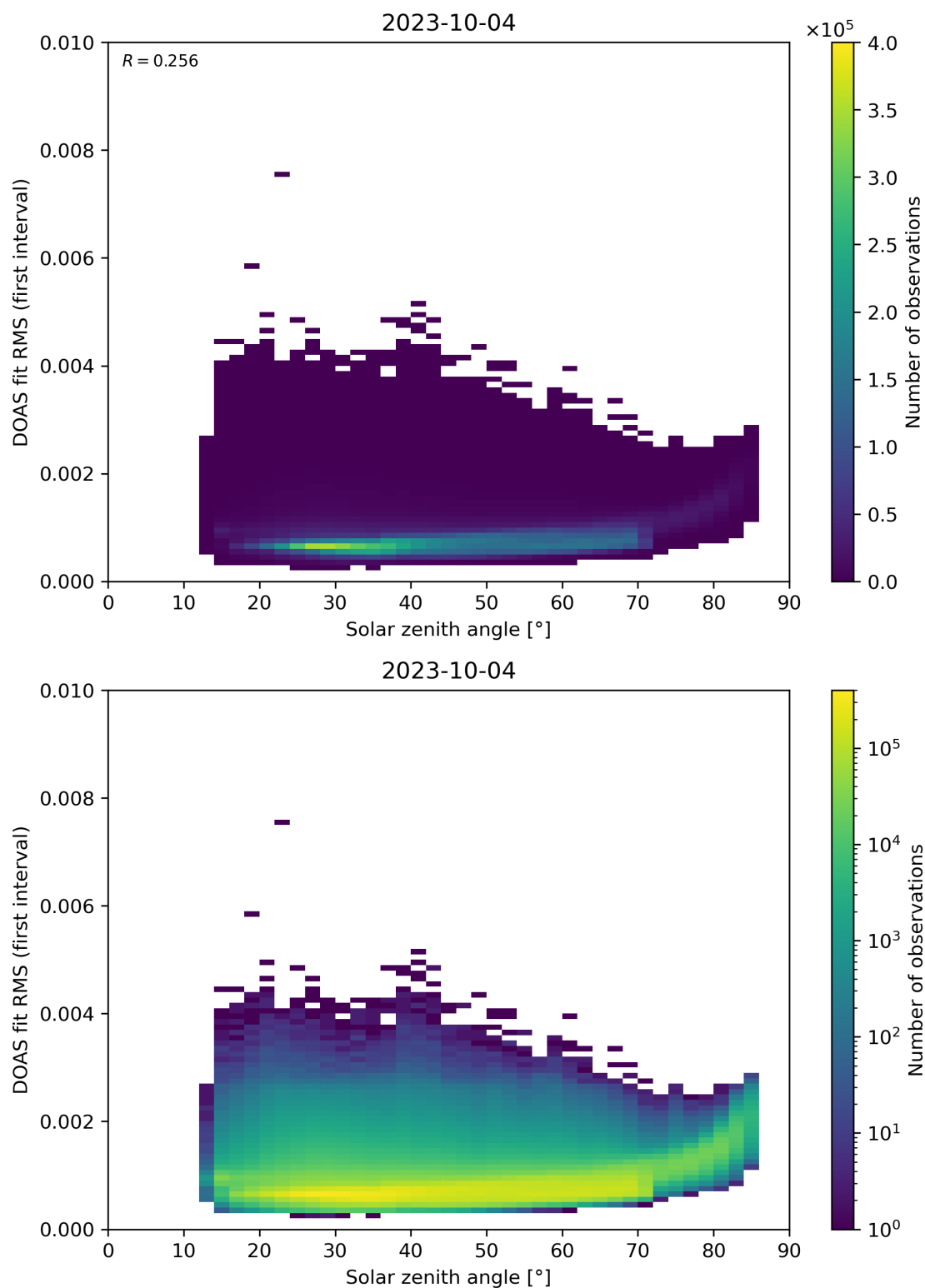
Figure 167: Scatter density plot of “Solar zenith angle” against “DOAS fit RMS (first interval)” for 2023-10-03 to 2023-10-05.
