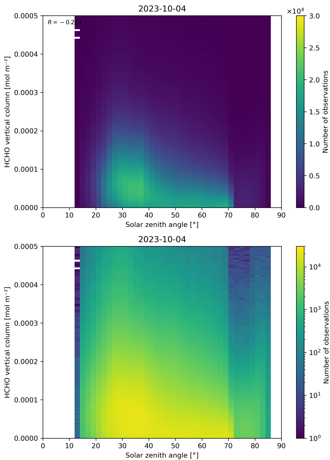
Figure 177: Scatter density plot of “Solar zenith angle” against “HCHO vertical column” for 2023-10-03 to 2023-10-05.
