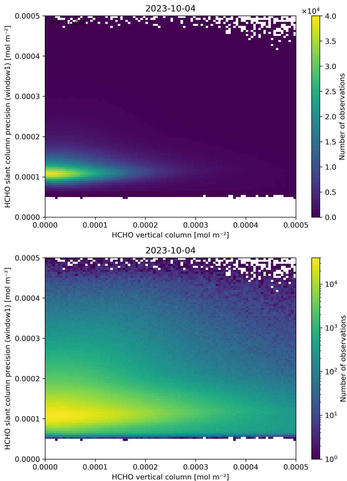
Figure 130: Scatter density plot of “HCHO vertical column” against “HCHO slant column precision (window1)” for 2023-10-03 to 2023-10-05.
