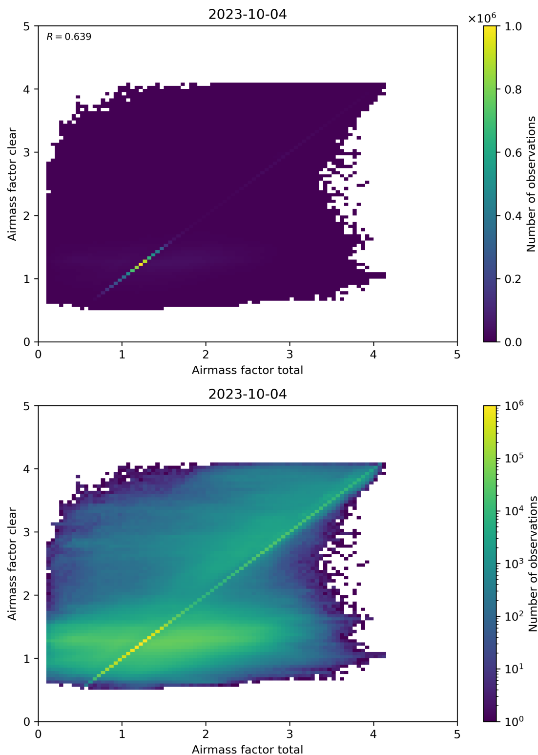
Figure 100: Scatter density plot of “Airmass factor total” against “Airmass factor clear” for 2023-10-03 to 2023-10-05.
