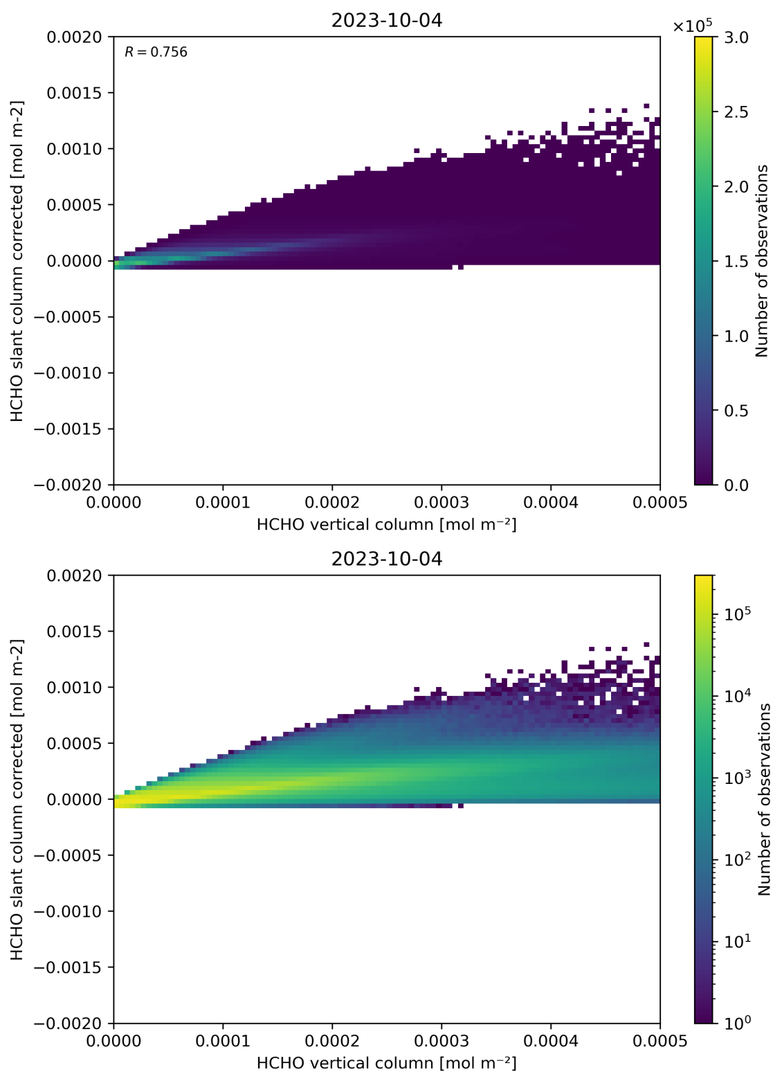
Figure 127: Scatter density plot of “HCHO vertical column” against “HCHO slant column corrected” for 2023-10-03 to 2023-10-05.
