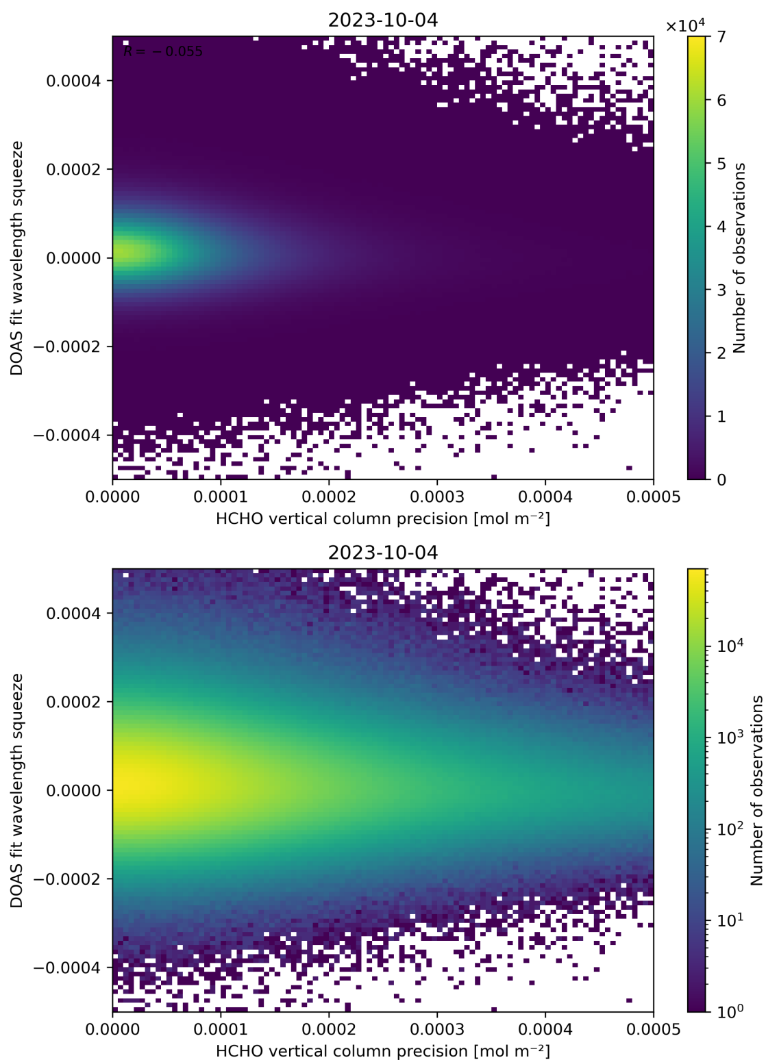
Figure 138: Scatter density plot of “HCHO vertical column precision” against “DOAS fit wavelength squeeze” for 2023-10-03 to 2023-10-05.
