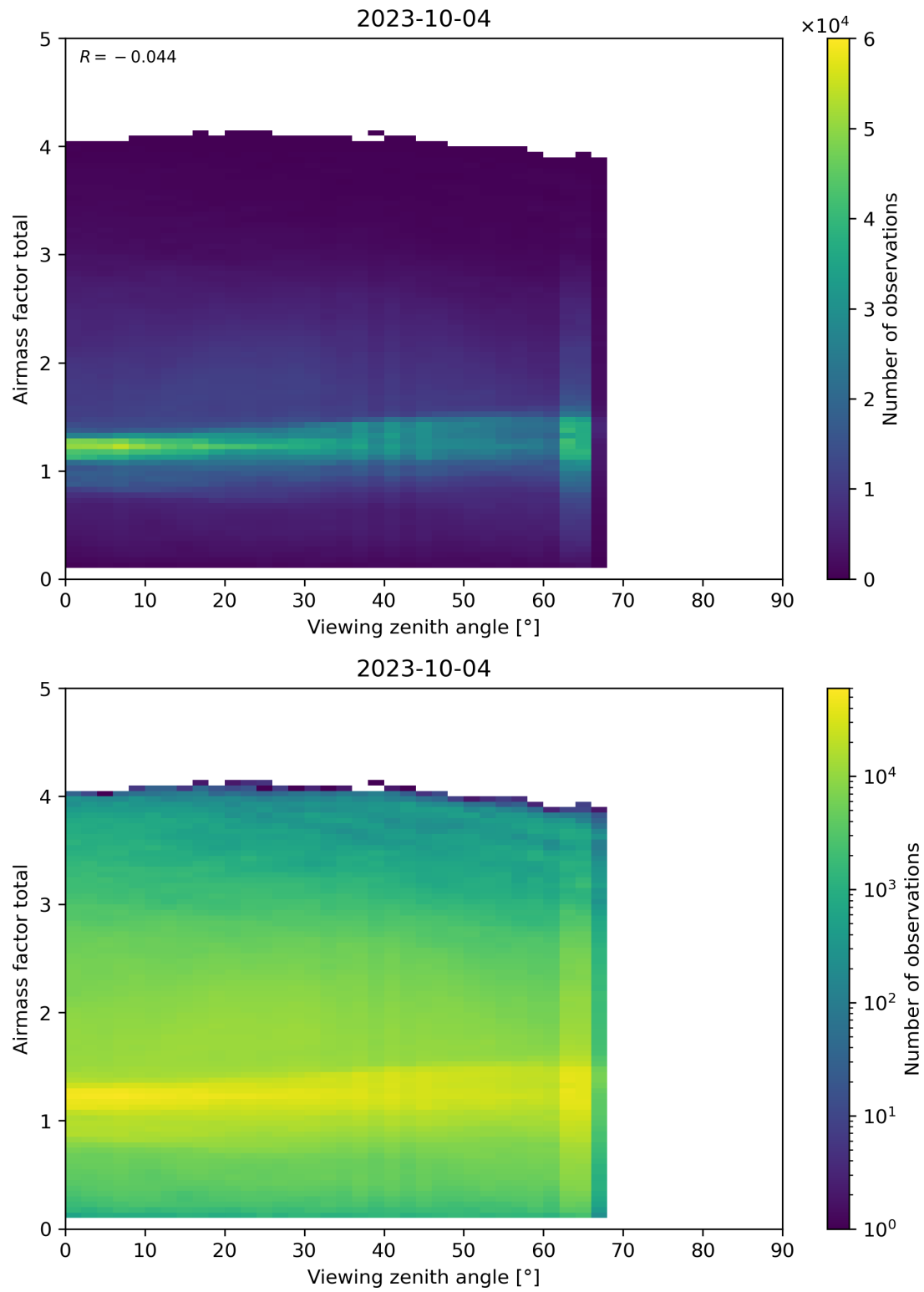
Figure 190: Scatter density plot of “Viewing zenith angle” against “Airmass factor total” for 2023-10-03 to 2023-10-05.
