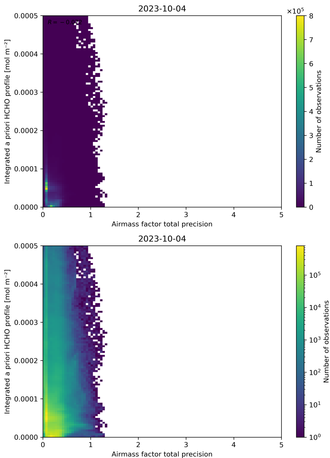
Figure 111: Scatter density plot of “Airmass factor total precision” against “Integrated a priori HCHO profile” for 2023-10-03 to 2023-10-05.
