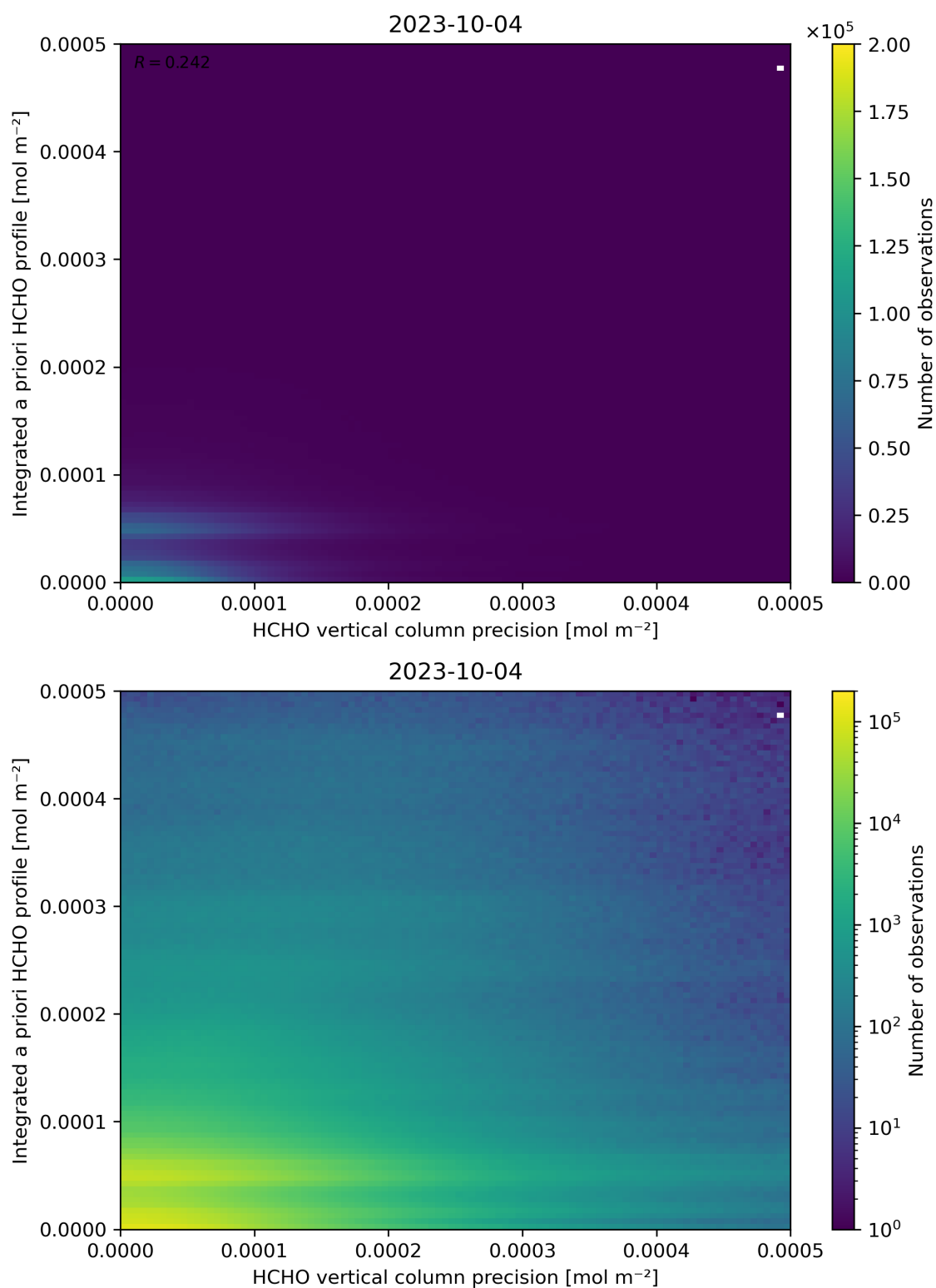
Figure 147: Scatter density plot of “HCHO vertical column precision” against “Integrated a priori HCHO profile” for 2023-10-03 to 2023-10-05.
