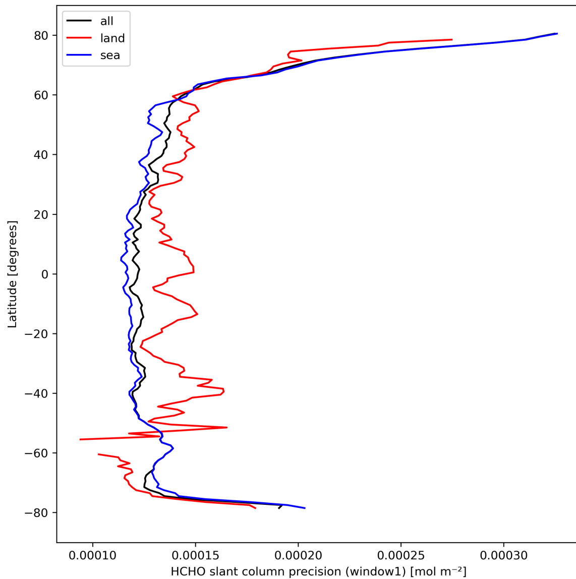
Figure 25: Zonal average of “HCHO slant column precision (window1)” for 2023-10-03 to 2023-10-05.
