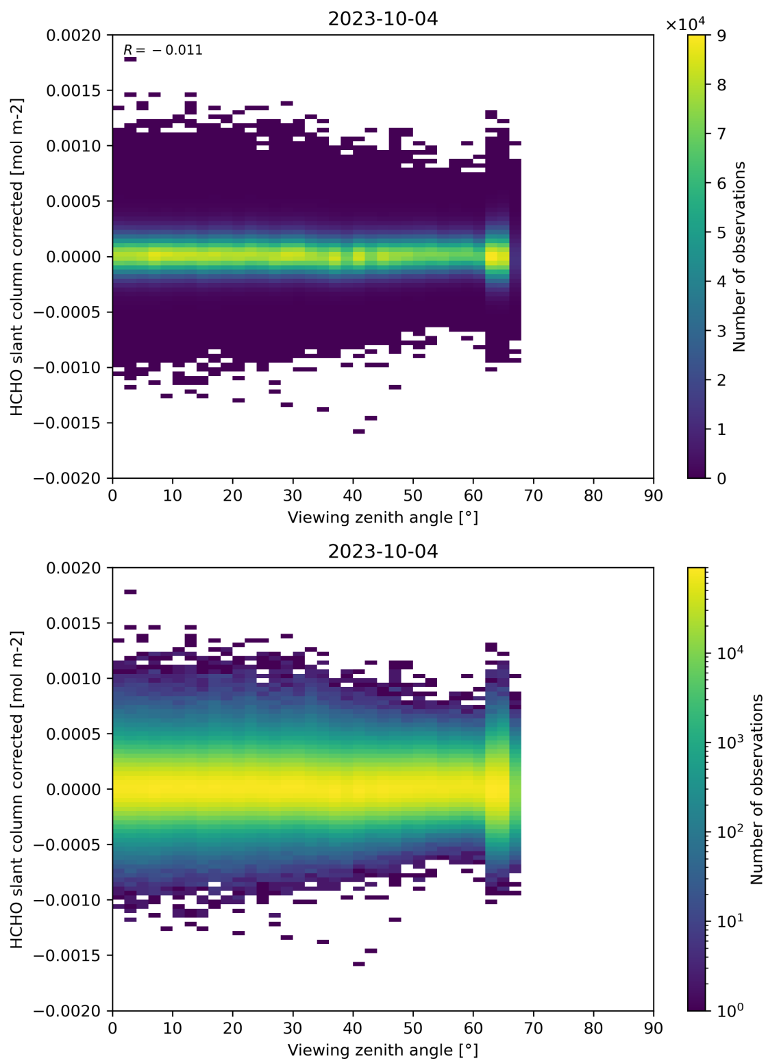
Figure 186: Scatter density plot of “Viewing zenith angle” against “HCHO slant column corrected” for 2023-10-03 to 2023-10-05.
