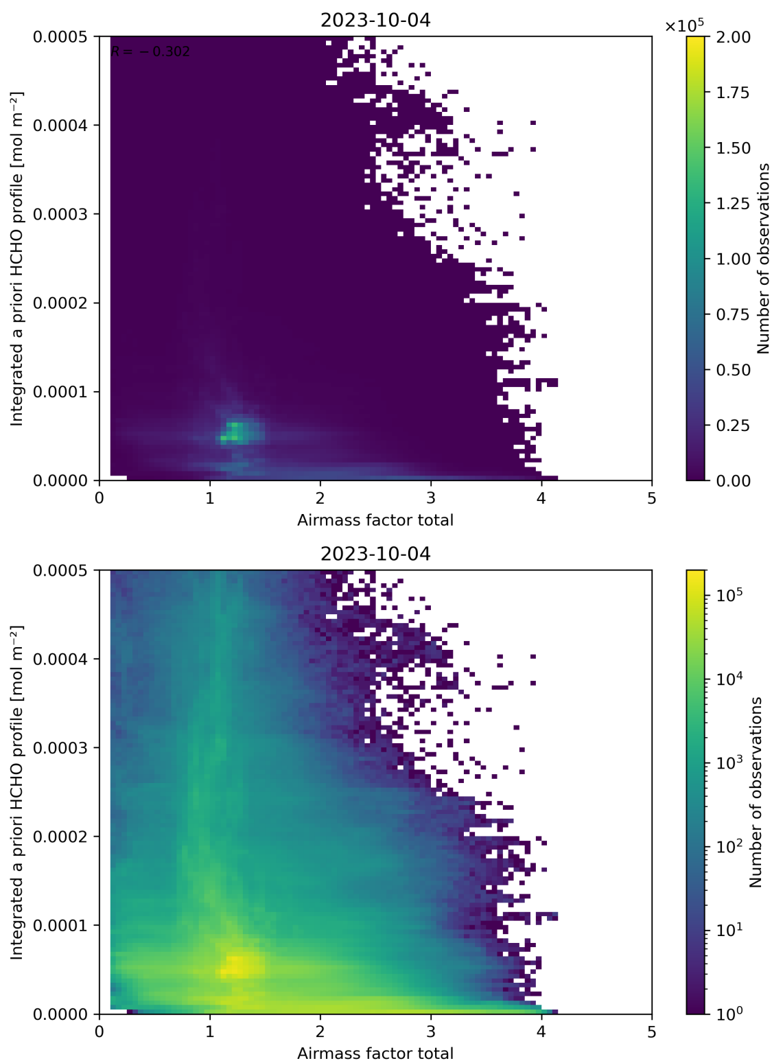
Figure 104: Scatter density plot of “Air mass factor total” against “Integrated a priori HCHO profile” for 2023-10-03 to 2023-10-05.
