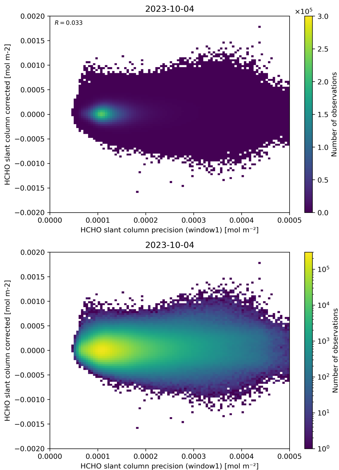
Figure 92: Scatter density plot of “HCHO slant column precision (window1)” against “HCHO slant column corrected” for 2023-10-03 to 2023-10-05.
