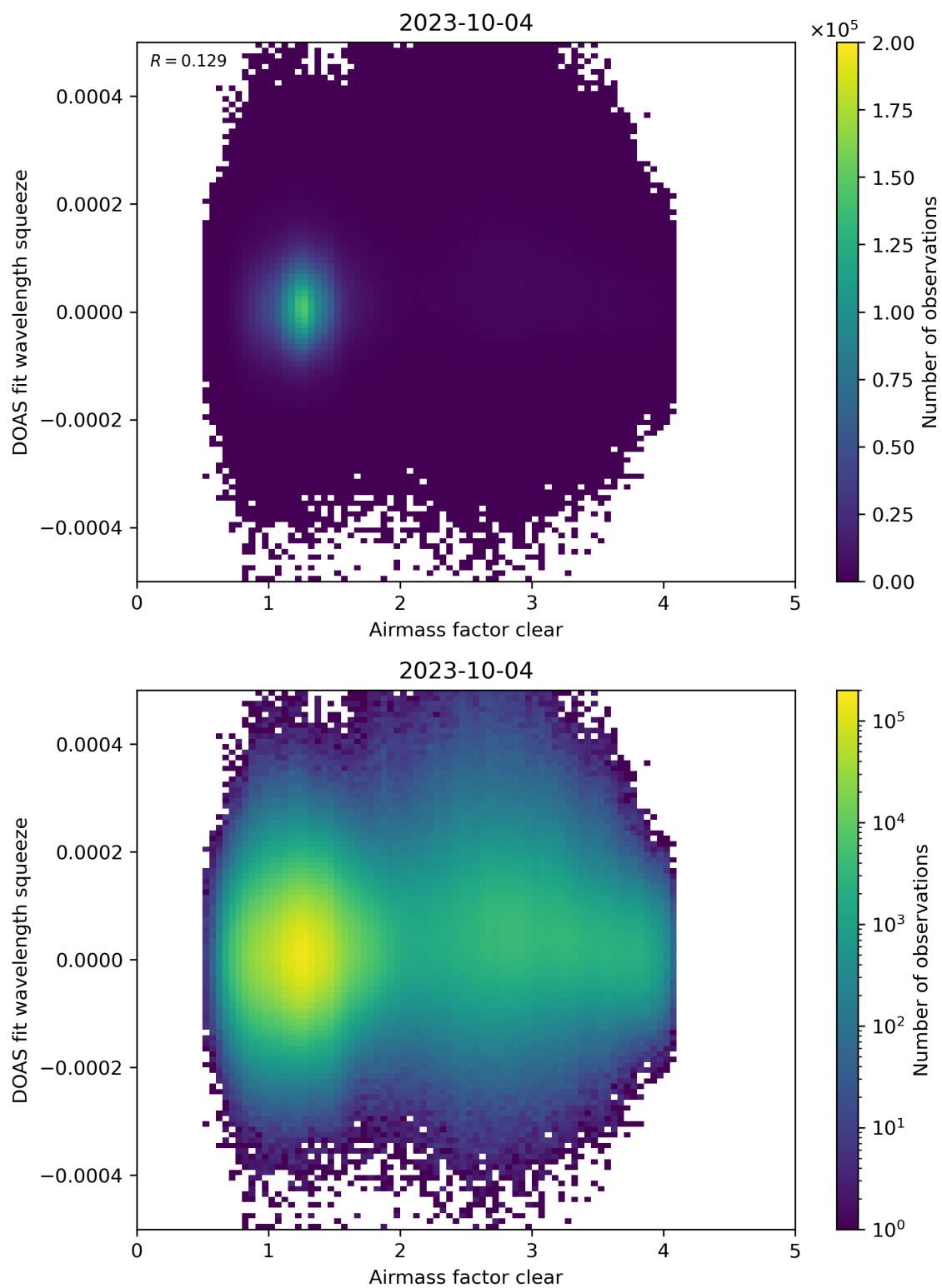
Figure 73: Scatter density plot of “Airmass factor clear” against “DOAS fit wavelength squeeze” for 2023-10-03 to 2023-10-05.
