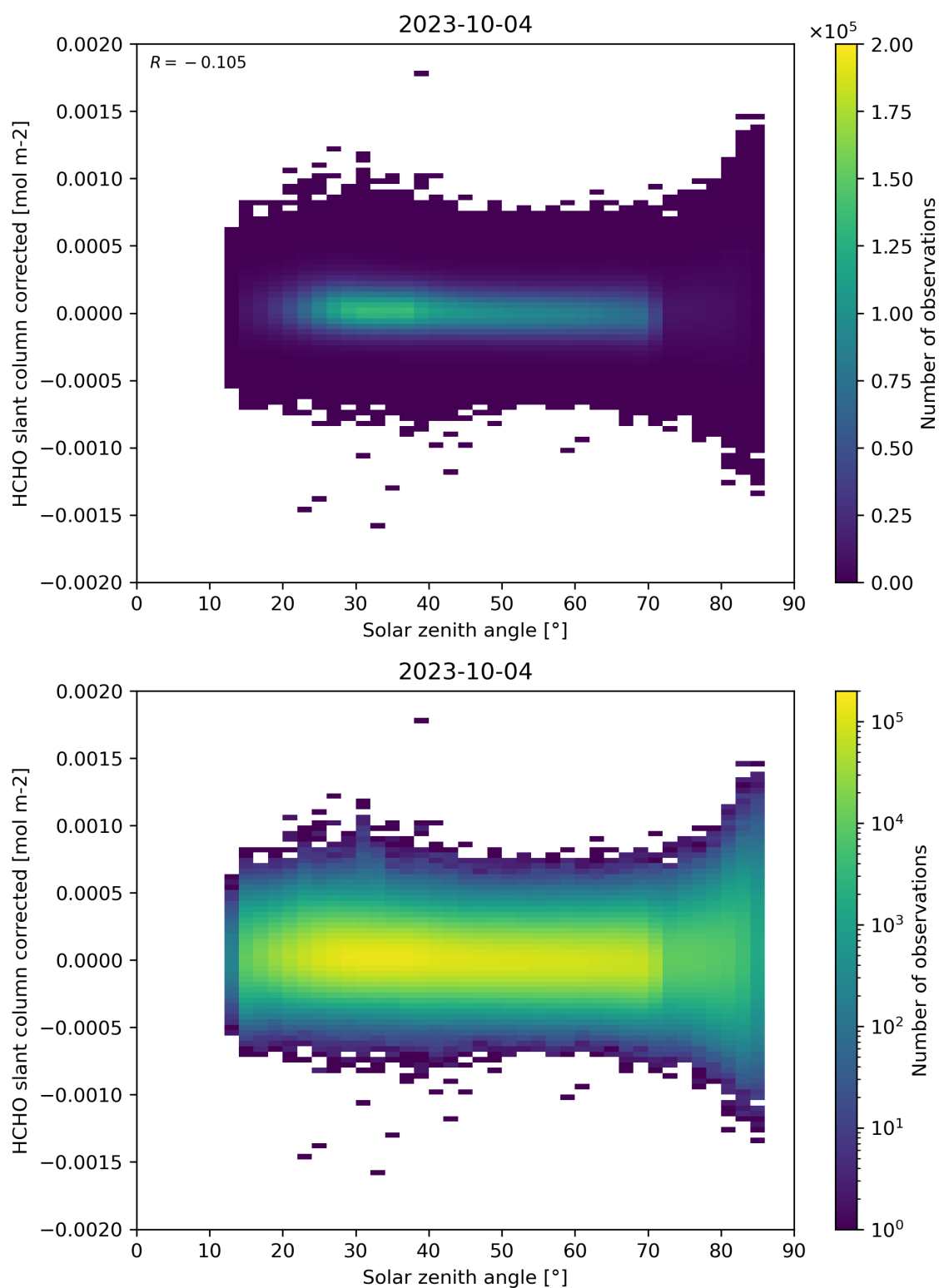
Figure 171: Scatter density plot of “Solar zenith angle” against “HCHO slant column corrected” for 2023-10-03 to 2023-10-05.
