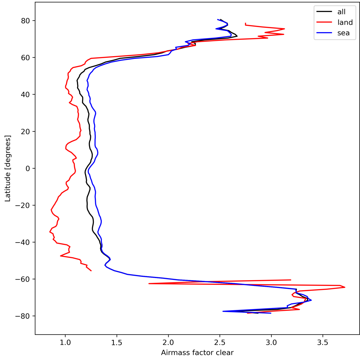
Figure 28: Zonal average of “Airmass factor clear” for 2023-10-03 to 2023-10-05.
