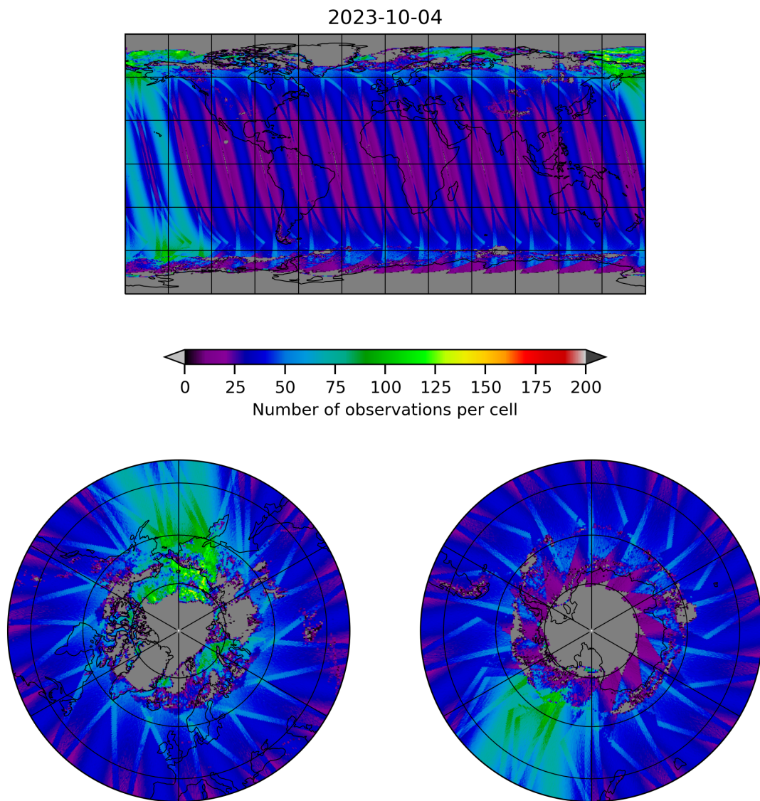
Figure 19: Map of the number of observations for 2023-10-03 to 2023-10-05
