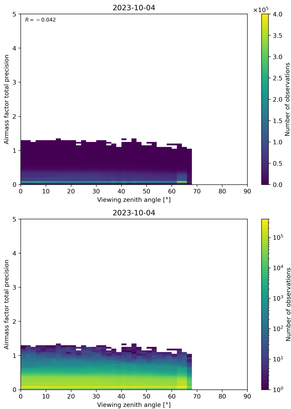
Figure 191: Scatter density plot of “Viewing zenith angle” against “Airmass factor total precision” for 2023-10-03 to 2023-10-05.
