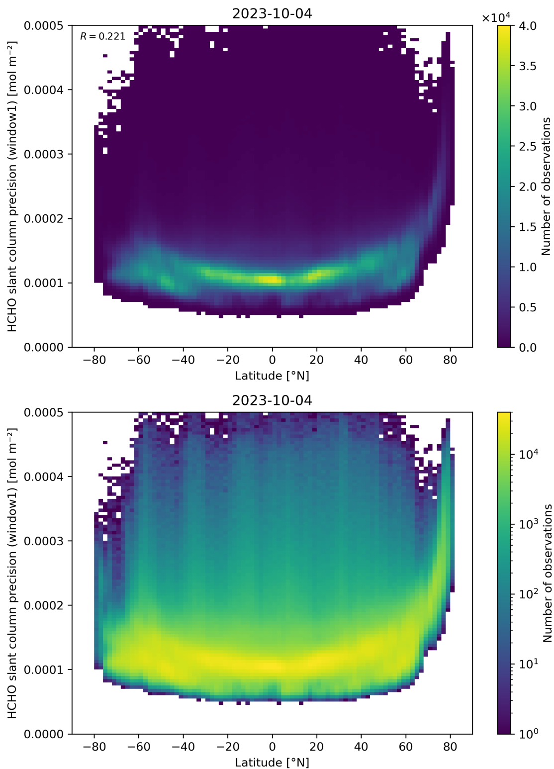
Figure 160: Scatter density plot of “Latitude” against “HCHO slant column precision (window1)” for 2023-10-03 to 2023-10-05.
