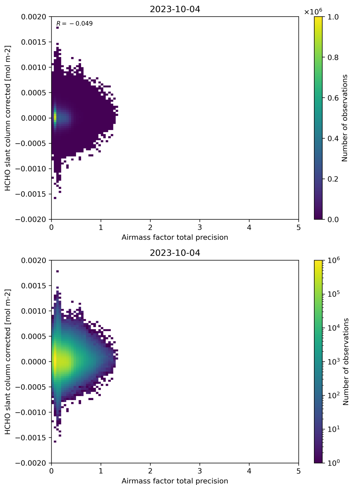
Figure 109: Scatter density plot of “Airmass factor total precision” against “HCHO slant column corrected” for 2023-10-03 to 2023-10-05.
