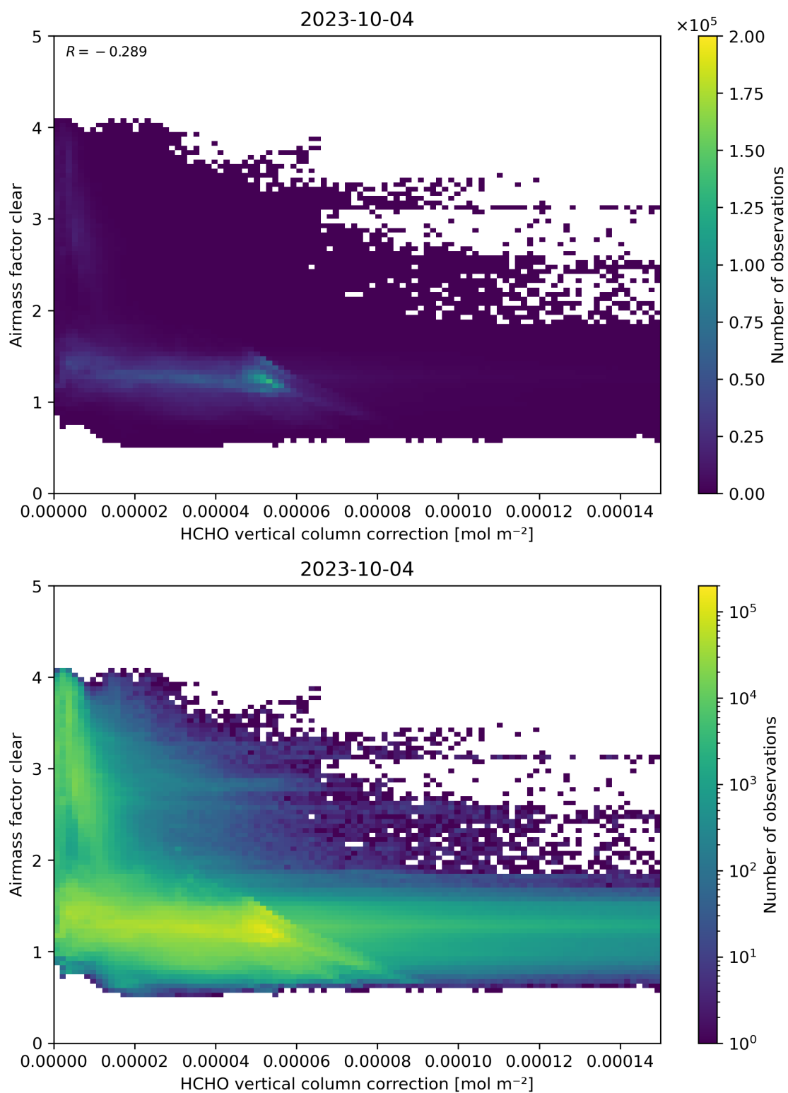
Figure 115: Scatter density plot of “HCHO vertical column correction” against “Airmass factor clear” for 2023-10-03 to 2023-10-05.
