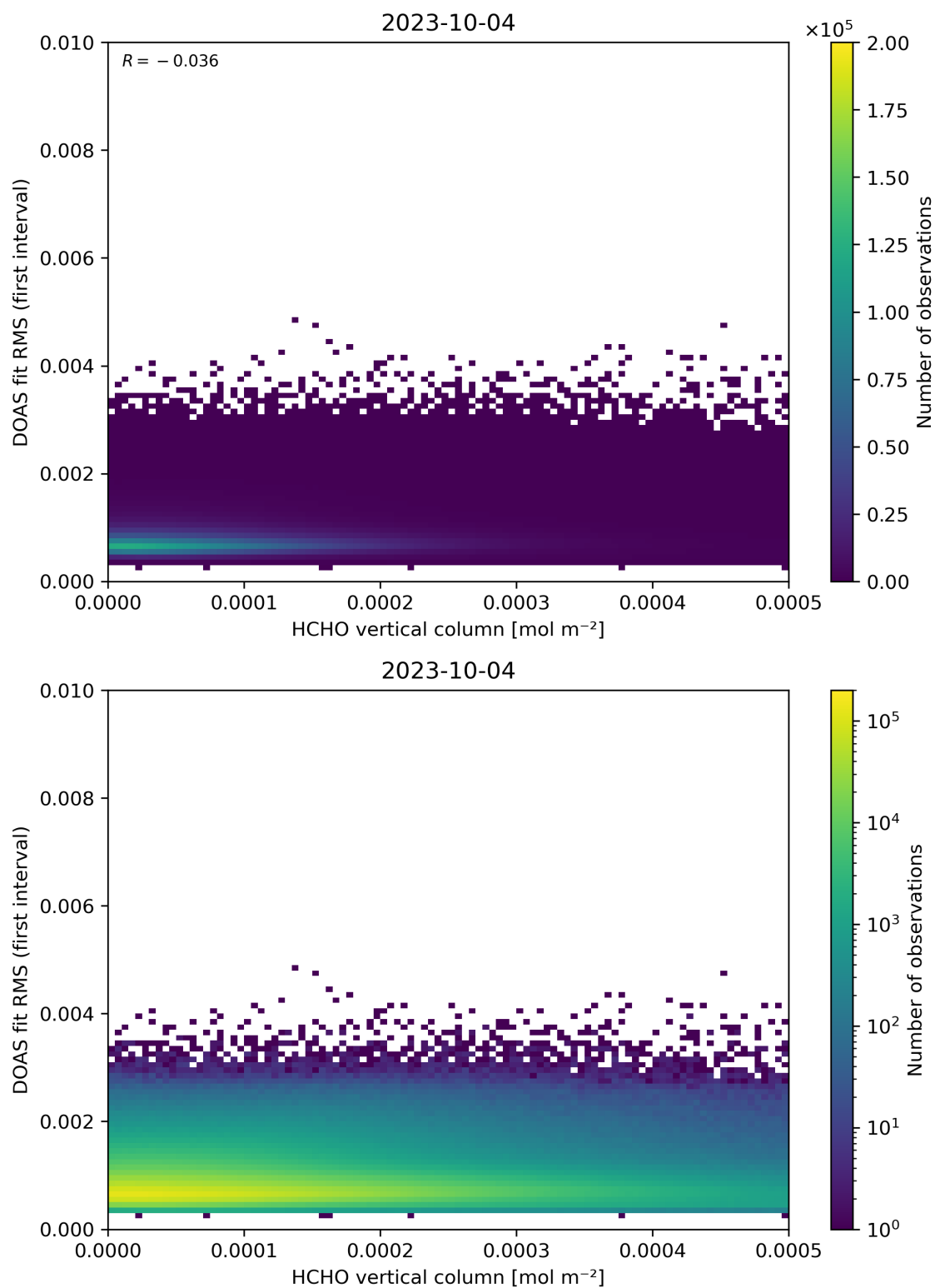
Figure 123: Scatter density plot of “HCHO vertical column” against “DOAS fit RMS (first interval)” for 2023-10-03 to 2023-10-05.
