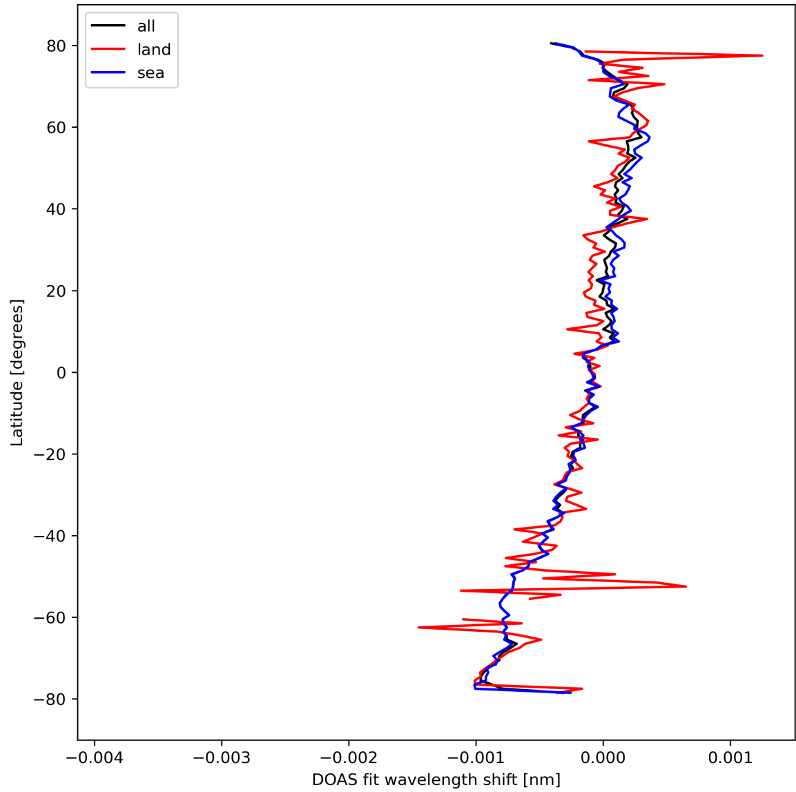
Figure 30: Zonal average of “DOAS fit wavelength shift” for 2023-10-03 to 2023-10-05.
