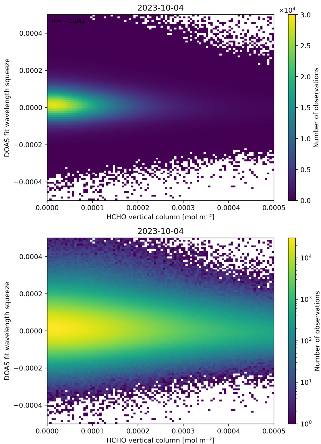
Figure 125: Scatter density plot of “HCHO vertical column” against “DOAS fit wavelength squeeze” for 2023-10-03 to 2023-10-05.
