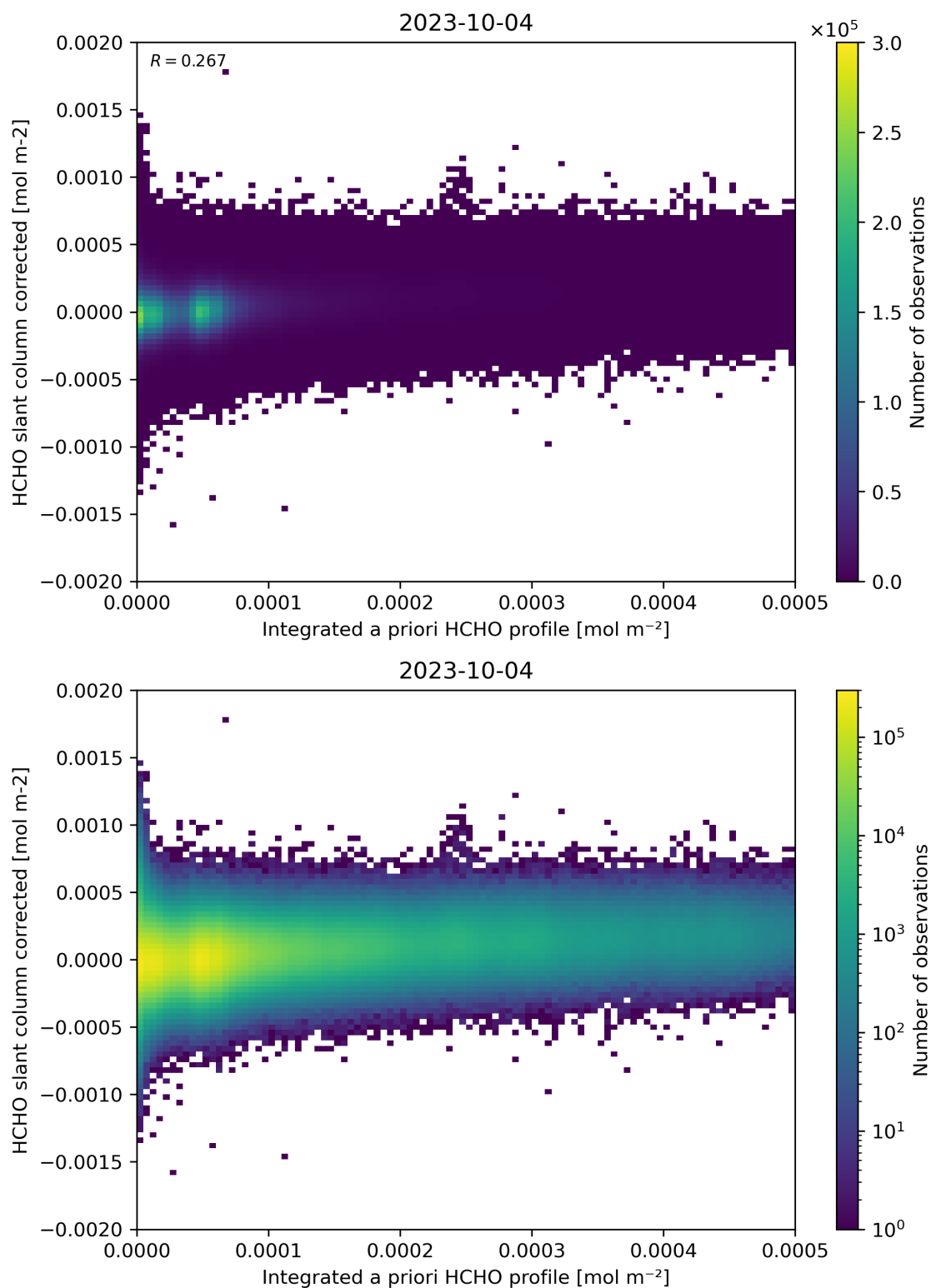
Figure 151: Scatter density plot of “Integrated a priori HCHO profile” against “HCHO slant column corrected” for 2023-10-03 to 2023-10-05.
