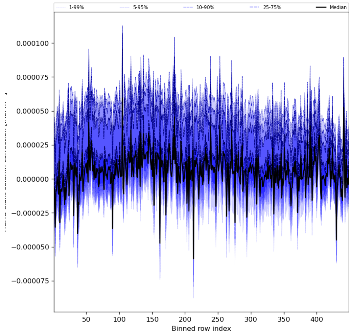
Figure 61: Along track statistics of “HCHO slant column correction” for 2023-10-03 to 2023-10-05
