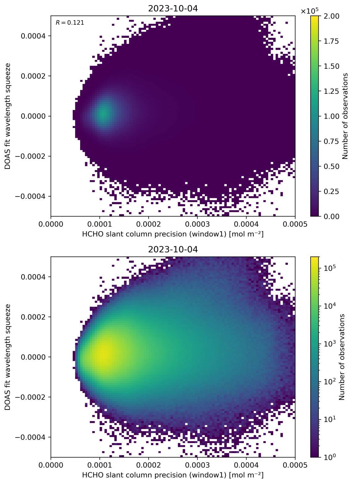
Figure 90: Scatter density plot of “HCHO slant column precision (window1)” against “DOAS fit wavelength squeeze” for 2023-10-03 to 2023-10-05.
