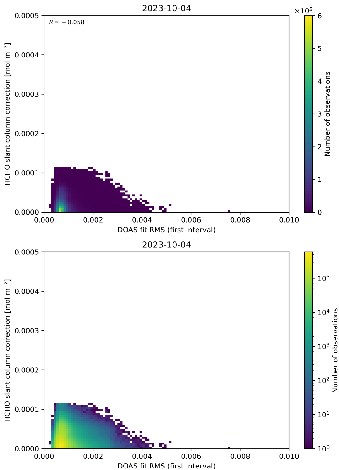
Figure 63: Scatter density plot of “DOAS fit RMS (first interval)” against “HCHO slant column correction” for 2023-10-03 to 2023-10-05.
