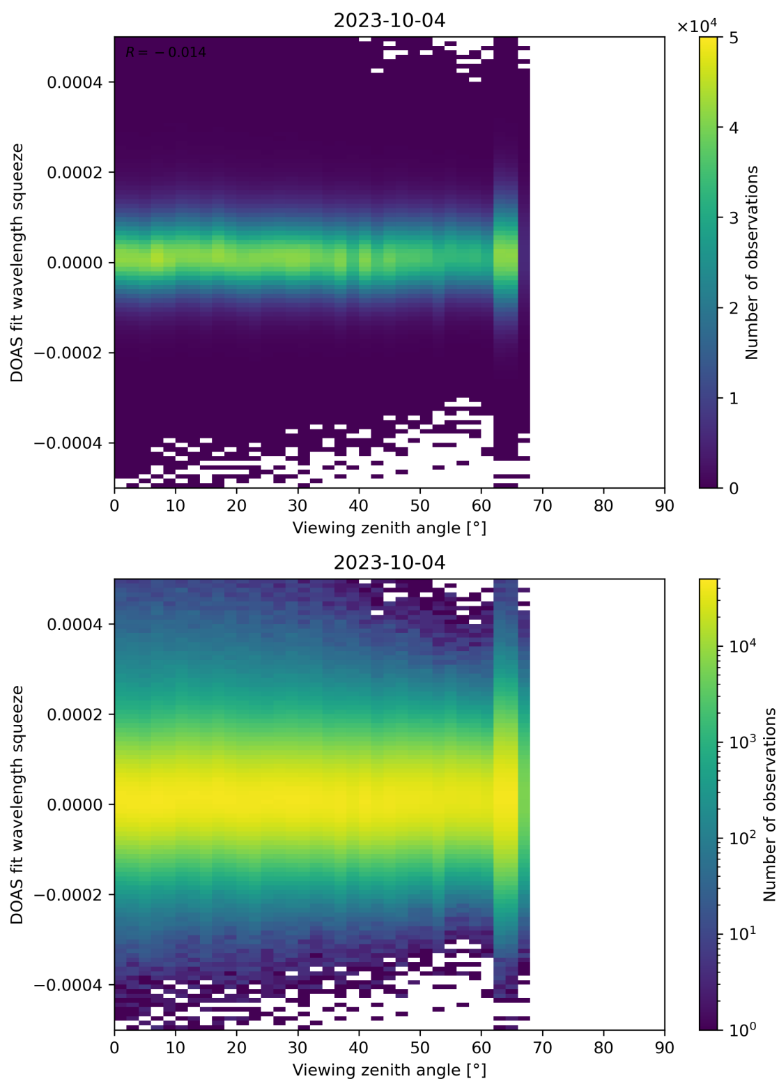
Figure 184: Scatter density plot of “Viewing zenith angle” against “DOAS fit wavelength squeeze” for 2023-10-03 to 2023-10-05.
