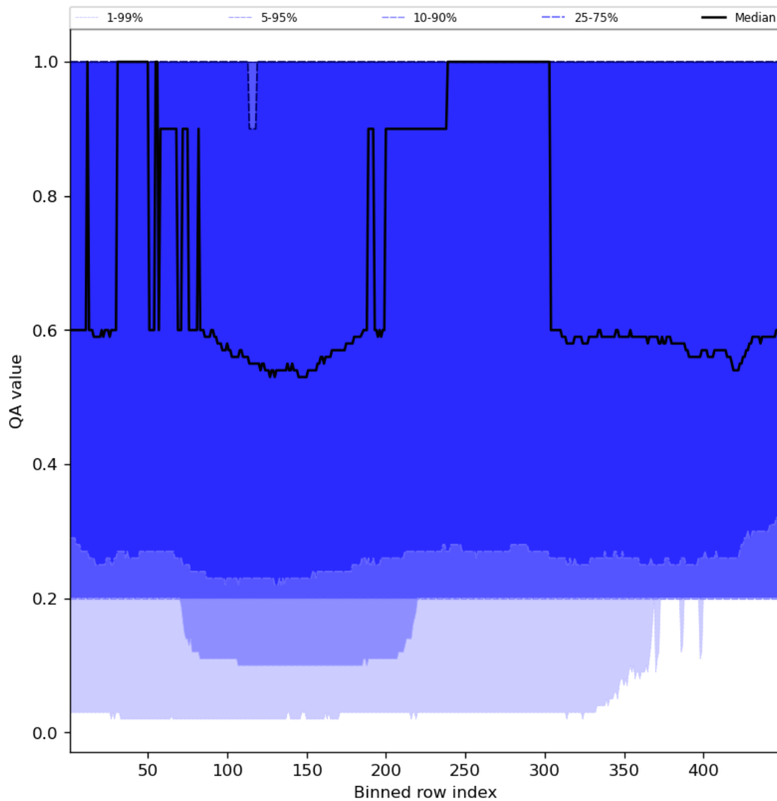
Figure 48: Along track statistics of “QA value” for 2023-10-03 to 2023-10-05
