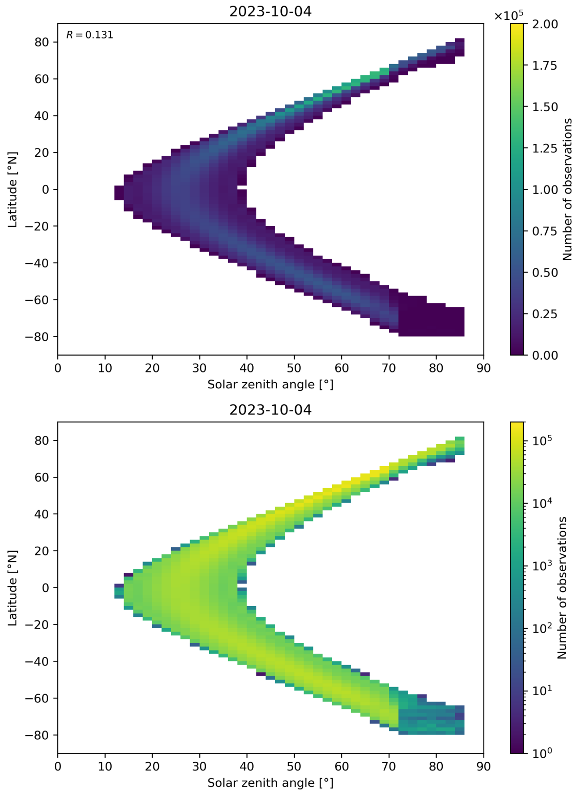
Figure 181: Scatter density plot of “Solar zenith angle” against “Latitude” for 2023-10-03 to 2023-10-05.
