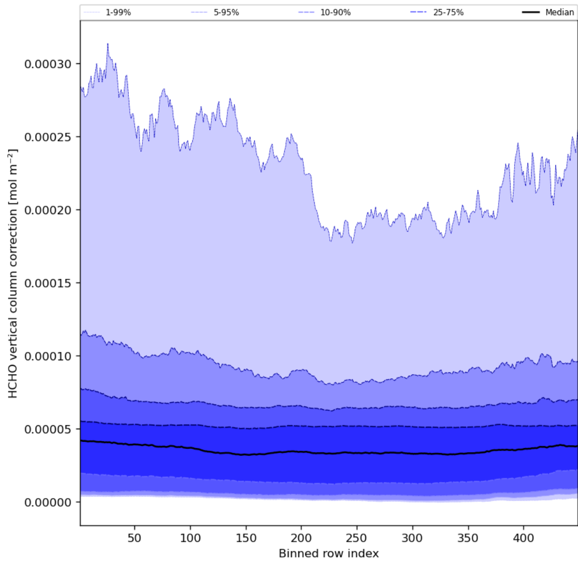
Figure 51: Along track statistics of “HCHO vertical column correction” for 2023-10-03 to 2023-10-05
