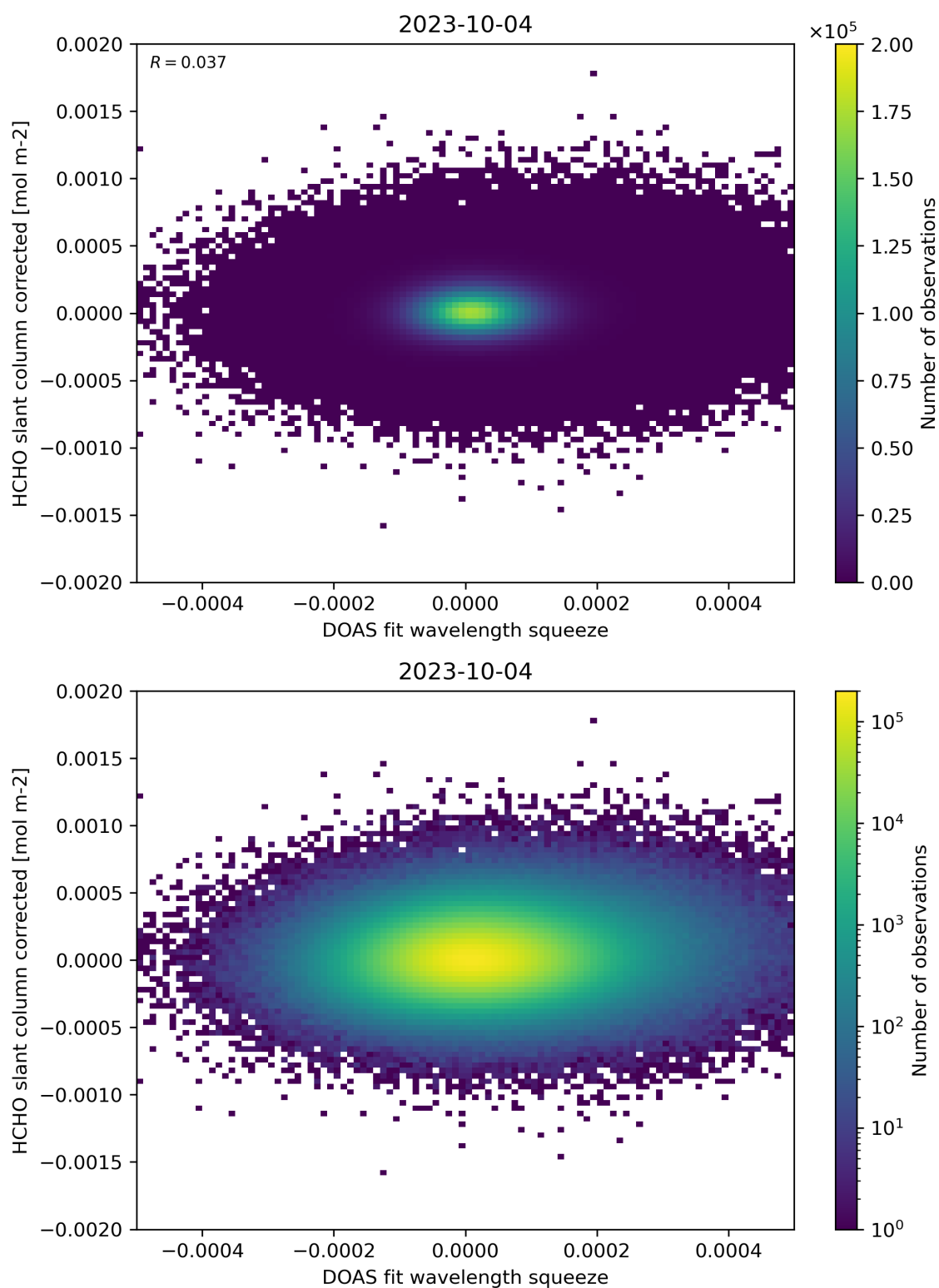
Figure 69: Scatter density plot of “DOAS fit wavelength squeeze” against “HCHO slant column corrected” for 2023-10-03 to 2023-10-05.
