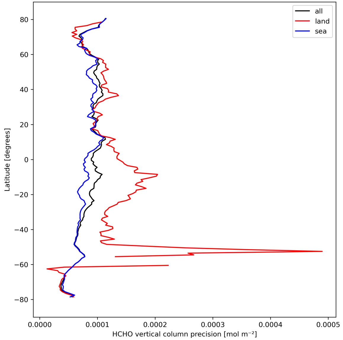
Figure 22: Zonal average of “HCHO vertical column precision” for 2023-10-03 to 2023-10-05.
