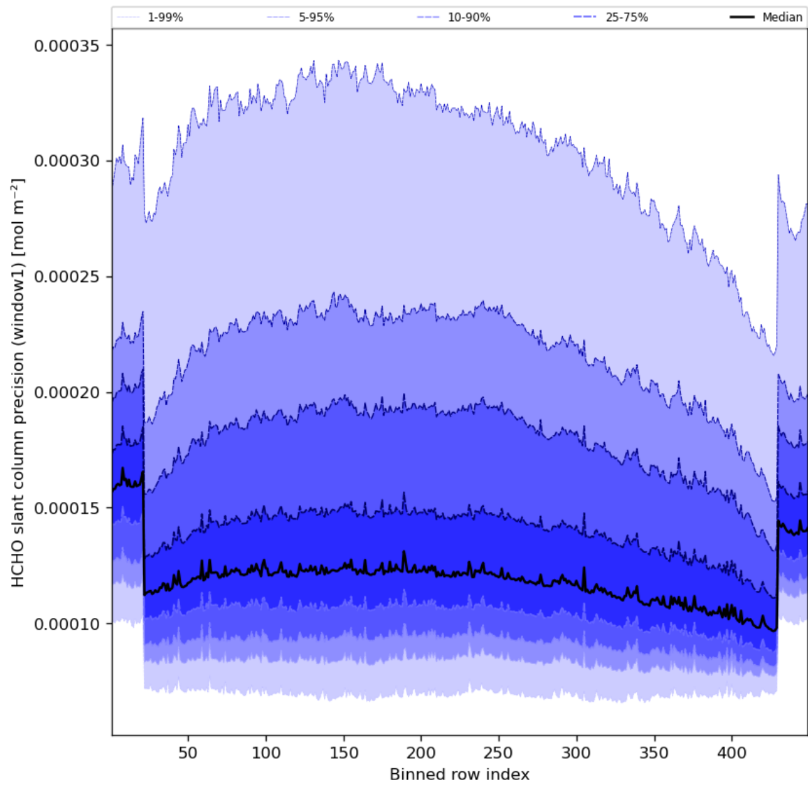
Figure 53: Along track statistics of “HCHO slant column precision (window1)” for 2023-10-03 to 2023-10-05
