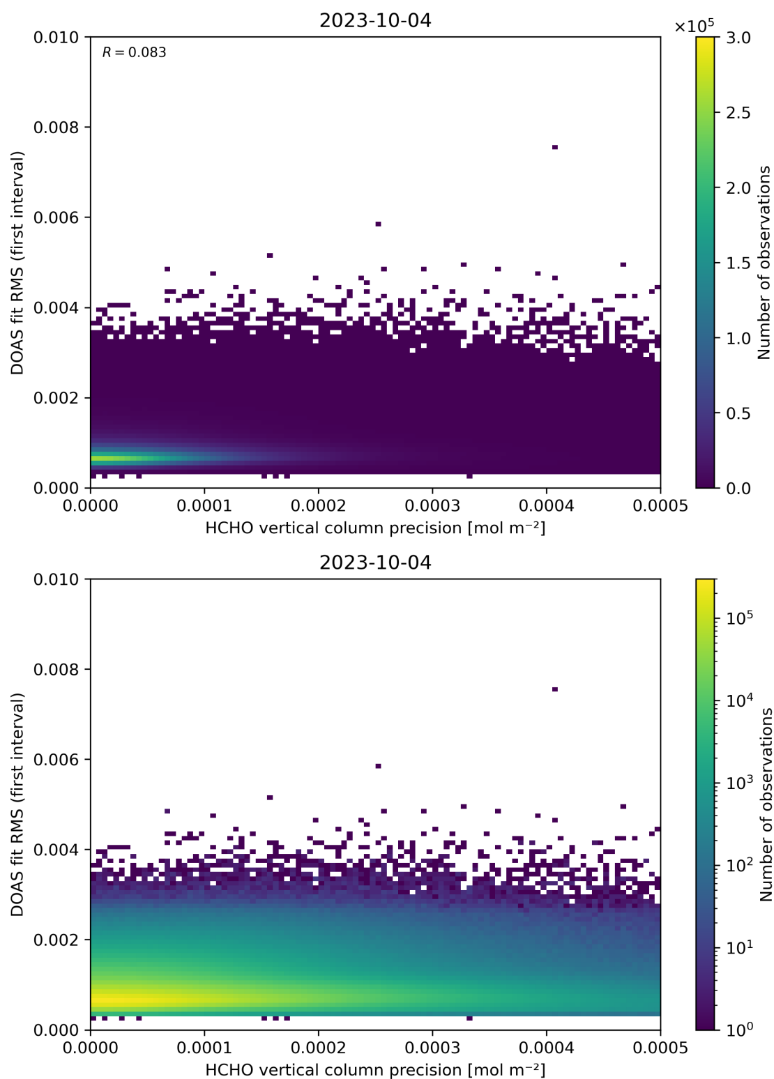
Figure 136: Scatter density plot of “HCHO vertical column precision” against “DOAS fit RMS (first interval)” for 2023-10-03 to 2023-10-05.
