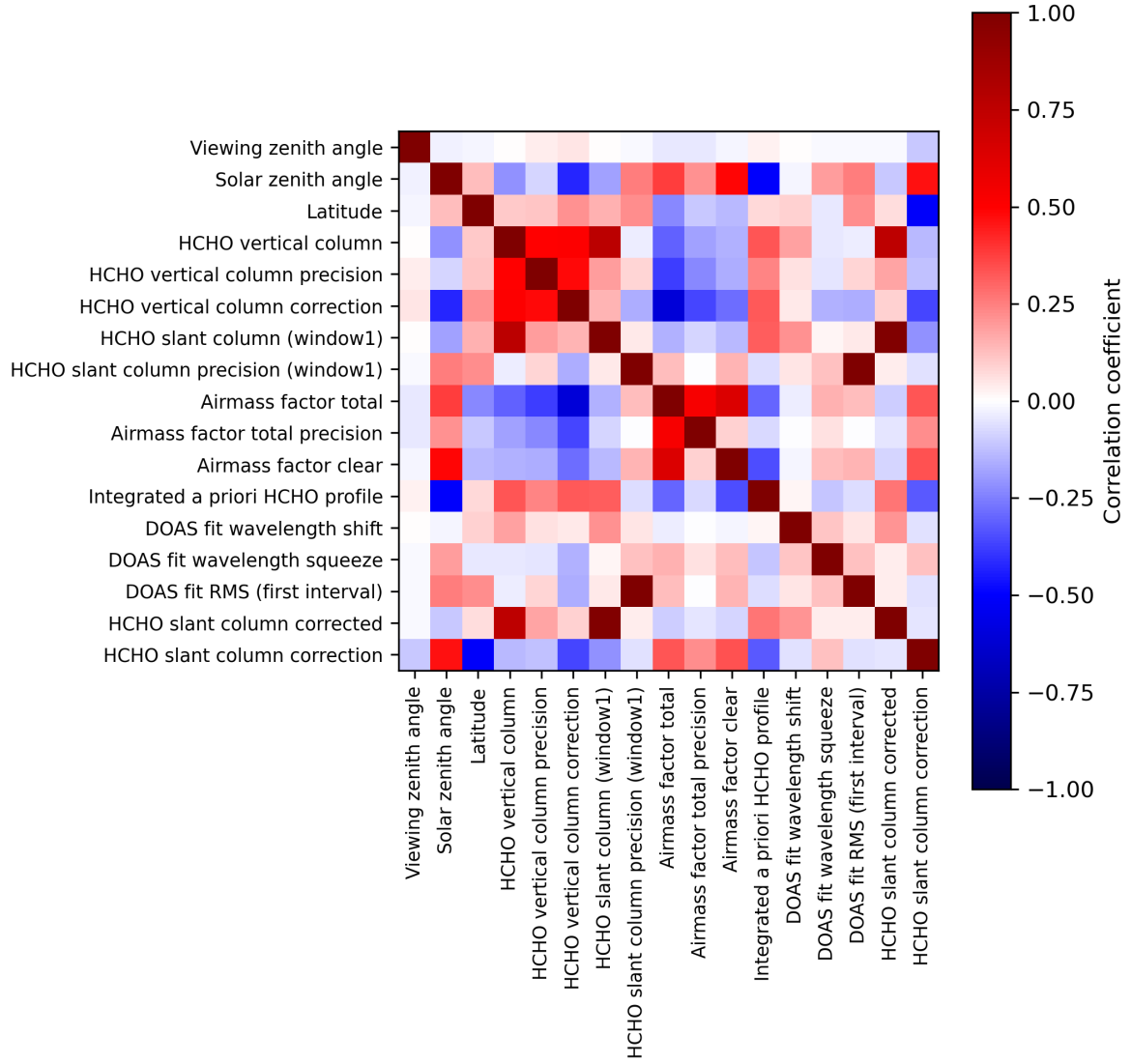
Figure 2: Map of correlation matrix for 2023-10-03 to 2023-10-05.
