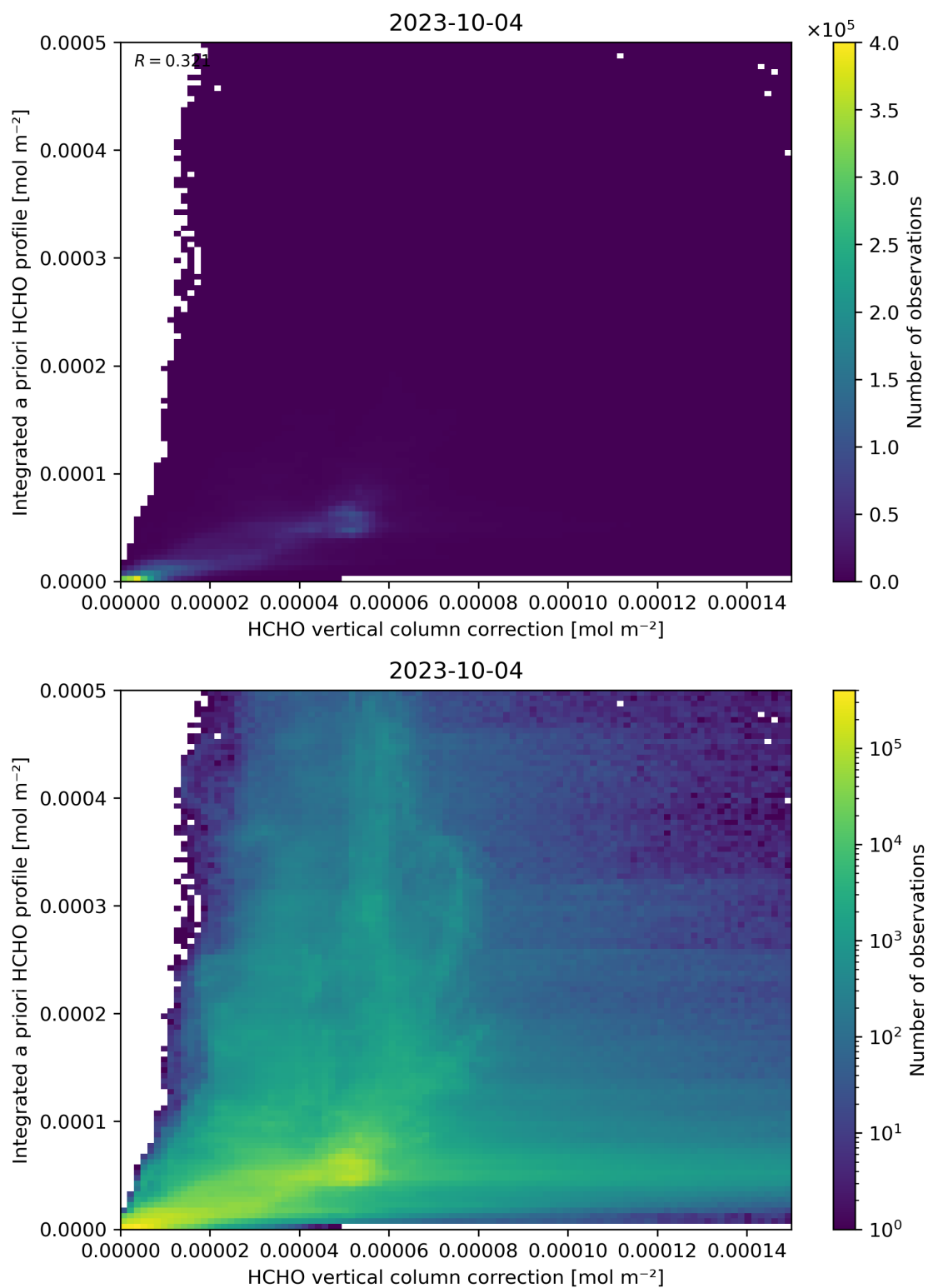
Figure 122: Scatter density plot of “HCHO vertical column correction” against “Integrated a priori HCHO profile” for 2023-10-03 to 2023-10-05.
