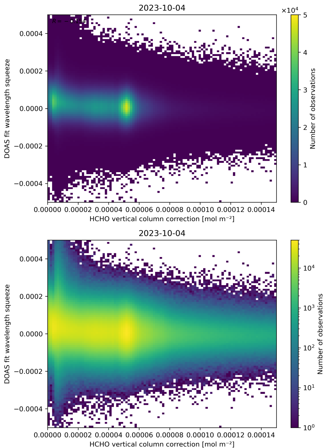
Figure 114: Scatter density plot of “HCHO vertical column correction” against “DOAS fit wavelength squeeze” for 2023-10-03 to 2023-10-05.
