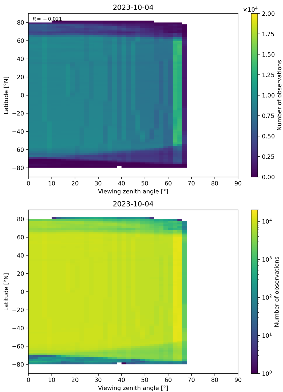
Figure 196: Scatter density plot of “Viewing zenith angle” against “Latitude” for 2023-10-03 to 2023-10-05.
