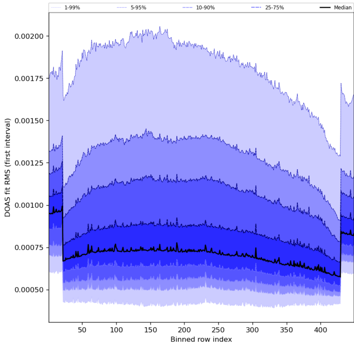
Figure 60: Along track statistics of “DOAS fit RMS (first interval)” for 2023-10-03 to 2023-10-05
