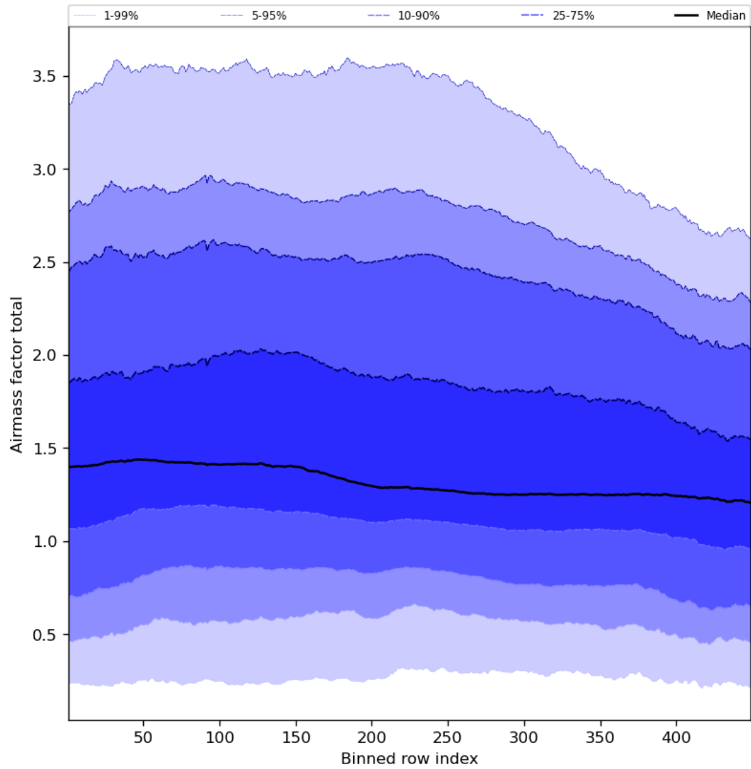
Figure 54: Along track statistics of “Airmass factor total” for 2023-10-03 to 2023-10-05
