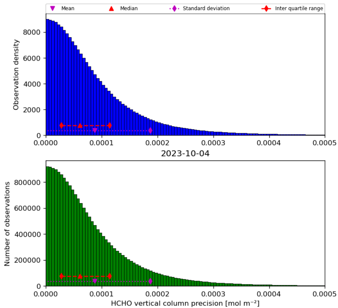
Figure 36: Histogram of “HCHO vertical column precision” for 2023-10-03 to 2023-10-05
