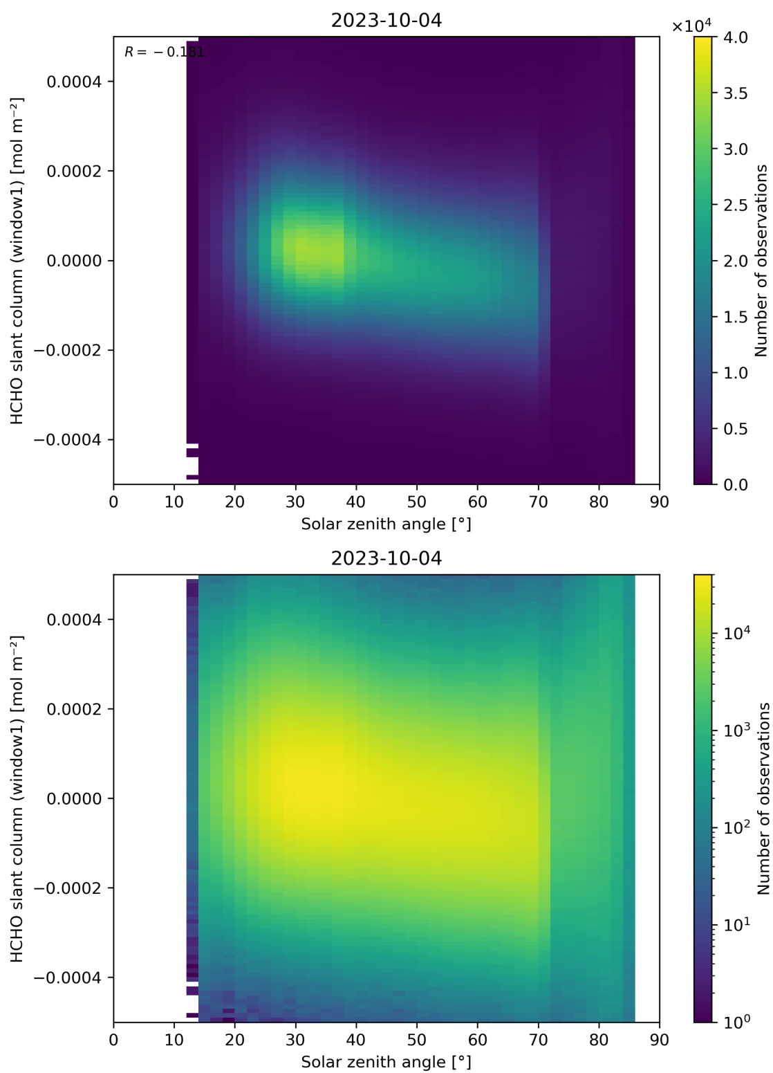
Figure 173: Scatter density plot of “Solar zenith angle” against “HCHO slant column (window1)” for 2023-10-03 to 2023-10-05.
