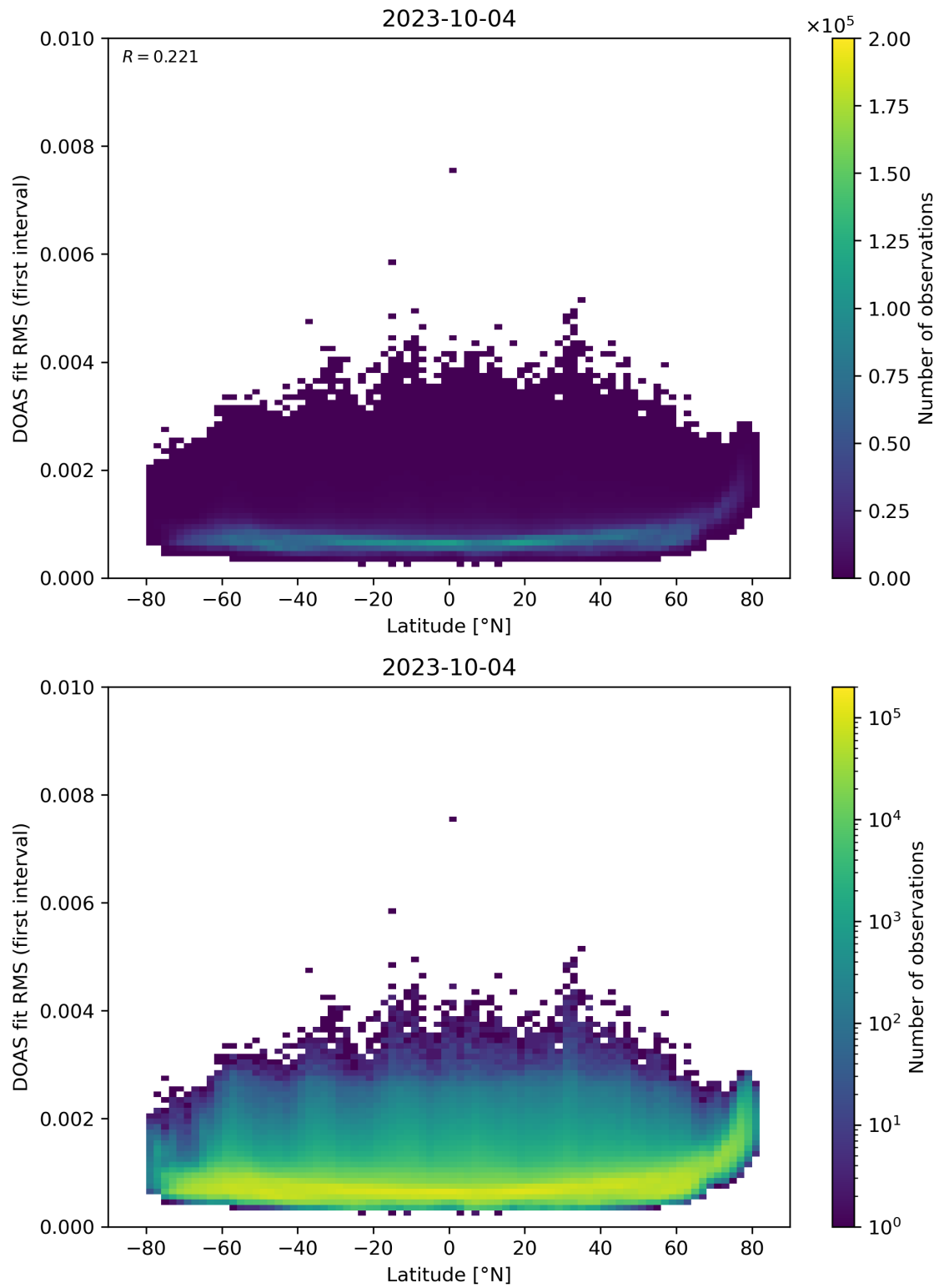
Figure 153: Scatter density plot of “Latitude” against “DOAS fit RMS (first interval)” for 2023-10-03 to 2023-10-05.
