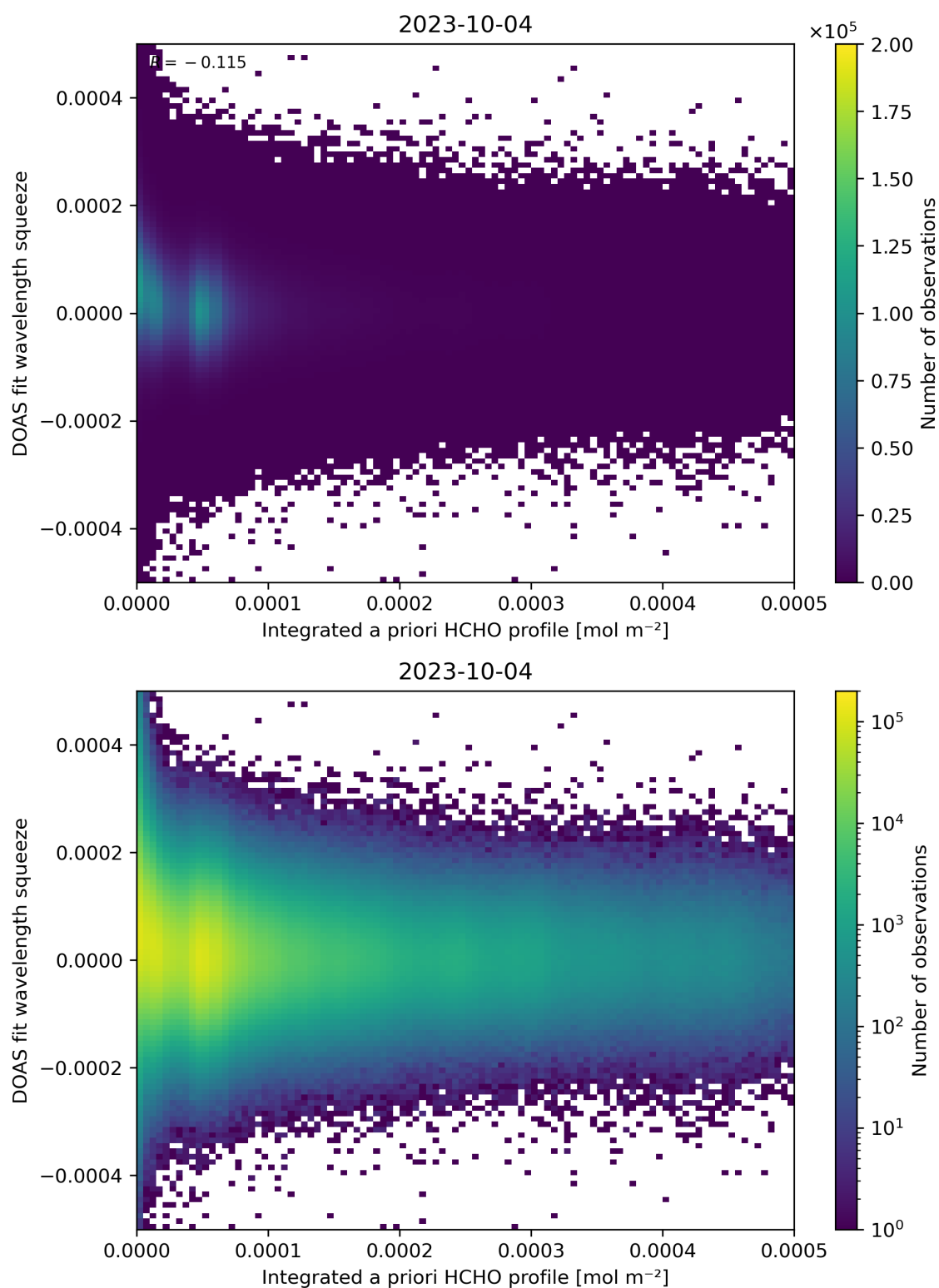
Figure 150: Scatter density plot of “Integrated a priori HCHO profile” against “DOAS fit wavelength squeeze” for 2023-10-03 to 2023-10-05.
