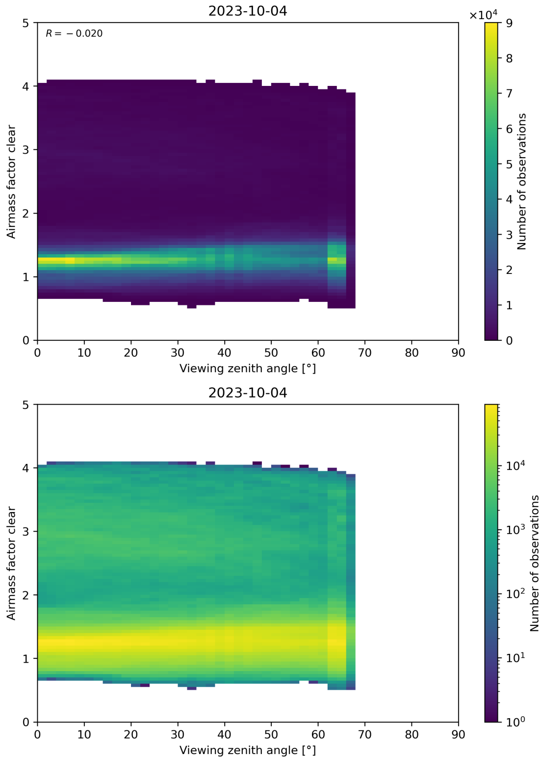
Figure 185: Scatter density plot of “Viewing zenith angle” against “Airmass factor clear” for 2023-10-03 to 2023-10-05.
