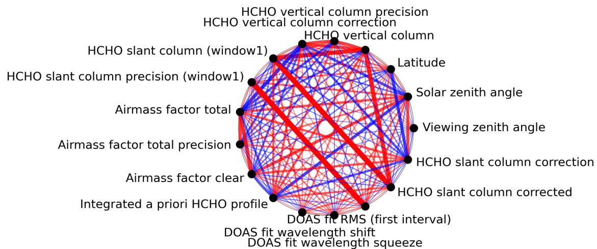
Figure 1: Map of correlation graph for 2023-10-03 to 2023-10-05.
