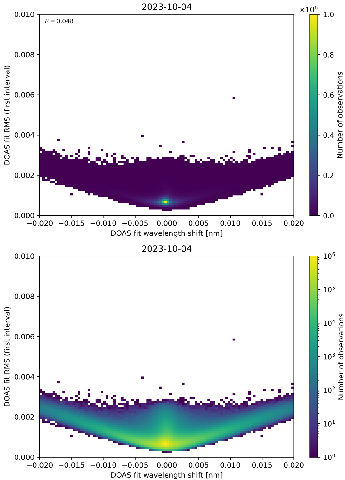
Figure 64: Scatter density plot of “DOAS fit wavelength shift” against “DOAS fit RMS (first interval)” for 2023-10-03 to 2023-10-05.
