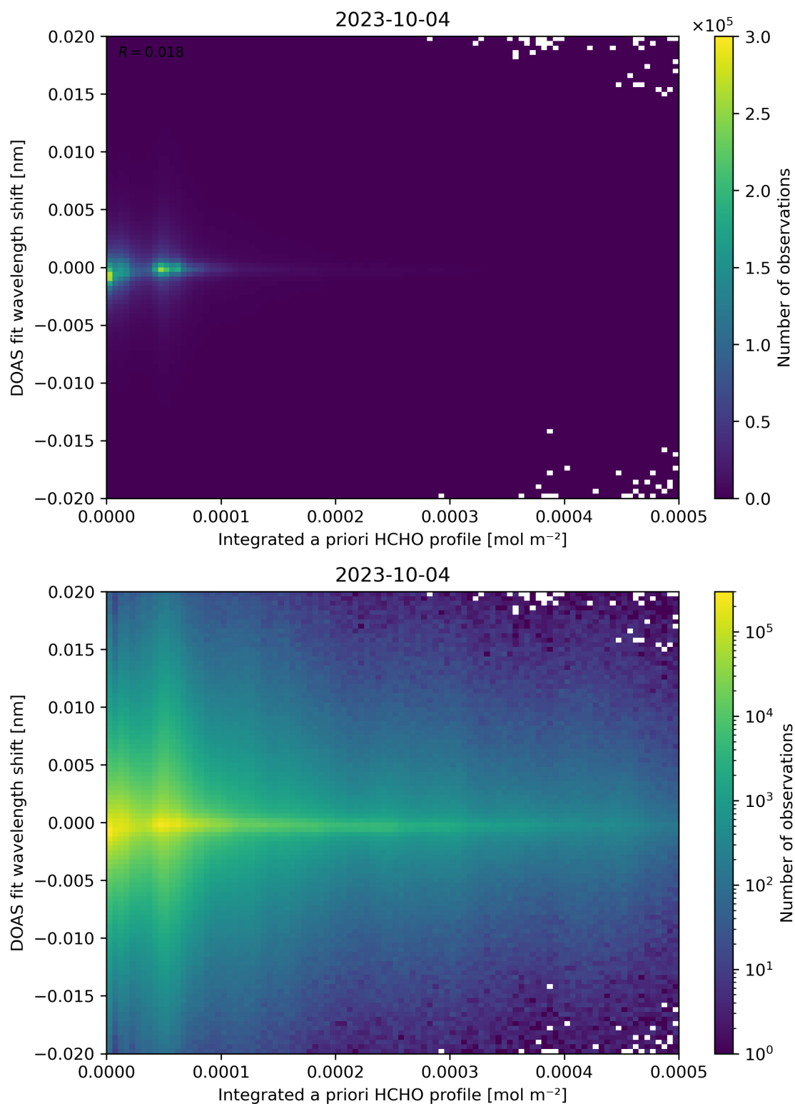
Figure 149: Scatter density plot of “Integrated a priori HCHO profile” against “DOAS fit wavelength shift” for 2023-10-03 to 2023-10-05.
