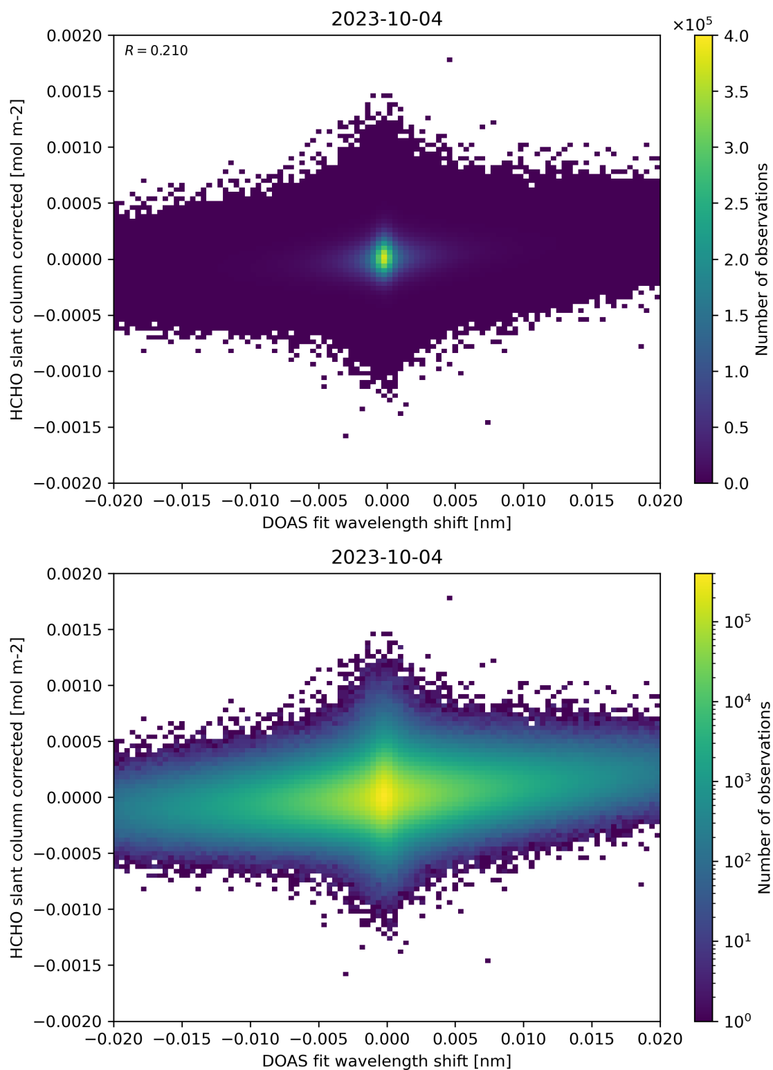
Figure 66: Scatter density plot of “DOAS fit wavelength shift” against “HCHO slant column corrected” for 2023-10-03 to 2023-10-05.
