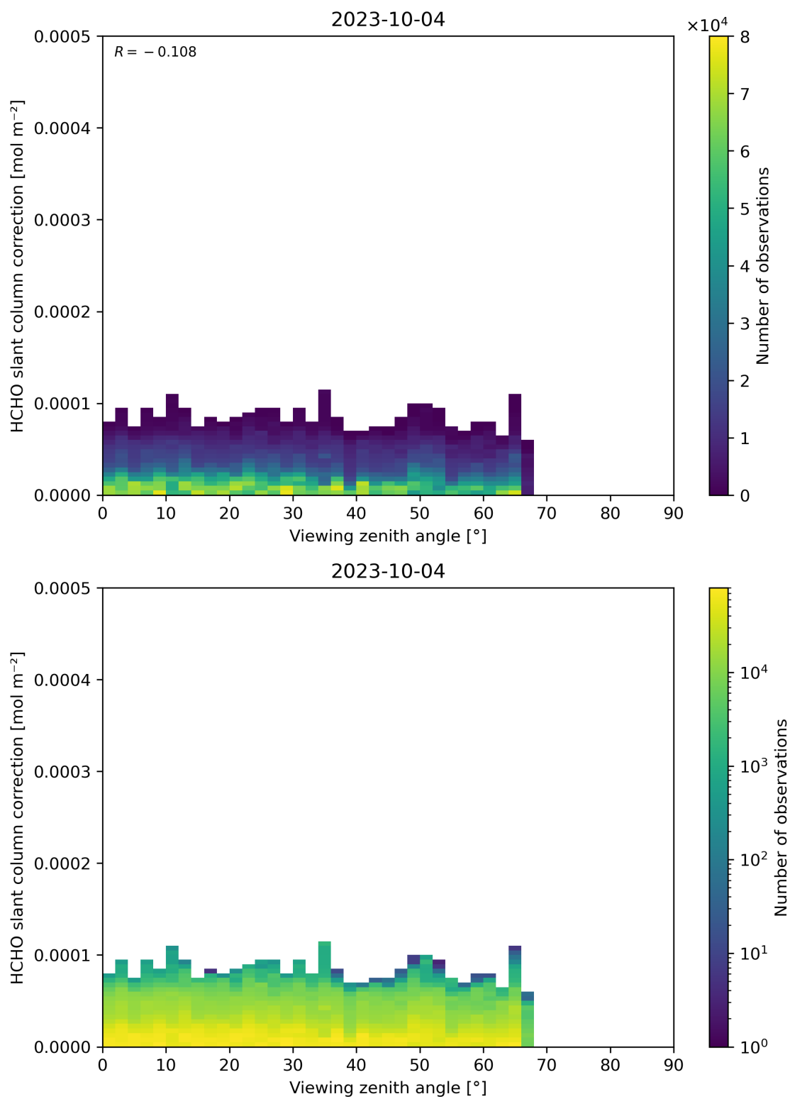
Figure 187: Scatter density plot of “Viewing zenith angle” against “HCHO slant column correction” for 2023-10-03 to 2023-10-05.
