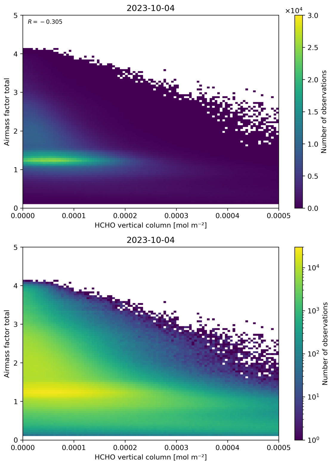
Figure 131: Scatter density plot of “HCHO vertical column” against “Airmass factor total” for 2023-10-03 to 2023-10-05.
