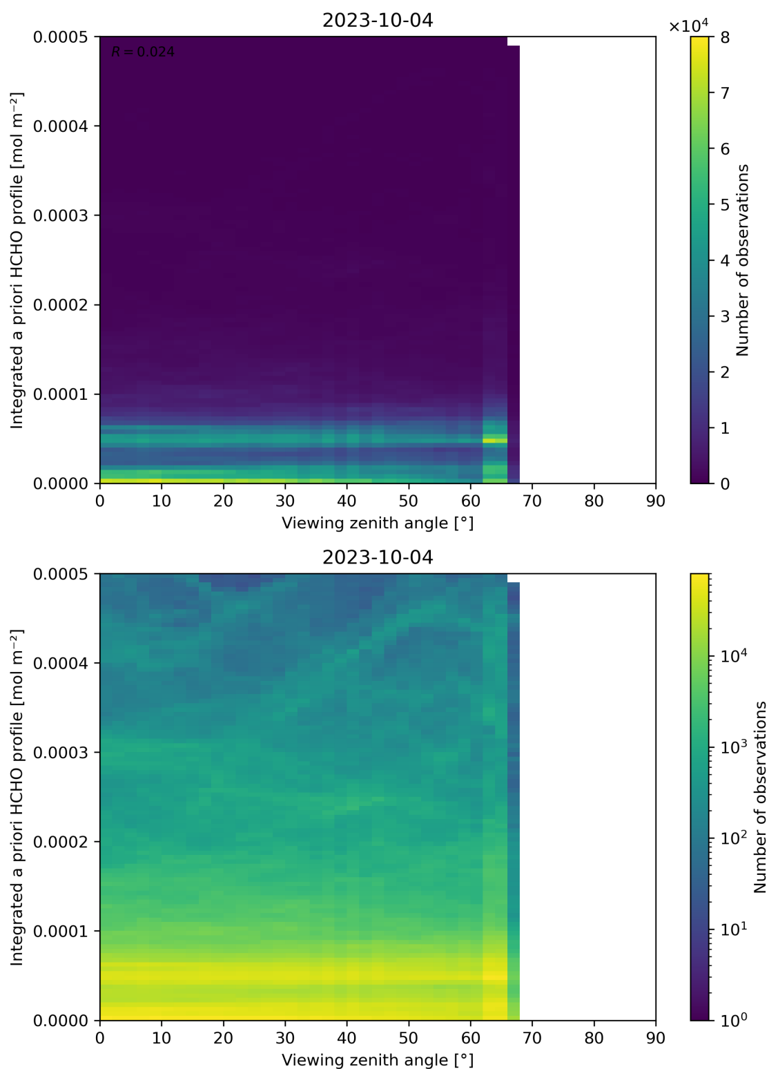
Figure 195: Scatter density plot of “Viewing zenith angle” against “Integrated a priori HCHO profile” for 2023-10-03 to 2023-10-05.
