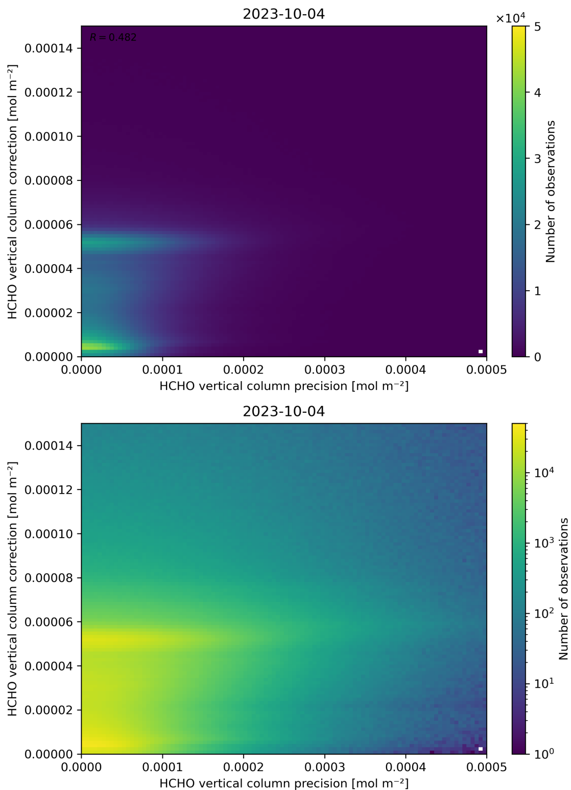
Figure 146: Scatter density plot of “HCHO vertical column precision” against “HCHO vertical column correction” for 2023-10-03 to 2023-10-05.
