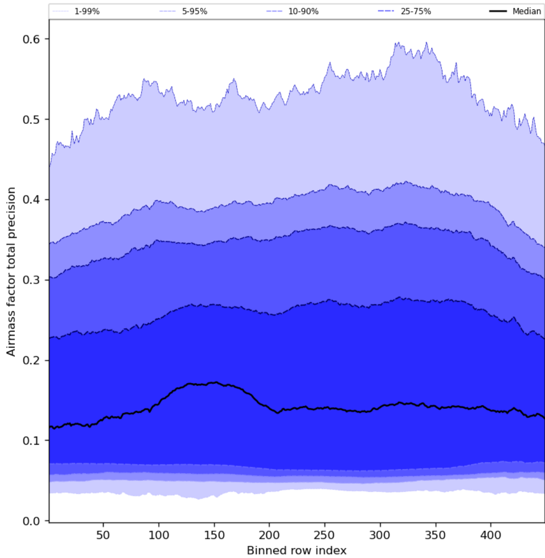
Figure 55: Along track statistics of “Airmass factor total precision” for 2023-10-03 to 2023-10-05
