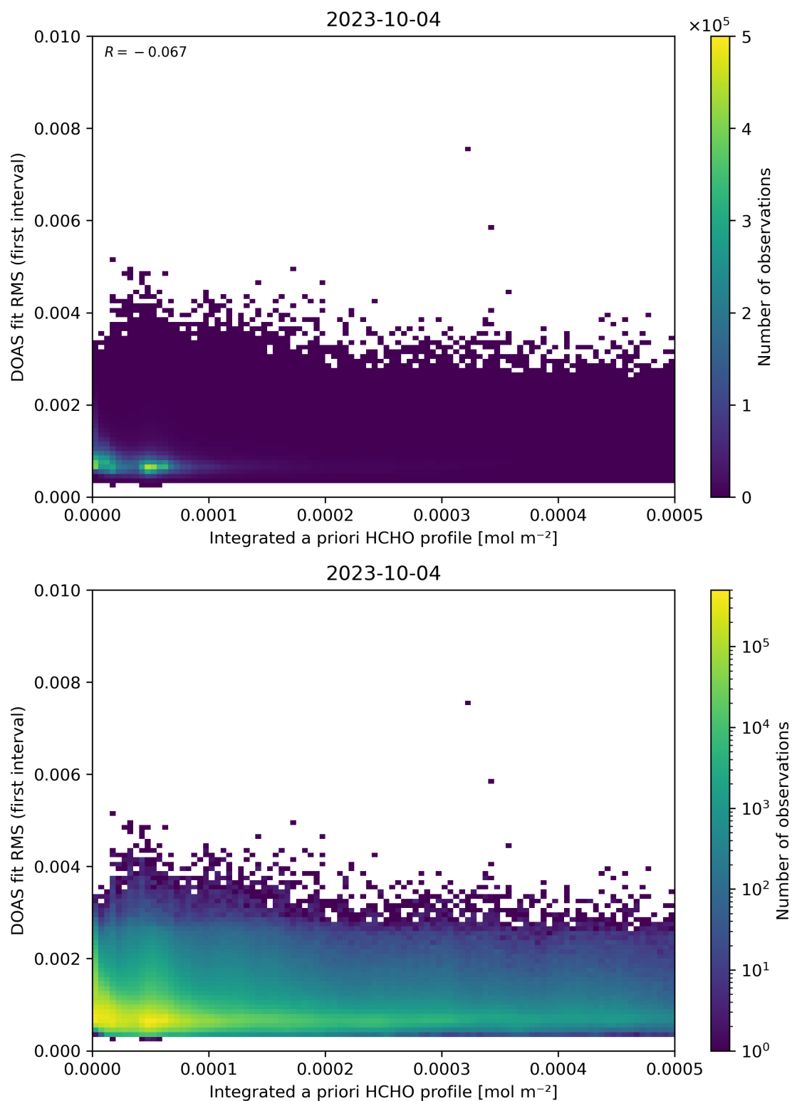
Figure 148: Scatter density plot of “Integrated a priori HCHO profile” against “DOAS fit RMS (first interval)” for 2023-10-03 to 2023-10-05.
