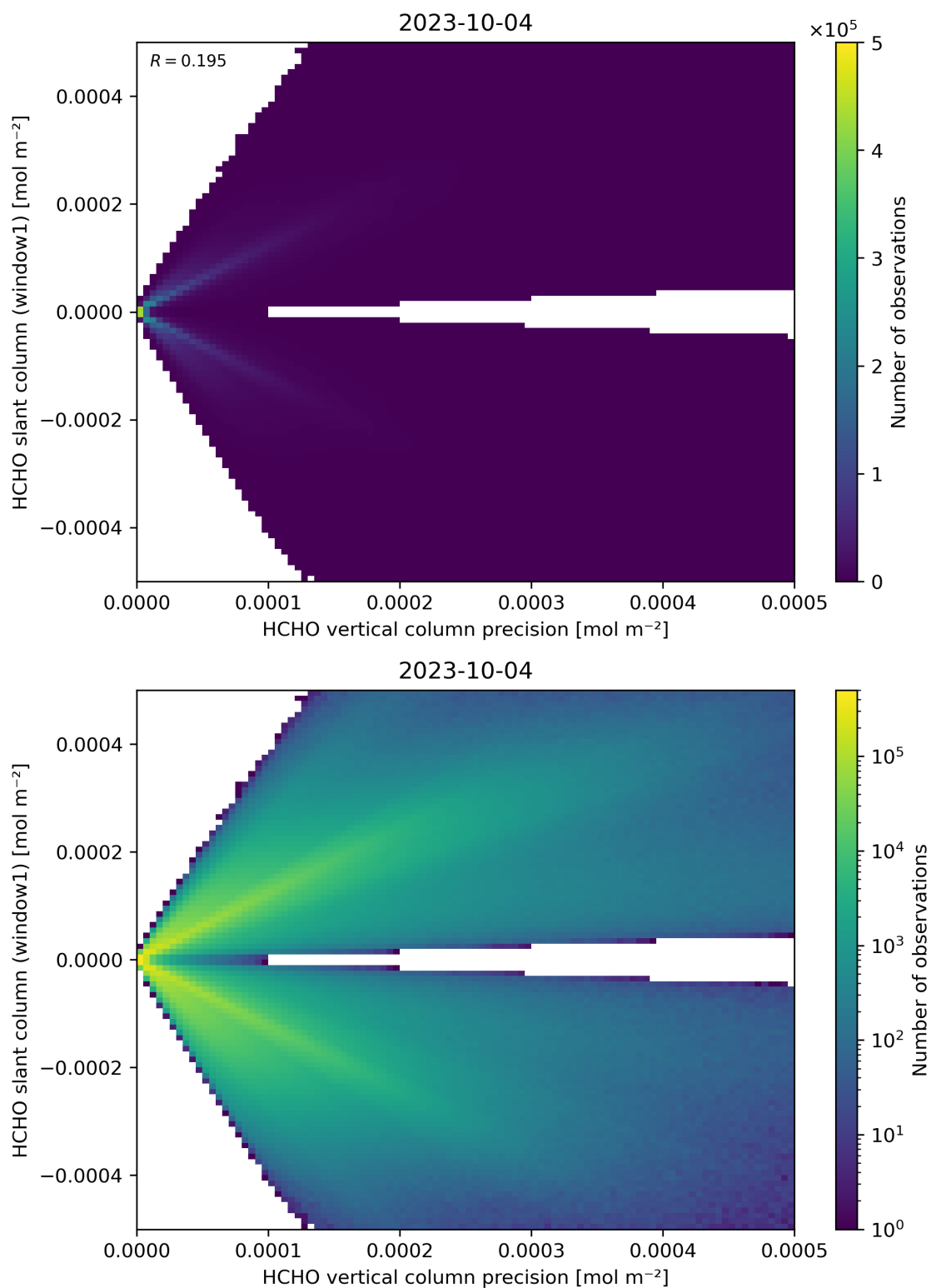
Figure 142: Scatter density plot of “HCHO vertical column precision” against “HCHO slant column (window1)” for 2023-10-03 to 2023-10-05.
