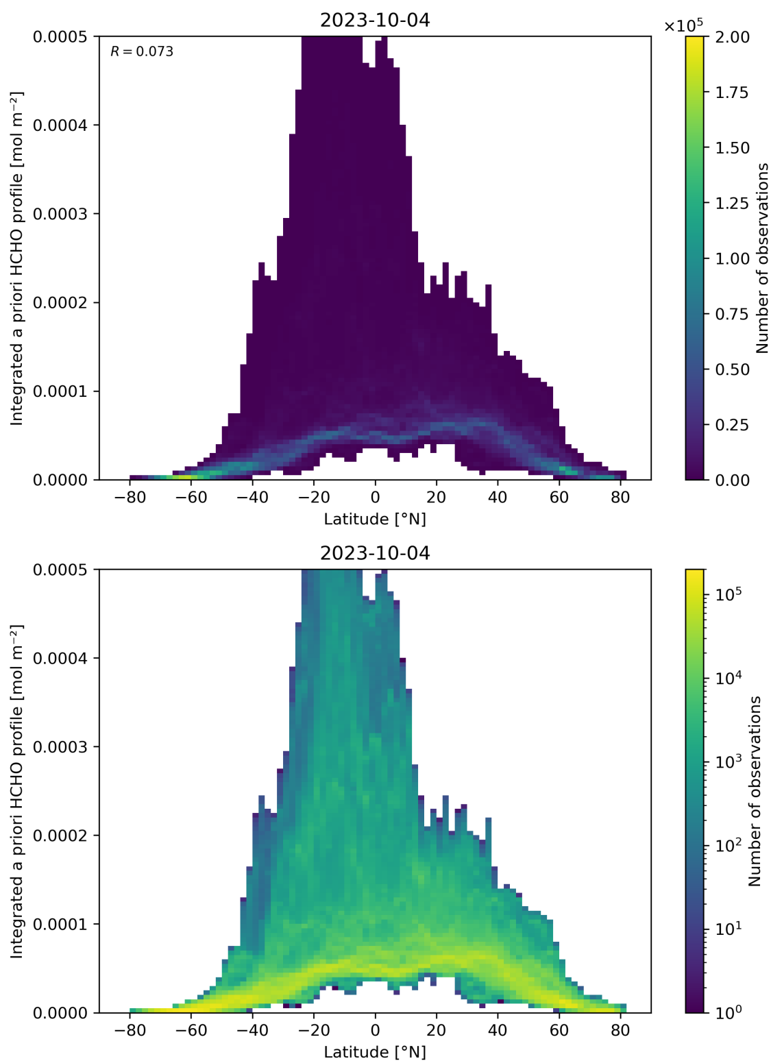
Figure 166: Scatter density plot of “Latitude” against “Integrated a priori HCHO profile” for 2023-10-03 to 2023-10-05.
