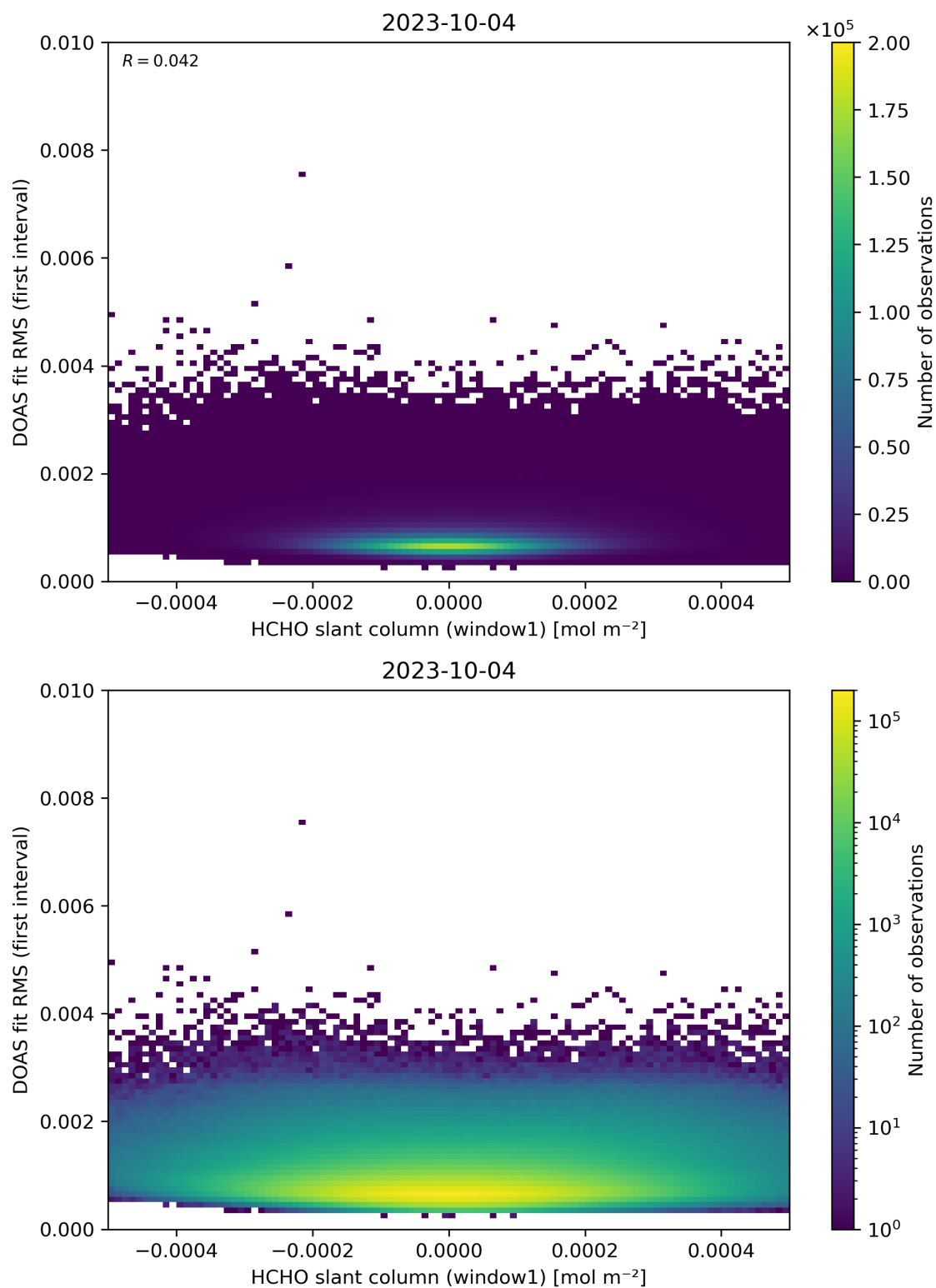
Figure 78: Scatter density plot of “HCHO slant column (window1)” against “DOAS fit RMS (first interval)” for 2023-10-03 to 2023-10-05.
