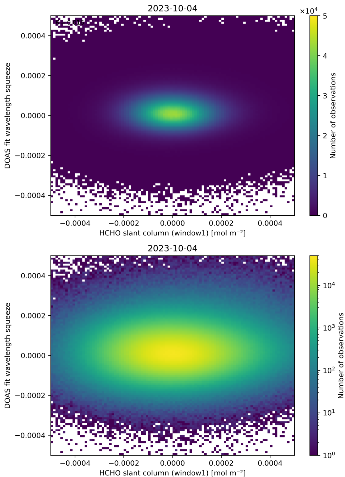
Figure 80: Scatter density plot of “HCHO slant column (window1)” against “DOAS fit wavelength squeeze” for 2023-10-03 to 2023-10-05.
