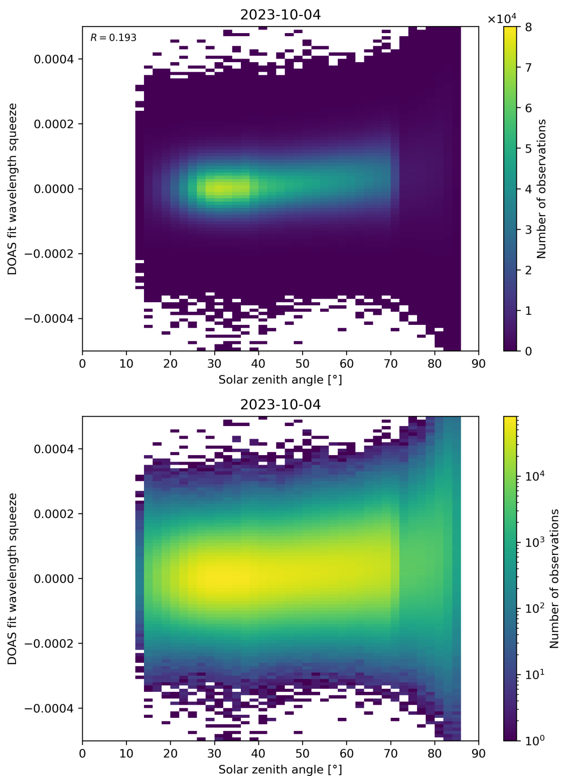
Figure 169: Scatter density plot of “Solar zenith angle” against “DOAS fit wavelength squeeze” for 2023-10-03 to 2023-10-05.
