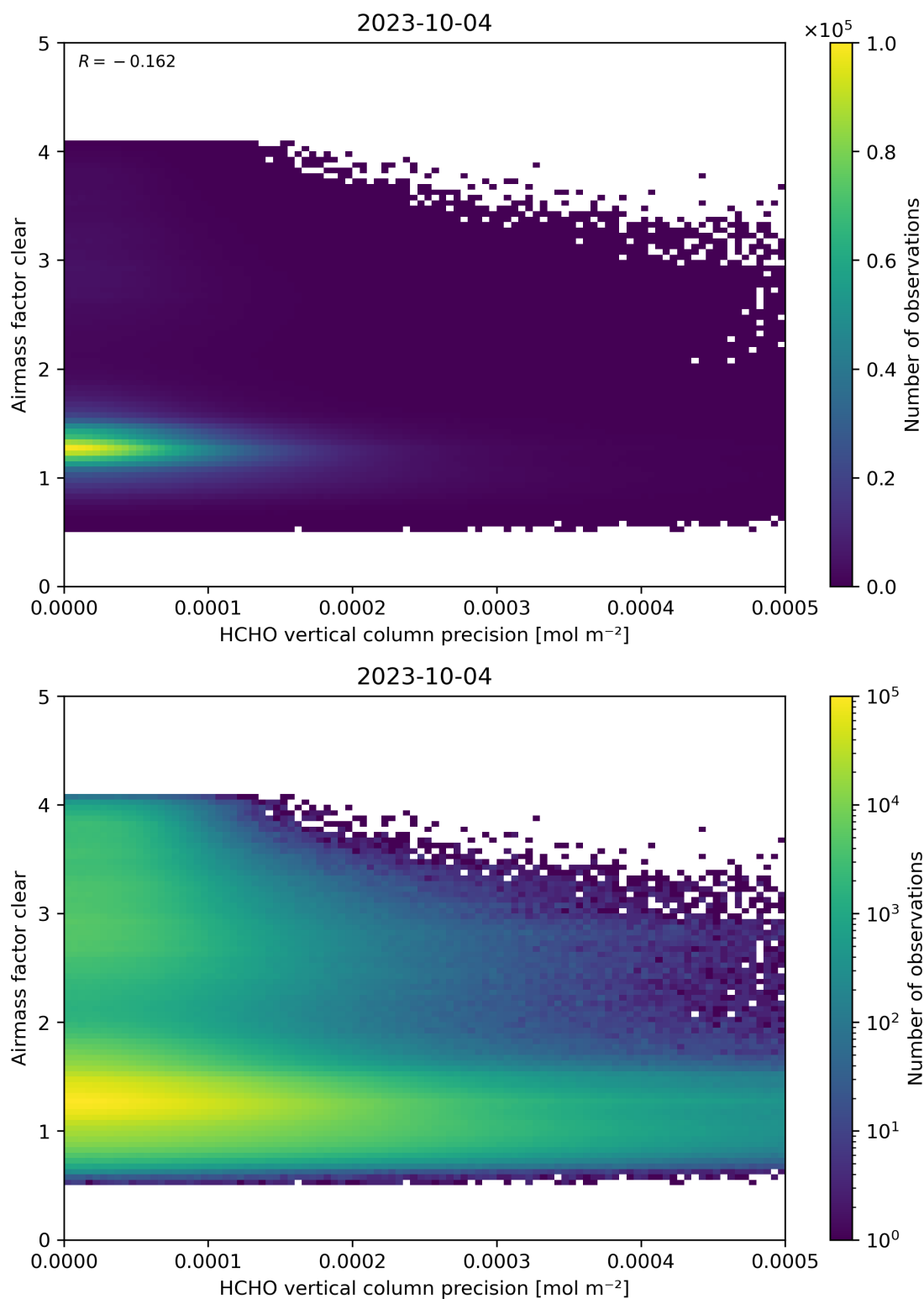
Figure 139: Scatter density plot of “HCHO vertical column precision” against “Airmass factor clear” for 2023-10-03 to 2023-10-05.
