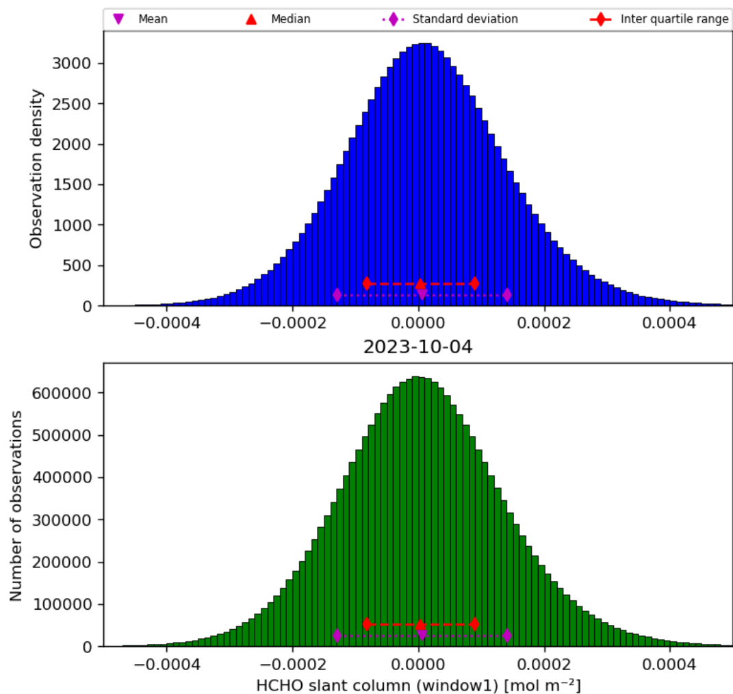
Figure 38: Histogram of “HCHO slant column (window1)” for 2023-10-03 to 2023-10-05
