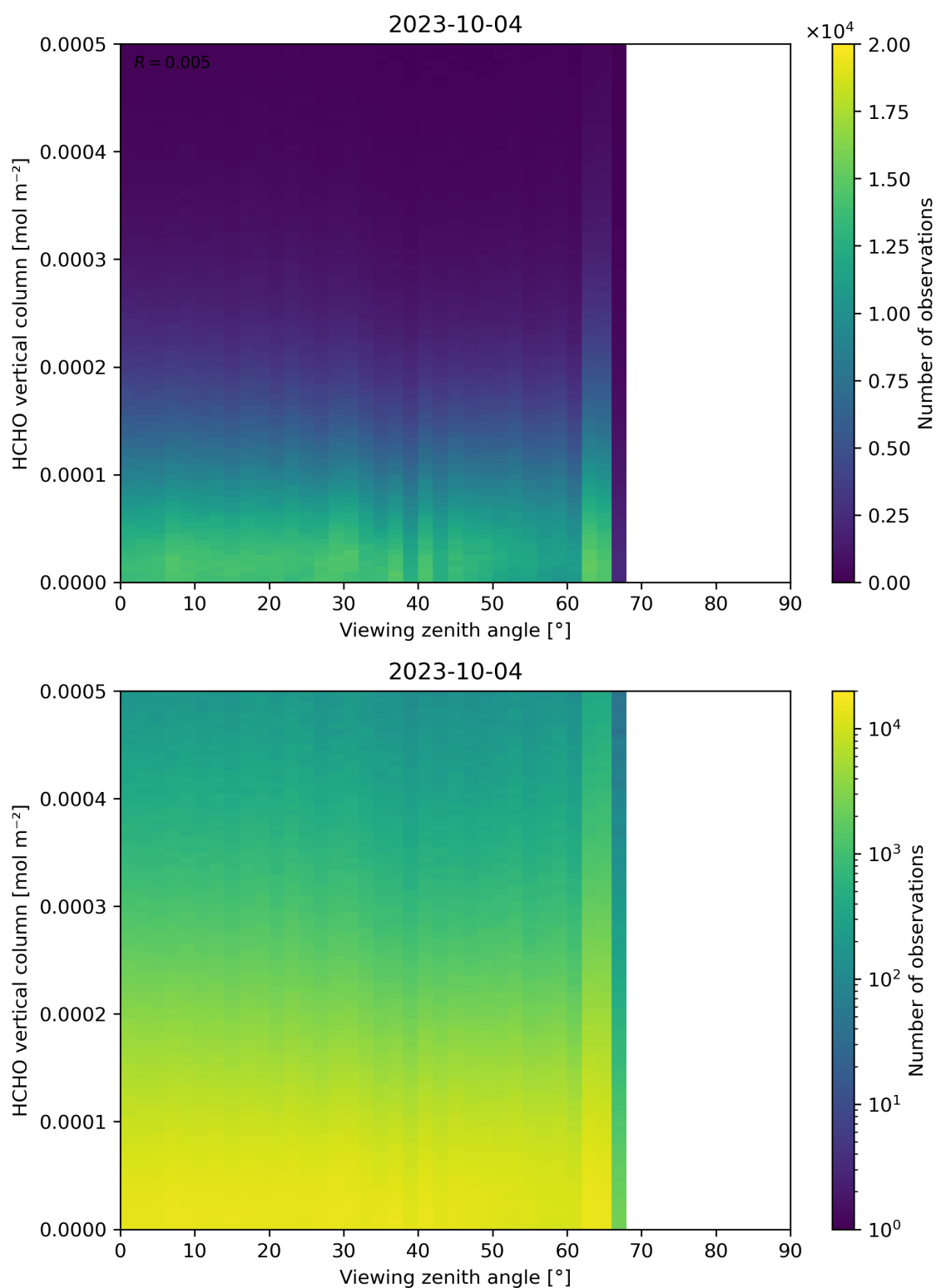
Figure 192: Scatter density plot of “Viewing zenith angle” against “HCHO vertical column” for 2023-10-03 to 2023-10-05.
