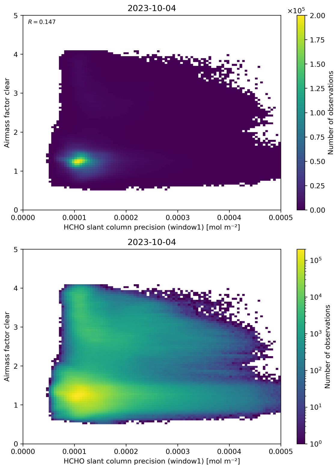
Figure 91: Scatter density plot of “HCHO slant column precision (window1)” against “Airmass factor clear” for 2023-10-03 to 2023-10-05.
