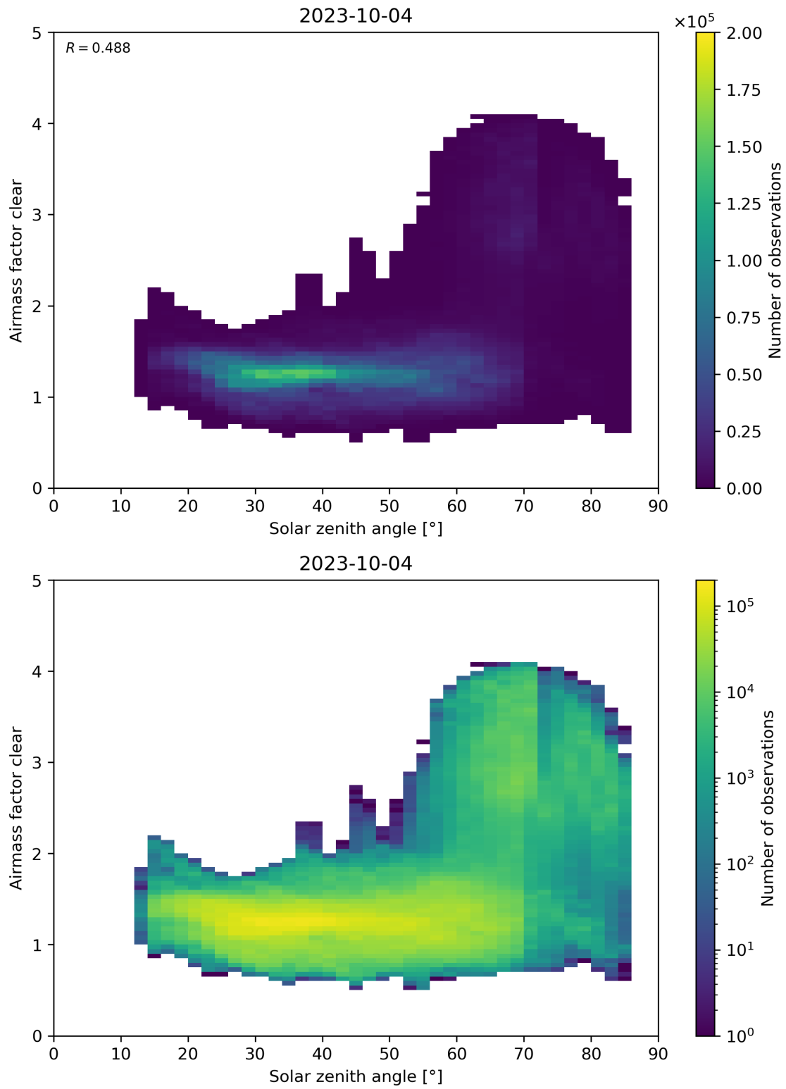
Figure 170: Scatter density plot of “Solar zenith angle” against “Airmass factor clear” for 2023-10-03 to 2023-10-05.
