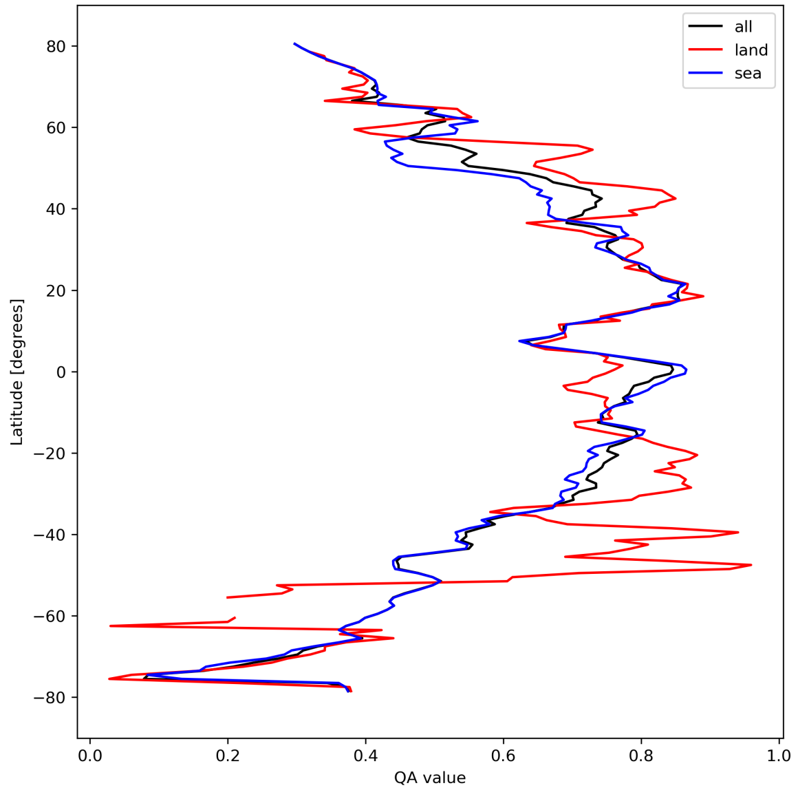
Figure 20: Zonal average of “QA value” for 2023-10-03 to 2023-10-05.
