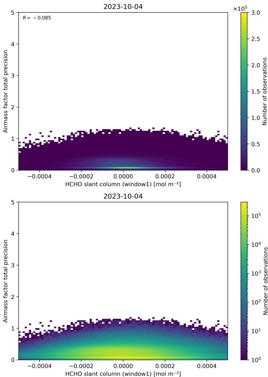
Figure 86: Scatter density plot of “HCHO slant column (window1)” against “Airmass factor total precision” for 2023-10-03 to 2023-10-05.
