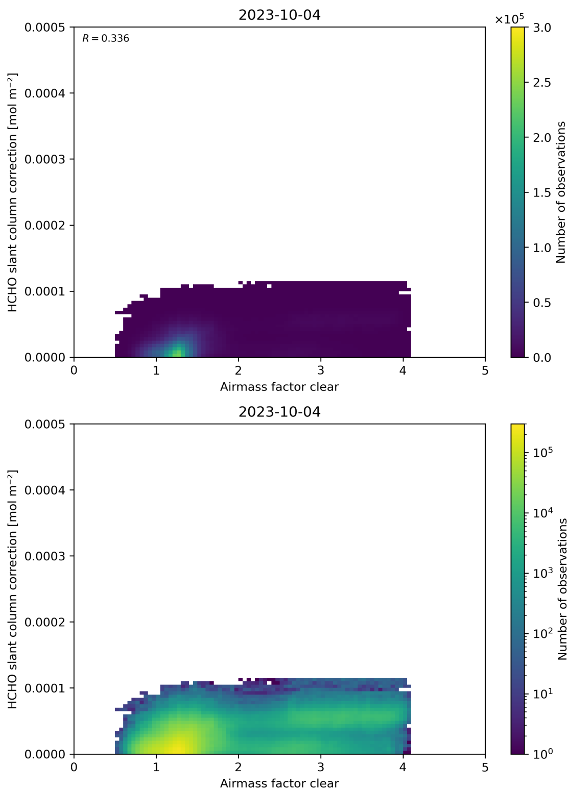
Figure 75: Scatter density plot of “Airmass factor clear” against “HCHO slant column correction” for 2023-10-03 to 2023-10-05.
