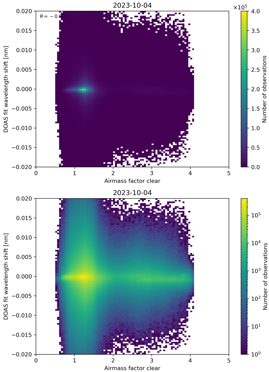
Figure 72: Scatter density plot of “Airmass factor clear” against “DOAS fit wavelength shift” for 2023-10-03 to 2023-10-05.
