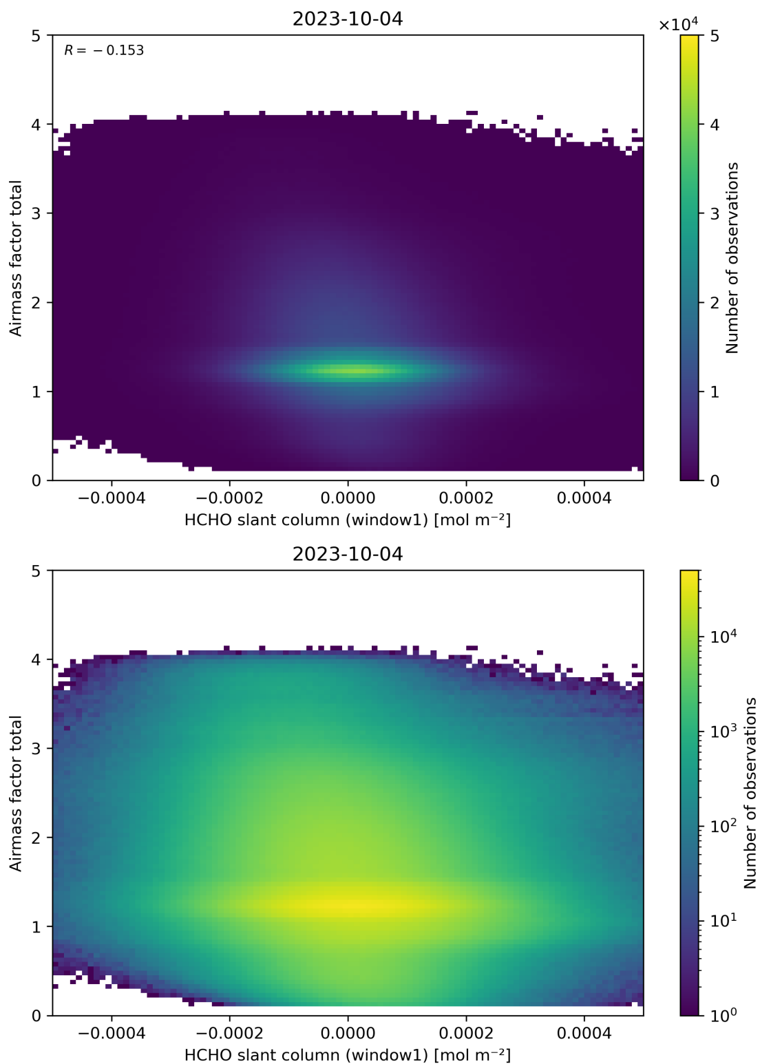
Figure 85: Scatter density plot of “HCHO slant column (window1)” against “Airmass factor total” for 2023-10-03 to 2023-10-05.
