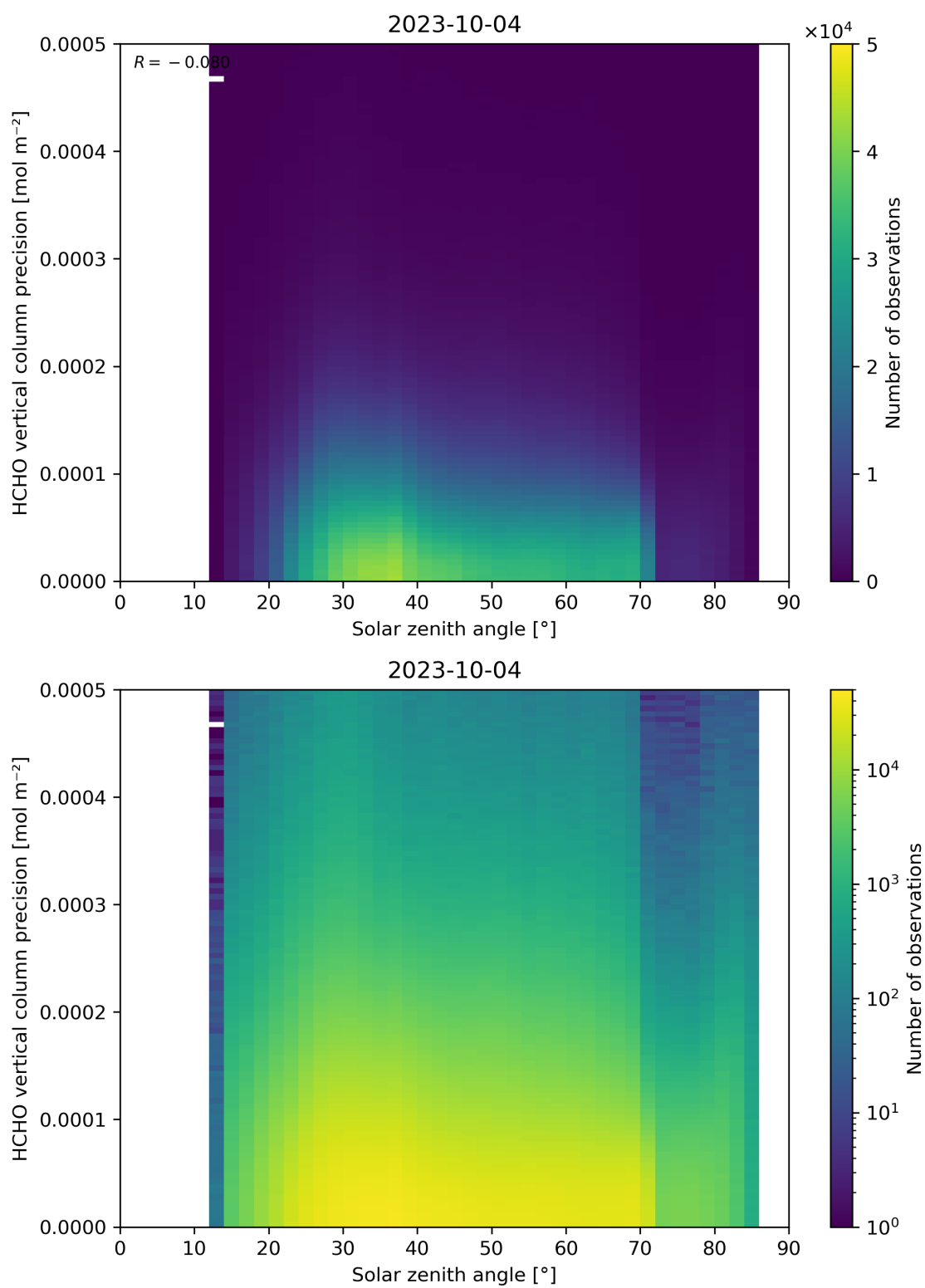
Figure 179: Scatter density plot of “Solar zenith angle” against “HCHO vertical column precision” for 2023-10-03 to 2023-10-05.
