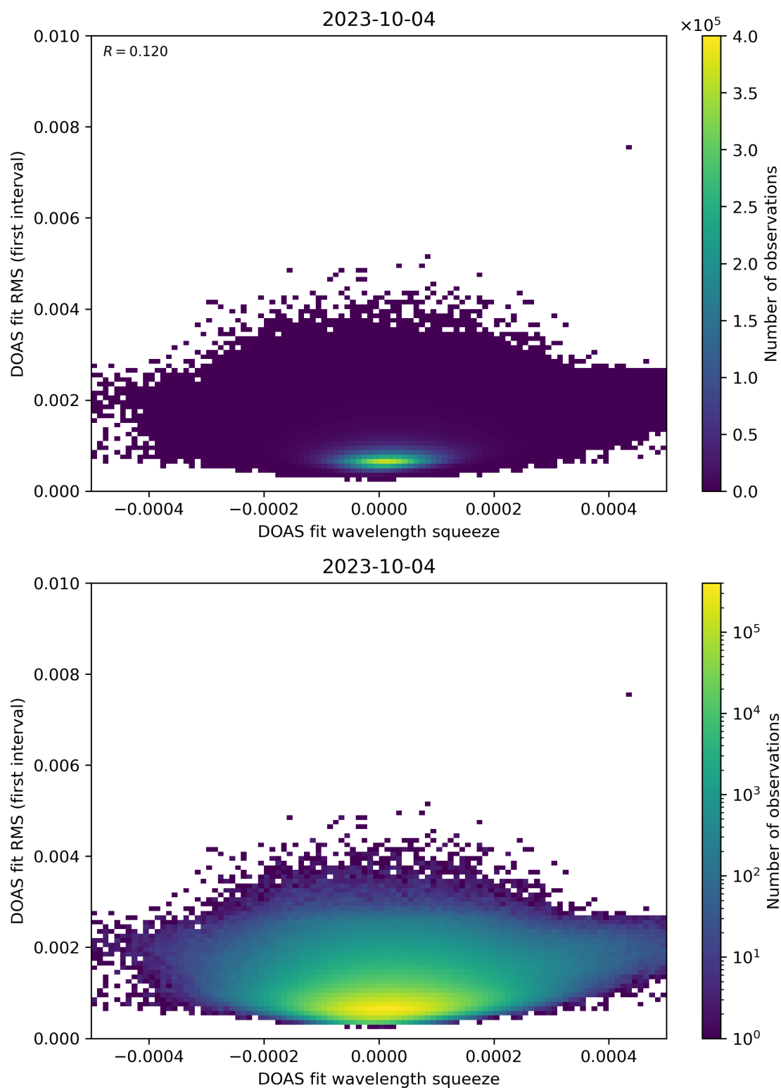
Figure 68: Scatter density plot of “DOAS fit wavelength squeeze” against “DOAS fit RMS (first interval)” for 2023-10-03 to 2023-10-05.
