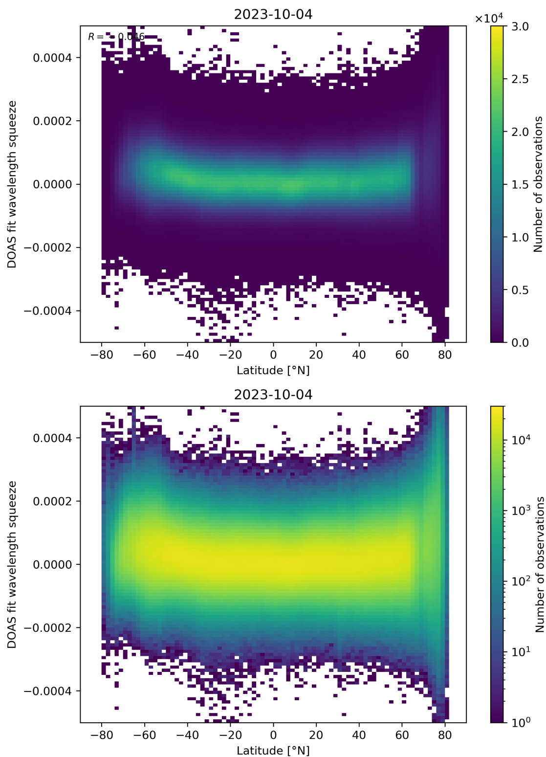
Figure 155: Scatter density plot of “Latitude” against “DOAS fit wavelength squeeze” for 2023-10-03 to 2023-10-05.
