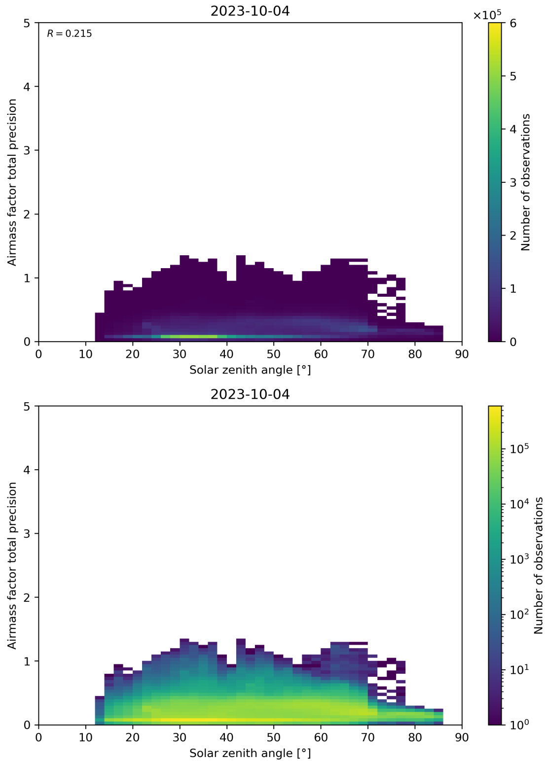
Figure 176: Scatter density plot of “Solar zenith angle” against “Airmass factor total precision” for 2023-10-03 to 2023-10-05.
