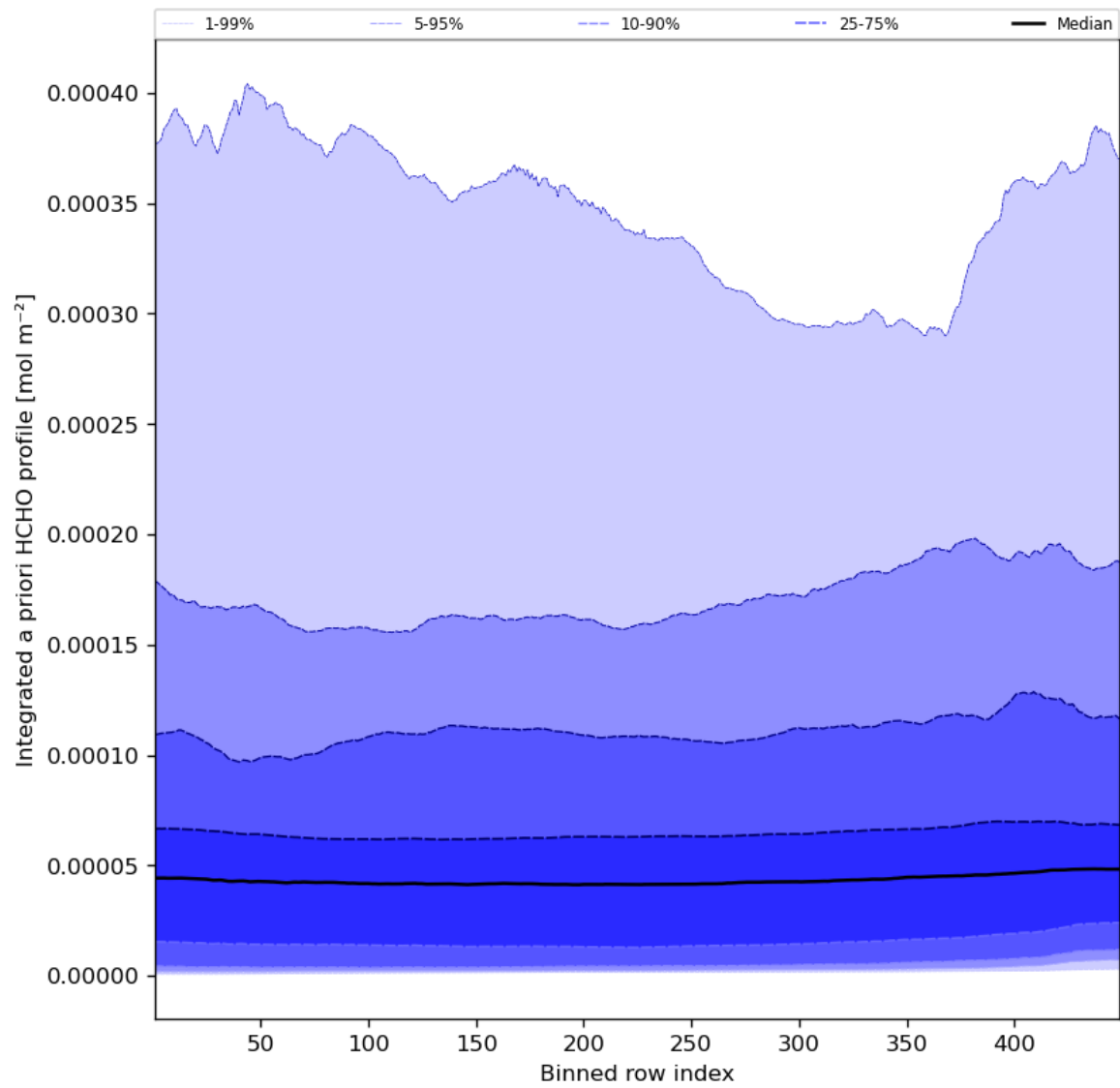
Figure 57: Along track statistics of “Integrated a priori HCHO profile” for 2023-10-03 to 2023-10-05
