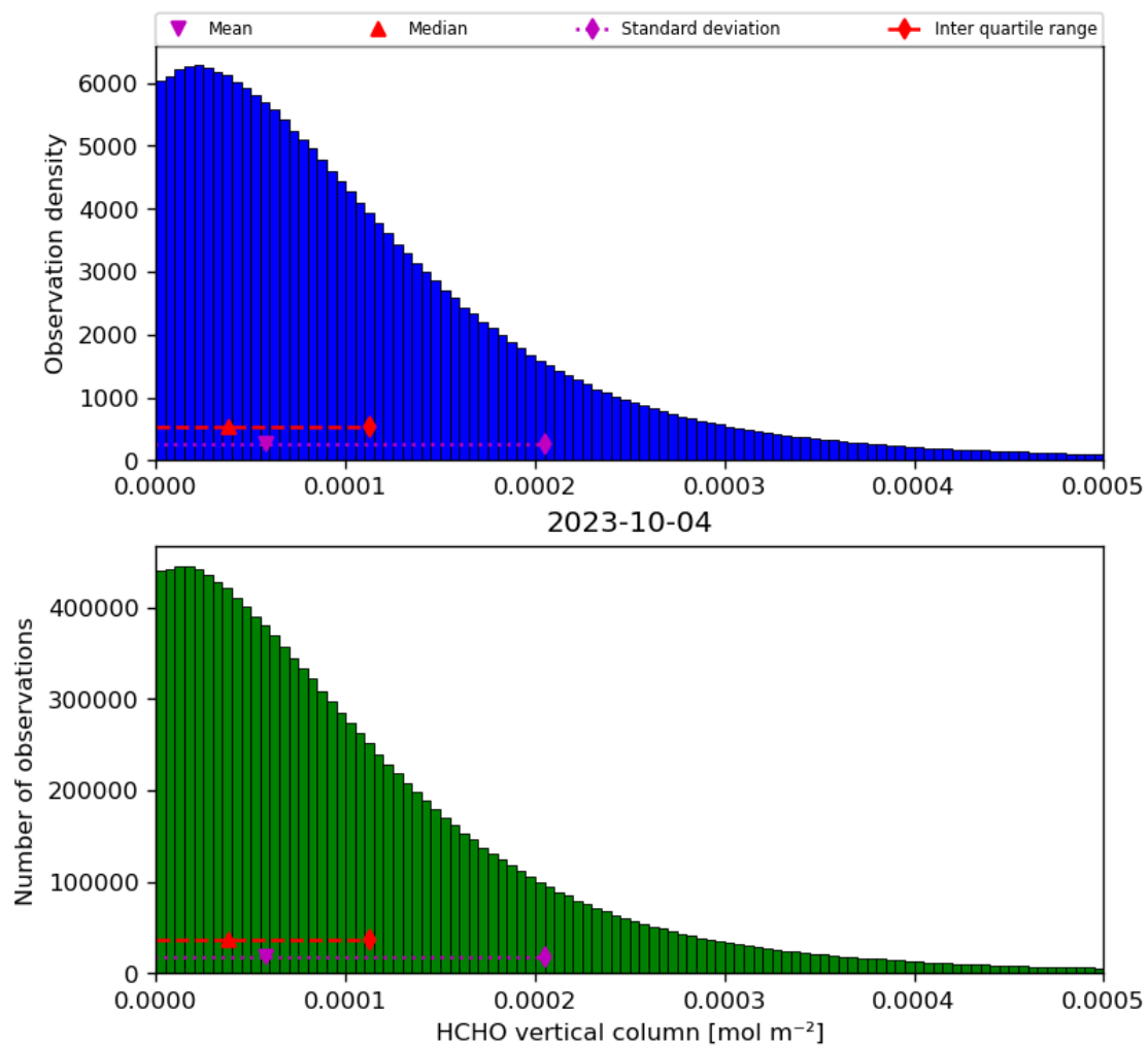
Figure 35: Histogram of “HCHO vertical column” for 2023-10-03 to 2023-10-05
