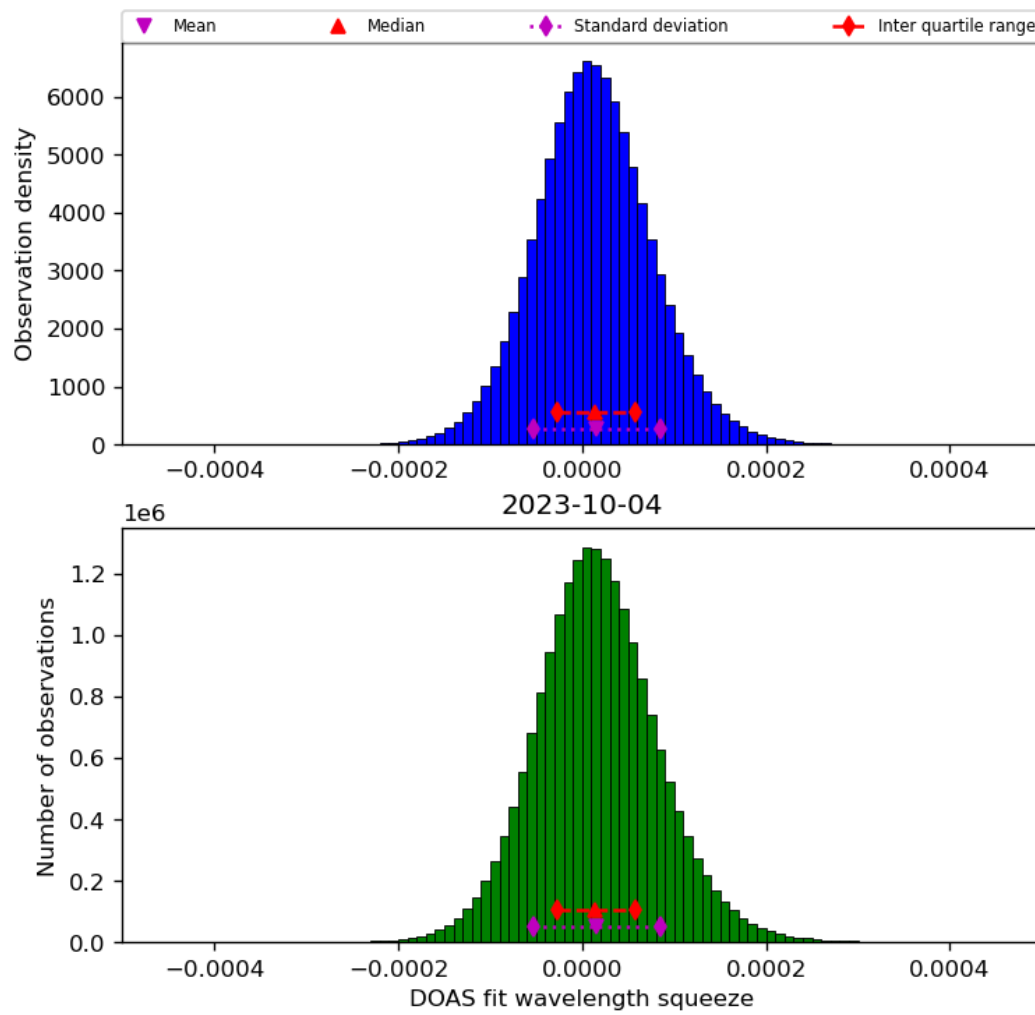
Figure 45: Histogram of “DOAS fit wavelength squeeze” for 2023-10-03 to 2023-10-05
