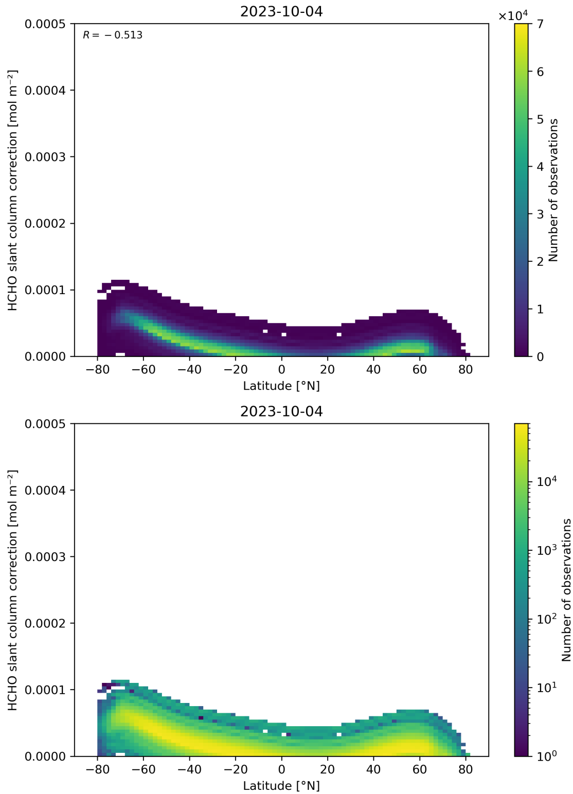
Figure 158: Scatter density plot of “Latitude” against “HCHO slant column correction” for 2023-10-03 to 2023-10-05.
