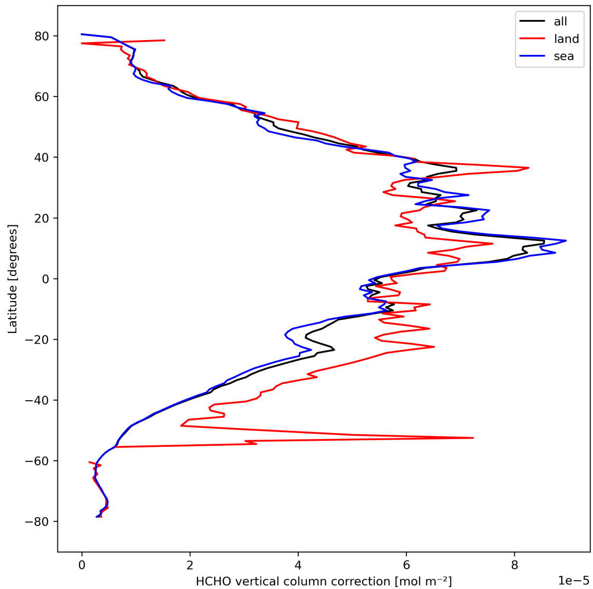
Figure 23: Zonal average of “HCHO vertical column correction” for 2023-10-03 to 2023-10-05.
