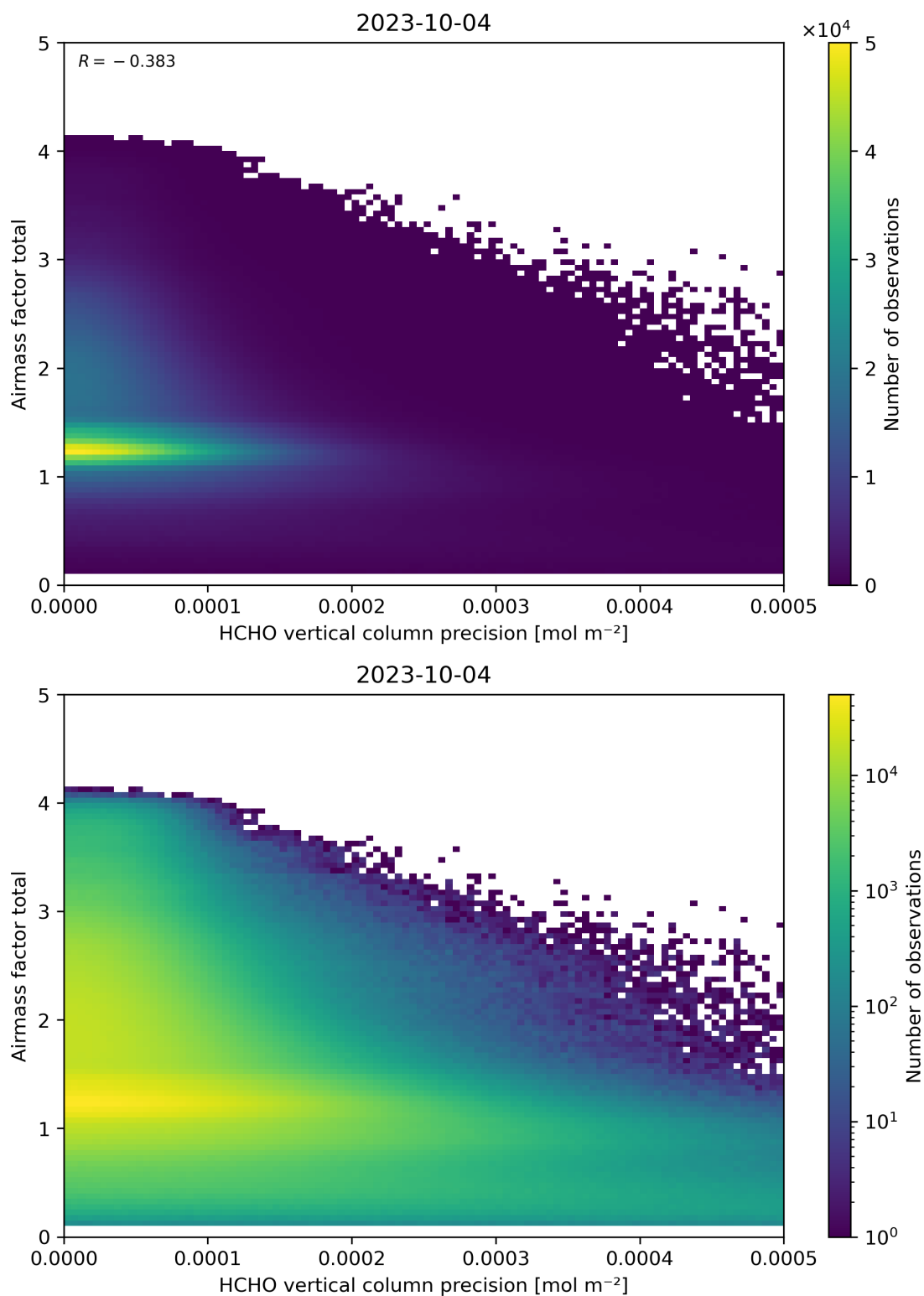
Figure 144: Scatter density plot of “HCHO vertical column precision” against “Airmass factor total” for 2023-10-03 to 2023-10-05.
