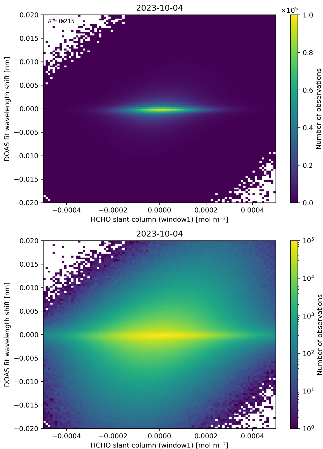
Figure 79: Scatter density plot of “HCHO slant column (window1)” against “DOAS fit wavelength shift” for 2023-10-03 to 2023-10-05.
