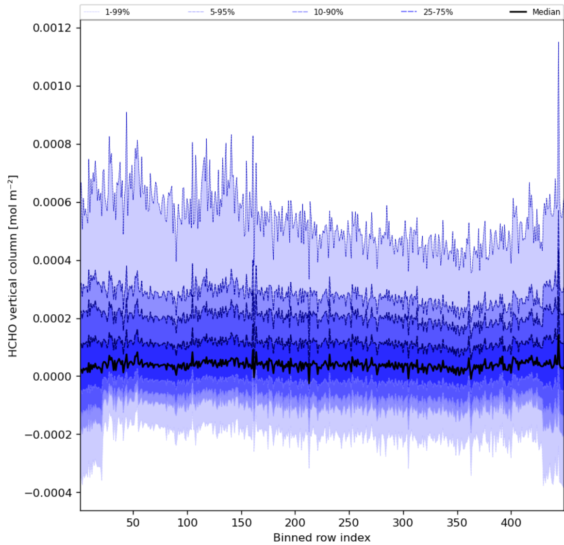
Figure 49: Along track statistics of “HCHO vertical column” for 2023-10-03 to 2023-10-05
