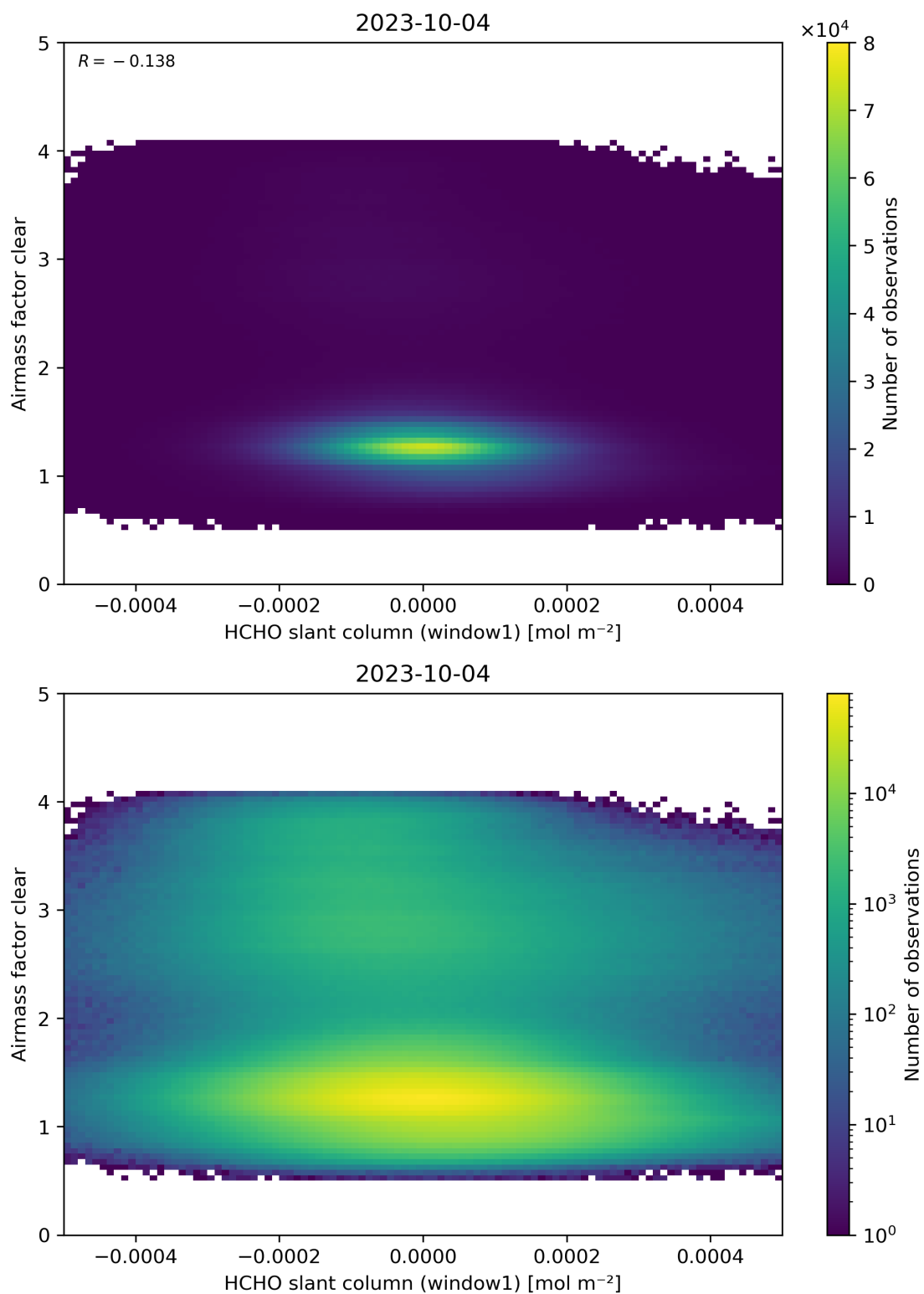
Figure 81: Scatter density plot of “HCHO slant column (window1)” against “Airmass factor clear” for 2023-10-03 to 2023-10-05.
