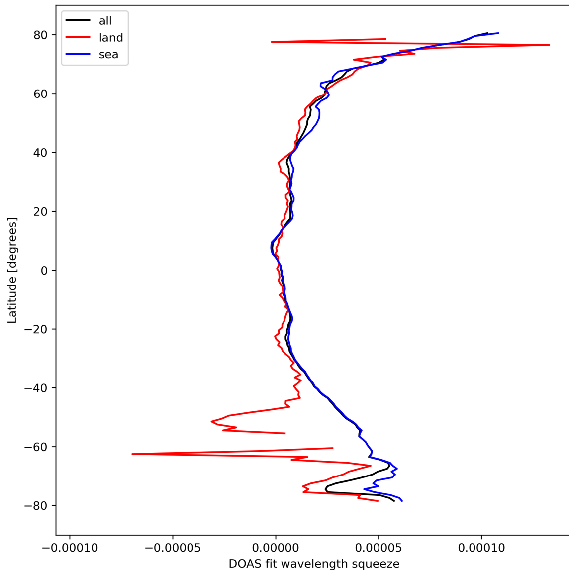
Figure 31: Zonal average of “DOAS fit wavelength squeeze” for 2023-10-03 to 2023-10-05.
