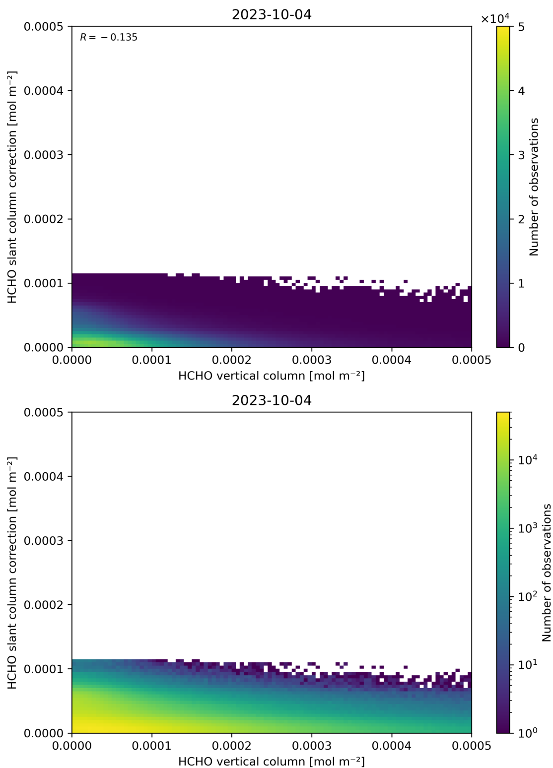
Figure 128: Scatter density plot of “HCHO vertical column” against “HCHO slant column correction” for 2023-10-03 to 2023-10-05.
