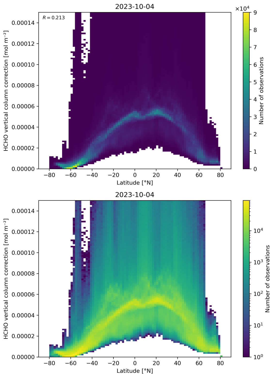
Figure 164: Scatter density plot of “Latitude” against “HCHO vertical column correction” for 2023-10-03 to 2023-10-05.
