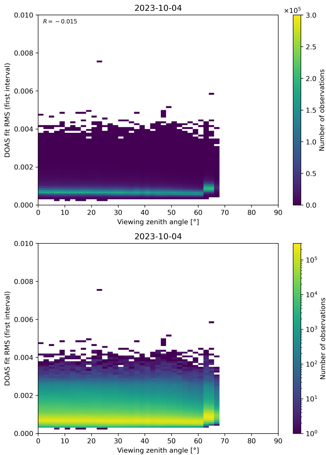
Figure 182: Scatter density plot of “Viewing zenith angle” against “DOAS fit RMS (first interval)” for 2023-10-03 to 2023-10-05.
