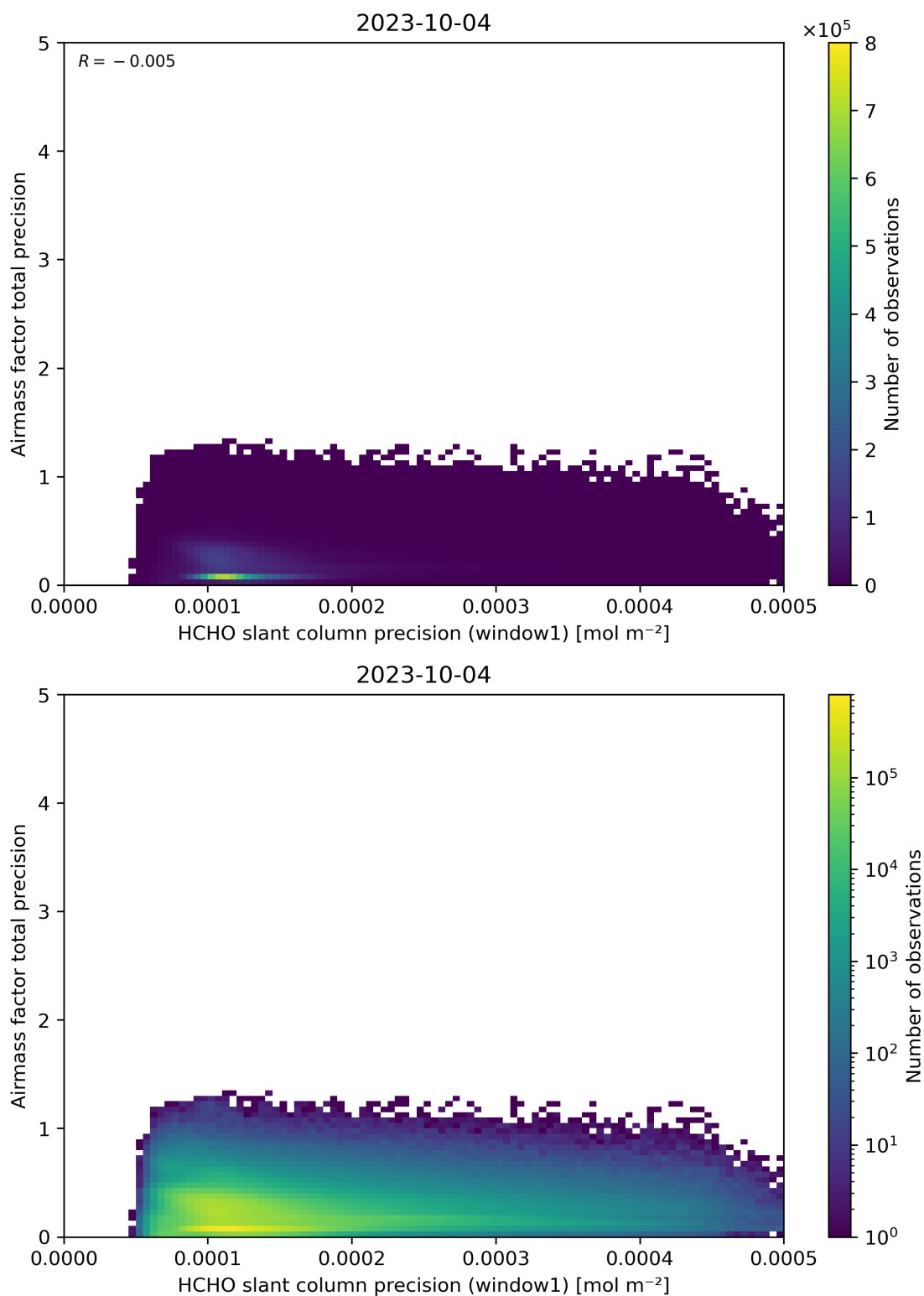
Figure 95: Scatter density plot of “HCHO slant column precision (window1)” against “Airmass factor total precision” for 2023-10-03 to 2023-10-05.
