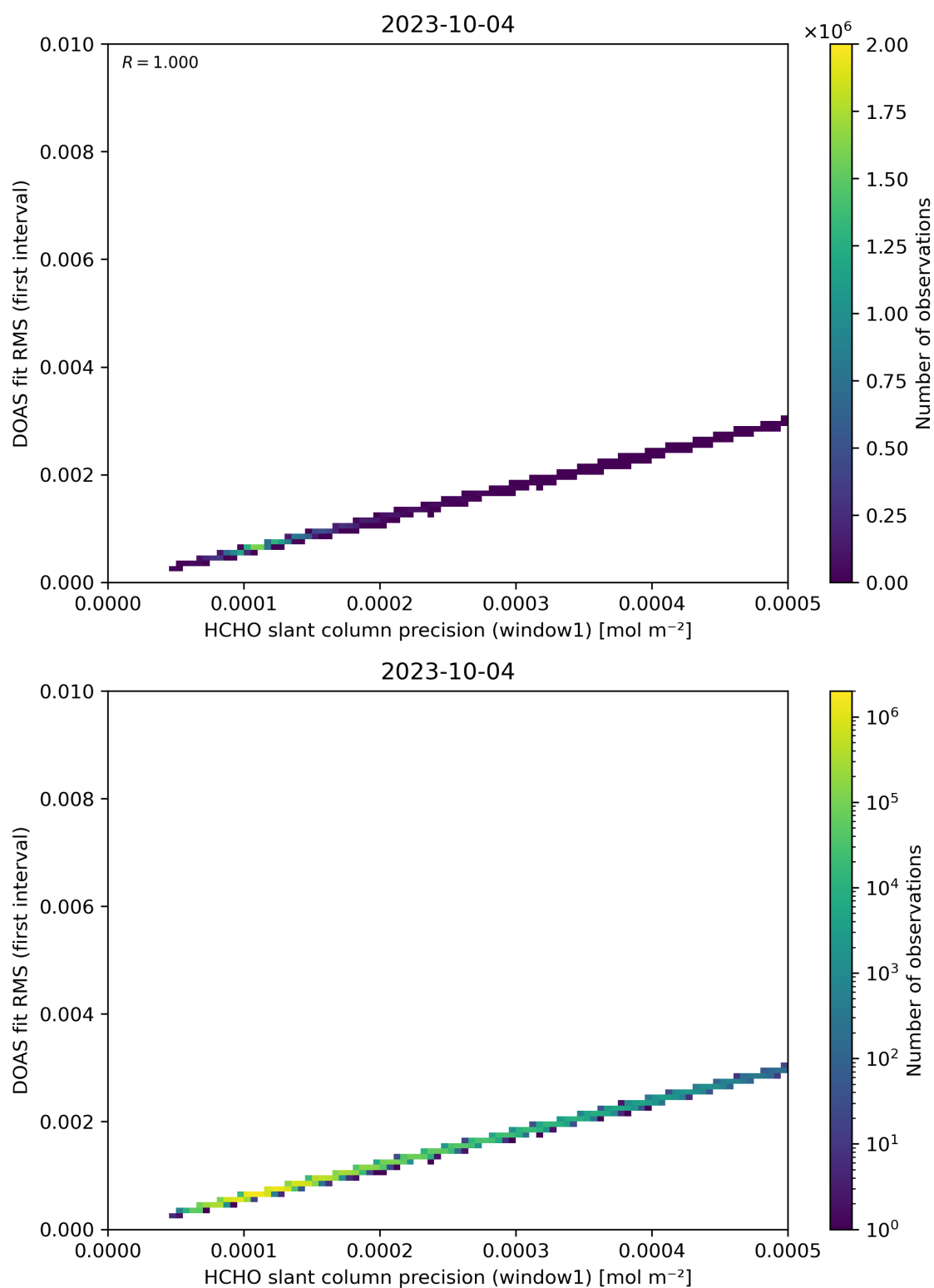
Figure 88: Scatter density plot of “HCHO slant column precision (window1)” against “DOAS fit RMS (first interval)” for 2023-10-03 to 2023-10-05.
