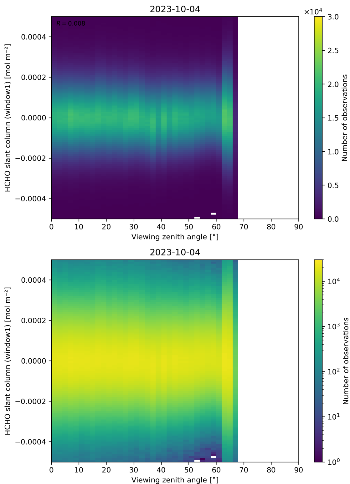
Figure 188: Scatter density plot of “Viewing zenith angle” against “HCHO slant column (window1)” for 2023-10-03 to 2023-10-05.
