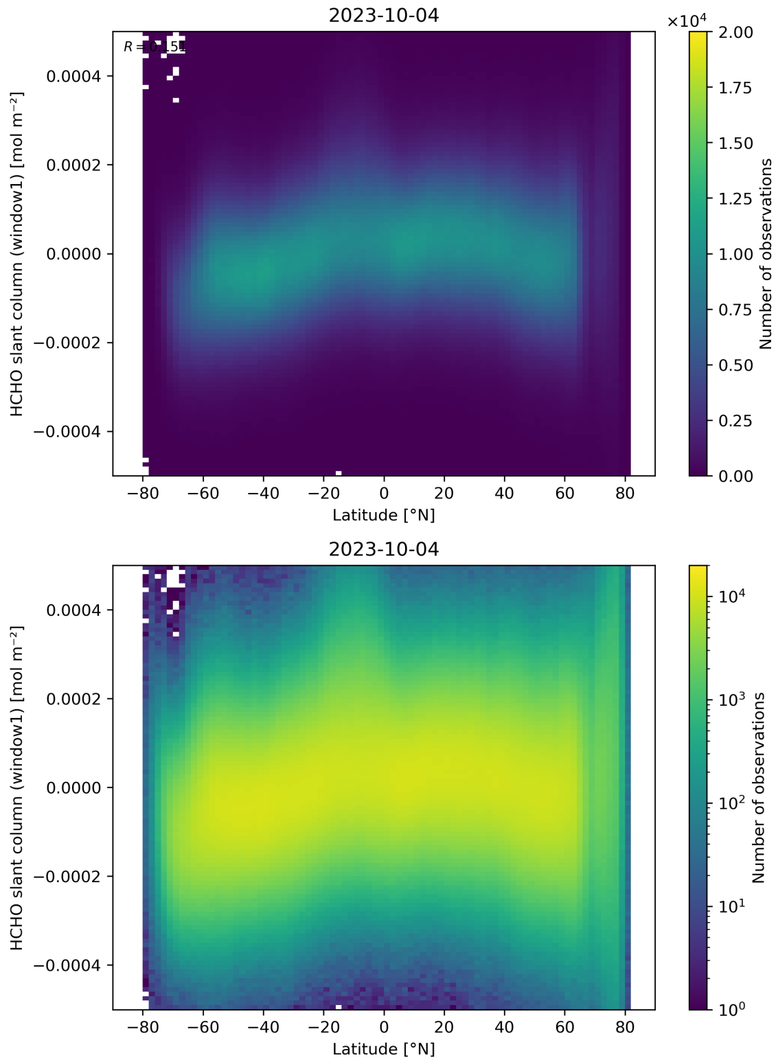
Figure 159: Scatter density plot of “Latitude” against “HCHO slant column (window1)” for 2023-10-03 to 2023-10-05.
