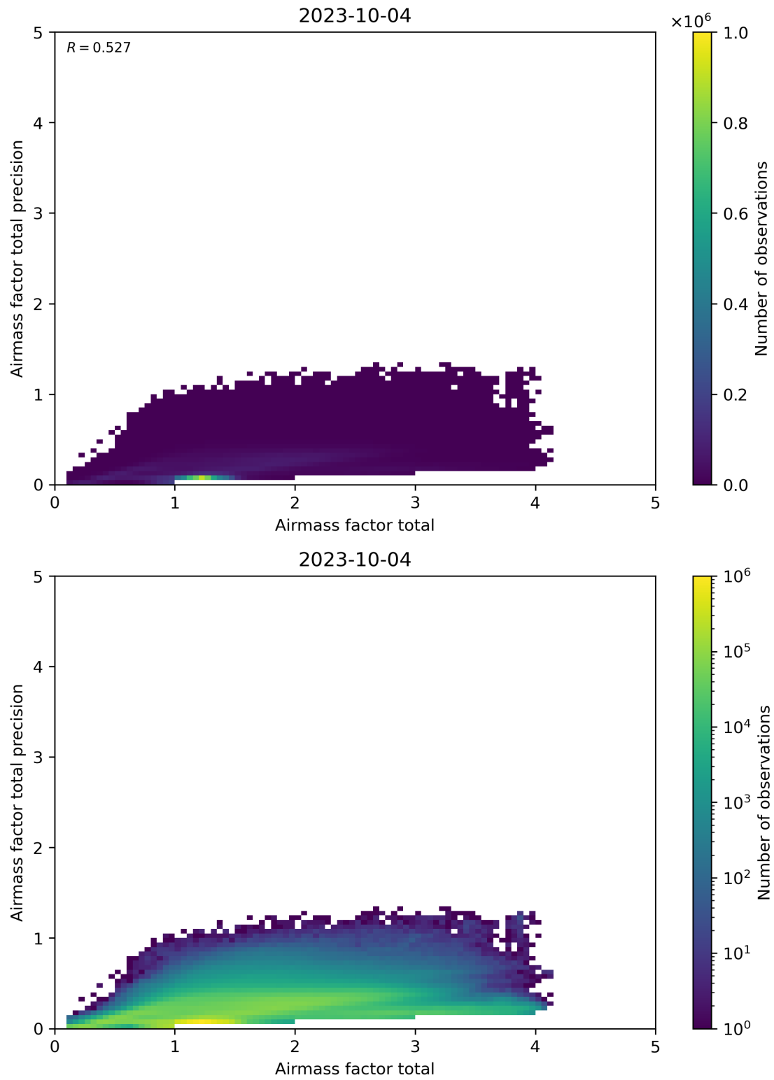
Figure 103: Scatter density plot of “Airmass factor total” against “Airmass factor total precision” for 2023-10-03 to 2023-10-05.
