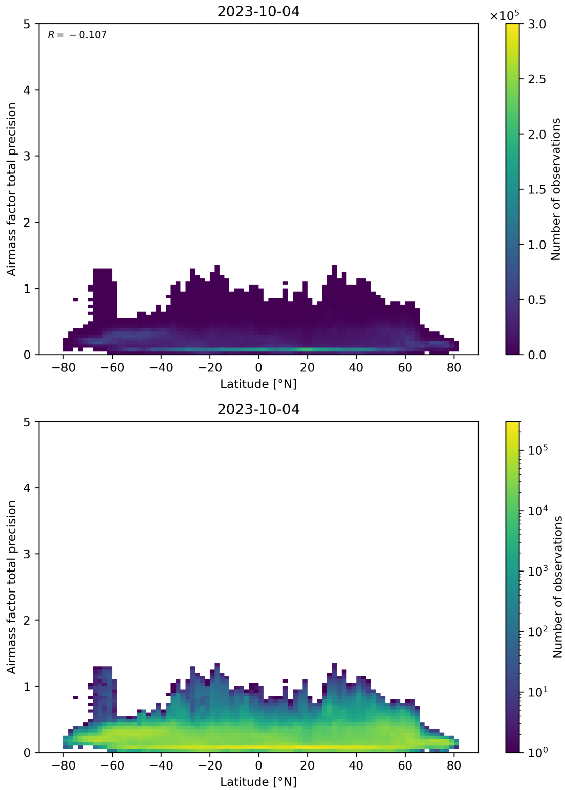
Figure 162: Scatter density plot of “Latitude” against “Airmass factor total precision” for 2023-10-03 to 2023-10-05.
