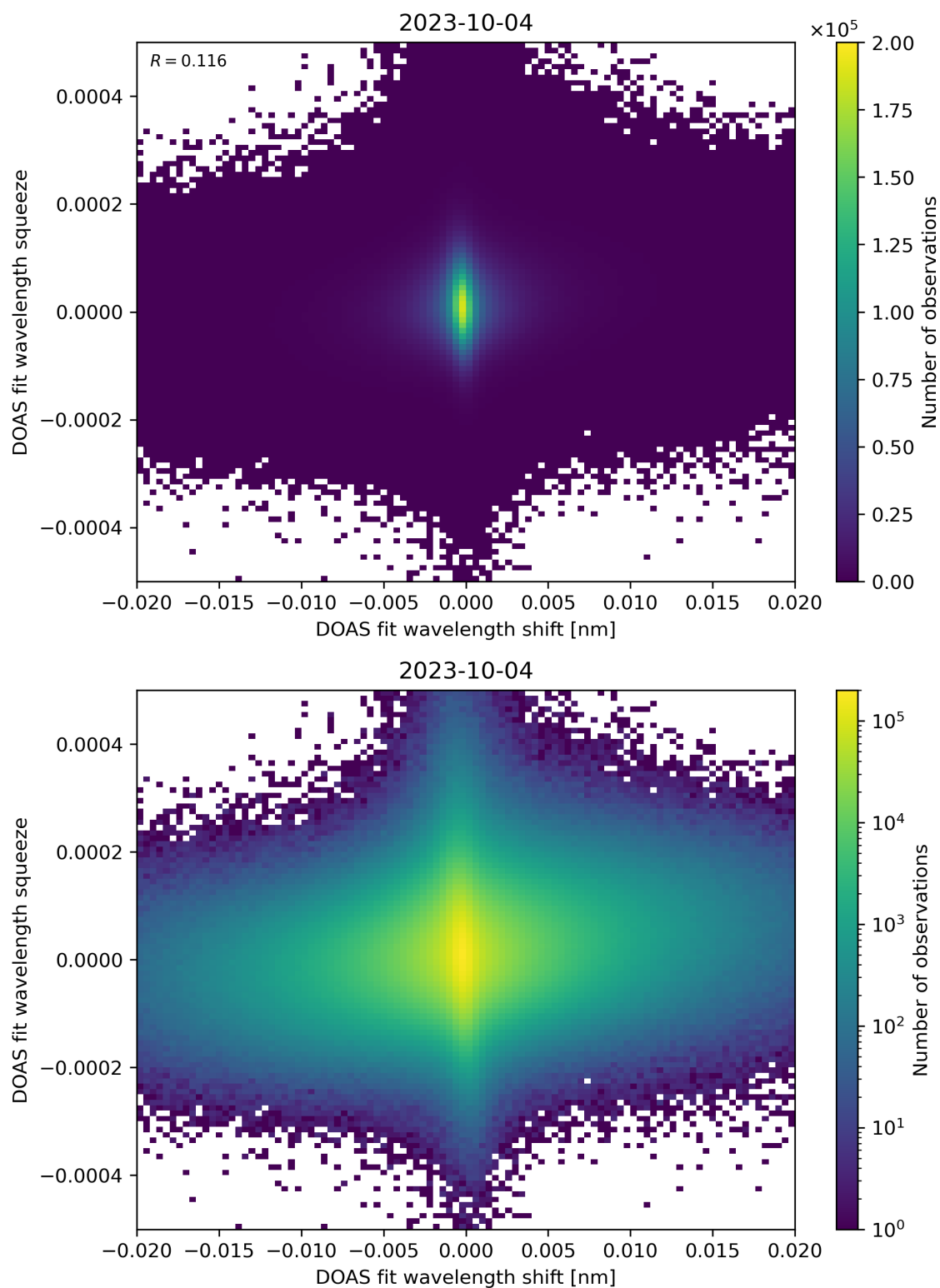
Figure 65: Scatter density plot of “DOAS fit wavelength shift” against “DOAS fit wavelength squeeze” for 2023-10-03 to 2023-10-05.
