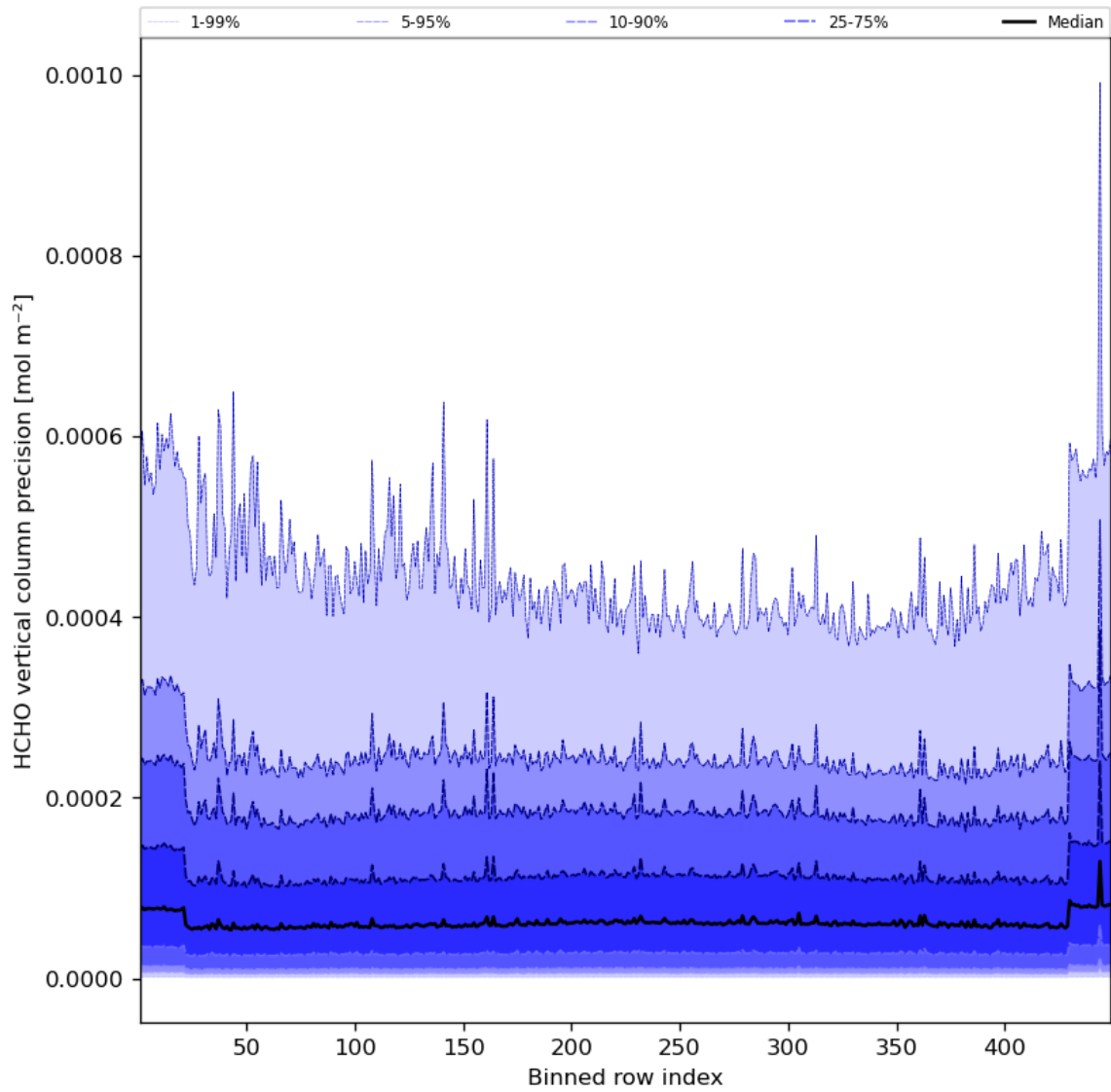
Figure 50: Along track statistics of “HCHO vertical column precision” for 2023-10-03 to 2023-10-05
