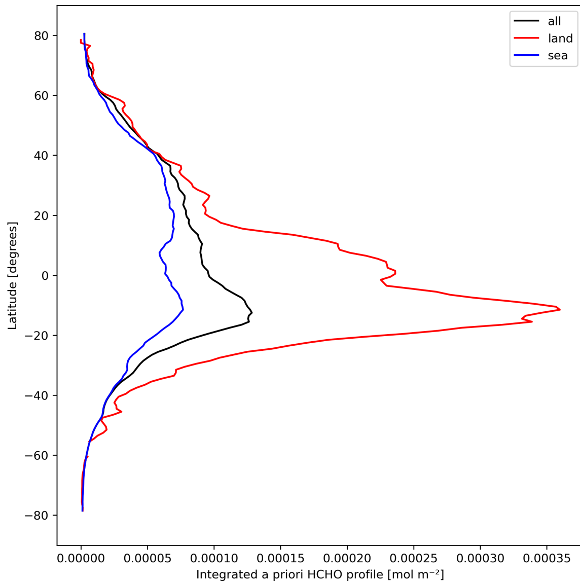
Figure 29: Zonal average of “Integrated a priori HCHO profile” for 2023-10-03 to 2023-10-05.
