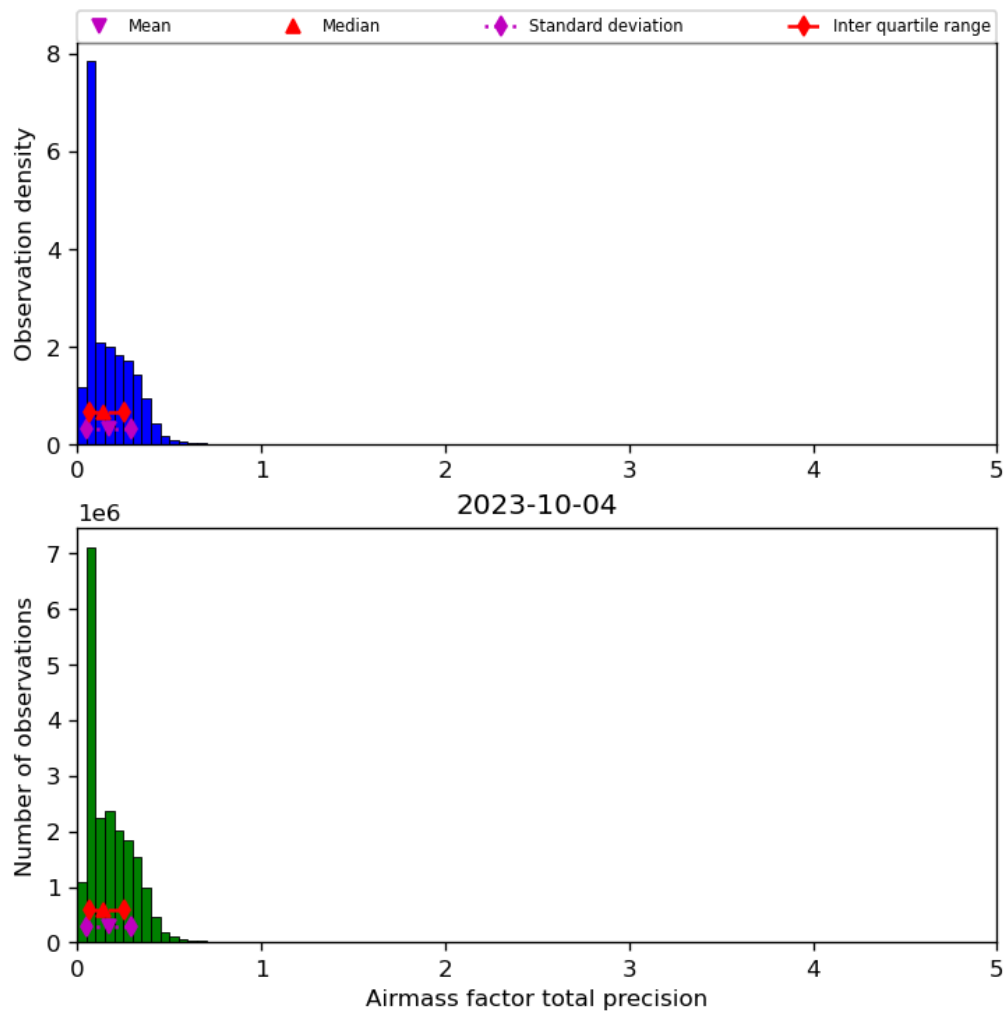
Figure 41: Histogram of “Airmass factor total precision” for 2023-10-03 to 2023-10-05
