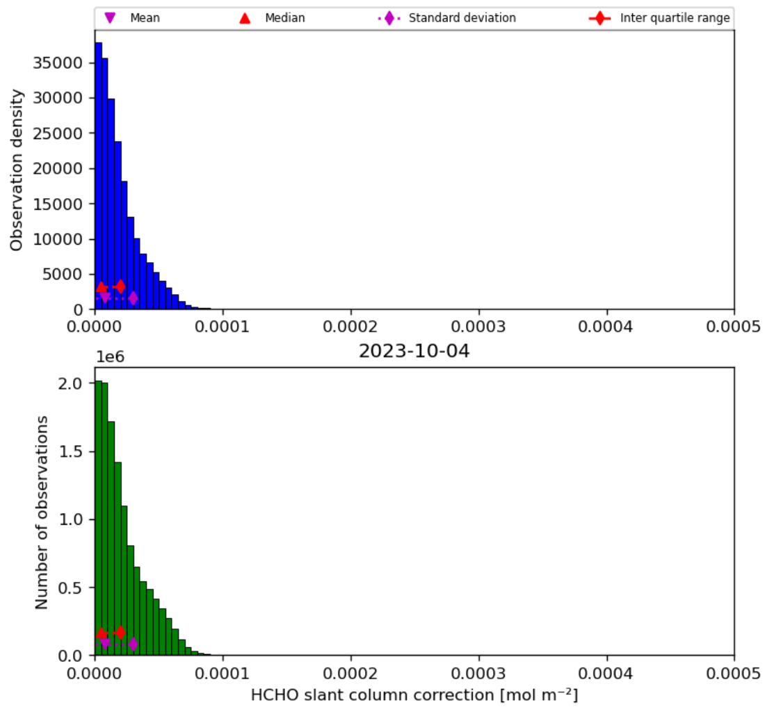
Figure 47: Histogram of “HCHO slant column correction” for 2023-10-03 to 2023-10-05
