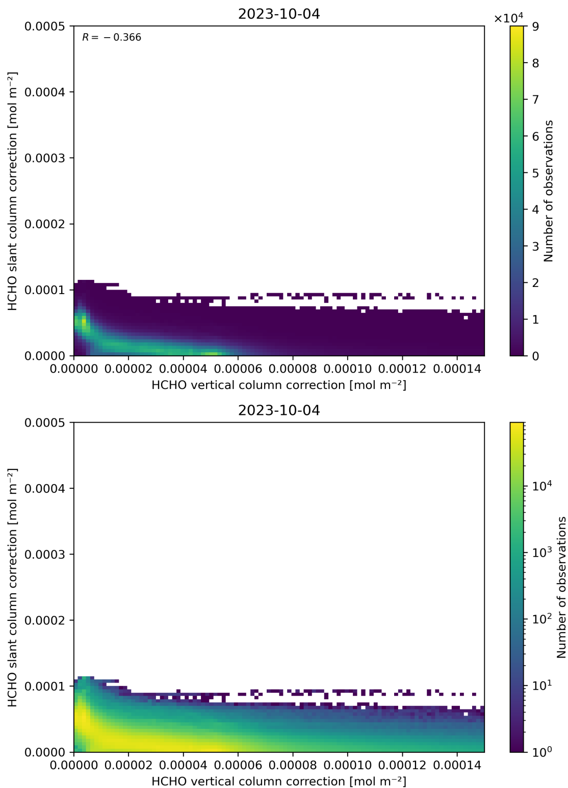
Figure 117: Scatter density plot of “HCHO vertical column correction” against “HCHO slant column correction” for 2023-10-03 to 2023-10-05.
