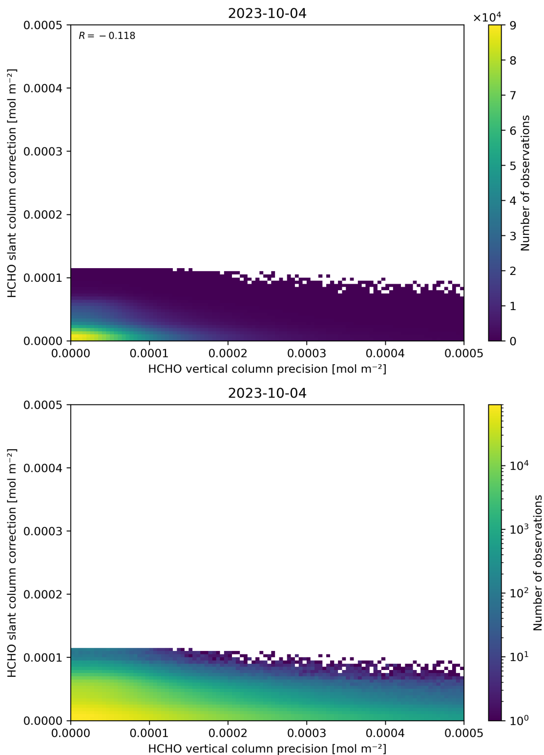
Figure 141: Scatter density plot of “HCHO vertical column precision” against “HCHO slant column correction” for 2023-10-03 to 2023-10-05.
