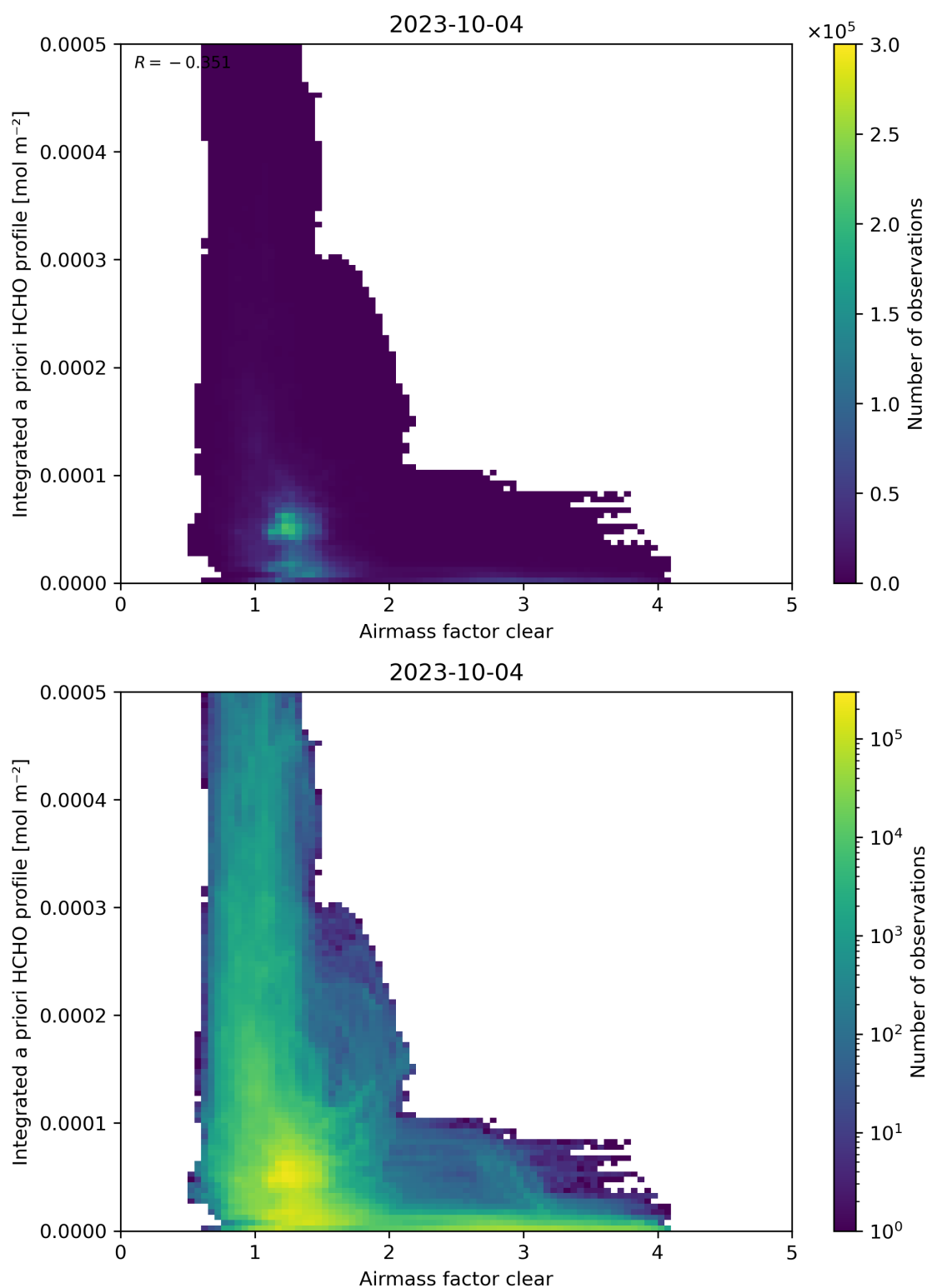
Figure 76: Scatter density plot of “Airmass factor clear” against “Integrated a priori HCHO profile” for 2023-10-03 to 2023-10-05.
