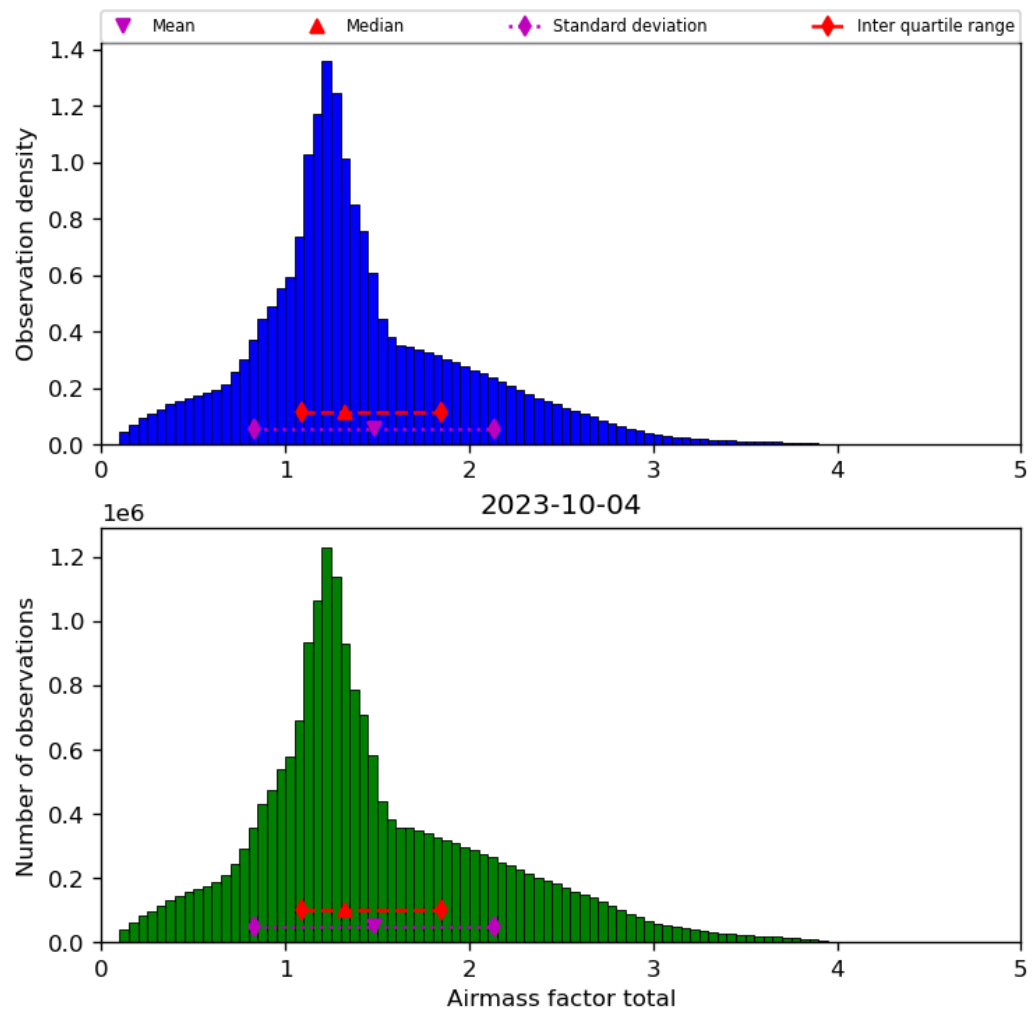
Figure 40: Histogram of “Airmass factor total” for 2023-10-03 to 2023-10-05
