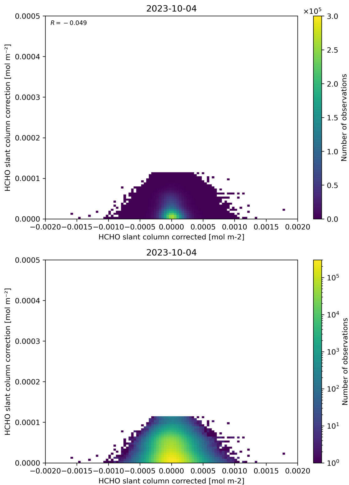
Figure 77: Scatter density plot of “HCHO slant column corrected” against “HCHO slant column correction” for 2023-10-03 to 2023-10-05.
