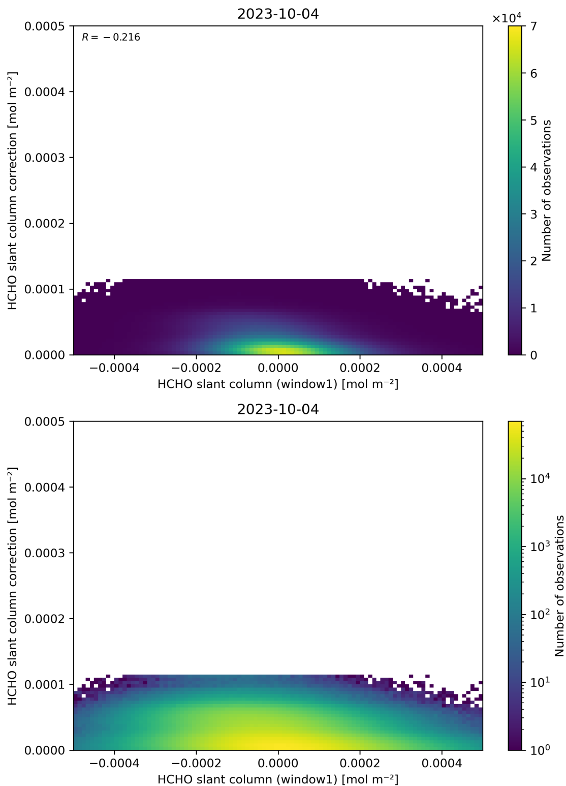
Figure 83: Scatter density plot of “HCHO slant column (window1)” against “HCHO slant column correction” for 2023-10-03 to 2023-10-05.
