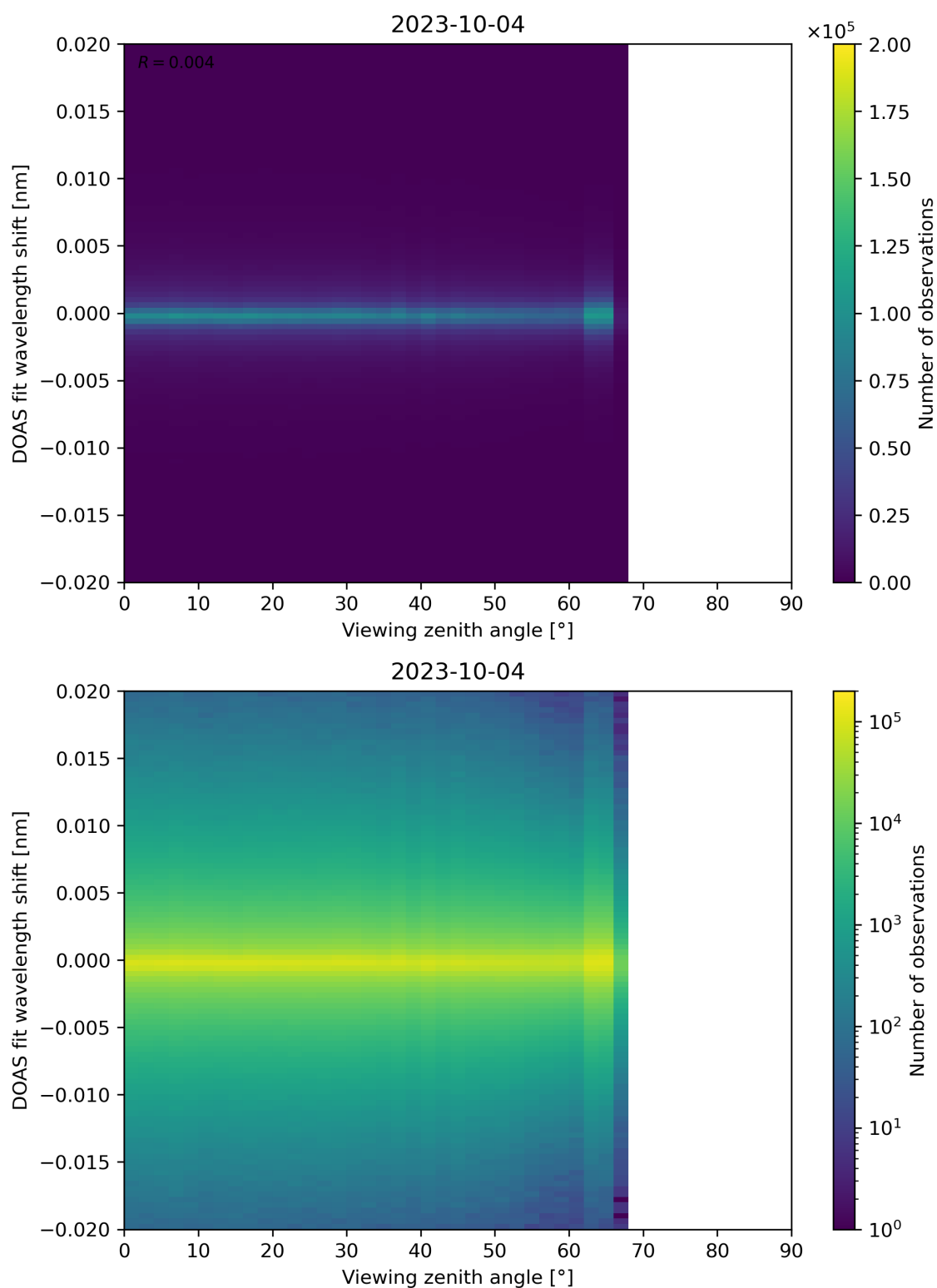
Figure 183: Scatter density plot of “Viewing zenith angle” against “DOAS fit wavelength shift” for 2023-10-03 to 2023-10-05.
