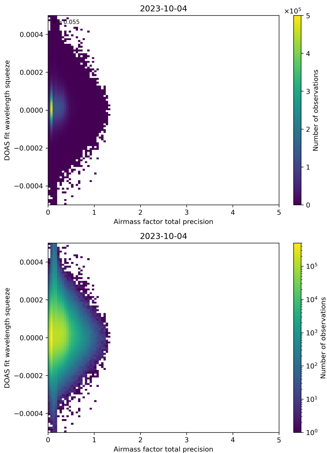
Figure 107: Scatter density plot of “Airmass factor total precision” against “DOAS fit wavelength squeeze” for 2023-10-03 to 2023-10-05.
