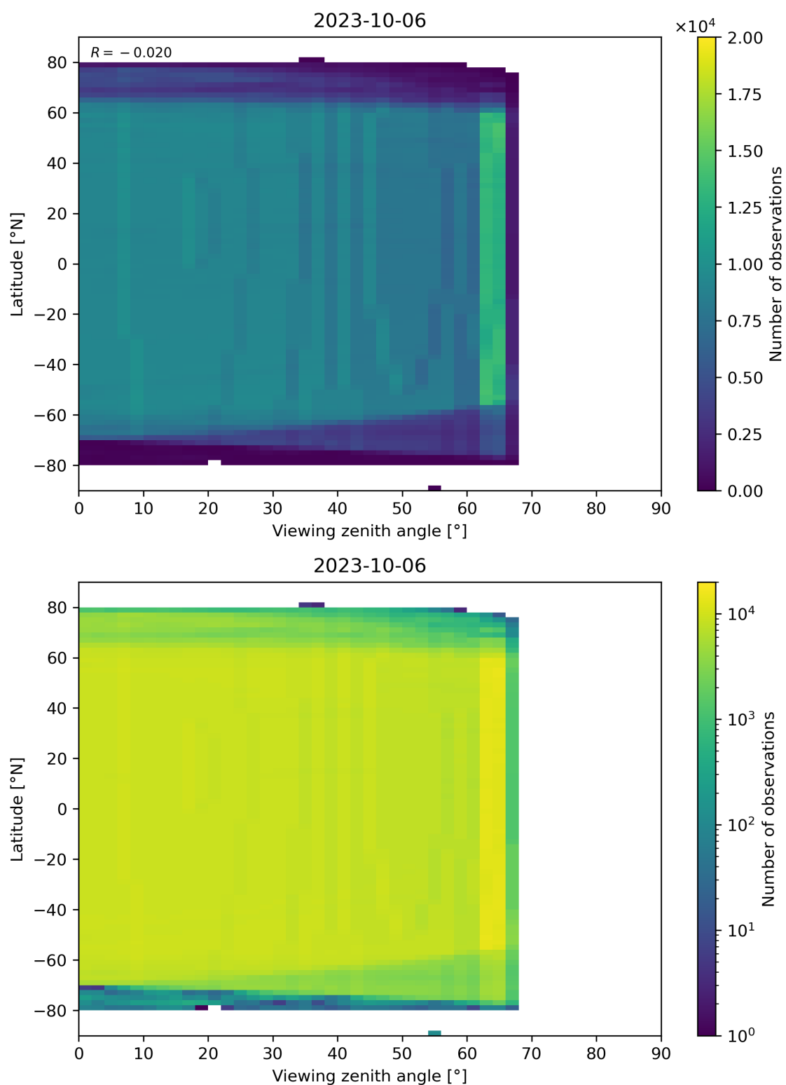
Figure 196: Scatter density plot of “Viewing zenith angle” against “Latitude” for 2023-10-06 to 2023-10-07.
