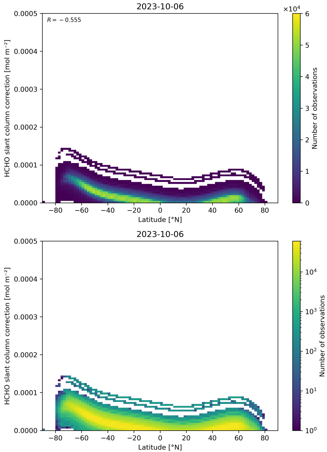
Figure 158: Scatter density plot of “Latitude” against “HCHO slant column correction” for 2023-10-06 to 2023-10-07.
