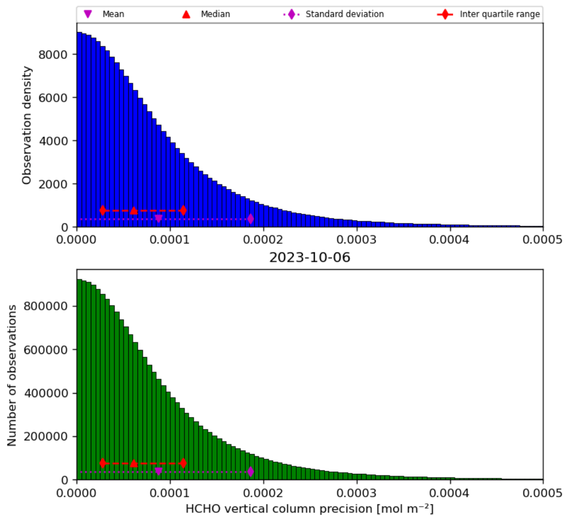
Figure 36: Histogram of “HCHO vertical column precision” for 2023-10-06 to 2023-10-07
