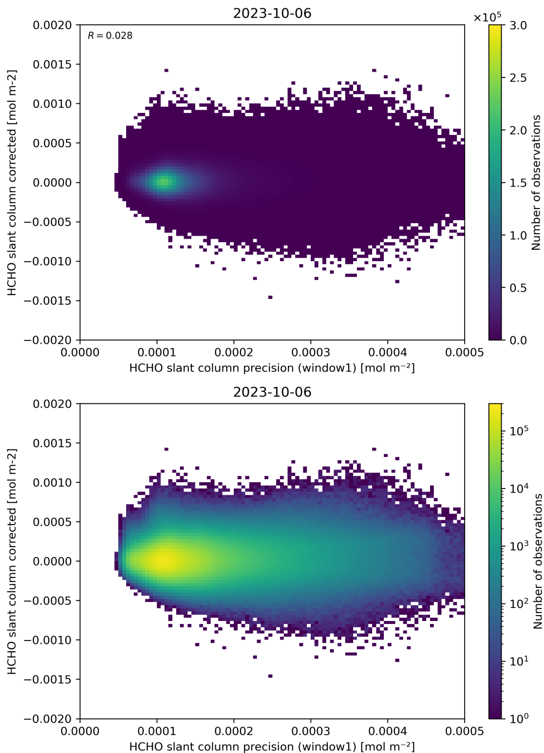
Figure 92: Scatter density plot of “HCHO slant column precision (window1)” against “HCHO slant column corrected” for 2023-10-06 to 2023-10-07.
