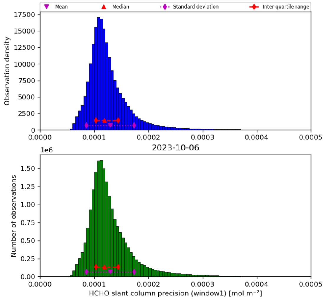
Figure 39: Histogram of “HCHO slant column precision (window1)” for 2023-10-06 to 2023-10-07
