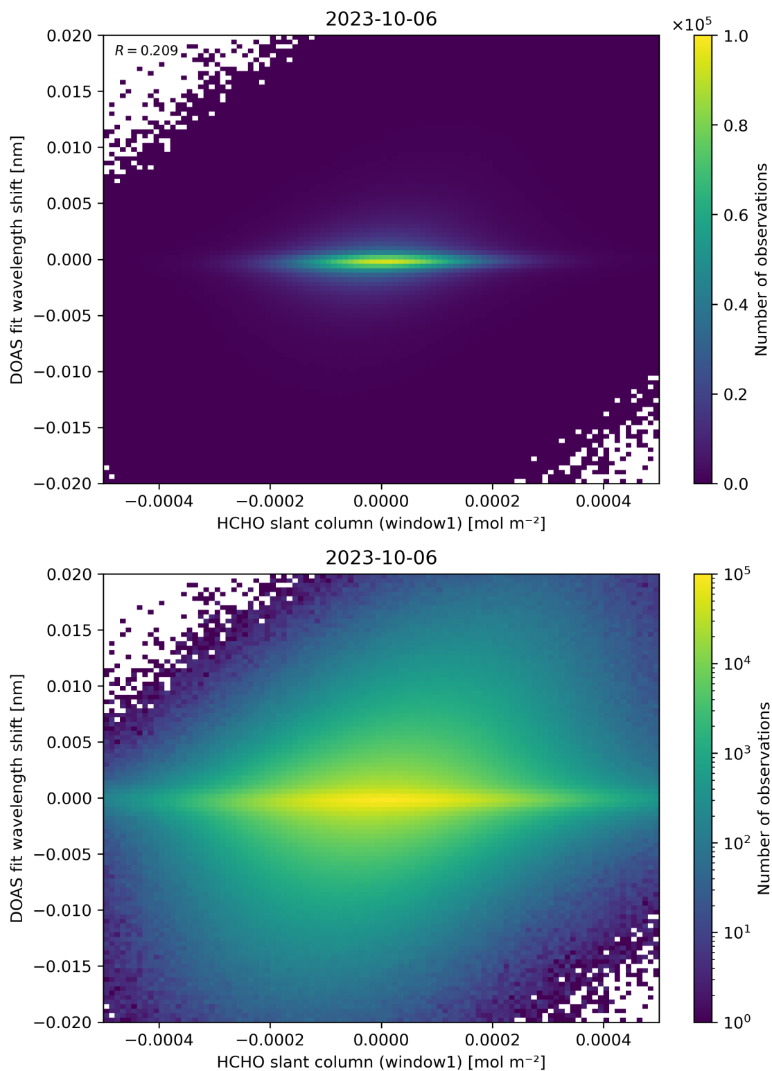
Figure 79: Scatter density plot of “HCHO slant column (window1)” against “DOAS fit wavelength shift” for 2023-10-06 to 2023-10-07.
