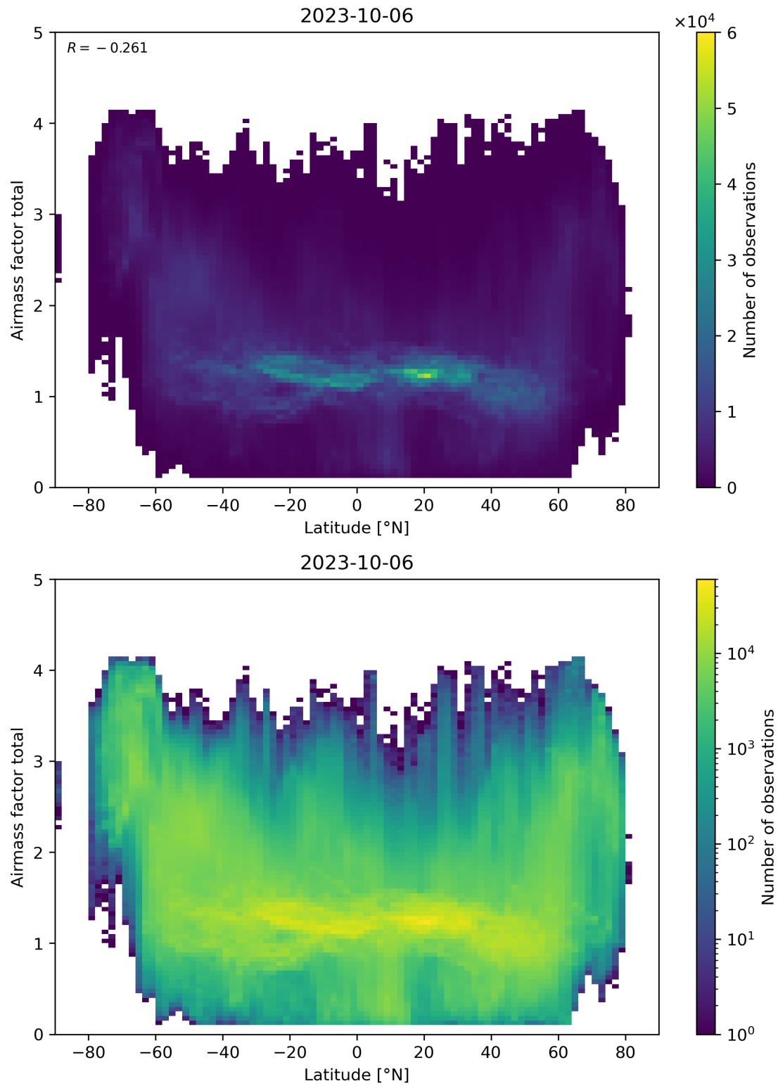
Figure 161: Scatter density plot of “Latitude” against “Airmass factor total” for 2023-10-06 to 2023-10-07.
