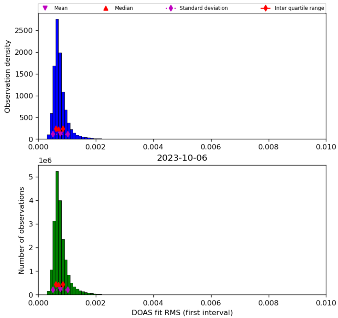
Figure 46: Histogram of “DOAS fit RMS (first interval)” for 2023-10-06 to 2023-10-07
