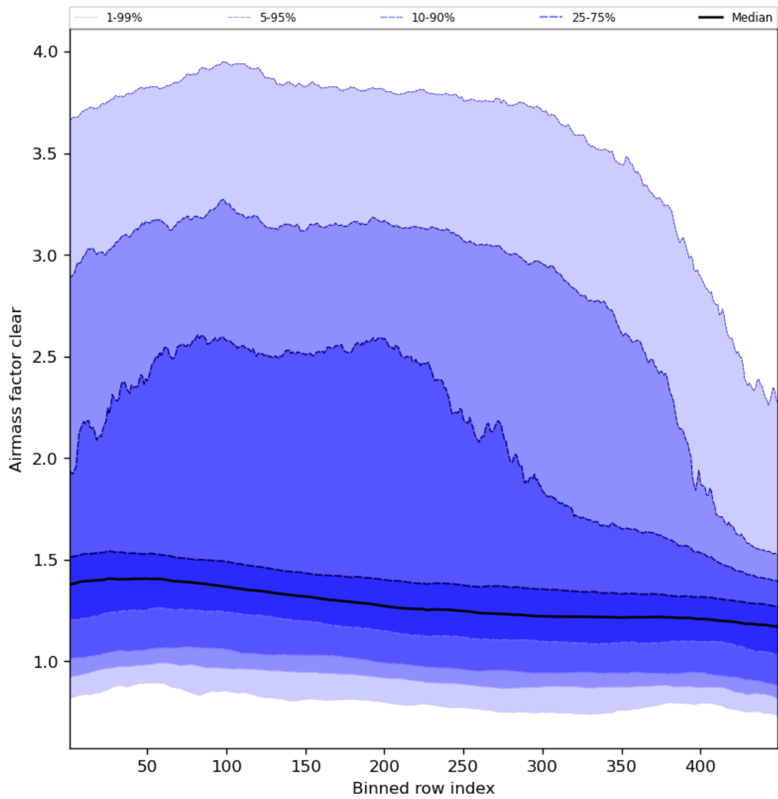
Figure 56: Along track statistics of “Airmass factor clear” for 2023-10-06 to 2023-10-07
