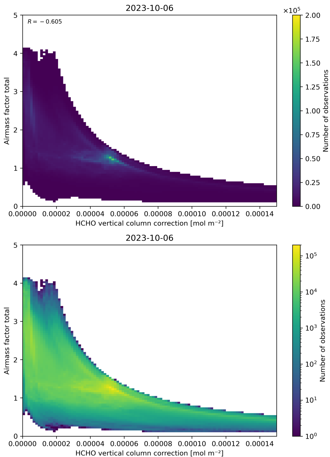
Figure 120: Scatter density plot of “HCHO vertical column correction” against “Airmass factor total” for 2023-10-06 to 2023-10-07.
