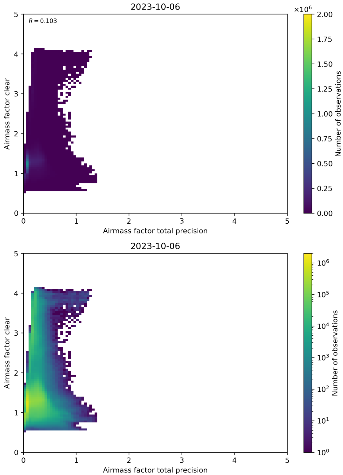
Figure 108: Scatter density plot of “Airmass factor total precision” against “Airmass factor clear” for 2023-10-06 to 2023-10-07.
