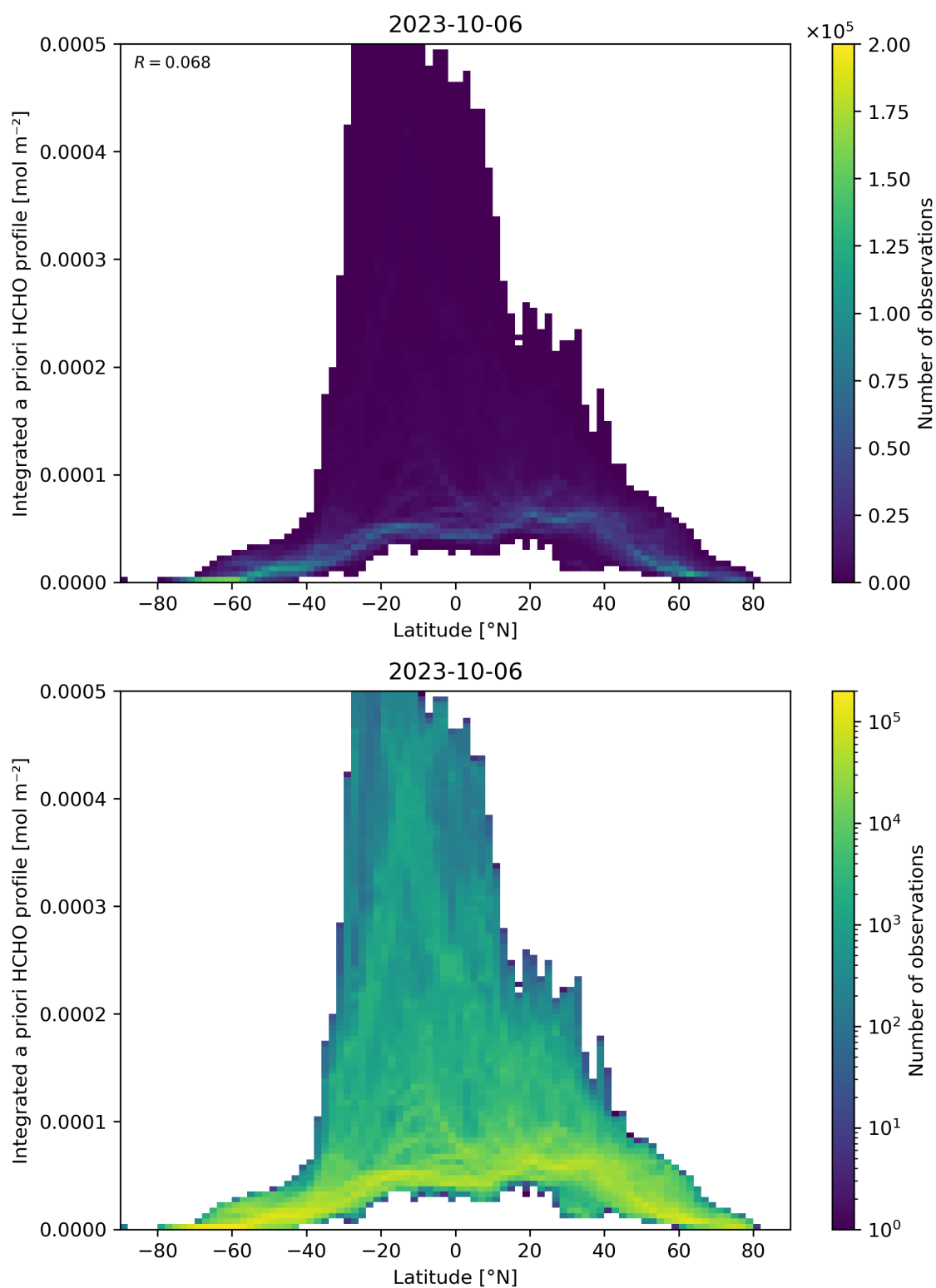
Figure 166: Scatter density plot of “Latitude” against “Integrated a priori HCHO profile” for 2023-10-06 to 2023-10-07.
