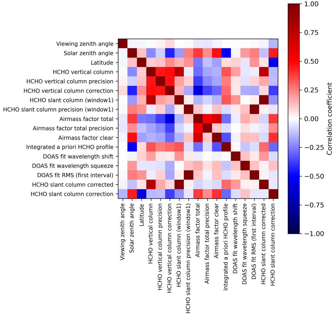
Figure 2: Map of correlation matrix for 2023-10-06 to 2023-10-07.
