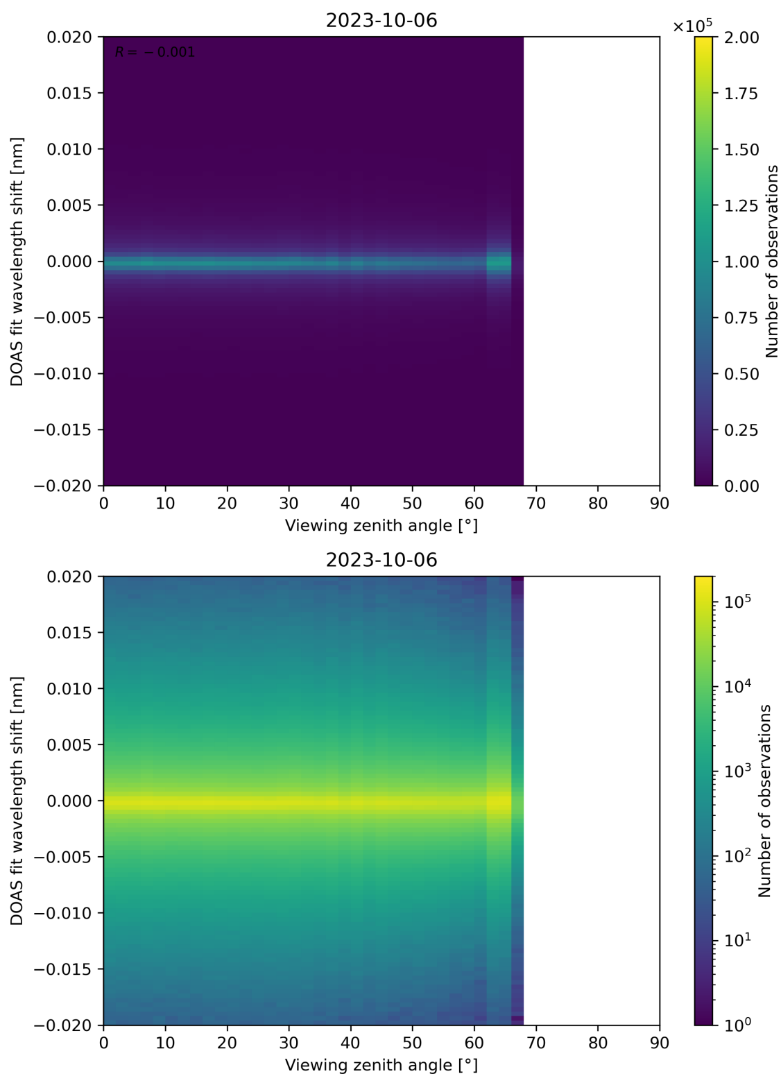
Figure 183: Scatter density plot of “Viewing zenith angle” against “DOAS fit wavelength shift” for 2023-10-06 to 2023-10-07.
