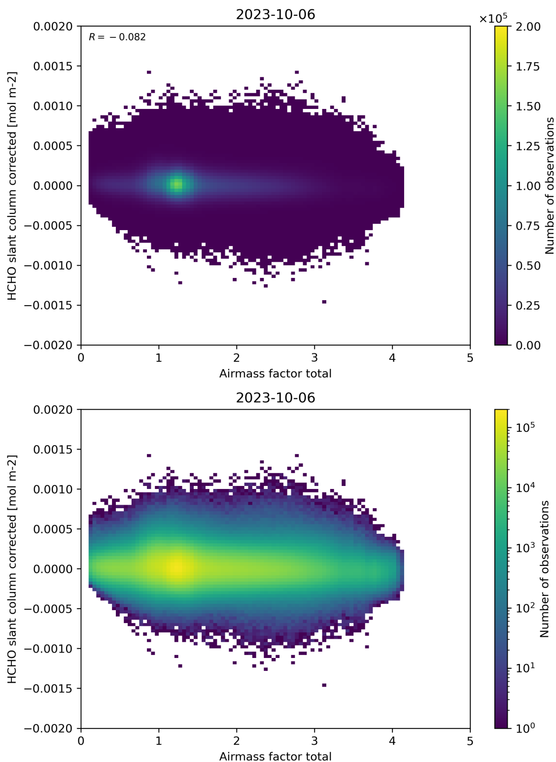
Figure 101: Scatter density plot of “Airmass factor total” against “HCHO slant column corrected” for 2023-10-06 to 2023-10-07.
