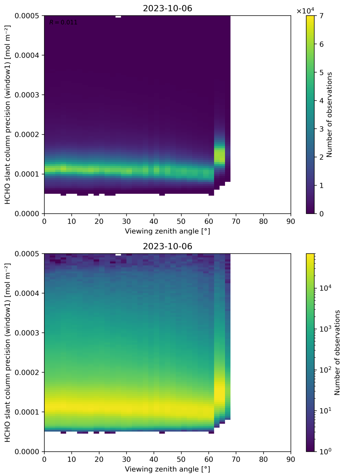
Figure 189: Scatter density plot of “Viewing zenith angle” against “HCHO slant column precision (window1)” for 2023-10-06 to 2023-10-07.
