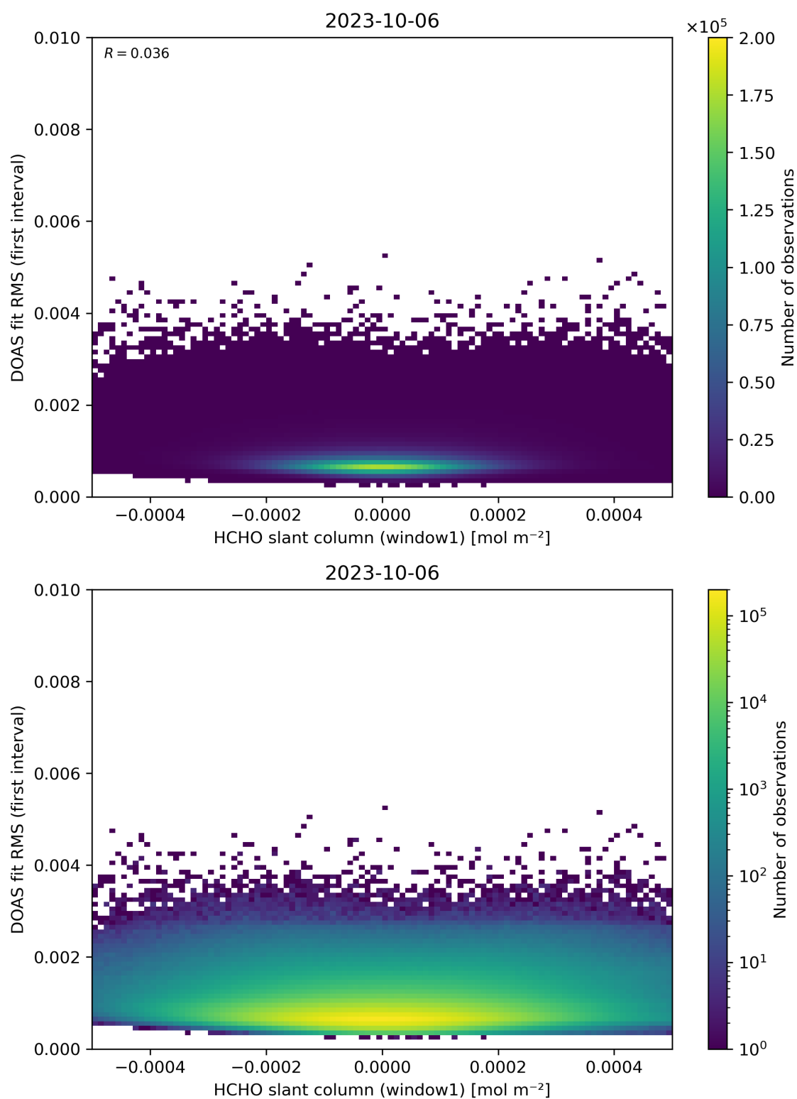
Figure 78: Scatter density plot of “HCHO slant column (window1)” against “DOAS fit RMS (first interval)” for 2023-10-06 to 2023-10-07.
