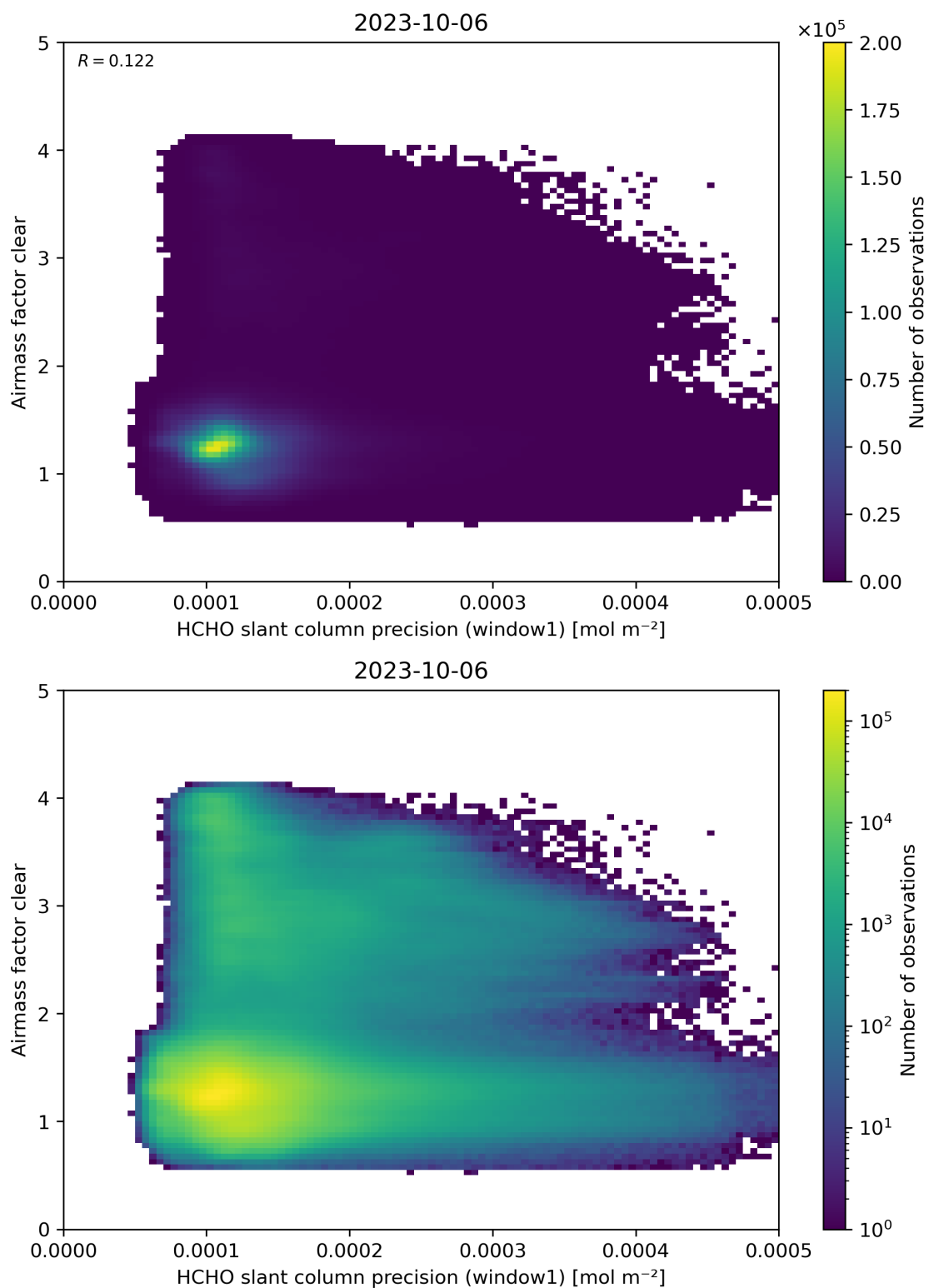
Figure 91: Scatter density plot of “HCHO slant column precision (window1)” against “Airmass factor clear” for 2023-10-06 to 2023-10-07.
