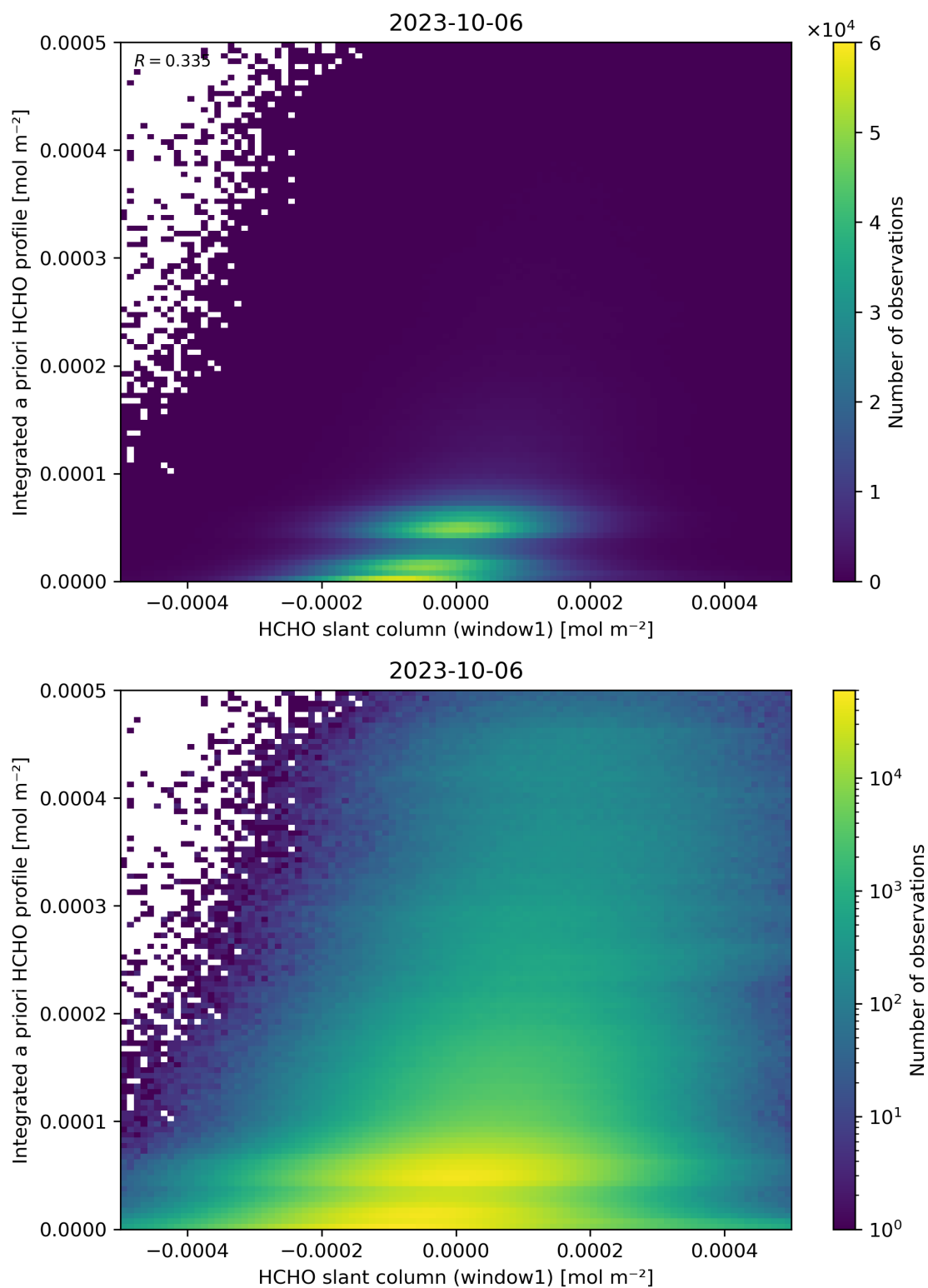
Figure 87: Scatter density plot of “HCHO slant column (window1)” against “Integrated a priori HCHO profile” for 2023-10-06 to 2023-10-07.
