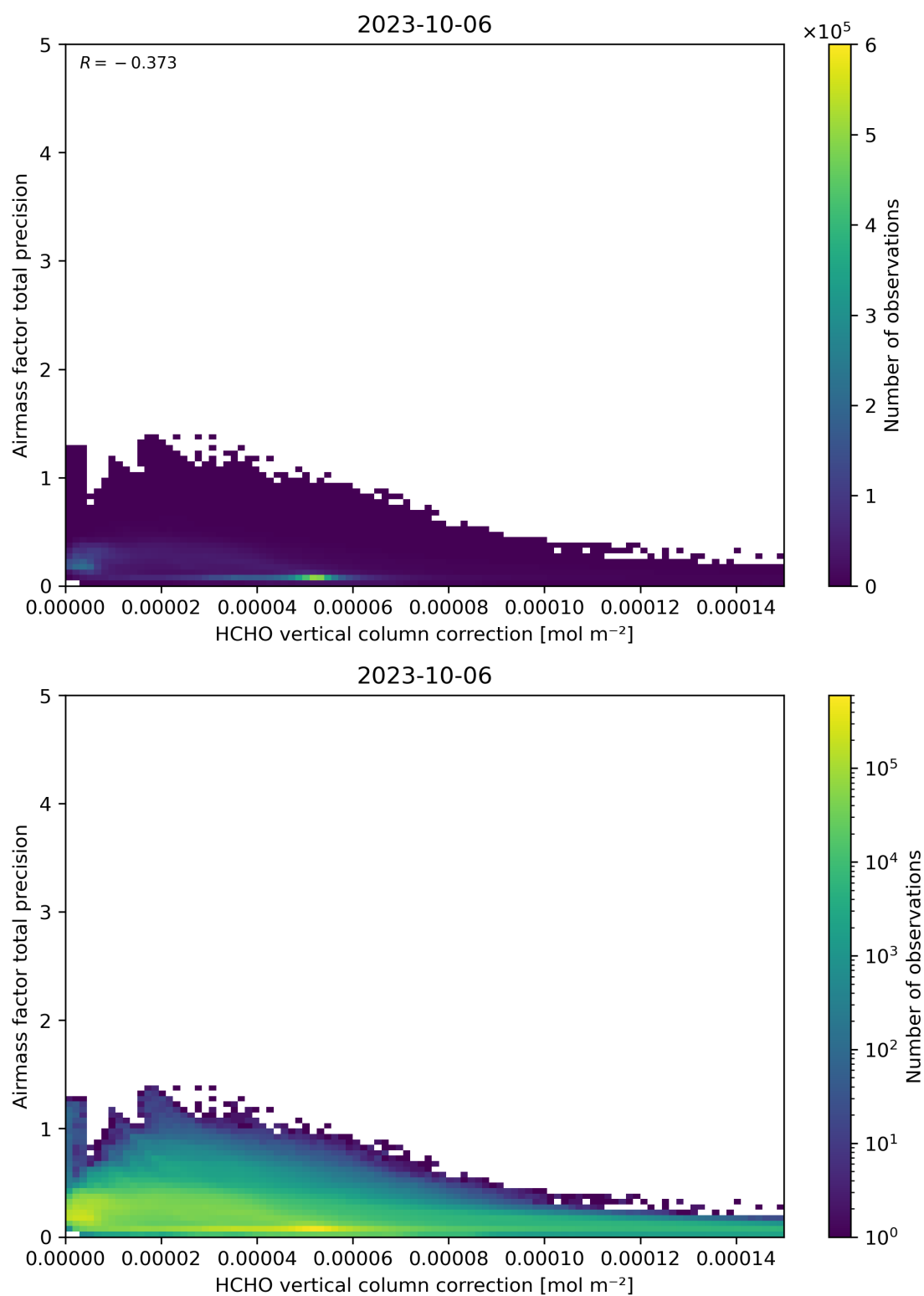
Figure 121: Scatter density plot of “HCHO vertical column correction” against “Air mass factor total precision” for 2023-10-06 to 2023-10-07.
