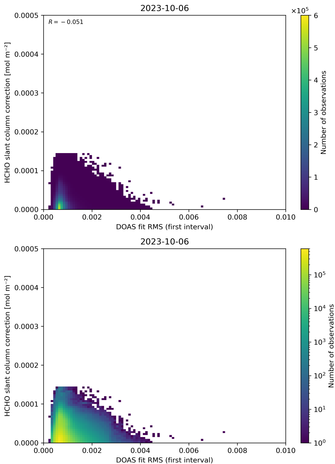
Figure 63: Scatter density plot of “DOAS fit RMS (first interval)” against “HCHO slant column correction” for 2023-10-06 to 2023-10-07.
