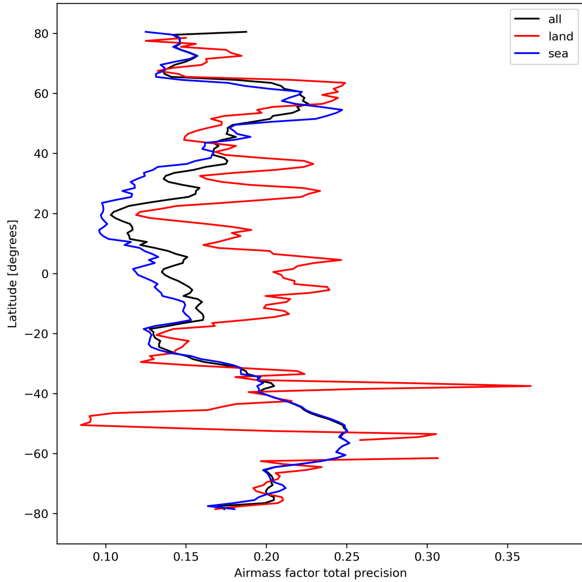
Figure 27: Zonal average of “Airmass factor total precision” for 2023-10-06 to 2023-10-07.
