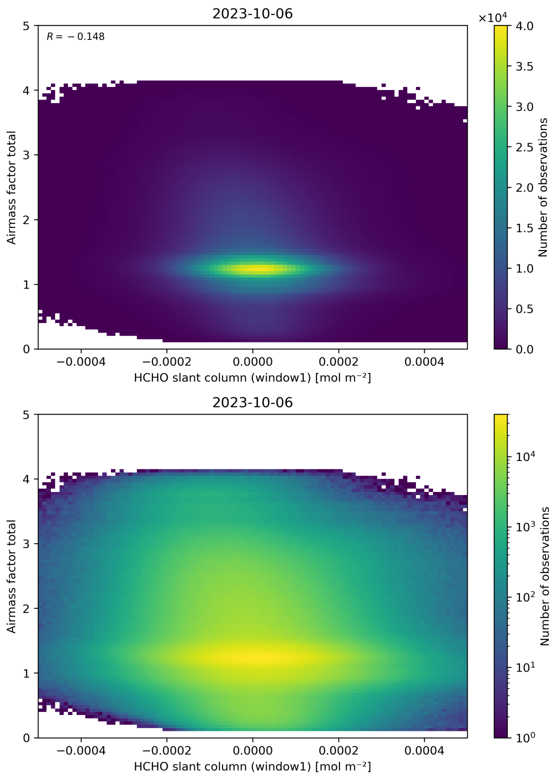
Figure 85: Scatter density plot of “HCHO slant column (window1)” against “Airmass factor total” for 2023-10-06 to 2023-10-07.
