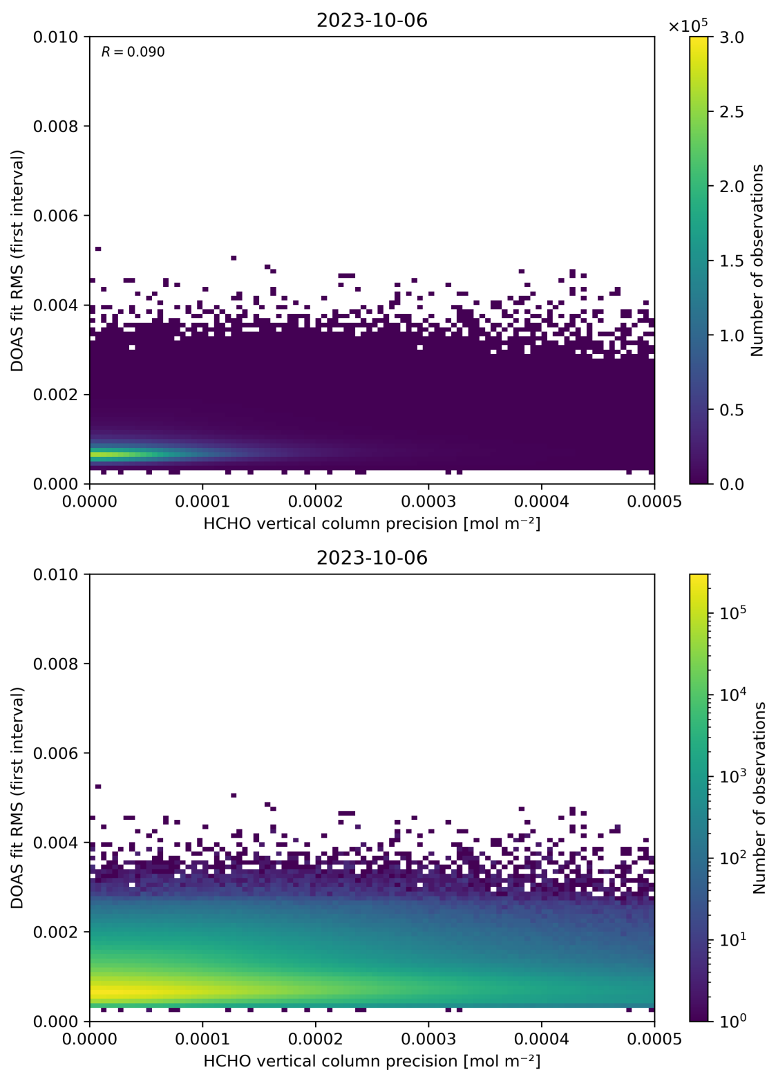
Figure 136: Scatter density plot of “HCHO vertical column precision” against “DOAS fit RMS (first interval)” for 2023-10-06 to 2023-10-07.
