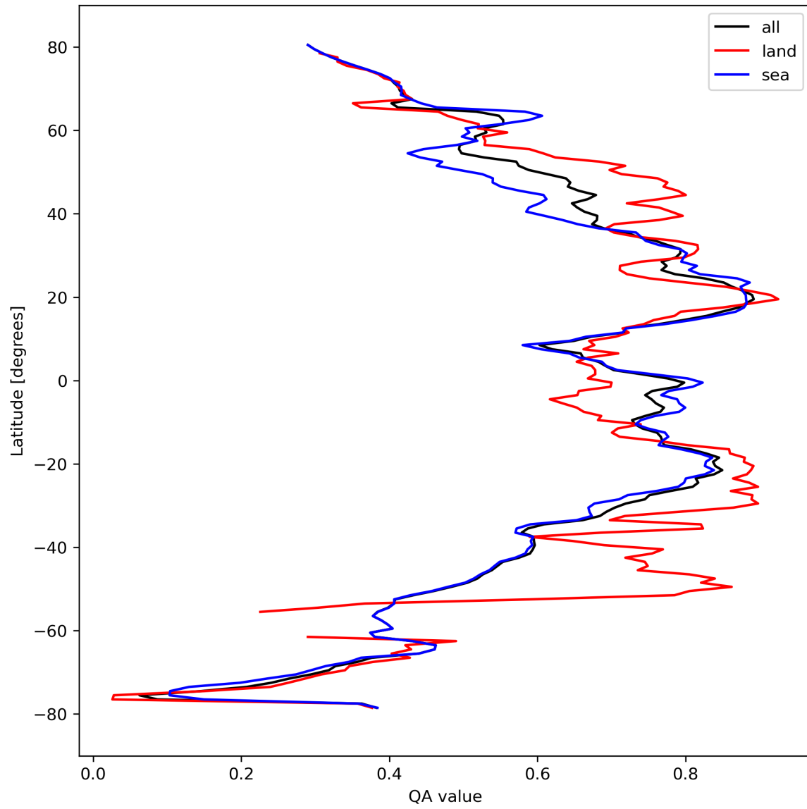
Figure 20: Zonal average of “QA value” for 2023-10-06 to 2023-10-07.
