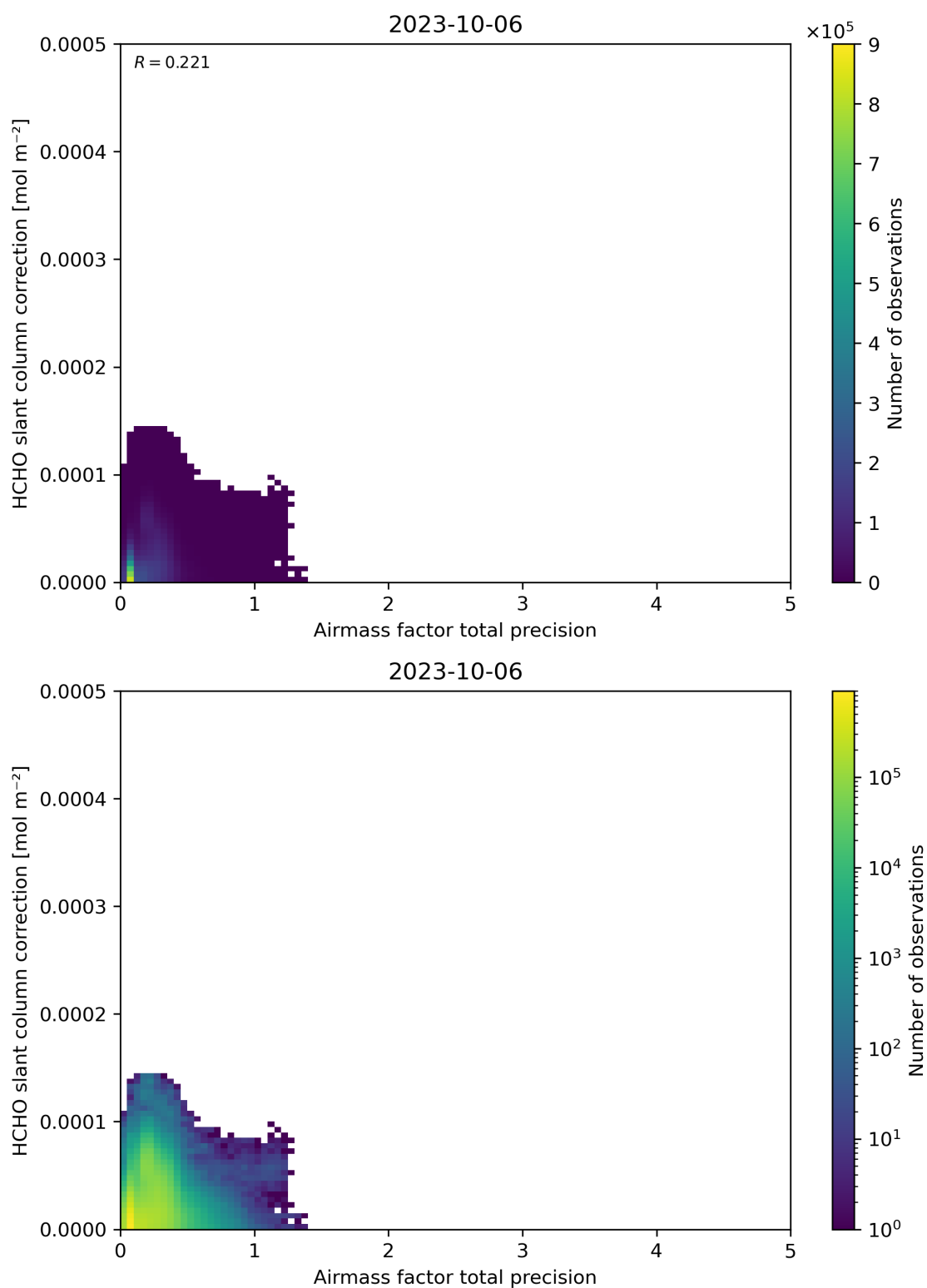
Figure 110: Scatter density plot of “Airmass factor total precision” against “HCHO slant column correction” for 2023-10-06 to 2023-10-07.
