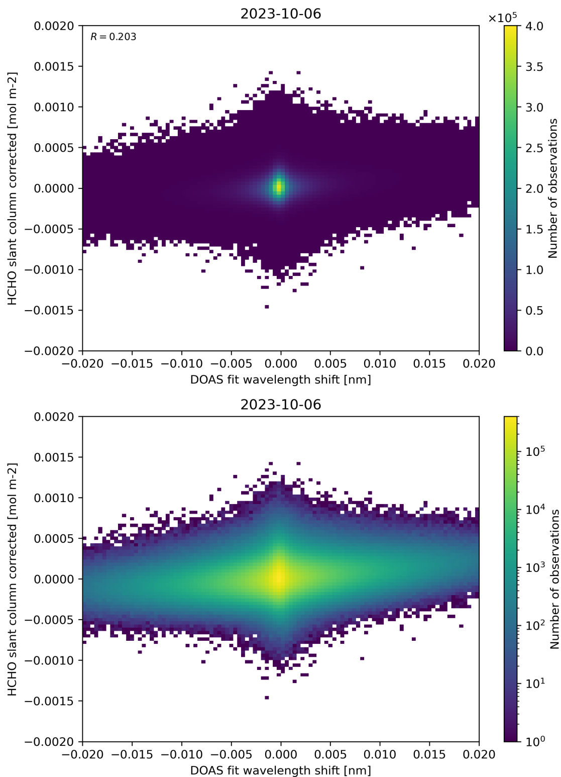
Figure 66: Scatter density plot of “DOAS fit wavelength shift” against “HCHO slant column corrected” for 2023-10-06 to 2023-10-07.
