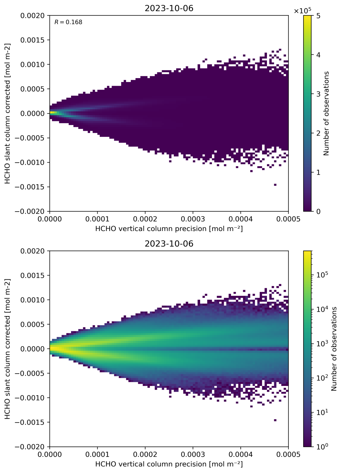
Figure 140: Scatter density plot of “HCHO vertical column precision” against “HCHO slant column corrected” for 2023-10-06 to 2023-10-07.
