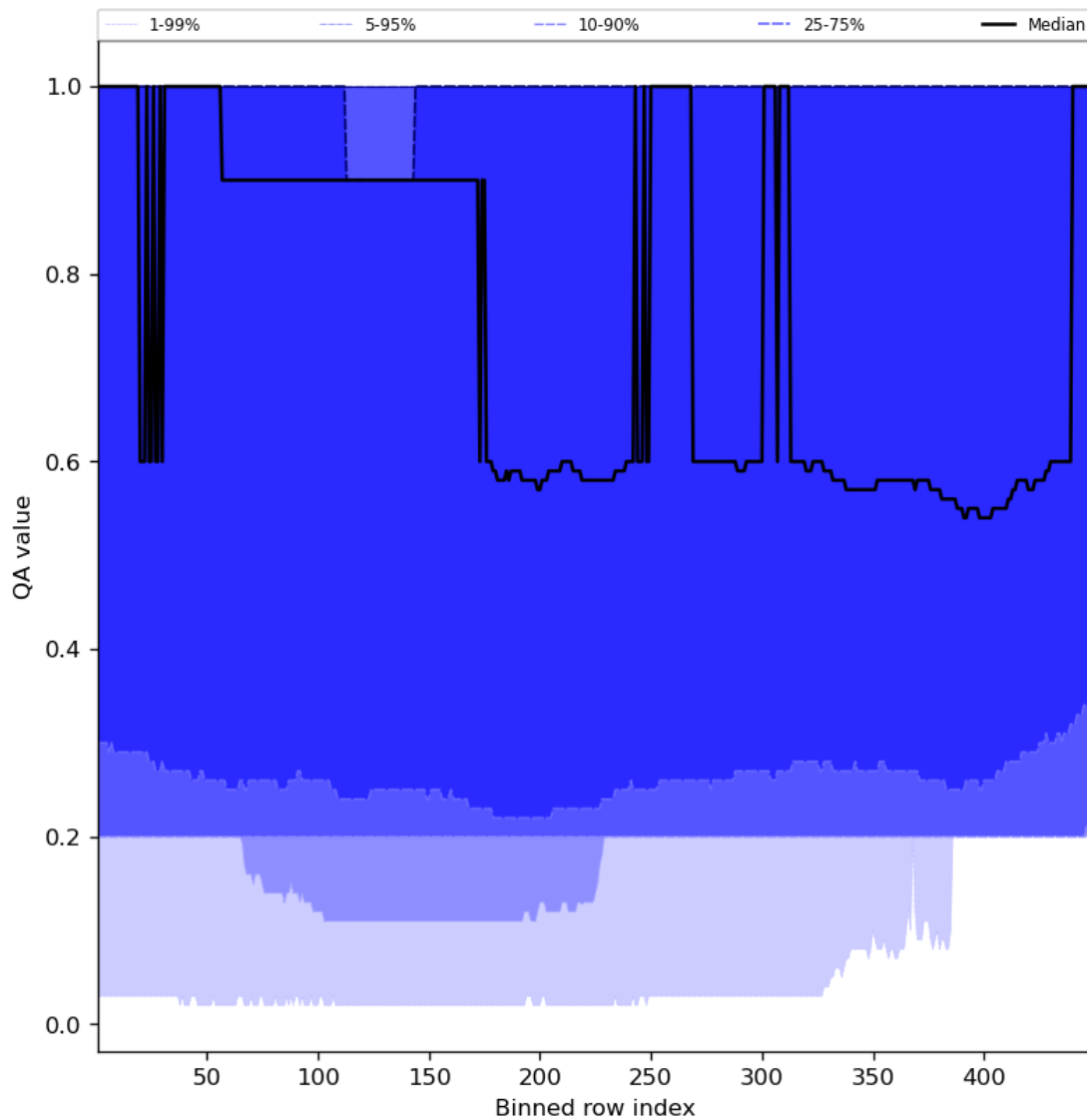
Figure 48: Along track statistics of “QA value” for 2023-10-06 to 2023-10-07
