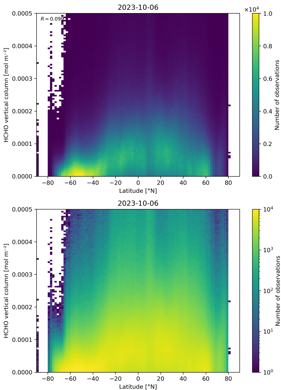
Figure 163: Scatter density plot of “Latitude” against “HCHO vertical column” for 2023-10-06 to 2023-10-07.
