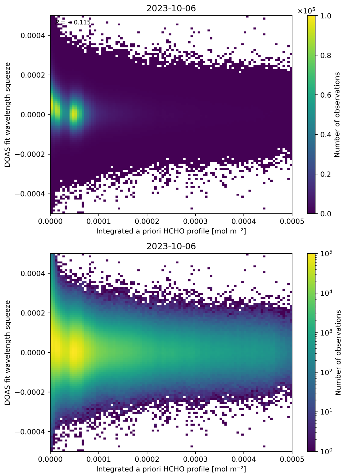
Figure 150: Scatter density plot of “Integrated a priori HCHO profile” against “DOAS fit wavelength squeeze” for 2023-10-06 to 2023-10-07.
