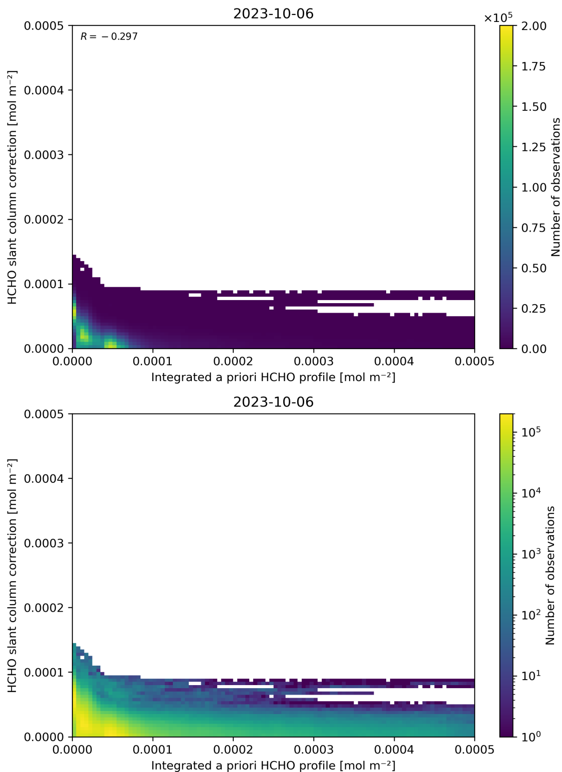
Figure 152: Scatter density plot of “Integrated a priori HCHO profile” against “HCHO slant column correction” for 2023-10-06 to 2023-10-07.
