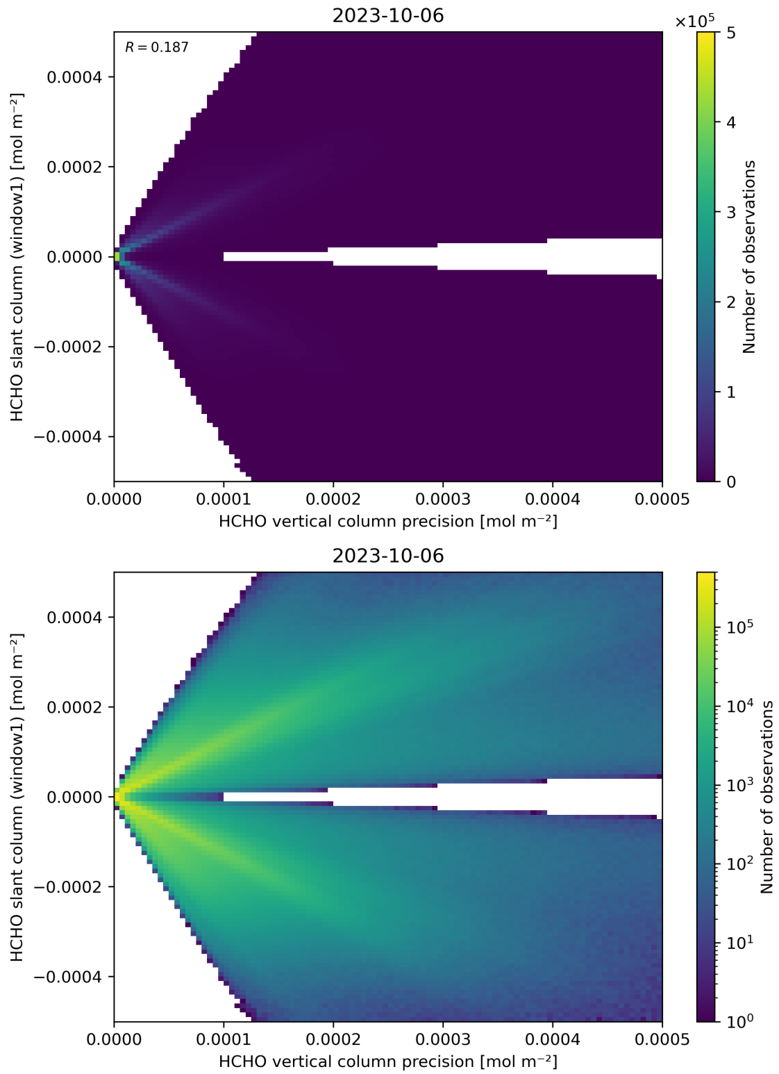
Figure 142: Scatter density plot of “HCHO vertical column precision” against “HCHO slant column (window1)” for 2023-10-06 to 2023-10-07.
