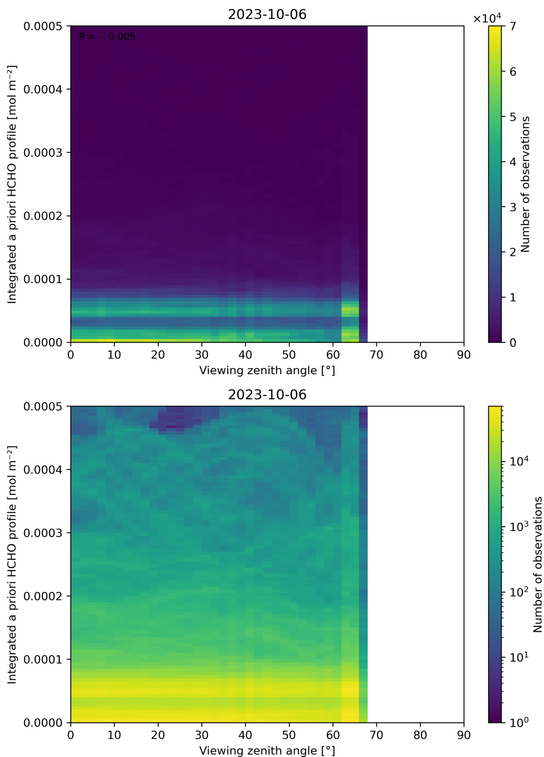
Figure 195: Scatter density plot of “Viewing zenith angle” against “Integrated a priori HCHO profile” for 2023-10-06 to 2023-10-07.
