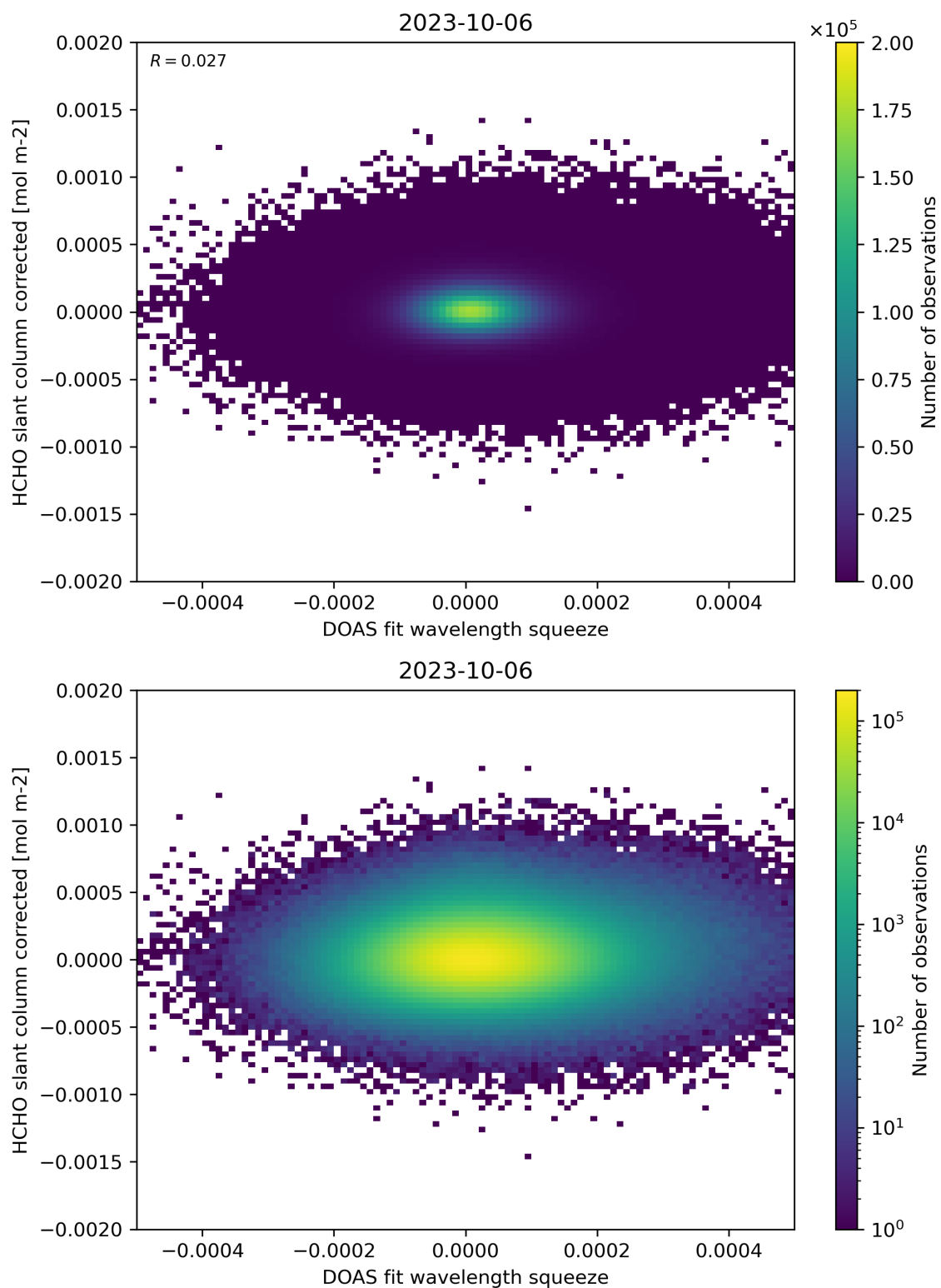
Figure 69: Scatter density plot of “DOAS fit wavelength squeeze” against “HCHO slant column corrected” for 2023-10-06 to 2023-10-07.
