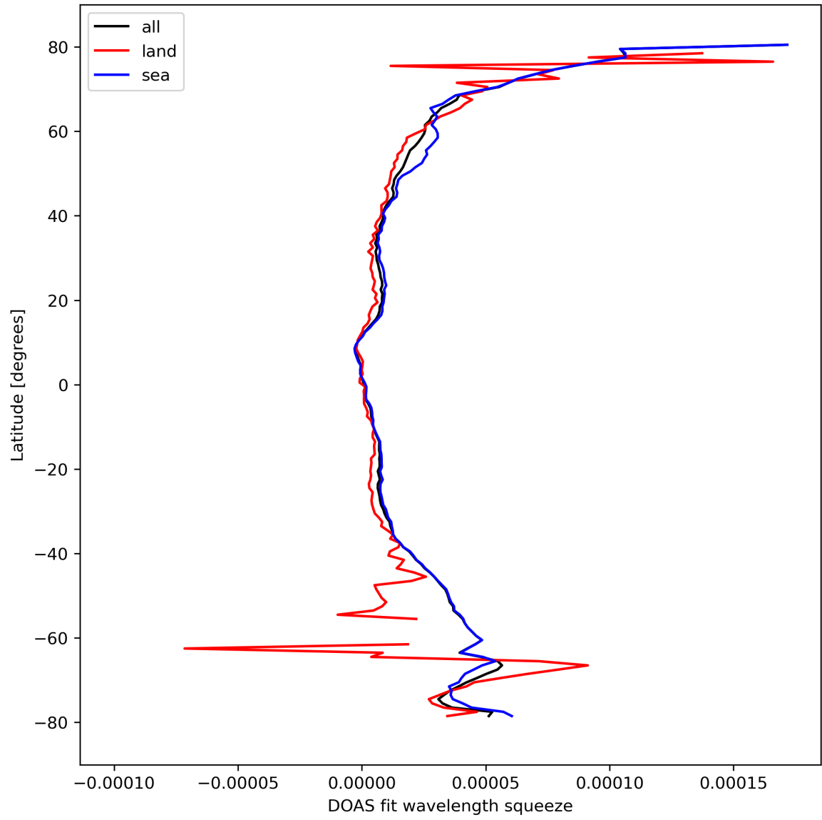
Figure 31: Zonal average of “DOAS fit wavelength squeeze” for 2023-10-06 to 2023-10-07.
