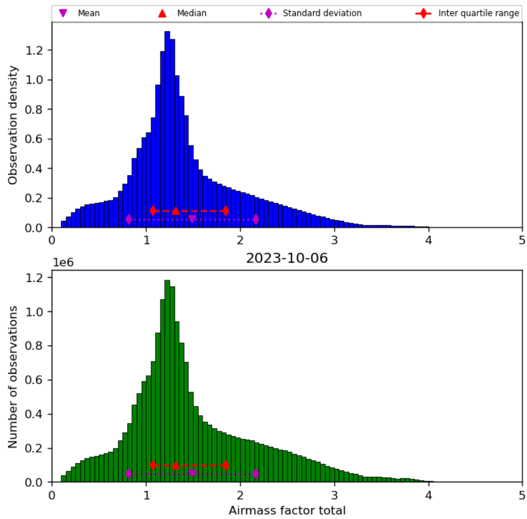
Figure 40: Histogram of “Airmass factor total” for 2023-10-06 to 2023-10-07
