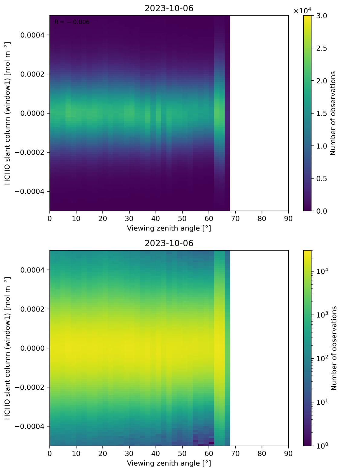
Figure 188: Scatter density plot of “Viewing zenith angle” against “HCHO slant column (window1)” for 2023-10-06 to 2023-10-07.
