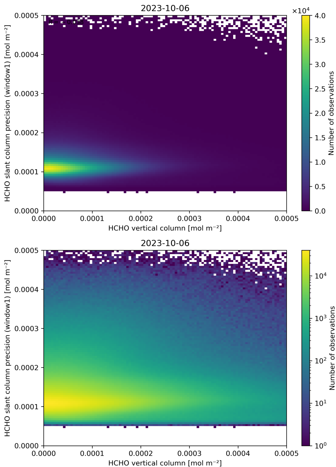
Figure 130: Scatter density plot of “HCHO vertical column” against “HCHO slant column precision (window1)” for 2023-10-06 to 2023-10-07.
