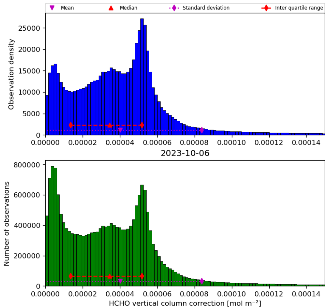
Figure 37: Histogram of “HCHO vertical column correction” for 2023-10-06 to 2023-10-07
