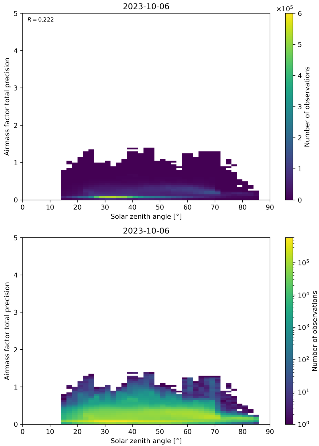
Figure 176: Scatter density plot of “Solar zenith angle” against “Airmass factor total precision” for 2023-10-06 to 2023-10-07.
