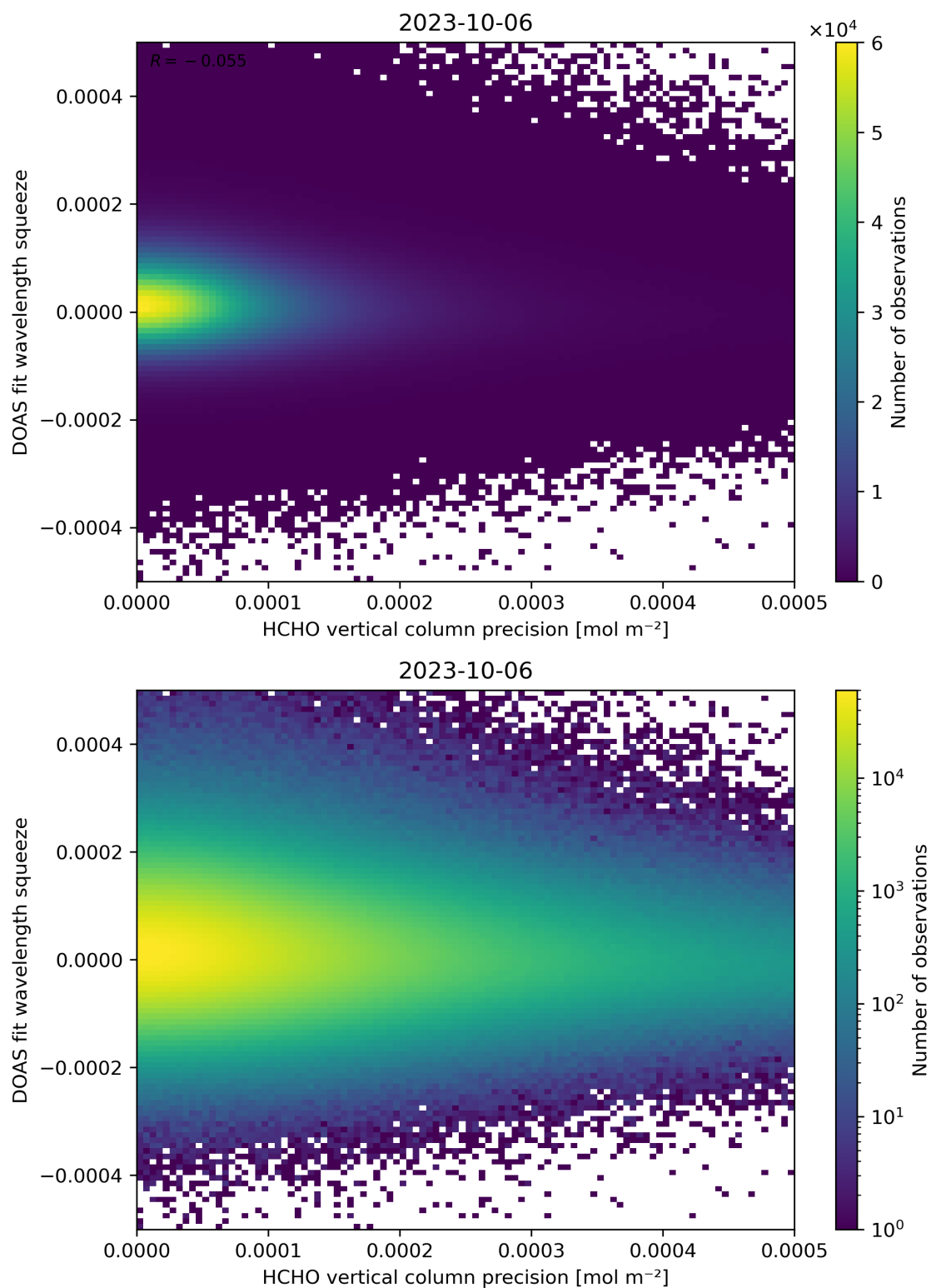
Figure 138: Scatter density plot of “HCHO vertical column precision” against “DOAS fit wavelength squeeze” for 2023-10-06 to 2023-10-07.
