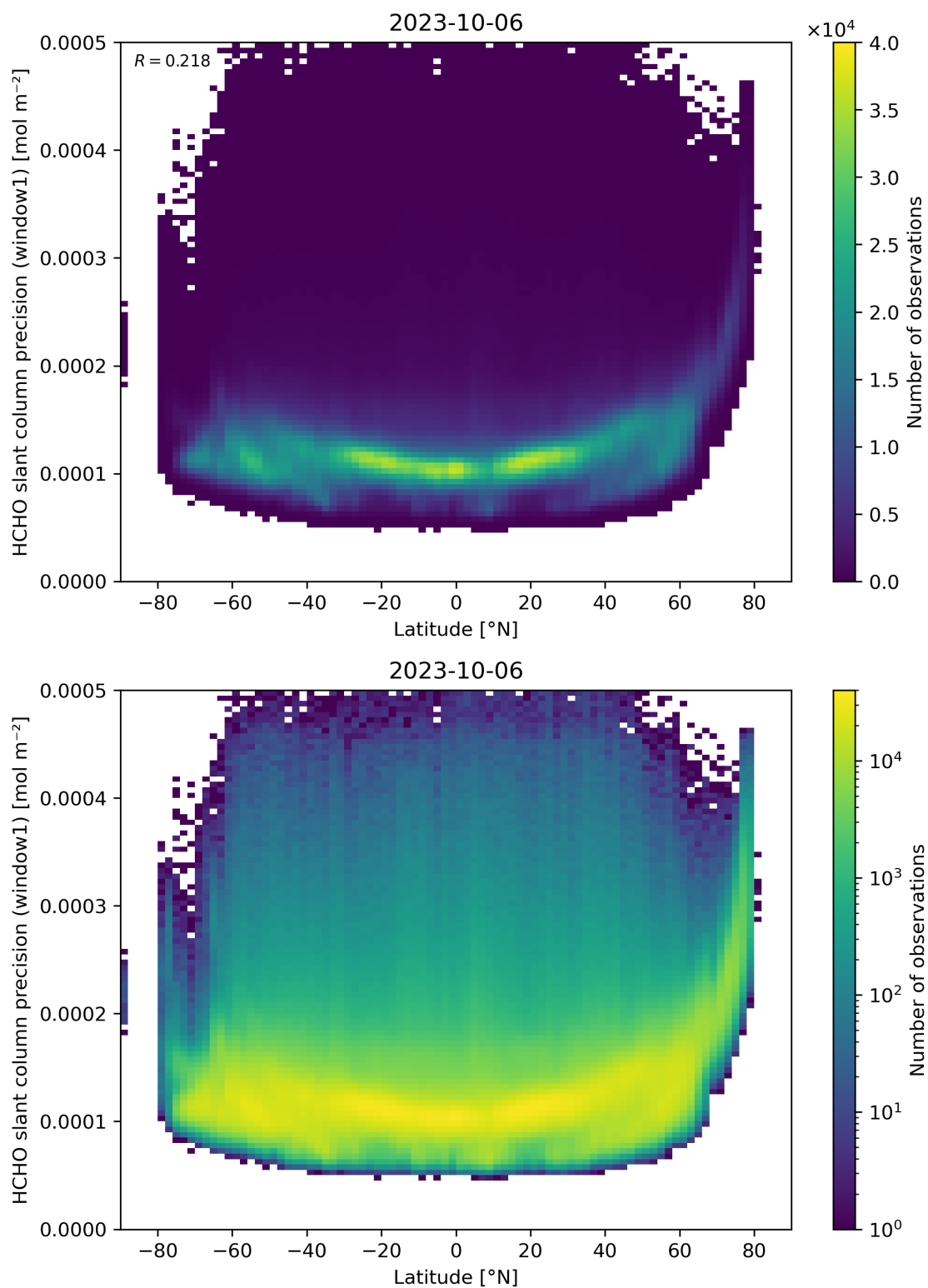
Figure 160: Scatter density plot of “Latitude” against “HCHO slant column precision (window1)” for 2023-10-06 to 2023-10-07.
