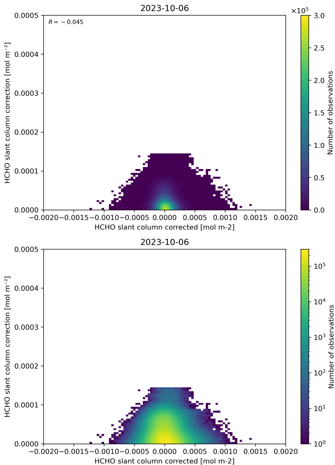
Figure 77: Scatter density plot of “HCHO slant column corrected” against “HCHO slant column correction” for 2023-10-06 to 2023-10-07.
