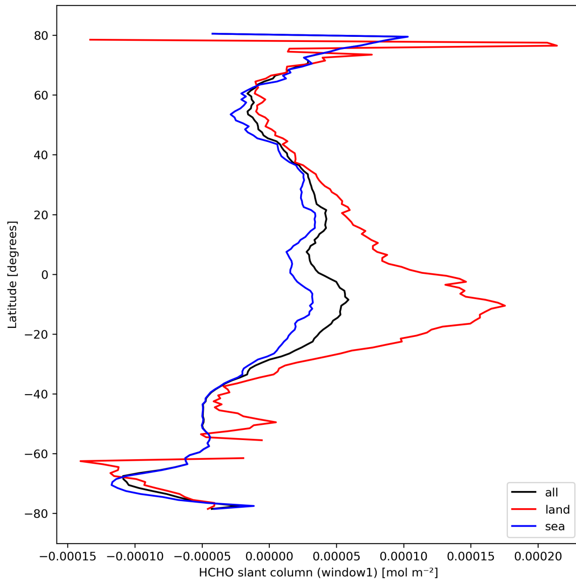
Figure 24: Zonal average of “HCHO slant column (window1)” for 2023-10-06 to 2023-10-07.
