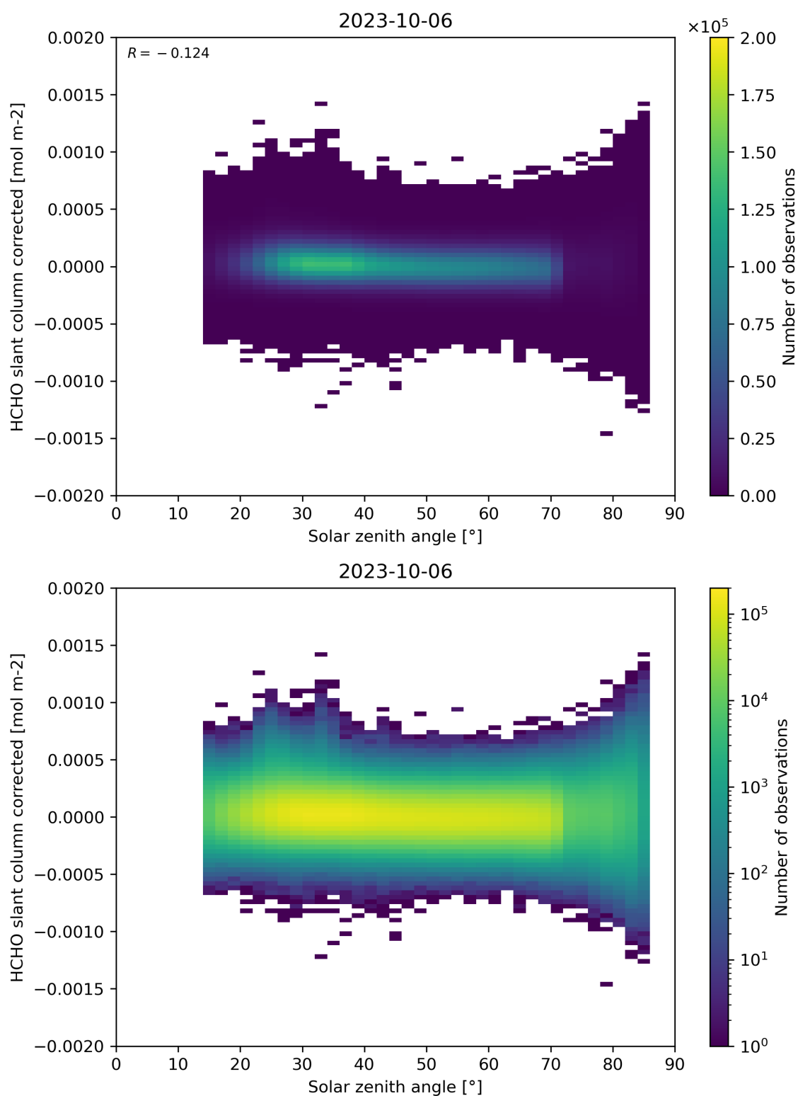
Figure 171: Scatter density plot of “Solar zenith angle” against “HCHO slant column corrected” for 2023-10-06 to 2023-10-07.
