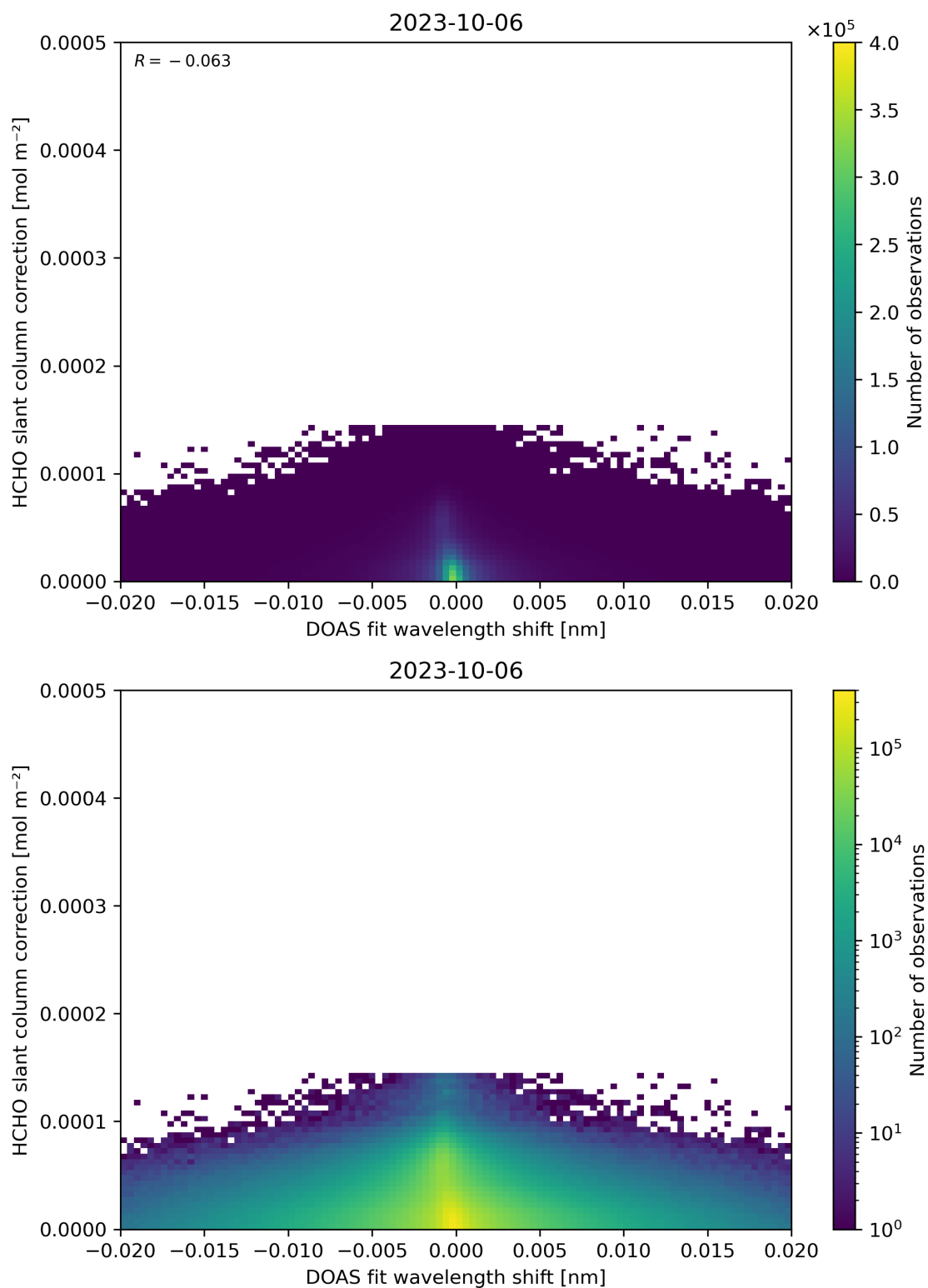
Figure 67: Scatter density plot of “DOAS fit wavelength shift” against “HCHO slant column correction” for 2023-10-06 to 2023-10-07.
