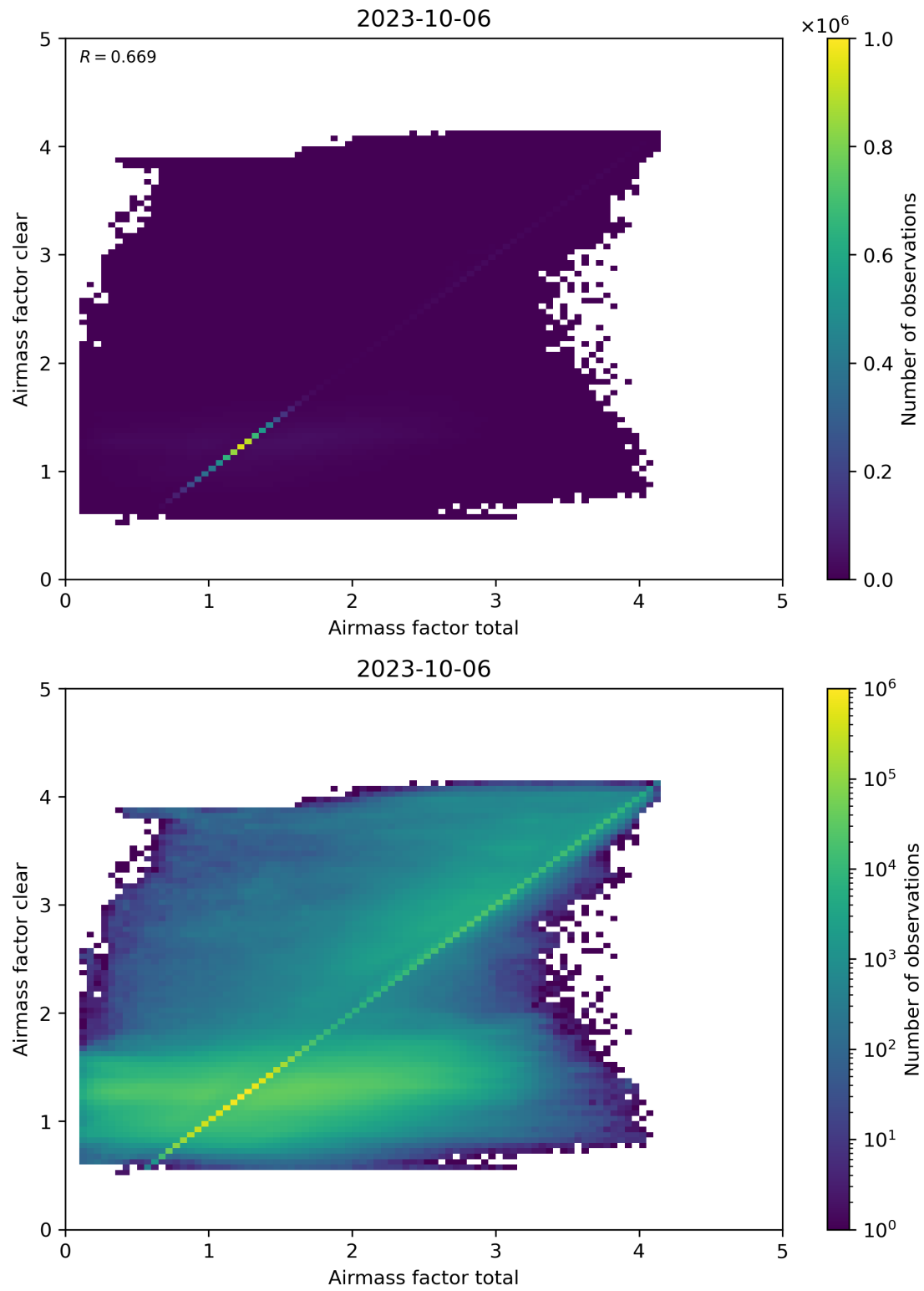
Figure 100: Scatter density plot of “Airmass factor total” against “Airmass factor clear” for 2023-10-06 to 2023-10-07.
