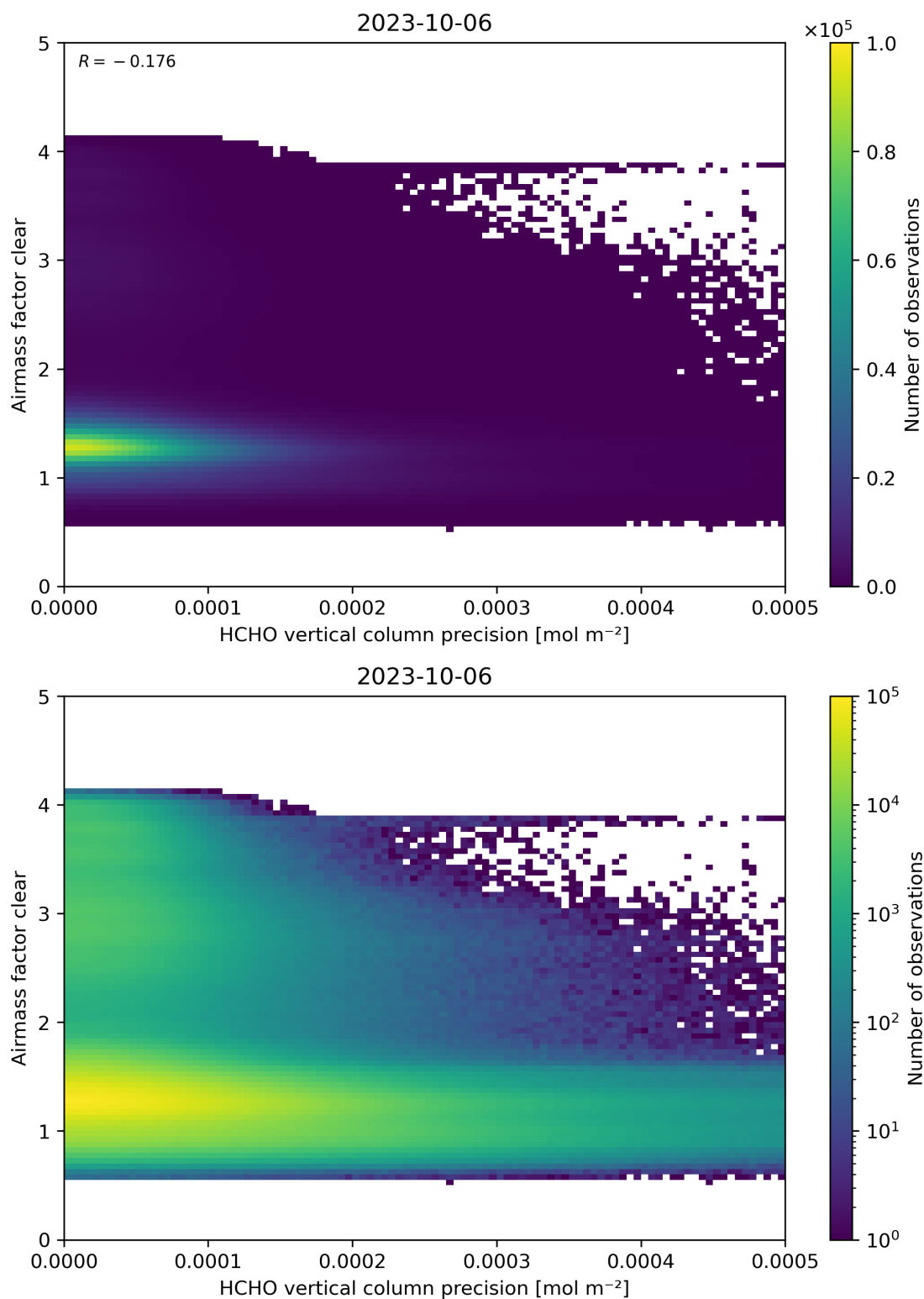
Figure 139: Scatter density plot of “HCHO vertical column precision” against “Airmass factor clear” for 2023-10-06 to 2023-10-07.
