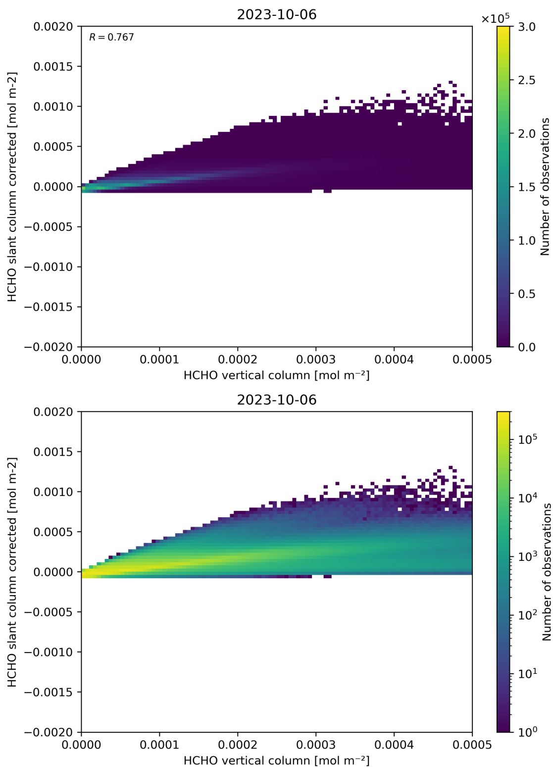
Figure 127: Scatter density plot of “HCHO vertical column” against “HCHO slant column corrected” for 2023-10-06 to 2023-10-07.
