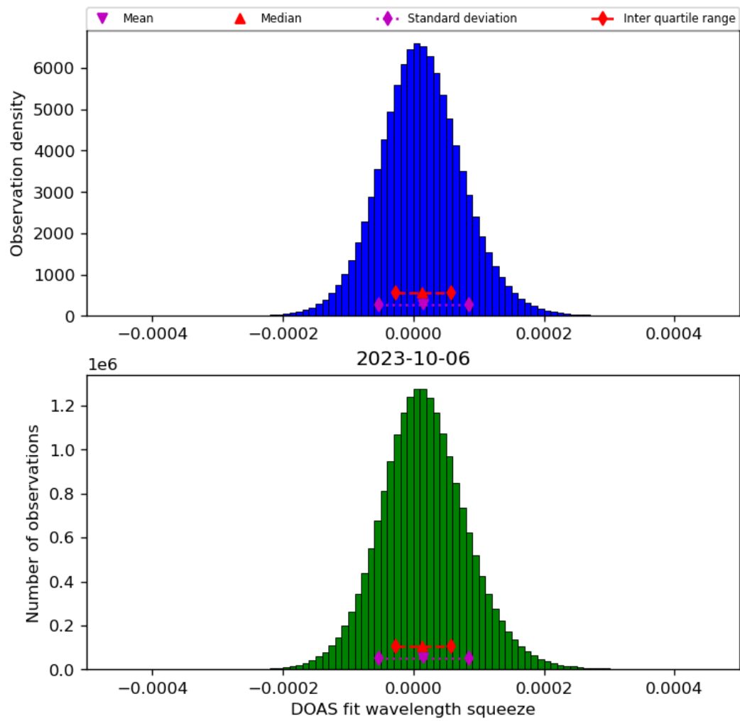
Figure 45: Histogram of “DOAS fit wavelength squeeze” for 2023-10-06 to 2023-10-07
