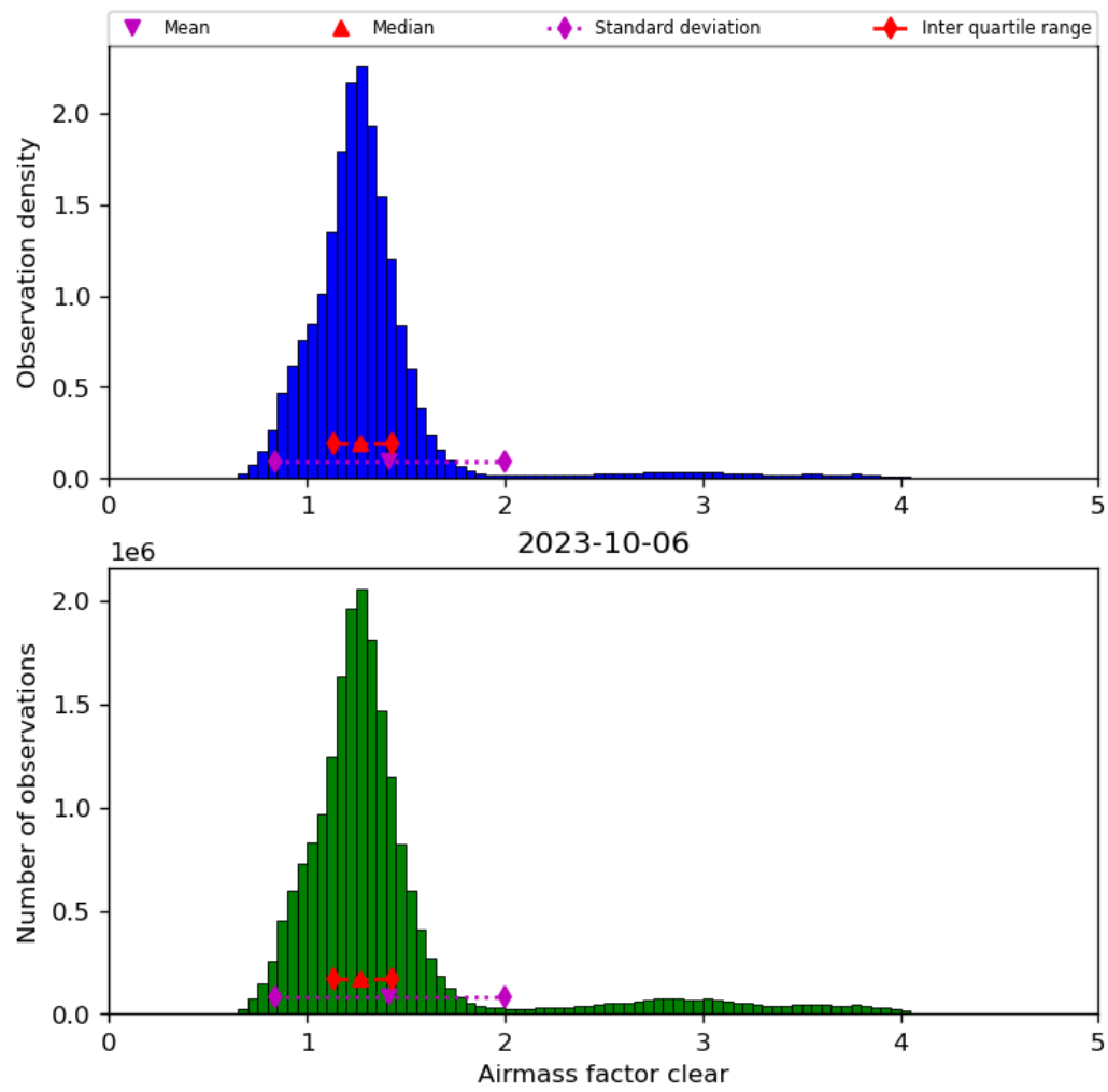
Figure 42: Histogram of “Airmass factor clear” for 2023-10-06 to 2023-10-07
