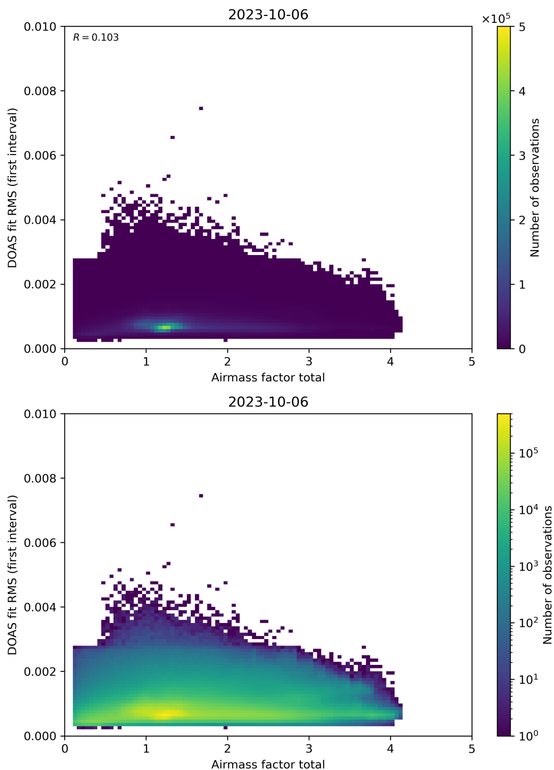
Figure 97: Scatter density plot of “Airmass factor total” against “DOAS fit RMS (first interval)” for 2023-10-06 to 2023-10-07.
