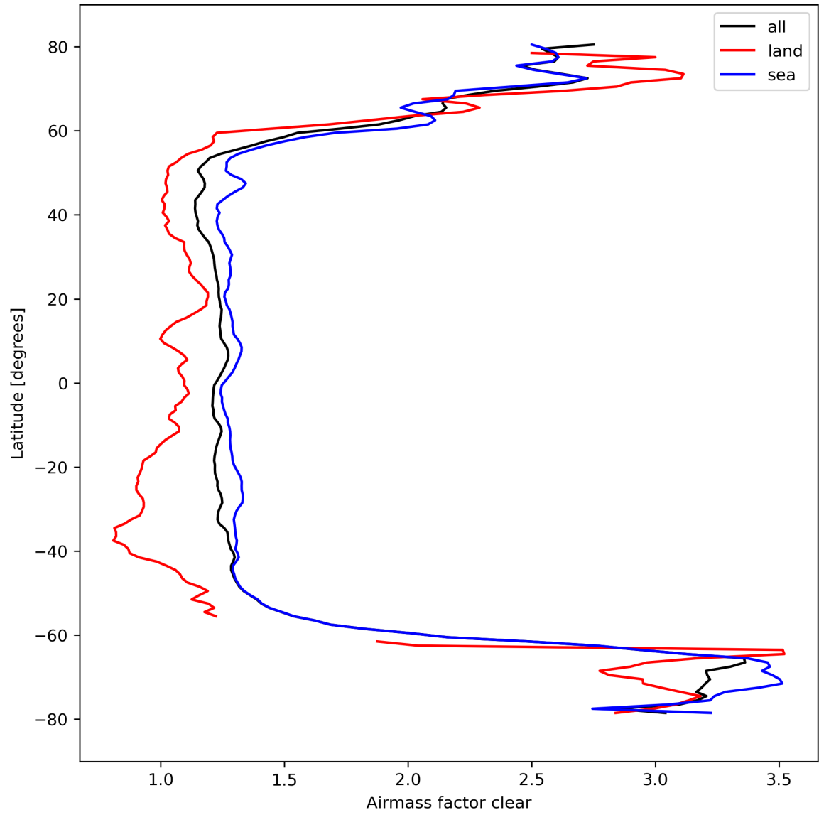
Figure 28: Zonal average of “Airmass factor clear” for 2023-10-06 to 2023-10-07.
