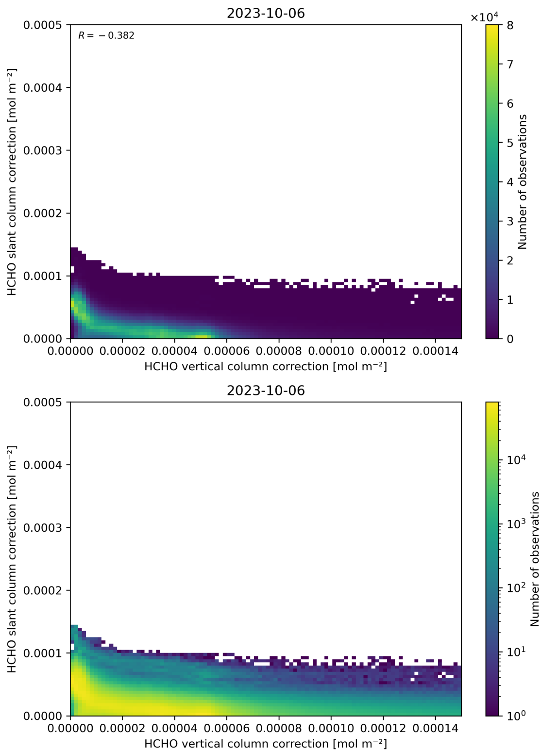
Figure 117: Scatter density plot of “HCHO vertical column correction” against “HCHO slant column correction” for 2023-10-06 to 2023-10-07.
