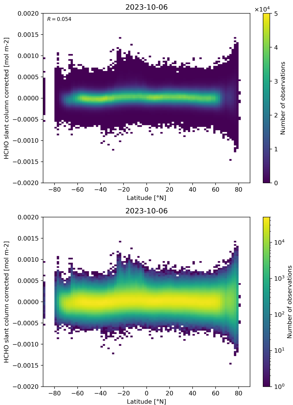
Figure 157: Scatter density plot of “Latitude” against “HCHO slant column corrected” for 2023-10-06 to 2023-10-07.
