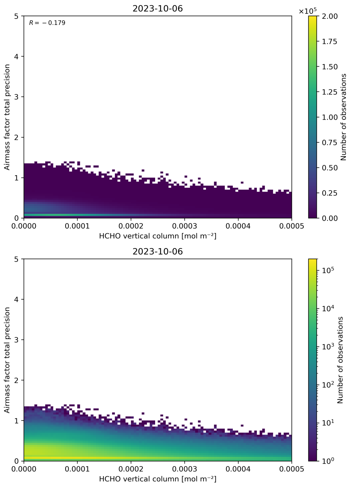
Figure 132: Scatter density plot of “HCHO vertical column” against “Airmass factor total precision” for 2023-10-06 to 2023-10-07.
