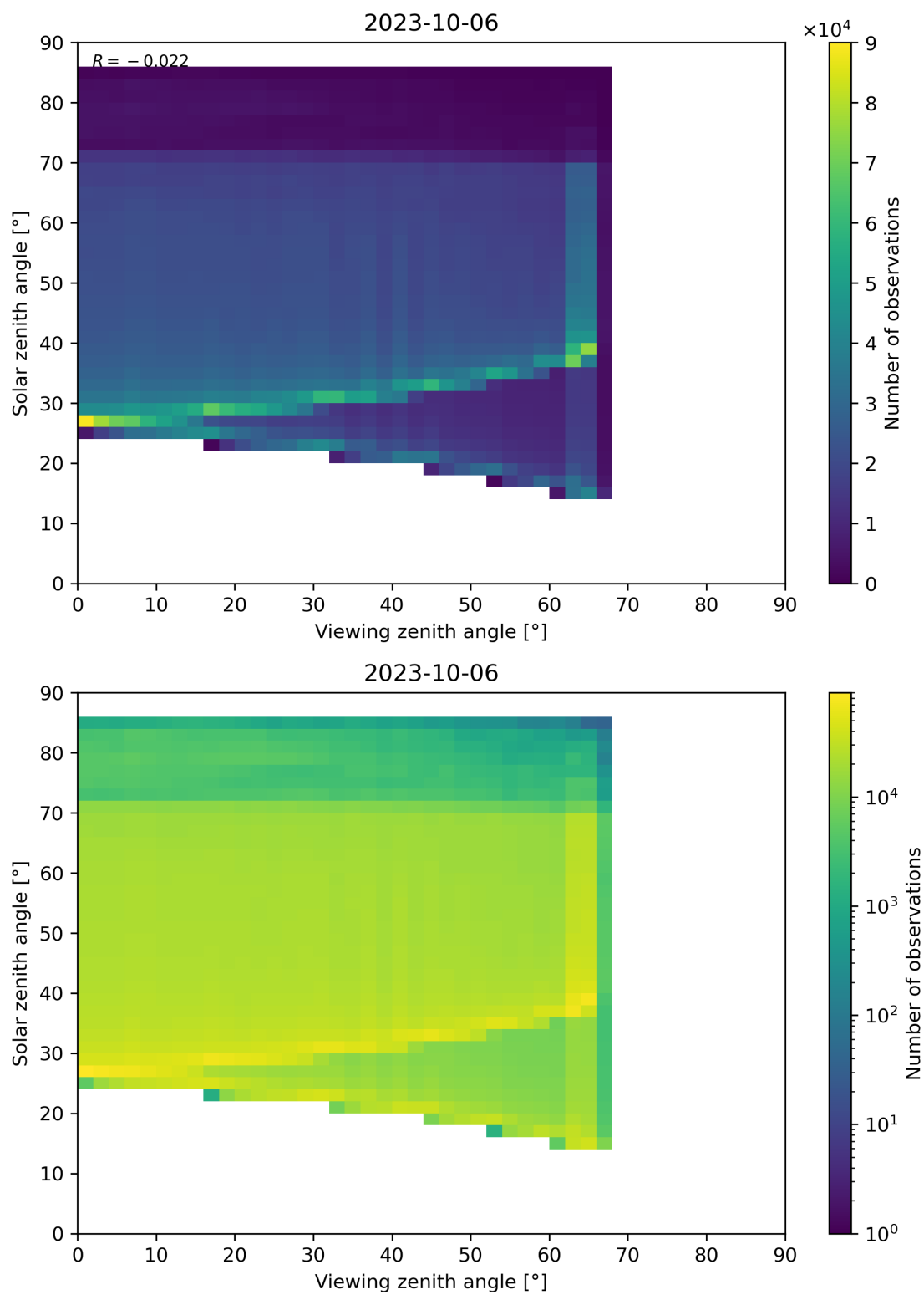
Figure 197: Scatter density plot of “Viewing zenith angle” against “Solar zenith angle” for 2023-10-06 to 2023-10-07.
