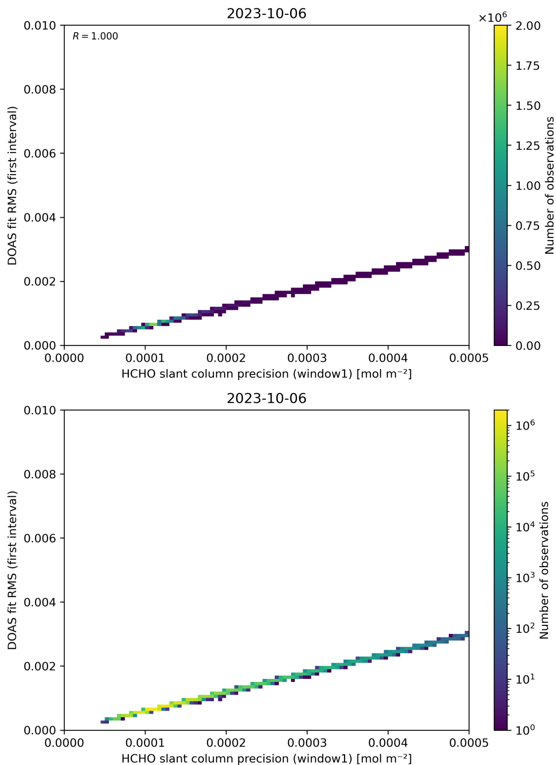
Figure 88: Scatter density plot of “HCHO slant column precision (window1)” against “DOAS fit RMS (first interval)” for 2023-10-06 to 2023-10-07.
