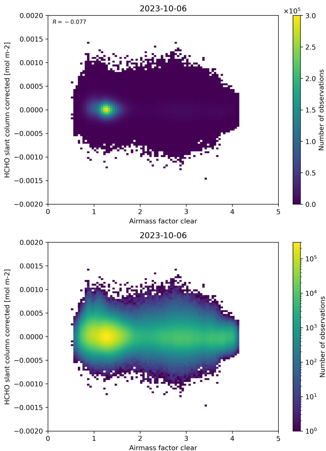
Figure 74: Scatter density plot of “Airmass factor clear” against “HCHO slant column corrected” for 2023-10-06 to 2023-10-07.
