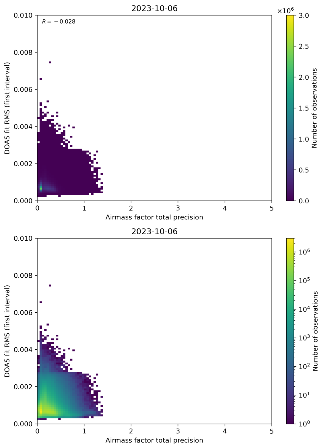
Figure 105: Scatter density plot of “Airmass factor total precision” against “DOAS fit RMS (first interval)” for 2023-10-06 to 2023-10-07.
