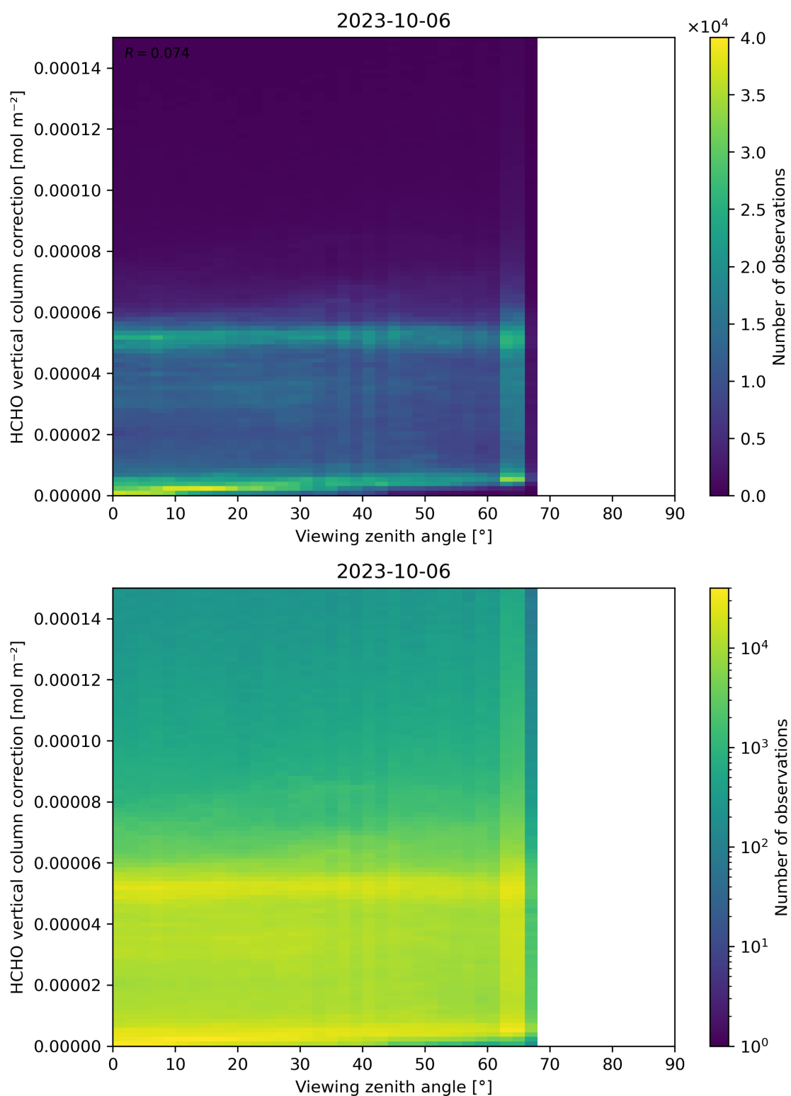
Figure 193: Scatter density plot of “Viewing zenith angle” against “HCHO vertical column correction” for 2023-10-06 to 2023-10-07.
