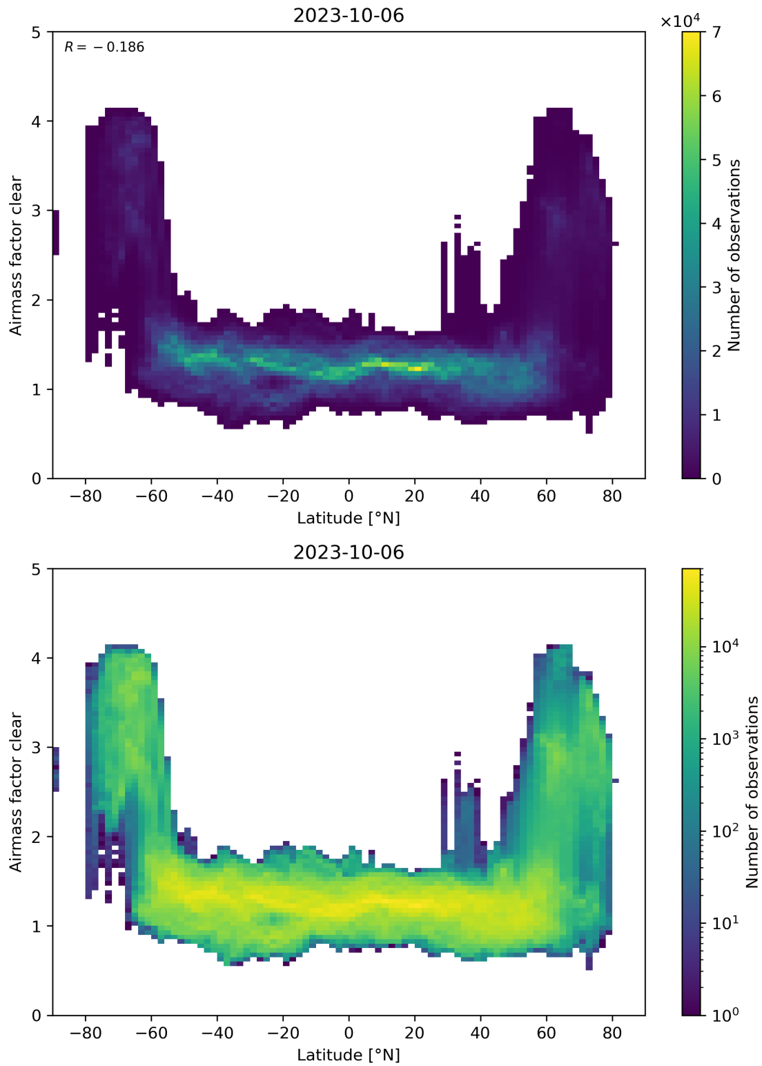
Figure 156: Scatter density plot of “Latitude” against “Airmass factor clear” for 2023-10-06 to 2023-10-07.
