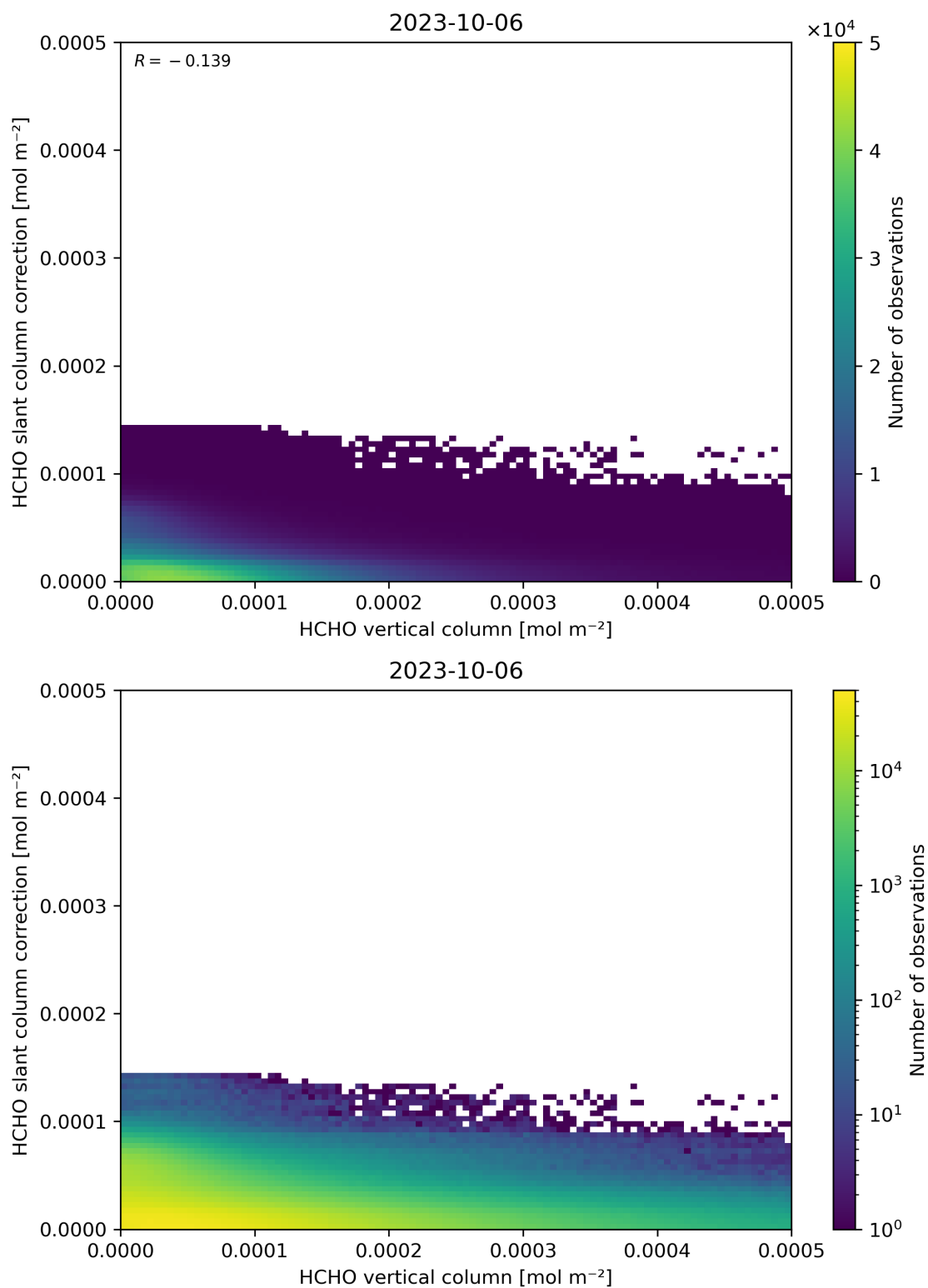
Figure 128: Scatter density plot of “HCHO vertical column” against “HCHO slant column correction” for 2023-10-06 to 2023-10-07.
