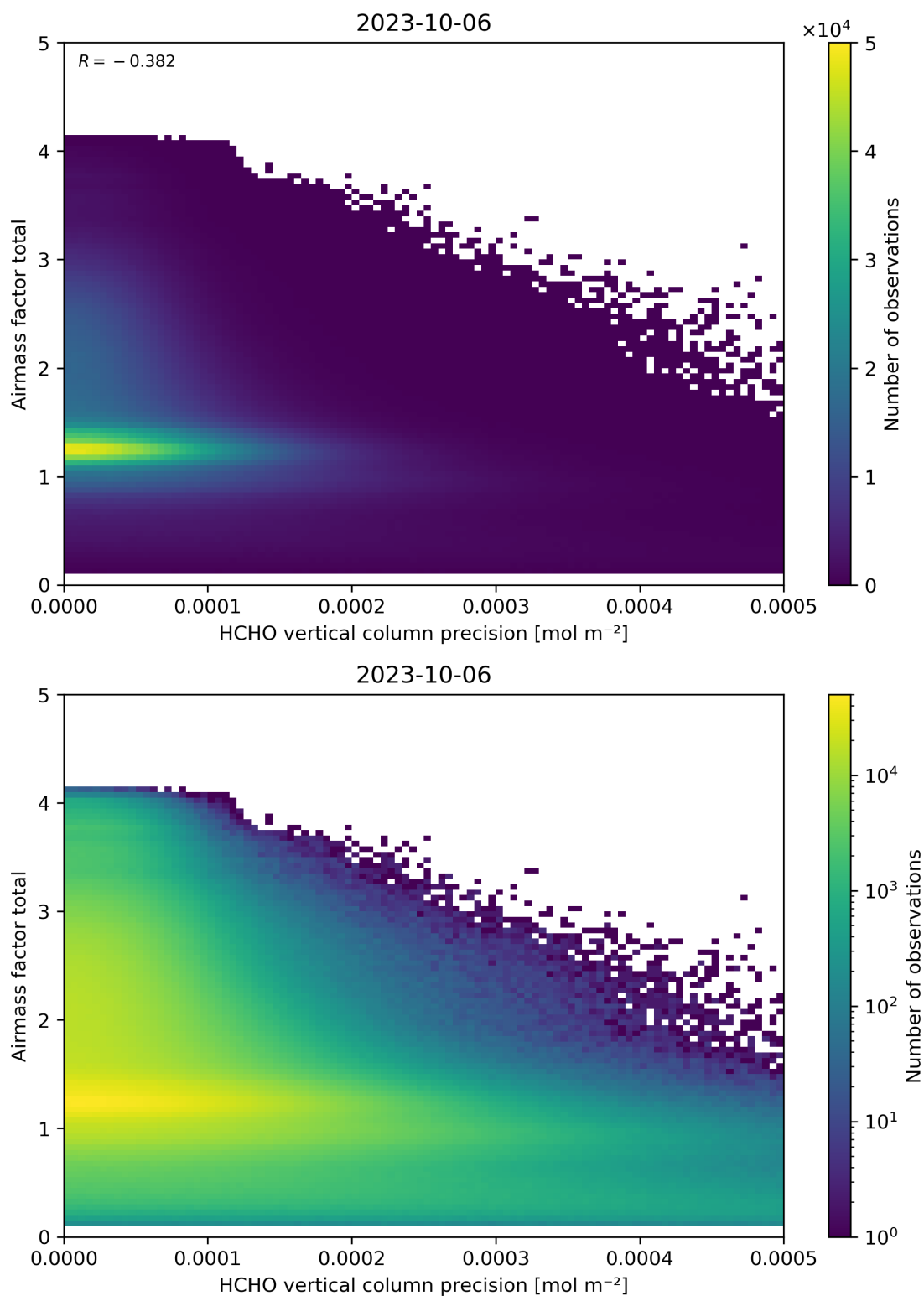
Figure 144: Scatter density plot of “HCHO vertical column precision” against “Airmass factor total” for 2023-10-06 to 2023-10-07.
