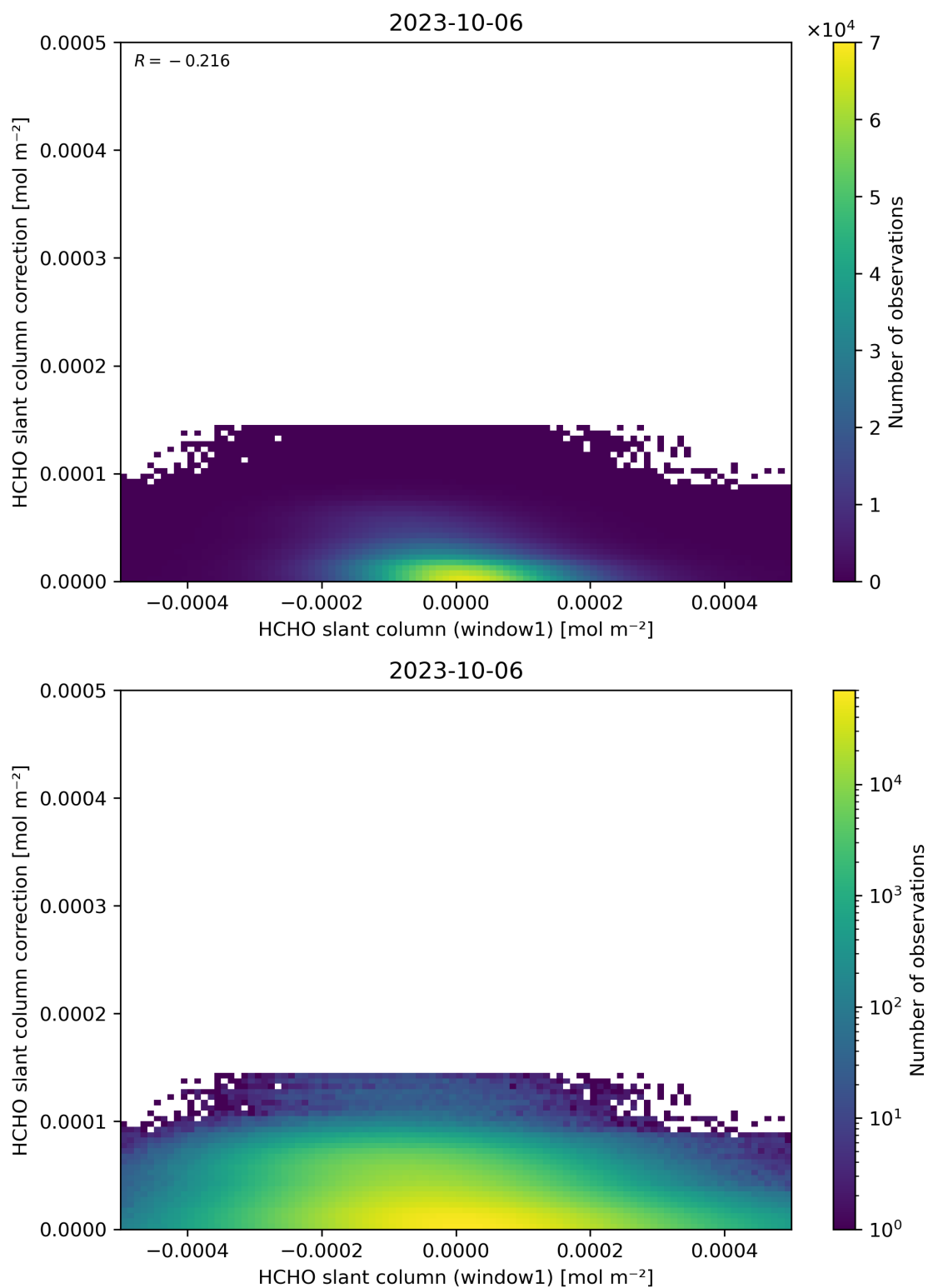
Figure 83: Scatter density plot of “HCHO slant column (window1)” against “HCHO slant column correction” for 2023-10-06 to 2023-10-07.
