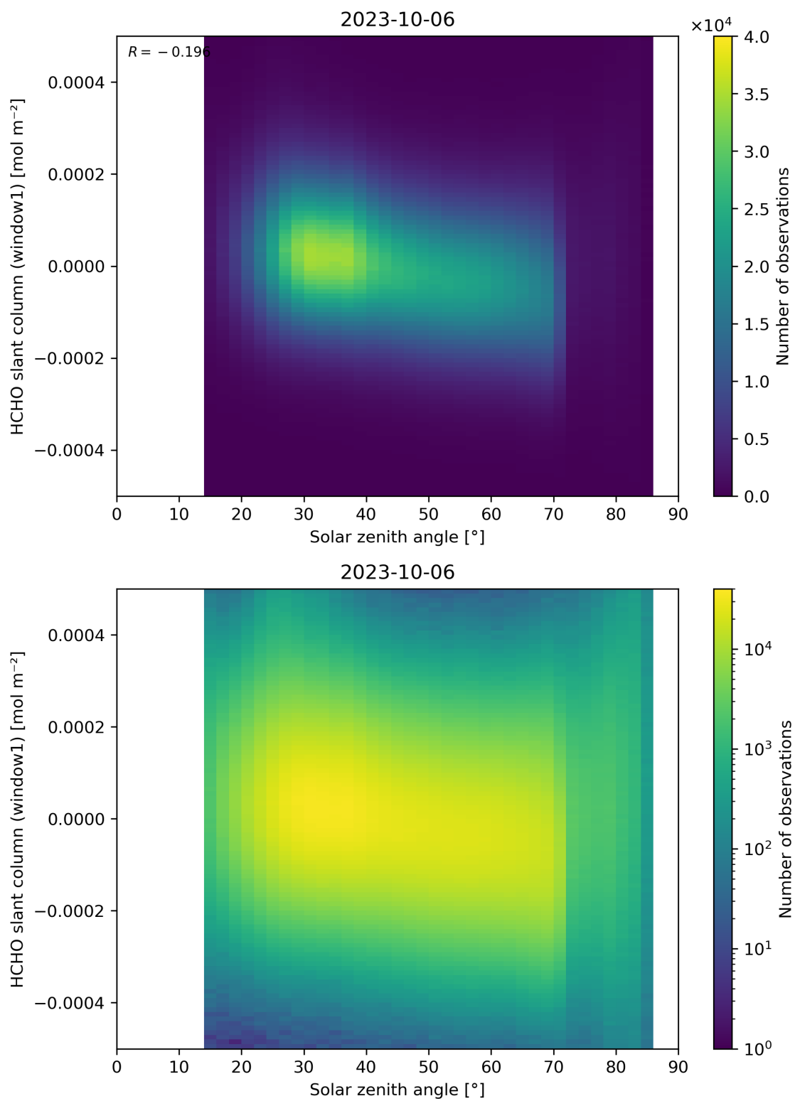
Figure 173: Scatter density plot of “Solar zenith angle” against “HCHO slant column (window1)” for 2023-10-06 to 2023-10-07.
