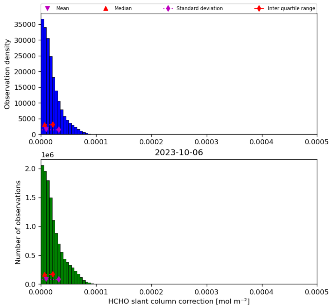
Figure 47: Histogram of “HCHO slant column correction” for 2023-10-06 to 2023-10-07
