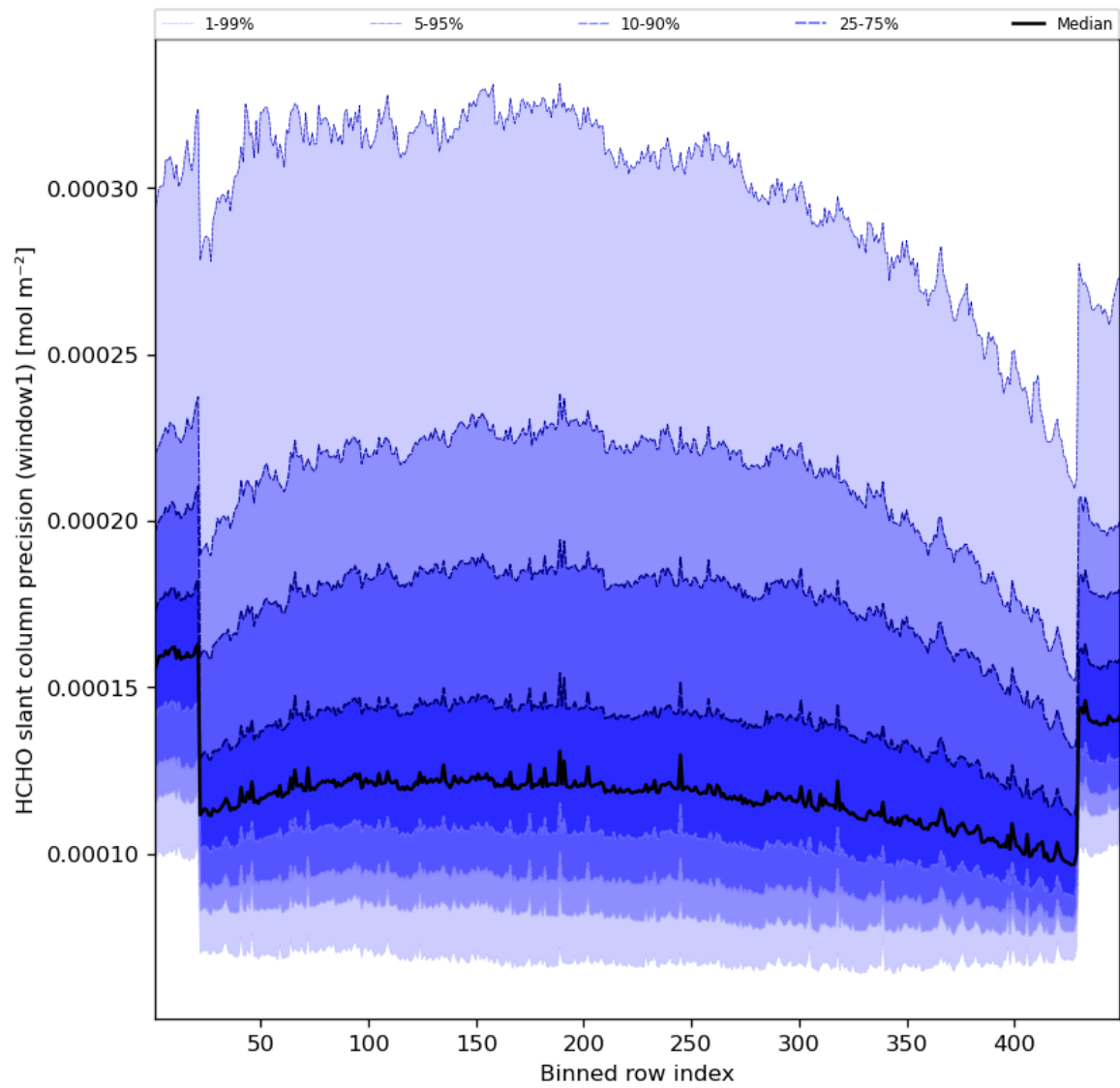
Figure 53: Along track statistics of “HCHO slant column precision (window1)” for 2023-10-06 to 2023-10-07
