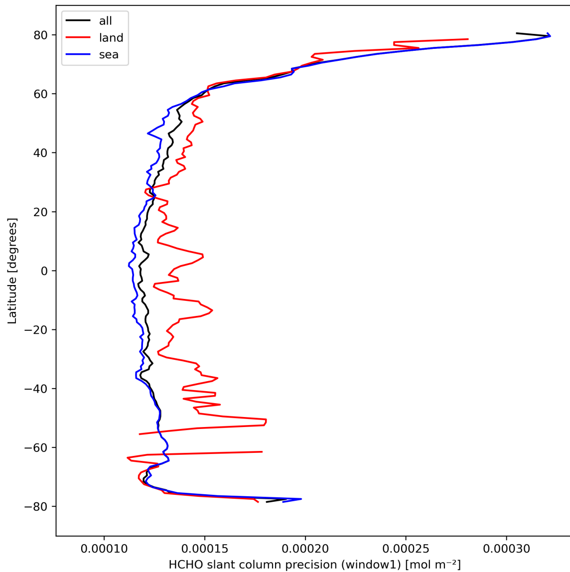
Figure 25: Zonal average of “HCHO slant column precision (window1)” for 2023-10-06 to 2023-10-07.
