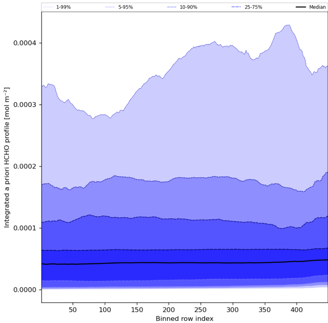
Figure 57: Along track statistics of “Integrated a priori HCHO profile” for 2023-10-06 to 2023-10-07
