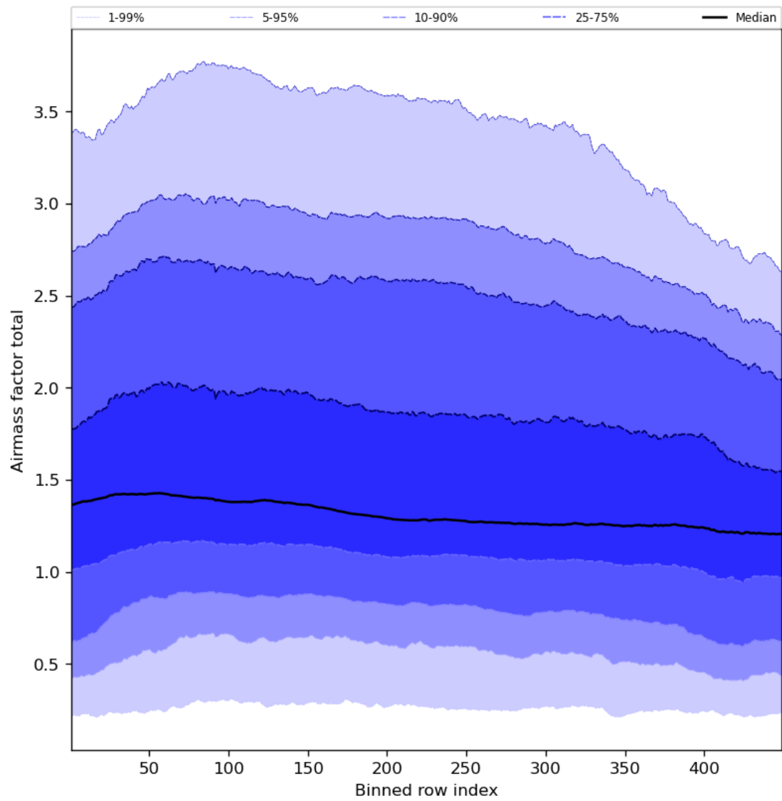
Figure 54: Along track statistics of “Airmass factor total” for 2023-10-06 to 2023-10-07
