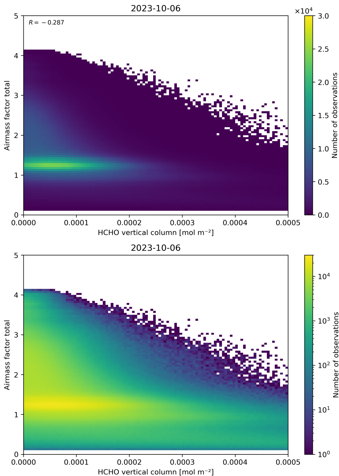
Figure 131: Scatter density plot of “HCHO vertical column” against “Airmass factor total” for 2023-10-06 to 2023-10-07.
