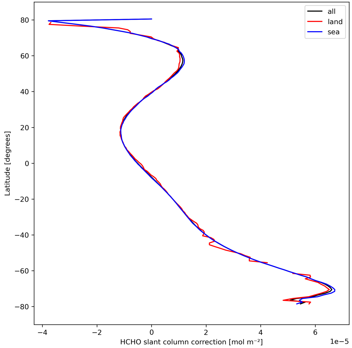
Figure 33: Zonal average of “HCHO slant column correction” for 2023-10-06 to 2023-10-07.
