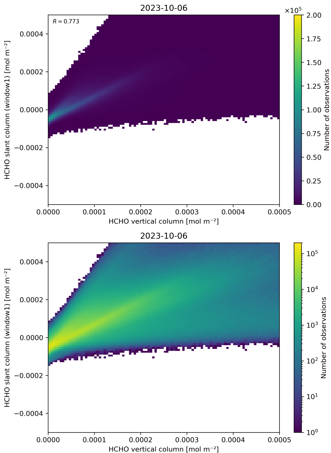
Figure 129: Scatter density plot of “HCHO vertical column” against “HCHO slant column (window1)” for 2023-10-06 to 2023-10-07.
