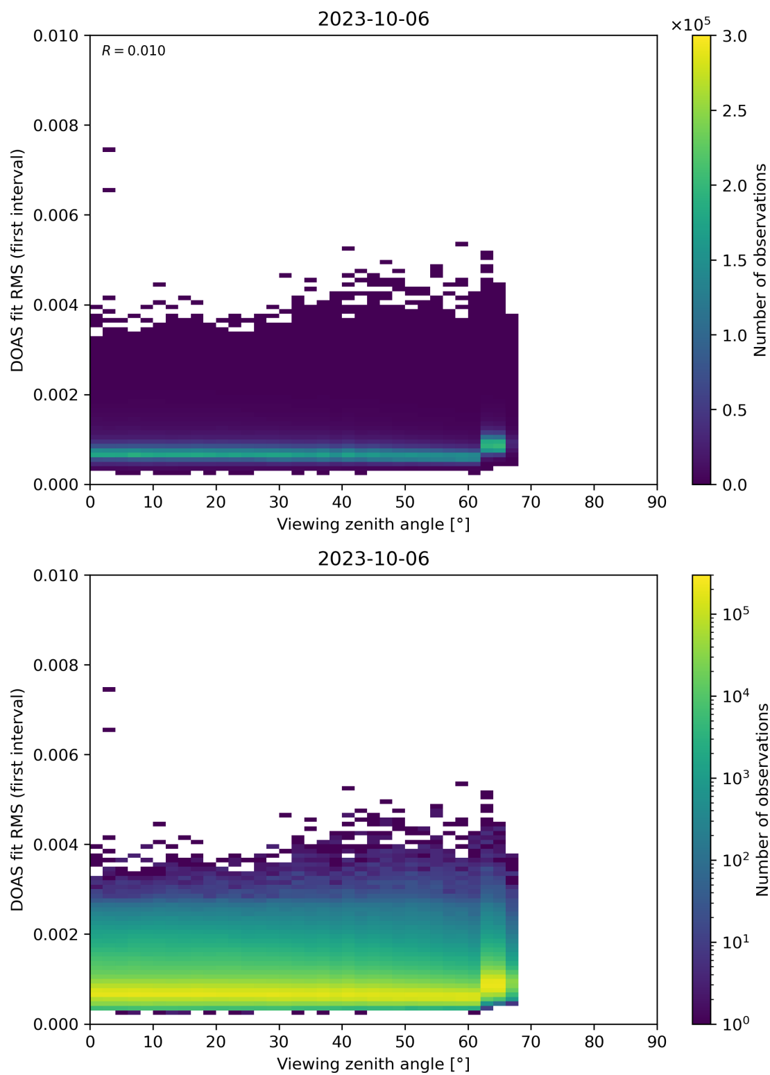
Figure 182: Scatter density plot of “Viewing zenith angle” against “DOAS fit RMS (first interval)” for 2023-10-06 to 2023-10-07.
