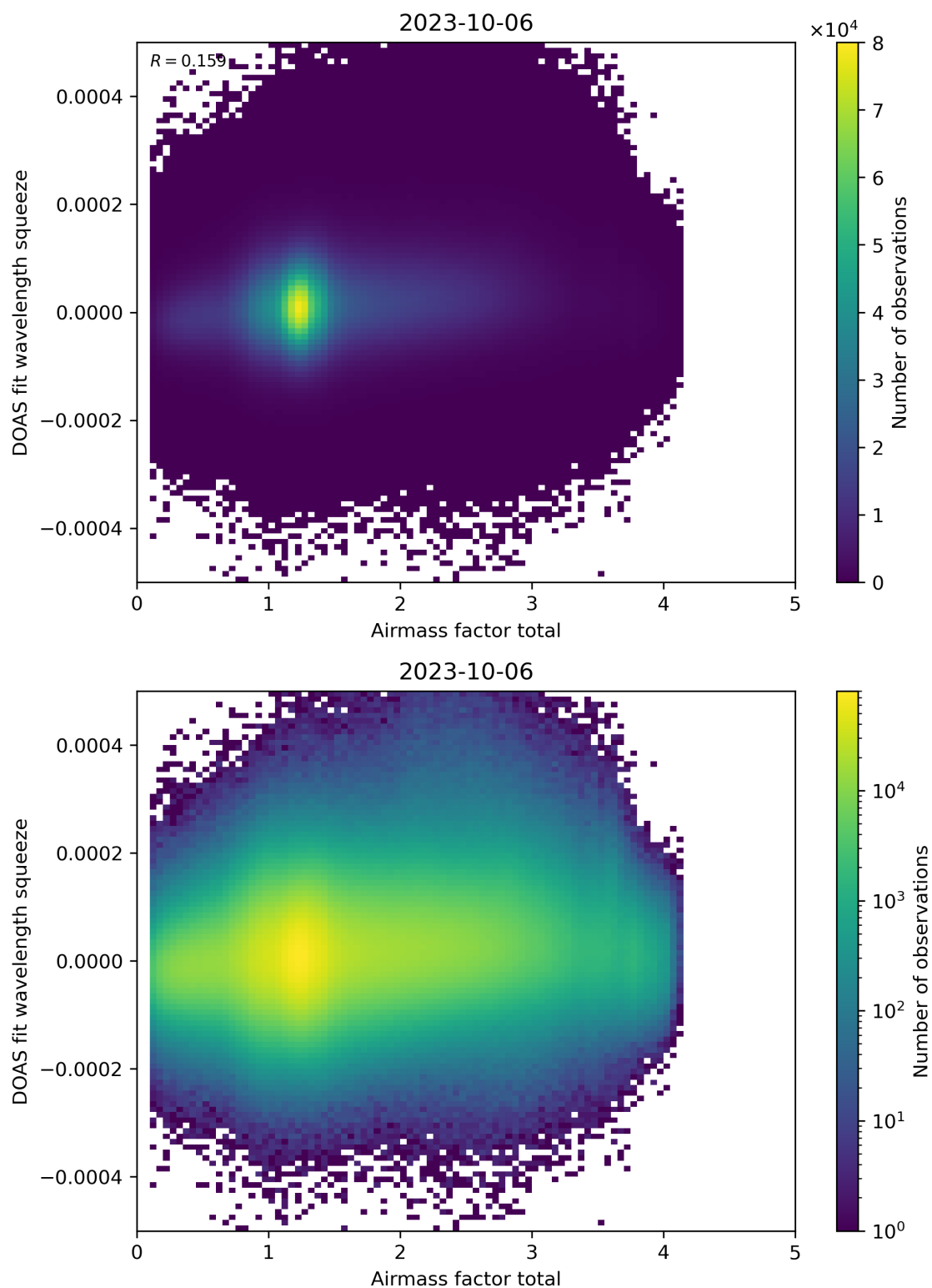
Figure 99: Scatter density plot of “Airmass factor total” against “DOAS fit wavelength squeeze” for 2023-10-06 to 2023-10-07.
