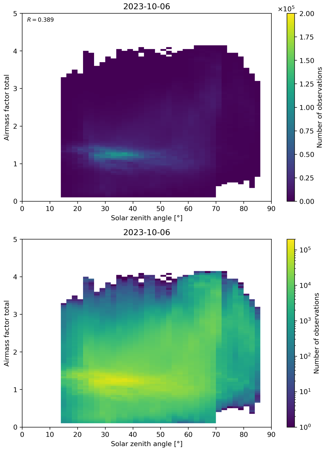
Figure 175: Scatter density plot of “Solar zenith angle” against “Airmass factor total” for 2023-10-06 to 2023-10-07.
