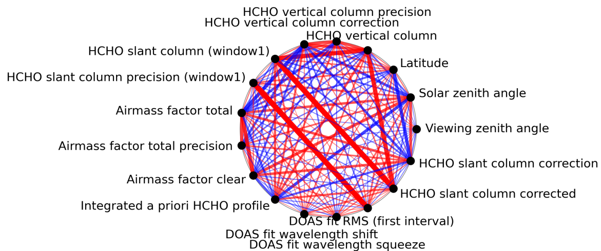
Figure 1: Map of correlation graph for 2023-10-06 to 2023-10-07.
