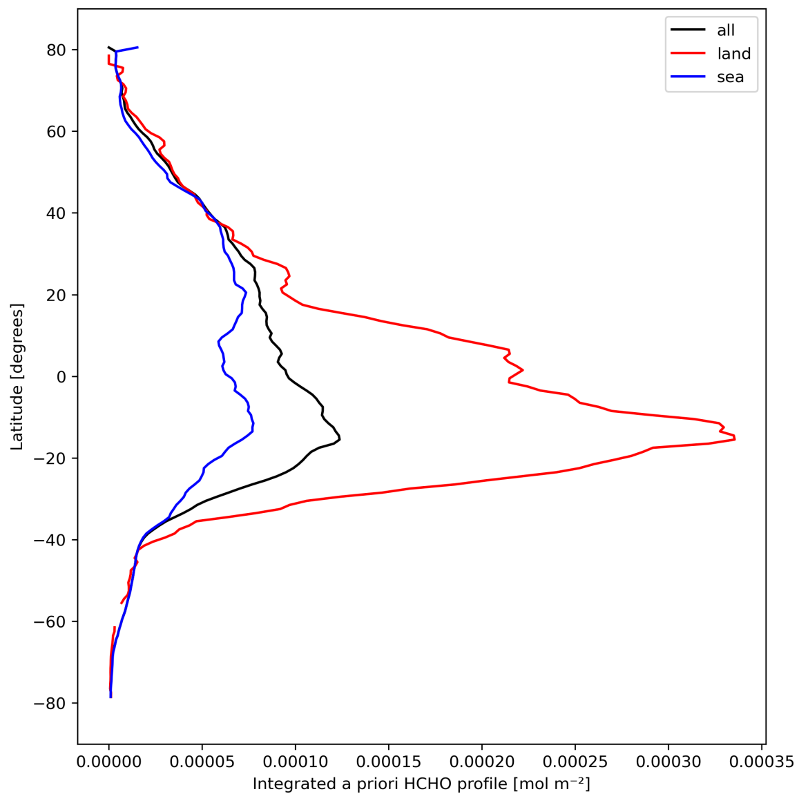
Figure 29: Zonal average of “Integrated a priori HCHO profile” for 2023-10-06 to 2023-10-07.
