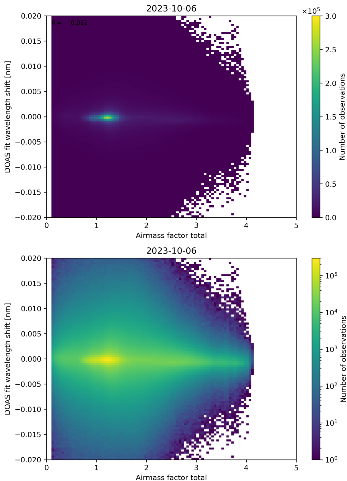
Figure 98: Scatter density plot of “Airmass factor total” against “DOAS fit wavelength shift” for 2023-10-06 to 2023-10-07.
