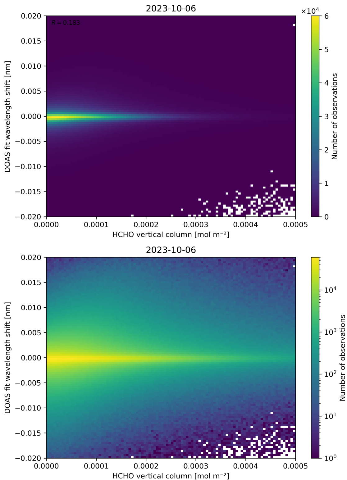
Figure 124: Scatter density plot of “HCHO vertical column” against “DOAS fit wavelength shift” for 2023-10-06 to 2023-10-07.
