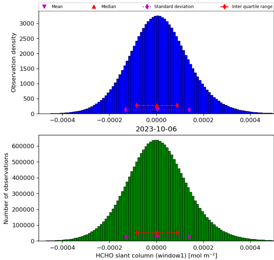
Figure 38: Histogram of “HCHO slant column (window1)” for 2023-10-06 to 2023-10-07
