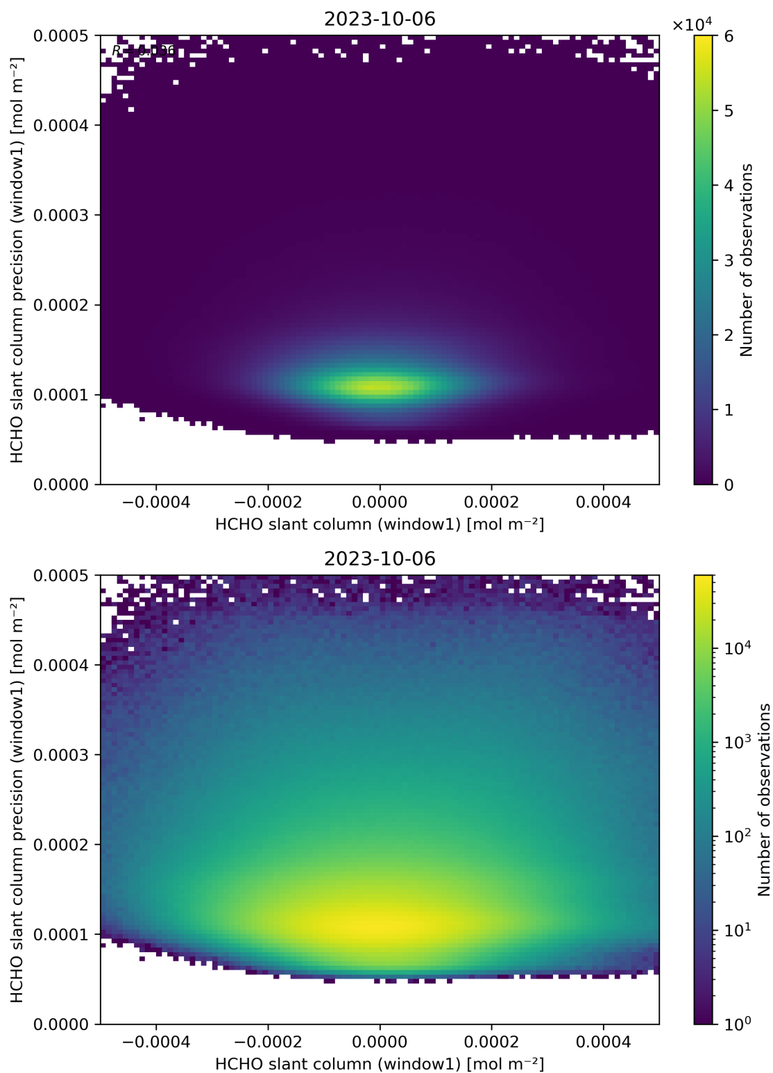
Figure 84: Scatter density plot of “HCHO slant column (window1)” against “HCHO slant column precision (window1)” for 2023-10-06 to 2023-10-07.
