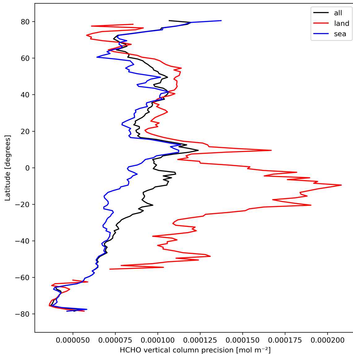
Figure 22: Zonal average of “HCHO vertical column precision” for 2023-10-06 to 2023-10-07.
