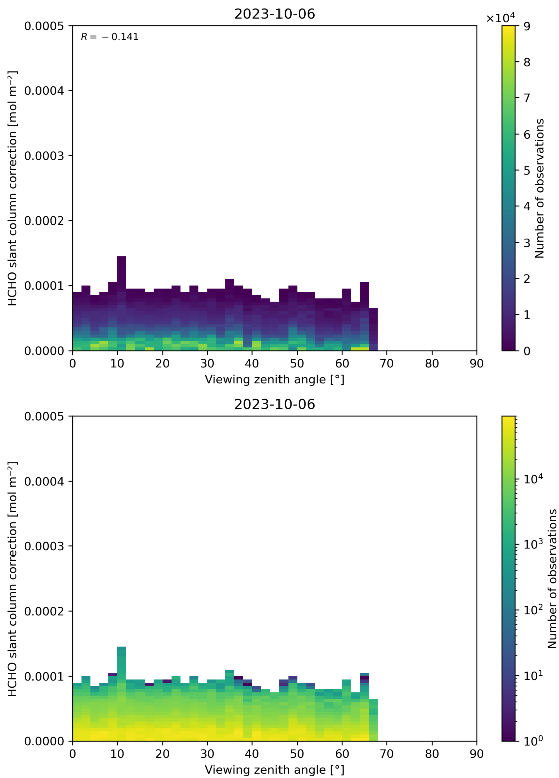
Figure 187: Scatter density plot of “Viewing zenith angle” against “HCHO slant column correction” for 2023-10-06 to 2023-10-07.
