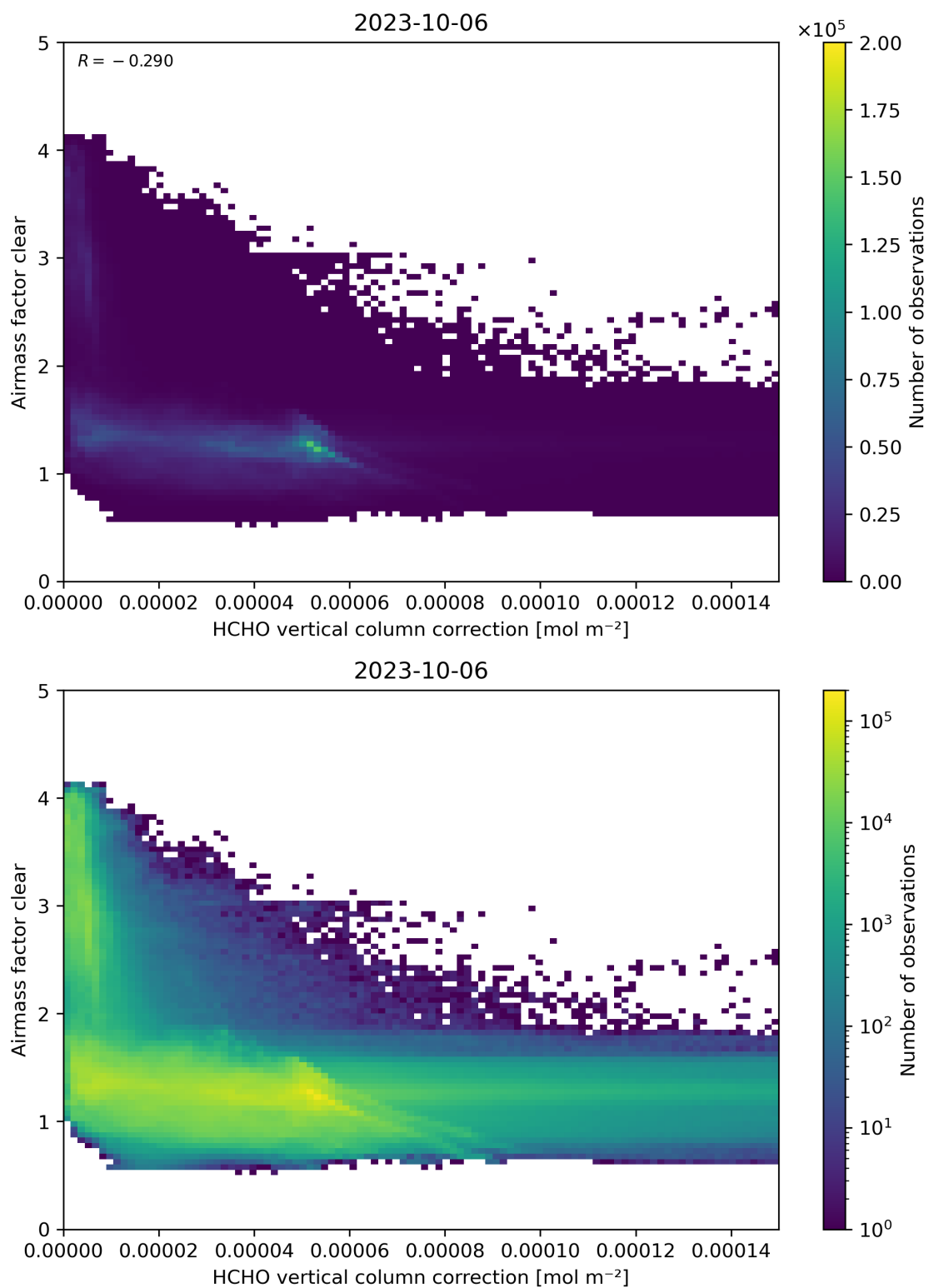
Figure 115: Scatter density plot of “HCHO vertical column correction” against “Airmass factor clear” for 2023-10-06 to 2023-10-07.
