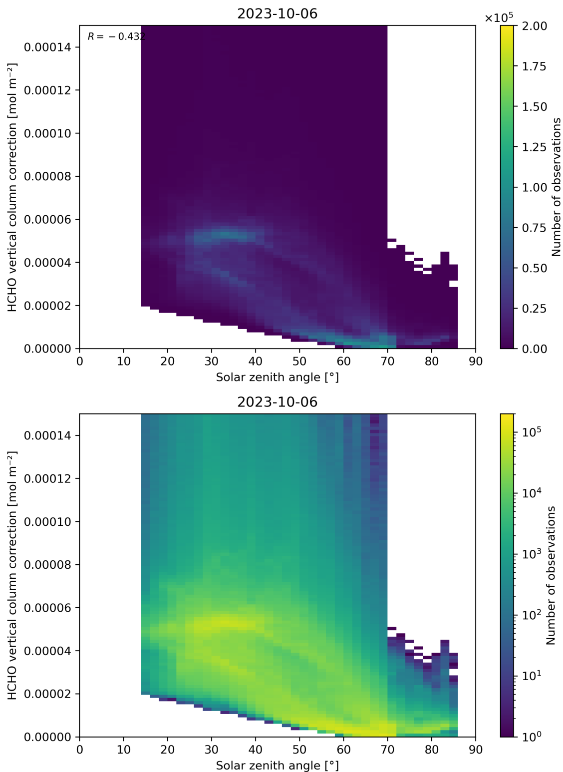
Figure 178: Scatter density plot of “Solar zenith angle” against “HCHO vertical column correction” for 2023-10-06 to 2023-10-07.
