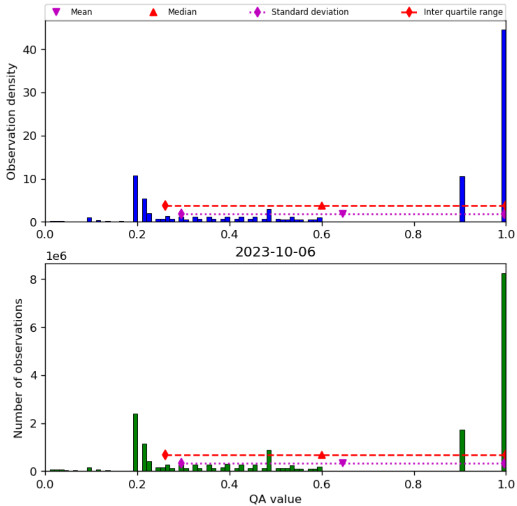
Figure 34: Histogram of “QA value” for 2023-10-06 to 2023-10-07
