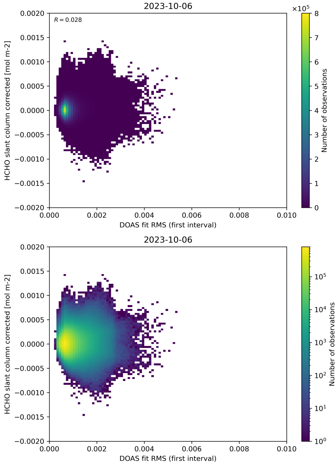
Figure 62: Scatter density plot of “DOAS fit RMS (first interval)” against “HCHO slant column corrected” for 2023-10-06 to 2023-10-07.
