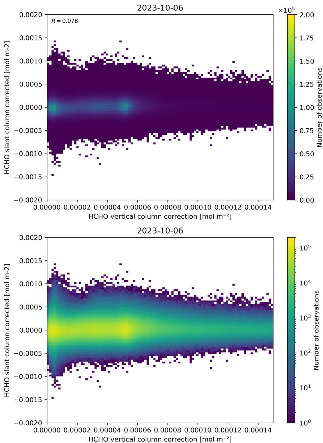
Figure 116: Scatter density plot of “HCHO vertical column correction” against “HCHO slant column corrected” for 2023-10-06 to 2023-10-07.
