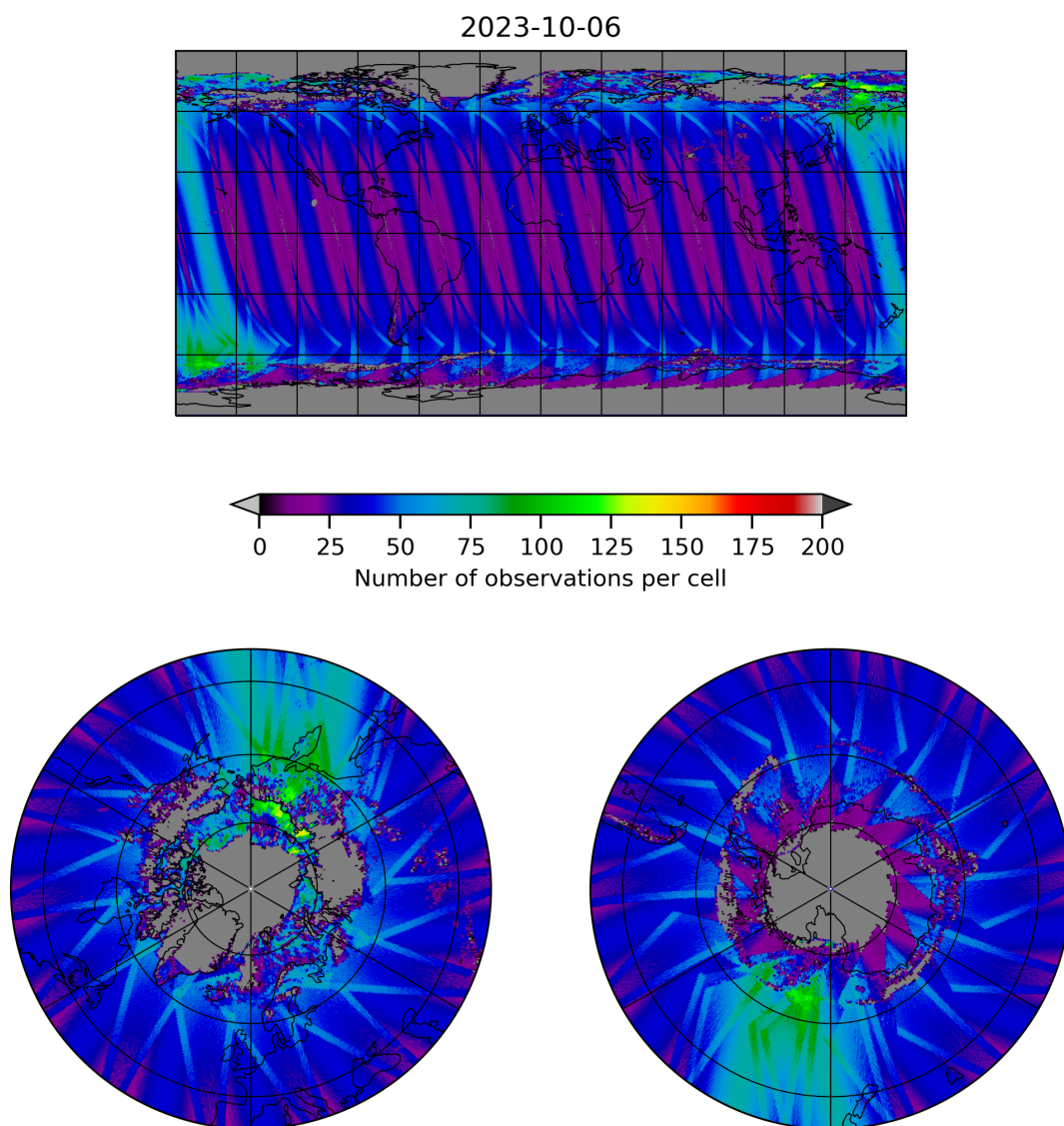
Figure 19: Map of the number of observations for 2023-10-06 to 2023-10-07
