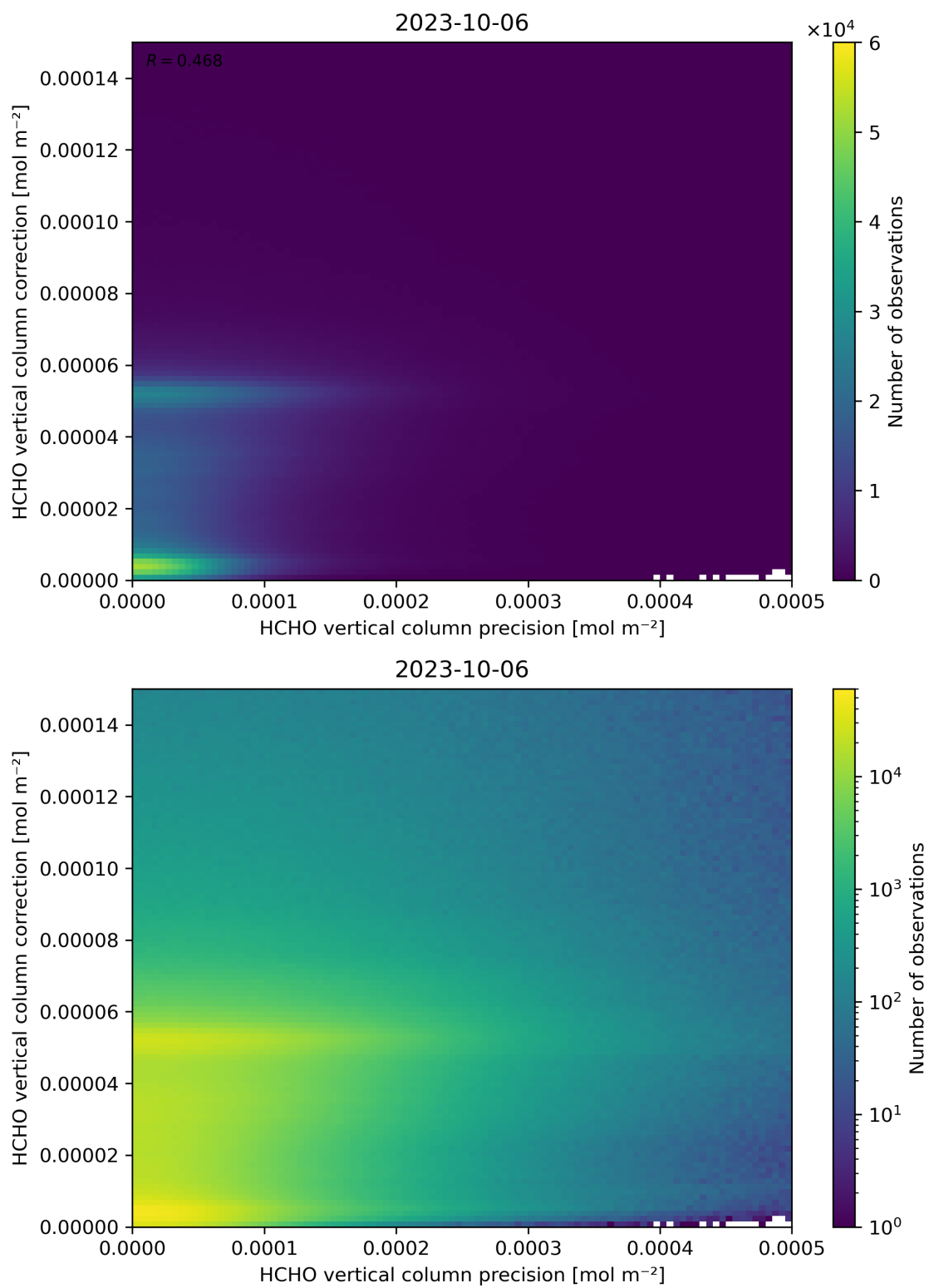
Figure 146: Scatter density plot of “HCHO vertical column precision” against “HCHO vertical column correction” for 2023-10-06 to 2023-10-07.
