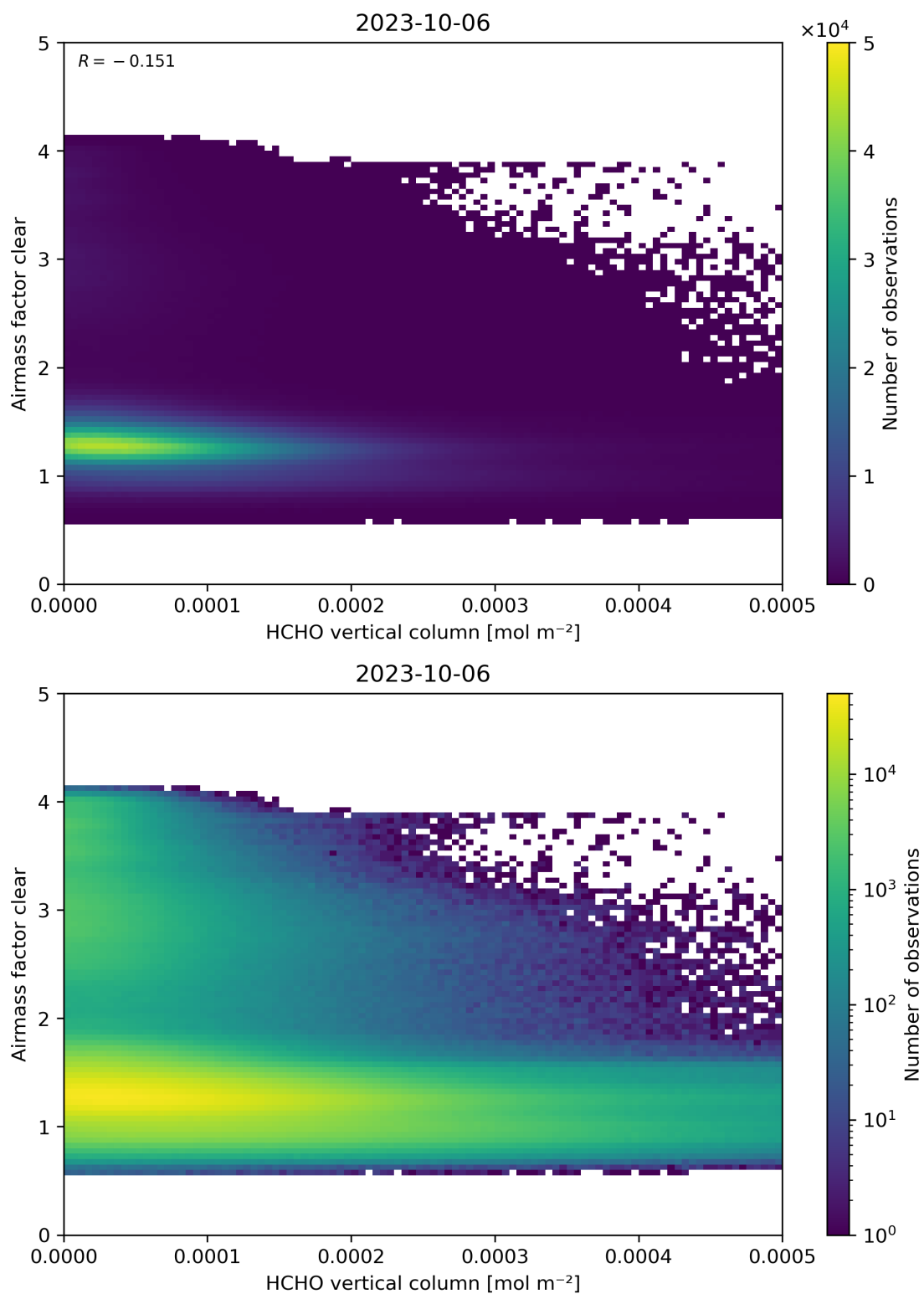
Figure 126: Scatter density plot of “HCHO vertical column” against “Airmass factor clear” for 2023-10-06 to 2023-10-07.
