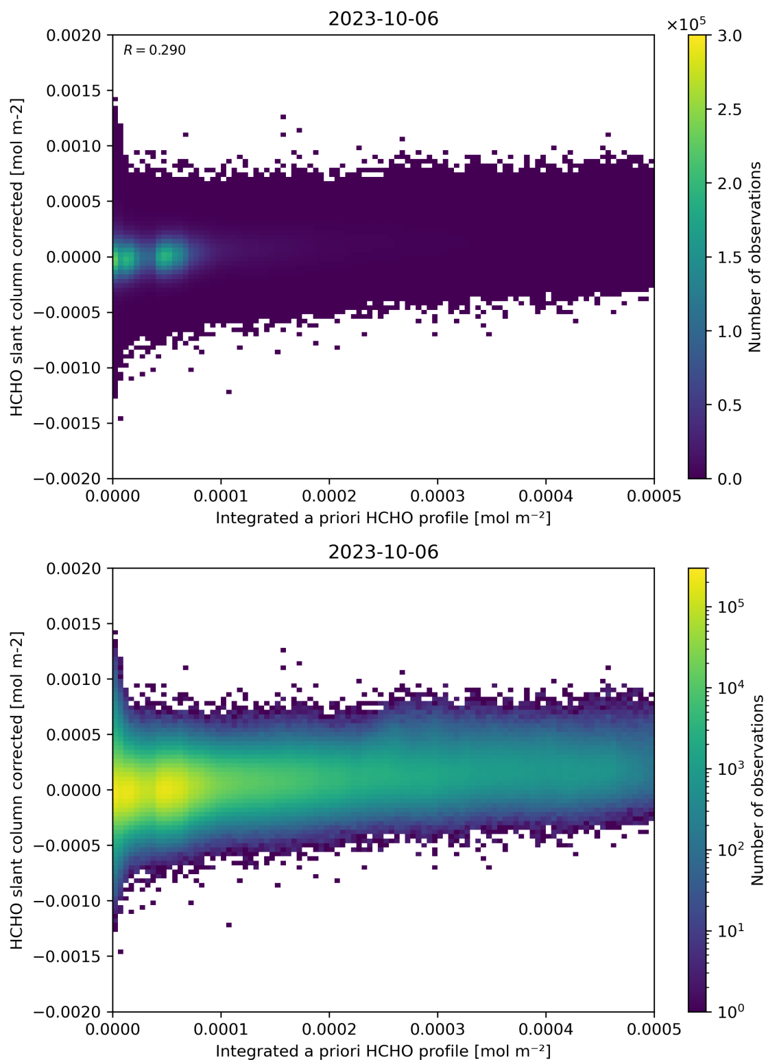
Figure 151: Scatter density plot of “Integrated a priori HCHO profile” against “HCHO slant column corrected” for 2023-10-06 to 2023-10-07.
