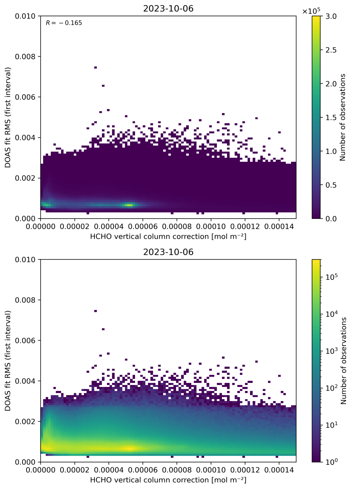
Figure 112: Scatter density plot of “HCHO vertical column correction” against “DOAS fit RMS (first interval)” for 2023-10-06 to 2023-10-07.
