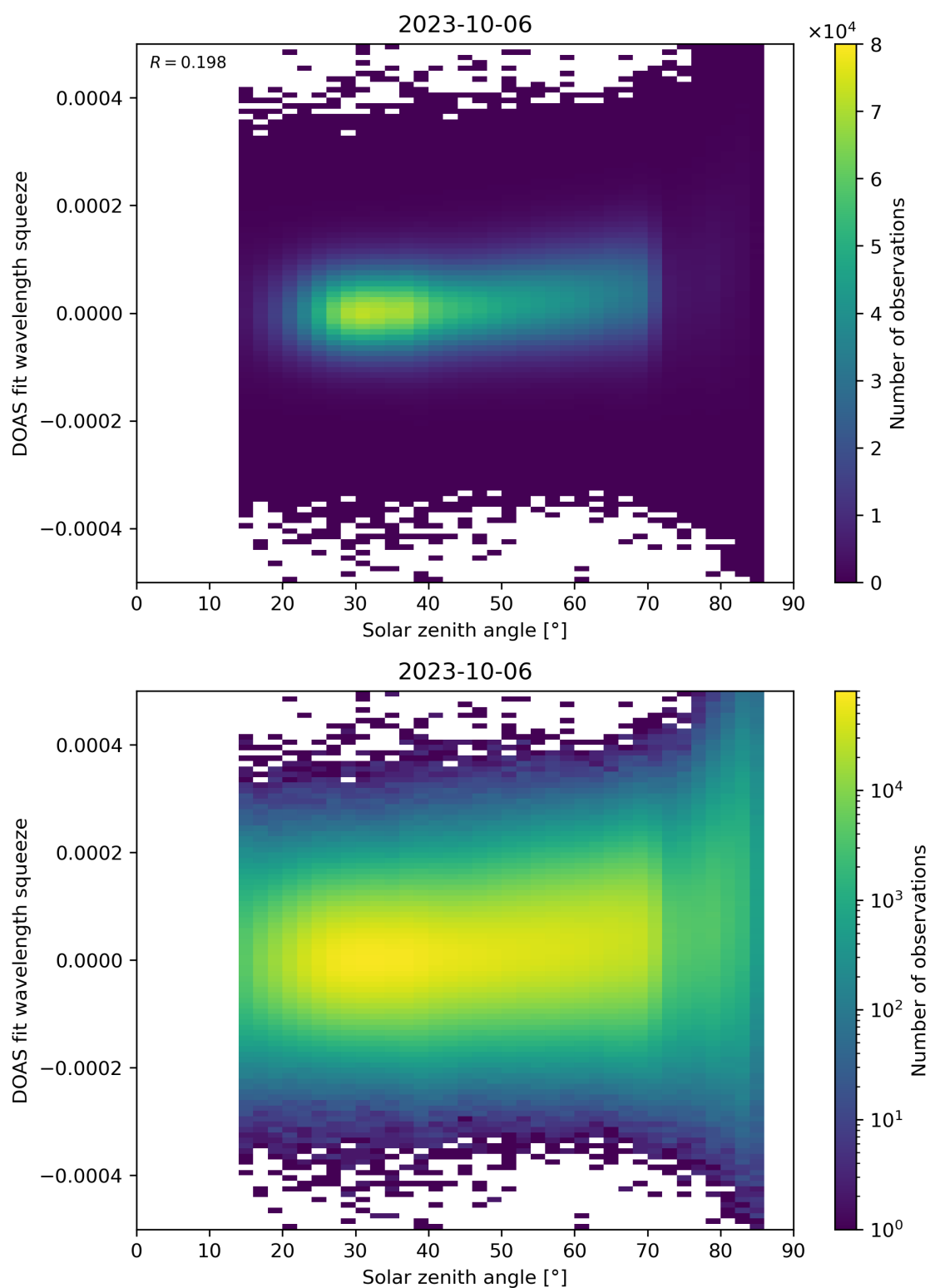
Figure 169: Scatter density plot of “Solar zenith angle” against “DOAS fit wavelength squeeze” for 2023-10-06 to 2023-10-07.
