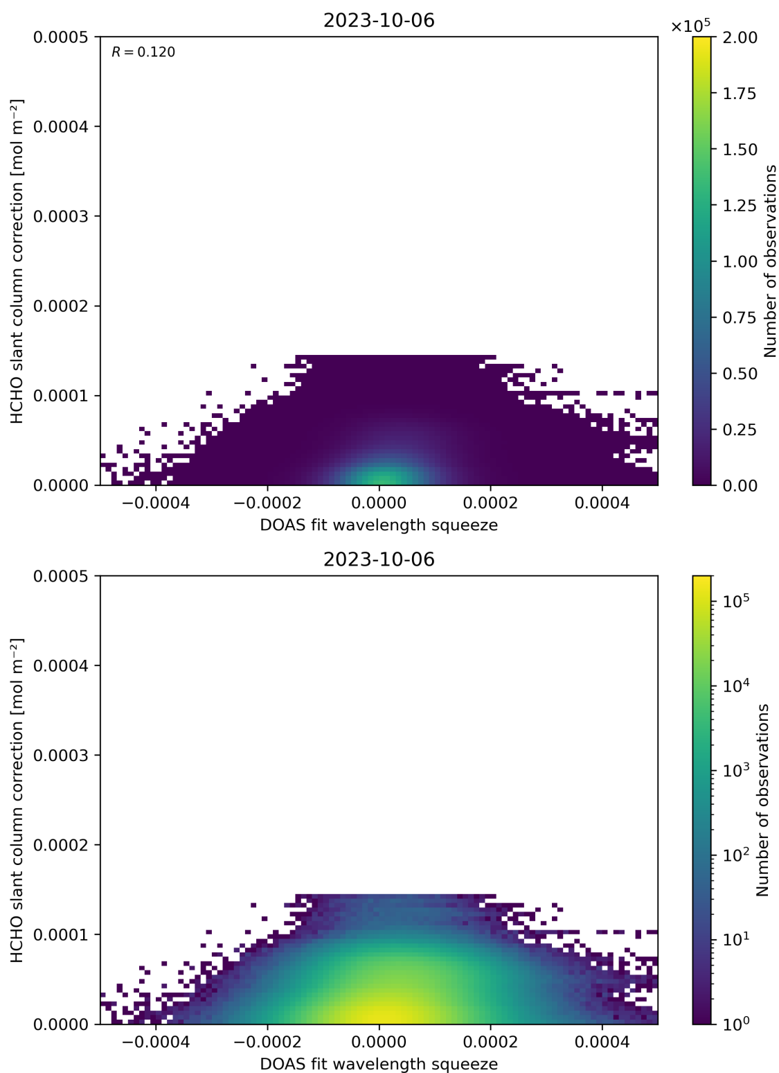
Figure 70: Scatter density plot of “DOAS fit wavelength squeeze” against “HCHO slant column correction” for 2023-10-06 to 2023-10-07.
