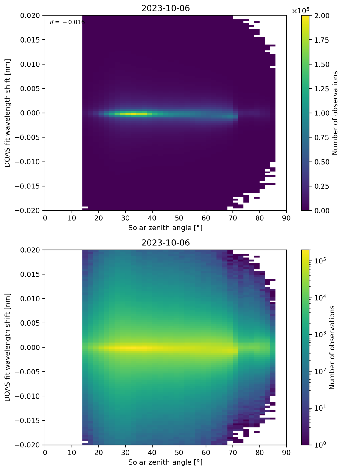
Figure 168: Scatter density plot of “Solar zenith angle” against “DOAS fit wavelength shift” for 2023-10-06 to 2023-10-07.
