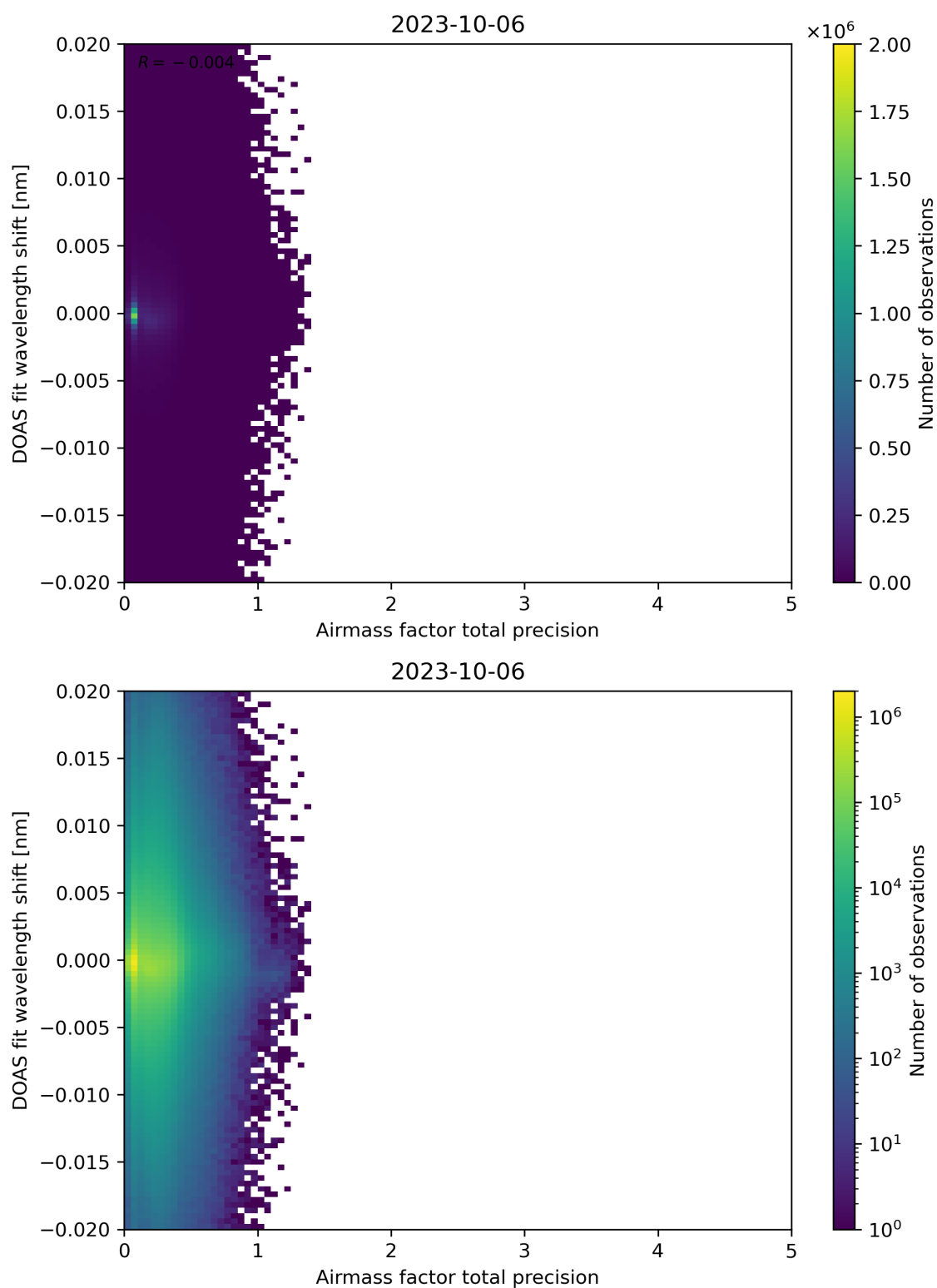
Figure 106: Scatter density plot of “Airmass factor total precision” against “DOAS fit wavelength shift” for 2023-10-06 to 2023-10-07.
