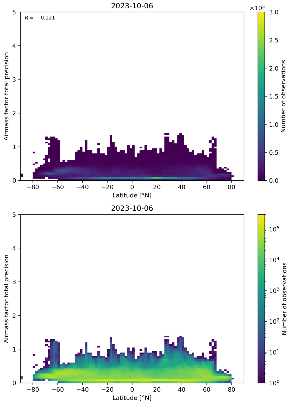
Figure 162: Scatter density plot of “Latitude” against “Airmass factor total precision” for 2023-10-06 to 2023-10-07.
