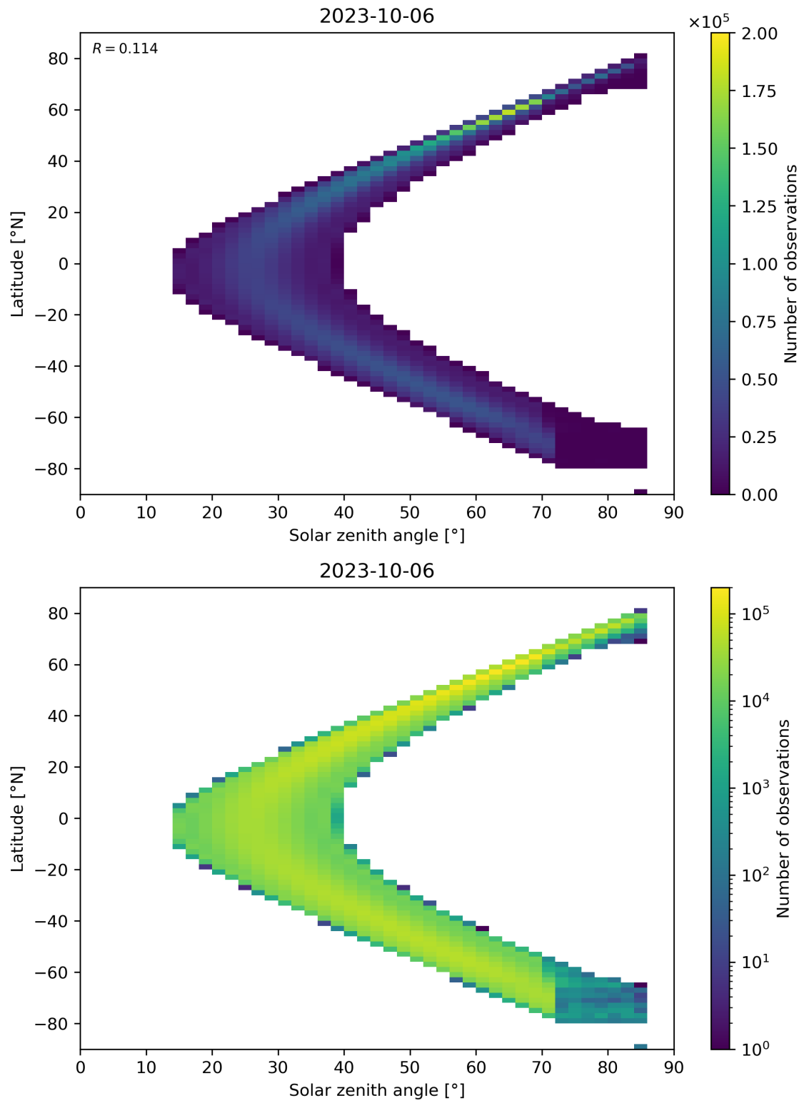
Figure 181: Scatter density plot of “Solar zenith angle” against “Latitude” for 2023-10-06 to 2023-10-07.
