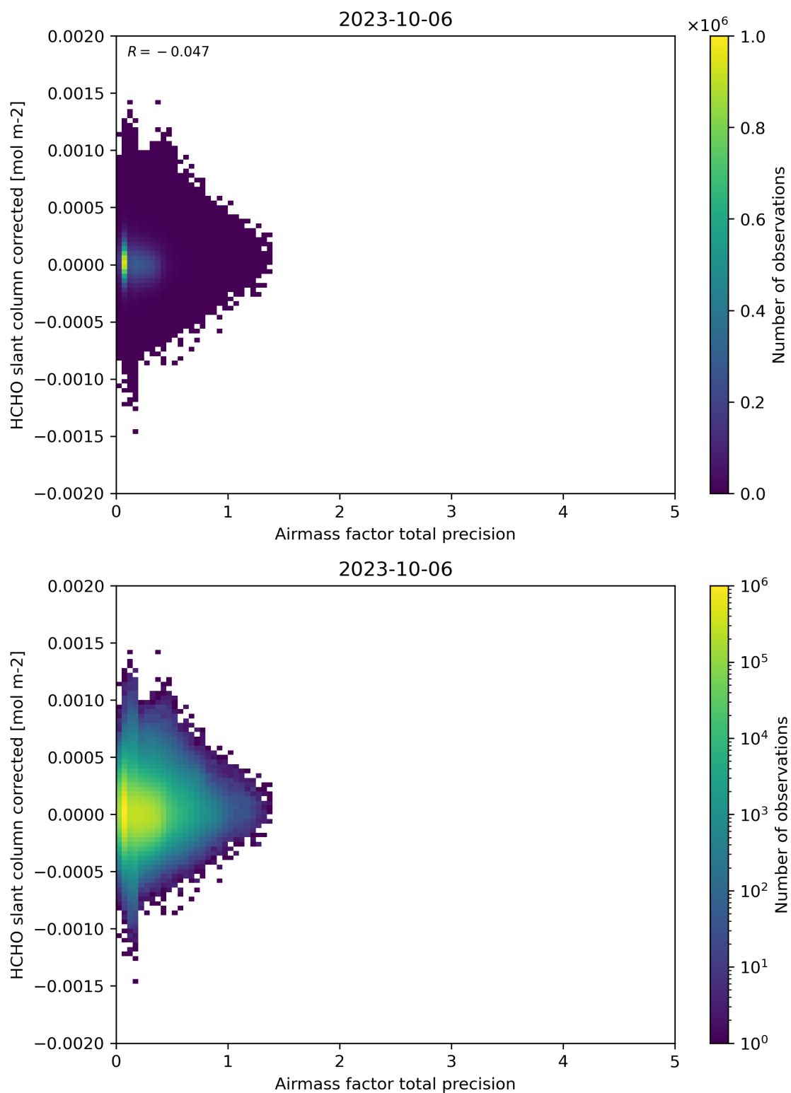
Figure 109: Scatter density plot of “Airmass factor total precision” against “HCHO slant column corrected” for 2023-10-06 to 2023-10-07.
