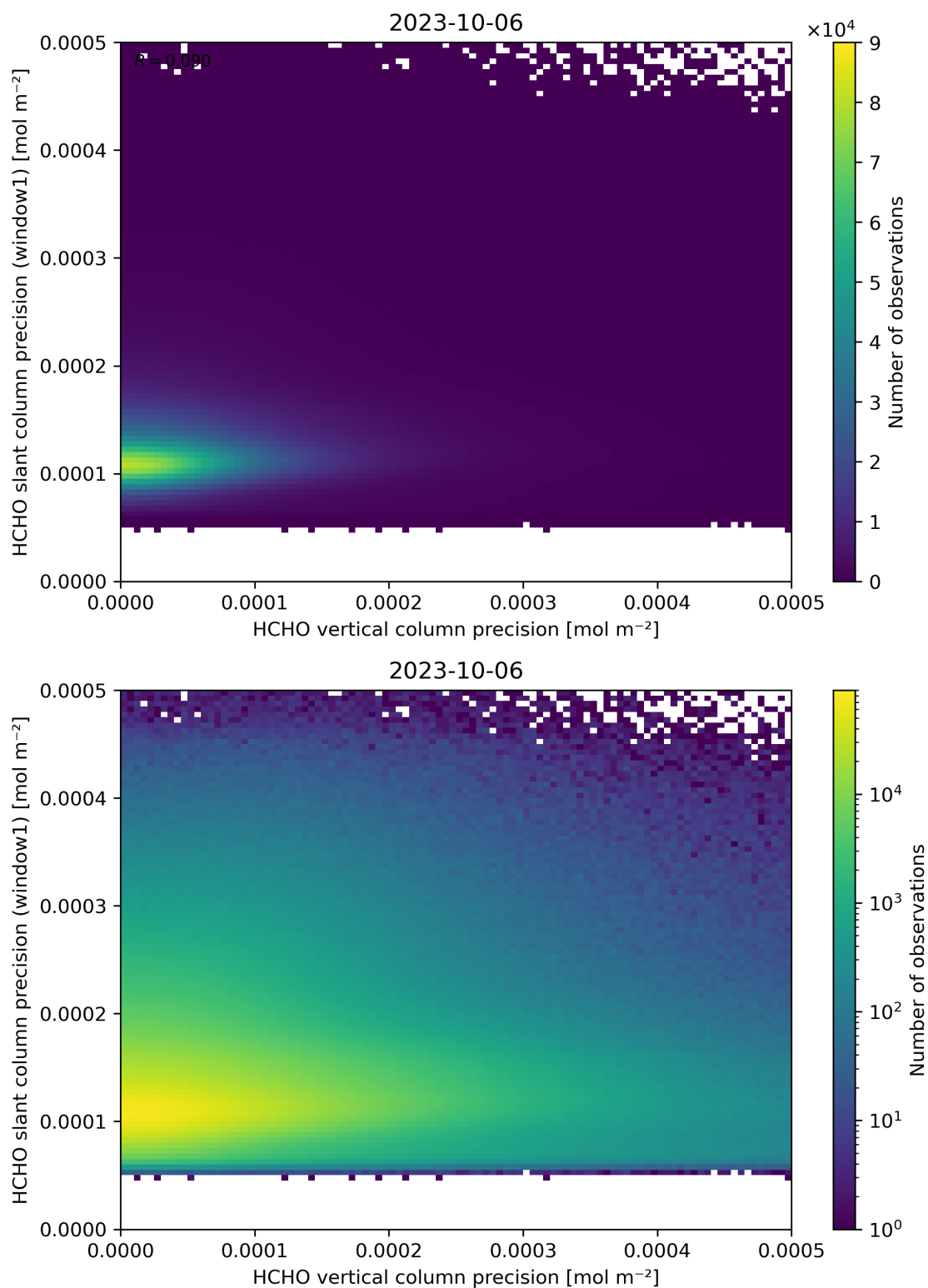
Figure 143: Scatter density plot of “HCHO vertical column precision” against “HCHO slant column precision (window1)” for 2023-10-06 to 2023-10-07.
