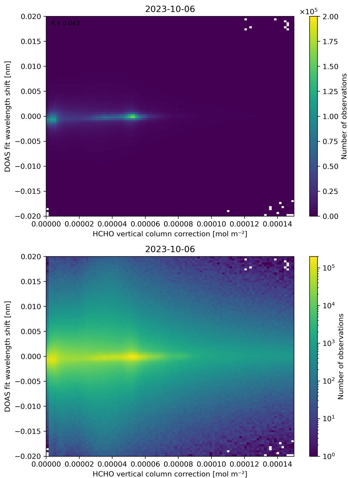
Figure 113: Scatter density plot of “HCHO vertical column correction” against “DOAS fit wavelength shift” for 2023-10-06 to 2023-10-07.
