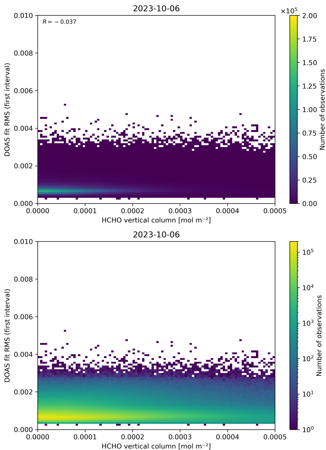
Figure 123: Scatter density plot of “HCHO vertical column” against “DOAS fit RMS (first interval)” for 2023-10-06 to 2023-10-07.
