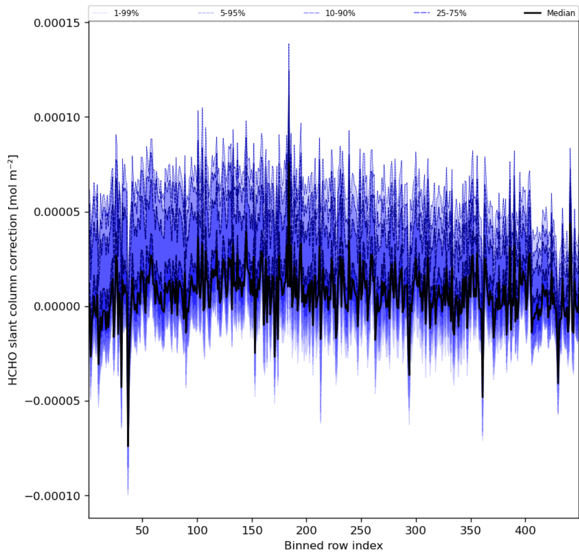
Figure 61: Along track statistics of “HCHO slant column correction” for 2023-10-06 to 2023-10-07
