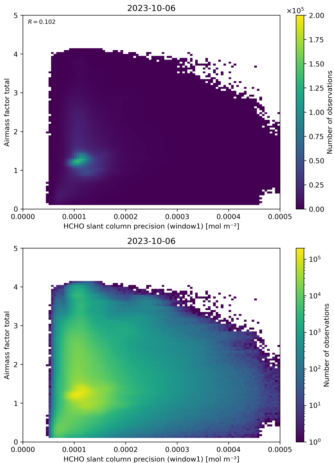
Figure 94: Scatter density plot of “HCHO slant column precision (window1)” against “Airmass factor total” for 2023-10-06 to 2023-10-07.
