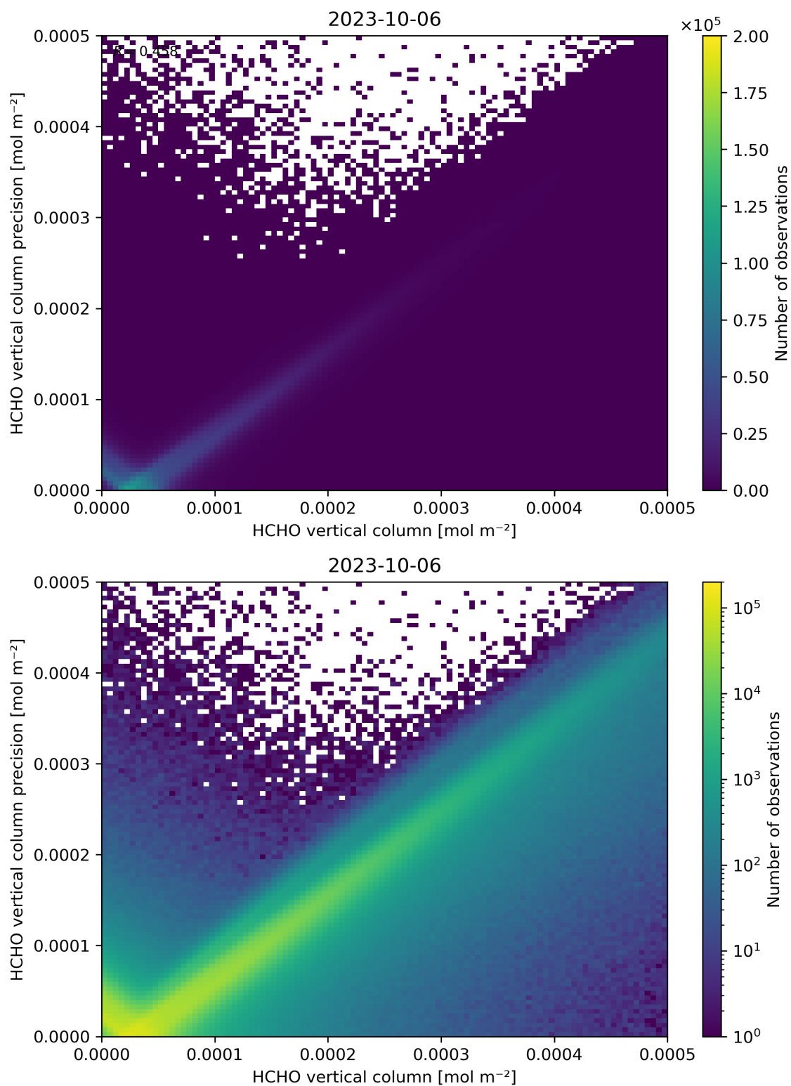
Figure 134: Scatter density plot of “HCHO vertical column” against “HCHO vertical column precision” for 2023-10-06 to 2023-10-07.
