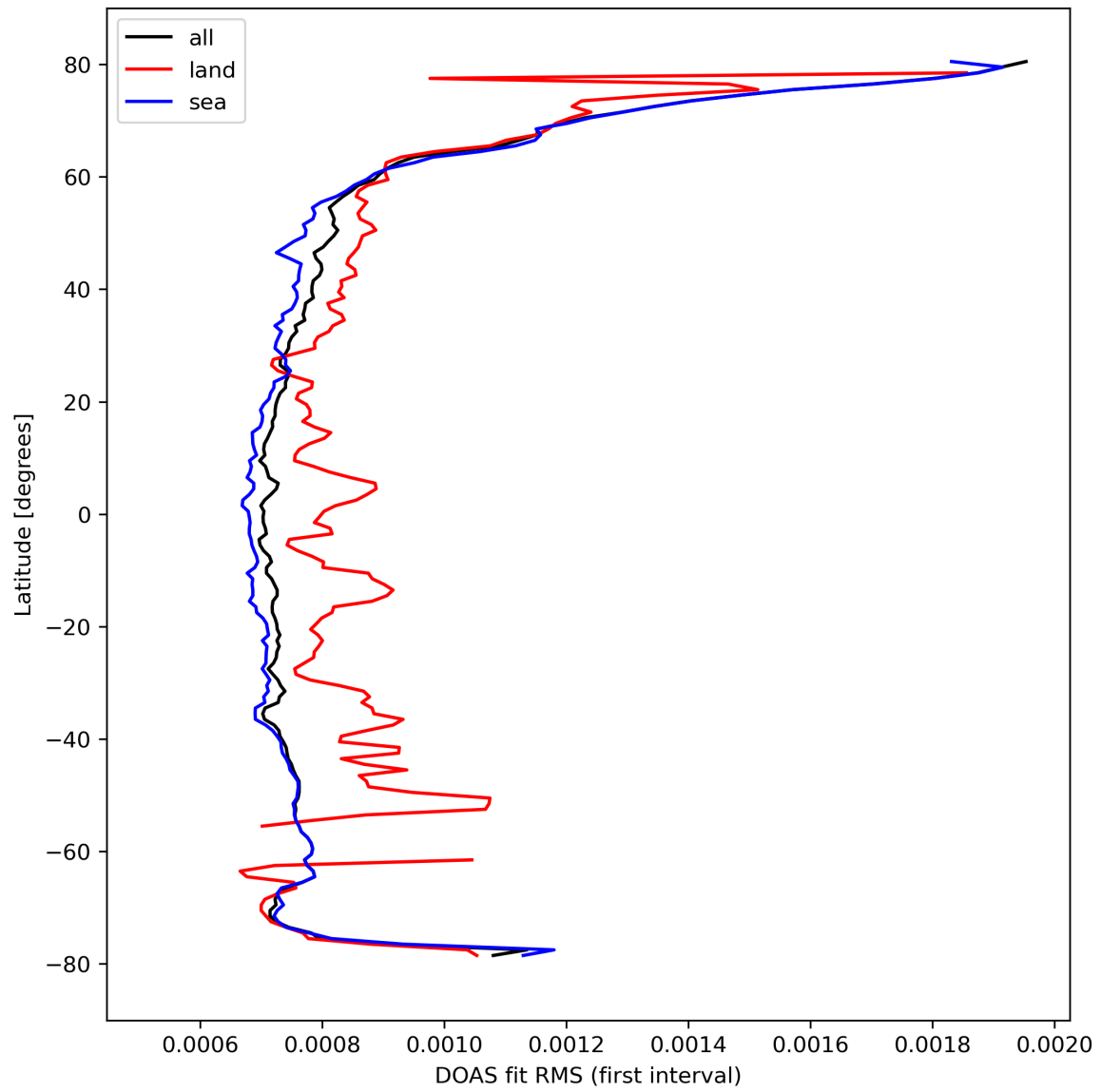
Figure 32: Zonal average of “DOAS fit RMS (first interval)” for 2023-10-06 to 2023-10-07.
