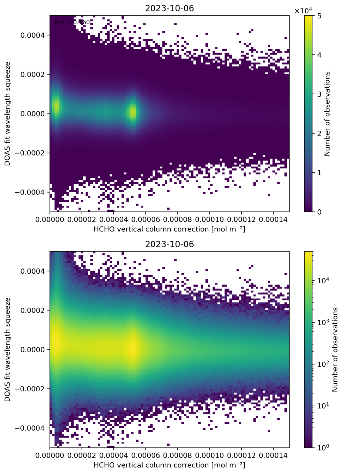
Figure 114: Scatter density plot of “HCHO vertical column correction” against “DOAS fit wavelength squeeze” for 2023-10-06 to 2023-10-07.
