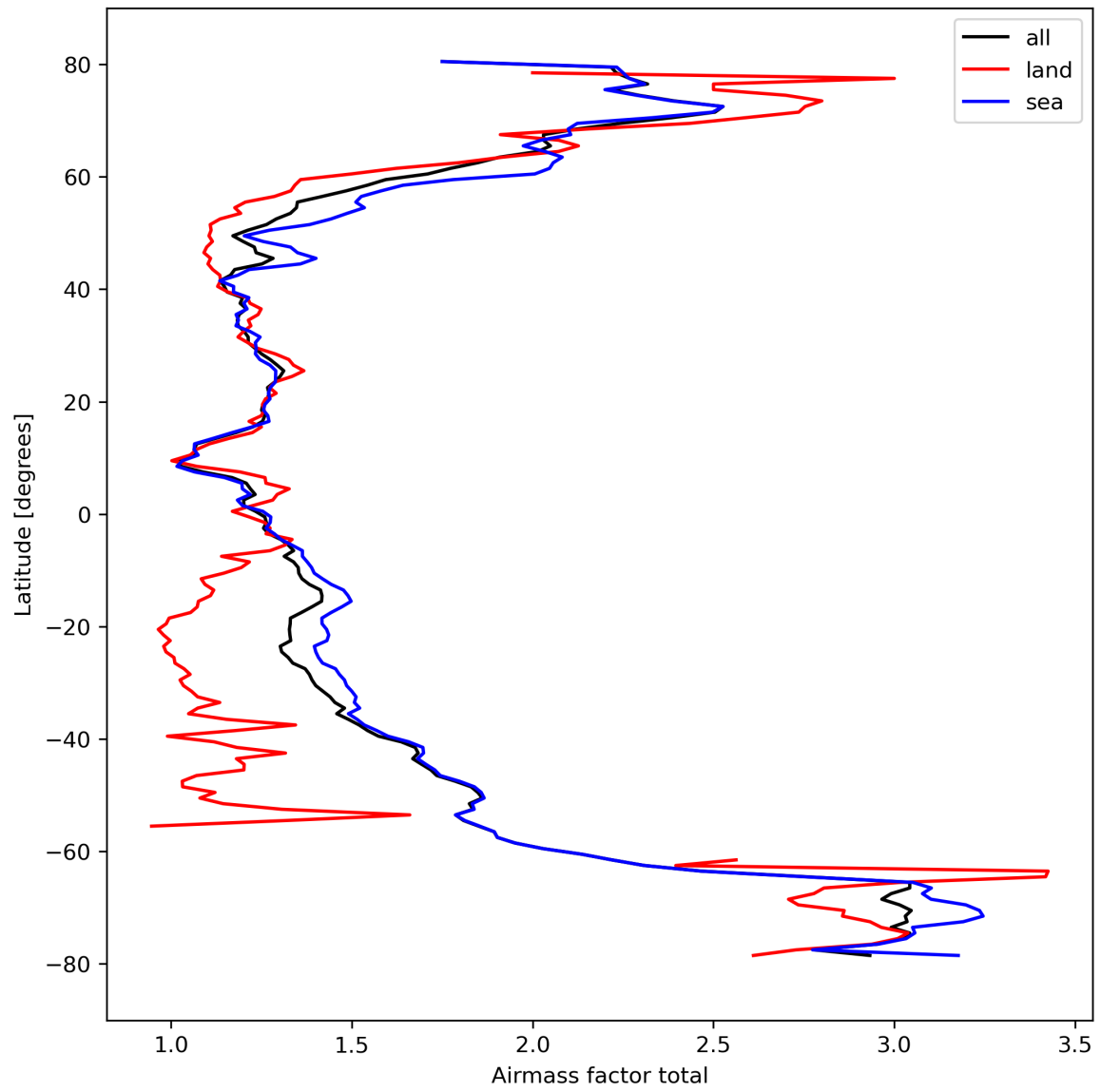
Figure 26: Zonal average of “Airmass factor total” for 2023-10-06 to 2023-10-07.
