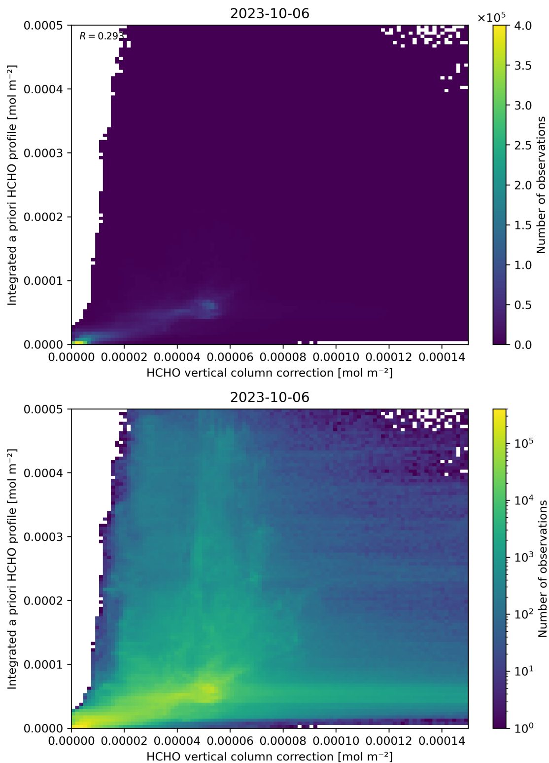
Figure 122: Scatter density plot of “HCHO vertical column correction” against “Integrated a priori HCHO profile” for 2023-10-06 to 2023-10-07.
