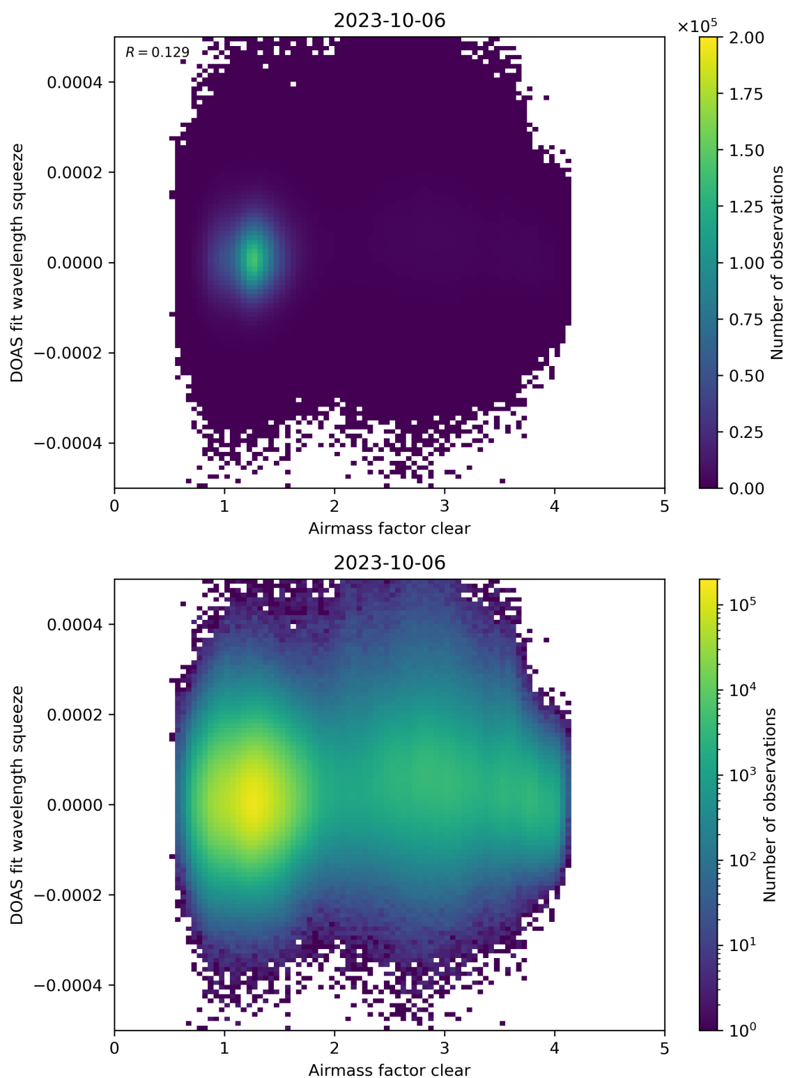
Figure 73: Scatter density plot of “Airmass factor clear” against “DOAS fit wavelength squeeze” for 2023-10-06 to 2023-10-07.
