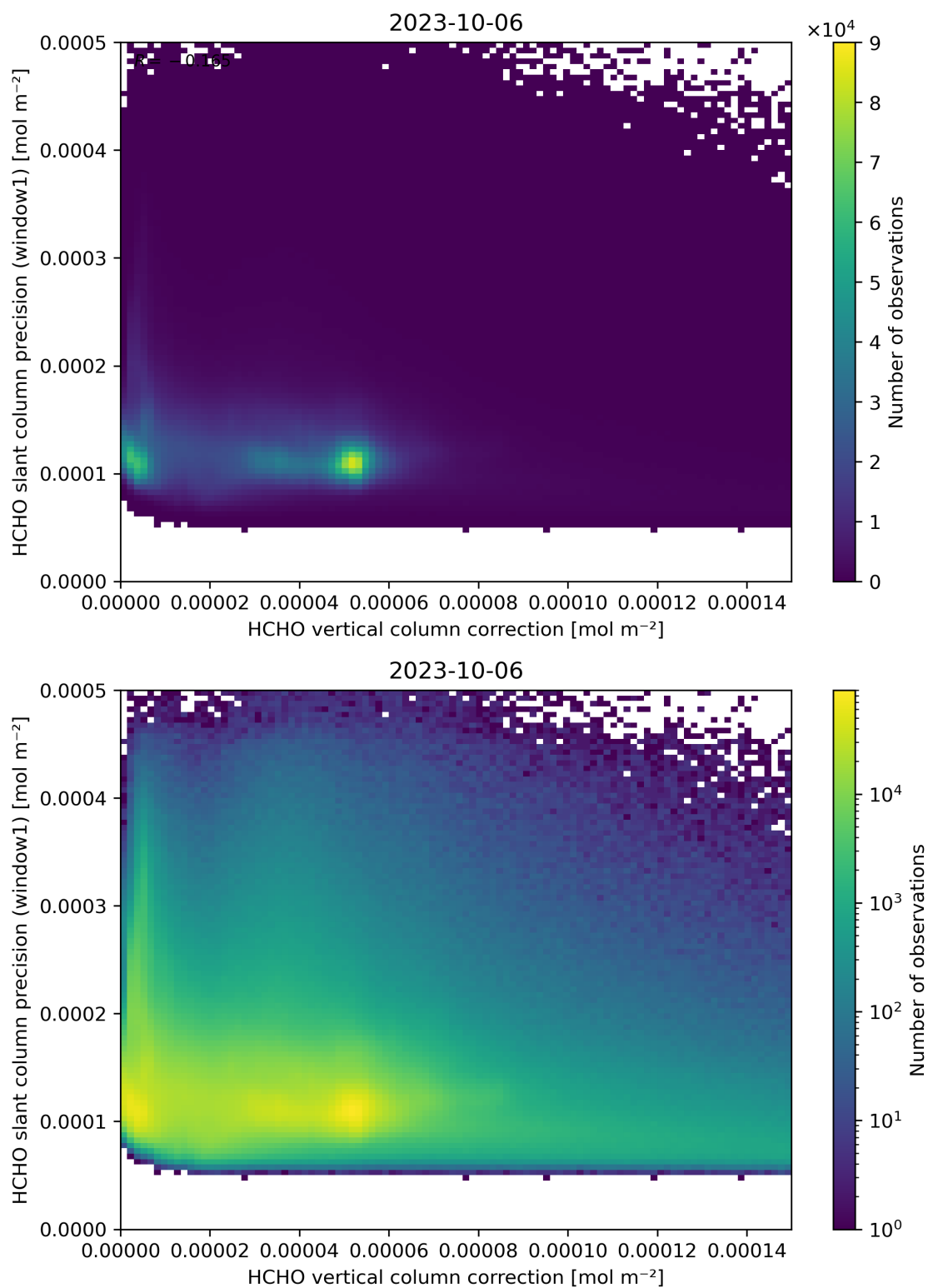
Figure 119: Scatter density plot of “HCHO vertical column correction” against “HCHO slant column precision (window1)” for 2023-10-06 to 2023-10-07.
