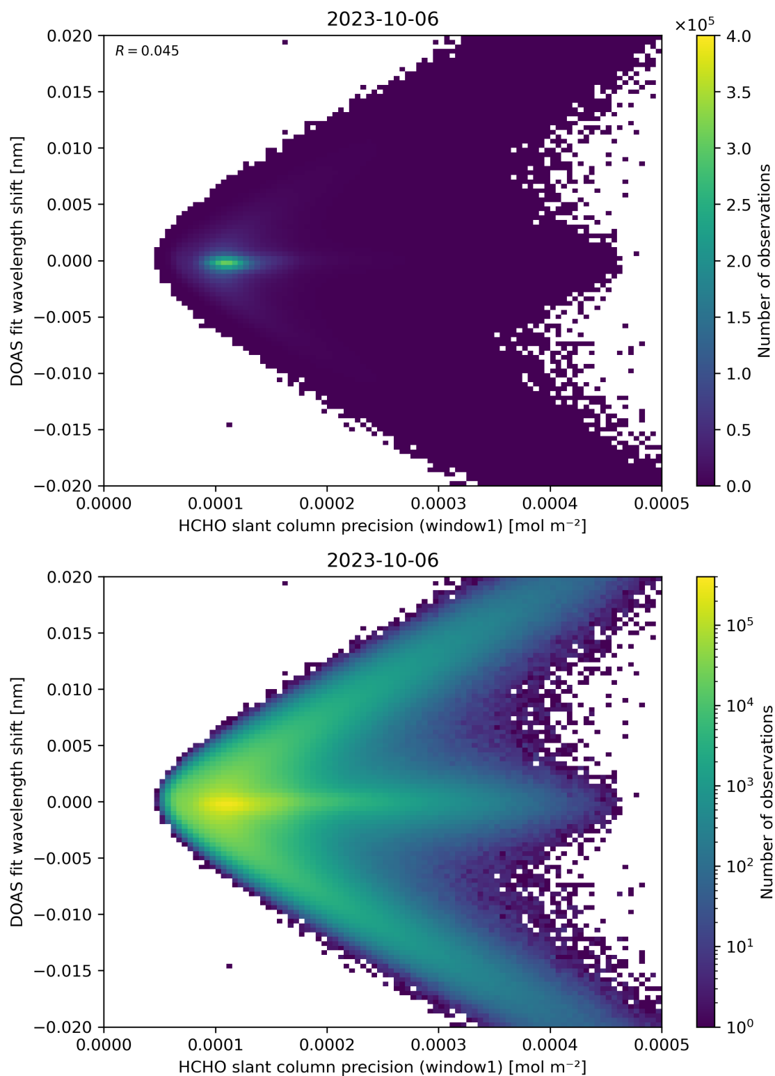
Figure 89: Scatter density plot of “HCHO slant column precision (window1)” against “DOAS fit wavelength shift” for 2023-10-06 to 2023-10-07.
