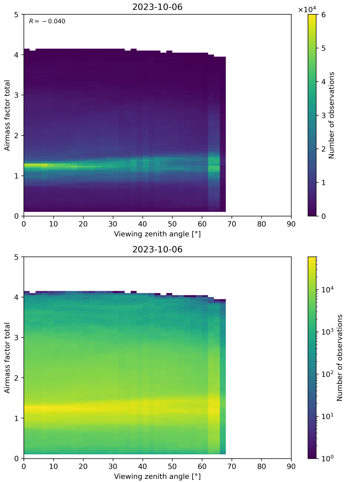
Figure 190: Scatter density plot of “Viewing zenith angle” against “Airmass factor total” for 2023-10-06 to 2023-10-07.
