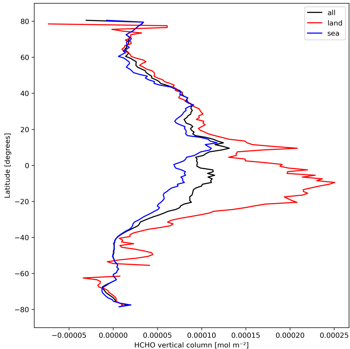
Figure 21: Zonal average of “HCHO vertical column” for 2023-10-06 to 2023-10-07.
