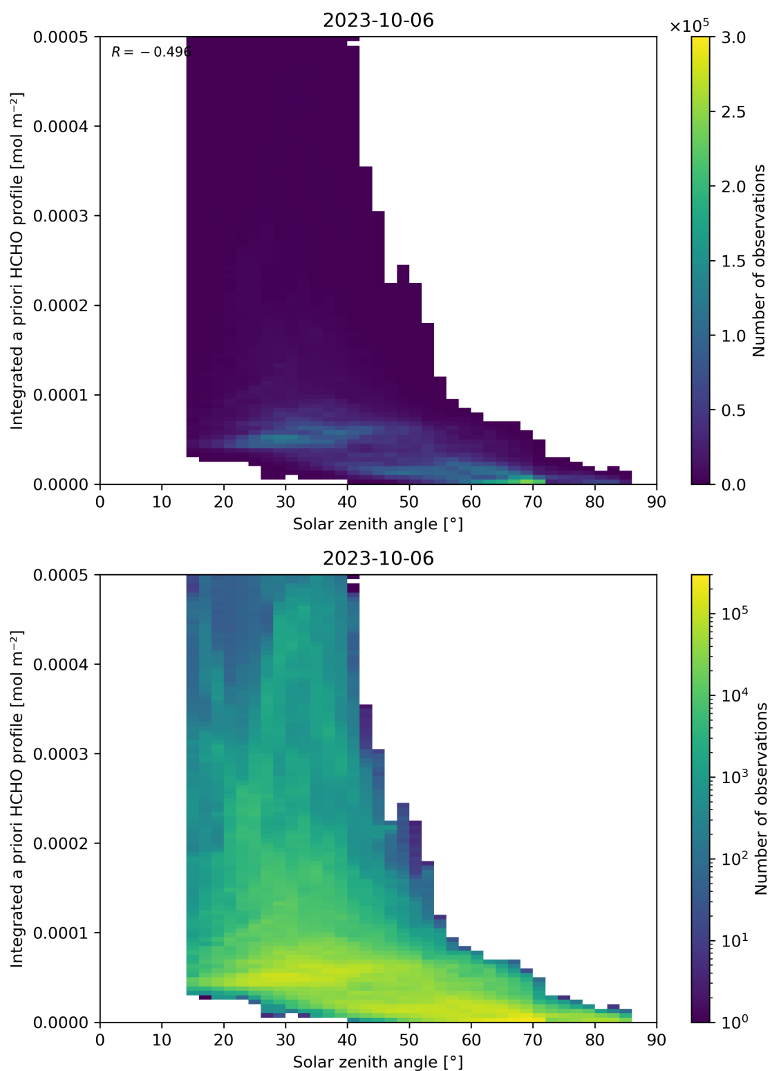
Figure 180: Scatter density plot of “Solar zenith angle” against “Integrated a priori HCHO profile” for 2023-10-06 to 2023-10-07.
