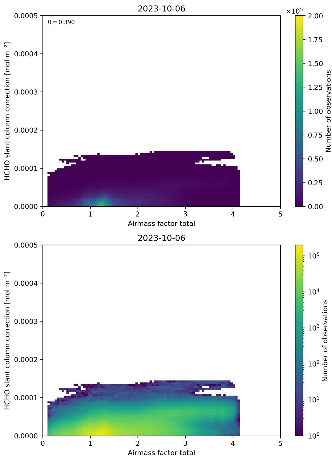
Figure 102: Scatter density plot of “Airmass factor total” against “HCHO slant column correction” for 2023-10-06 to 2023-10-07.
