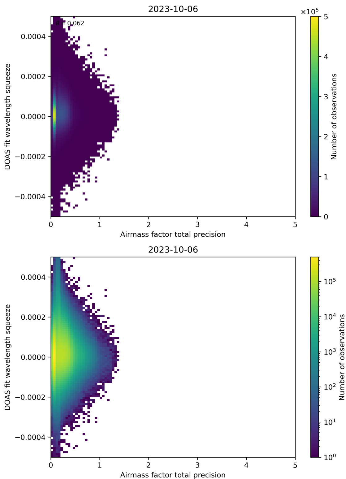
Figure 107: Scatter density plot of “Airmass factor total precision” against “DOAS fit wavelength squeeze” for 2023-10-06 to 2023-10-07.
