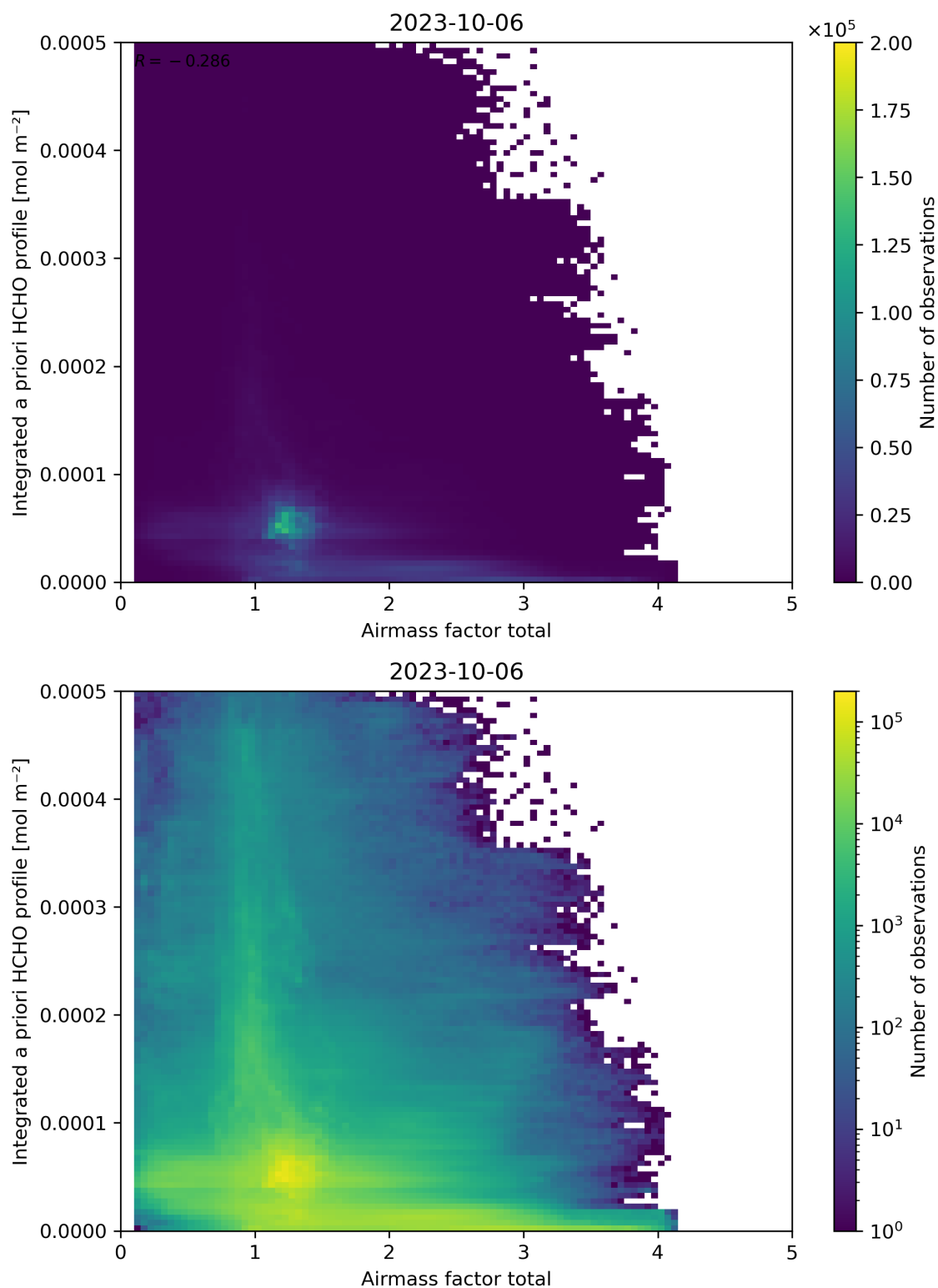
Figure 104: Scatter density plot of “Air mass factor total” against “Integrated a priori HCHO profile” for 2023-10-06 to 2023-10-07.
