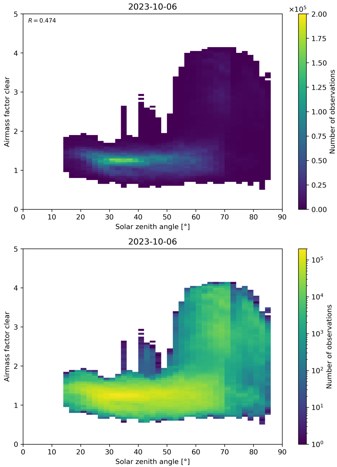
Figure 170: Scatter density plot of “Solar zenith angle” against “Airmass factor clear” for 2023-10-06 to 2023-10-07.
