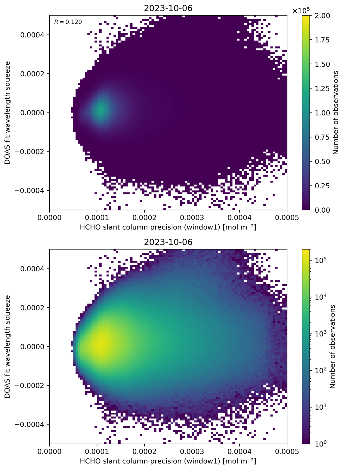
Figure 90: Scatter density plot of “HCHO slant column precision (window1)” against “DOAS fit wavelength squeeze” for 2023-10-06 to 2023-10-07.
