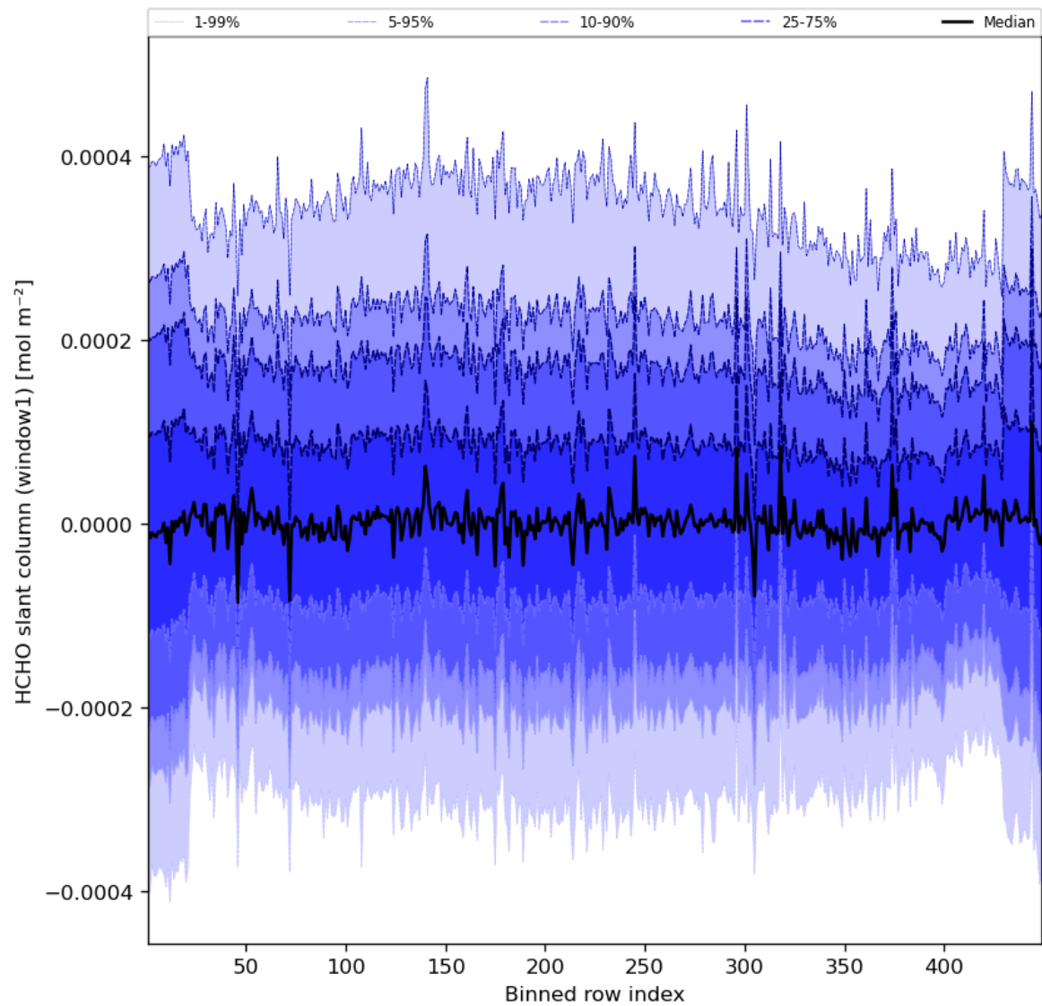
Figure 52: Along track statistics of “HCHO slant column (window1)” for 2023-10-06 to 2023-10-07
