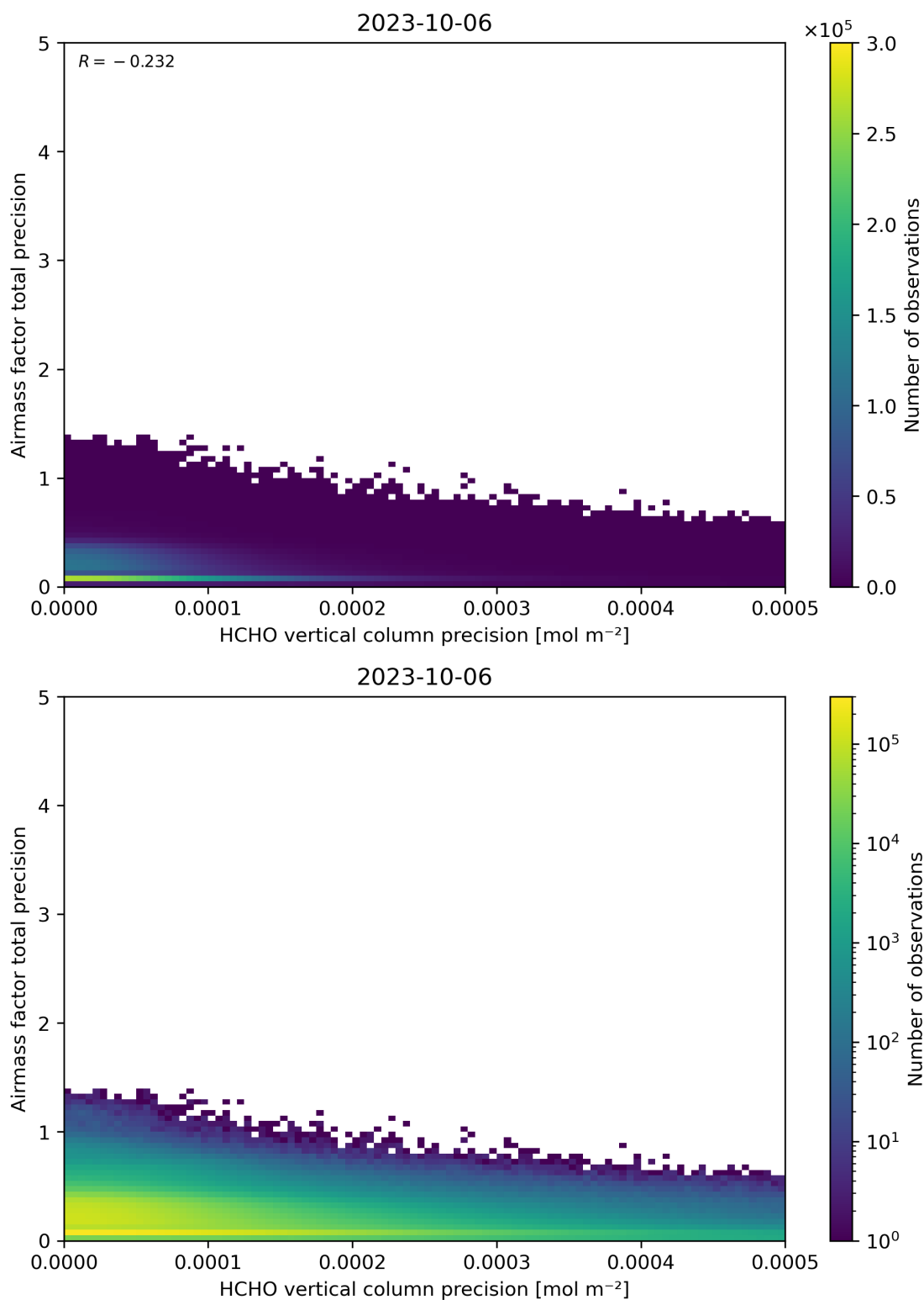
Figure 145: Scatter density plot of “HCHO vertical column precision” against “Airmass factor total precision” for 2023-10-06 to 2023-10-07.
