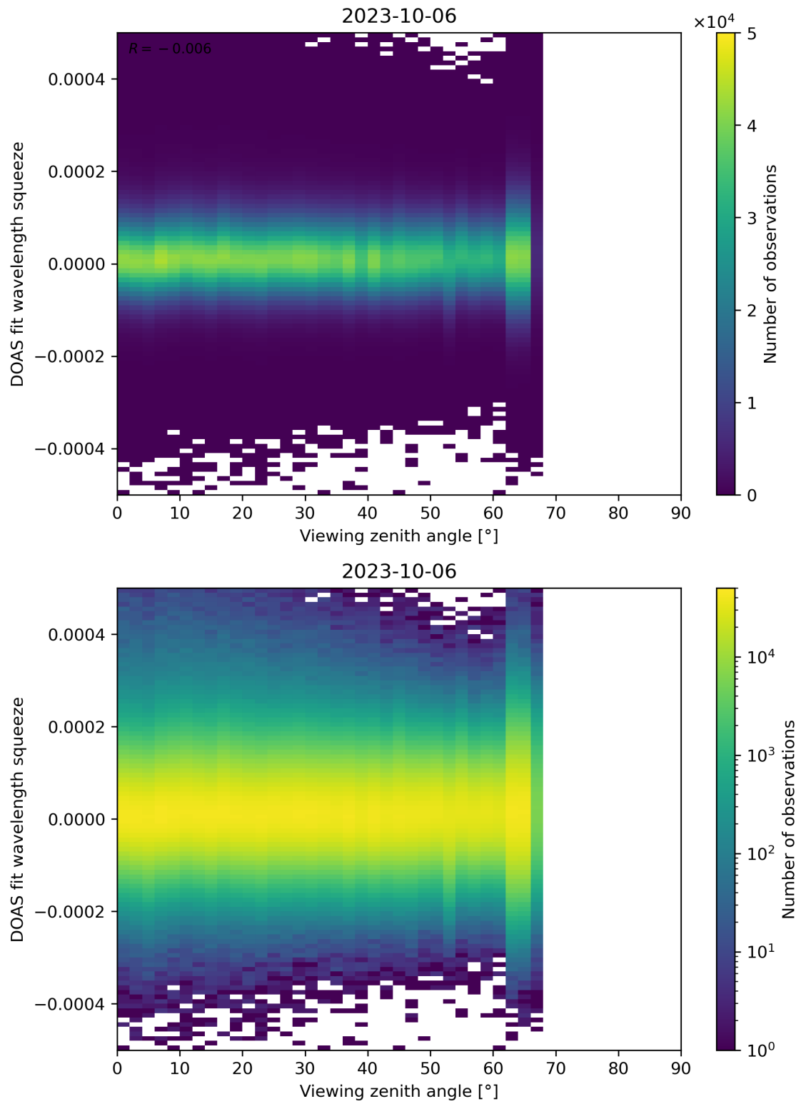
Figure 184: Scatter density plot of “Viewing zenith angle” against “DOAS fit wavelength squeeze” for 2023-10-06 to 2023-10-07.
