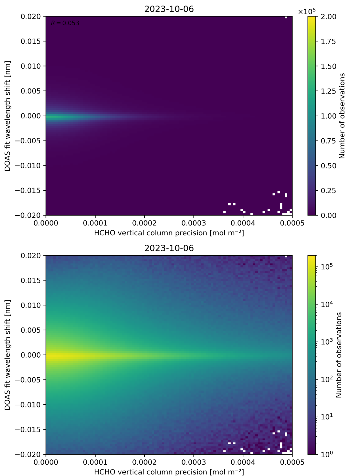
Figure 137: Scatter density plot of “HCHO vertical column precision” against “DOAS fit wavelength shift” for 2023-10-06 to 2023-10-07.
