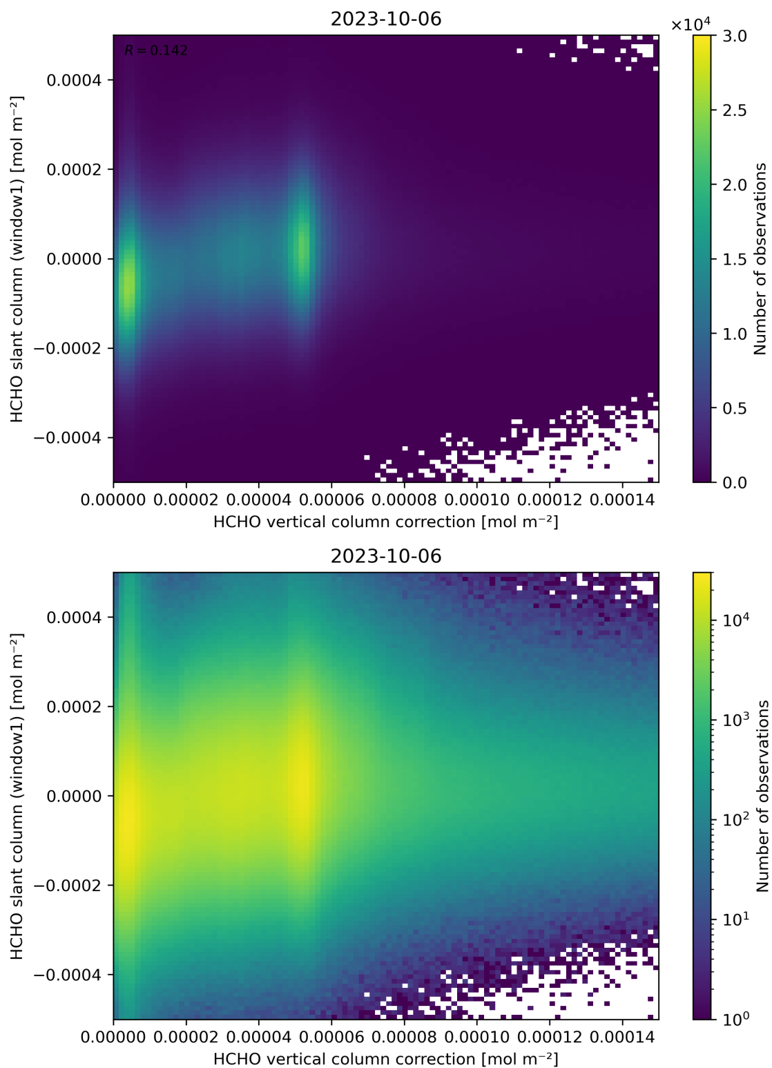
Figure 118: Scatter density plot of “HCHO vertical column correction” against “HCHO slant column (window1)” for 2023-10-06 to 2023-10-07.
