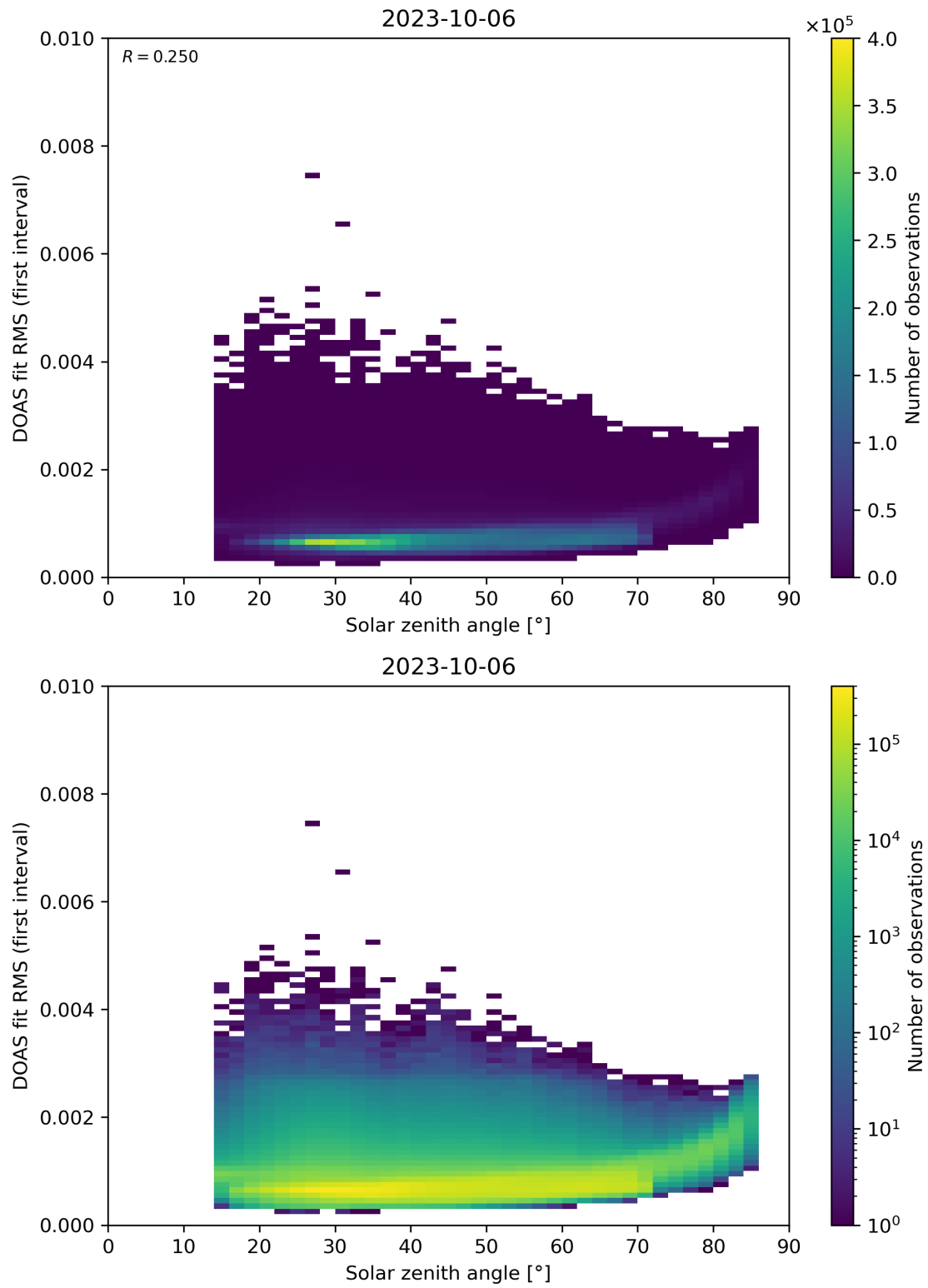
Figure 167: Scatter density plot of “Solar zenith angle” against “DOAS fit RMS (first interval)” for 2023-10-06 to 2023-10-07.
