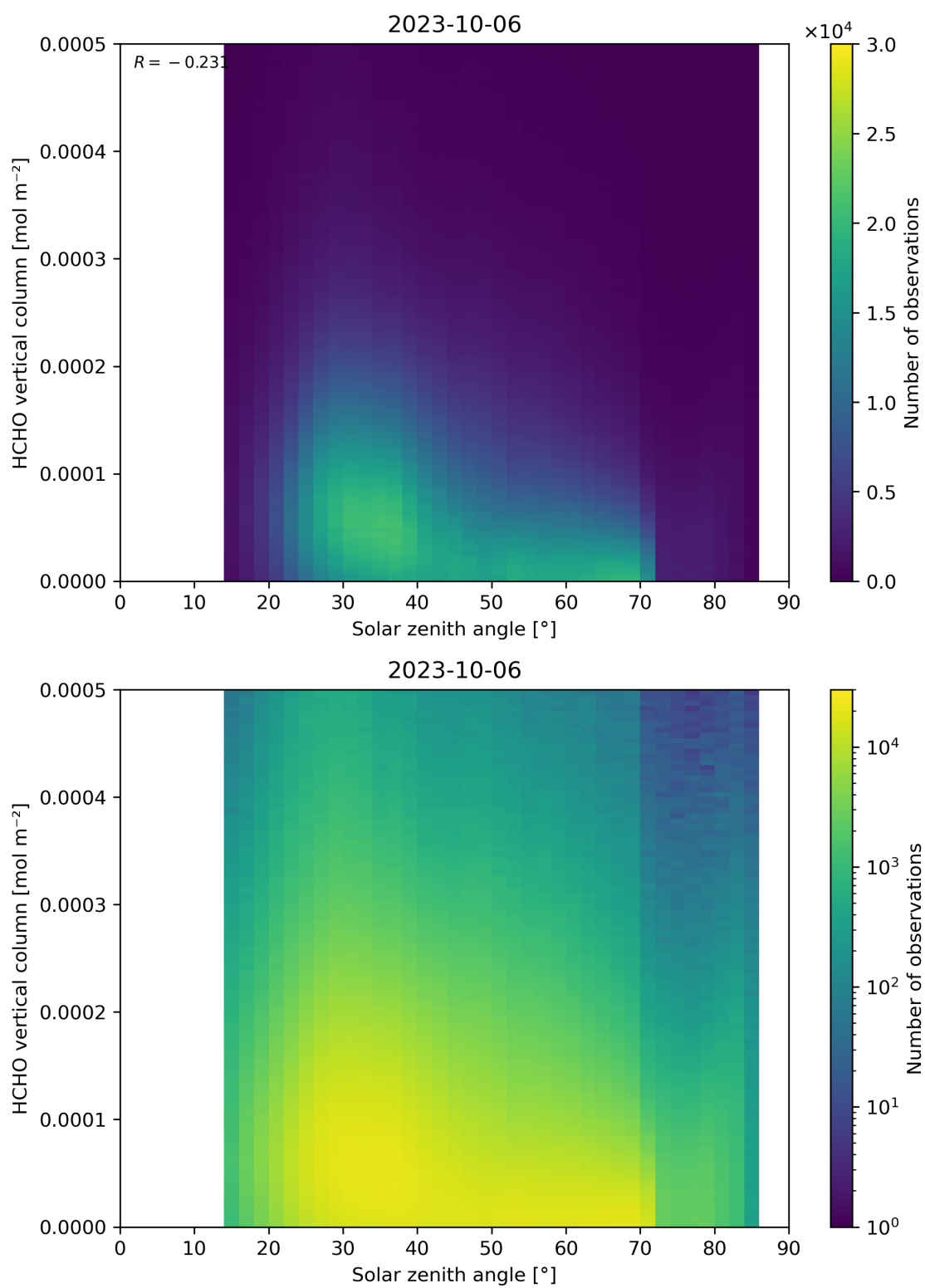
Figure 177: Scatter density plot of “Solar zenith angle” against “HCHO vertical column” for 2023-10-06 to 2023-10-07.
