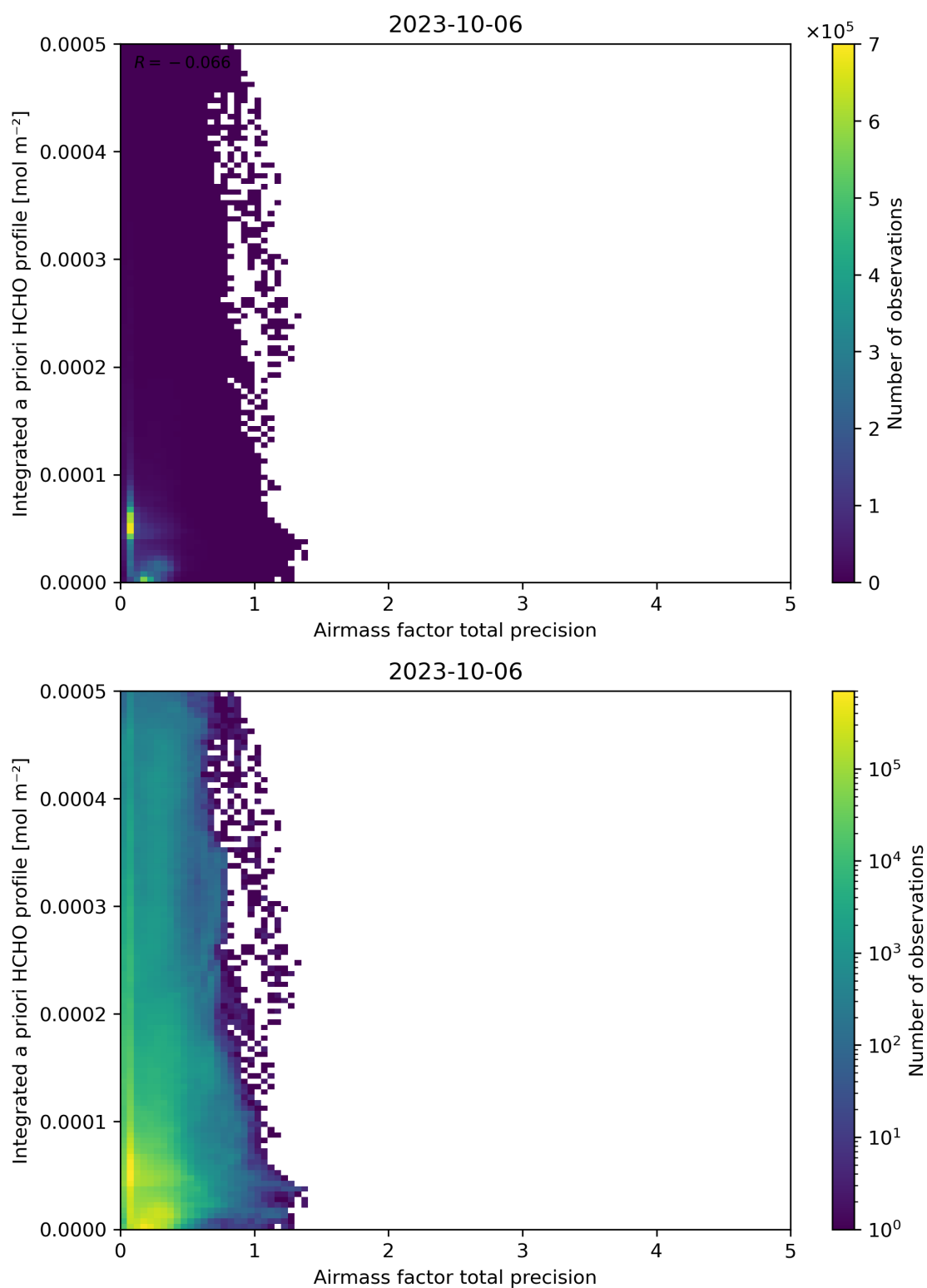
Figure 111: Scatter density plot of “Airmass factor total precision” against “Integrated a priori HCHO profile” for 2023-10-06 to 2023-10-07.
