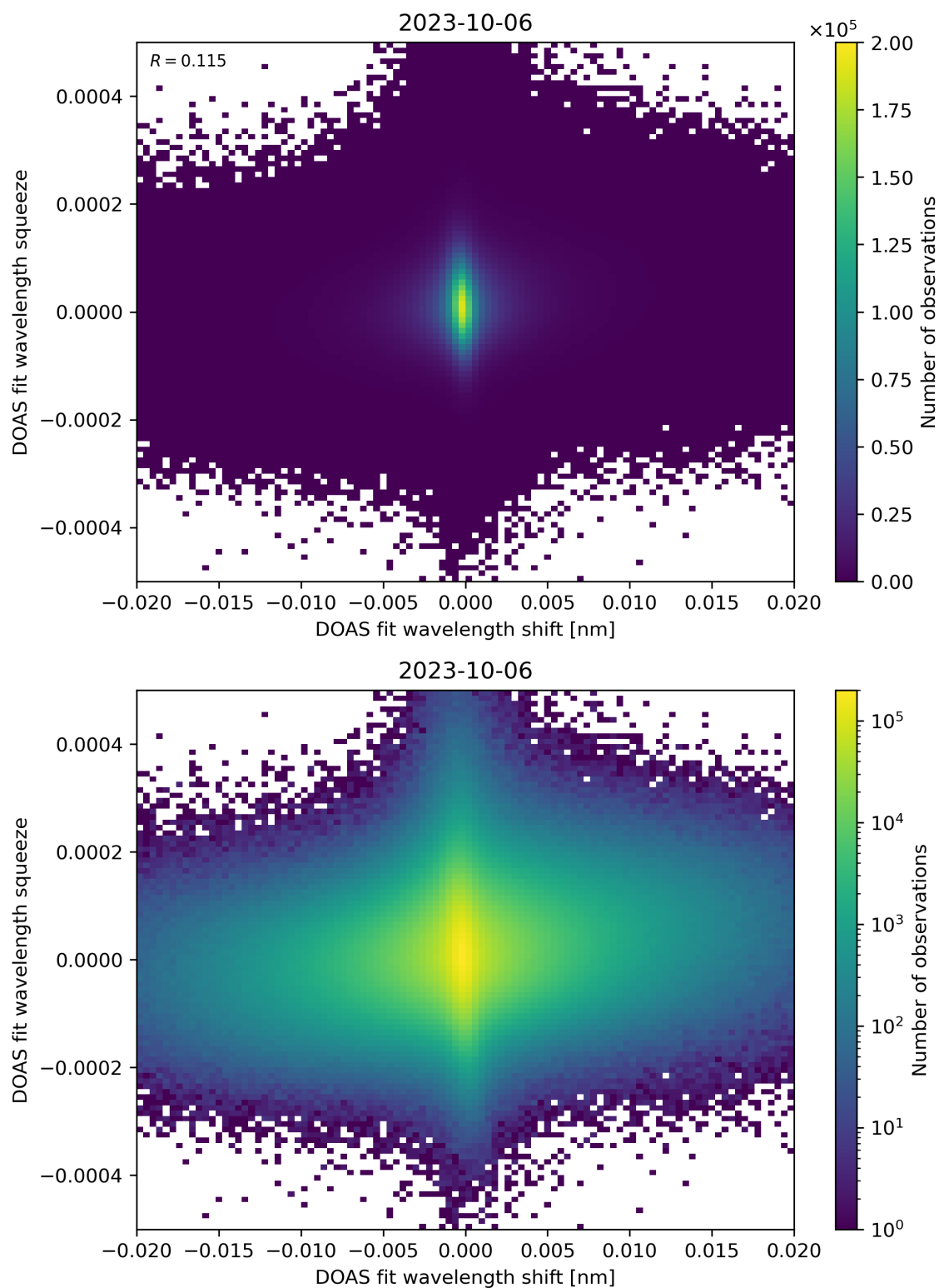
Figure 65: Scatter density plot of “DOAS fit wavelength shift” against “DOAS fit wavelength squeeze” for 2023-10-06 to 2023-10-07.
