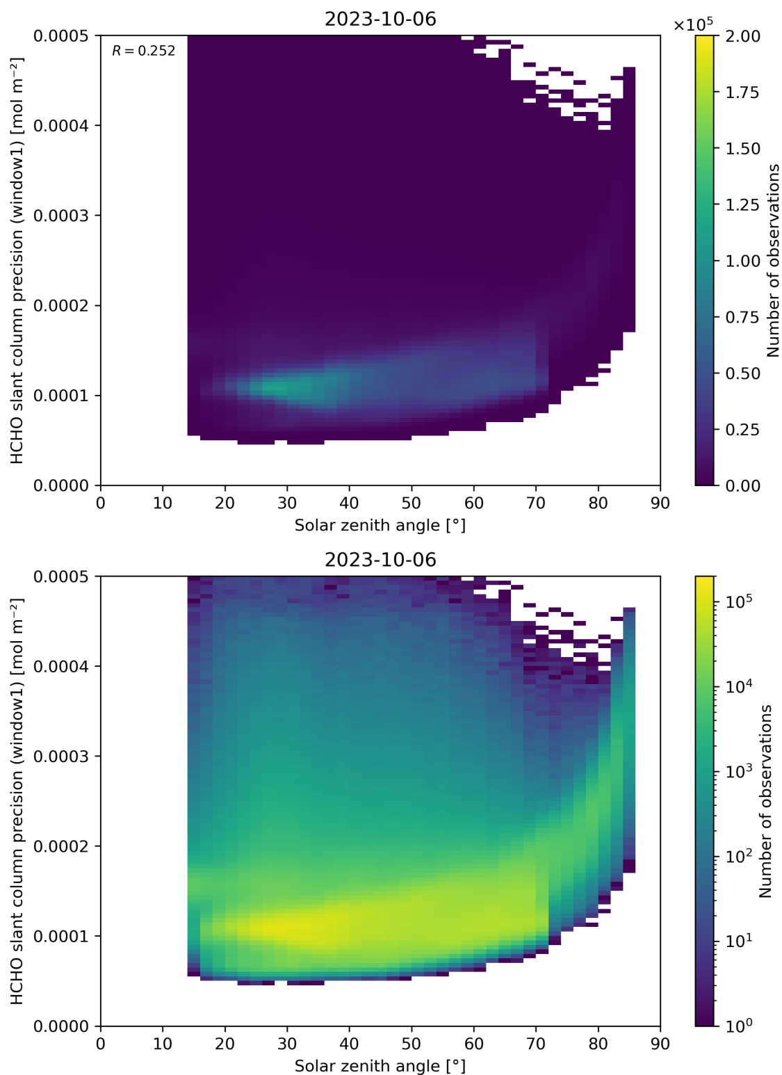
Figure 174: Scatter density plot of “Solar zenith angle” against “HCHO slant column precision (window1)” for 2023-10-06 to 2023-10-07.
