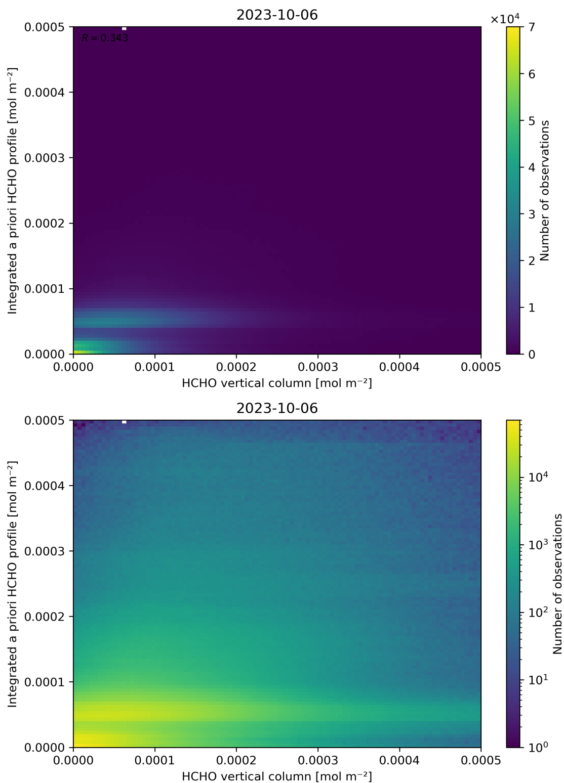
Figure 135: Scatter density plot of “HCHO vertical column” against “Integrated a priori HCHO profile” for 2023-10-06 to 2023-10-07.
