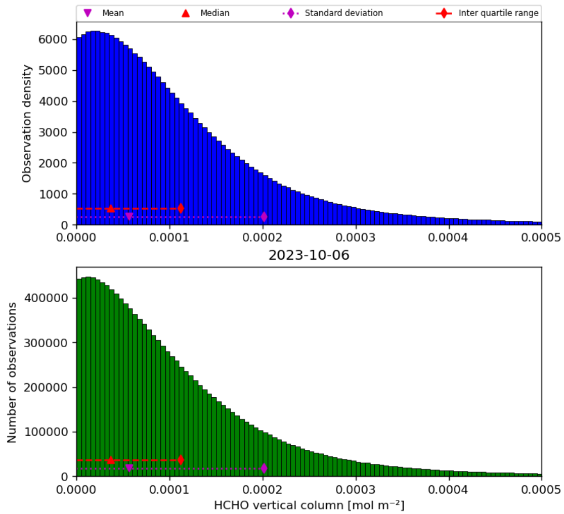
Figure 35: Histogram of “HCHO vertical column” for 2023-10-06 to 2023-10-07
