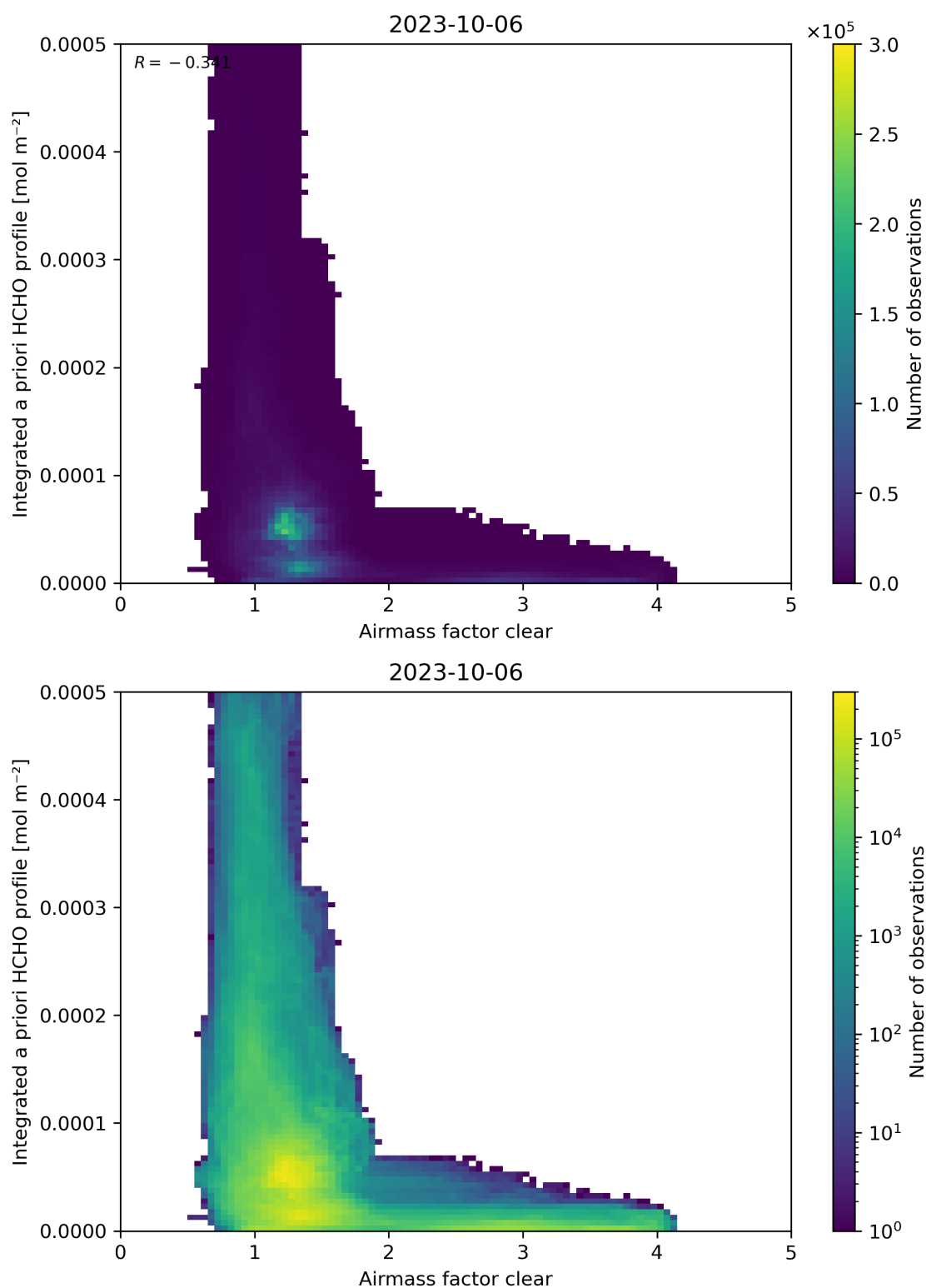
Figure 76: Scatter density plot of “Airmass factor clear” against “Integrated a priori HCHO profile” for 2023-10-06 to 2023-10-07.
