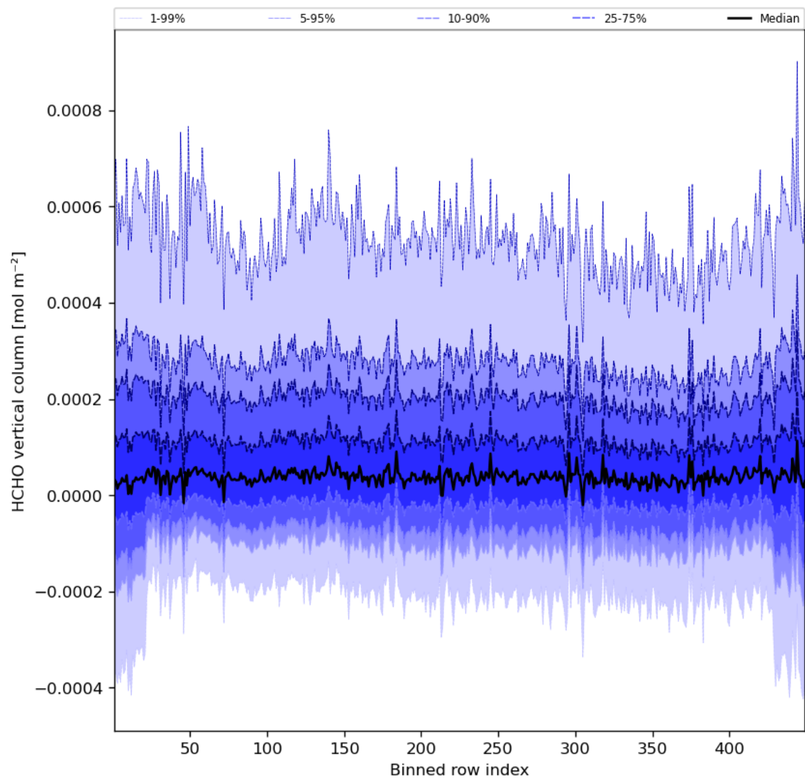
Figure 49: Along track statistics of “HCHO vertical column” for 2023-10-06 to 2023-10-07
