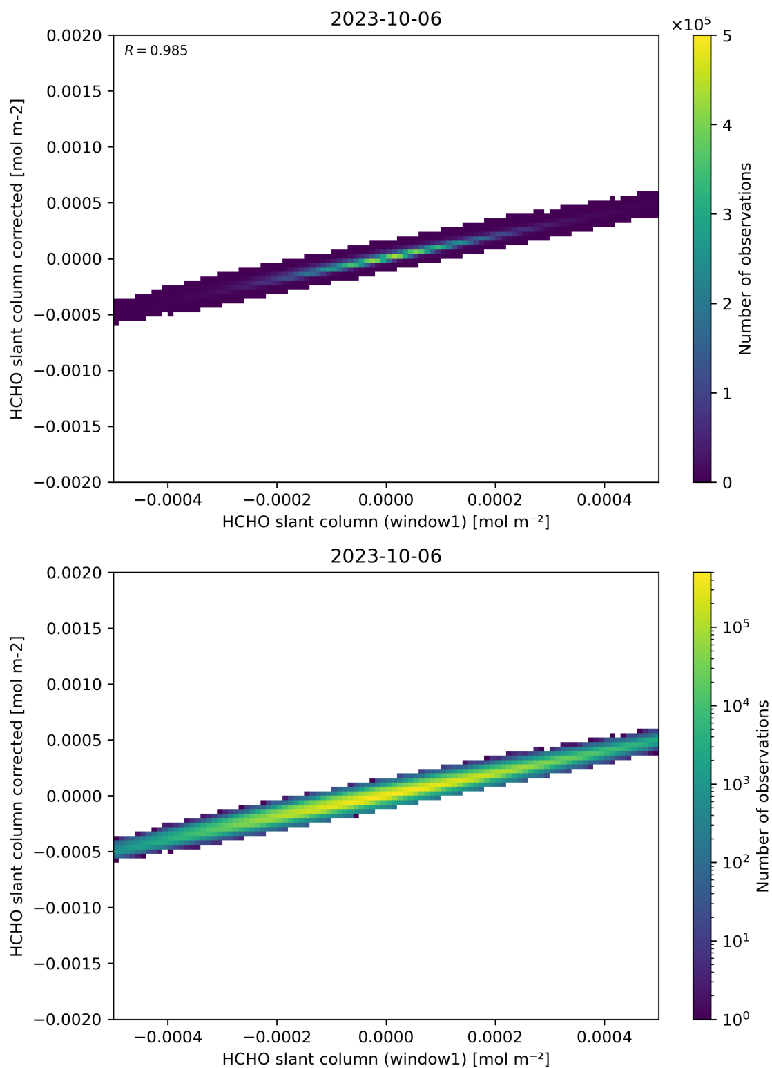
Figure 82: Scatter density plot of “HCHO slant column (window1)” against “HCHO slant column corrected” for 2023-10-06 to 2023-10-07.
