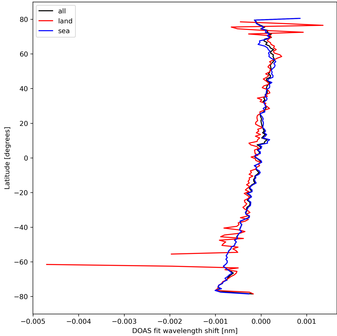
Figure 30: Zonal average of “DOAS fit wavelength shift” for 2023-10-06 to 2023-10-07.
