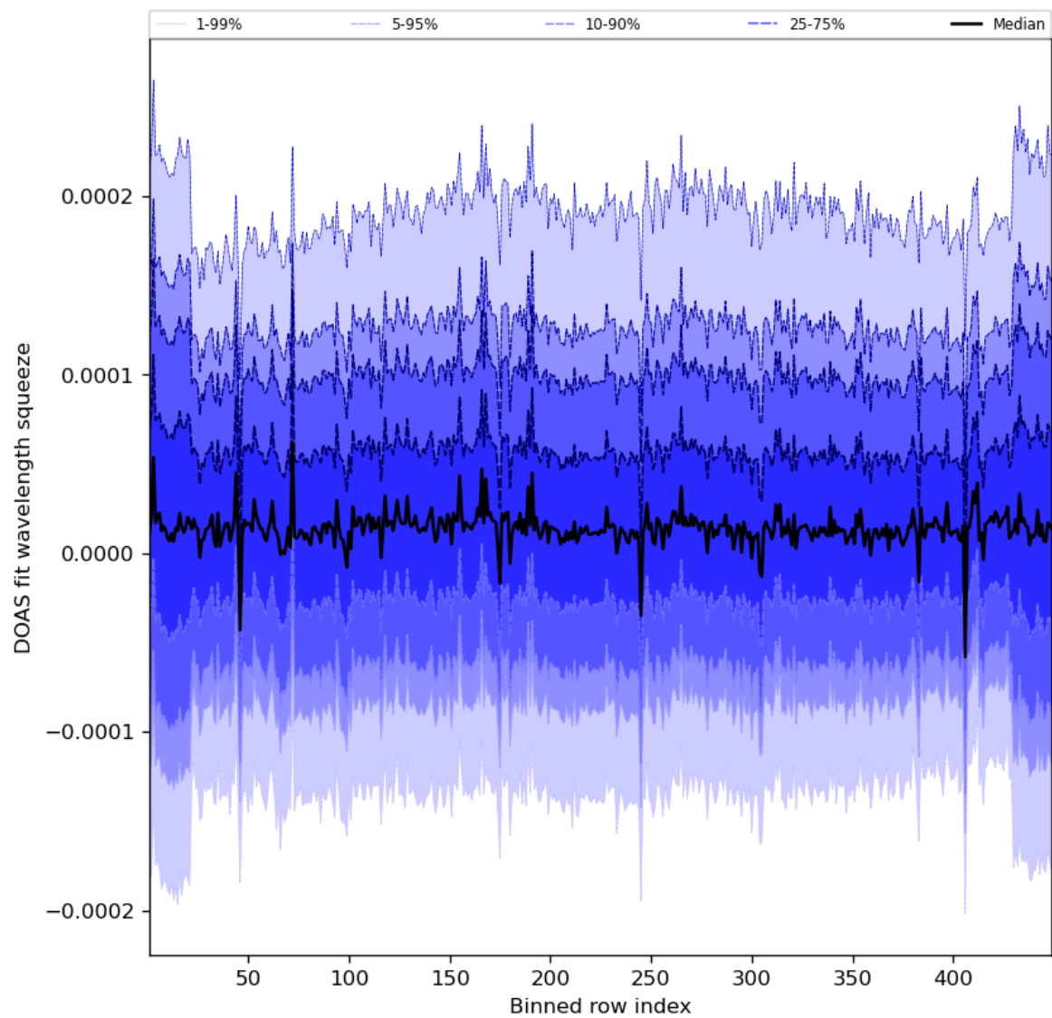
Figure 59: Along track statistics of “DOAS fit wavelength squeeze” for 2023-10-06 to 2023-10-07
