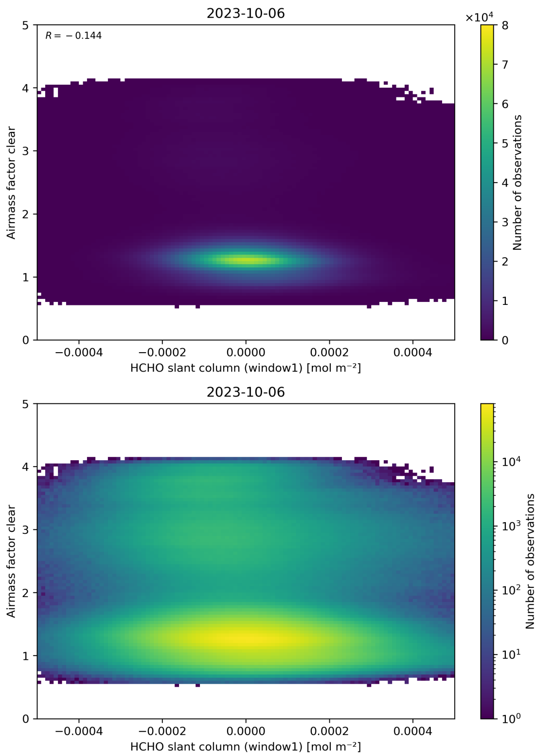
Figure 81: Scatter density plot of “HCHO slant column (window1)” against “Airmass factor clear” for 2023-10-06 to 2023-10-07.
