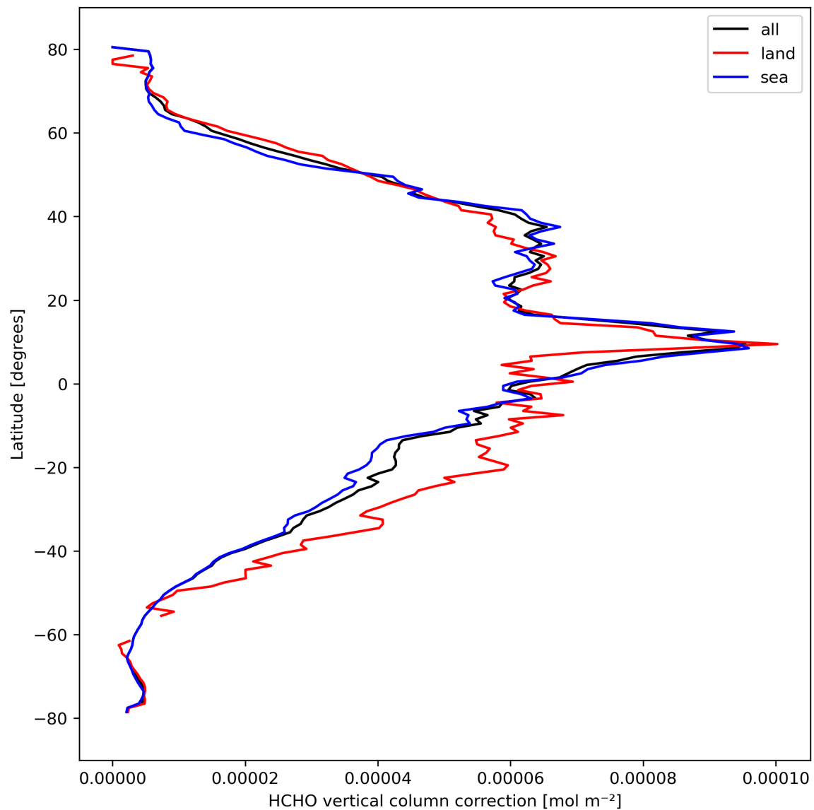
Figure 23: Zonal average of “HCHO vertical column correction” for 2023-10-06 to 2023-10-07.
