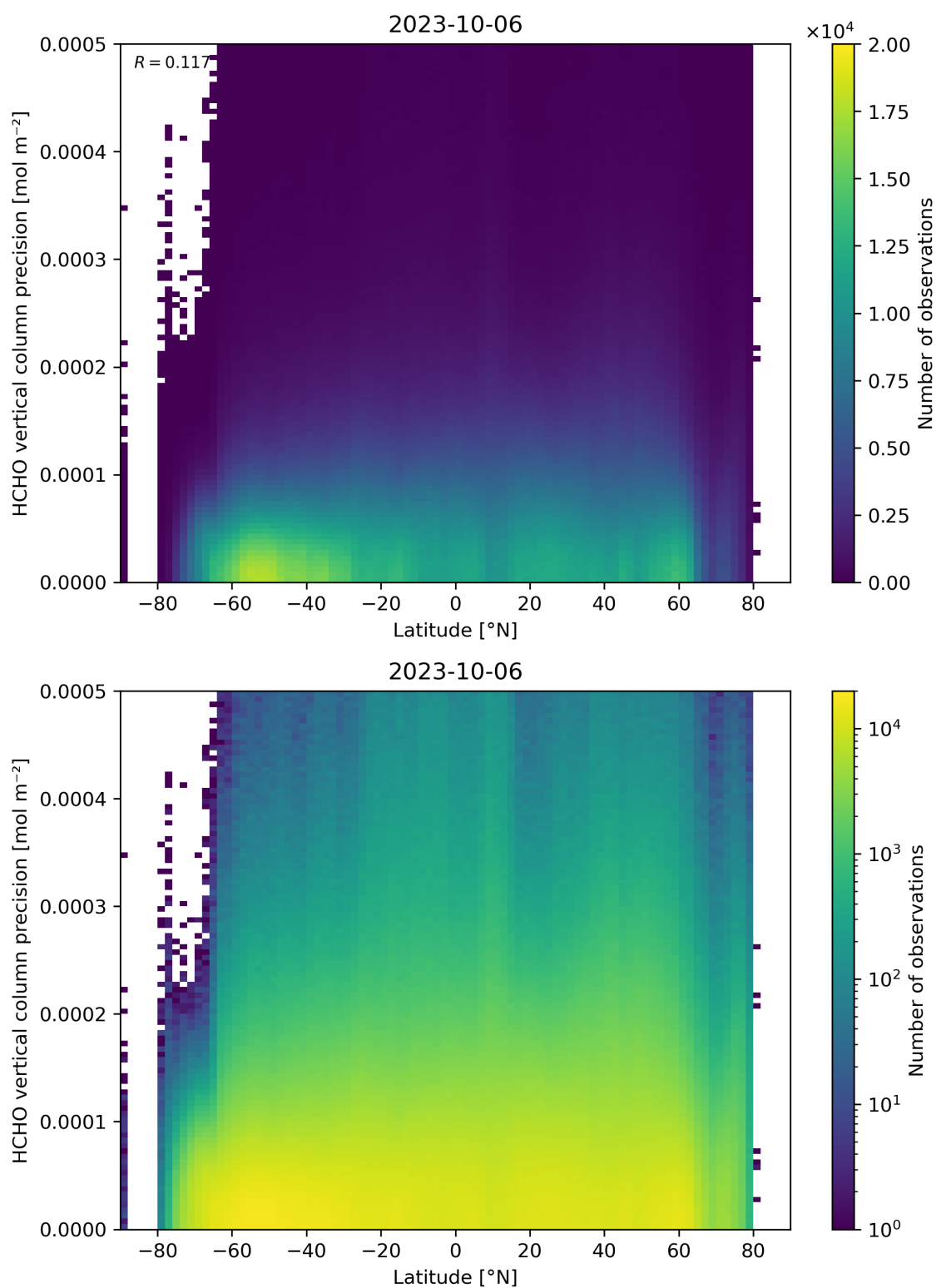
Figure 165: Scatter density plot of “Latitude” against “HCHO vertical column precision” for 2023-10-06 to 2023-10-07.
