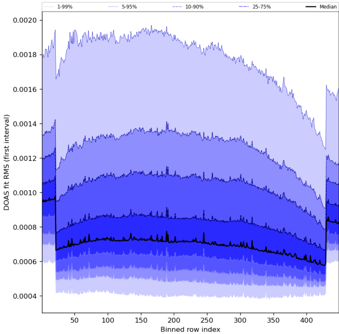
Figure 60: Along track statistics of “DOAS fit RMS (first interval)” for 2023-10-06 to 2023-10-07
