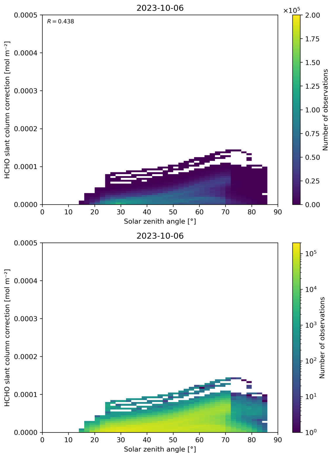
Figure 172: Scatter density plot of “Solar zenith angle” against “HCHO slant column correction” for 2023-10-06 to 2023-10-07.
