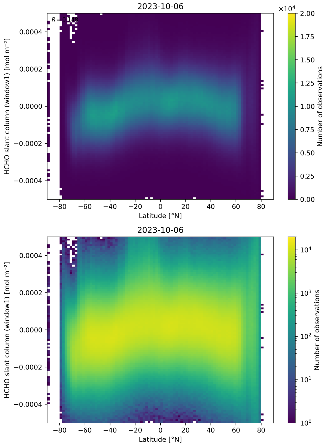
Figure 159: Scatter density plot of “Latitude” against “HCHO slant column (window1)” for 2023-10-06 to 2023-10-07.
