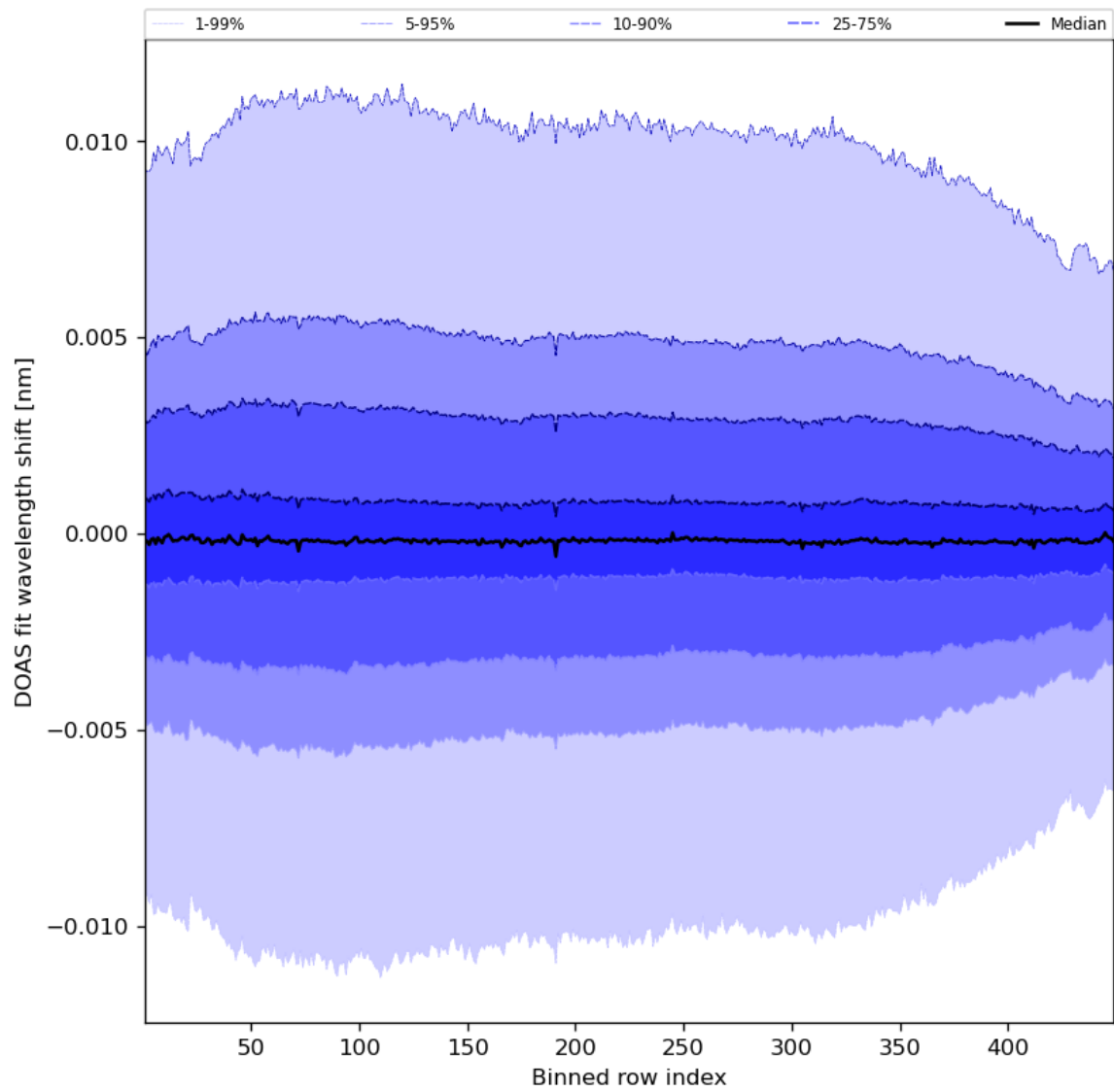
Figure 58: Along track statistics of “DOAS fit wavelength shift” for 2023-10-06 to 2023-10-07
