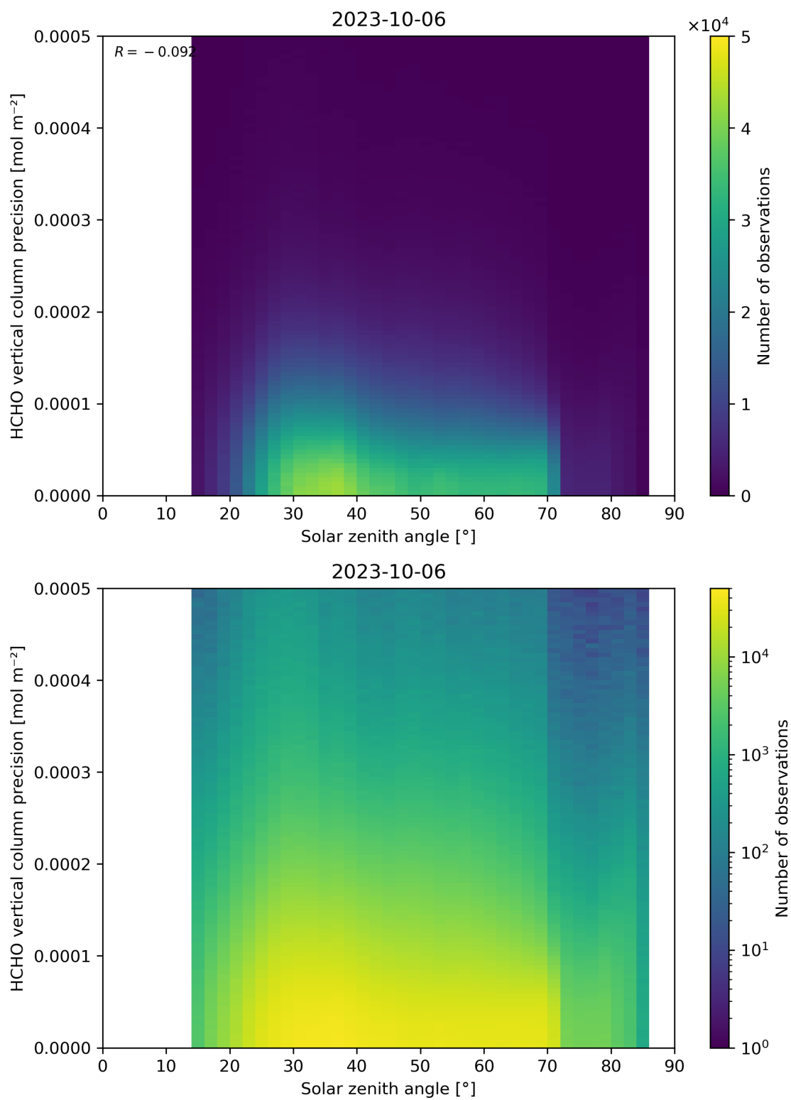
Figure 179: Scatter density plot of “Solar zenith angle” against “HCHO vertical column precision” for 2023-10-06 to 2023-10-07.
