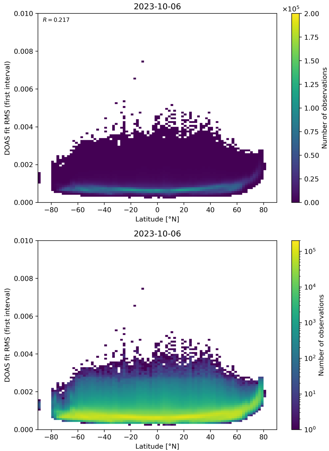
Figure 153: Scatter density plot of “Latitude” against “DOAS fit RMS (first interval)” for 2023-10-06 to 2023-10-07.
