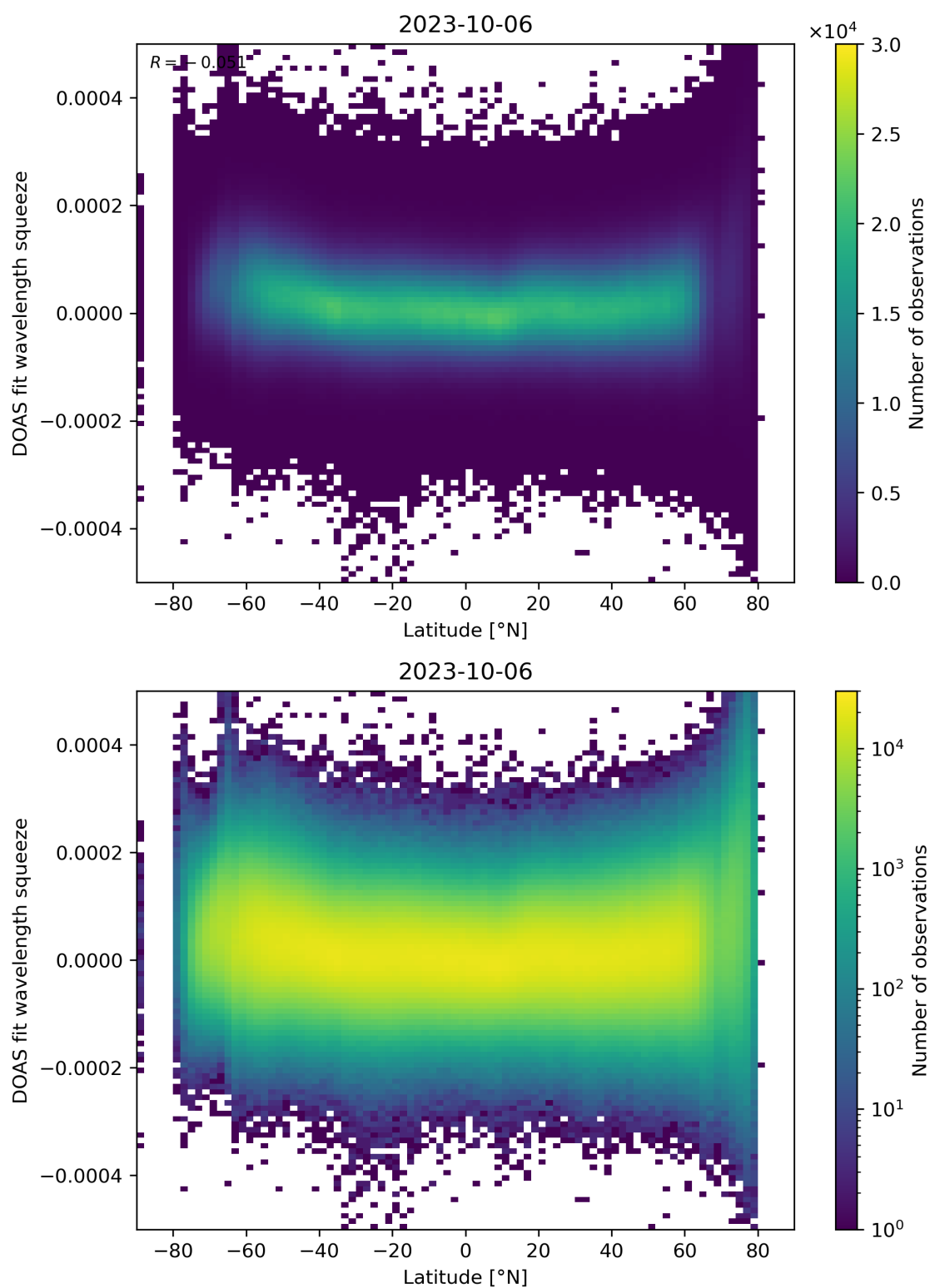
Figure 155: Scatter density plot of “Latitude” against “DOAS fit wavelength squeeze” for 2023-10-06 to 2023-10-07.
