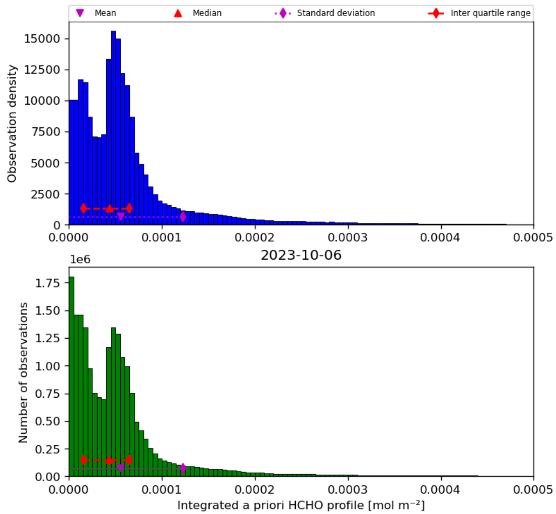
Figure 43: Histogram of “Integrated a priori HCHO profile” for 2023-10-06 to 2023-10-07
