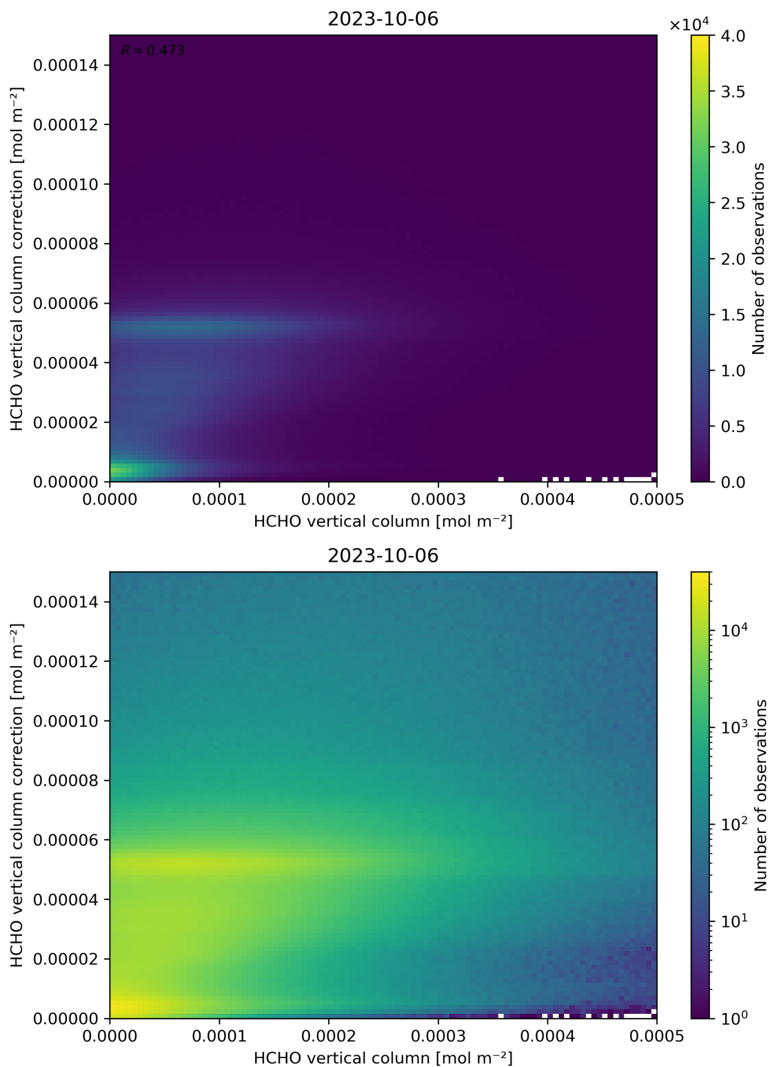
Figure 133: Scatter density plot of “HCHO vertical column” against “HCHO vertical column correction” for 2023-10-06 to 2023-10-07.
