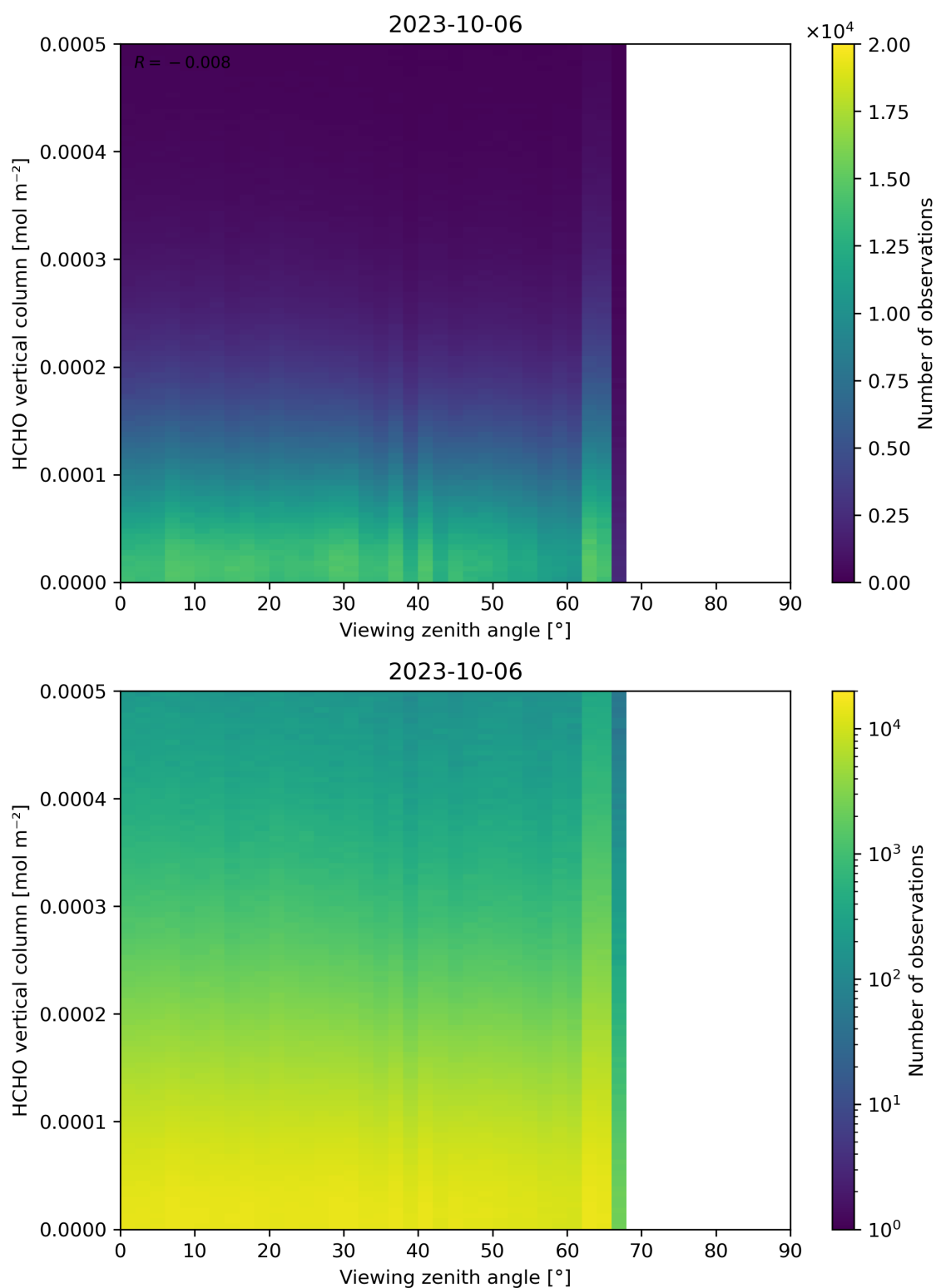
Figure 192: Scatter density plot of “Viewing zenith angle” against “HCHO vertical column” for 2023-10-06 to 2023-10-07.
