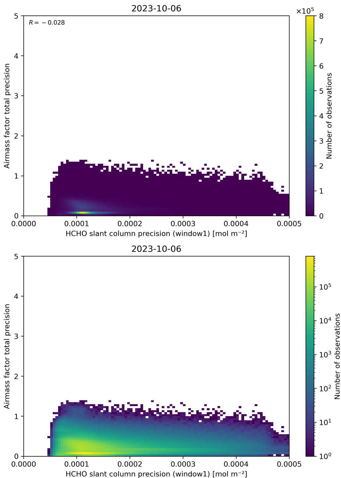
Figure 95: Scatter density plot of “HCHO slant column precision (window1)” against “Airmass factor total precision” for 2023-10-06 to 2023-10-07.
