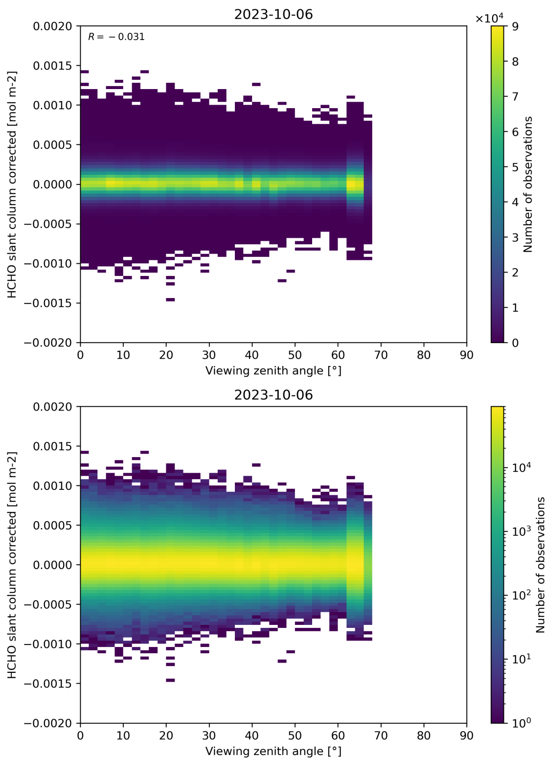
Figure 186: Scatter density plot of “Viewing zenith angle” against “HCHO slant column corrected” for 2023-10-06 to 2023-10-07.
