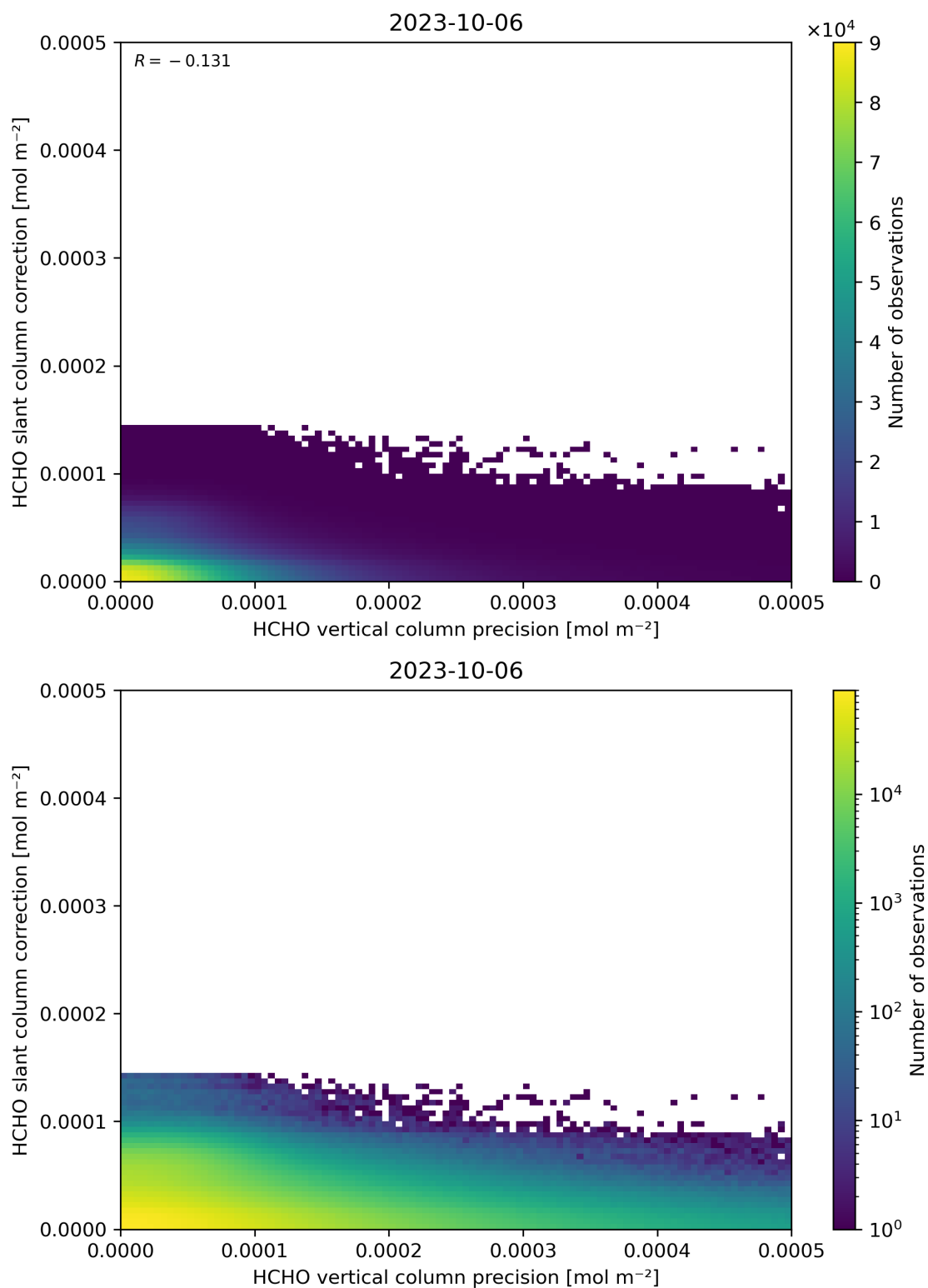
Figure 141: Scatter density plot of “HCHO vertical column precision” against “HCHO slant column correction” for 2023-10-06 to 2023-10-07.
