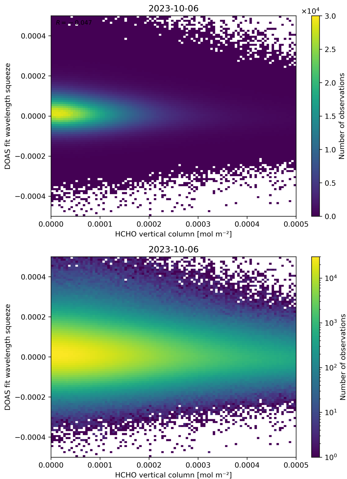
Figure 125: Scatter density plot of “HCHO vertical column” against “DOAS fit wavelength squeeze” for 2023-10-06 to 2023-10-07.
