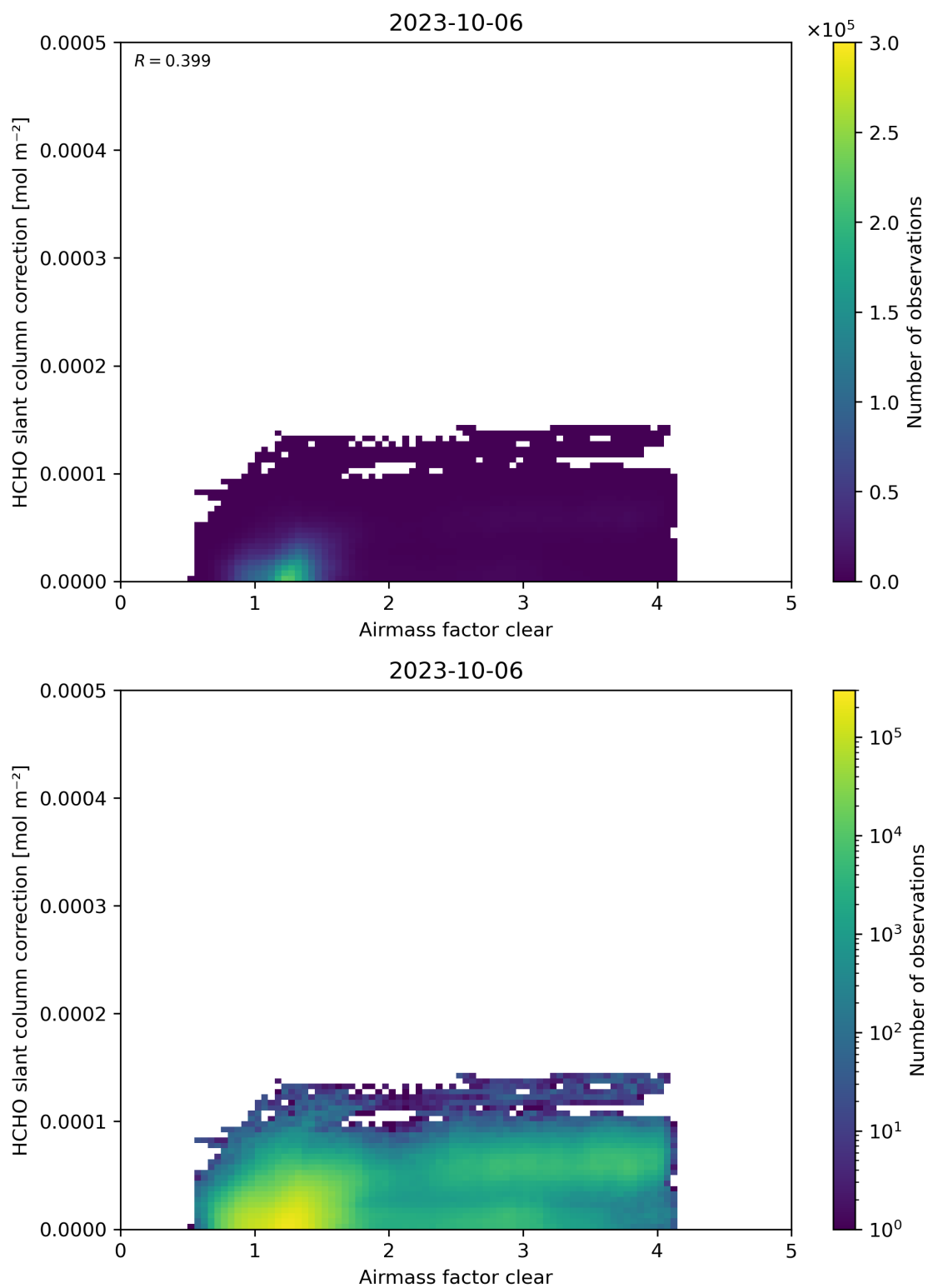
Figure 75: Scatter density plot of “Airmass factor clear” against “HCHO slant column correction” for 2023-10-06 to 2023-10-07.
