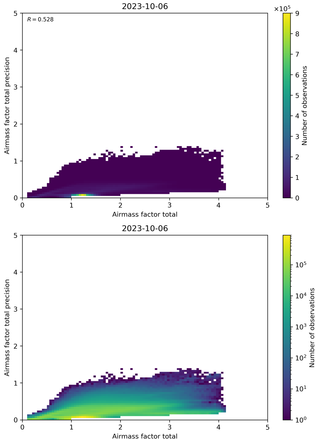
Figure 103: Scatter density plot of “Airmass factor total” against “Airmass factor total precision” for 2023-10-06 to 2023-10-07.
