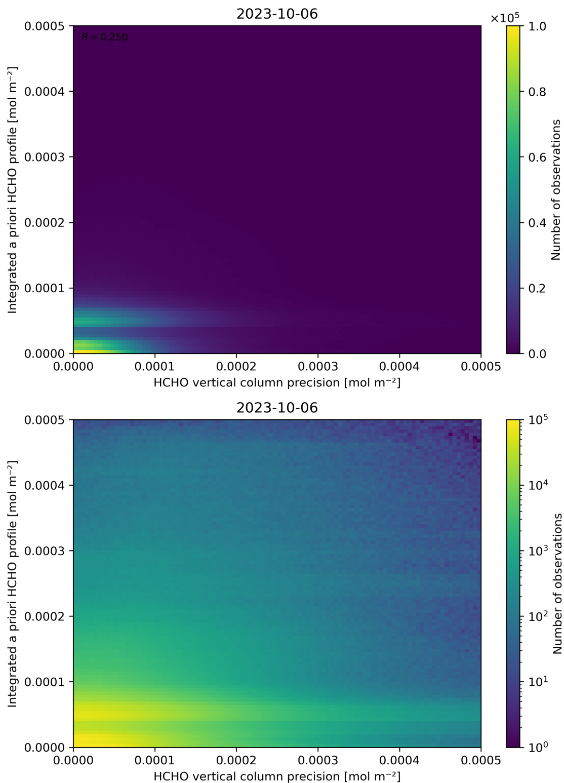
Figure 147: Scatter density plot of “HCHO vertical column precision” against “Integrated a priori HCHO profile” for 2023-10-06 to 2023-10-07.
