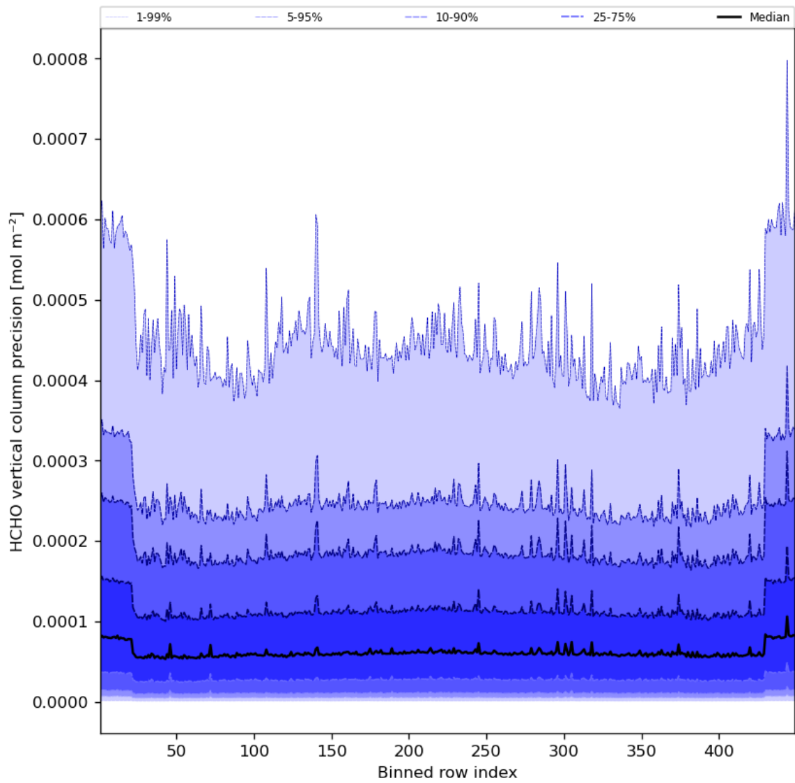
Figure 50: Along track statistics of "HCHO vertical column precision" for 2023-10-06 to 2023-10-07
