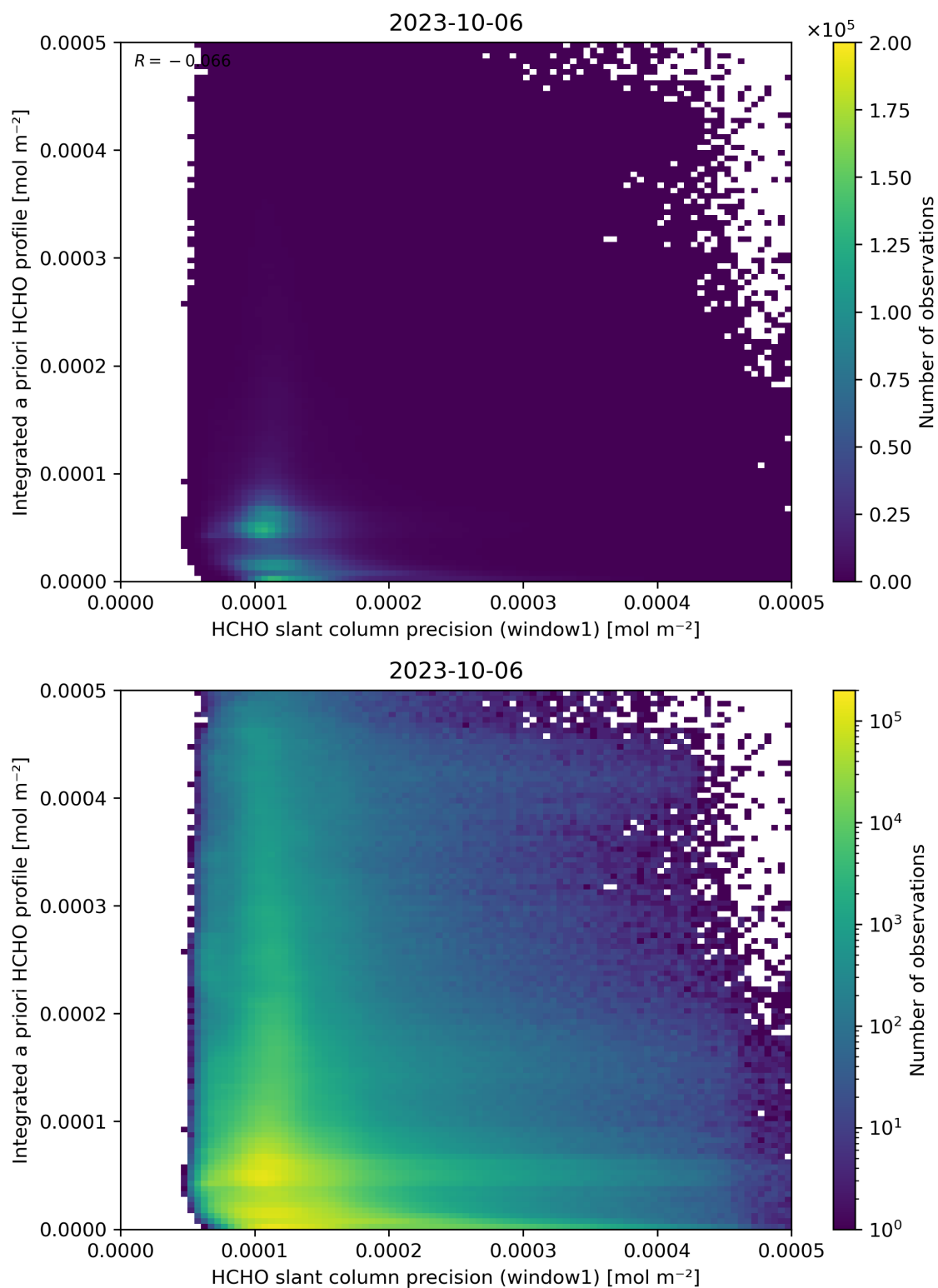
Figure 96: Scatter density plot of “HCHO slant column precision (window1)” against “Integrated a priori HCHO profile” for 2023-10-06 to 2023-10-07.
