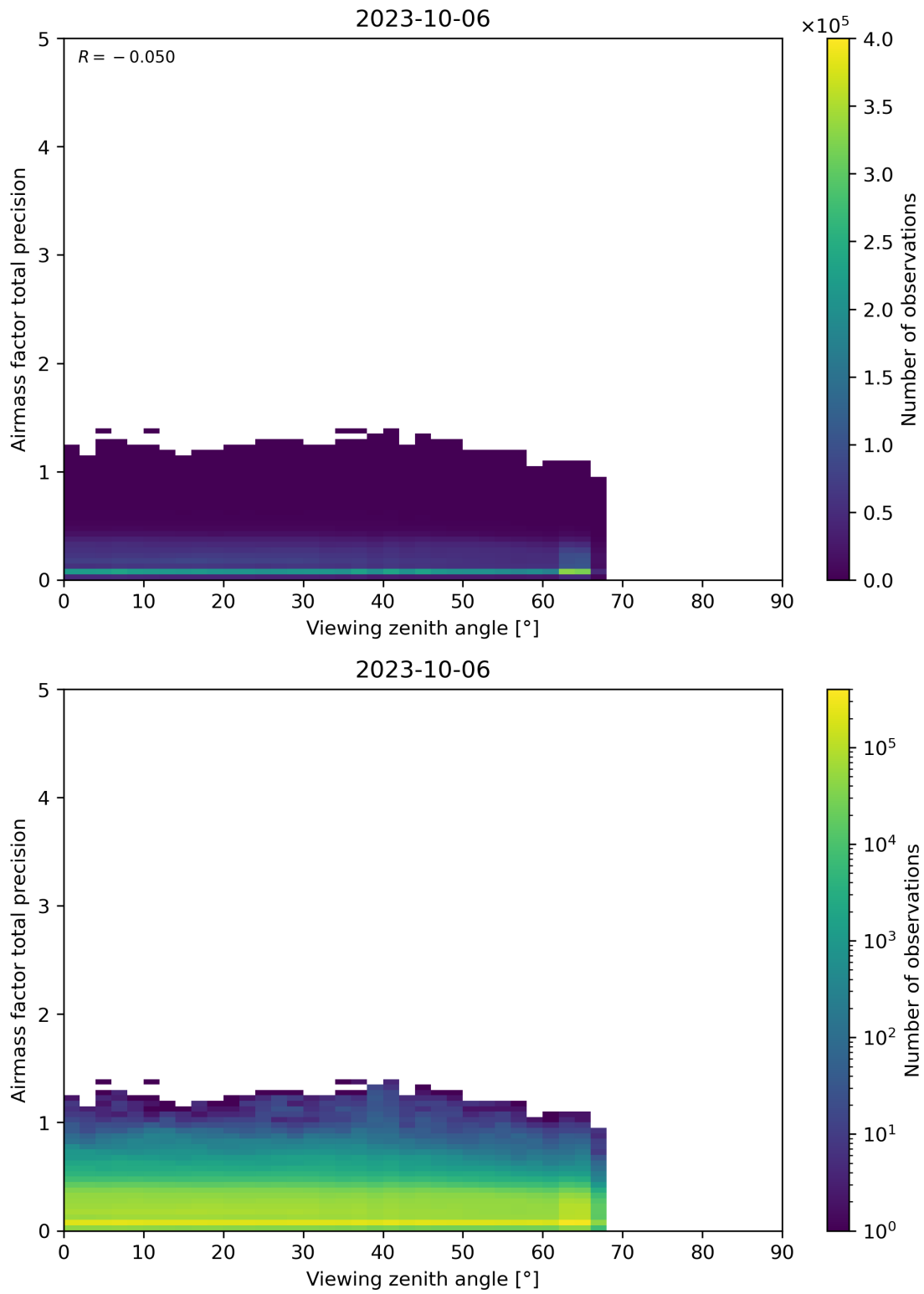
Figure 191: Scatter density plot of “Viewing zenith angle” against “Airmass factor total precision” for 2023-10-06 to 2023-10-07.
