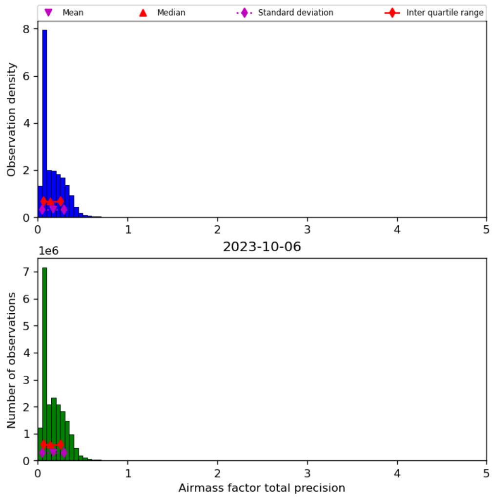
Figure 41: Histogram of “Airmass factor total precision” for 2023-10-06 to 2023-10-07
