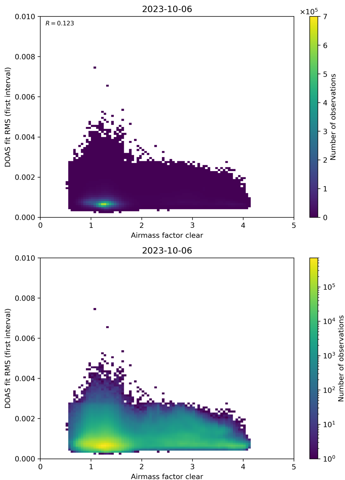
Figure 71: Scatter density plot of “Airmass factor clear” against “DOAS fit RMS (first interval)” for 2023-10-06 to 2023-10-07.
