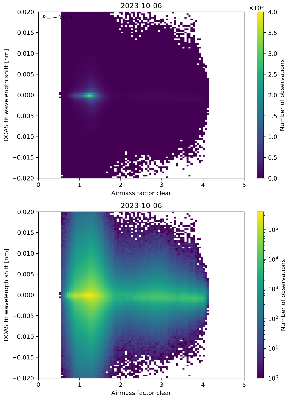
Figure 72: Scatter density plot of “Airmass factor clear” against “DOAS fit wavelength shift” for 2023-10-06 to 2023-10-07.
