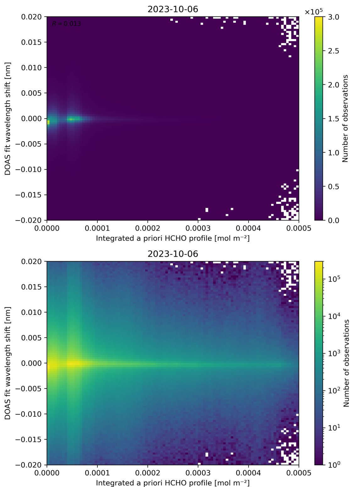
Figure 149: Scatter density plot of “Integrated a priori HCHO profile” against “DOAS fit wavelength shift” for 2023-10-06 to 2023-10-07.
