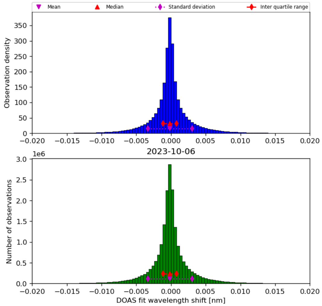
Figure 44: Histogram of “DOAS fit wavelength shift” for 2023-10-06 to 2023-10-07
