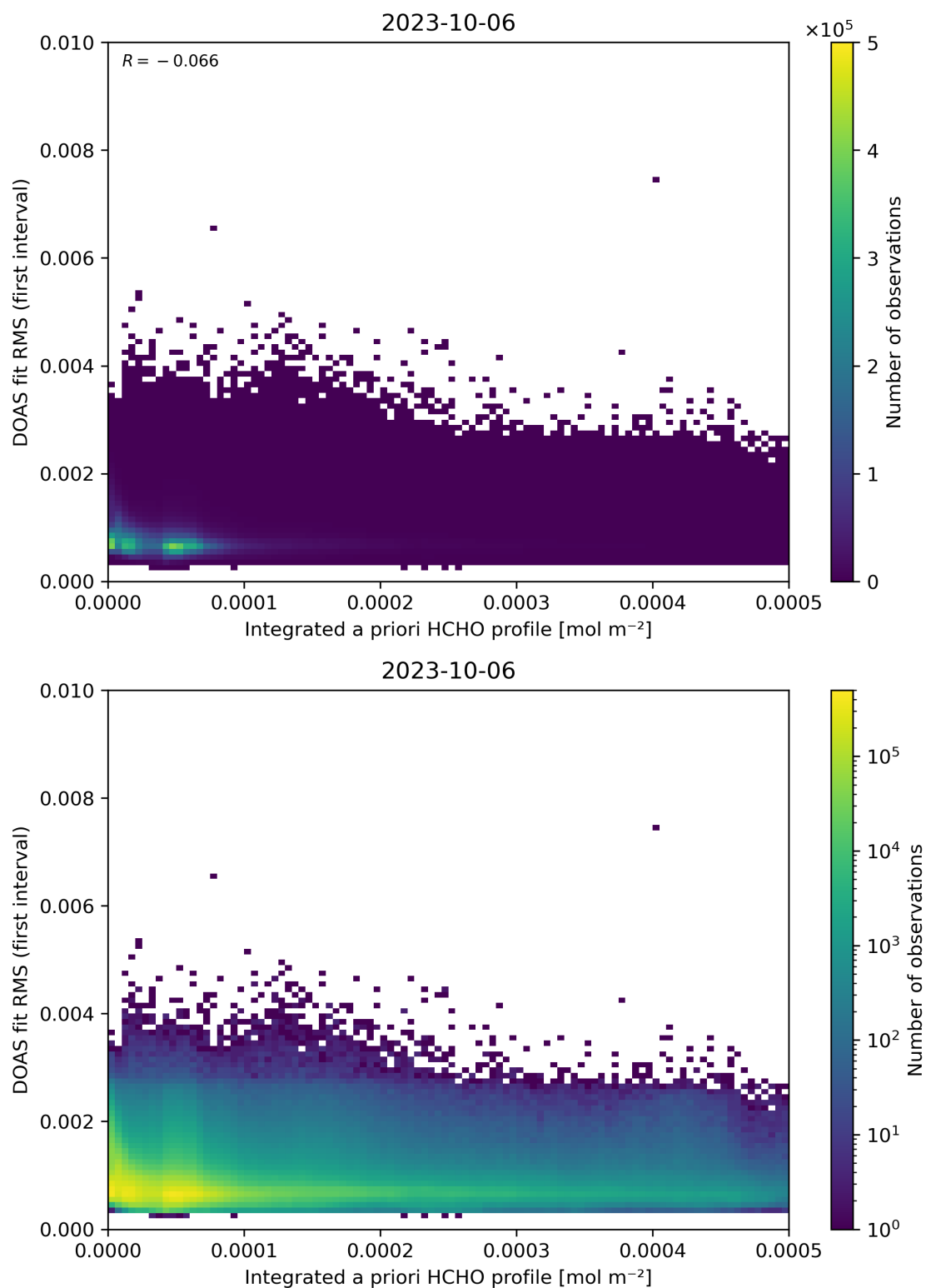
Figure 148: Scatter density plot of “Integrated a priori HCHO profile” against “DOAS fit RMS (first interval)” for 2023-10-06 to 2023-10-07.
