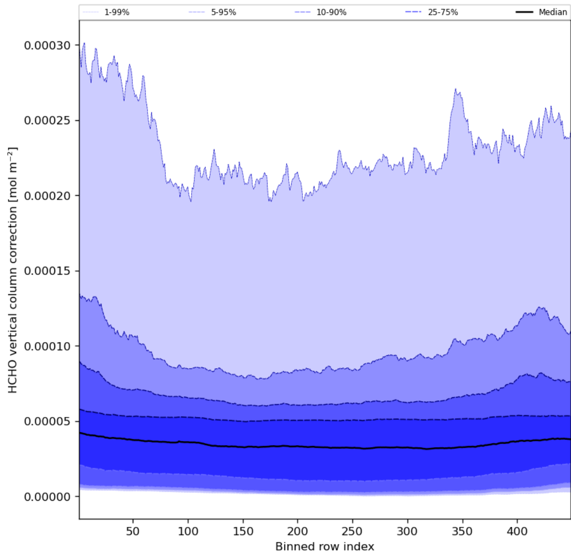
Figure 51: Along track statistics of “HCHO vertical column correction” for 2023-10-06 to 2023-10-07
