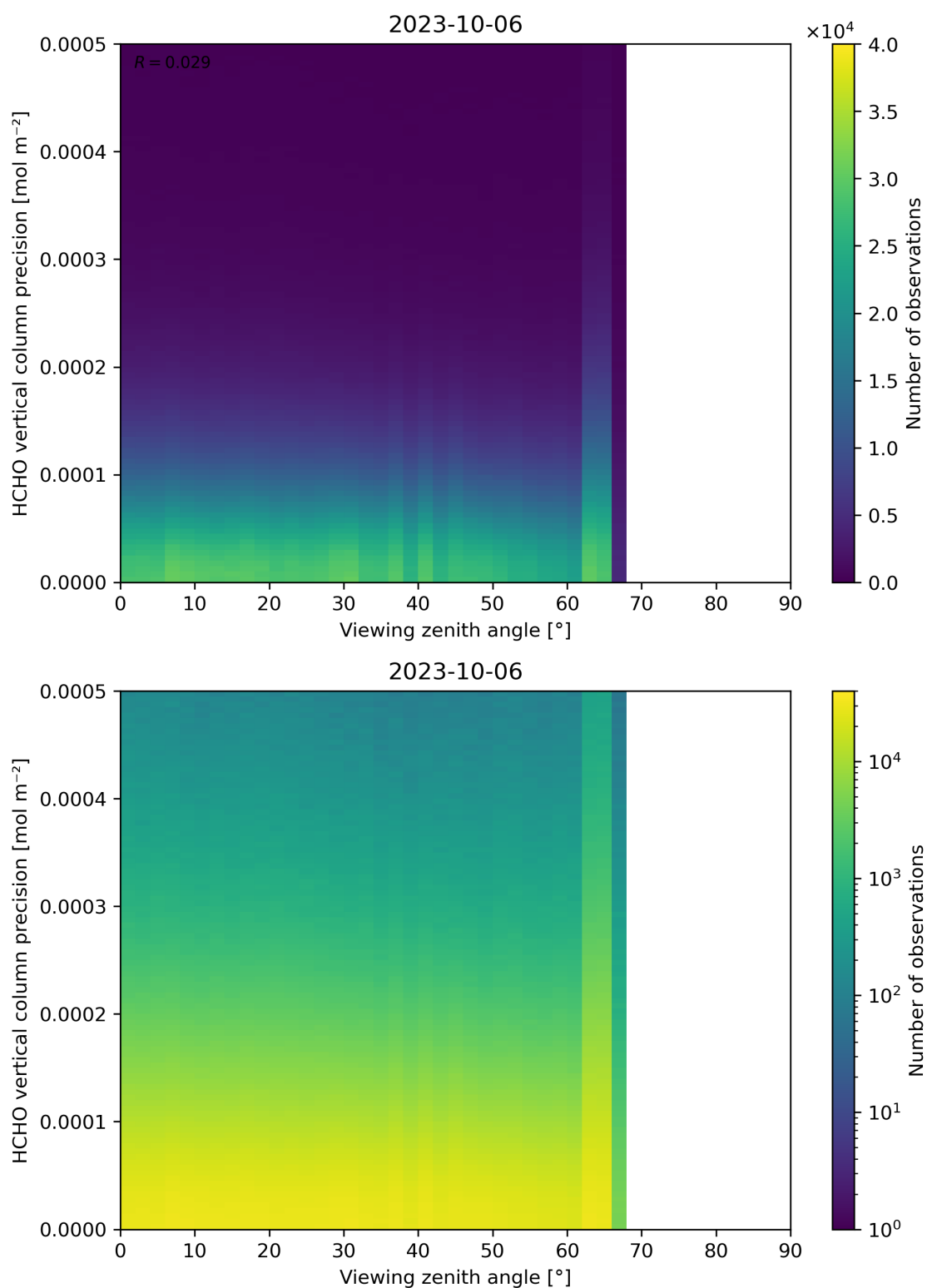
Figure 194: Scatter density plot of “Viewing zenith angle” against “HCHO vertical column precision” for 2023-10-06 to 2023-10-07.
