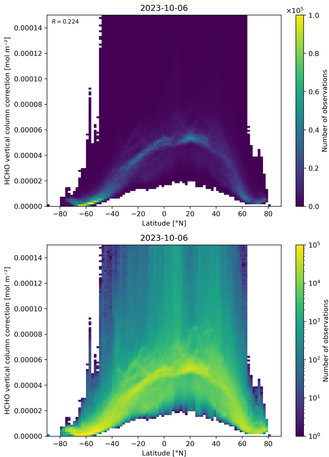
Figure 164: Scatter density plot of “Latitude” against “HCHO vertical column correction” for 2023-10-06 to 2023-10-07.
