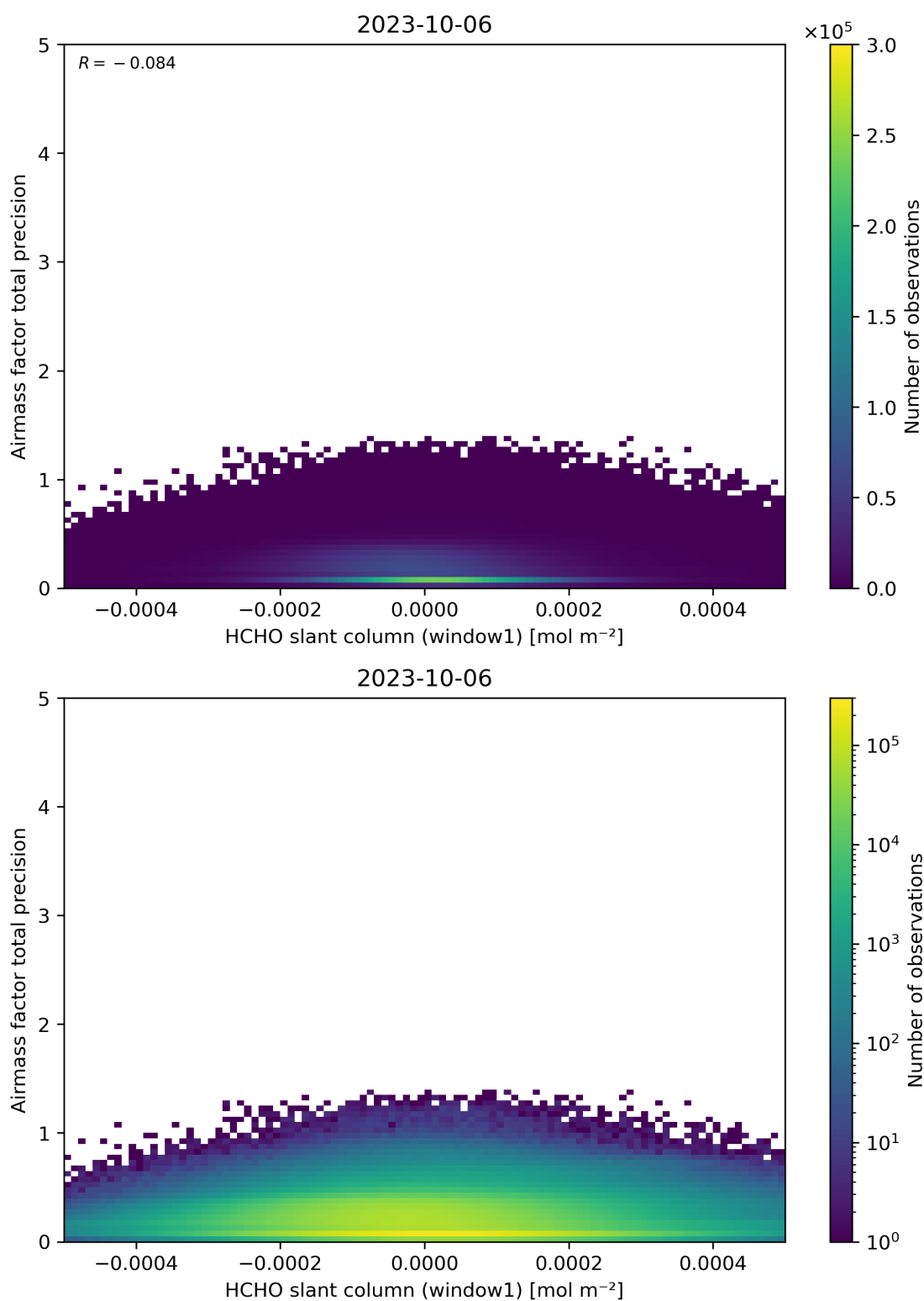
Figure 86: Scatter density plot of “HCHO slant column (window1)” against “Airmass factor total precision” for 2023-10-06 to 2023-10-07.
