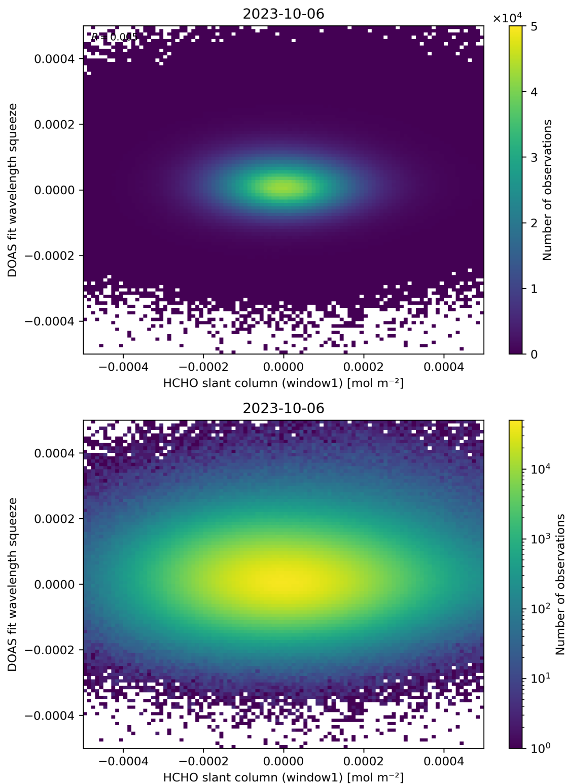
Figure 80: Scatter density plot of “HCHO slant column (window1)” against “DOAS fit wavelength squeeze” for 2023-10-06 to 2023-10-07.
