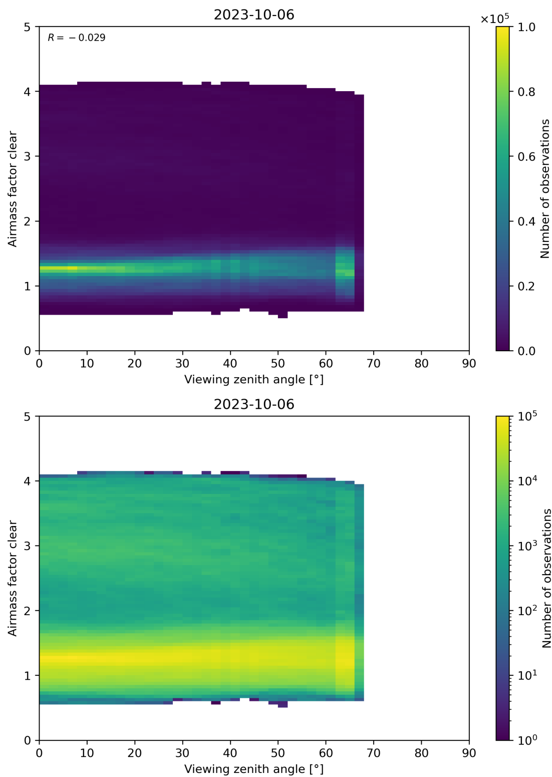
Figure 185: Scatter density plot of “Viewing zenith angle” against “Airmass factor clear” for 2023-10-06 to 2023-10-07.
