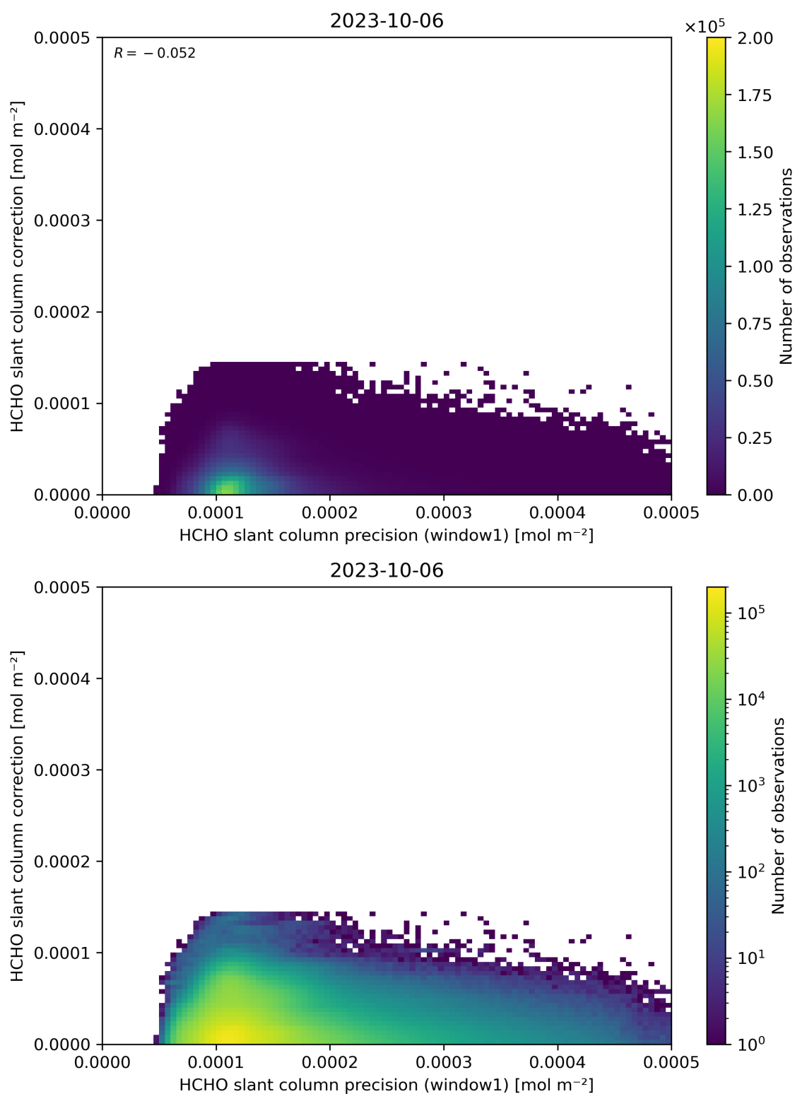
Figure 93: Scatter density plot of “HCHO slant column precision (window1)” against “HCHO slant column correction” for 2023-10-06 to 2023-10-07.
