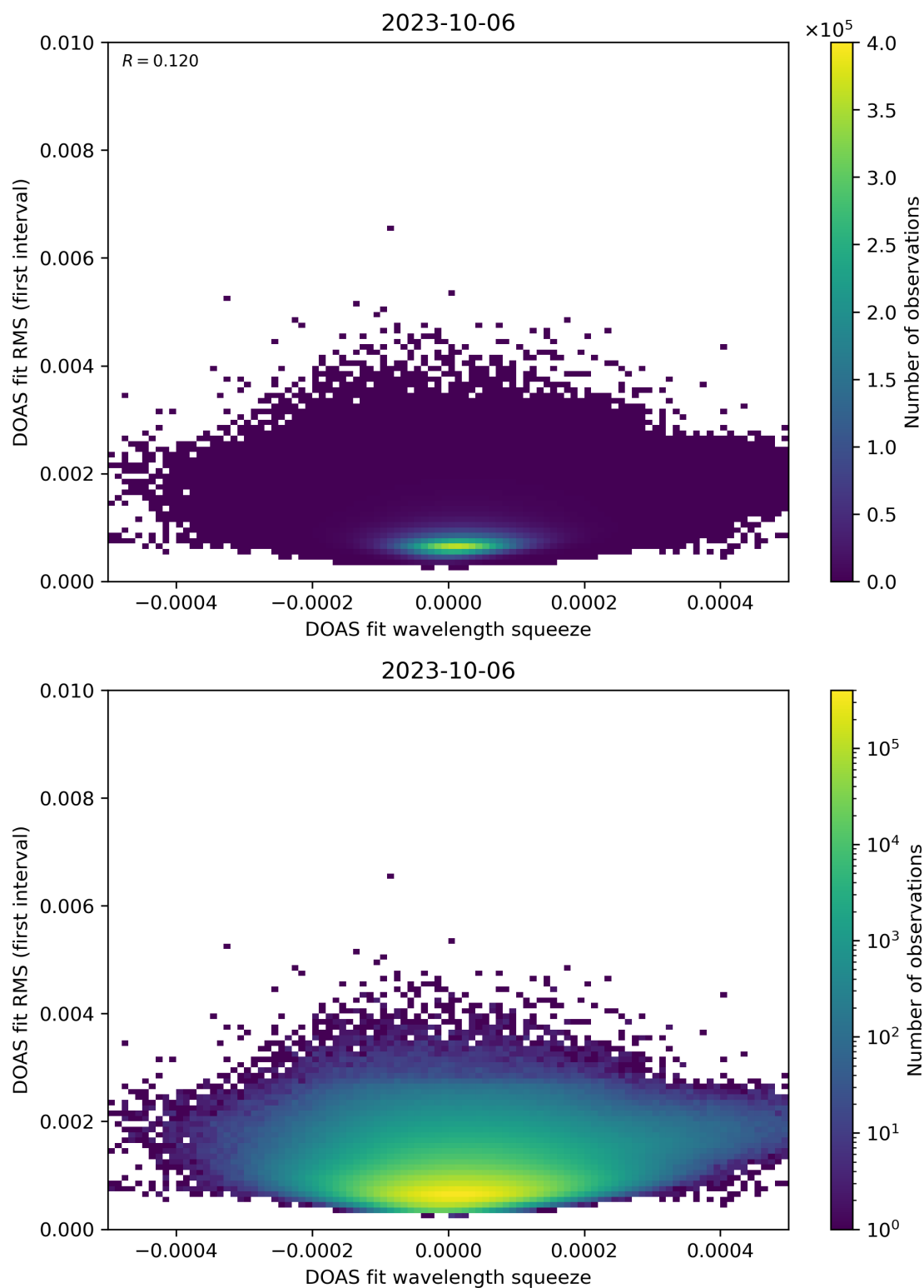
Figure 68: Scatter density plot of “DOAS fit wavelength squeeze” against “DOAS fit RMS (first interval)” for 2023-10-06 to 2023-10-07.
