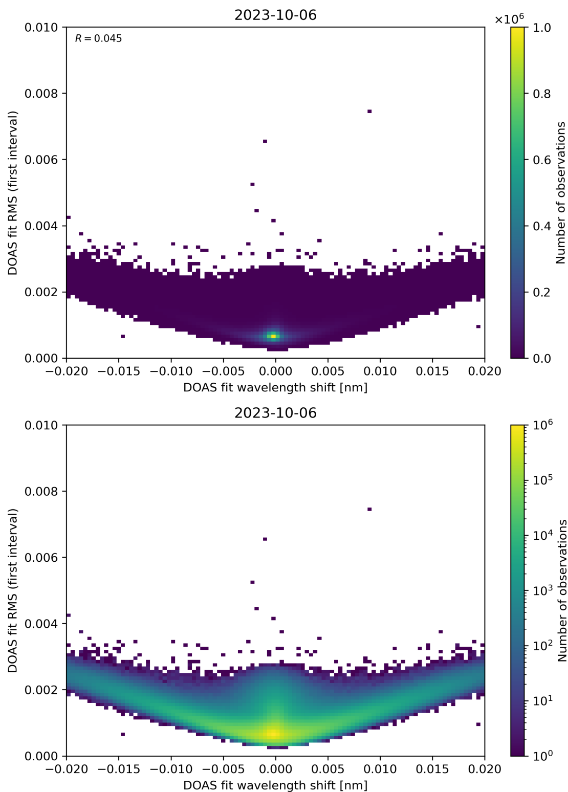
Figure 64: Scatter density plot of “DOAS fit wavelength shift” against “DOAS fit RMS (first interval)” for 2023-10-06 to 2023-10-07.
