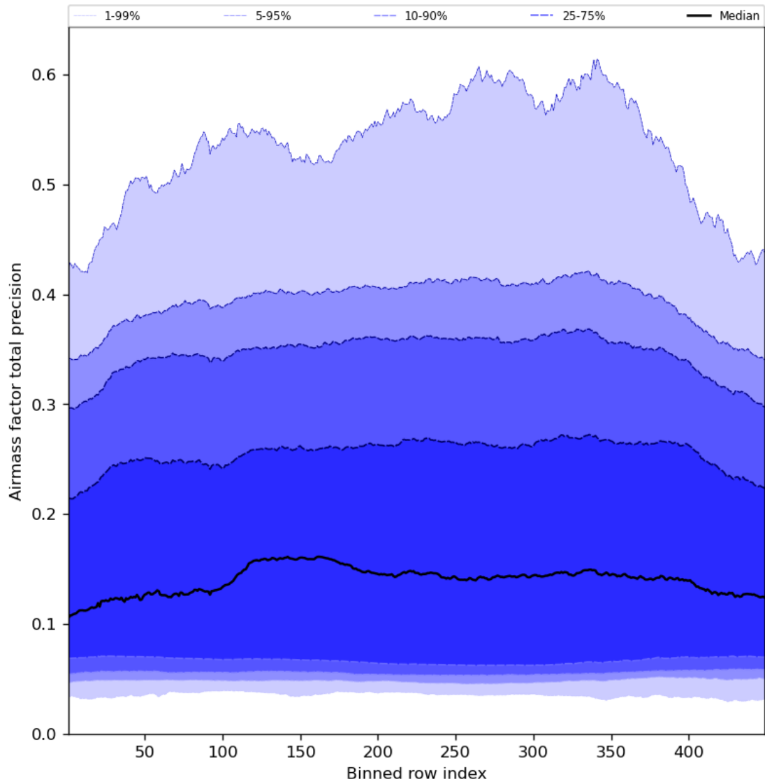
Figure 55: Along track statistics of “Airmass factor total precision” for 2023-10-06 to 2023-10-07
