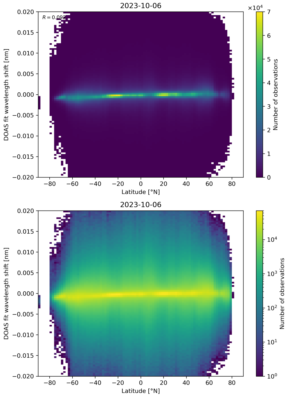
Figure 154: Scatter density plot of “Latitude” against “DOAS fit wavelength shift” for 2023-10-06 to 2023-10-07.
