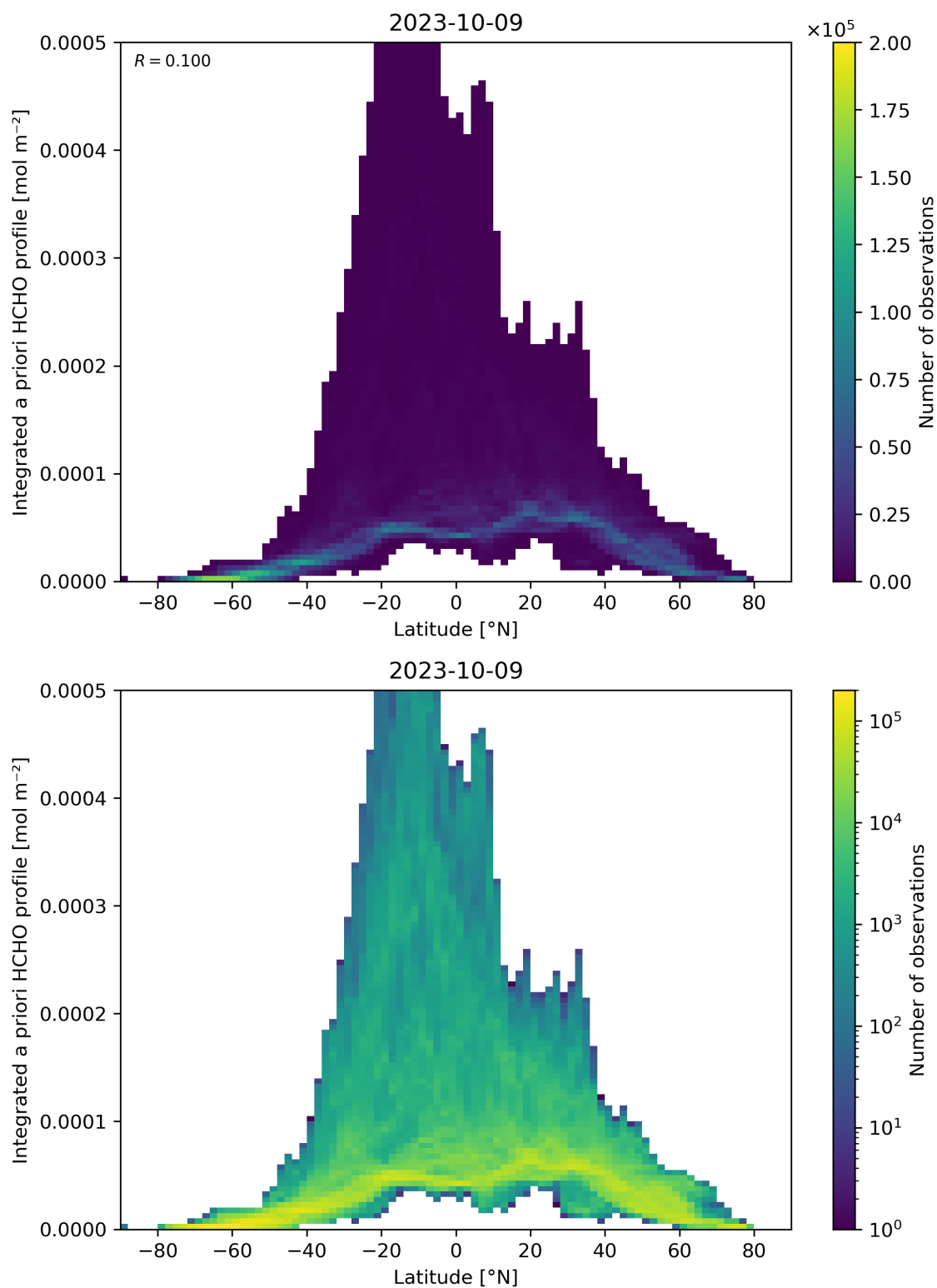
Figure 166: Scatter density plot of “Latitude” against “Integrated a priori HCHO profile” for 2023-10-08 to 2023-10-10.
