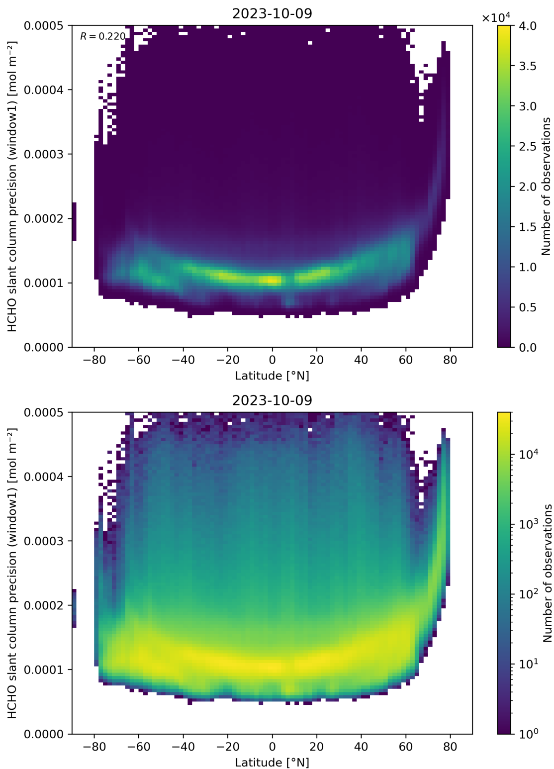
Figure 160: Scatter density plot of “Latitude” against “HCHO slant column precision (window1)” for 2023-10-08 to 2023-10-10.
