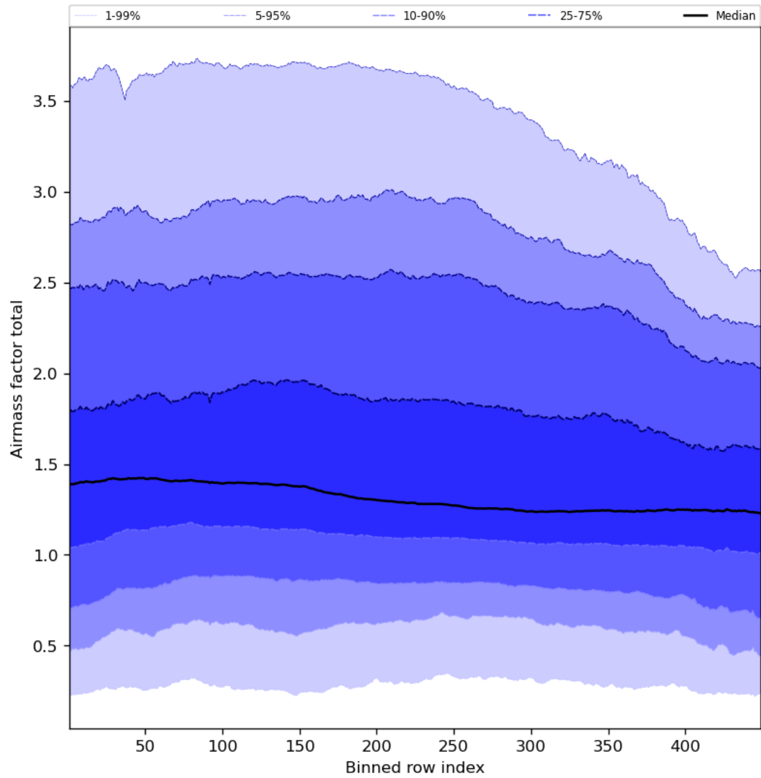
Figure 54: Along track statistics of “Airmass factor total” for 2023-10-08 to 2023-10-10
