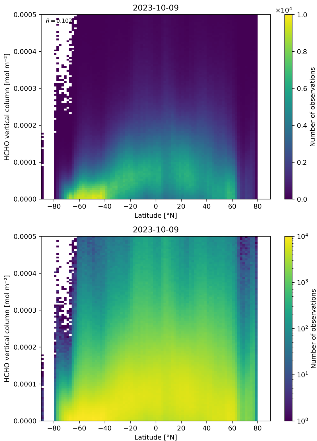
Figure 163: Scatter density plot of “Latitude” against “HCHO vertical column” for 2023-10-08 to 2023-10-10.
