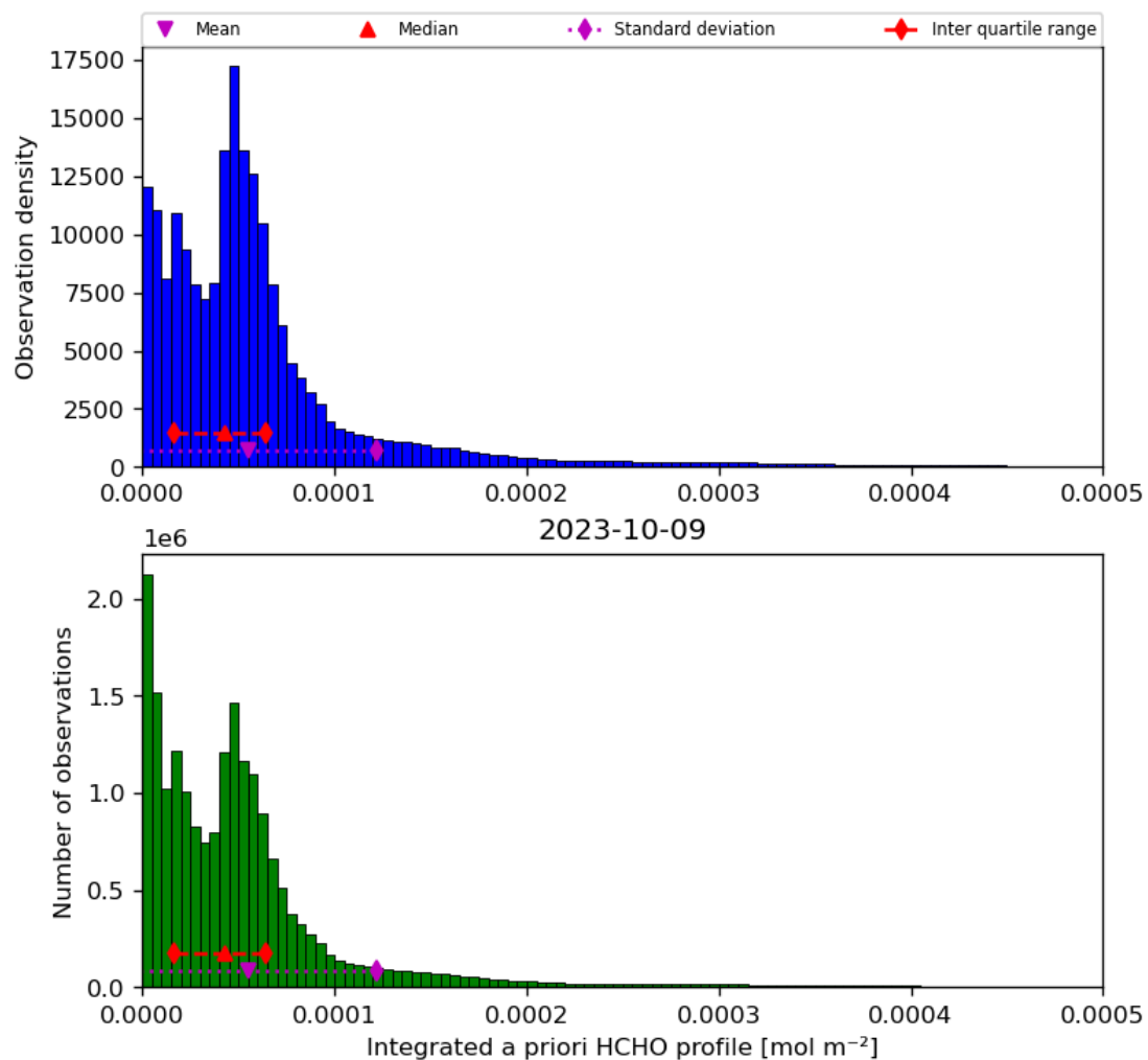
Figure 43: Histogram of “Integrated a priori HCHO profile” for 2023-10-08 to 2023-10-10
