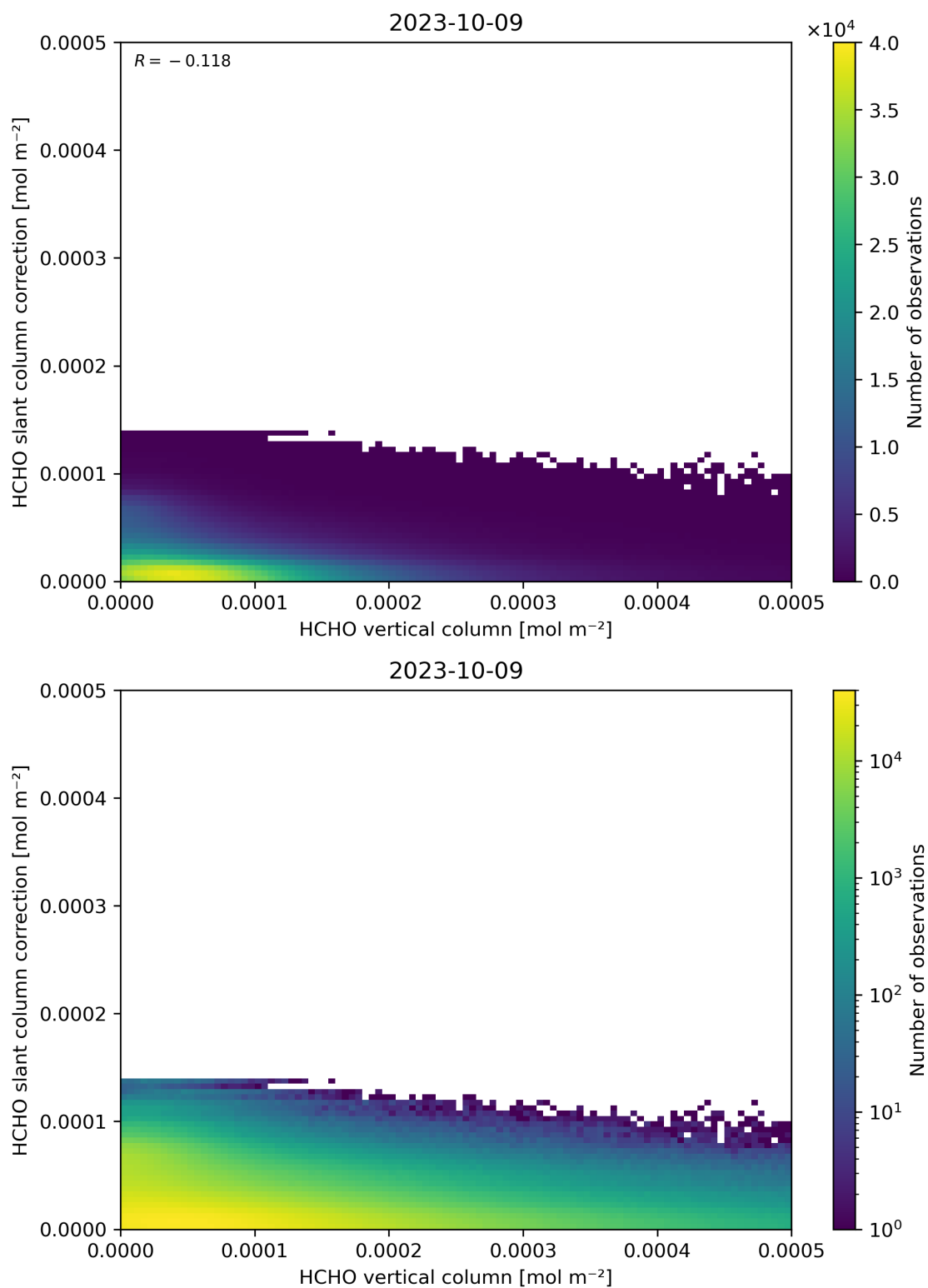
Figure 128: Scatter density plot of “HCHO vertical column” against “HCHO slant column correction” for 2023-10-08 to 2023-10-10.
