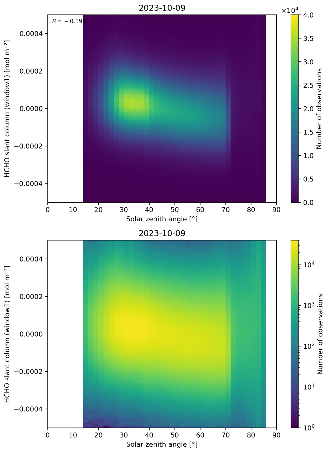
Figure 173: Scatter density plot of “Solar zenith angle” against “HCHO slant column (window1)” for 2023-10-08 to 2023-10-10.
