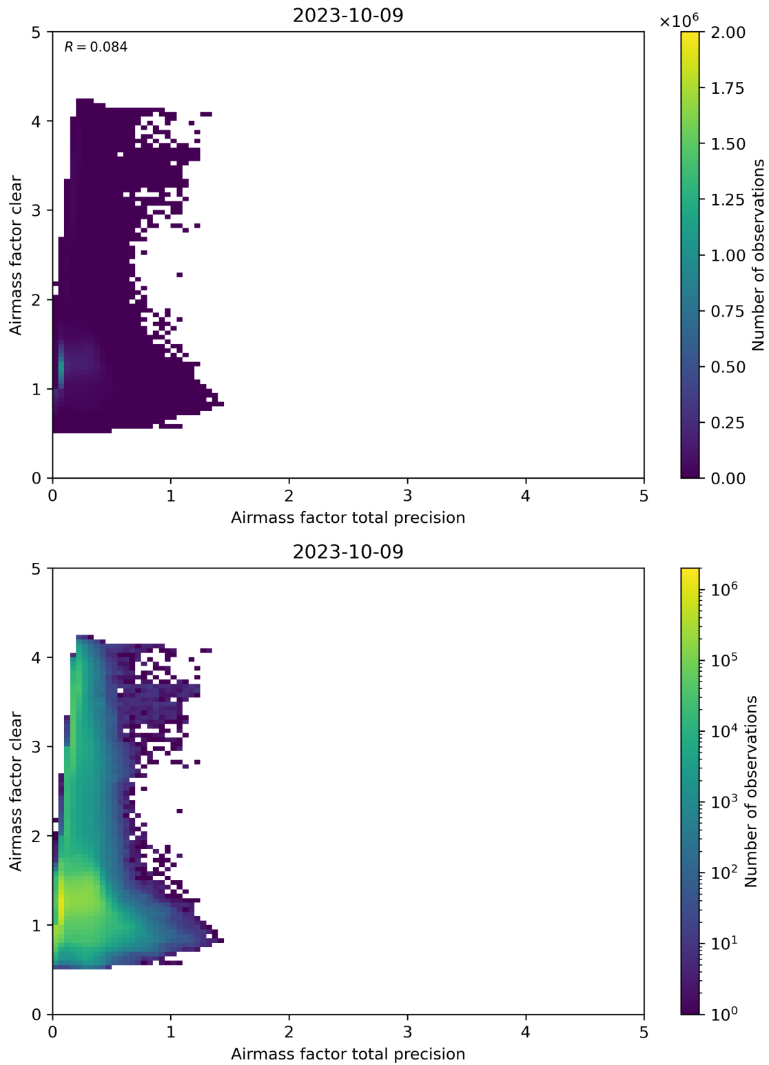
Figure 108: Scatter density plot of “Airmass factor total precision” against “Airmass factor clear” for 2023-10-08 to 2023-10-10.
