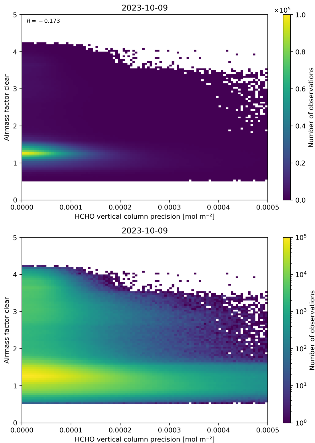
Figure 139: Scatter density plot of “HCHO vertical column precision” against “Airmass factor clear” for 2023-10-08 to 2023-10-10.
