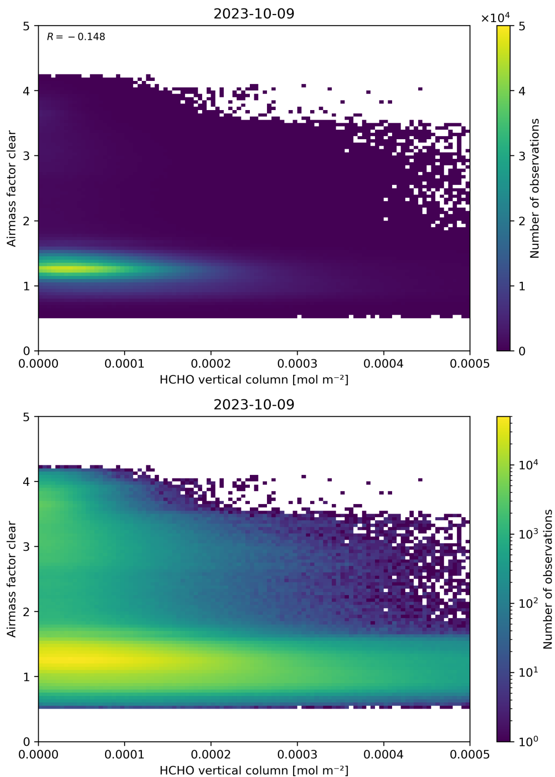
Figure 126: Scatter density plot of “HCHO vertical column” against “Airmass factor clear” for 2023-10-08 to 2023-10-10.
