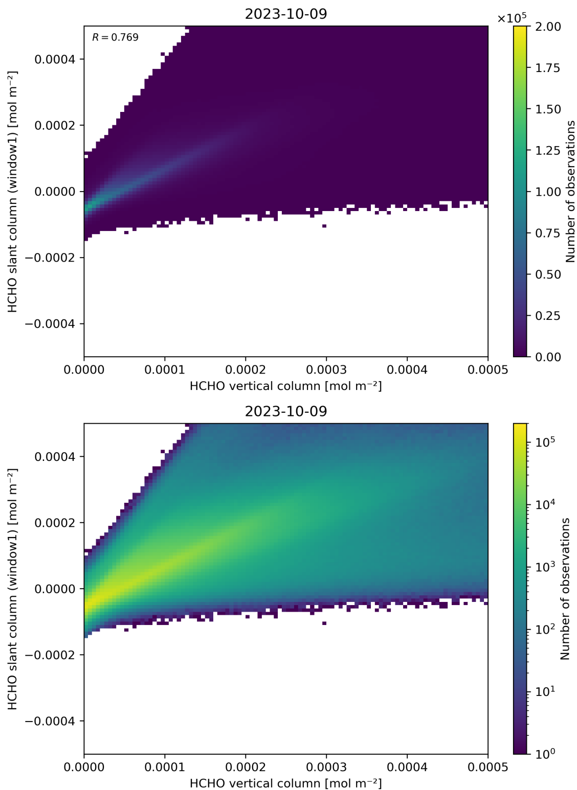
Figure 129: Scatter density plot of “HCHO vertical column” against “HCHO slant column (window1)” for 2023-10-08 to 2023-10-10.
