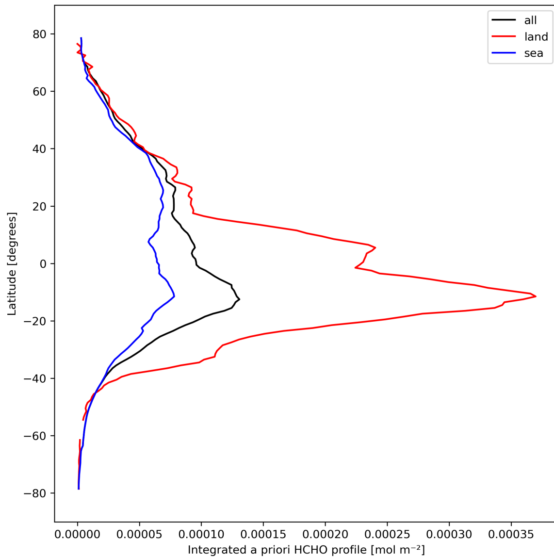
Figure 29: Zonal average of “Integrated a priori HCHO profile” for 2023-10-08 to 2023-10-10.
