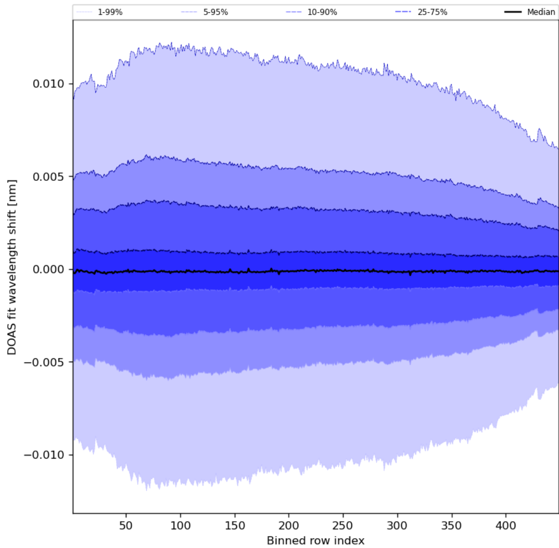
Figure 58: Along track statistics of “DOAS fit wavelength shift” for 2023-10-08 to 2023-10-10
