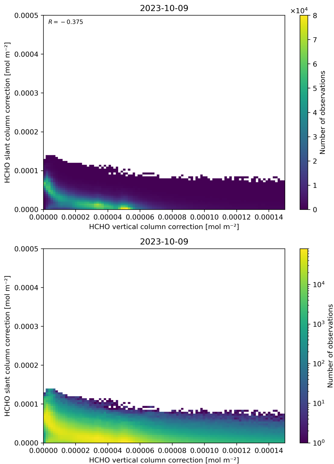
Figure 117: Scatter density plot of “HCHO vertical column correction” against “HCHO slant column correction” for 2023-10-08 to 2023-10-10.
