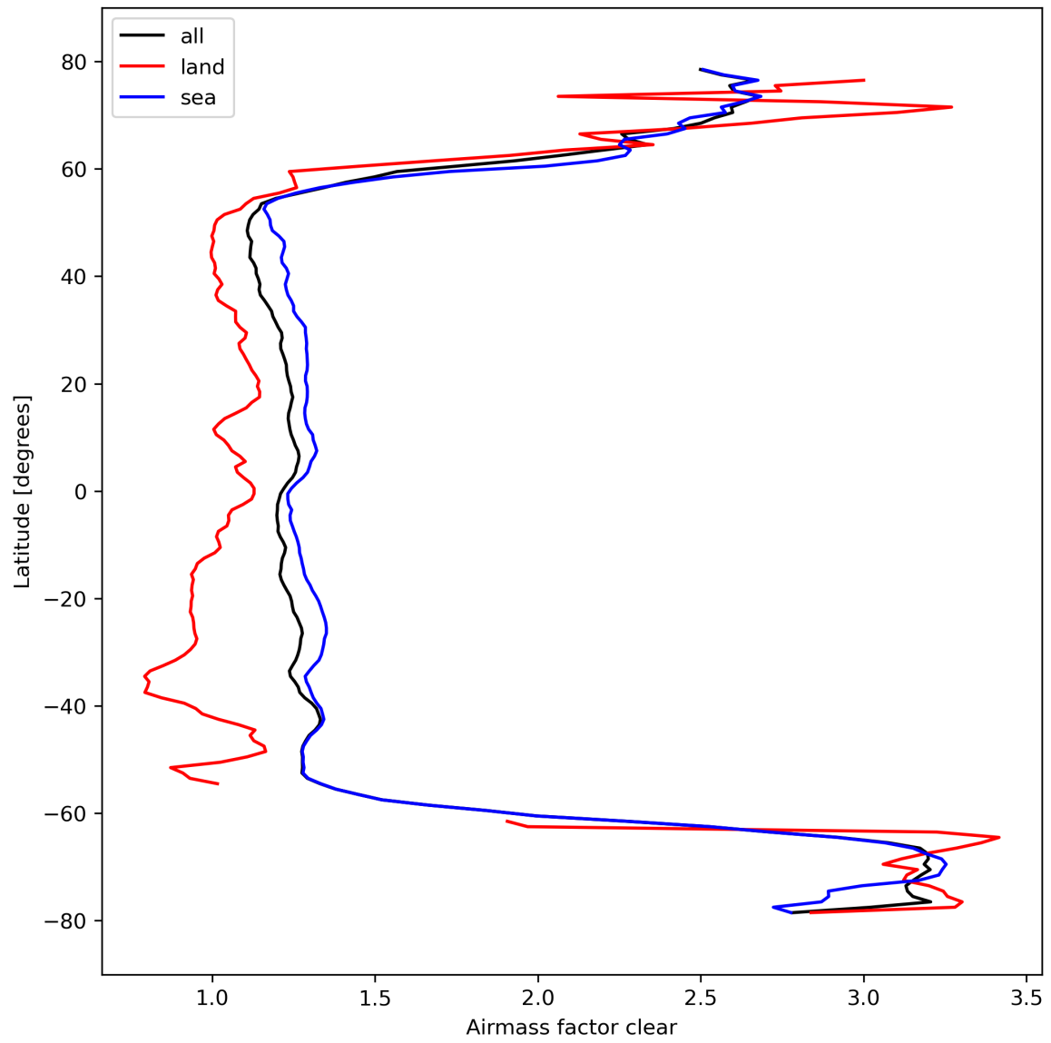
Figure 28: Zonal average of “Airmass factor clear” for 2023-10-08 to 2023-10-10.
