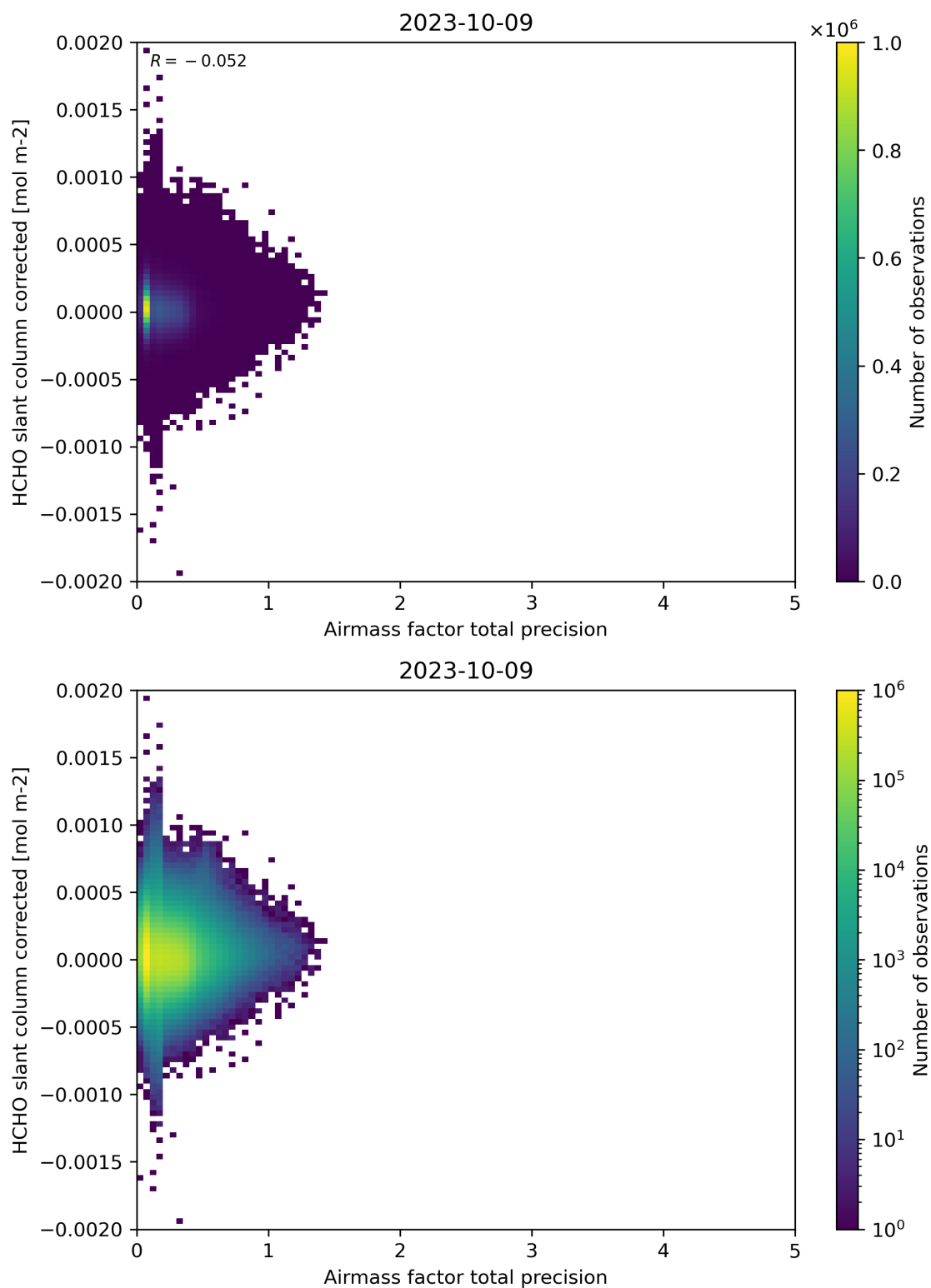
Figure 109: Scatter density plot of “Airmass factor total precision” against “HCHO slant column corrected” for 2023-10-08 to 2023-10-10.
