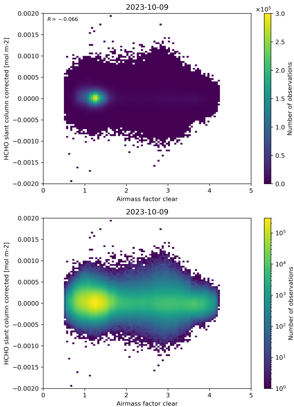
Figure 74: Scatter density plot of “Airmass factor clear” against “HCHO slant column corrected” for 2023-10-08 to 2023-10-10.
