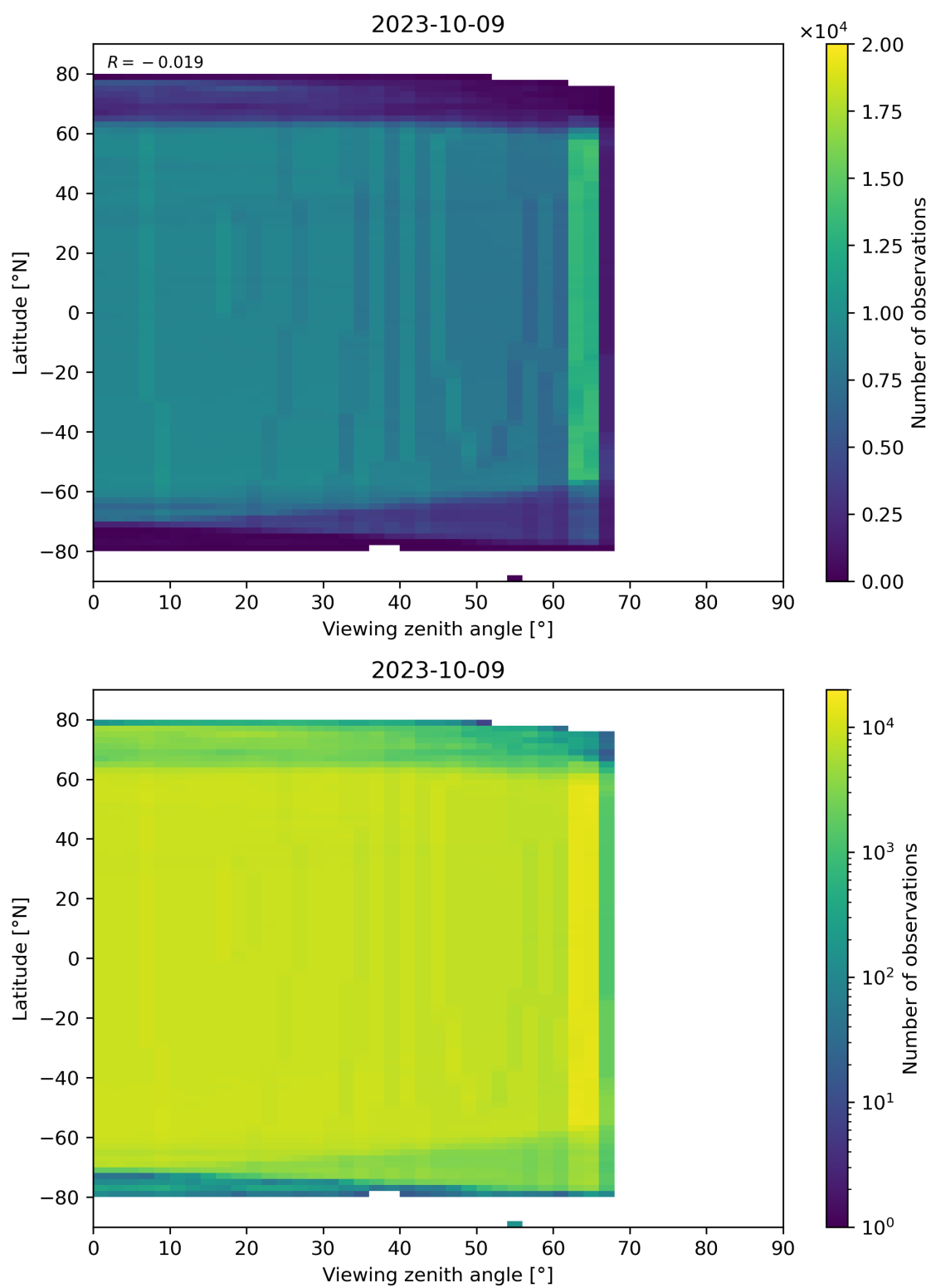
Figure 196: Scatter density plot of “Viewing zenith angle” against “Latitude” for 2023-10-08 to 2023-10-10.
