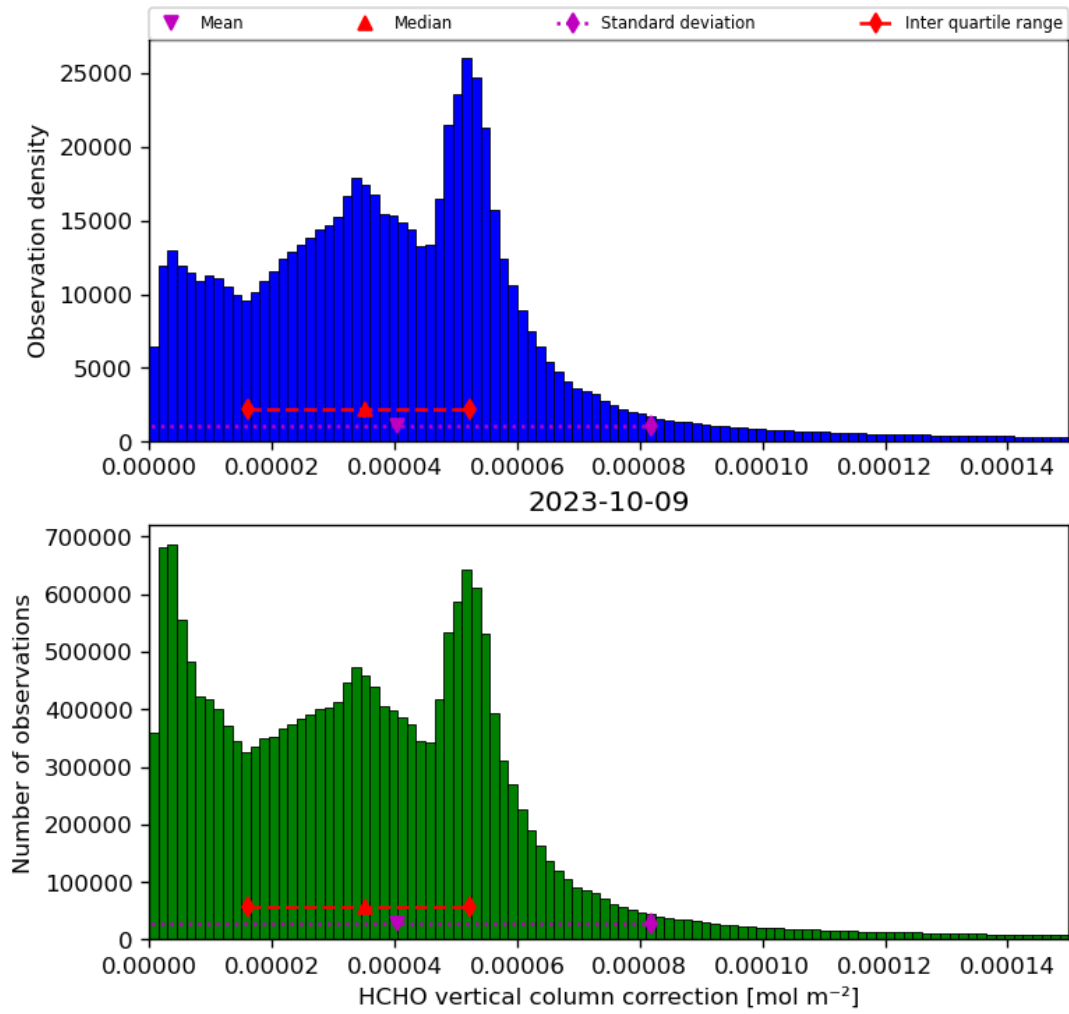
Figure 37: Histogram of “HCHO vertical column correction” for 2023-10-08 to 2023-10-10
