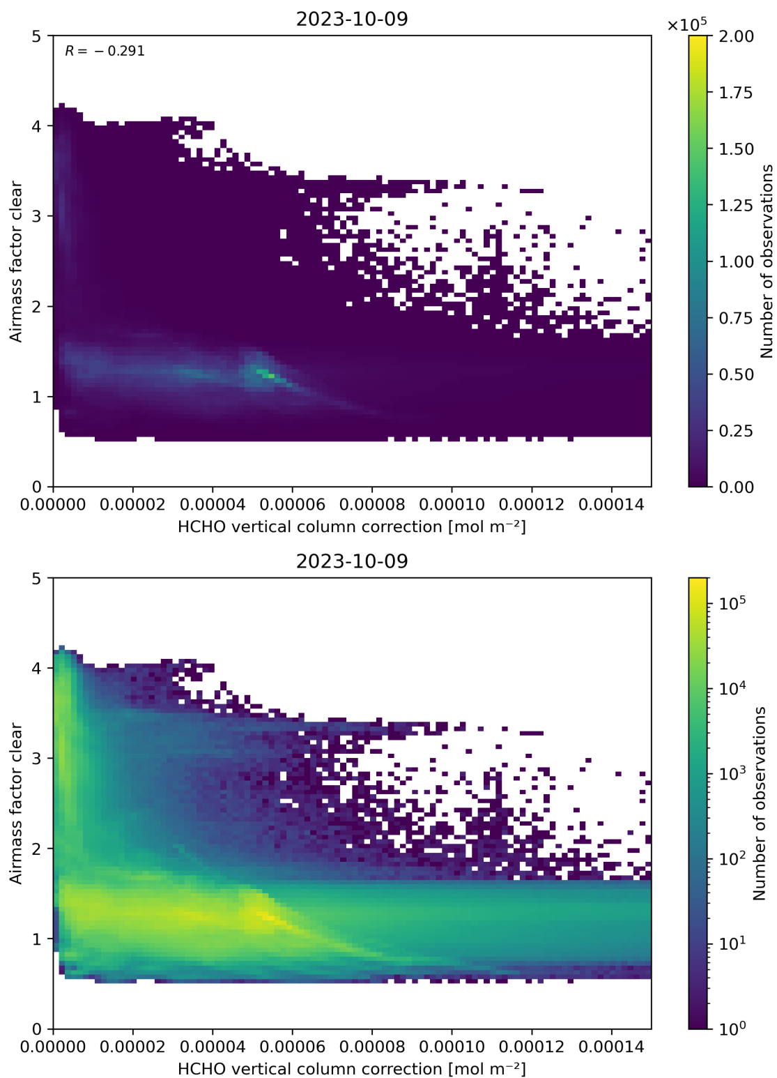
Figure 115: Scatter density plot of “HCHO vertical column correction” against “Airmass factor clear” for 2023-10-08 to 2023-10-10.
