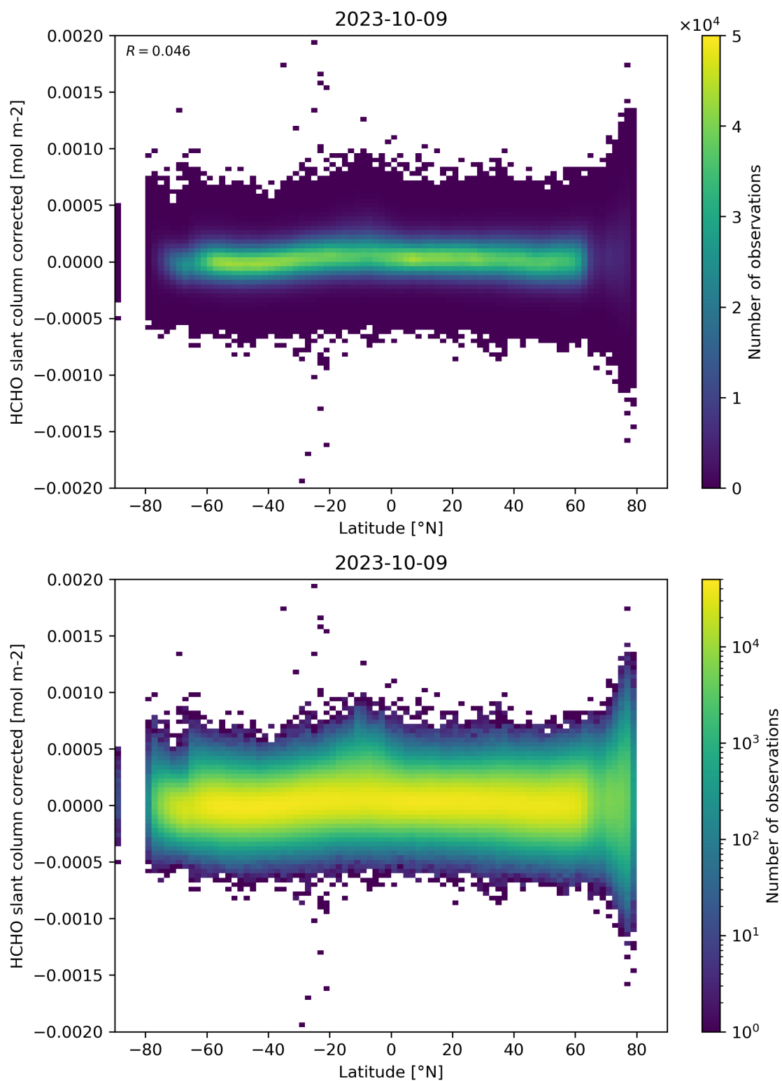
Figure 157: Scatter density plot of “Latitude” against “HCHO slant column corrected” for 2023-10-08 to 2023-10-10.
