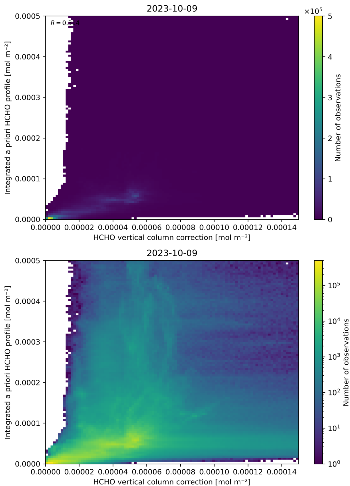
Figure 122: Scatter density plot of “HCHO vertical column correction” against “Integrated a priori HCHO profile” for 2023-10-08 to 2023-10-10.
