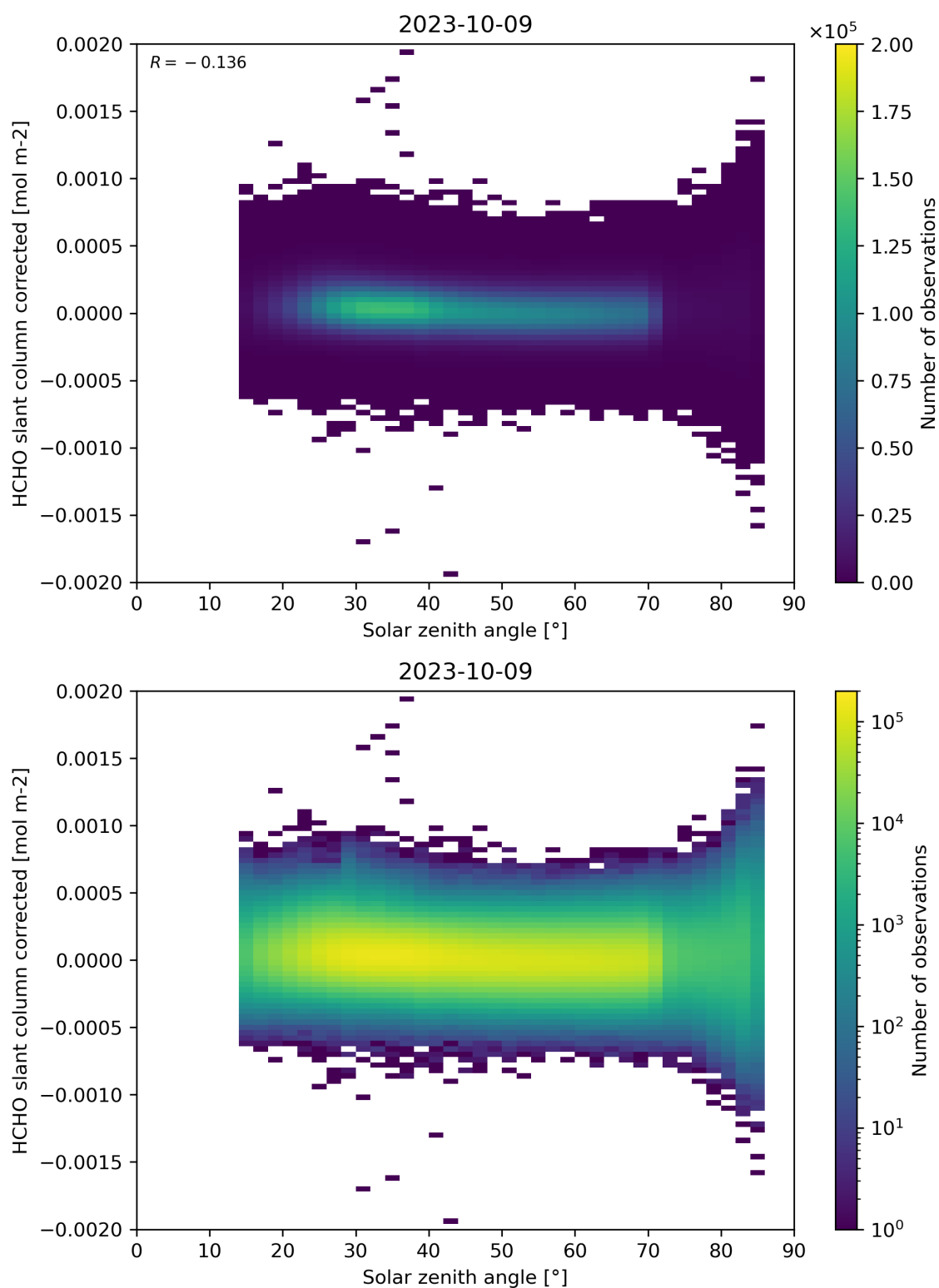
Figure 171: Scatter density plot of “Solar zenith angle” against “HCHO slant column corrected” for 2023-10-08 to 2023-10-10.
