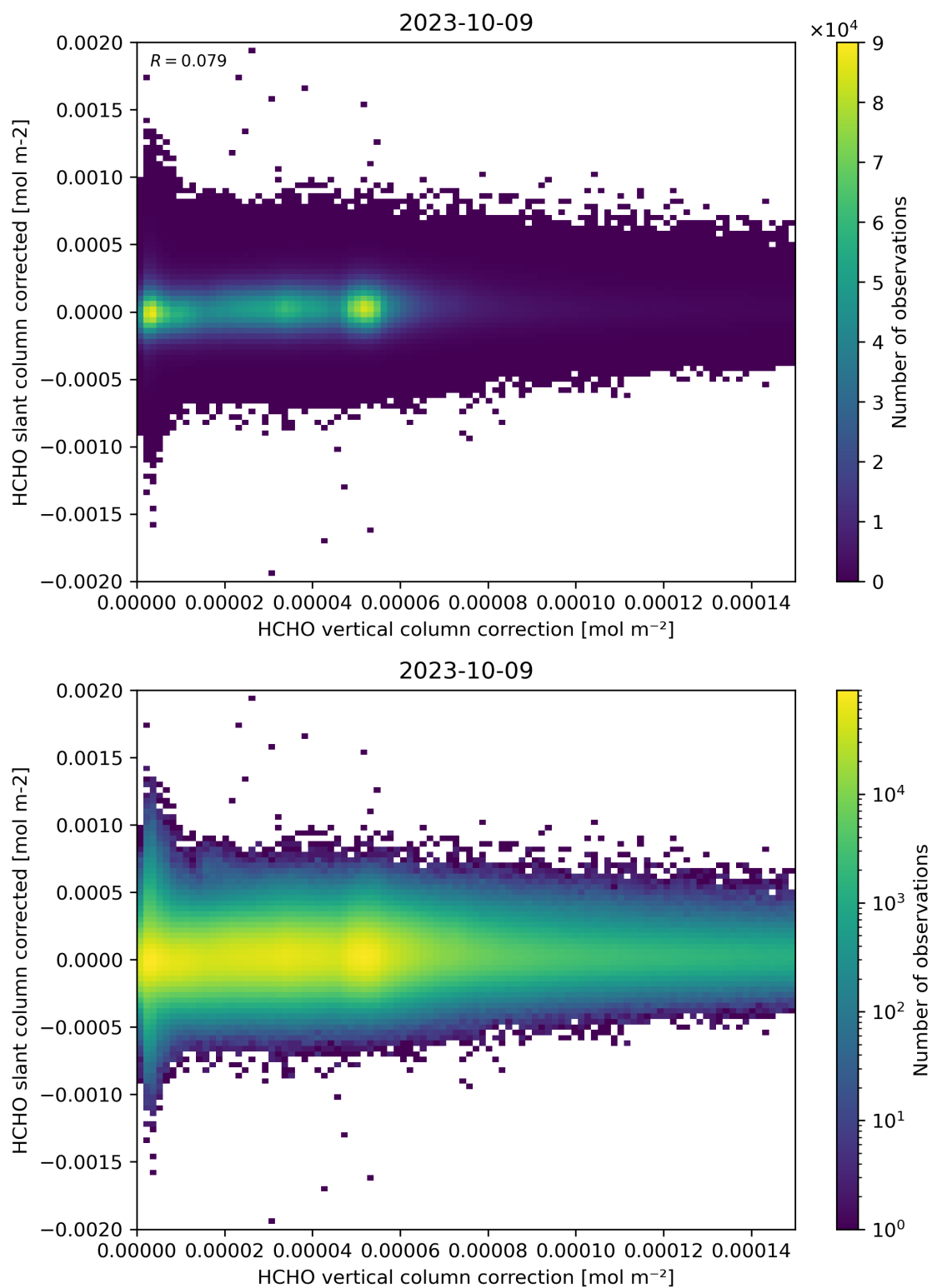
Figure 116: Scatter density plot of “HCHO vertical column correction” against “HCHO slant column corrected” for 2023-10-08 to 2023-10-10.
