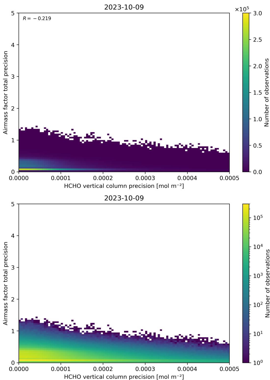
Figure 145: Scatter density plot of “HCHO vertical column precision” against “Airmass factor total precision” for 2023-10-08 to 2023-10-10.
