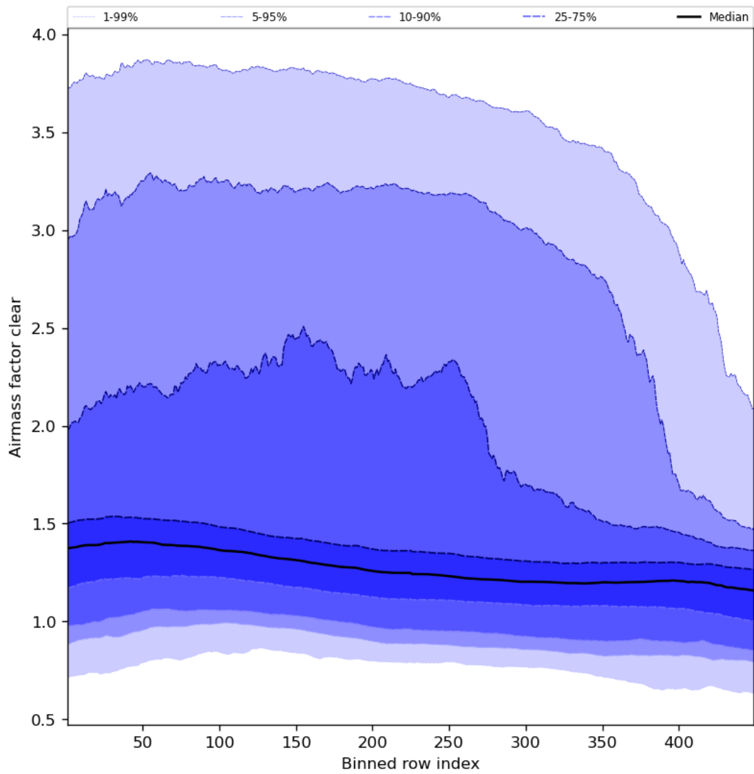
Figure 56: Along track statistics of “Airmass factor clear” for 2023-10-08 to 2023-10-10
