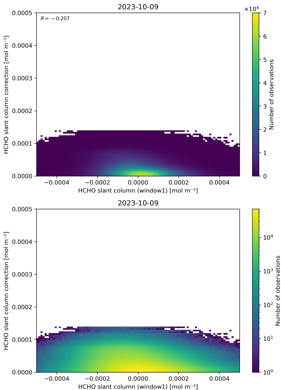
Figure 83: Scatter density plot of “HCHO slant column (window1)” against “HCHO slant column correction” for 2023-10-08 to 2023-10-10.
