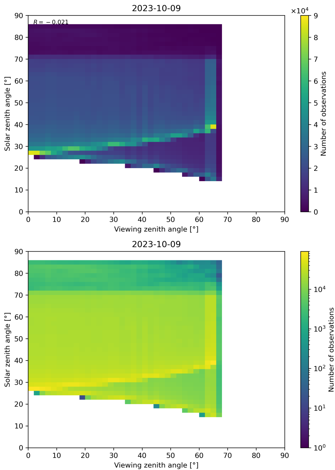
Figure 197: Scatter density plot of “Viewing zenith angle” against “Solar zenith angle” for 2023-10-08 to 2023-10-10.
