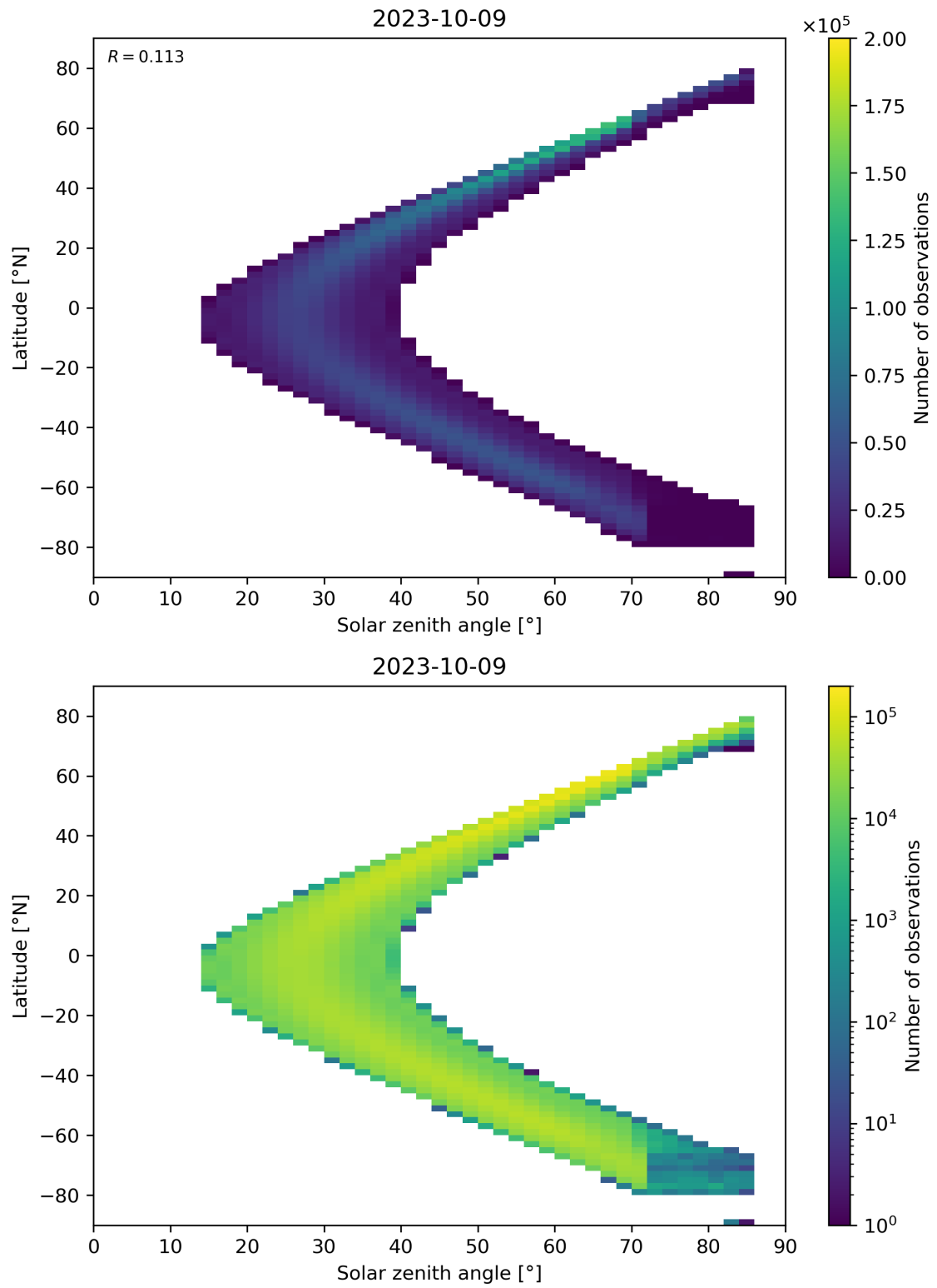
Figure 181: Scatter density plot of “Solar zenith angle” against “Latitude” for 2023-10-08 to 2023-10-10.
