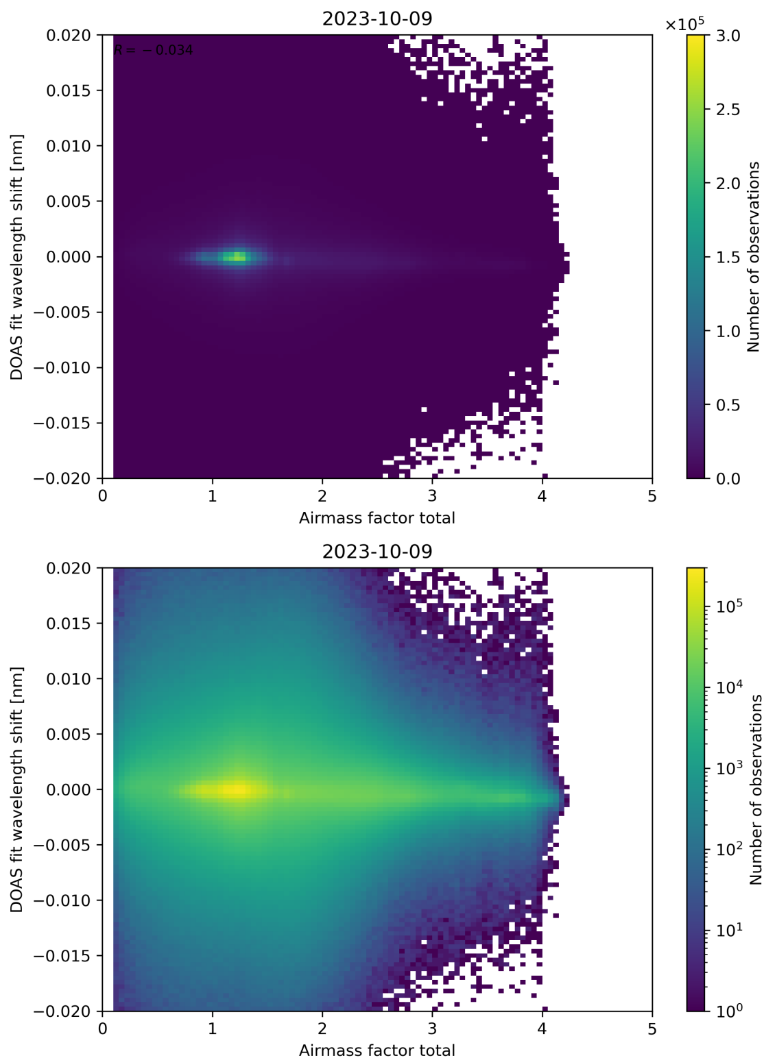
Figure 98: Scatter density plot of “Airmass factor total” against “DOAS fit wavelength shift” for 2023-10-08 to 2023-10-10.
