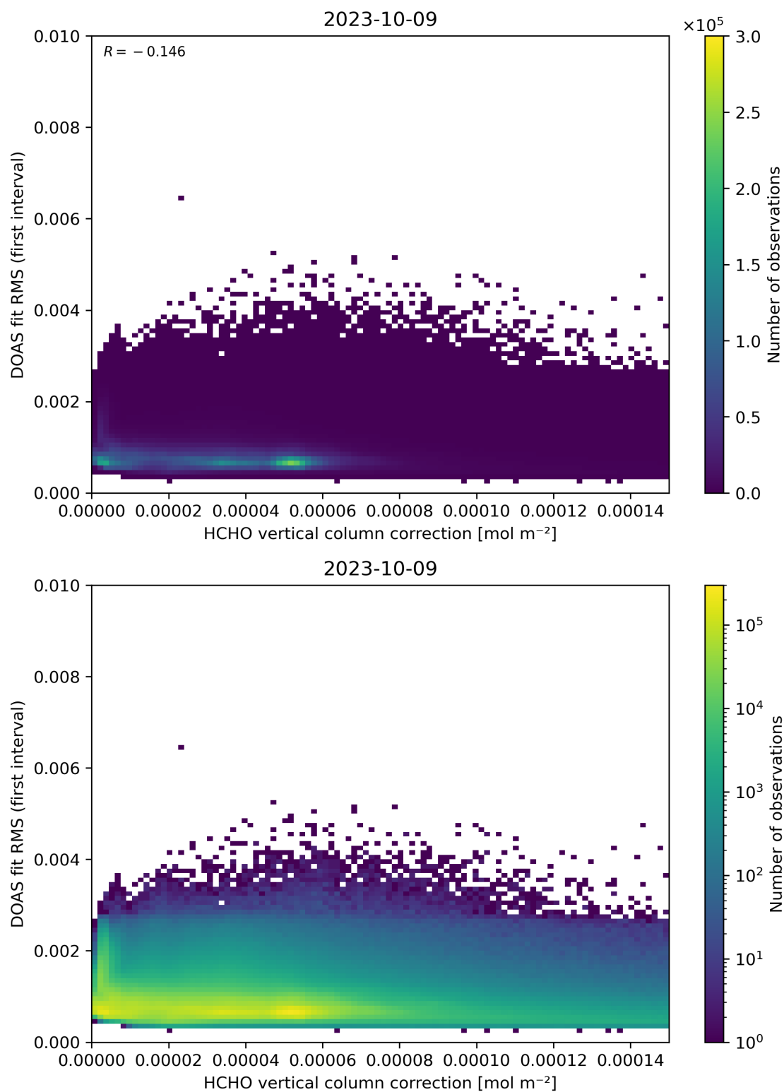
Figure 112: Scatter density plot of “HCHO vertical column correction” against “DOAS fit RMS (first interval)” for 2023-10-08 to 2023-10-10.
