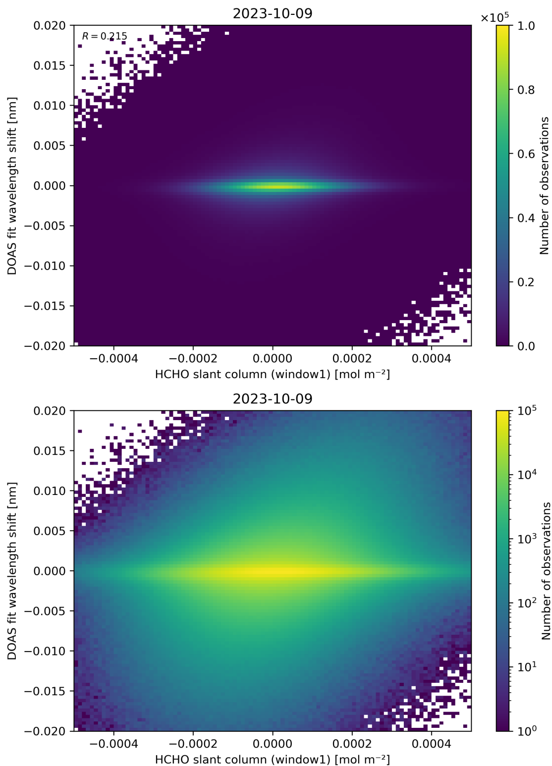
Figure 79: Scatter density plot of “HCHO slant column (window1)” against “DOAS fit wavelength shift” for 2023-10-08 to 2023-10-10.
