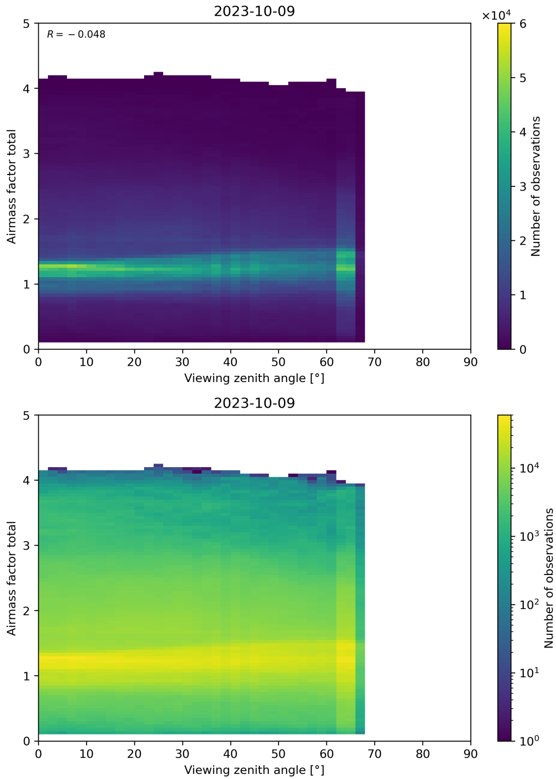
Figure 190: Scatter density plot of “Viewing zenith angle” against “Airmass factor total” for 2023-10-08 to 2023-10-10.
