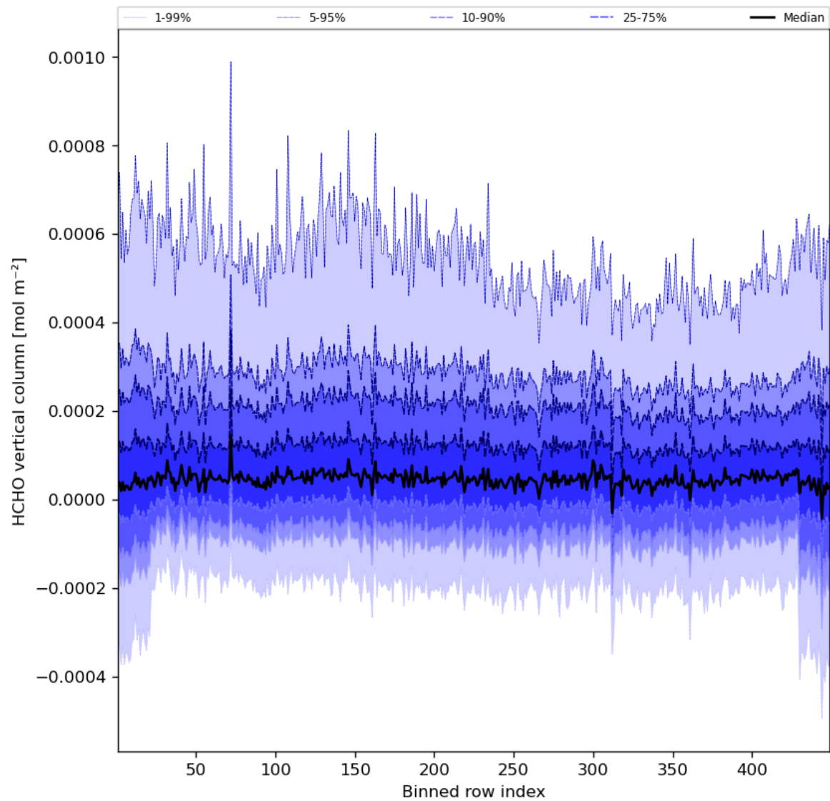
Figure 49: Along track statistics of “HCHO vertical column” for 2023-10-08 to 2023-10-10
