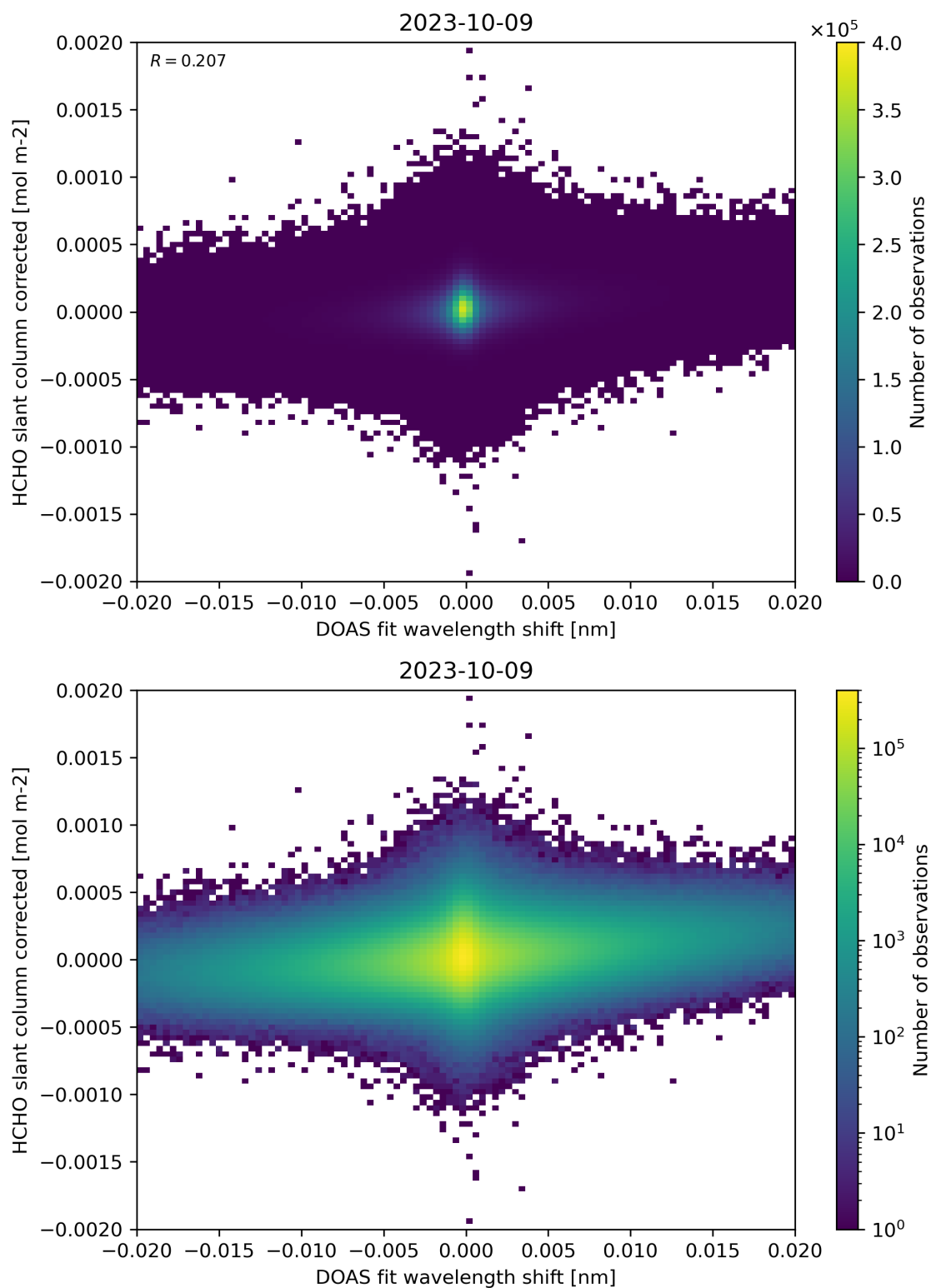
Figure 66: Scatter density plot of “DOAS fit wavelength shift” against “HCHO slant column corrected” for 2023-10-08 to 2023-10-10.
