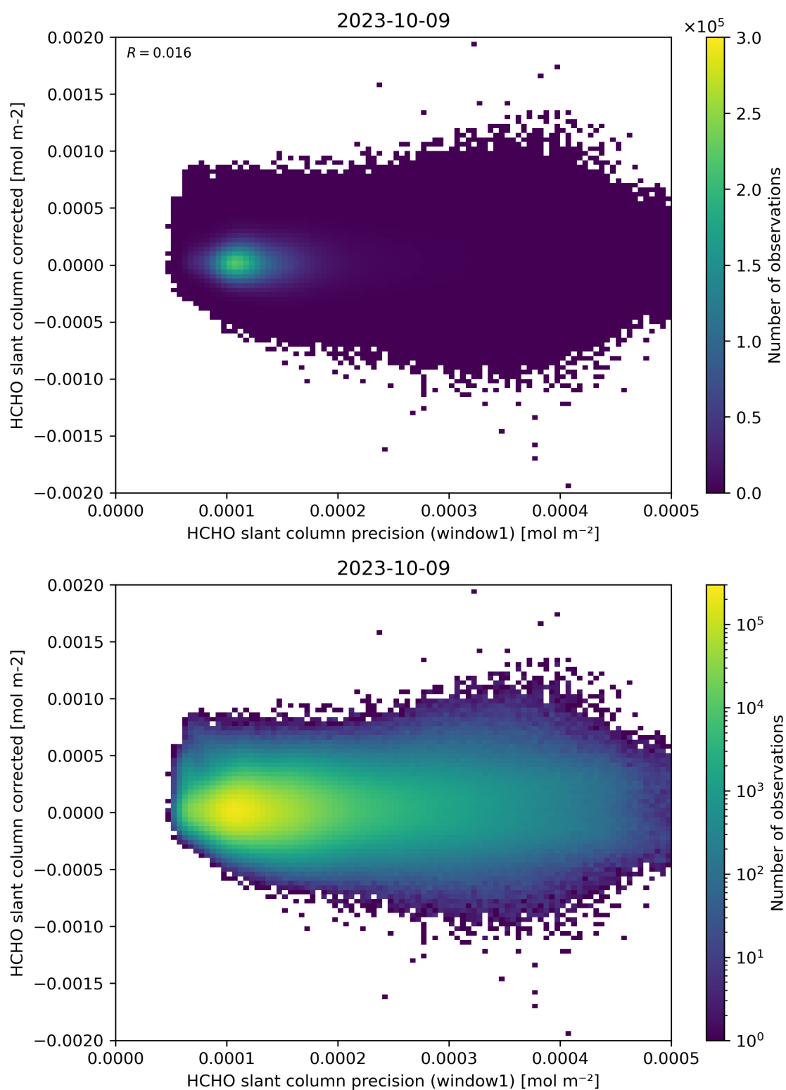
Figure 92: Scatter density plot of “HCHO slant column precision (window1)” against “HCHO slant column corrected” for 2023-10-08 to 2023-10-10.
