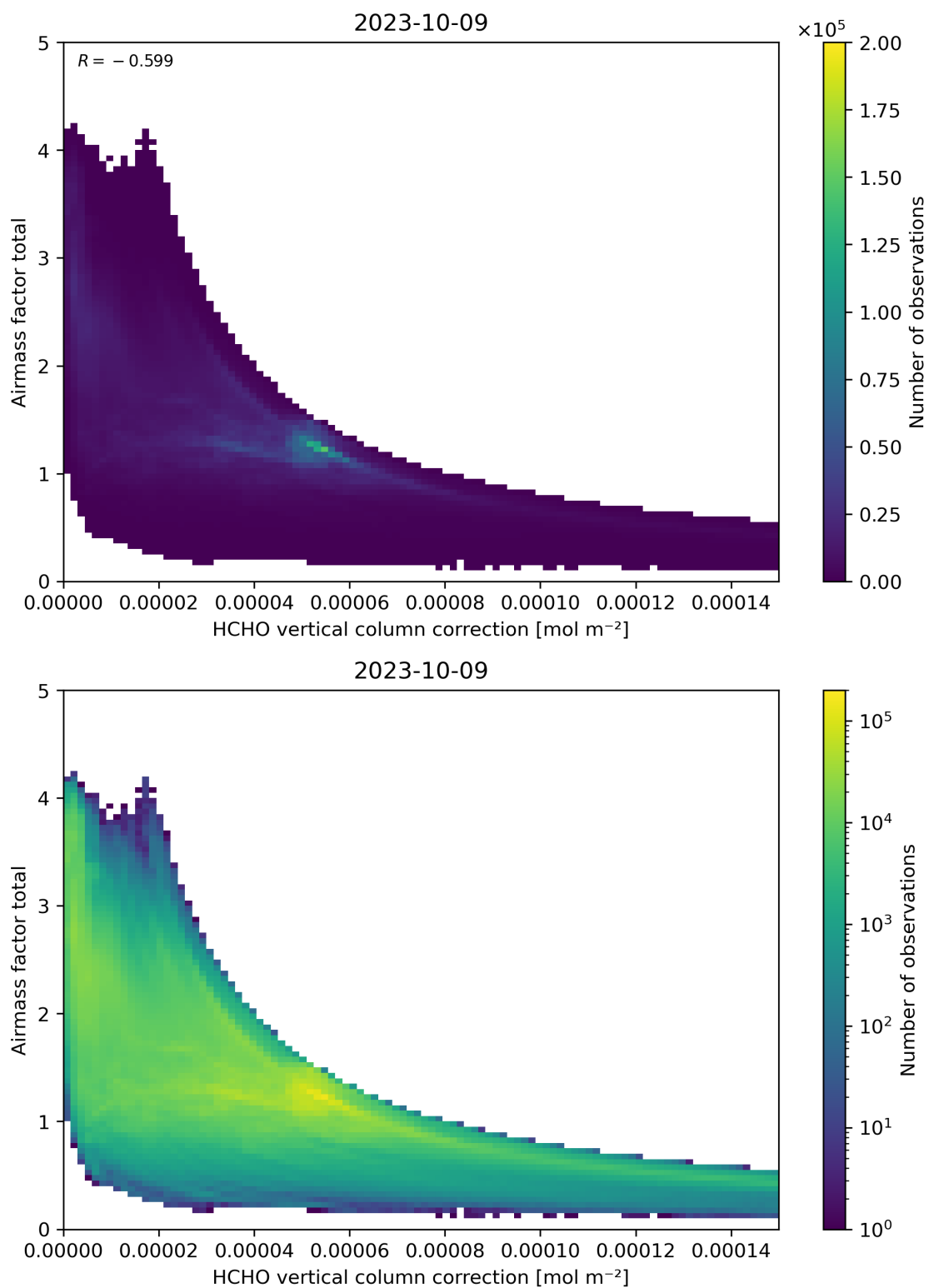
Figure 120: Scatter density plot of “HCHO vertical column correction” against “Airmass factor total” for 2023-10-08 to 2023-10-10.
