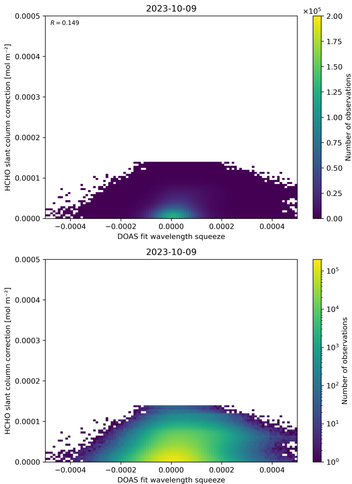
Figure 70: Scatter density plot of “DOAS fit wavelength squeeze” against “HCHO slant column correction” for 2023-10-08 to 2023-10-10.
