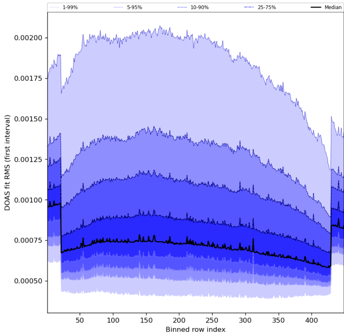
Figure 60: Along track statistics of “DOAS fit RMS (first interval)” for 2023-10-08 to 2023-10-10
