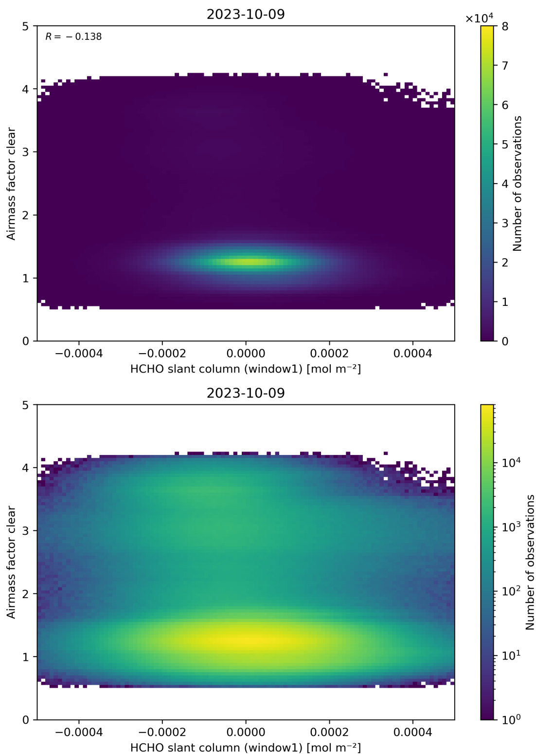
Figure 81: Scatter density plot of “HCHO slant column (window1)” against “Airmass factor clear” for 2023-10-08 to 2023-10-10.
