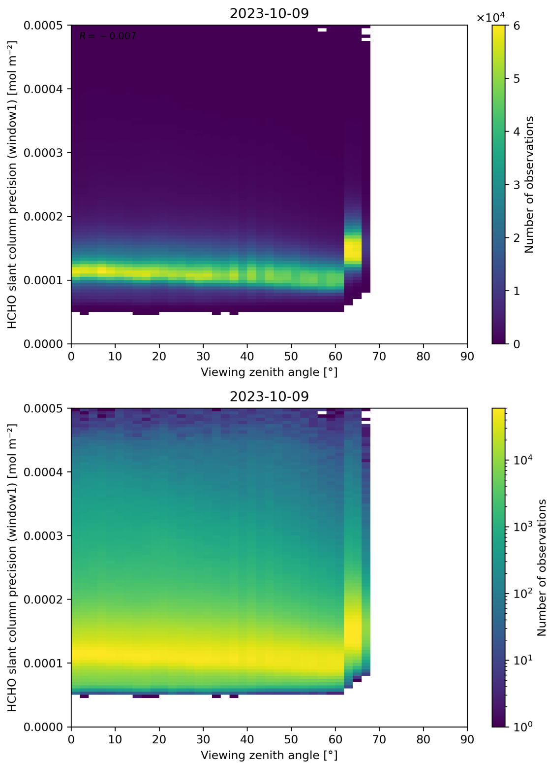
Figure 189: Scatter density plot of “Viewing zenith angle” against “HCHO slant column precision (window1)” for 2023-10-08 to 2023-10-10.
