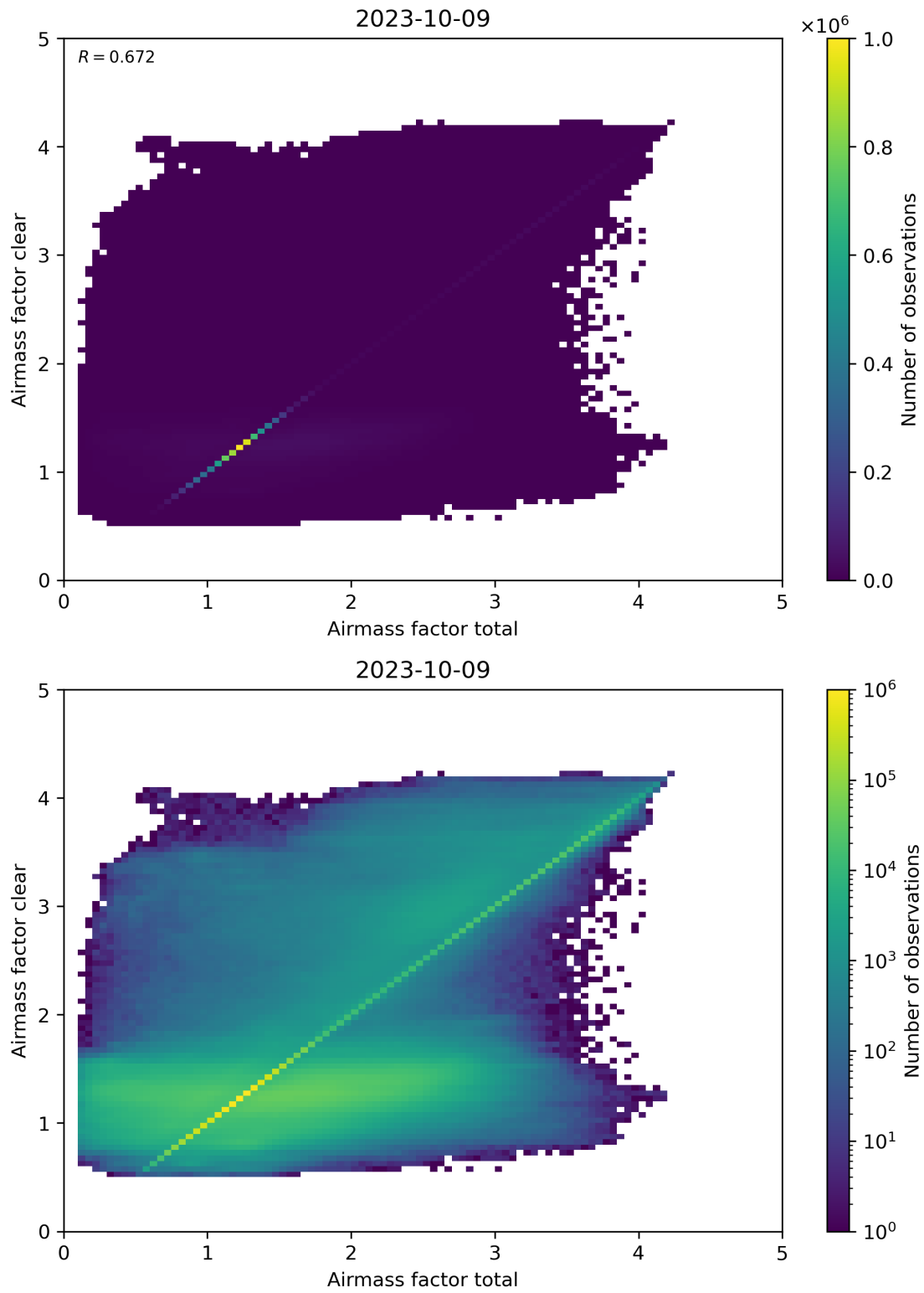
Figure 100: Scatter density plot of “Airmass factor total” against “Airmass factor clear” for 2023-10-08 to 2023-10-10.
