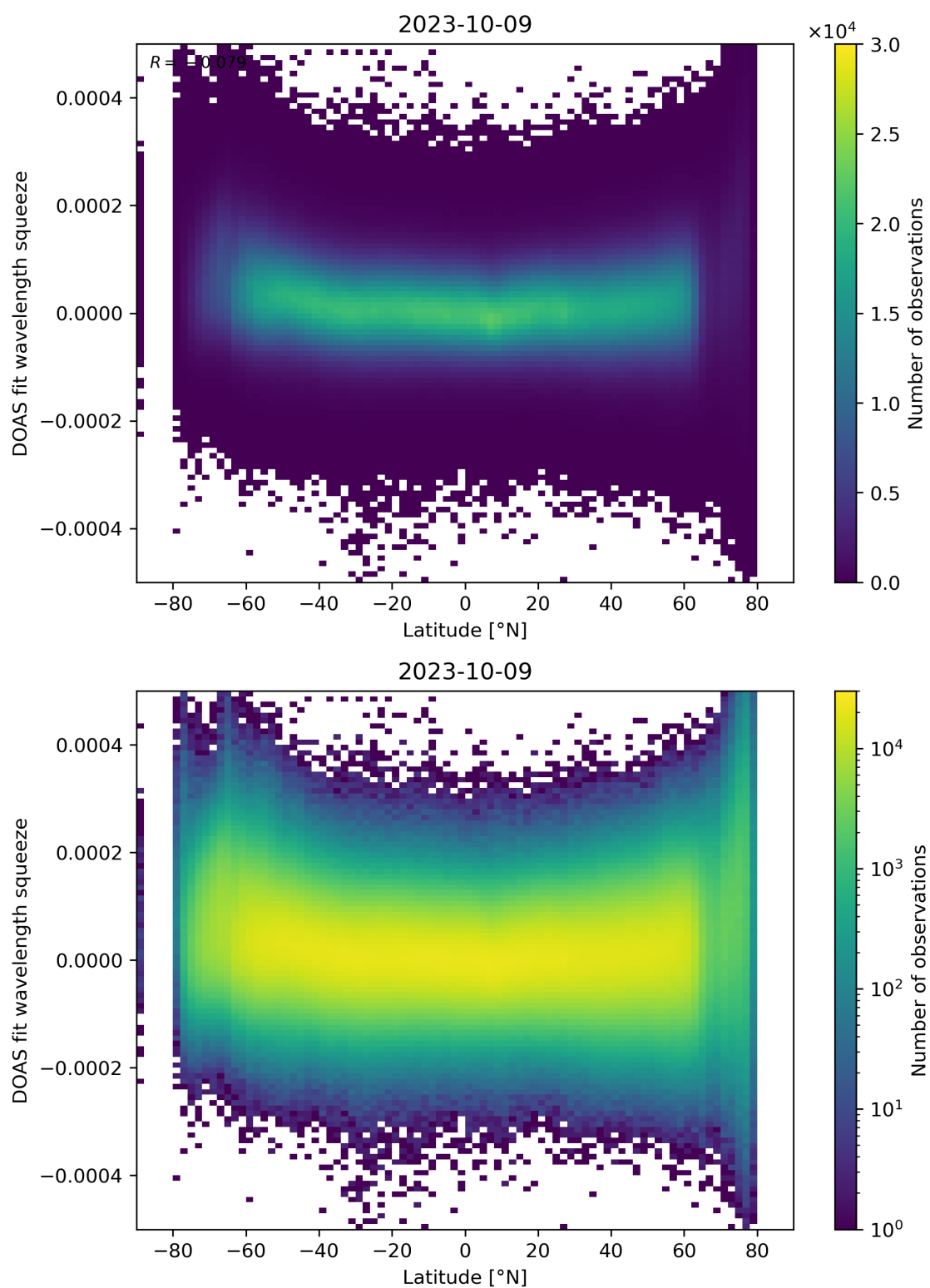
Figure 155: Scatter density plot of “Latitude” against “DOAS fit wavelength squeeze” for 2023-10-08 to 2023-10-10.
