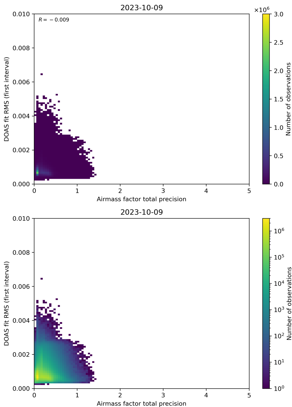
Figure 105: Scatter density plot of “Airmass factor total precision” against “DOAS fit RMS (first interval)” for 2023-10-08 to 2023-10-10.
