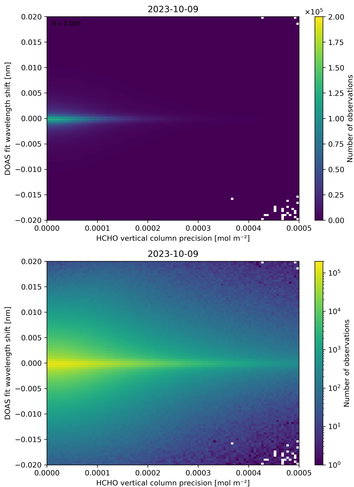
Figure 137: Scatter density plot of “HCHO vertical column precision” against “DOAS fit wavelength shift” for 2023-10-08 to 2023-10-10.
