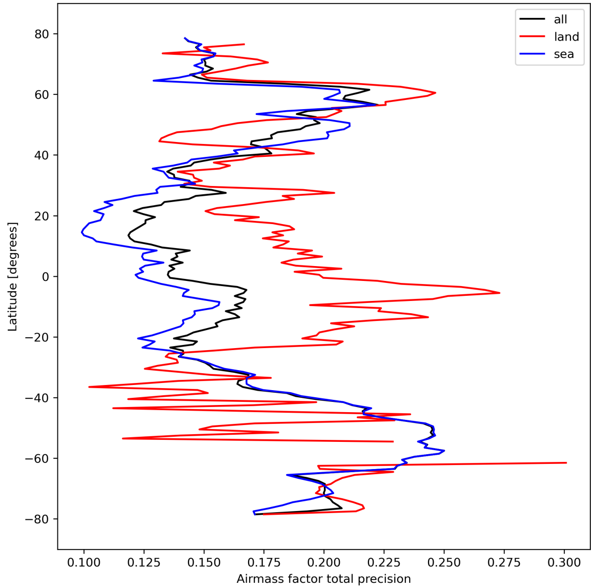
Figure 27: Zonal average of “Airmass factor total precision” for 2023-10-08 to 2023-10-10.
