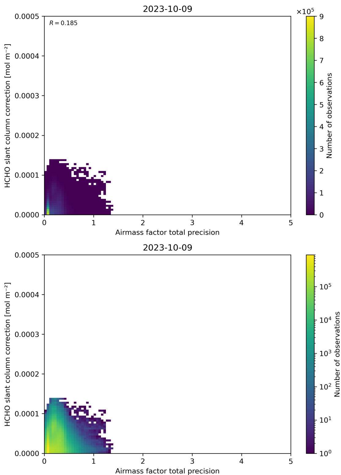
Figure 110: Scatter density plot of “Airmass factor total precision” against “HCHO slant column correction” for 2023-10-08 to 2023-10-10.
