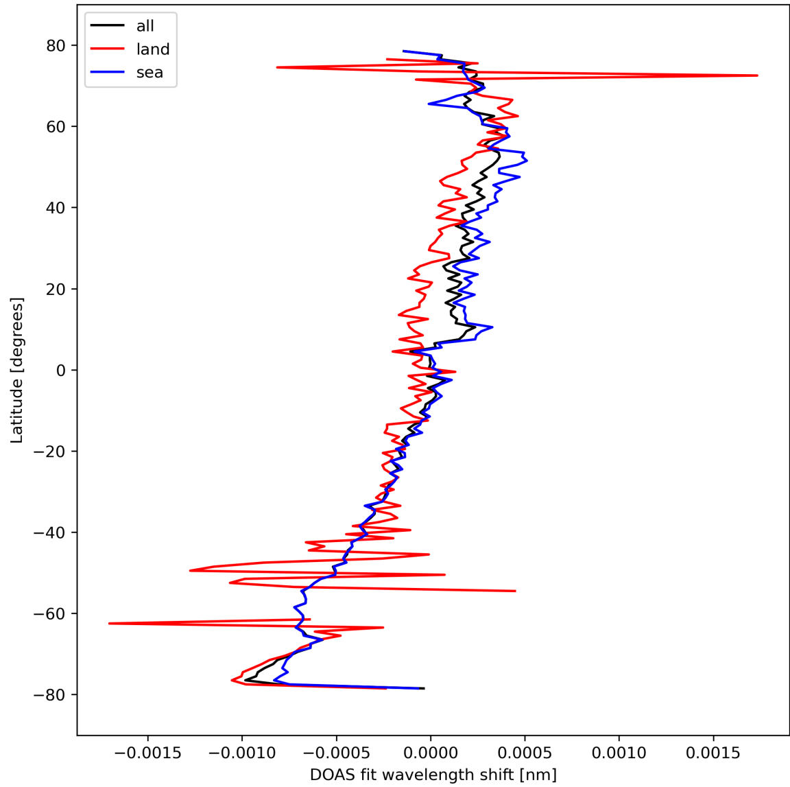
Figure 30: Zonal average of "DOAS fit wavelength shift" for 2023-10-08 to 2023-10-10.
