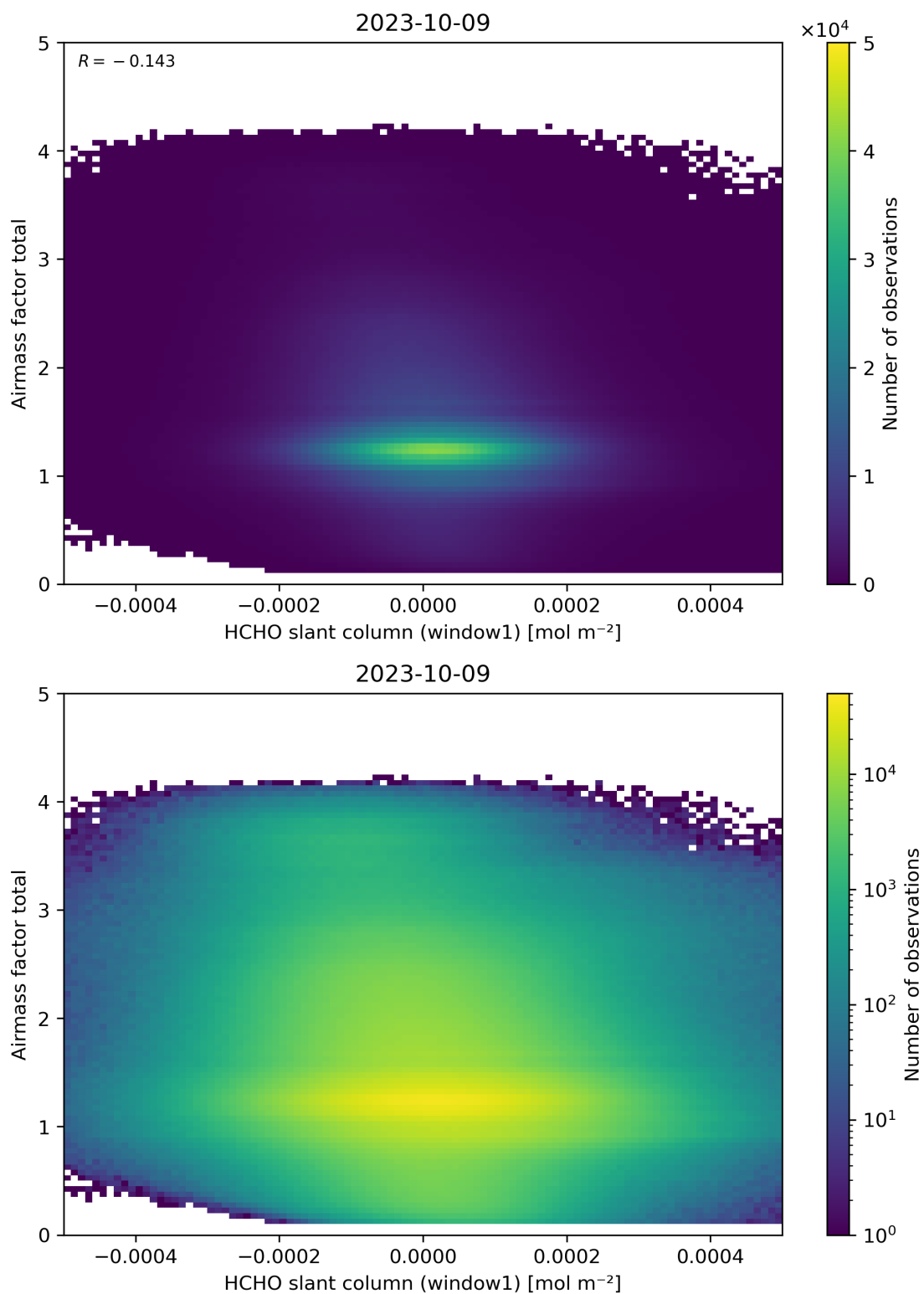
Figure 85: Scatter density plot of “HCHO slant column (window1)” against “Airmass factor total” for 2023-10-08 to 2023-10-10.
