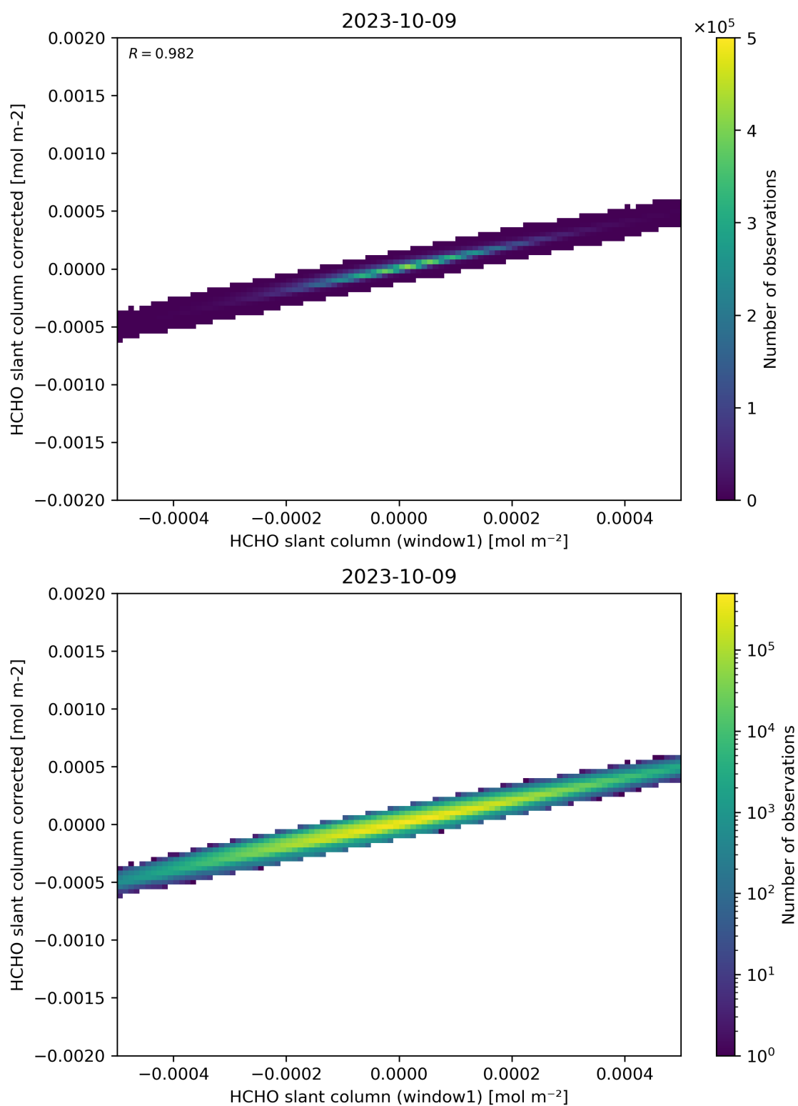
Figure 82: Scatter density plot of “HCHO slant column (window1)” against “HCHO slant column corrected” for 2023-10-08 to 2023-10-10.
