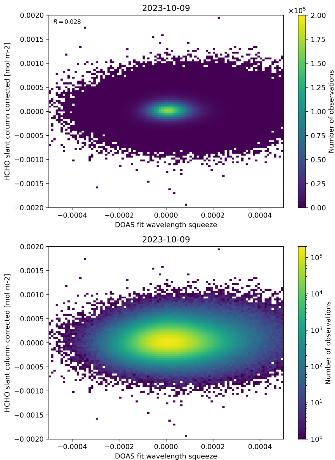
Figure 69: Scatter density plot of “DOAS fit wavelength squeeze” against “HCHO slant column corrected” for 2023-10-08 to 2023-10-10.
