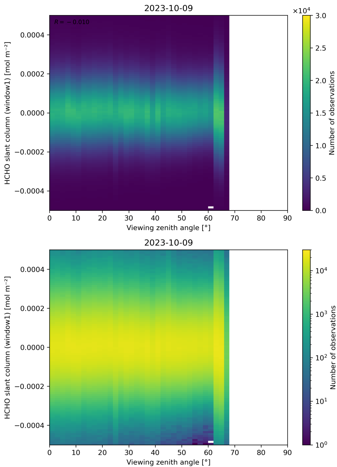
Figure 188: Scatter density plot of “Viewing zenith angle” against “HCHO slant column (window1)” for 2023-10-08 to 2023-10-10.
