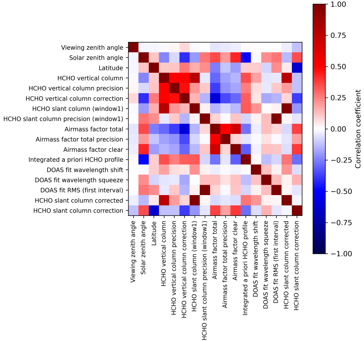
Figure 2: Map of correlation matrix for 2023-10-08 to 2023-10-10.
