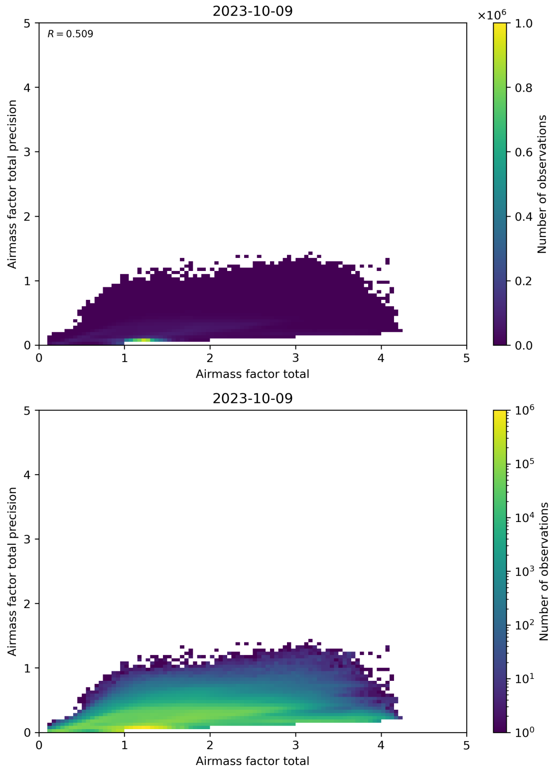
Figure 103: Scatter density plot of “Airmass factor total” against “Airmass factor total precision” for 2023-10-08 to 2023-10-10.
