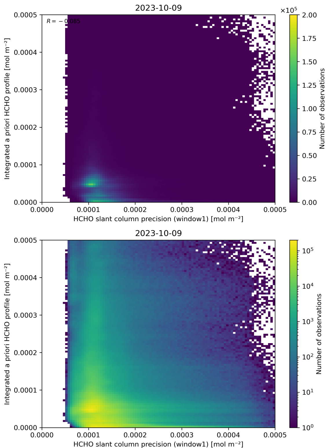
Figure 96: Scatter density plot of “HCHO slant column precision (window1)” against “Integrated a priori HCHO profile” for 2023-10-08 to 2023-10-10.
