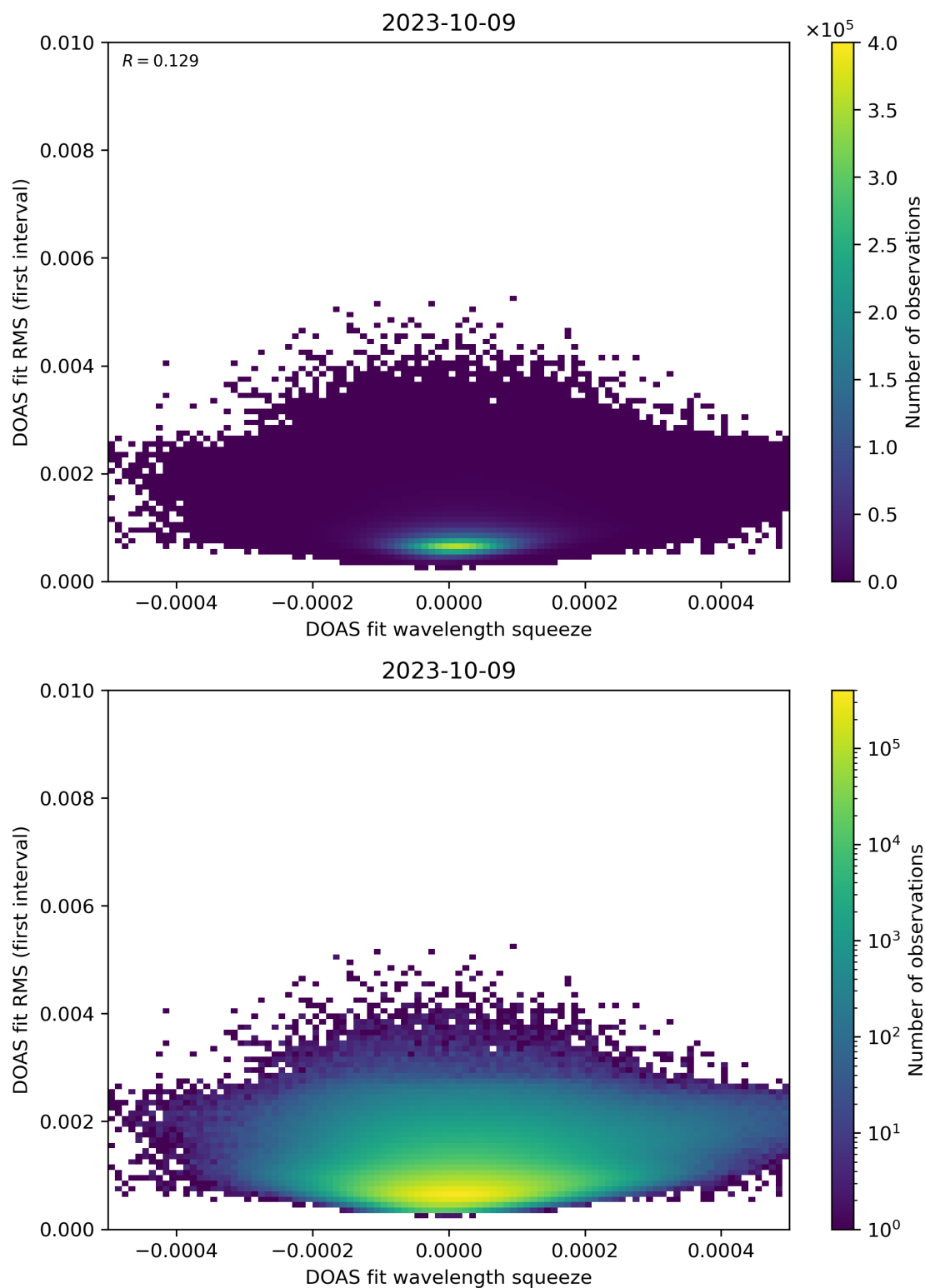
Figure 68: Scatter density plot of “DOAS fit wavelength squeeze” against “DOAS fit RMS (first interval)” for 2023-10-08 to 2023-10-10.
