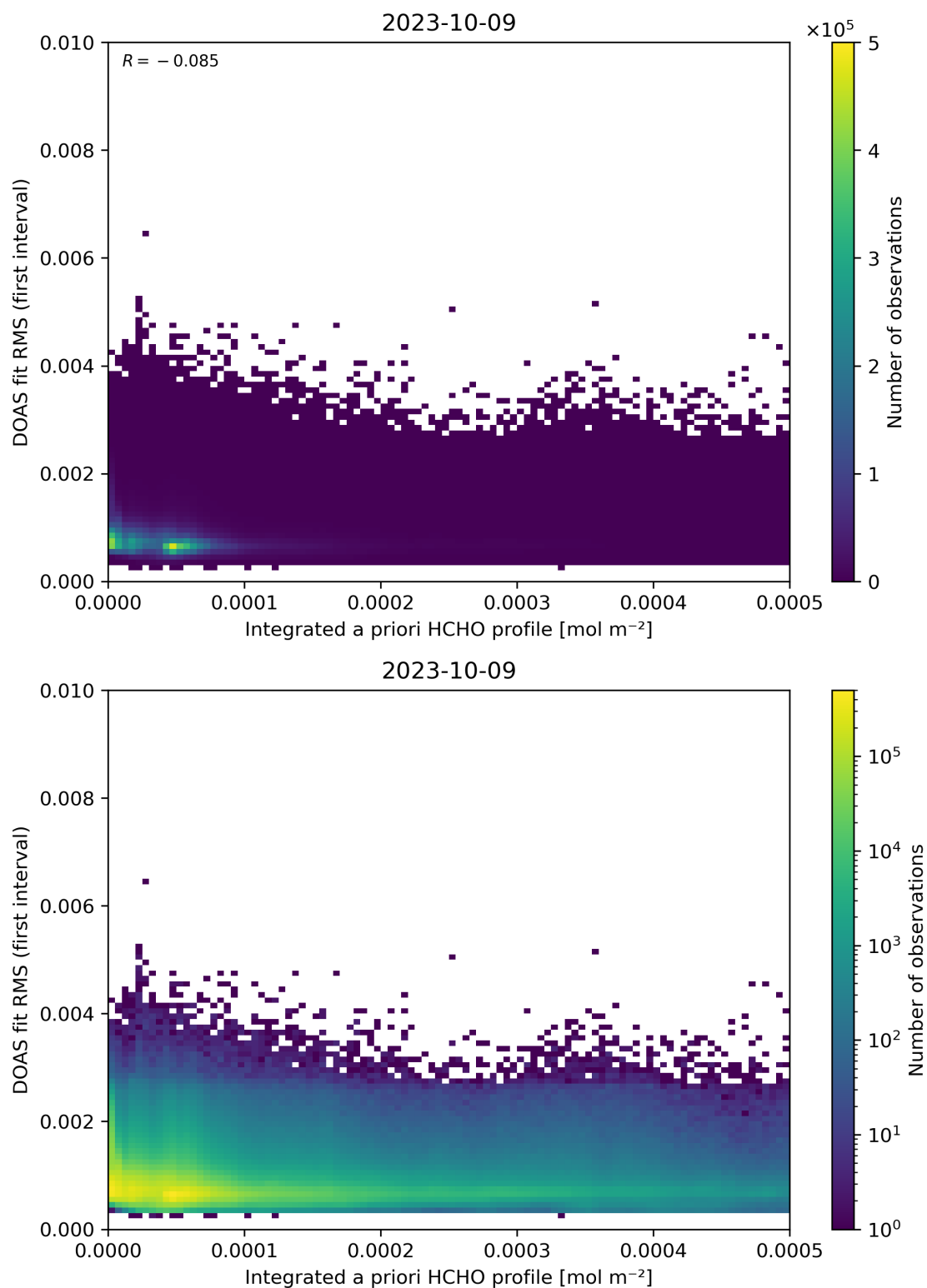
Figure 148: Scatter density plot of “Integrated a priori HCHO profile” against “DOAS fit RMS (first interval)” for 2023-10-08 to 2023-10-10.
