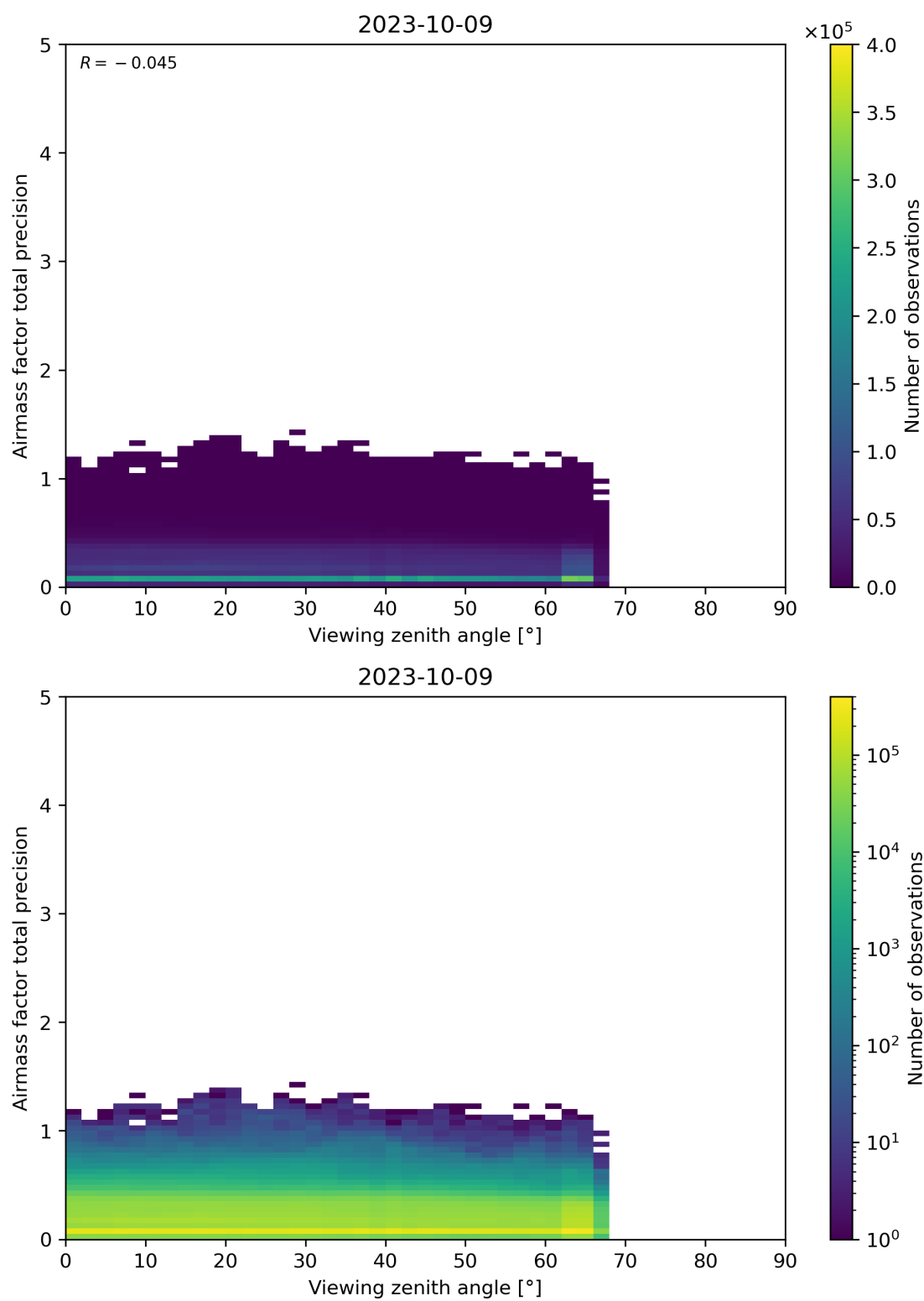
Figure 191: Scatter density plot of “Viewing zenith angle” against “Airmass factor total precision” for 2023-10-08 to 2023-10-10.
