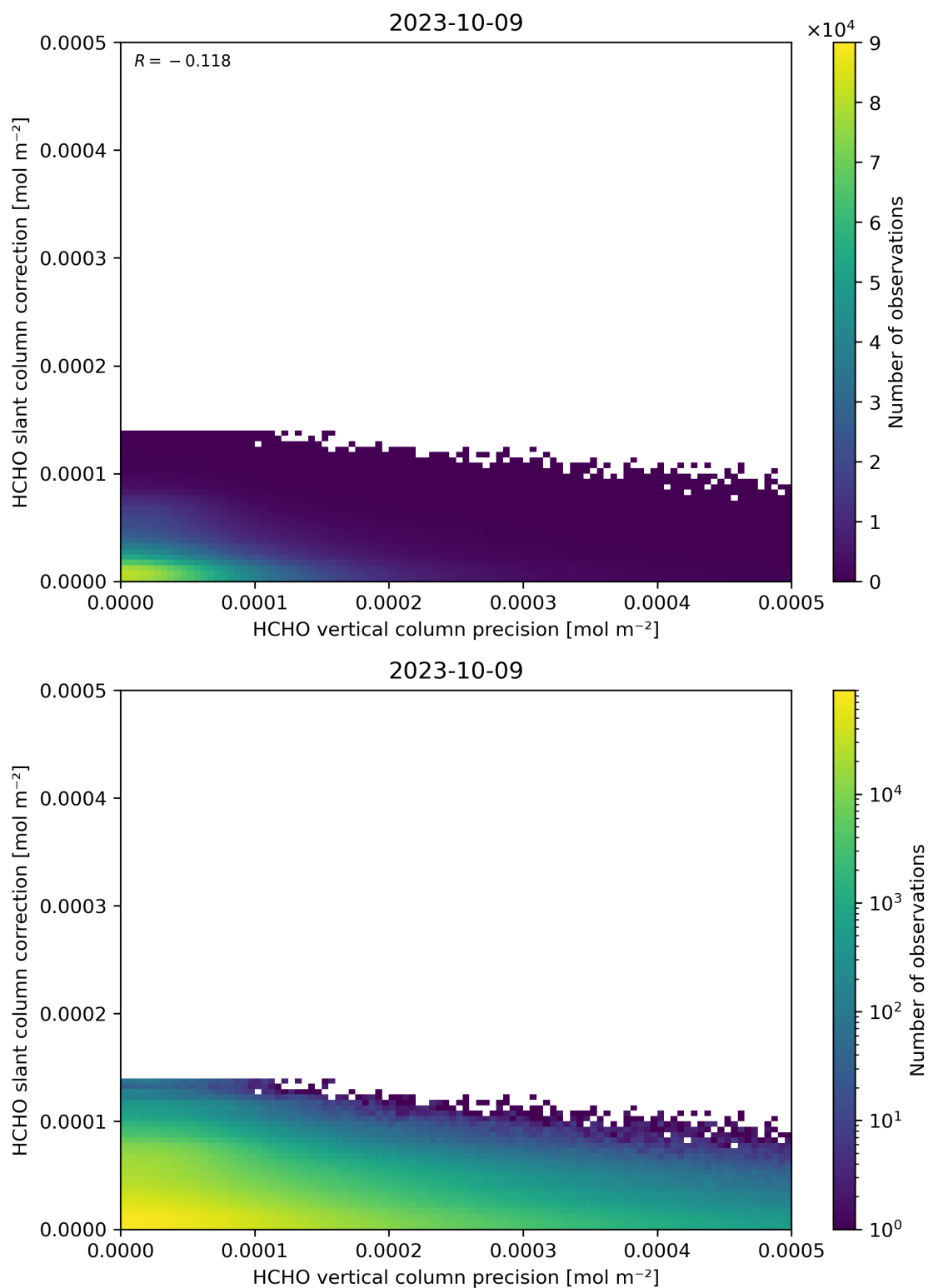
Figure 141: Scatter density plot of “HCHO vertical column precision” against “HCHO slant column correction” for 2023-10-08 to 2023-10-10.
