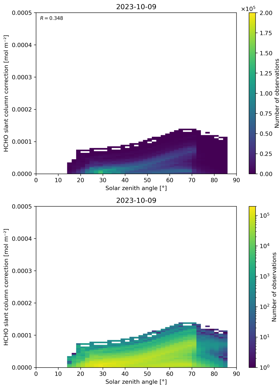
Figure 172: Scatter density plot of “Solar zenith angle” against “HCHO slant column correction” for 2023-10-08 to 2023-10-10.
