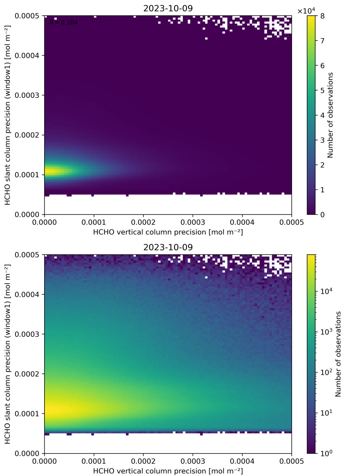
Figure 143: Scatter density plot of “HCHO vertical column precision” against “HCHO slant column precision (window1)” for 2023-10-08 to 2023-10-10.
