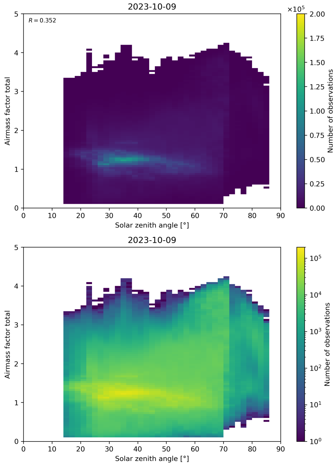
Figure 175: Scatter density plot of “Solar zenith angle” against “Airmass factor total” for 2023-10-08 to 2023-10-10.
