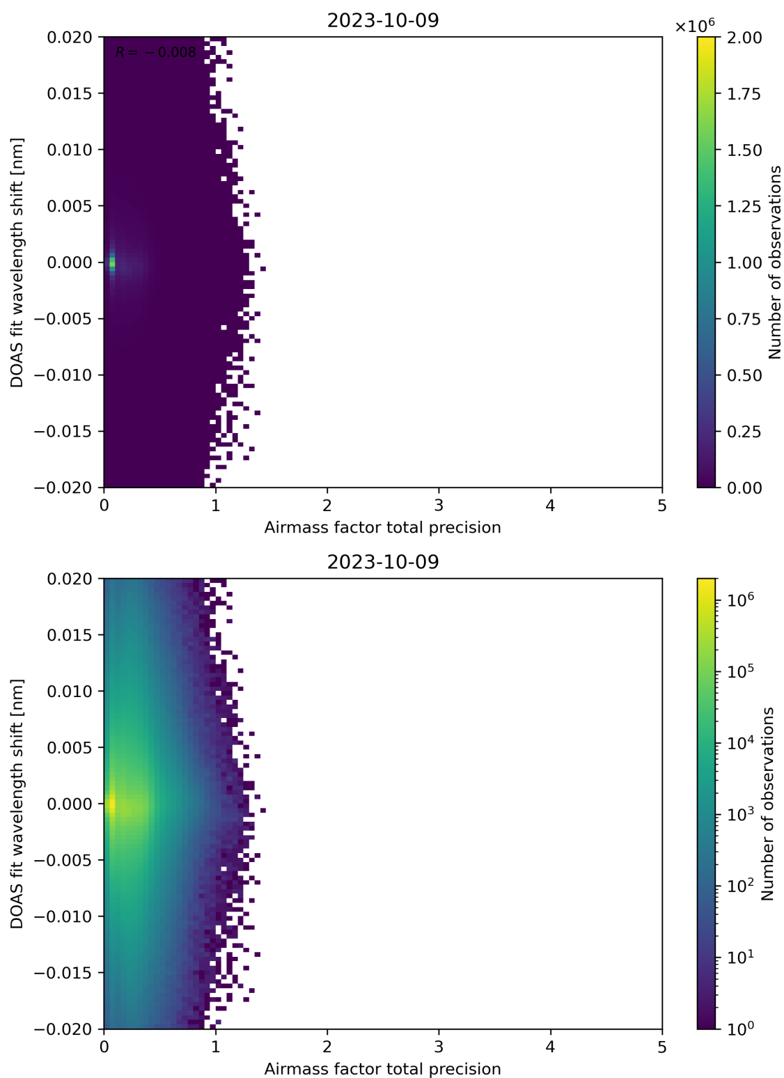
Figure 106: Scatter density plot of “Airmass factor total precision” against “DOAS fit wavelength shift” for 2023-10-08 to 2023-10-10.
