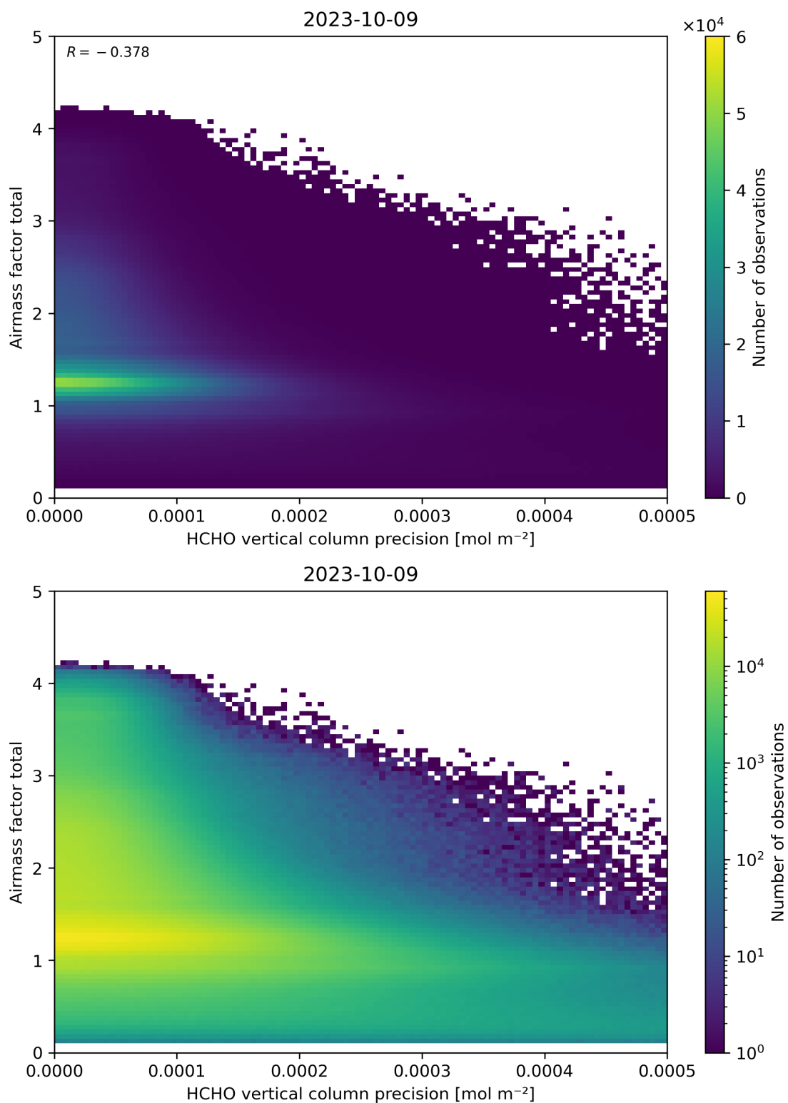
Figure 144: Scatter density plot of “HCHO vertical column precision” against “Airmass factor total” for 2023-10-08 to 2023-10-10.
