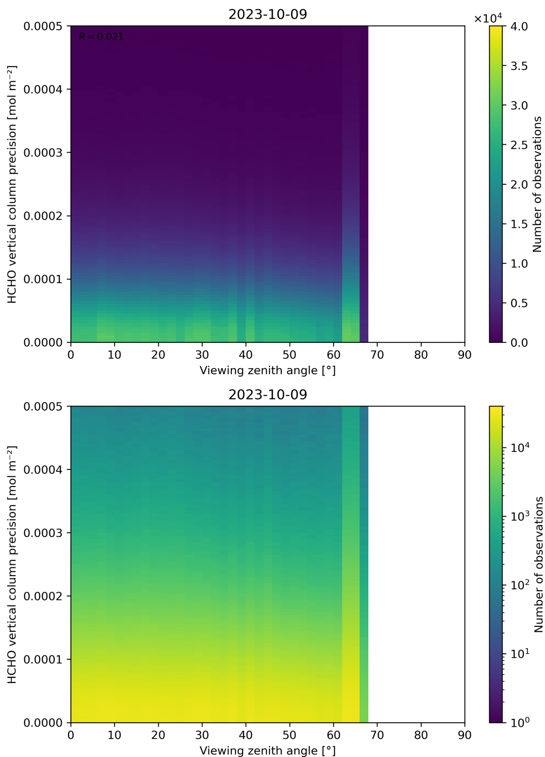
Figure 194: Scatter density plot of “Viewing zenith angle” against “HCHO vertical column precision” for 2023-10-08 to 2023-10-10.
