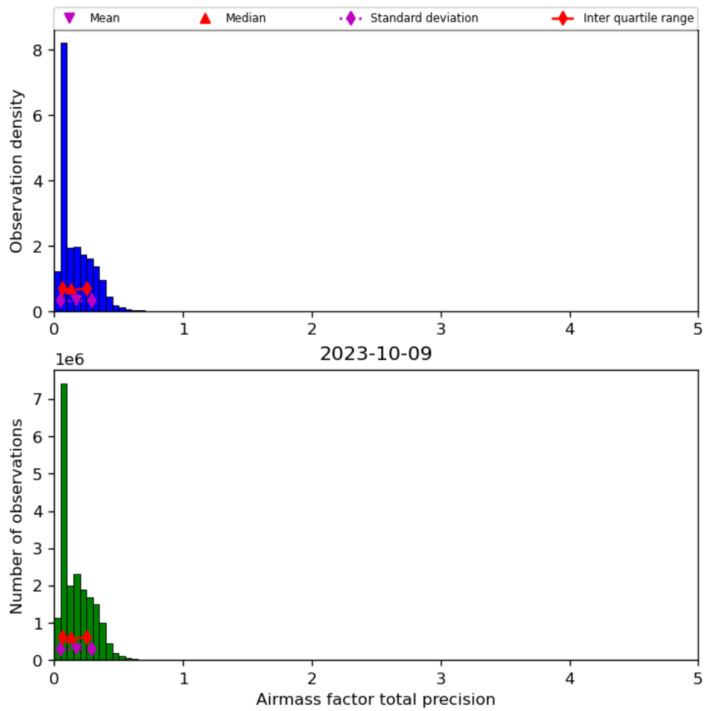
Figure 41: Histogram of “Airmass factor total precision” for 2023-10-08 to 2023-10-10
