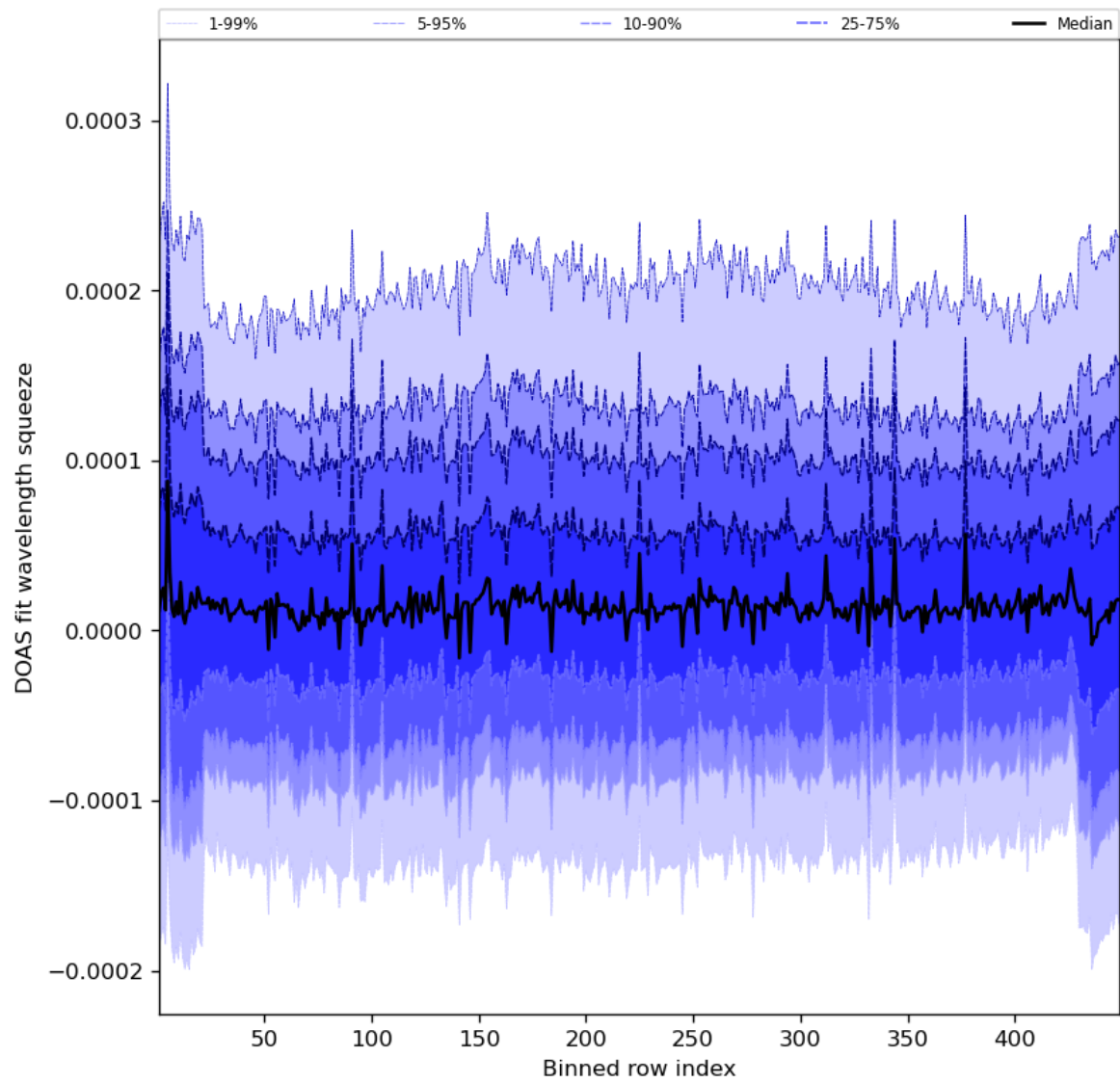
Figure 59: Along track statistics of “DOAS fit wavelength squeeze” for 2023-10-08 to 2023-10-10
