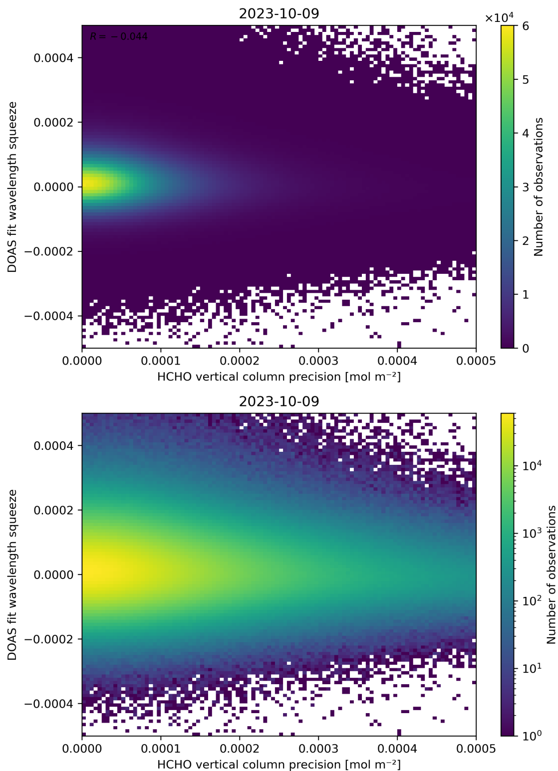
Figure 138: Scatter density plot of “HCHO vertical column precision” against “DOAS fit wavelength squeeze” for 2023-10-08 to 2023-10-10.
