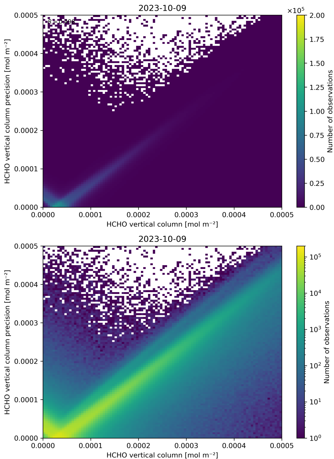
Figure 134: Scatter density plot of “HCHO vertical column” against “HCHO vertical column precision” for 2023-10-08 to 2023-10-10.
