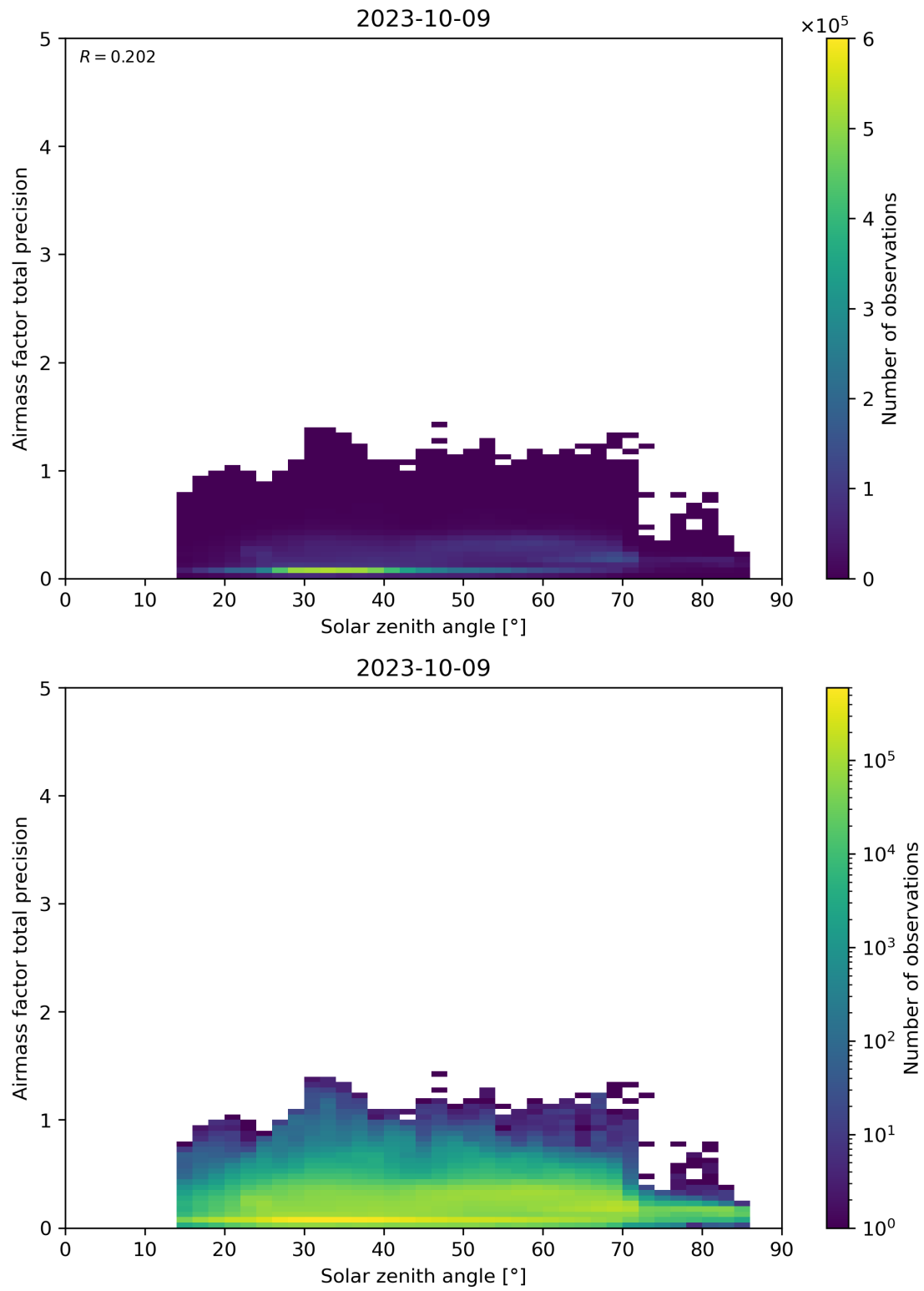
Figure 176: Scatter density plot of “Solar zenith angle” against “Airmass factor total precision” for 2023-10-08 to 2023-10-10.
