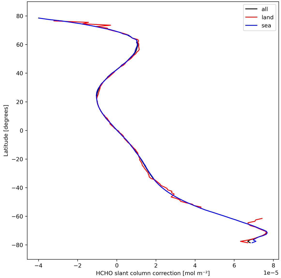
Figure 33: Zonal average of “HCHO slant column correction” for 2023-10-08 to 2023-10-10.
