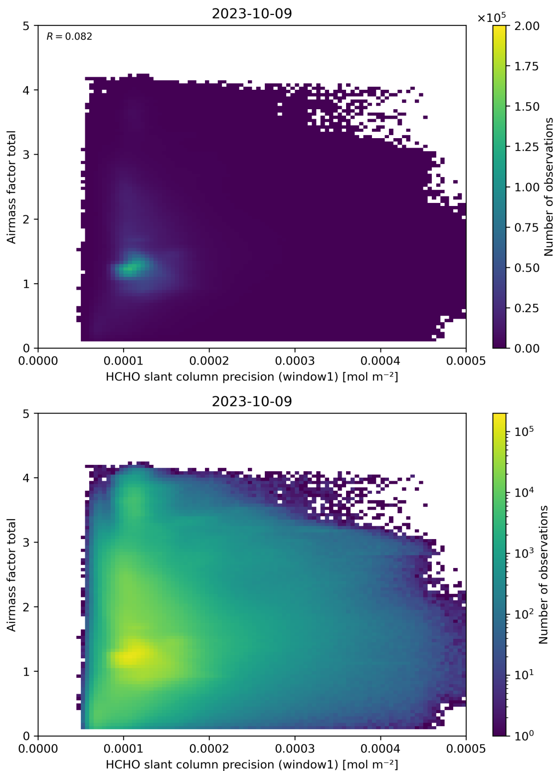
Figure 94: Scatter density plot of “HCHO slant column precision (window1)” against “Airmass factor total” for 2023-10-08 to 2023-10-10.
