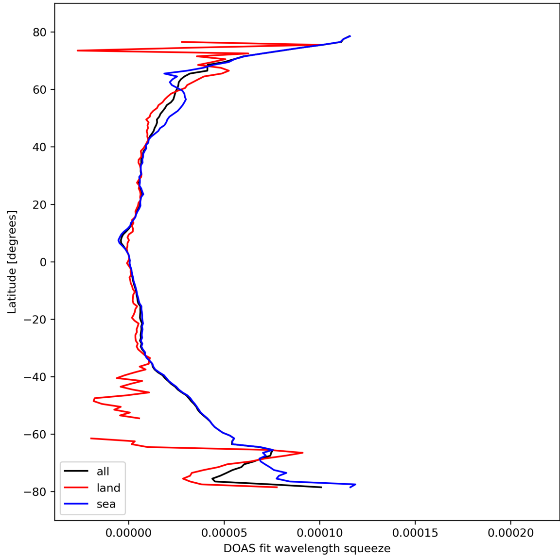
Figure 31: Zonal average of “DOAS fit wavelength squeeze” for 2023-10-08 to 2023-10-10.
