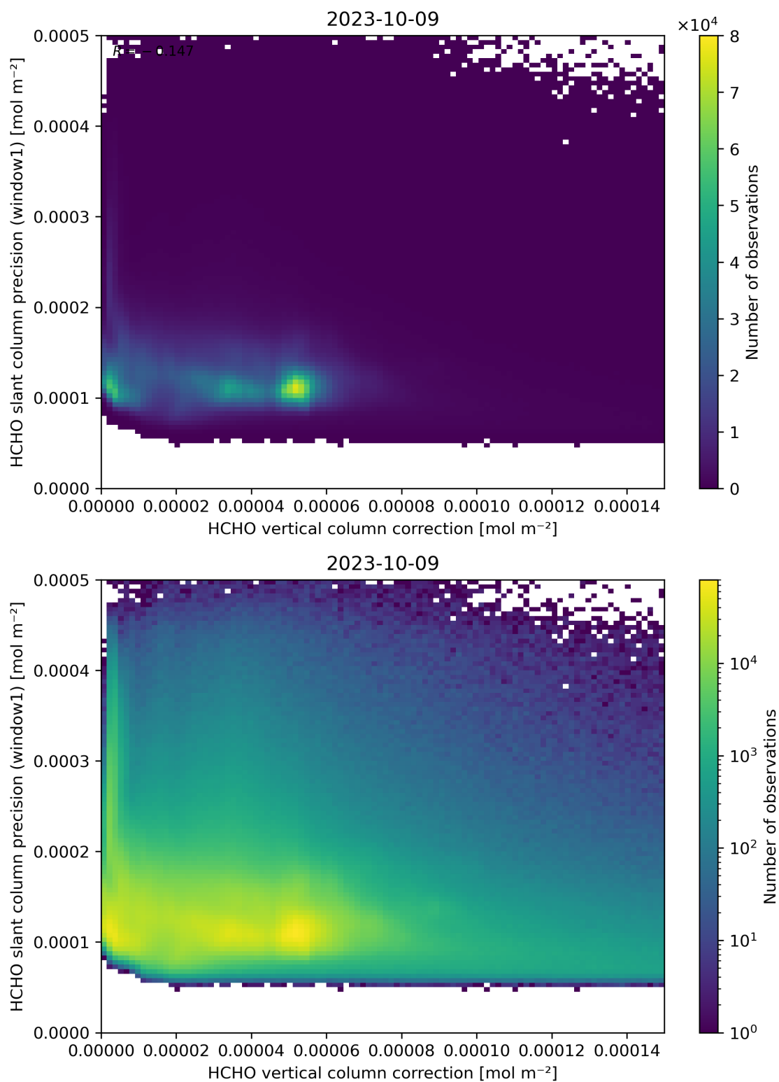
Figure 119: Scatter density plot of “HCHO vertical column correction” against “HCHO slant column precision (window1)” for 2023-10-08 to 2023-10-10.
