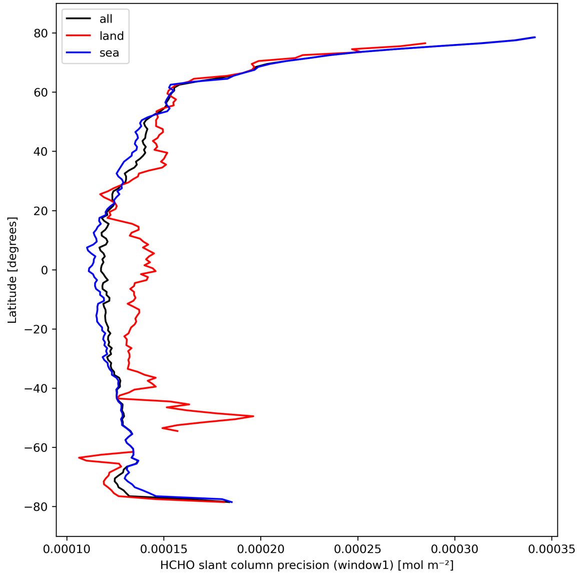
Figure 25: Zonal average of “HCHO slant column precision (window1)” for 2023-10-08 to 2023-10-10.
