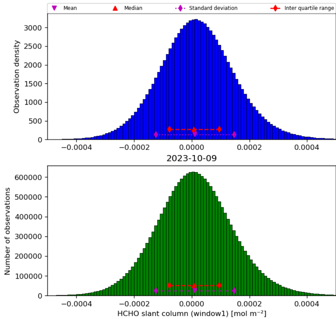
Figure 38: Histogram of “HCHO slant column (window1)” for 2023-10-08 to 2023-10-10
