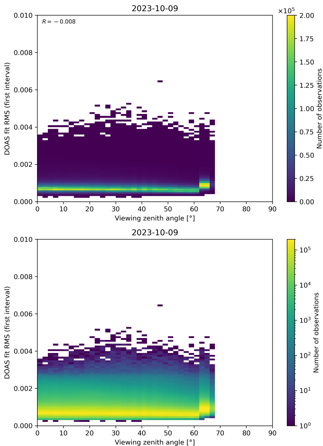
Figure 182: Scatter density plot of “Viewing zenith angle” against “DOAS fit RMS (first interval)” for 2023-10-08 to 2023-10-10.
