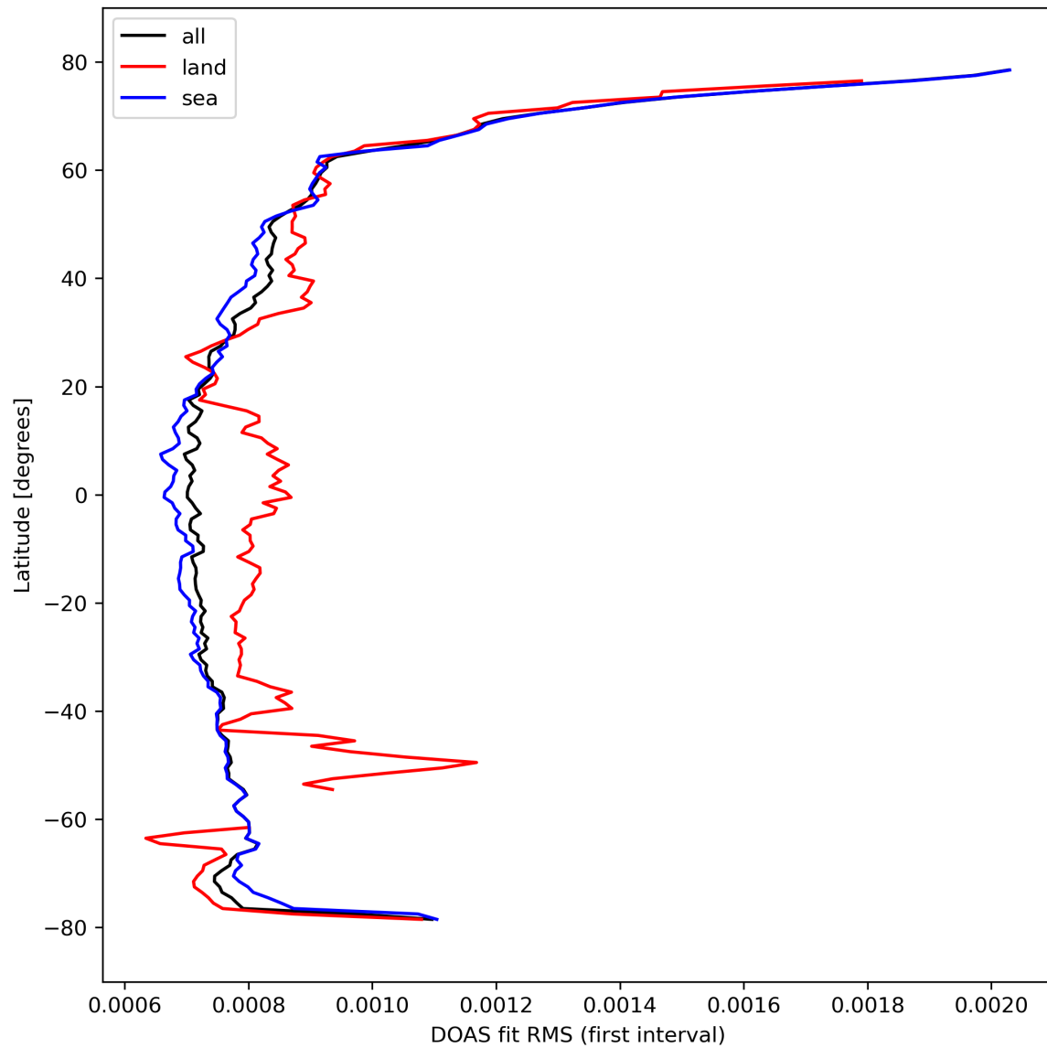
Figure 32: Zonal average of “DOAS fit RMS (first interval)” for 2023-10-08 to 2023-10-10.
