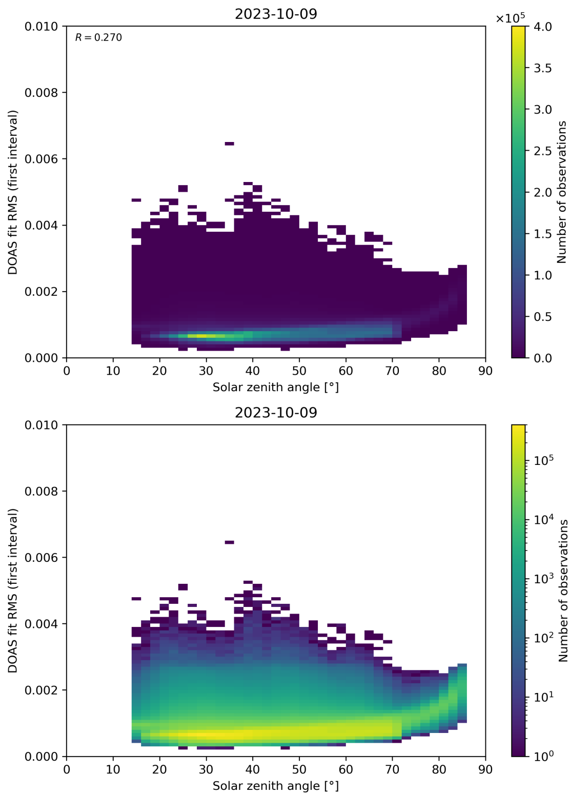
Figure 167: Scatter density plot of “Solar zenith angle” against “DOAS fit RMS (first interval)” for 2023-10-08 to 2023-10-10.
