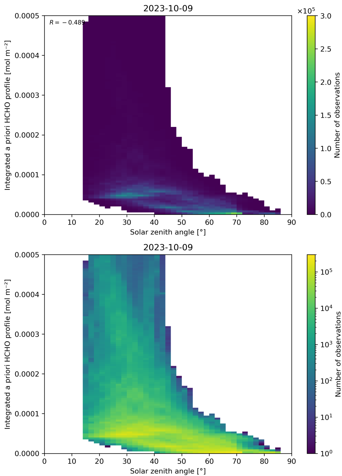
Figure 180: Scatter density plot of “Solar zenith angle” against “Integrated a priori HCHO profile” for 2023-10-08 to 2023-10-10.
