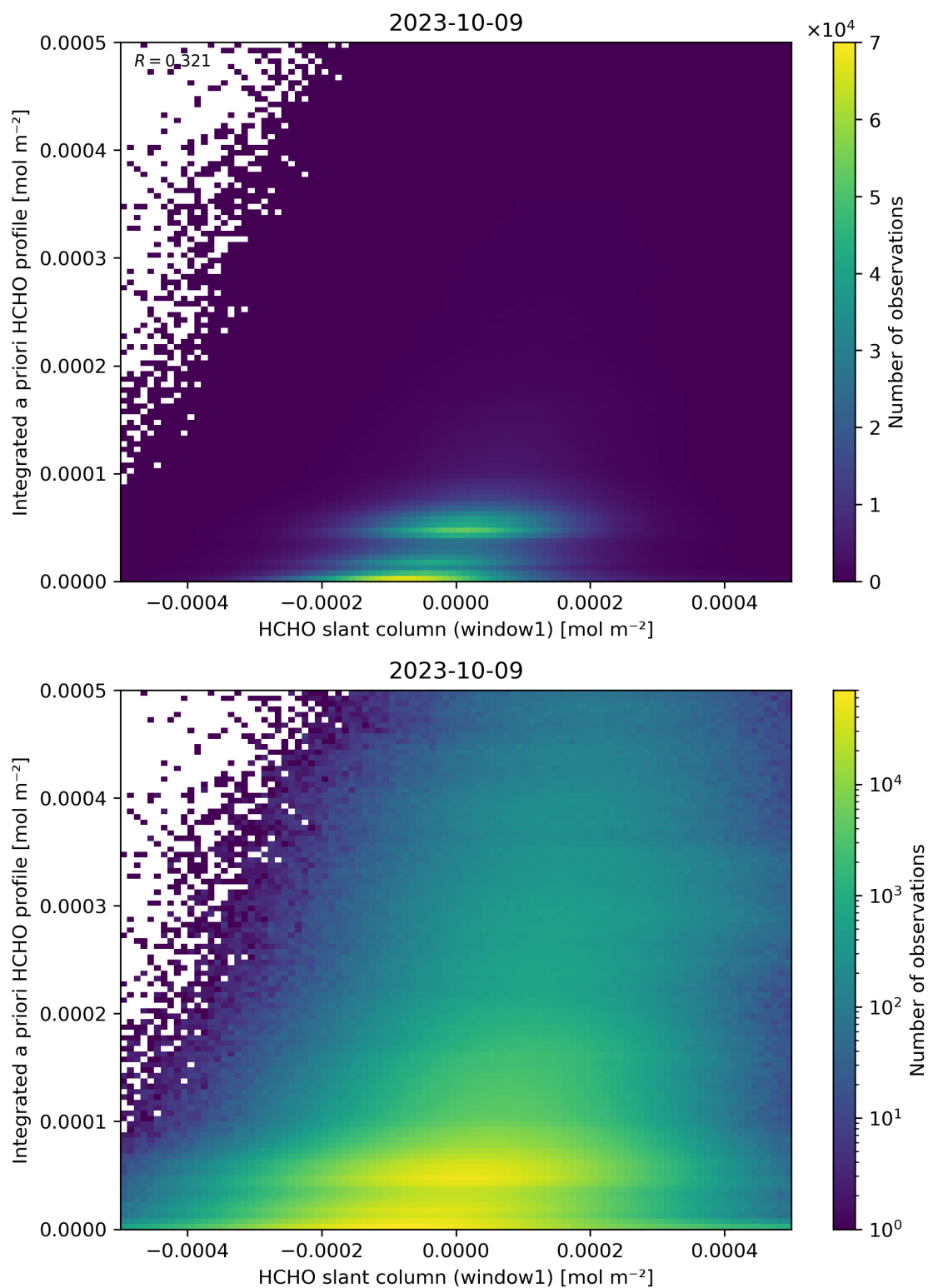
Figure 87: Scatter density plot of “HCHO slant column (window1)” against “Integrated a priori HCHO profile” for 2023-10-08 to 2023-10-10.
