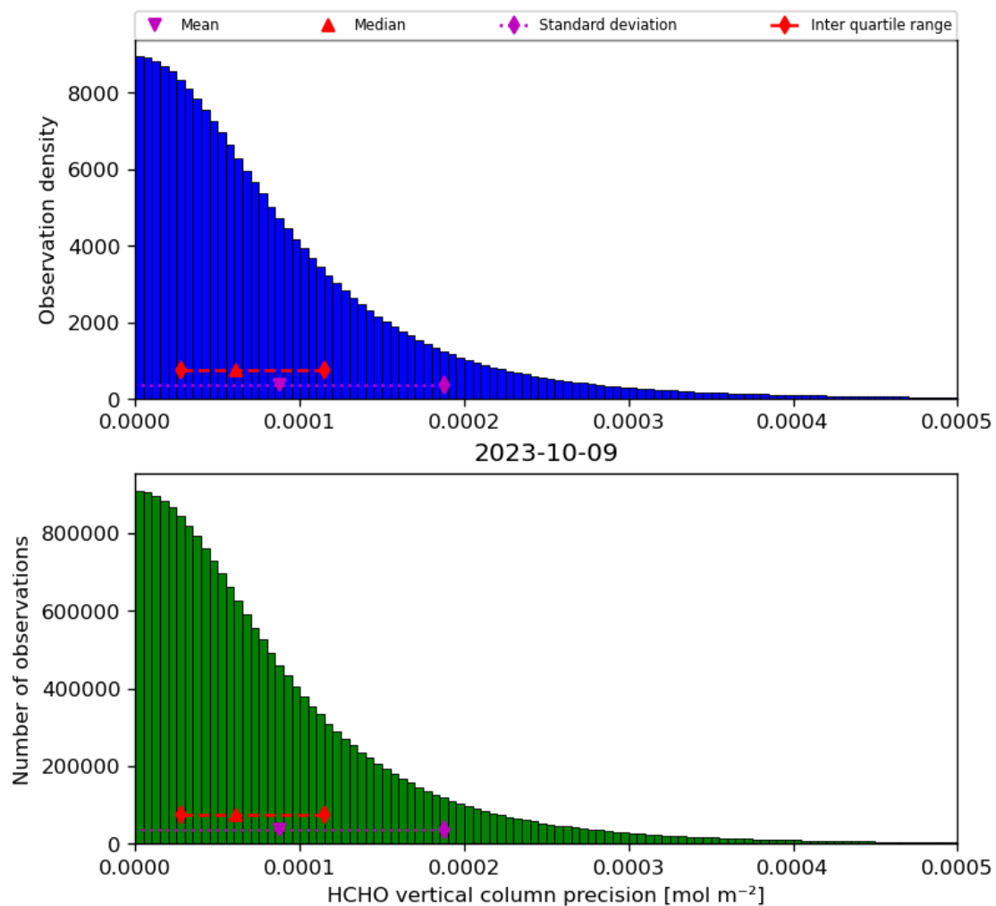
Figure 36: Histogram of “HCHO vertical column precision” for 2023-10-08 to 2023-10-10
