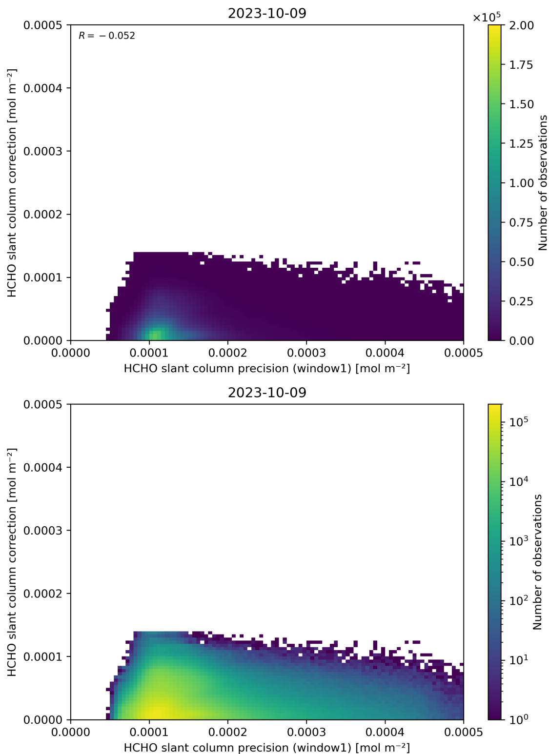
Figure 93: Scatter density plot of “HCHO slant column precision (window1)” against “HCHO slant column correction” for 2023-10-08 to 2023-10-10.
