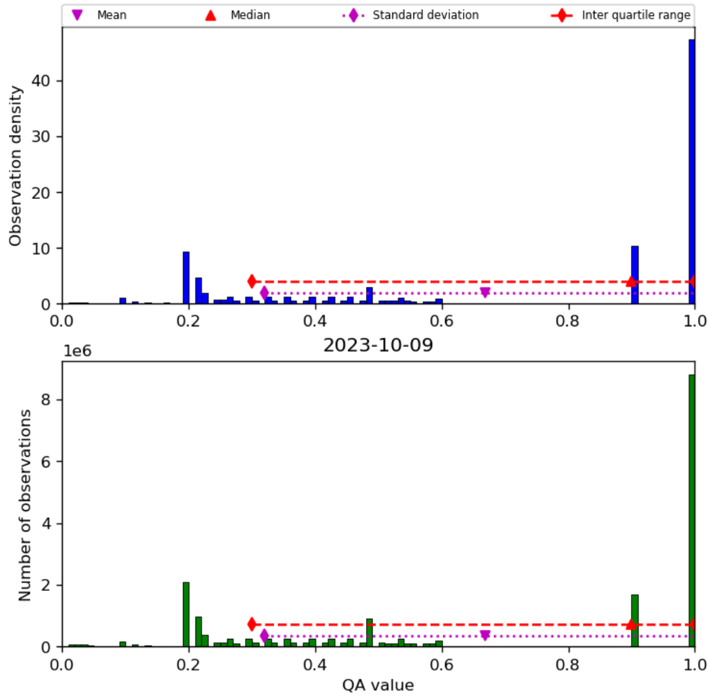
Figure 34: Histogram of “QA value” for 2023-10-08 to 2023-10-10
