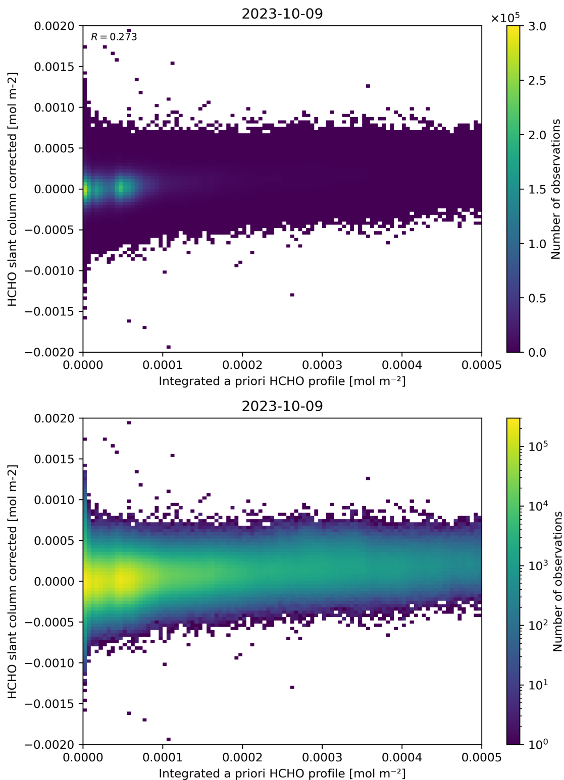
Figure 151: Scatter density plot of “Integrated a priori HCHO profile” against “HCHO slant column corrected” for 2023-10-08 to 2023-10-10.
