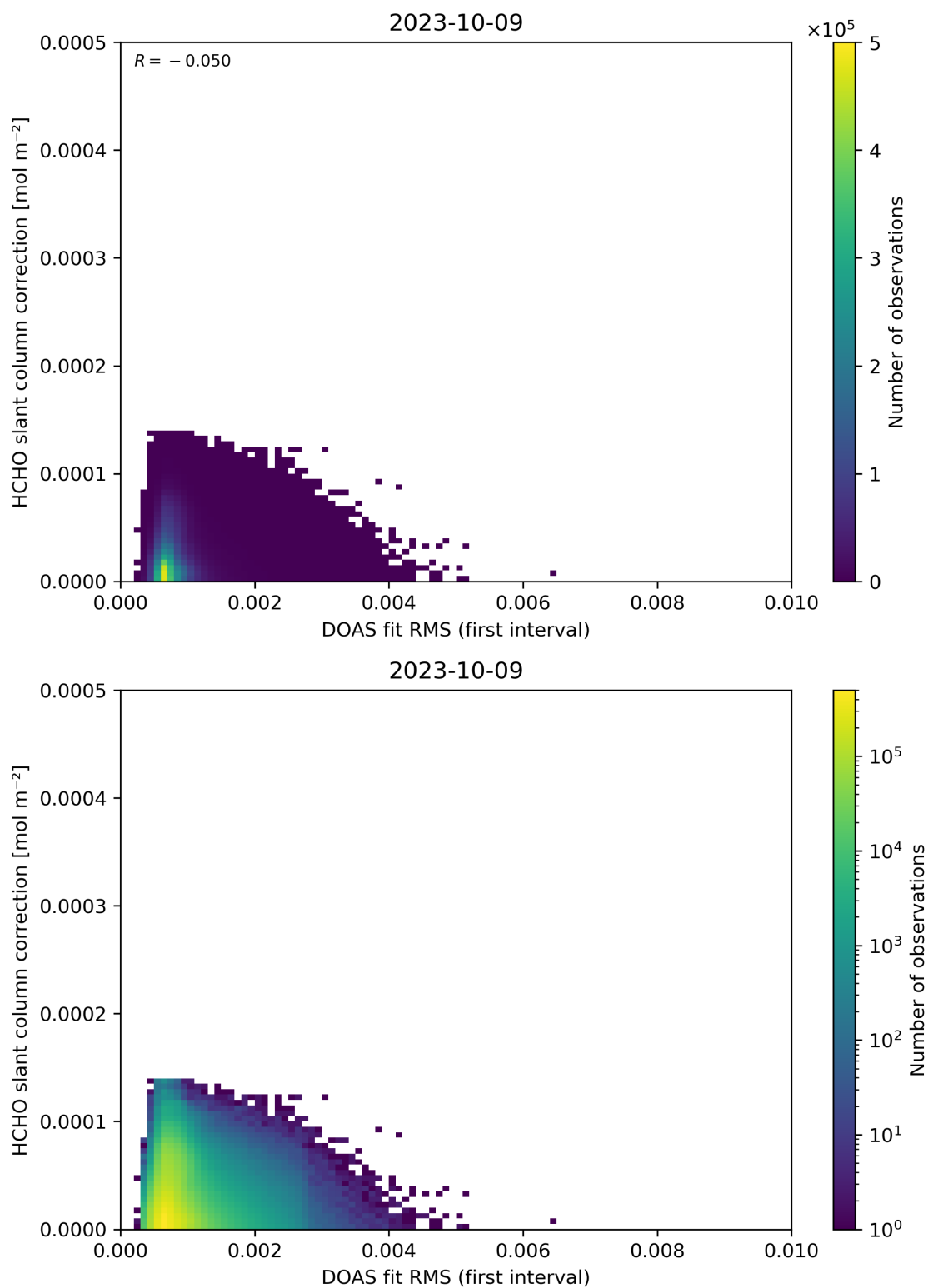
Figure 63: Scatter density plot of “DOAS fit RMS (first interval)” against “HCHO slant column correction” for 2023-10-08 to 2023-10-10.
