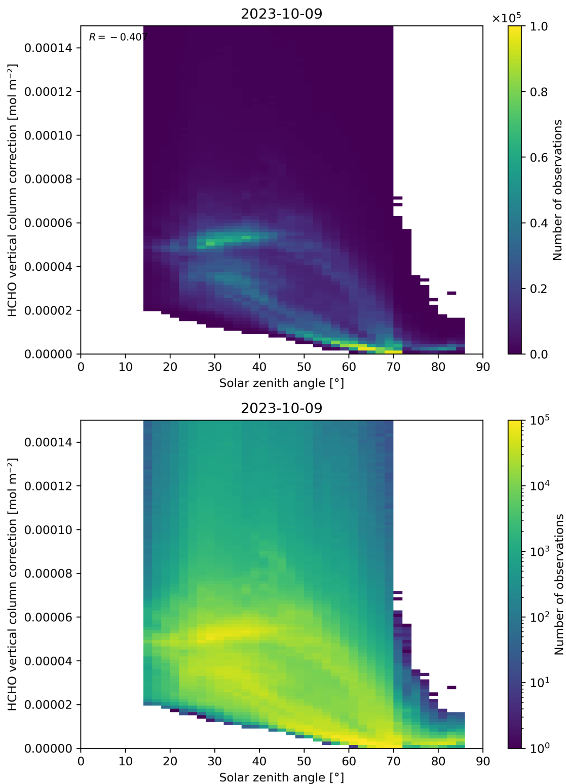
Figure 178: Scatter density plot of “Solar zenith angle” against “HCHO vertical column correction” for 2023-10-08 to 2023-10-10.
