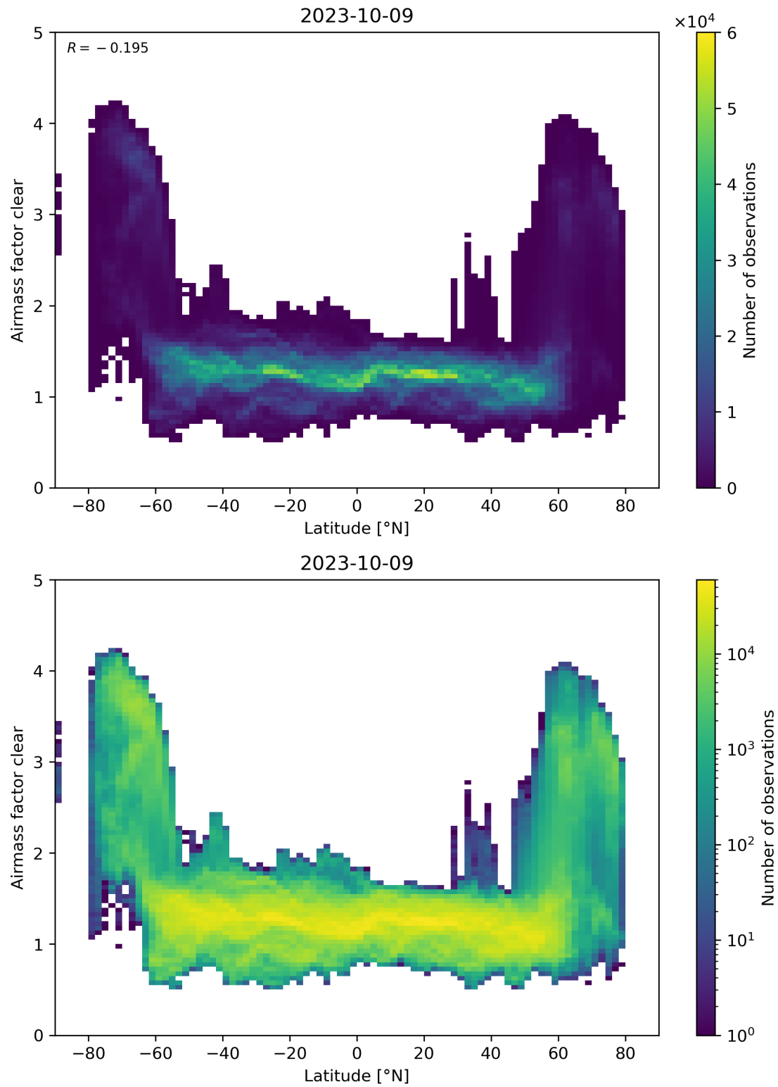
Figure 156: Scatter density plot of “Latitude” against “Airmass factor clear” for 2023-10-08 to 2023-10-10.
