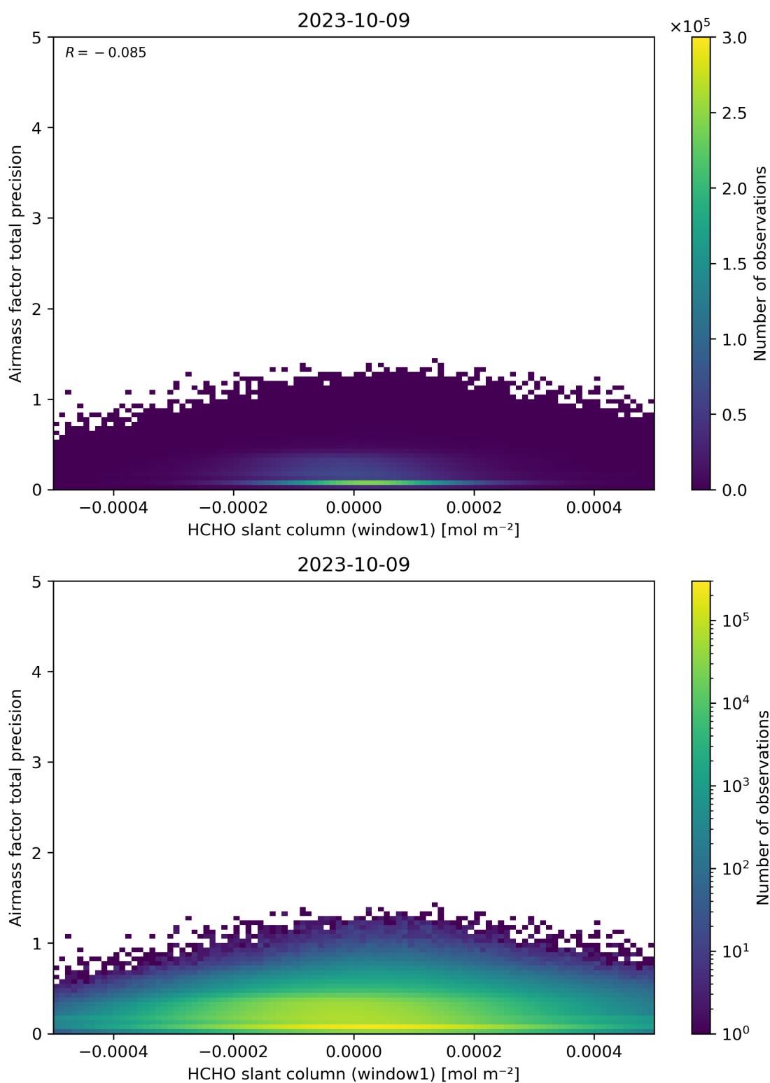
Figure 86: Scatter density plot of “HCHO slant column (window1)” against “Airmass factor total precision” for 2023-10-08 to 2023-10-10.
