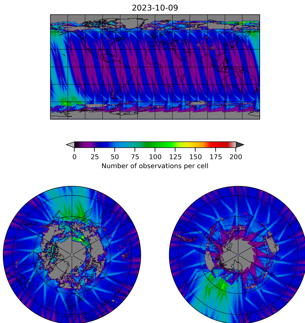
Figure 19: Map of the number of observations for 2023-10-08 to 2023-10-10
