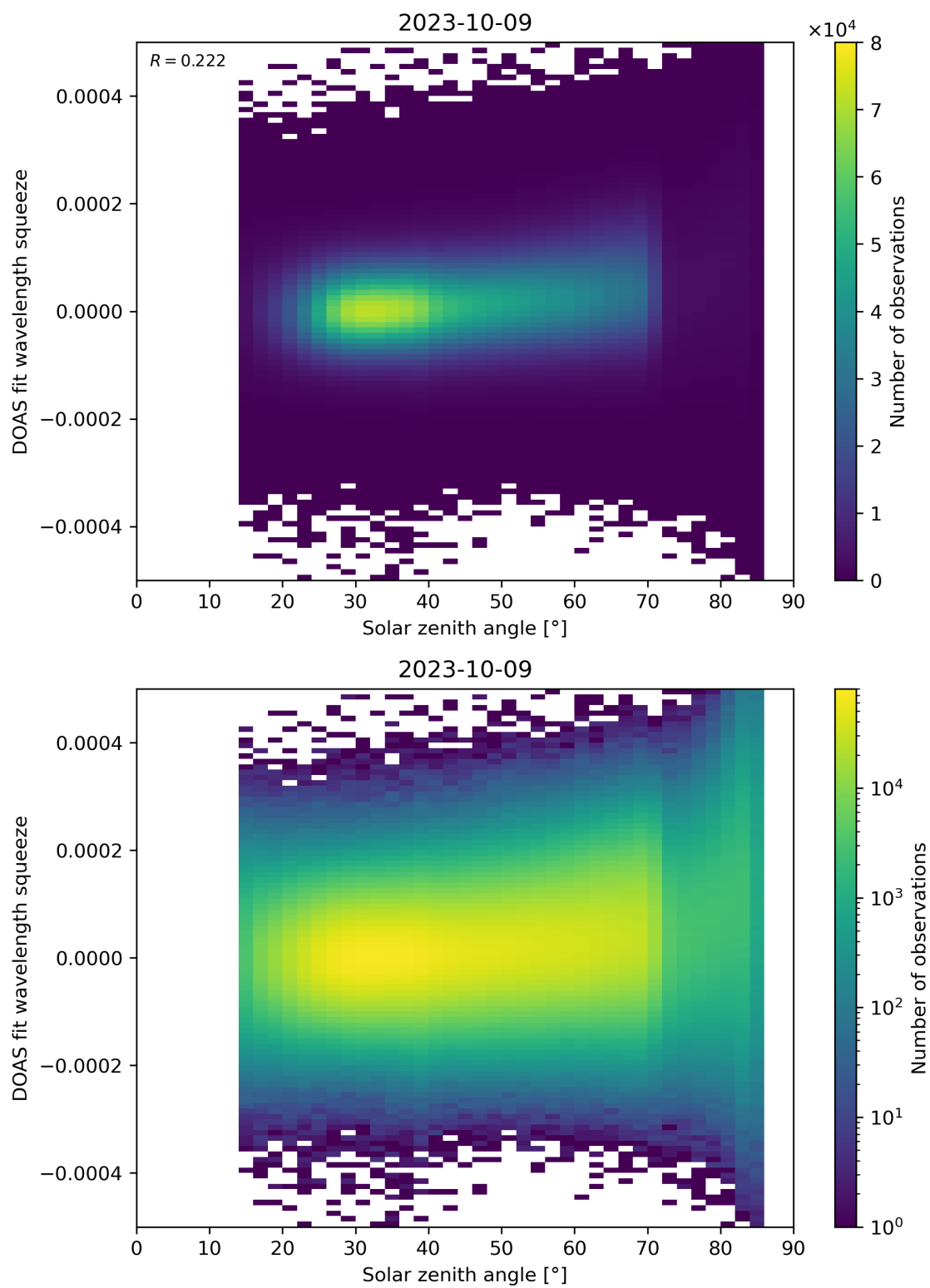
Figure 169: Scatter density plot of “Solar zenith angle” against “DOAS fit wavelength squeeze” for 2023-10-08 to 2023-10-10.
