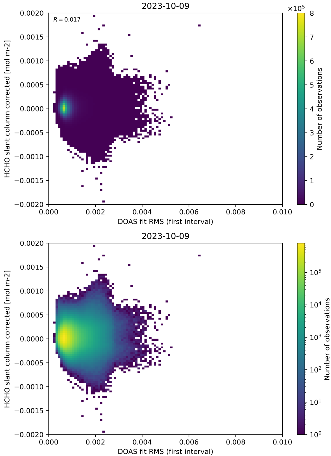
Figure 62: Scatter density plot of “DOAS fit RMS (first interval)” against “HCHO slant column corrected” for 2023-10-08 to 2023-10-10.
