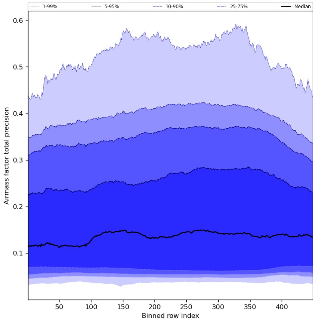
Figure 55: Along track statistics of “Airmass factor total precision” for 2023-10-08 to 2023-10-10
