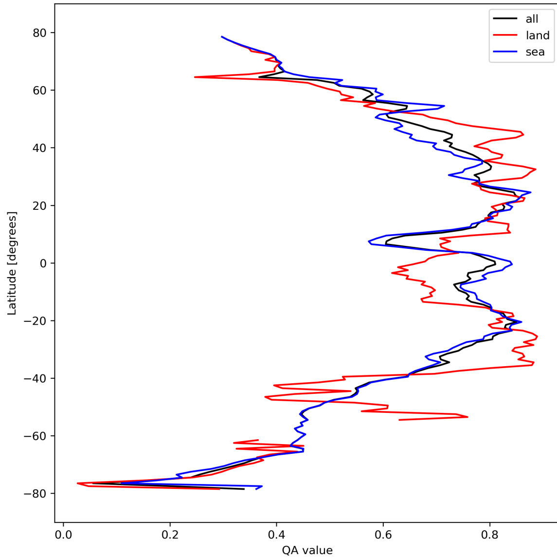
Figure 20: Zonal average of “QA value” for 2023-10-08 to 2023-10-10.
