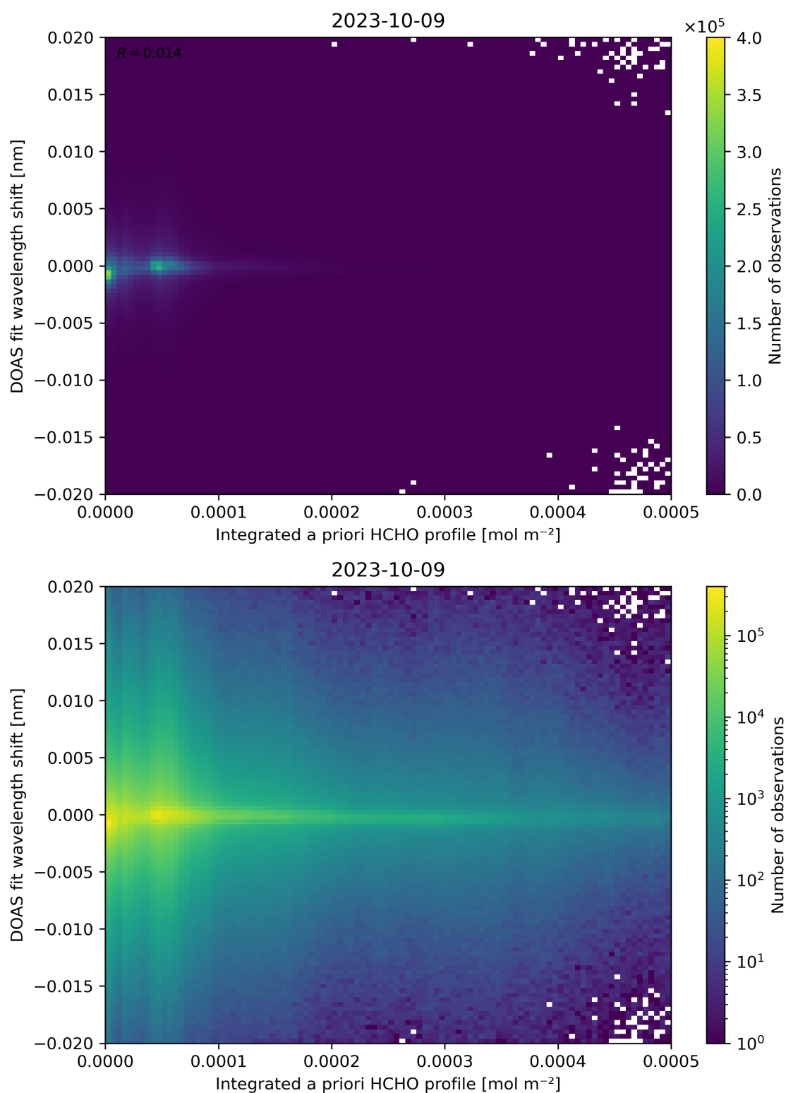
Figure 149: Scatter density plot of “Integrated a priori HCHO profile” against “DOAS fit wavelength shift” for 2023-10-08 to 2023-10-10.
