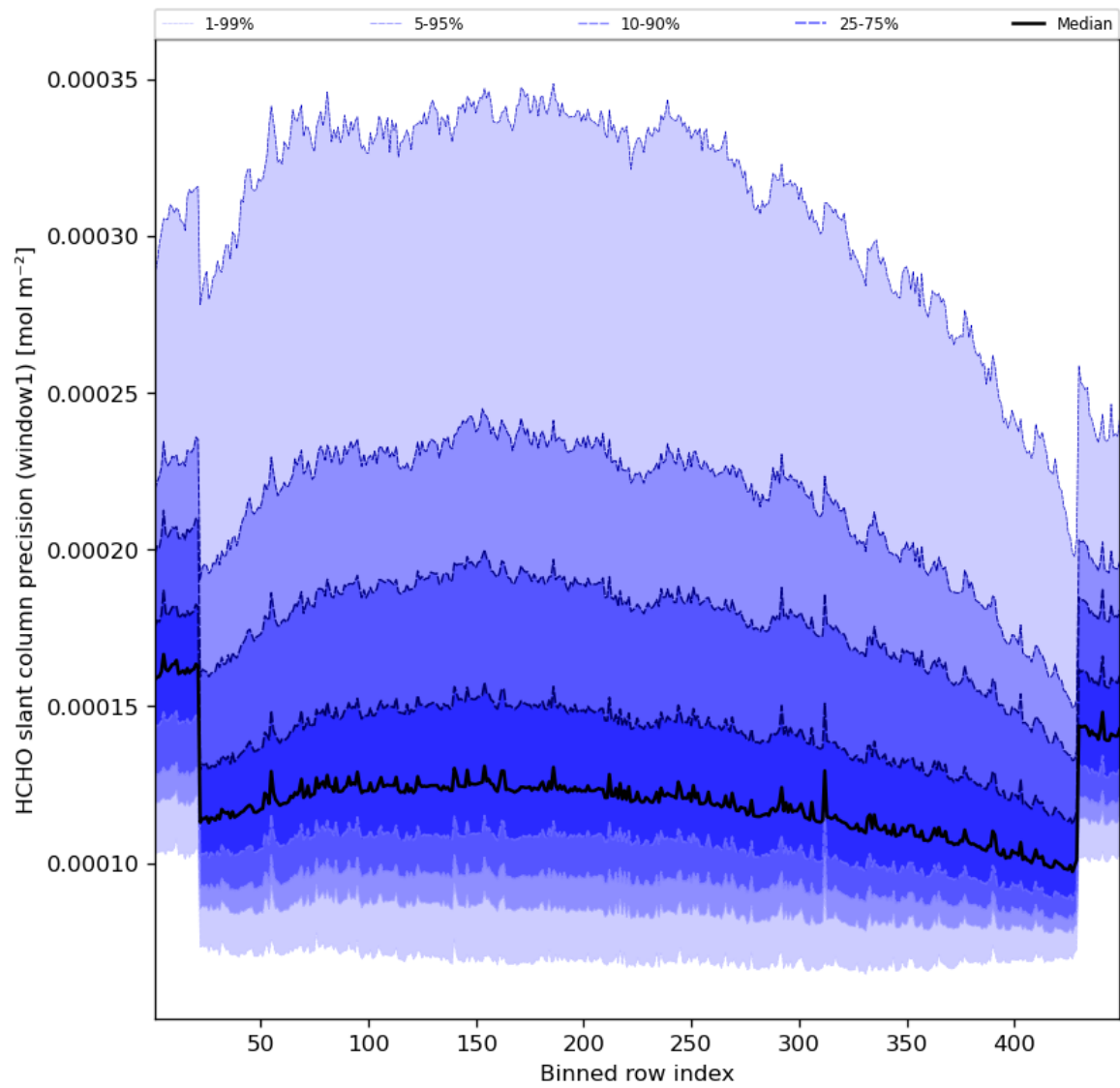
Figure 53: Along track statistics of “HCHO slant column precision (window1)” for 2023-10-08 to 2023-10-10
