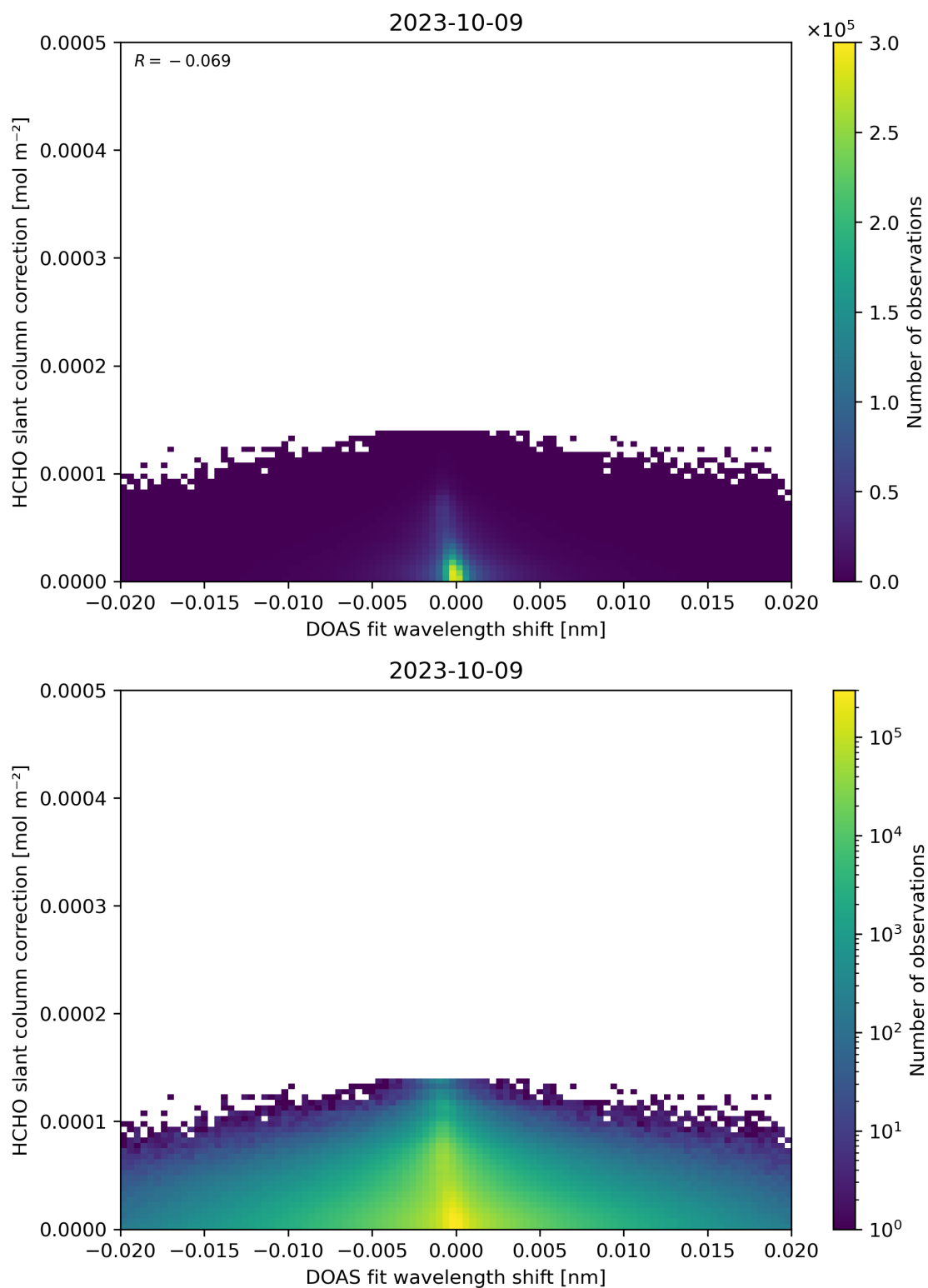
Figure 67: Scatter density plot of “DOAS fit wavelength shift” against “HCHO slant column correction” for 2023-10-08 to 2023-10-10.
