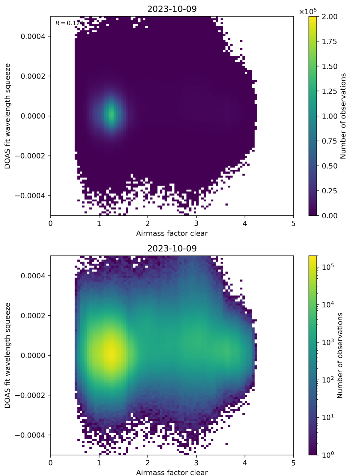
Figure 73: Scatter density plot of “Airmass factor clear” against “DOAS fit wavelength squeeze” for 2023-10-08 to 2023-10-10.
