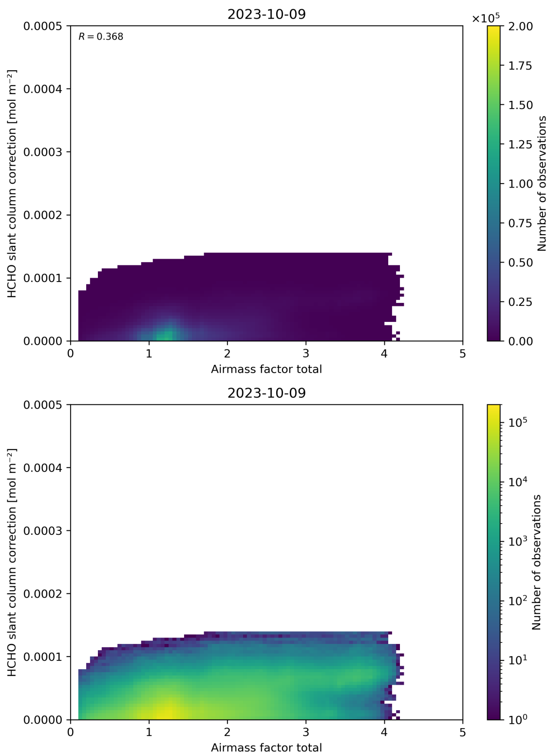
Figure 102: Scatter density plot of “Airmass factor total” against “HCHO slant column correction” for 2023-10-08 to 2023-10-10.
