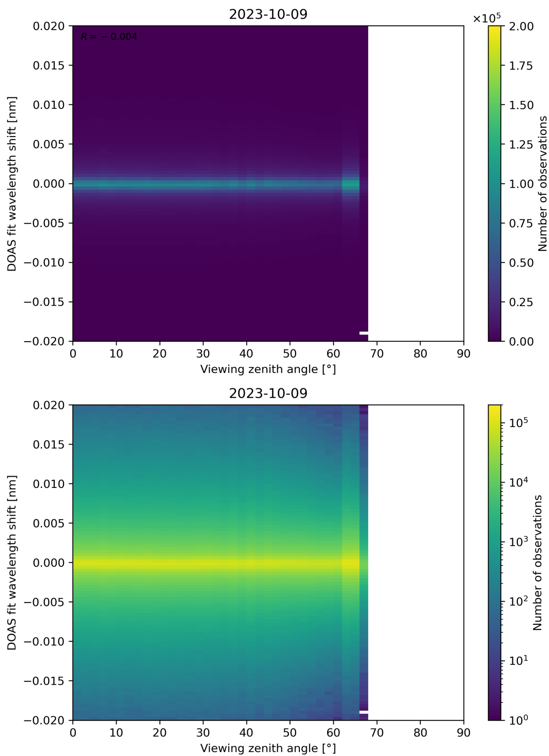
Figure 183: Scatter density plot of “Viewing zenith angle” against “DOAS fit wavelength shift” for 2023-10-08 to 2023-10-10.
