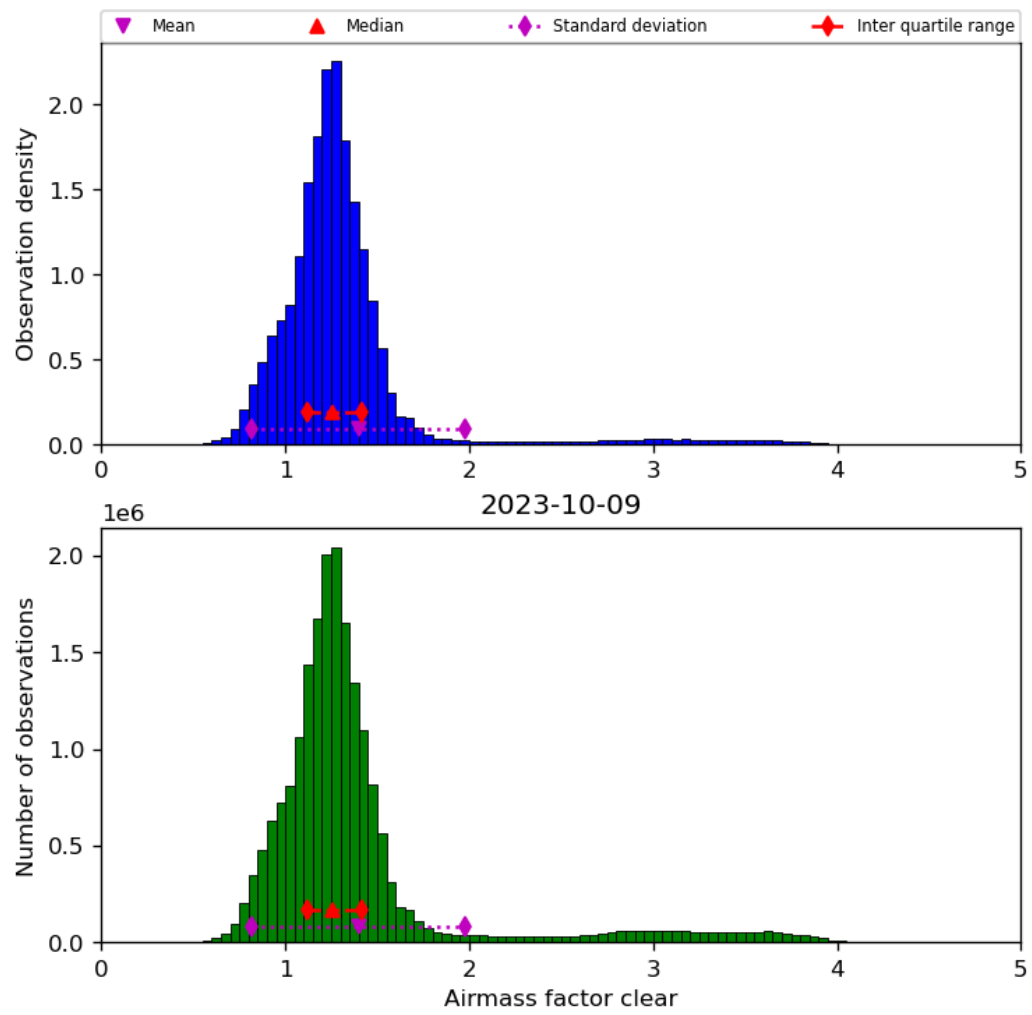
Figure 42: Histogram of “Airmass factor clear” for 2023-10-08 to 2023-10-10
