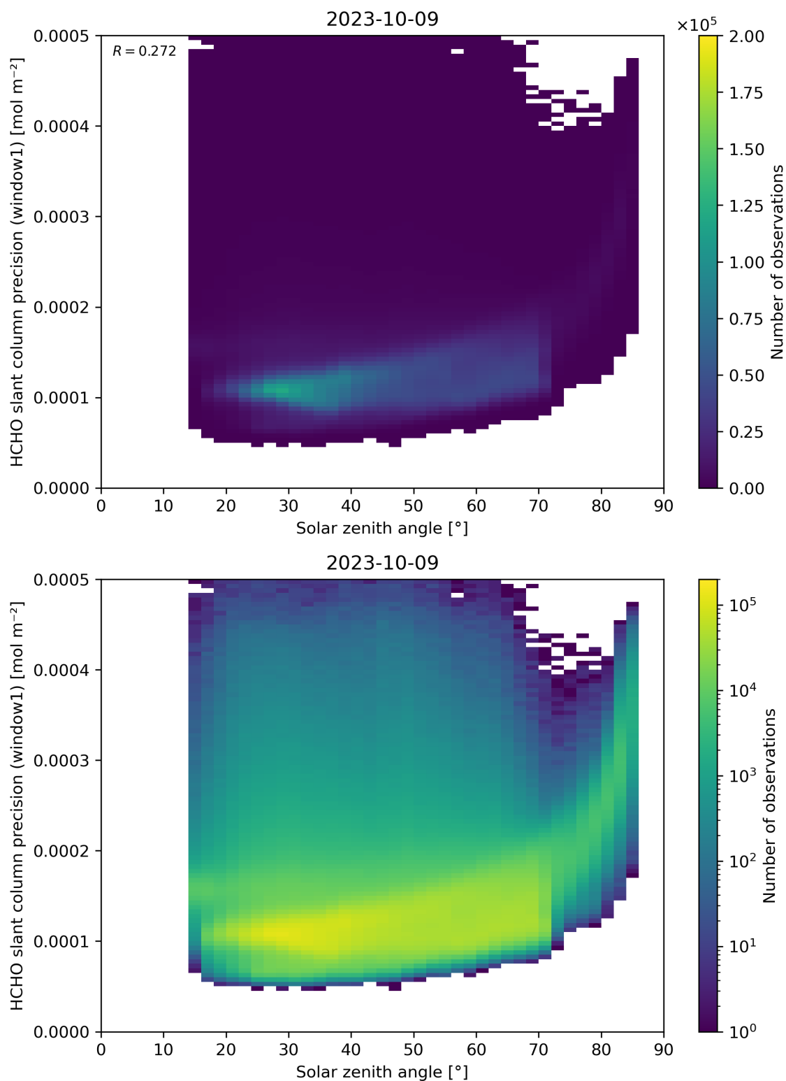
Figure 174: Scatter density plot of “Solar zenith angle” against “HCHO slant column precision (window1)” for 2023-10-08 to 2023-10-10.
