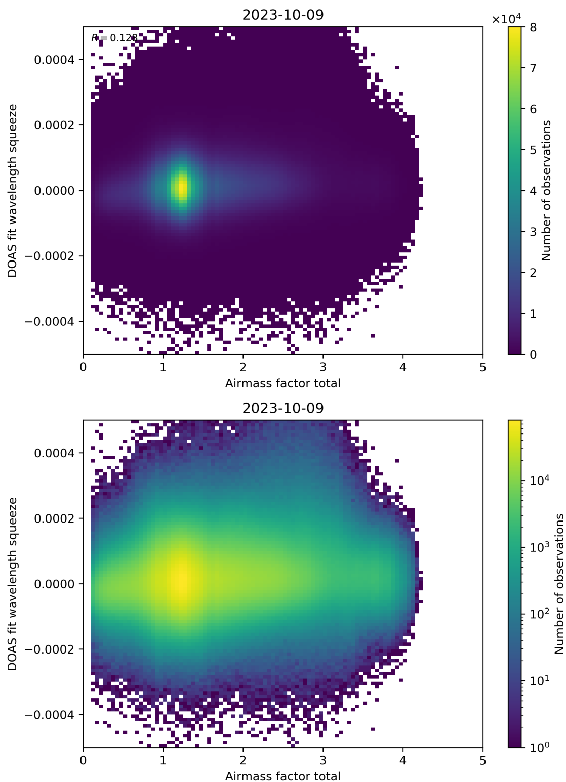
Figure 99: Scatter density plot of “Airmass factor total” against “DOAS fit wavelength squeeze” for 2023-10-08 to 2023-10-10.
