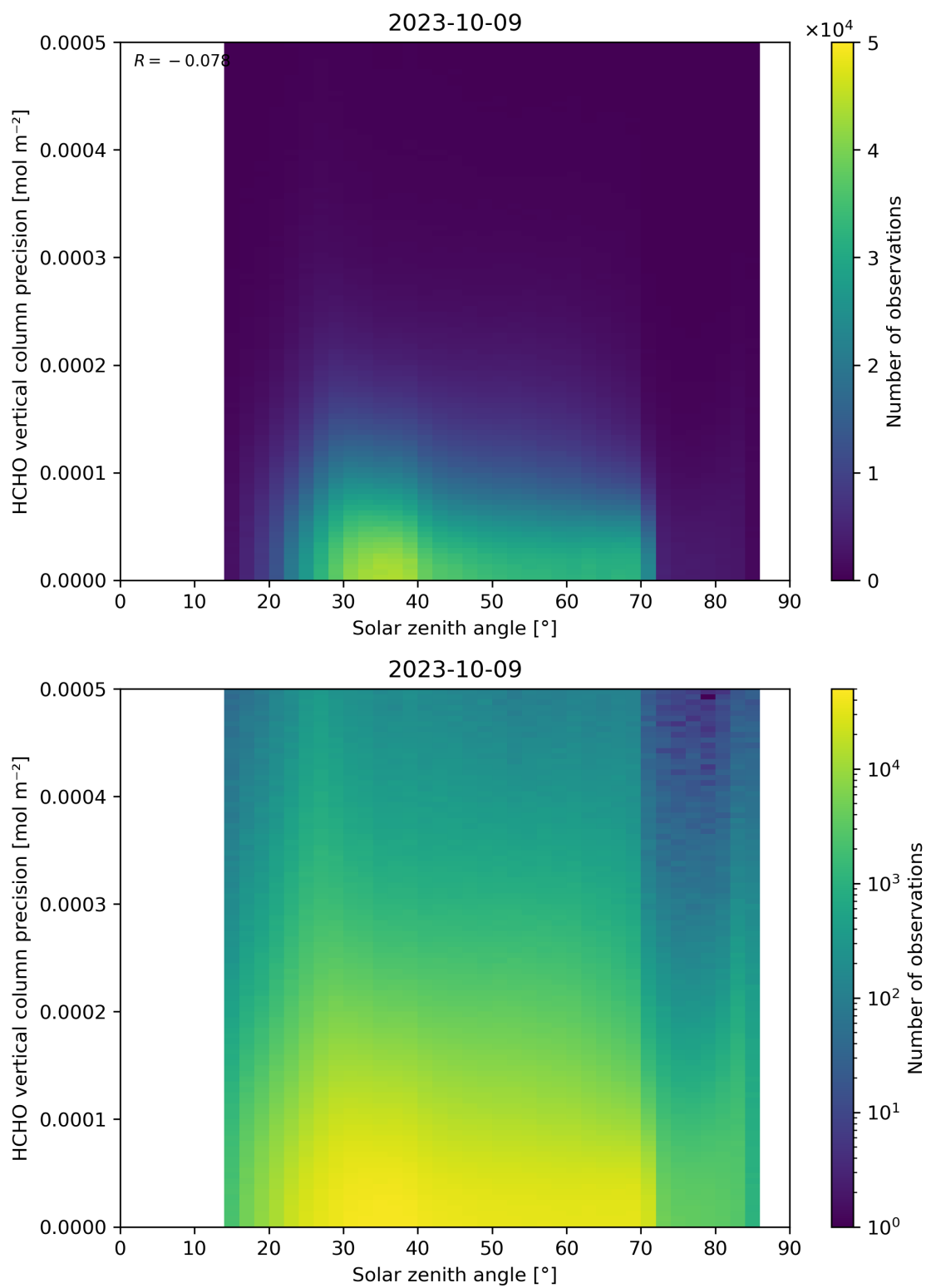
Figure 179: Scatter density plot of “Solar zenith angle” against “HCHO vertical column precision” for 2023-10-08 to 2023-10-10.
