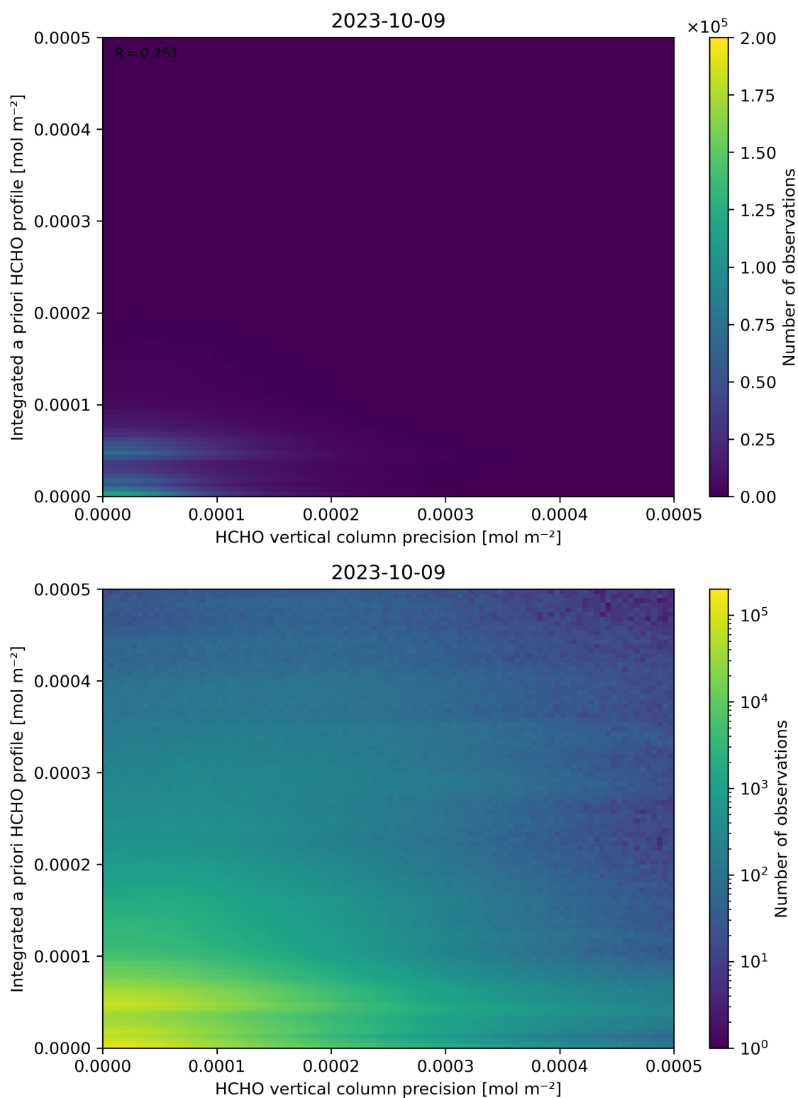
Figure 147: Scatter density plot of “HCHO vertical column precision” against “Integrated a priori HCHO profile” for 2023-10-08 to 2023-10-10.
