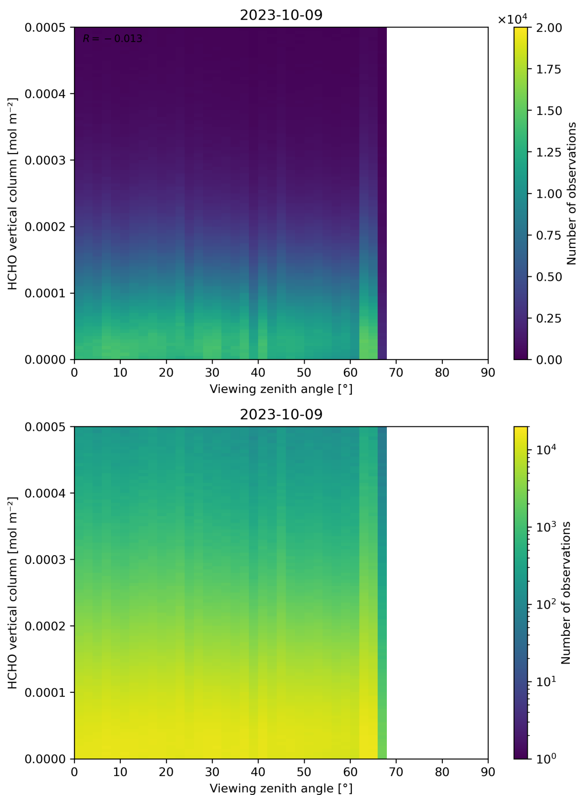
Figure 192: Scatter density plot of “Viewing zenith angle” against “HCHO vertical column” for 2023-10-08 to 2023-10-10.
