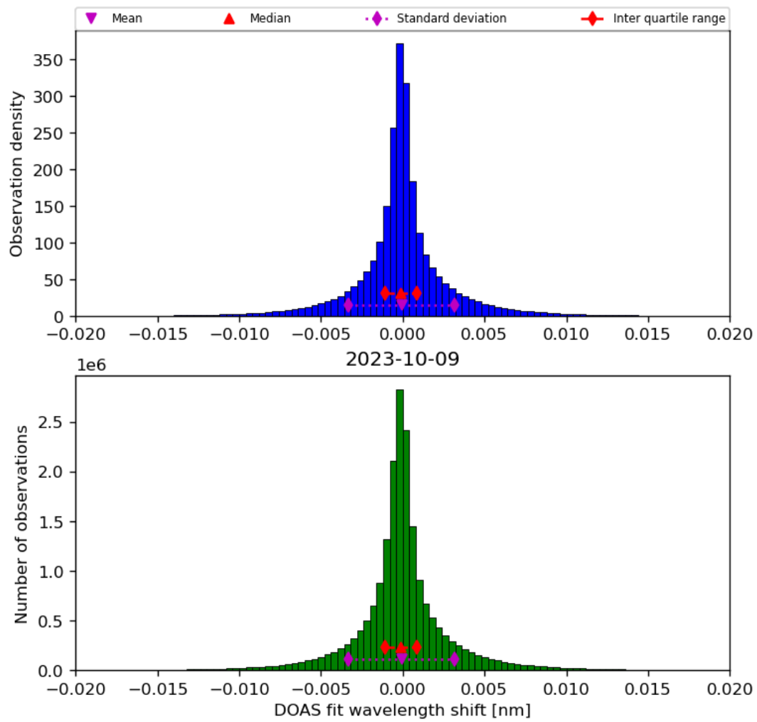
Figure 44: Histogram of “DOAS fit wavelength shift” for 2023-10-08 to 2023-10-10
