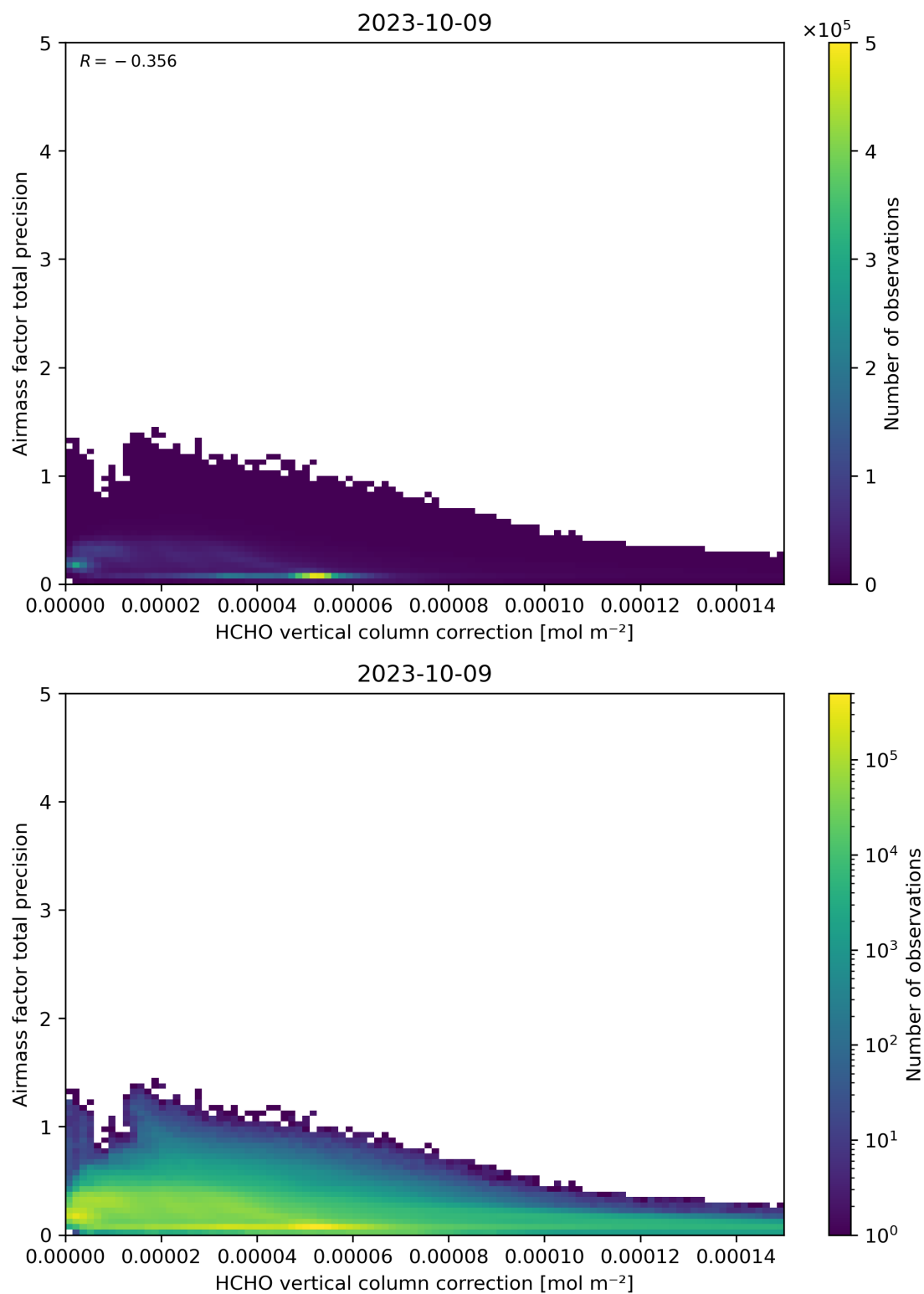
Figure 121: Scatter density plot of “HCHO vertical column correction” against “Airmass factor total precision” for 2023-10-08 to 2023-10-10.
