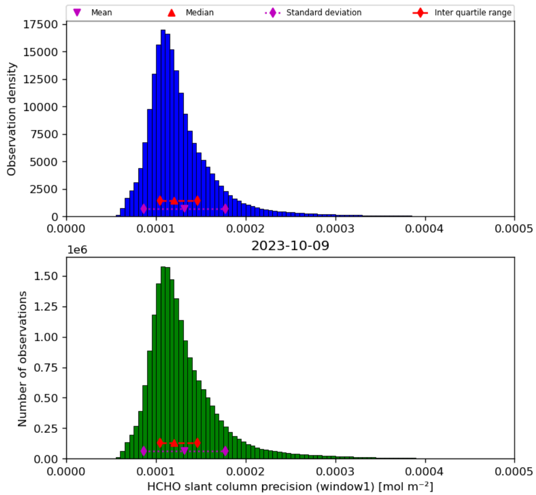
Figure 39: Histogram of “HCHO slant column precision (window1)” for 2023-10-08 to 2023-10-10
