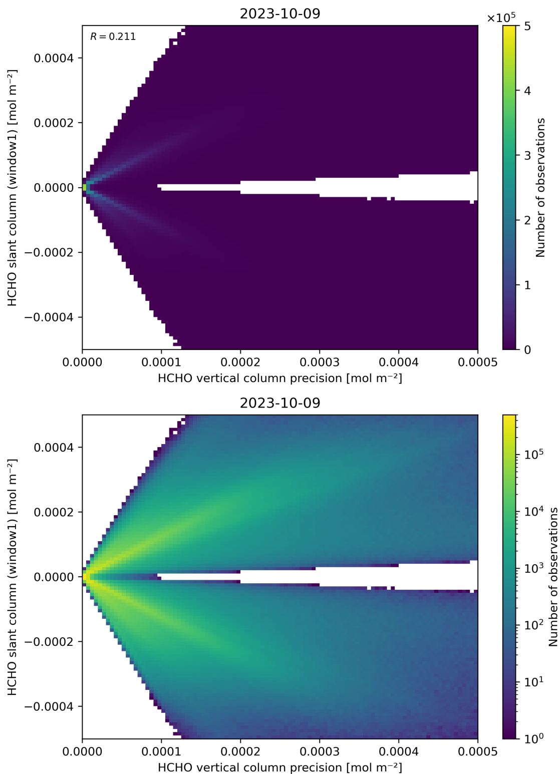
Figure 142: Scatter density plot of “HCHO vertical column precision” against “HCHO slant column (window1)” for 2023-10-08 to 2023-10-10.
