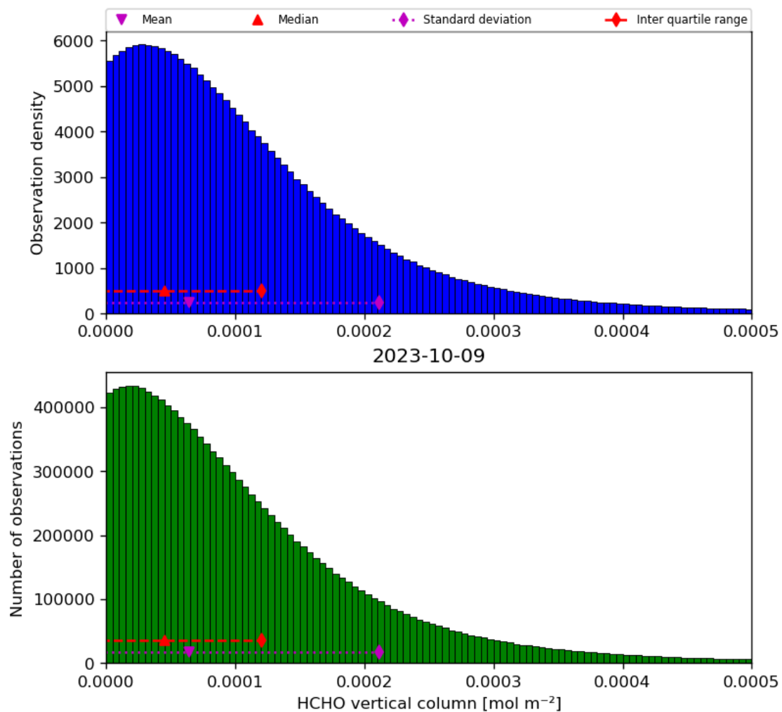
Figure 35: Histogram of “HCHO vertical column” for 2023-10-08 to 2023-10-10
