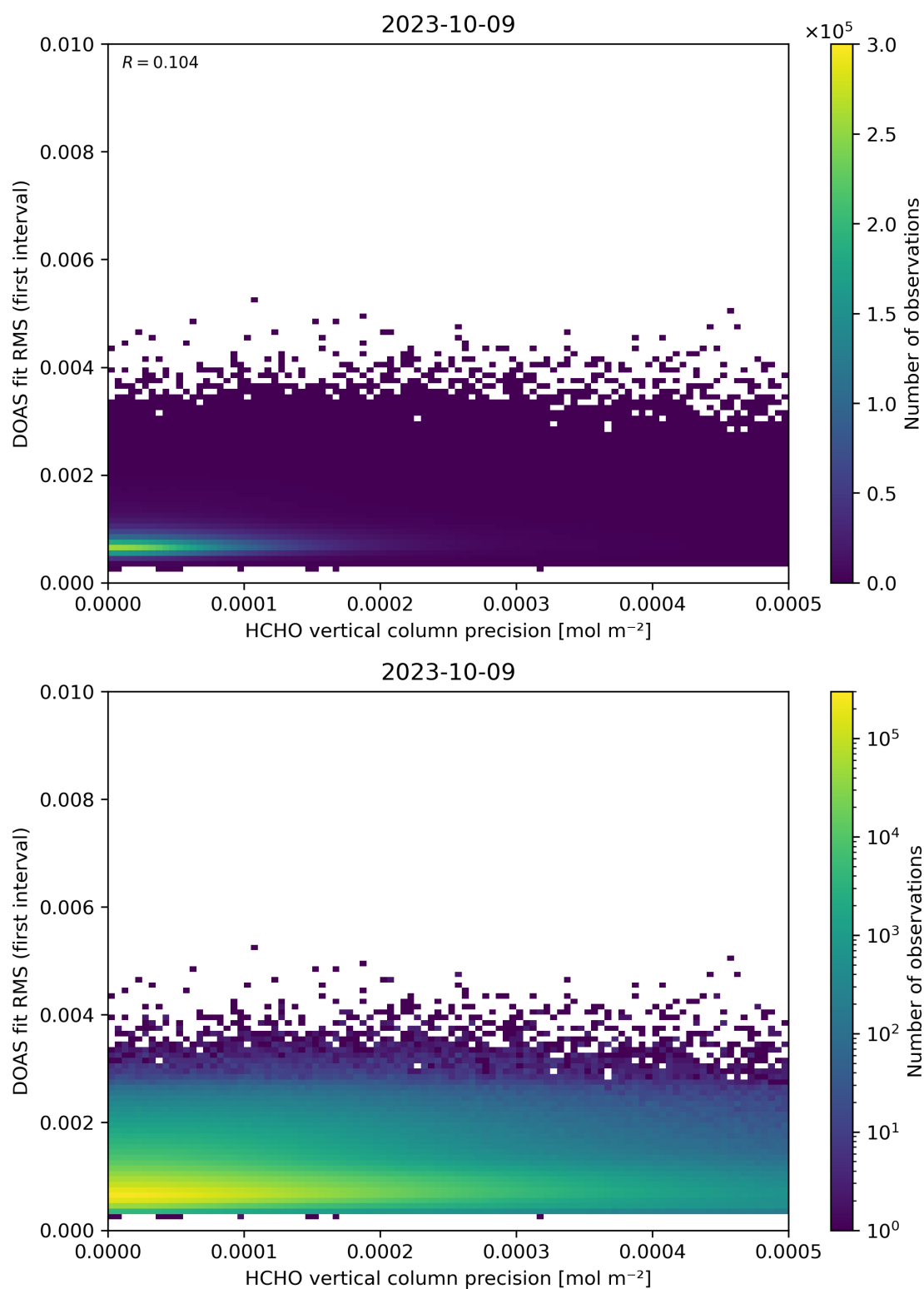
Figure 136: Scatter density plot of “HCHO vertical column precision” against “DOAS fit RMS (first interval)” for 2023-10-08 to 2023-10-10.
