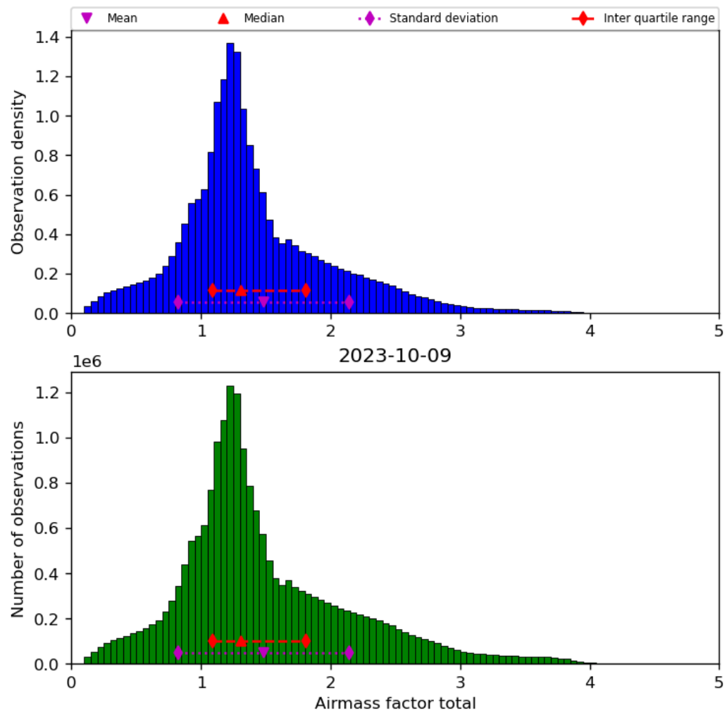
Figure 40: Histogram of “Airmass factor total” for 2023-10-08 to 2023-10-10
