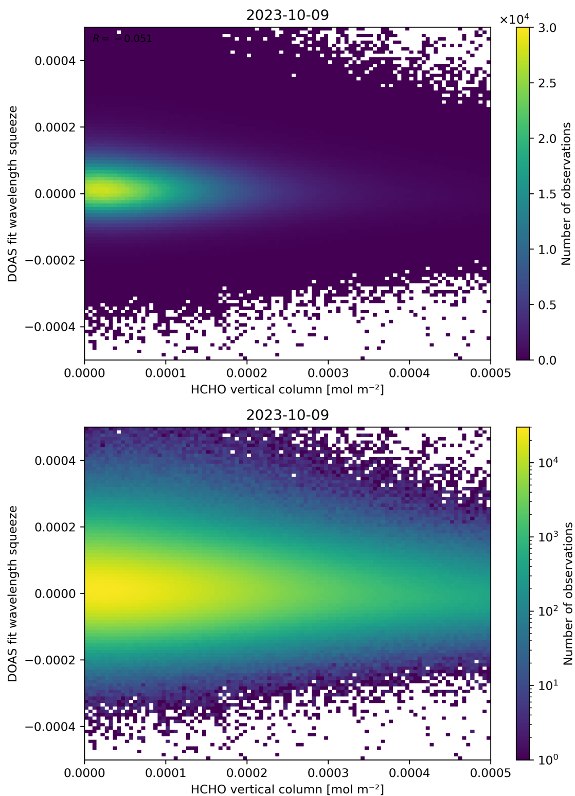
Figure 125: Scatter density plot of “HCHO vertical column” against “DOAS fit wavelength squeeze” for 2023-10-08 to 2023-10-10.
