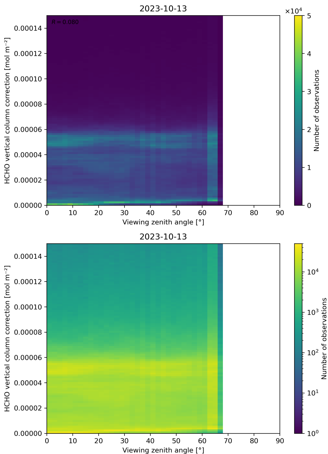
Figure 193: Scatter density plot of “Viewing zenith angle” against “HCHO vertical column correction” for 2023-10-12 to 2023-10-14.
