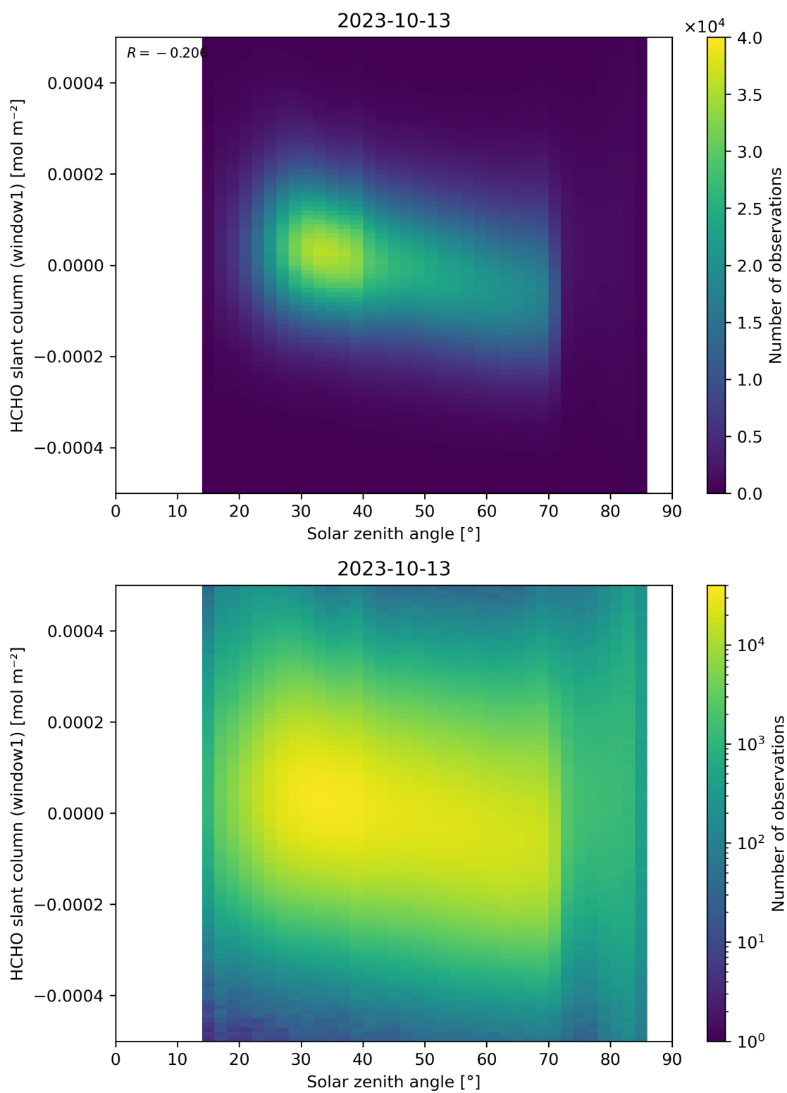
Figure 173: Scatter density plot of “Solar zenith angle” against “HCHO slant column (window1)” for 2023-10-12 to 2023-10-14.
