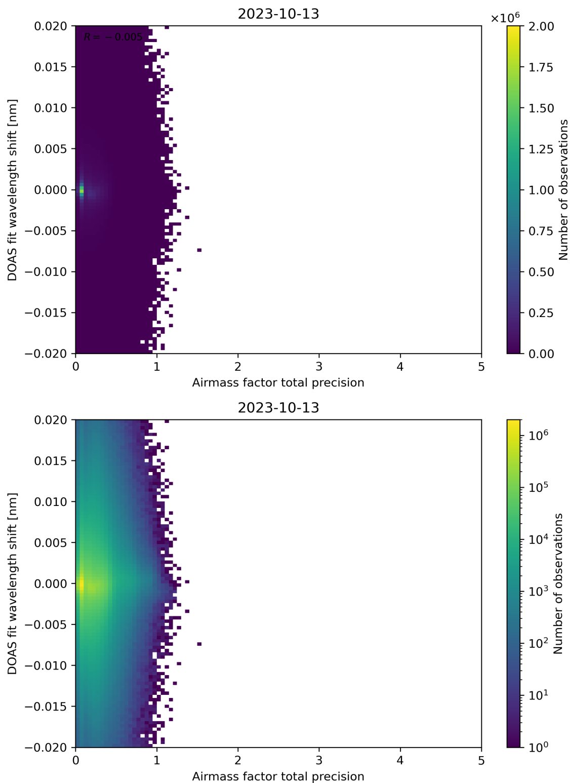
Figure 106: Scatter density plot of “Airmass factor total precision” against “DOAS fit wavelength shift” for 2023-10-12 to 2023-10-14.
