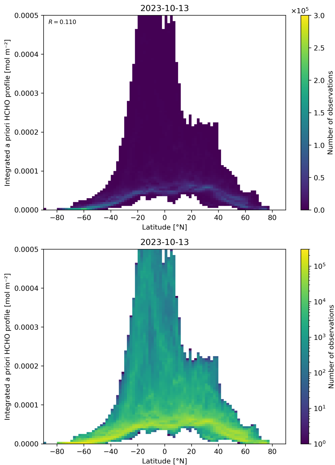
Figure 166: Scatter density plot of “Latitude” against “Integrated a priori HCHO profile” for 2023-10-12 to 2023-10-14.
