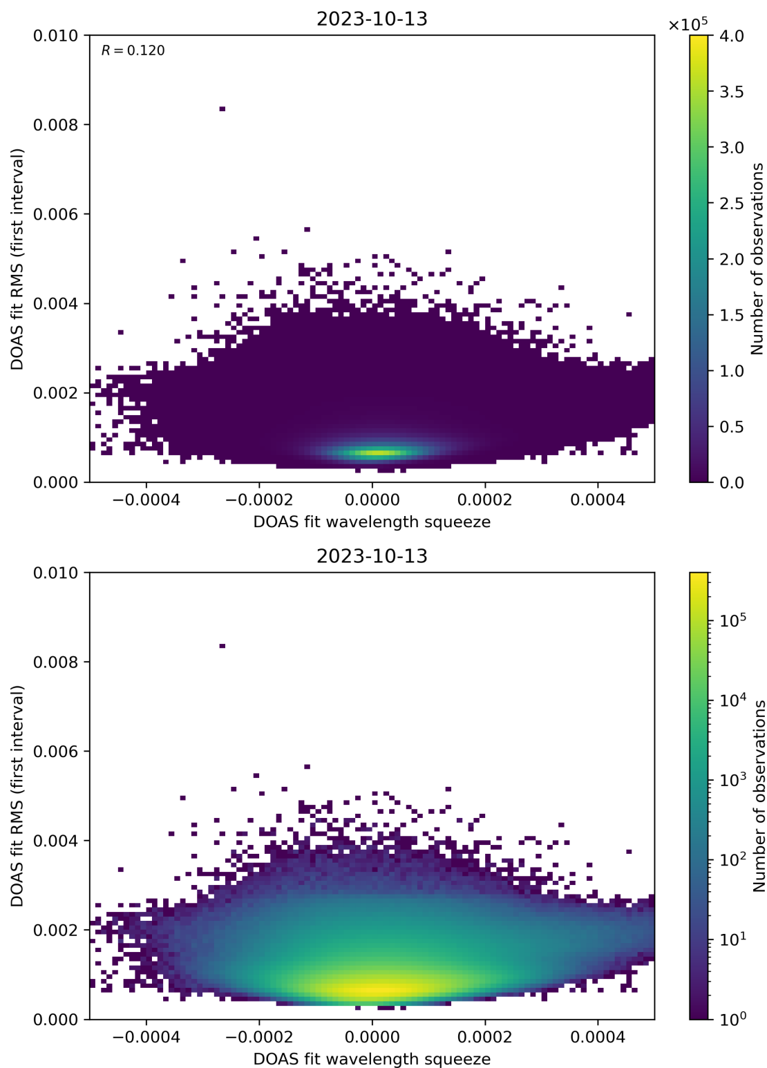
Figure 68: Scatter density plot of “DOAS fit wavelength squeeze” against “DOAS fit RMS (first interval)” for 2023-10-12 to 2023-10-14.
