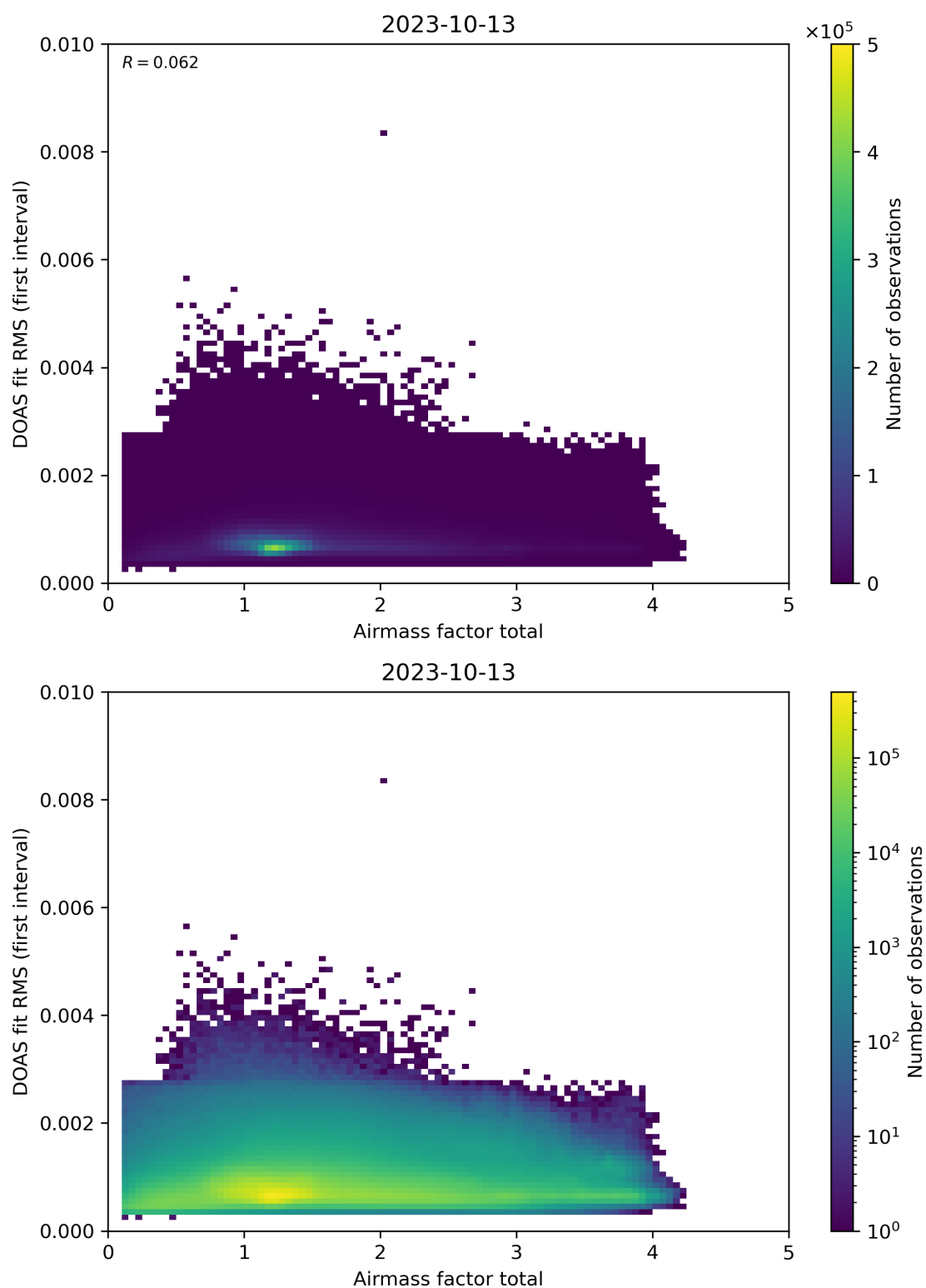
Figure 97: Scatter density plot of “Airmass factor total” against “DOAS fit RMS (first interval)” for 2023-10-12 to 2023-10-14.
