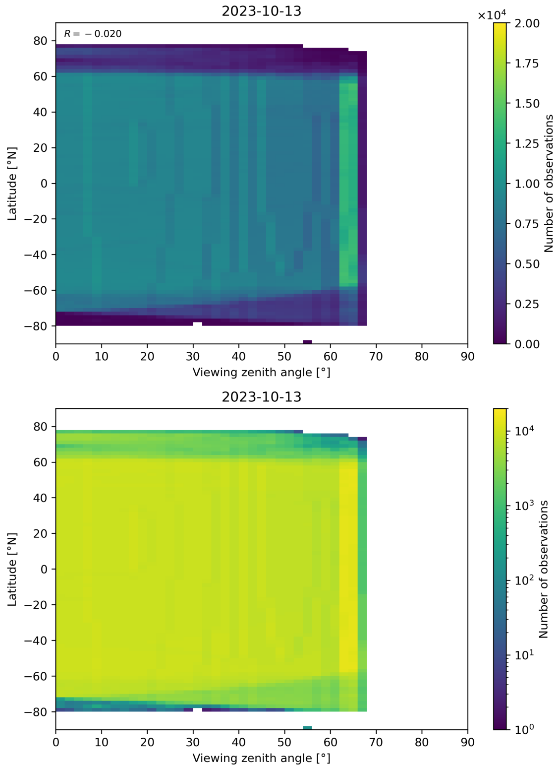
Figure 196: Scatter density plot of “Viewing zenith angle” against “Latitude” for 2023-10-12 to 2023-10-14.
