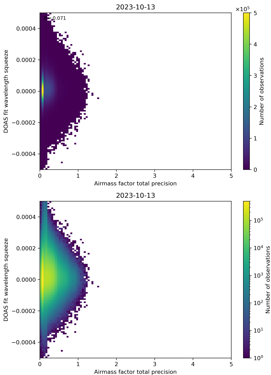
Figure 107: Scatter density plot of “Airmass factor total precision” against “DOAS fit wavelength squeeze” for 2023-10-12 to 2023-10-14.
