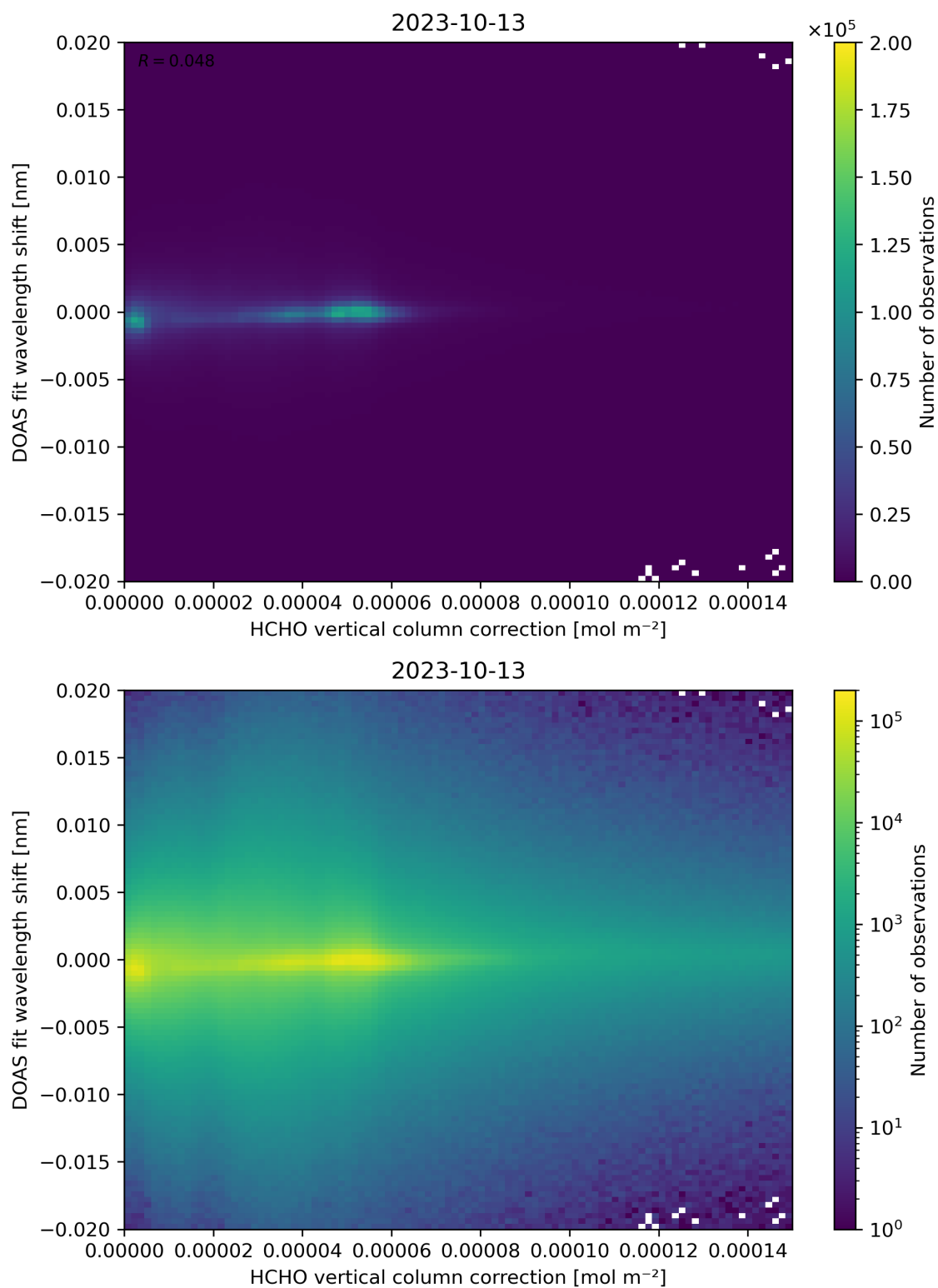
Figure 113: Scatter density plot of “HCHO vertical column correction” against “DOAS fit wavelength shift” for 2023-10-12 to 2023-10-14.
