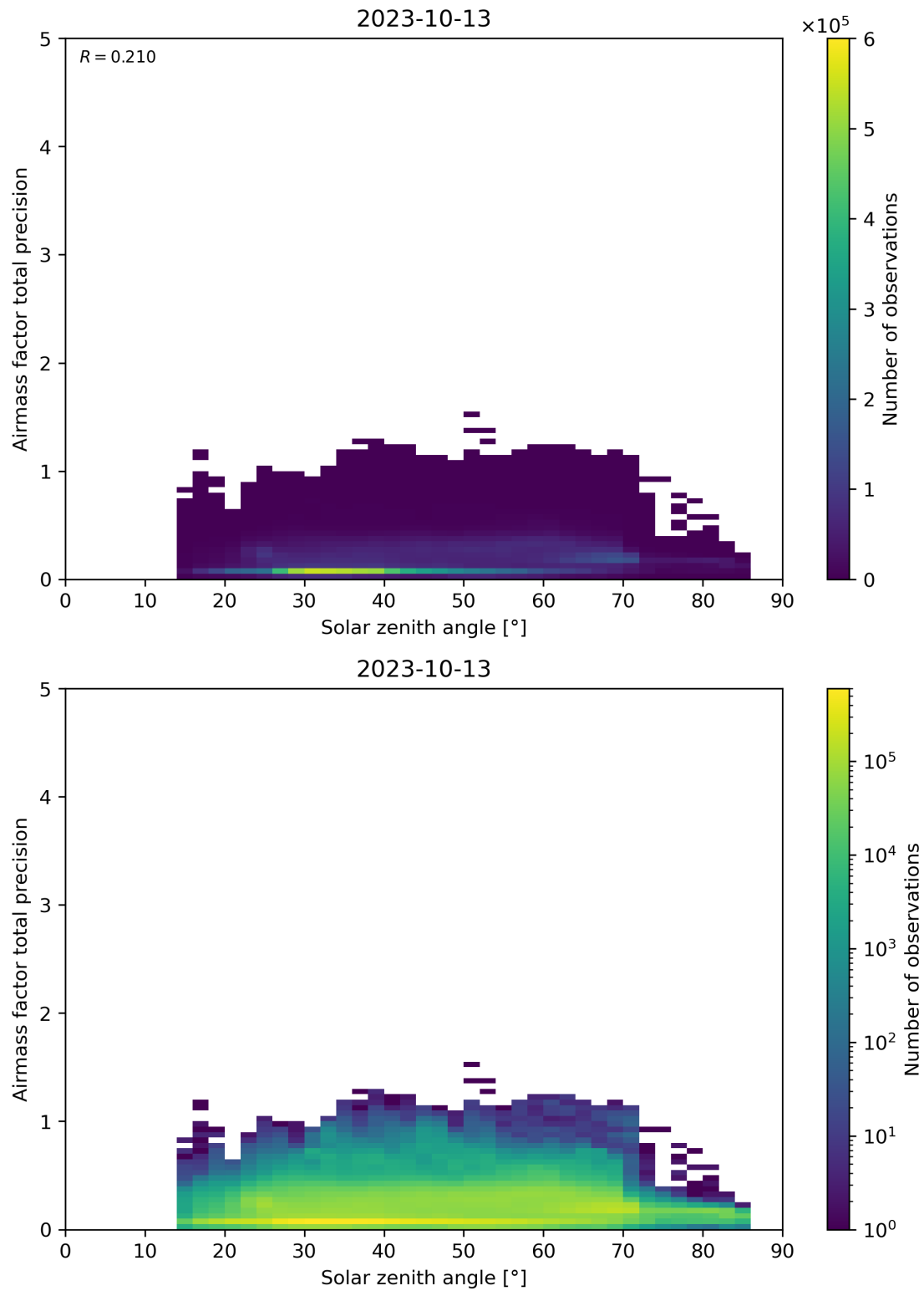
Figure 176: Scatter density plot of “Solar zenith angle” against “Airmass factor total precision” for 2023-10-12 to 2023-10-14.
