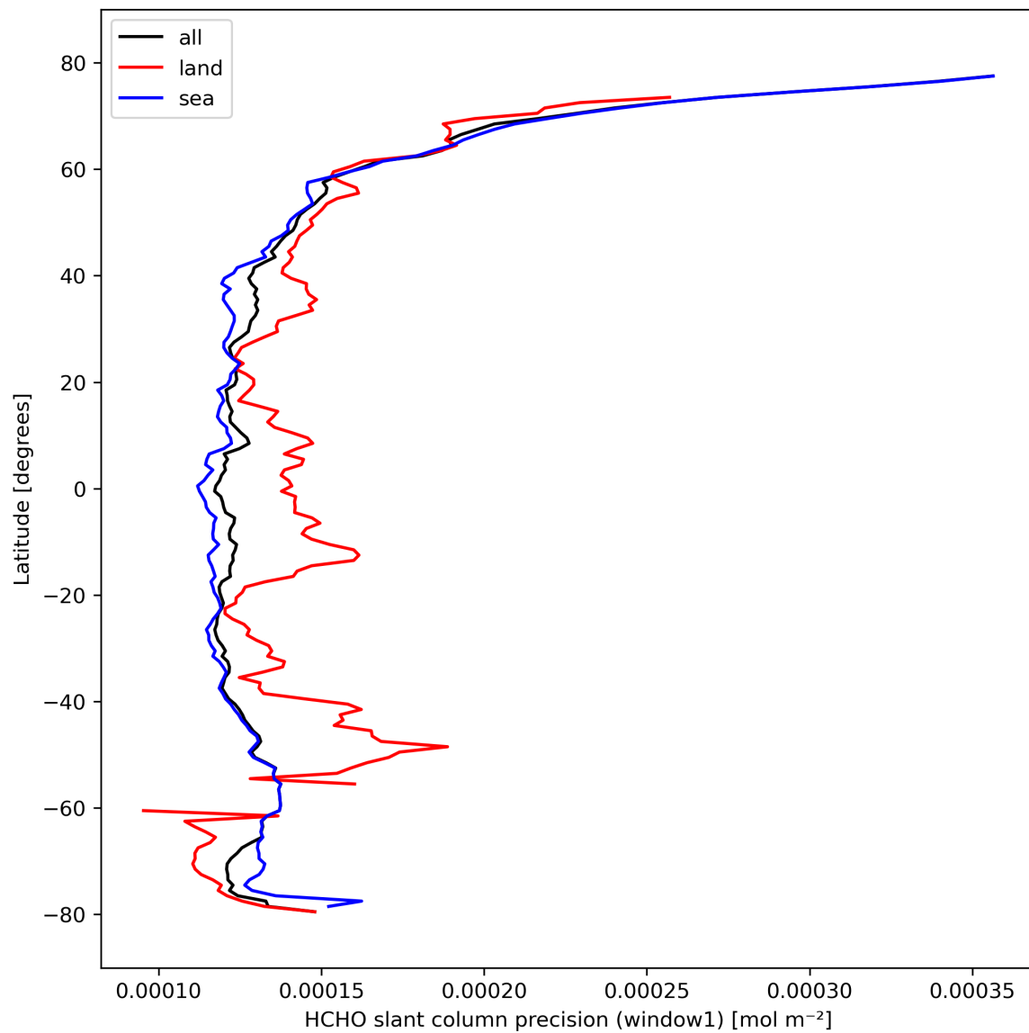
Figure 25: Zonal average of “HCHO slant column precision (window1)” for 2023-10-12 to 2023-10-14.
