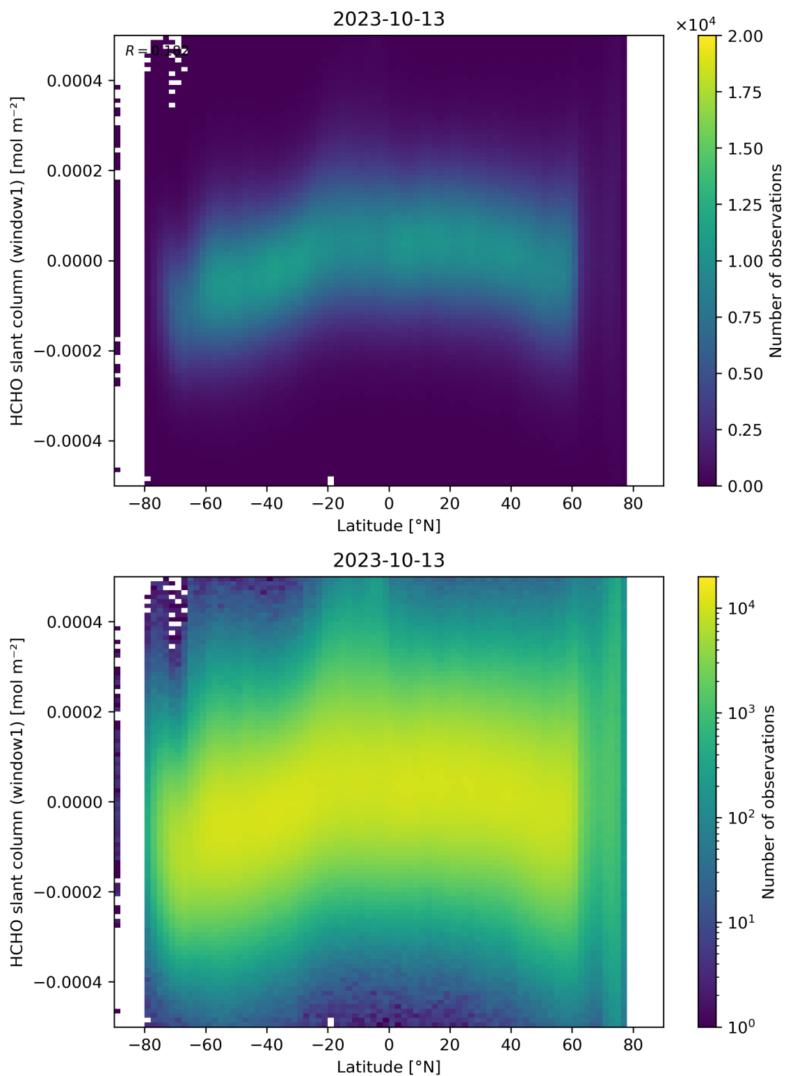
Figure 159: Scatter density plot of “Latitude” against “HCHO slant column (window1)” for 2023-10-12 to 2023-10-14.
