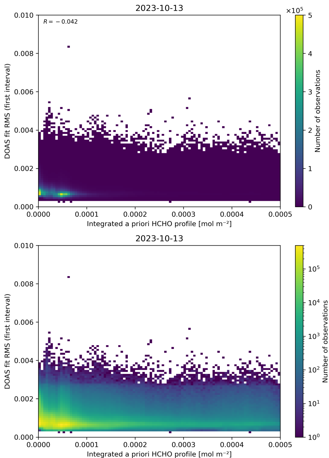
Figure 148: Scatter density plot of “Integrated a priori HCHO profile” against “DOAS fit RMS (first interval)” for 2023-10-12 to 2023-10-14.
