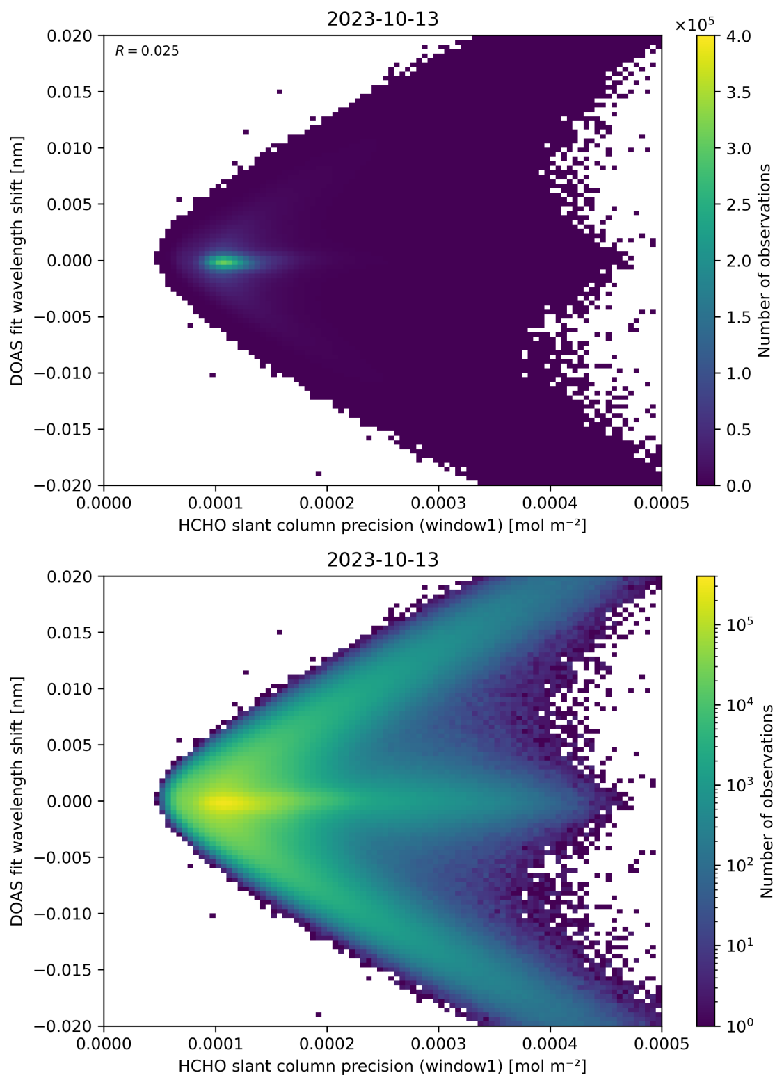
Figure 89: Scatter density plot of “HCHO slant column precision (window1)” against “DOAS fit wavelength shift” for 2023-10-12 to 2023-10-14.
