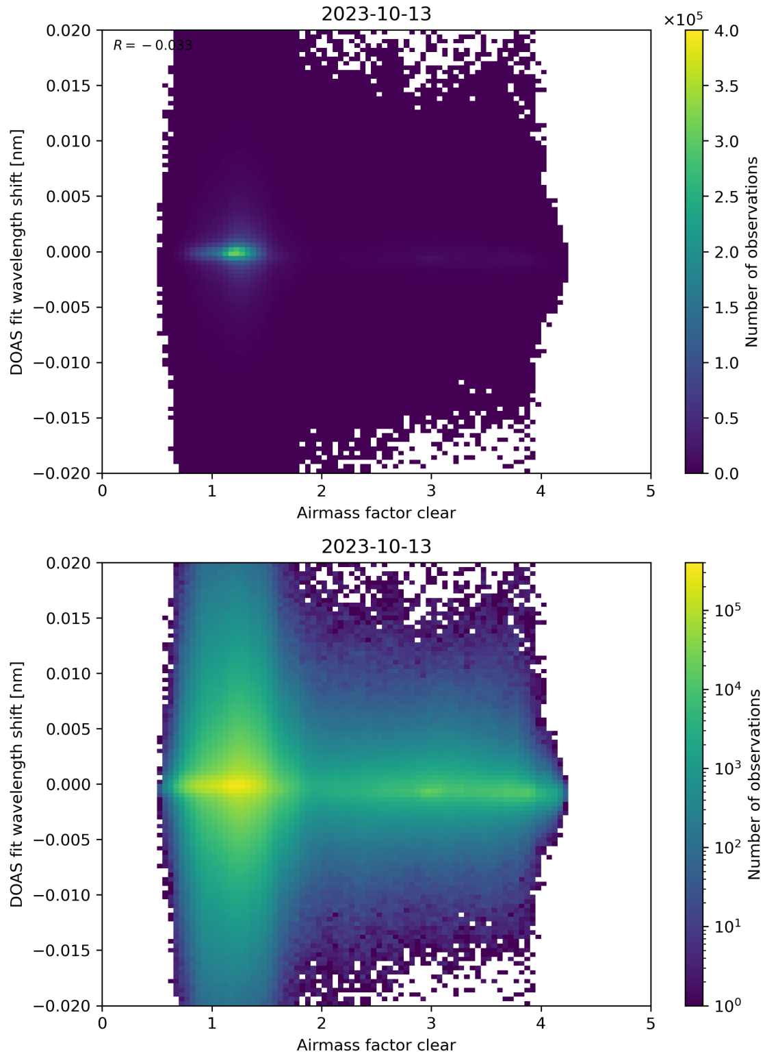
Figure 72: Scatter density plot of “Airmass factor clear” against “DOAS fit wavelength shift” for 2023-10-12 to 2023-10-14.
