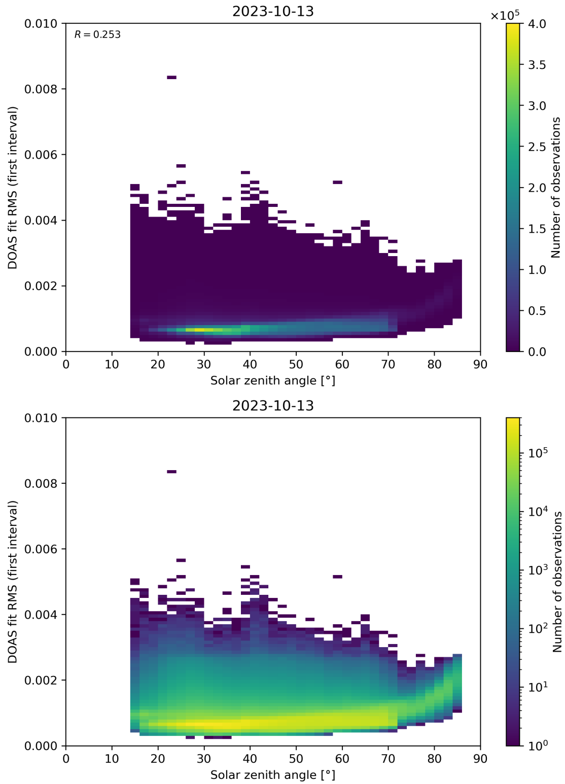
Figure 167: Scatter density plot of “Solar zenith angle” against “DOAS fit RMS (first interval)” for 2023-10-12 to 2023-10-14.
