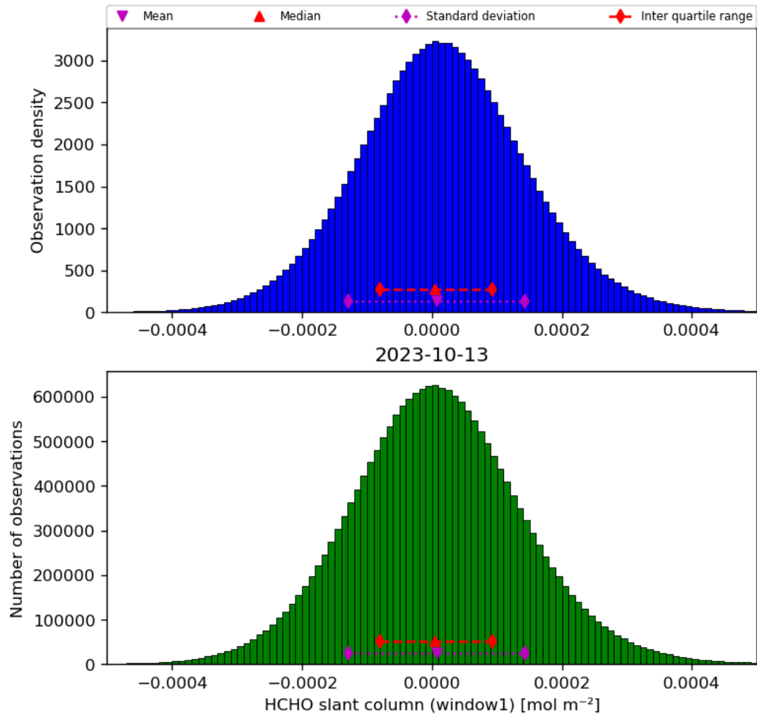
Figure 38: Histogram of “HCHO slant column (window1)” for 2023-10-12 to 2023-10-14
