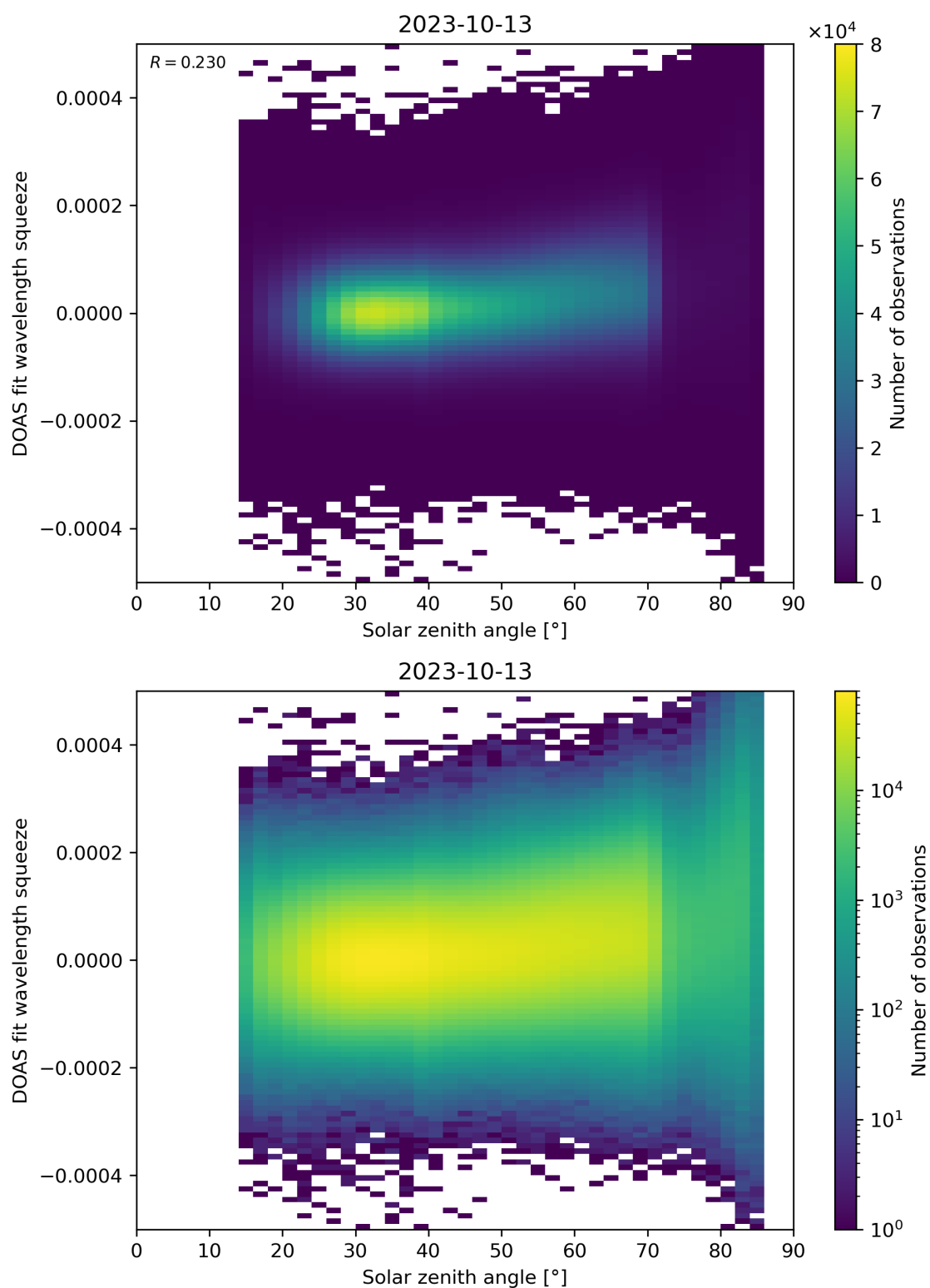
Figure 169: Scatter density plot of “Solar zenith angle” against “DOAS fit wavelength squeeze” for 2023-10-12 to 2023-10-14.
