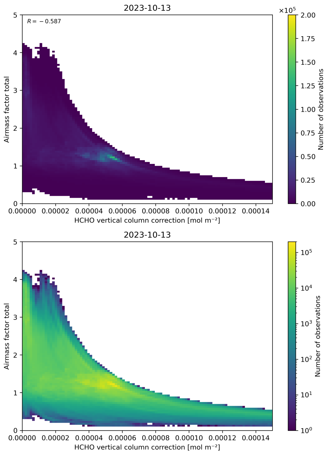
Figure 120: Scatter density plot of “HCHO vertical column correction” against “Airmass factor total” for 2023-10-12 to 2023-10-14.
