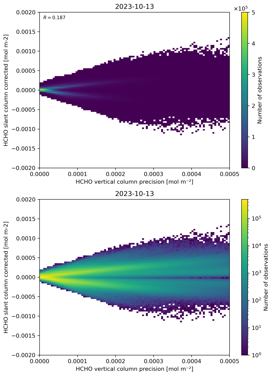
Figure 140: Scatter density plot of “HCHO vertical column precision” against “HCHO slant column corrected” for 2023-10-12 to 2023-10-14.
