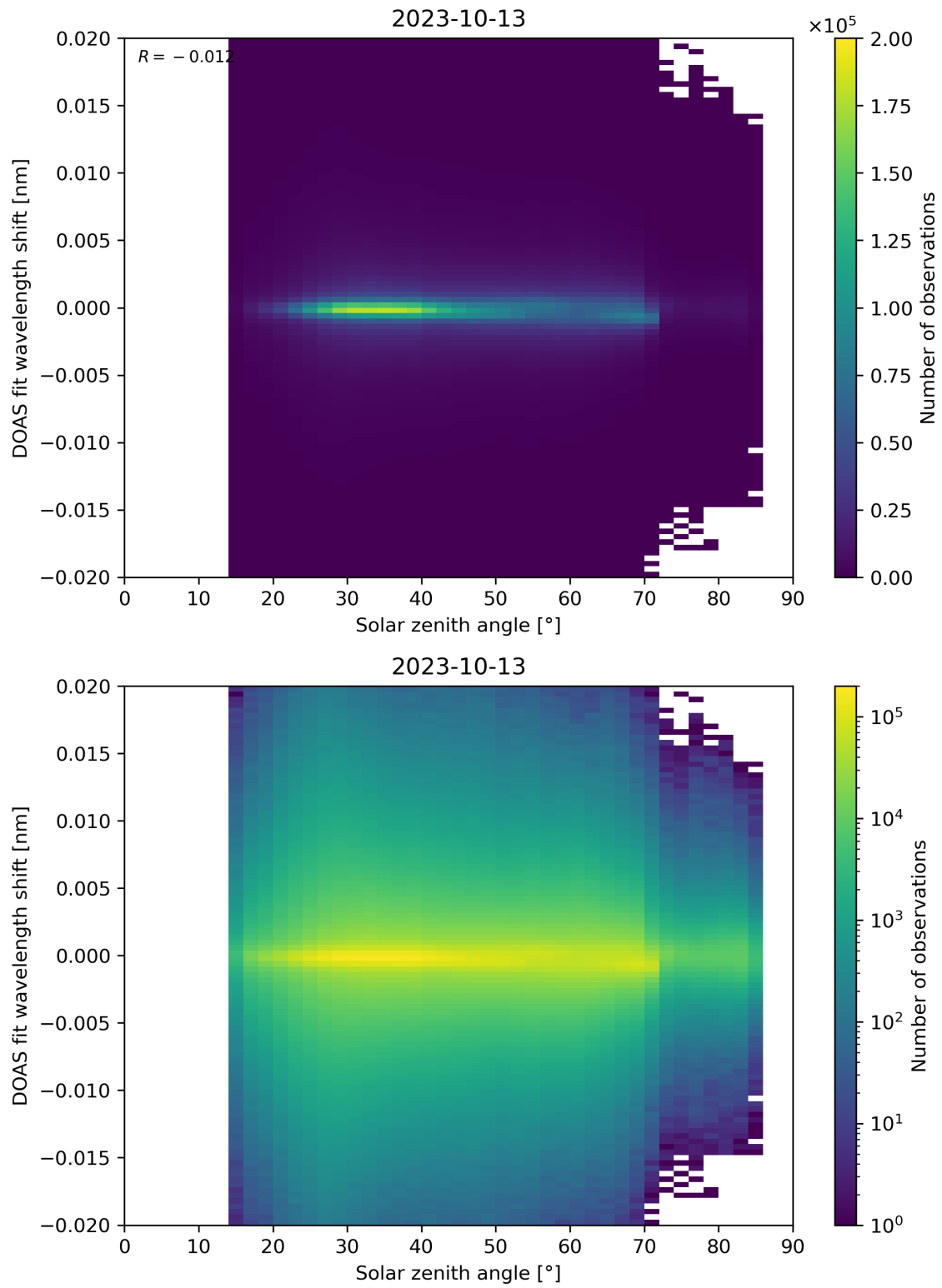
Figure 168: Scatter density plot of “Solar zenith angle” against “DOAS fit wavelength shift” for 2023-10-12 to 2023-10-14.
