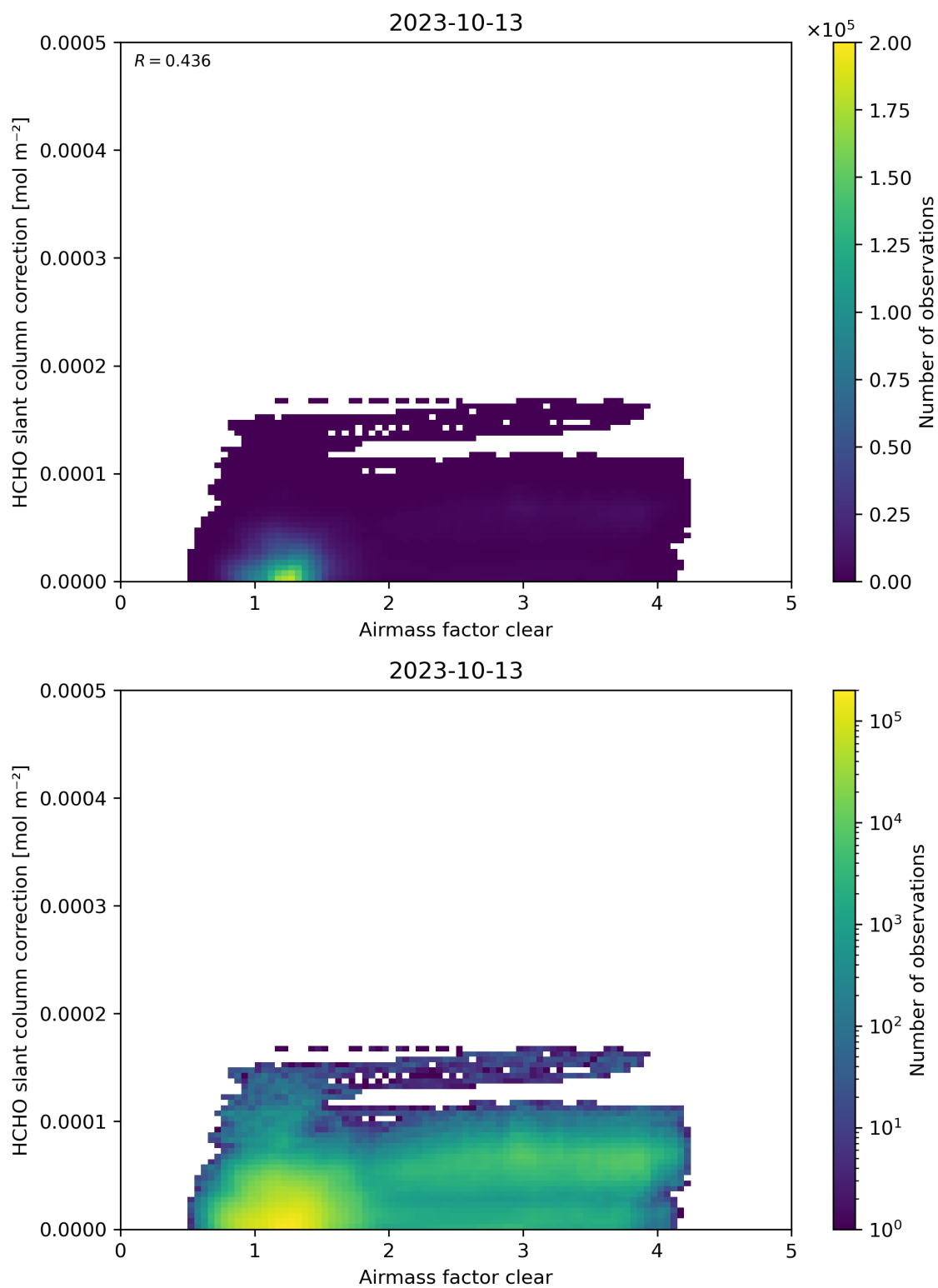
Figure 75: Scatter density plot of “Airmass factor clear” against “HCHO slant column correction” for 2023-10-12 to 2023-10-14.
