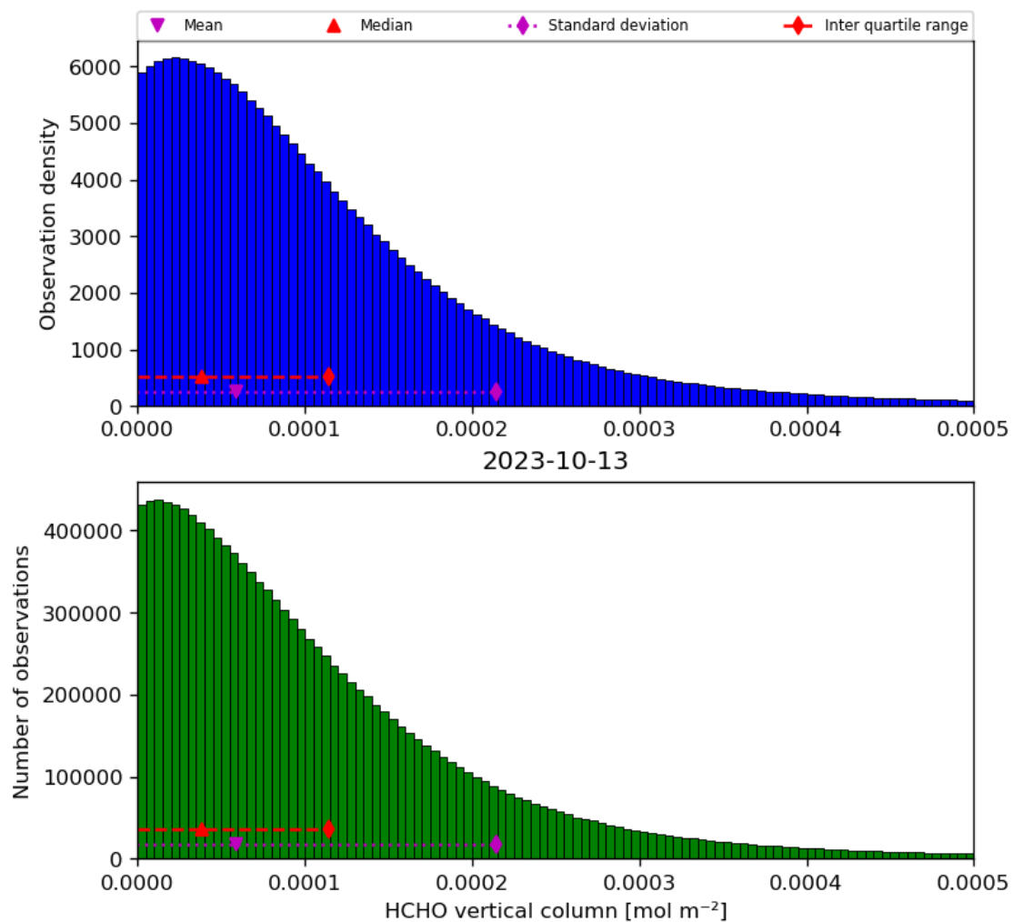
Figure 35: Histogram of “HCHO vertical column” for 2023-10-12 to 2023-10-14
