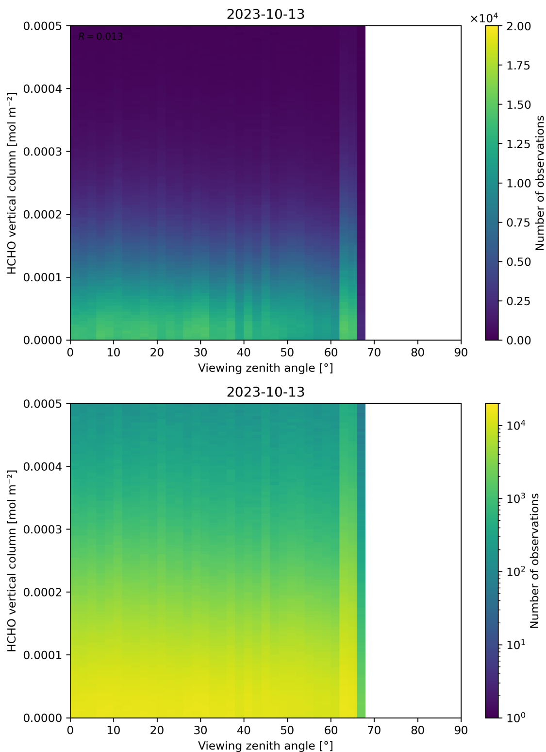
Figure 192: Scatter density plot of “Viewing zenith angle” against “HCHO vertical column” for 2023-10-12 to 2023-10-14.
