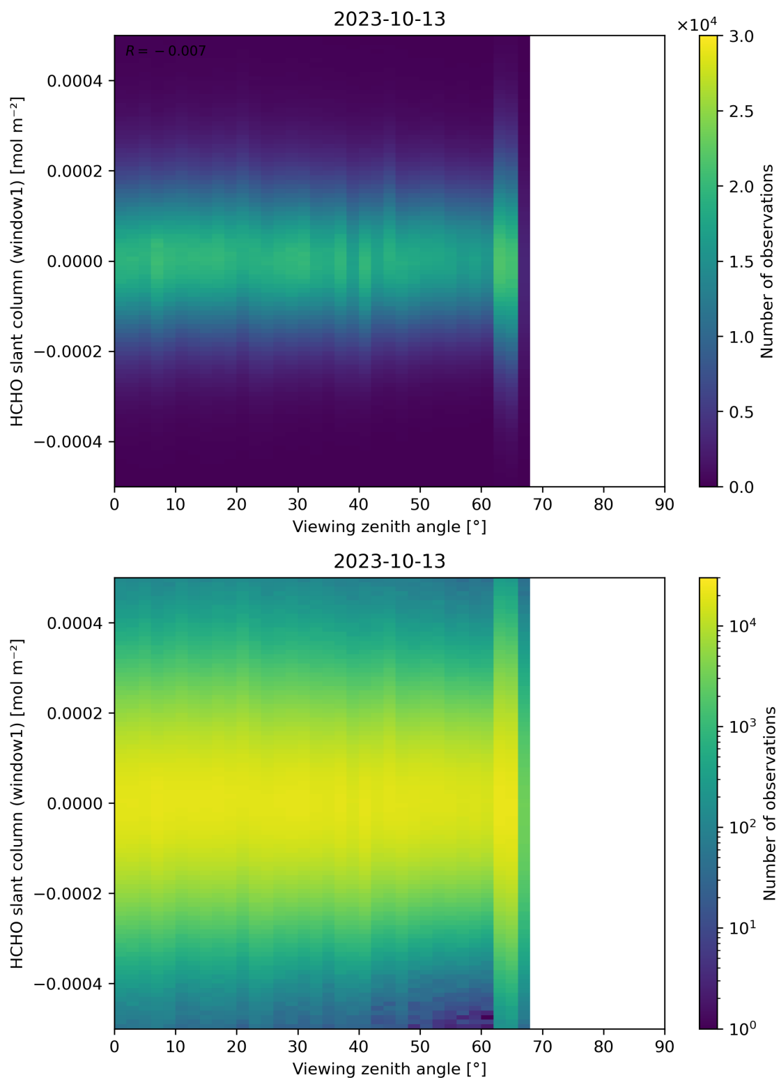
Figure 188: Scatter density plot of “Viewing zenith angle” against “HCHO slant column (window1)” for 2023-10-12 to 2023-10-14.
