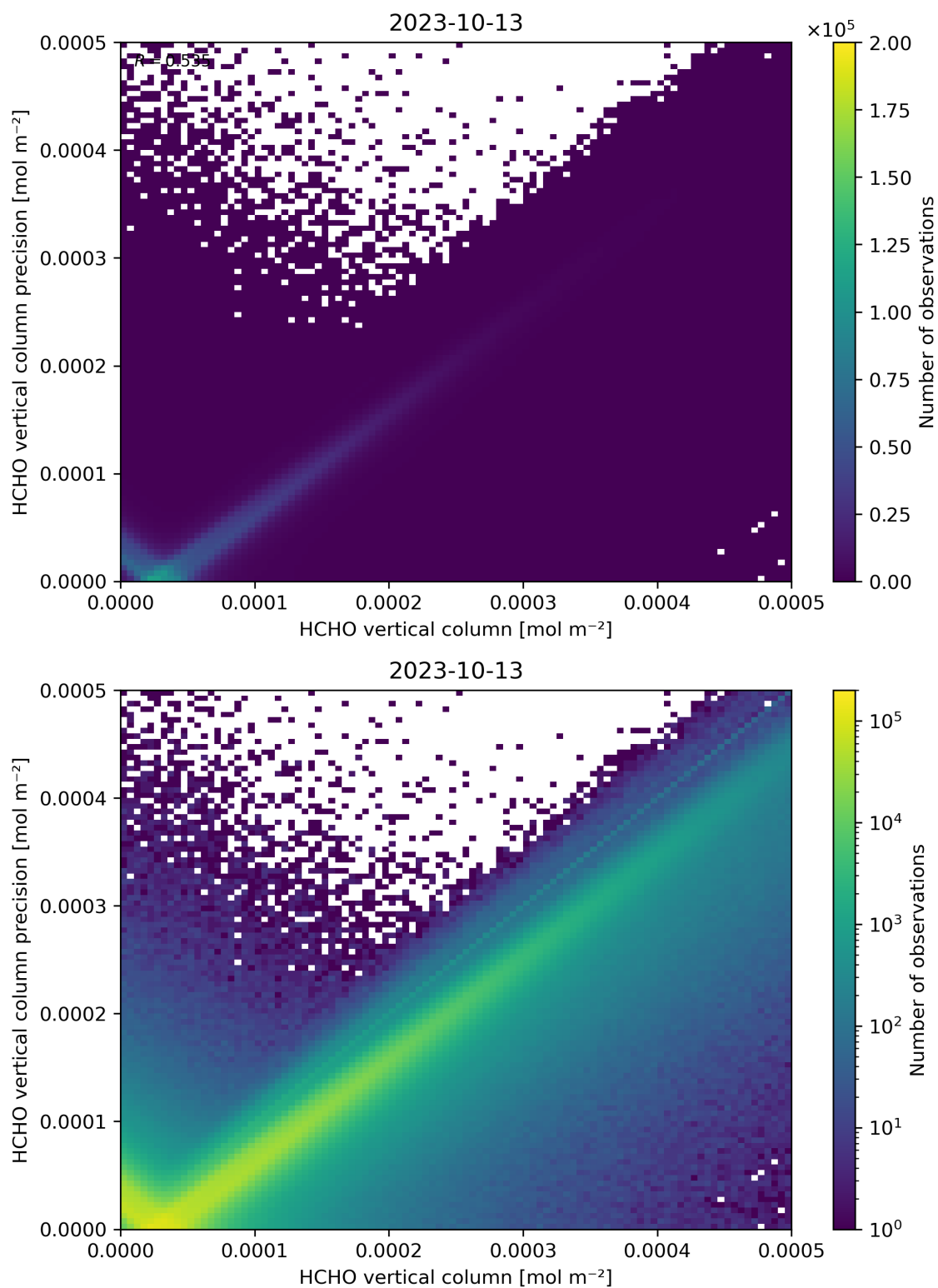
Figure 134: Scatter density plot of “HCHO vertical column” against “HCHO vertical column precision” for 2023-10-12 to 2023-10-14.
