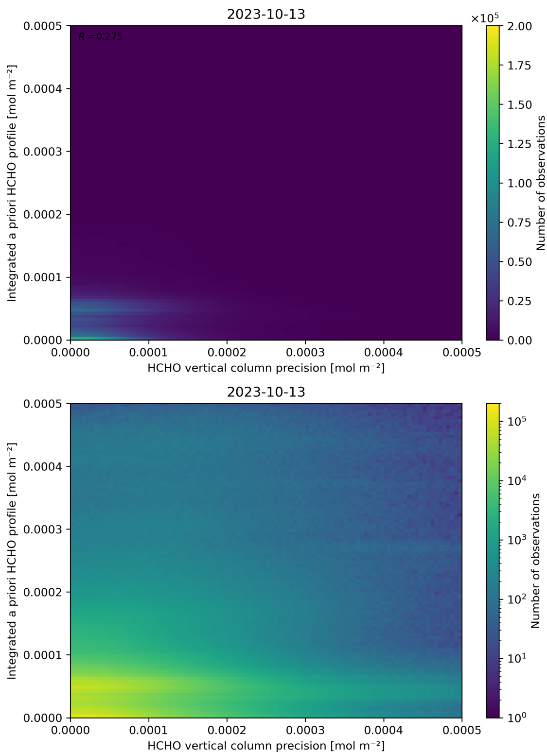
Figure 147: Scatter density plot of “HCHO vertical column precision” against “Integrated a priori HCHO profile” for 2023-10-12 to 2023-10-14.
