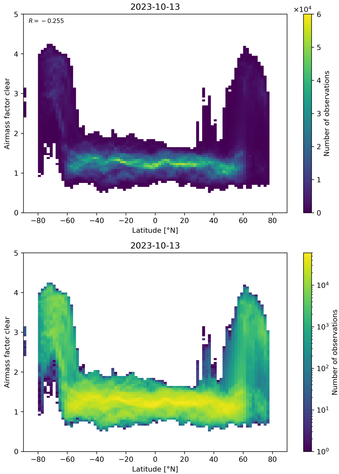
Figure 156: Scatter density plot of “Latitude” against “Airmass factor clear” for 2023-10-12 to 2023-10-14.
