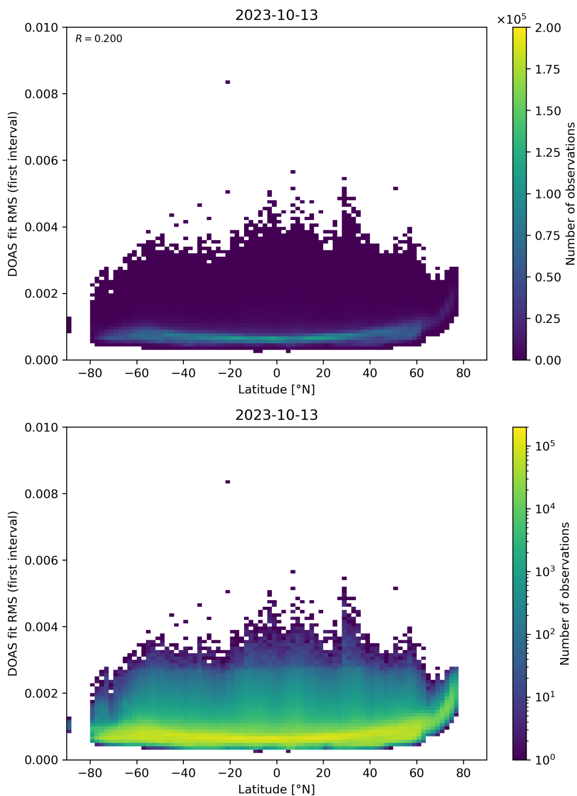
Figure 153: Scatter density plot of “Latitude” against “DOAS fit RMS (first interval)” for 2023-10-12 to 2023-10-14.
