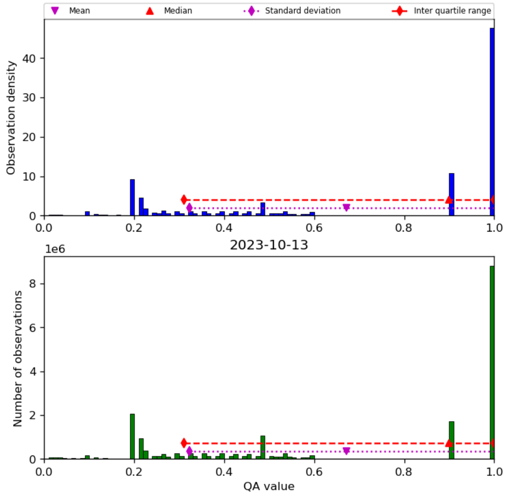
Figure 34: Histogram of “QA value” for 2023-10-12 to 2023-10-14
