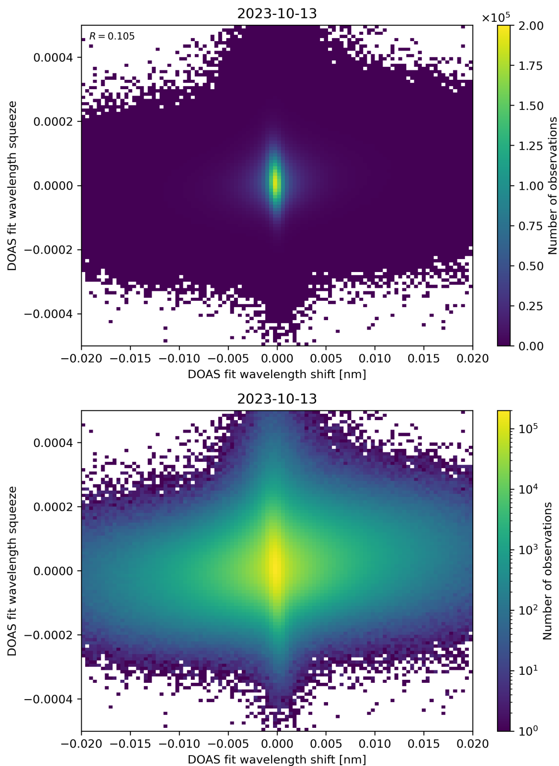
Figure 65: Scatter density plot of “DOAS fit wavelength shift” against “DOAS fit wavelength squeeze” for 2023-10-12 to 2023-10-14.
