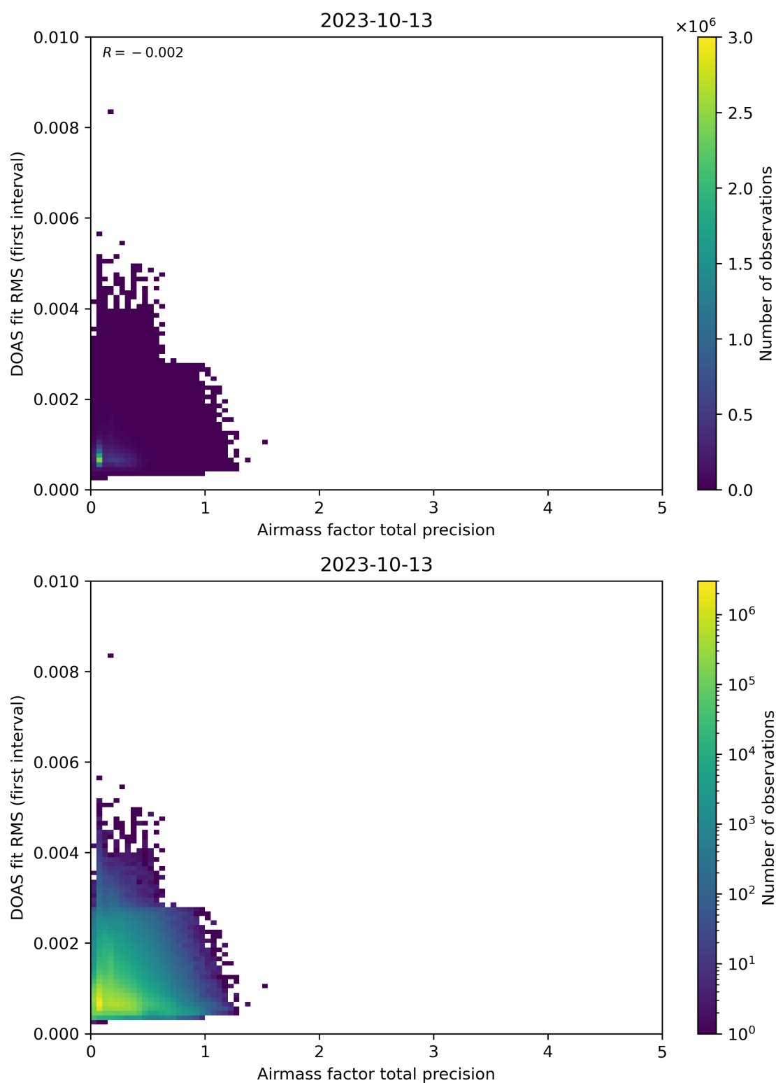
Figure 105: Scatter density plot of “Airmass factor total precision” against “DOAS fit RMS (first interval)” for 2023-10-12 to 2023-10-14.
