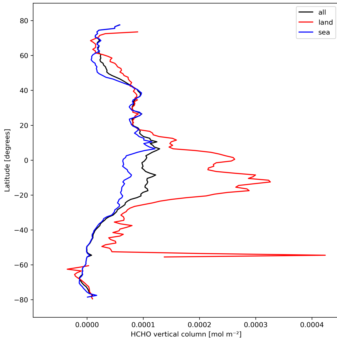
Figure 21: Zonal average of “HCHO vertical column” for 2023-10-12 to 2023-10-14.
