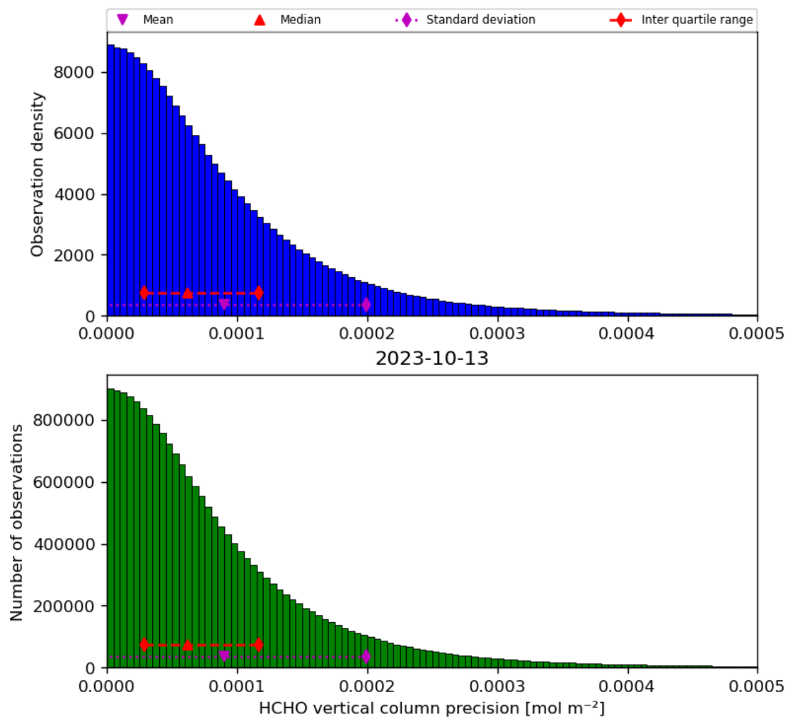
Figure 36: Histogram of “HCHO vertical column precision” for 2023-10-12 to 2023-10-14
