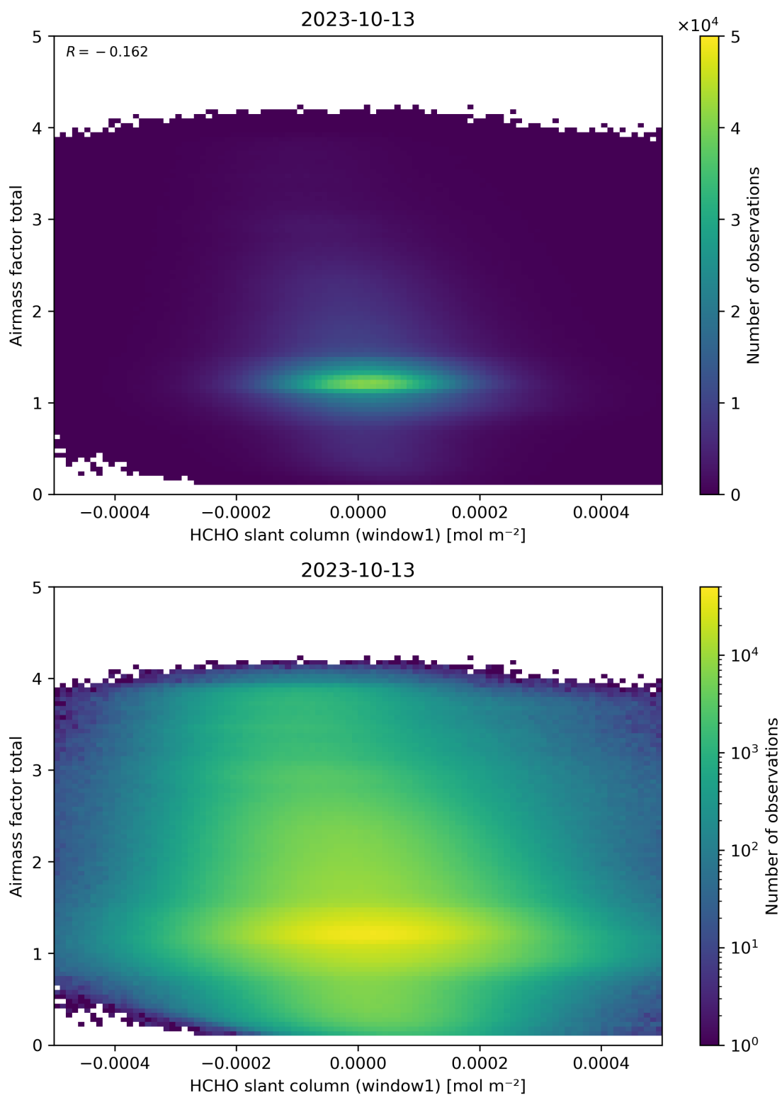
Figure 85: Scatter density plot of “HCHO slant column (window1)” against “Airmass factor total” for 2023-10-12 to 2023-10-14.
