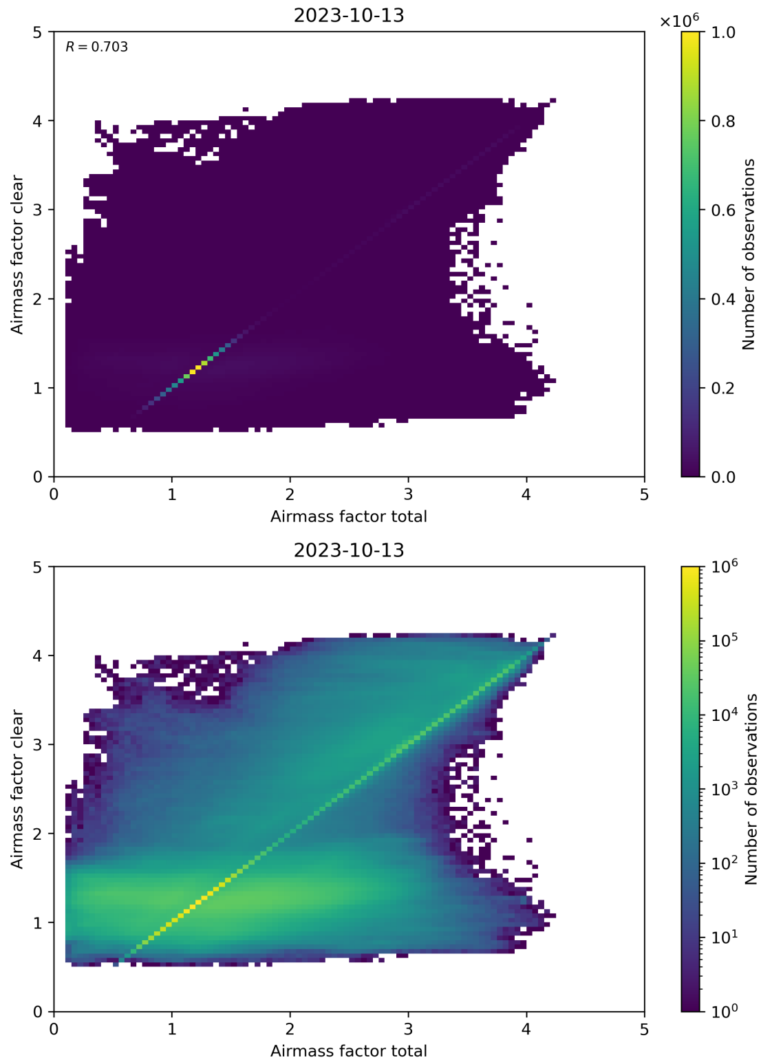
Figure 100: Scatter density plot of “Airmass factor total” against “Airmass factor clear” for 2023-10-12 to 2023-10-14.
