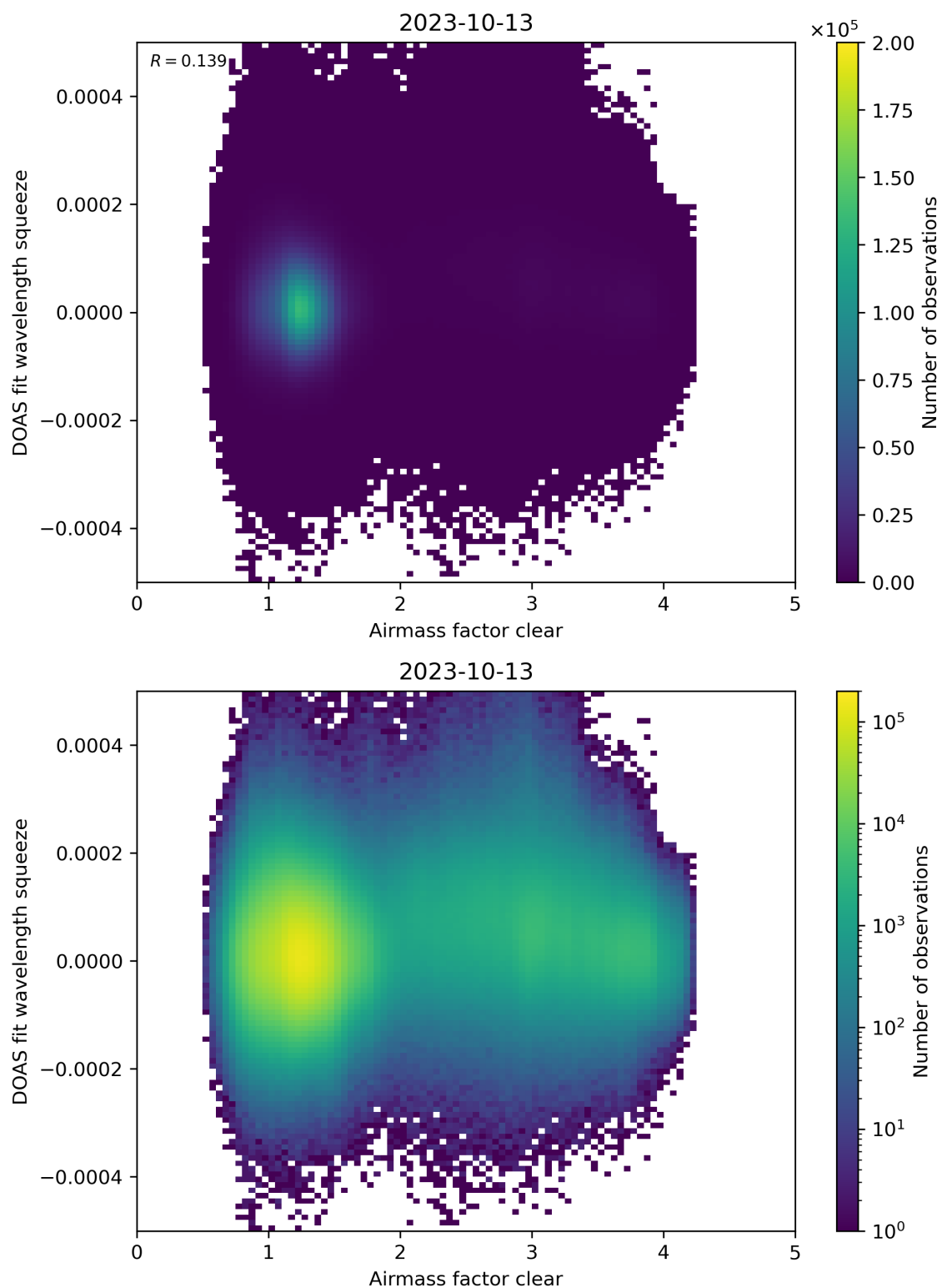
Figure 73: Scatter density plot of “Airmass factor clear” against “DOAS fit wavelength squeeze” for 2023-10-12 to 2023-10-14.
