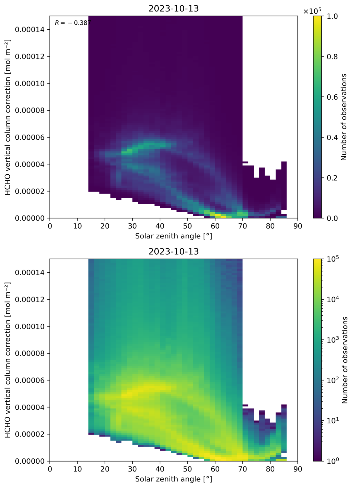
Figure 178: Scatter density plot of “Solar zenith angle” against “HCHO vertical column correction” for 2023-10-12 to 2023-10-14.
