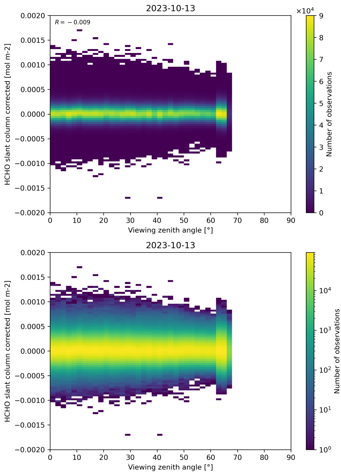
Figure 186: Scatter density plot of “Viewing zenith angle” against “HCHO slant column corrected” for 2023-10-12 to 2023-10-14.
