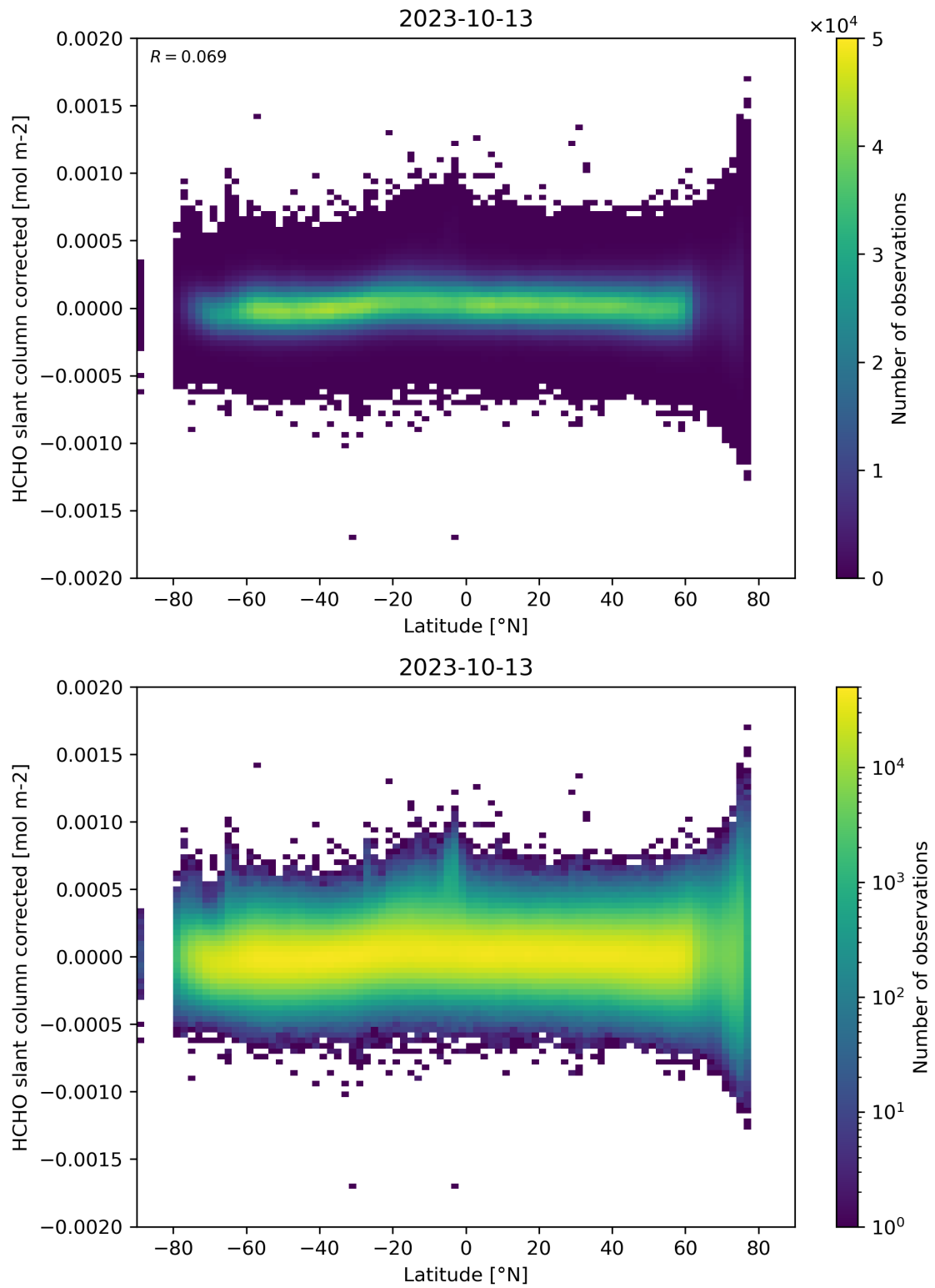
Figure 157: Scatter density plot of “Latitude” against “HCHO slant column corrected” for 2023-10-12 to 2023-10-14.
