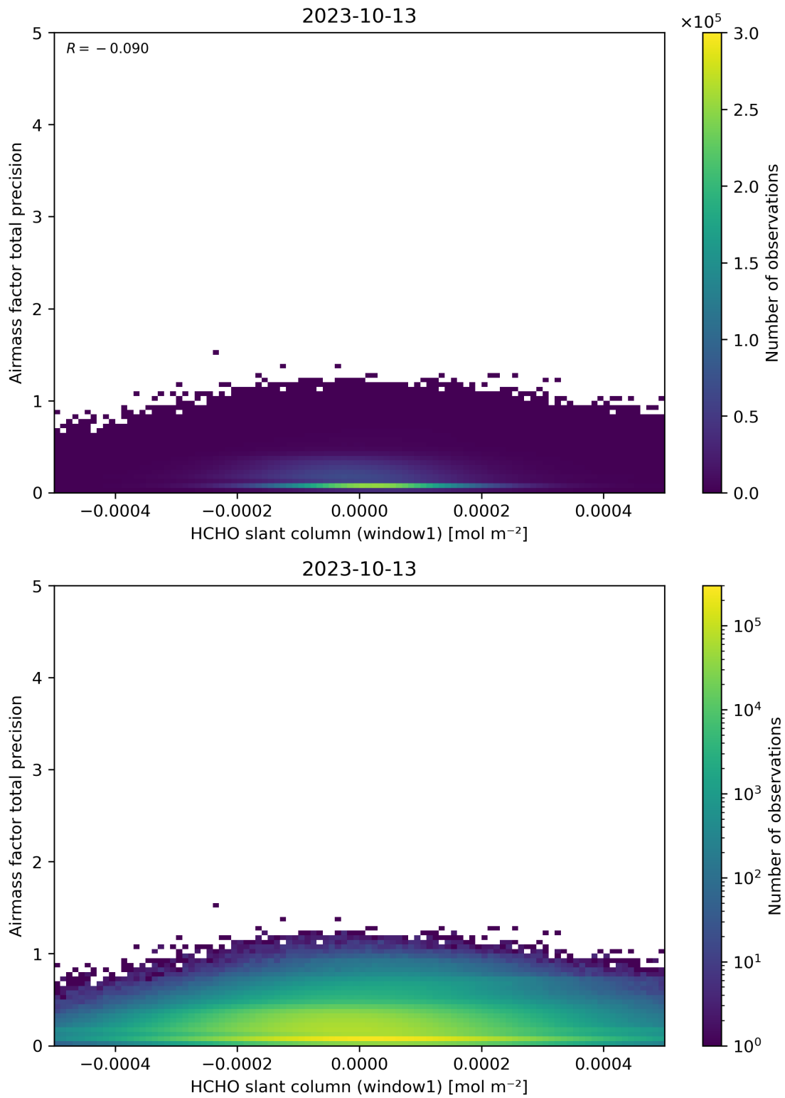
Figure 86: Scatter density plot of “HCHO slant column (window1)” against “Airmass factor total precision” for 2023-10-12 to 2023-10-14.
