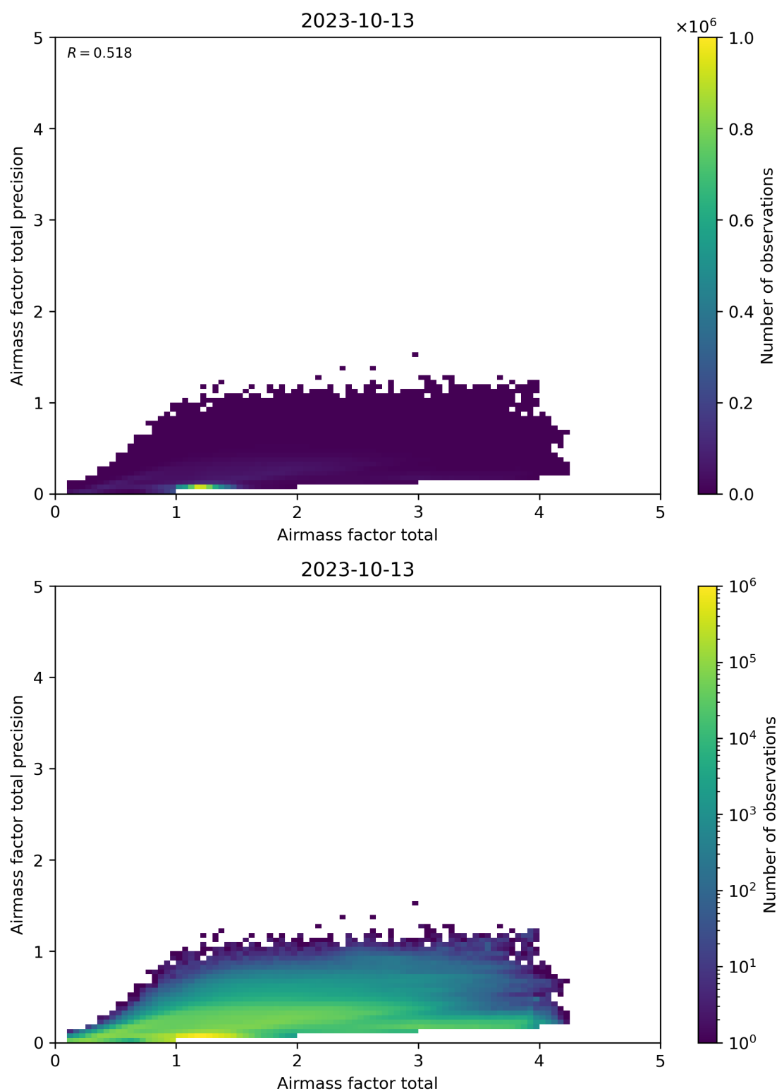
Figure 103: Scatter density plot of “Airmass factor total” against “Airmass factor total precision” for 2023-10-12 to 2023-10-14.
