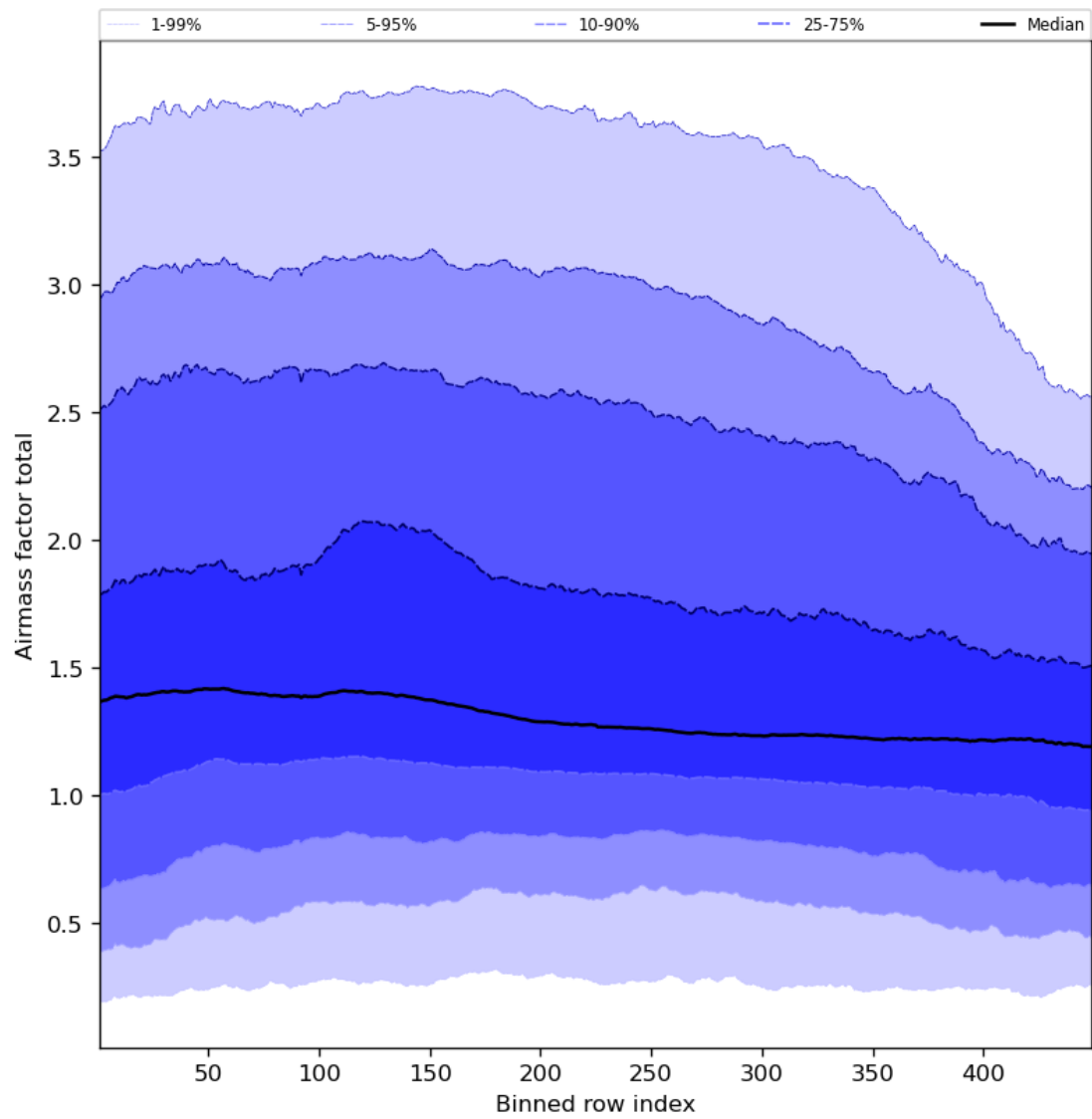
Figure 54: Along track statistics of “Airmass factor total” for 2023-10-12 to 2023-10-14
