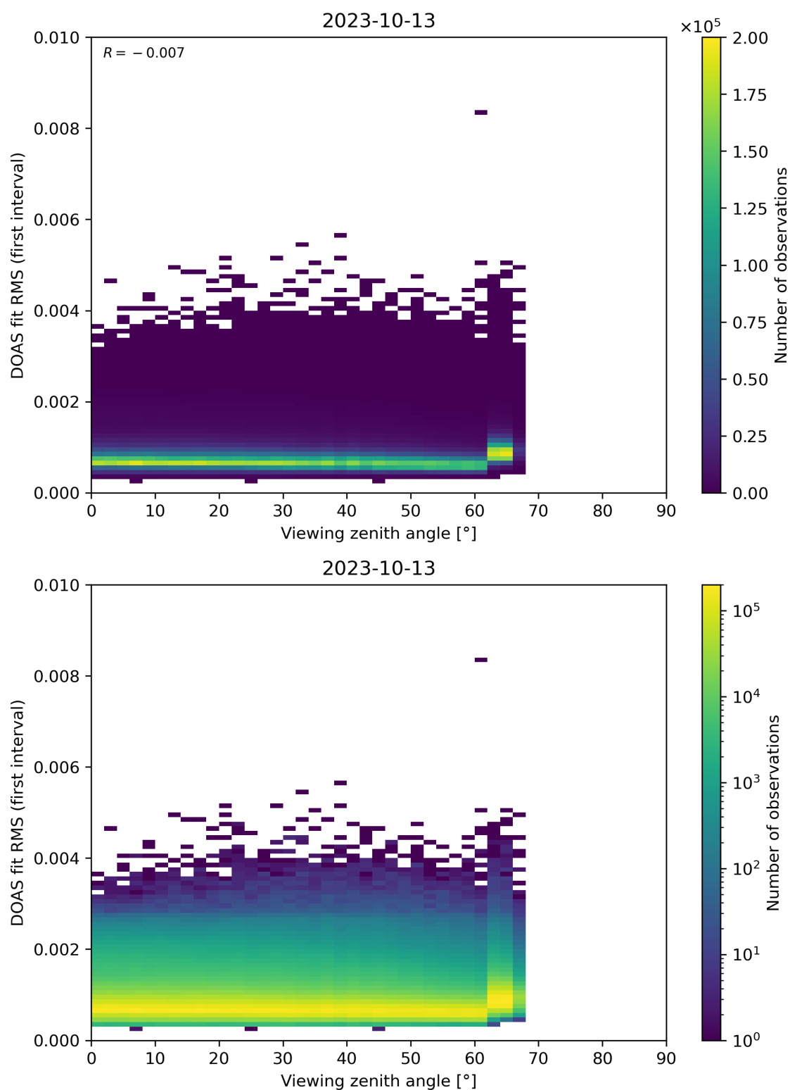
Figure 182: Scatter density plot of “Viewing zenith angle” against “DOAS fit RMS (first interval)” for 2023-10-12 to 2023-10-14.
