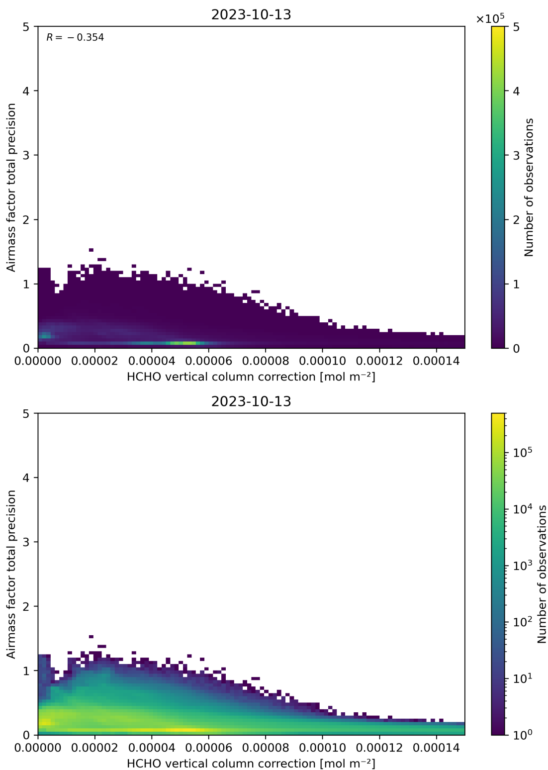
Figure 121: Scatter density plot of “HCHO vertical column correction” against “Airmass factor total precision” for 2023-10-12 to 2023-10-14.
