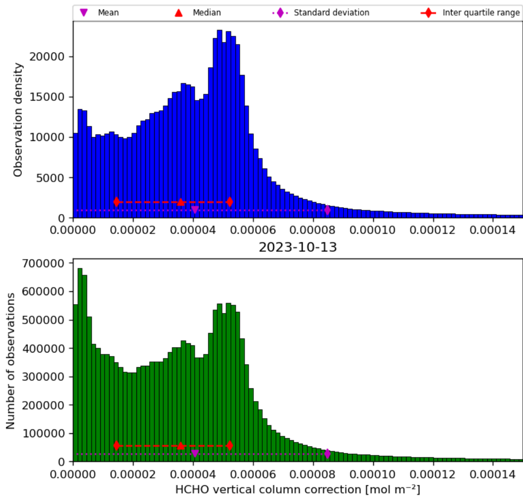
Figure 37: Histogram of “HCHO vertical column correction” for 2023-10-12 to 2023-10-14
