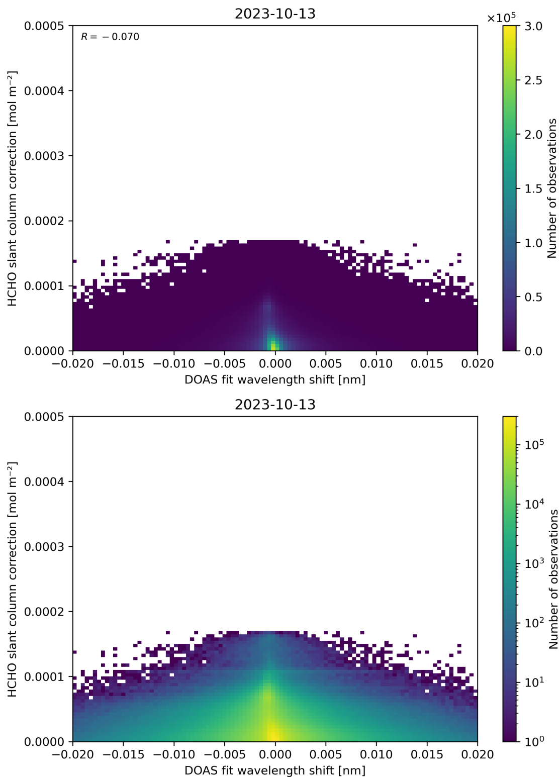
Figure 67: Scatter density plot of “DOAS fit wavelength shift” against “HCHO slant column correction” for 2023-10-12 to 2023-10-14.
