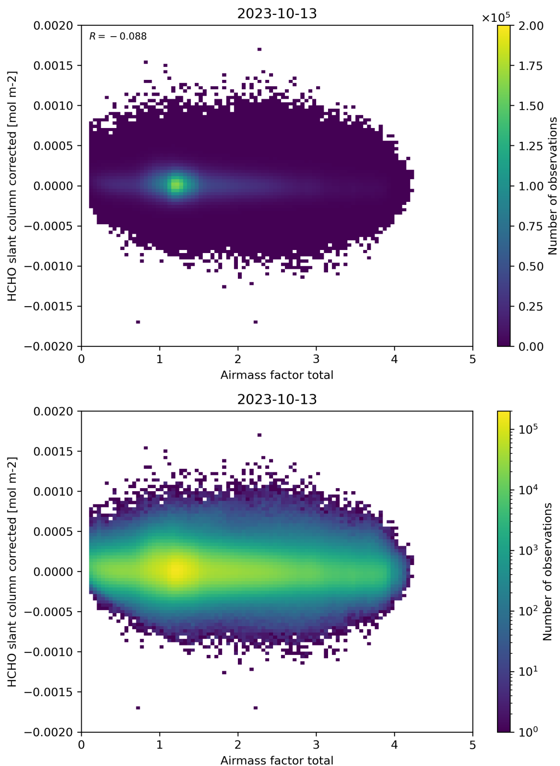
Figure 101: Scatter density plot of “Airmass factor total” against “HCHO slant column corrected” for 2023-10-12 to 2023-10-14.
