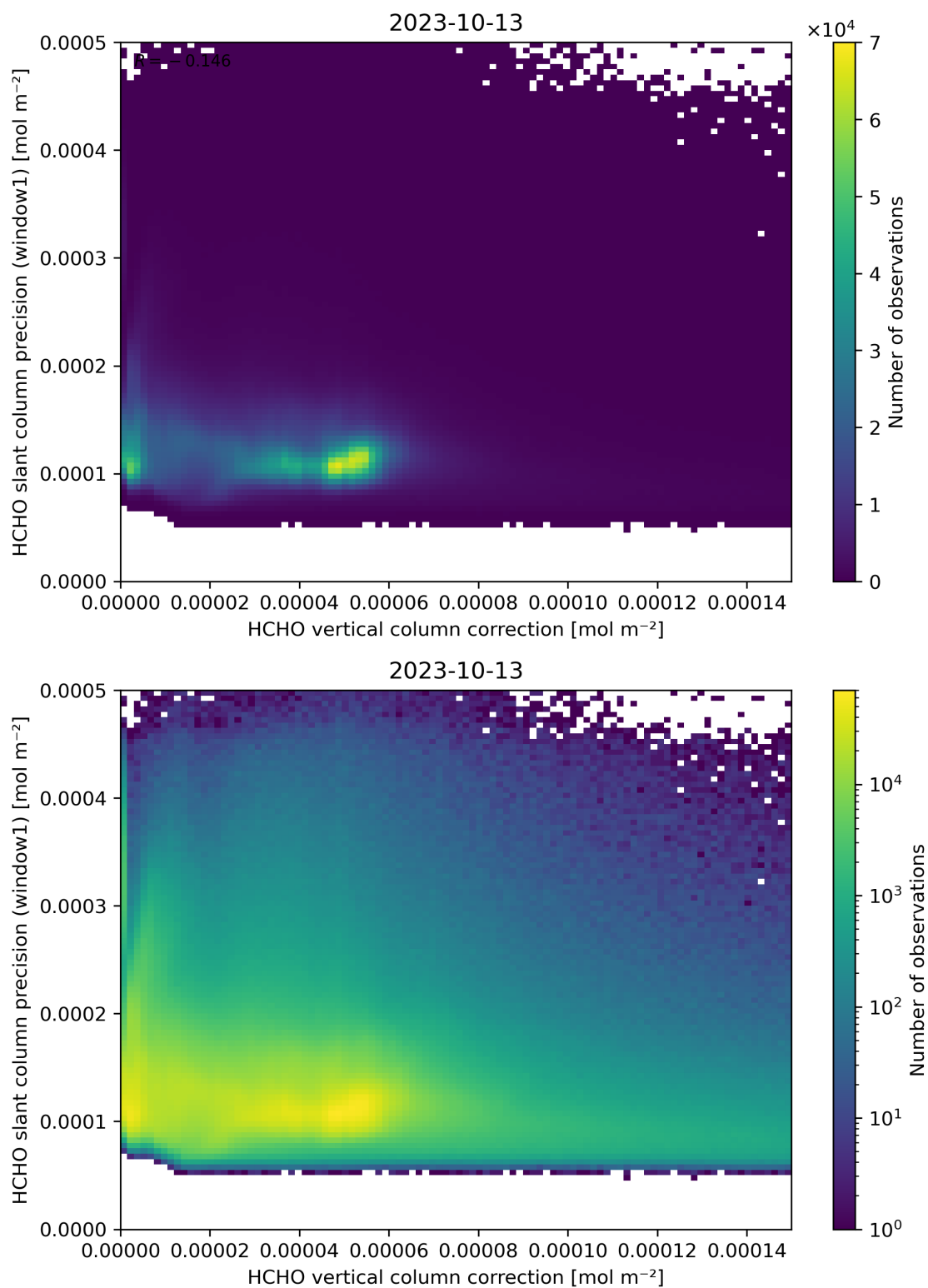
Figure 119: Scatter density plot of “HCHO vertical column correction” against “HCHO slant column precision (window1)” for 2023-10-12 to 2023-10-14.
