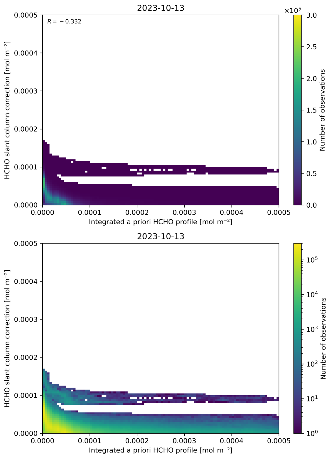
Figure 152: Scatter density plot of “Integrated a priori HCHO profile” against “HCHO slant column correction” for 2023-10-12 to 2023-10-14.
