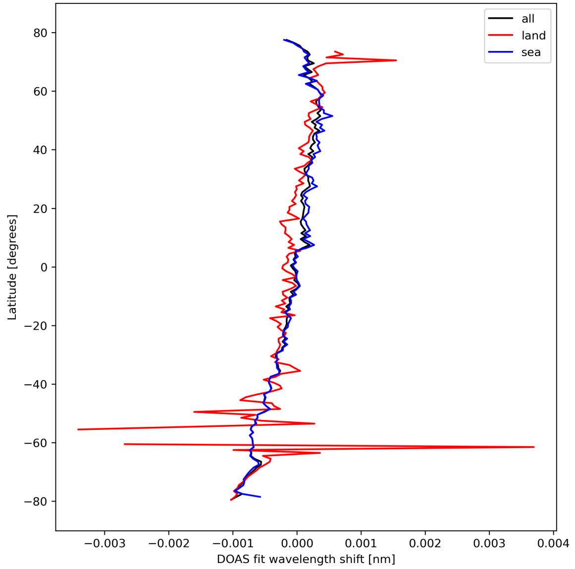
Figure 30: Zonal average of “DOAS fit wavelength shift” for 2023-10-12 to 2023-10-14.
