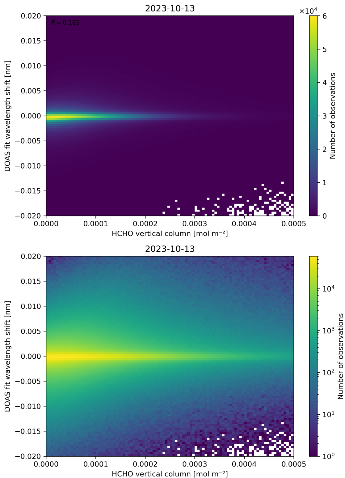
Figure 124: Scatter density plot of “HCHO vertical column” against “DOAS fit wavelength shift” for 2023-10-12 to 2023-10-14.
