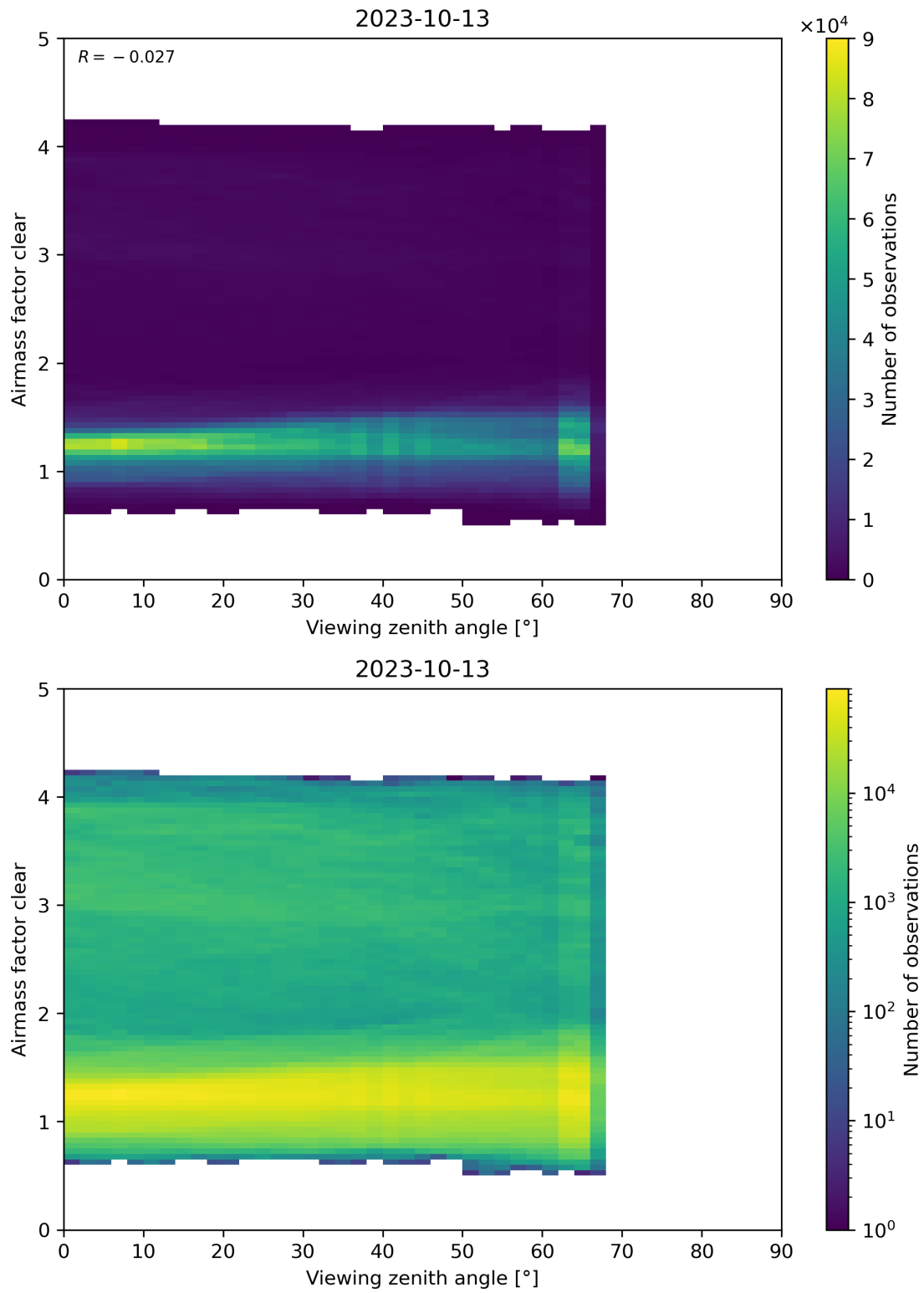
Figure 185: Scatter density plot of “Viewing zenith angle” against “Airmass factor clear” for 2023-10-12 to 2023-10-14.
