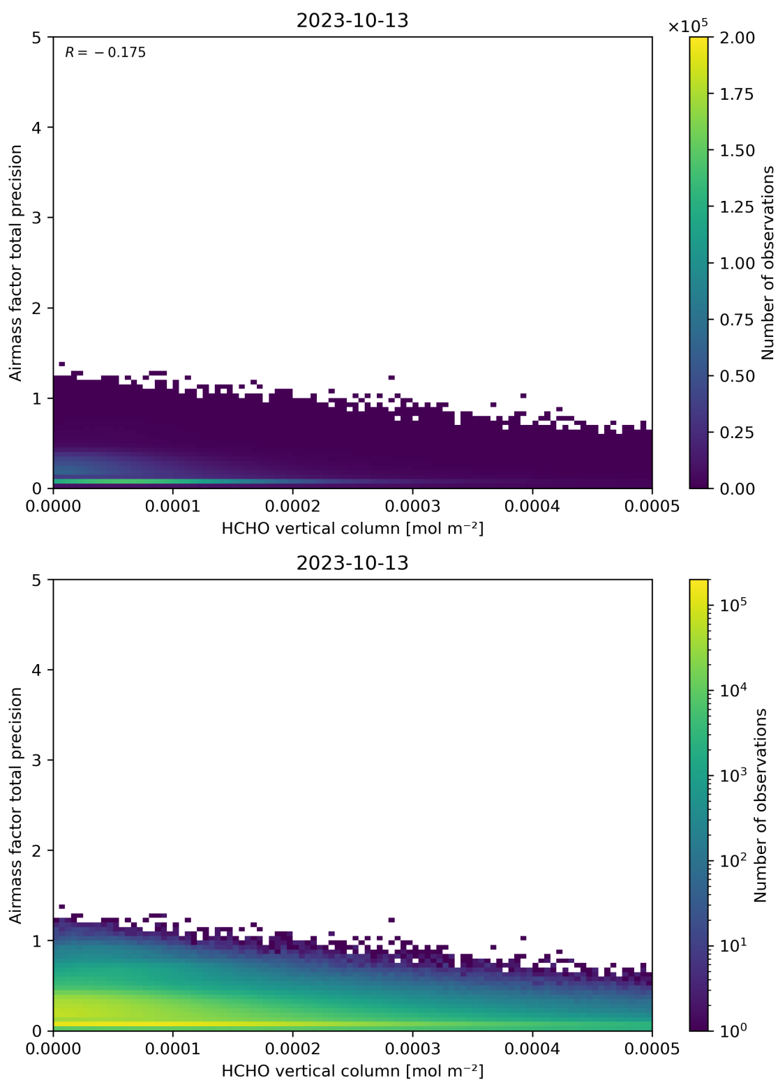
Figure 132: Scatter density plot of “HCHO vertical column” against “Airmass factor total precision” for 2023-10-12 to 2023-10-14.
