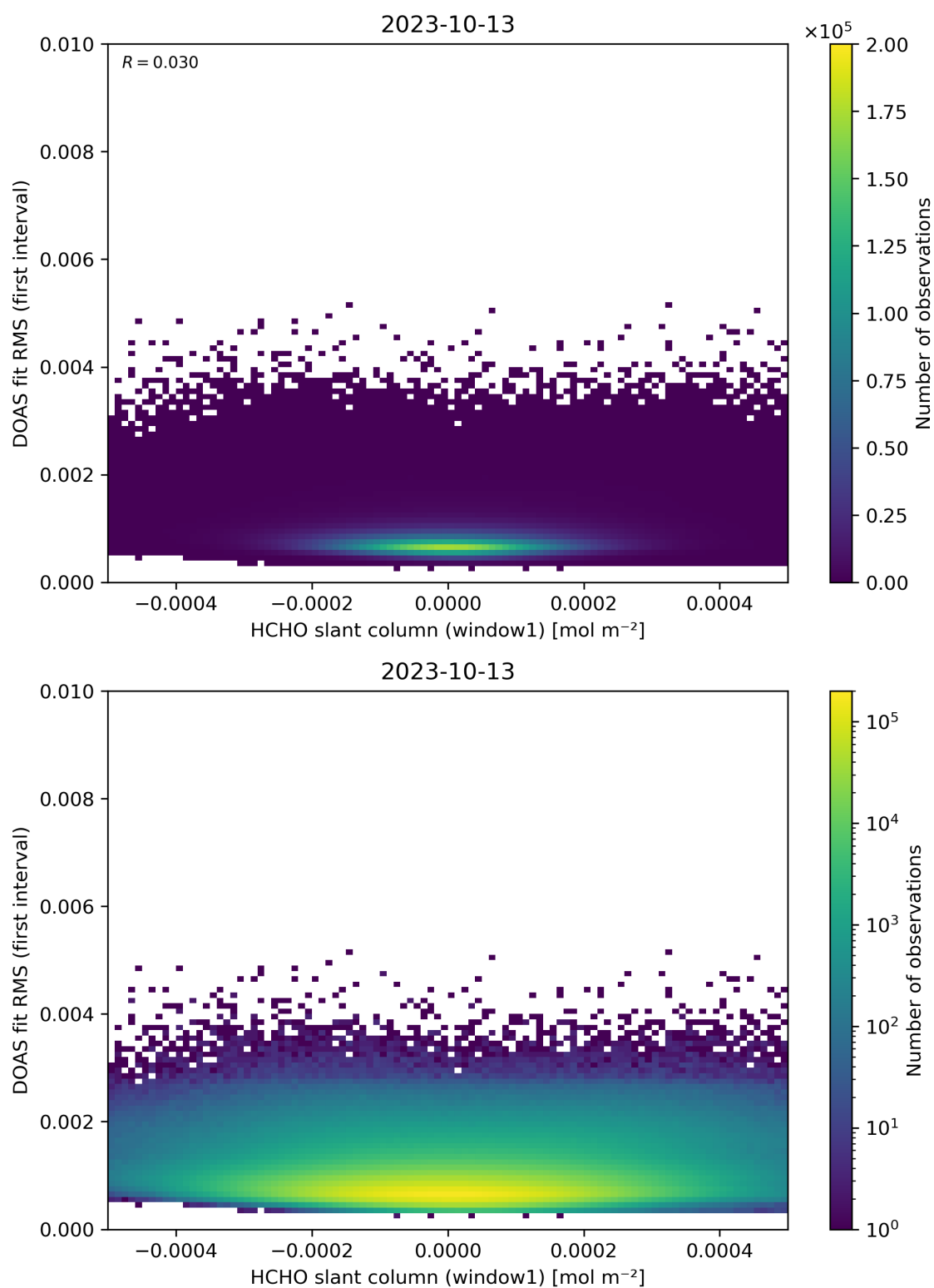
Figure 78: Scatter density plot of “HCHO slant column (window1)” against “DOAS fit RMS (first interval)” for 2023-10-12 to 2023-10-14.
