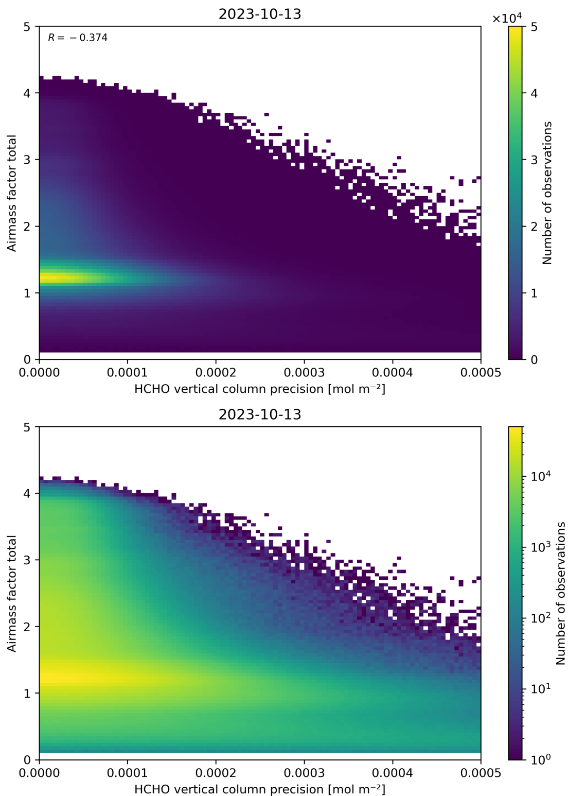
Figure 144: Scatter density plot of “HCHO vertical column precision” against “Airmass factor total” for 2023-10-12 to 2023-10-14.
