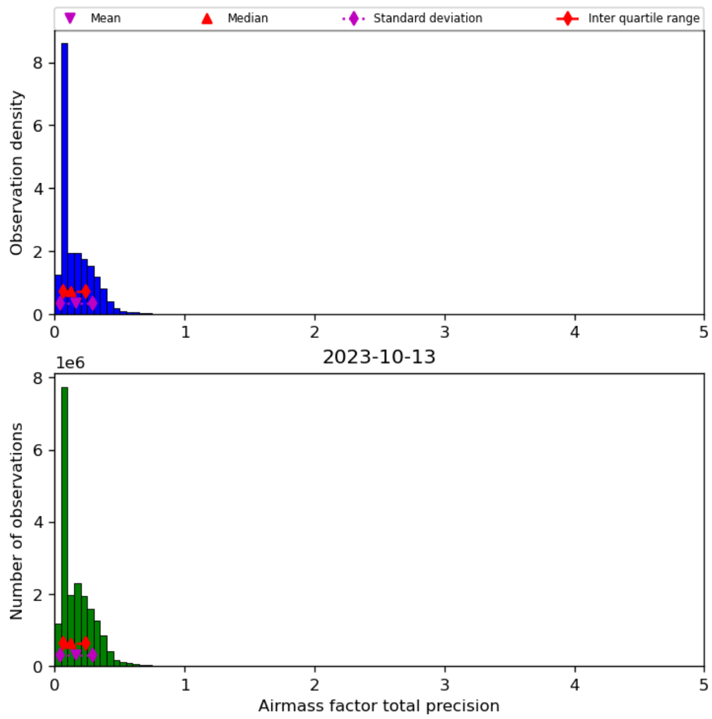
Figure 41: Histogram of “Airmass factor total precision” for 2023-10-12 to 2023-10-14
