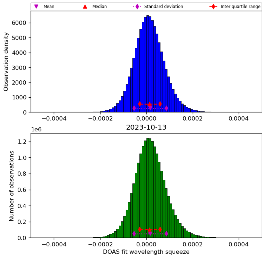
Figure 45: Histogram of “DOAS fit wavelength squeeze” for 2023-10-12 to 2023-10-14
