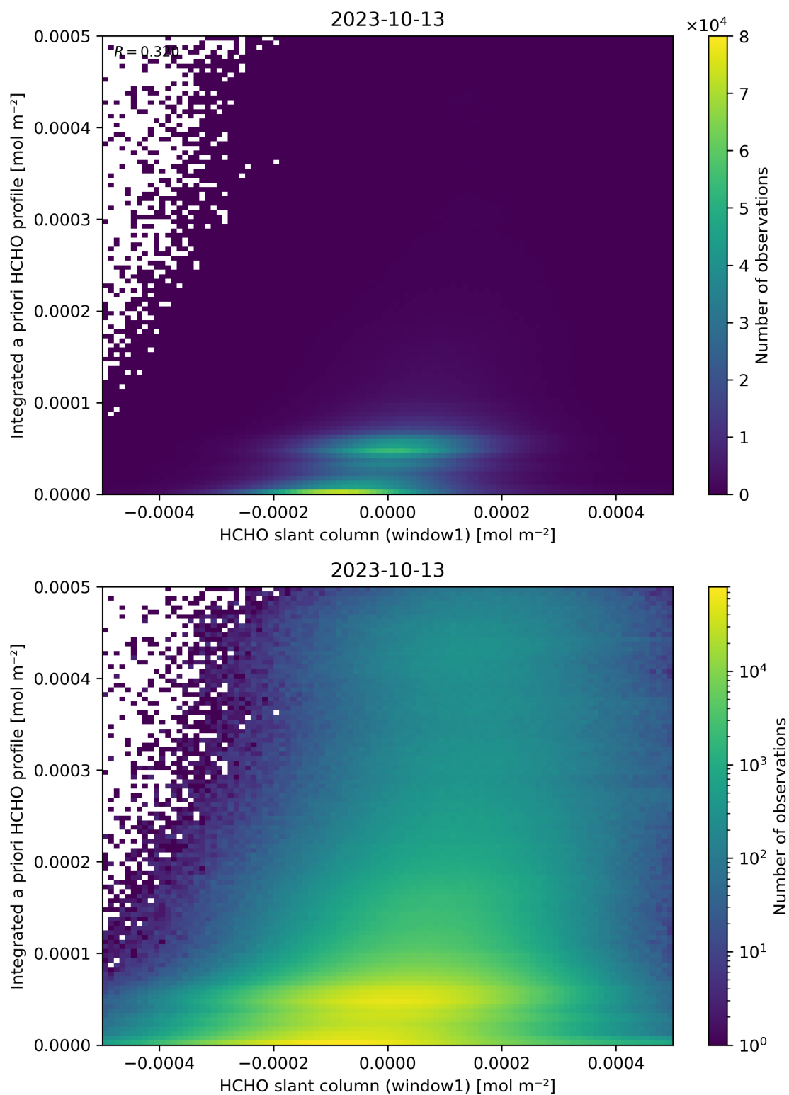
Figure 87: Scatter density plot of “HCHO slant column (window1)” against “Integrated a priori HCHO profile” for 2023-10-12 to 2023-10-14.
