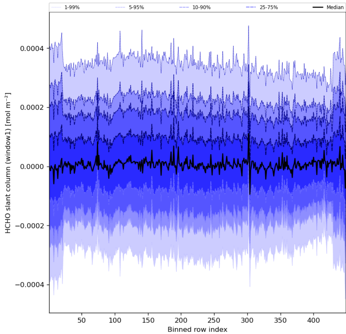
Figure 52: Along track statistics of “HCHO slant column (window1)” for 2023-10-12 to 2023-10-14
