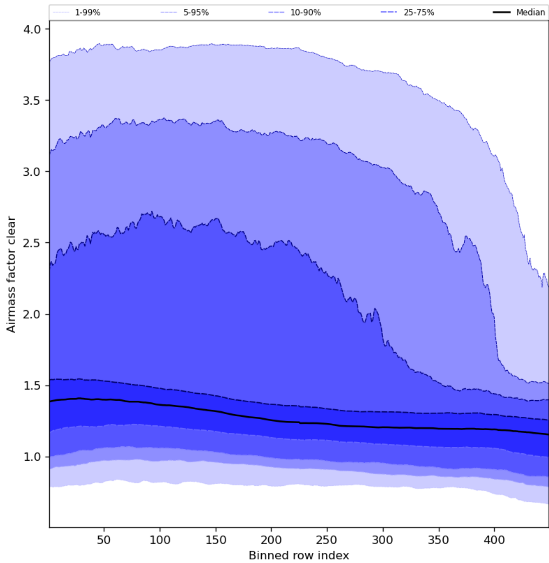
Figure 56: Along track statistics of “Air mass factor clear” for 2023-10-12 to 2023-10-14
