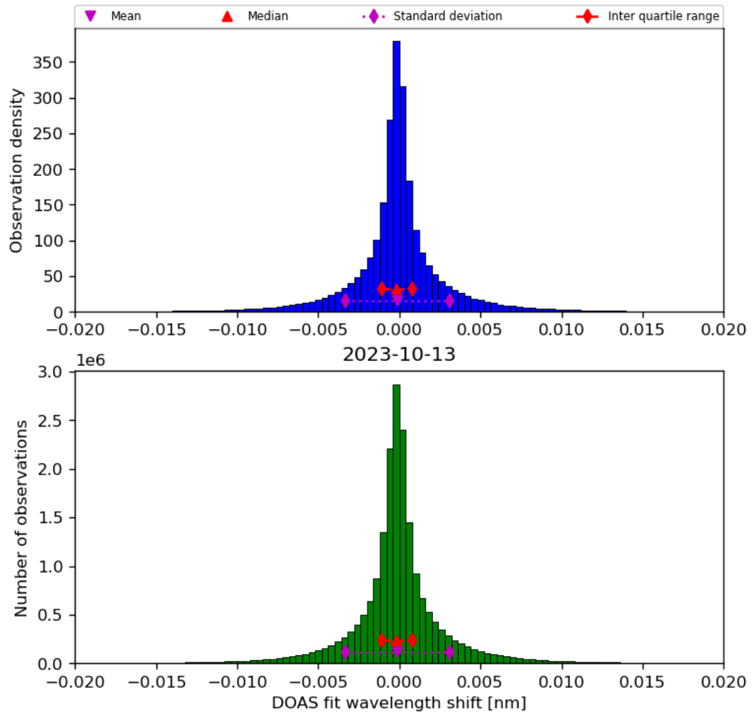
Figure 44: Histogram of “DOAS fit wavelength shift” for 2023-10-12 to 2023-10-14
