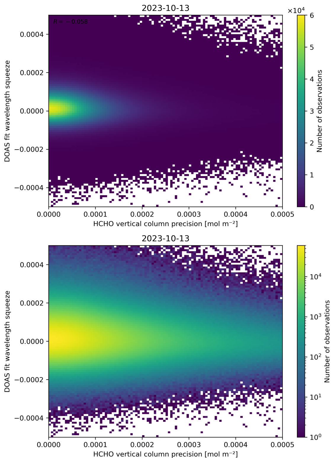
Figure 138: Scatter density plot of “HCHO vertical column precision” against “DOAS fit wavelength squeeze” for 2023-10-12 to 2023-10-14.
