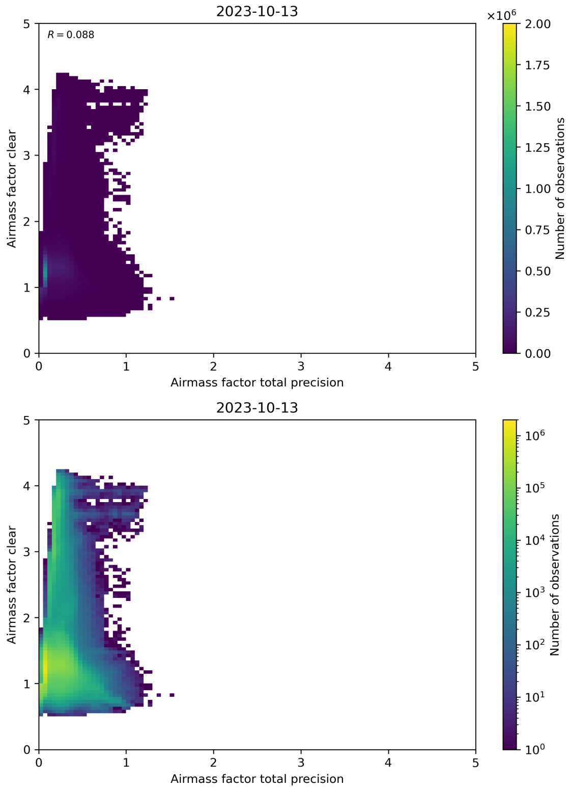
Figure 108: Scatter density plot of “Airmass factor total precision” against “Airmass factor clear” for 2023-10-12 to 2023-10-14.
