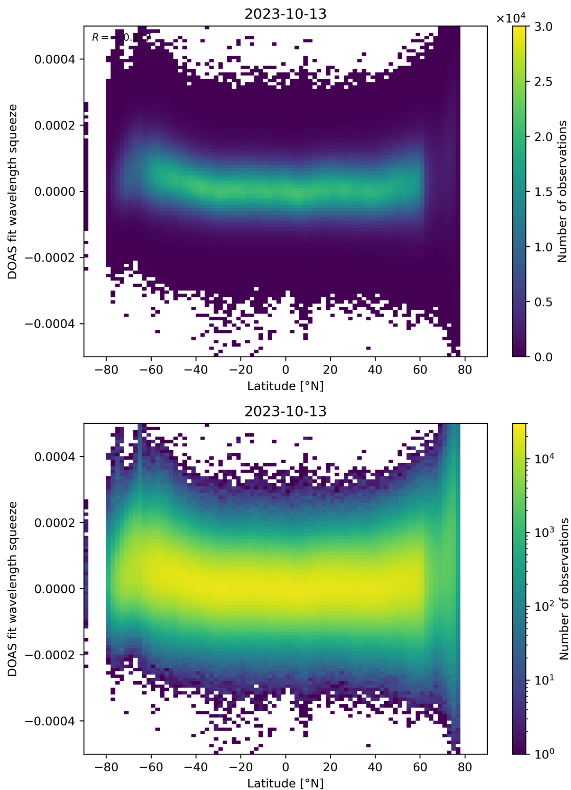
Figure 155: Scatter density plot of “Latitude” against “DOAS fit wavelength squeeze” for 2023-10-12 to 2023-10-14.
