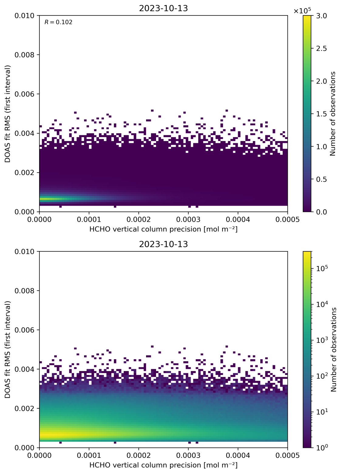
Figure 136: Scatter density plot of “HCHO vertical column precision” against “DOAS fit RMS (first interval)” for 2023-10-12 to 2023-10-14.
