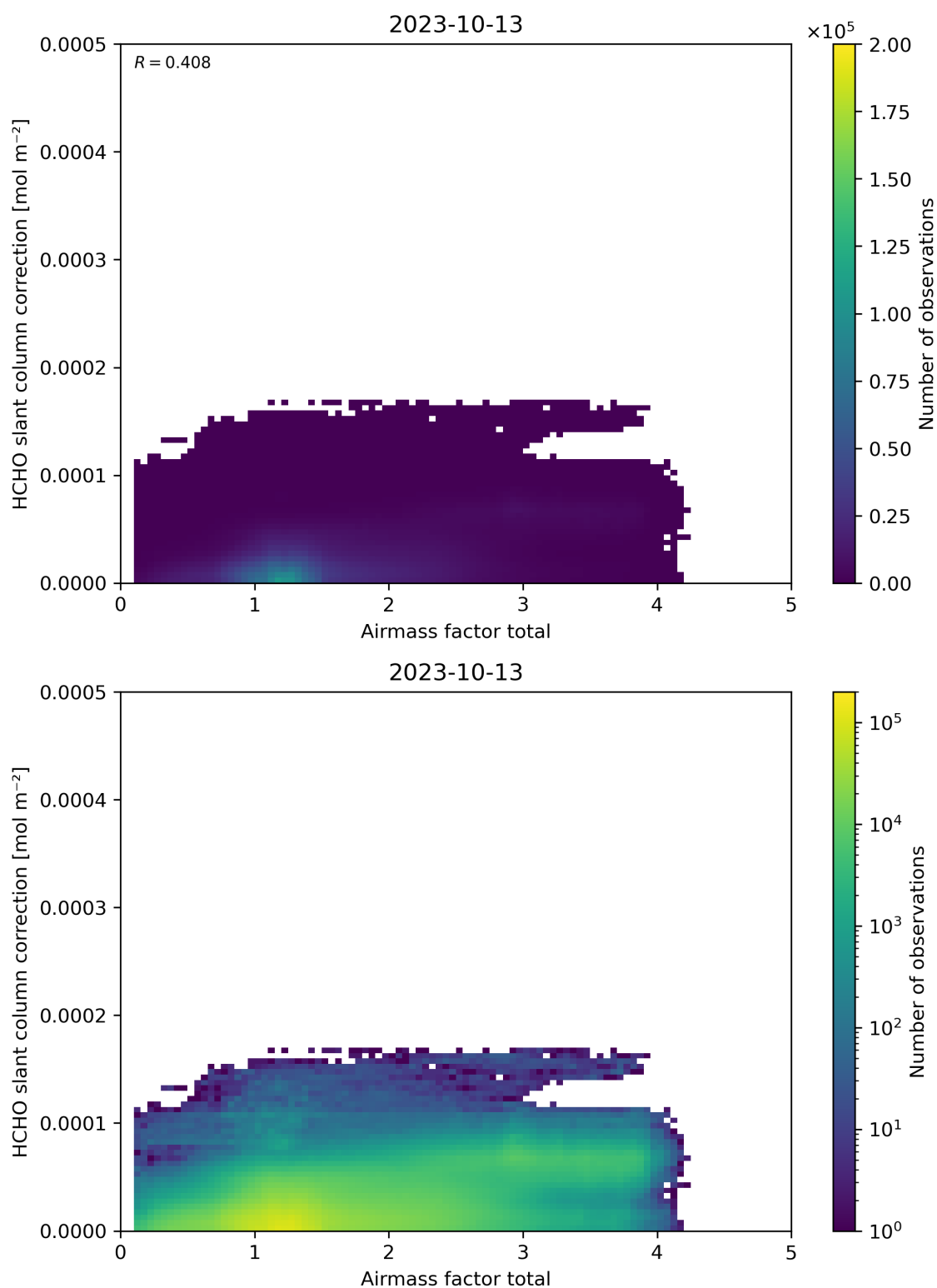
Figure 102: Scatter density plot of “Airmass factor total” against “HCHO slant column correction” for 2023-10-12 to 2023-10-14.
