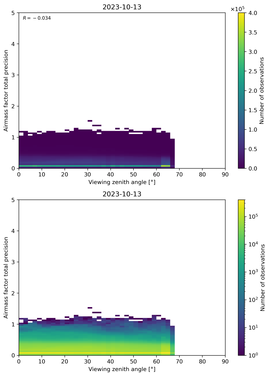
Figure 191: Scatter density plot of “Viewing zenith angle” against “Airmass factor total precision” for 2023-10-12 to 2023-10-14.
