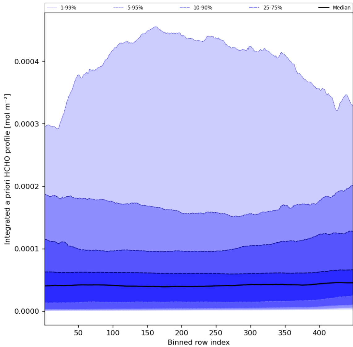
Figure 57: Along track statistics of “Integrated a priori HCHO profile” for 2023-10-12 to 2023-10-14
