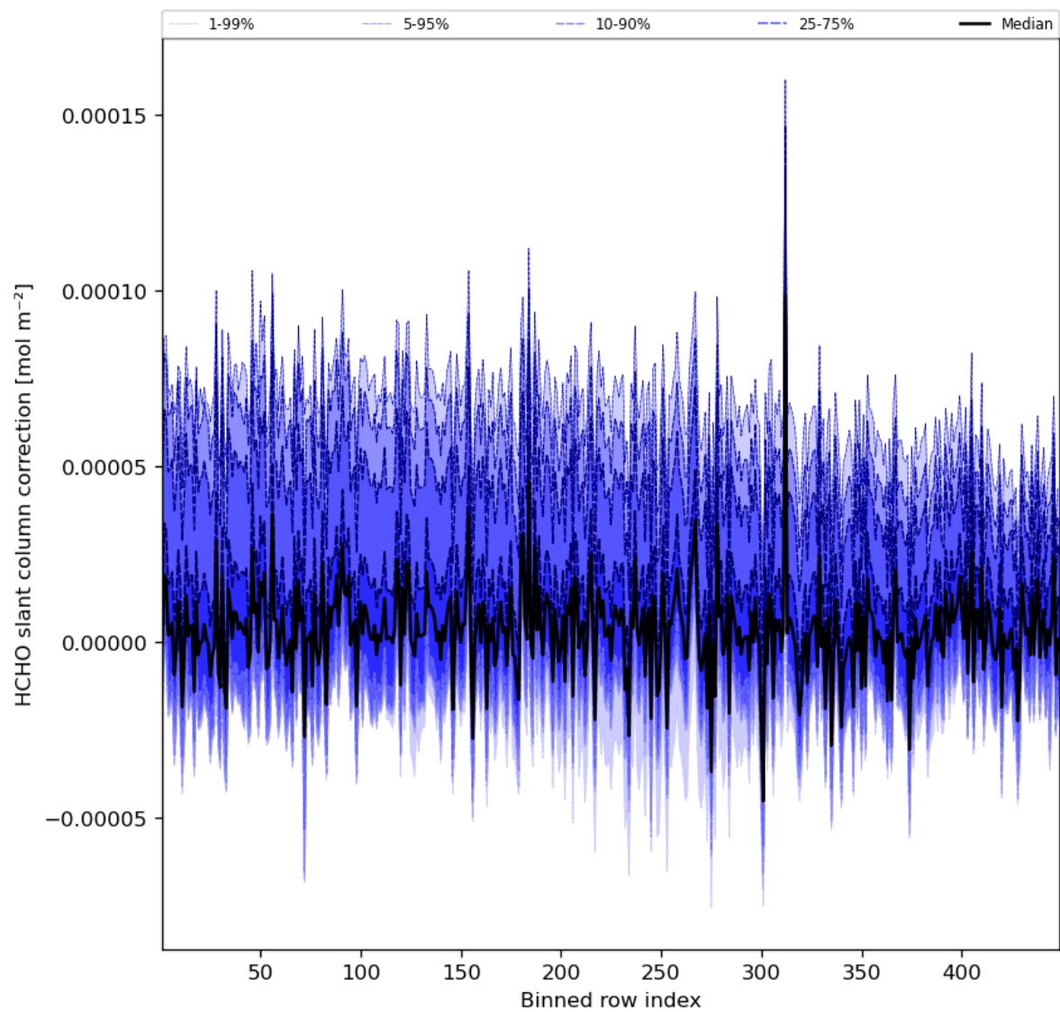
Figure 61: Along track statistics of “HCHO slant column correction” for 2023-10-12 to 2023-10-14
