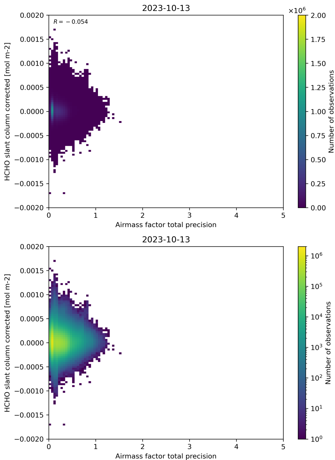
Figure 109: Scatter density plot of “Airmass factor total precision” against “HCHO slant column corrected” for 2023-10-12 to 2023-10-14.
