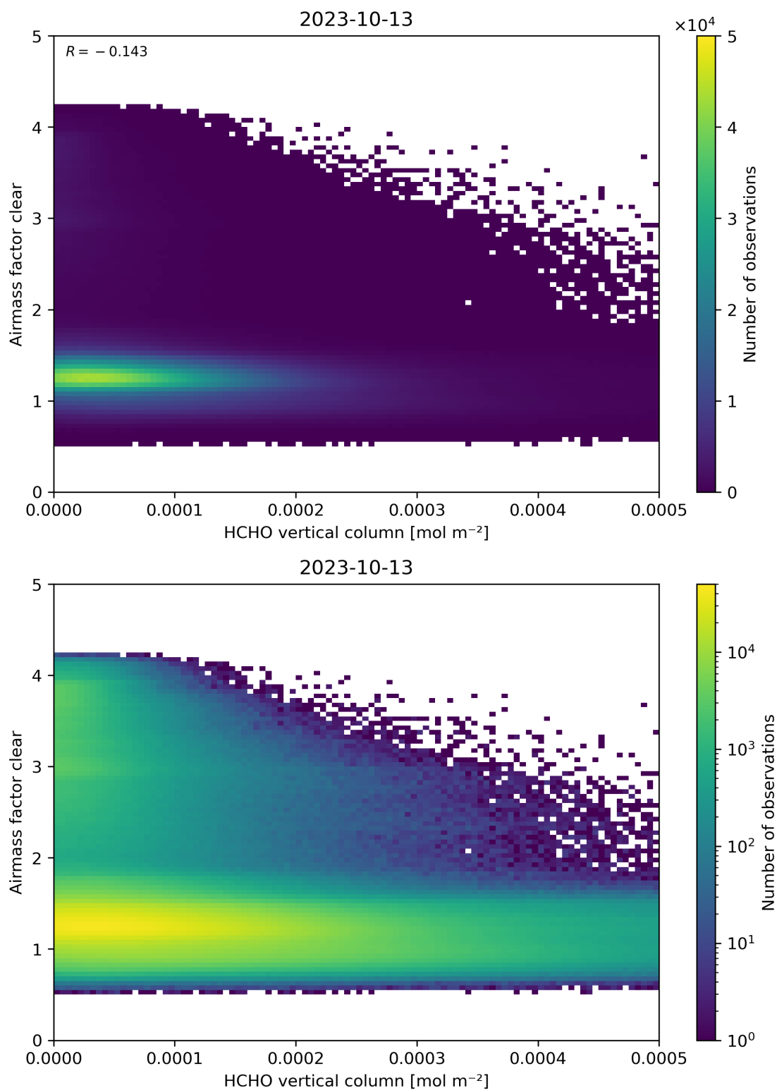
Figure 126: Scatter density plot of “HCHO vertical column” against “Airmass factor clear” for 2023-10-12 to 2023-10-14.
