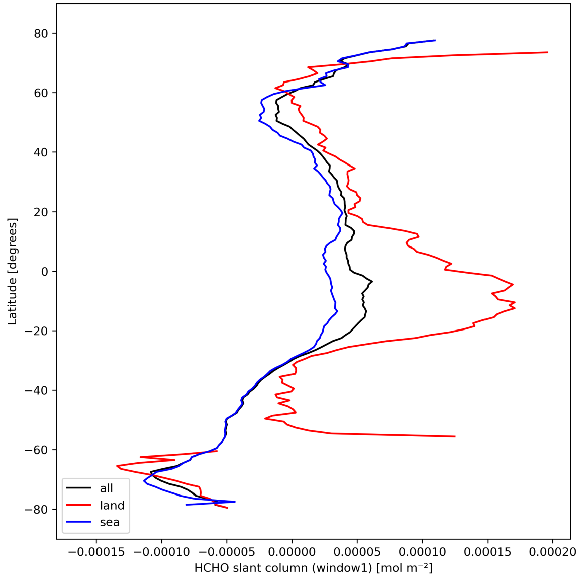
Figure 24: Zonal average of “HCHO slant column (window1)” for 2023-10-12 to 2023-10-14.
