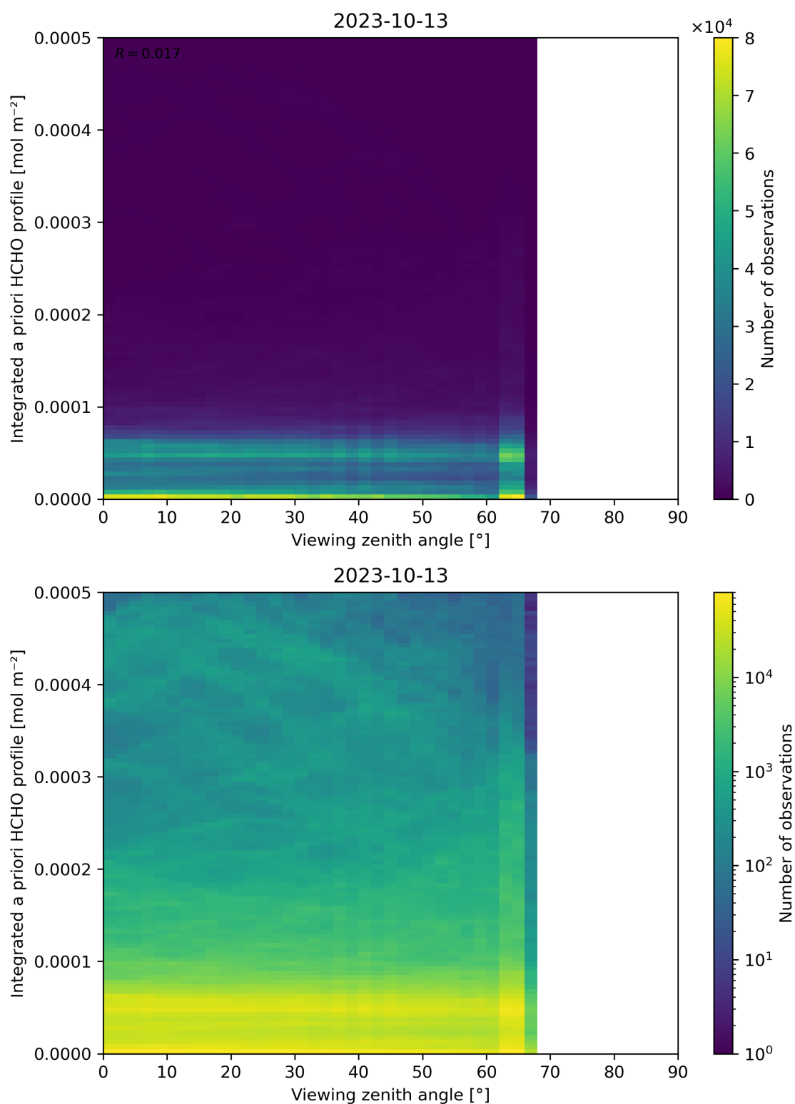
Figure 195: Scatter density plot of “Viewing zenith angle” against “Integrated a priori HCHO profile” for 2023-10-12 to 2023-10-14.
