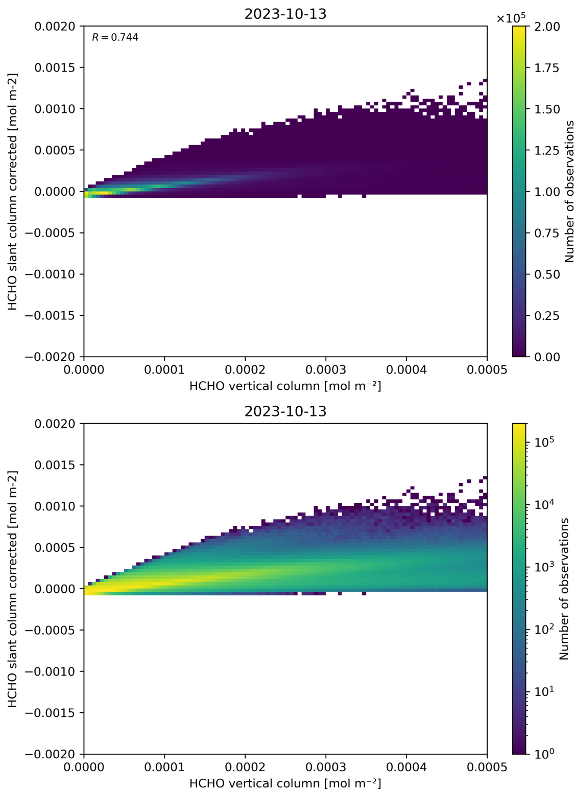
Figure 127: Scatter density plot of “HCHO vertical column” against “HCHO slant column corrected” for 2023-10-12 to 2023-10-14.
