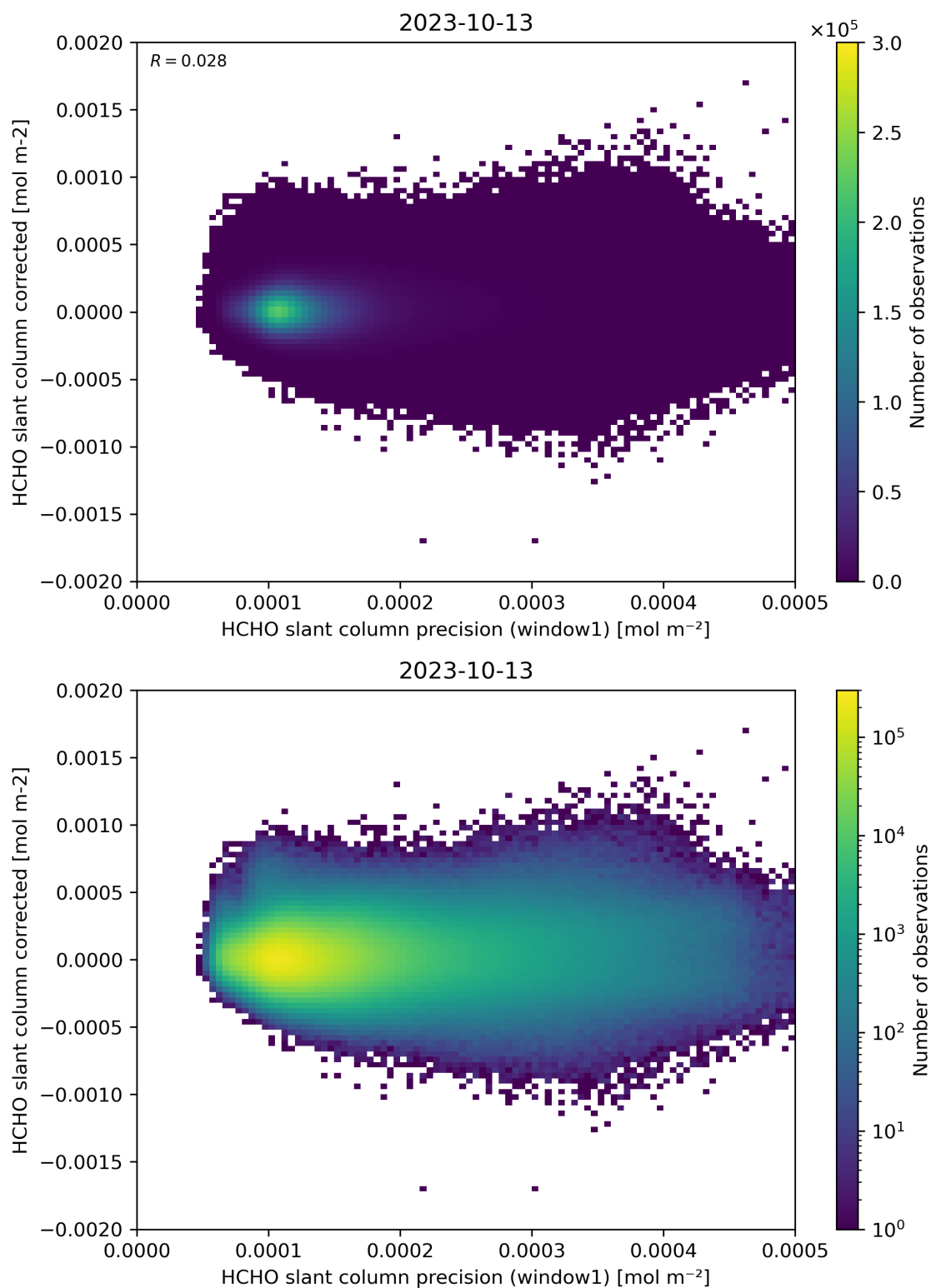
Figure 92: Scatter density plot of “HCHO slant column precision (window1)” against “HCHO slant column corrected” for 2023-10-12 to 2023-10-14.
