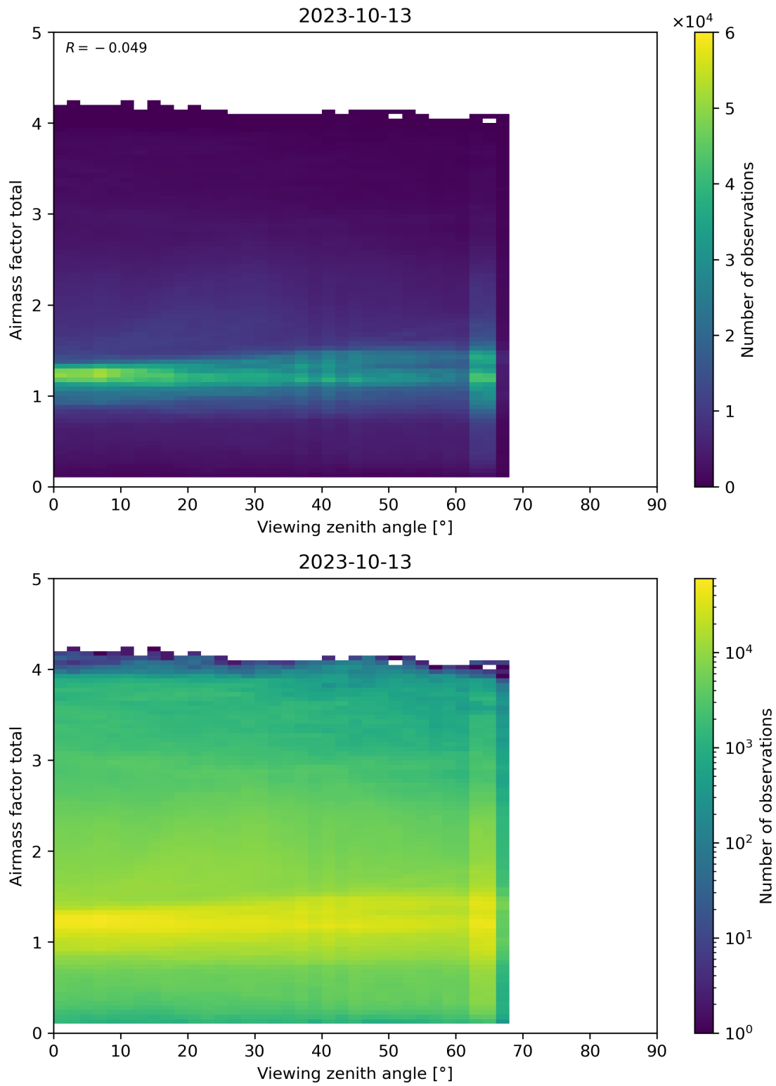
Figure 190: Scatter density plot of “Viewing zenith angle” against “Airmass factor total” for 2023-10-12 to 2023-10-14.
