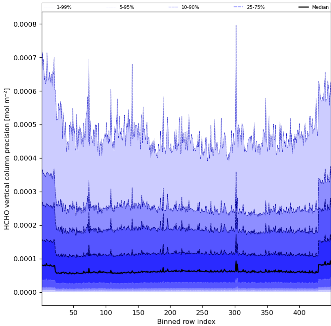
Figure 50: Along track statistics of “HCHO vertical column precision” for 2023-10-12 to 2023-10-14
