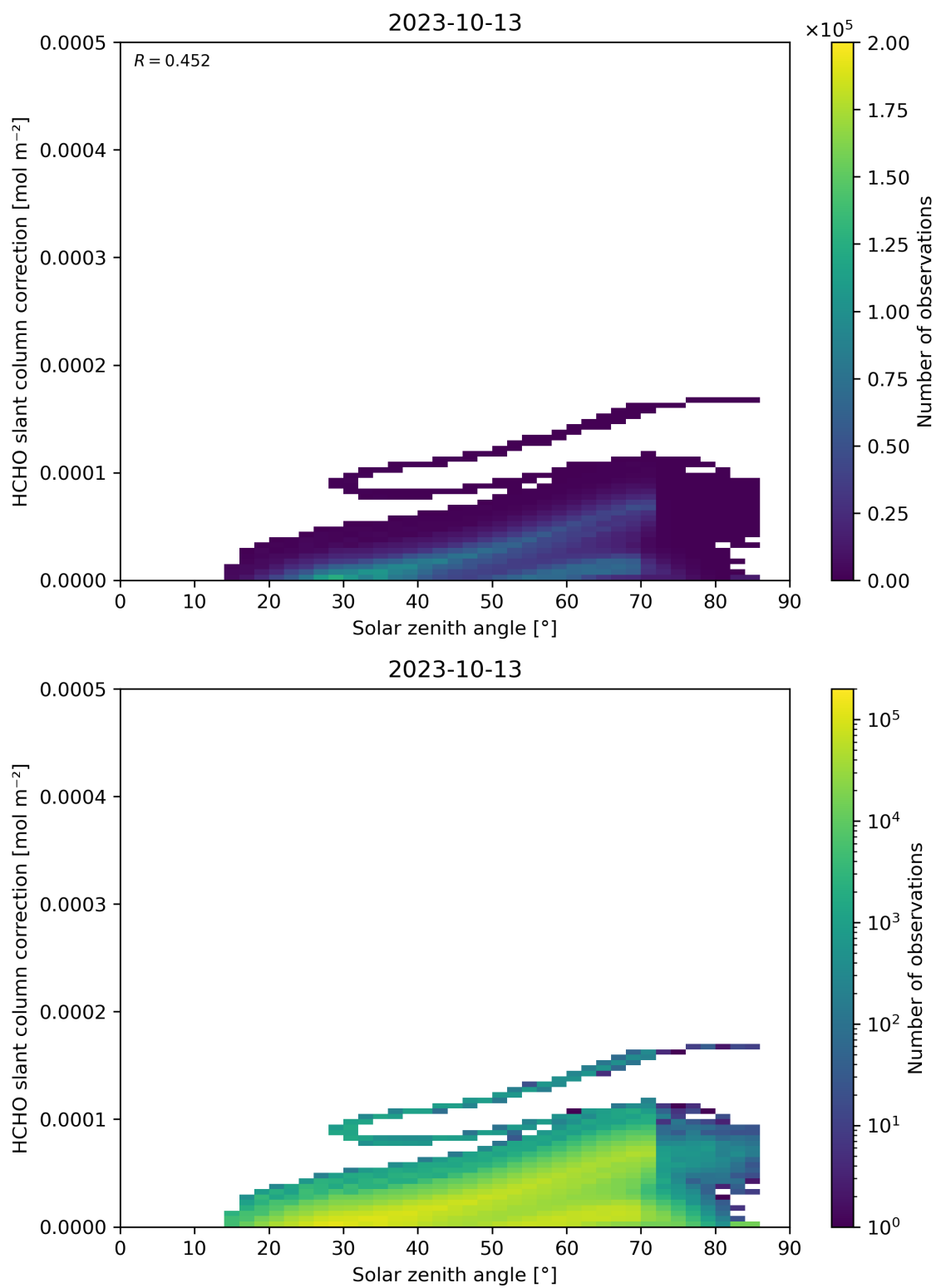
Figure 172: Scatter density plot of “Solar zenith angle” against “HCHO slant column correction” for 2023-10-12 to 2023-10-14.
