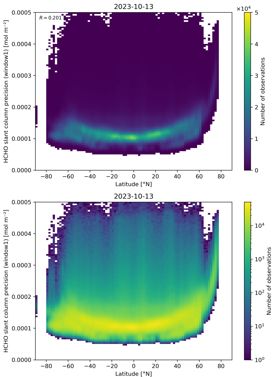
Figure 160: Scatter density plot of “Latitude” against “HCHO slant column precision (window1)” for 2023-10-12 to 2023-10-14.
