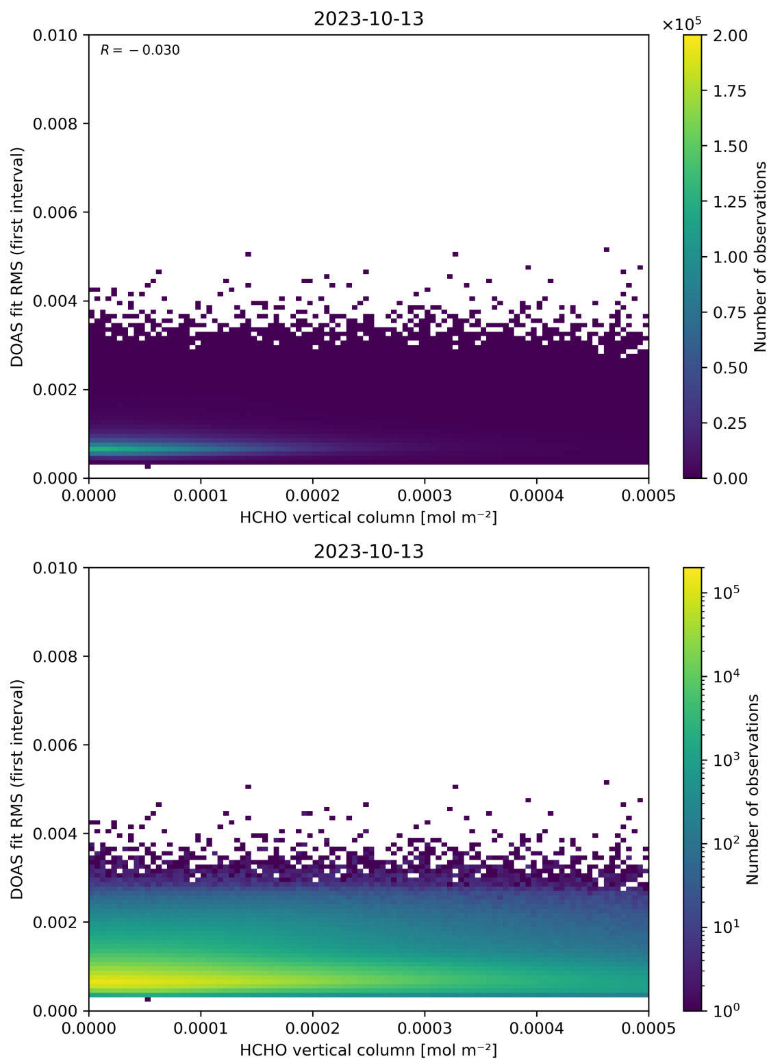
Figure 123: Scatter density plot of “HCHO vertical column” against “DOAS fit RMS (first interval)” for 2023-10-12 to 2023-10-14.
