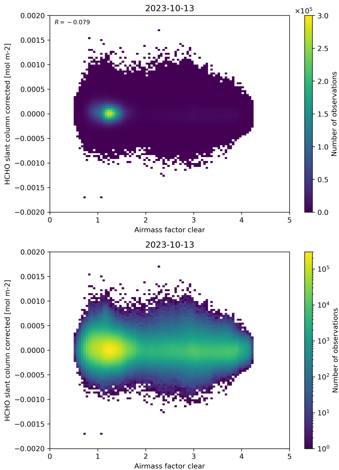
Figure 74: Scatter density plot of “Airmass factor clear” against “HCHO slant column corrected” for 2023-10-12 to 2023-10-14.
