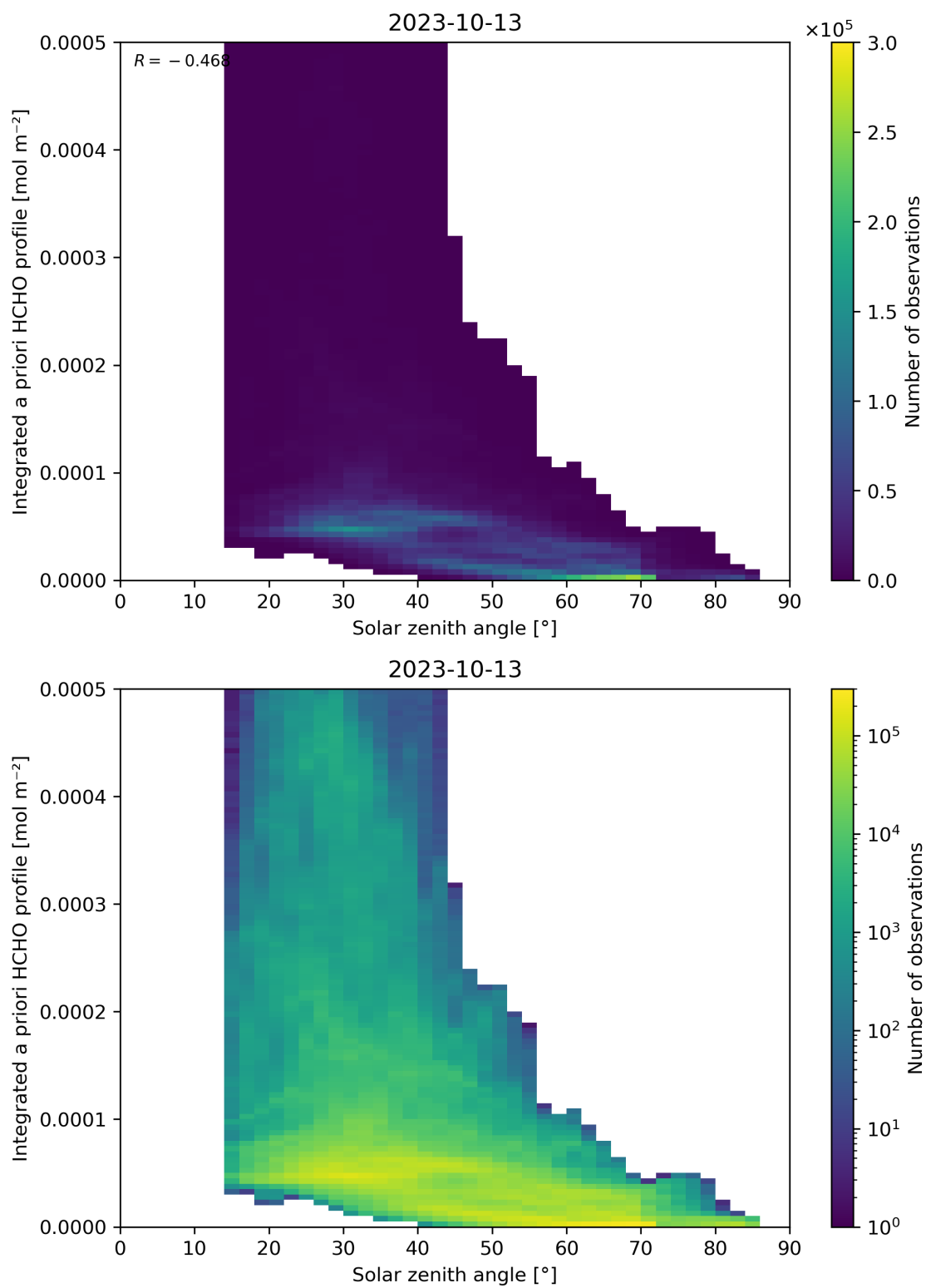
Figure 180: Scatter density plot of “Solar zenith angle” against “Integrated a priori HCHO profile” for 2023-10-12 to 2023-10-14.
