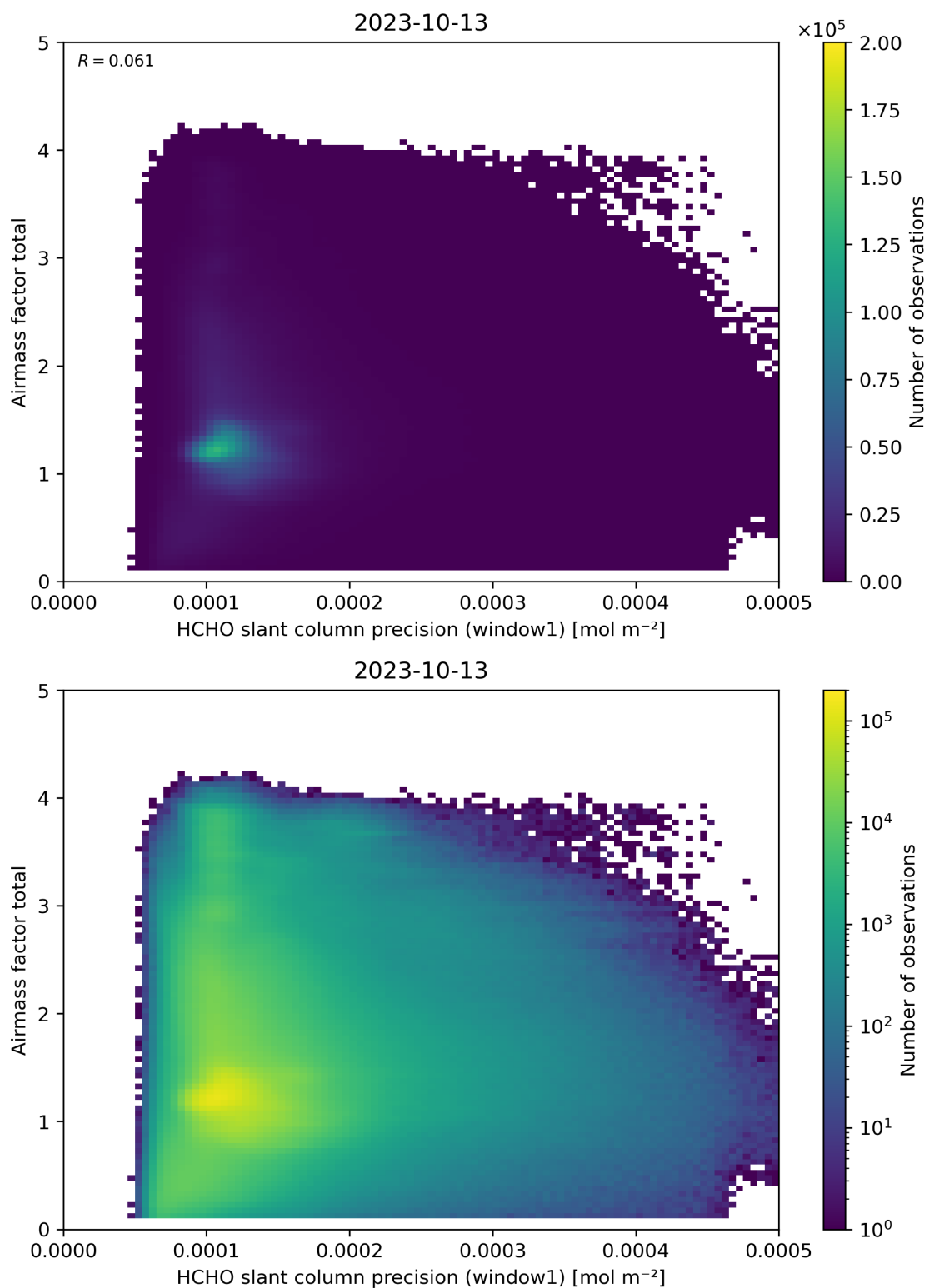
Figure 94: Scatter density plot of “HCHO slant column precision (window1)” against “Airmass factor total” for 2023-10-12 to 2023-10-14.
