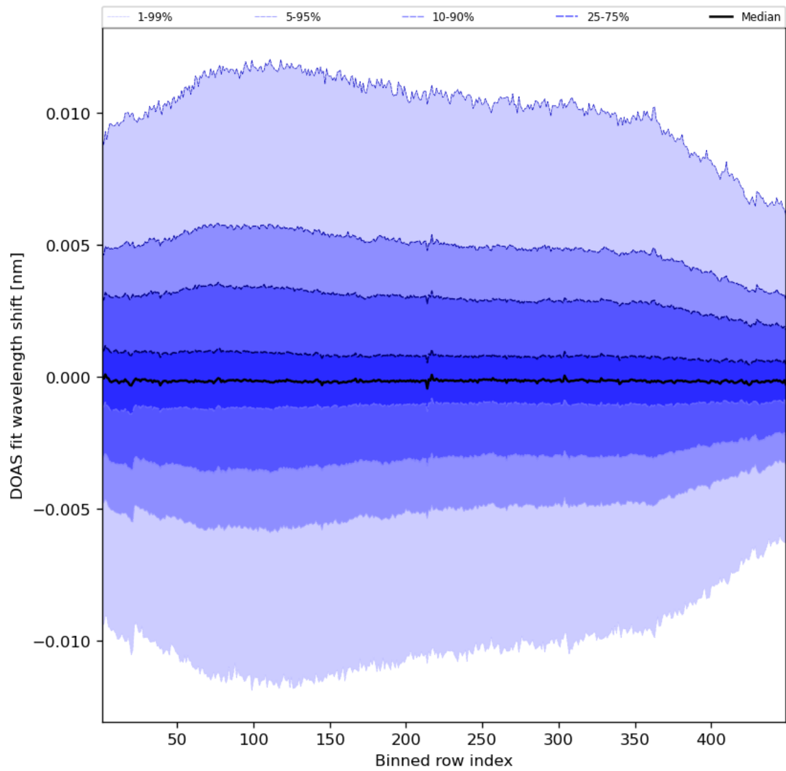
Figure 58: Along track statistics of “DOAS fit wavelength shift” for 2023-10-12 to 2023-10-14
