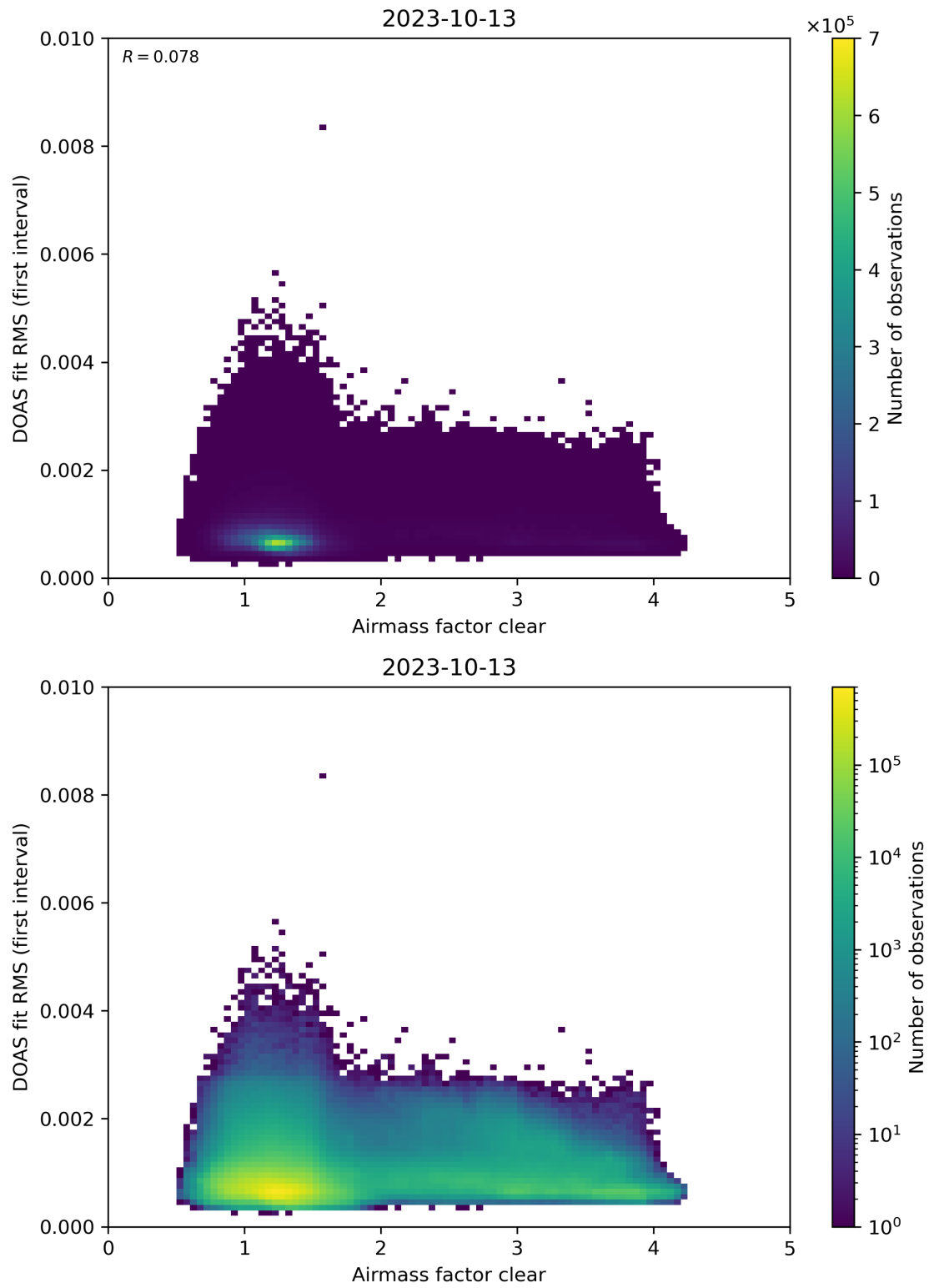
Figure 71: Scatter density plot of “Airmass factor clear” against “DOAS fit RMS (first interval)” for 2023-10-12 to 2023-10-14.
