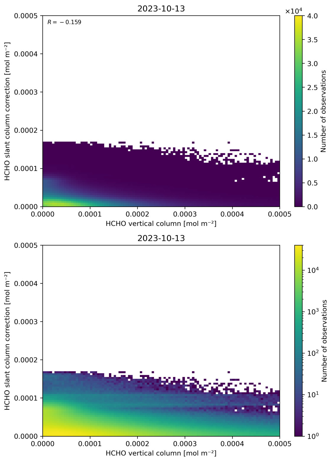
Figure 128: Scatter density plot of “HCHO vertical column” against “HCHO slant column correction” for 2023-10-12 to 2023-10-14.
