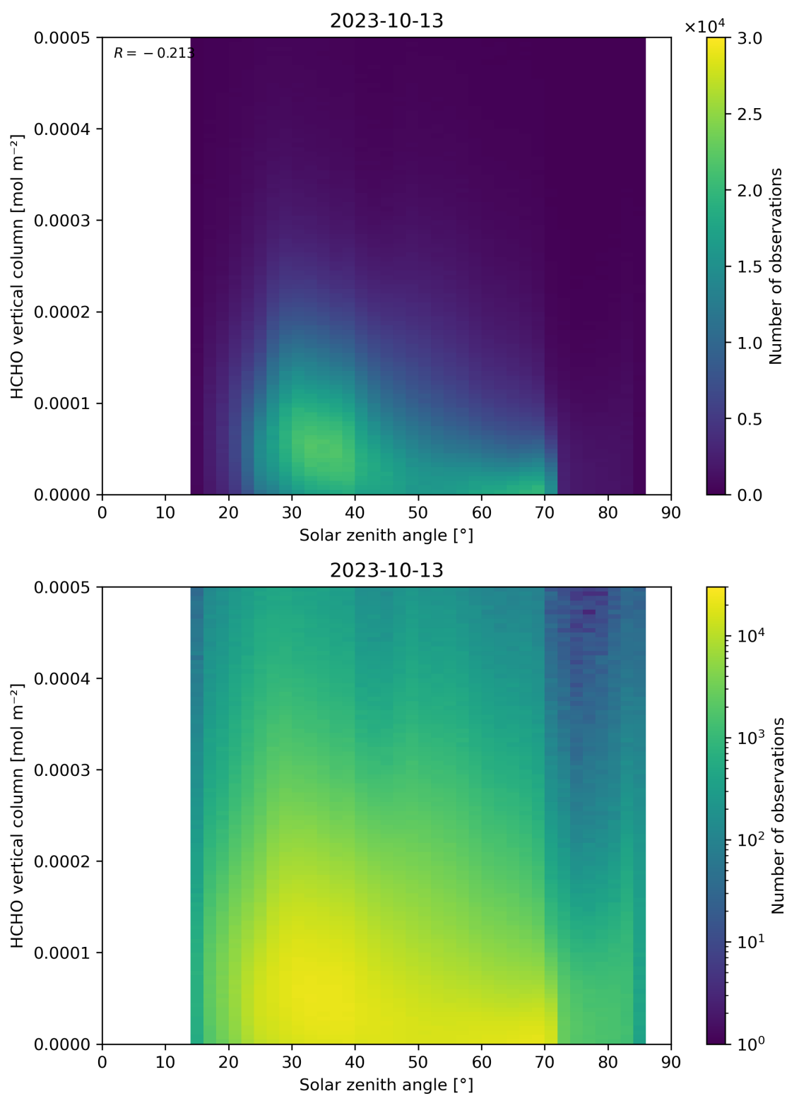
Figure 177: Scatter density plot of “Solar zenith angle” against “HCHO vertical column” for 2023-10-12 to 2023-10-14.
