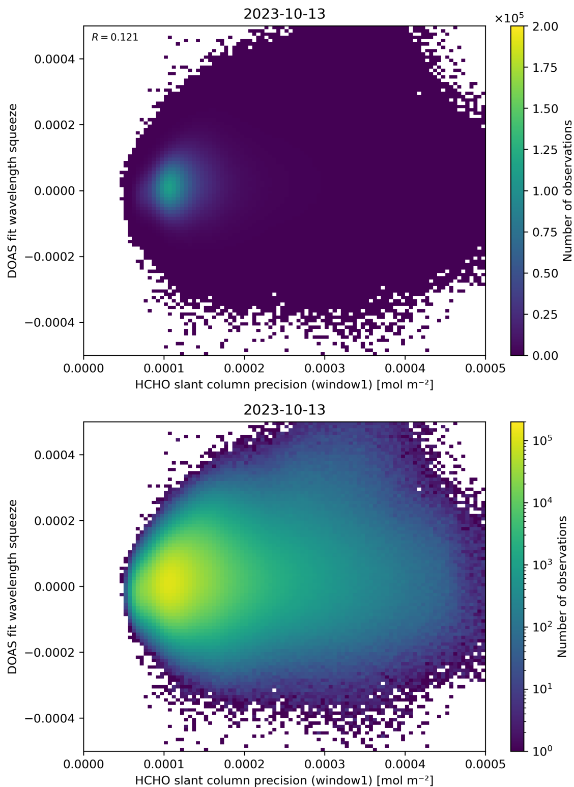
Figure 90: Scatter density plot of “HCHO slant column precision (window1)” against “DOAS fit wavelength squeeze” for 2023-10-12 to 2023-10-14.
