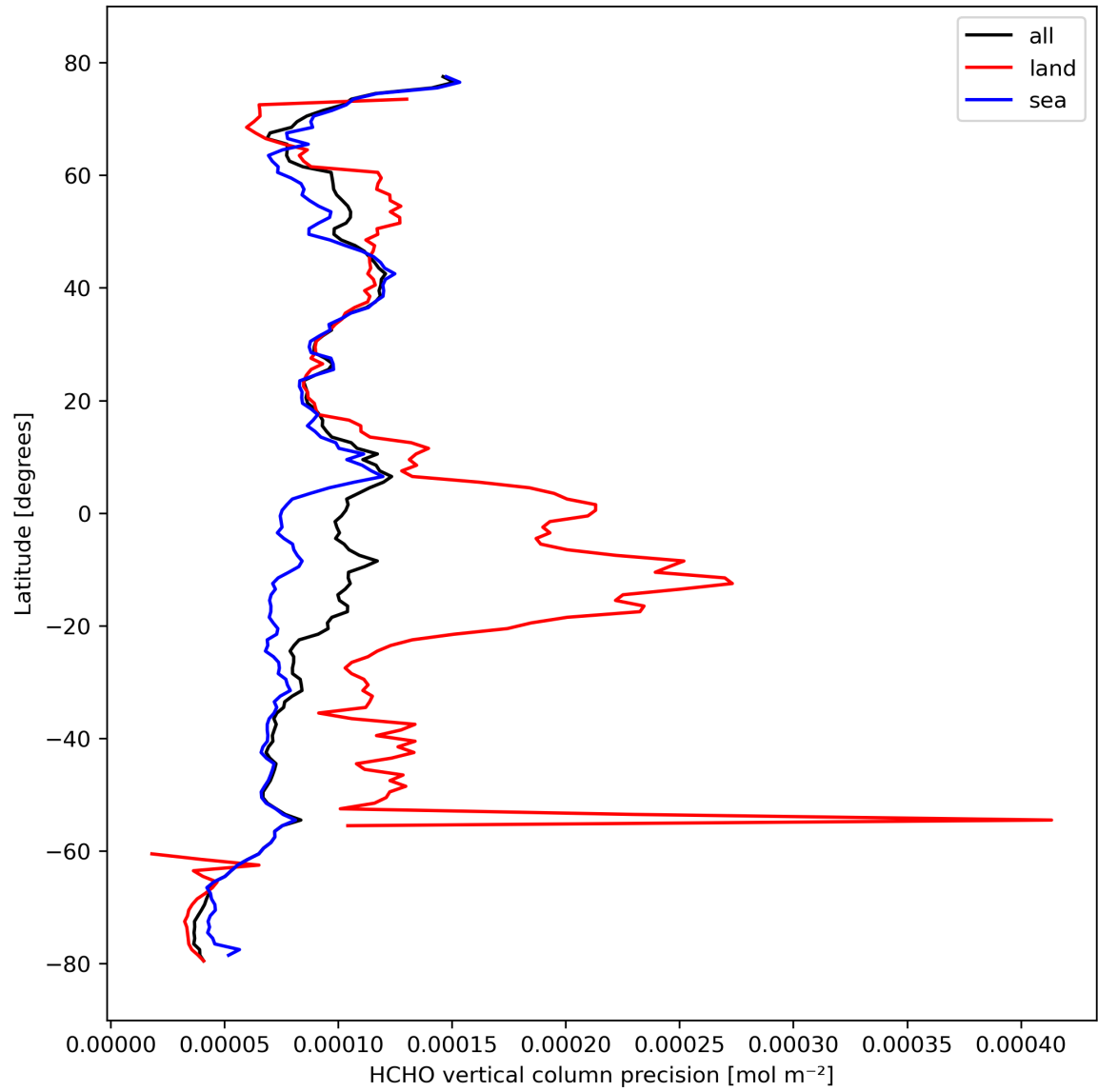
Figure 22: Zonal average of “HCHO vertical column precision” for 2023-10-12 to 2023-10-14.
