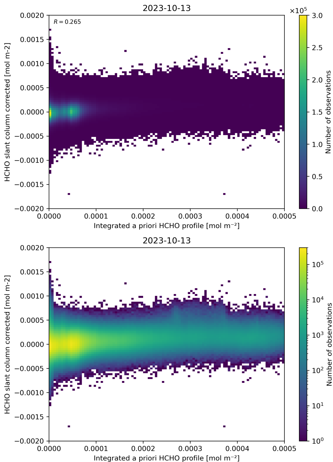
Figure 151: Scatter density plot of “Integrated a priori HCHO profile” against “HCHO slant column corrected” for 2023-10-12 to 2023-10-14.
