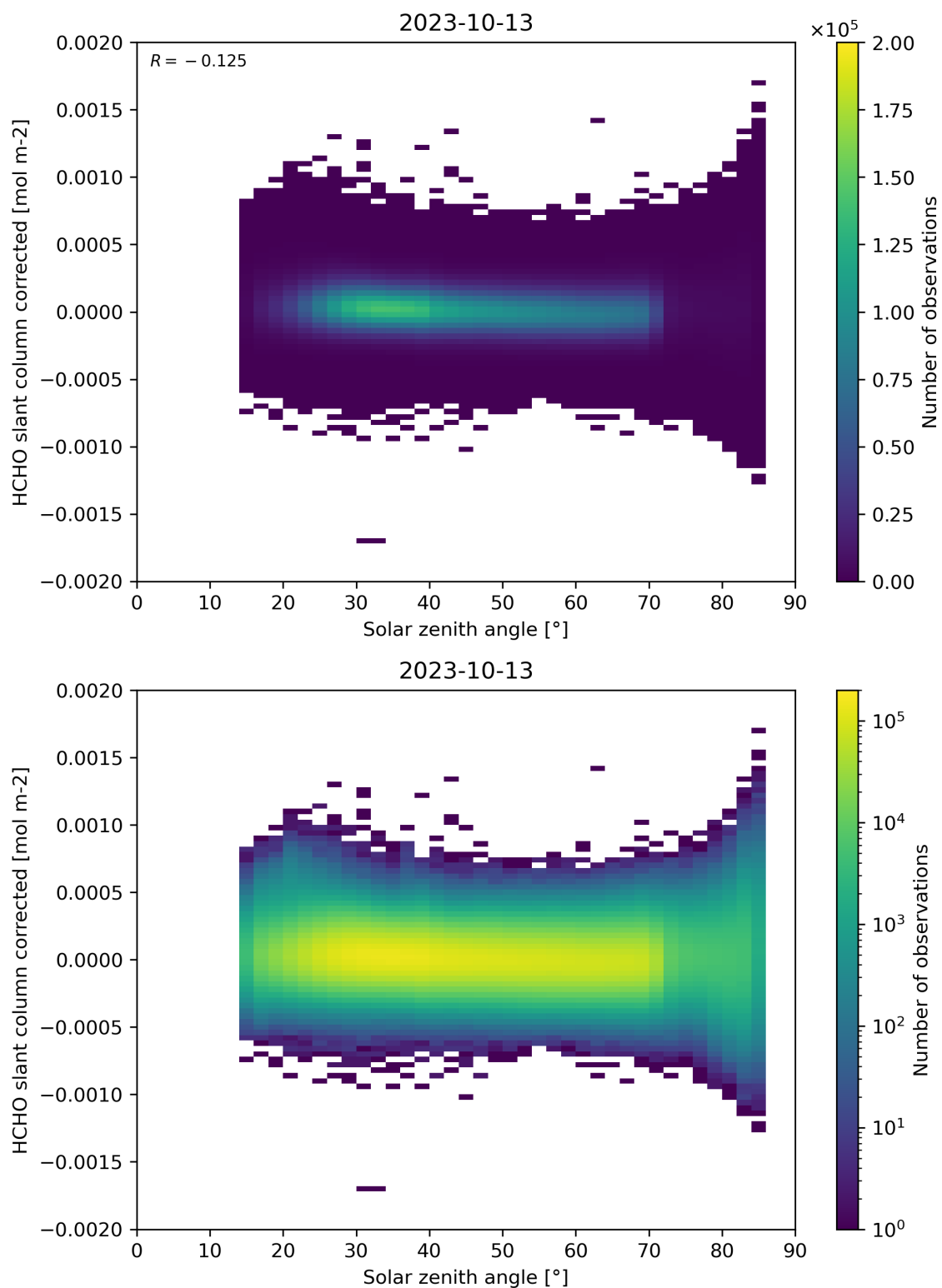
Figure 171: Scatter density plot of “Solar zenith angle” against “HCHO slant column corrected” for 2023-10-12 to 2023-10-14.
