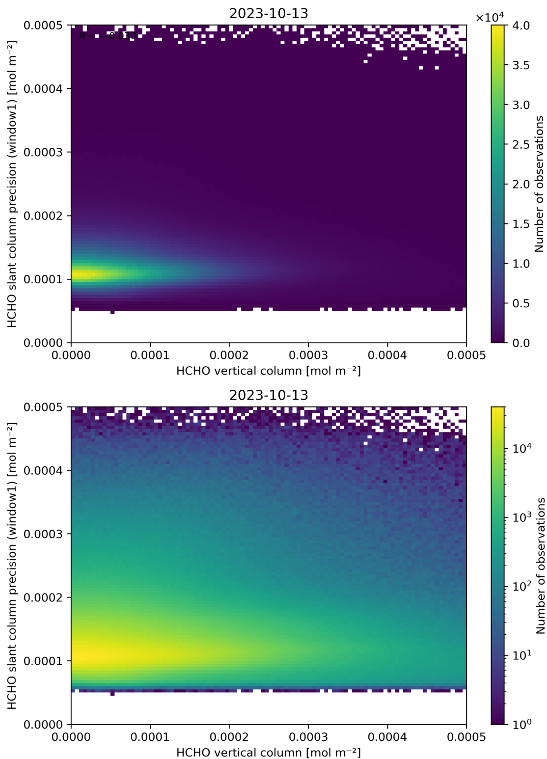
Figure 130: Scatter density plot of “HCHO vertical column” against “HCHO slant column precision (window1)” for 2023-10-12 to 2023-10-14.
