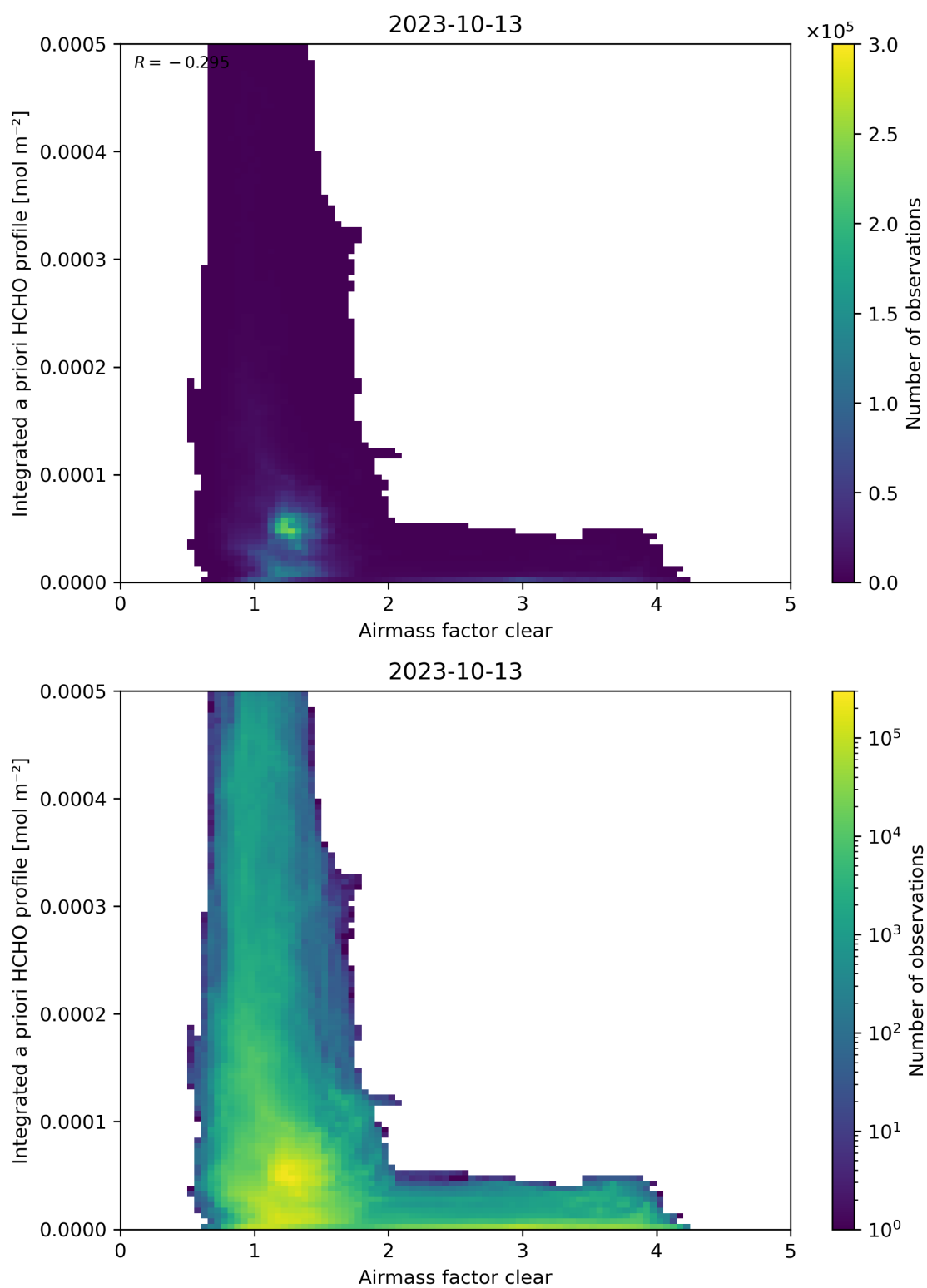
Figure 76: Scatter density plot of “Airmass factor clear” against “Integrated a priori HCHO profile” for 2023-10-12 to 2023-10-14.
