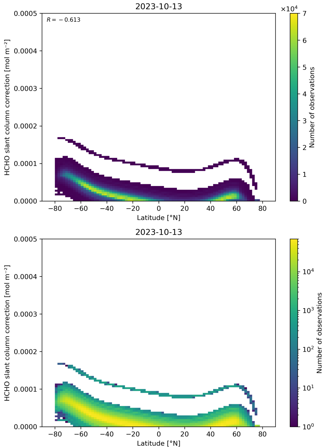
Figure 158: Scatter density plot of “Latitude” against “HCHO slant column correction” for 2023-10-12 to 2023-10-14.
