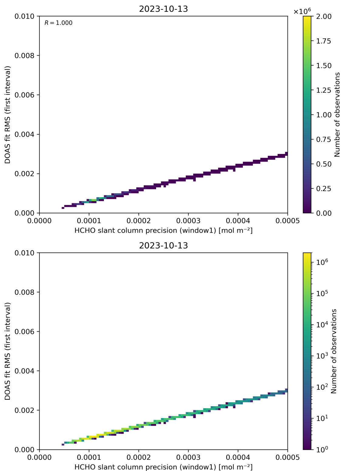
Figure 88: Scatter density plot of “HCHO slant column precision (window1)” against “DOAS fit RMS (first interval)” for 2023-10-12 to 2023-10-14.
