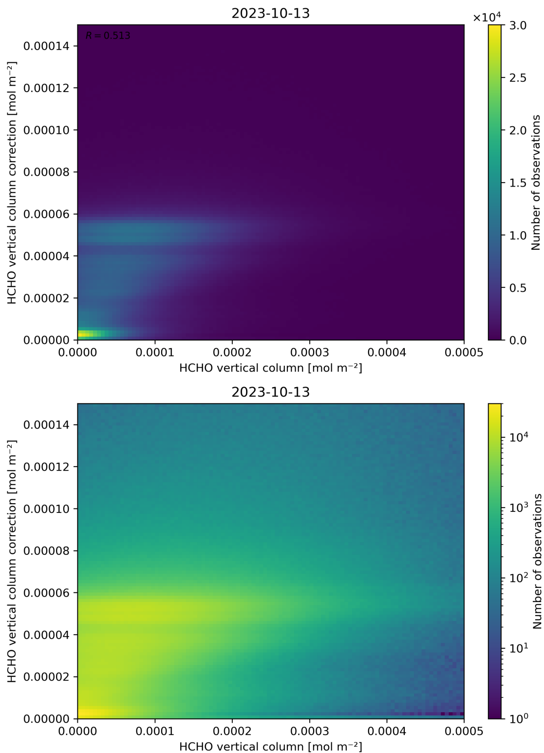
Figure 133: Scatter density plot of “HCHO vertical column” against “HCHO vertical column correction” for 2023-10-12 to 2023-10-14.
