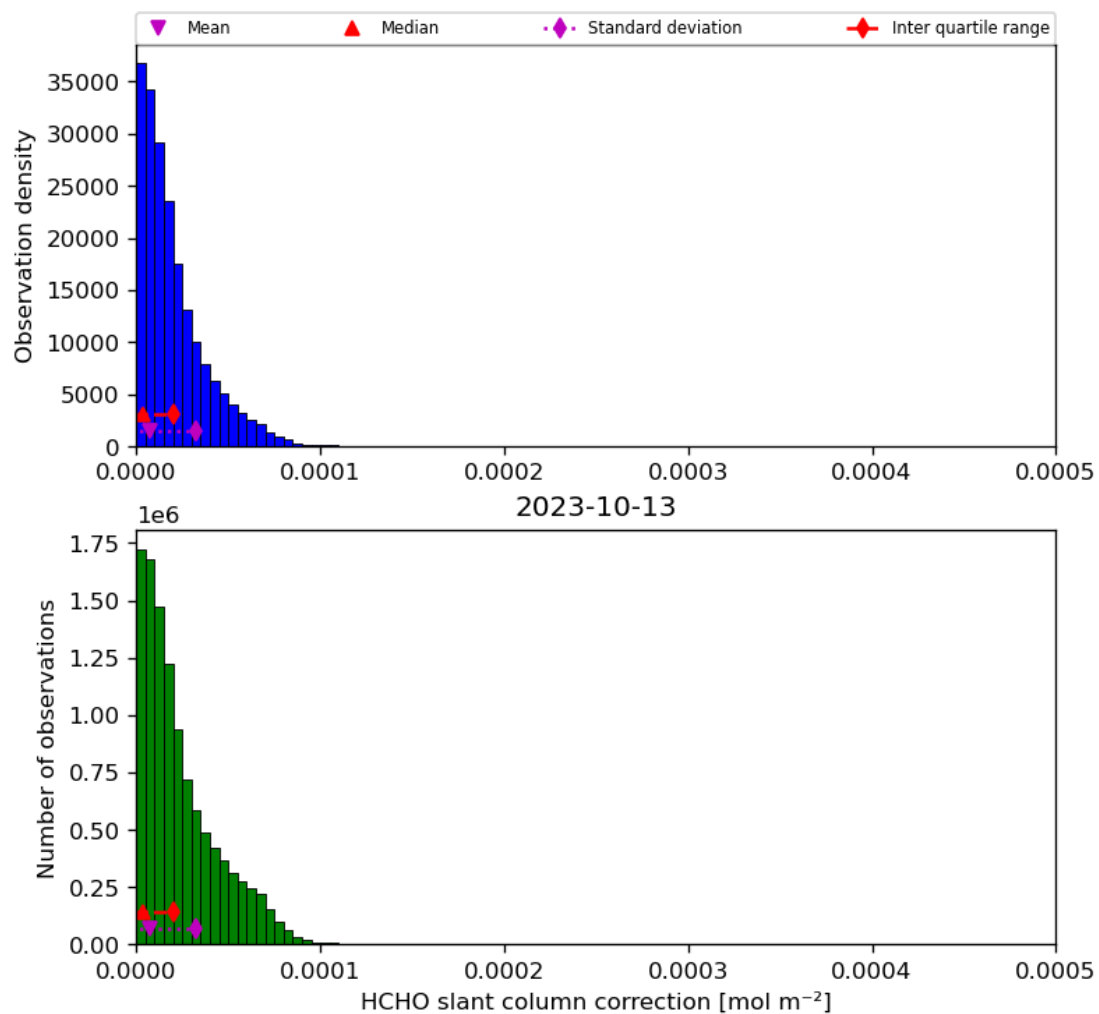
Figure 47: Histogram of “HCHO slant column correction” for 2023-10-12 to 2023-10-14
