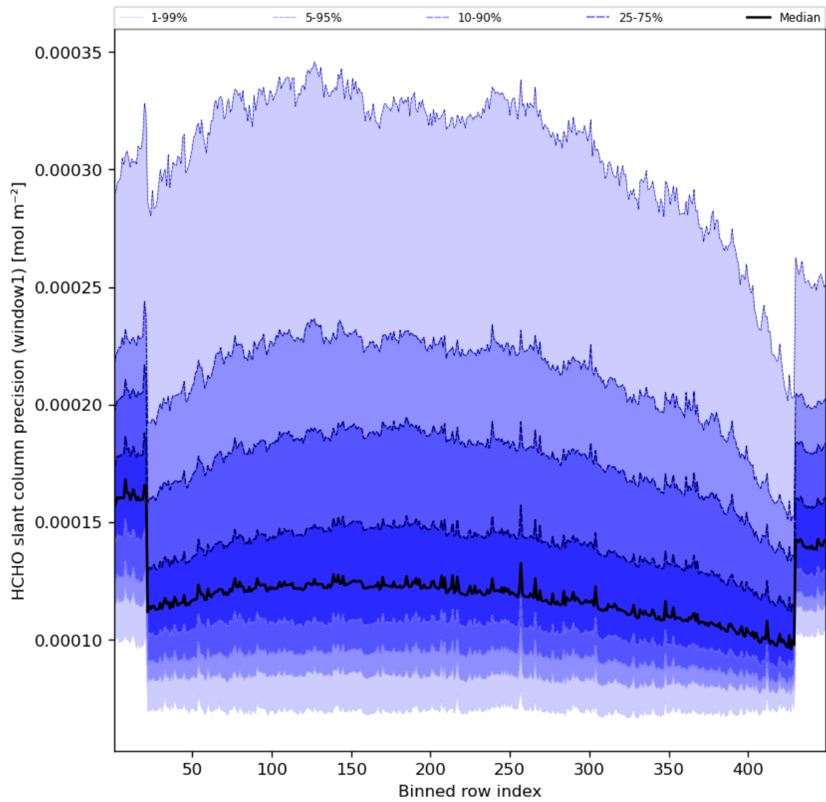
Figure 53: Along track statistics of “HCHO slant column precision (window1)” for 2023-10-12 to 2023-10-14
