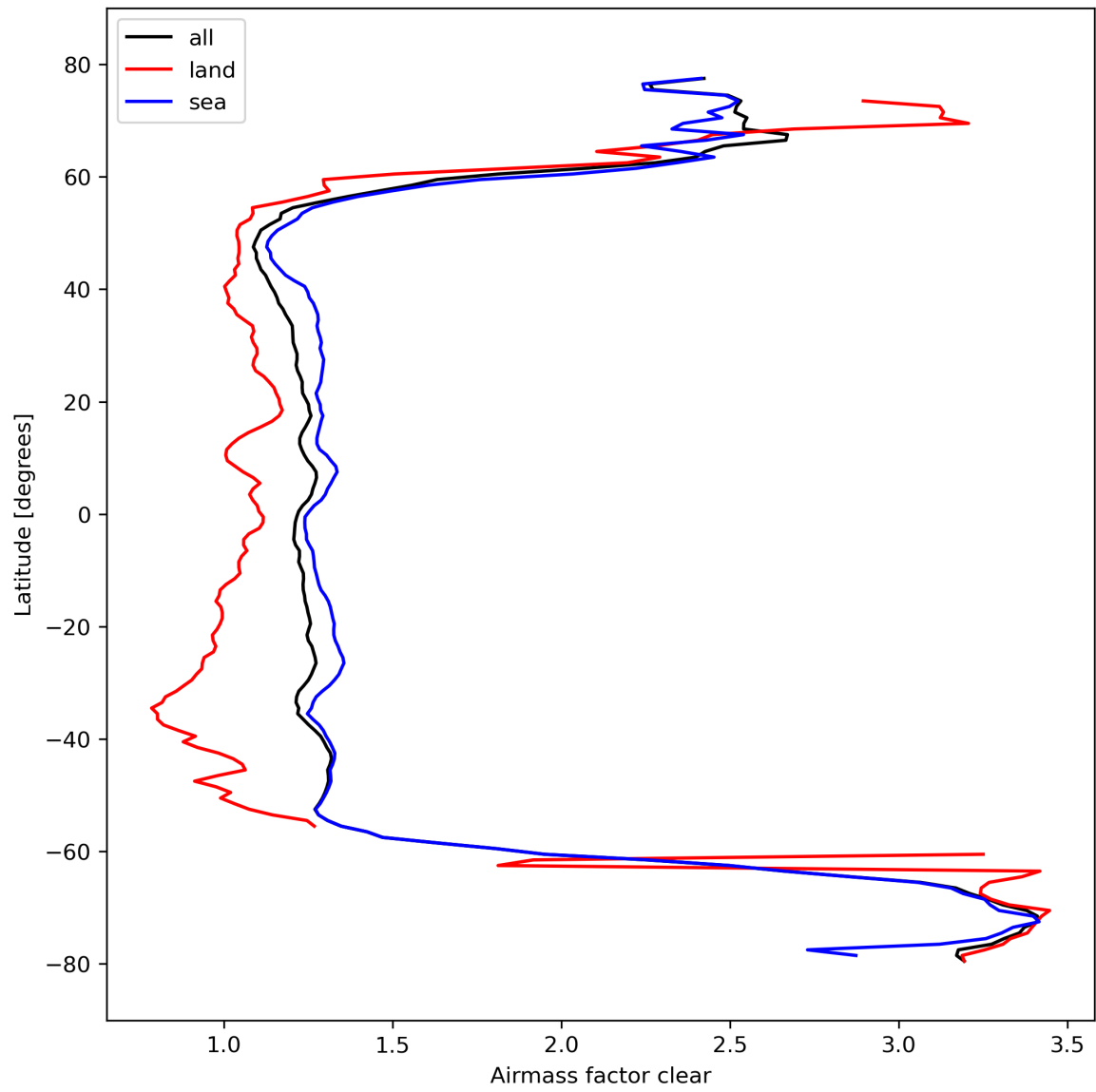
Figure 28: Zonal average of “Airmass factor clear” for 2023-10-12 to 2023-10-14.
