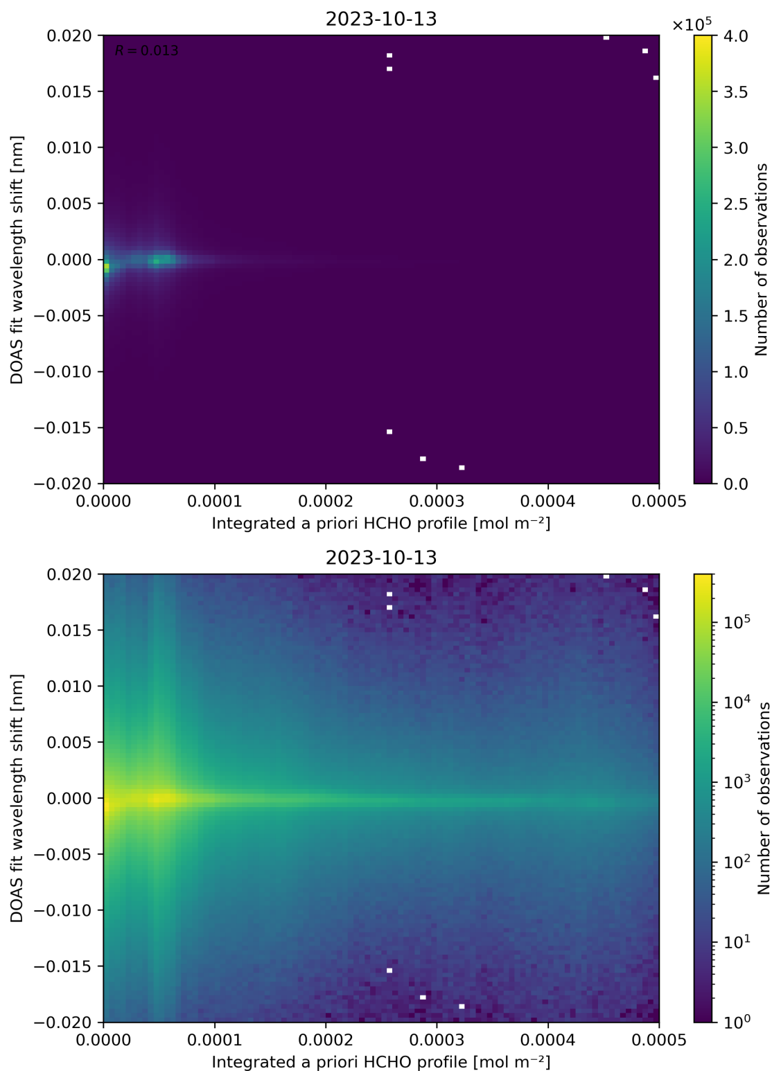
Figure 149: Scatter density plot of “Integrated a priori HCHO profile” against “DOAS fit wavelength shift” for 2023-10-12 to 2023-10-14.
