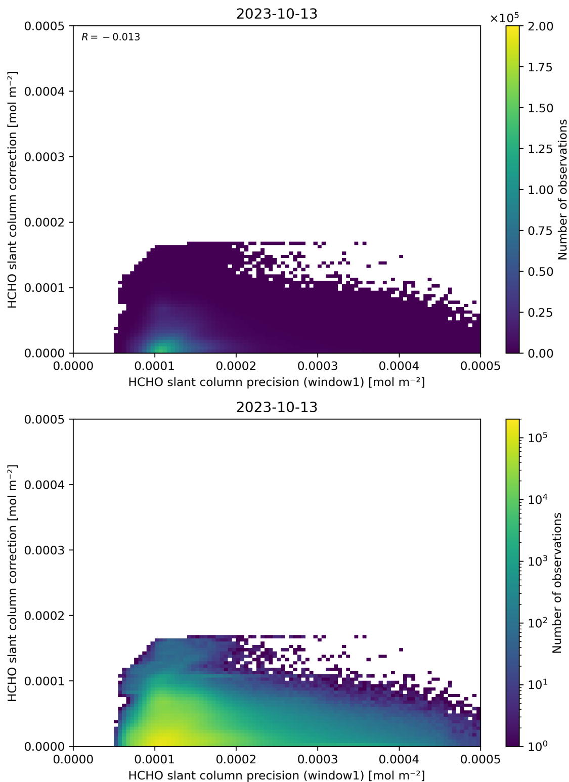
Figure 93: Scatter density plot of “HCHO slant column precision (window1)” against “HCHO slant column correction” for 2023-10-12 to 2023-10-14.
