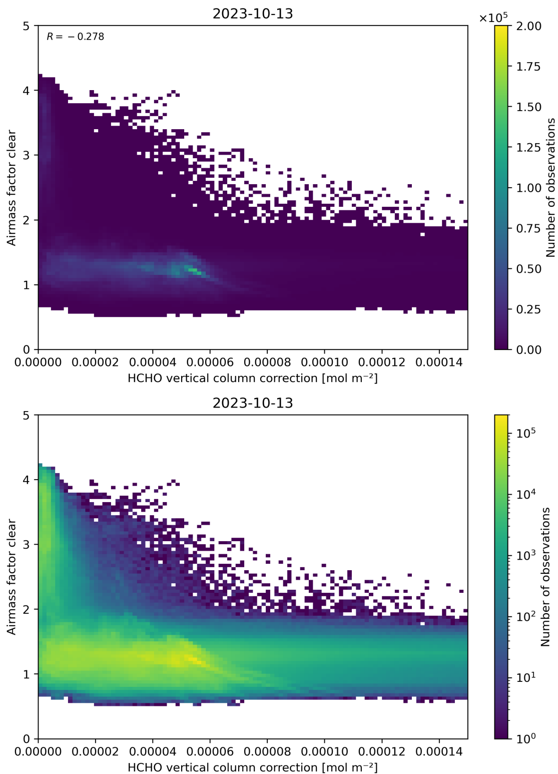
Figure 115: Scatter density plot of “HCHO vertical column correction” against “Airmass factor clear” for 2023-10-12 to 2023-10-14.
