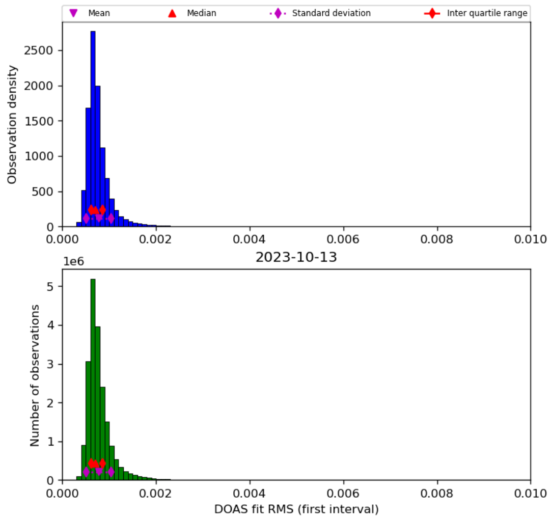
Figure 46: Histogram of “DOAS fit RMS (first interval)” for 2023-10-12 to 2023-10-14
