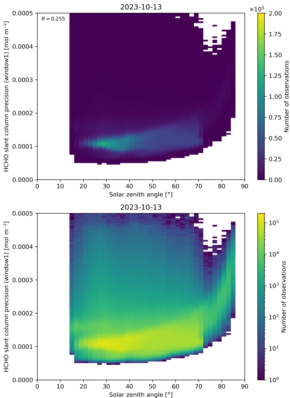
Figure 174: Scatter density plot of “Solar zenith angle” against “HCHO slant column precision (window1)” for 2023-10-12 to 2023-10-14.
