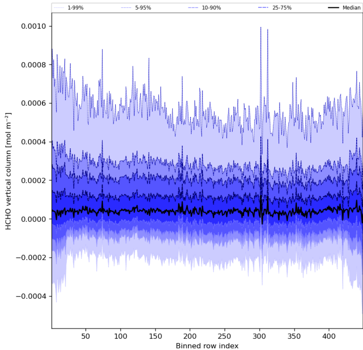
Figure 49: Along track statistics of “HCHO vertical column” for 2023-10-12 to 2023-10-14
