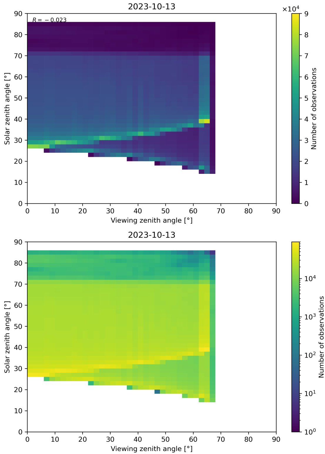
Figure 197: Scatter density plot of “Viewing zenith angle” against “Solar zenith angle” for 2023-10-12 to 2023-10-14.
