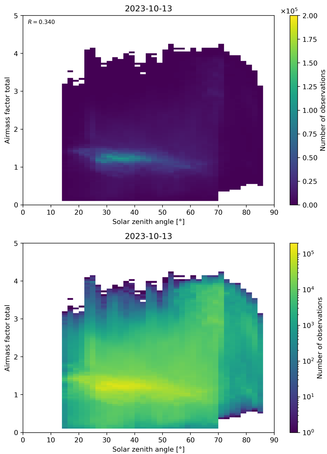
Figure 175: Scatter density plot of “Solar zenith angle” against “Airmass factor total” for 2023-10-12 to 2023-10-14.
