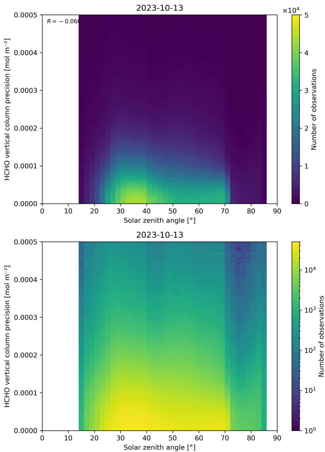
Figure 179: Scatter density plot of “Solar zenith angle” against “HCHO vertical column precision” for 2023-10-12 to 2023-10-14.
