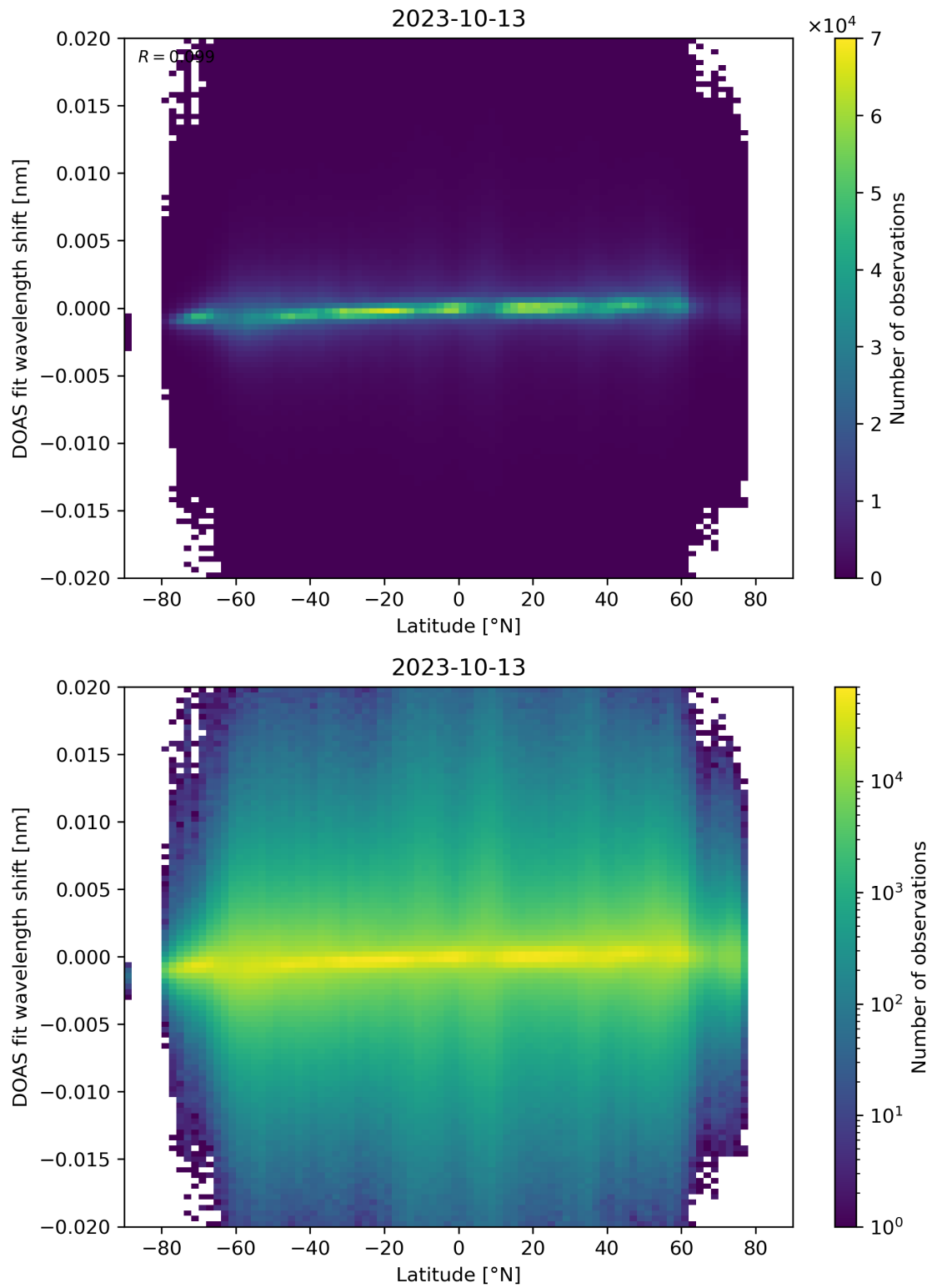
Figure 154: Scatter density plot of “Latitude” against “DOAS fit wavelength shift” for 2023-10-12 to 2023-10-14.
