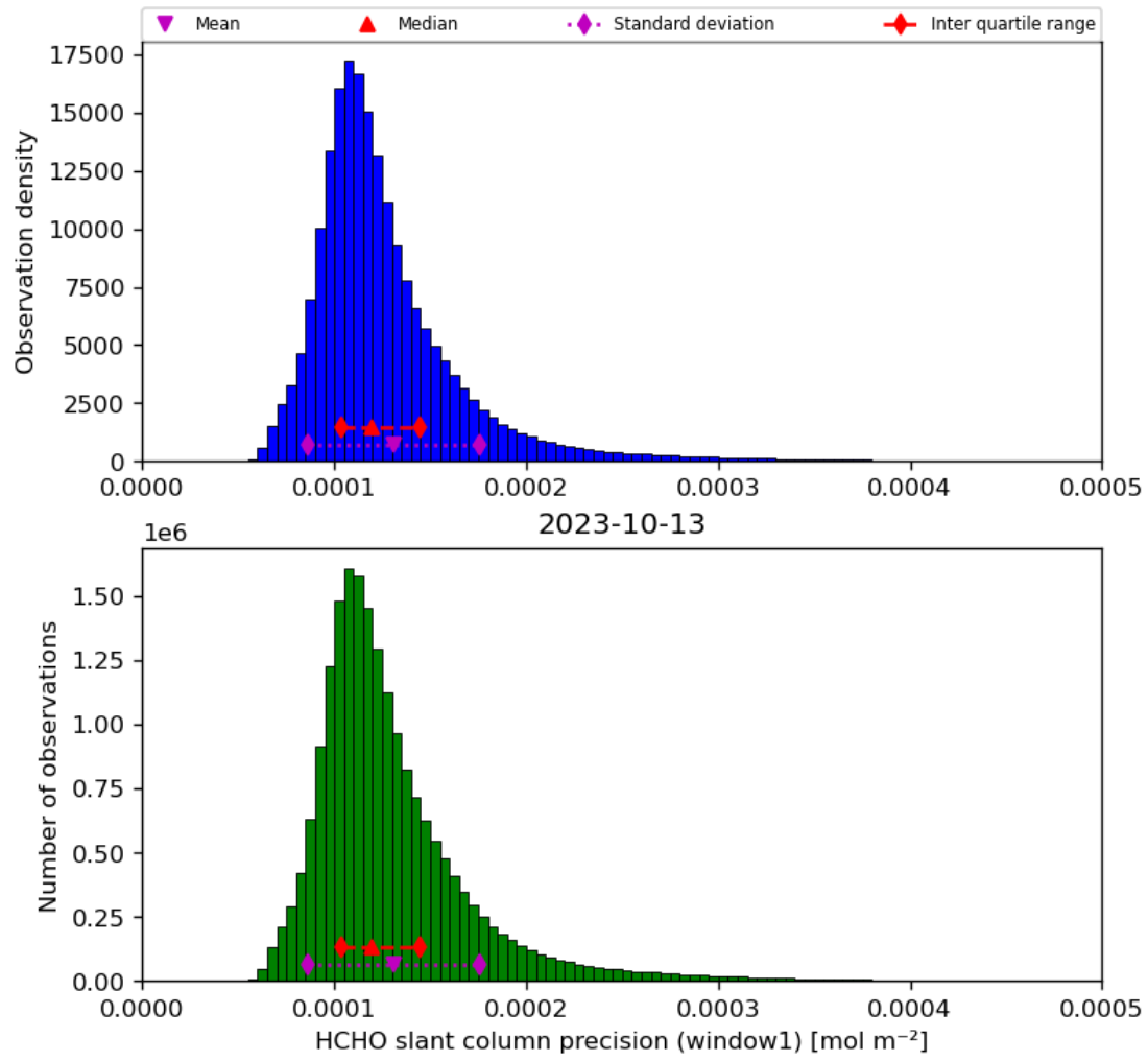
Figure 39: Histogram of “HCHO slant column precision (window1)” for 2023-10-12 to 2023-10-14
