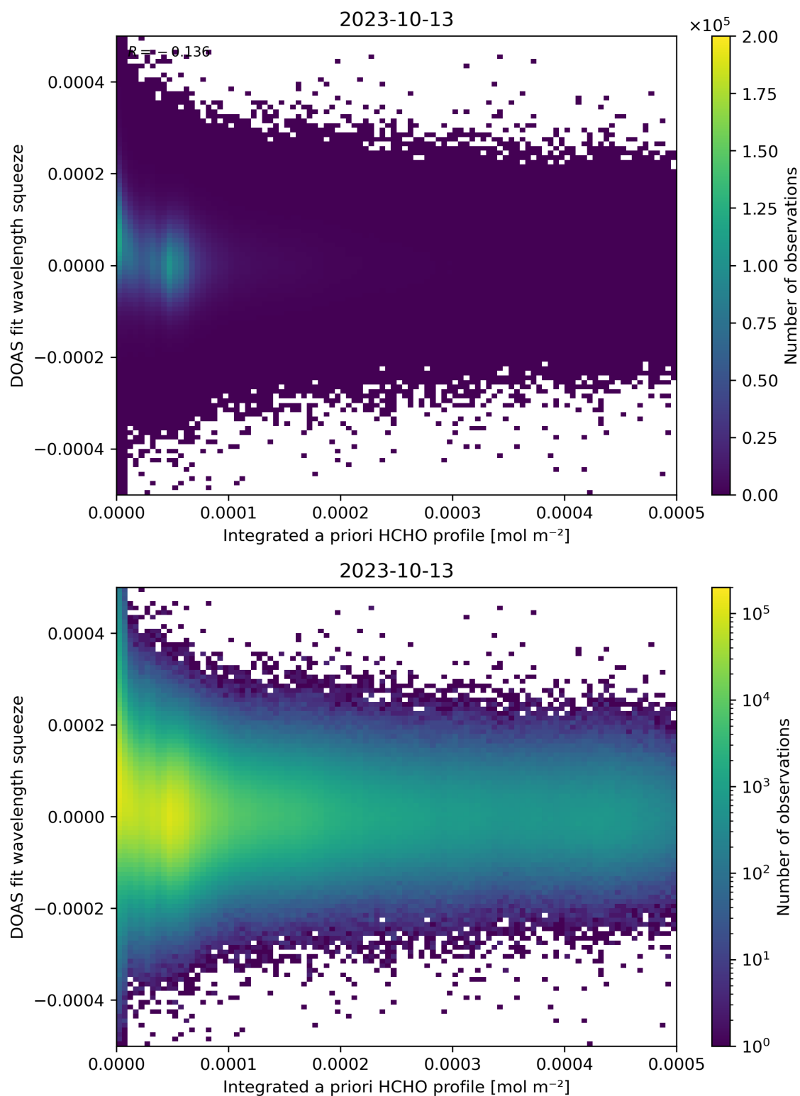
Figure 150: Scatter density plot of “Integrated a priori HCHO profile” against “DOAS fit wavelength squeeze” for 2023-10-12 to 2023-10-14.
