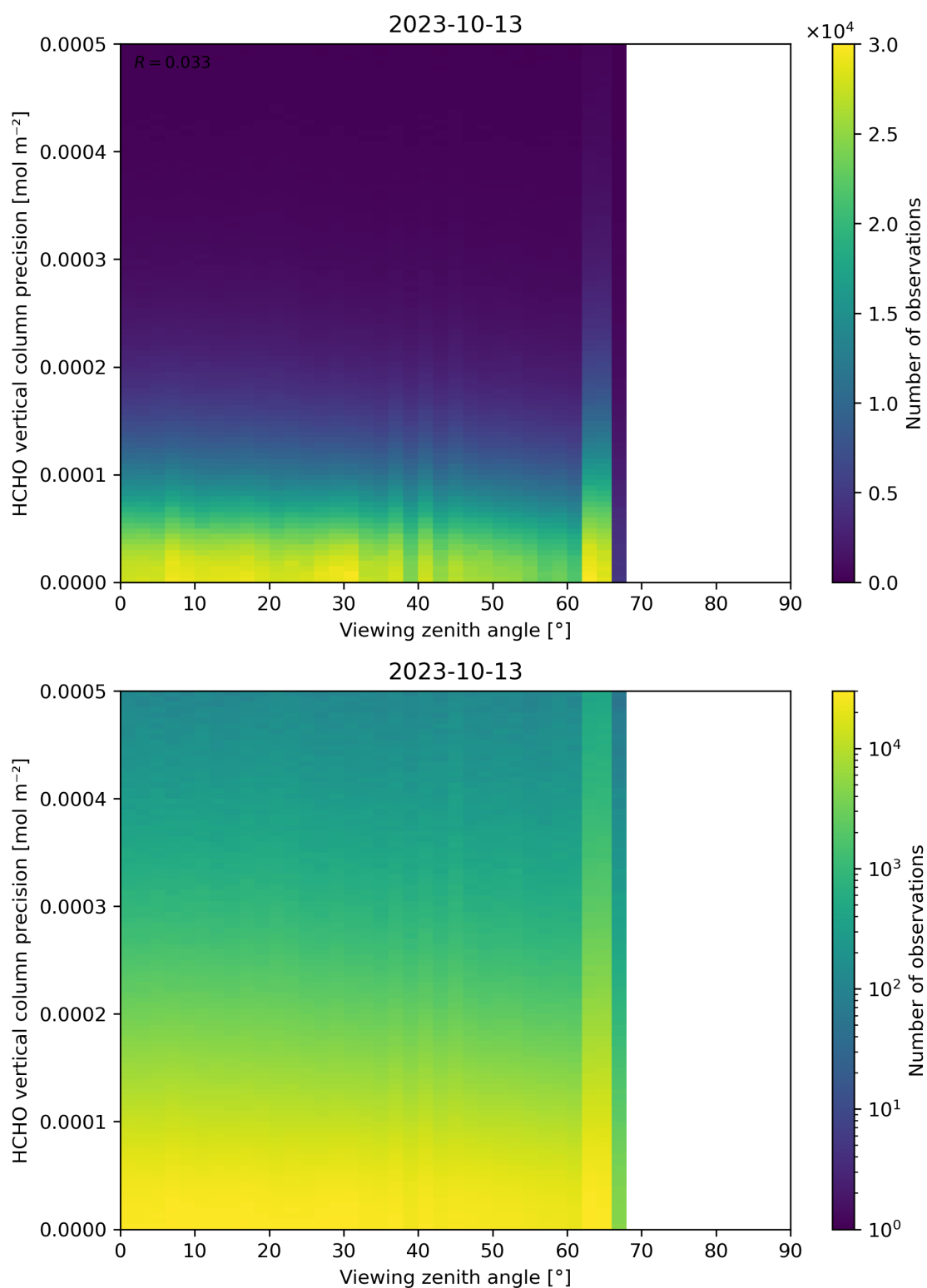
Figure 194: Scatter density plot of “Viewing zenith angle” against “HCHO vertical column precision” for 2023-10-12 to 2023-10-14.
