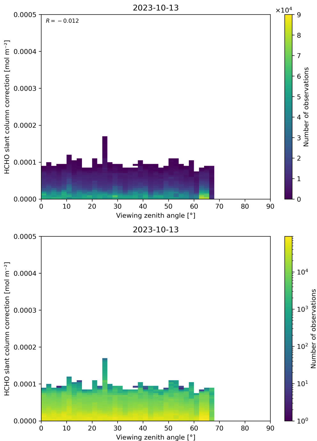
Figure 187: Scatter density plot of “Viewing zenith angle” against “HCHO slant column correction” for 2023-10-12 to 2023-10-14.
