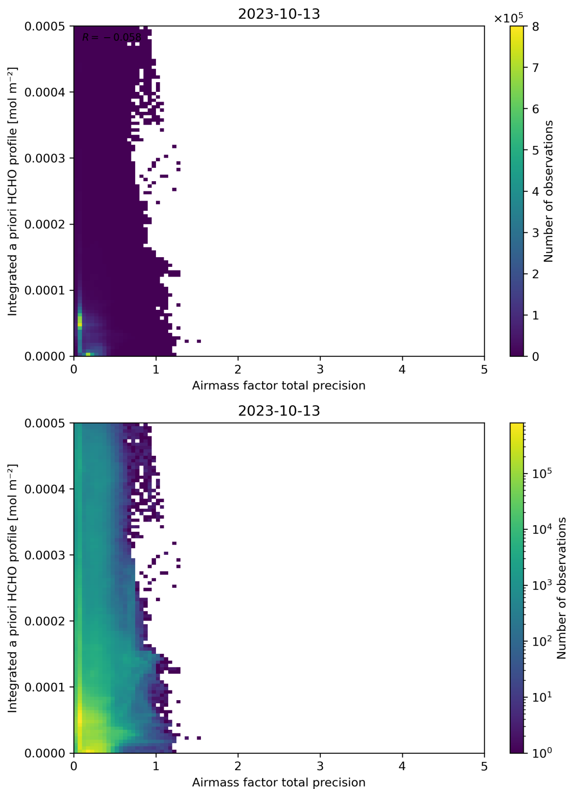
Figure 111: Scatter density plot of “Airmass factor total precision” against “Integrated a priori HCHO profile” for 2023-10-12 to 2023-10-14.
