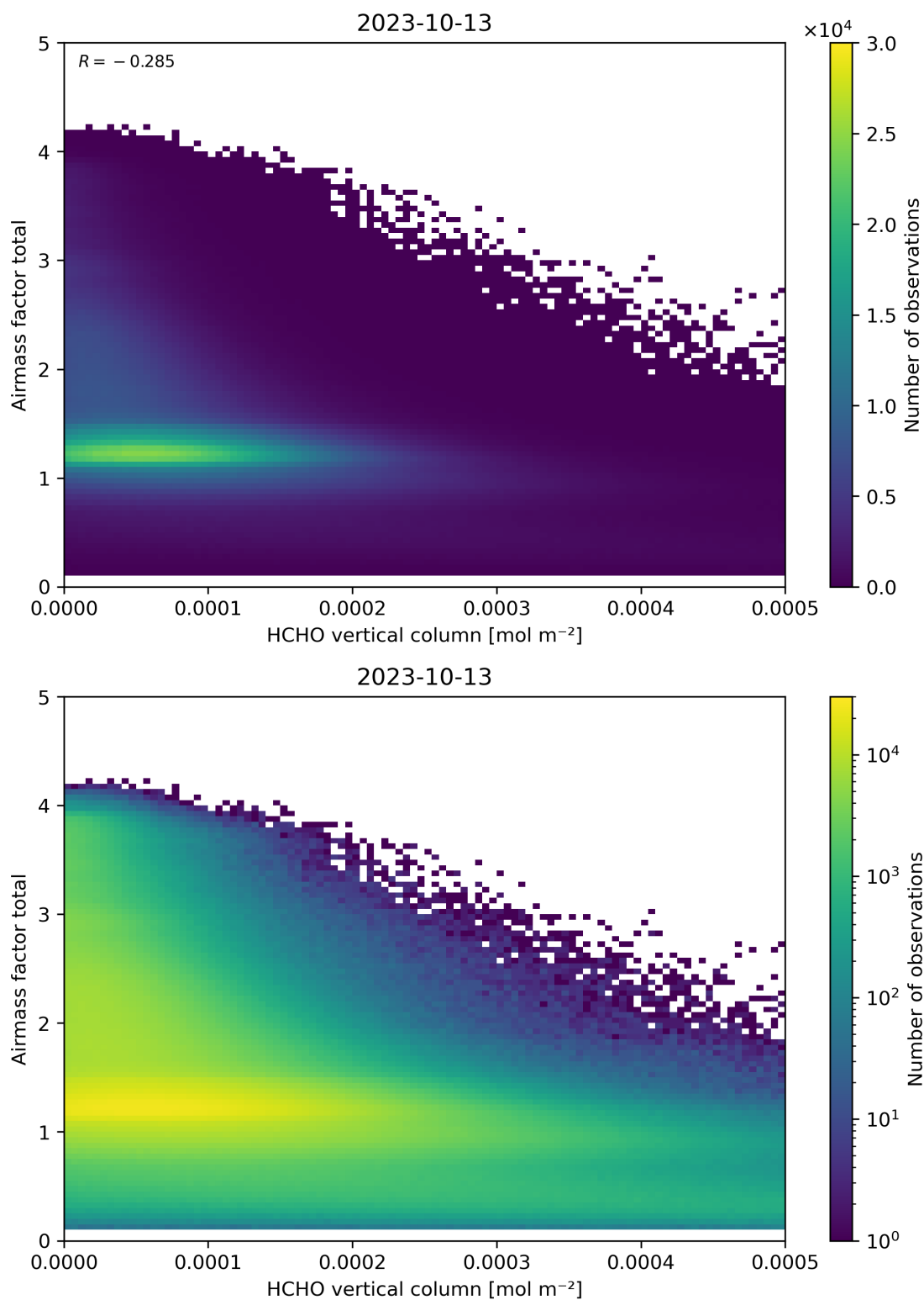
Figure 131: Scatter density plot of “HCHO vertical column” against “Airmass factor total” for 2023-10-12 to 2023-10-14.
