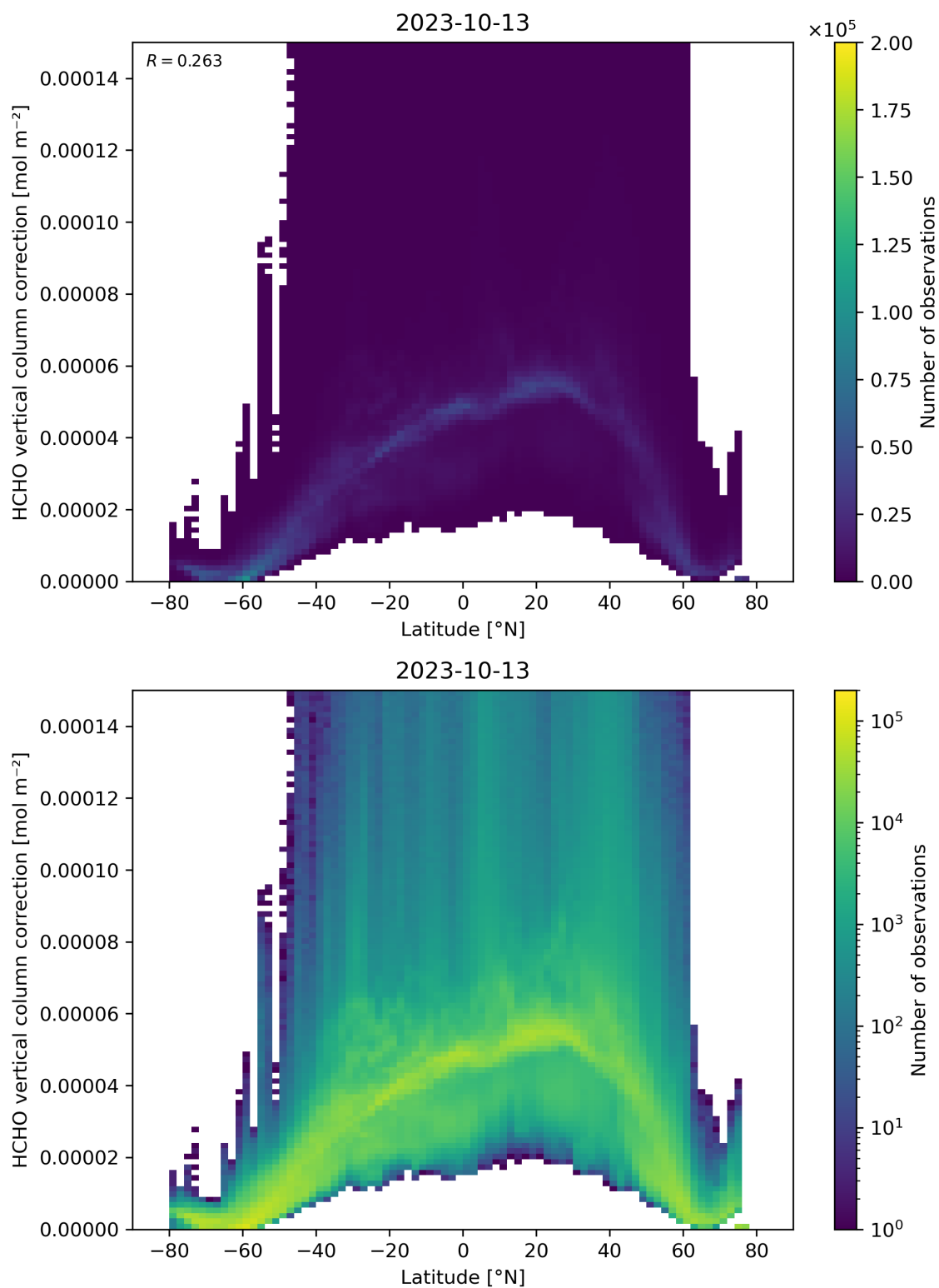
Figure 164: Scatter density plot of “Latitude” against “HCHO vertical column correction” for 2023-10-12 to 2023-10-14.
