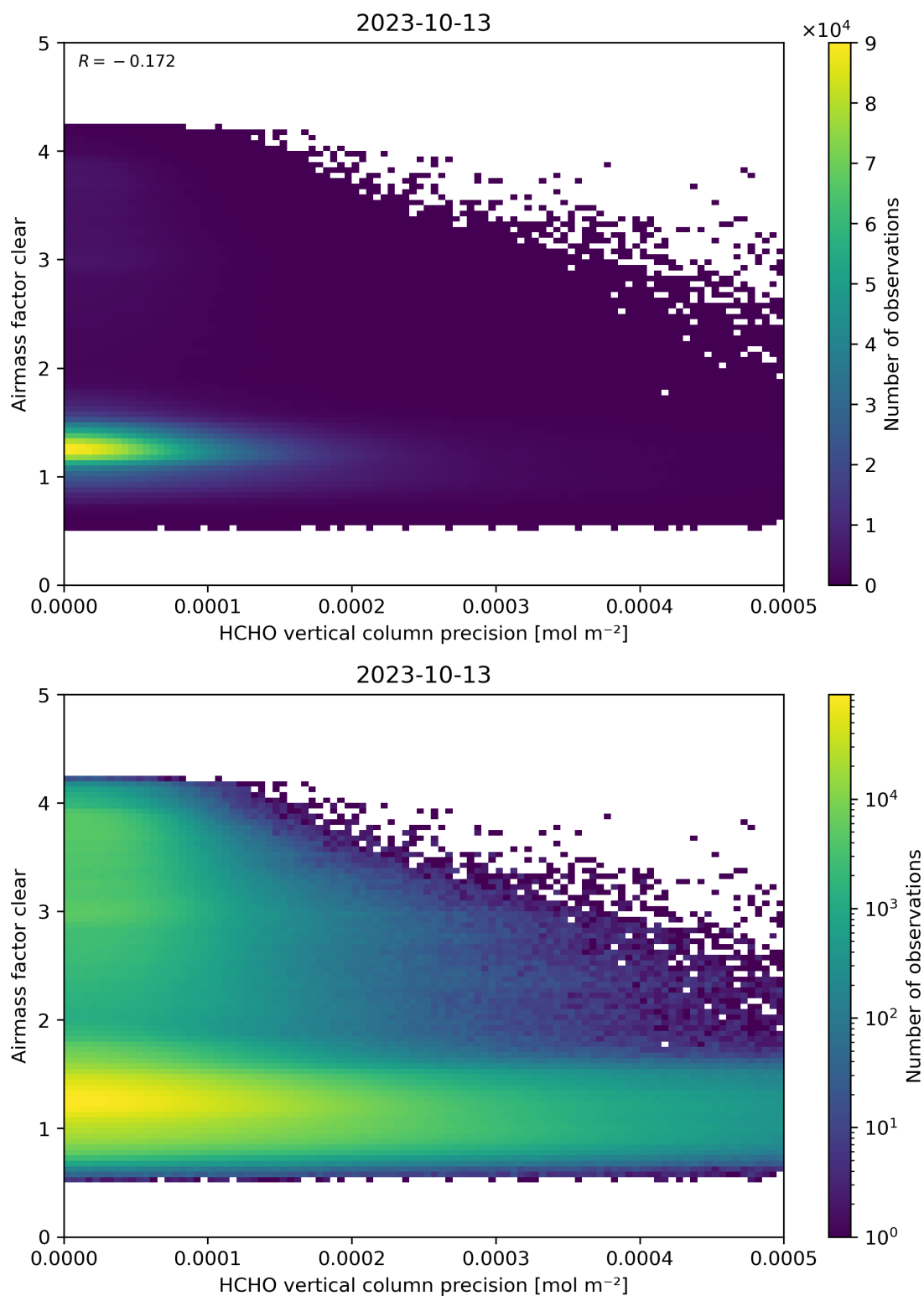
Figure 139: Scatter density plot of “HCHO vertical column precision” against “Airmass factor clear” for 2023-10-12 to 2023-10-14.
