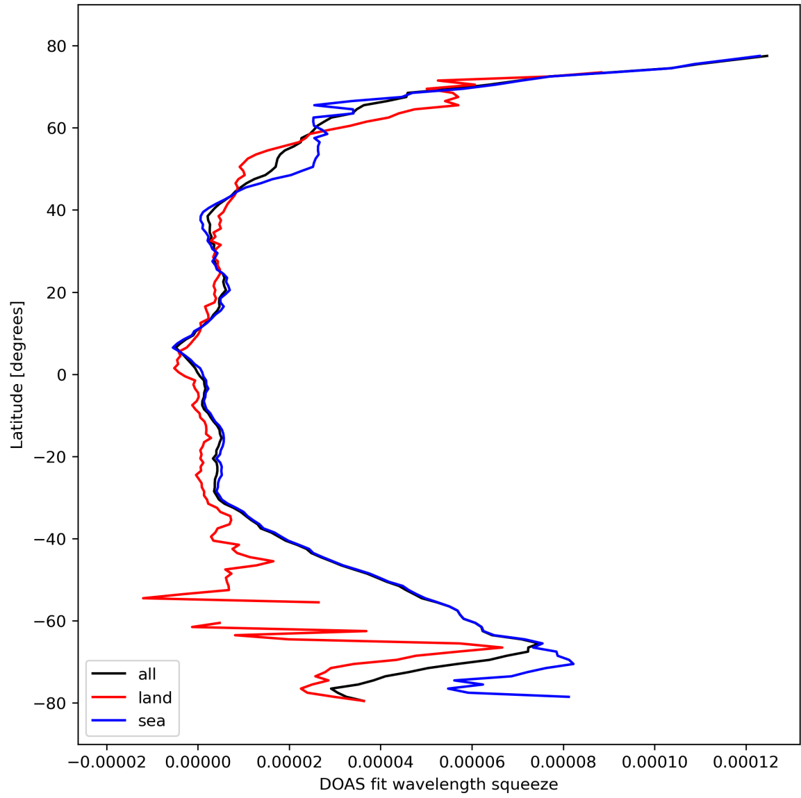
Figure 31: Zonal average of “DOAS fit wavelength squeeze” for 2023-10-12 to 2023-10-14.
