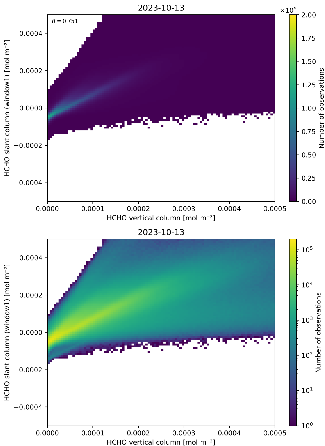
Figure 129: Scatter density plot of “HCHO vertical column” against “HCHO slant column (window1)” for 2023-10-12 to 2023-10-14.
