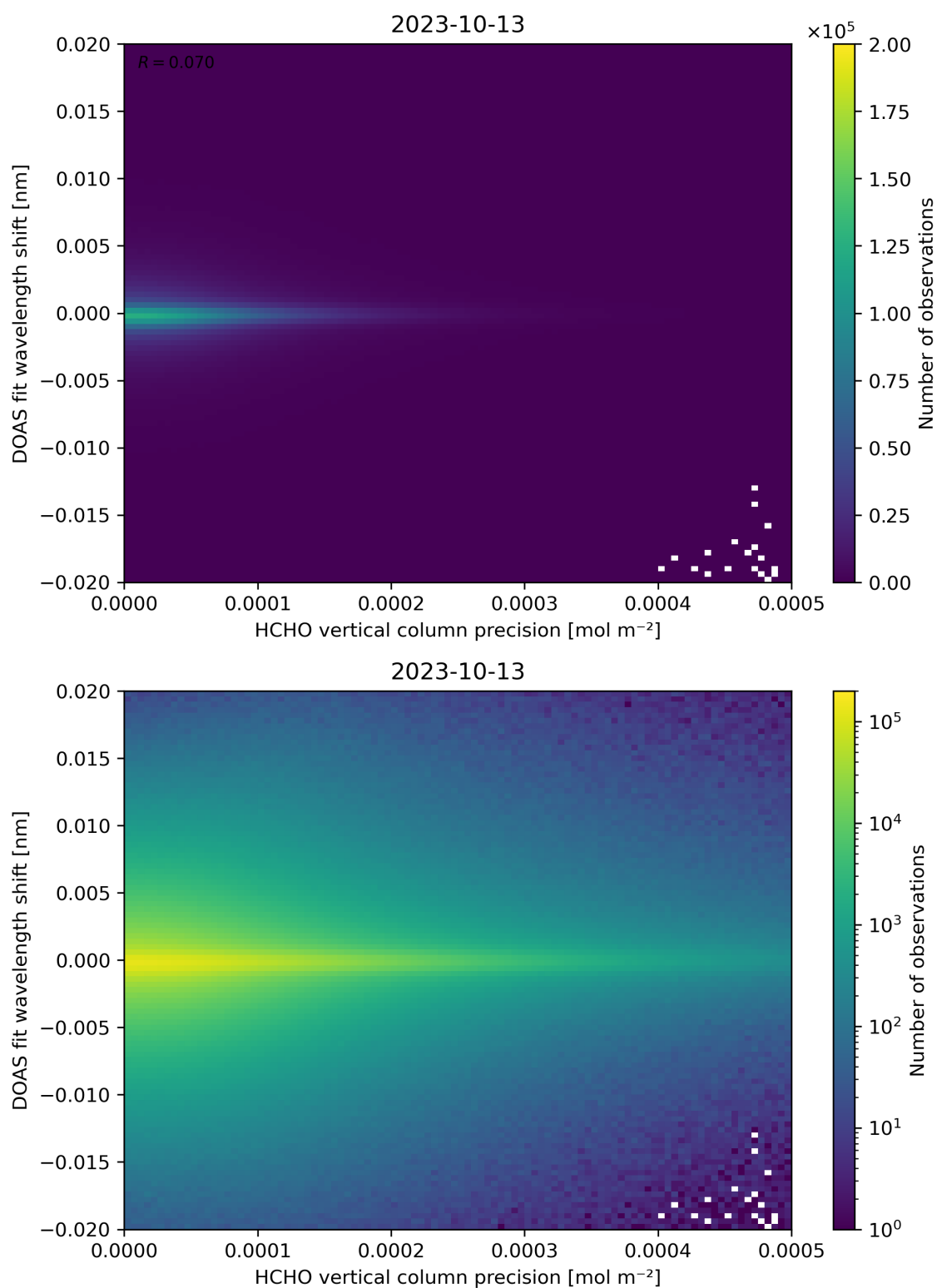
Figure 137: Scatter density plot of “HCHO vertical column precision” against “DOAS fit wavelength shift” for 2023-10-12 to 2023-10-14.
