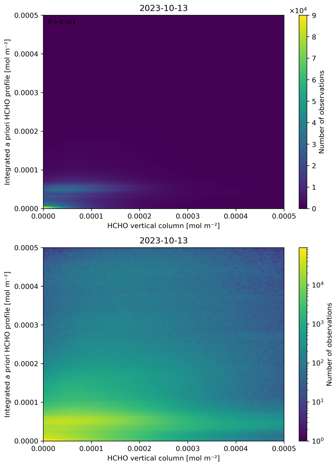
Figure 135: Scatter density plot of “HCHO vertical column” against “Integrated a priori HCHO profile” for 2023-10-12 to 2023-10-14.
