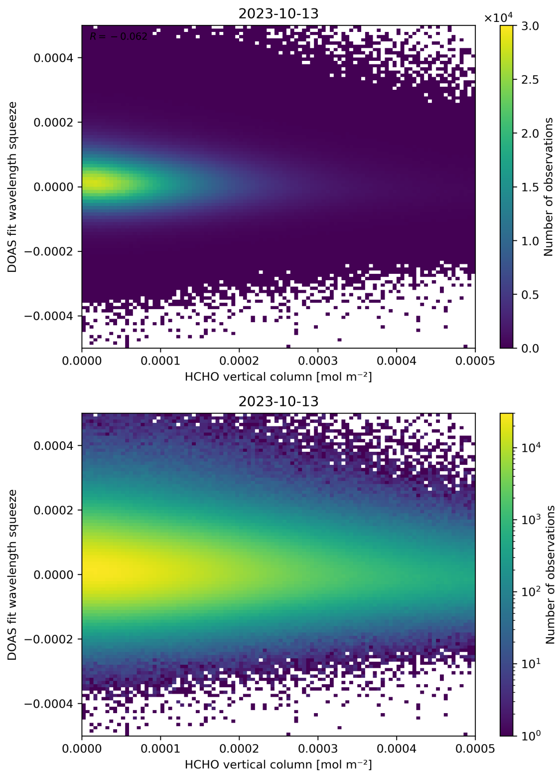
Figure 125: Scatter density plot of “HCHO vertical column” against “DOAS fit wavelength squeeze” for 2023-10-12 to 2023-10-14.
