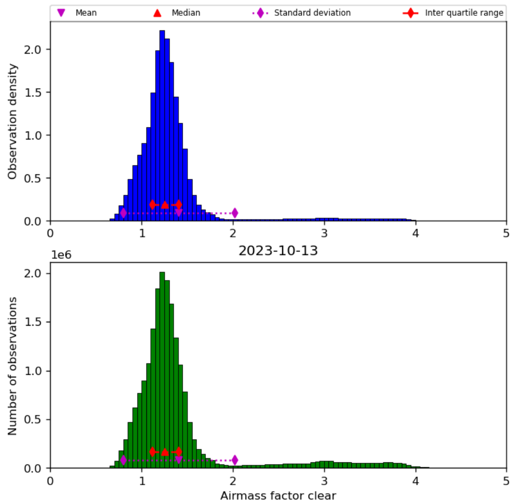
Figure 42: Histogram of “Airmass factor clear” for 2023-10-12 to 2023-10-14
