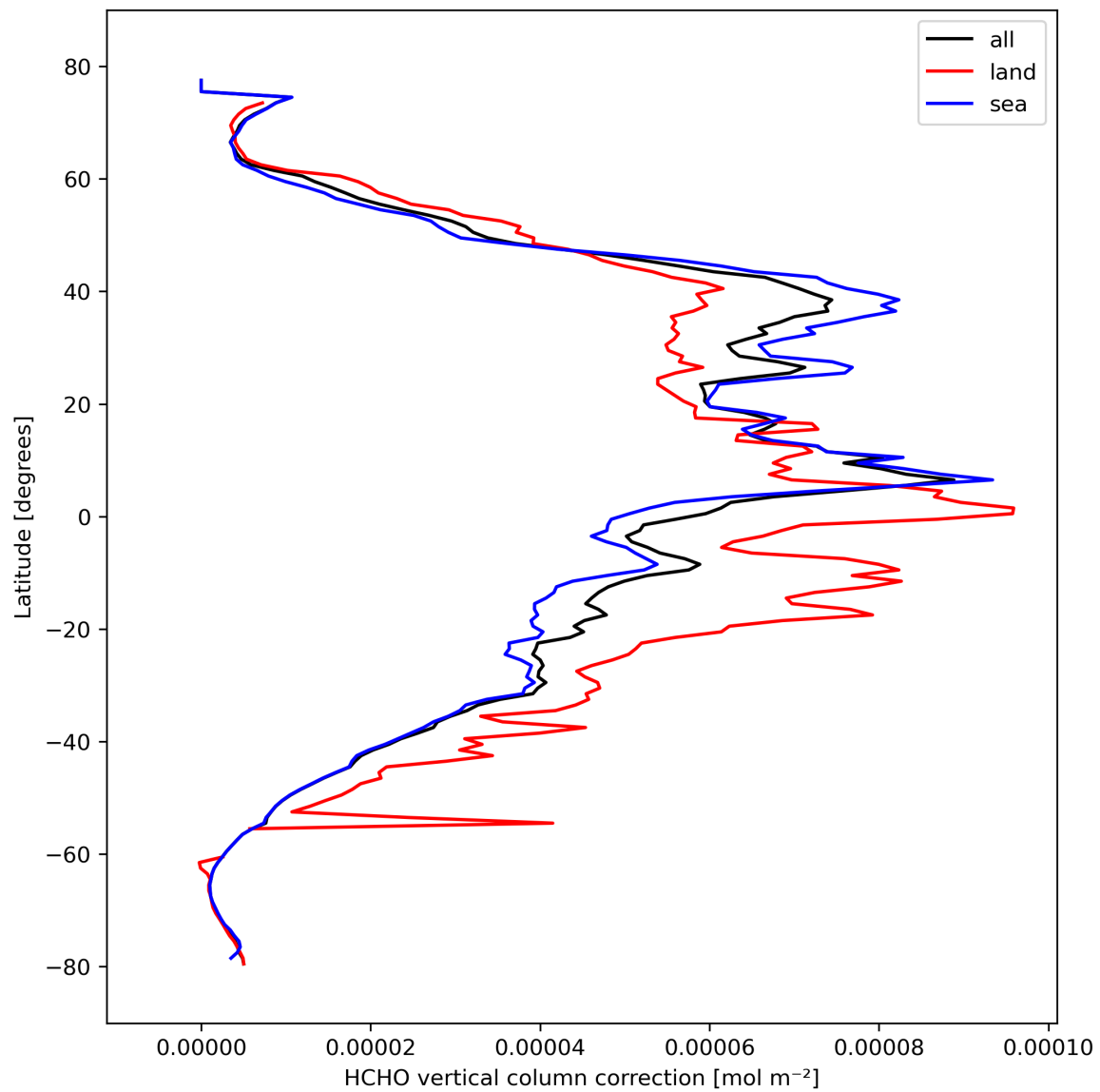
Figure 23: Zonal average of “HCHO vertical column correction” for 2023-10-12 to 2023-10-14.
