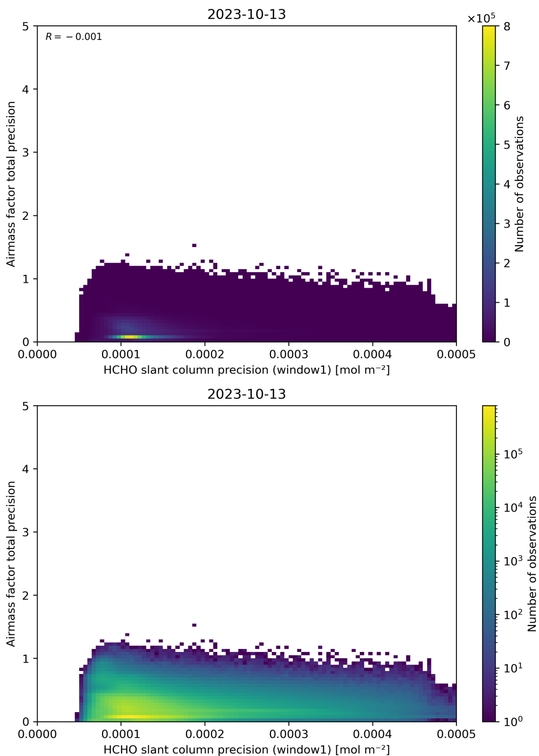
Figure 95: Scatter density plot of “HCHO slant column precision (window1)” against “Airmass factor total precision” for 2023-10-12 to 2023-10-14.
