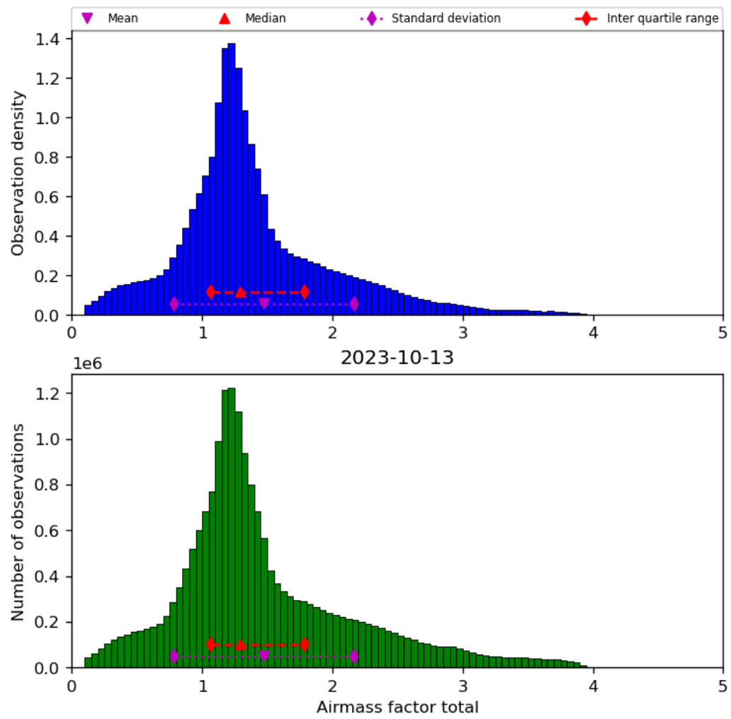
Figure 40: Histogram of “Airmass factor total” for 2023-10-12 to 2023-10-14
