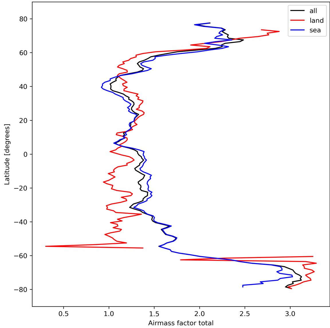
Figure 26: Zonal average of “Airmass factor total” for 2023-10-12 to 2023-10-14.
