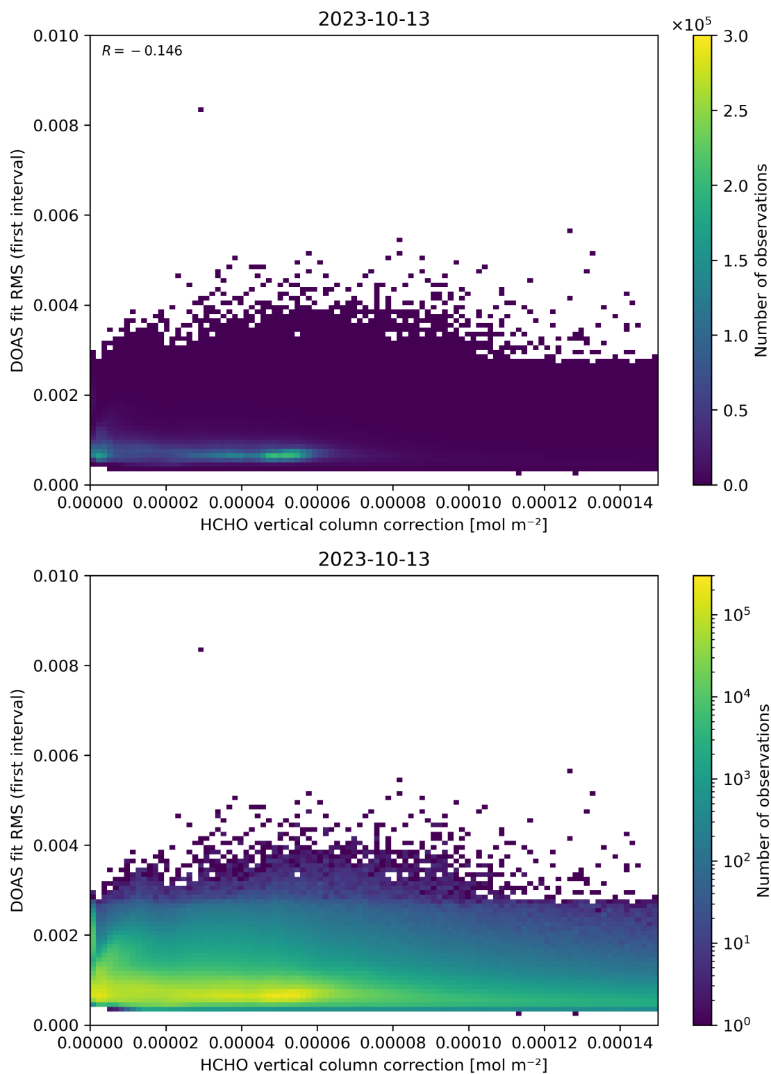
Figure 112: Scatter density plot of “HCHO vertical column correction” against “DOAS fit RMS (first interval)” for 2023-10-12 to 2023-10-14.
