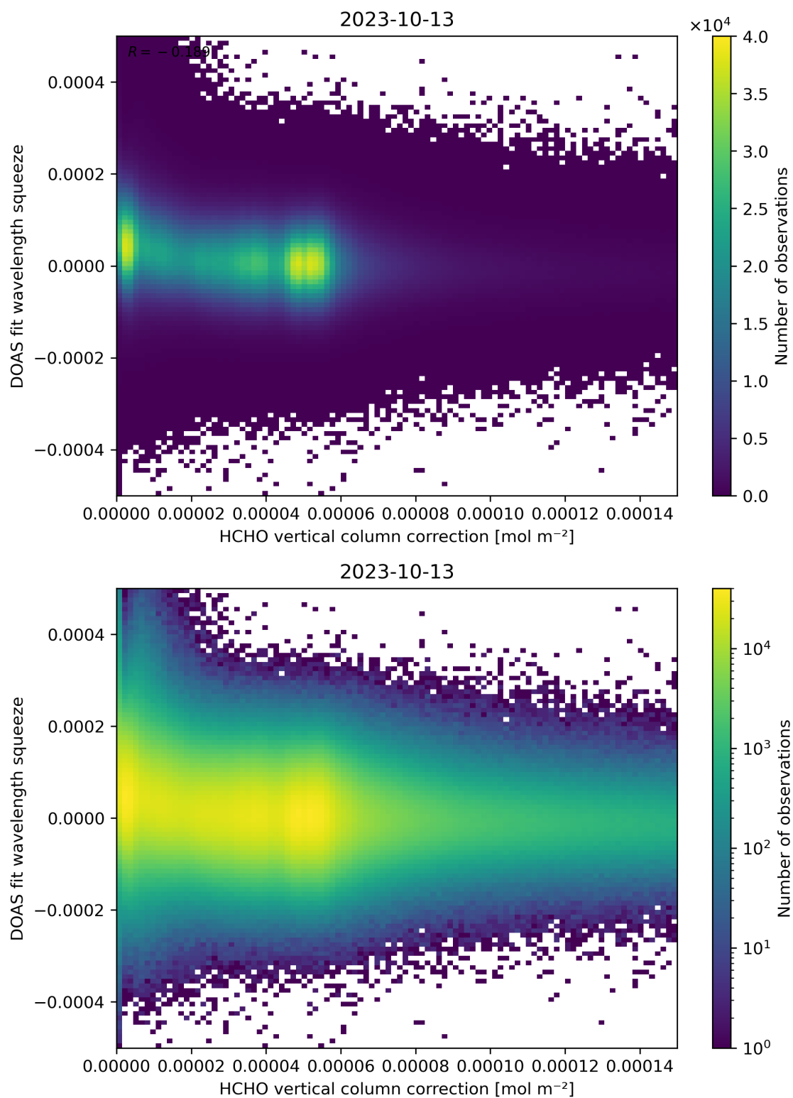
Figure 114: Scatter density plot of “HCHO vertical column correction” against “DOAS fit wavelength squeeze” for 2023-10-12 to 2023-10-14.
