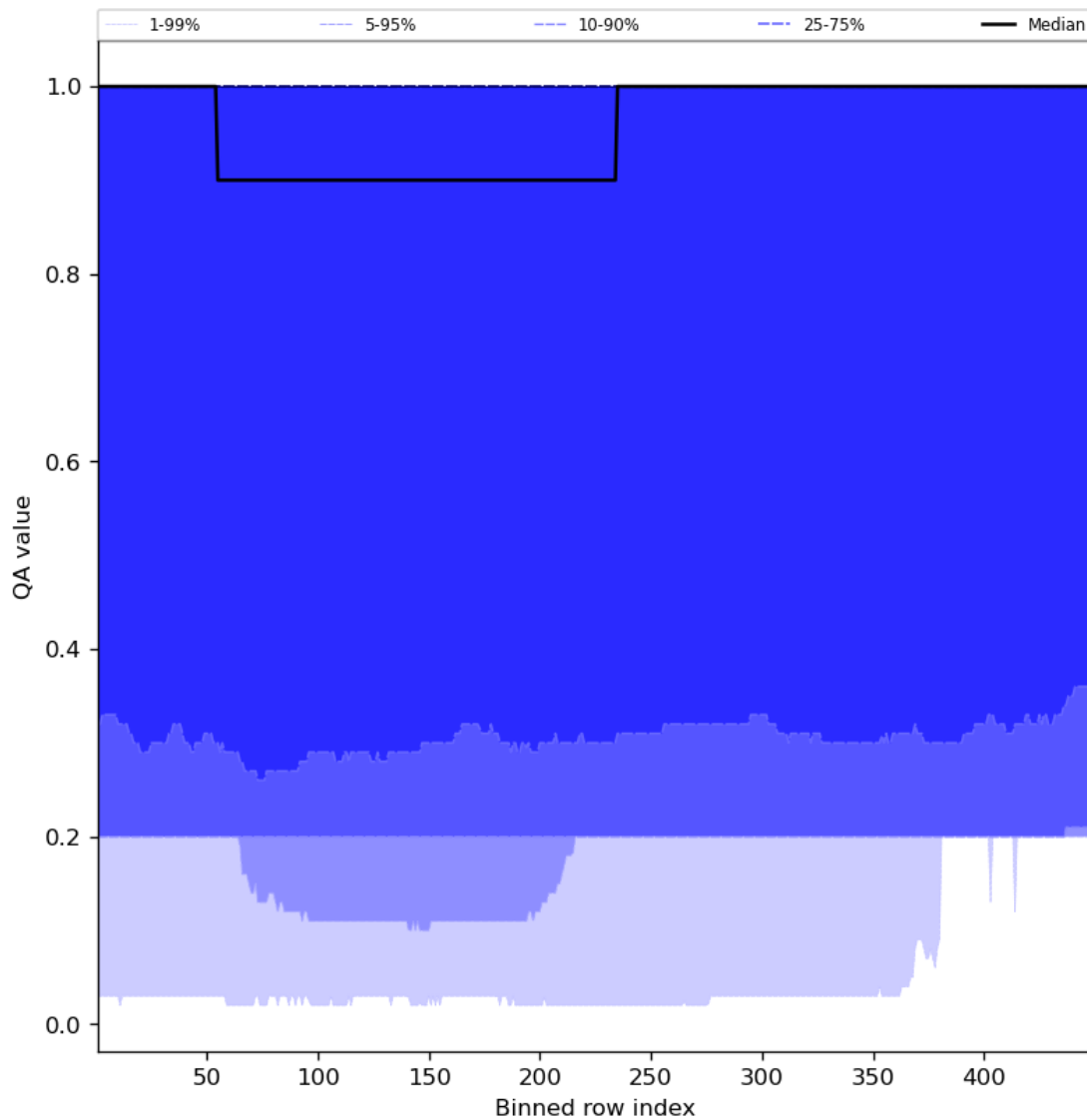
Figure 48: Along track statistics of “QA value” for 2023-10-12 to 2023-10-14
