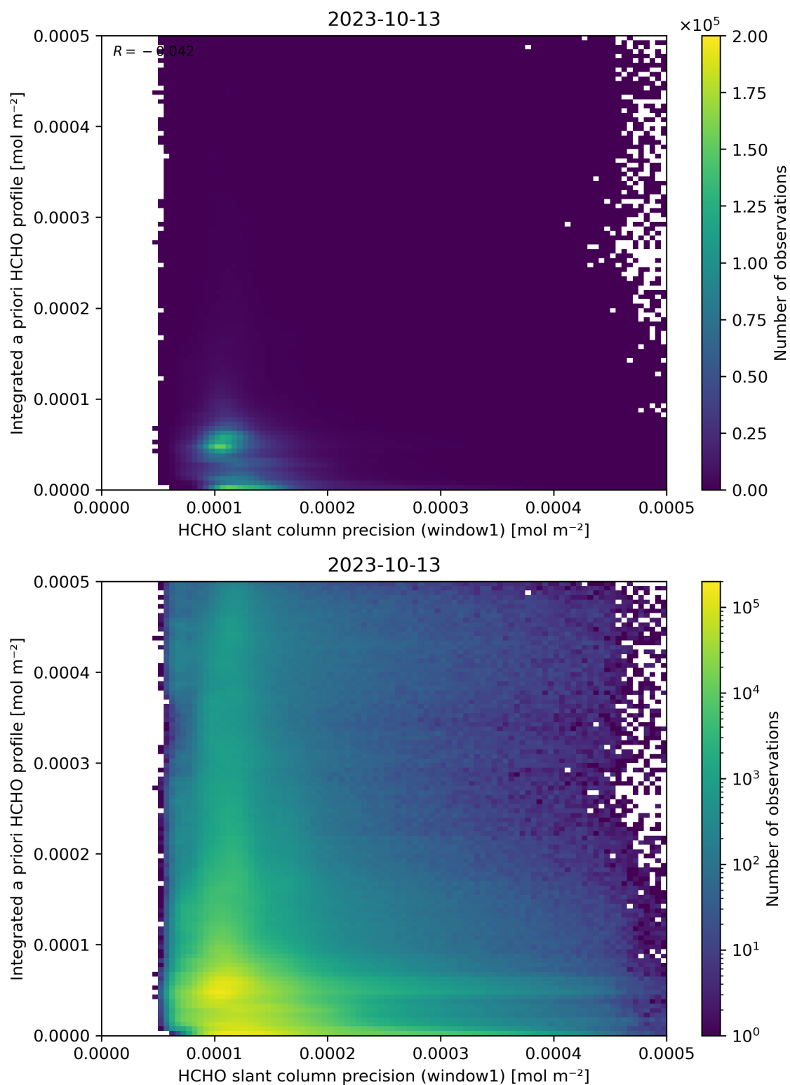
Figure 96: Scatter density plot of “HCHO slant column precision (window1)” against “Integrated a priori HCHO profile” for 2023-10-12 to 2023-10-14.
