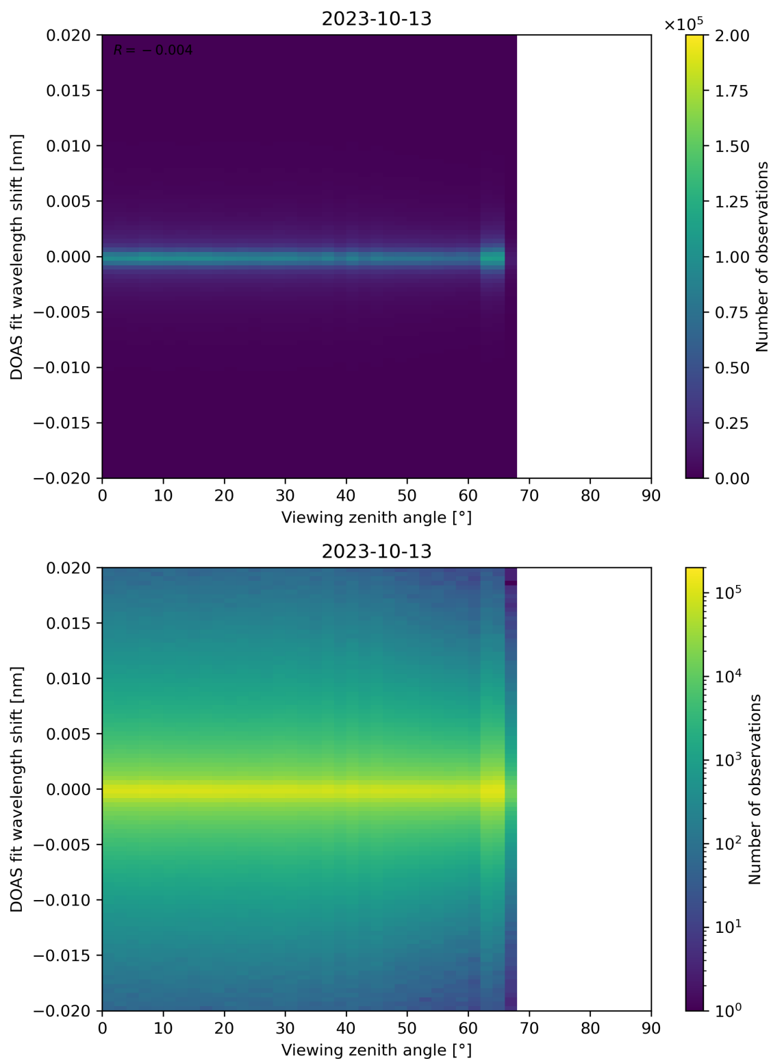
Figure 183: Scatter density plot of “Viewing zenith angle” against “DOAS fit wavelength shift” for 2023-10-12 to 2023-10-14.
