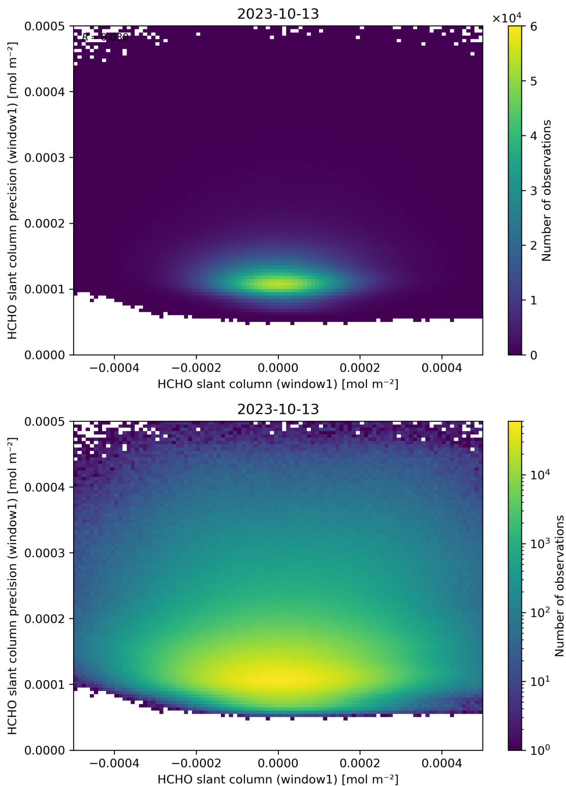
Figure 84: Scatter density plot of “HCHO slant column (window1)” against “HCHO slant column precision (window1)” for 2023-10-12 to 2023-10-14.
