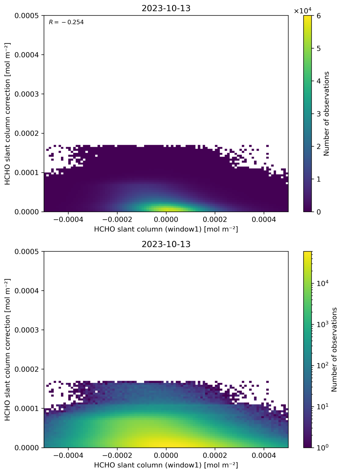
Figure 83: Scatter density plot of “HCHO slant column (window1)” against “HCHO slant column correction” for 2023-10-12 to 2023-10-14.
