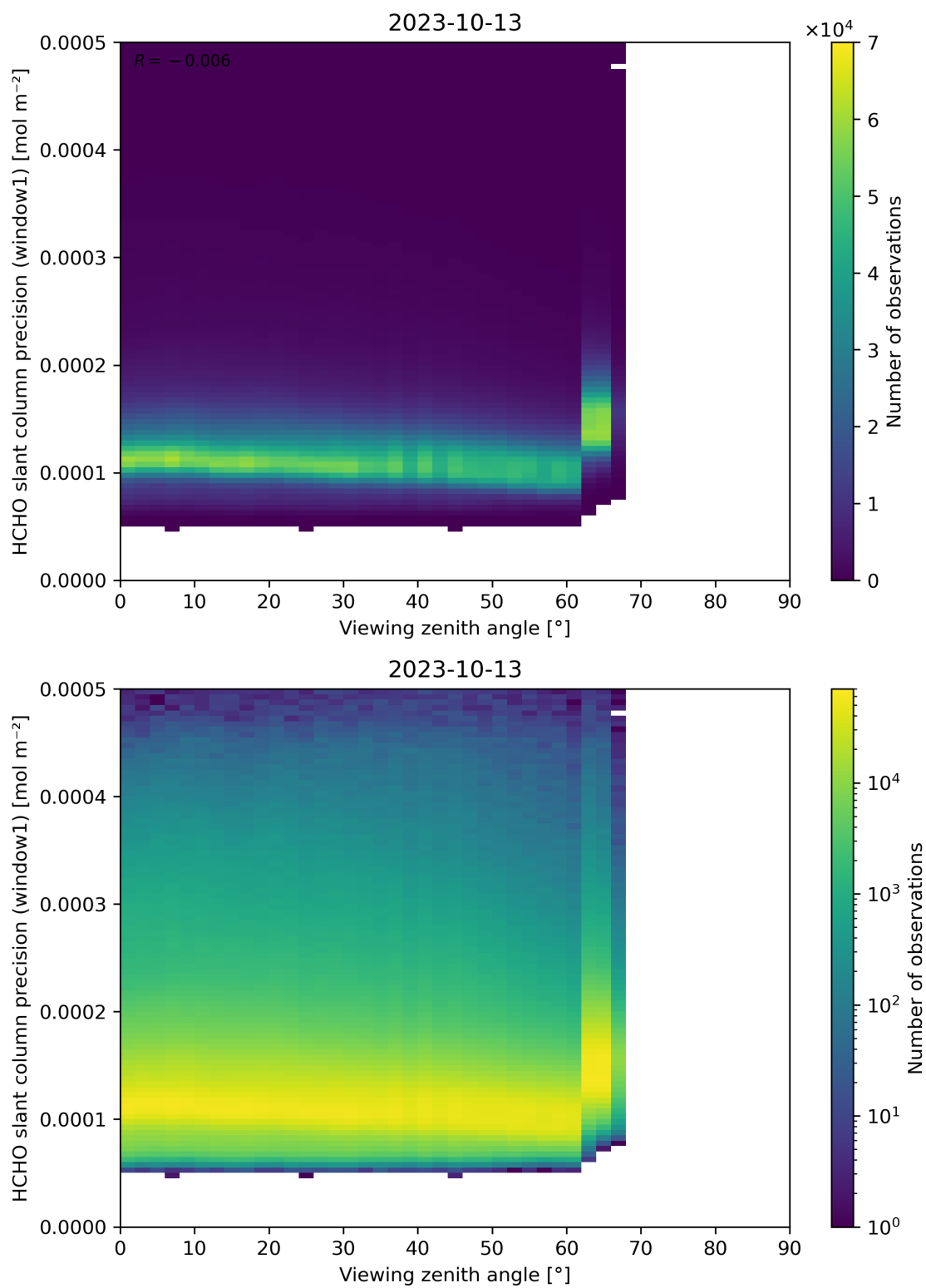
Figure 189: Scatter density plot of “Viewing zenith angle” against “HCHO slant column precision (window1)” for 2023-10-12 to 2023-10-14.
