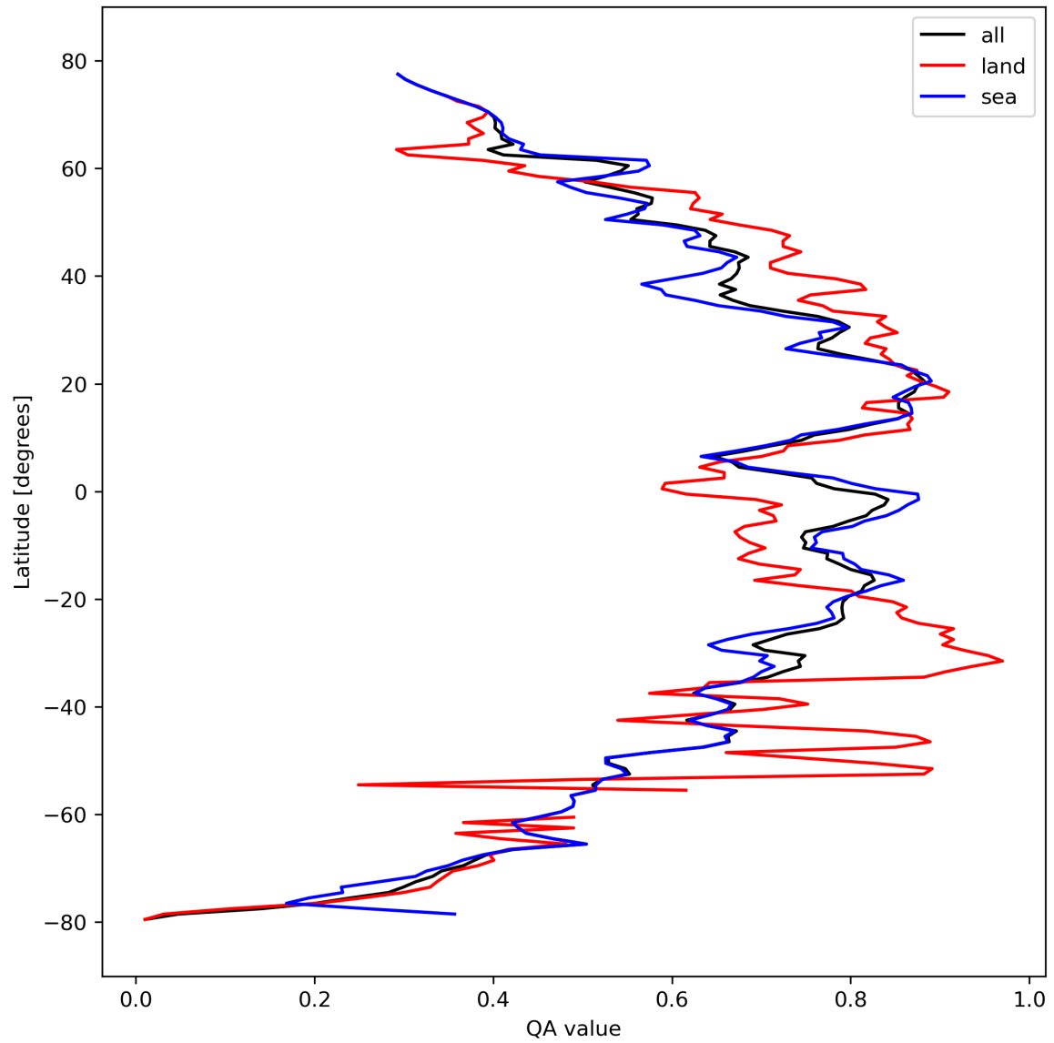
Figure 20: Zonal average of “QA value” for 2023-10-12 to 2023-10-14.
