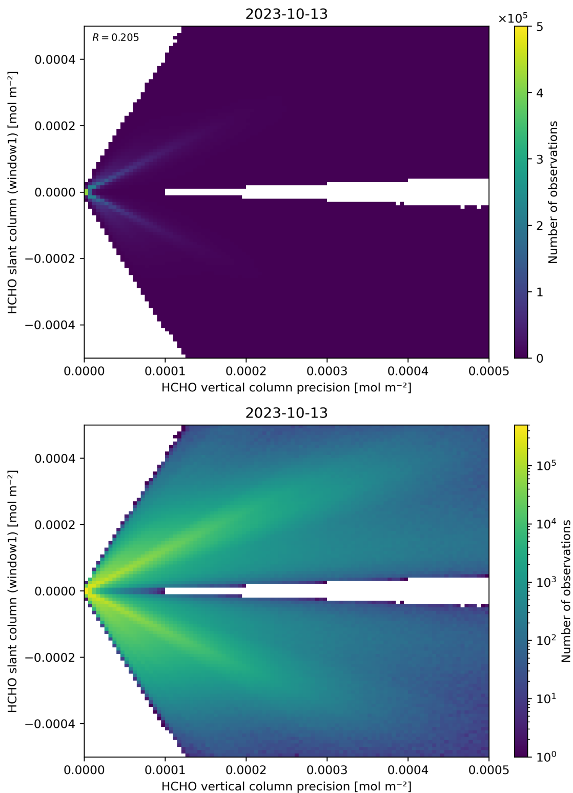
Figure 142: Scatter density plot of “HCHO vertical column precision” against “HCHO slant column (window1)” for 2023-10-12 to 2023-10-14.
