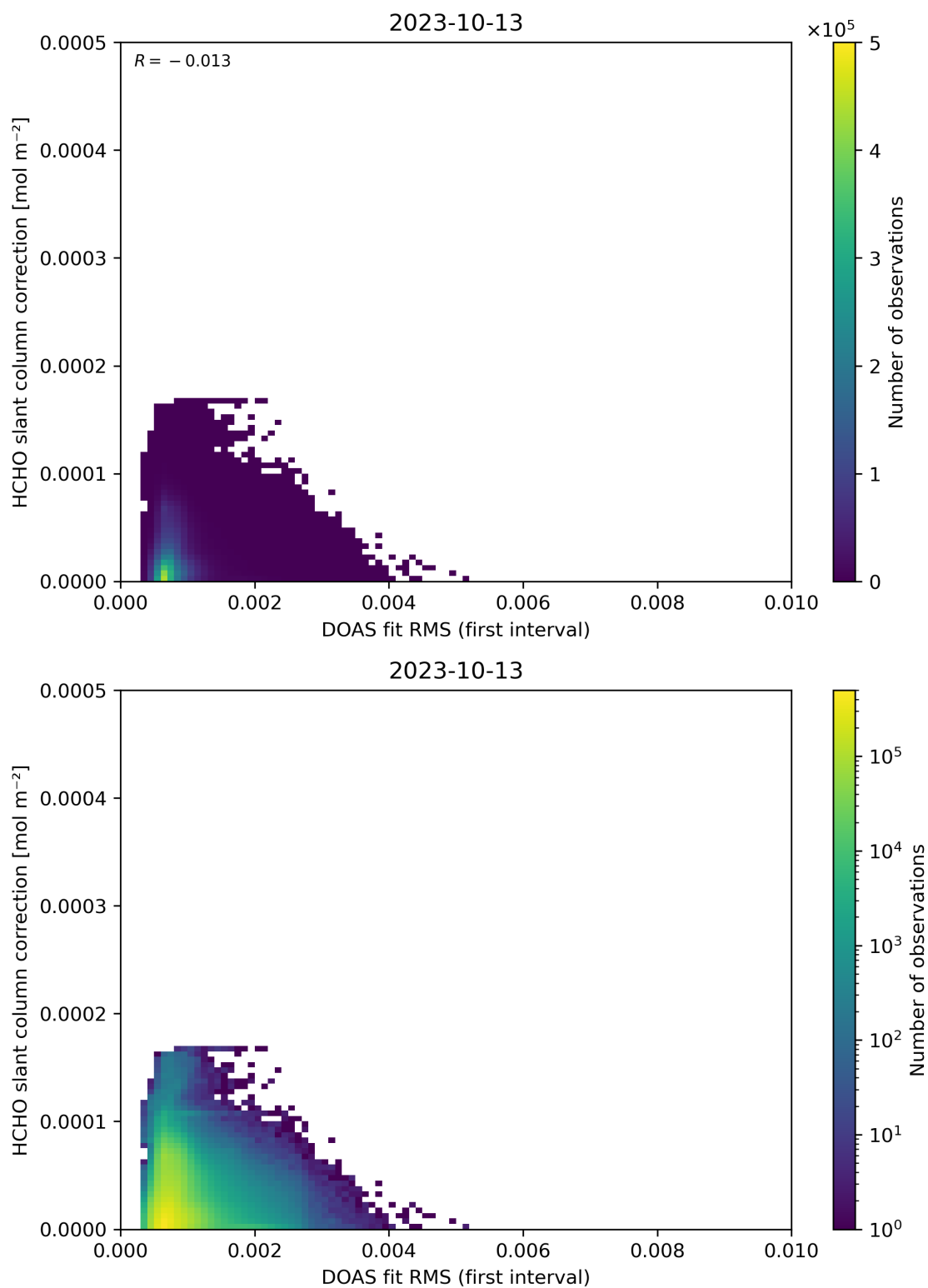
Figure 63: Scatter density plot of “DOAS fit RMS (first interval)” against “HCHO slant column correction” for 2023-10-12 to 2023-10-14.
