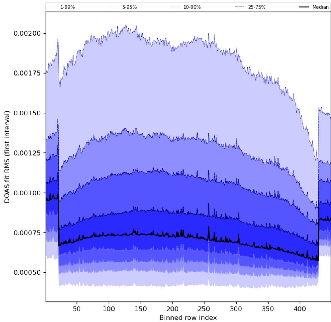
Figure 60: Along track statistics of “DOAS fit RMS (first interval)” for 2023-10-12 to 2023-10-14
