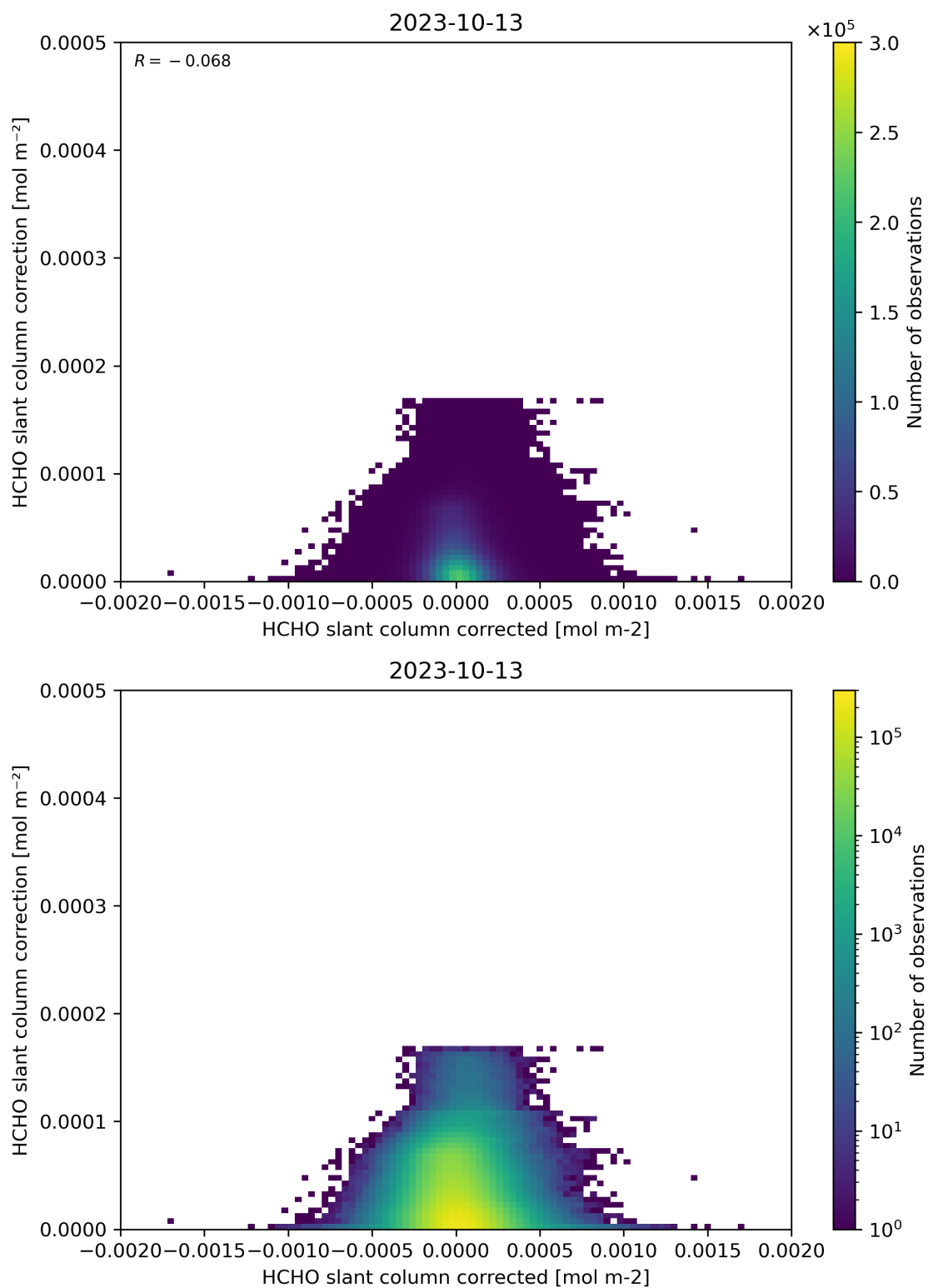
Figure 77: Scatter density plot of “HCHO slant column corrected” against “HCHO slant column correction” for 2023-10-12 to 2023-10-14.
