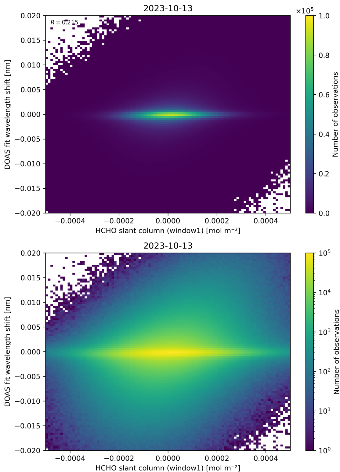
Figure 79: Scatter density plot of “HCHO slant column (window1)” against “DOAS fit wavelength shift” for 2023-10-12 to 2023-10-14.
