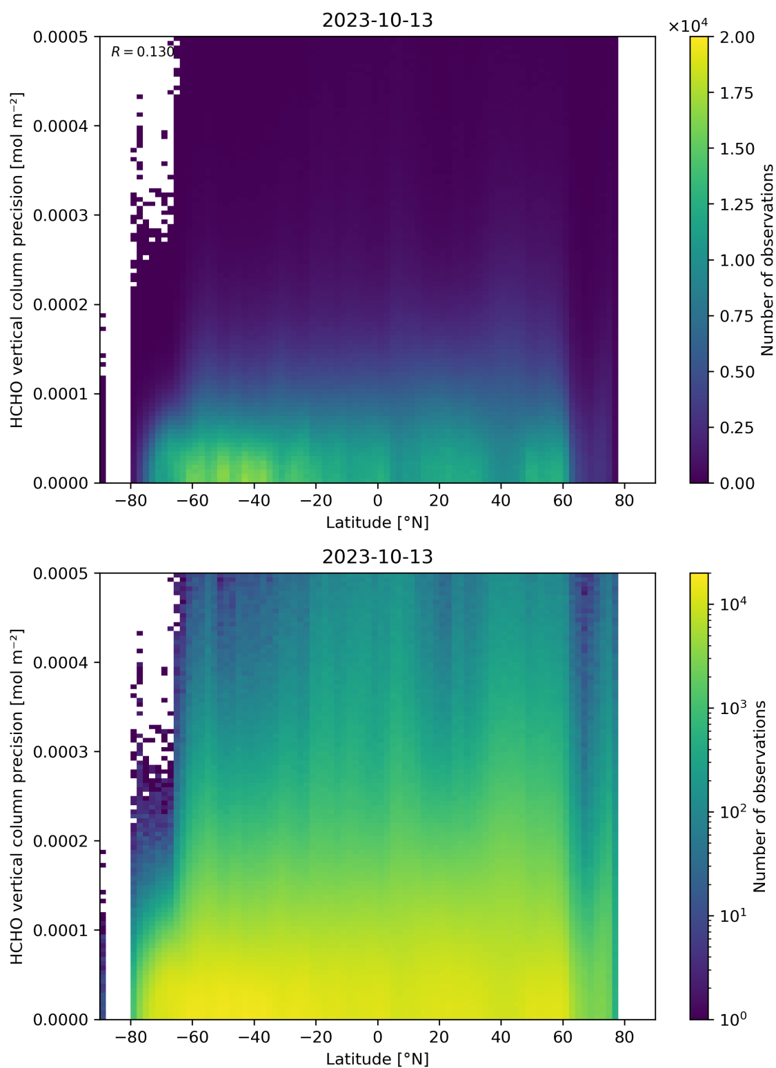
Figure 165: Scatter density plot of “Latitude” against “HCHO vertical column precision” for 2023-10-12 to 2023-10-14.
