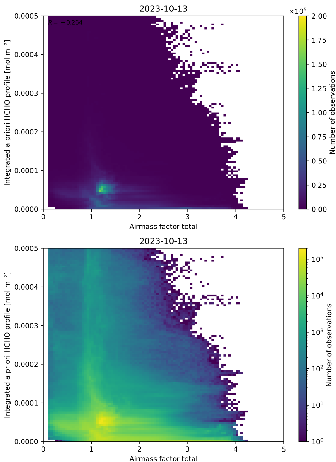
Figure 104: Scatter density plot of “Airmass factor total” against “Integrated a priori HCHO profile” for 2023-10-12 to 2023-10-14.
