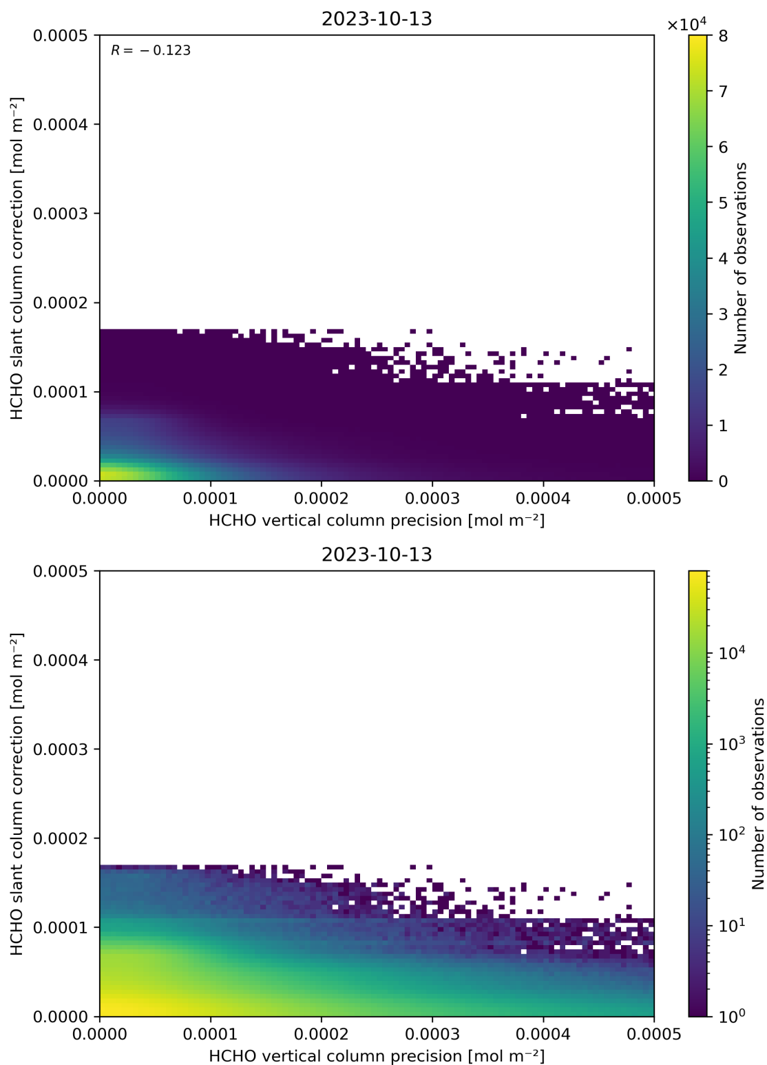
Figure 141: Scatter density plot of “HCHO vertical column precision” against “HCHO slant column correction” for 2023-10-12 to 2023-10-14.
