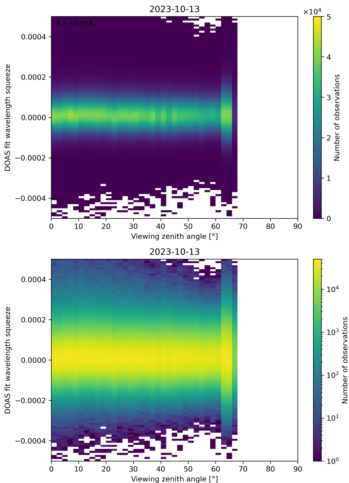
Figure 184: Scatter density plot of “Viewing zenith angle” against “DOAS fit wavelength squeeze” for 2023-10-12 to 2023-10-14.
