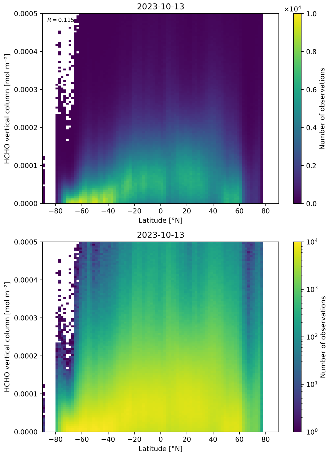
Figure 163: Scatter density plot of “Latitude” against “HCHO vertical column” for 2023-10-12 to 2023-10-14.
