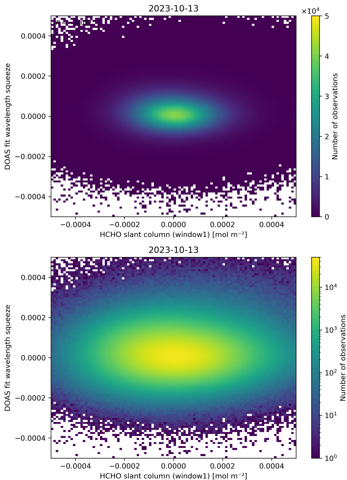
Figure 80: Scatter density plot of “HCHO slant column (window1)” against “DOAS fit wavelength squeeze” for 2023-10-12 to 2023-10-14.
