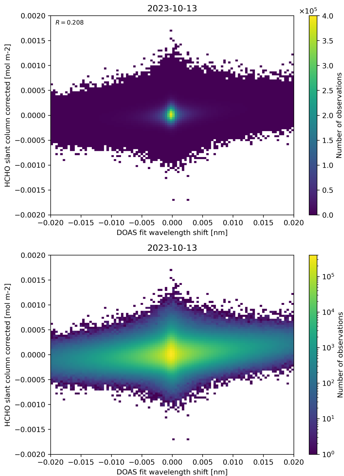
Figure 66: Scatter density plot of “DOAS fit wavelength shift” against “HCHO slant column corrected” for 2023-10-12 to 2023-10-14.
