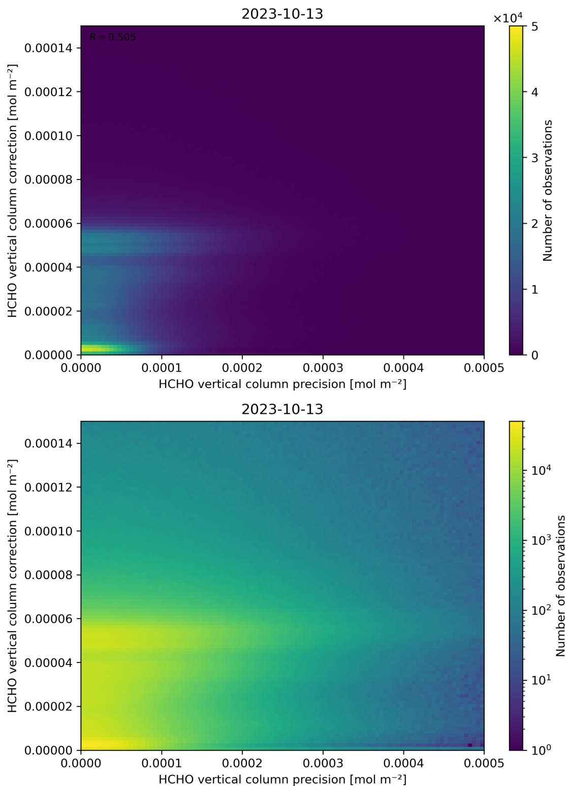
Figure 146: Scatter density plot of “HCHO vertical column precision” against “HCHO vertical column correction” for 2023-10-12 to 2023-10-14.
