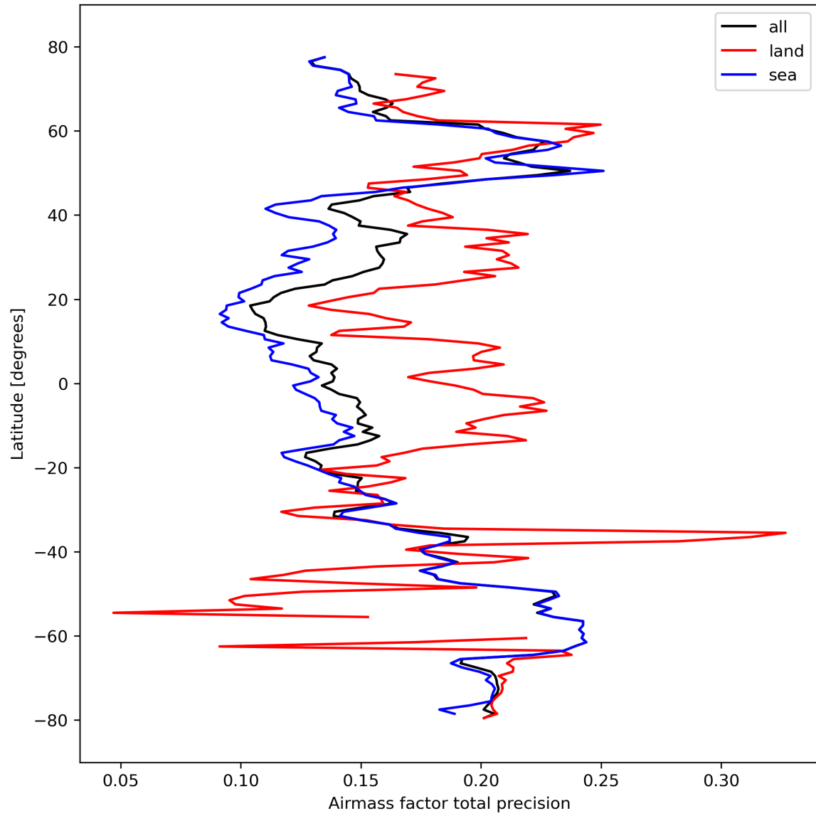
Figure 27: Zonal average of “Airmass factor total precision” for 2023-10-12 to 2023-10-14.
