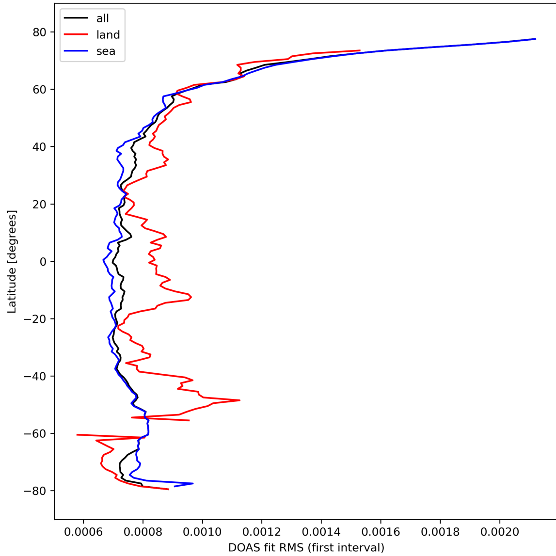
Figure 32: Zonal average of “DOAS fit RMS (first interval)” for 2023-10-12 to 2023-10-14.
