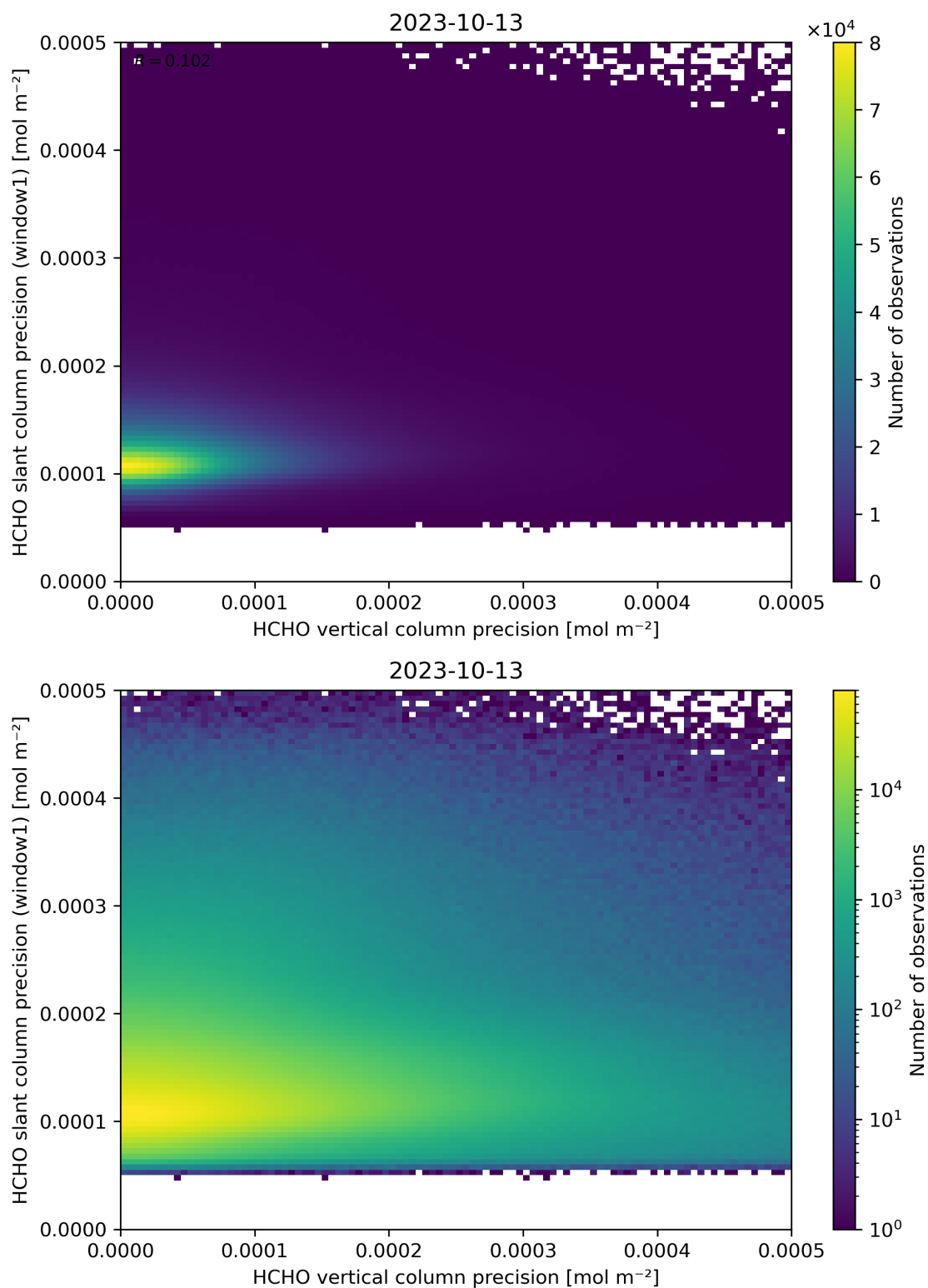
Figure 143: Scatter density plot of “HCHO vertical column precision” against “HCHO slant column precision (window1)” for 2023-10-12 to 2023-10-14.
