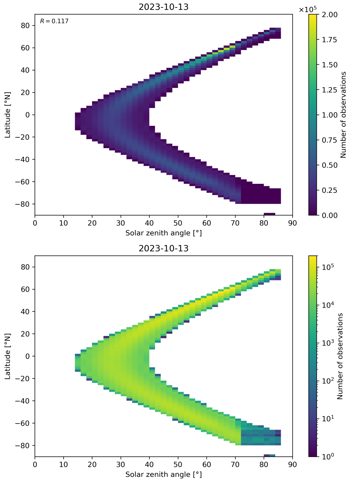
Figure 181: Scatter density plot of “Solar zenith angle” against “Latitude” for 2023-10-12 to 2023-10-14.
