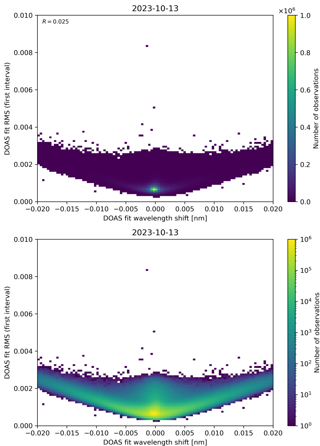
Figure 64: Scatter density plot of “DOAS fit wavelength shift” against “DOAS fit RMS (first interval)” for 2023-10-12 to 2023-10-14.
