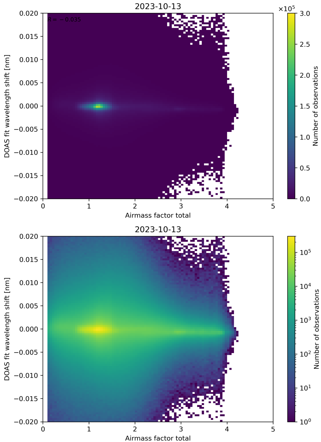
Figure 98: Scatter density plot of “Airmass factor total” against “DOAS fit wavelength shift” for 2023-10-12 to 2023-10-14.
