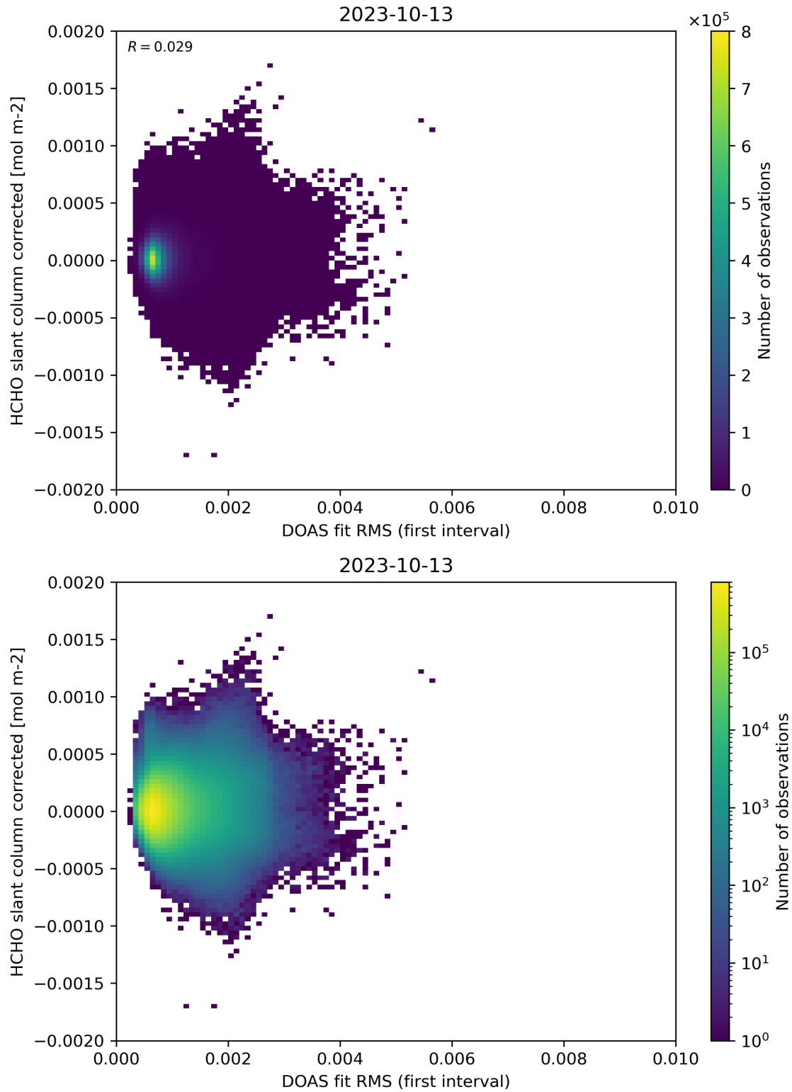
Figure 62: Scatter density plot of “DOAS fit RMS (first interval)” against “HCHO slant column corrected” for 2023-10-12 to 2023-10-14.
