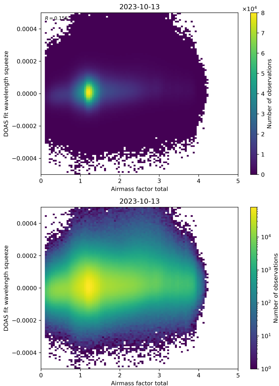
Figure 99: Scatter density plot of “Airmass factor total” against “DOAS fit wavelength squeeze” for 2023-10-12 to 2023-10-14.
