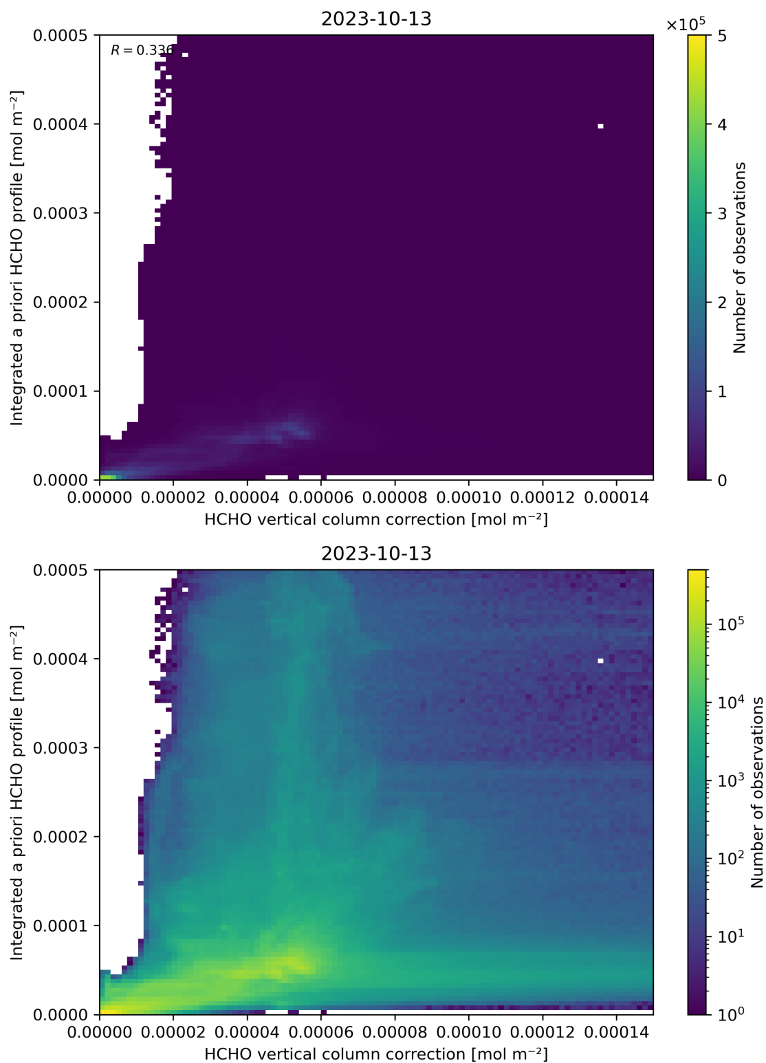
Figure 122: Scatter density plot of “HCHO vertical column correction” against “Integrated a priori HCHO profile” for 2023-10-12 to 2023-10-14.
