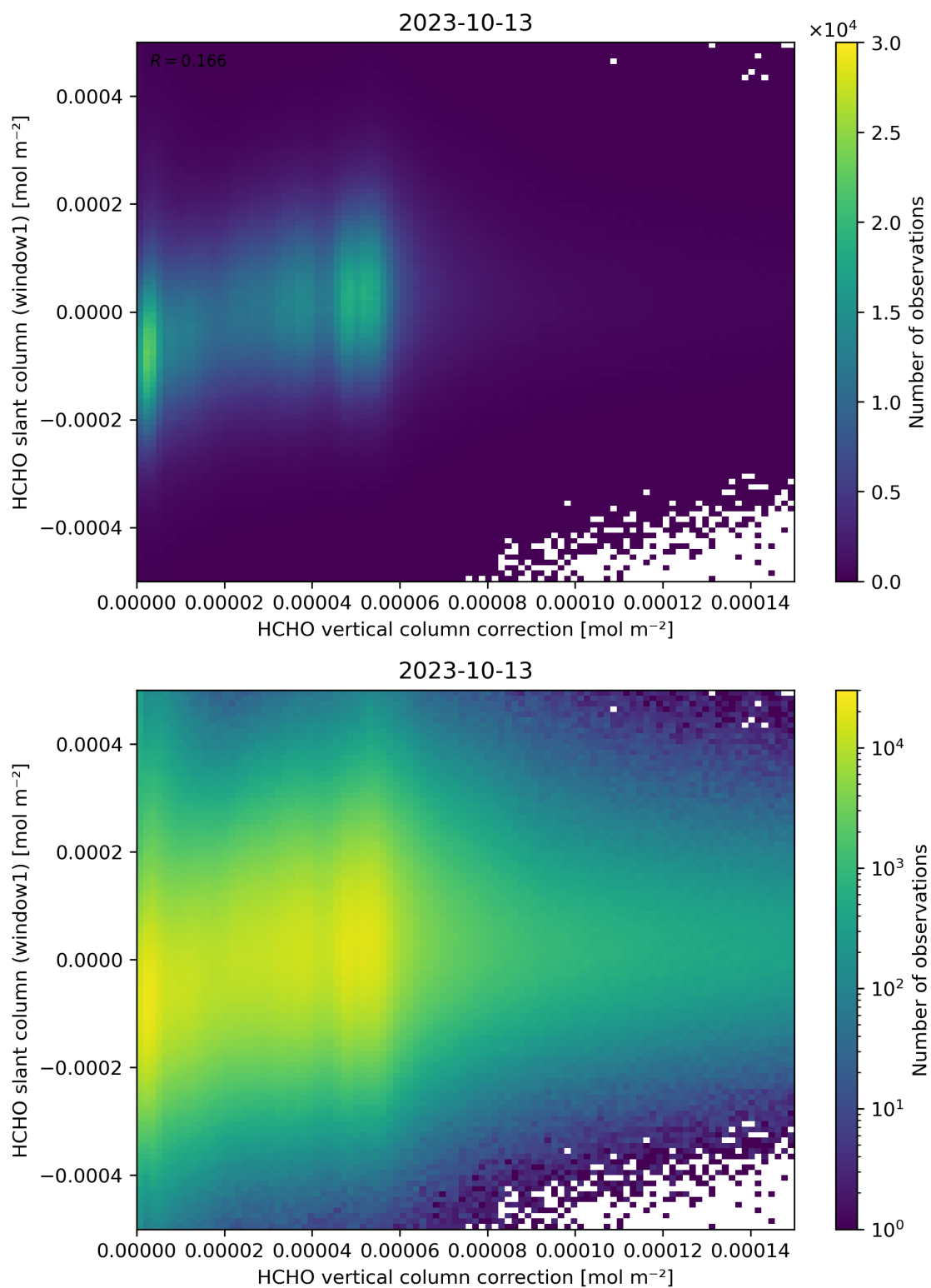
Figure 118: Scatter density plot of “HCHO vertical column correction” against “HCHO slant column (window1)” for 2023-10-12 to 2023-10-14.
