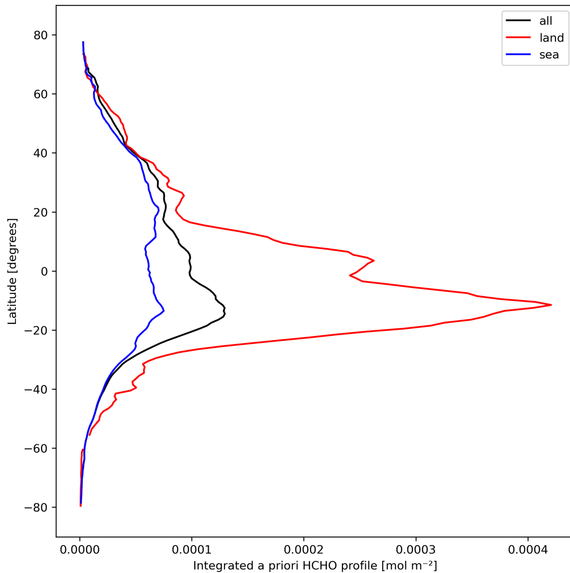
Figure 29: Zonal average of “Integrated a priori HCHO profile” for 2023-10-12 to 2023-10-14.
