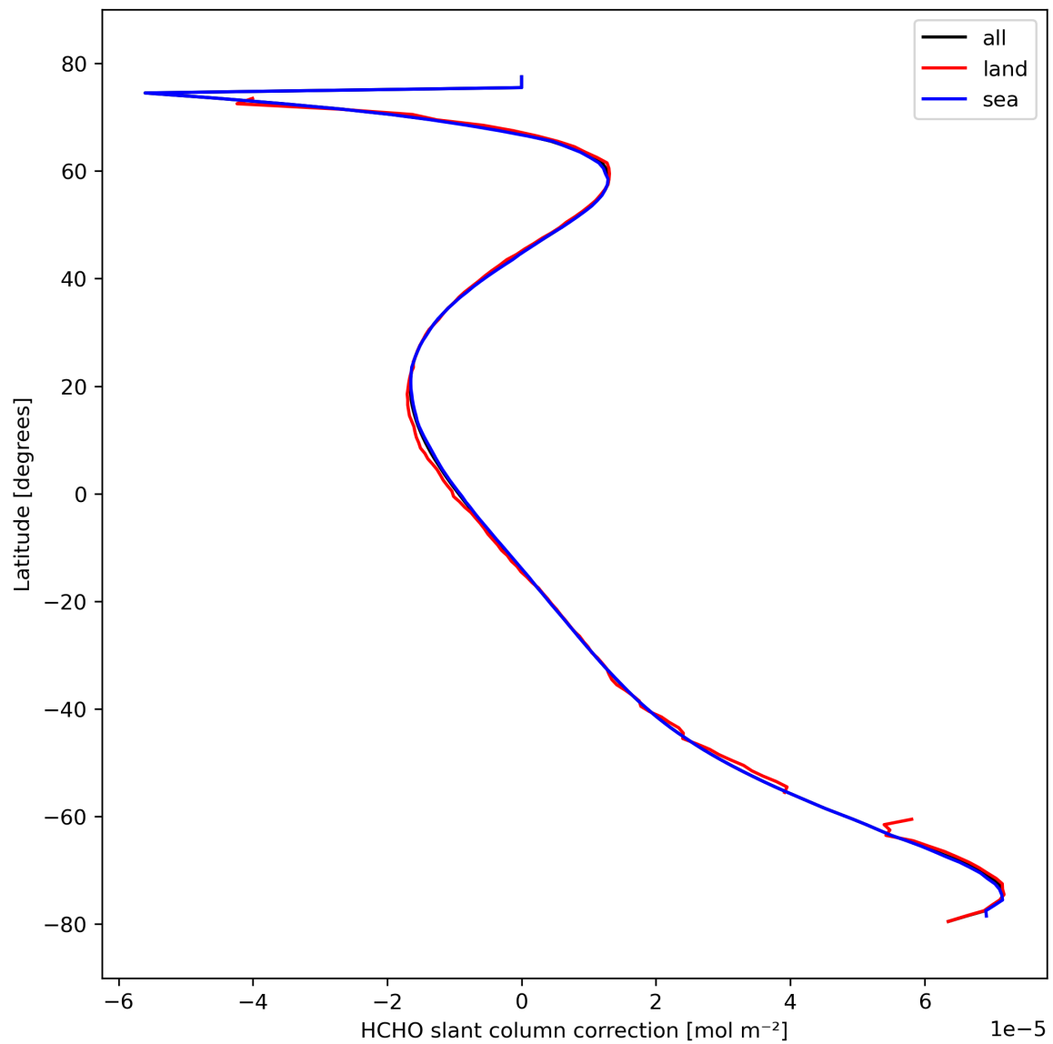
Figure 33: Zonal average of “HCHO slant column correction” for 2023-10-12 to 2023-10-14.
