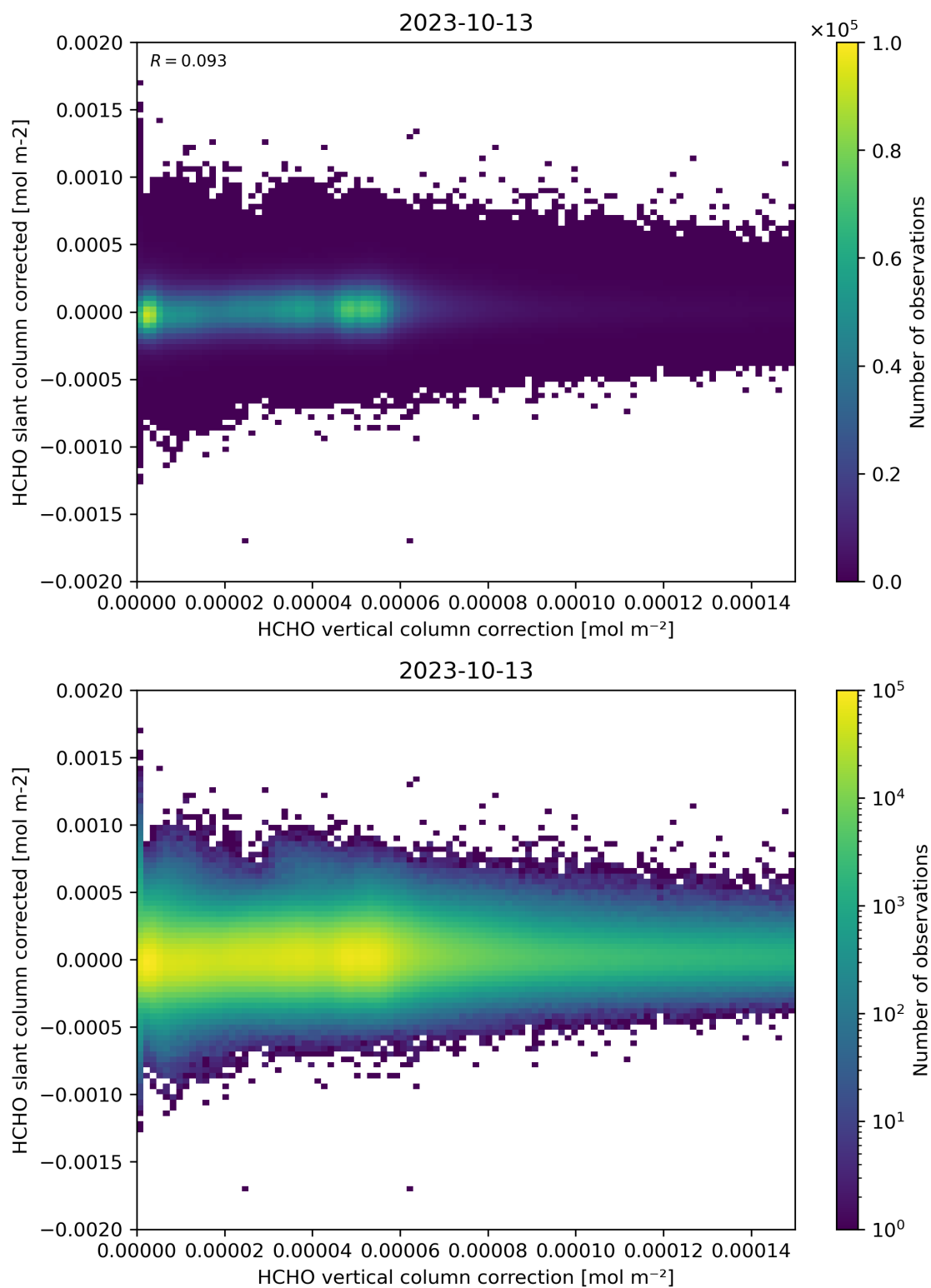
Figure 116: Scatter density plot of “HCHO vertical column correction” against “HCHO slant column corrected” for 2023-10-12 to 2023-10-14.
