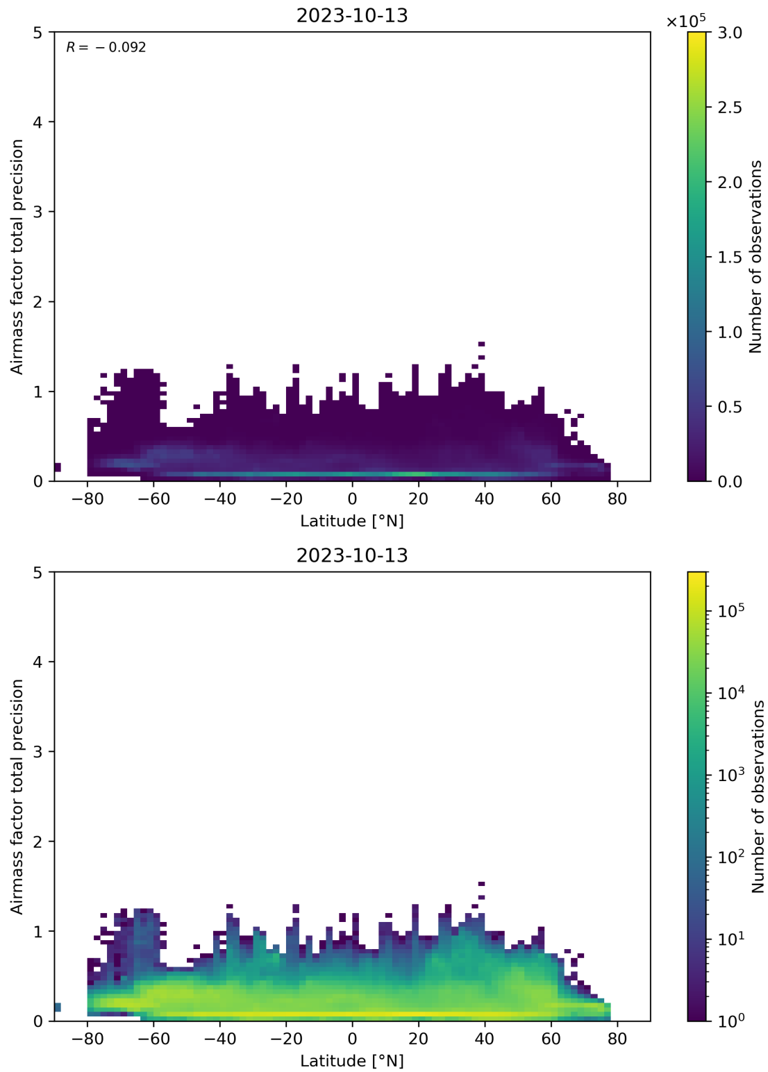
Figure 162: Scatter density plot of “Latitude” against “Airmass factor total precision” for 2023-10-12 to 2023-10-14.
