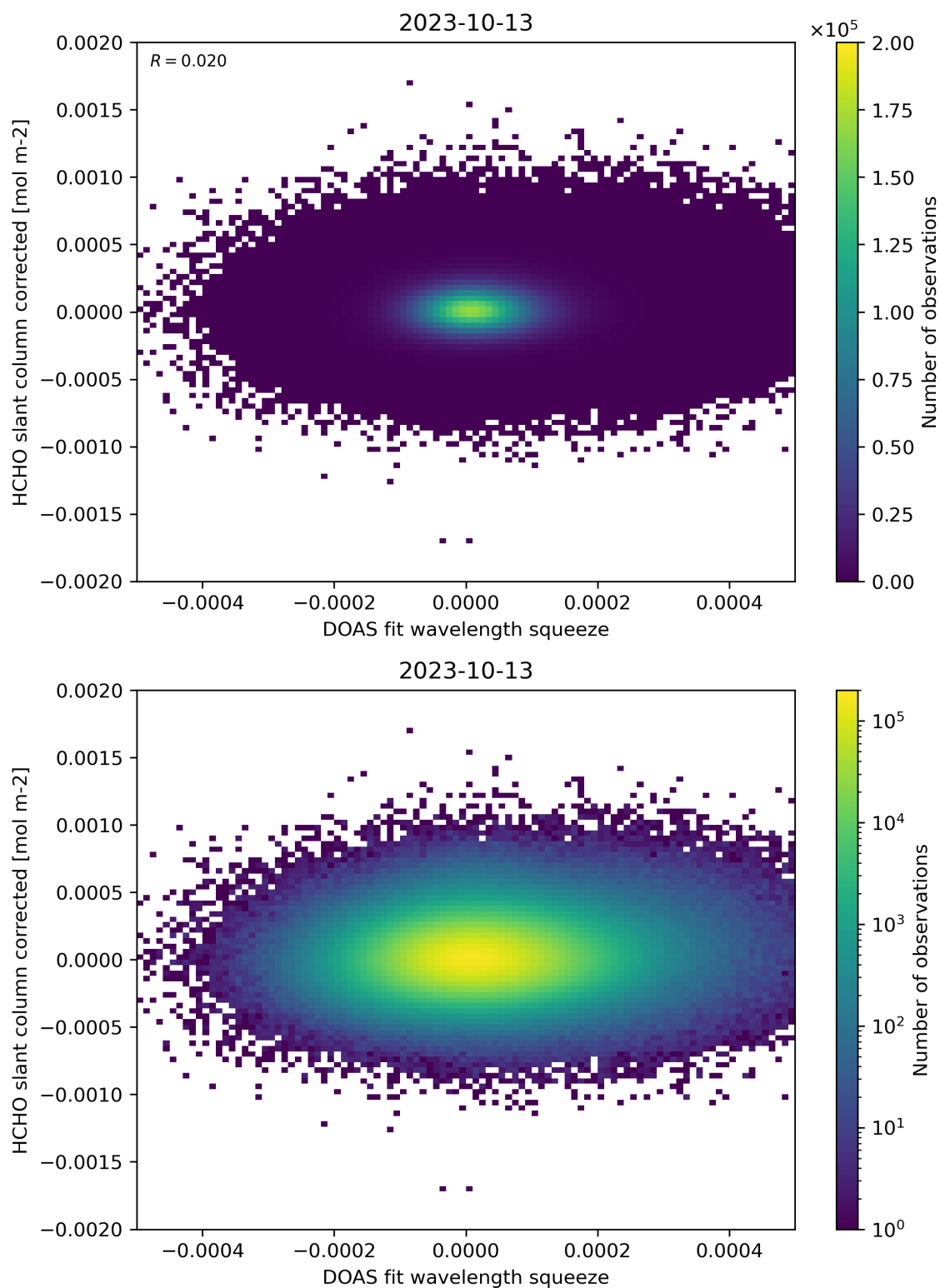
Figure 69: Scatter density plot of “DOAS fit wavelength squeeze” against “HCHO slant column corrected” for 2023-10-12 to 2023-10-14.
