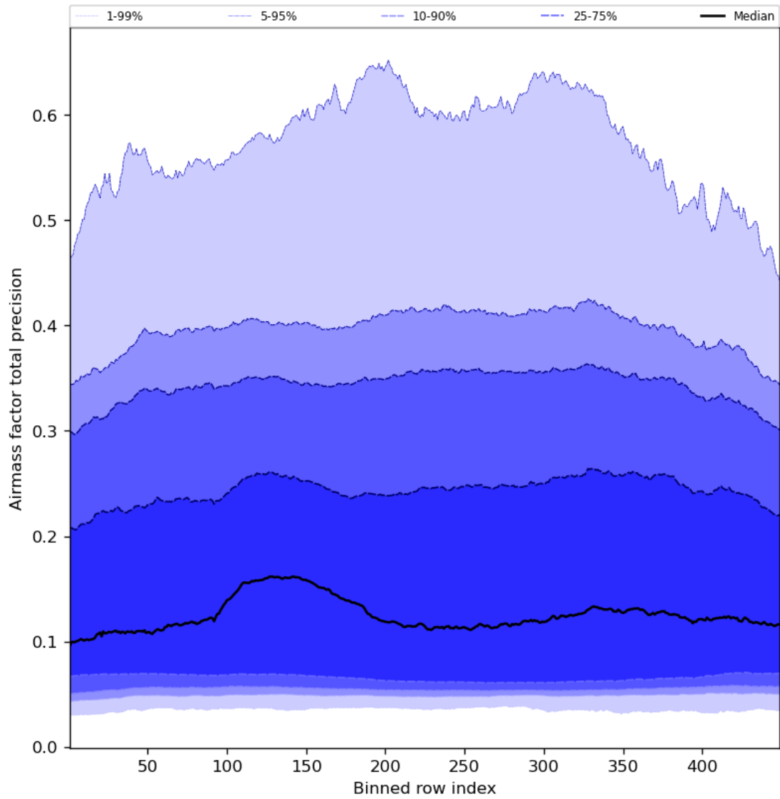
Figure 55: Along track statistics of “Airmass factor total precision” for 2023-10-12 to 2023-10-14
