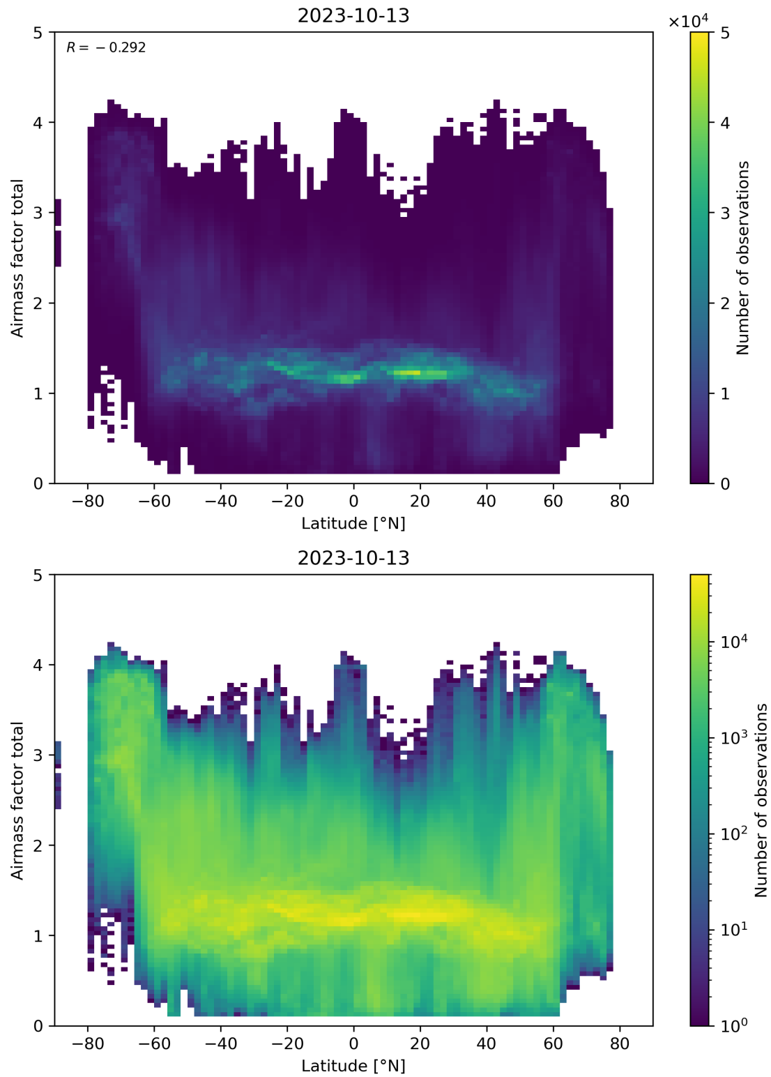
Figure 161: Scatter density plot of “Latitude” against “Airmass factor total” for 2023-10-12 to 2023-10-14.
