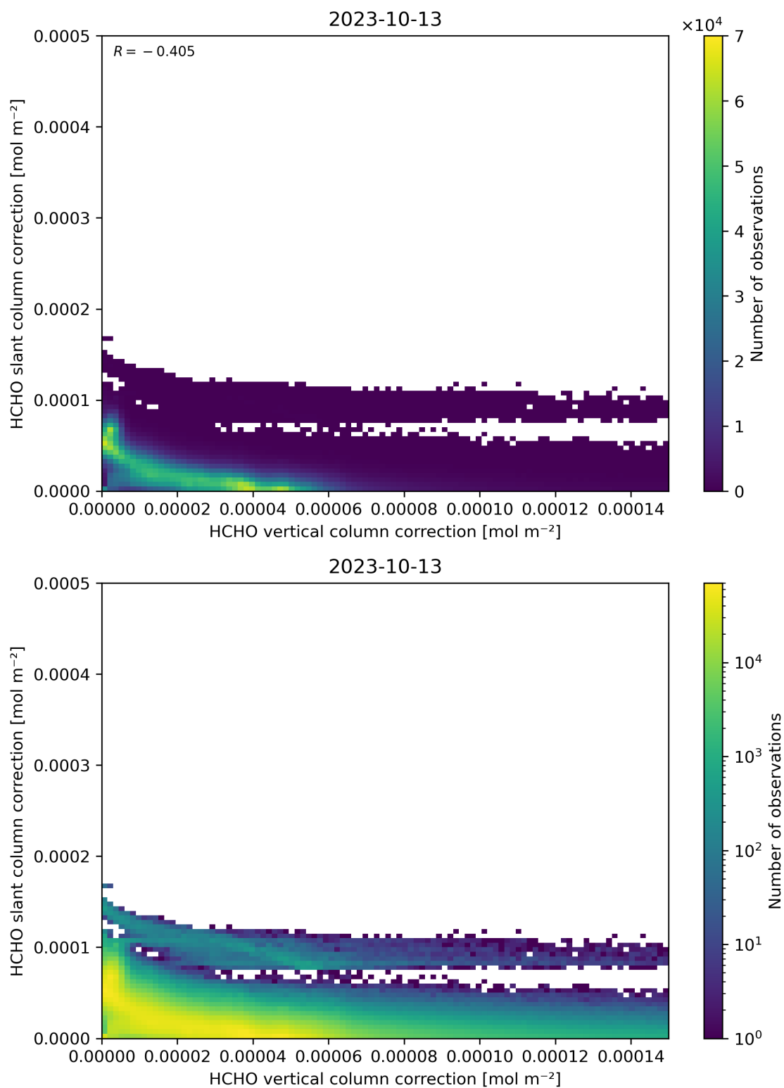
Figure 117: Scatter density plot of “HCHO vertical column correction” against “HCHO slant column correction” for 2023-10-12 to 2023-10-14.
