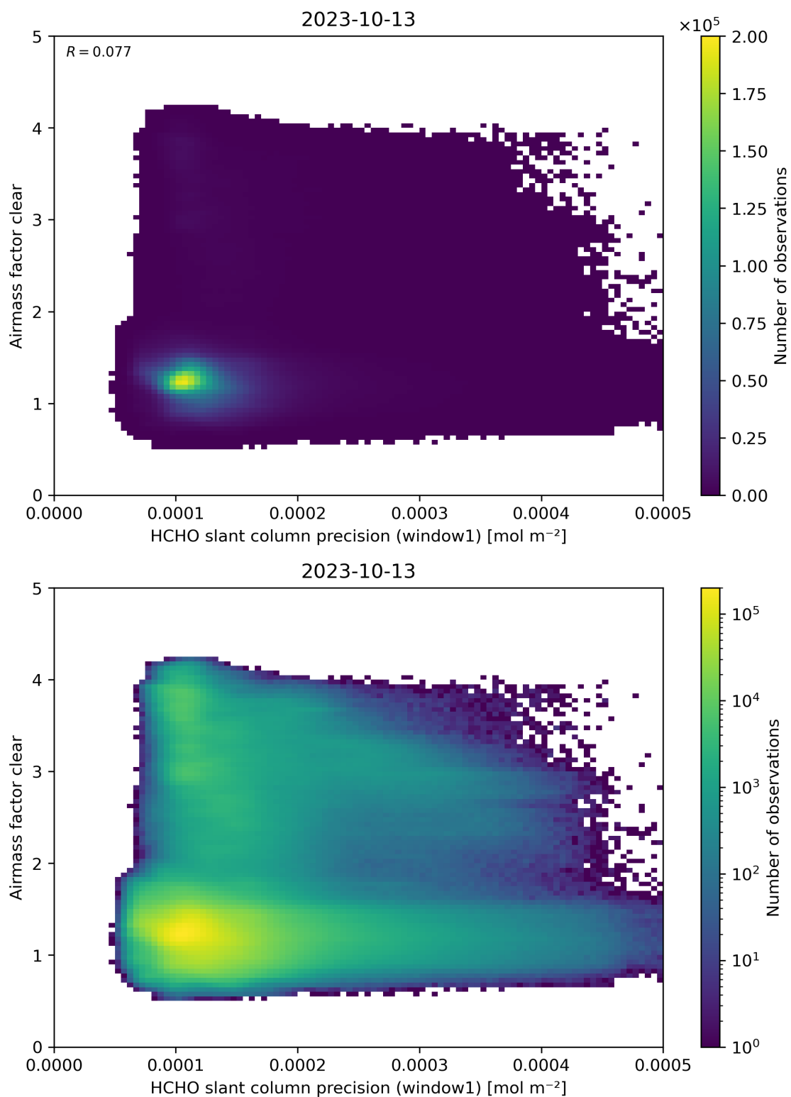
Figure 91: Scatter density plot of “HCHO slant column precision (window1)” against “Airmass factor clear” for 2023-10-12 to 2023-10-14.
