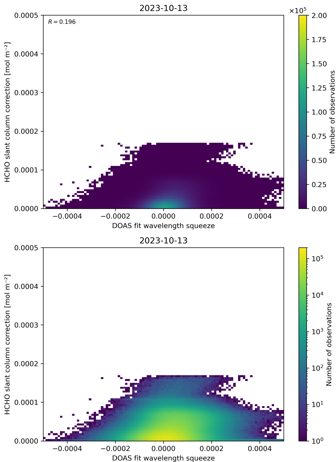
Figure 70: Scatter density plot of “DOAS fit wavelength squeeze” against “HCHO slant column correction” for 2023-10-12 to 2023-10-14.
