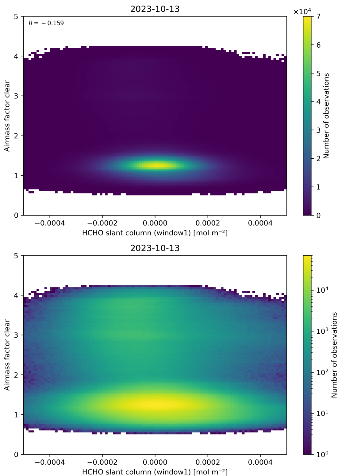
Figure 81: Scatter density plot of “HCHO slant column (window1)” against “Airmass factor clear” for 2023-10-12 to 2023-10-14.
