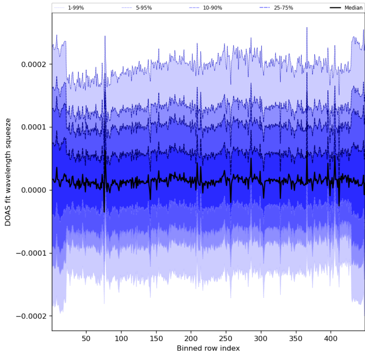
Figure 59: Along track statistics of “DOAS fit wavelength squeeze” for 2023-10-12 to 2023-10-14
