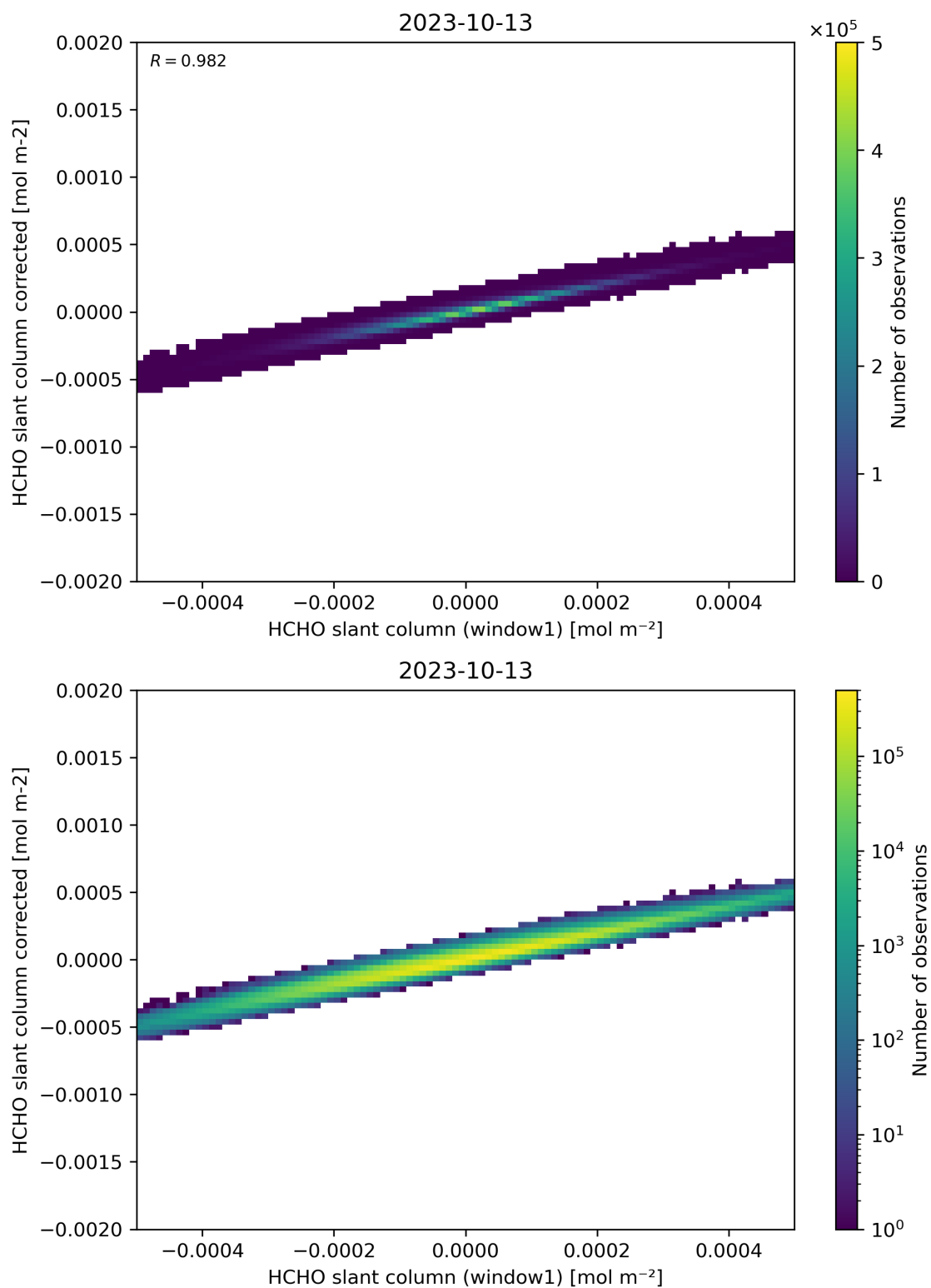
Figure 82: Scatter density plot of “HCHO slant column (window1)” against “HCHO slant column corrected” for 2023-10-12 to 2023-10-14.
