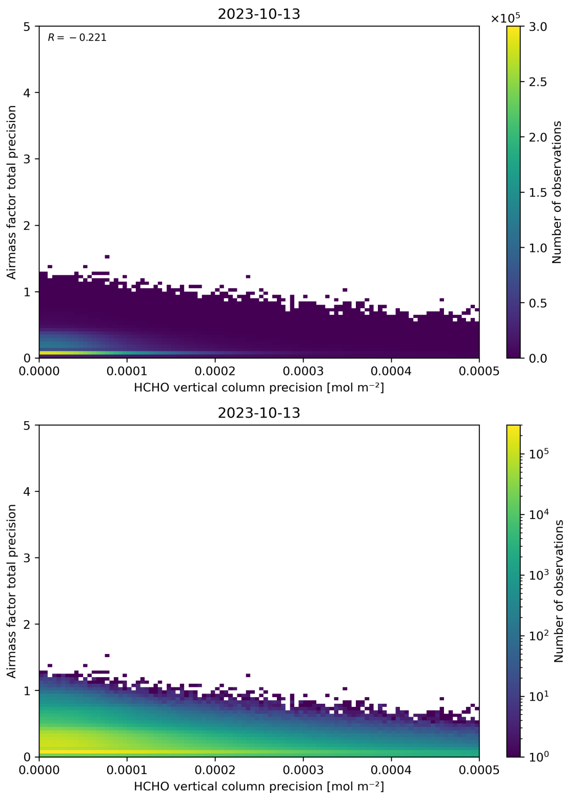
Figure 145: Scatter density plot of “HCHO vertical column precision” against “Airmass factor total precision” for 2023-10-12 to 2023-10-14.
