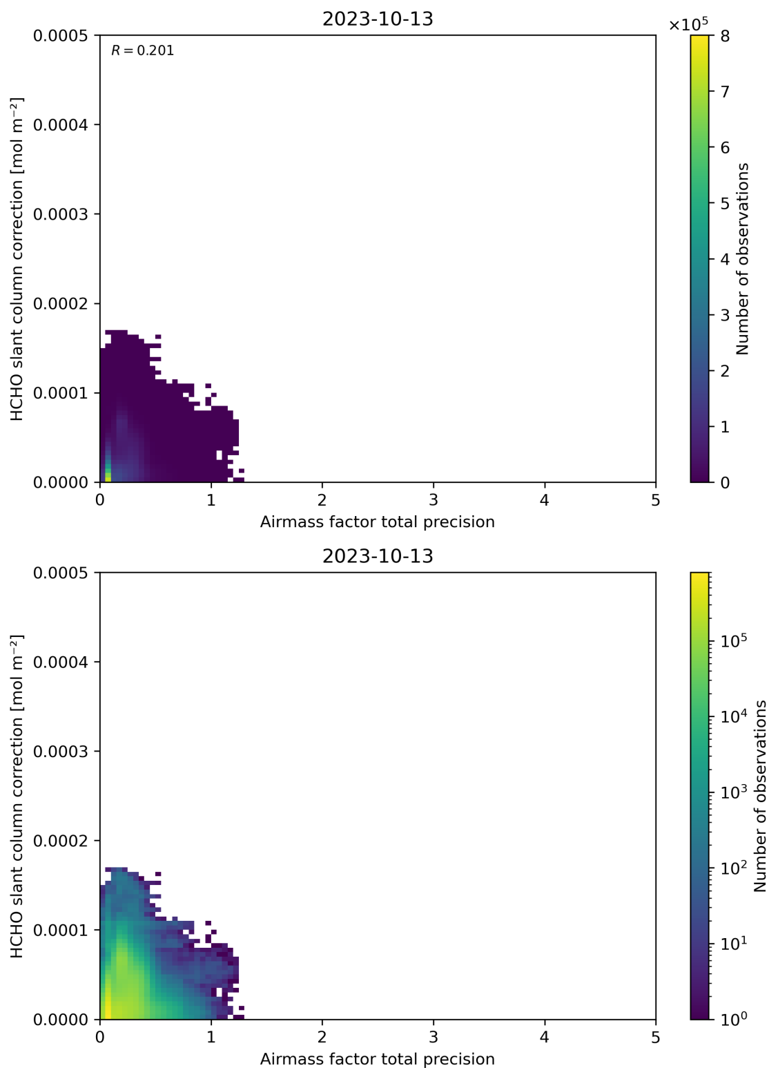
Figure 110: Scatter density plot of “Airmass factor total precision” against “HCHO slant column correction” for 2023-10-12 to 2023-10-14.
