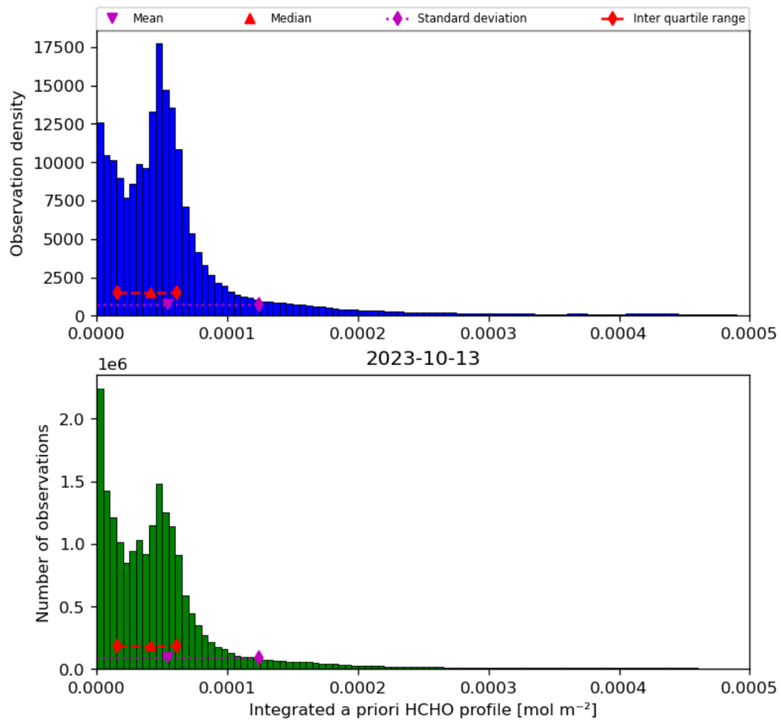
Figure 43: Histogram of “Integrated a priori HCHO profile” for 2023-10-12 to 2023-10-14
