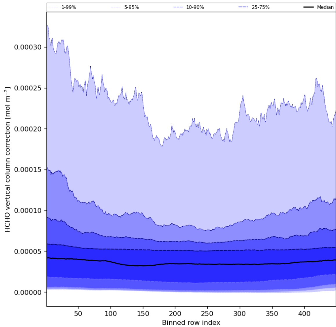
Figure 51: Along track statistics of “HCHO vertical column correction” for 2023-10-12 to 2023-10-14
