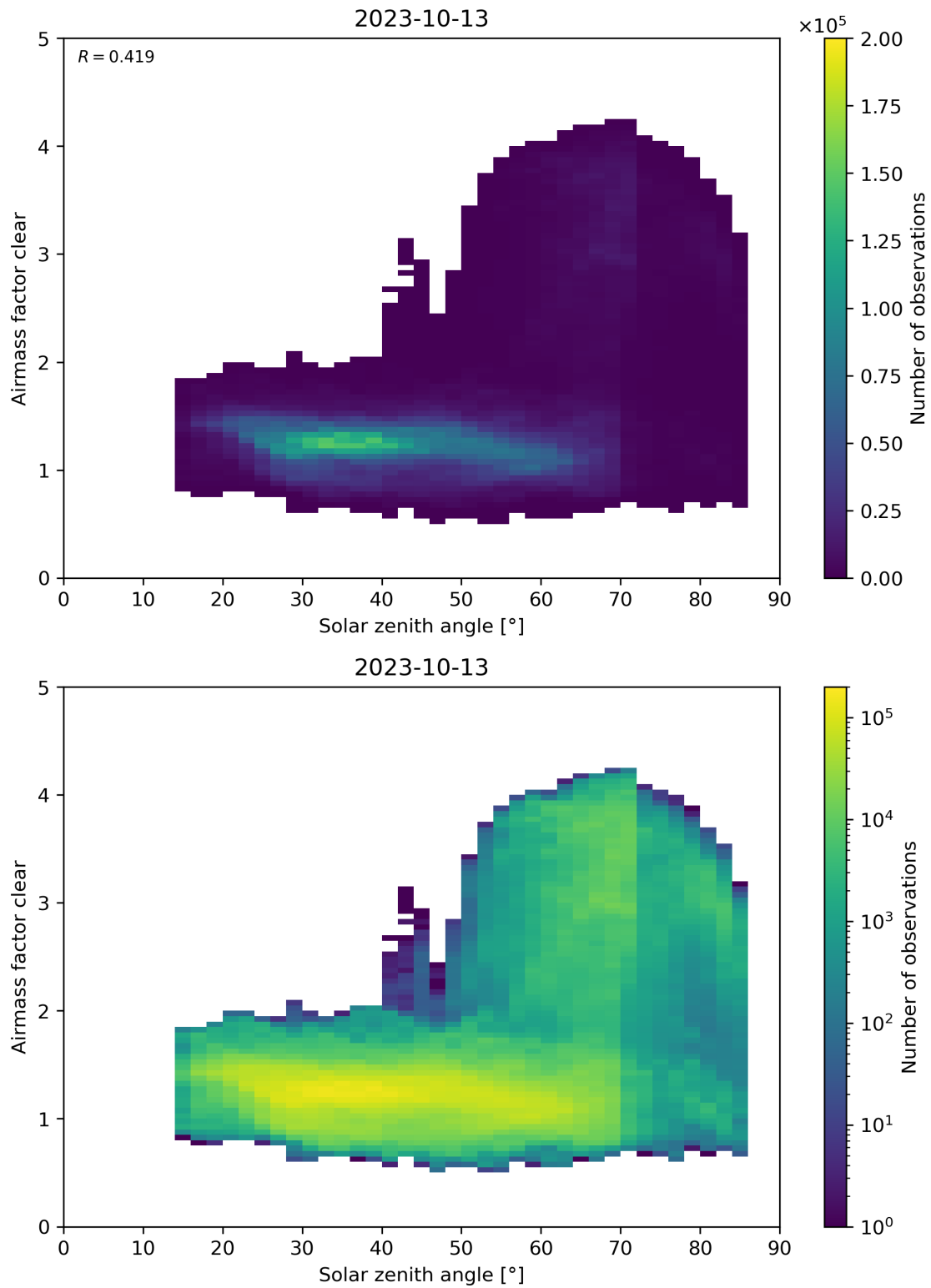
Figure 170: Scatter density plot of “Solar zenith angle” against “Airmass factor clear” for 2023-10-12 to 2023-10-14.
