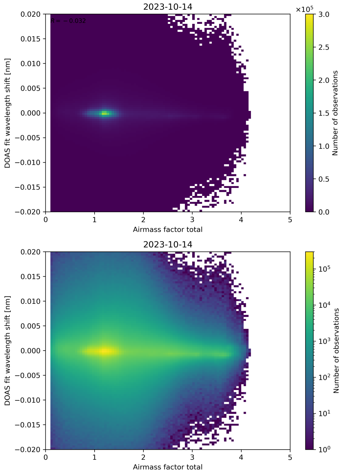
Figure 98: Scatter density plot of “Airmass factor total” against “DOAS fit wavelength shift” for 2023-10-13 to 2023-10-15.
