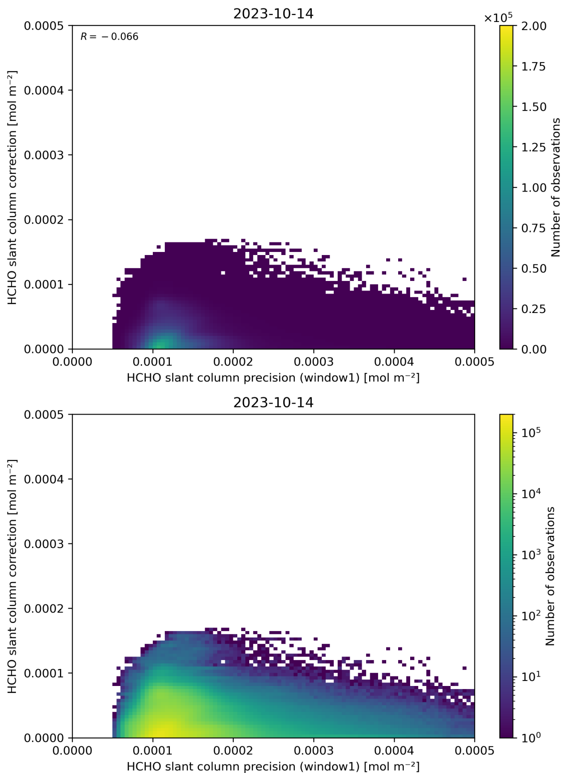
Figure 93: Scatter density plot of “HCHO slant column precision (window1)” against “HCHO slant column correction” for 2023-10-13 to 2023-10-15.
