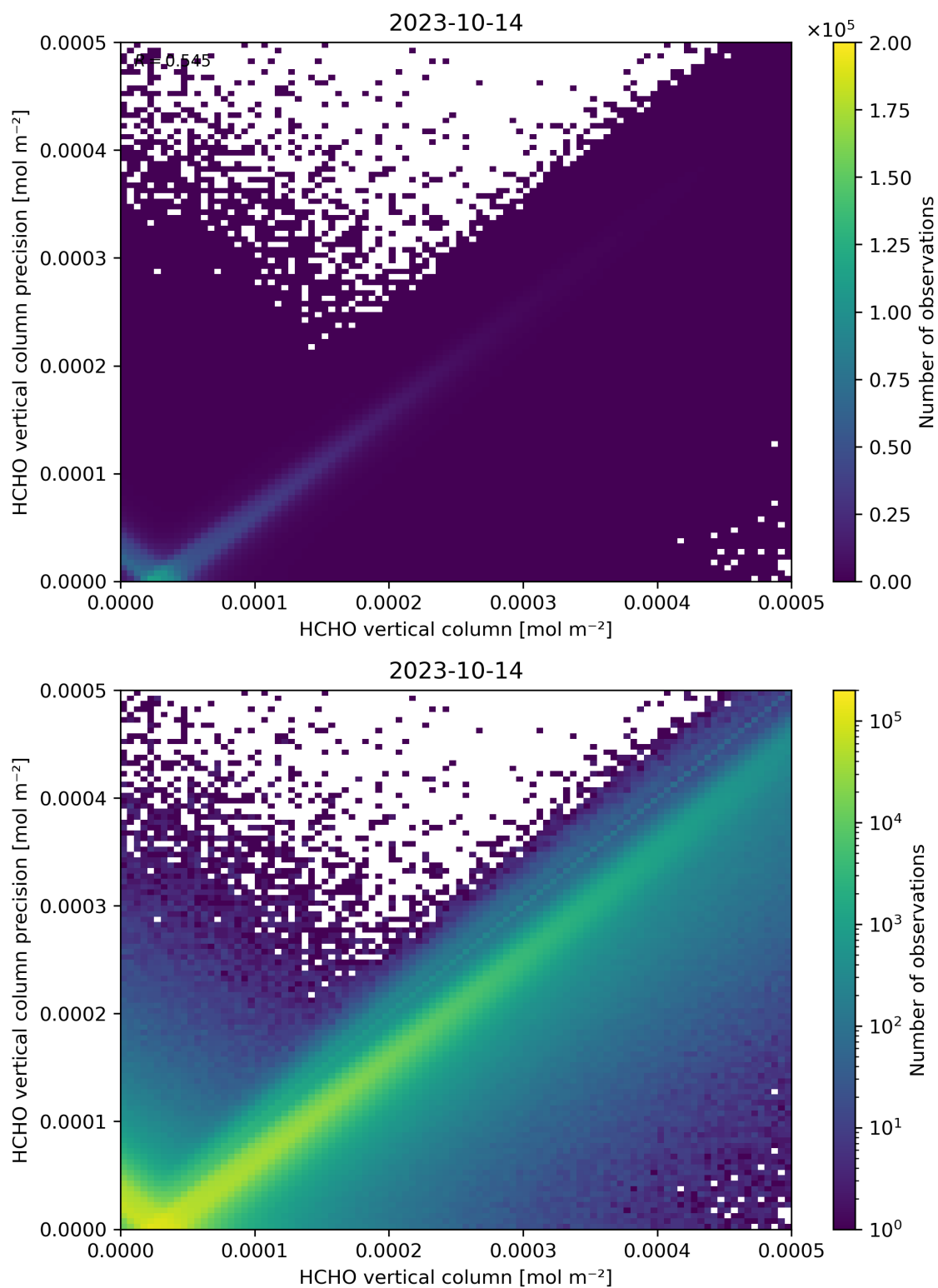
Figure 134: Scatter density plot of “HCHO vertical column” against “HCHO vertical column precision” for 2023-10-13 to 2023-10-15.
