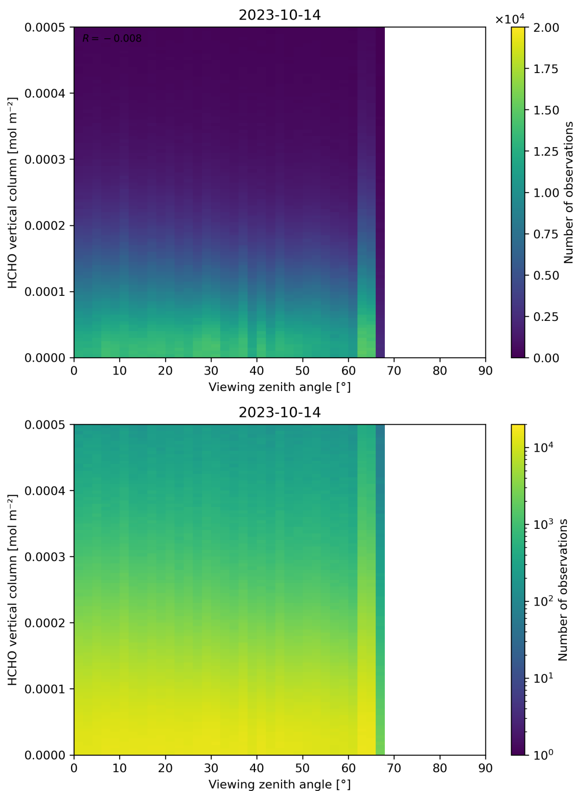
Figure 192: Scatter density plot of “Viewing zenith angle” against “HCHO vertical column” for 2023-10-13 to 2023-10-15.
