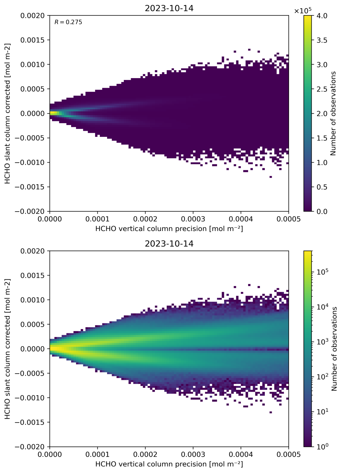
Figure 140: Scatter density plot of “HCHO vertical column precision” against “HCHO slant column corrected” for 2023-10-13 to 2023-10-15.
