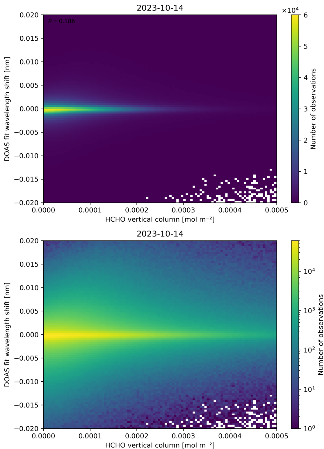
Figure 124: Scatter density plot of “HCHO vertical column” against “DOAS fit wavelength shift” for 2023-10-13 to 2023-10-15.
