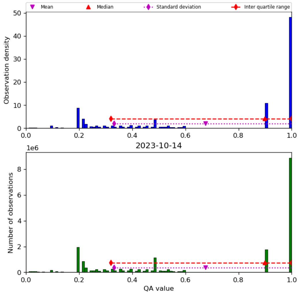
Figure 34: Histogram of “QA value” for 2023-10-13 to 2023-10-15
