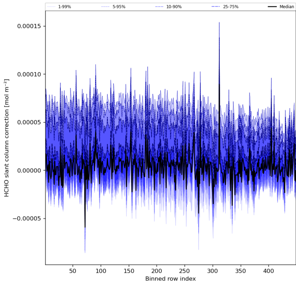
Figure 61: Along track statistics of “HCHO slant column correction” for 2023-10-13 to 2023-10-15
