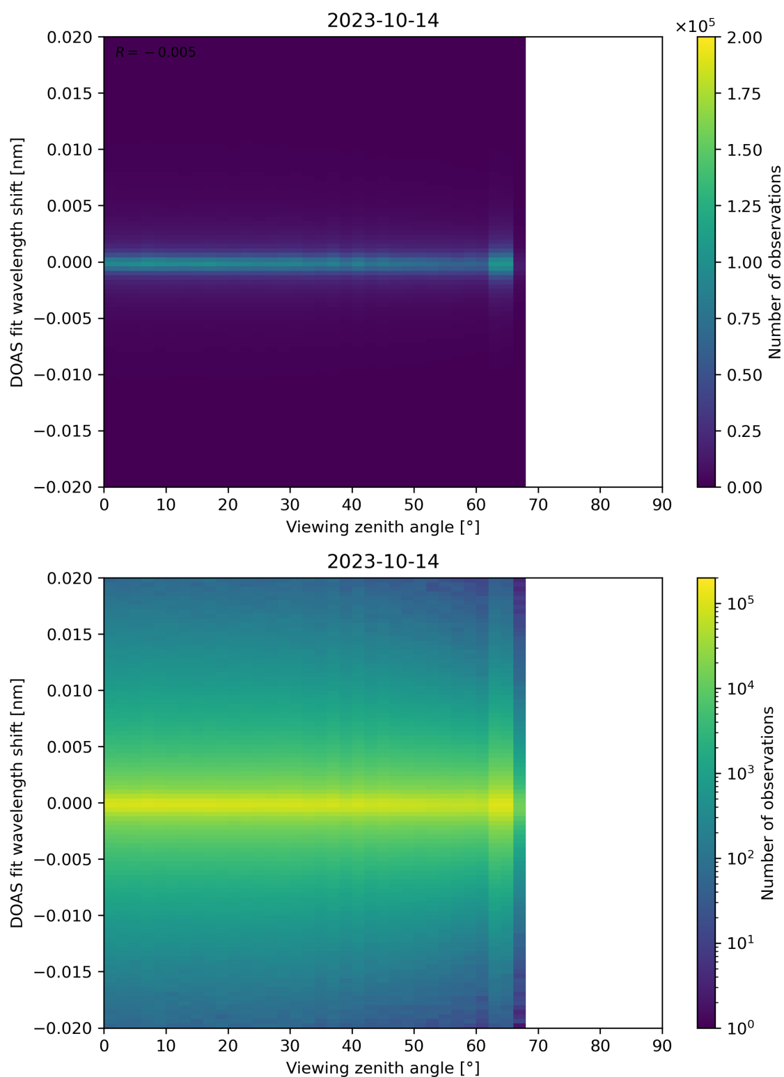
Figure 183: Scatter density plot of “Viewing zenith angle” against “DOAS fit wavelength shift” for 2023-10-13 to 2023-10-15.
