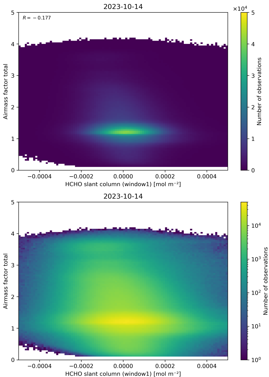
Figure 85: Scatter density plot of “HCHO slant column (window1)” against “Airmass factor total” for 2023-10-13 to 2023-10-15.
