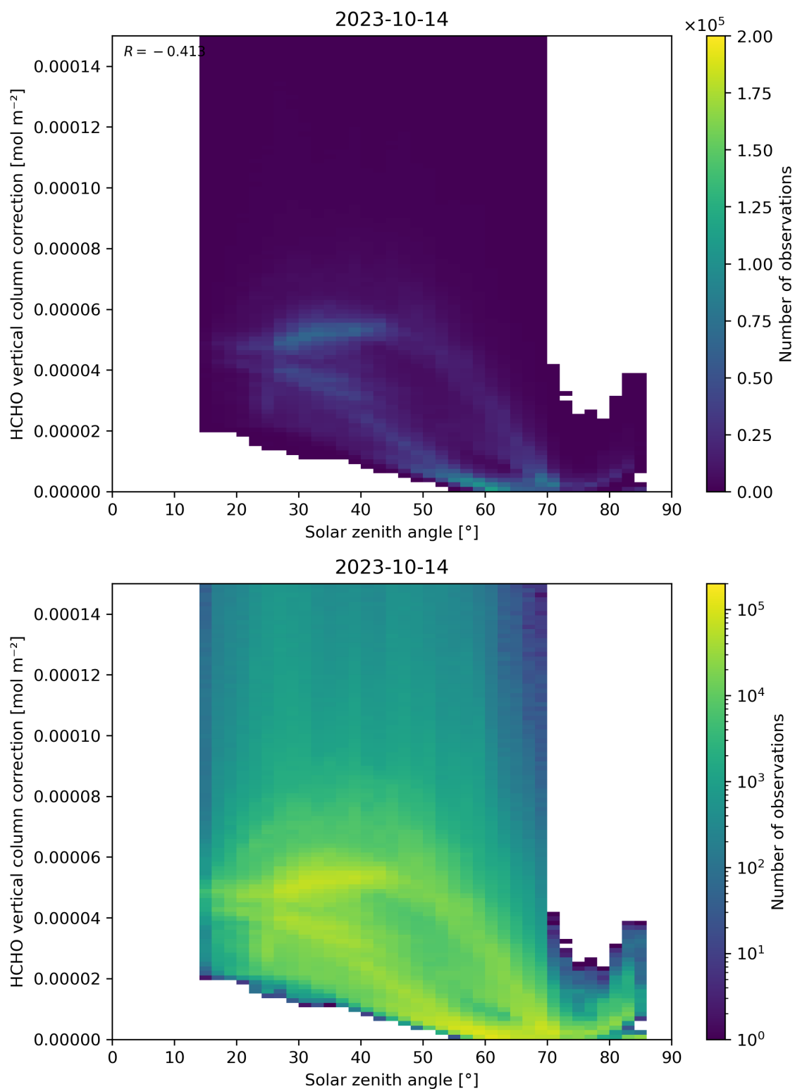
Figure 178: Scatter density plot of “Solar zenith angle” against “HCHO vertical column correction” for 2023-10-13 to 2023-10-15.
