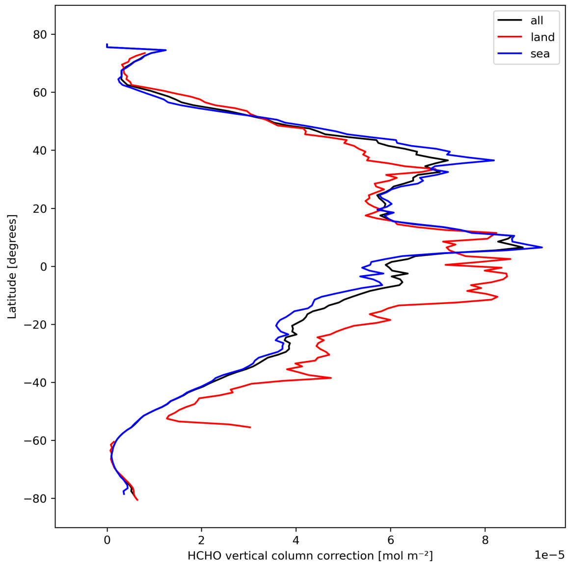
Figure 23: Zonal average of “HCHO vertical column correction” for 2023-10-13 to 2023-10-15.
