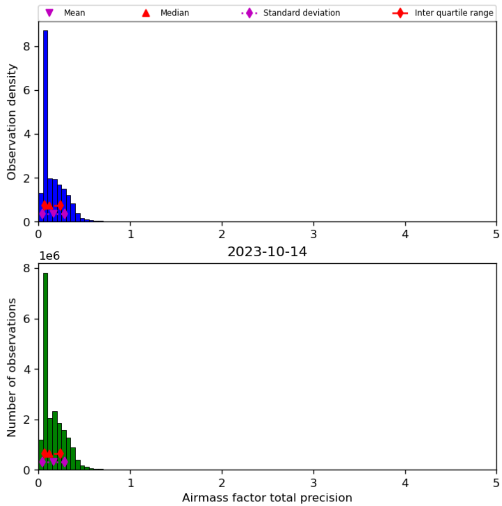
Figure 41: Histogram of “Airmass factor total precision” for 2023-10-13 to 2023-10-15
