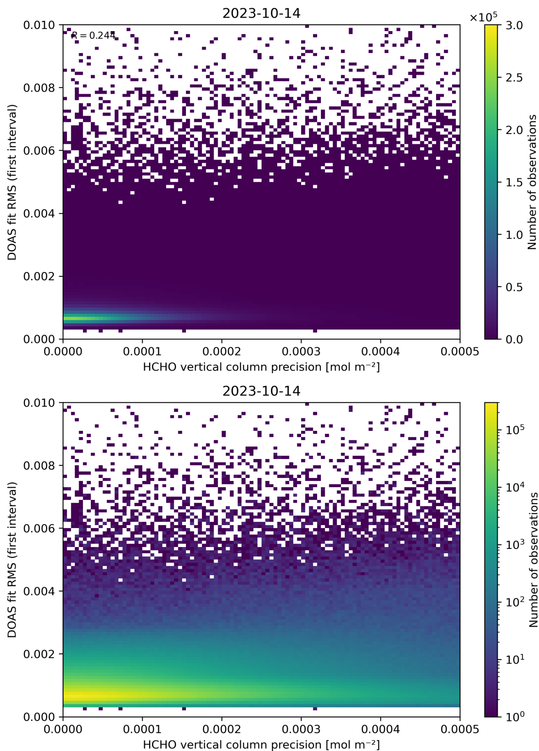
Figure 136: Scatter density plot of “HCHO vertical column precision” against “DOAS fit RMS (first interval)” for 2023-10-13 to 2023-10-15.
