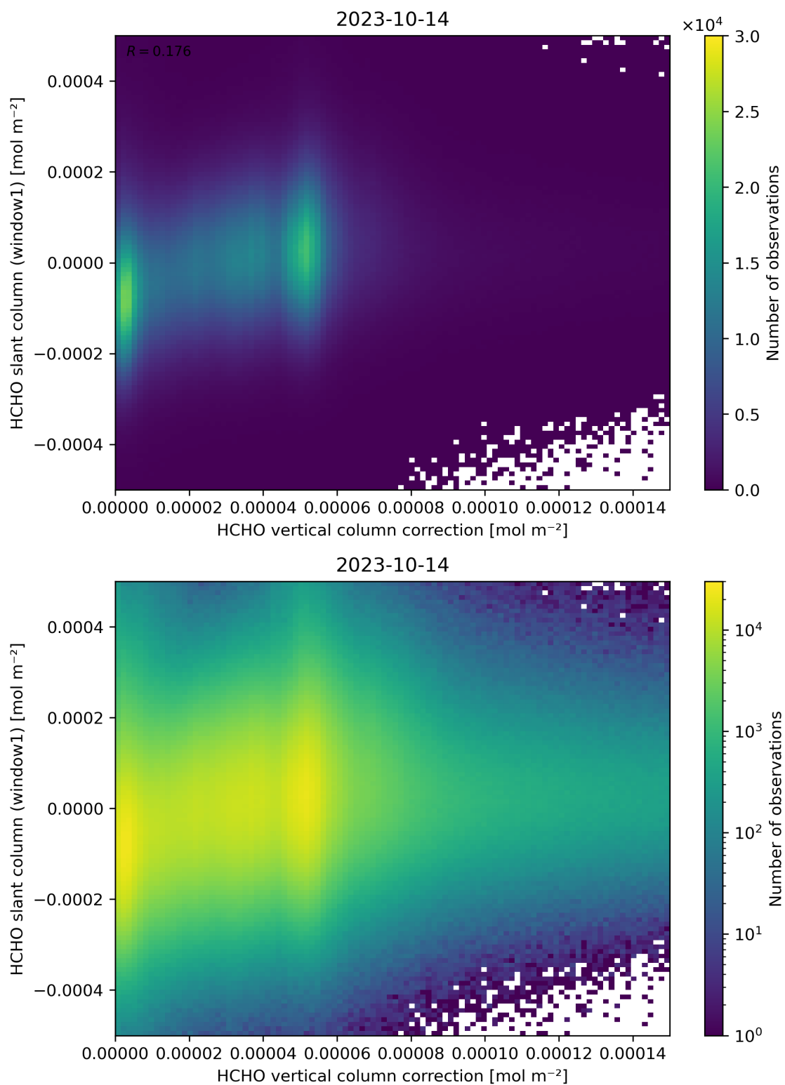
Figure 118: Scatter density plot of “HCHO vertical column correction” against “HCHO slant column (window1)” for 2023-10-13 to 2023-10-15.
