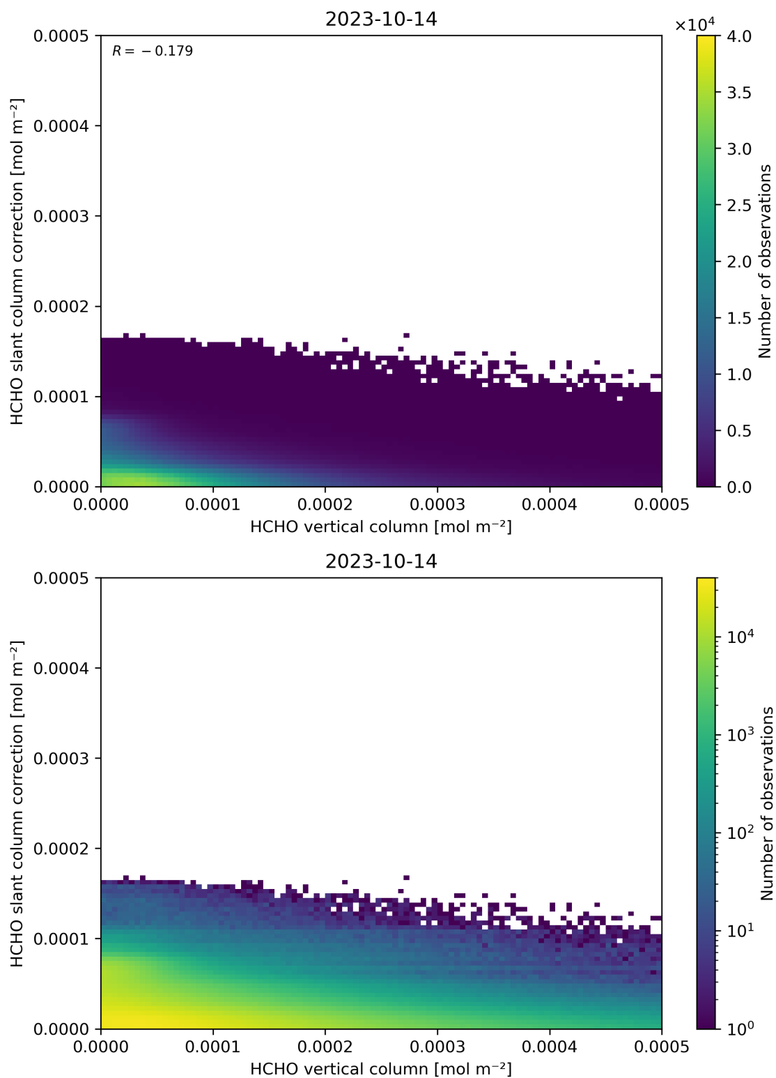
Figure 128: Scatter density plot of “HCHO vertical column” against “HCHO slant column correction” for 2023-10-13 to 2023-10-15.
