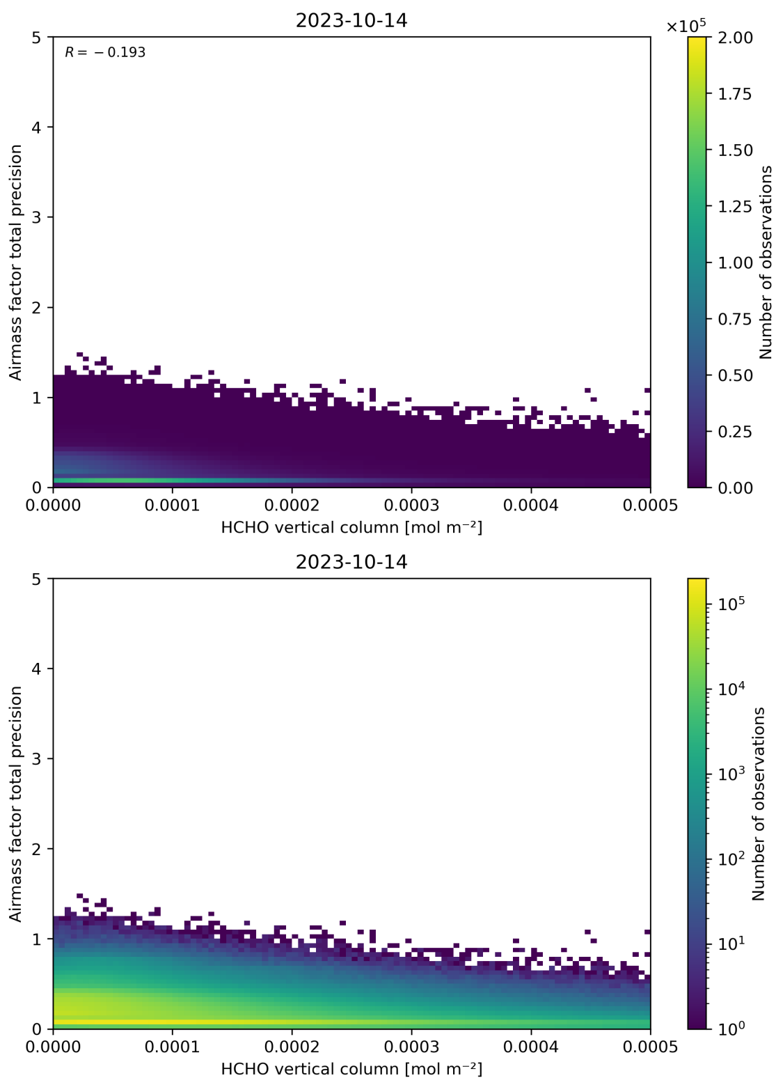
Figure 132: Scatter density plot of “HCHO vertical column” against “Airmass factor total precision” for 2023-10-13 to 2023-10-15.
