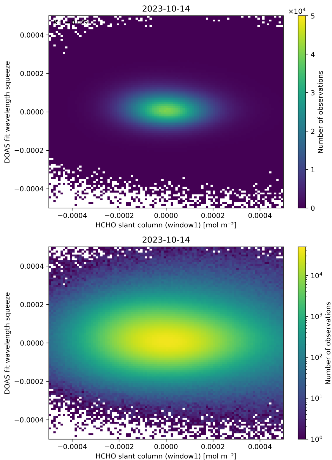
Figure 80: Scatter density plot of “HCHO slant column (window1)” against “DOAS fit wavelength squeeze” for 2023-10-13 to 2023-10-15.
