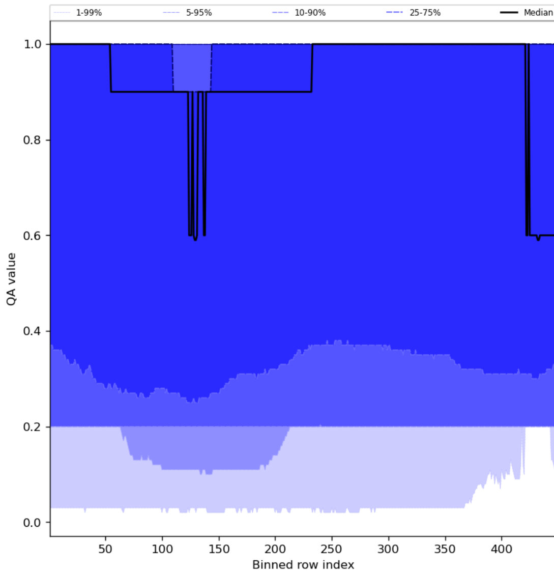
Figure 48: Along track statistics of “QA value” for 2023-10-13 to 2023-10-15
