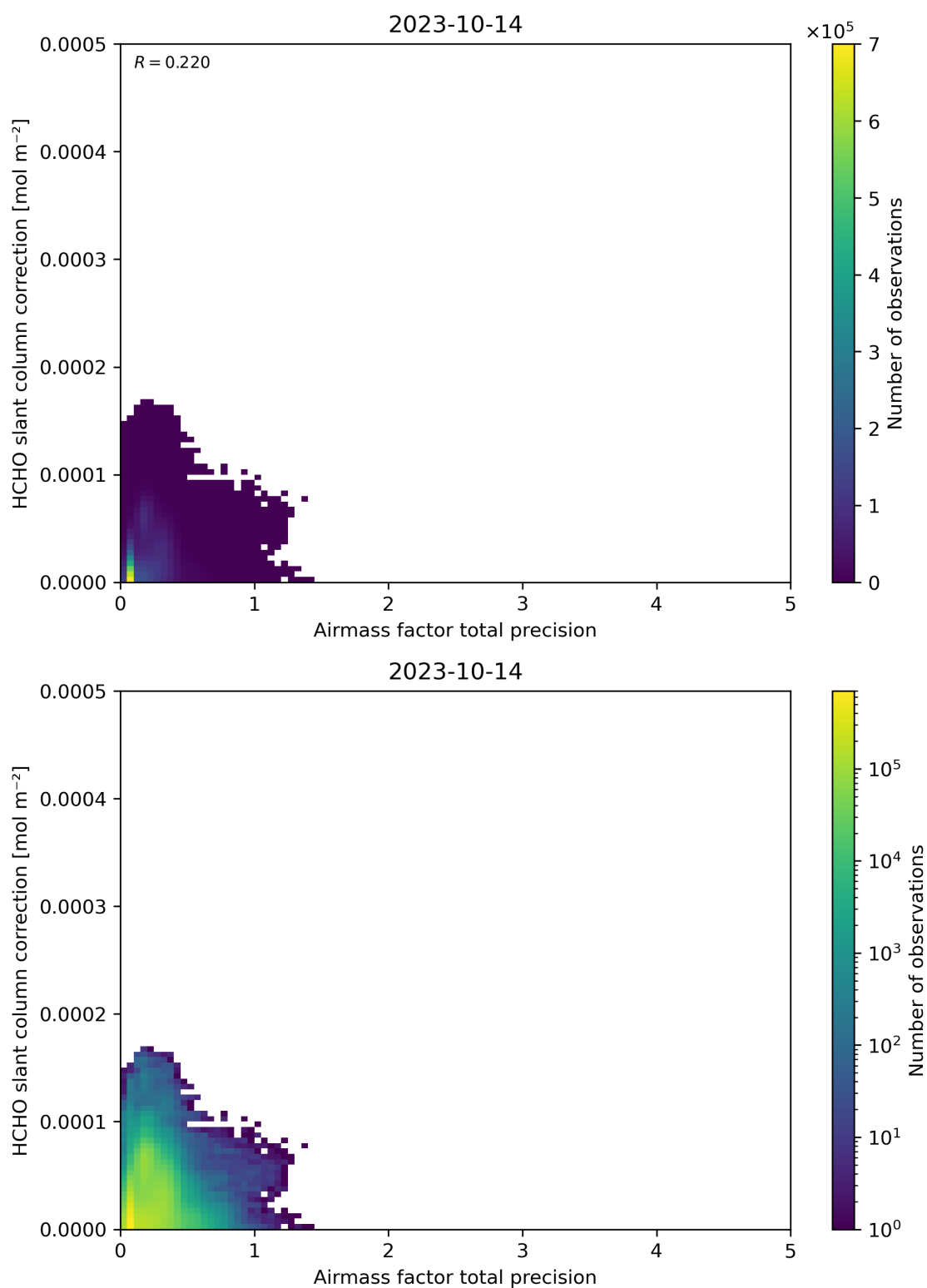
Figure 110: Scatter density plot of “Airmass factor total precision” against “HCHO slant column correction” for 2023-10-13 to 2023-10-15.
