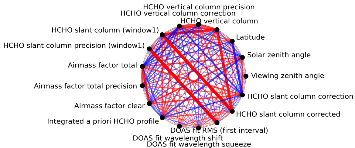
Figure 1: Map of correlation graph for 2023-10-13 to 2023-10-15.
