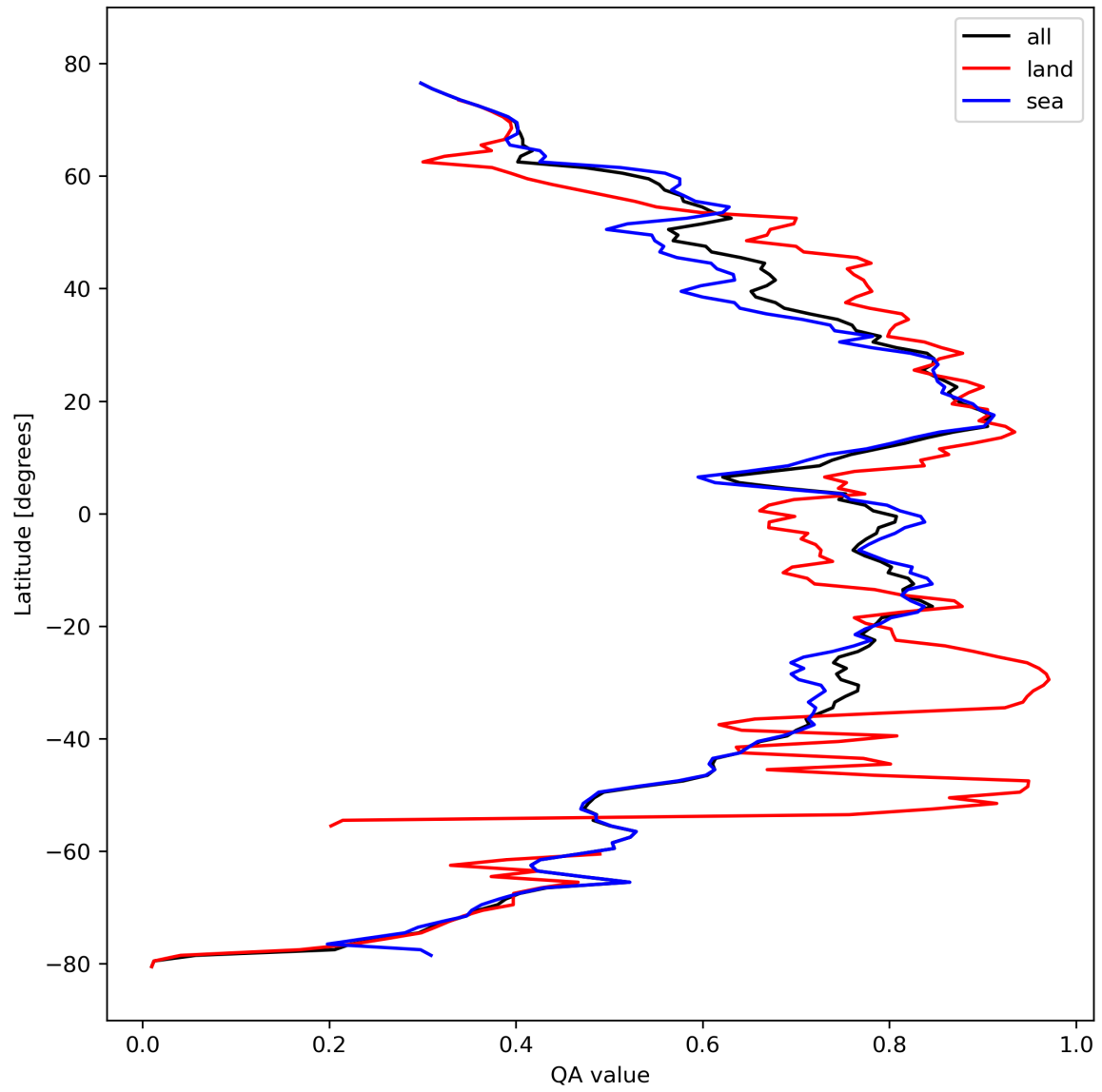
Figure 20: Zonal average of “QA value” for 2023-10-13 to 2023-10-15.
