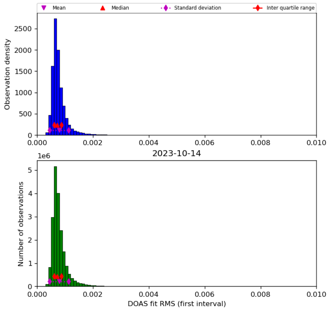
Figure 46: Histogram of “DOAS fit RMS (first interval)” for 2023-10-13 to 2023-10-15
