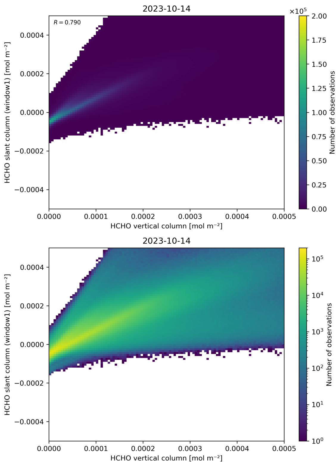
Figure 129: Scatter density plot of “HCHO vertical column” against “HCHO slant column (window1)” for 2023-10-13 to 2023-10-15.
