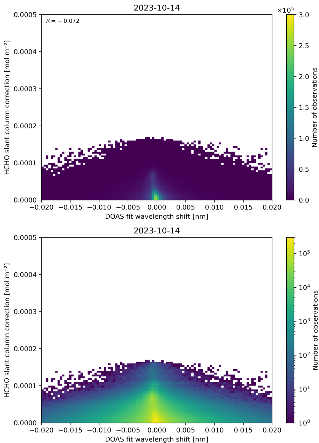
Figure 67: Scatter density plot of “DOAS fit wavelength shift” against “HCHO slant column correction” for 2023-10-13 to 2023-10-15.
