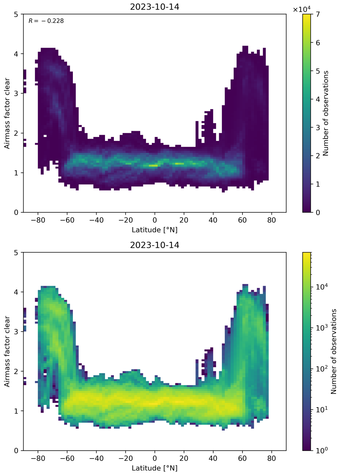
Figure 156: Scatter density plot of “Latitude” against “Airmass factor clear” for 2023-10-13 to 2023-10-15.
