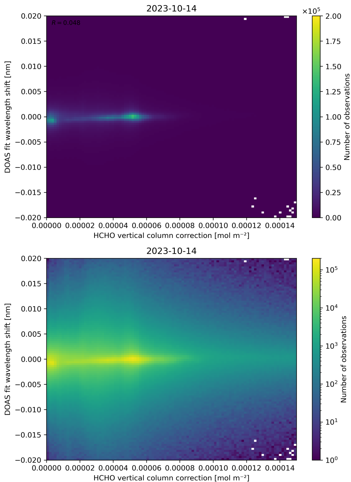
Figure 113: Scatter density plot of “HCHO vertical column correction” against “DOAS fit wavelength shift” for 2023-10-13 to 2023-10-15.
