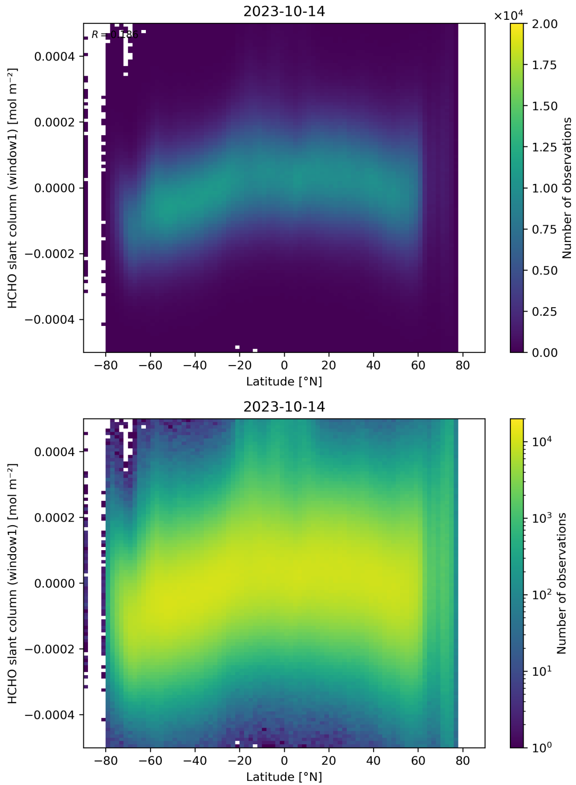
Figure 159: Scatter density plot of “Latitude” against “HCHO slant column (window1)” for 2023-10-13 to 2023-10-15.
