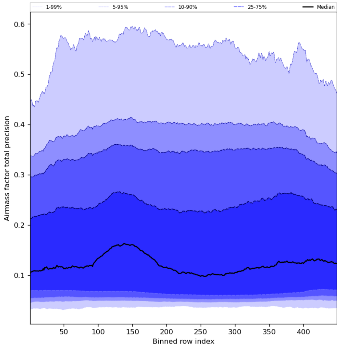
Figure 55: Along track statistics of “Airmass factor total precision” for 2023-10-13 to 2023-10-15
