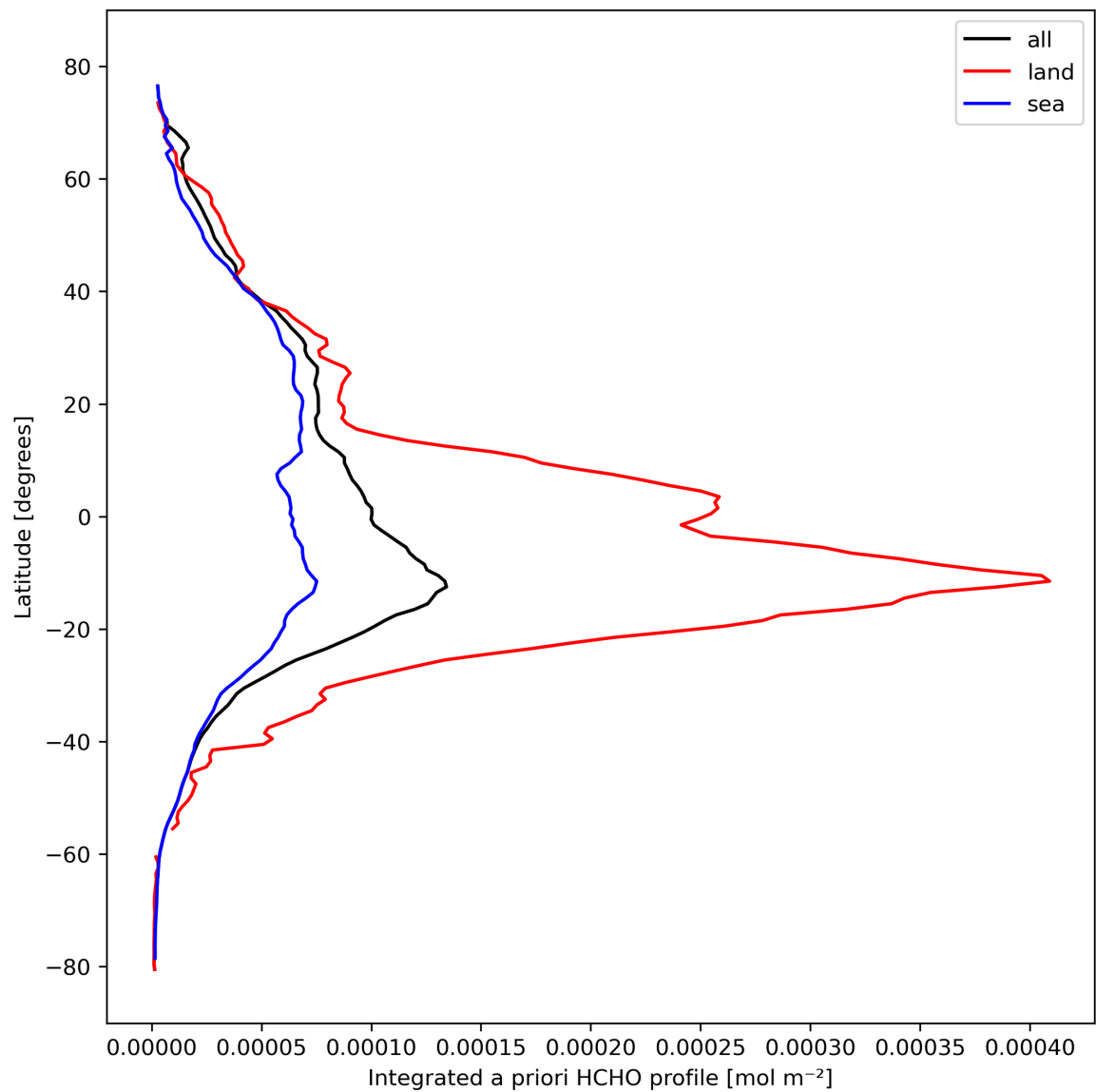
Figure 29: Zonal average of “Integrated a priori HCHO profile” for 2023-10-13 to 2023-10-15.
