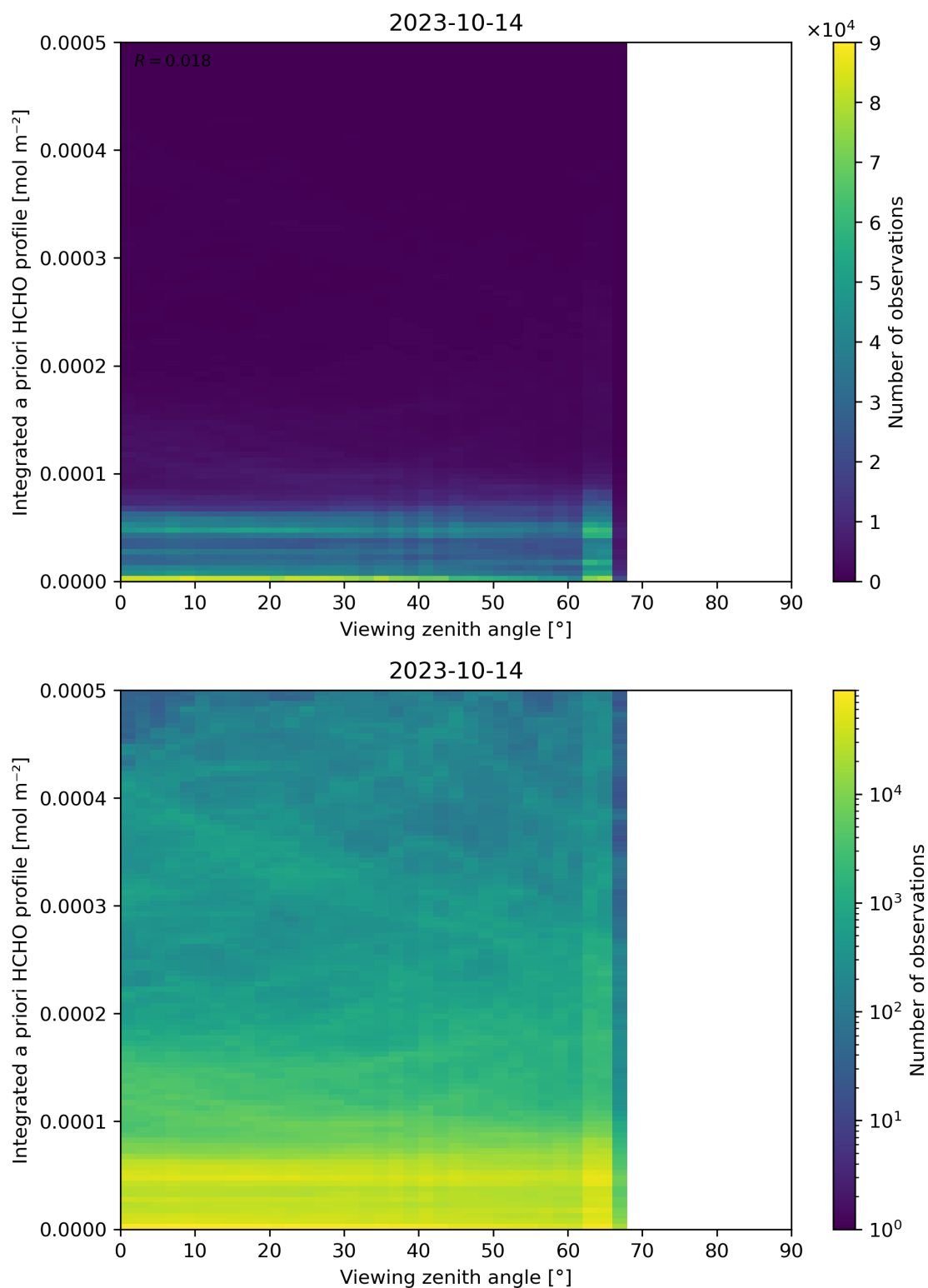
Figure 195: Scatter density plot of “Viewing zenith angle” against “Integrated a priori HCHO profile” for 2023-10-13 to 2023-10-15.
