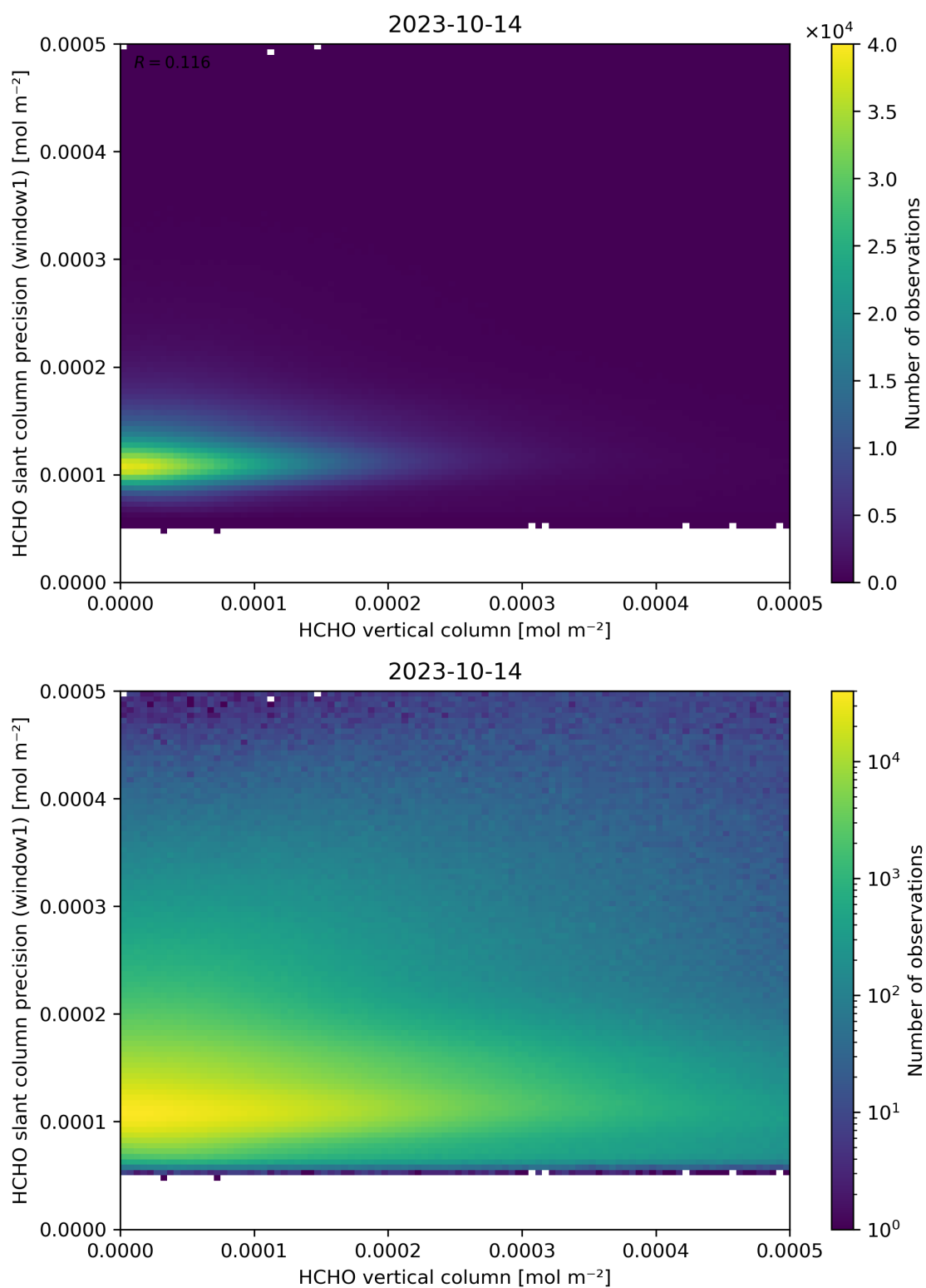
Figure 130: Scatter density plot of “HCHO vertical column” against “HCHO slant column precision (window1)” for 2023-10-13 to 2023-10-15.
