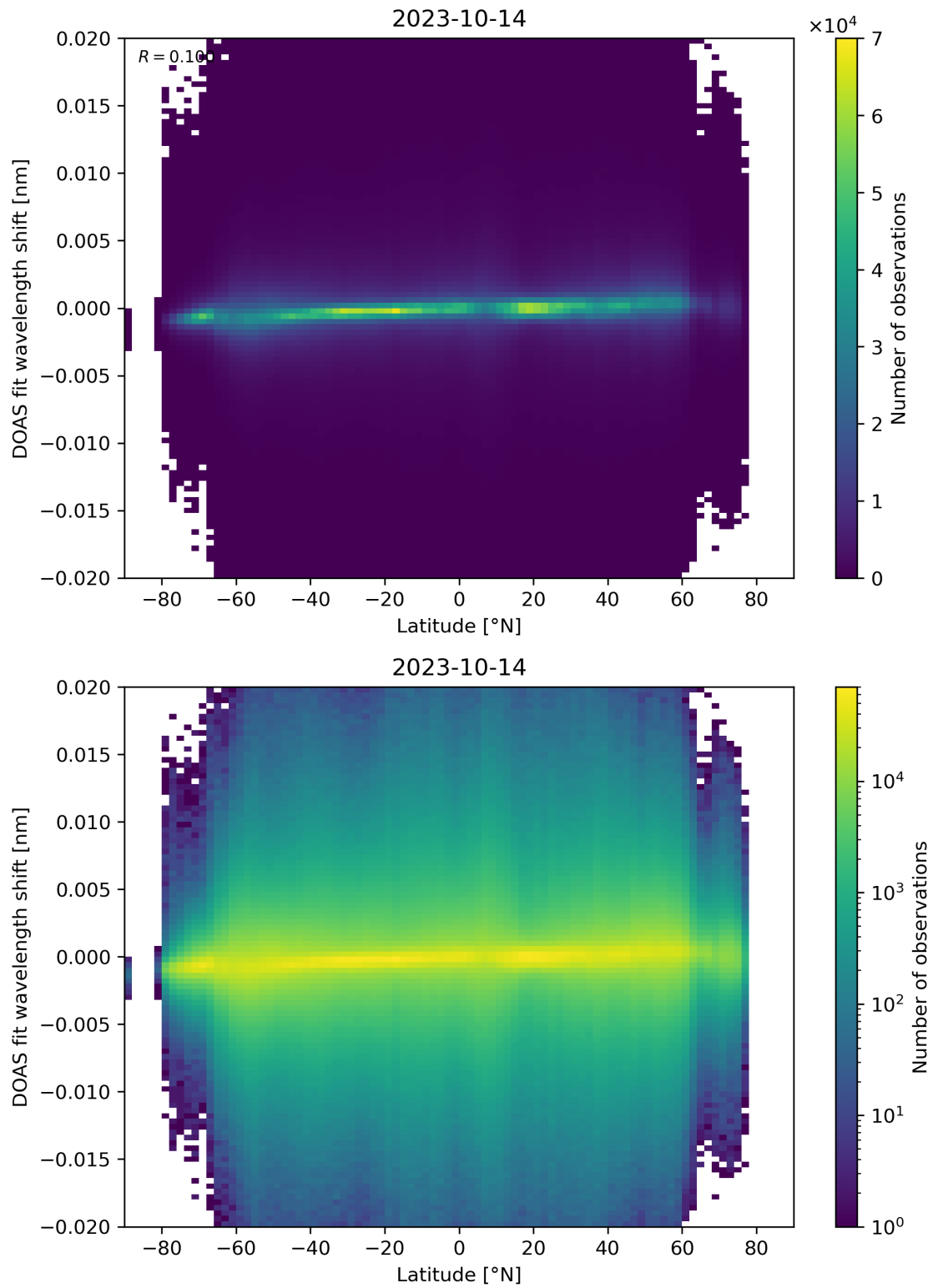
Figure 154: Scatter density plot of “Latitude” against “DOAS fit wavelength shift” for 2023-10-13 to 2023-10-15.
