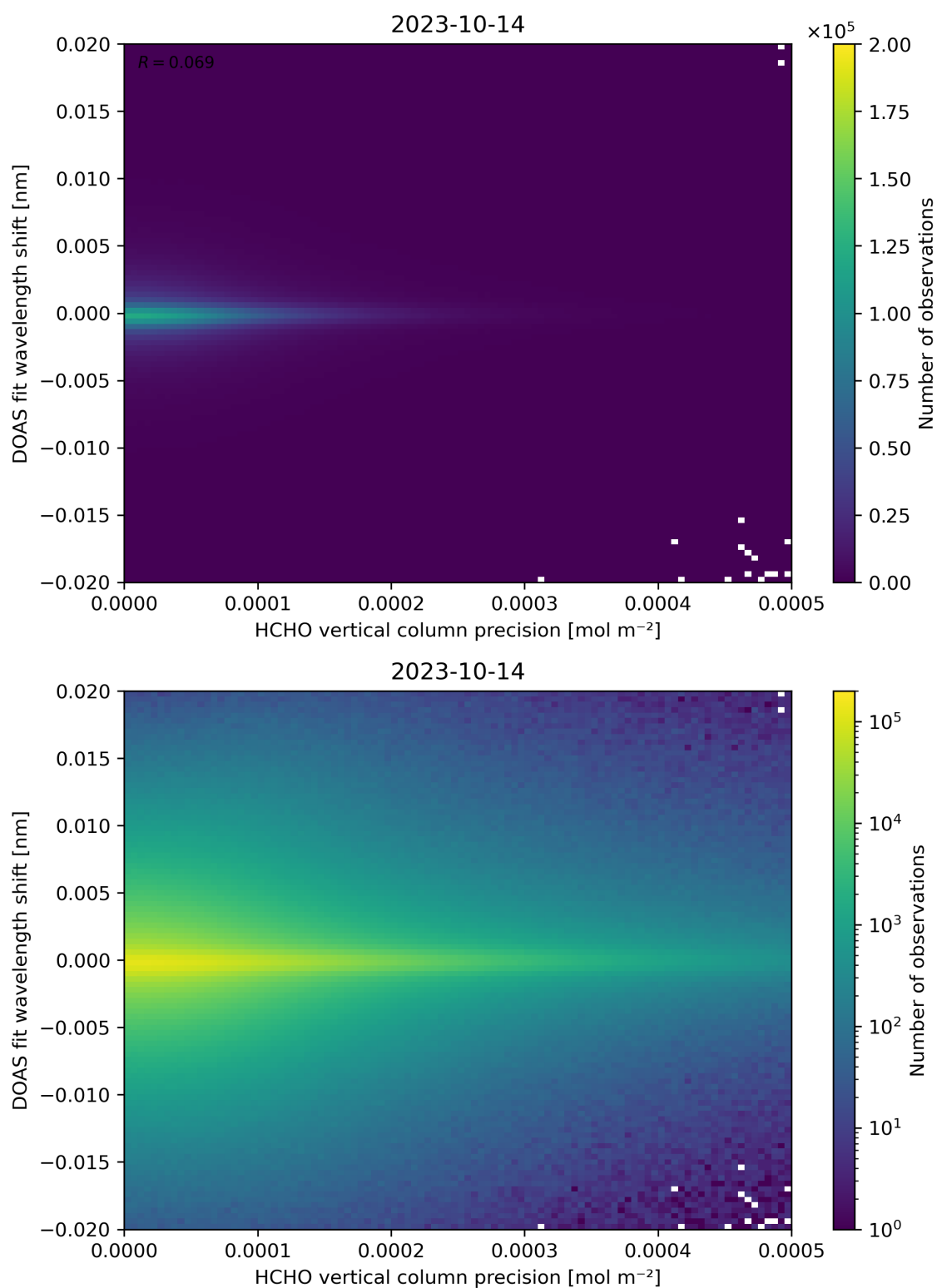
Figure 137: Scatter density plot of “HCHO vertical column precision” against “DOAS fit wavelength shift” for 2023-10-13 to 2023-10-15.
