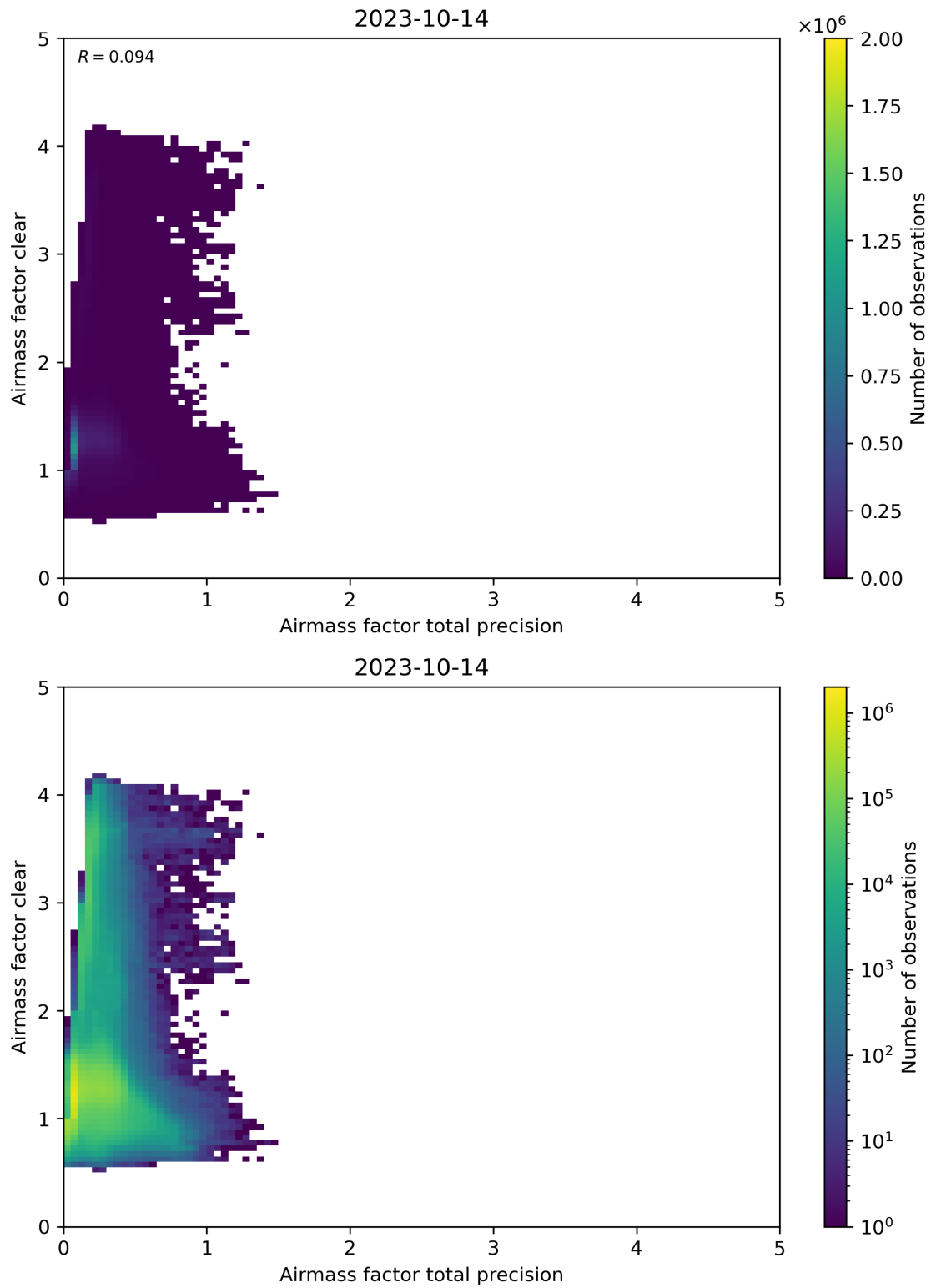
Figure 108: Scatter density plot of “Airmass factor total precision” against “Airmass factor clear” for 2023-10-13 to 2023-10-15.
