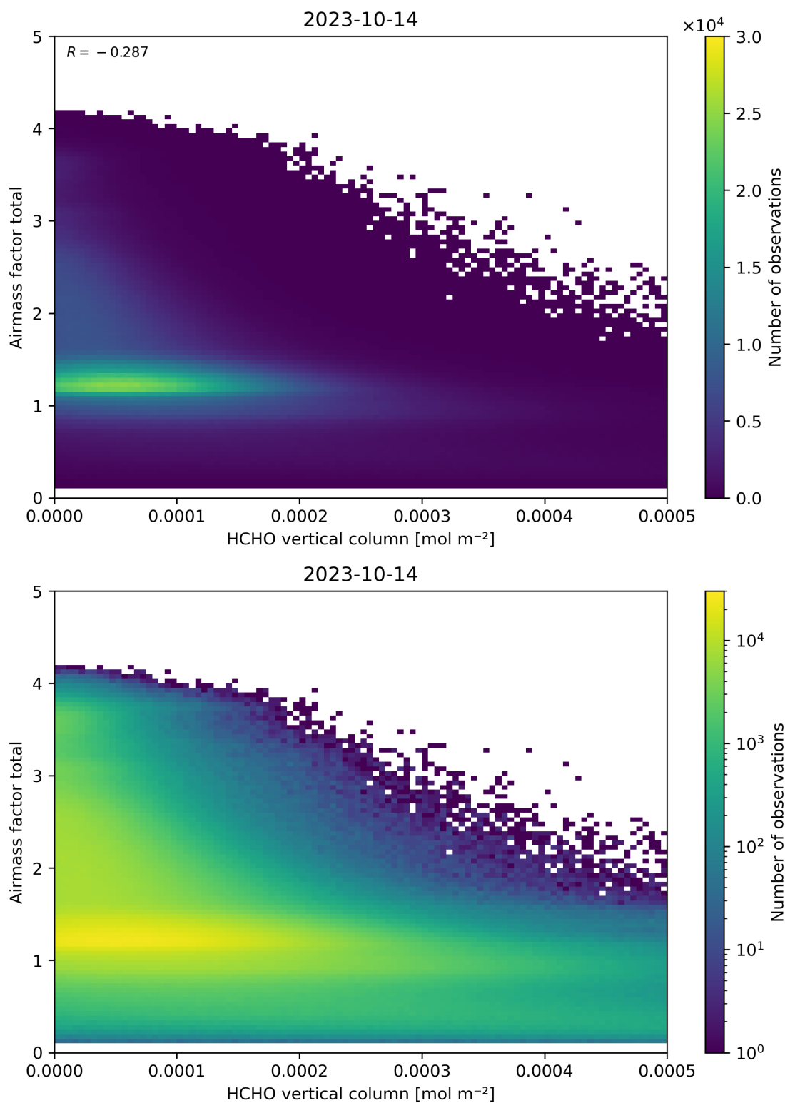
Figure 131: Scatter density plot of “HCHO vertical column” against “Airmass factor total” for 2023-10-13 to 2023-10-15.
