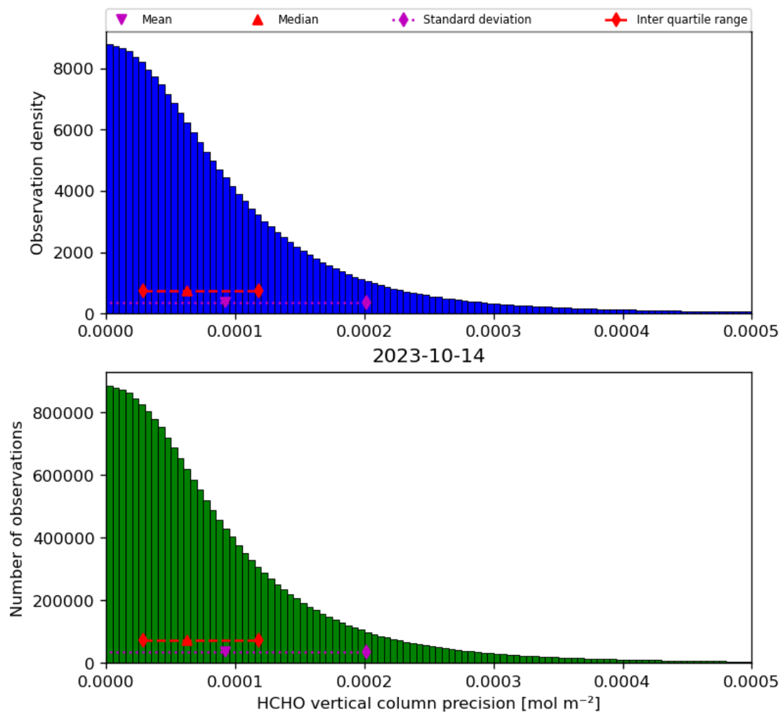
Figure 36: Histogram of “HCHO vertical column precision” for 2023-10-13 to 2023-10-15
