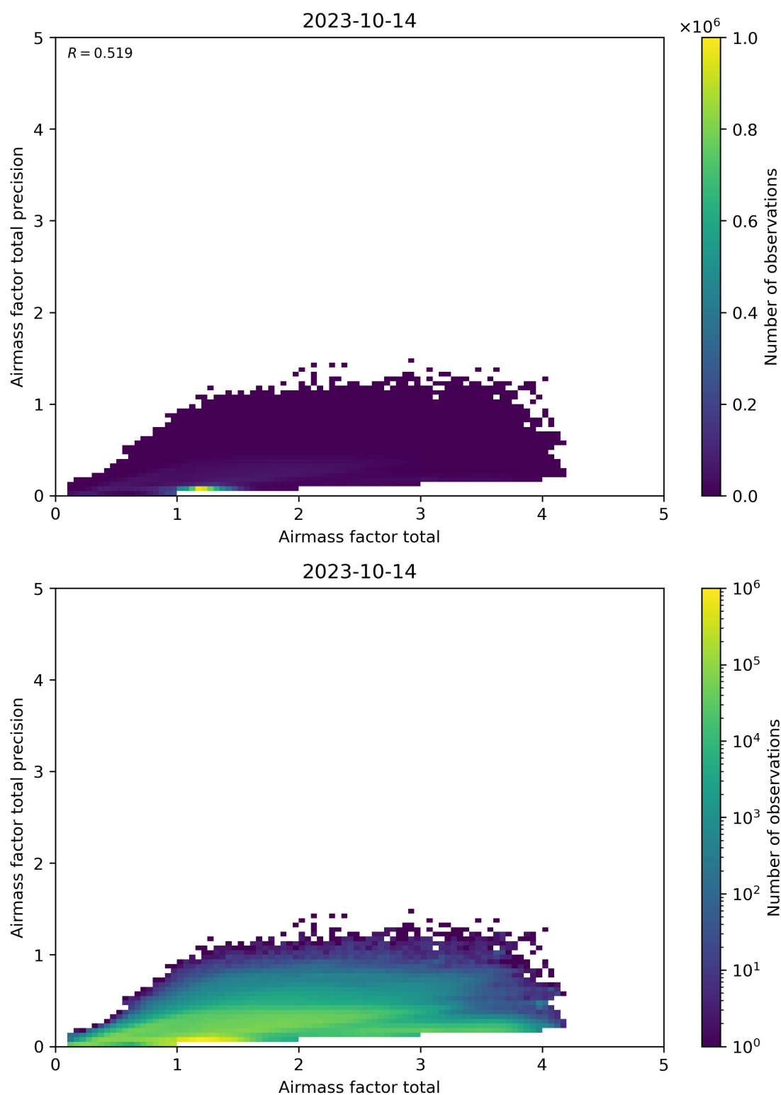
Figure 103: Scatter density plot of “Airmass factor total” against “Airmass factor total precision” for 2023-10-13 to 2023-10-15.
