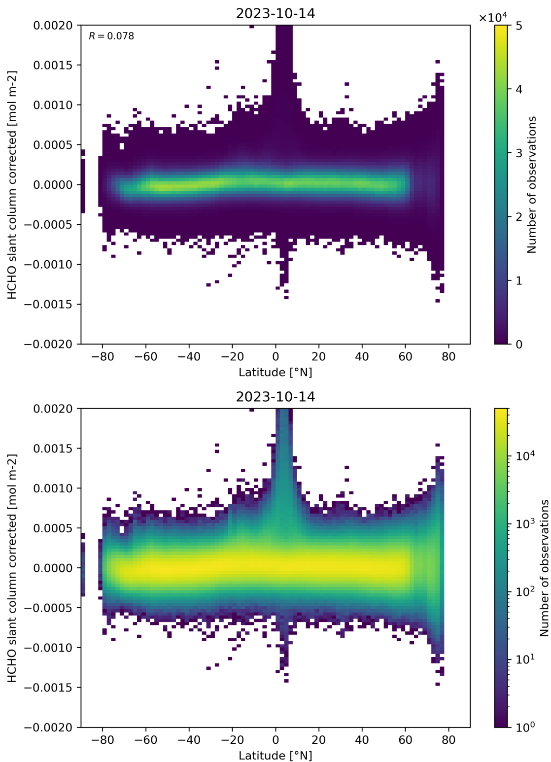
Figure 157: Scatter density plot of “Latitude” against “HCHO slant column corrected” for 2023-10-13 to 2023-10-15.
