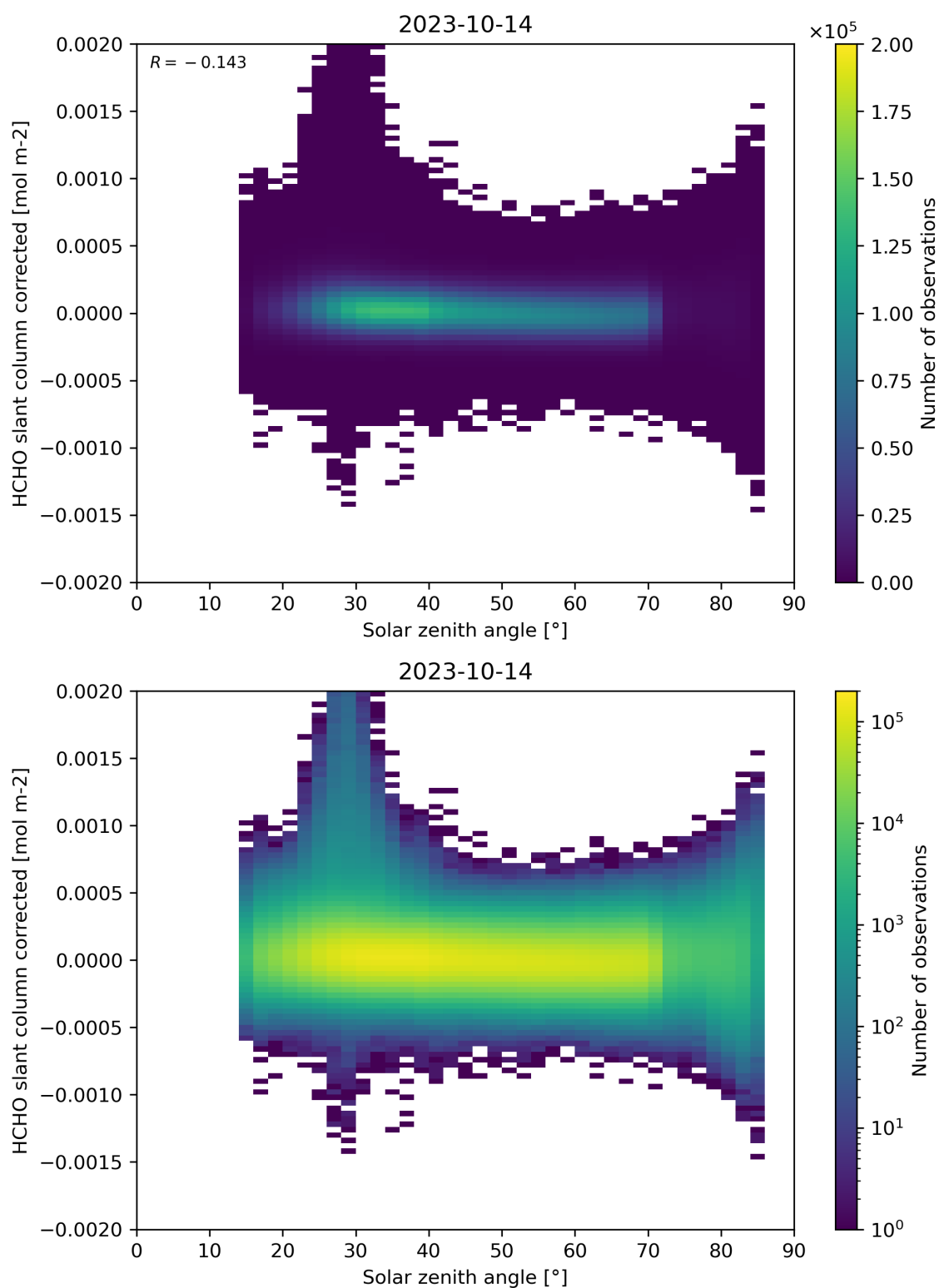
Figure 171: Scatter density plot of “Solar zenith angle” against “HCHO slant column corrected” for 2023-10-13 to 2023-10-15.
