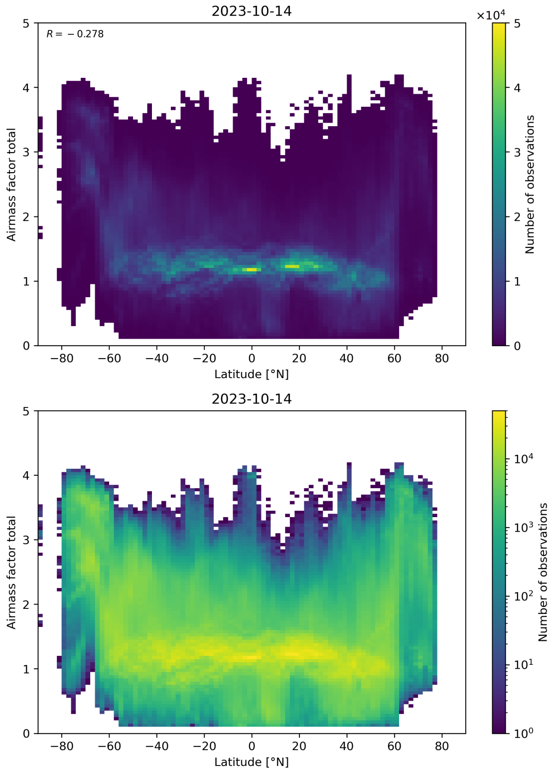
Figure 161: Scatter density plot of “Latitude” against “Airmass factor total” for 2023-10-13 to 2023-10-15.
