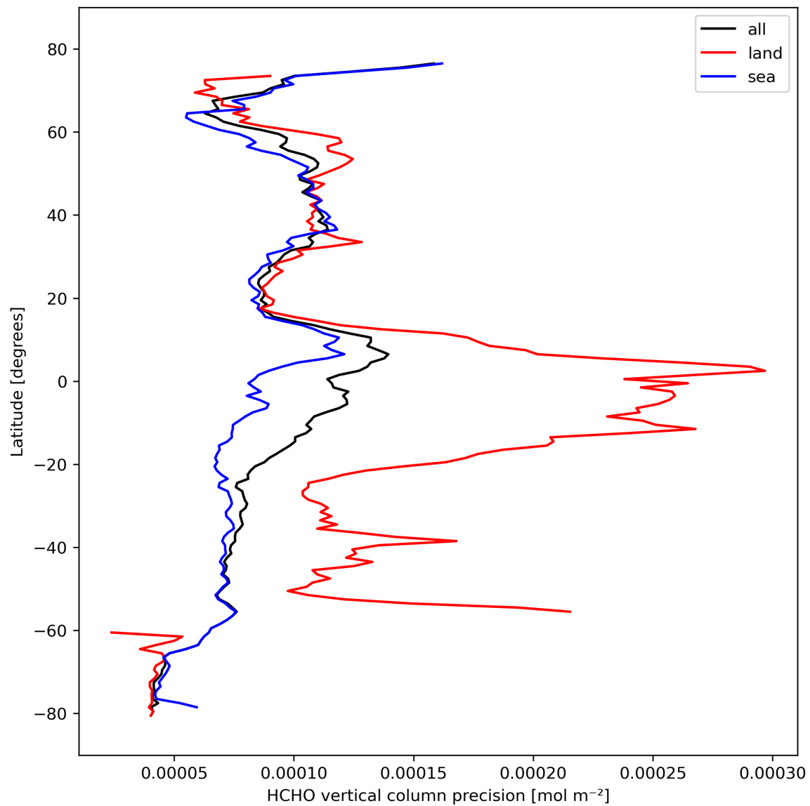
Figure 22: Zonal average of “HCHO vertical column precision” for 2023-10-13 to 2023-10-15.
