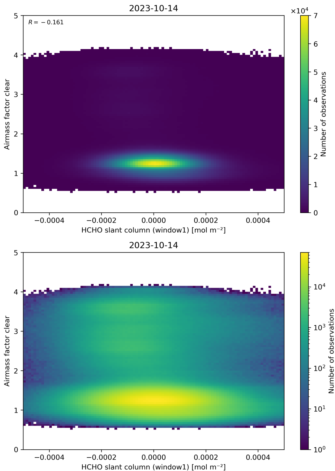
Figure 81: Scatter density plot of “HCHO slant column (window1)” against “Airmass factor clear” for 2023-10-13 to 2023-10-15.
