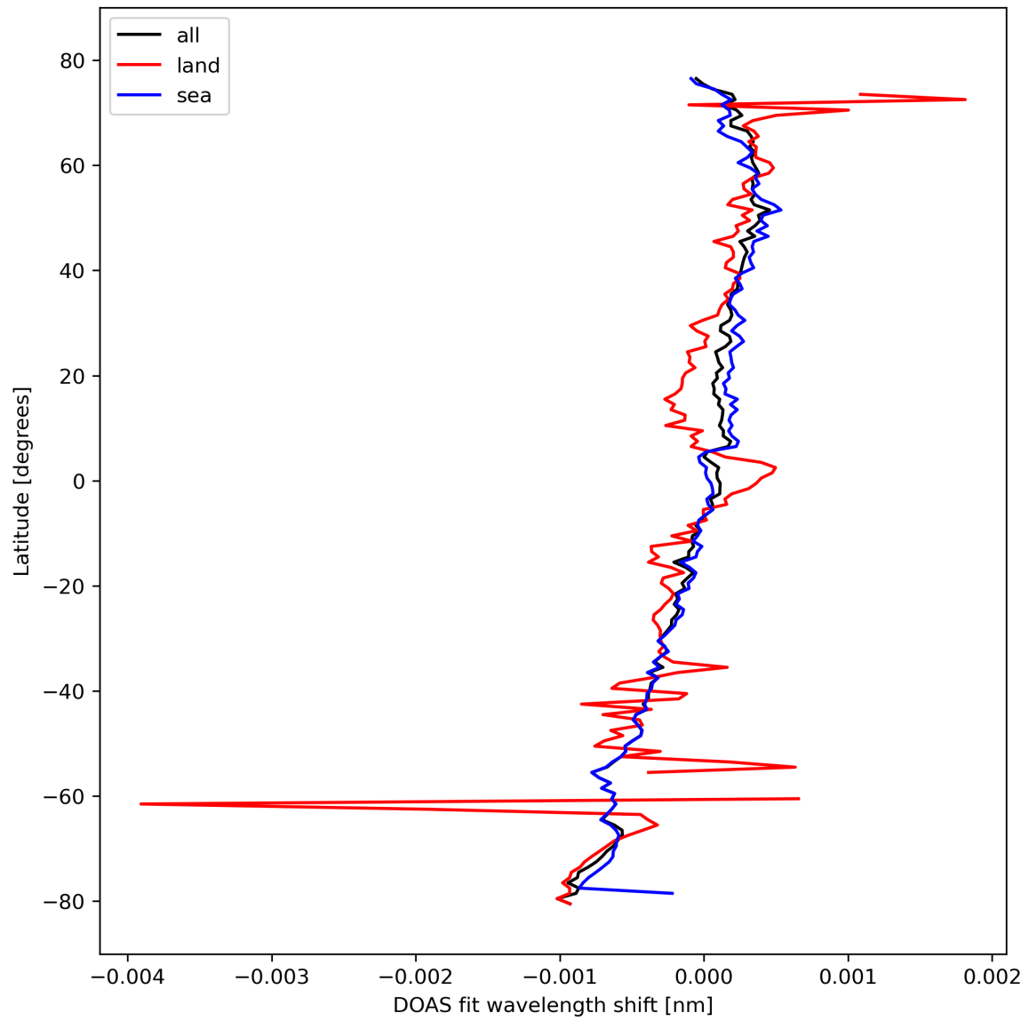
Figure 30: Zonal average of “DOAS fit wavelength shift” for 2023-10-13 to 2023-10-15.
