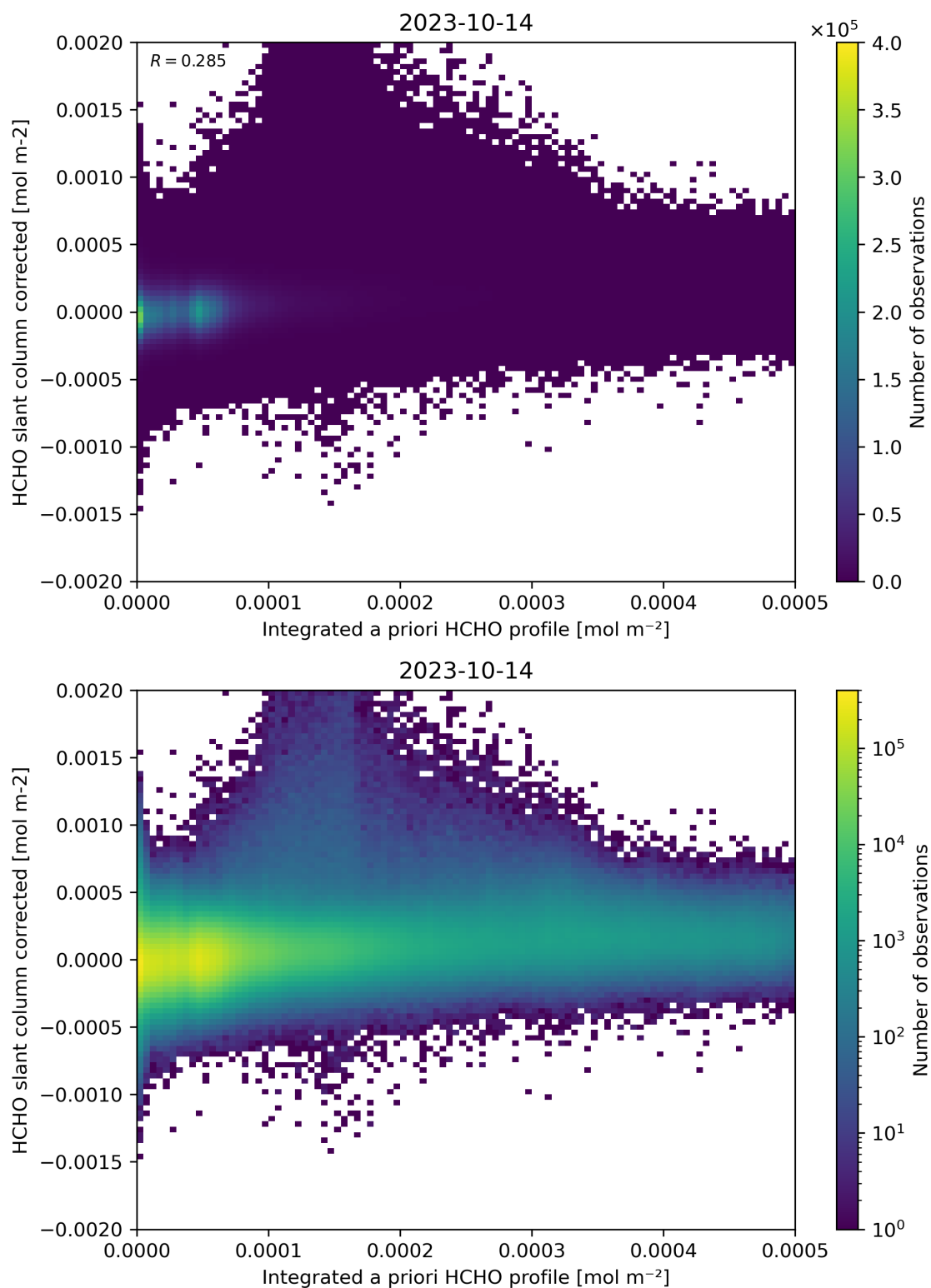
Figure 151: Scatter density plot of “Integrated a priori HCHO profile” against “HCHO slant column corrected” for 2023-10-13 to 2023-10-15.
