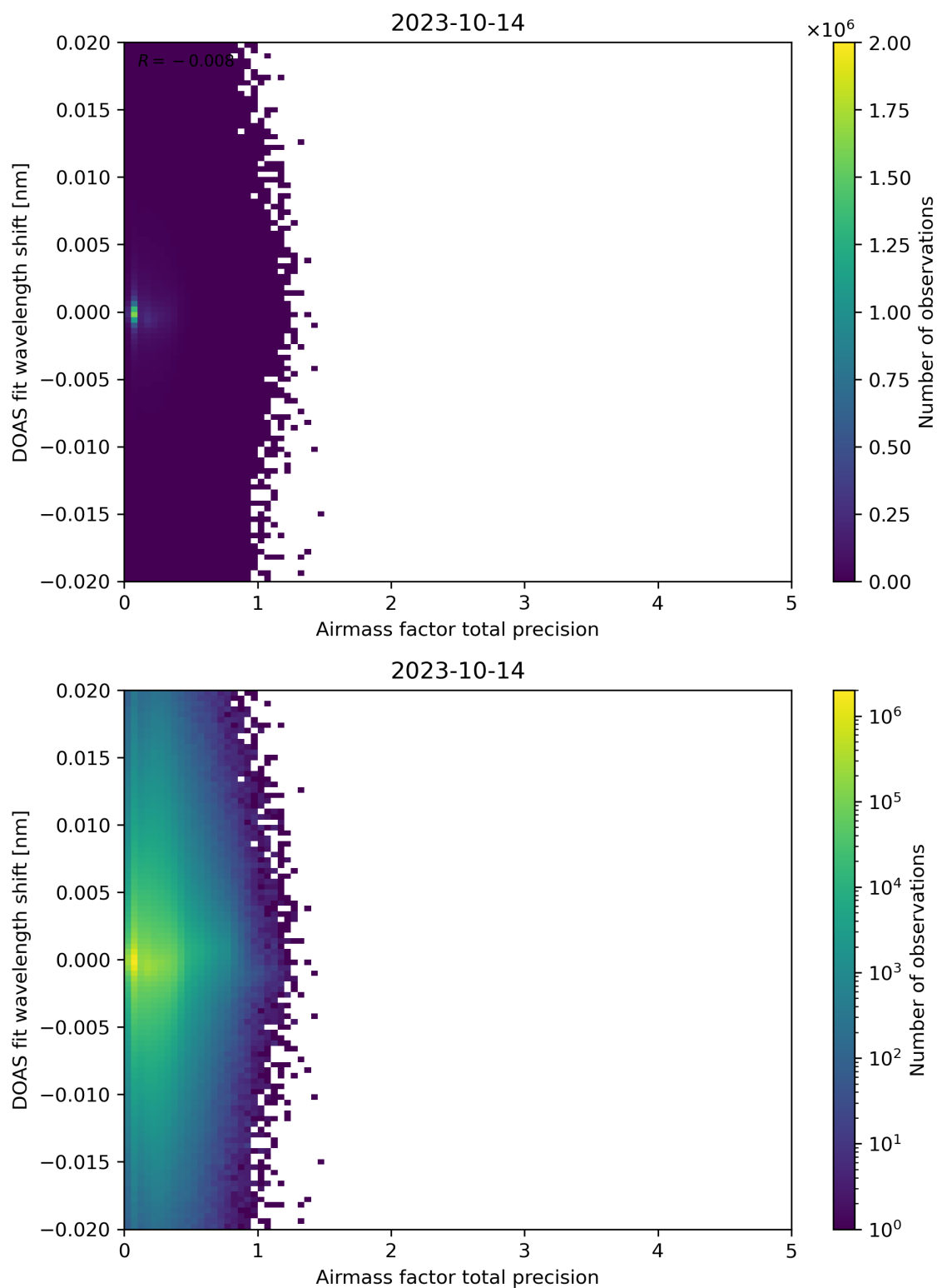
Figure 106: Scatter density plot of “Airmass factor total precision” against “DOAS fit wavelength shift” for 2023-10-13 to 2023-10-15.
