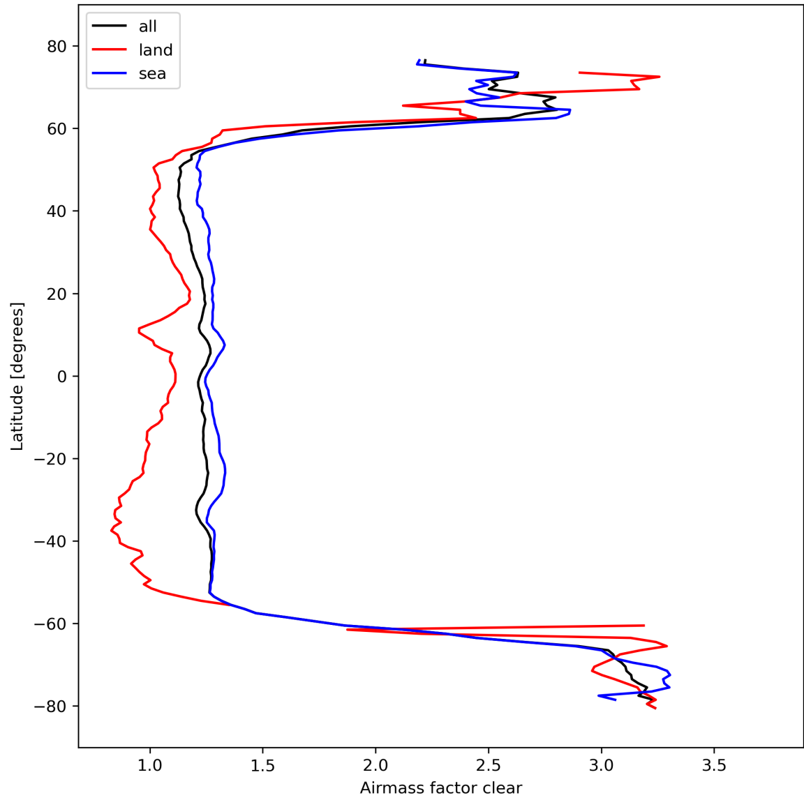
Figure 28: Zonal average of “Airmass factor clear” for 2023-10-13 to 2023-10-15.
