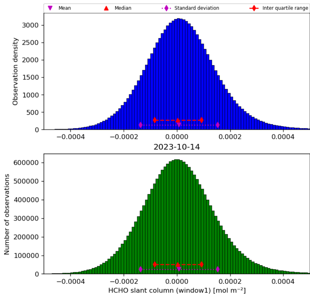
Figure 38: Histogram of “HCHO slant column (window1)” for 2023-10-13 to 2023-10-15
