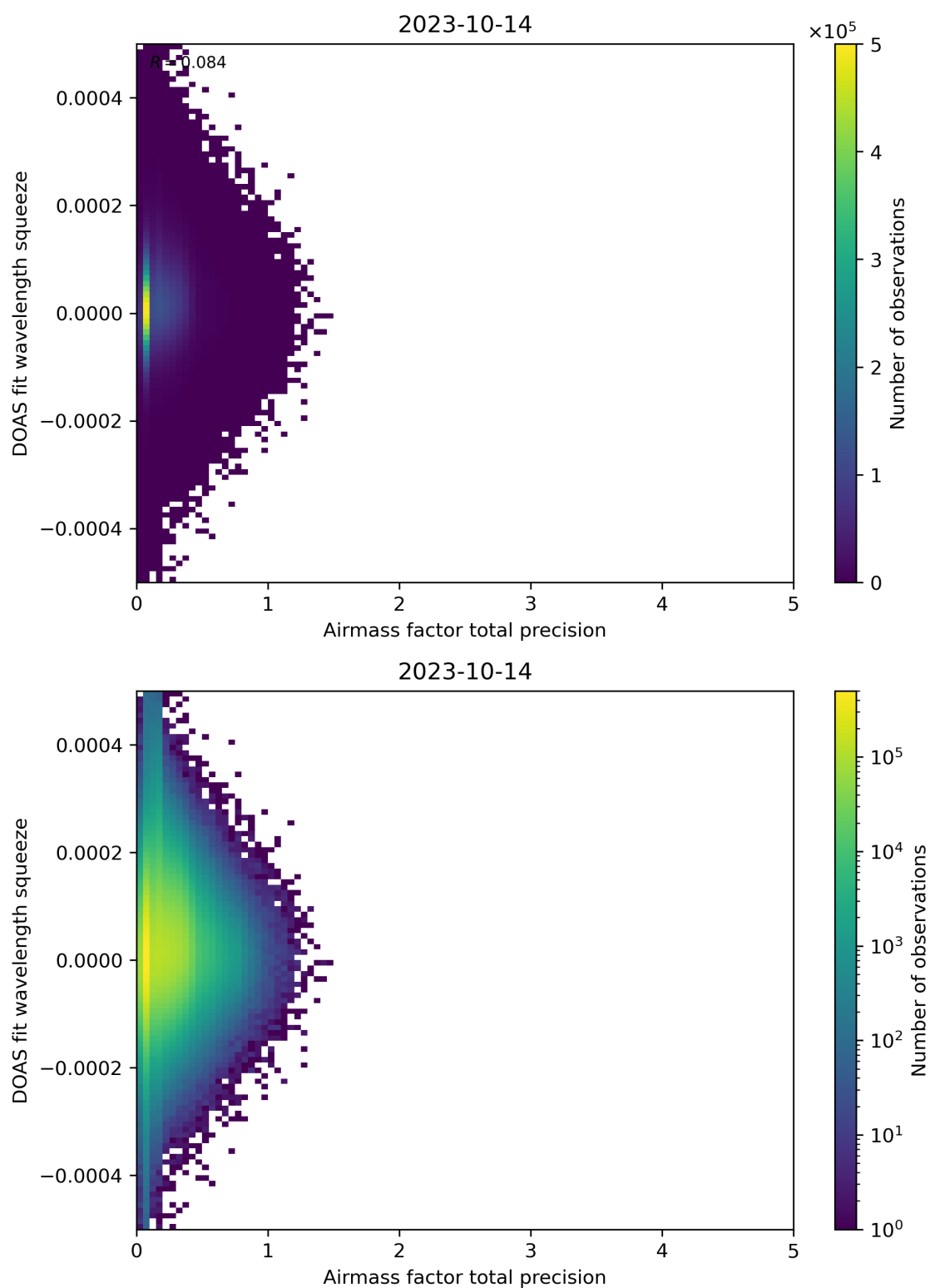
Figure 107: Scatter density plot of “Airmass factor total precision” against “DOAS fit wavelength squeeze” for 2023-10-13 to 2023-10-15.
