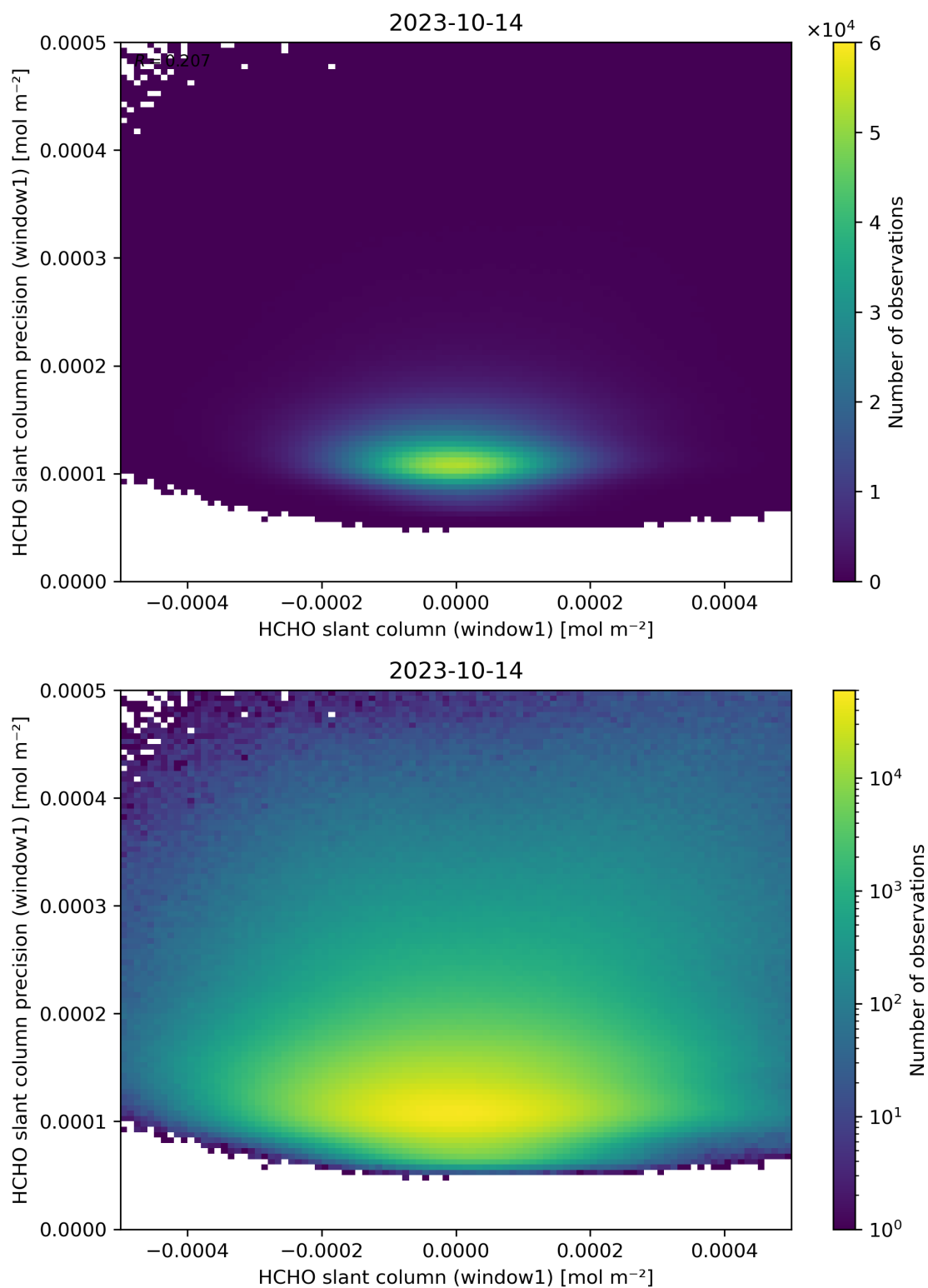
Figure 84: Scatter density plot of “HCHO slant column (window1)” against “HCHO slant column precision (window1)” for 2023-10-13 to 2023-10-15.
