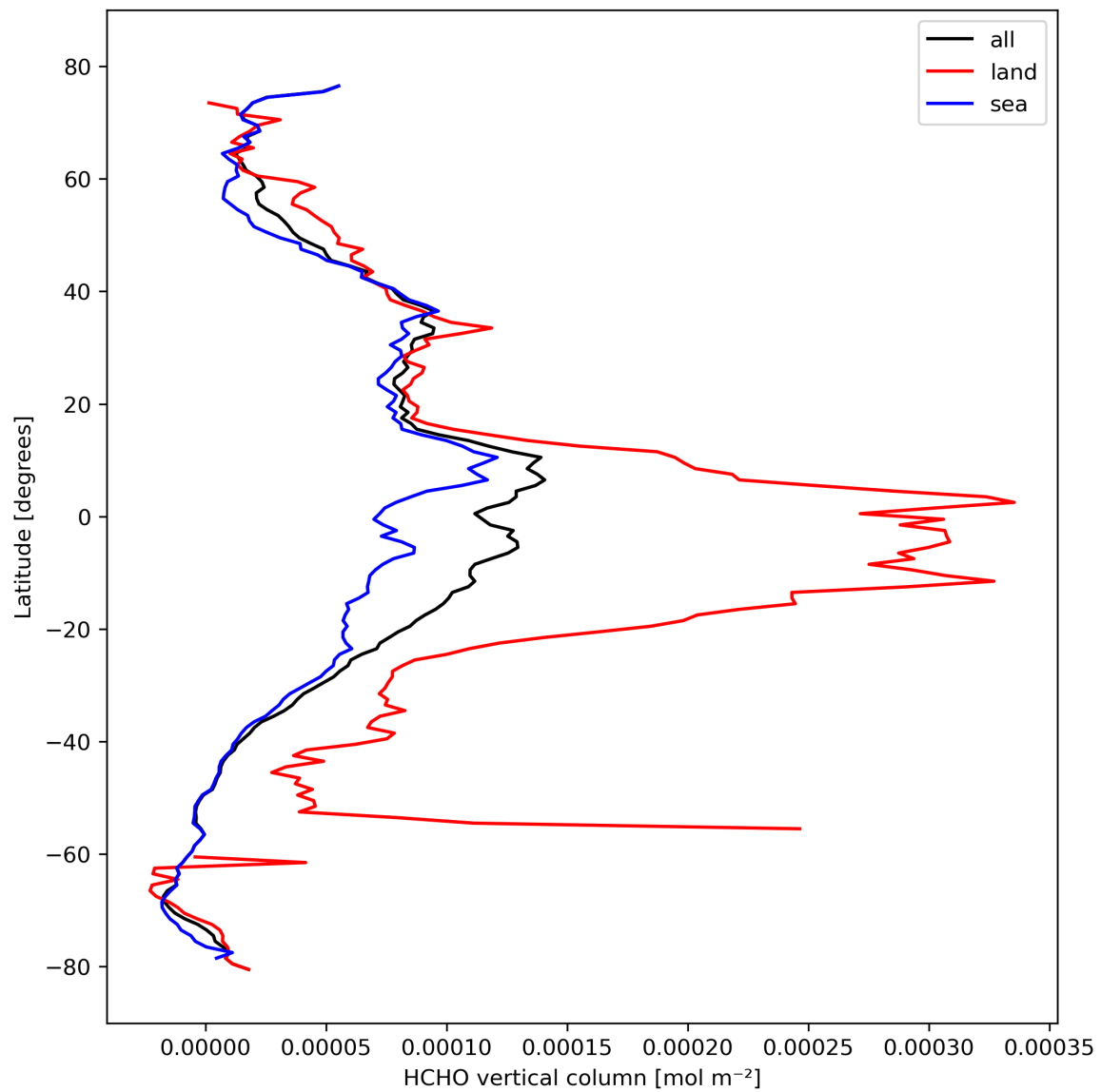
Figure 21: Zonal average of “HCHO vertical column” for 2023-10-13 to 2023-10-15.
