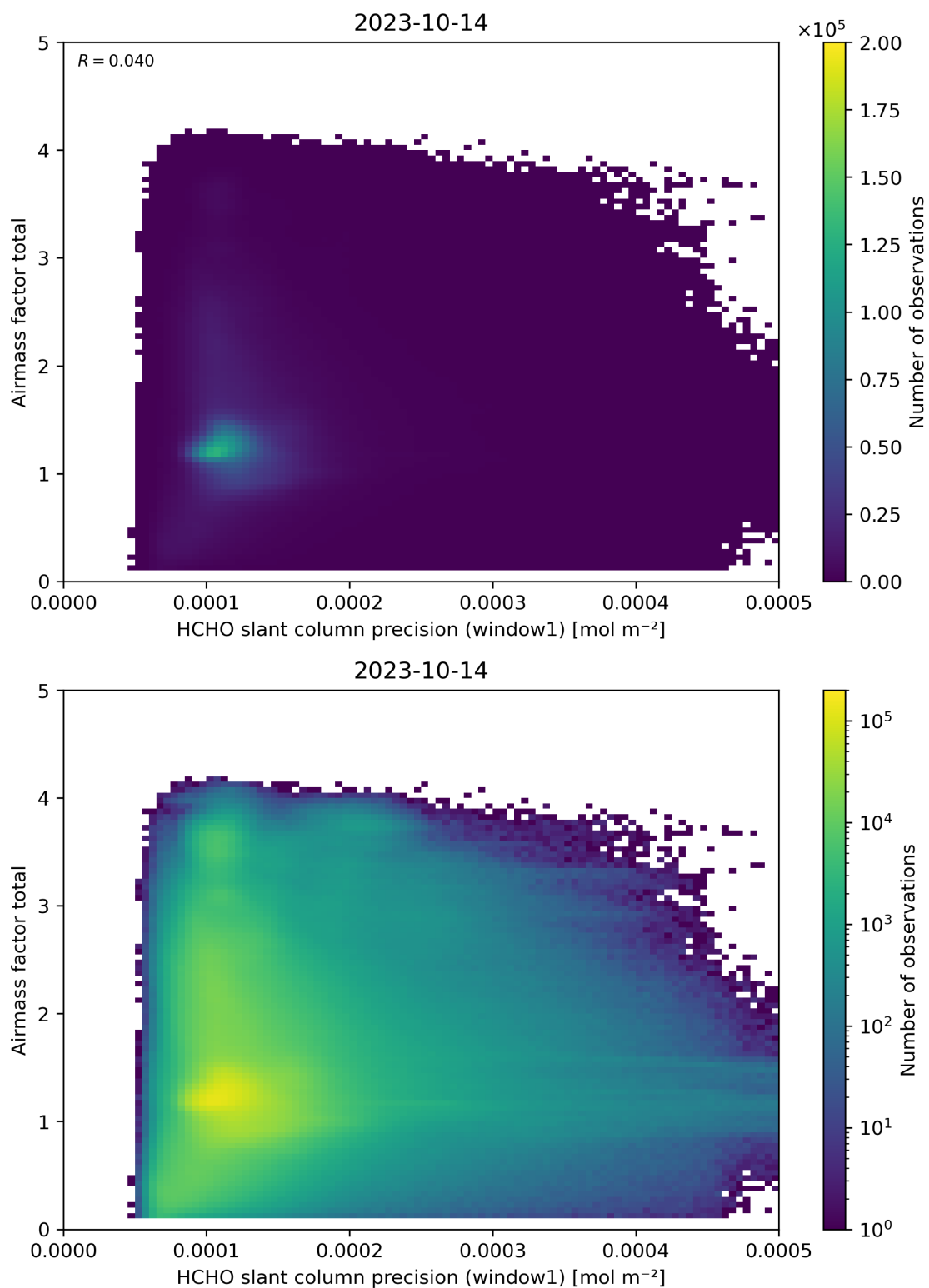
Figure 94: Scatter density plot of “HCHO slant column precision (window1)” against “Airmass factor total” for 2023-10-13 to 2023-10-15.
