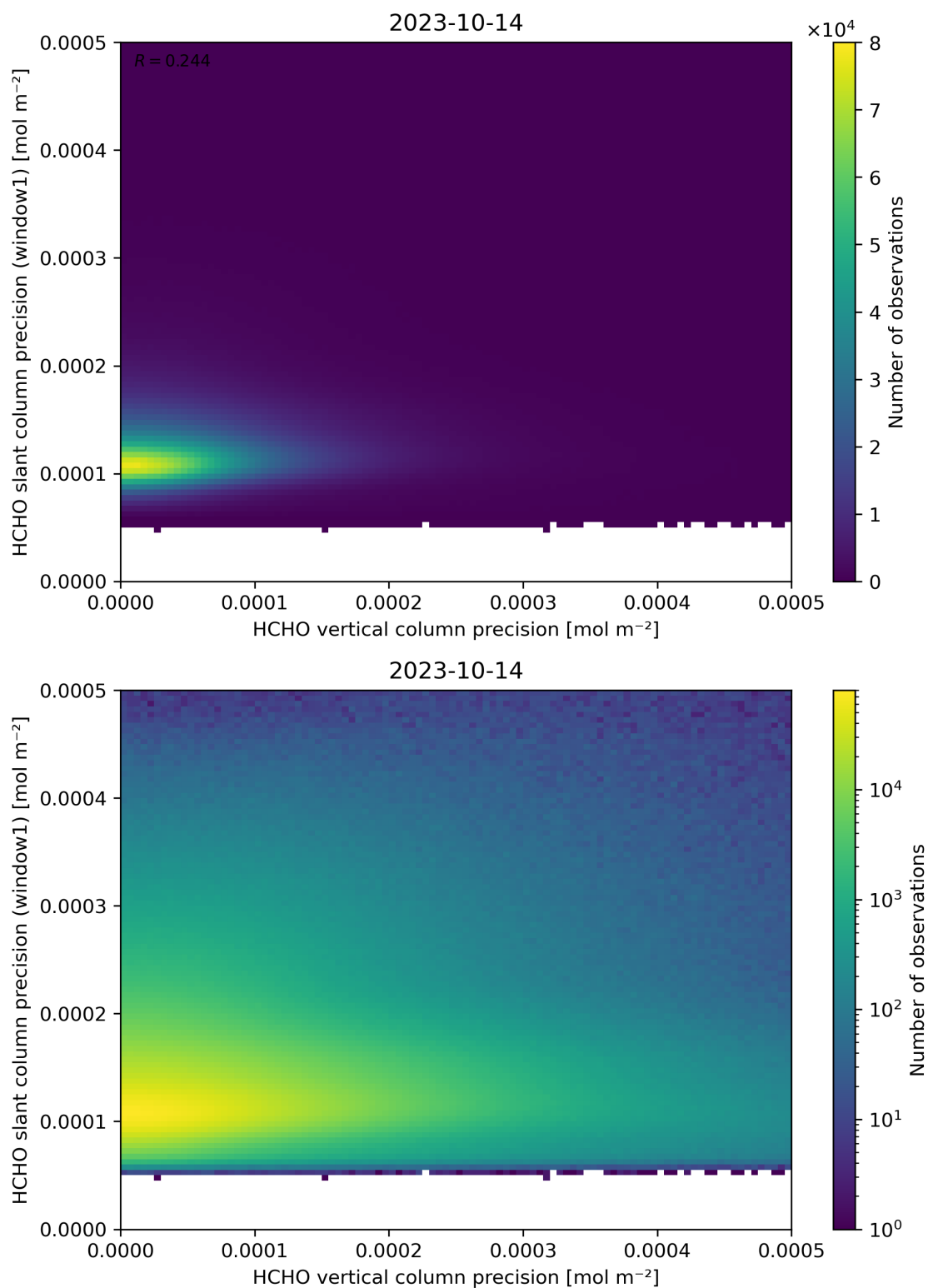
Figure 143: Scatter density plot of “HCHO vertical column precision” against “HCHO slant column precision (window1)” for 2023-10-13 to 2023-10-15.
