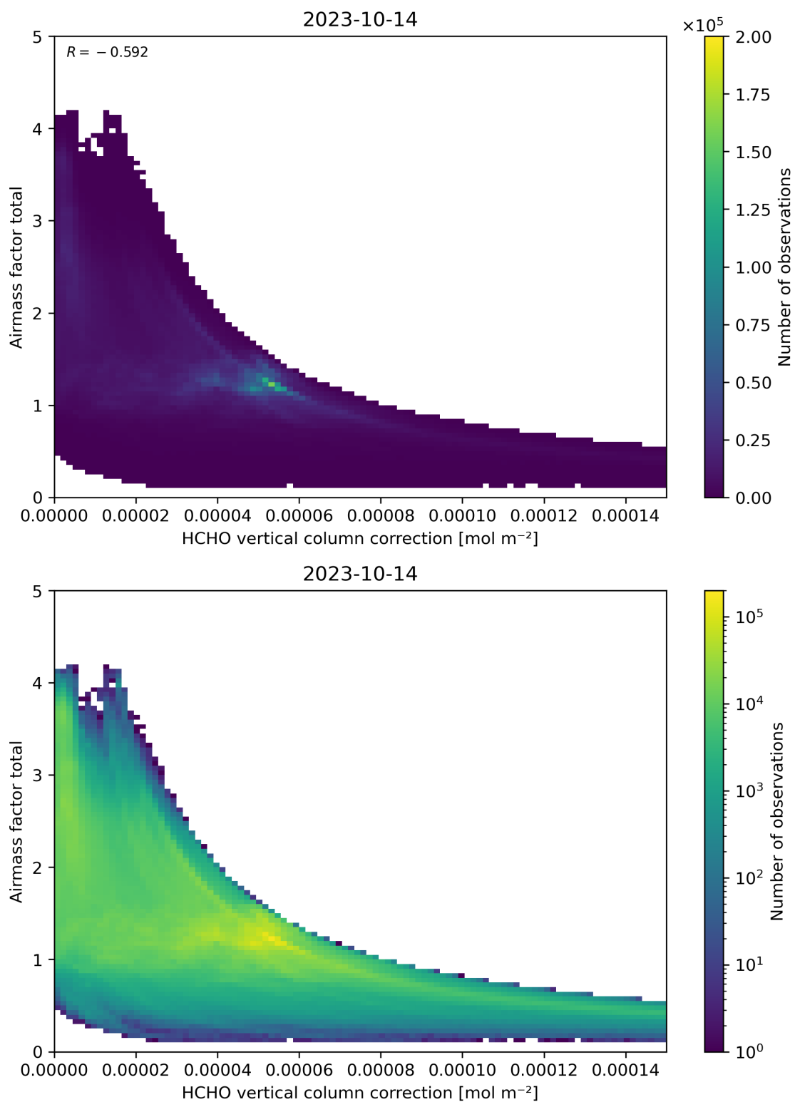
Figure 120: Scatter density plot of “HCHO vertical column correction” against “Airmass factor total” for 2023-10-13 to 2023-10-15.
