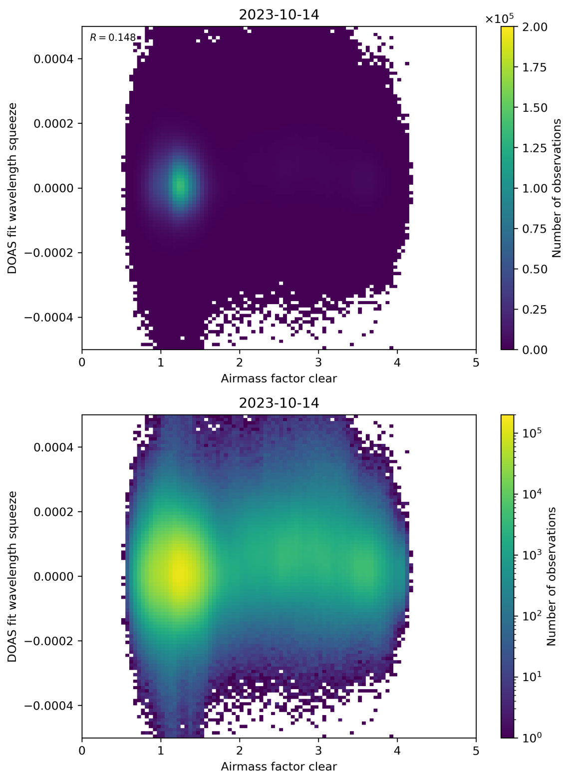
Figure 73: Scatter density plot of “Airmass factor clear” against “DOAS fit wavelength squeeze” for 2023-10-13 to 2023-10-15.
