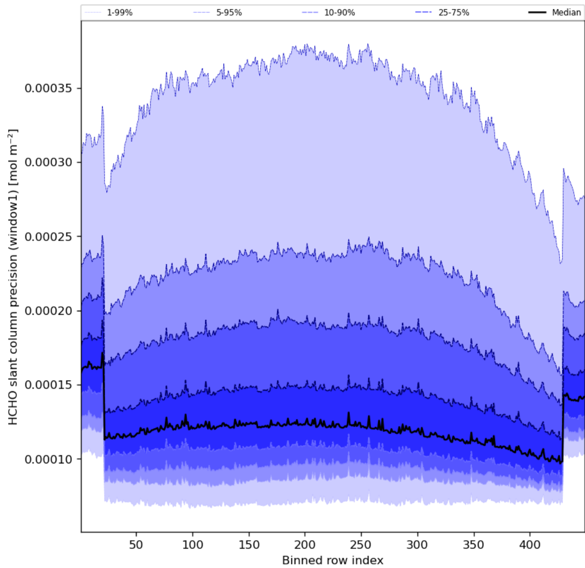
Figure 53: Along track statistics of “HCHO slant column precision (window1)” for 2023-10-13 to 2023-10-15
