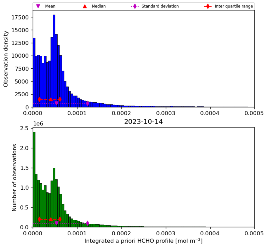
Figure 43: Histogram of “Integrated a priori HCHO profile” for 2023-10-13 to 2023-10-15
