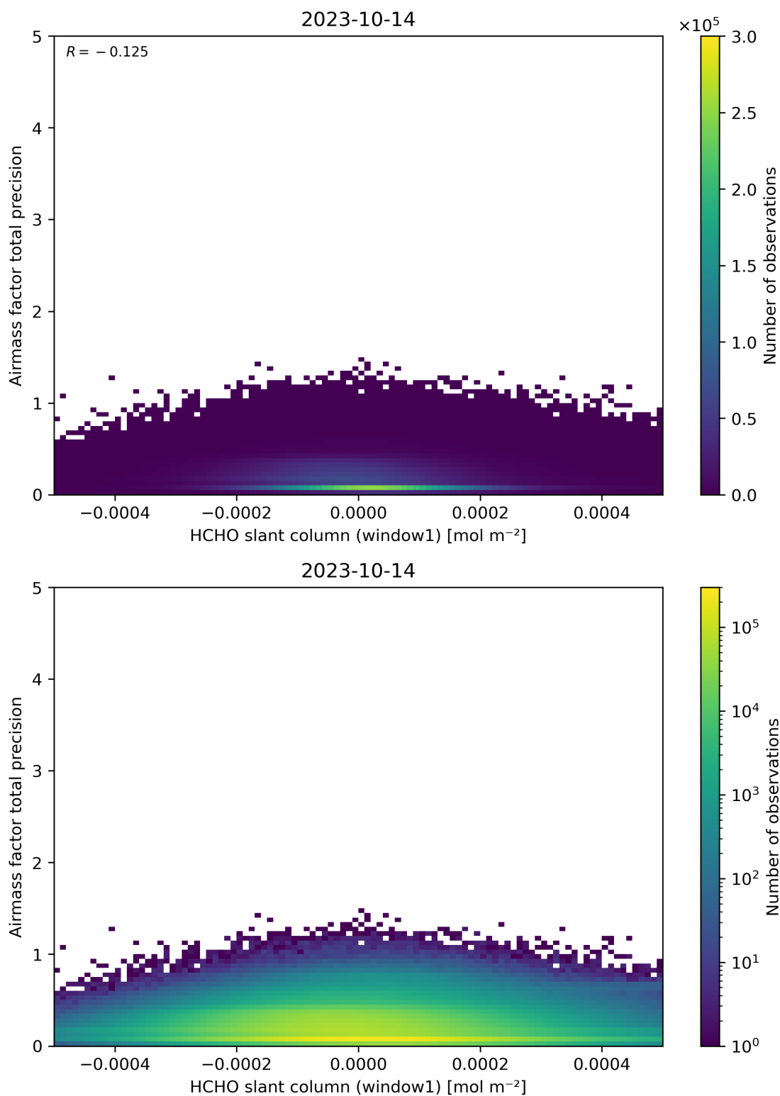
Figure 86: Scatter density plot of “HCHO slant column (window1)” against “Airmass factor total precision” for 2023-10-13 to 2023-10-15.
