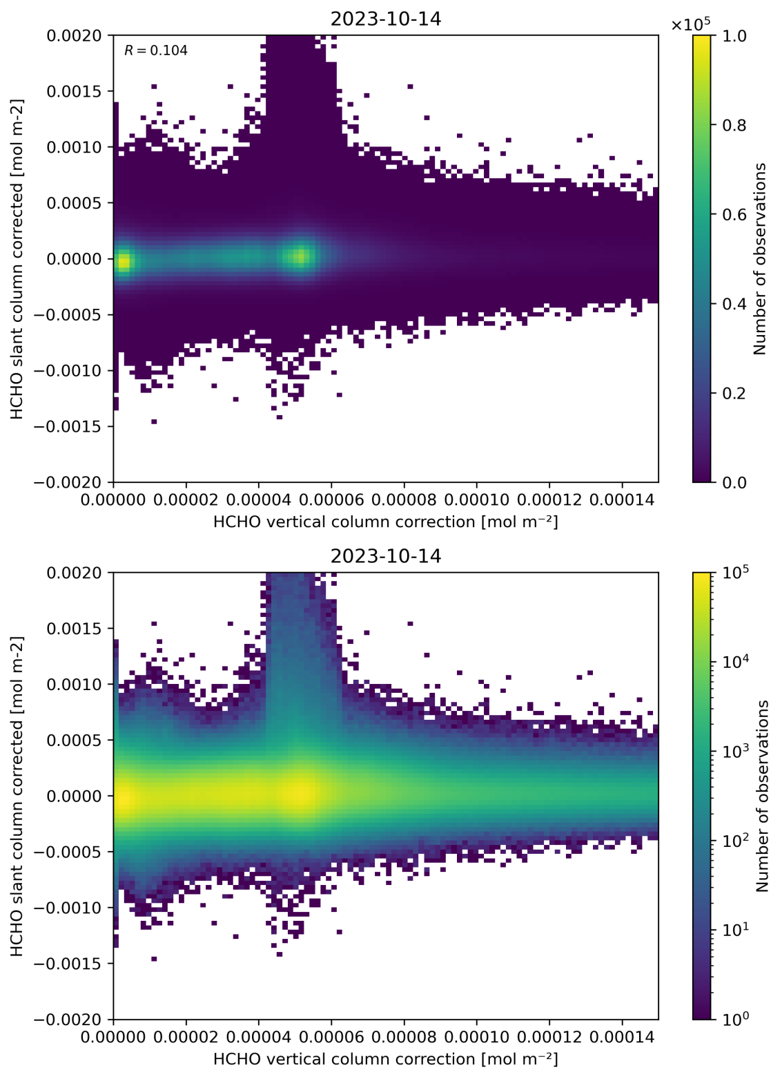
Figure 116: Scatter density plot of “HCHO vertical column correction” against “HCHO slant column corrected” for 2023-10-13 to 2023-10-15.
