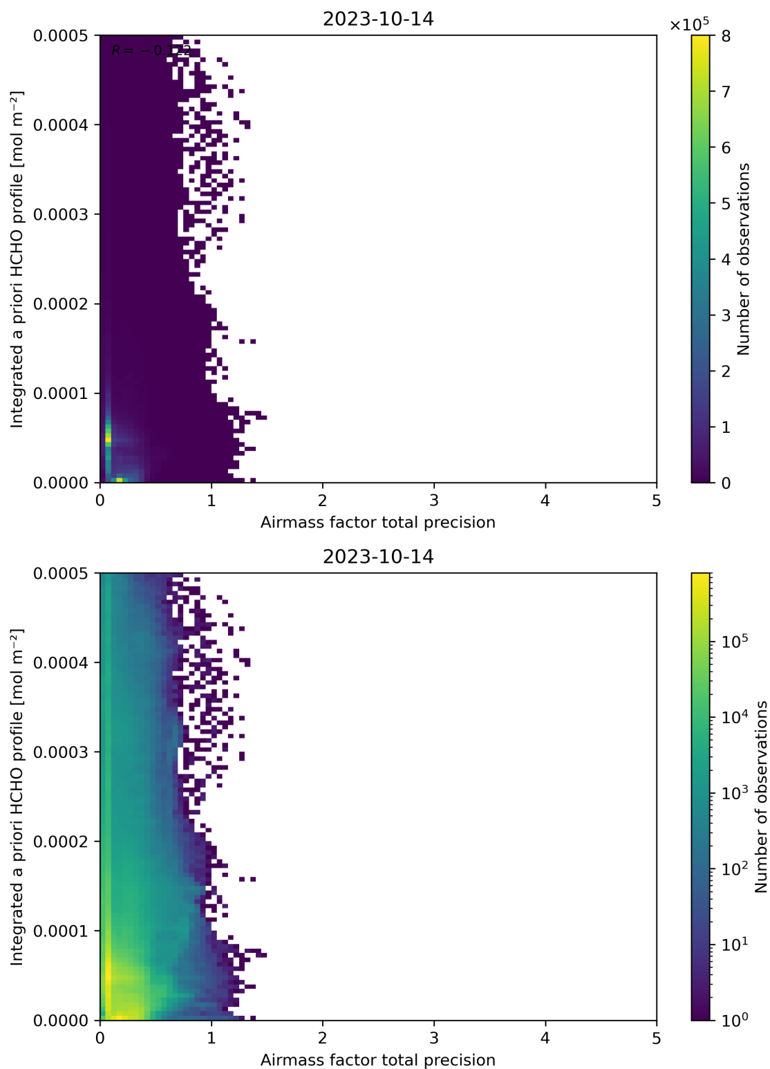
Figure 111: Scatter density plot of “Airmass factor total precision” against “Integrated a priori HCHO profile” for 2023-10-13 to 2023-10-15.
