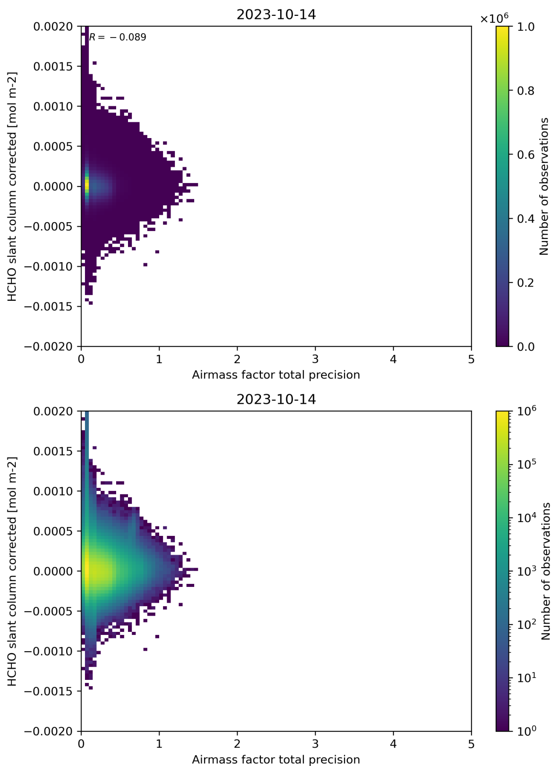
Figure 109: Scatter density plot of “Airmass factor total precision” against “HCHO slant column corrected” for 2023-10-13 to 2023-10-15.
