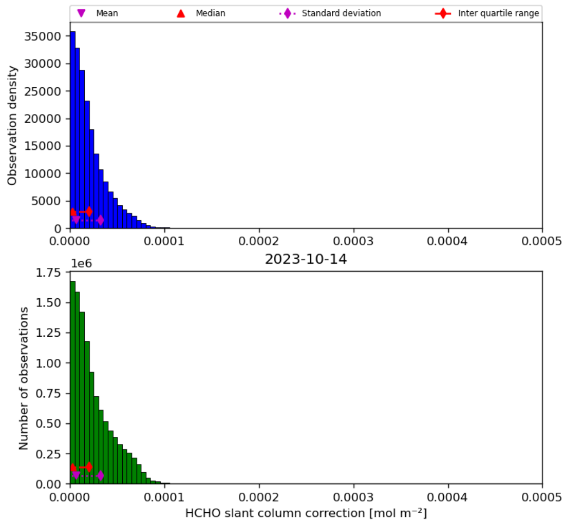
Figure 47: Histogram of “HCHO slant column correction” for 2023-10-13 to 2023-10-15
