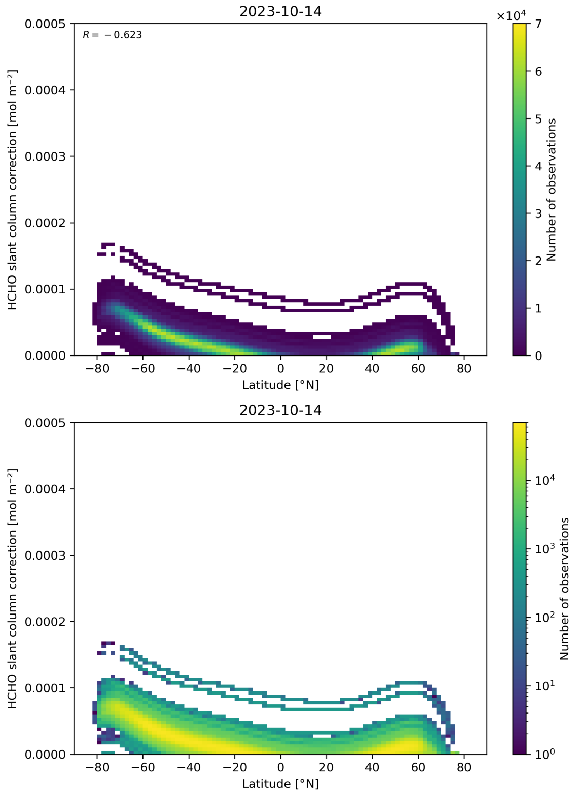
Figure 158: Scatter density plot of “Latitude” against “HCHO slant column correction” for 2023-10-13 to 2023-10-15.
