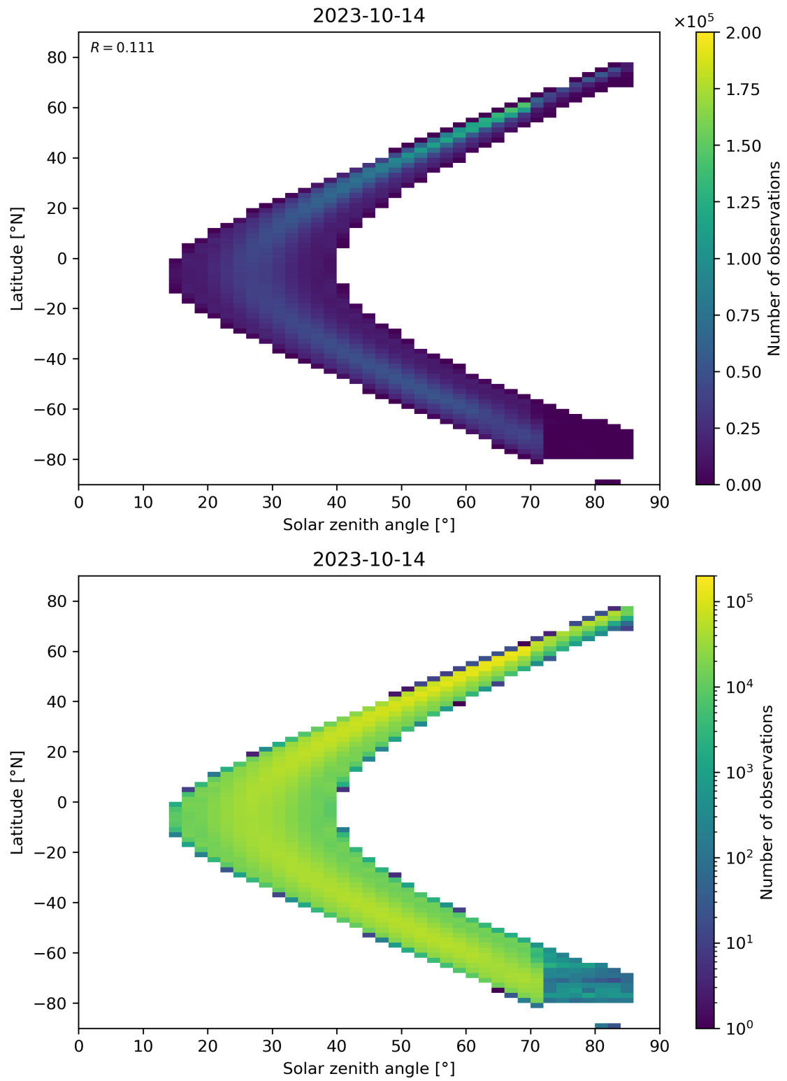
Figure 181: Scatter density plot of “Solar zenith angle” against “Latitude” for 2023-10-13 to 2023-10-15.
