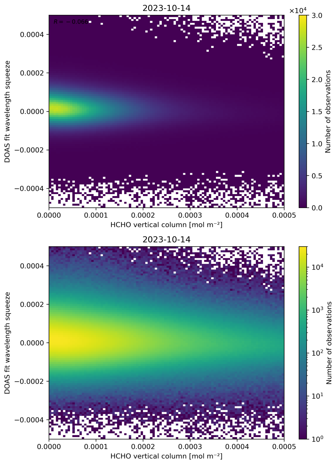
Figure 125: Scatter density plot of “HCHO vertical column” against “DOAS fit wavelength squeeze” for 2023-10-13 to 2023-10-15.
