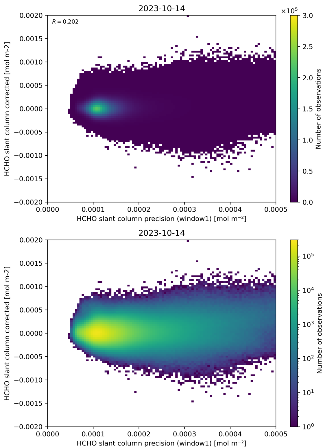
Figure 92: Scatter density plot of “HCHO slant column precision (window1)” against “HCHO slant column corrected” for 2023-10-13 to 2023-10-15.
