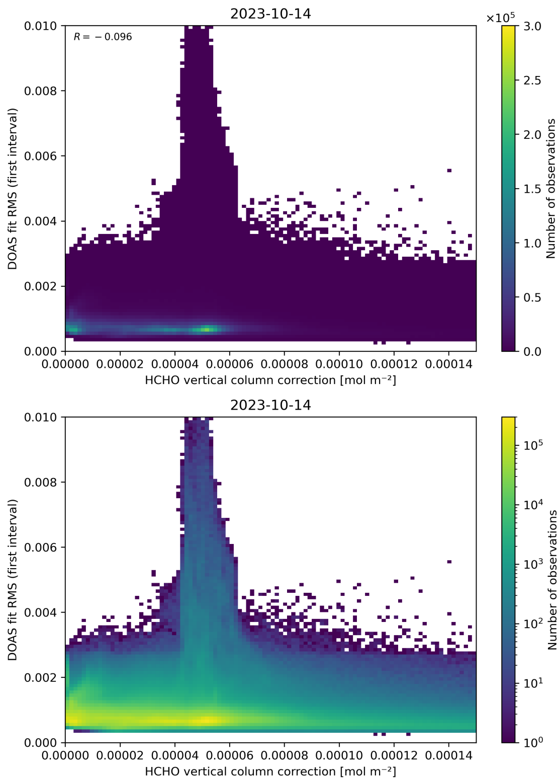
Figure 112: Scatter density plot of “HCHO vertical column correction” against “DOAS fit RMS (first interval)” for 2023-10-13 to 2023-10-15.
