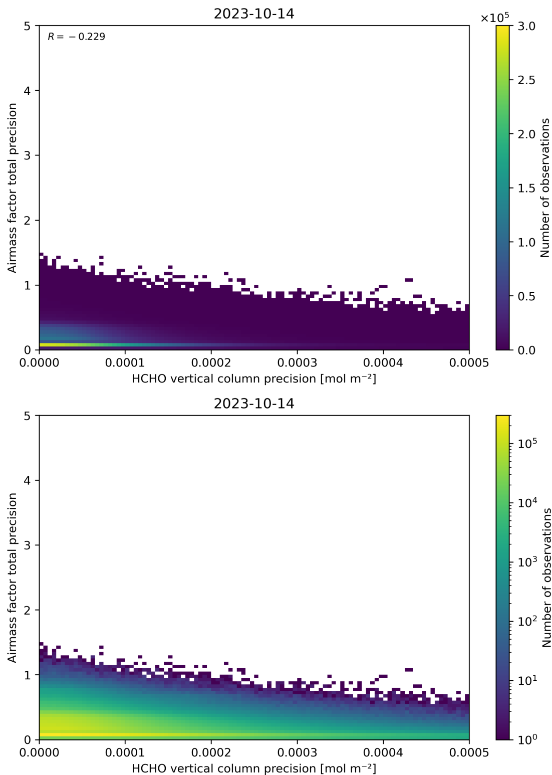
Figure 145: Scatter density plot of “HCHO vertical column precision” against “Airmass factor total precision” for 2023-10-13 to 2023-10-15.
