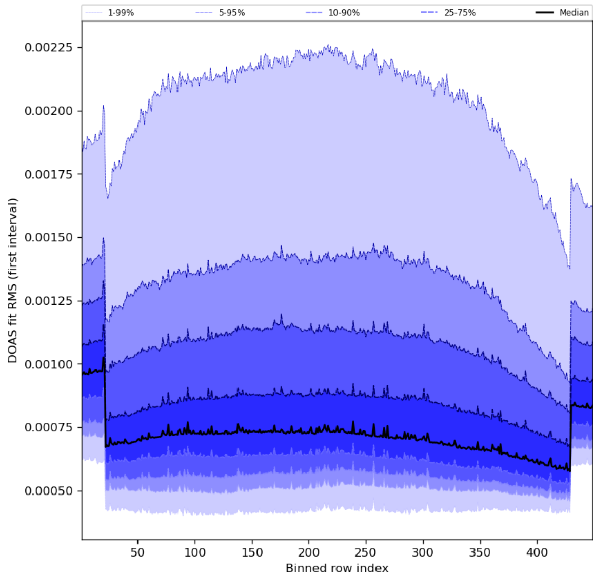
Figure 60: Along track statistics of “DOAS fit RMS (first interval)” for 2023-10-13 to 2023-10-15
