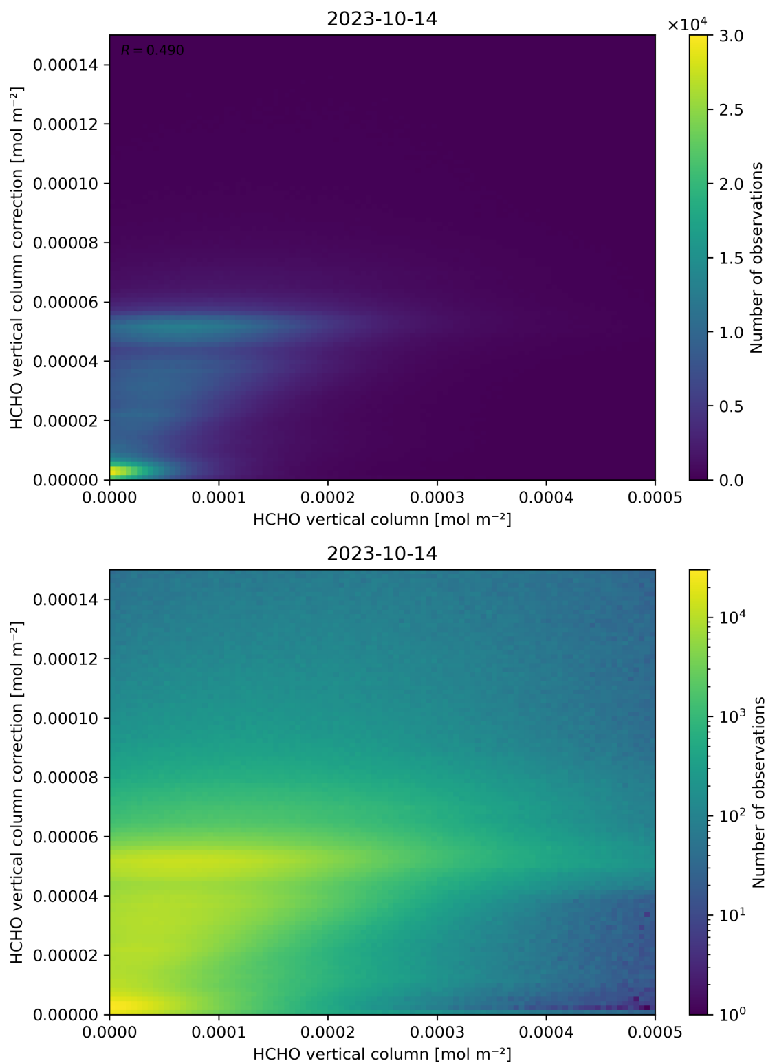
Figure 133: Scatter density plot of “HCHO vertical column” against “HCHO vertical column correction” for 2023-10-13 to 2023-10-15.
