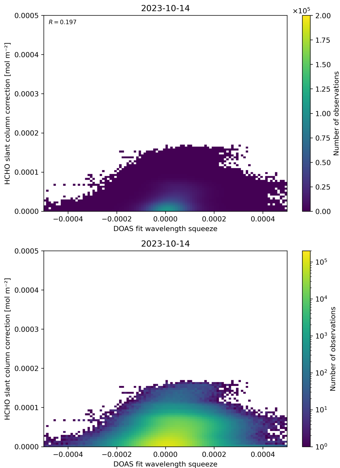
Figure 70: Scatter density plot of “DOAS fit wavelength squeeze” against “HCHO slant column correction” for 2023-10-13 to 2023-10-15.
