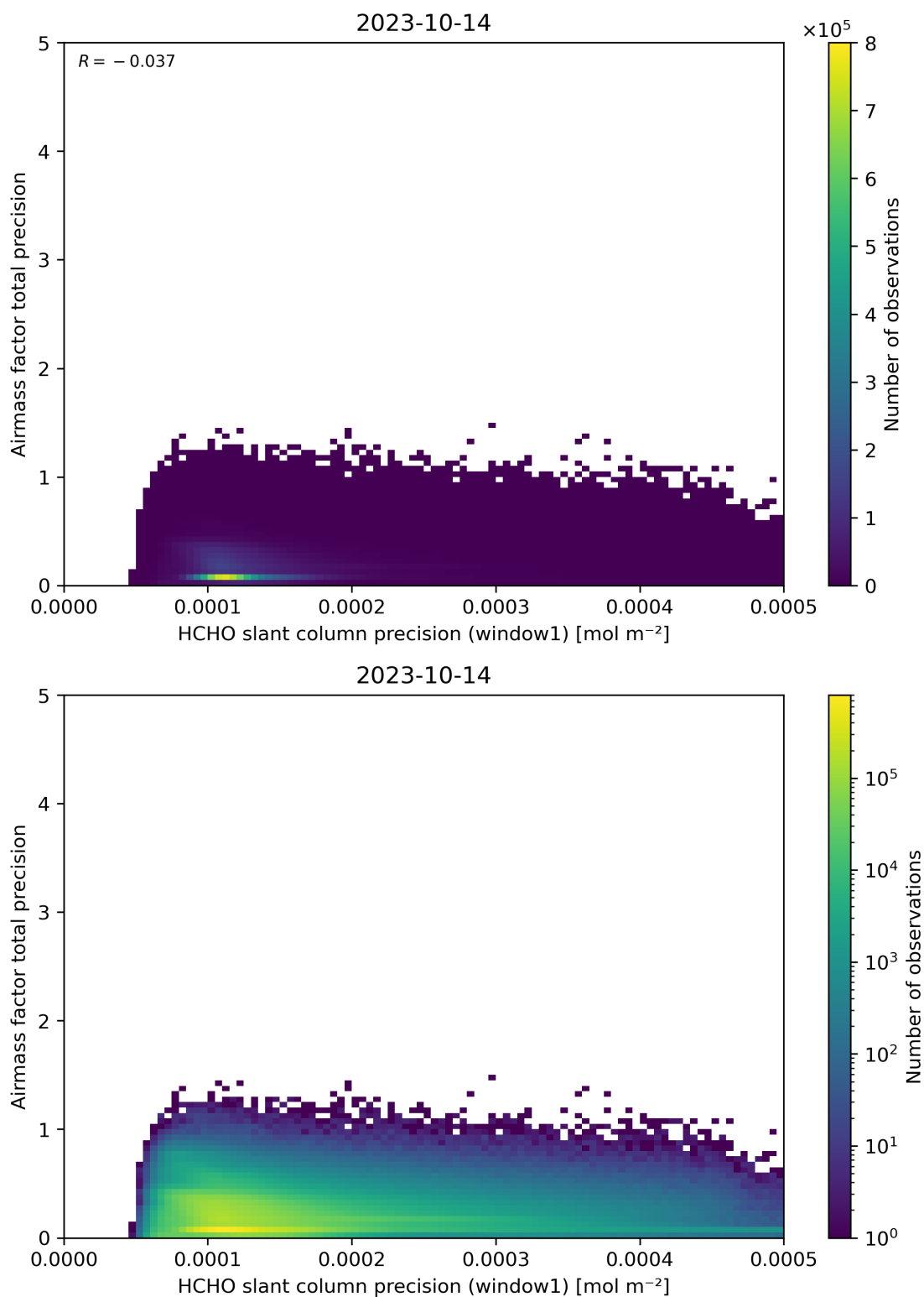
Figure 95: Scatter density plot of “HCHO slant column precision (window1)” against “Airmass factor total precision” for 2023-10-13 to 2023-10-15.
