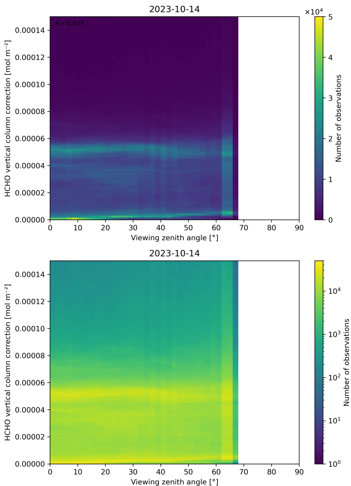
Figure 193: Scatter density plot of “Viewing zenith angle” against “HCHO vertical column correction” for 2023-10-13 to 2023-10-15.
