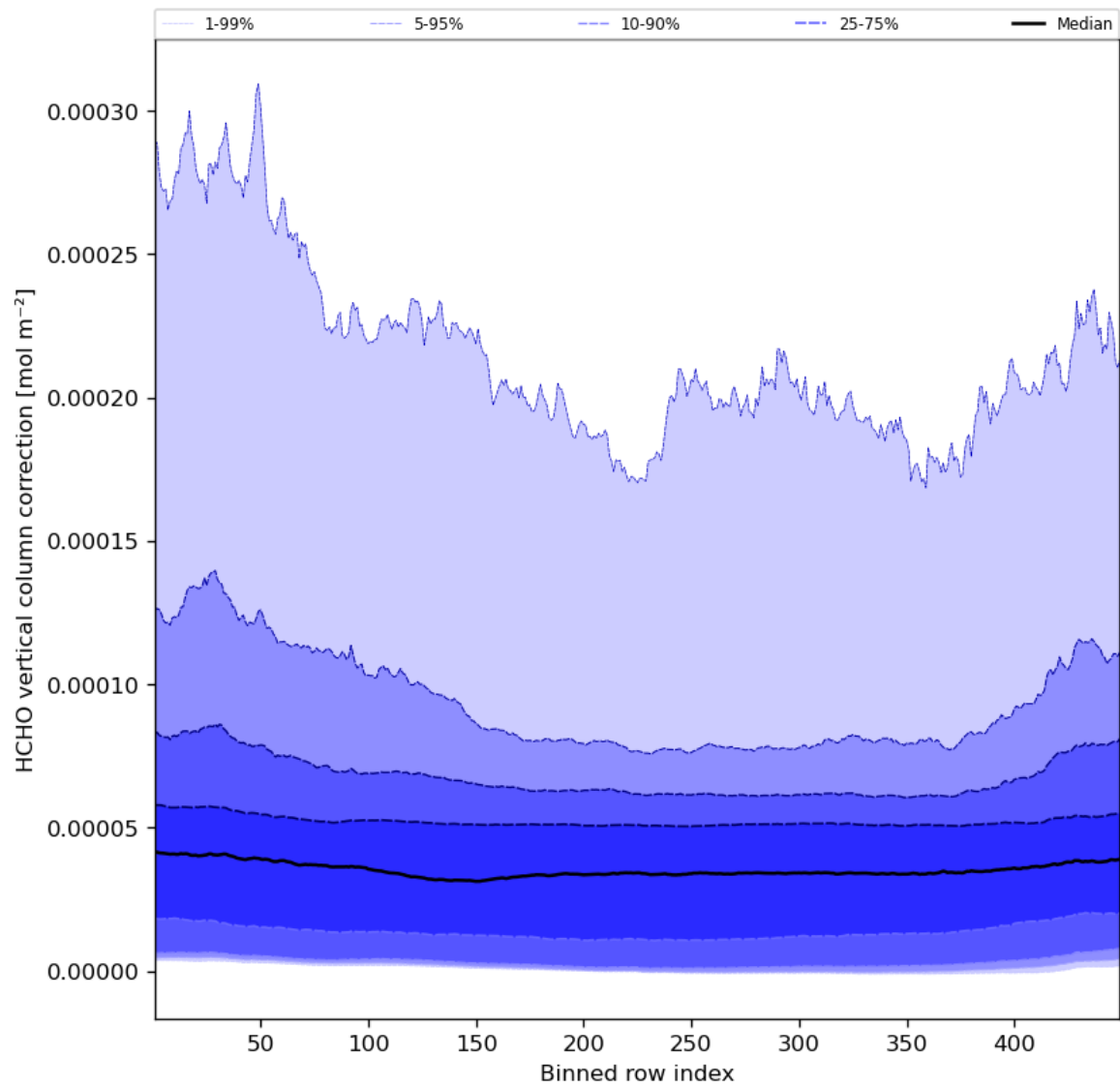
Figure 51: Along track statistics of “HCHO vertical column correction” for 2023-10-13 to 2023-10-15
