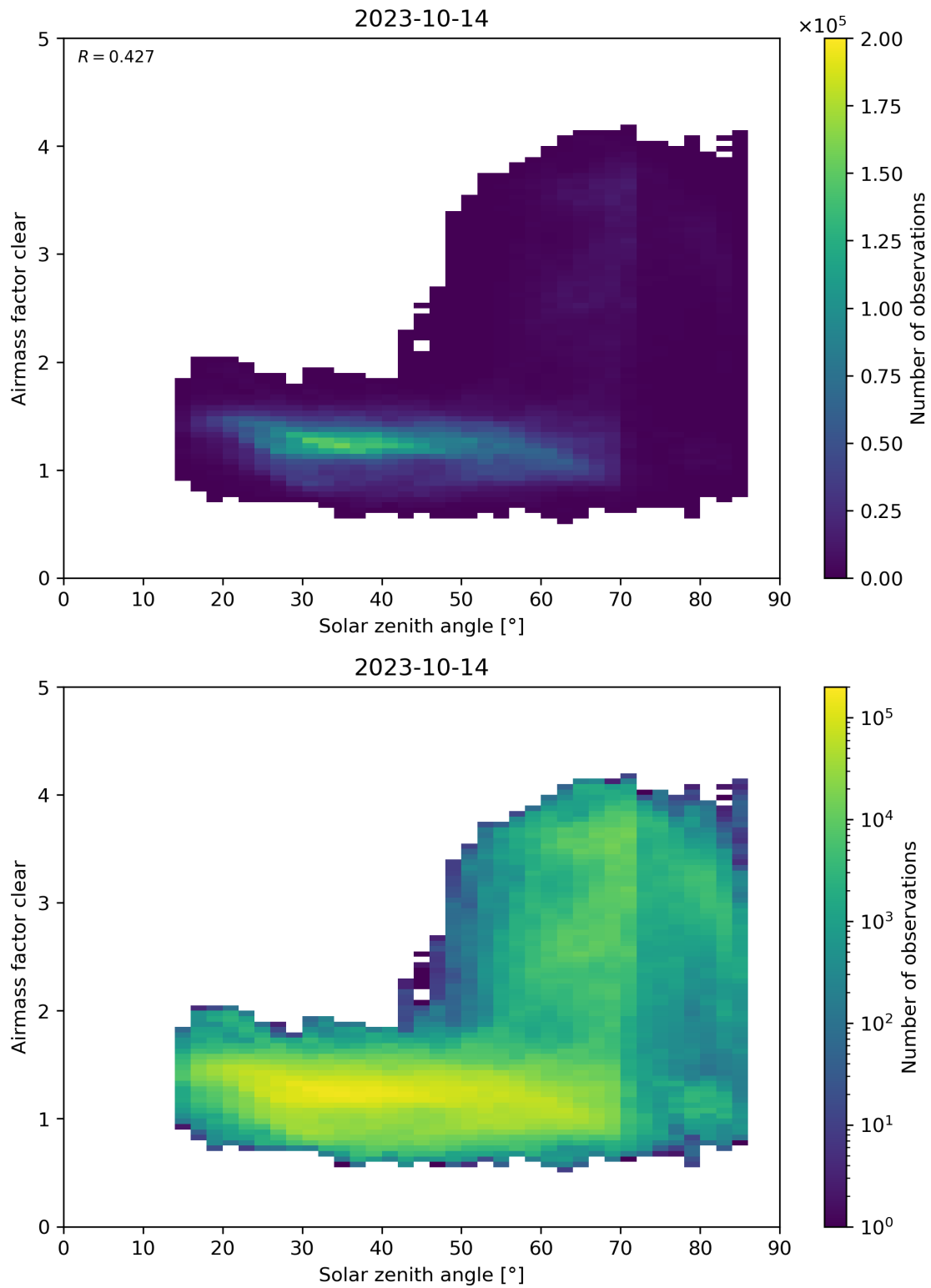
Figure 170: Scatter density plot of “Solar zenith angle” against “Airmass factor clear” for 2023-10-13 to 2023-10-15.
