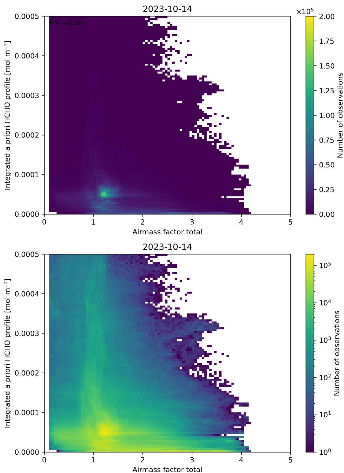
Figure 104: Scatter density plot of “Airmass factor total” against “Integrated a priori HCHO profile” for 2023-10-13 to 2023-10-15.
