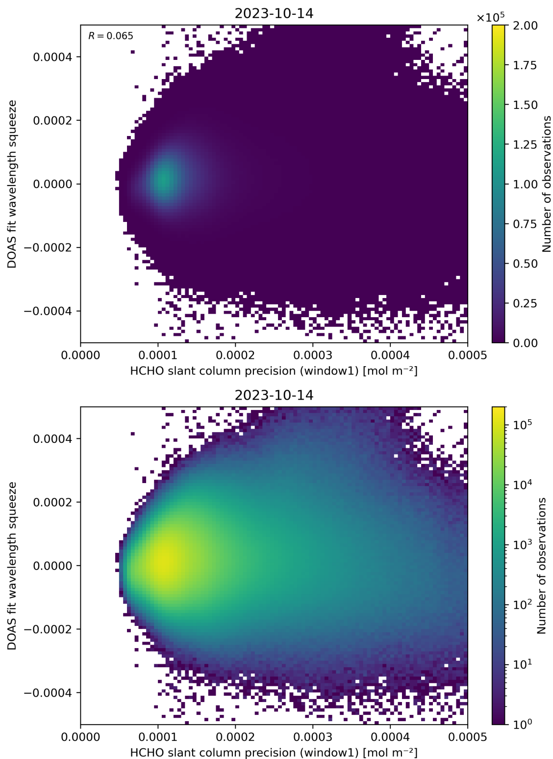
Figure 90: Scatter density plot of “HCHO slant column precision (window1)” against “DOAS fit wavelength squeeze” for 2023-10-13 to 2023-10-15.
