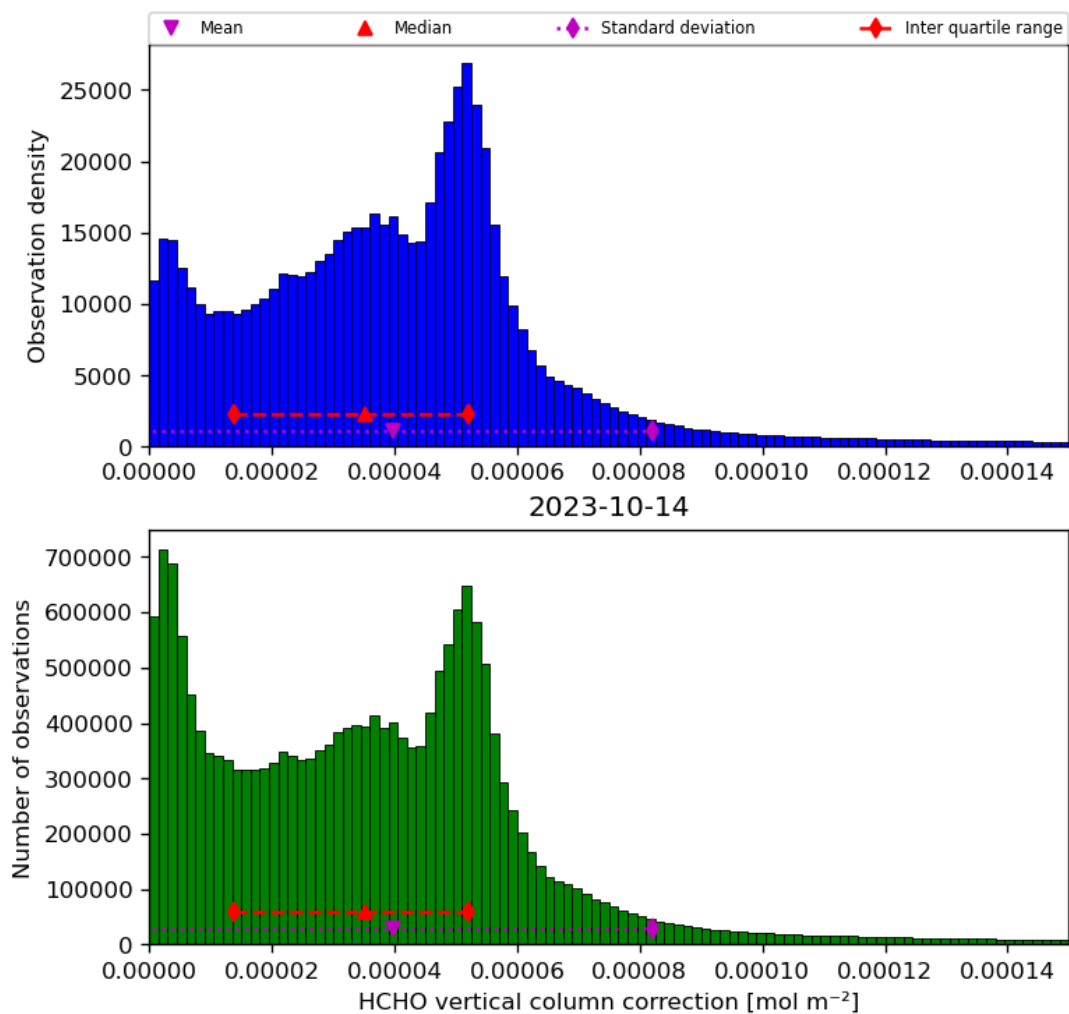
Figure 37: Histogram of “HCHO vertical column correction” for 2023-10-13 to 2023-10-15
