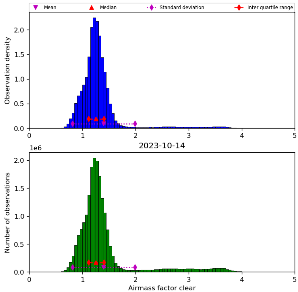
Figure 42: Histogram of “Airmass factor clear” for 2023-10-13 to 2023-10-15
