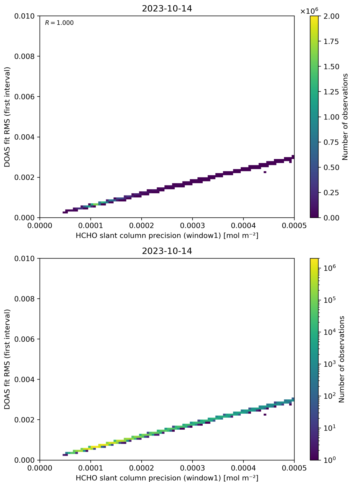
Figure 88: Scatter density plot of “HCHO slant column precision (window1)” against “DOAS fit RMS (first interval)” for 2023-10-13 to 2023-10-15.
