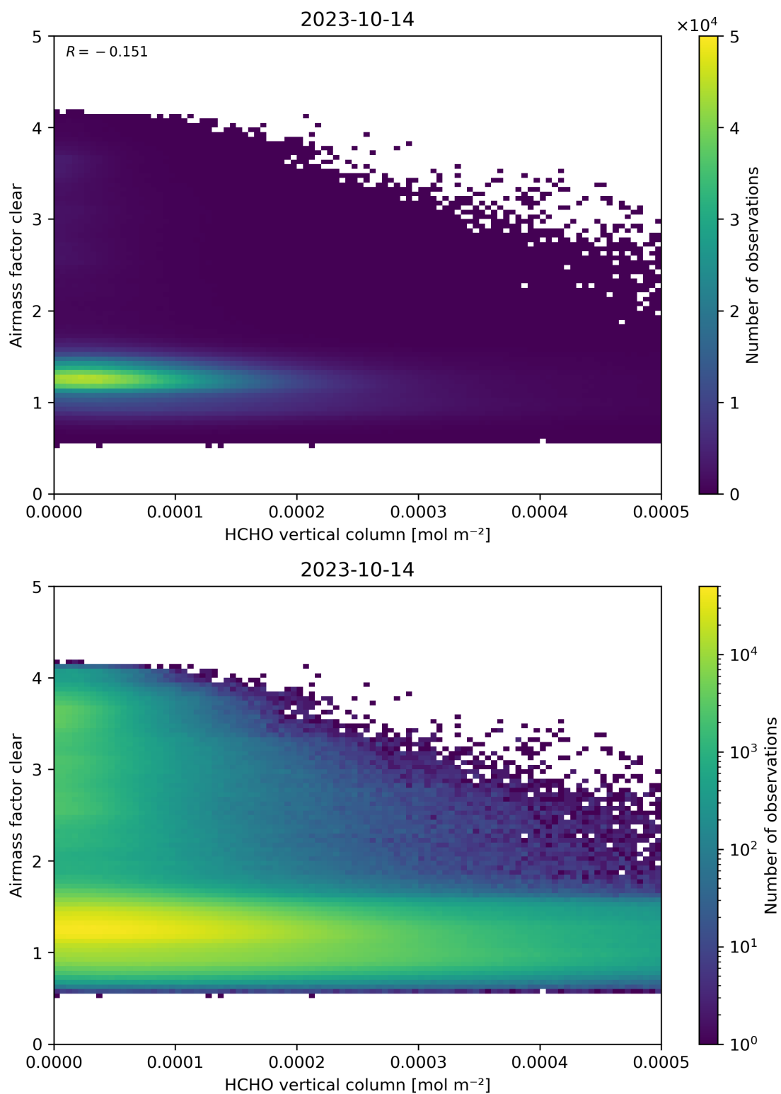
Figure 126: Scatter density plot of “HCHO vertical column” against “Airmass factor clear” for 2023-10-13 to 2023-10-15.
