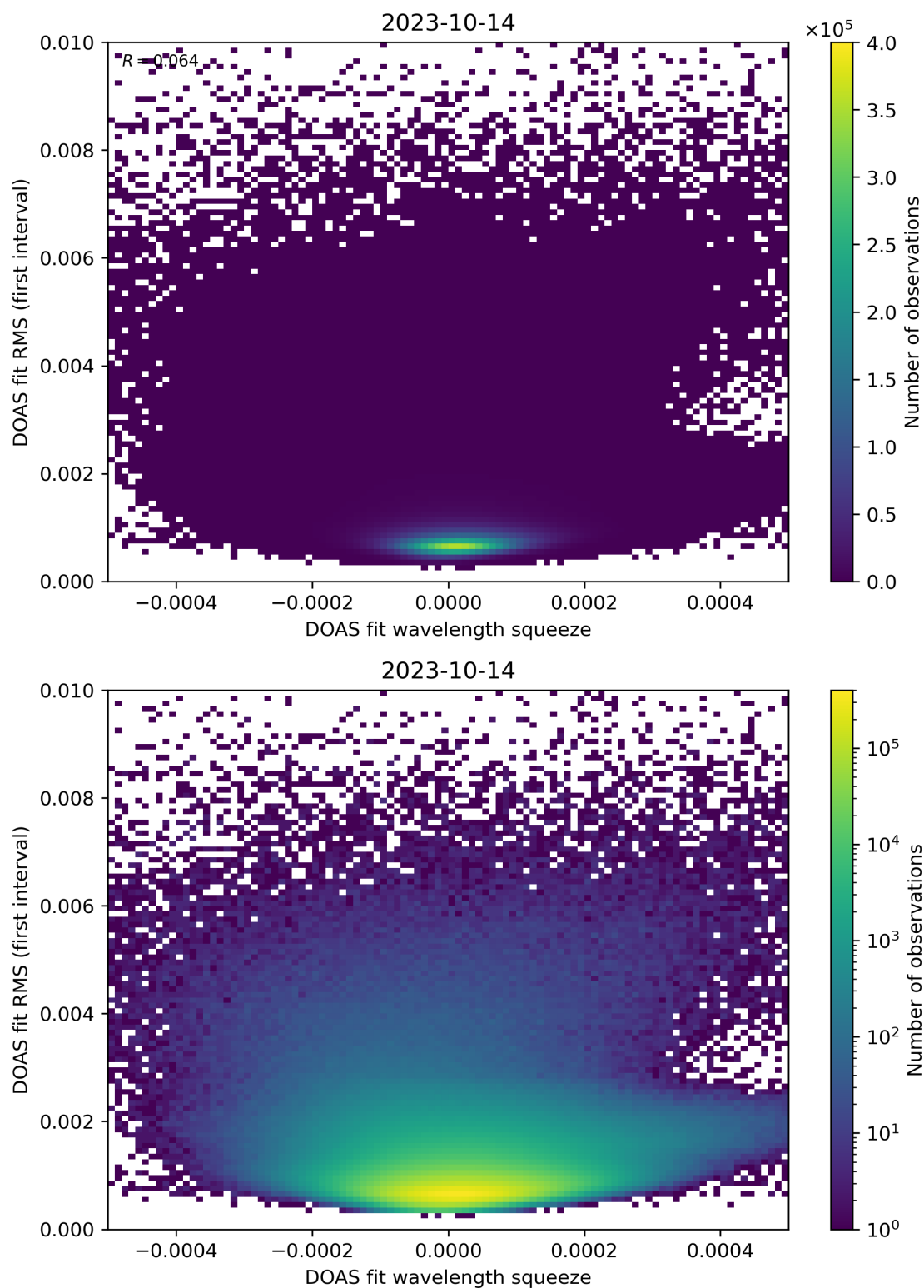
Figure 68: Scatter density plot of “DOAS fit wavelength squeeze” against “DOAS fit RMS (first interval)” for 2023-10-13 to 2023-10-15.
