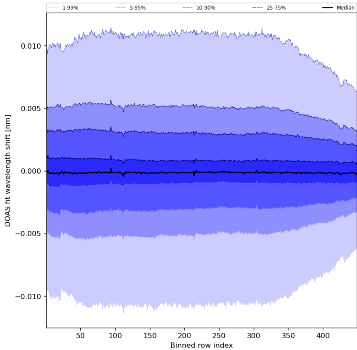
Figure 58: Along track statistics of “DOAS fit wavelength shift” for 2023-10-13 to 2023-10-15
