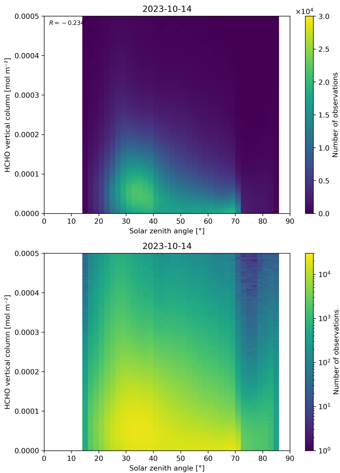
Figure 177: Scatter density plot of “Solar zenith angle” against “HCHO vertical column” for 2023-10-13 to 2023-10-15.
