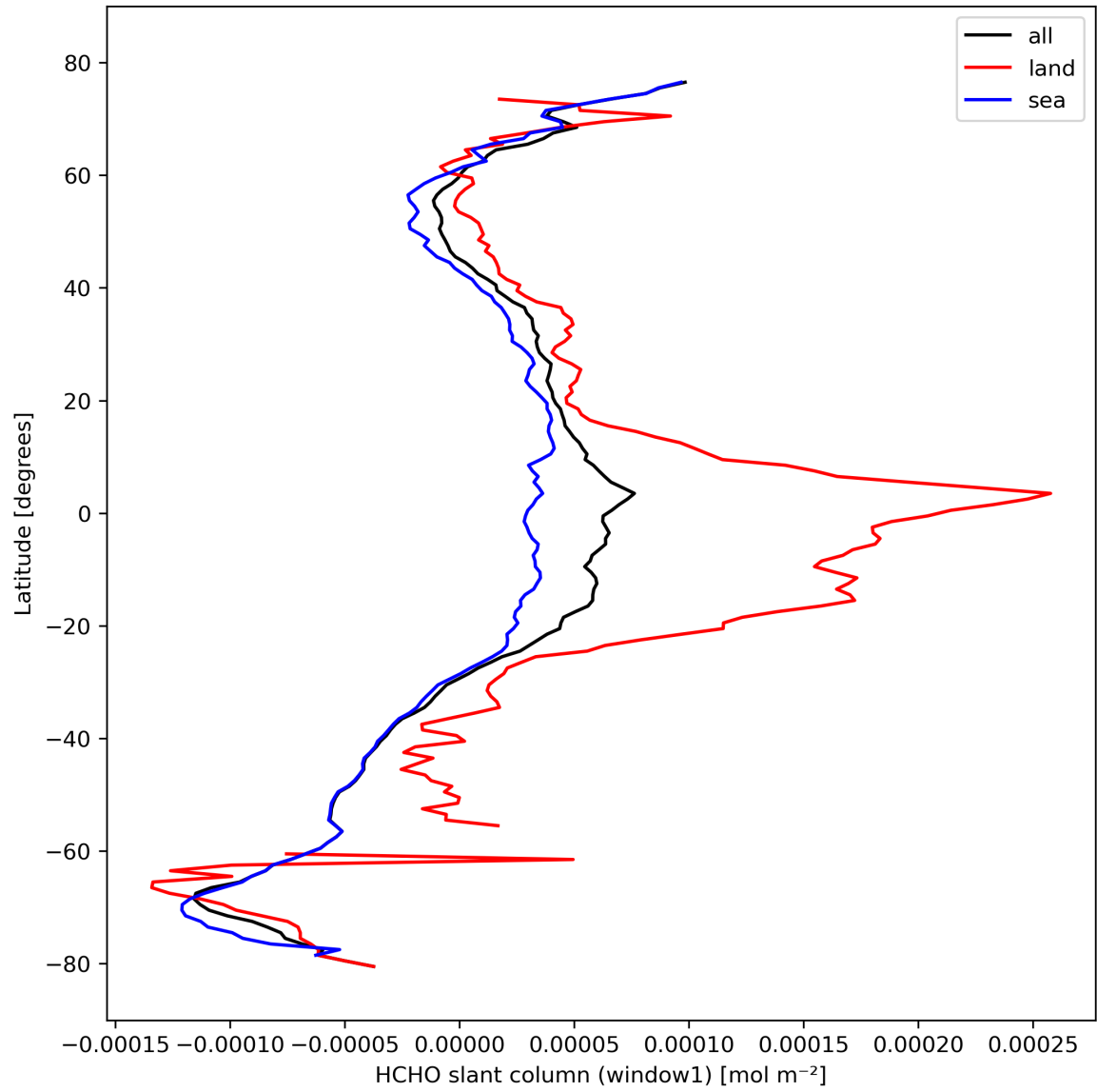
Figure 24: Zonal average of “HCHO slant column (window1)” for 2023-10-13 to 2023-10-15.
