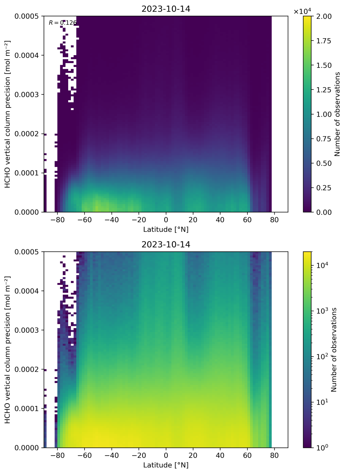
Figure 165: Scatter density plot of “Latitude” against “HCHO vertical column precision” for 2023-10-13 to 2023-10-15.
