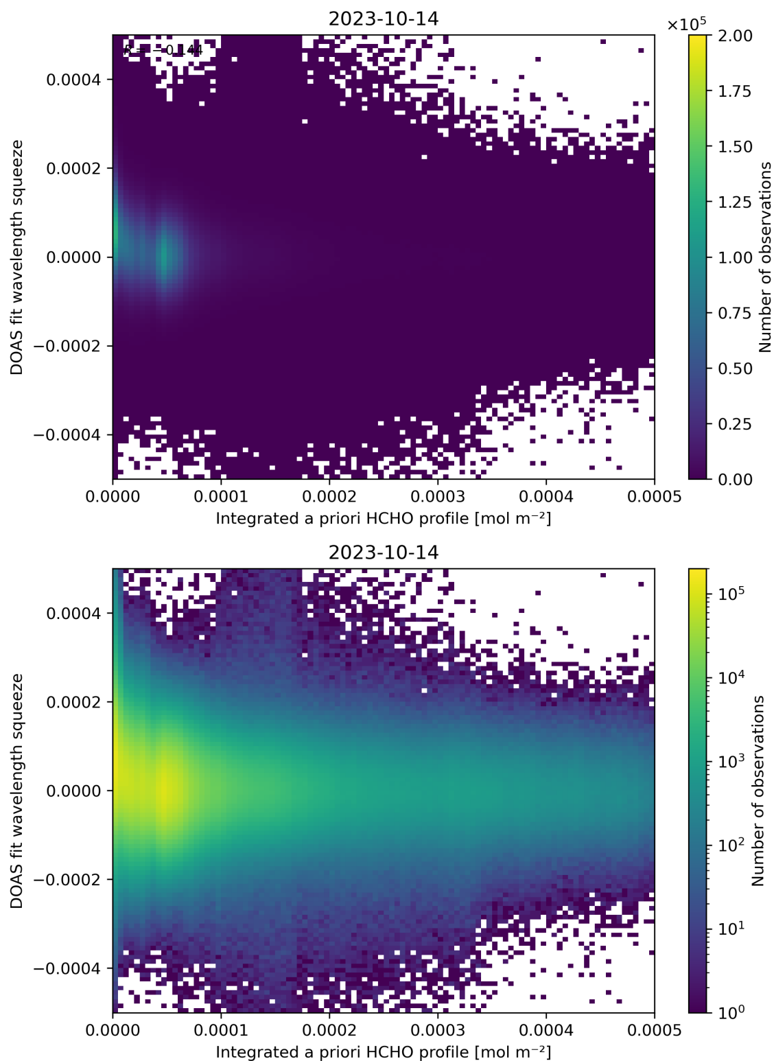
Figure 150: Scatter density plot of “Integrated a priori HCHO profile” against “DOAS fit wavelength squeeze” for 2023-10-13 to 2023-10-15.
