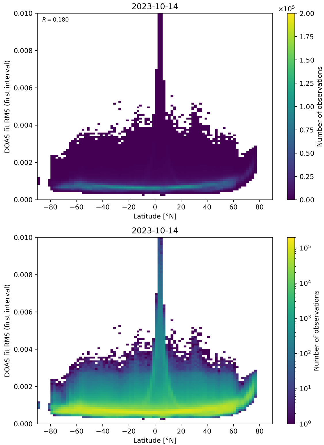
Figure 153: Scatter density plot of “Latitude” against “DOAS fit RMS (first interval)” for 2023-10-13 to 2023-10-15.
