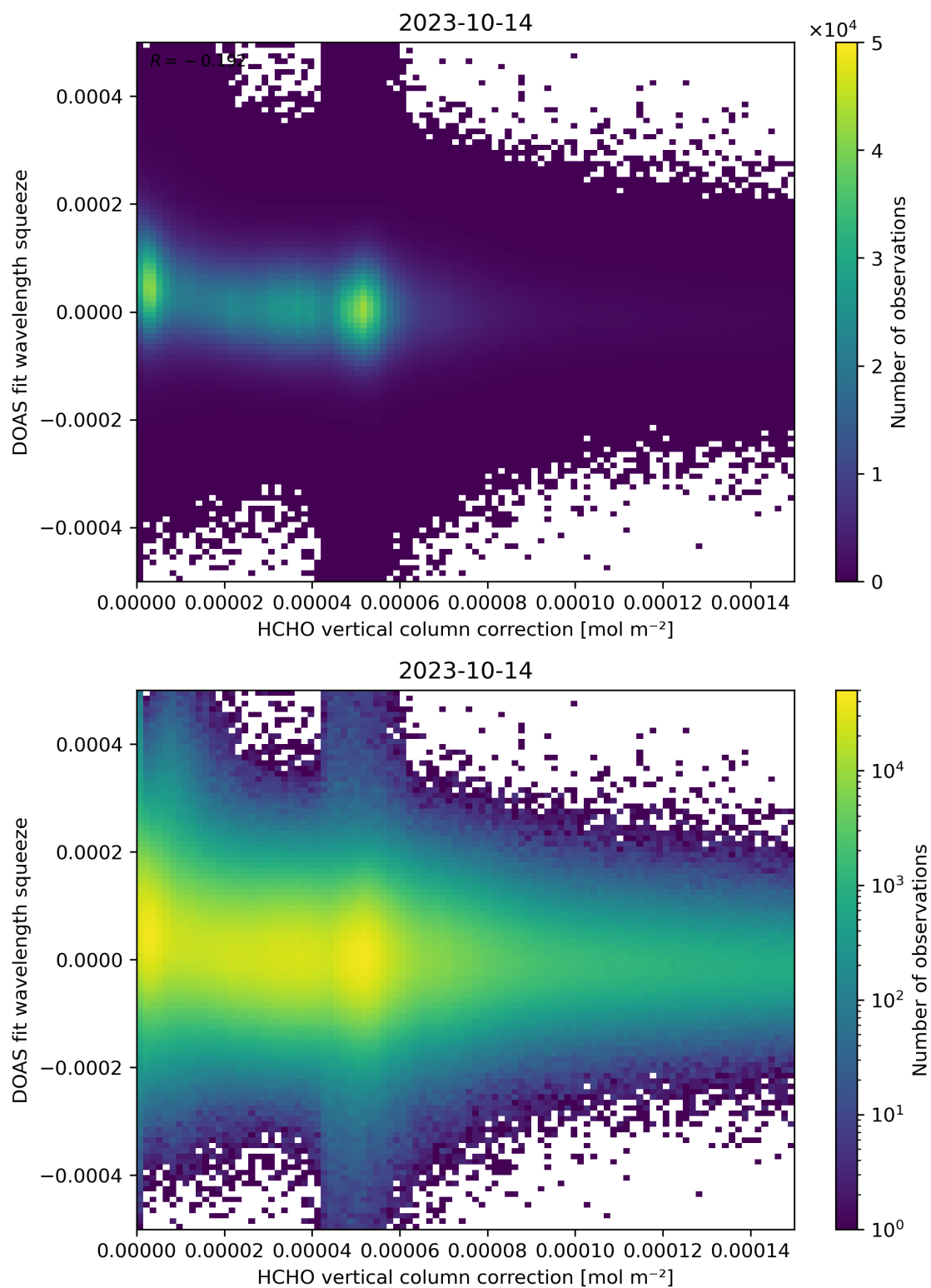
Figure 114: Scatter density plot of “HCHO vertical column correction” against “DOAS fit wavelength squeeze” for 2023-10-13 to 2023-10-15.
