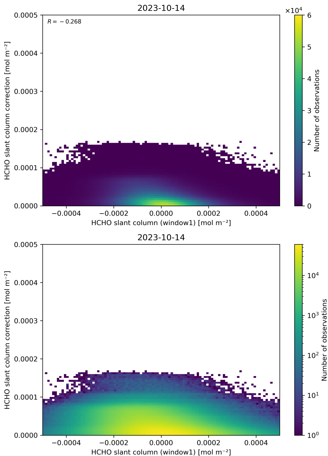
Figure 83: Scatter density plot of “HCHO slant column (window1)” against “HCHO slant column correction” for 2023-10-13 to 2023-10-15.
