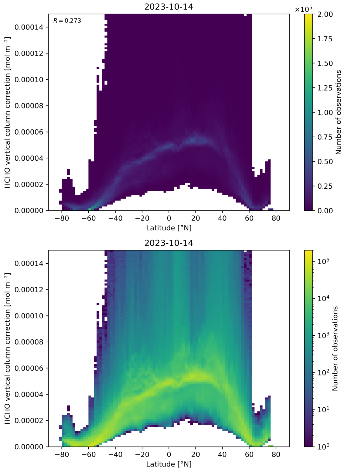
Figure 164: Scatter density plot of “Latitude” against “HCHO vertical column correction” for 2023-10-13 to 2023-10-15.
