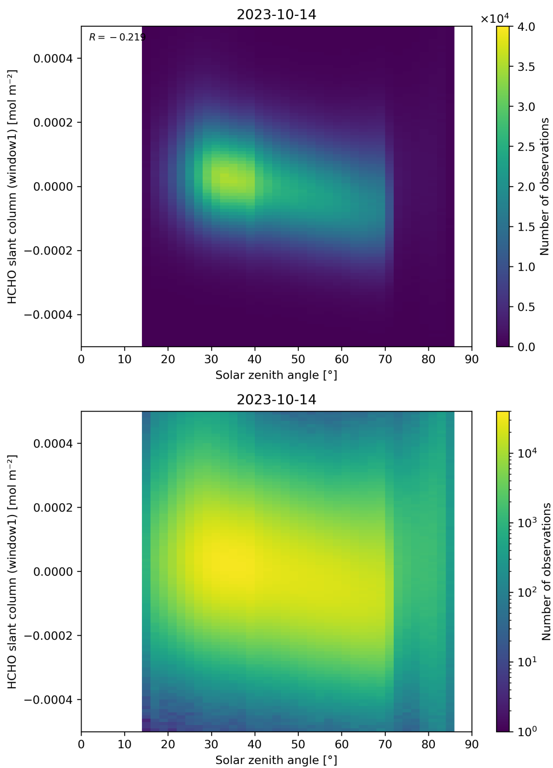
Figure 173: Scatter density plot of “Solar zenith angle” against “HCHO slant column (window1)” for 2023-10-13 to 2023-10-15.
