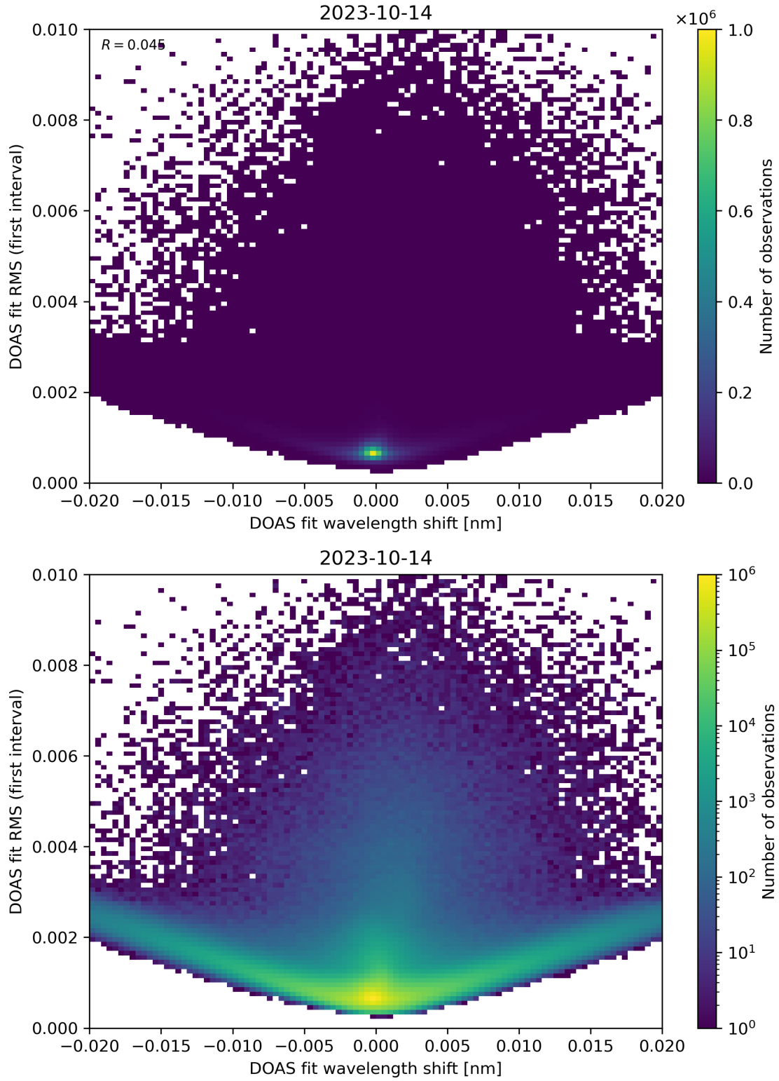
Figure 64: Scatter density plot of “DOAS fit wavelength shift” against “DOAS fit RMS (first interval)” for 2023-10-13 to 2023-10-15.
