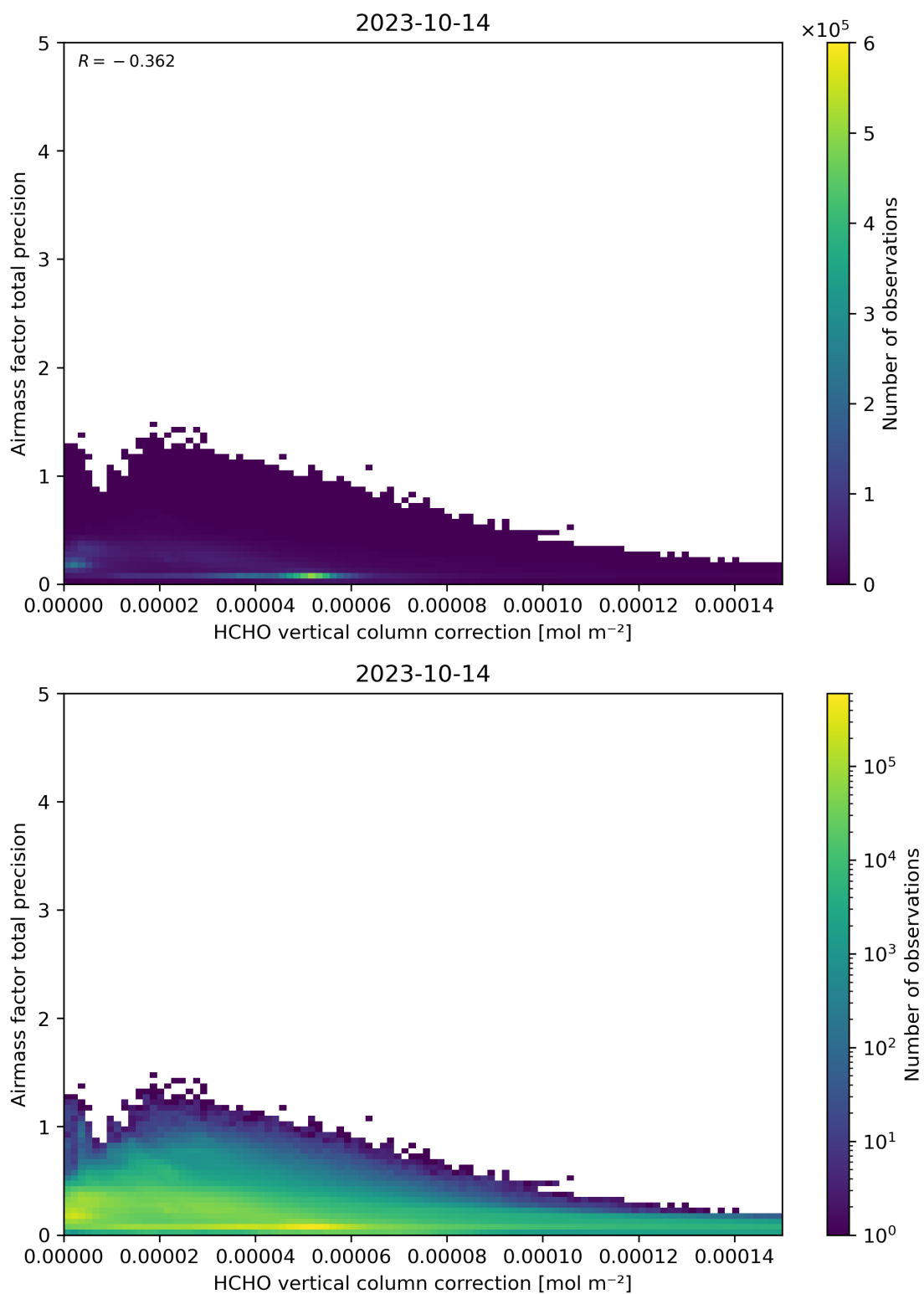
Figure 121: Scatter density plot of “HCHO vertical column correction” against “Airmass factor total precision” for 2023-10-13 to 2023-10-15.
