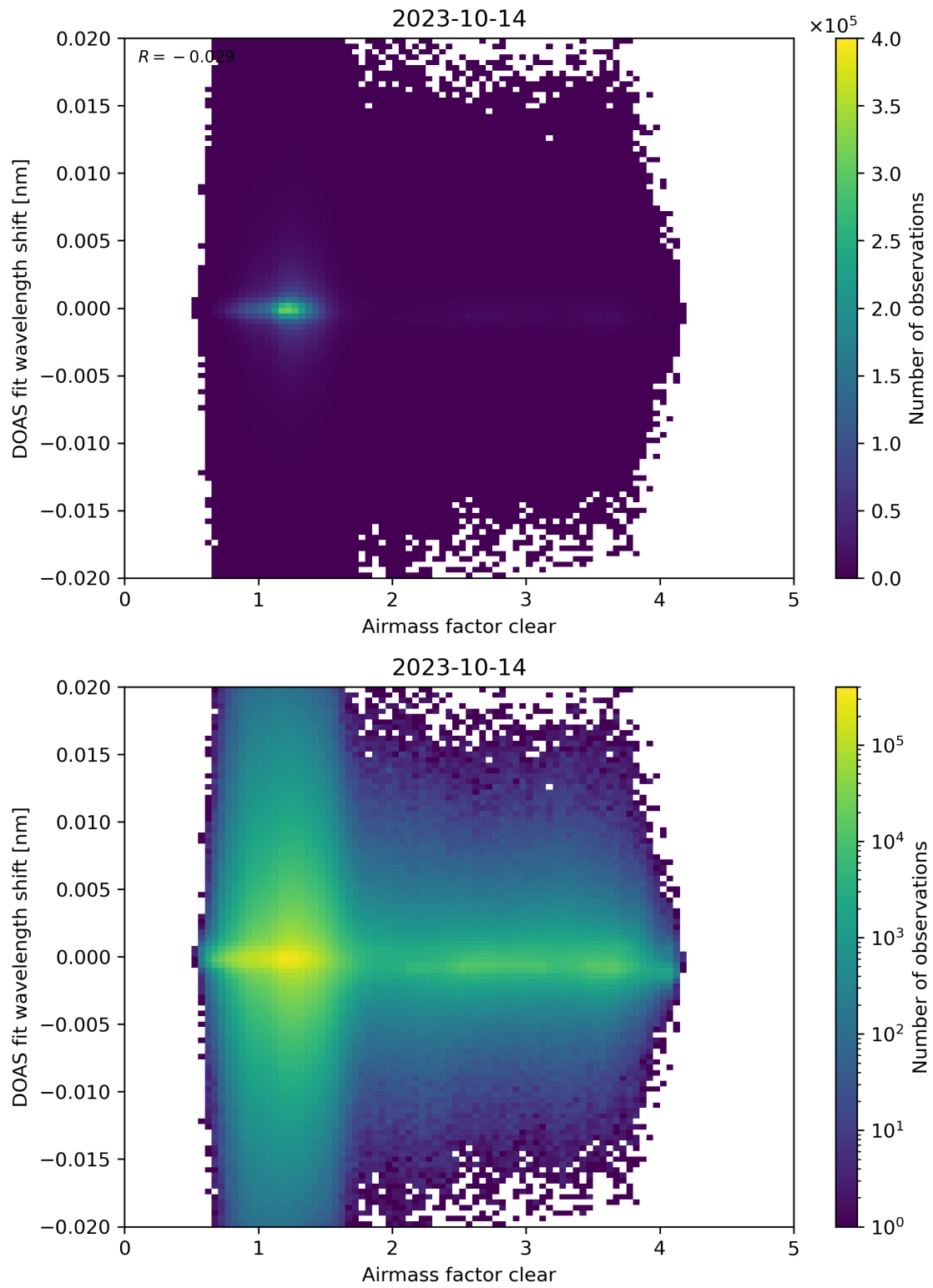
Figure 72: Scatter density plot of “Airmass factor clear” against “DOAS fit wavelength shift” for 2023-10-13 to 2023-10-15.
