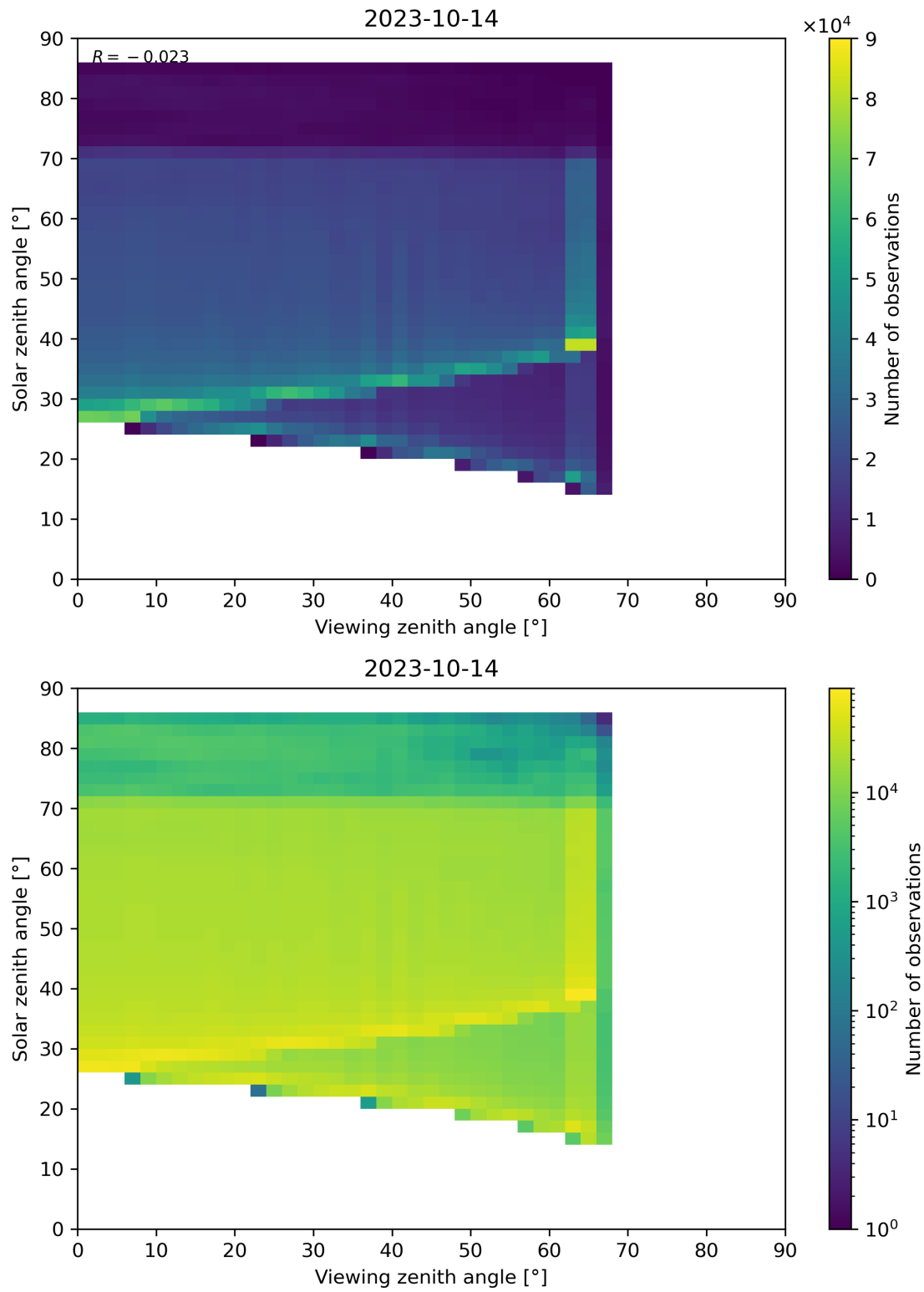
Figure 197: Scatter density plot of “Viewing zenith angle” against “Solar zenith angle” for 2023-10-13 to 2023-10-15.
