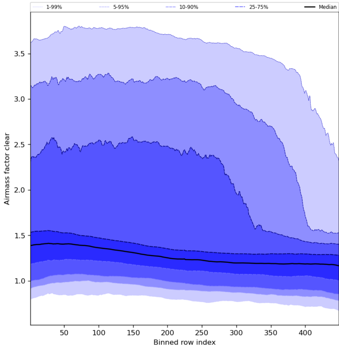
Figure 56: Along track statistics of “Airmass factor clear” for 2023-10-13 to 2023-10-15
