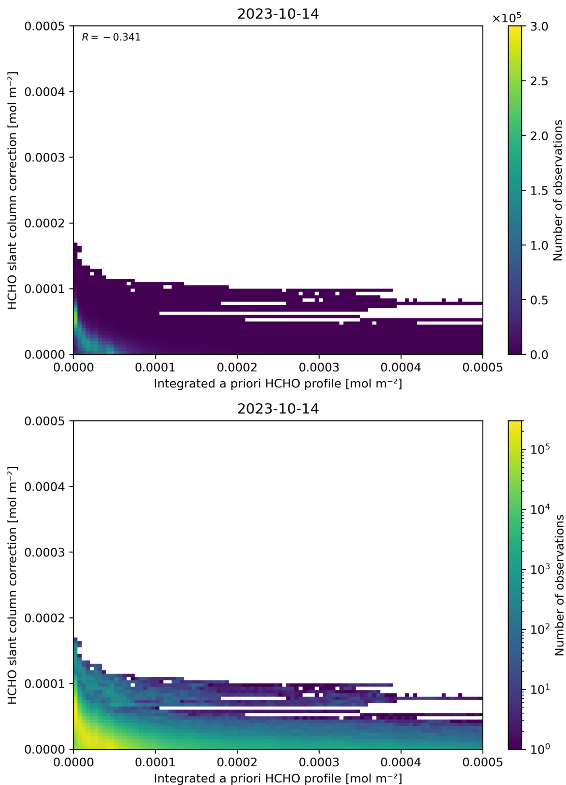
Figure 152: Scatter density plot of “Integrated a priori HCHO profile” against “HCHO slant column correction” for 2023-10-13 to 2023-10-15.
