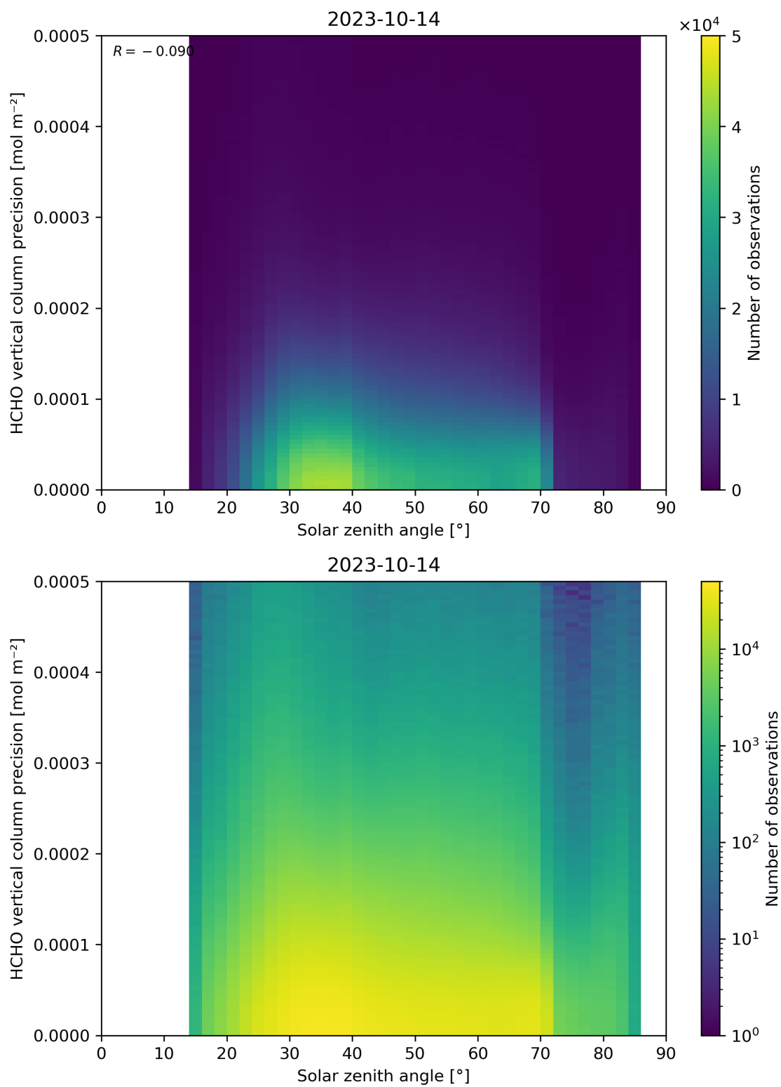
Figure 179: Scatter density plot of “Solar zenith angle” against “HCHO vertical column precision” for 2023-10-13 to 2023-10-15.
