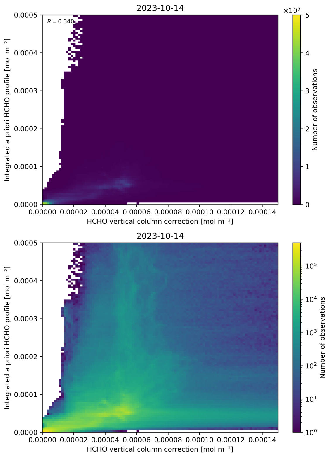
Figure 122: Scatter density plot of “HCHO vertical column correction” against “Integrated a priori HCHO profile” for 2023-10-13 to 2023-10-15.
