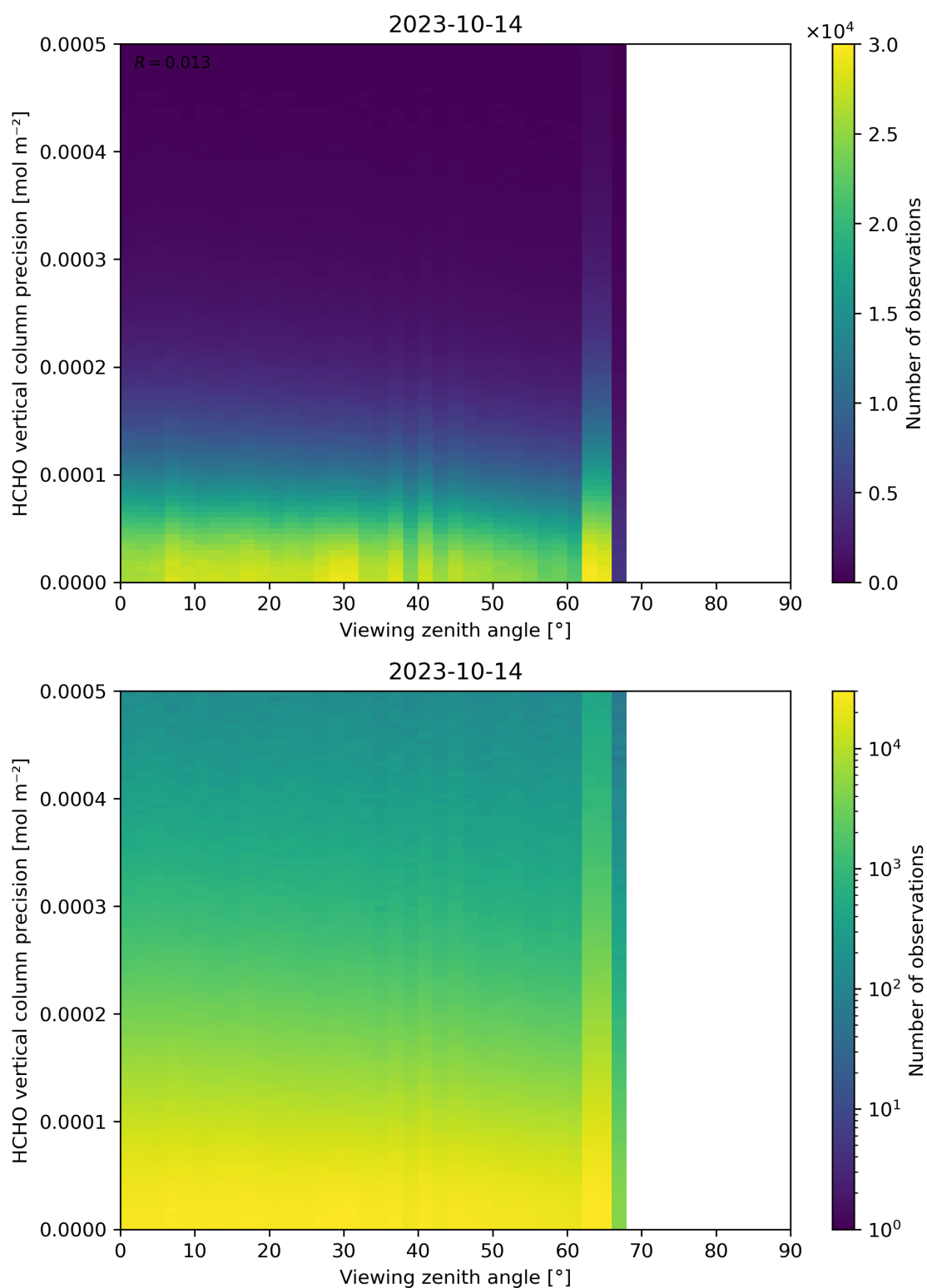
Figure 194: Scatter density plot of “Viewing zenith angle” against “HCHO vertical column precision” for 2023-10-13 to 2023-10-15.
