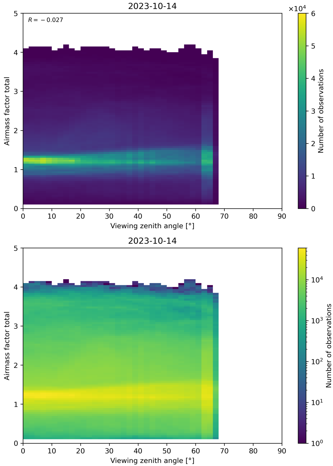
Figure 190: Scatter density plot of “Viewing zenith angle” against “Airmass factor total” for 2023-10-13 to 2023-10-15.
