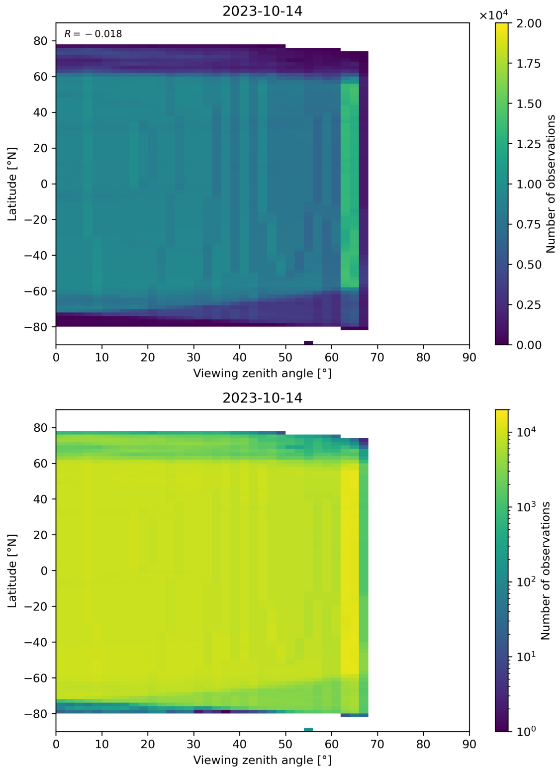
Figure 196: Scatter density plot of “Viewing zenith angle” against “Latitude” for 2023-10-13 to 2023-10-15.
