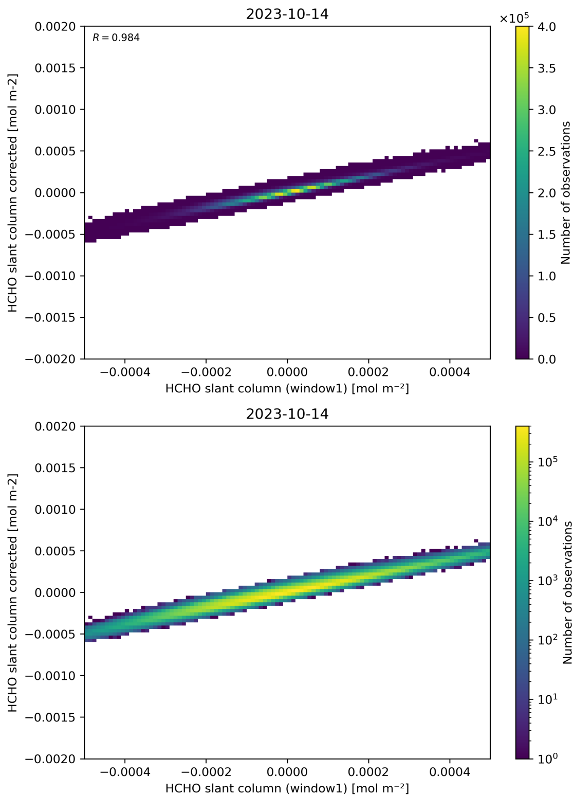
Figure 82: Scatter density plot of “HCHO slant column (window1)” against “HCHO slant column corrected” for 2023-10-13 to 2023-10-15.
