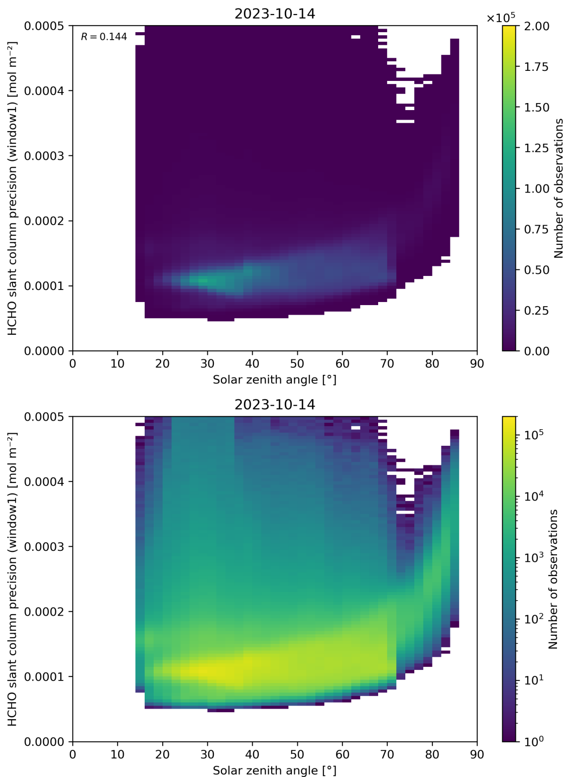
Figure 174: Scatter density plot of “Solar zenith angle” against “HCHO slant column precision (window1)” for 2023-10-13 to 2023-10-15.
