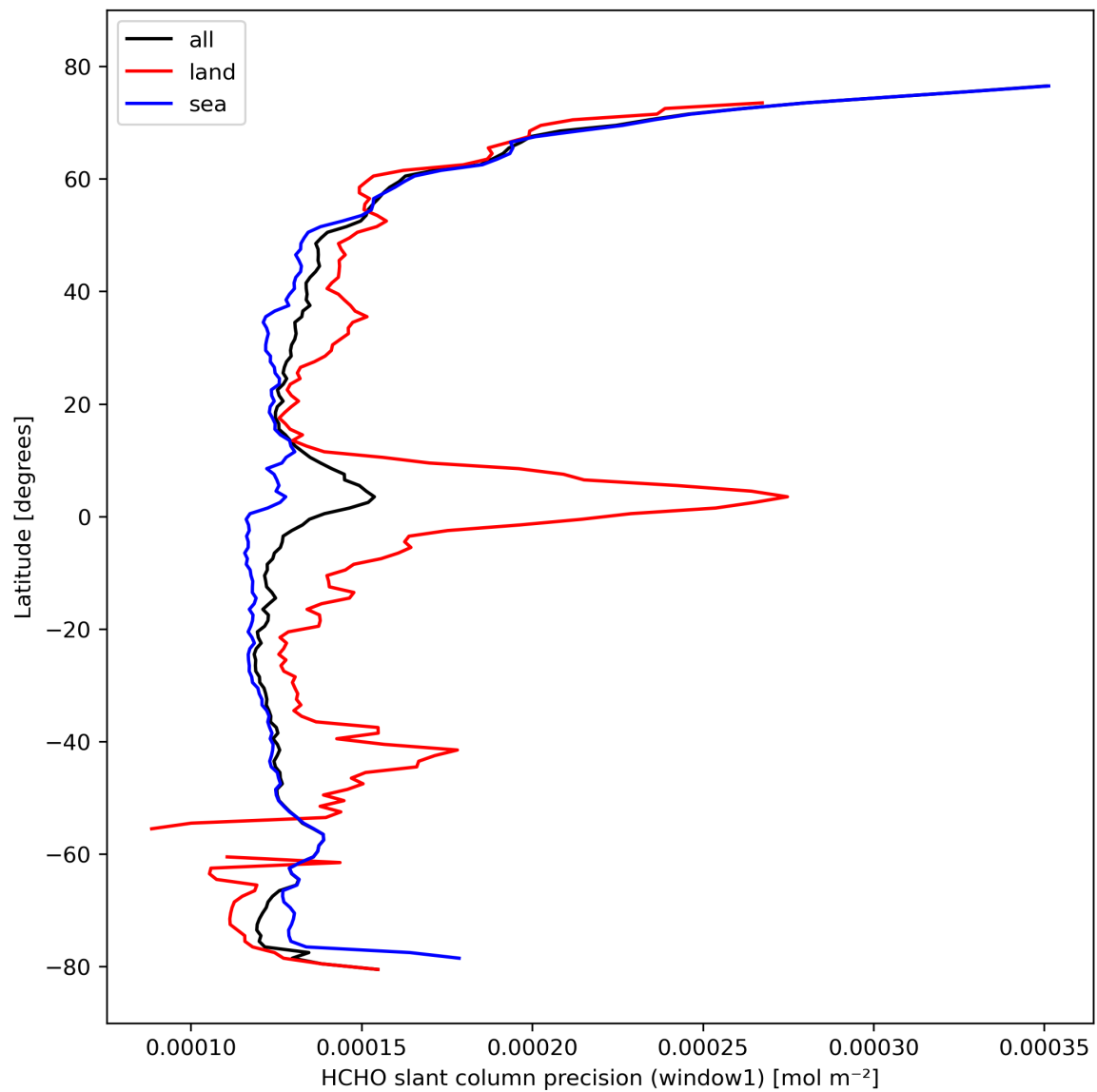
Figure 25: Zonal average of “HCHO slant column precision (window1)” for 2023-10-13 to 2023-10-15.
