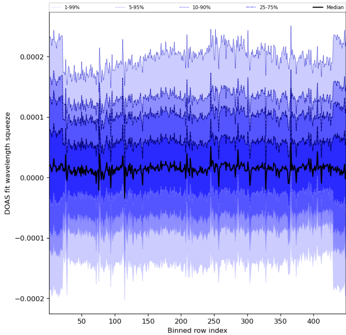
Figure 59: Along track statistics of “DOAS fit wavelength squeeze” for 2023-10-13 to 2023-10-15
