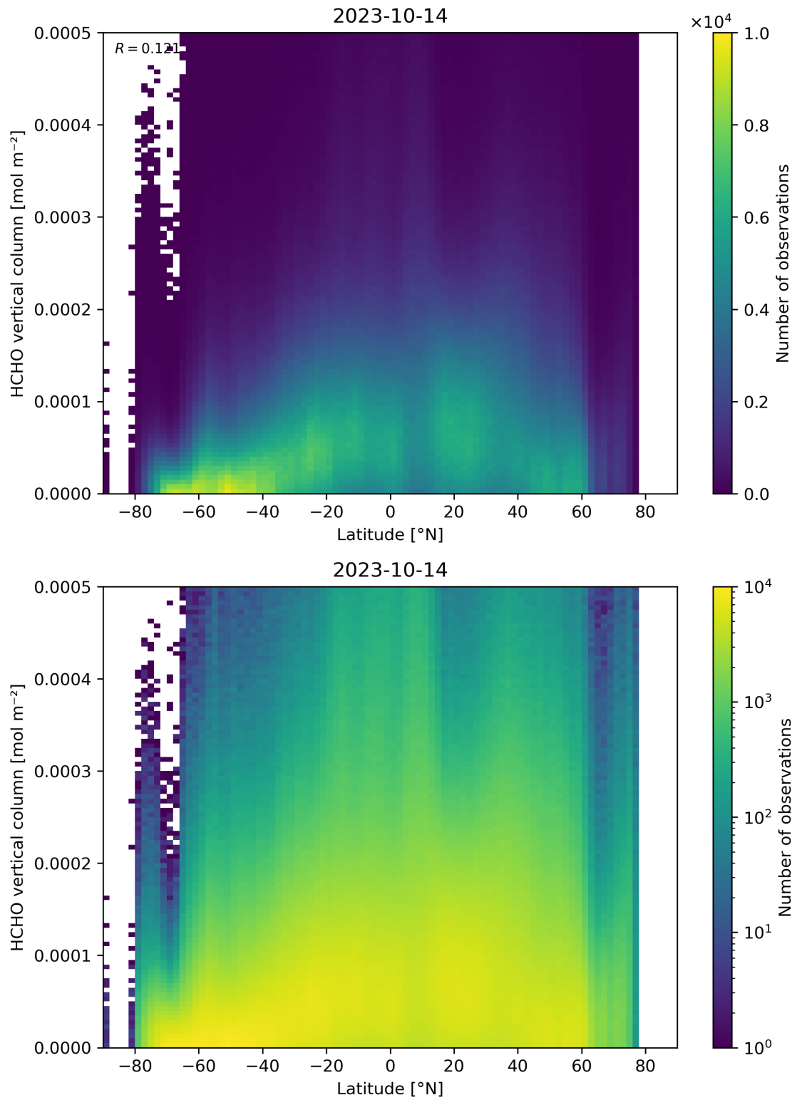
Figure 163: Scatter density plot of “Latitude” against “HCHO vertical column” for 2023-10-13 to 2023-10-15.
