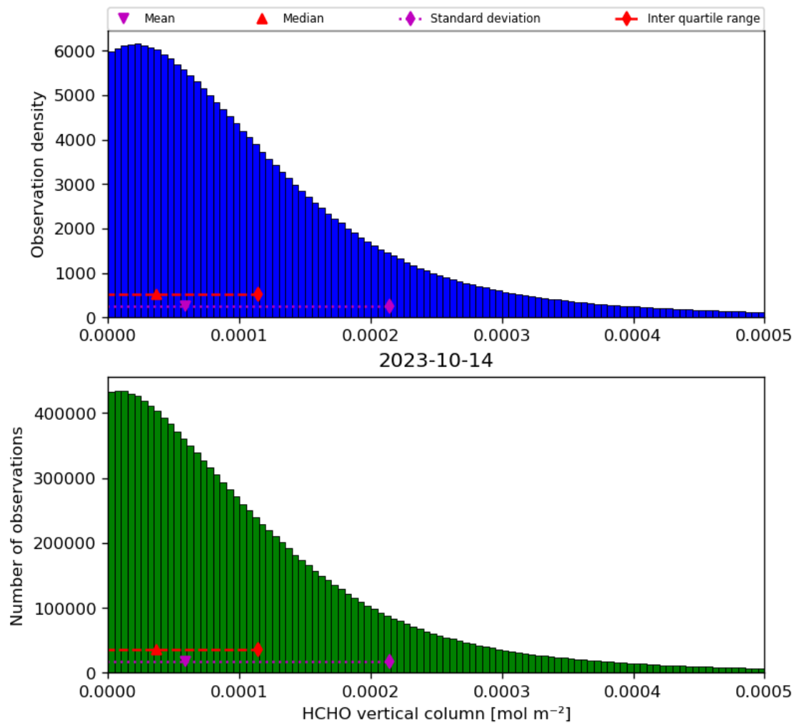
Figure 35: Histogram of “HCHO vertical column” for 2023-10-13 to 2023-10-15
