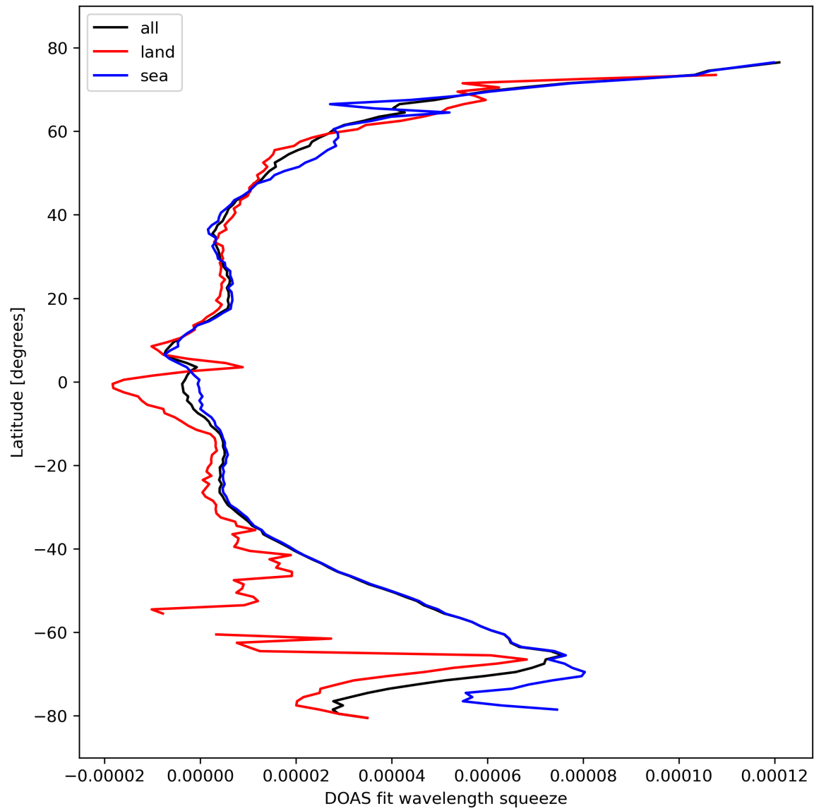
Figure 31: Zonal average of “DOAS fit wavelength squeeze” for 2023-10-13 to 2023-10-15.
