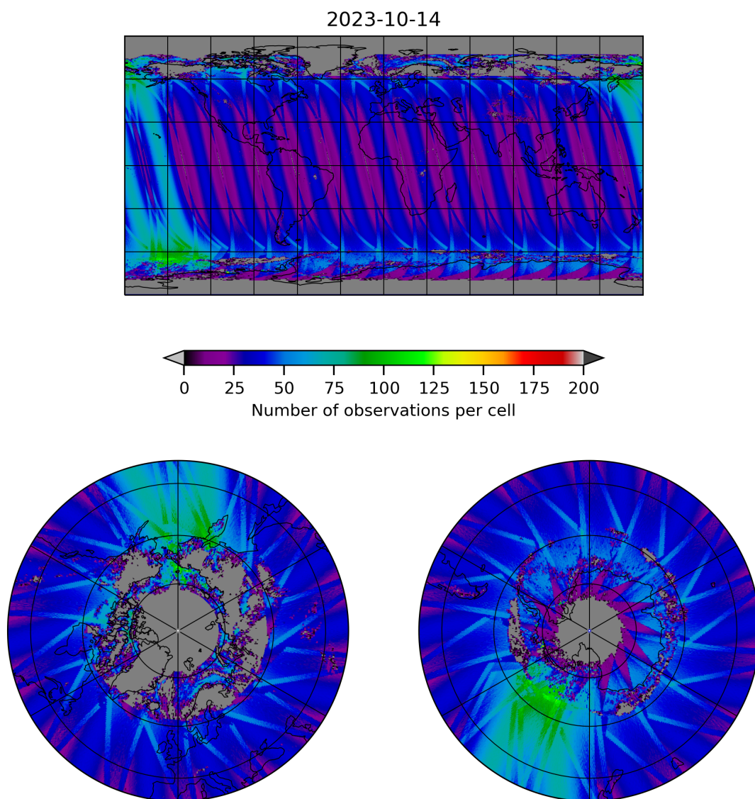
Figure 19: Map of the number of observations for 2023-10-13 to 2023-10-15
