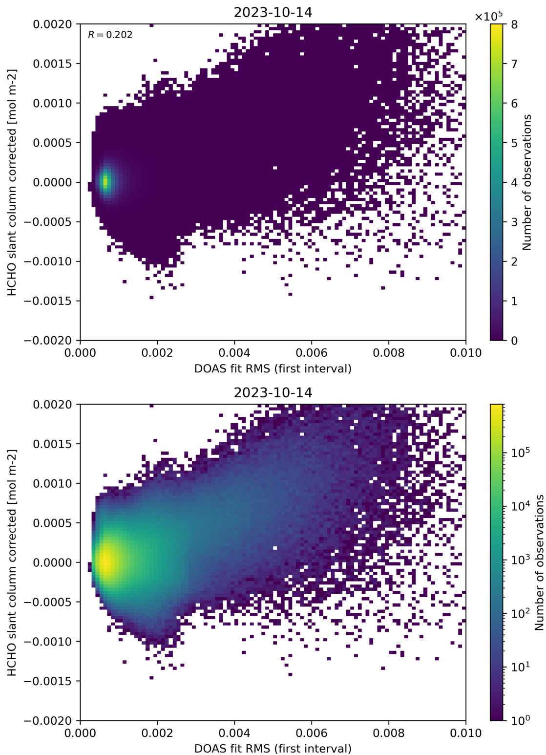
Figure 62: Scatter density plot of “DOAS fit RMS (first interval)” against “HCHO slant column corrected” for 2023-10-13 to 2023-10-15.
