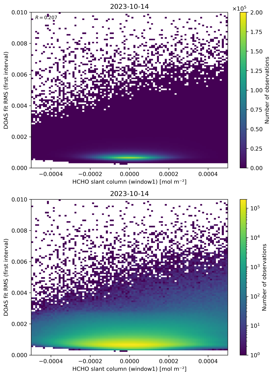
Figure 78: Scatter density plot of “HCHO slant column (window1)” against “DOAS fit RMS (first interval)” for 2023-10-13 to 2023-10-15.
