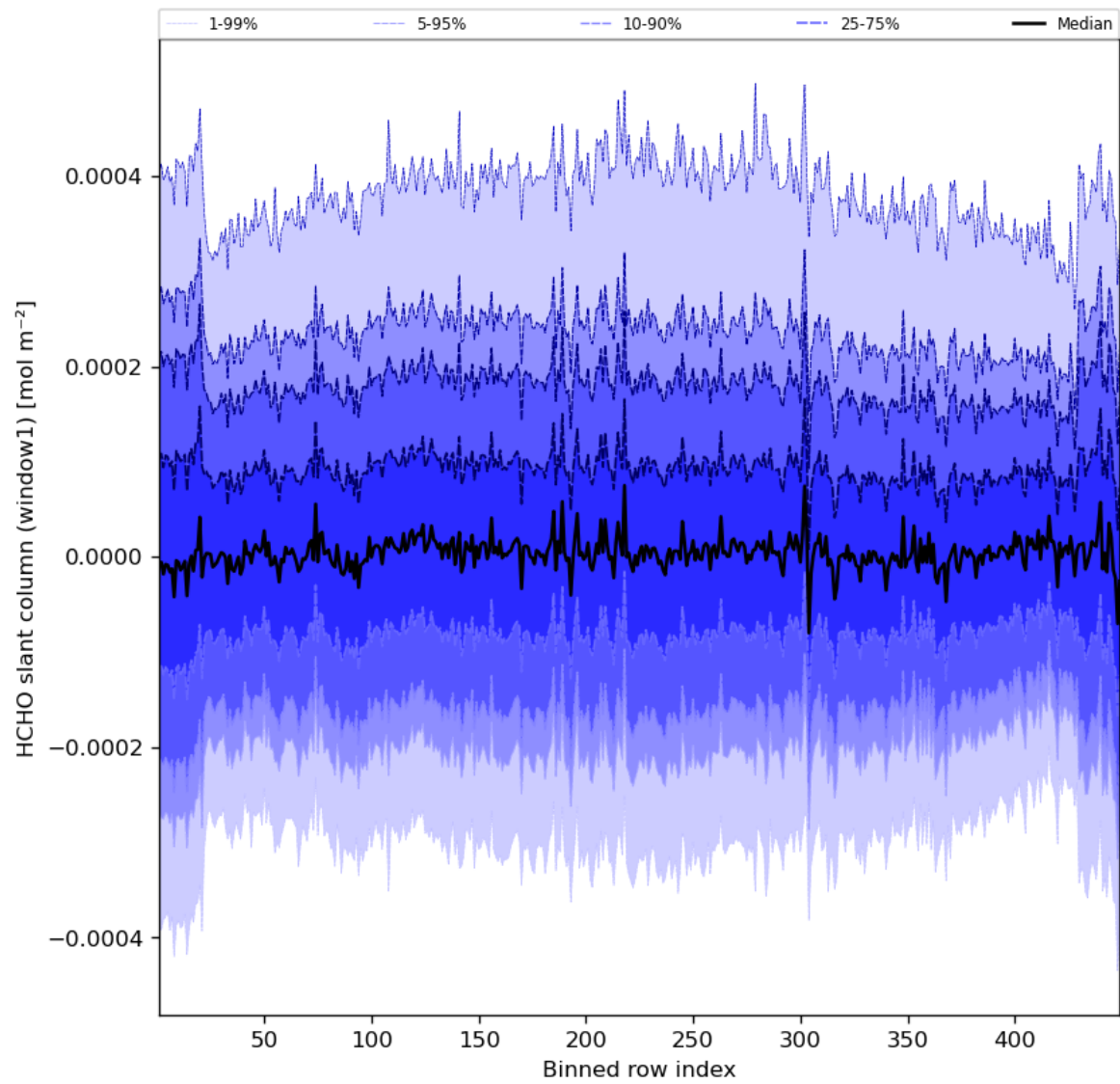
Figure 52: Along track statistics of “HCHO slant column (window1)” for 2023-10-13 to 2023-10-15
