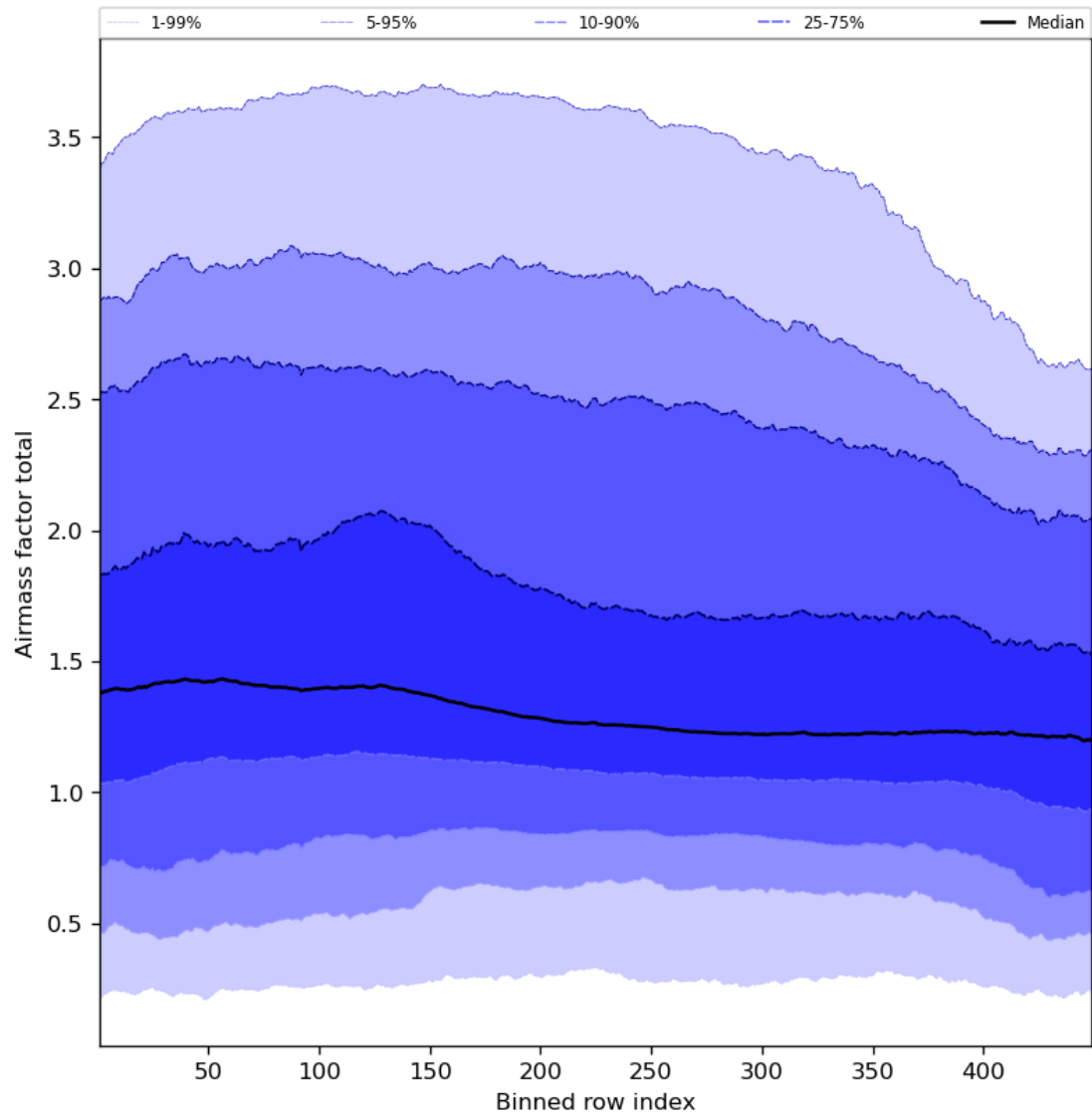
Figure 54: Along track statistics of “Airmass factor total” for 2023-10-13 to 2023-10-15
