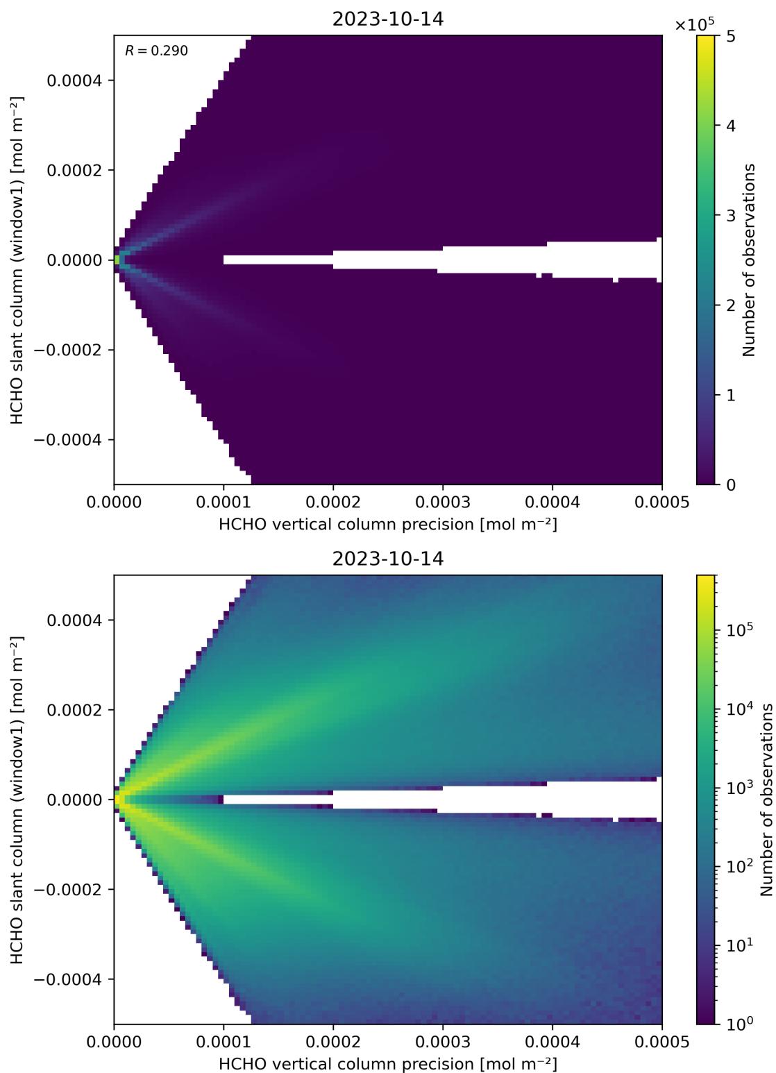
Figure 142: Scatter density plot of “HCHO vertical column precision” against “HCHO slant column (window1)” for 2023-10-13 to 2023-10-15.
