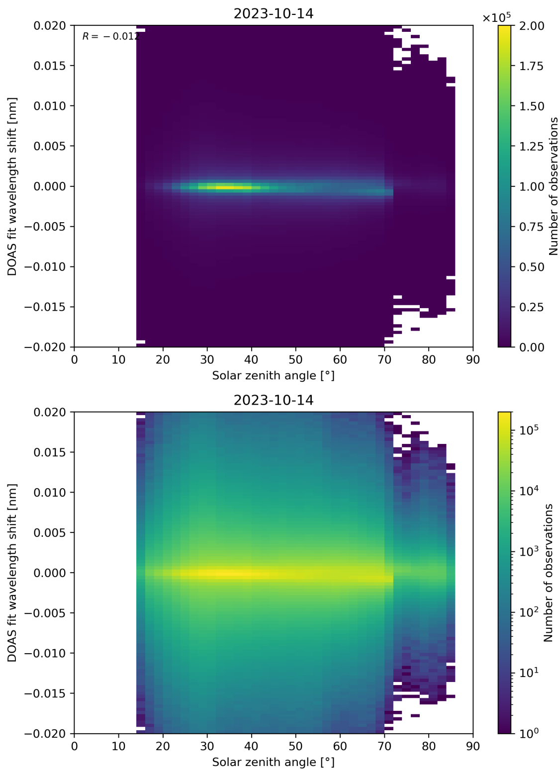
Figure 168: Scatter density plot of “Solar zenith angle” against “DOAS fit wavelength shift” for 2023-10-13 to 2023-10-15.
