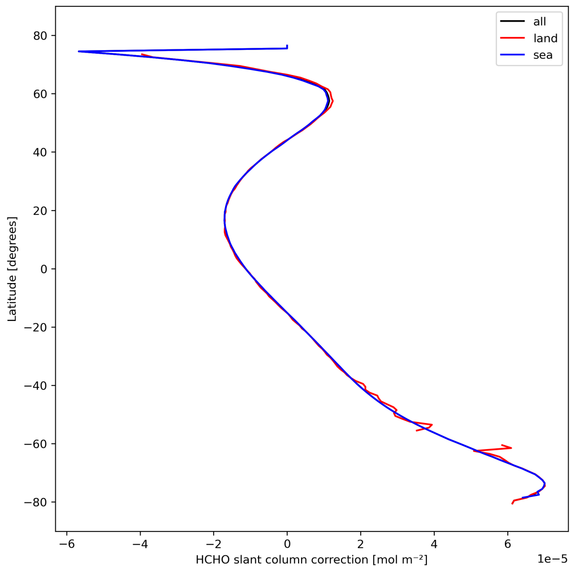
Figure 33: Zonal average of “HCHO slant column correction” for 2023-10-13 to 2023-10-15.
