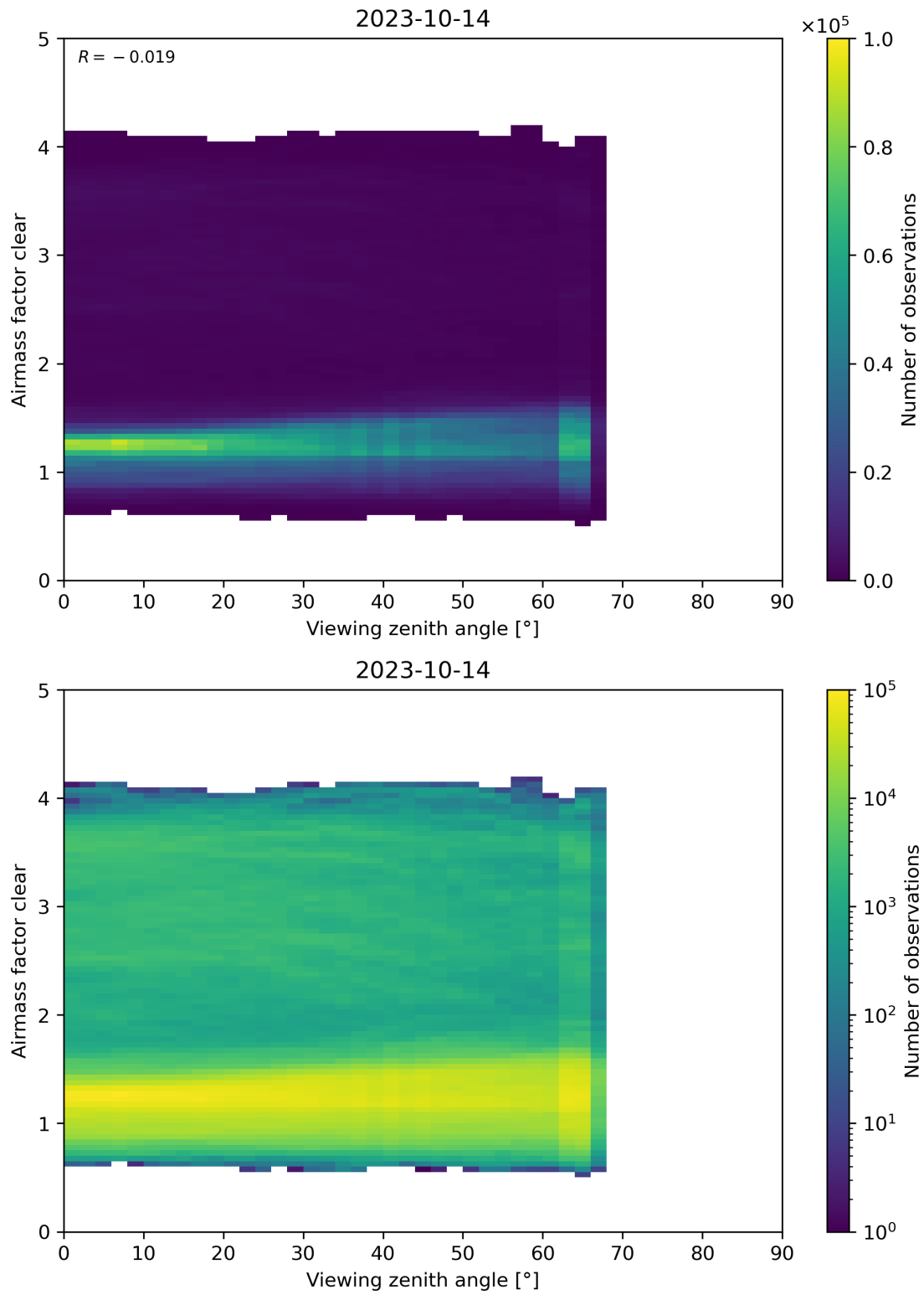
Figure 185: Scatter density plot of “Viewing zenith angle” against “Airmass factor clear” for 2023-10-13 to 2023-10-15.
