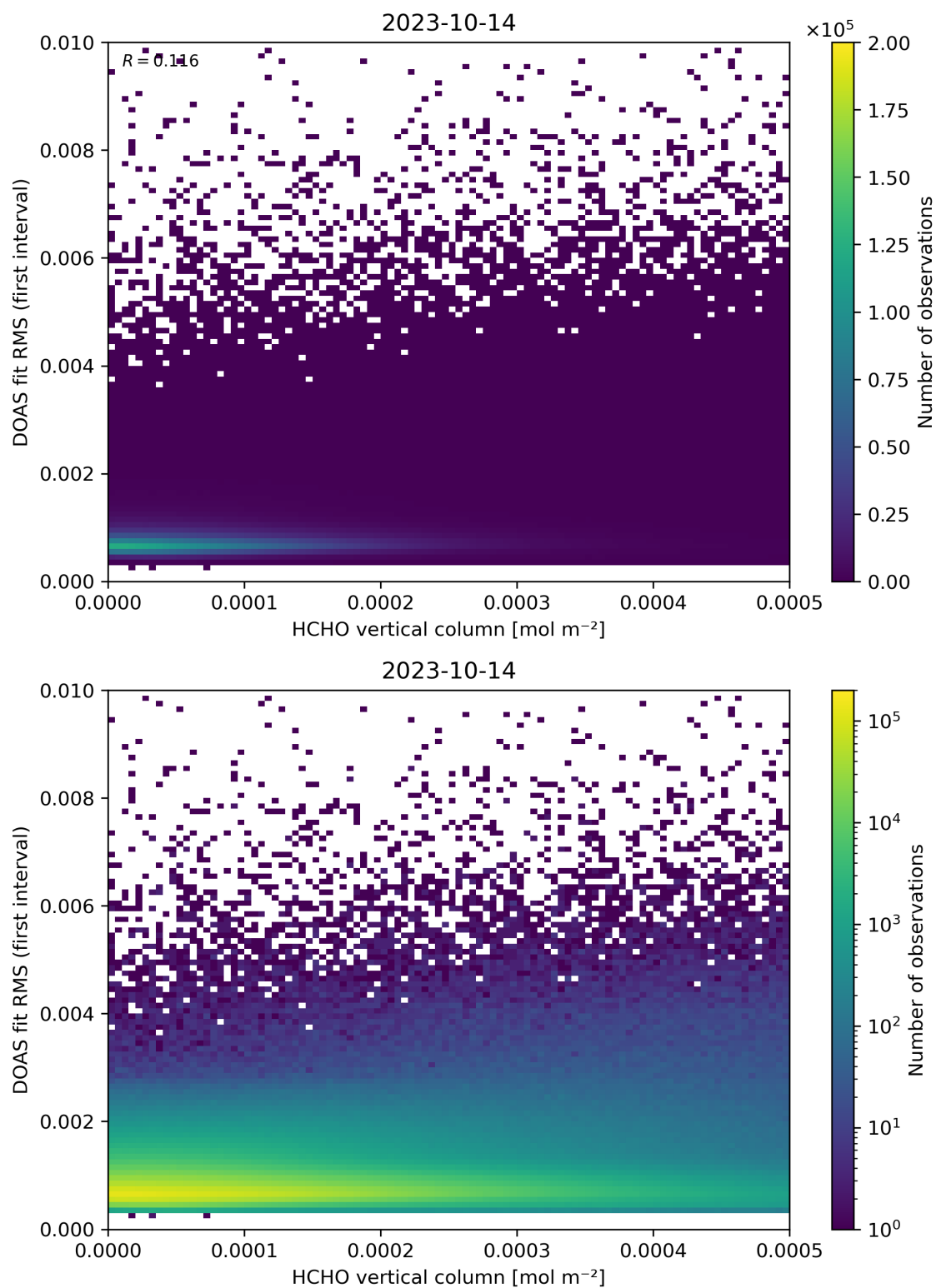
Figure 123: Scatter density plot of “HCHO vertical column” against “DOAS fit RMS (first interval)” for 2023-10-13 to 2023-10-15.
