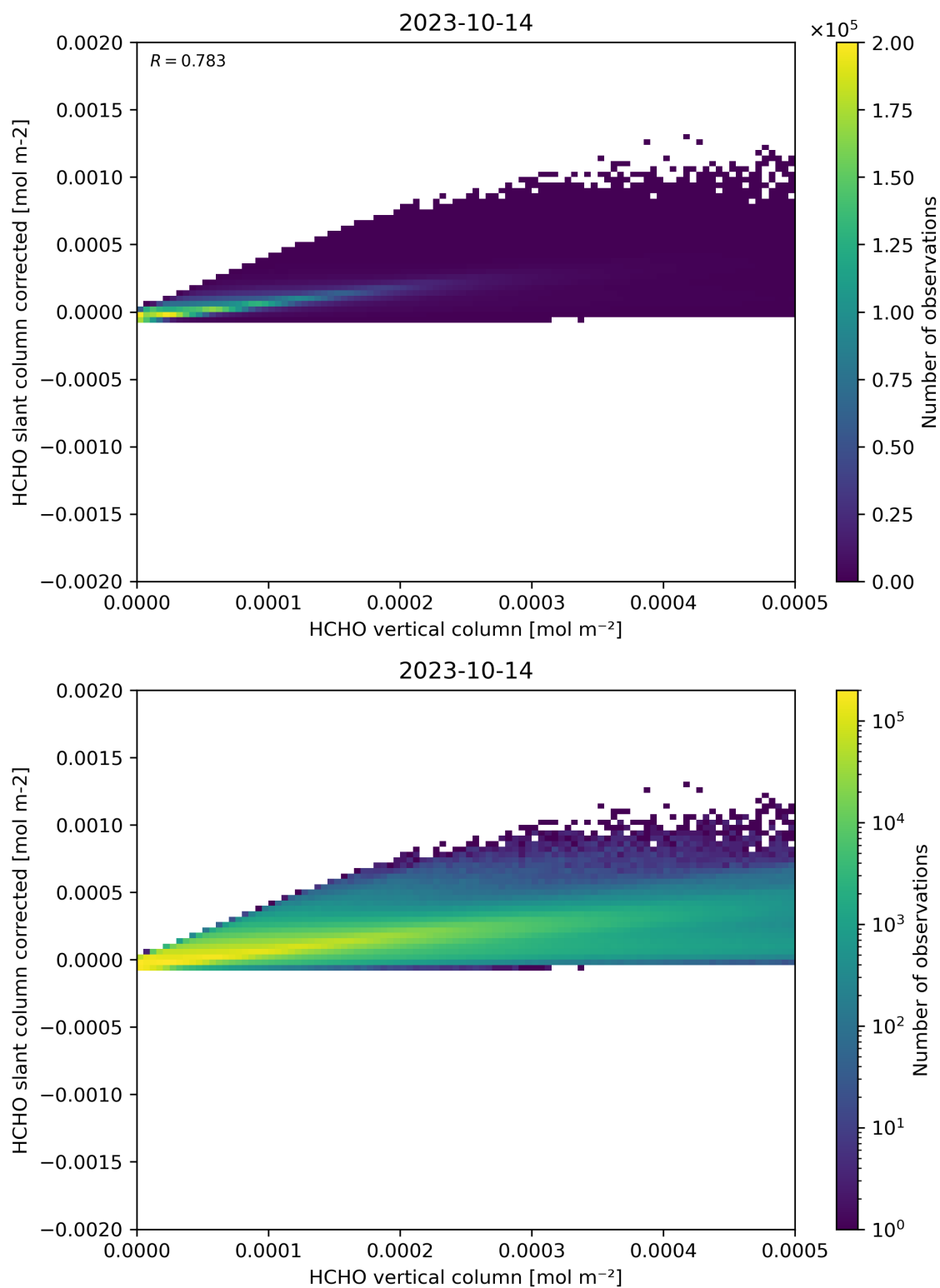
Figure 127: Scatter density plot of “HCHO vertical column” against “HCHO slant column corrected” for 2023-10-13 to 2023-10-15.
