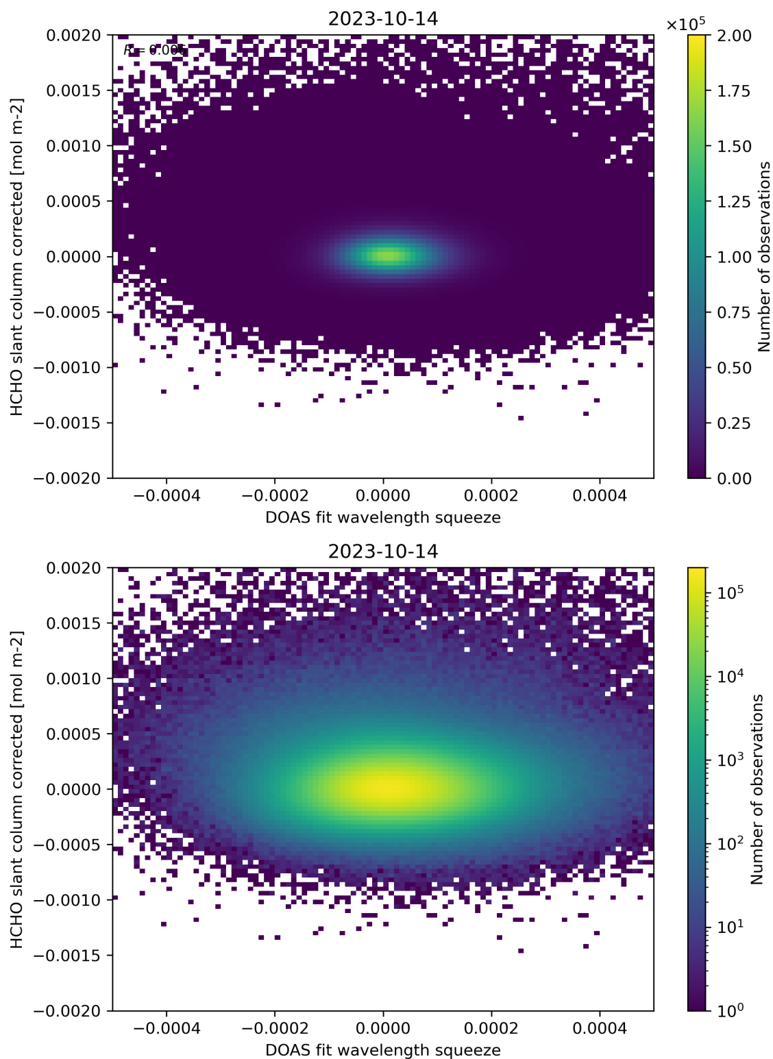
Figure 69: Scatter density plot of “DOAS fit wavelength squeeze” against “HCHO slant column corrected” for 2023-10-13 to 2023-10-15.
