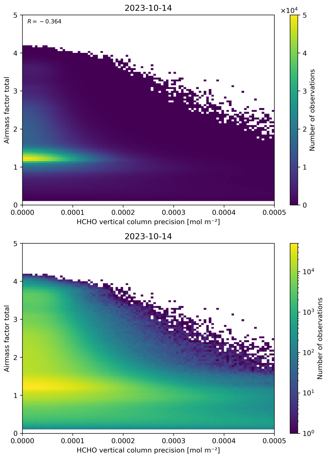
Figure 144: Scatter density plot of “HCHO vertical column precision” against “Airmass factor total” for 2023-10-13 to 2023-10-15.
