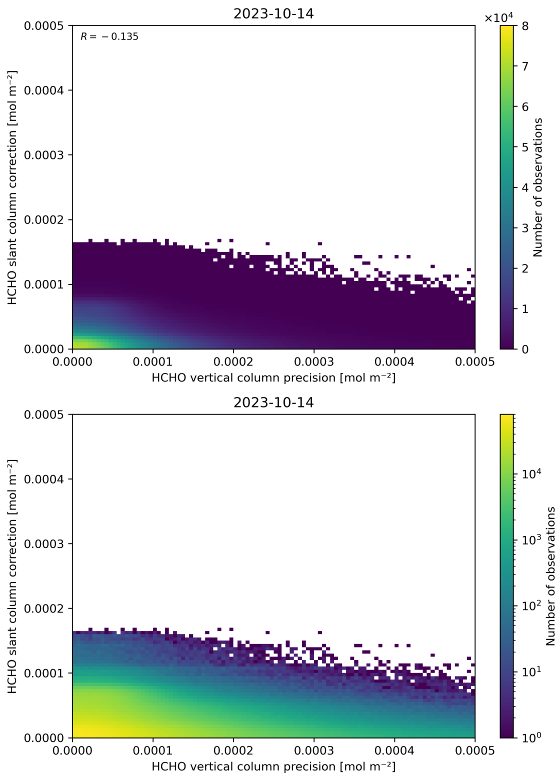
Figure 141: Scatter density plot of “HCHO vertical column precision” against “HCHO slant column correction” for 2023-10-13 to 2023-10-15.
