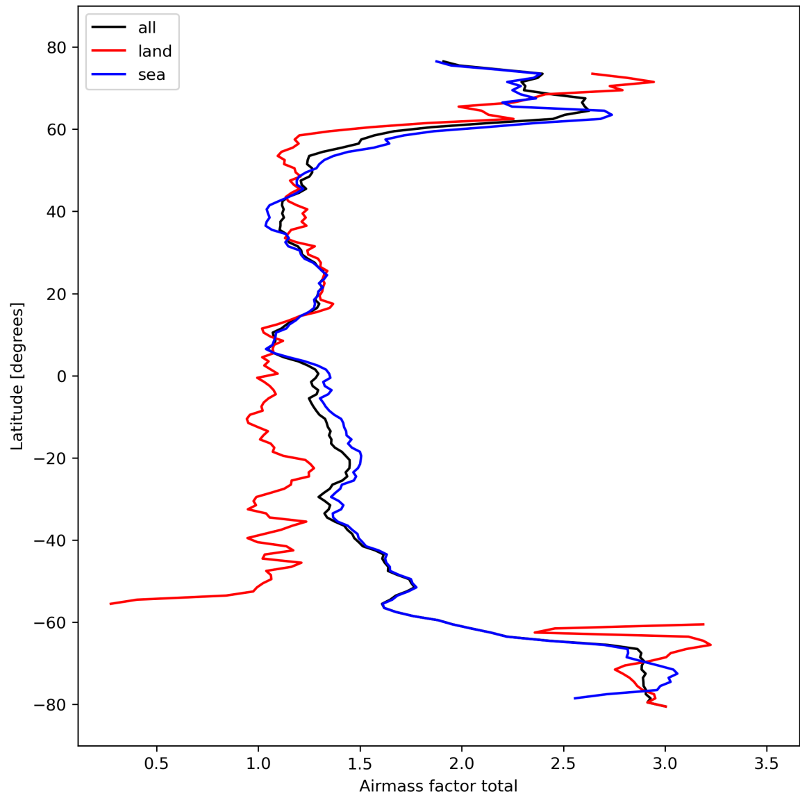
Figure 26: Zonal average of “Airmass factor total” for 2023-10-13 to 2023-10-15.
