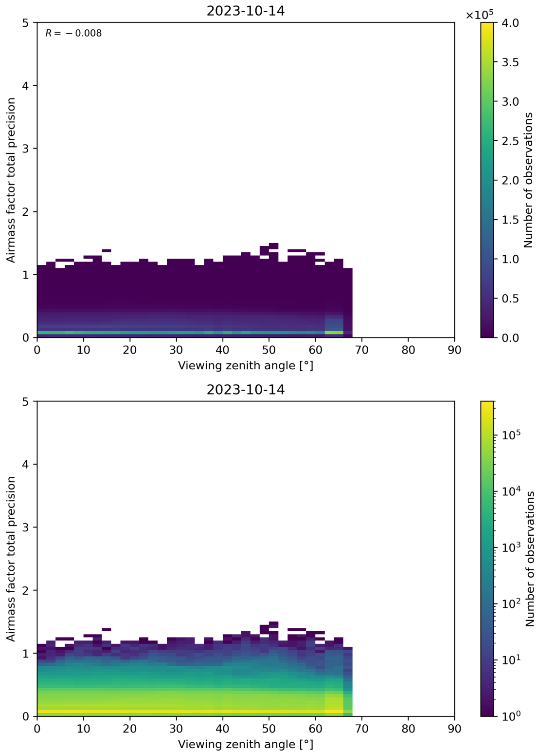
Figure 191: Scatter density plot of “Viewing zenith angle” against “Airmass factor total precision” for 2023-10-13 to 2023-10-15.
