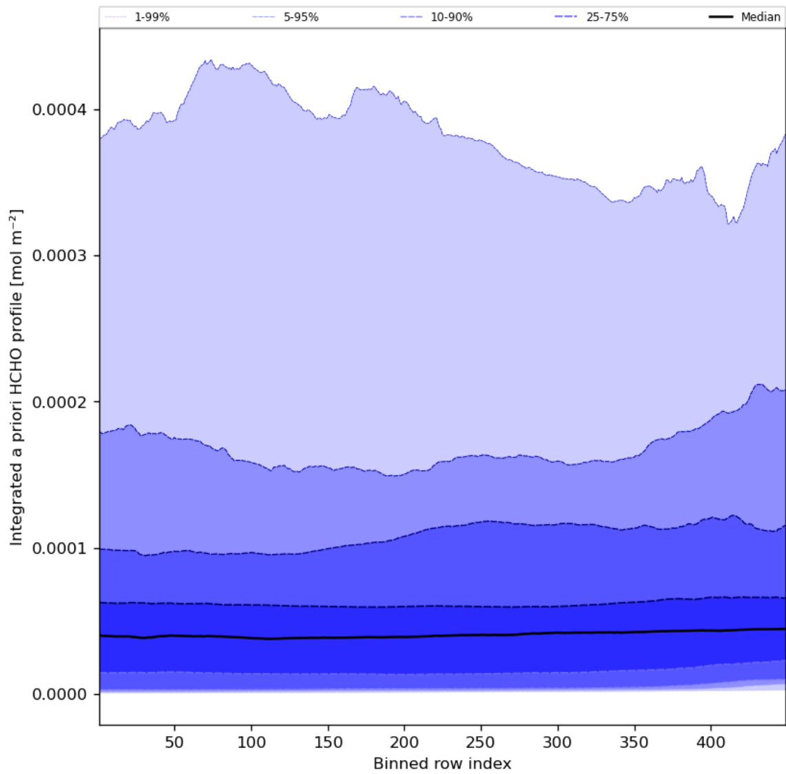
Figure 57: Along track statistics of “Integrated a priori HCHO profile” for 2023-10-13 to 2023-10-15
