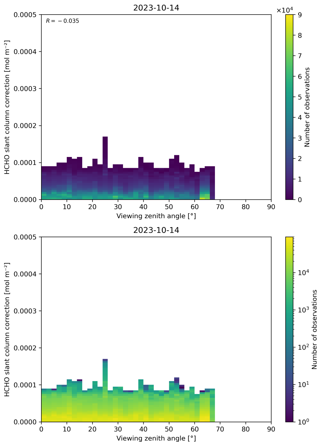
Figure 187: Scatter density plot of “Viewing zenith angle” against “HCHO slant column correction” for 2023-10-13 to 2023-10-15.
