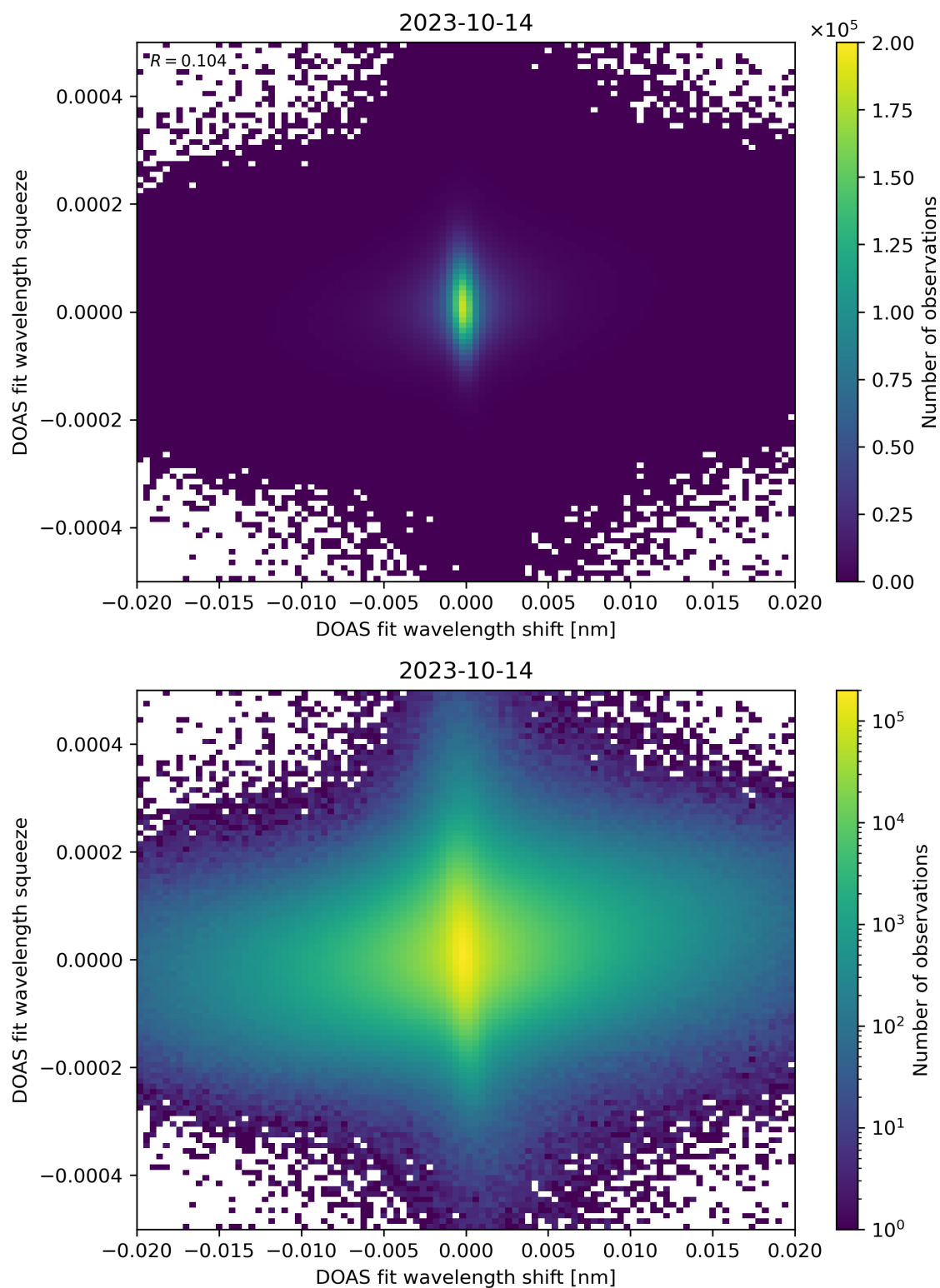
Figure 65: Scatter density plot of “DOAS fit wavelength shift” against “DOAS fit wavelength squeeze” for 2023-10-13 to 2023-10-15.
