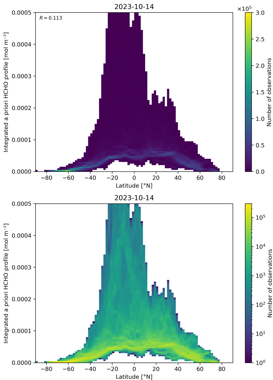
Figure 166: Scatter density plot of “Latitude” against “Integrated a priori HCHO profile” for 2023-10-13 to 2023-10-15.
