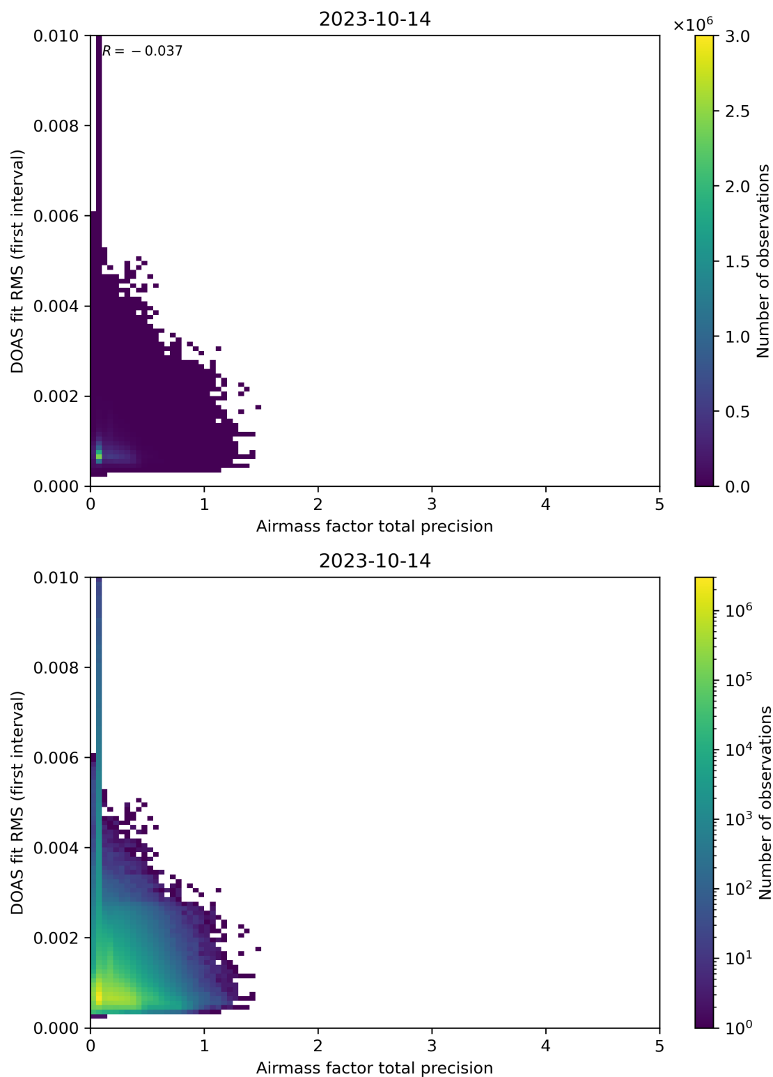
Figure 105: Scatter density plot of “Airmass factor total precision” against “DOAS fit RMS (first interval)” for 2023-10-13 to 2023-10-15.
