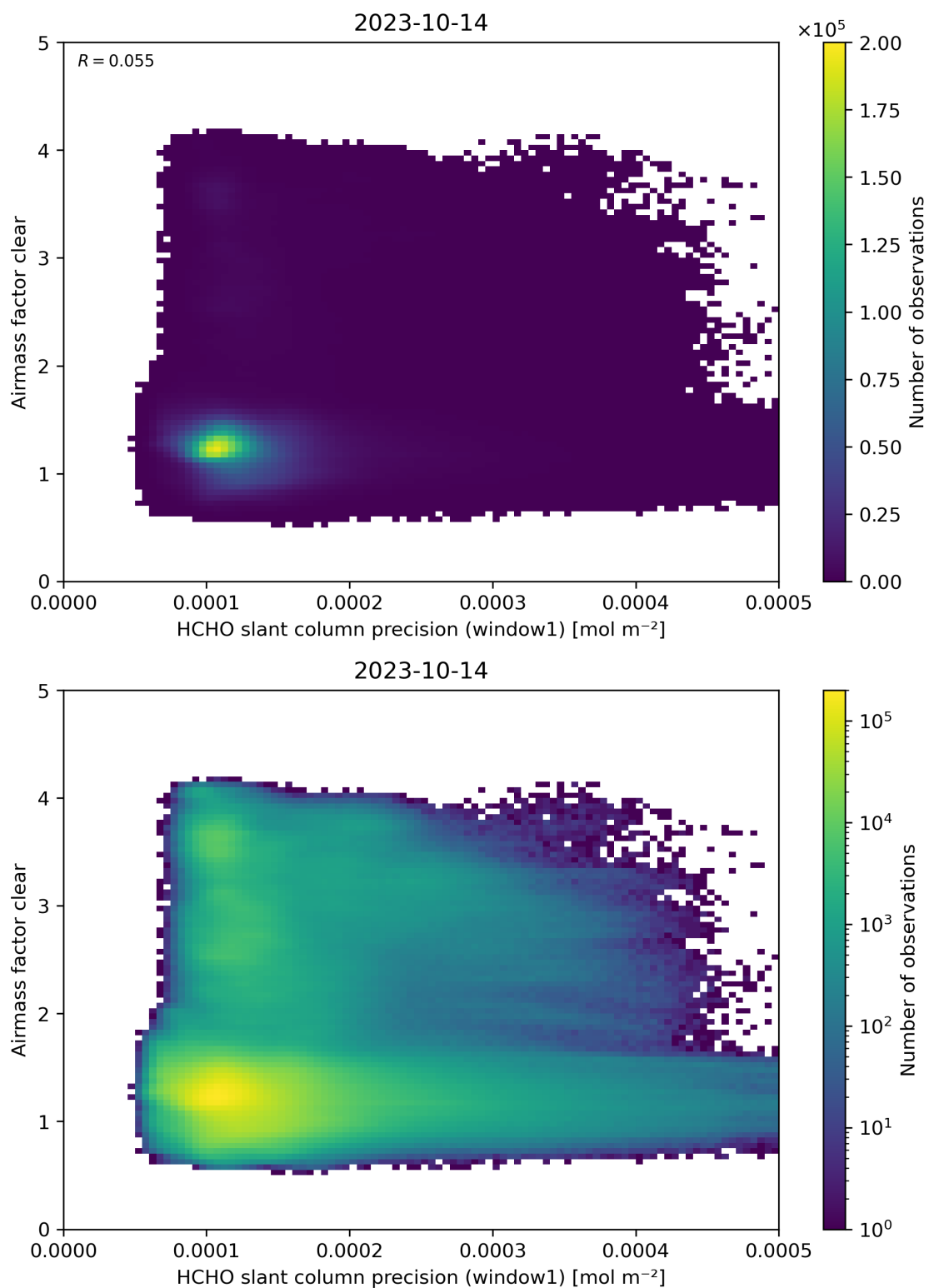
Figure 91: Scatter density plot of “HCHO slant column precision (window1)” against “Airmass factor clear” for 2023-10-13 to 2023-10-15.
