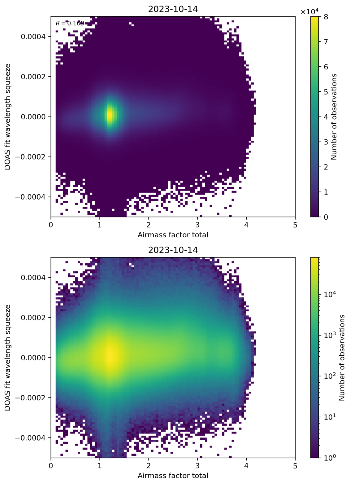
Figure 99: Scatter density plot of “Airmass factor total” against “DOAS fit wavelength squeeze” for 2023-10-13 to 2023-10-15.
