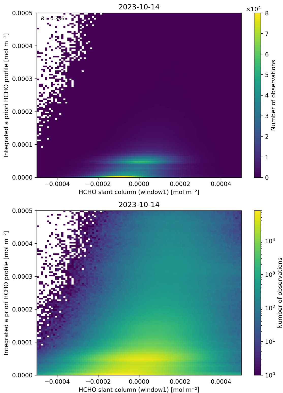
Figure 87: Scatter density plot of “HCHO slant column (window1)” against “Integrated a priori HCHO profile” for 2023-10-13 to 2023-10-15.
