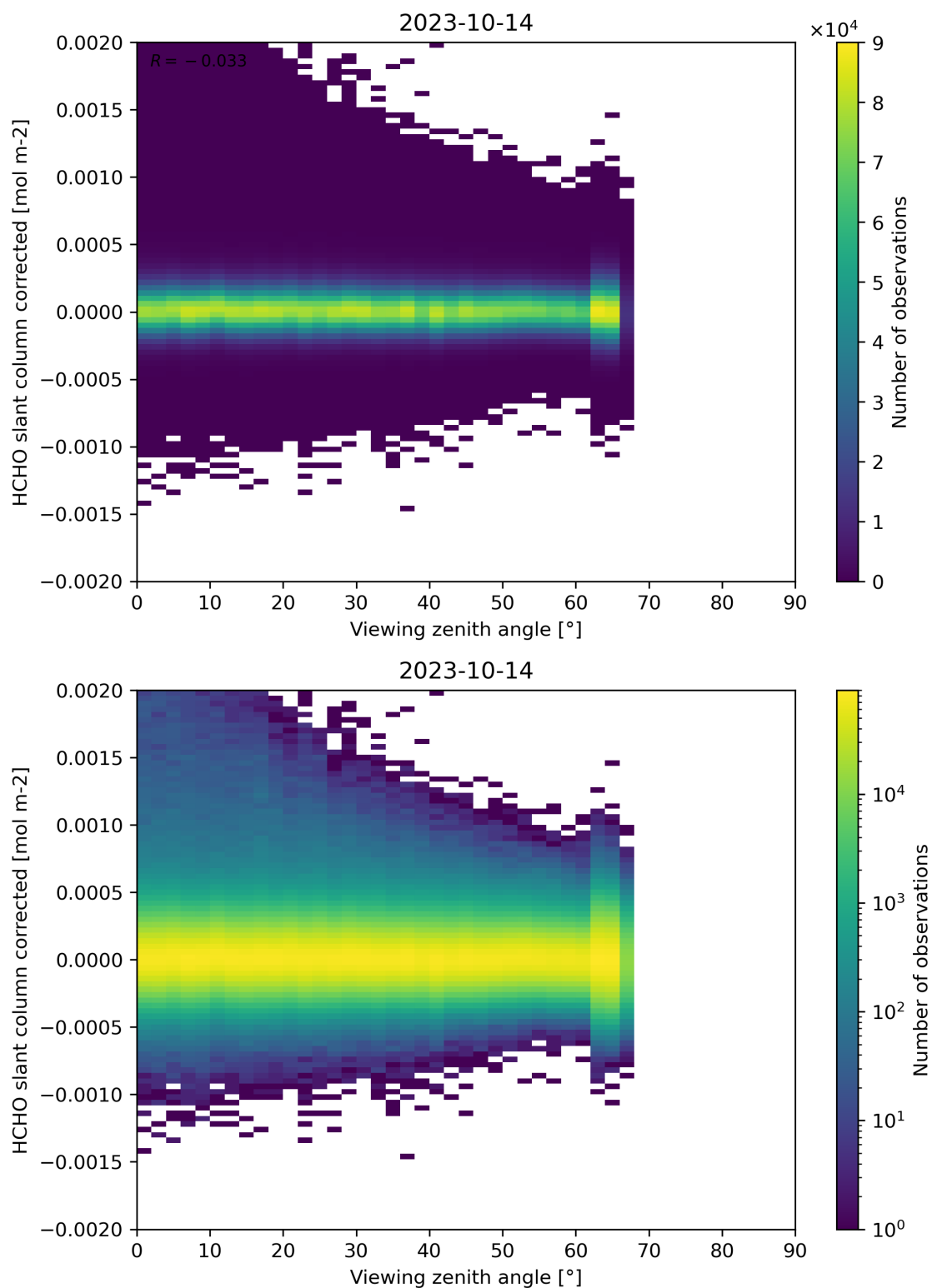
Figure 186: Scatter density plot of “Viewing zenith angle” against “HCHO slant column corrected” for 2023-10-13 to 2023-10-15.
