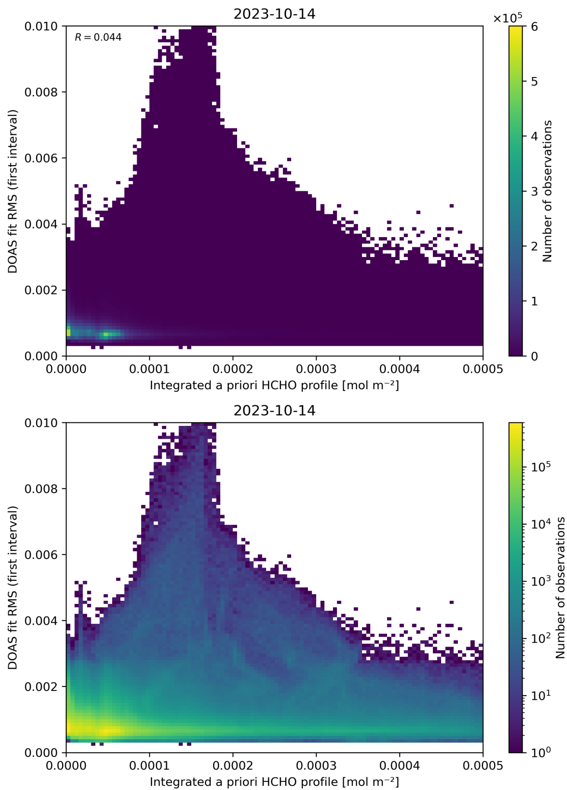
Figure 148: Scatter density plot of “Integrated a priori HCHO profile” against “DOAS fit RMS (first interval)” for 2023-10-13 to 2023-10-15.
