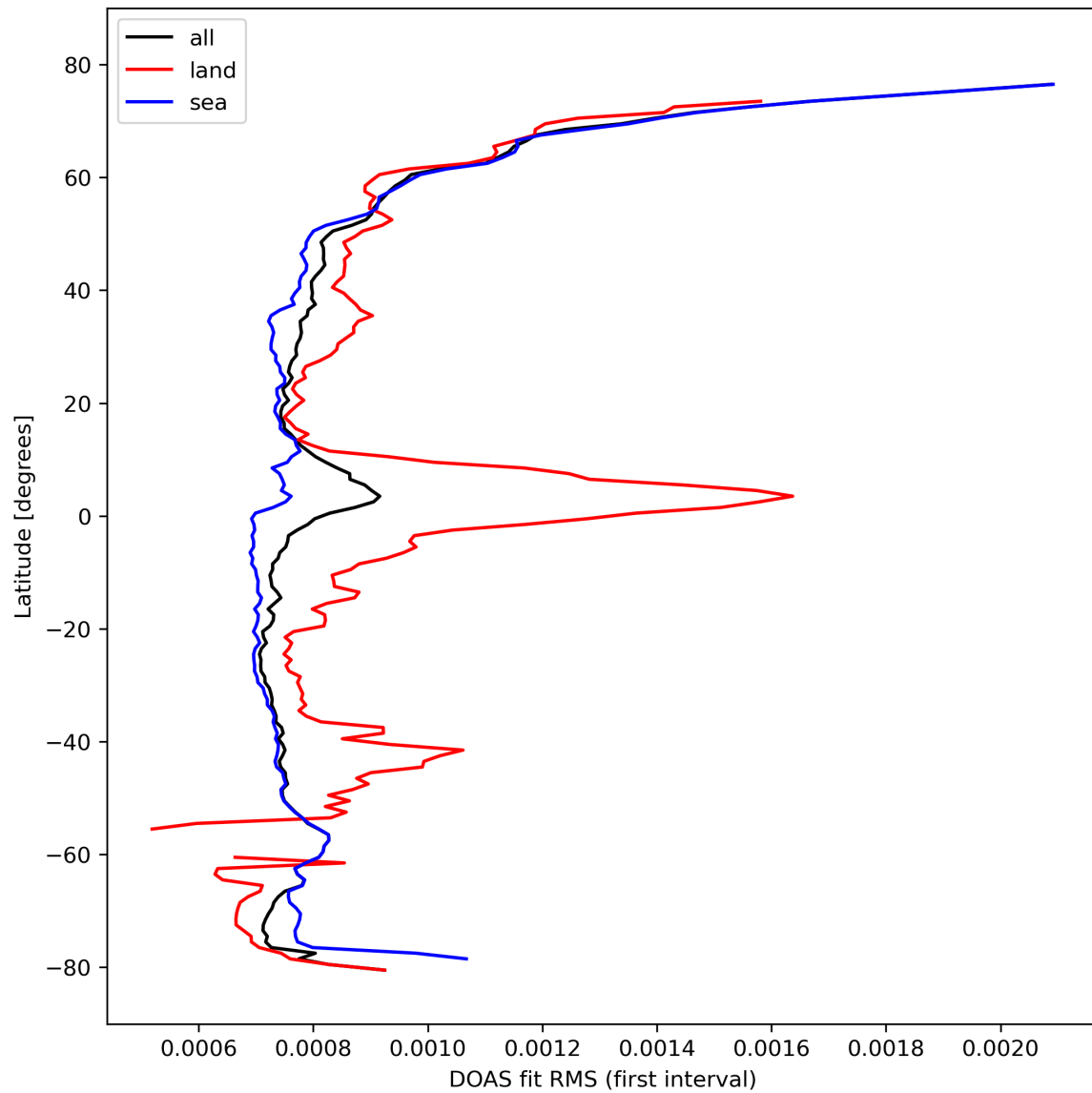
Figure 32: Zonal average of “DOAS fit RMS (first interval)” for 2023-10-13 to 2023-10-15.
