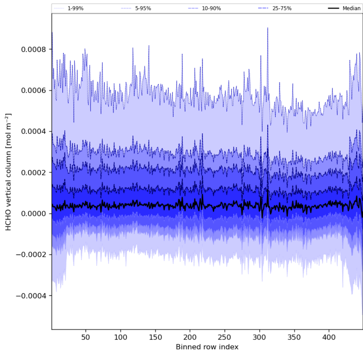
Figure 49: Along track statistics of “HCHO vertical column” for 2023-10-13 to 2023-10-15
