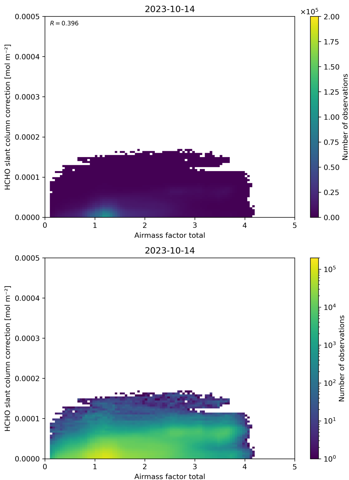
Figure 102: Scatter density plot of “Airmass factor total” against “HCHO slant column correction” for 2023-10-13 to 2023-10-15.
