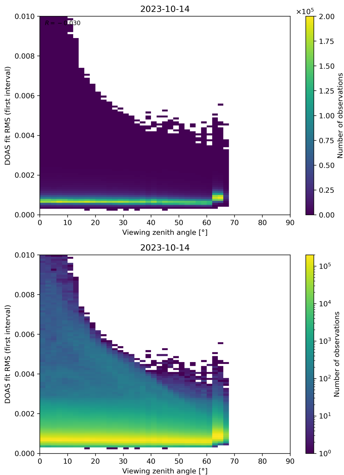
Figure 182: Scatter density plot of “Viewing zenith angle” against “DOAS fit RMS (first interval)” for 2023-10-13 to 2023-10-15.
