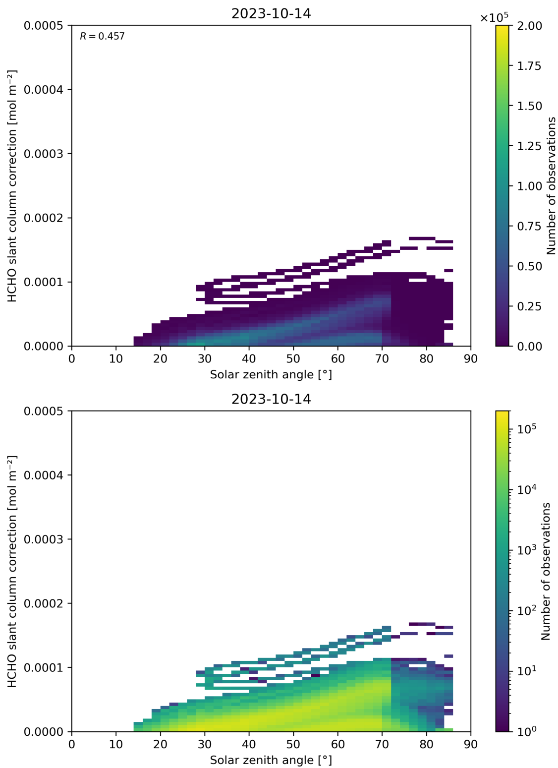
Figure 172: Scatter density plot of “Solar zenith angle” against “HCHO slant column correction” for 2023-10-13 to 2023-10-15.
