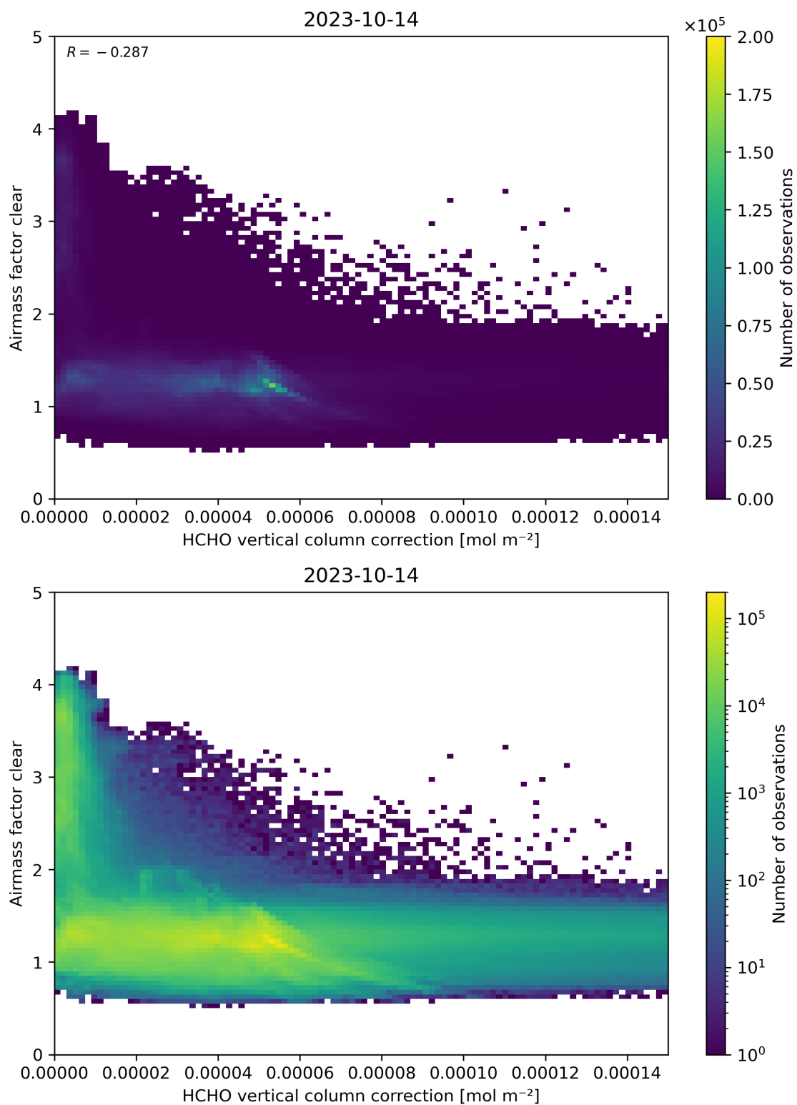
Figure 115: Scatter density plot of “HCHO vertical column correction” against “Airmass factor clear” for 2023-10-13 to 2023-10-15.
