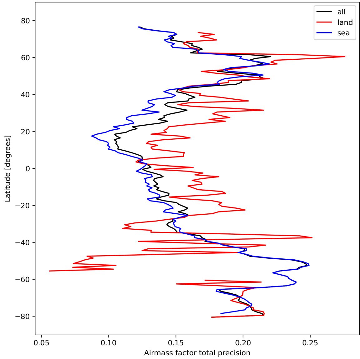
Figure 27: Zonal average of “Airmass factor total precision” for 2023-10-13 to 2023-10-15.
