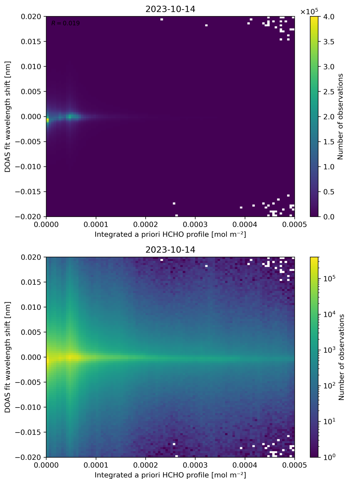
Figure 149: Scatter density plot of “Integrated a priori HCHO profile” against “DOAS fit wavelength shift” for 2023-10-13 to 2023-10-15.
