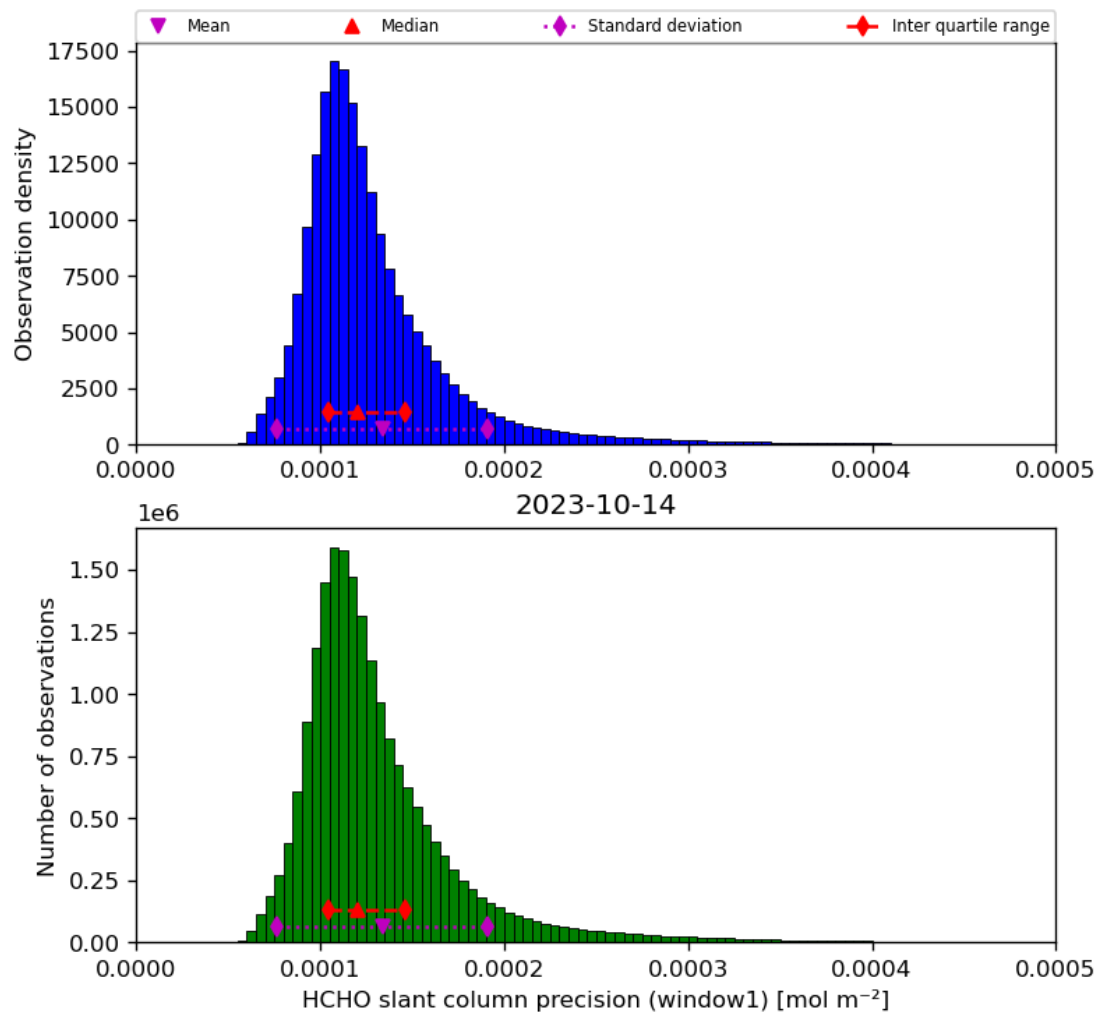
Figure 39: Histogram of “HCHO slant column precision (window1)” for 2023-10-13 to 2023-10-15
