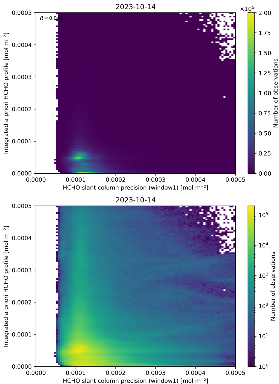
Figure 96: Scatter density plot of “HCHO slant column precision (window1)” against “Integrated a priori HCHO profile” for 2023-10-13 to 2023-10-15.
