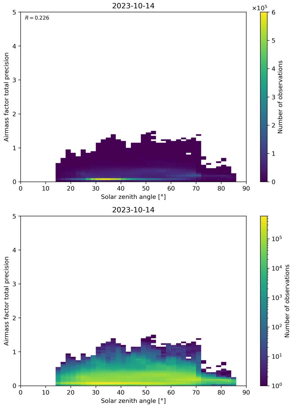
Figure 176: Scatter density plot of “Solar zenith angle” against “Airmass factor total precision” for 2023-10-13 to 2023-10-15.
