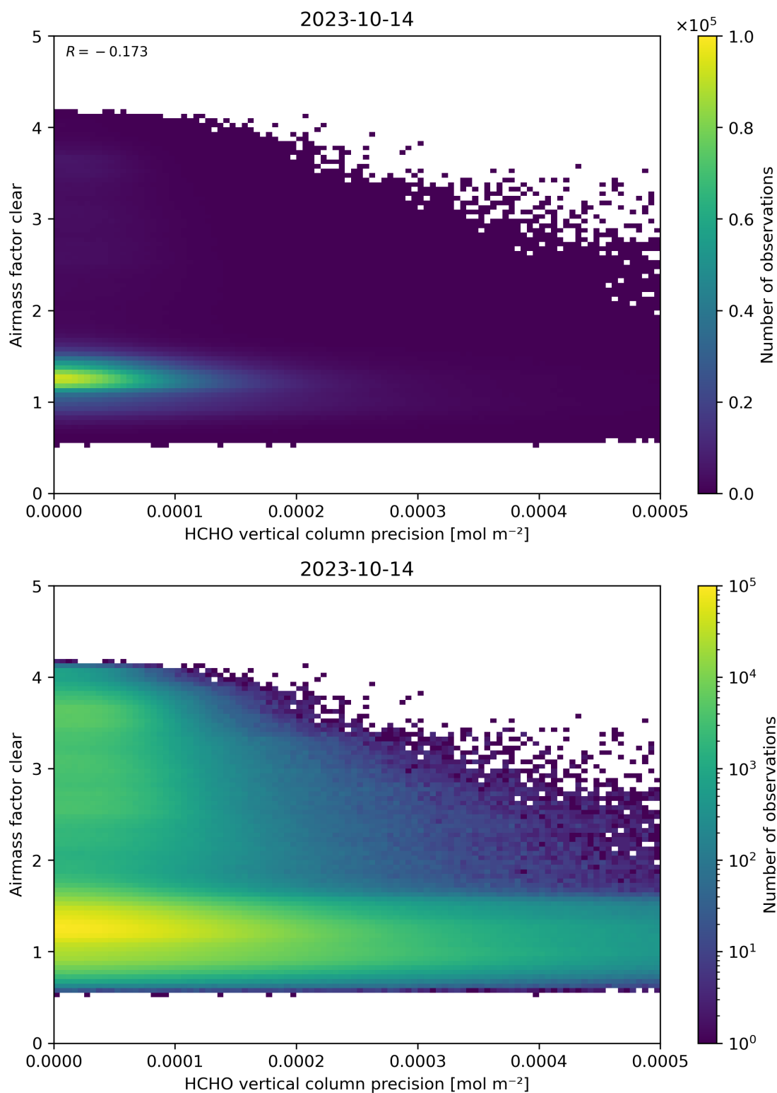
Figure 139: Scatter density plot of “HCHO vertical column precision” against “Airmass factor clear” for 2023-10-13 to 2023-10-15.
