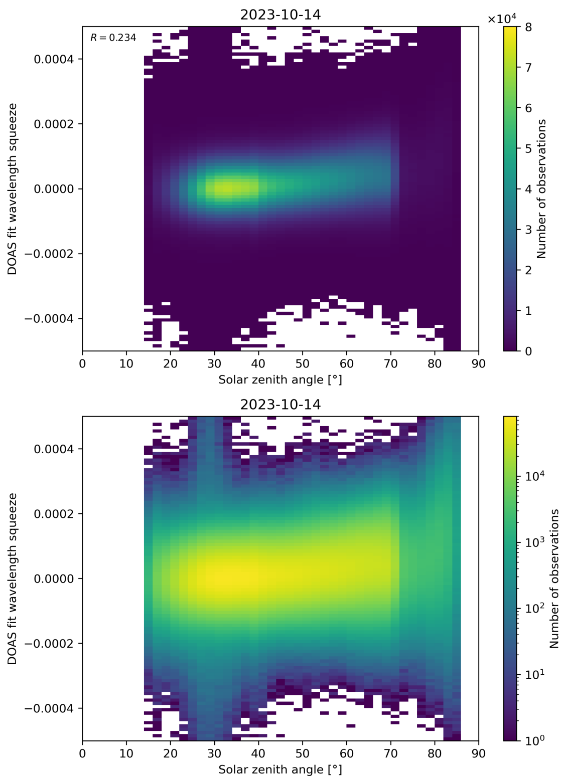
Figure 169: Scatter density plot of “Solar zenith angle” against “DOAS fit wavelength squeeze” for 2023-10-13 to 2023-10-15.
