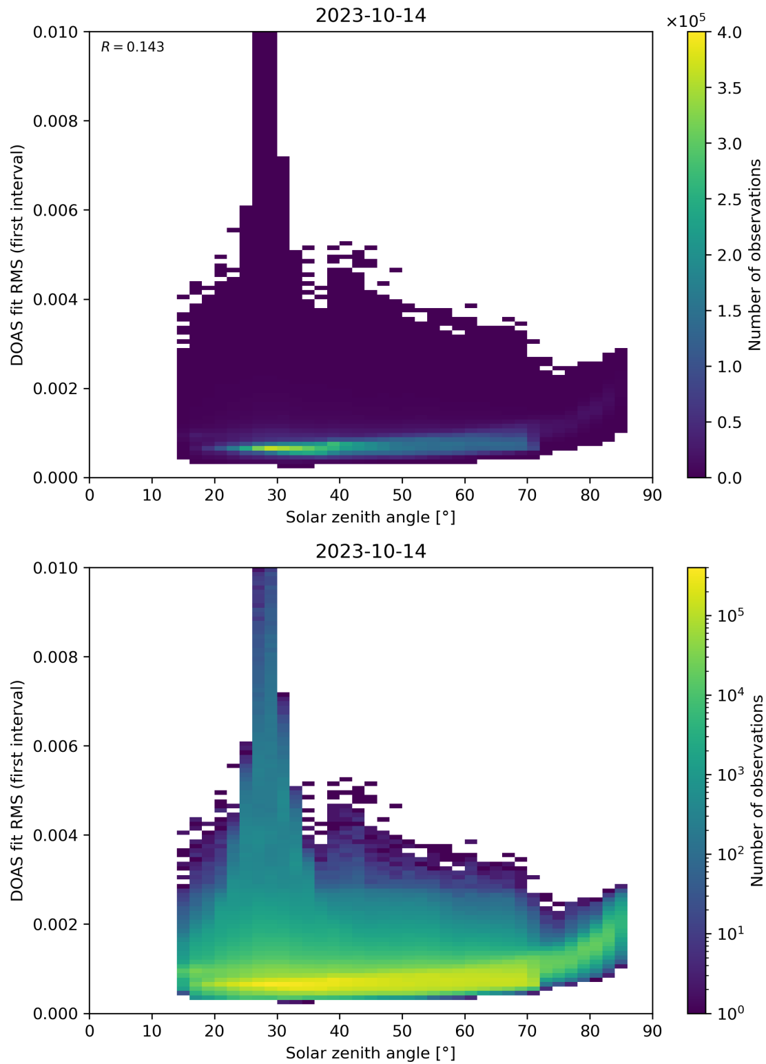
Figure 167: Scatter density plot of “Solar zenith angle” against “DOAS fit RMS (first interval)” for 2023-10-13 to 2023-10-15.
