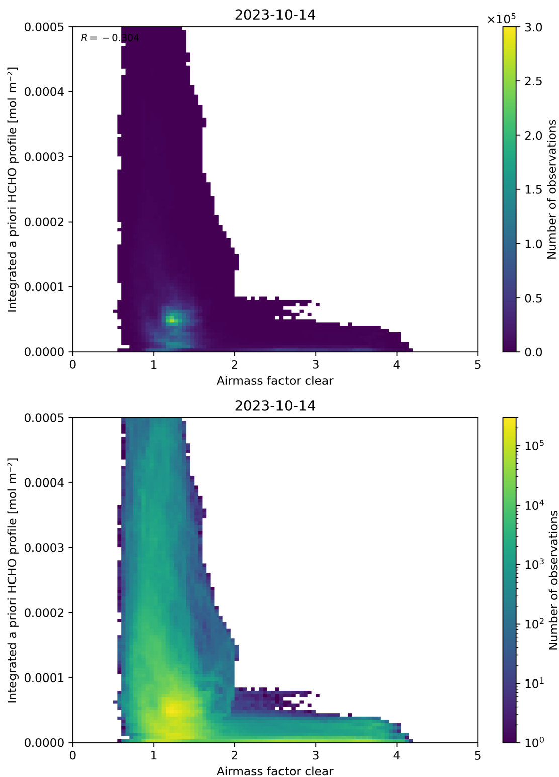
Figure 76: Scatter density plot of “Airmass factor clear” against “Integrated a priori HCHO profile” for 2023-10-13 to 2023-10-15.
