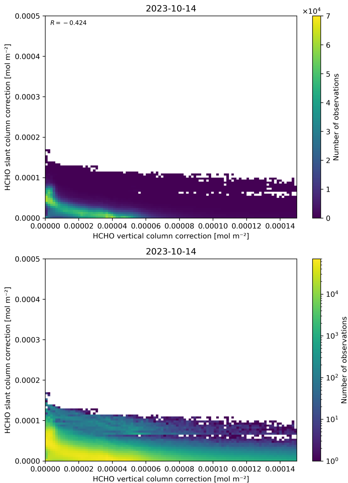
Figure 117: Scatter density plot of “HCHO vertical column correction” against “HCHO slant column correction” for 2023-10-13 to 2023-10-15.
