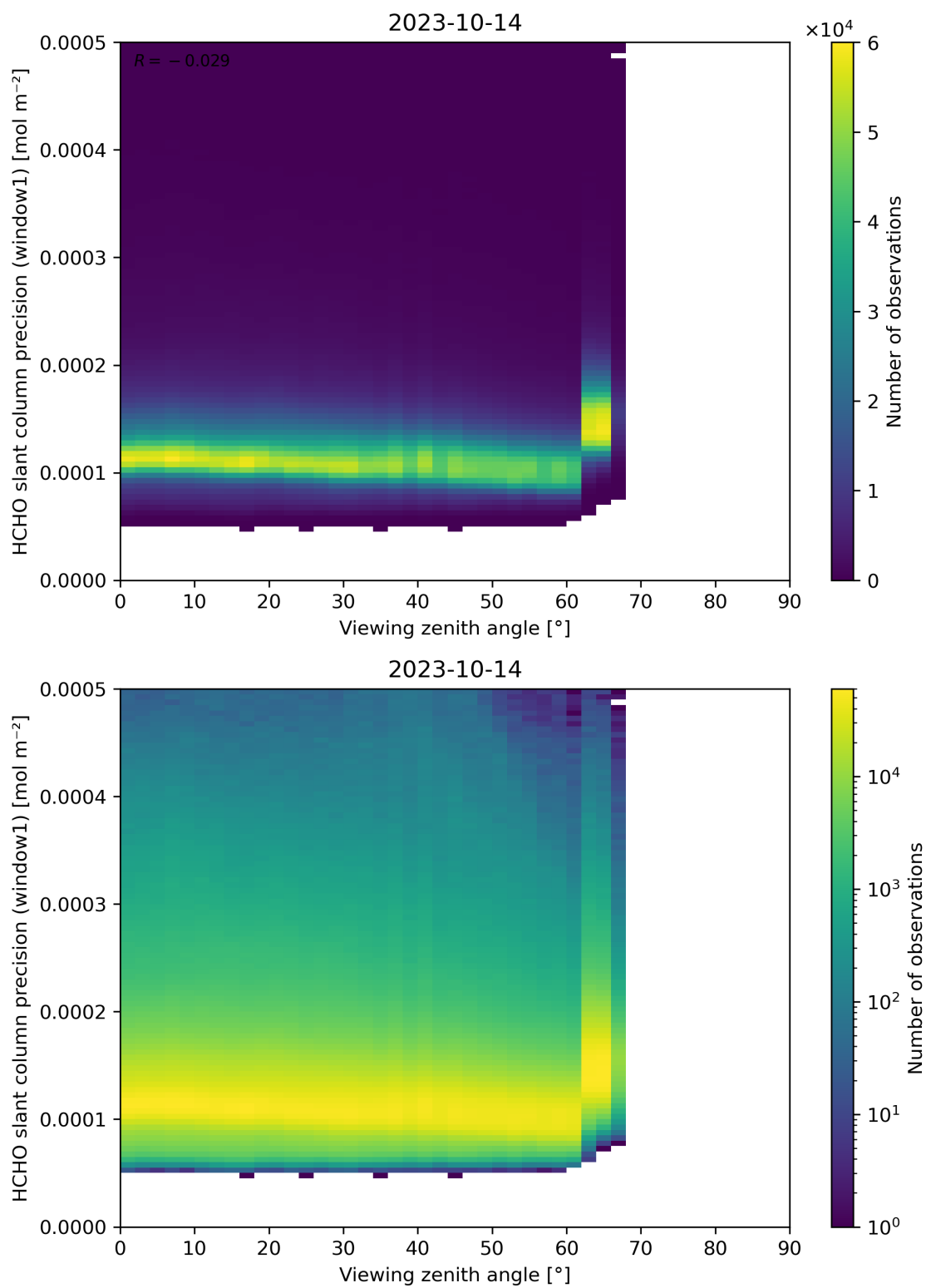
Figure 189: Scatter density plot of “Viewing zenith angle” against “HCHO slant column precision (window1)” for 2023-10-13 to 2023-10-15.
