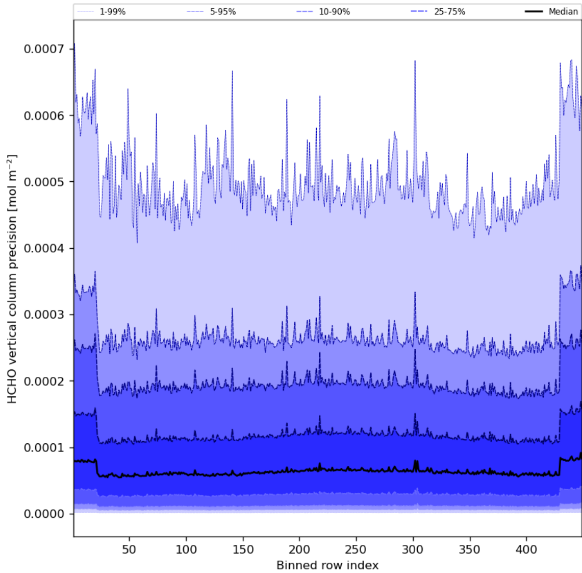
Figure 50: Along track statistics of “HCHO vertical column precision” for 2023-10-13 to 2023-10-15
