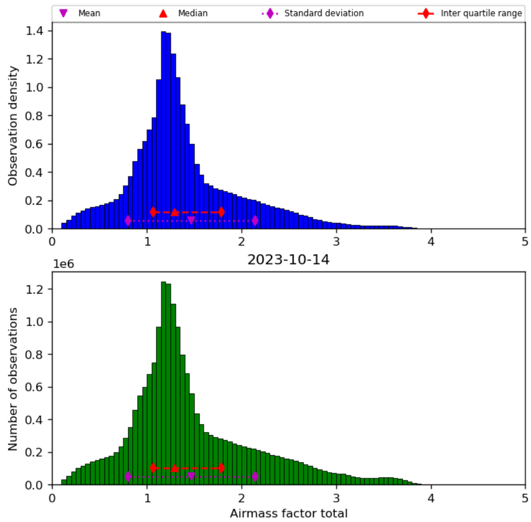
Figure 40: Histogram of “Airmass factor total” for 2023-10-13 to 2023-10-15
