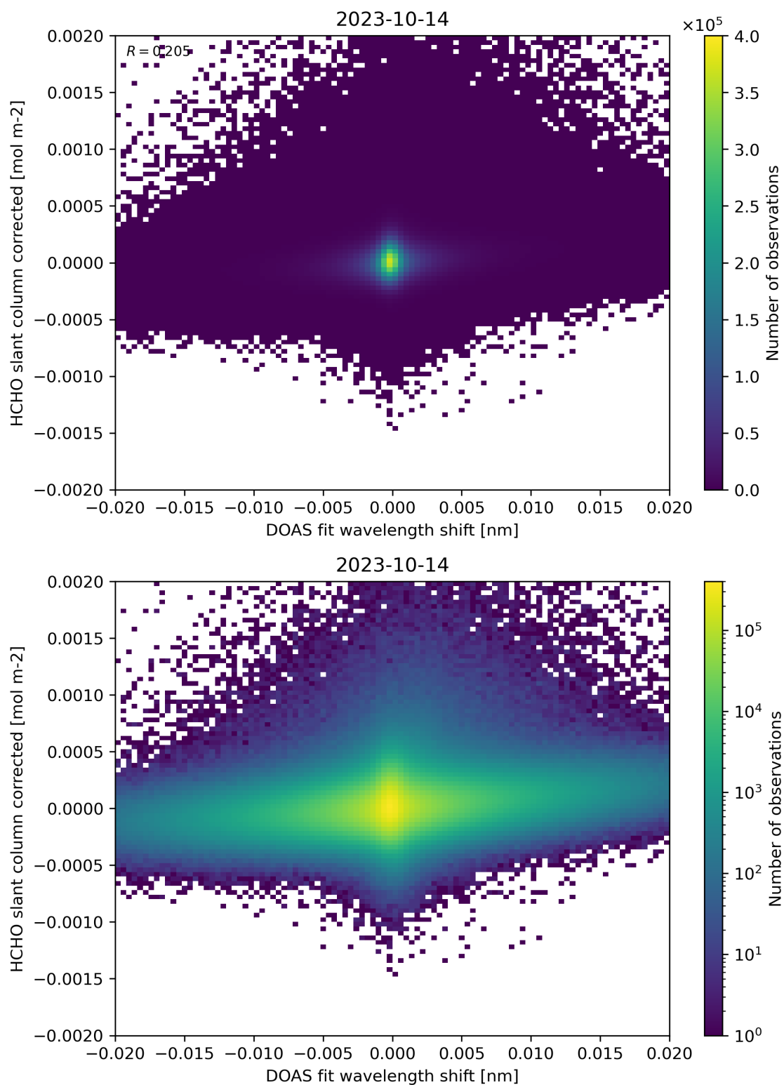
Figure 66: Scatter density plot of “DOAS fit wavelength shift” against “HCHO slant column corrected” for 2023-10-13 to 2023-10-15.
