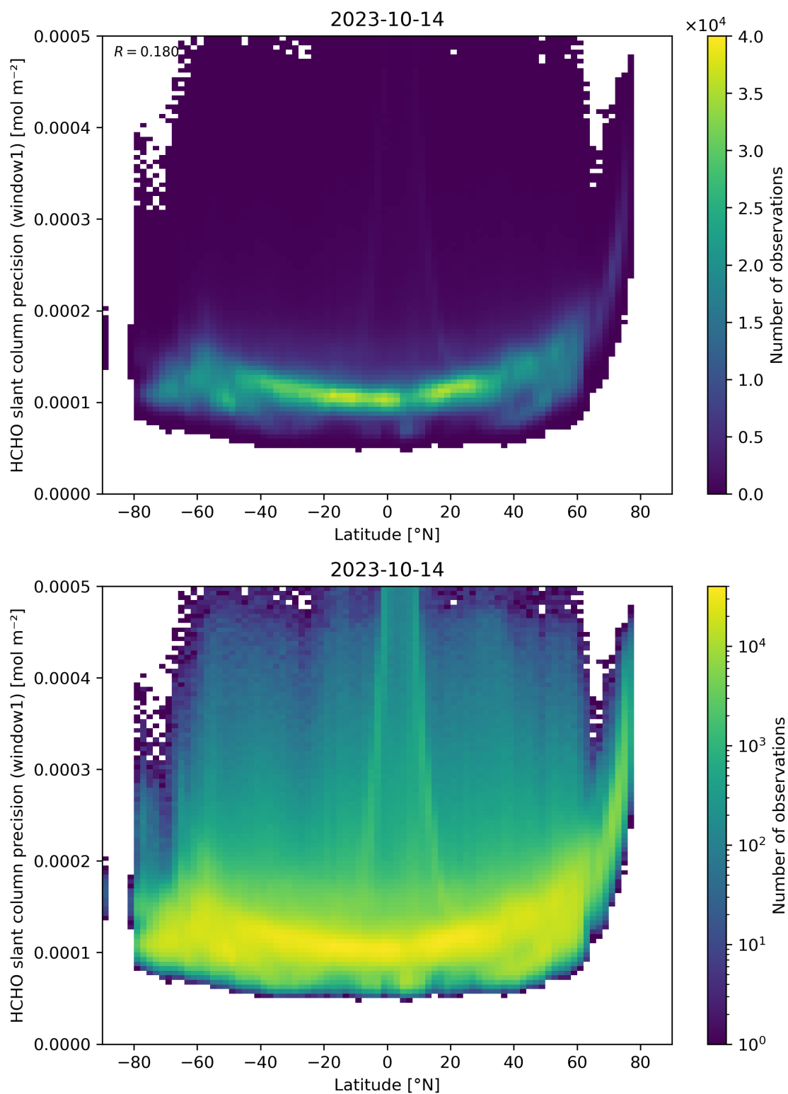
Figure 160: Scatter density plot of “Latitude” against “HCHO slant column precision (window1)” for 2023-10-13 to 2023-10-15.
