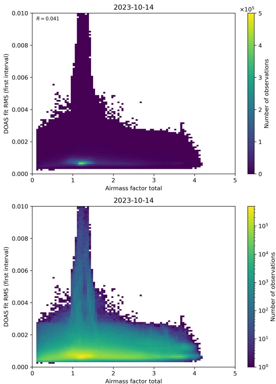
Figure 97: Scatter density plot of “Airmass factor total” against “DOAS fit RMS (first interval)” for 2023-10-13 to 2023-10-15.
