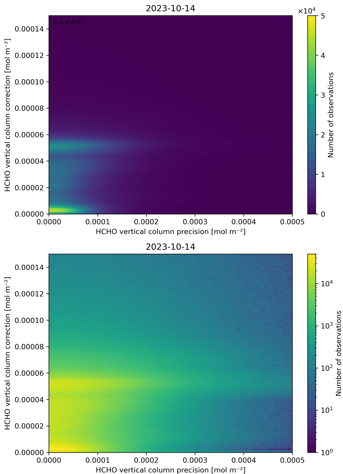
Figure 146: Scatter density plot of “HCHO vertical column precision” against “HCHO vertical column correction” for 2023-10-13 to 2023-10-15.
