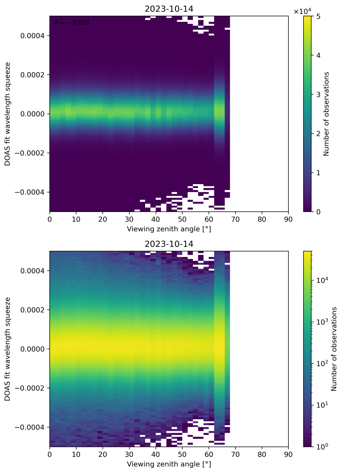
Figure 184: Scatter density plot of “Viewing zenith angle” against “DOAS fit wavelength squeeze” for 2023-10-13 to 2023-10-15.
