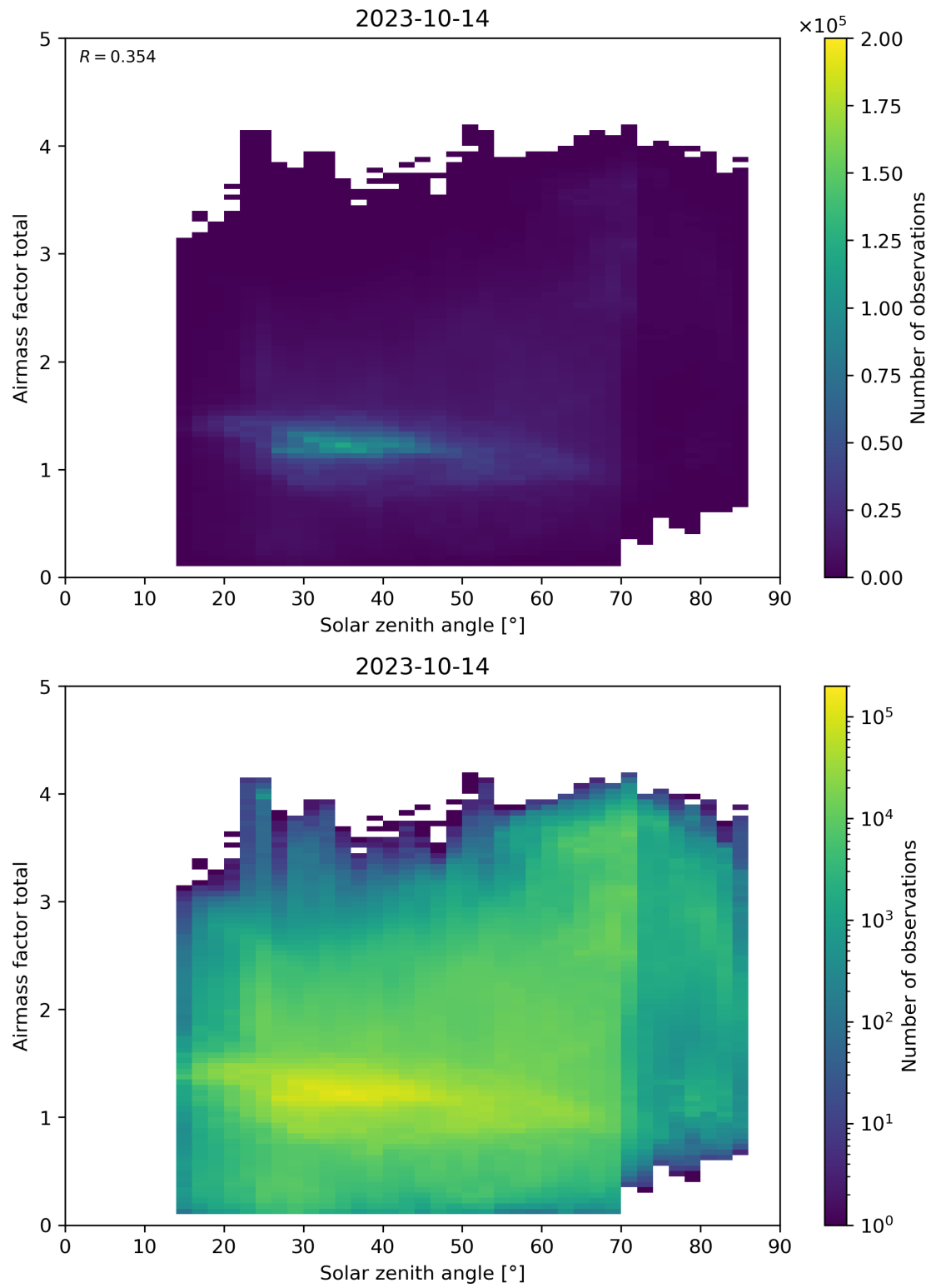
Figure 175: Scatter density plot of “Solar zenith angle” against “Airmass factor total” for 2023-10-13 to 2023-10-15.
