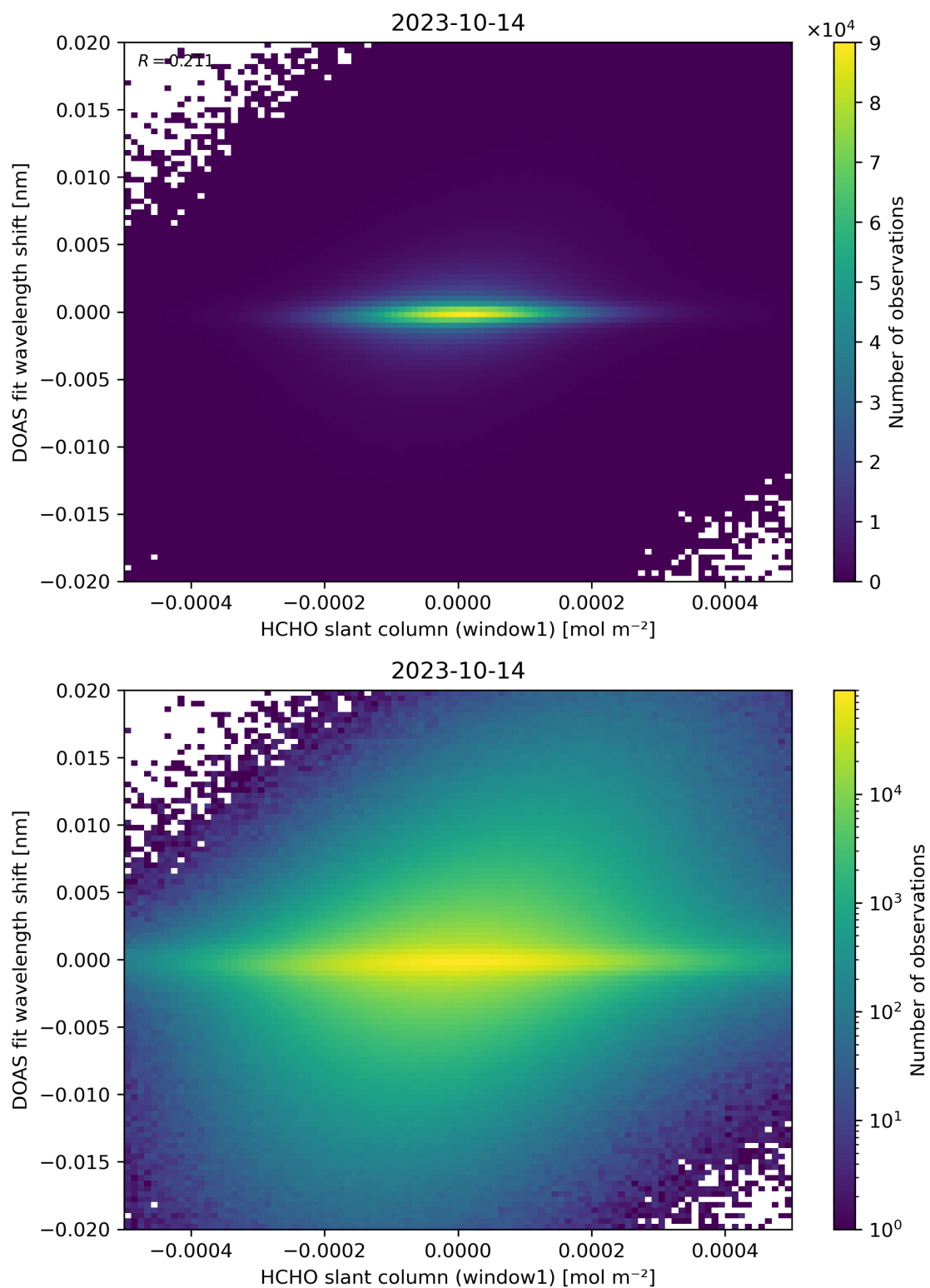
Figure 79: Scatter density plot of “HCHO slant column (window1)” against “DOAS fit wavelength shift” for 2023-10-13 to 2023-10-15.
