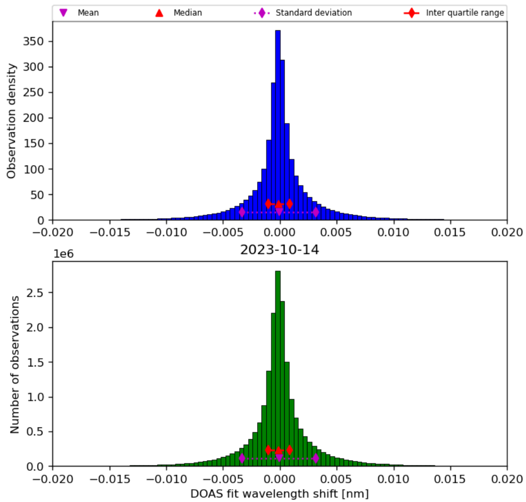
Figure 44: Histogram of “DOAS fit wavelength shift” for 2023-10-13 to 2023-10-15
