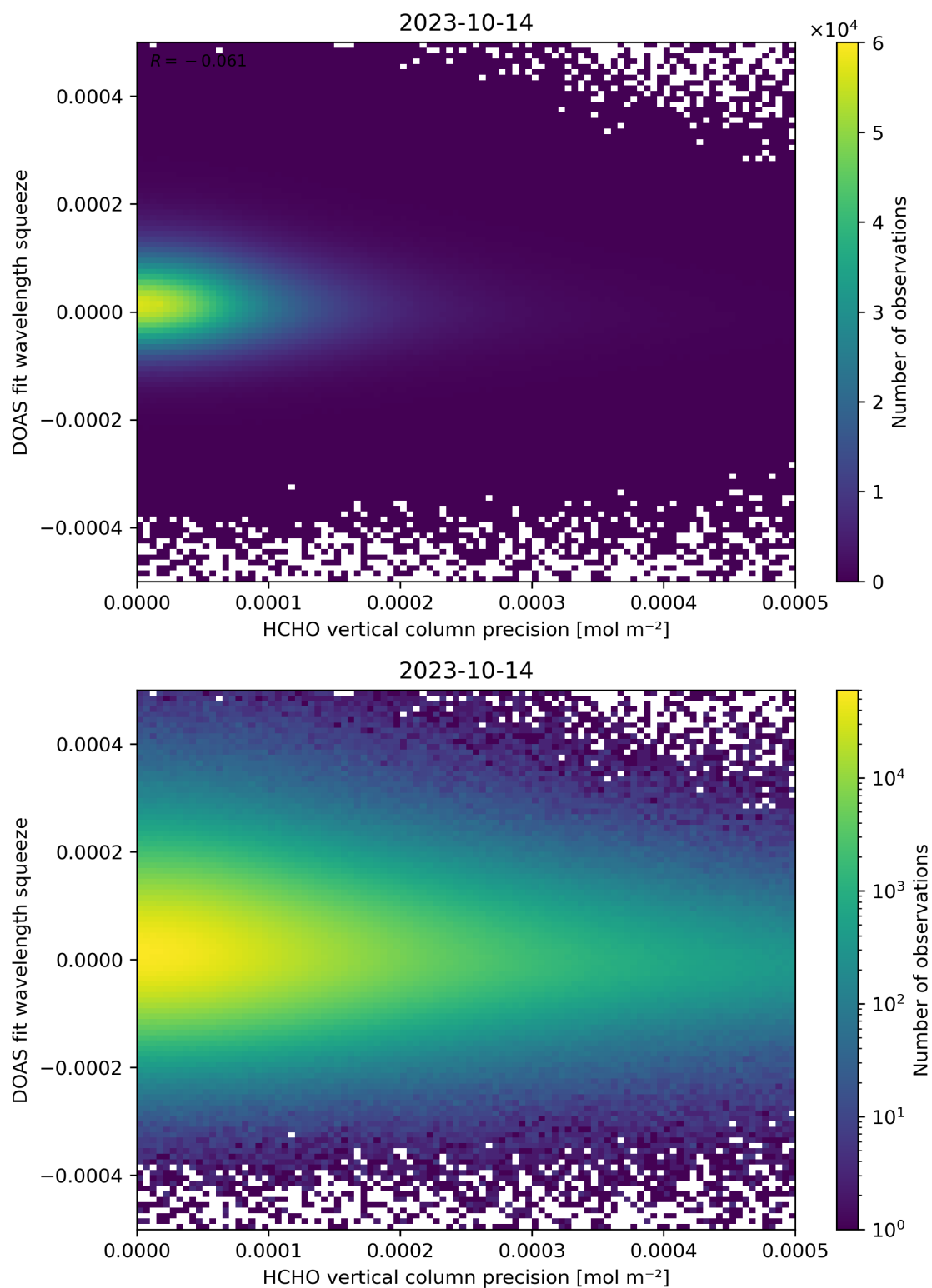
Figure 138: Scatter density plot of “HCHO vertical column precision” against “DOAS fit wavelength squeeze” for 2023-10-13 to 2023-10-15.
