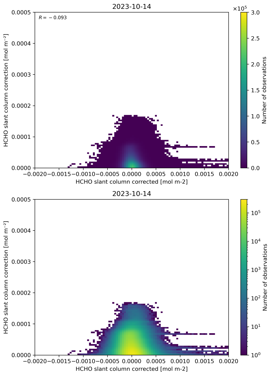
Figure 77: Scatter density plot of “HCHO slant column corrected” against “HCHO slant column correction” for 2023-10-13 to 2023-10-15.
