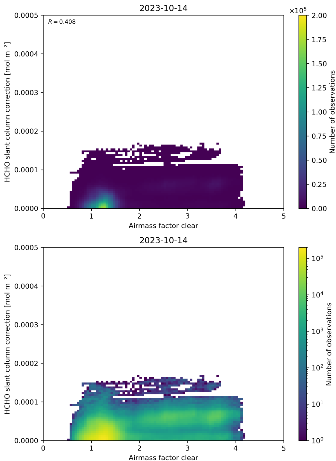
Figure 75: Scatter density plot of “Airmass factor clear” against “HCHO slant column correction” for 2023-10-13 to 2023-10-15.
