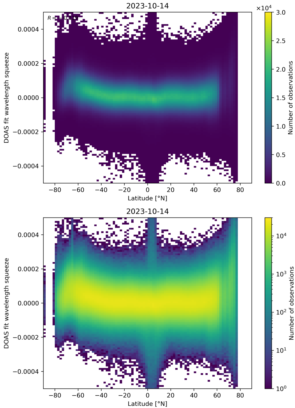
Figure 155: Scatter density plot of “Latitude” against “DOAS fit wavelength squeeze” for 2023-10-13 to 2023-10-15.
