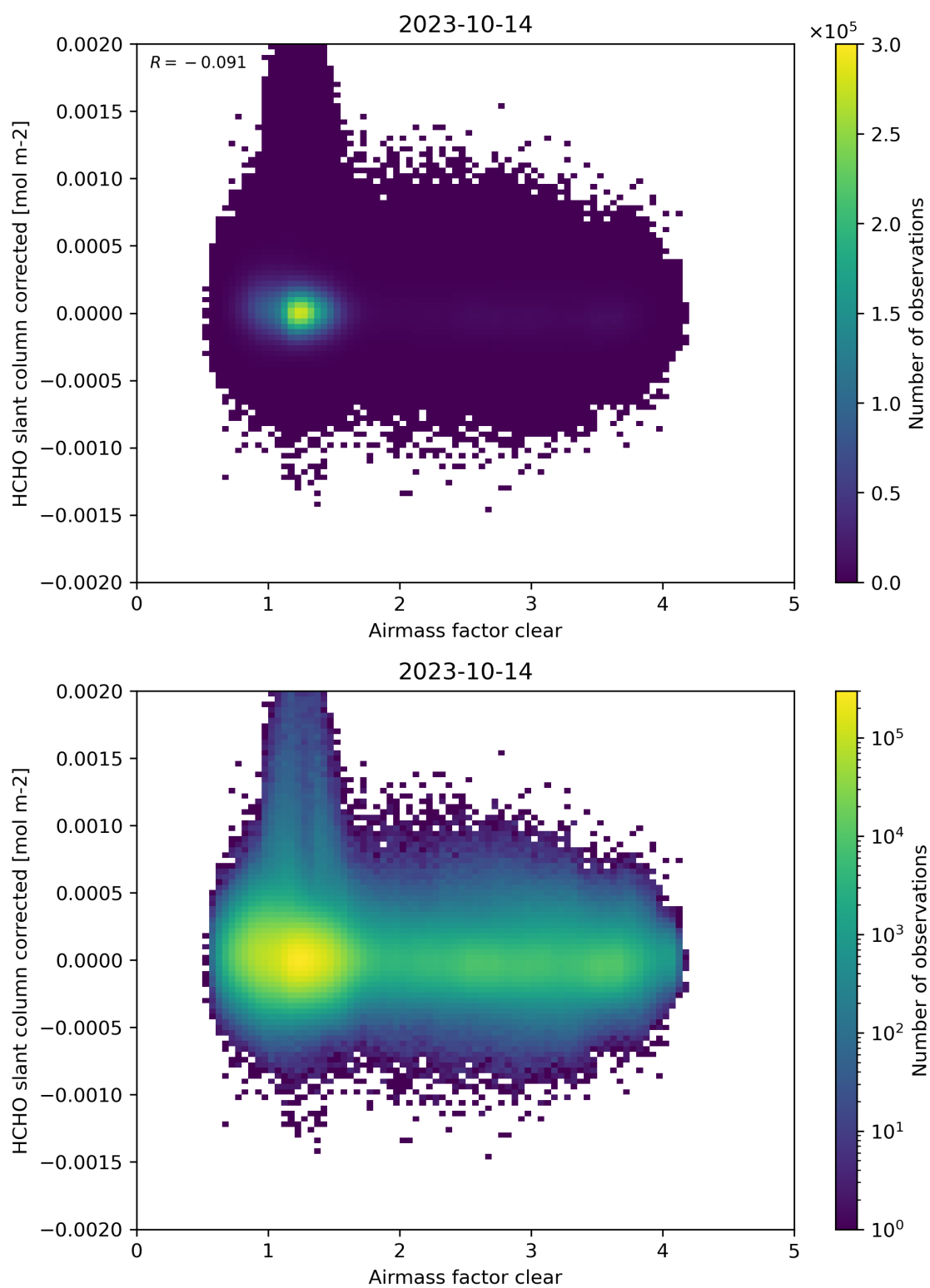
Figure 74: Scatter density plot of “Airmass factor clear” against “HCHO slant column corrected” for 2023-10-13 to 2023-10-15.
