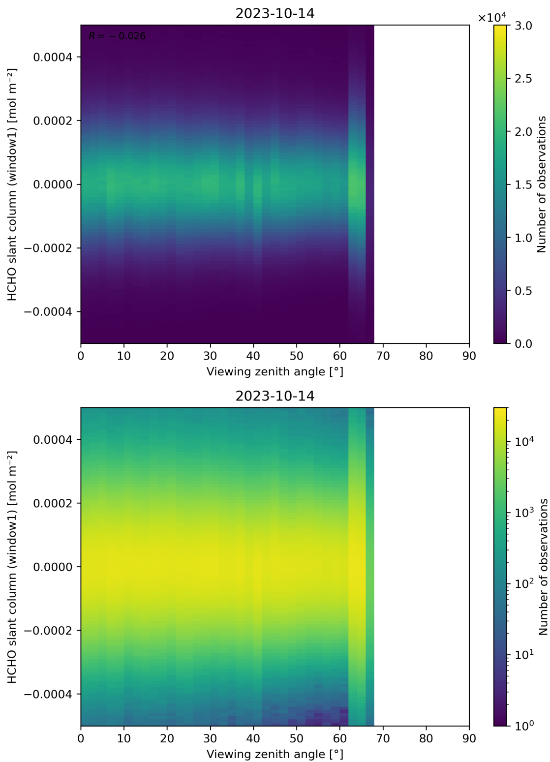
Figure 188: Scatter density plot of “Viewing zenith angle” against “HCHO slant column (window1)” for 2023-10-13 to 2023-10-15.
