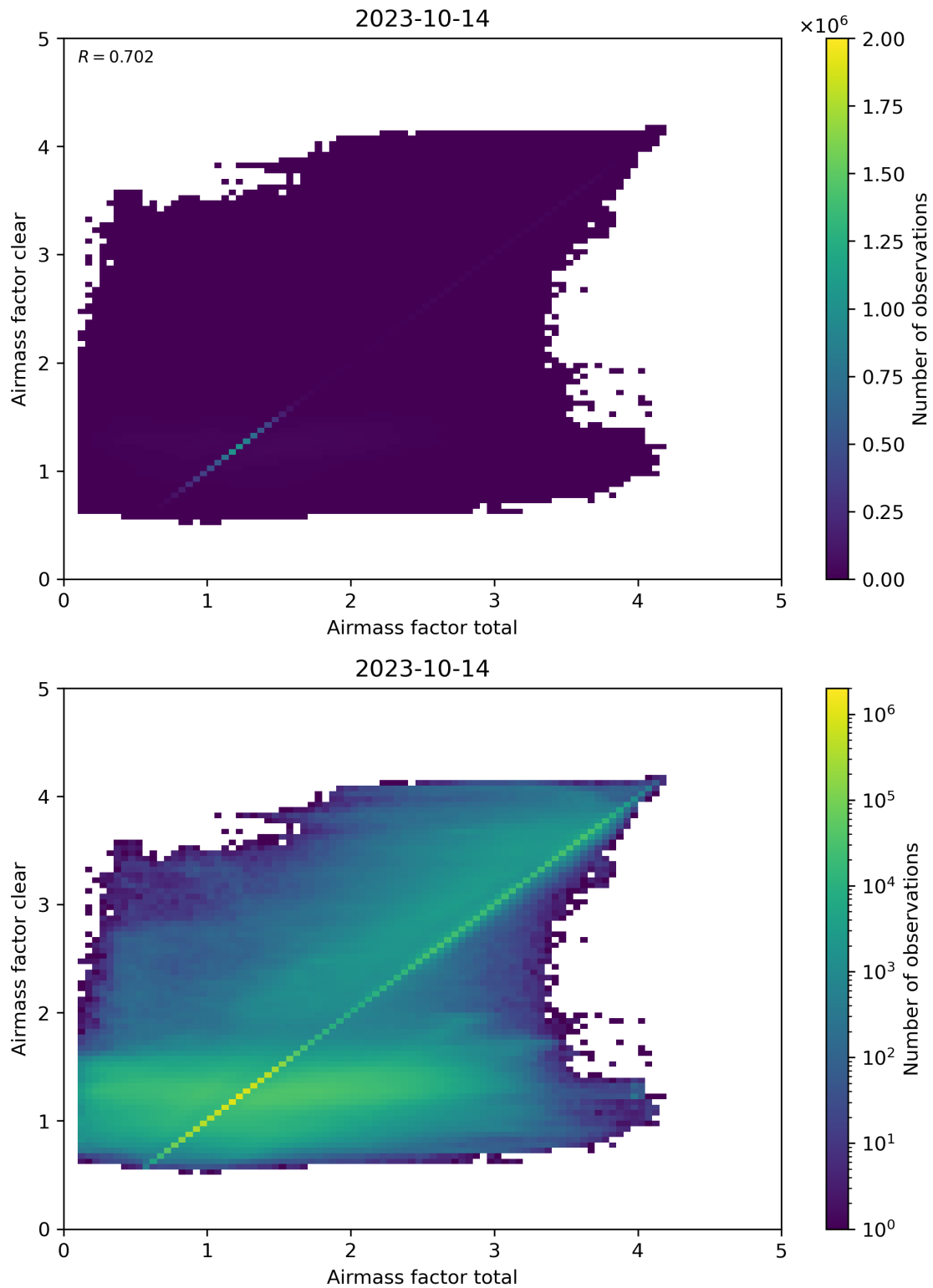
Figure 100: Scatter density plot of “Airmass factor total” against “Airmass factor clear” for 2023-10-13 to 2023-10-15.
