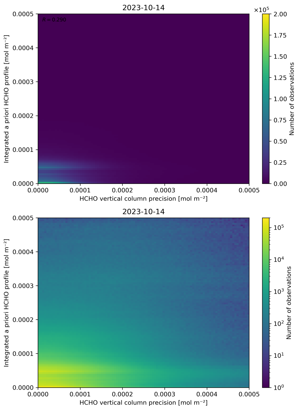
Figure 147: Scatter density plot of “HCHO vertical column precision” against “Integrated a priori HCHO profile” for 2023-10-13 to 2023-10-15.
