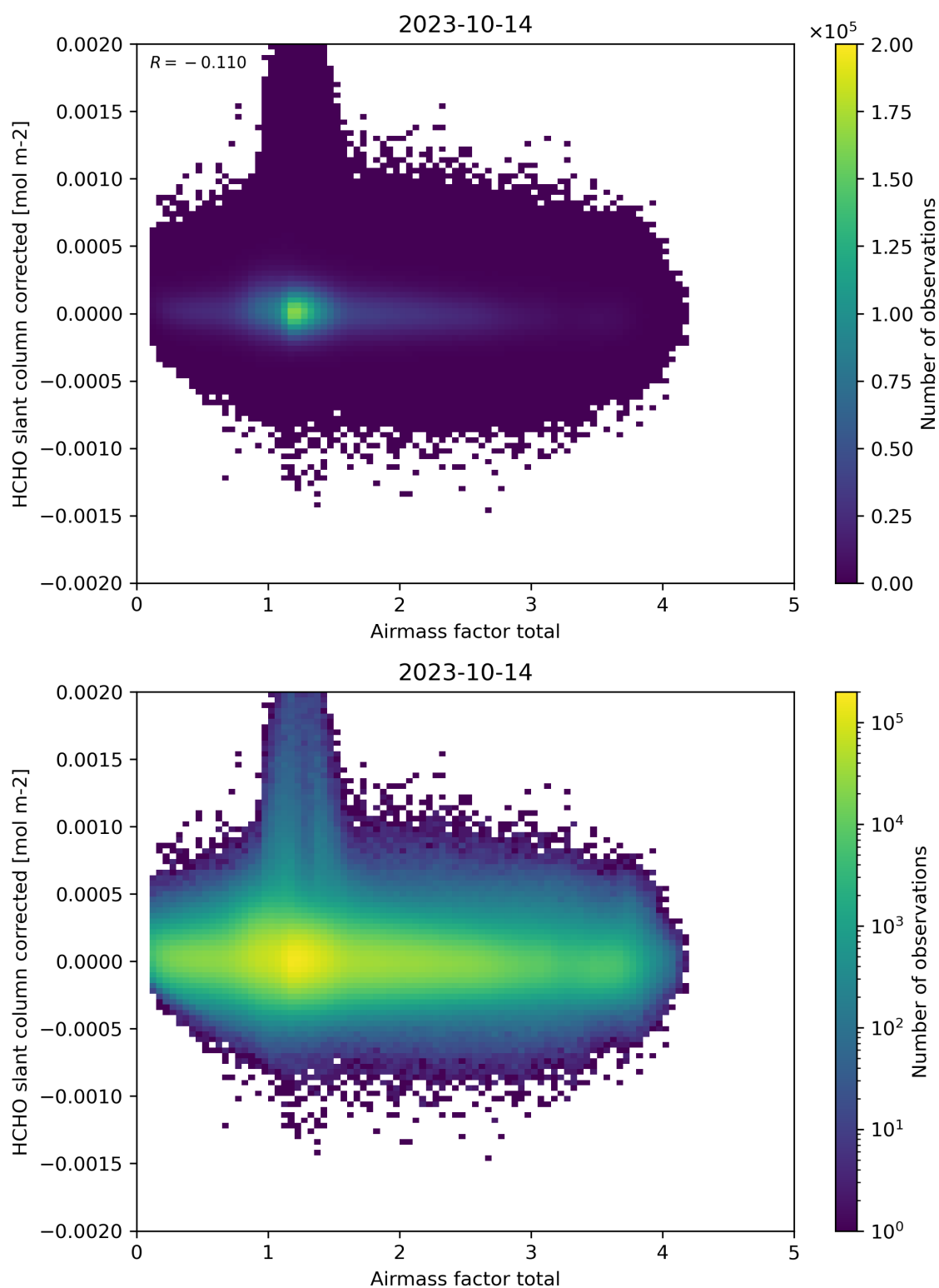
Figure 101: Scatter density plot of “Airmass factor total” against “HCHO slant column corrected” for 2023-10-13 to 2023-10-15.
