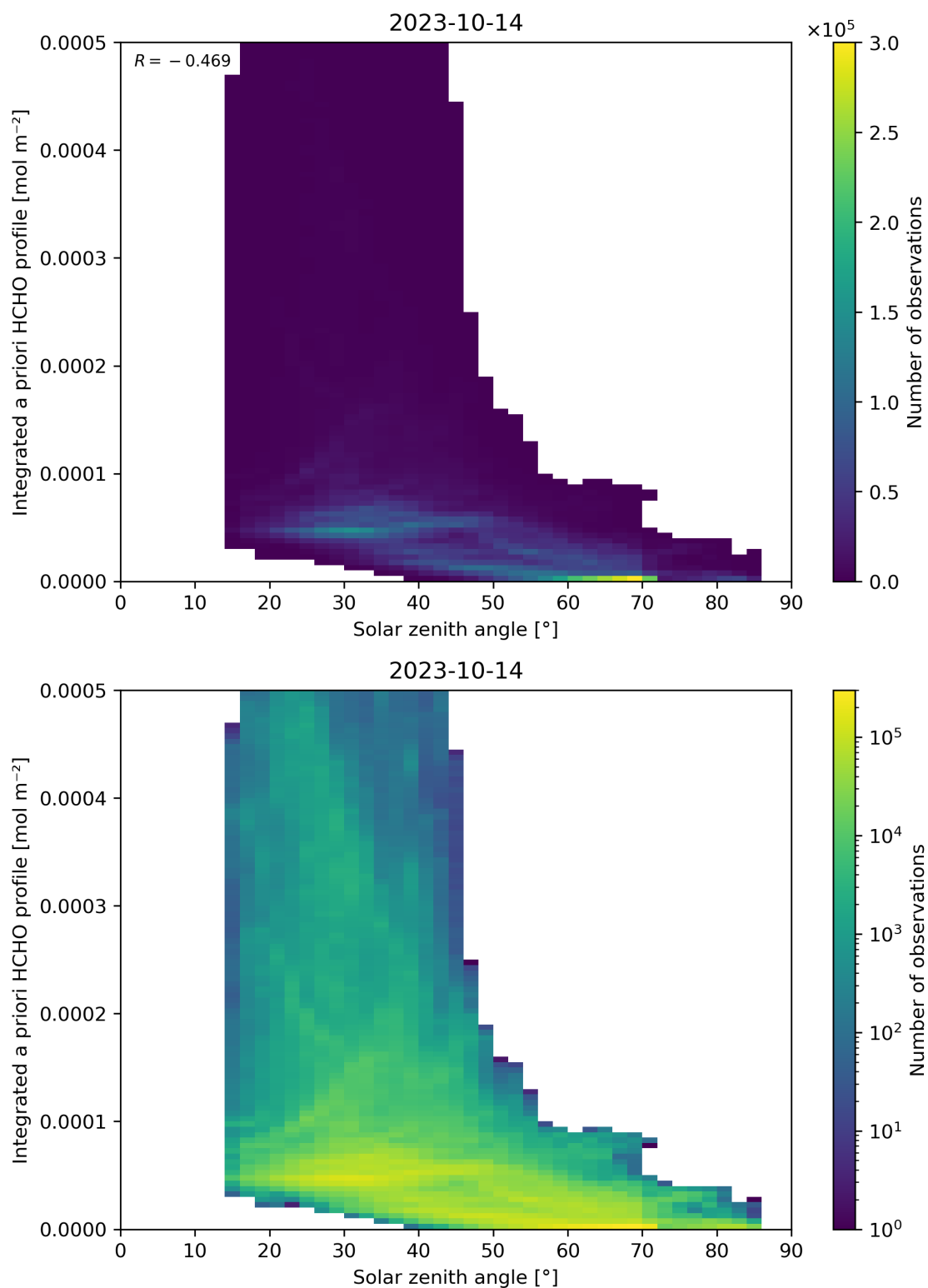
Figure 180: Scatter density plot of “Solar zenith angle” against “Integrated a priori HCHO profile” for 2023-10-13 to 2023-10-15.
