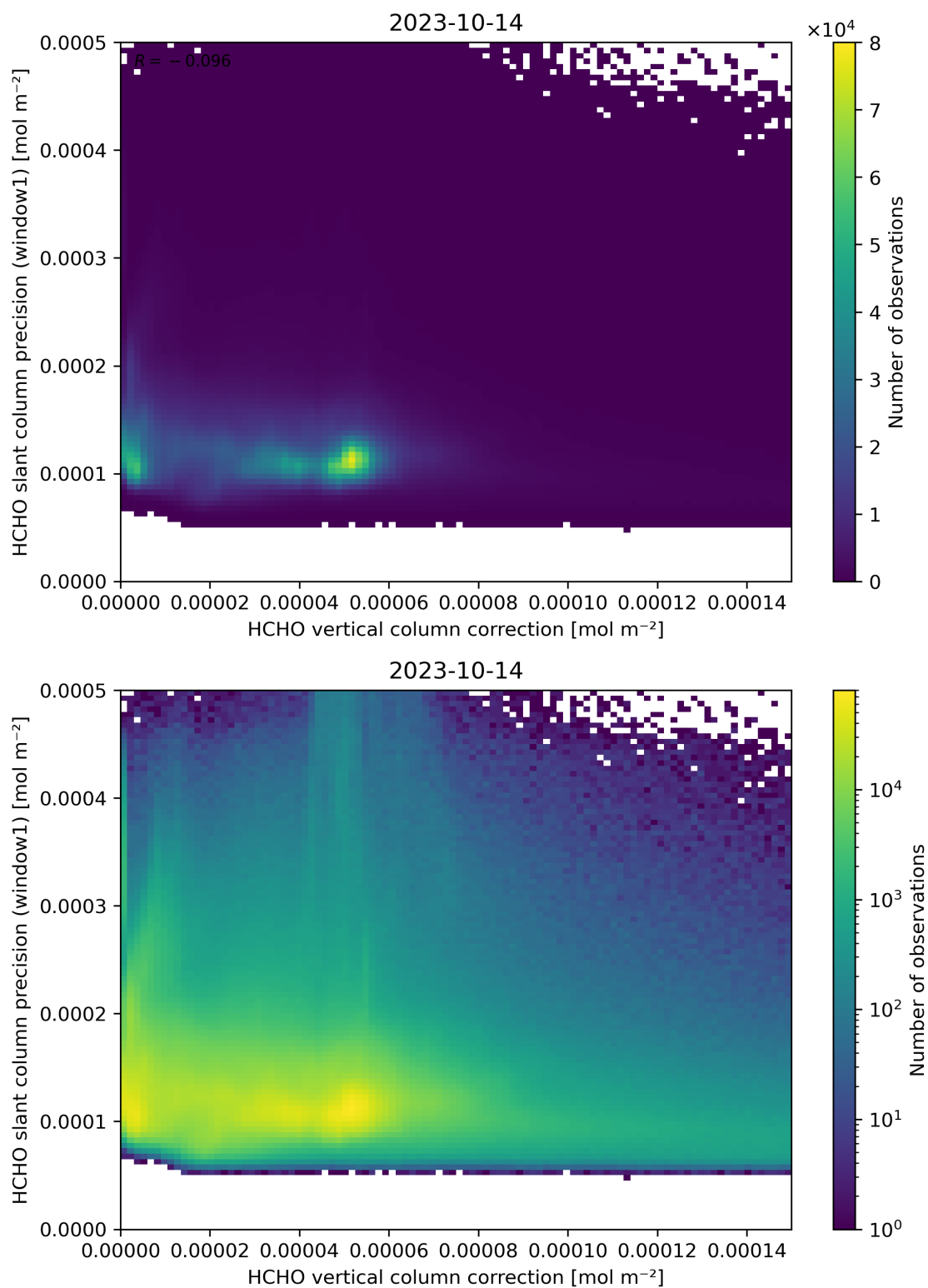
Figure 119: Scatter density plot of “HCHO vertical column correction” against “HCHO slant column precision (window1)” for 2023-10-13 to 2023-10-15.
