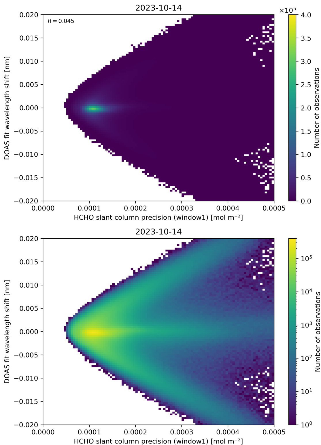
Figure 89: Scatter density plot of “HCHO slant column precision (window1)” against “DOAS fit wavelength shift” for 2023-10-13 to 2023-10-15.
