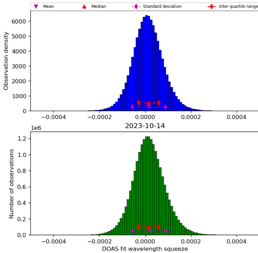
Figure 45: Histogram of “DOAS fit wavelength squeeze” for 2023-10-13 to 2023-10-15
