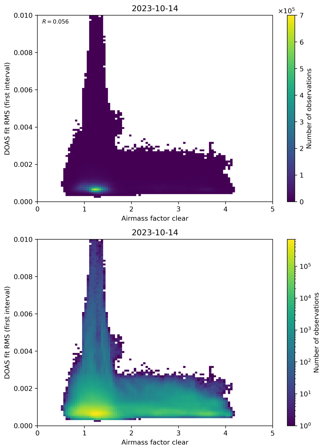
Figure 71: Scatter density plot of “Airmass factor clear” against “DOAS fit RMS (first interval)” for 2023-10-13 to 2023-10-15.
