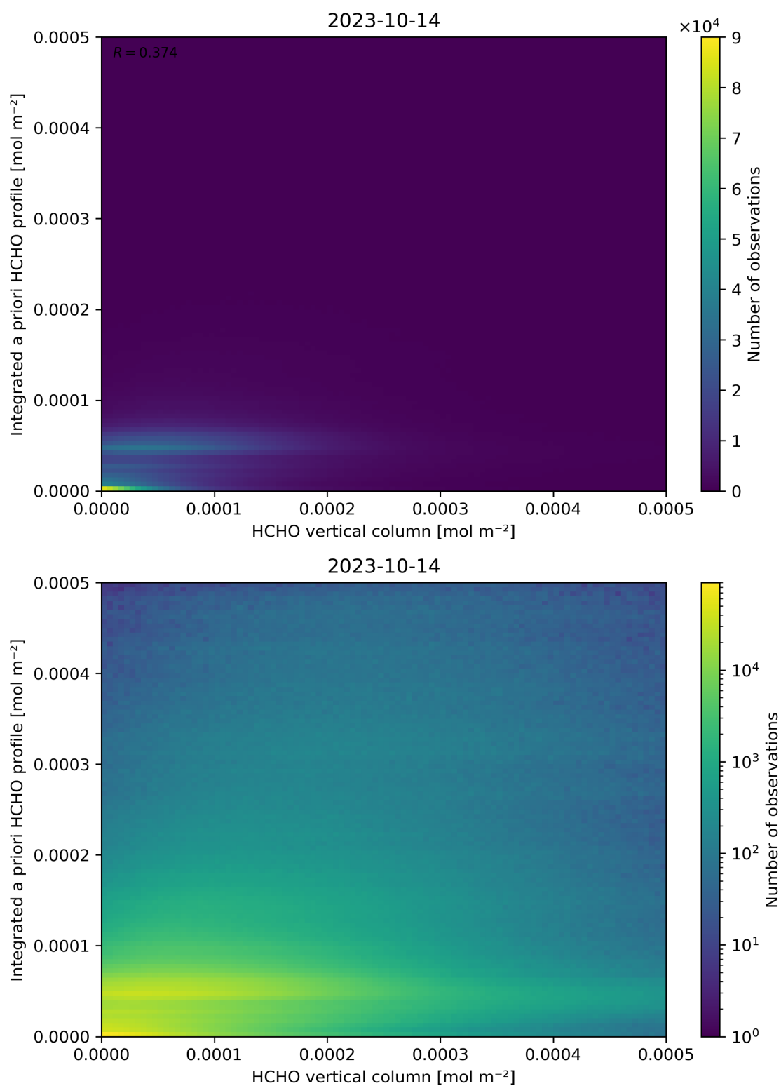
Figure 135: Scatter density plot of “HCHO vertical column” against “Integrated a priori HCHO profile” for 2023-10-13 to 2023-10-15.
