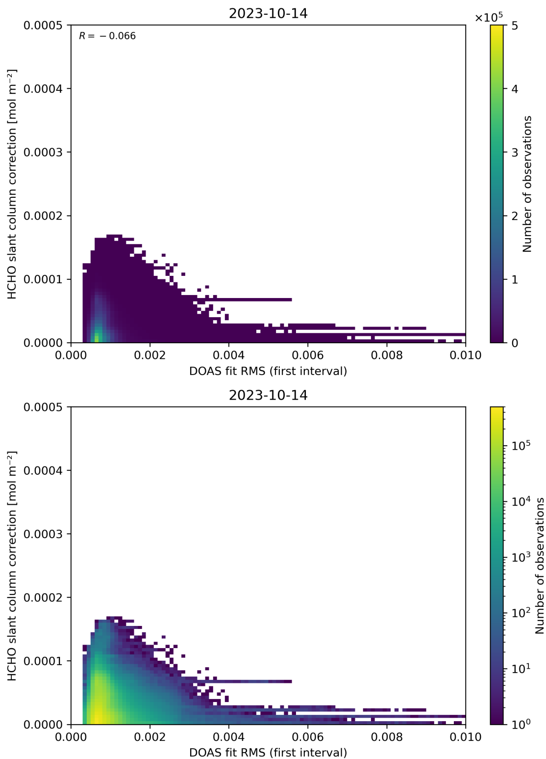
Figure 63: Scatter density plot of “DOAS fit RMS (first interval)” against “HCHO slant column correction” for 2023-10-13 to 2023-10-15.
