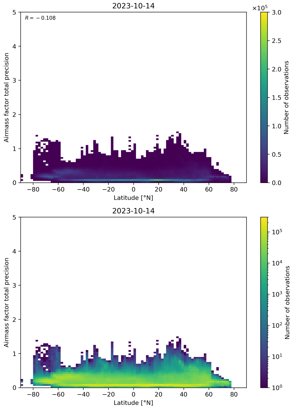
Figure 162: Scatter density plot of “Latitude” against “Airmass factor total precision” for 2023-10-13 to 2023-10-15.
