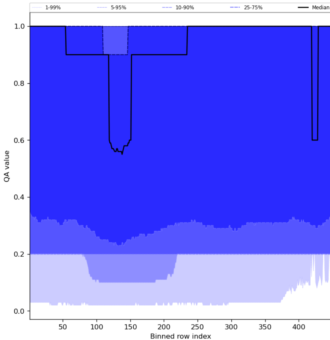
Figure 48: Along track statistics of “QA value” for 2023-10-14 to 2023-10-16
