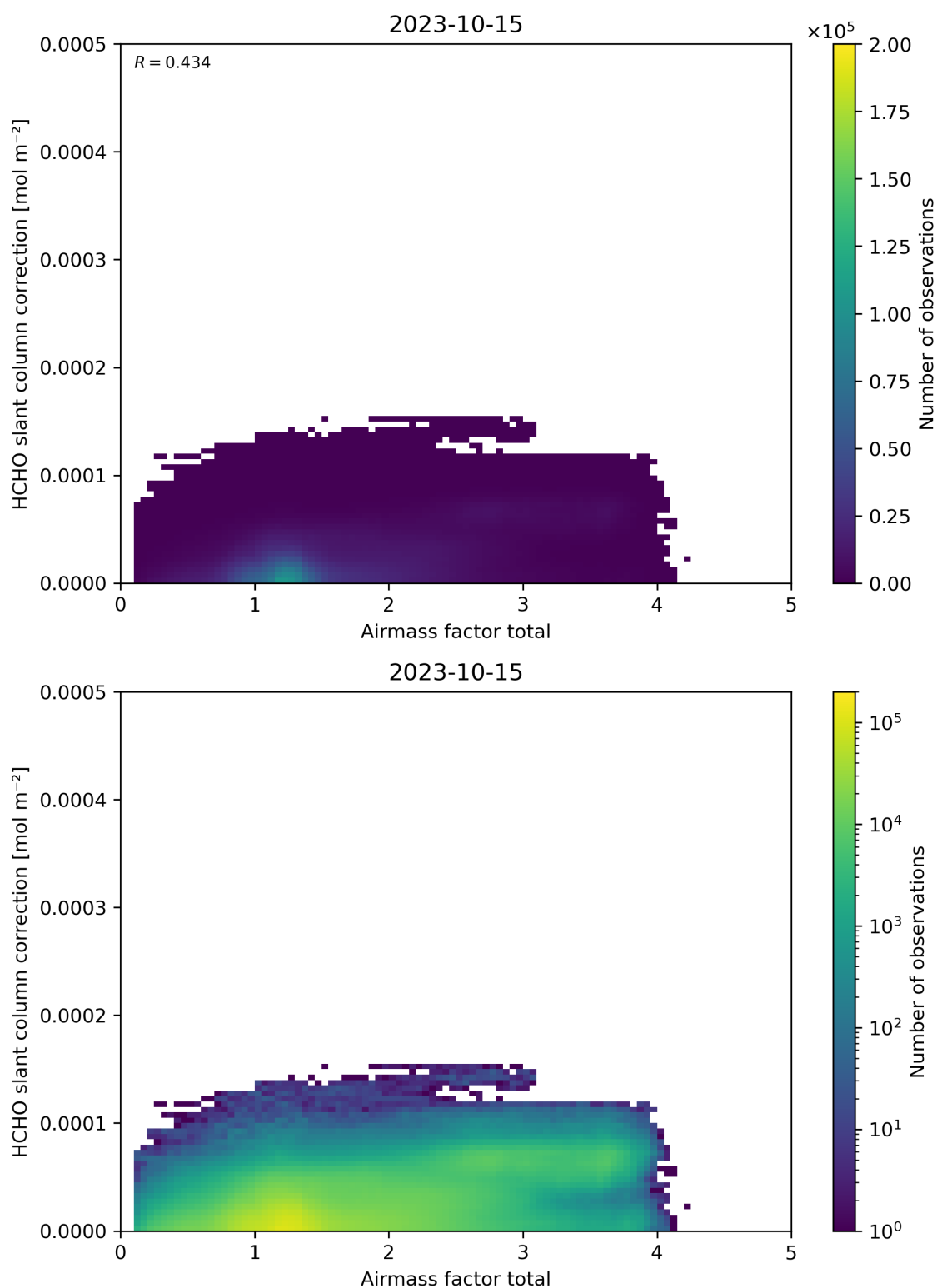
Figure 102: Scatter density plot of “Airmass factor total” against “HCHO slant column correction” for 2023-10-14 to 2023-10-16.
