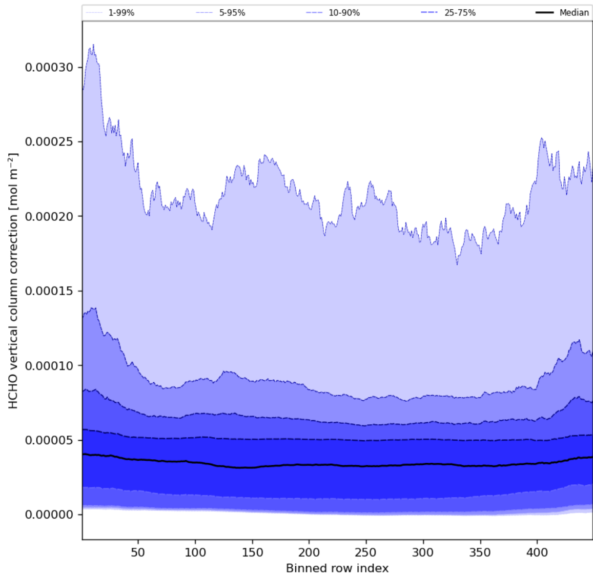
Figure 51: Along track statistics of “HCHO vertical column correction” for 2023-10-14 to 2023-10-16
