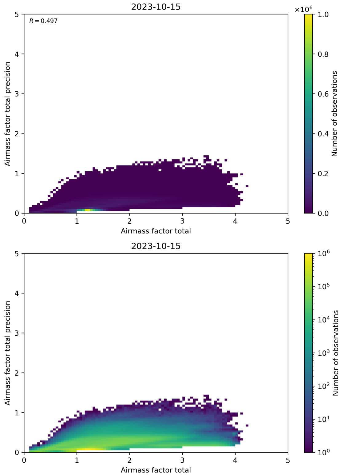
Figure 103: Scatter density plot of “Airmass factor total” against “Airmass factor total precision” for 2023-10-14 to 2023-10-16.
