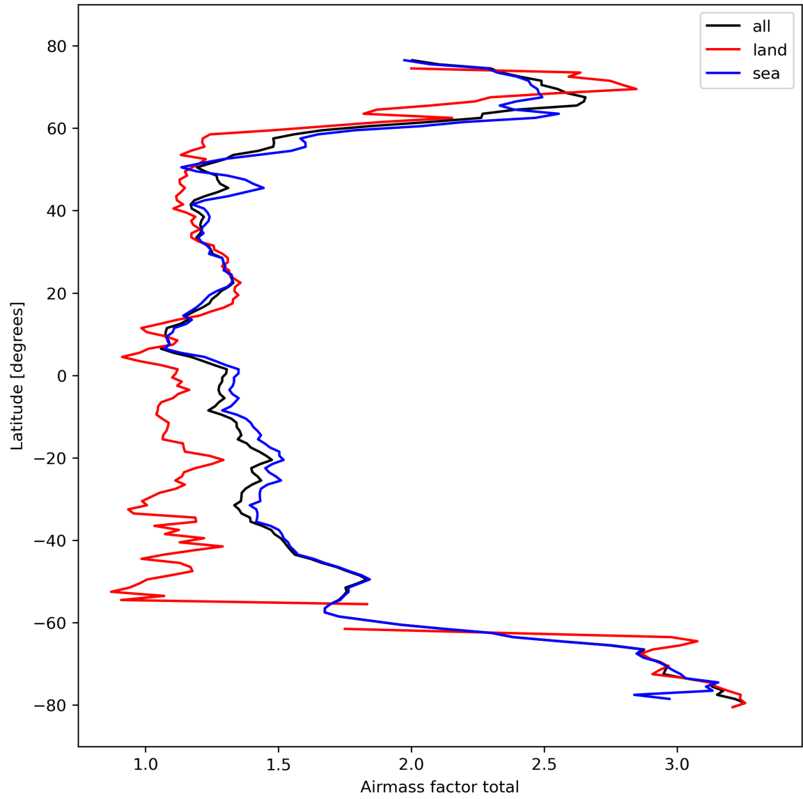
Figure 26: Zonal average of “Airmass factor total” for 2023-10-14 to 2023-10-16.
