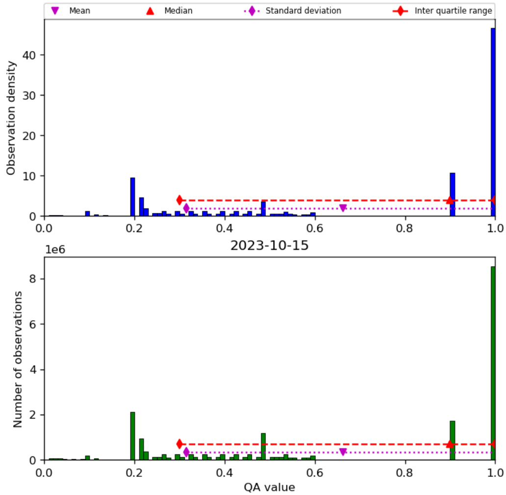
Figure 34: Histogram of “QA value” for 2023-10-14 to 2023-10-16
