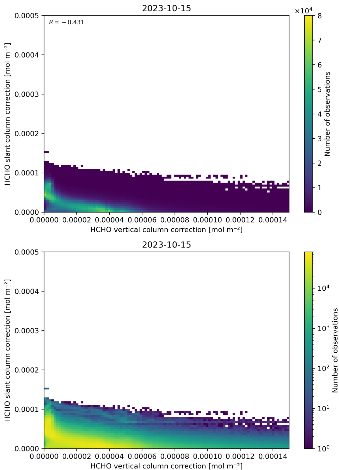
Figure 117: Scatter density plot of “HCHO vertical column correction” against “HCHO slant column correction” for 2023-10-14 to 2023-10-16.
