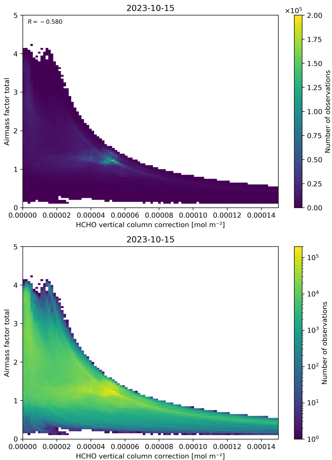
Figure 120: Scatter density plot of “HCHO vertical column correction” against “Airmass factor total” for 2023-10-14 to 2023-10-16.
