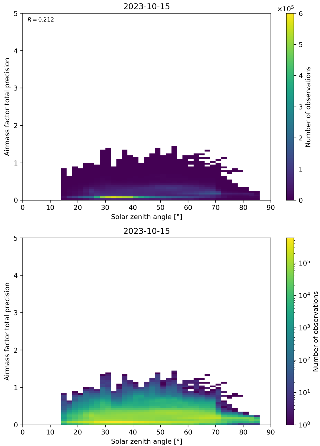
Figure 176: Scatter density plot of “Solar zenith angle” against “Airmass factor total precision” for 2023-10-14 to 2023-10-16.
