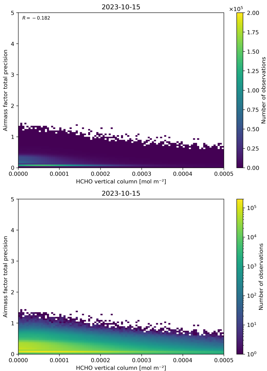
Figure 132: Scatter density plot of “HCHO vertical column” against “Airmass factor total precision” for 2023-10-14 to 2023-10-16.
