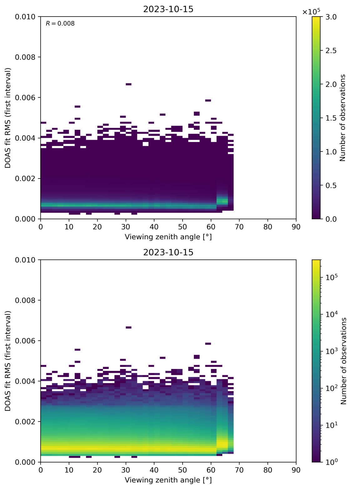
Figure 182: Scatter density plot of “Viewing zenith angle” against “DOAS fit RMS (first interval)” for 2023-10-14 to 2023-10-16.
