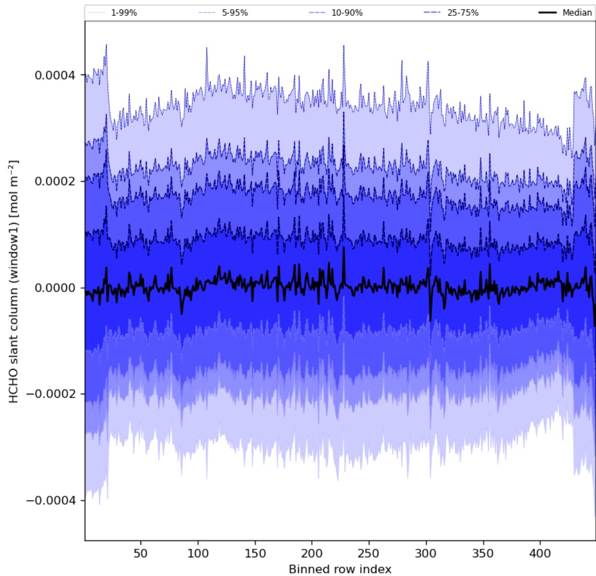
Figure 52: Along track statistics of “HCHO slant column (window1)” for 2023-10-14 to 2023-10-16
