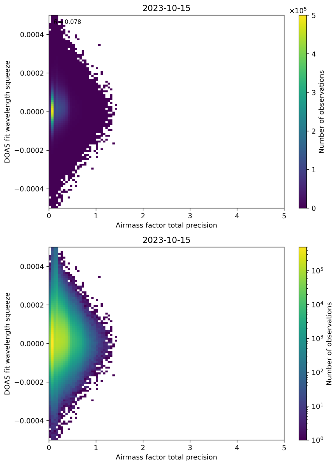
Figure 107: Scatter density plot of “Airmass factor total precision” against “DOAS fit wavelength squeeze” for 2023-10-14 to 2023-10-16.
