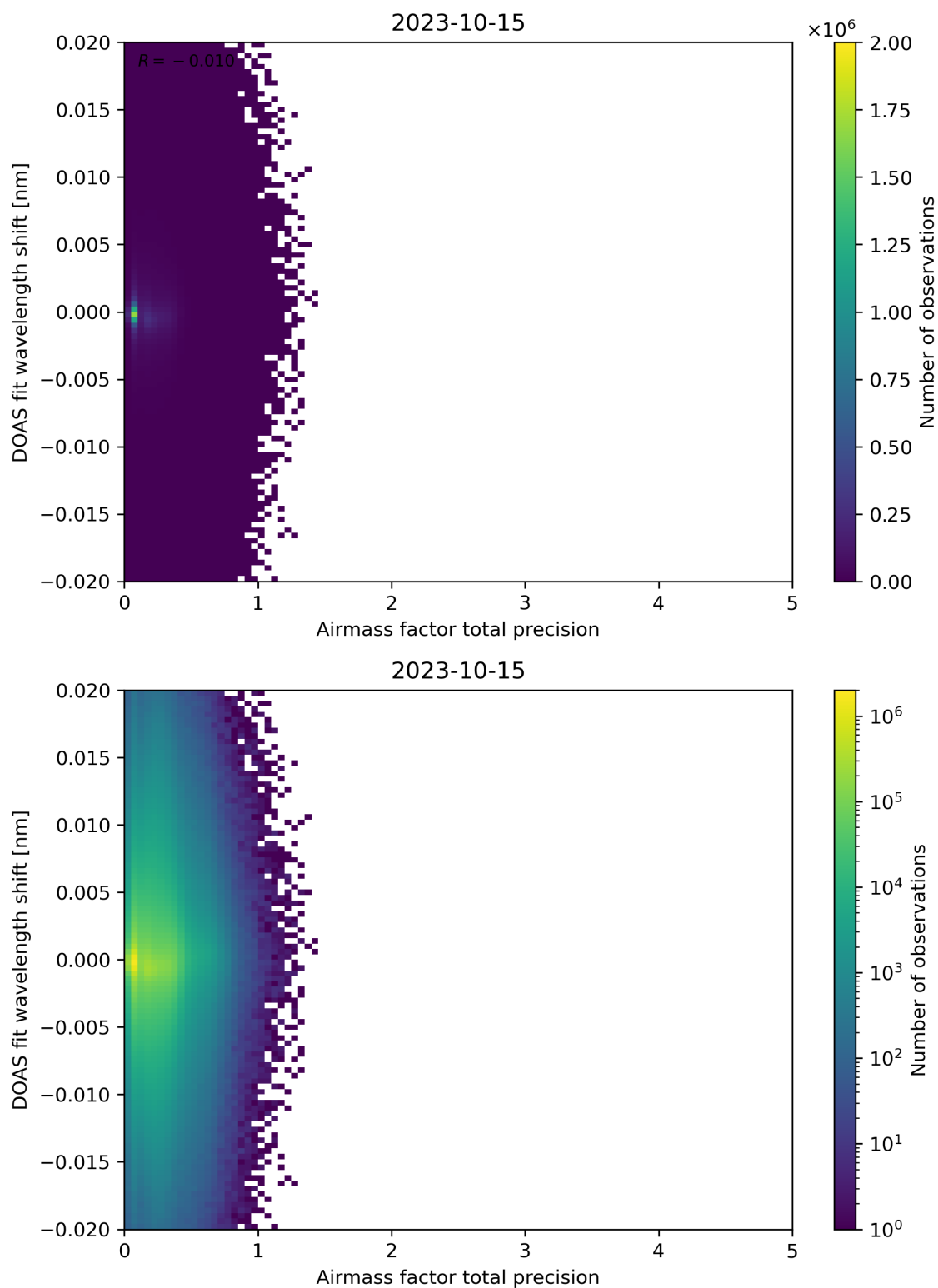
Figure 106: Scatter density plot of “Airmass factor total precision” against “DOAS fit wavelength shift” for 2023-10-14 to 2023-10-16.
