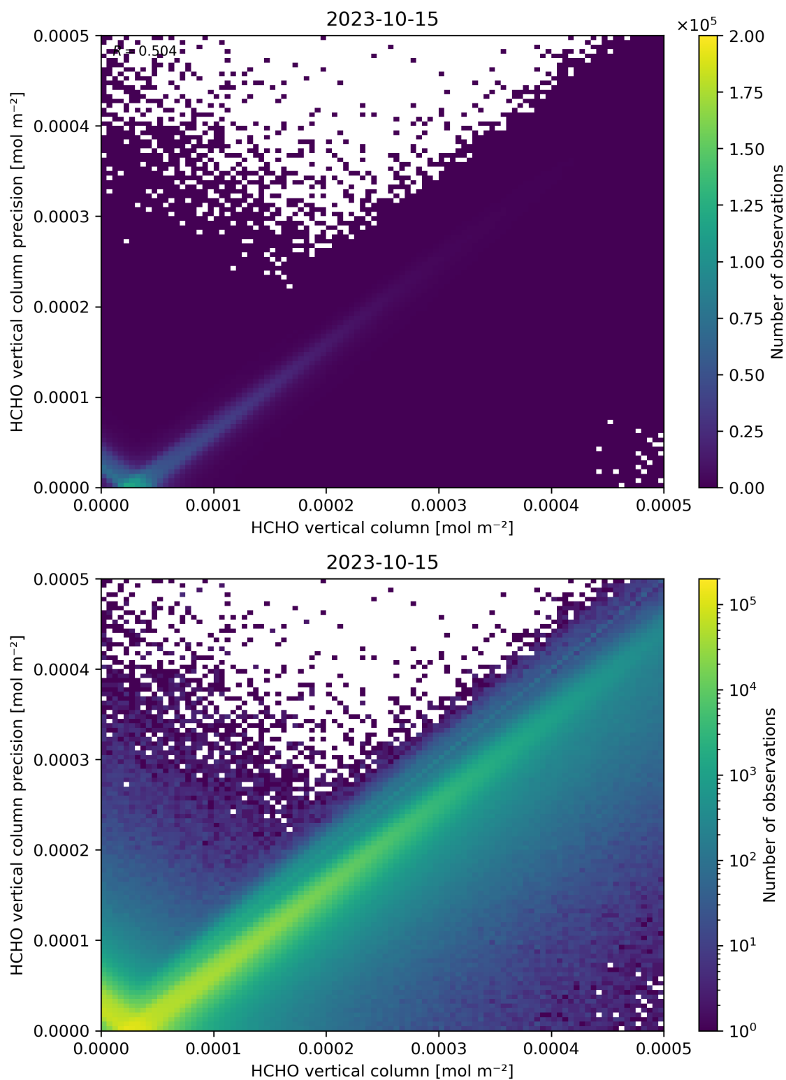
Figure 134: Scatter density plot of “HCHO vertical column” against “HCHO vertical column precision” for 2023-10-14 to 2023-10-16.
