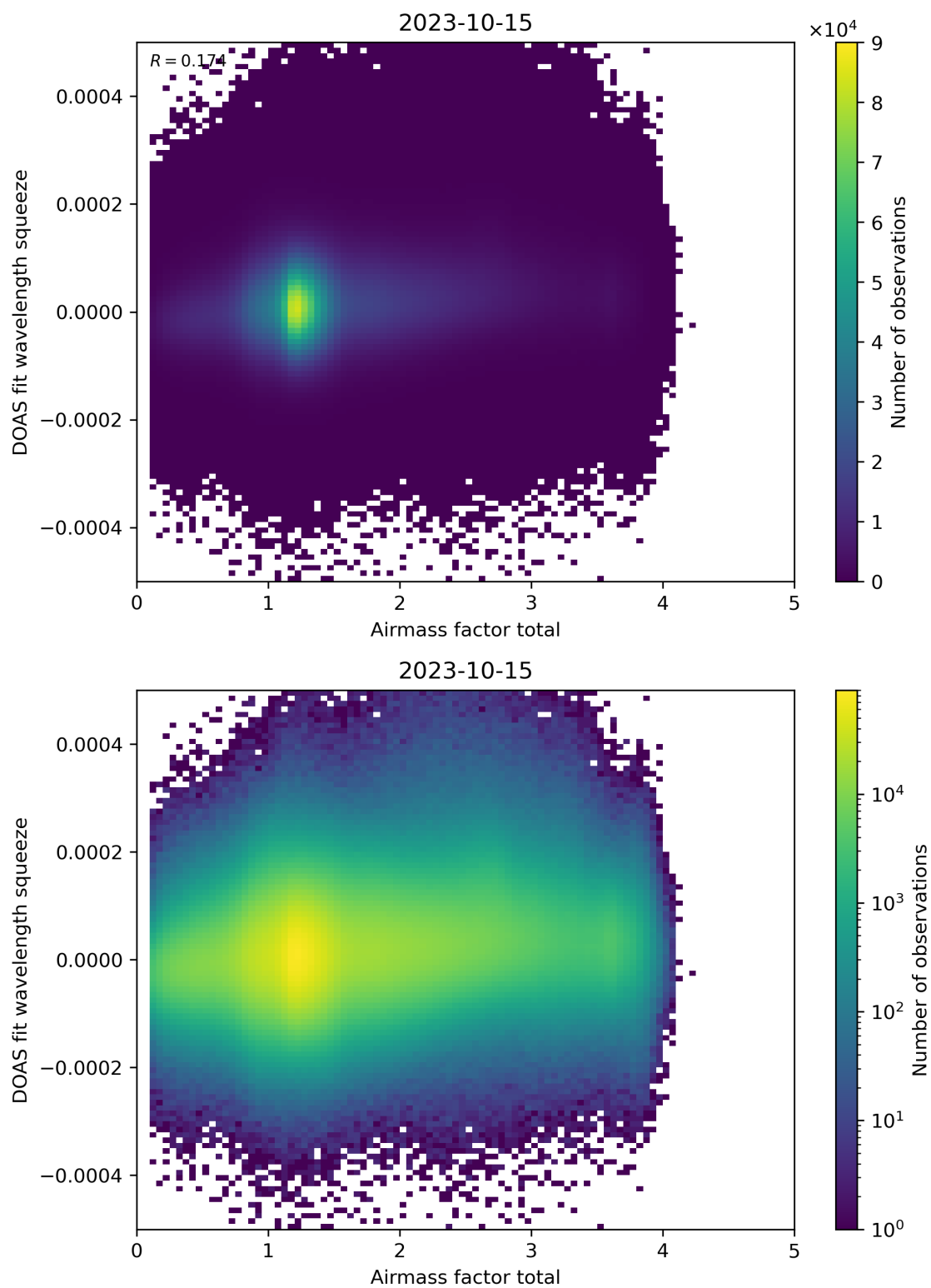
Figure 99: Scatter density plot of “Airmass factor total” against “DOAS fit wavelength squeeze” for 2023-10-14 to 2023-10-16.
