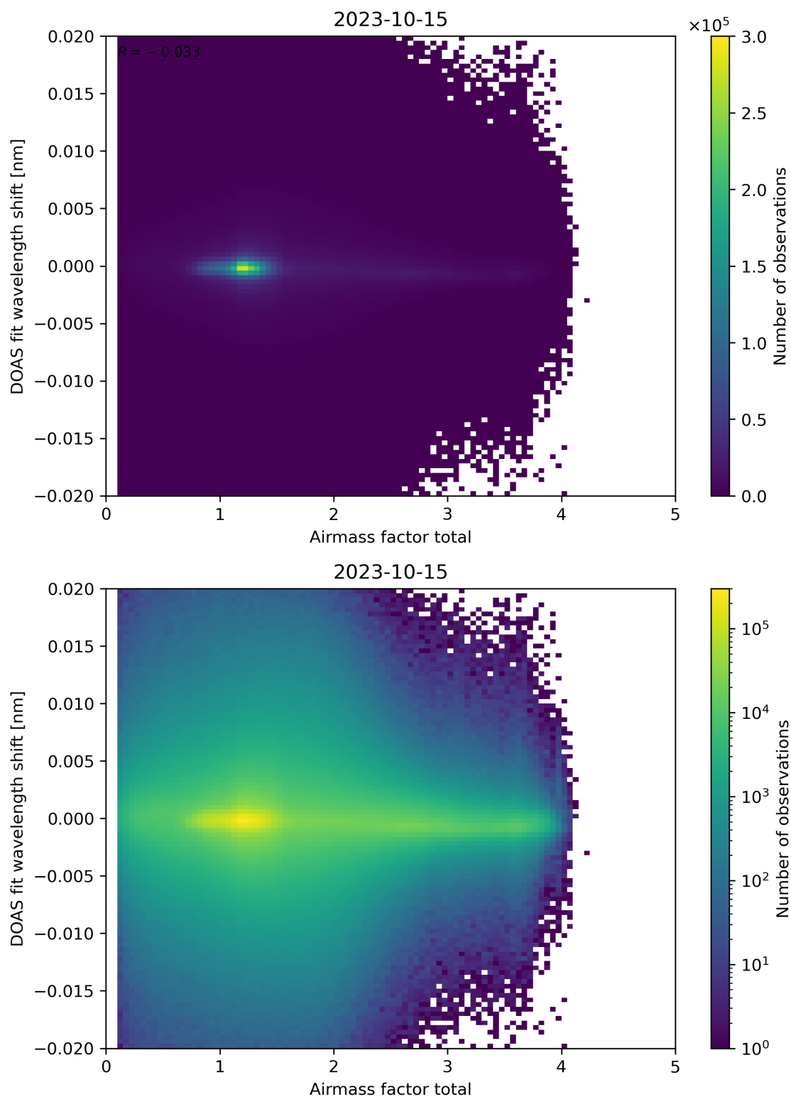
Figure 98: Scatter density plot of “Airmass factor total” against “DOAS fit wavelength shift” for 2023-10-14 to 2023-10-16.
