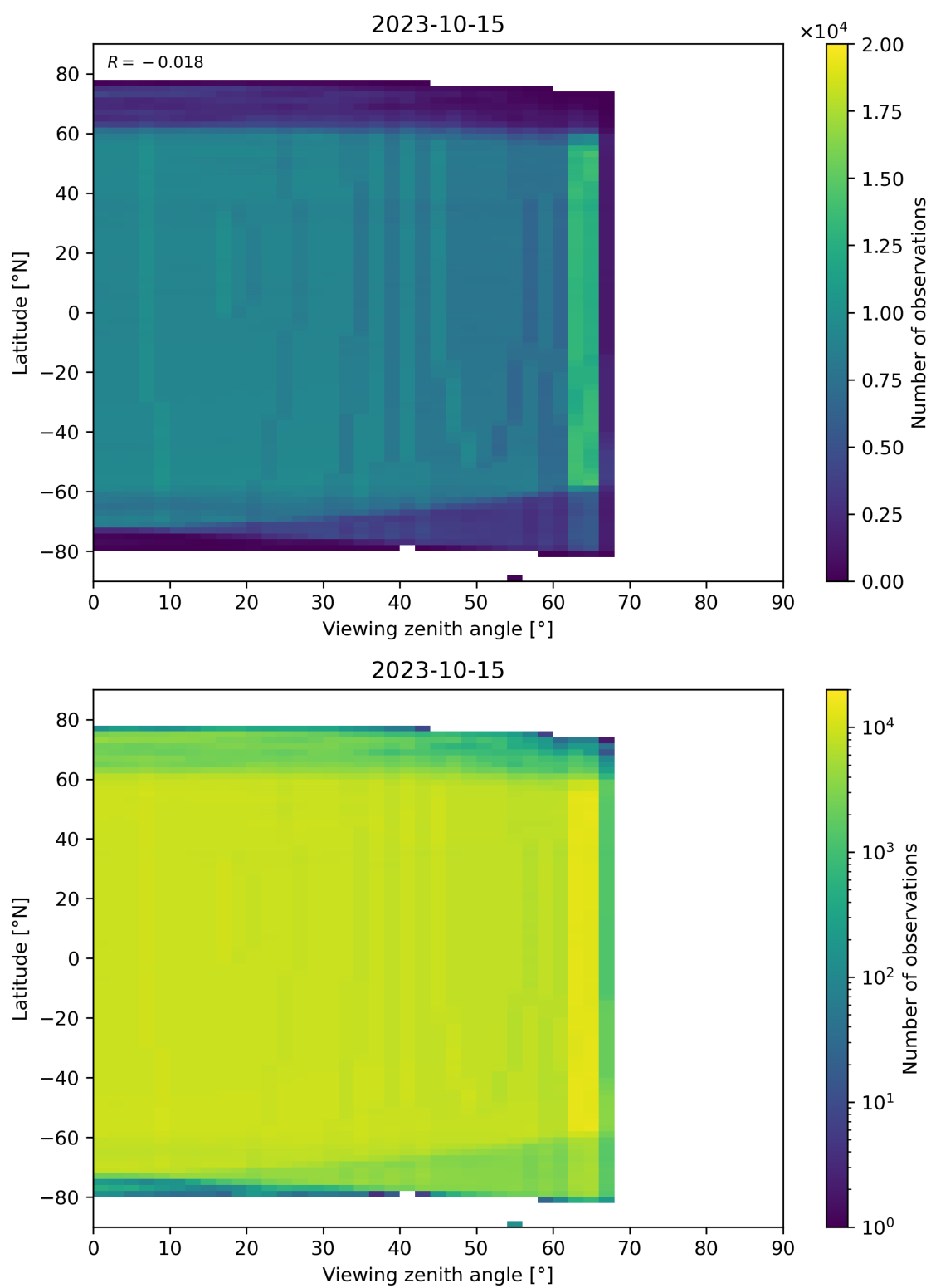
Figure 196: Scatter density plot of “Viewing zenith angle” against “Latitude” for 2023-10-14 to 2023-10-16.
