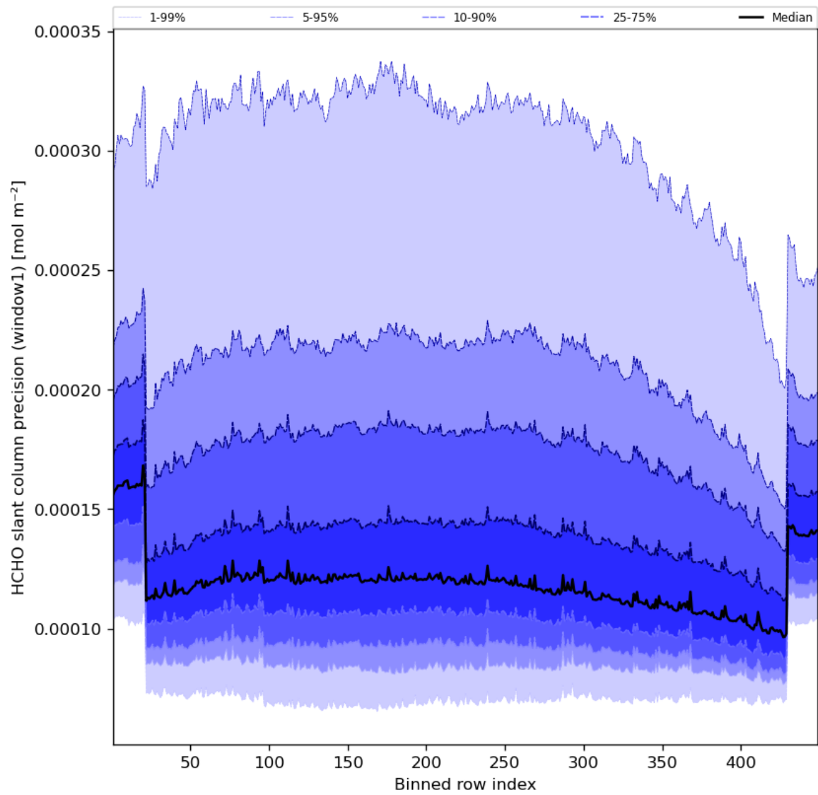
Figure 53: Along track statistics of “HCHO slant column precision (window1)” for 2023-10-14 to 2023-10-16
