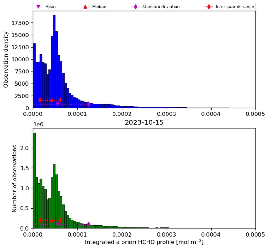
Figure 43: Histogram of “Integrated a priori HCHO profile” for 2023-10-14 to 2023-10-16
