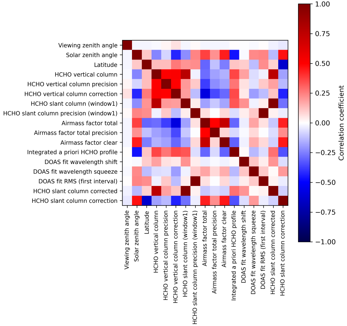
Figure 2: Map of correlation matrix for 2023-10-14 to 2023-10-16.
