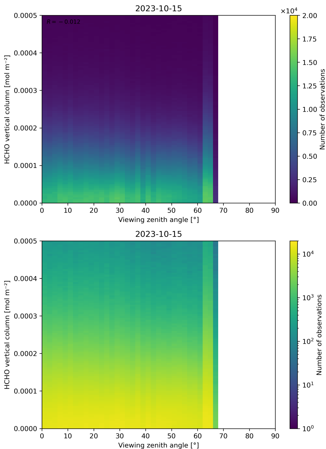
Figure 192: Scatter density plot of “Viewing zenith angle” against “HCHO vertical column” for 2023-10-14 to 2023-10-16.
