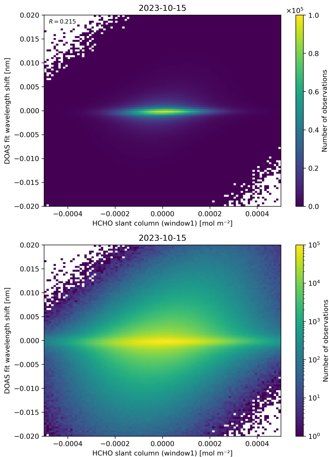
Figure 79: Scatter density plot of “HCHO slant column (window1)” against “DOAS fit wavelength shift” for 2023-10-14 to 2023-10-16.
