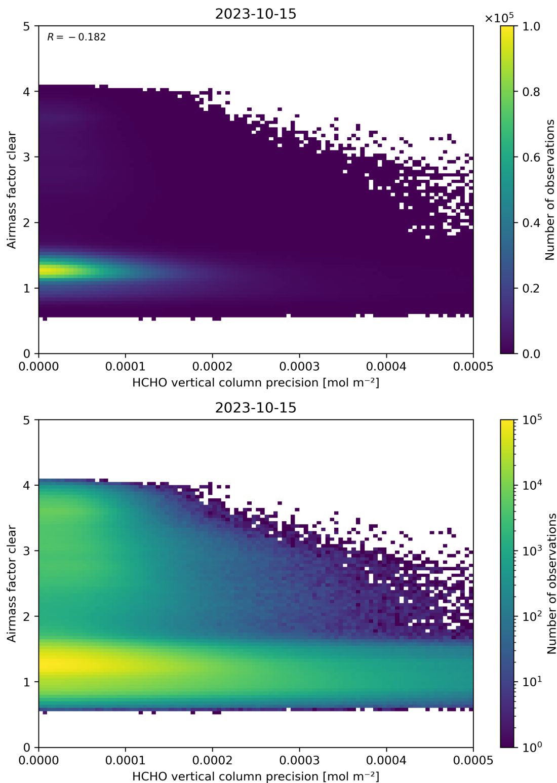
Figure 139: Scatter density plot of “HCHO vertical column precision” against “Airmass factor clear” for 2023-10-14 to 2023-10-16.
