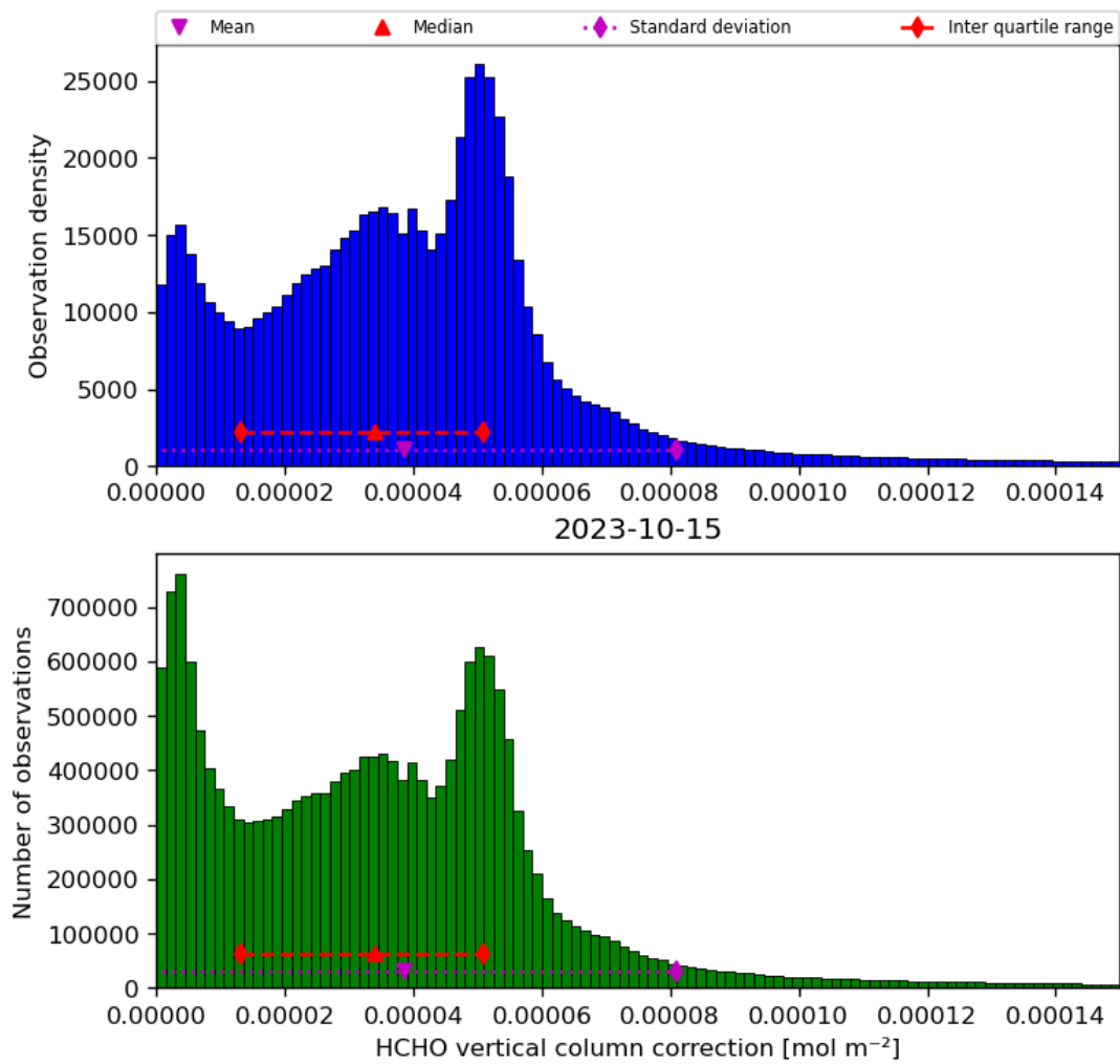
Figure 37: Histogram of “HCHO vertical column correction” for 2023-10-14 to 2023-10-16
