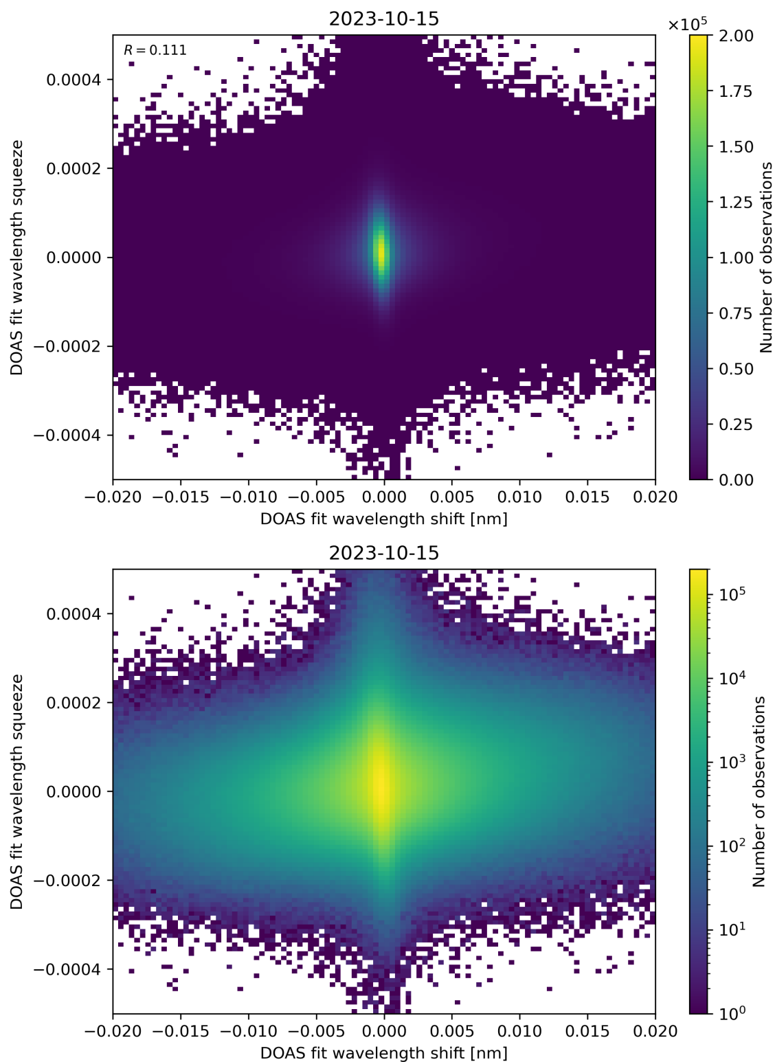
Figure 65: Scatter density plot of “DOAS fit wavelength shift” against “DOAS fit wavelength squeeze” for 2023-10-14 to 2023-10-16.
