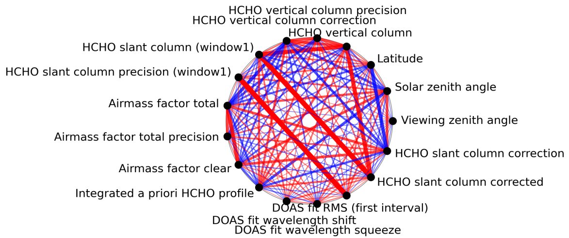
Figure 1: Map of correlation graph for 2023-10-14 to 2023-10-16.
