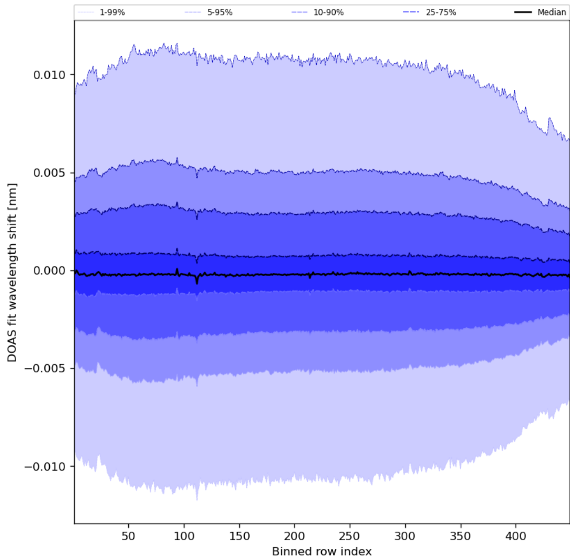
Figure 58: Along track statistics of “DOAS fit wavelength shift” for 2023-10-14 to 2023-10-16
