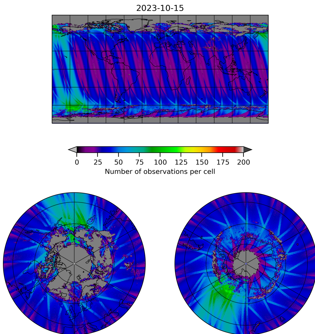
Figure 19: Map of the number of observations for 2023-10-14 to 2023-10-16
