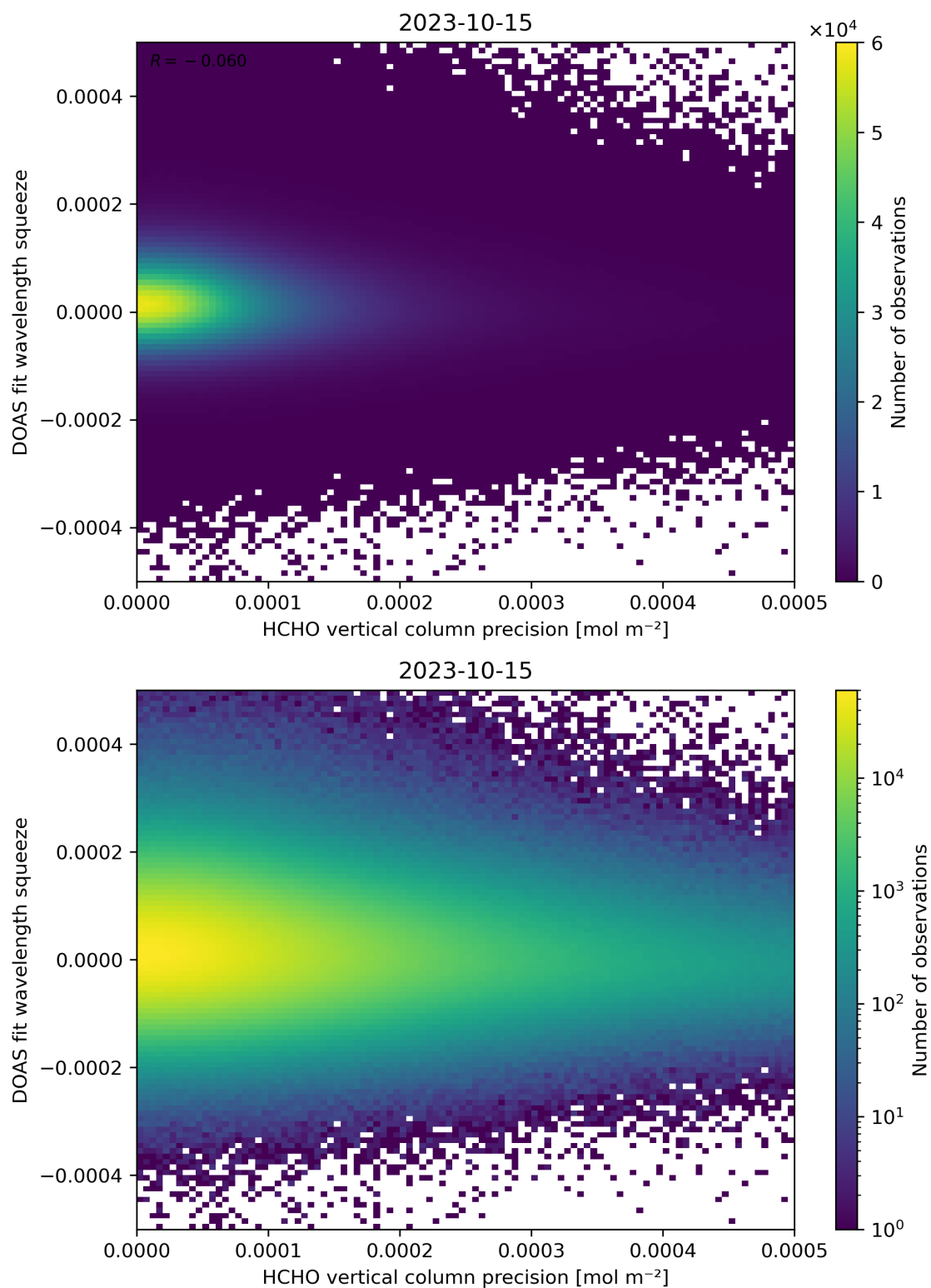
Figure 138: Scatter density plot of “HCHO vertical column precision” against “DOAS fit wavelength squeeze” for 2023-10-14 to 2023-10-16.
