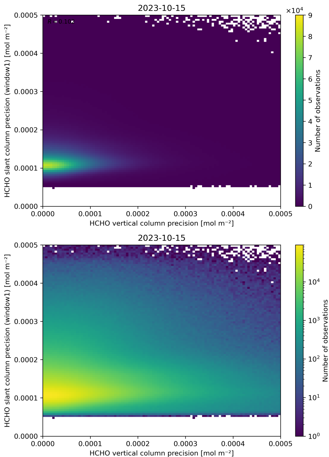
Figure 143: Scatter density plot of “HCHO vertical column precision” against “HCHO slant column precision (window1)” for 2023-10-14 to 2023-10-16.
