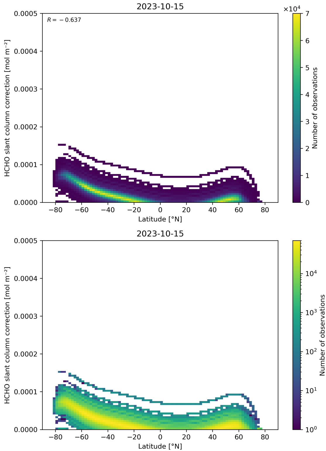
Figure 158: Scatter density plot of “Latitude” against “HCHO slant column correction” for 2023-10-14 to 2023-10-16.
