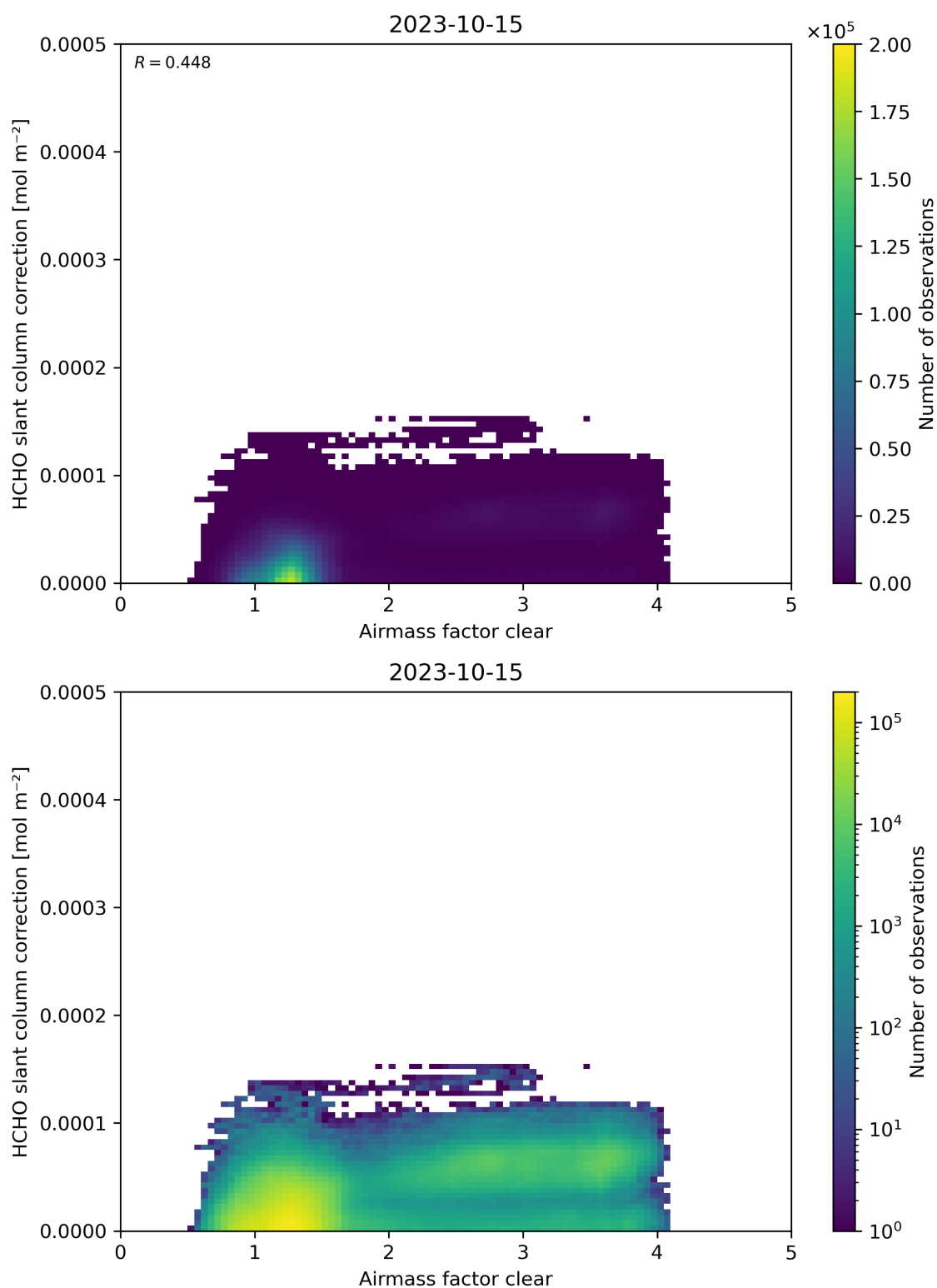
Figure 75: Scatter density plot of “Airmass factor clear” against “HCHO slant column correction” for 2023-10-14 to 2023-10-16.
