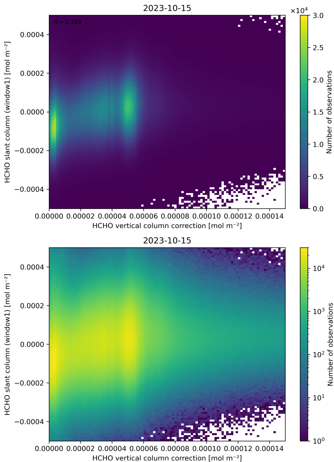
Figure 118: Scatter density plot of “HCHO vertical column correction” against “HCHO slant column (window1)” for 2023-10-14 to 2023-10-16.
