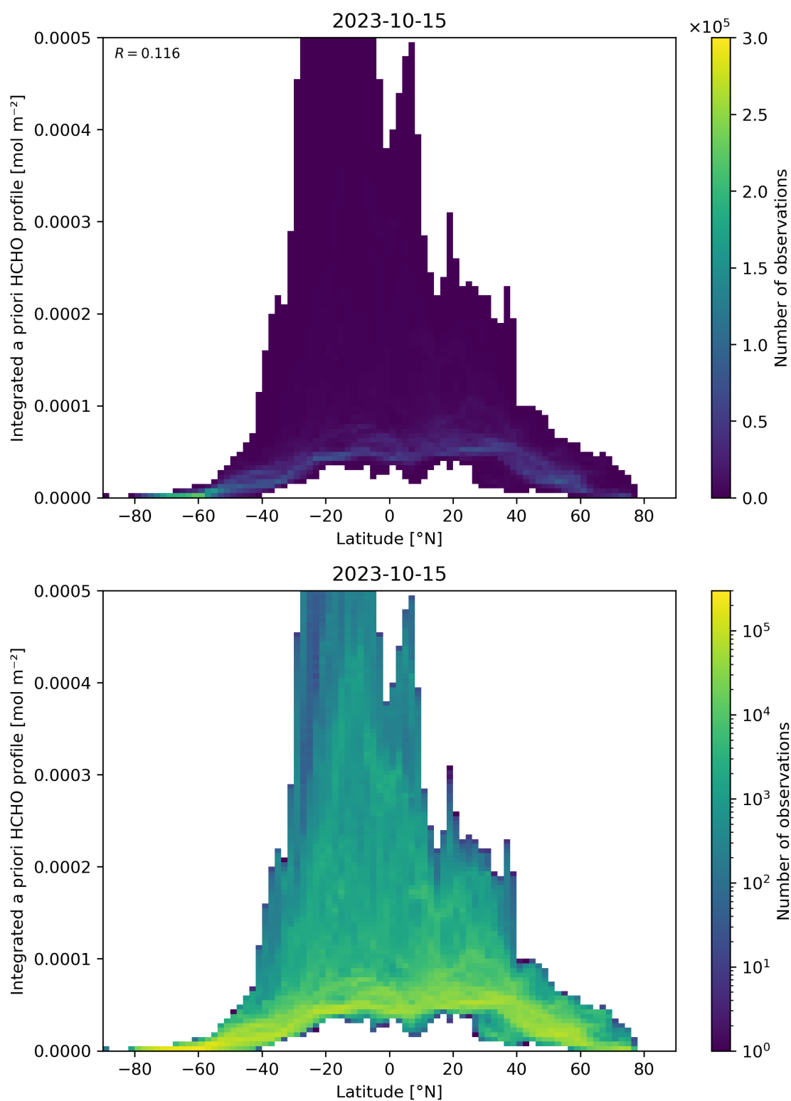
Figure 166: Scatter density plot of “Latitude” against “Integrated a priori HCHO profile” for 2023-10-14 to 2023-10-16.
