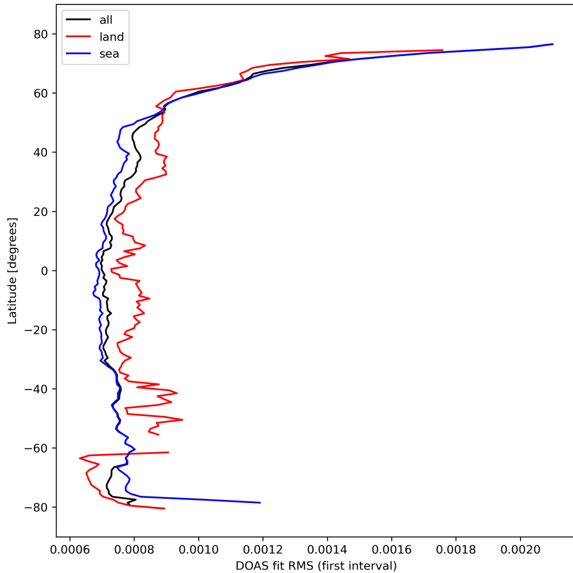
Figure 32: Zonal average of “DOAS fit RMS (first interval)” for 2023-10-14 to 2023-10-16.
