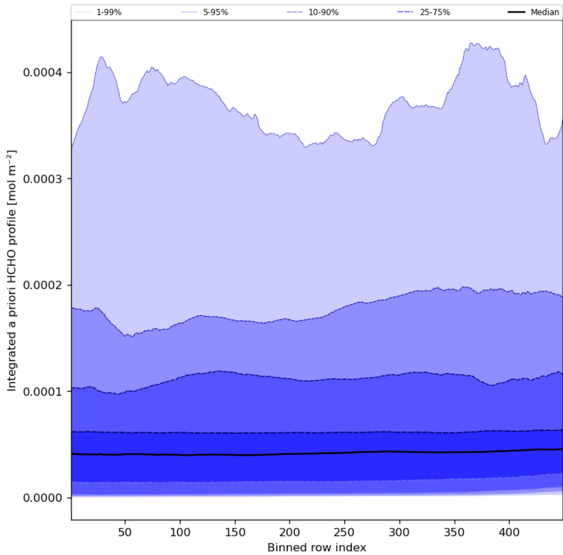
Figure 57: Along track statistics of “Integrated a priori HCHO profile” for 2023-10-14 to 2023-10-16
