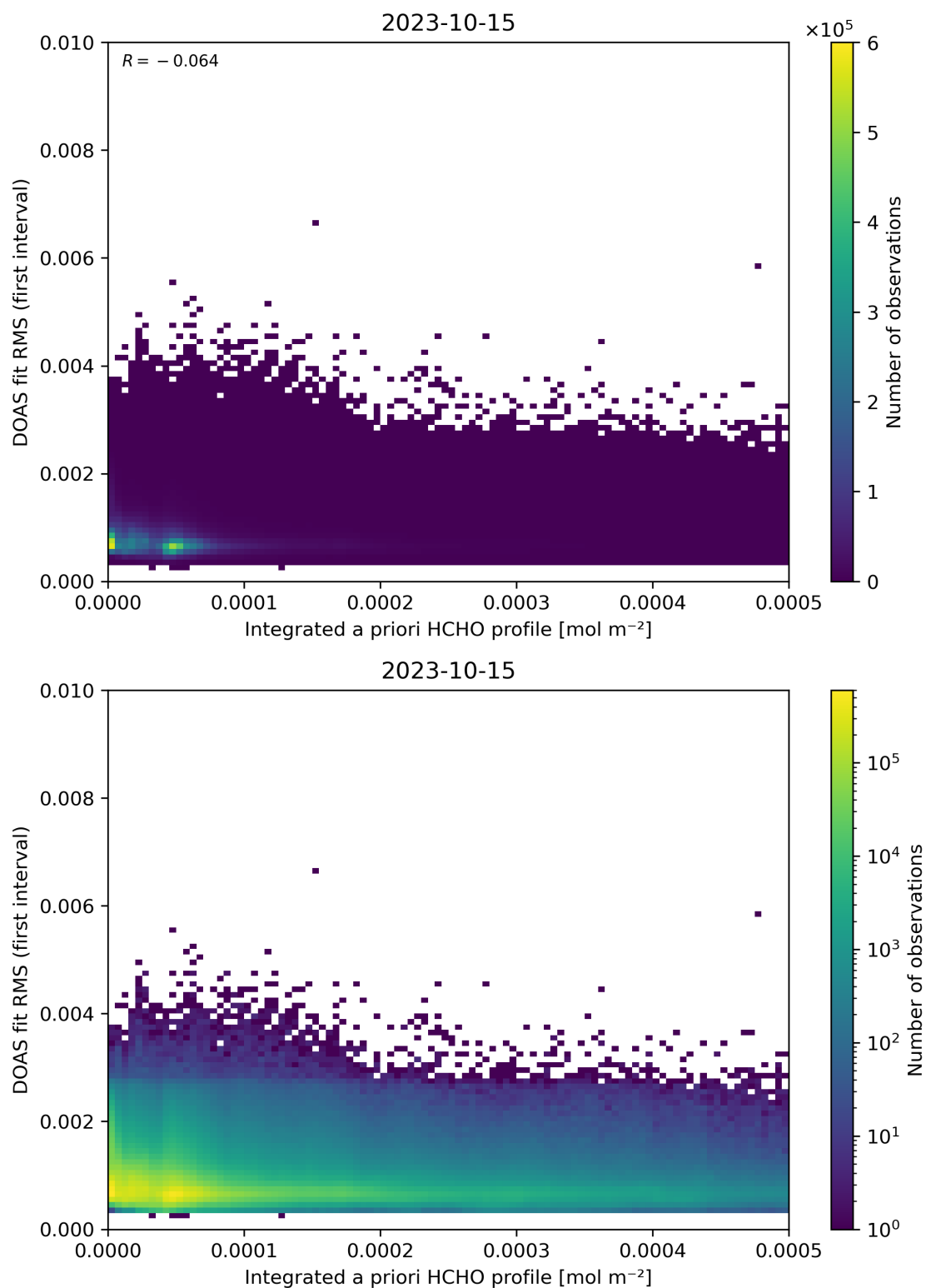
Figure 148: Scatter density plot of “Integrated a priori HCHO profile” against “DOAS fit RMS (first interval)” for 2023-10-14 to 2023-10-16.
