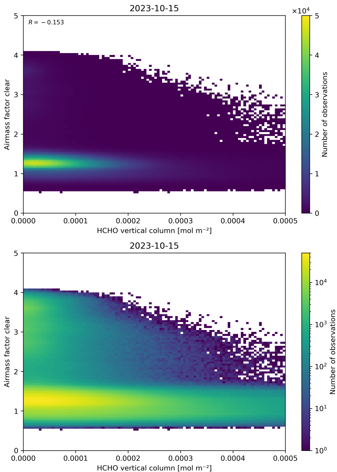
Figure 126: Scatter density plot of “HCHO vertical column” against “Airmass factor clear” for 2023-10-14 to 2023-10-16.
