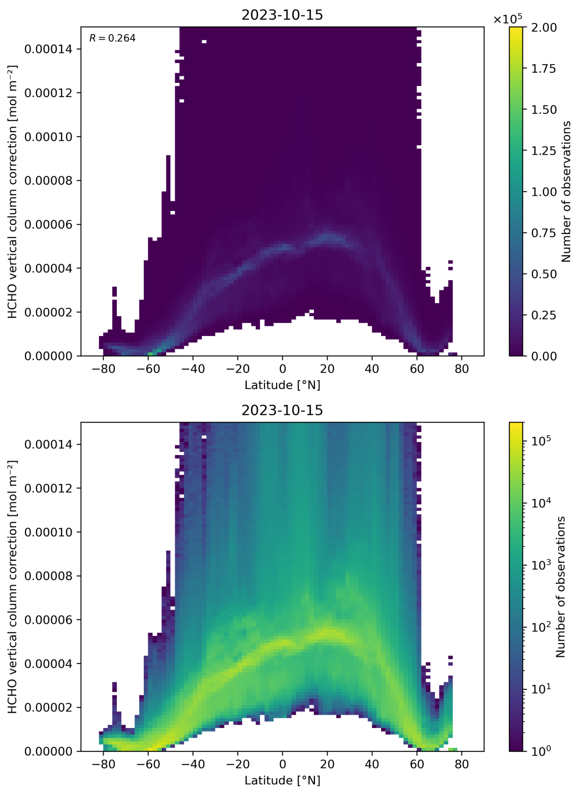
Figure 164: Scatter density plot of “Latitude” against “HCHO vertical column correction” for 2023-10-14 to 2023-10-16.
