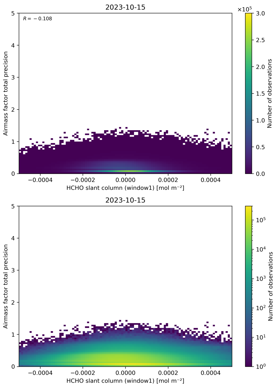
Figure 86: Scatter density plot of “HCHO slant column (window1)” against “Airmass factor total precision” for 2023-10-14 to 2023-10-16.
