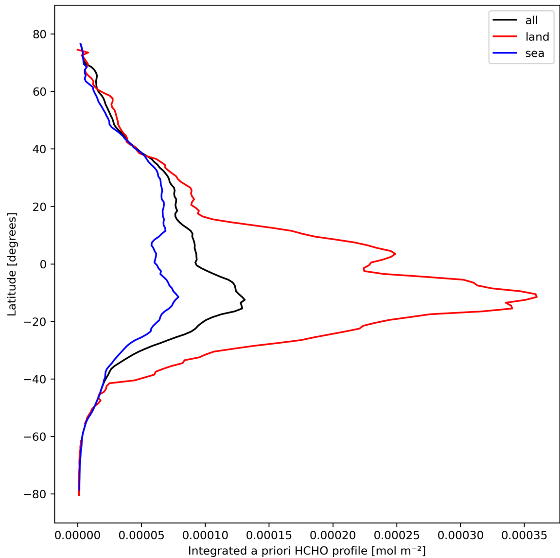
Figure 29: Zonal average of “Integrated a priori HCHO profile” for 2023-10-14 to 2023-10-16.
