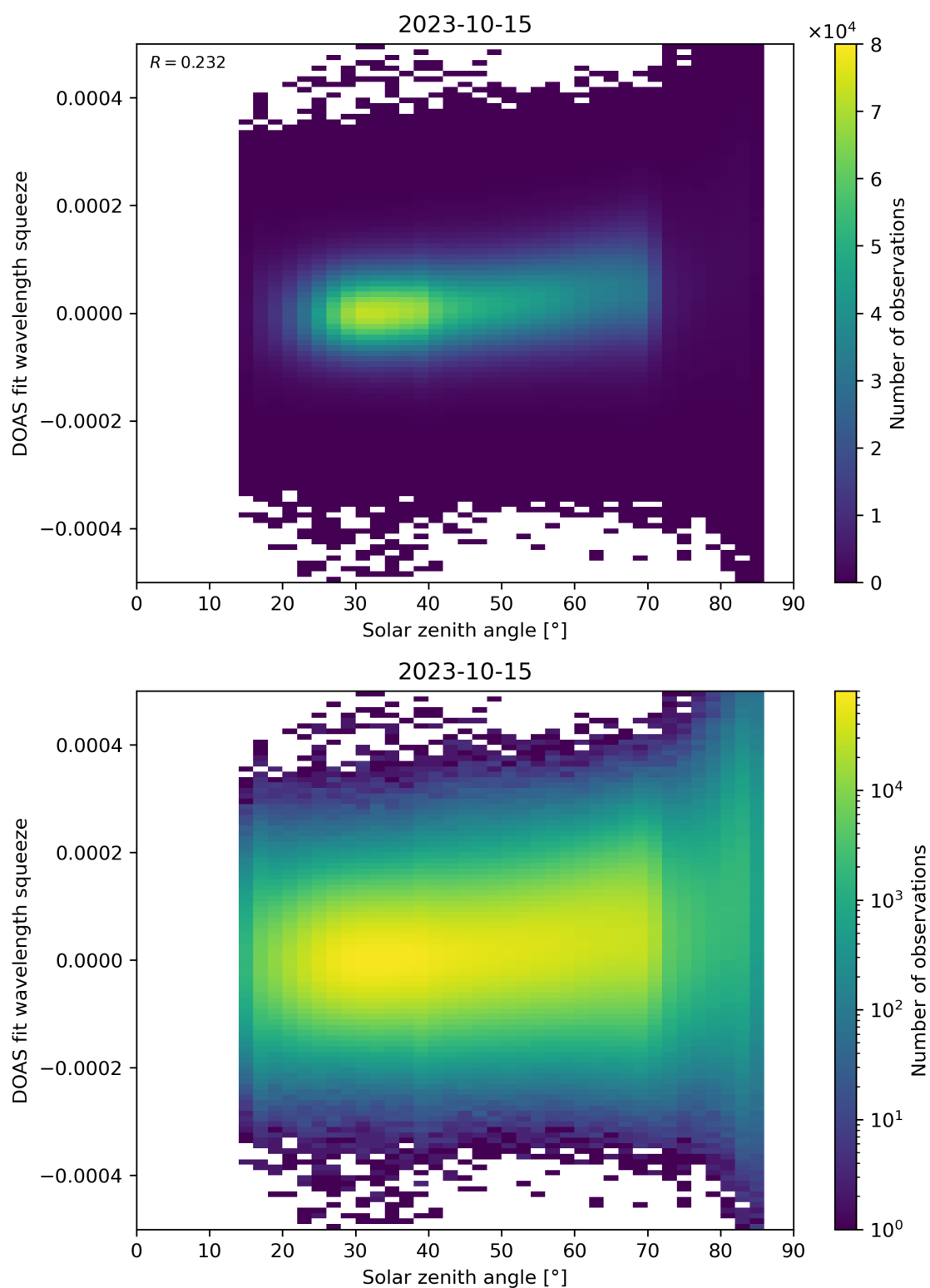
Figure 169: Scatter density plot of “Solar zenith angle” against “DOAS fit wavelength squeeze” for 2023-10-14 to 2023-10-16.
