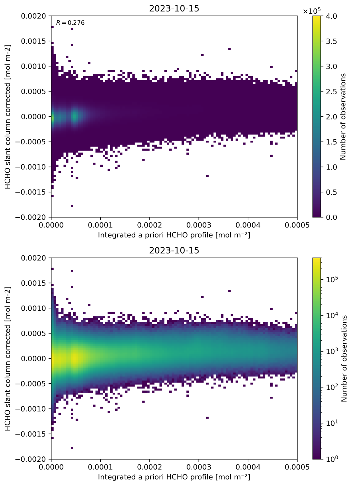
Figure 151: Scatter density plot of “Integrated a priori HCHO profile” against “HCHO slant column corrected” for 2023-10-14 to 2023-10-16.
