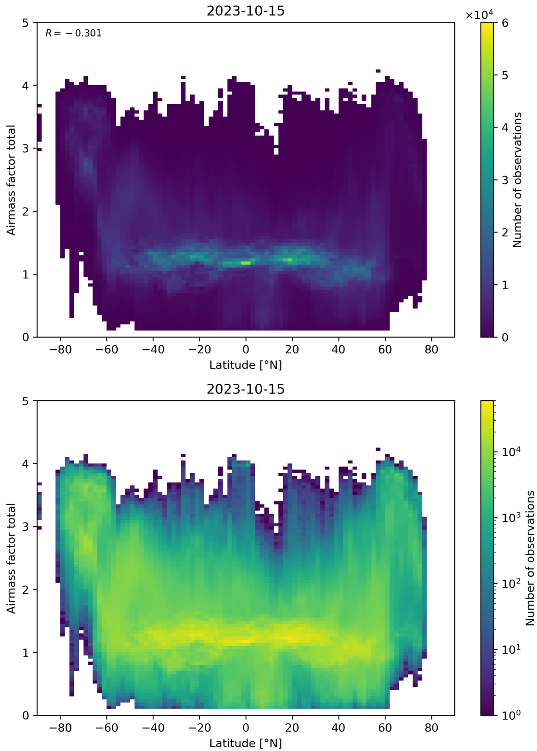
Figure 161: Scatter density plot of “Latitude” against “Airmass factor total” for 2023-10-14 to 2023-10-16.
