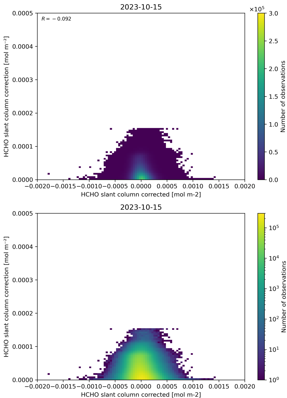
Figure 77: Scatter density plot of “HCHO slant column corrected” against “HCHO slant column correction” for 2023-10-14 to 2023-10-16.
