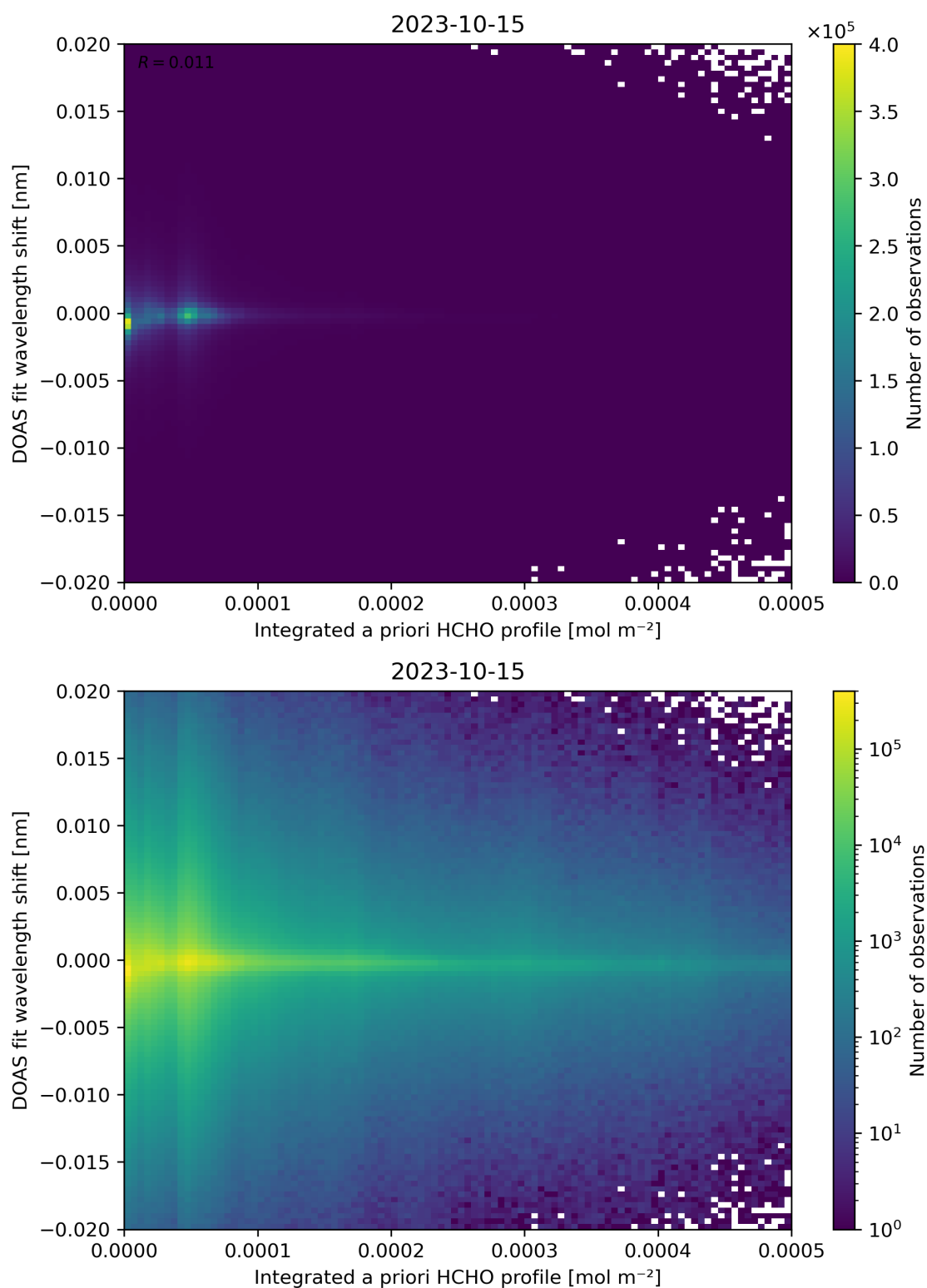
Figure 149: Scatter density plot of “Integrated a priori HCHO profile” against “DOAS fit wavelength shift” for 2023-10-14 to 2023-10-16.
