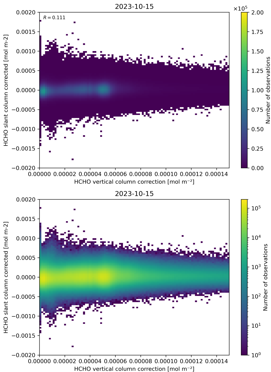
Figure 116: Scatter density plot of “HCHO vertical column correction” against “HCHO slant column corrected” for 2023-10-14 to 2023-10-16.
