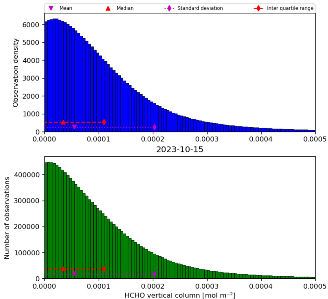
Figure 35: Histogram of “HCHO vertical column” for 2023-10-14 to 2023-10-16
