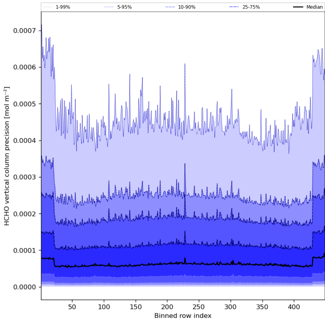
Figure 50: Along track statistics of “HCHO vertical column precision” for 2023-10-14 to 2023-10-16
