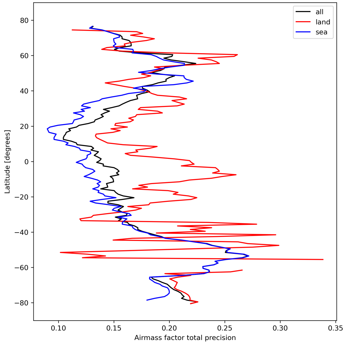
Figure 27: Zonal average of “Airmass factor total precision” for 2023-10-14 to 2023-10-16.
