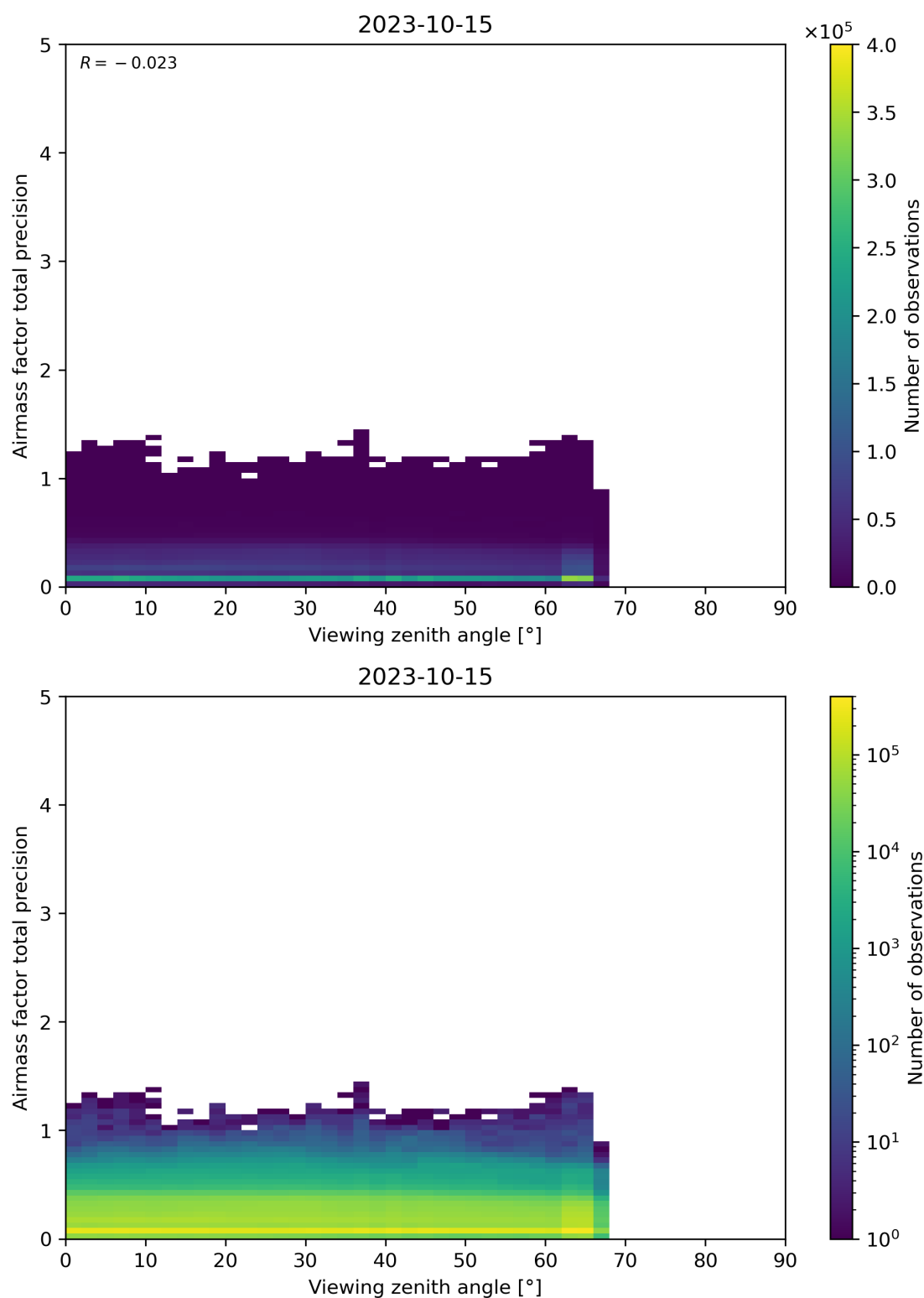
Figure 191: Scatter density plot of “Viewing zenith angle” against “Airmass factor total precision” for 2023-10-14 to 2023-10-16.
