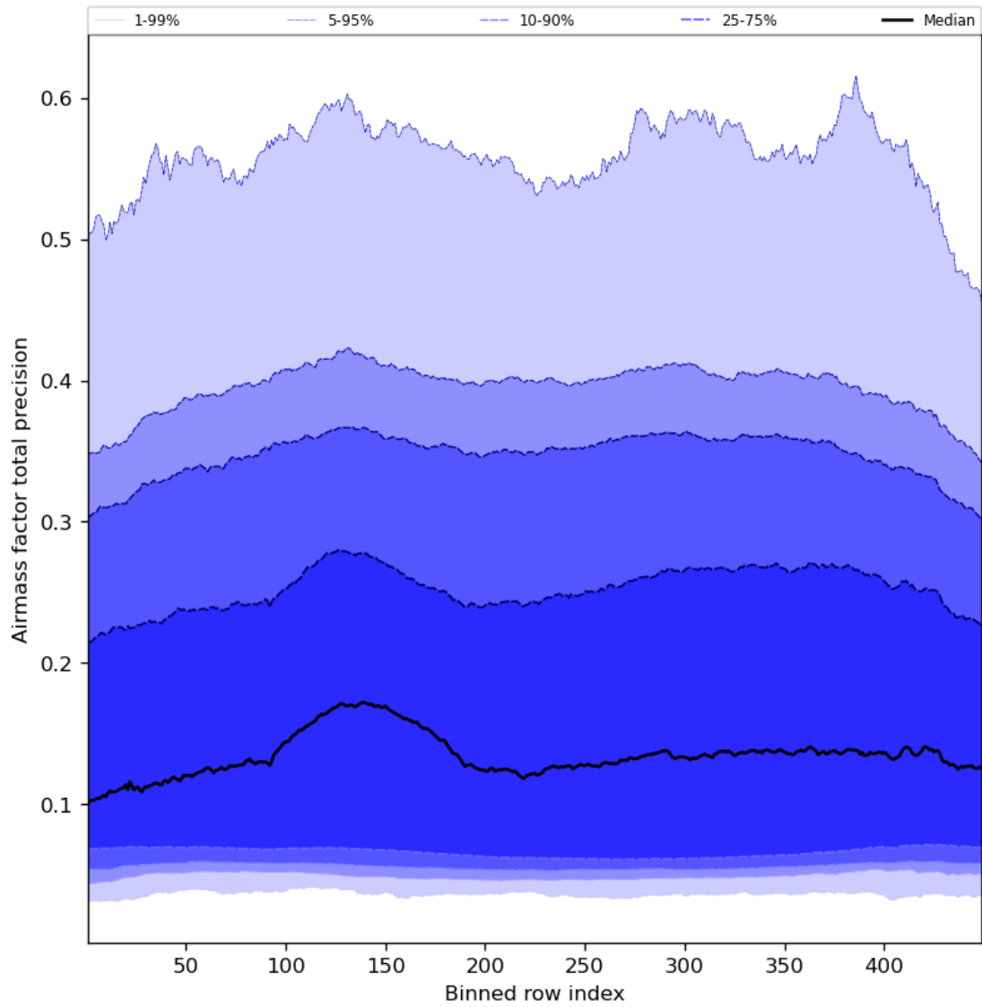
Figure 55: Along track statistics of “Airmass factor total precision” for 2023-10-14 to 2023-10-16
