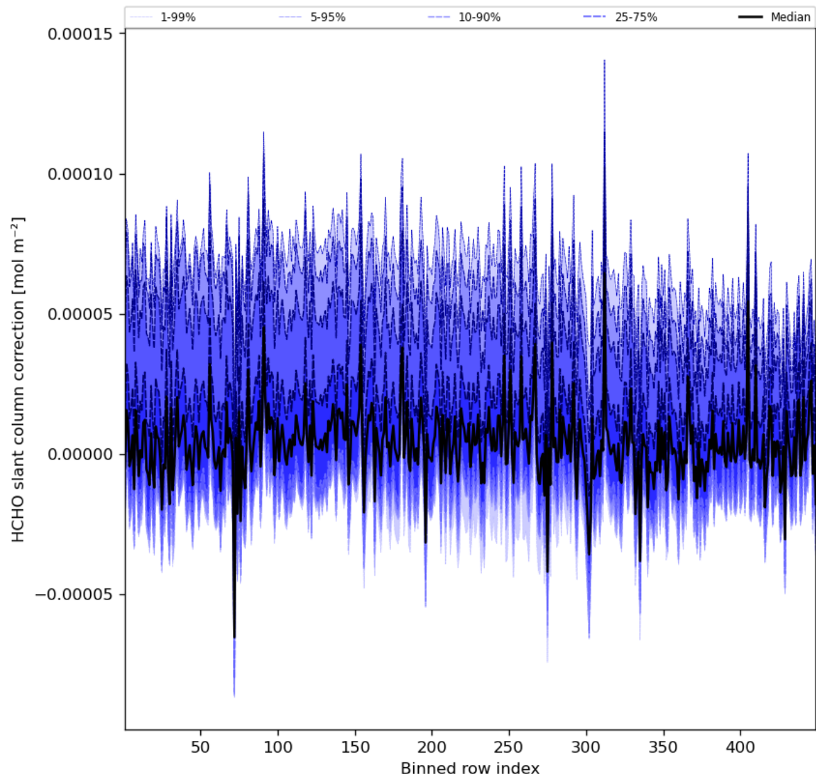
Figure 61: Along track statistics of “HCHO slant column correction” for 2023-10-14 to 2023-10-16
