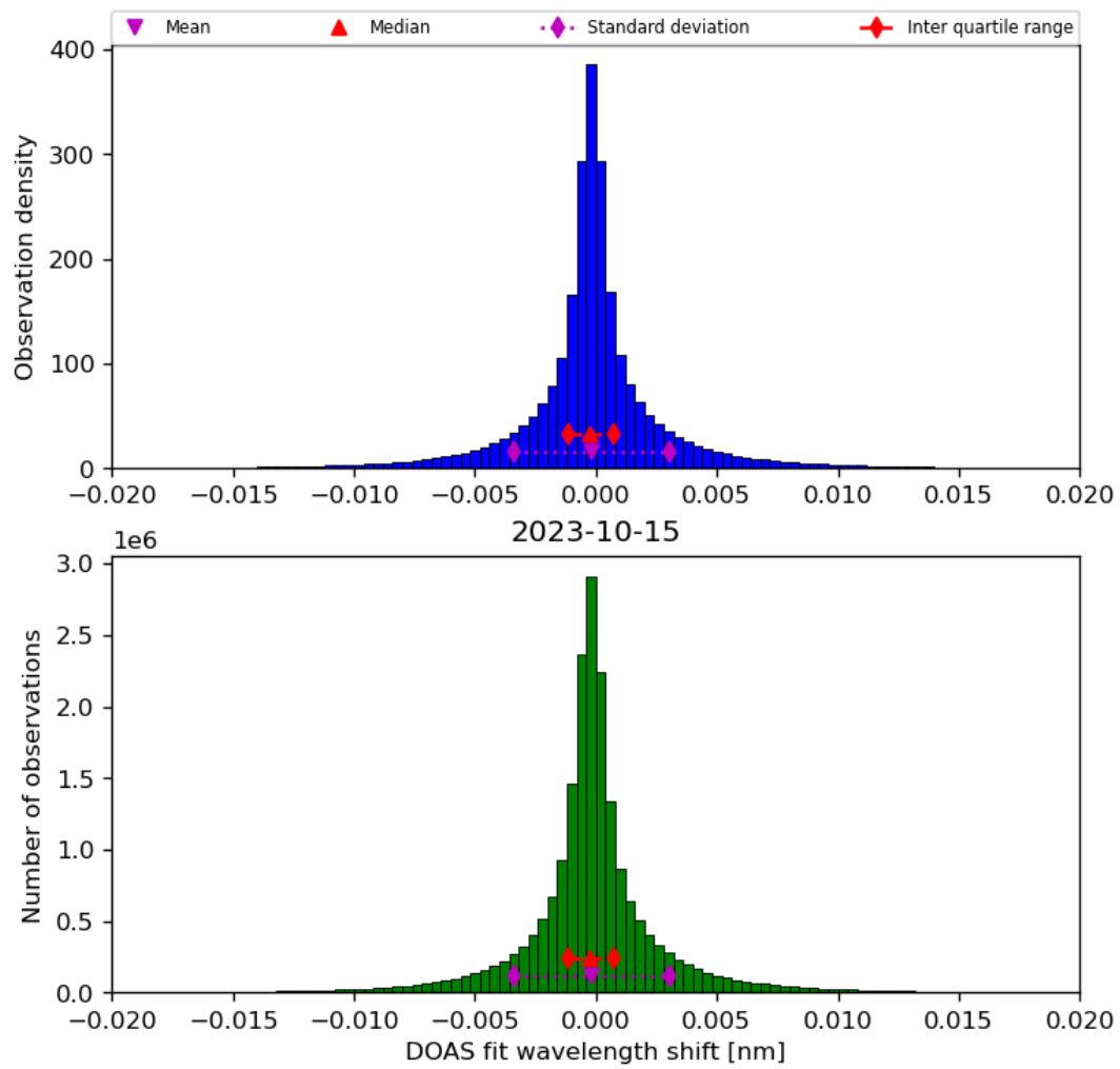
Figure 44: Histogram of “DOAS fit wavelength shift” for 2023-10-14 to 2023-10-16
