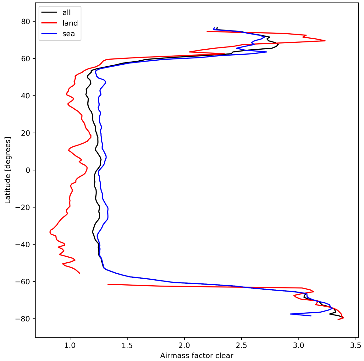
Figure 28: Zonal average of “Airmass factor clear” for 2023-10-14 to 2023-10-16.
