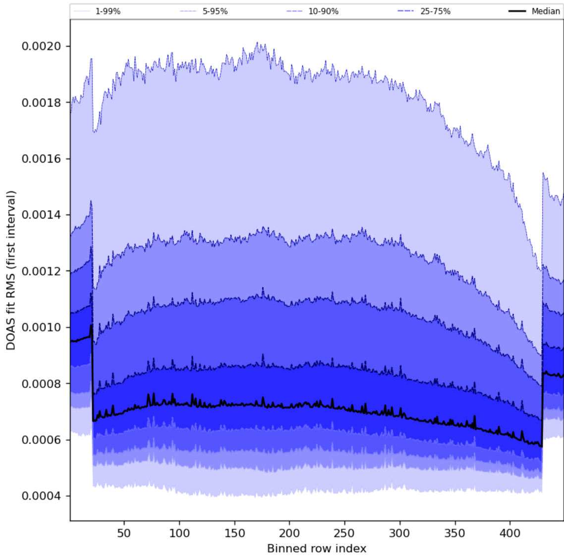
Figure 60: Along track statistics of “DOAS fit RMS (first interval)” for 2023-10-14 to 2023-10-16
