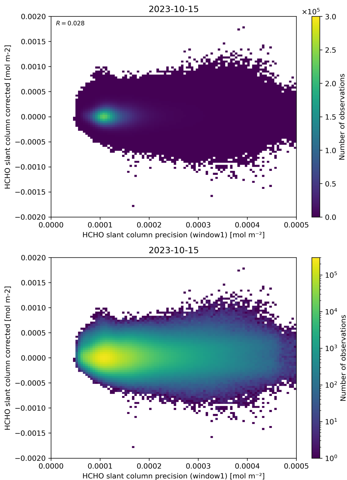
Figure 92: Scatter density plot of “HCHO slant column precision (window1)” against “HCHO slant column corrected” for 2023-10-14 to 2023-10-16.
