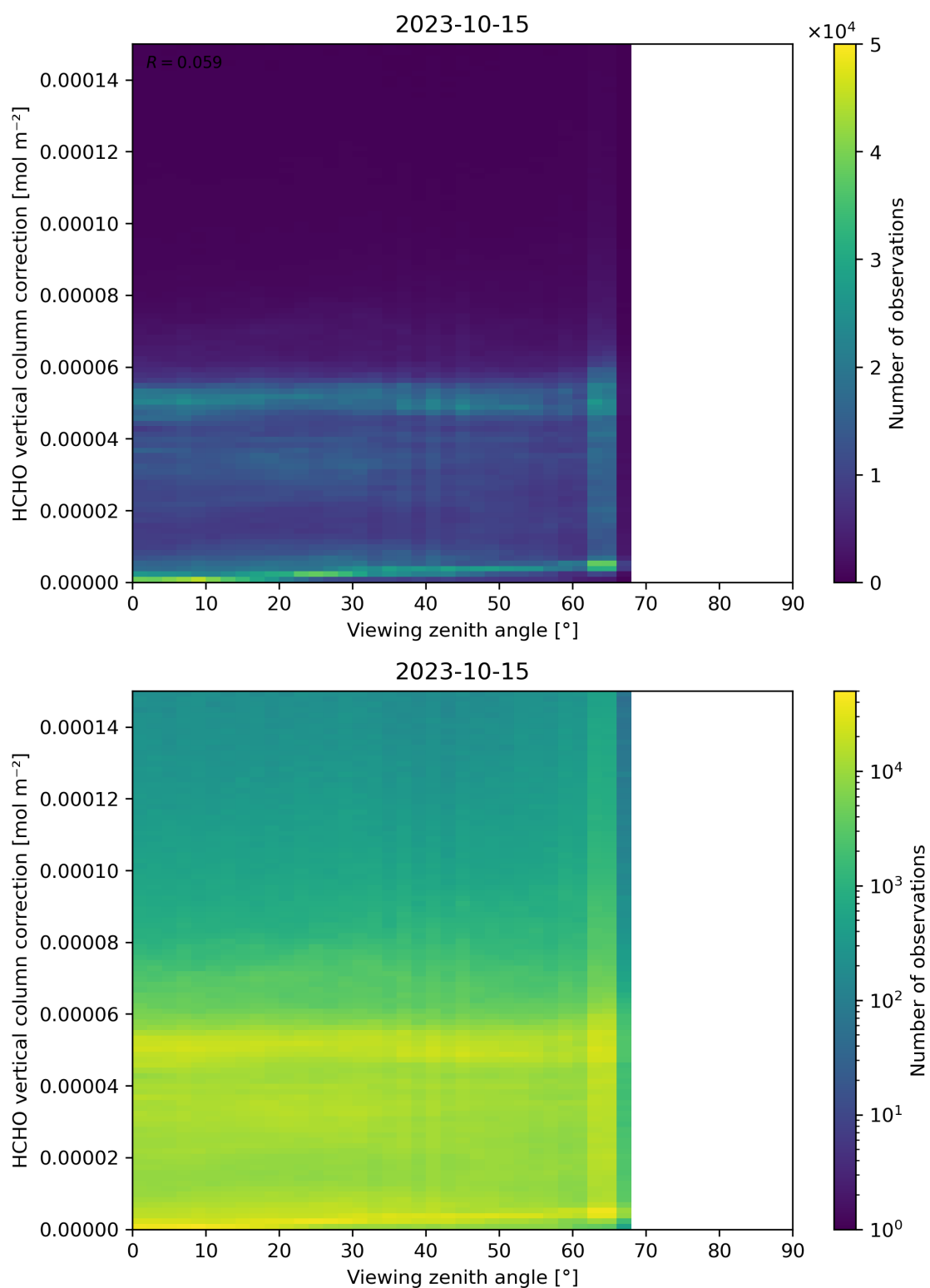
Figure 193: Scatter density plot of “Viewing zenith angle” against “HCHO vertical column correction” for 2023-10-14 to 2023-10-16.
