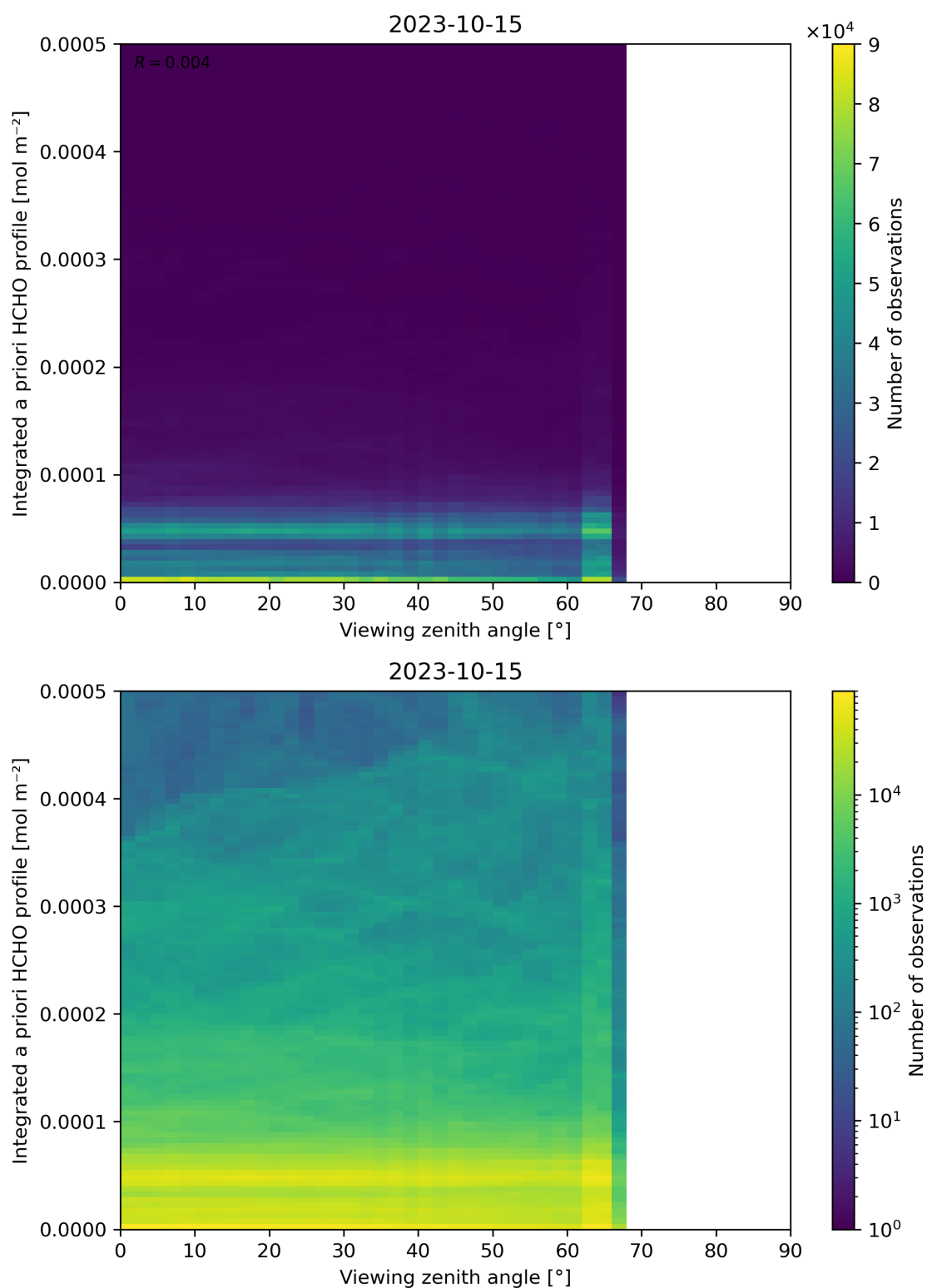
Figure 195: Scatter density plot of “Viewing zenith angle” against “Integrated a priori HCHO profile” for 2023-10-14 to 2023-10-16.
