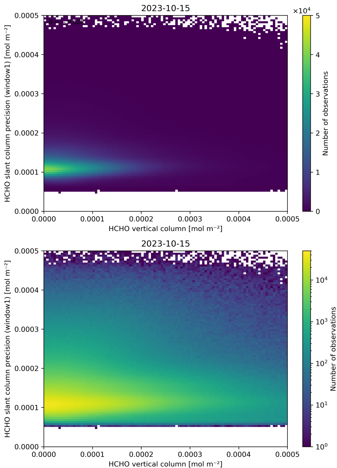
Figure 130: Scatter density plot of “HCHO vertical column” against “HCHO slant column precision (window1)” for 2023-10-14 to 2023-10-16.
