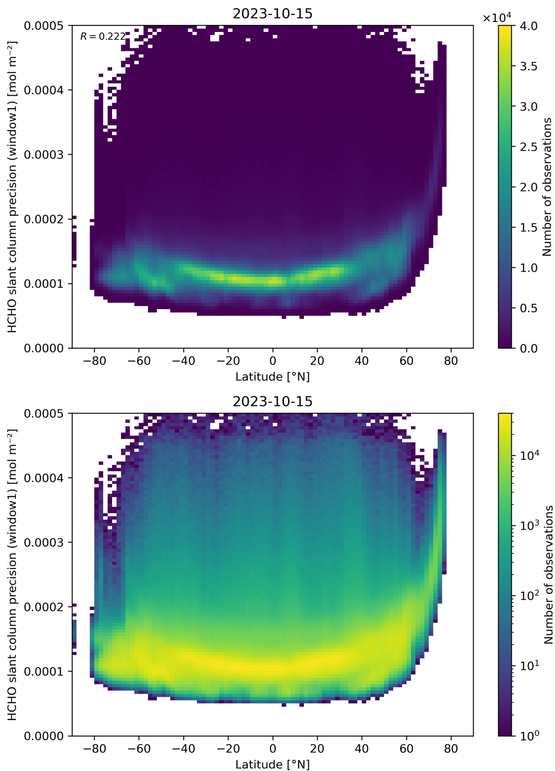
Figure 160: Scatter density plot of “Latitude” against “HCHO slant column precision (window1)” for 2023-10-14 to 2023-10-16.
