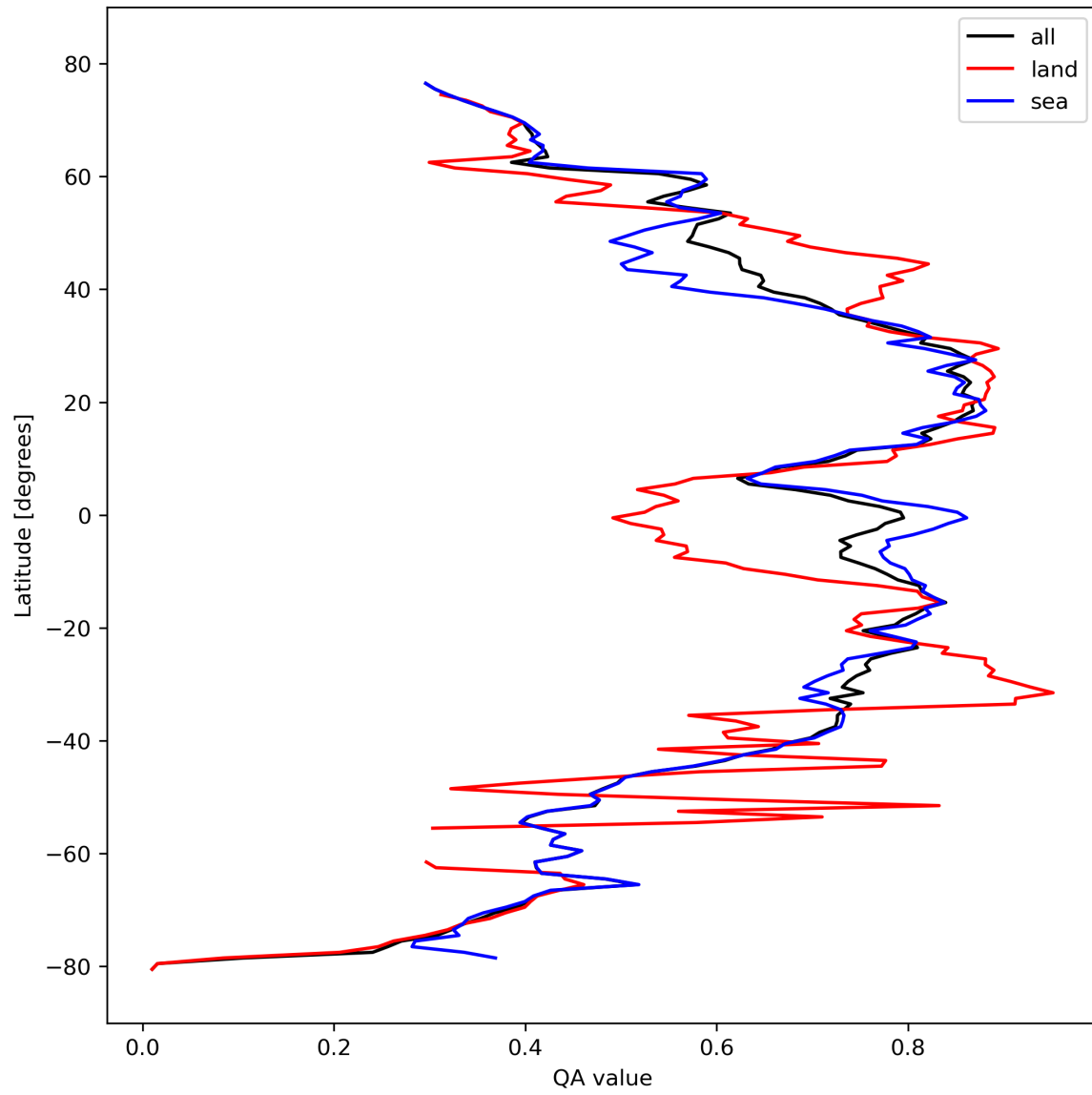
Figure 20: Zonal average of “QA value” for 2023-10-14 to 2023-10-16.
