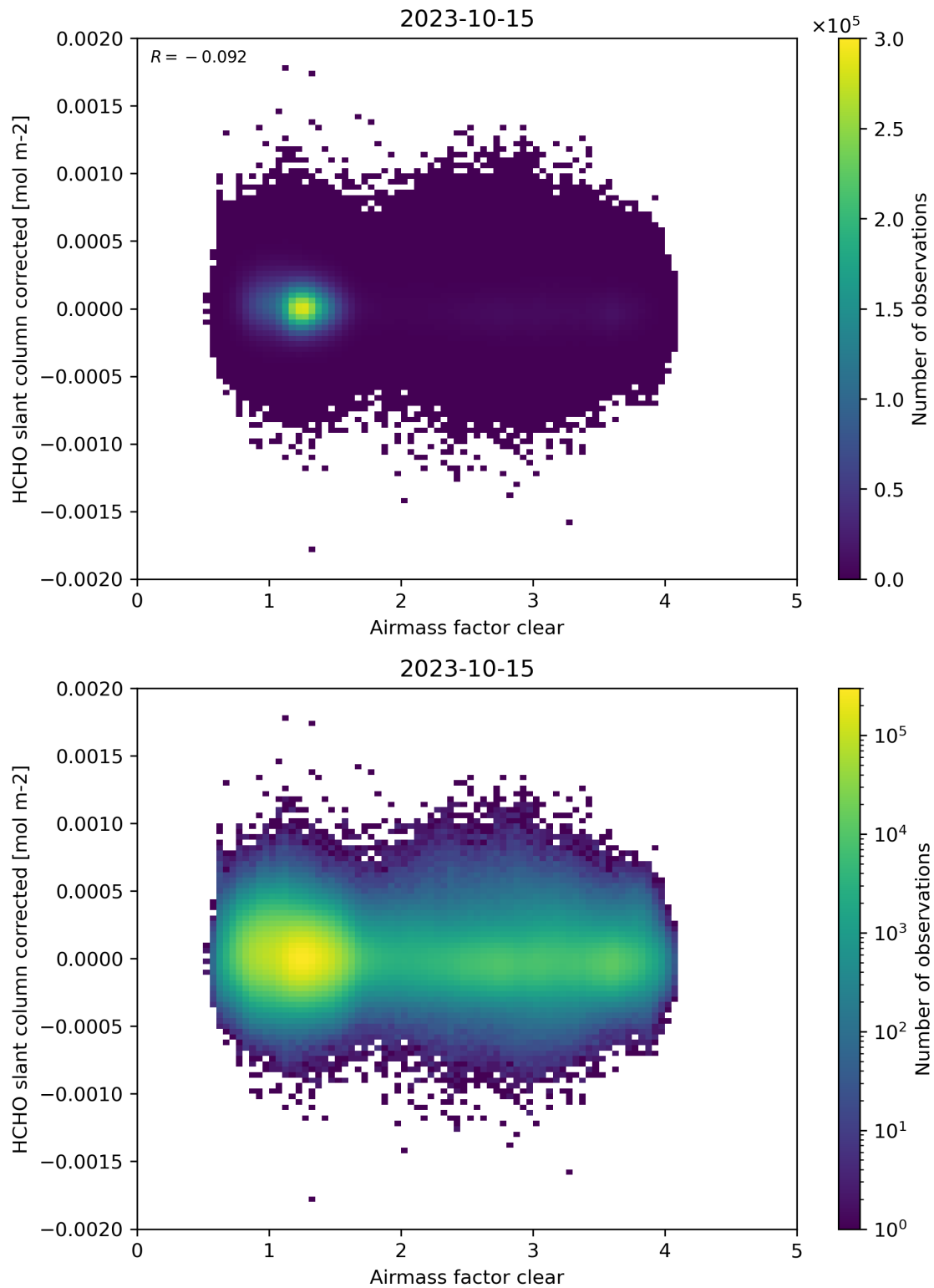
Figure 74: Scatter density plot of “Airmass factor clear” against “HCHO slant column corrected” for 2023-10-14 to 2023-10-16.
