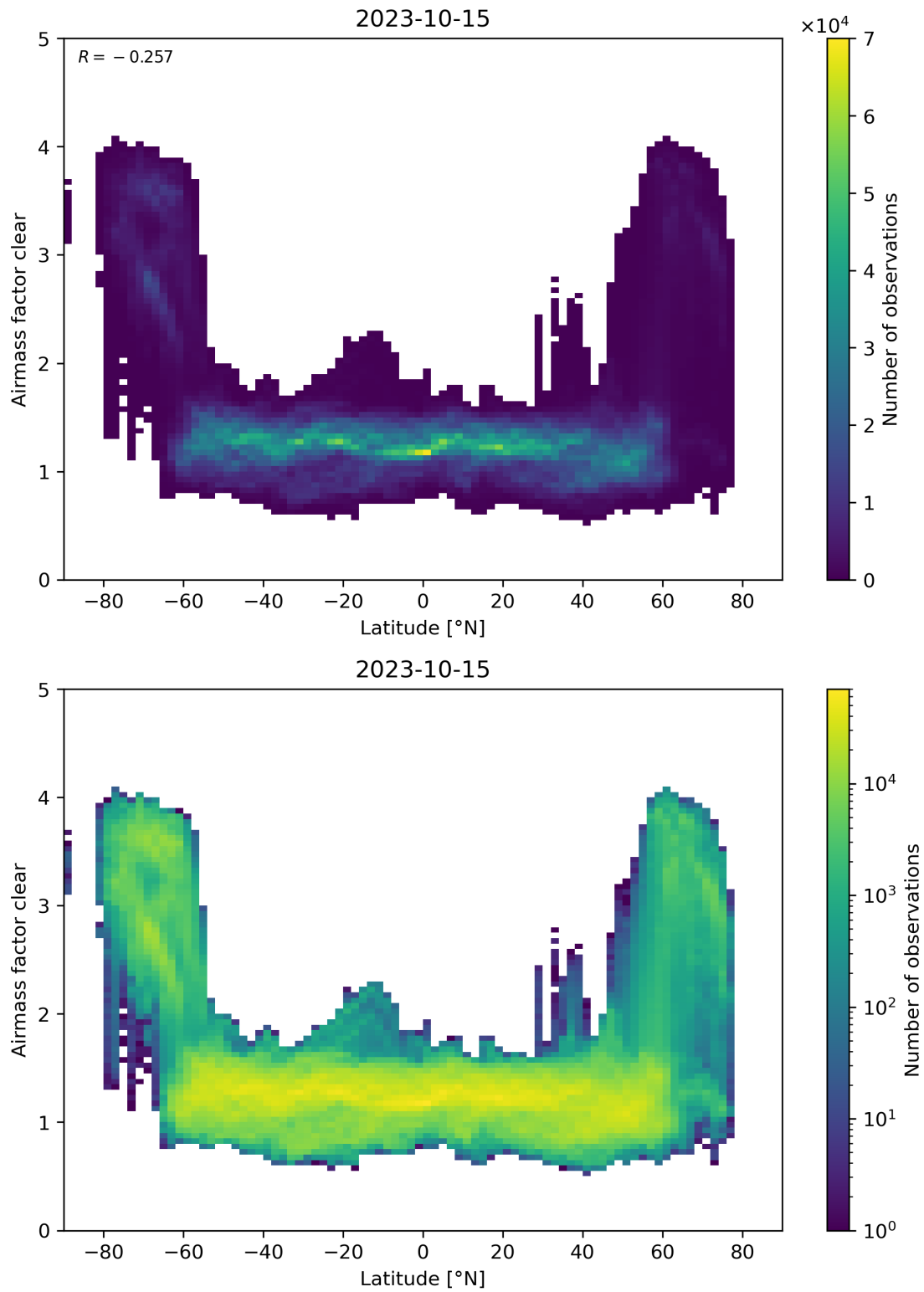
Figure 156: Scatter density plot of “Latitude” against “Airmass factor clear” for 2023-10-14 to 2023-10-16.
