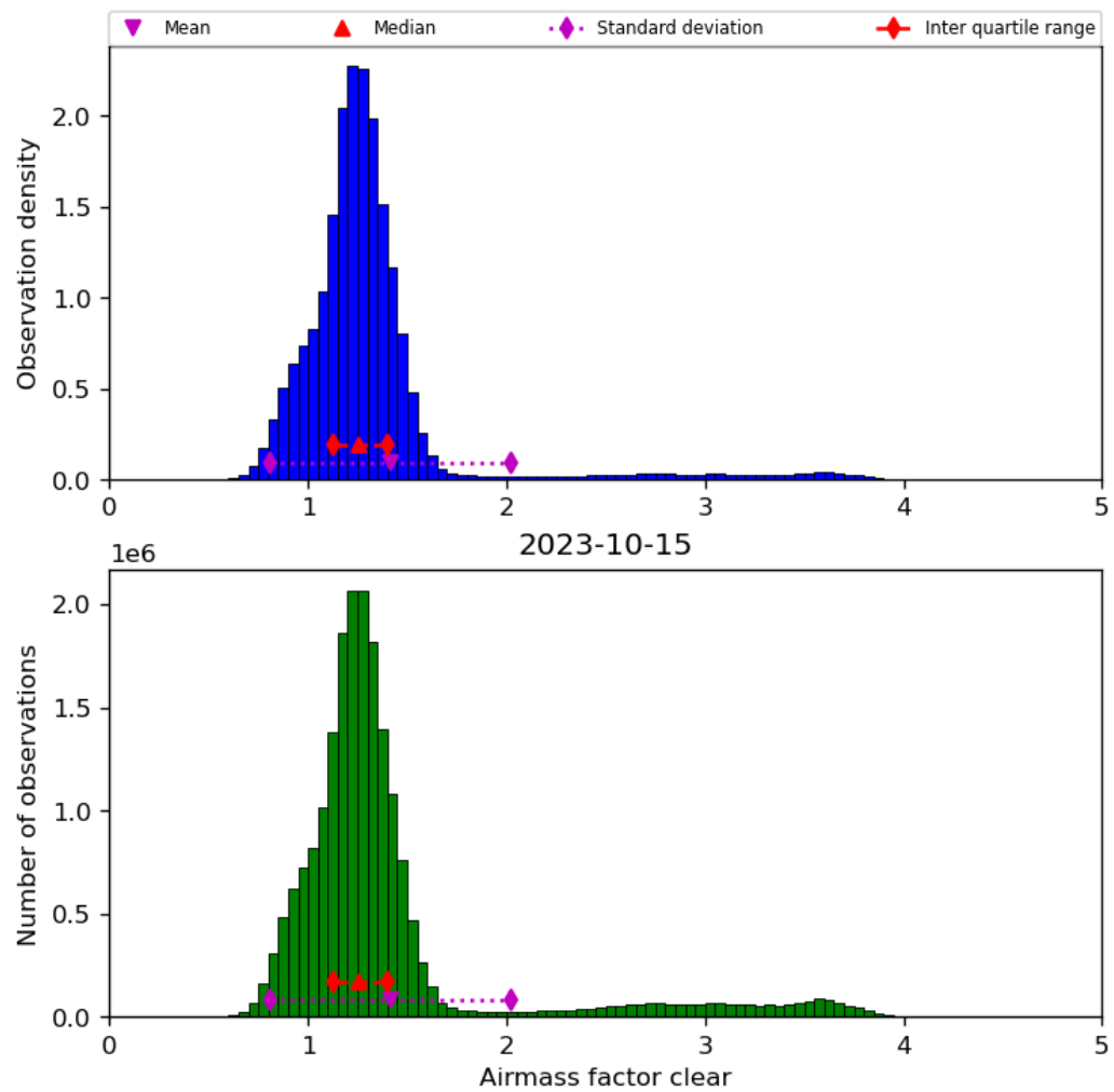
Figure 42: Histogram of “Airmass factor clear” for 2023-10-14 to 2023-10-16
