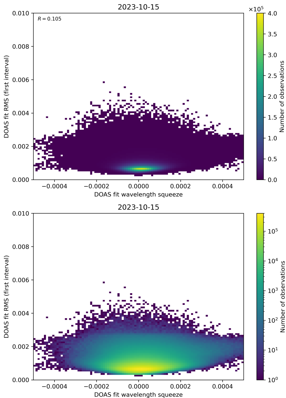
Figure 68: Scatter density plot of “DOAS fit wavelength squeeze” against “DOAS fit RMS (first interval)” for 2023-10-14 to 2023-10-16.
