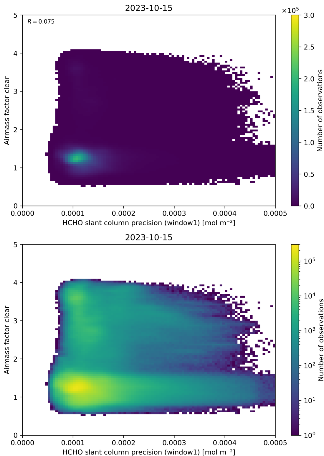
Figure 91: Scatter density plot of “HCHO slant column precision (window1)” against “Airmass factor clear” for 2023-10-14 to 2023-10-16.
