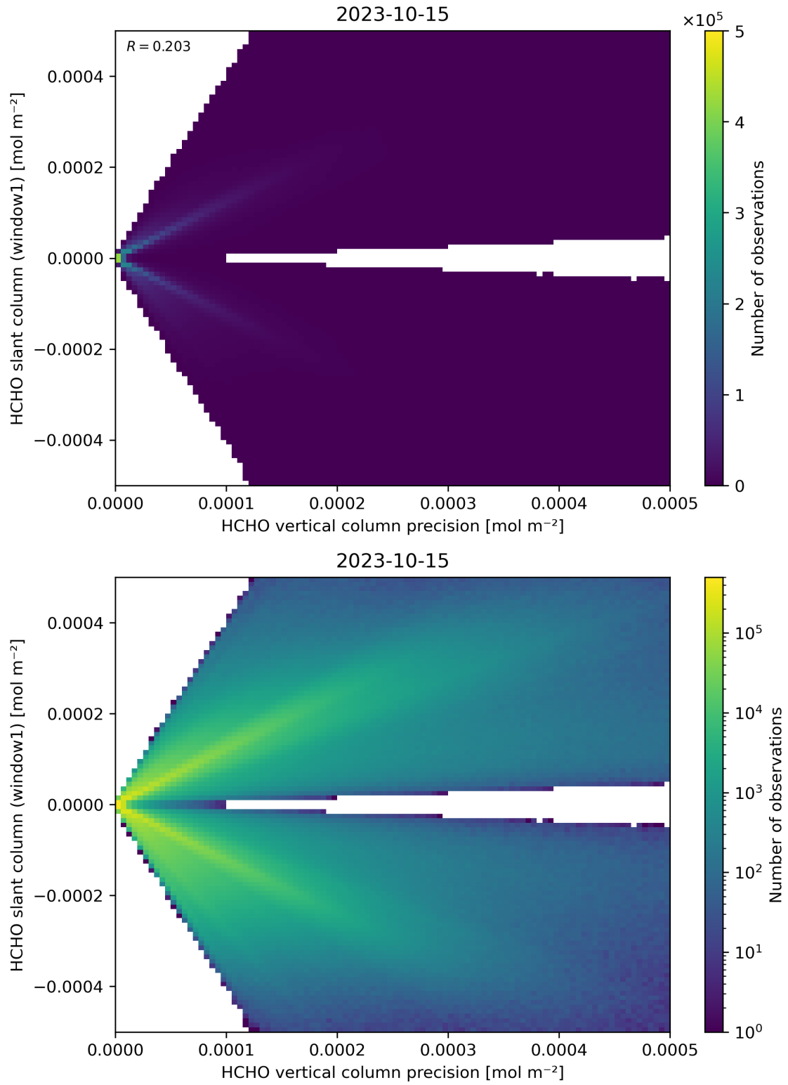
Figure 142: Scatter density plot of “HCHO vertical column precision” against “HCHO slant column (window1)” for 2023-10-14 to 2023-10-16.
