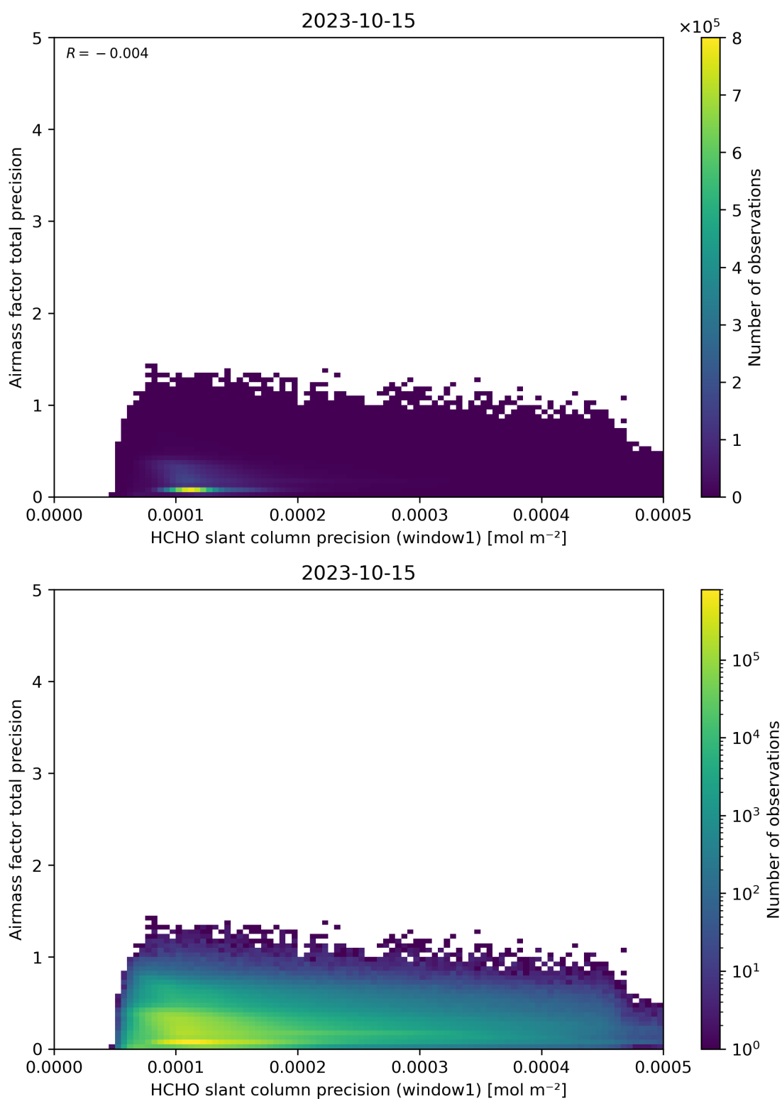
Figure 95: Scatter density plot of “HCHO slant column precision (window1)” against “Airmass factor total precision” for 2023-10-14 to 2023-10-16.
