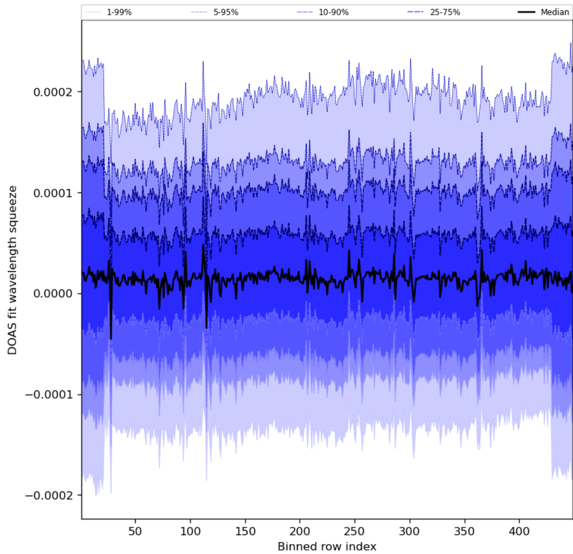
Figure 59: Along track statistics of “DOAS fit wavelength squeeze” for 2023-10-14 to 2023-10-16
