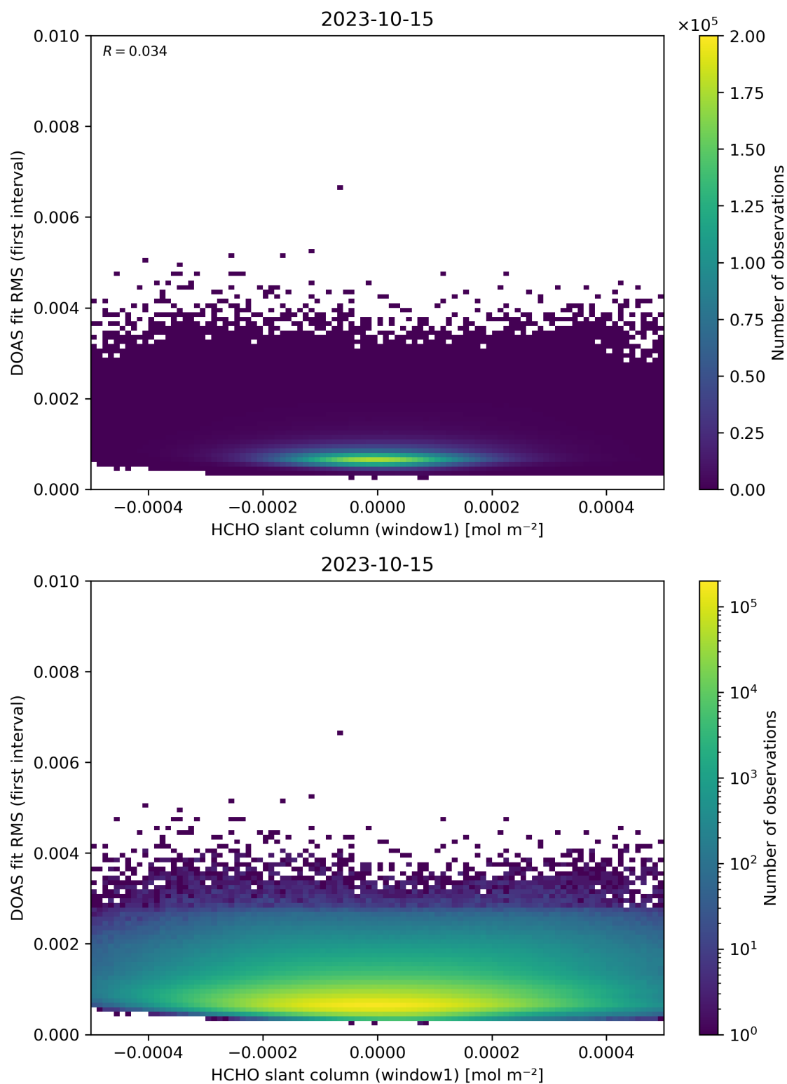
Figure 78: Scatter density plot of “HCHO slant column (window1)” against “DOAS fit RMS (first interval)” for 2023-10-14 to 2023-10-16.
