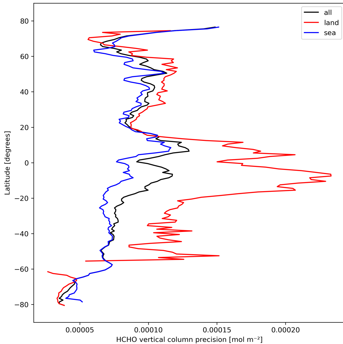
Figure 22: Zonal average of “HCHO vertical column precision” for 2023-10-14 to 2023-10-16.
