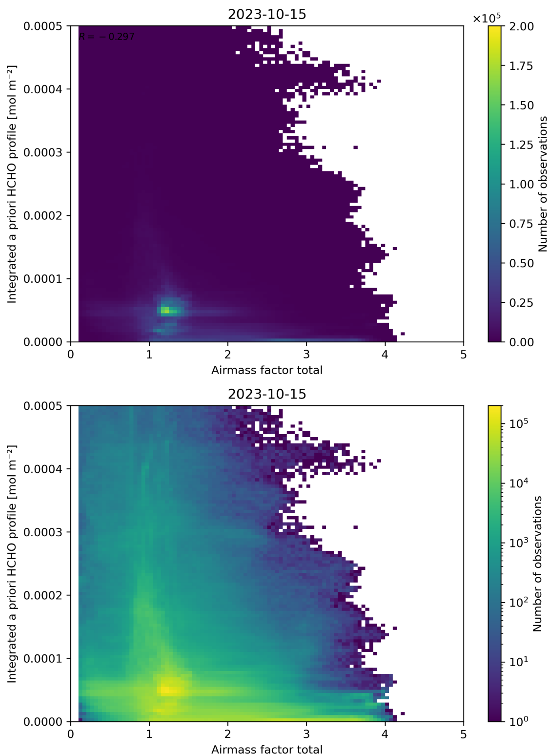
Figure 104: Scatter density plot of “Airmass factor total” against “Integrated a priori HCHO profile” for 2023-10-14 to 2023-10-16.
