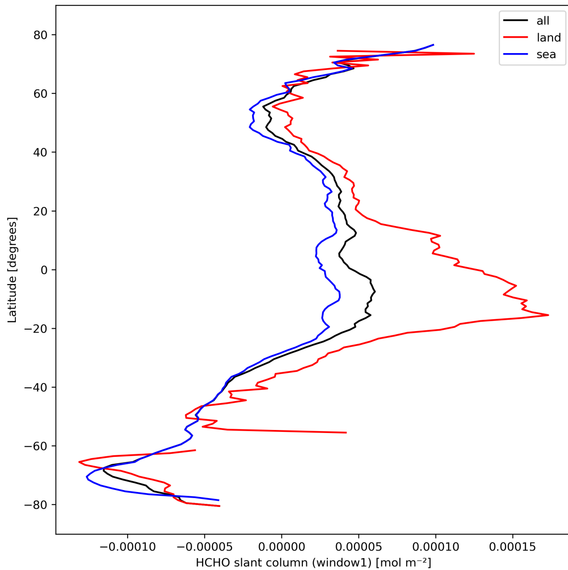
Figure 24: Zonal average of “HCHO slant column (window1)” for 2023-10-14 to 2023-10-16.
