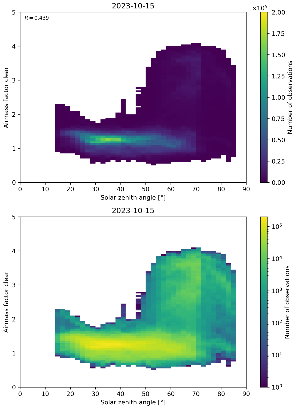
Figure 170: Scatter density plot of “Solar zenith angle” against “Airmass factor clear” for 2023-10-14 to 2023-10-16.
