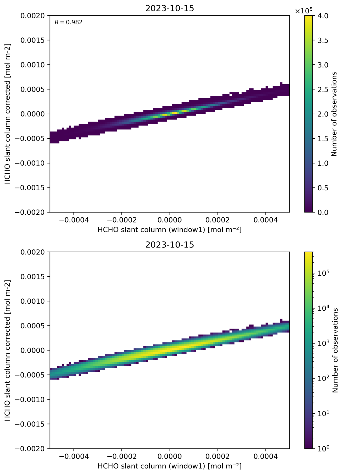
Figure 82: Scatter density plot of “HCHO slant column (window1)” against “HCHO slant column corrected” for 2023-10-14 to 2023-10-16.
