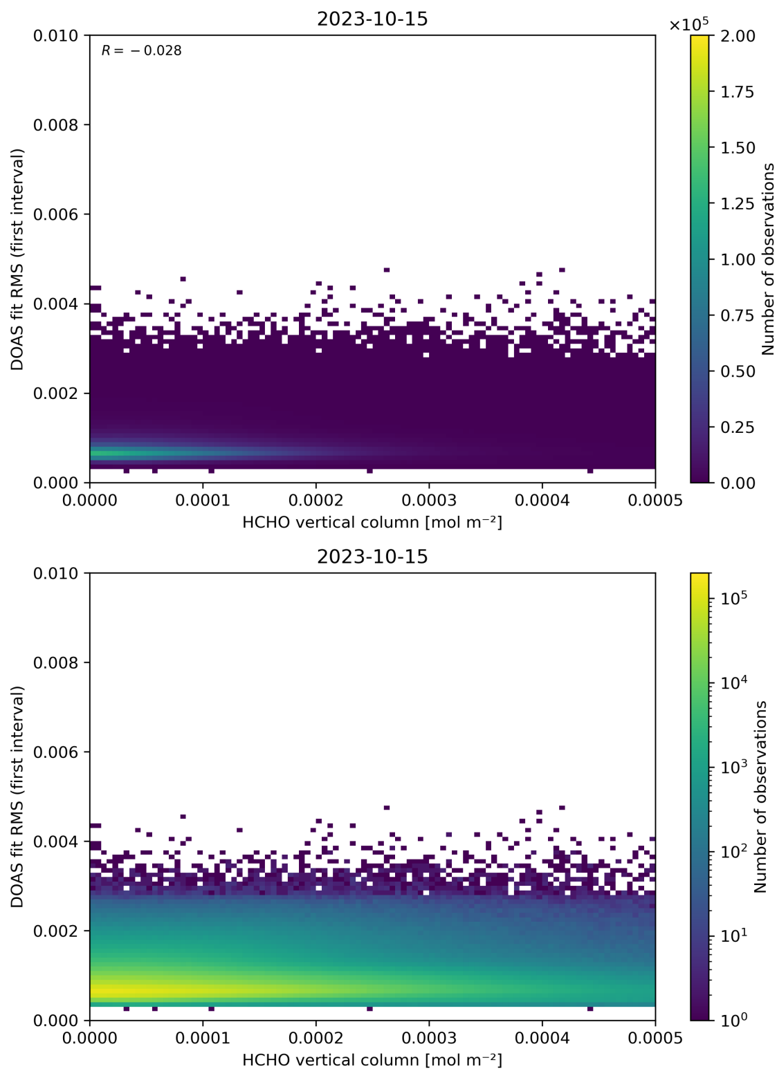
Figure 123: Scatter density plot of “HCHO vertical column” against “DOAS fit RMS (first interval)” for 2023-10-14 to 2023-10-16.
