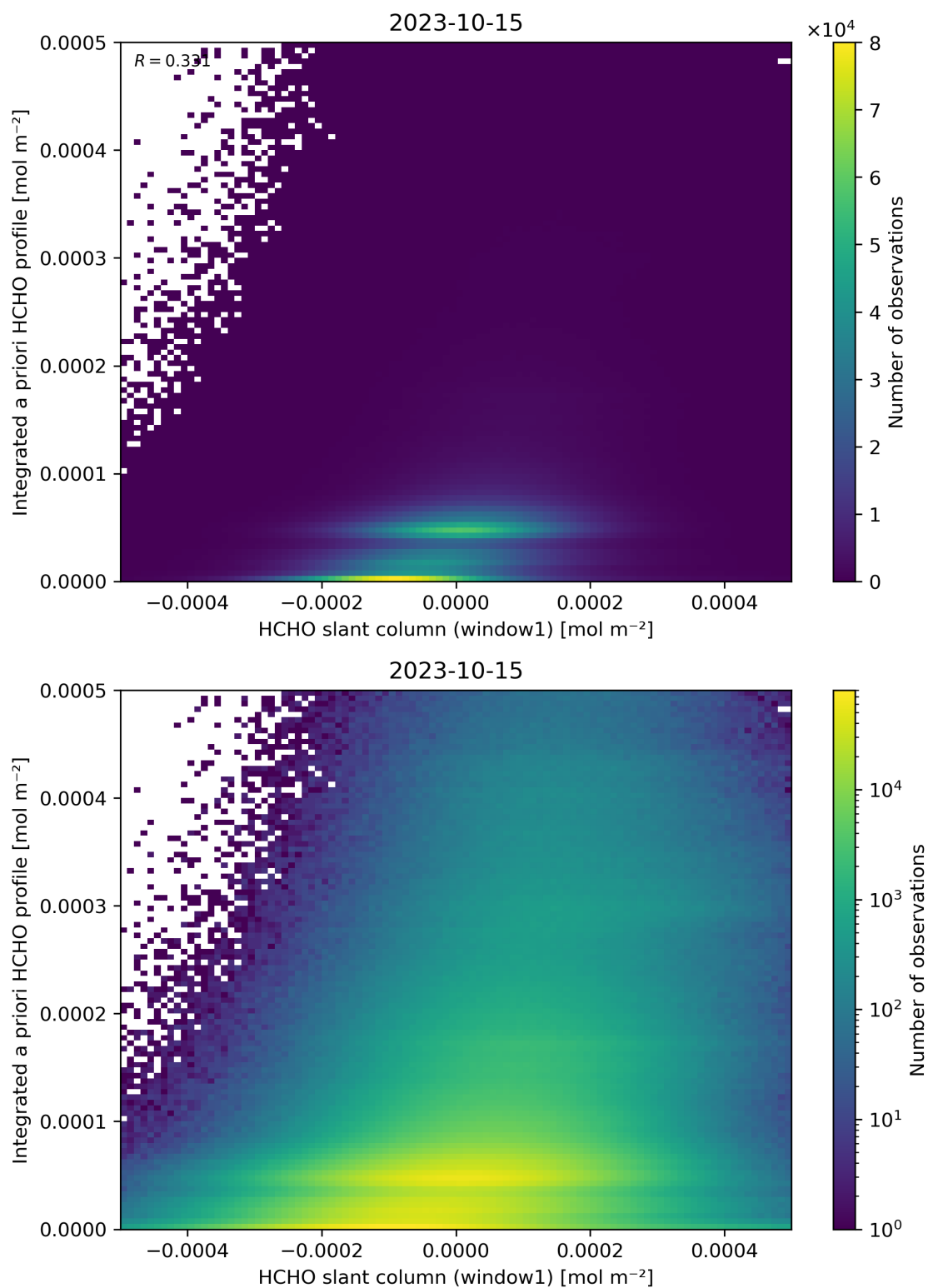
Figure 87: Scatter density plot of “HCHO slant column (window1)” against “Integrated a priori HCHO profile” for 2023-10-14 to 2023-10-16.
