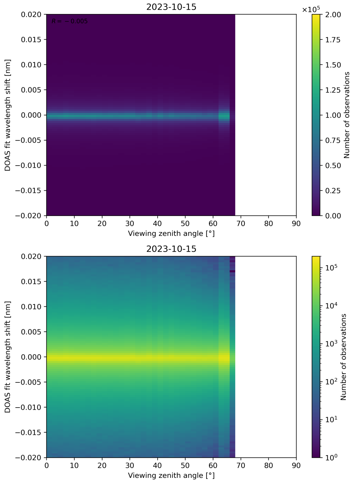
Figure 183: Scatter density plot of “Viewing zenith angle” against “DOAS fit wavelength shift” for 2023-10-14 to 2023-10-16.
