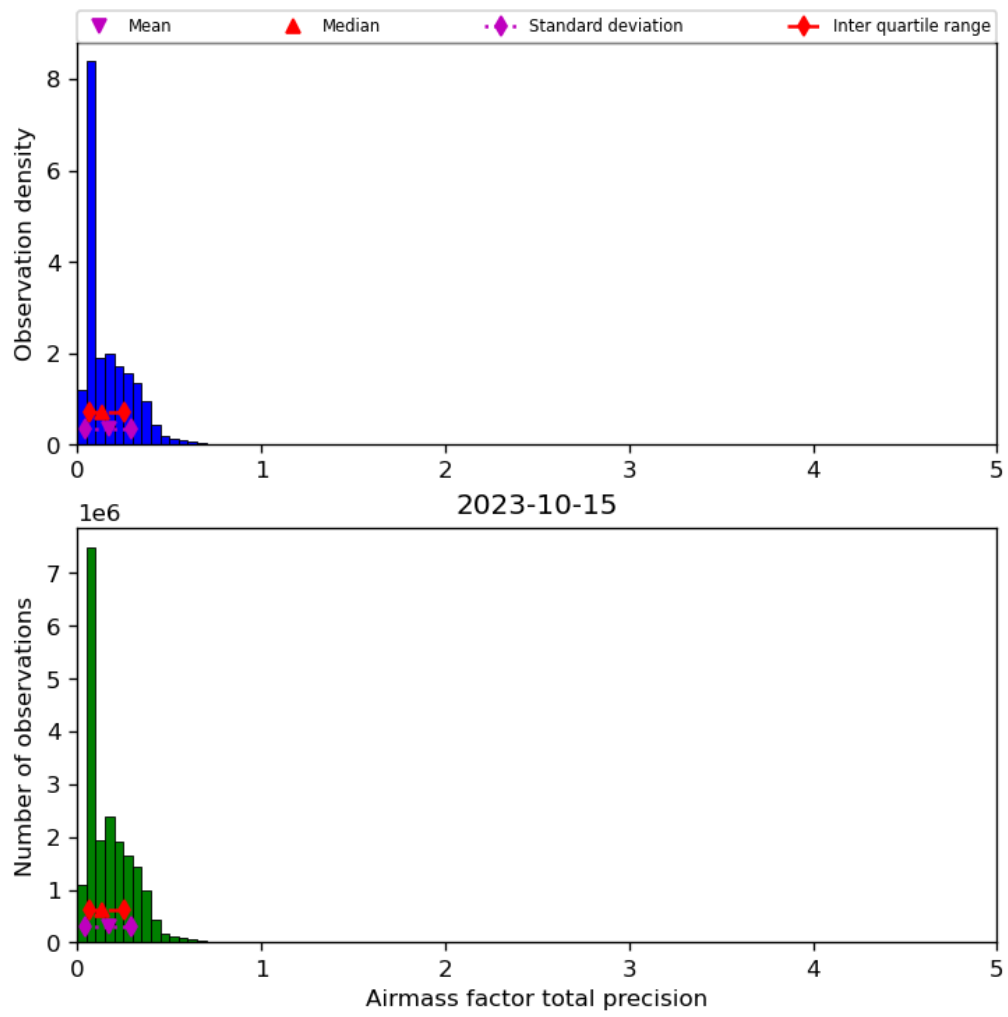
Figure 41: Histogram of “Airmass factor total precision” for 2023-10-14 to 2023-10-16
