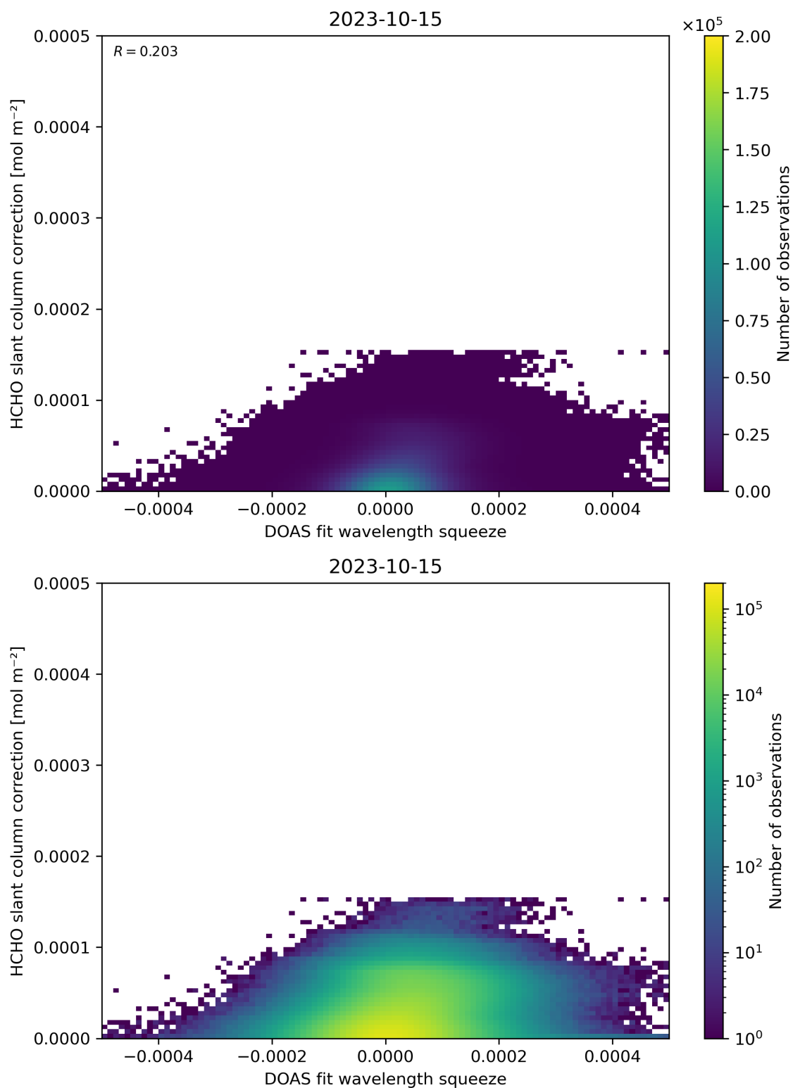
Figure 70: Scatter density plot of “DOAS fit wavelength squeeze” against “HCHO slant column correction” for 2023-10-14 to 2023-10-16.
