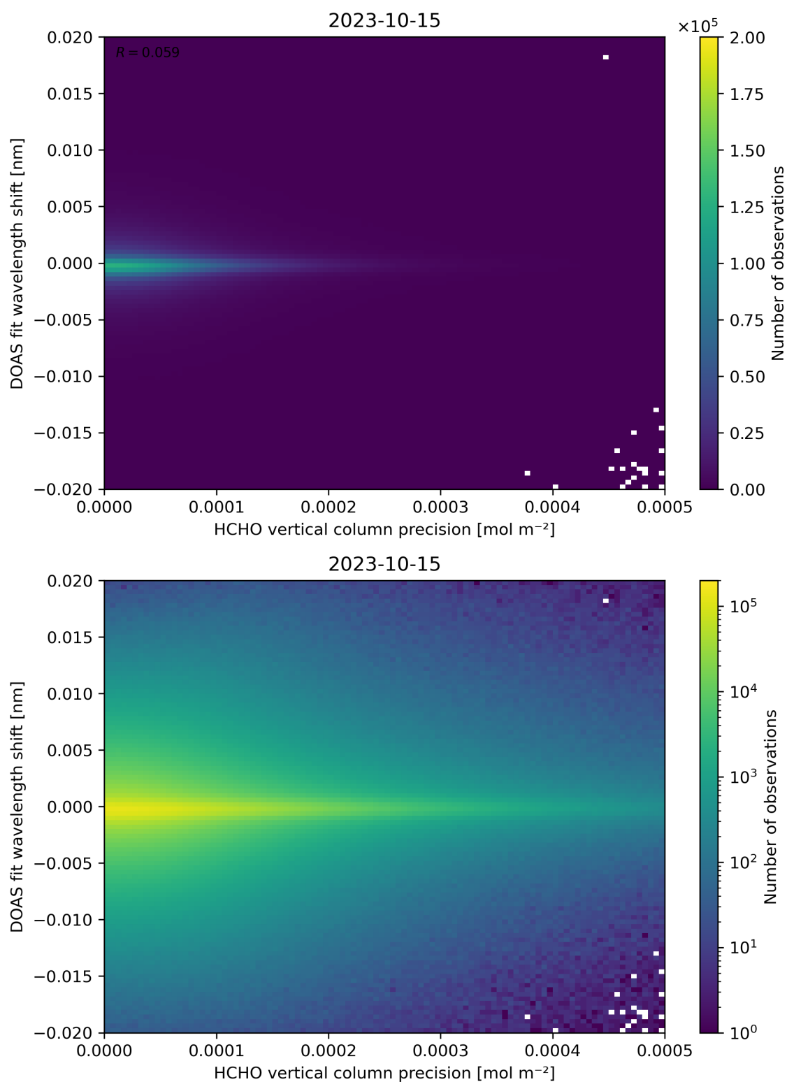
Figure 137: Scatter density plot of “HCHO vertical column precision” against “DOAS fit wavelength shift” for 2023-10-14 to 2023-10-16.
