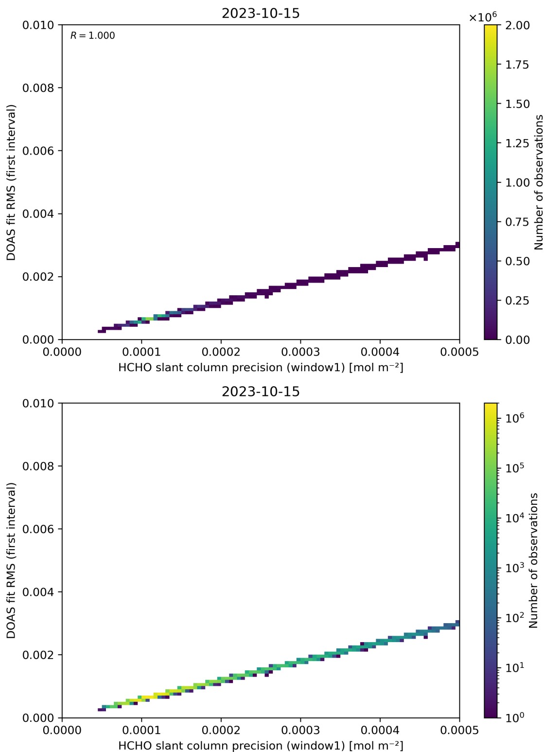
Figure 88: Scatter density plot of “HCHO slant column precision (window1)” against “DOAS fit RMS (first interval)” for 2023-10-14 to 2023-10-16.
