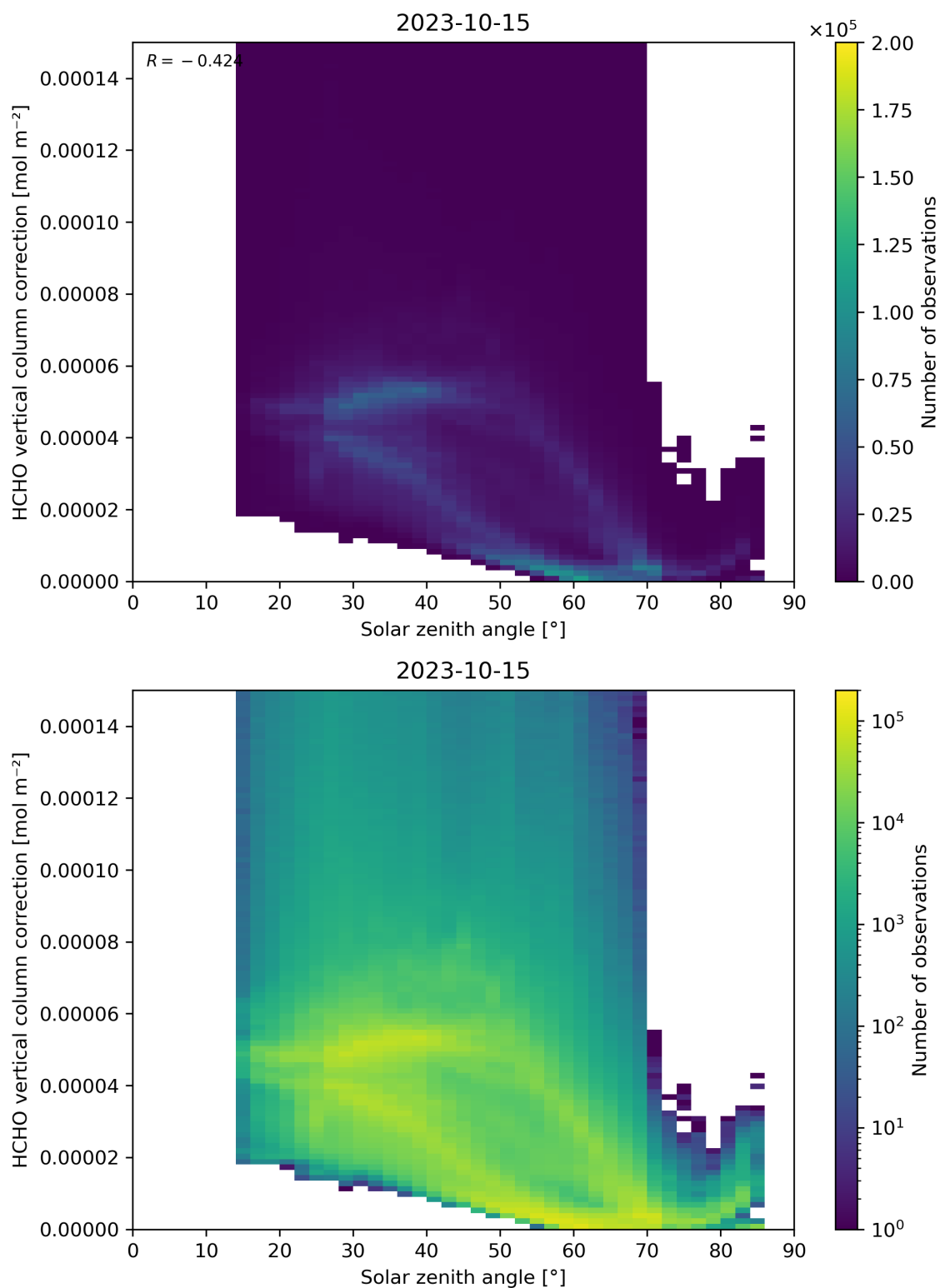
Figure 178: Scatter density plot of “Solar zenith angle” against “HCHO vertical column correction” for 2023-10-14 to 2023-10-16.
