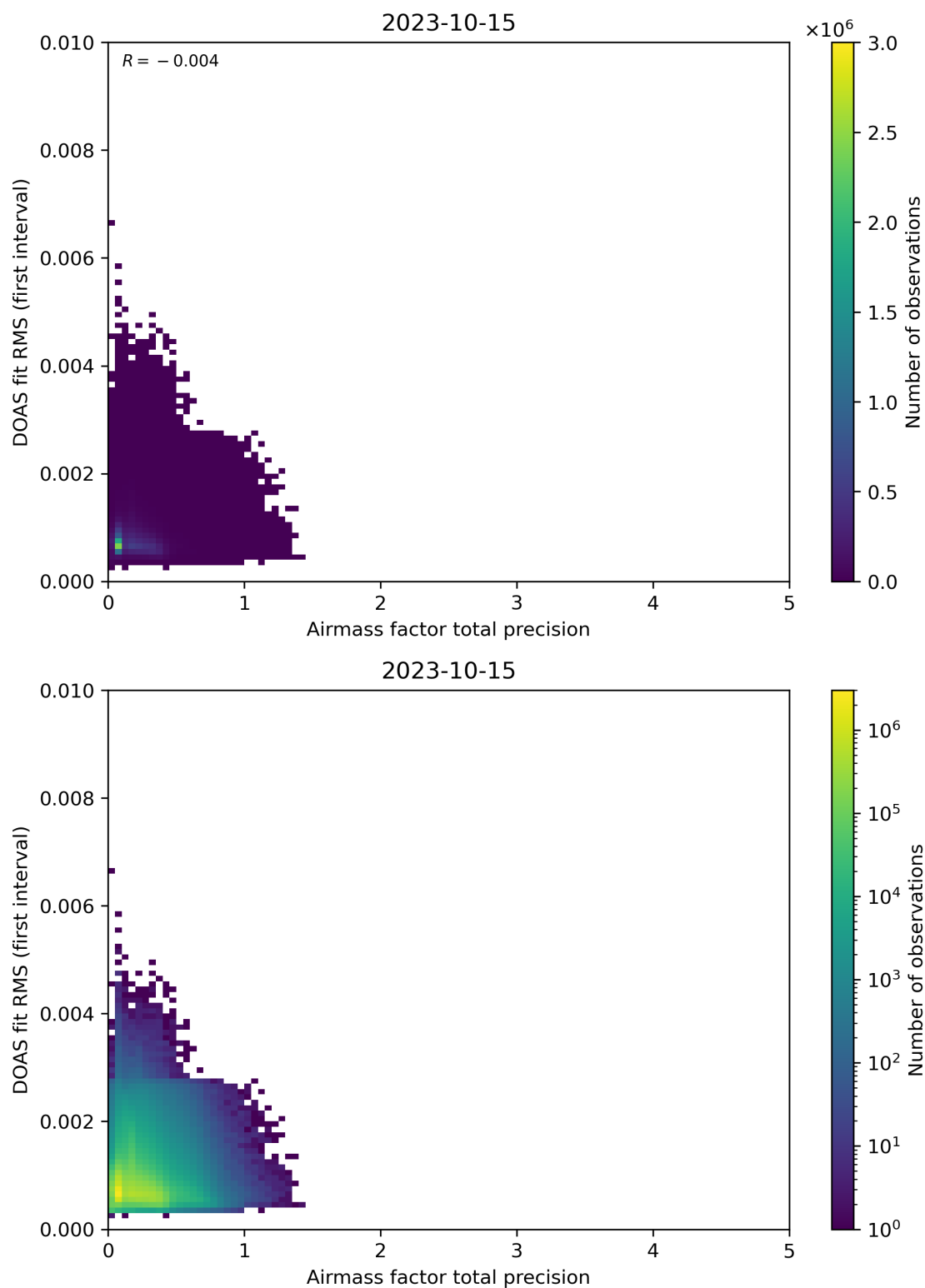
Figure 105: Scatter density plot of “Airmass factor total precision” against “DOAS fit RMS (first interval)” for 2023-10-14 to 2023-10-16.
