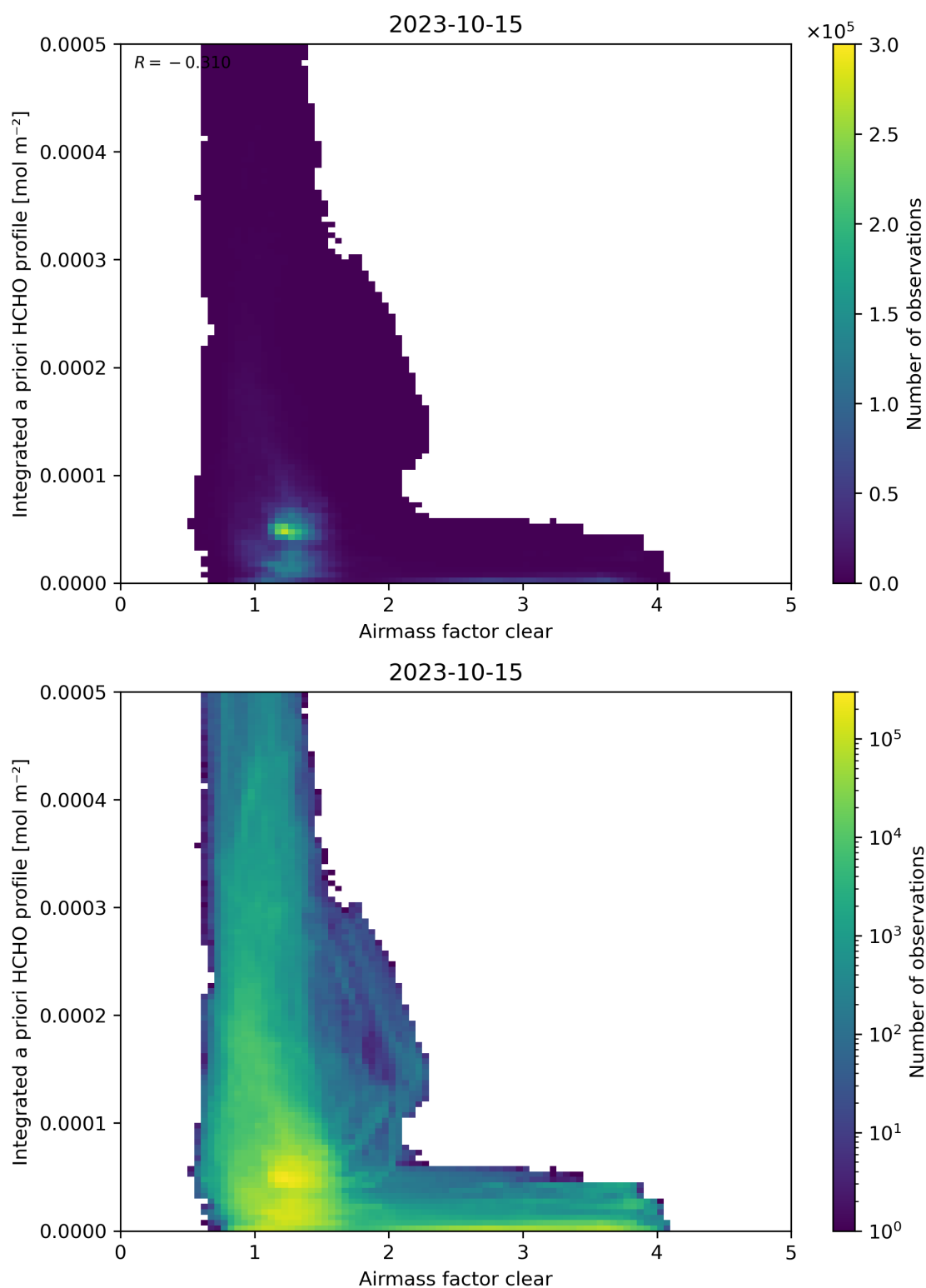
Figure 76: Scatter density plot of “Airmass factor clear” against “Integrated a priori HCHO profile” for 2023-10-14 to 2023-10-16.
