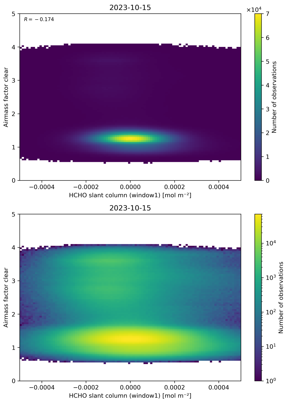
Figure 81: Scatter density plot of “HCHO slant column (window1)” against “Airmass factor clear” for 2023-10-14 to 2023-10-16.
