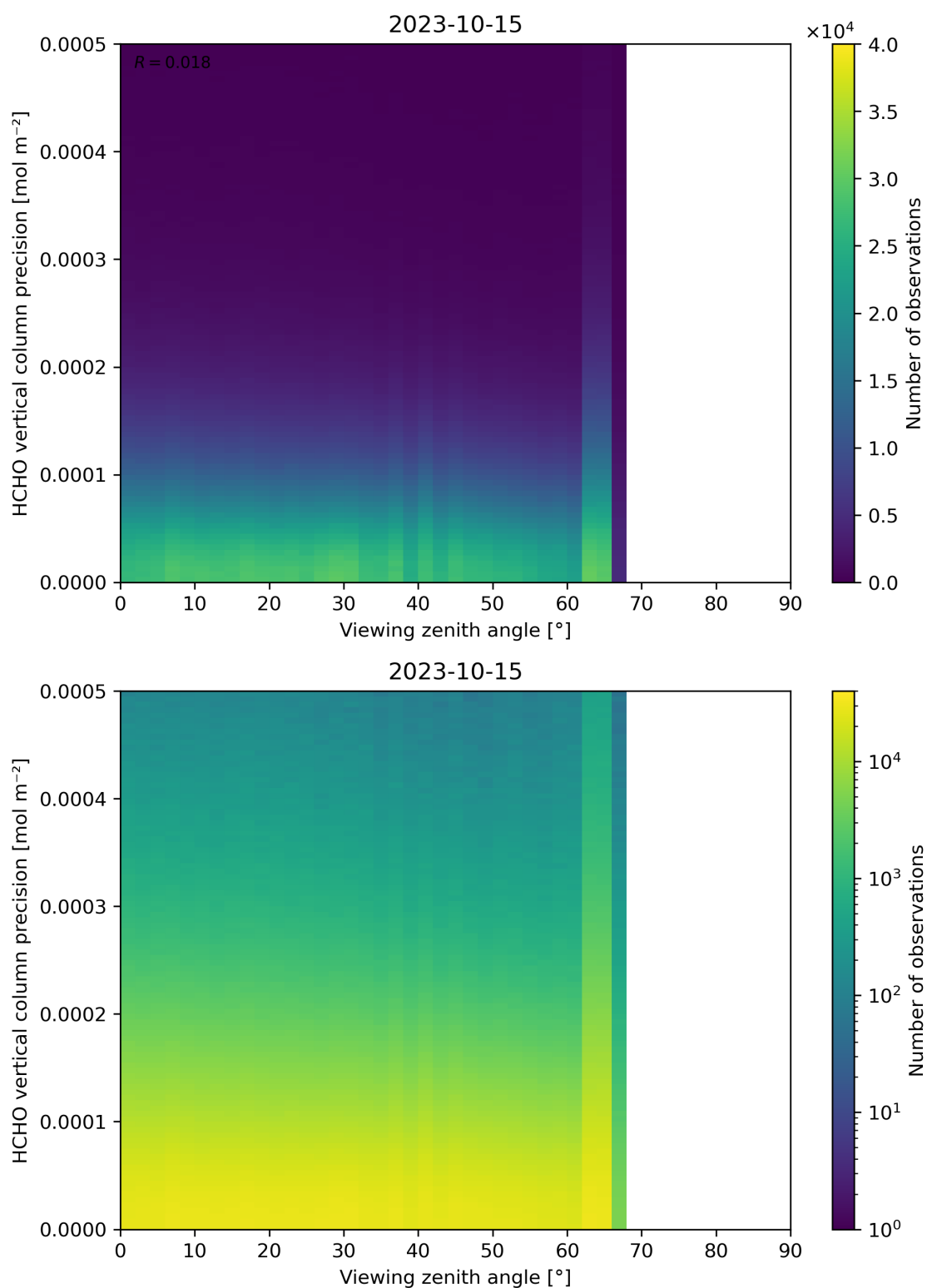
Figure 194: Scatter density plot of “Viewing zenith angle” against “HCHO vertical column precision” for 2023-10-14 to 2023-10-16.
