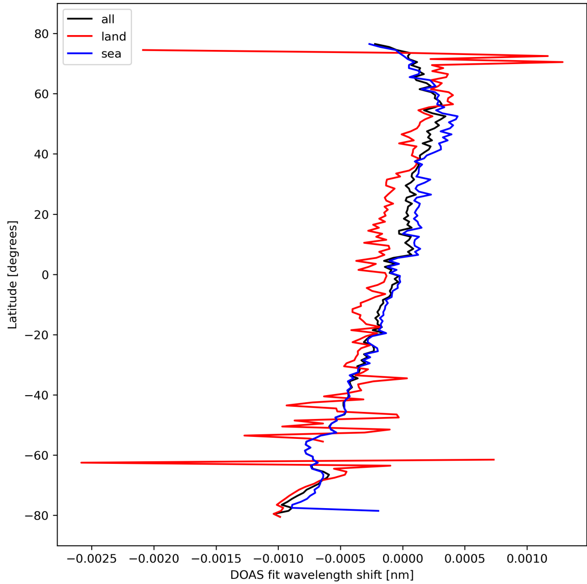
Figure 30: Zonal average of “DOAS fit wavelength shift” for 2023-10-14 to 2023-10-16.
