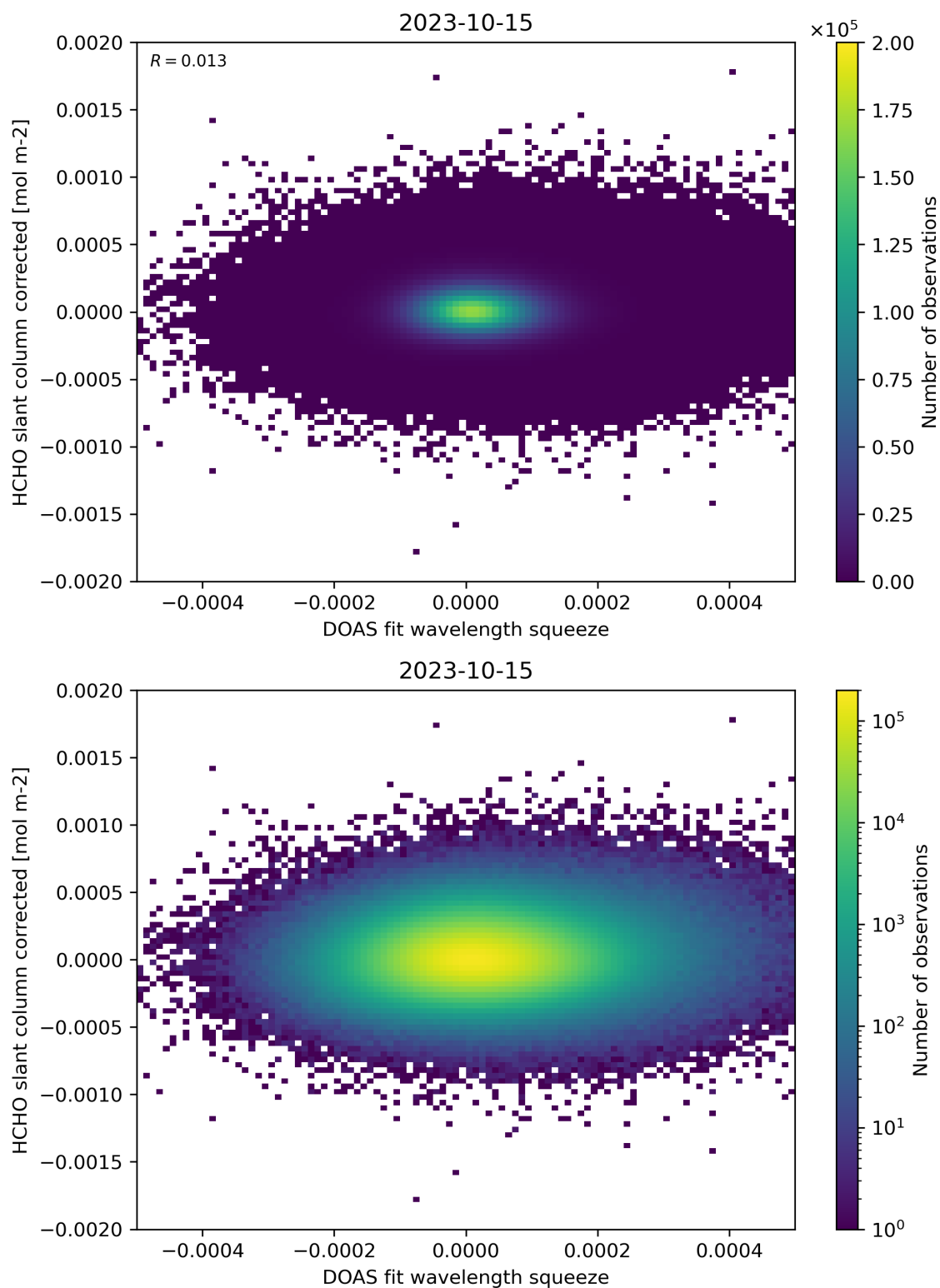
Figure 69: Scatter density plot of “DOAS fit wavelength squeeze” against “HCHO slant column corrected” for 2023-10-14 to 2023-10-16.
