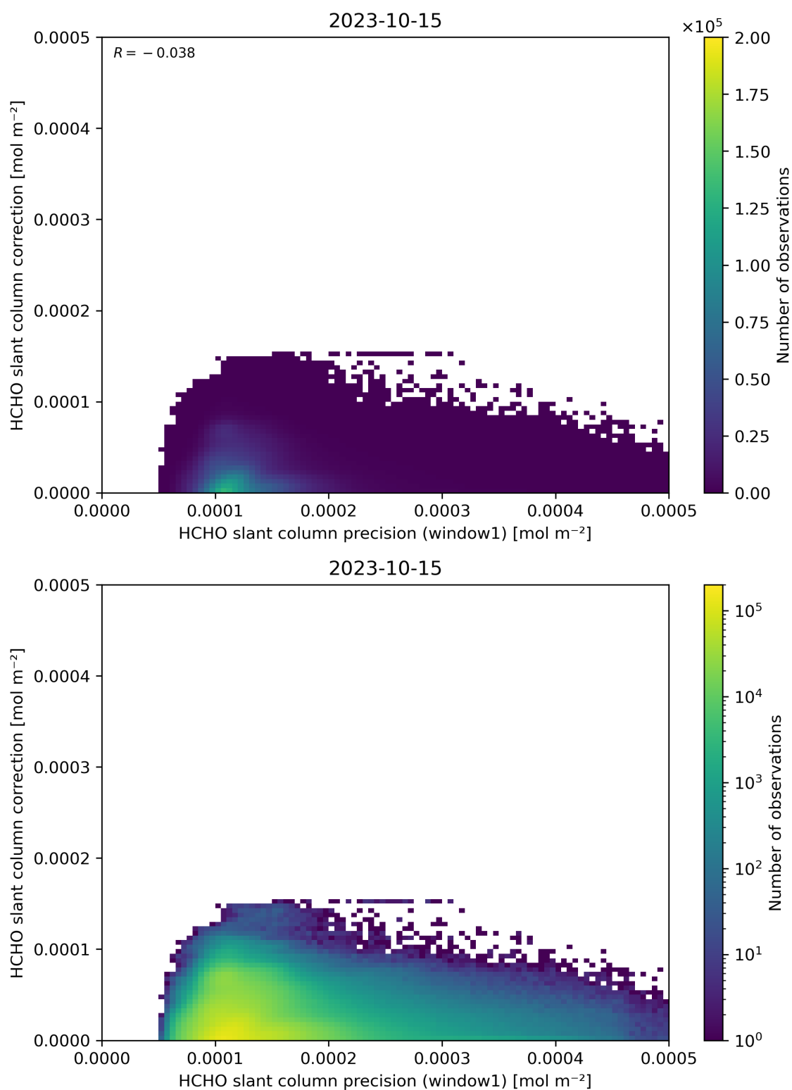
Figure 93: Scatter density plot of “HCHO slant column precision (window1)” against “HCHO slant column correction” for 2023-10-14 to 2023-10-16.
