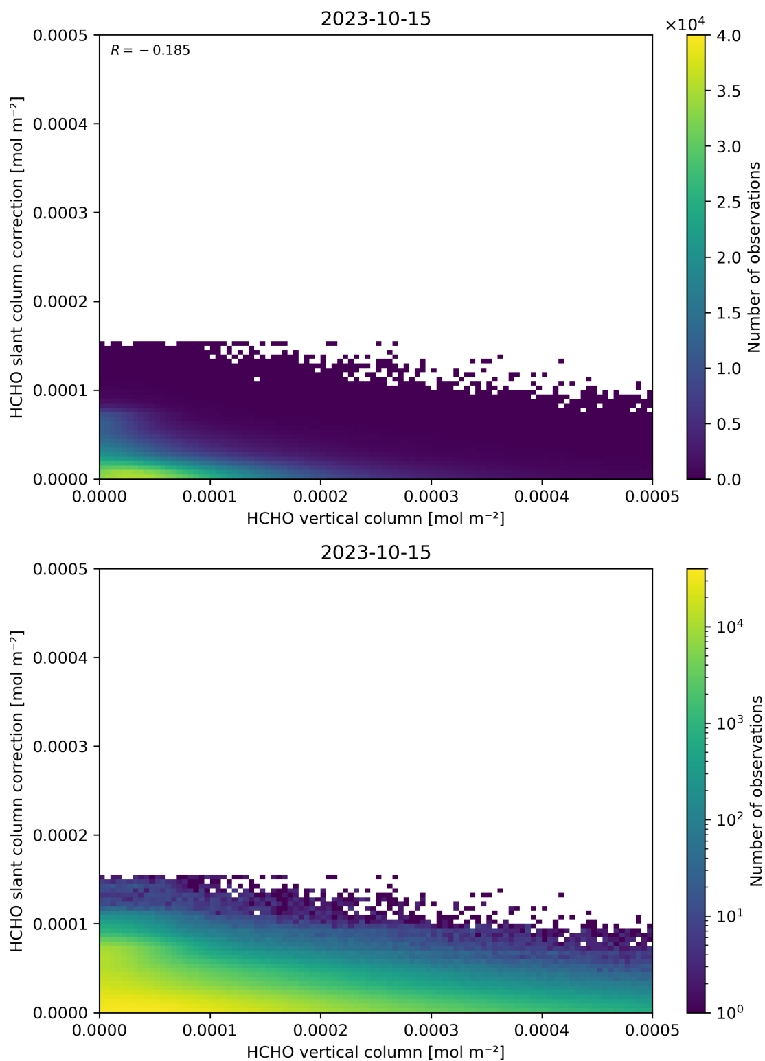
Figure 128: Scatter density plot of “HCHO vertical column” against “HCHO slant column correction” for 2023-10-14 to 2023-10-16.
