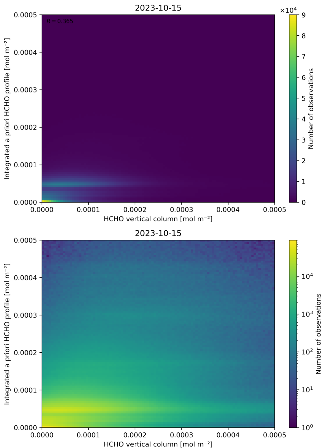
Figure 135: Scatter density plot of “HCHO vertical column” against “Integrated a priori HCHO profile” for 2023-10-14 to 2023-10-16.
