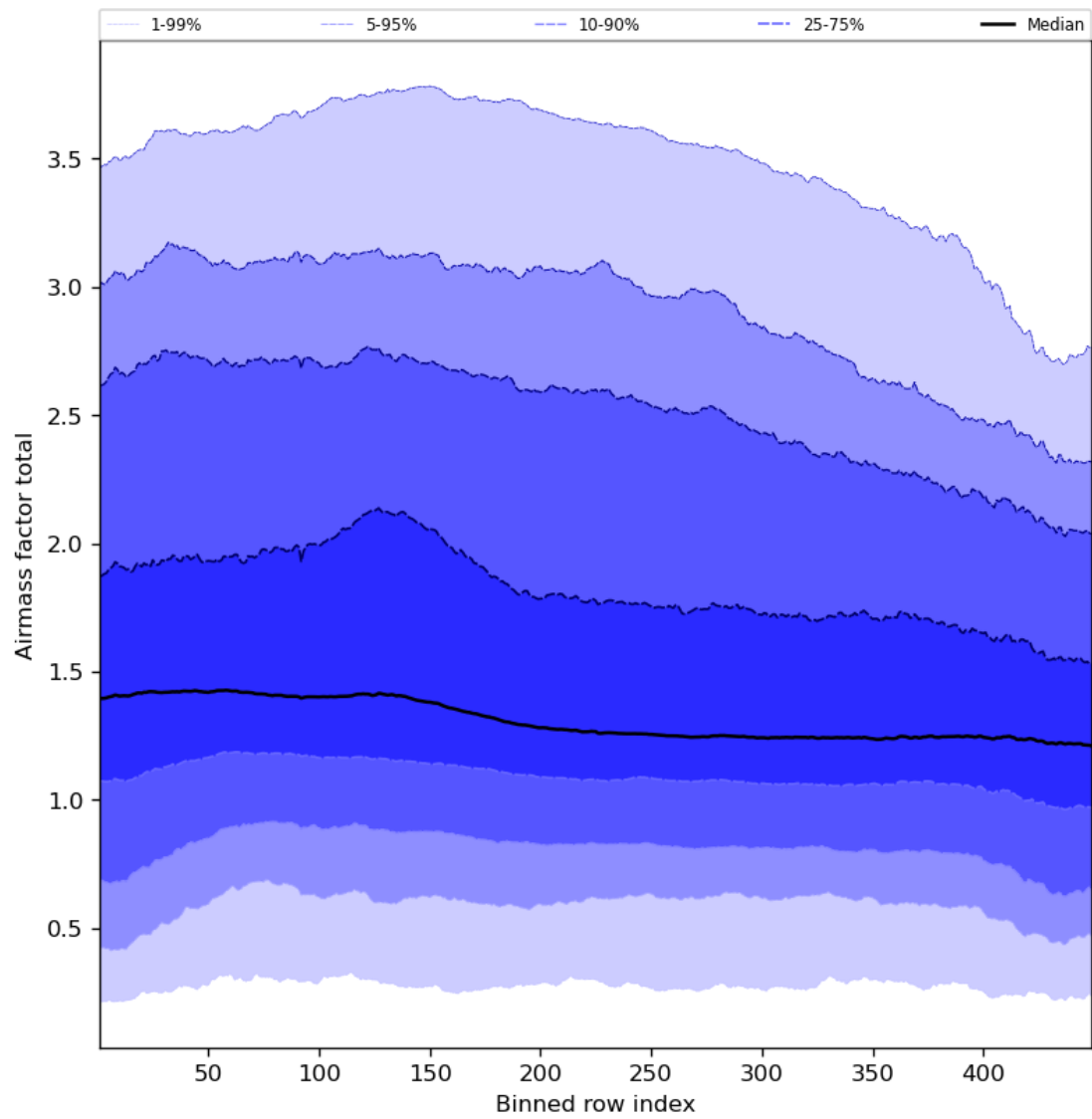
Figure 54: Along track statistics of “Airmass factor total” for 2023-10-14 to 2023-10-16
