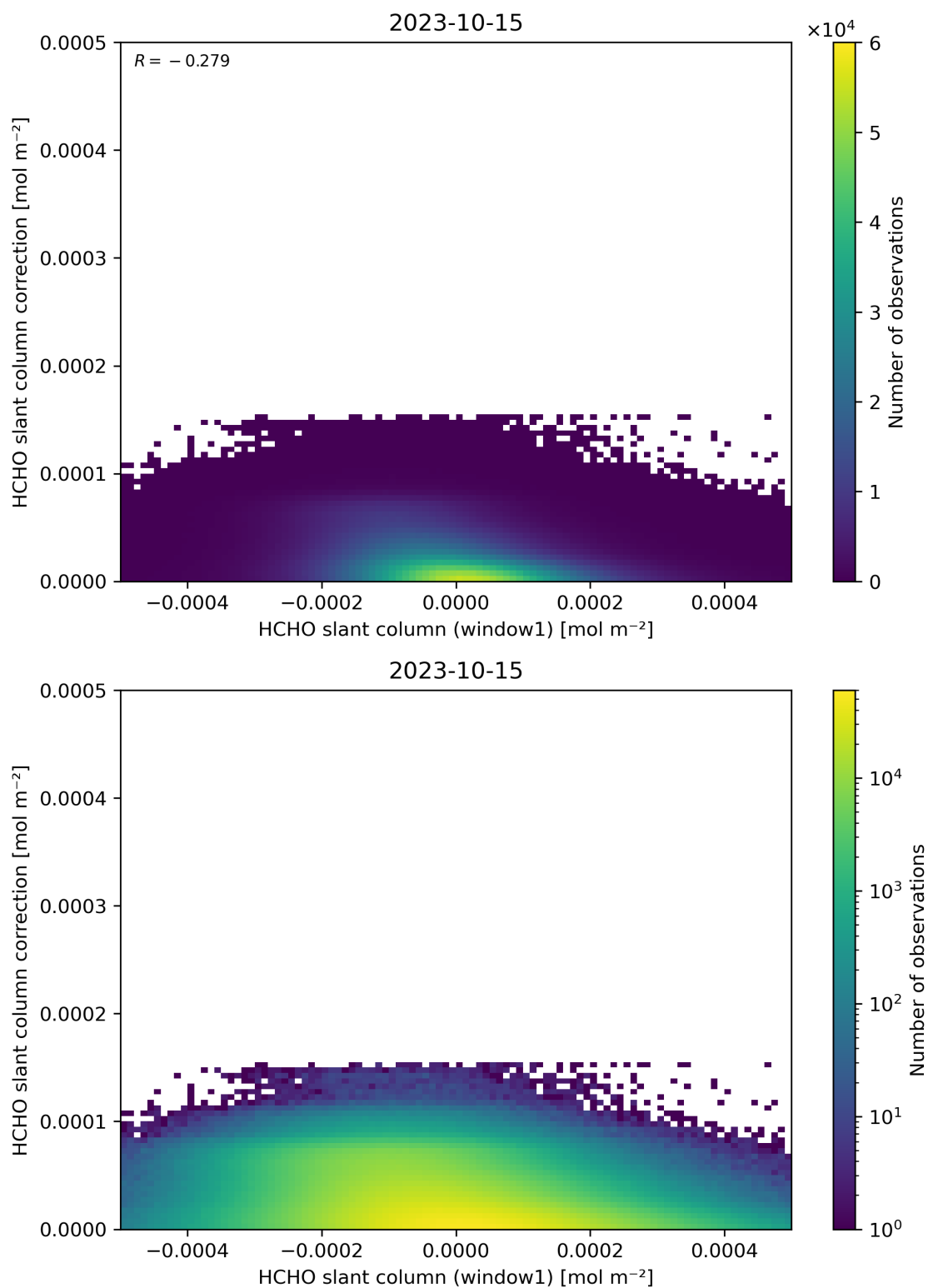
Figure 83: Scatter density plot of “HCHO slant column (window1)” against “HCHO slant column correction” for 2023-10-14 to 2023-10-16.
