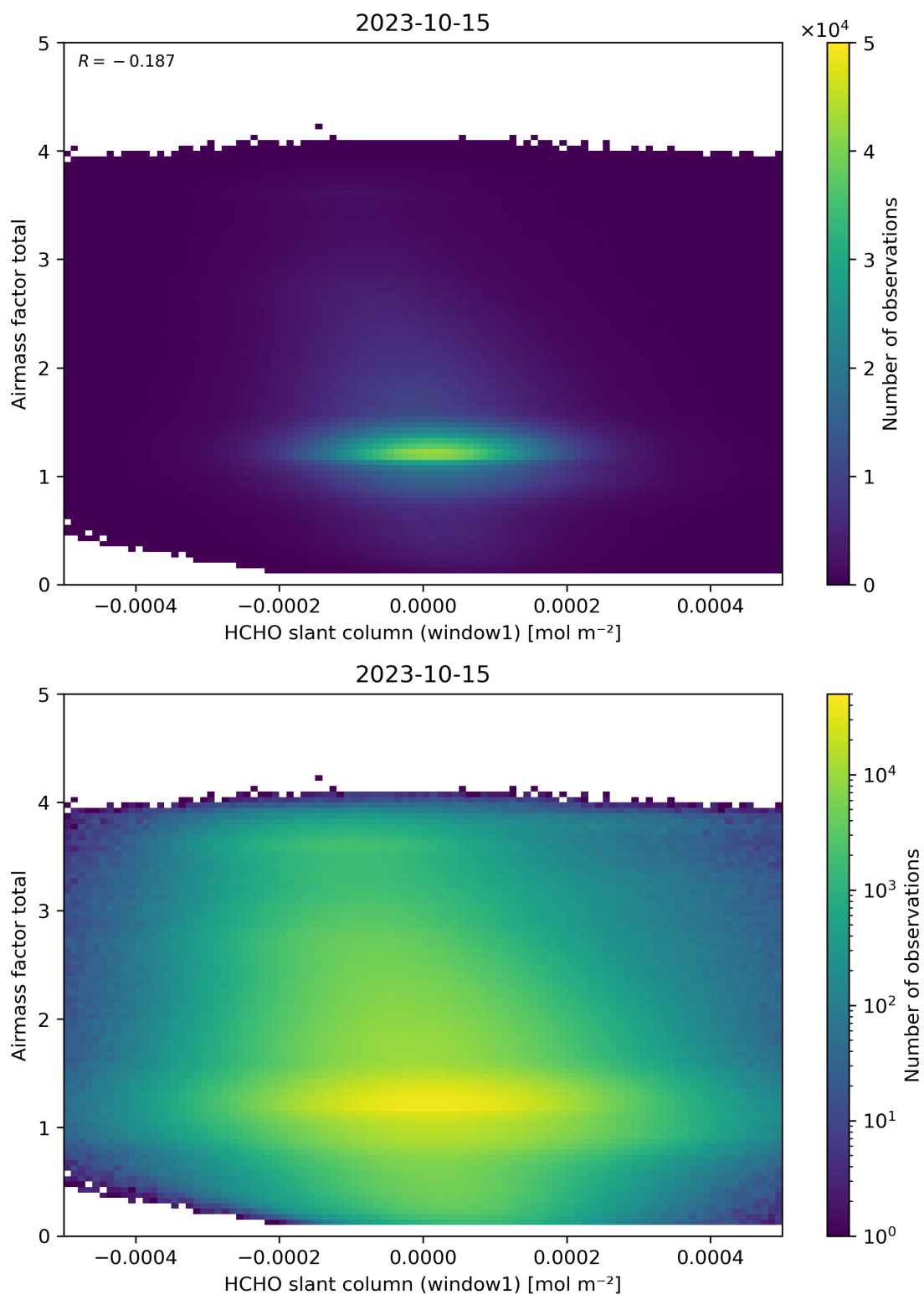
Figure 85: Scatter density plot of “HCHO slant column (window1)” against “Airmass factor total” for 2023-10-14 to 2023-10-16.
