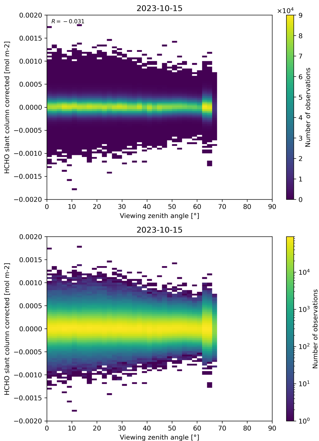
Figure 186: Scatter density plot of “Viewing zenith angle” against “HCHO slant column corrected” for 2023-10-14 to 2023-10-16.
