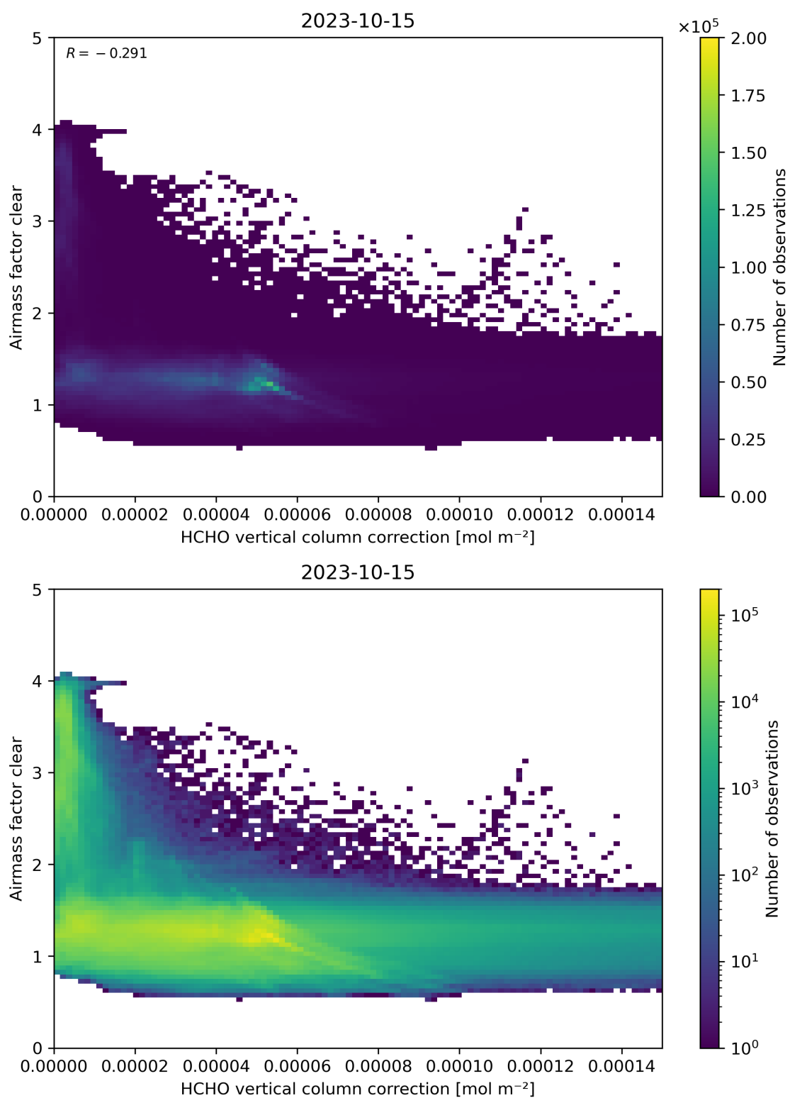
Figure 115: Scatter density plot of “HCHO vertical column correction” against “Airmass factor clear” for 2023-10-14 to 2023-10-16.
