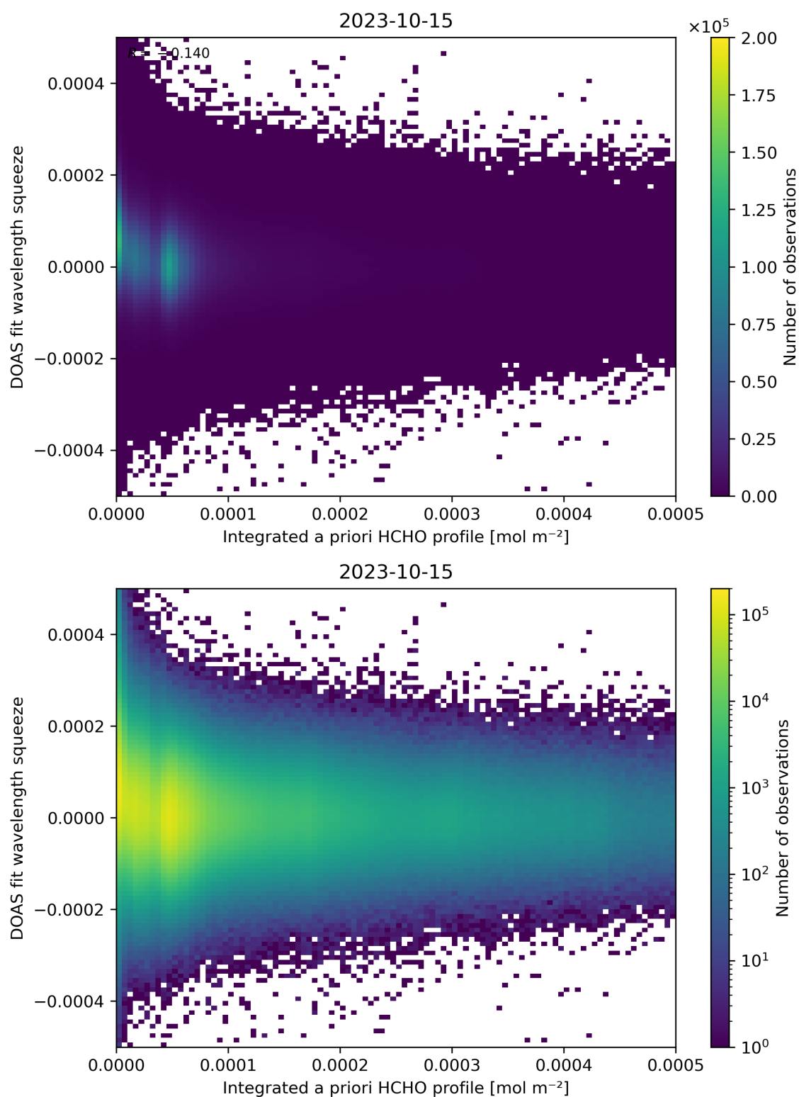
Figure 150: Scatter density plot of “Integrated a priori HCHO profile” against “DOAS fit wavelength squeeze” for 2023-10-14 to 2023-10-16.
