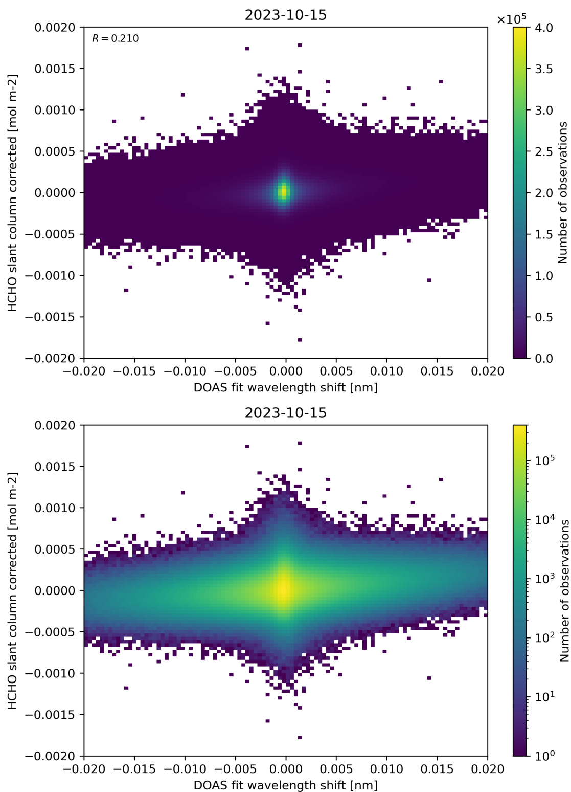
Figure 66: Scatter density plot of “DOAS fit wavelength shift” against “HCHO slant column corrected” for 2023-10-14 to 2023-10-16.
