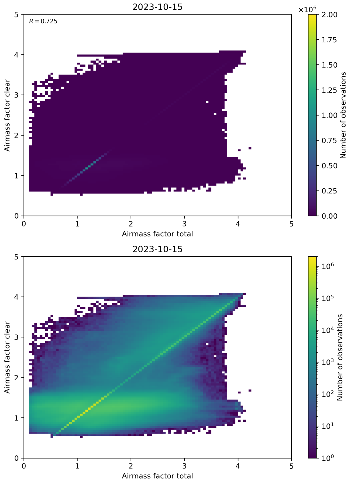
Figure 100: Scatter density plot of “Airmass factor total” against “Airmass factor clear” for 2023-10-14 to 2023-10-16.
