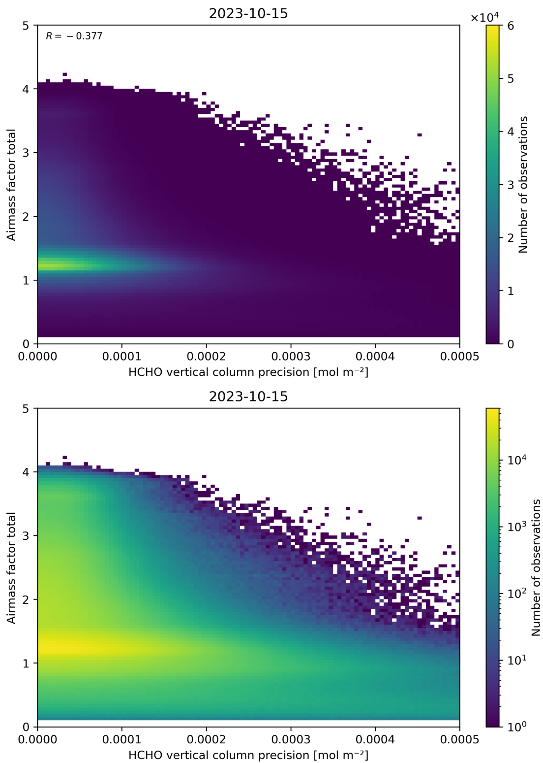
Figure 144: Scatter density plot of “HCHO vertical column precision” against “Airmass factor total” for 2023-10-14 to 2023-10-16.
