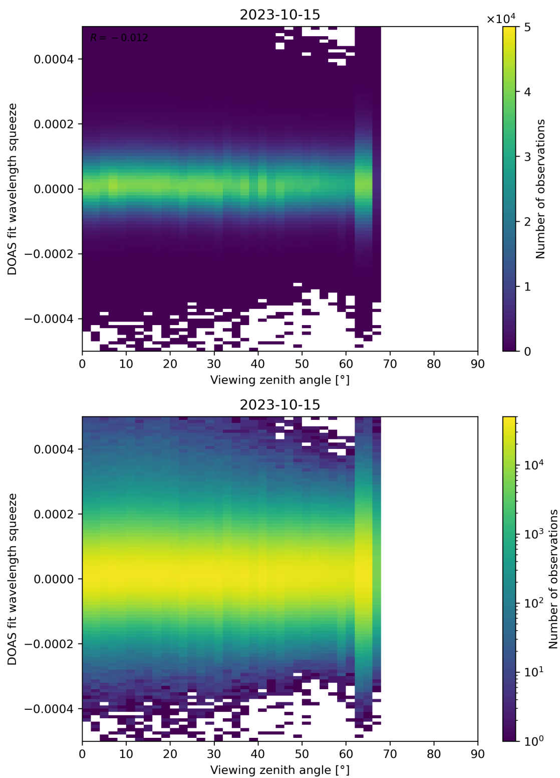
Figure 184: Scatter density plot of “Viewing zenith angle” against “DOAS fit wavelength squeeze” for 2023-10-14 to 2023-10-16.
