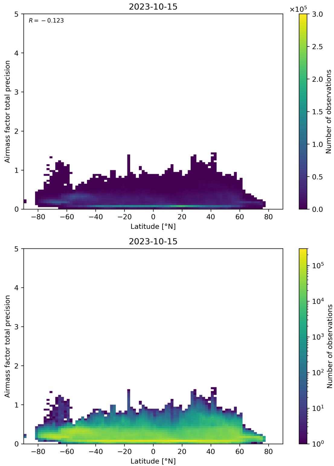
Figure 162: Scatter density plot of “Latitude” against “Airmass factor total precision” for 2023-10-14 to 2023-10-16.
