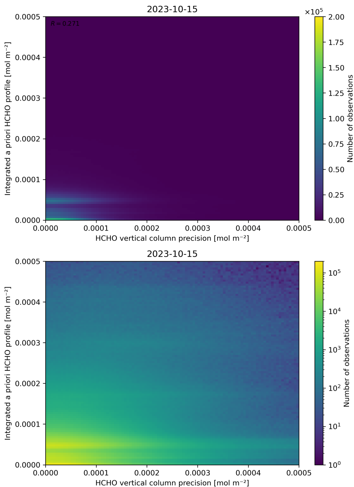
Figure 147: Scatter density plot of “HCHO vertical column precision” against “Integrated a priori HCHO profile” for 2023-10-14 to 2023-10-16.
