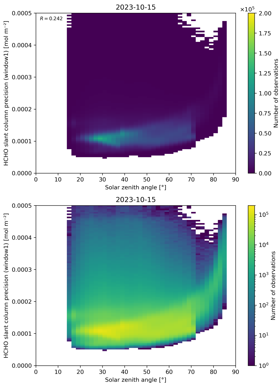
Figure 174: Scatter density plot of “Solar zenith angle” against “HCHO slant column precision (window1)” for 2023-10-14 to 2023-10-16.
