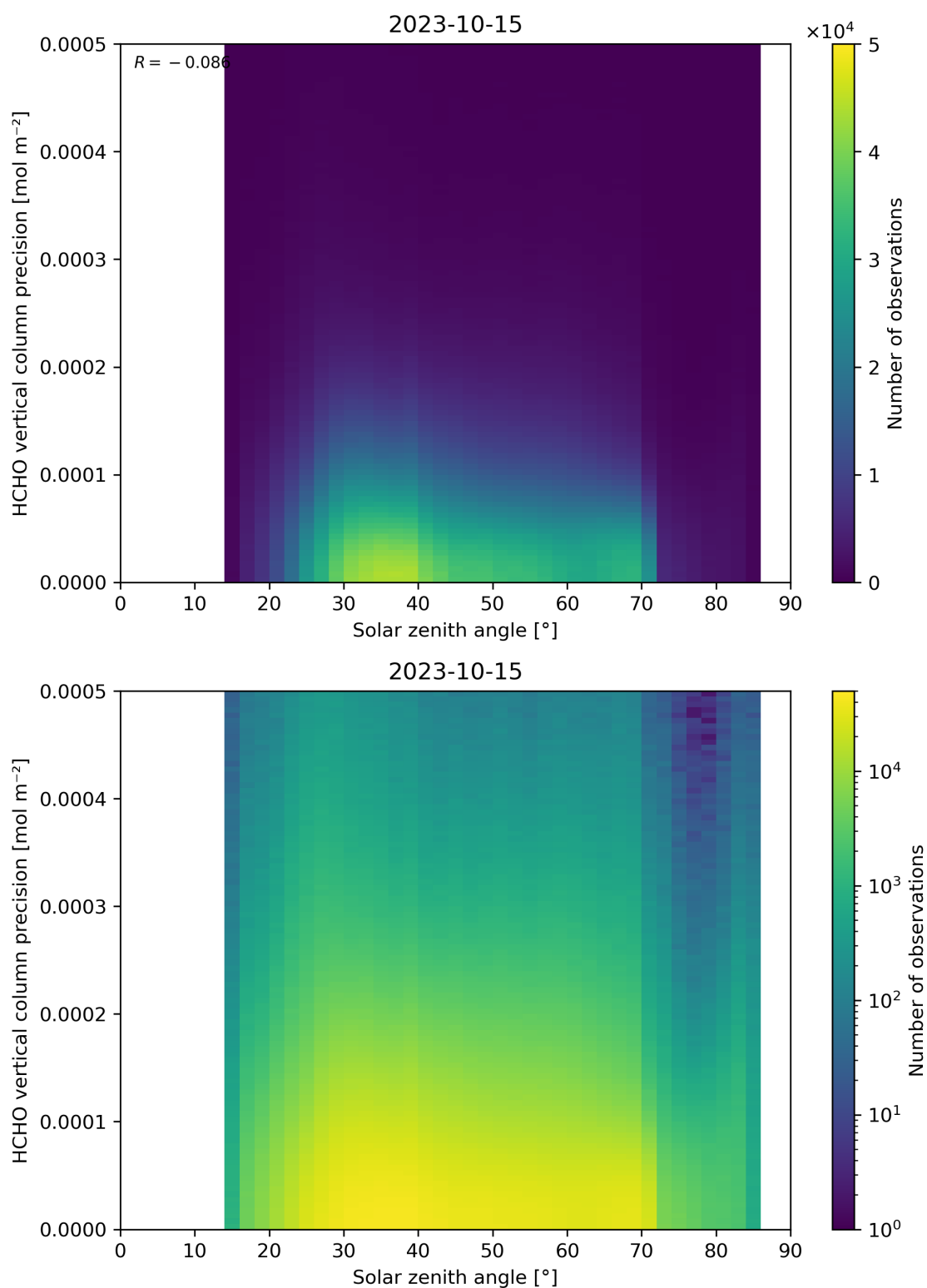
Figure 179: Scatter density plot of “Solar zenith angle” against “HCHO vertical column precision” for 2023-10-14 to 2023-10-16.
