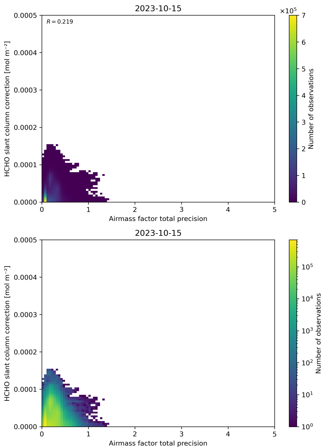
Figure 110: Scatter density plot of “Airmass factor total precision” against “HCHO slant column correction” for 2023-10-14 to 2023-10-16.
