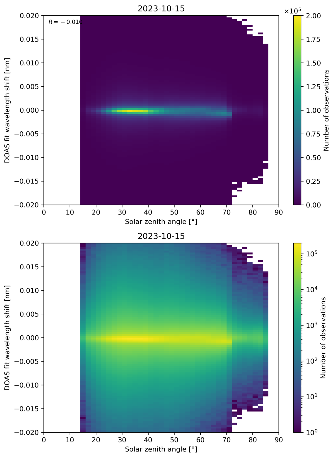
Figure 168: Scatter density plot of “Solar zenith angle” against “DOAS fit wavelength shift” for 2023-10-14 to 2023-10-16.
