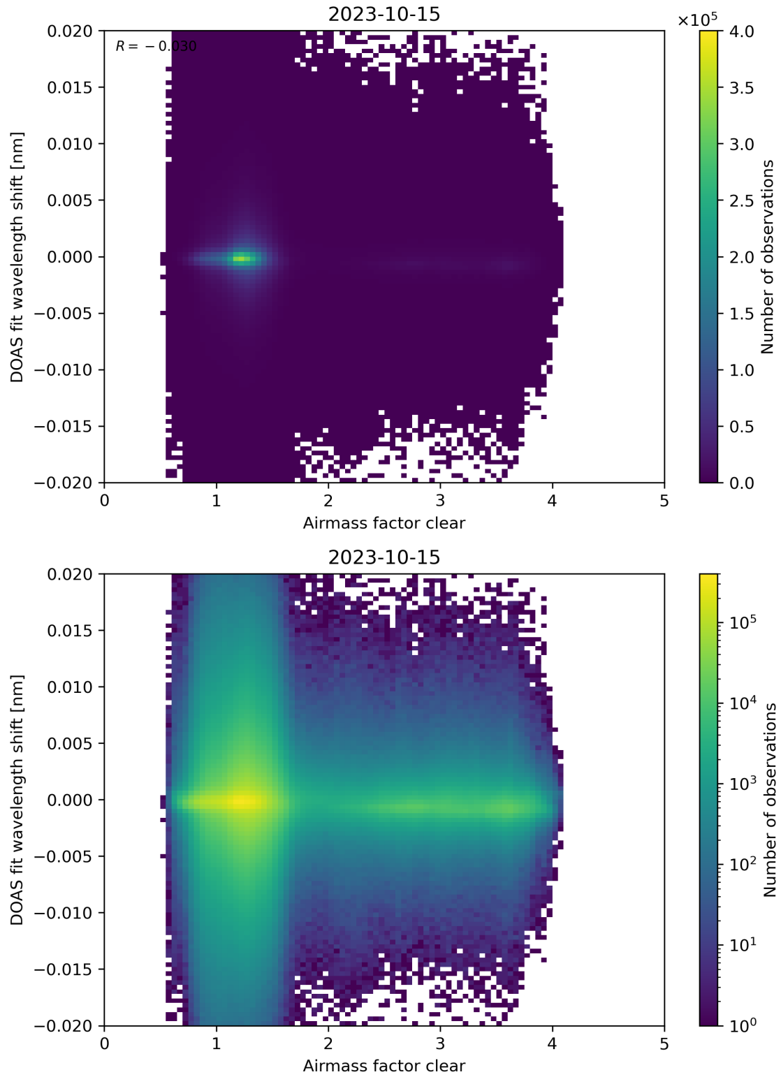
Figure 72: Scatter density plot of “Airmass factor clear” against “DOAS fit wavelength shift” for 2023-10-14 to 2023-10-16.
