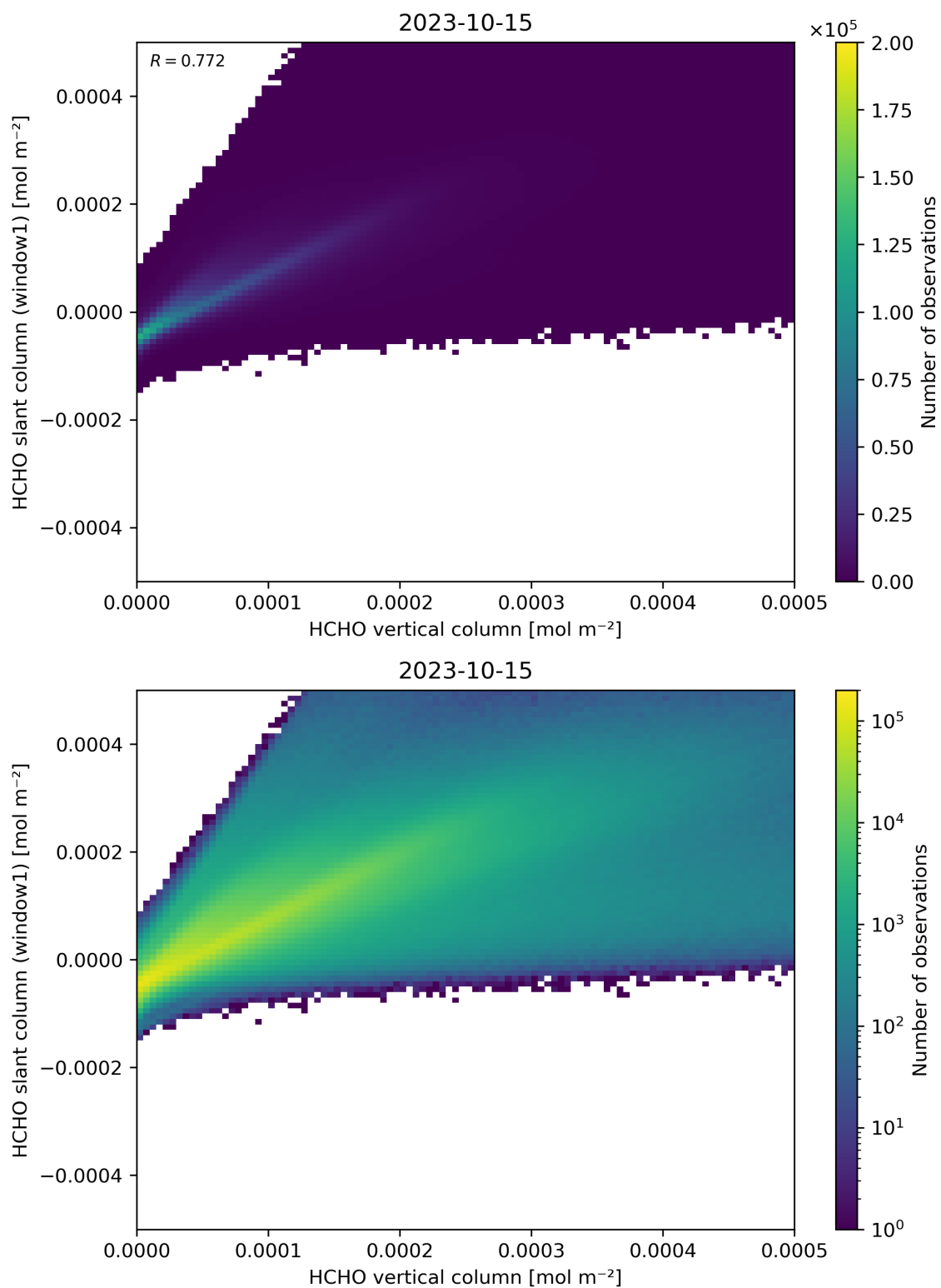
Figure 129: Scatter density plot of “HCHO vertical column” against “HCHO slant column (window1)” for 2023-10-14 to 2023-10-16.
