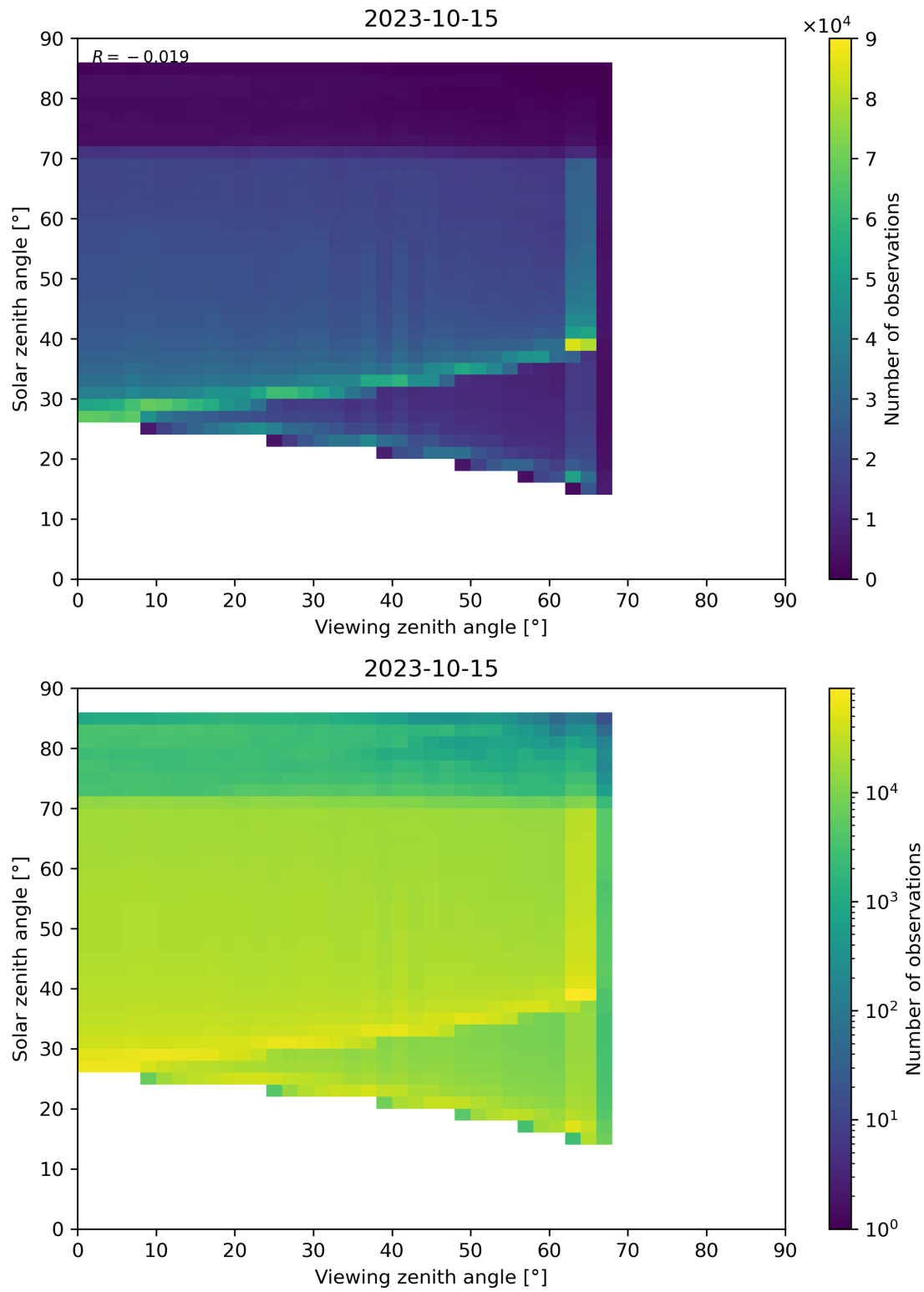
Figure 197: Scatter density plot of “Viewing zenith angle” against “Solar zenith angle” for 2023-10-14 to 2023-10-16.
