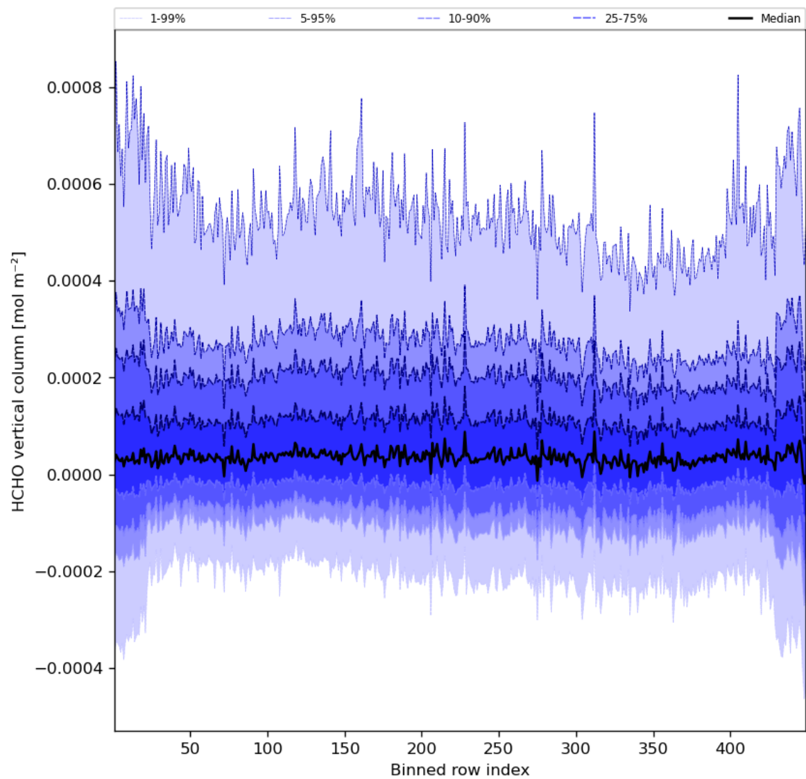
Figure 49: Along track statistics of “HCHO vertical column” for 2023-10-14 to 2023-10-16
