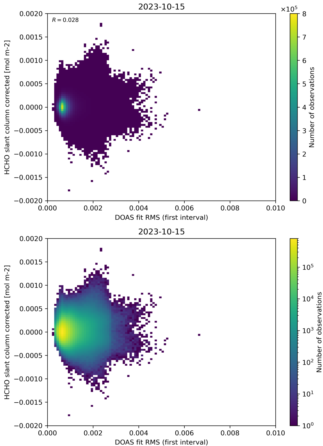
Figure 62: Scatter density plot of “DOAS fit RMS (first interval)” against “HCHO slant column corrected” for 2023-10-14 to 2023-10-16.
