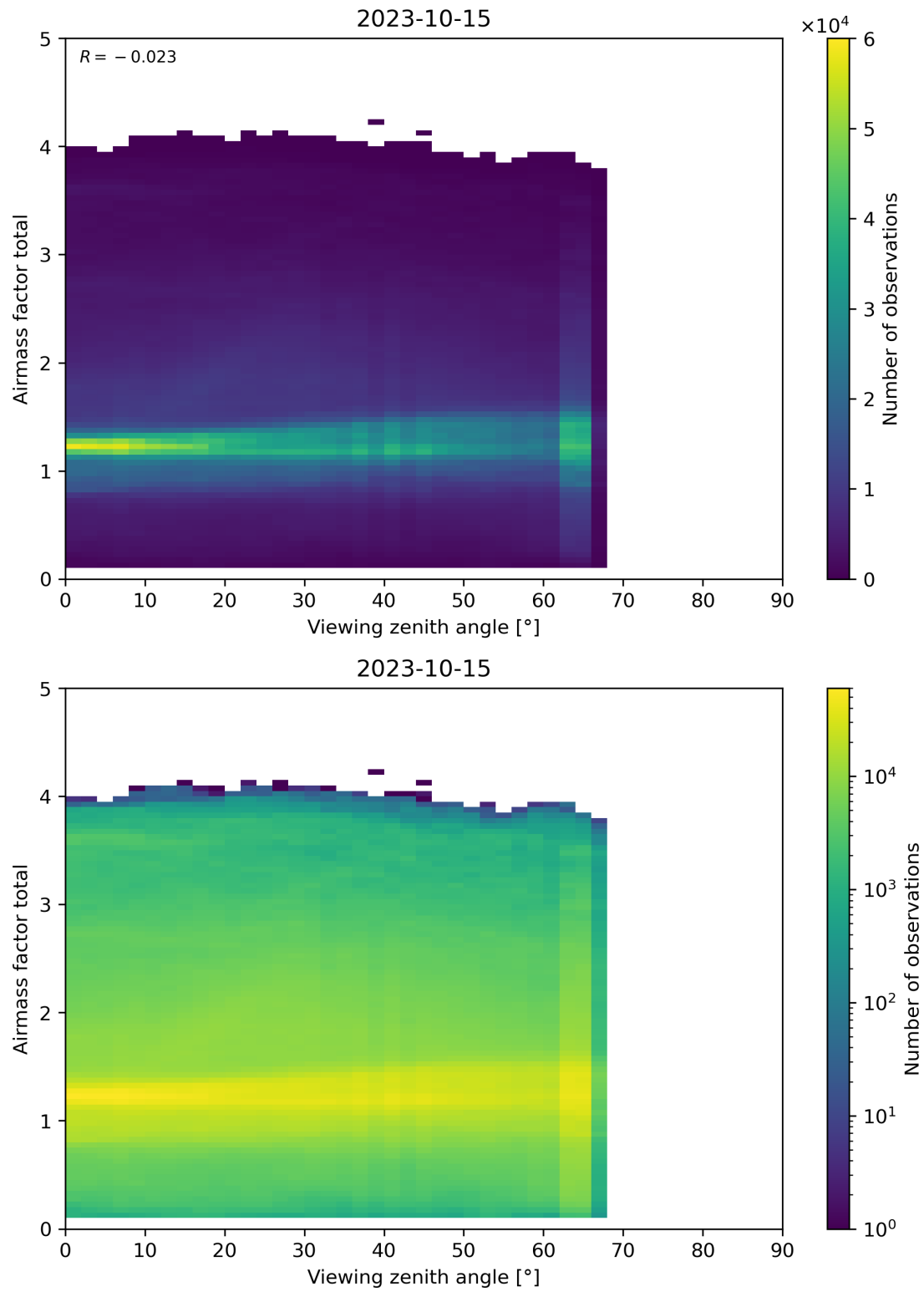
Figure 190: Scatter density plot of “Viewing zenith angle” against “Airmass factor total” for 2023-10-14 to 2023-10-16.
