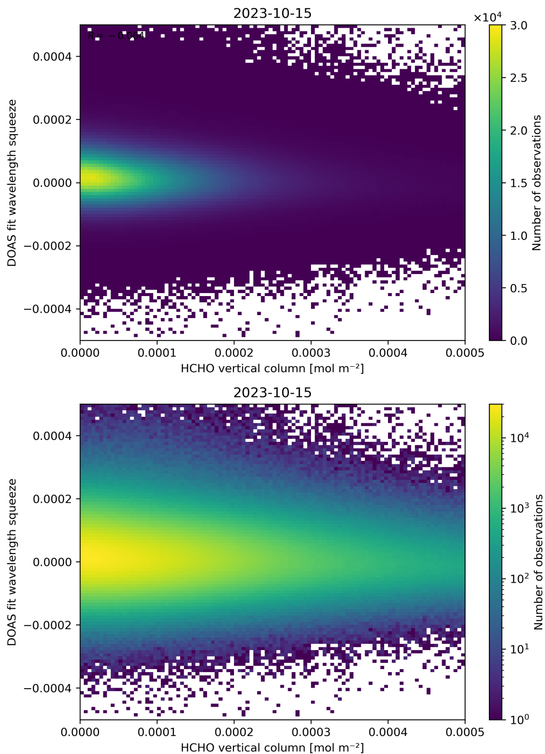
Figure 125: Scatter density plot of “HCHO vertical column” against “DOAS fit wavelength squeeze” for 2023-10-14 to 2023-10-16.
