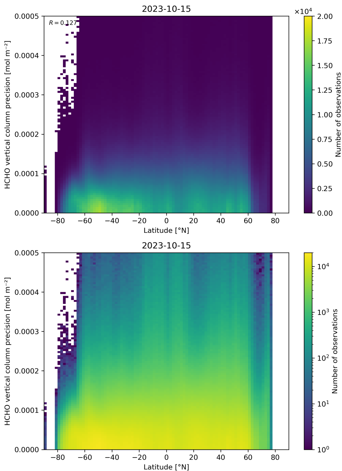
Figure 165: Scatter density plot of “Latitude” against “HCHO vertical column precision” for 2023-10-14 to 2023-10-16.
