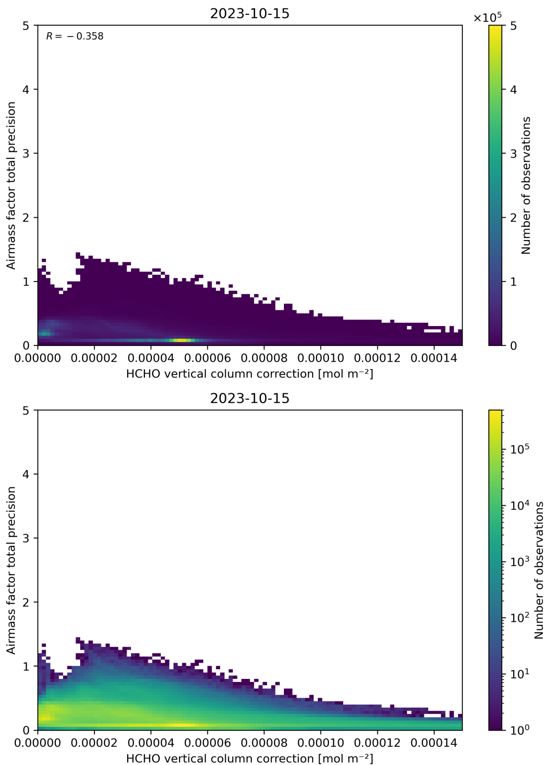
Figure 121: Scatter density plot of “HCHO vertical column correction” against “Airmass factor total precision” for 2023-10-14 to 2023-10-16.
