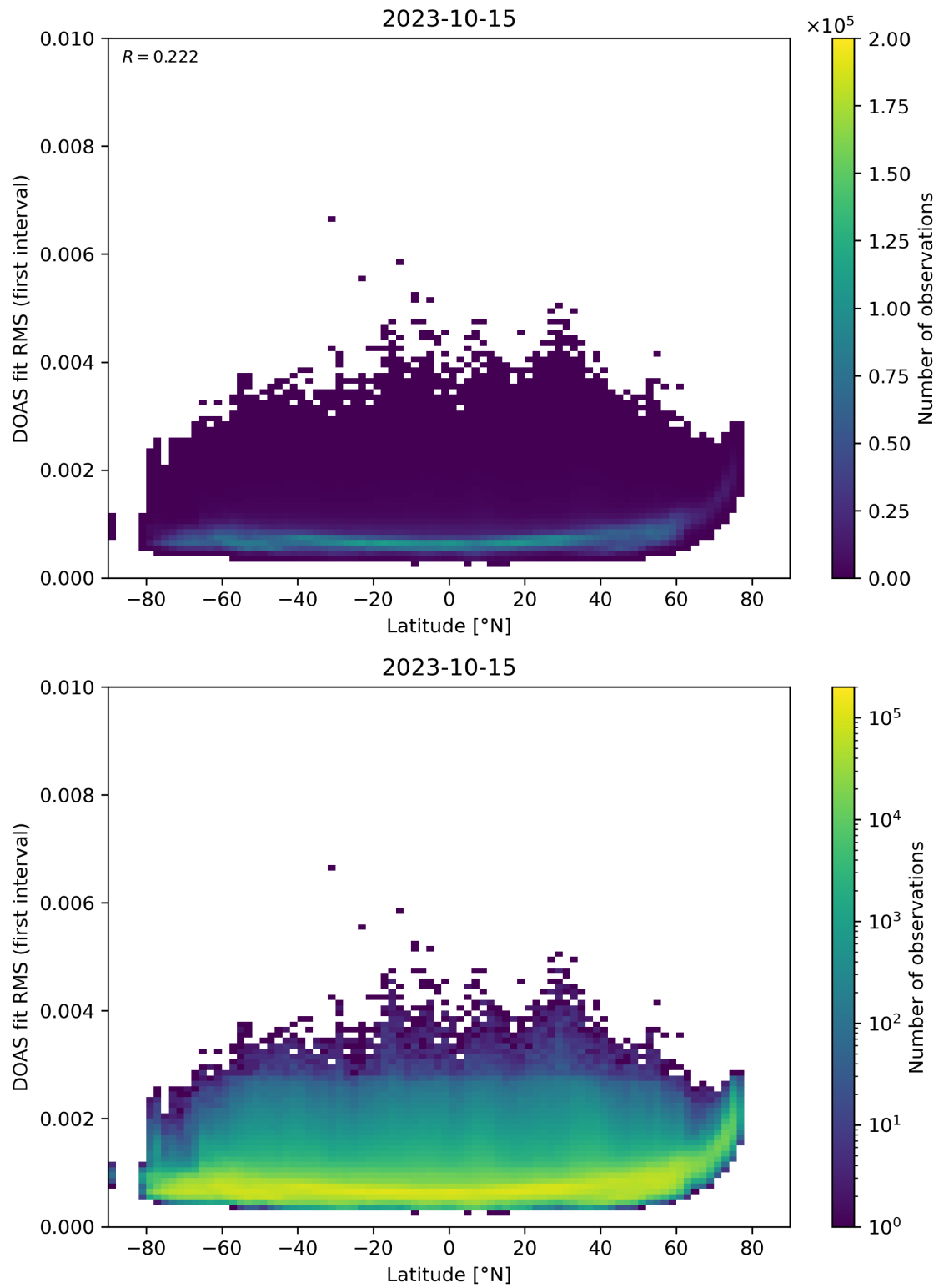
Figure 153: Scatter density plot of “Latitude” against “DOAS fit RMS (first interval)” for 2023-10-14 to 2023-10-16.
