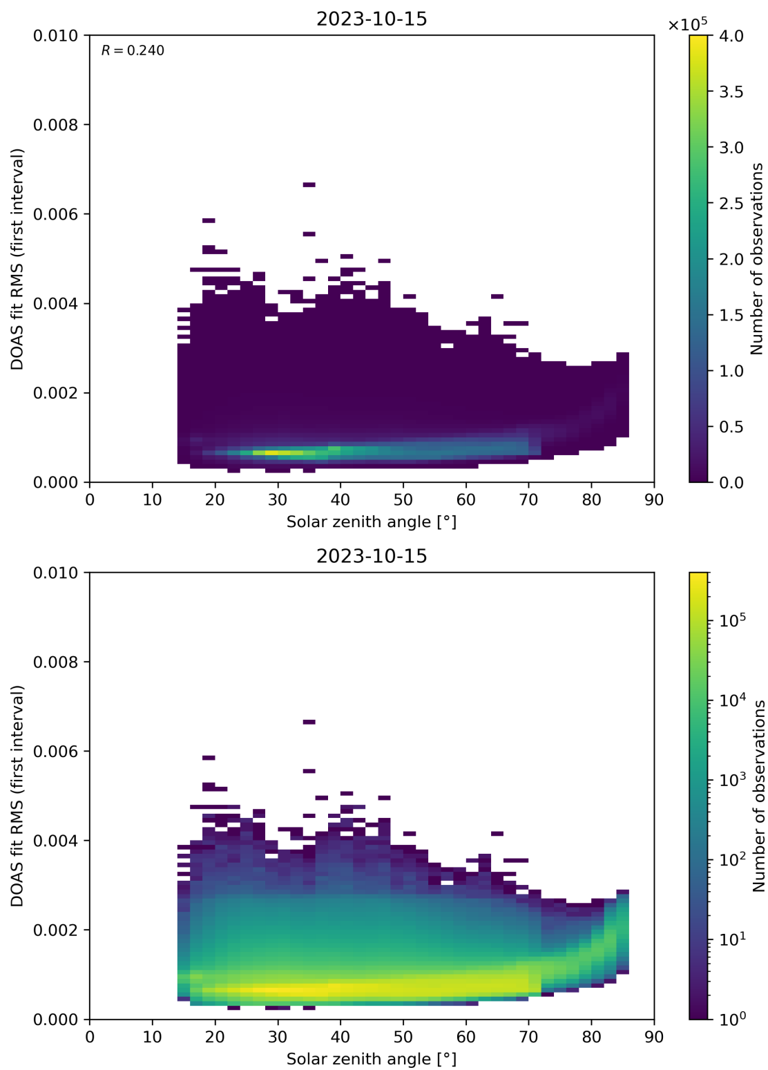
Figure 167: Scatter density plot of “Solar zenith angle” against “DOAS fit RMS (first interval)” for 2023-10-14 to 2023-10-16.
