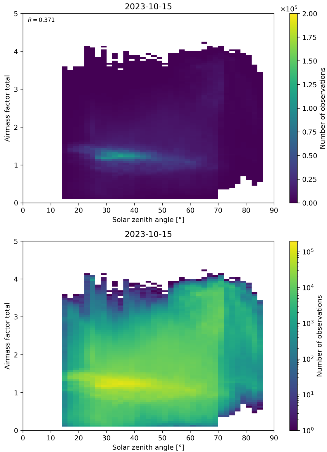
Figure 175: Scatter density plot of “Solar zenith angle” against “Airmass factor total” for 2023-10-14 to 2023-10-16.
