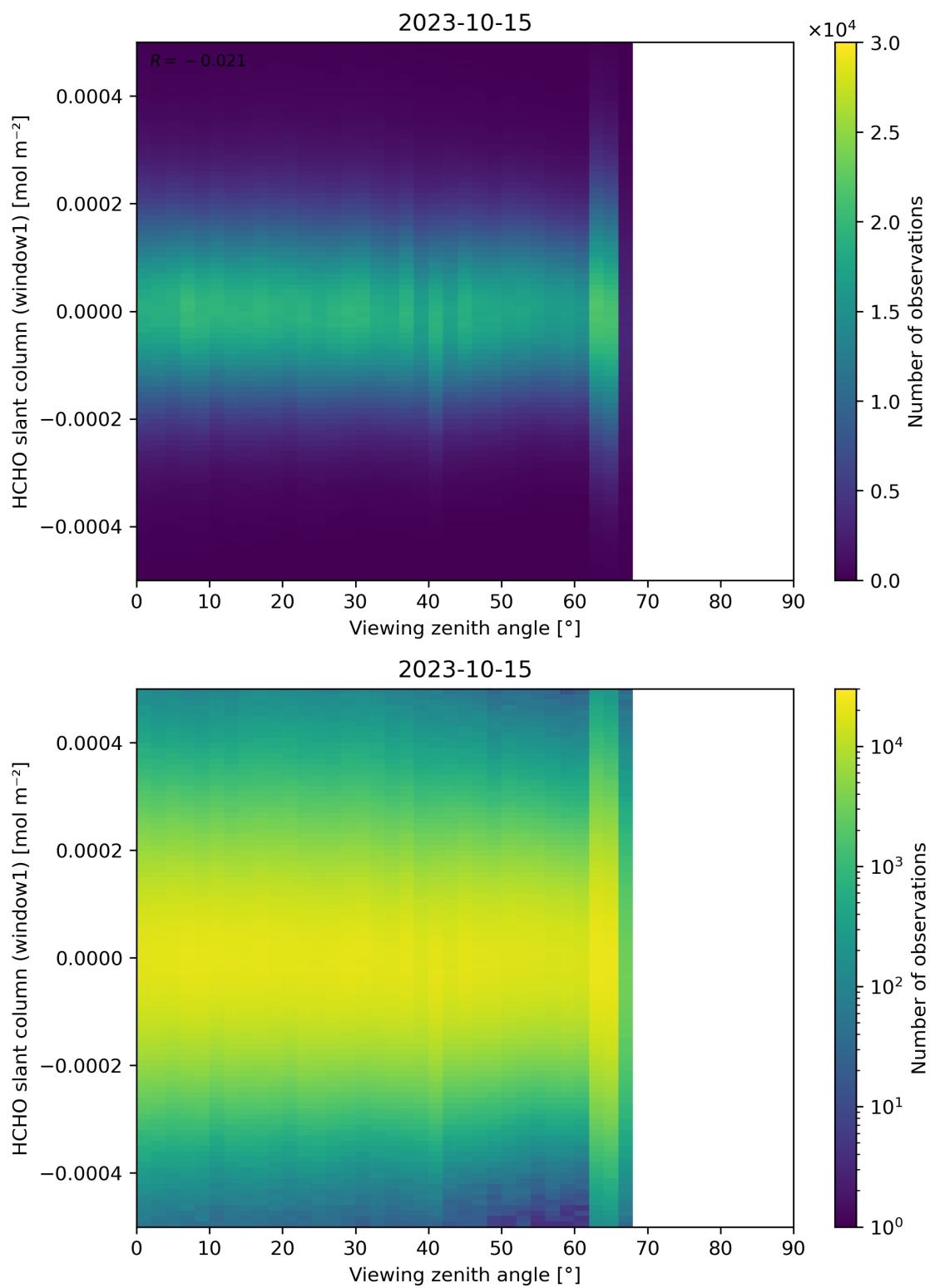
Figure 188: Scatter density plot of “Viewing zenith angle” against “HCHO slant column (window1)” for 2023-10-14 to 2023-10-16.
