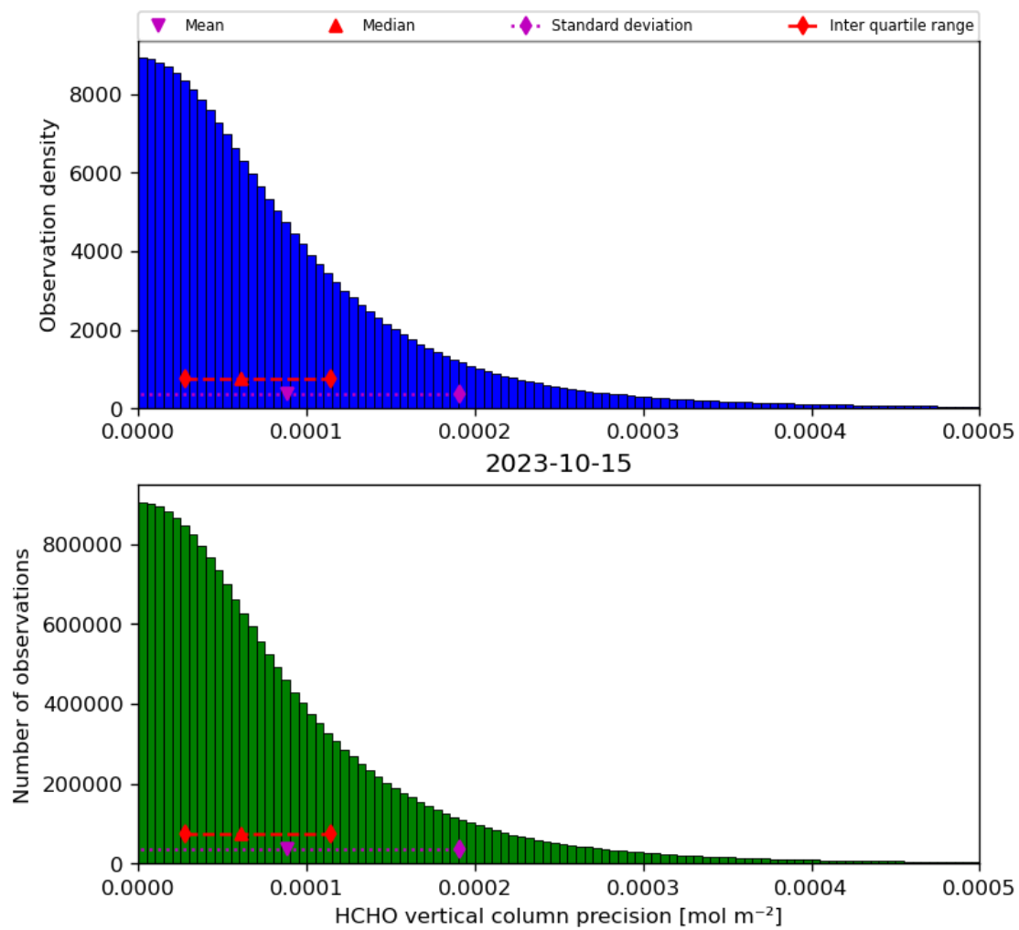
Figure 36: Histogram of “HCHO vertical column precision” for 2023-10-14 to 2023-10-16
