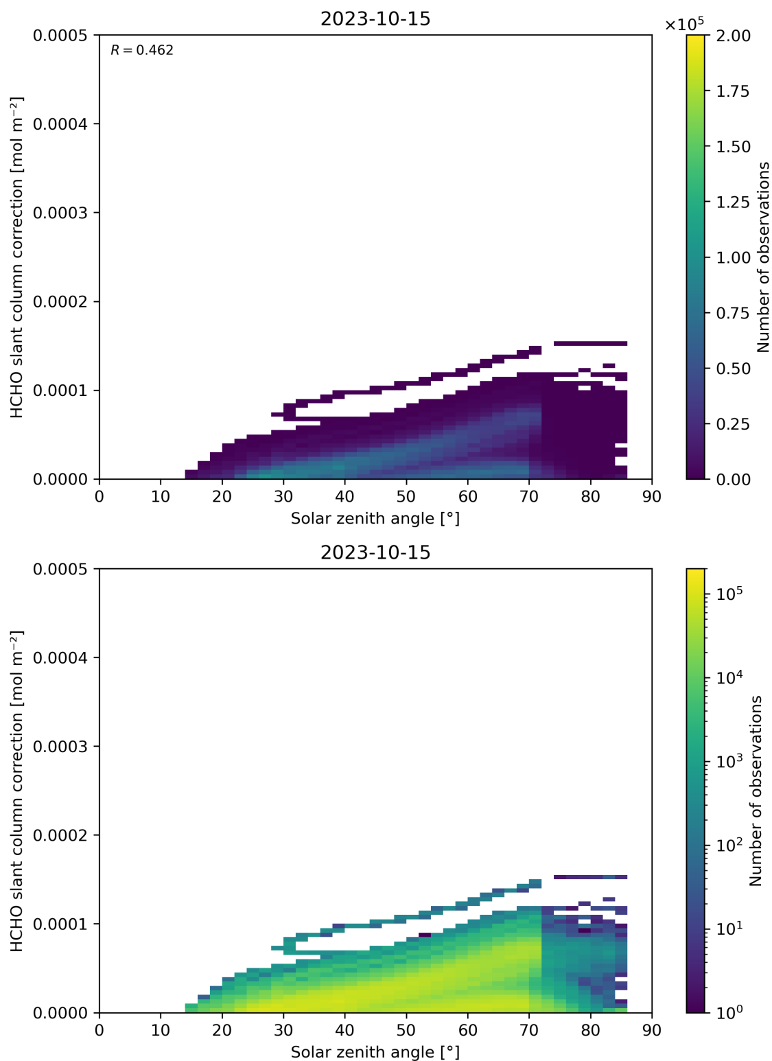
Figure 172: Scatter density plot of “Solar zenith angle” against “HCHO slant column correction” for 2023-10-14 to 2023-10-16.
