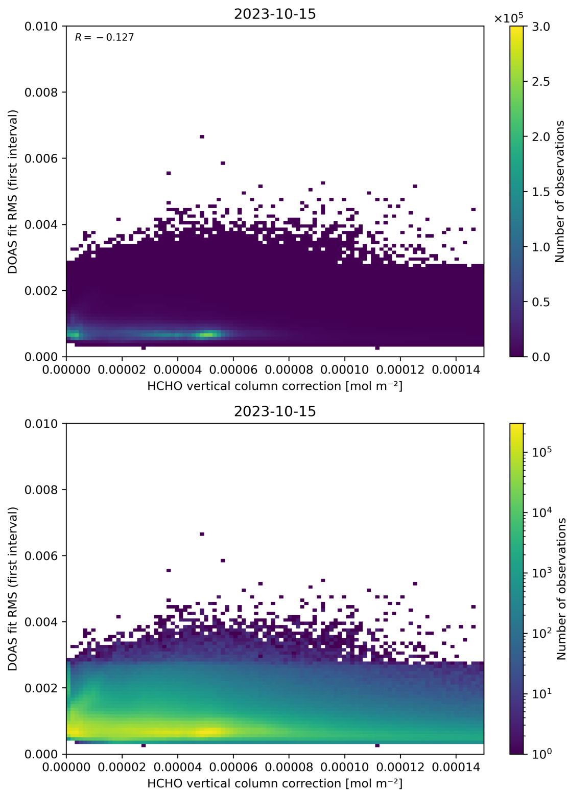
Figure 112: Scatter density plot of “HCHO vertical column correction” against “DOAS fit RMS (first interval)” for 2023-10-14 to 2023-10-16.
