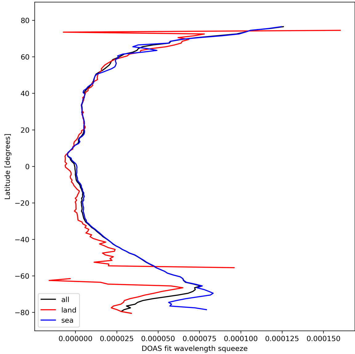
Figure 31: Zonal average of “DOAS fit wavelength squeeze” for 2023-10-14 to 2023-10-16.
