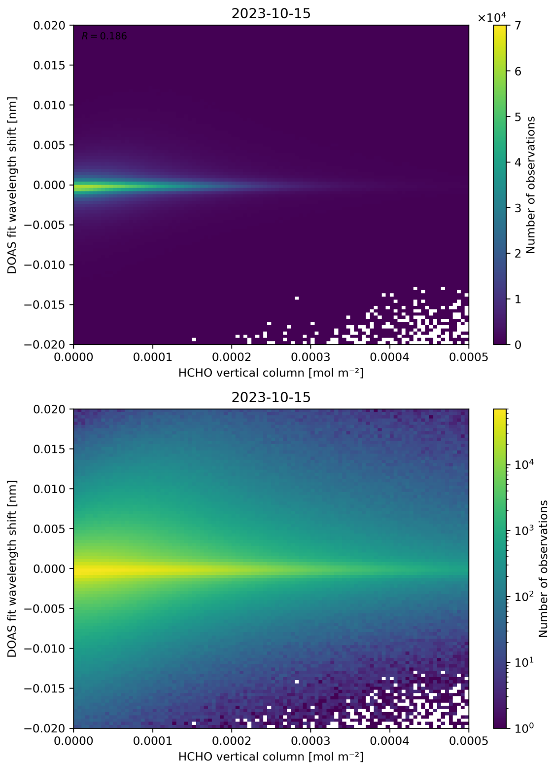
Figure 124: Scatter density plot of “HCHO vertical column” against “DOAS fit wavelength shift” for 2023-10-14 to 2023-10-16.
