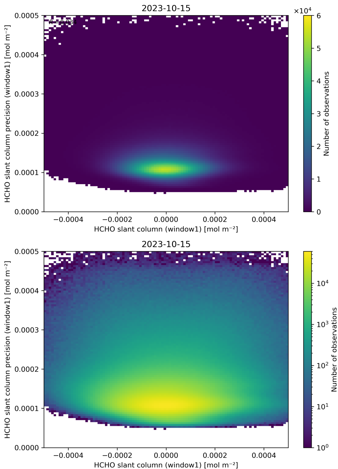
Figure 84: Scatter density plot of “HCHO slant column (window1)” against “HCHO slant column precision (window1)” for 2023-10-14 to 2023-10-16.
