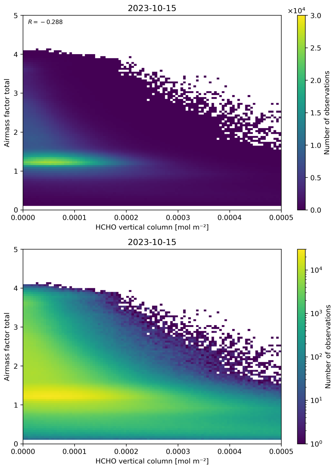
Figure 131: Scatter density plot of “HCHO vertical column” against “Airmass factor total” for 2023-10-14 to 2023-10-16.
