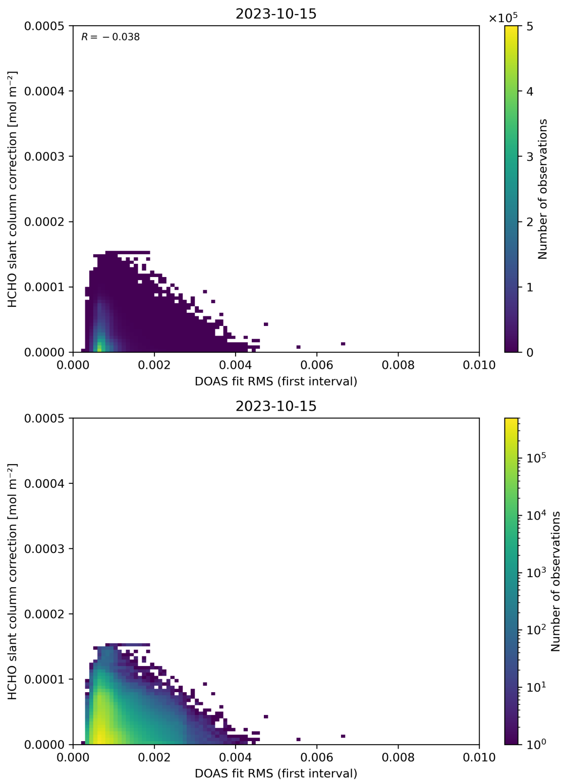
Figure 63: Scatter density plot of “DOAS fit RMS (first interval)” against “HCHO slant column correction” for 2023-10-14 to 2023-10-16.
