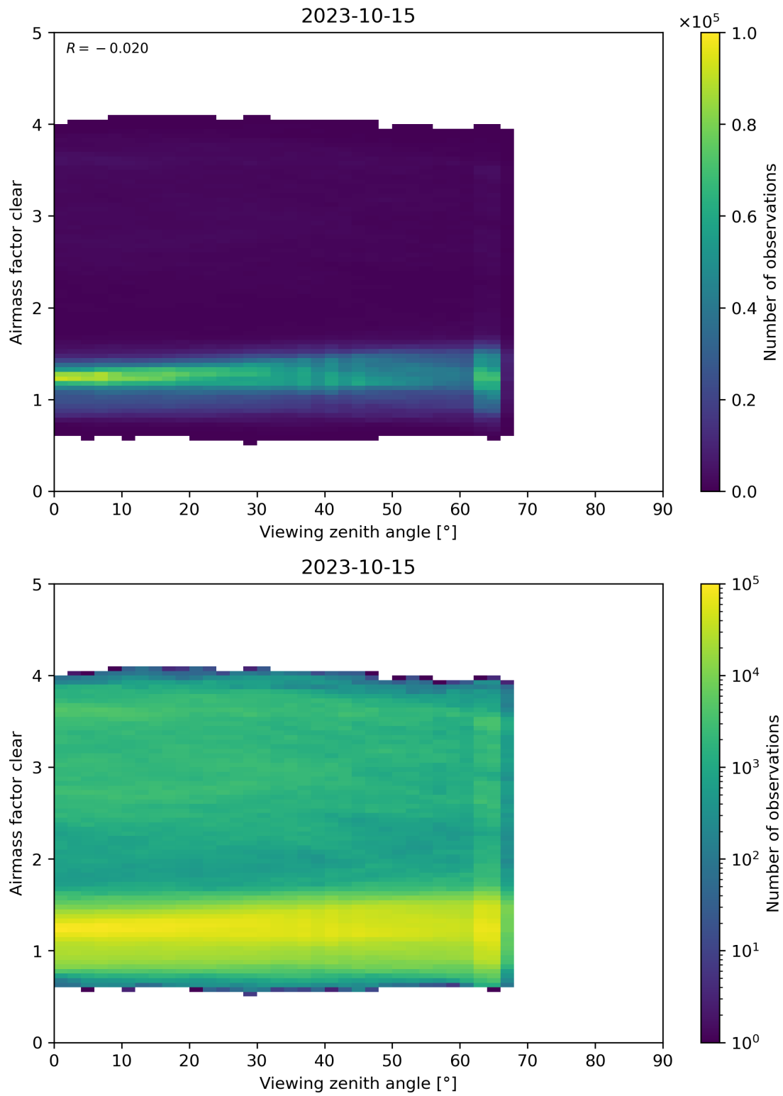
Figure 185: Scatter density plot of “Viewing zenith angle” against “Airmass factor clear” for 2023-10-14 to 2023-10-16.
