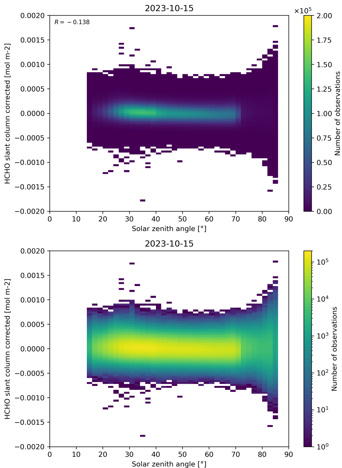
Figure 171: Scatter density plot of “Solar zenith angle” against “HCHO slant column corrected” for 2023-10-14 to 2023-10-16.
