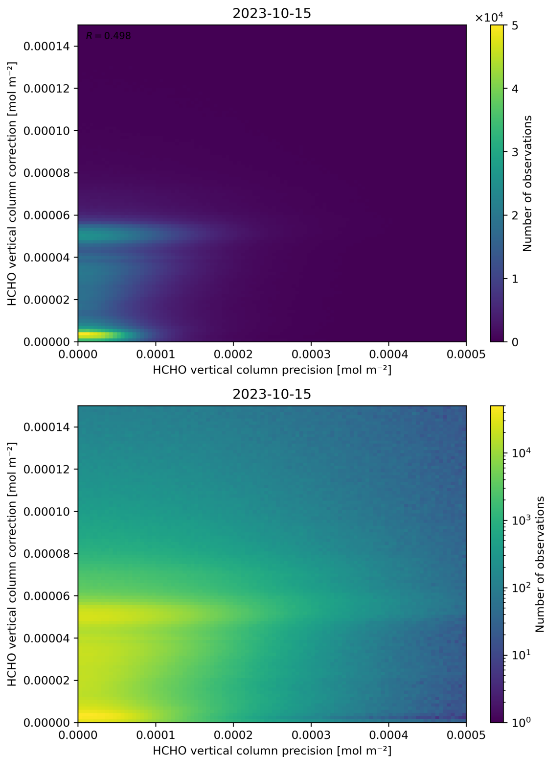
Figure 146: Scatter density plot of “HCHO vertical column precision” against “HCHO vertical column correction” for 2023-10-14 to 2023-10-16.
