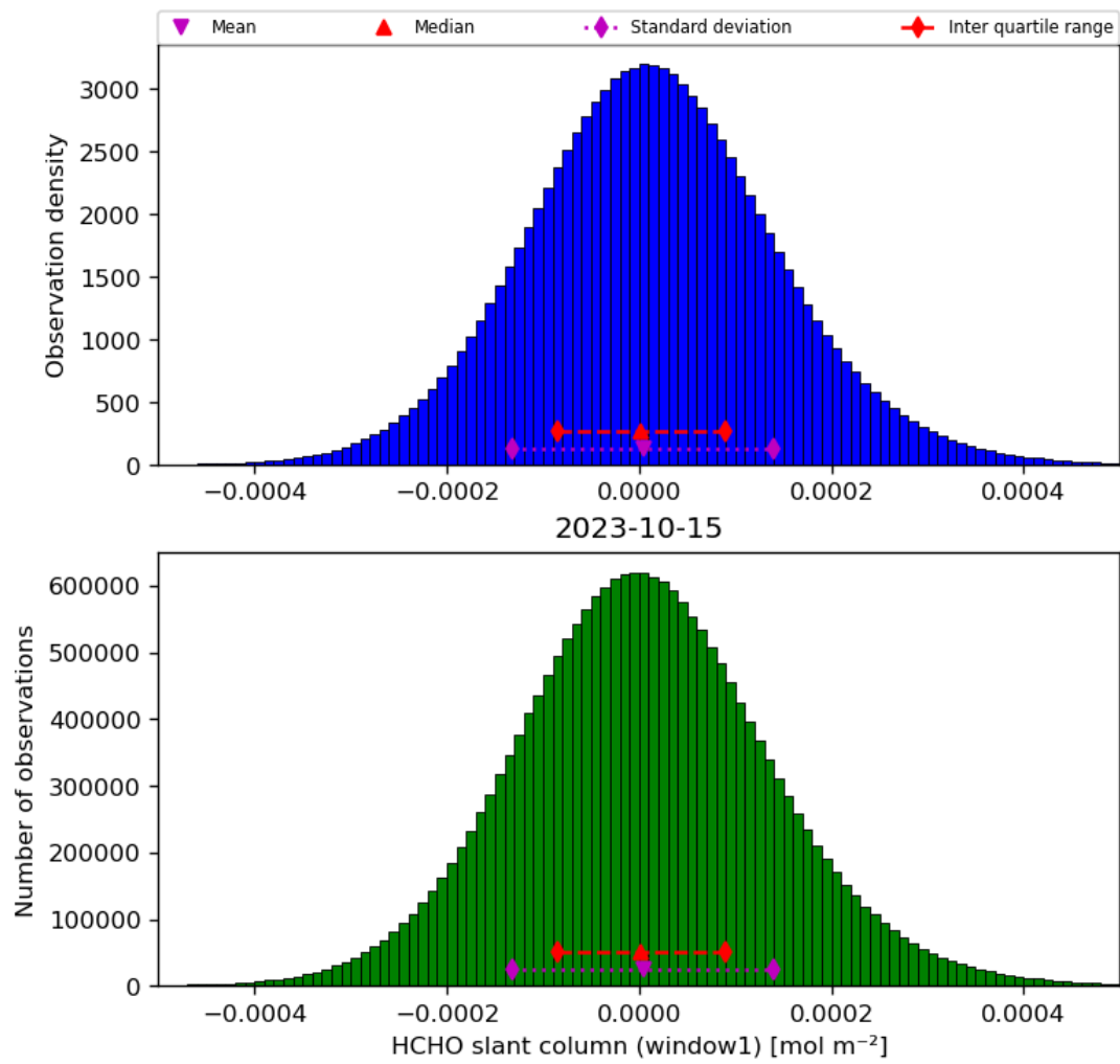
Figure 38: Histogram of “HCHO slant column (window1)” for 2023-10-14 to 2023-10-16
