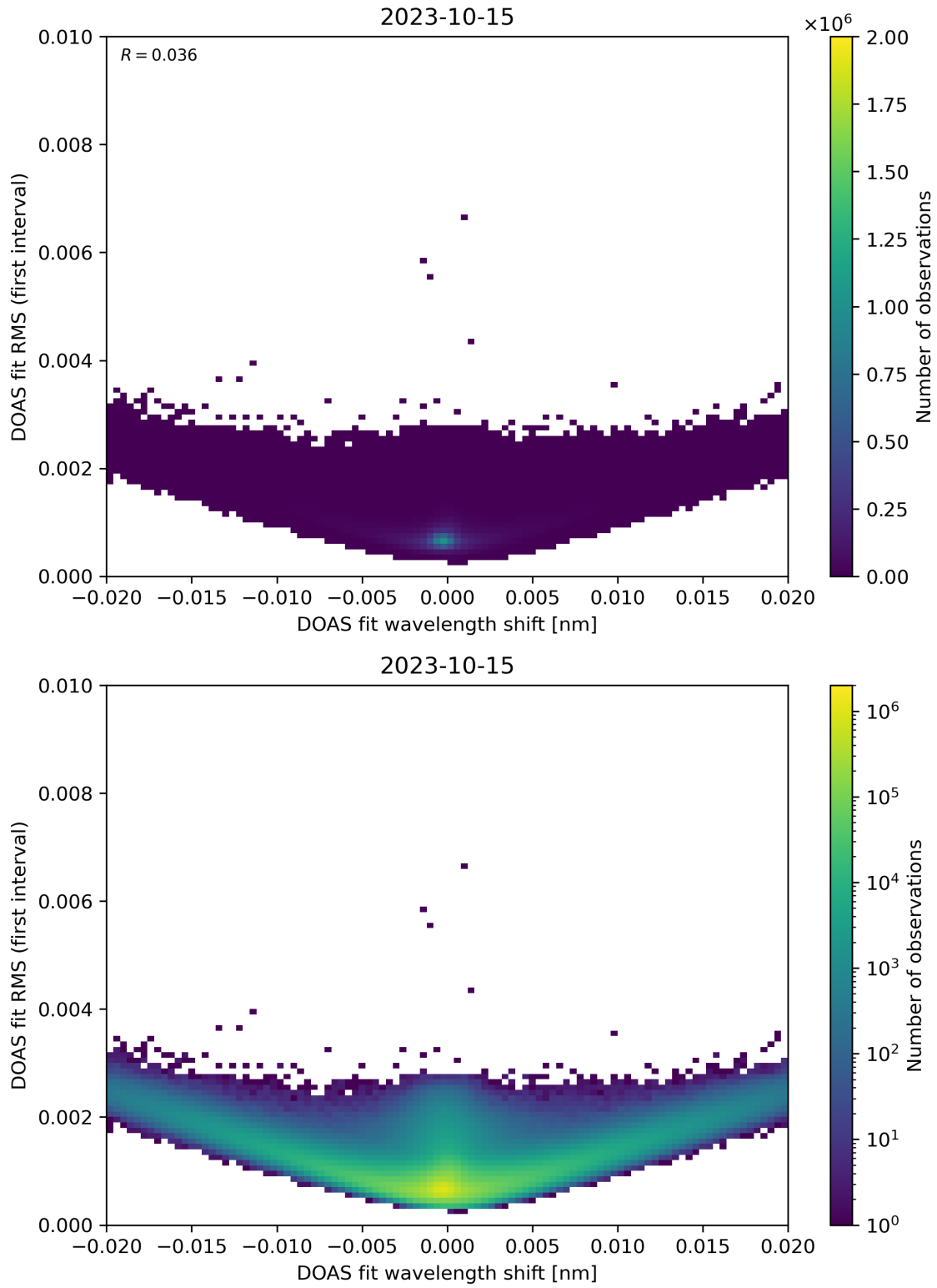
Figure 64: Scatter density plot of “DOAS fit wavelength shift” against “DOAS fit RMS (first interval)” for 2023-10-14 to 2023-10-16.
