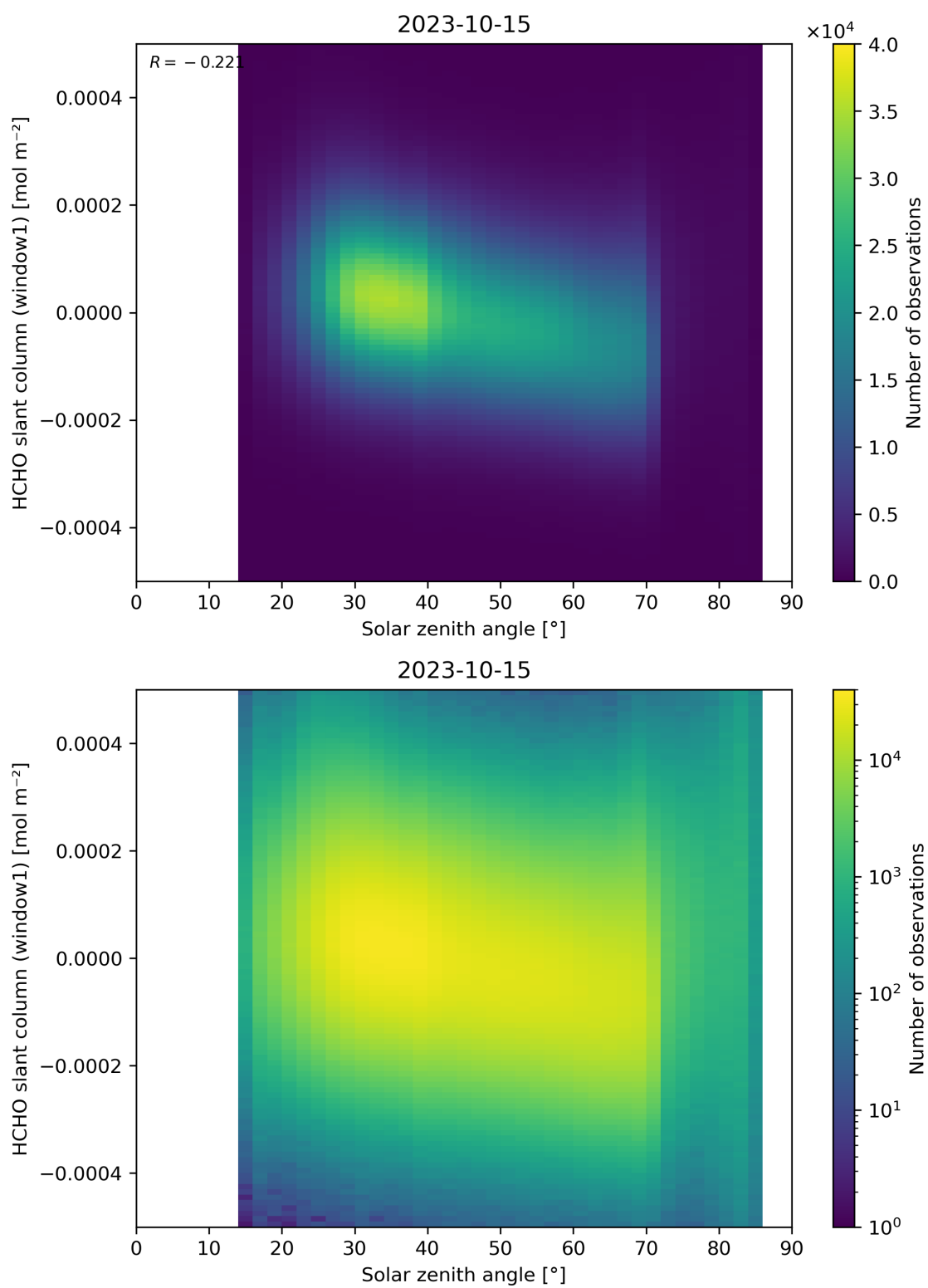
Figure 173: Scatter density plot of “Solar zenith angle” against “HCHO slant column (window1)” for 2023-10-14 to 2023-10-16.
