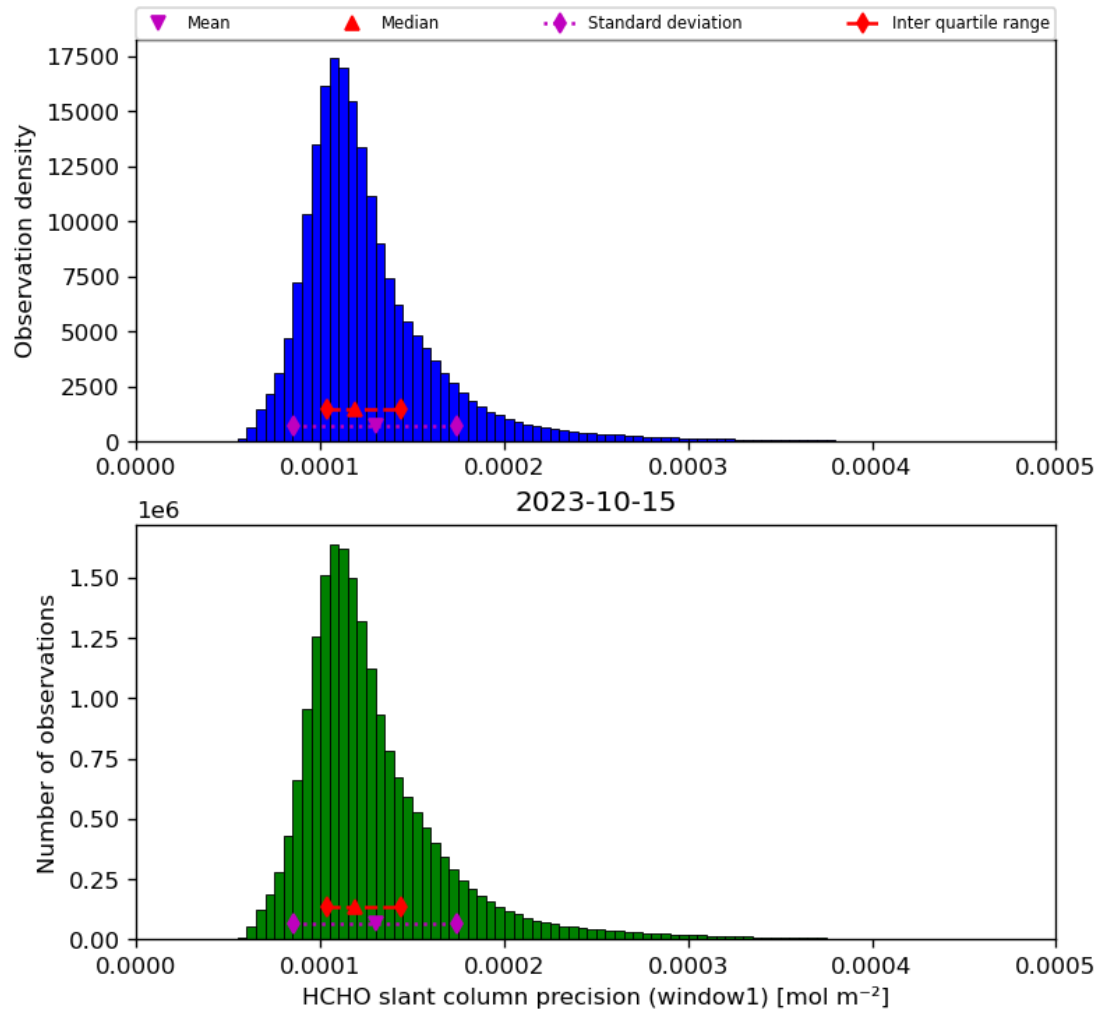
Figure 39: Histogram of “HCHO slant column precision (window1)” for 2023-10-14 to 2023-10-16
