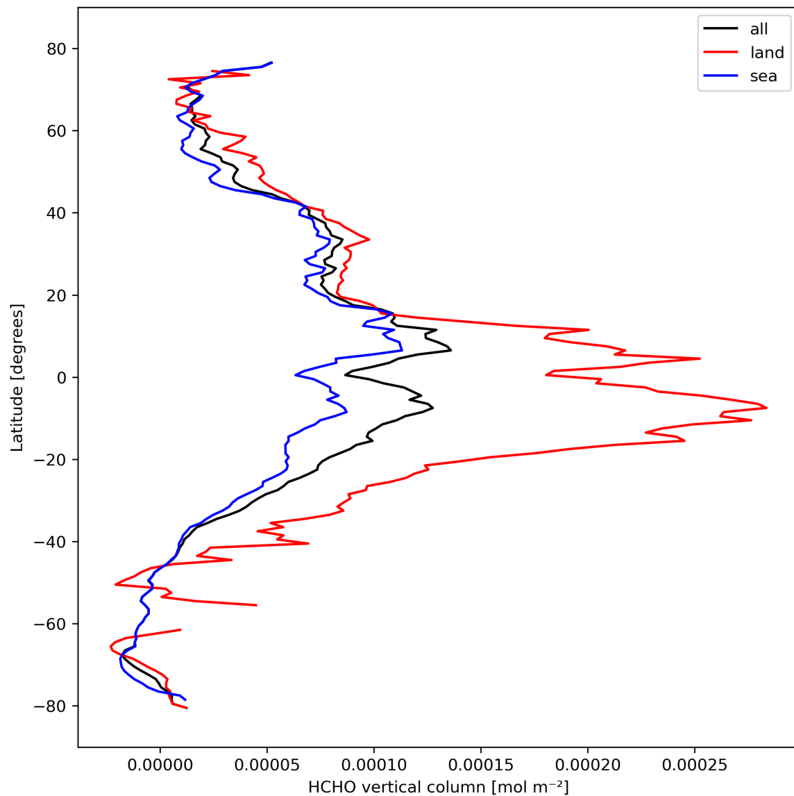
Figure 21: Zonal average of “HCHO vertical column” for 2023-10-14 to 2023-10-16.
