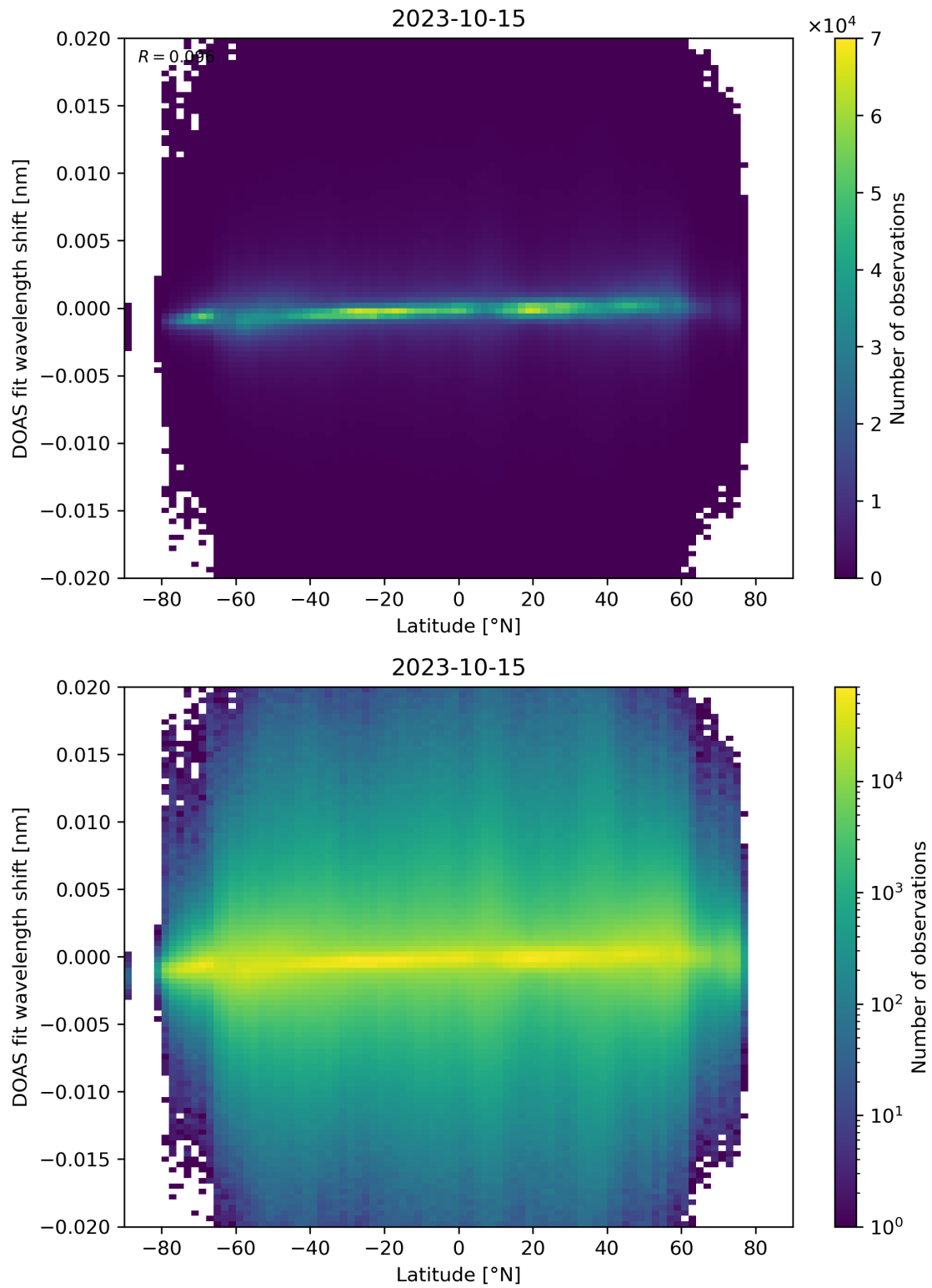
Figure 154: Scatter density plot of “Latitude” against “DOAS fit wavelength shift” for 2023-10-14 to 2023-10-16.
