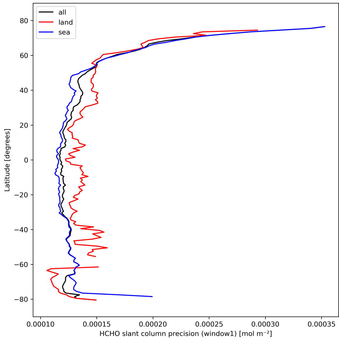
Figure 25: Zonal average of "HCHO slant column precision (window1)" for 2023-10-14 to 2023-10-16.
