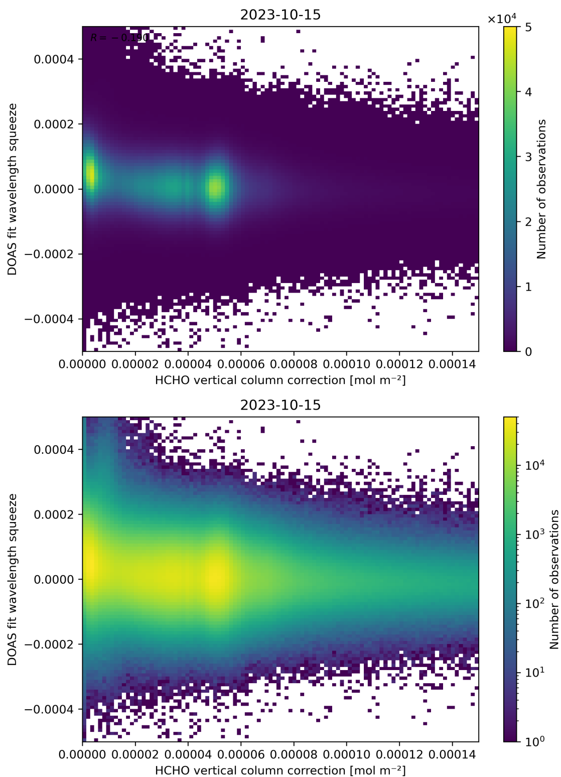
Figure 114: Scatter density plot of “HCHO vertical column correction” against “DOAS fit wavelength squeeze” for 2023-10-14 to 2023-10-16.
