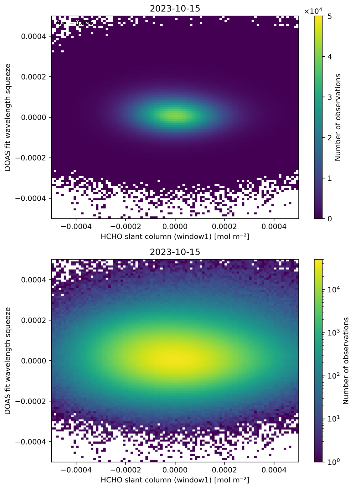
Figure 80: Scatter density plot of “HCHO slant column (window1)” against “DOAS fit wavelength squeeze” for 2023-10-14 to 2023-10-16.
