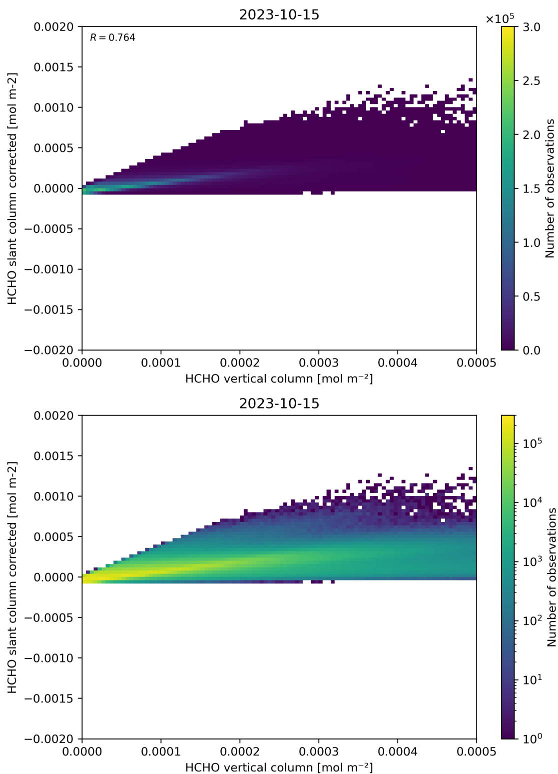
Figure 127: Scatter density plot of “HCHO vertical column” against “HCHO slant column corrected” for 2023-10-14 to 2023-10-16.
