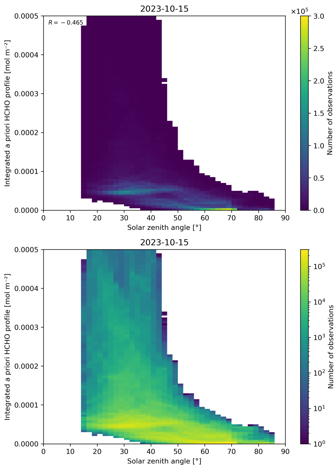
Figure 180: Scatter density plot of “Solar zenith angle” against “Integrated a priori HCHO profile” for 2023-10-14 to 2023-10-16.
