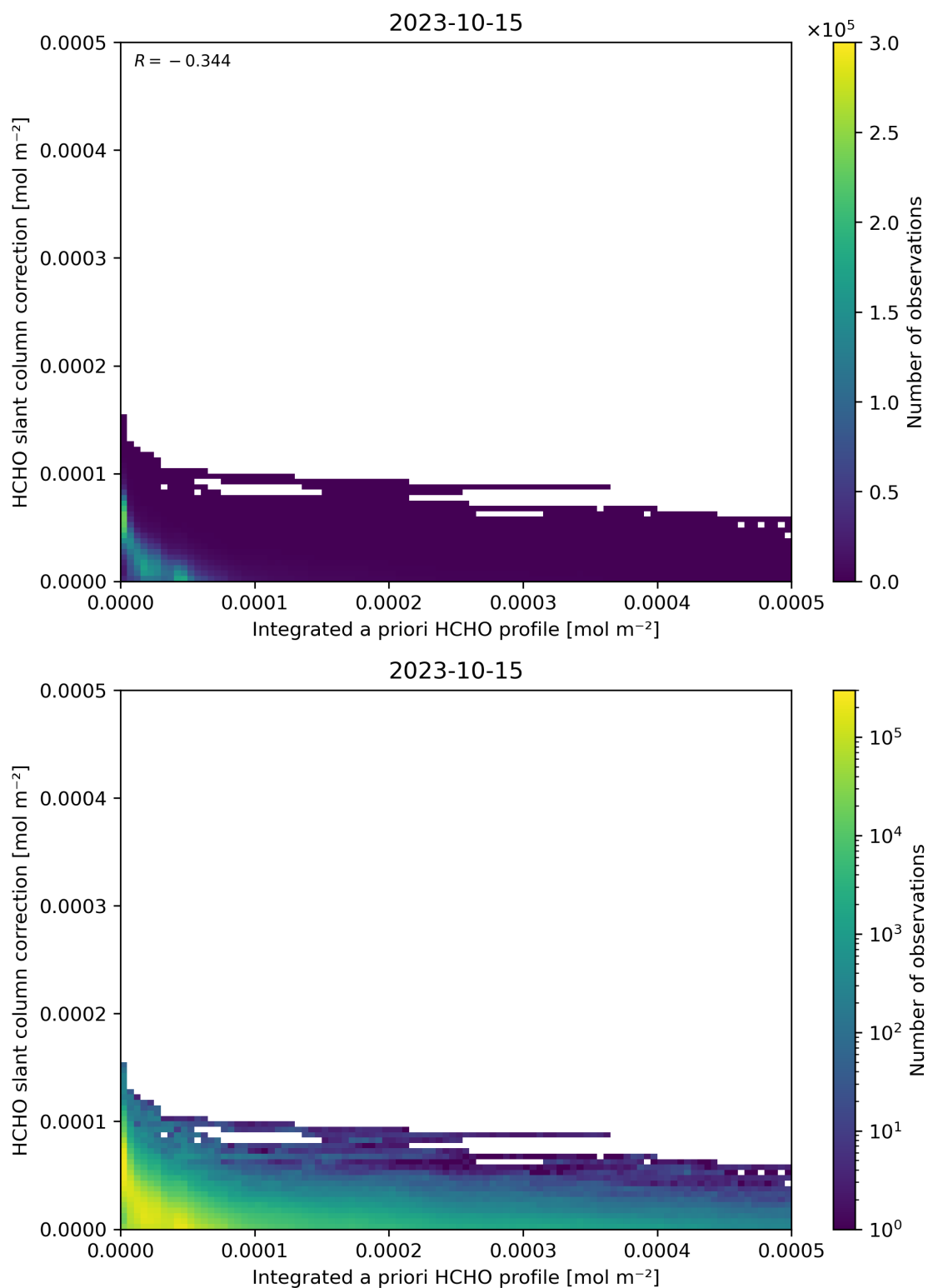
Figure 152: Scatter density plot of “Integrated a priori HCHO profile” against “HCHO slant column correction” for 2023-10-14 to 2023-10-16.
