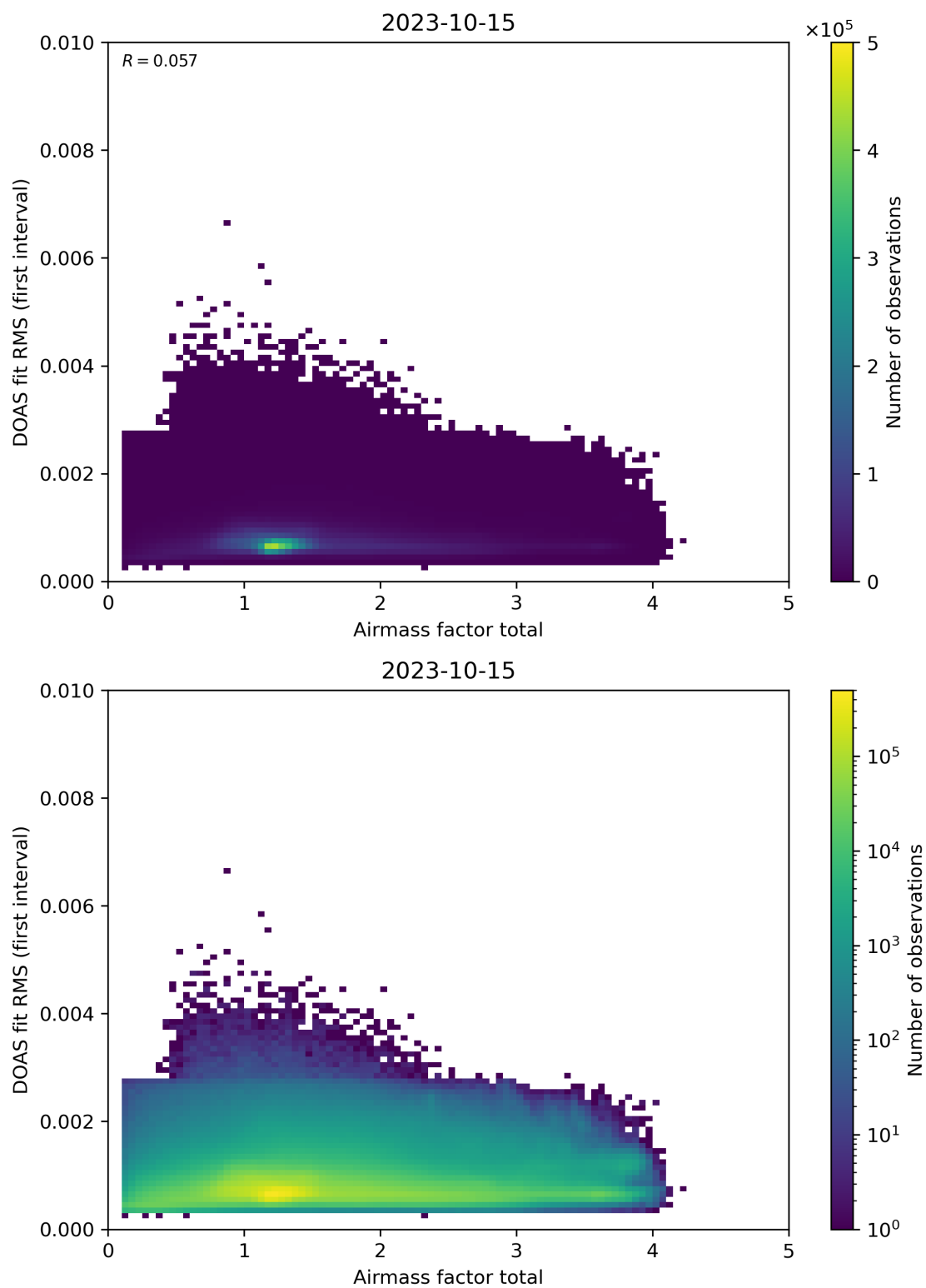
Figure 97: Scatter density plot of “Airmass factor total” against “DOAS fit RMS (first interval)” for 2023-10-14 to 2023-10-16.
