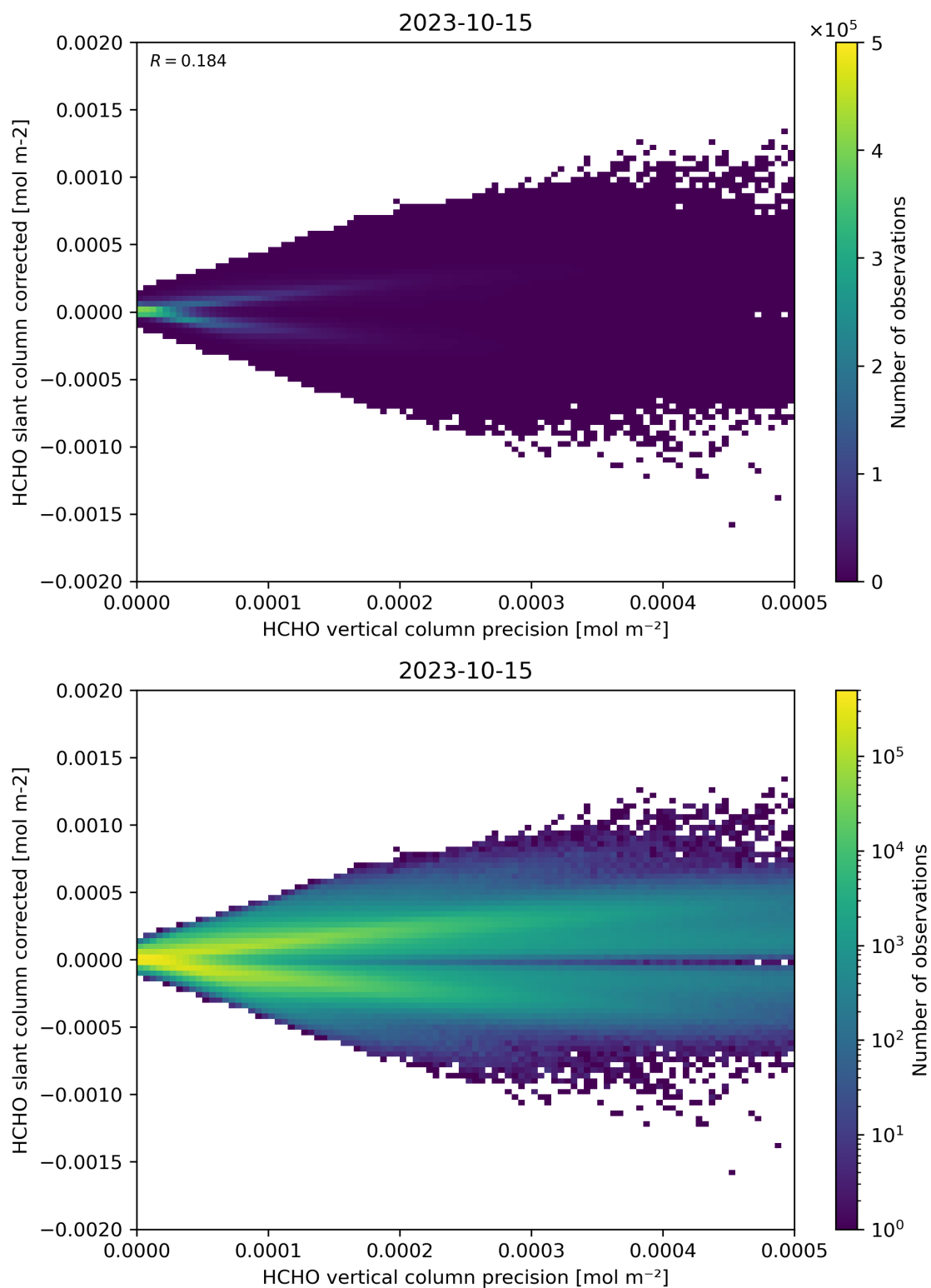
Figure 140: Scatter density plot of “HCHO vertical column precision” against “HCHO slant column corrected” for 2023-10-14 to 2023-10-16.
