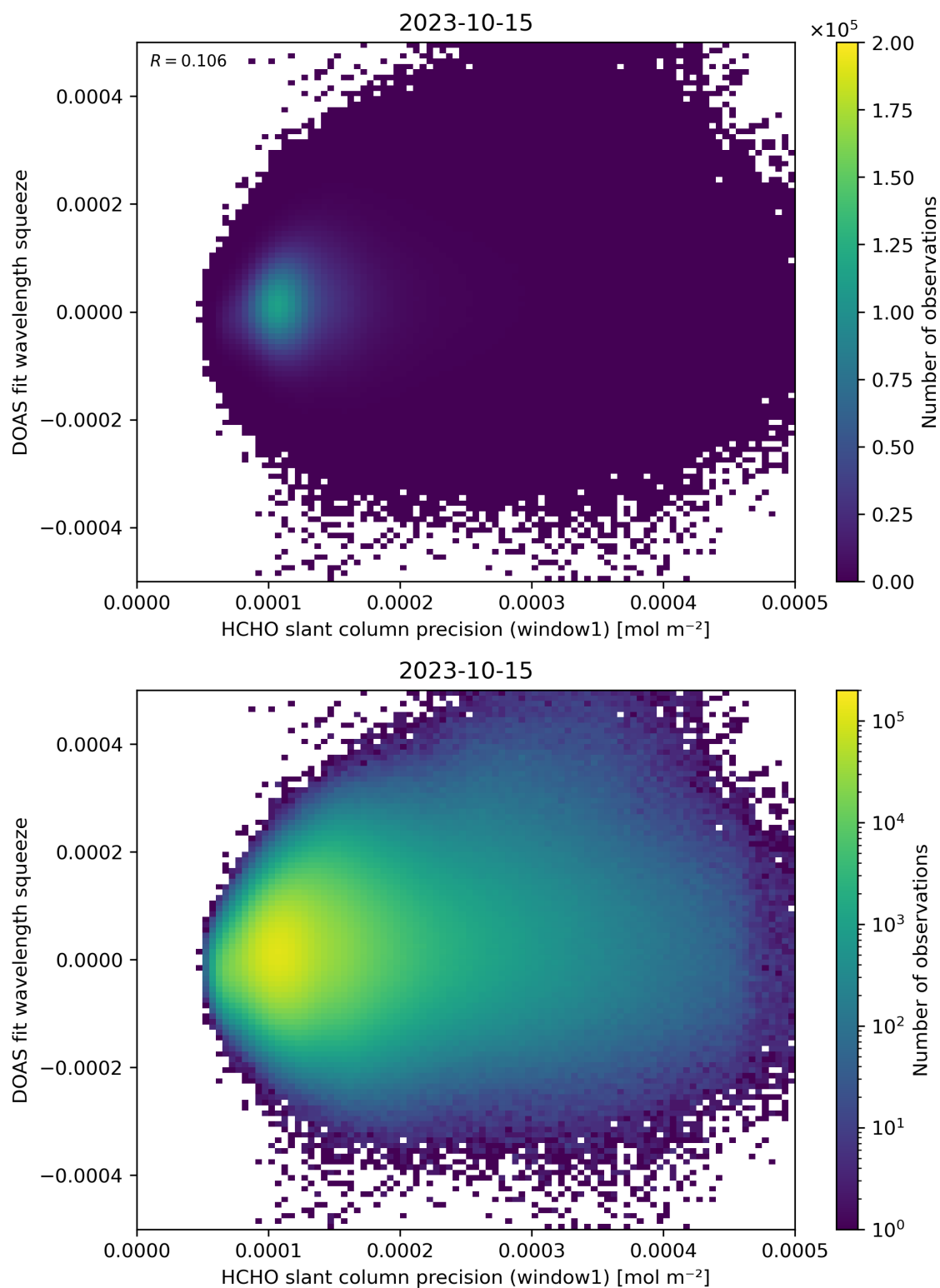
Figure 90: Scatter density plot of “HCHO slant column precision (window1)” against “DOAS fit wavelength squeeze” for 2023-10-14 to 2023-10-16.
