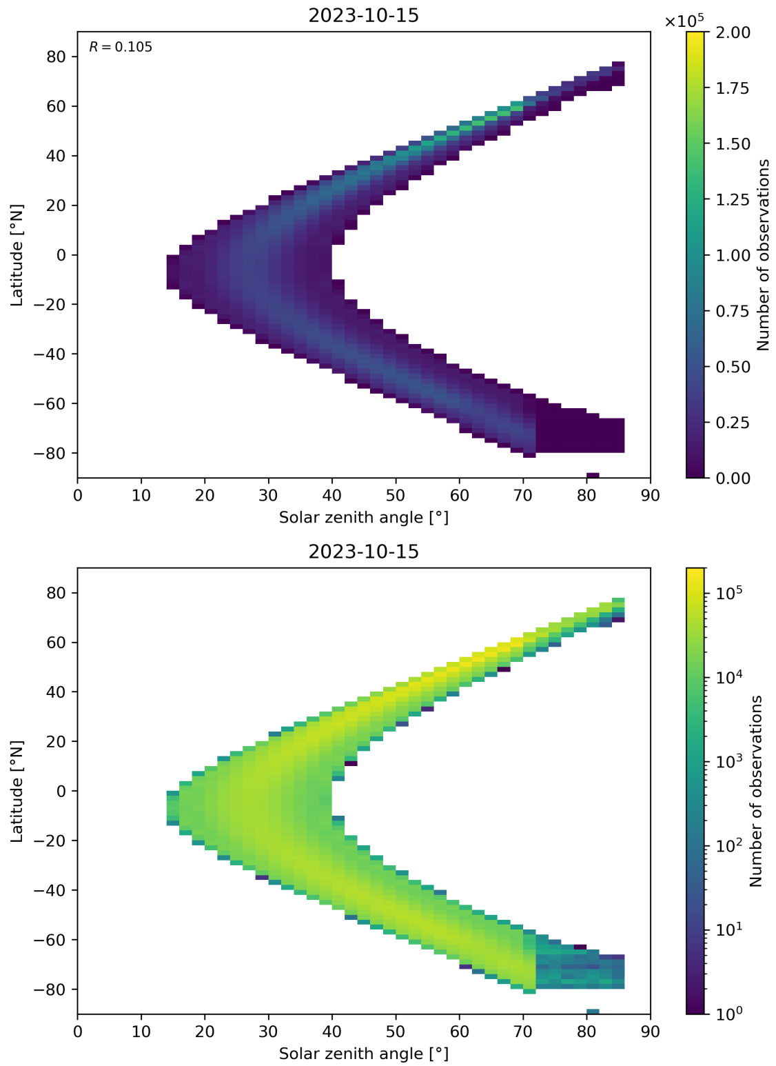
Figure 181: Scatter density plot of “Solar zenith angle” against “Latitude” for 2023-10-14 to 2023-10-16.
