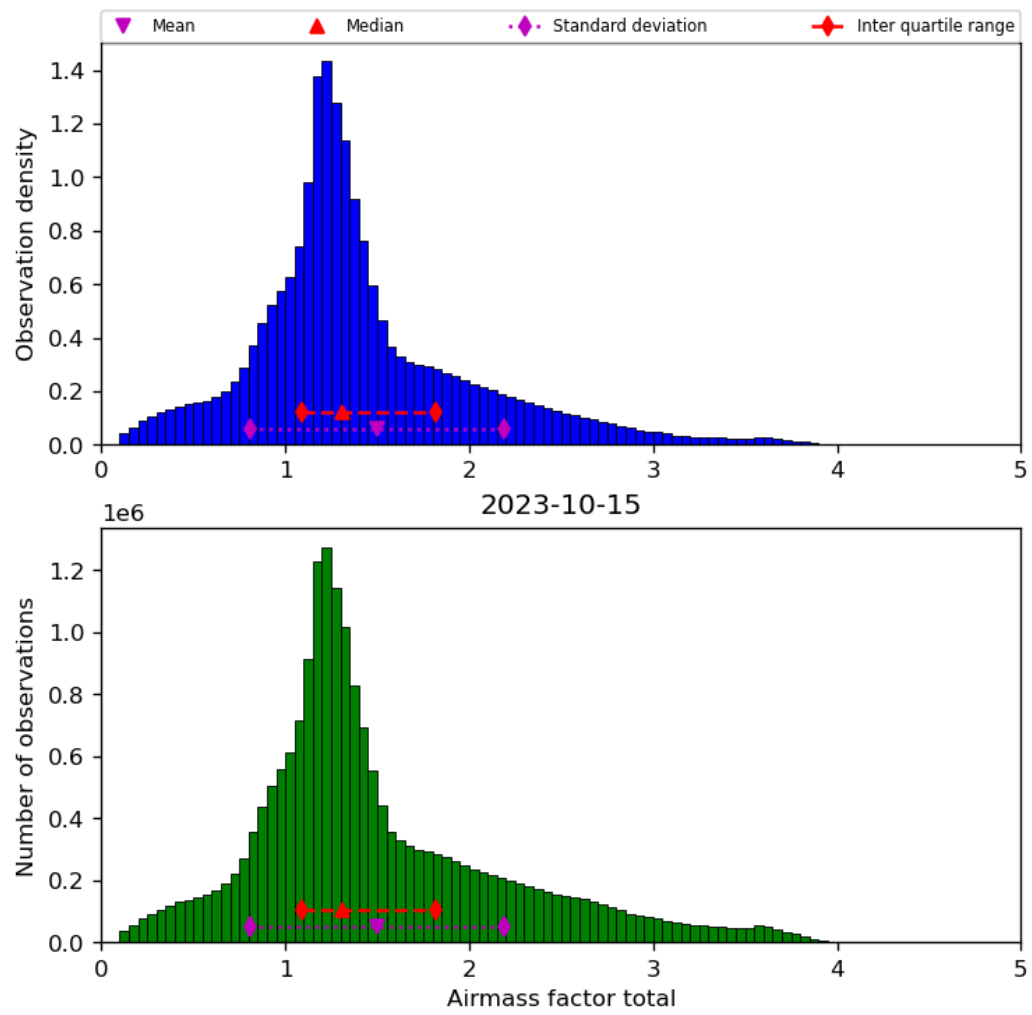
Figure 40: Histogram of “Airmass factor total” for 2023-10-14 to 2023-10-16
