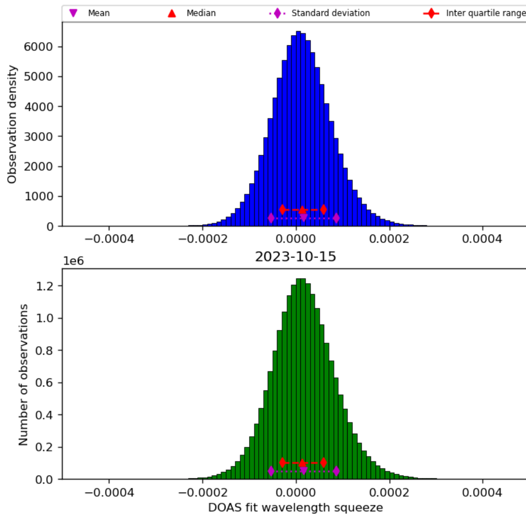
Figure 45: Histogram of “DOAS fit wavelength squeeze” for 2023-10-14 to 2023-10-16
