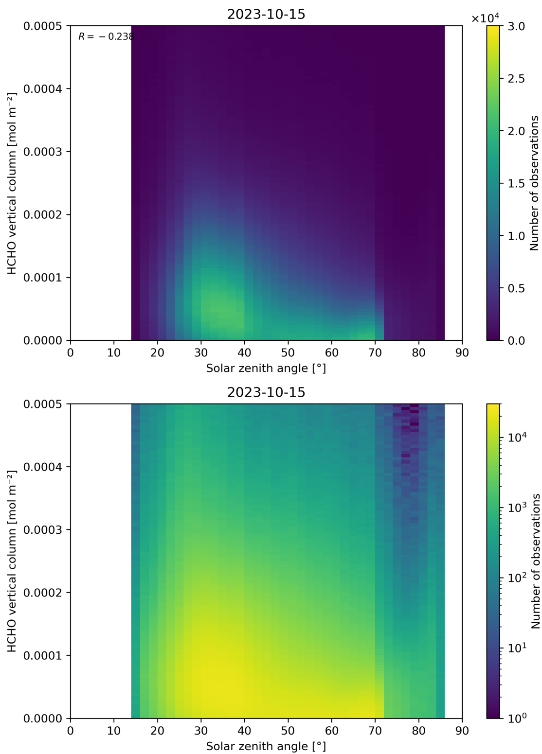
Figure 177: Scatter density plot of “Solar zenith angle” against “HCHO vertical column” for 2023-10-14 to 2023-10-16.
