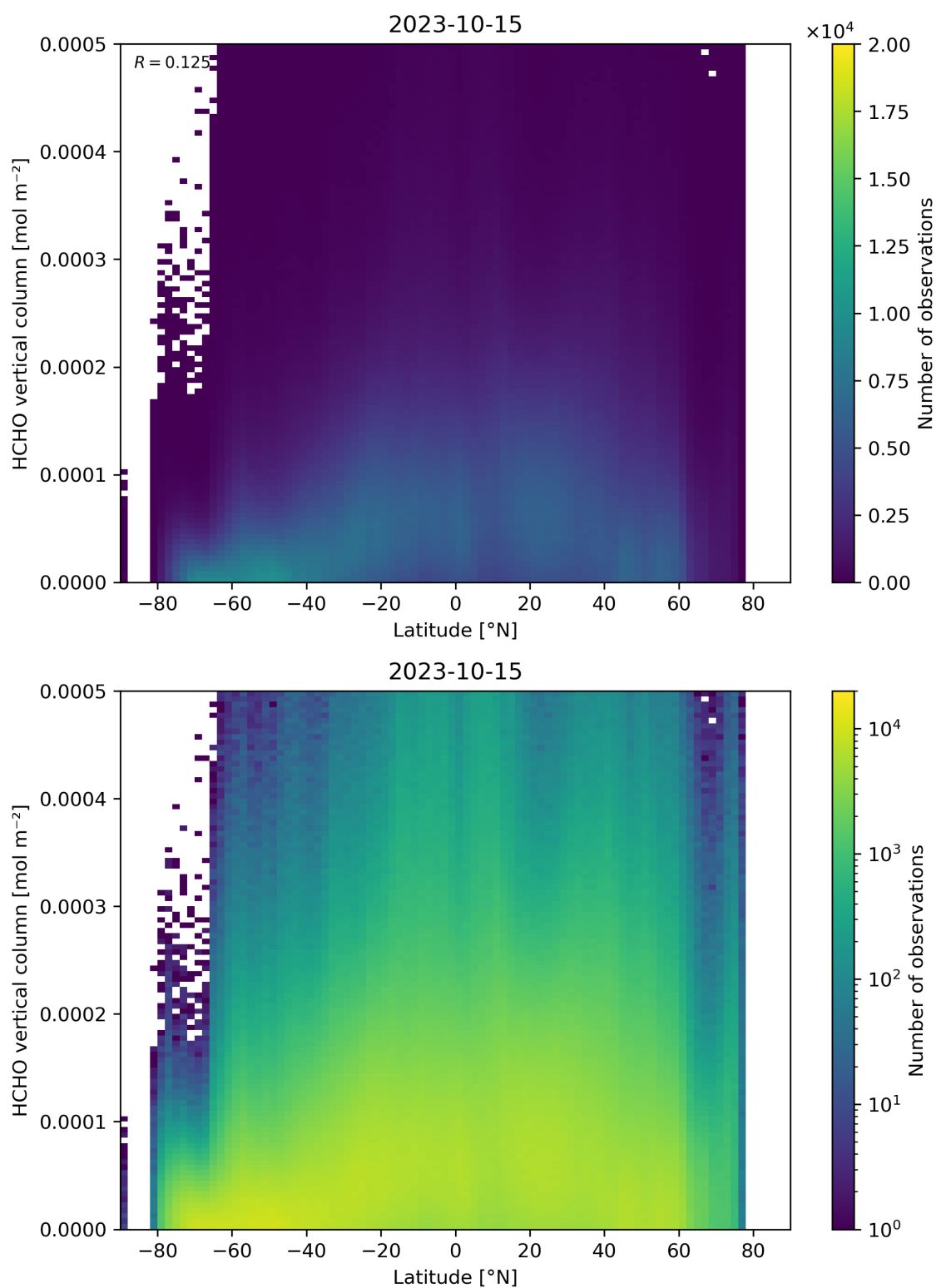
Figure 163: Scatter density plot of “Latitude” against “HCHO vertical column” for 2023-10-14 to 2023-10-16.
