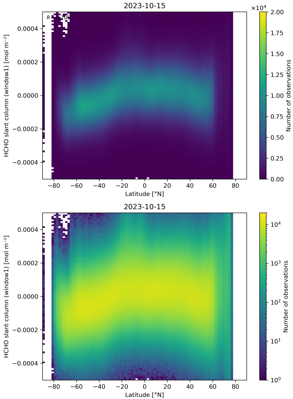
Figure 159: Scatter density plot of “Latitude” against “HCHO slant column (window1)” for 2023-10-14 to 2023-10-16.
