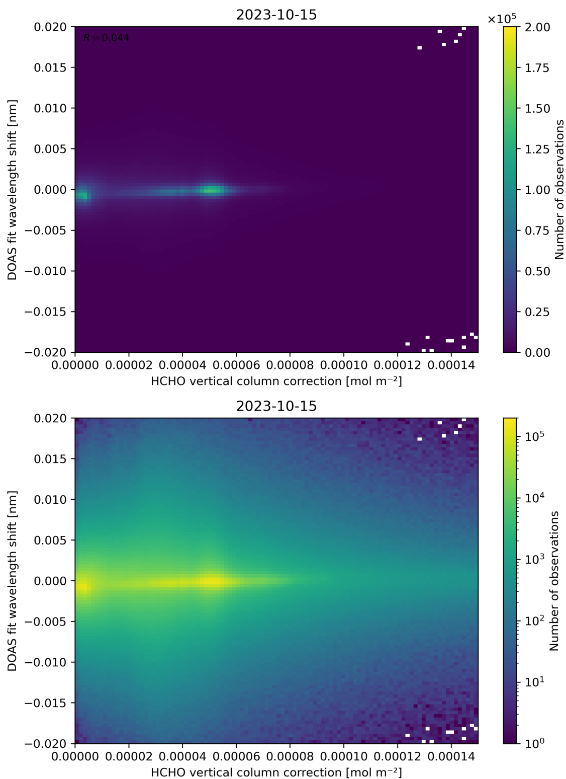
Figure 113: Scatter density plot of “HCHO vertical column correction” against “DOAS fit wavelength shift” for 2023-10-14 to 2023-10-16.
