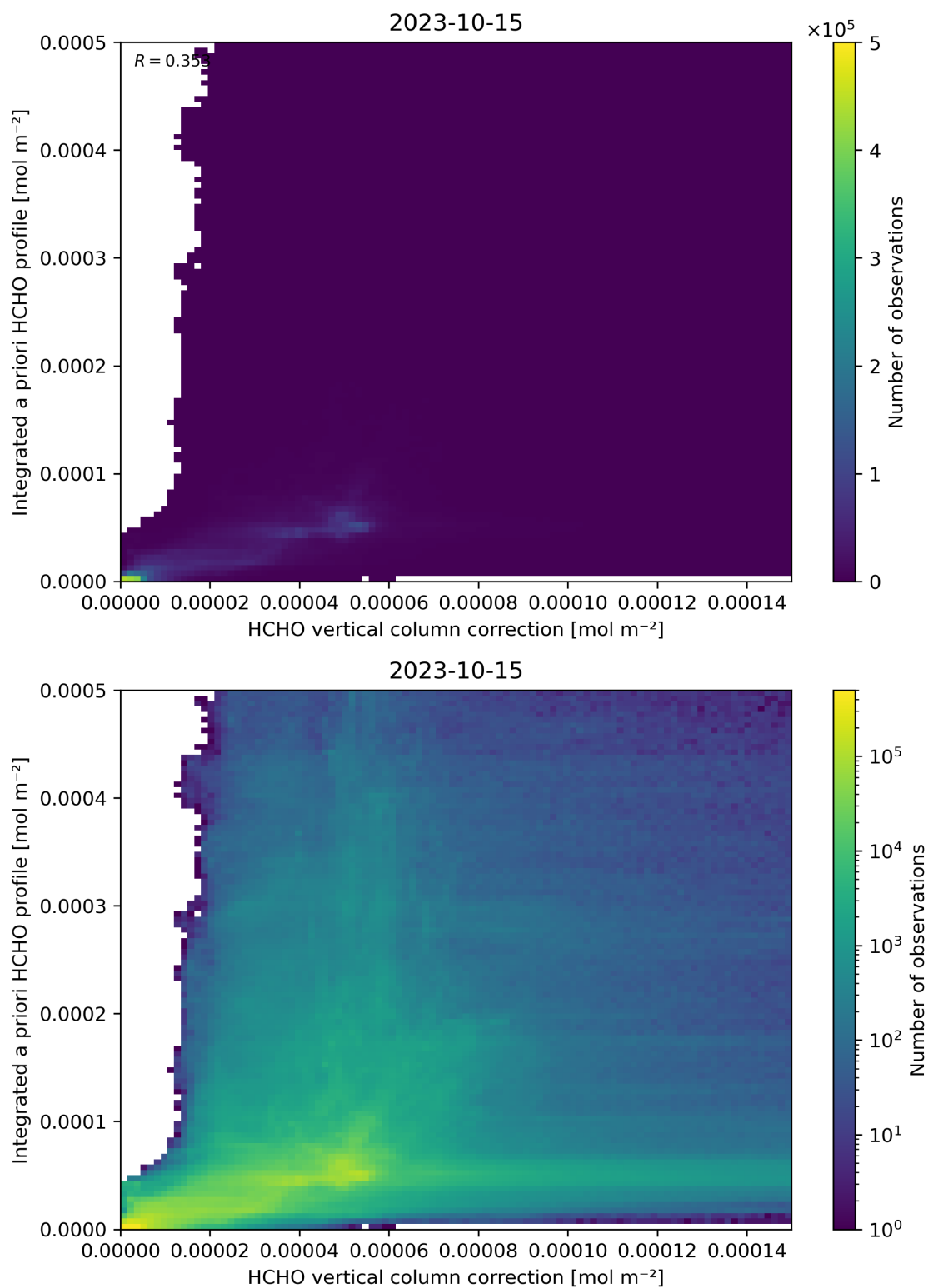
Figure 122: Scatter density plot of “HCHO vertical column correction” against “Integrated a priori HCHO profile” for 2023-10-14 to 2023-10-16.
