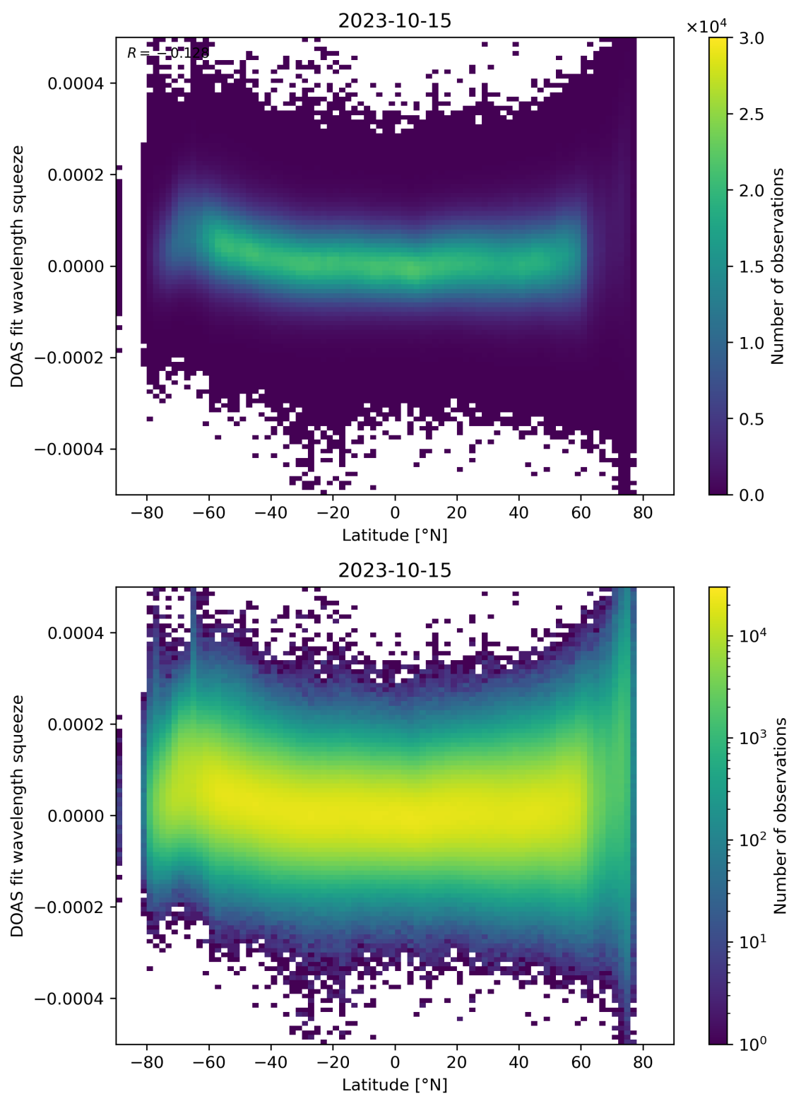
Figure 155: Scatter density plot of “Latitude” against “DOAS fit wavelength squeeze” for 2023-10-14 to 2023-10-16.
