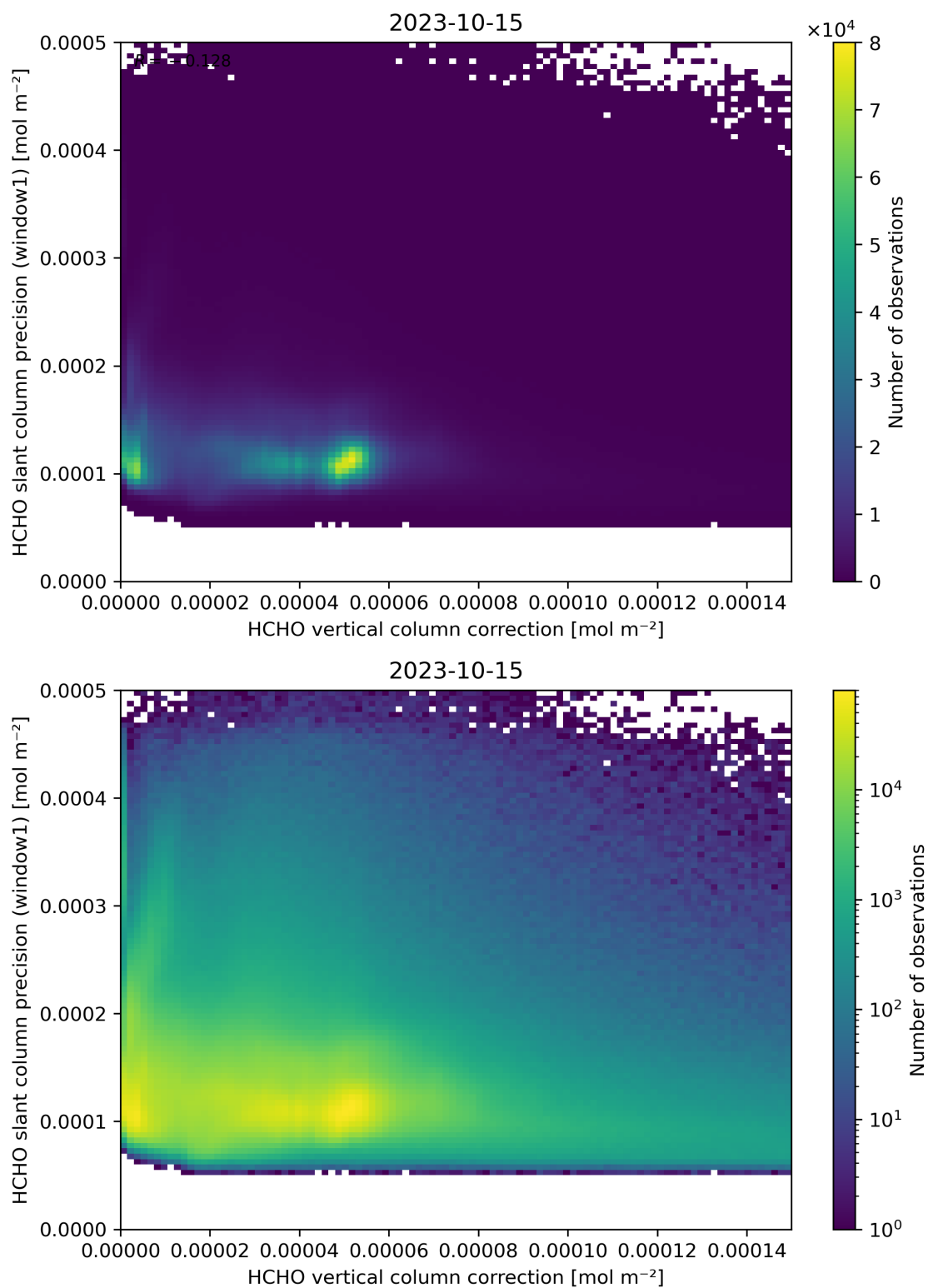
Figure 119: Scatter density plot of “HCHO vertical column correction” against “HCHO slant column precision (window1)” for 2023-10-14 to 2023-10-16.
