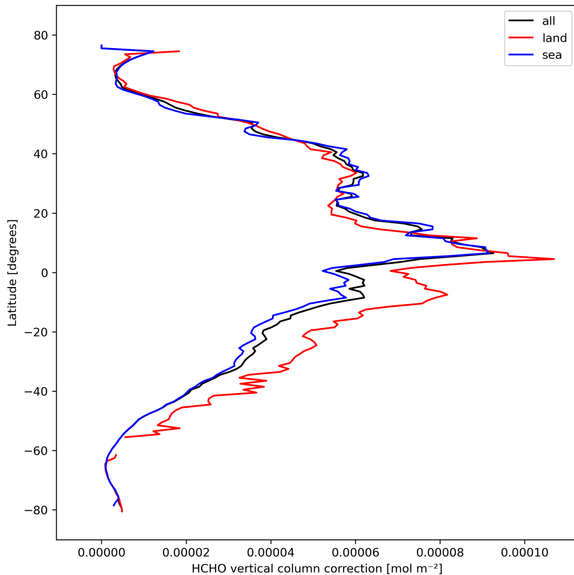
Figure 23: Zonal average of “HCHO vertical column correction” for 2023-10-14 to 2023-10-16.
