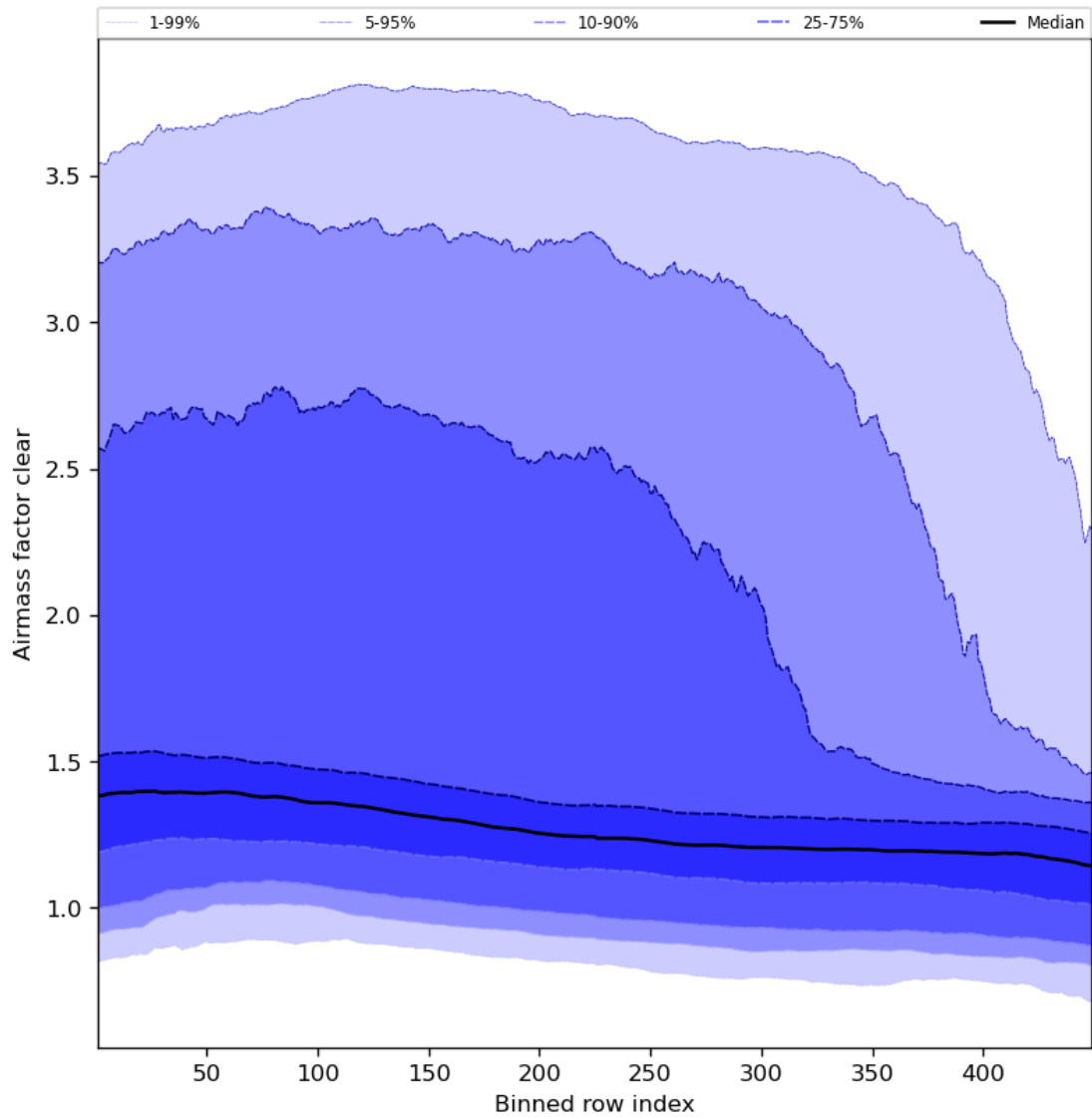
Figure 56: Along track statistics of “Airmass factor clear” for 2023-10-14 to 2023-10-16
