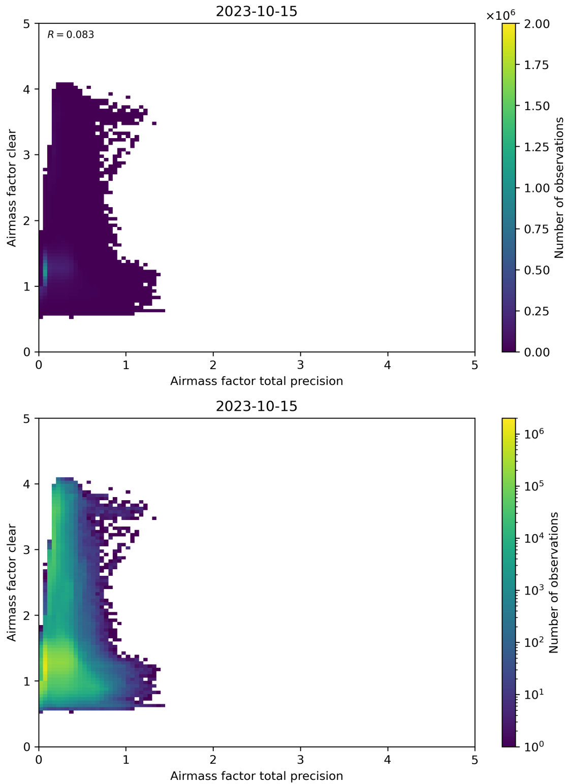
Figure 108: Scatter density plot of “Airmass factor total precision” against “Airmass factor clear” for 2023-10-14 to 2023-10-16.
