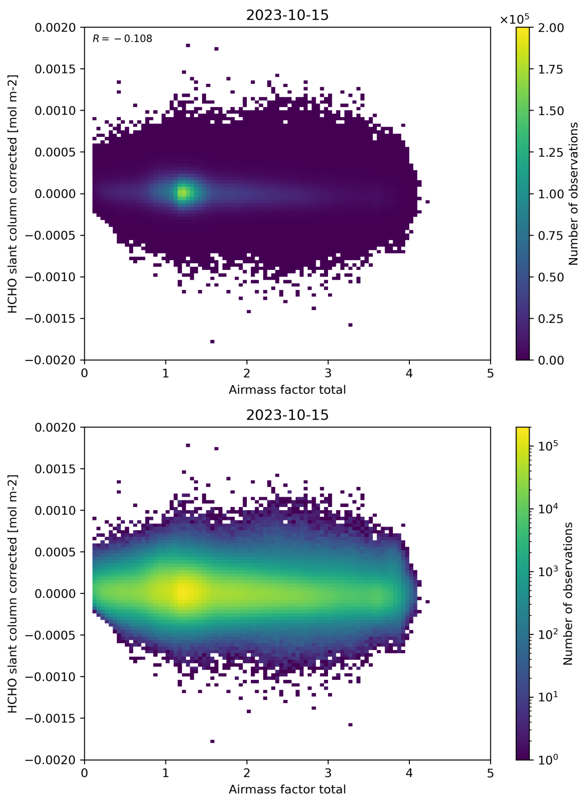
Figure 101: Scatter density plot of “Airmass factor total” against “HCHO slant column corrected” for 2023-10-14 to 2023-10-16.
