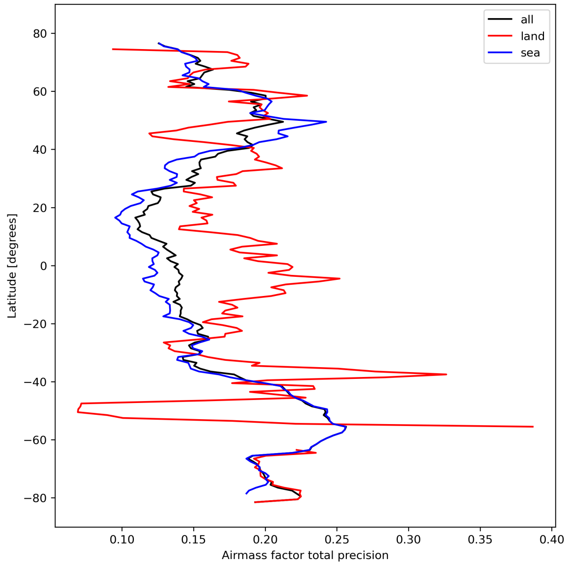
Figure 27: Zonal average of “Airmass factor total precision” for 2023-10-15 to 2023-10-17.
