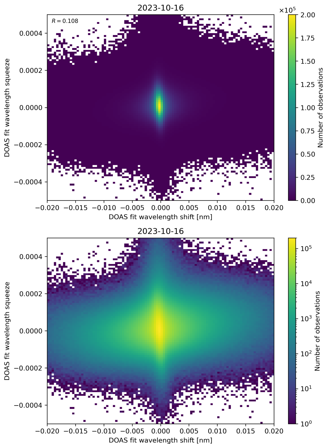
Figure 65: Scatter density plot of “DOAS fit wavelength shift” against “DOAS fit wavelength squeeze” for 2023-10-15 to 2023-10-17.
