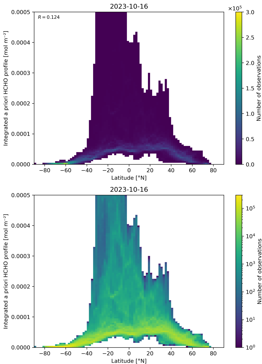
Figure 166: Scatter density plot of “Latitude” against “Integrated a priori HCHO profile” for 2023-10-15 to 2023-10-17.
