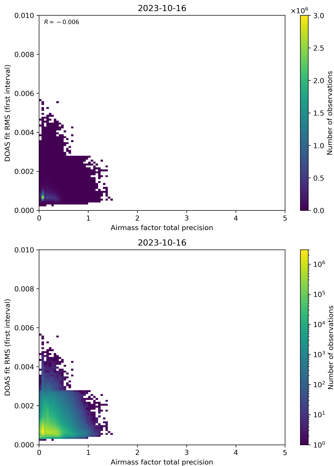
Figure 105: Scatter density plot of “Airmass factor total precision” against “DOAS fit RMS (first interval)” for 2023-10-15 to 2023-10-17.
