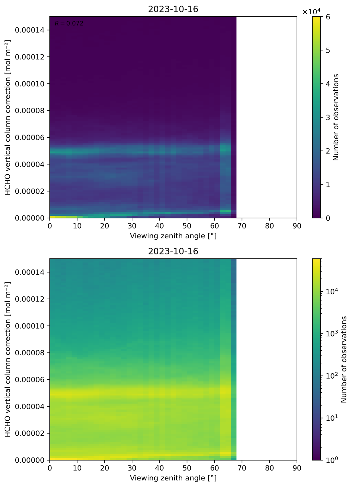
Figure 193: Scatter density plot of “Viewing zenith angle” against “HCHO vertical column correction” for 2023-10-15 to 2023-10-17.
