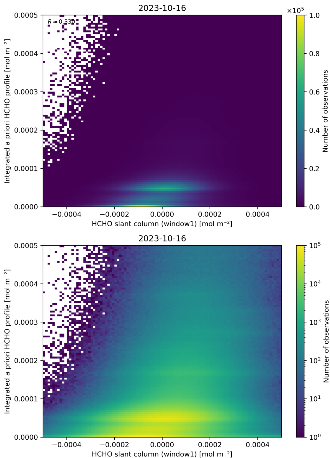
Figure 87: Scatter density plot of “HCHO slant column (window1)” against “Integrated a priori HCHO profile” for 2023-10-15 to 2023-10-17.
