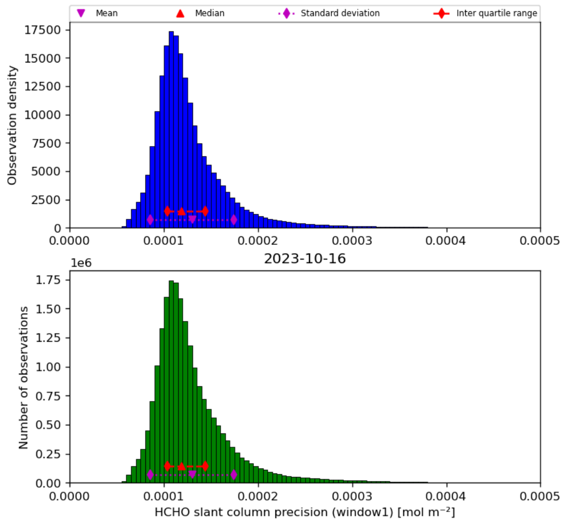
Figure 39: Histogram of “HCHO slant column precision (window1)” for 2023-10-15 to 2023-10-17
