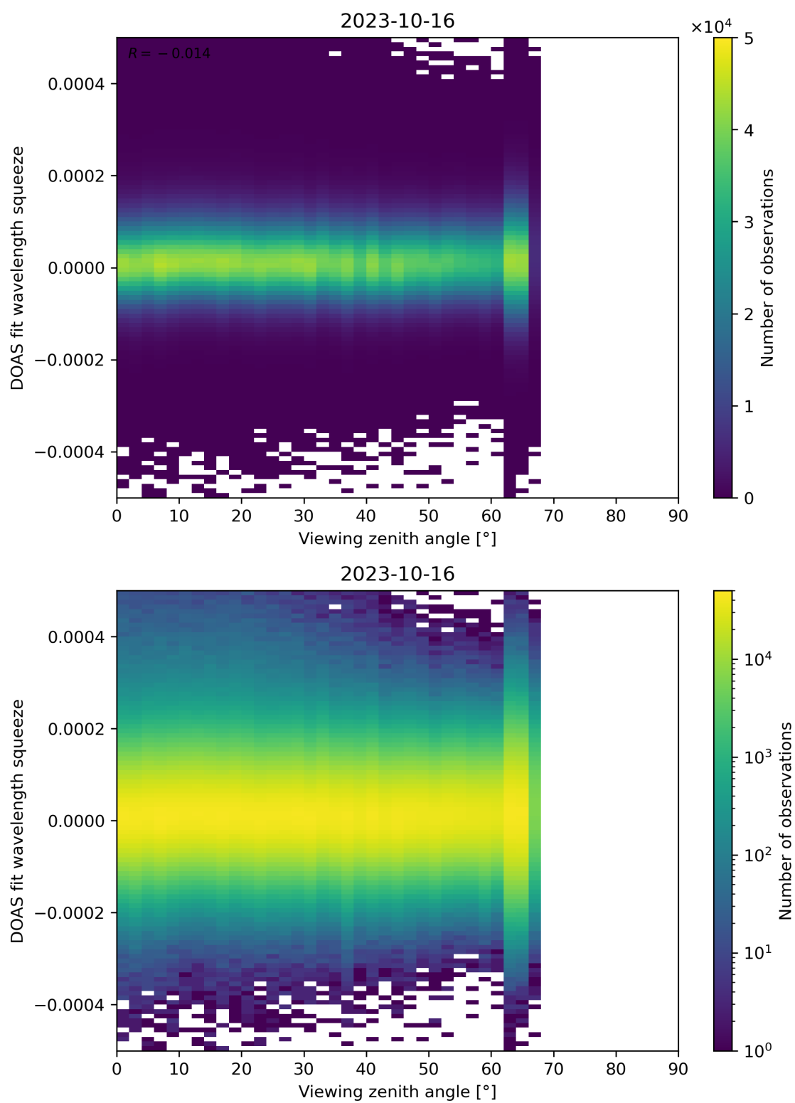
Figure 184: Scatter density plot of “Viewing zenith angle” against “DOAS fit wavelength squeeze” for 2023-10-15 to 2023-10-17.
