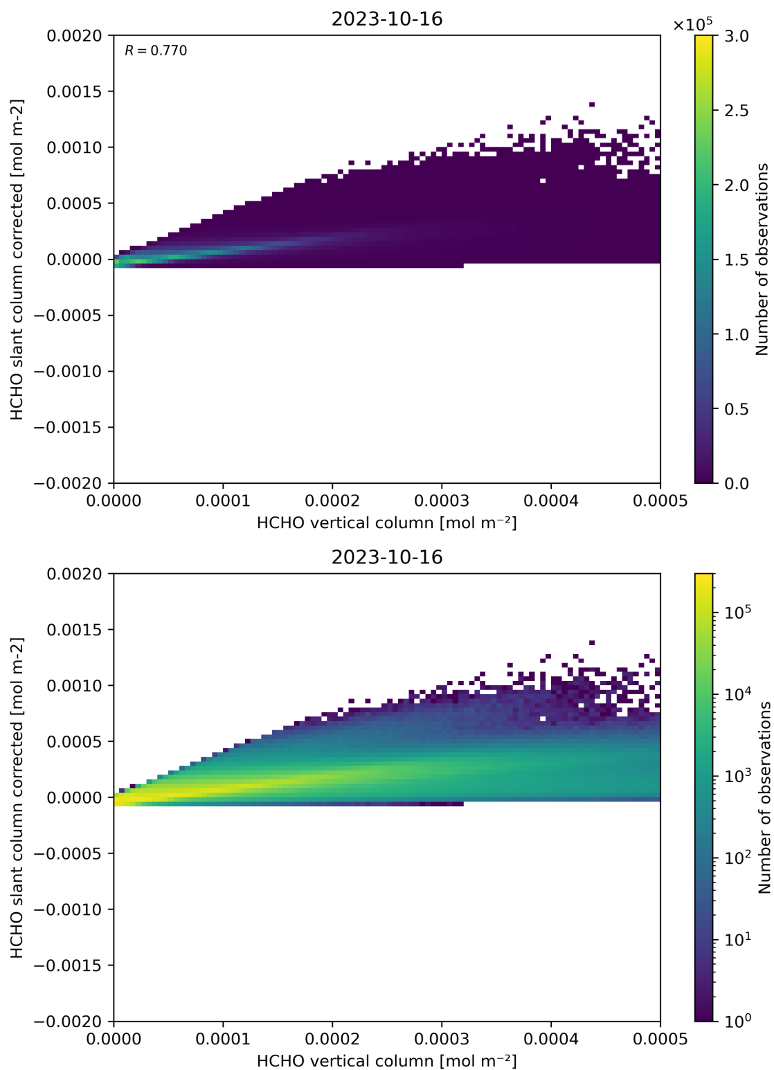
Figure 127: Scatter density plot of “HCHO vertical column” against “HCHO slant column corrected” for 2023-10-15 to 2023-10-17.
