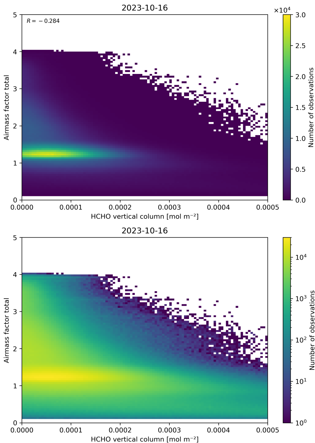
Figure 131: Scatter density plot of “HCHO vertical column” against “Airmass factor total” for 2023-10-15 to 2023-10-17.
