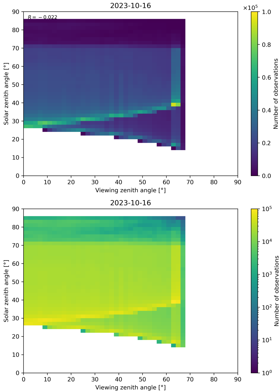
Figure 197: Scatter density plot of “Viewing zenith angle” against “Solar zenith angle” for 2023-10-15 to 2023-10-17.
