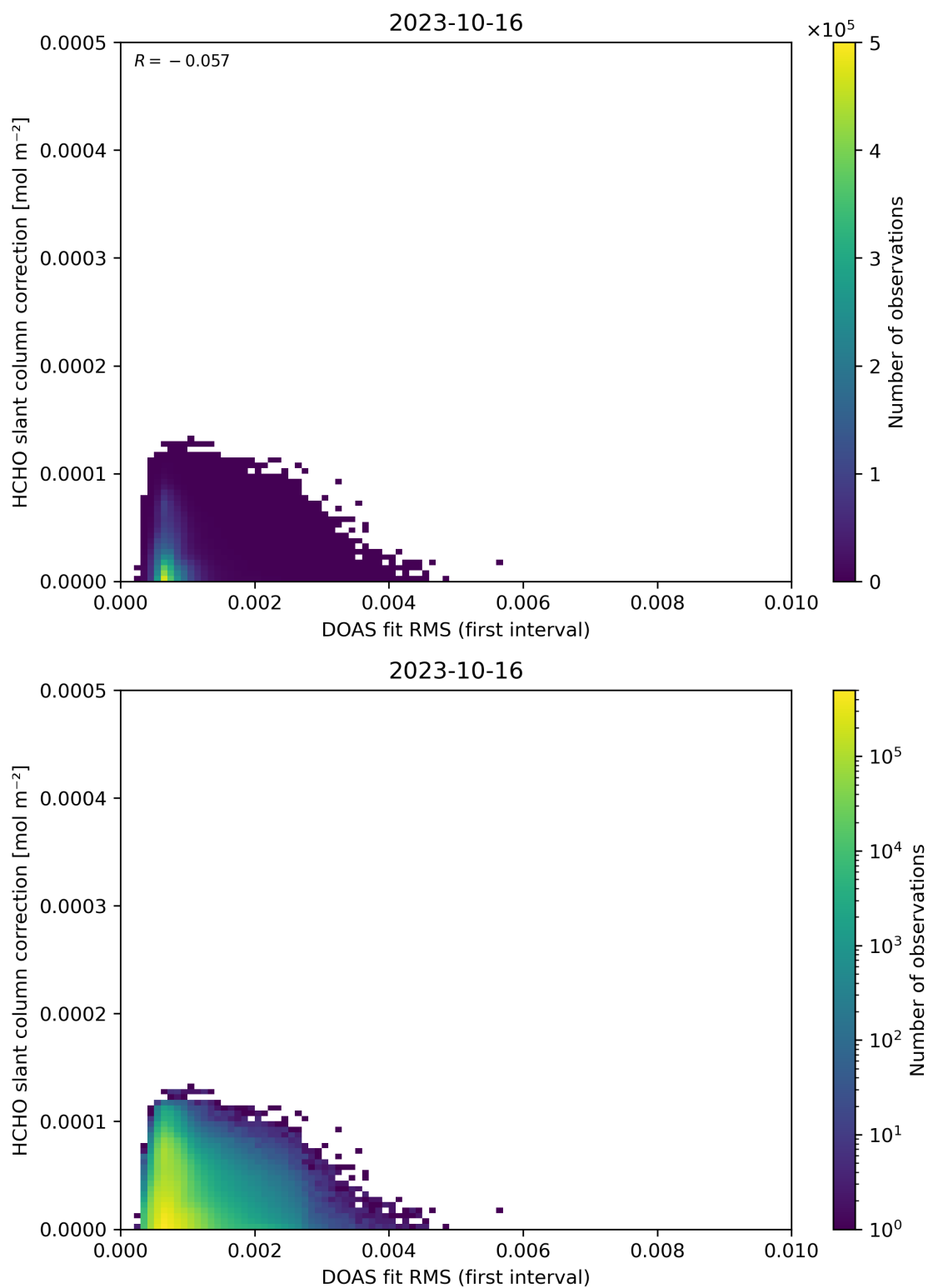
Figure 63: Scatter density plot of “DOAS fit RMS (first interval)” against “HCHO slant column correction” for 2023-10-15 to 2023-10-17.
