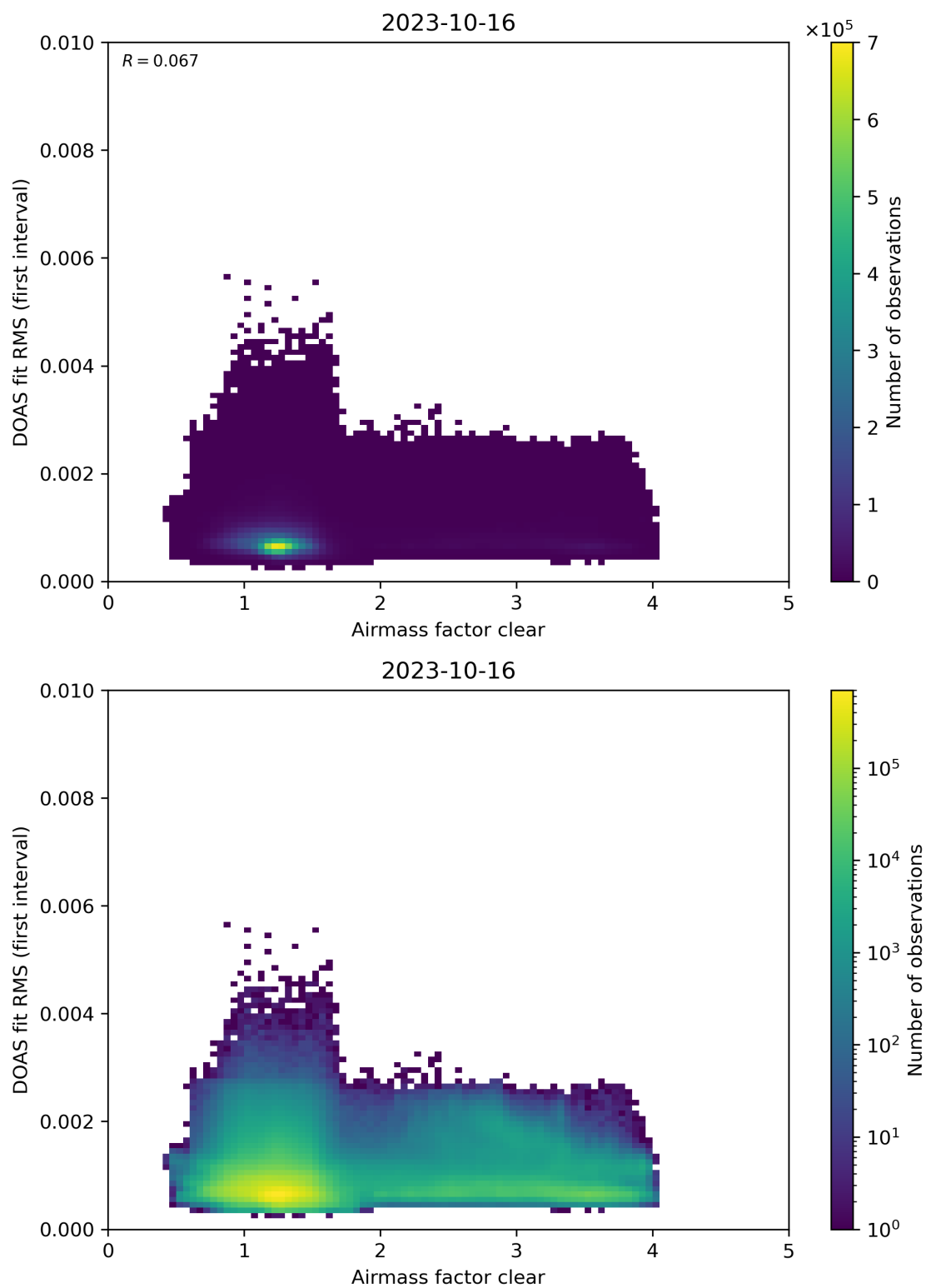
Figure 71: Scatter density plot of “Airmass factor clear” against “DOAS fit RMS (first interval)” for 2023-10-15 to 2023-10-17.
