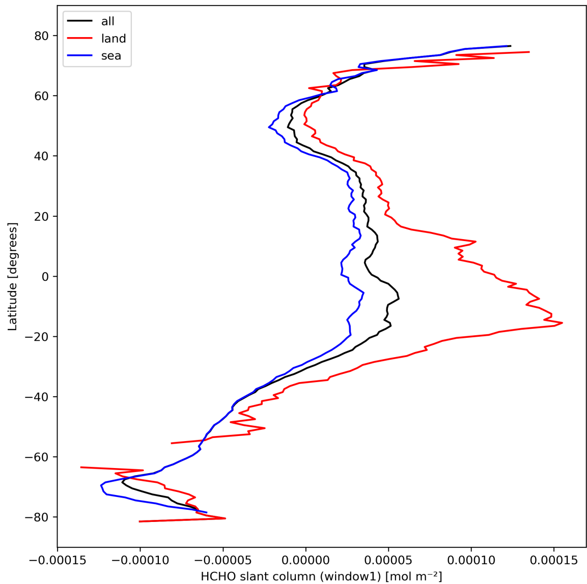
Figure 24: Zonal average of “HCHO slant column (window1)” for 2023-10-15 to 2023-10-17.
