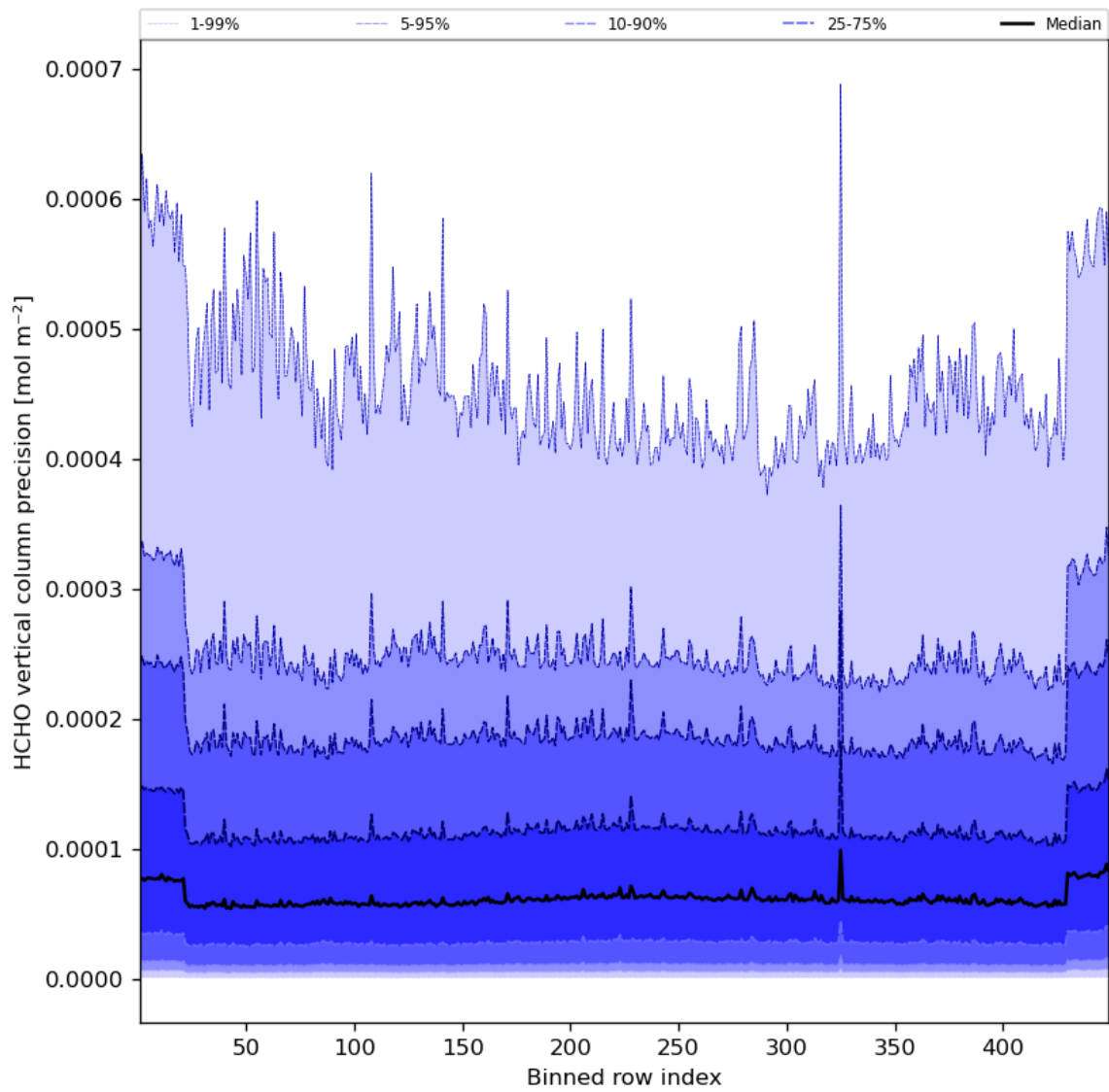
Figure 50: Along track statistics of “HCHO vertical column precision” for 2023-10-15 to 2023-10-17
