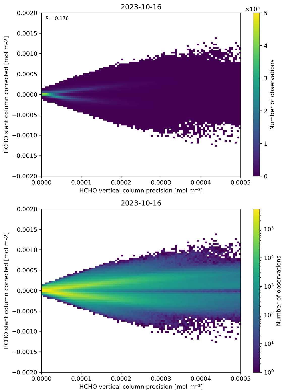
Figure 140: Scatter density plot of “HCHO vertical column precision” against “HCHO slant column corrected” for 2023-10-15 to 2023-10-17.
