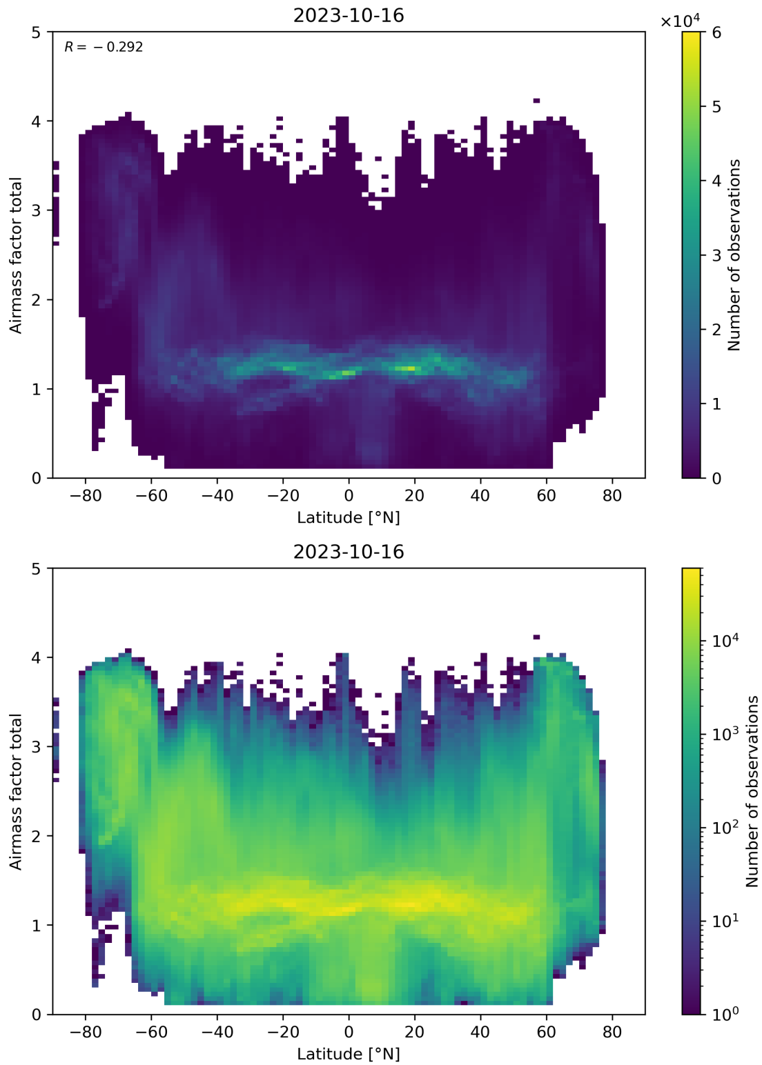
Figure 161: Scatter density plot of “Latitude” against “Airmass factor total” for 2023-10-15 to 2023-10-17.
