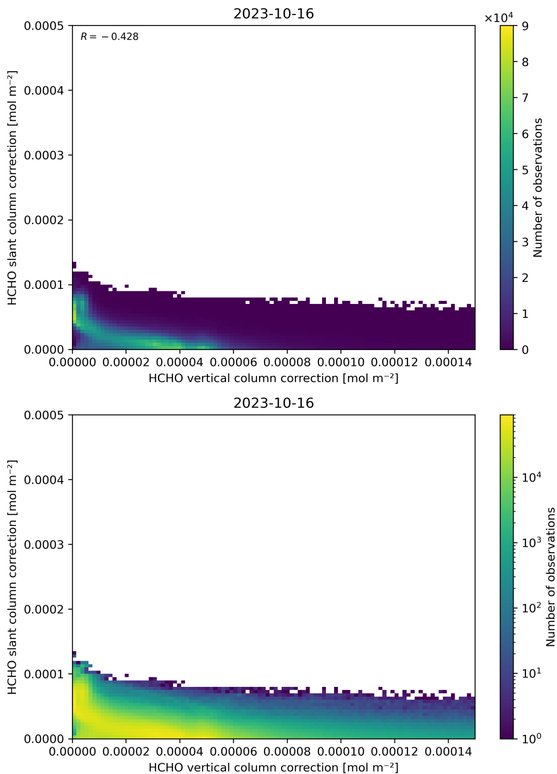
Figure 117: Scatter density plot of “HCHO vertical column correction” against “HCHO slant column correction” for 2023-10-15 to 2023-10-17.
