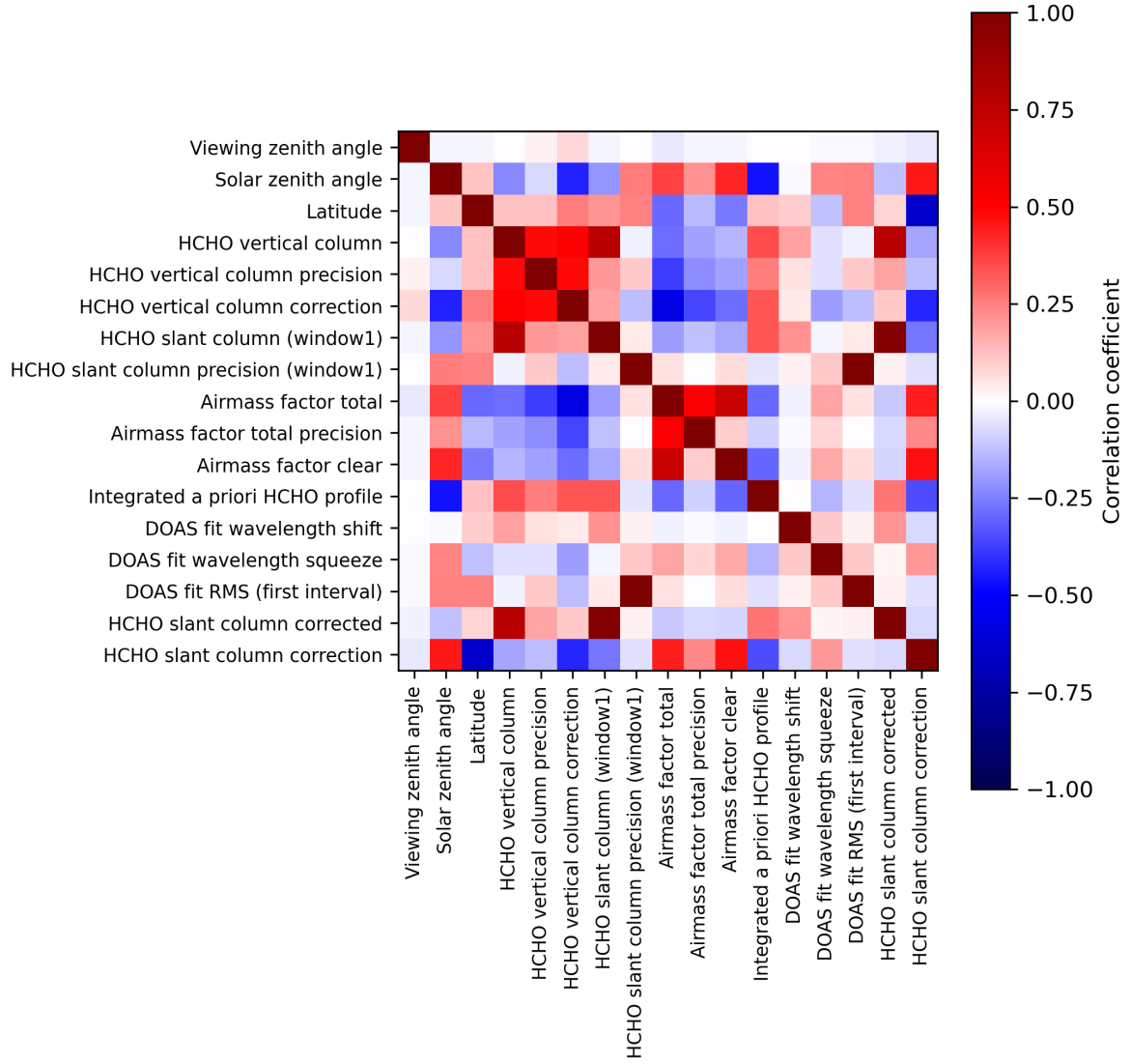
Figure 2: Map of correlation matrix for 2023-10-15 to 2023-10-17.
