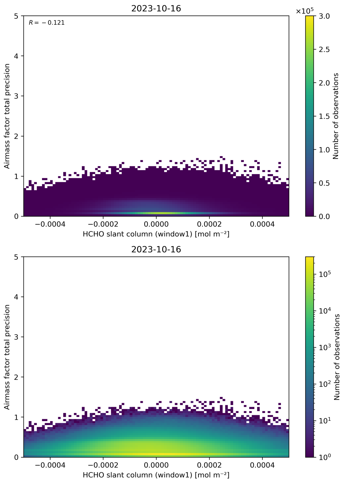
Figure 86: Scatter density plot of “HCHO slant column (window1)” against “Airmass factor total precision” for 2023-10-15 to 2023-10-17.
