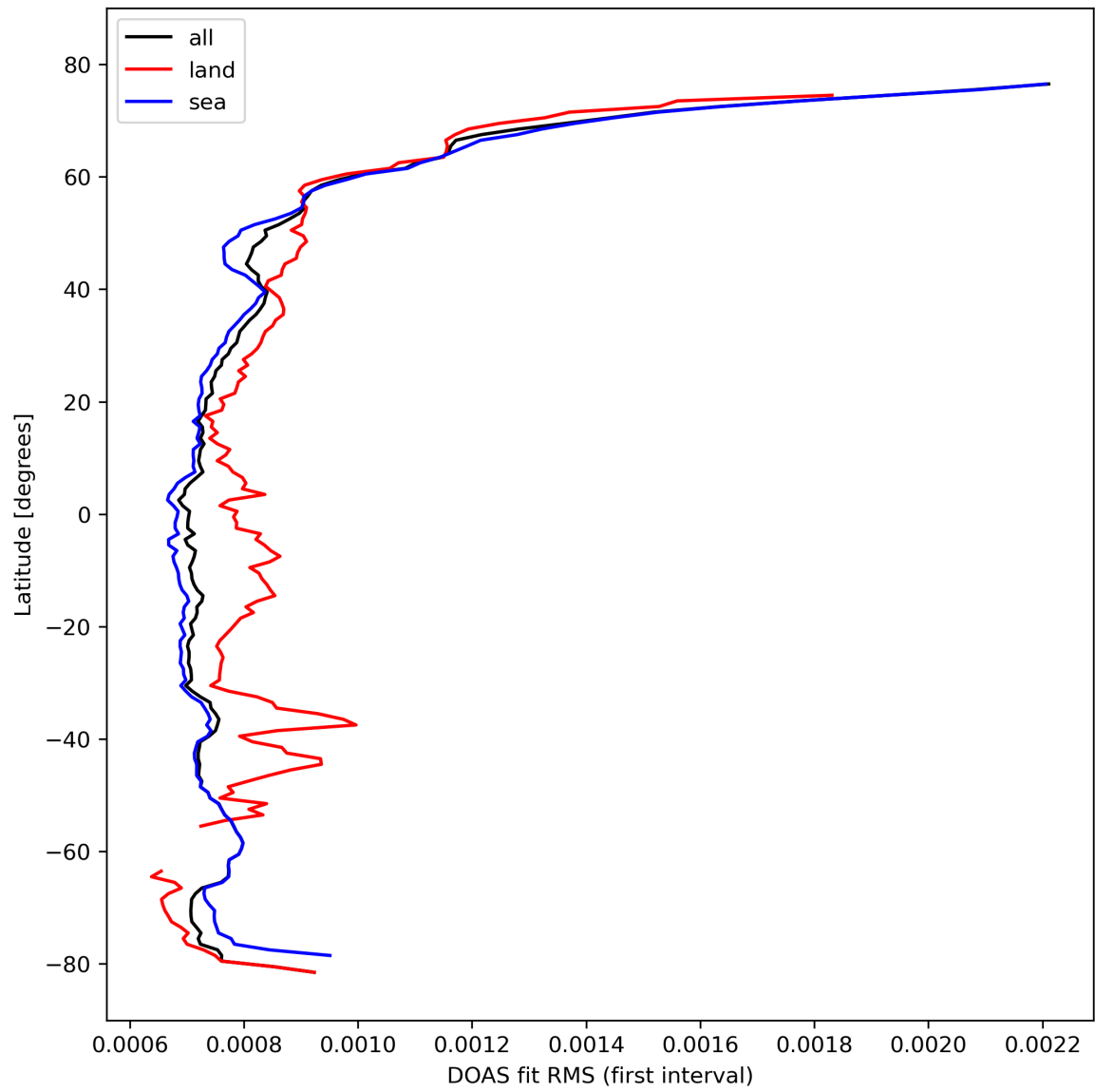
Figure 32: Zonal average of “DOAS fit RMS (first interval)” for 2023-10-15 to 2023-10-17.
