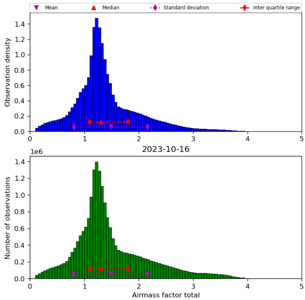
Figure 40: Histogram of “Airmass factor total” for 2023-10-15 to 2023-10-17
