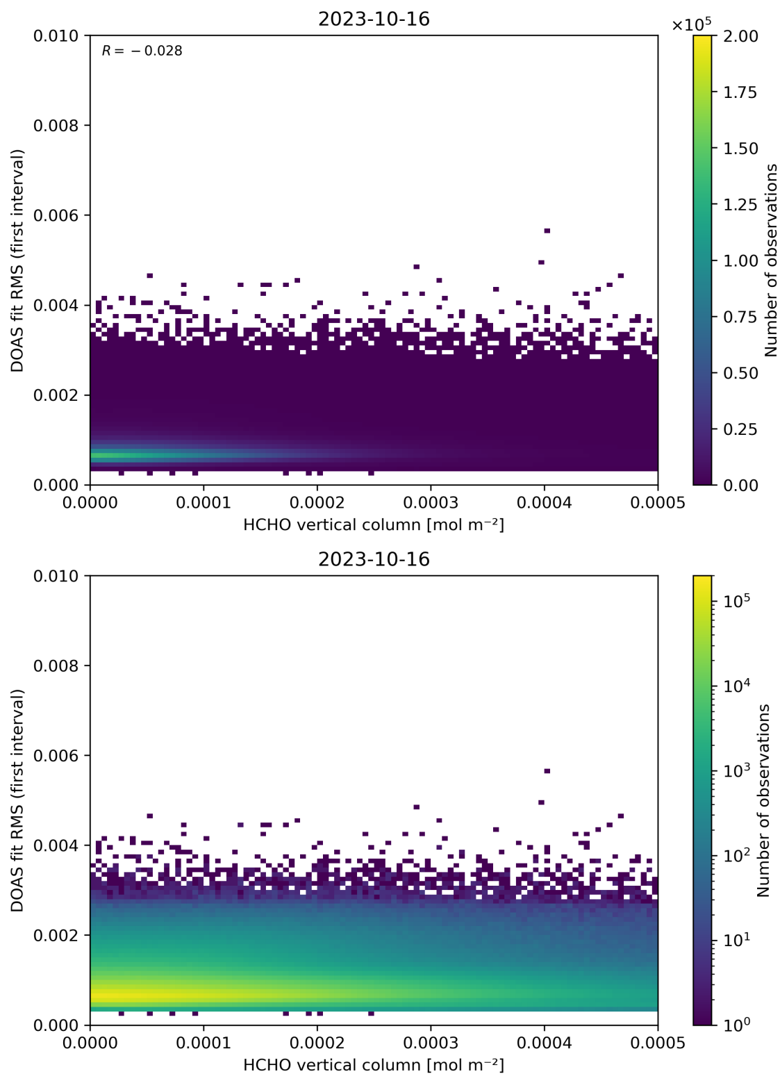
Figure 123: Scatter density plot of “HCHO vertical column” against “DOAS fit RMS (first interval)” for 2023-10-15 to 2023-10-17.
