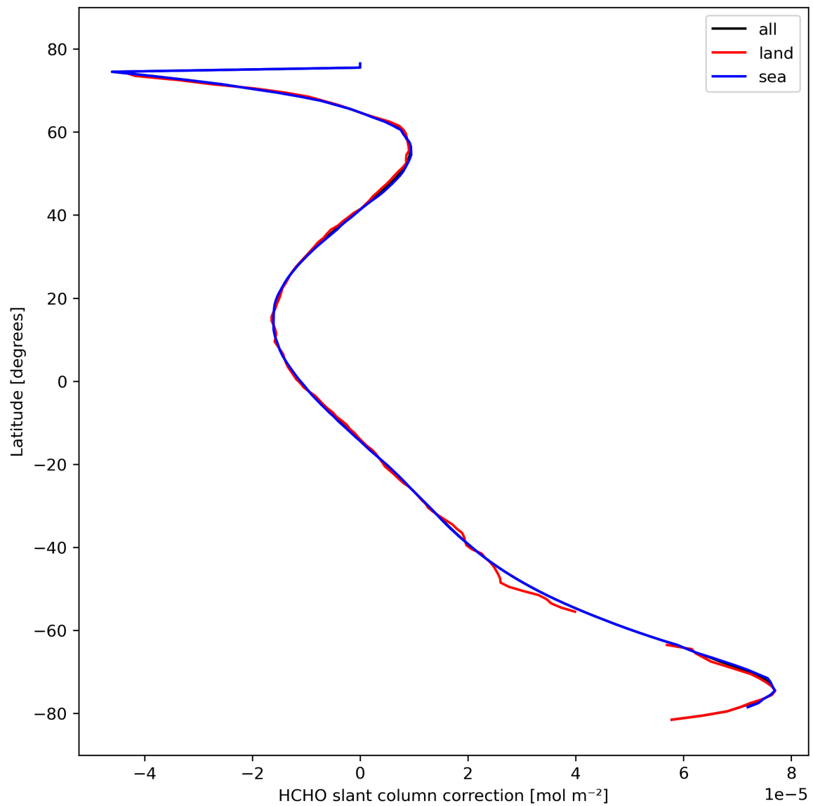
Figure 33: Zonal average of “HCHO slant column correction” for 2023-10-15 to 2023-10-17.
