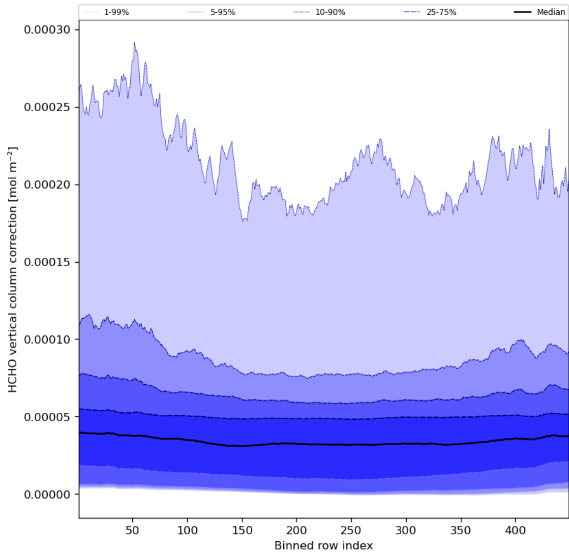
Figure 51: Along track statistics of “HCHO vertical column correction” for 2023-10-15 to 2023-10-17
