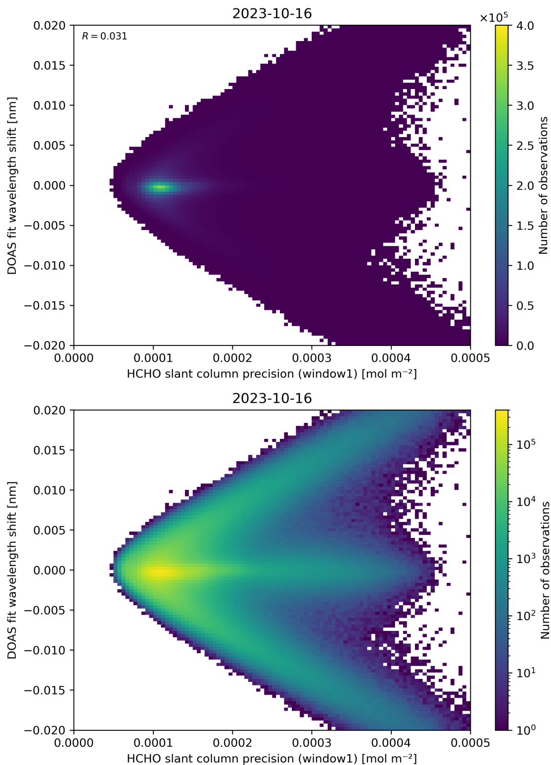
Figure 89: Scatter density plot of “HCHO slant column precision (window1)” against “DOAS fit wavelength shift” for 2023-10-15 to 2023-10-17.
