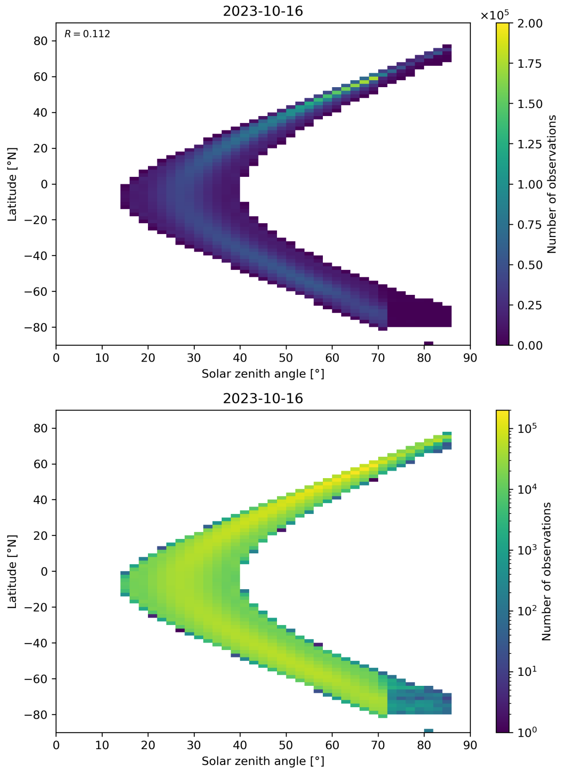
Figure 181: Scatter density plot of “Solar zenith angle” against “Latitude” for 2023-10-15 to 2023-10-17.
