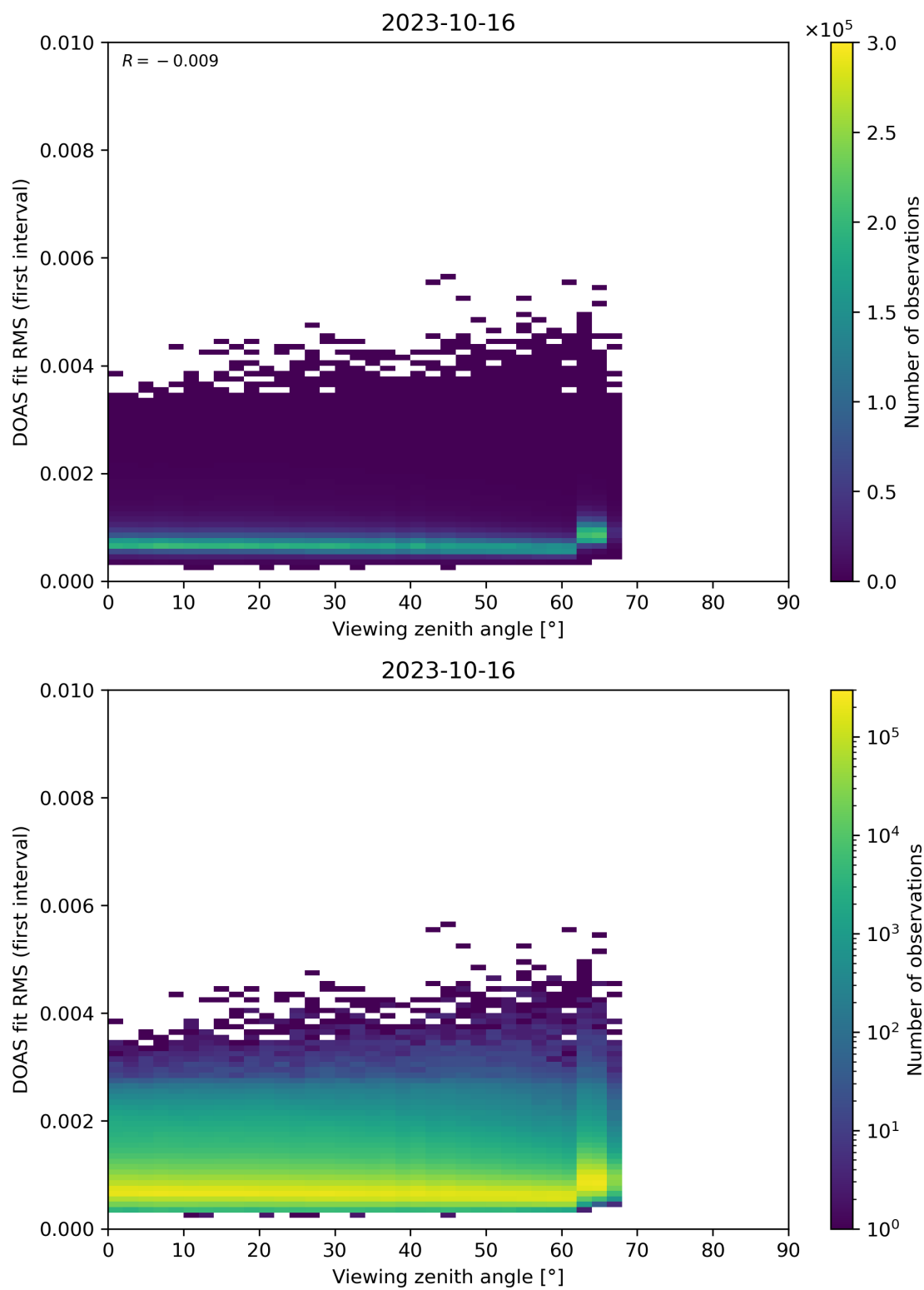
Figure 182: Scatter density plot of “Viewing zenith angle” against “DOAS fit RMS (first interval)” for 2023-10-15 to 2023-10-17.
