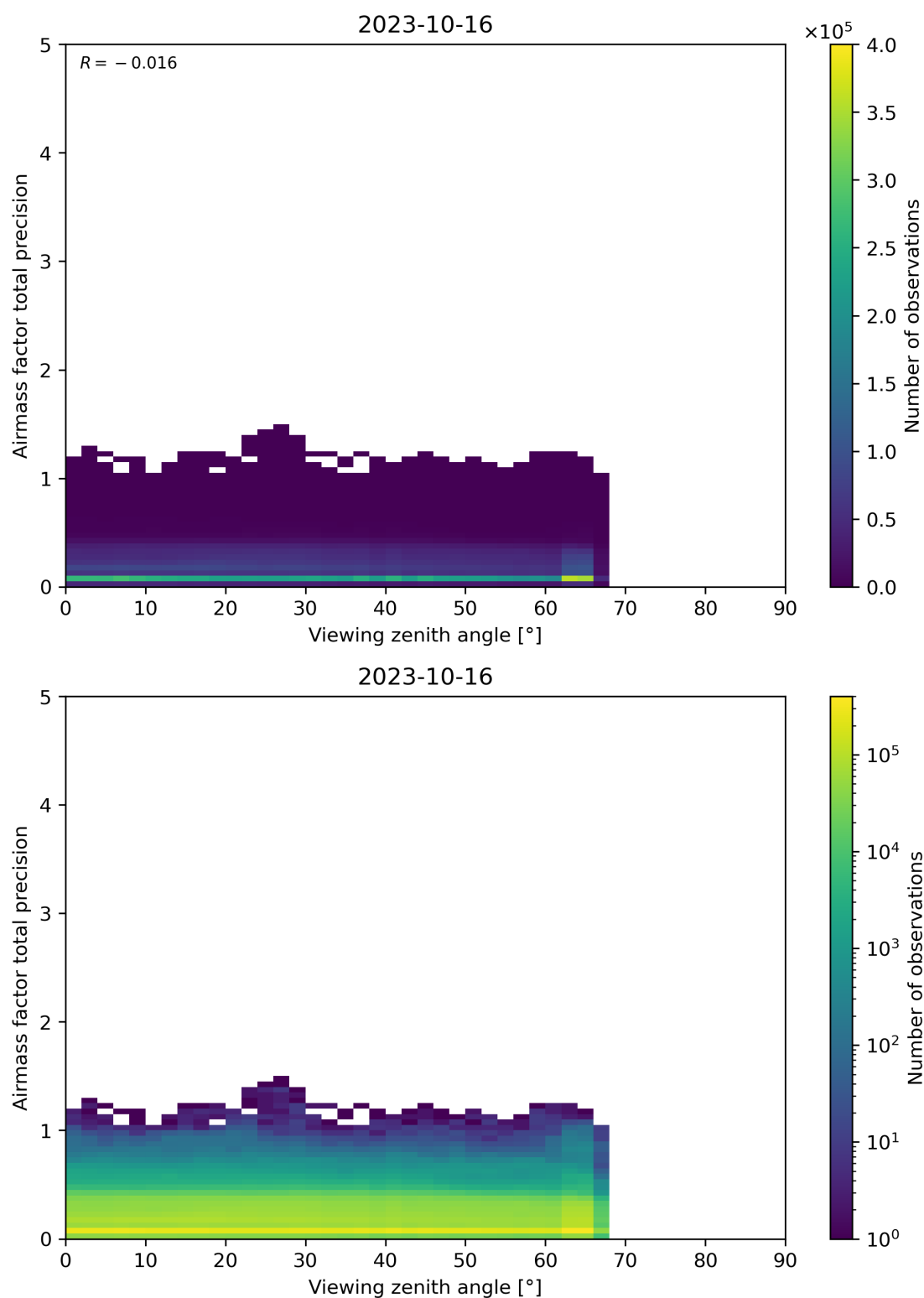
Figure 191: Scatter density plot of “Viewing zenith angle” against “Airmass factor total precision” for 2023-10-15 to 2023-10-17.
