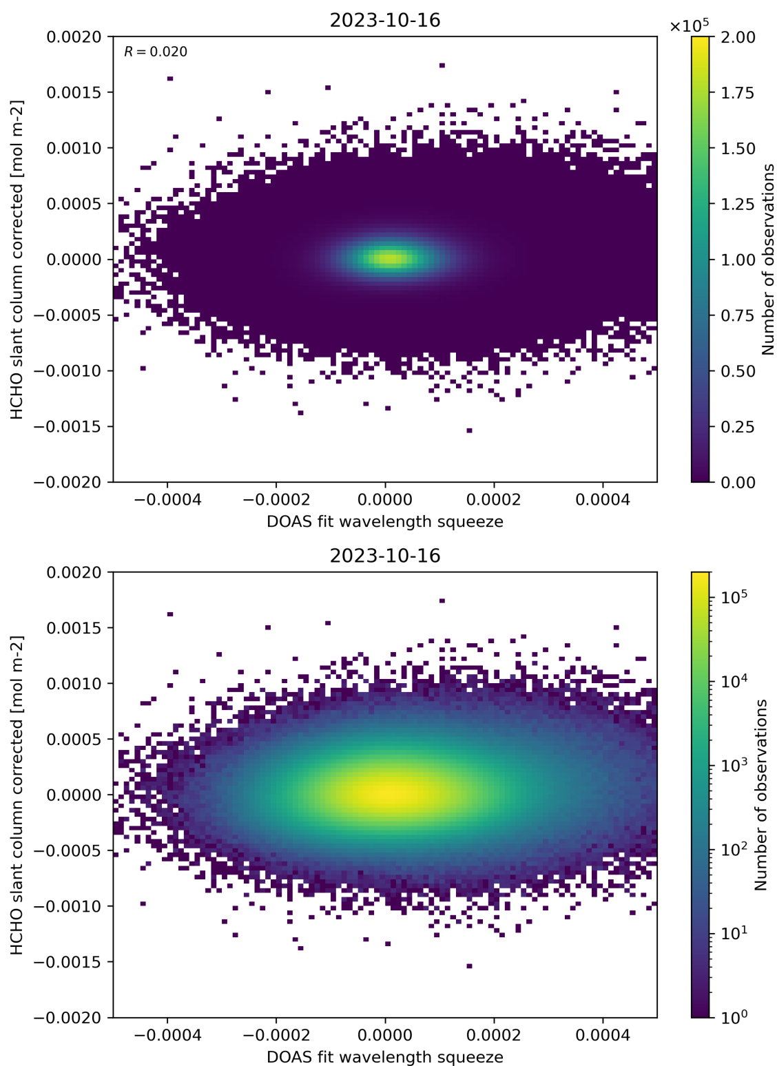
Figure 69: Scatter density plot of “DOAS fit wavelength squeeze” against “HCHO slant column corrected” for 2023-10-15 to 2023-10-17.
