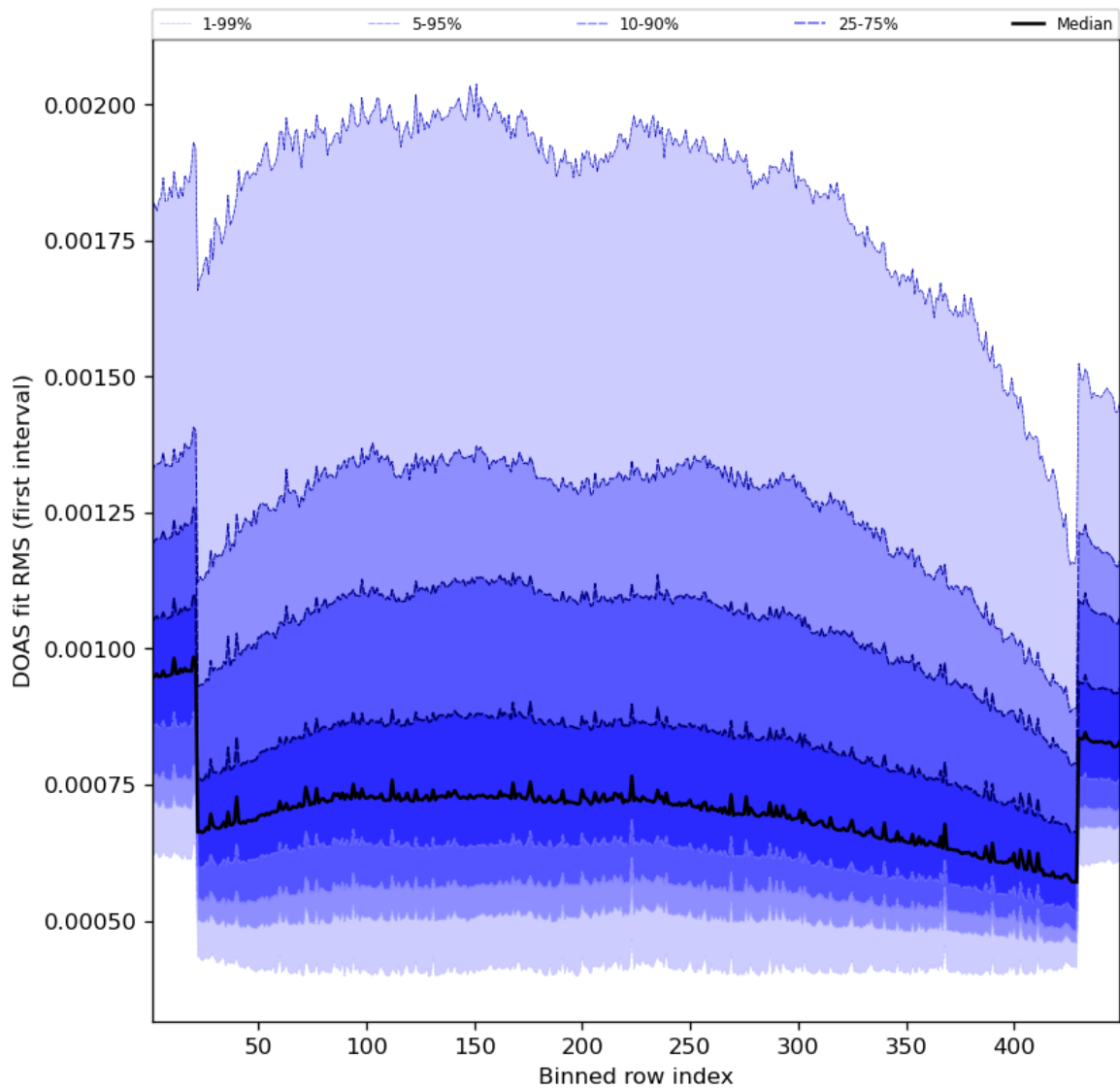
Figure 60: Along track statistics of “DOAS fit RMS (first interval)” for 2023-10-15 to 2023-10-17
