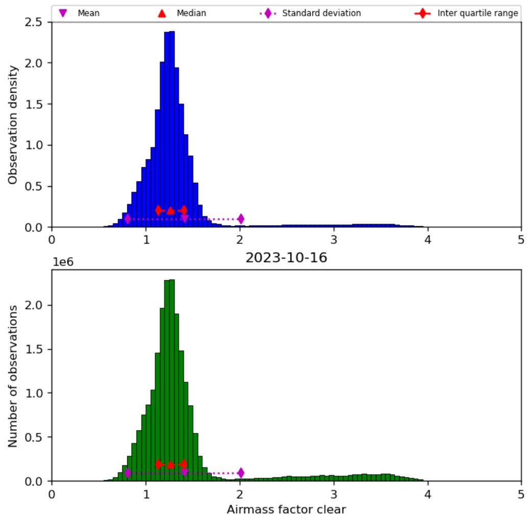
Figure 42: Histogram of “Airmass factor clear” for 2023-10-15 to 2023-10-17
