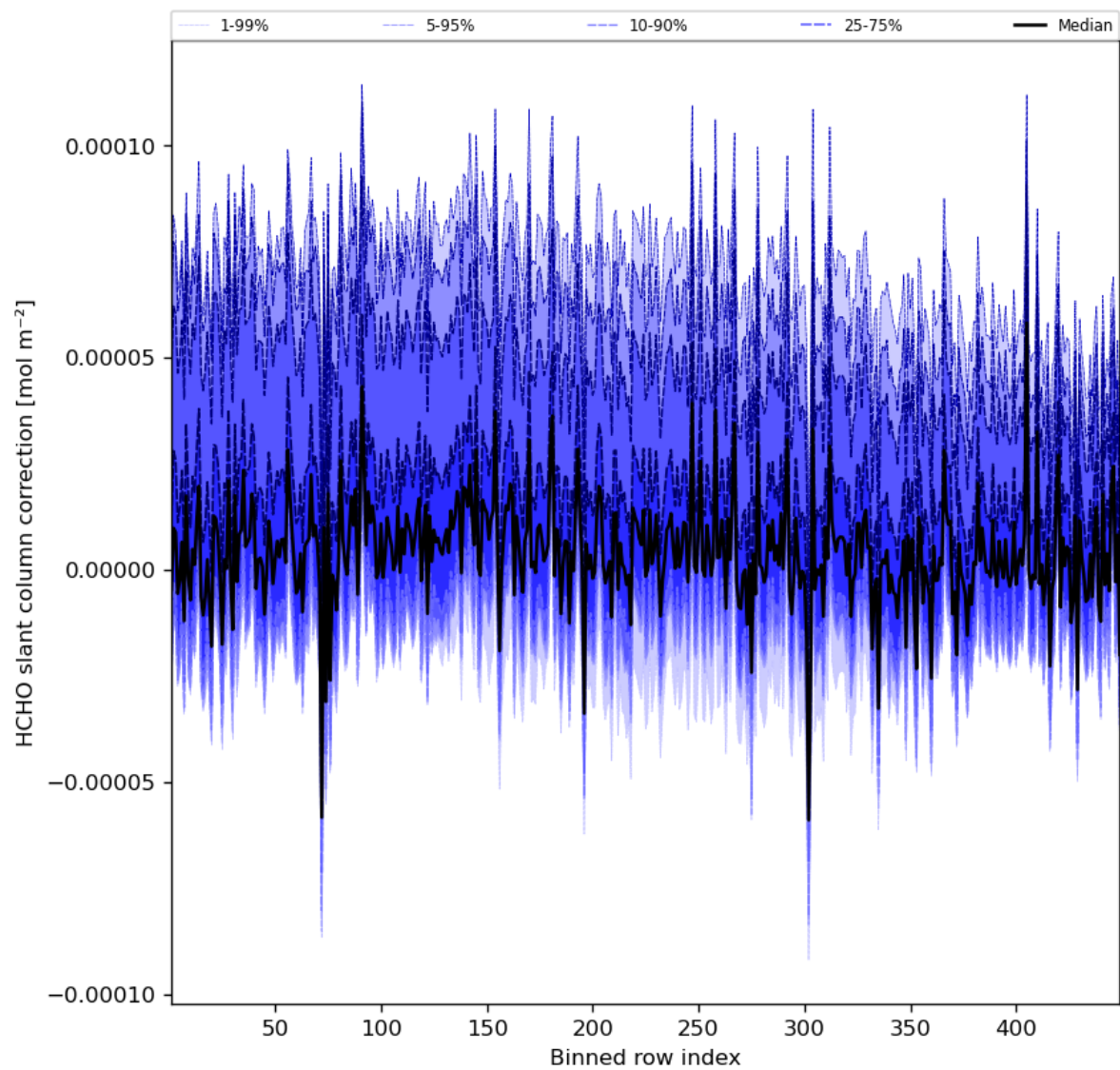
Figure 61: Along track statistics of “HCHO slant column correction” for 2023-10-15 to 2023-10-17
