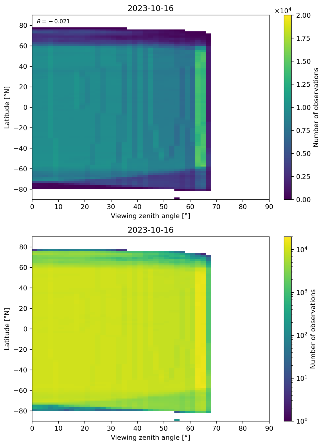
Figure 196: Scatter density plot of “Viewing zenith angle” against “Latitude” for 2023-10-15 to 2023-10-17.
