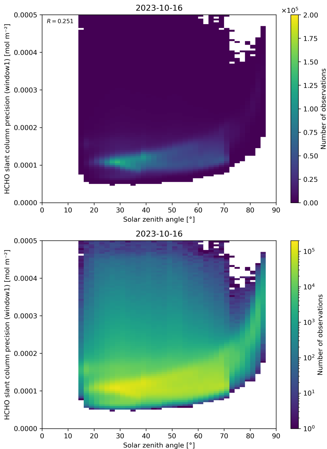
Figure 174: Scatter density plot of “Solar zenith angle” against “HCHO slant column precision (window1)” for 2023-10-15 to 2023-10-17.
