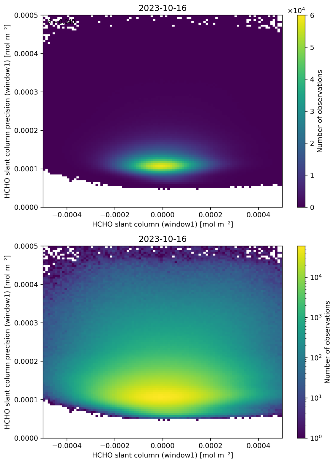
Figure 84: Scatter density plot of “HCHO slant column (window1)” against “HCHO slant column precision (window1)” for 2023-10-15 to 2023-10-17.
