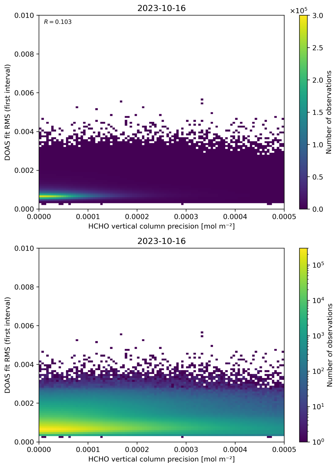
Figure 136: Scatter density plot of “HCHO vertical column precision” against “DOAS fit RMS (first interval)” for 2023-10-15 to 2023-10-17.
