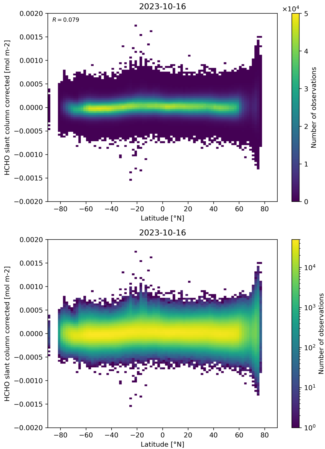
Figure 157: Scatter density plot of “Latitude” against “HCHO slant column corrected” for 2023-10-15 to 2023-10-17.
