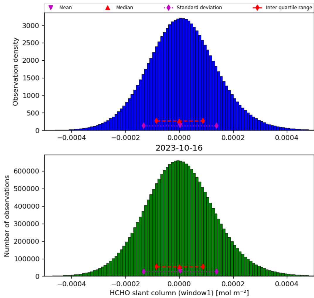
Figure 38: Histogram of “HCHO slant column (window1)” for 2023-10-15 to 2023-10-17
