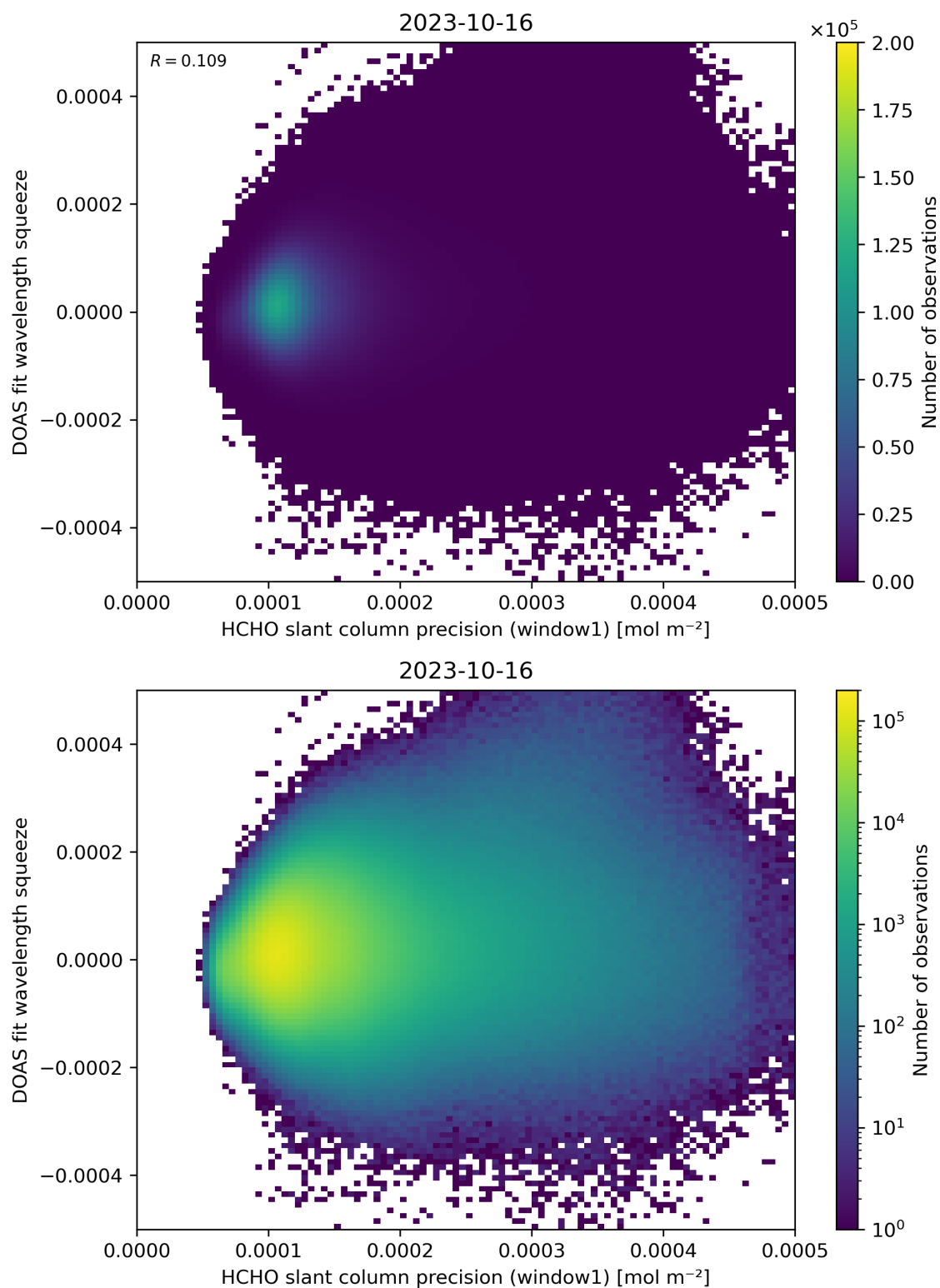
Figure 90: Scatter density plot of “HCHO slant column precision (window1)” against “DOAS fit wavelength squeeze” for 2023-10-15 to 2023-10-17.
