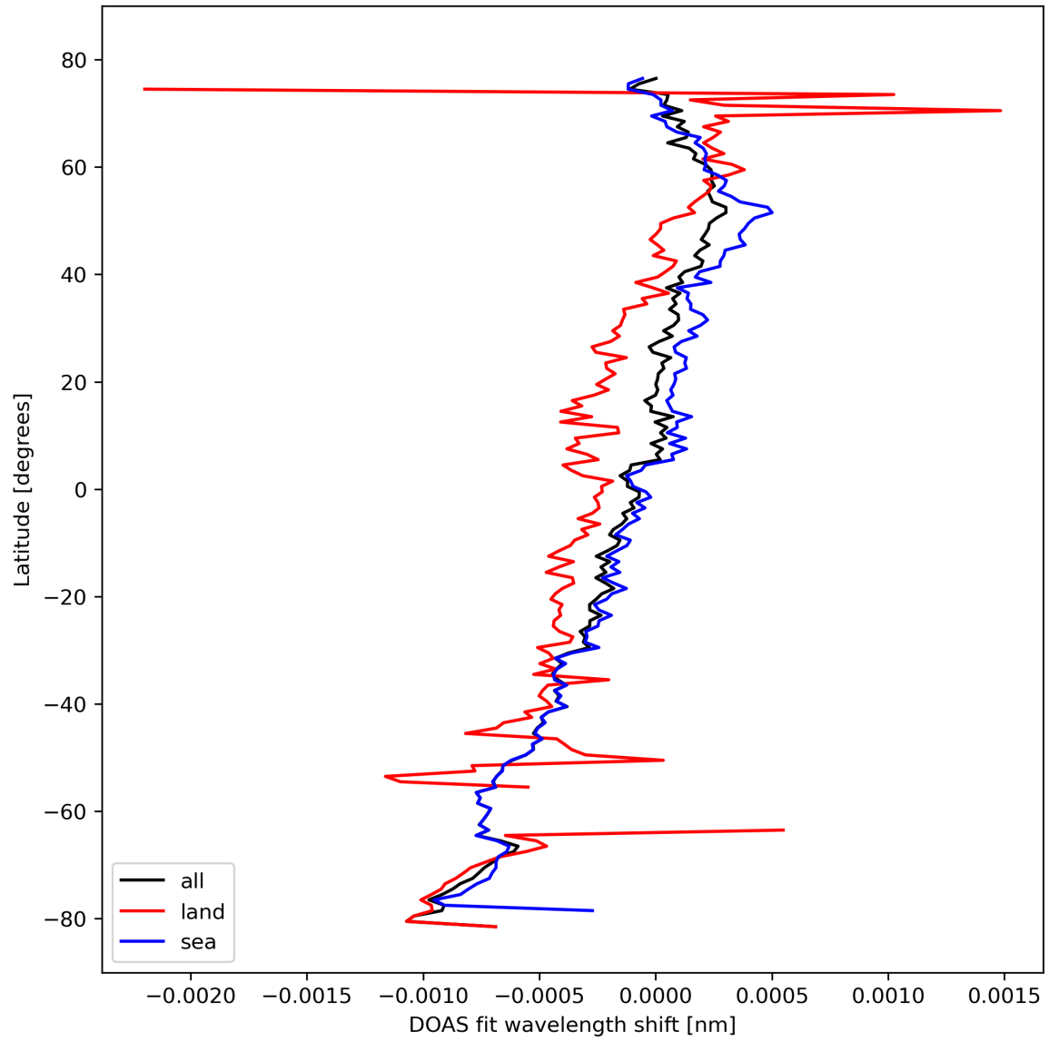
Figure 30: Zonal average of “DOAS fit wavelength shift” for 2023-10-15 to 2023-10-17.
