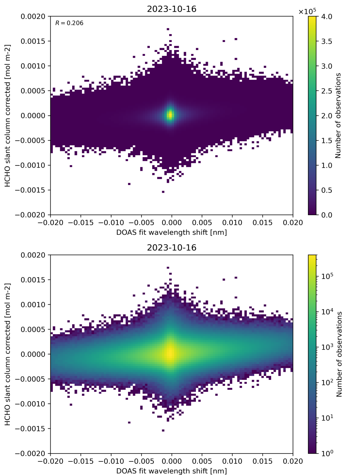
Figure 66: Scatter density plot of “DOAS fit wavelength shift” against “HCHO slant column corrected” for 2023-10-15 to 2023-10-17.
