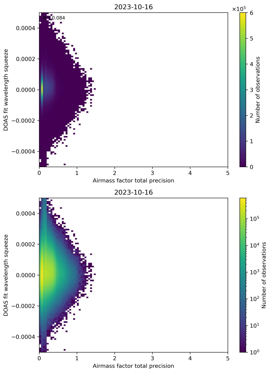
Figure 107: Scatter density plot of “Airmass factor total precision” against “DOAS fit wavelength squeeze” for 2023-10-15 to 2023-10-17.
