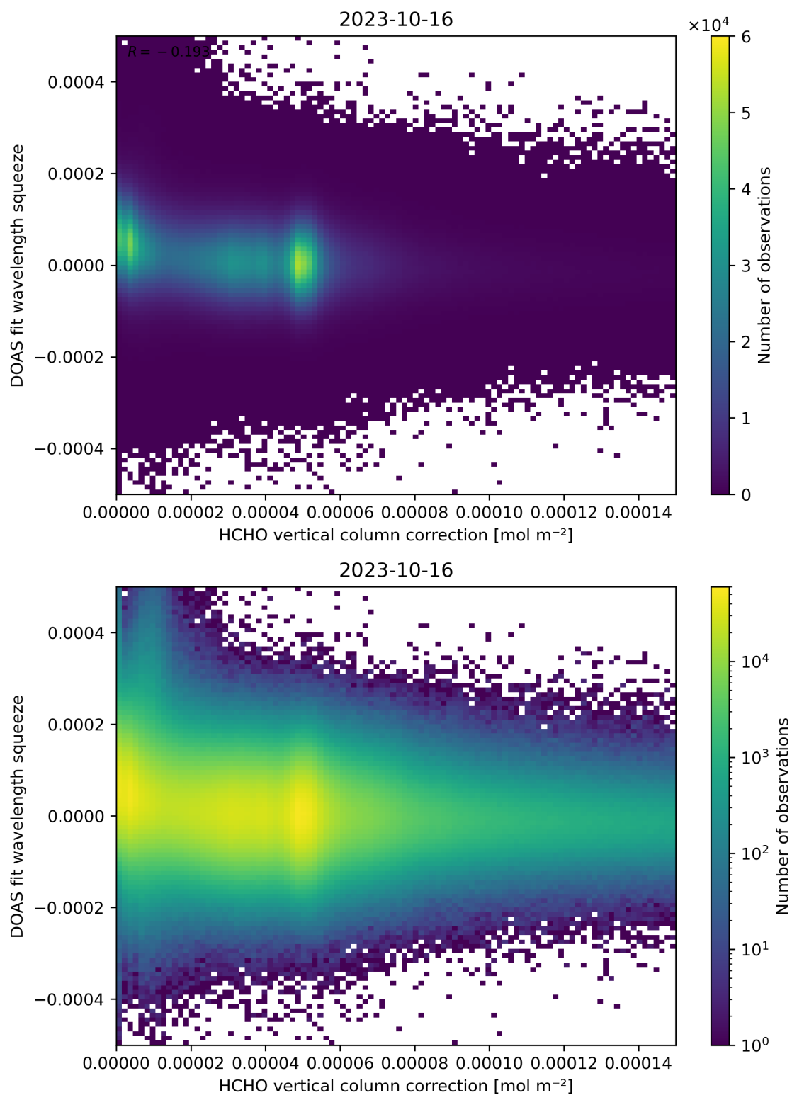
Figure 114: Scatter density plot of “HCHO vertical column correction” against “DOAS fit wavelength squeeze” for 2023-10-15 to 2023-10-17.
