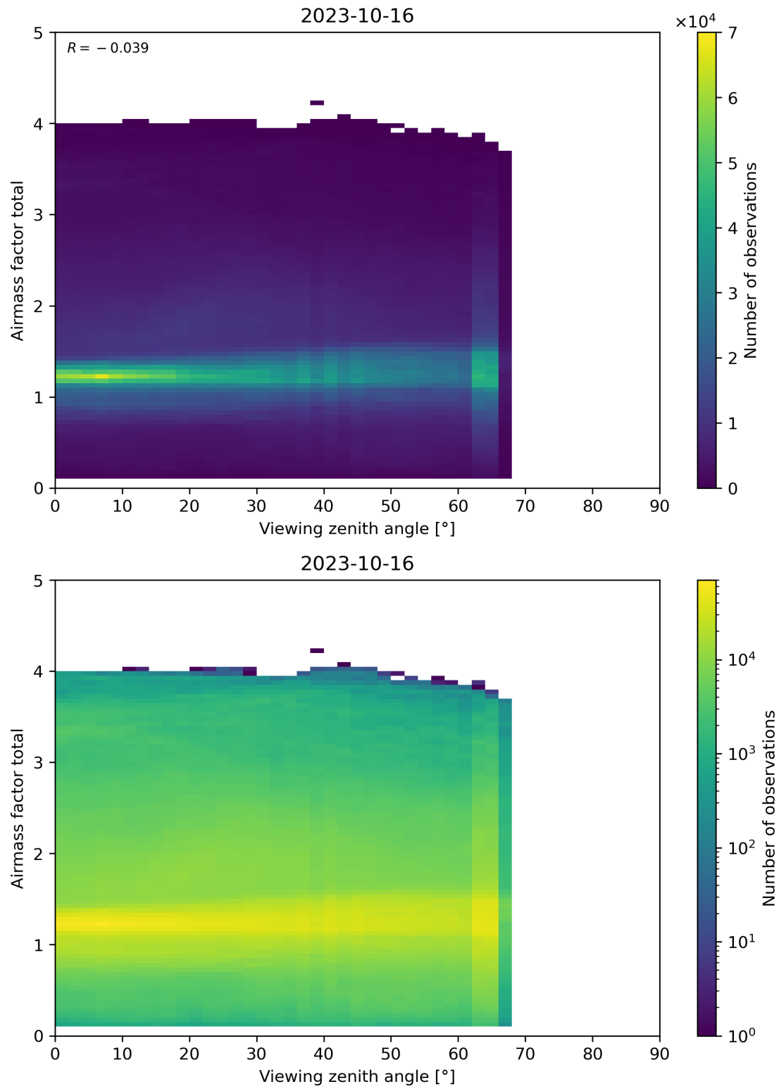
Figure 190: Scatter density plot of “Viewing zenith angle” against “Airmass factor total” for 2023-10-15 to 2023-10-17.
