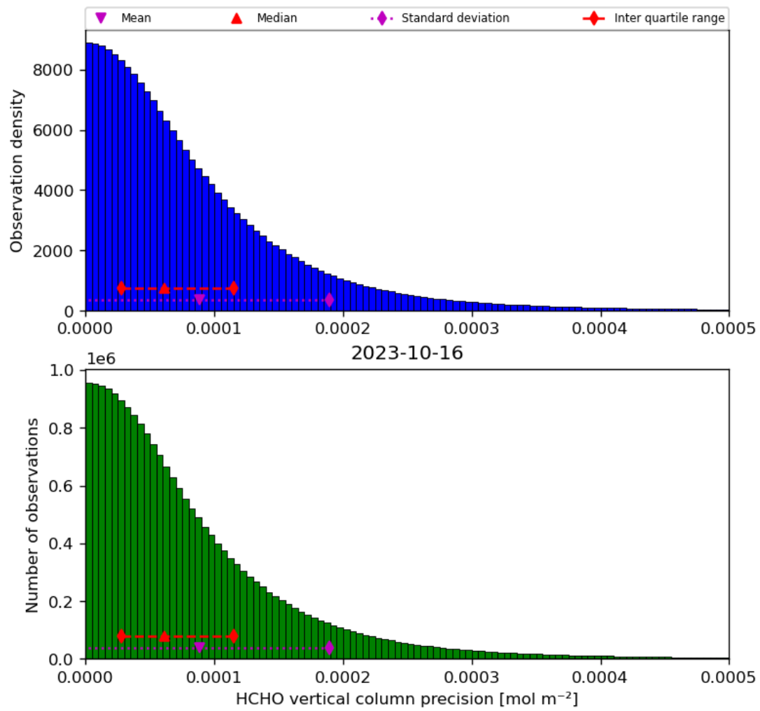
Figure 36: Histogram of “HCHO vertical column precision” for 2023-10-15 to 2023-10-17
