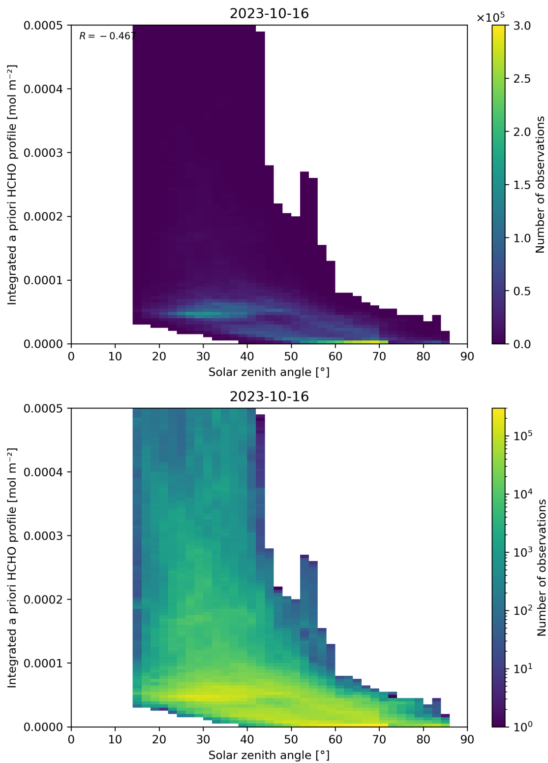
Figure 180: Scatter density plot of “Solar zenith angle” against “Integrated a priori HCHO profile” for 2023-10-15 to 2023-10-17.
