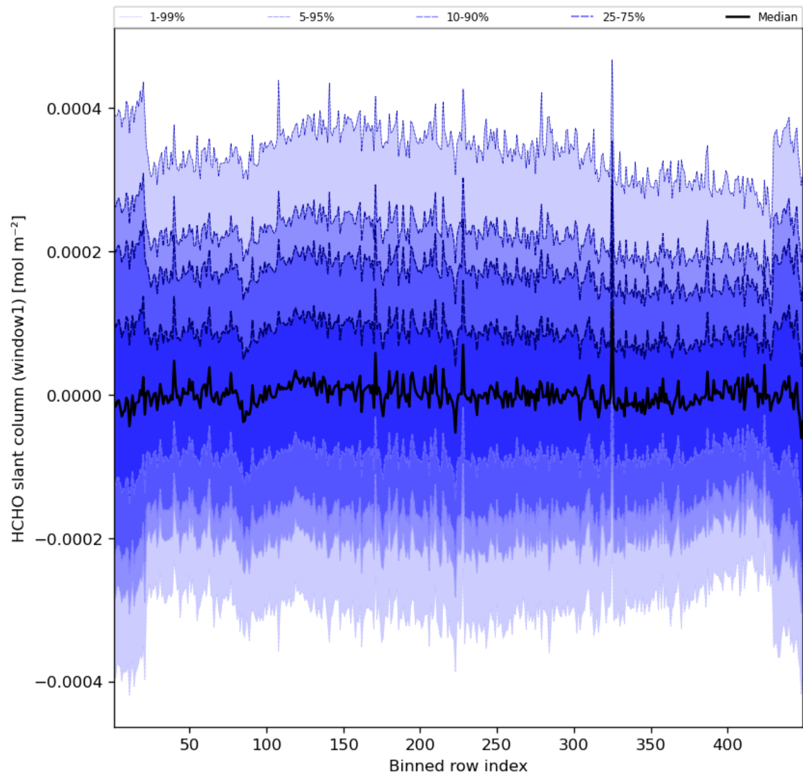
Figure 52: Along track statistics of “HCHO slant column (window1)” for 2023-10-15 to 2023-10-17
