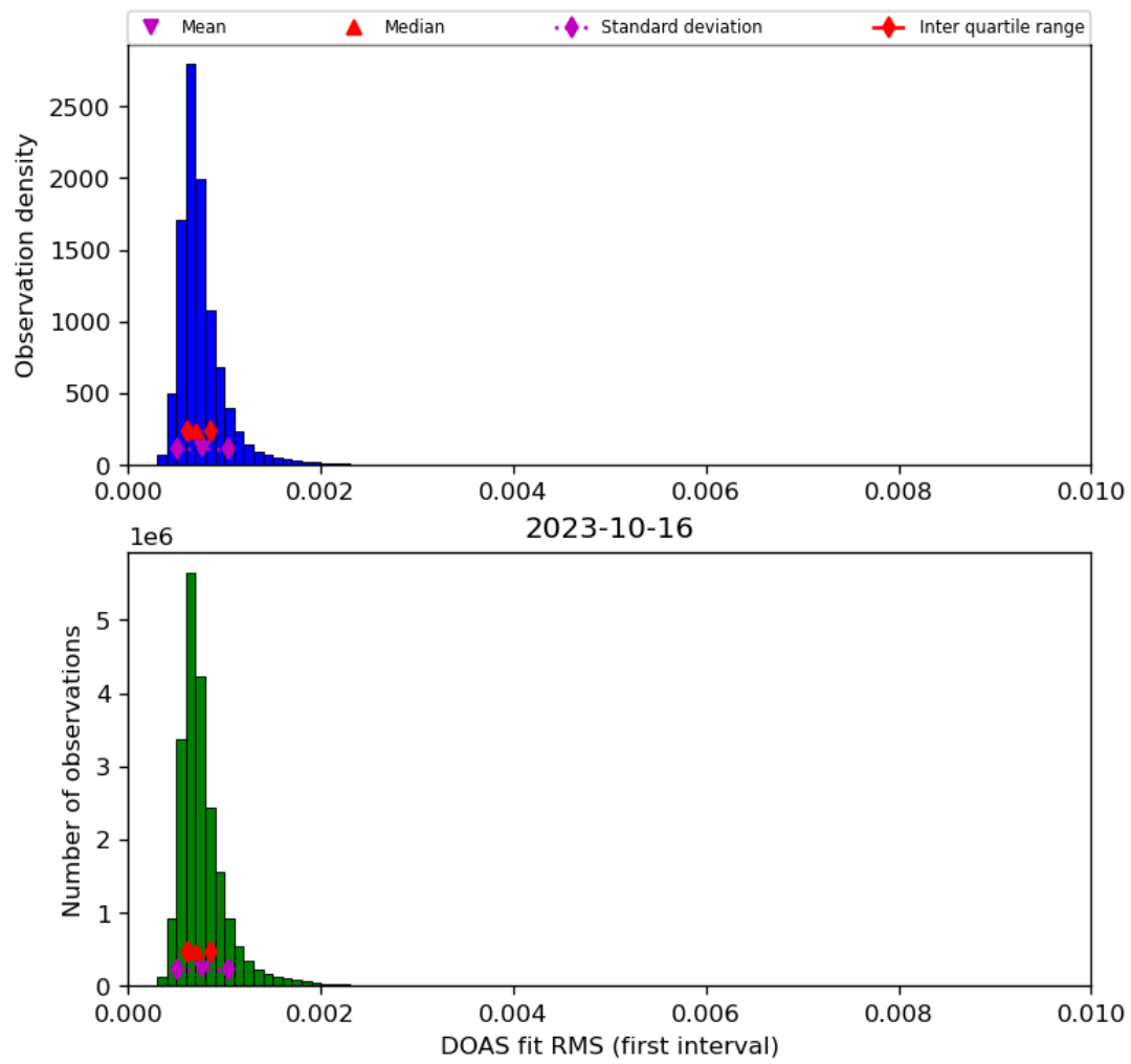
Figure 46: Histogram of “DOAS fit RMS (first interval)” for 2023-10-15 to 2023-10-17
