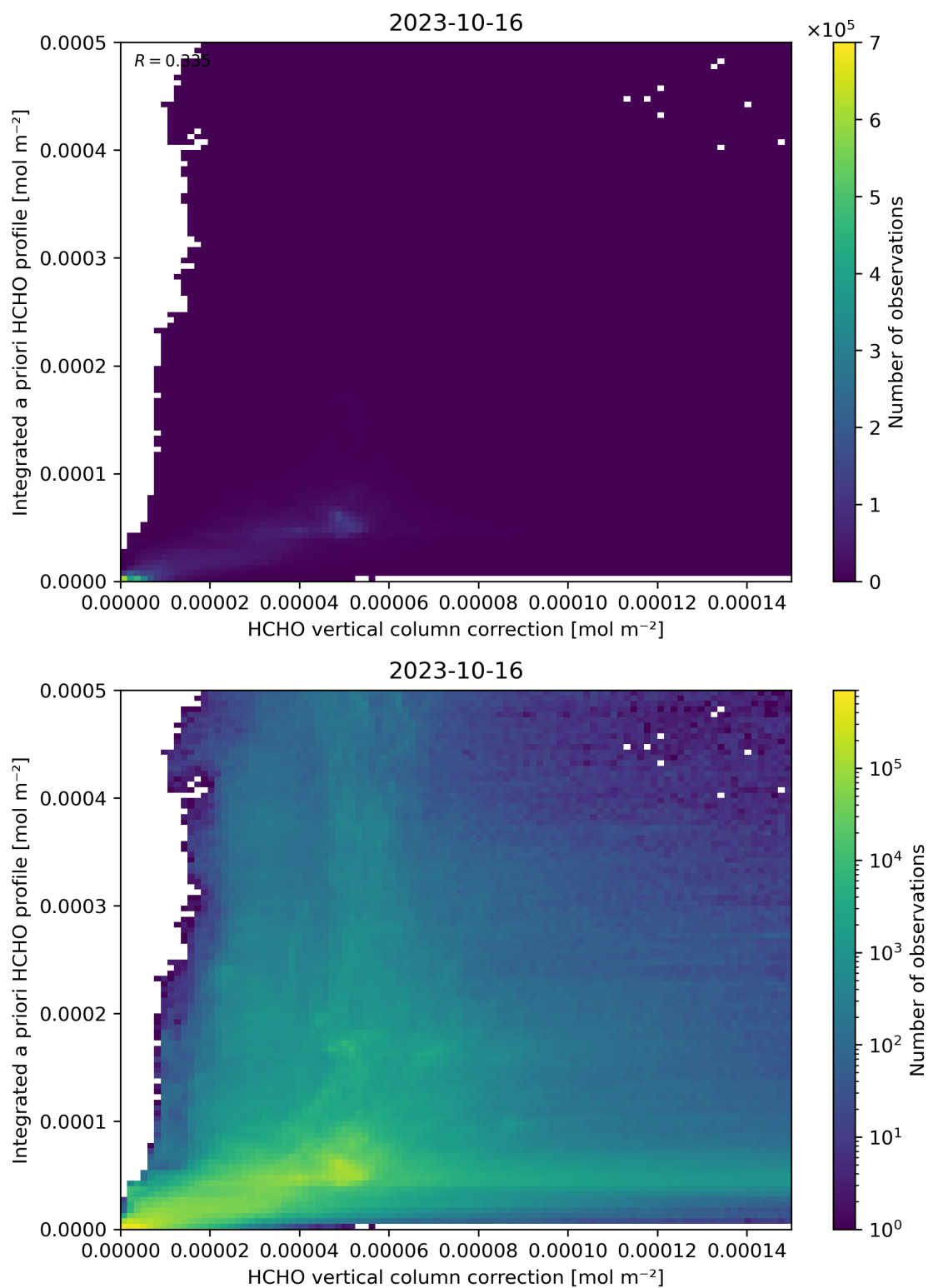
Figure 122: Scatter density plot of “HCHO vertical column correction” against “Integrated a priori HCHO profile” for 2023-10-15 to 2023-10-17.
