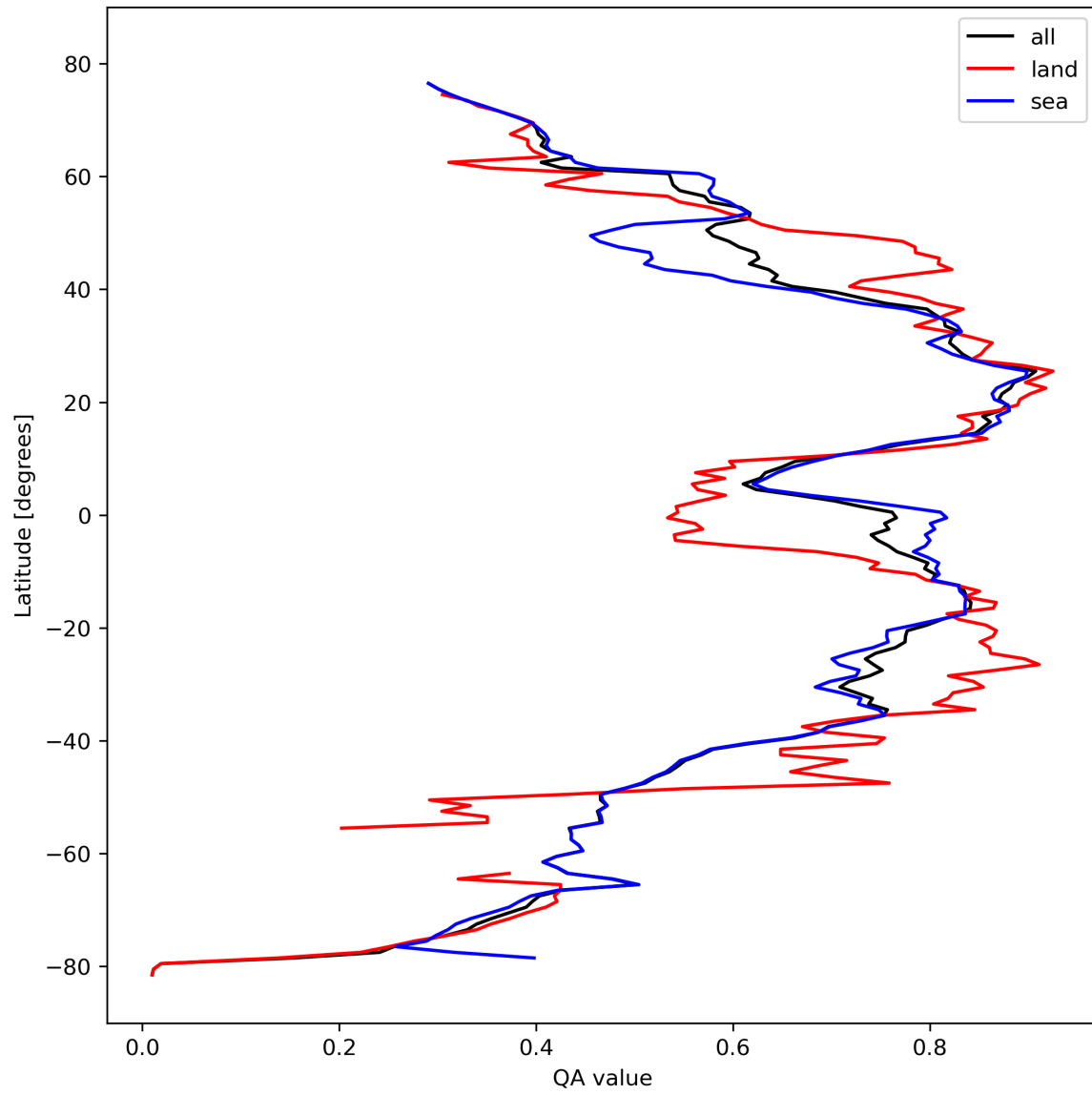
Figure 20: Zonal average of “QA value” for 2023-10-15 to 2023-10-17.
