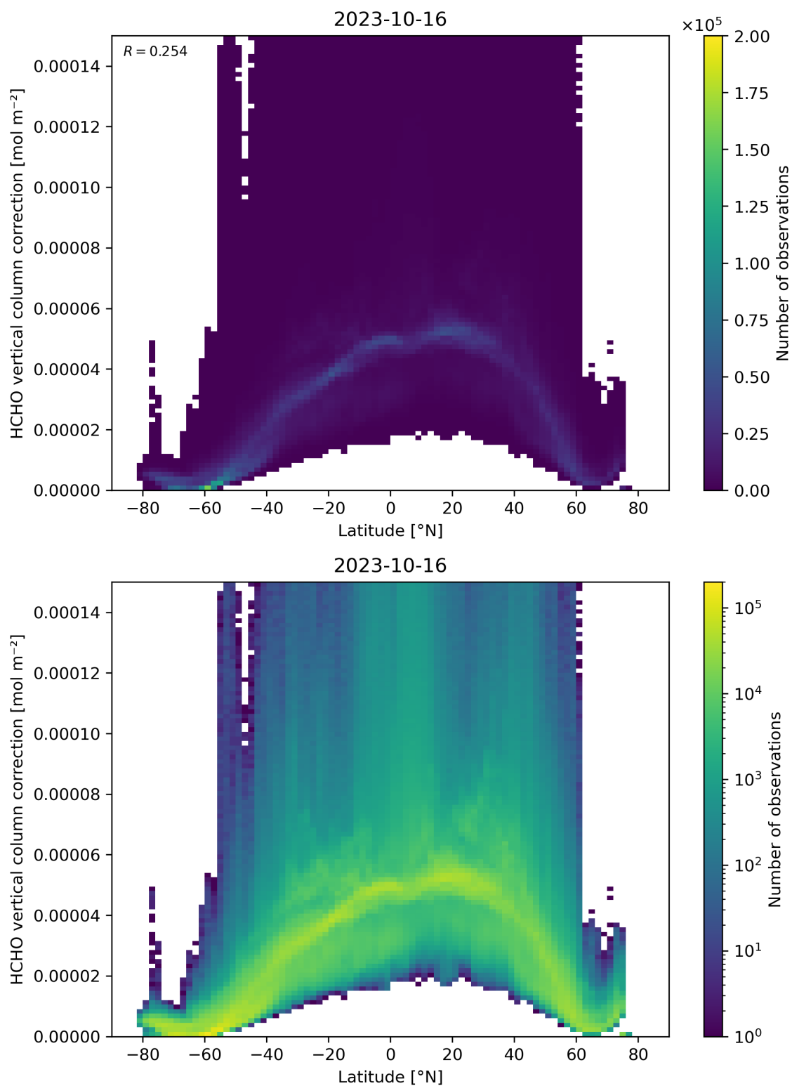
Figure 164: Scatter density plot of “Latitude” against “HCHO vertical column correction” for 2023-10-15 to 2023-10-17.
