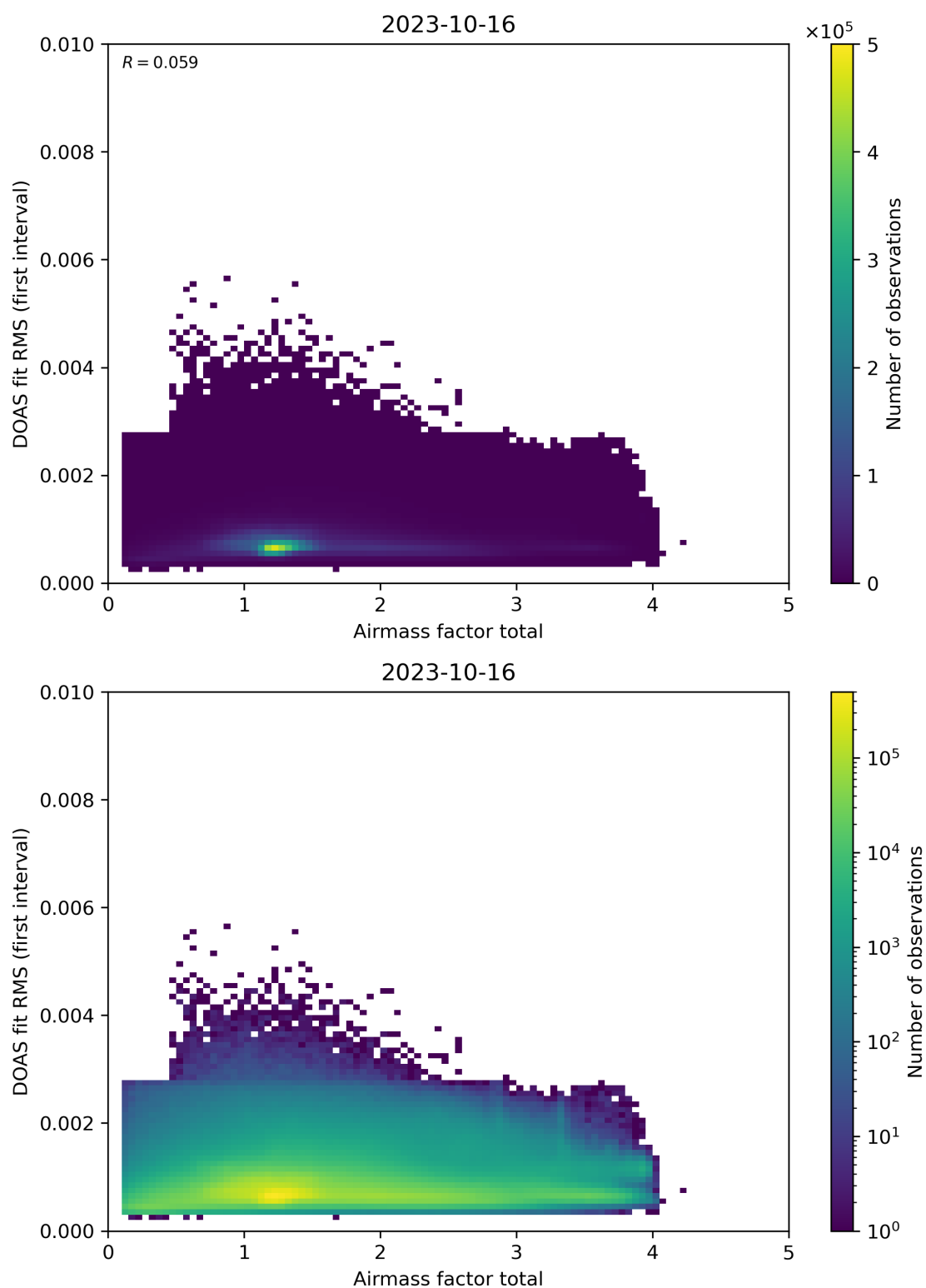
Figure 97: Scatter density plot of “Airmass factor total” against “DOAS fit RMS (first interval)” for 2023-10-15 to 2023-10-17.
