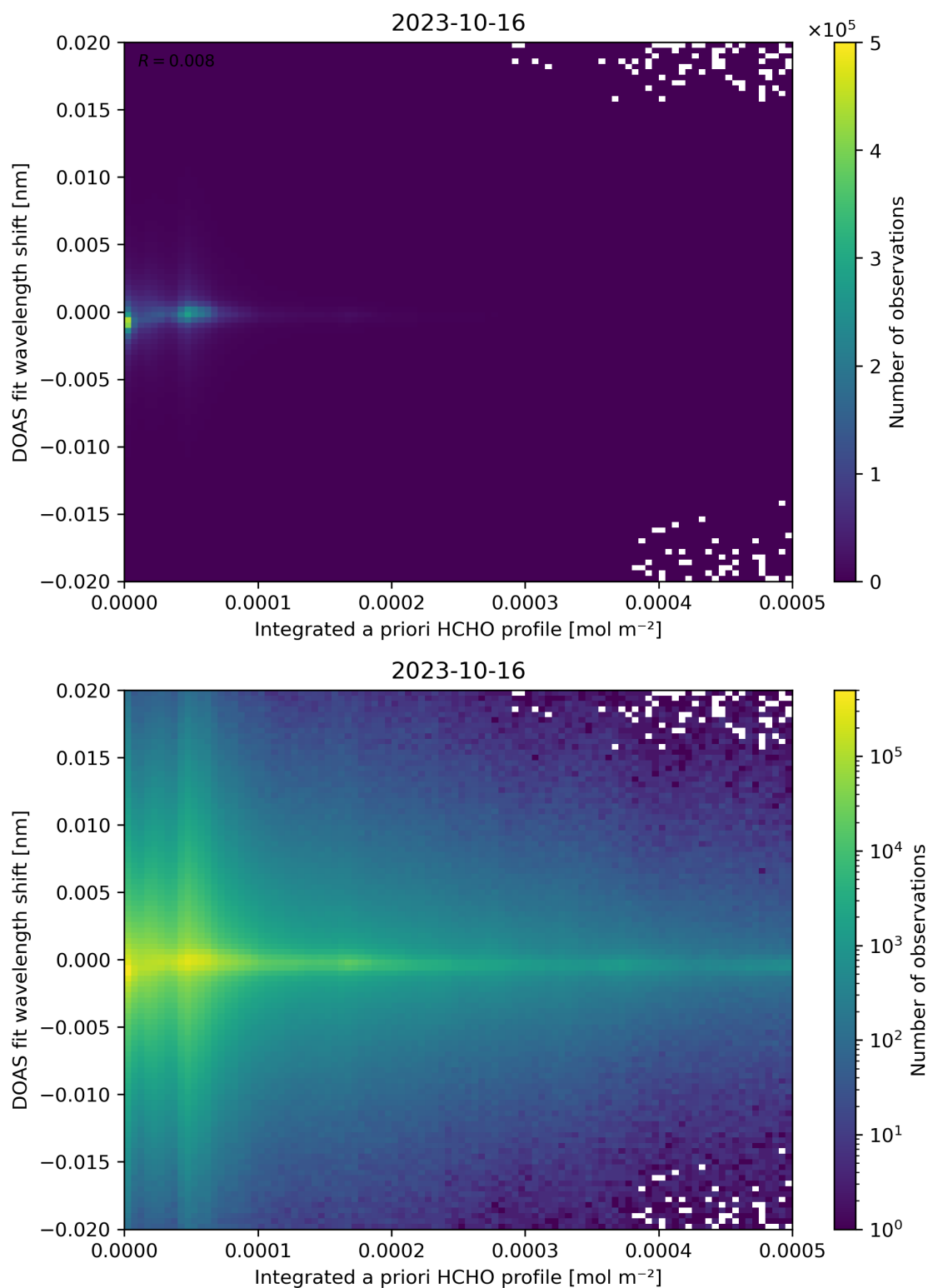
Figure 149: Scatter density plot of “Integrated a priori HCHO profile” against “DOAS fit wavelength shift” for 2023-10-15 to 2023-10-17.
