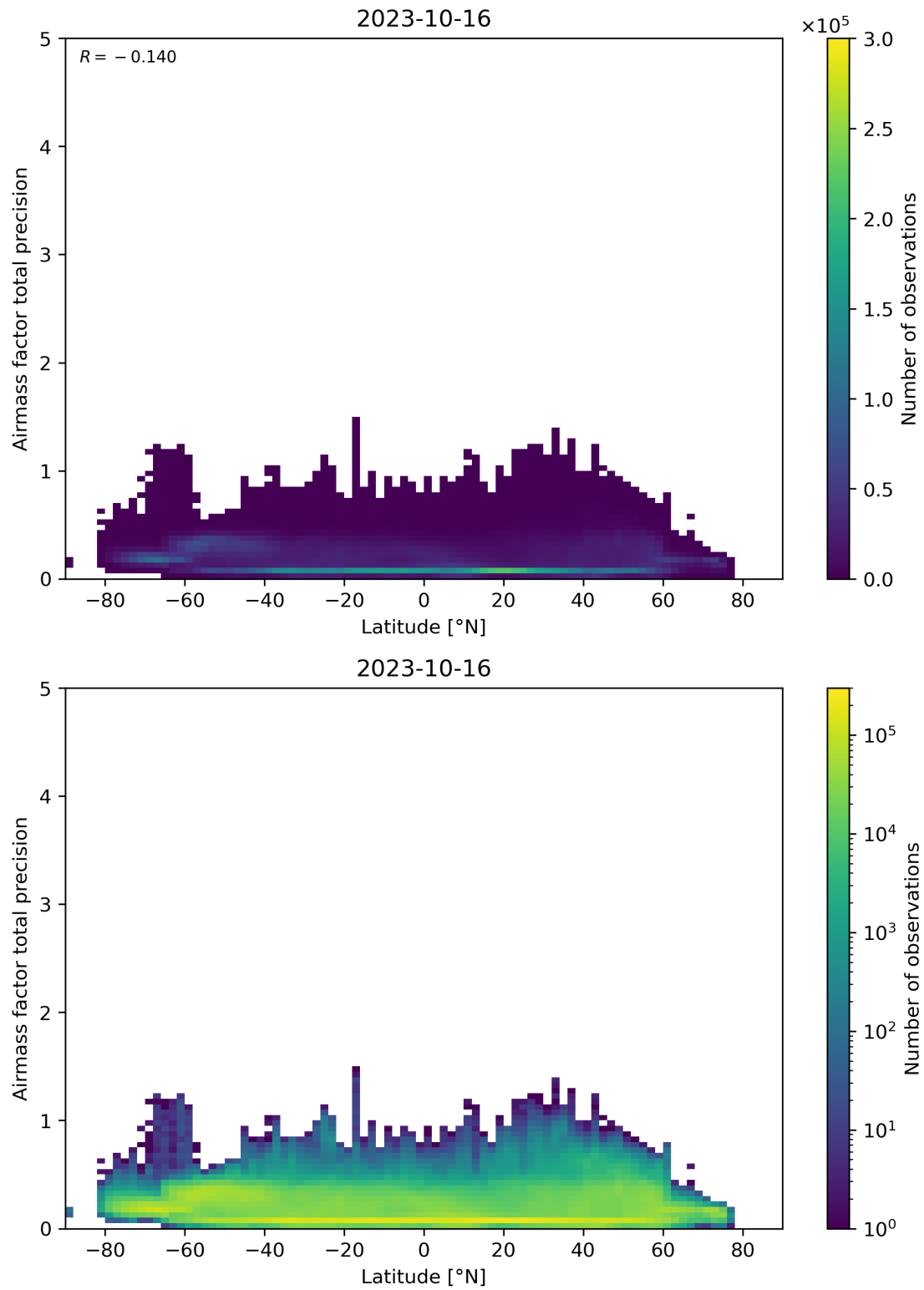
Figure 162: Scatter density plot of “Latitude” against “Airmass factor total precision” for 2023-10-15 to 2023-10-17.
