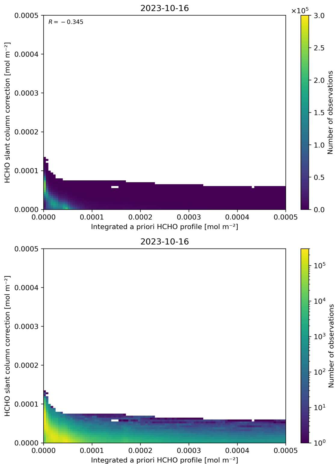
Figure 152: Scatter density plot of “Integrated a priori HCHO profile” against “HCHO slant column correction” for 2023-10-15 to 2023-10-17.
