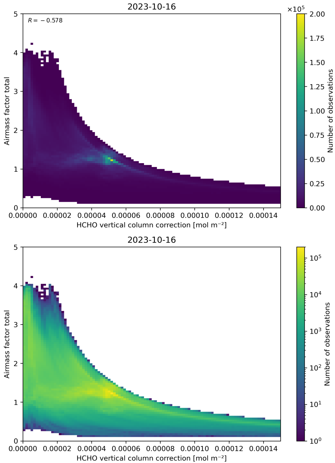
Figure 120: Scatter density plot of “HCHO vertical column correction” against “Airmass factor total” for 2023-10-15 to 2023-10-17.
