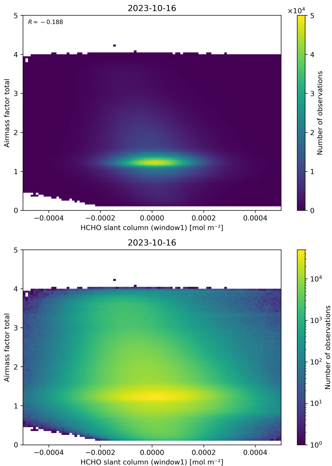
Figure 85: Scatter density plot of “HCHO slant column (window1)” against “Airmass factor total” for 2023-10-15 to 2023-10-17.
