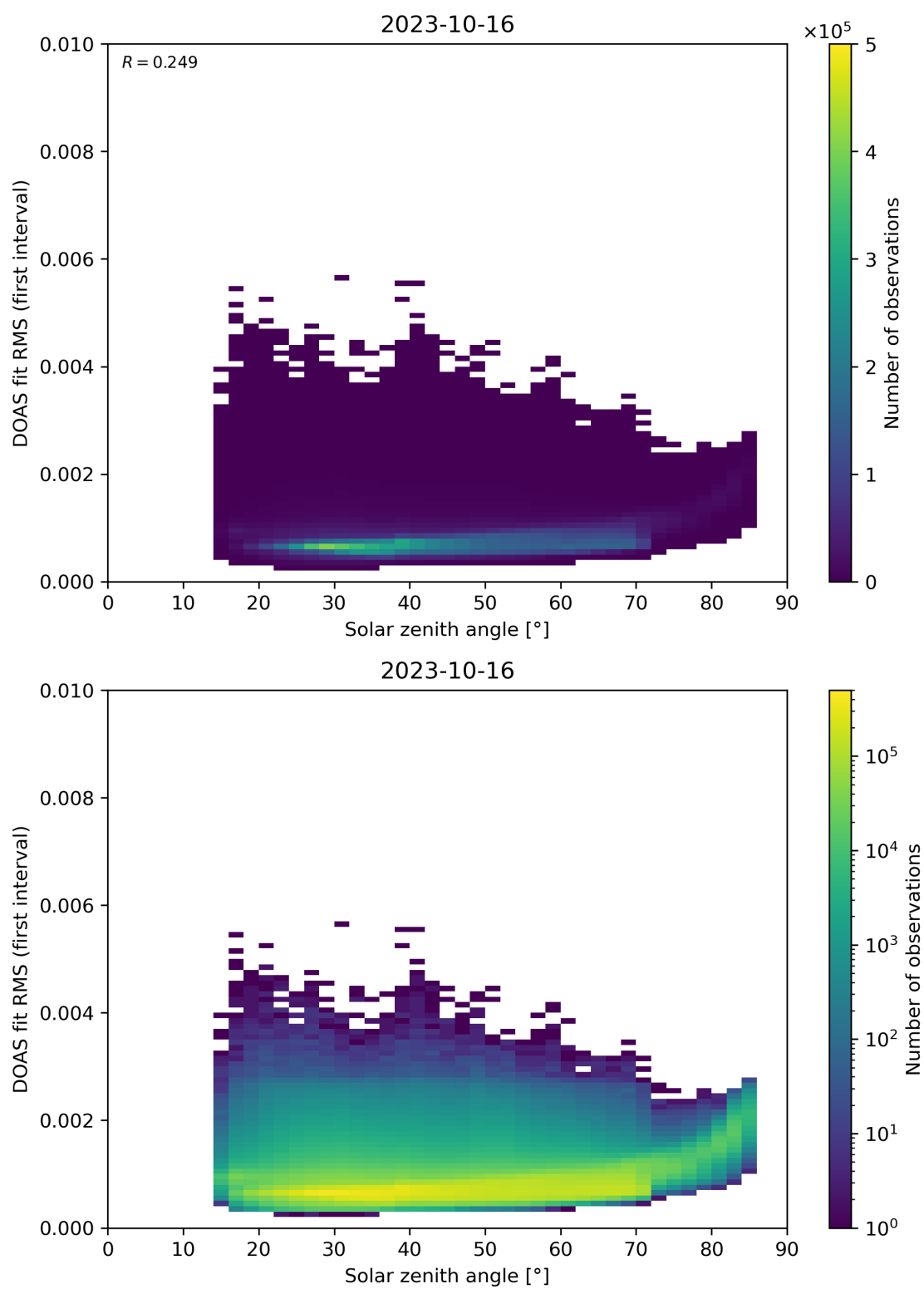
Figure 167: Scatter density plot of “Solar zenith angle” against “DOAS fit RMS (first interval)” for 2023-10-15 to 2023-10-17.
