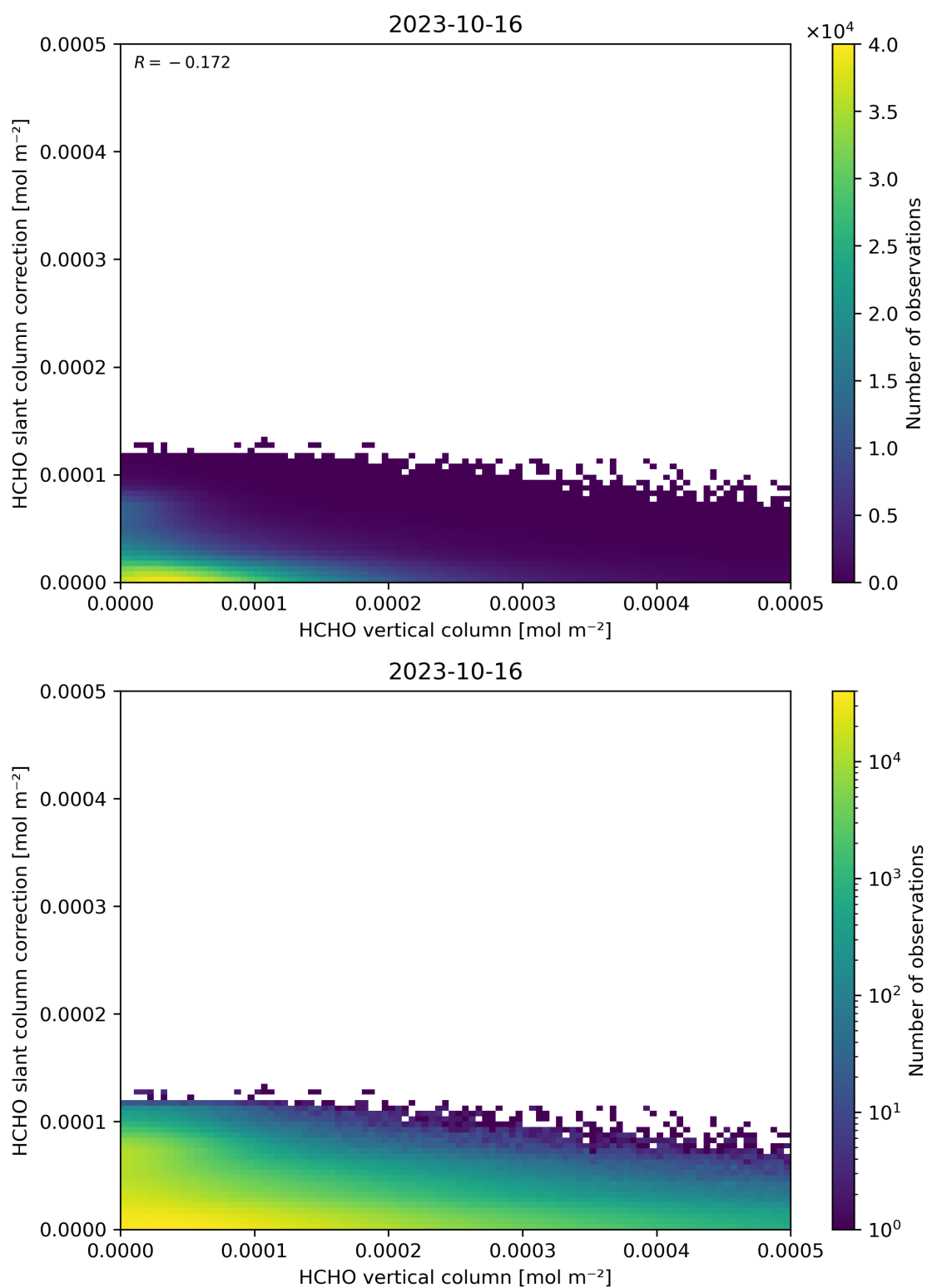
Figure 128: Scatter density plot of “HCHO vertical column” against “HCHO slant column correction” for 2023-10-15 to 2023-10-17.
