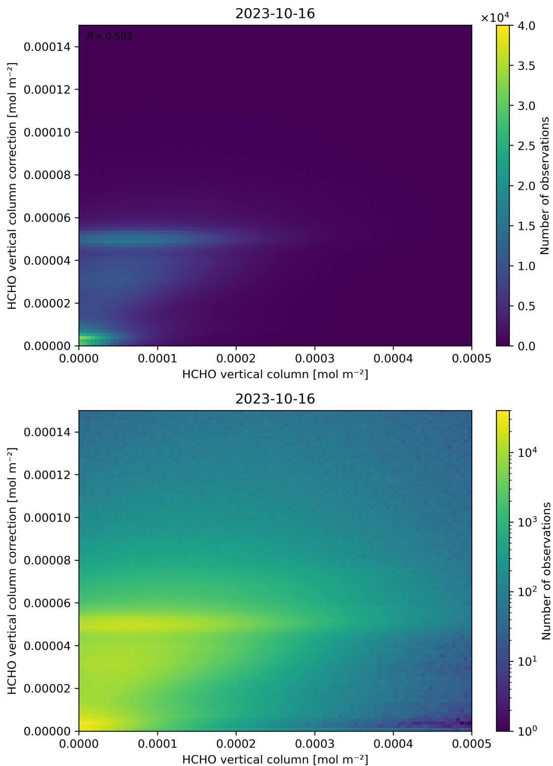
Figure 133: Scatter density plot of “HCHO vertical column” against “HCHO vertical column correction” for 2023-10-15 to 2023-10-17.
