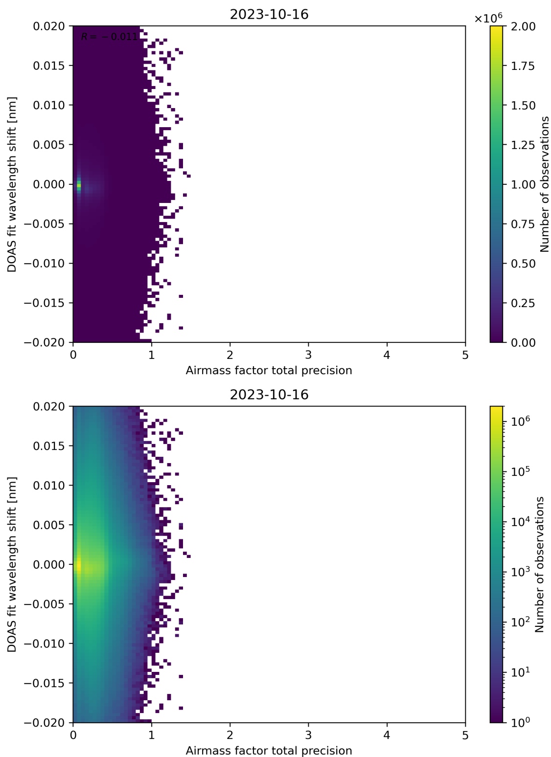
Figure 106: Scatter density plot of “Airmass factor total precision” against “DOAS fit wavelength shift” for 2023-10-15 to 2023-10-17.
