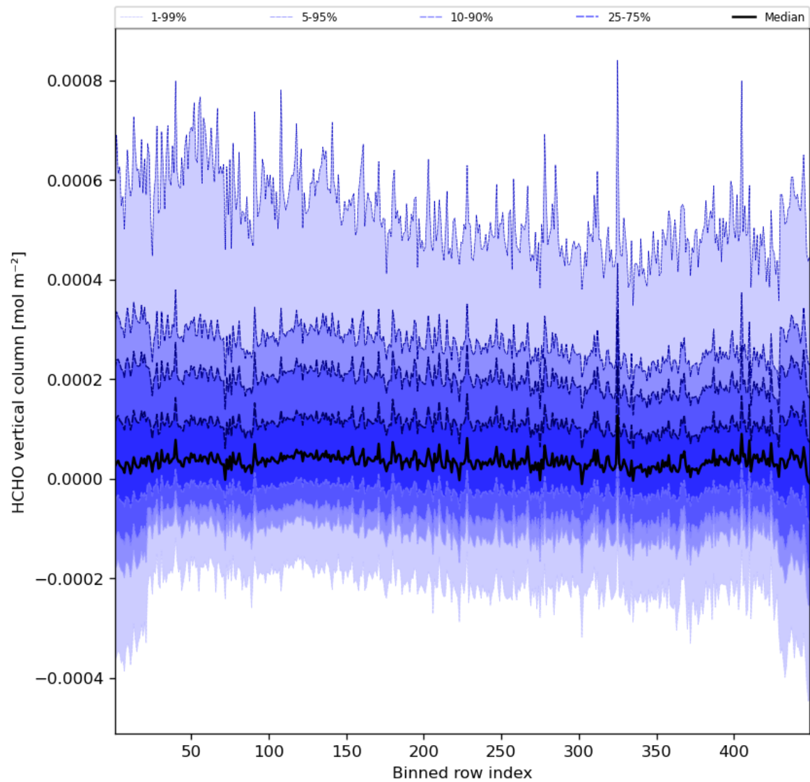
Figure 49: Along track statistics of “HCHO vertical column” for 2023-10-15 to 2023-10-17
