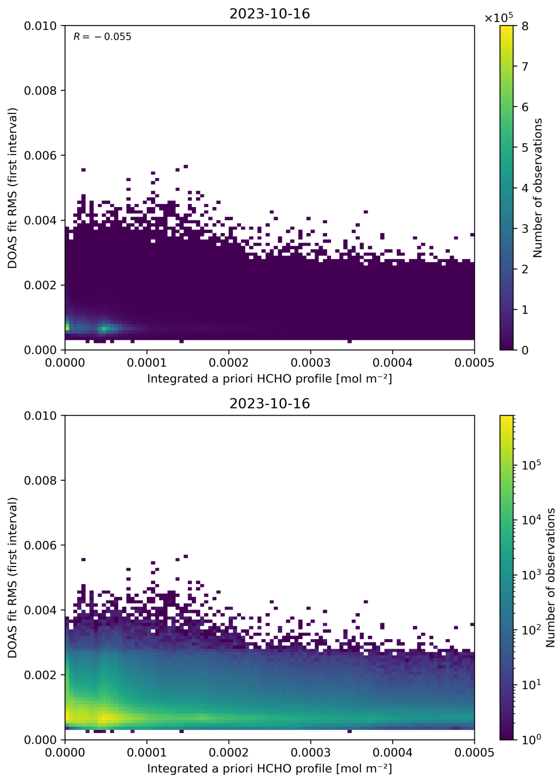
Figure 148: Scatter density plot of “Integrated a priori HCHO profile” against “DOAS fit RMS (first interval)” for 2023-10-15 to 2023-10-17.
