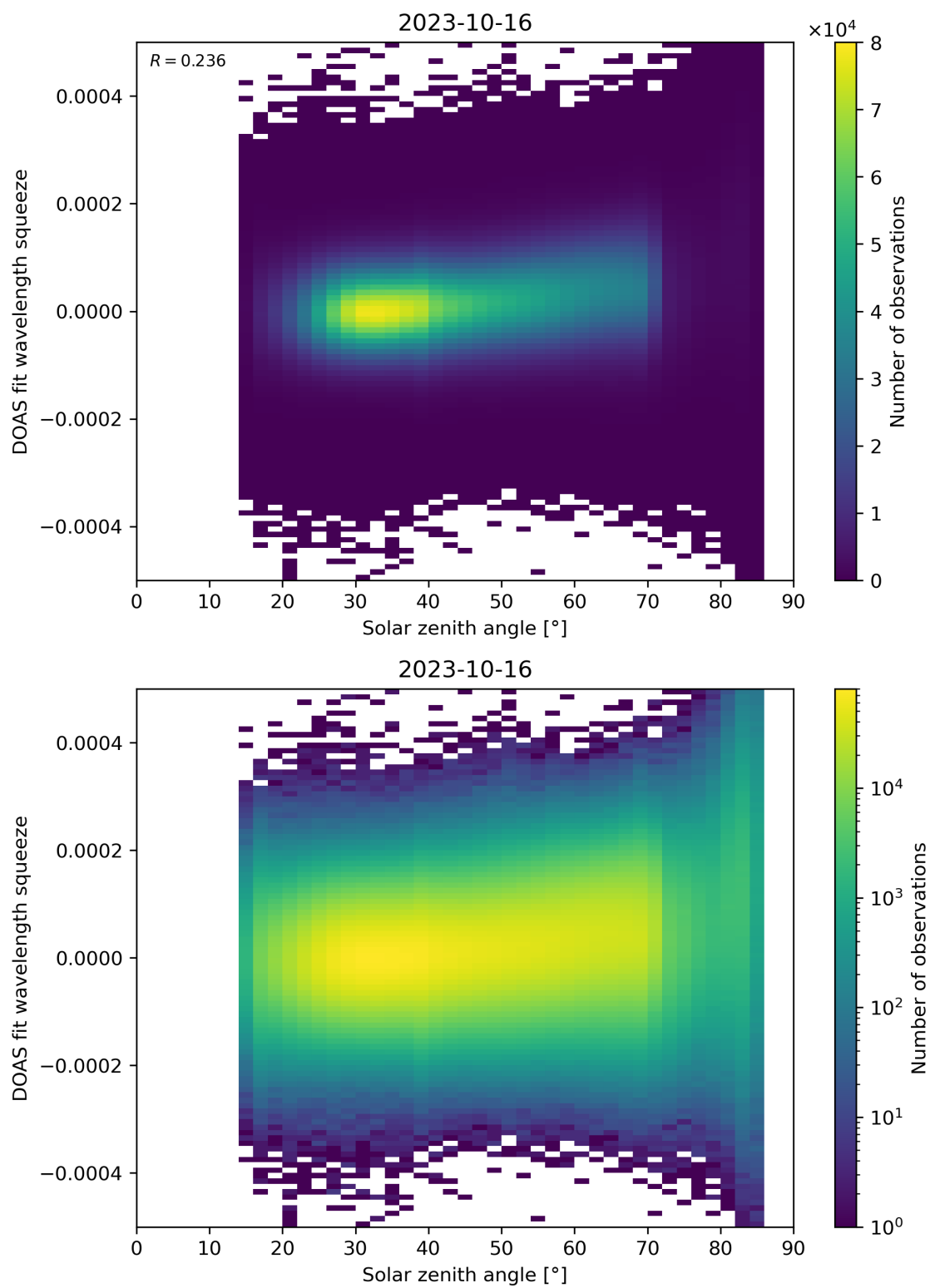
Figure 169: Scatter density plot of “Solar zenith angle” against “DOAS fit wavelength squeeze” for 2023-10-15 to 2023-10-17.
