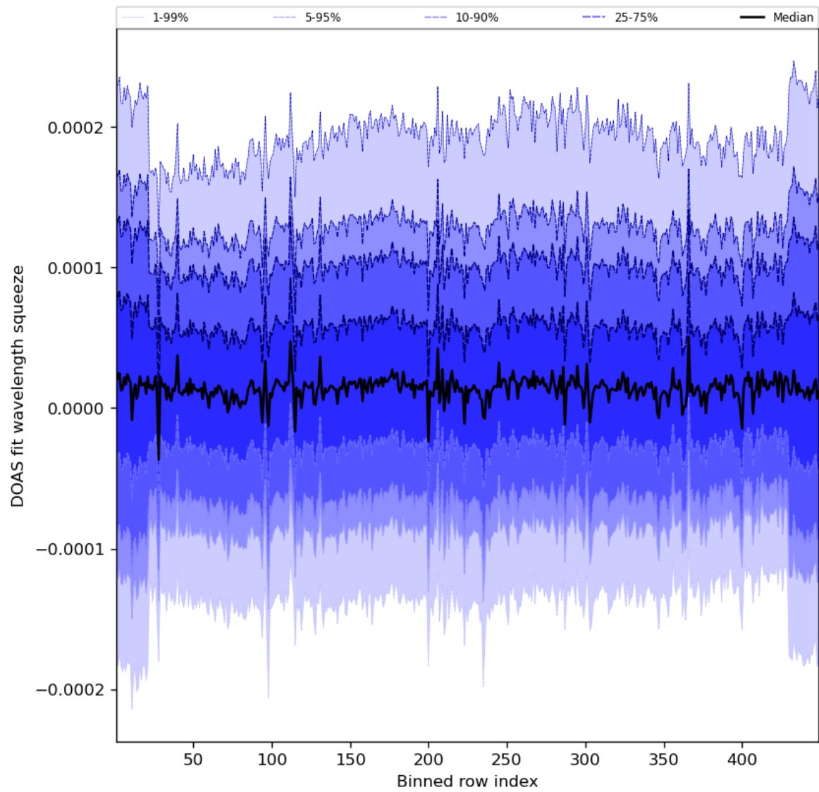
Figure 59: Along track statistics of “DOAS fit wavelength squeeze” for 2023-10-15 to 2023-10-17
