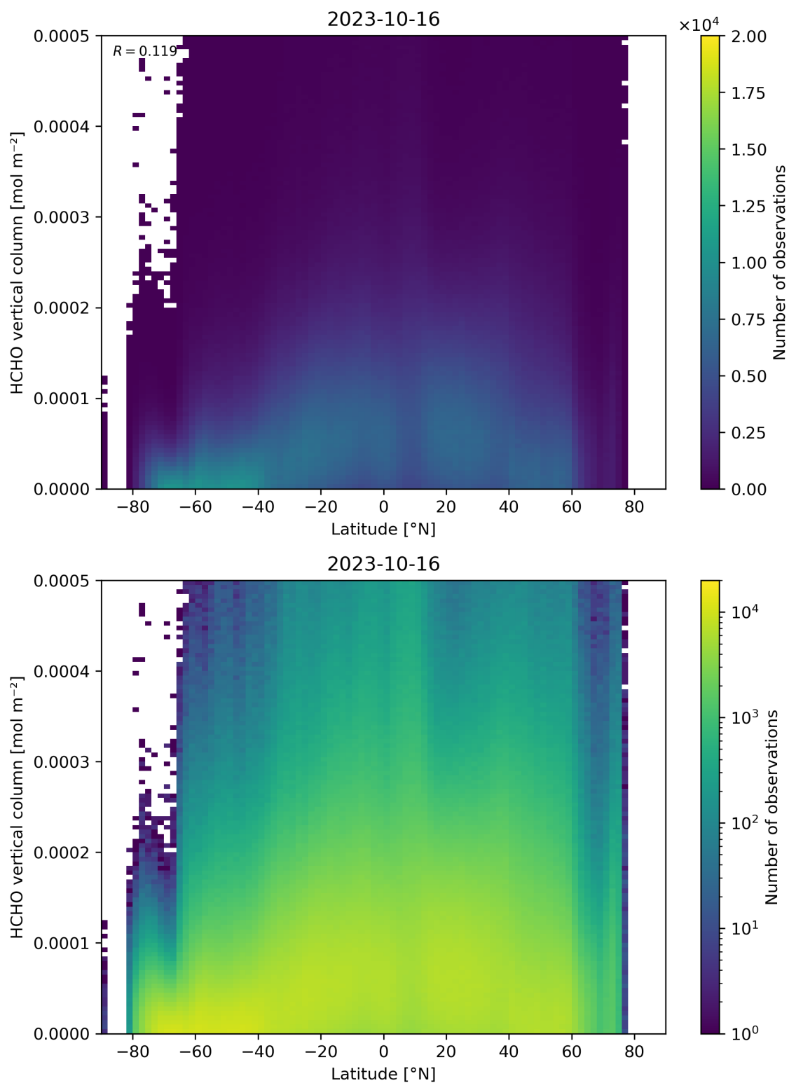
Figure 163: Scatter density plot of “Latitude” against “HCHO vertical column” for 2023-10-15 to 2023-10-17.
