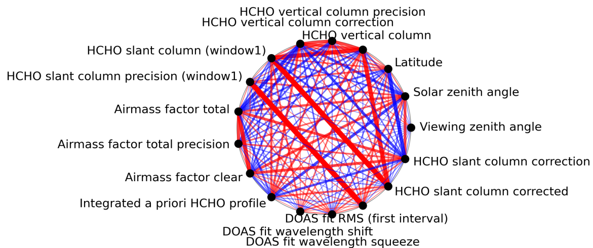
Figure 1: Map of correlation graph for 2023-10-15 to 2023-10-17.
