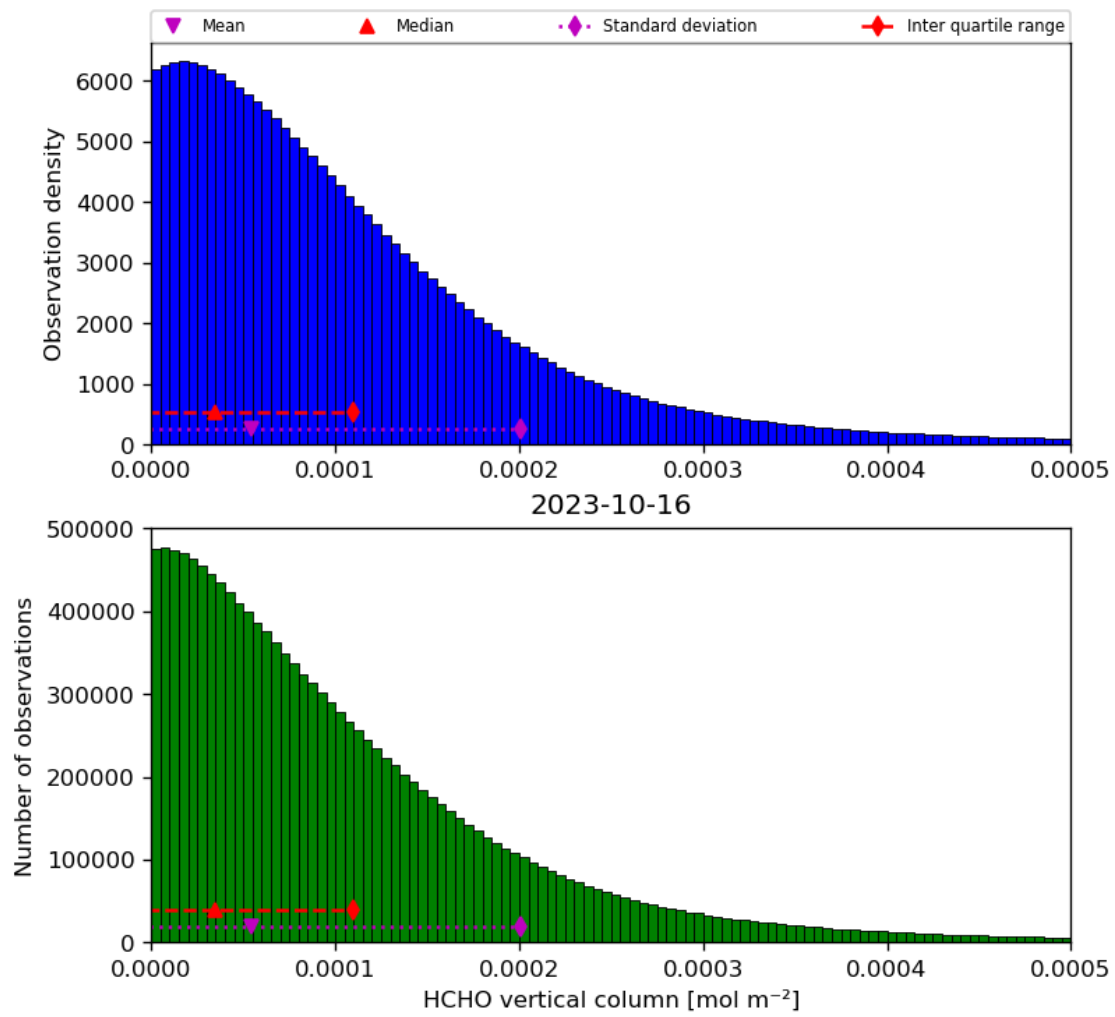
Figure 35: Histogram of “HCHO vertical column” for 2023-10-15 to 2023-10-17
