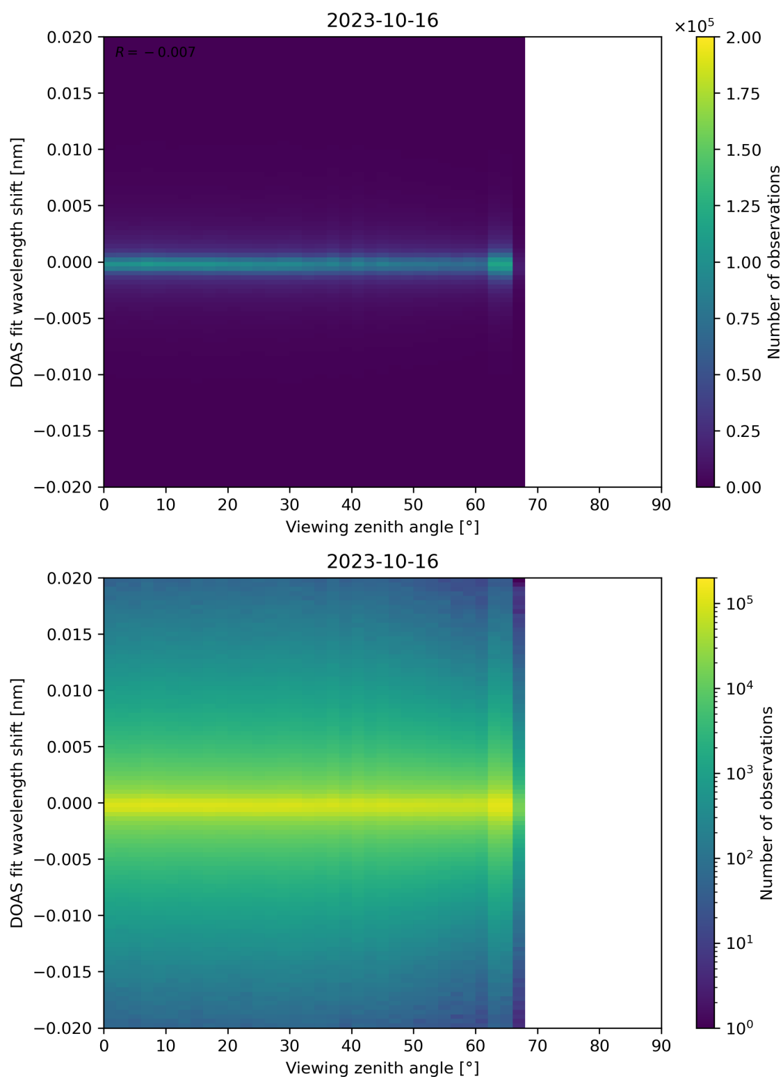
Figure 183: Scatter density plot of “Viewing zenith angle” against “DOAS fit wavelength shift” for 2023-10-15 to 2023-10-17.
