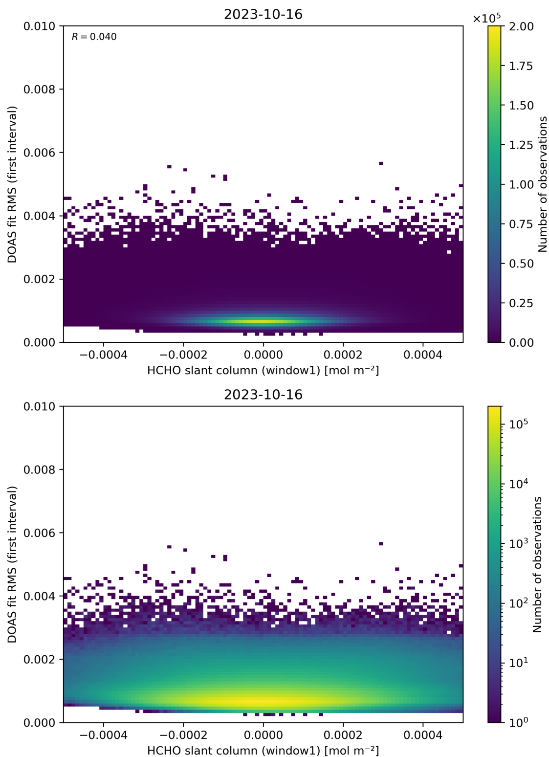
Figure 78: Scatter density plot of “HCHO slant column (window1)” against “DOAS fit RMS (first interval)” for 2023-10-15 to 2023-10-17.
