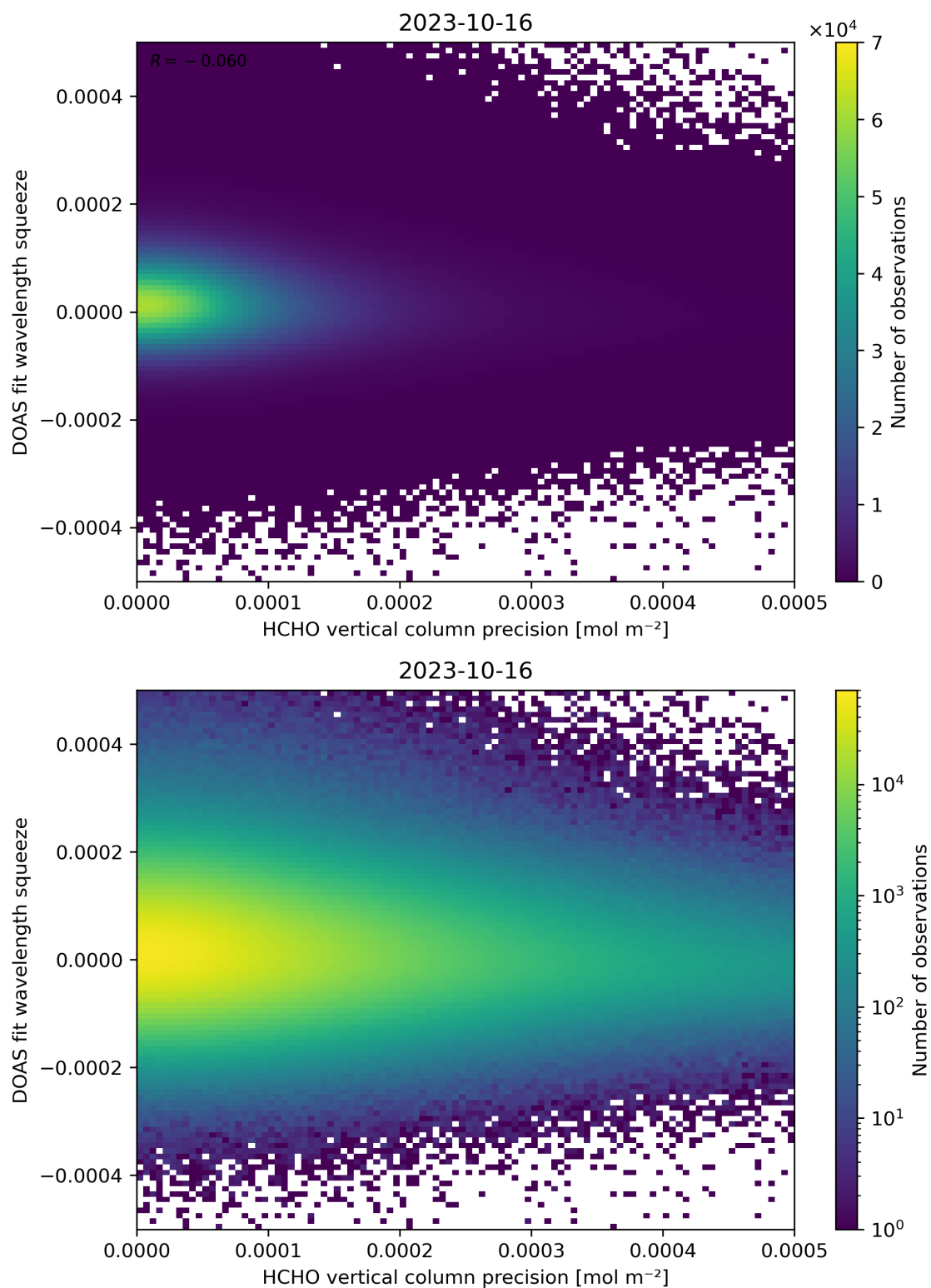
Figure 138: Scatter density plot of “HCHO vertical column precision” against “DOAS fit wavelength squeeze” for 2023-10-15 to 2023-10-17.
