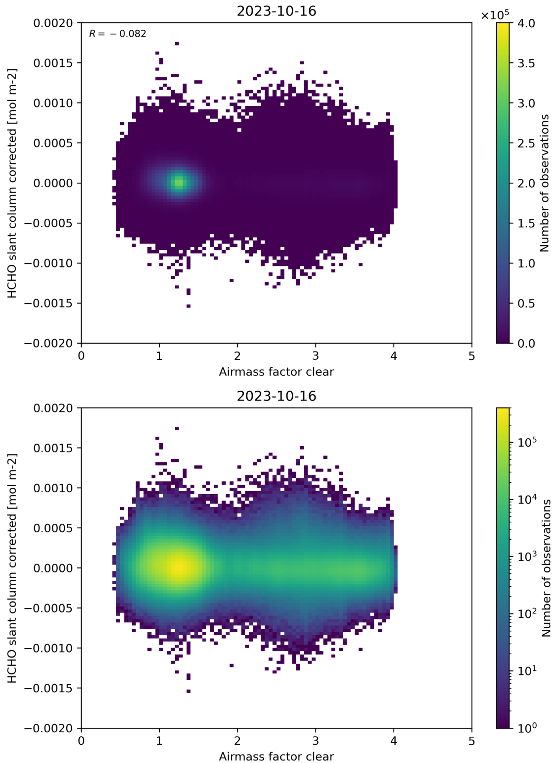
Figure 74: Scatter density plot of “Airmass factor clear” against “HCHO slant column corrected” for 2023-10-15 to 2023-10-17.
