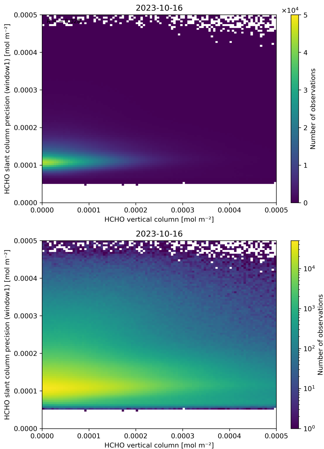
Figure 130: Scatter density plot of “HCHO vertical column” against “HCHO slant column precision (window1)” for 2023-10-15 to 2023-10-17.
