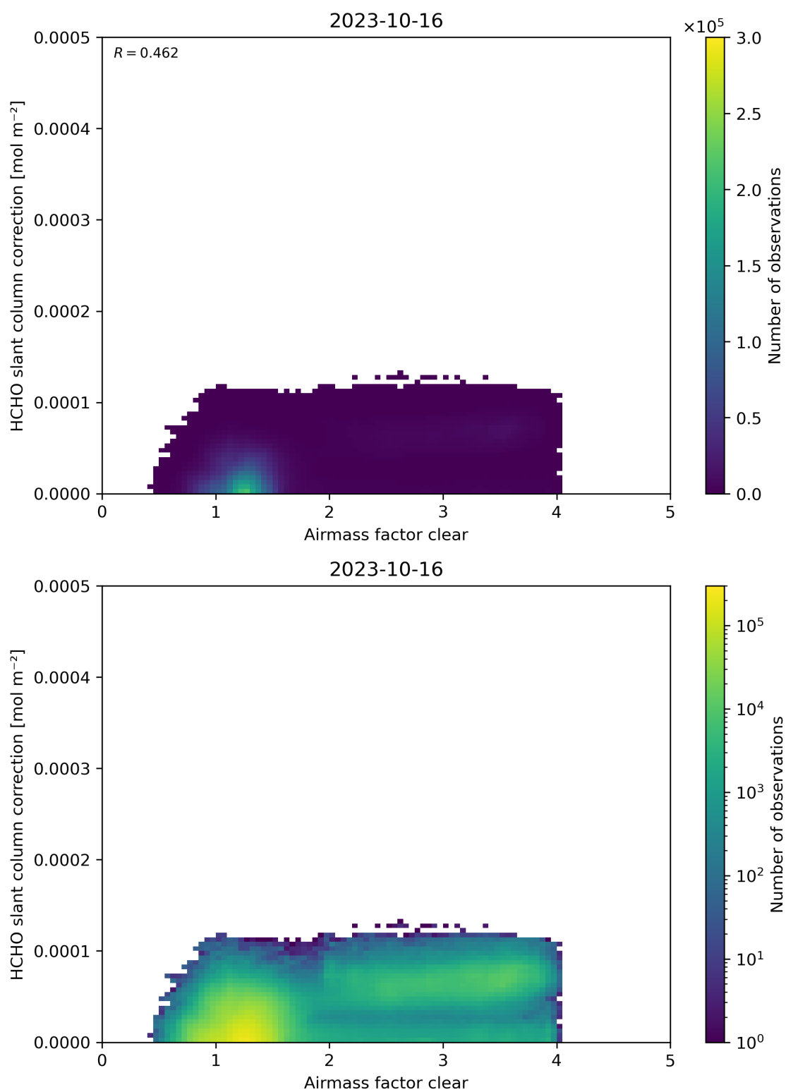
Figure 75: Scatter density plot of “Airmass factor clear” against “HCHO slant column correction” for 2023-10-15 to 2023-10-17.
