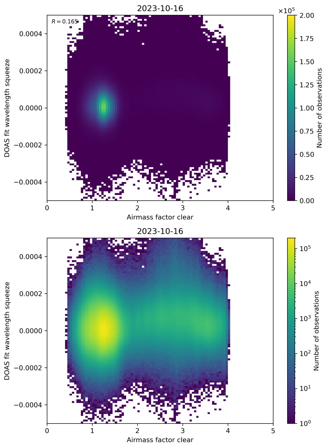
Figure 73: Scatter density plot of “Airmass factor clear” against “DOAS fit wavelength squeeze” for 2023-10-15 to 2023-10-17.
