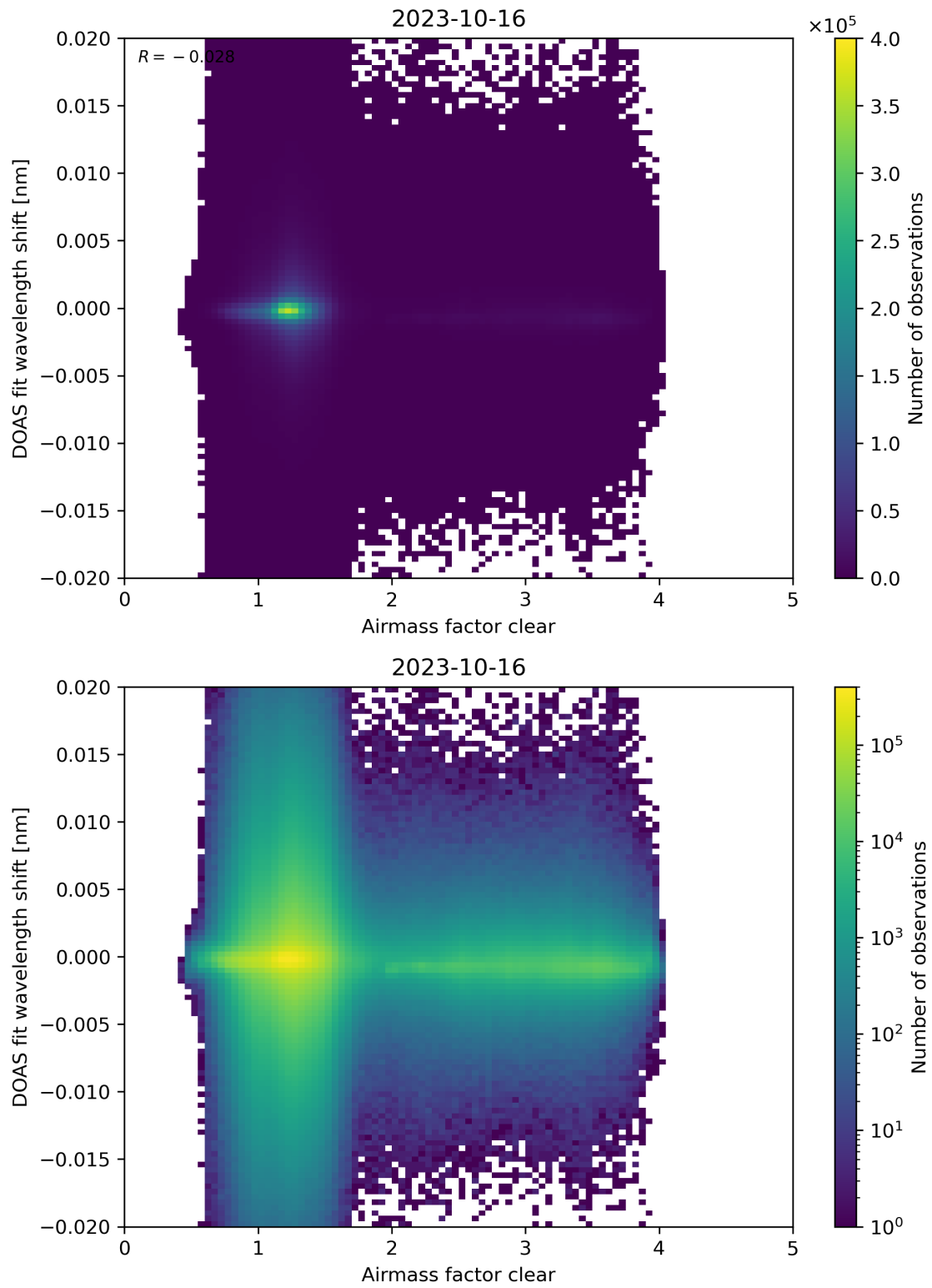
Figure 72: Scatter density plot of “Airmass factor clear” against “DOAS fit wavelength shift” for 2023-10-15 to 2023-10-17.
