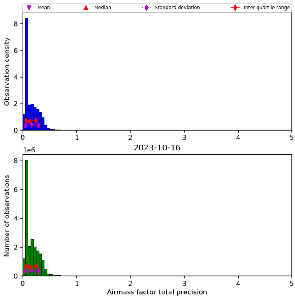
Figure 41: Histogram of “Airmass factor total precision” for 2023-10-15 to 2023-10-17
