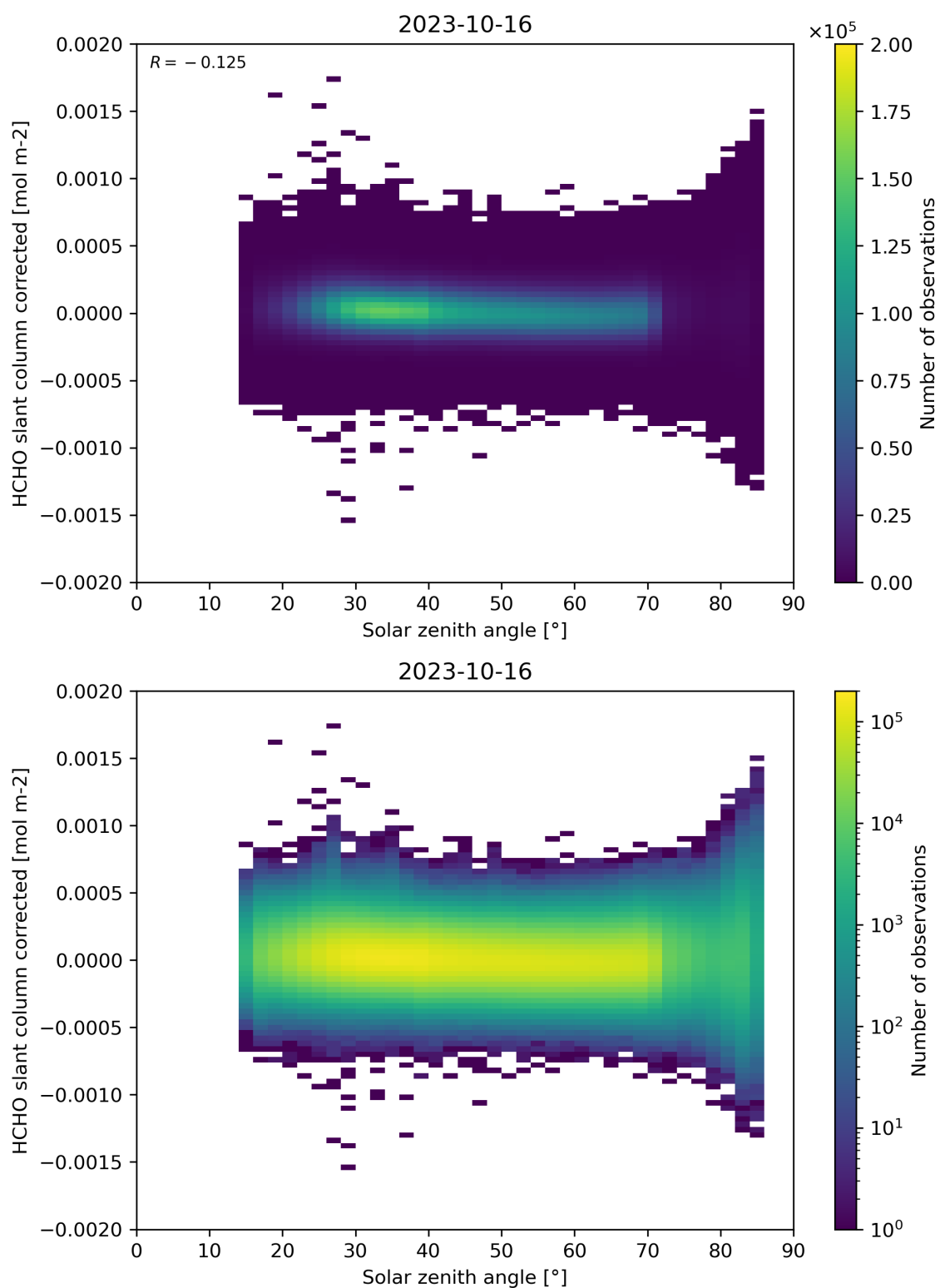
Figure 171: Scatter density plot of “Solar zenith angle” against “HCHO slant column corrected” for 2023-10-15 to 2023-10-17.
