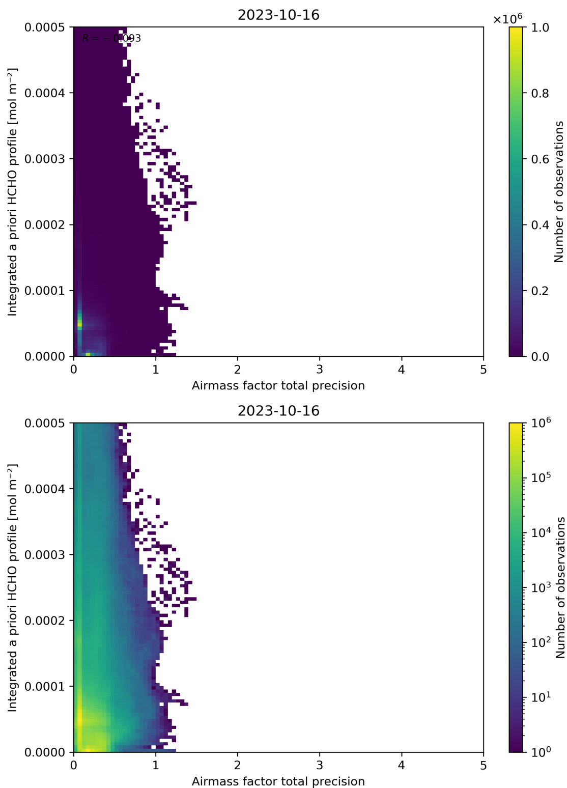
Figure 111: Scatter density plot of “Airmass factor total precision” against “Integrated a priori HCHO profile” for 2023-10-15 to 2023-10-17.
