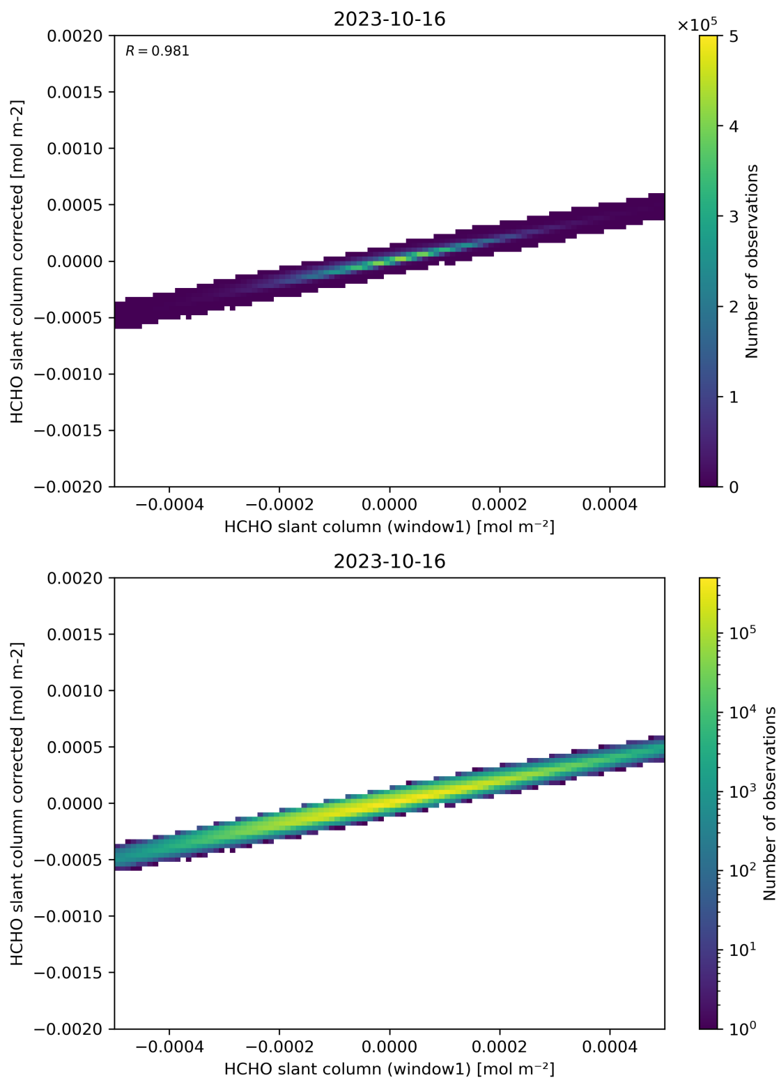
Figure 82: Scatter density plot of “HCHO slant column (window1)” against “HCHO slant column corrected” for 2023-10-15 to 2023-10-17.
