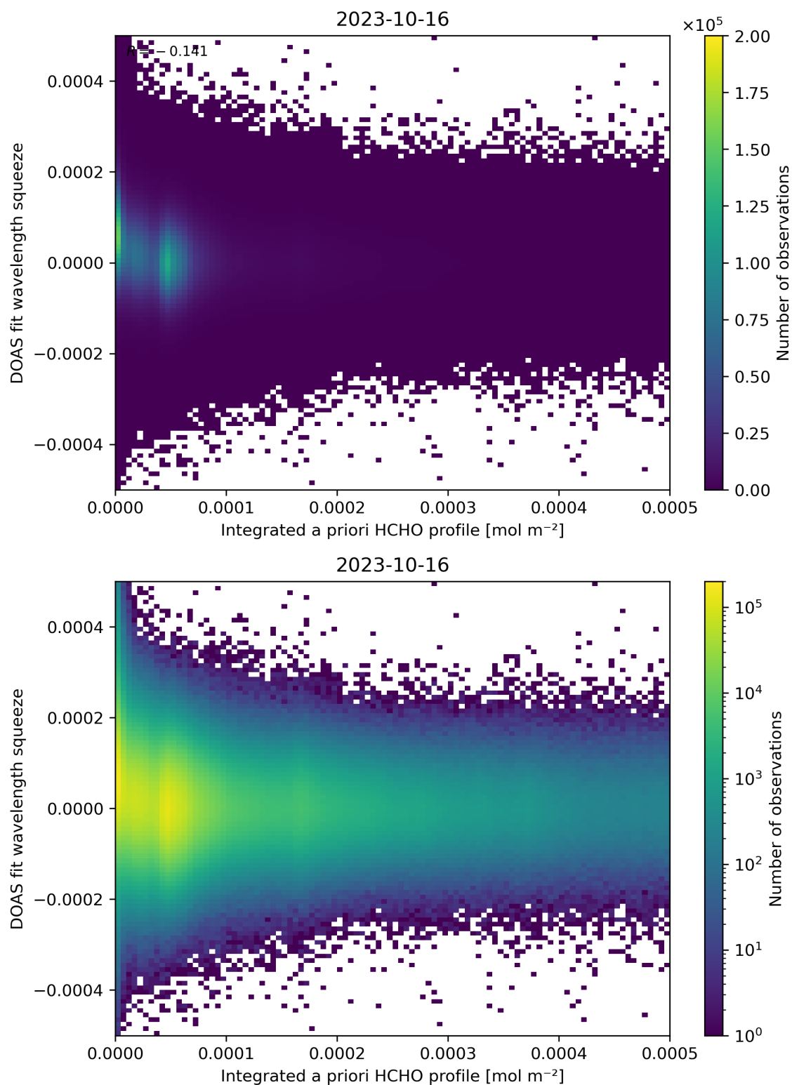
Figure 150: Scatter density plot of “Integrated a priori HCHO profile” against “DOAS fit wavelength squeeze” for 2023-10-15 to 2023-10-17.
