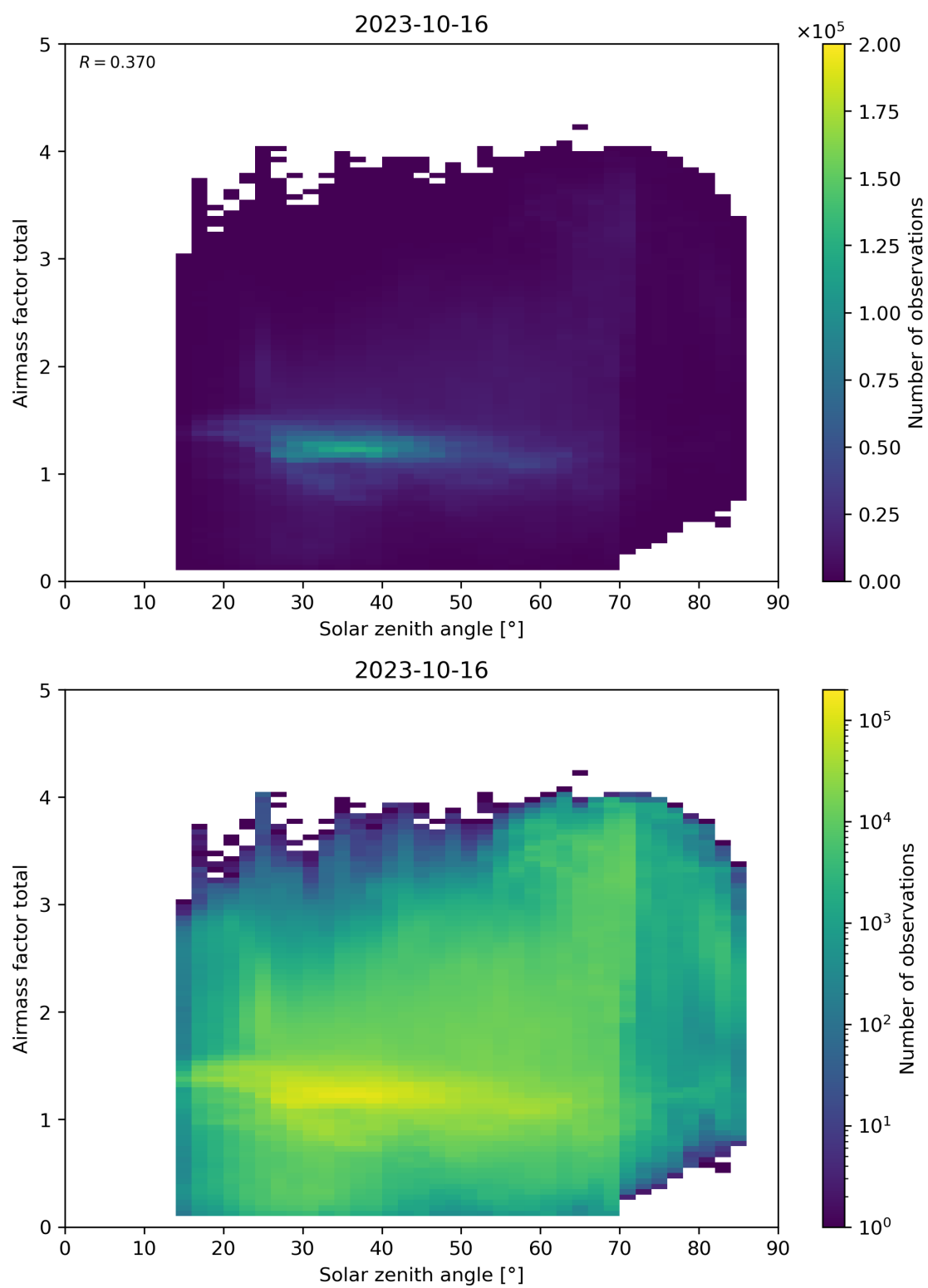
Figure 175: Scatter density plot of “Solar zenith angle” against “Airmass factor total” for 2023-10-15 to 2023-10-17.
