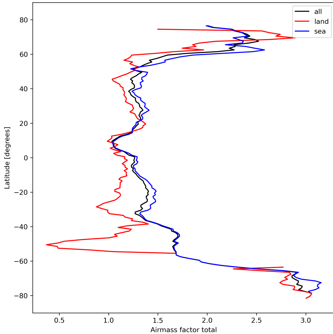
Figure 26: Zonal average of “Airmass factor total” for 2023-10-15 to 2023-10-17.
