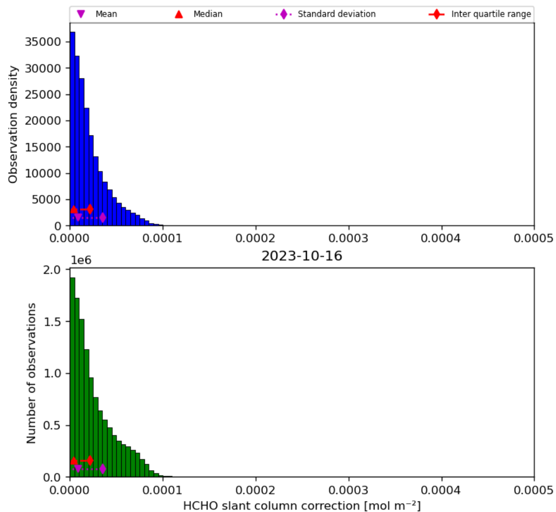
Figure 47: Histogram of “HCHO slant column correction” for 2023-10-15 to 2023-10-17
