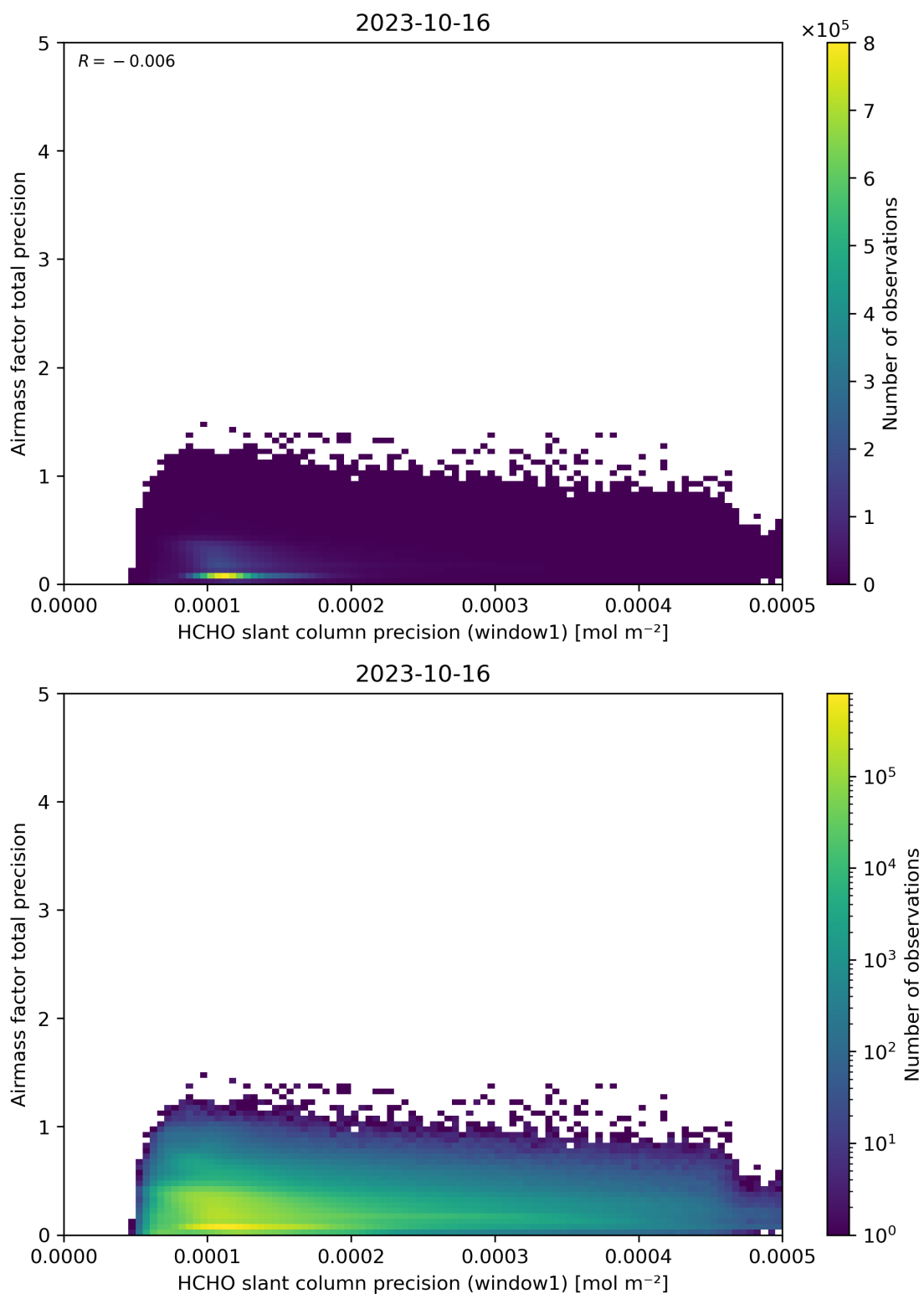
Figure 95: Scatter density plot of “HCHO slant column precision (window1)” against “Airmass factor total precision” for 2023-10-15 to 2023-10-17.
