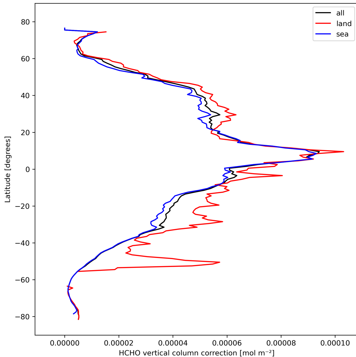
Figure 23: Zonal average of “HCHO vertical column correction” for 2023-10-15 to 2023-10-17.
