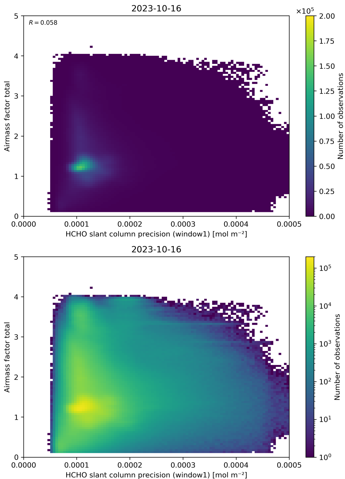
Figure 94: Scatter density plot of “HCHO slant column precision (window1)” against “Airmass factor total” for 2023-10-15 to 2023-10-17.
