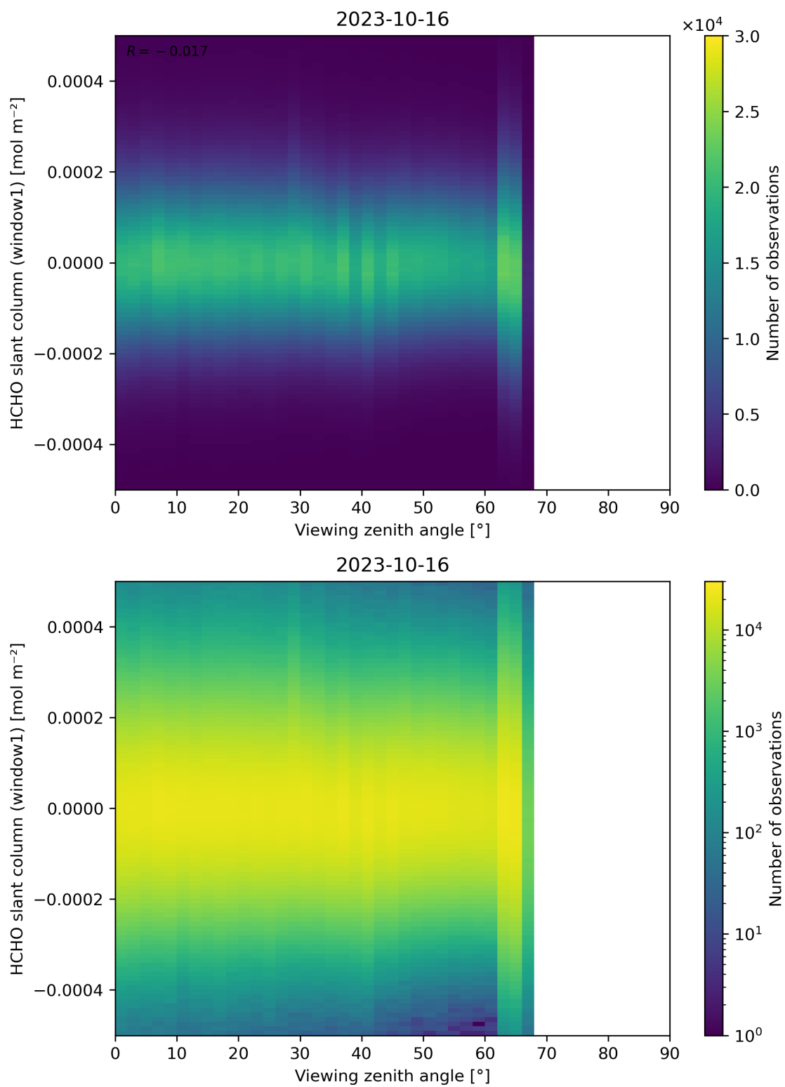
Figure 188: Scatter density plot of “Viewing zenith angle” against “HCHO slant column (window1)” for 2023-10-15 to 2023-10-17.
