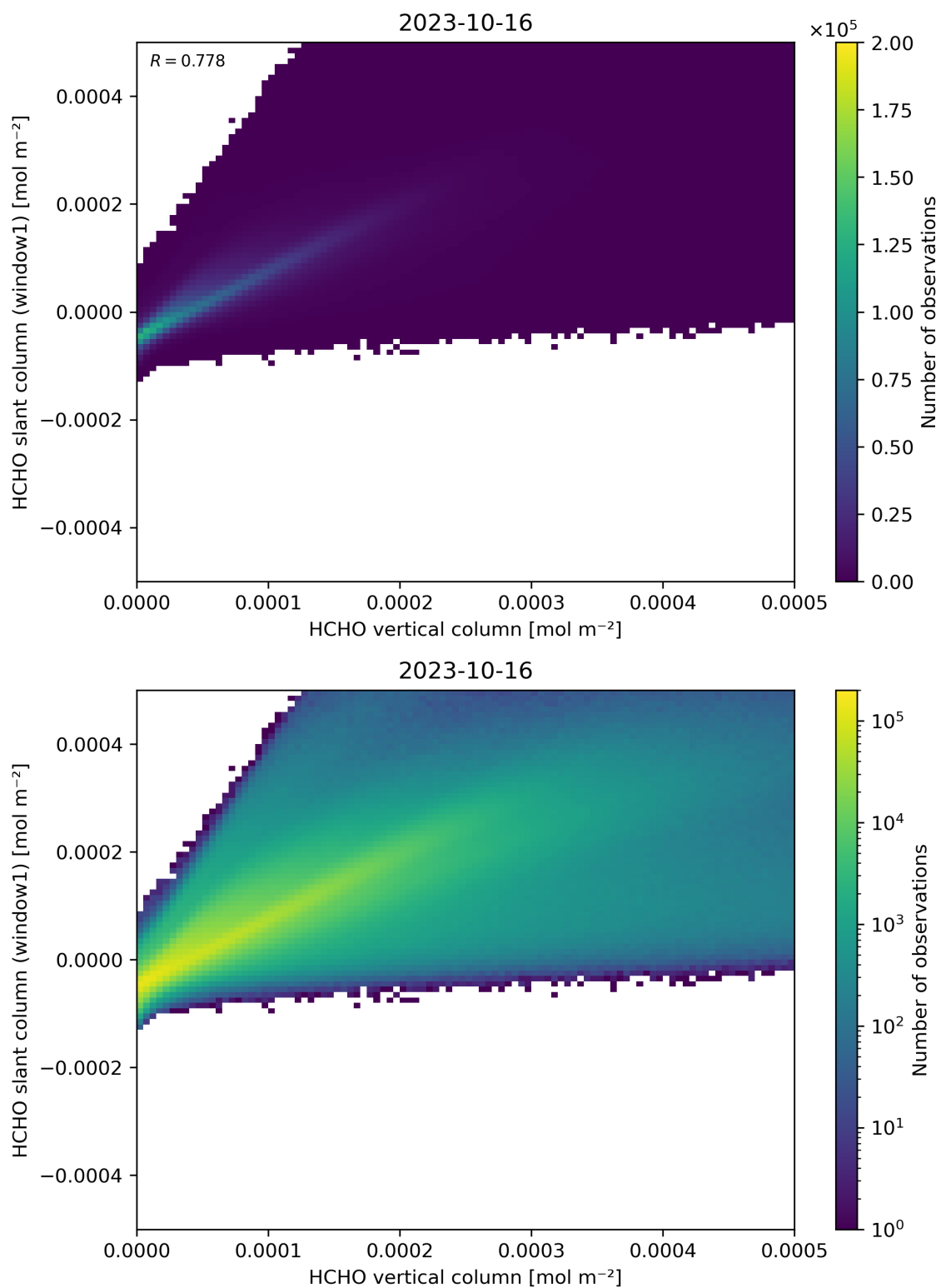
Figure 129: Scatter density plot of “HCHO vertical column” against “HCHO slant column (window1)” for 2023-10-15 to 2023-10-17.
