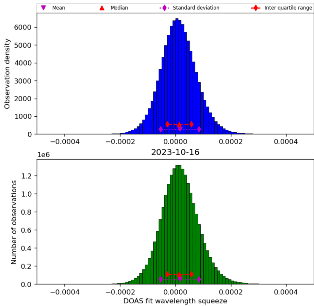
Figure 45: Histogram of “DOAS fit wavelength squeeze” for 2023-10-15 to 2023-10-17
