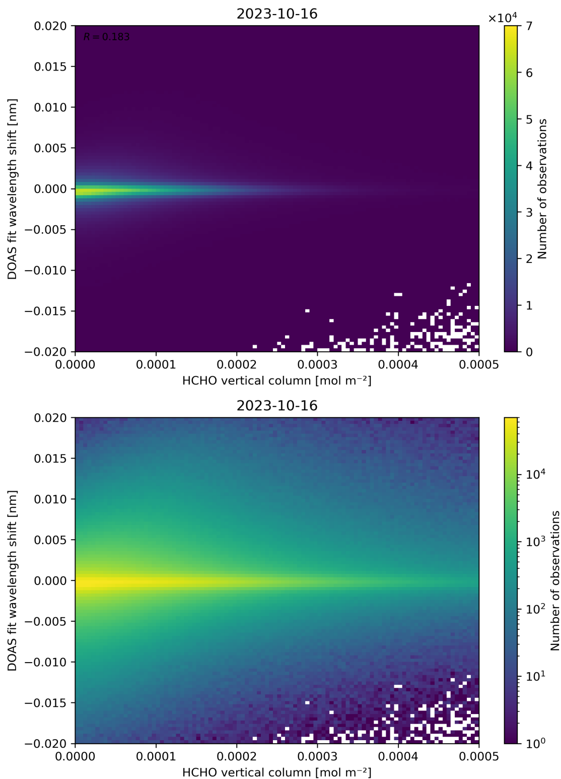
Figure 124: Scatter density plot of “HCHO vertical column” against “DOAS fit wavelength shift” for 2023-10-15 to 2023-10-17.
