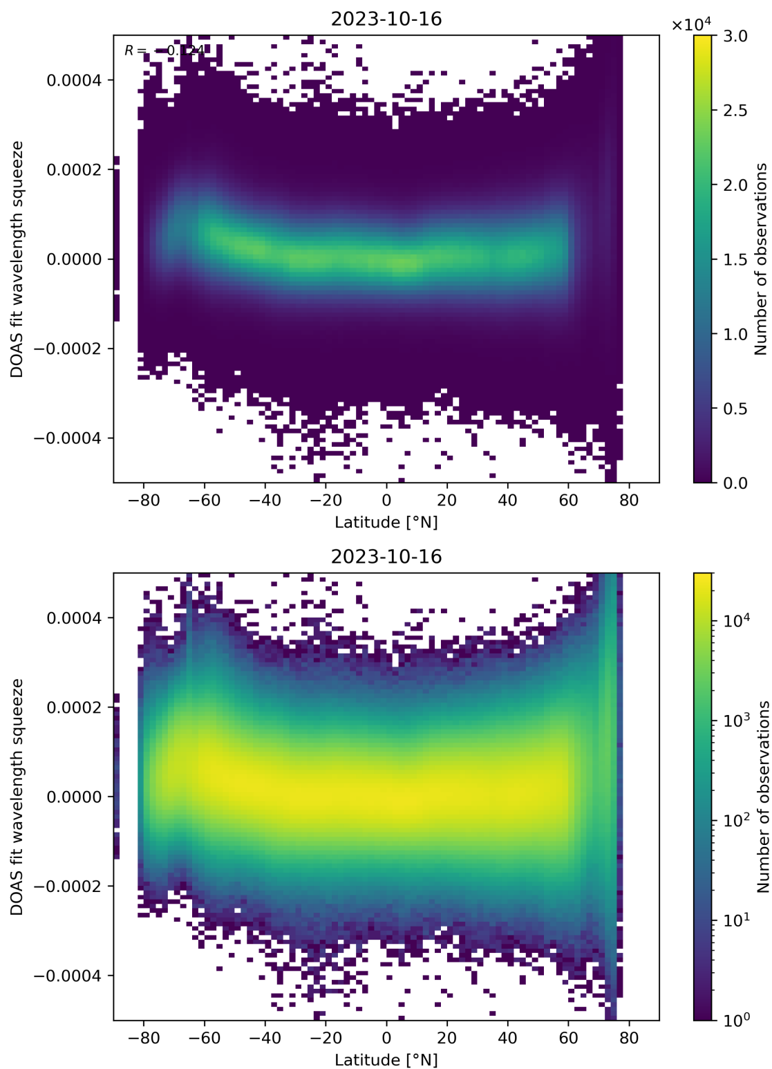
Figure 155: Scatter density plot of “Latitude” against “DOAS fit wavelength squeeze” for 2023-10-15 to 2023-10-17.
