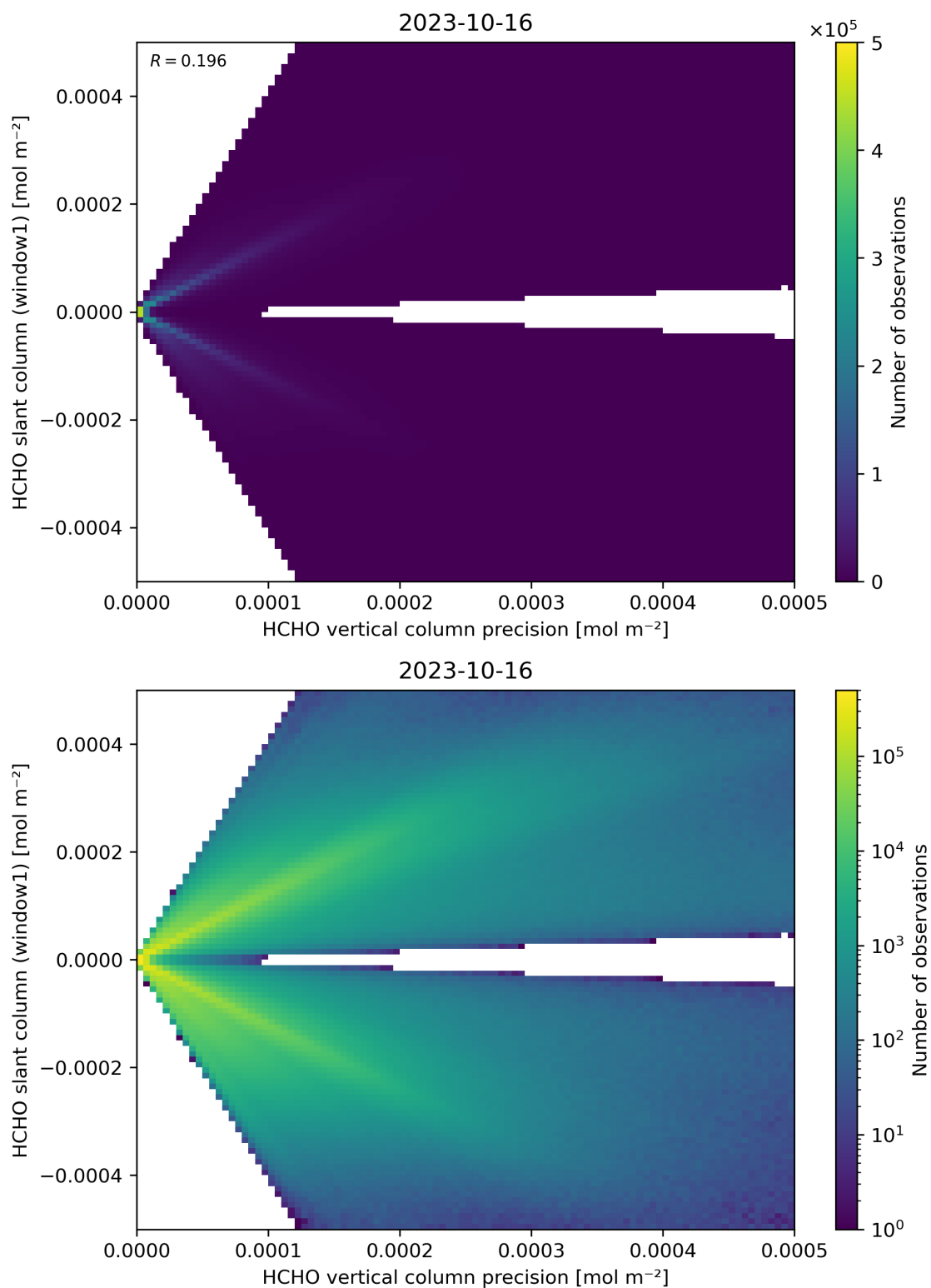
Figure 142: Scatter density plot of “HCHO vertical column precision” against “HCHO slant column (window1)” for 2023-10-15 to 2023-10-17.
