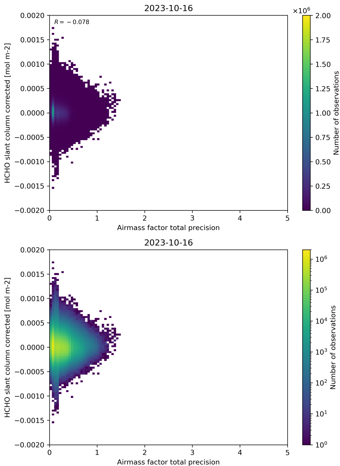
Figure 109: Scatter density plot of “Airmass factor total precision” against “HCHO slant column corrected” for 2023-10-15 to 2023-10-17.
