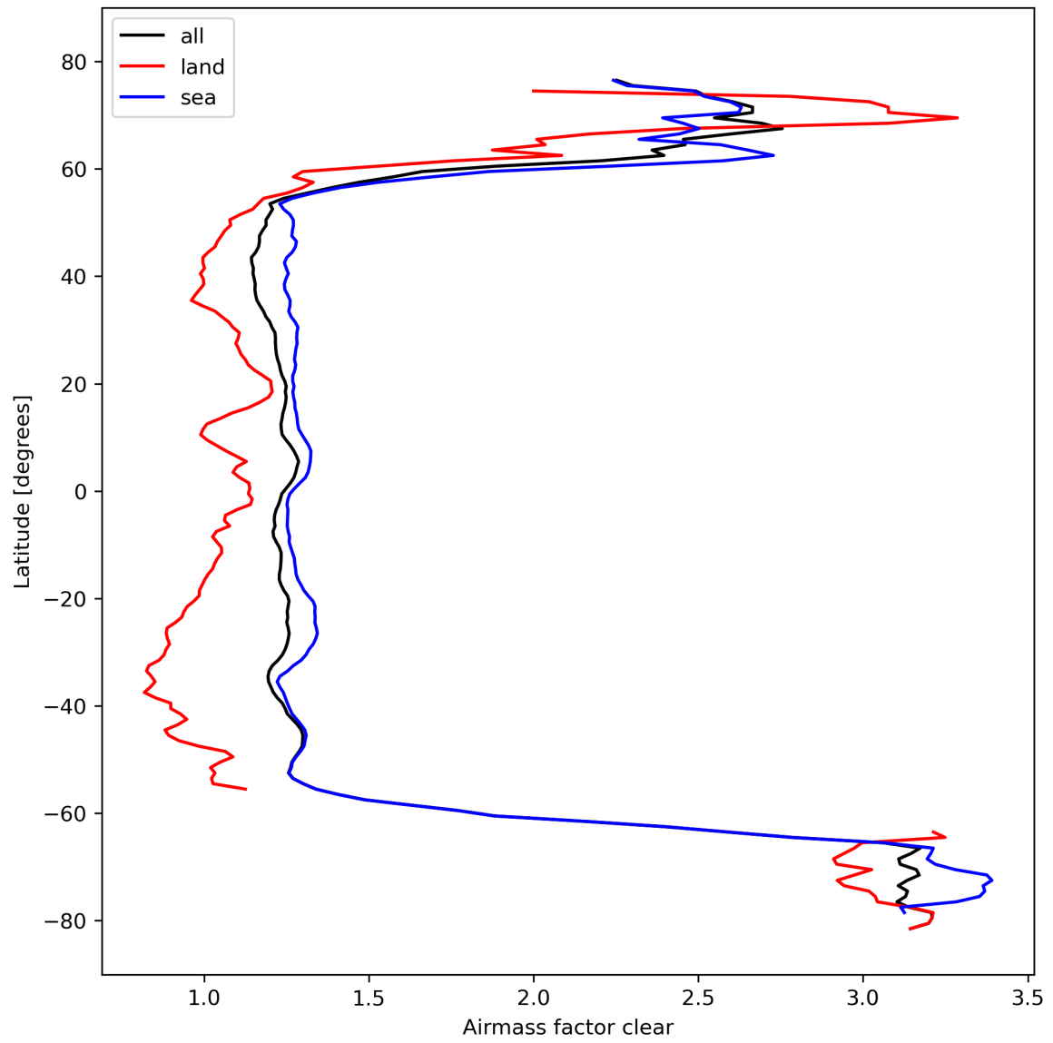
Figure 28: Zonal average of “Airmass factor clear” for 2023-10-15 to 2023-10-17.
