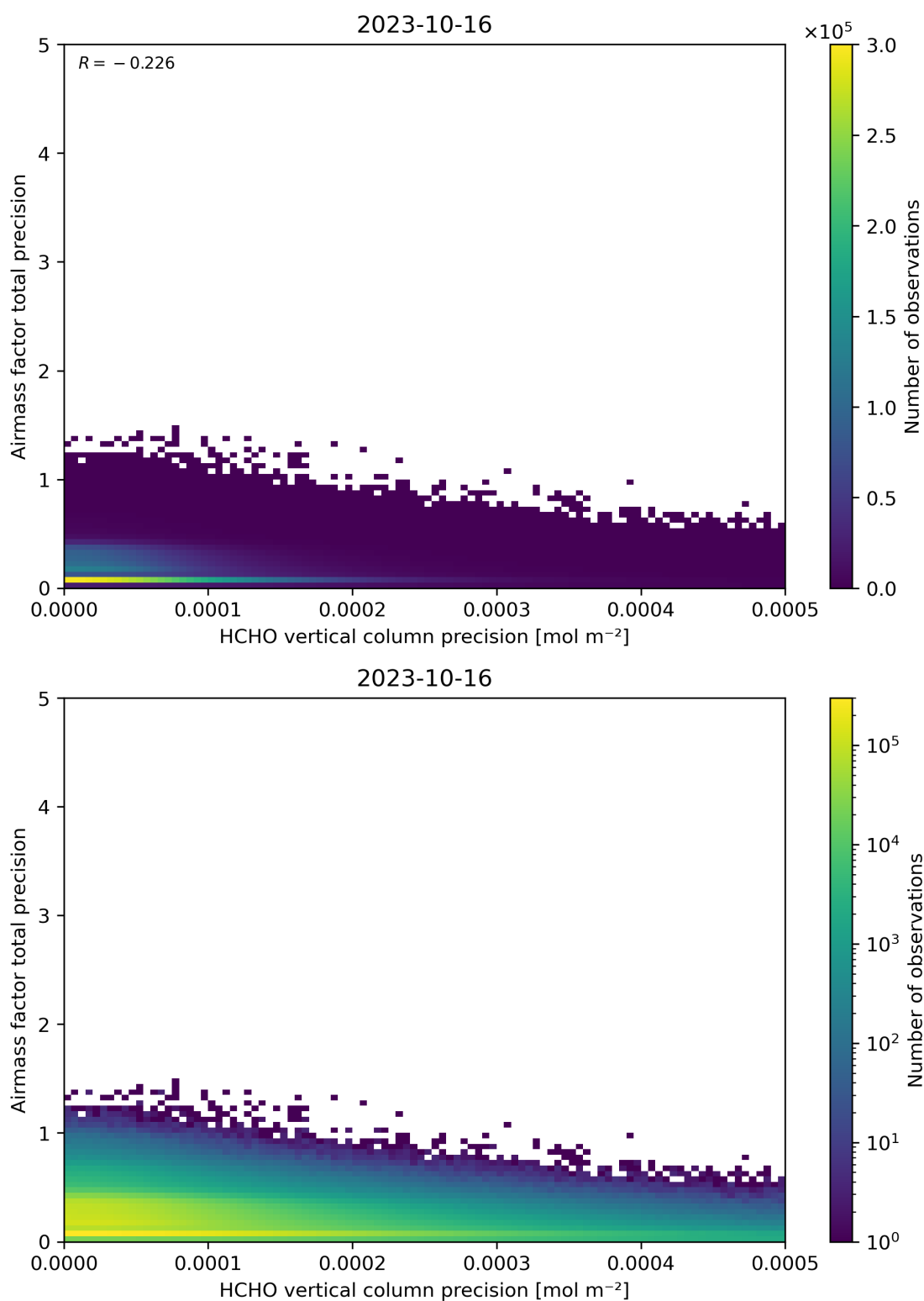
Figure 145: Scatter density plot of “HCHO vertical column precision” against “Airmass factor total precision” for 2023-10-15 to 2023-10-17.
