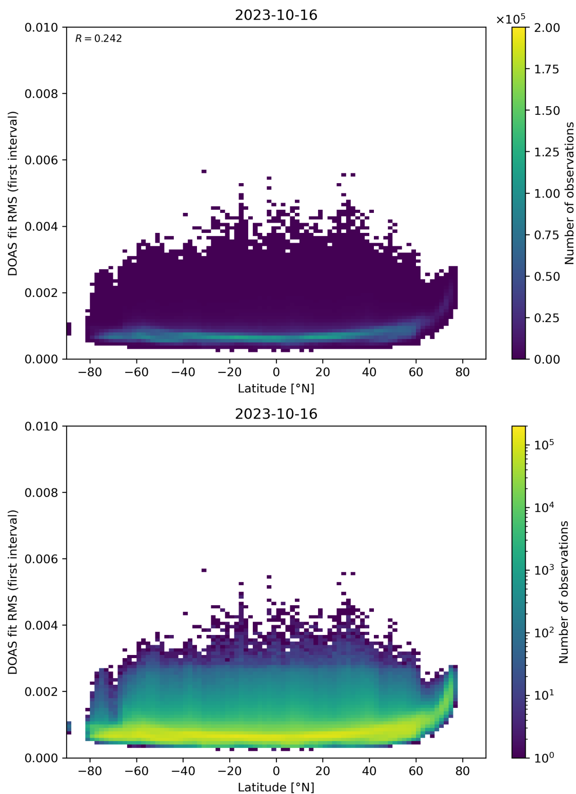
Figure 153: Scatter density plot of “Latitude” against “DOAS fit RMS (first interval)” for 2023-10-15 to 2023-10-17.
