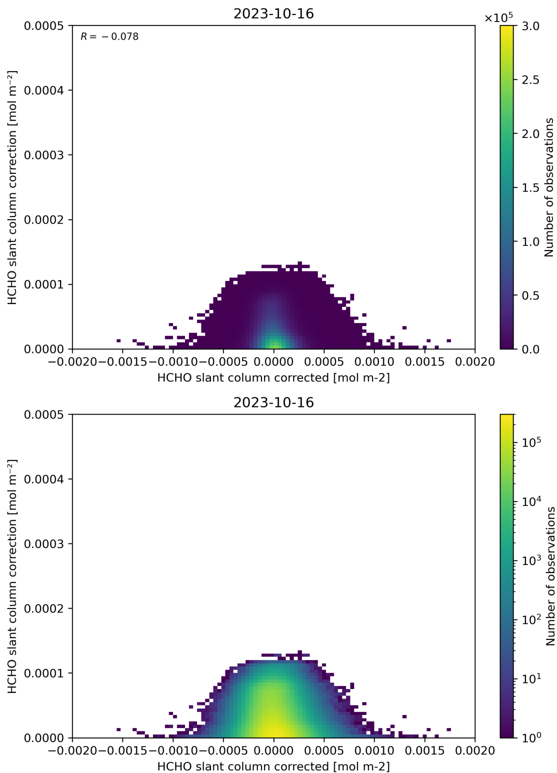
Figure 77: Scatter density plot of “HCHO slant column corrected” against “HCHO slant column correction” for 2023-10-15 to 2023-10-17.
