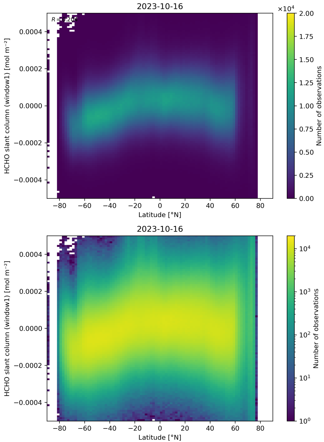
Figure 159: Scatter density plot of “Latitude” against “HCHO slant column (window1)” for 2023-10-15 to 2023-10-17.
