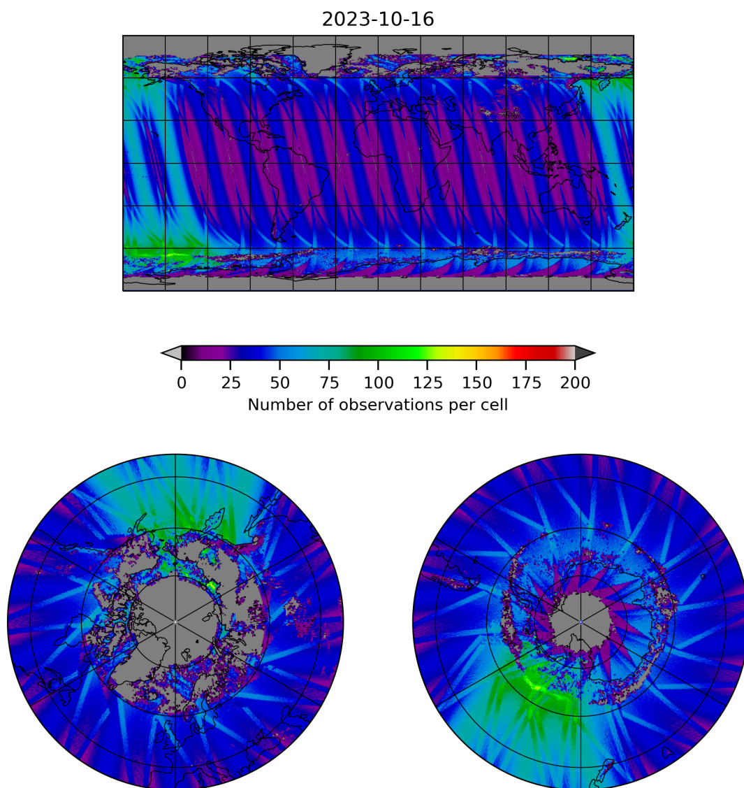
Figure 19: Map of the number of observations for 2023-10-15 to 2023-10-17
