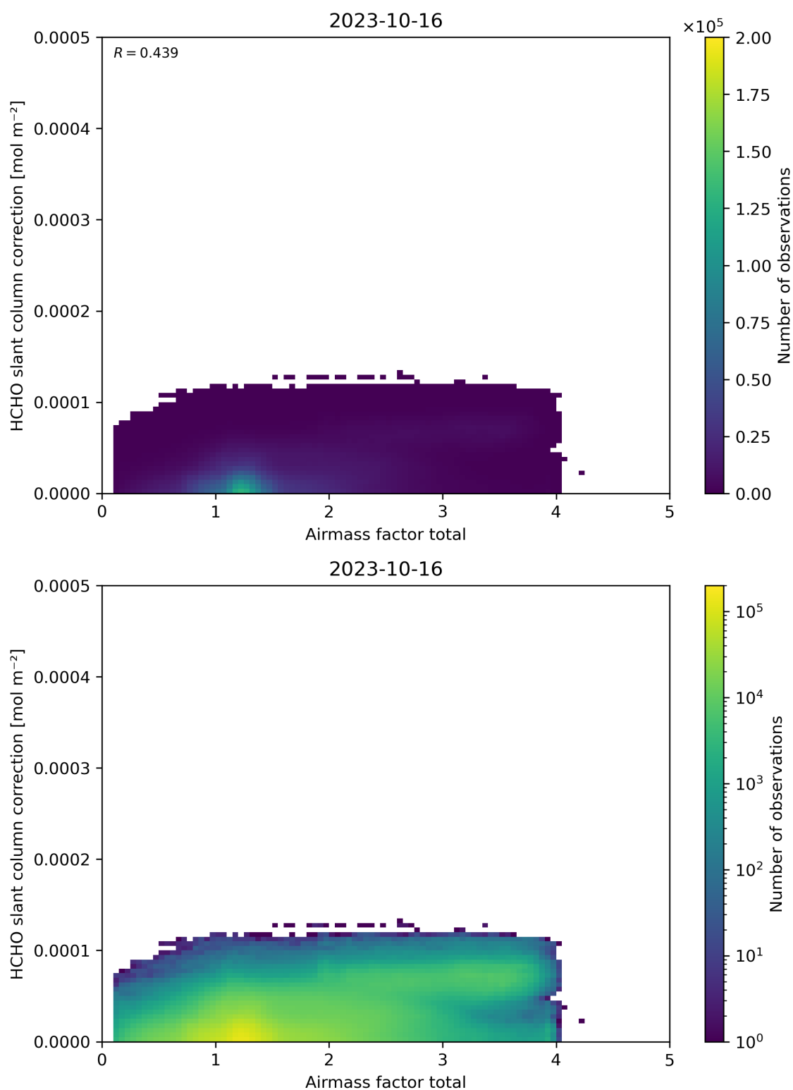
Figure 102: Scatter density plot of “Airmass factor total” against “HCHO slant column correction” for 2023-10-15 to 2023-10-17.
