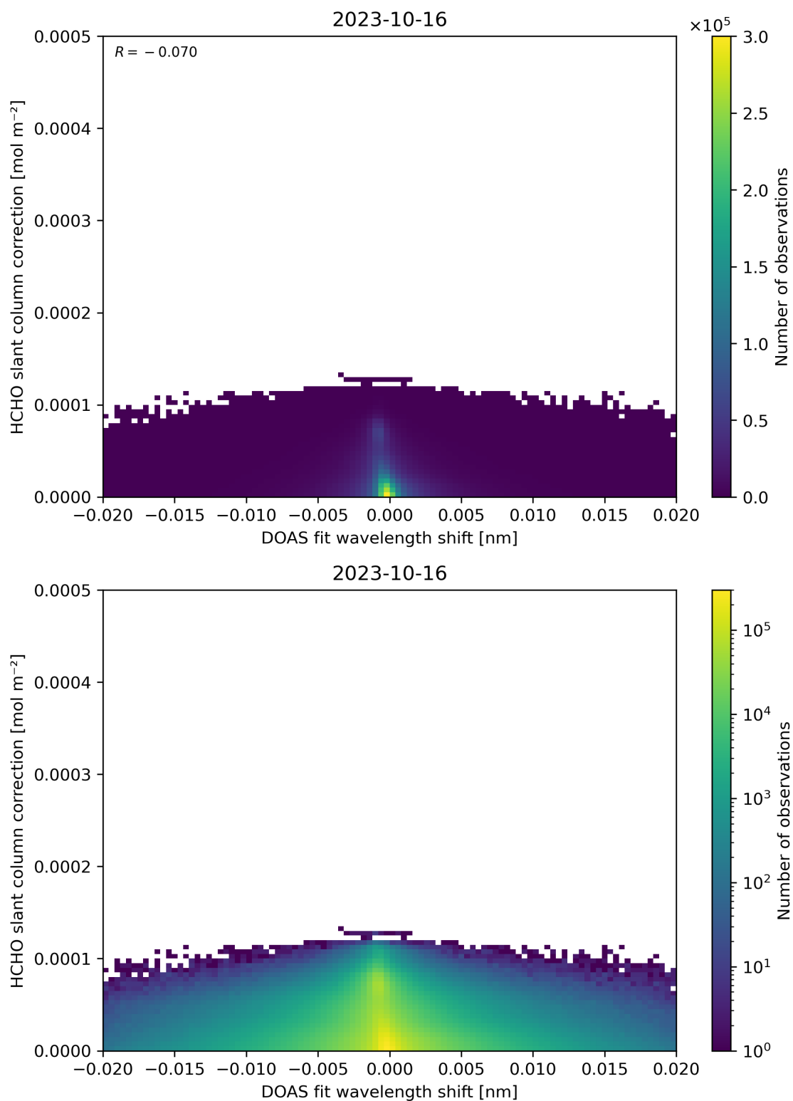
Figure 67: Scatter density plot of “DOAS fit wavelength shift” against “HCHO slant column correction” for 2023-10-15 to 2023-10-17.
