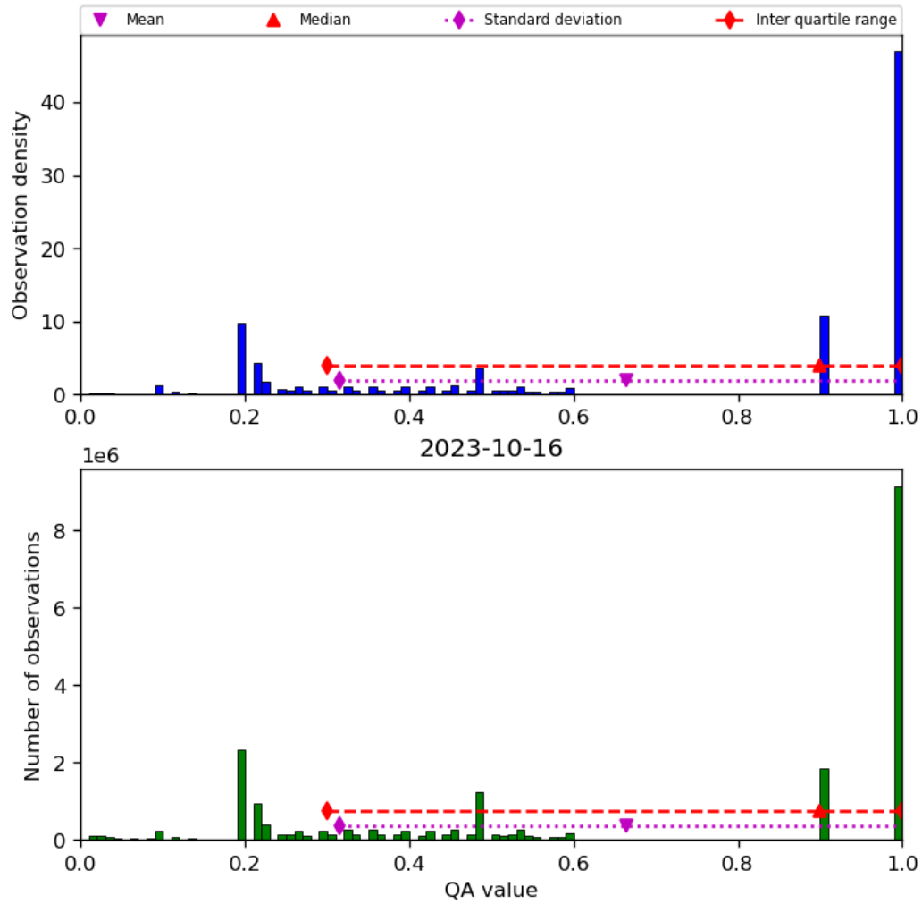
Figure 34: Histogram of “QA value” for 2023-10-15 to 2023-10-17
