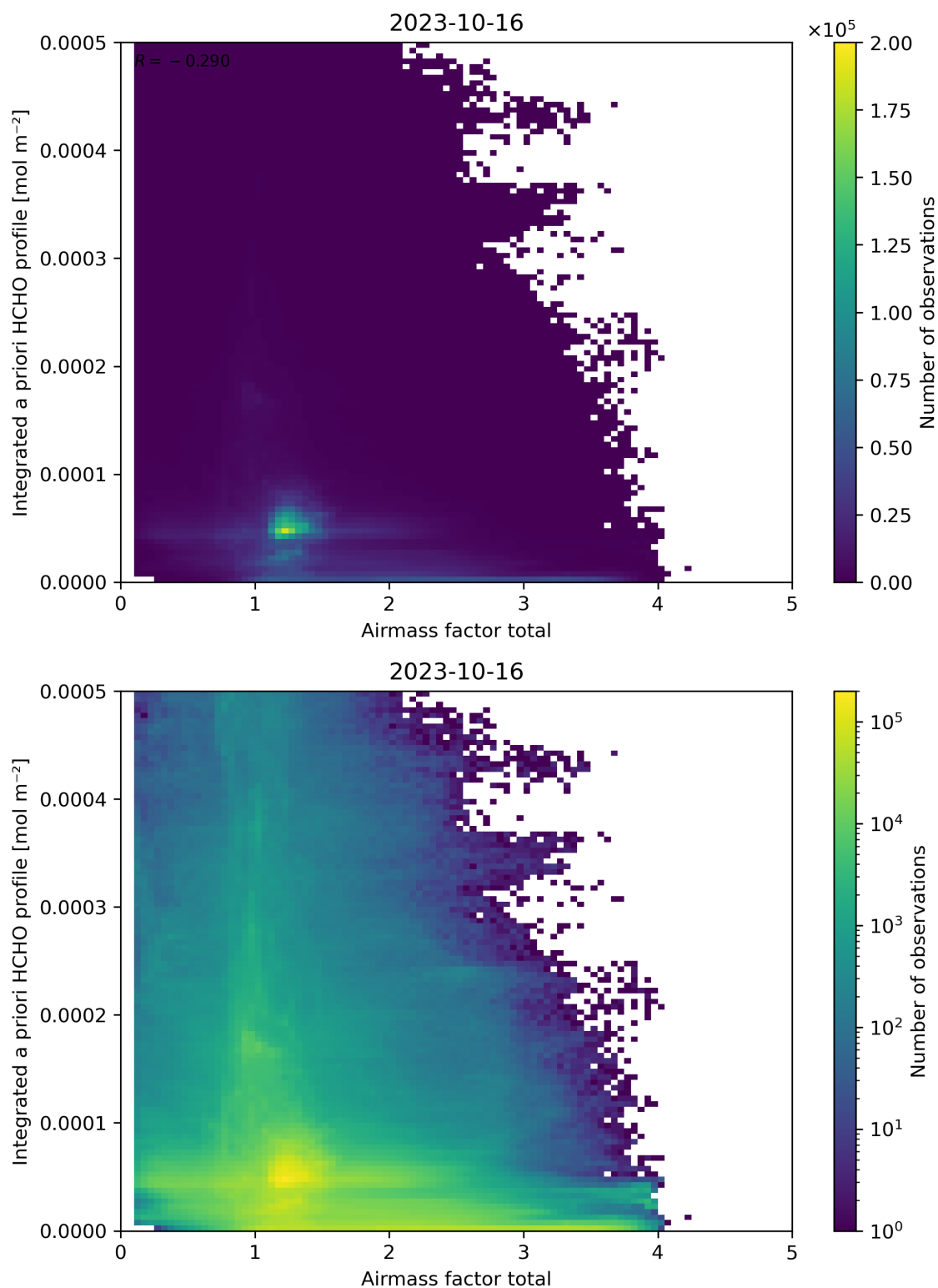
Figure 104: Scatter density plot of “Airmass factor total” against “Integrated a priori HCHO profile” for 2023-10-15 to 2023-10-17.
