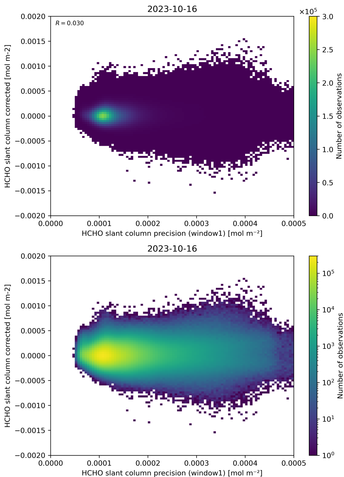
Figure 92: Scatter density plot of “HCHO slant column precision (window1)” against “HCHO slant column corrected” for 2023-10-15 to 2023-10-17.
