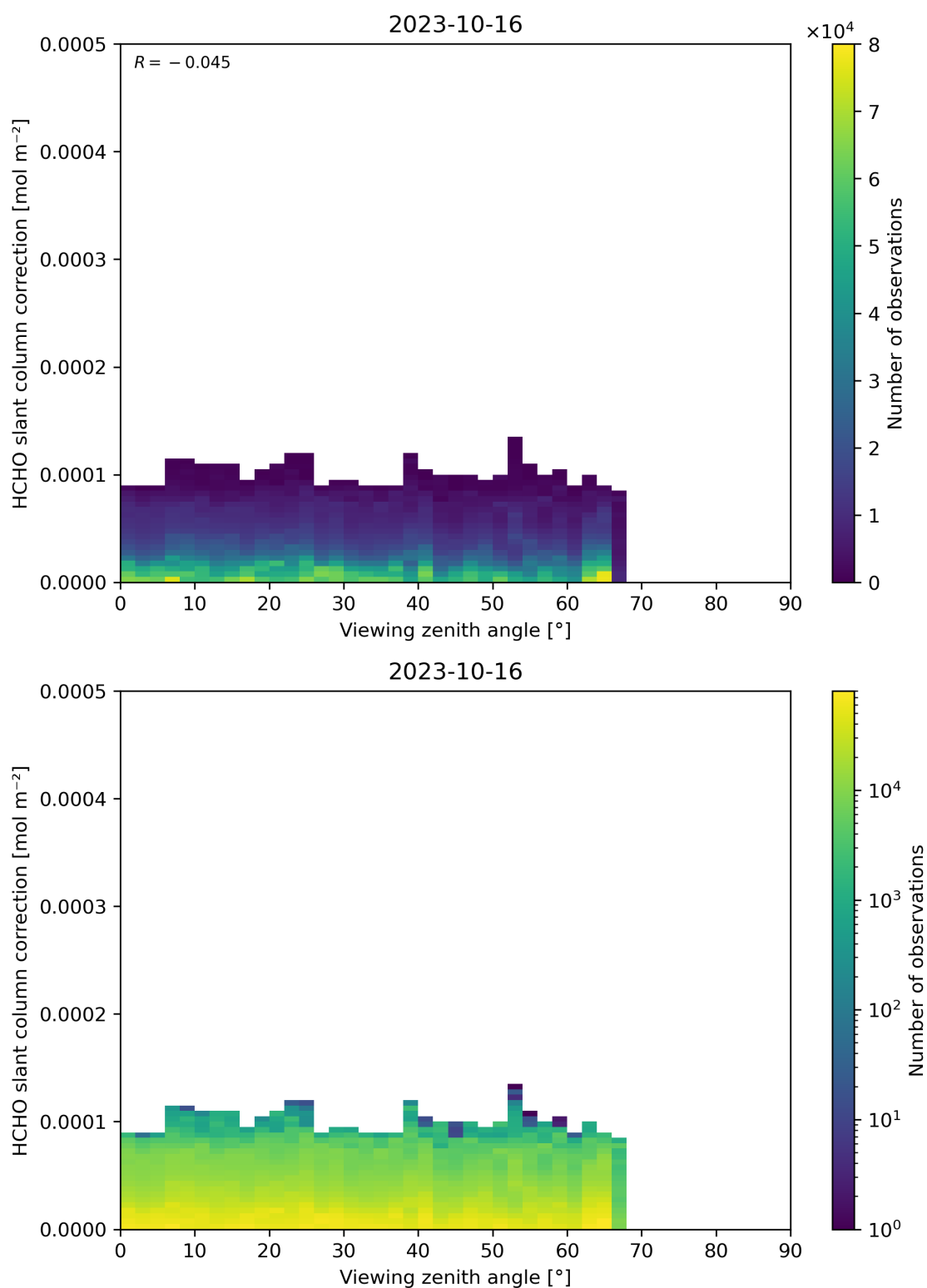
Figure 187: Scatter density plot of “Viewing zenith angle” against “HCHO slant column correction” for 2023-10-15 to 2023-10-17.
