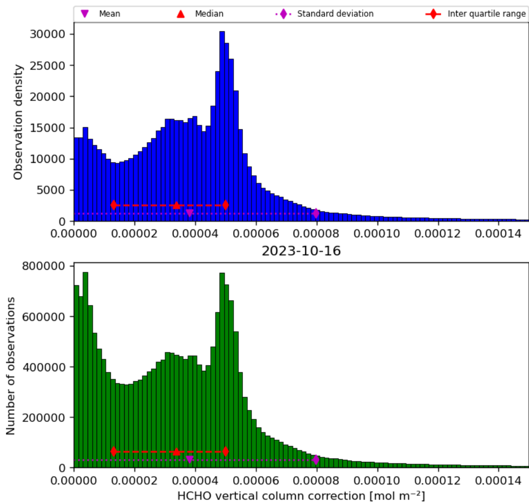
Figure 37: Histogram of “HCHO vertical column correction” for 2023-10-15 to 2023-10-17
