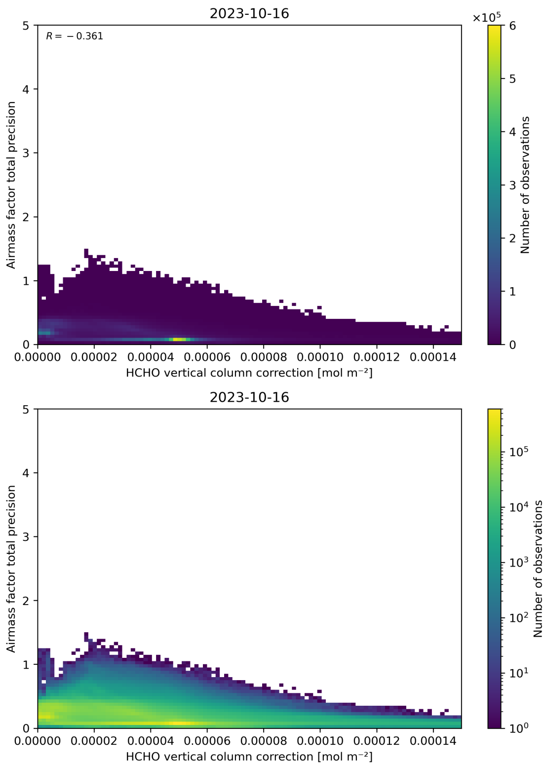
Figure 121: Scatter density plot of “HCHO vertical column correction” against “Airmass factor total precision” for 2023-10-15 to 2023-10-17.
