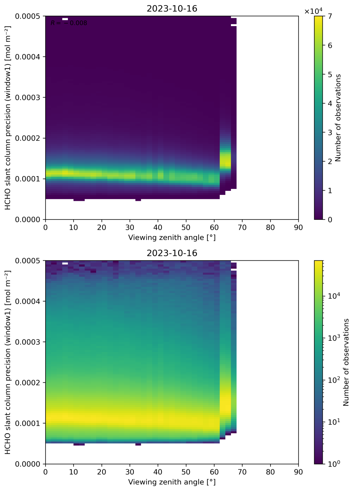
Figure 189: Scatter density plot of “Viewing zenith angle” against “HCHO slant column precision (window1)” for 2023-10-15 to 2023-10-17.
