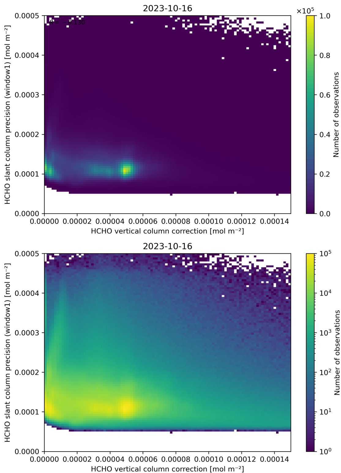
Figure 119: Scatter density plot of “HCHO vertical column correction” against “HCHO slant column precision (window1)” for 2023-10-15 to 2023-10-17.
