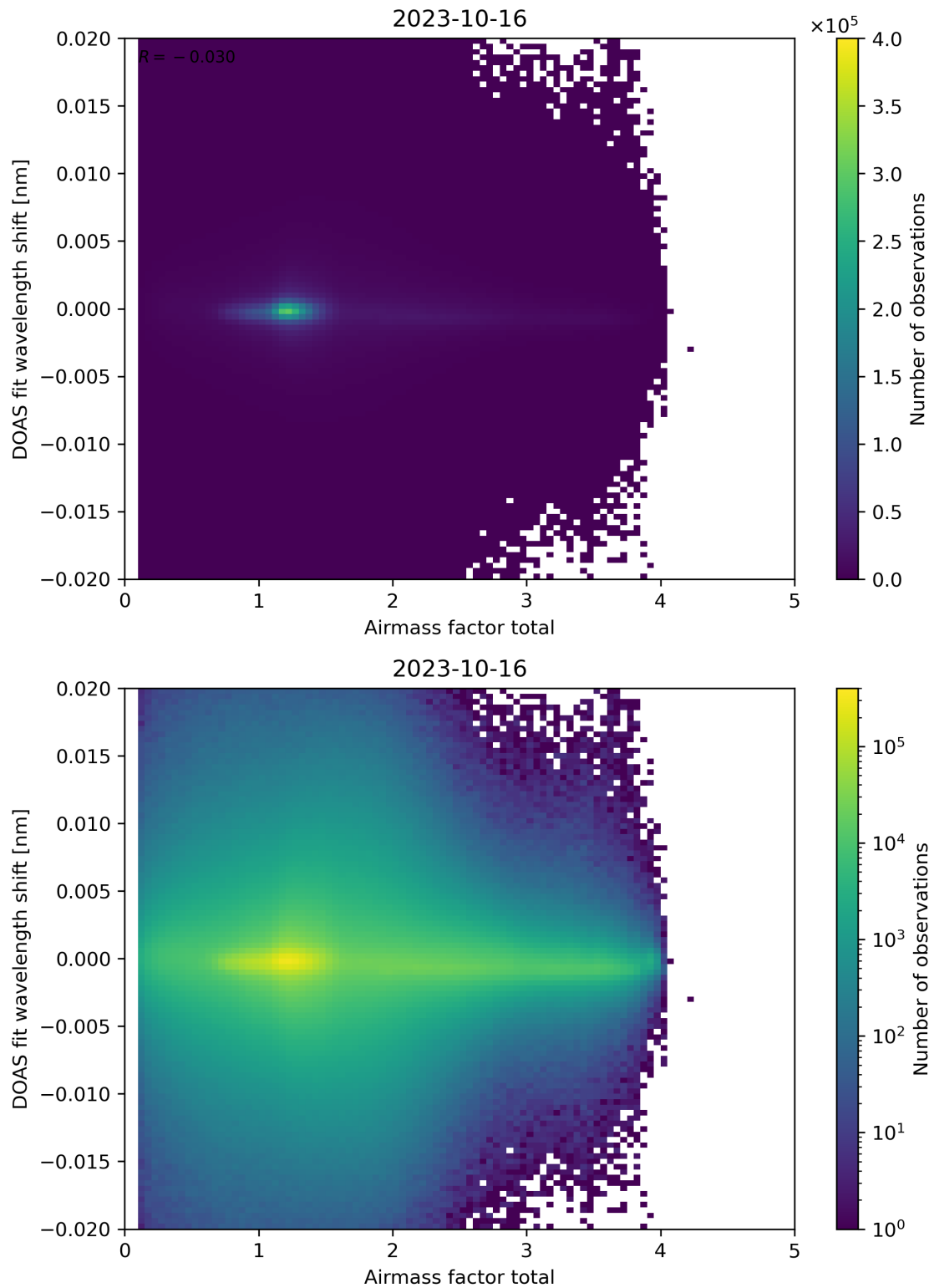
Figure 98: Scatter density plot of “Airmass factor total” against “DOAS fit wavelength shift” for 2023-10-15 to 2023-10-17.
