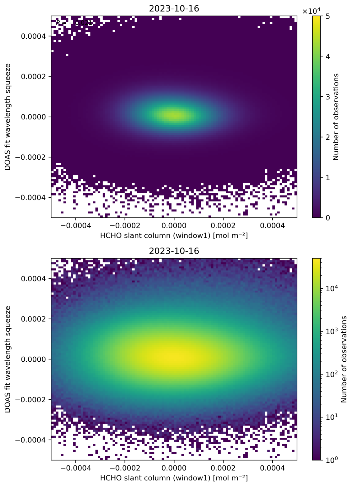
Figure 80: Scatter density plot of “HCHO slant column (window1)” against “DOAS fit wavelength squeeze” for 2023-10-15 to 2023-10-17.
