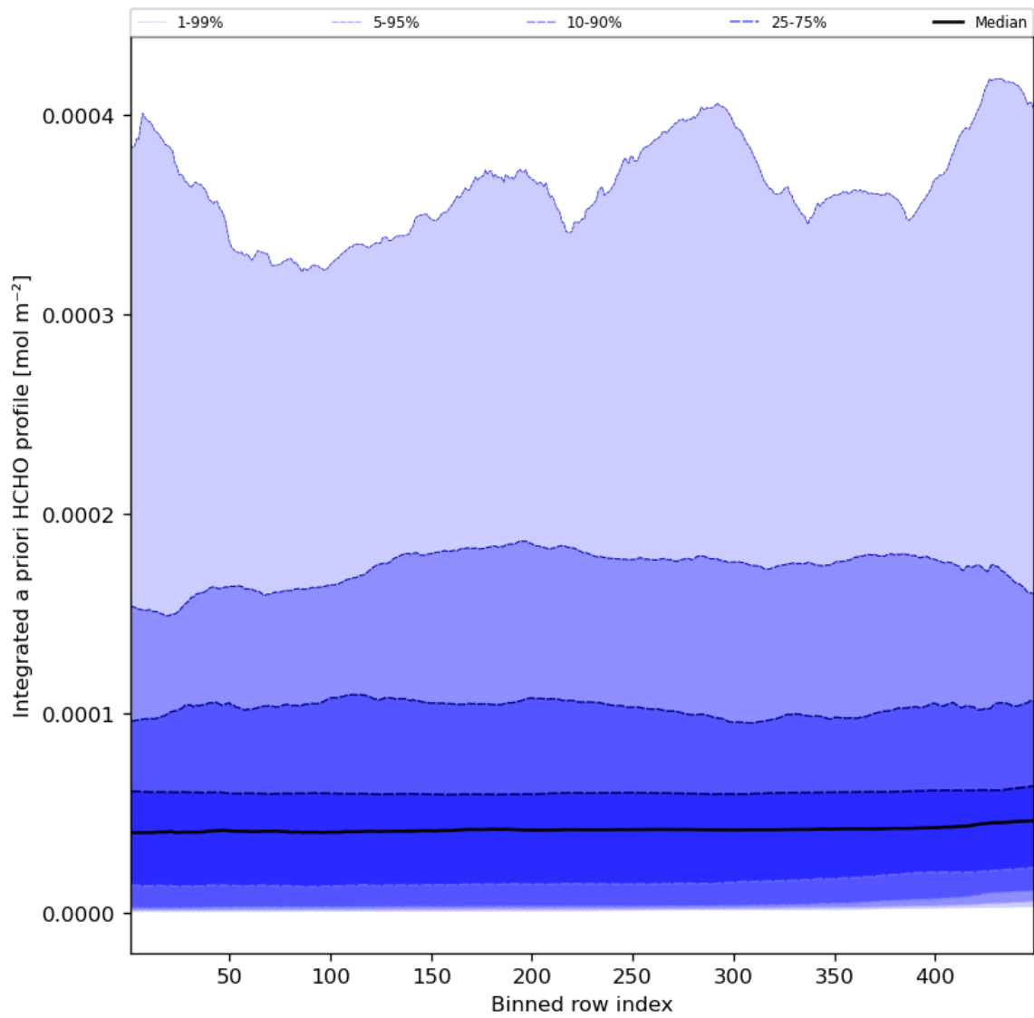
Figure 57: Along track statistics of “Integrated a priori HCHO profile” for 2023-10-15 to 2023-10-17
