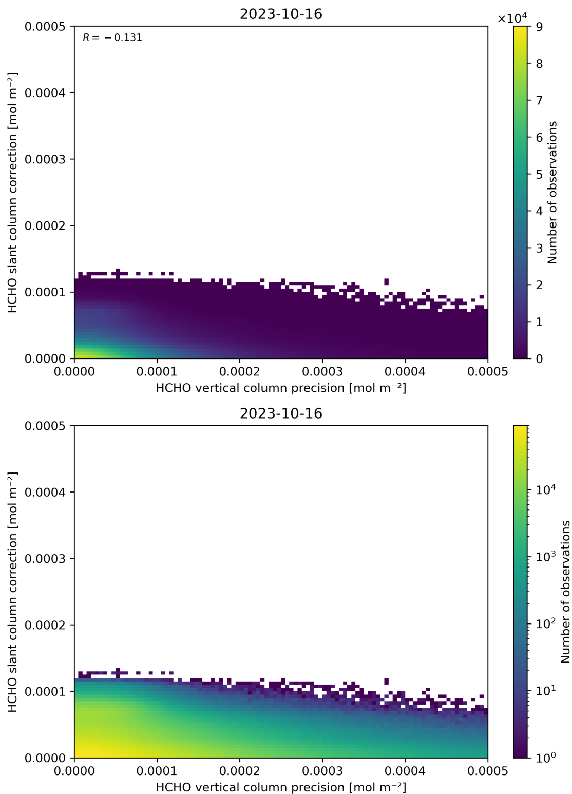
Figure 141: Scatter density plot of “HCHO vertical column precision” against “HCHO slant column correction” for 2023-10-15 to 2023-10-17.
