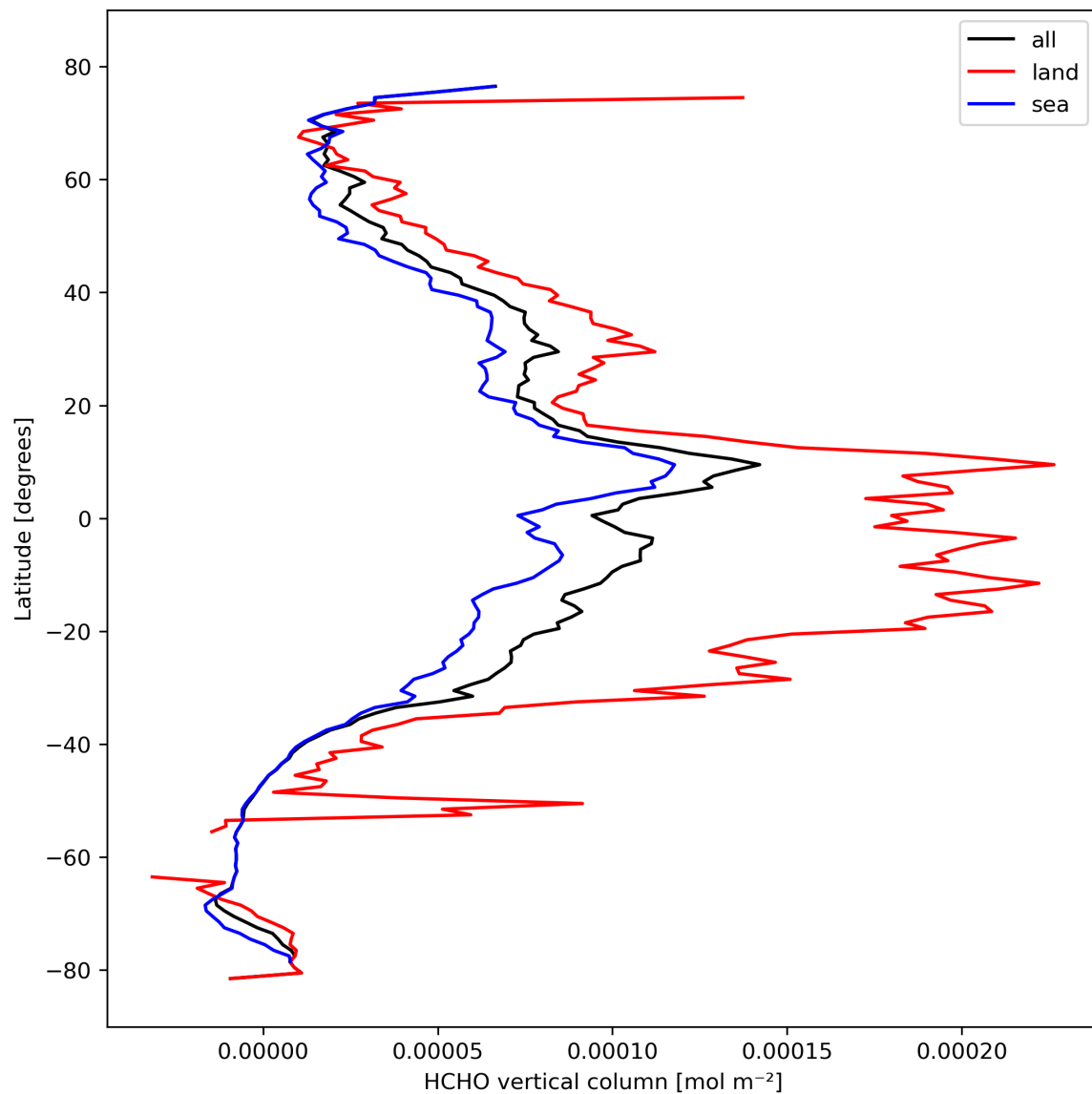
Figure 21: Zonal average of “HCHO vertical column” for 2023-10-15 to 2023-10-17.
