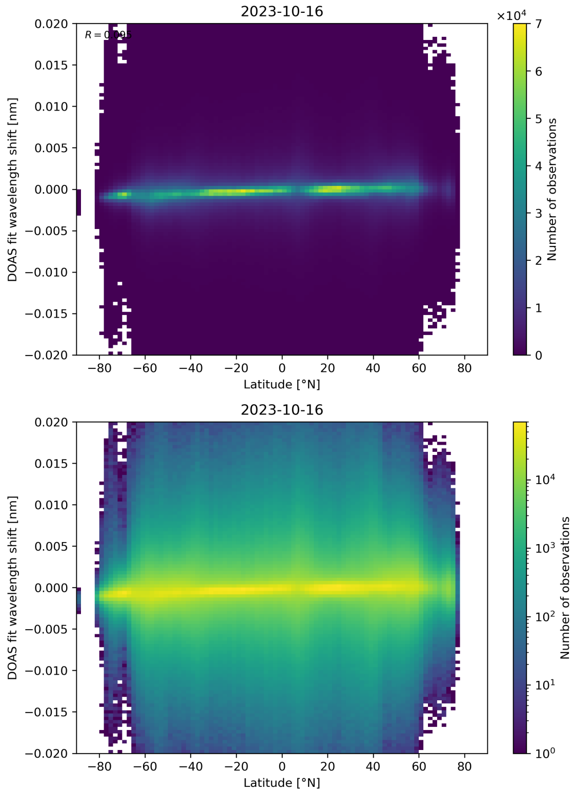
Figure 154: Scatter density plot of “Latitude” against “DOAS fit wavelength shift” for 2023-10-15 to 2023-10-17.
