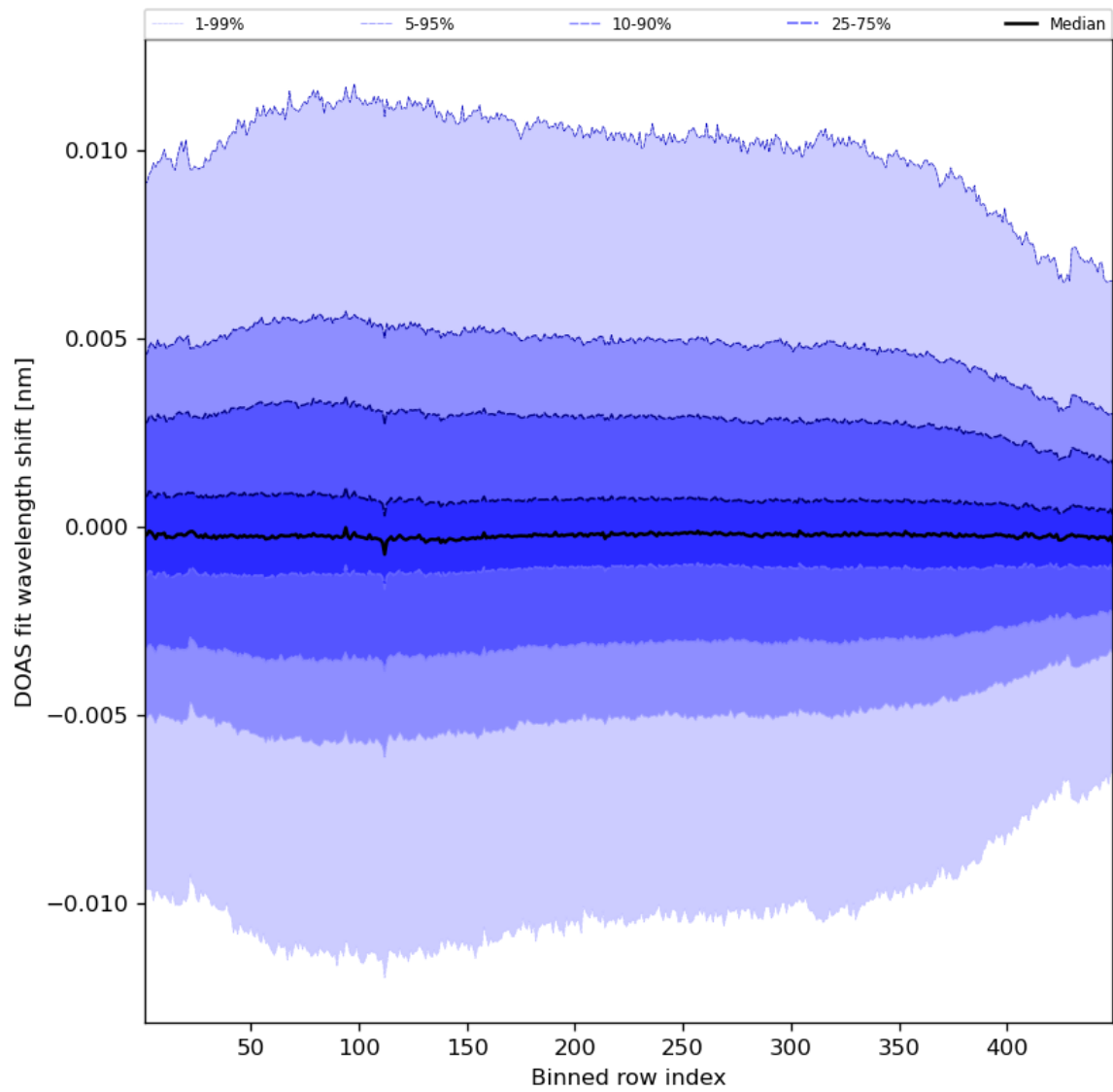
Figure 58: Along track statistics of “DOAS fit wavelength shift” for 2023-10-15 to 2023-10-17
