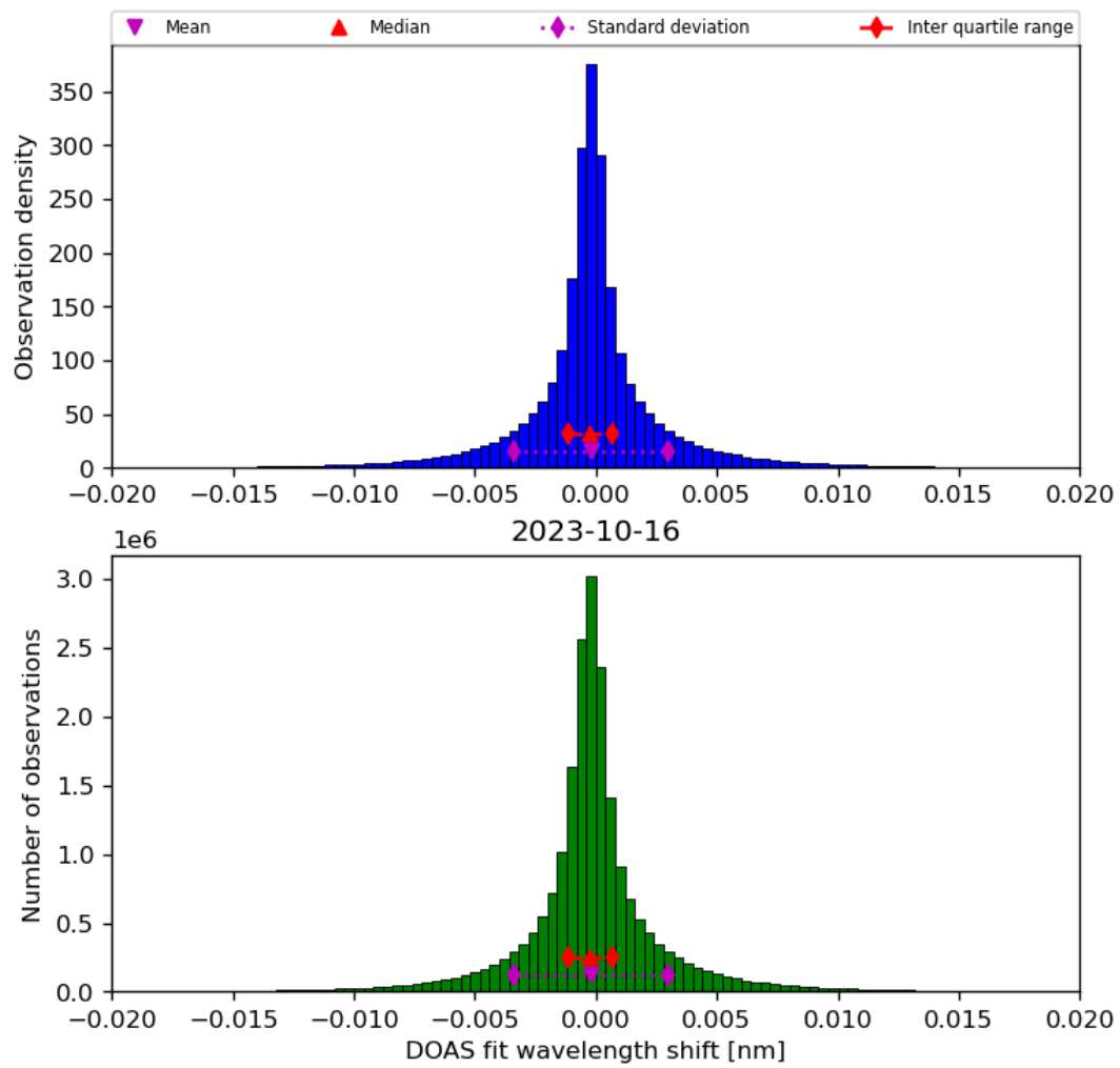
Figure 44: Histogram of “DOAS fit wavelength shift” for 2023-10-15 to 2023-10-17
