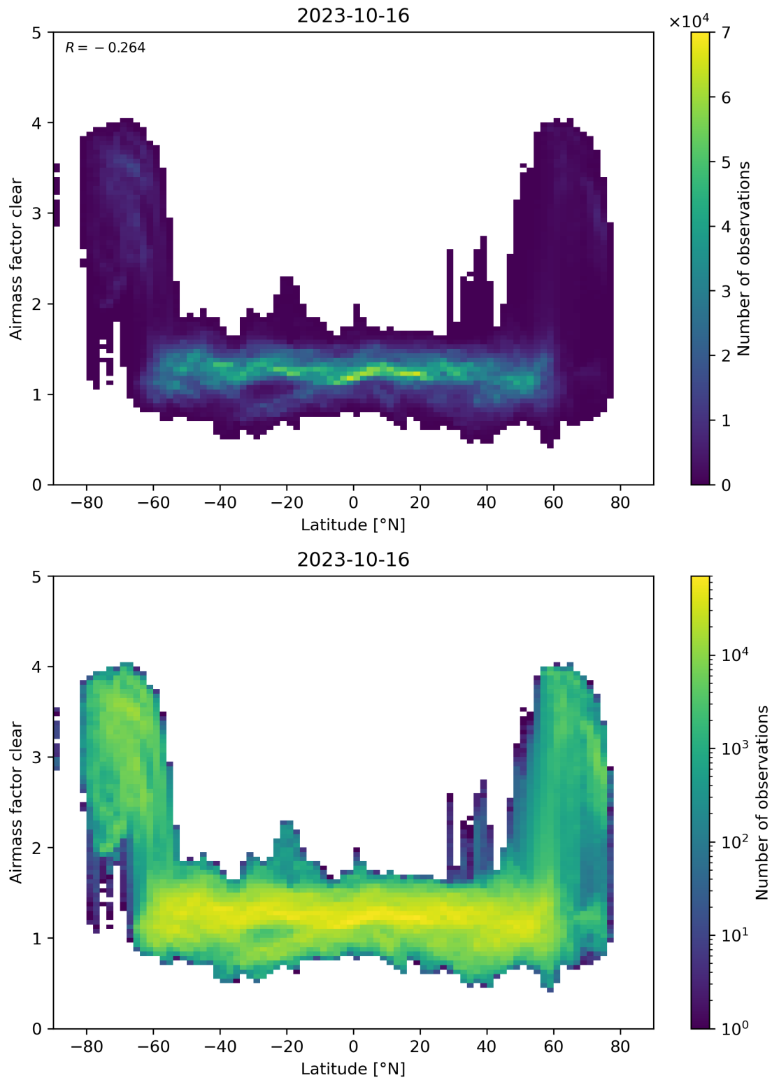
Figure 156: Scatter density plot of “Latitude” against “Airmass factor clear” for 2023-10-15 to 2023-10-17.
