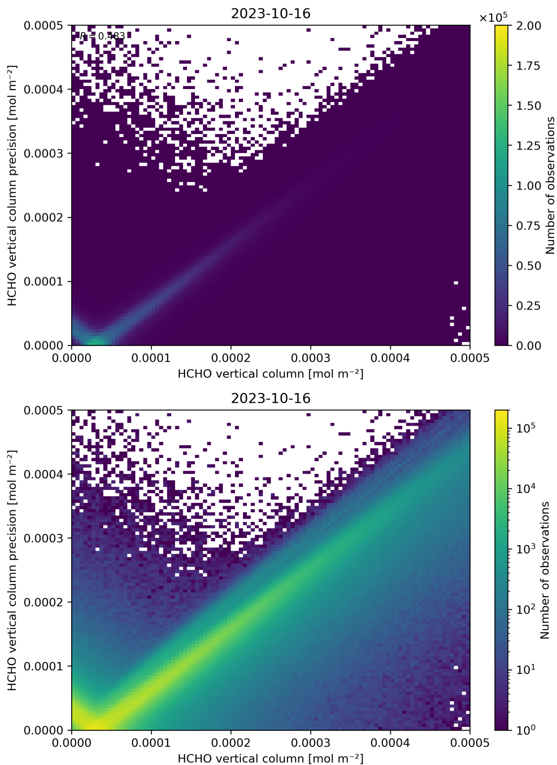
Figure 134: Scatter density plot of “HCHO vertical column” against “HCHO vertical column precision” for 2023-10-15 to 2023-10-17.
