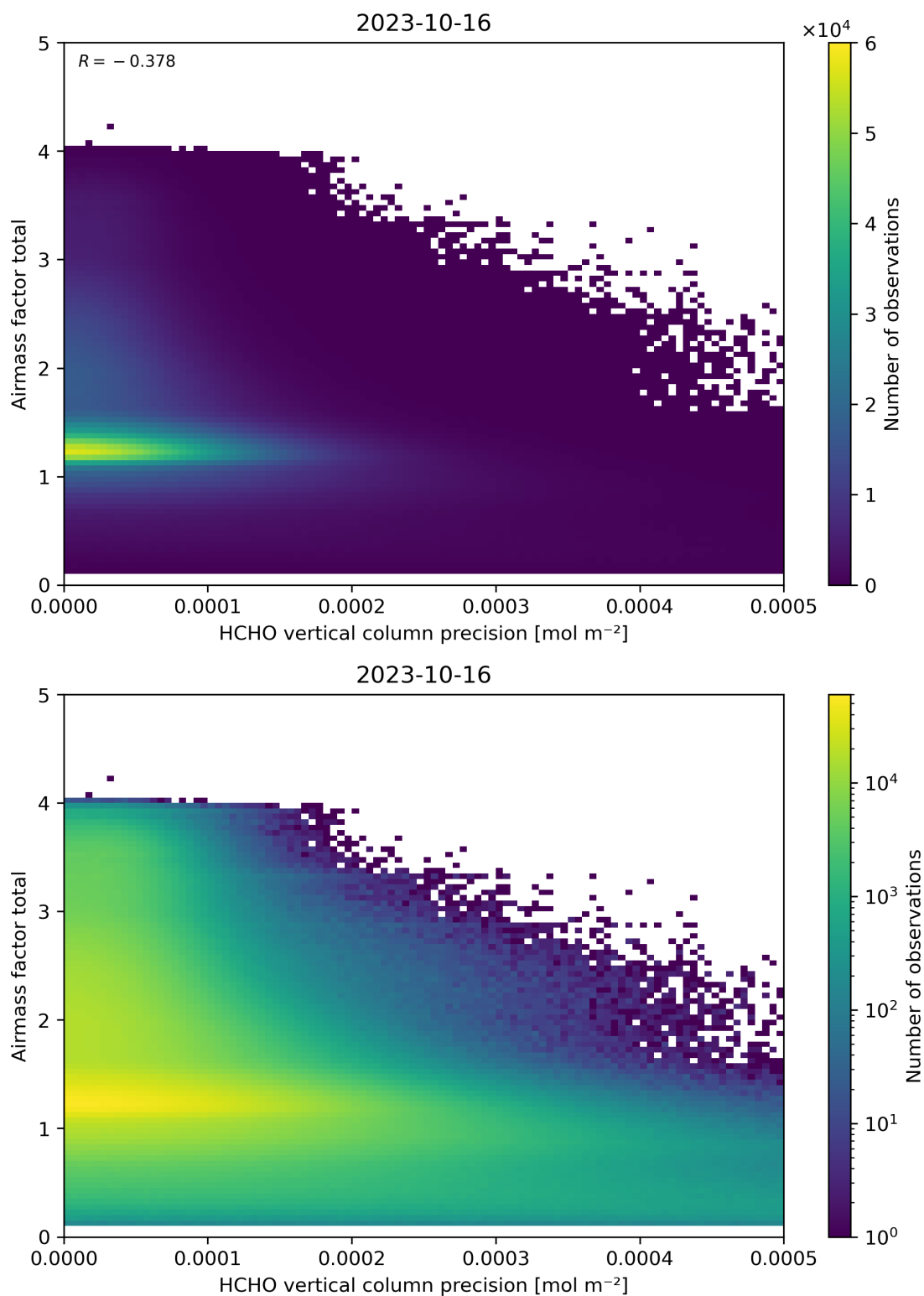
Figure 144: Scatter density plot of “HCHO vertical column precision” against “Airmass factor total” for 2023-10-15 to 2023-10-17.
