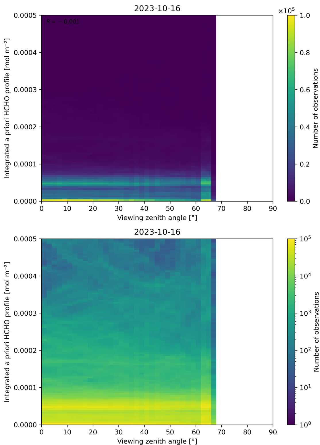
Figure 195: Scatter density plot of “Viewing zenith angle” against “Integrated a priori HCHO profile” for 2023-10-15 to 2023-10-17.
