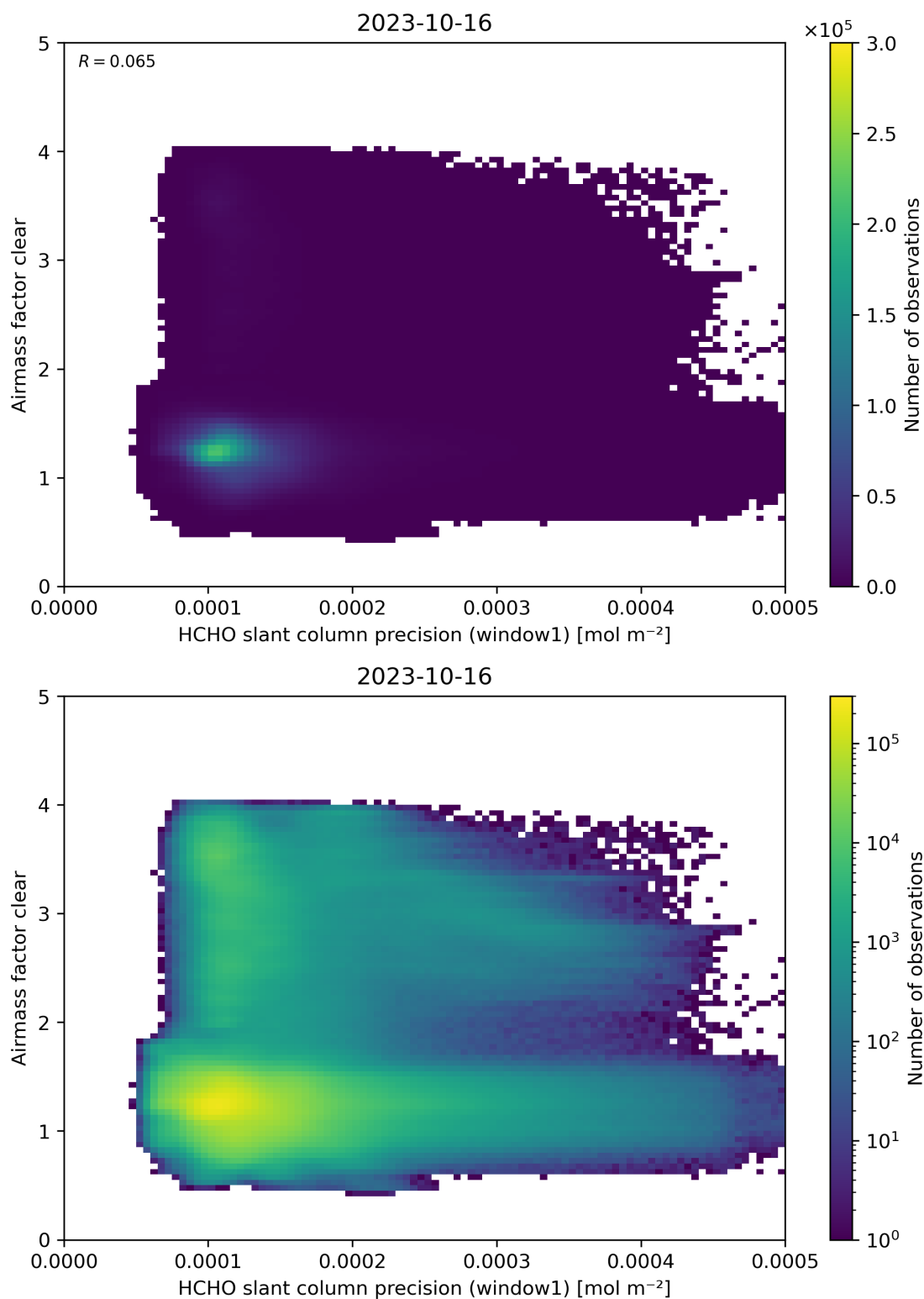
Figure 91: Scatter density plot of “HCHO slant column precision (window1)” against “Airmass factor clear” for 2023-10-15 to 2023-10-17.
