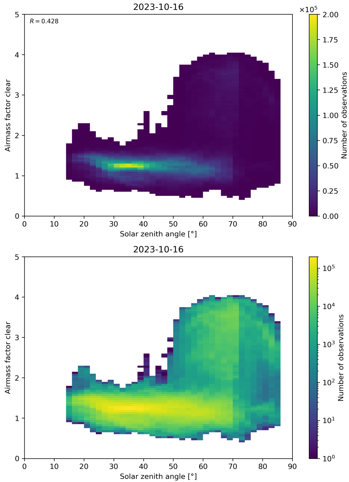
Figure 170: Scatter density plot of “Solar zenith angle” against “Airmass factor clear” for 2023-10-15 to 2023-10-17.
