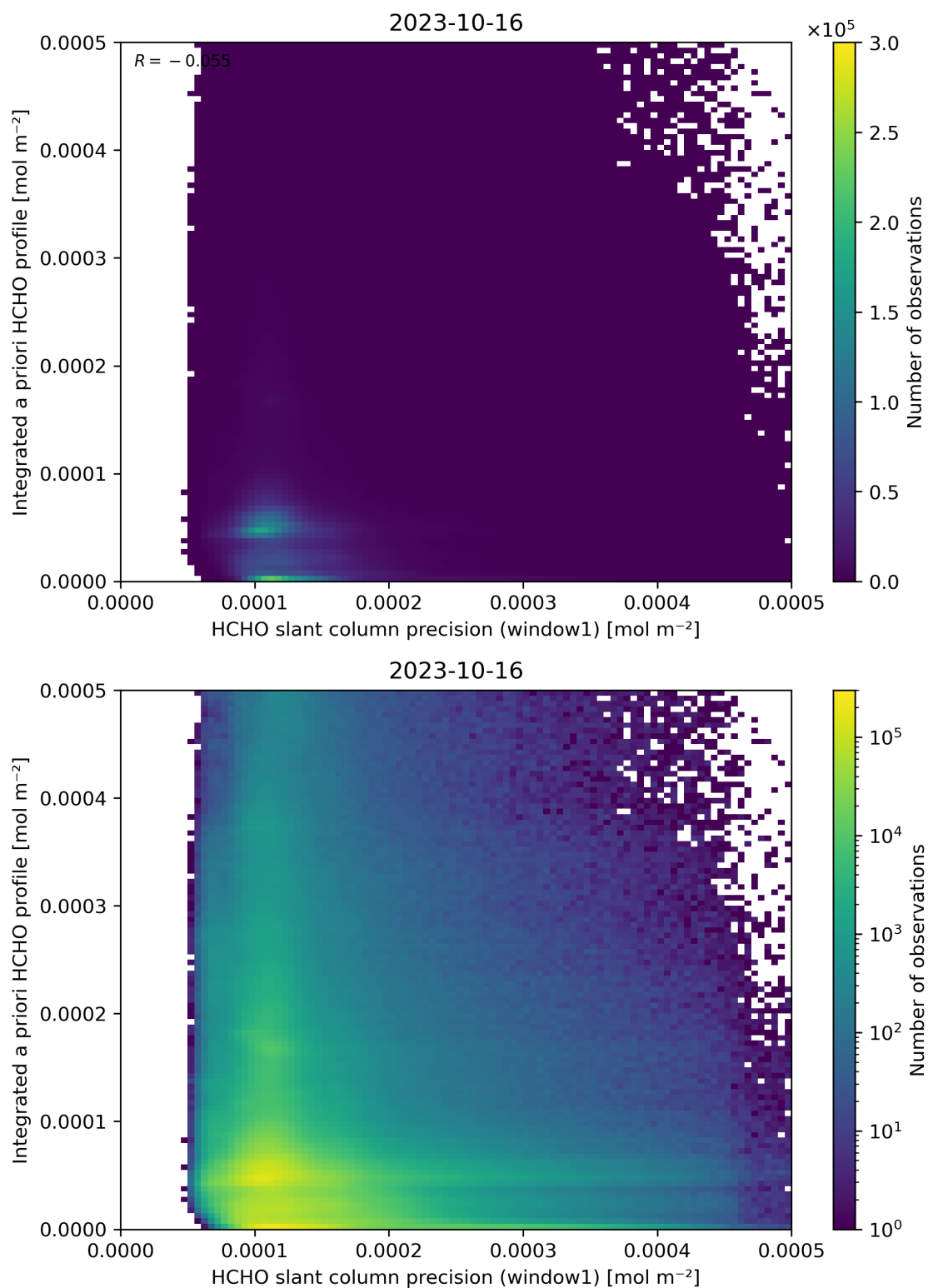
Figure 96: Scatter density plot of “HCHO slant column precision (window1)” against “Integrated a priori HCHO profile” for 2023-10-15 to 2023-10-17.
