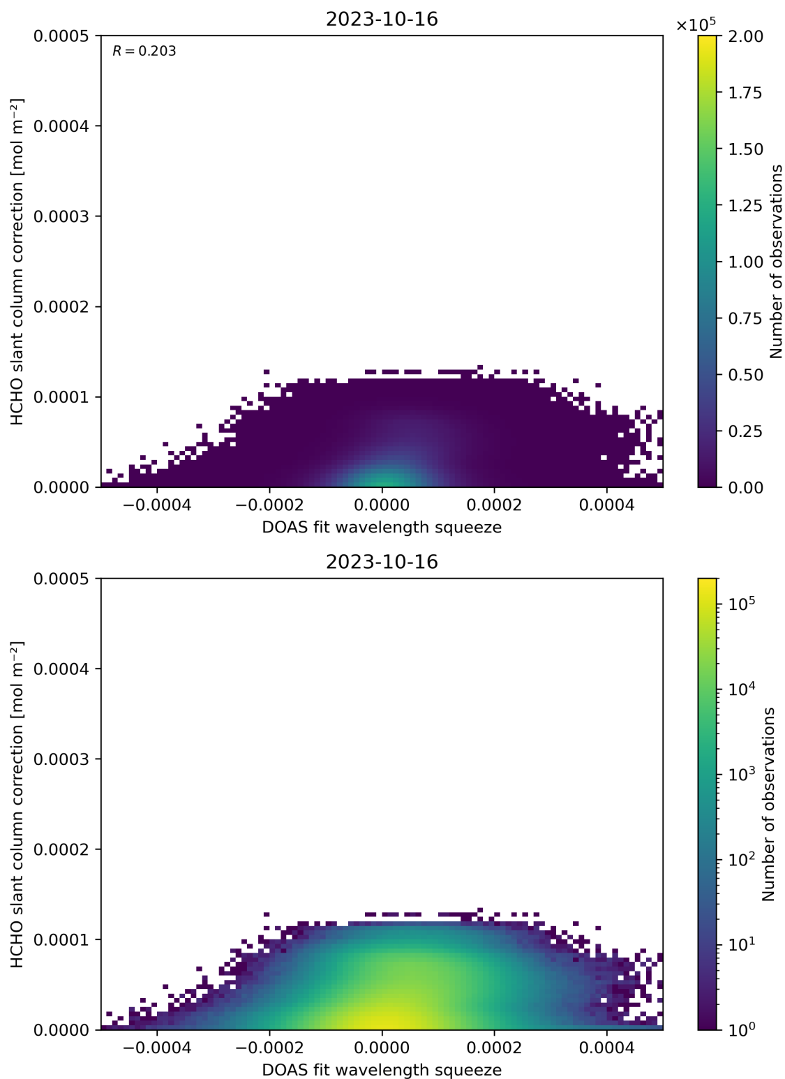
Figure 70: Scatter density plot of “DOAS fit wavelength squeeze” against “HCHO slant column correction” for 2023-10-15 to 2023-10-17.
