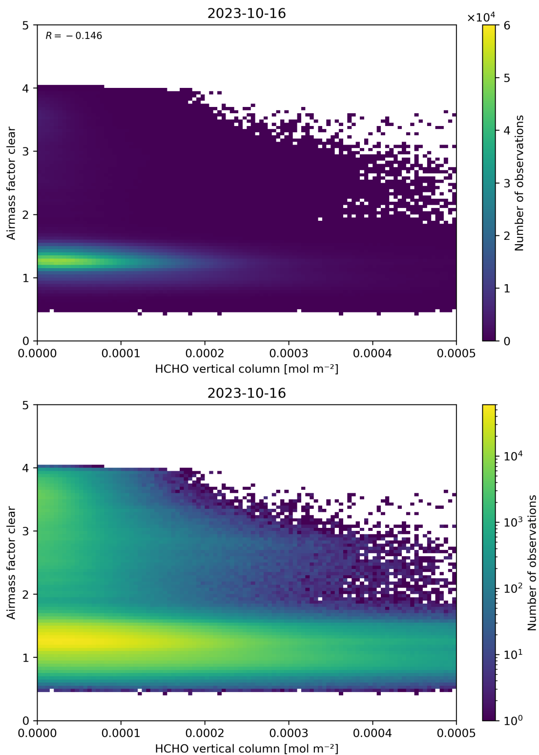
Figure 126: Scatter density plot of “HCHO vertical column” against “Airmass factor clear” for 2023-10-15 to 2023-10-17.
