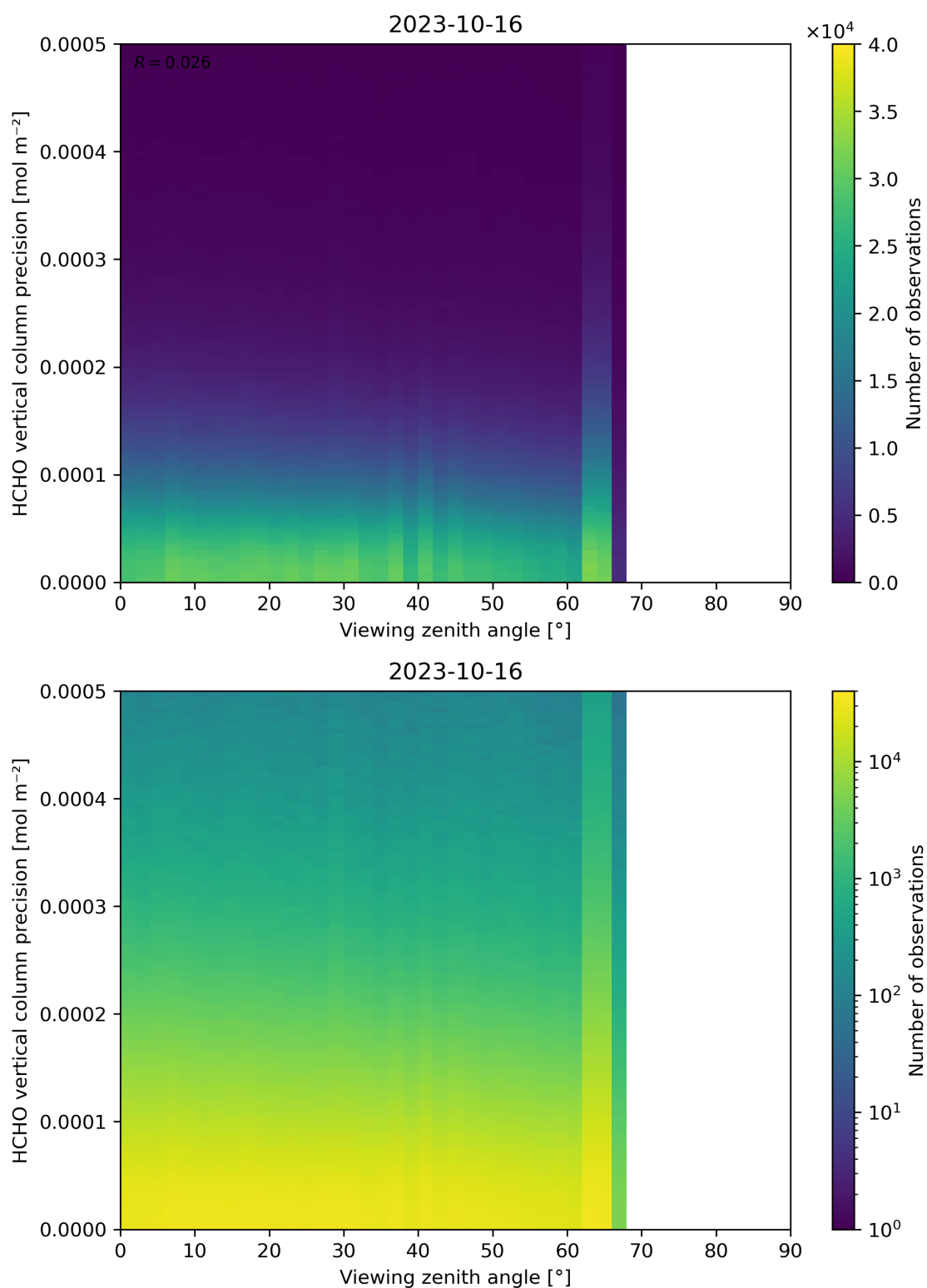
Figure 194: Scatter density plot of “Viewing zenith angle” against “HCHO vertical column precision” for 2023-10-15 to 2023-10-17.
