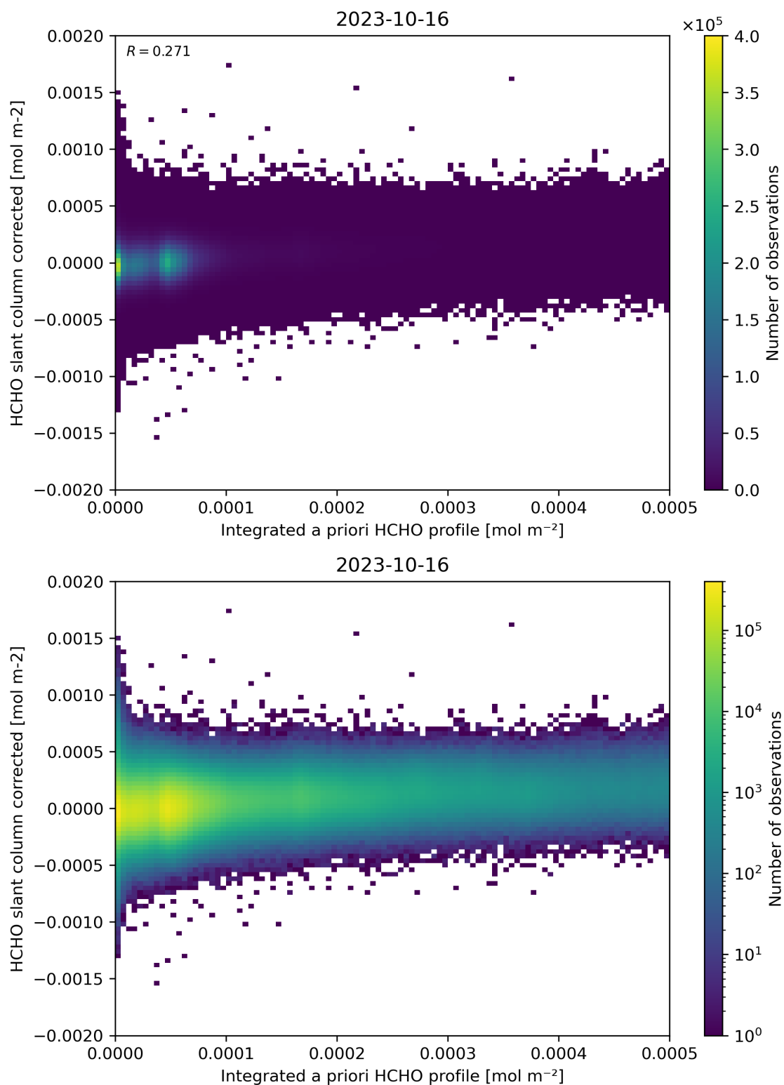
Figure 151: Scatter density plot of “Integrated a priori HCHO profile” against “HCHO slant column corrected” for 2023-10-15 to 2023-10-17.
