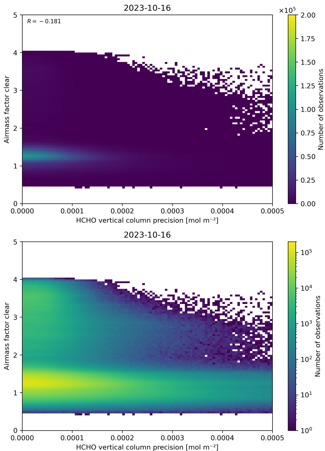
Figure 139: Scatter density plot of “HCHO vertical column precision” against “Airmass factor clear” for 2023-10-15 to 2023-10-17.
