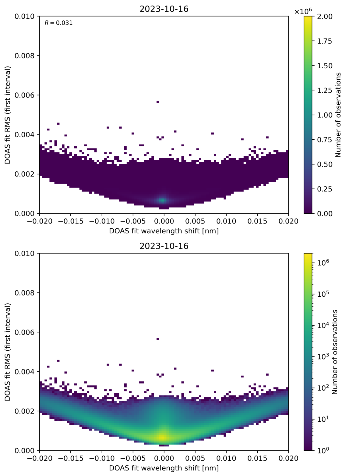
Figure 64: Scatter density plot of “DOAS fit wavelength shift” against “DOAS fit RMS (first interval)” for 2023-10-15 to 2023-10-17.
