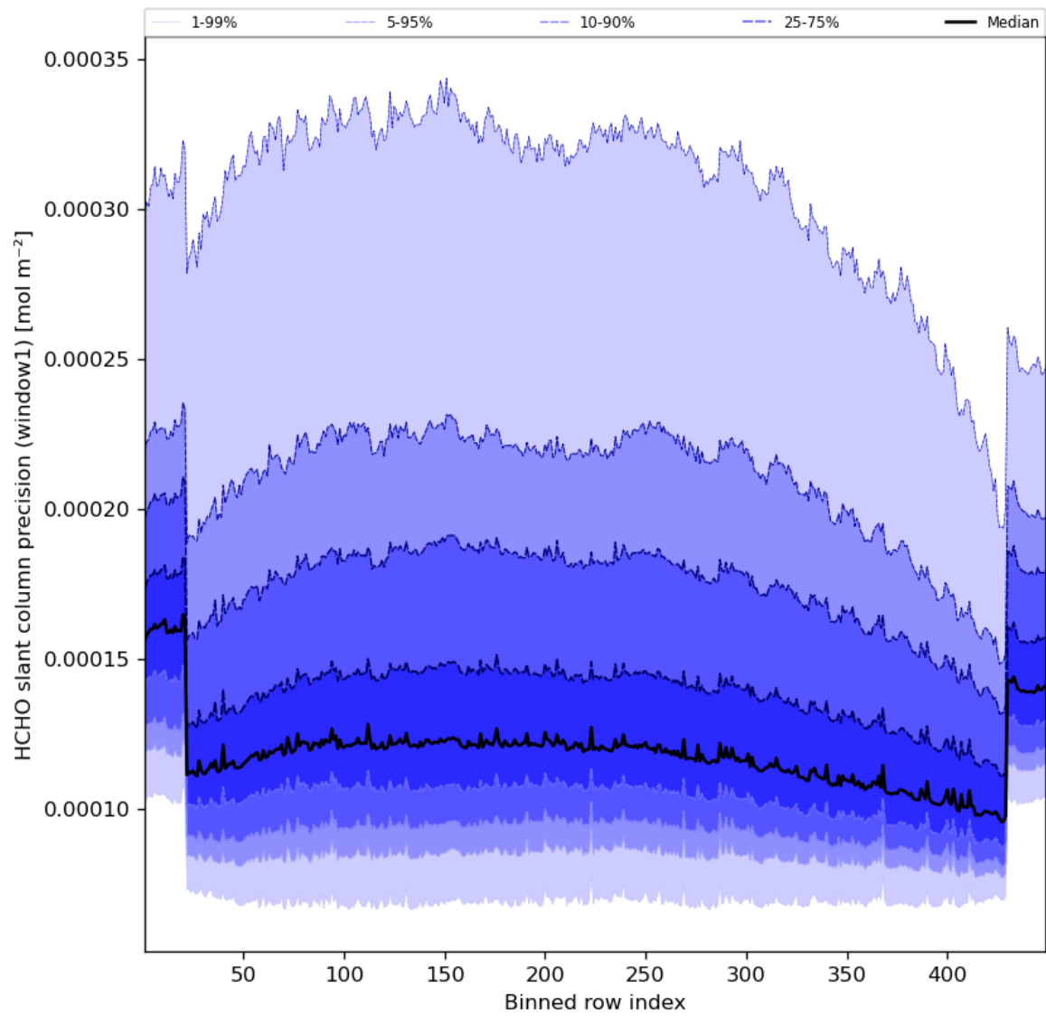
Figure 53: Along track statistics of “HCHO slant column precision (window1)” for 2023-10-15 to 2023-10-17
