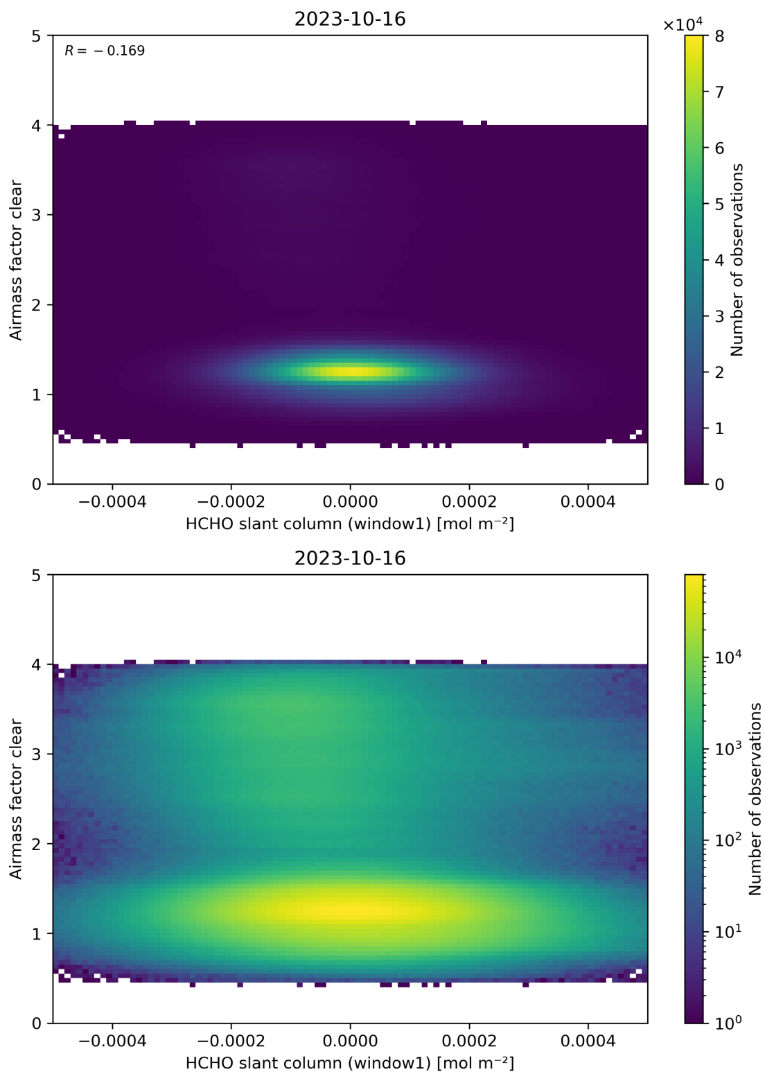
Figure 81: Scatter density plot of “HCHO slant column (window1)” against “Airmass factor clear” for 2023-10-15 to 2023-10-17.
