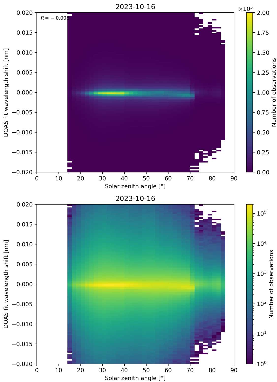
Figure 168: Scatter density plot of “Solar zenith angle” against “DOAS fit wavelength shift” for 2023-10-15 to 2023-10-17.
