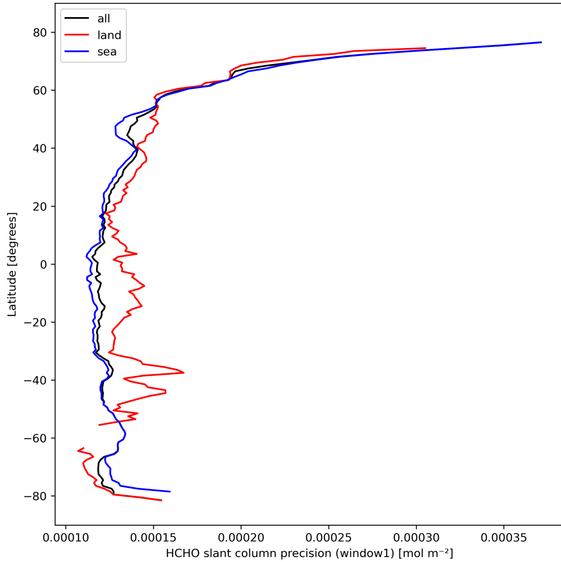
Figure 25: Zonal average of “HCHO slant column precision (window1)” for 2023-10-15 to 2023-10-17.
