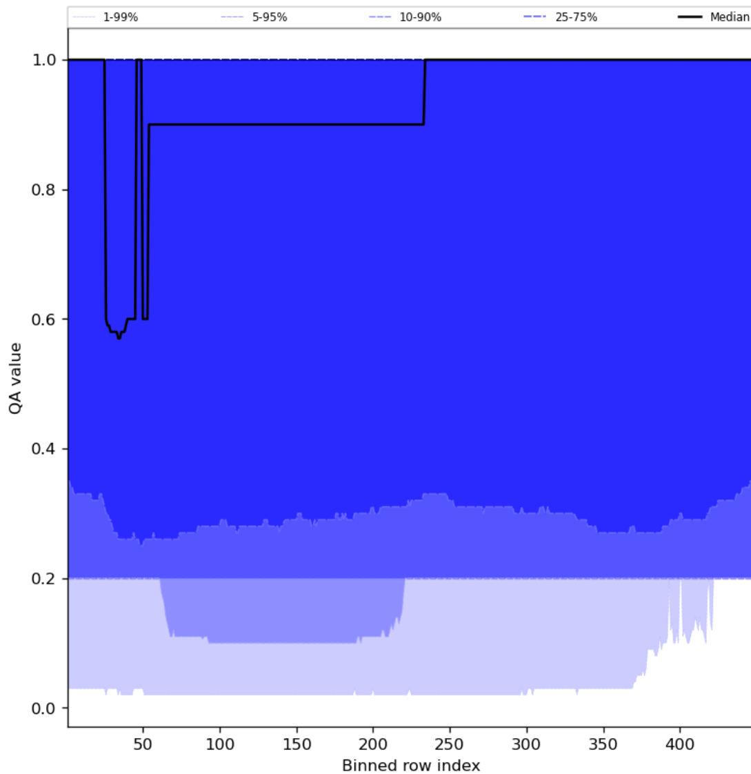
Figure 48: Along track statistics of “QA value” for 2023-10-15 to 2023-10-17
