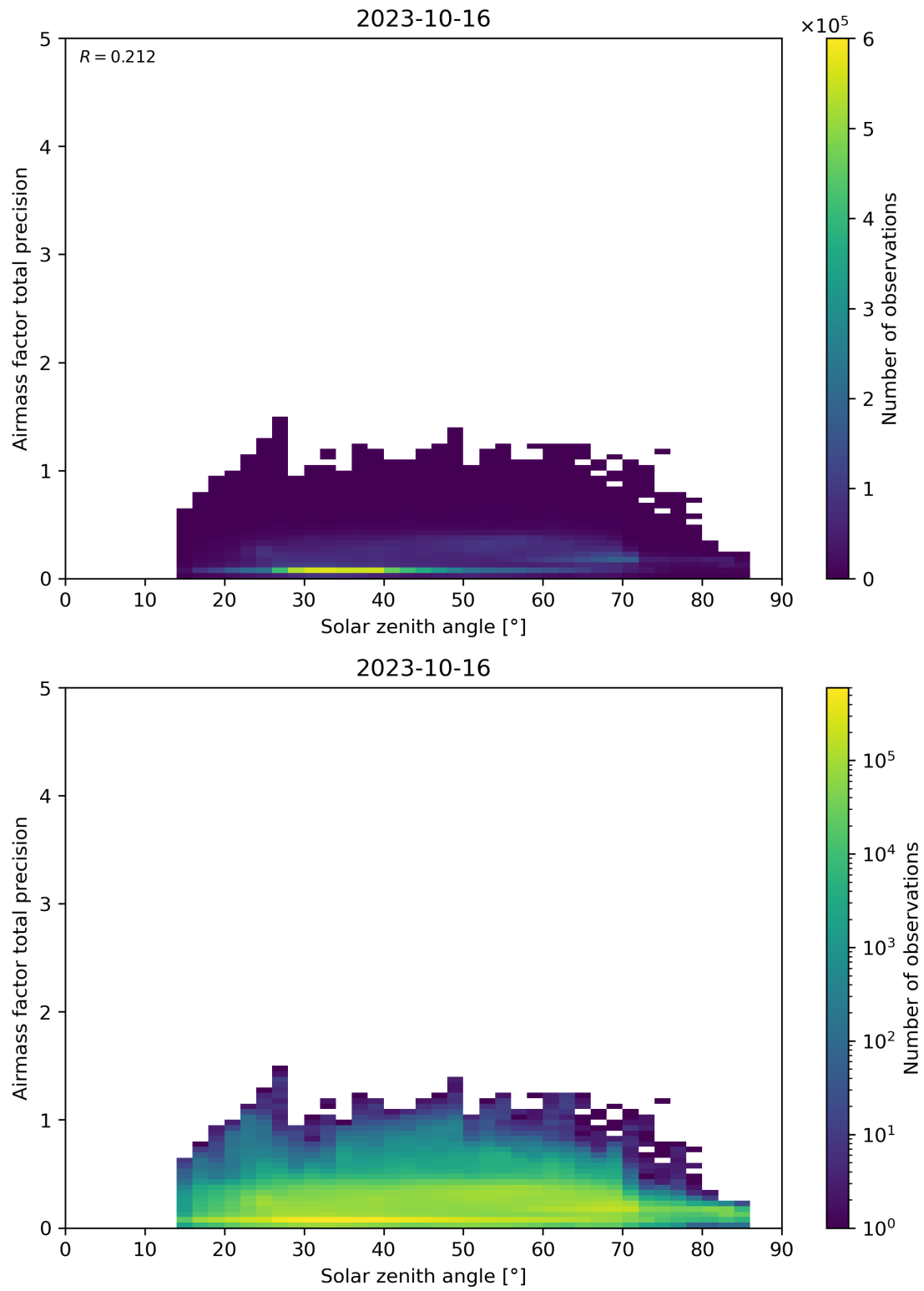
Figure 176: Scatter density plot of “Solar zenith angle” against “Airmass factor total precision” for 2023-10-15 to 2023-10-17.
