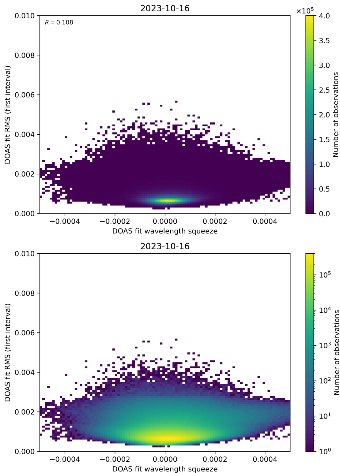
Figure 68: Scatter density plot of “DOAS fit wavelength squeeze” against “DOAS fit RMS (first interval)” for 2023-10-15 to 2023-10-17.
