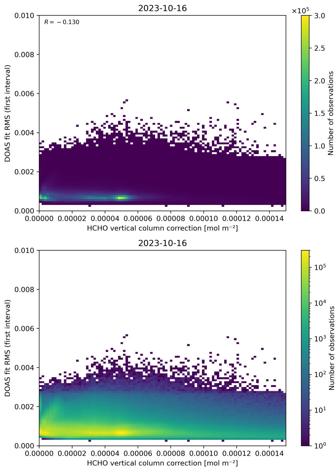
Figure 112: Scatter density plot of “HCHO vertical column correction” against “DOAS fit RMS (first interval)” for 2023-10-15 to 2023-10-17.
