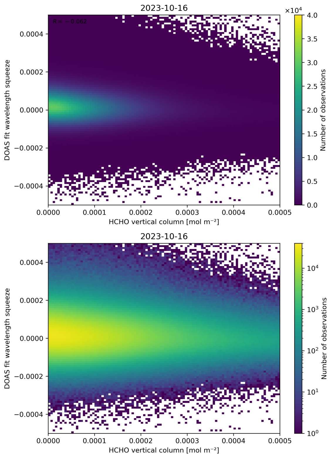
Figure 125: Scatter density plot of “HCHO vertical column” against “DOAS fit wavelength squeeze” for 2023-10-15 to 2023-10-17.
