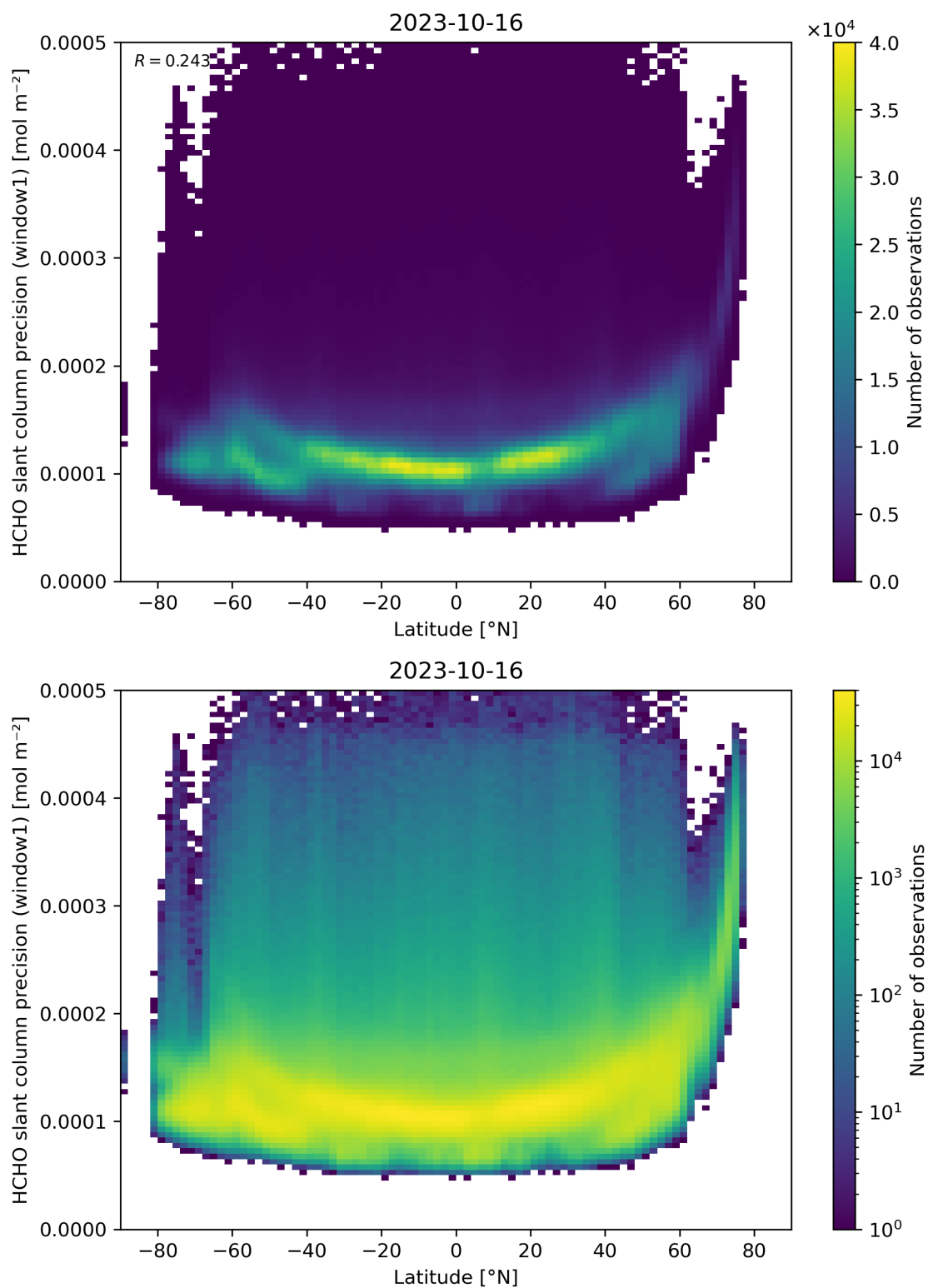
Figure 160: Scatter density plot of “Latitude” against “HCHO slant column precision (window1)” for 2023-10-15 to 2023-10-17.
