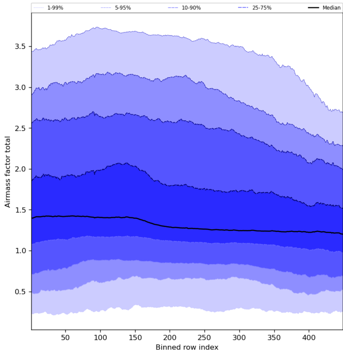
Figure 54: Along track statistics of “Airmass factor total” for 2023-10-15 to 2023-10-17
