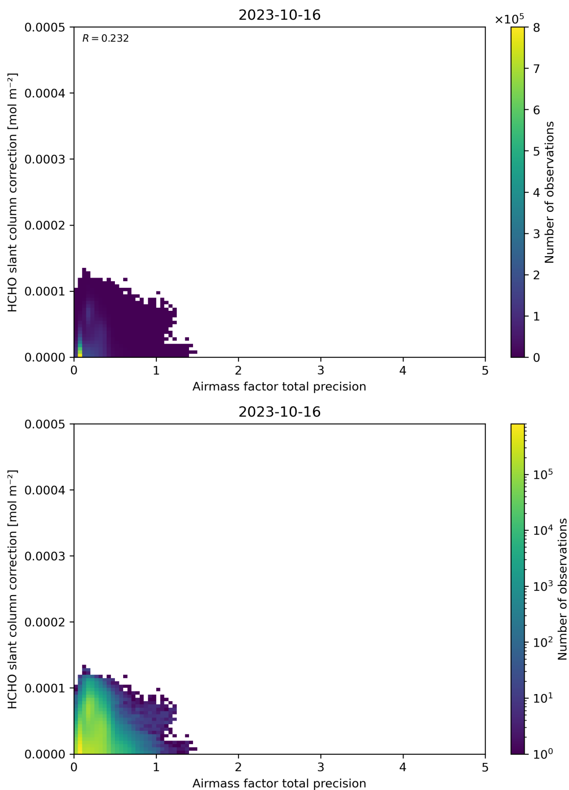
Figure 110: Scatter density plot of “Airmass factor total precision” against “HCHO slant column correction” for 2023-10-15 to 2023-10-17.
