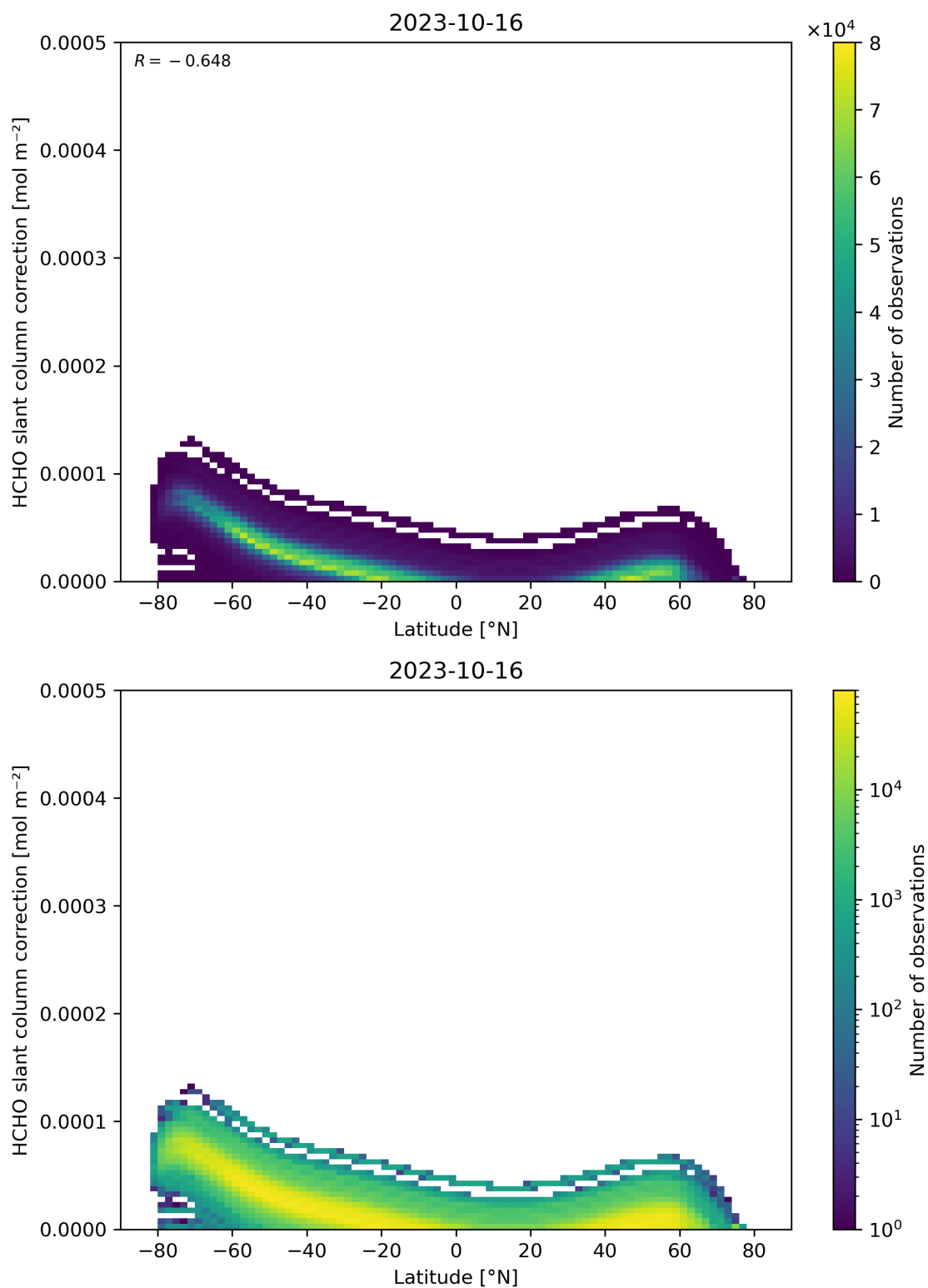
Figure 158: Scatter density plot of “Latitude” against “HCHO slant column correction” for 2023-10-15 to 2023-10-17.
