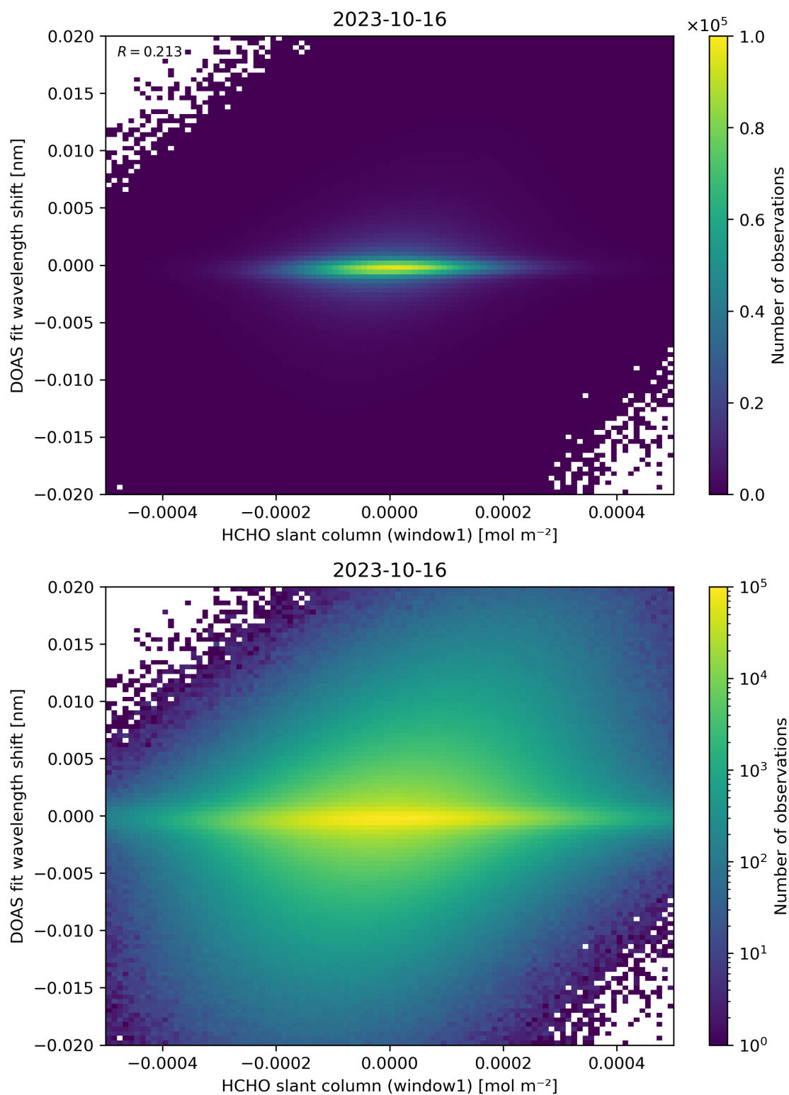
Figure 79: Scatter density plot of “HCHO slant column (window1)” against “DOAS fit wavelength shift” for 2023-10-15 to 2023-10-17.
