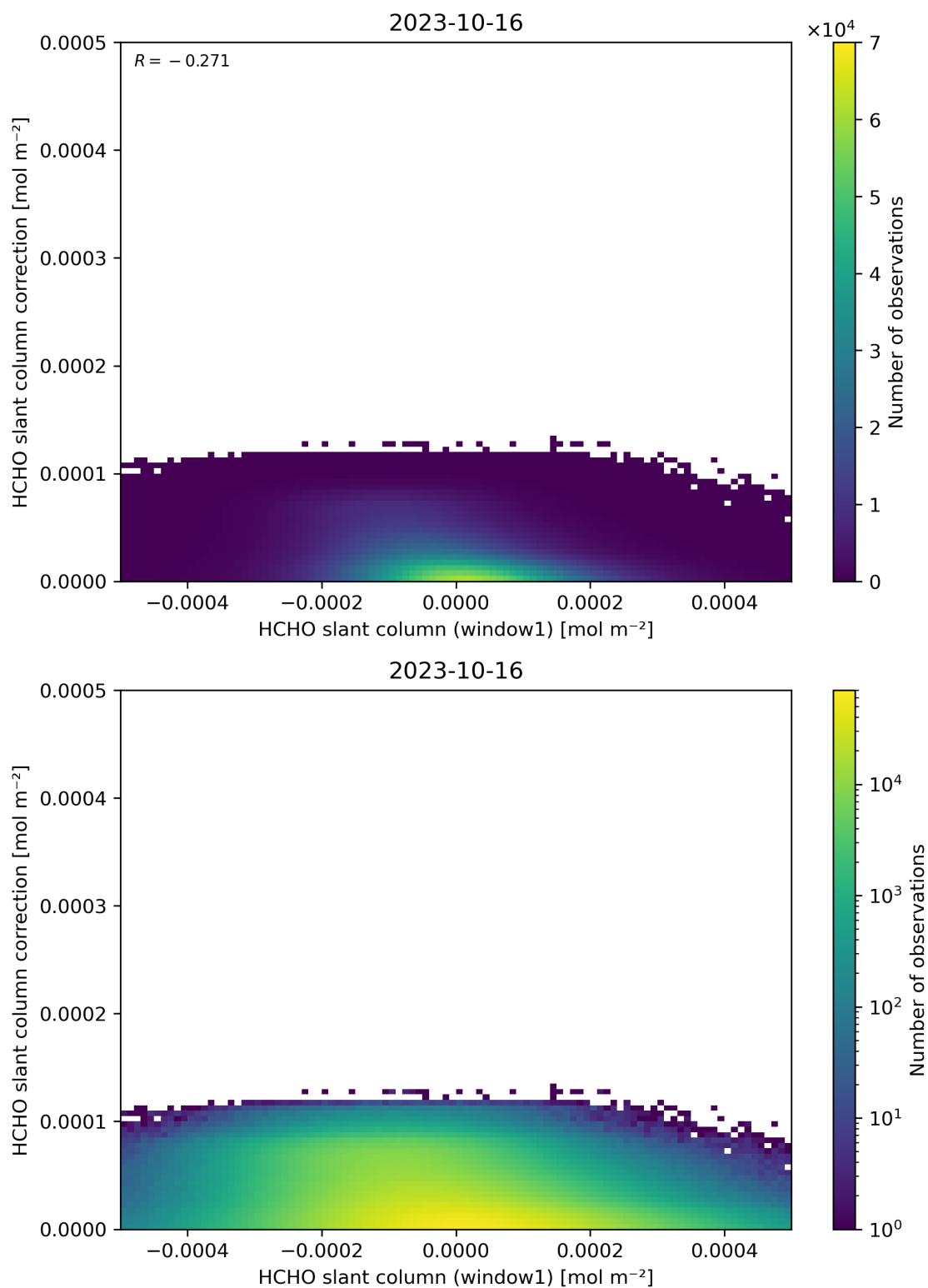
Figure 83: Scatter density plot of “HCHO slant column (window1)” against “HCHO slant column correction” for 2023-10-15 to 2023-10-17.
