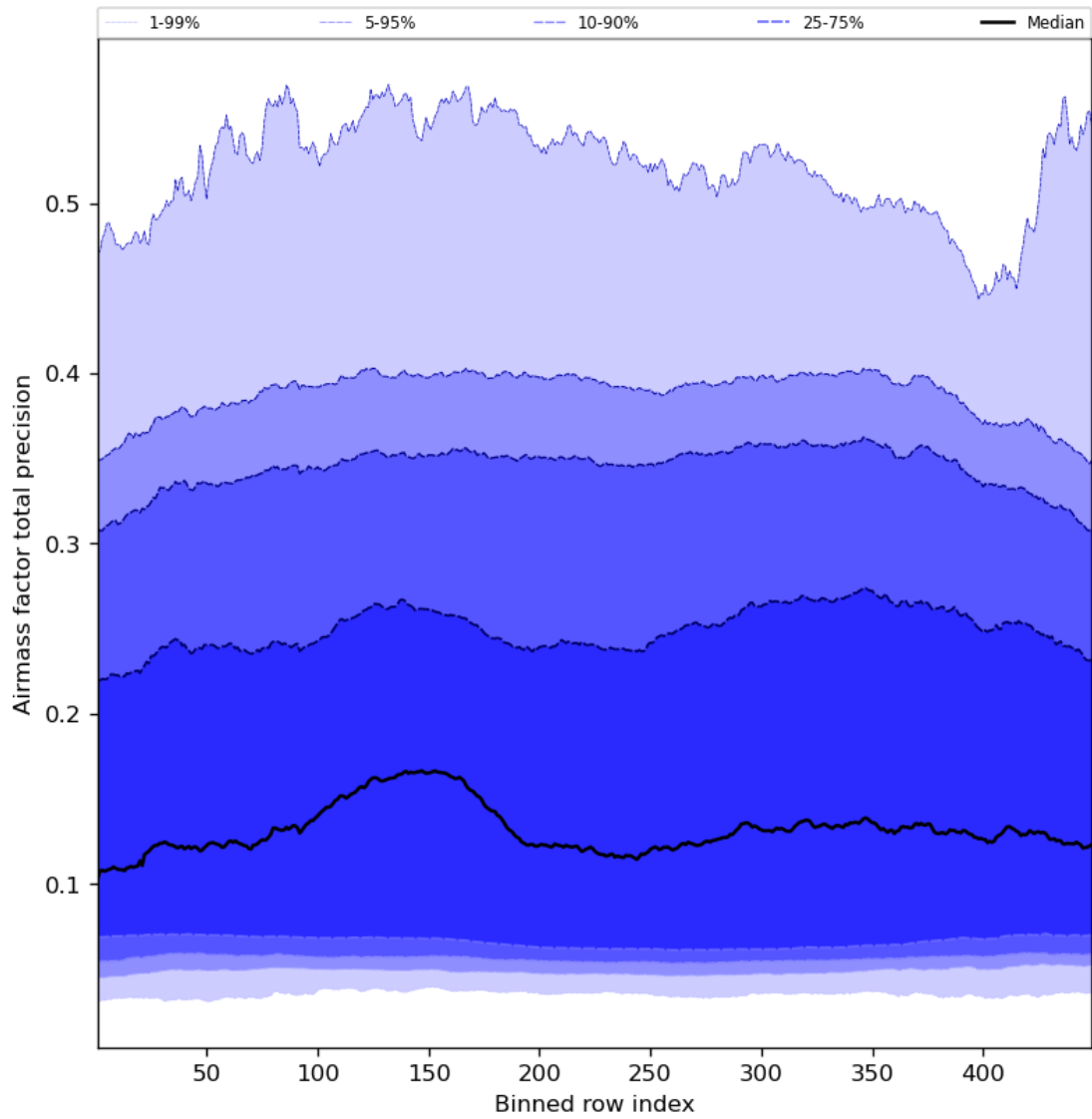
Figure 55: Along track statistics of “Airmass factor total precision” for 2023-10-15 to 2023-10-17
