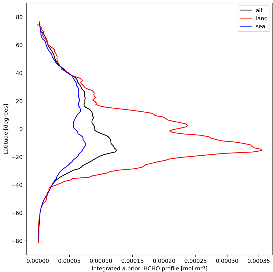
Figure 29: Zonal average of “Integrated a priori HCHO profile” for 2023-10-15 to 2023-10-17.
