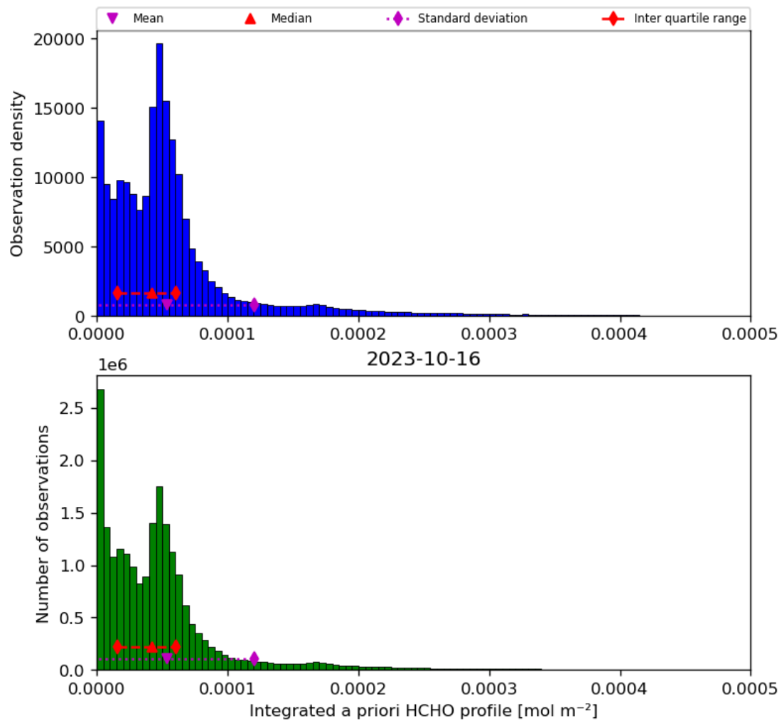
Figure 43: Histogram of “Integrated a priori HCHO profile” for 2023-10-15 to 2023-10-17
