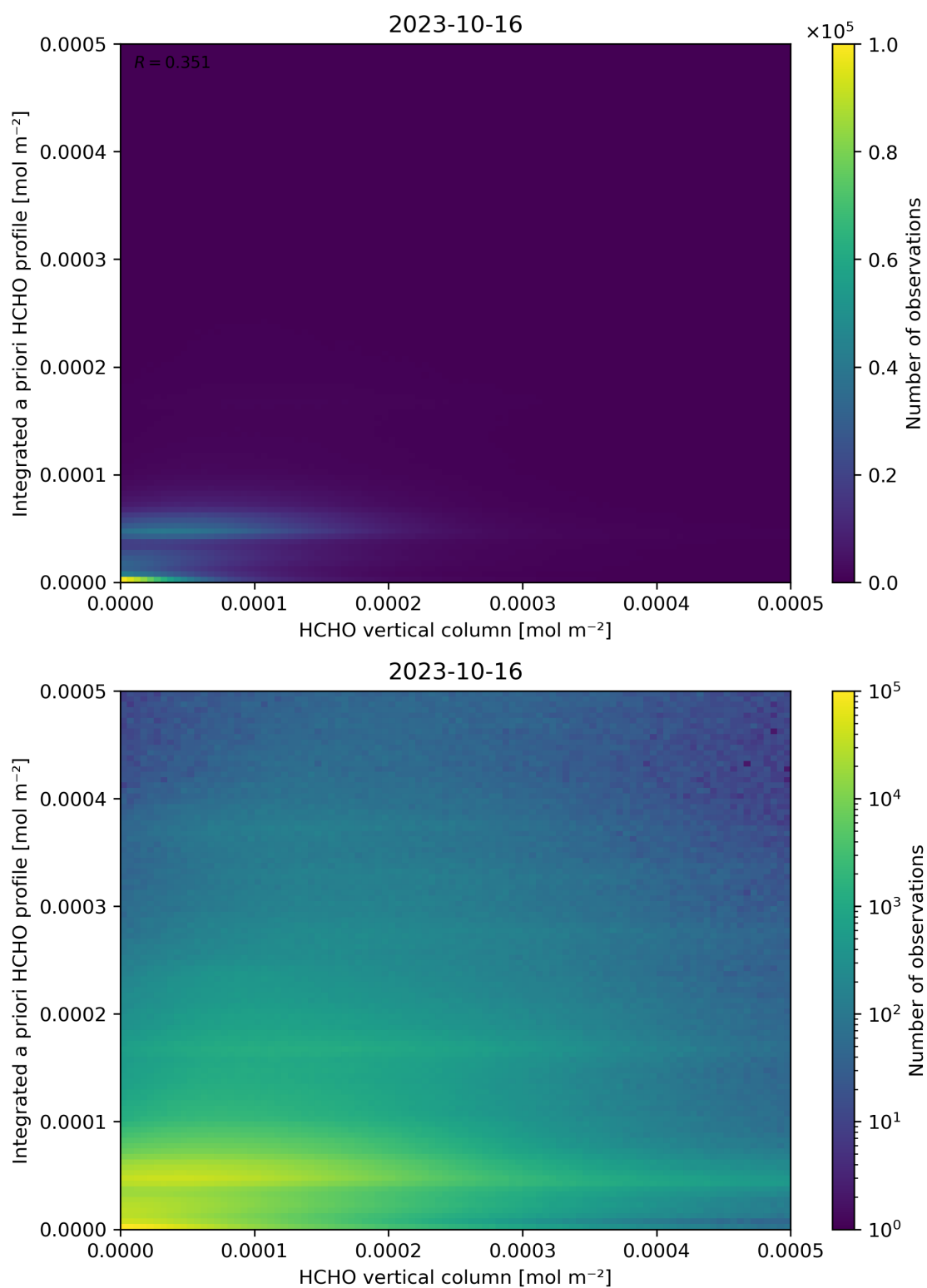
Figure 135: Scatter density plot of “HCHO vertical column” against “Integrated a priori HCHO profile” for 2023-10-15 to 2023-10-17.
