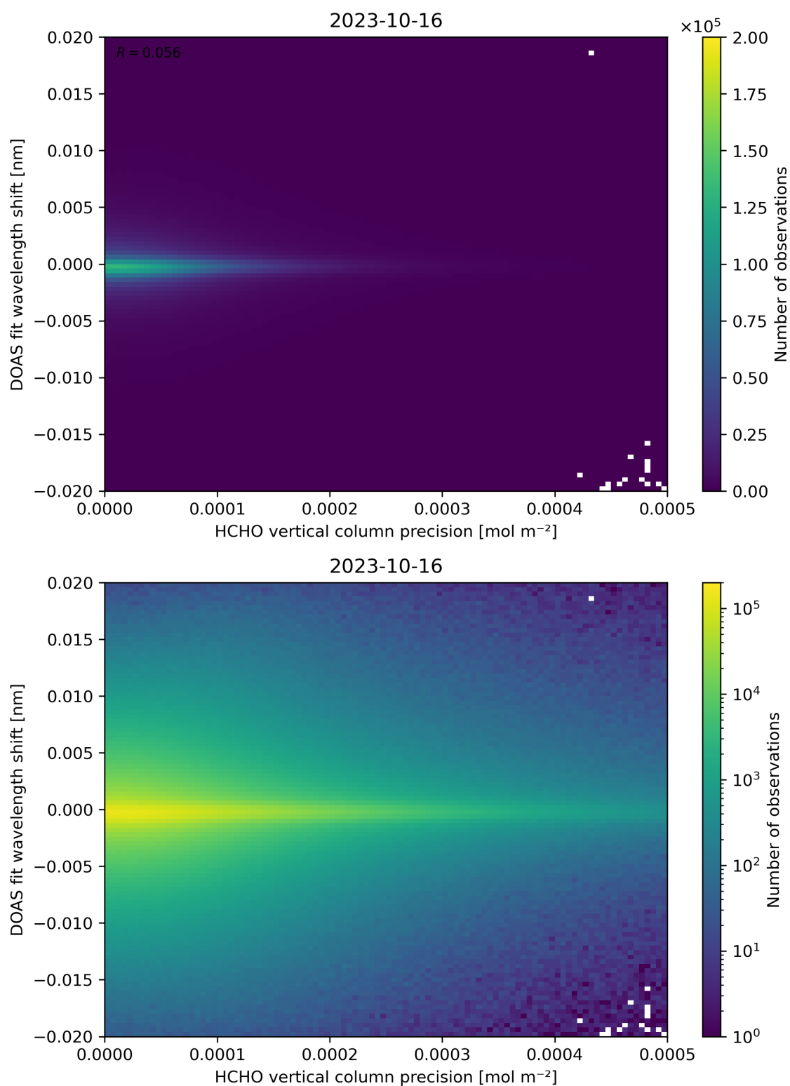
Figure 137: Scatter density plot of “HCHO vertical column precision” against “DOAS fit wavelength shift” for 2023-10-15 to 2023-10-17.
