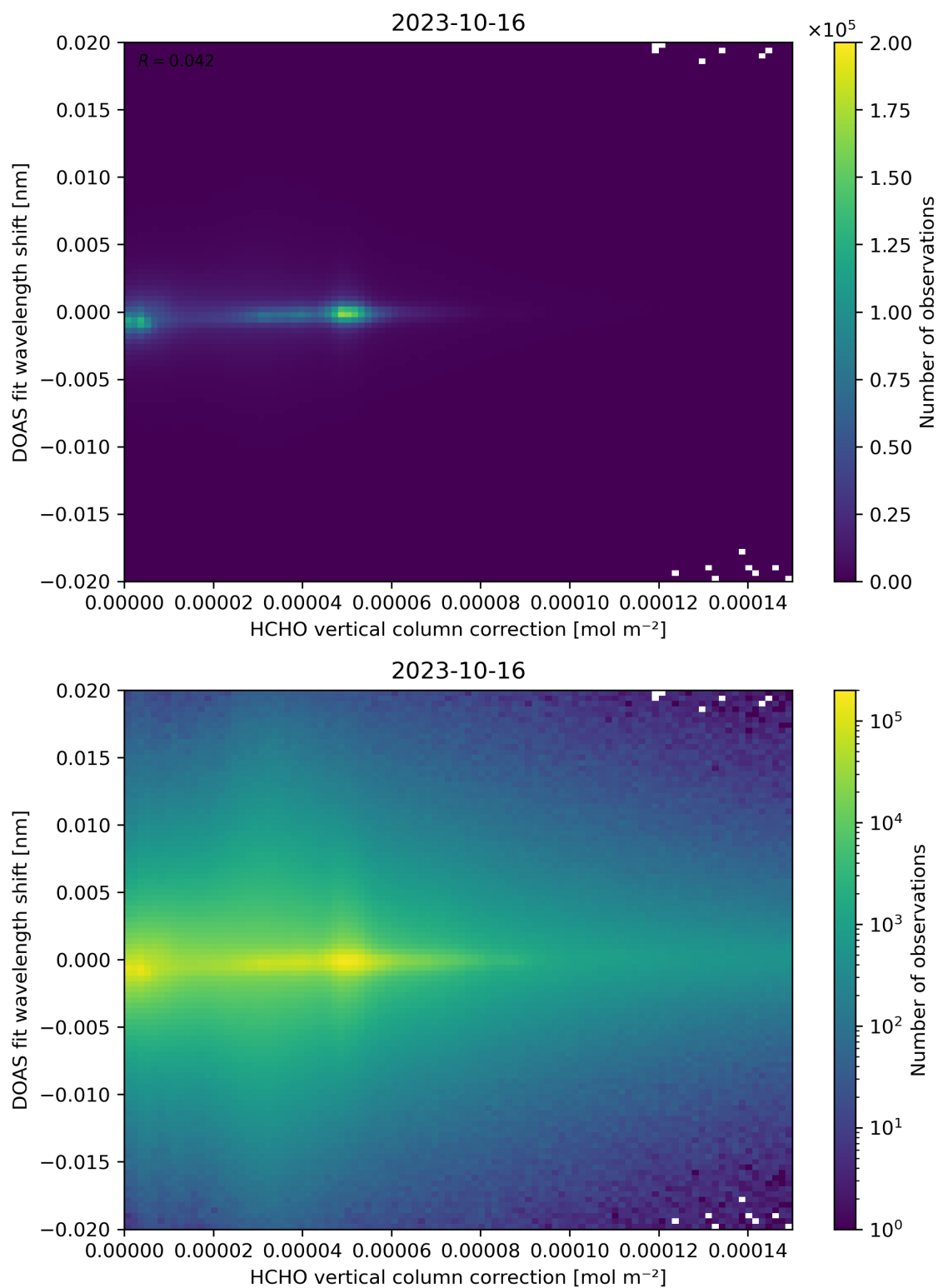
Figure 113: Scatter density plot of “HCHO vertical column correction” against “DOAS fit wavelength shift” for 2023-10-15 to 2023-10-17.
