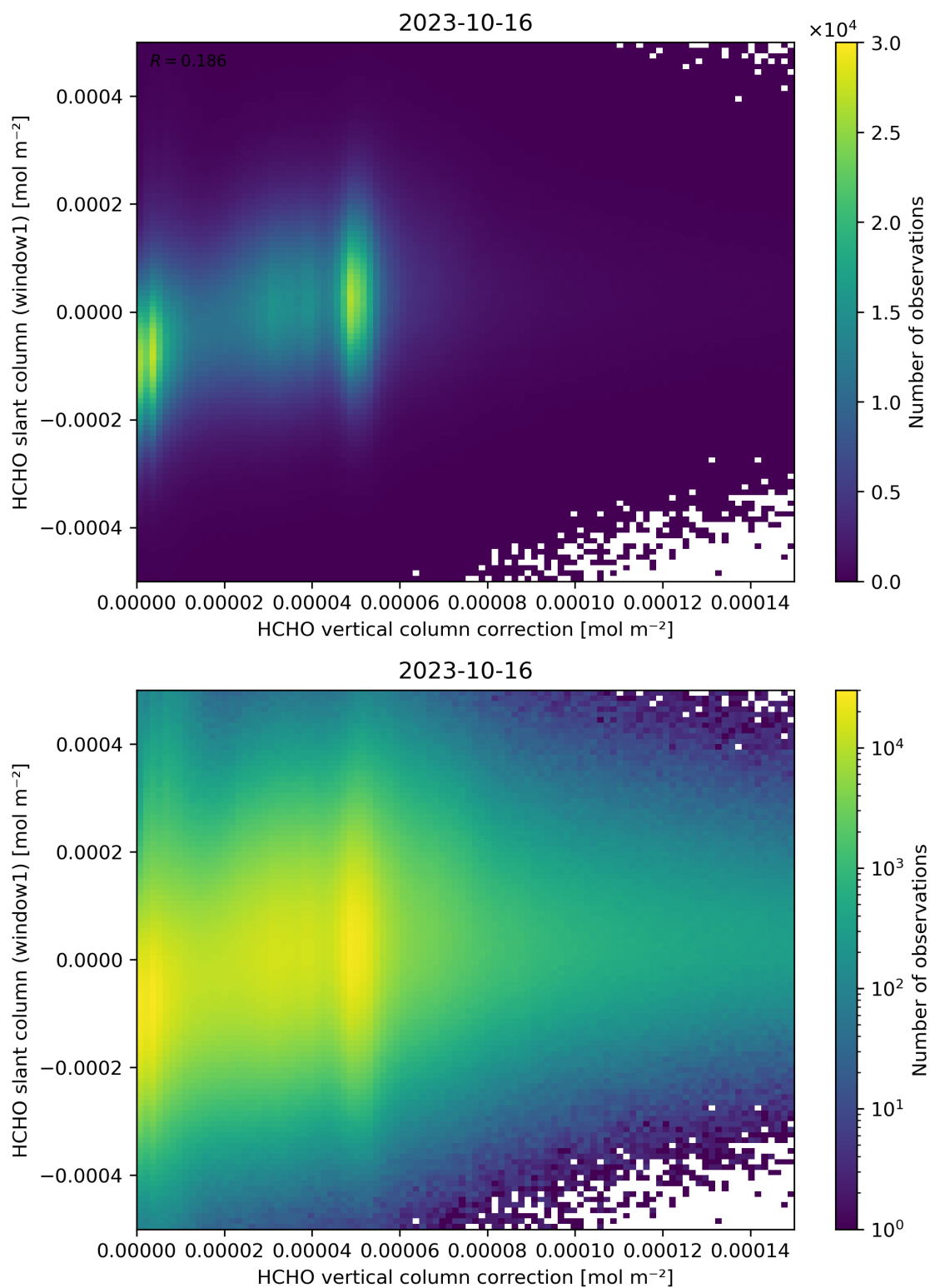
Figure 118: Scatter density plot of “HCHO vertical column correction” against “HCHO slant column (window1)” for 2023-10-15 to 2023-10-17.
