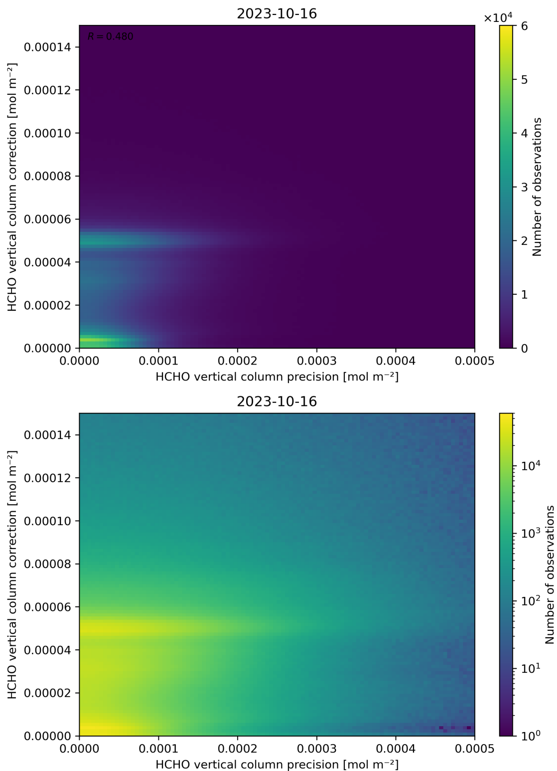
Figure 146: Scatter density plot of “HCHO vertical column precision” against “HCHO vertical column correction” for 2023-10-15 to 2023-10-17.
