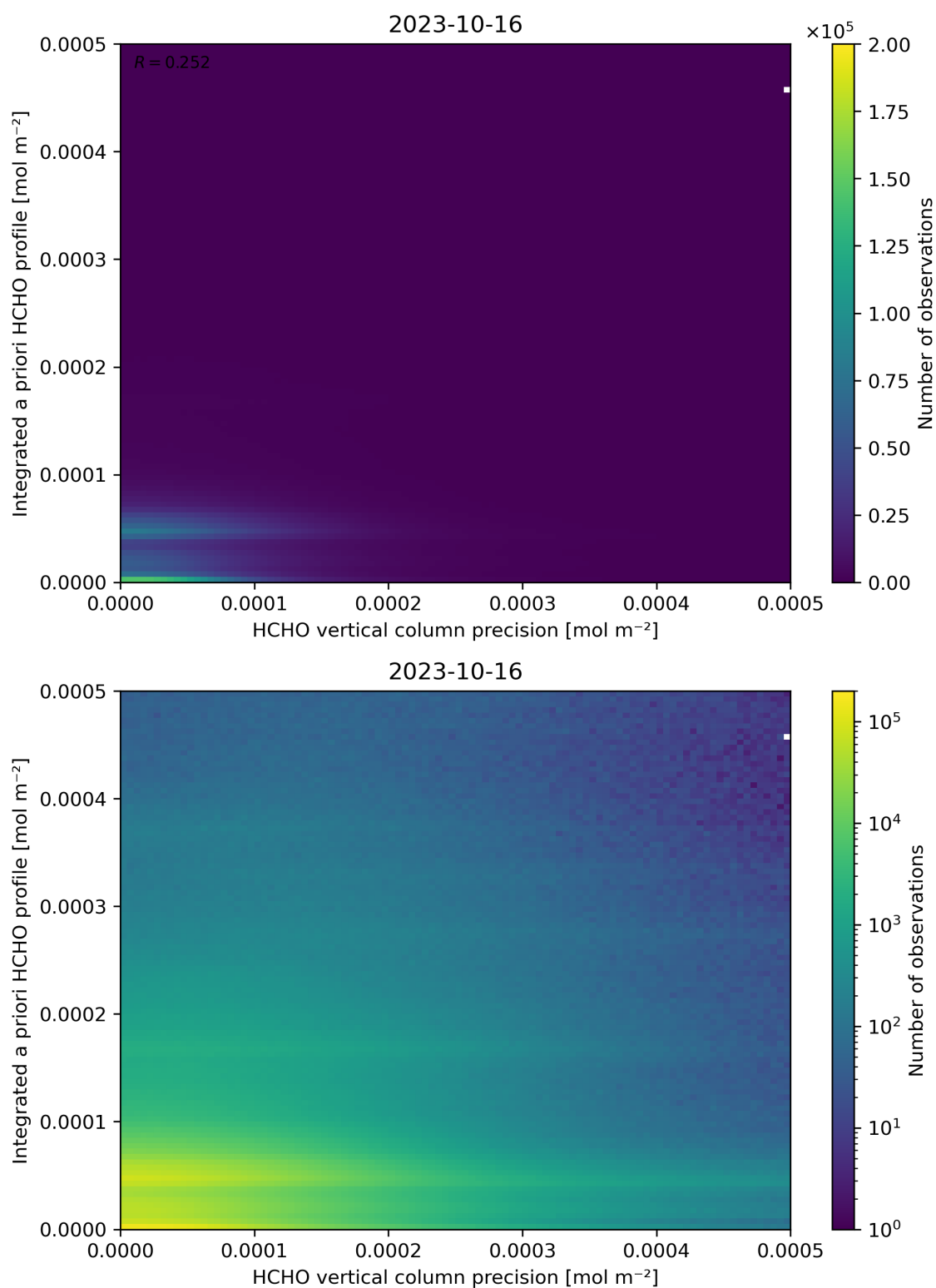
Figure 147: Scatter density plot of “HCHO vertical column precision” against “Integrated a priori HCHO profile” for 2023-10-15 to 2023-10-17.
