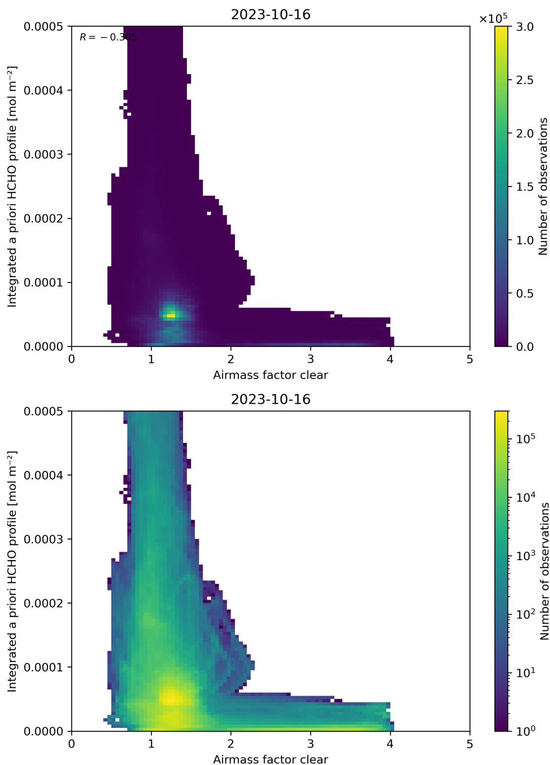
Figure 76: Scatter density plot of “Airmass factor clear” against “Integrated a priori HCHO profile” for 2023-10-15 to 2023-10-17.
