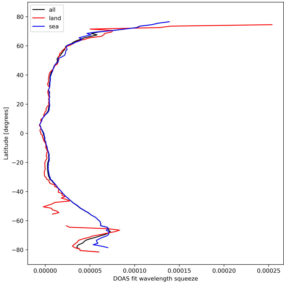
Figure 31: Zonal average of “DOAS fit wavelength squeeze” for 2023-10-15 to 2023-10-17.
