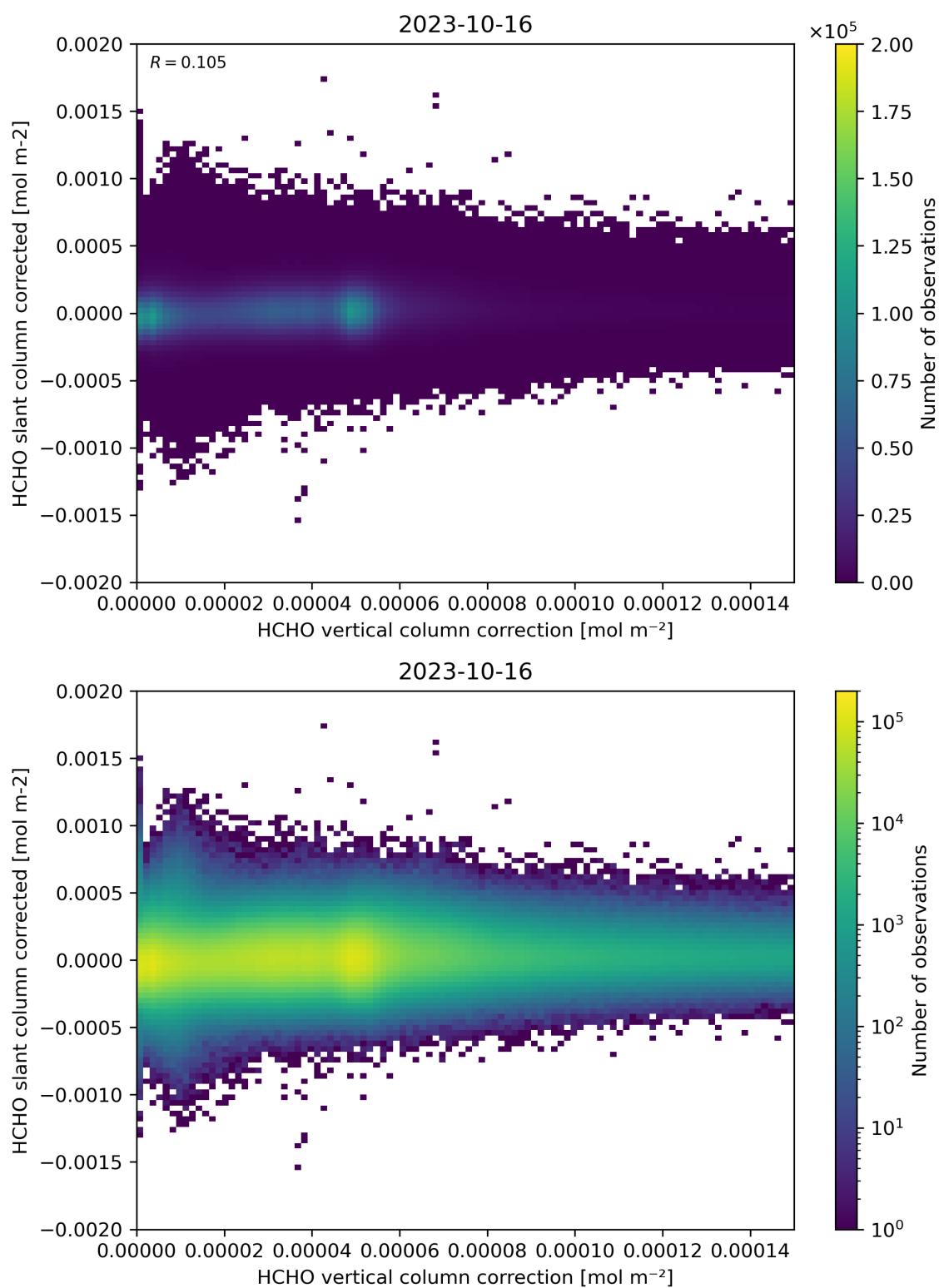
Figure 116: Scatter density plot of “HCHO vertical column correction” against “HCHO slant column corrected” for 2023-10-15 to 2023-10-17.
