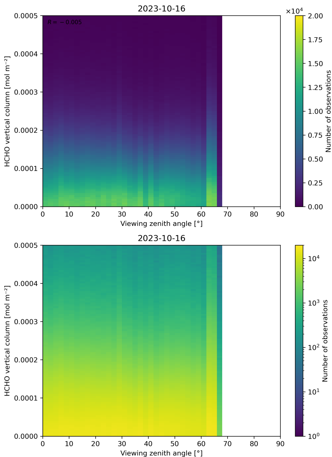
Figure 192: Scatter density plot of “Viewing zenith angle” against “HCHO vertical column” for 2023-10-15 to 2023-10-17.
