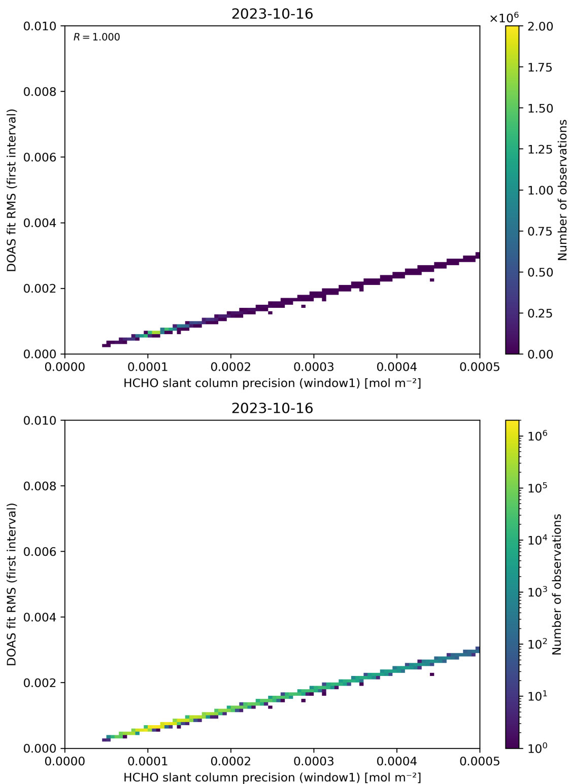
Figure 88: Scatter density plot of “HCHO slant column precision (window1)” against “DOAS fit RMS (first interval)” for 2023-10-15 to 2023-10-17.
