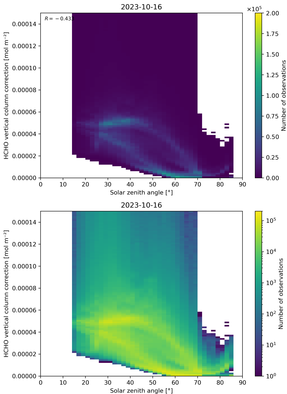
Figure 178: Scatter density plot of “Solar zenith angle” against “HCHO vertical column correction” for 2023-10-15 to 2023-10-17.
