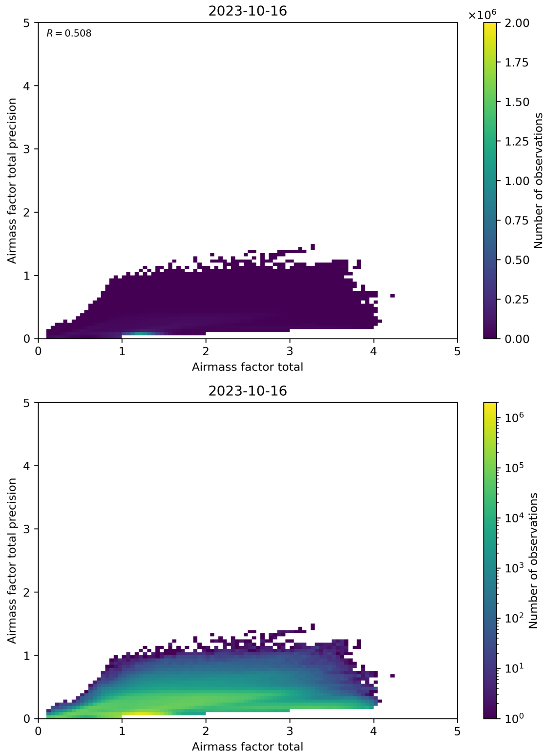
Figure 103: Scatter density plot of “Airmass factor total” against “Airmass factor total precision” for 2023-10-15 to 2023-10-17.
