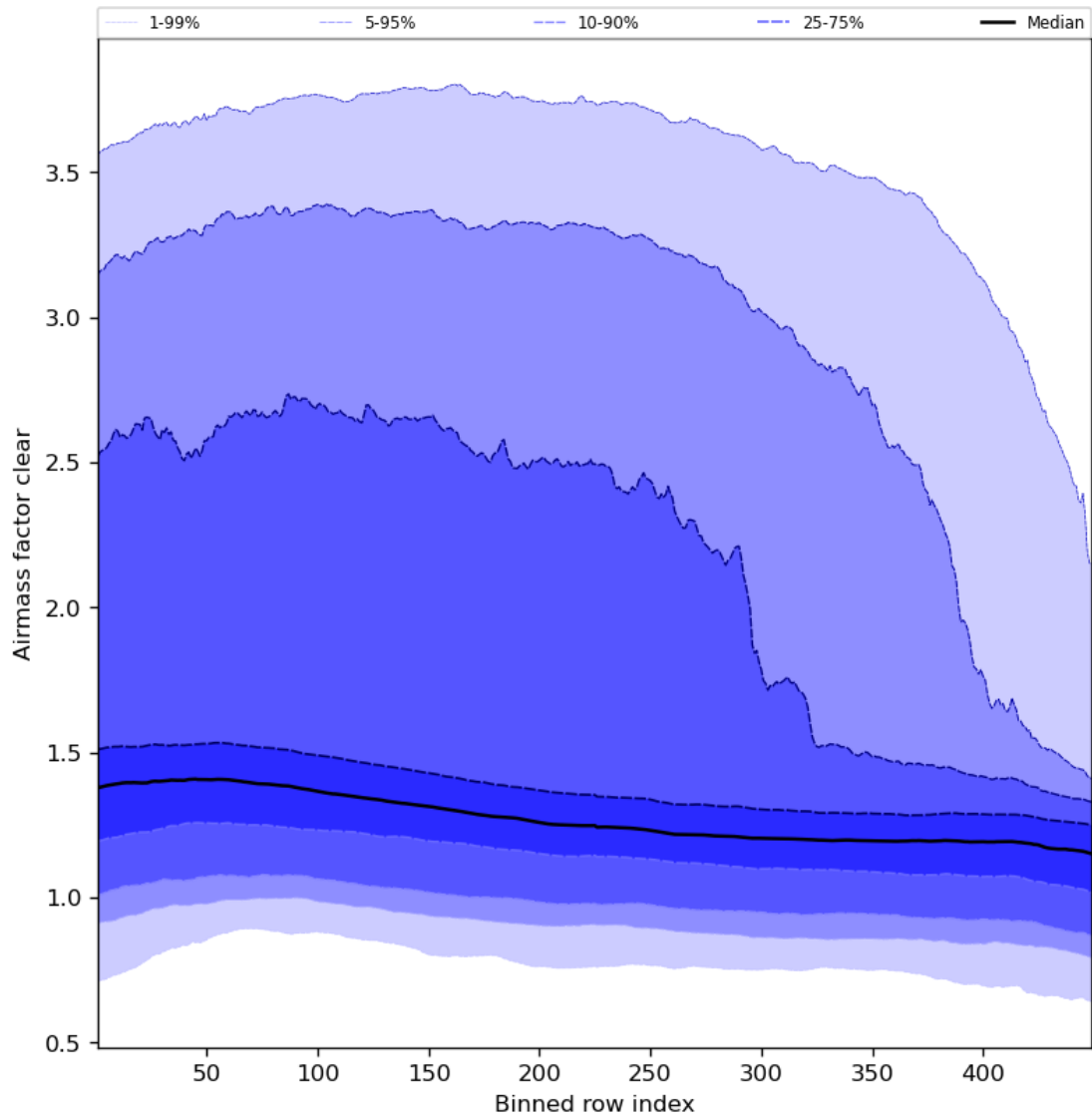
Figure 56: Along track statistics of “Airmass factor clear” for 2023-10-15 to 2023-10-17
