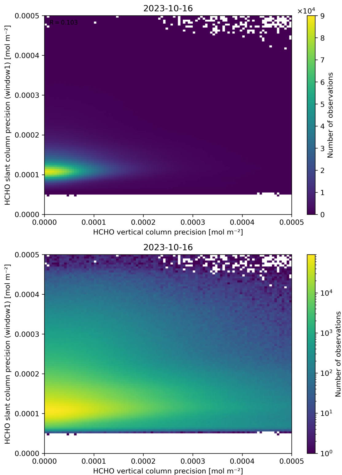
Figure 143: Scatter density plot of “HCHO vertical column precision” against “HCHO slant column precision (window1)” for 2023-10-15 to 2023-10-17.
