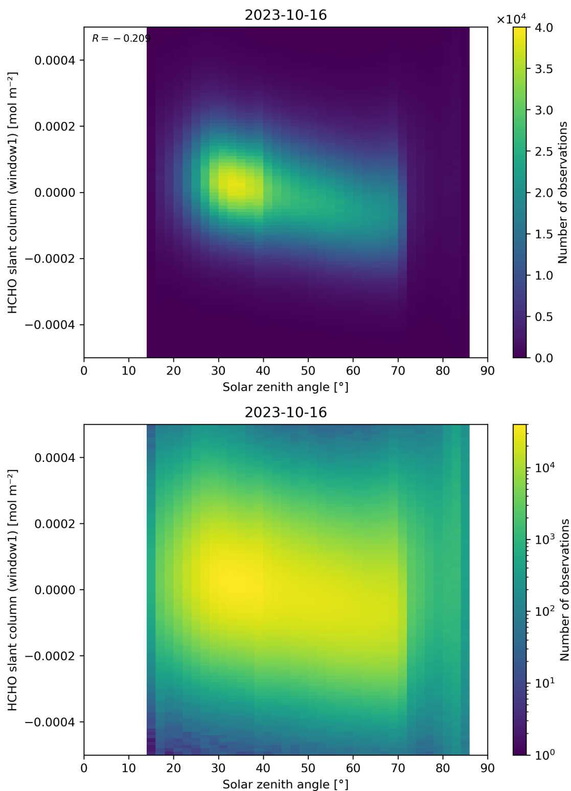
Figure 173: Scatter density plot of “Solar zenith angle” against “HCHO slant column (window1)” for 2023-10-15 to 2023-10-17.
