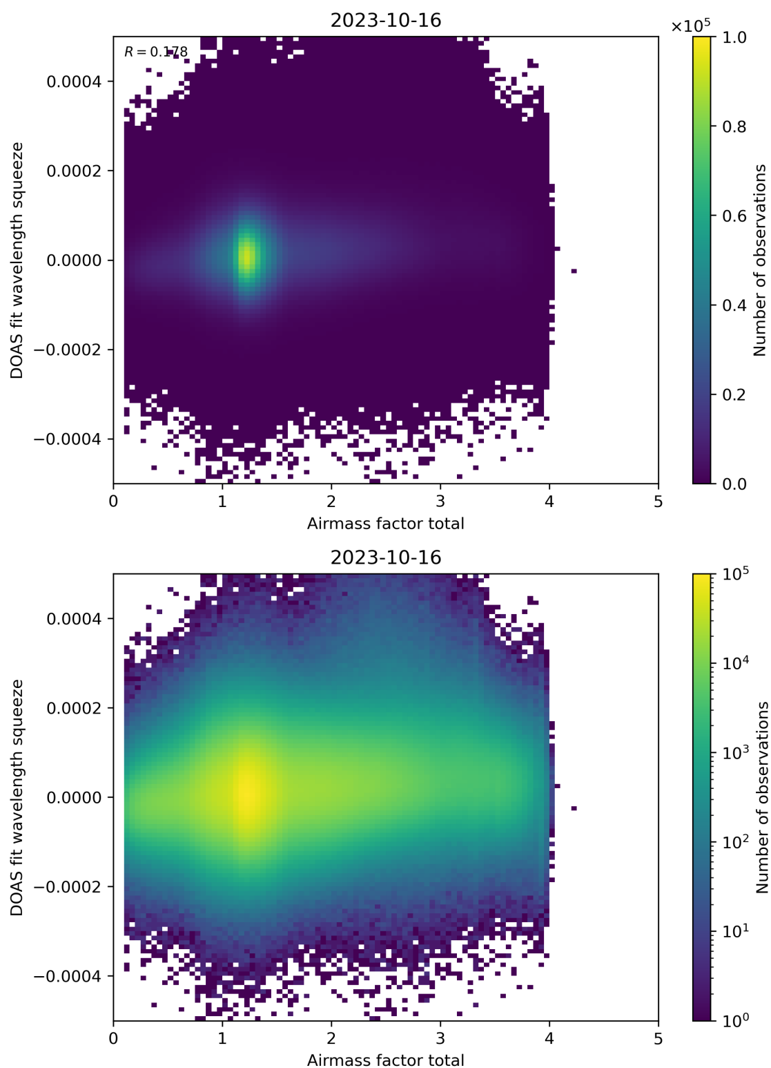
Figure 99: Scatter density plot of “Airmass factor total” against “DOAS fit wavelength squeeze” for 2023-10-15 to 2023-10-17.
