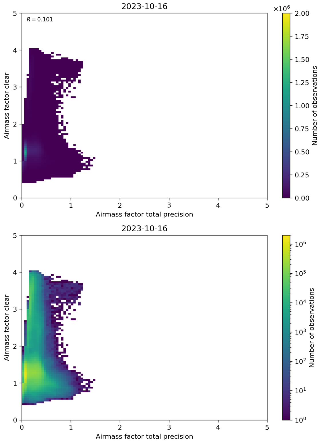
Figure 108: Scatter density plot of “Airmass factor total precision” against “Airmass factor clear” for 2023-10-15 to 2023-10-17.
