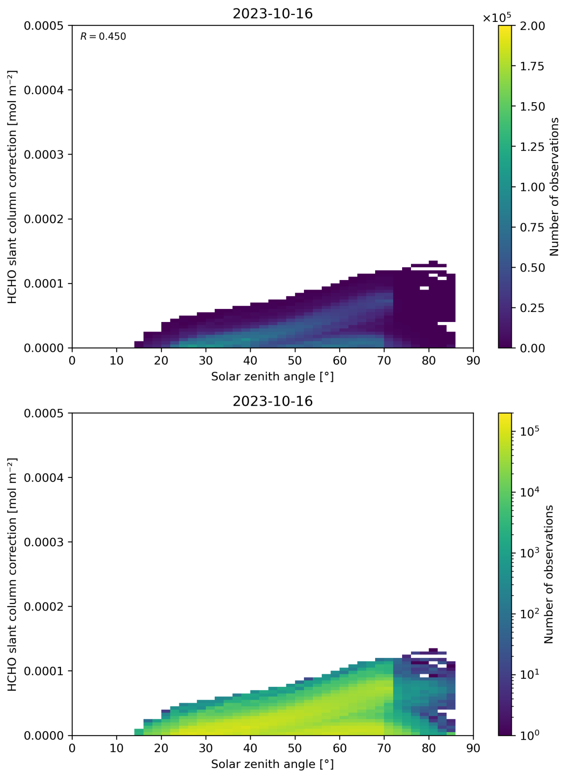
Figure 172: Scatter density plot of “Solar zenith angle” against “HCHO slant column correction” for 2023-10-15 to 2023-10-17.
