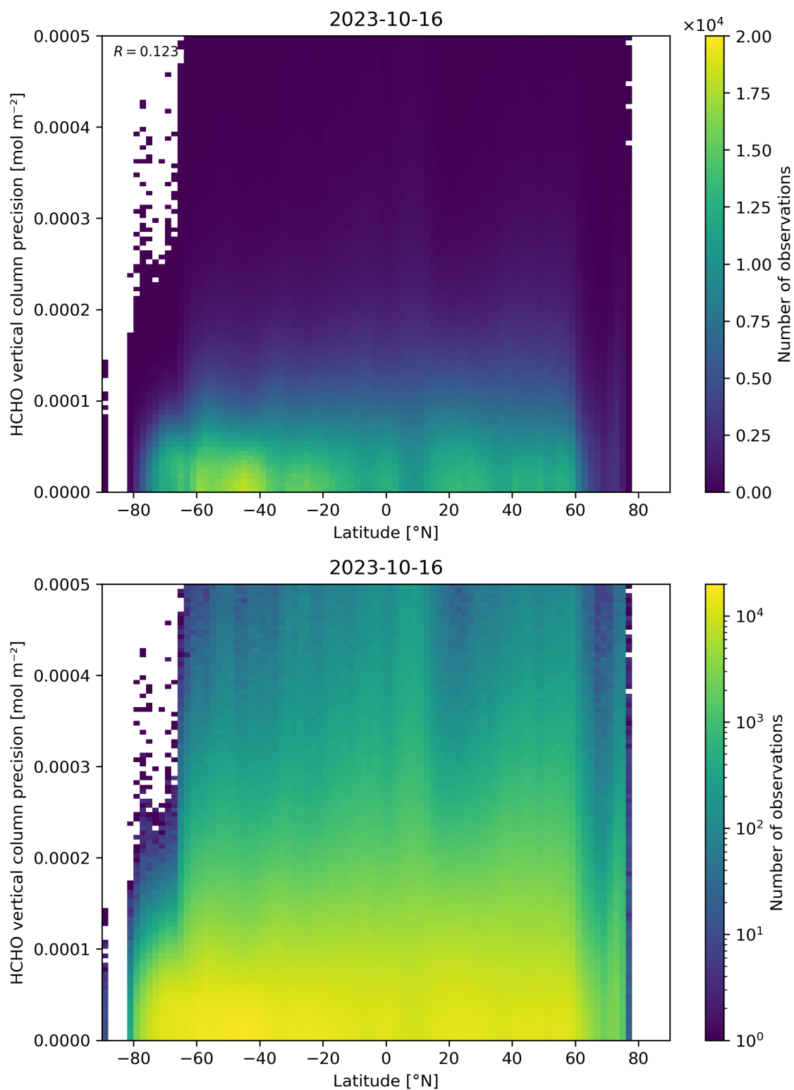
Figure 165: Scatter density plot of “Latitude” against “HCHO vertical column precision” for 2023-10-15 to 2023-10-17.
