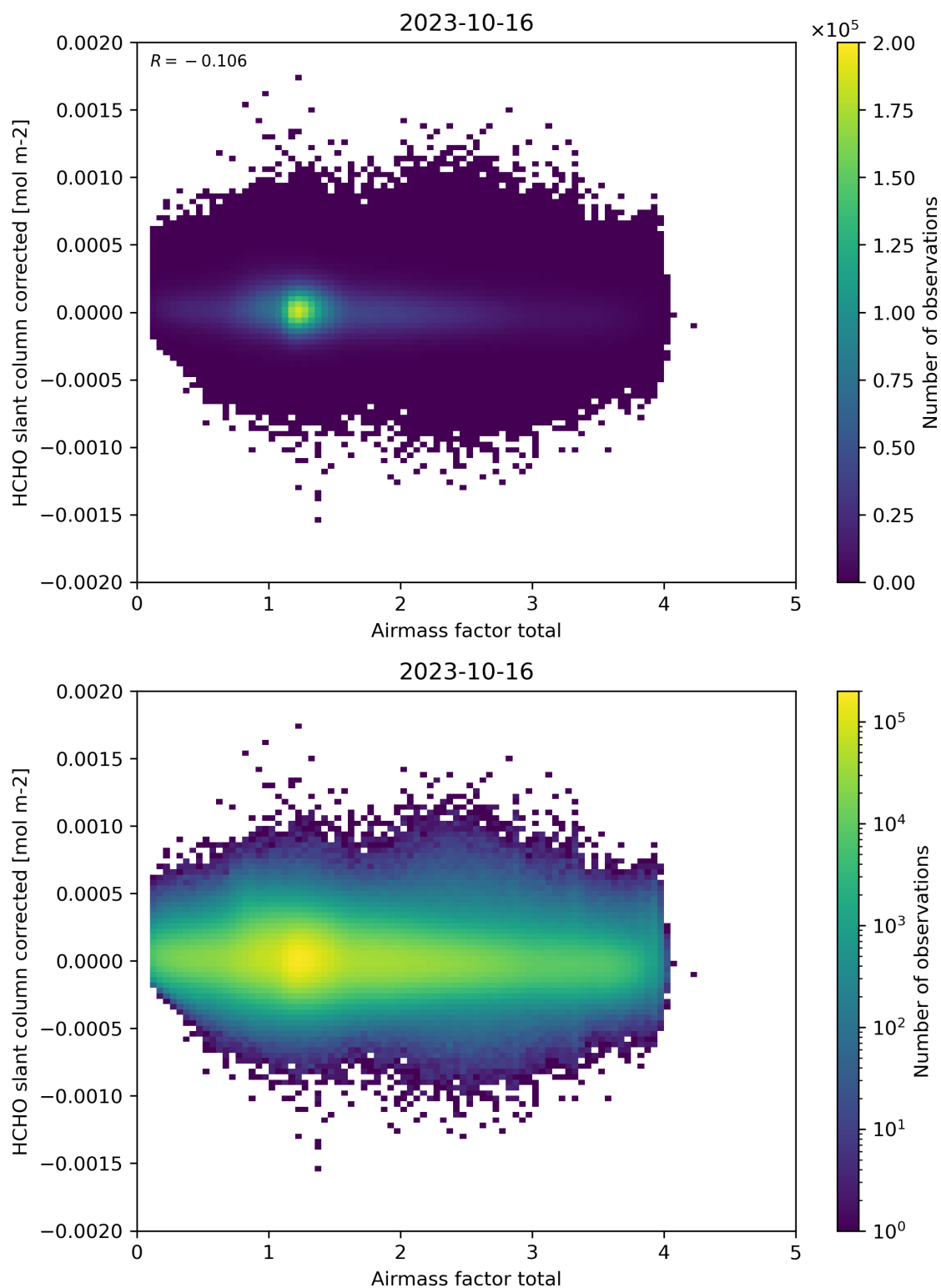
Figure 101: Scatter density plot of “Airmass factor total” against “HCHO slant column corrected” for 2023-10-15 to 2023-10-17.
