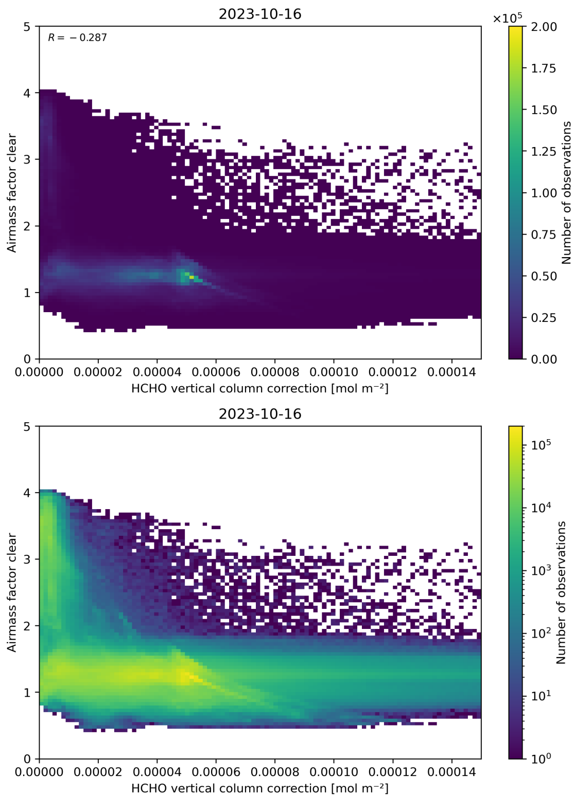
Figure 115: Scatter density plot of “HCHO vertical column correction” against “Airmass factor clear” for 2023-10-15 to 2023-10-17.
