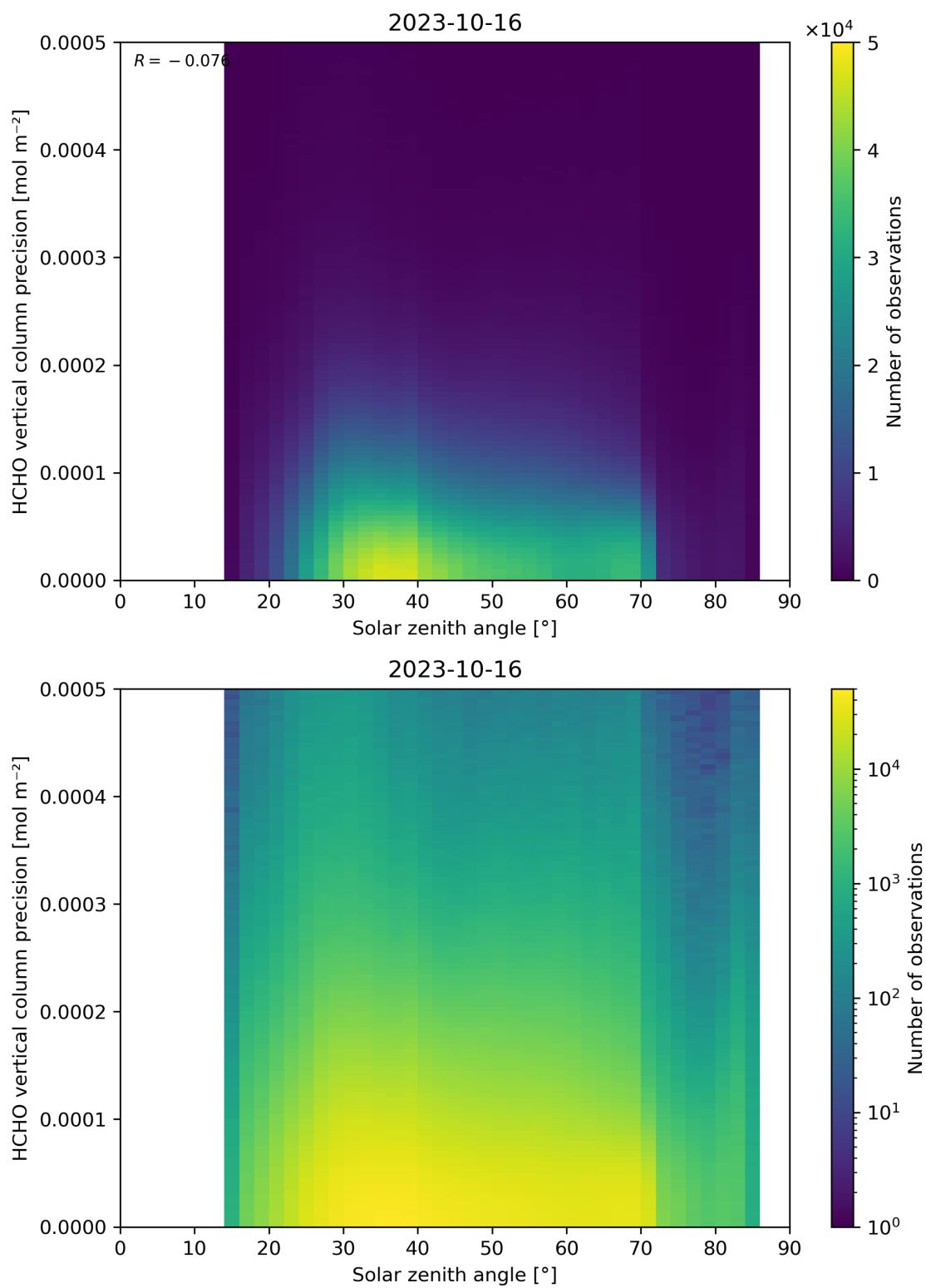
Figure 179: Scatter density plot of “Solar zenith angle” against “HCHO vertical column precision” for 2023-10-15 to 2023-10-17.
