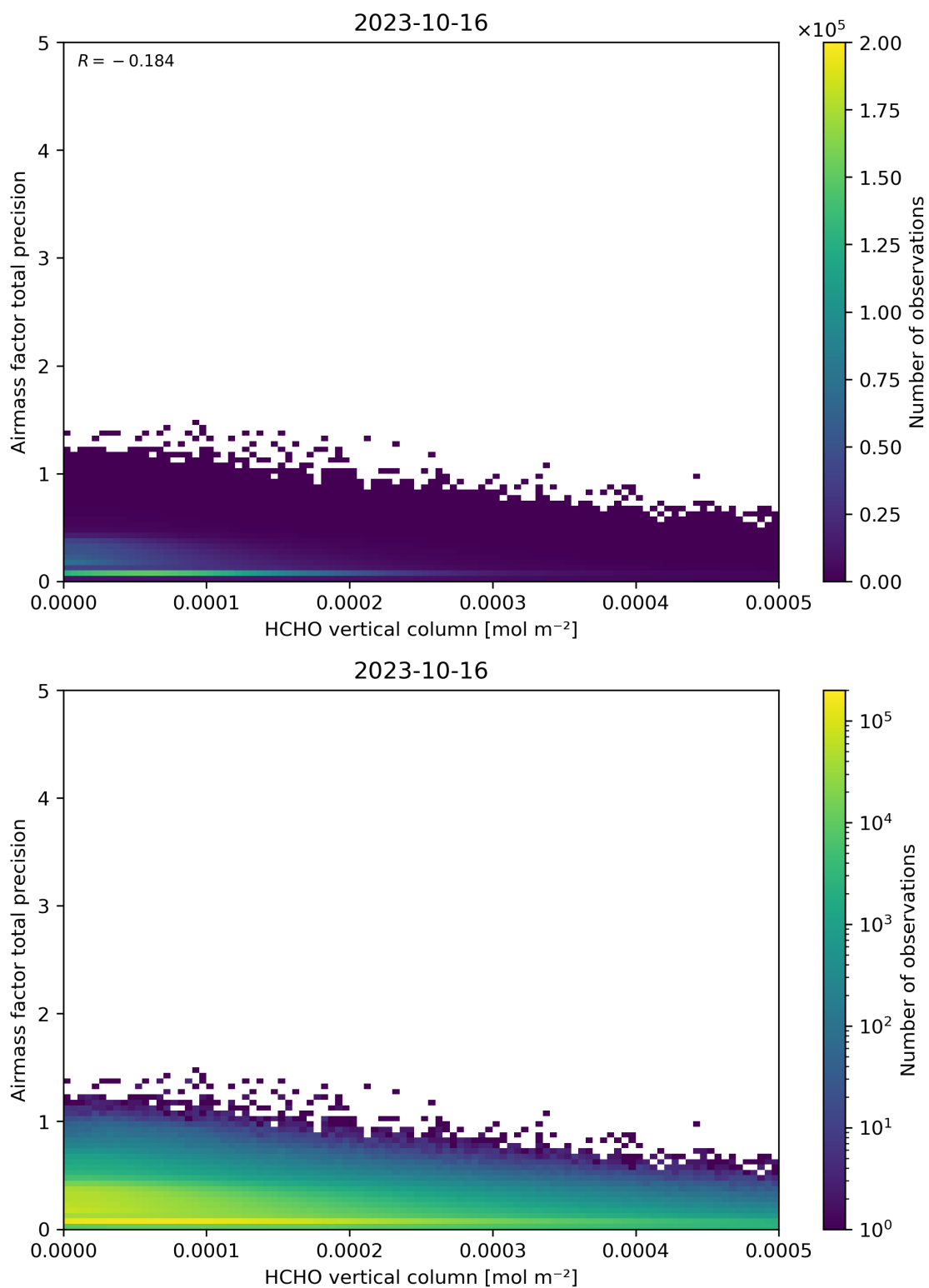
Figure 132: Scatter density plot of “HCHO vertical column” against “Airmass factor total precision” for 2023-10-15 to 2023-10-17.
