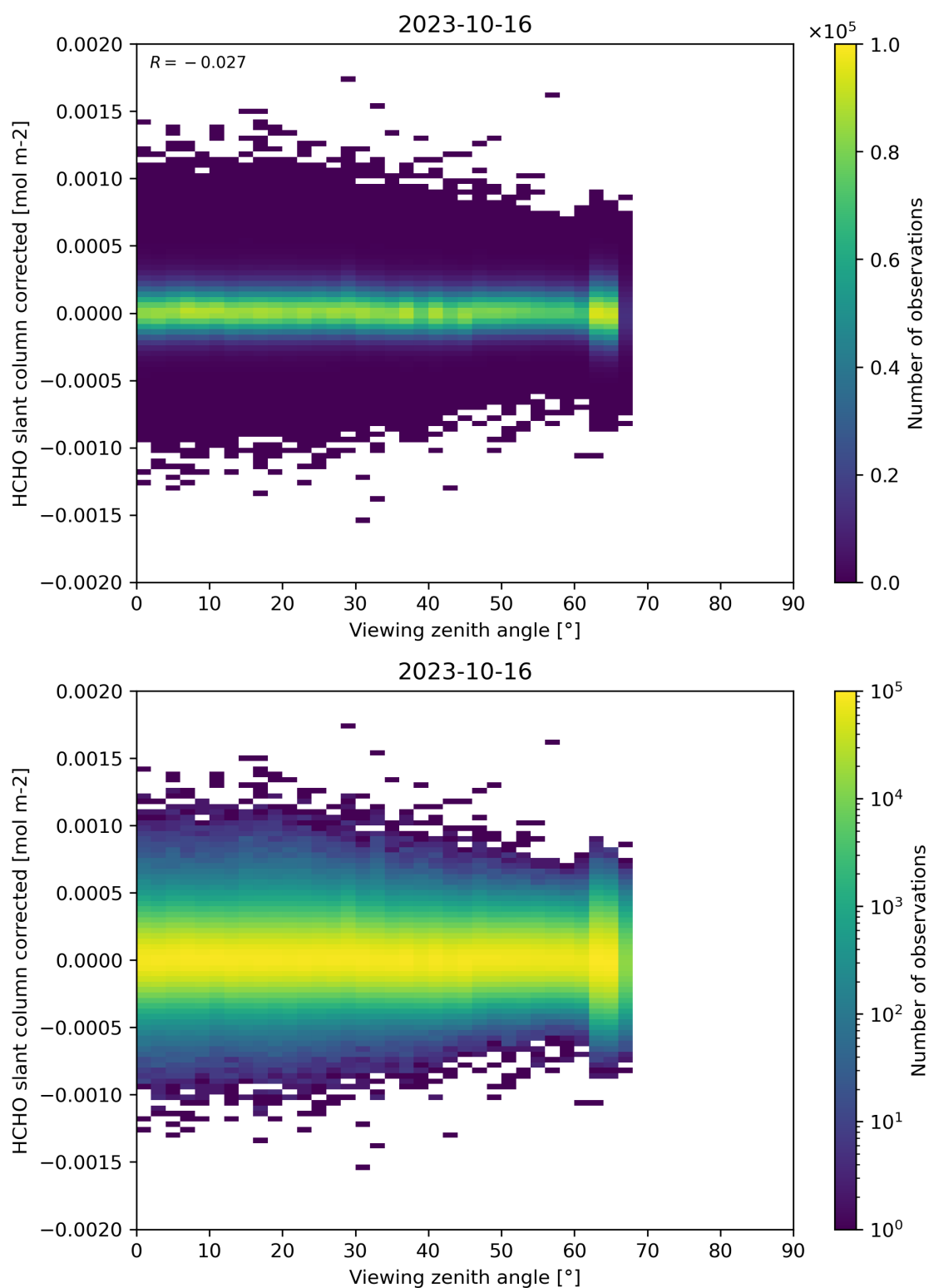
Figure 186: Scatter density plot of “Viewing zenith angle” against “HCHO slant column corrected” for 2023-10-15 to 2023-10-17.
