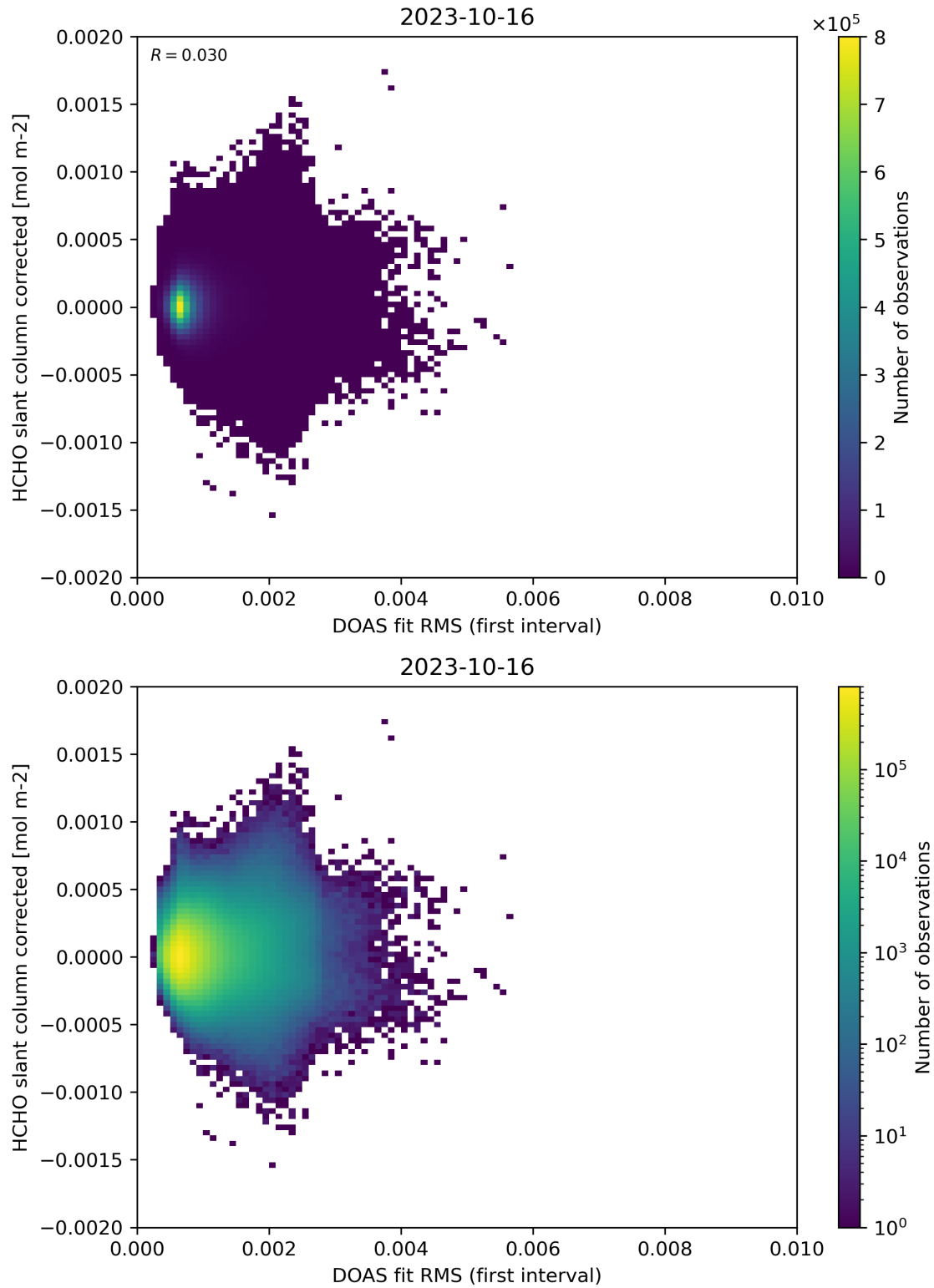
Figure 62: Scatter density plot of “DOAS fit RMS (first interval)” against “HCHO slant column corrected” for 2023-10-15 to 2023-10-17.
