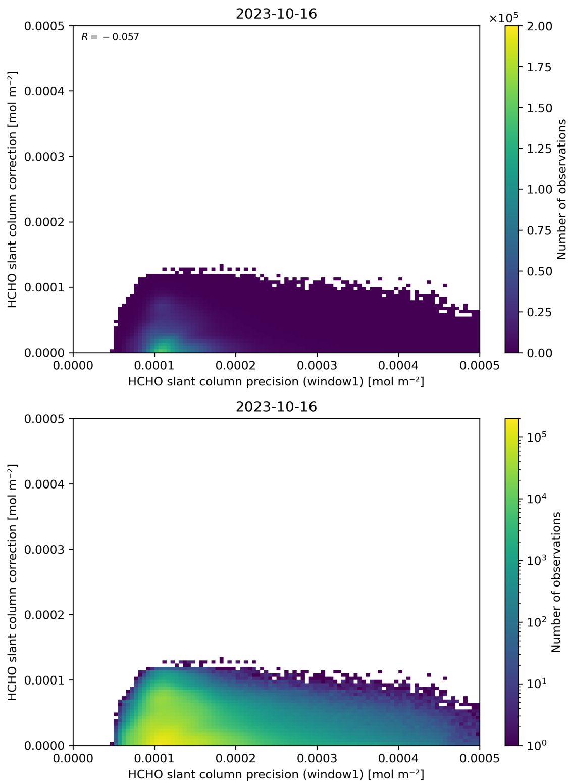
Figure 93: Scatter density plot of “HCHO slant column precision (window1)” against “HCHO slant column correction” for 2023-10-15 to 2023-10-17.
