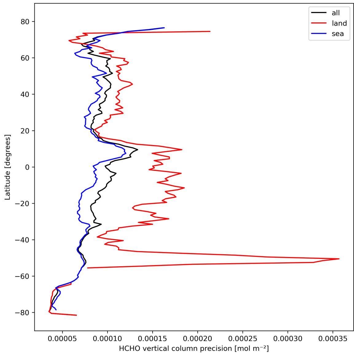
Figure 22: Zonal average of “HCHO vertical column precision” for 2023-10-15 to 2023-10-17.
