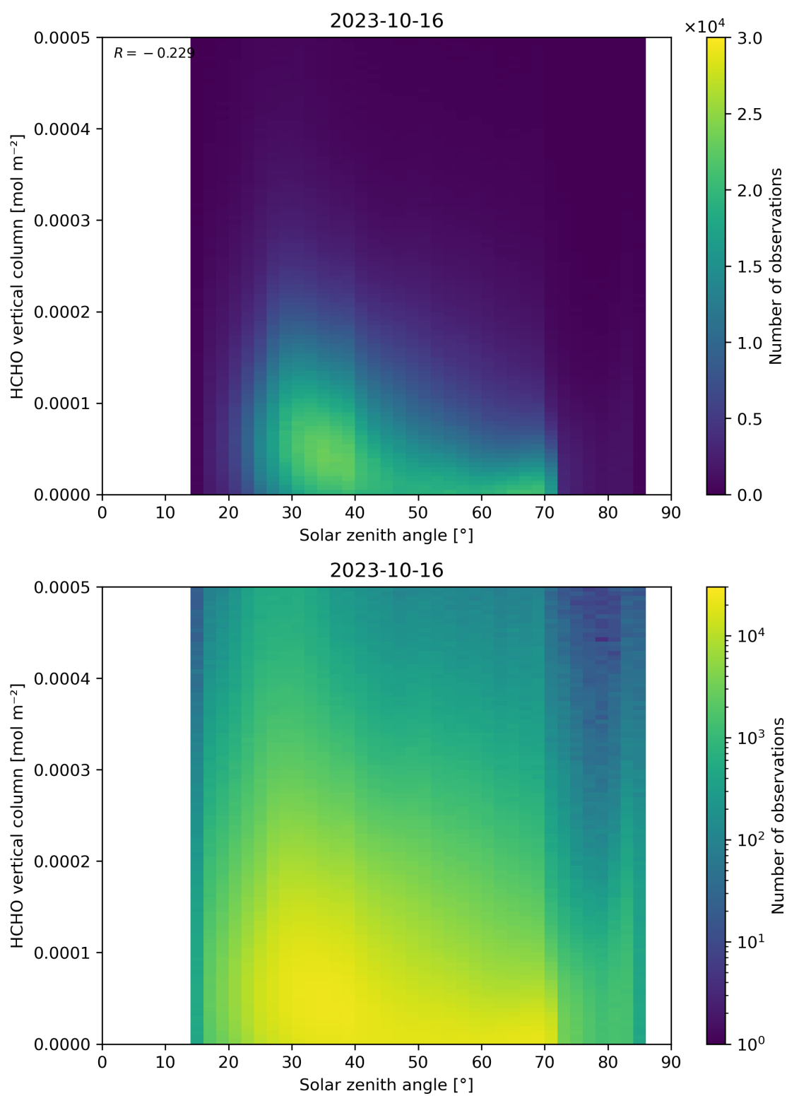
Figure 177: Scatter density plot of “Solar zenith angle” against “HCHO vertical column” for 2023-10-15 to 2023-10-17.
