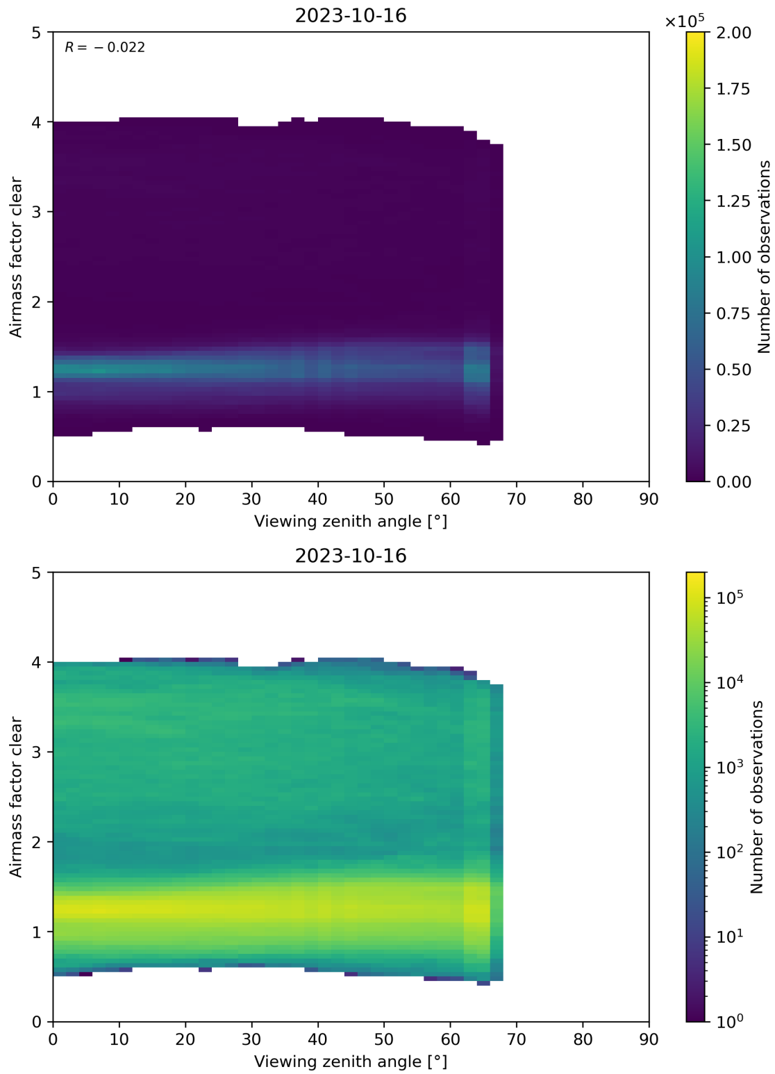
Figure 185: Scatter density plot of “Viewing zenith angle” against “Airmass factor clear” for 2023-10-15 to 2023-10-17.
