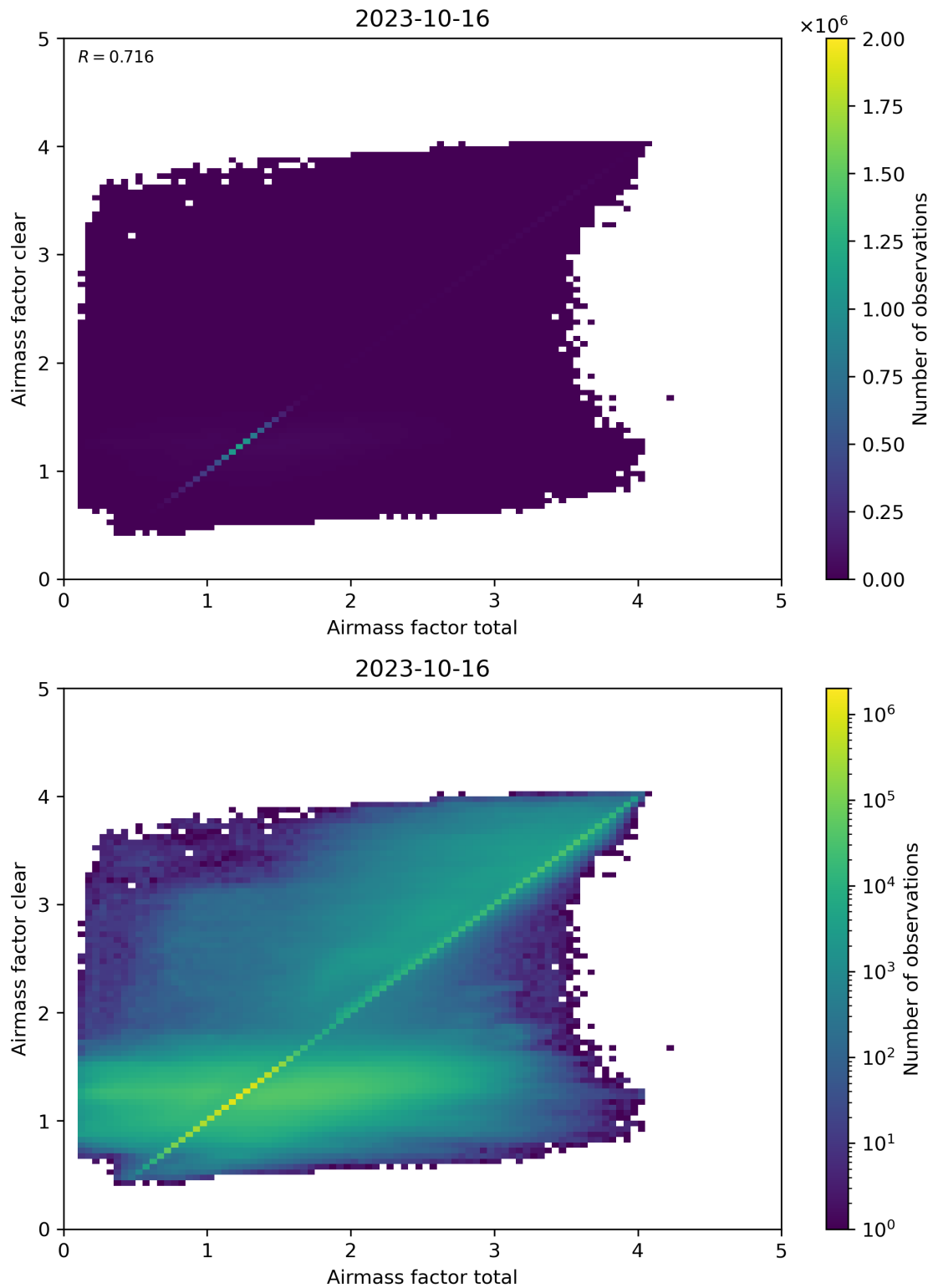
Figure 100: Scatter density plot of “Airmass factor total” against “Airmass factor clear” for 2023-10-15 to 2023-10-17.
