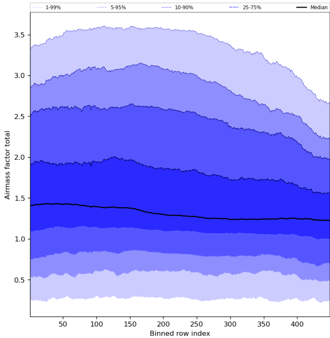
Figure 54: Along track statistics of “Airmass factor total” for 2023-10-17 to 2023-10-18
