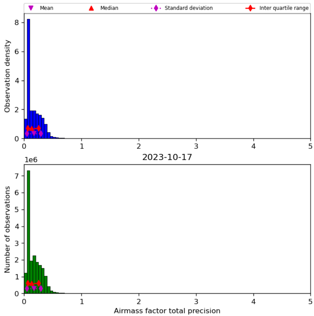
Figure 41: Histogram of “Airmass factor total precision” for 2023-10-17 to 2023-10-18
