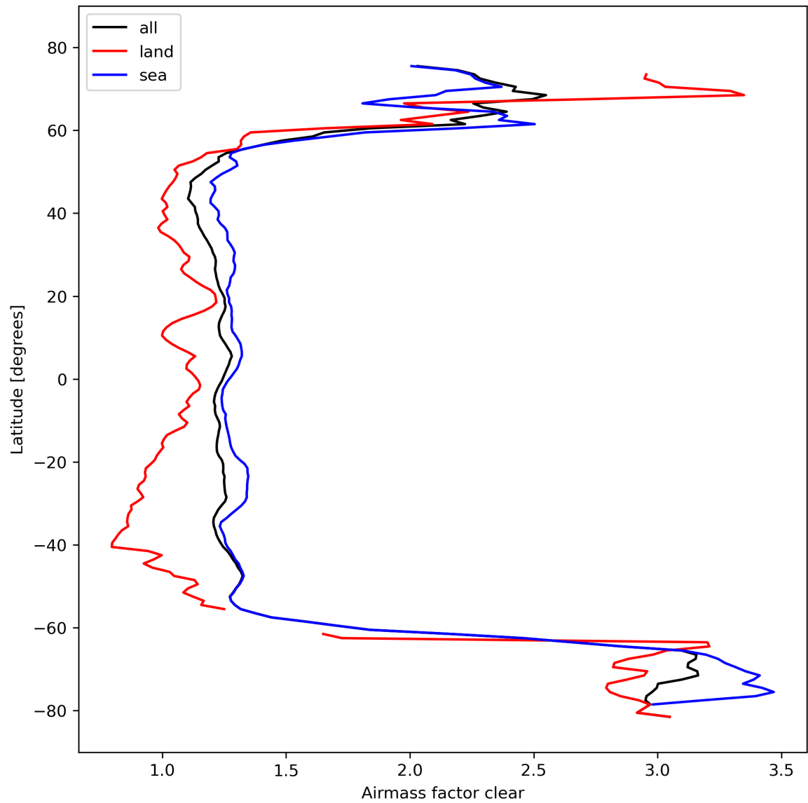
Figure 28: Zonal average of “Airmass factor clear” for 2023-10-17 to 2023-10-18.
