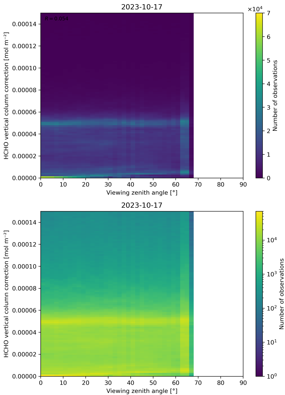
Figure 193: Scatter density plot of “Viewing zenith angle” against “HCHO vertical column correction” for 2023-10-17 to 2023-10-18.
