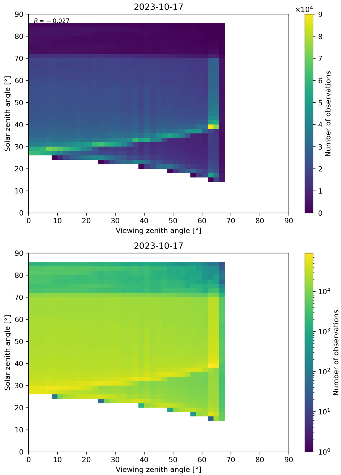
Figure 197: Scatter density plot of “Viewing zenith angle” against “Solar zenith angle” for 2023-10-17 to 2023-10-18.
