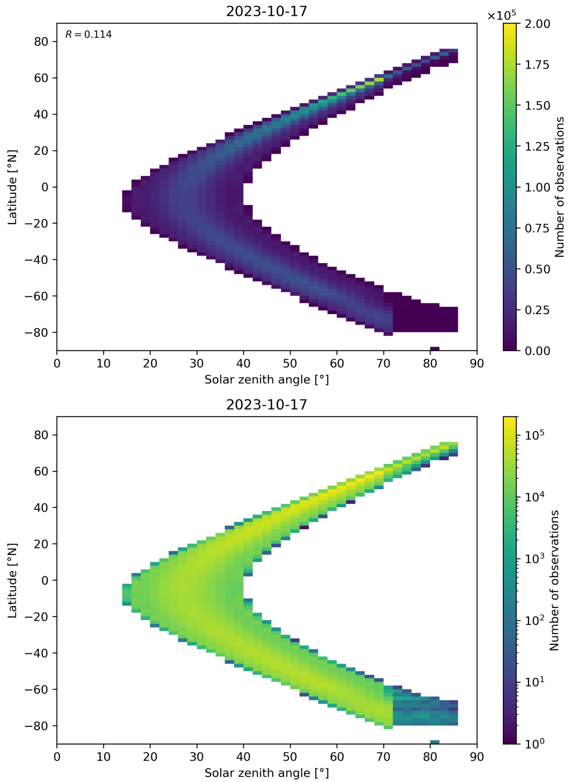
Figure 181: Scatter density plot of “Solar zenith angle” against “Latitude” for 2023-10-17 to 2023-10-18.
