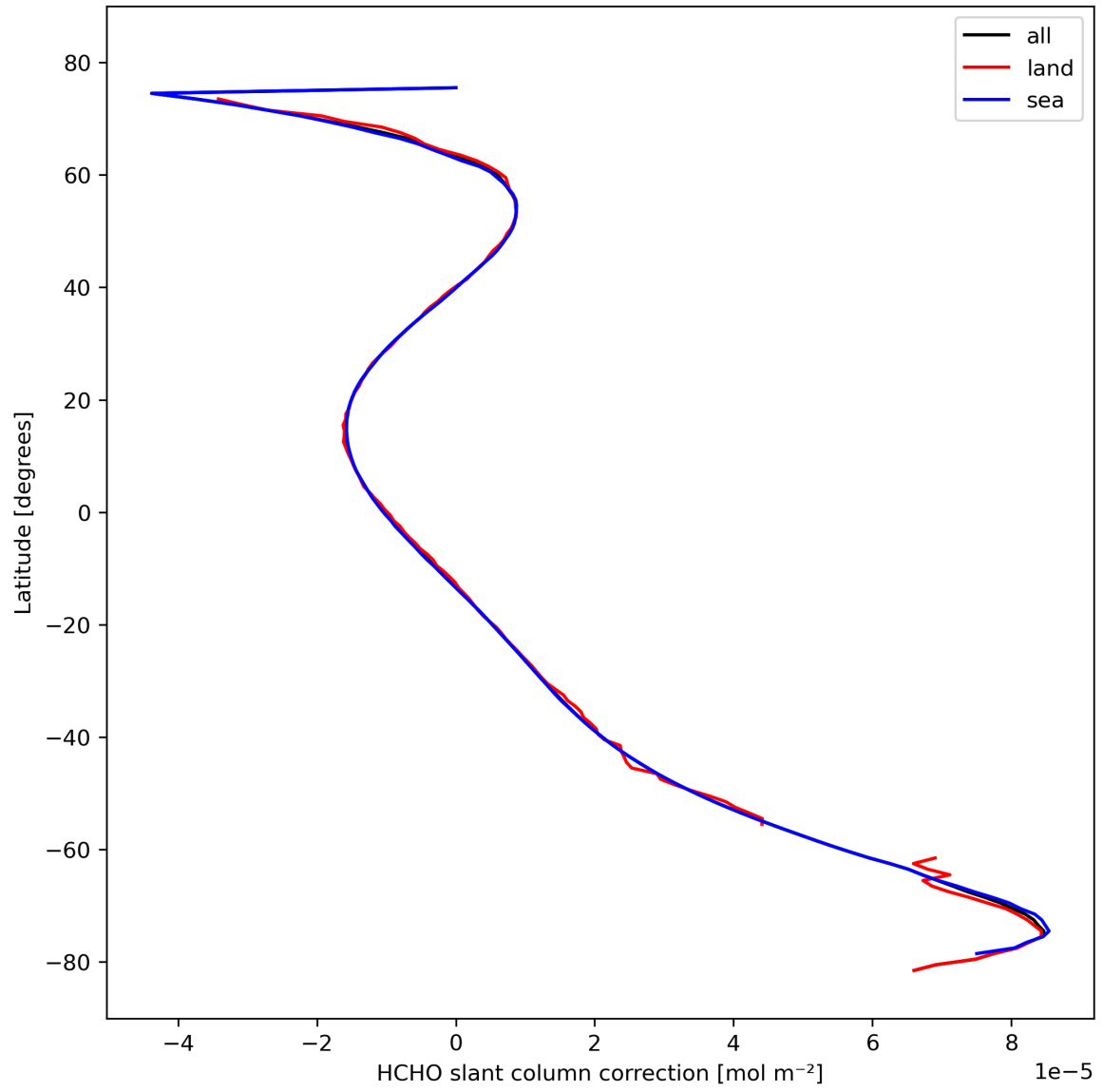
Figure 33: Zonal average of “HCHO slant column correction” for 2023-10-17 to 2023-10-18.
