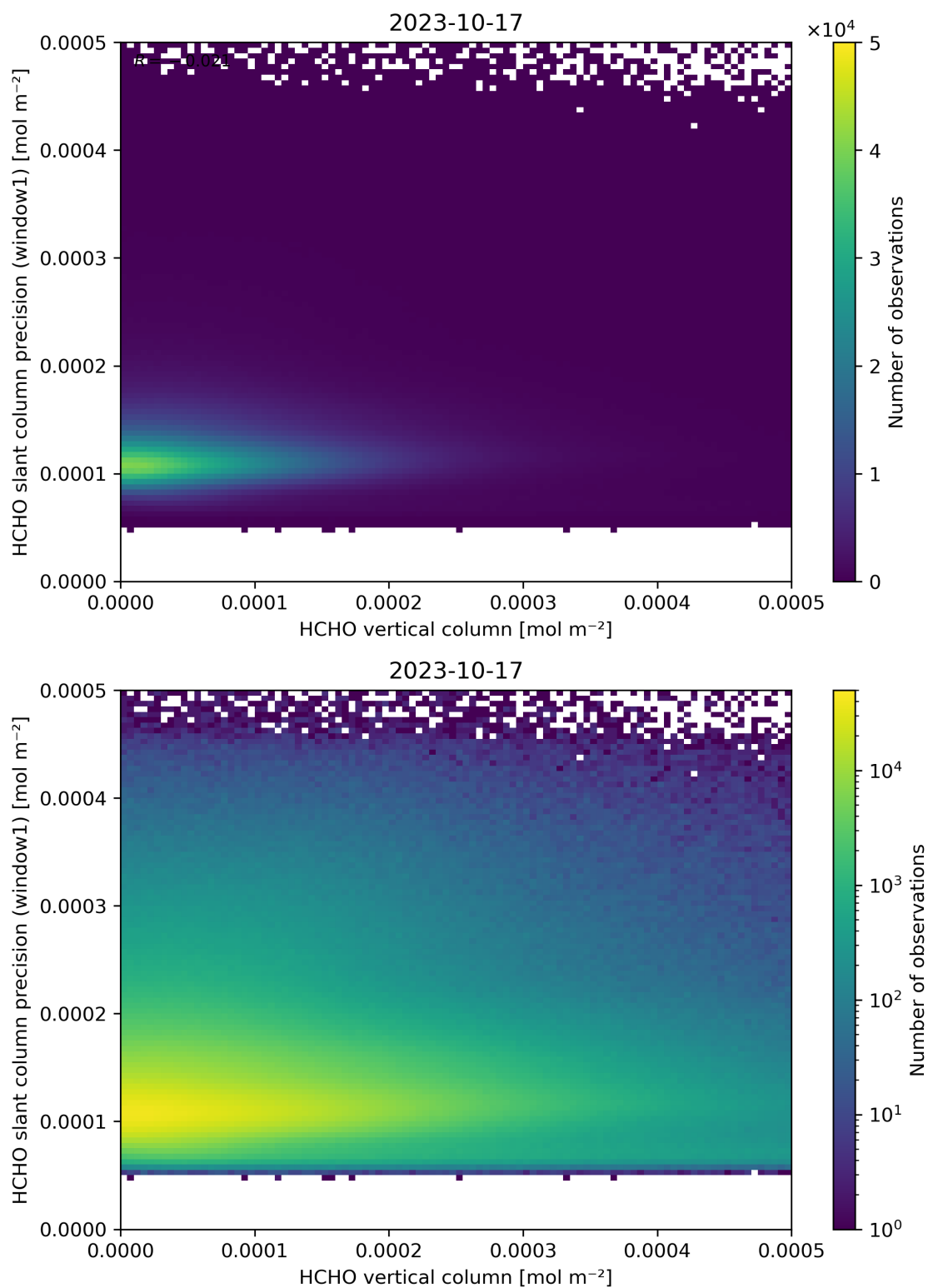
Figure 130: Scatter density plot of “HCHO vertical column” against “HCHO slant column precision (window1)” for 2023-10-17 to 2023-10-18.
