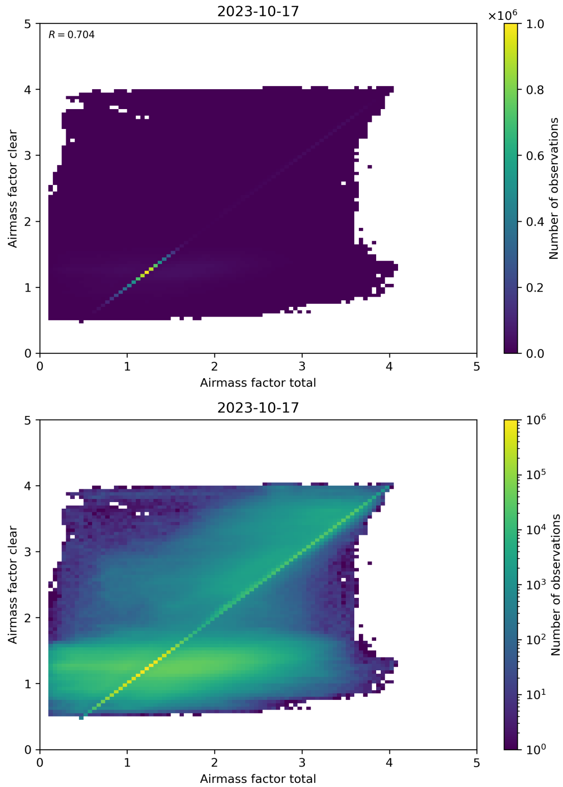
Figure 100: Scatter density plot of “Airmass factor total” against “Airmass factor clear” for 2023-10-17 to 2023-10-18.
