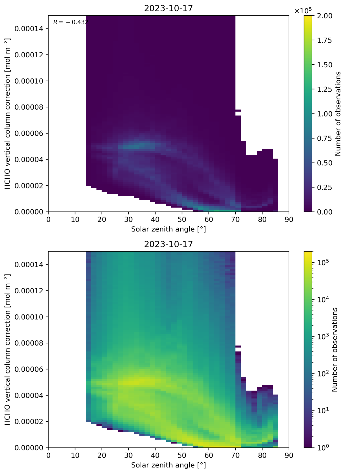
Figure 178: Scatter density plot of “Solar zenith angle” against “HCHO vertical column correction” for 2023-10-17 to 2023-10-18.
