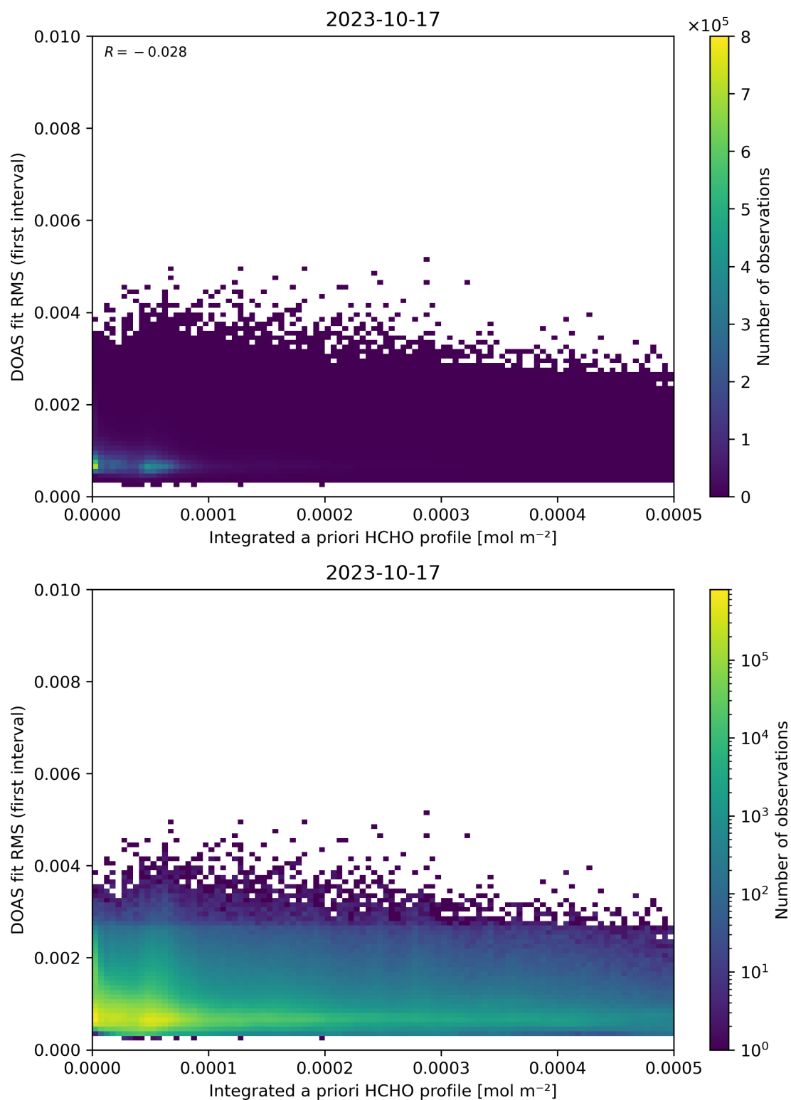
Figure 148: Scatter density plot of “Integrated a priori HCHO profile” against “DOAS fit RMS (first interval)” for 2023-10-17 to 2023-10-18.
