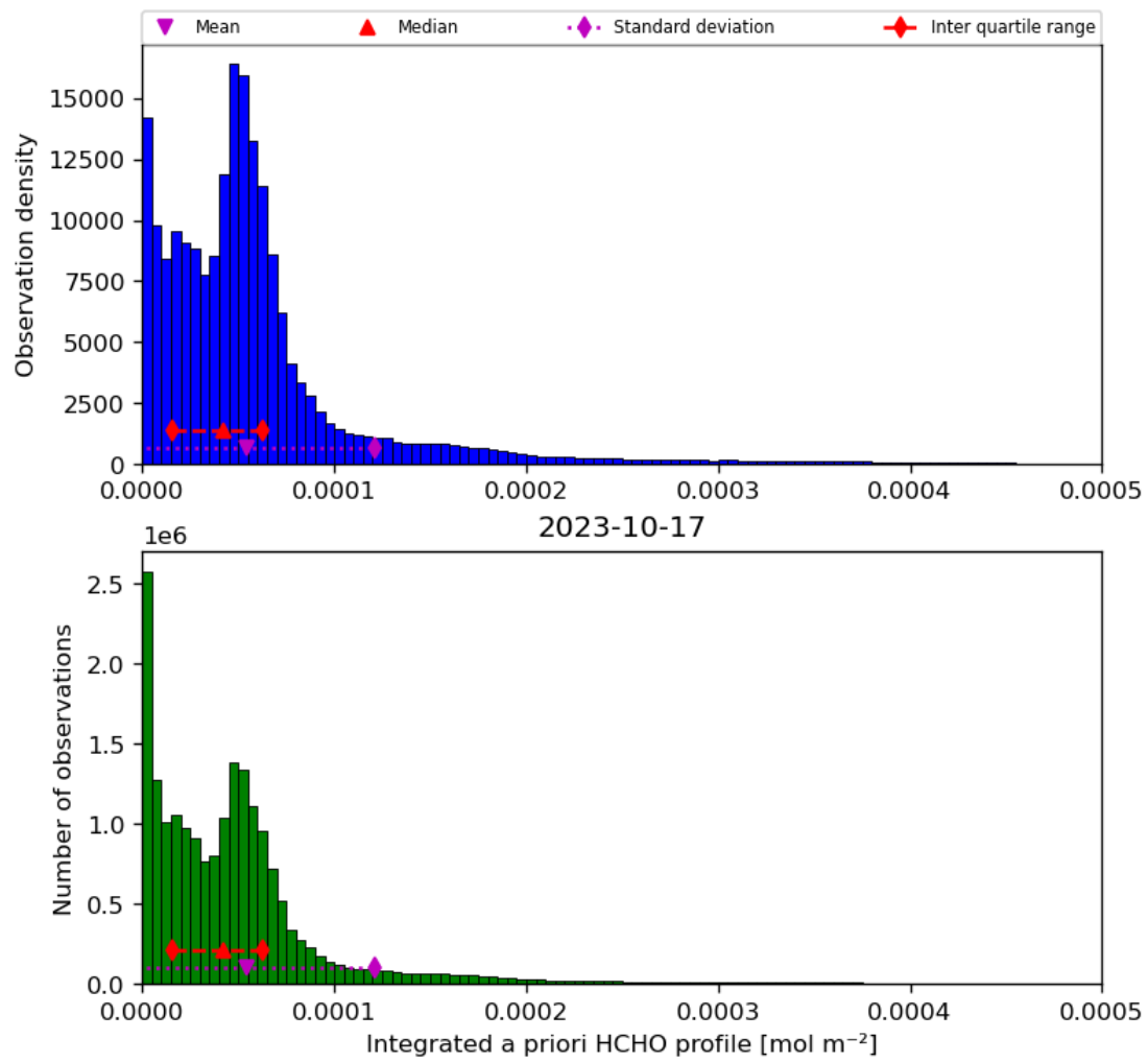
Figure 43: Histogram of “Integrated a priori HCHO profile” for 2023-10-17 to 2023-10-18
