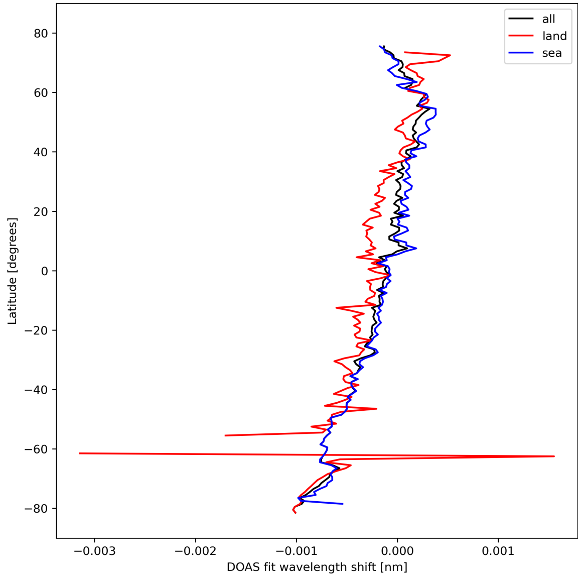
Figure 30: Zonal average of “DOAS fit wavelength shift” for 2023-10-17 to 2023-10-18.
