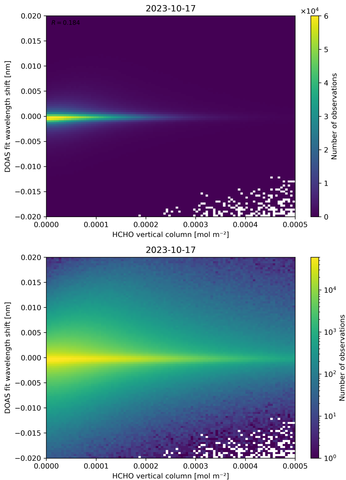
Figure 124: Scatter density plot of “HCHO vertical column” against “DOAS fit wavelength shift” for 2023-10-17 to 2023-10-18.
