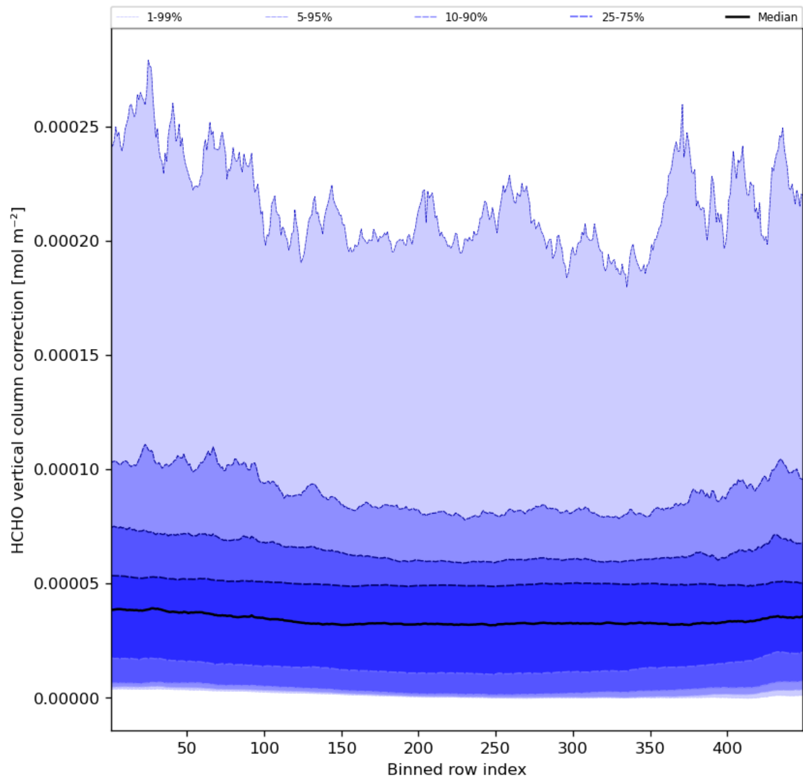
Figure 51: Along track statistics of “HCHO vertical column correction” for 2023-10-17 to 2023-10-18
