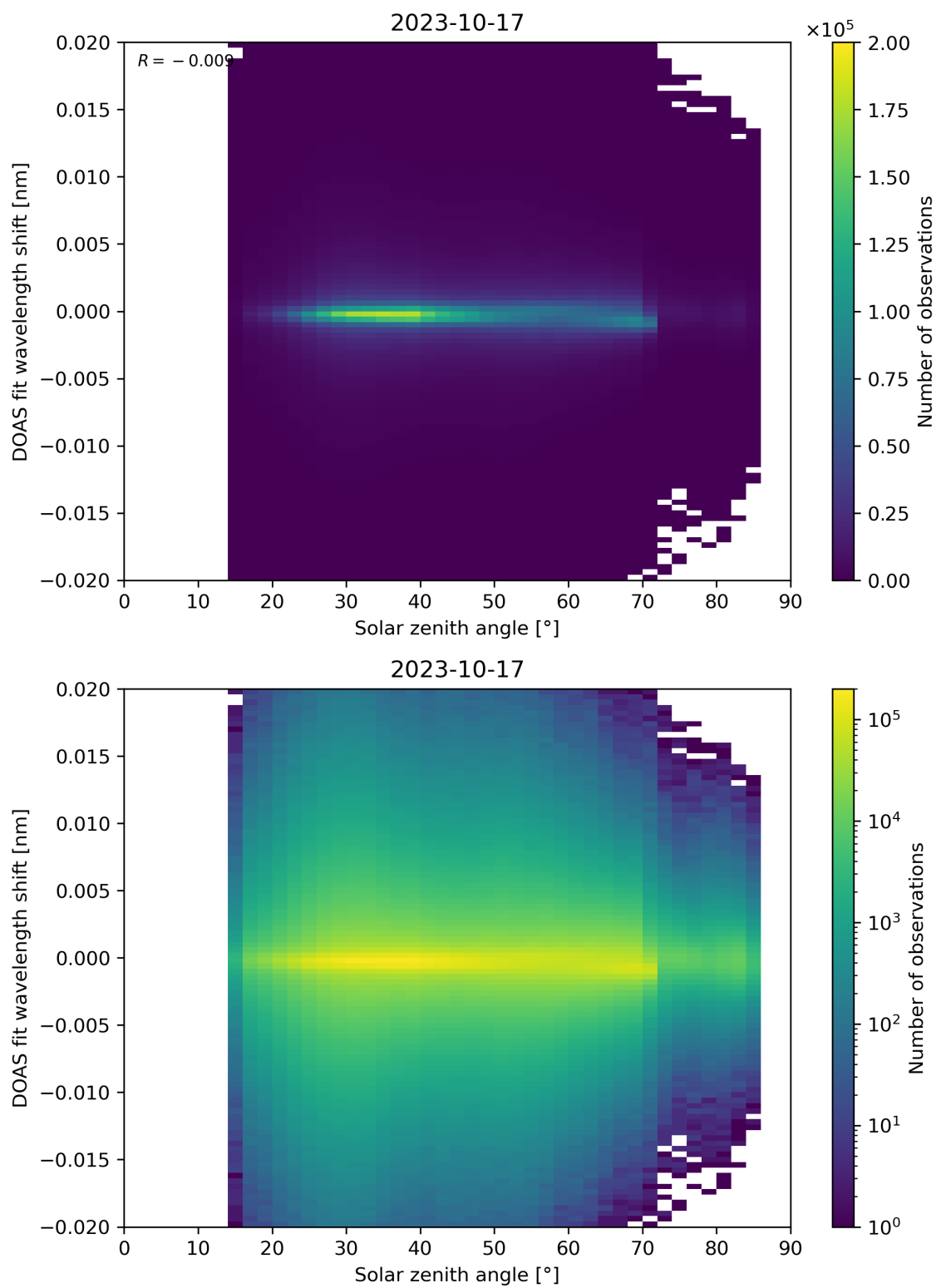
Figure 168: Scatter density plot of “Solar zenith angle” against “DOAS fit wavelength shift” for 2023-10-17 to 2023-10-18.
