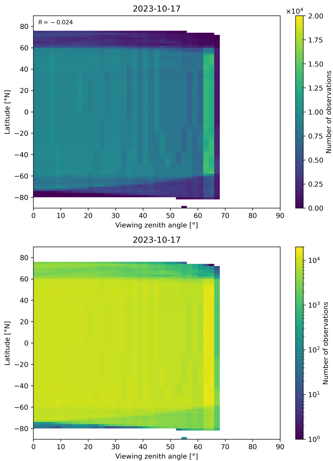
Figure 196: Scatter density plot of “Viewing zenith angle” against “Latitude” for 2023-10-17 to 2023-10-18.
