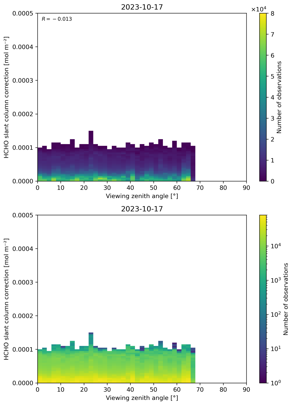
Figure 187: Scatter density plot of “Viewing zenith angle” against “HCHO slant column correction” for 2023-10-17 to 2023-10-18.
