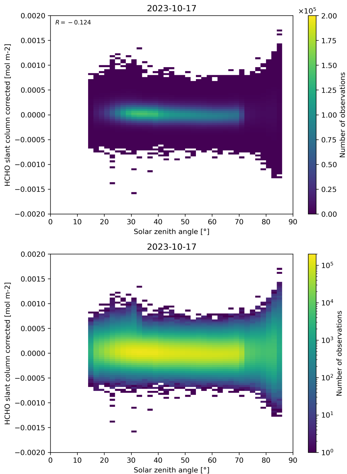
Figure 171: Scatter density plot of “Solar zenith angle” against “HCHO slant column corrected” for 2023-10-17 to 2023-10-18.
