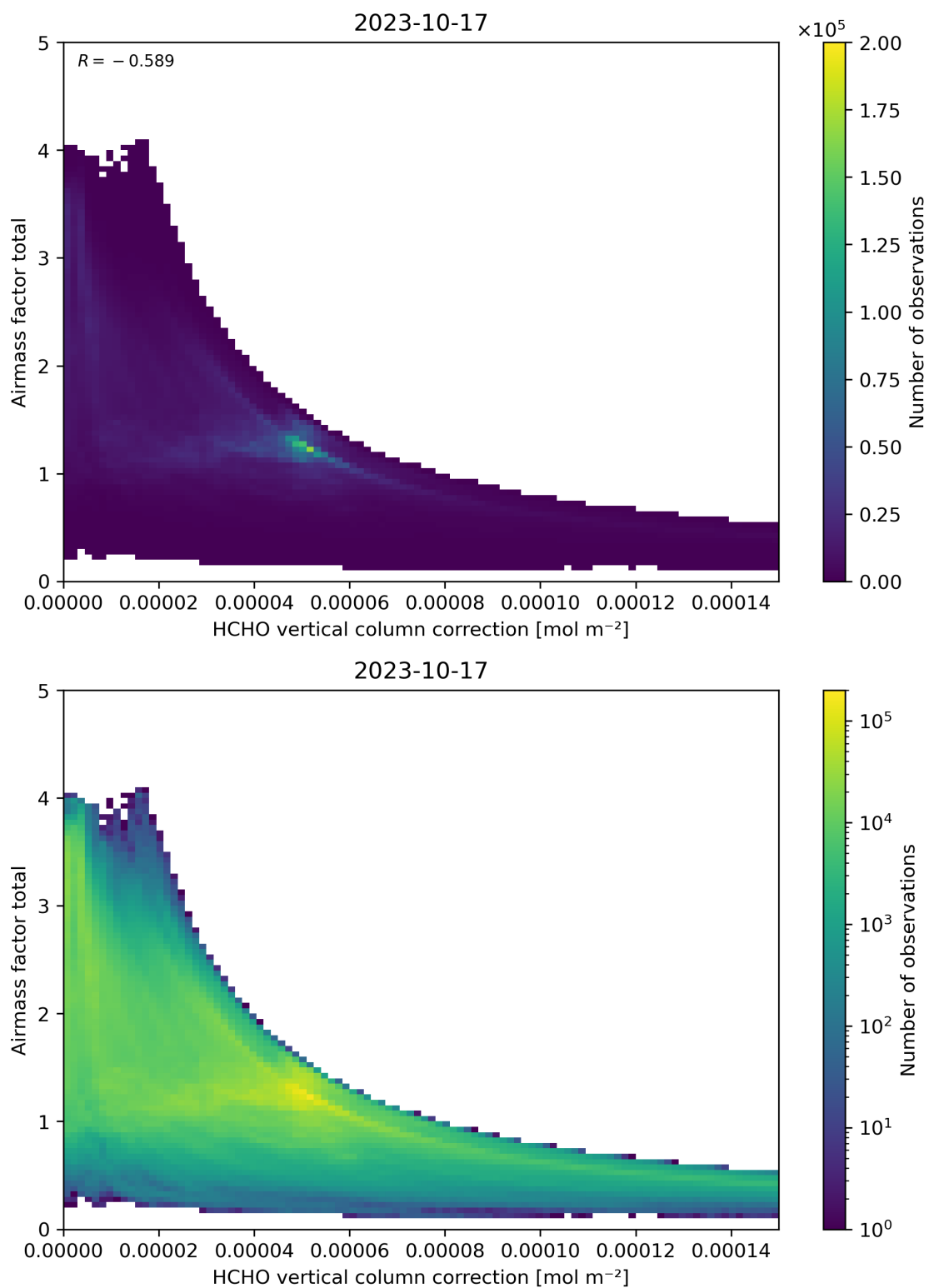
Figure 120: Scatter density plot of “HCHO vertical column correction” against “Airmass factor total” for 2023-10-17 to 2023-10-18.
