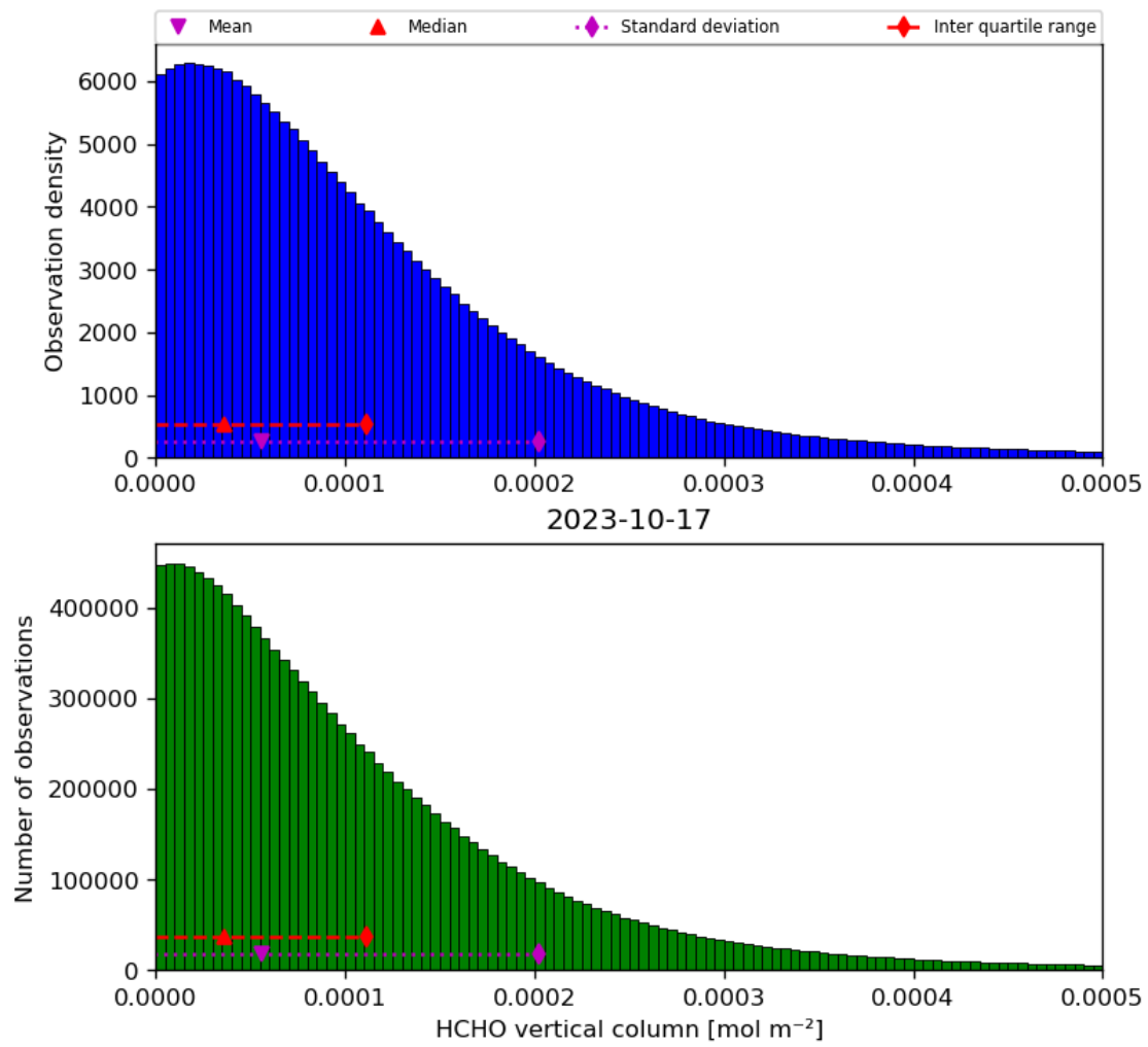
Figure 35: Histogram of “HCHO vertical column” for 2023-10-17 to 2023-10-18
