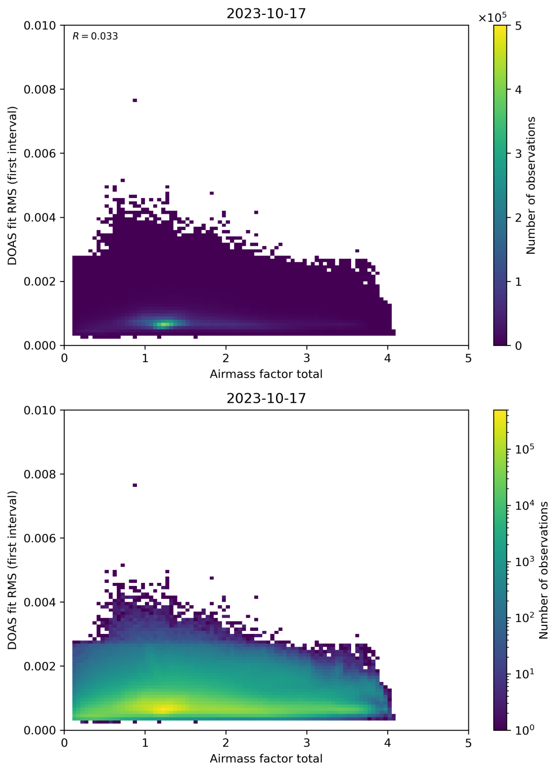
Figure 97: Scatter density plot of “Airmass factor total” against “DOAS fit RMS (first interval)” for 2023-10-17 to 2023-10-18.
