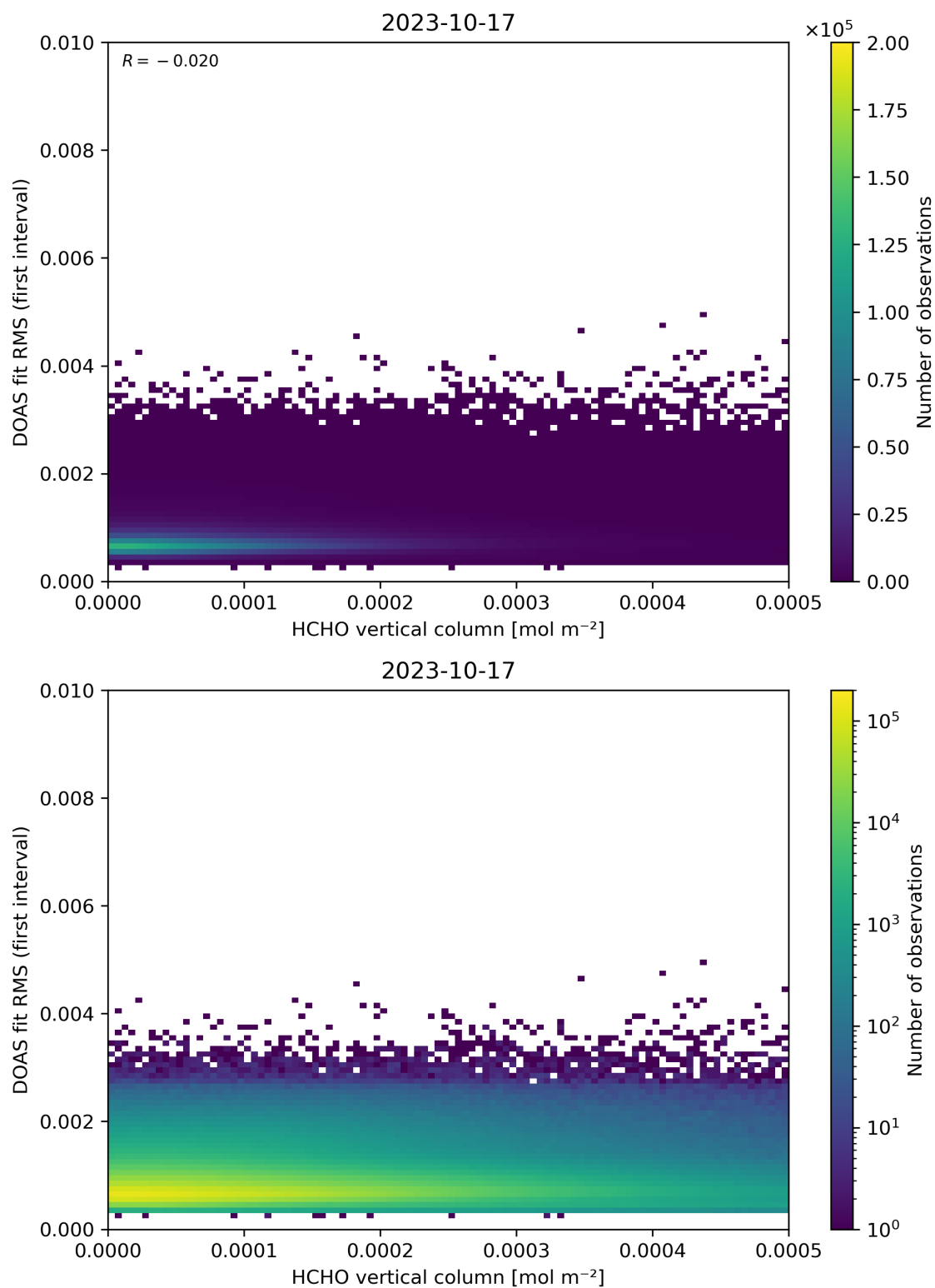
Figure 123: Scatter density plot of “HCHO vertical column” against “DOAS fit RMS (first interval)” for 2023-10-17 to 2023-10-18.
