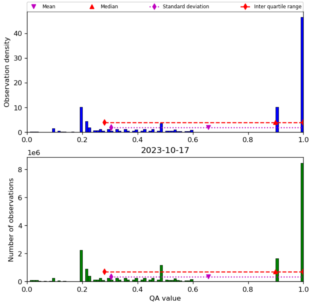
Figure 34: Histogram of “QA value” for 2023-10-17 to 2023-10-18
