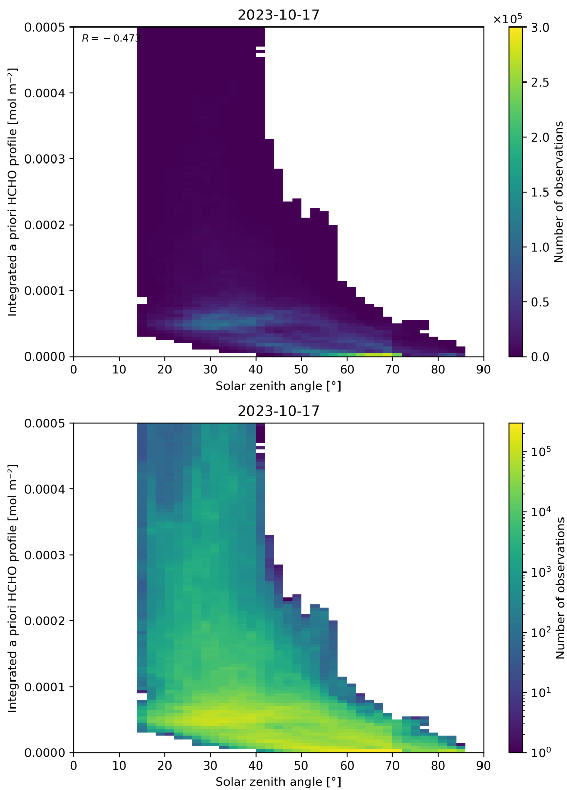
Figure 180: Scatter density plot of “Solar zenith angle” against “Integrated a priori HCHO profile” for 2023-10-17 to 2023-10-18.
