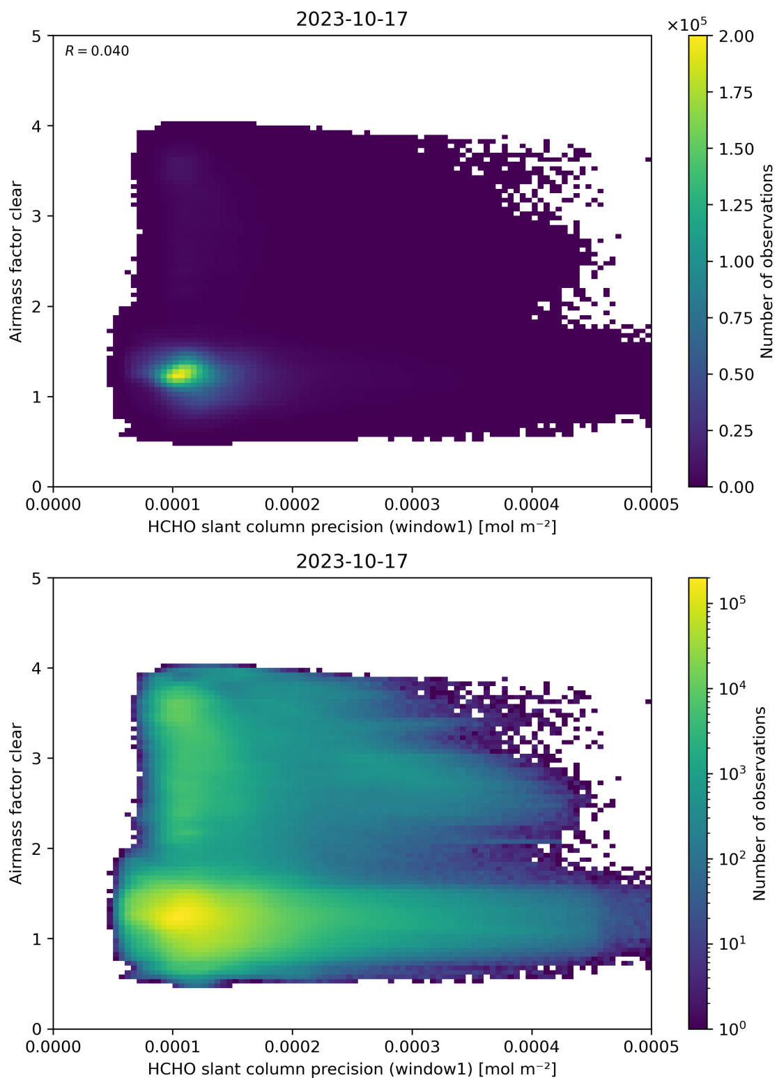
Figure 91: Scatter density plot of “HCHO slant column precision (window1)” against “Airmass factor clear” for 2023-10-17 to 2023-10-18.
