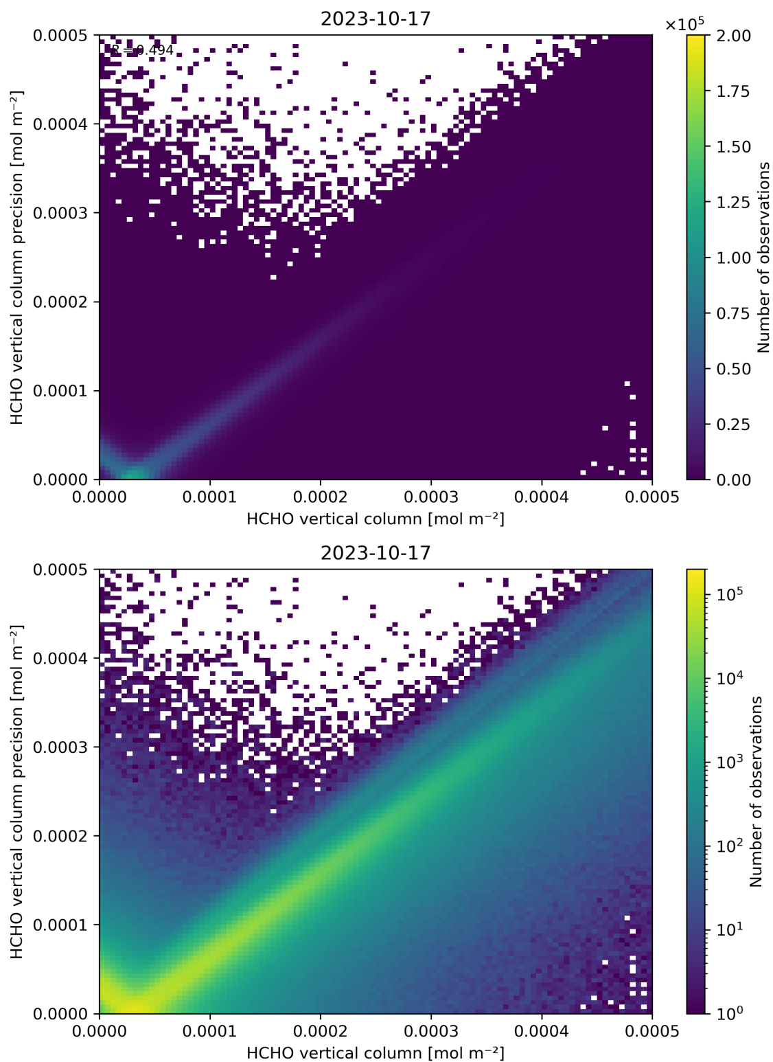
Figure 134: Scatter density plot of “HCHO vertical column” against “HCHO vertical column precision” for 2023-10-17 to 2023-10-18.
