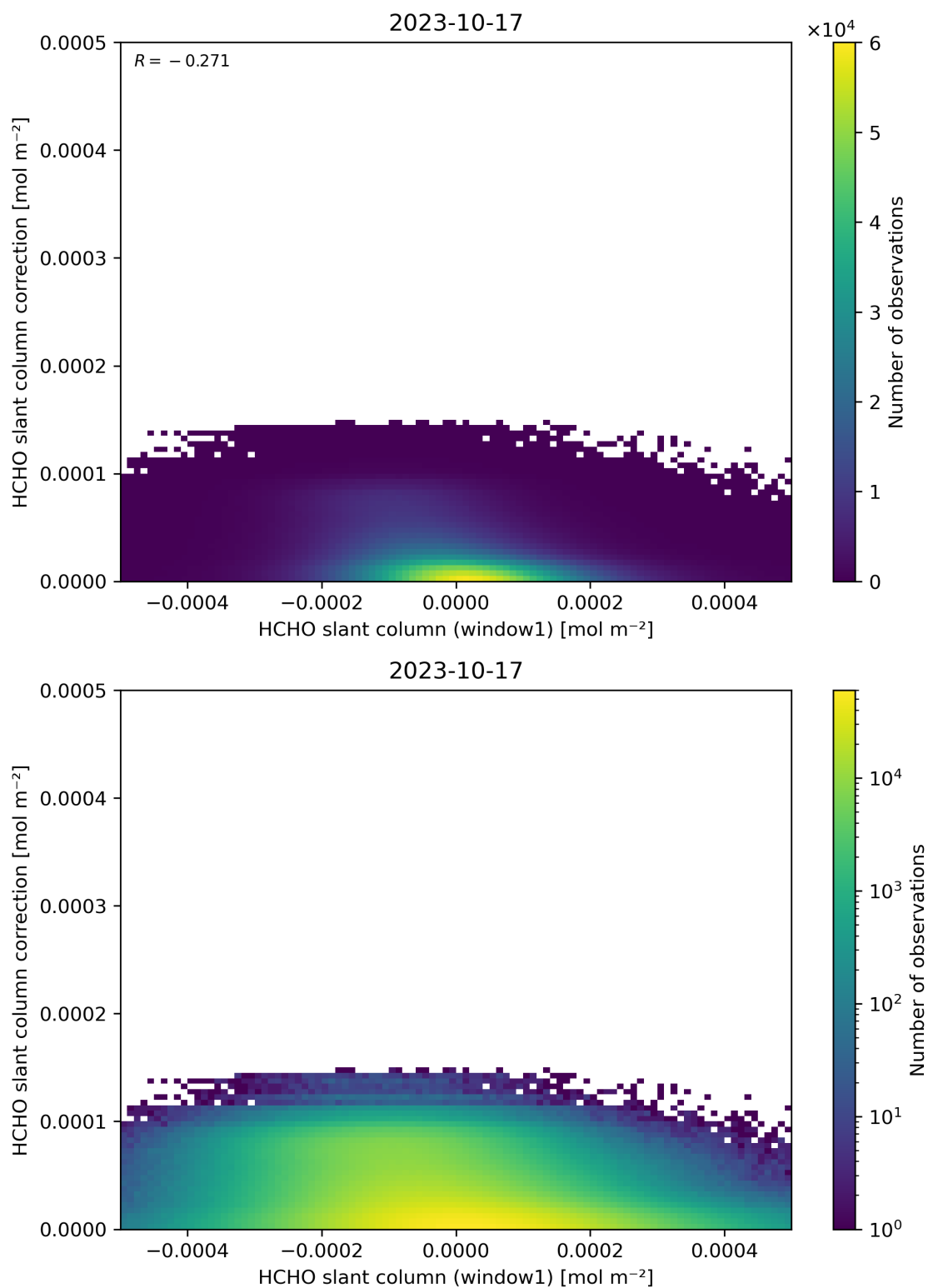
Figure 83: Scatter density plot of “HCHO slant column (window1)” against “HCHO slant column correction” for 2023-10-17 to 2023-10-18.
