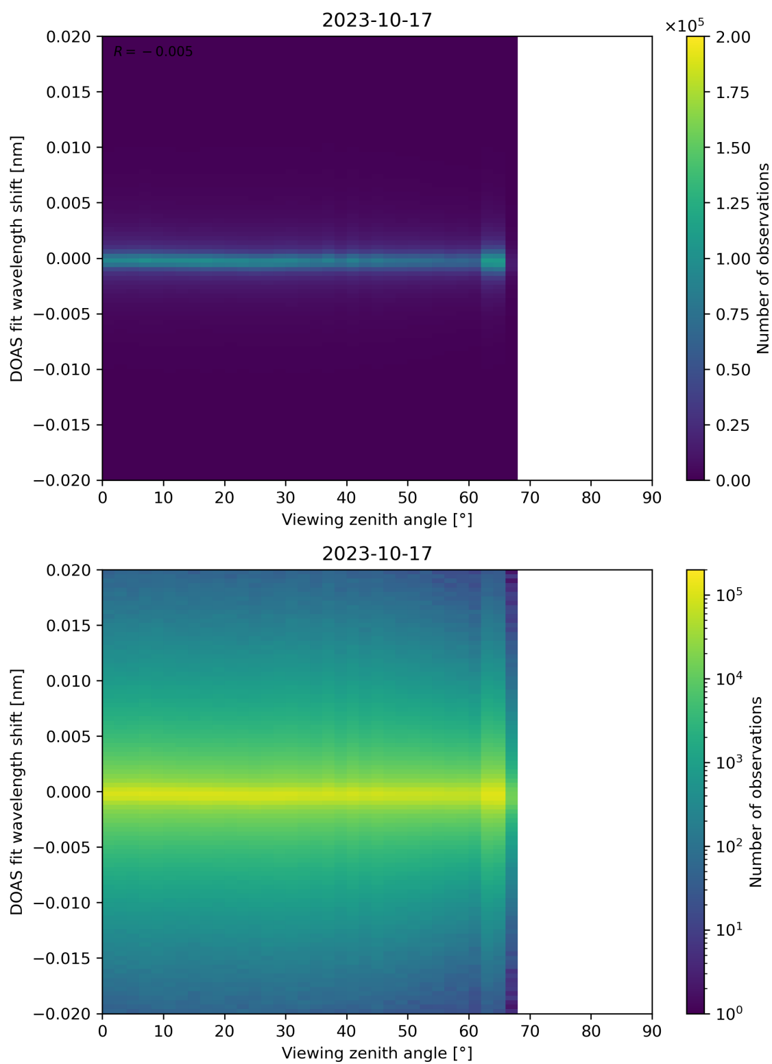
Figure 183: Scatter density plot of “Viewing zenith angle” against “DOAS fit wavelength shift” for 2023-10-17 to 2023-10-18.
