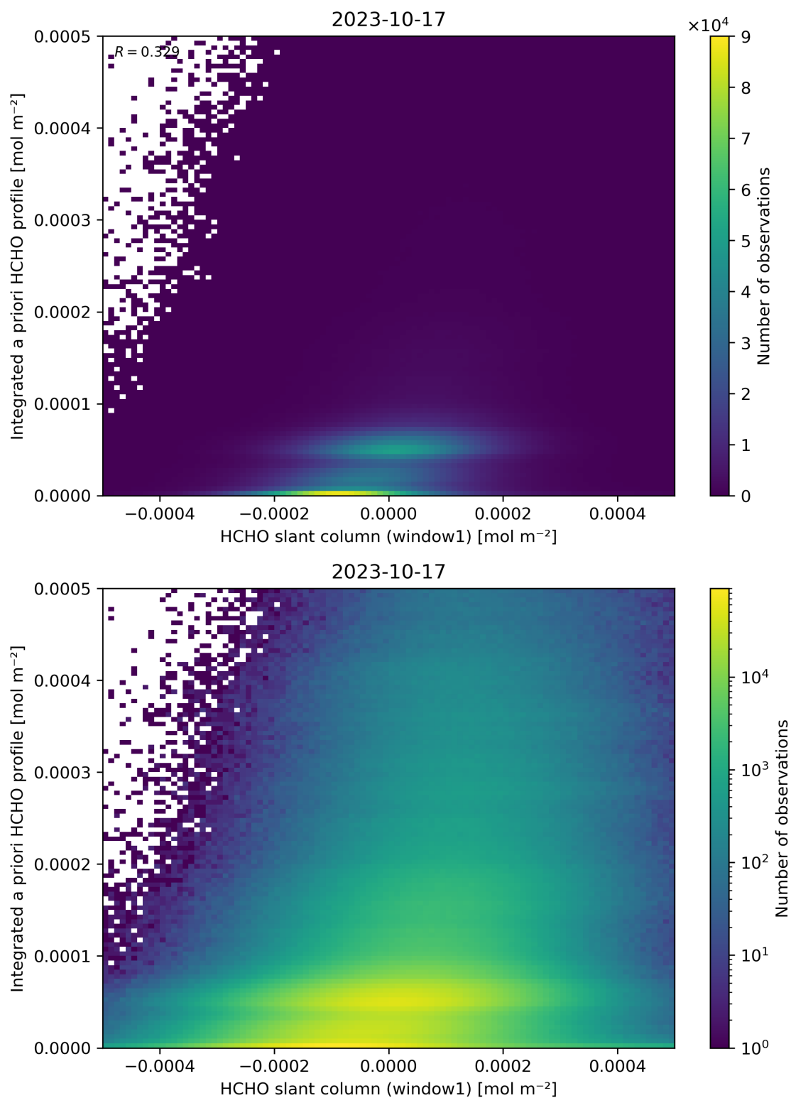
Figure 87: Scatter density plot of “HCHO slant column (window1)” against “Integrated a priori HCHO profile” for 2023-10-17 to 2023-10-18.
