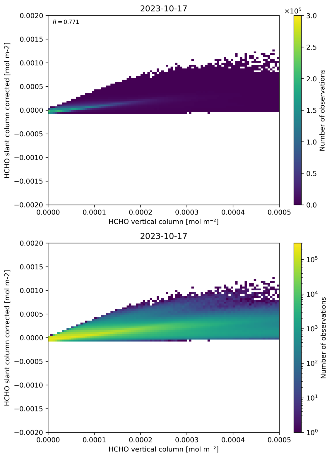
Figure 127: Scatter density plot of “HCHO vertical column” against “HCHO slant column corrected” for 2023-10-17 to 2023-10-18.
