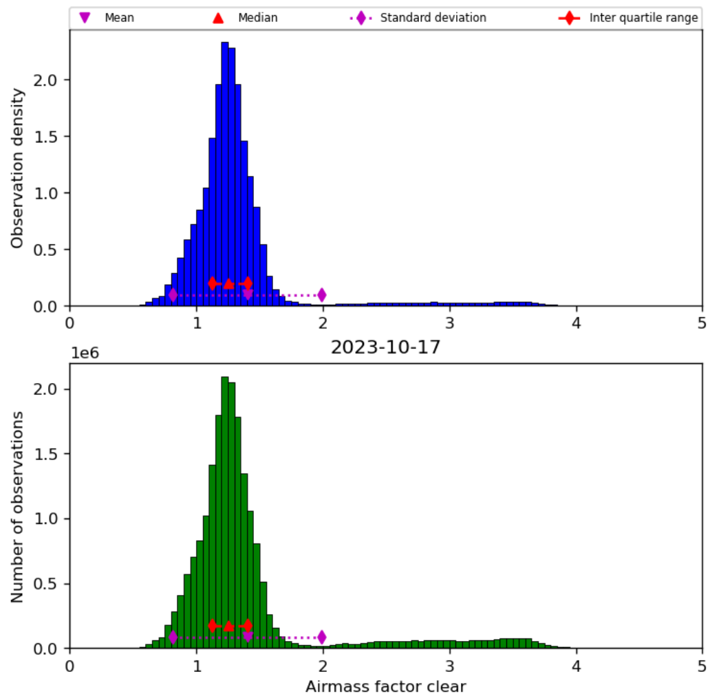
Figure 42: Histogram of “Airmass factor clear” for 2023-10-17 to 2023-10-18
