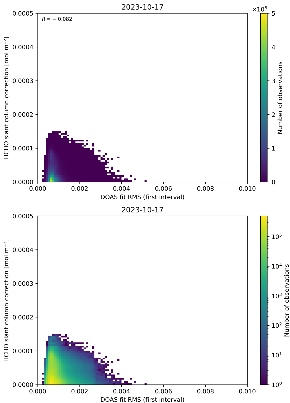
Figure 63: Scatter density plot of “DOAS fit RMS (first interval)” against “HCHO slant column correction” for 2023-10-17 to 2023-10-18.
