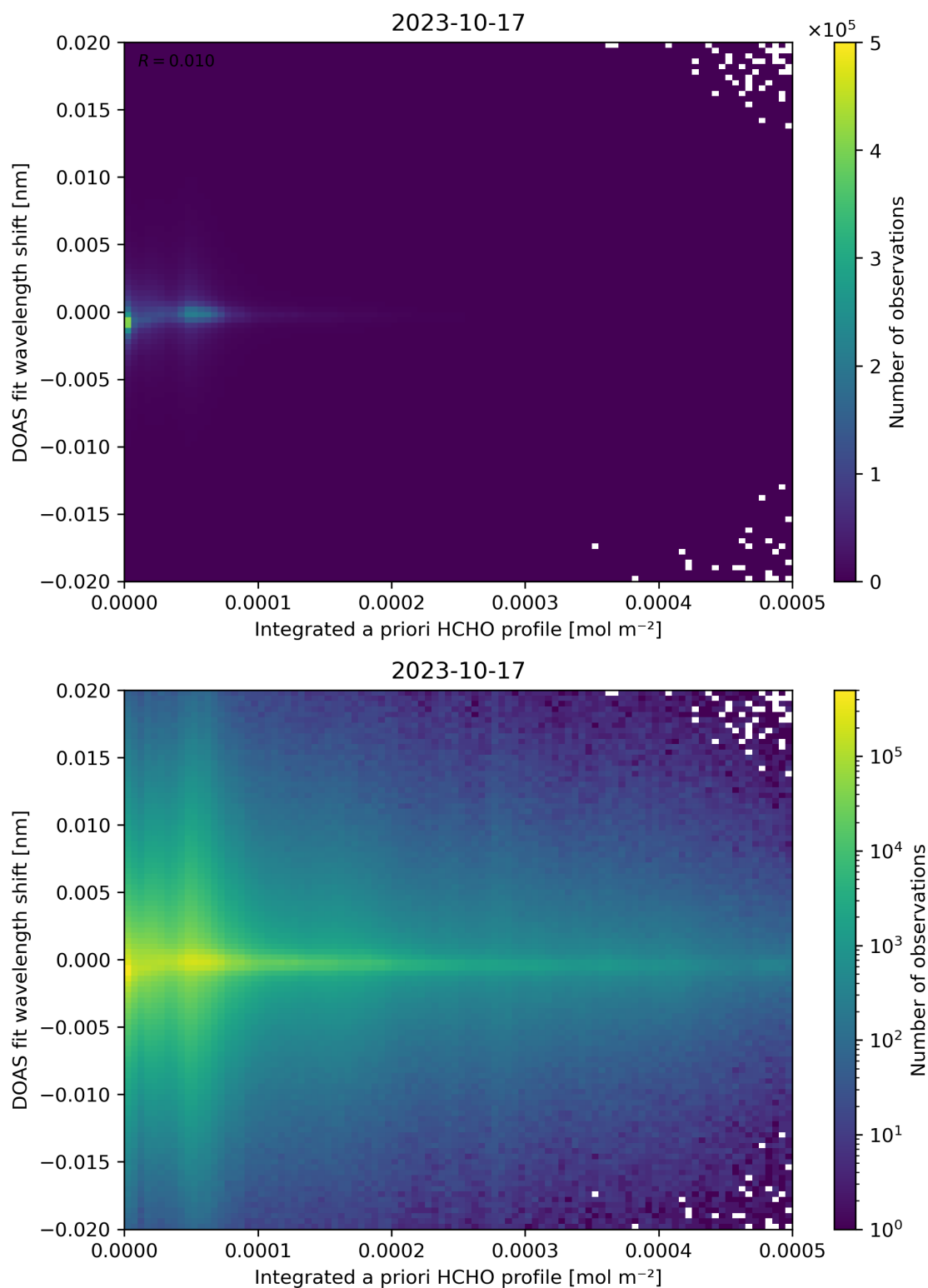
Figure 149: Scatter density plot of “Integrated a priori HCHO profile” against “DOAS fit wavelength shift” for 2023-10-17 to 2023-10-18.
