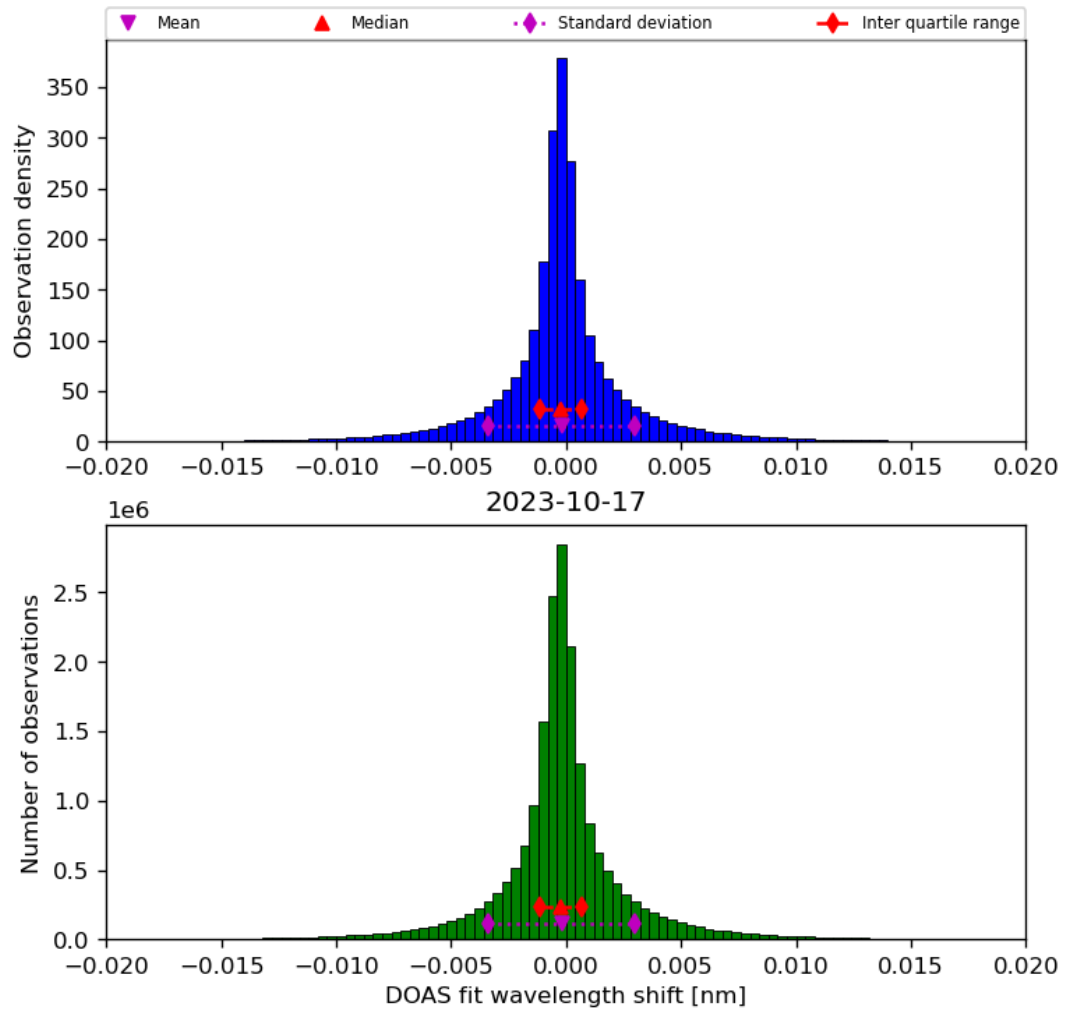
Figure 44: Histogram of “DOAS fit wavelength shift” for 2023-10-17 to 2023-10-18
