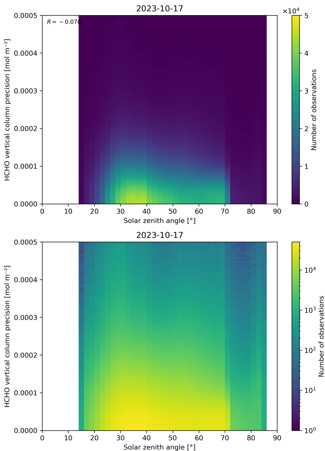
Figure 179: Scatter density plot of “Solar zenith angle” against “HCHO vertical column precision” for 2023-10-17 to 2023-10-18.
