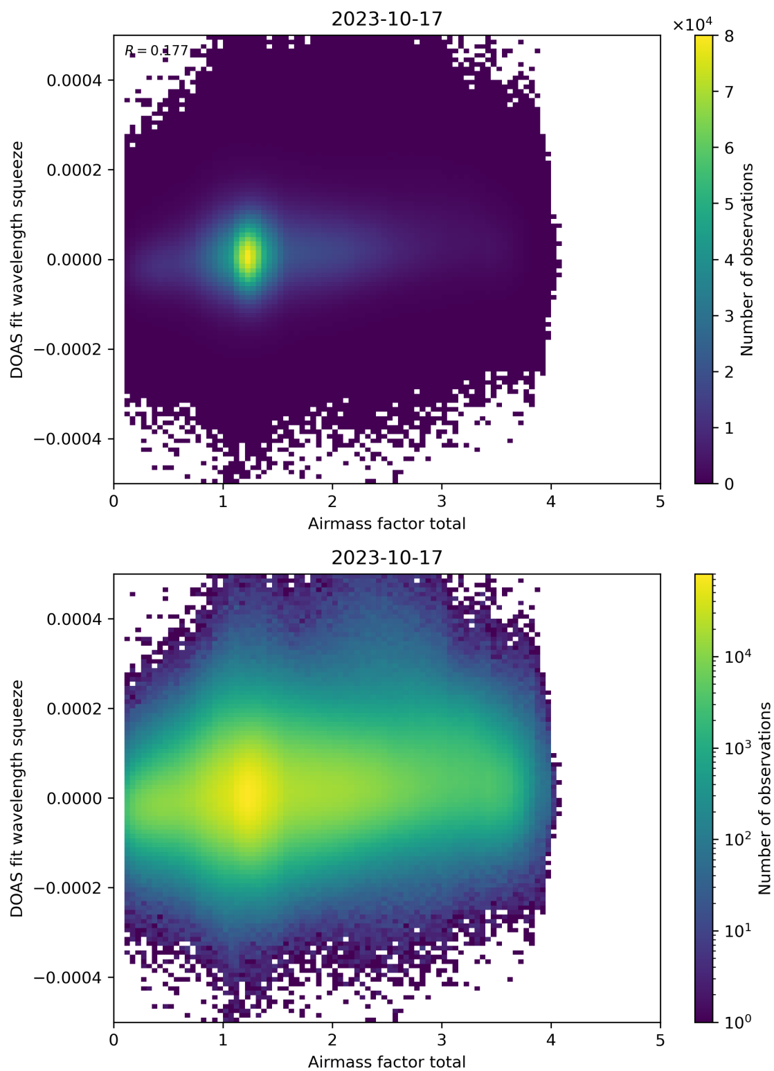
Figure 99: Scatter density plot of “Airmass factor total” against “DOAS fit wavelength squeeze” for 2023-10-17 to 2023-10-18.
