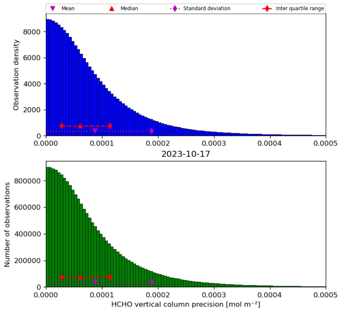
Figure 36: Histogram of “HCHO vertical column precision” for 2023-10-17 to 2023-10-18
