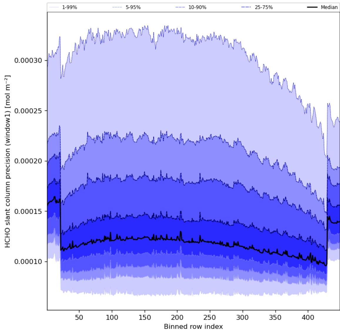
Figure 53: Along track statistics of “HCHO slant column precision (window1)” for 2023-10-17 to 2023-10-18
