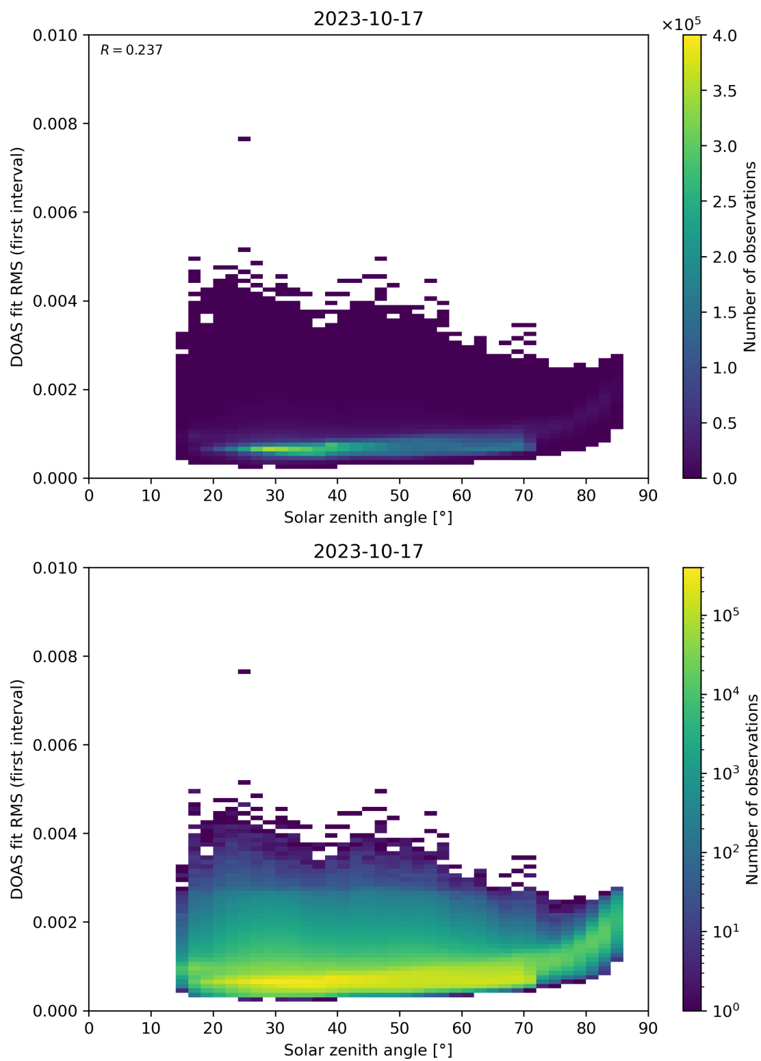
Figure 167: Scatter density plot of “Solar zenith angle” against “DOAS fit RMS (first interval)” for 2023-10-17 to 2023-10-18.
