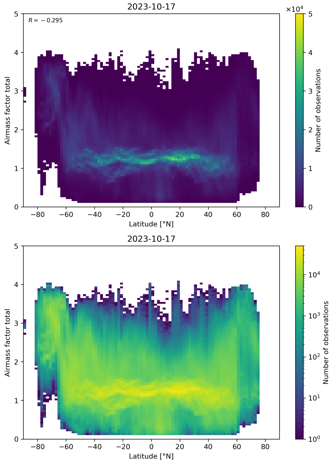
Figure 161: Scatter density plot of “Latitude” against “Airmass factor total” for 2023-10-17 to 2023-10-18.
