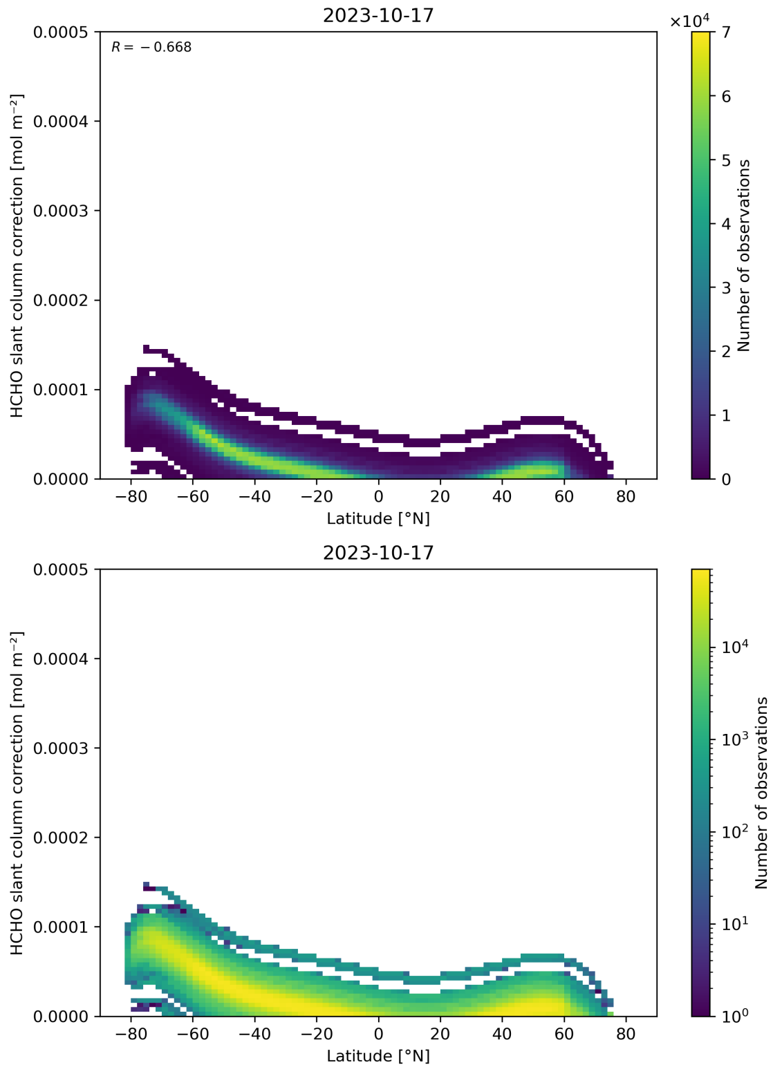
Figure 158: Scatter density plot of “Latitude” against “HCHO slant column correction” for 2023-10-17 to 2023-10-18.
