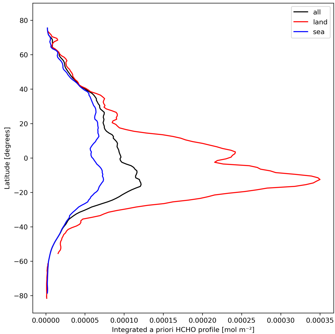
Figure 29: Zonal average of “Integrated a priori HCHO profile” for 2023-10-17 to 2023-10-18.
