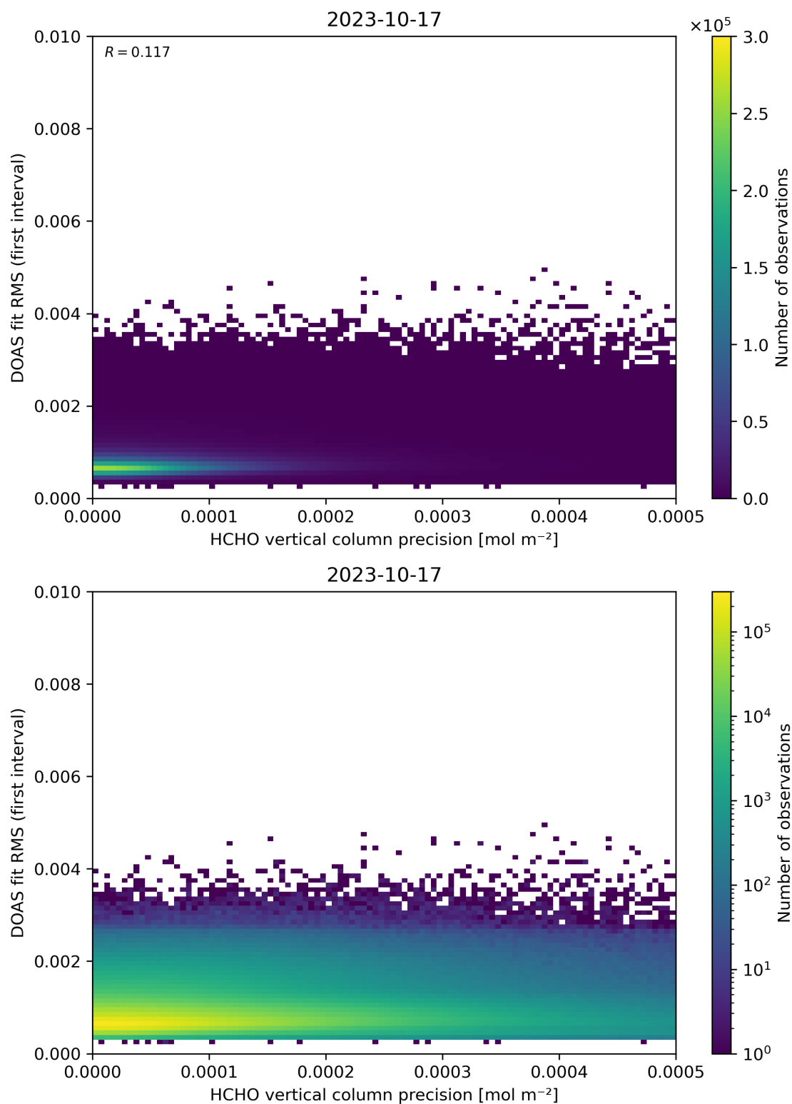
Figure 136: Scatter density plot of “HCHO vertical column precision” against “DOAS fit RMS (first interval)” for 2023-10-17 to 2023-10-18.
