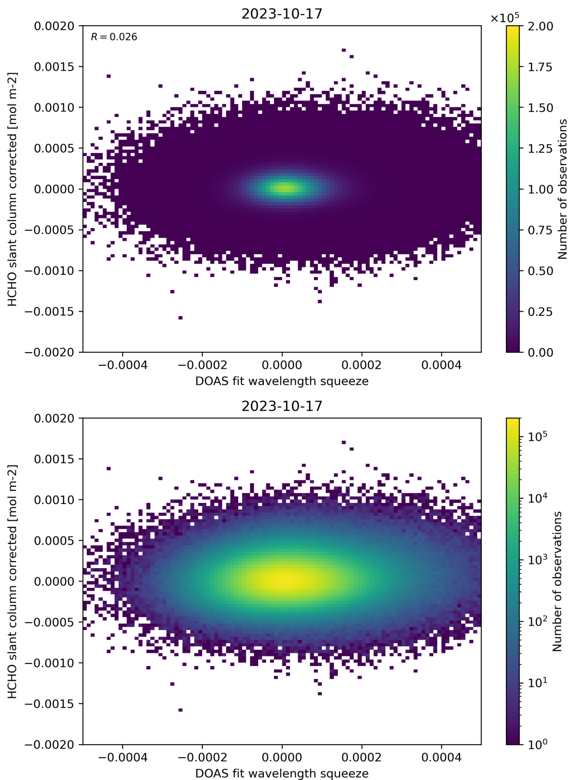
Figure 69: Scatter density plot of “DOAS fit wavelength squeeze” against “HCHO slant column corrected” for 2023-10-17 to 2023-10-18.
