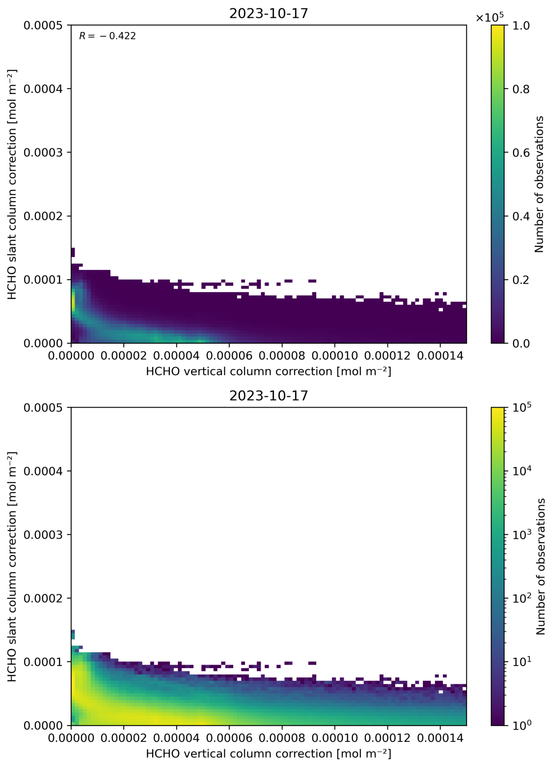
Figure 117: Scatter density plot of “HCHO vertical column correction” against “HCHO slant column correction” for 2023-10-17 to 2023-10-18.
