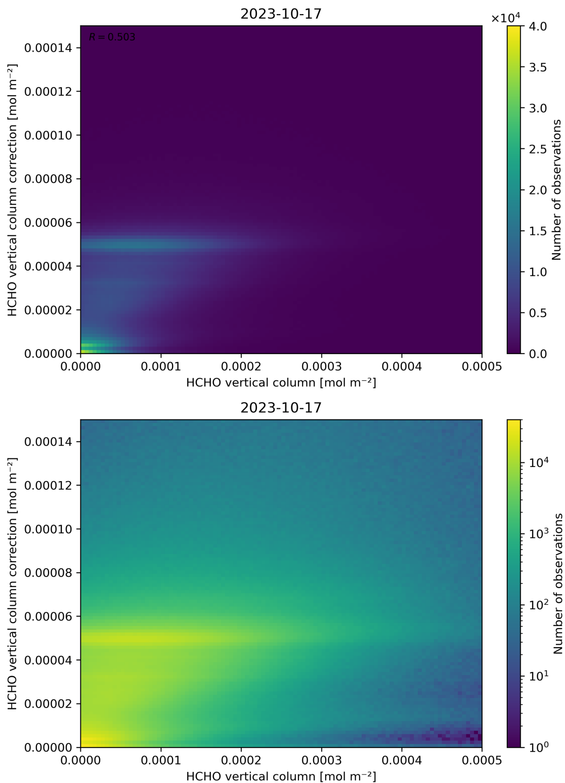
Figure 133: Scatter density plot of “HCHO vertical column” against “HCHO vertical column correction” for 2023-10-17 to 2023-10-18.
