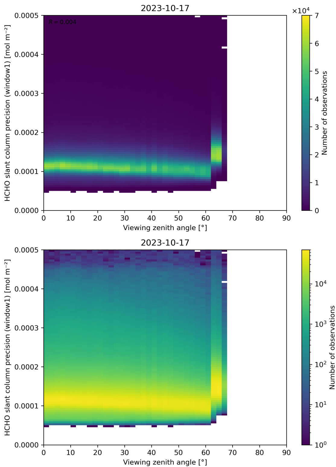
Figure 189: Scatter density plot of “Viewing zenith angle” against “HCHO slant column precision (window1)” for 2023-10-17 to 2023-10-18.
