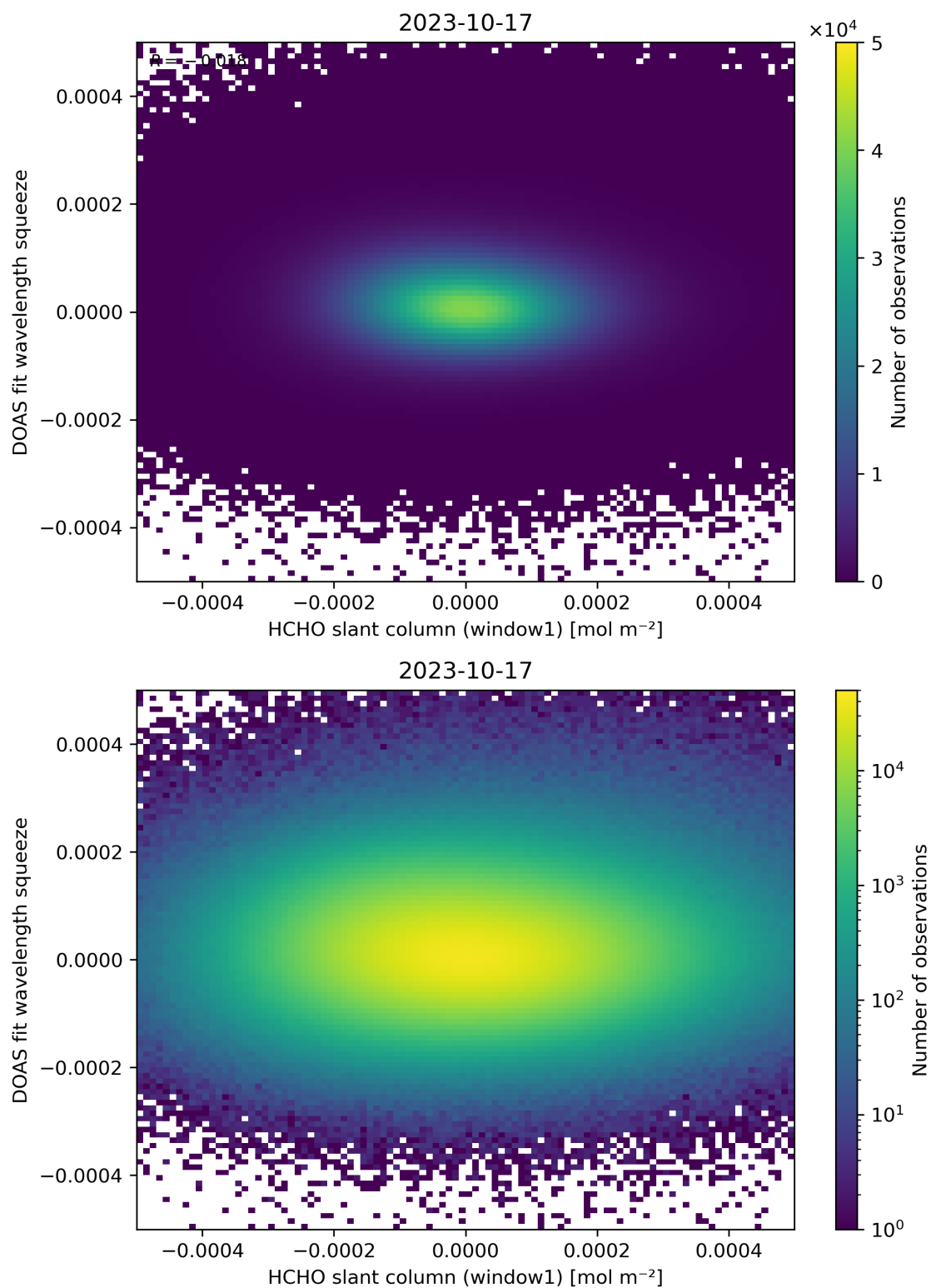
Figure 80: Scatter density plot of “HCHO slant column (window1)” against “DOAS fit wavelength squeeze” for 2023-10-17 to 2023-10-18.
