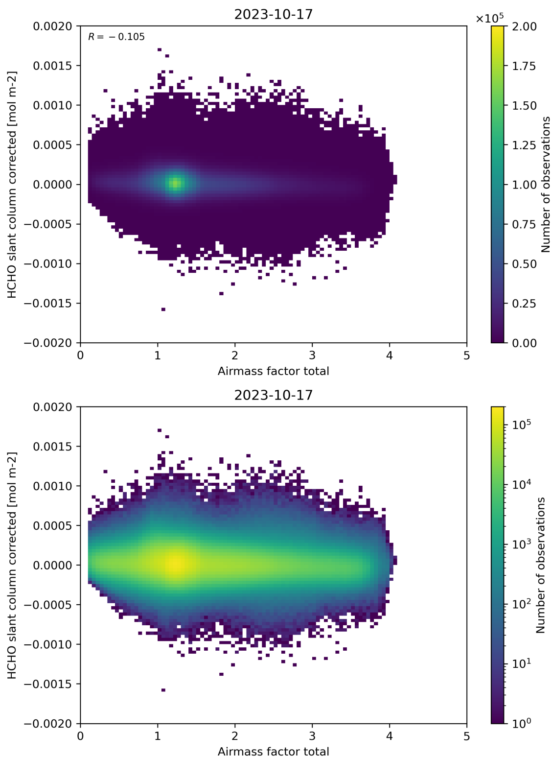
Figure 101: Scatter density plot of “Airmass factor total” against “HCHO slant column corrected” for 2023-10-17 to 2023-10-18.
