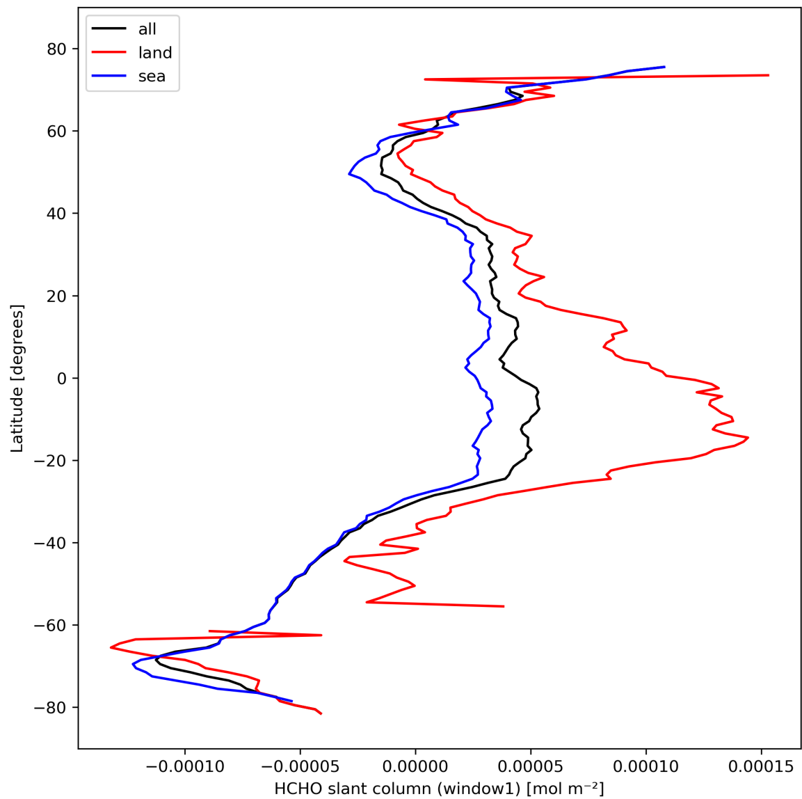
Figure 24: Zonal average of “HCHO slant column (window1)” for 2023-10-17 to 2023-10-18.
