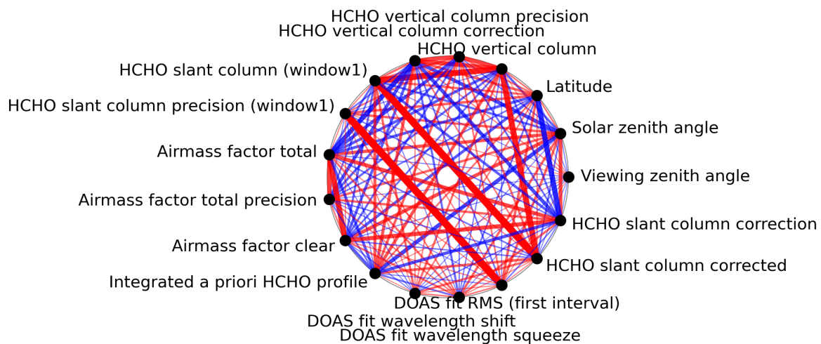
Figure 1: Map of correlation graph for 2023-10-17 to 2023-10-18.
