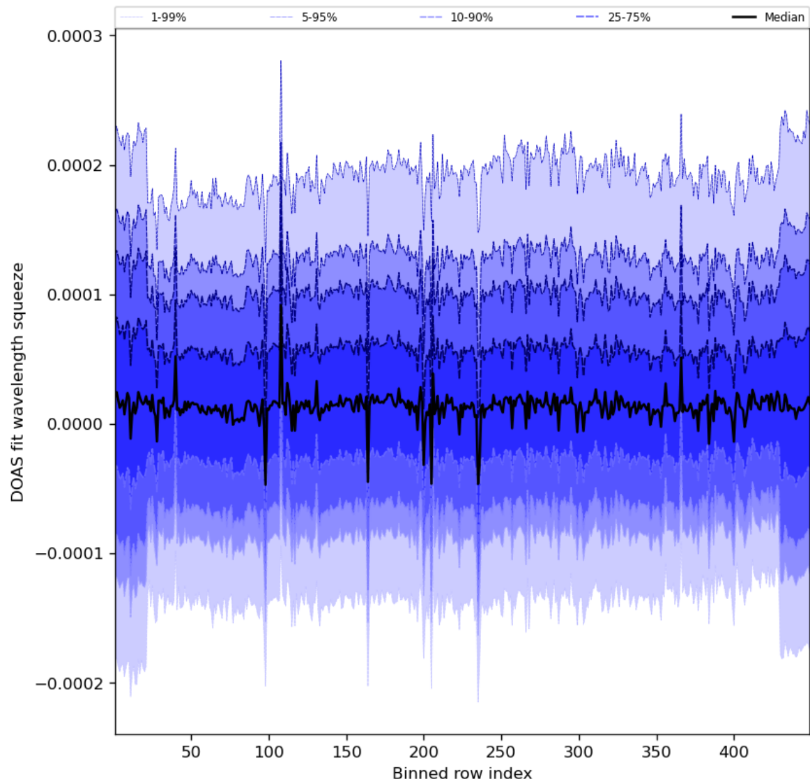
Figure 59: Along track statistics of “DOAS fit wavelength squeeze” for 2023-10-17 to 2023-10-18
