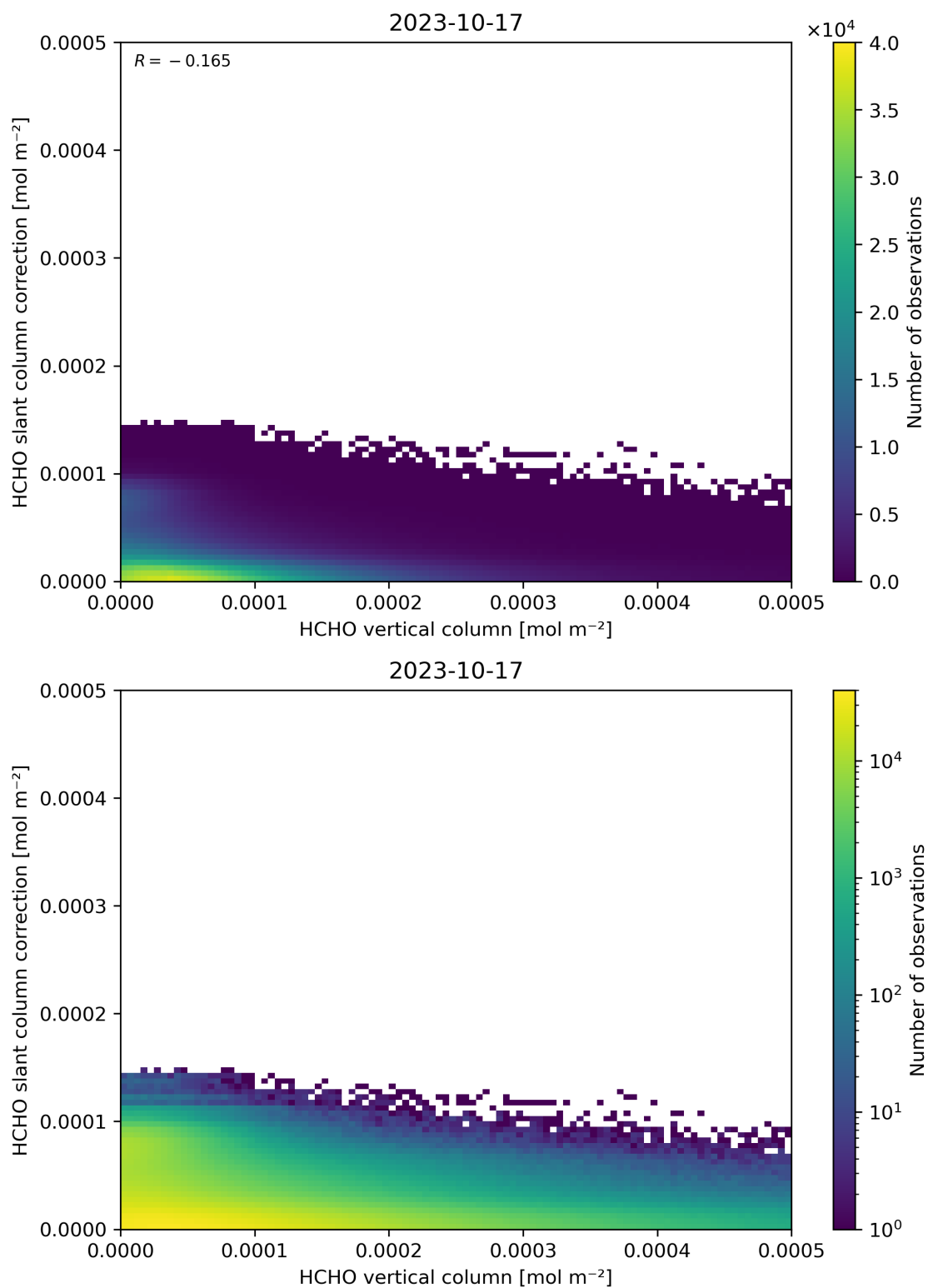
Figure 128: Scatter density plot of “HCHO vertical column” against “HCHO slant column correction” for 2023-10-17 to 2023-10-18.
