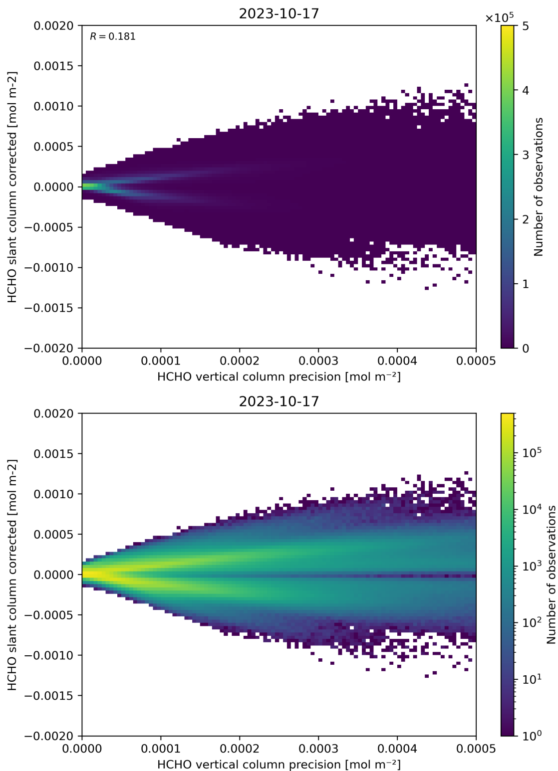
Figure 140: Scatter density plot of “HCHO vertical column precision” against “HCHO slant column corrected” for 2023-10-17 to 2023-10-18.
