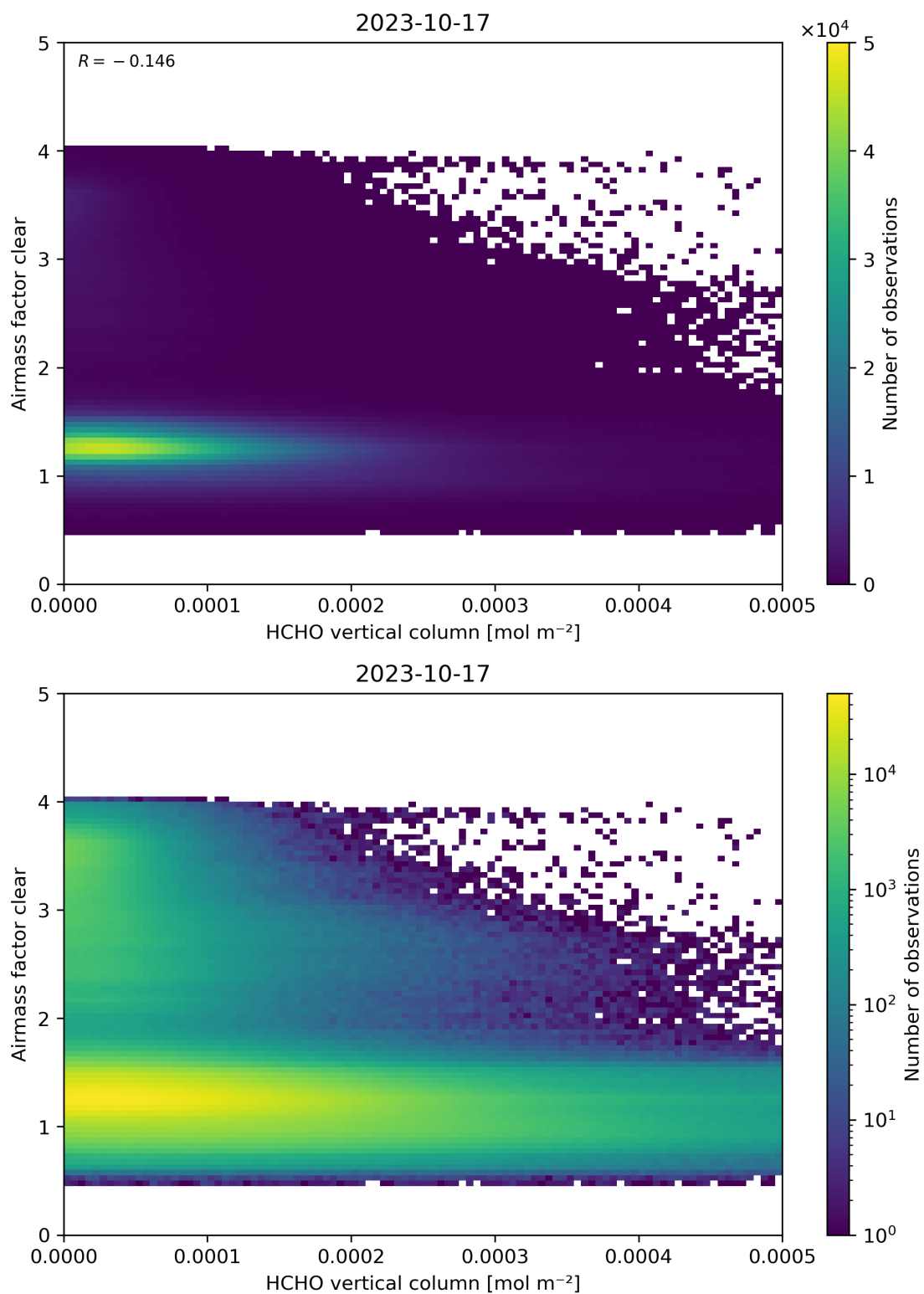
Figure 126: Scatter density plot of “HCHO vertical column” against “Airmass factor clear” for 2023-10-17 to 2023-10-18.
