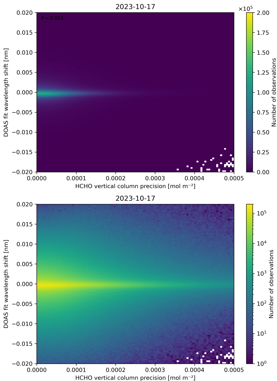
Figure 137: Scatter density plot of “HCHO vertical column precision” against “DOAS fit wavelength shift” for 2023-10-17 to 2023-10-18.
