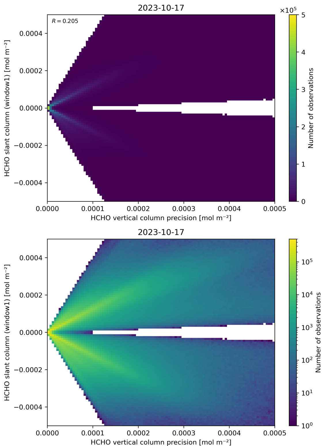
Figure 142: Scatter density plot of “HCHO vertical column precision” against “HCHO slant column (window1)” for 2023-10-17 to 2023-10-18.
