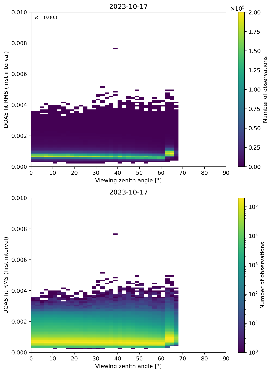
Figure 182: Scatter density plot of “Viewing zenith angle” against “DOAS fit RMS (first interval)” for 2023-10-17 to 2023-10-18.
