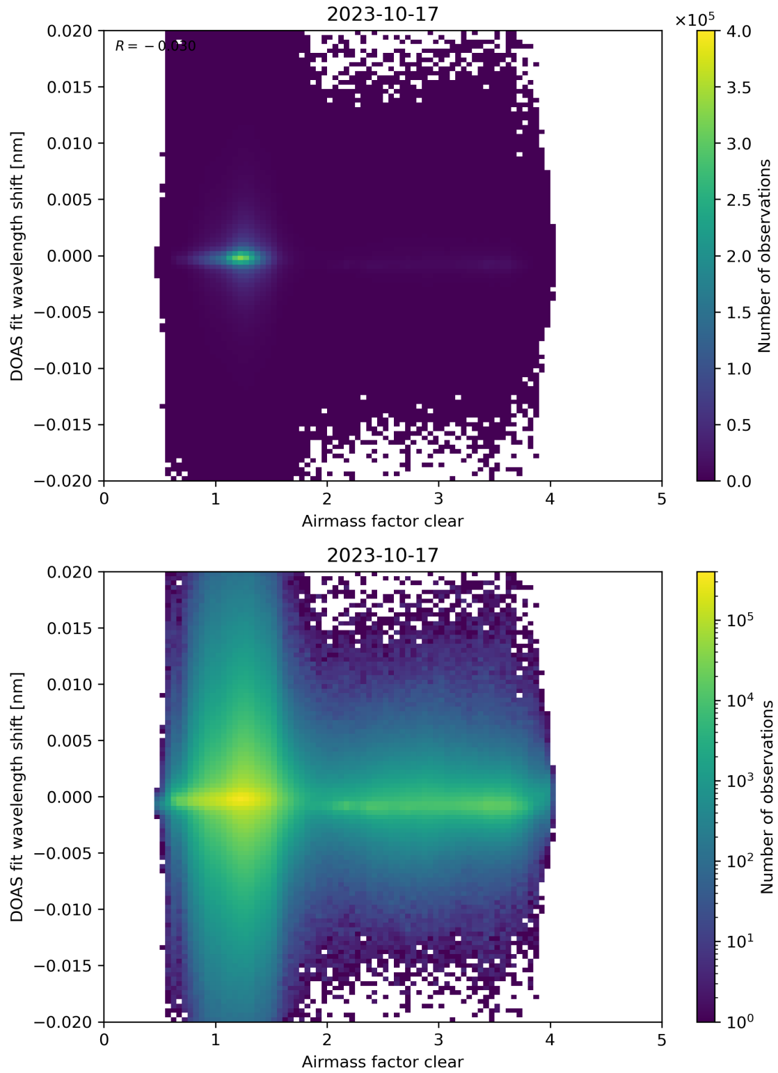
Figure 72: Scatter density plot of “Airmass factor clear” against “DOAS fit wavelength shift” for 2023-10-17 to 2023-10-18.
