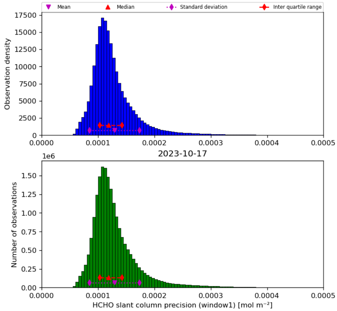
Figure 39: Histogram of “HCHO slant column precision (window1)” for 2023-10-17 to 2023-10-18
