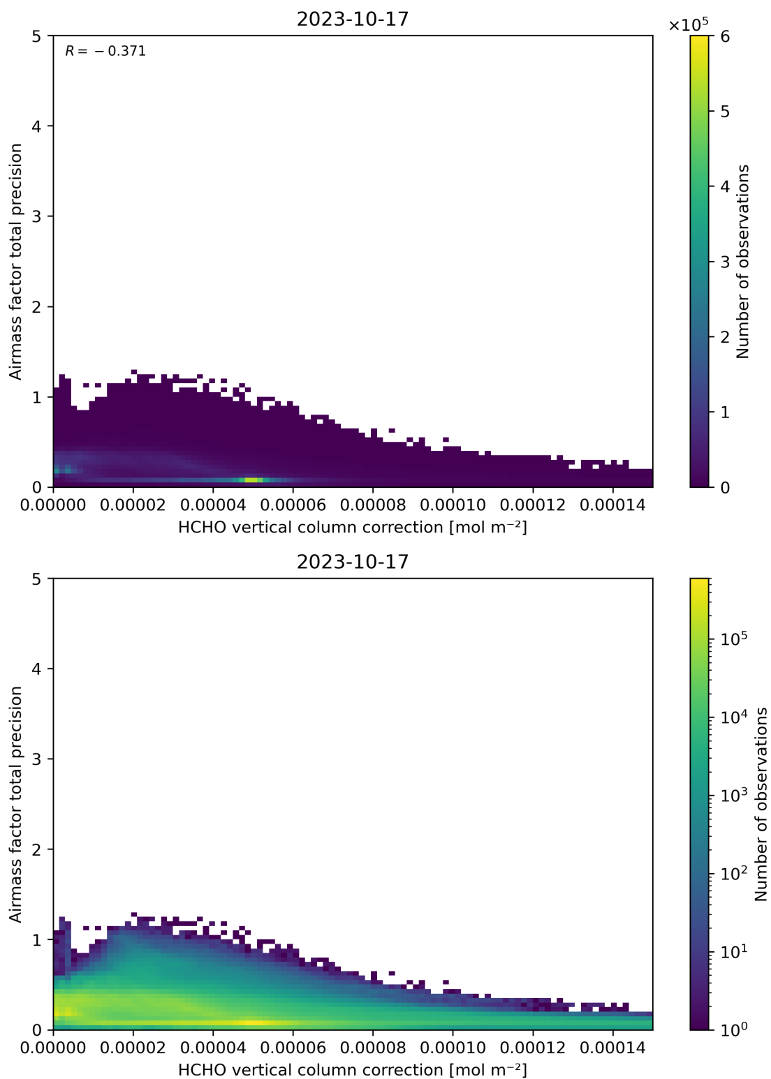
Figure 121: Scatter density plot of “HCHO vertical column correction” against “Airmass factor total precision” for 2023-10-17 to 2023-10-18.
