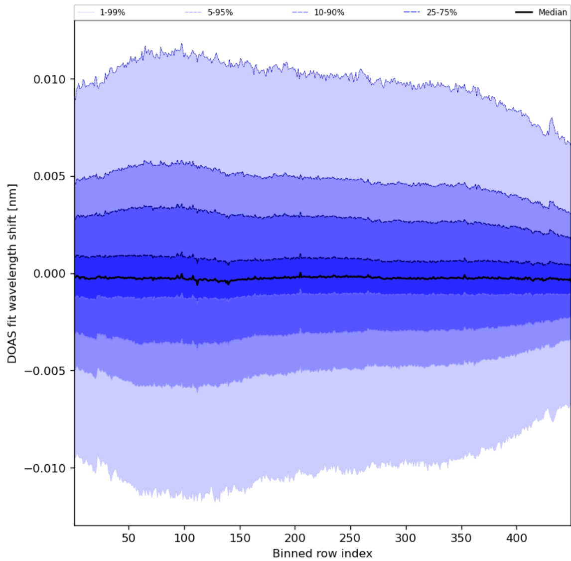
Figure 58: Along track statistics of “DOAS fit wavelength shift” for 2023-10-17 to 2023-10-18
