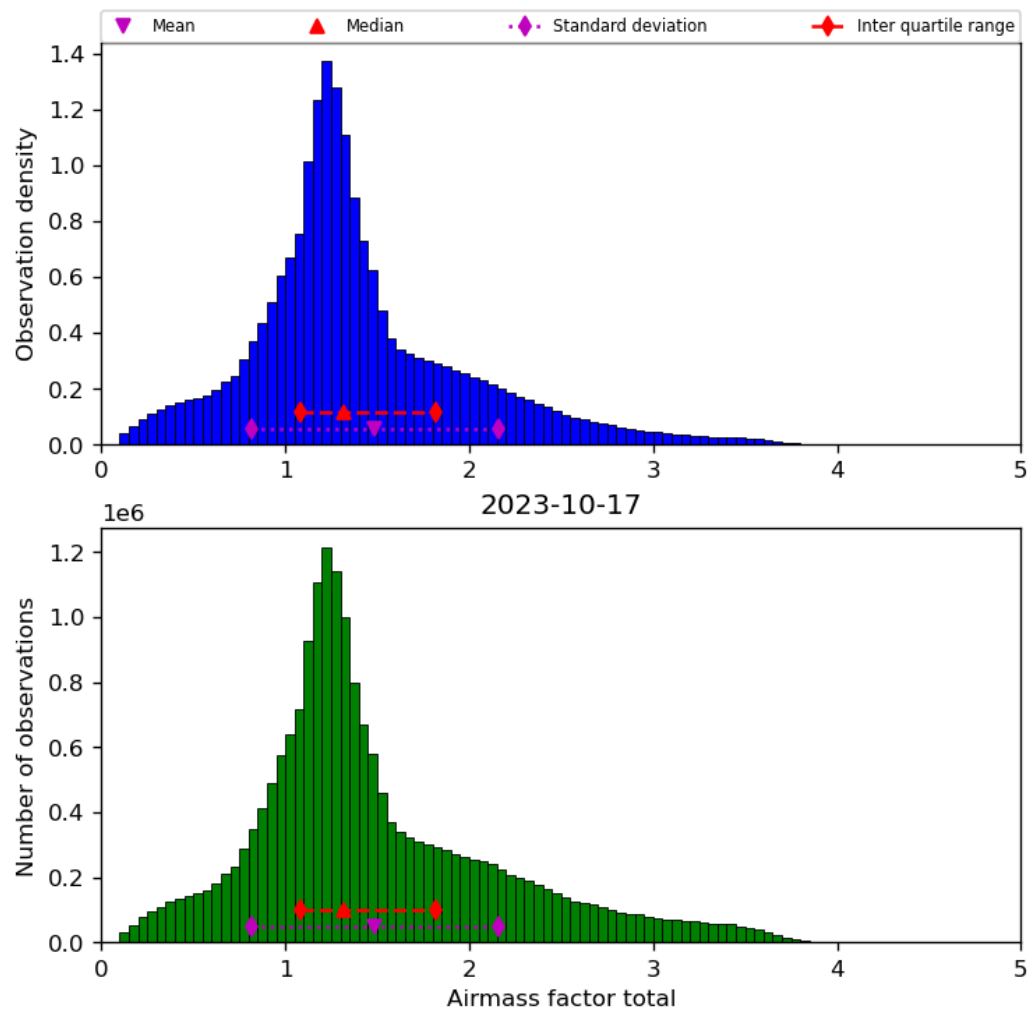
Figure 40: Histogram of “Airmass factor total” for 2023-10-17 to 2023-10-18
