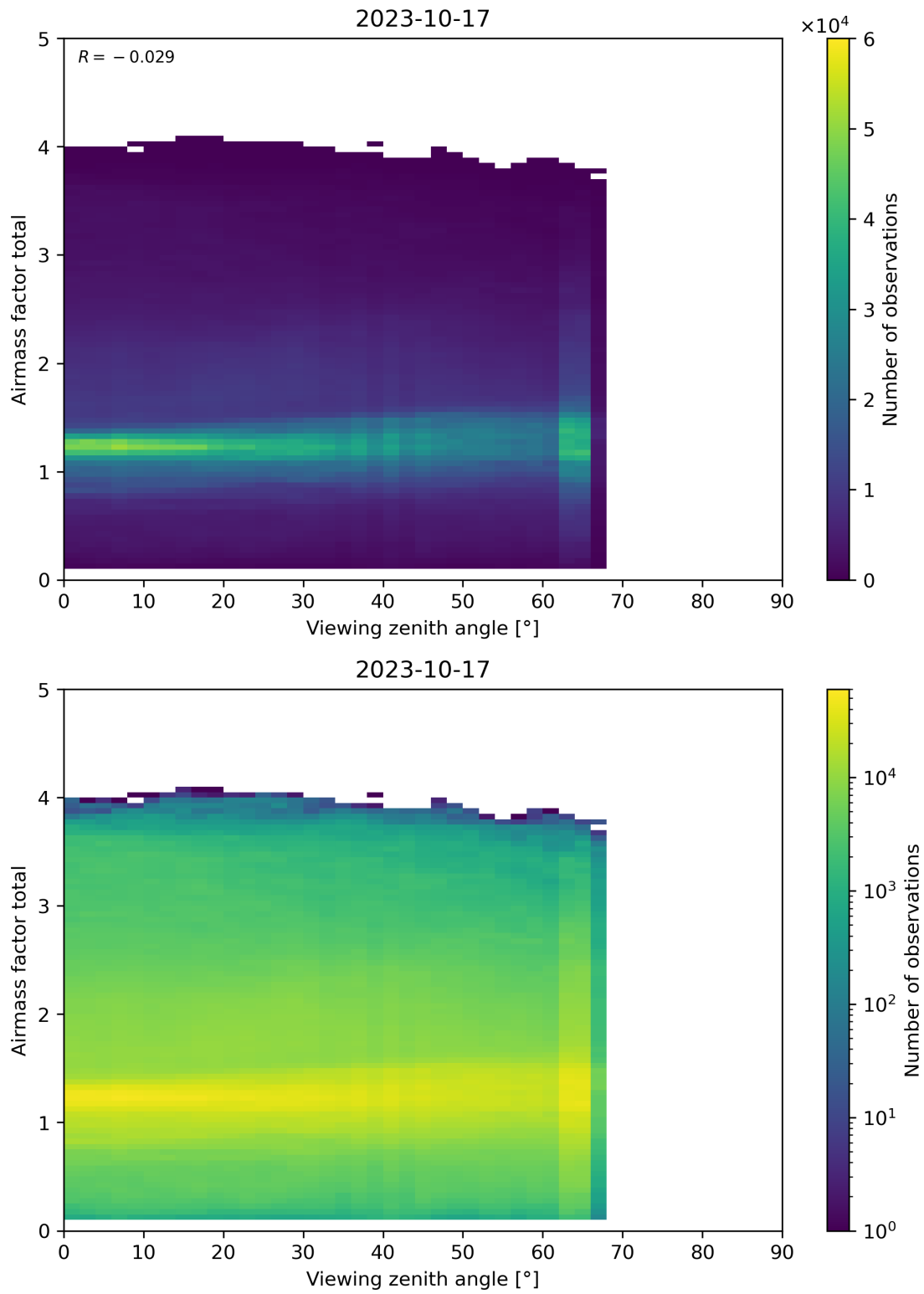
Figure 190: Scatter density plot of “Viewing zenith angle” against “Airmass factor total” for 2023-10-17 to 2023-10-18.
