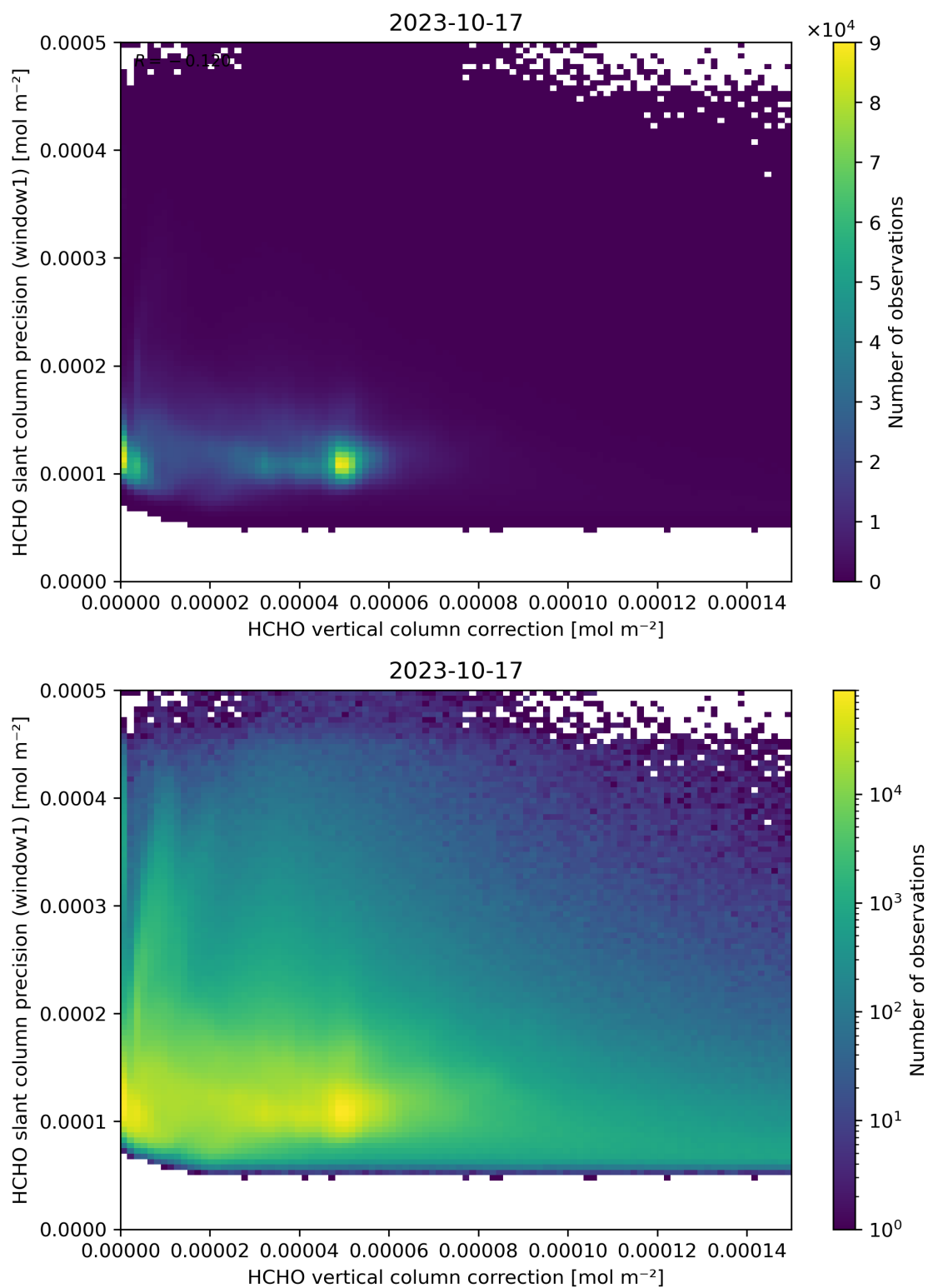
Figure 119: Scatter density plot of “HCHO vertical column correction” against “HCHO slant column precision (window1)” for 2023-10-17 to 2023-10-18.
