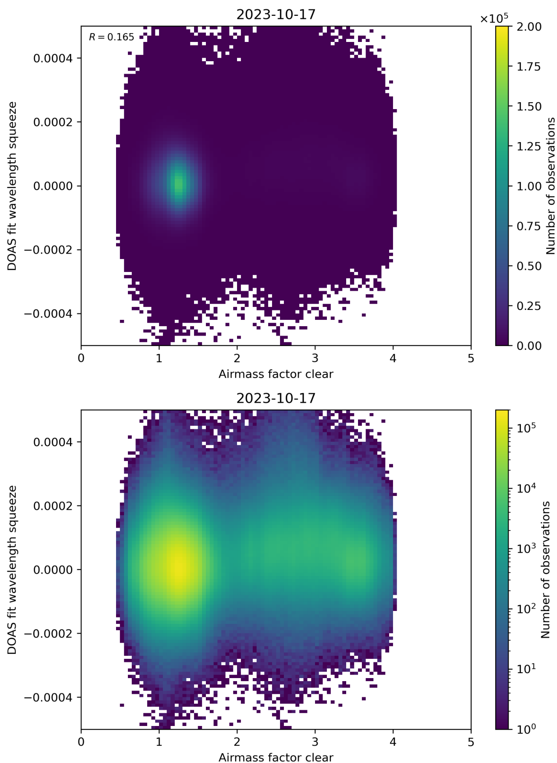
Figure 73: Scatter density plot of “Airmass factor clear” against “DOAS fit wavelength squeeze” for 2023-10-17 to 2023-10-18.
