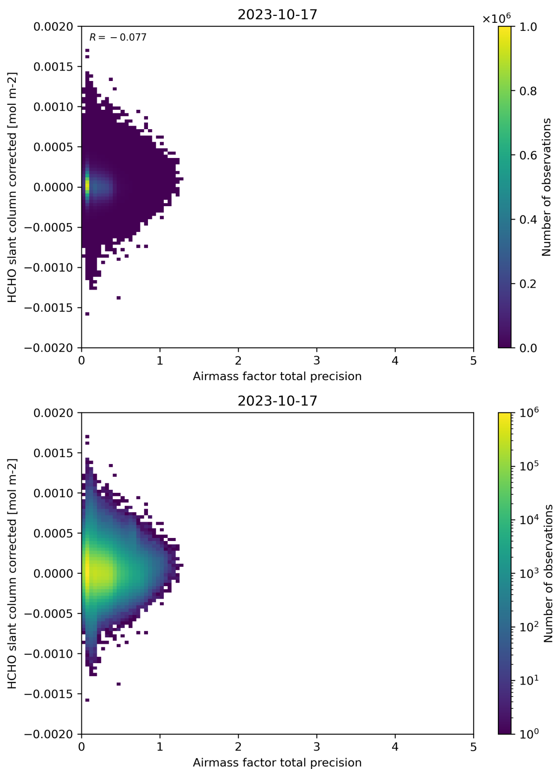
Figure 109: Scatter density plot of “Airmass factor total precision” against “HCHO slant column corrected” for 2023-10-17 to 2023-10-18.
