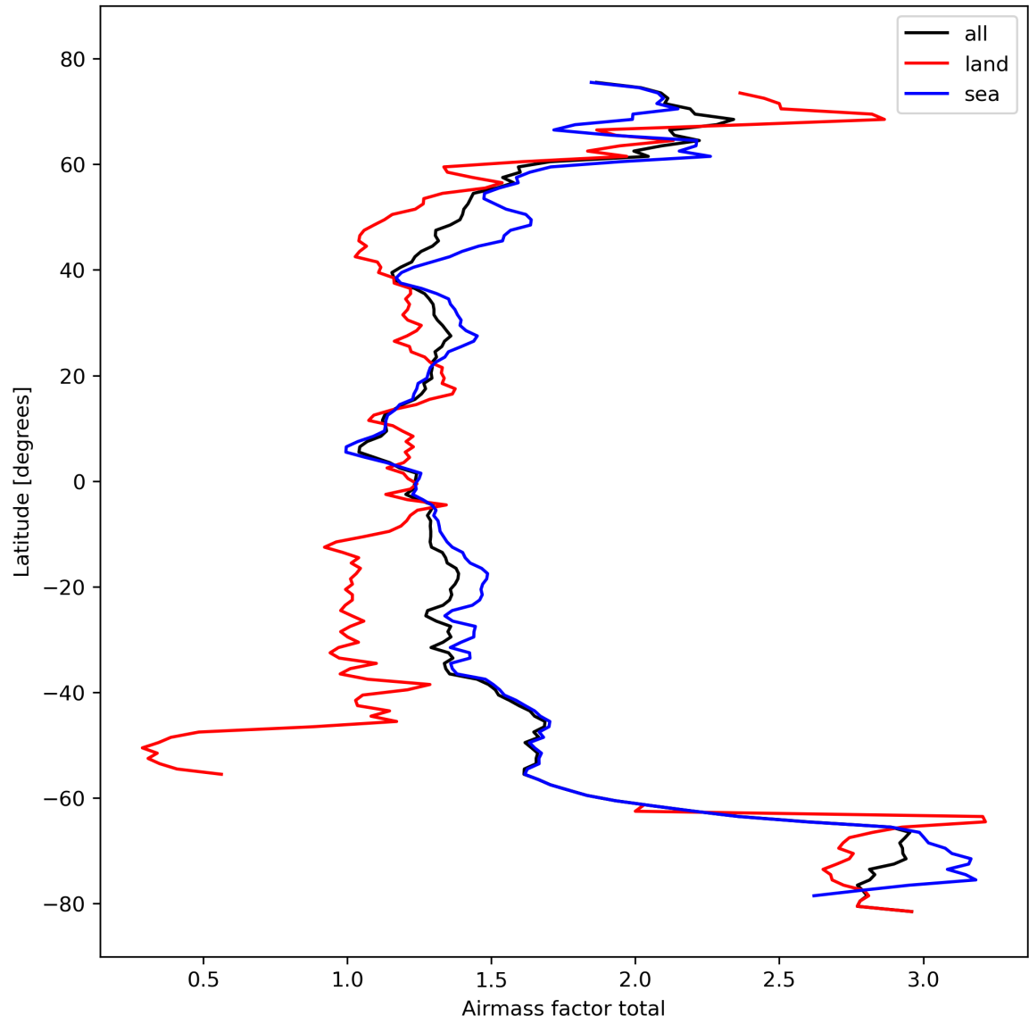
Figure 26: Zonal average of “Airmass factor total” for 2023-10-17 to 2023-10-18.
