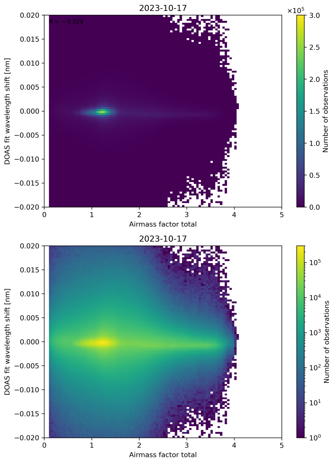
Figure 98: Scatter density plot of “Airmass factor total” against “DOAS fit wavelength shift” for 2023-10-17 to 2023-10-18.
