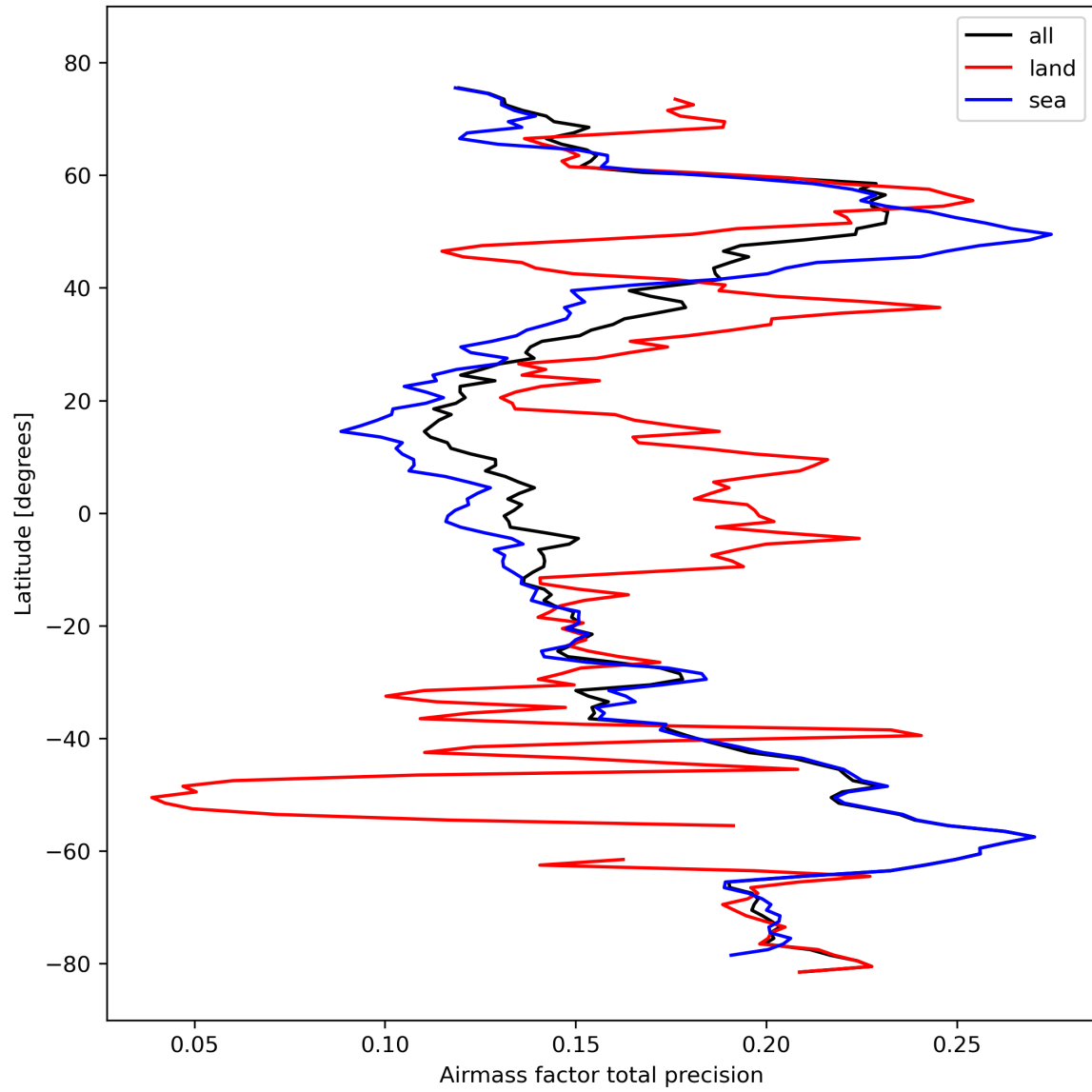
Figure 27: Zonal average of “Airmass factor total precision” for 2023-10-17 to 2023-10-18.
