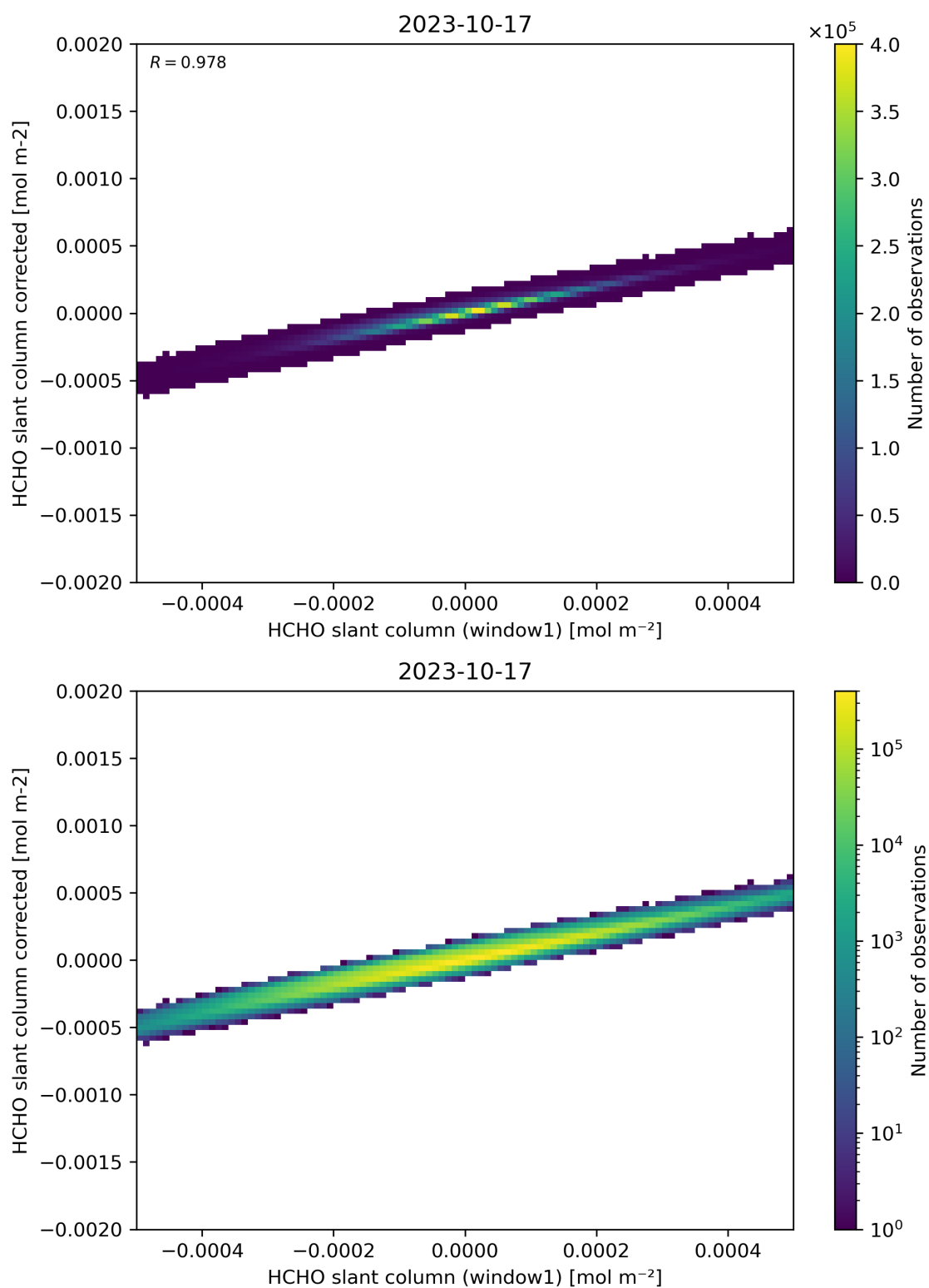
Figure 82: Scatter density plot of “HCHO slant column (window1)” against “HCHO slant column corrected” for 2023-10-17 to 2023-10-18.
