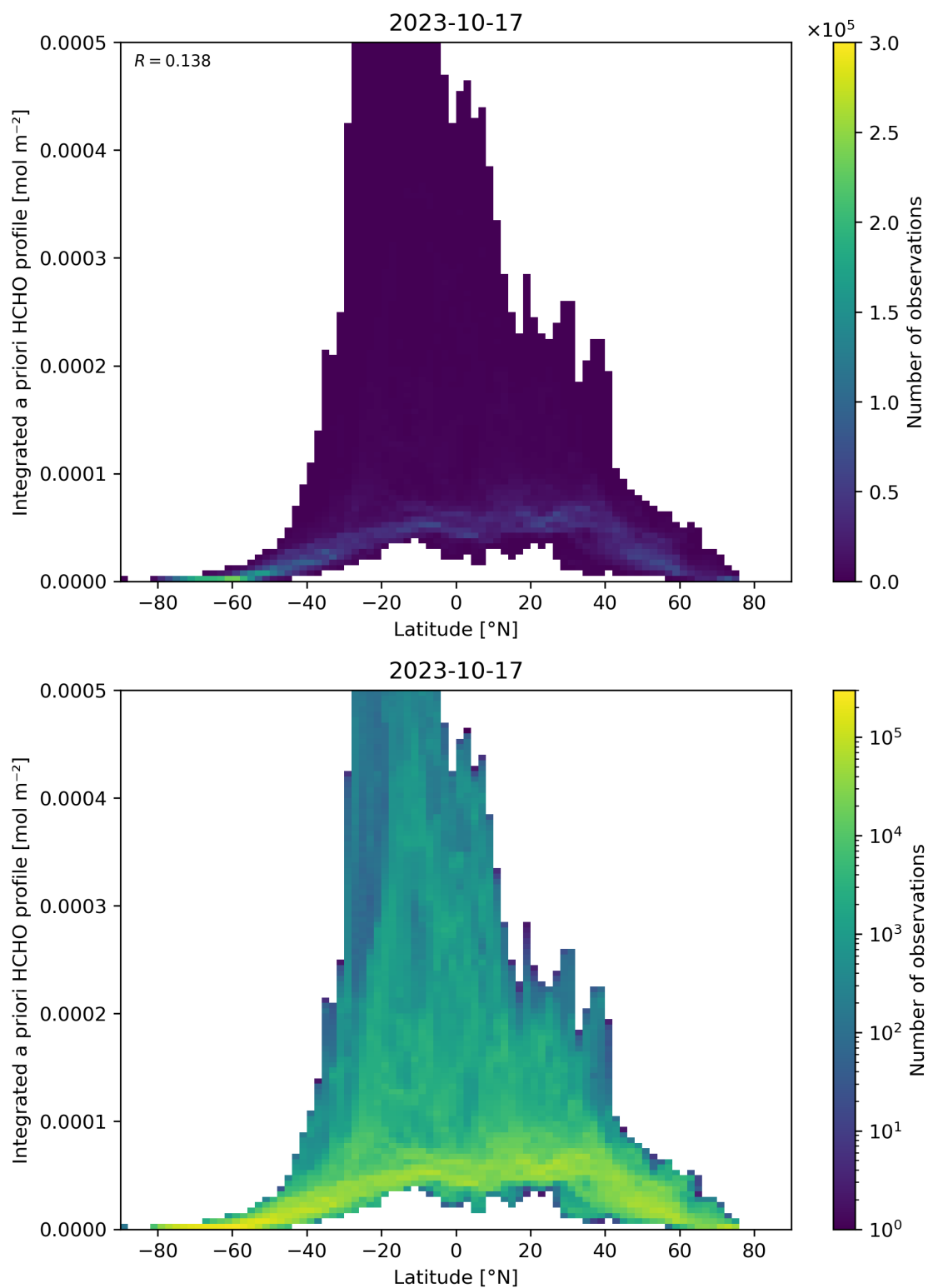
Figure 166: Scatter density plot of “Latitude” against “Integrated a priori HCHO profile” for 2023-10-17 to 2023-10-18.
