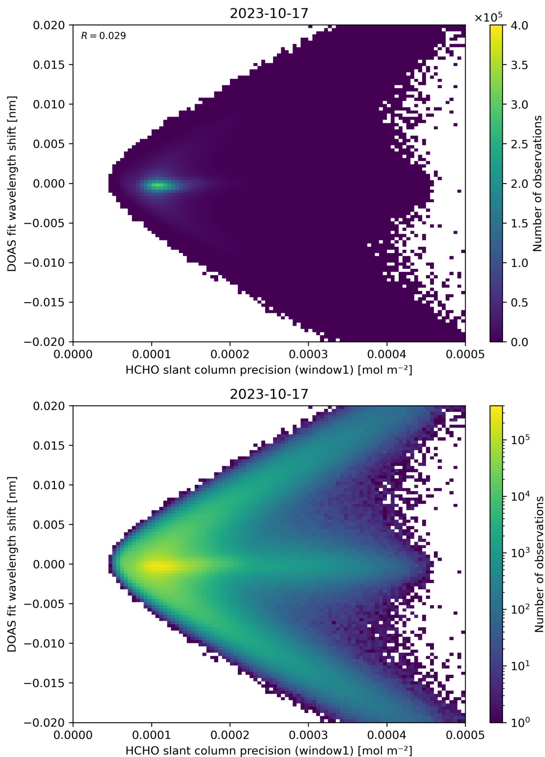
Figure 89: Scatter density plot of “HCHO slant column precision (window1)” against “DOAS fit wavelength shift” for 2023-10-17 to 2023-10-18.
