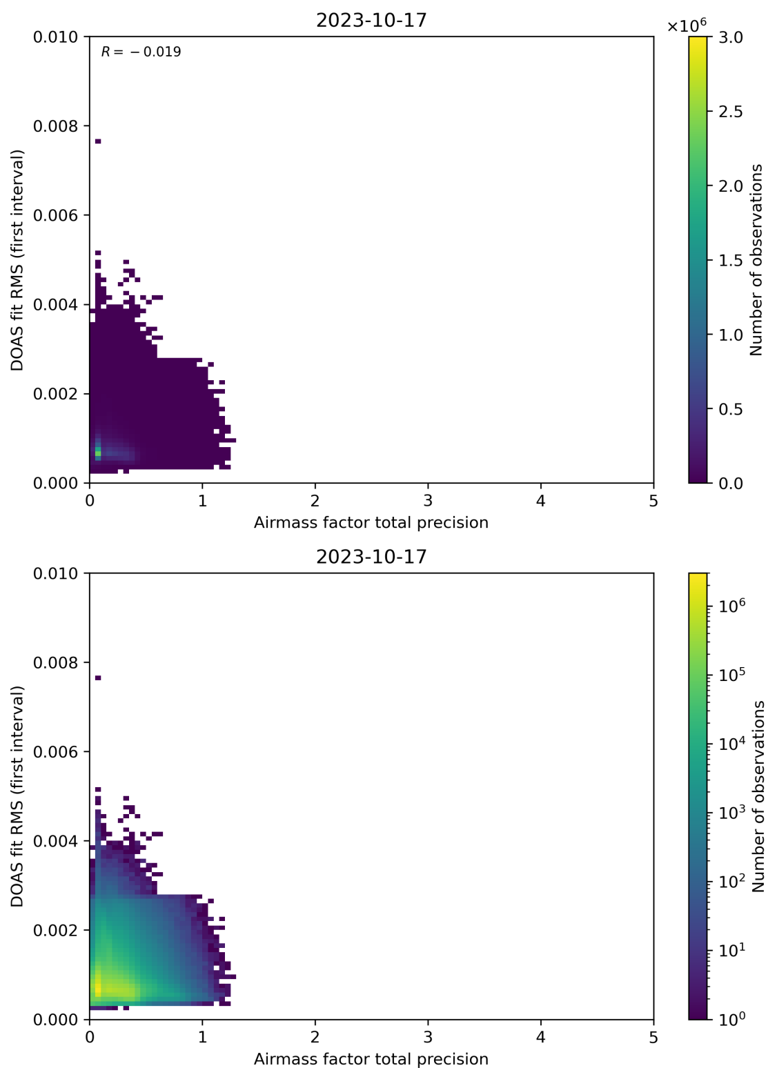
Figure 105: Scatter density plot of “Airmass factor total precision” against “DOAS fit RMS (first interval)” for 2023-10-17 to 2023-10-18.
