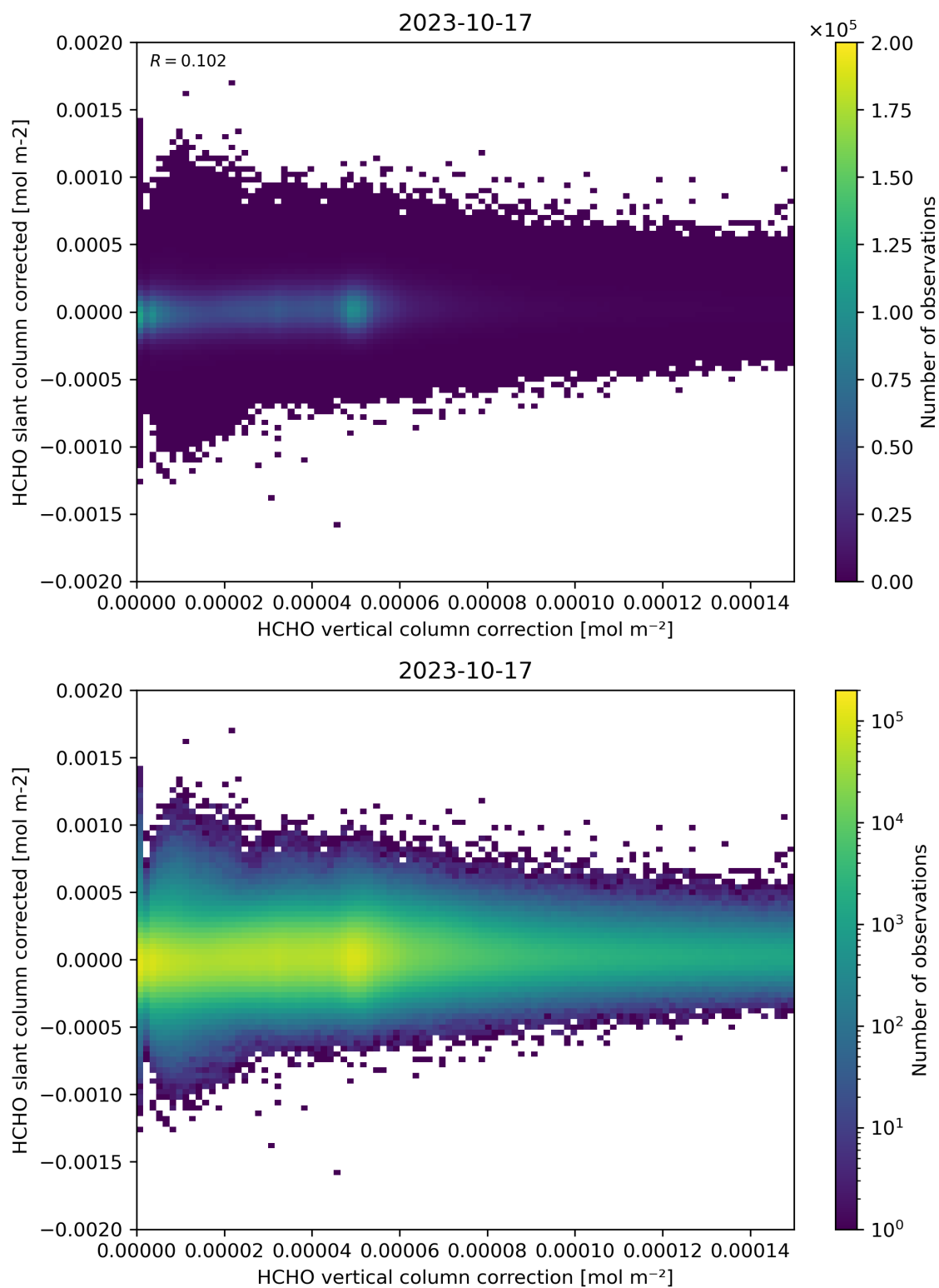
Figure 116: Scatter density plot of “HCHO vertical column correction” against “HCHO slant column corrected” for 2023-10-17 to 2023-10-18.
