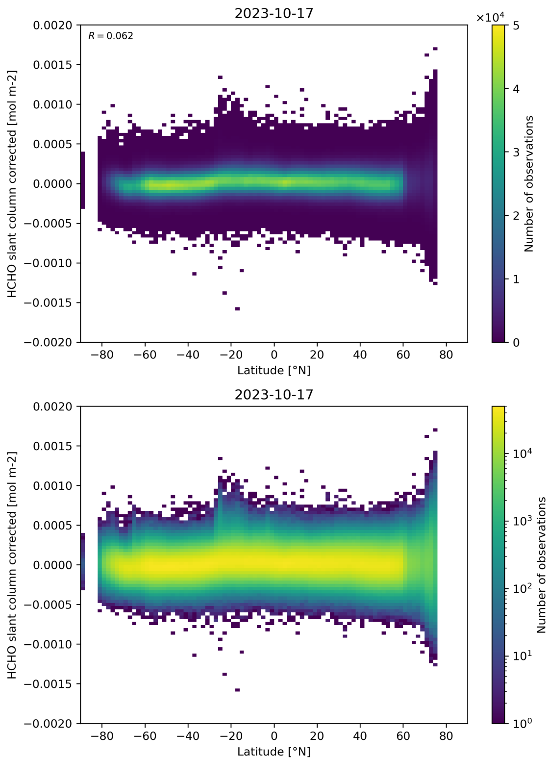
Figure 157: Scatter density plot of “Latitude” against “HCHO slant column corrected” for 2023-10-17 to 2023-10-18.
