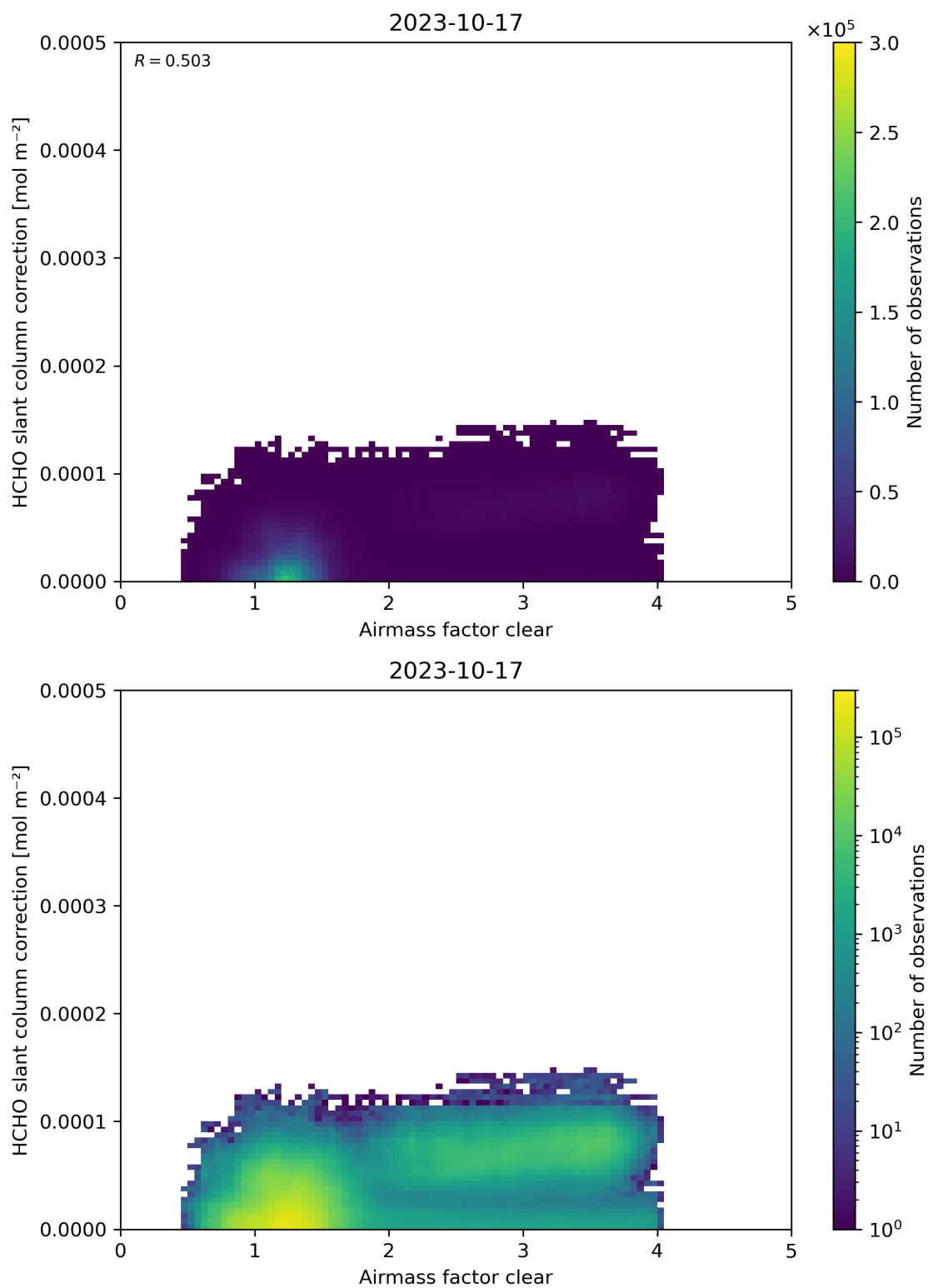
Figure 75: Scatter density plot of “Airmass factor clear” against “HCHO slant column correction” for 2023-10-17 to 2023-10-18.
