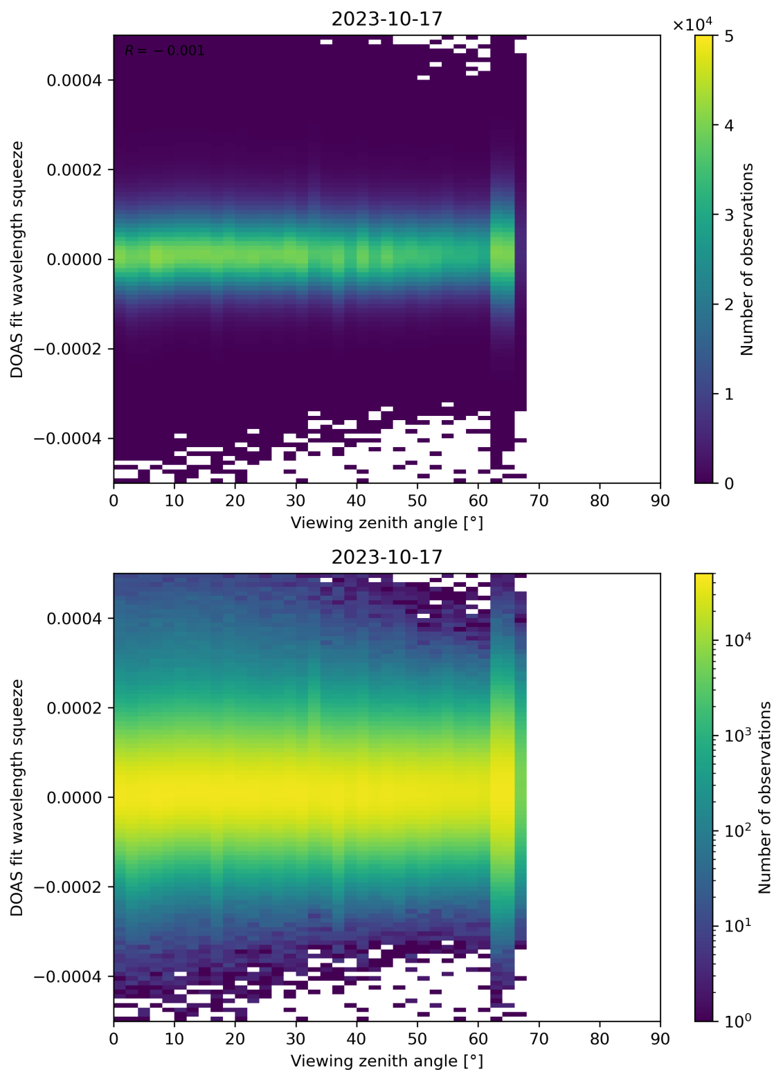
Figure 184: Scatter density plot of “Viewing zenith angle” against “DOAS fit wavelength squeeze” for 2023-10-17 to 2023-10-18.
