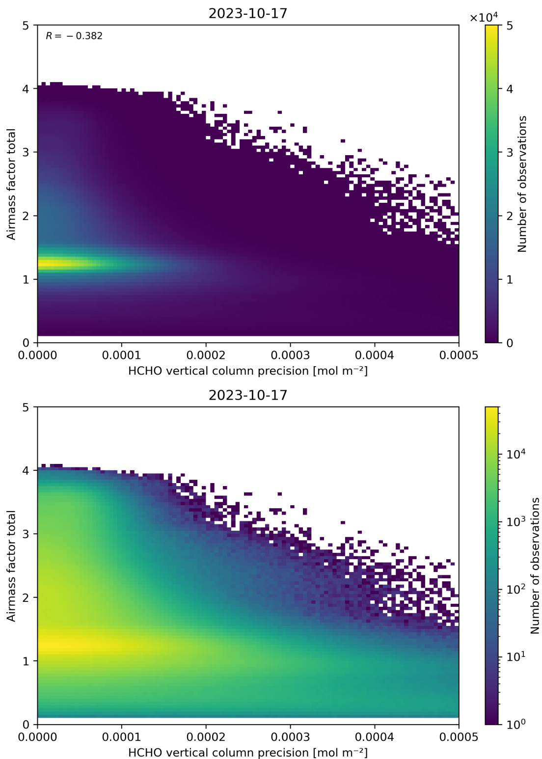
Figure 144: Scatter density plot of “HCHO vertical column precision” against “Airmass factor total” for 2023-10-17 to 2023-10-18.
