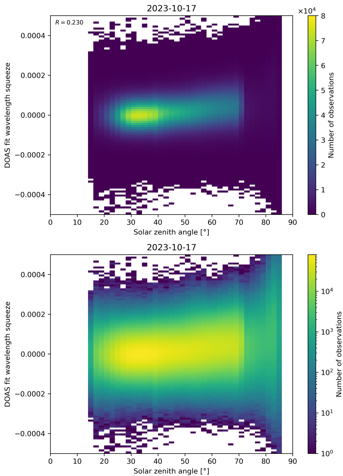
Figure 169: Scatter density plot of “Solar zenith angle” against “DOAS fit wavelength squeeze” for 2023-10-17 to 2023-10-18.
