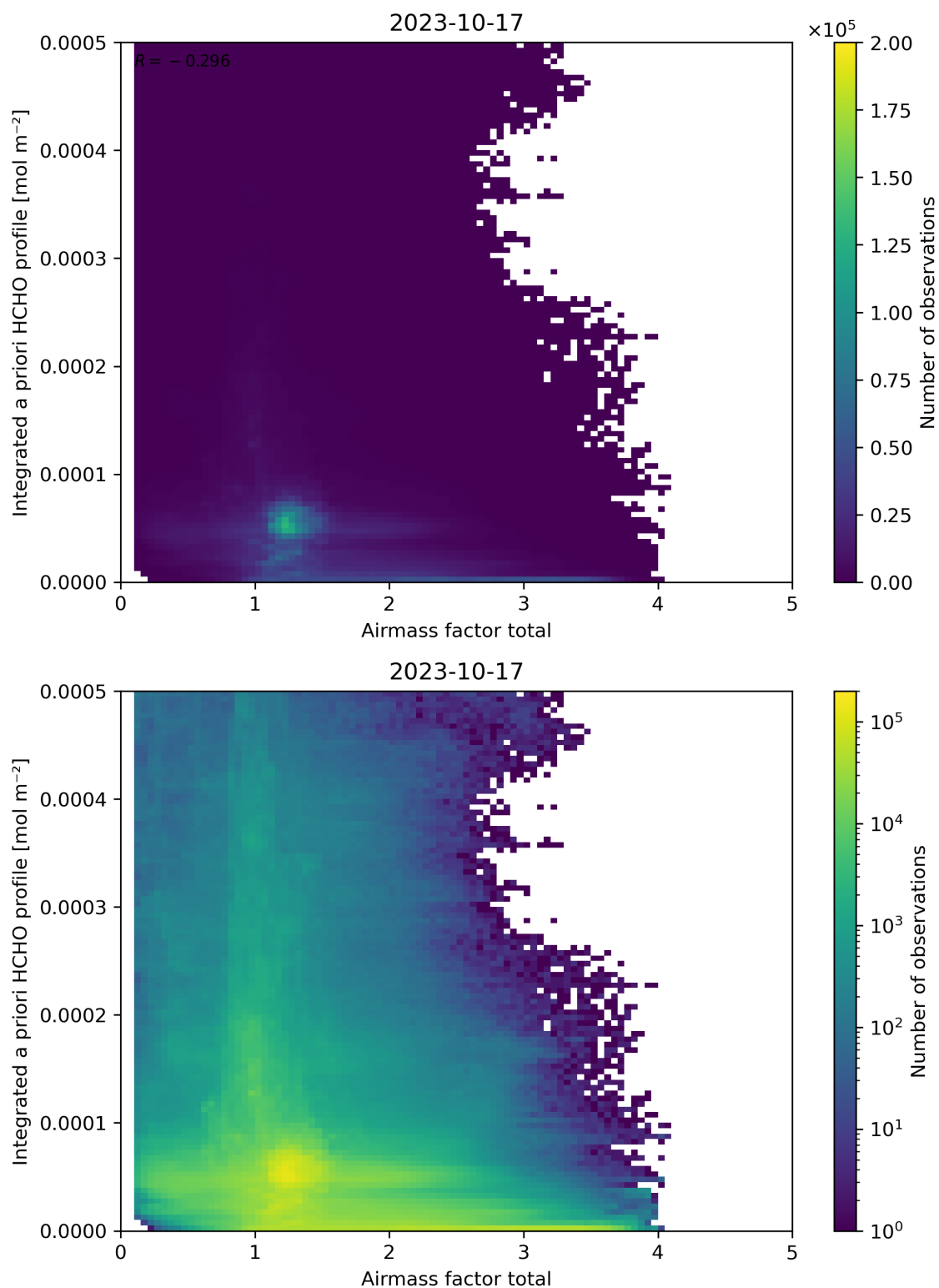
Figure 104: Scatter density plot of “Airmass factor total” against “Integrated a priori HCHO profile” for 2023-10-17 to 2023-10-18.
