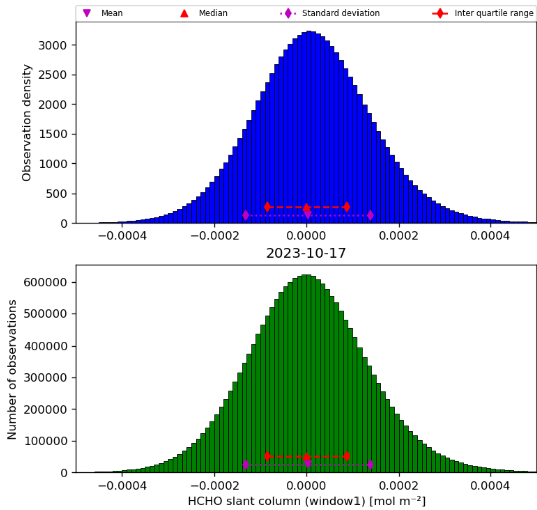
Figure 38: Histogram of “HCHO slant column (window1)” for 2023-10-17 to 2023-10-18
