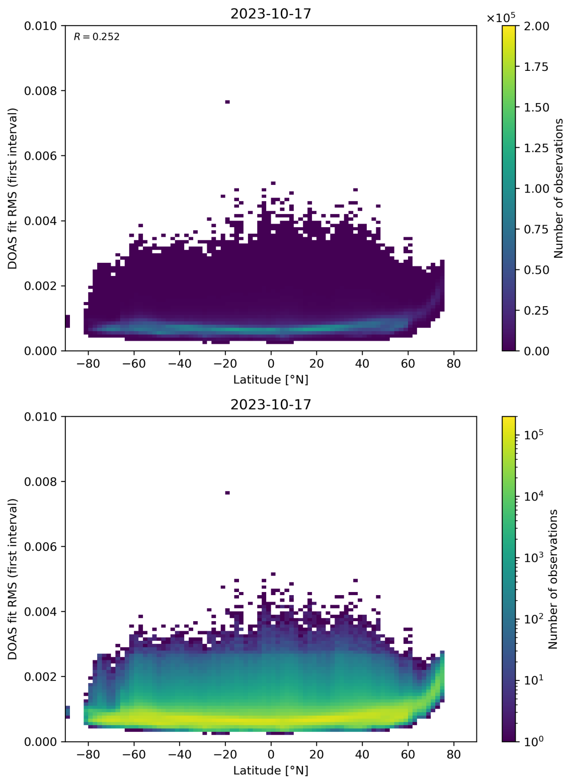
Figure 153: Scatter density plot of “Latitude” against “DOAS fit RMS (first interval)” for 2023-10-17 to 2023-10-18.
