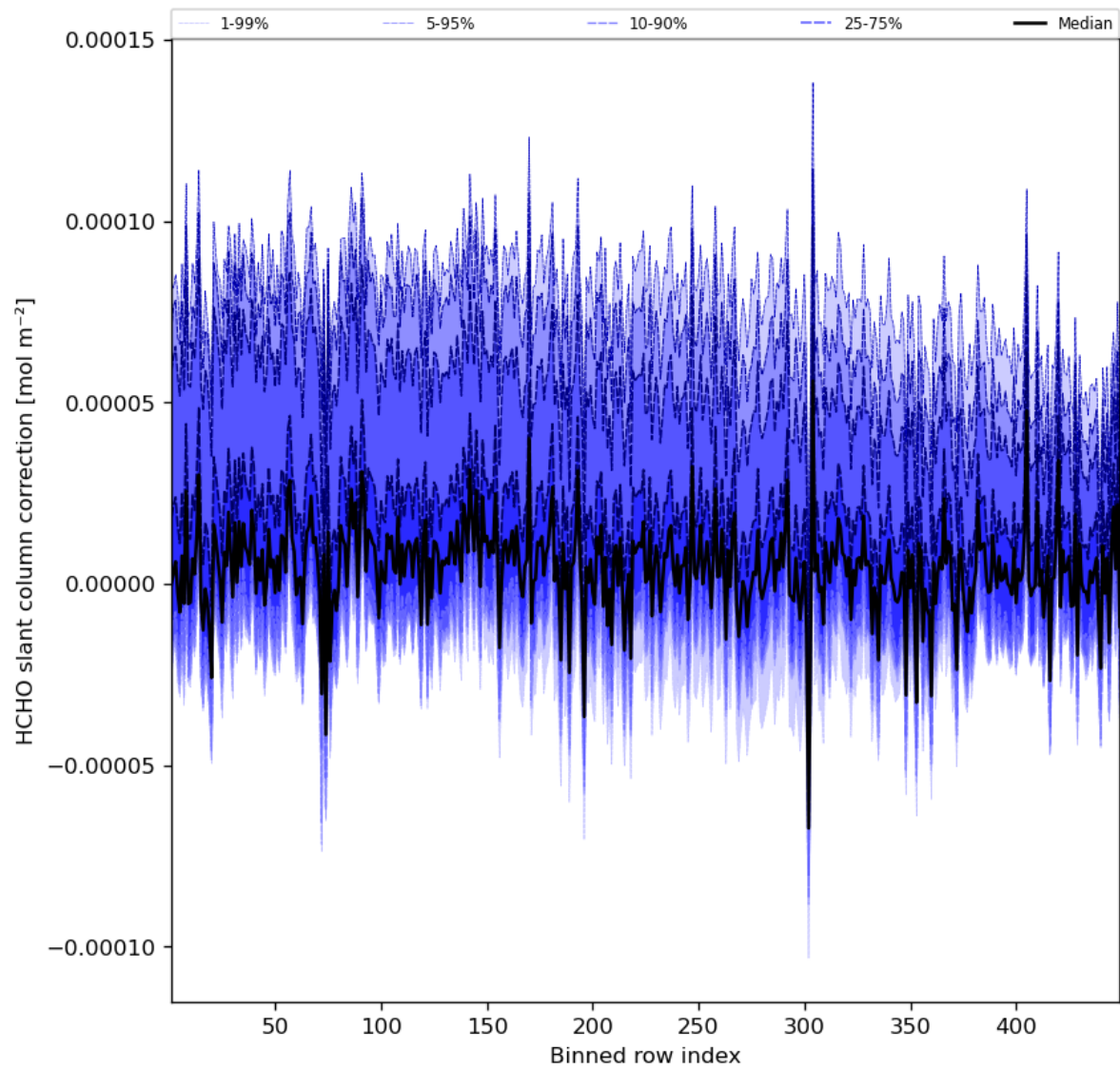
Figure 61: Along track statistics of “HCHO slant column correction” for 2023-10-17 to 2023-10-18
