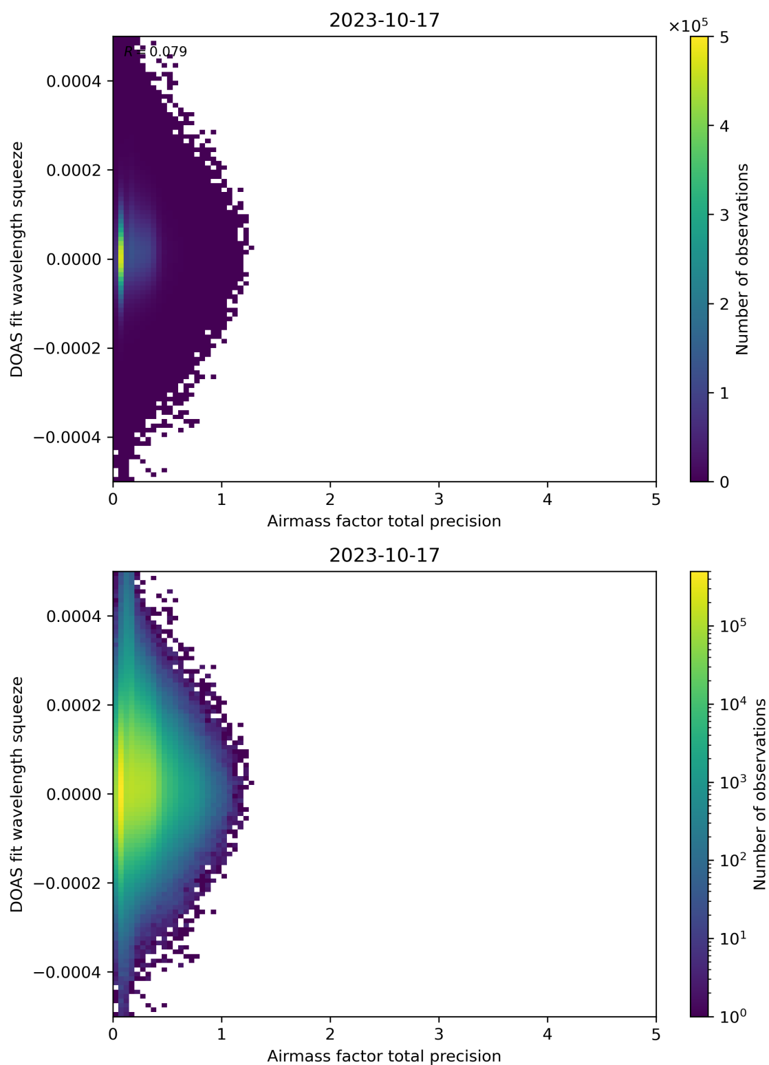
Figure 107: Scatter density plot of “Airmass factor total precision” against “DOAS fit wavelength squeeze” for 2023-10-17 to 2023-10-18.
