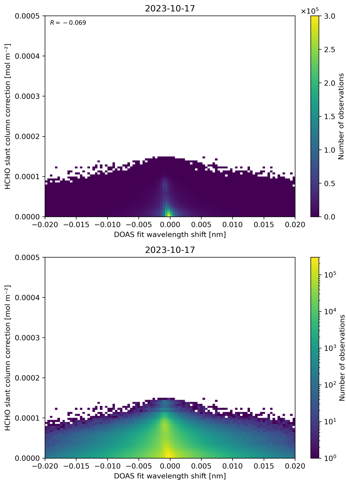
Figure 67: Scatter density plot of “DOAS fit wavelength shift” against “HCHO slant column correction” for 2023-10-17 to 2023-10-18.
