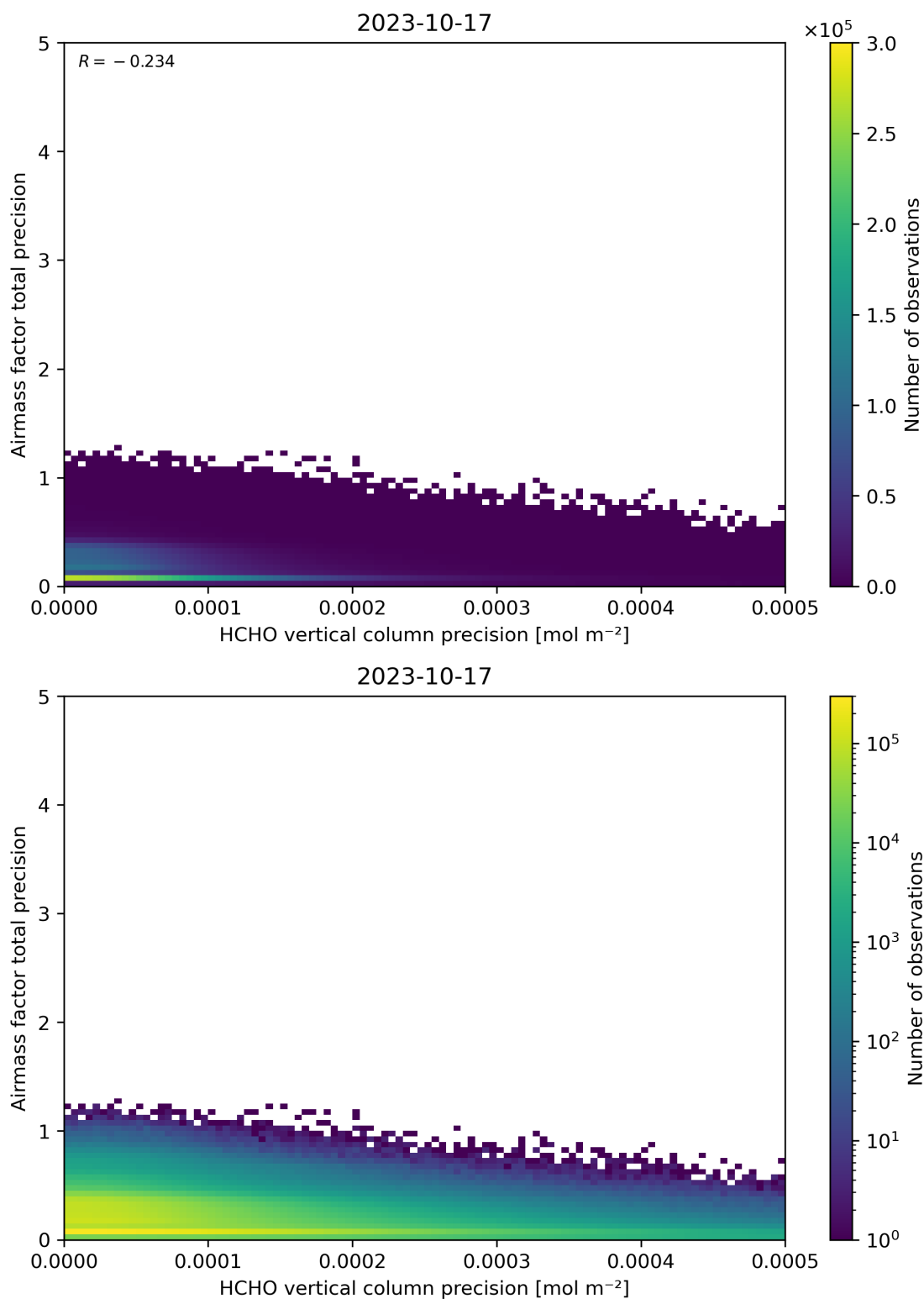
Figure 145: Scatter density plot of “HCHO vertical column precision” against “Airmass factor total precision” for 2023-10-17 to 2023-10-18.
