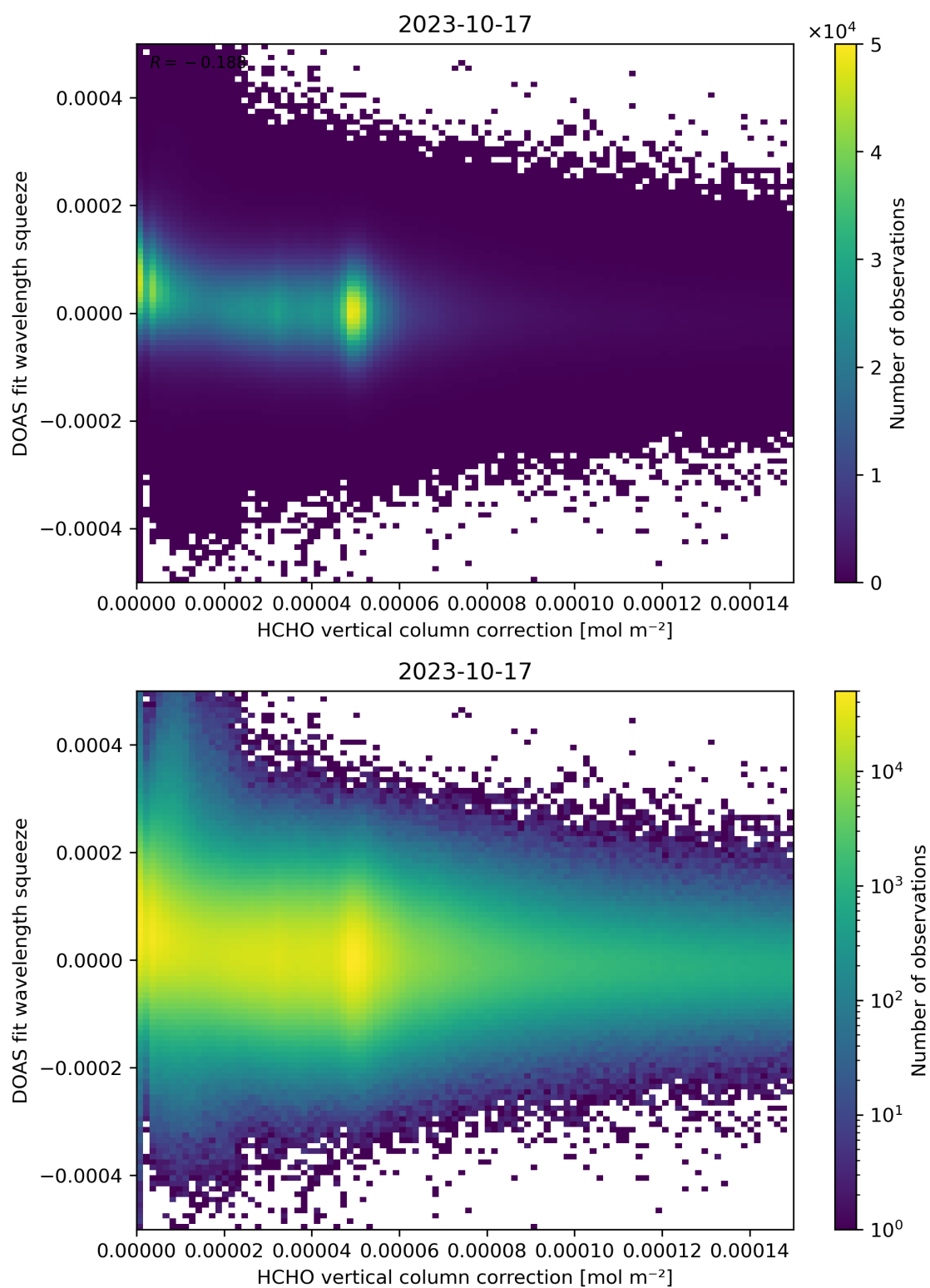
Figure 114: Scatter density plot of “HCHO vertical column correction” against “DOAS fit wavelength squeeze” for 2023-10-17 to 2023-10-18.
