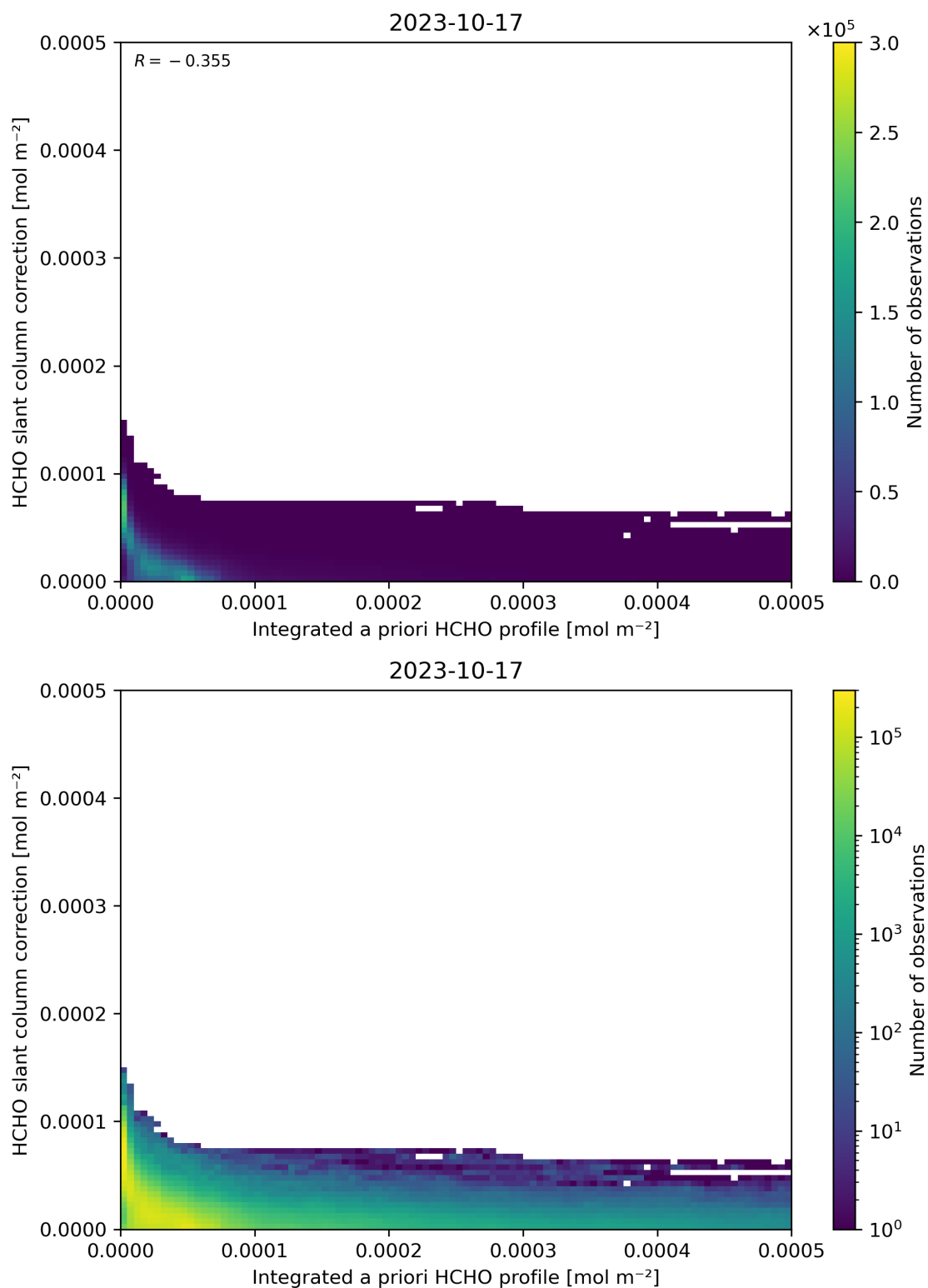
Figure 152: Scatter density plot of “Integrated a priori HCHO profile” against “HCHO slant column correction” for 2023-10-17 to 2023-10-18.
