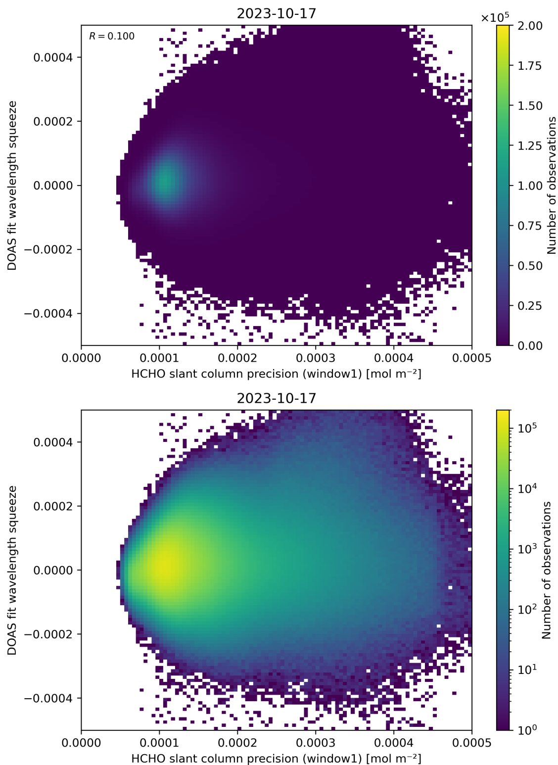
Figure 90: Scatter density plot of “HCHO slant column precision (window1)” against “DOAS fit wavelength squeeze” for 2023-10-17 to 2023-10-18.
