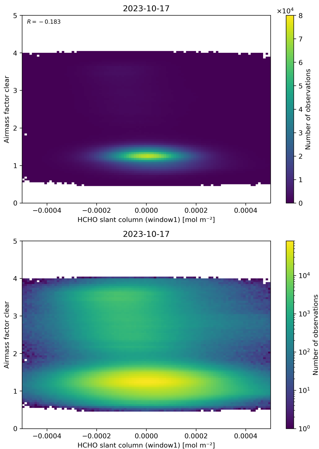
Figure 81: Scatter density plot of “HCHO slant column (window1)” against “Airmass factor clear” for 2023-10-17 to 2023-10-18.
