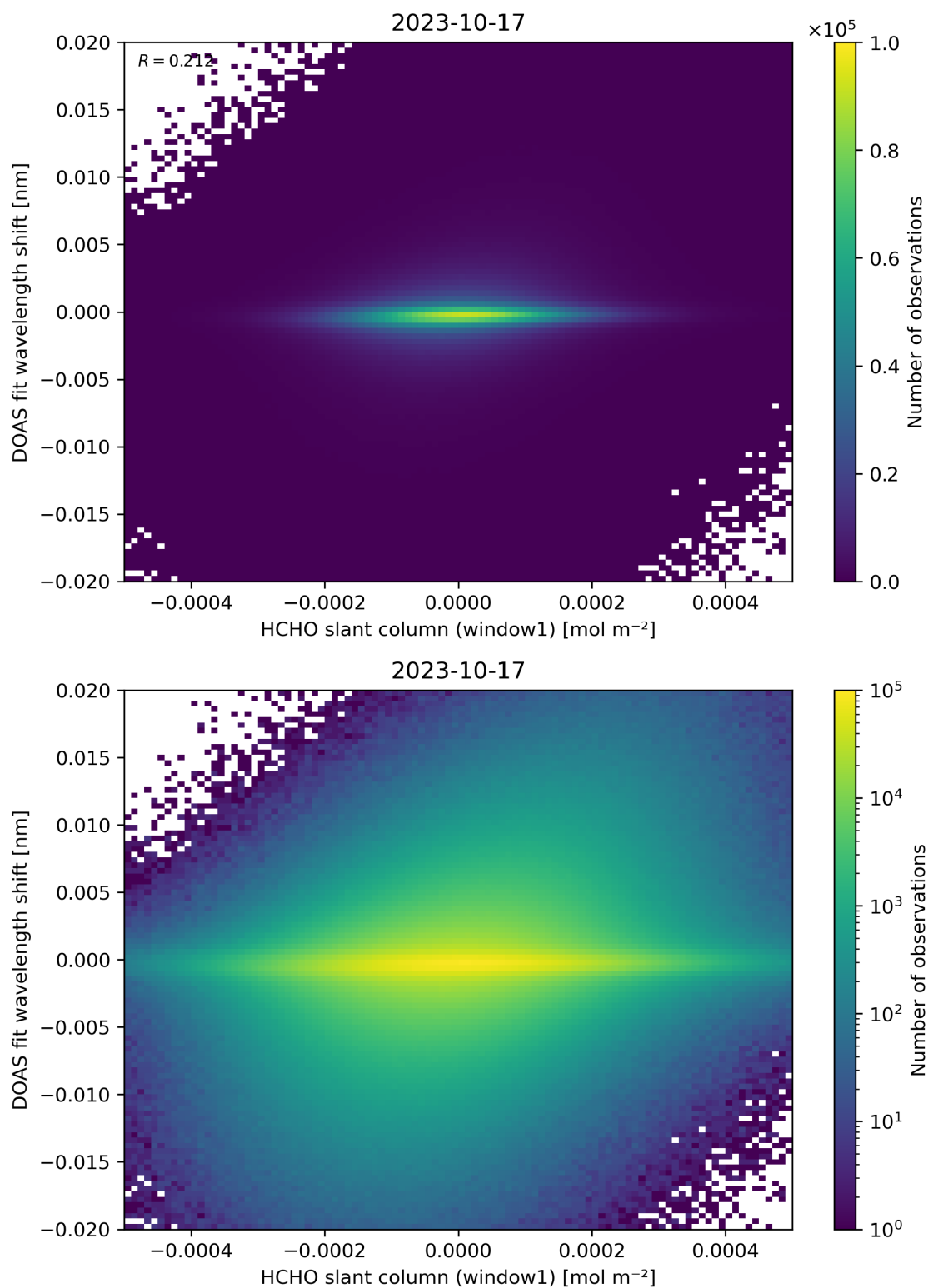
Figure 79: Scatter density plot of “HCHO slant column (window1)” against “DOAS fit wavelength shift” for 2023-10-17 to 2023-10-18.
