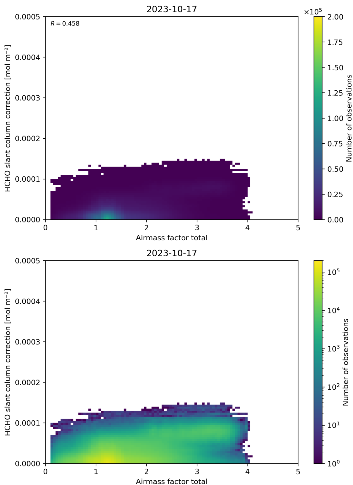
Figure 102: Scatter density plot of “Airmass factor total” against “HCHO slant column correction” for 2023-10-17 to 2023-10-18.
