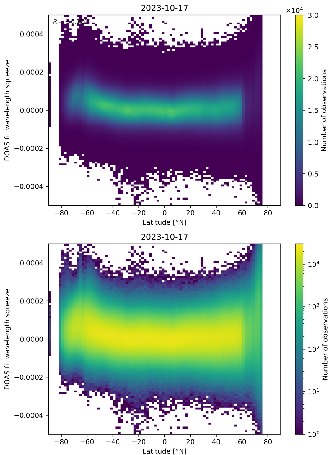
Figure 155: Scatter density plot of “Latitude” against “DOAS fit wavelength squeeze” for 2023-10-17 to 2023-10-18.
