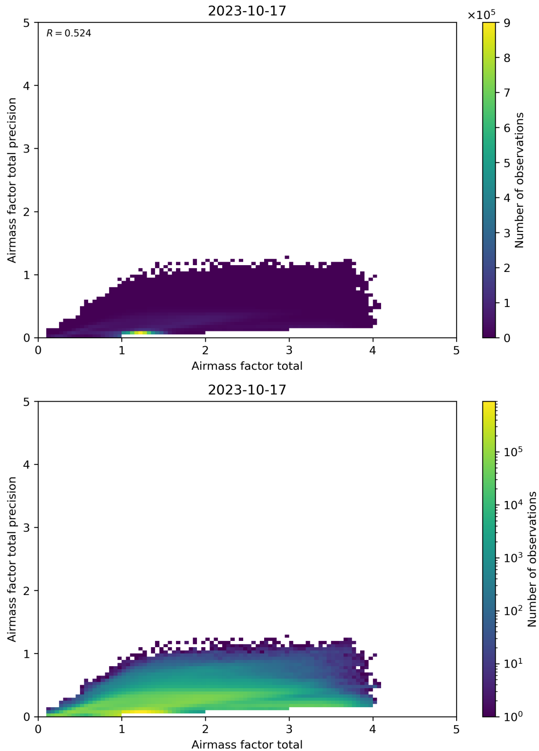
Figure 103: Scatter density plot of “Airmass factor total” against “Airmass factor total precision” for 2023-10-17 to 2023-10-18.
