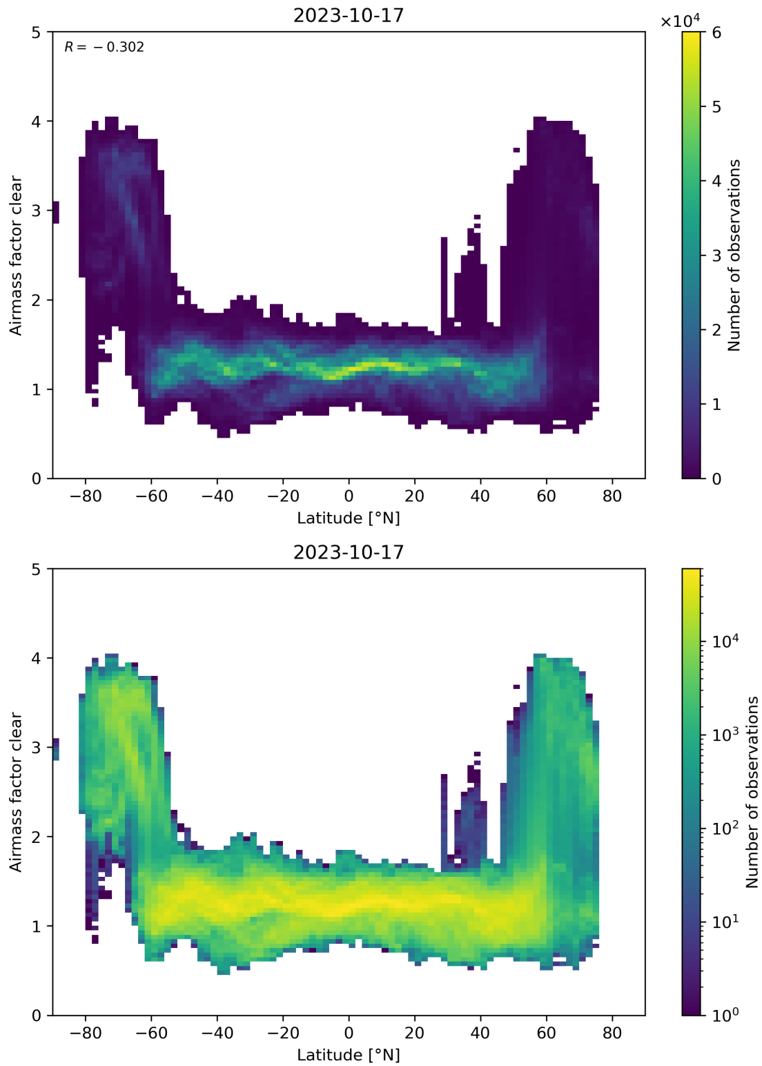
Figure 156: Scatter density plot of “Latitude” against “Airmass factor clear” for 2023-10-17 to 2023-10-18.
