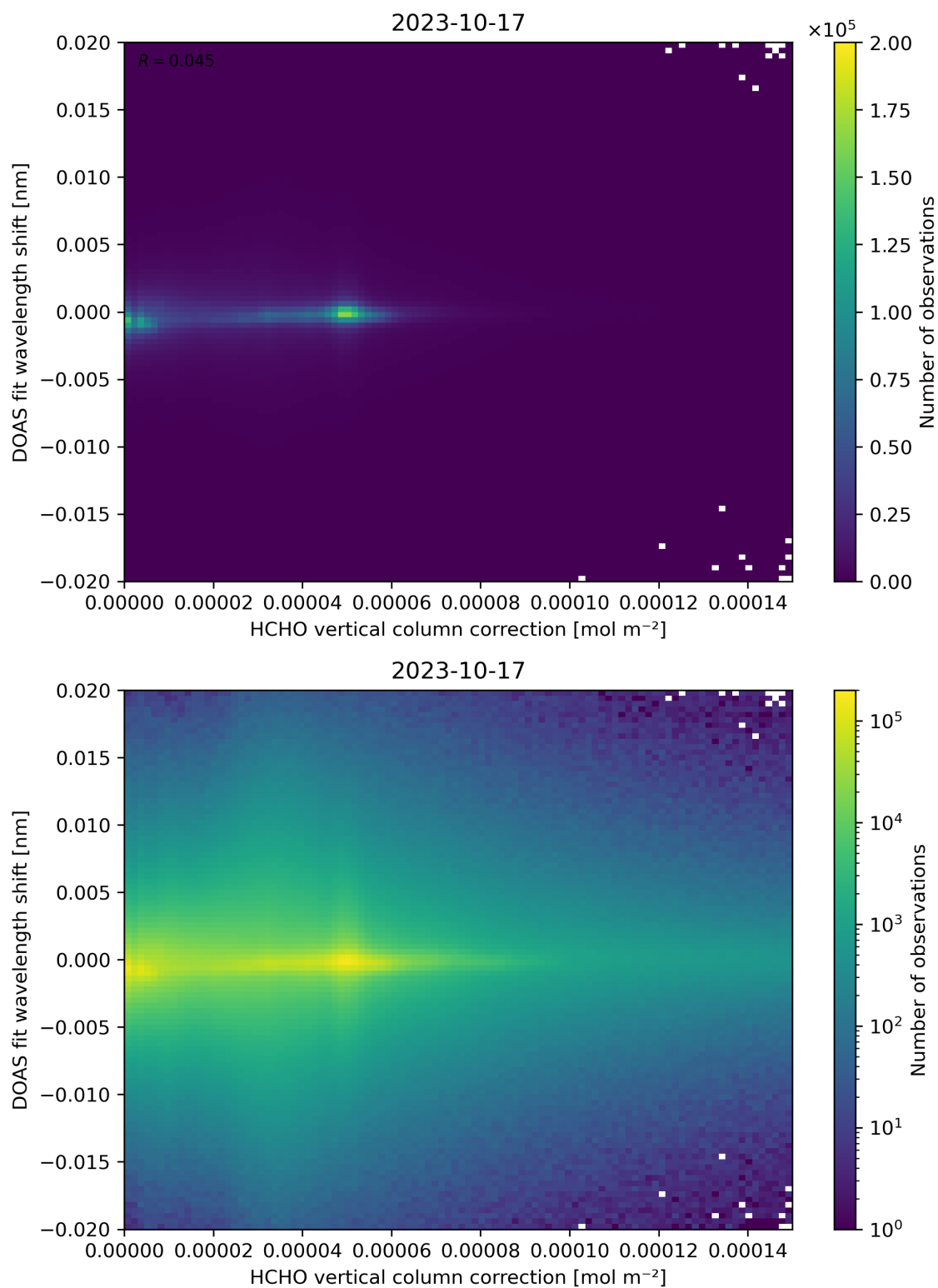
Figure 113: Scatter density plot of “HCHO vertical column correction” against “DOAS fit wavelength shift” for 2023-10-17 to 2023-10-18.
