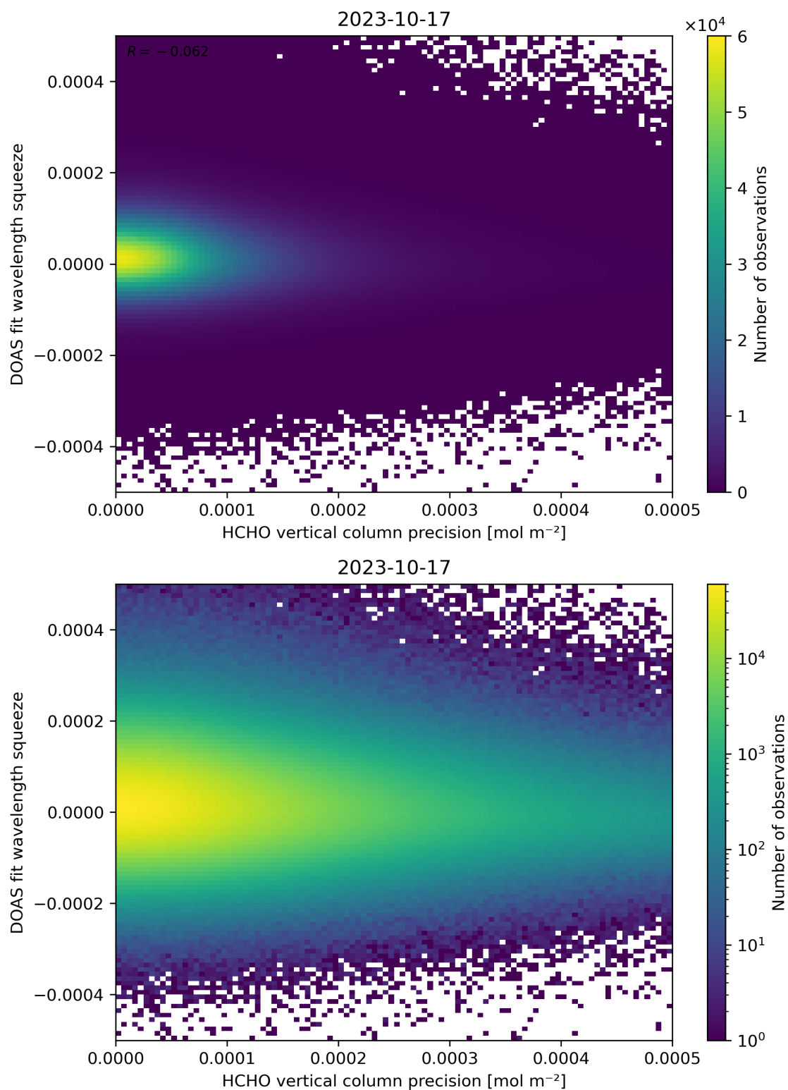
Figure 138: Scatter density plot of “HCHO vertical column precision” against “DOAS fit wavelength squeeze” for 2023-10-17 to 2023-10-18.
