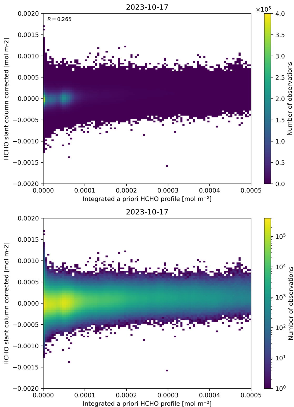
Figure 151: Scatter density plot of “Integrated a priori HCHO profile” against “HCHO slant column corrected” for 2023-10-17 to 2023-10-18.
