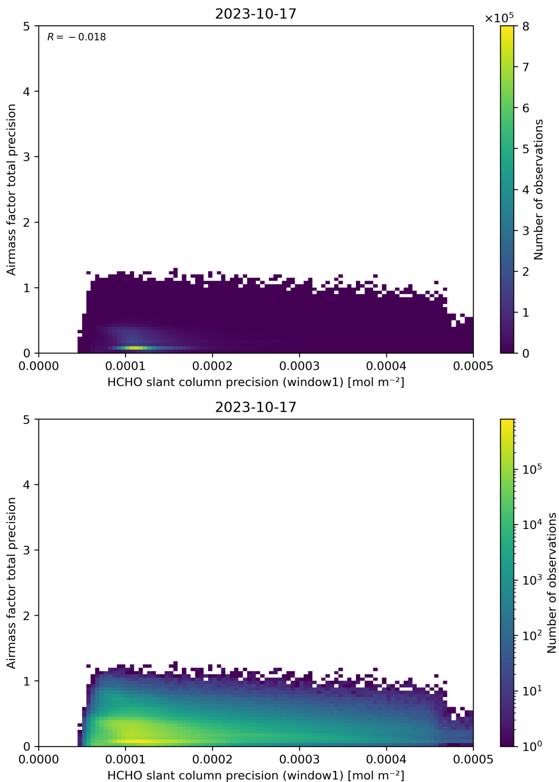
Figure 95: Scatter density plot of “HCHO slant column precision (window1)” against “Airmass factor total precision” for 2023-10-17 to 2023-10-18.
