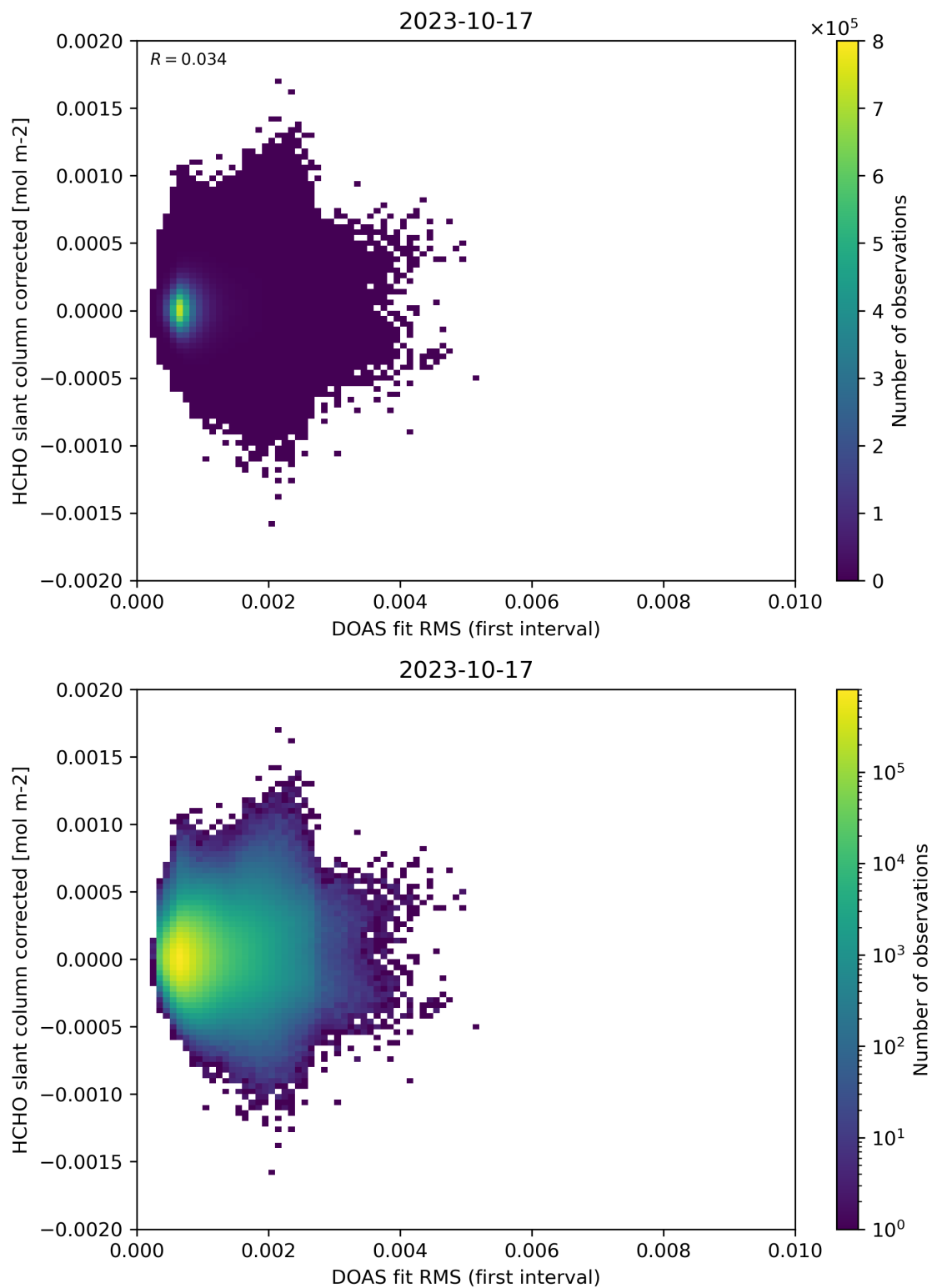
Figure 62: Scatter density plot of “DOAS fit RMS (first interval)” against “HCHO slant column corrected” for 2023-10-17 to 2023-10-18.
