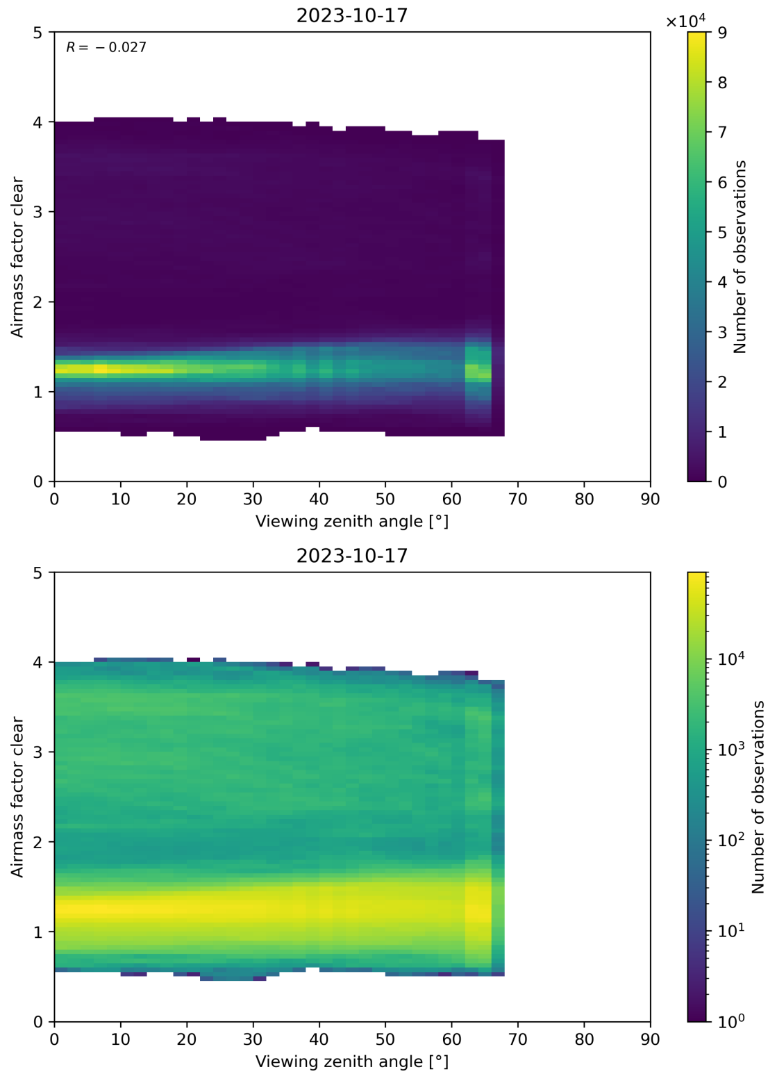
Figure 185: Scatter density plot of “Viewing zenith angle” against “Airmass factor clear” for 2023-10-17 to 2023-10-18.
