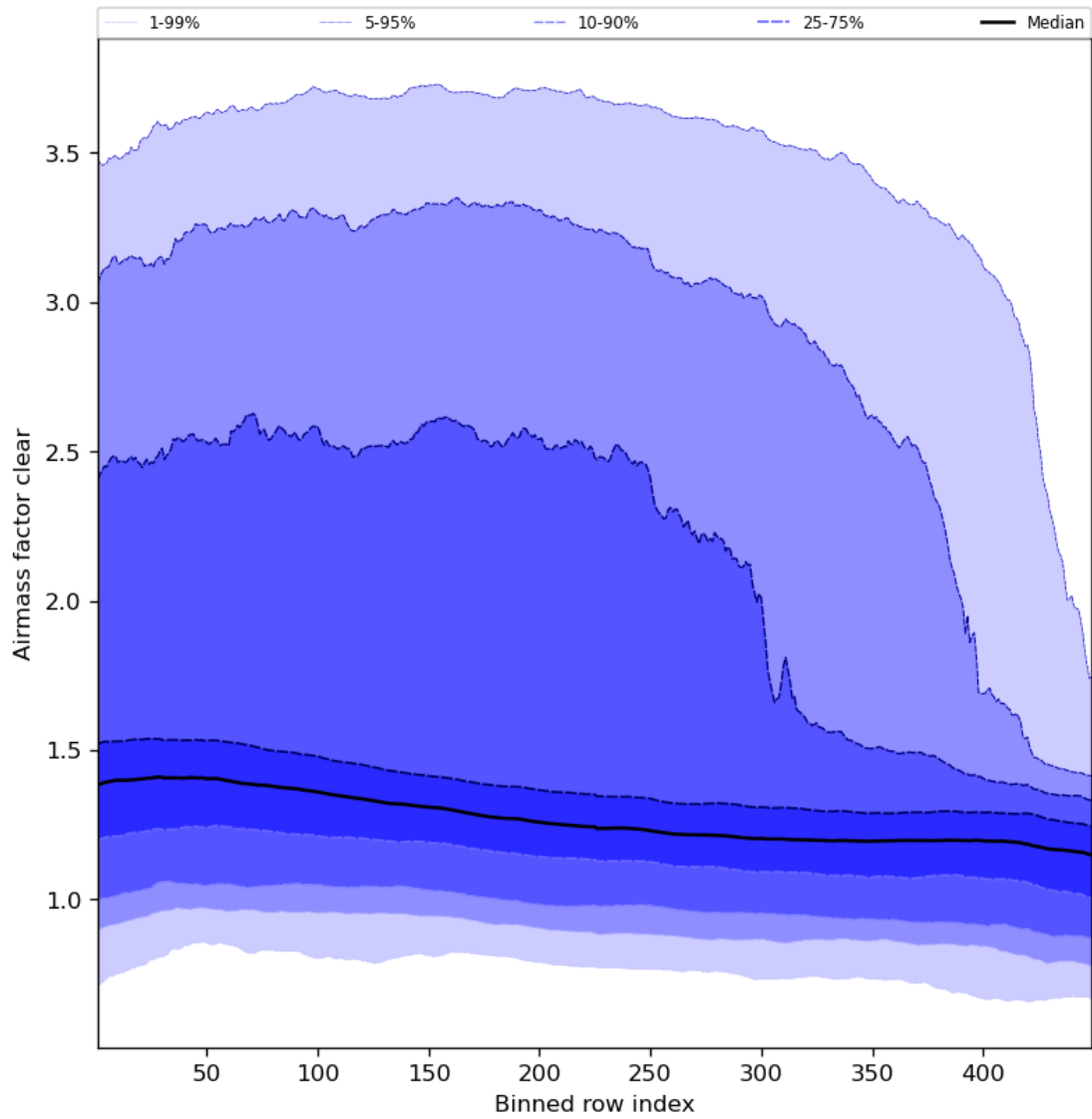
Figure 56: Along track statistics of “Airmass factor clear” for 2023-10-17 to 2023-10-18
