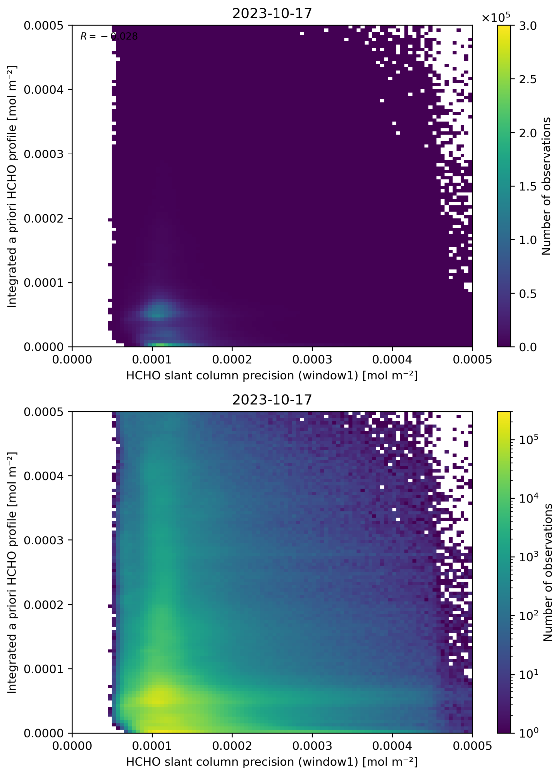
Figure 96: Scatter density plot of “HCHO slant column precision (window1)” against “Integrated a priori HCHO profile” for 2023-10-17 to 2023-10-18.
