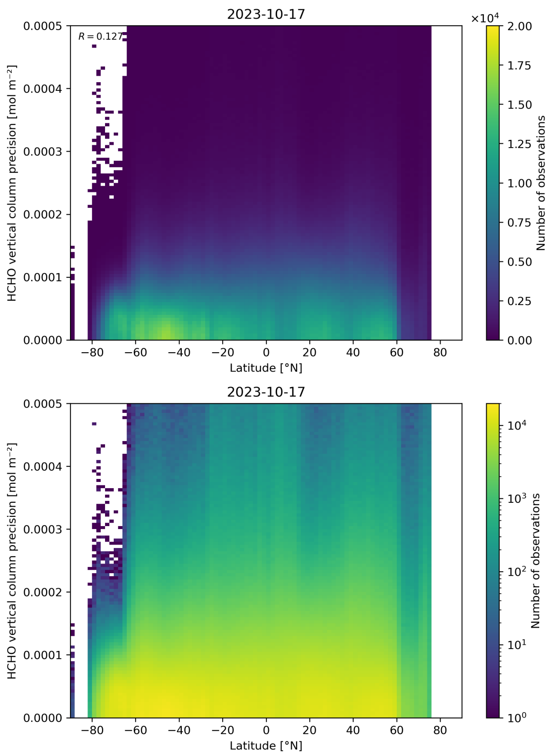
Figure 165: Scatter density plot of “Latitude” against “HCHO vertical column precision” for 2023-10-17 to 2023-10-18.
