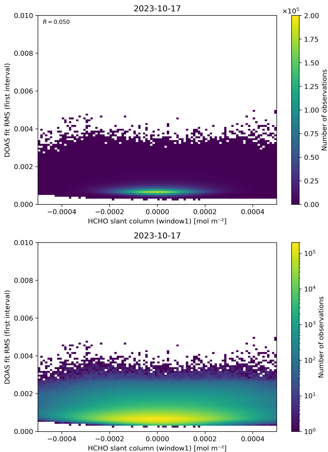
Figure 78: Scatter density plot of “HCHO slant column (window1)” against “DOAS fit RMS (first interval)” for 2023-10-17 to 2023-10-18.
