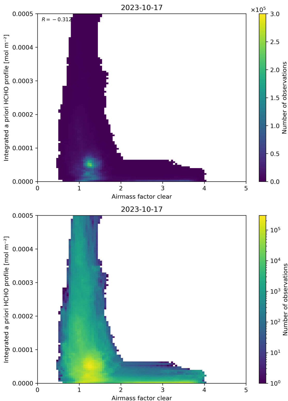
Figure 76: Scatter density plot of “Airmass factor clear” against “Integrated a priori HCHO profile” for 2023-10-17 to 2023-10-18.
