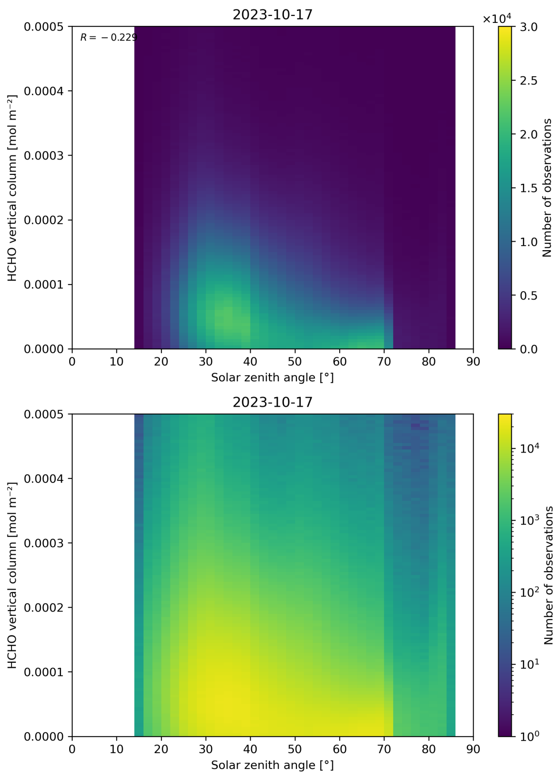
Figure 177: Scatter density plot of “Solar zenith angle” against “HCHO vertical column” for 2023-10-17 to 2023-10-18.
