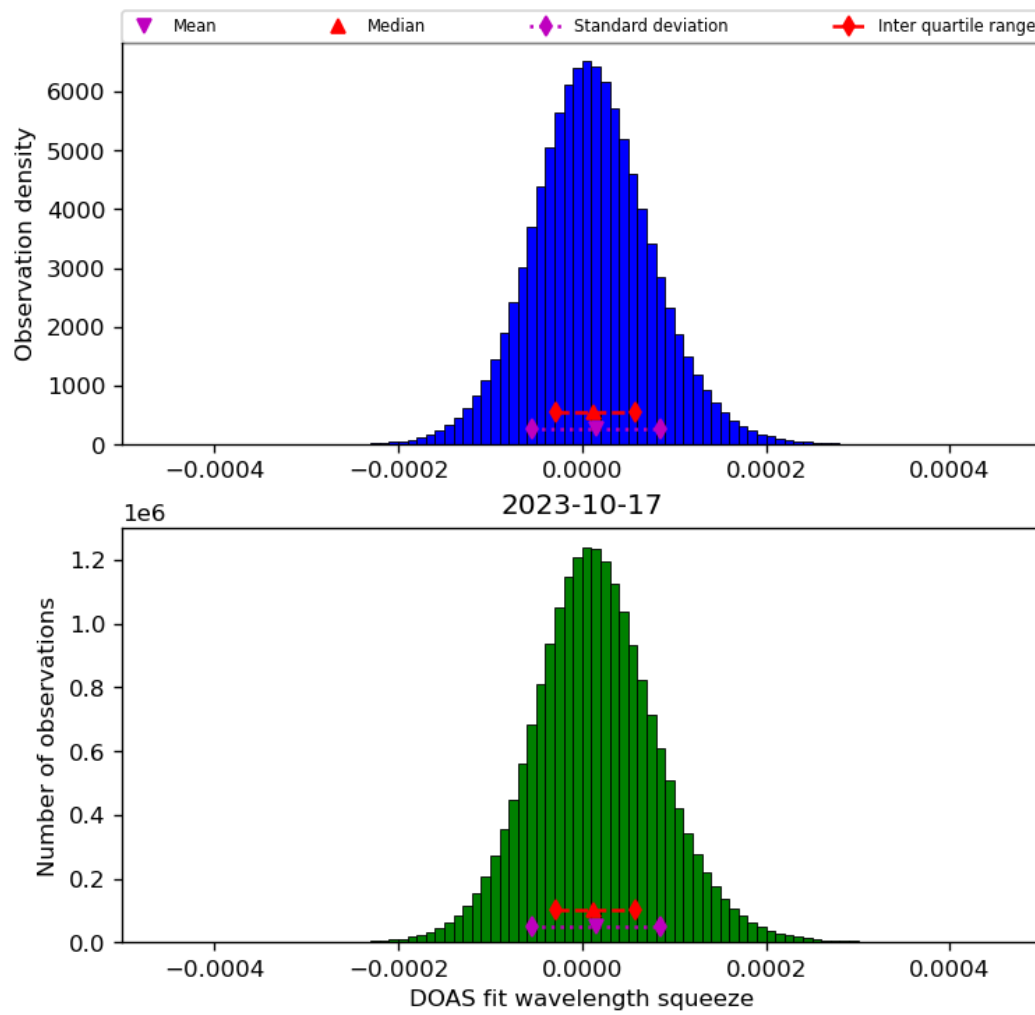
Figure 45: Histogram of “DOAS fit wavelength squeeze” for 2023-10-17 to 2023-10-18
