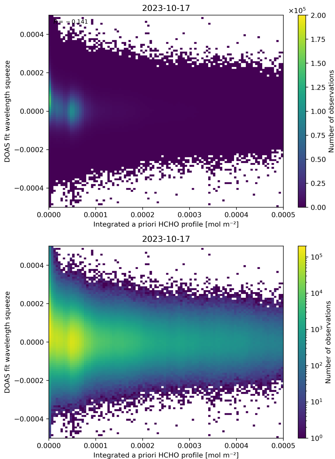
Figure 150: Scatter density plot of “Integrated a priori HCHO profile” against “DOAS fit wavelength squeeze” for 2023-10-17 to 2023-10-18.
