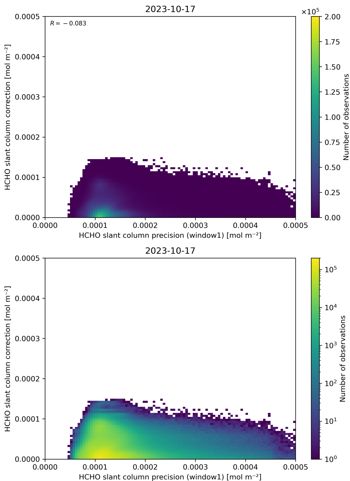
Figure 93: Scatter density plot of “HCHO slant column precision (window1)” against “HCHO slant column correction” for 2023-10-17 to 2023-10-18.
