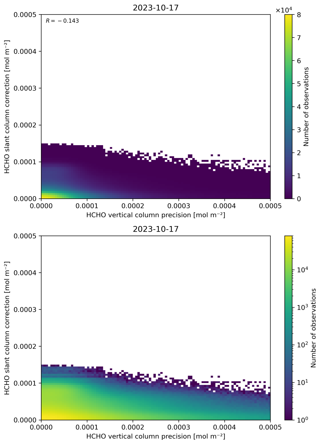
Figure 141: Scatter density plot of “HCHO vertical column precision” against “HCHO slant column correction” for 2023-10-17 to 2023-10-18.
