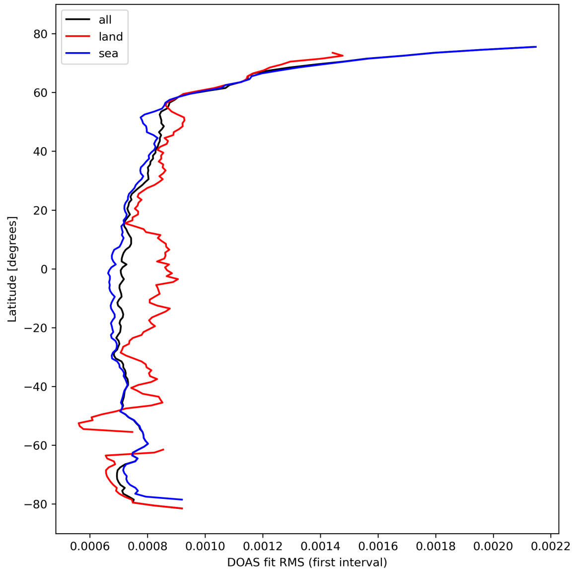
Figure 32: Zonal average of “DOAS fit RMS (first interval)” for 2023-10-17 to 2023-10-18.
