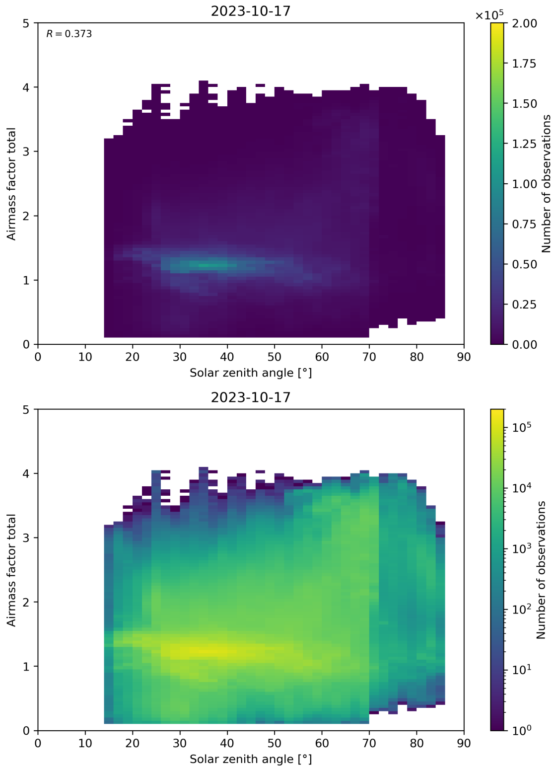
Figure 175: Scatter density plot of “Solar zenith angle” against “Airmass factor total” for 2023-10-17 to 2023-10-18.
