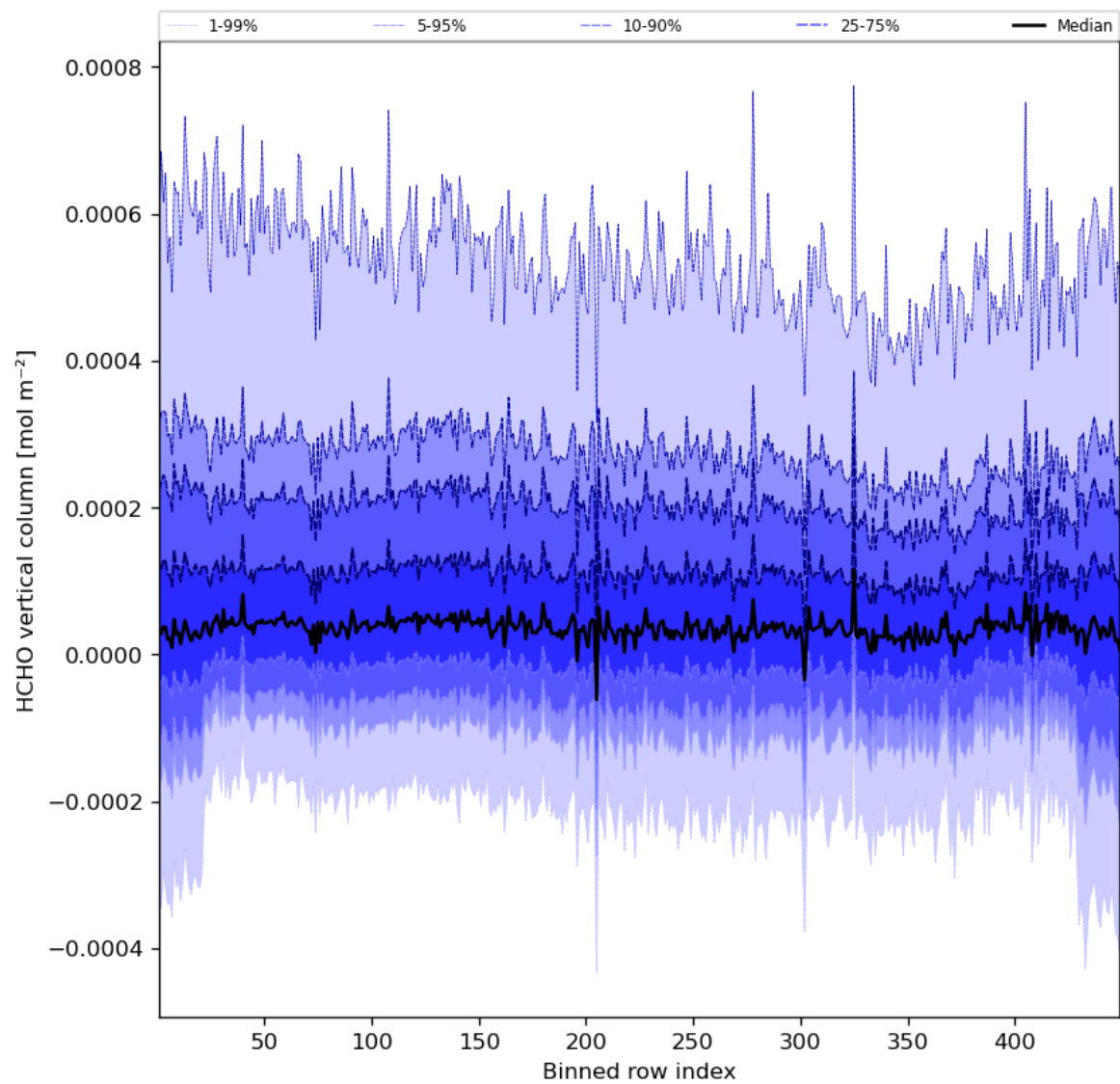
Figure 49: Along track statistics of “HCHO vertical column” for 2023-10-17 to 2023-10-18
