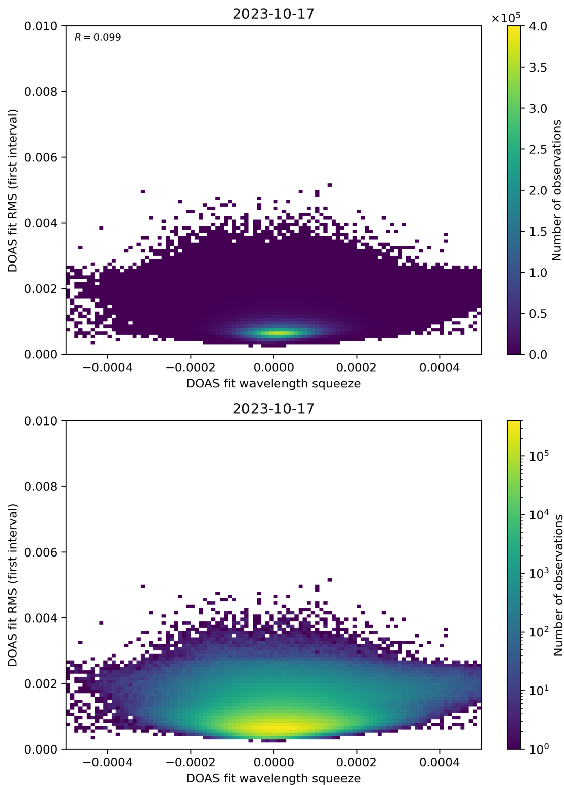
Figure 68: Scatter density plot of “DOAS fit wavelength squeeze” against “DOAS fit RMS (first interval)” for 2023-10-17 to 2023-10-18.
