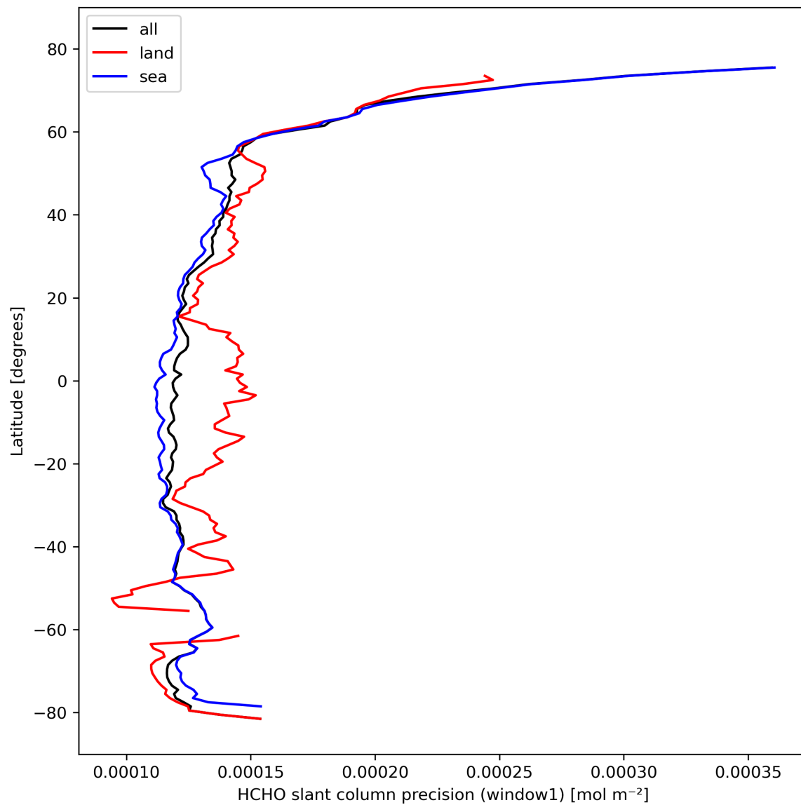
Figure 25: Zonal average of “HCHO slant column precision (window1)” for 2023-10-17 to 2023-10-18.
