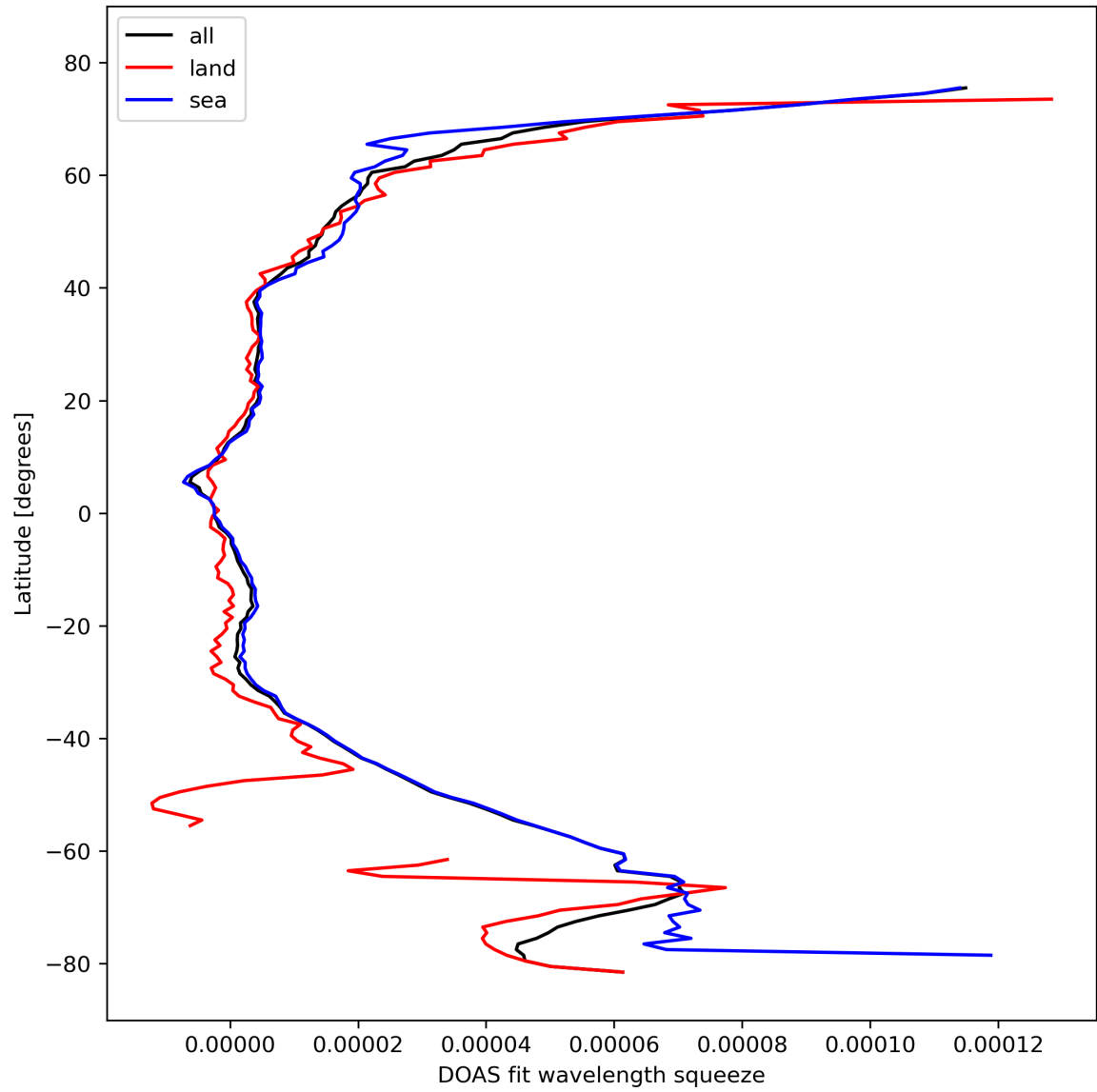
Figure 31: Zonal average of “DOAS fit wavelength squeeze” for 2023-10-17 to 2023-10-18.
