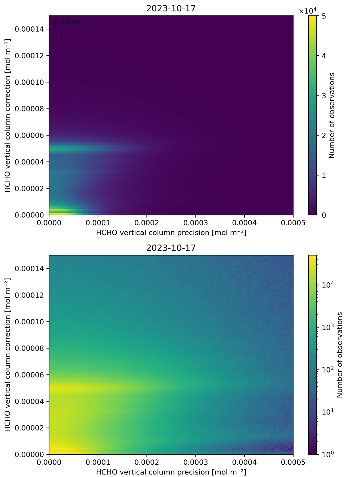
Figure 146: Scatter density plot of “HCHO vertical column precision” against “HCHO vertical column correction” for 2023-10-17 to 2023-10-18.
