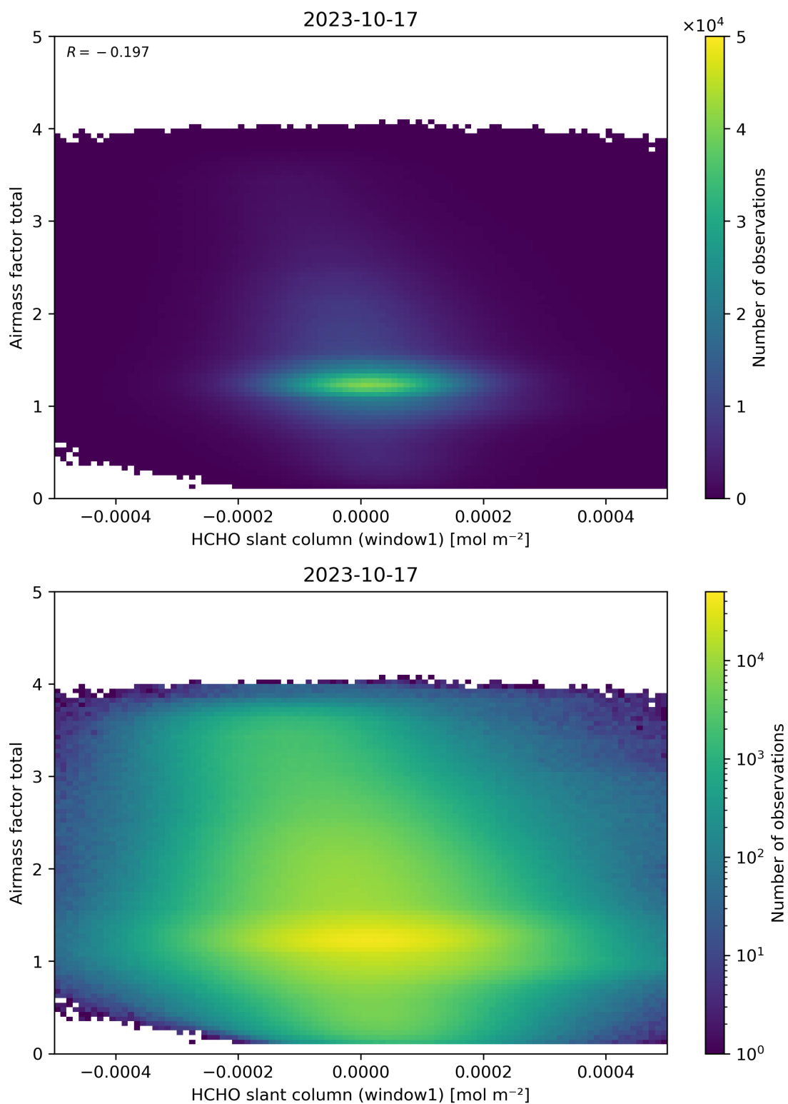
Figure 85: Scatter density plot of “HCHO slant column (window1)” against “Airmass factor total” for 2023-10-17 to 2023-10-18.
