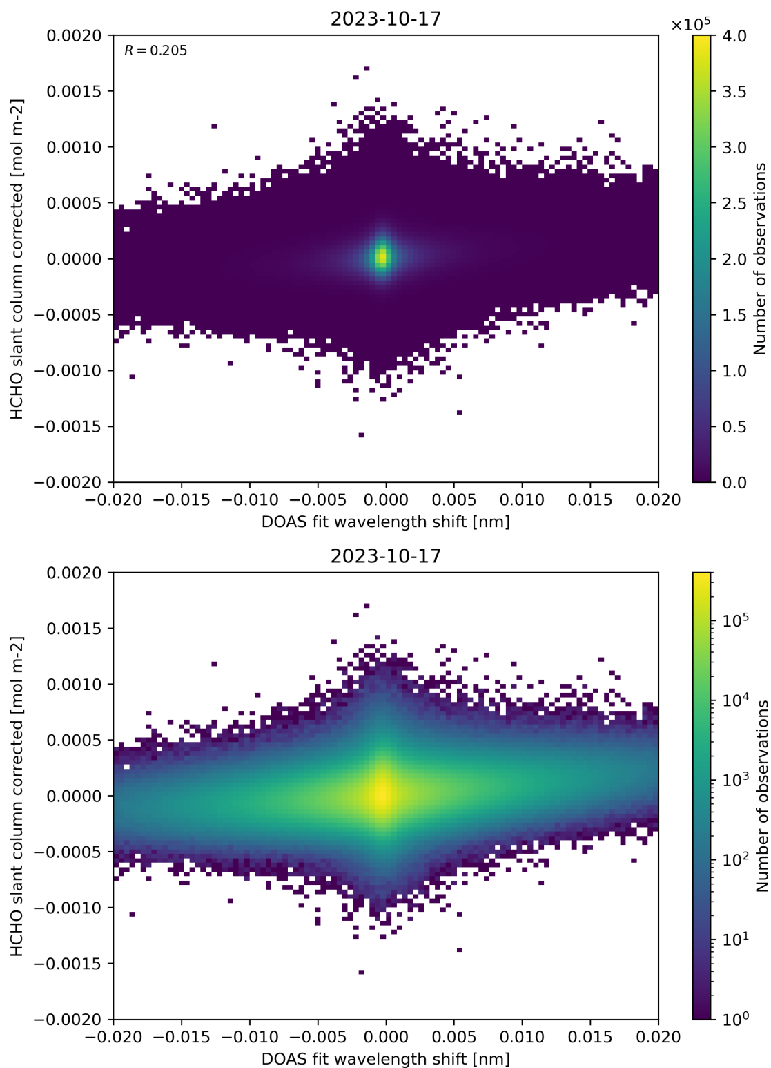
Figure 66: Scatter density plot of “DOAS fit wavelength shift” against “HCHO slant column corrected” for 2023-10-17 to 2023-10-18.
