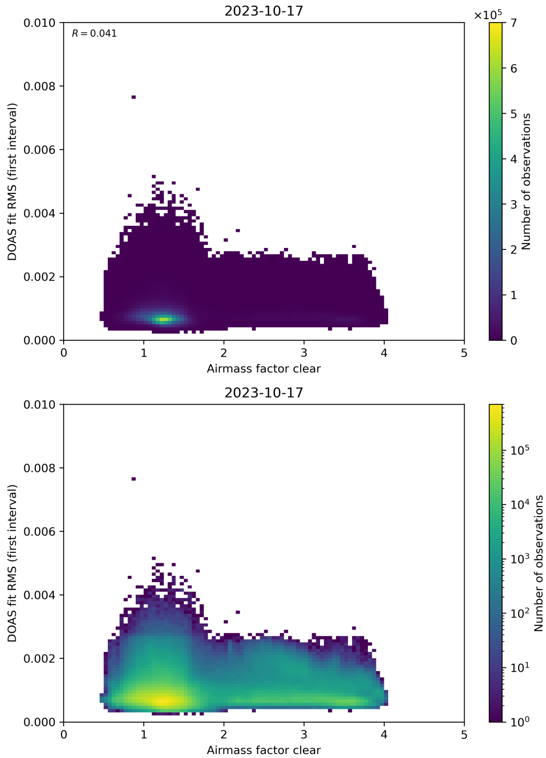
Figure 71: Scatter density plot of “Airmass factor clear” against “DOAS fit RMS (first interval)” for 2023-10-17 to 2023-10-18.
