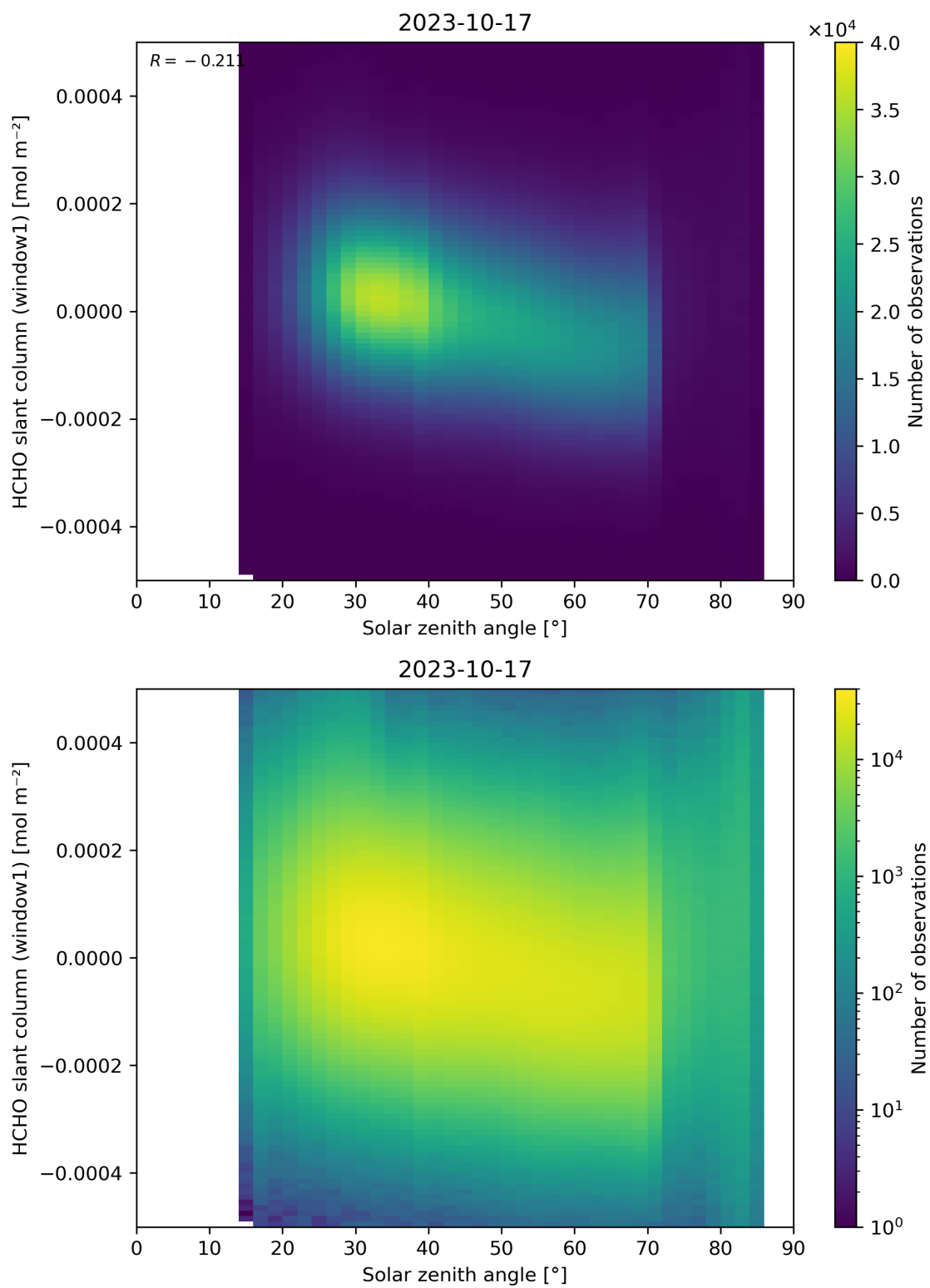
Figure 173: Scatter density plot of “Solar zenith angle” against “HCHO slant column (window1)” for 2023-10-17 to 2023-10-18.
