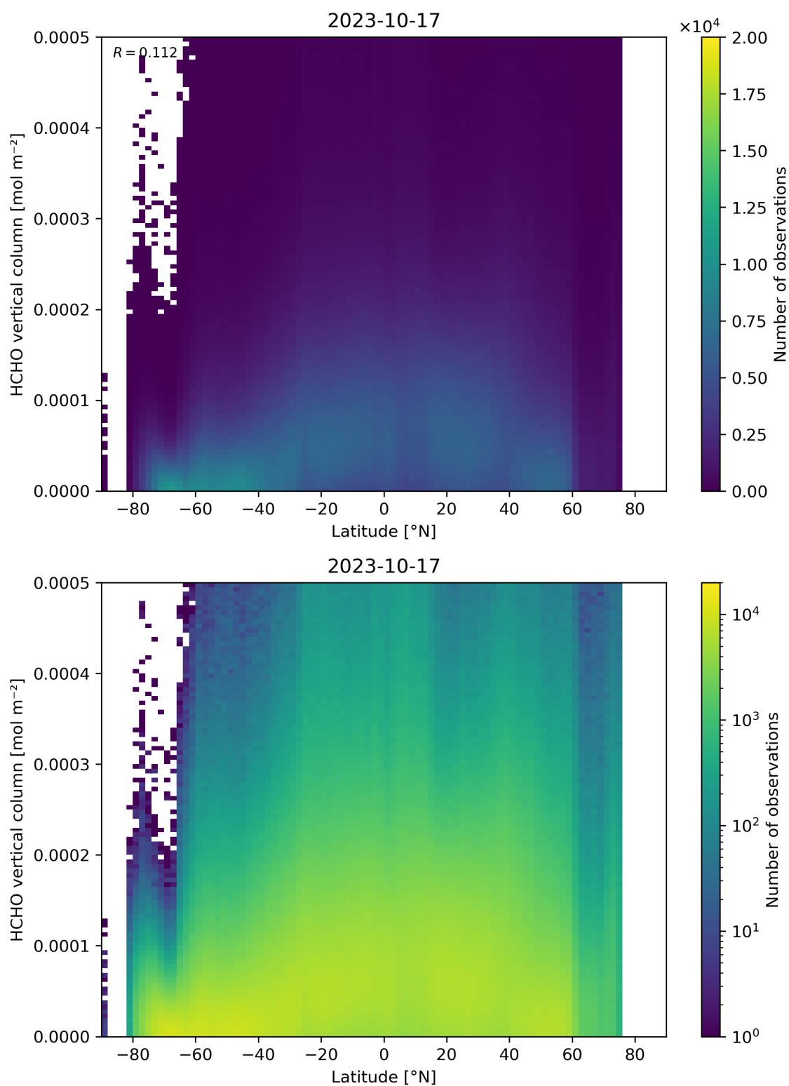
Figure 163: Scatter density plot of “Latitude” against “HCHO vertical column” for 2023-10-17 to 2023-10-18.
