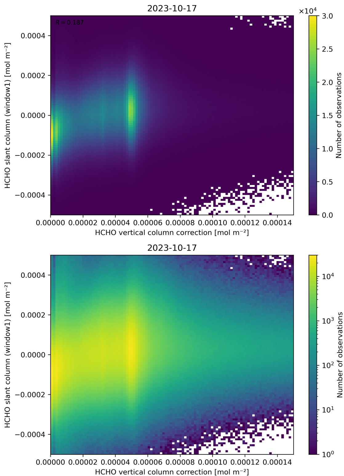
Figure 118: Scatter density plot of “HCHO vertical column correction” against “HCHO slant column (window1)” for 2023-10-17 to 2023-10-18.
