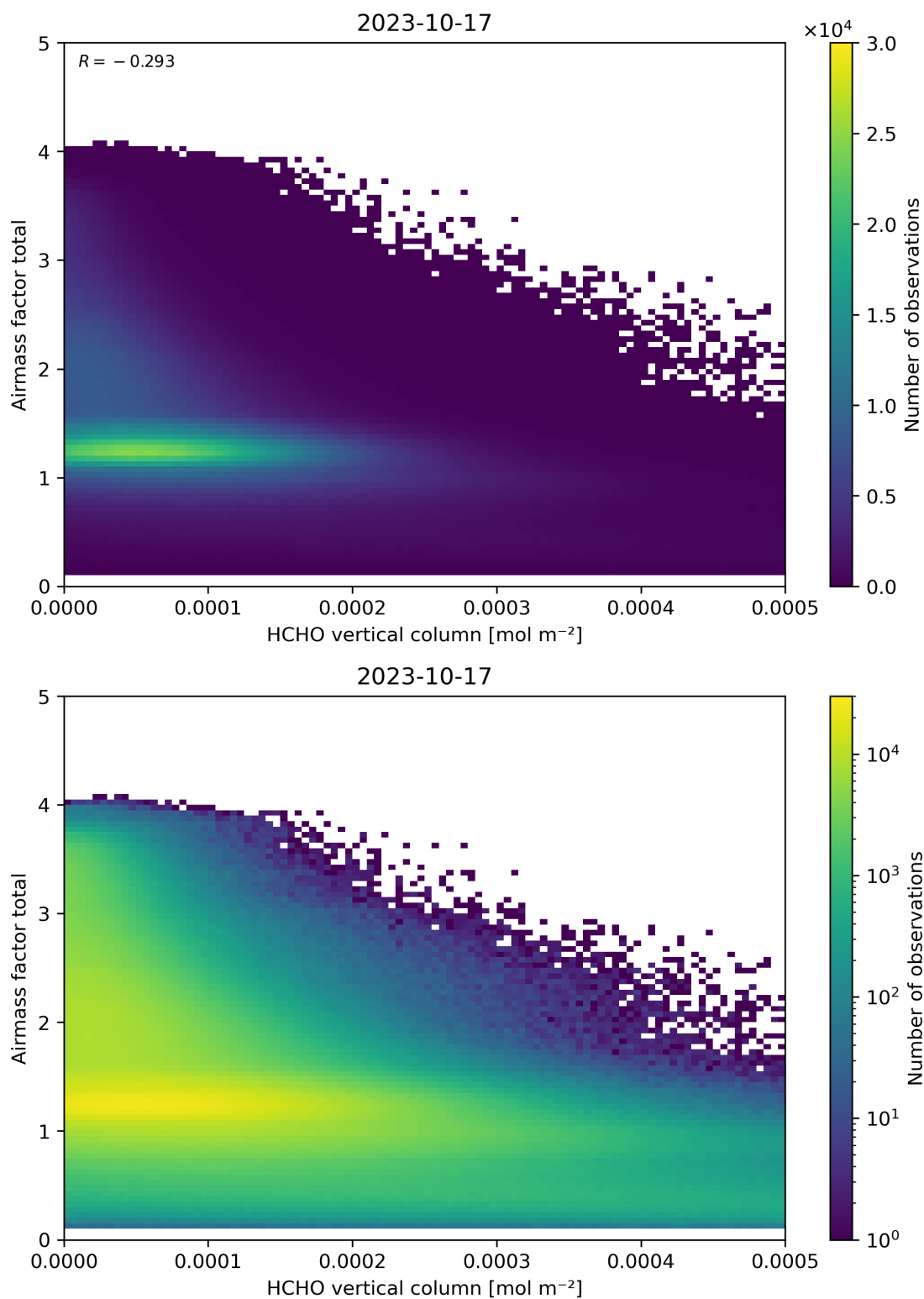
Figure 131: Scatter density plot of “HCHO vertical column” against “Airmass factor total” for 2023-10-17 to 2023-10-18.
