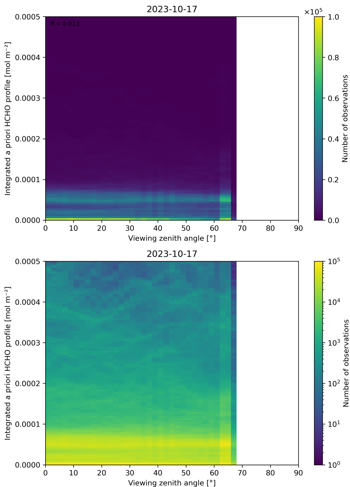
Figure 195: Scatter density plot of “Viewing zenith angle” against “Integrated a priori HCHO profile” for 2023-10-17 to 2023-10-18.
