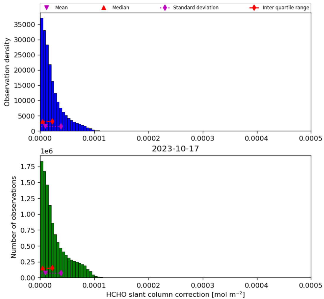
Figure 47: Histogram of “HCHO slant column correction” for 2023-10-17 to 2023-10-18
