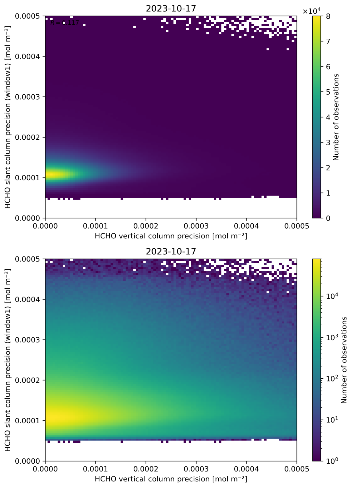
Figure 143: Scatter density plot of “HCHO vertical column precision” against “HCHO slant column precision (window1)” for 2023-10-17 to 2023-10-18.
