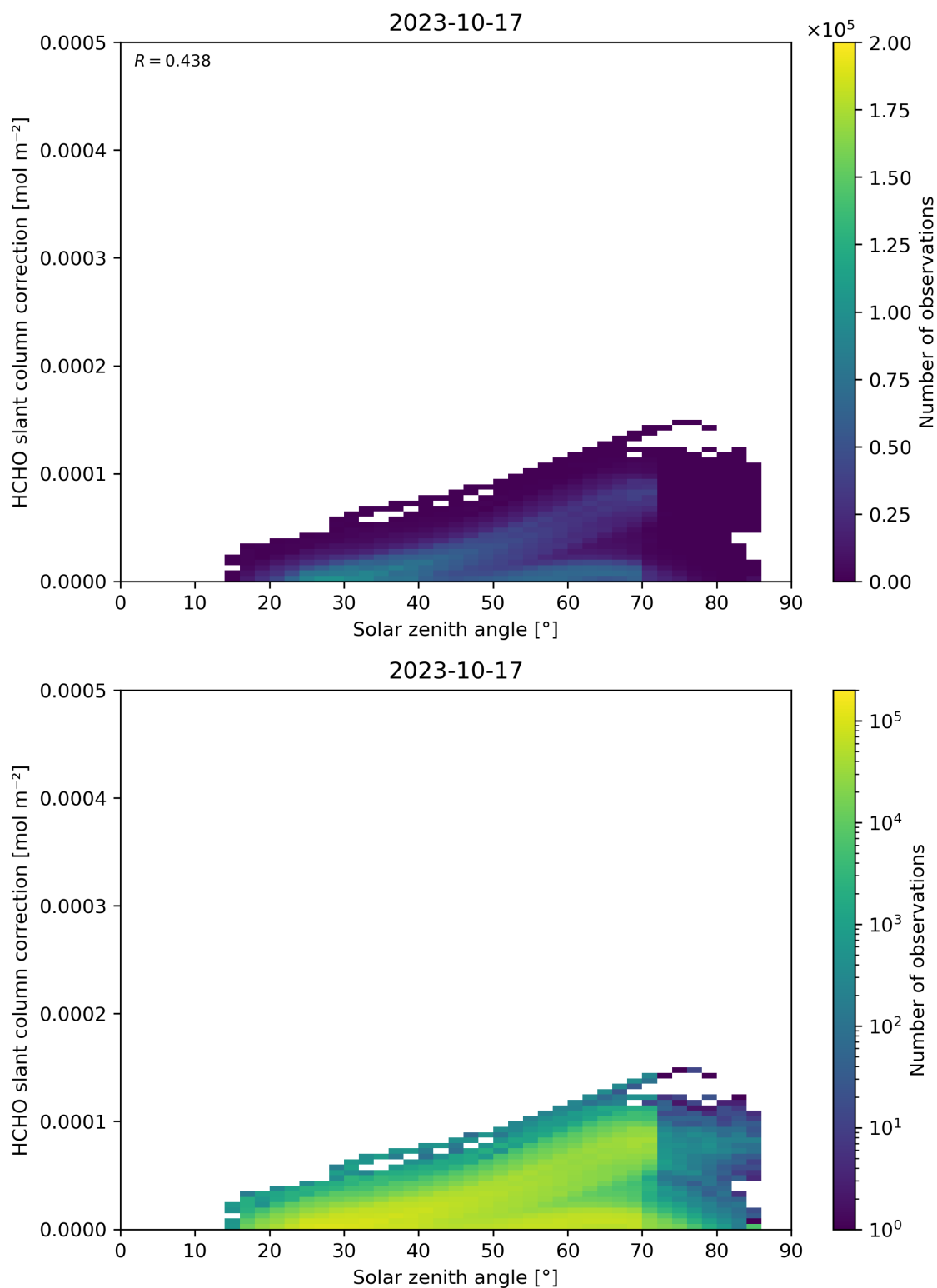
Figure 172: Scatter density plot of “Solar zenith angle” against “HCHO slant column correction” for 2023-10-17 to 2023-10-18.
