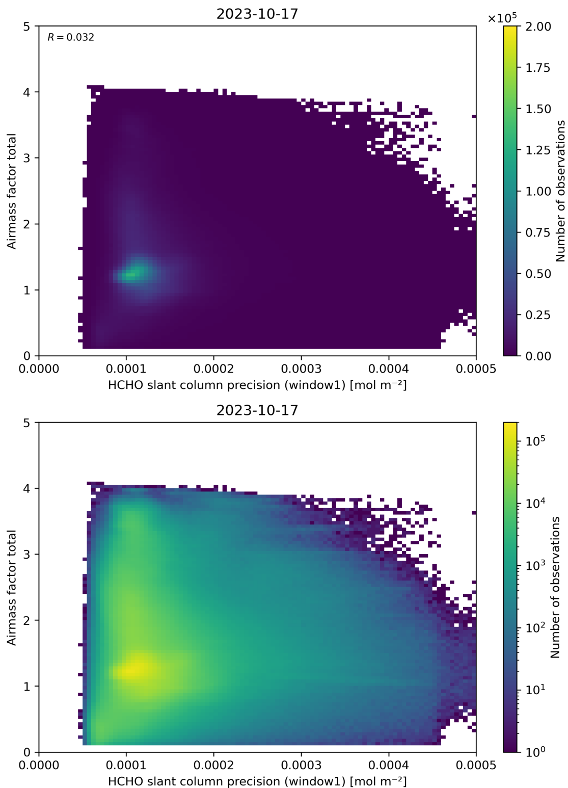
Figure 94: Scatter density plot of “HCHO slant column precision (window1)” against “Airmass factor total” for 2023-10-17 to 2023-10-18.
