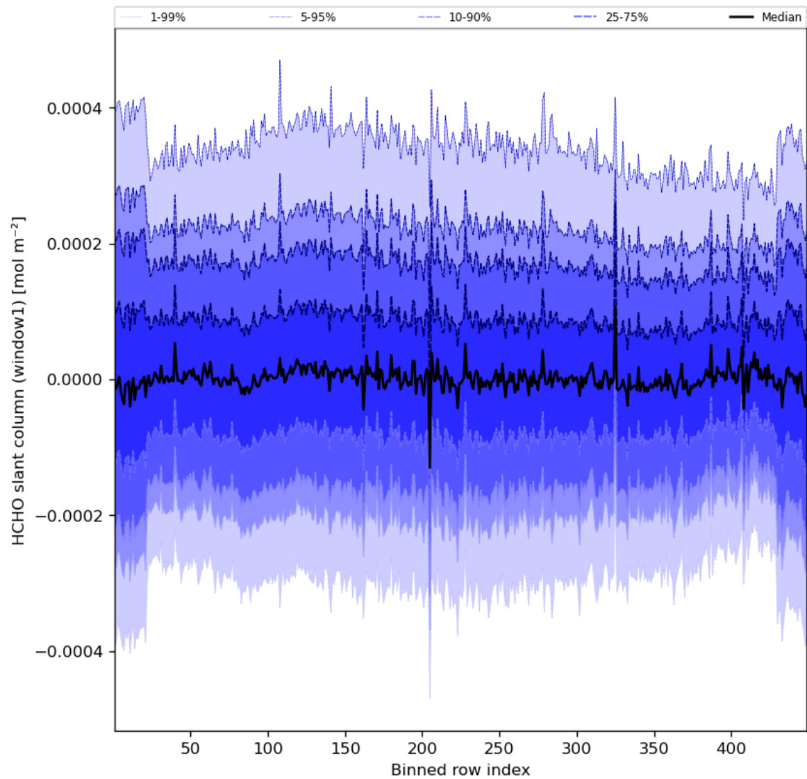
Figure 52: Along track statistics of “HCHO slant column (window1)” for 2023-10-17 to 2023-10-18
