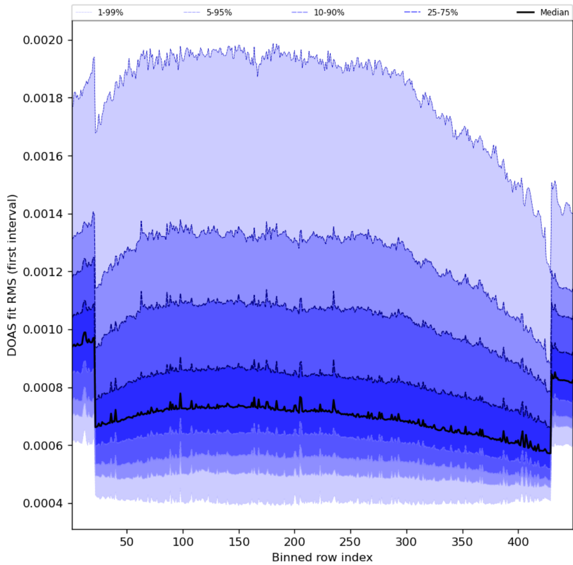
Figure 60: Along track statistics of “DOAS fit RMS (first interval)” for 2023-10-17 to 2023-10-18
