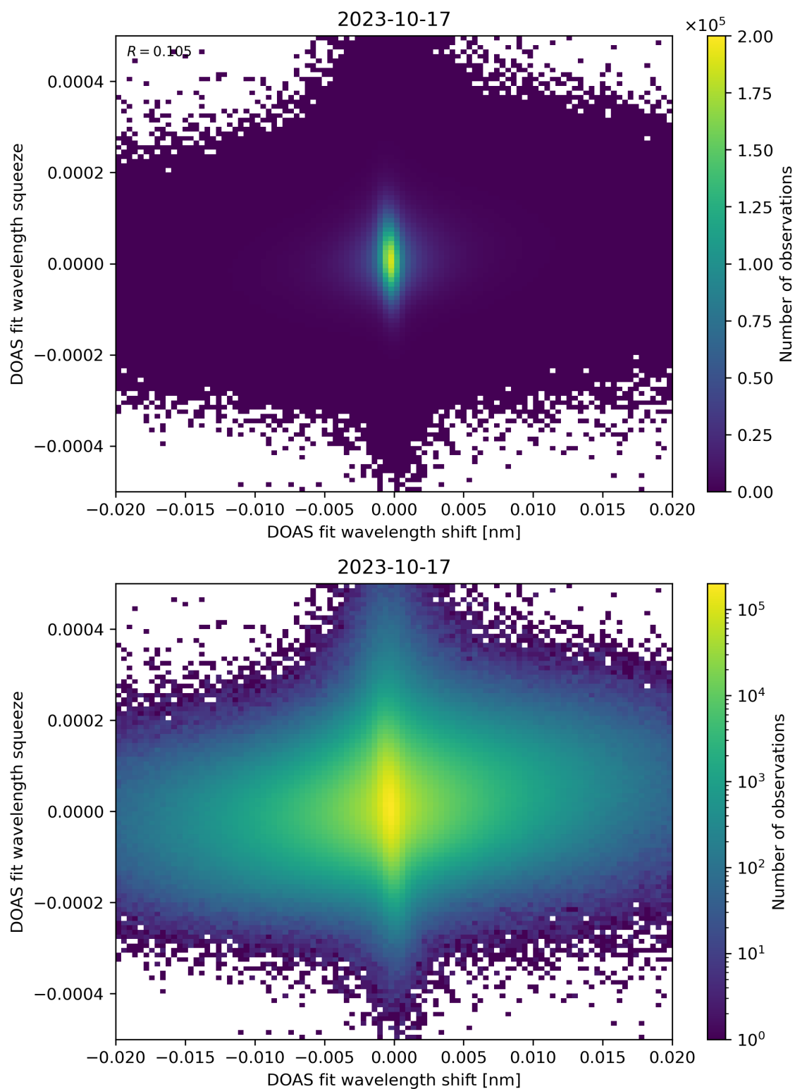
Figure 65: Scatter density plot of “DOAS fit wavelength shift” against “DOAS fit wavelength squeeze” for 2023-10-17 to 2023-10-18.
