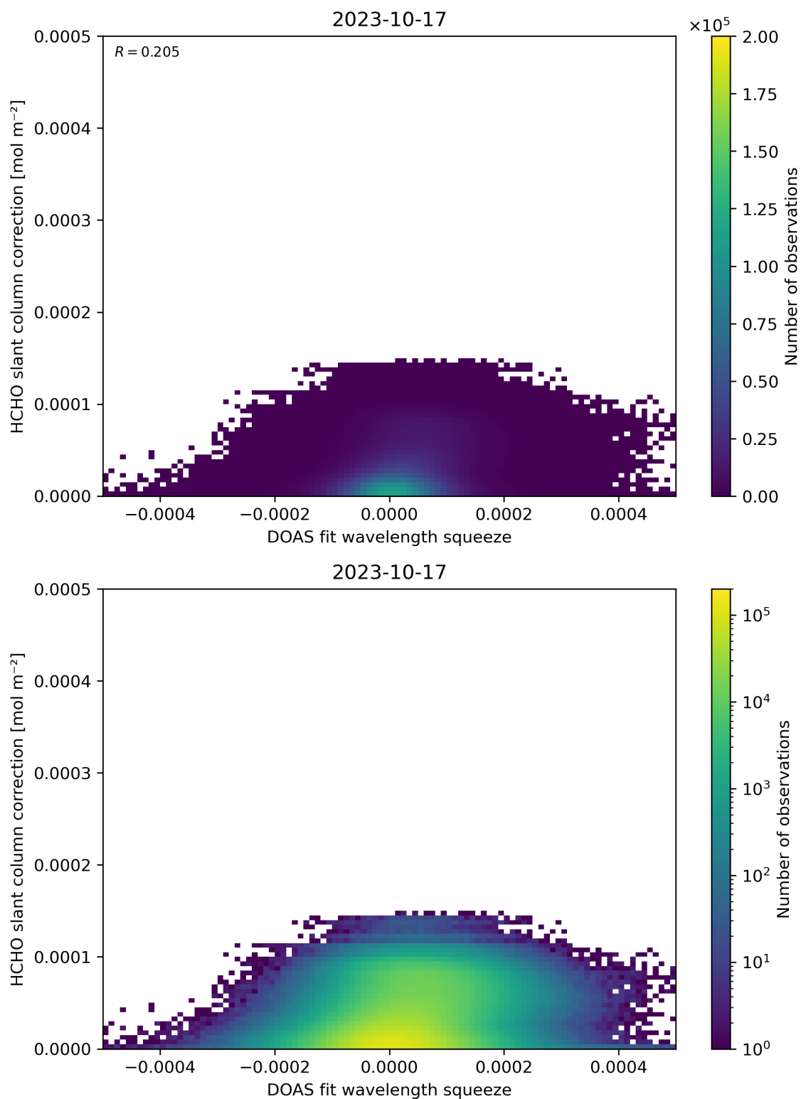
Figure 70: Scatter density plot of “DOAS fit wavelength squeeze” against “HCHO slant column correction” for 2023-10-17 to 2023-10-18.
