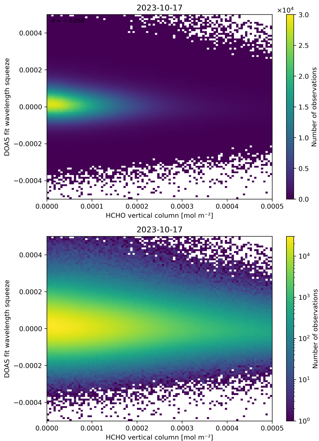
Figure 125: Scatter density plot of “HCHO vertical column” against “DOAS fit wavelength squeeze” for 2023-10-17 to 2023-10-18.
