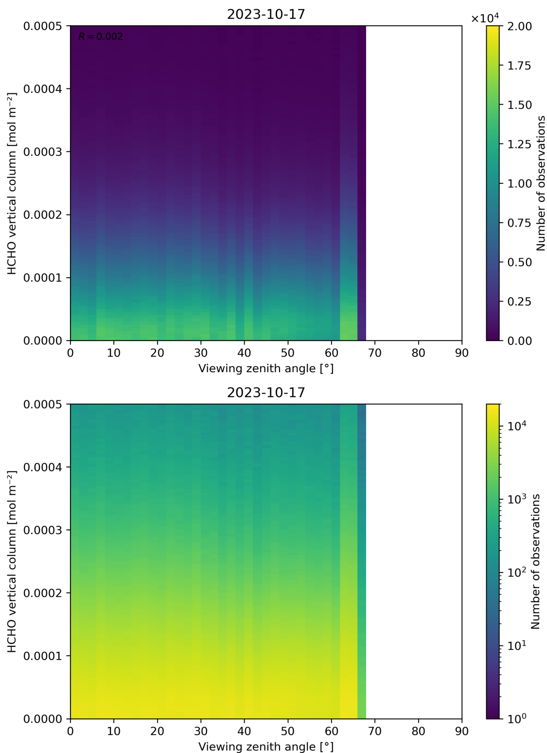
Figure 192: Scatter density plot of “Viewing zenith angle” against “HCHO vertical column” for 2023-10-17 to 2023-10-18.
