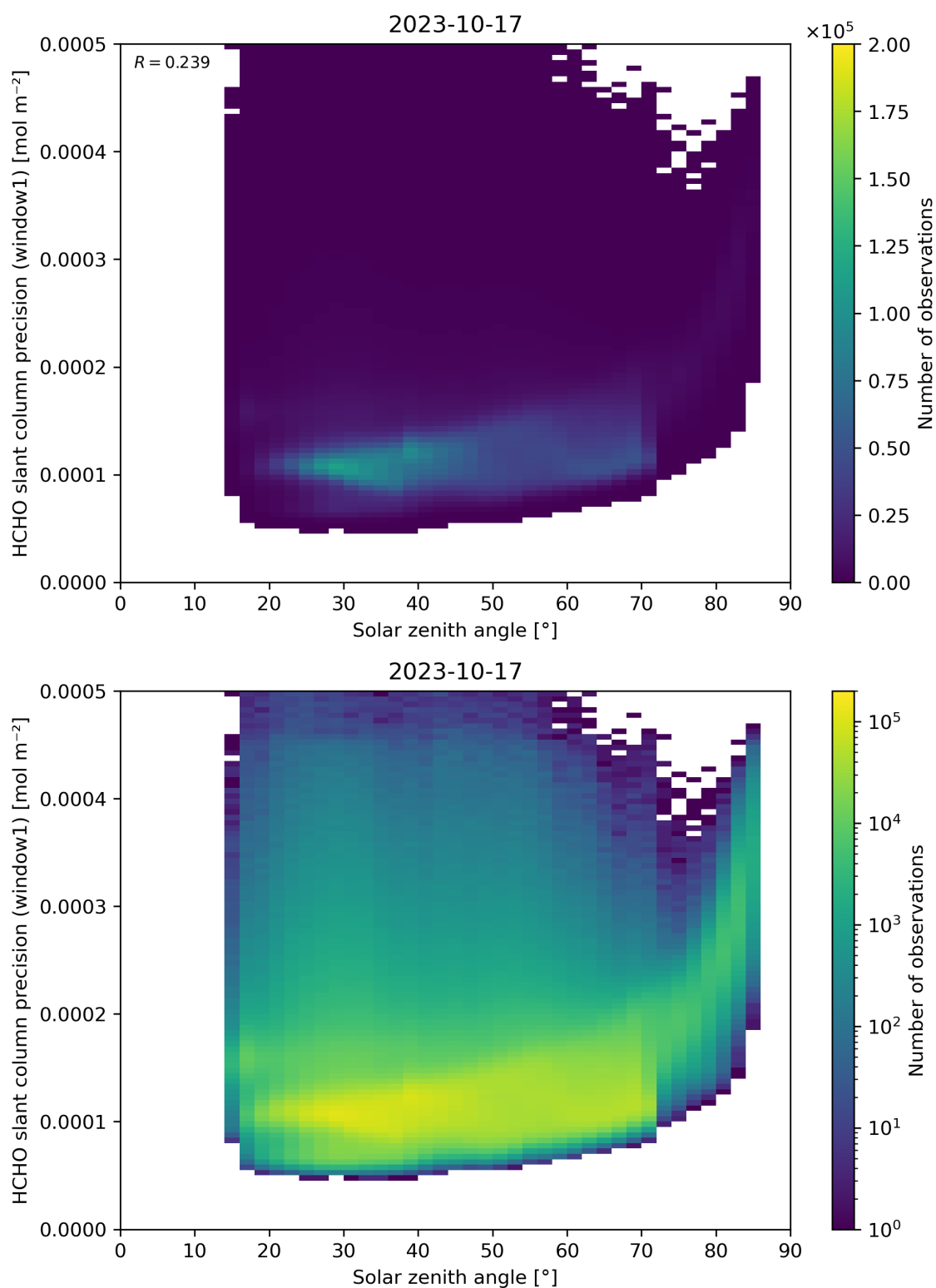
Figure 174: Scatter density plot of “Solar zenith angle” against “HCHO slant column precision (window1)” for 2023-10-17 to 2023-10-18.
