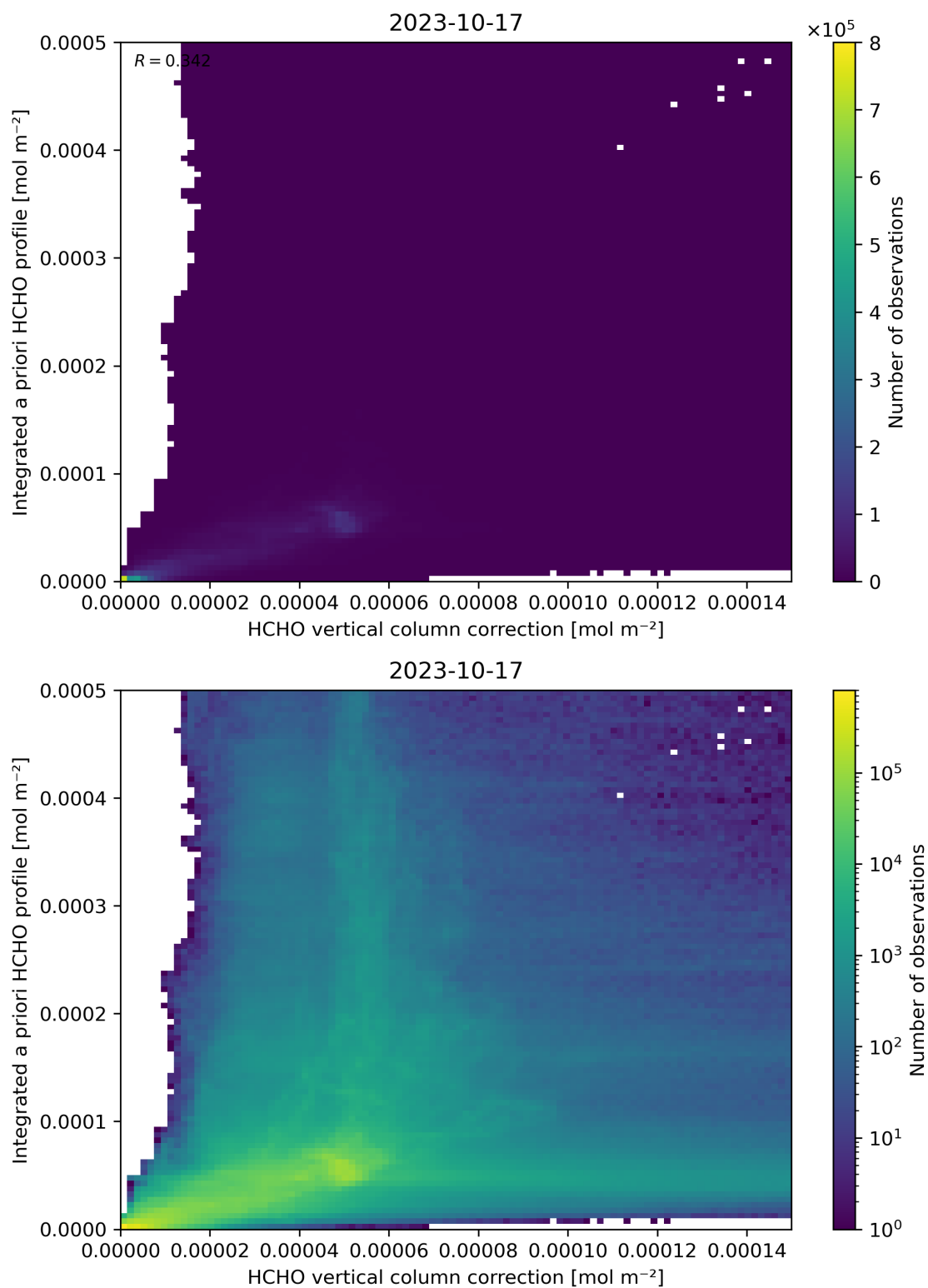
Figure 122: Scatter density plot of “HCHO vertical column correction” against “Integrated a priori HCHO profile” for 2023-10-17 to 2023-10-18.
