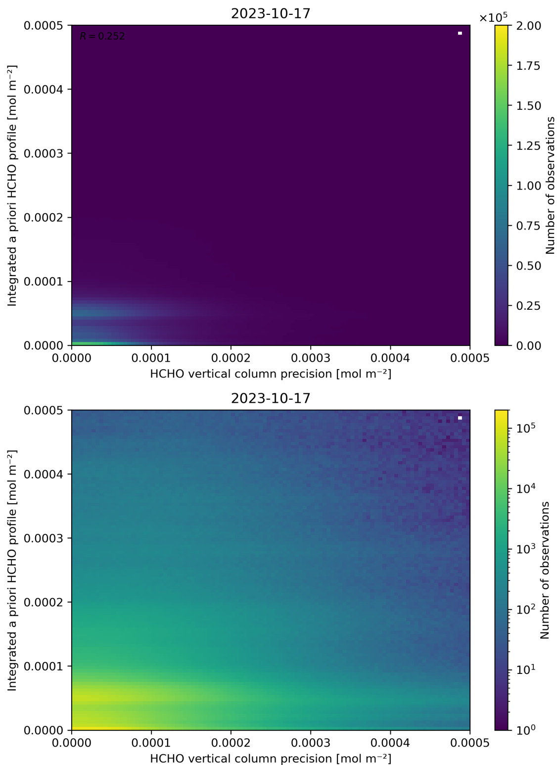
Figure 147: Scatter density plot of “HCHO vertical column precision” against “Integrated a priori HCHO profile” for 2023-10-17 to 2023-10-18.
