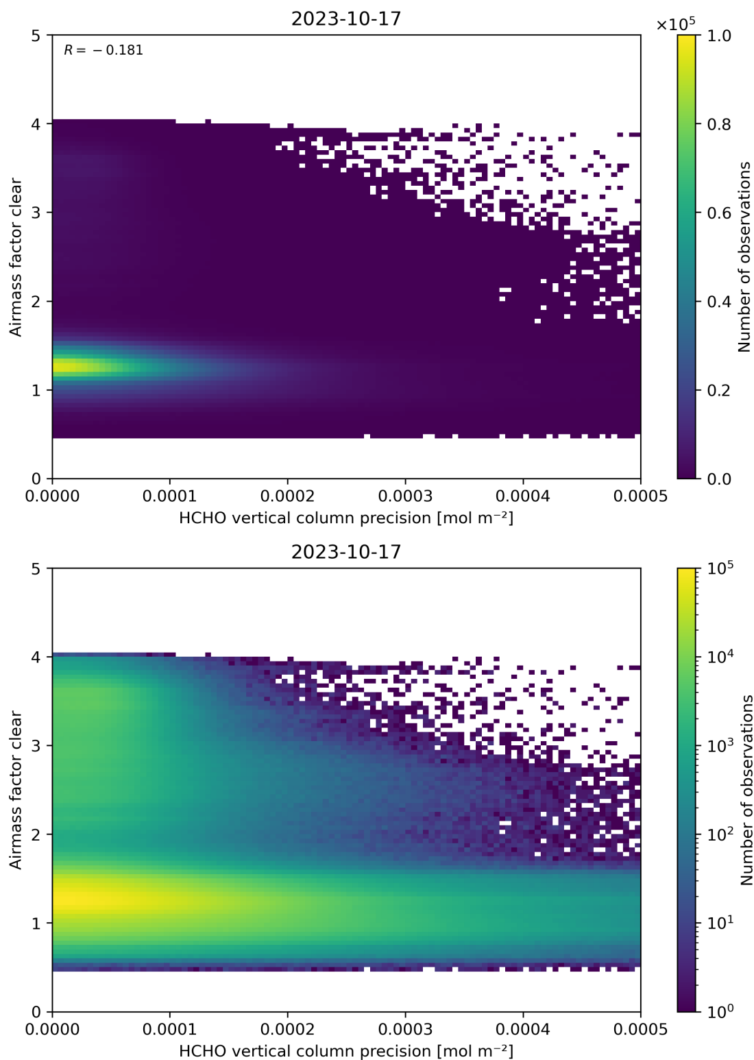
Figure 139: Scatter density plot of “HCHO vertical column precision” against “Airmass factor clear” for 2023-10-17 to 2023-10-18.
