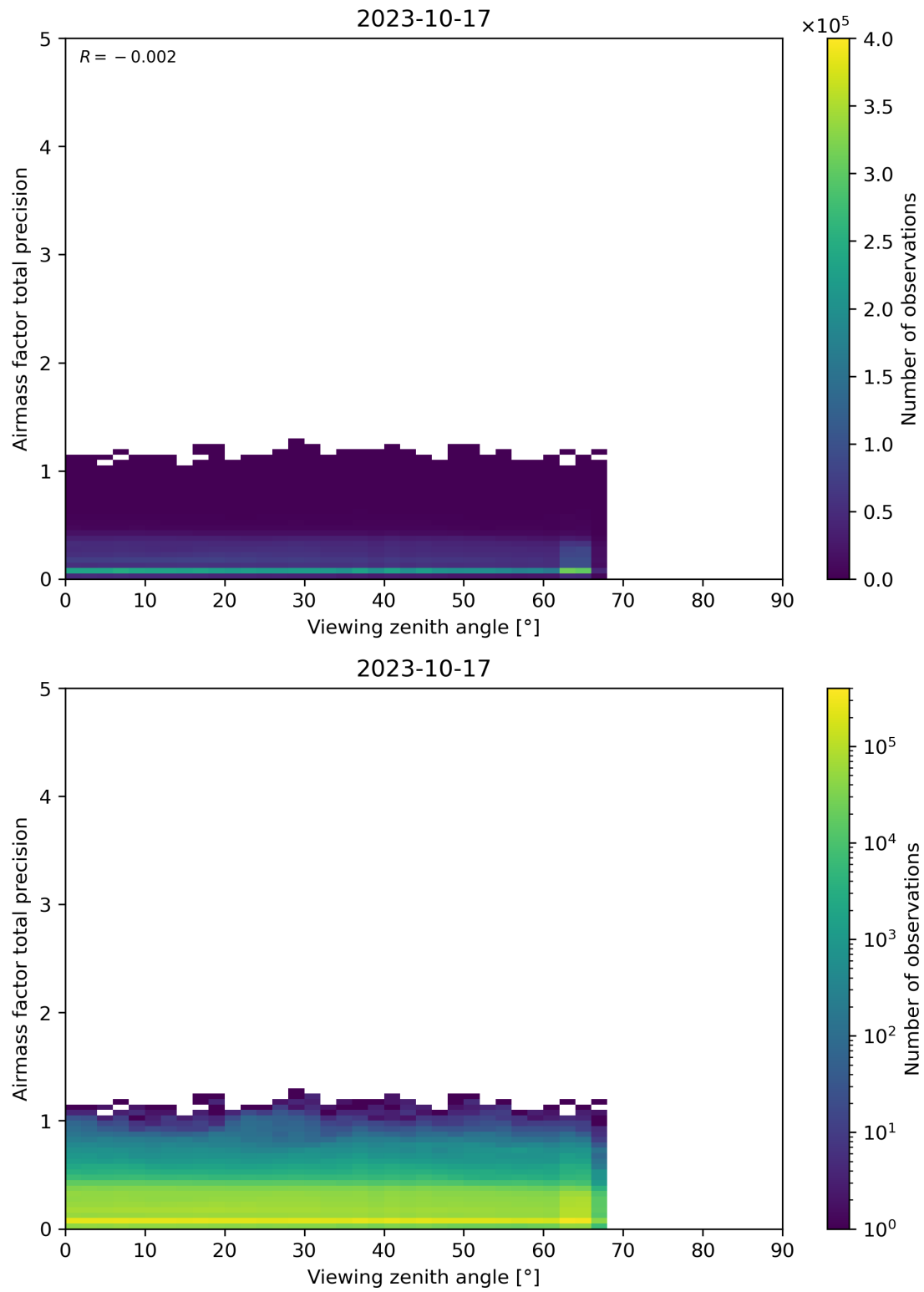
Figure 191: Scatter density plot of “Viewing zenith angle” against “Airmass factor total precision” for 2023-10-17 to 2023-10-18.
