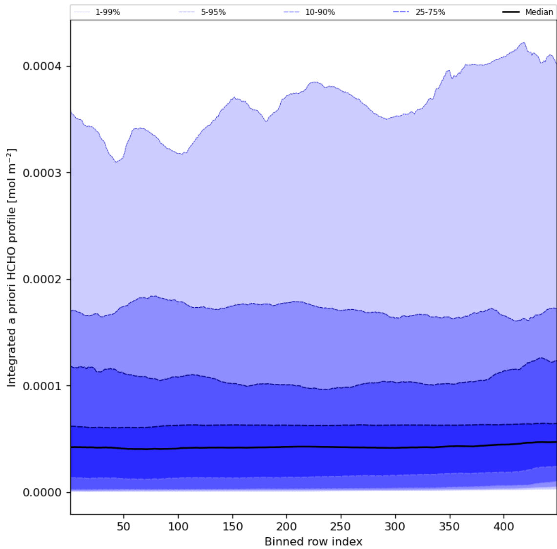
Figure 57: Along track statistics of "Integrated a priori HCHO profile" for 2023-10-17 to 2023-10-18
