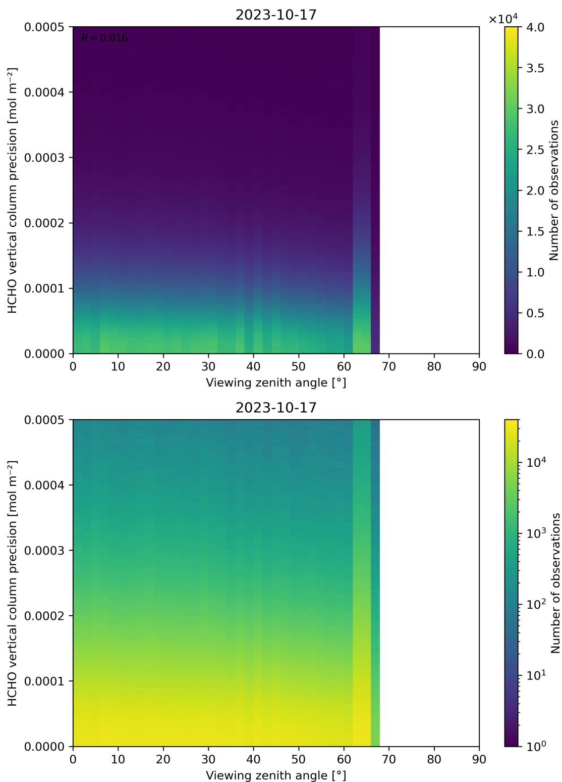
Figure 194: Scatter density plot of “Viewing zenith angle” against “HCHO vertical column precision” for 2023-10-17 to 2023-10-18.
