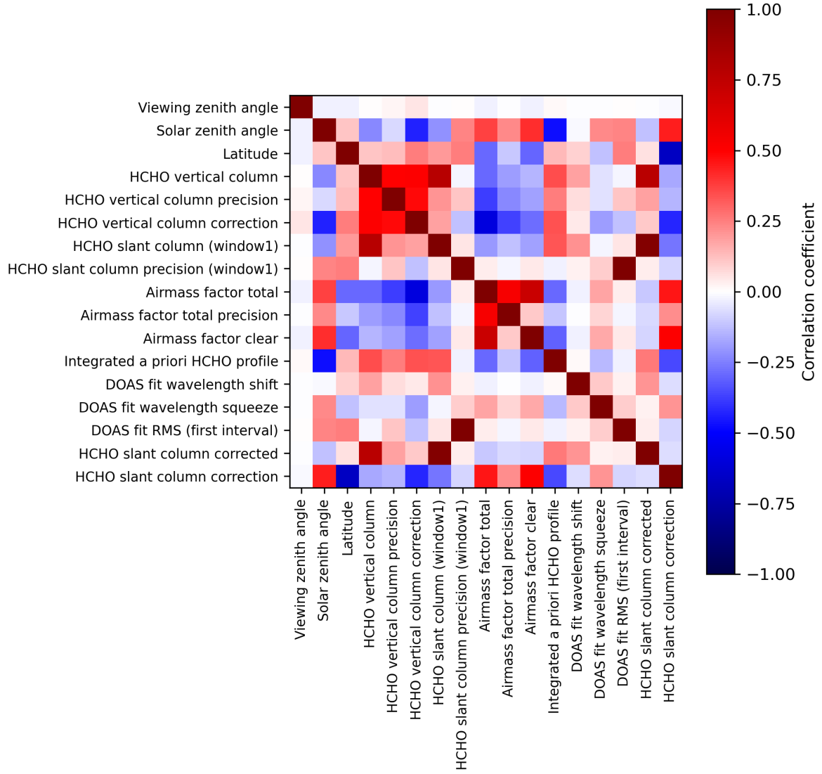
Figure 2: Map of correlation matrix for 2023-10-17 to 2023-10-18.
