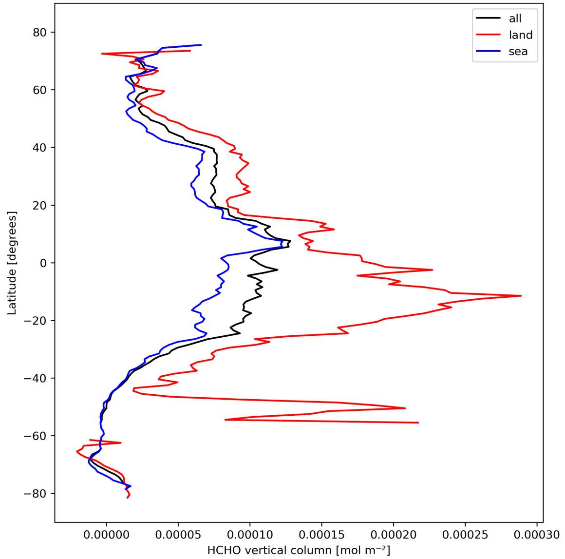
Figure 21: Zonal average of “HCHO vertical column” for 2023-10-17 to 2023-10-18.
