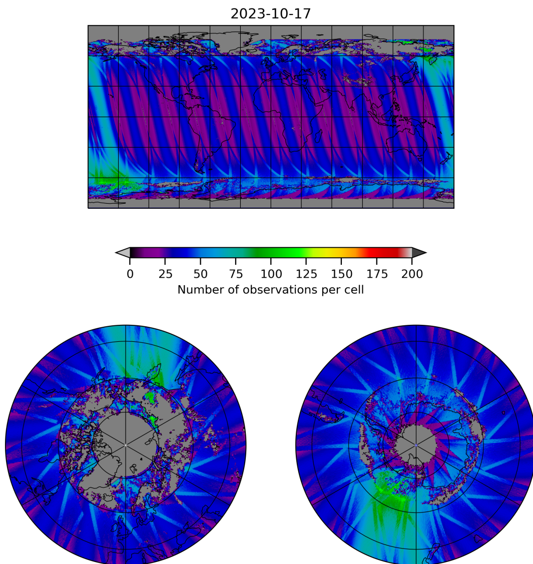
Figure 19: Map of the number of observations for 2023-10-17 to 2023-10-18
