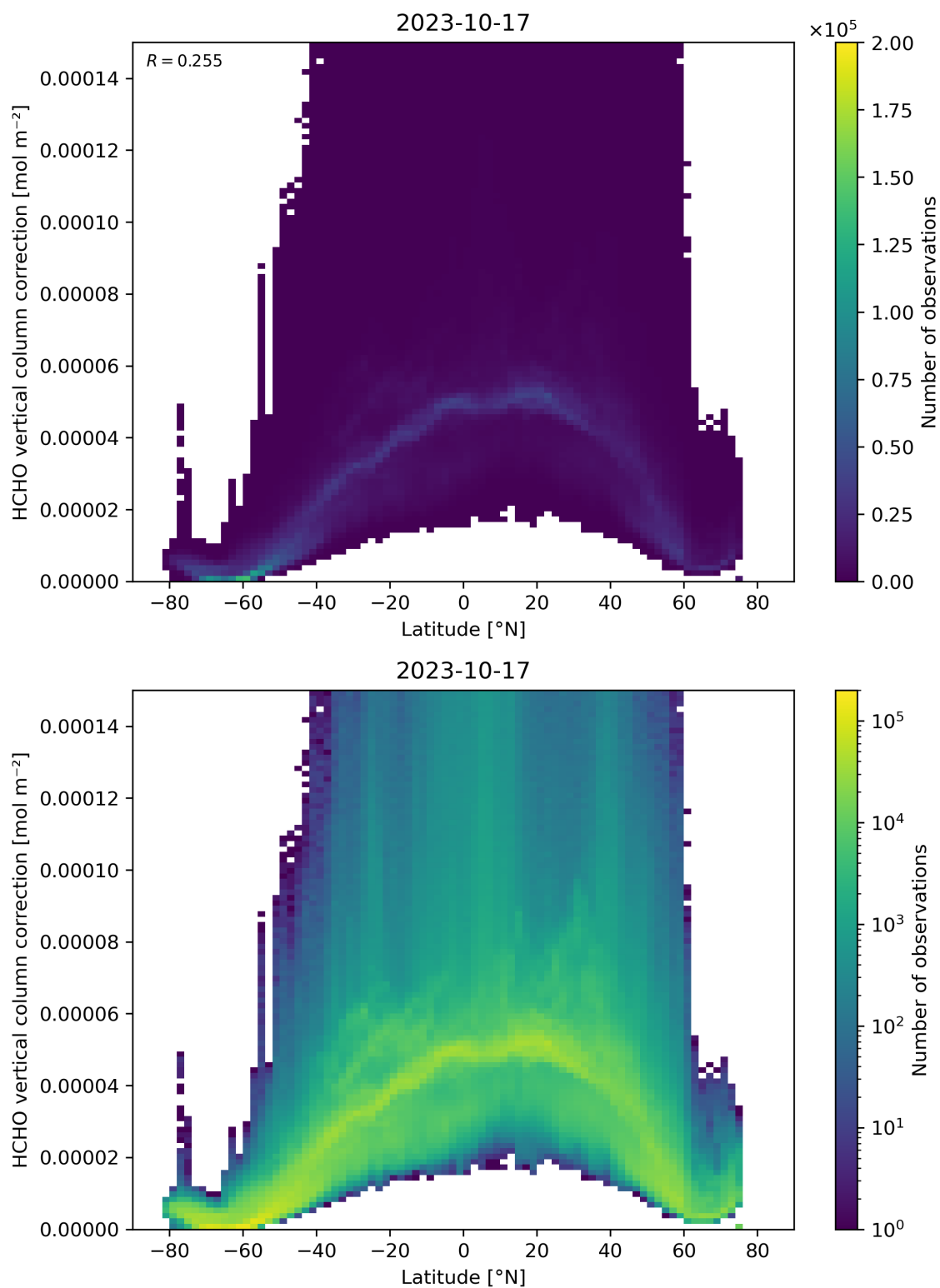
Figure 164: Scatter density plot of “Latitude” against “HCHO vertical column correction” for 2023-10-17 to 2023-10-18.
