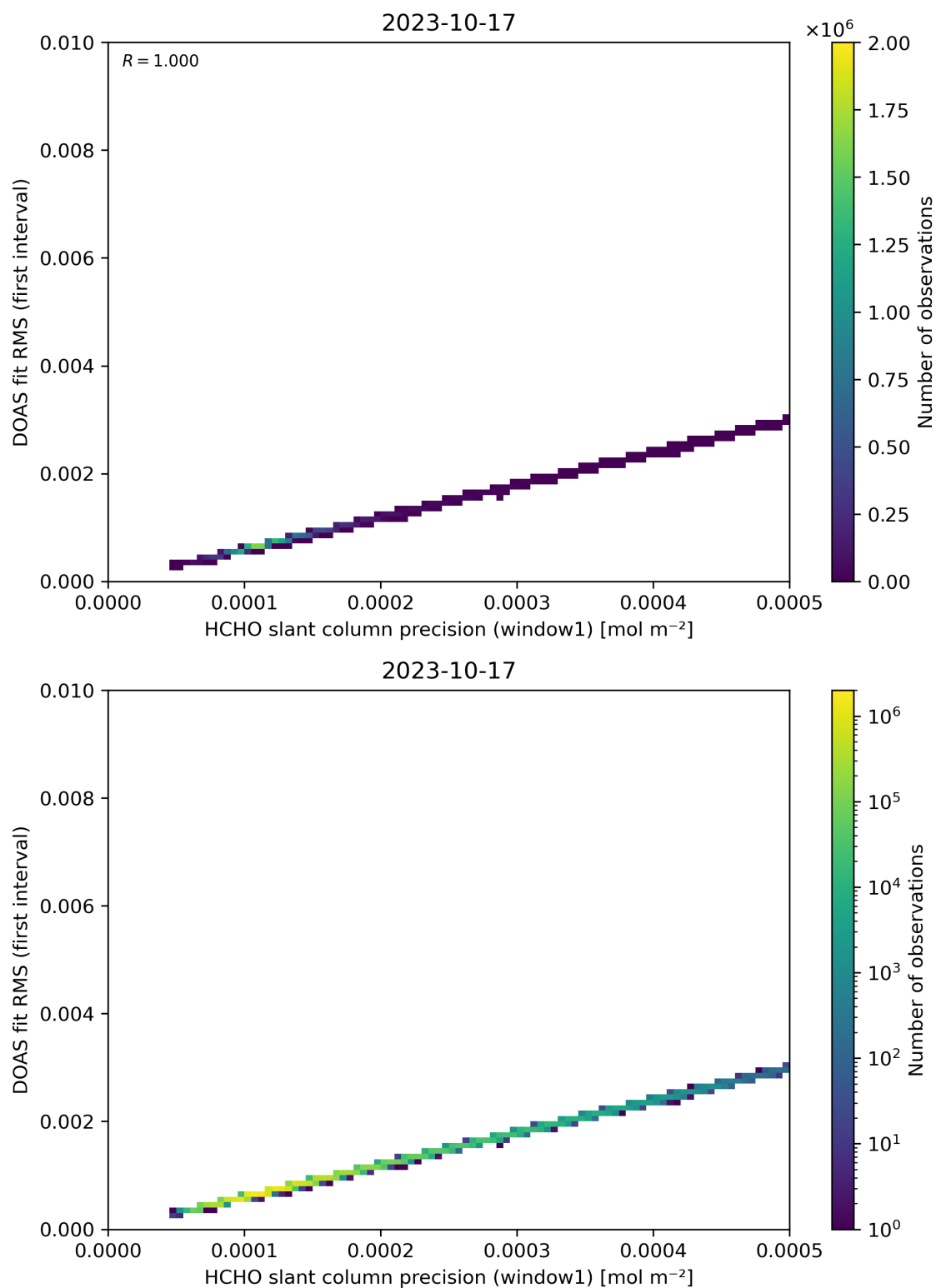
Figure 88: Scatter density plot of “HCHO slant column precision (window1)” against “DOAS fit RMS (first interval)” for 2023-10-17 to 2023-10-18.
