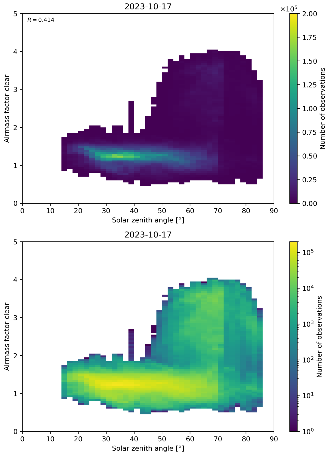
Figure 170: Scatter density plot of “Solar zenith angle” against “Airmass factor clear” for 2023-10-17 to 2023-10-18.
