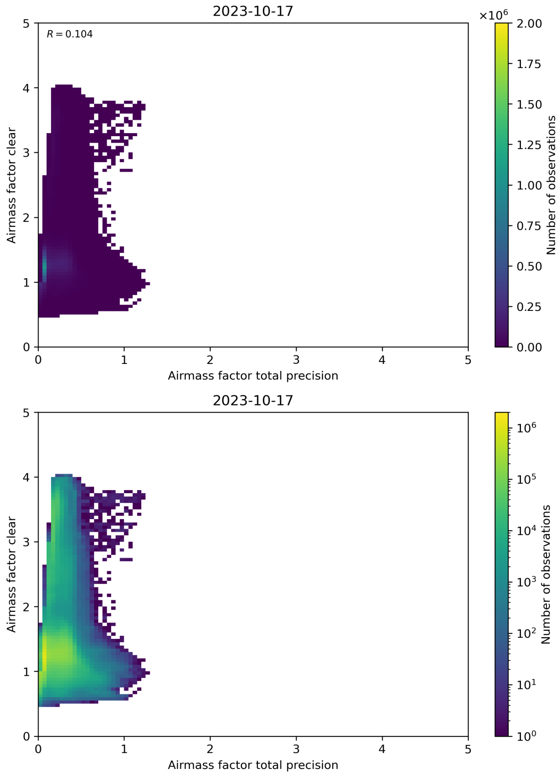
Figure 108: Scatter density plot of “Airmass factor total precision” against “Airmass factor clear” for 2023-10-17 to 2023-10-18.
