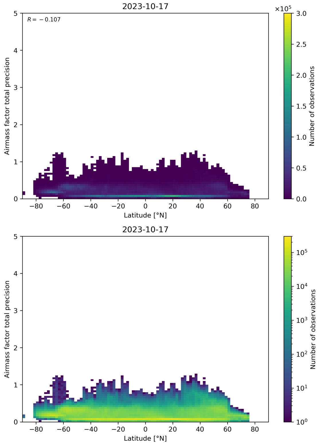
Figure 162: Scatter density plot of “Latitude” against “Airmass factor total precision” for 2023-10-17 to 2023-10-18.
