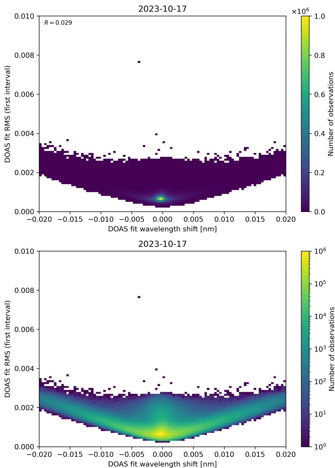
Figure 64: Scatter density plot of “DOAS fit wavelength shift” against “DOAS fit RMS (first interval)” for 2023-10-17 to 2023-10-18.
