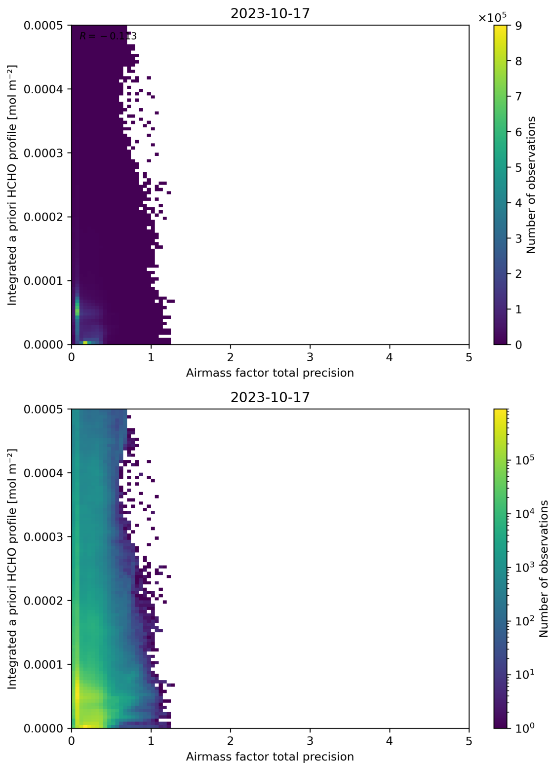
Figure 111: Scatter density plot of “Airmass factor total precision” against “Integrated a priori HCHO profile” for 2023-10-17 to 2023-10-18.
