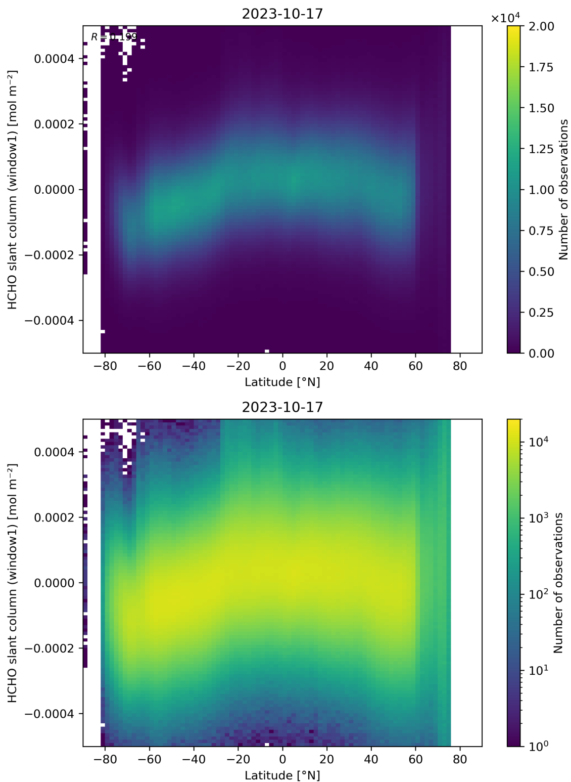
Figure 159: Scatter density plot of “Latitude” against “HCHO slant column (window1)” for 2023-10-17 to 2023-10-18.
