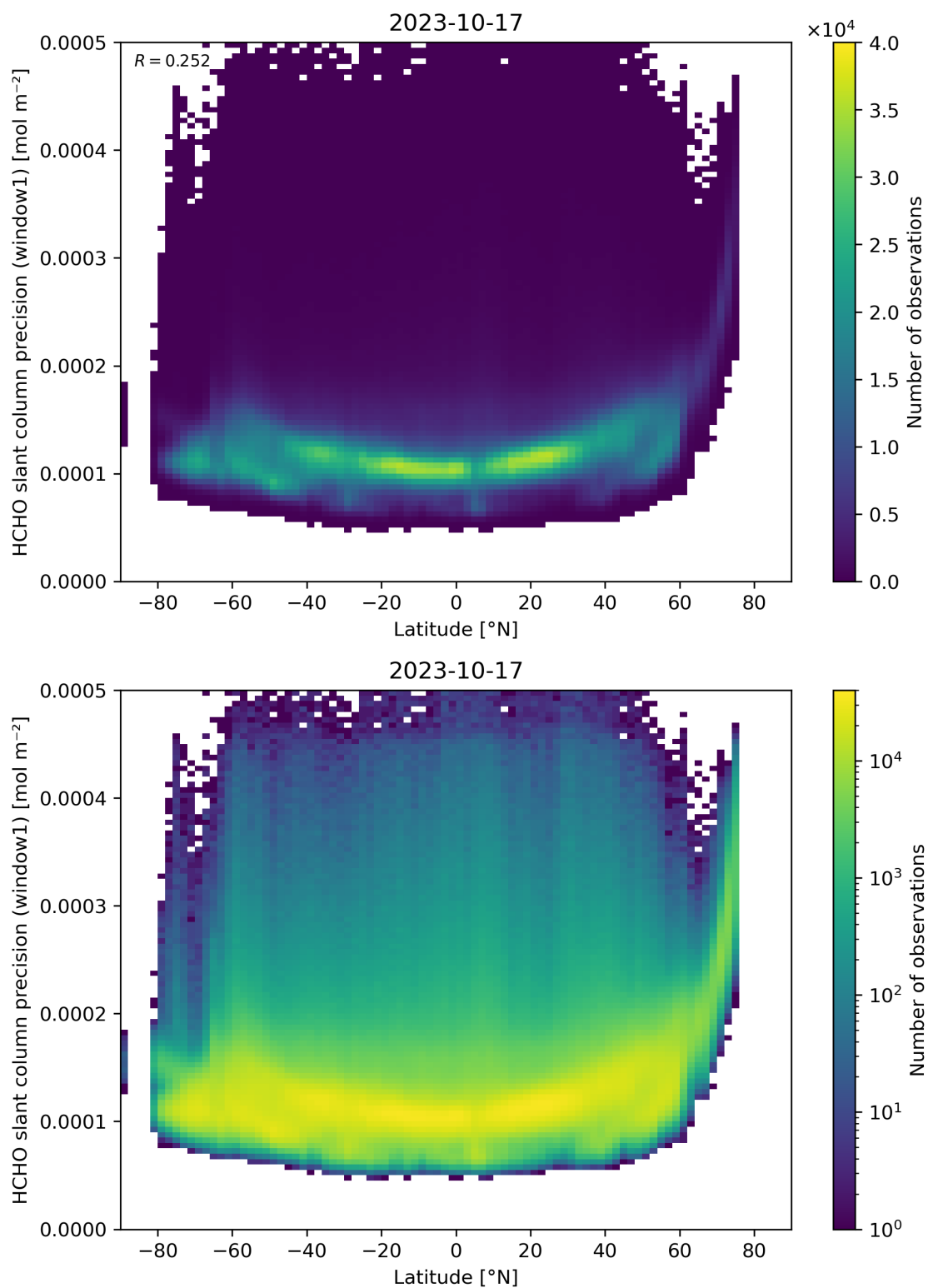
Figure 160: Scatter density plot of “Latitude” against “HCHO slant column precision (window1)” for 2023-10-17 to 2023-10-18.
