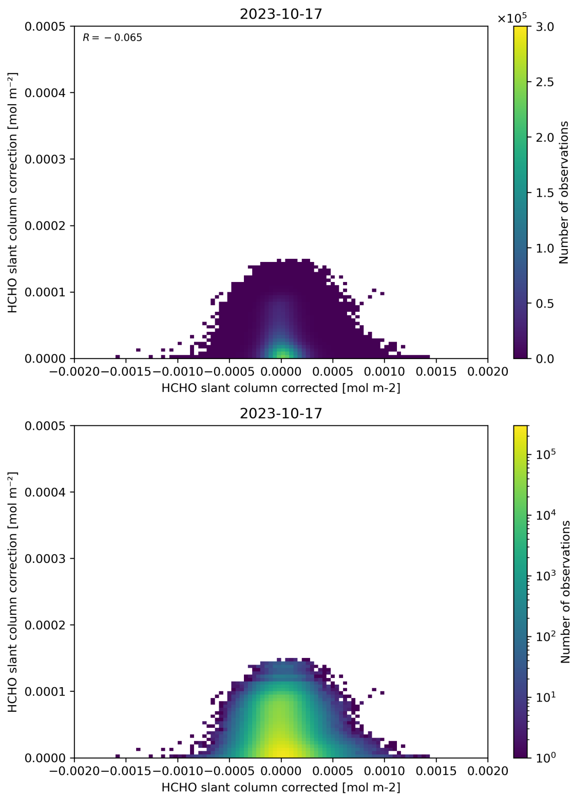
Figure 77: Scatter density plot of “HCHO slant column corrected” against “HCHO slant column correction” for 2023-10-17 to 2023-10-18.
