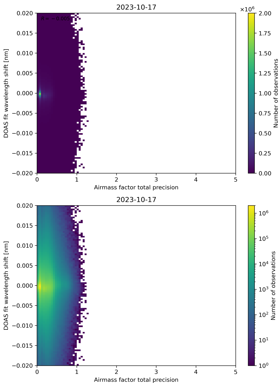
Figure 106: Scatter density plot of “Airmass factor total precision” against “DOAS fit wavelength shift” for 2023-10-17 to 2023-10-18.
