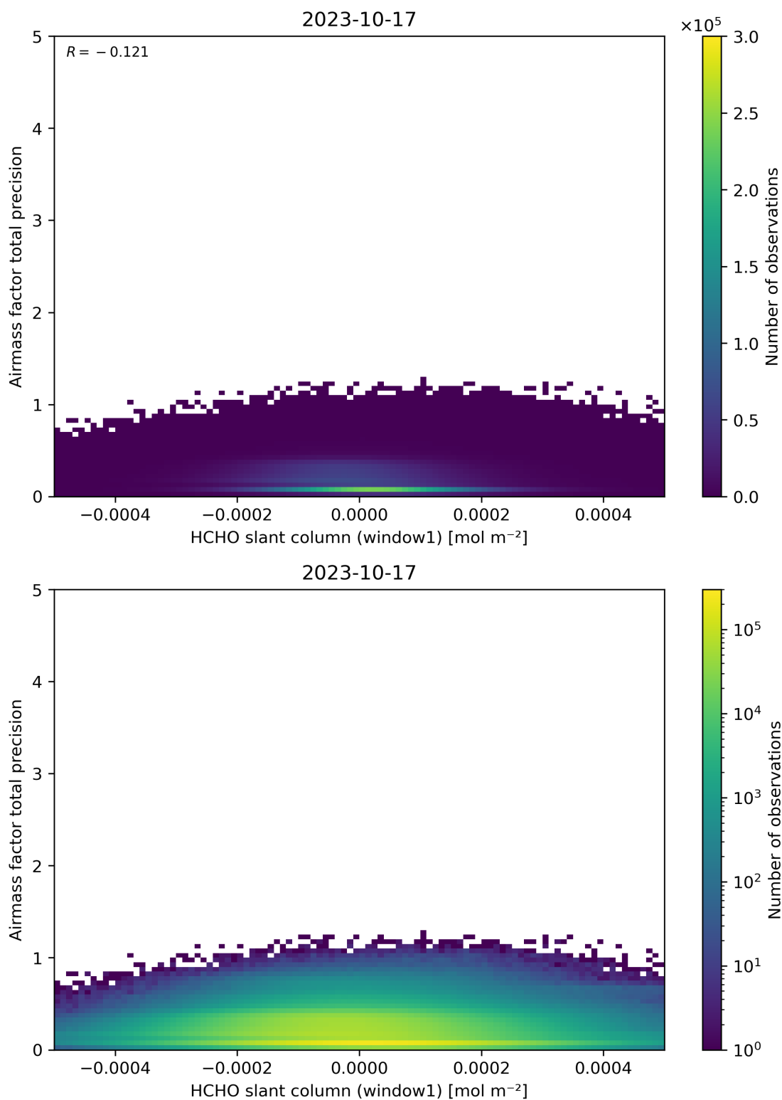
Figure 86: Scatter density plot of “HCHO slant column (window1)” against “Airmass factor total precision” for 2023-10-17 to 2023-10-18.
