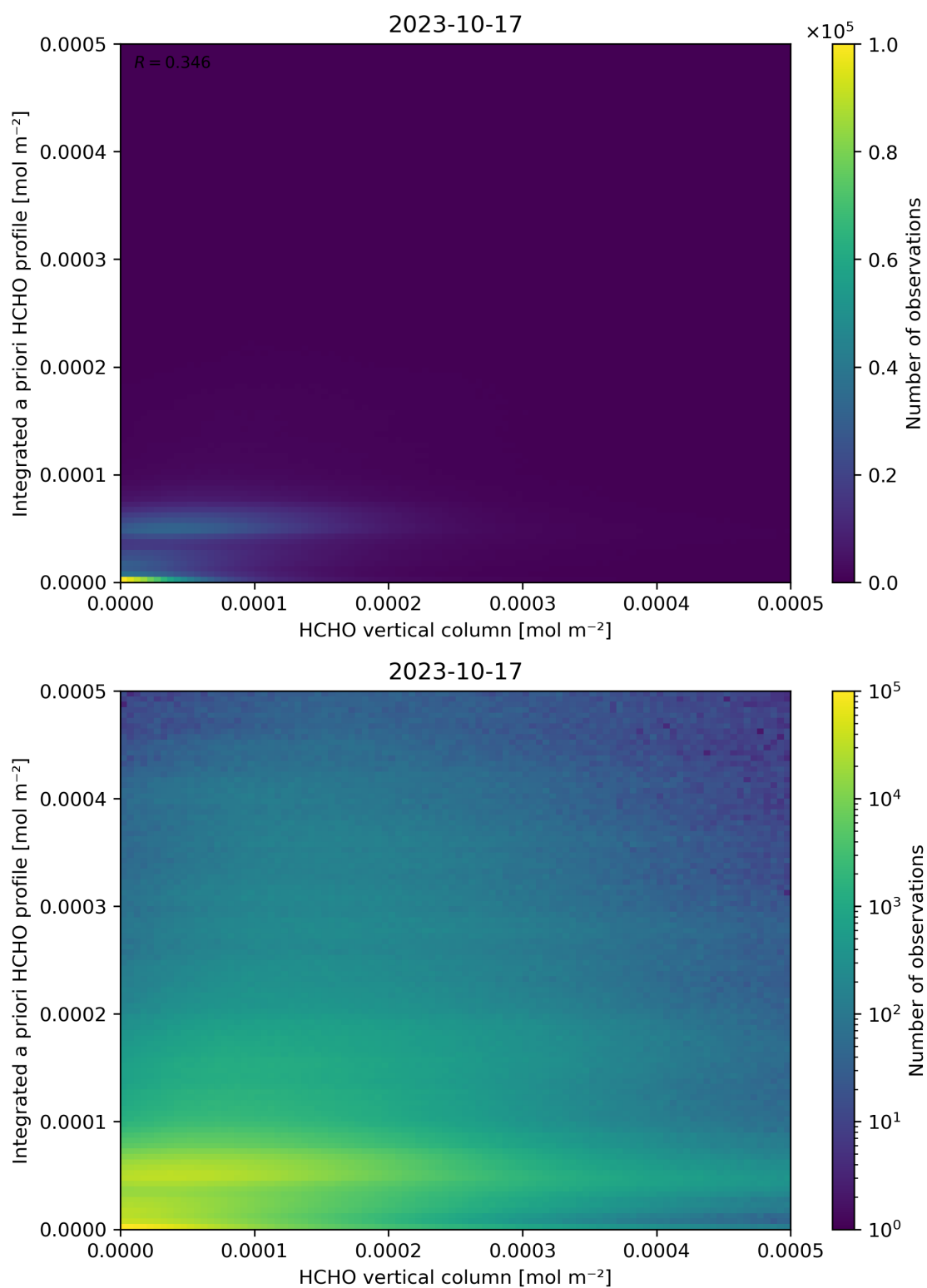
Figure 135: Scatter density plot of “HCHO vertical column” against “Integrated a priori HCHO profile” for 2023-10-17 to 2023-10-18.
