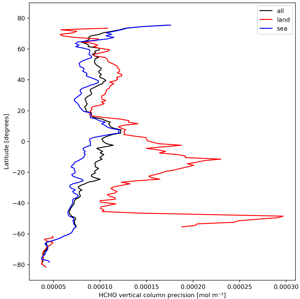
Figure 22: Zonal average of “HCHO vertical column precision” for 2023-10-17 to 2023-10-18.
