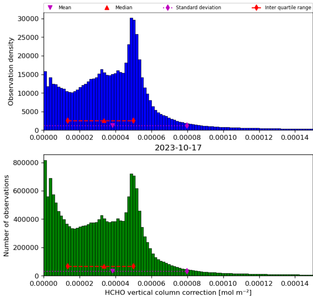
Figure 37: Histogram of “HCHO vertical column correction” for 2023-10-17 to 2023-10-18
