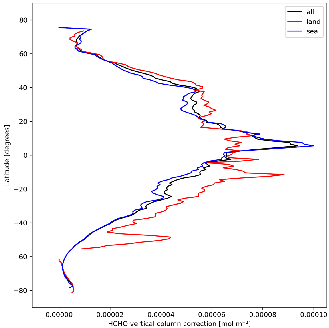
Figure 23: Zonal average of “HCHO vertical column correction” for 2023-10-17 to 2023-10-18.
