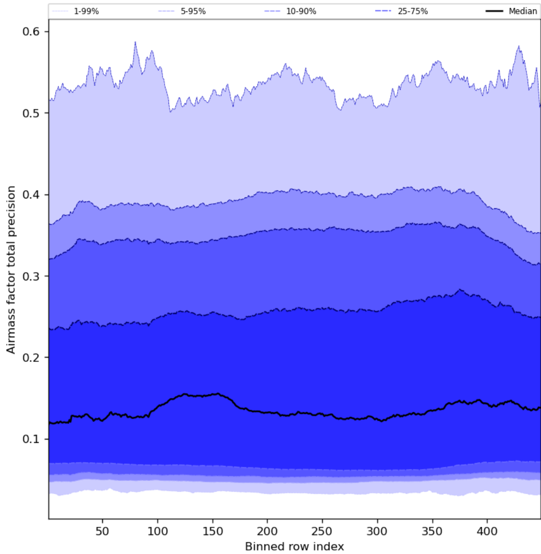
Figure 55: Along track statistics of “Airmass factor total precision” for 2023-10-17 to 2023-10-18
