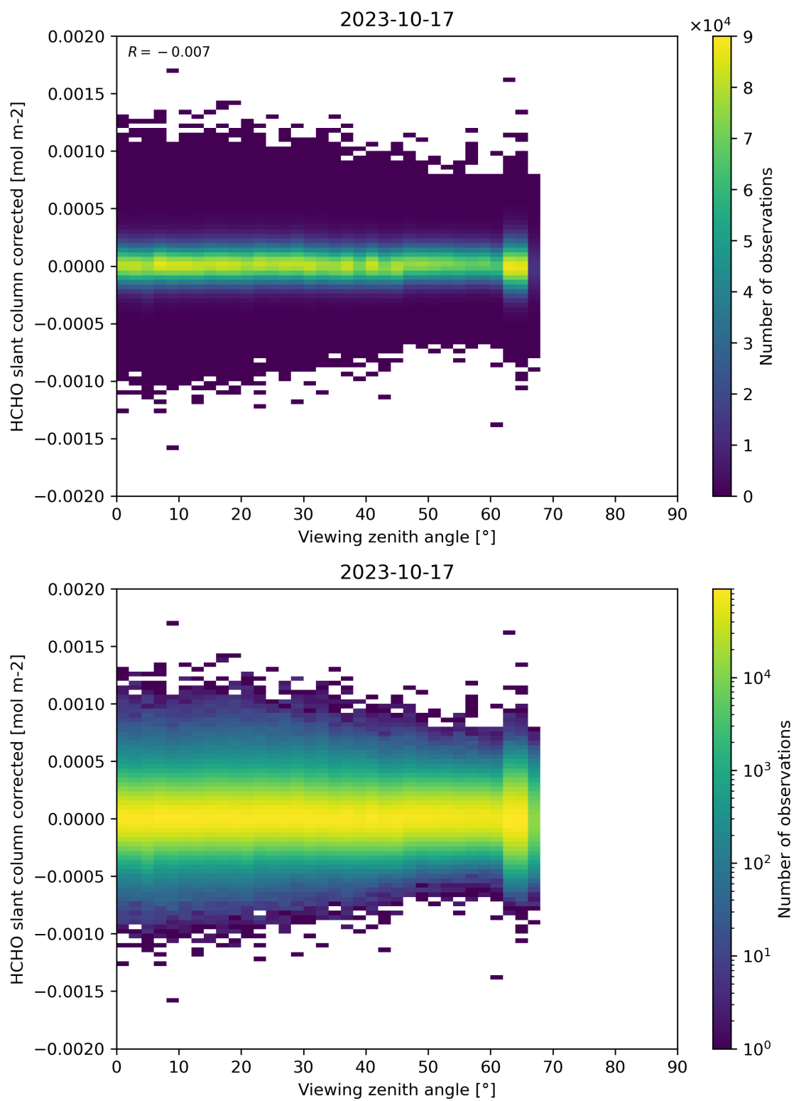
Figure 186: Scatter density plot of “Viewing zenith angle” against “HCHO slant column corrected” for 2023-10-17 to 2023-10-18.
