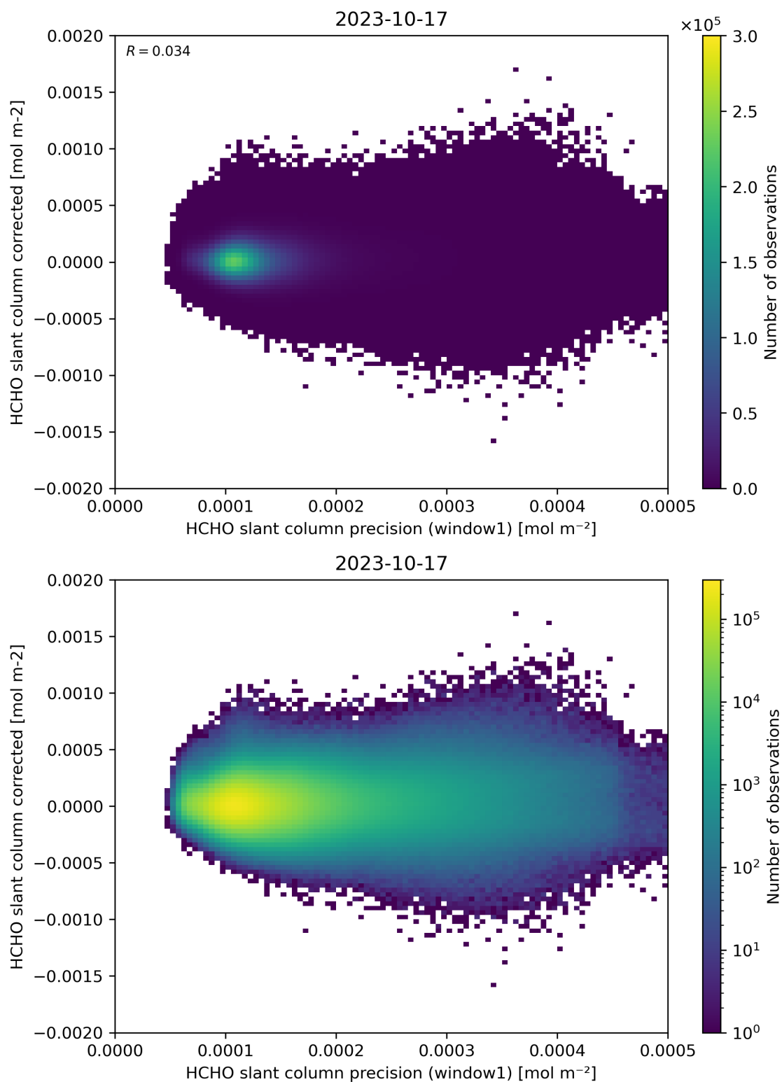
Figure 92: Scatter density plot of “HCHO slant column precision (window1)” against “HCHO slant column corrected” for 2023-10-17 to 2023-10-18.
