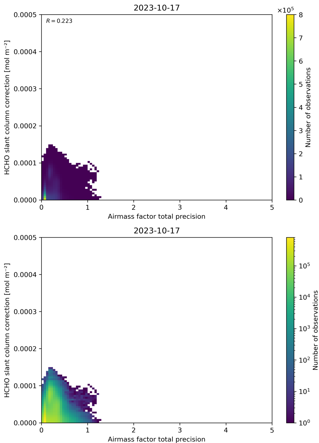
Figure 110: Scatter density plot of “Airmass factor total precision” against “HCHO slant column correction” for 2023-10-17 to 2023-10-18.
