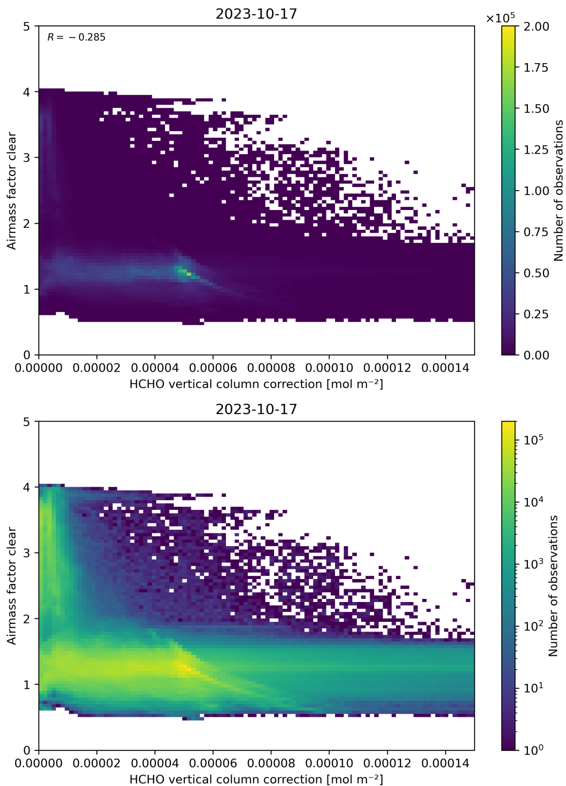
Figure 115: Scatter density plot of “HCHO vertical column correction” against “Airmass factor clear” for 2023-10-17 to 2023-10-18.
