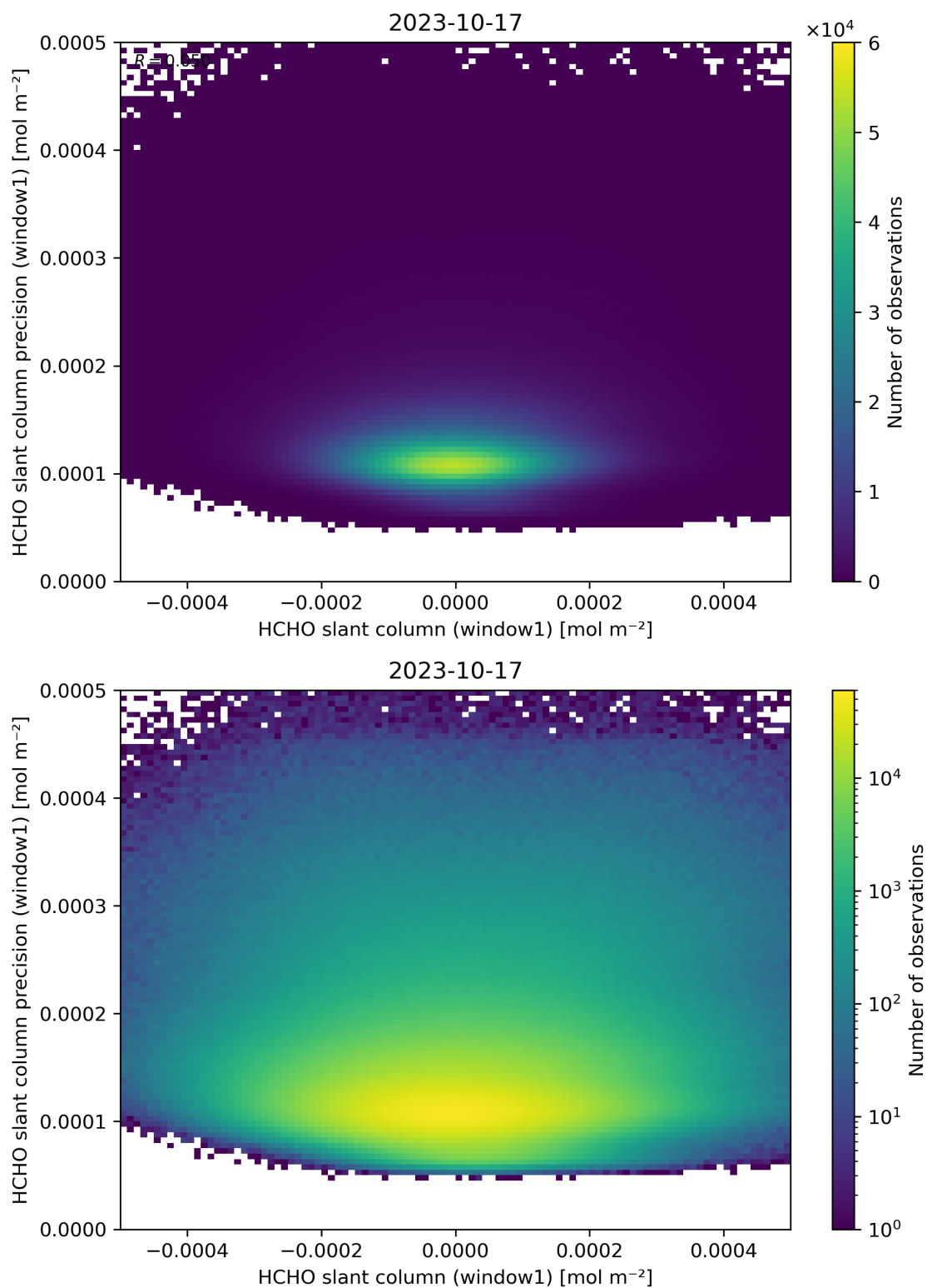
Figure 84: Scatter density plot of “HCHO slant column (window1)” against “HCHO slant column precision (window1)” for 2023-10-17 to 2023-10-18.
