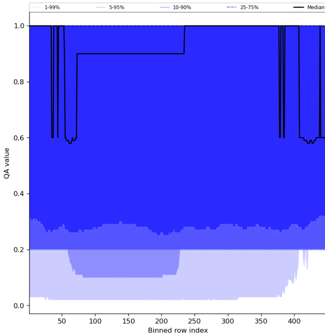
Figure 48: Along track statistics of “QA value” for 2023-10-17 to 2023-10-18
