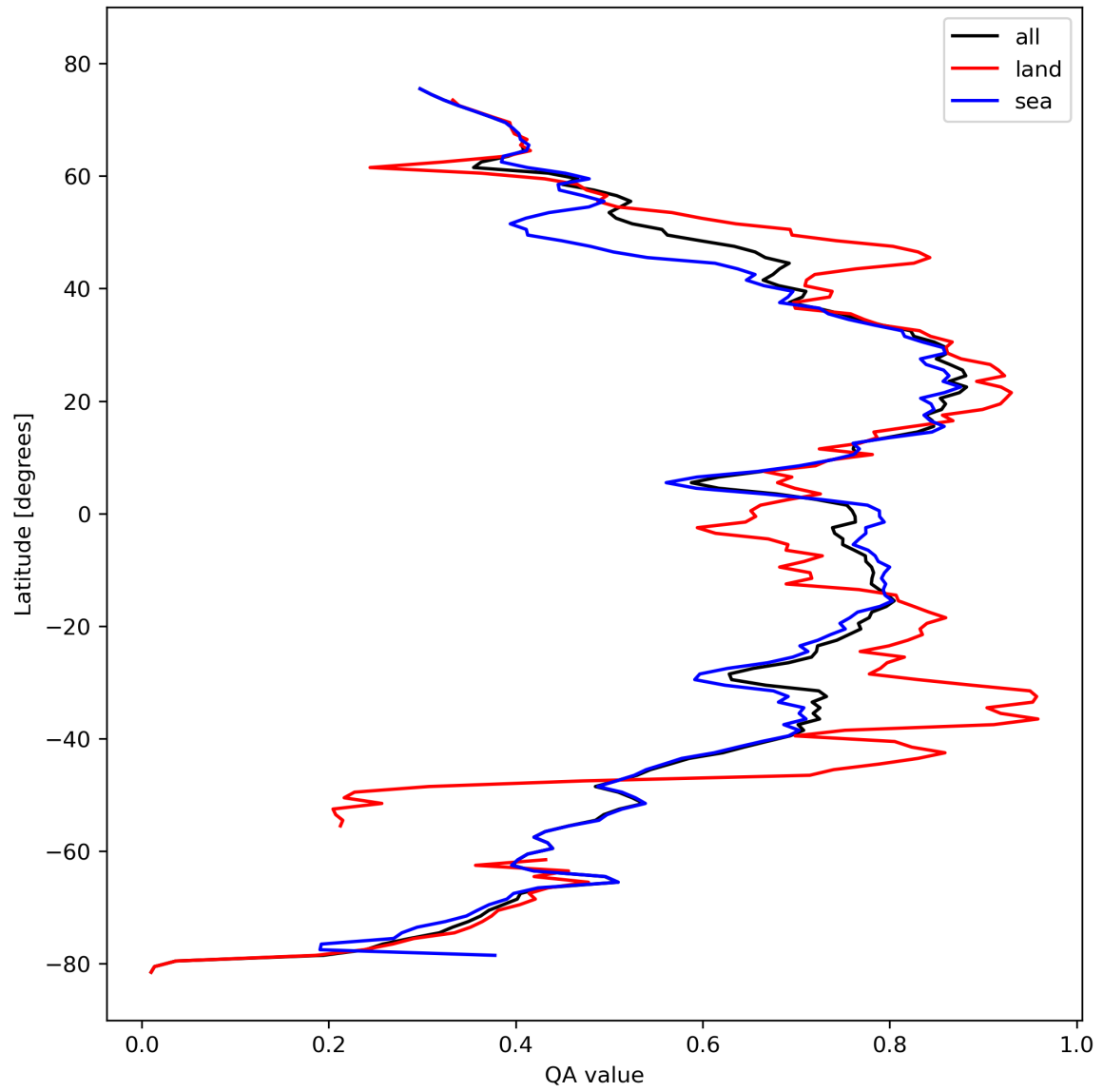
Figure 20: Zonal average of “QA value” for 2023-10-17 to 2023-10-18.
