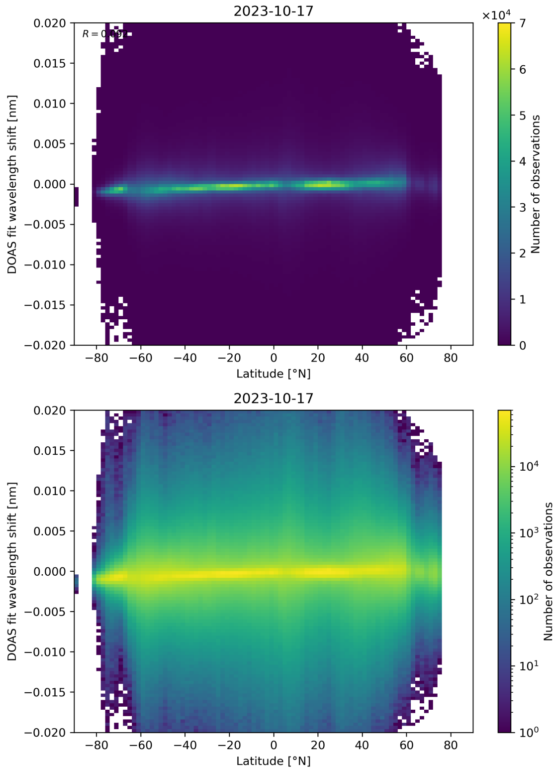
Figure 154: Scatter density plot of “Latitude” against “DOAS fit wavelength shift” for 2023-10-17 to 2023-10-18.
