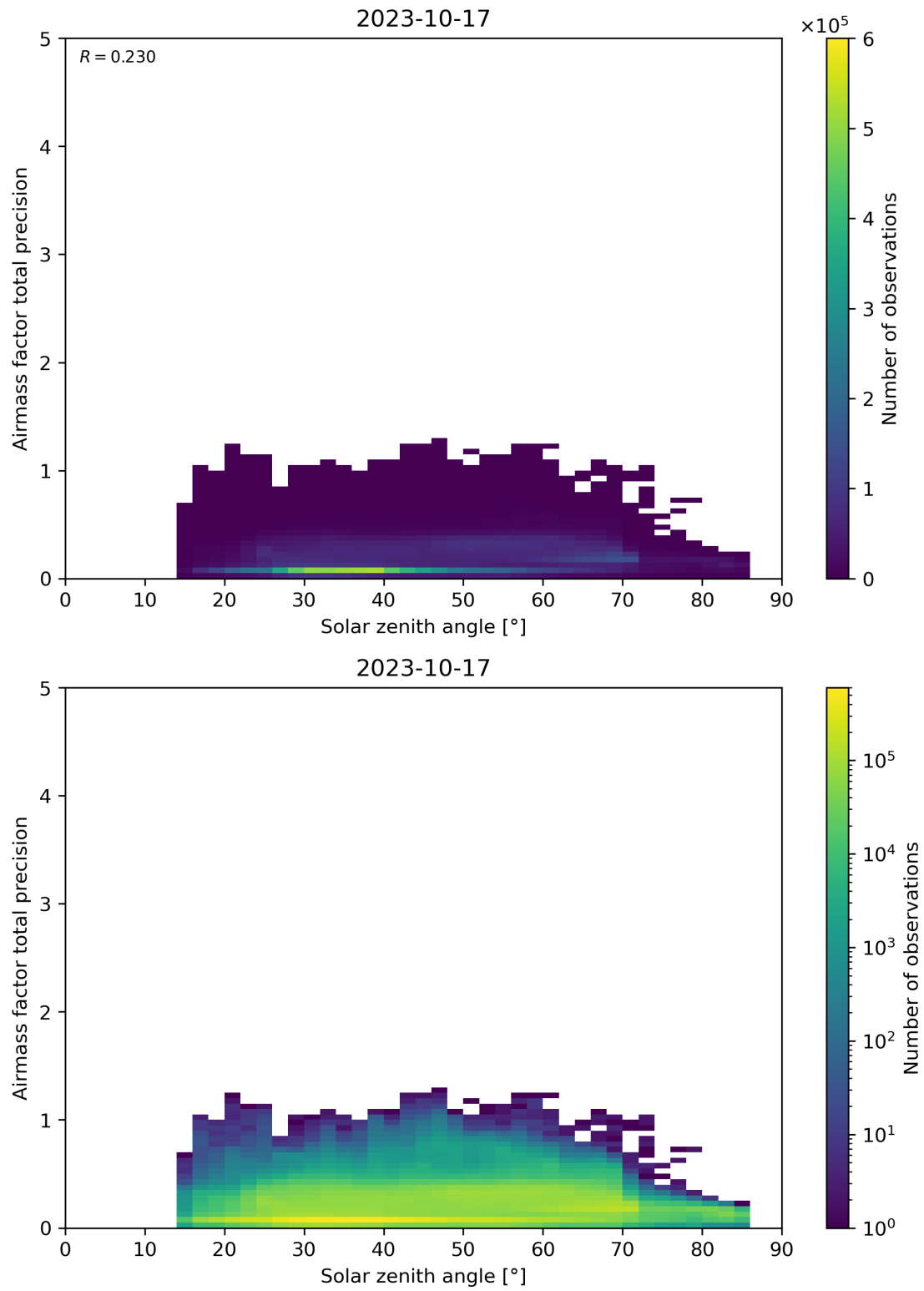
Figure 176: Scatter density plot of “Solar zenith angle” against “Airmass factor total precision” for 2023-10-17 to 2023-10-18.
