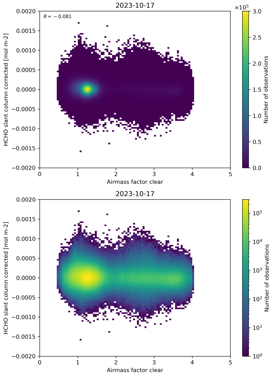
Figure 74: Scatter density plot of “Airmass factor clear” against “HCHO slant column corrected” for 2023-10-17 to 2023-10-18.
