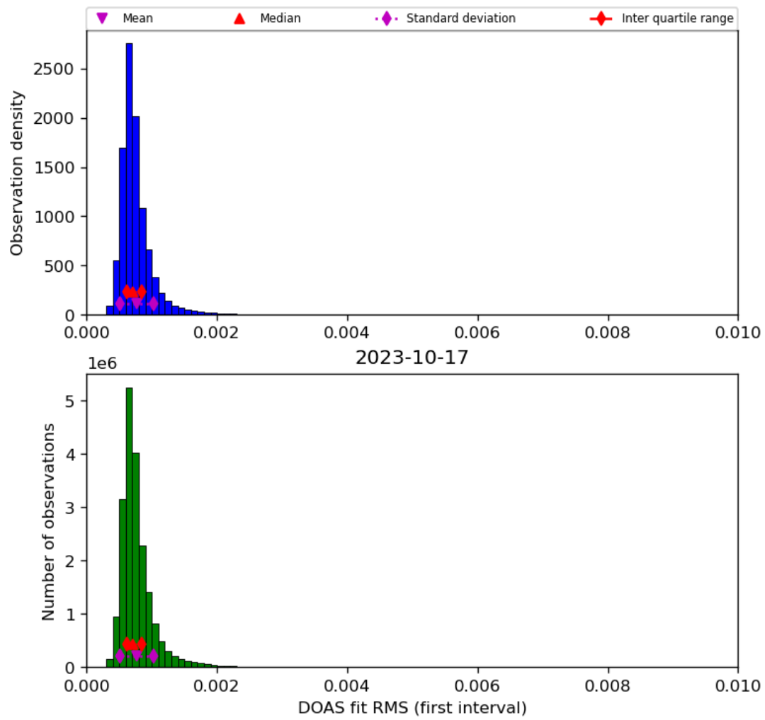
Figure 46: Histogram of “DOAS fit RMS (first interval)” for 2023-10-17 to 2023-10-18
