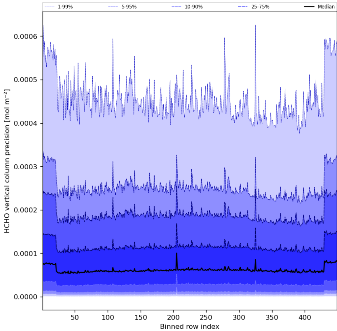
Figure 50: Along track statistics of “HCHO vertical column precision” for 2023-10-17 to 2023-10-18
