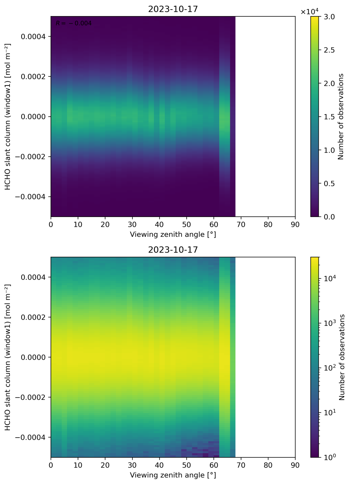
Figure 188: Scatter density plot of “Viewing zenith angle” against “HCHO slant column (window1)” for 2023-10-17 to 2023-10-18.
