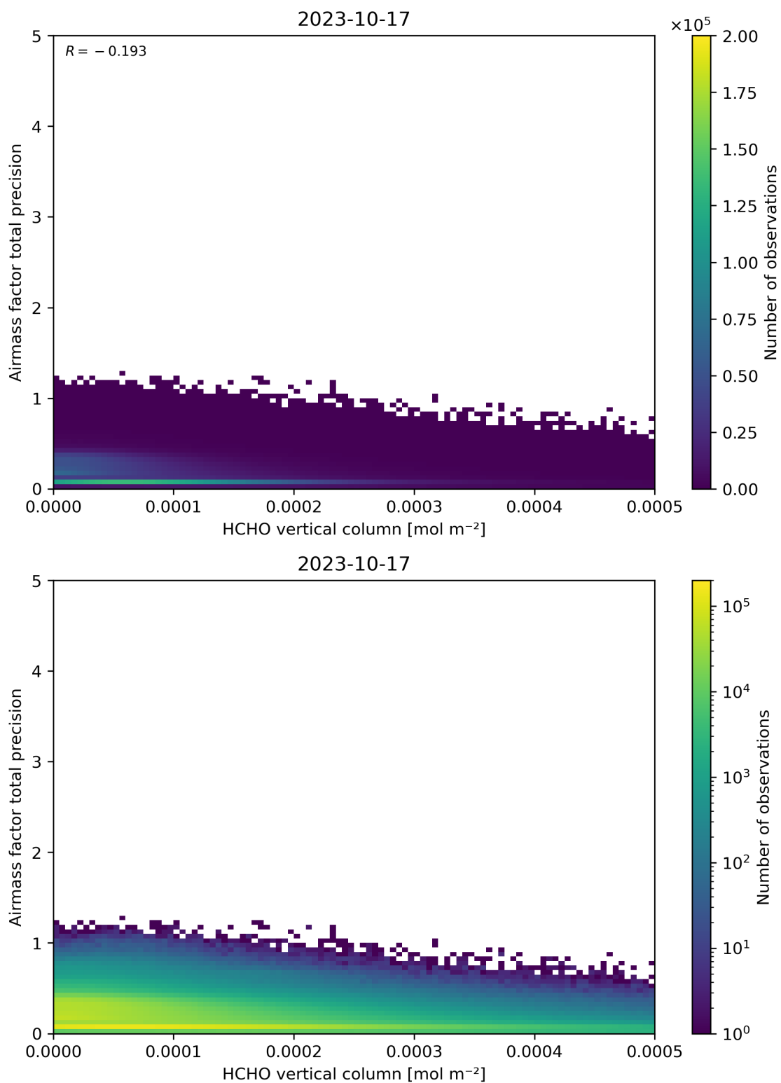
Figure 132: Scatter density plot of “HCHO vertical column” against “Airmass factor total precision” for 2023-10-17 to 2023-10-18.
