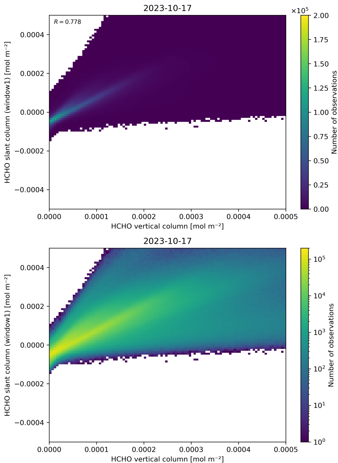
Figure 129: Scatter density plot of “HCHO vertical column” against “HCHO slant column (window1)” for 2023-10-17 to 2023-10-18.
