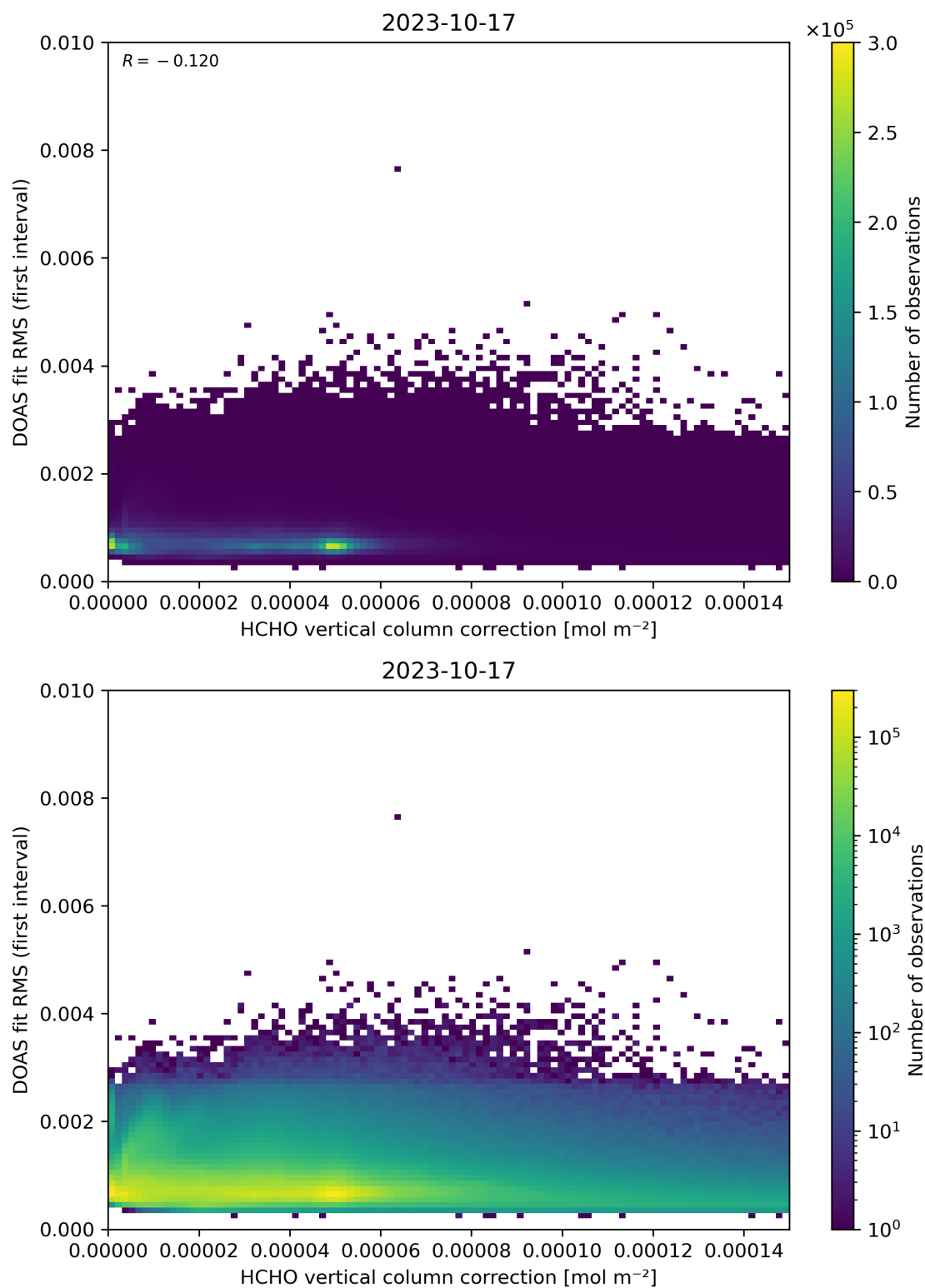
Figure 112: Scatter density plot of “HCHO vertical column correction” against “DOAS fit RMS (first interval)” for 2023-10-17 to 2023-10-18.
