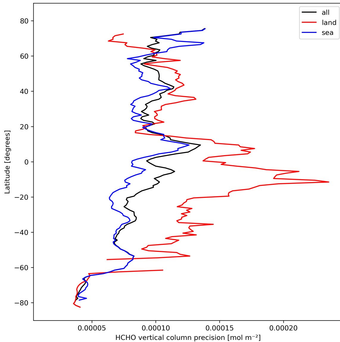
Figure 22: Zonal average of “HCHO vertical column precision” for 2023-10-18 to 2023-10-20.
