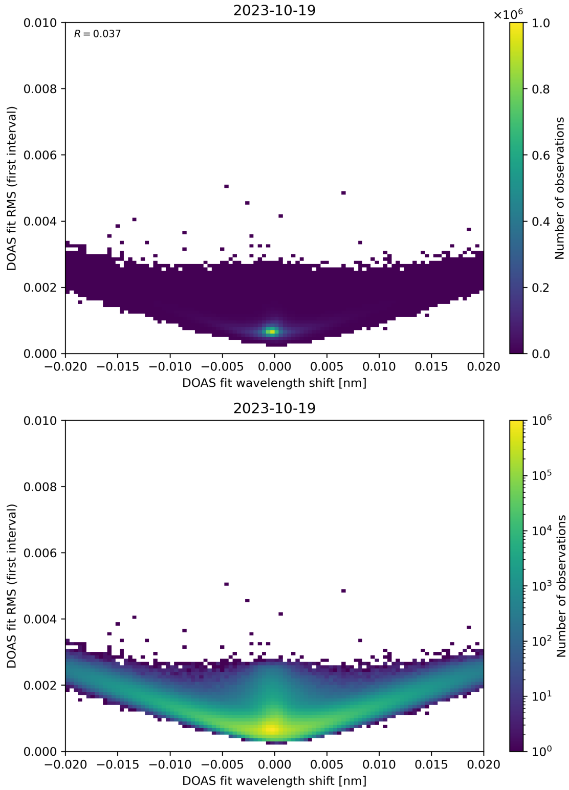
Figure 64: Scatter density plot of “DOAS fit wavelength shift” against “DOAS fit RMS (first interval)” for 2023-10-18 to 2023-10-20.
