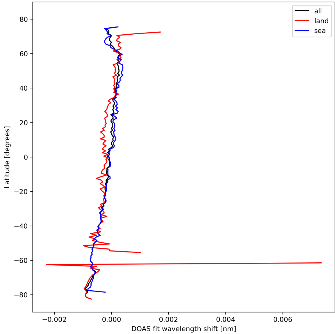
Figure 30: Zonal average of “DOAS fit wavelength shift” for 2023-10-18 to 2023-10-20.
