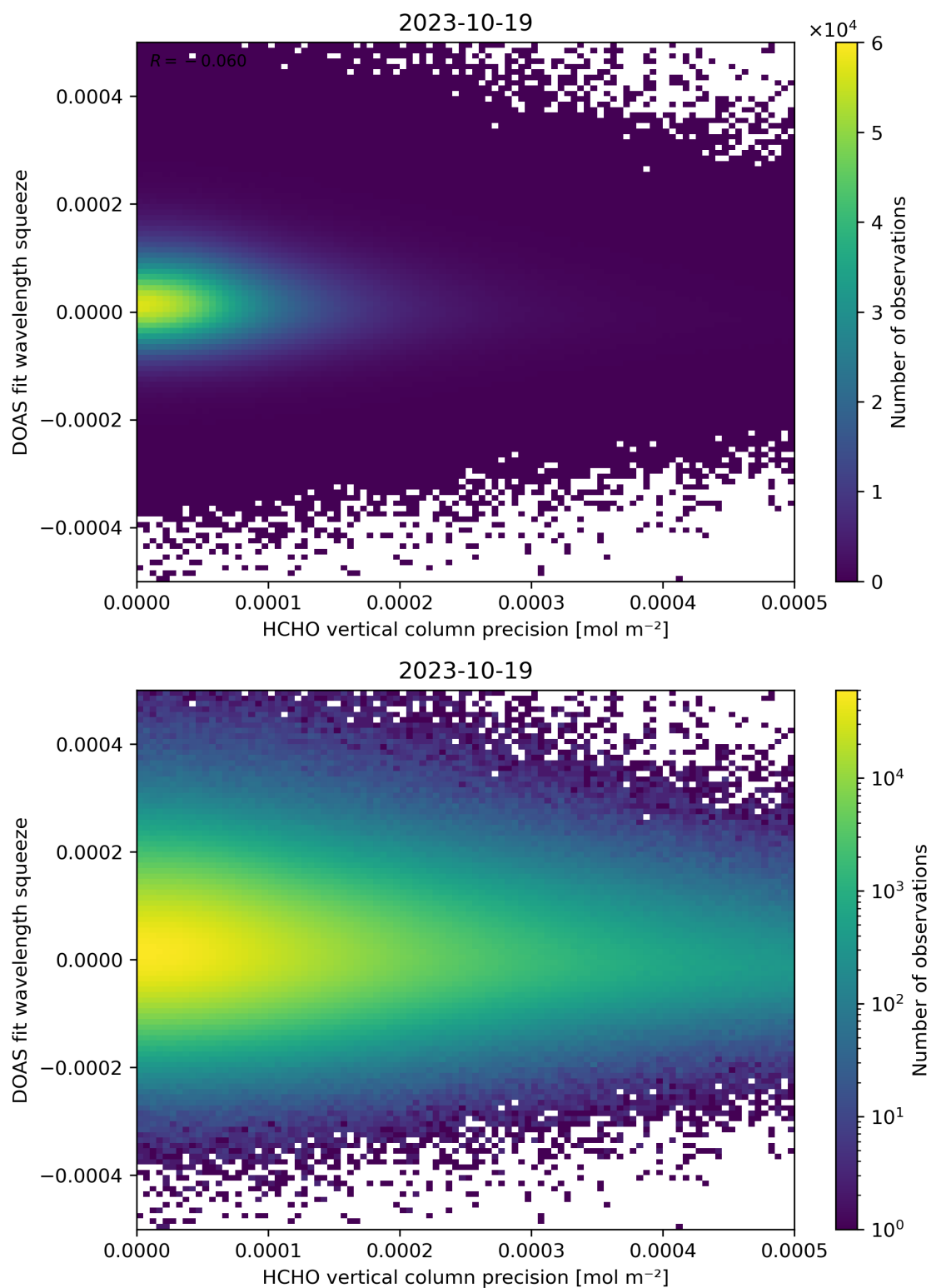
Figure 138: Scatter density plot of “HCHO vertical column precision” against “DOAS fit wavelength squeeze” for 2023-10-18 to 2023-10-20.
