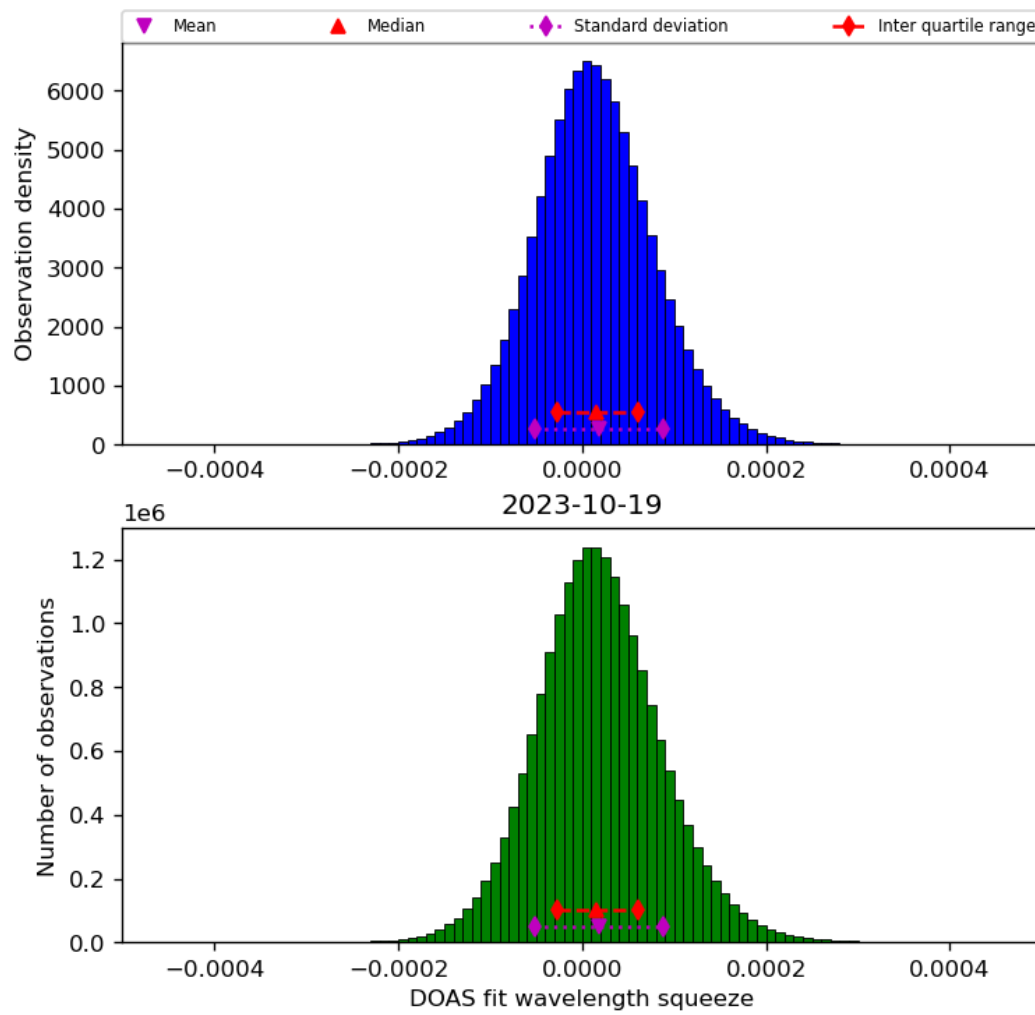
Figure 45: Histogram of “DOAS fit wavelength squeeze” for 2023-10-18 to 2023-10-20
