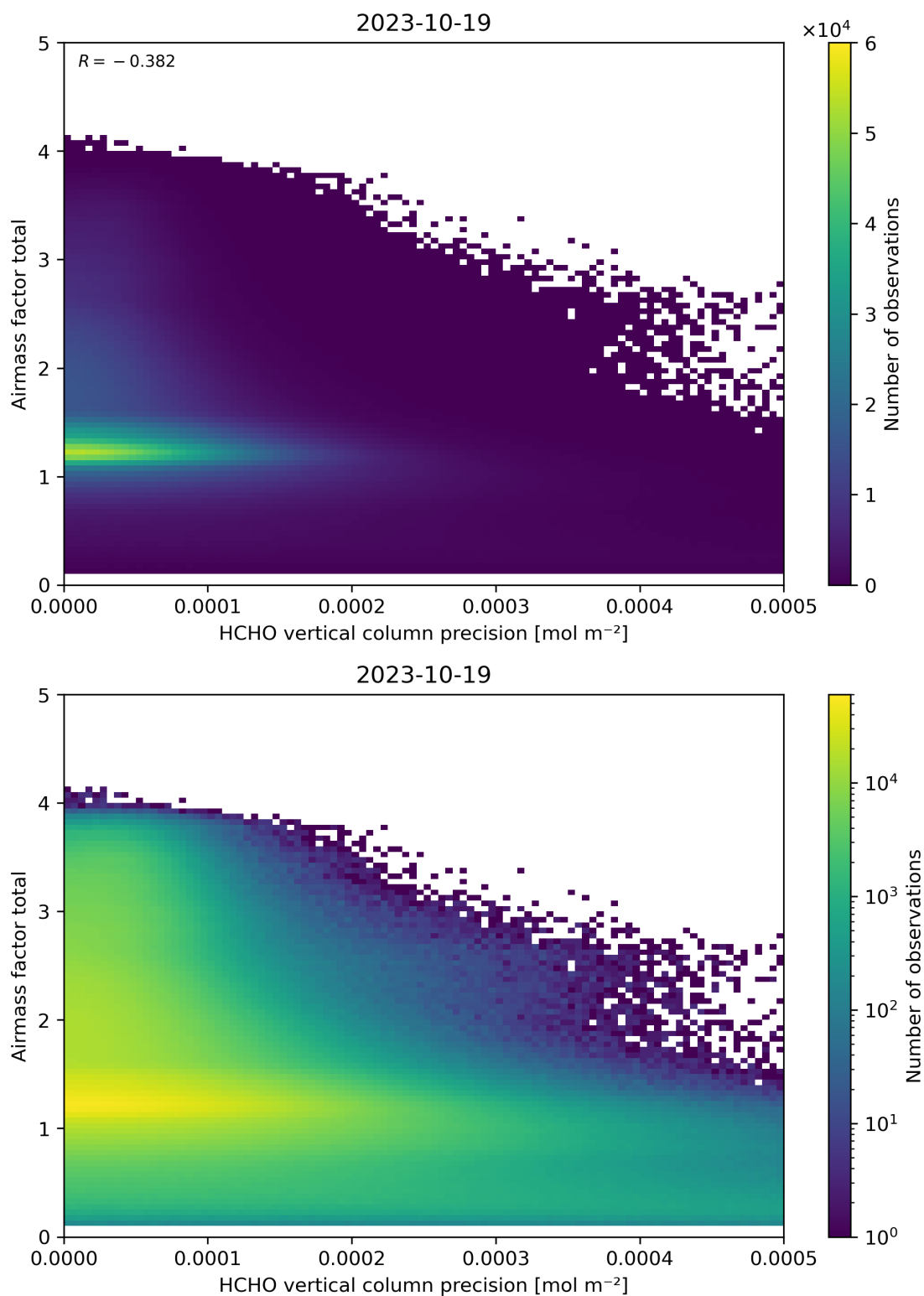
Figure 144: Scatter density plot of “HCHO vertical column precision” against “Airmass factor total” for 2023-10-18 to 2023-10-20.
