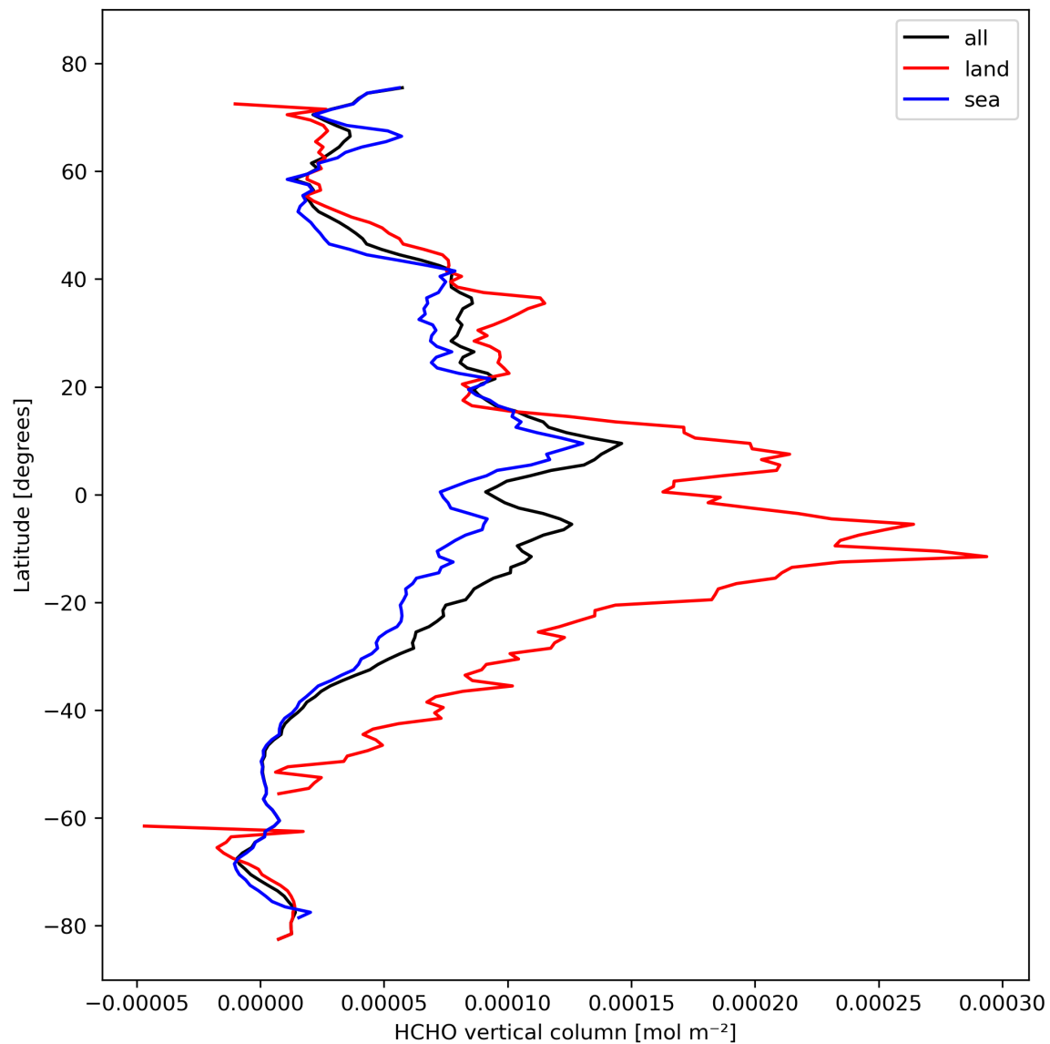
Figure 21: Zonal average of “HCHO vertical column” for 2023-10-18 to 2023-10-20.
