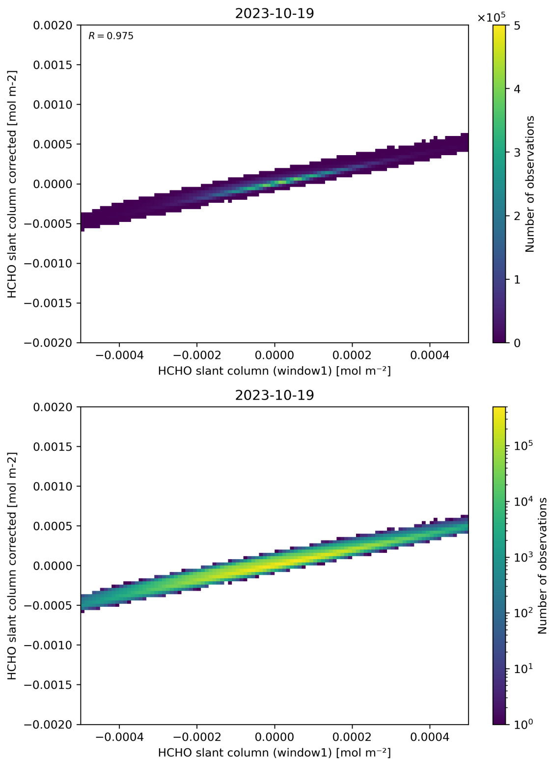
Figure 82: Scatter density plot of “HCHO slant column (window1)” against “HCHO slant column corrected” for 2023-10-18 to 2023-10-20.
