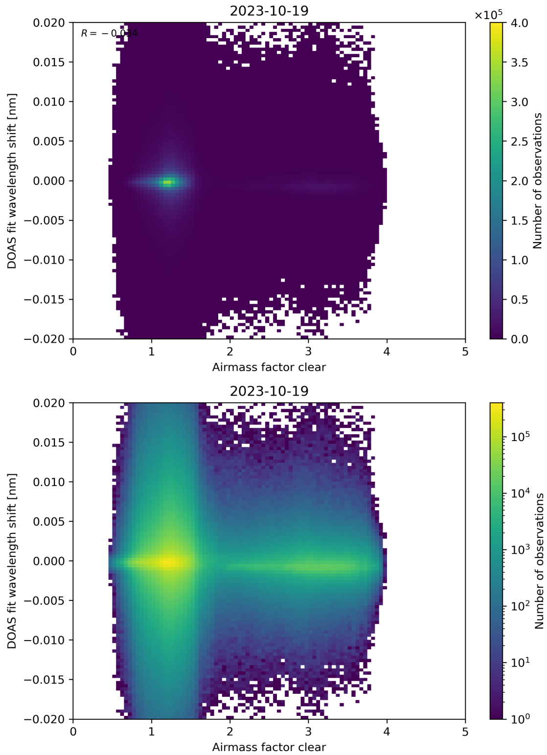
Figure 72: Scatter density plot of “Airmass factor clear” against “DOAS fit wavelength shift” for 2023-10-18 to 2023-10-20.
