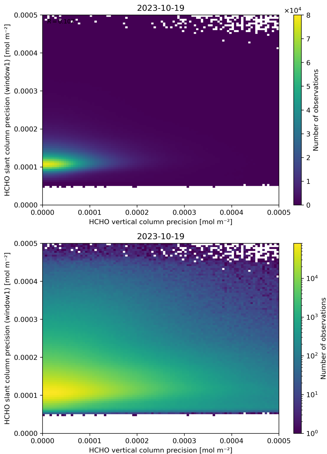
Figure 143: Scatter density plot of “HCHO vertical column precision” against “HCHO slant column precision (window1)” for 2023-10-18 to 2023-10-20.
