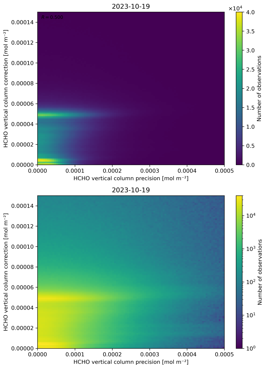
Figure 146: Scatter density plot of “HCHO vertical column precision” against “HCHO vertical column correction” for 2023-10-18 to 2023-10-20.
