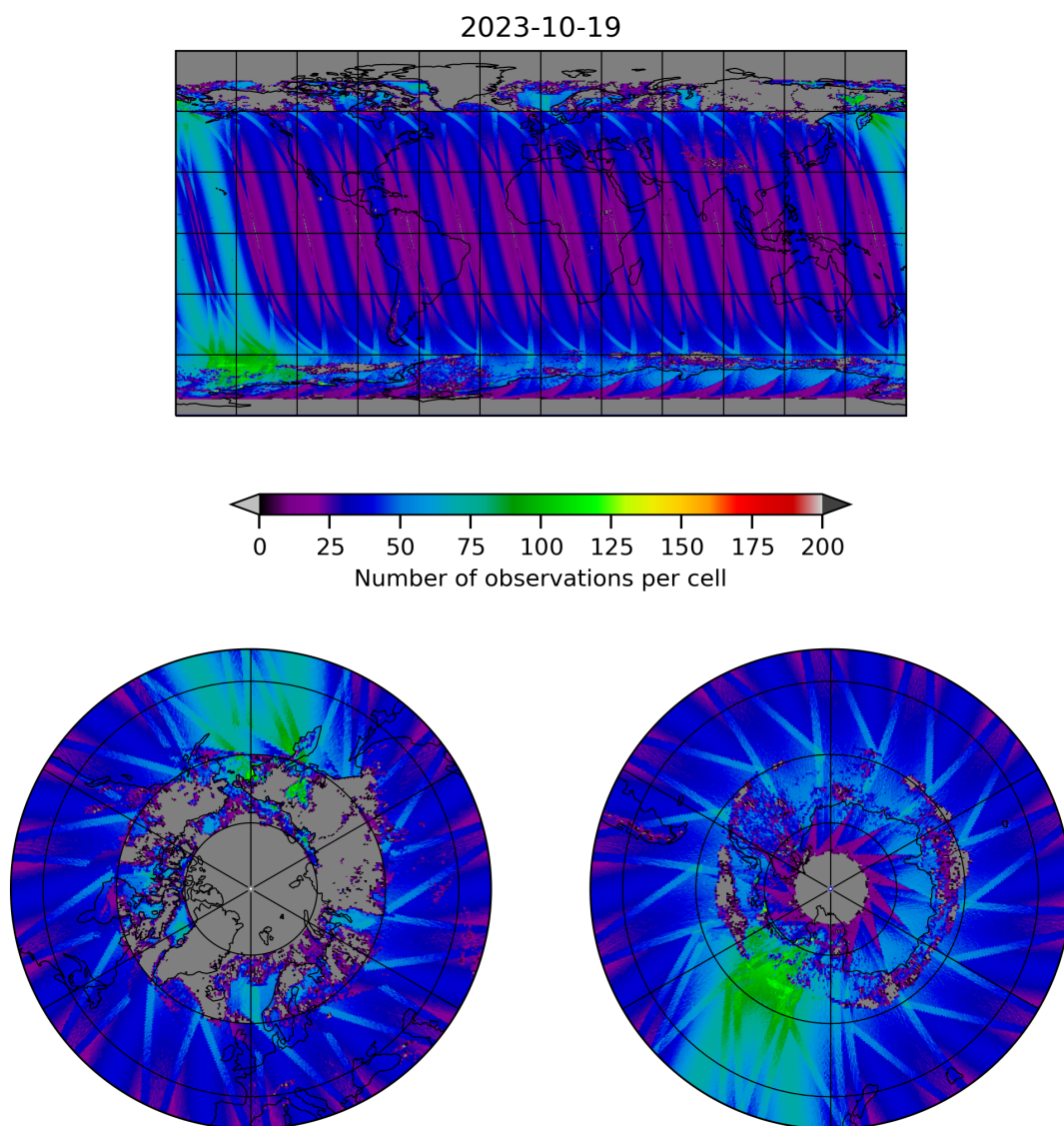
Figure 19: Map of the number of observations for 2023-10-18 to 2023-10-20
