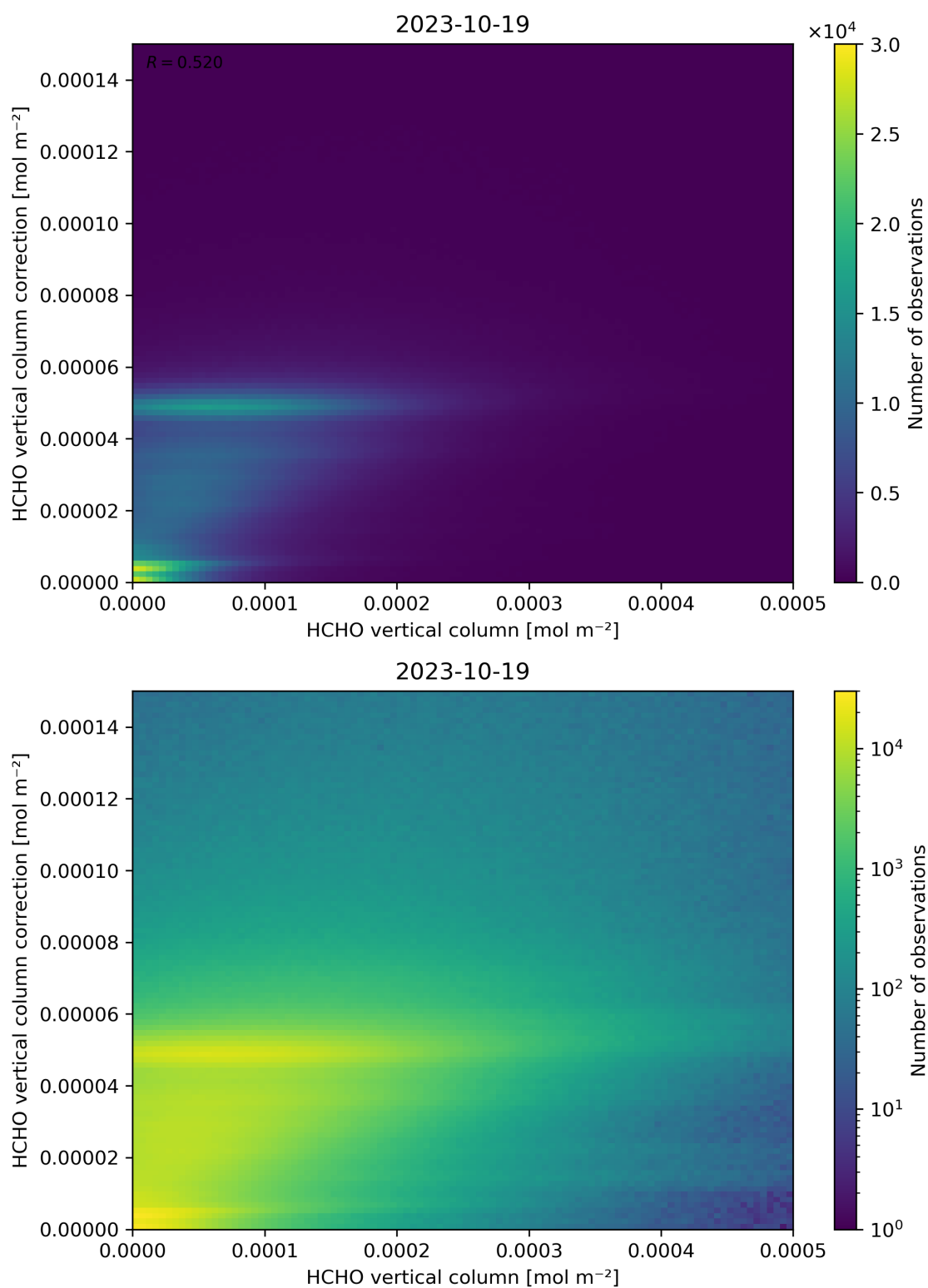
Figure 133: Scatter density plot of “HCHO vertical column” against “HCHO vertical column correction” for 2023-10-18 to 2023-10-20.
