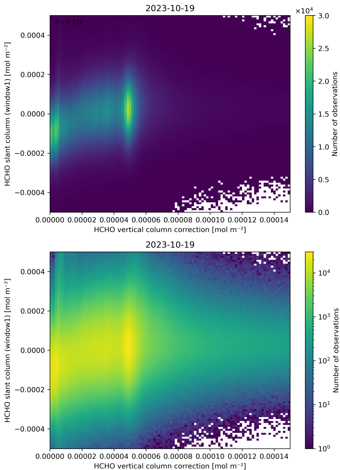
Figure 118: Scatter density plot of “HCHO vertical column correction” against “HCHO slant column (window1)” for 2023-10-18 to 2023-10-20.
