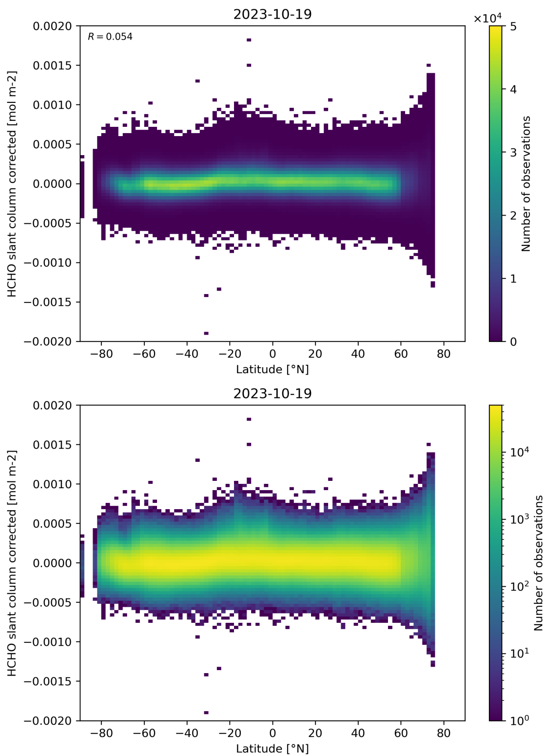
Figure 157: Scatter density plot of “Latitude” against “HCHO slant column corrected” for 2023-10-18 to 2023-10-20.
