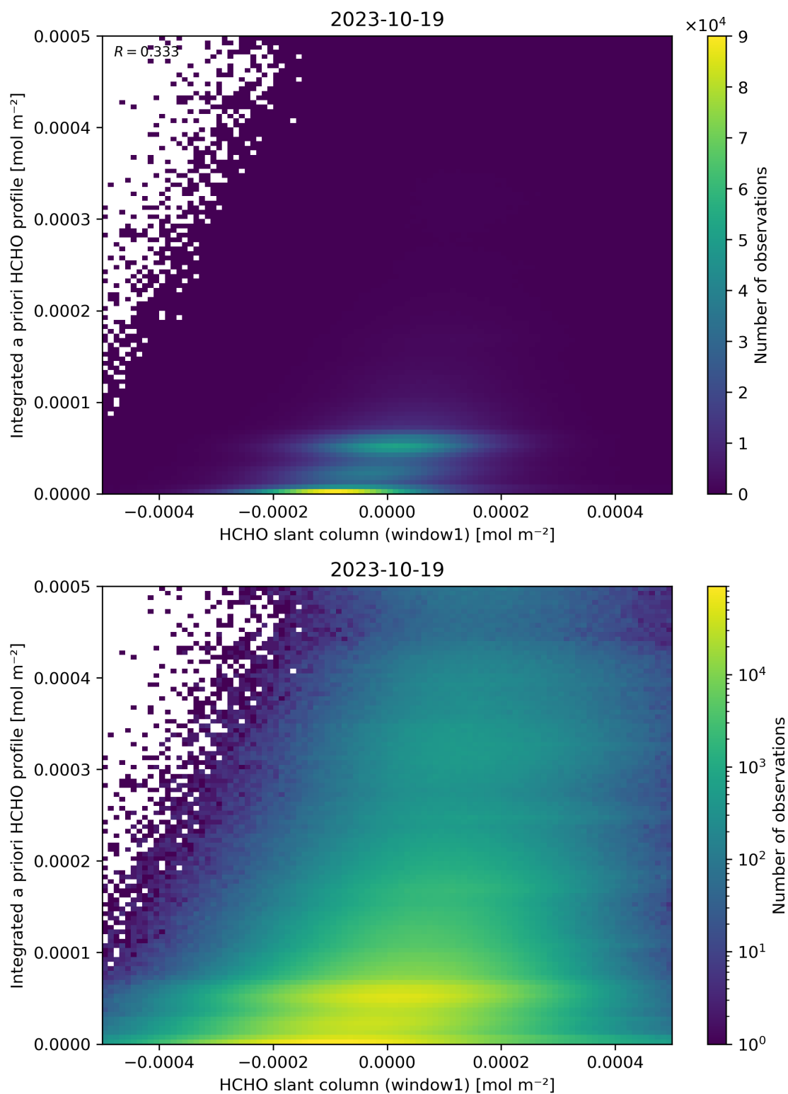
Figure 87: Scatter density plot of “HCHO slant column (window1)” against “Integrated a priori HCHO profile” for 2023-10-18 to 2023-10-20.
