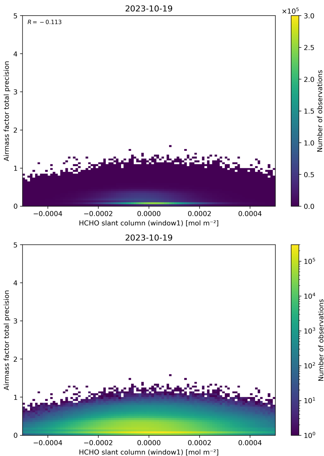
Figure 86: Scatter density plot of “HCHO slant column (window1)” against “Airmass factor total precision” for 2023-10-18 to 2023-10-20.
