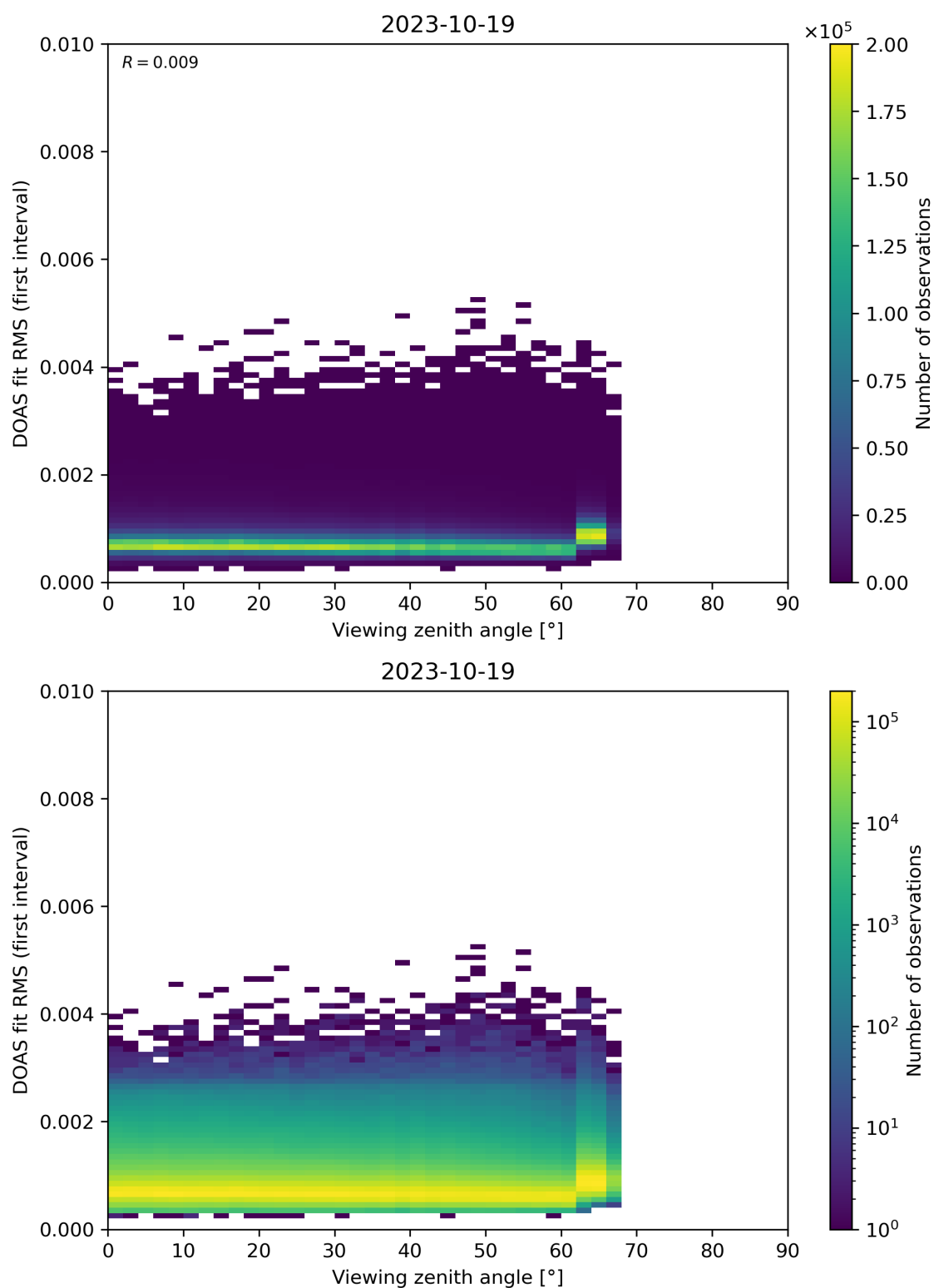
Figure 182: Scatter density plot of “Viewing zenith angle” against “DOAS fit RMS (first interval)” for 2023-10-18 to 2023-10-20.
