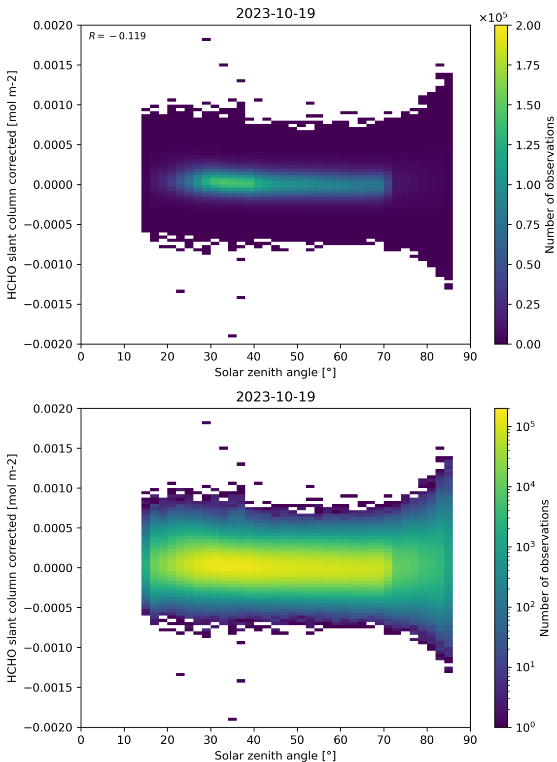
Figure 171: Scatter density plot of “Solar zenith angle” against “HCHO slant column corrected” for 2023-10-18 to 2023-10-20.
