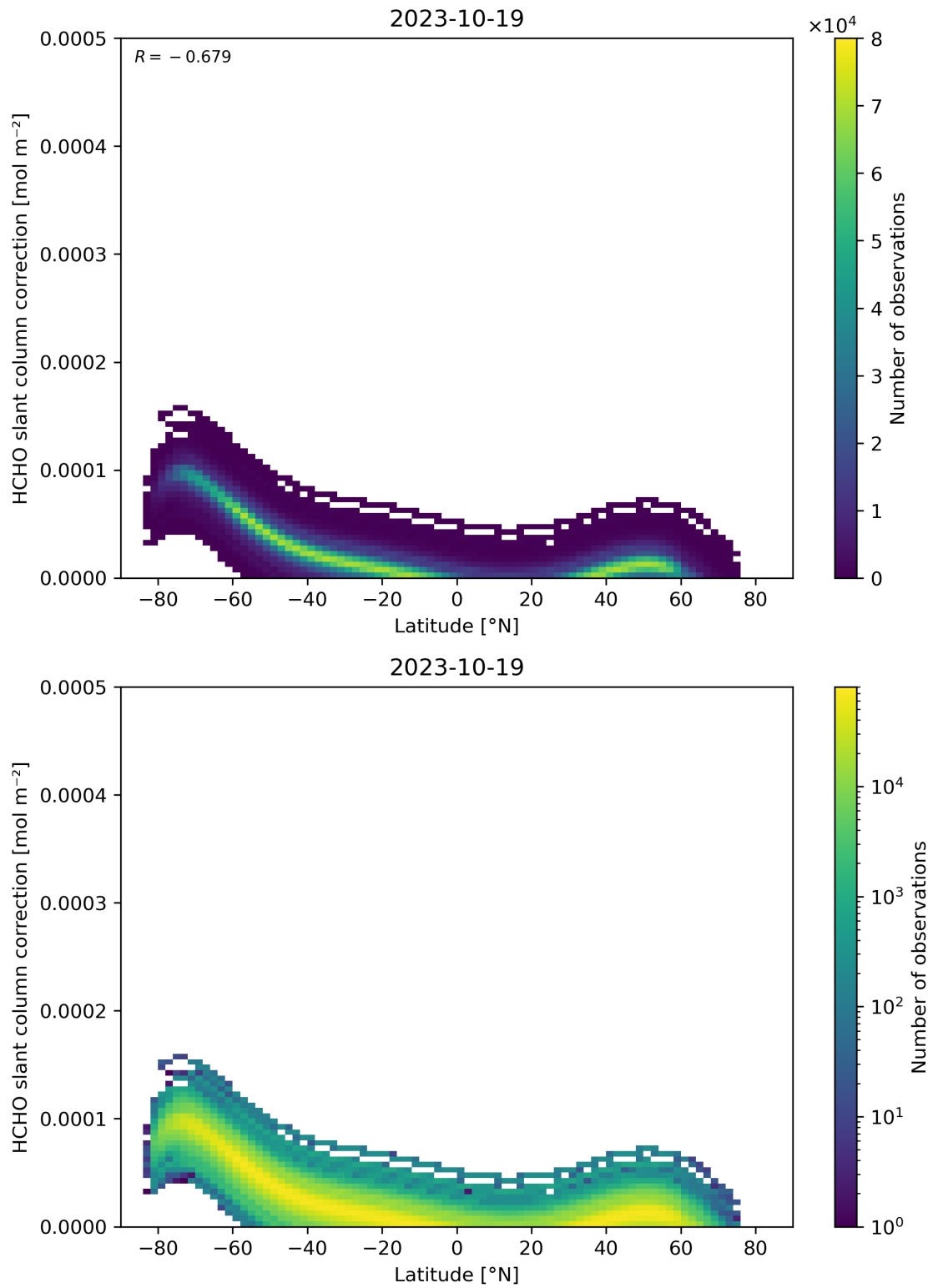
Figure 158: Scatter density plot of “Latitude” against “HCHO slant column correction” for 2023-10-18 to 2023-10-20.
