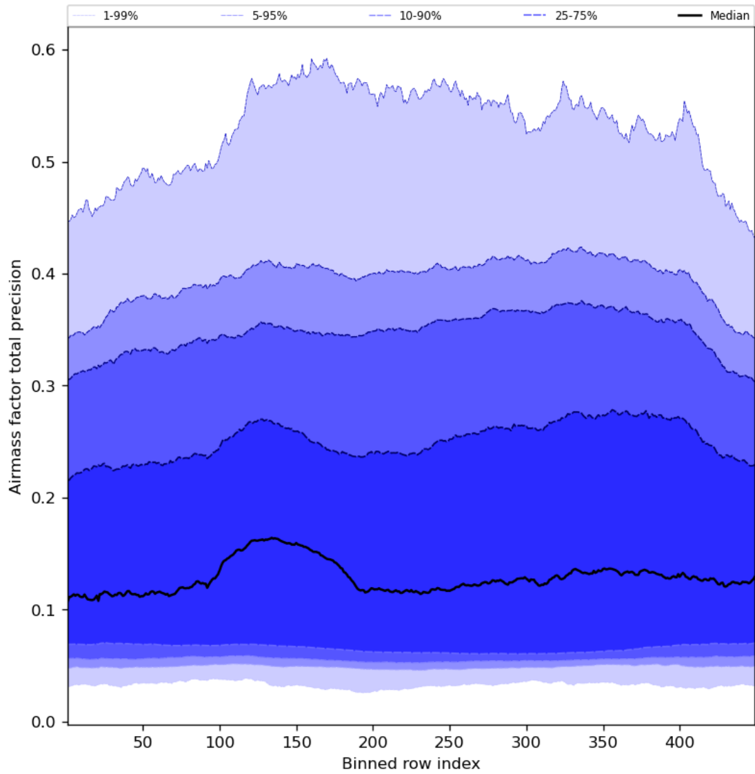
Figure 55: Along track statistics of “Airmass factor total precision” for 2023-10-18 to 2023-10-20
