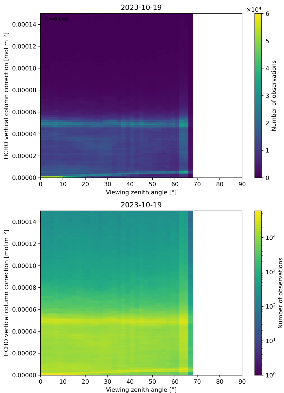
Figure 193: Scatter density plot of “Viewing zenith angle” against “HCHO vertical column correction” for 2023-10-18 to 2023-10-20.
