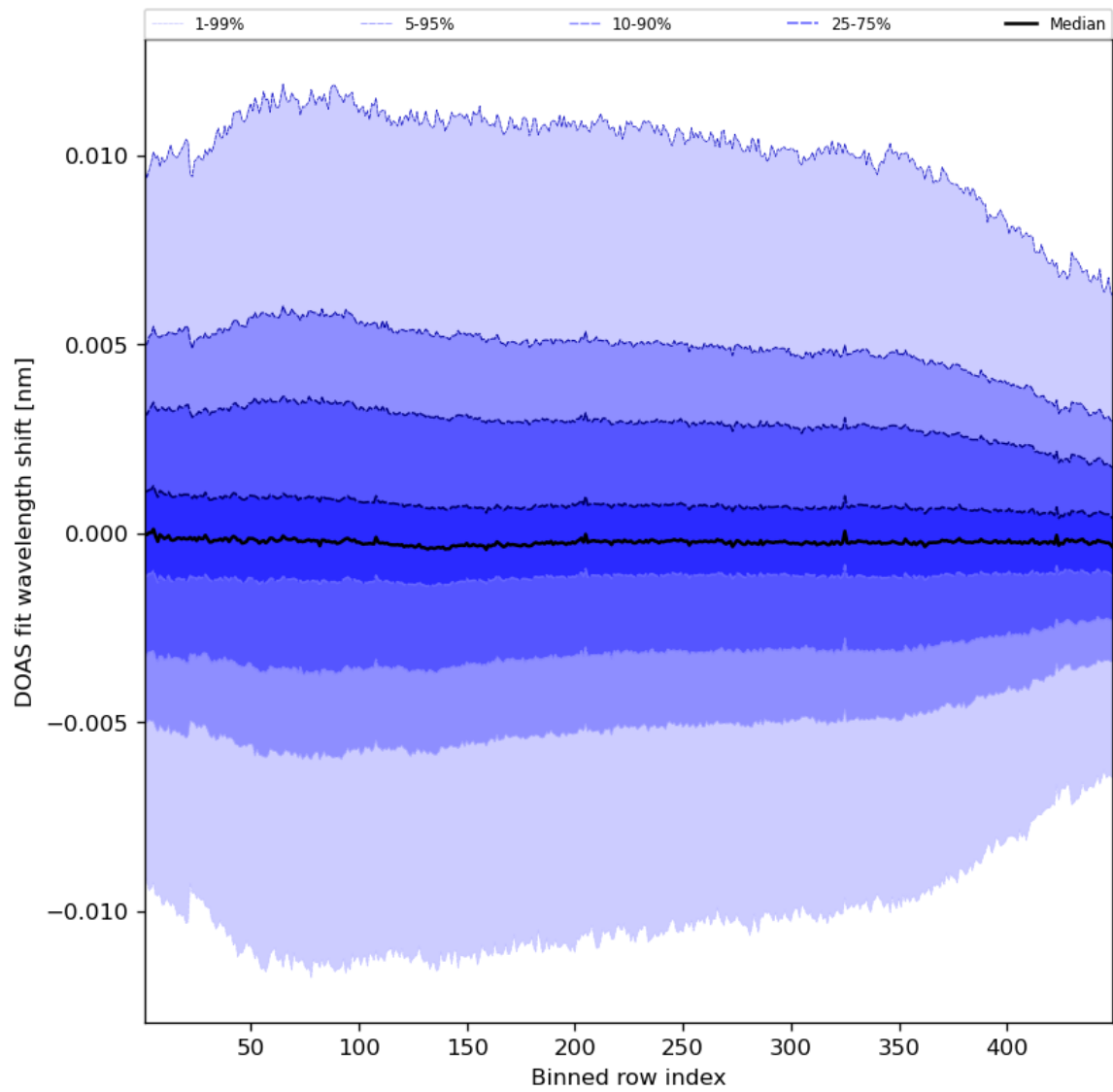
Figure 58: Along track statistics of “DOAS fit wavelength shift” for 2023-10-18 to 2023-10-20
