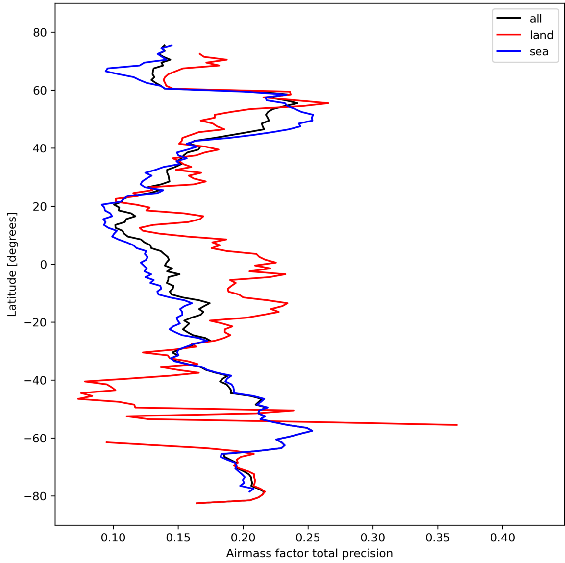
Figure 27: Zonal average of “Airmass factor total precision” for 2023-10-18 to 2023-10-20.
