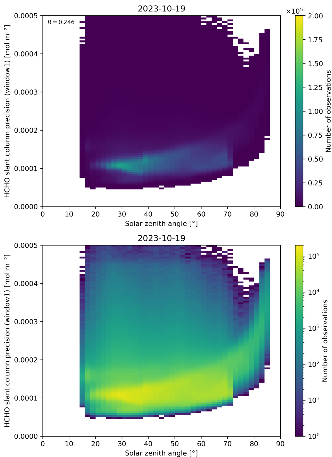
Figure 174: Scatter density plot of “Solar zenith angle” against “HCHO slant column precision (window1)” for 2023-10-18 to 2023-10-20.
