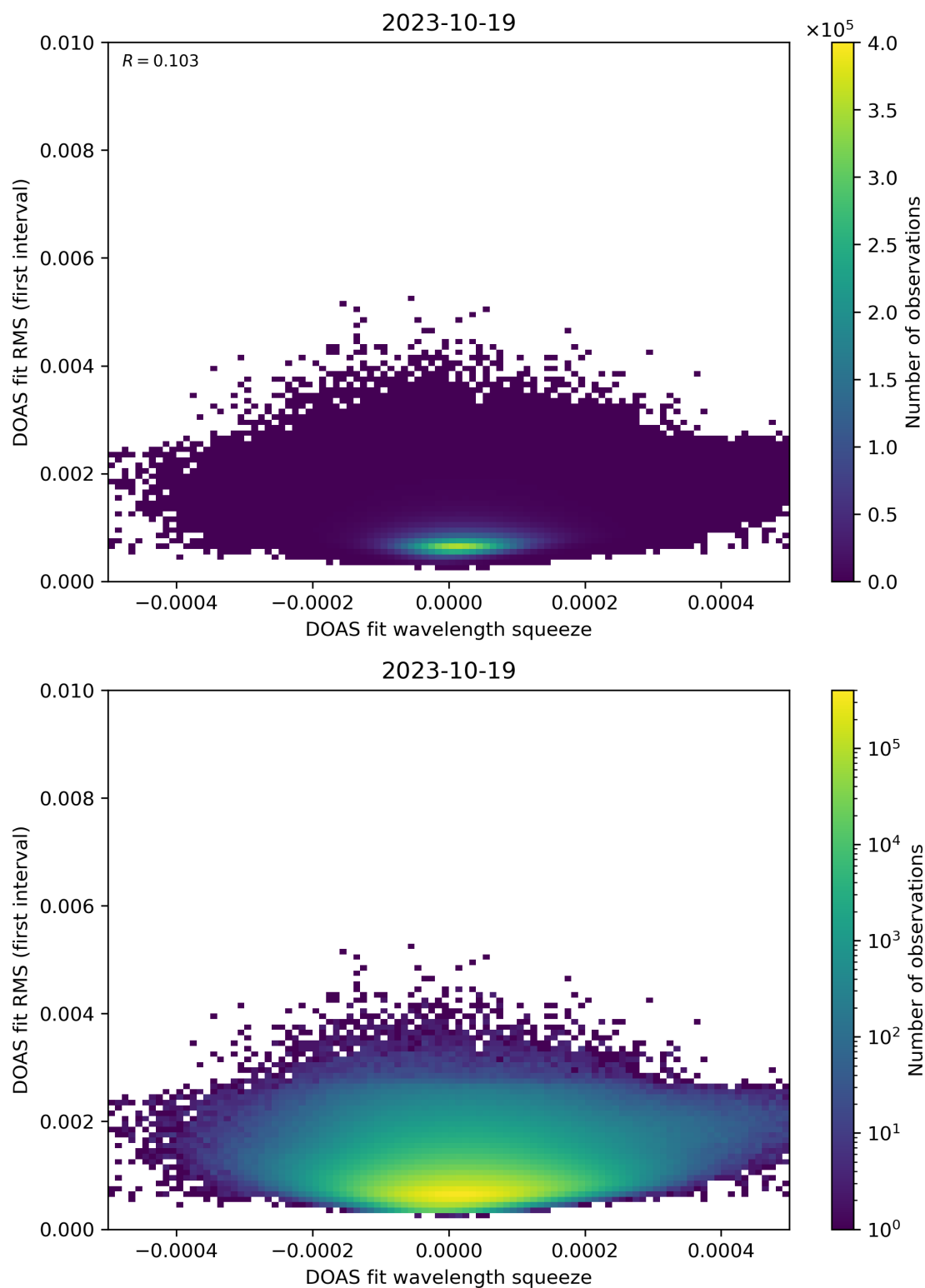
Figure 68: Scatter density plot of “DOAS fit wavelength squeeze” against “DOAS fit RMS (first interval)” for 2023-10-18 to 2023-10-20.
