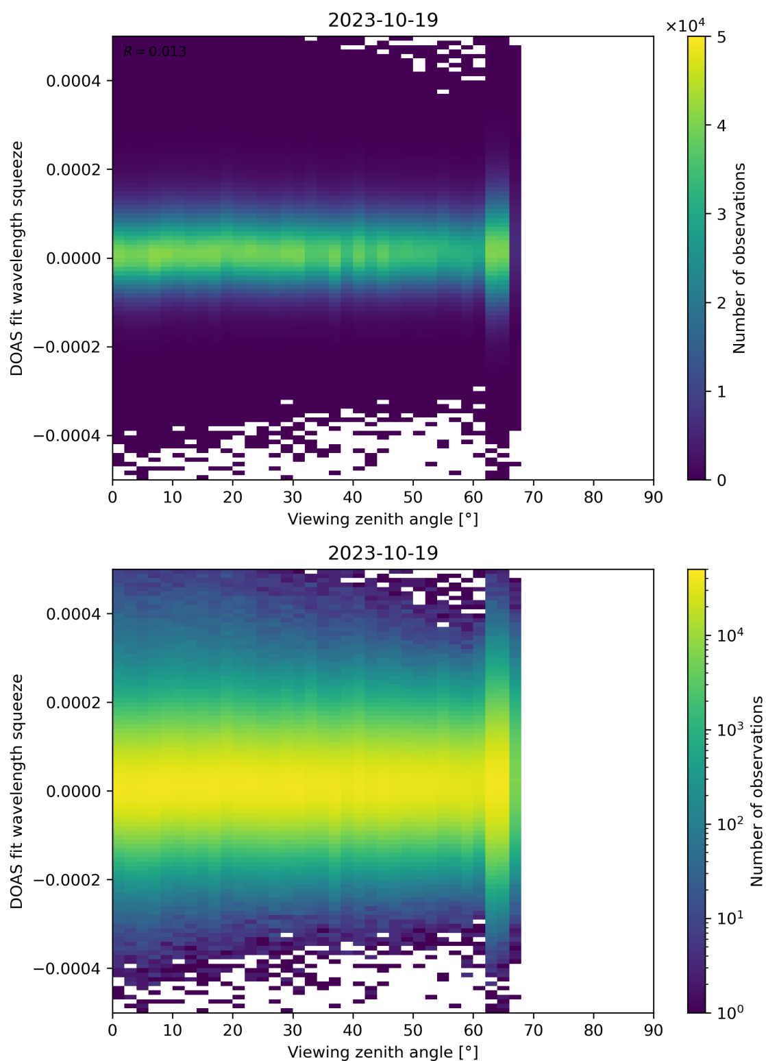
Figure 184: Scatter density plot of “Viewing zenith angle” against “DOAS fit wavelength squeeze” for 2023-10-18 to 2023-10-20.
