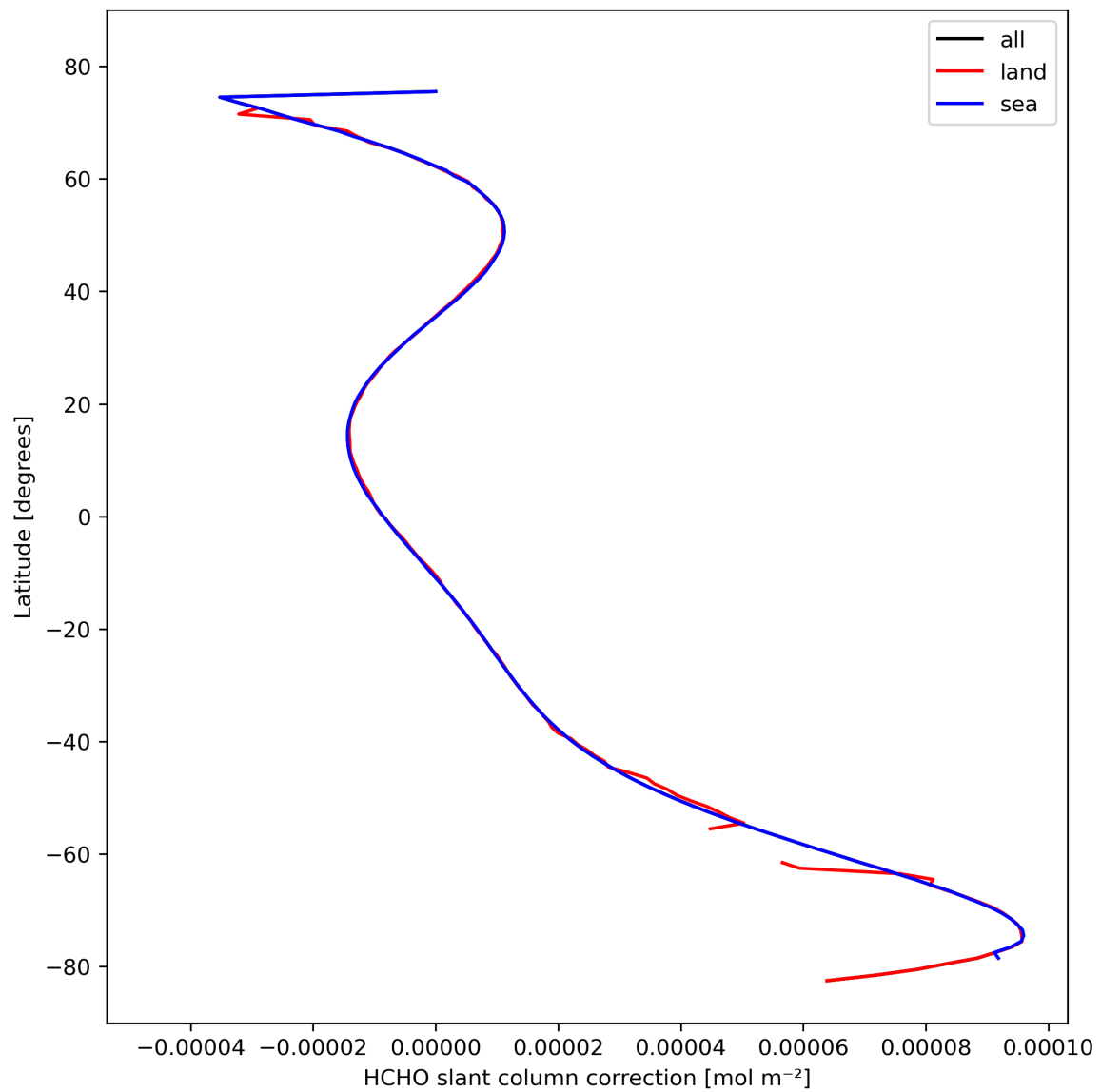
Figure 33: Zonal average of “HCHO slant column correction” for 2023-10-18 to 2023-10-20.
