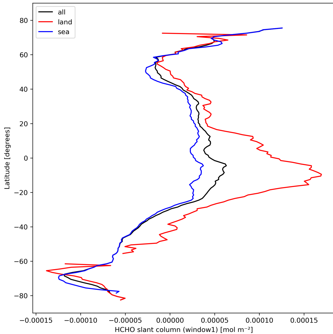
Figure 24: Zonal average of “HCHO slant column (window1)” for 2023-10-18 to 2023-10-20.
