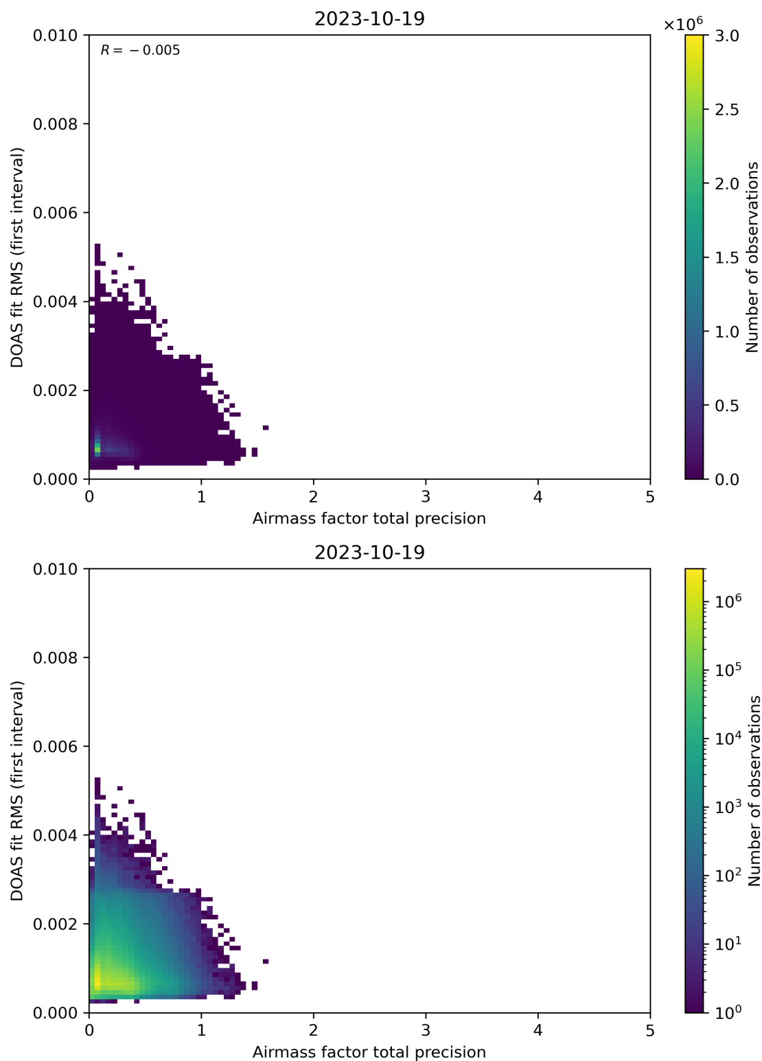
Figure 105: Scatter density plot of “Airmass factor total precision” against “DOAS fit RMS (first interval)” for 2023-10-18 to 2023-10-20.
