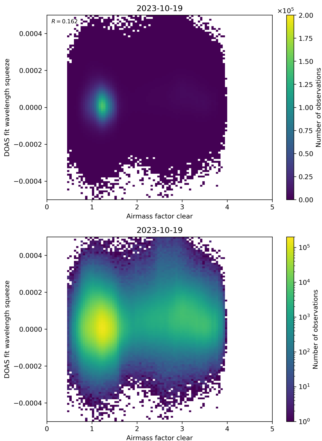
Figure 73: Scatter density plot of “Airmass factor clear” against “DOAS fit wavelength squeeze” for 2023-10-18 to 2023-10-20.
