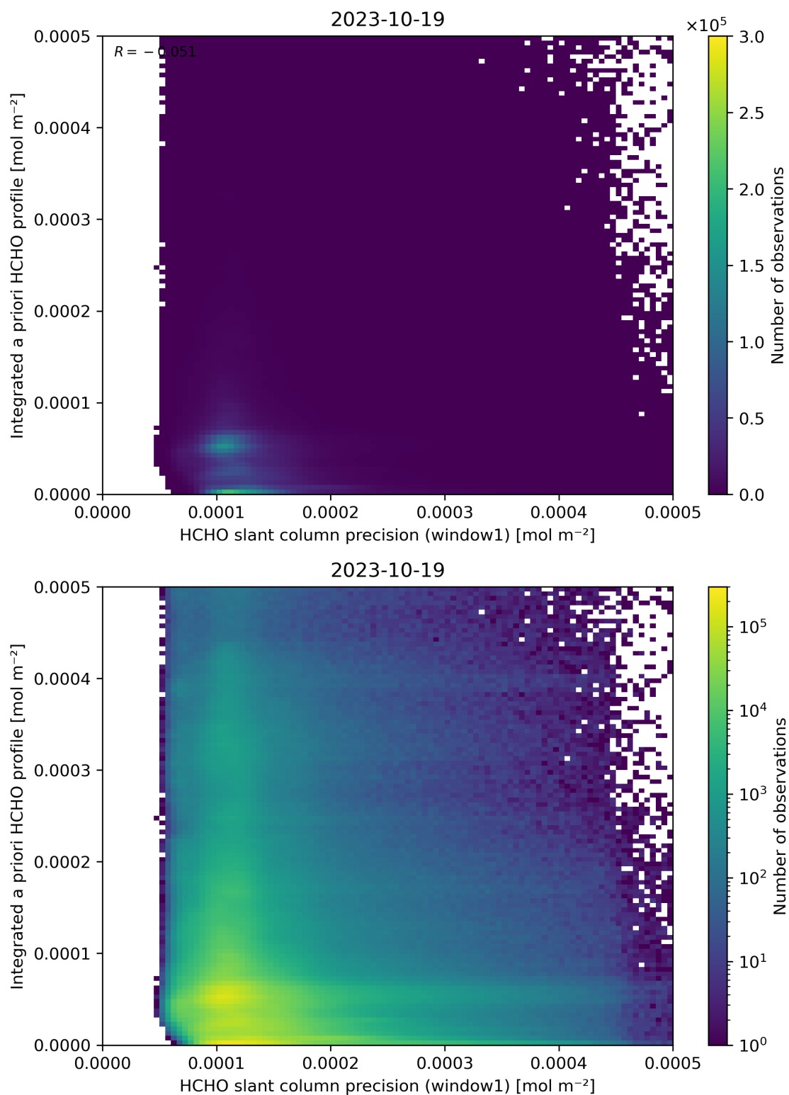
Figure 96: Scatter density plot of “HCHO slant column precision (window1)” against “Integrated a priori HCHO profile” for 2023-10-18 to 2023-10-20.
