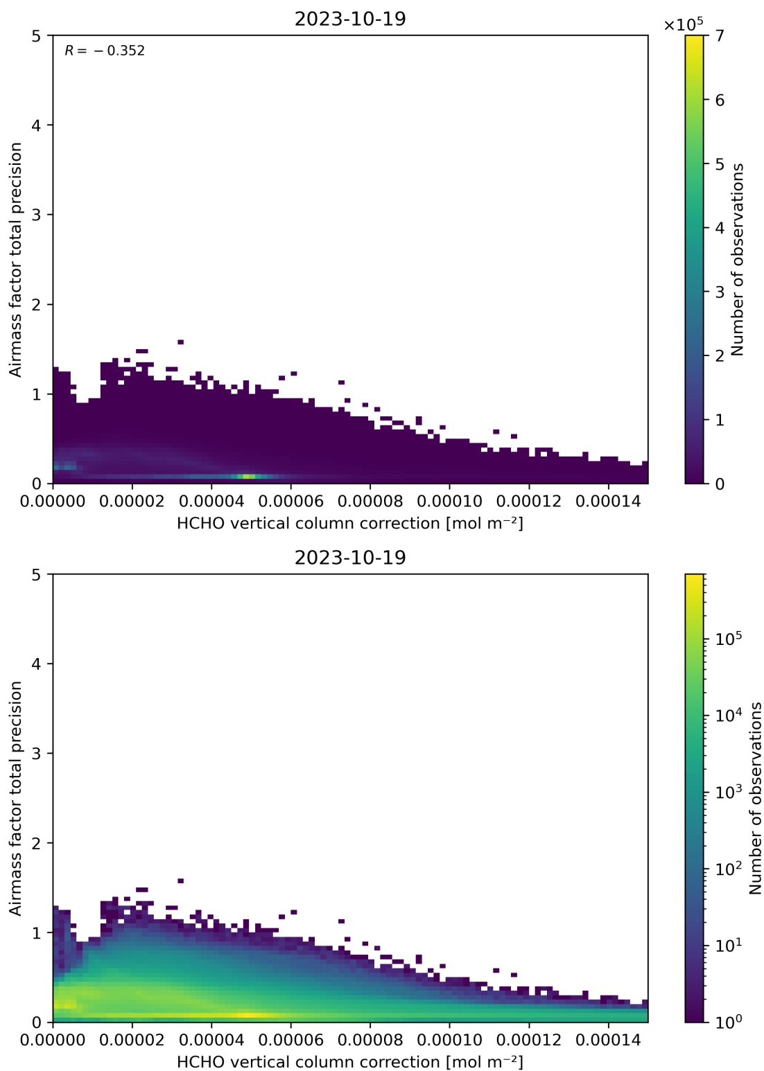
Figure 121: Scatter density plot of “HCHO vertical column correction” against “Airmass factor total precision” for 2023-10-18 to 2023-10-20.
