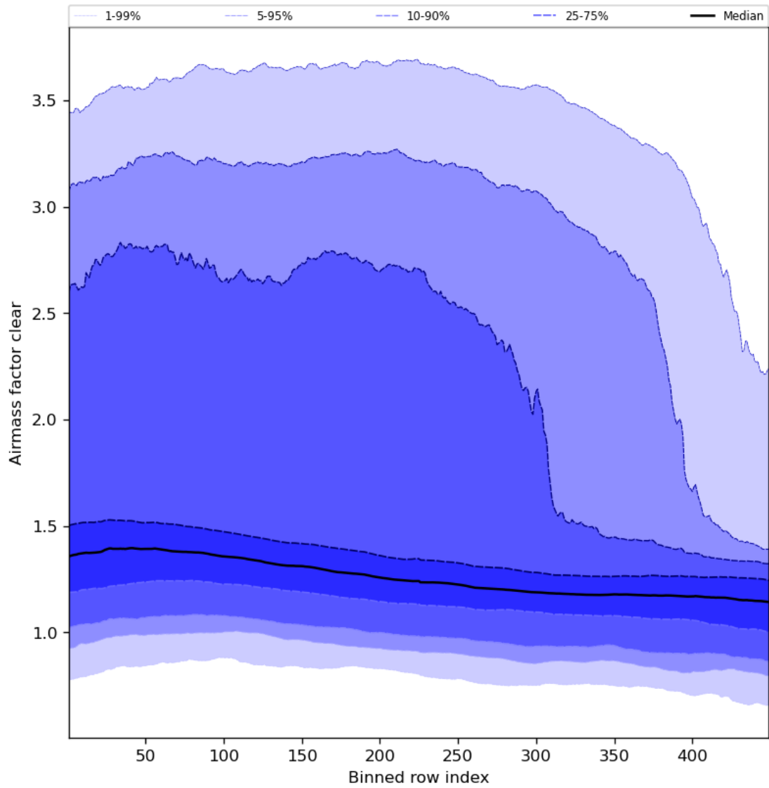
Figure 56: Along track statistics of “Airmass factor clear” for 2023-10-18 to 2023-10-20
