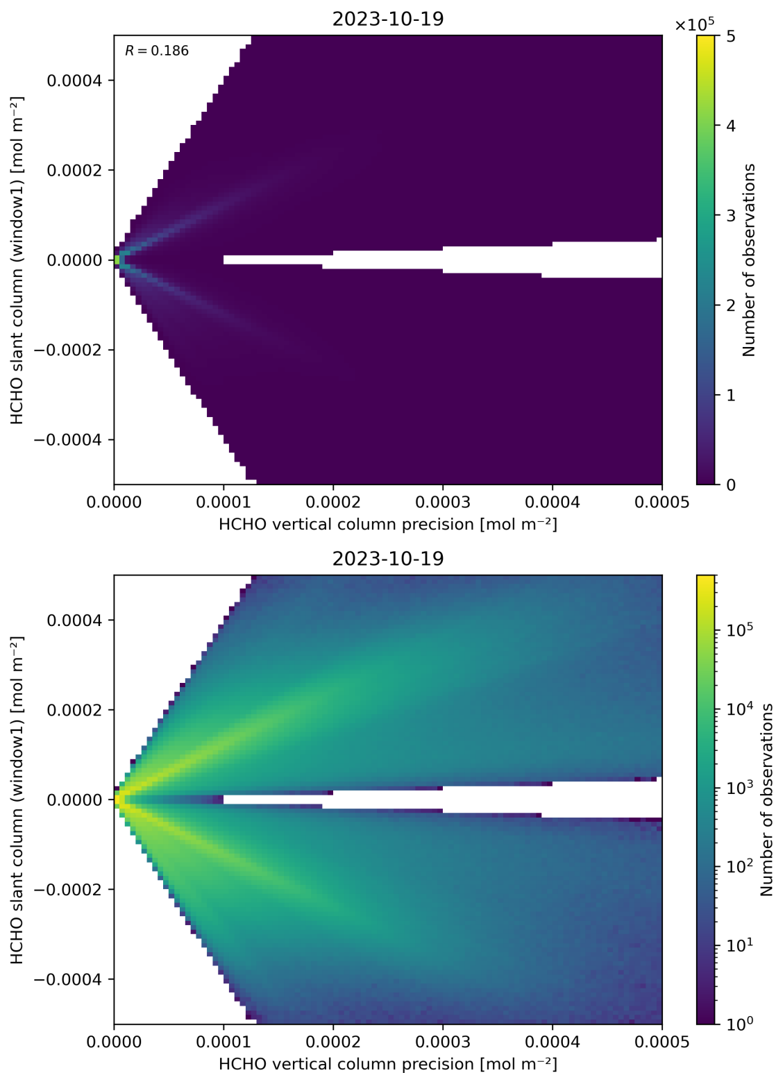
Figure 142: Scatter density plot of “HCHO vertical column precision” against “HCHO slant column (window1)” for 2023-10-18 to 2023-10-20.
