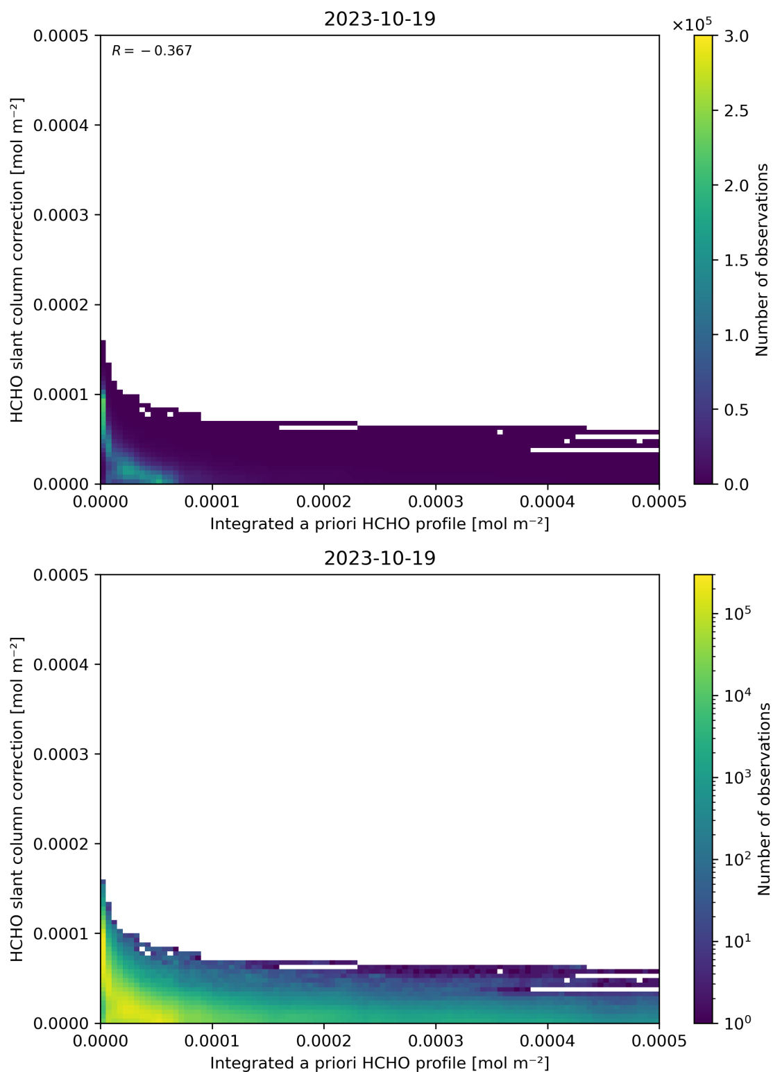
Figure 152: Scatter density plot of “Integrated a priori HCHO profile” against “HCHO slant column correction” for 2023-10-18 to 2023-10-20.
