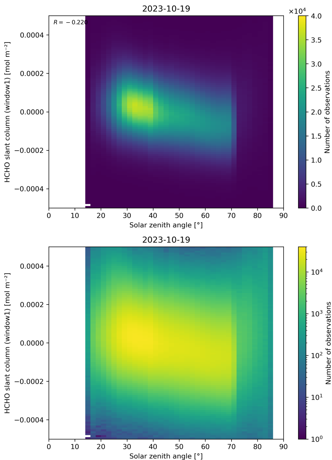
Figure 173: Scatter density plot of “Solar zenith angle” against “HCHO slant column (window1)” for 2023-10-18 to 2023-10-20.
