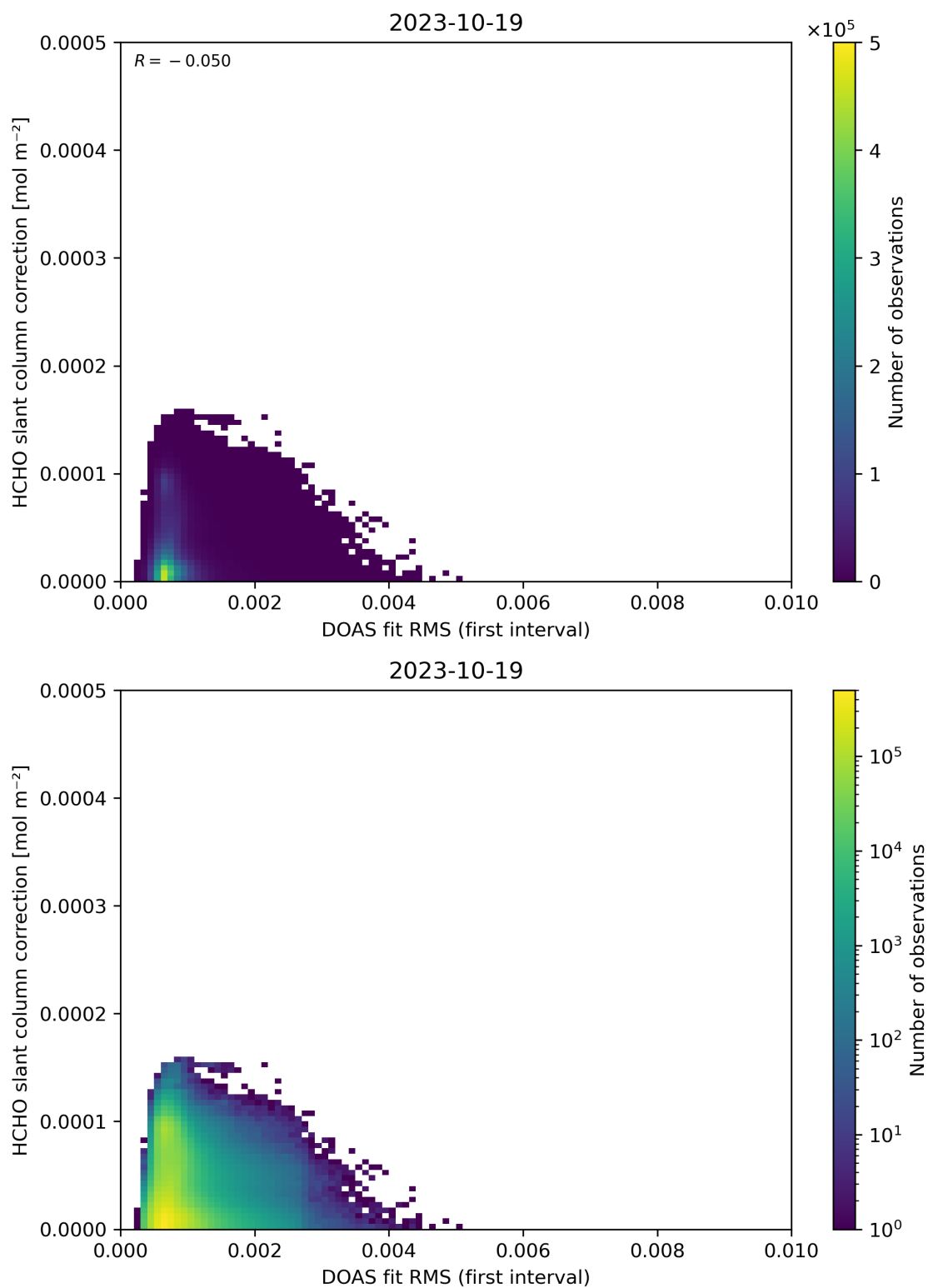
Figure 63: Scatter density plot of “DOAS fit RMS (first interval)” against “HCHO slant column correction” for 2023-10-18 to 2023-10-20.
