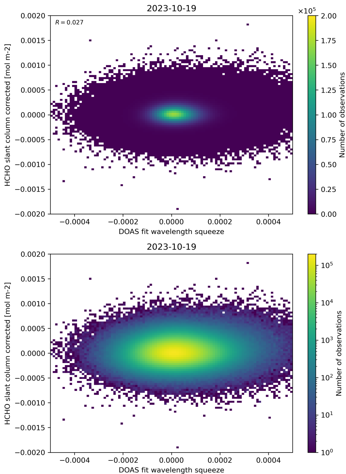
Figure 69: Scatter density plot of “DOAS fit wavelength squeeze” against “HCHO slant column corrected” for 2023-10-18 to 2023-10-20.
