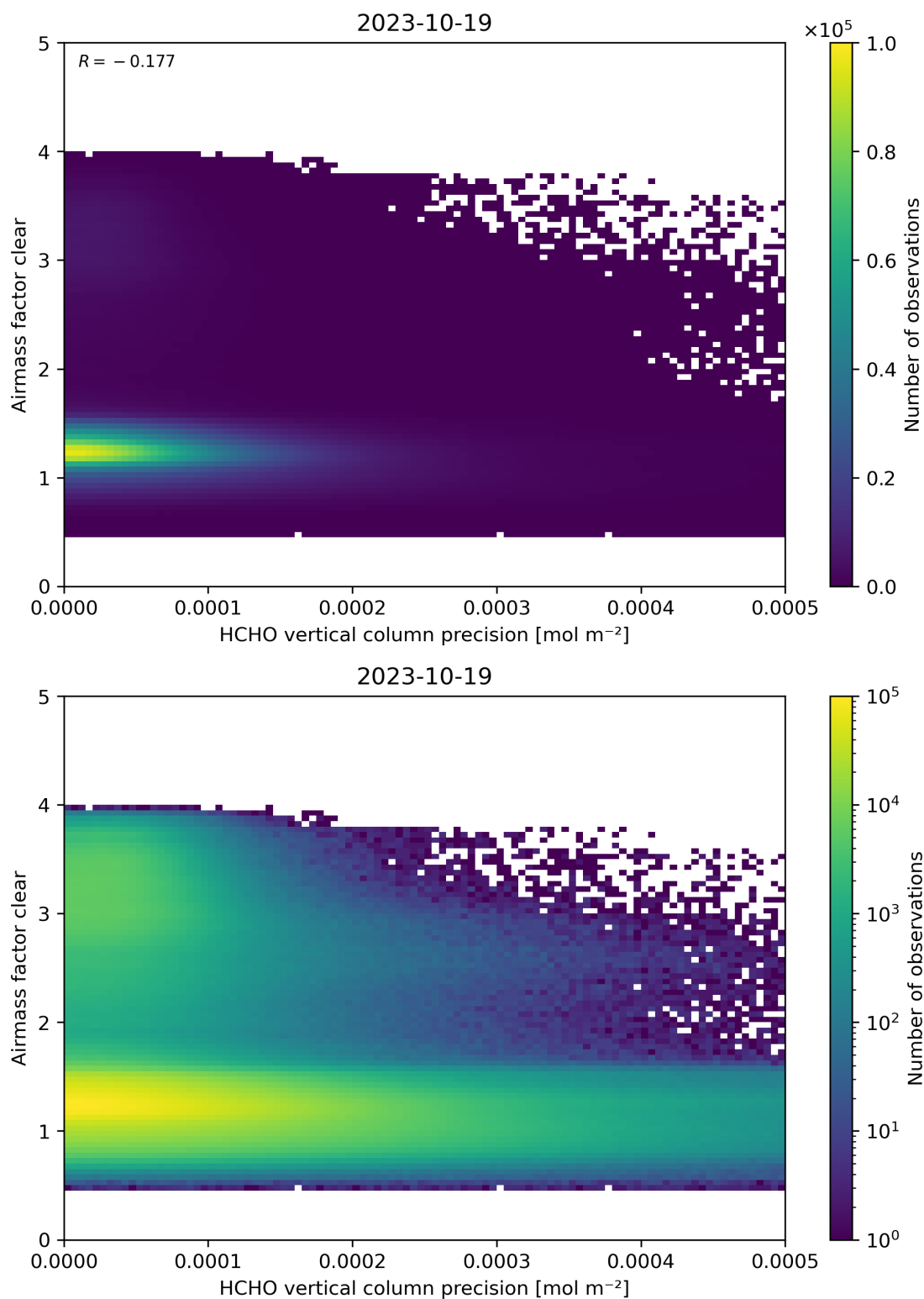
Figure 139: Scatter density plot of “HCHO vertical column precision” against “Airmass factor clear” for 2023-10-18 to 2023-10-20.
