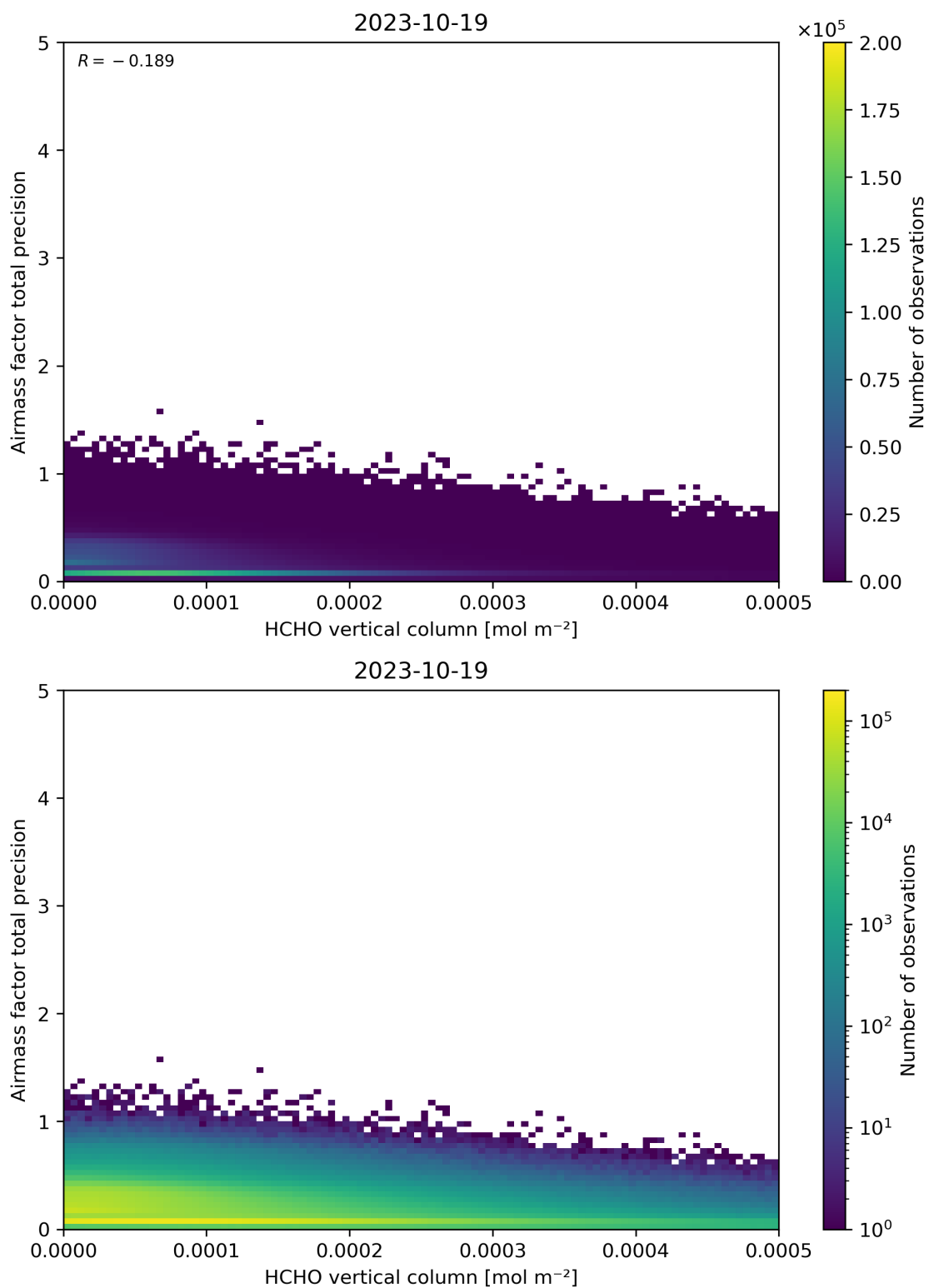
Figure 132: Scatter density plot of “HCHO vertical column” against “Airmass factor total precision” for 2023-10-18 to 2023-10-20.
