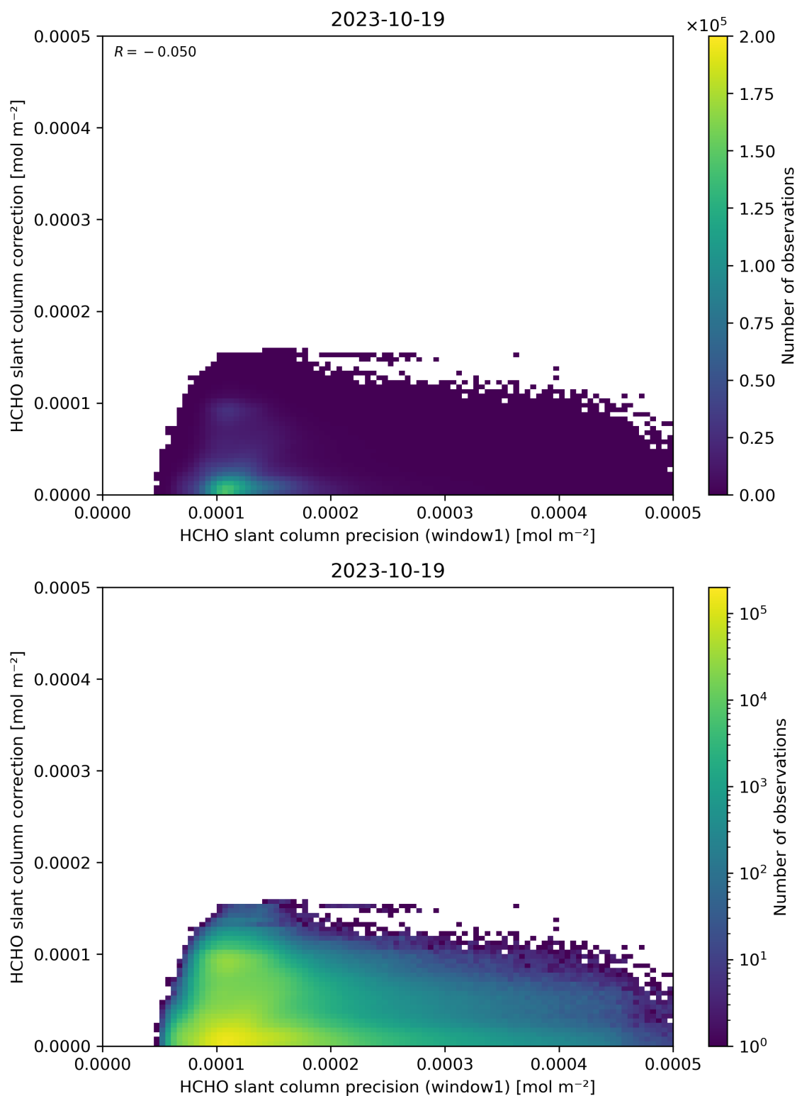
Figure 93: Scatter density plot of “HCHO slant column precision (window1)” against “HCHO slant column correction” for 2023-10-18 to 2023-10-20.
