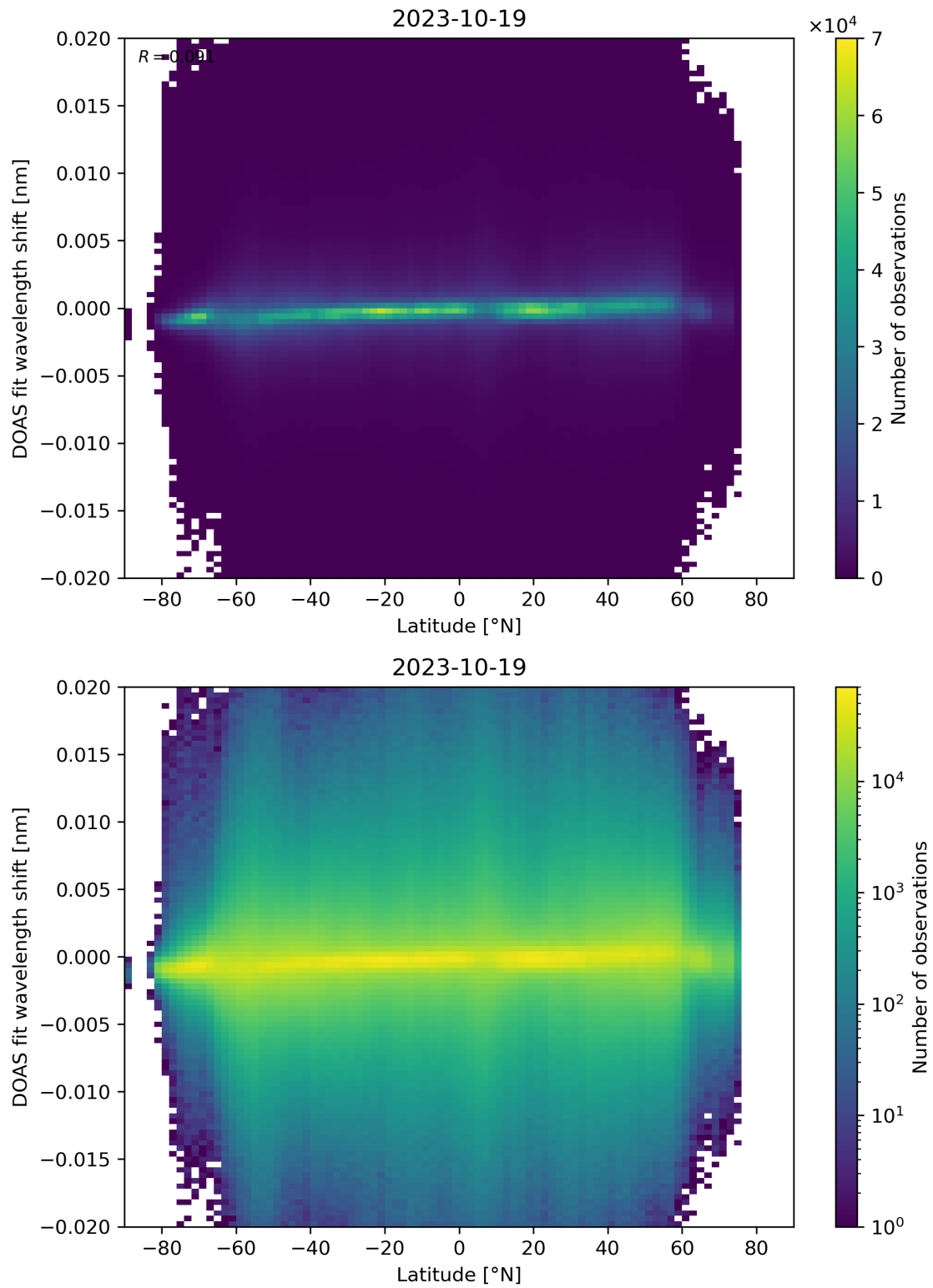
Figure 154: Scatter density plot of “Latitude” against “DOAS fit wavelength shift” for 2023-10-18 to 2023-10-20.
