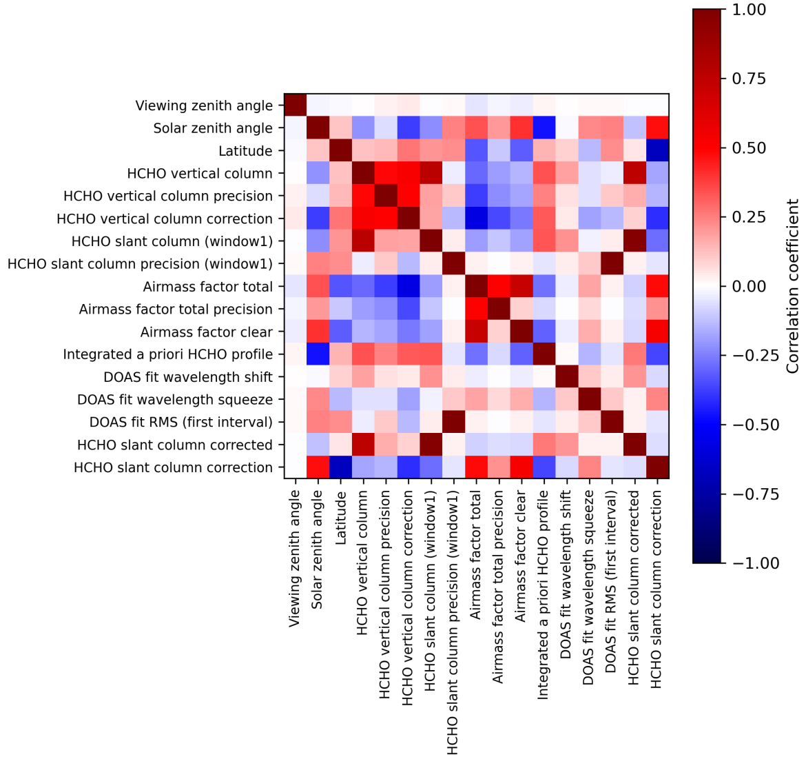
Figure 2: Map of correlation matrix for 2023-10-18 to 2023-10-20.
