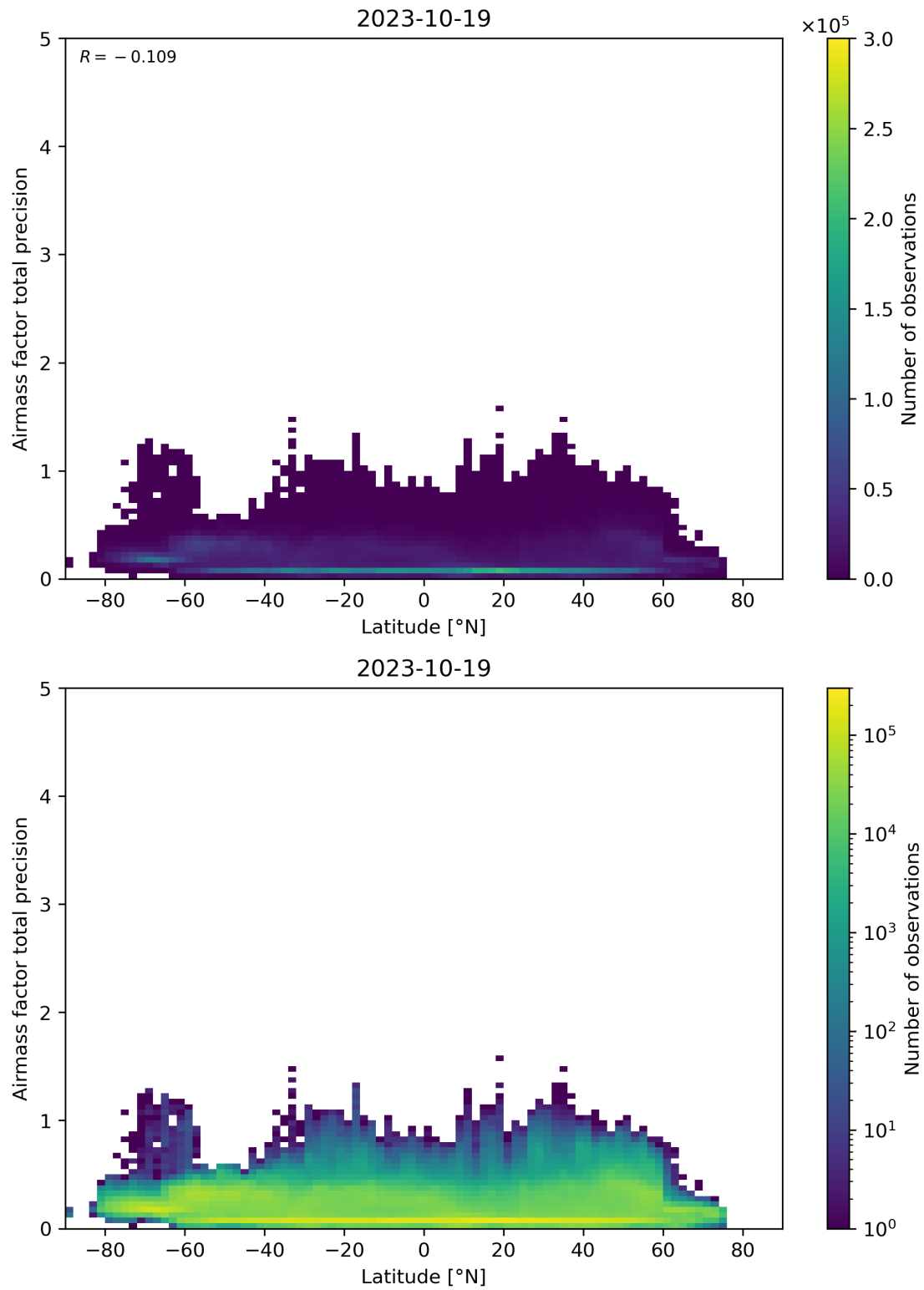
Figure 162: Scatter density plot of “Latitude” against “Airmass factor total precision” for 2023-10-18 to 2023-10-20.
