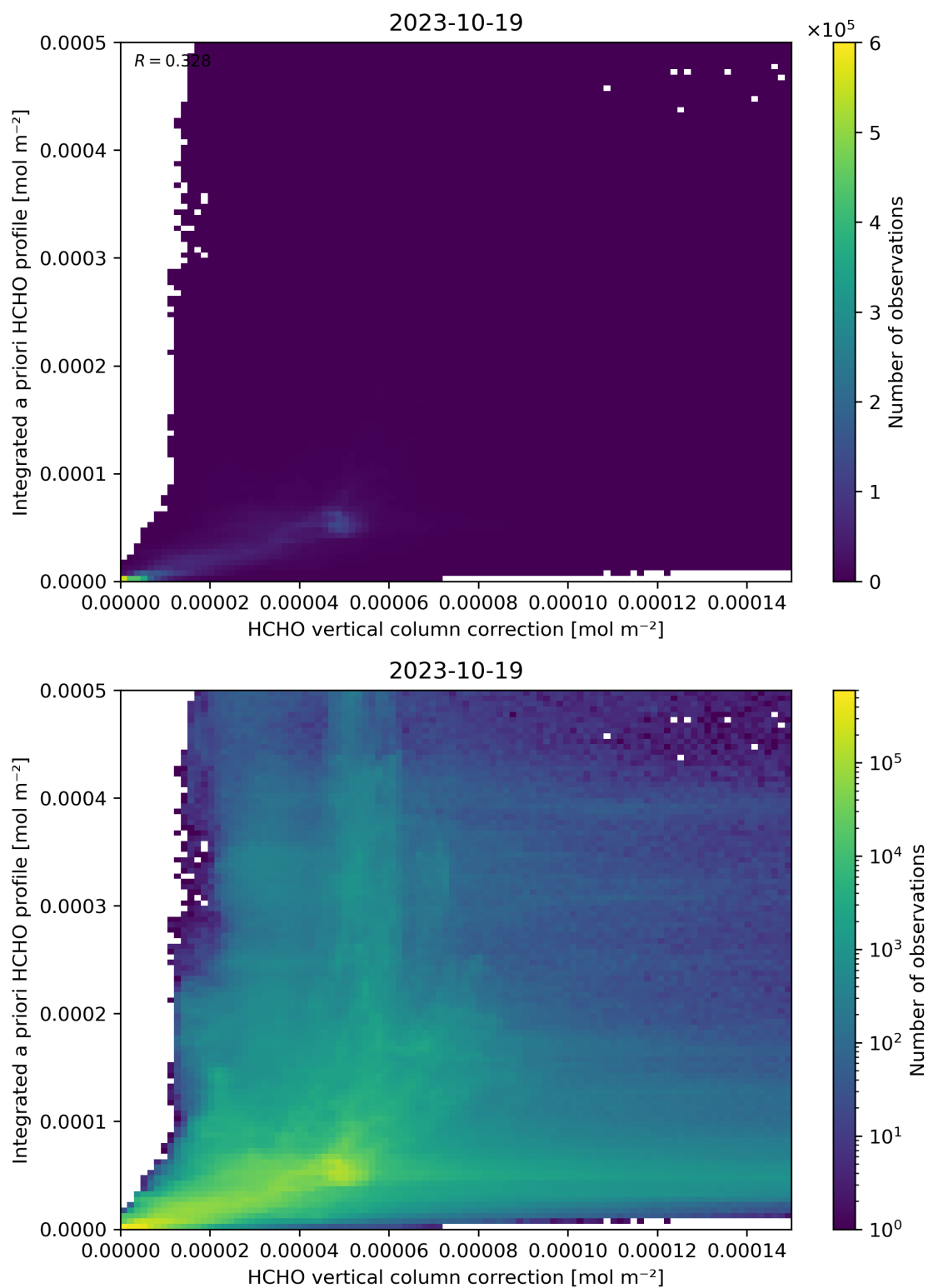
Figure 122: Scatter density plot of “HCHO vertical column correction” against “Integrated a priori HCHO profile” for 2023-10-18 to 2023-10-20.
