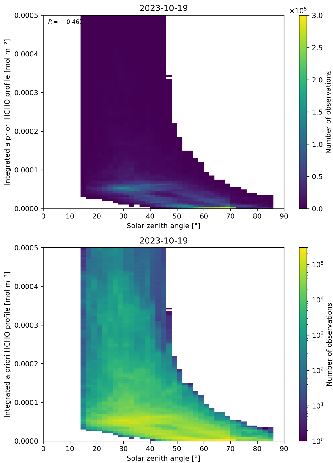
Figure 180: Scatter density plot of “Solar zenith angle” against “Integrated a priori HCHO profile” for 2023-10-18 to 2023-10-20.
