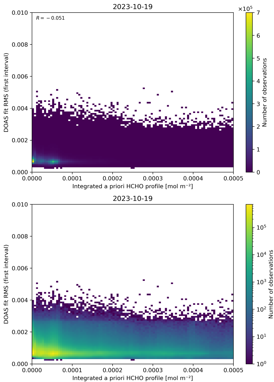
Figure 148: Scatter density plot of “Integrated a priori HCHO profile” against “DOAS fit RMS (first interval)” for 2023-10-18 to 2023-10-20.
