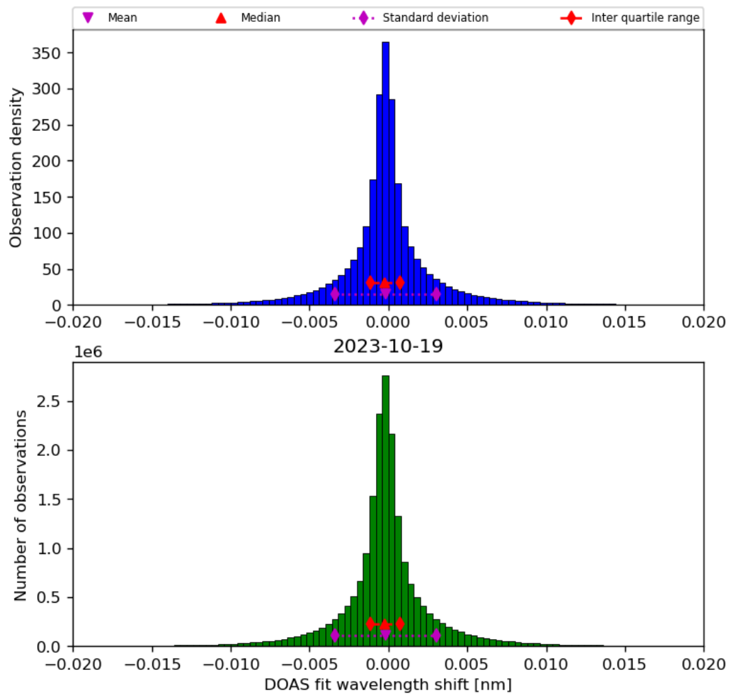
Figure 44: Histogram of “DOAS fit wavelength shift” for 2023-10-18 to 2023-10-20
