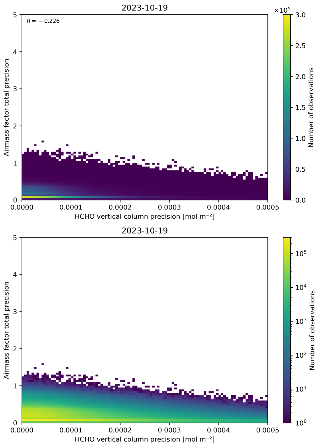
Figure 145: Scatter density plot of “HCHO vertical column precision” against “Airmass factor total precision” for 2023-10-18 to 2023-10-20.
