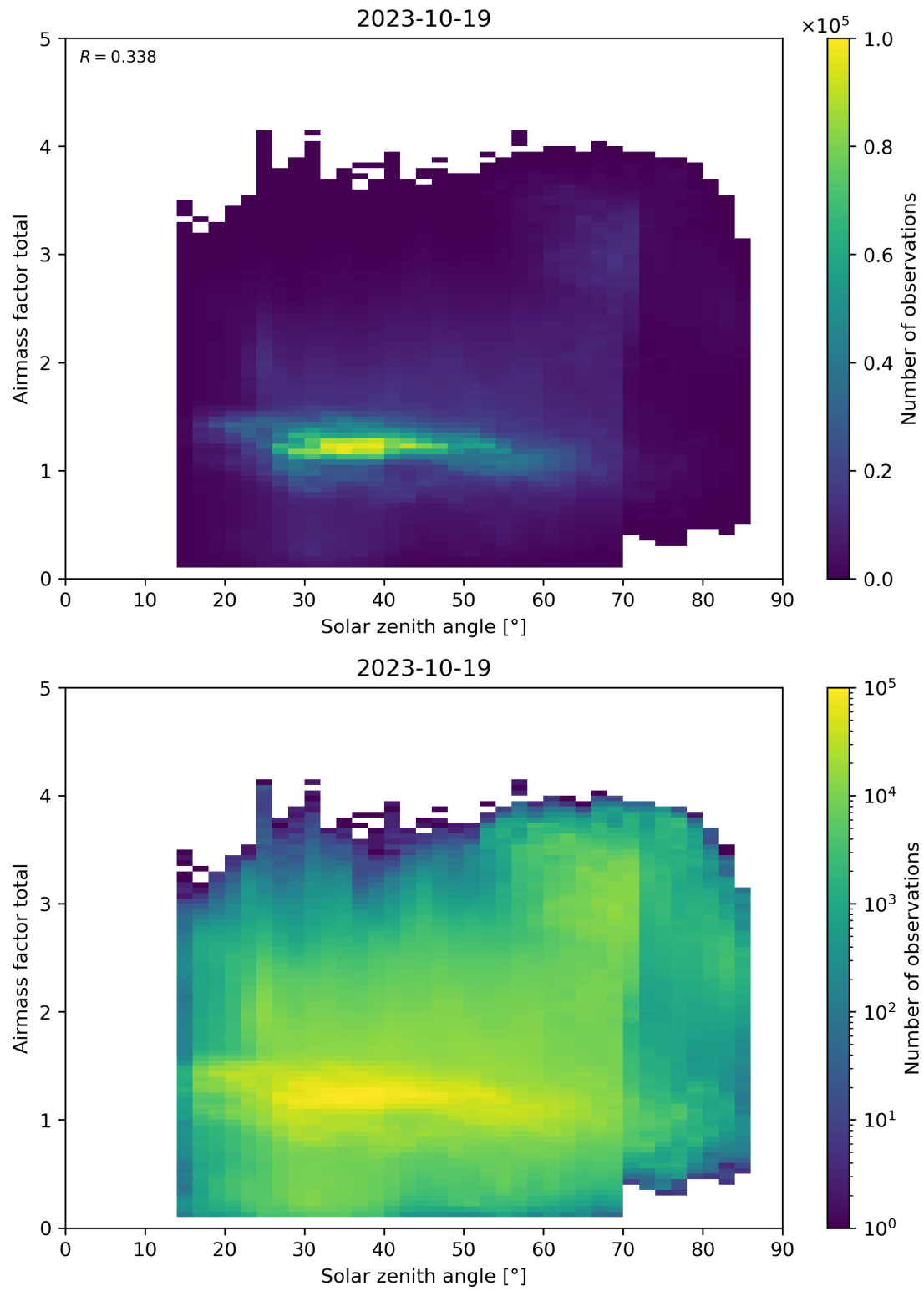
Figure 175: Scatter density plot of “Solar zenith angle” against “Airmass factor total” for 2023-10-18 to 2023-10-20.
