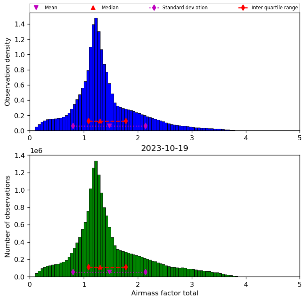
Figure 40: Histogram of “Airmass factor total” for 2023-10-18 to 2023-10-20
