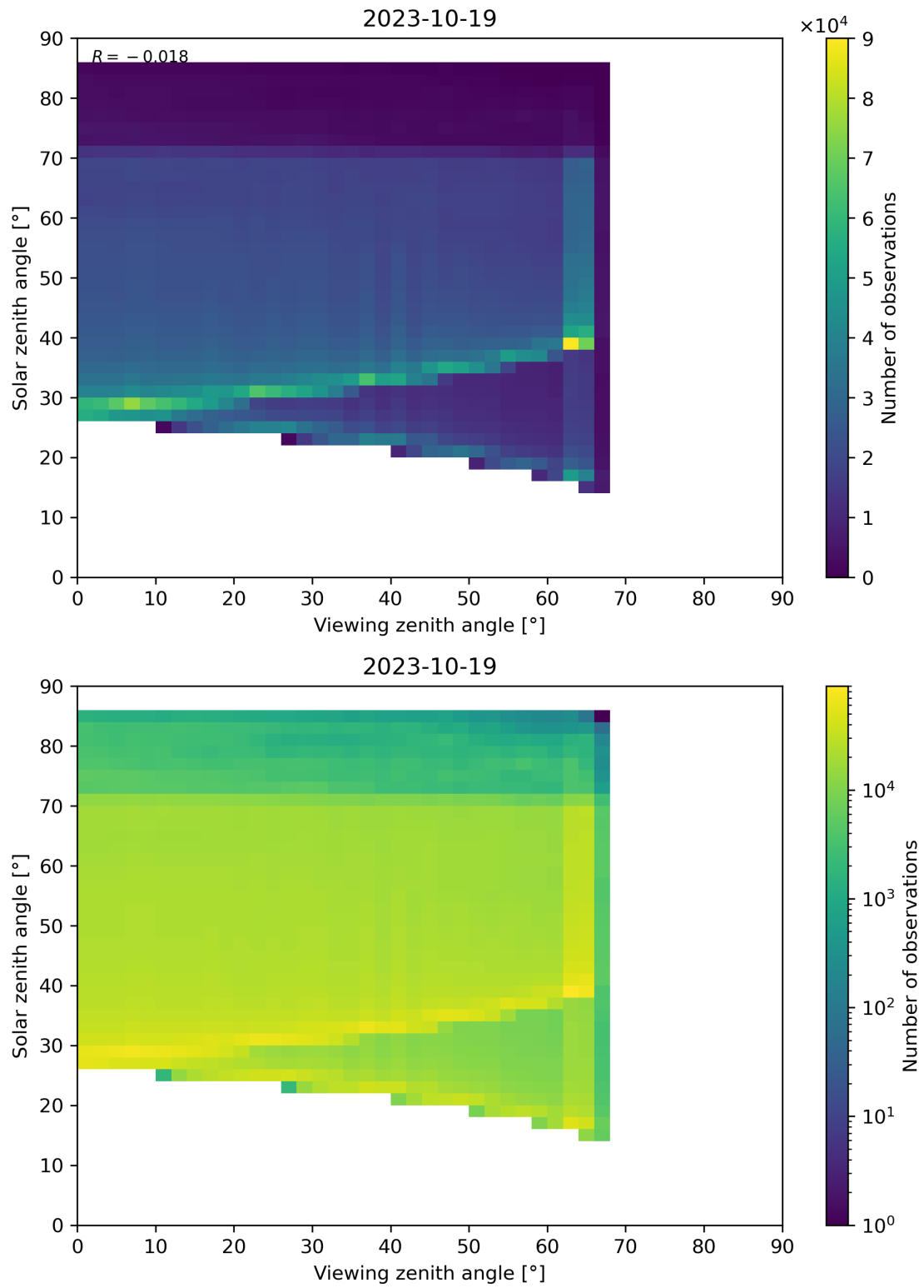
Figure 197: Scatter density plot of “Viewing zenith angle” against “Solar zenith angle” for 2023-10-18 to 2023-10-20.
