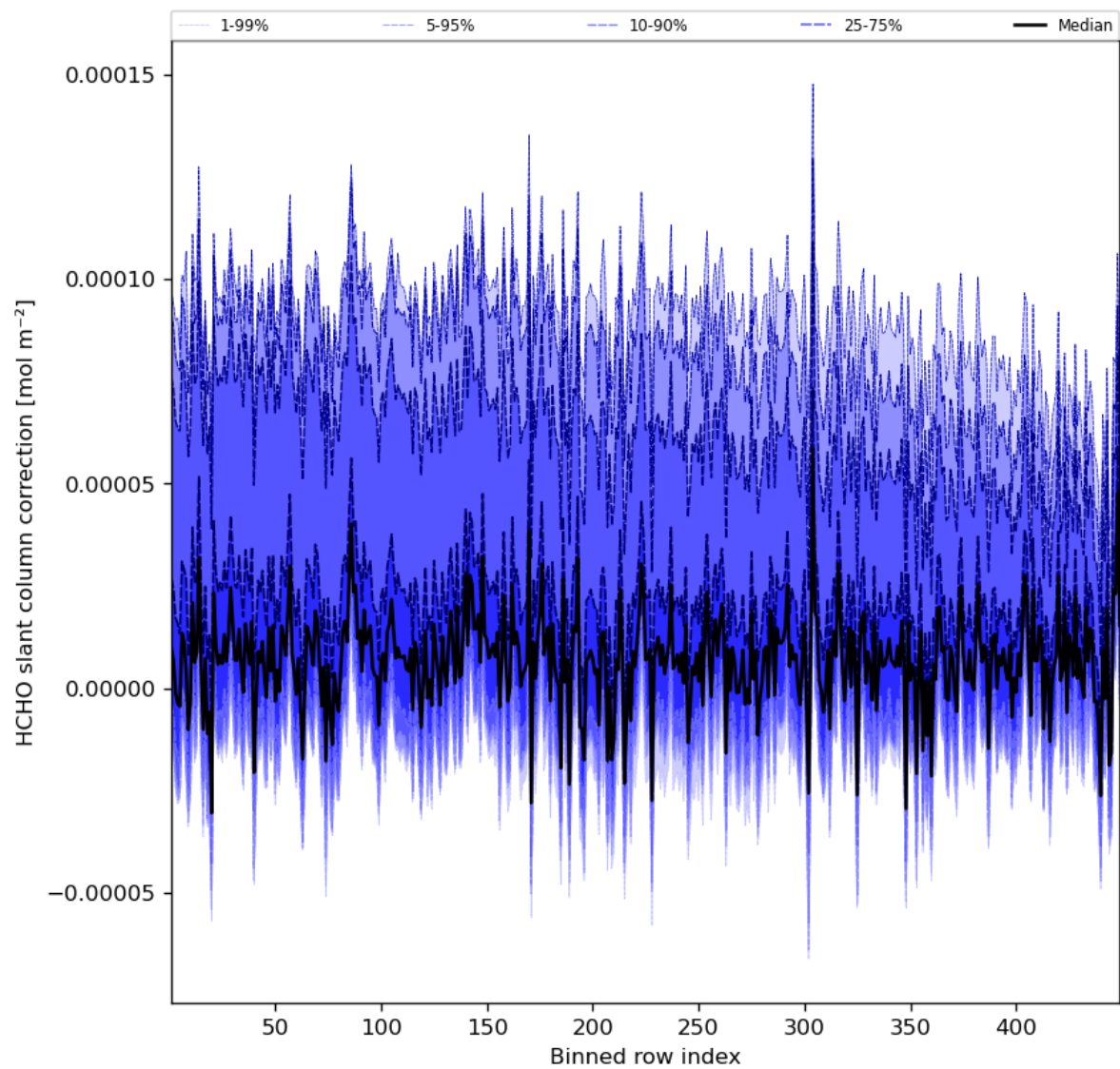
Figure 61: Along track statistics of “HCHO slant column correction” for 2023-10-18 to 2023-10-20
