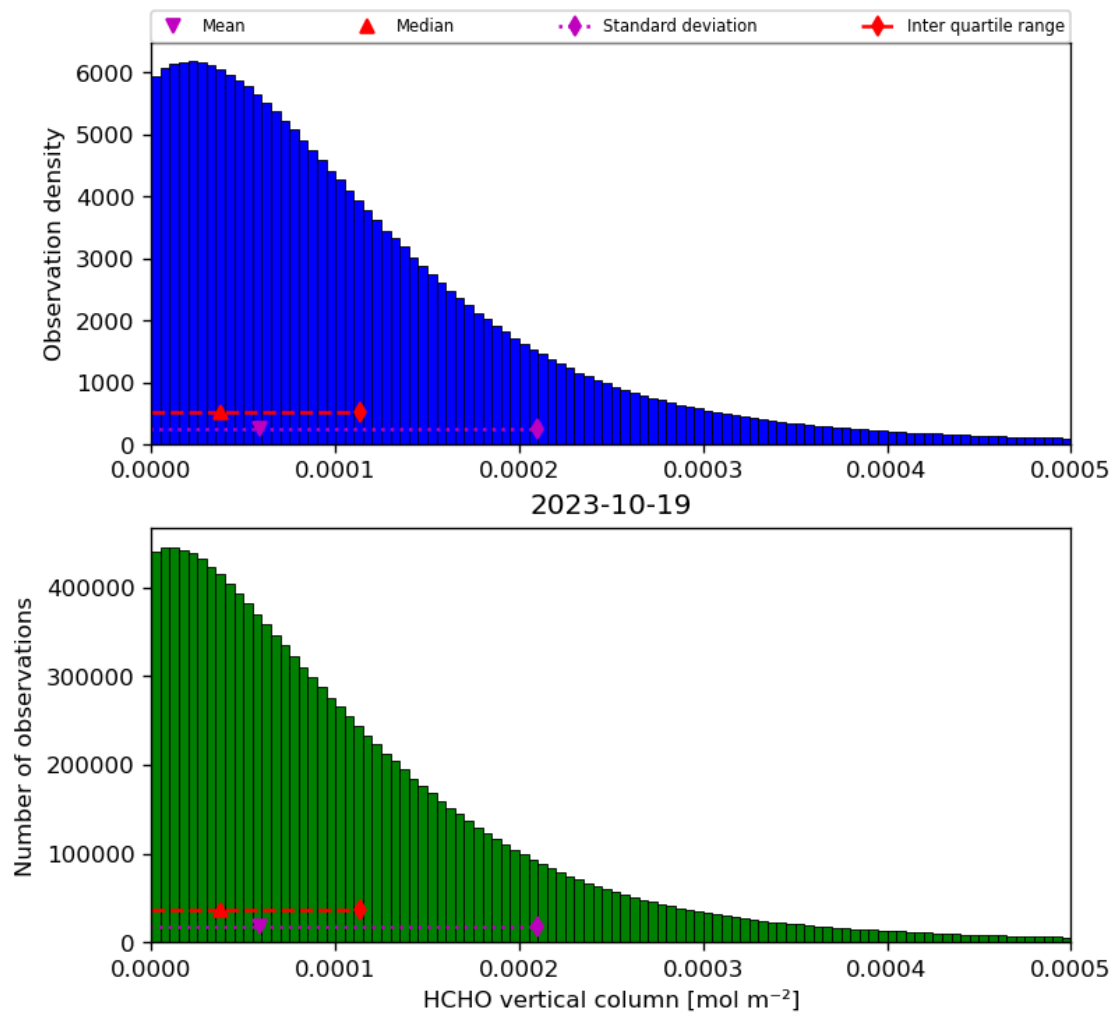
Figure 35: Histogram of “HCHO vertical column” for 2023-10-18 to 2023-10-20
