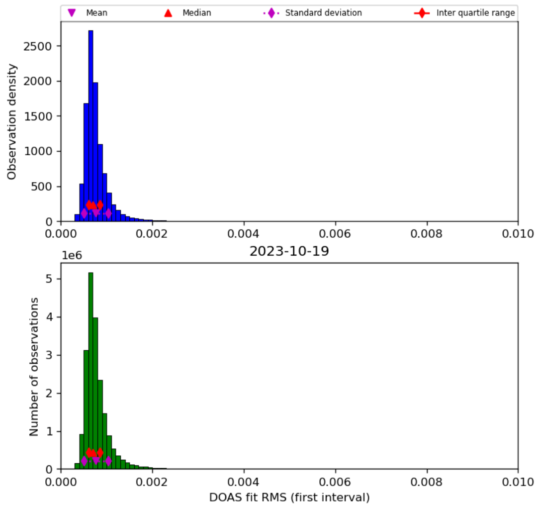
Figure 46: Histogram of “DOAS fit RMS (first interval)” for 2023-10-18 to 2023-10-20
