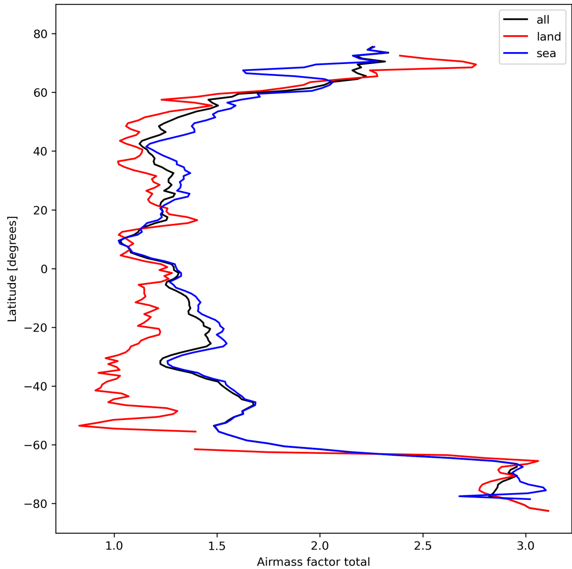
Figure 26: Zonal average of “Airmass factor total” for 2023-10-18 to 2023-10-20.
