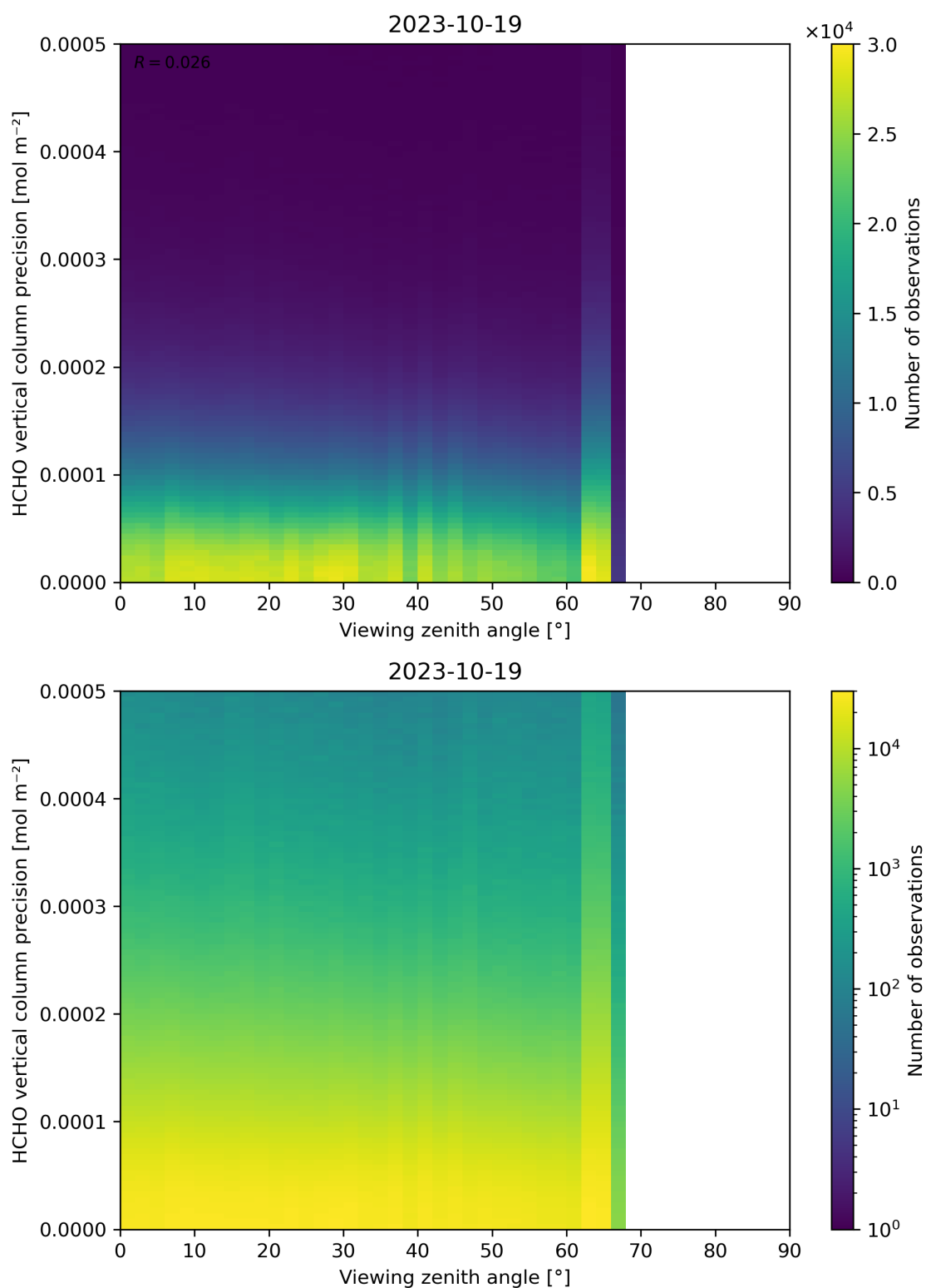
Figure 194: Scatter density plot of “Viewing zenith angle” against “HCHO vertical column precision” for 2023-10-18 to 2023-10-20.
