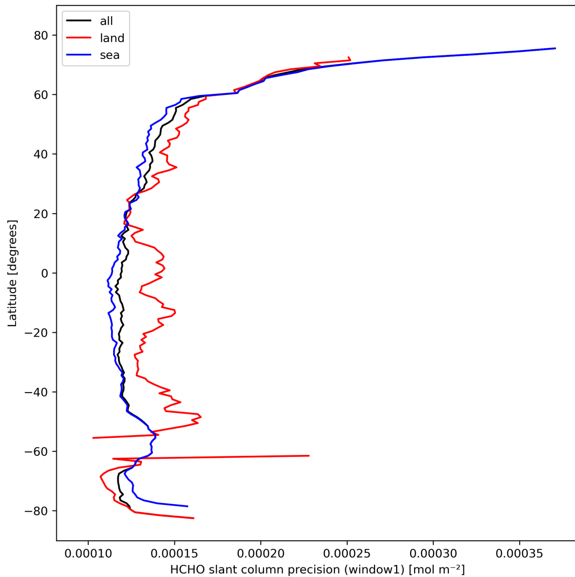
Figure 25: Zonal average of “HCHO slant column precision (window1)” for 2023-10-18 to 2023-10-20.
