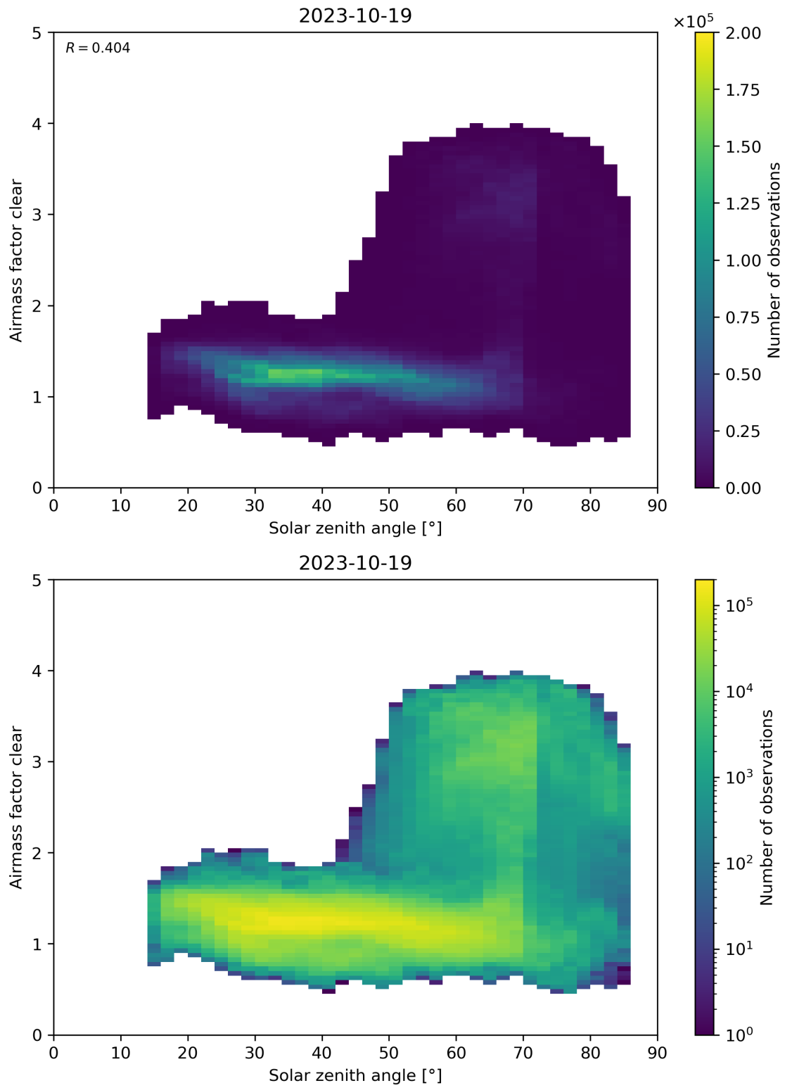
Figure 170: Scatter density plot of “Solar zenith angle” against “Airmass factor clear” for 2023-10-18 to 2023-10-20.
