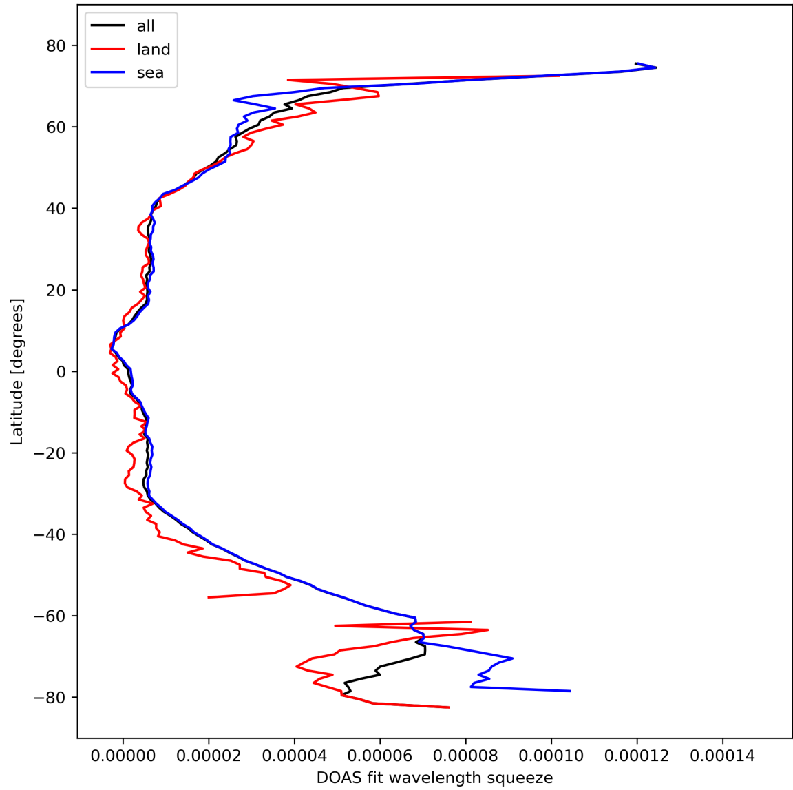
Figure 31: Zonal average of “DOAS fit wavelength squeeze” for 2023-10-18 to 2023-10-20.
