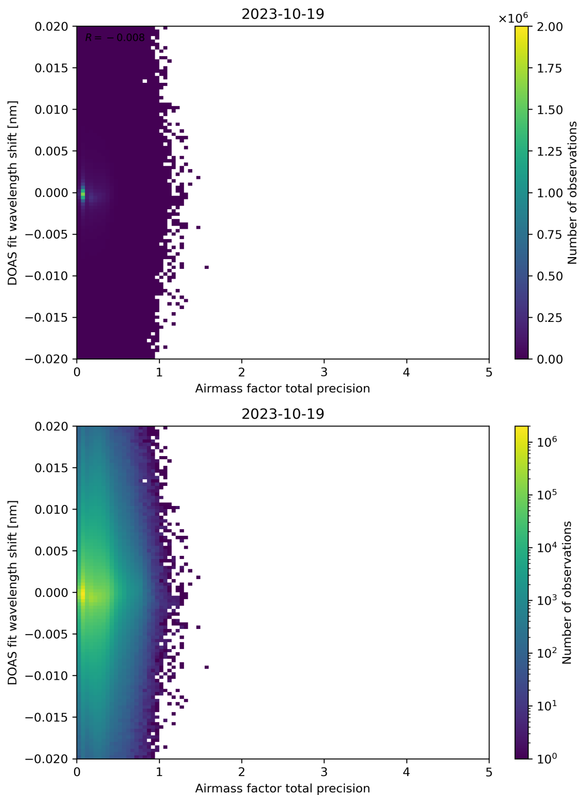
Figure 106: Scatter density plot of “Airmass factor total precision” against “DOAS fit wavelength shift” for 2023-10-18 to 2023-10-20.
