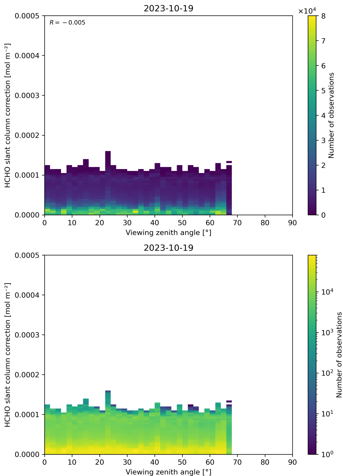
Figure 187: Scatter density plot of “Viewing zenith angle” against “HCHO slant column correction” for 2023-10-18 to 2023-10-20.
