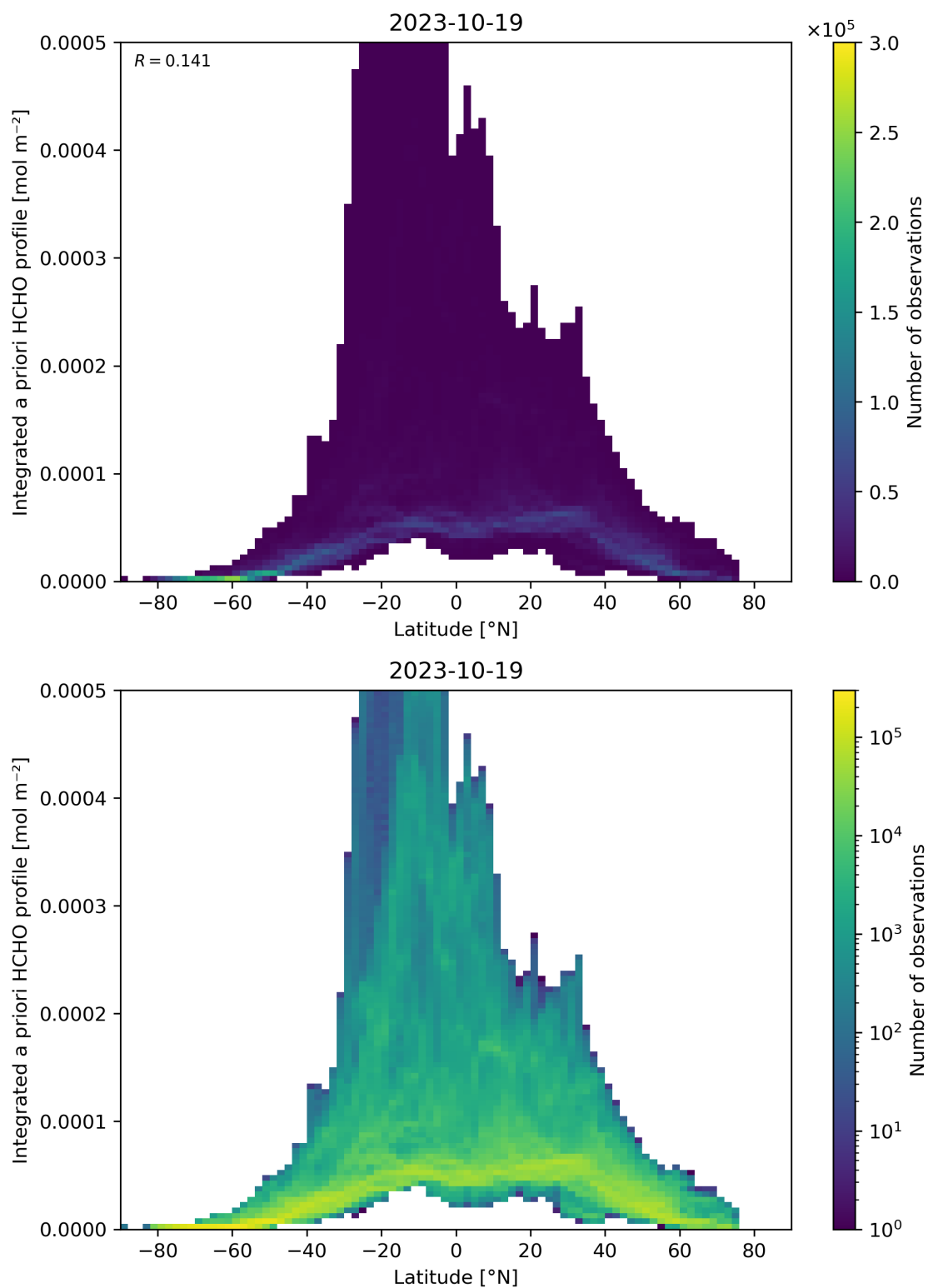
Figure 166: Scatter density plot of “Latitude” against “Integrated a priori HCHO profile” for 2023-10-18 to 2023-10-20.
