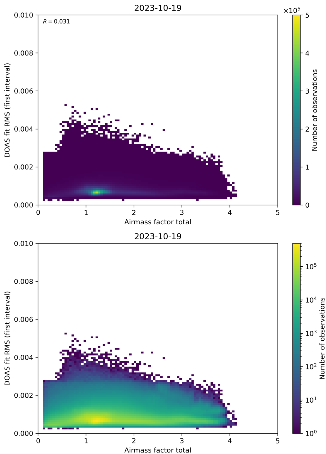
Figure 97: Scatter density plot of “Airmass factor total” against “DOAS fit RMS (first interval)” for 2023-10-18 to 2023-10-20.
