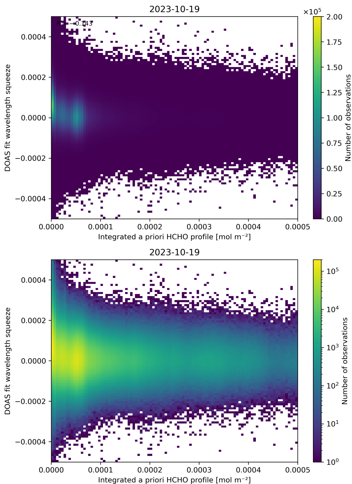
Figure 150: Scatter density plot of “Integrated a priori HCHO profile” against “DOAS fit wavelength squeeze” for 2023-10-18 to 2023-10-20.
