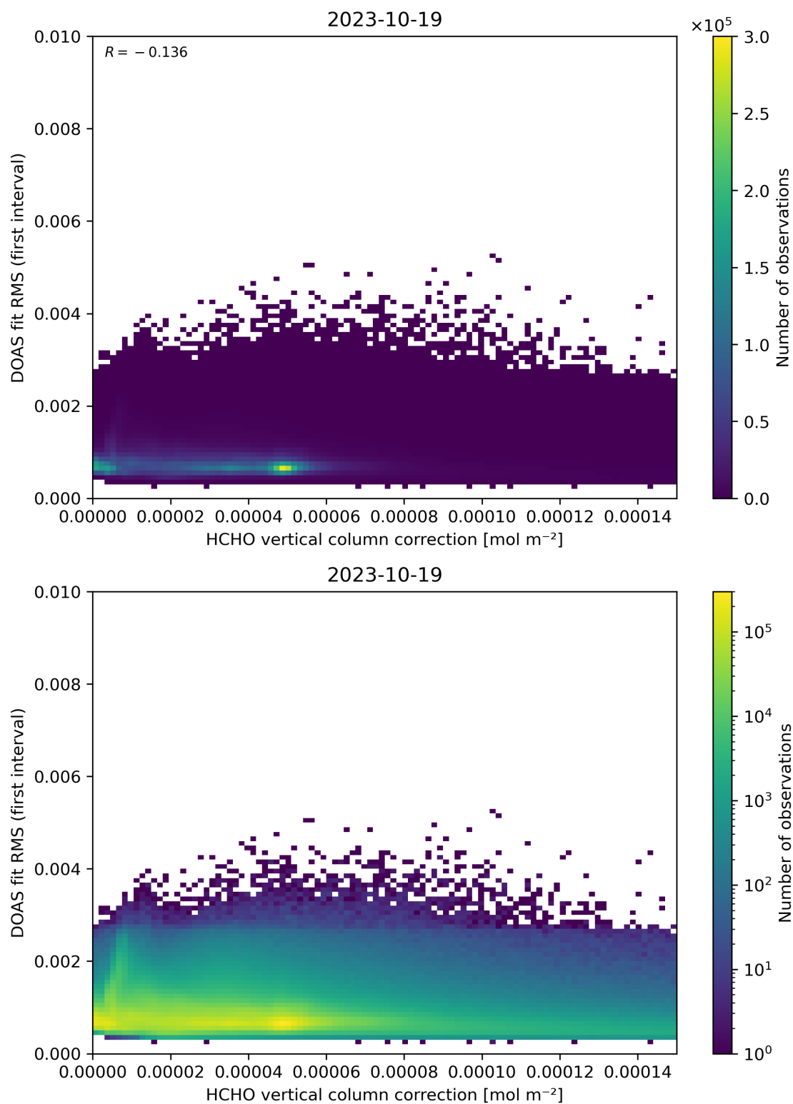
Figure 112: Scatter density plot of “HCHO vertical column correction” against “DOAS fit RMS (first interval)” for 2023-10-18 to 2023-10-20.
