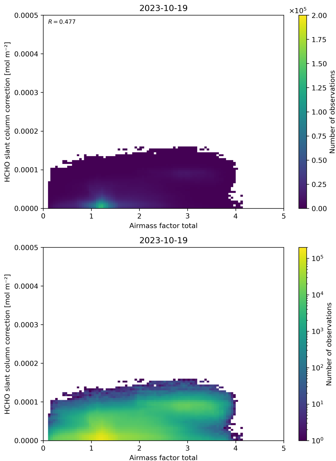
Figure 102: Scatter density plot of “Airmass factor total” against “HCHO slant column correction” for 2023-10-18 to 2023-10-20.
