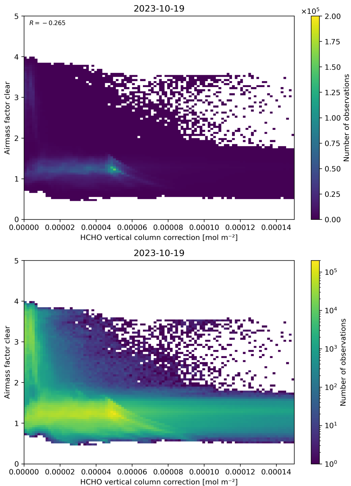
Figure 115: Scatter density plot of “HCHO vertical column correction” against “Airmass factor clear” for 2023-10-18 to 2023-10-20.
