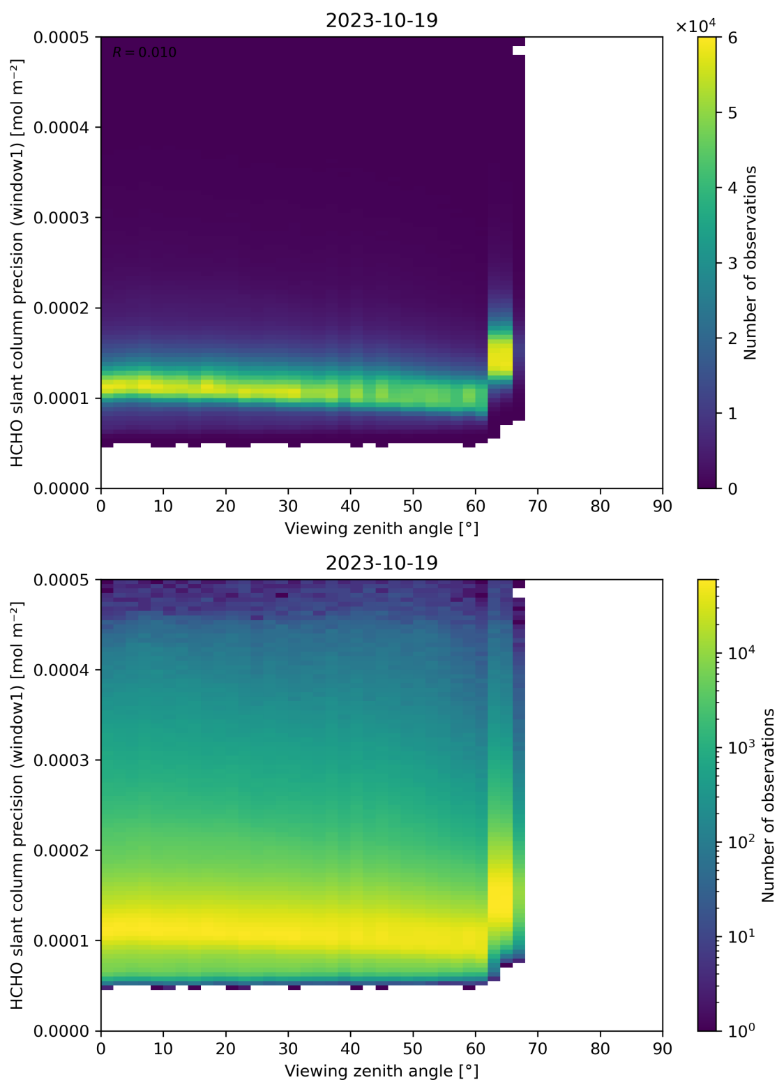
Figure 189: Scatter density plot of “Viewing zenith angle” against “HCHO slant column precision (window1)” for 2023-10-18 to 2023-10-20.
