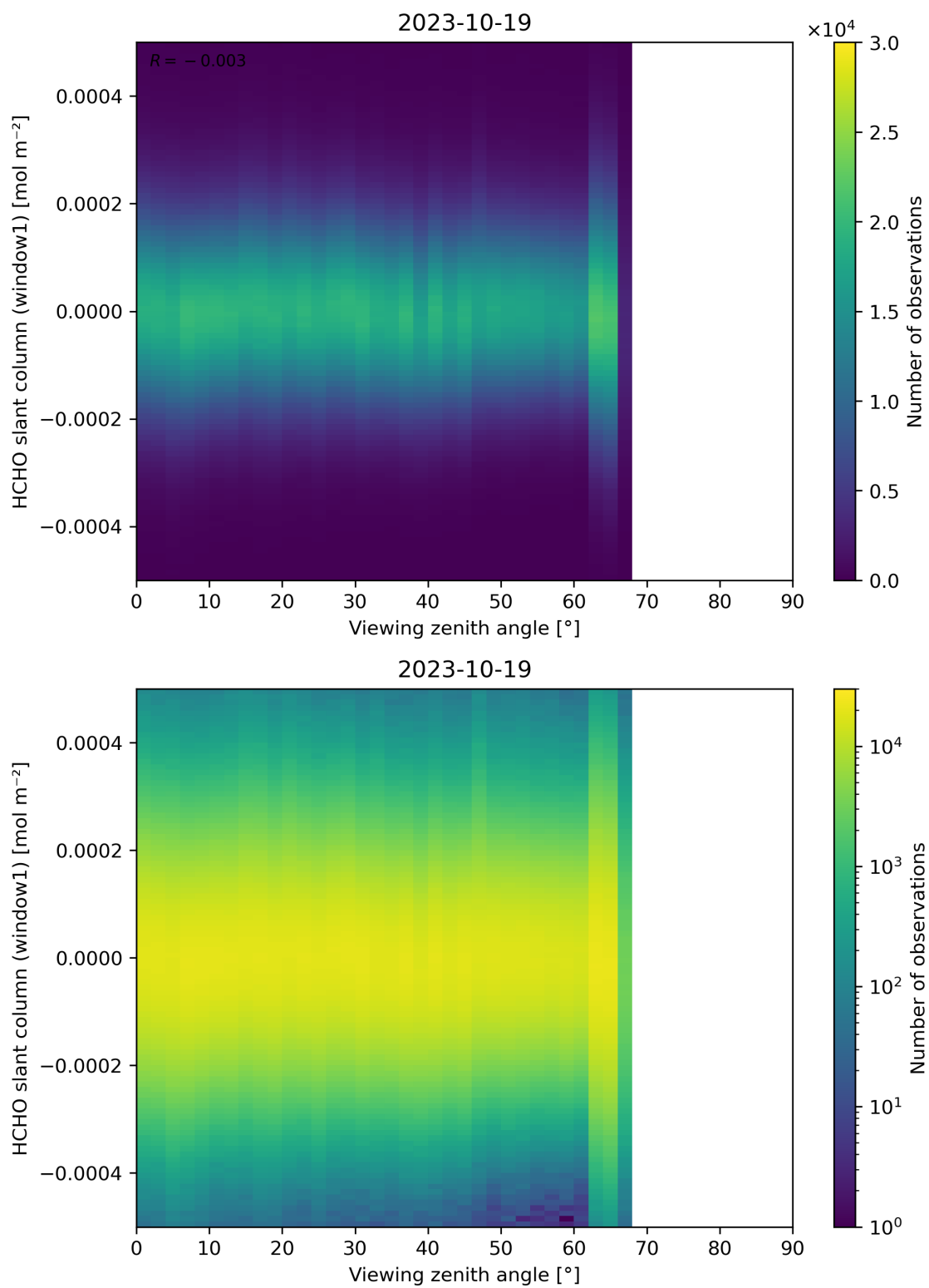
Figure 188: Scatter density plot of “Viewing zenith angle” against “HCHO slant column (window1)” for 2023-10-18 to 2023-10-20.
