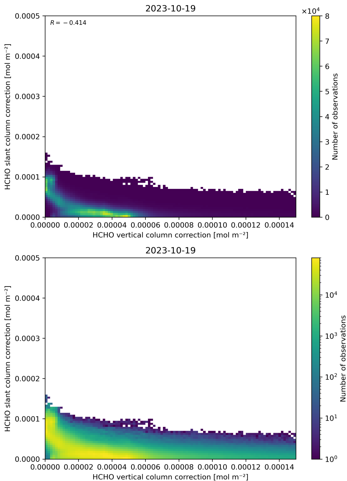
Figure 117: Scatter density plot of “HCHO vertical column correction” against “HCHO slant column correction” for 2023-10-18 to 2023-10-20.
