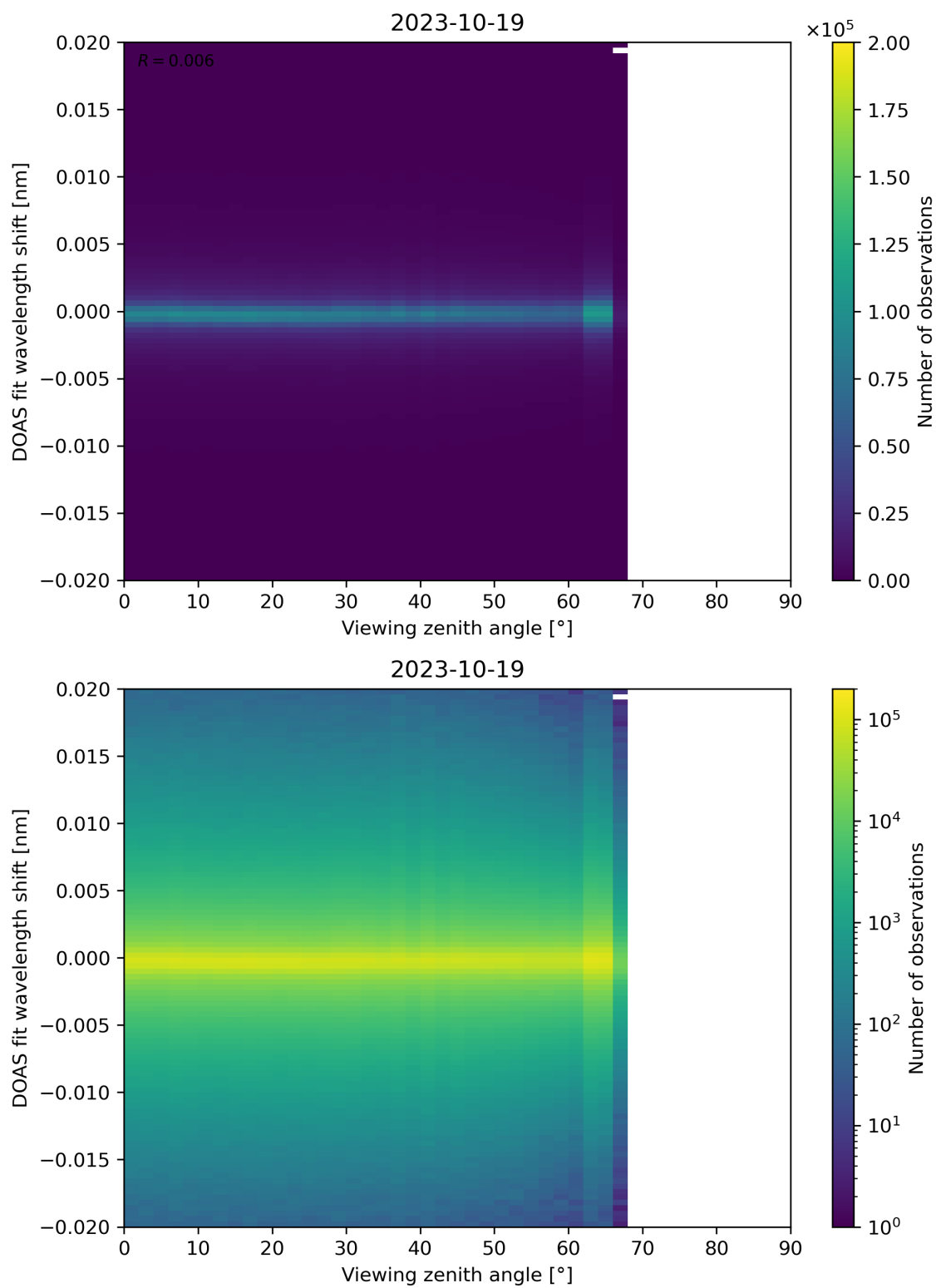
Figure 183: Scatter density plot of “Viewing zenith angle” against “DOAS fit wavelength shift” for 2023-10-18 to 2023-10-20.
