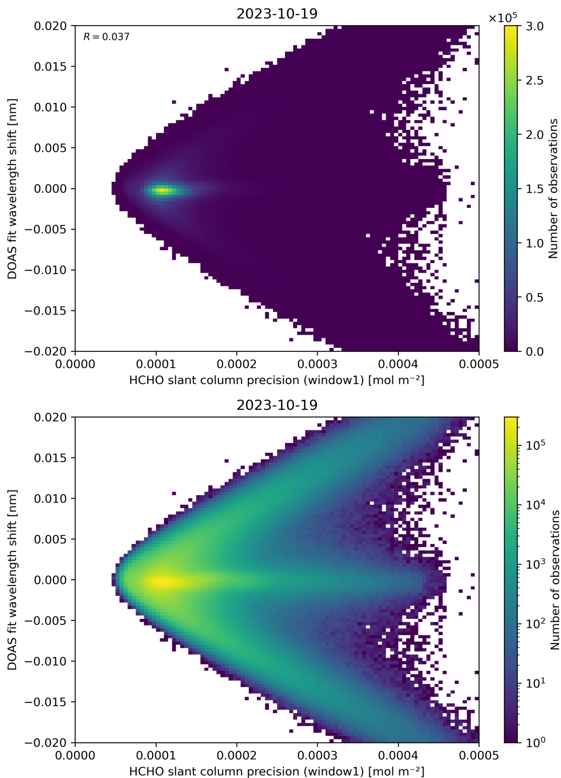
Figure 89: Scatter density plot of “HCHO slant column precision (window1)” against “DOAS fit wavelength shift” for 2023-10-18 to 2023-10-20.
