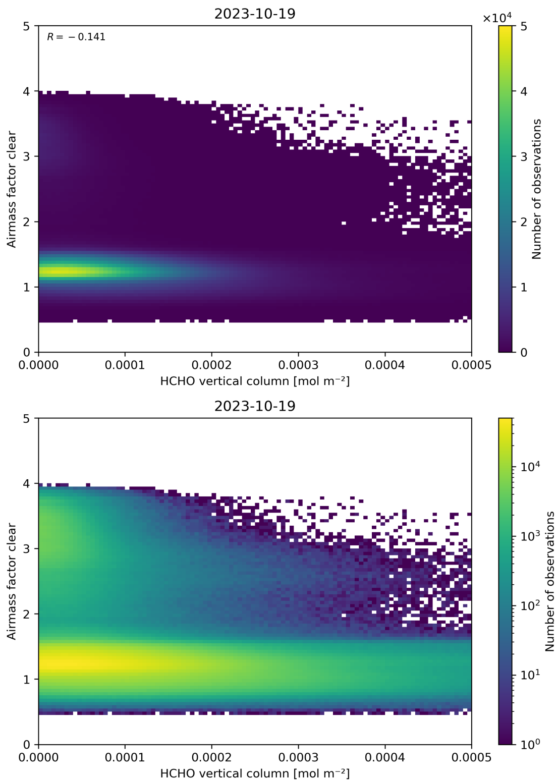
Figure 126: Scatter density plot of “HCHO vertical column” against “Airmass factor clear” for 2023-10-18 to 2023-10-20.
