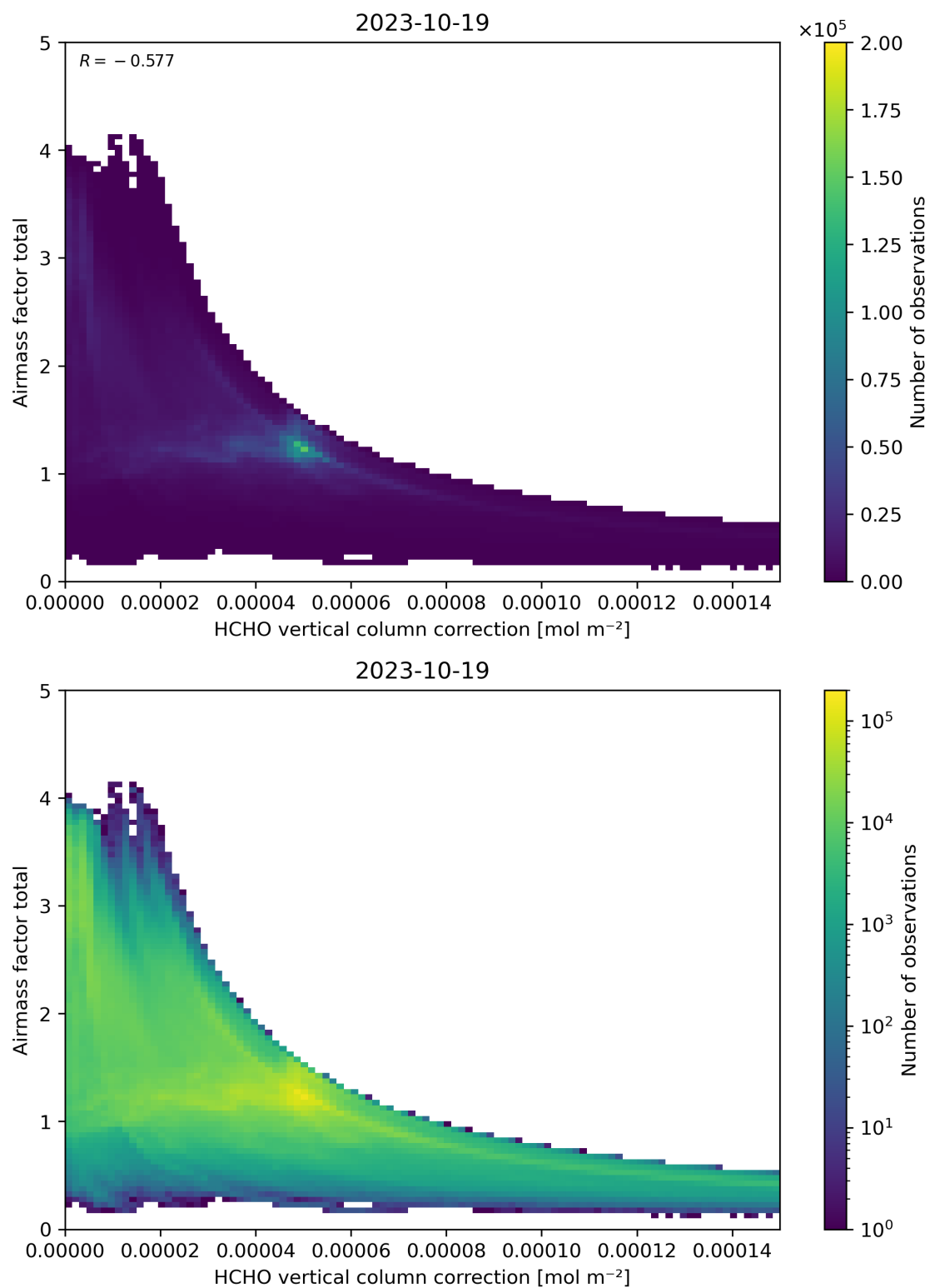
Figure 120: Scatter density plot of “HCHO vertical column correction” against “Airmass factor total” for 2023-10-18 to 2023-10-20.
