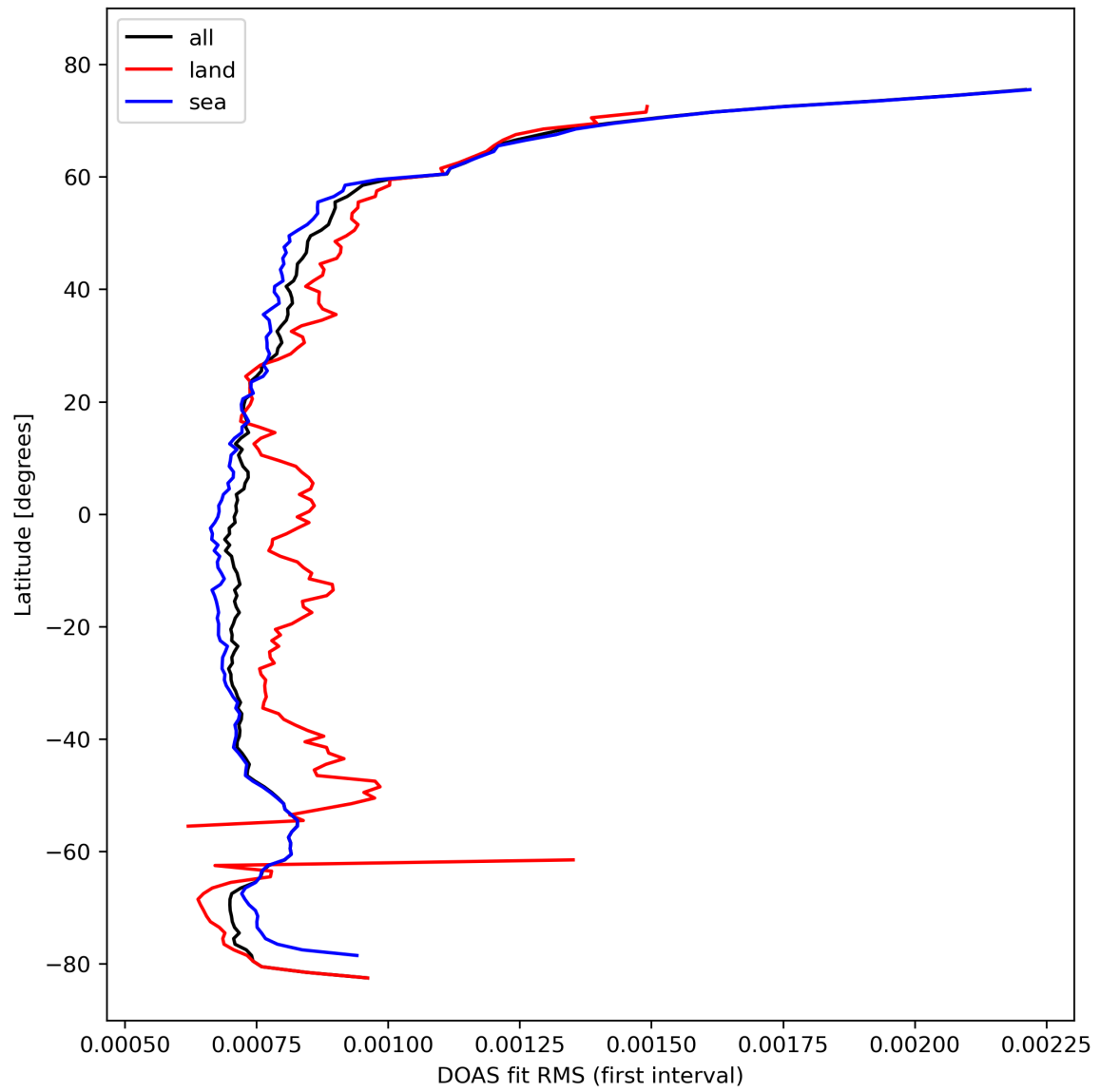
Figure 32: Zonal average of “DOAS fit RMS (first interval)” for 2023-10-18 to 2023-10-20.
