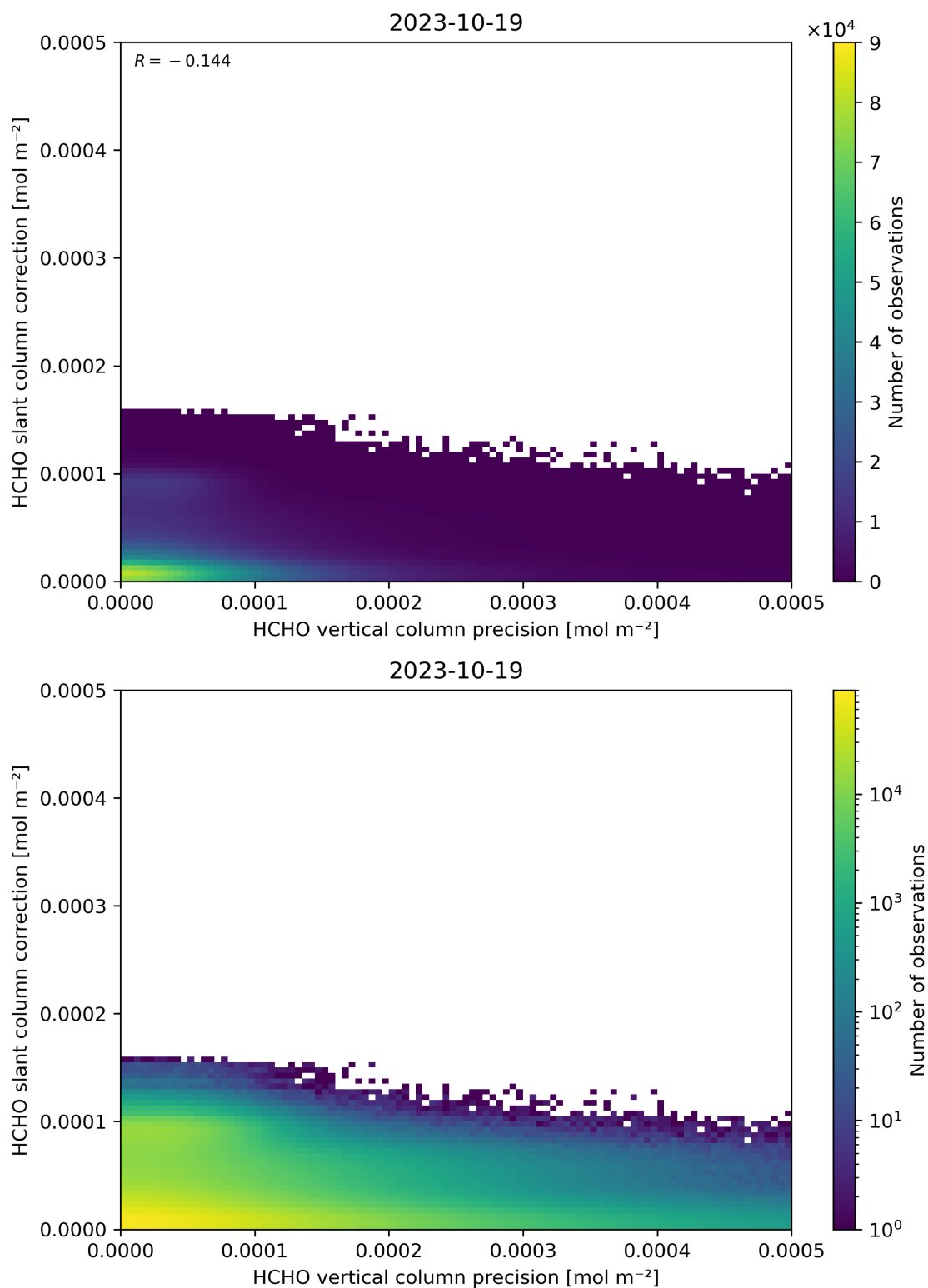
Figure 141: Scatter density plot of “HCHO vertical column precision” against “HCHO slant column correction” for 2023-10-18 to 2023-10-20.
