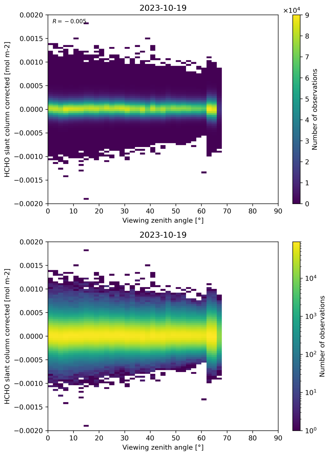
Figure 186: Scatter density plot of “Viewing zenith angle” against “HCHO slant column corrected” for 2023-10-18 to 2023-10-20.
