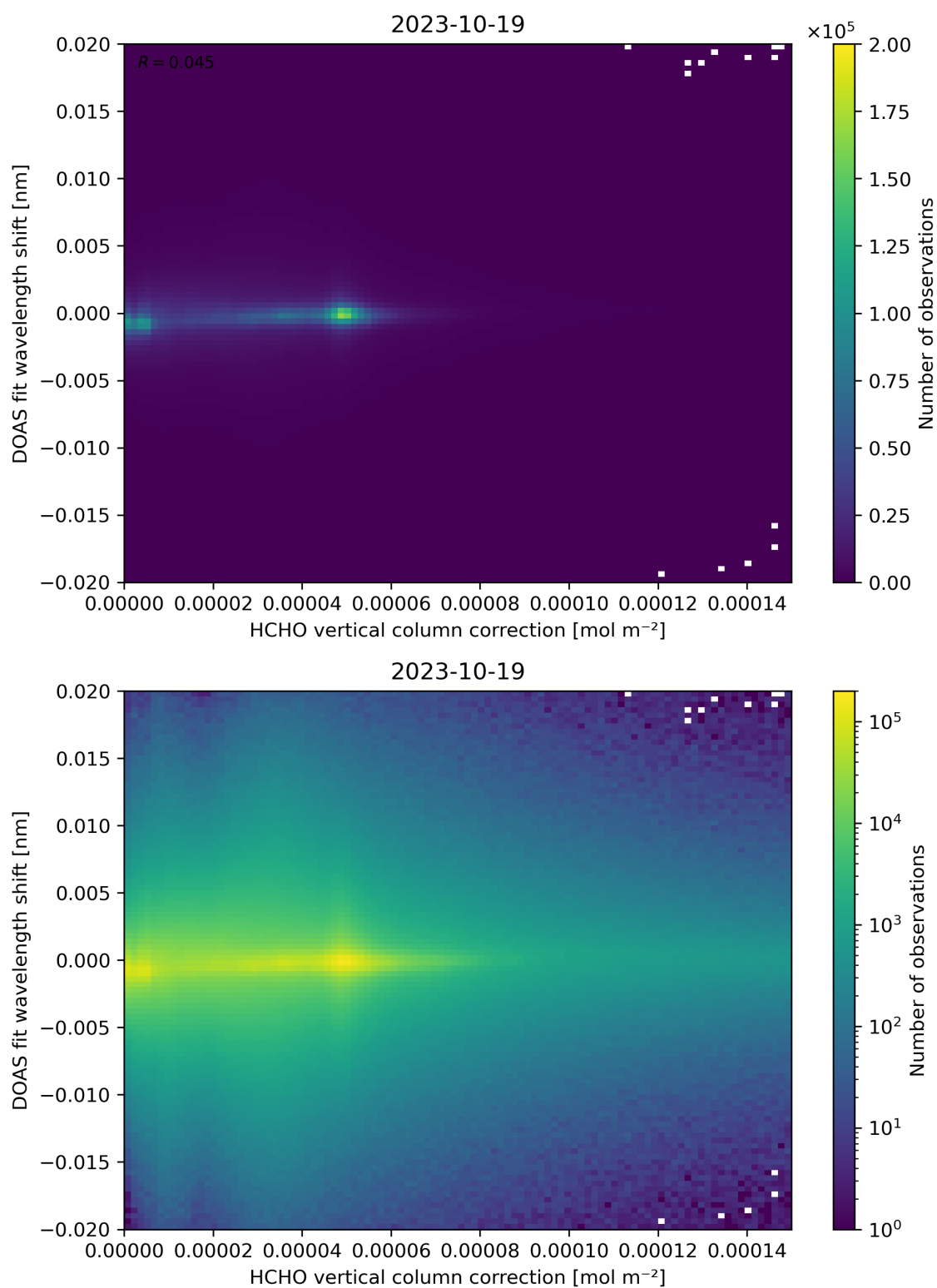
Figure 113: Scatter density plot of “HCHO vertical column correction” against “DOAS fit wavelength shift” for 2023-10-18 to 2023-10-20.
