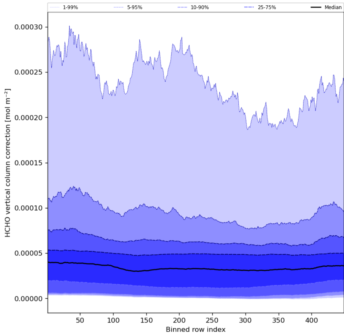
Figure 51: Along track statistics of “HCHO vertical column correction” for 2023-10-18 to 2023-10-20
