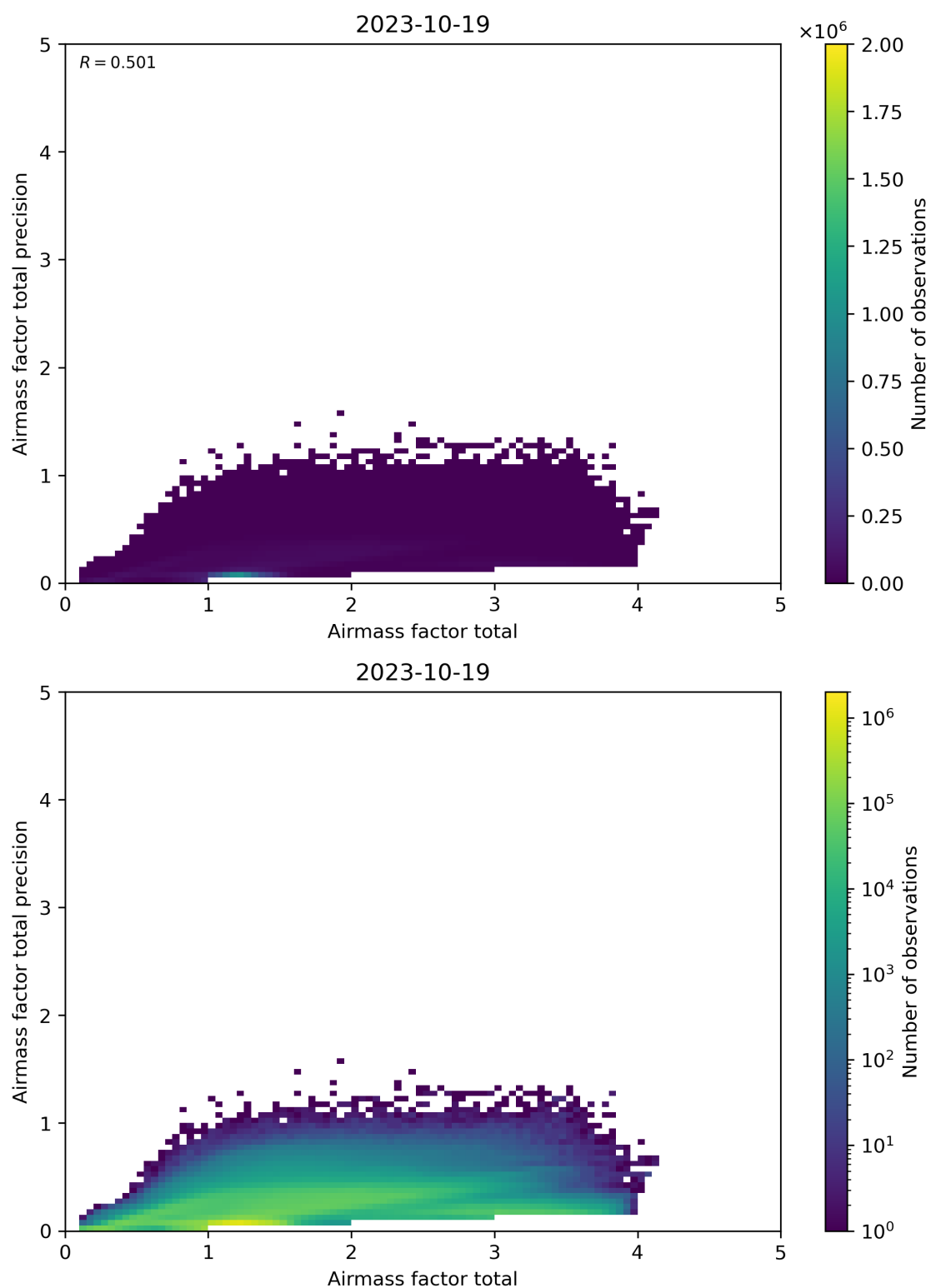
Figure 103: Scatter density plot of “Airmass factor total” against “Airmass factor total precision” for 2023-10-18 to 2023-10-20.
