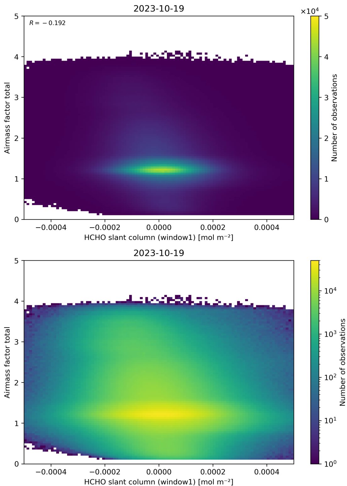
Figure 85: Scatter density plot of “HCHO slant column (window1)” against “Airmass factor total” for 2023-10-18 to 2023-10-20.
