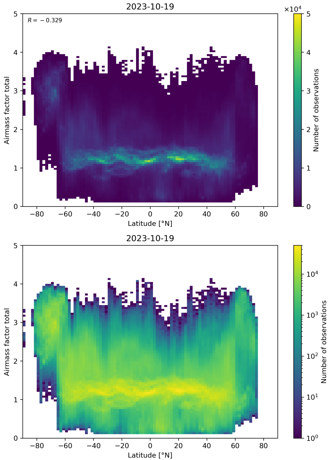
Figure 161: Scatter density plot of “Latitude” against “Airmass factor total” for 2023-10-18 to 2023-10-20.
