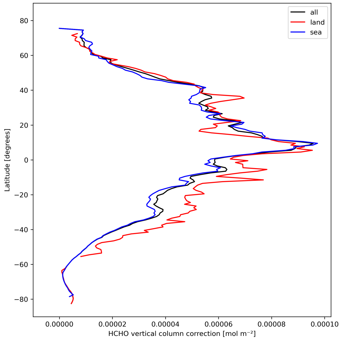
Figure 23: Zonal average of “HCHO vertical column correction” for 2023-10-18 to 2023-10-20.
