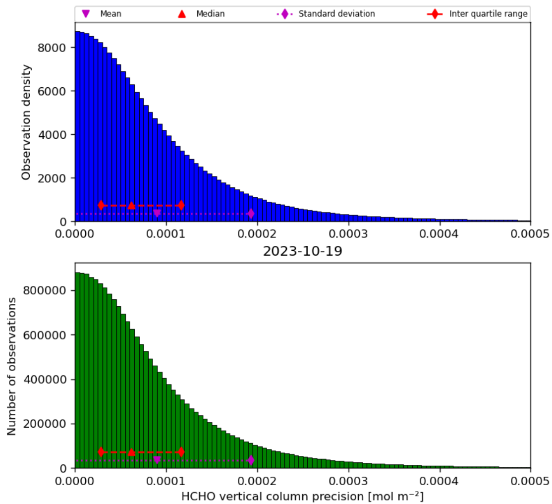
Figure 36: Histogram of “HCHO vertical column precision” for 2023-10-18 to 2023-10-20
