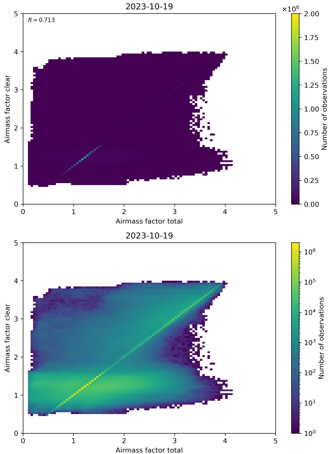
Figure 100: Scatter density plot of “Airmass factor total” against “Airmass factor clear” for 2023-10-18 to 2023-10-20.
