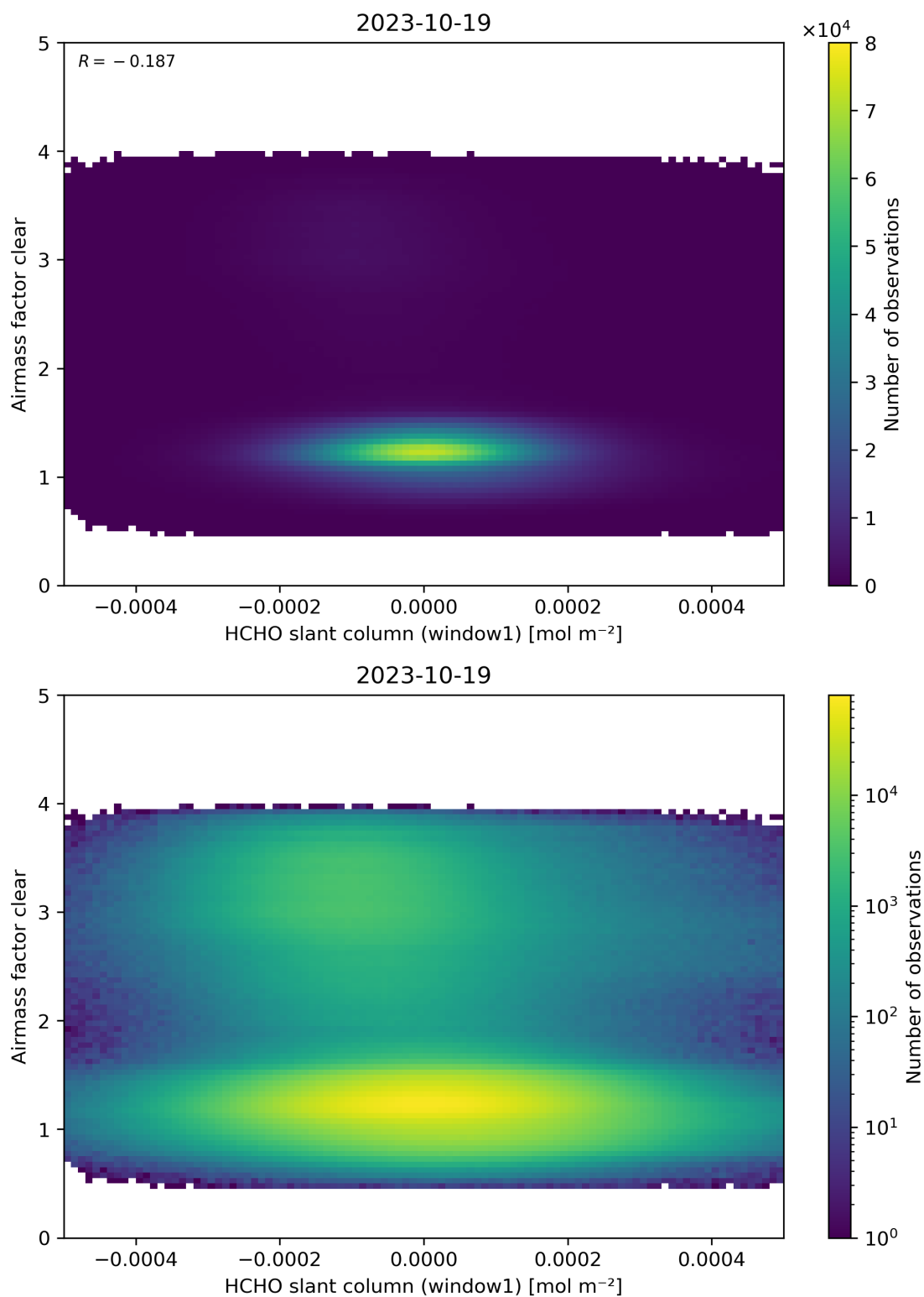
Figure 81: Scatter density plot of “HCHO slant column (window1)” against “Airmass factor clear” for 2023-10-18 to 2023-10-20.
