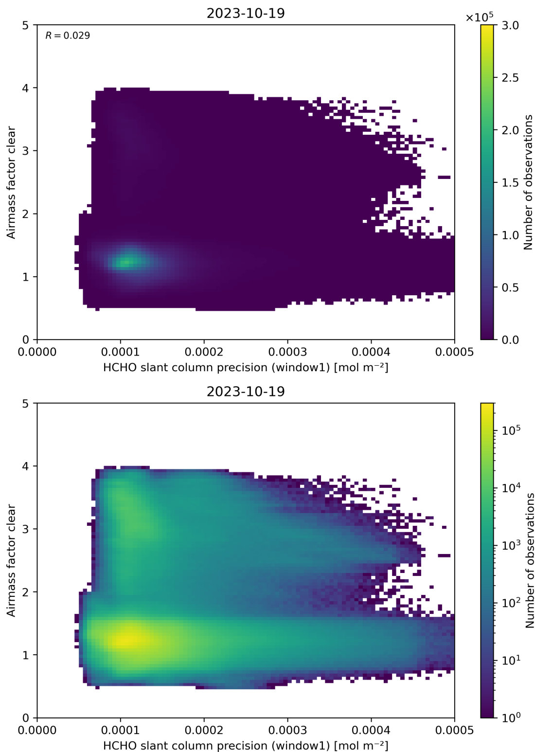
Figure 91: Scatter density plot of “HCHO slant column precision (window1)” against “Airmass factor clear” for 2023-10-18 to 2023-10-20.
