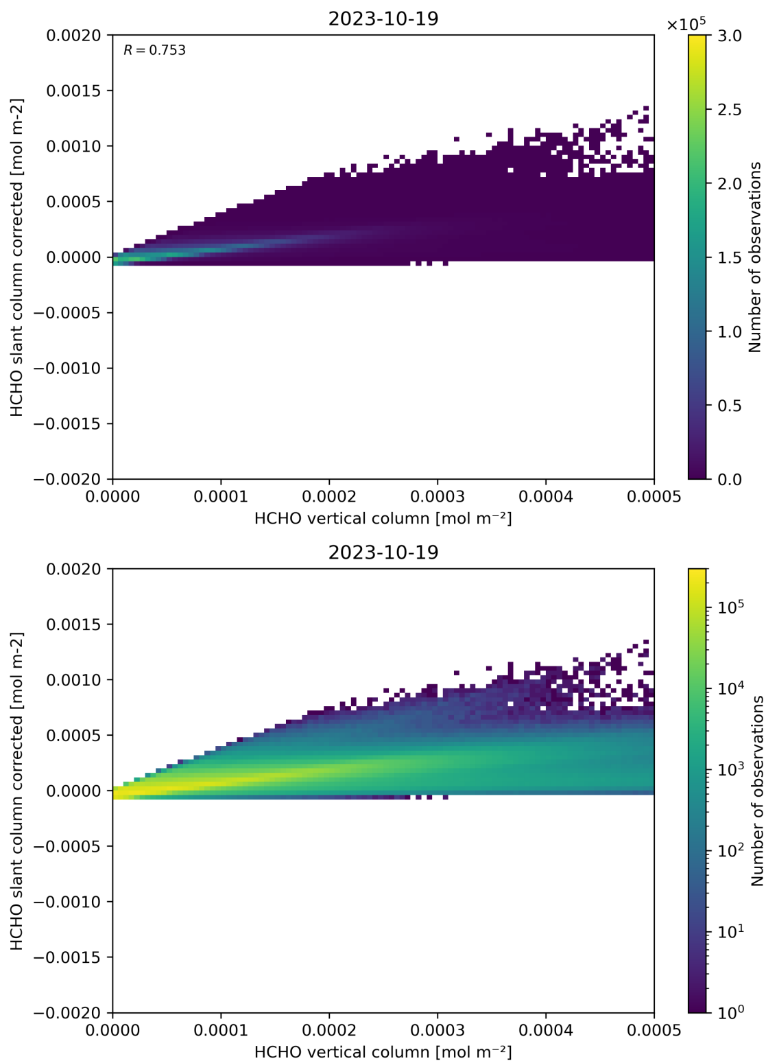
Figure 127: Scatter density plot of “HCHO vertical column” against “HCHO slant column corrected” for 2023-10-18 to 2023-10-20.
