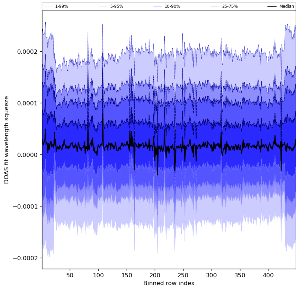
Figure 59: Along track statistics of “DOAS fit wavelength squeeze” for 2023-10-18 to 2023-10-20
