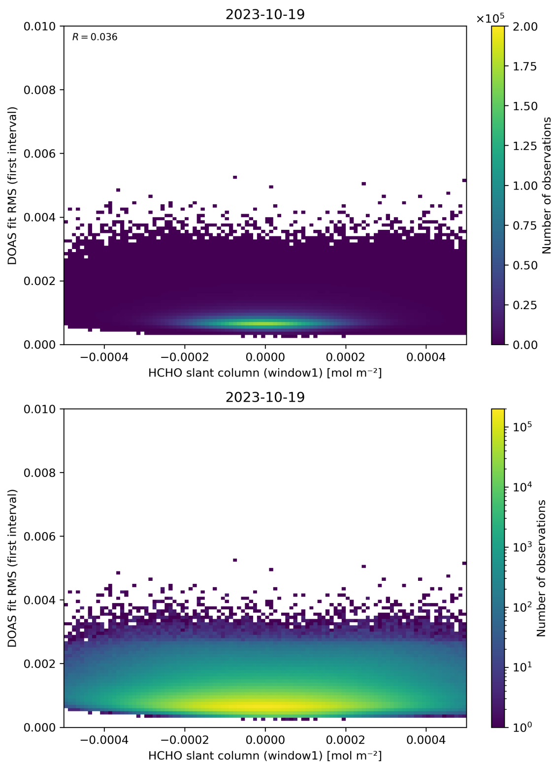
Figure 78: Scatter density plot of “HCHO slant column (window1)” against “DOAS fit RMS (first interval)” for 2023-10-18 to 2023-10-20.
