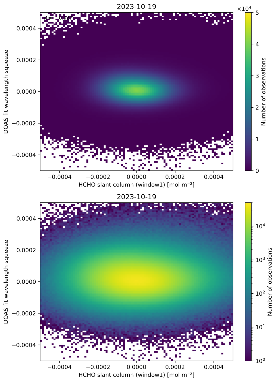
Figure 80: Scatter density plot of “HCHO slant column (window1)” against “DOAS fit wavelength squeeze” for 2023-10-18 to 2023-10-20.
