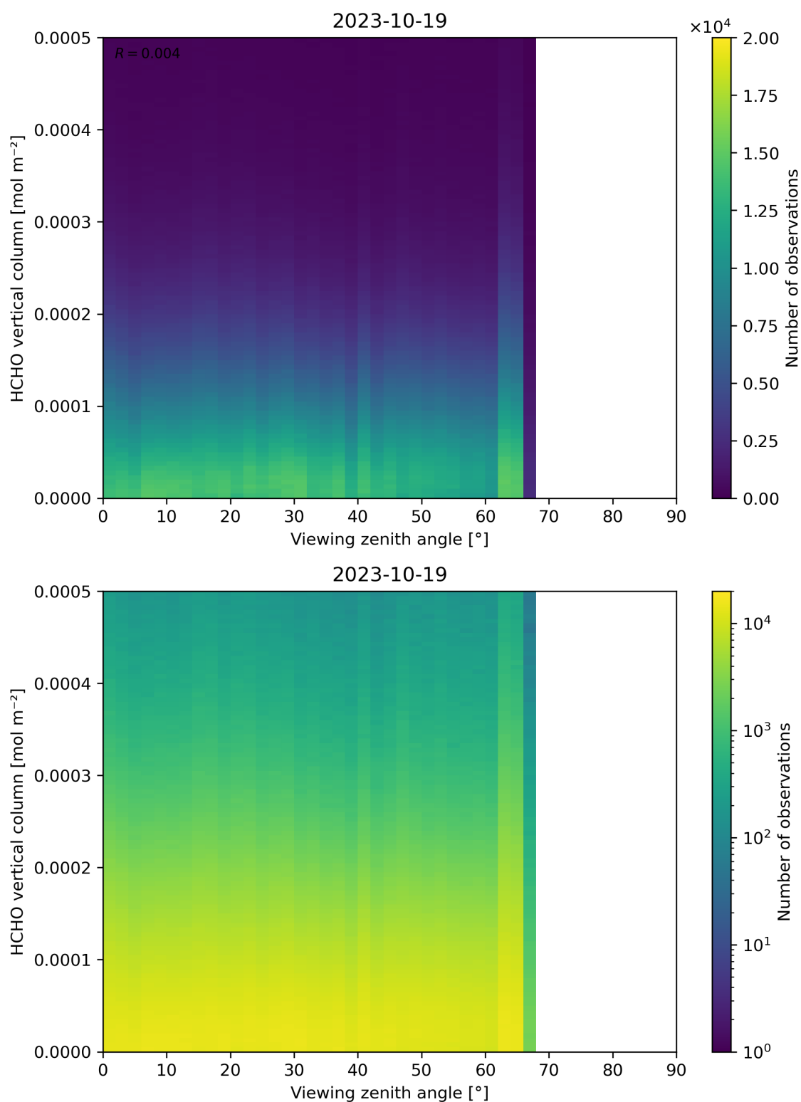
Figure 192: Scatter density plot of “Viewing zenith angle” against “HCHO vertical column” for 2023-10-18 to 2023-10-20.
