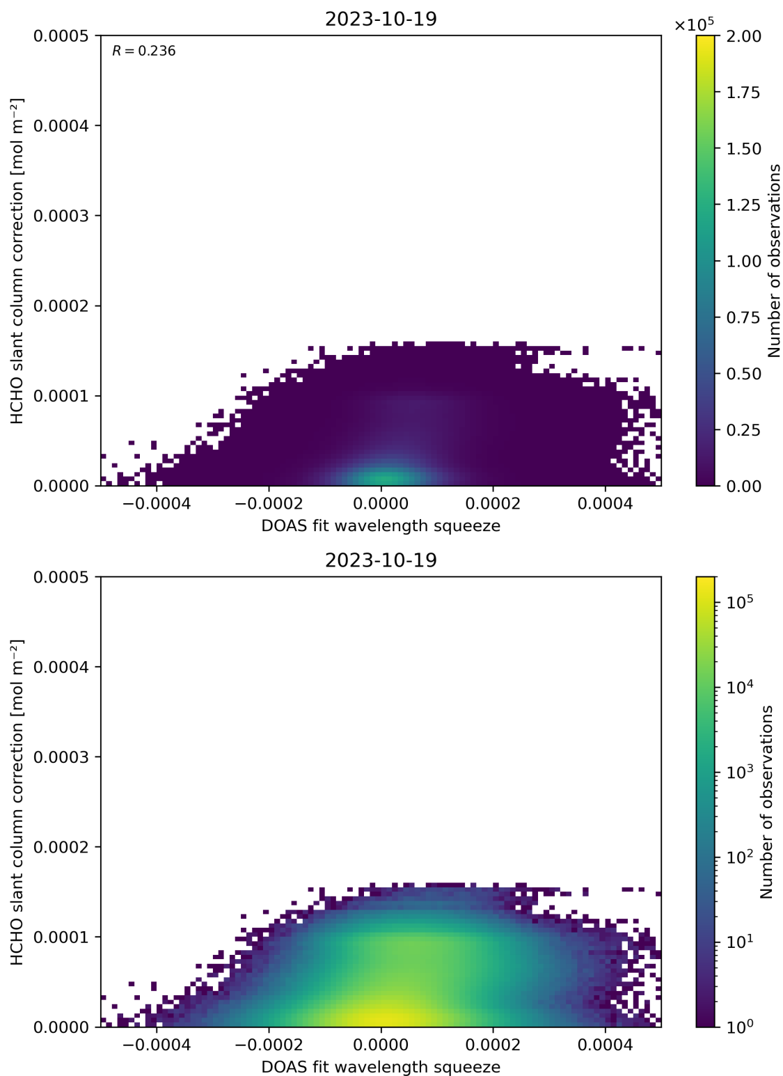
Figure 70: Scatter density plot of “DOAS fit wavelength squeeze” against “HCHO slant column correction” for 2023-10-18 to 2023-10-20.
