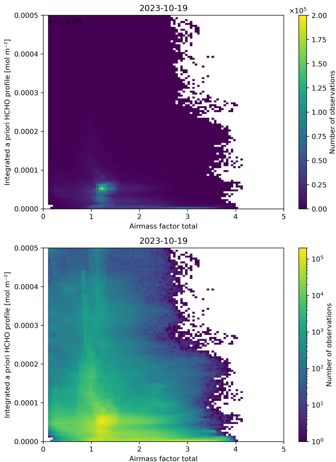
Figure 104: Scatter density plot of “Airmass factor total” against “Integrated a priori HCHO profile” for 2023-10-18 to 2023-10-20.
