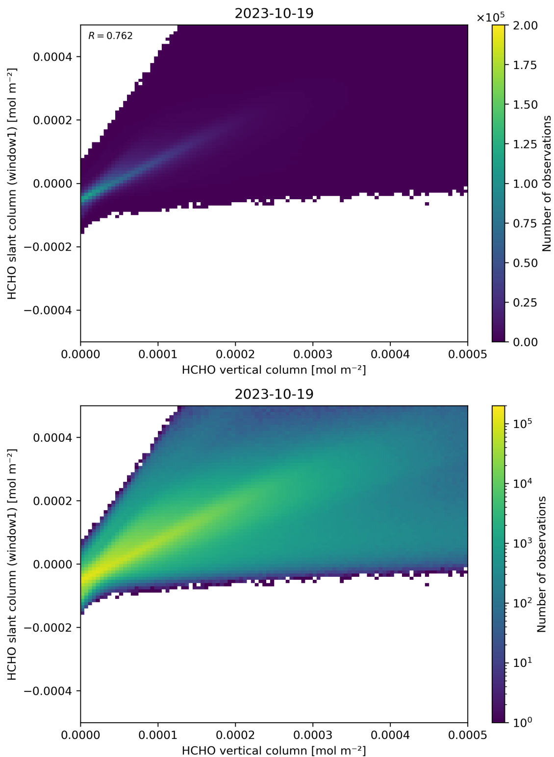
Figure 129: Scatter density plot of “HCHO vertical column” against “HCHO slant column (window1)” for 2023-10-18 to 2023-10-20.
