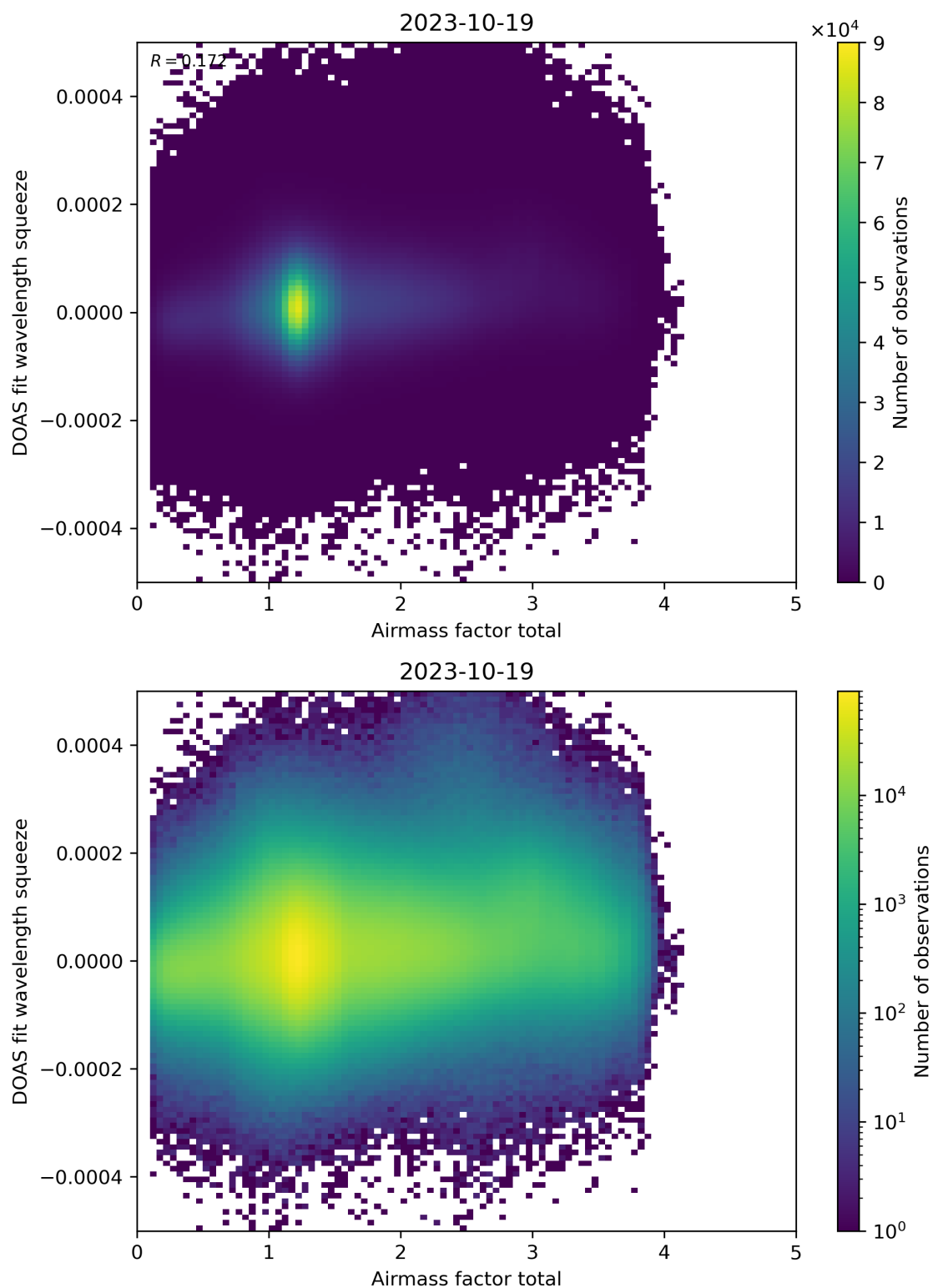
Figure 99: Scatter density plot of “Airmass factor total” against “DOAS fit wavelength squeeze” for 2023-10-18 to 2023-10-20.
