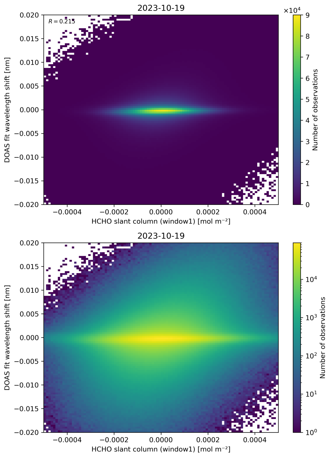
Figure 79: Scatter density plot of “HCHO slant column (window1)” against “DOAS fit wavelength shift” for 2023-10-18 to 2023-10-20.
