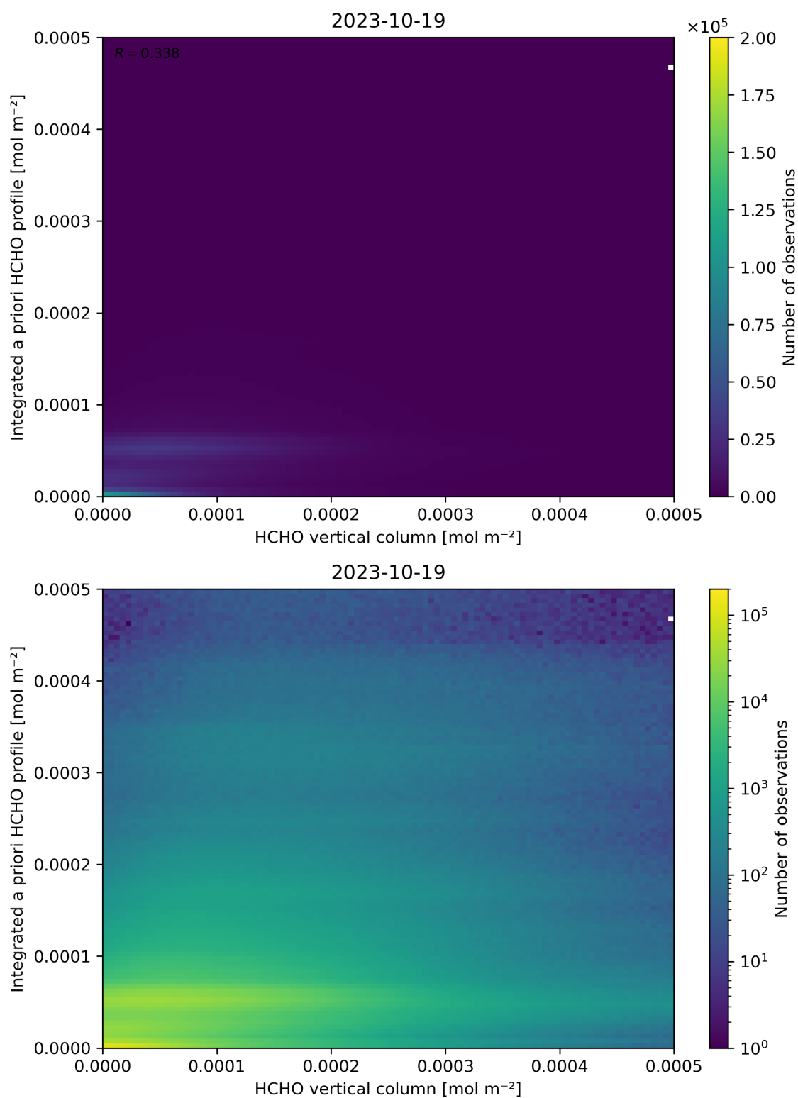
Figure 135: Scatter density plot of “HCHO vertical column” against “Integrated a priori HCHO profile” for 2023-10-18 to 2023-10-20.
