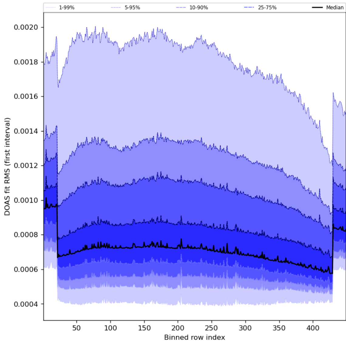
Figure 60: Along track statistics of “DOAS fit RMS (first interval)” for 2023-10-18 to 2023-10-20
