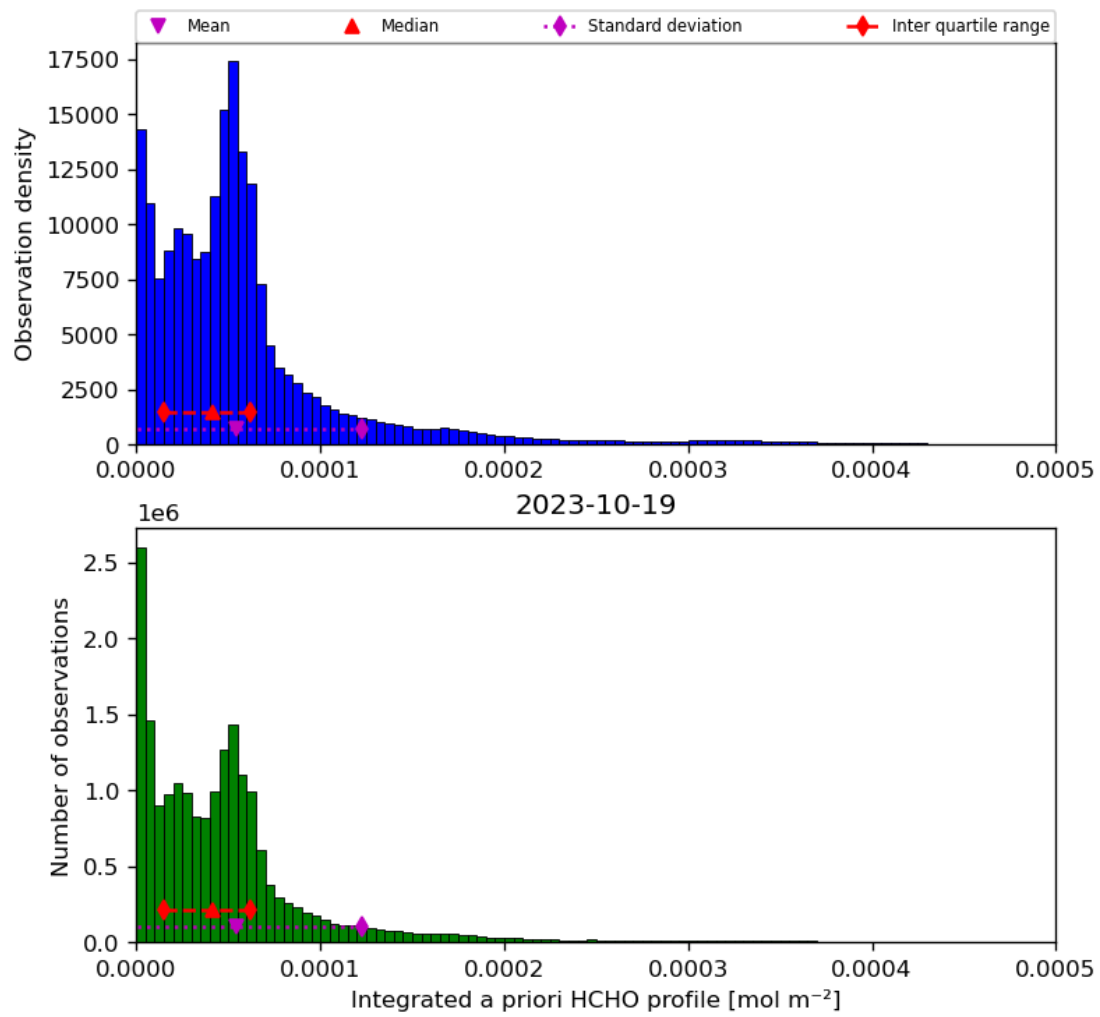
Figure 43: Histogram of “Integrated a priori HCHO profile” for 2023-10-18 to 2023-10-20
