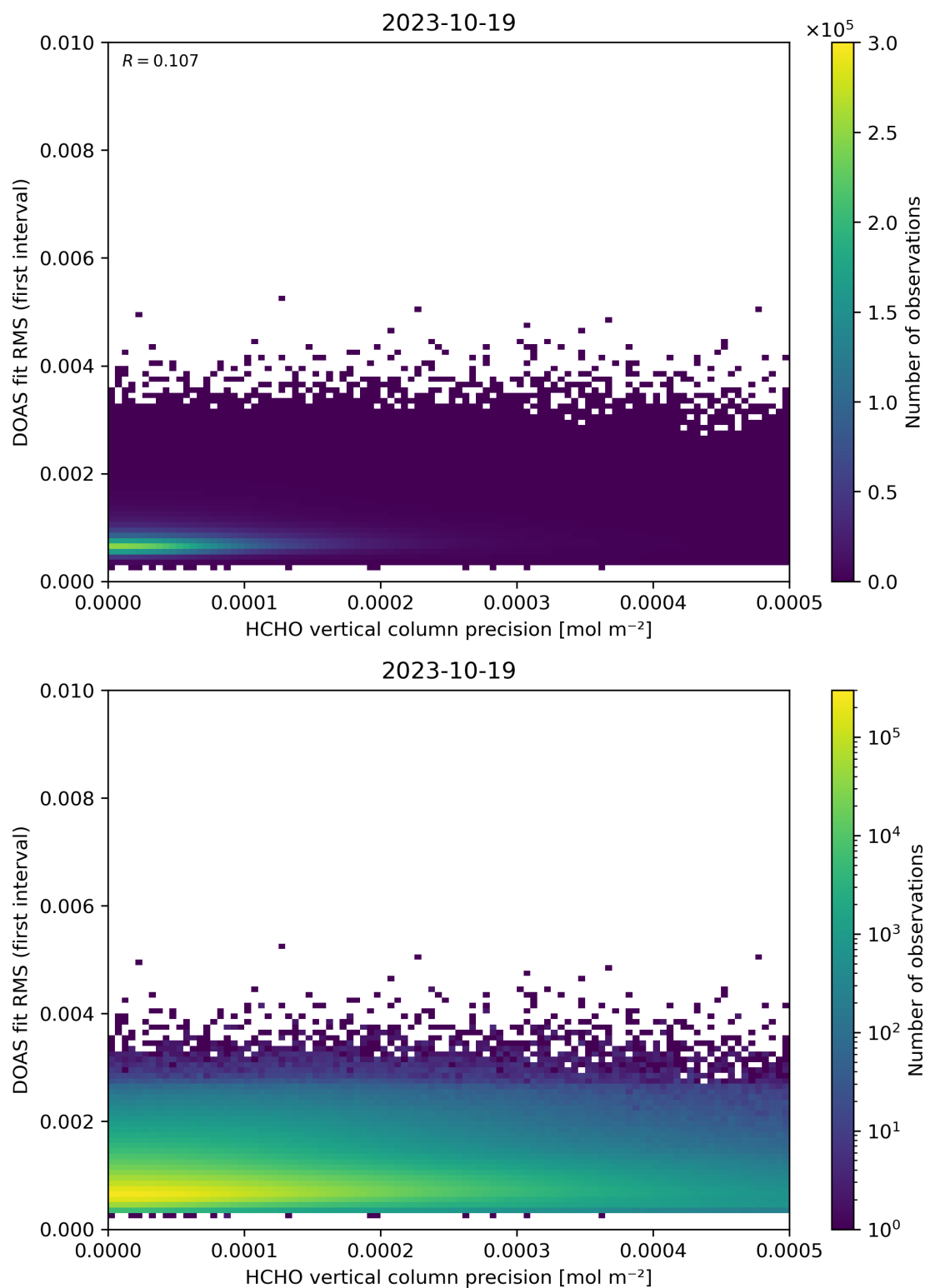
Figure 136: Scatter density plot of “HCHO vertical column precision” against “DOAS fit RMS (first interval)” for 2023-10-18 to 2023-10-20.
