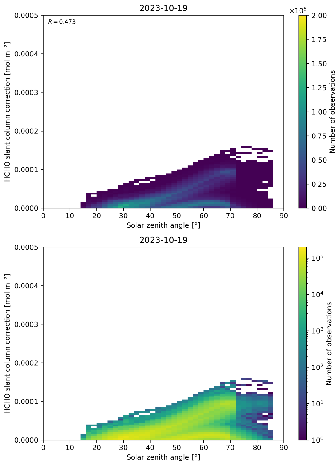
Figure 172: Scatter density plot of “Solar zenith angle” against “HCHO slant column correction” for 2023-10-18 to 2023-10-20.
