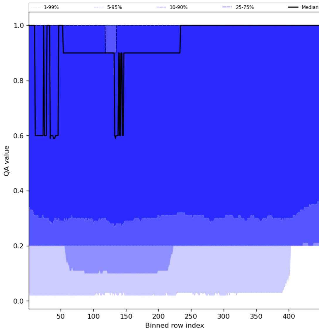
Figure 48: Along track statistics of “QA value” for 2023-10-18 to 2023-10-20
