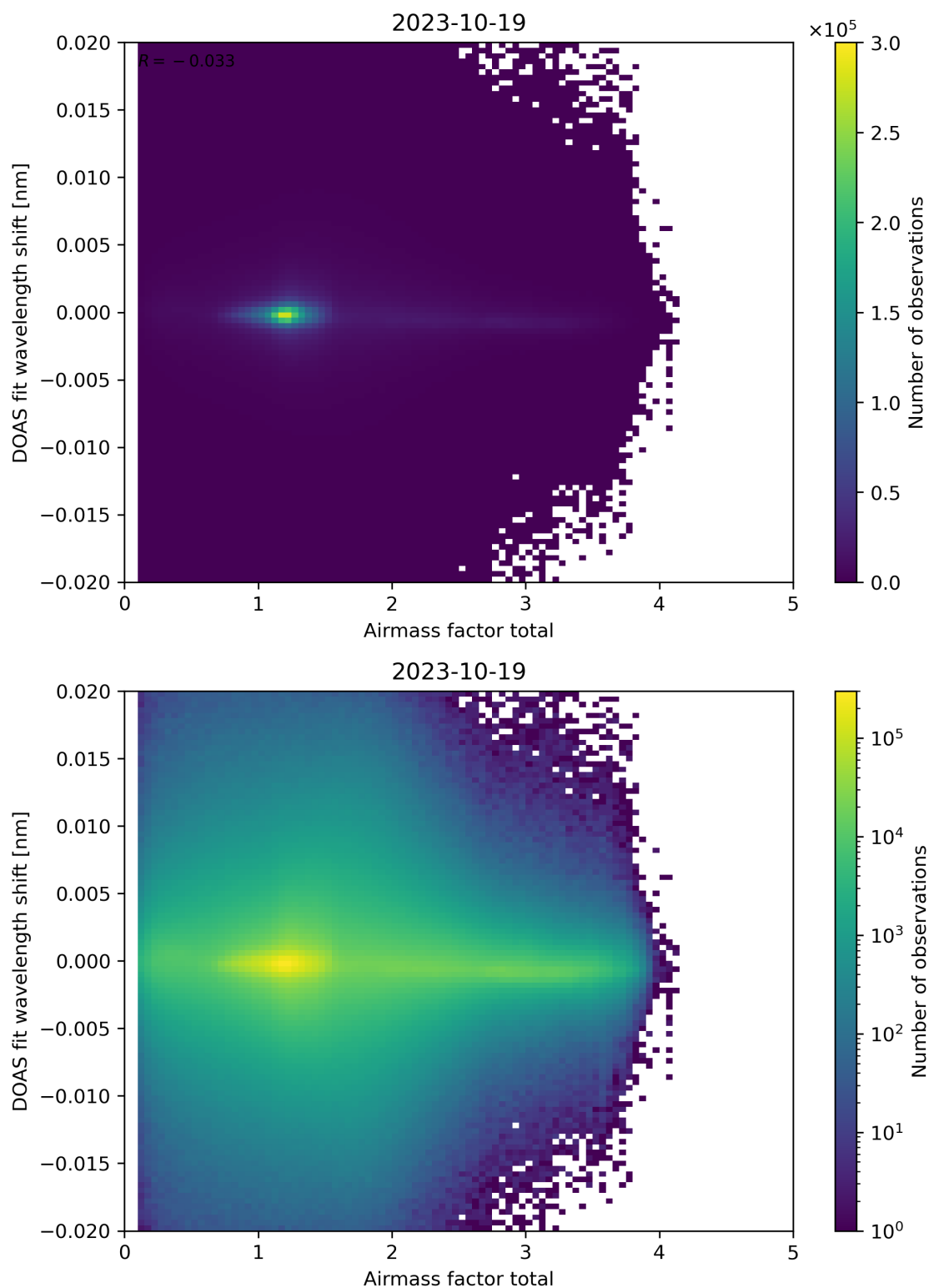
Figure 98: Scatter density plot of “Airmass factor total” against “DOAS fit wavelength shift” for 2023-10-18 to 2023-10-20.
