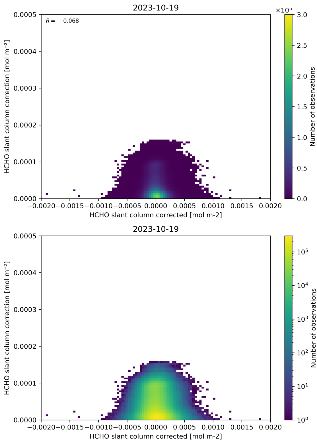
Figure 77: Scatter density plot of “HCHO slant column corrected” against “HCHO slant column correction” for 2023-10-18 to 2023-10-20.
