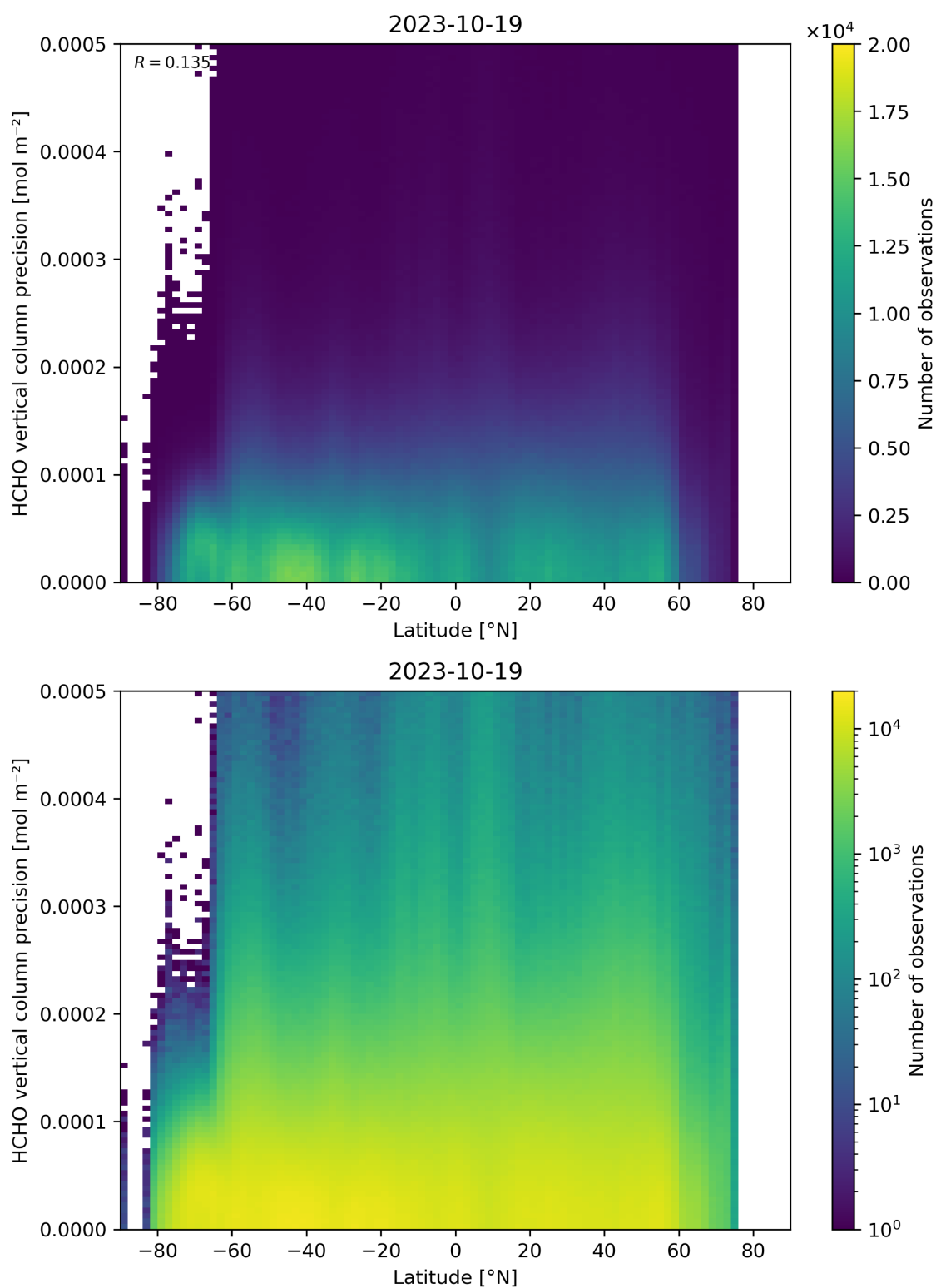
Figure 165: Scatter density plot of “Latitude” against “HCHO vertical column precision” for 2023-10-18 to 2023-10-20.
