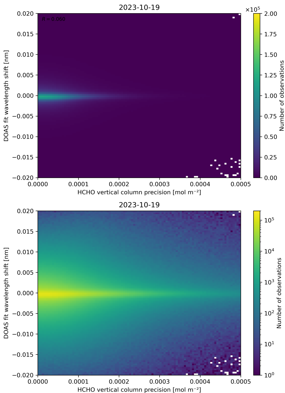
Figure 137: Scatter density plot of “HCHO vertical column precision” against “DOAS fit wavelength shift” for 2023-10-18 to 2023-10-20.
