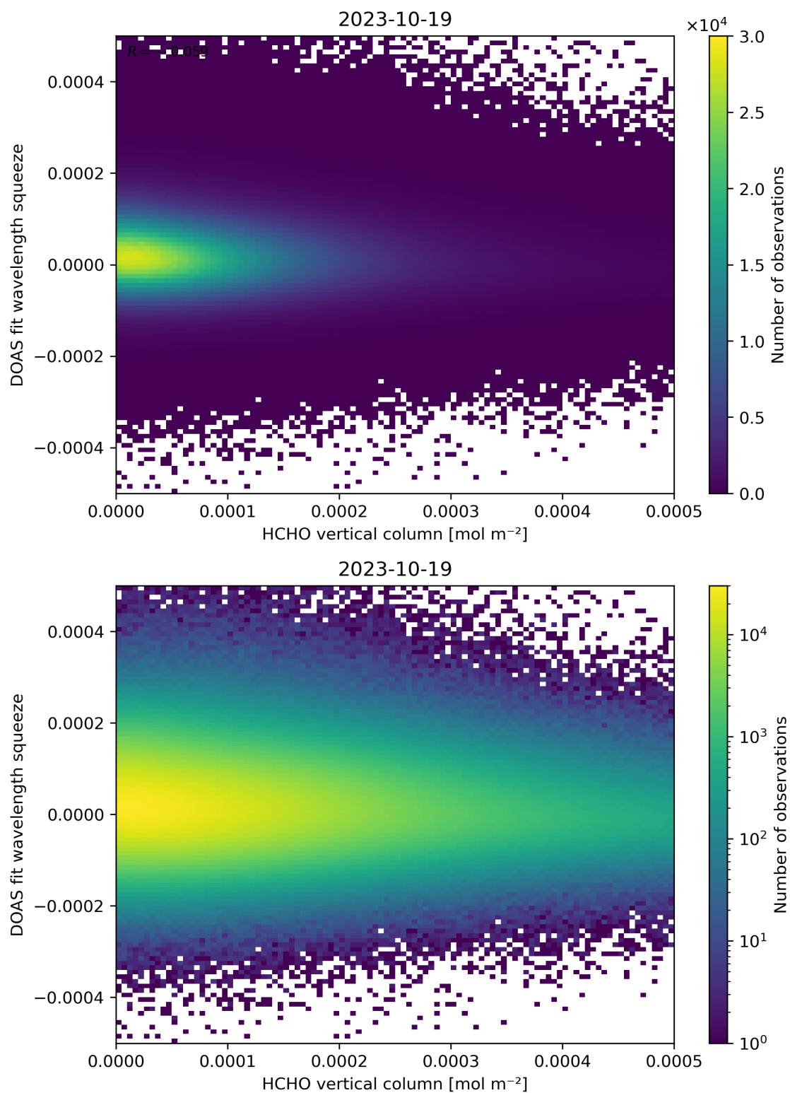
Figure 125: Scatter density plot of “HCHO vertical column” against “DOAS fit wavelength squeeze” for 2023-10-18 to 2023-10-20.
