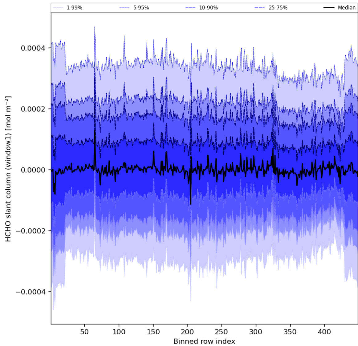
Figure 52: Along track statistics of “HCHO slant column (window1)” for 2023-10-18 to 2023-10-20
