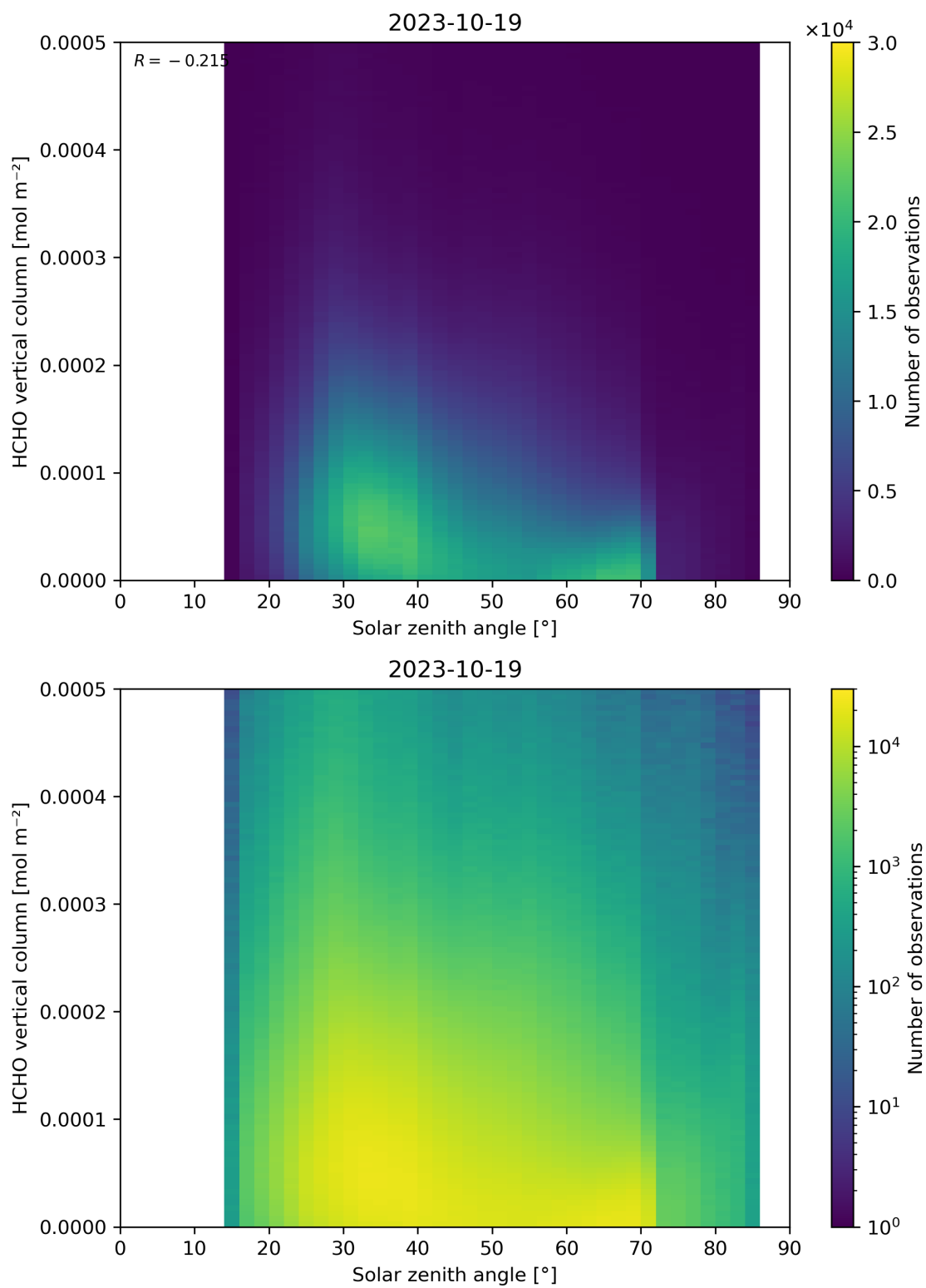
Figure 177: Scatter density plot of “Solar zenith angle” against “HCHO vertical column” for 2023-10-18 to 2023-10-20.
