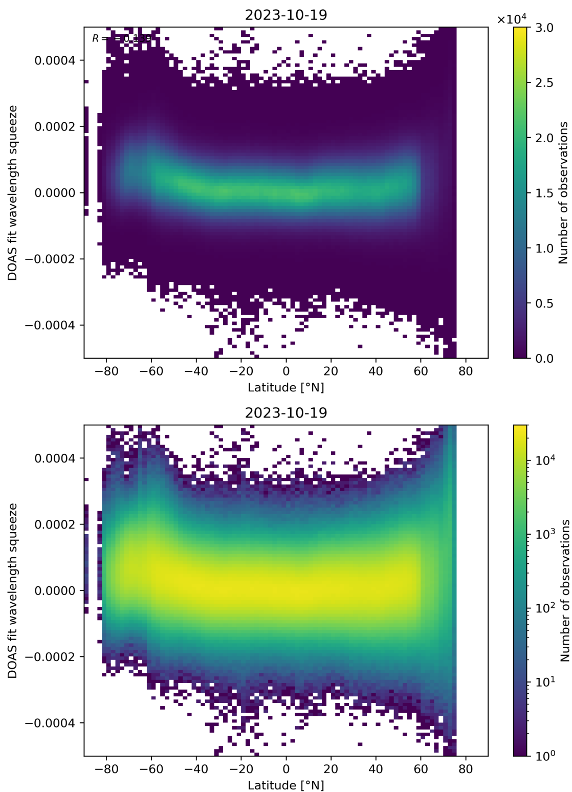
Figure 155: Scatter density plot of “Latitude” against “DOAS fit wavelength squeeze” for 2023-10-18 to 2023-10-20.
