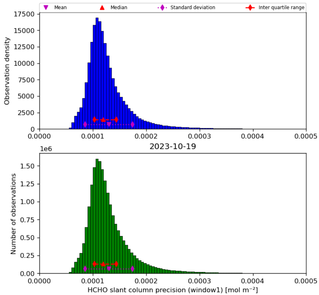
Figure 39: Histogram of “HCHO slant column precision (window1)” for 2023-10-18 to 2023-10-20
