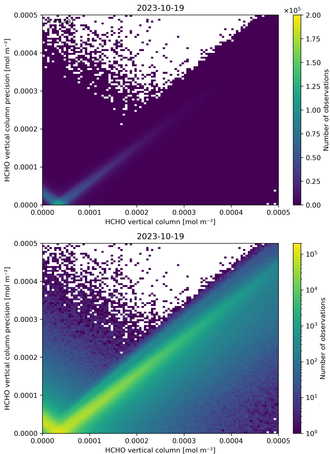
Figure 134: Scatter density plot of “HCHO vertical column” against “HCHO vertical column precision” for 2023-10-18 to 2023-10-20.
