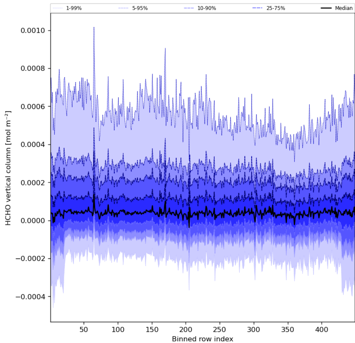
Figure 49: Along track statistics of “HCHO vertical column” for 2023-10-18 to 2023-10-20
