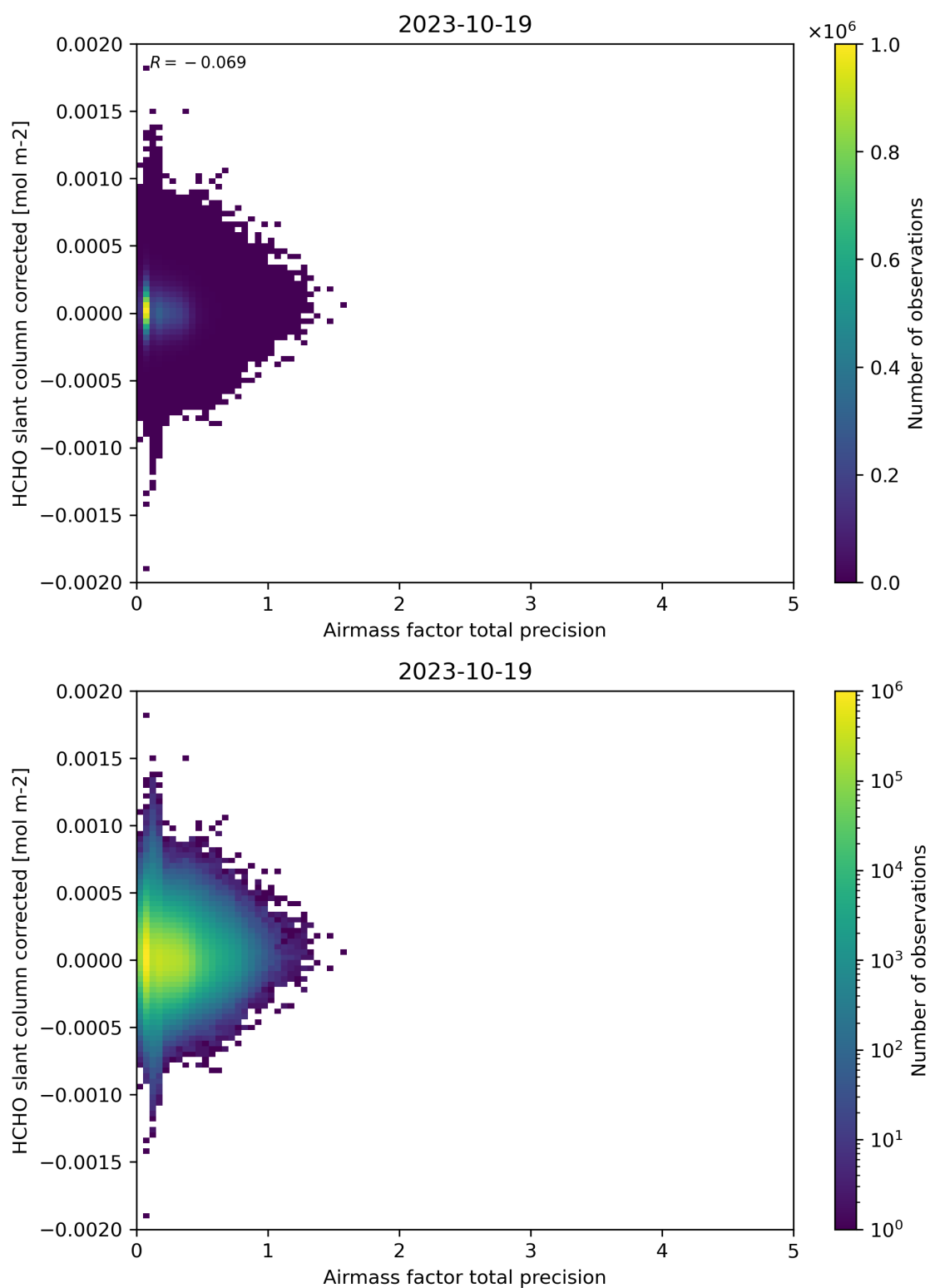
Figure 109: Scatter density plot of “Airmass factor total precision” against “HCHO slant column corrected” for 2023-10-18 to 2023-10-20.
