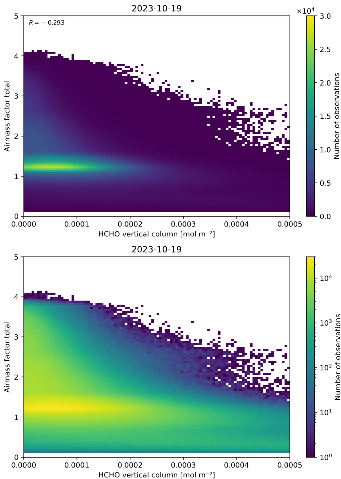
Figure 131: Scatter density plot of “HCHO vertical column” against “Airmass factor total” for 2023-10-18 to 2023-10-20.
