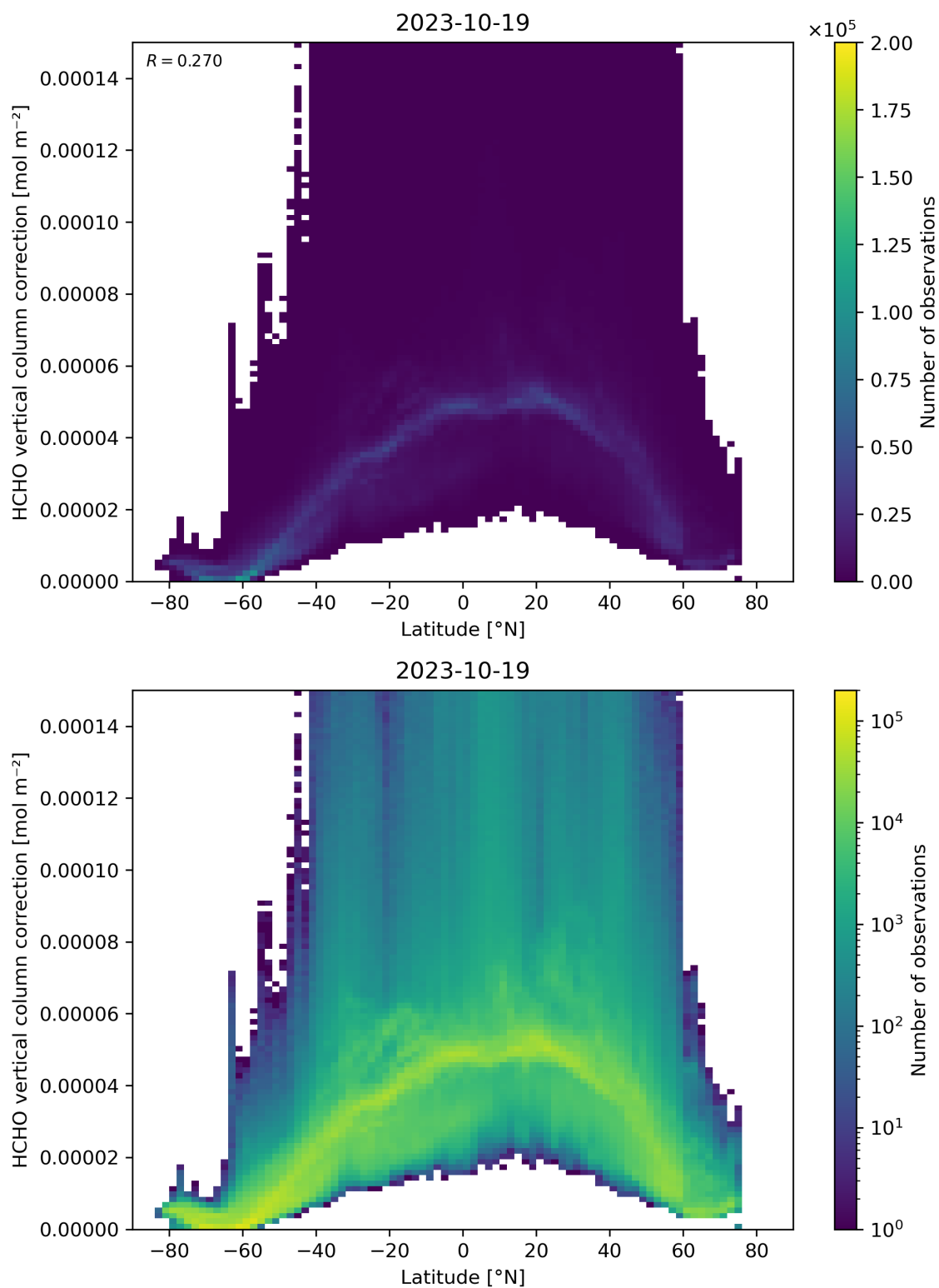
Figure 164: Scatter density plot of “Latitude” against “HCHO vertical column correction” for 2023-10-18 to 2023-10-20.
