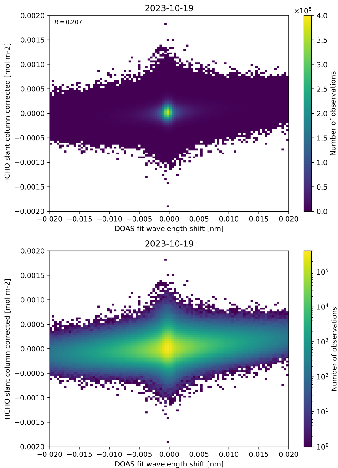
Figure 66: Scatter density plot of “DOAS fit wavelength shift” against “HCHO slant column corrected” for 2023-10-18 to 2023-10-20.
