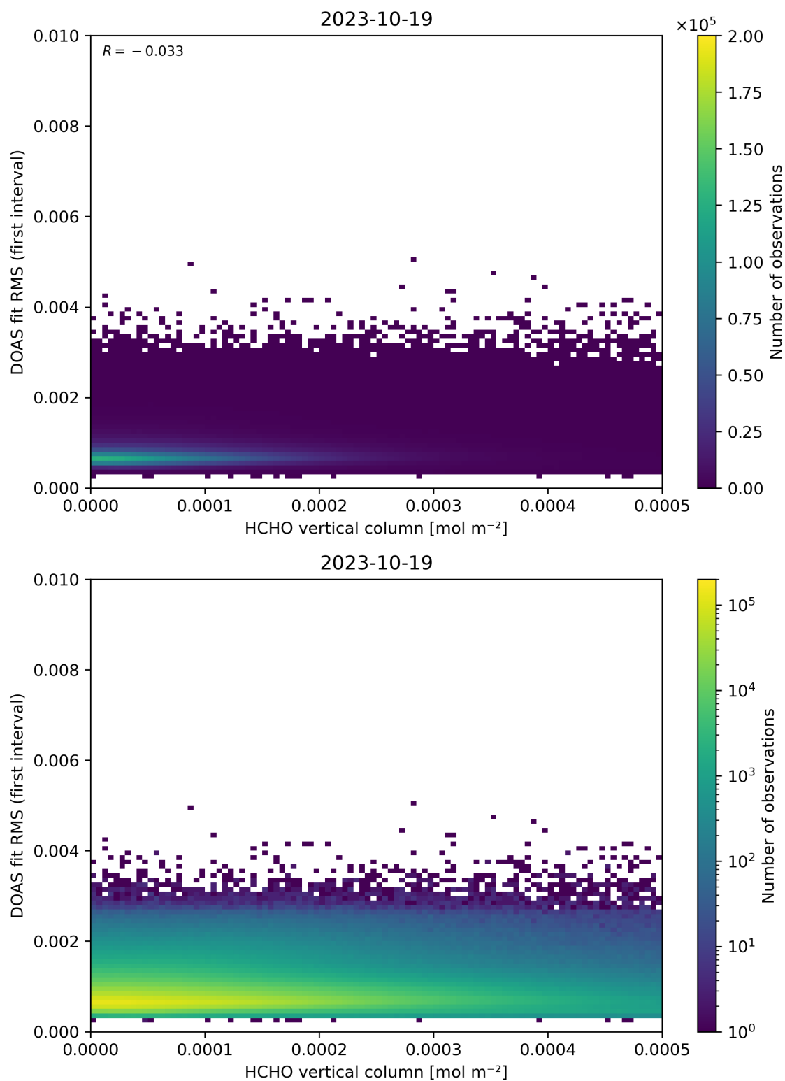
Figure 123: Scatter density plot of “HCHO vertical column” against “DOAS fit RMS (first interval)” for 2023-10-18 to 2023-10-20.
