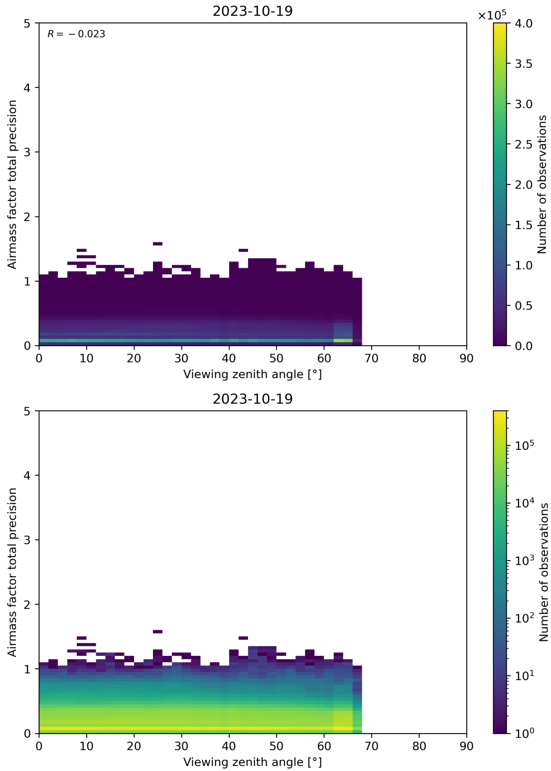
Figure 191: Scatter density plot of “Viewing zenith angle” against “Airmass factor total precision” for 2023-10-18 to 2023-10-20.
