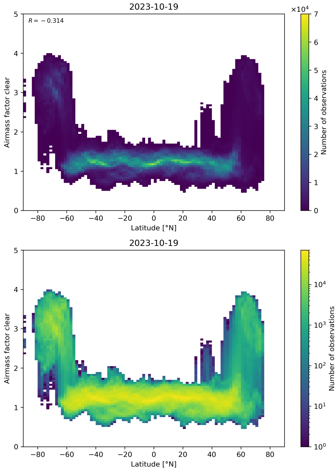
Figure 156: Scatter density plot of “Latitude” against “Airmass factor clear” for 2023-10-18 to 2023-10-20.
