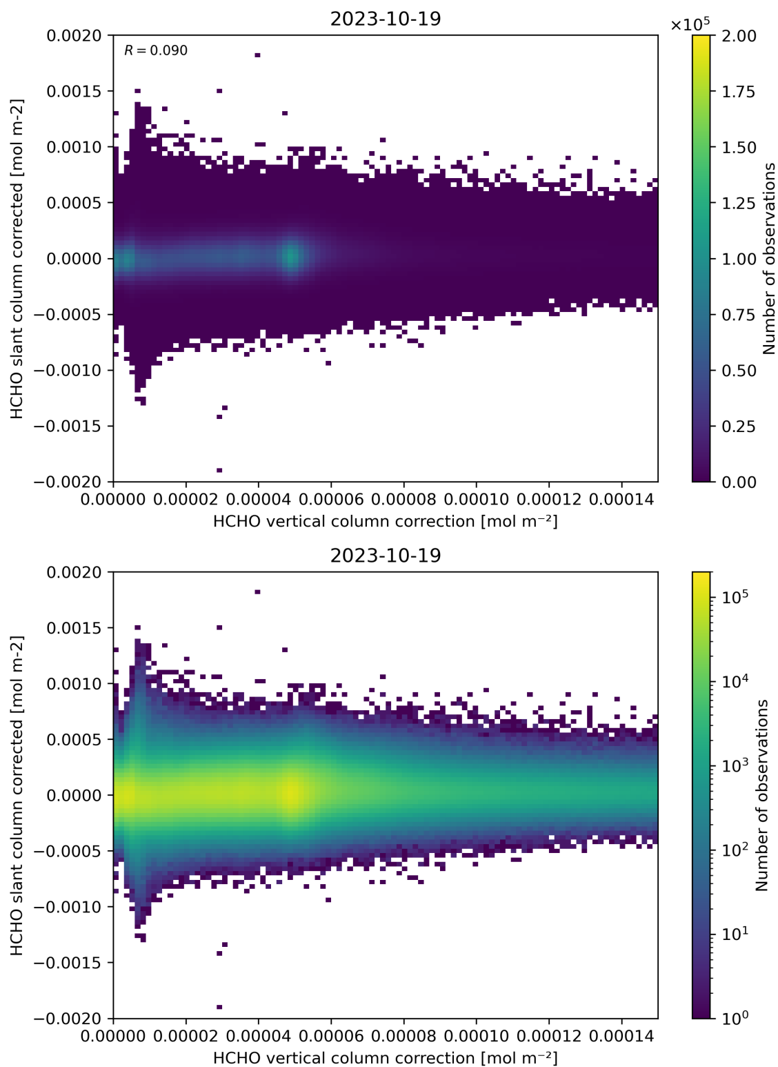
Figure 116: Scatter density plot of “HCHO vertical column correction” against “HCHO slant column corrected” for 2023-10-18 to 2023-10-20.
