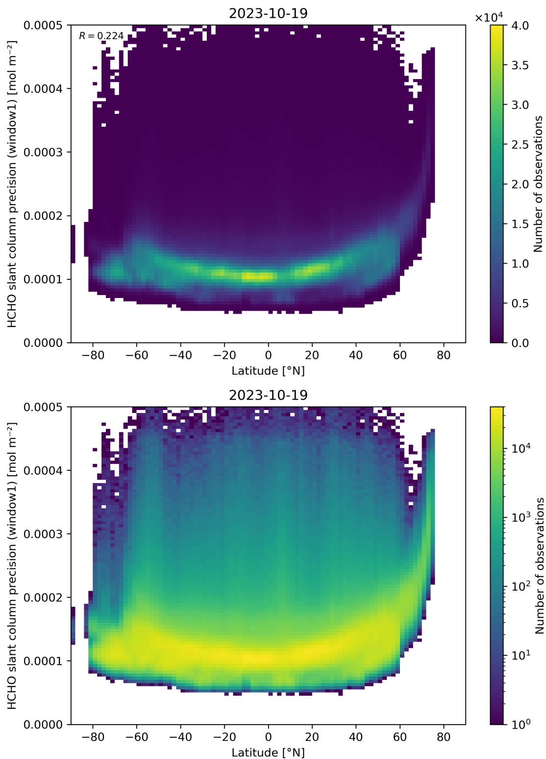
Figure 160: Scatter density plot of “Latitude” against “HCHO slant column precision (window1)” for 2023-10-18 to 2023-10-20.
