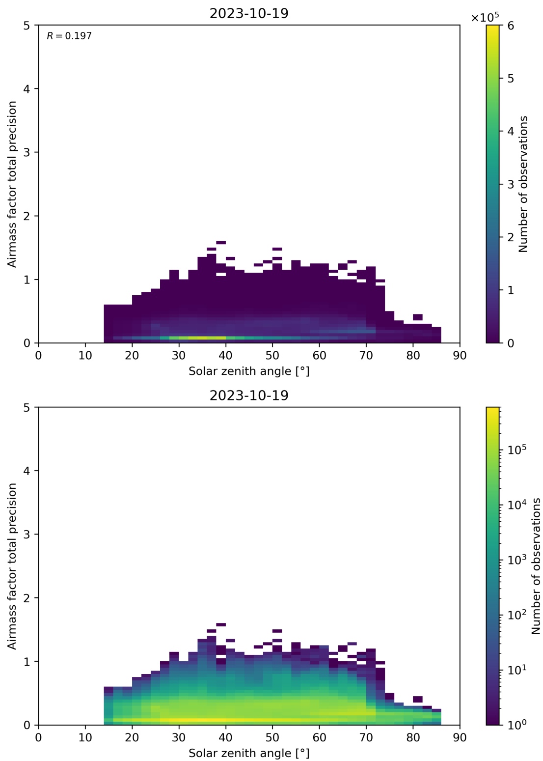
Figure 176: Scatter density plot of “Solar zenith angle” against “Airmass factor total precision” for 2023-10-18 to 2023-10-20.
