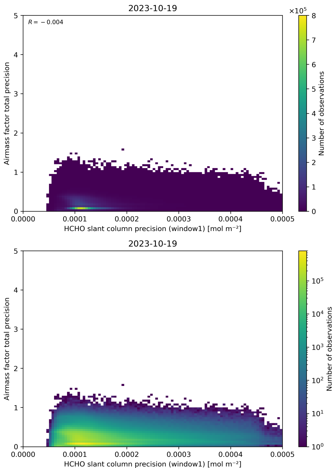
Figure 95: Scatter density plot of “HCHO slant column precision (window1)” against “Airmass factor total precision” for 2023-10-18 to 2023-10-20.
