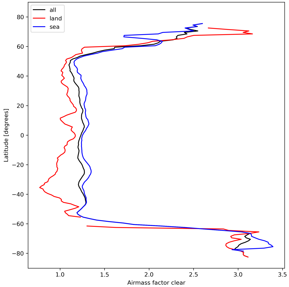
Figure 28: Zonal average of “Airmass factor clear” for 2023-10-18 to 2023-10-20.
