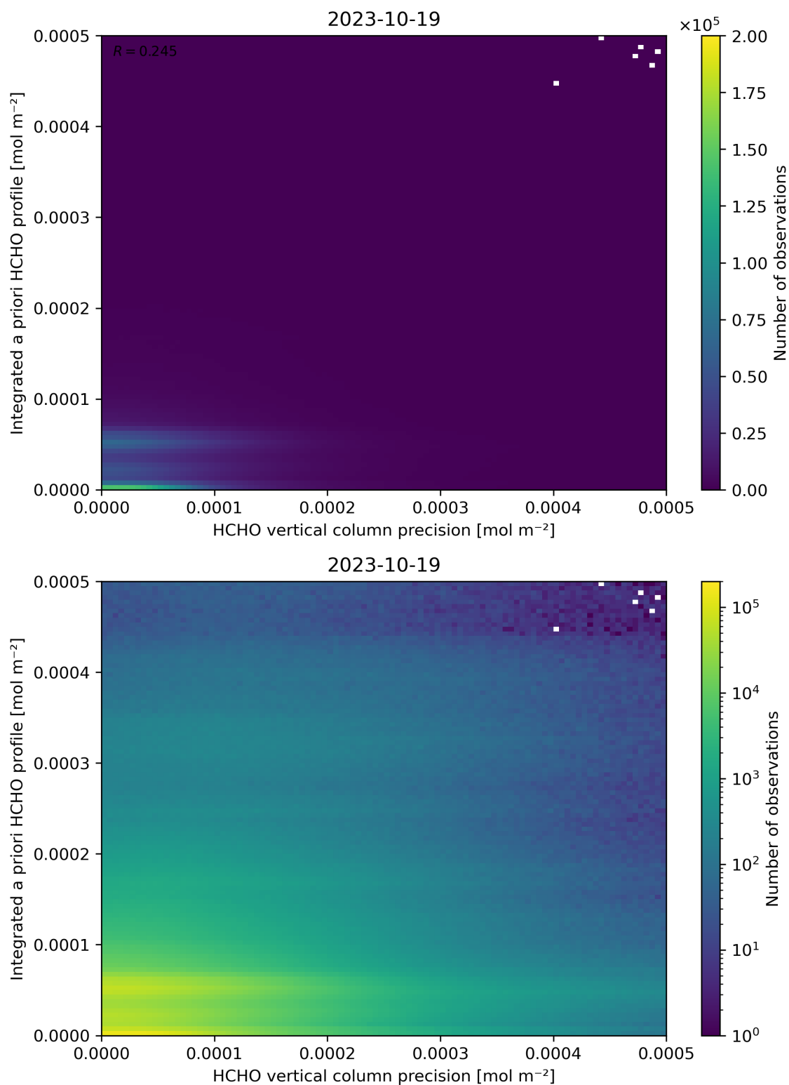
Figure 147: Scatter density plot of “HCHO vertical column precision” against “Integrated a priori HCHO profile” for 2023-10-18 to 2023-10-20.
