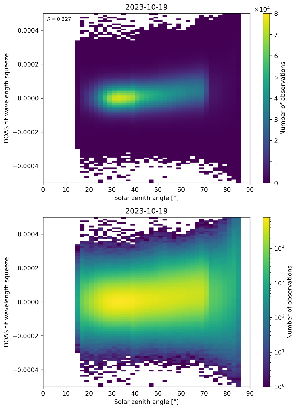
Figure 169: Scatter density plot of “Solar zenith angle” against “DOAS fit wavelength squeeze” for 2023-10-18 to 2023-10-20.
