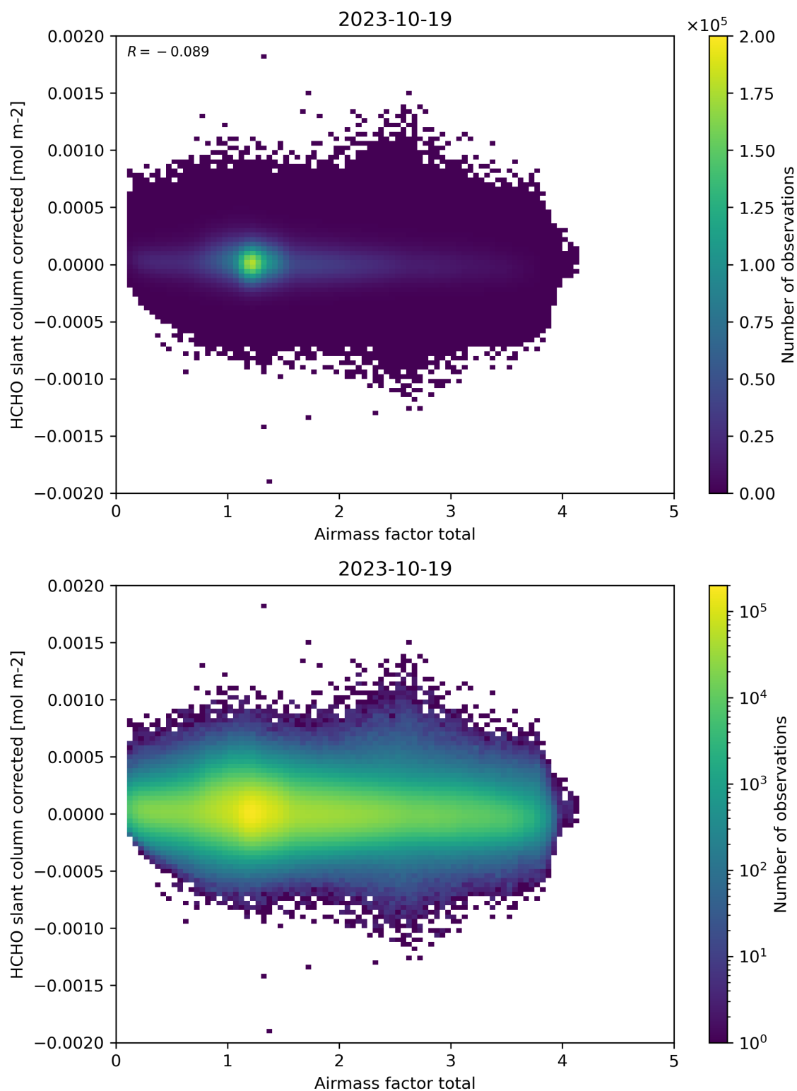
Figure 101: Scatter density plot of “Airmass factor total” against “HCHO slant column corrected” for 2023-10-18 to 2023-10-20.
