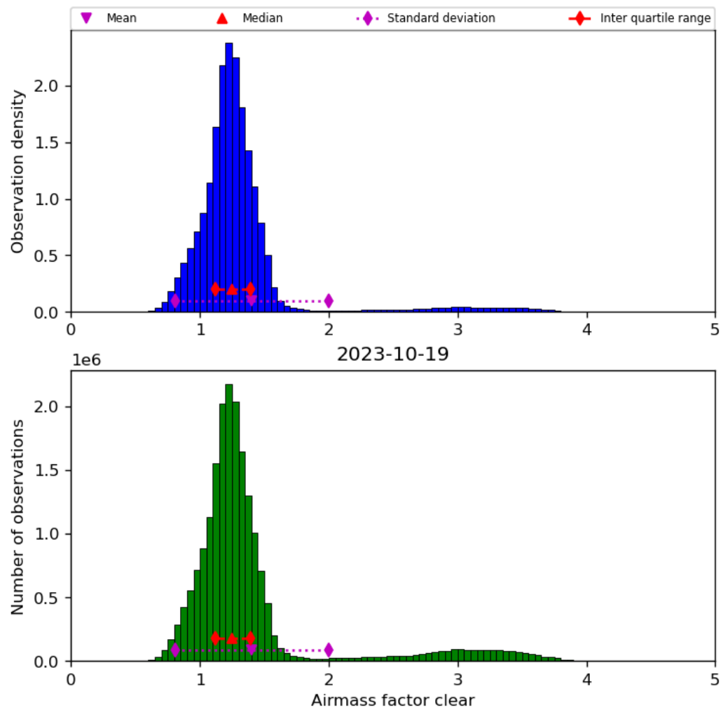
Figure 42: Histogram of “Airmass factor clear” for 2023-10-18 to 2023-10-20
