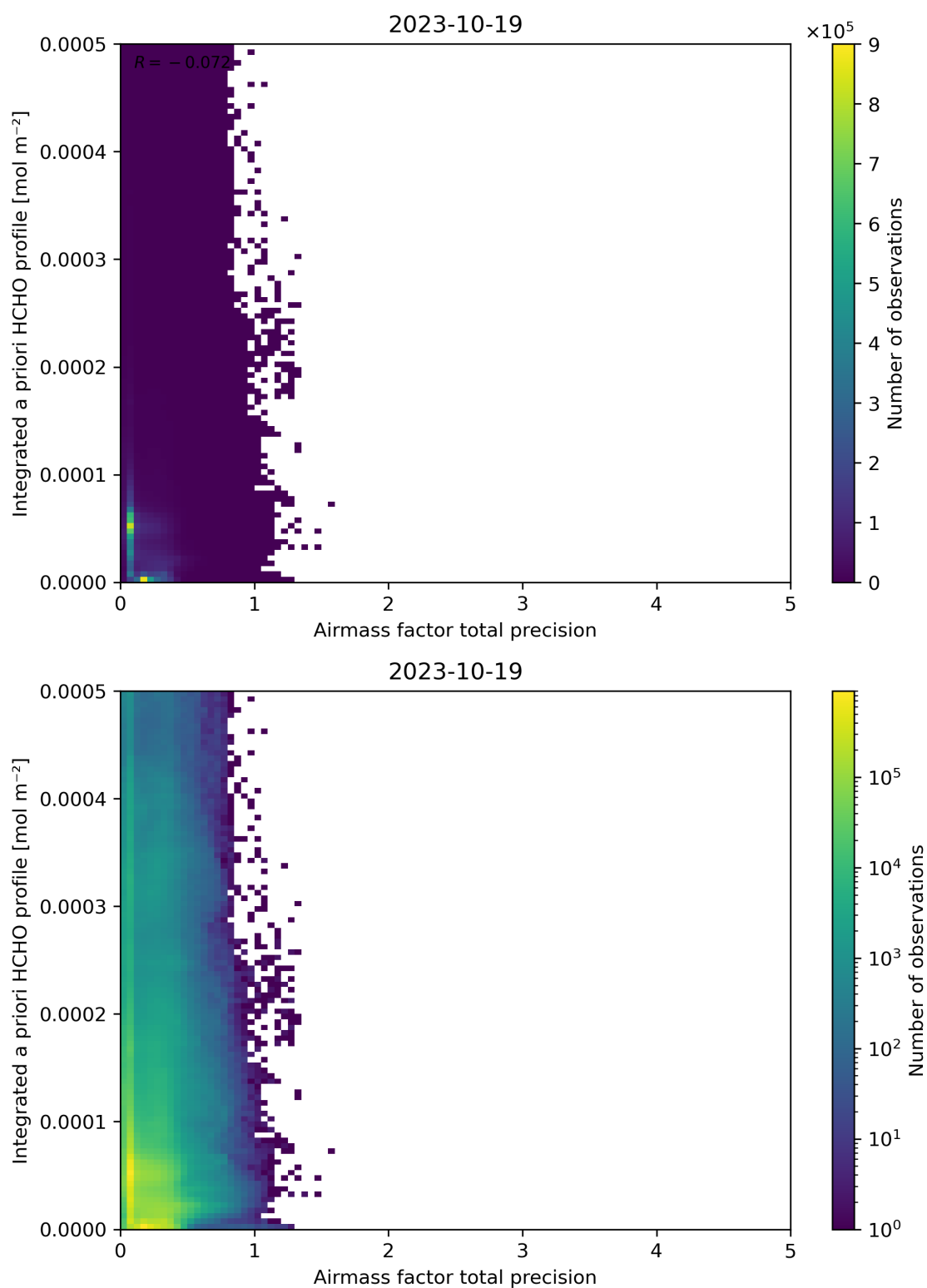
Figure 111: Scatter density plot of “Airmass factor total precision” against “Integrated a priori HCHO profile” for 2023-10-18 to 2023-10-20.
