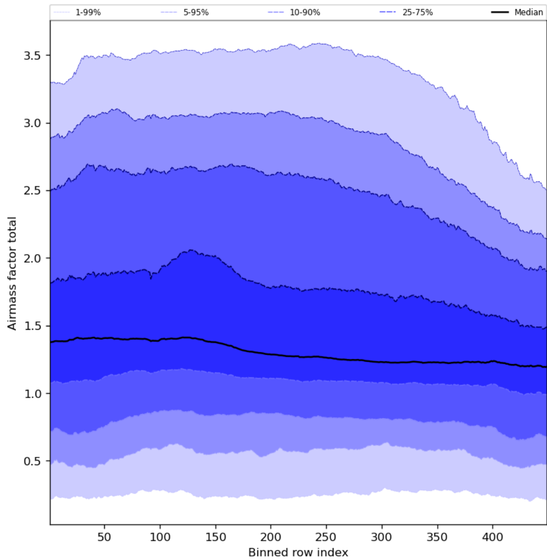
Figure 54: Along track statistics of “Airmass factor total” for 2023-10-18 to 2023-10-20
