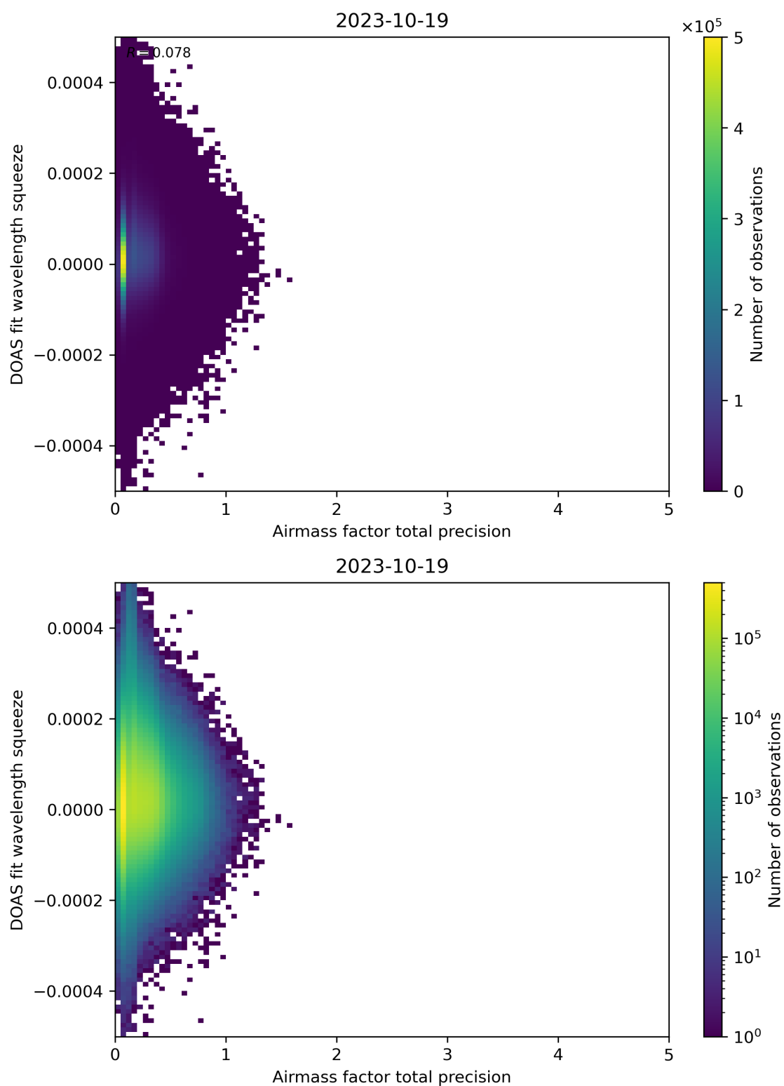
Figure 107: Scatter density plot of “Airmass factor total precision” against “DOAS fit wavelength squeeze” for 2023-10-18 to 2023-10-20.
