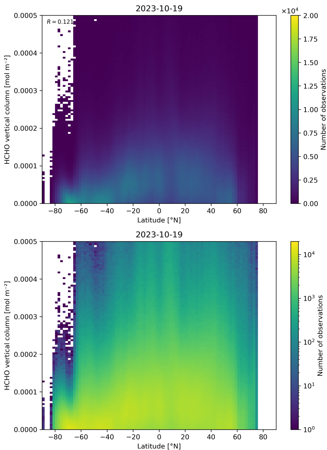
Figure 163: Scatter density plot of “Latitude” against “HCHO vertical column” for 2023-10-18 to 2023-10-20.
