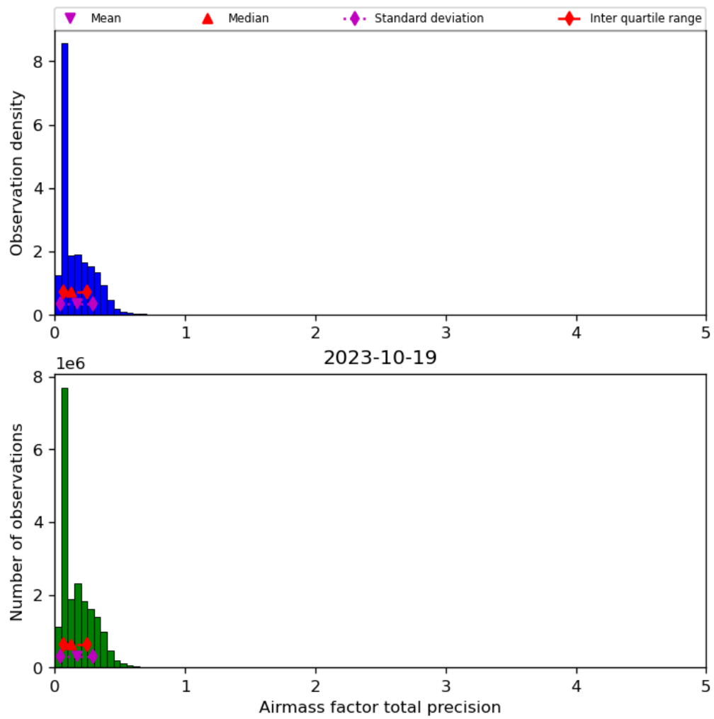
Figure 41: Histogram of “Airmass factor total precision” for 2023-10-18 to 2023-10-20
