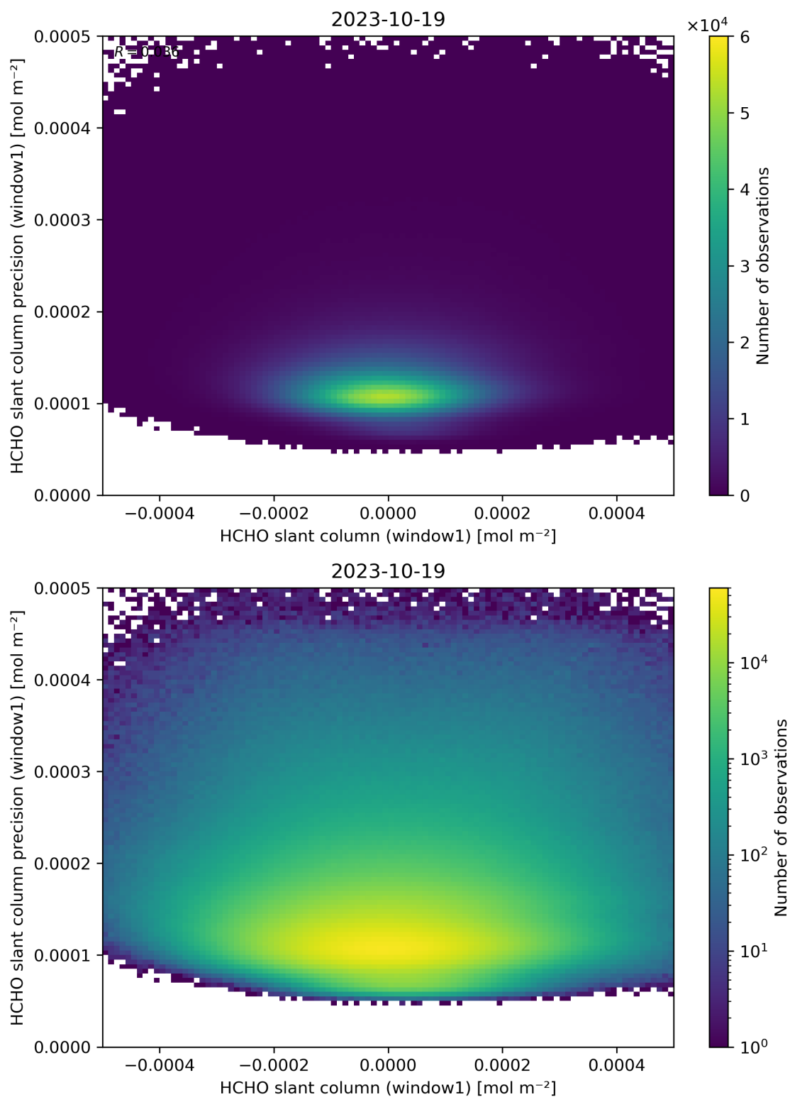
Figure 84: Scatter density plot of “HCHO slant column (window1)” against “HCHO slant column precision (window1)” for 2023-10-18 to 2023-10-20.
