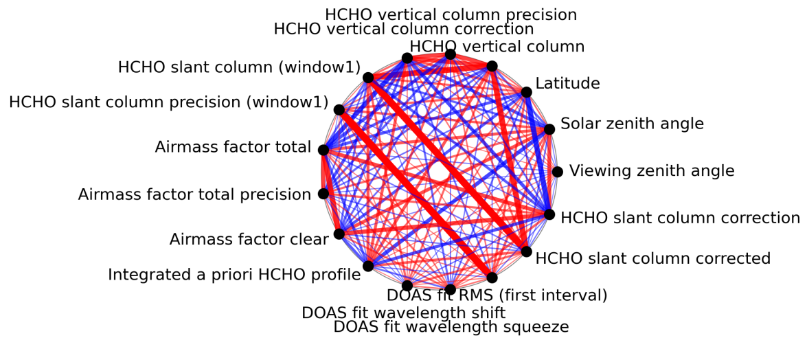
Figure 1: Map of correlation graph for 2023-10-18 to 2023-10-20.
