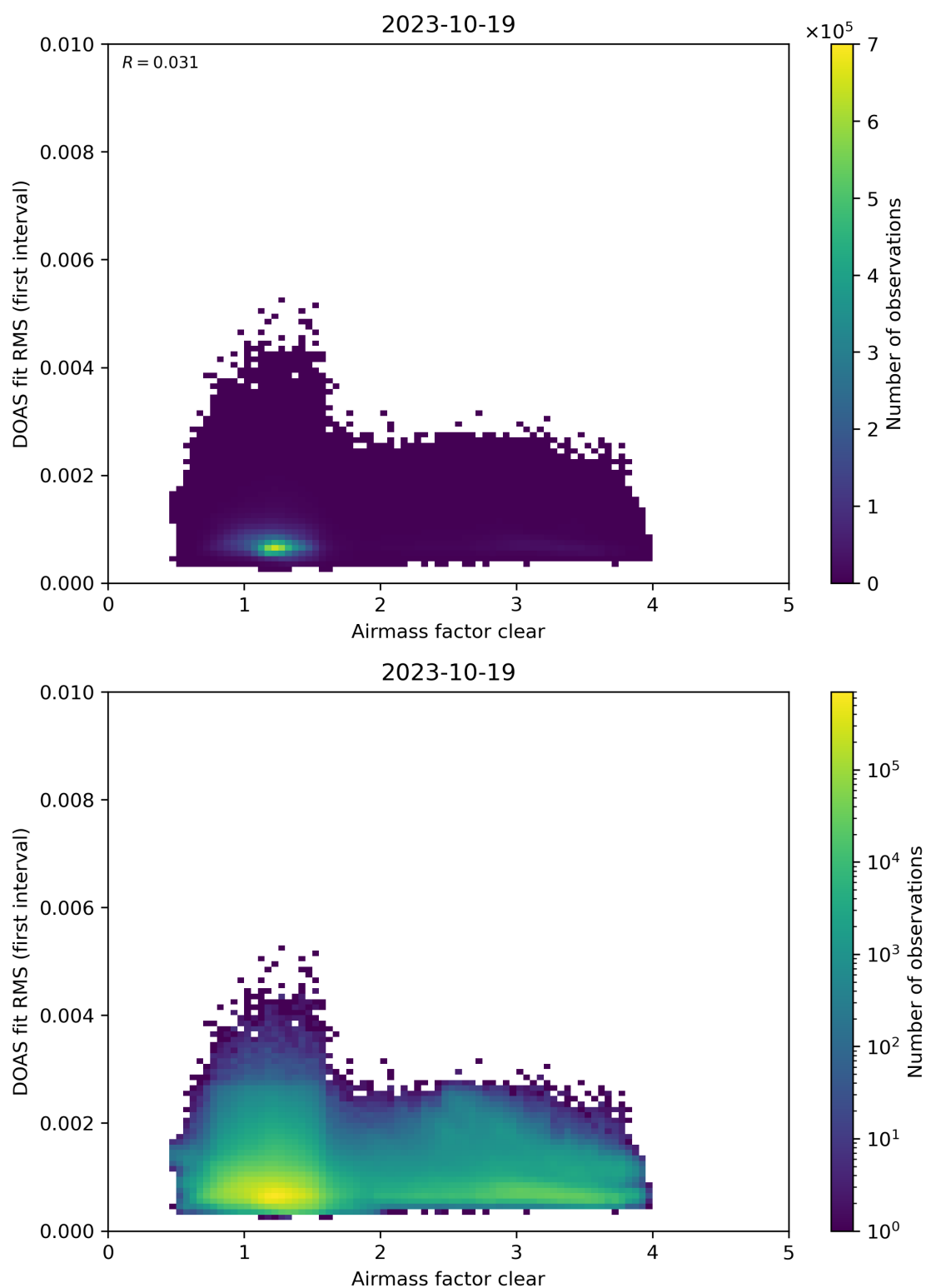
Figure 71: Scatter density plot of “Airmass factor clear” against “DOAS fit RMS (first interval)” for 2023-10-18 to 2023-10-20.
