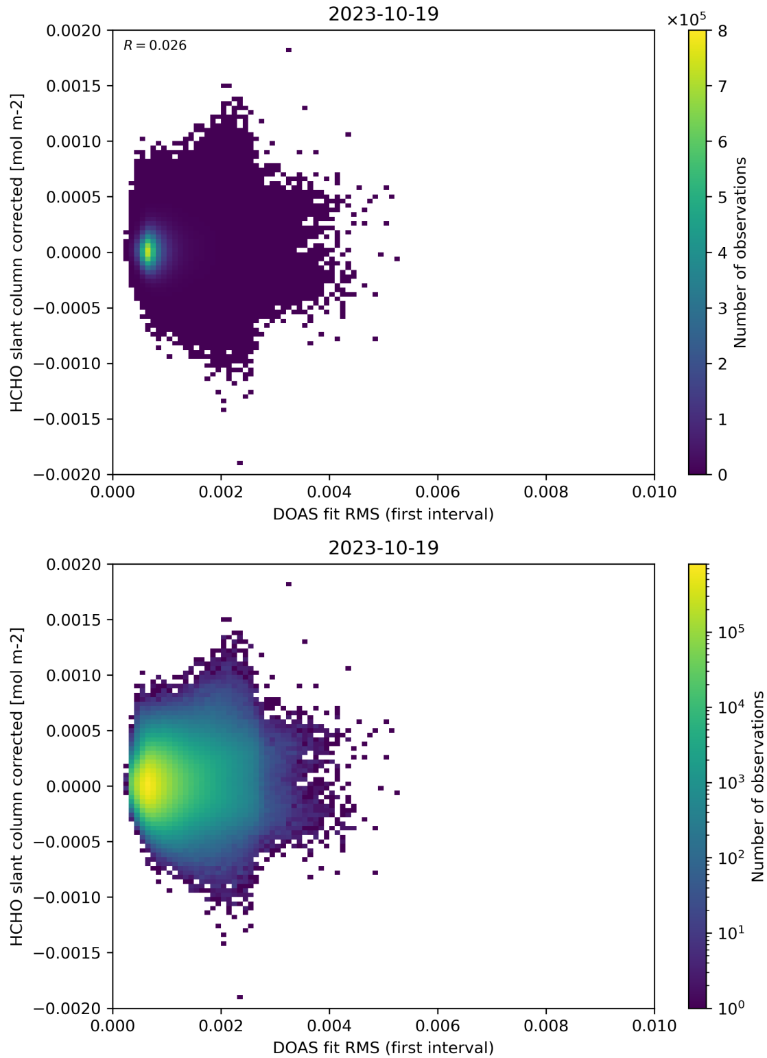
Figure 62: Scatter density plot of “DOAS fit RMS (first interval)” against “HCHO slant column corrected” for 2023-10-18 to 2023-10-20.
