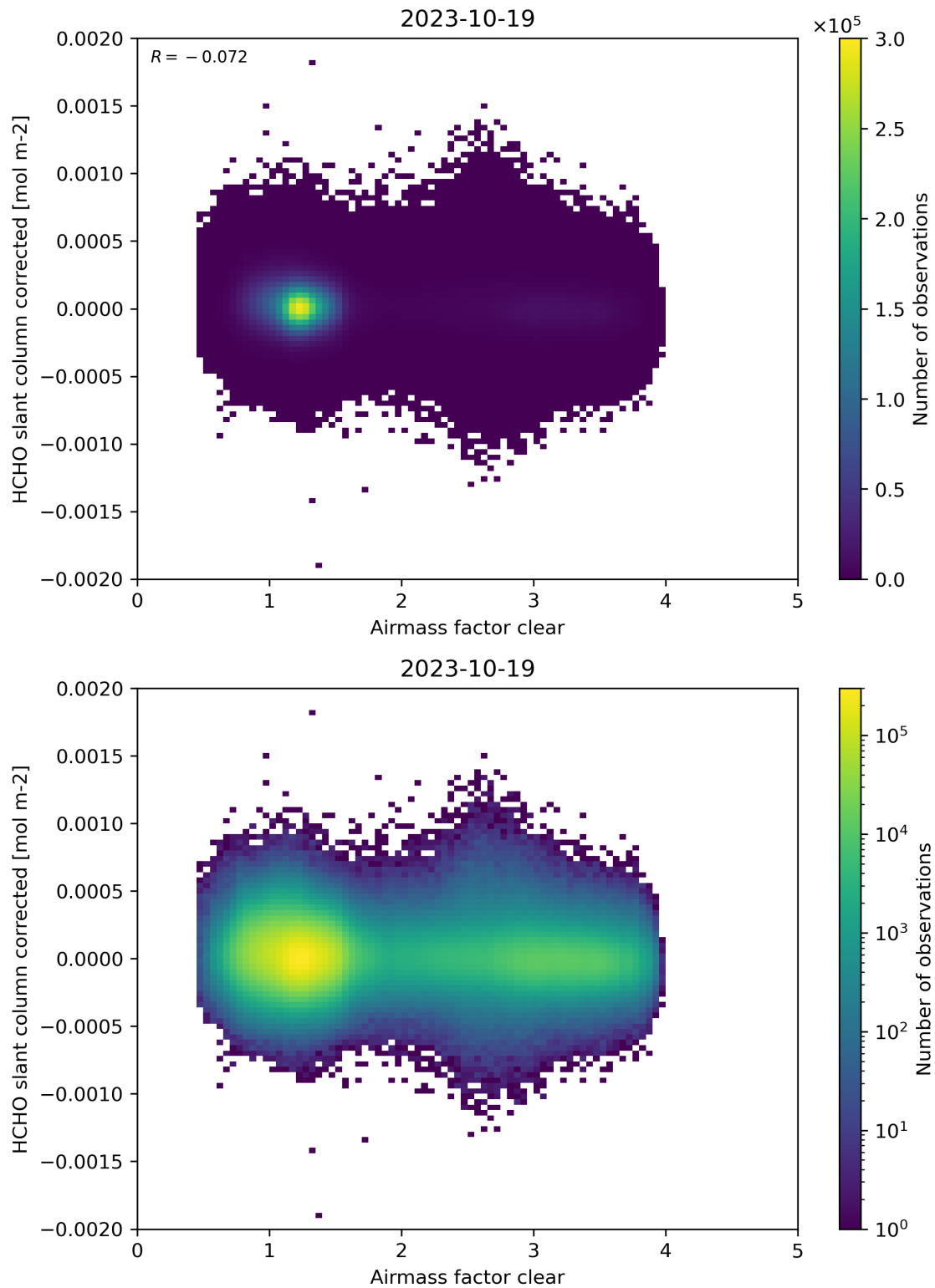
Figure 74: Scatter density plot of “Airmass factor clear” against “HCHO slant column corrected” for 2023-10-18 to 2023-10-20.
