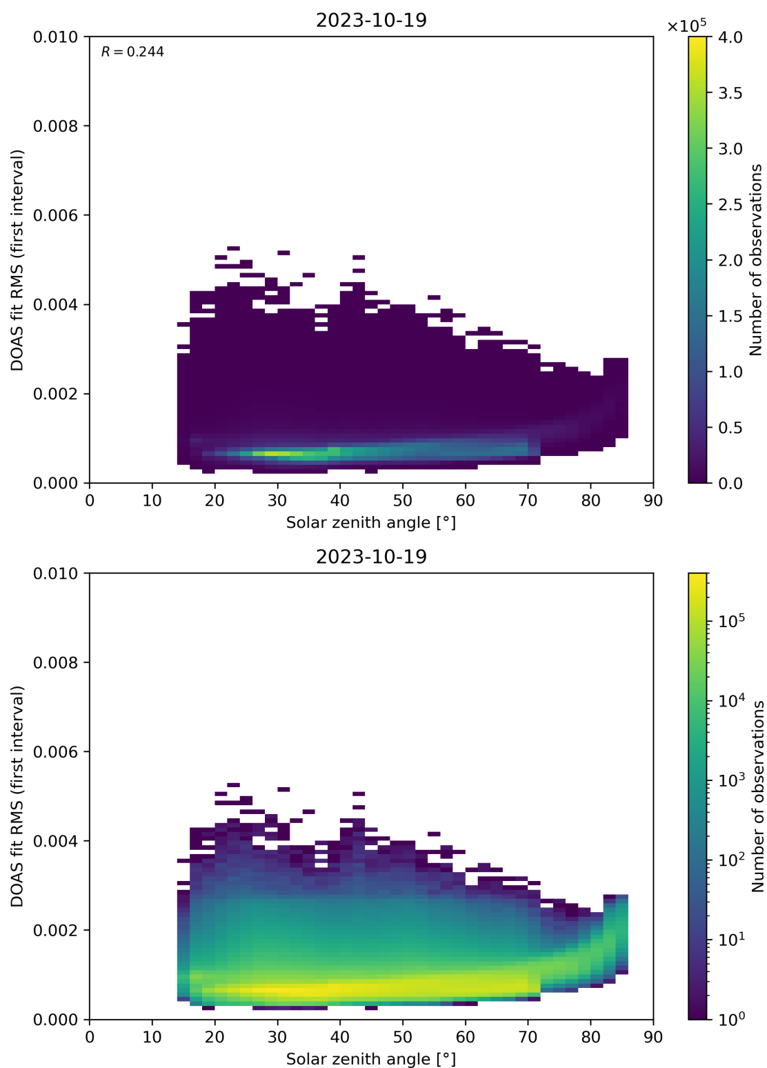
Figure 167: Scatter density plot of “Solar zenith angle” against “DOAS fit RMS (first interval)” for 2023-10-18 to 2023-10-20.
