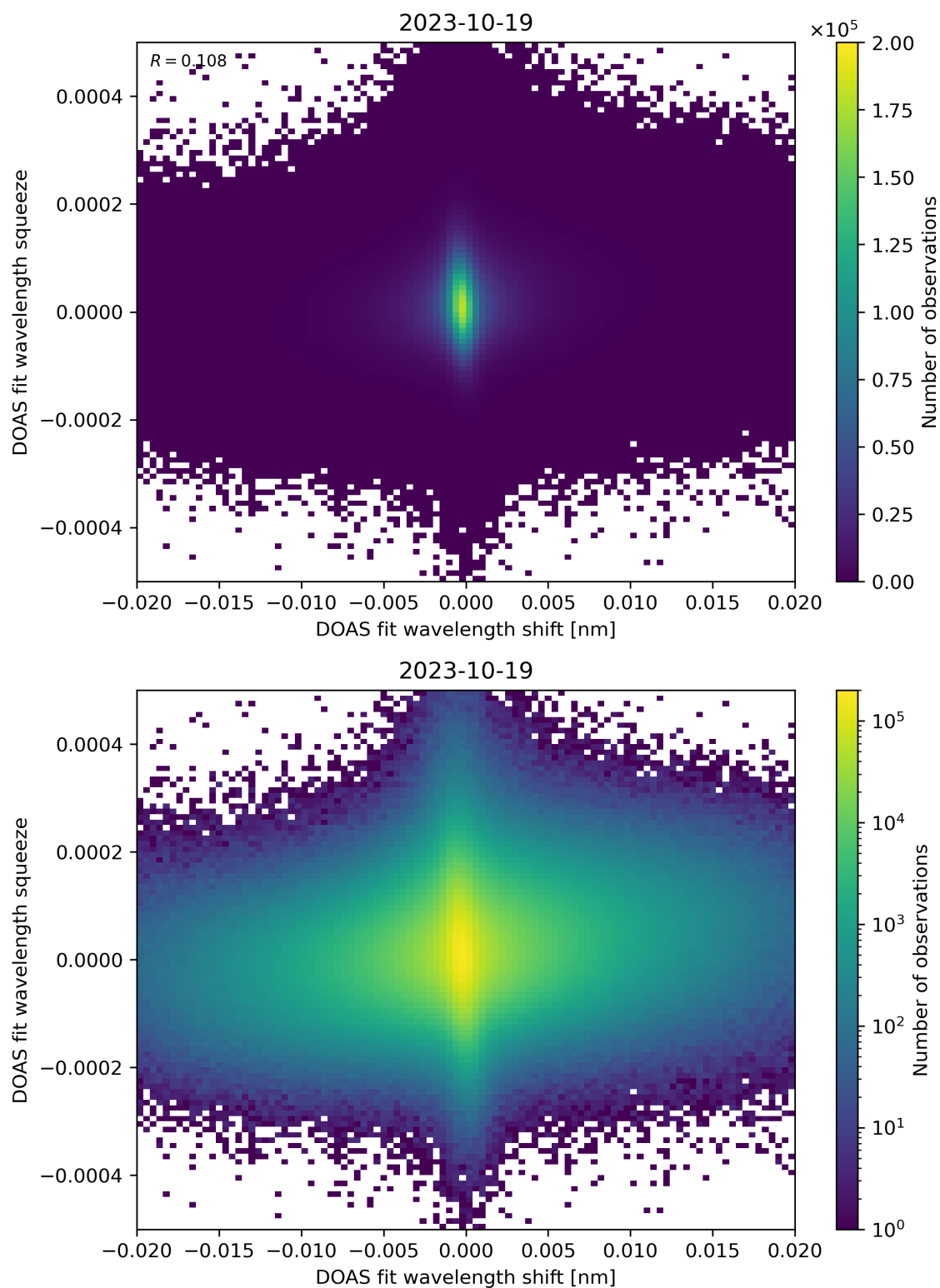
Figure 65: Scatter density plot of “DOAS fit wavelength shift” against “DOAS fit wavelength squeeze” for 2023-10-18 to 2023-10-20.
