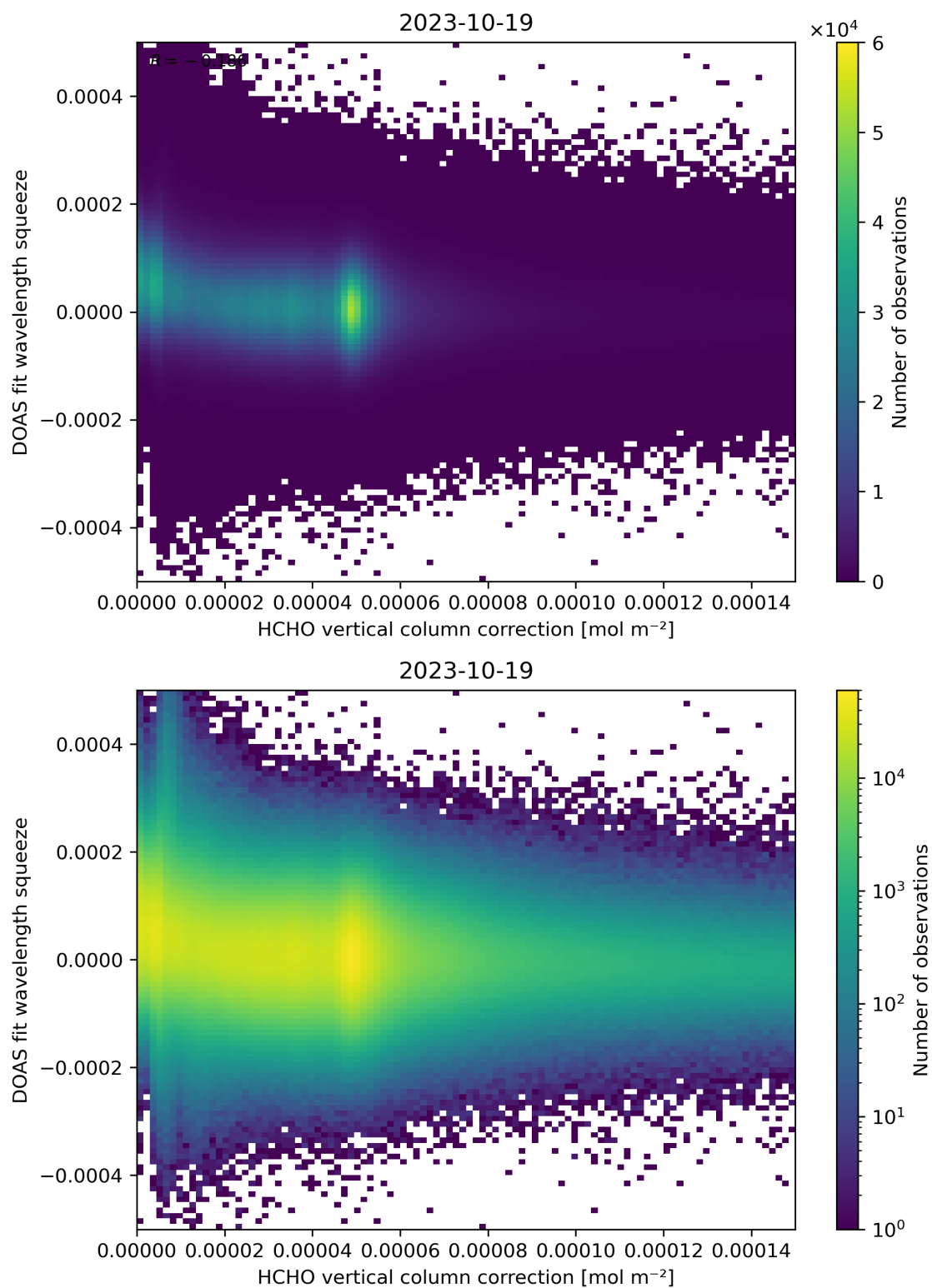
Figure 114: Scatter density plot of “HCHO vertical column correction” against “DOAS fit wavelength squeeze” for 2023-10-18 to 2023-10-20.
