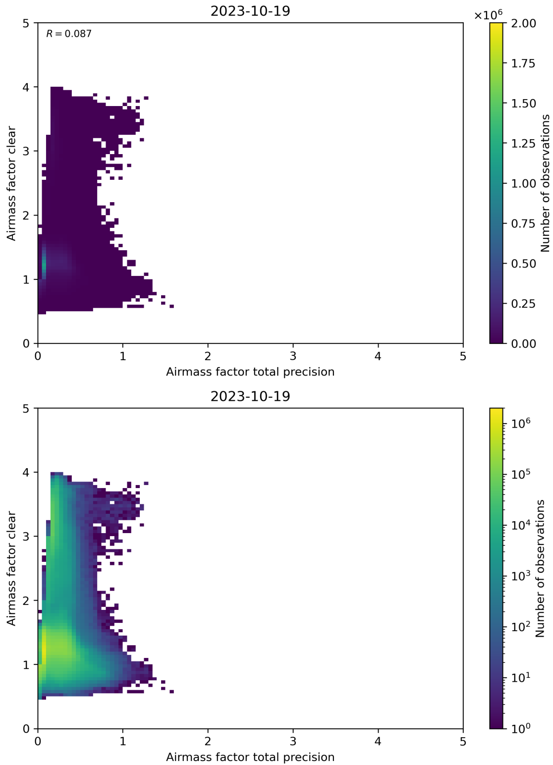
Figure 108: Scatter density plot of “Airmass factor total precision” against “Airmass factor clear” for 2023-10-18 to 2023-10-20.
