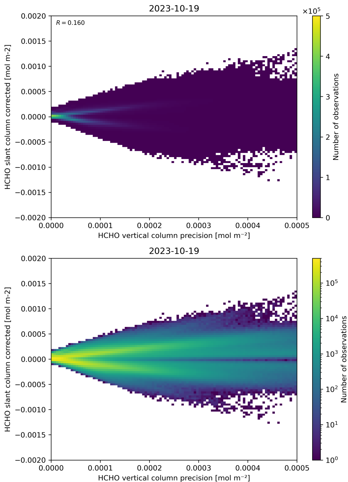
Figure 140: Scatter density plot of “HCHO vertical column precision” against “HCHO slant column corrected” for 2023-10-18 to 2023-10-20.
