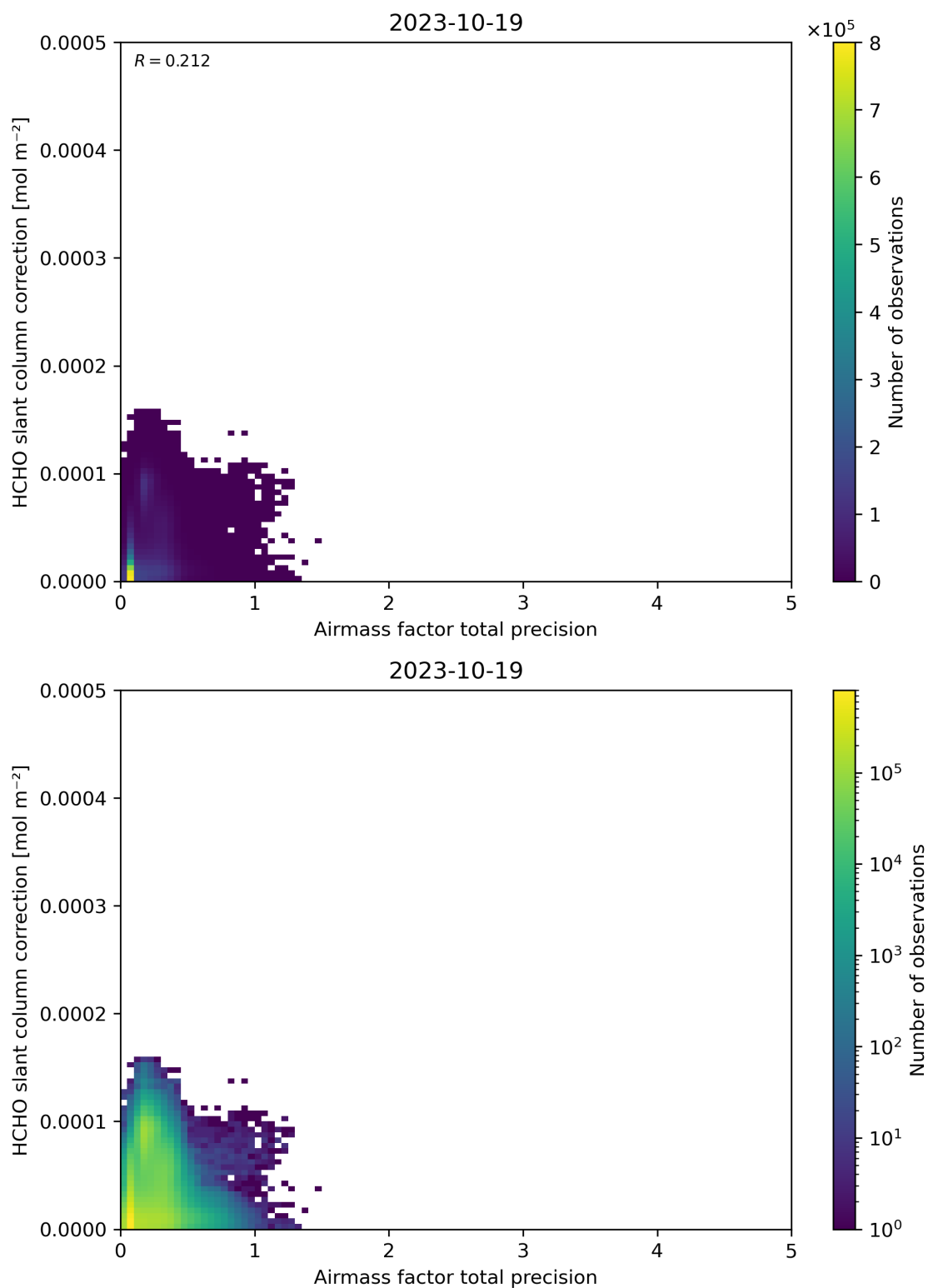
Figure 110: Scatter density plot of “Airmass factor total precision” against “HCHO slant column correction” for 2023-10-18 to 2023-10-20.
