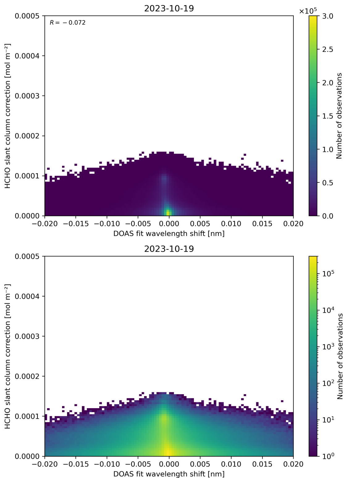
Figure 67: Scatter density plot of “DOAS fit wavelength shift” against “HCHO slant column correction” for 2023-10-18 to 2023-10-20.
