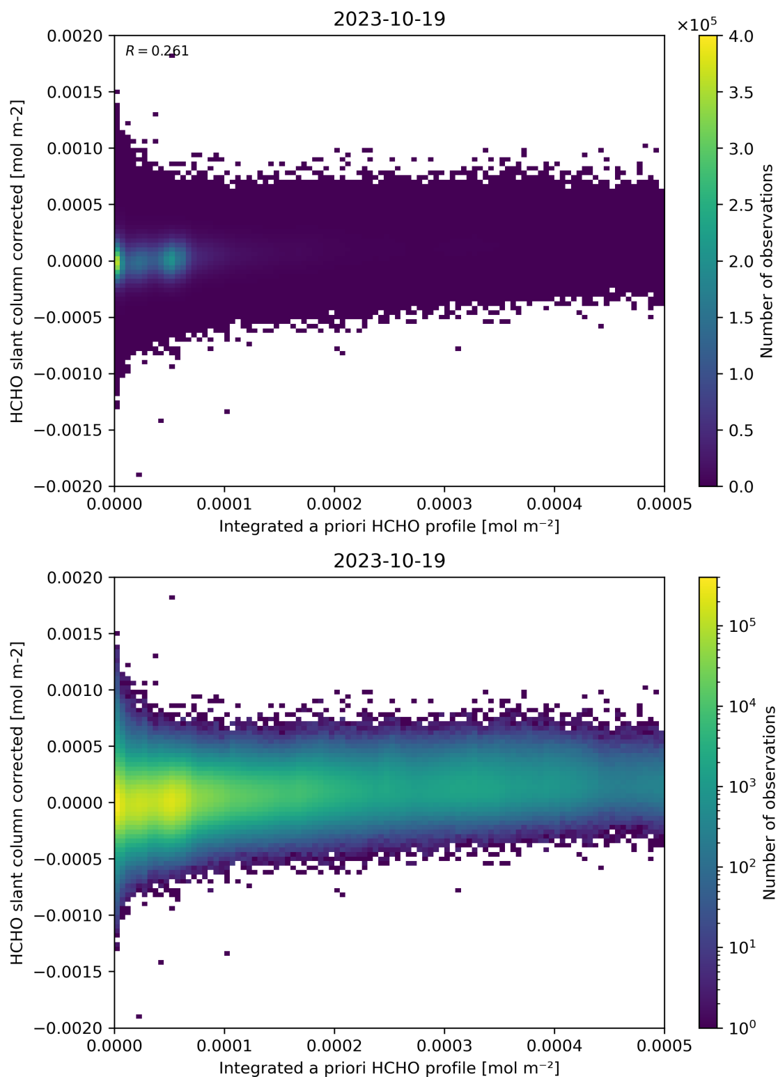
Figure 151: Scatter density plot of “Integrated a priori HCHO profile” against “HCHO slant column corrected” for 2023-10-18 to 2023-10-20.
