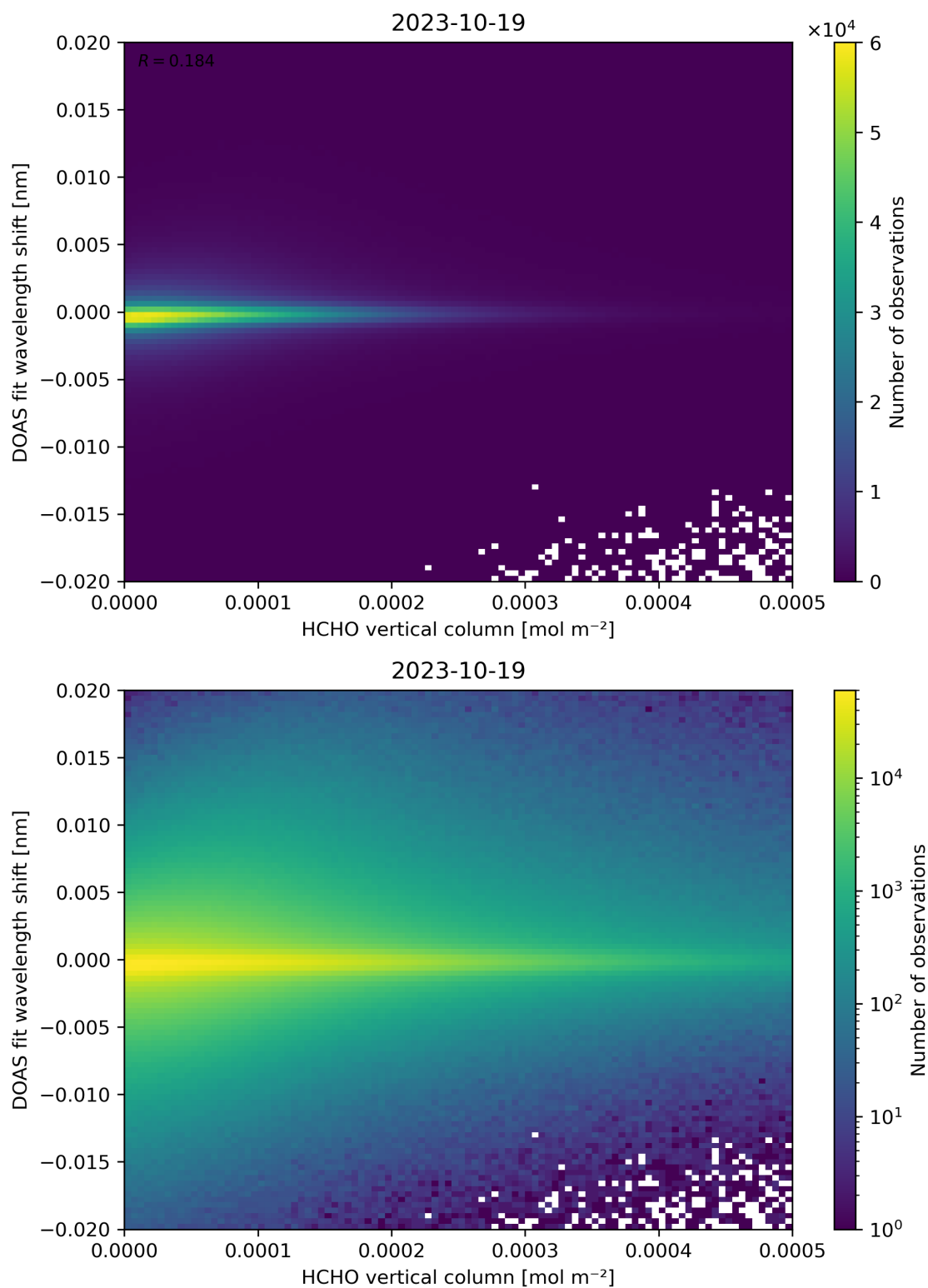
Figure 124: Scatter density plot of “HCHO vertical column” against “DOAS fit wavelength shift” for 2023-10-18 to 2023-10-20.
