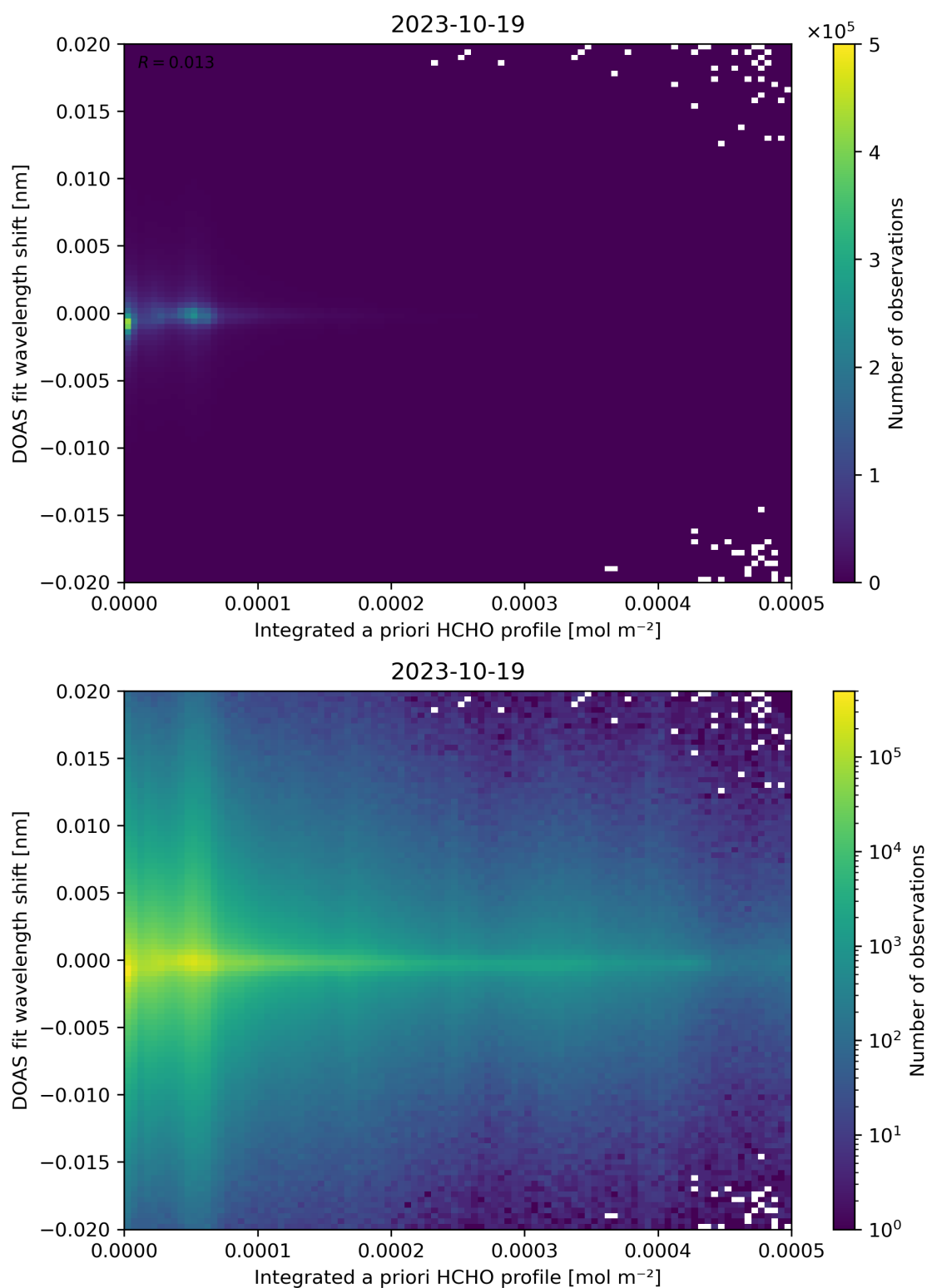
Figure 149: Scatter density plot of “Integrated a priori HCHO profile” against “DOAS fit wavelength shift” for 2023-10-18 to 2023-10-20.
