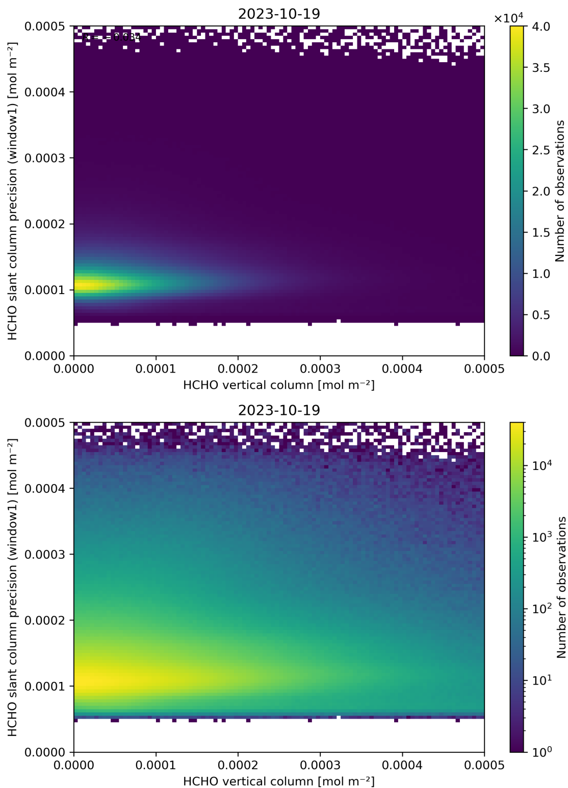
Figure 130: Scatter density plot of “HCHO vertical column” against “HCHO slant column precision (window1)” for 2023-10-18 to 2023-10-20.
