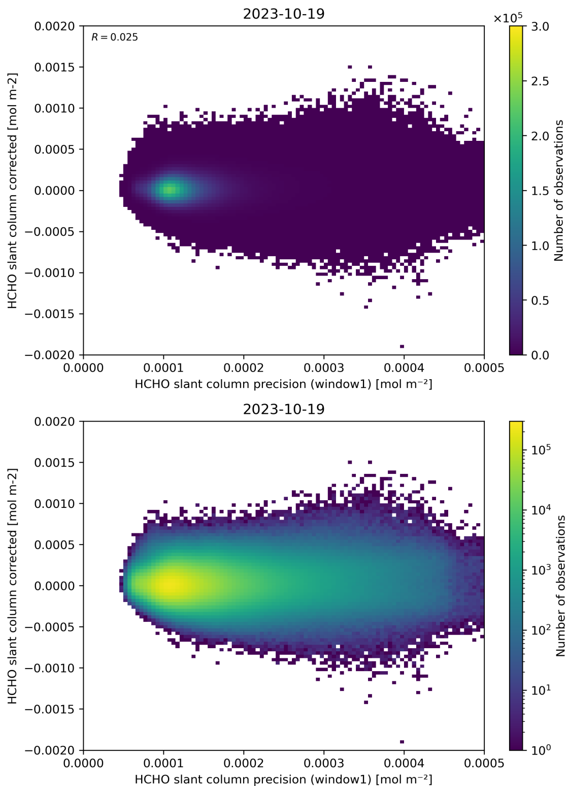
Figure 92: Scatter density plot of “HCHO slant column precision (window1)” against “HCHO slant column corrected” for 2023-10-18 to 2023-10-20.
