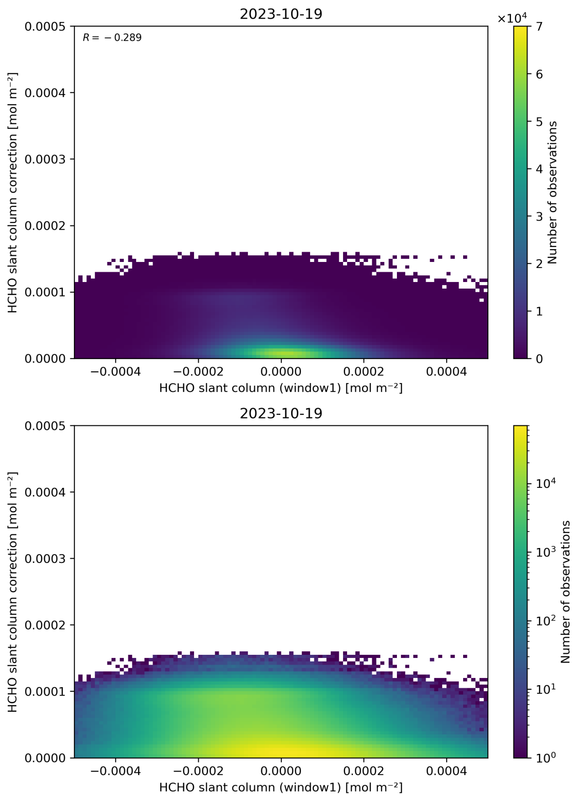
Figure 83: Scatter density plot of “HCHO slant column (window1)” against “HCHO slant column correction” for 2023-10-18 to 2023-10-20.
