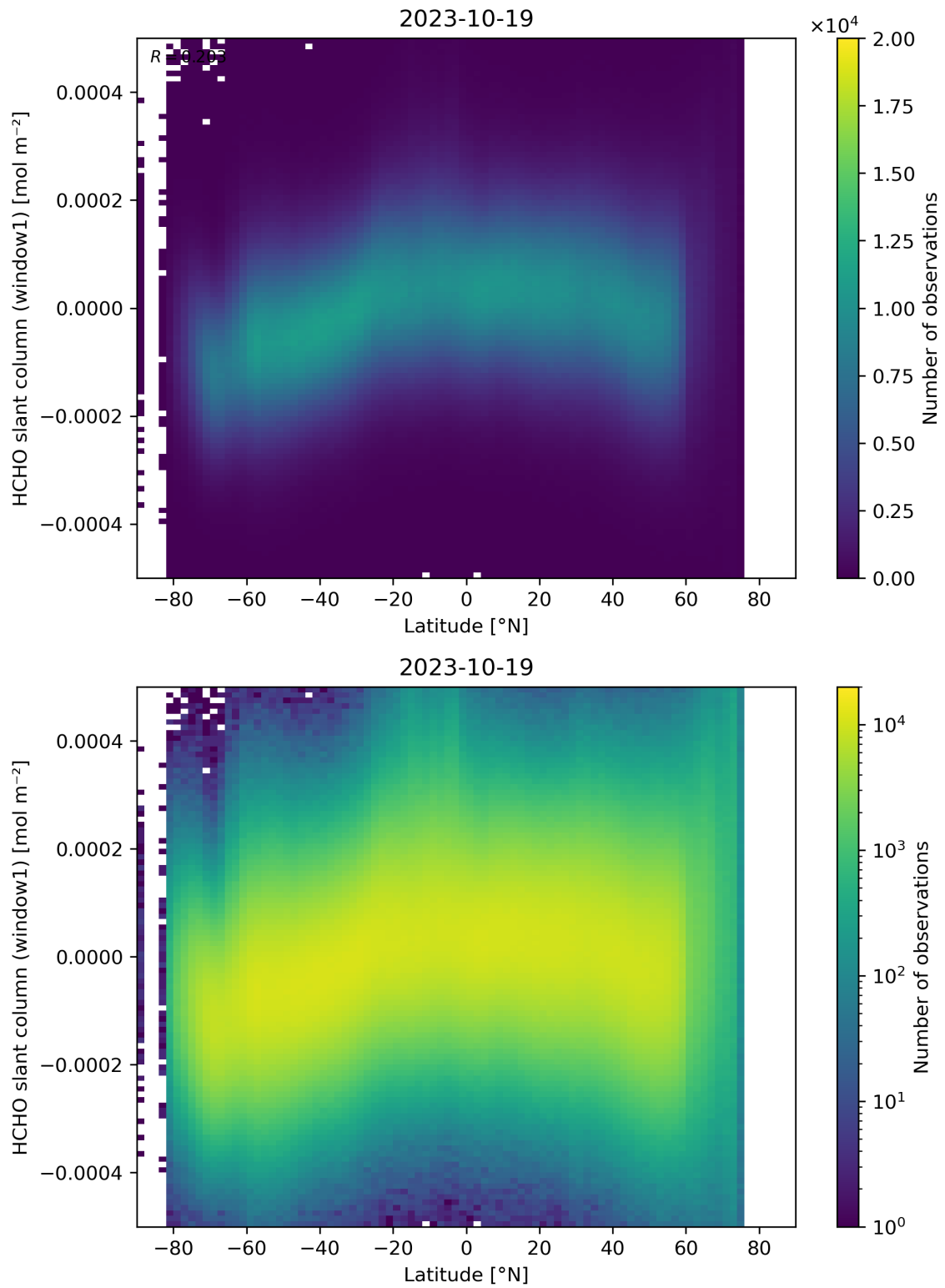
Figure 159: Scatter density plot of “Latitude” against “HCHO slant column (window1)” for 2023-10-18 to 2023-10-20.
