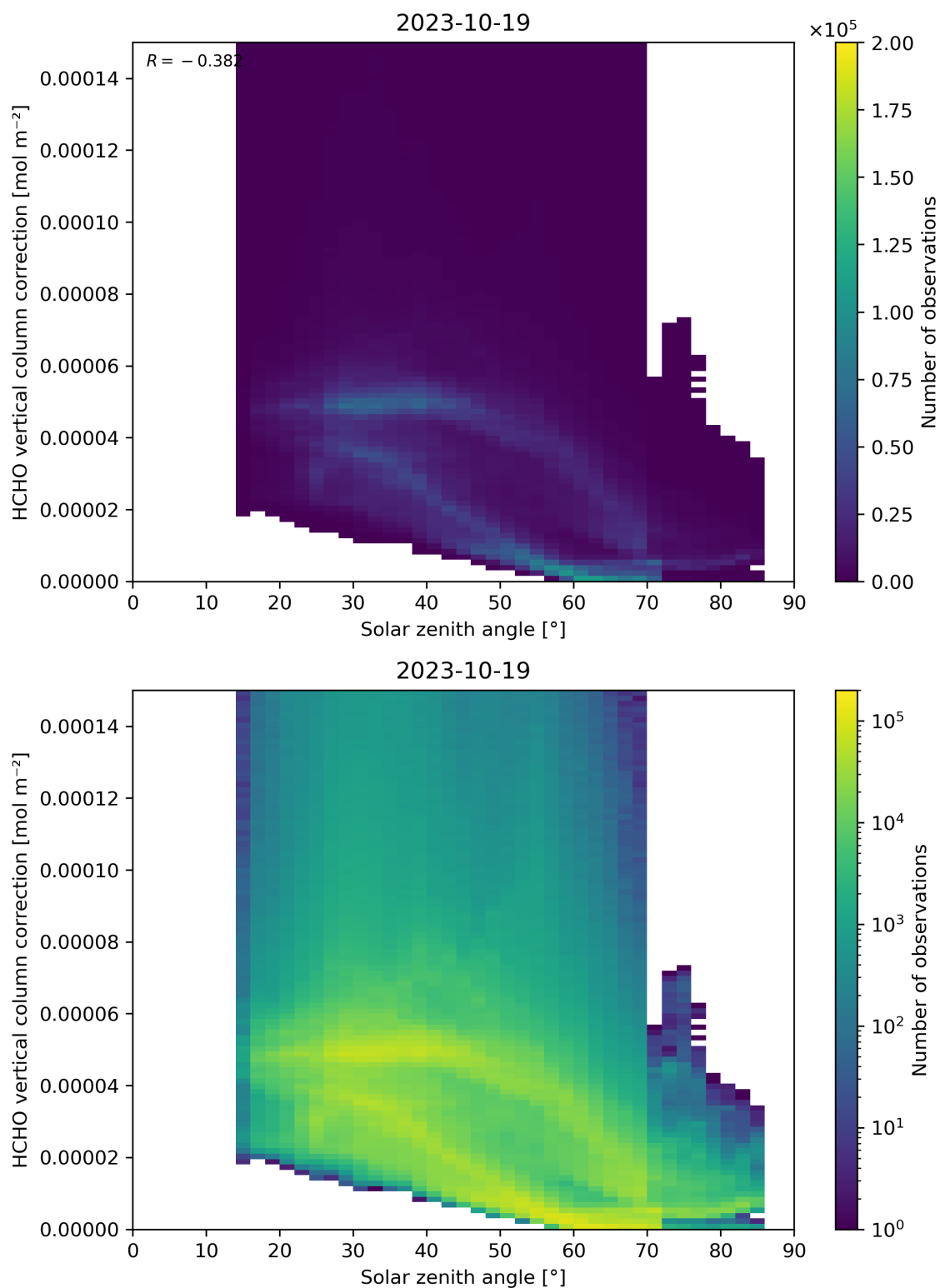
Figure 178: Scatter density plot of “Solar zenith angle” against “HCHO vertical column correction” for 2023-10-18 to 2023-10-20.
