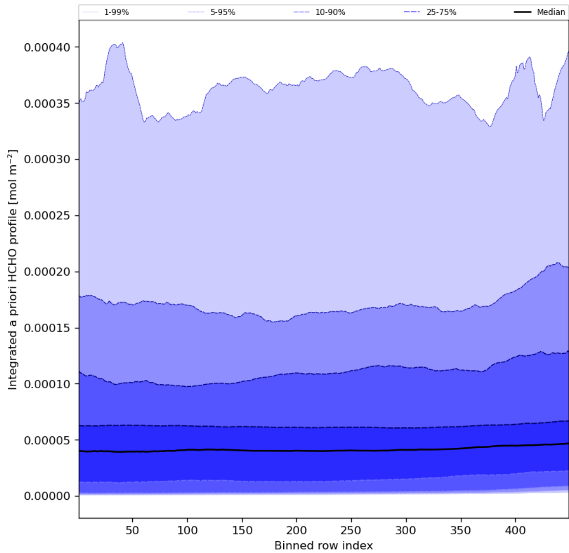
Figure 57: Along track statistics of “Integrated a priori HCHO profile” for 2023-10-18 to 2023-10-20
