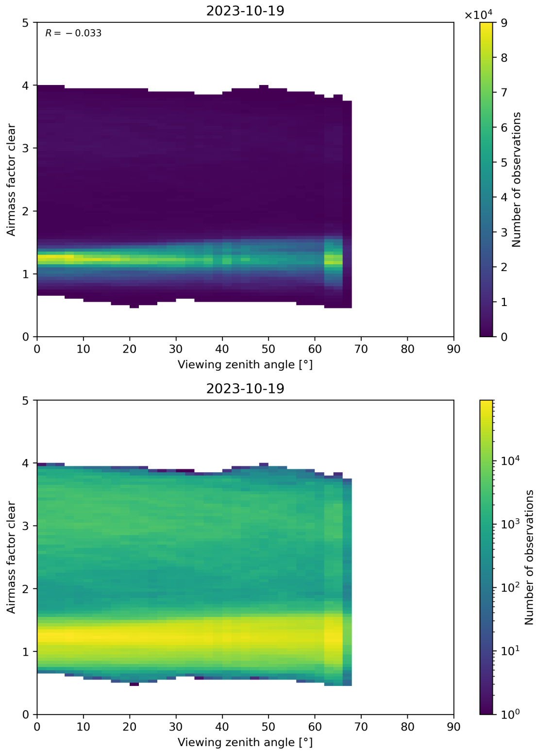
Figure 185: Scatter density plot of “Viewing zenith angle” against “Airmass factor clear” for 2023-10-18 to 2023-10-20.
