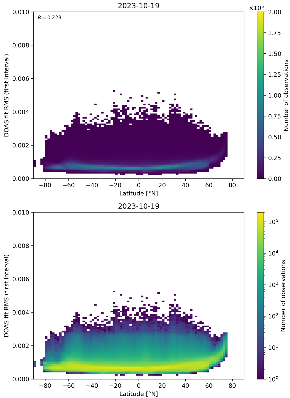
Figure 153: Scatter density plot of “Latitude” against “DOAS fit RMS (first interval)” for 2023-10-18 to 2023-10-20.
