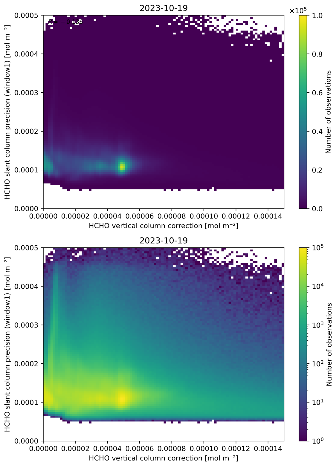
Figure 119: Scatter density plot of “HCHO vertical column correction” against “HCHO slant column precision (window1)” for 2023-10-18 to 2023-10-20.
