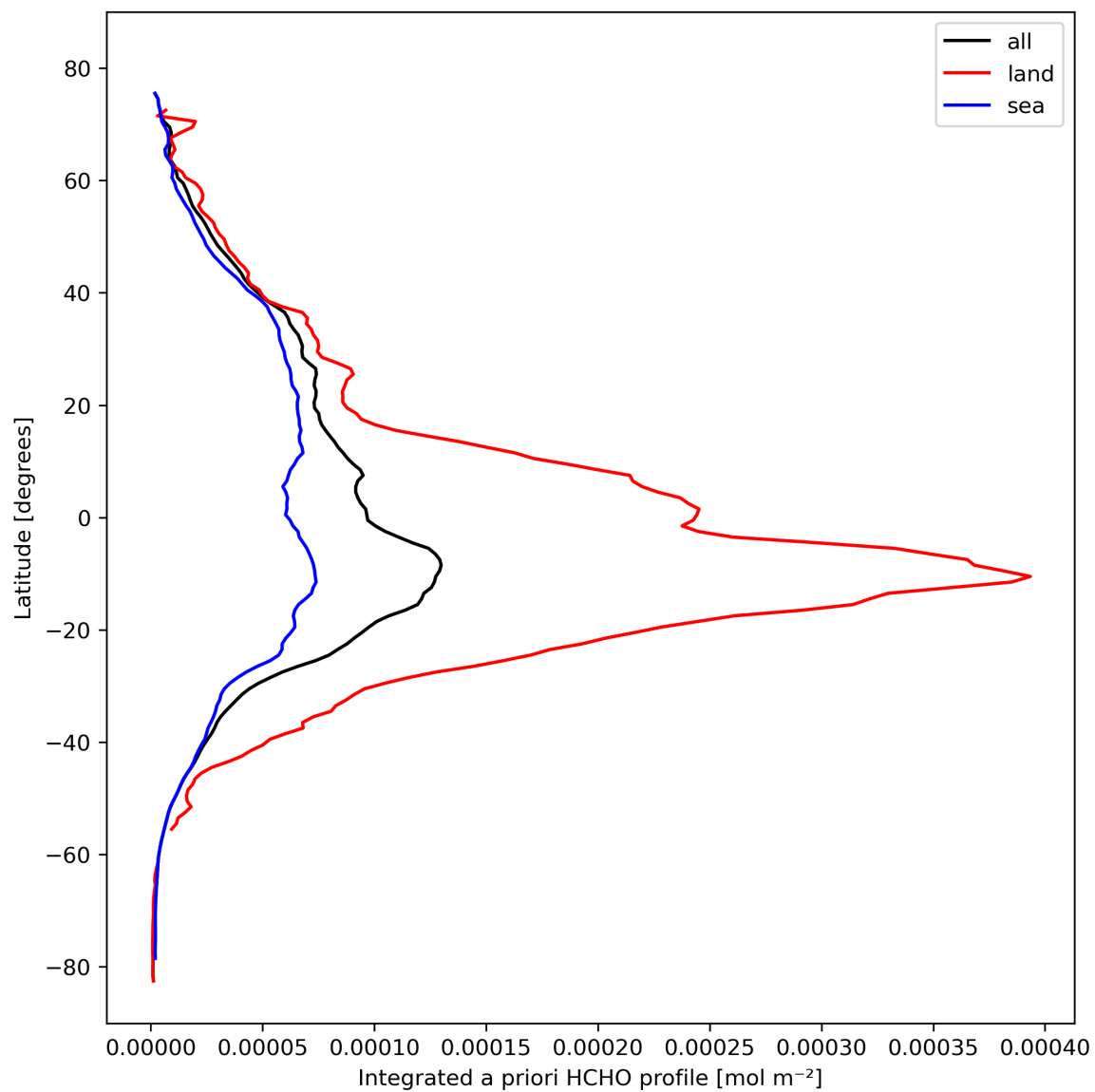
Figure 29: Zonal average of “Integrated a priori HCHO profile” for 2023-10-18 to 2023-10-20.
