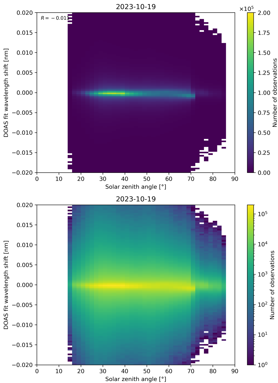
Figure 168: Scatter density plot of “Solar zenith angle” against “DOAS fit wavelength shift” for 2023-10-18 to 2023-10-20.
