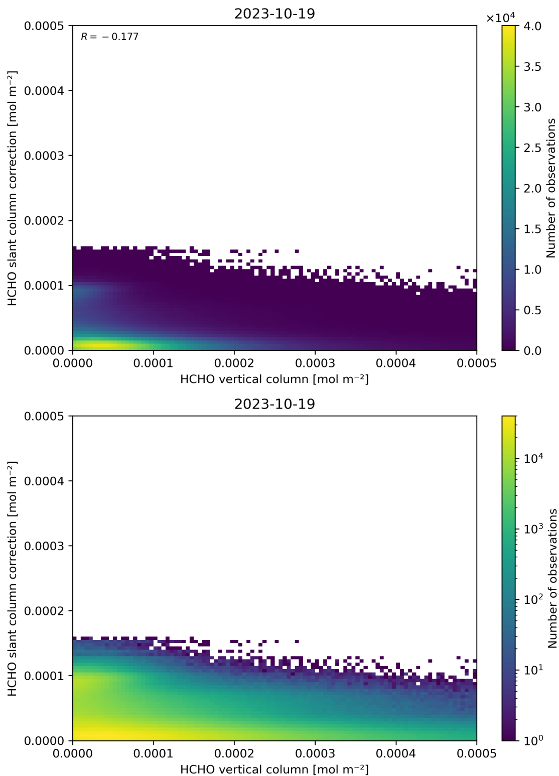
Figure 128: Scatter density plot of “HCHO vertical column” against “HCHO slant column correction” for 2023-10-18 to 2023-10-20.
