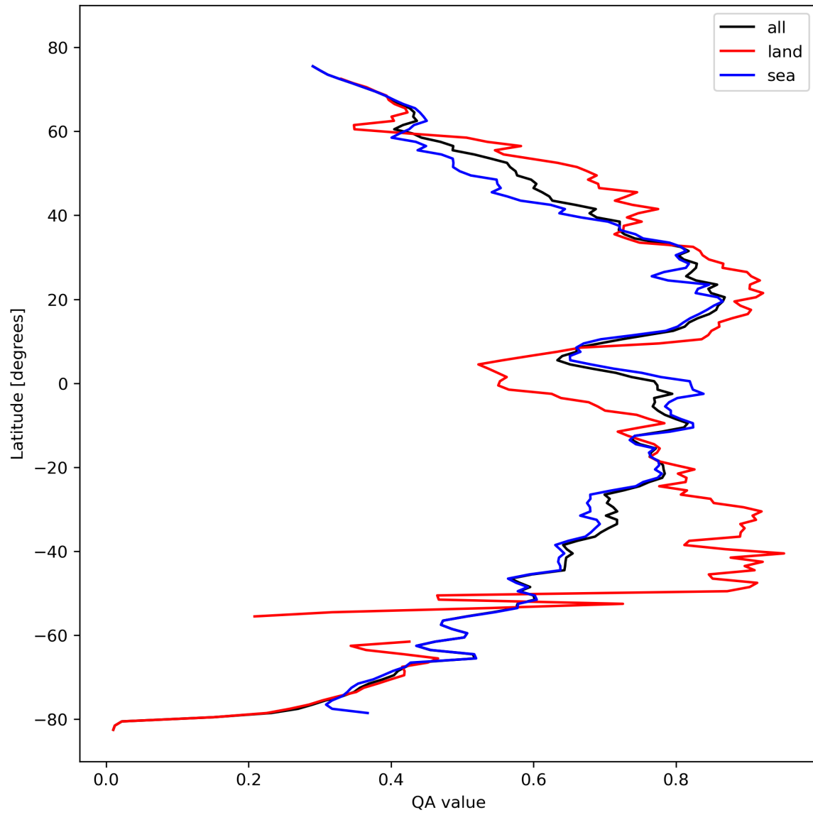
Figure 20: Zonal average of “QA value” for 2023-10-18 to 2023-10-20.
