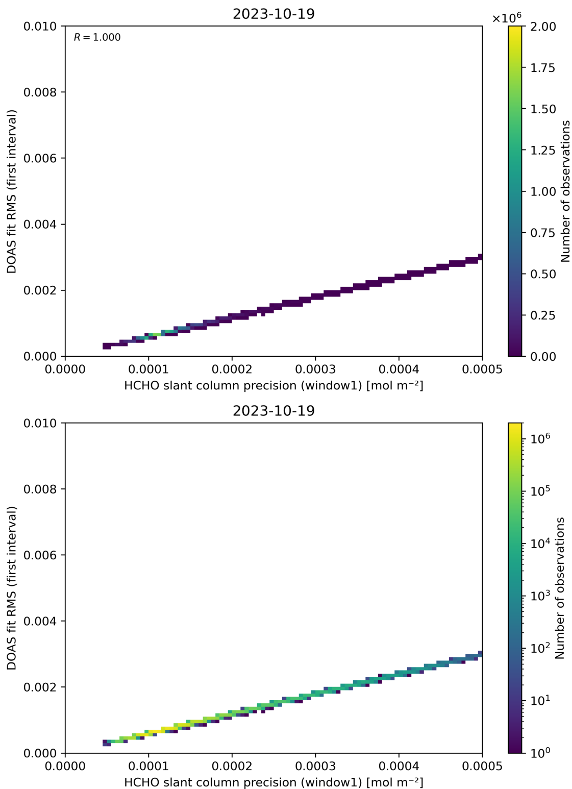
Figure 88: Scatter density plot of “HCHO slant column precision (window1)” against “DOAS fit RMS (first interval)” for 2023-10-18 to 2023-10-20.
