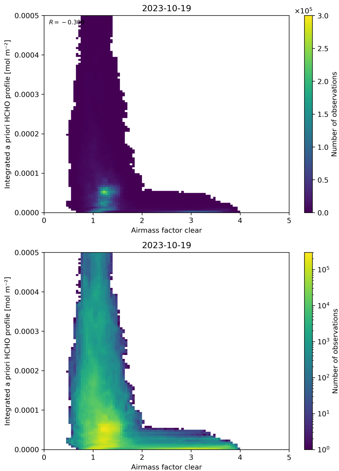
Figure 76: Scatter density plot of “Airmass factor clear” against “Integrated a priori HCHO profile” for 2023-10-18 to 2023-10-20.
