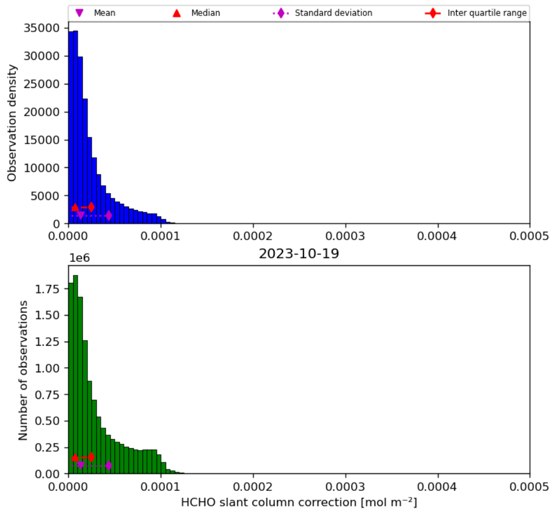
Figure 47: Histogram of “HCHO slant column correction” for 2023-10-18 to 2023-10-20
