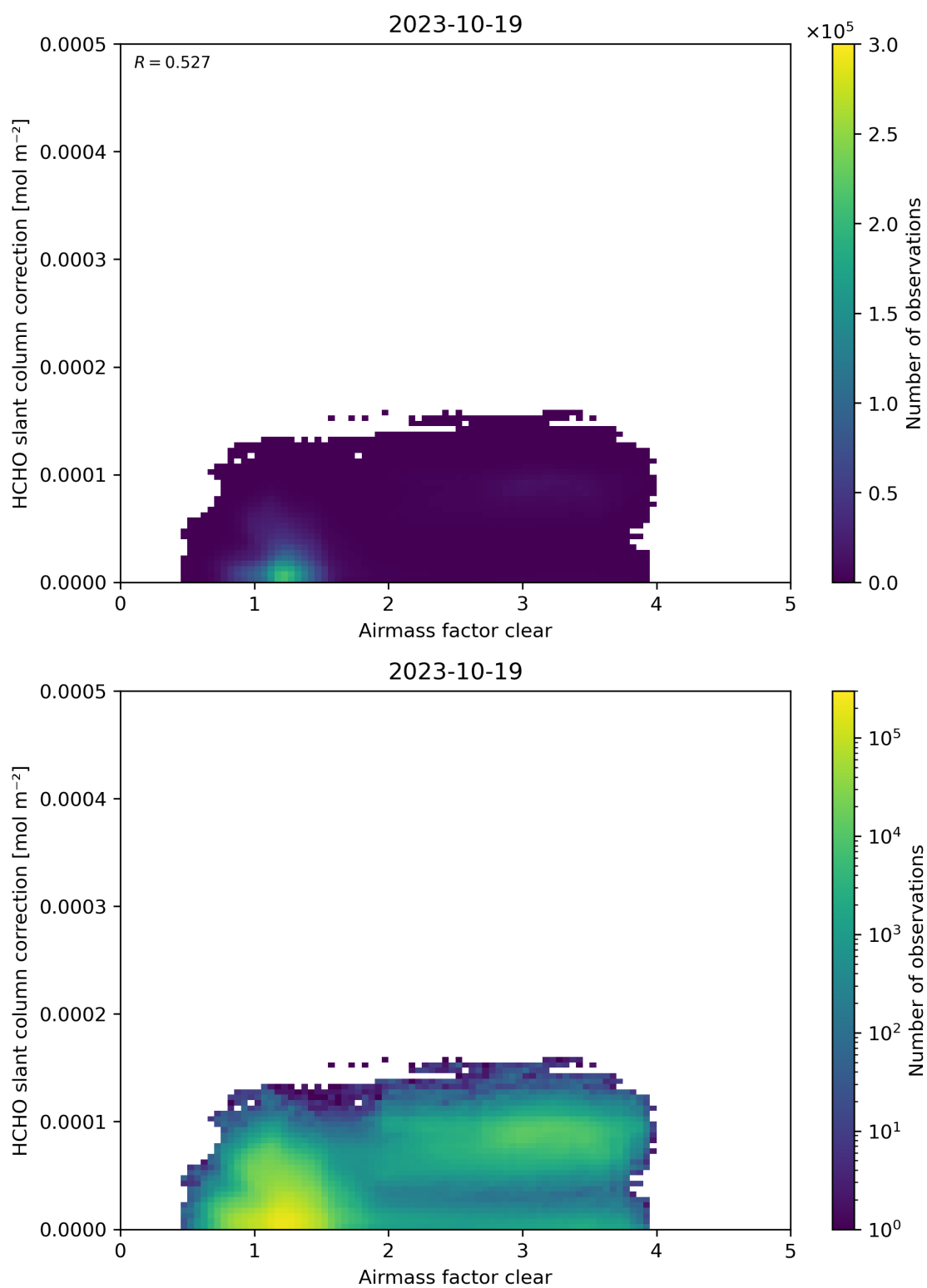
Figure 75: Scatter density plot of “Airmass factor clear” against “HCHO slant column correction” for 2023-10-18 to 2023-10-20.
