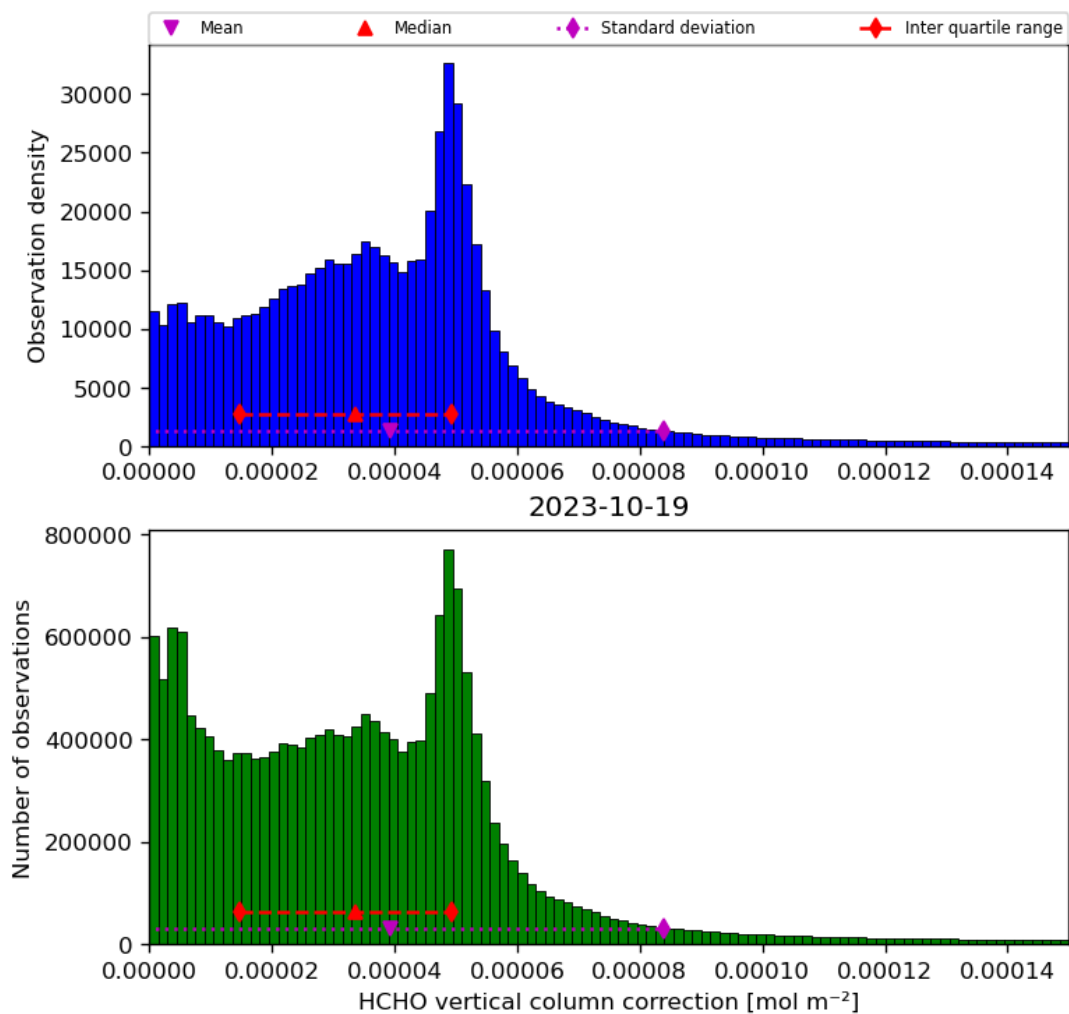
Figure 37: Histogram of “HCHO vertical column correction” for 2023-10-18 to 2023-10-20
