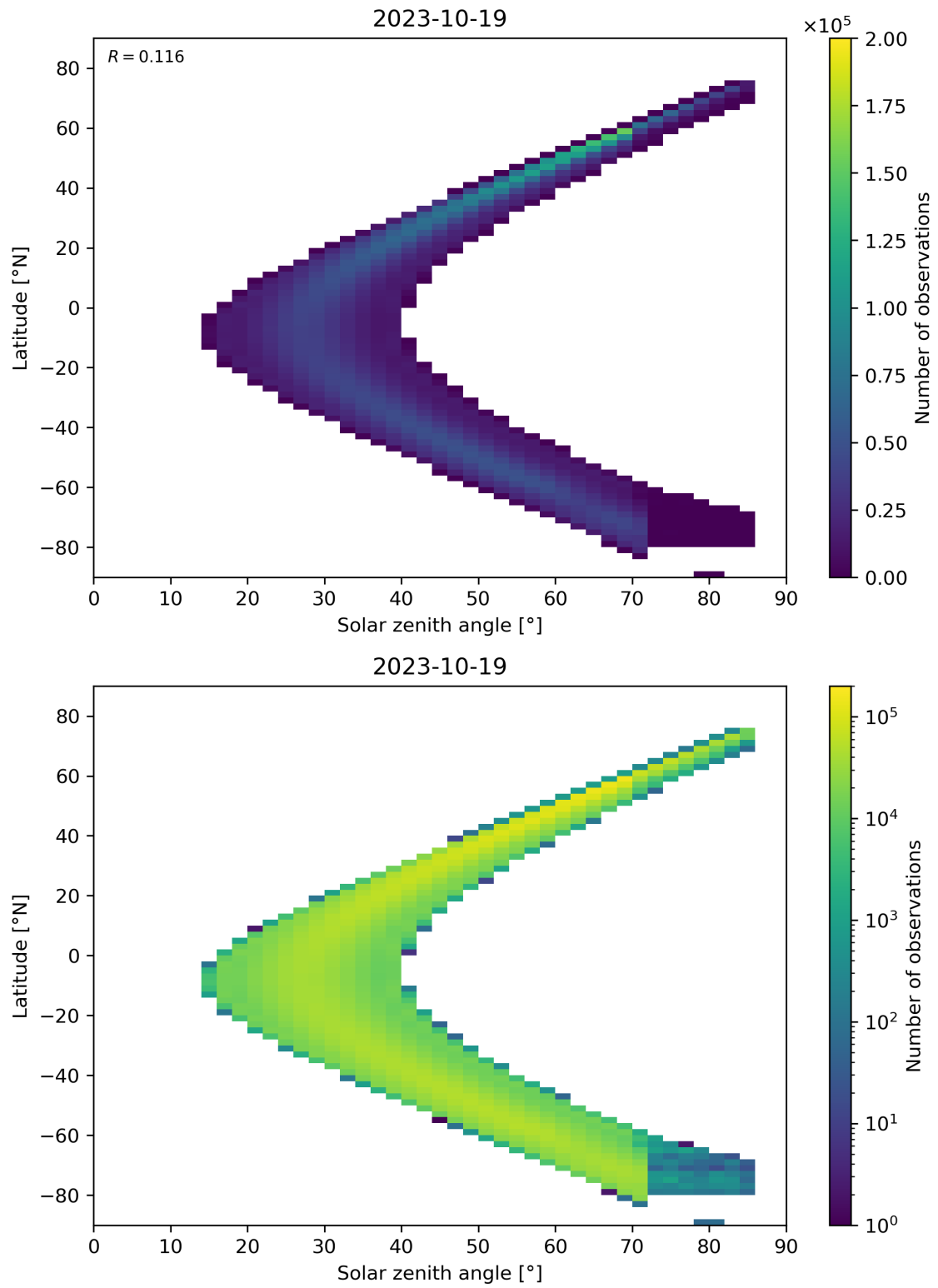
Figure 181: Scatter density plot of “Solar zenith angle” against “Latitude” for 2023-10-18 to 2023-10-20.
