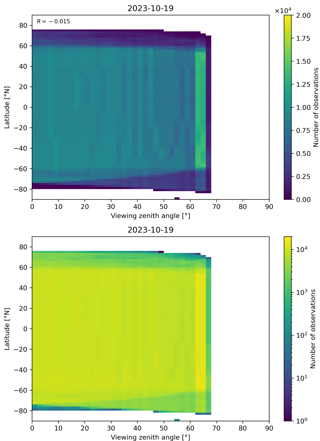
Figure 196: Scatter density plot of “Viewing zenith angle” against “Latitude” for 2023-10-18 to 2023-10-20.
