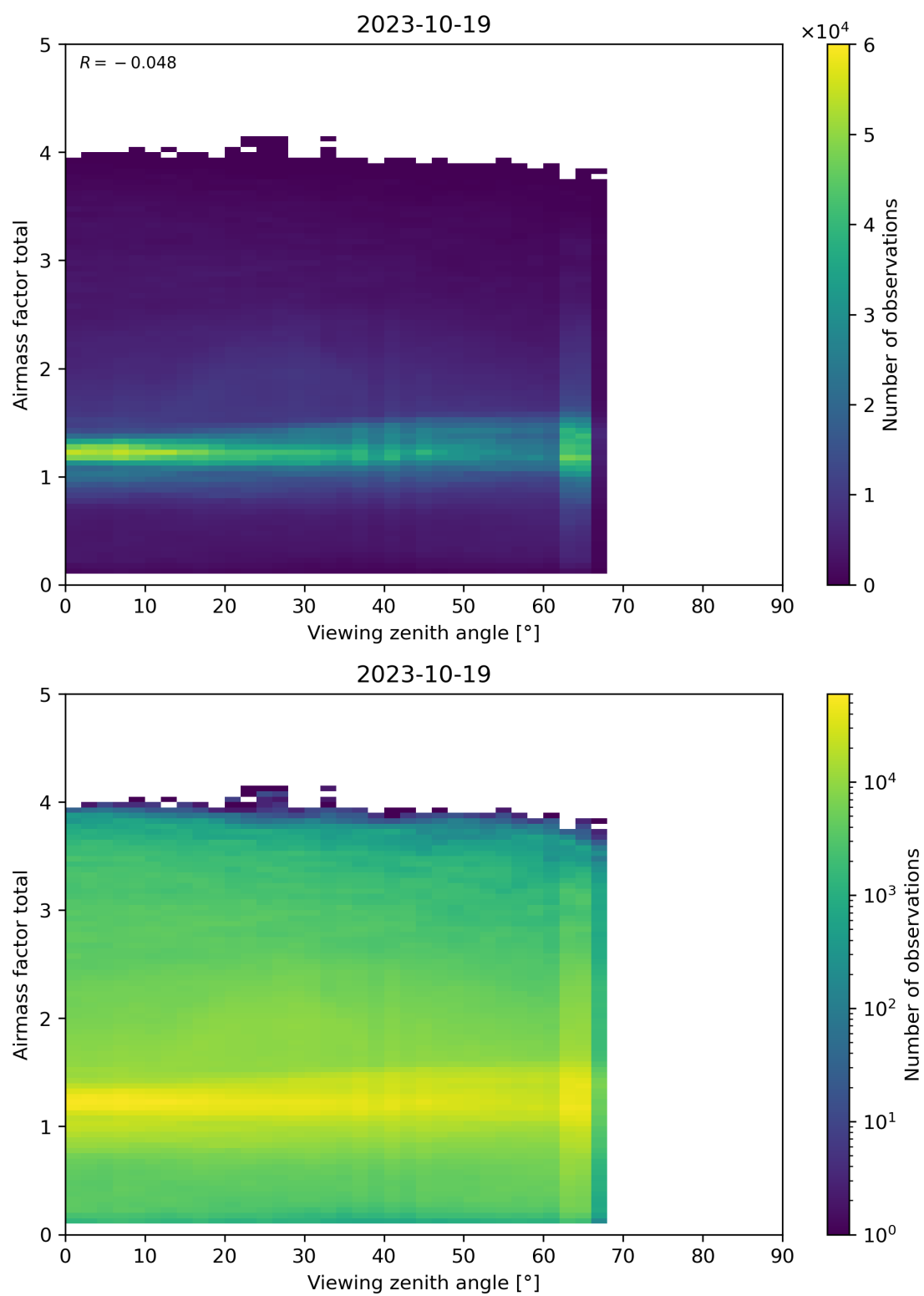
Figure 190: Scatter density plot of “Viewing zenith angle” against “Airmass factor total” for 2023-10-18 to 2023-10-20.
