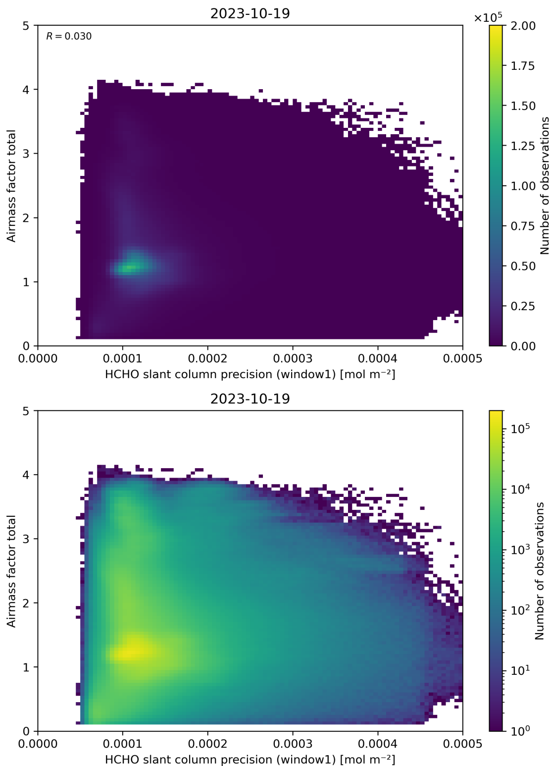
Figure 94: Scatter density plot of “HCHO slant column precision (window1)” against “Airmass factor total” for 2023-10-18 to 2023-10-20.
