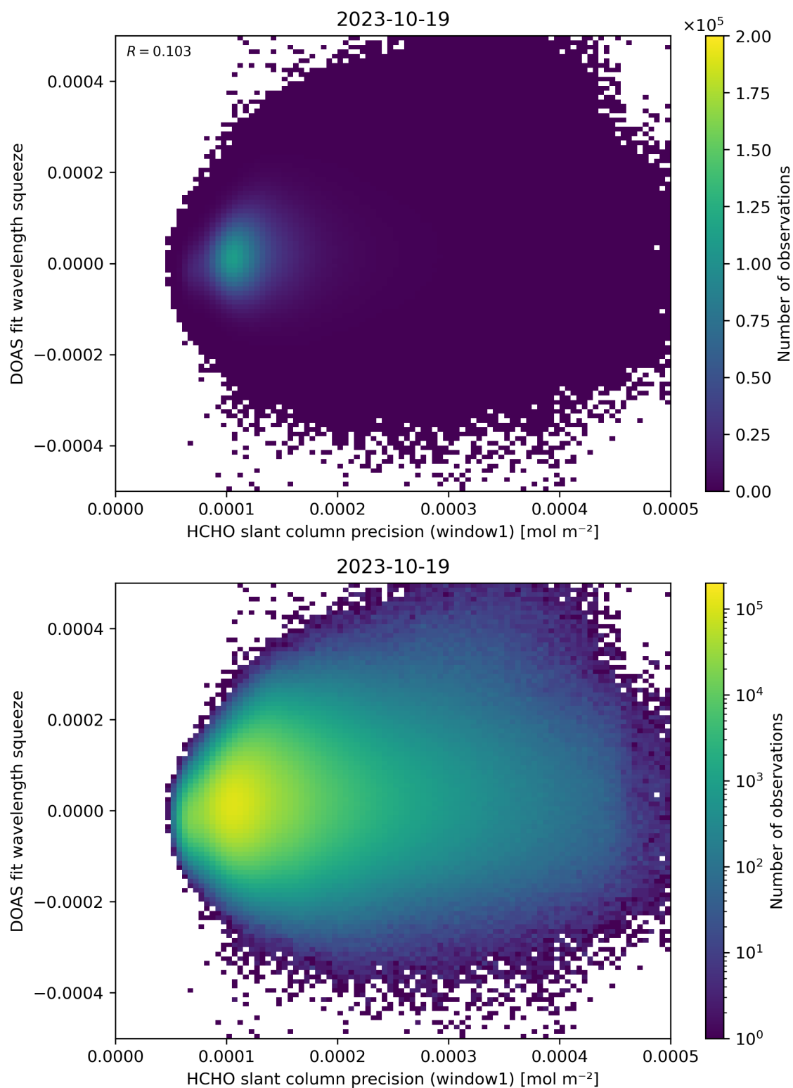
Figure 90: Scatter density plot of “HCHO slant column precision (window1)” against “DOAS fit wavelength squeeze” for 2023-10-18 to 2023-10-20.
