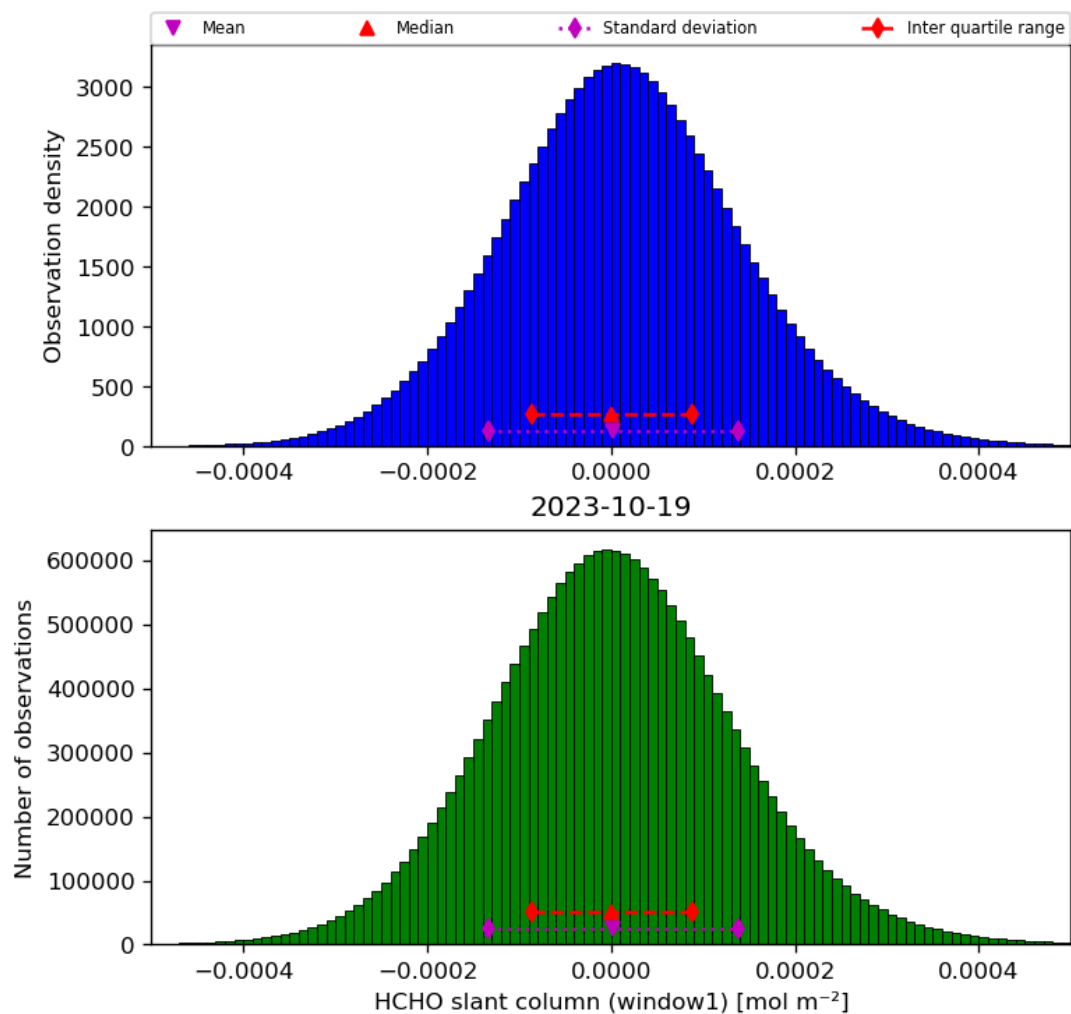
Figure 38: Histogram of “HCHO slant column (window1)” for 2023-10-18 to 2023-10-20
