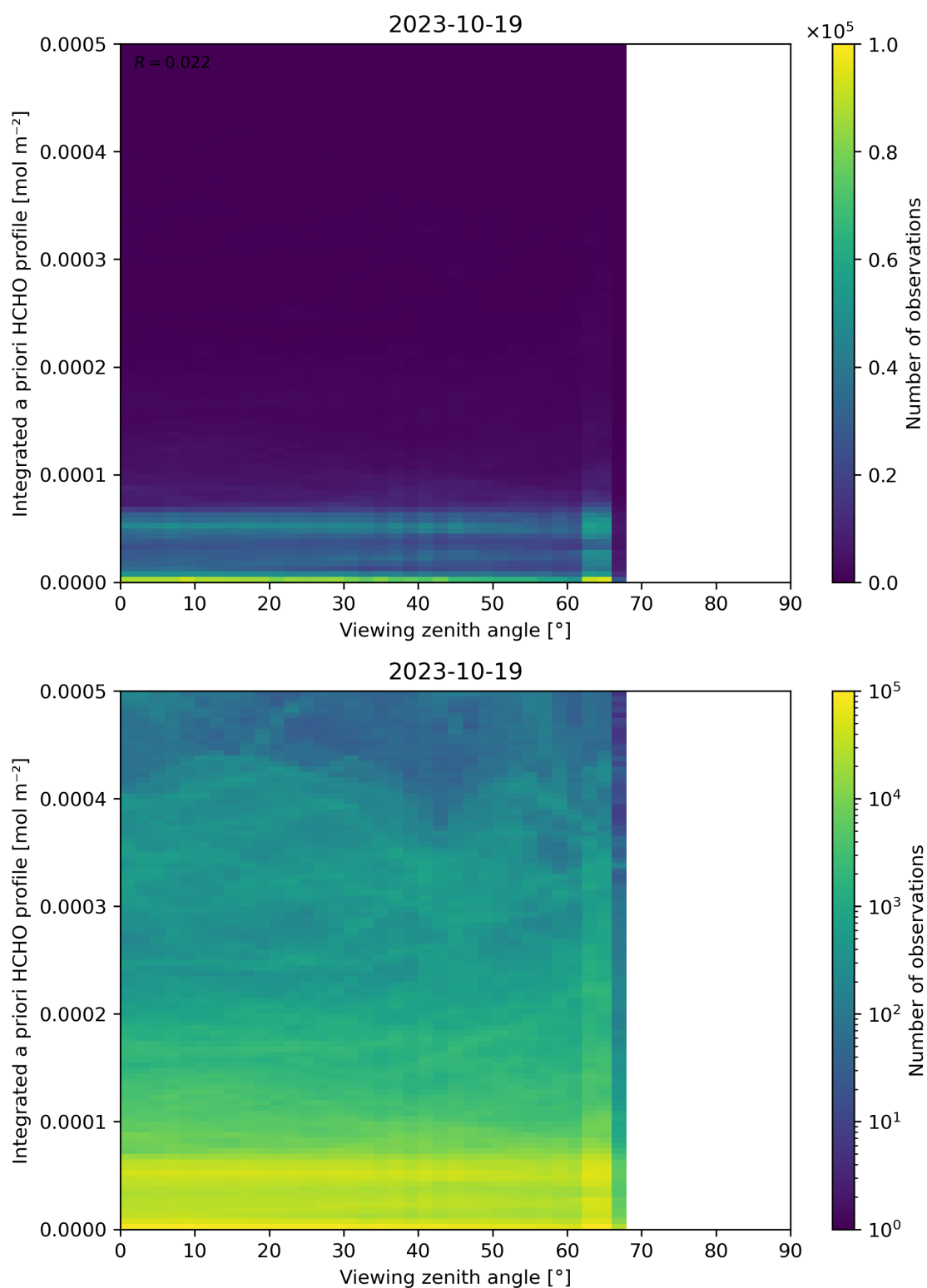
Figure 195: Scatter density plot of “Viewing zenith angle” against “Integrated a priori HCHO profile” for 2023-10-18 to 2023-10-20.
