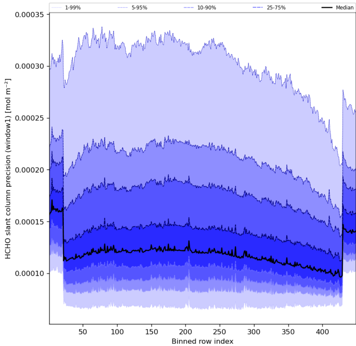
Figure 53: Along track statistics of “HCHO slant column precision (window1)” for 2023-10-18 to 2023-10-20
