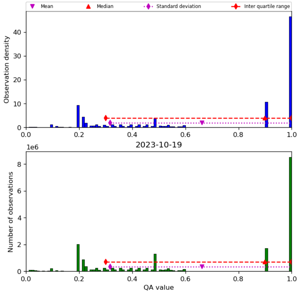
Figure 34: Histogram of “QA value” for 2023-10-18 to 2023-10-20
