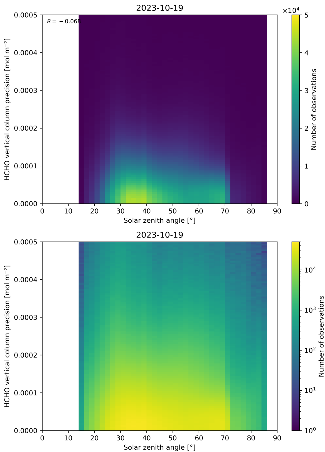
Figure 179: Scatter density plot of “Solar zenith angle” against “HCHO vertical column precision” for 2023-10-18 to 2023-10-20.
