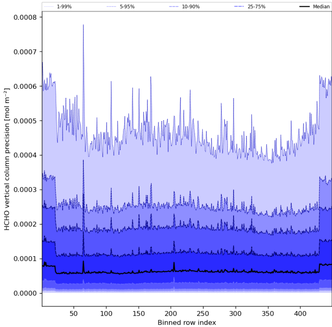
Figure 50: Along track statistics of “HCHO vertical column precision” for 2023-10-18 to 2023-10-20
