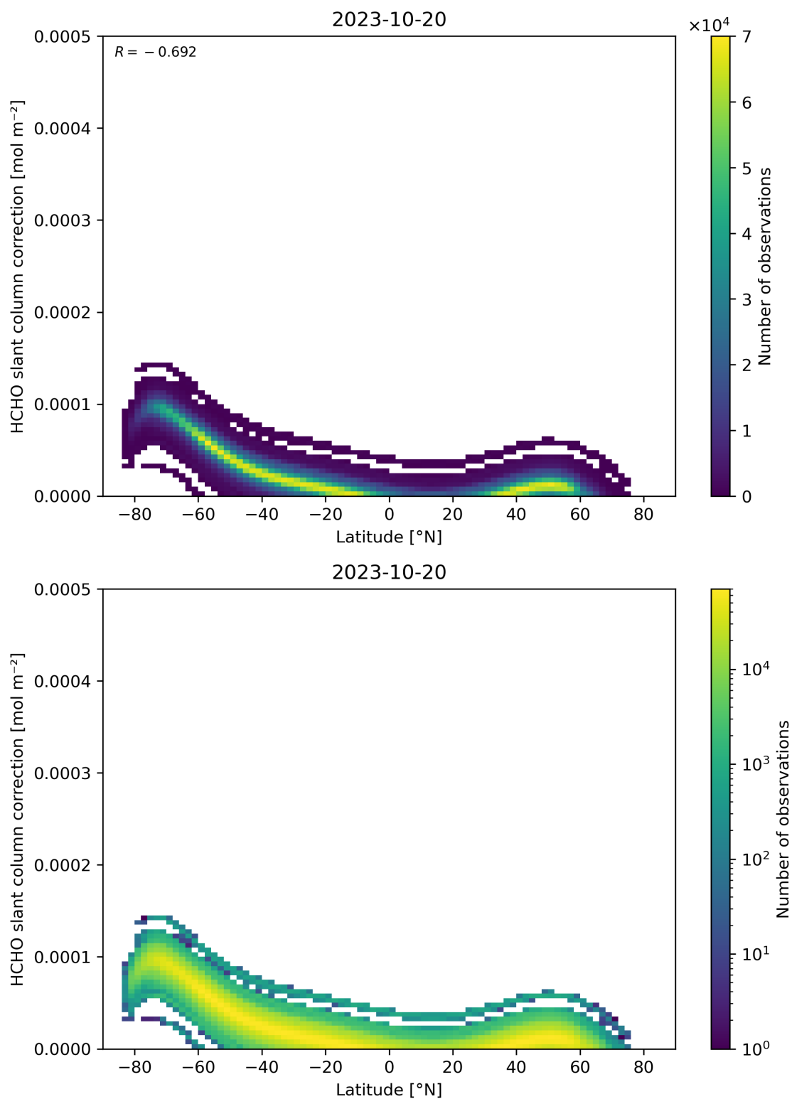
Figure 158: Scatter density plot of “Latitude” against “HCHO slant column correction” for 2023-10-19 to 2023-10-21.
