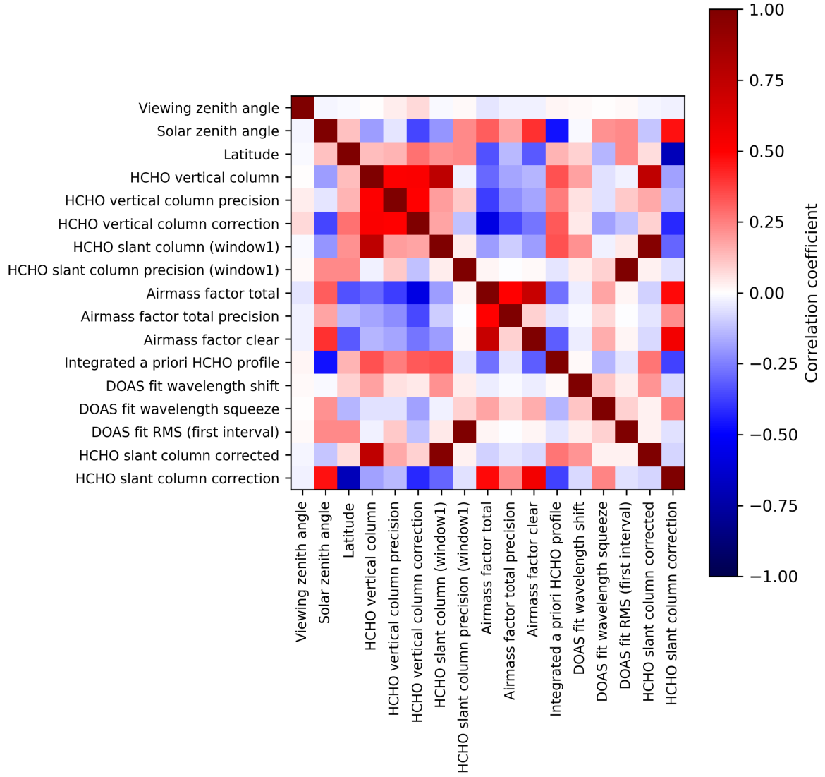
Figure 2: Map of correlation matrix for 2023-10-19 to 2023-10-21.
