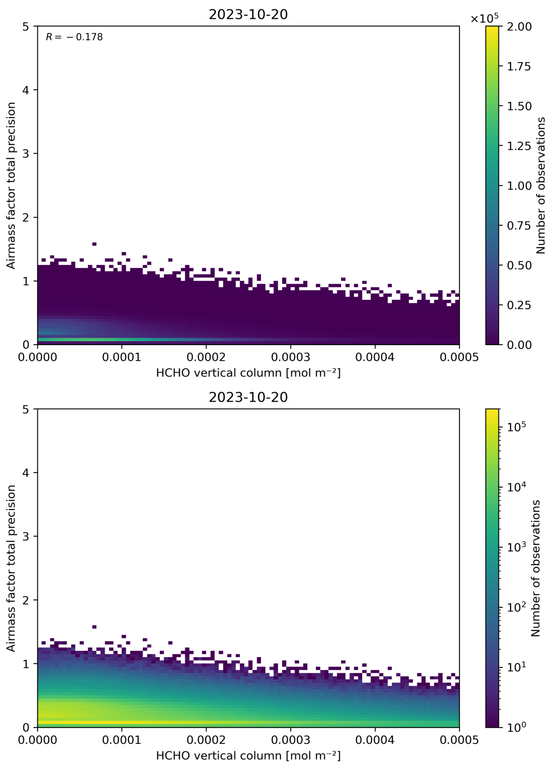
Figure 132: Scatter density plot of “HCHO vertical column” against “Airmass factor total precision” for 2023-10-19 to 2023-10-21.
