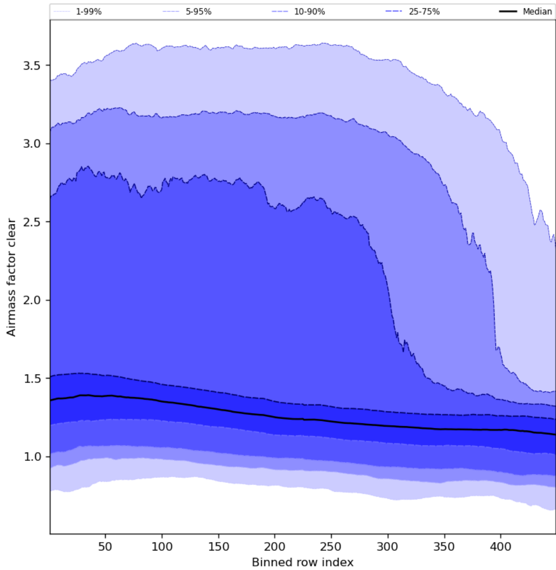
Figure 56: Along track statistics of “Airmass factor clear” for 2023-10-19 to 2023-10-21
