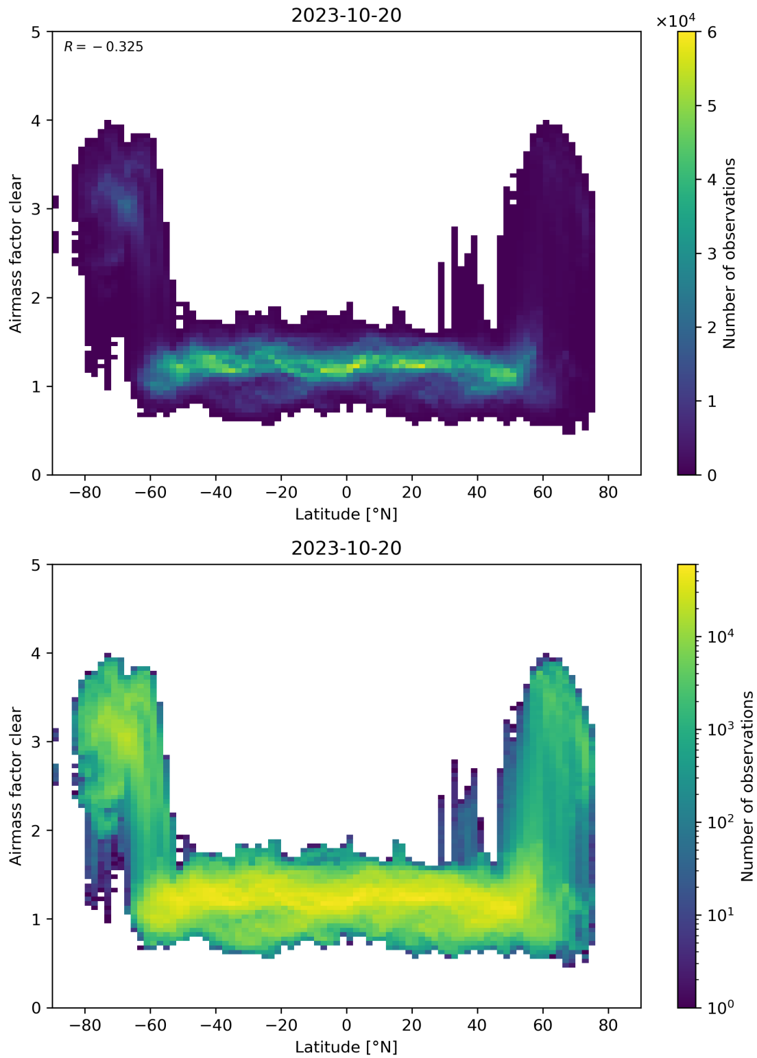
Figure 156: Scatter density plot of “Latitude” against “Airmass factor clear” for 2023-10-19 to 2023-10-21.
