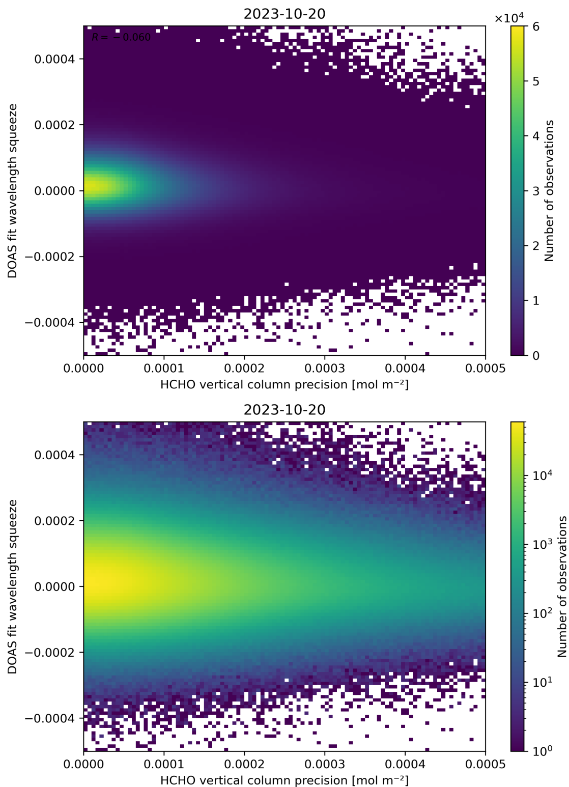
Figure 138: Scatter density plot of “HCHO vertical column precision” against “DOAS fit wavelength squeeze” for 2023-10-19 to 2023-10-21.
