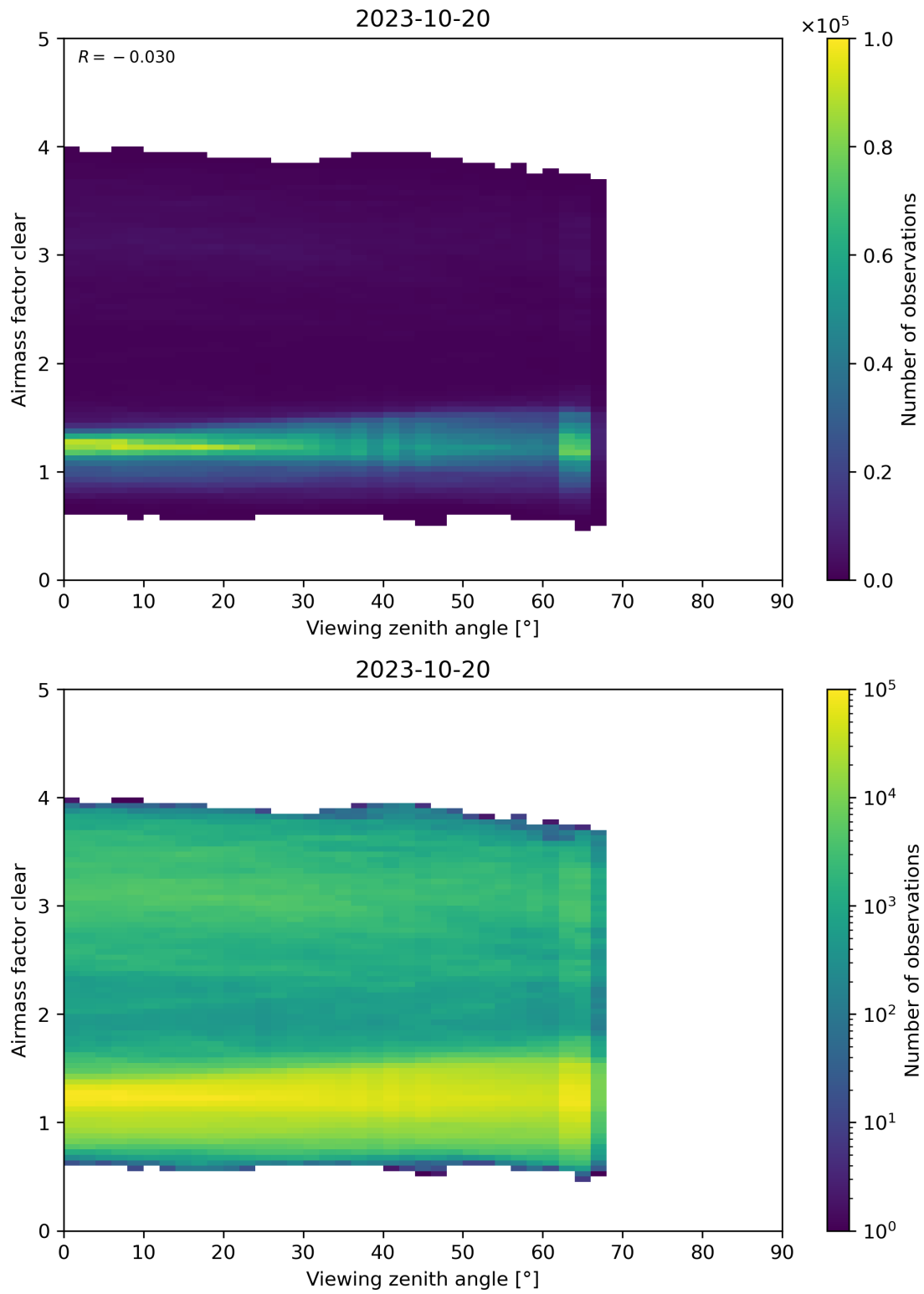
Figure 185: Scatter density plot of “Viewing zenith angle” against “Airmass factor clear” for 2023-10-19 to 2023-10-21.
