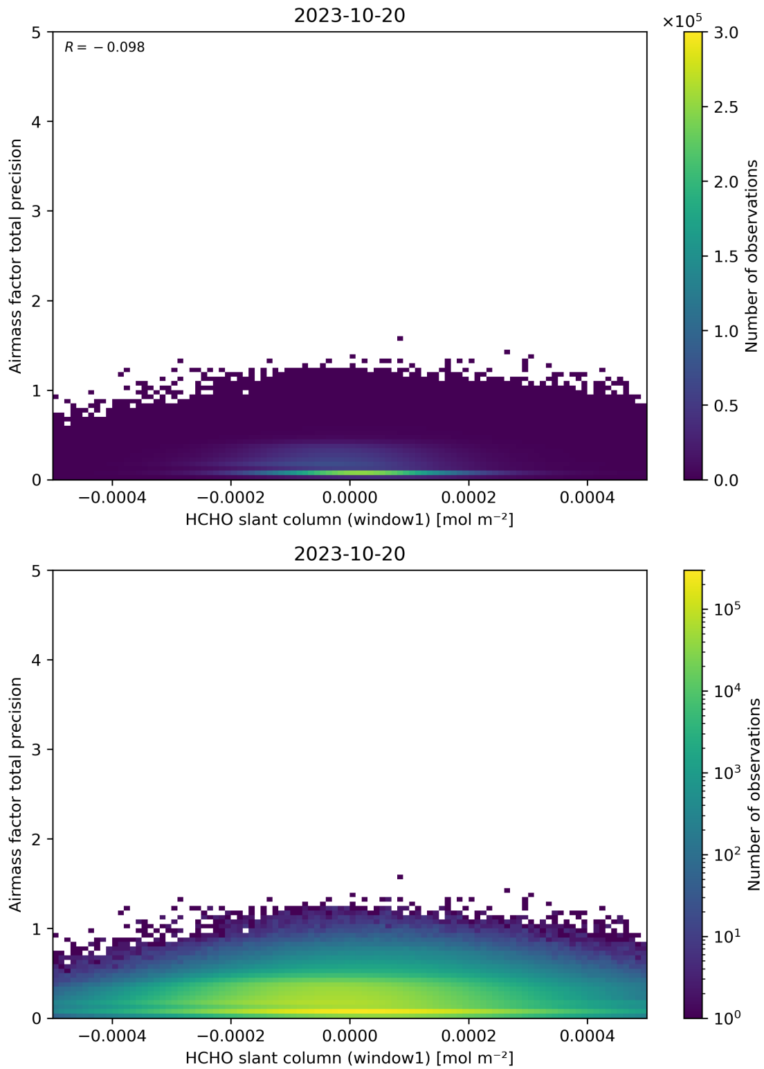
Figure 86: Scatter density plot of “HCHO slant column (window1)” against “Airmass factor total precision” for 2023-10-19 to 2023-10-21.
