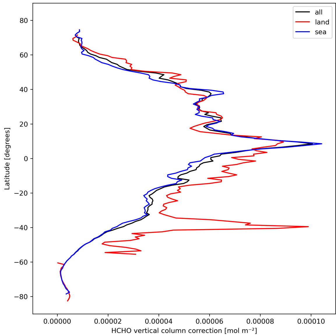
Figure 23: Zonal average of “HCHO vertical column correction” for 2023-10-19 to 2023-10-21.
