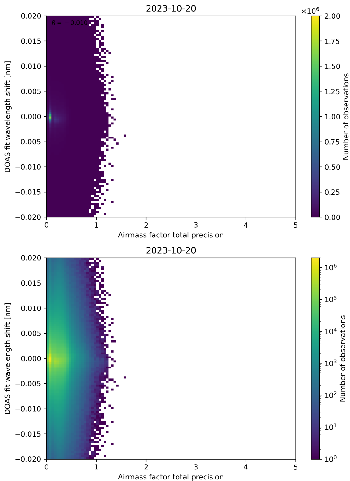
Figure 106: Scatter density plot of “Airmass factor total precision” against “DOAS fit wavelength shift” for 2023-10-19 to 2023-10-21.
