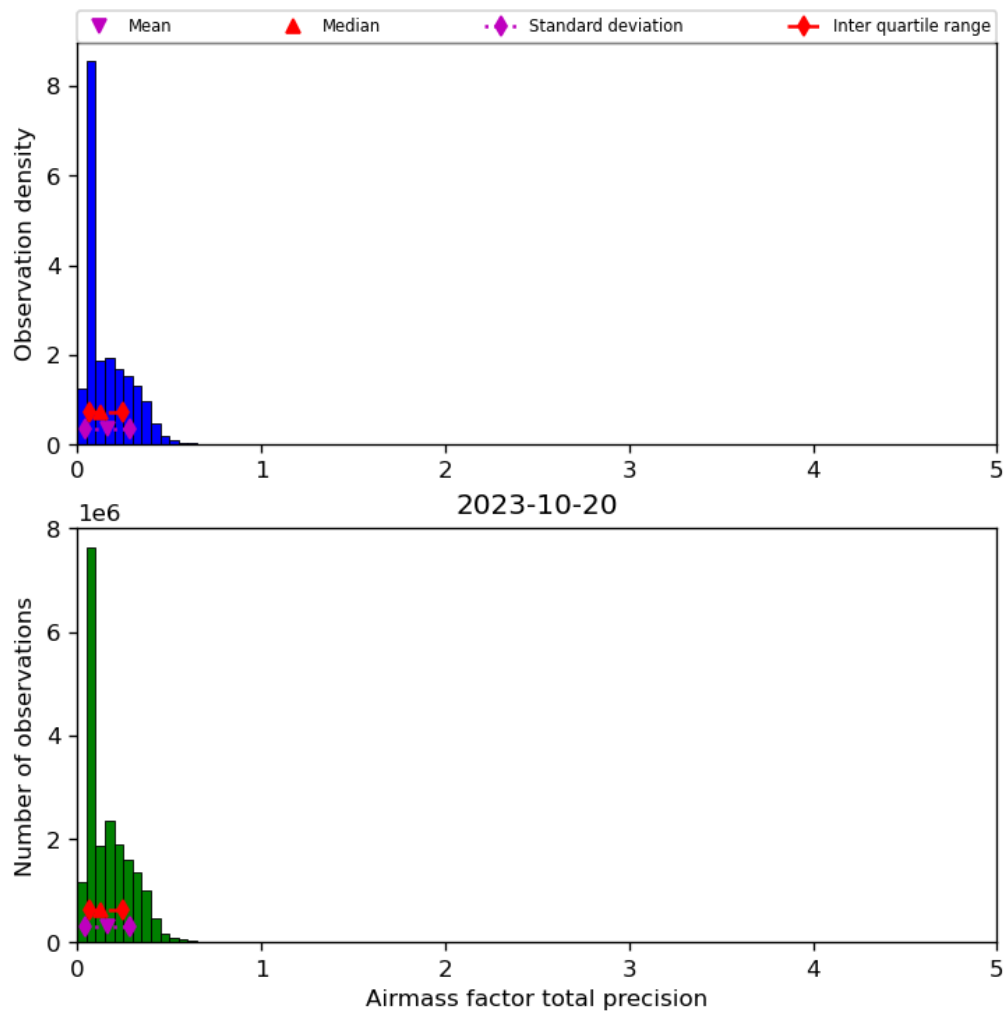
Figure 41: Histogram of “Airmass factor total precision” for 2023-10-19 to 2023-10-21
