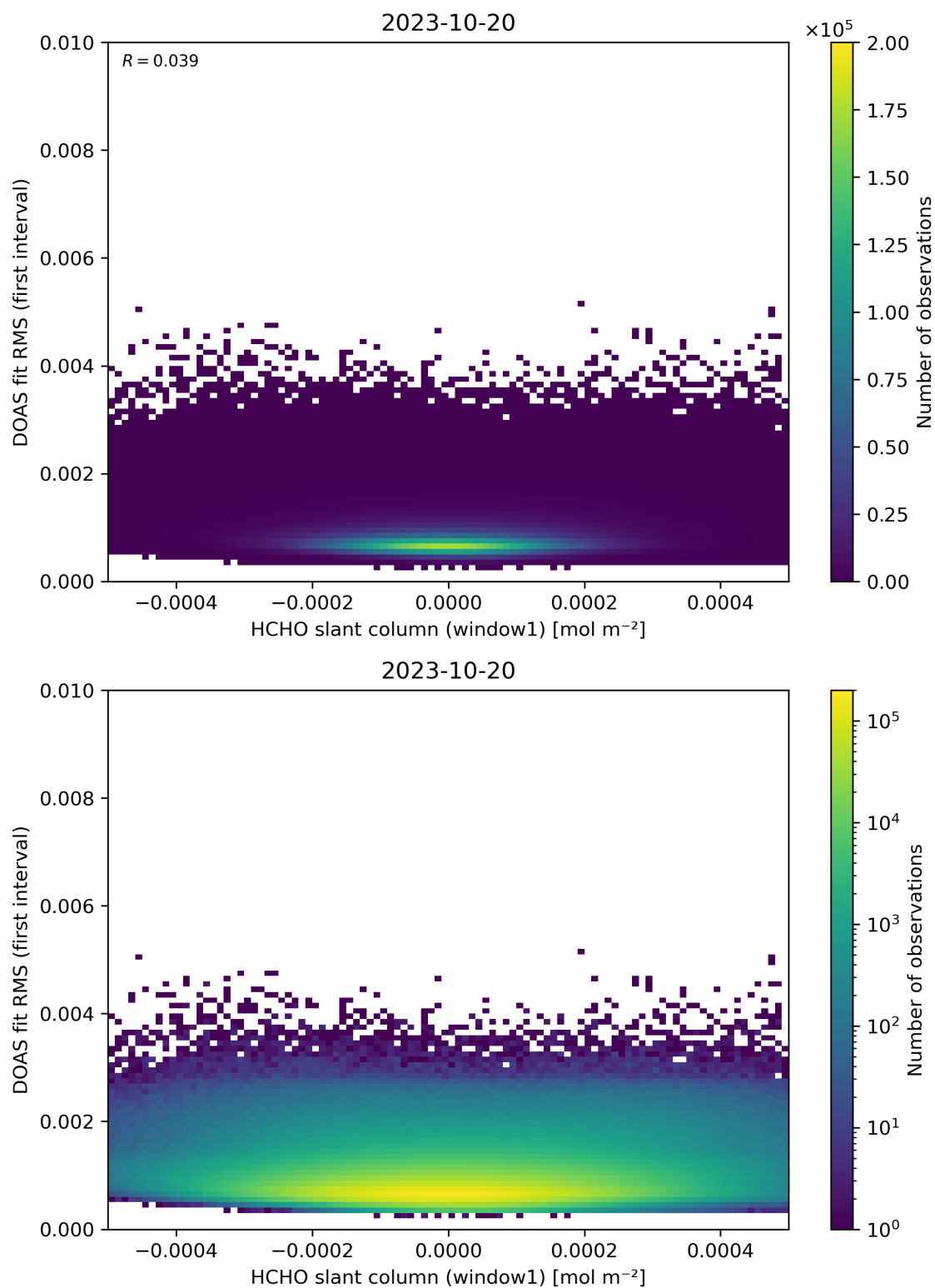
Figure 78: Scatter density plot of “HCHO slant column (window1)” against “DOAS fit RMS (first interval)” for 2023-10-19 to 2023-10-21.
