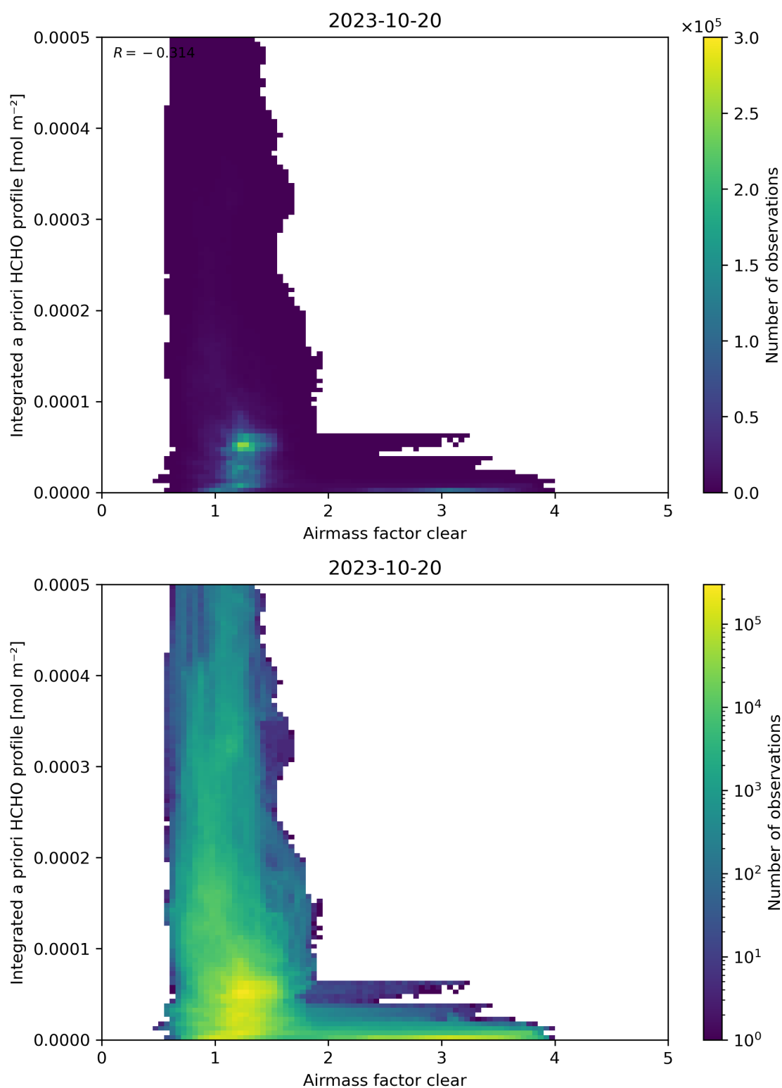
Figure 76: Scatter density plot of “Airmass factor clear” against “Integrated a priori HCHO profile” for 2023-10-19 to 2023-10-21.
