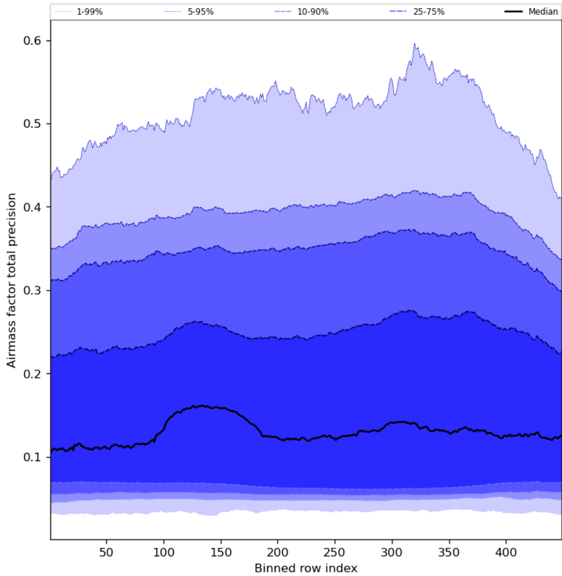
Figure 55: Along track statistics of “Airmass factor total precision” for 2023-10-19 to 2023-10-21
