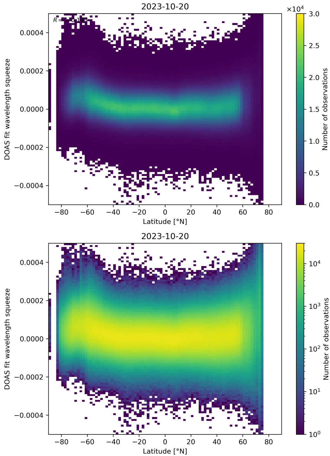
Figure 155: Scatter density plot of “Latitude” against “DOAS fit wavelength squeeze” for 2023-10-19 to 2023-10-21.
