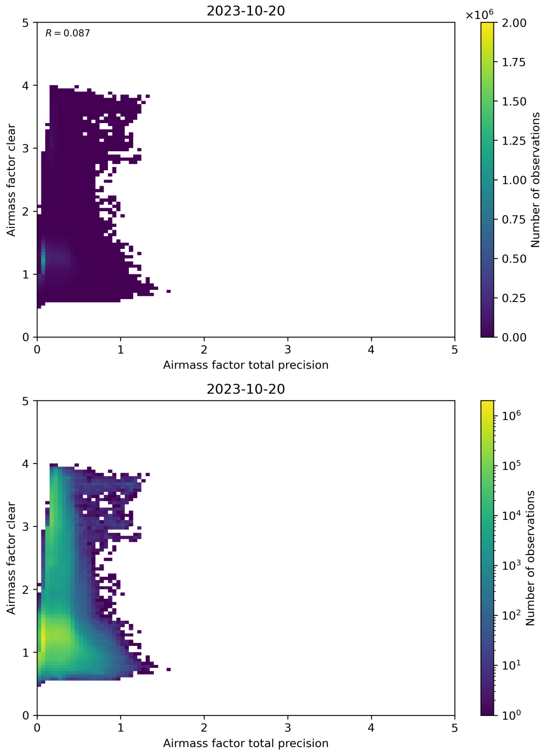
Figure 108: Scatter density plot of “Airmass factor total precision” against “Airmass factor clear” for 2023-10-19 to 2023-10-21.
