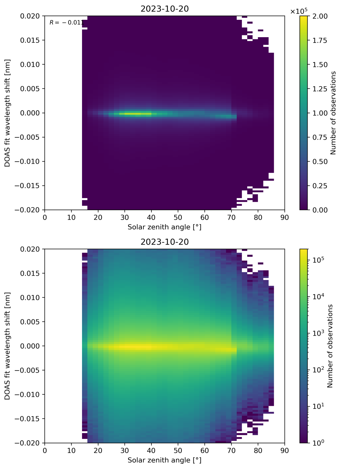
Figure 168: Scatter density plot of “Solar zenith angle” against “DOAS fit wavelength shift” for 2023-10-19 to 2023-10-21.
