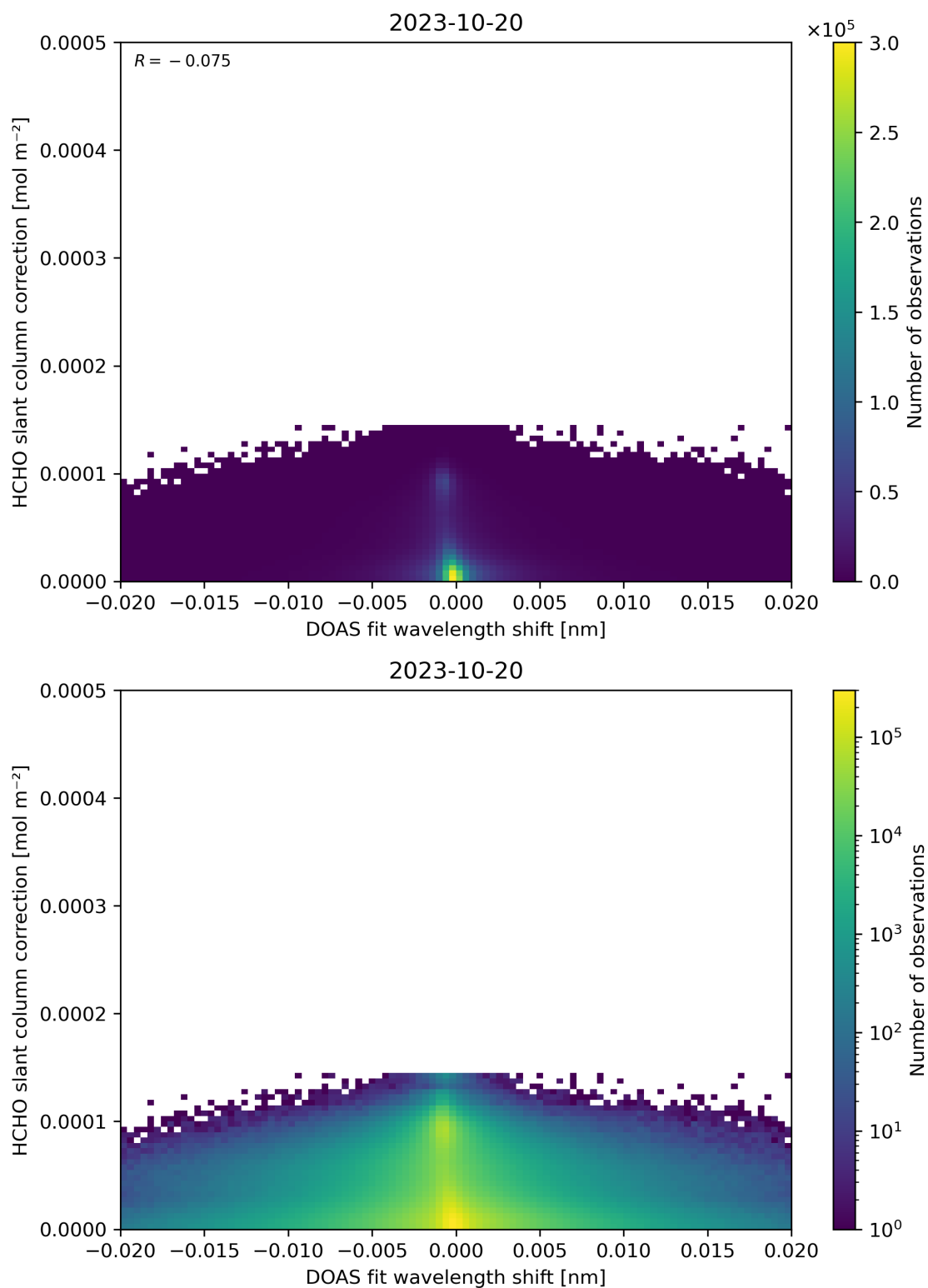
Figure 67: Scatter density plot of “DOAS fit wavelength shift” against “HCHO slant column correction” for 2023-10-19 to 2023-10-21.
