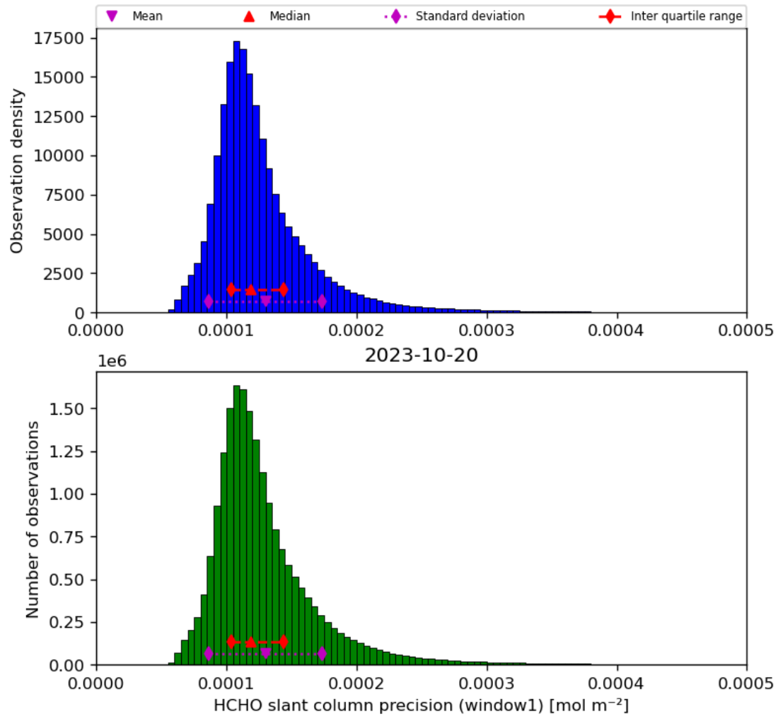
Figure 39: Histogram of “HCHO slant column precision (window1)” for 2023-10-19 to 2023-10-21
