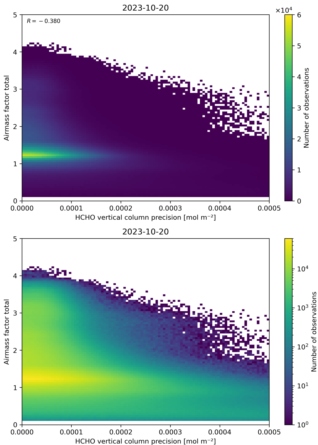
Figure 144: Scatter density plot of “HCHO vertical column precision” against “Airmass factor total” for 2023-10-19 to 2023-10-21.
