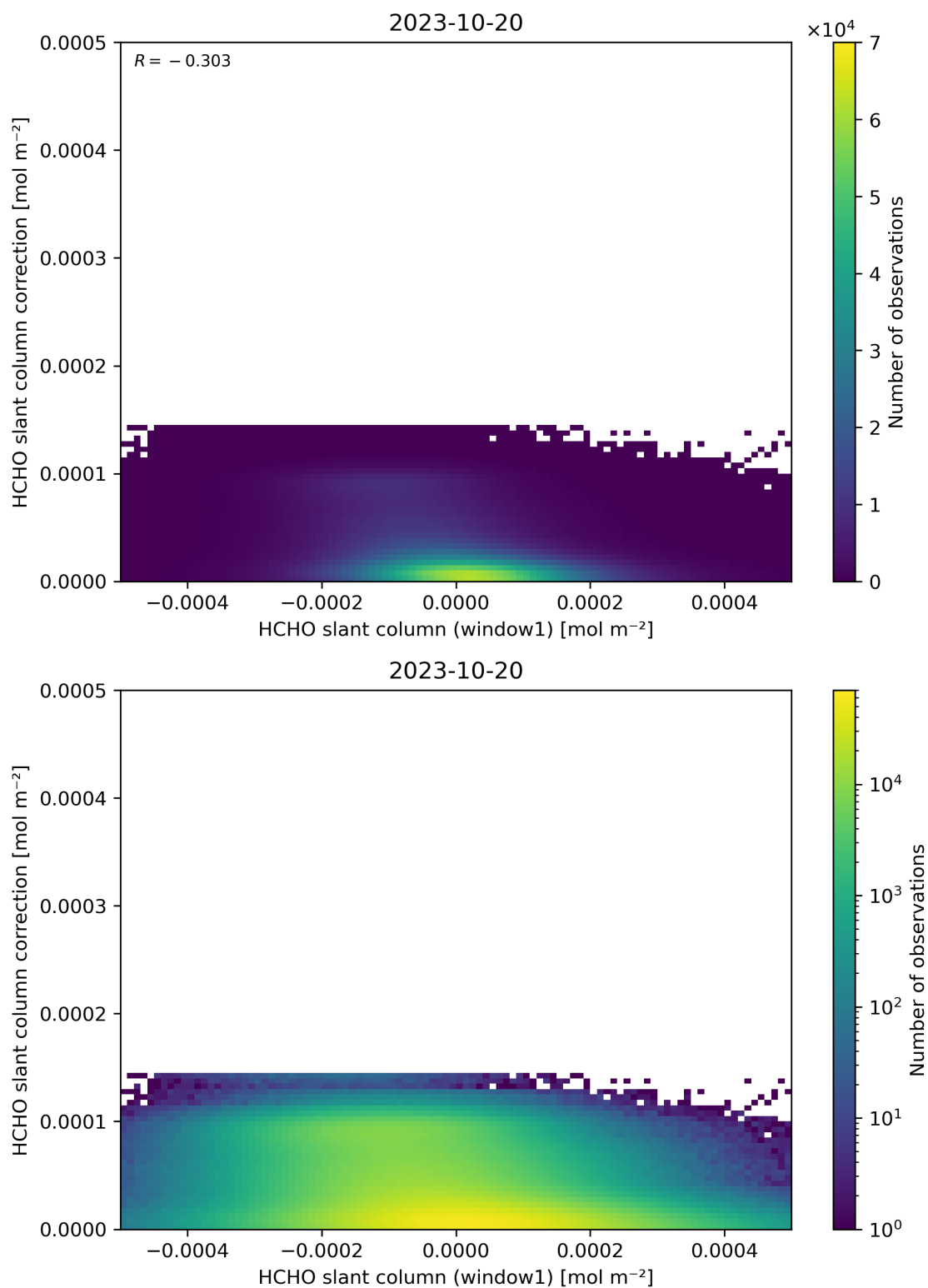
Figure 83: Scatter density plot of “HCHO slant column (window1)” against “HCHO slant column correction” for 2023-10-19 to 2023-10-21.
