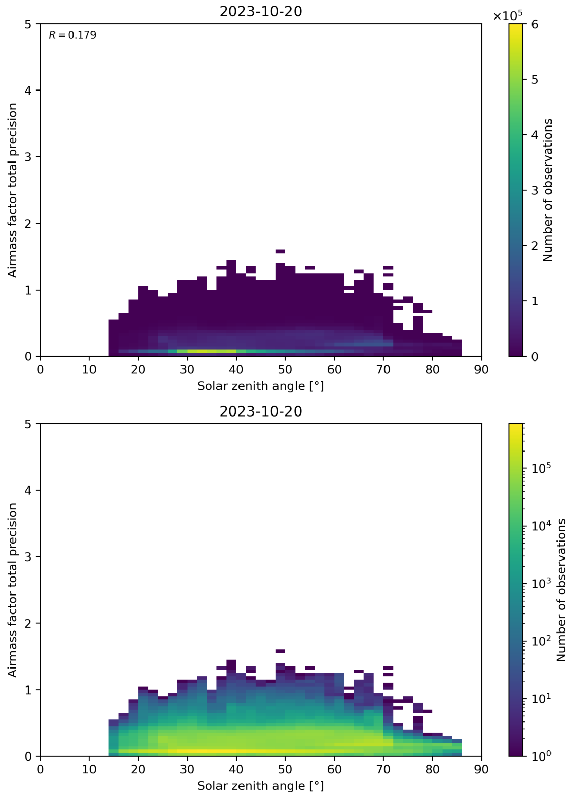
Figure 176: Scatter density plot of “Solar zenith angle” against “Airmass factor total precision” for 2023-10-19 to 2023-10-21.
