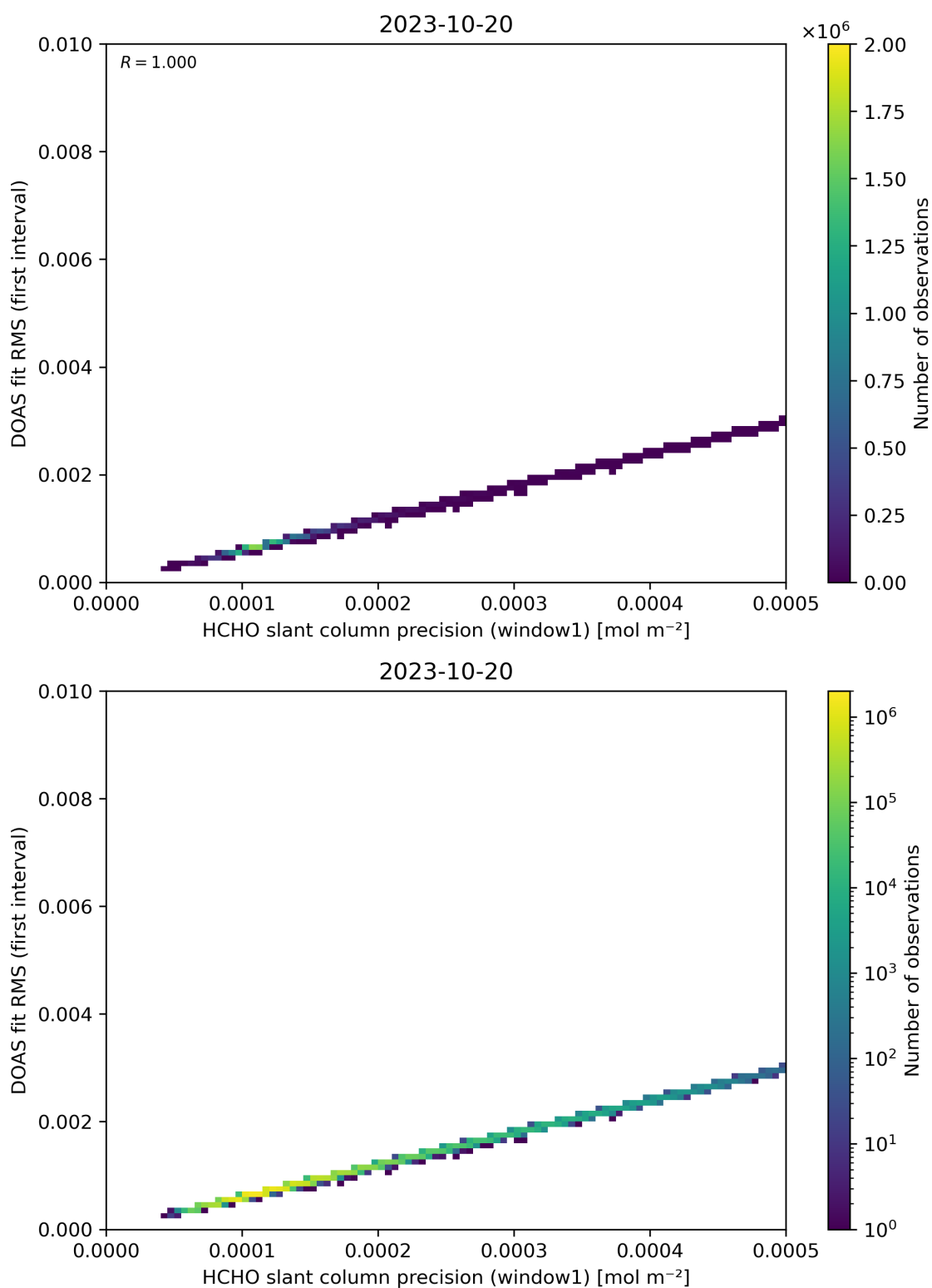
Figure 88: Scatter density plot of “HCHO slant column precision (window1)” against “DOAS fit RMS (first interval)” for 2023-10-19 to 2023-10-21.
