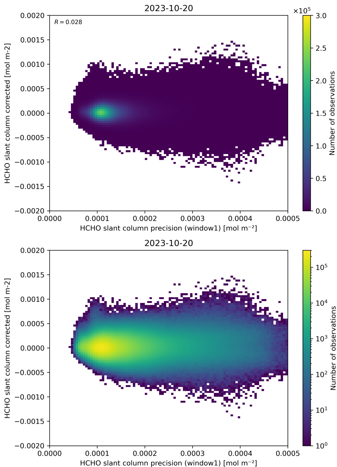
Figure 92: Scatter density plot of “HCHO slant column precision (window1)” against “HCHO slant column corrected” for 2023-10-19 to 2023-10-21.
