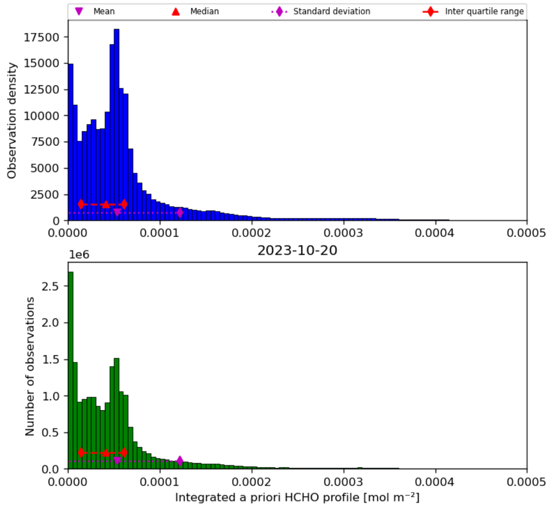
Figure 43: Histogram of “Integrated a priori HCHO profile” for 2023-10-19 to 2023-10-21
