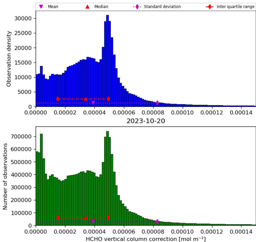
Figure 37: Histogram of “HCHO vertical column correction” for 2023-10-19 to 2023-10-21
