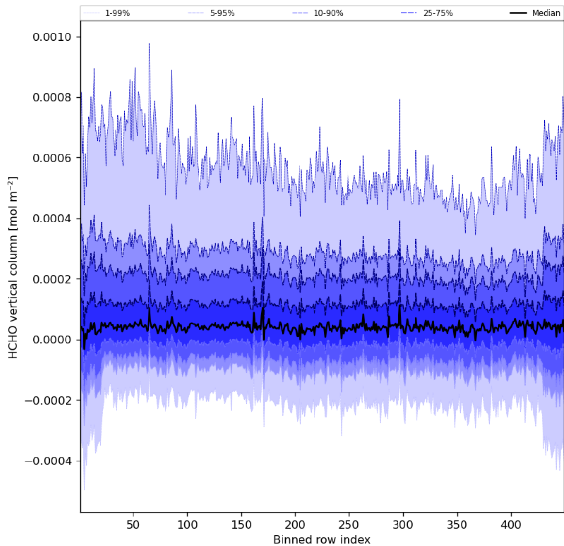
Figure 49: Along track statistics of “HCHO vertical column” for 2023-10-19 to 2023-10-21
