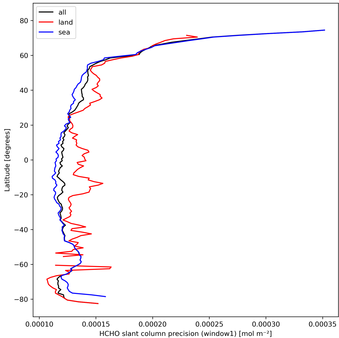
Figure 25: Zonal average of “HCHO slant column precision (window1)” for 2023-10-19 to 2023-10-21.
