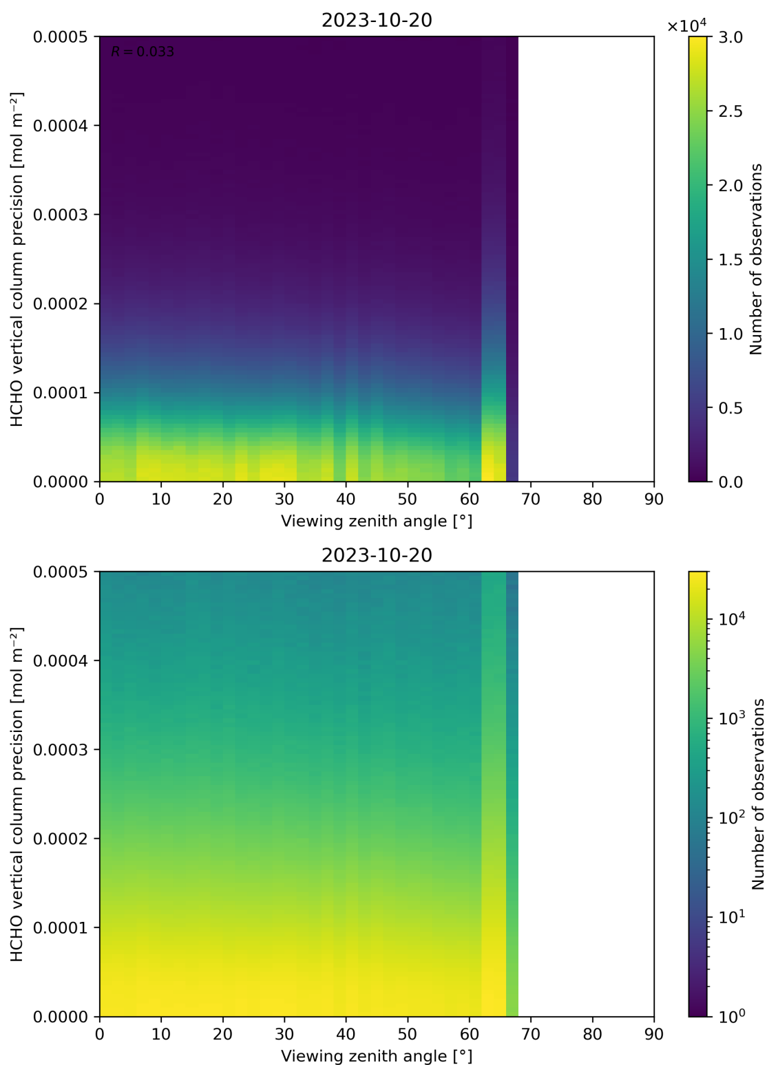
Figure 194: Scatter density plot of “Viewing zenith angle” against “HCHO vertical column precision” for 2023-10-19 to 2023-10-21.
