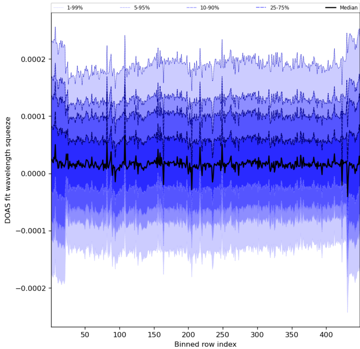
Figure 59: Along track statistics of “DOAS fit wavelength squeeze” for 2023-10-19 to 2023-10-21
