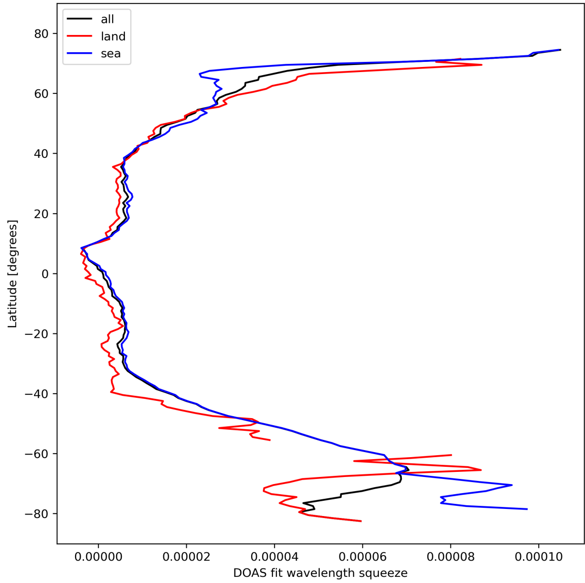
Figure 31: Zonal average of “DOAS fit wavelength squeeze” for 2023-10-19 to 2023-10-21.
