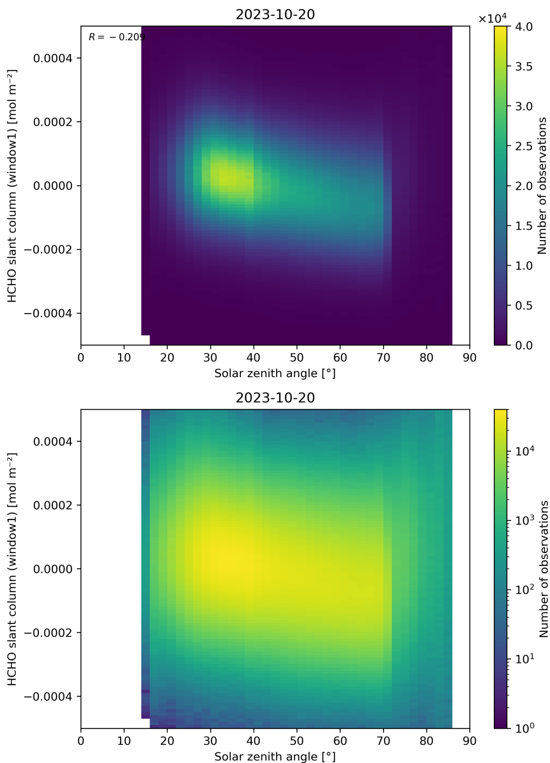
Figure 173: Scatter density plot of “Solar zenith angle” against “HCHO slant column (window1)” for 2023-10-19 to 2023-10-21.
