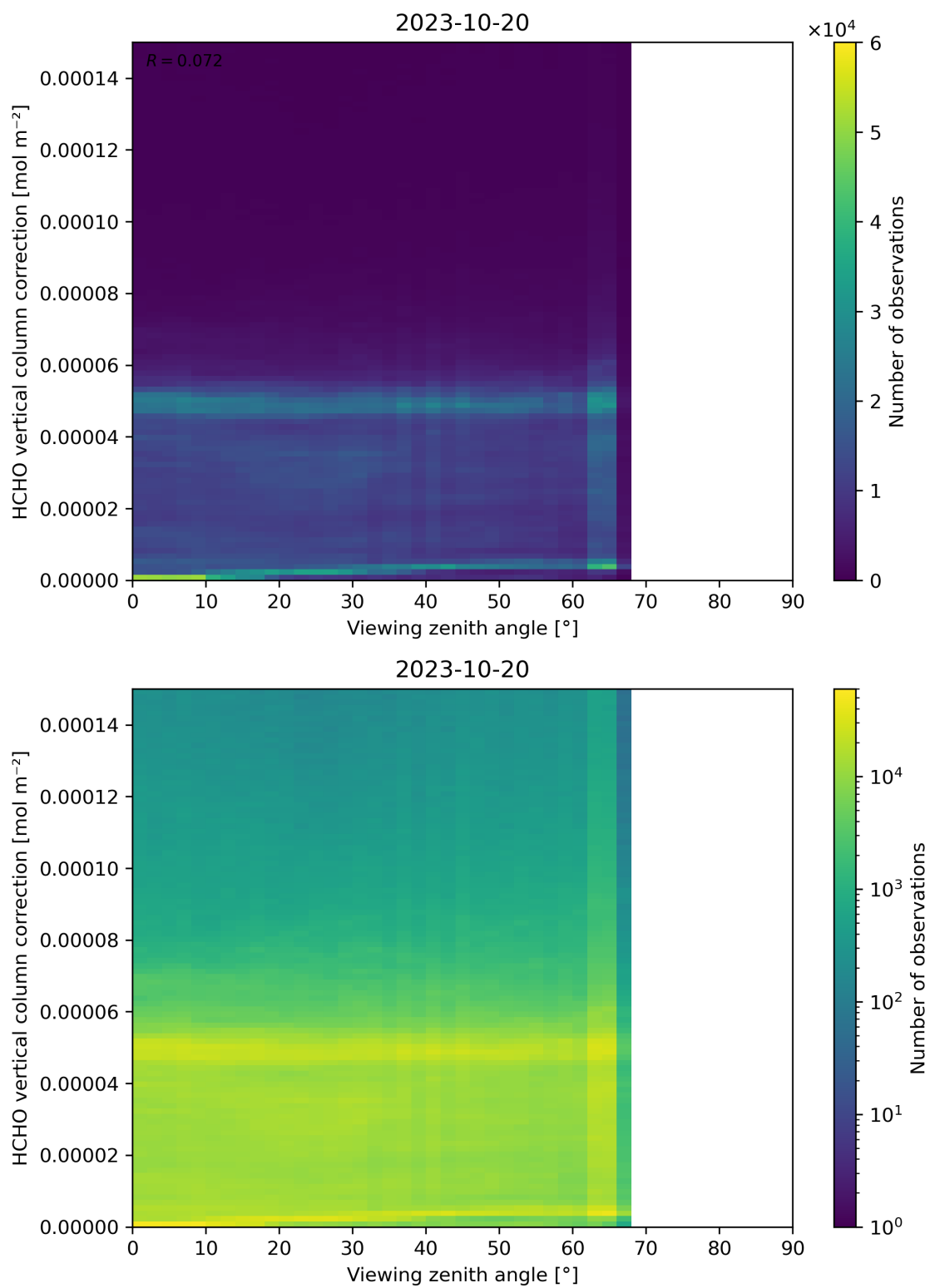
Figure 193: Scatter density plot of “Viewing zenith angle” against “HCHO vertical column correction” for 2023-10-19 to 2023-10-21.
