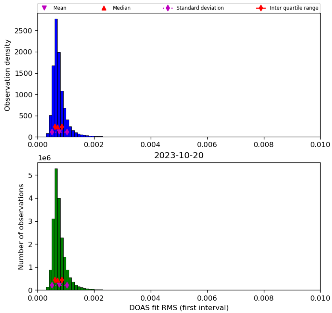
Figure 46: Histogram of “DOAS fit RMS (first interval)” for 2023-10-19 to 2023-10-21
