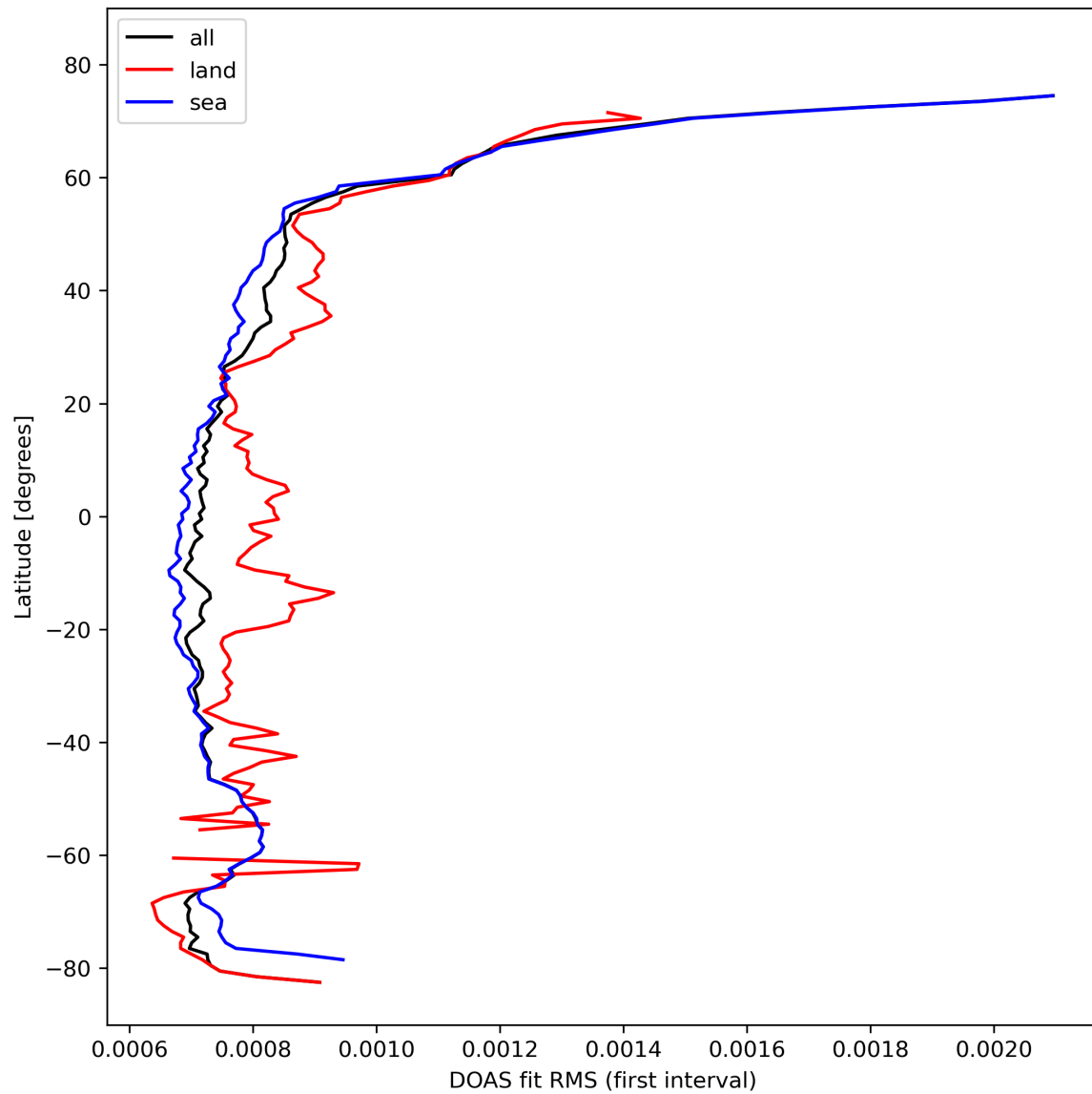
Figure 32: Zonal average of “DOAS fit RMS (first interval)” for 2023-10-19 to 2023-10-21.
