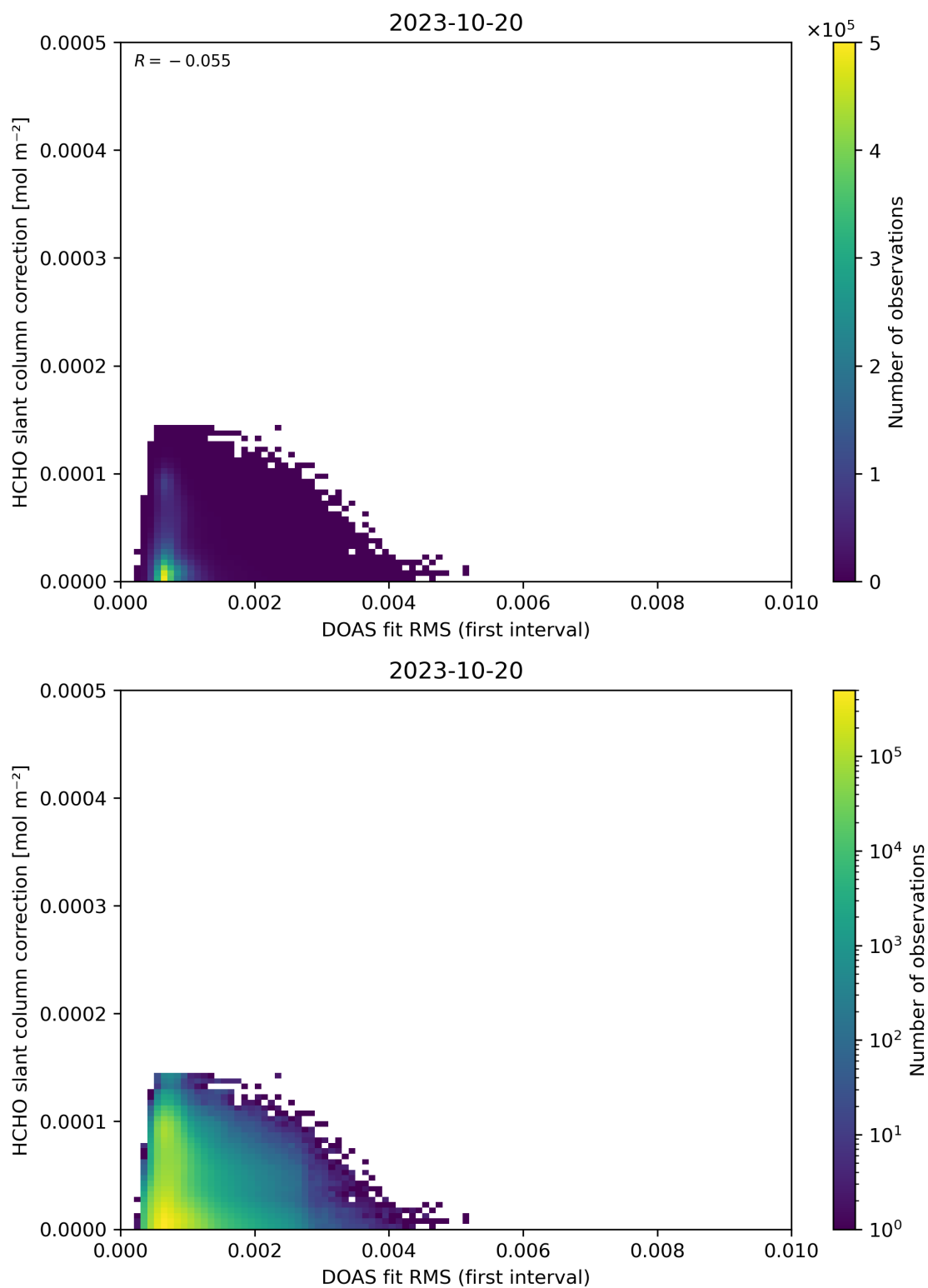
Figure 63: Scatter density plot of “DOAS fit RMS (first interval)” against “HCHO slant column correction” for 2023-10-19 to 2023-10-21.
