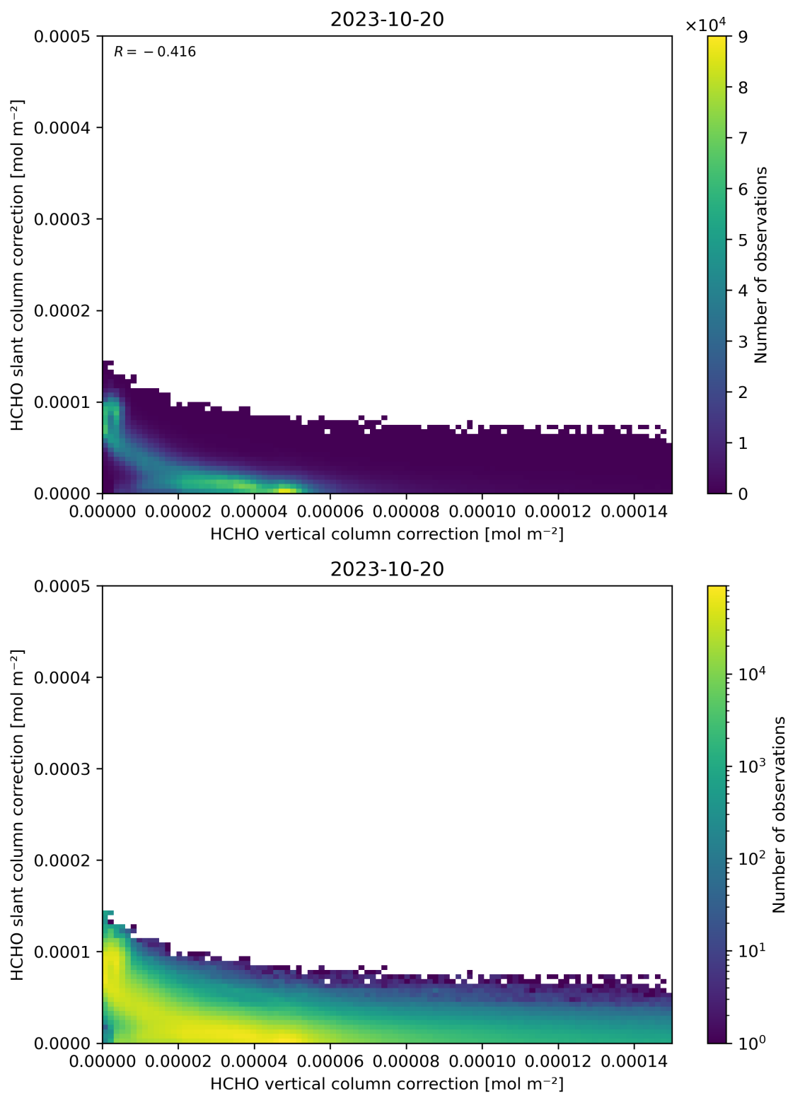
Figure 117: Scatter density plot of “HCHO vertical column correction” against “HCHO slant column correction” for 2023-10-19 to 2023-10-21.
