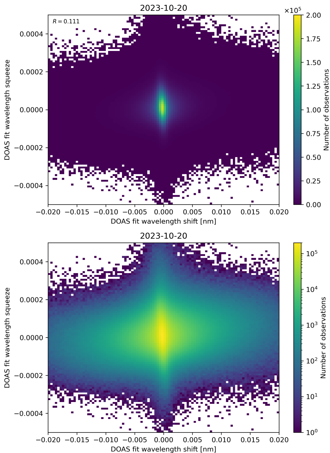
Figure 65: Scatter density plot of “DOAS fit wavelength shift” against “DOAS fit wavelength squeeze” for 2023-10-19 to 2023-10-21.
