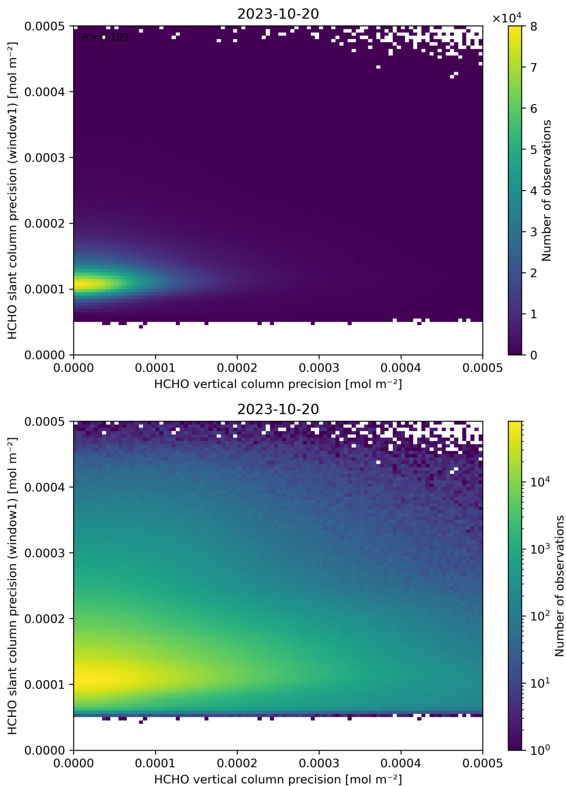
Figure 143: Scatter density plot of “HCHO vertical column precision” against “HCHO slant column precision (window1)” for 2023-10-19 to 2023-10-21.
