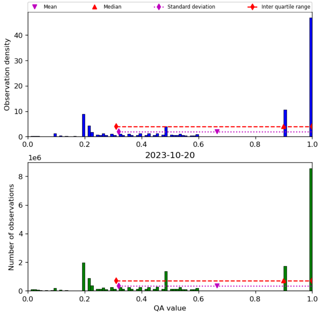
Figure 34: Histogram of “QA value” for 2023-10-19 to 2023-10-21
