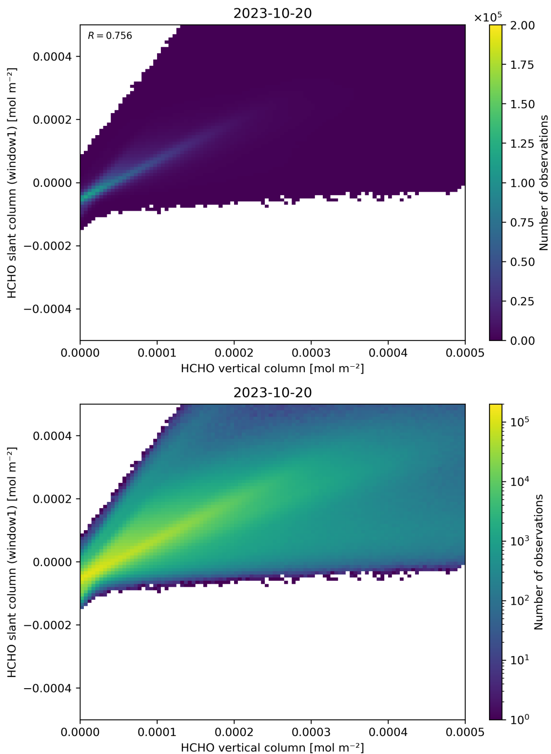
Figure 129: Scatter density plot of “HCHO vertical column” against “HCHO slant column (window1)” for 2023-10-19 to 2023-10-21.
