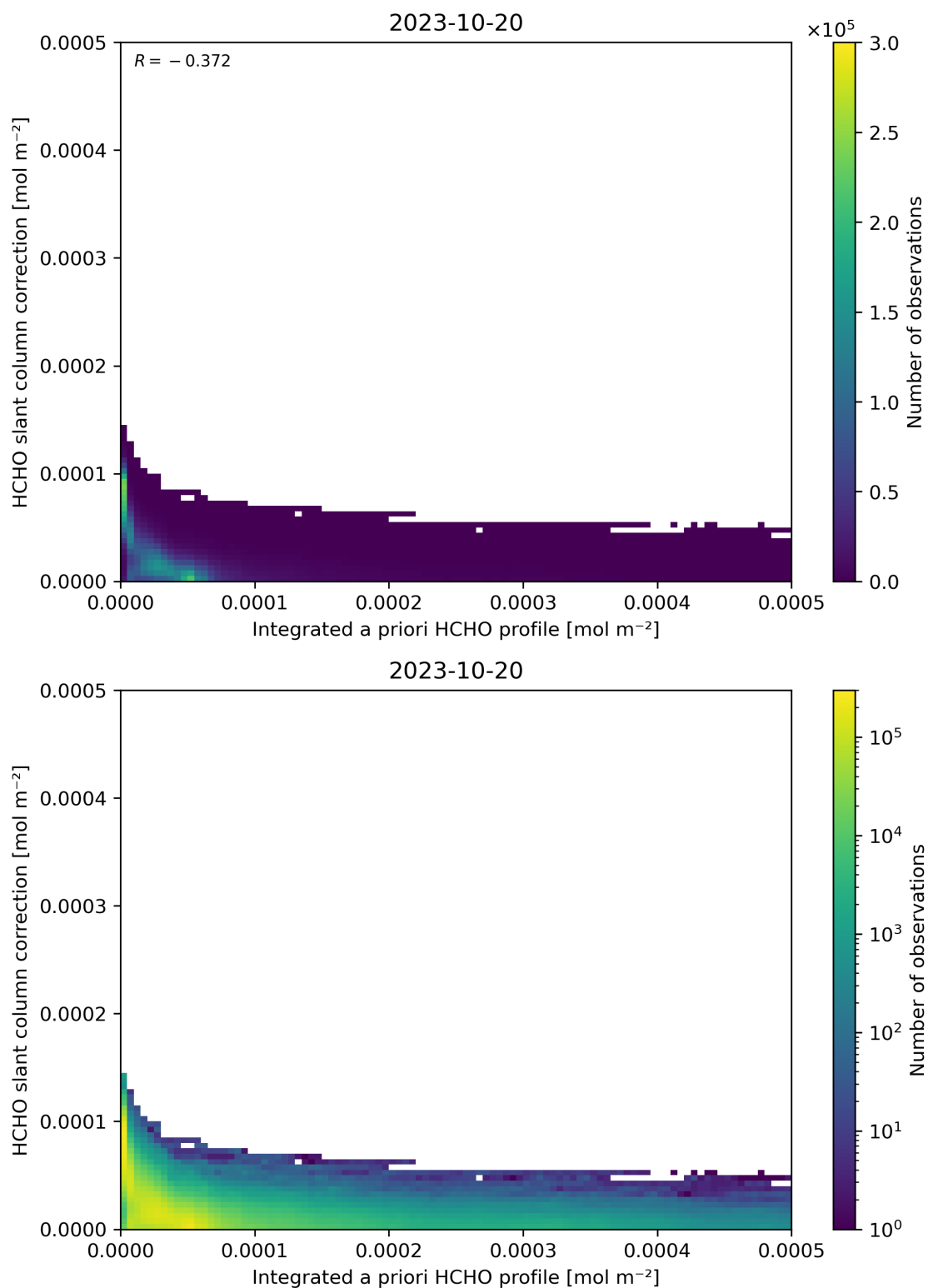
Figure 152: Scatter density plot of “Integrated a priori HCHO profile” against “HCHO slant column correction” for 2023-10-19 to 2023-10-21.
