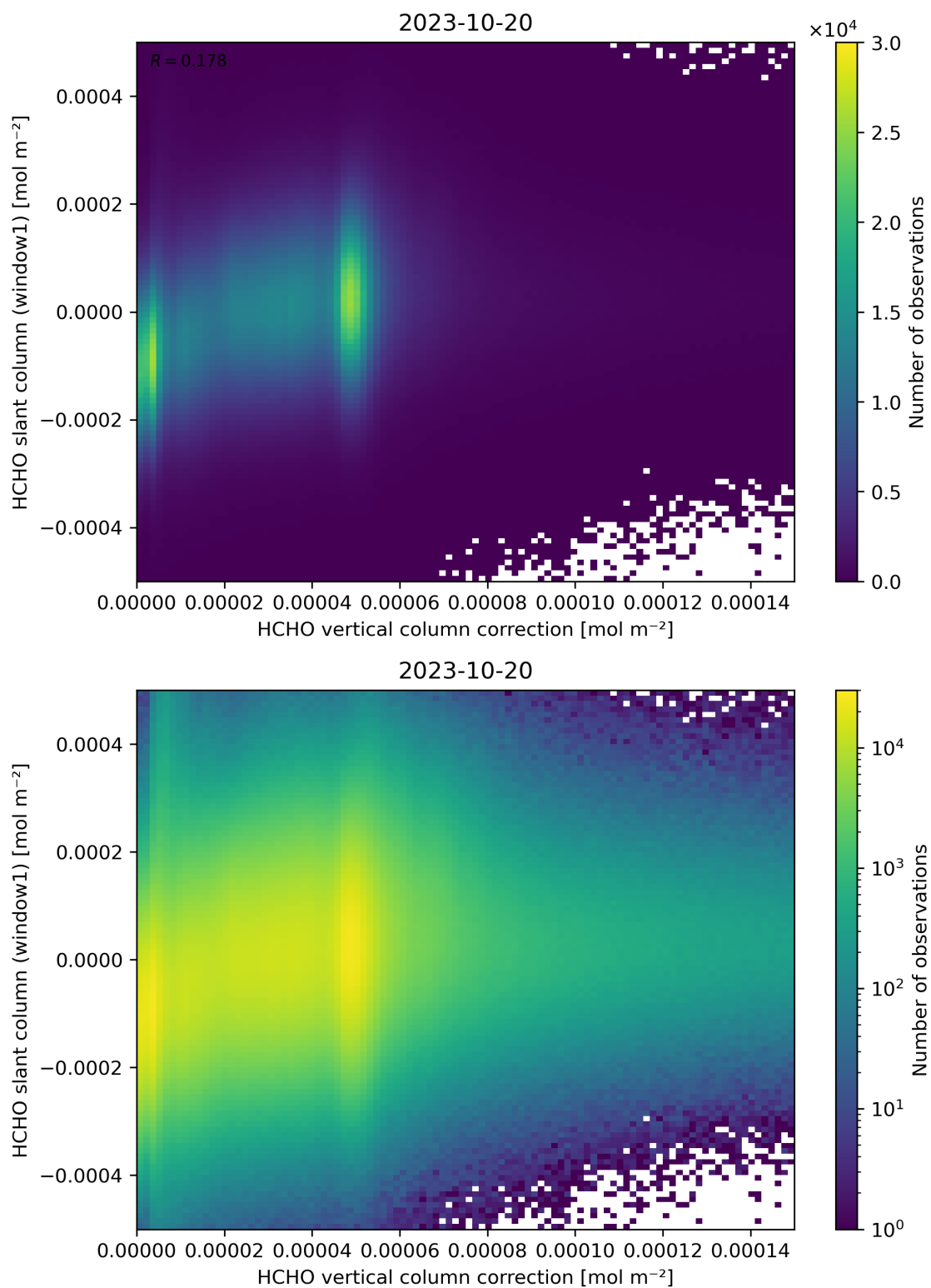
Figure 118: Scatter density plot of “HCHO vertical column correction” against “HCHO slant column (window1)” for 2023-10-19 to 2023-10-21.
