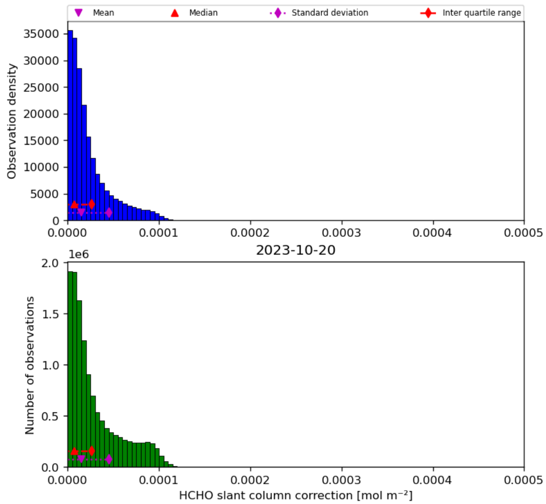
Figure 47: Histogram of “HCHO slant column correction” for 2023-10-19 to 2023-10-21
