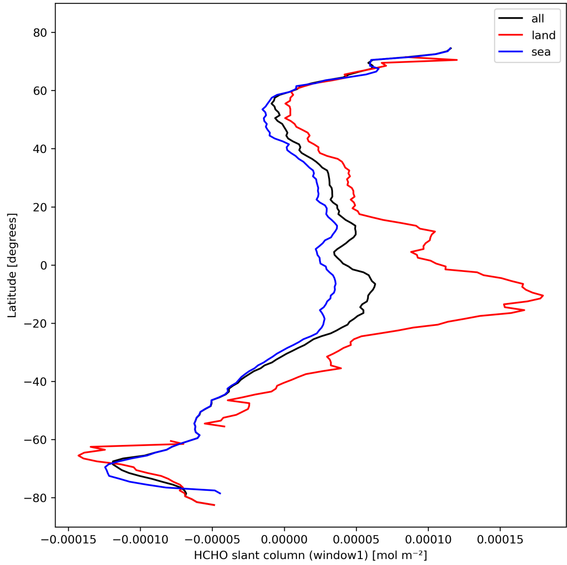
Figure 24: Zonal average of “HCHO slant column (window1)” for 2023-10-19 to 2023-10-21.
