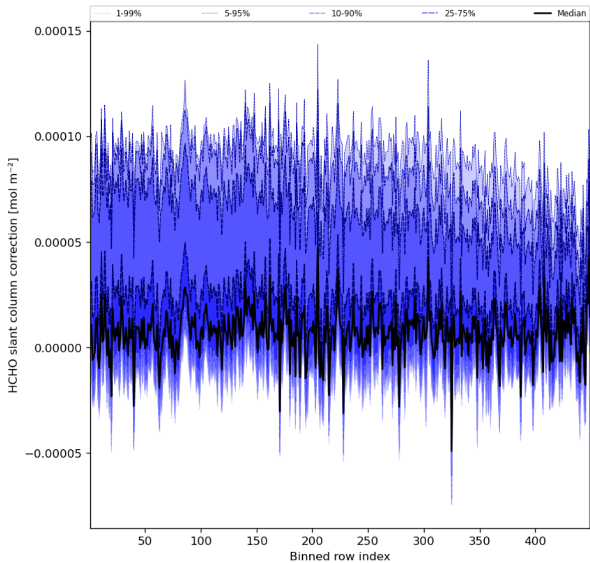
Figure 61: Along track statistics of “HCHO slant column correction” for 2023-10-19 to 2023-10-21
