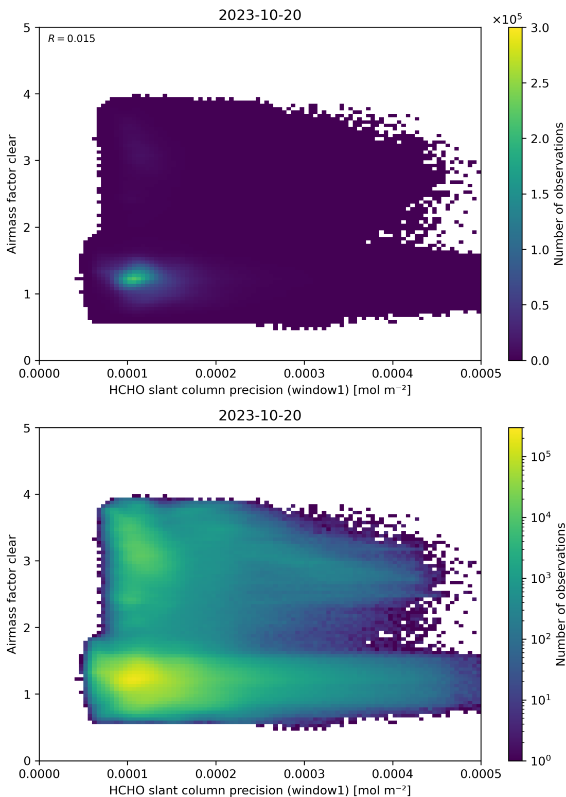
Figure 91: Scatter density plot of “HCHO slant column precision (window1)” against “Airmass factor clear” for 2023-10-19 to 2023-10-21.
