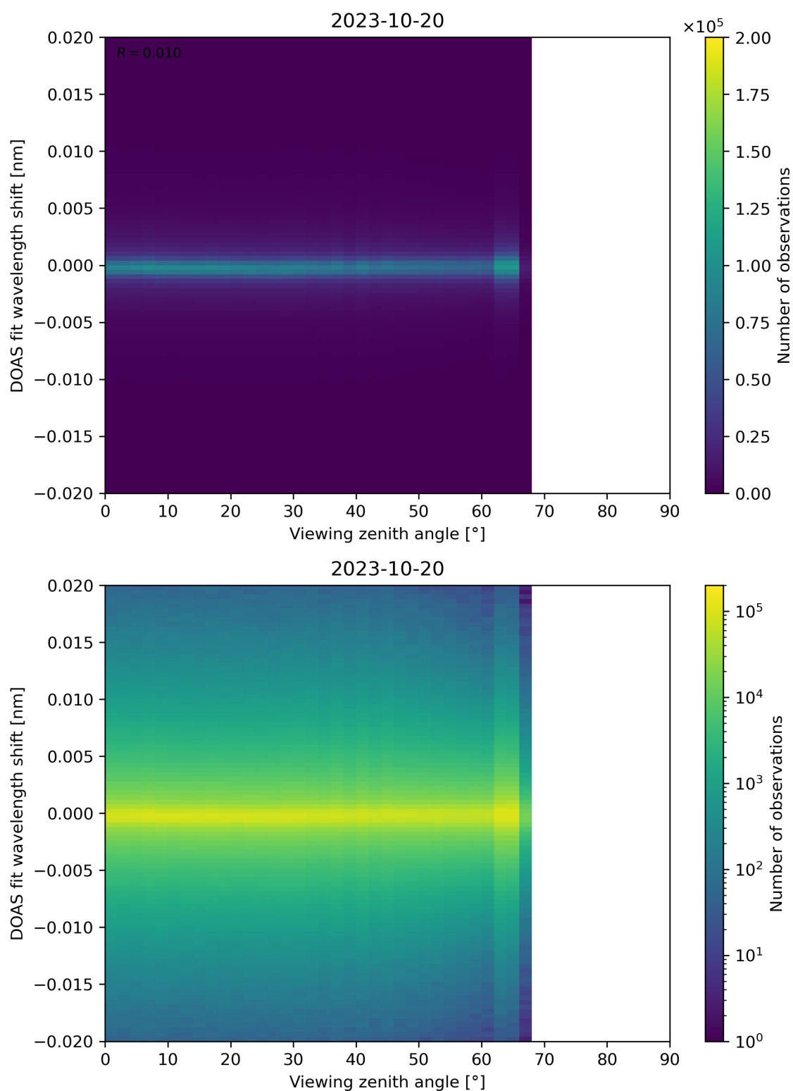
Figure 183: Scatter density plot of “Viewing zenith angle” against “DOAS fit wavelength shift” for 2023-10-19 to 2023-10-21.
