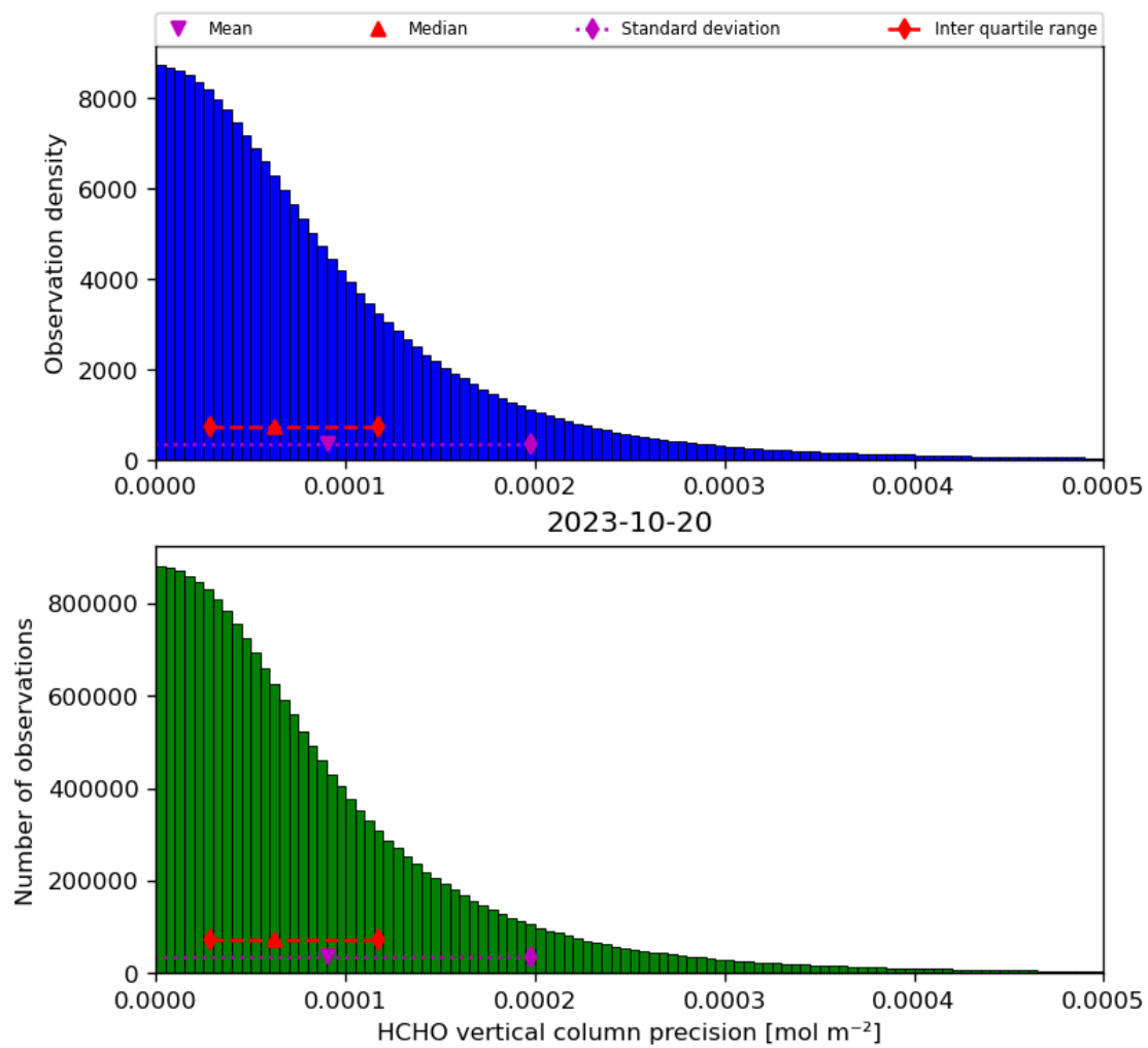
Figure 36: Histogram of “HCHO vertical column precision” for 2023-10-19 to 2023-10-21
