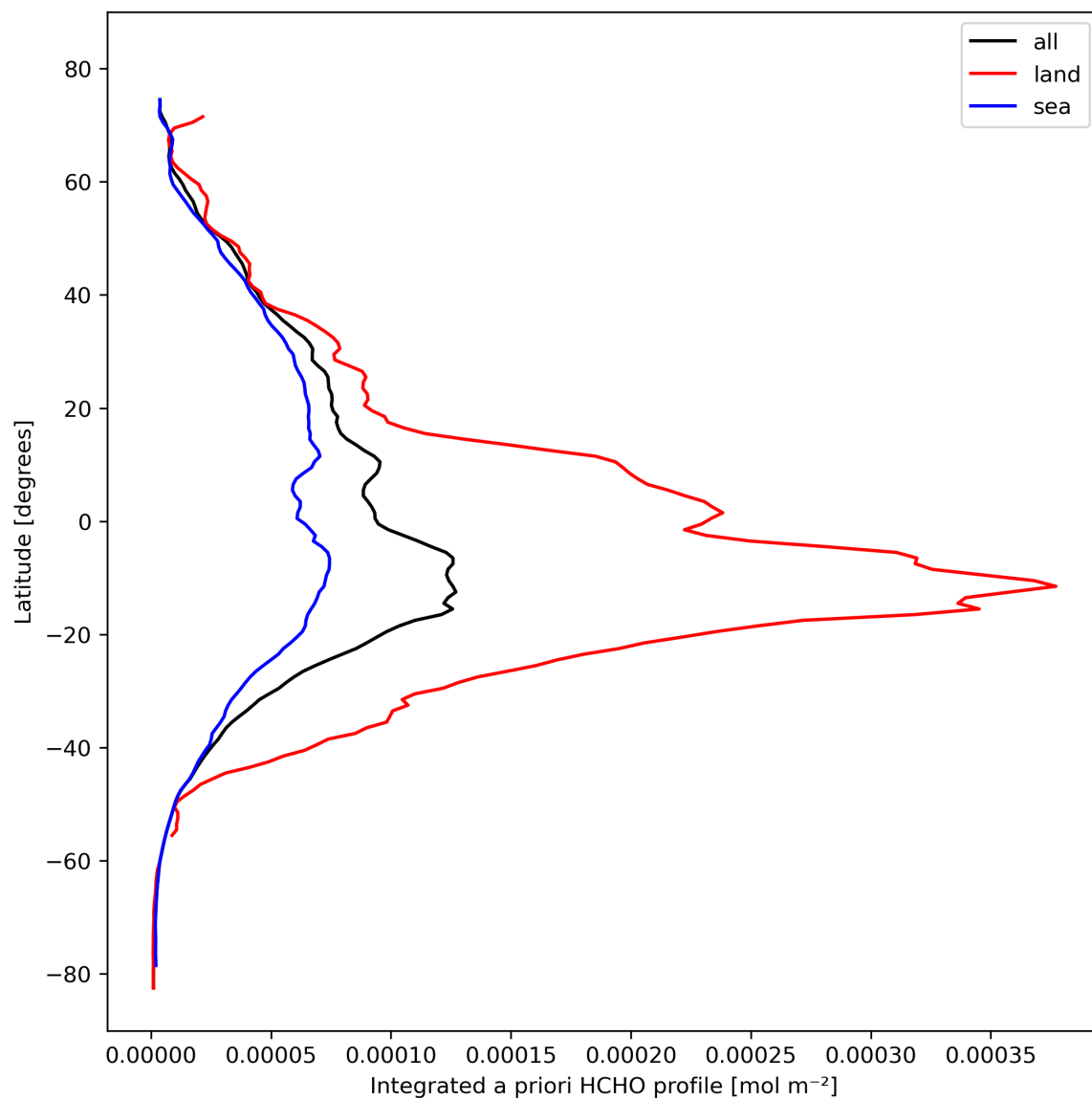
Figure 29: Zonal average of “Integrated a priori HCHO profile” for 2023-10-19 to 2023-10-21.
