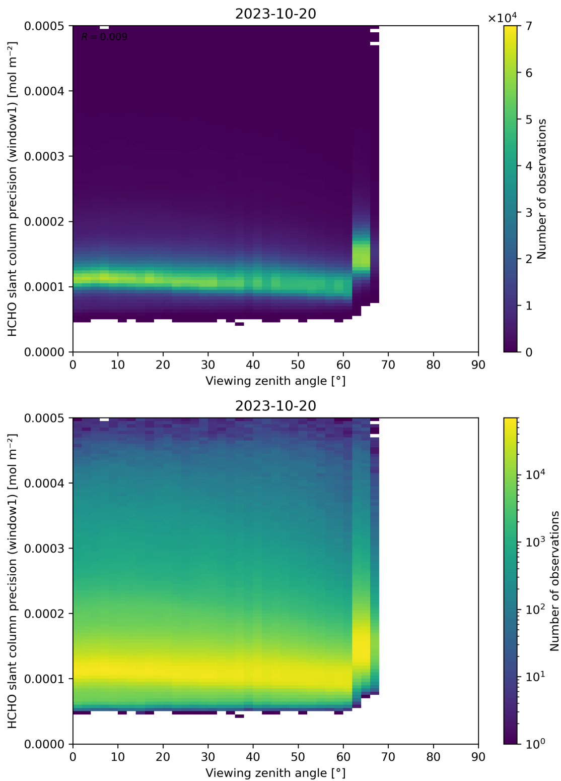
Figure 189: Scatter density plot of “Viewing zenith angle” against “HCHO slant column precision (window1)” for 2023-10-19 to 2023-10-21.
