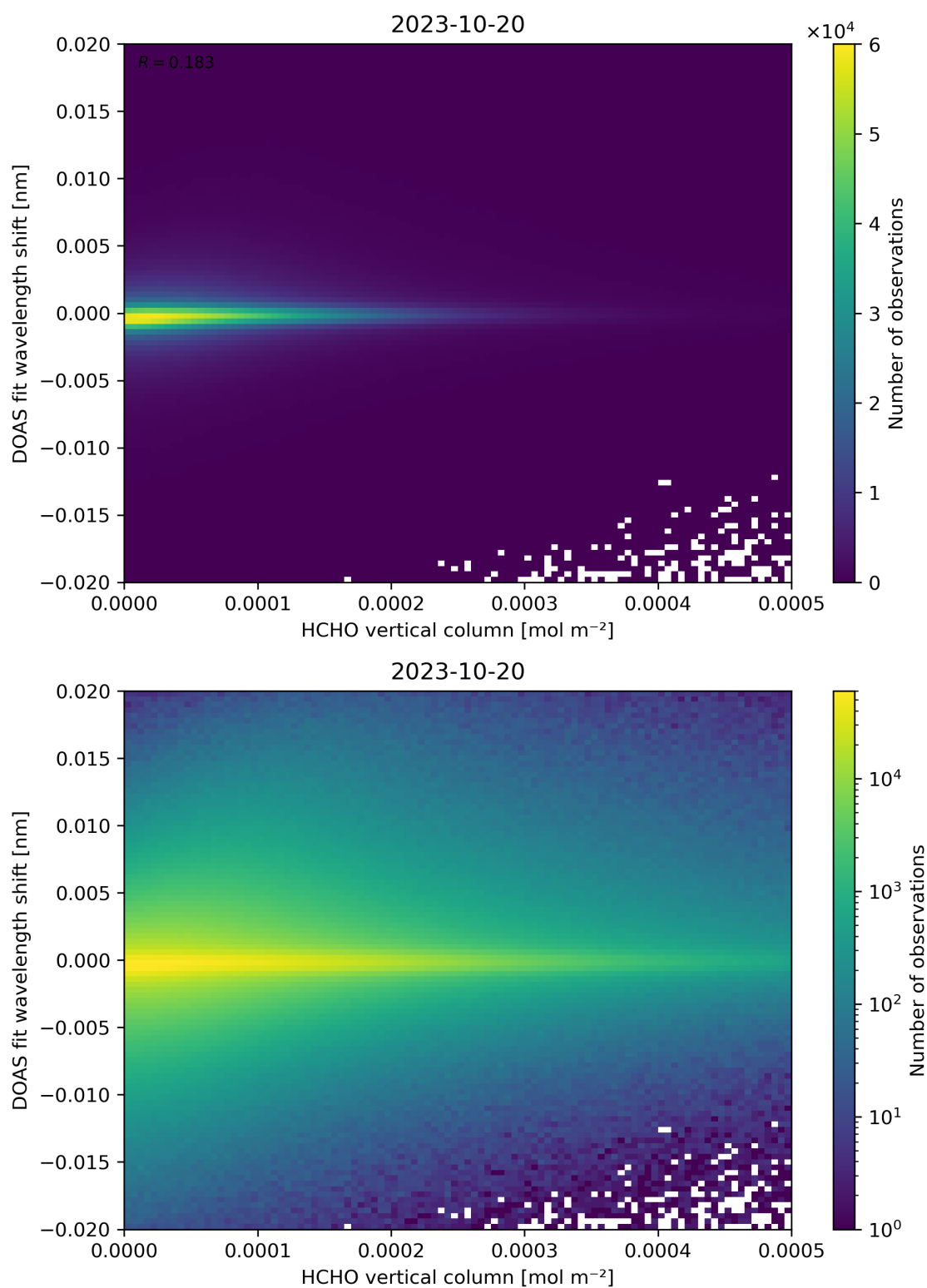
Figure 124: Scatter density plot of “HCHO vertical column” against “DOAS fit wavelength shift” for 2023-10-19 to 2023-10-21.
