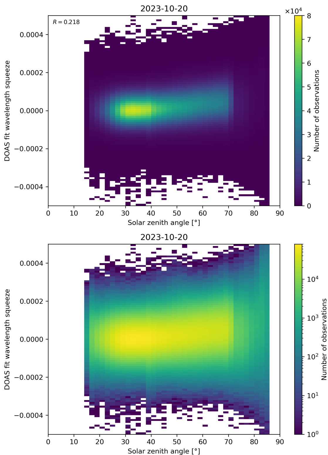
Figure 169: Scatter density plot of “Solar zenith angle” against “DOAS fit wavelength squeeze” for 2023-10-19 to 2023-10-21.
