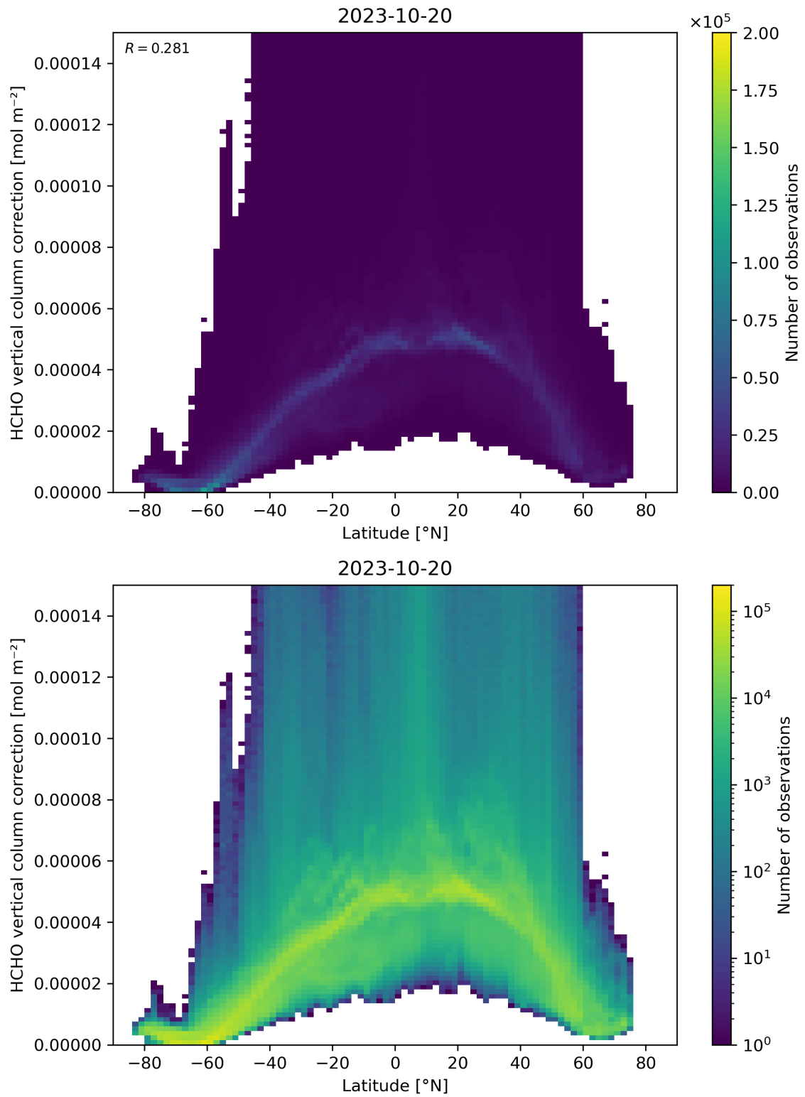
Figure 164: Scatter density plot of “Latitude” against “HCHO vertical column correction” for 2023-10-19 to 2023-10-21.
