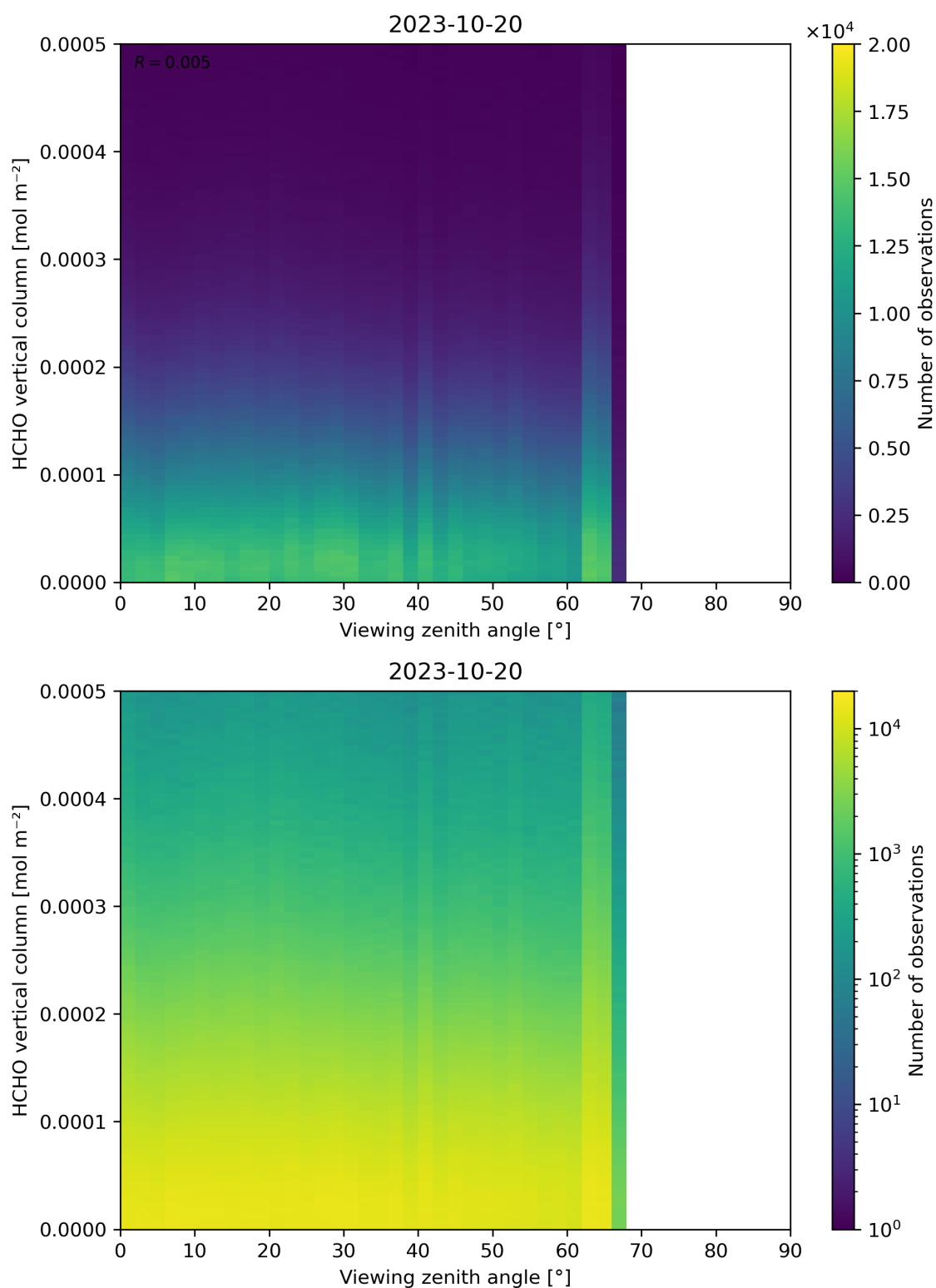
Figure 192: Scatter density plot of “Viewing zenith angle” against “HCHO vertical column” for 2023-10-19 to 2023-10-21.
