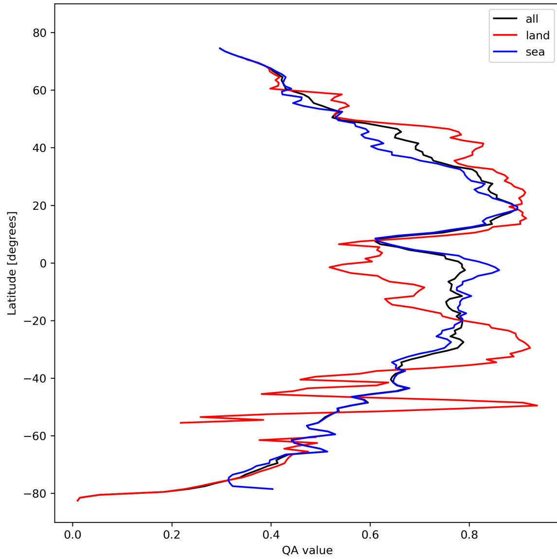
Figure 20: Zonal average of “QA value” for 2023-10-19 to 2023-10-21.
