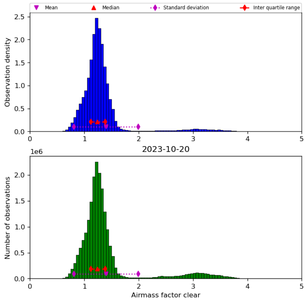
Figure 42: Histogram of “Airmass factor clear” for 2023-10-19 to 2023-10-21
