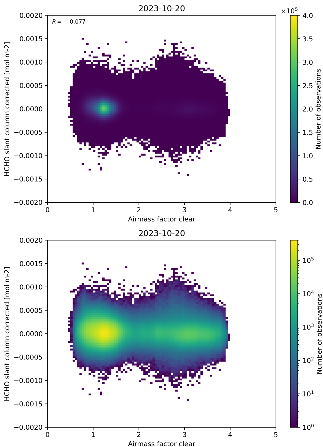
Figure 74: Scatter density plot of “Airmass factor clear” against “HCHO slant column corrected” for 2023-10-19 to 2023-10-21.
