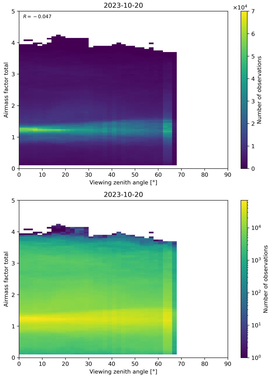
Figure 190: Scatter density plot of “Viewing zenith angle” against “Airmass factor total” for 2023-10-19 to 2023-10-21.
