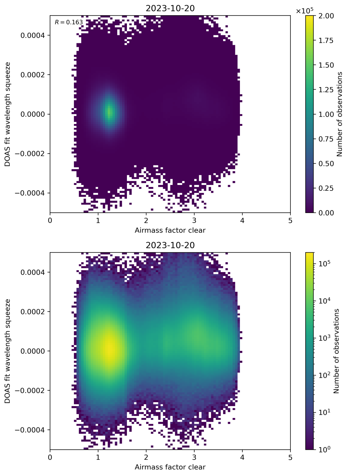
Figure 73: Scatter density plot of “Airmass factor clear” against “DOAS fit wavelength squeeze” for 2023-10-19 to 2023-10-21.
