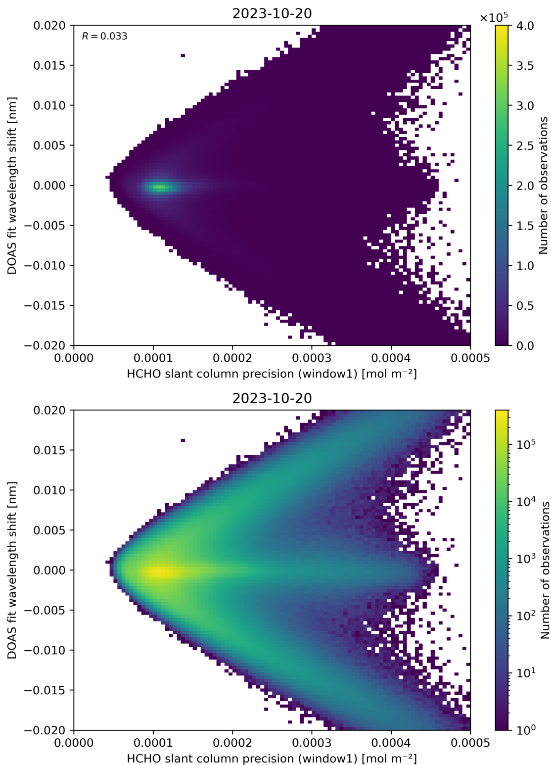
Figure 89: Scatter density plot of “HCHO slant column precision (window1)” against “DOAS fit wavelength shift” for 2023-10-19 to 2023-10-21.
