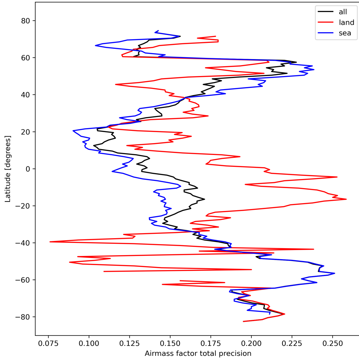
Figure 27: Zonal average of “Airmass factor total precision” for 2023-10-19 to 2023-10-21.
