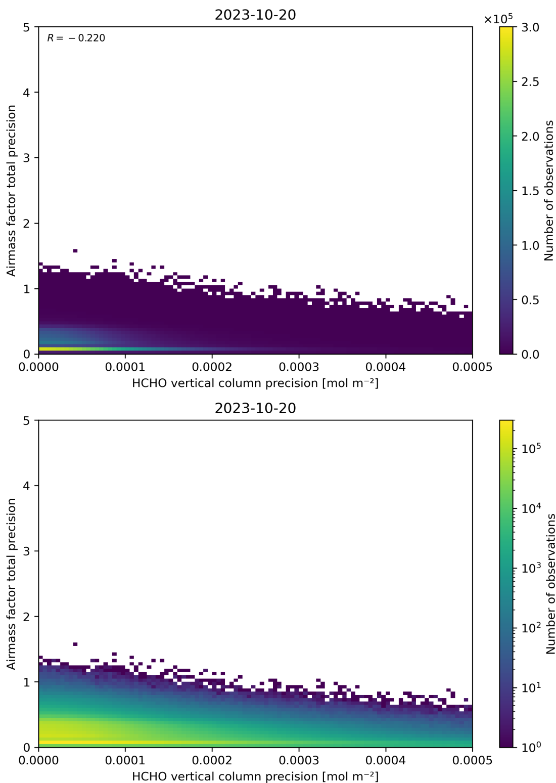
Figure 145: Scatter density plot of “HCHO vertical column precision” against “Airmass factor total precision” for 2023-10-19 to 2023-10-21.
