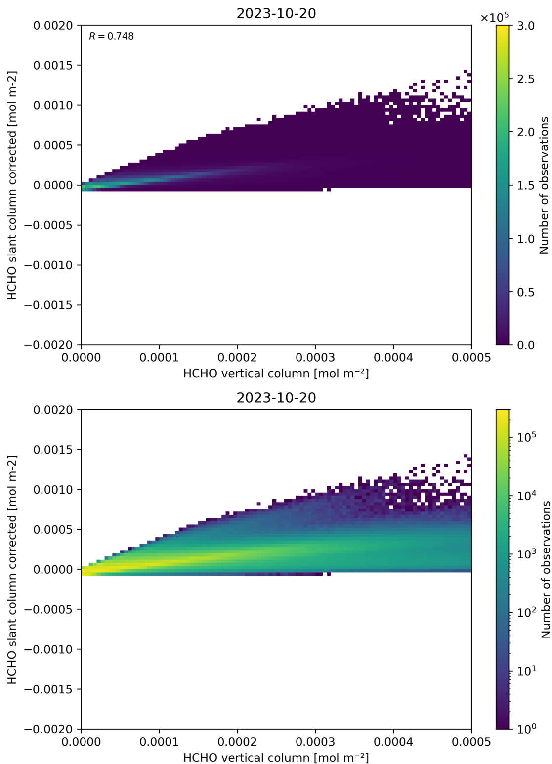
Figure 127: Scatter density plot of “HCHO vertical column” against “HCHO slant column corrected” for 2023-10-19 to 2023-10-21.
