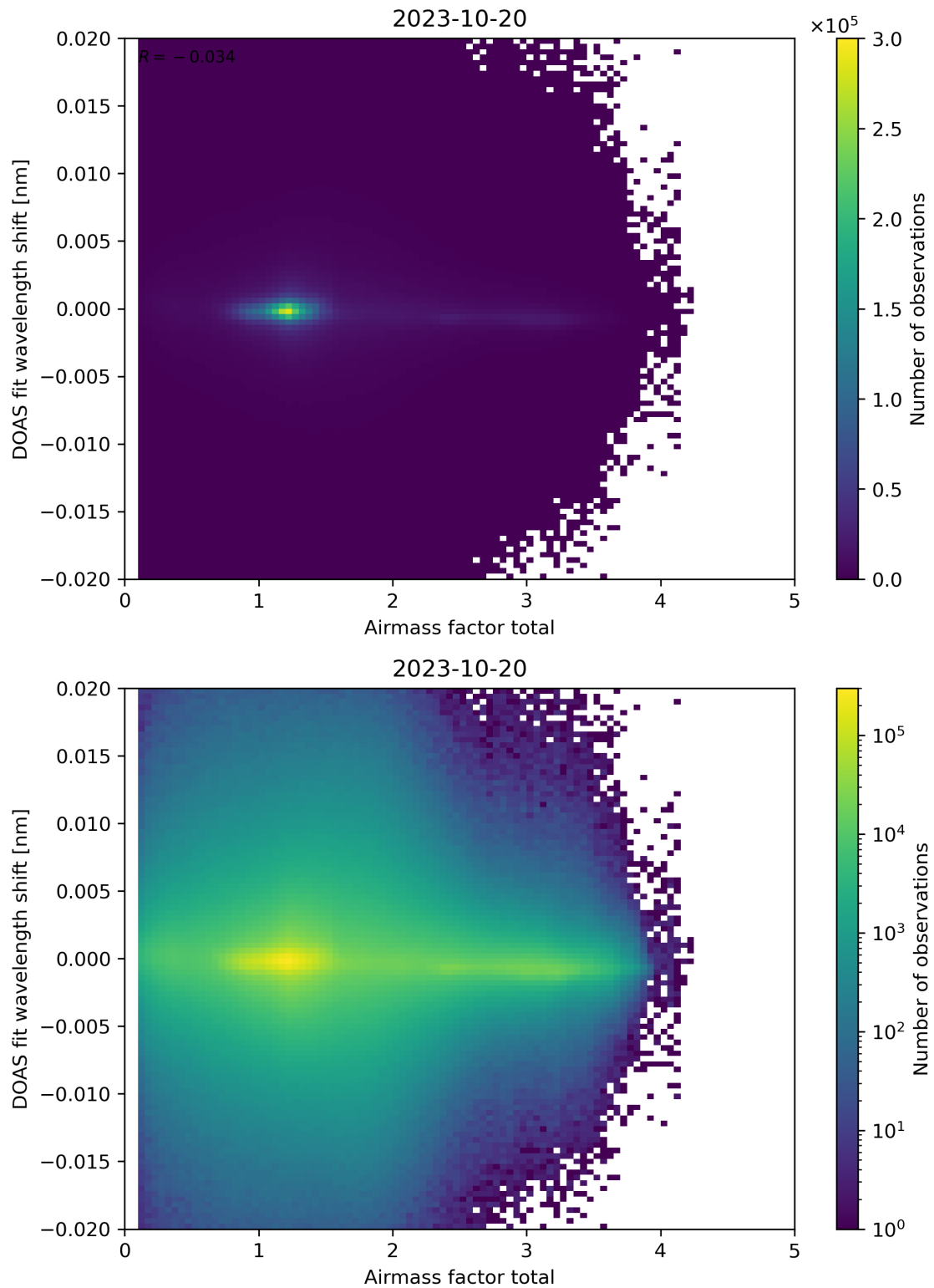
Figure 98: Scatter density plot of “Airmass factor total” against “DOAS fit wavelength shift” for 2023-10-19 to 2023-10-21.
