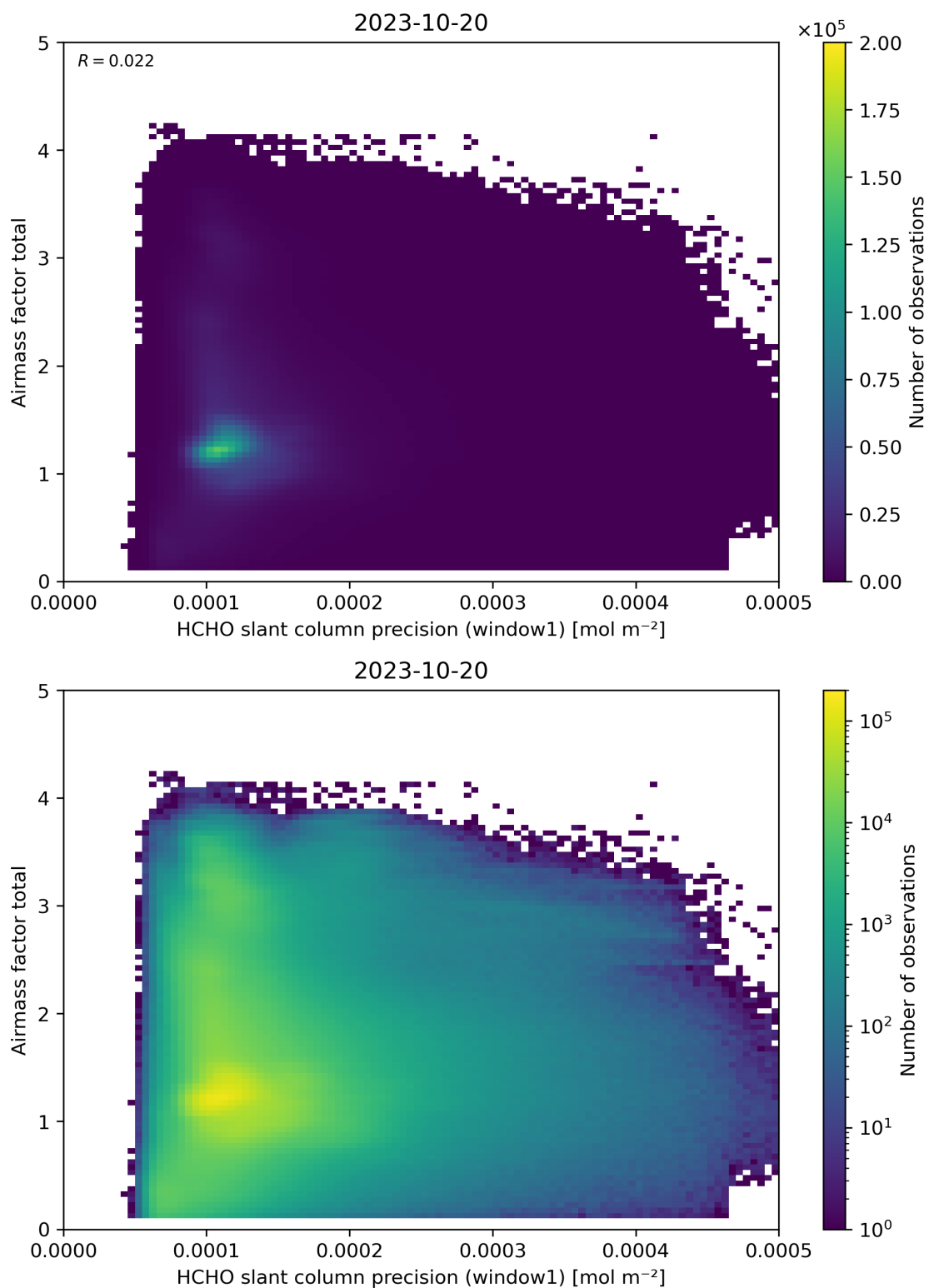
Figure 94: Scatter density plot of “HCHO slant column precision (window1)” against “Airmass factor total” for 2023-10-19 to 2023-10-21.
