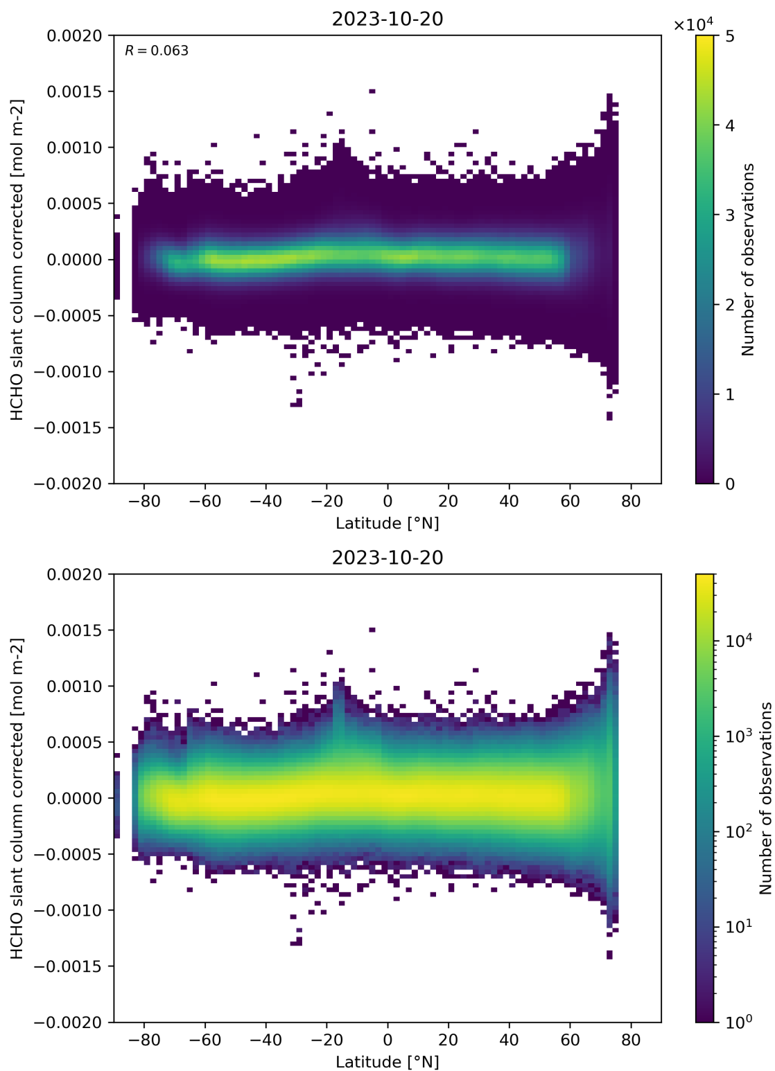
Figure 157: Scatter density plot of “Latitude” against “HCHO slant column corrected” for 2023-10-19 to 2023-10-21.
