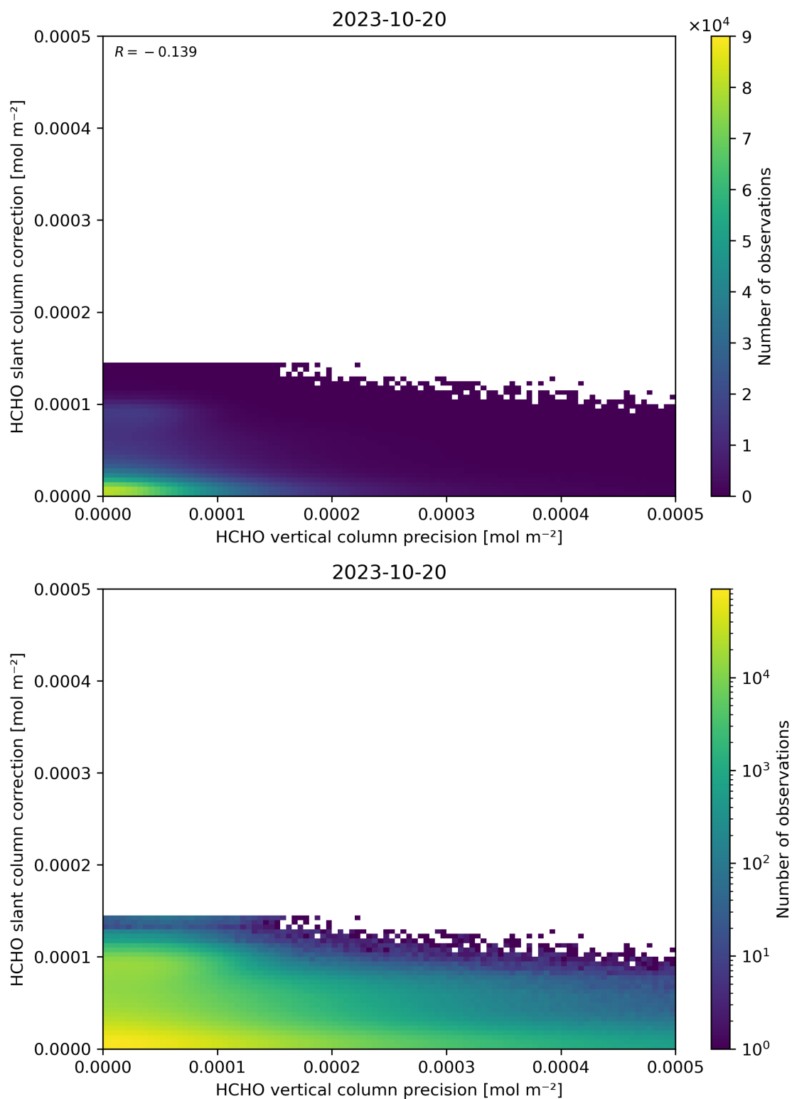
Figure 141: Scatter density plot of “HCHO vertical column precision” against “HCHO slant column correction” for 2023-10-19 to 2023-10-21.
