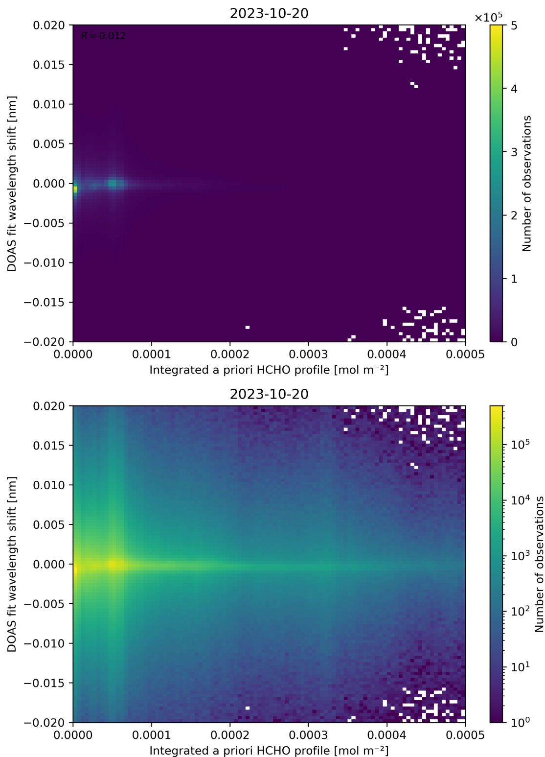
Figure 149: Scatter density plot of “Integrated a priori HCHO profile” against “DOAS fit wavelength shift” for 2023-10-19 to 2023-10-21.
