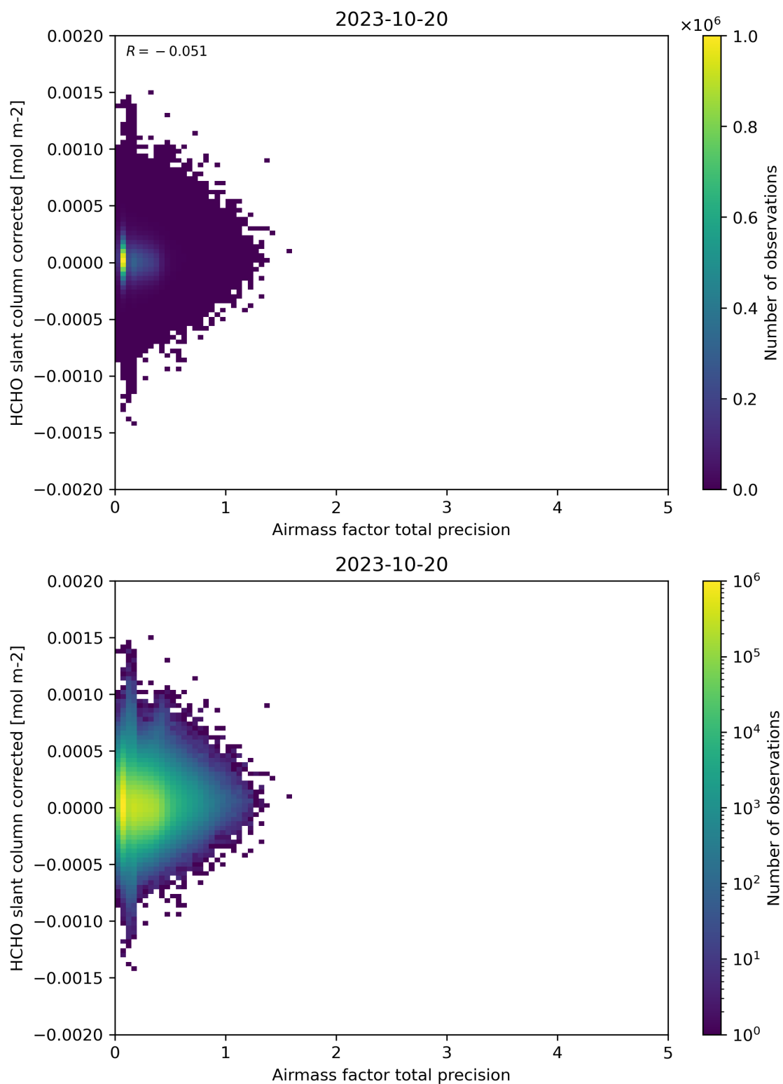
Figure 109: Scatter density plot of “Airmass factor total precision” against “HCHO slant column corrected” for 2023-10-19 to 2023-10-21.
