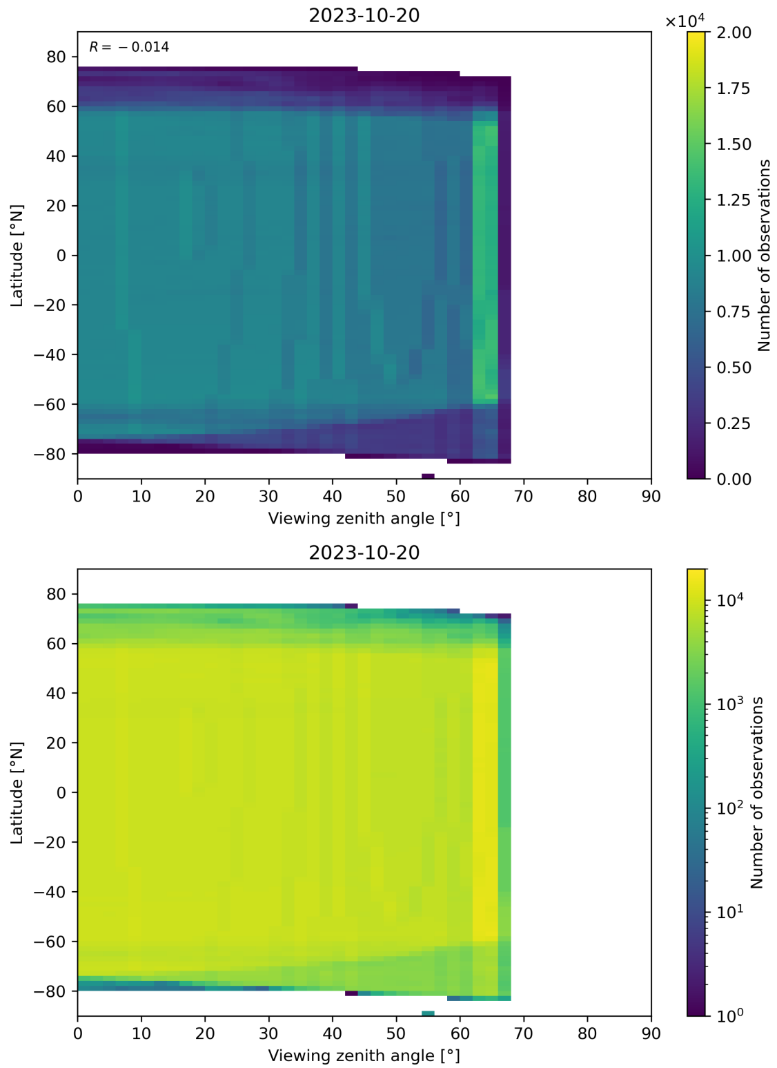
Figure 196: Scatter density plot of “Viewing zenith angle” against “Latitude” for 2023-10-19 to 2023-10-21.
