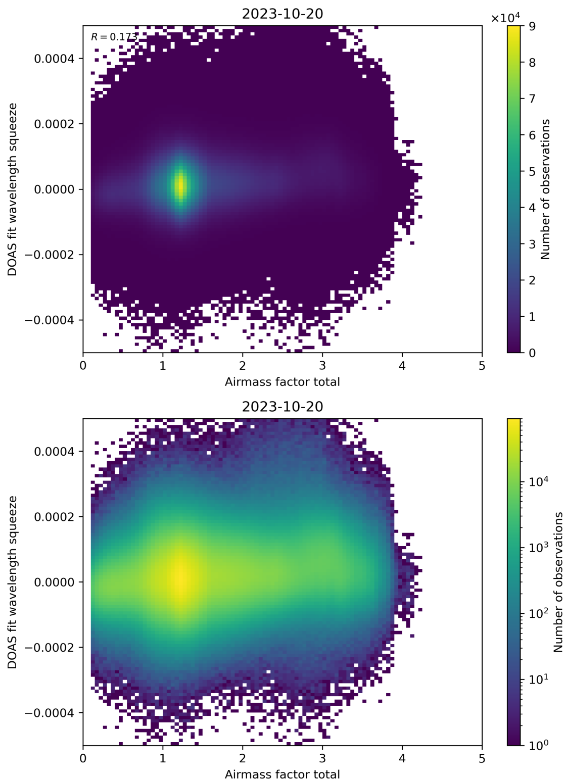
Figure 99: Scatter density plot of “Airmass factor total” against “DOAS fit wavelength squeeze” for 2023-10-19 to 2023-10-21.
