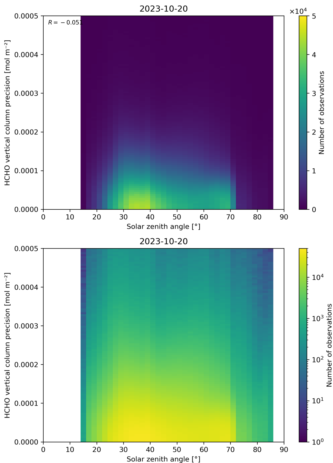
Figure 179: Scatter density plot of “Solar zenith angle” against “HCHO vertical column precision” for 2023-10-19 to 2023-10-21.
