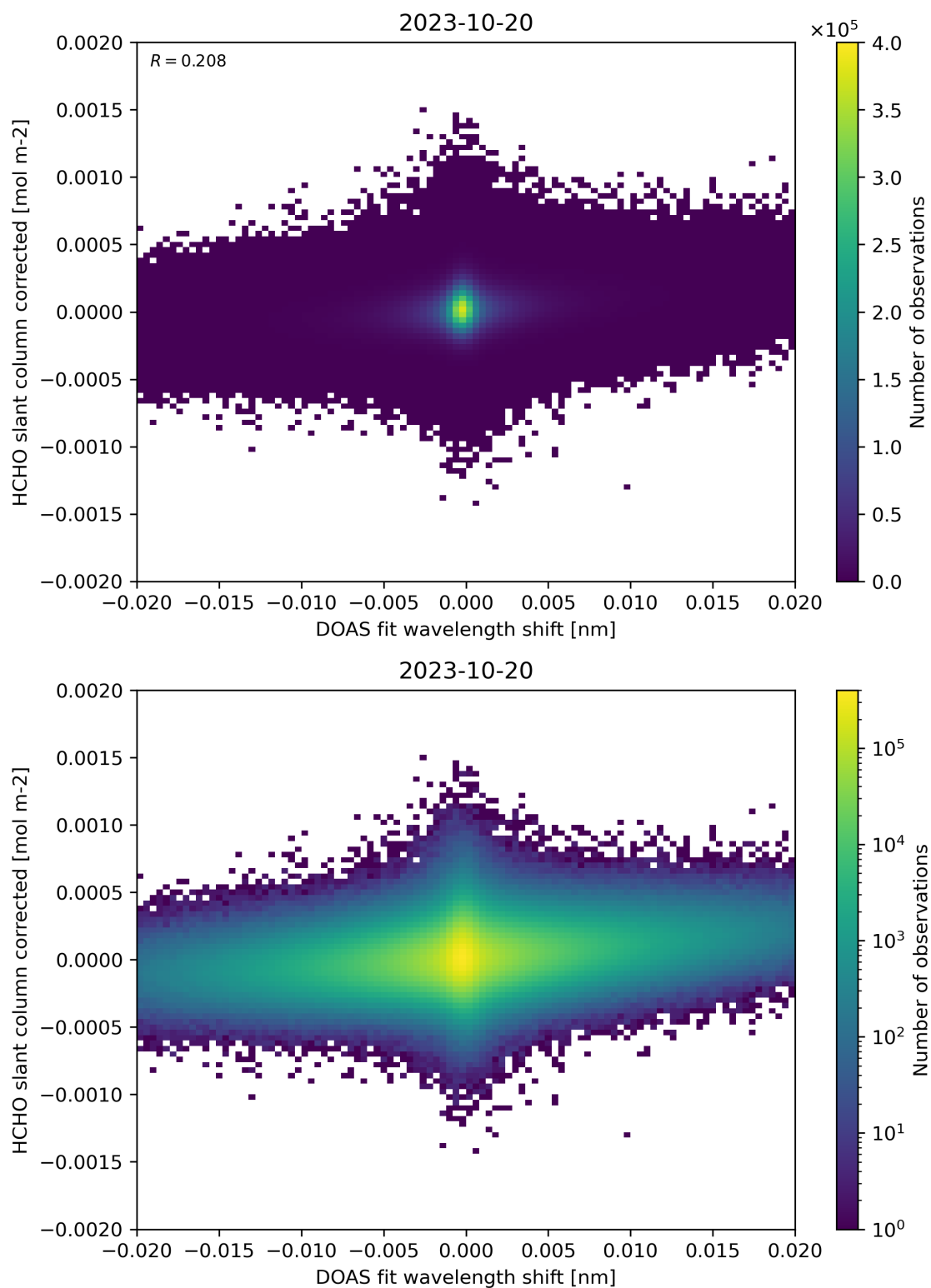
Figure 66: Scatter density plot of “DOAS fit wavelength shift” against “HCHO slant column corrected” for 2023-10-19 to 2023-10-21.
