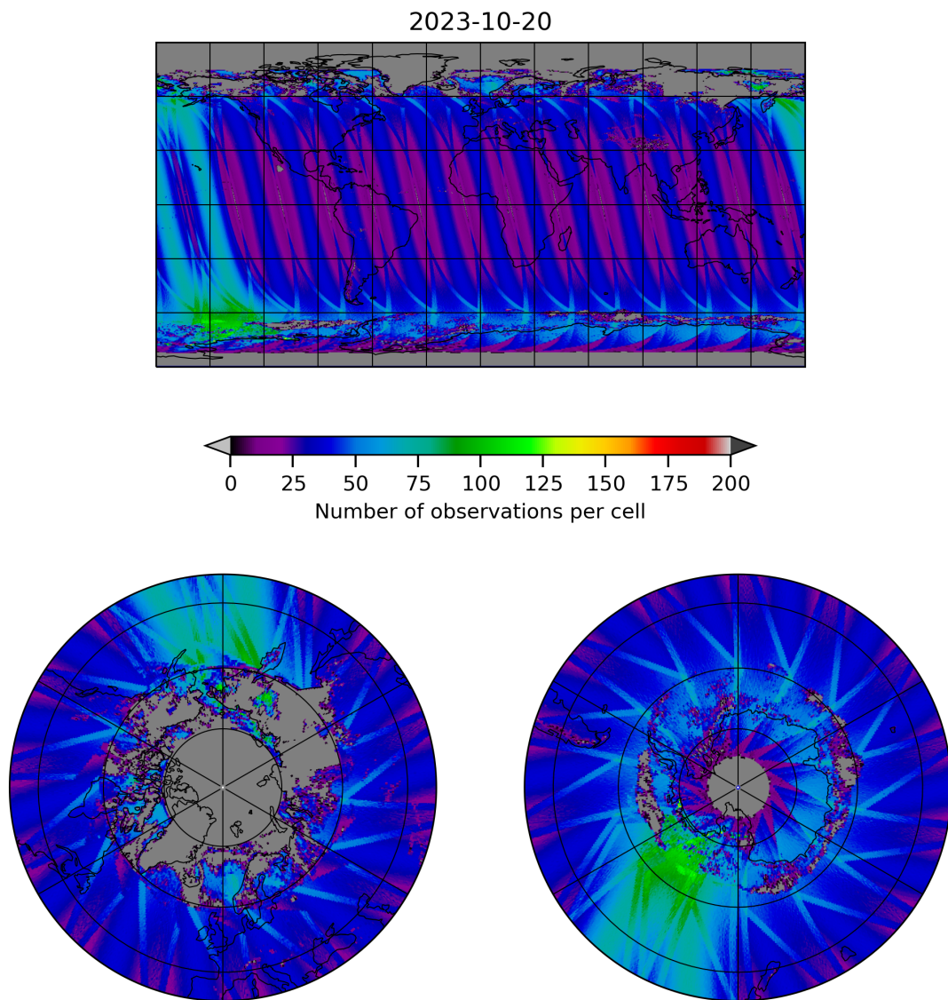
Figure 19: Map of the number of observations for 2023-10-19 to 2023-10-21
