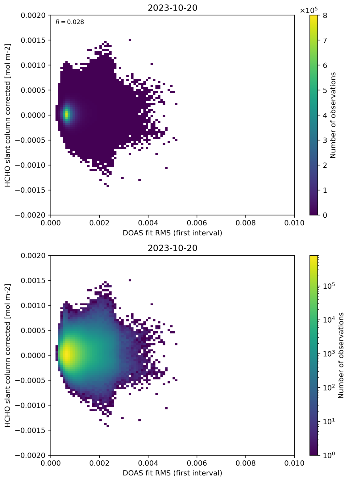
Figure 62: Scatter density plot of “DOAS fit RMS (first interval)” against “HCHO slant column corrected” for 2023-10-19 to 2023-10-21.
