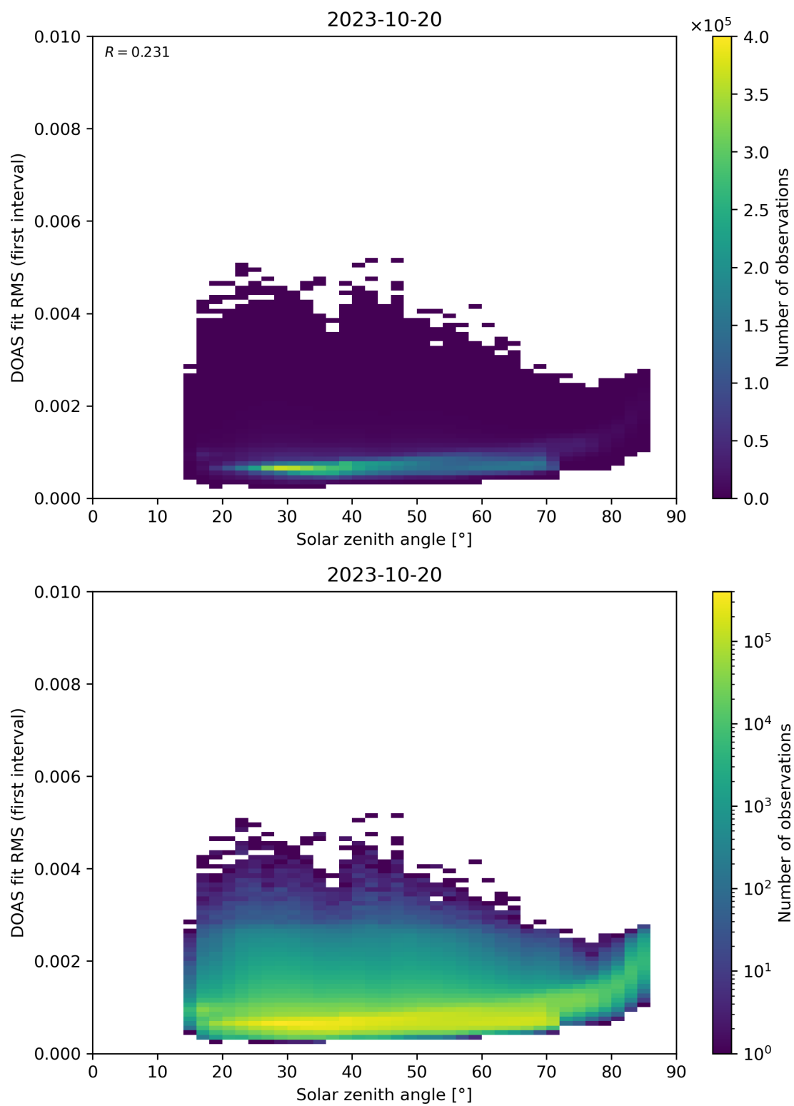
Figure 167: Scatter density plot of “Solar zenith angle” against “DOAS fit RMS (first interval)” for 2023-10-19 to 2023-10-21.
