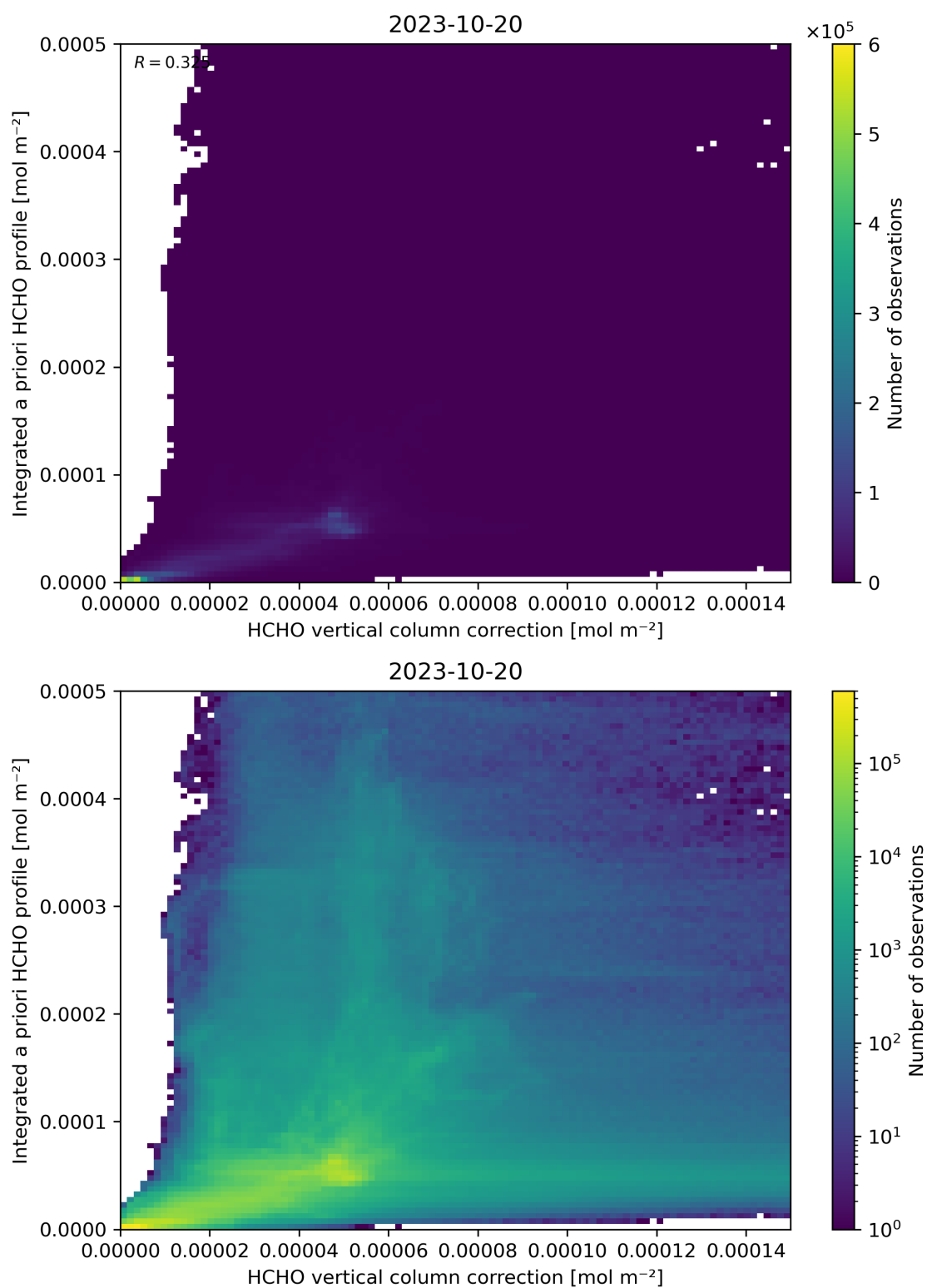
Figure 122: Scatter density plot of “HCHO vertical column correction” against “Integrated a priori HCHO profile” for 2023-10-19 to 2023-10-21.
