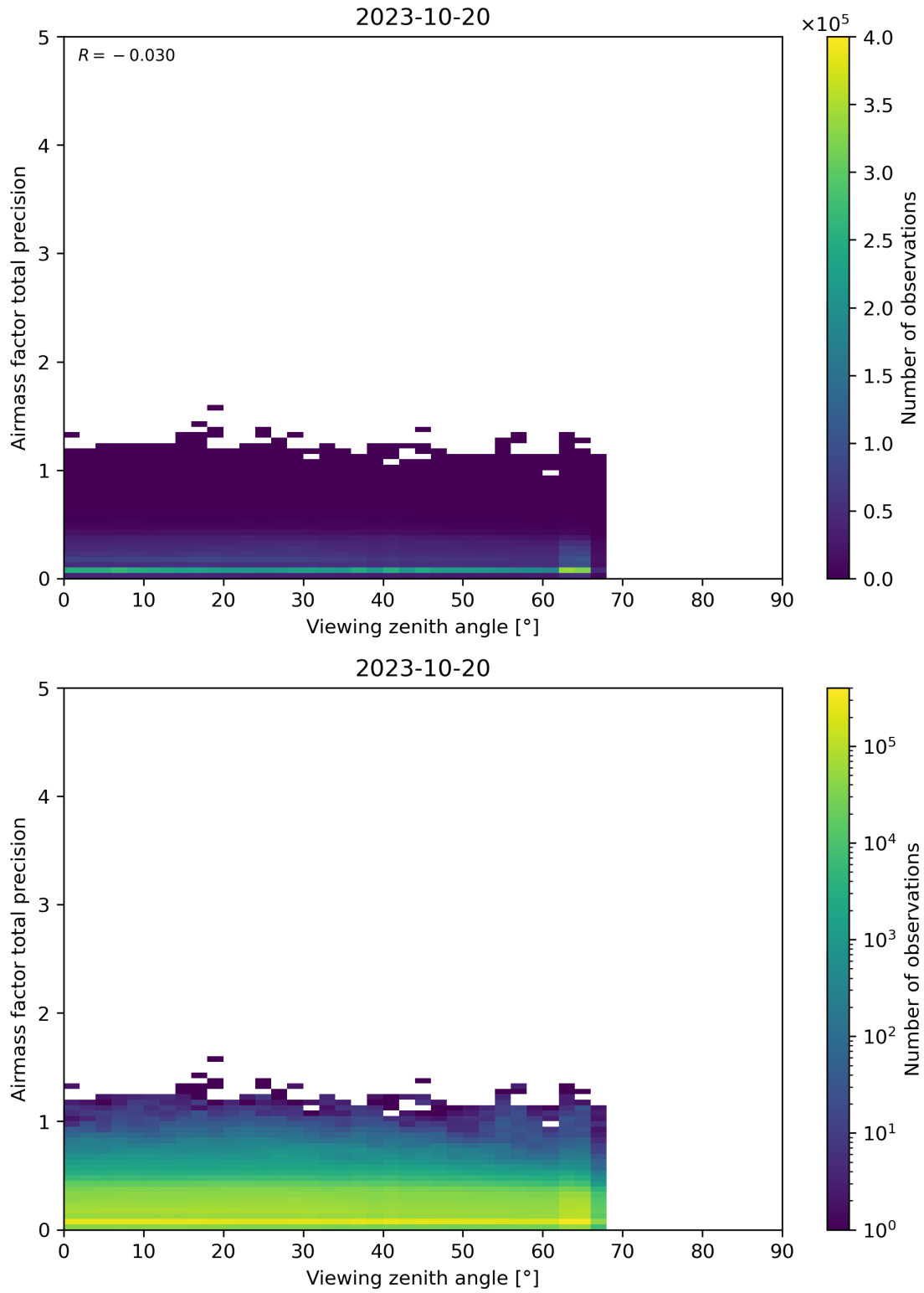
Figure 191: Scatter density plot of “Viewing zenith angle” against “Airmass factor total precision” for 2023-10-19 to 2023-10-21.
