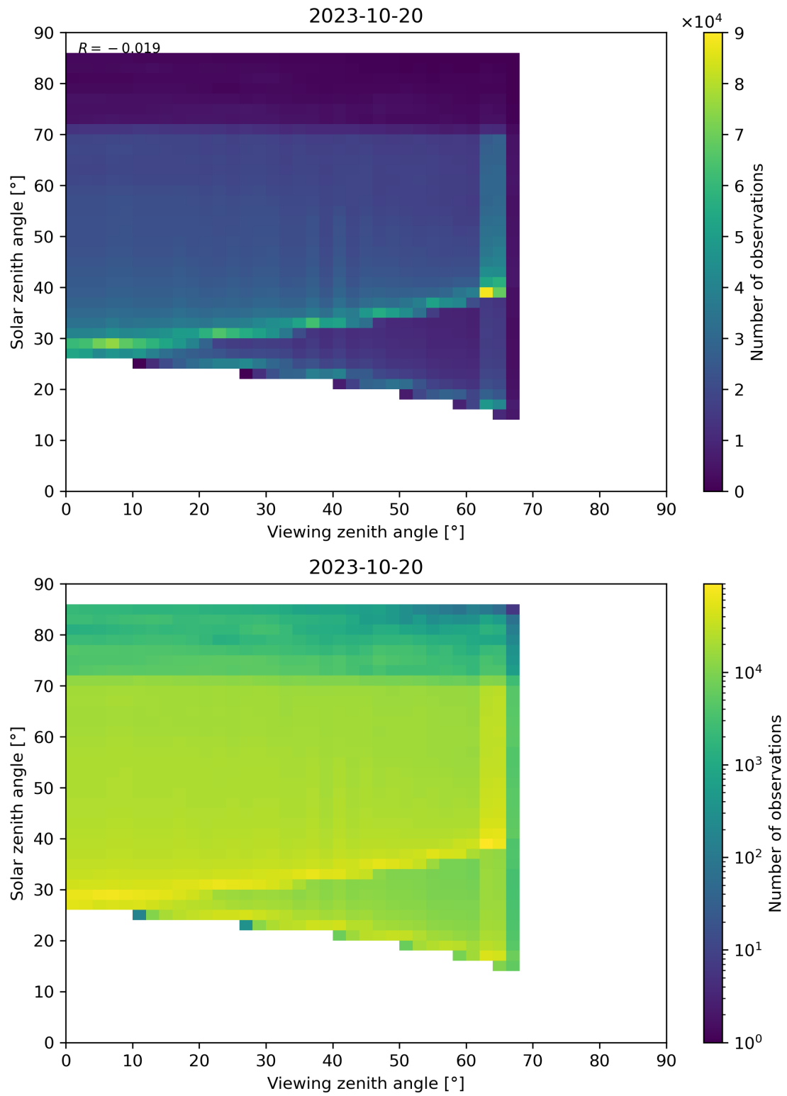
Figure 197: Scatter density plot of “Viewing zenith angle” against “Solar zenith angle” for 2023-10-19 to 2023-10-21.
