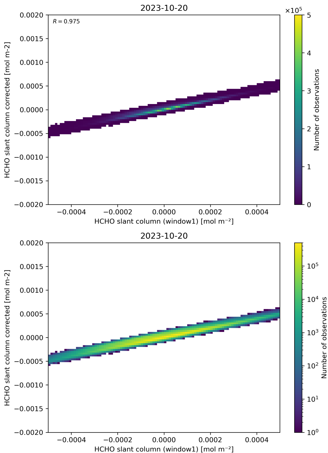
Figure 82: Scatter density plot of “HCHO slant column (window1)” against “HCHO slant column corrected” for 2023-10-19 to 2023-10-21.
