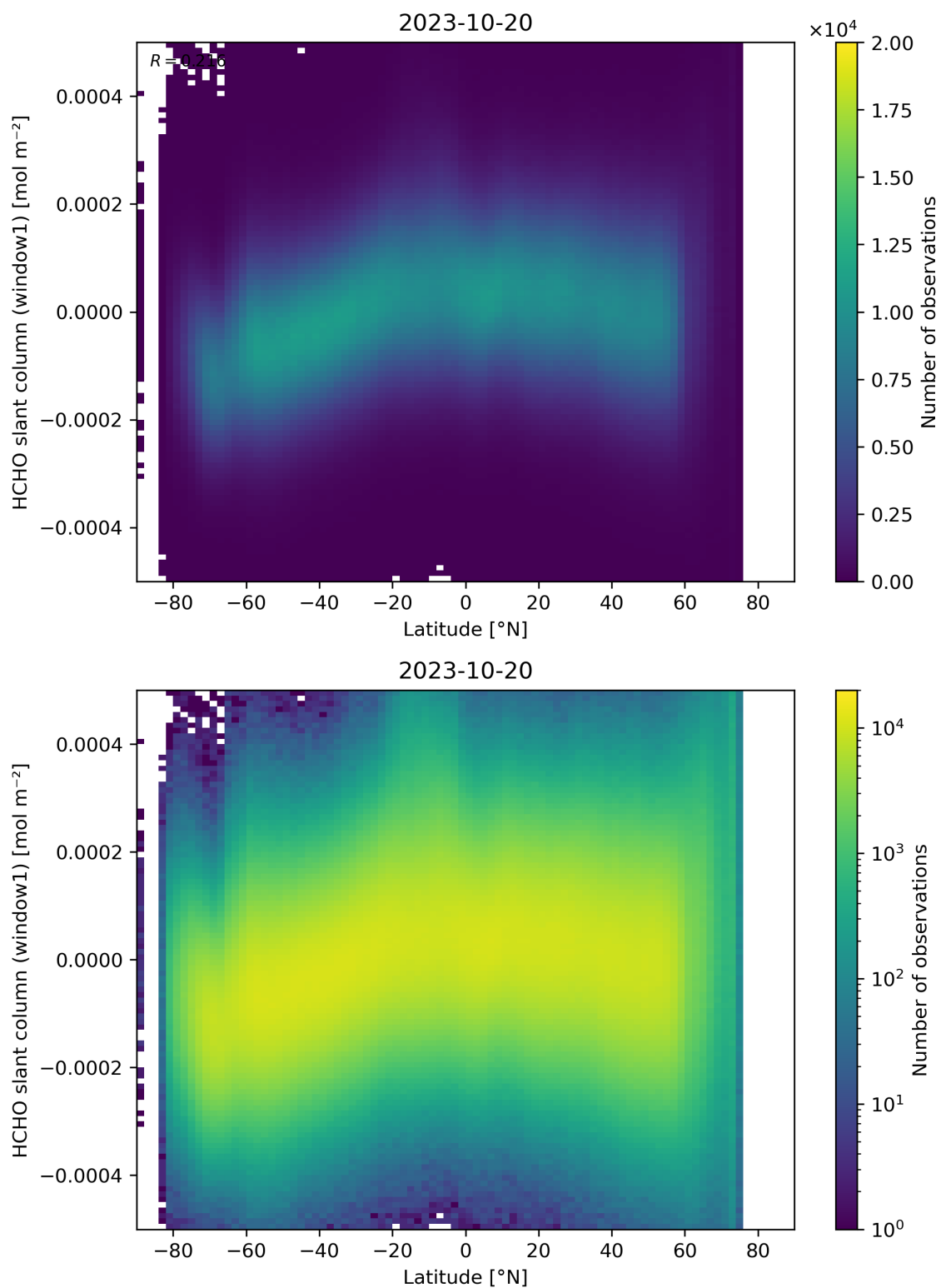
Figure 159: Scatter density plot of “Latitude” against “HCHO slant column (window1)” for 2023-10-19 to 2023-10-21.
