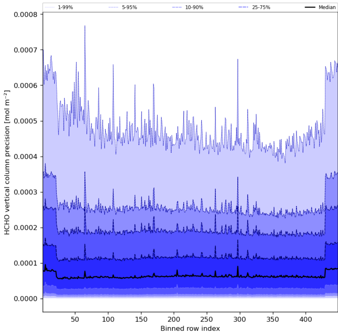
Figure 50: Along track statistics of “HCHO vertical column precision” for 2023-10-19 to 2023-10-21
