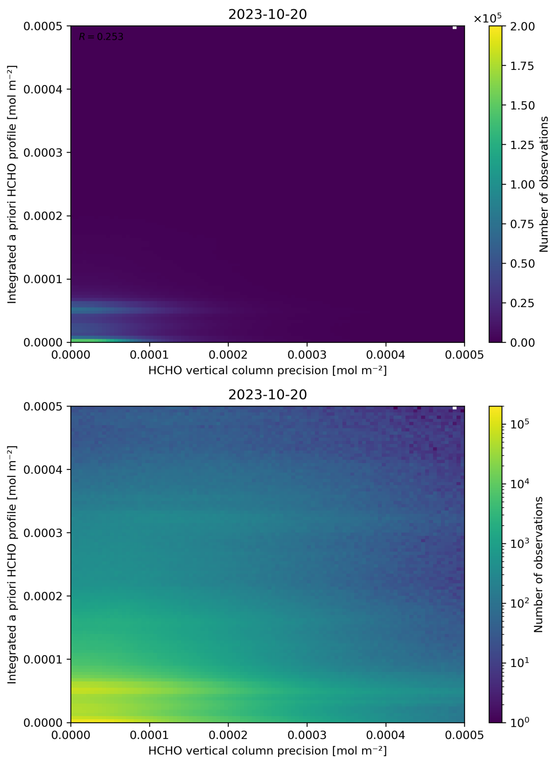
Figure 147: Scatter density plot of “HCHO vertical column precision” against “Integrated a priori HCHO profile” for 2023-10-19 to 2023-10-21.
