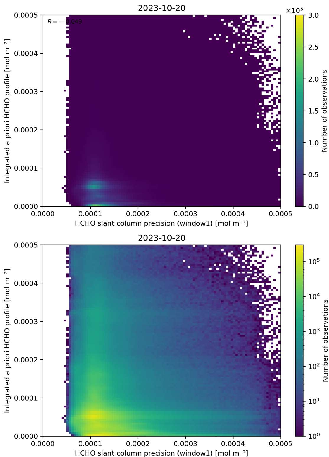
Figure 96: Scatter density plot of “HCHO slant column precision (window1)” against “Integrated a priori HCHO profile” for 2023-10-19 to 2023-10-21.
