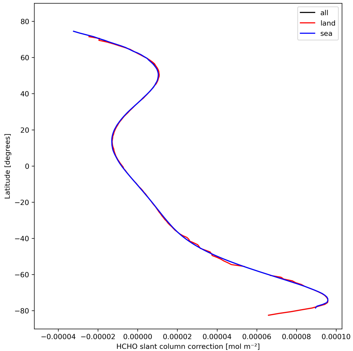
Figure 33: Zonal average of “HCHO slant column correction” for 2023-10-19 to 2023-10-21.
