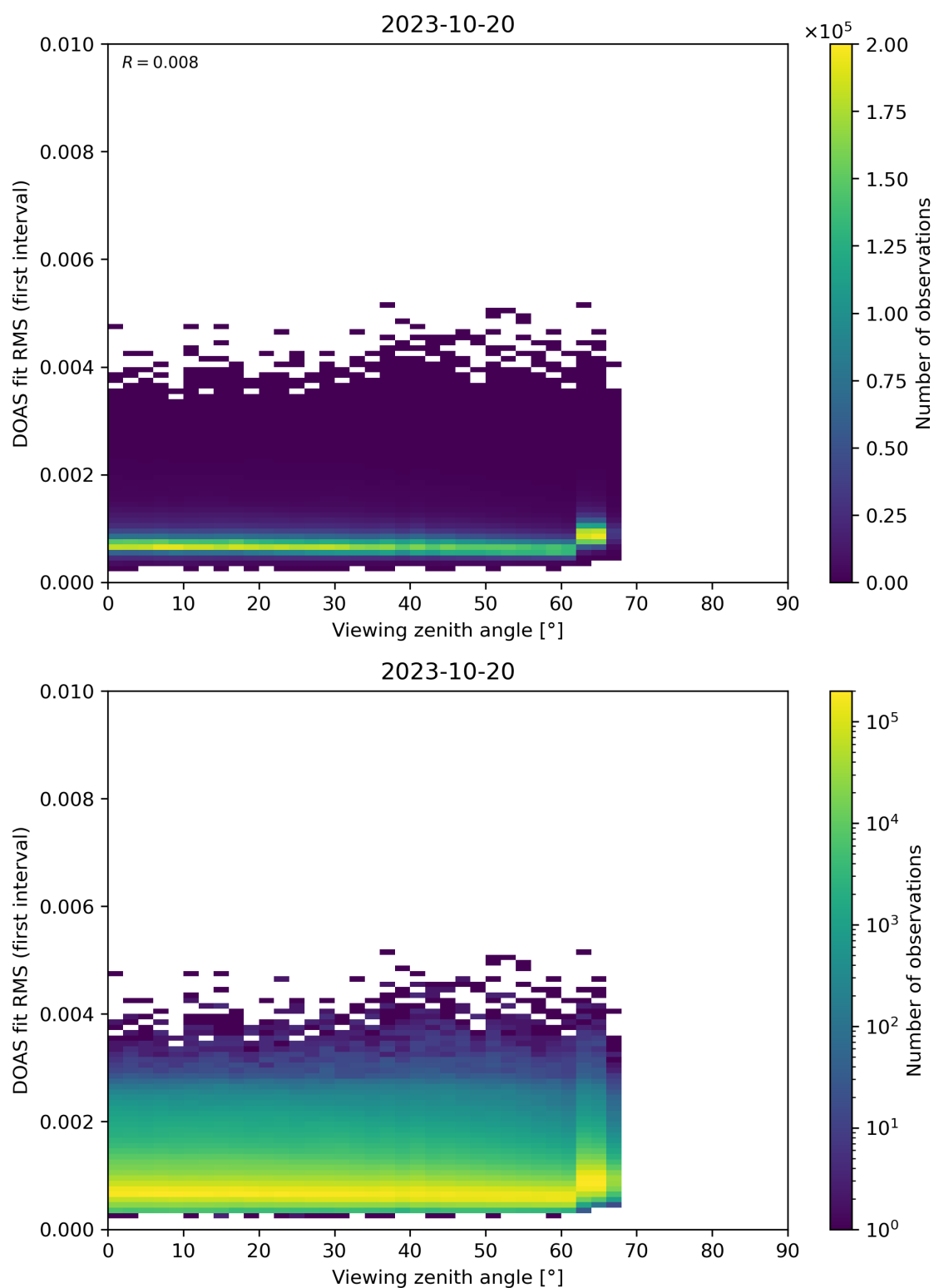
Figure 182: Scatter density plot of “Viewing zenith angle” against “DOAS fit RMS (first interval)” for 2023-10-19 to 2023-10-21.
