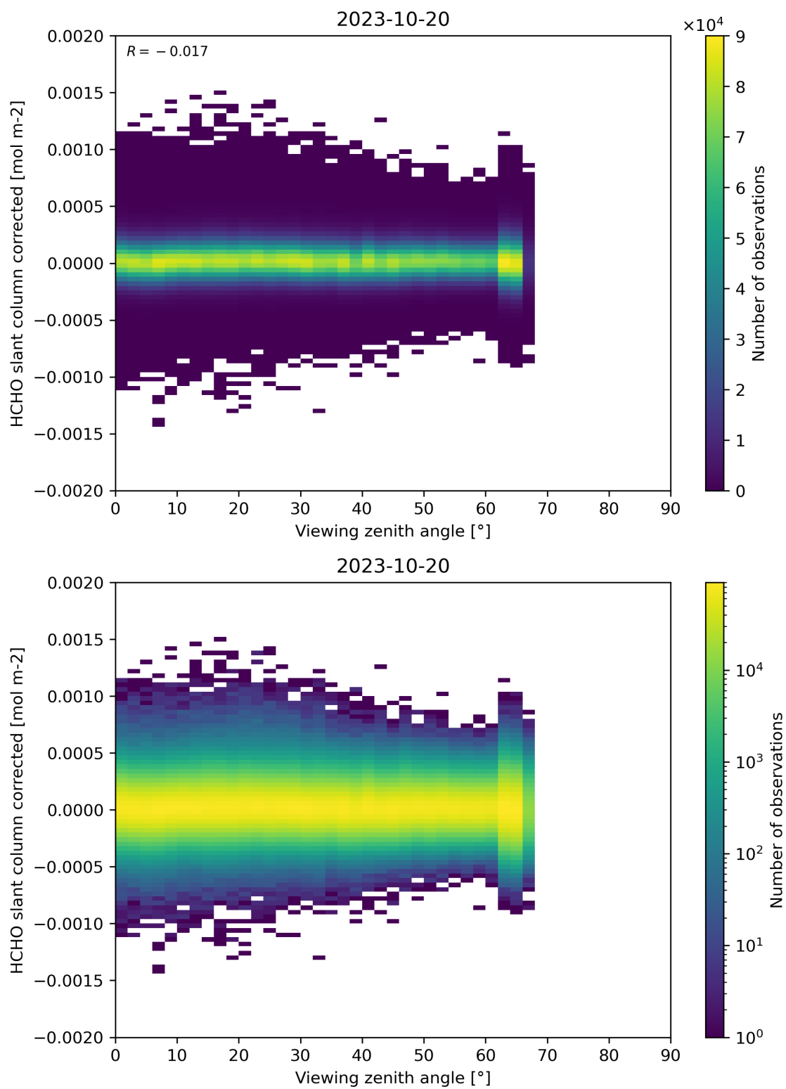
Figure 186: Scatter density plot of “Viewing zenith angle” against “HCHO slant column corrected” for 2023-10-19 to 2023-10-21.
