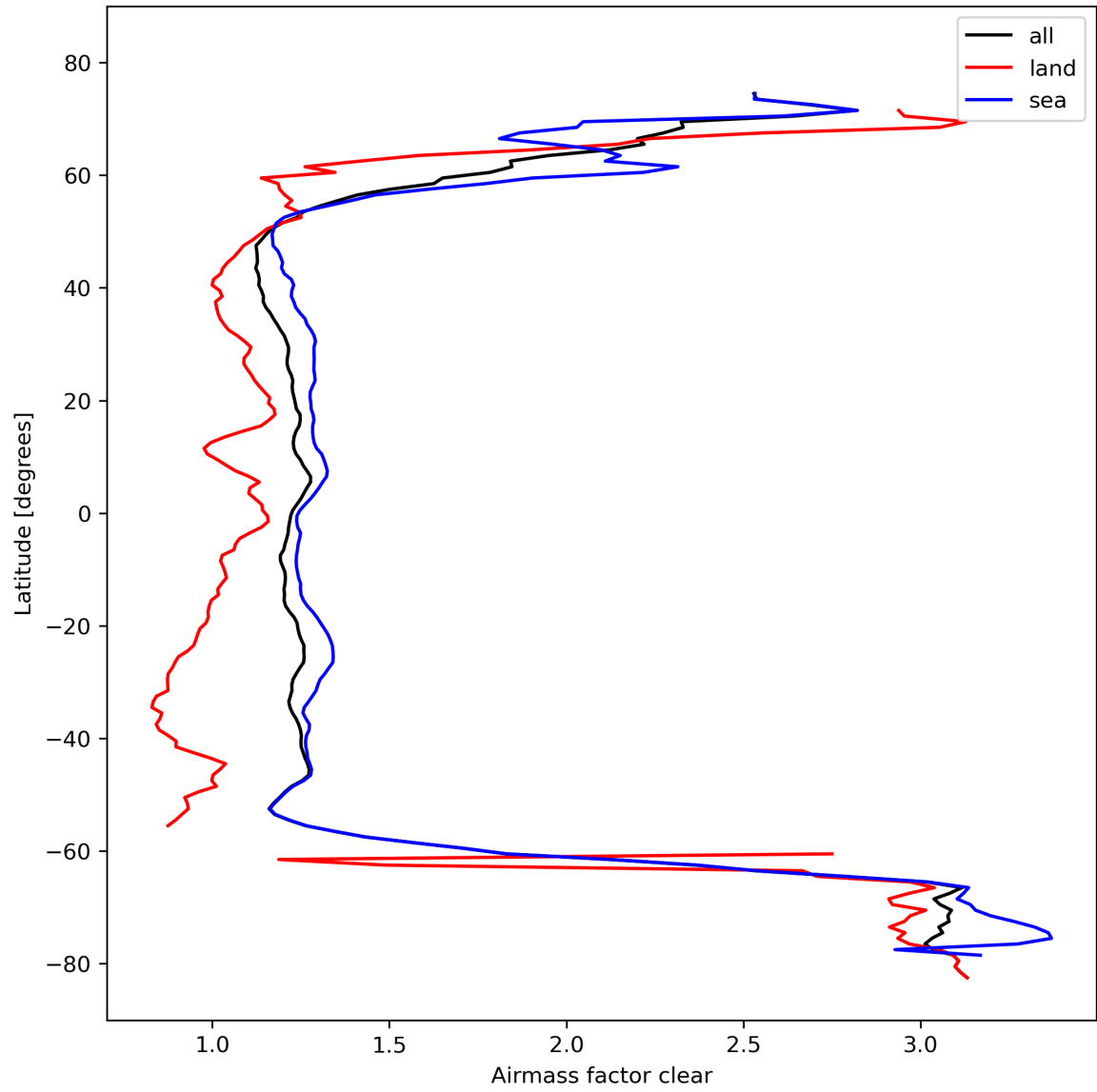
Figure 28: Zonal average of “Airmass factor clear” for 2023-10-19 to 2023-10-21.
