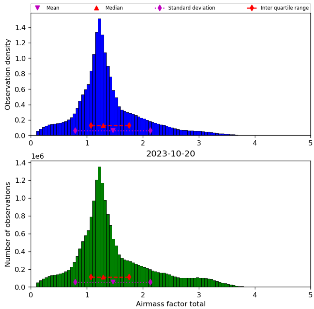
Figure 40: Histogram of “Airmass factor total” for 2023-10-19 to 2023-10-21
