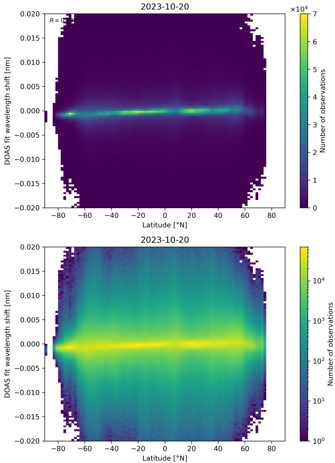
Figure 154: Scatter density plot of “Latitude” against “DOAS fit wavelength shift” for 2023-10-19 to 2023-10-21.
