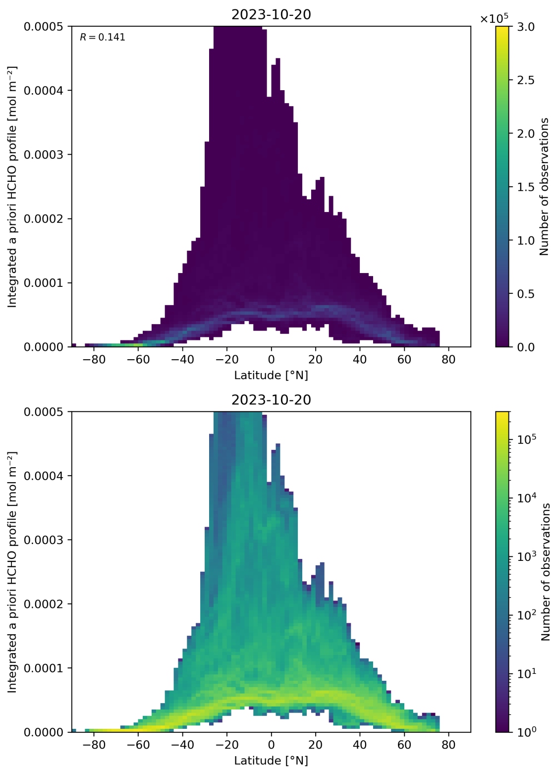
Figure 166: Scatter density plot of “Latitude” against “Integrated a priori HCHO profile” for 2023-10-19 to 2023-10-21.
