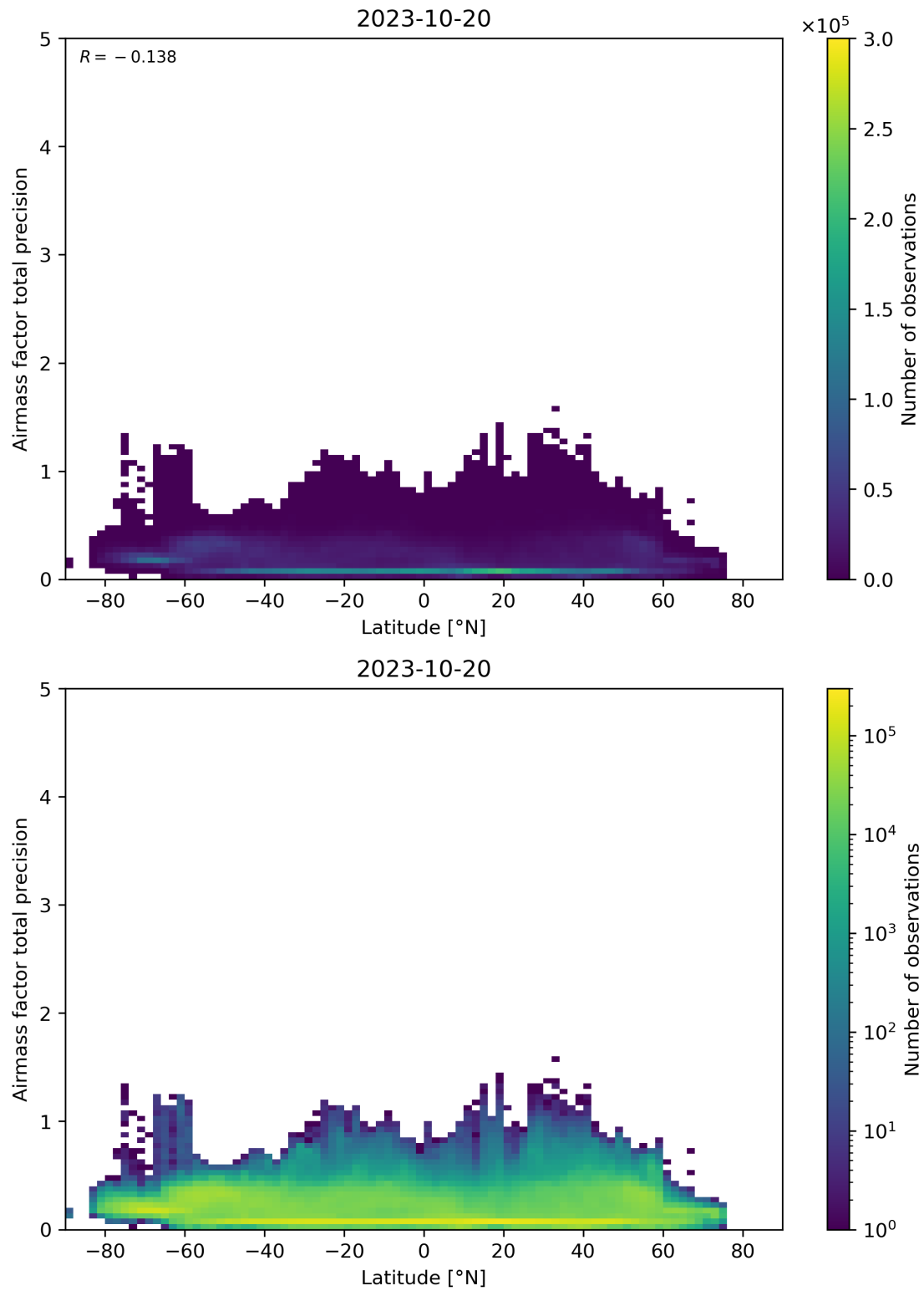
Figure 162: Scatter density plot of “Latitude” against “Airmass factor total precision” for 2023-10-19 to 2023-10-21.
