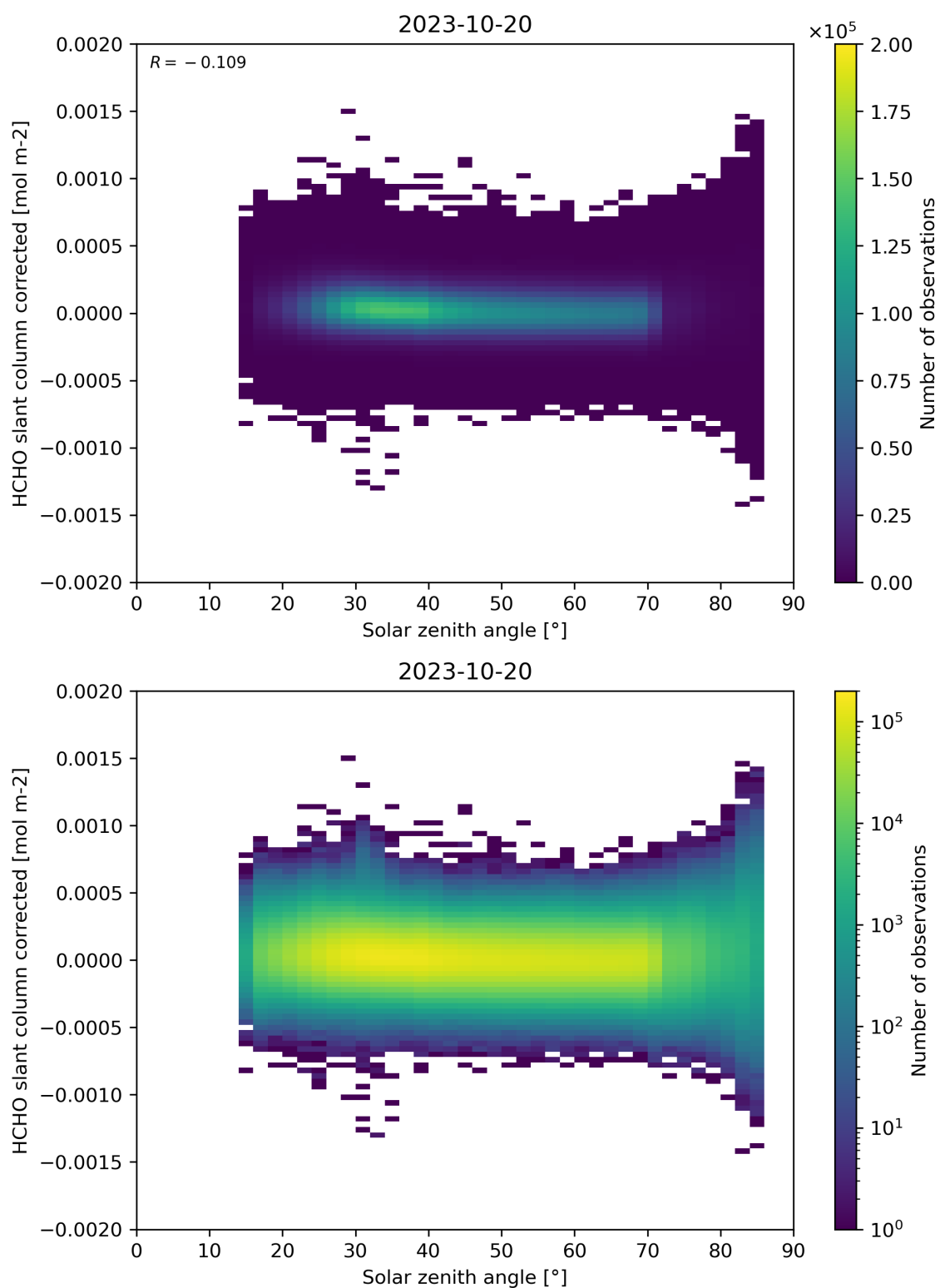
Figure 171: Scatter density plot of “Solar zenith angle” against “HCHO slant column corrected” for 2023-10-19 to 2023-10-21.
