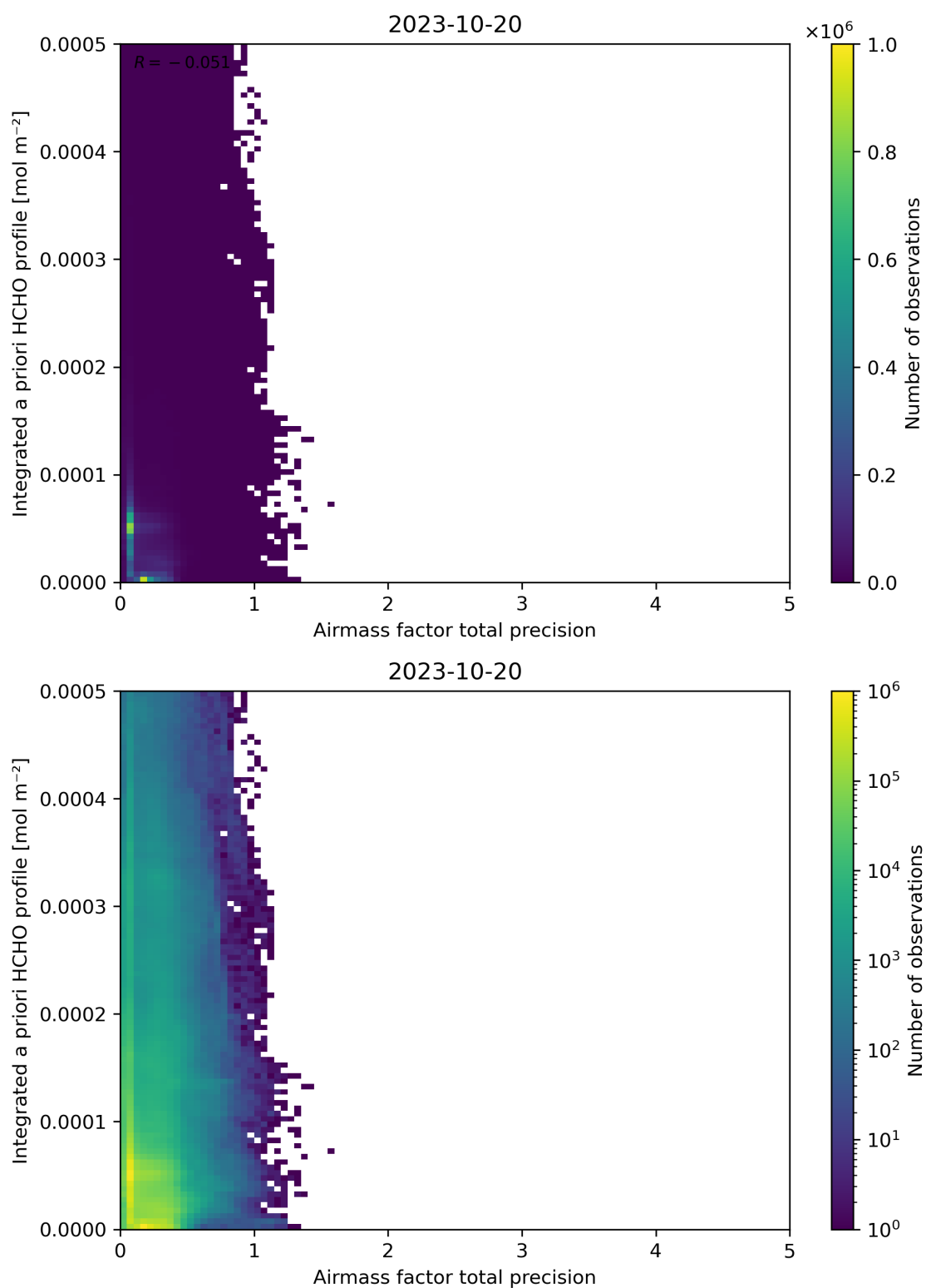
Figure 111: Scatter density plot of “Airmass factor total precision” against “Integrated a priori HCHO profile” for 2023-10-19 to 2023-10-21.
