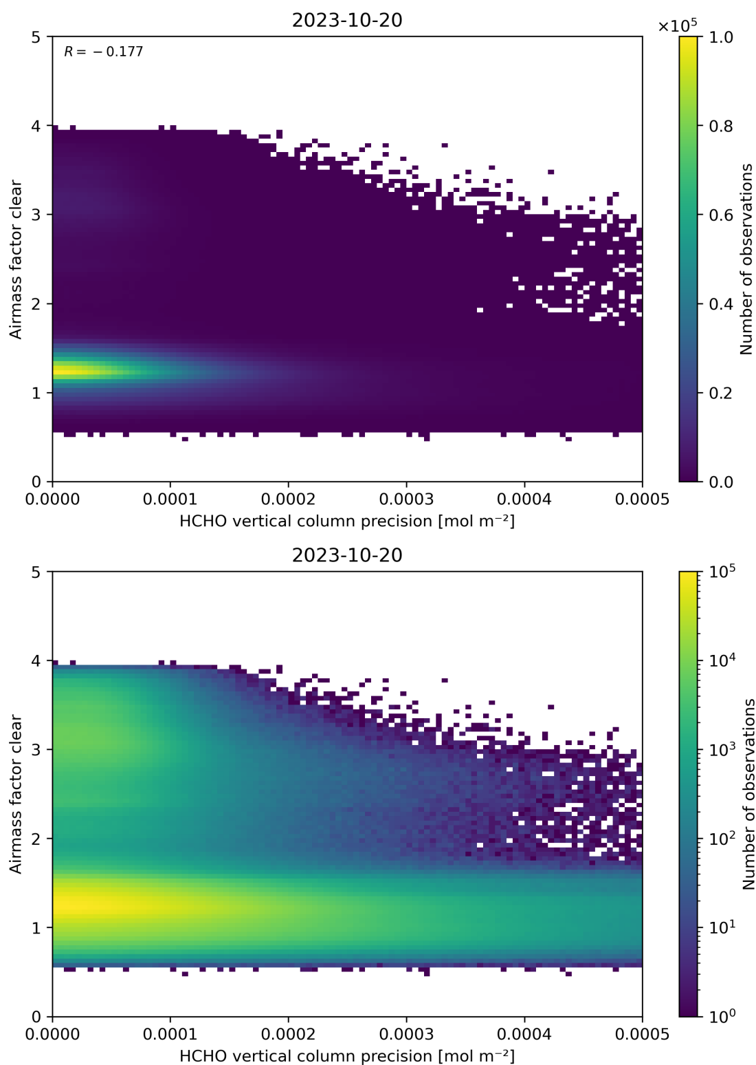
Figure 139: Scatter density plot of “HCHO vertical column precision” against “Airmass factor clear” for 2023-10-19 to 2023-10-21.
