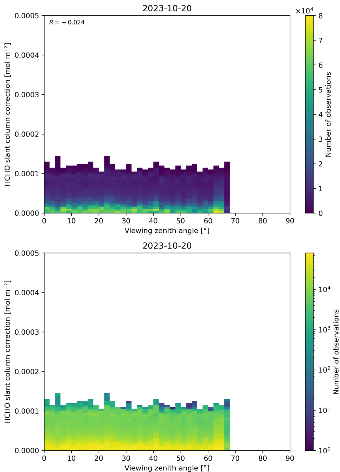
Figure 187: Scatter density plot of “Viewing zenith angle” against “HCHO slant column correction” for 2023-10-19 to 2023-10-21.
