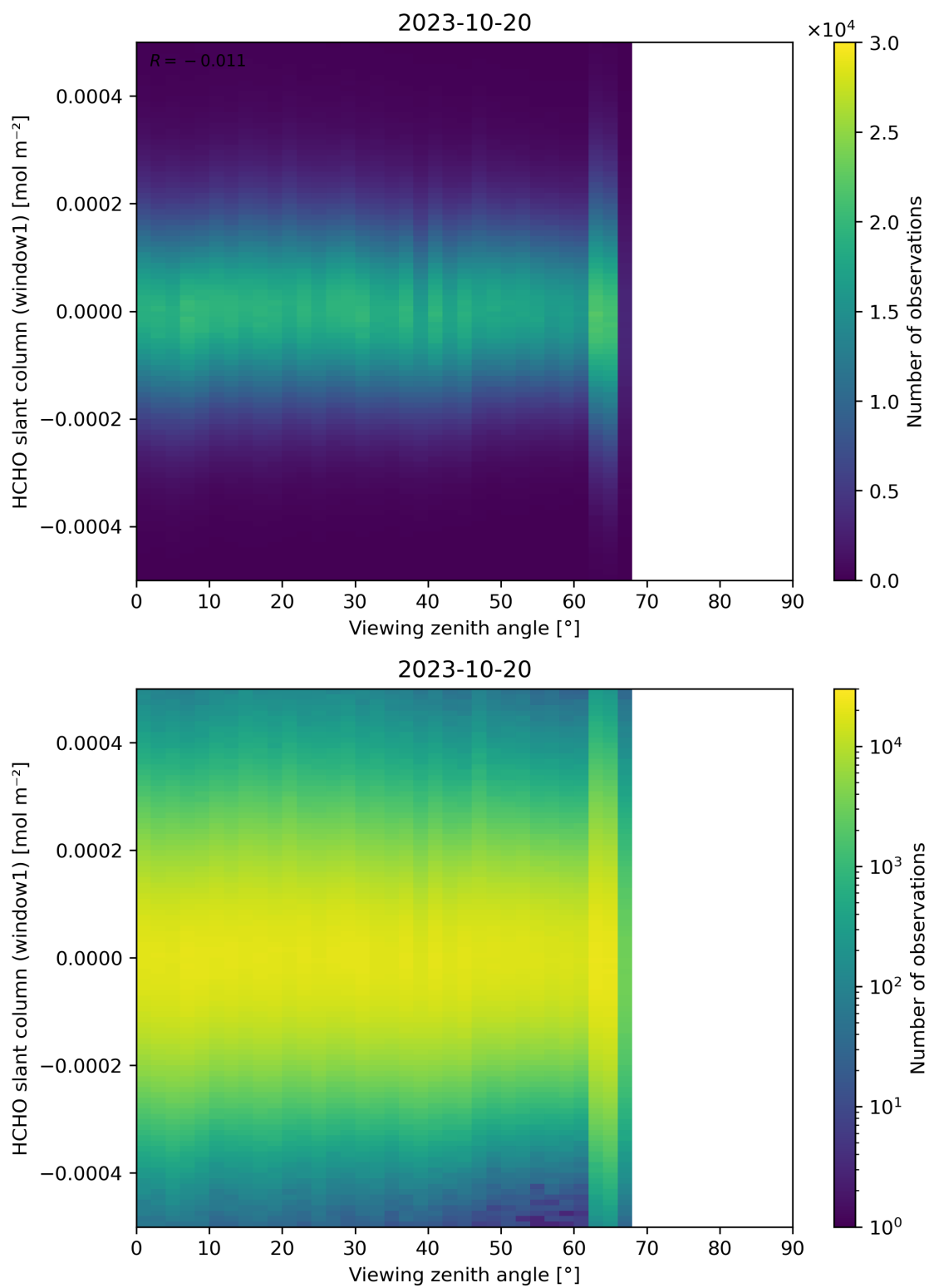
Figure 188: Scatter density plot of “Viewing zenith angle” against “HCHO slant column (window1)” for 2023-10-19 to 2023-10-21.
