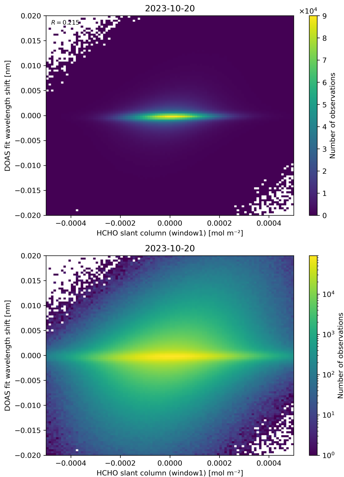
Figure 79: Scatter density plot of “HCHO slant column (window1)” against “DOAS fit wavelength shift” for 2023-10-19 to 2023-10-21.
