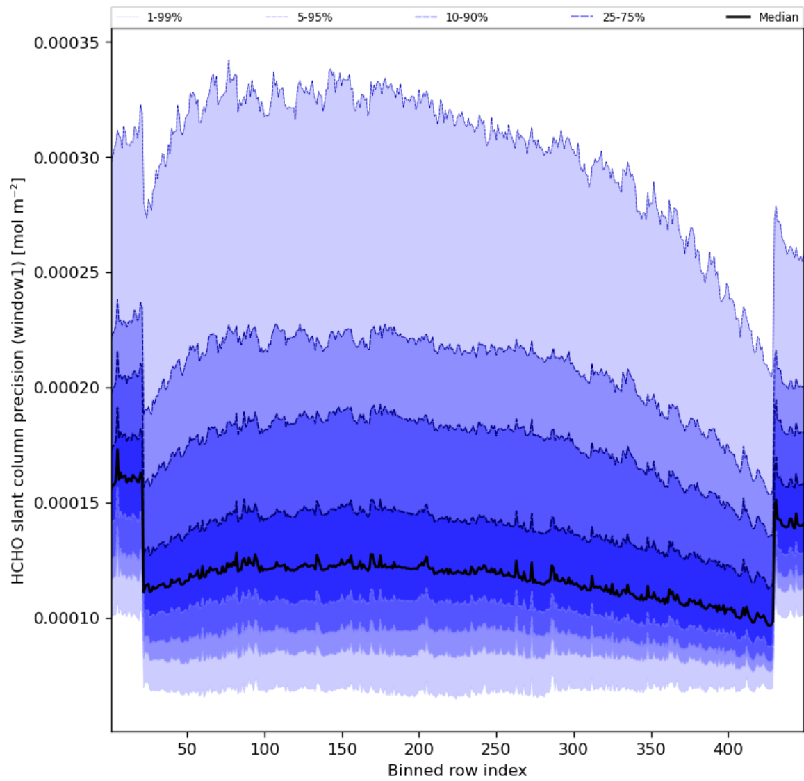
Figure 53: Along track statistics of “HCHO slant column precision (window1)” for 2023-10-19 to 2023-10-21
