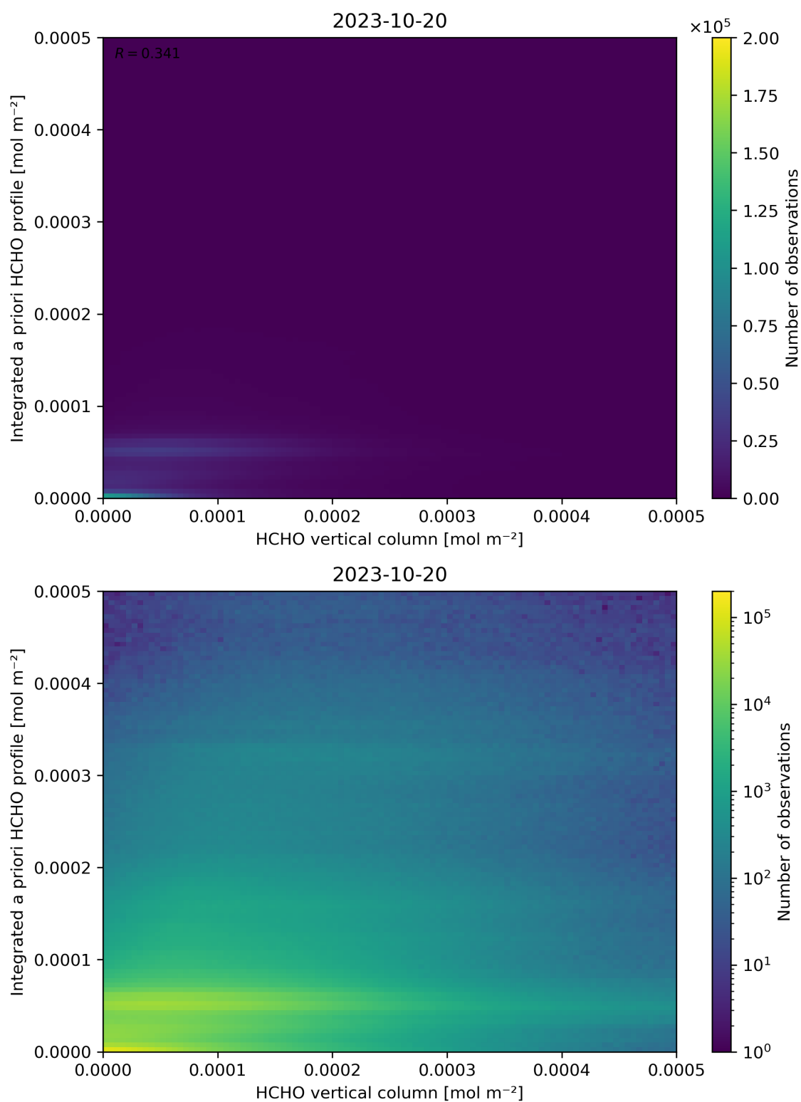
Figure 135: Scatter density plot of “HCHO vertical column” against “Integrated a priori HCHO profile” for 2023-10-19 to 2023-10-21.
