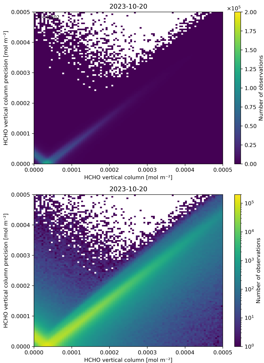
Figure 134: Scatter density plot of “HCHO vertical column” against “HCHO vertical column precision” for 2023-10-19 to 2023-10-21.
