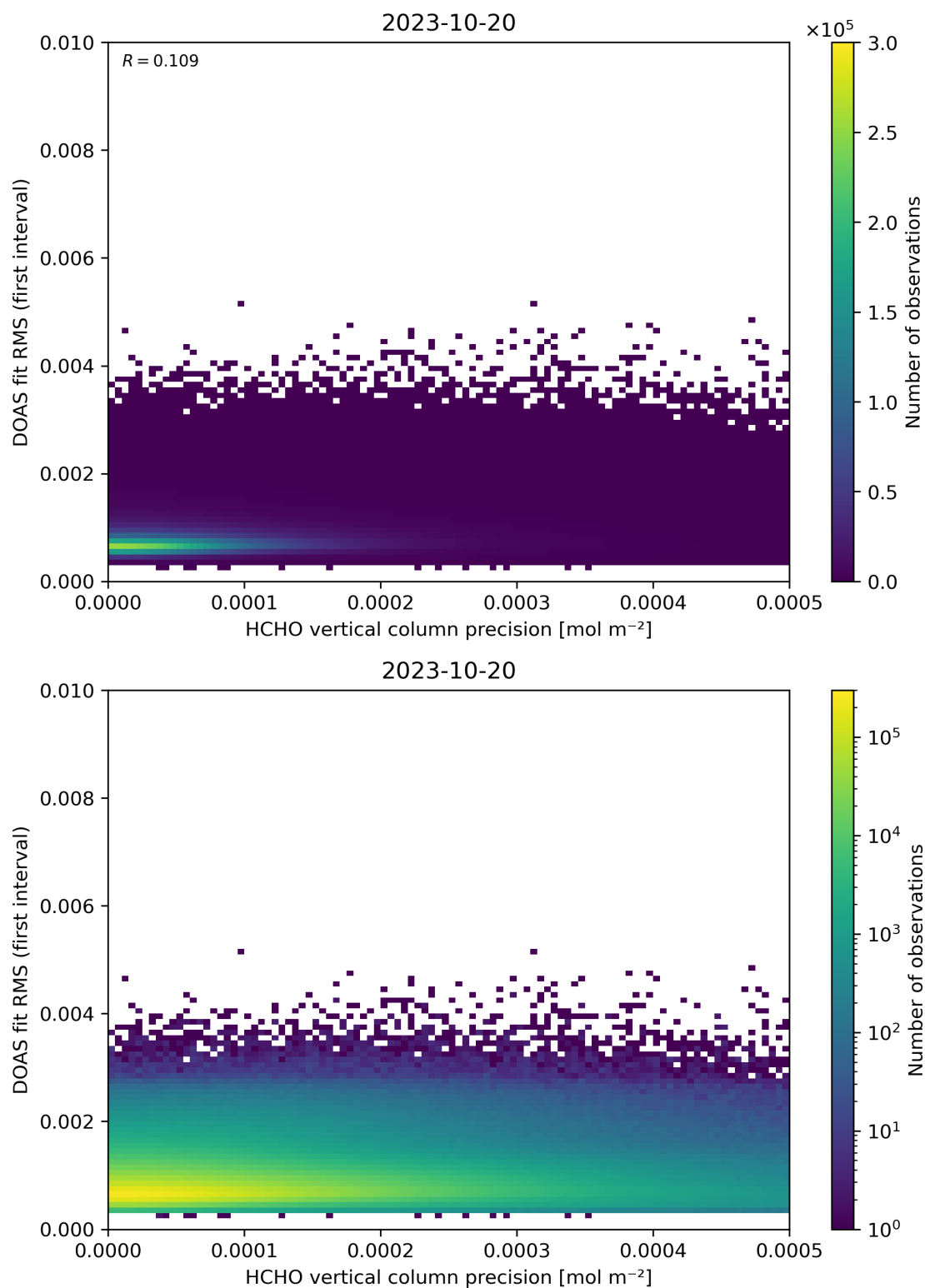
Figure 136: Scatter density plot of “HCHO vertical column precision” against “DOAS fit RMS (first interval)” for 2023-10-19 to 2023-10-21.
