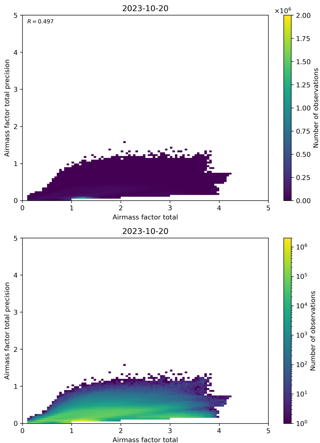
Figure 103: Scatter density plot of “Airmass factor total” against “Airmass factor total precision” for 2023-10-19 to 2023-10-21.
