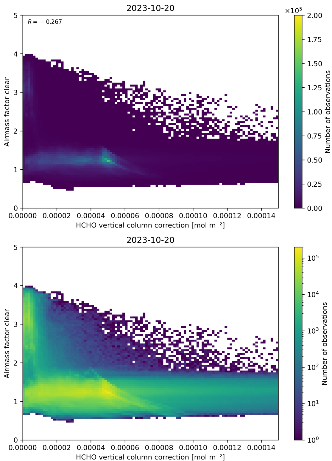
Figure 115: Scatter density plot of “HCHO vertical column correction” against “Airmass factor clear” for 2023-10-19 to 2023-10-21.
