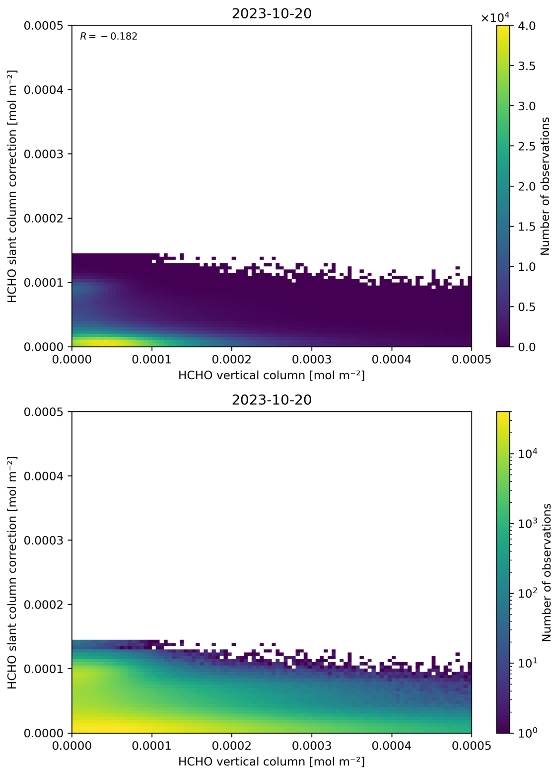
Figure 128: Scatter density plot of “HCHO vertical column” against “HCHO slant column correction” for 2023-10-19 to 2023-10-21.
