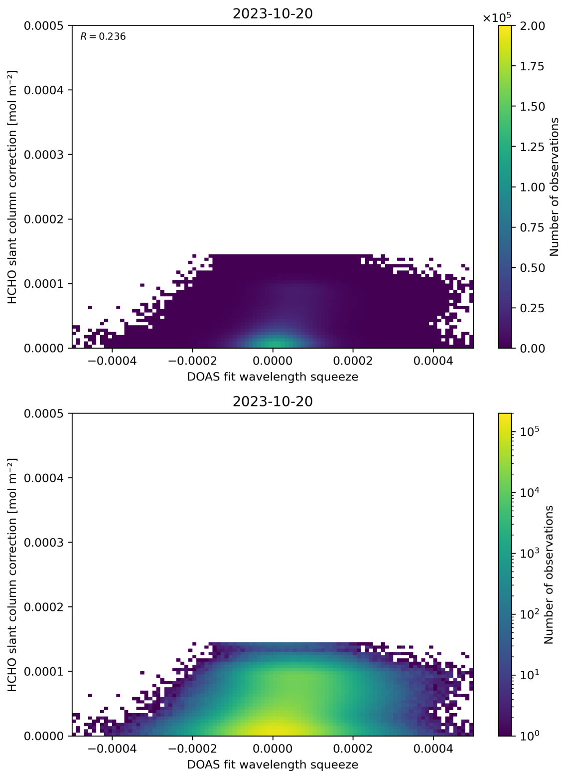
Figure 70: Scatter density plot of “DOAS fit wavelength squeeze” against “HCHO slant column correction” for 2023-10-19 to 2023-10-21.
