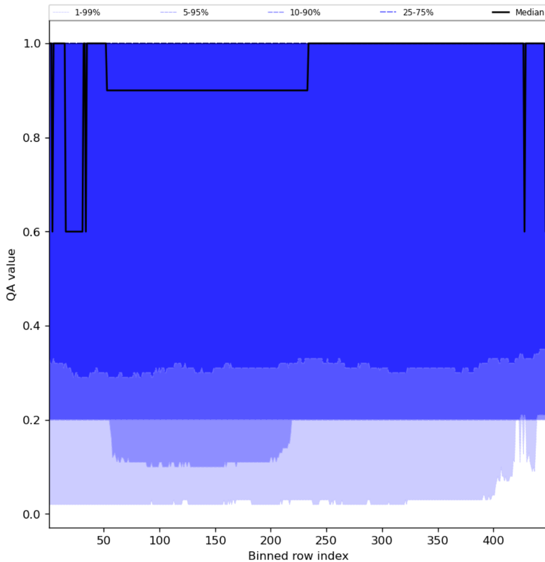
Figure 48: Along track statistics of “QA value” for 2023-10-19 to 2023-10-21
