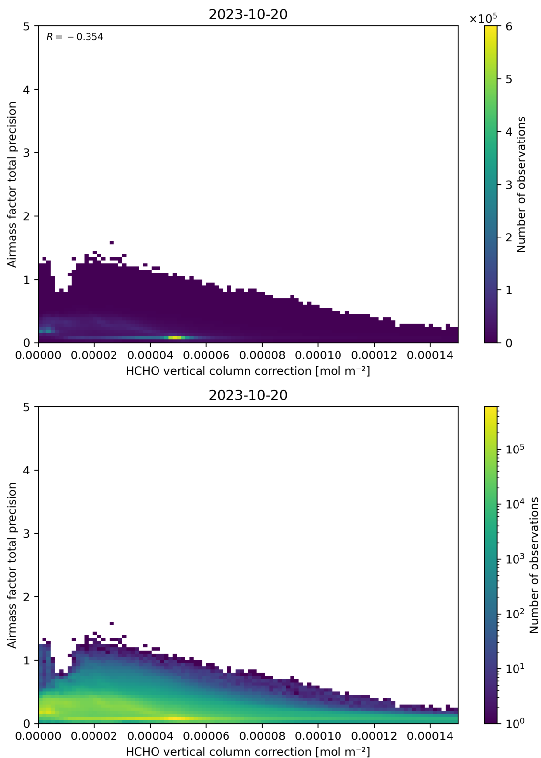
Figure 121: Scatter density plot of “HCHO vertical column correction” against “Airmass factor total precision” for 2023-10-19 to 2023-10-21.
