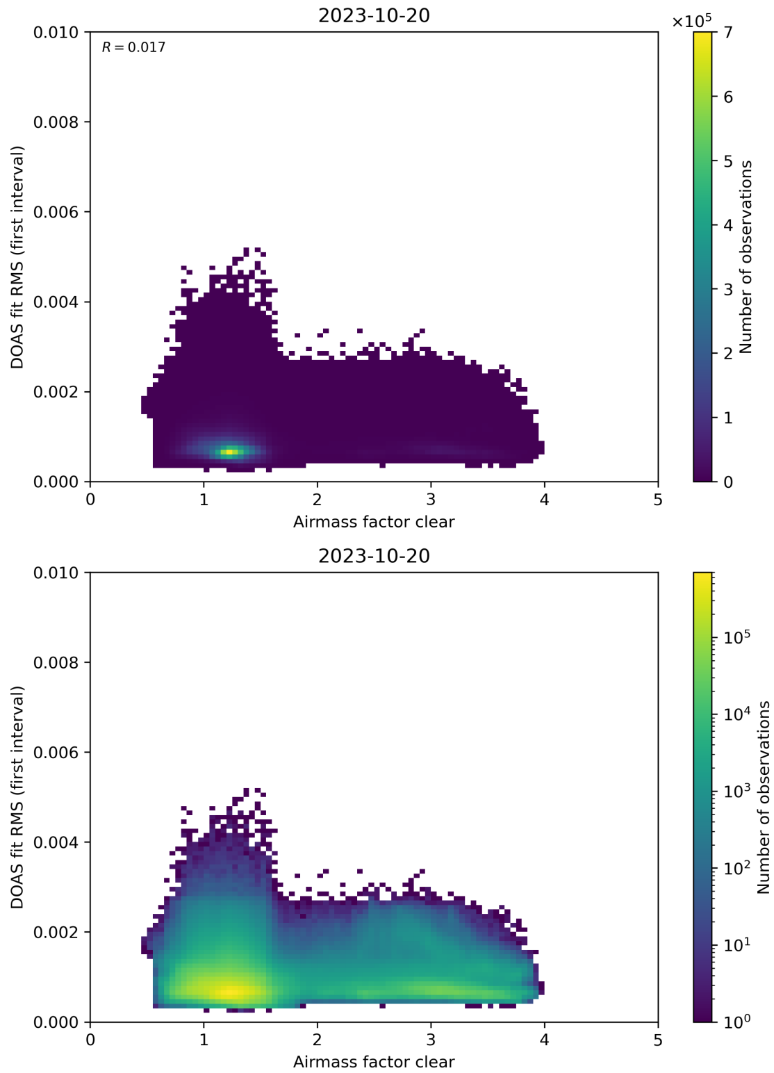
Figure 71: Scatter density plot of “Airmass factor clear” against “DOAS fit RMS (first interval)” for 2023-10-19 to 2023-10-21.
