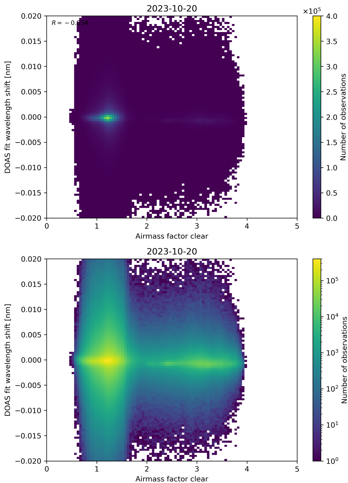
Figure 72: Scatter density plot of “Airmass factor clear” against “DOAS fit wavelength shift” for 2023-10-19 to 2023-10-21.
