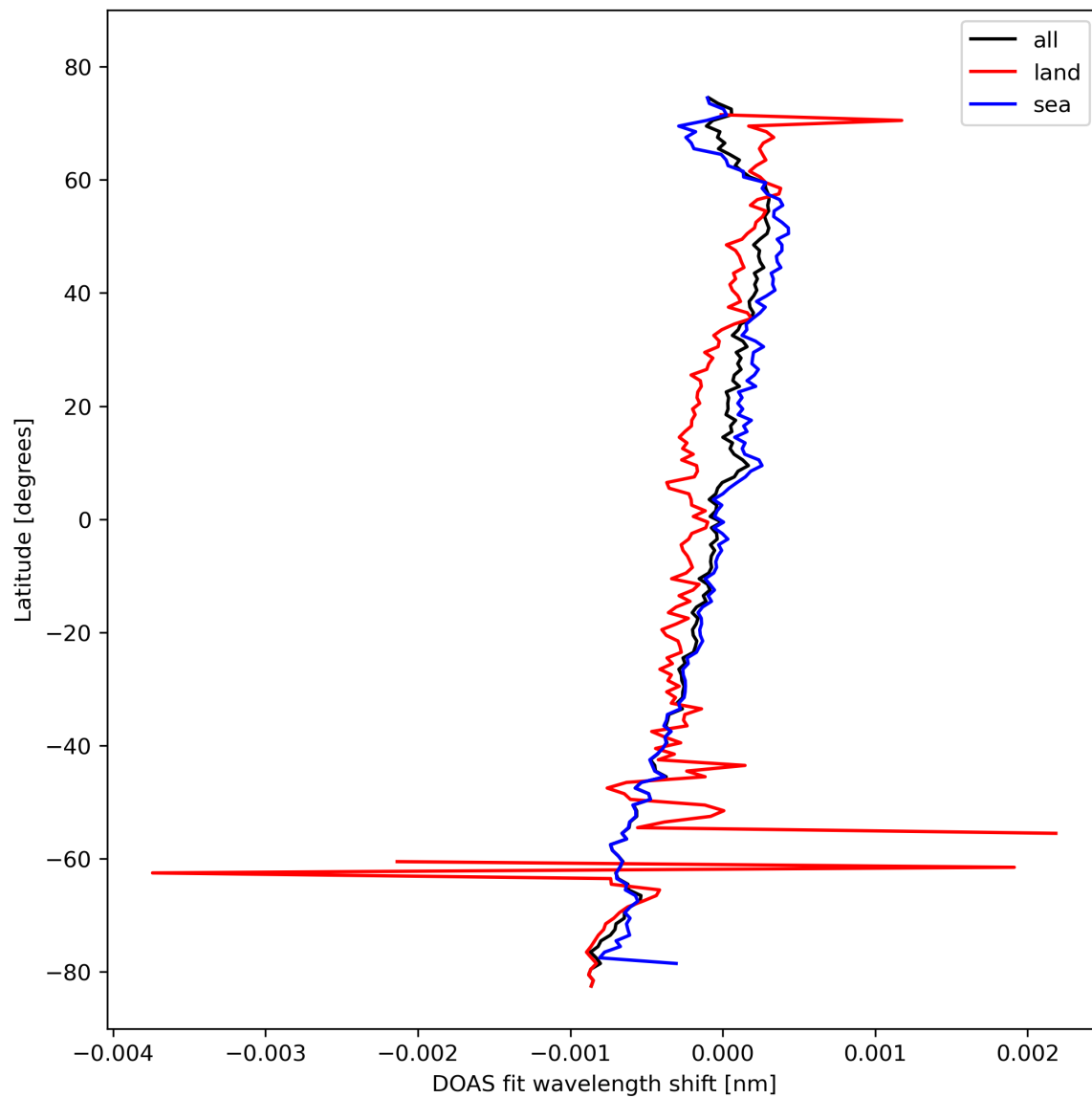
Figure 30: Zonal average of "DOAS fit wavelength shift" for 2023-10-19 to 2023-10-21.
