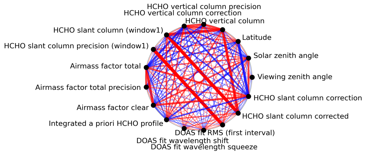
Figure 1: Map of correlation graph for 2023-10-19 to 2023-10-21.
