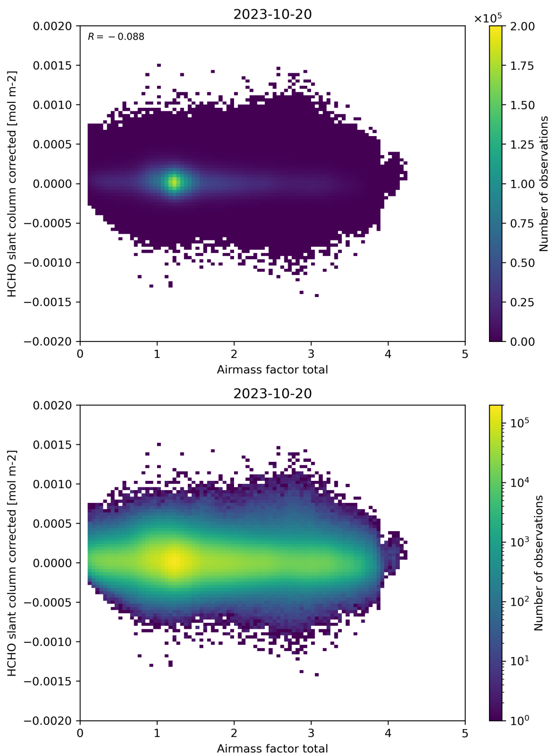
Figure 101: Scatter density plot of “Airmass factor total” against “HCHO slant column corrected” for 2023-10-19 to 2023-10-21.
