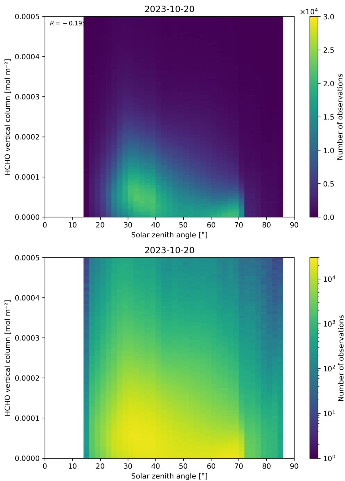
Figure 177: Scatter density plot of “Solar zenith angle” against “HCHO vertical column” for 2023-10-19 to 2023-10-21.
