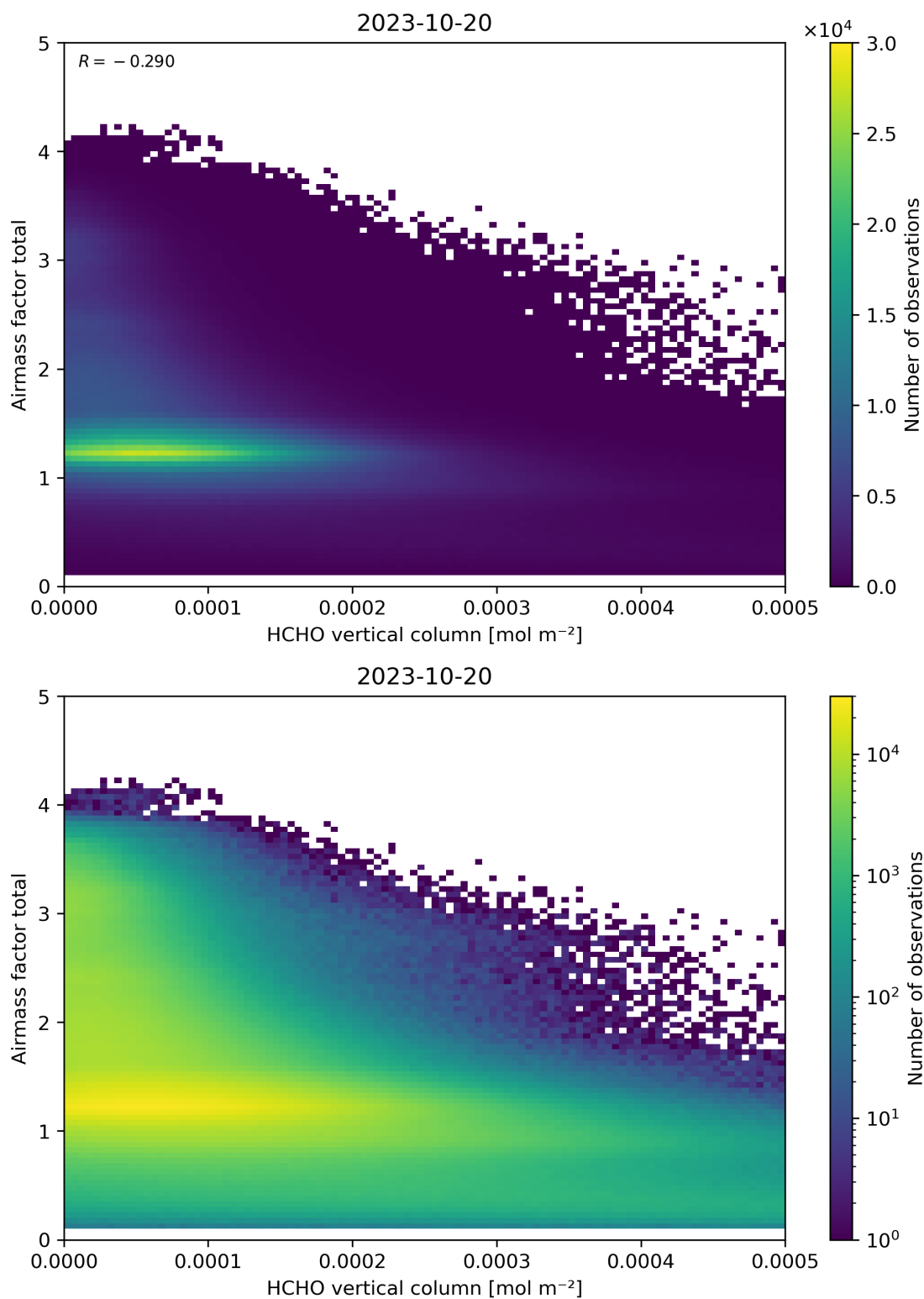
Figure 131: Scatter density plot of “HCHO vertical column” against “Airmass factor total” for 2023-10-19 to 2023-10-21.
