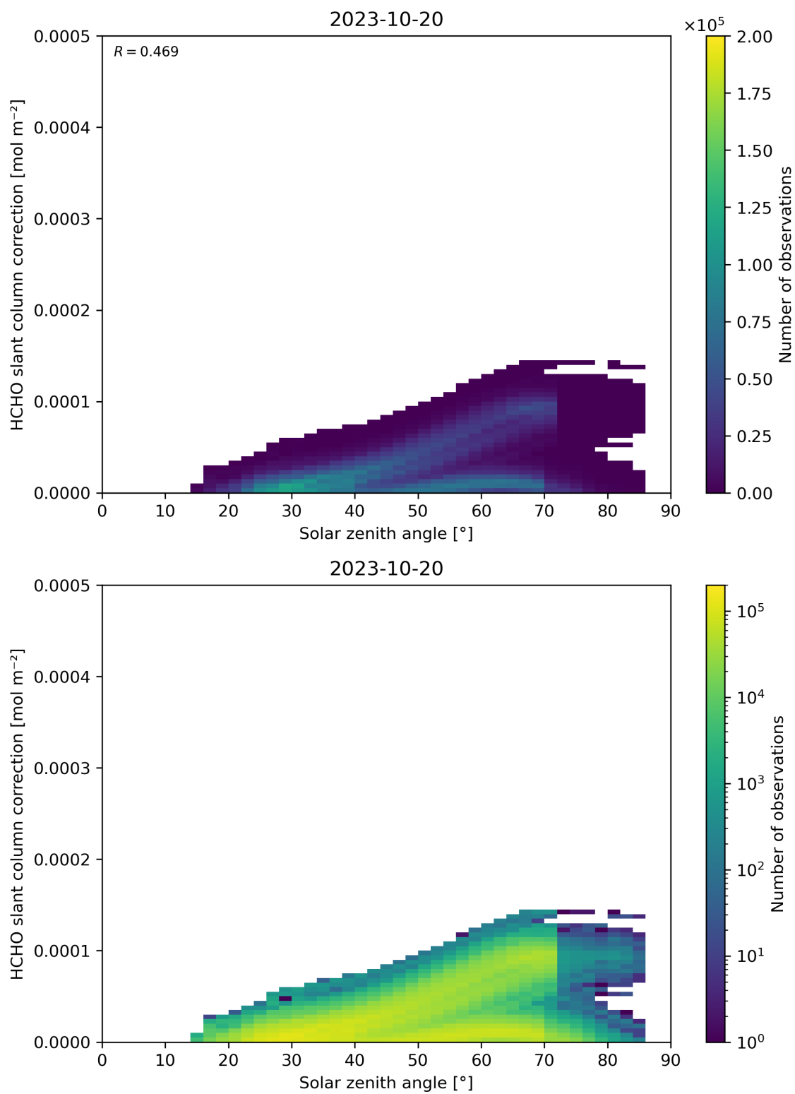
Figure 172: Scatter density plot of “Solar zenith angle” against “HCHO slant column correction” for 2023-10-19 to 2023-10-21.
