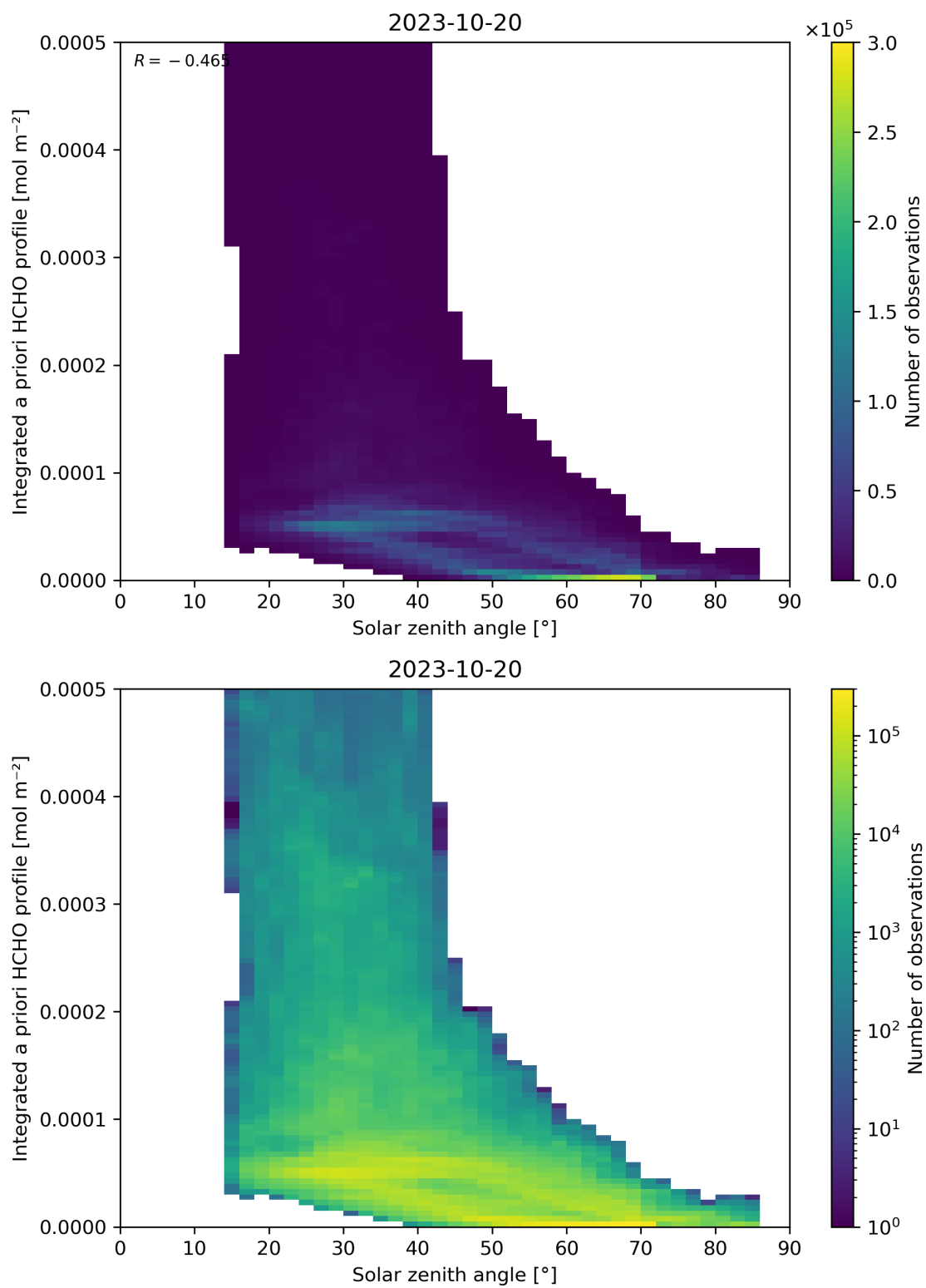
Figure 180: Scatter density plot of “Solar zenith angle” against “Integrated a priori HCHO profile” for 2023-10-19 to 2023-10-21.
