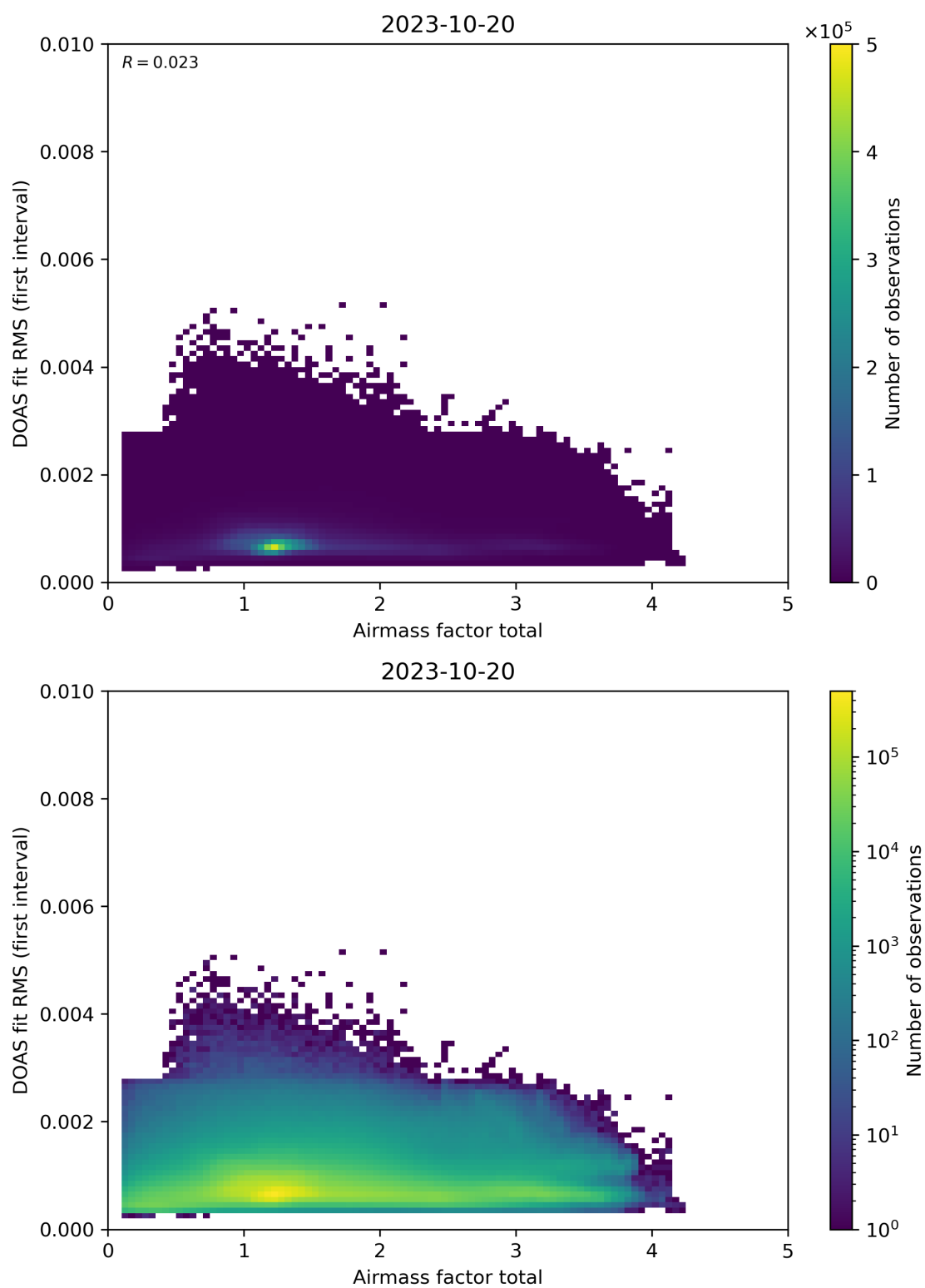
Figure 97: Scatter density plot of “Airmass factor total” against “DOAS fit RMS (first interval)” for 2023-10-19 to 2023-10-21.
