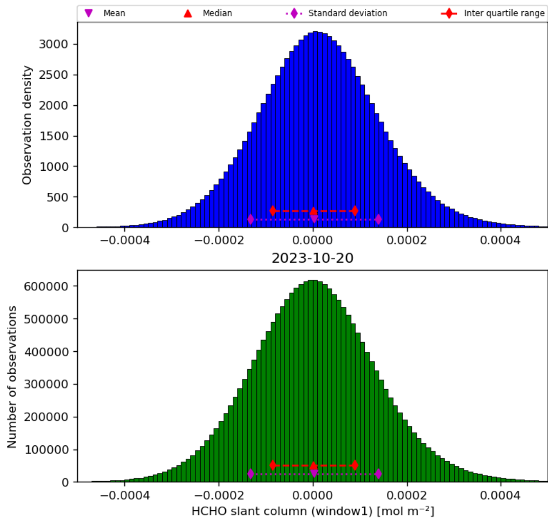
Figure 38: Histogram of “HCHO slant column (window1)” for 2023-10-19 to 2023-10-21
