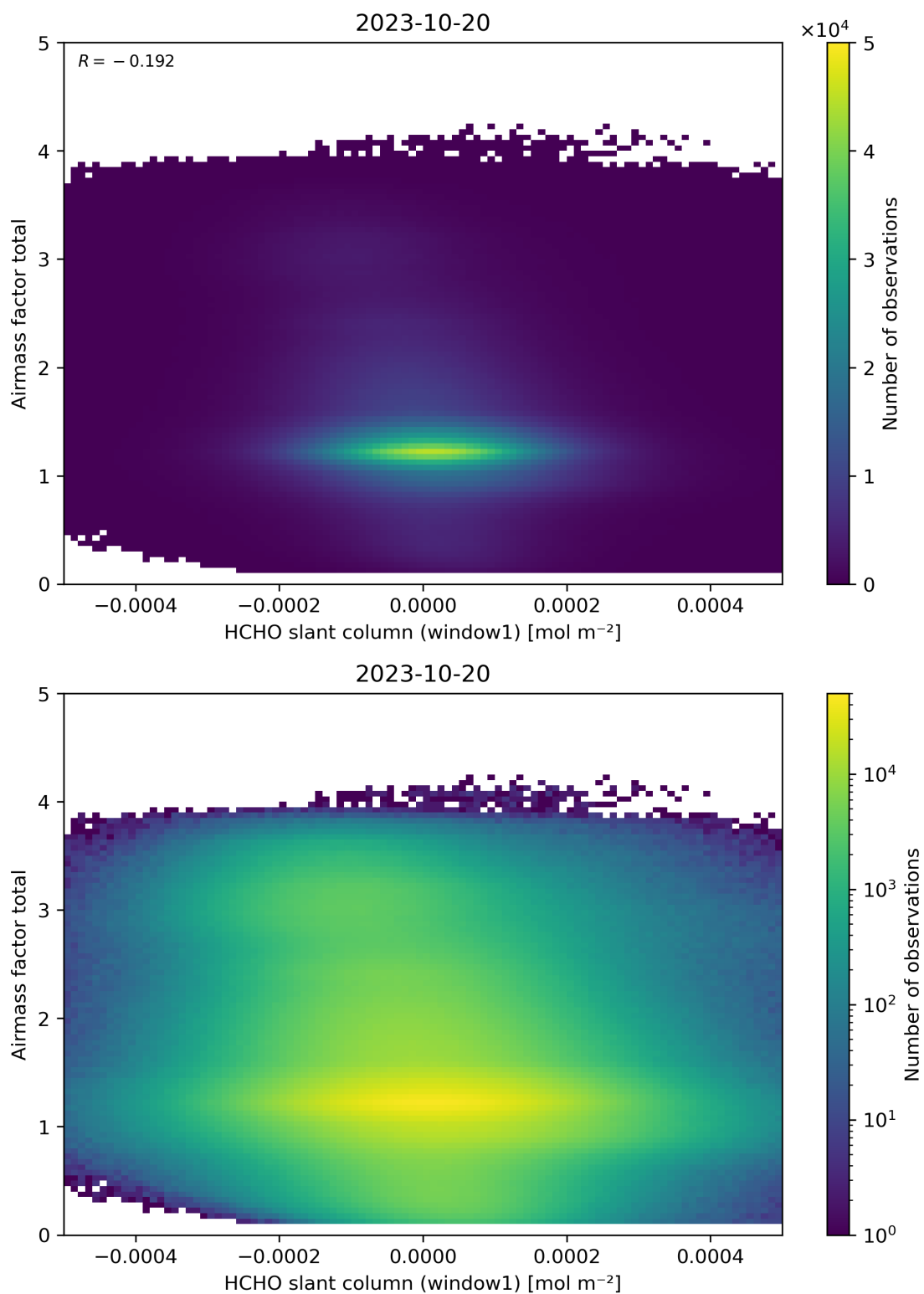
Figure 85: Scatter density plot of “HCHO slant column (window1)” against “Airmass factor total” for 2023-10-19 to 2023-10-21.
