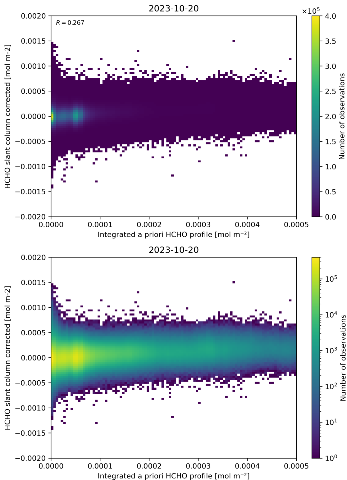
Figure 151: Scatter density plot of “Integrated a priori HCHO profile” against “HCHO slant column corrected” for 2023-10-19 to 2023-10-21.
