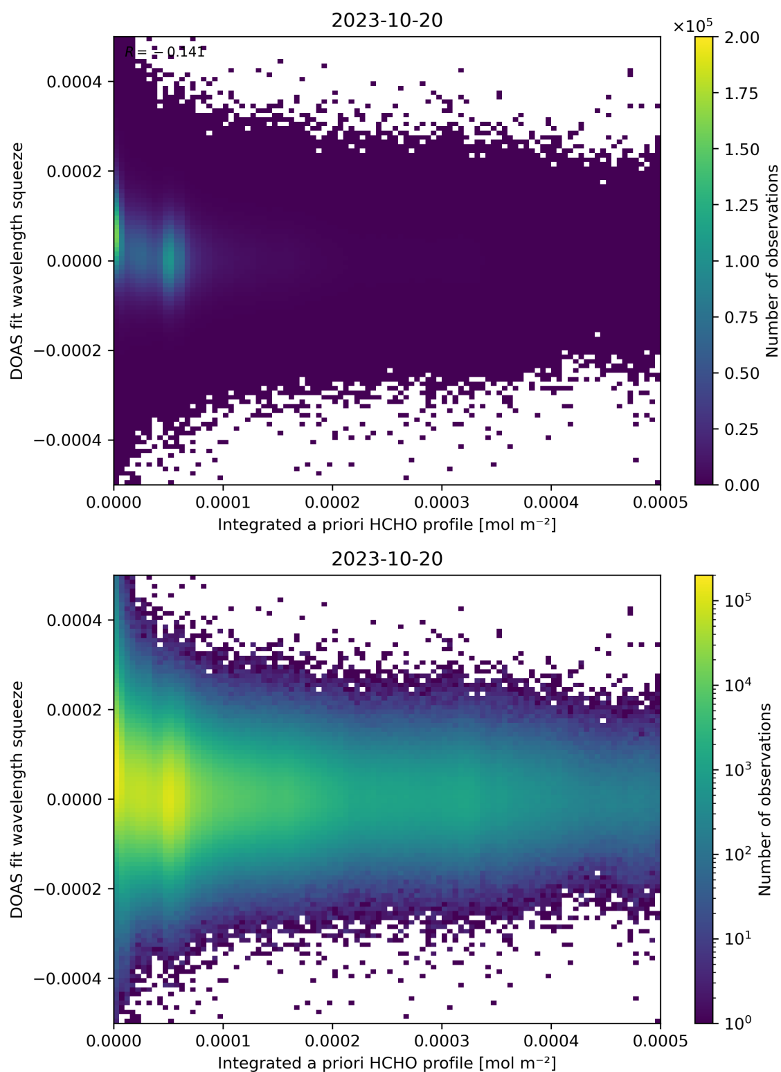
Figure 150: Scatter density plot of “Integrated a priori HCHO profile” against “DOAS fit wavelength squeeze” for 2023-10-19 to 2023-10-21.
