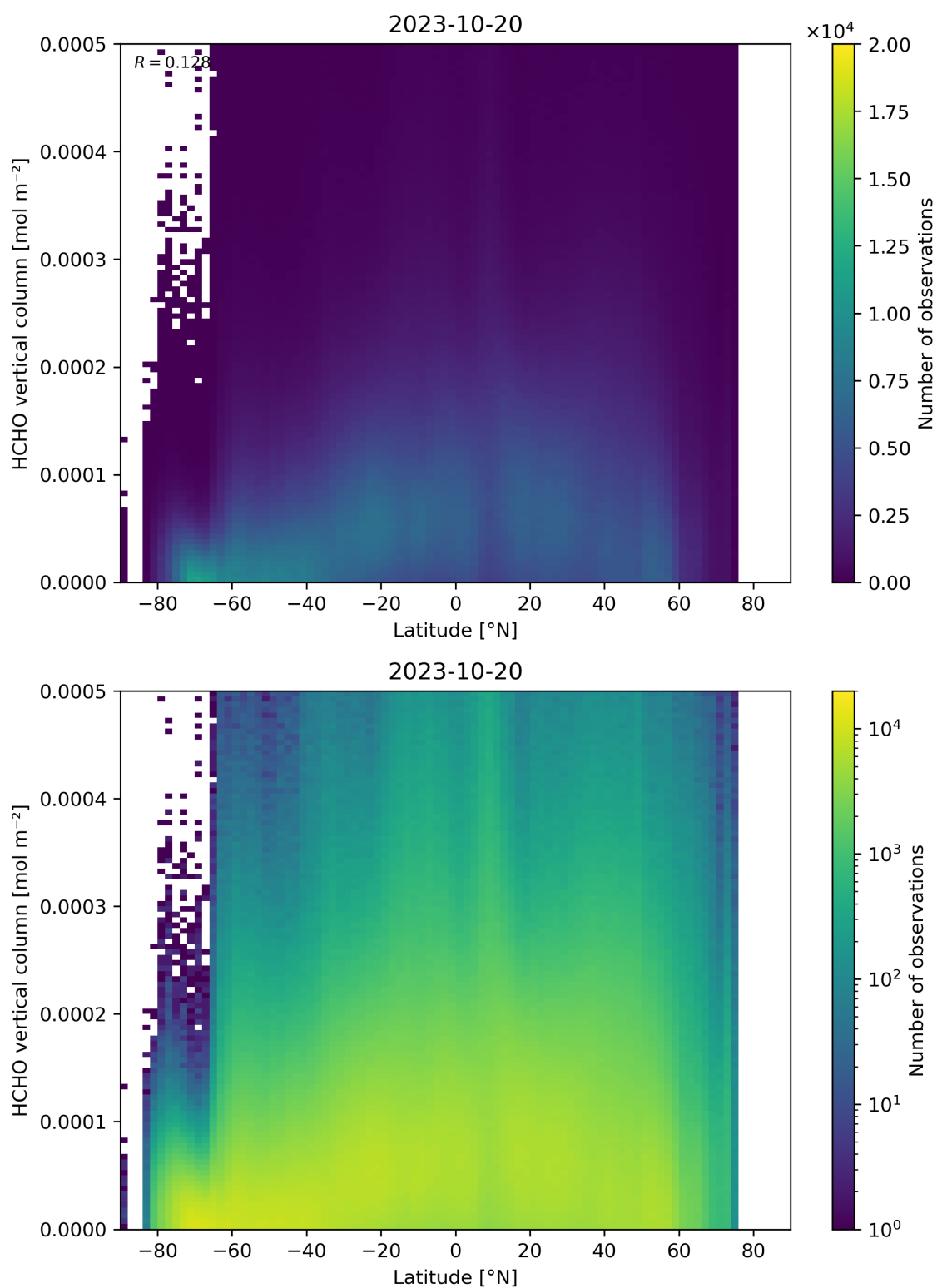
Figure 163: Scatter density plot of “Latitude” against “HCHO vertical column” for 2023-10-19 to 2023-10-21.
