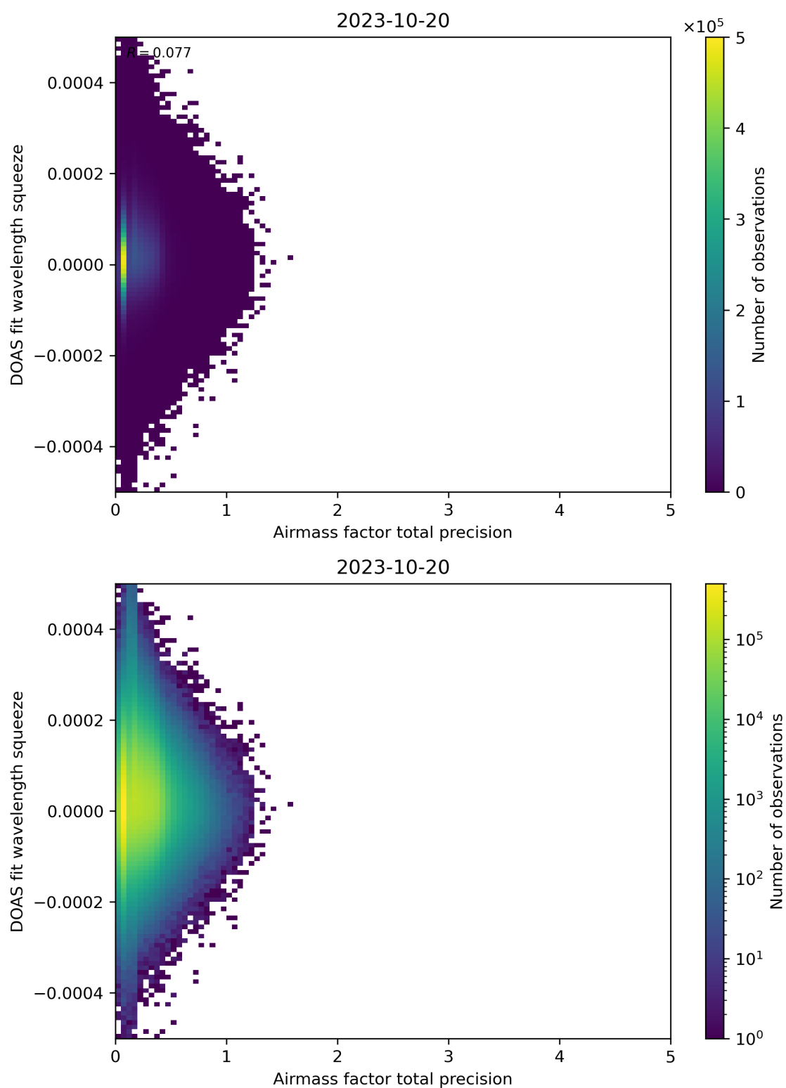
Figure 107: Scatter density plot of “Airmass factor total precision” against “DOAS fit wavelength squeeze” for 2023-10-19 to 2023-10-21.
