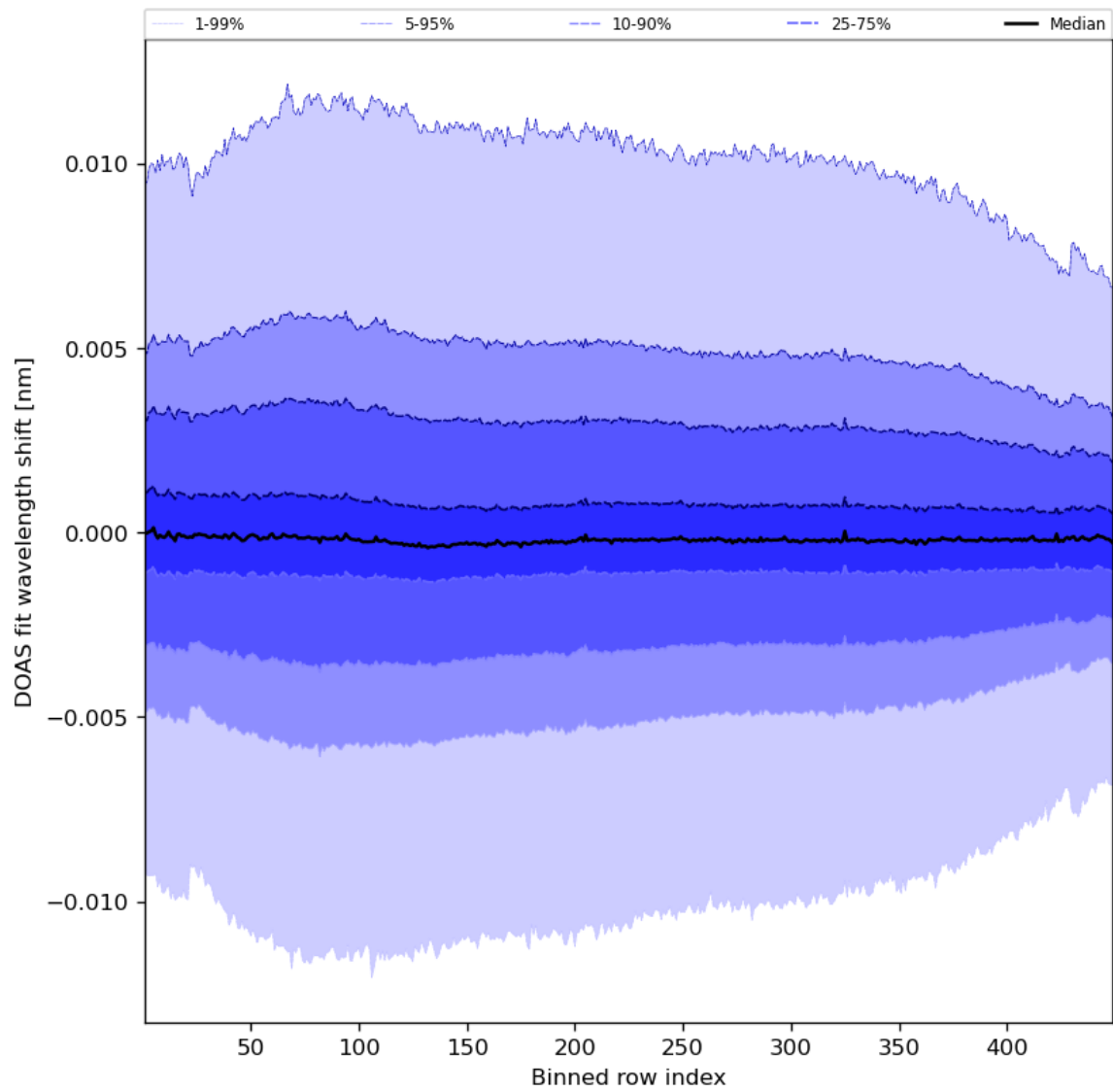
Figure 58: Along track statistics of “DOAS fit wavelength shift” for 2023-10-19 to 2023-10-21
