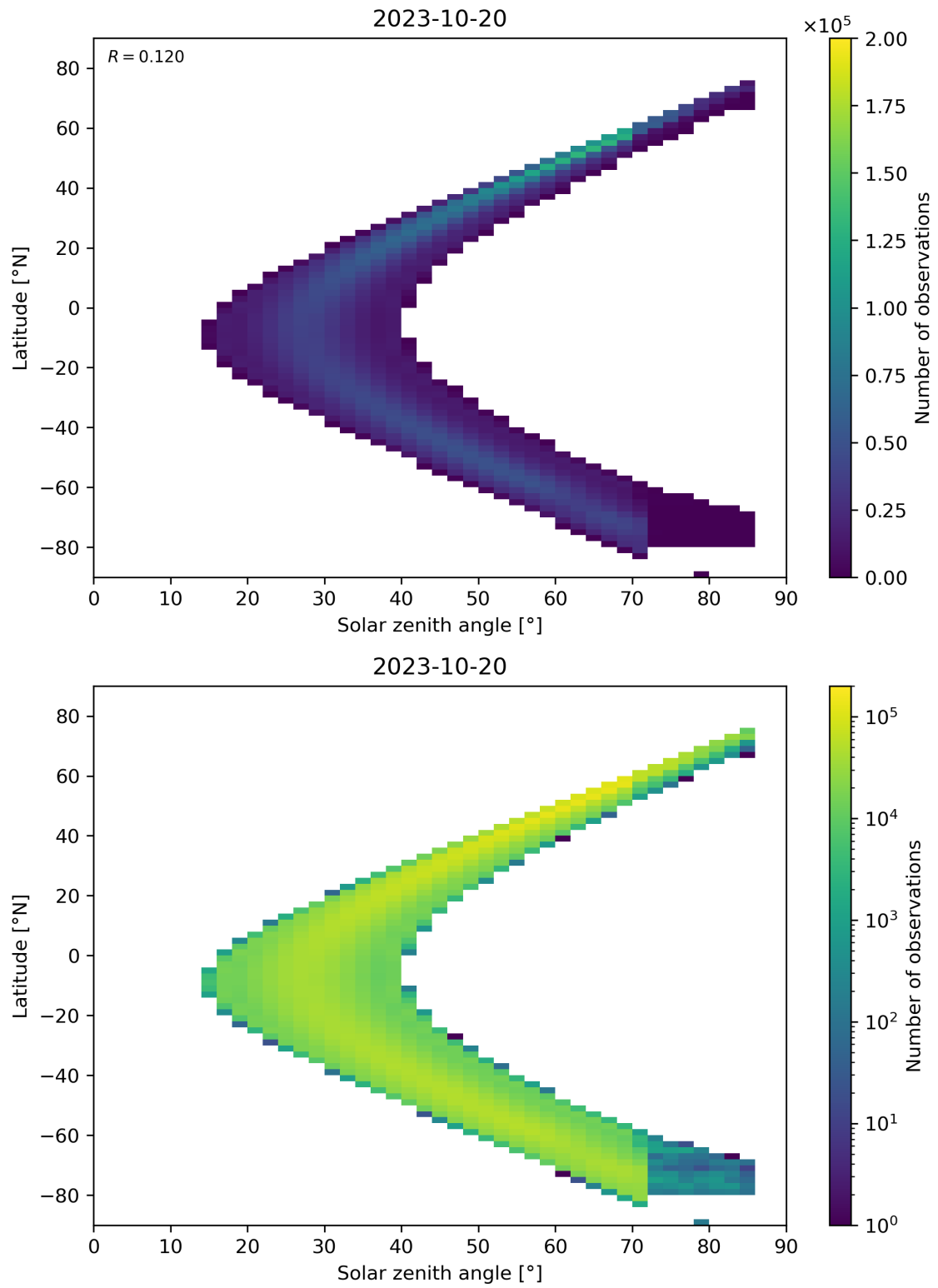
Figure 181: Scatter density plot of “Solar zenith angle” against “Latitude” for 2023-10-19 to 2023-10-21.
