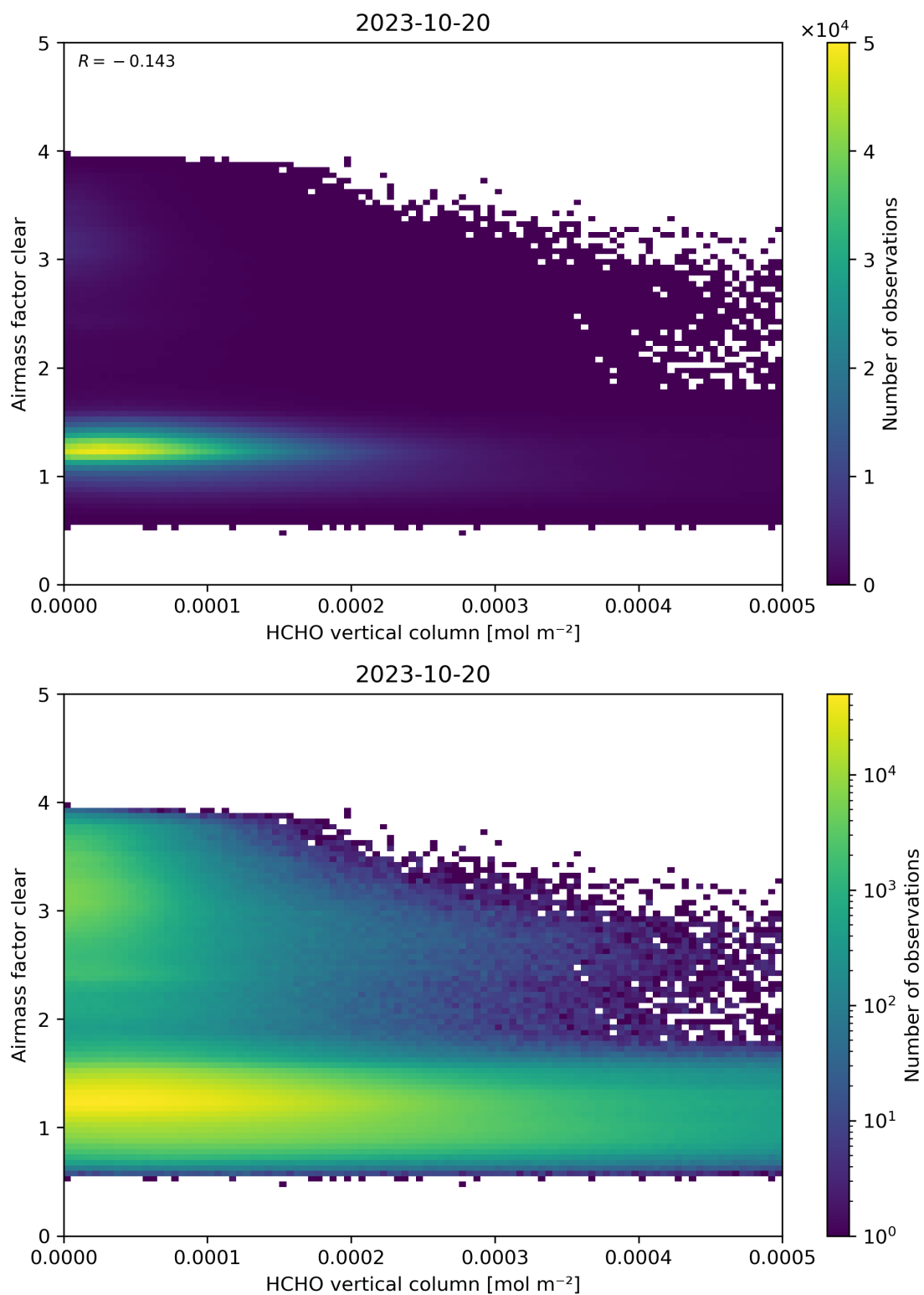
Figure 126: Scatter density plot of “HCHO vertical column” against “Airmass factor clear” for 2023-10-19 to 2023-10-21.
