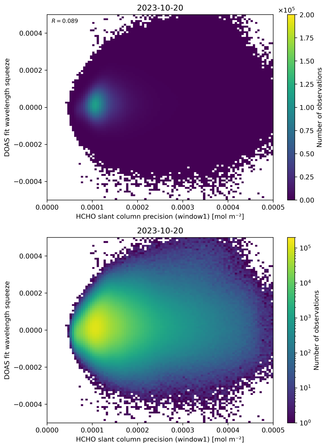
Figure 90: Scatter density plot of “HCHO slant column precision (window1)” against “DOAS fit wavelength squeeze” for 2023-10-19 to 2023-10-21.
