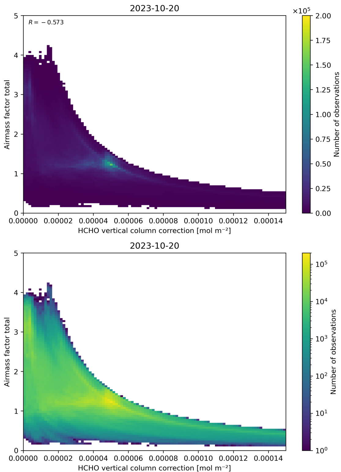
Figure 120: Scatter density plot of “HCHO vertical column correction” against “Airmass factor total” for 2023-10-19 to 2023-10-21.
