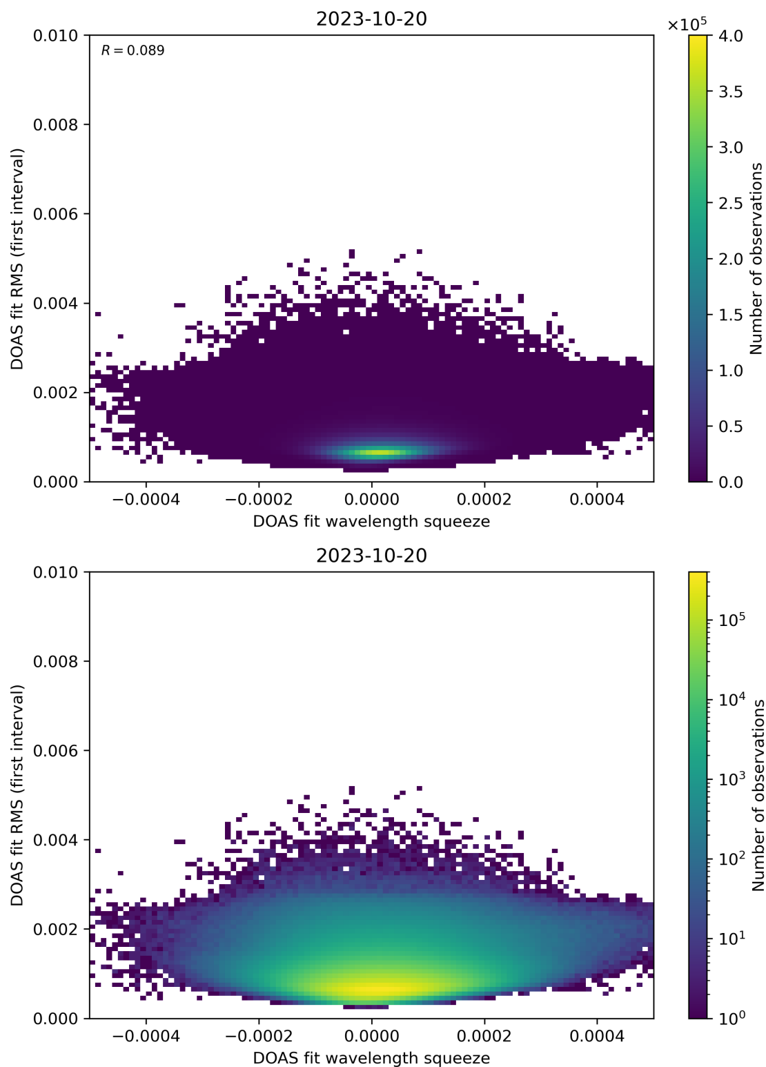
Figure 68: Scatter density plot of “DOAS fit wavelength squeeze” against “DOAS fit RMS (first interval)” for 2023-10-19 to 2023-10-21.
