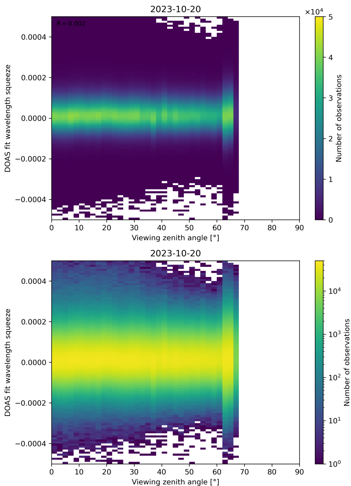
Figure 184: Scatter density plot of “Viewing zenith angle” against “DOAS fit wavelength squeeze” for 2023-10-19 to 2023-10-21.
