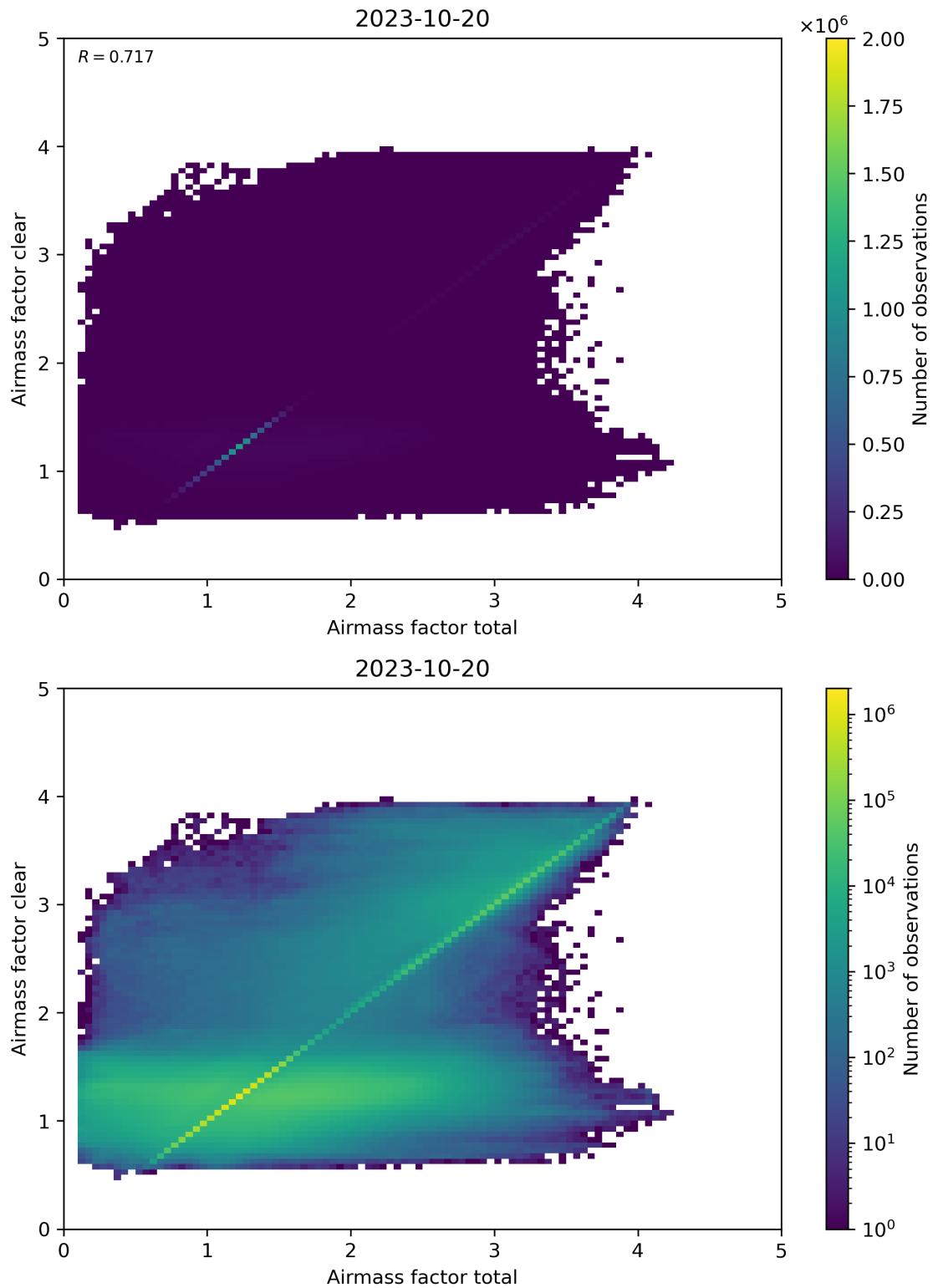
Figure 100: Scatter density plot of “Airmass factor total” against “Airmass factor clear” for 2023-10-19 to 2023-10-21.
