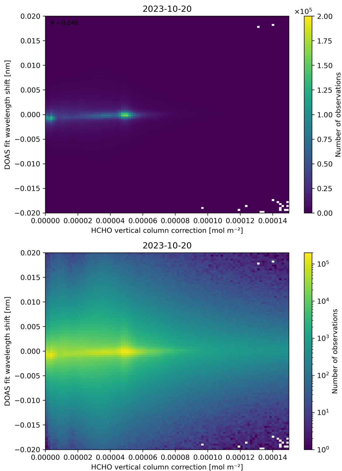
Figure 113: Scatter density plot of “HCHO vertical column correction” against “DOAS fit wavelength shift” for 2023-10-19 to 2023-10-21.
