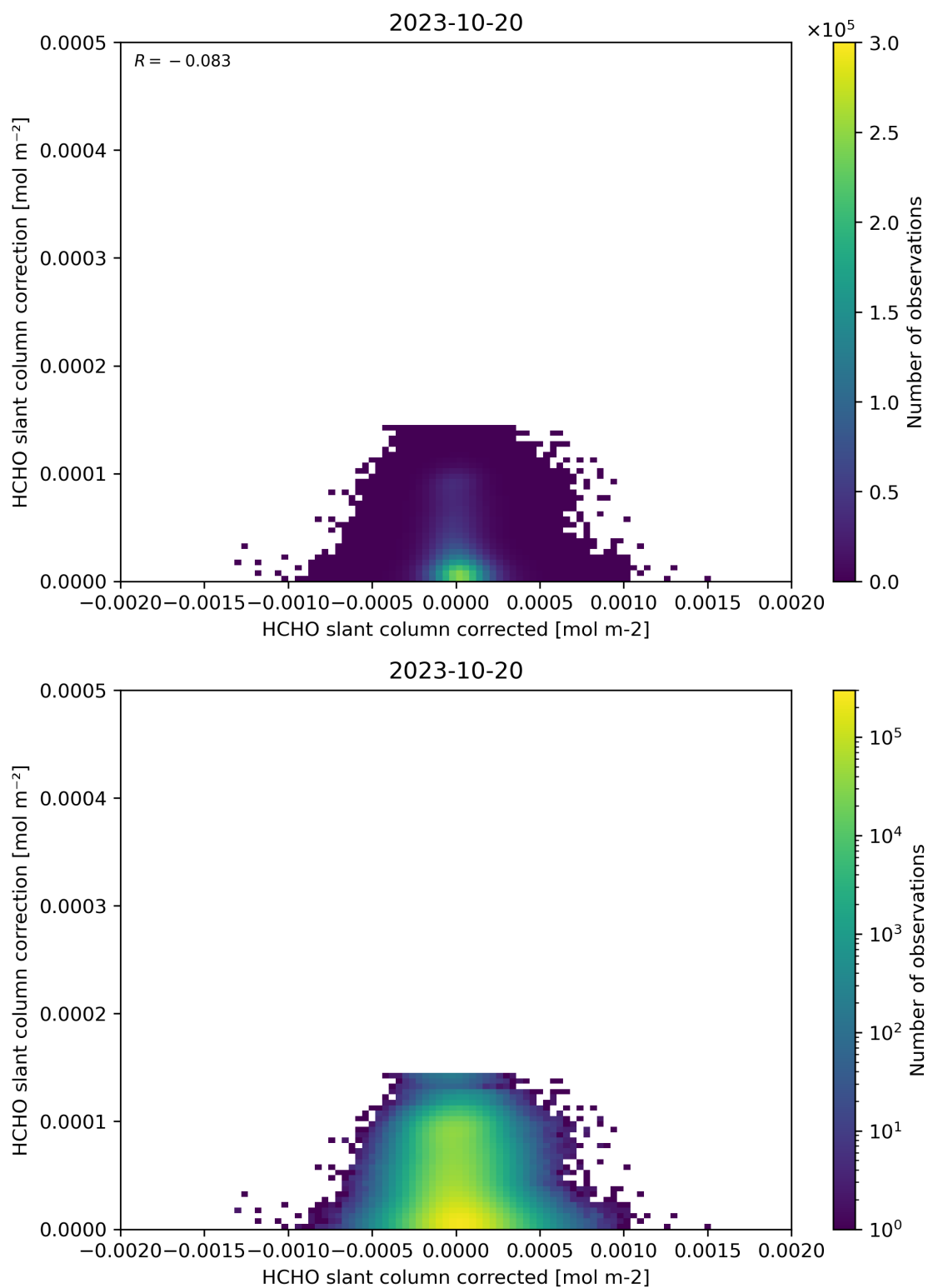
Figure 77: Scatter density plot of “HCHO slant column corrected” against “HCHO slant column correction” for 2023-10-19 to 2023-10-21.
