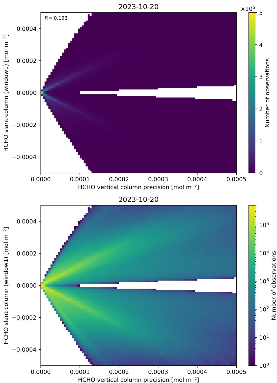
Figure 142: Scatter density plot of “HCHO vertical column precision” against “HCHO slant column (window1)” for 2023-10-19 to 2023-10-21.
