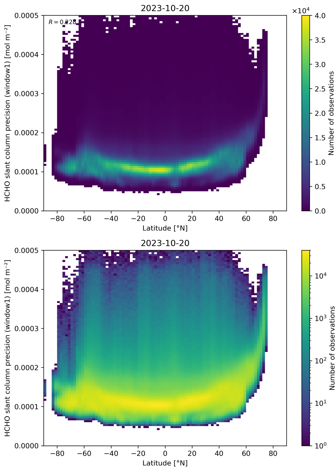
Figure 160: Scatter density plot of “Latitude” against “HCHO slant column precision (window1)” for 2023-10-19 to 2023-10-21.
