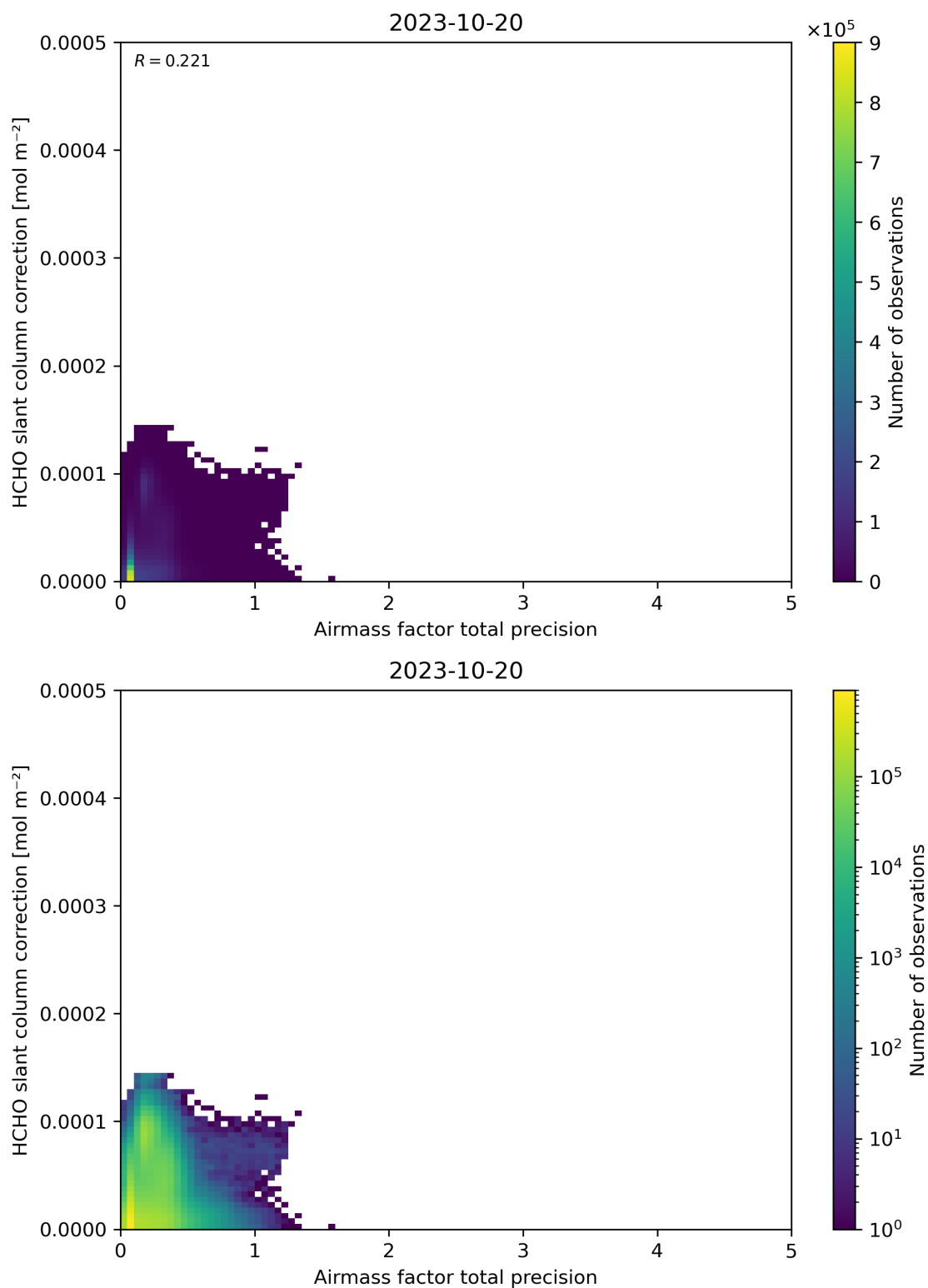
Figure 110: Scatter density plot of “Airmass factor total precision” against “HCHO slant column correction” for 2023-10-19 to 2023-10-21.
