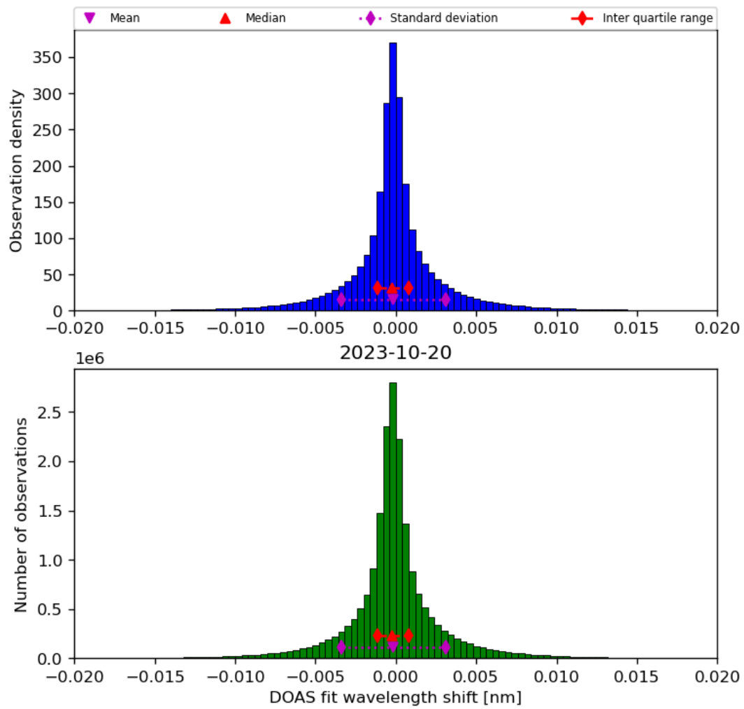
Figure 44: Histogram of “DOAS fit wavelength shift” for 2023-10-19 to 2023-10-21
