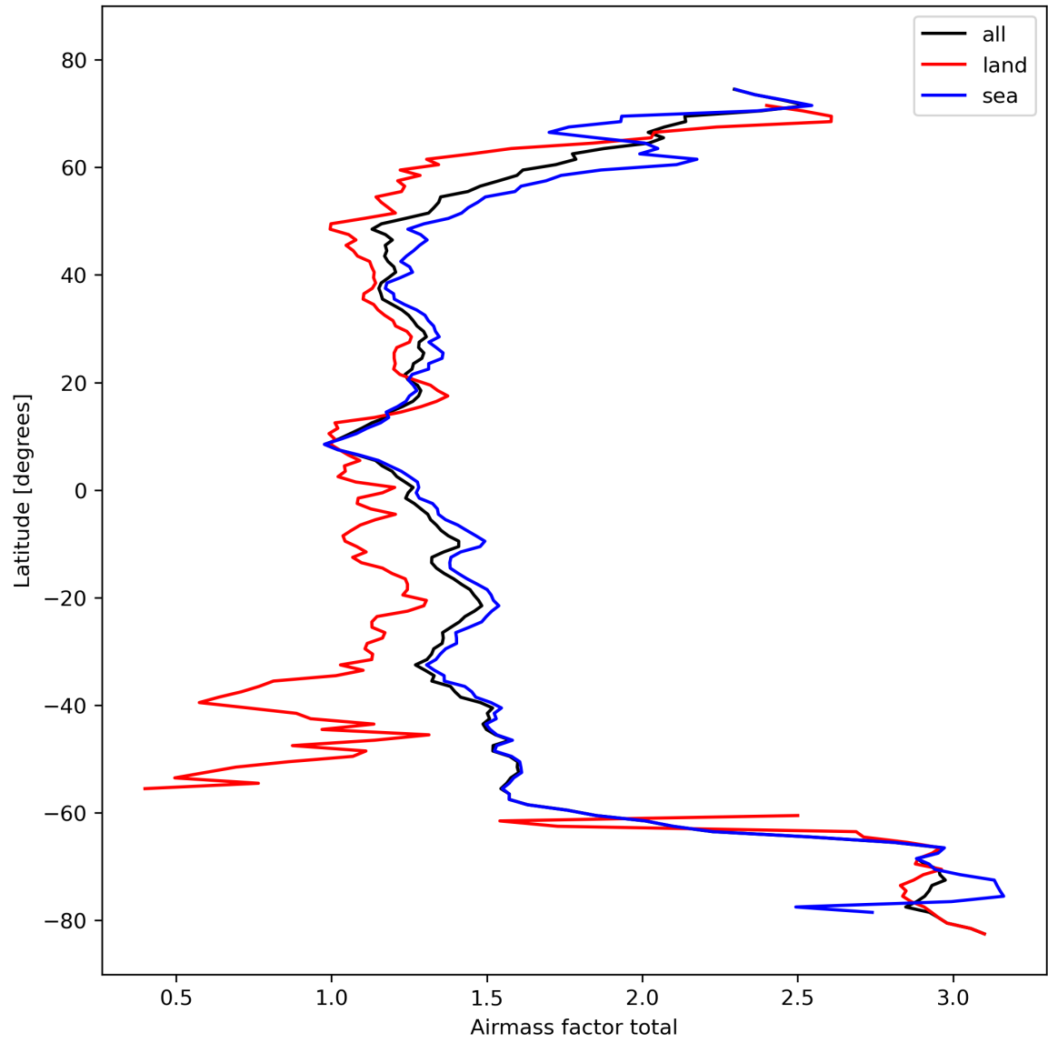
Figure 26: Zonal average of “Airmass factor total” for 2023-10-19 to 2023-10-21.
