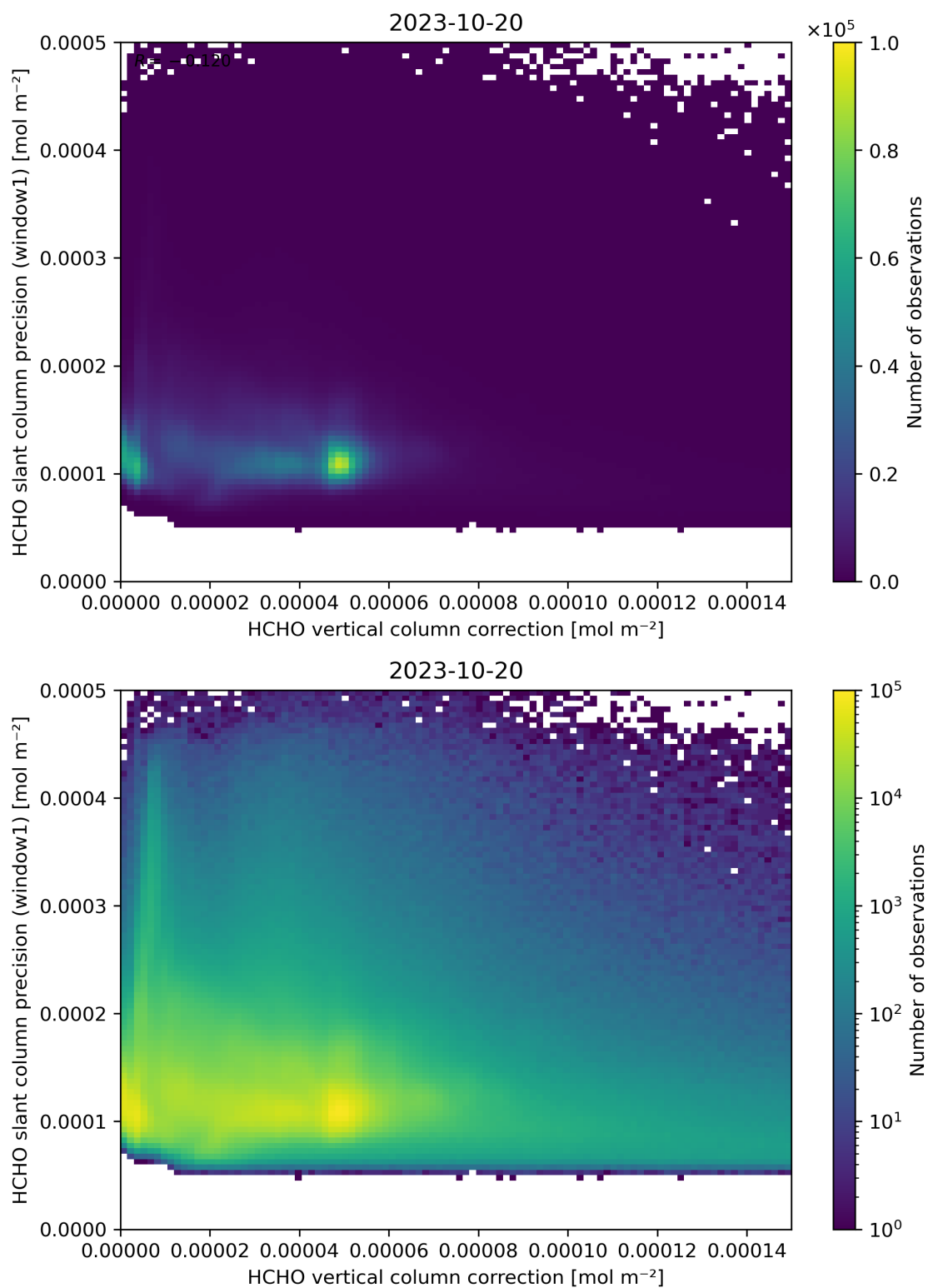
Figure 119: Scatter density plot of “HCHO vertical column correction” against “HCHO slant column precision (window1)” for 2023-10-19 to 2023-10-21.
