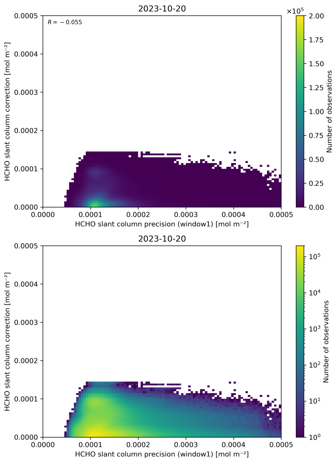
Figure 93: Scatter density plot of “HCHO slant column precision (window1)” against “HCHO slant column correction” for 2023-10-19 to 2023-10-21.
