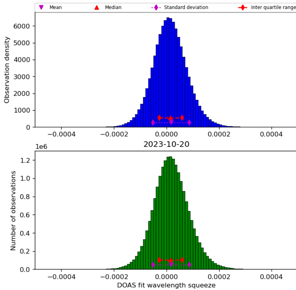
Figure 45: Histogram of “DOAS fit wavelength squeeze” for 2023-10-19 to 2023-10-21
