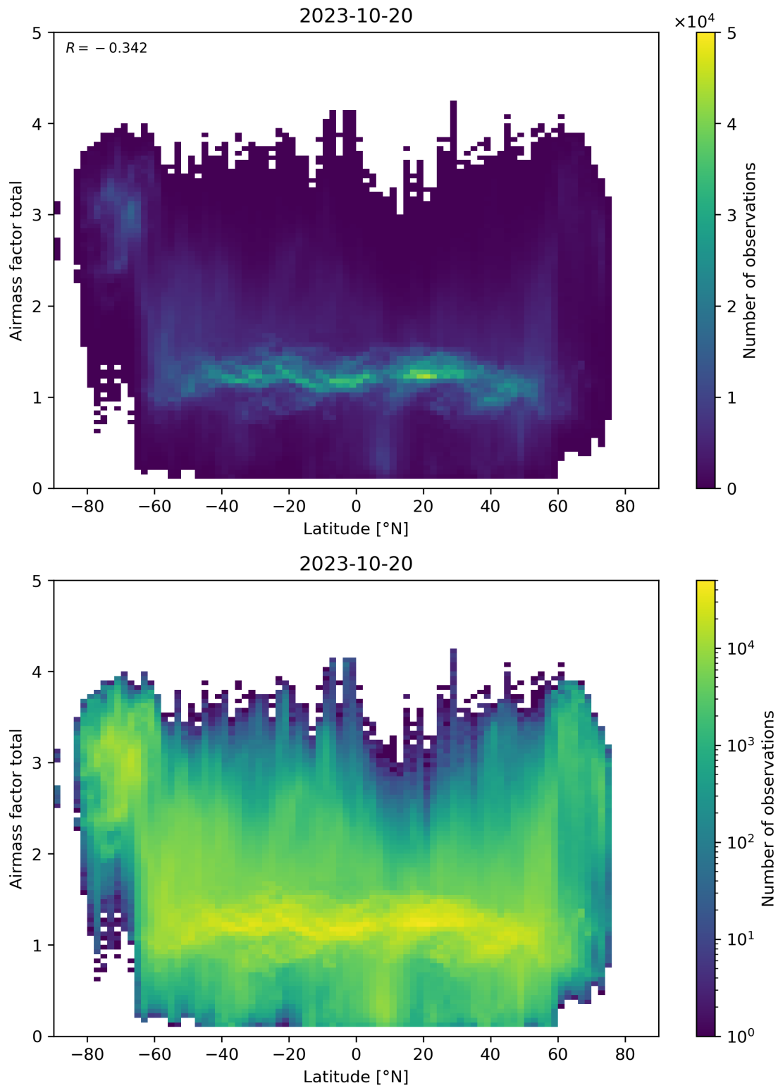
Figure 161: Scatter density plot of “Latitude” against “Airmass factor total” for 2023-10-19 to 2023-10-21.
