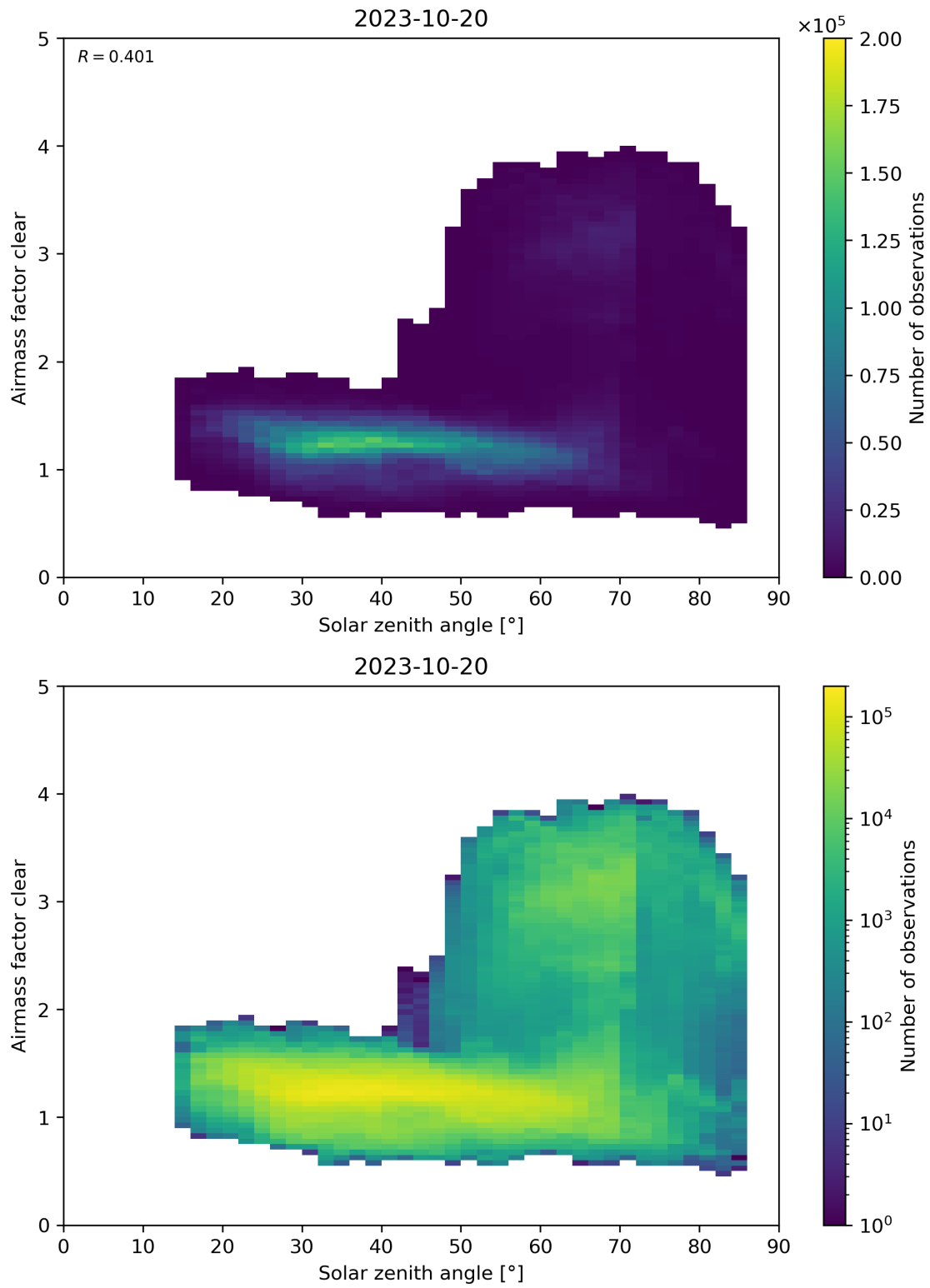
Figure 170: Scatter density plot of “Solar zenith angle” against “Airmass factor clear” for 2023-10-19 to 2023-10-21.
