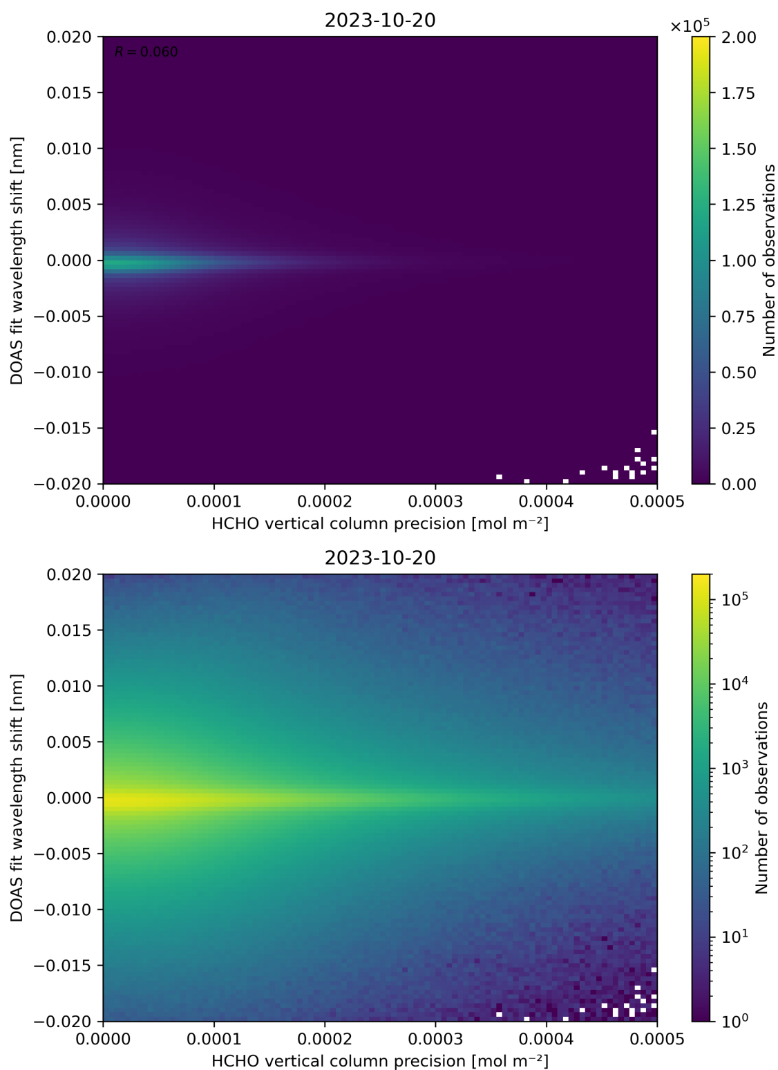
Figure 137: Scatter density plot of “HCHO vertical column precision” against “DOAS fit wavelength shift” for 2023-10-19 to 2023-10-21.
