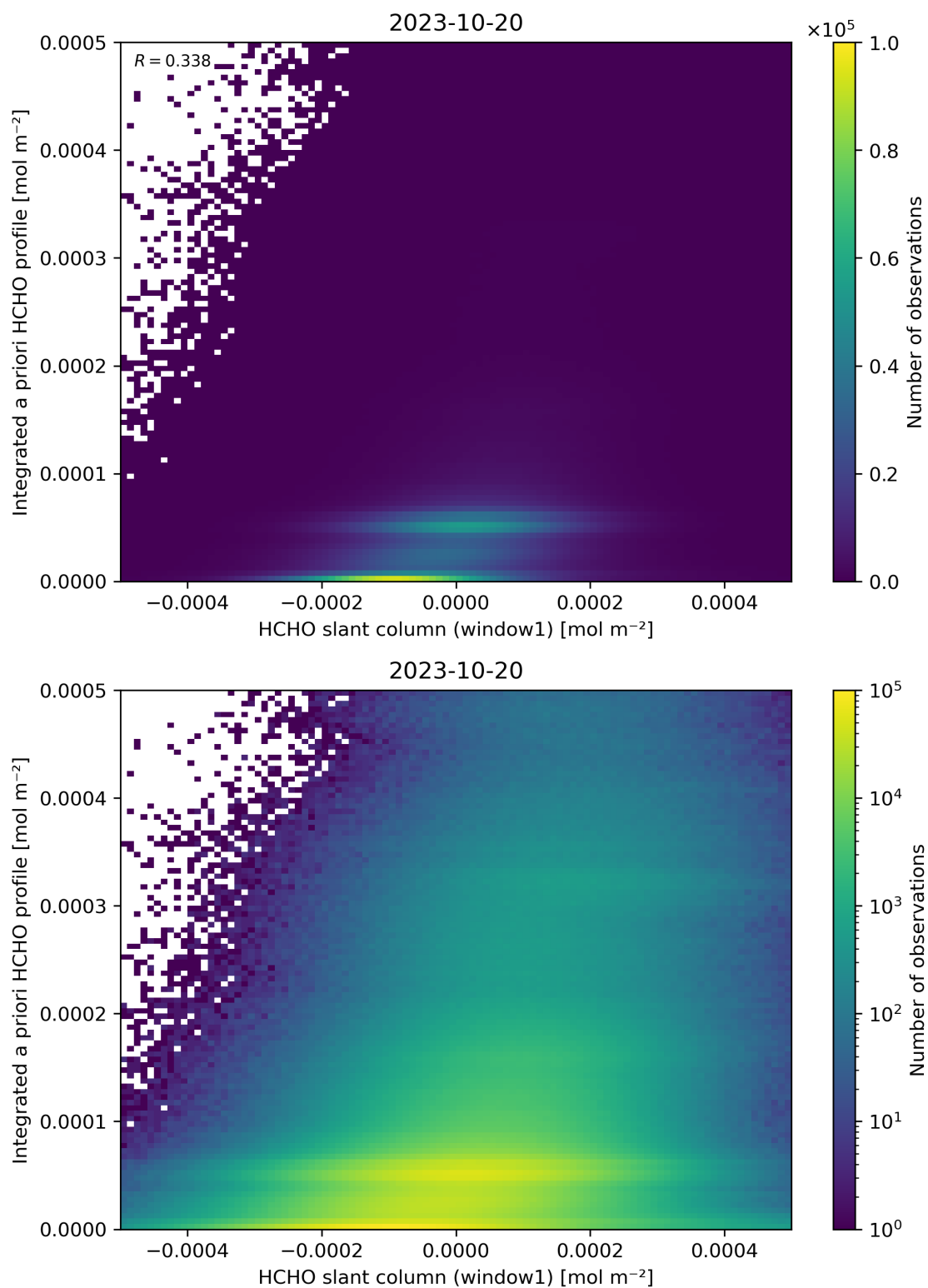
Figure 87: Scatter density plot of “HCHO slant column (window1)” against “Integrated a priori HCHO profile” for 2023-10-19 to 2023-10-21.
