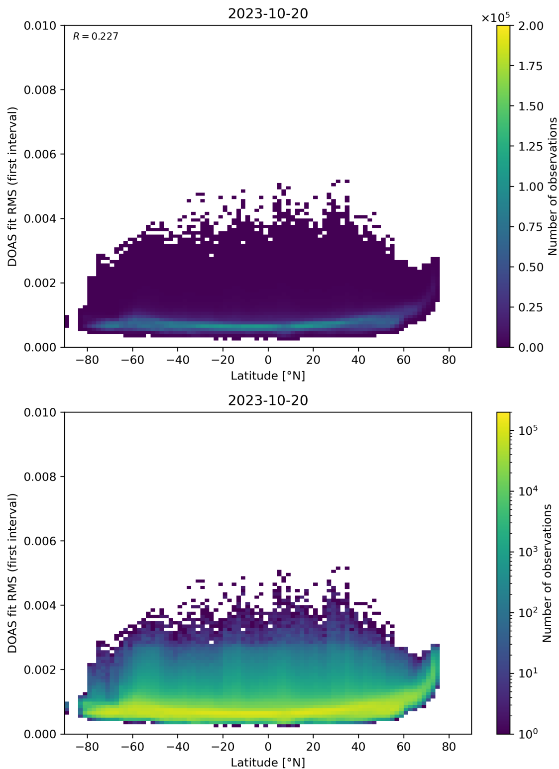
Figure 153: Scatter density plot of “Latitude” against “DOAS fit RMS (first interval)” for 2023-10-19 to 2023-10-21.
