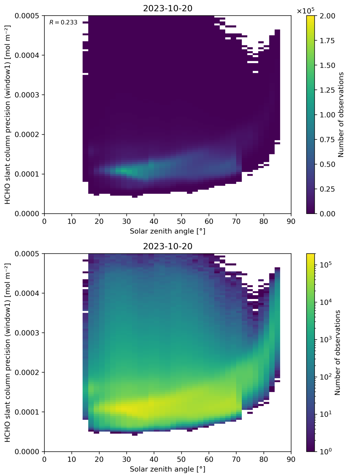
Figure 174: Scatter density plot of “Solar zenith angle” against “HCHO slant column precision (window1)” for 2023-10-19 to 2023-10-21.
