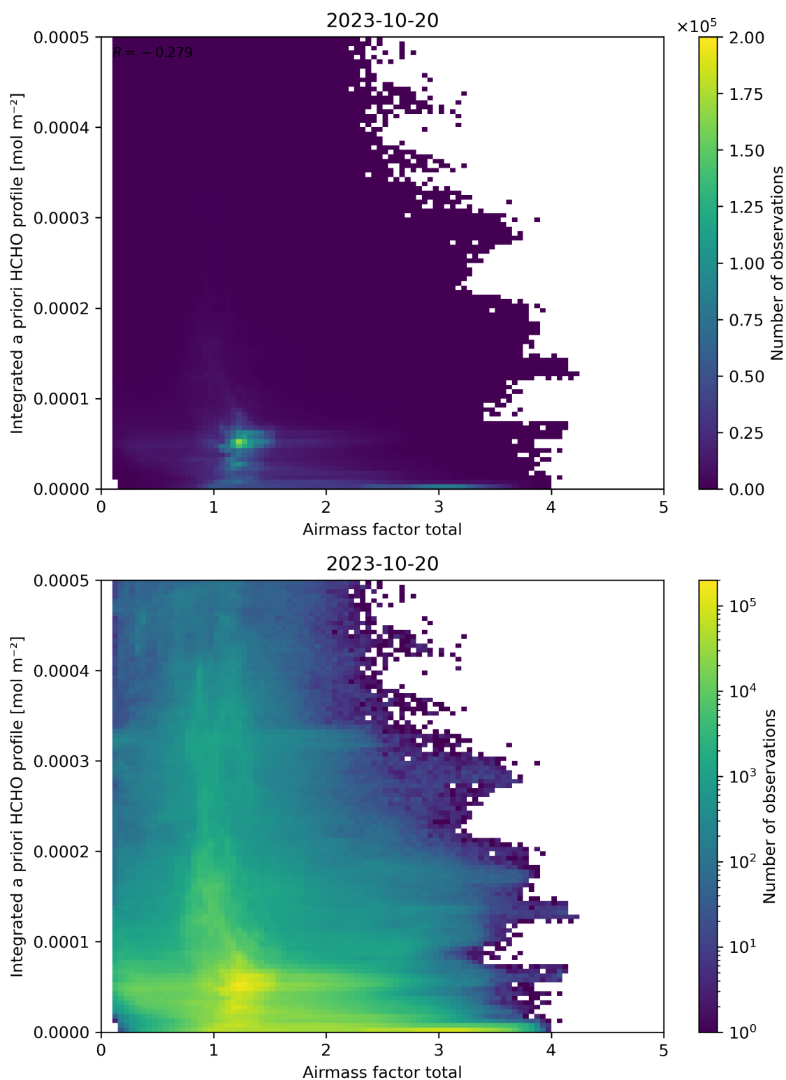
Figure 104: Scatter density plot of “Airmass factor total” against “Integrated a priori HCHO profile” for 2023-10-19 to 2023-10-21.
