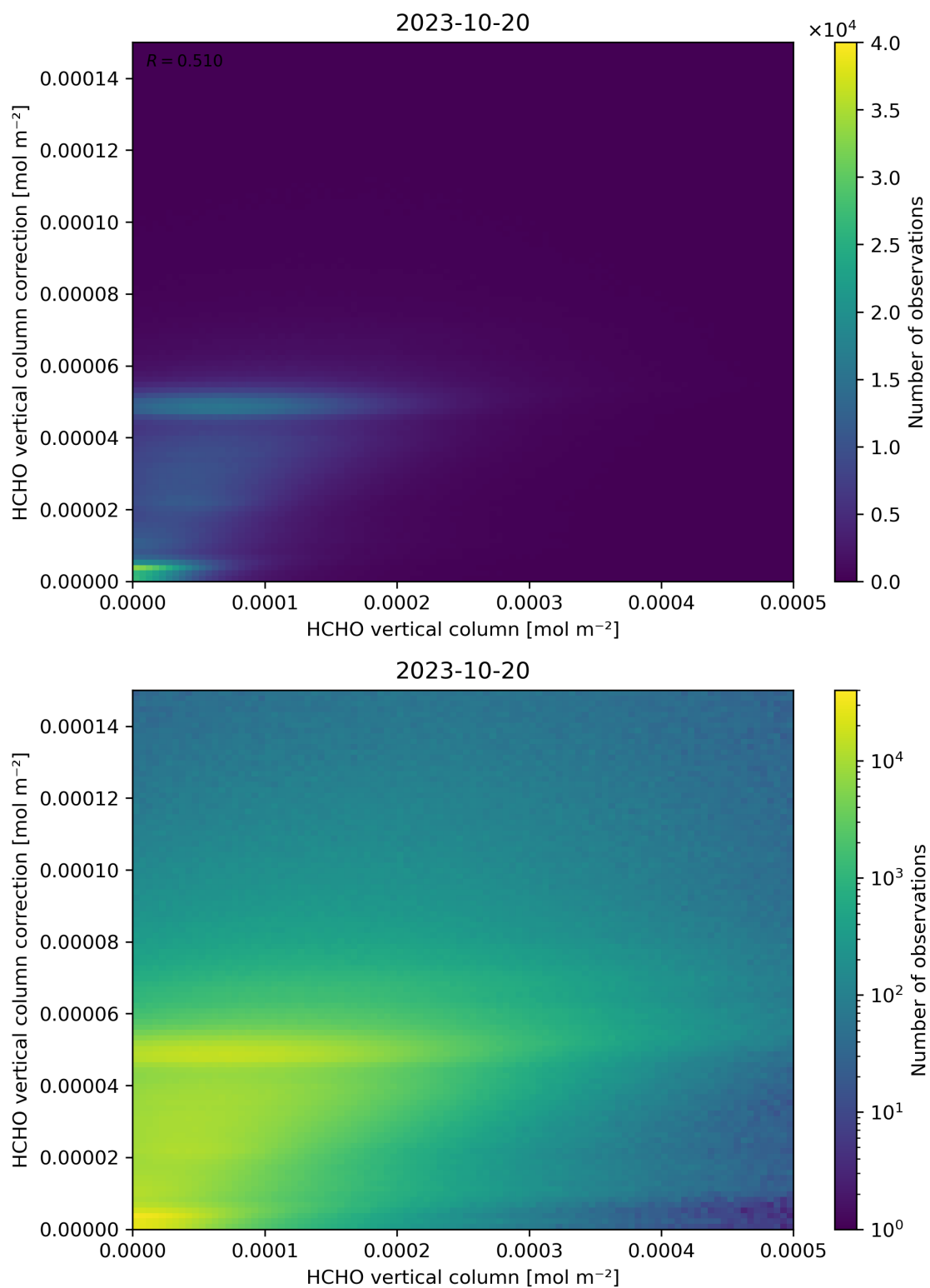
Figure 133: Scatter density plot of “HCHO vertical column” against “HCHO vertical column correction” for 2023-10-19 to 2023-10-21.
