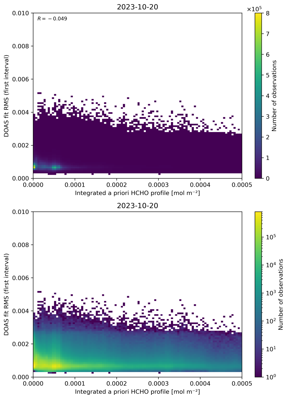
Figure 148: Scatter density plot of “Integrated a priori HCHO profile” against “DOAS fit RMS (first interval)” for 2023-10-19 to 2023-10-21.
