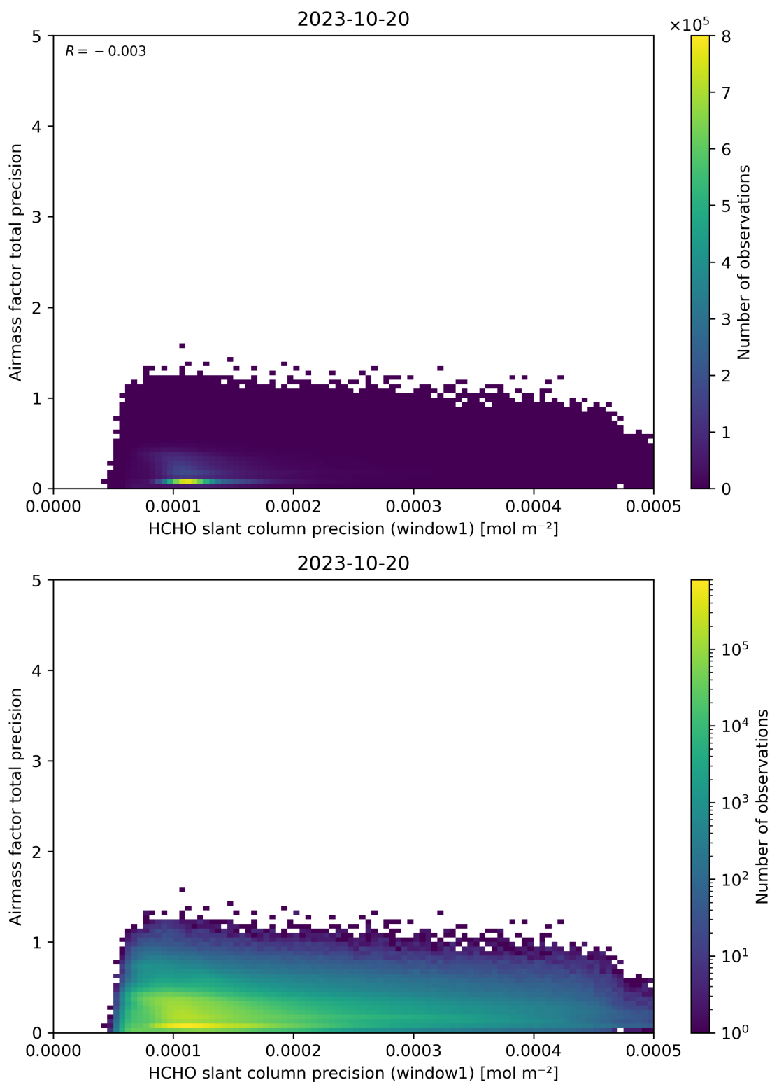
Figure 95: Scatter density plot of “HCHO slant column precision (window1)” against “Airmass factor total precision” for 2023-10-19 to 2023-10-21.
