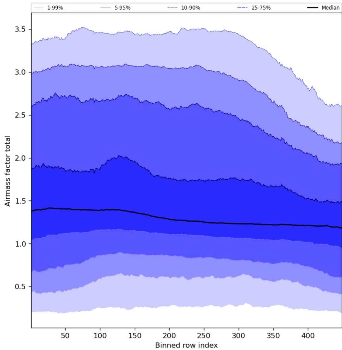
Figure 54: Along track statistics of “Airmass factor total” for 2023-10-19 to 2023-10-21
