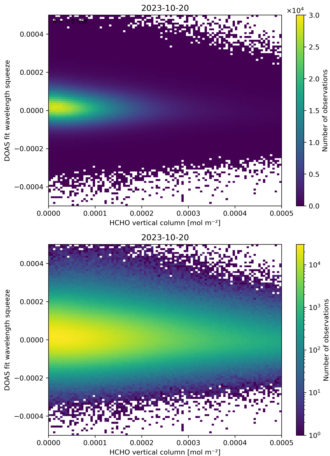
Figure 125: Scatter density plot of “HCHO vertical column” against “DOAS fit wavelength squeeze” for 2023-10-19 to 2023-10-21.
