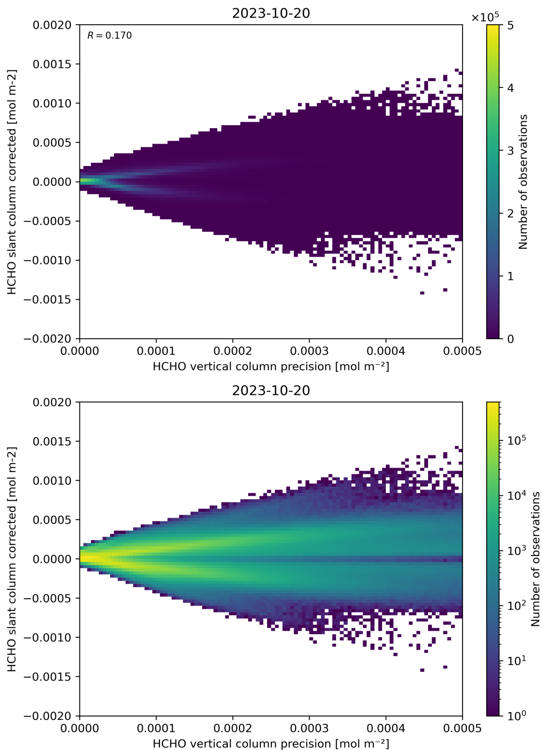
Figure 140: Scatter density plot of “HCHO vertical column precision” against “HCHO slant column corrected” for 2023-10-19 to 2023-10-21.
