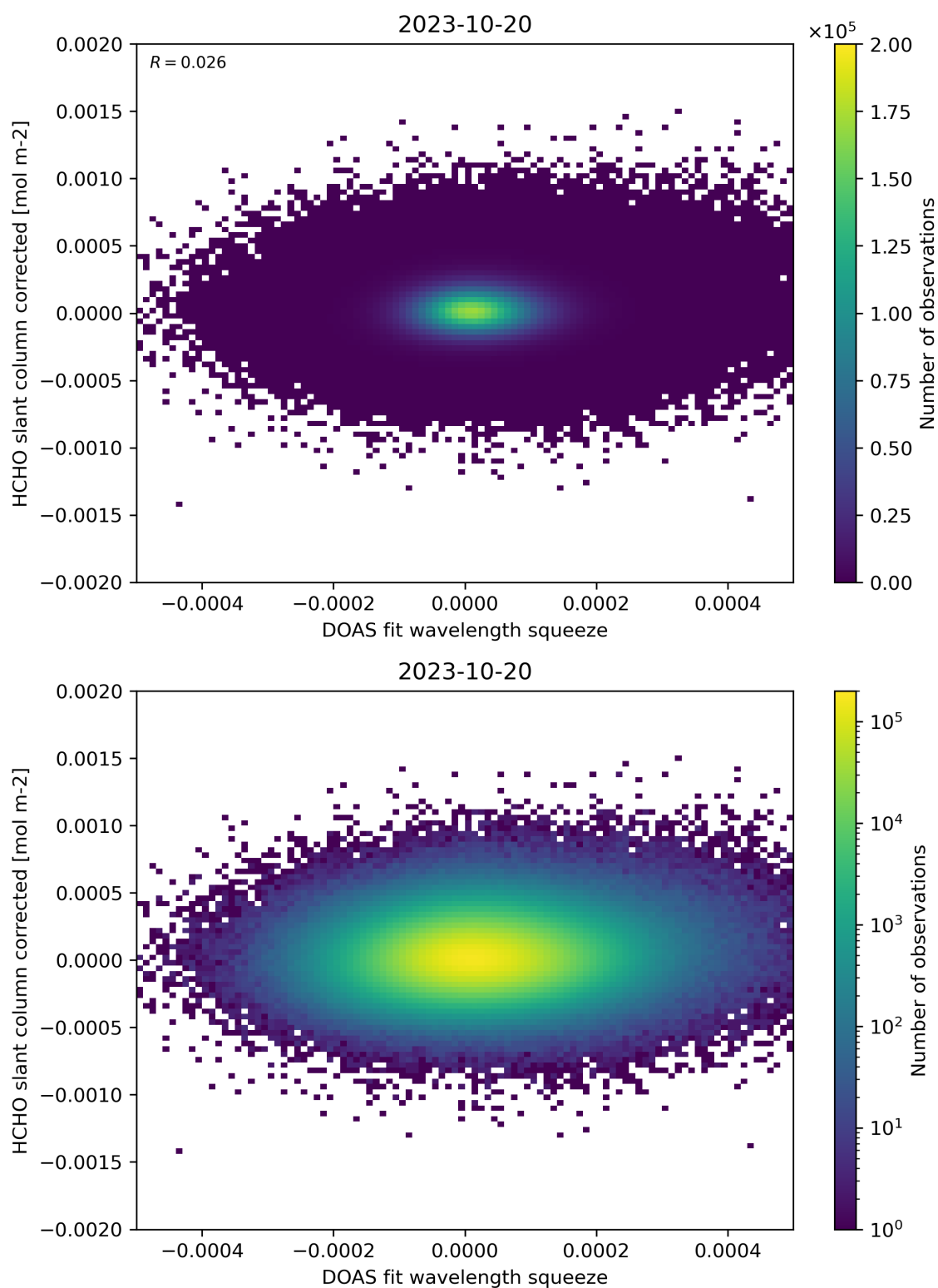
Figure 69: Scatter density plot of “DOAS fit wavelength squeeze” against “HCHO slant column corrected” for 2023-10-19 to 2023-10-21.
