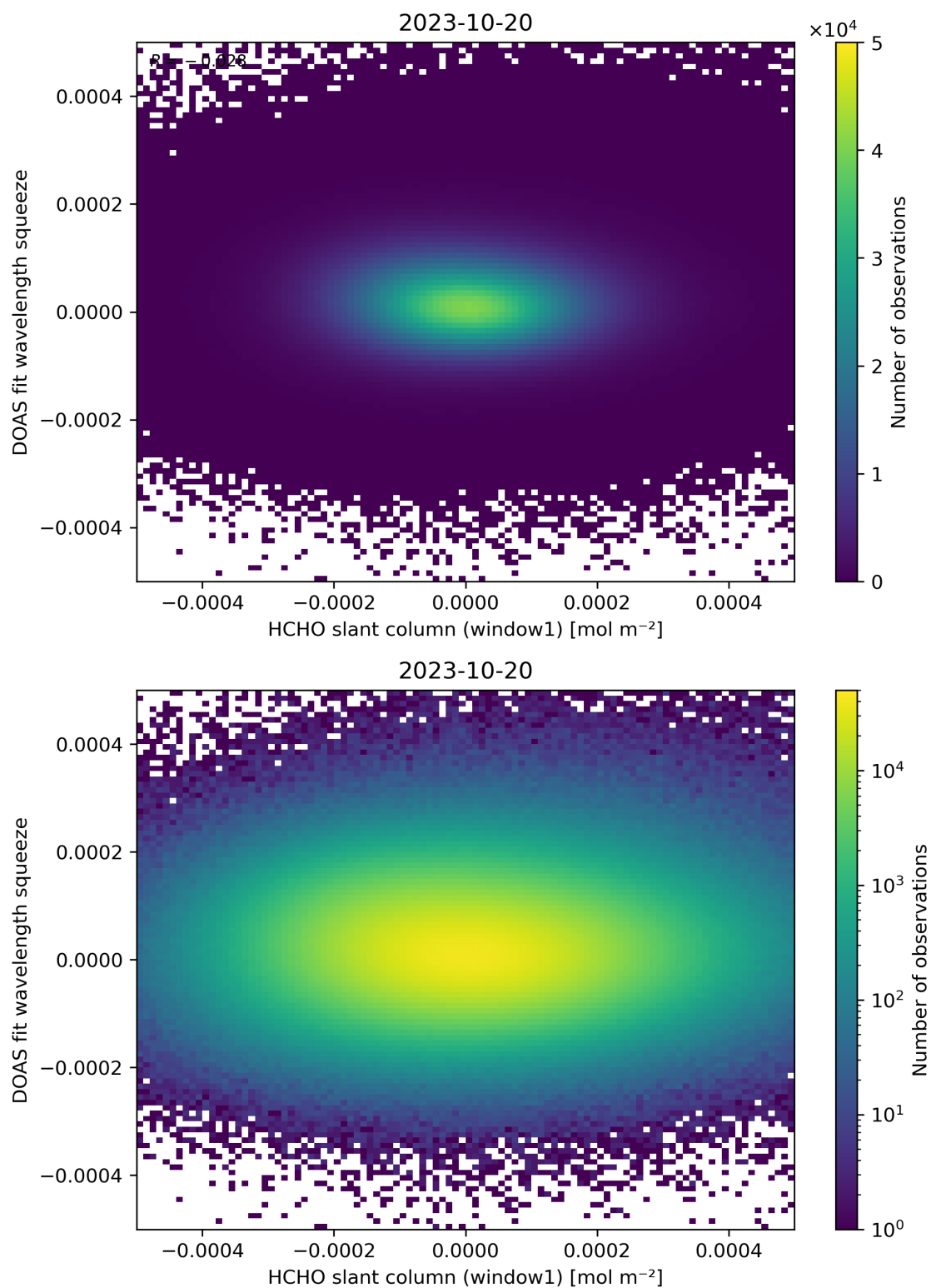
Figure 80: Scatter density plot of “HCHO slant column (window1)” against “DOAS fit wavelength squeeze” for 2023-10-19 to 2023-10-21.
