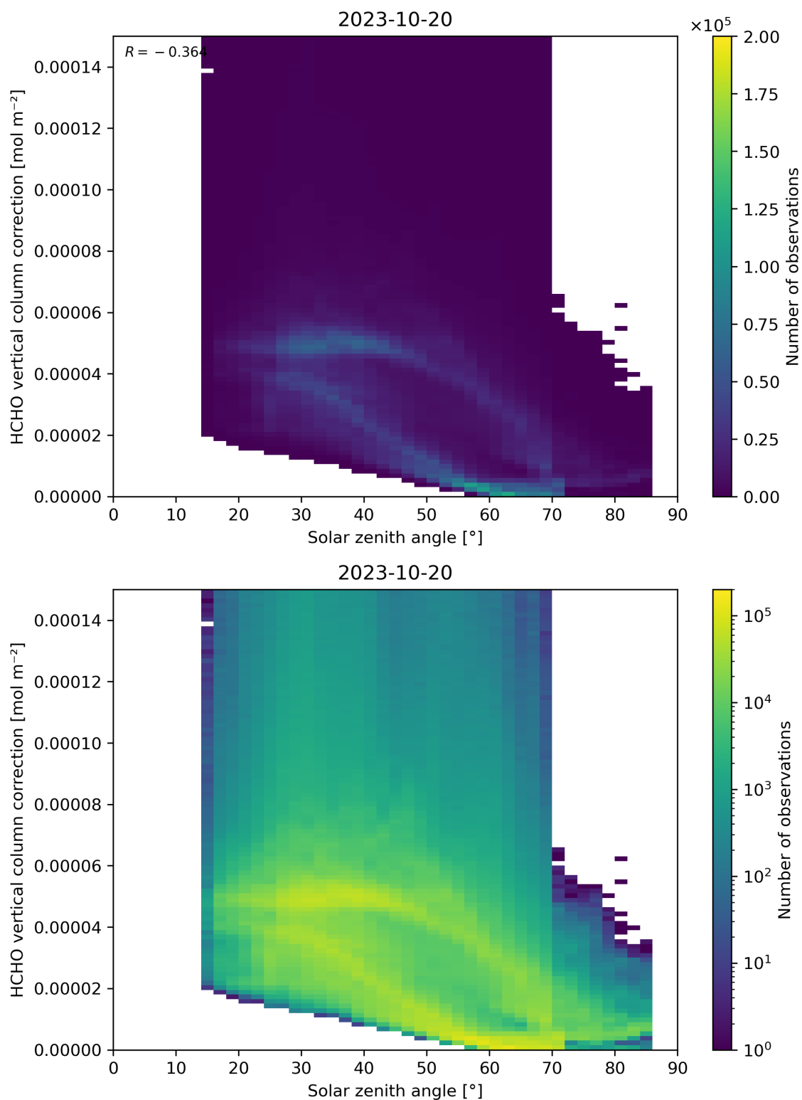
Figure 178: Scatter density plot of “Solar zenith angle” against “HCHO vertical column correction” for 2023-10-19 to 2023-10-21.
