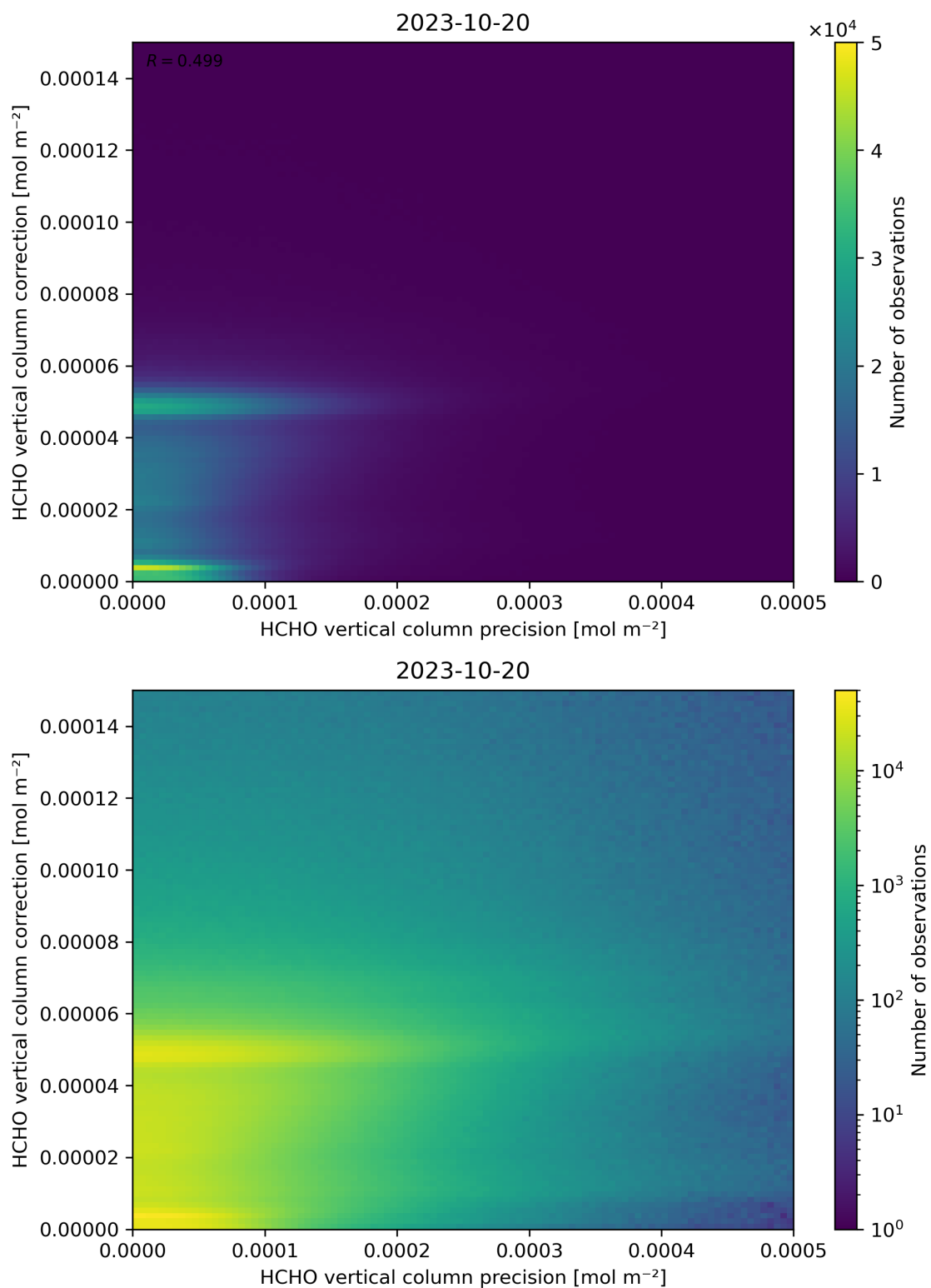
Figure 146: Scatter density plot of “HCHO vertical column precision” against “HCHO vertical column correction” for 2023-10-19 to 2023-10-21.
