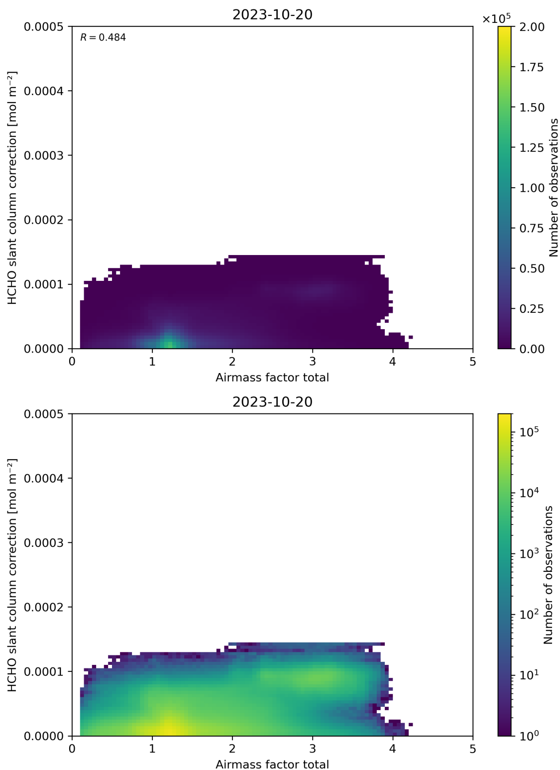
Figure 102: Scatter density plot of “Airmass factor total” against “HCHO slant column correction” for 2023-10-19 to 2023-10-21.
