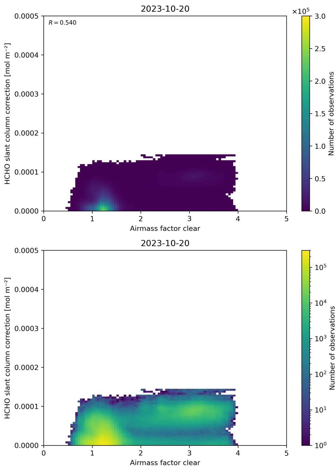
Figure 75: Scatter density plot of “Airmass factor clear” against “HCHO slant column correction” for 2023-10-19 to 2023-10-21.
