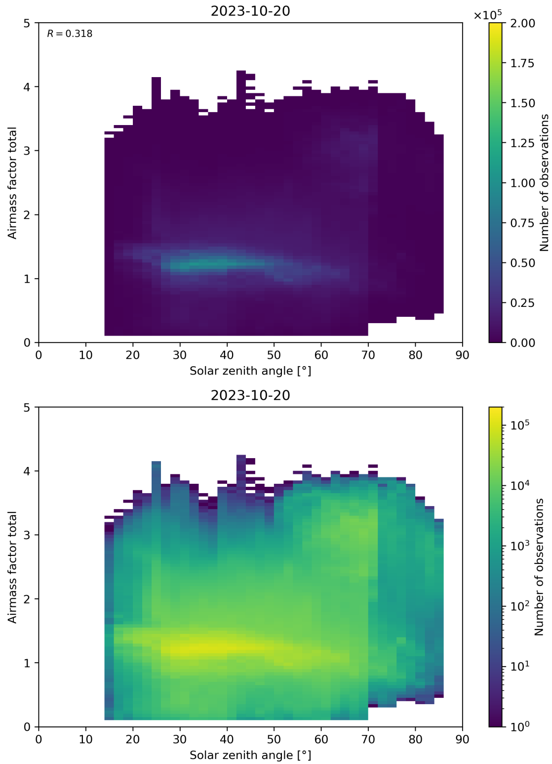
Figure 175: Scatter density plot of “Solar zenith angle” against “Airmass factor total” for 2023-10-19 to 2023-10-21.
