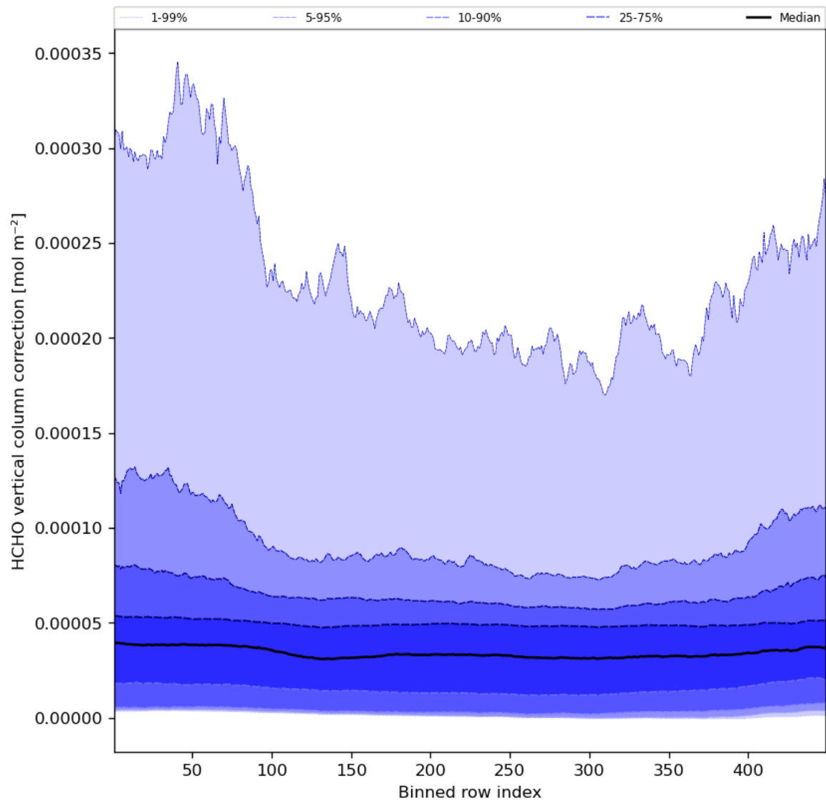
Figure 51: Along track statistics of “HCHO vertical column correction” for 2023-10-19 to 2023-10-21
