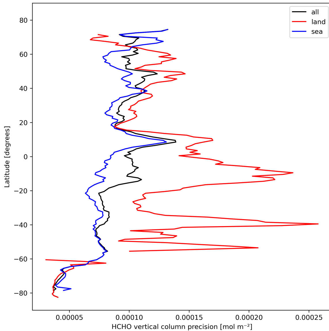
Figure 22: Zonal average of “HCHO vertical column precision” for 2023-10-19 to 2023-10-21.
