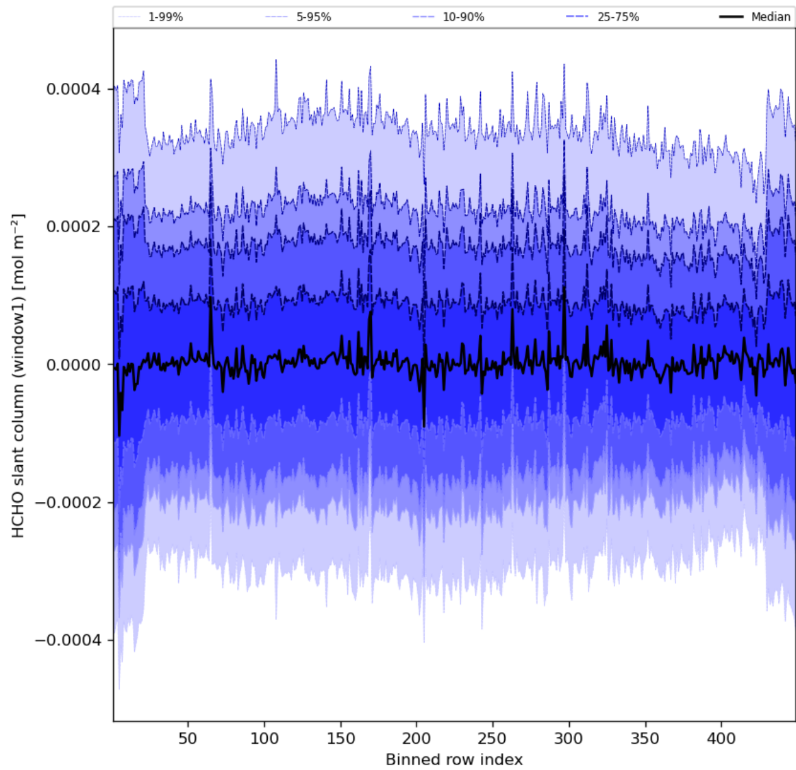
Figure 52: Along track statistics of “HCHO slant column (window1)” for 2023-10-19 to 2023-10-21
