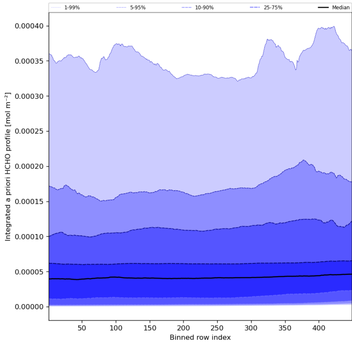
Figure 57: Along track statistics of "Integrated a priori HCHO profile" for 2023-10-19 to 2023-10-21
