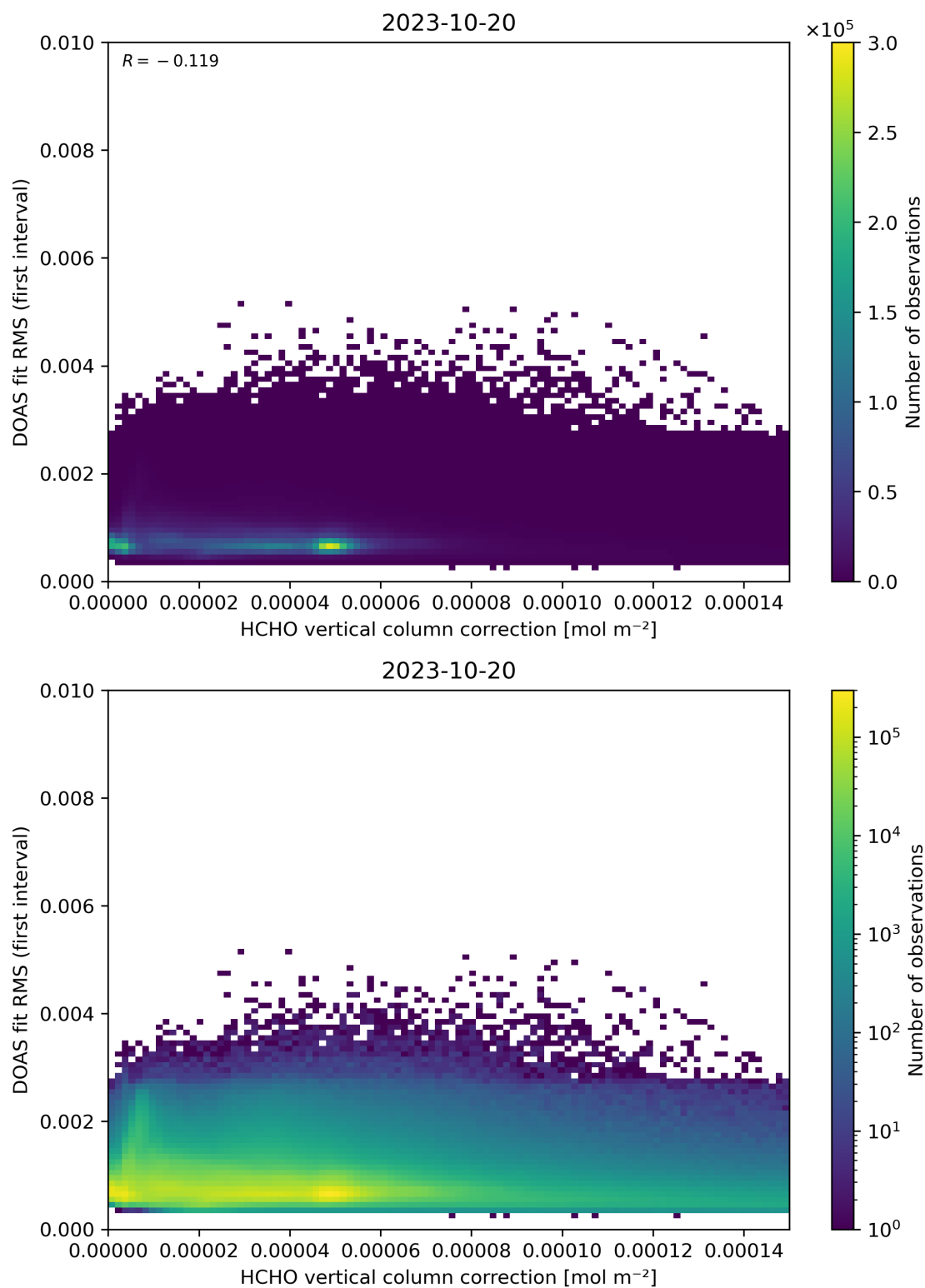
Figure 112: Scatter density plot of “HCHO vertical column correction” against “DOAS fit RMS (first interval)” for 2023-10-19 to 2023-10-21.
