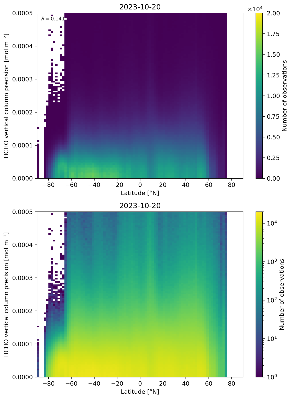
Figure 165: Scatter density plot of “Latitude” against “HCHO vertical column precision” for 2023-10-19 to 2023-10-21.
