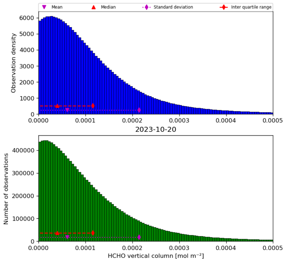
Figure 35: Histogram of “HCHO vertical column” for 2023-10-19 to 2023-10-21
