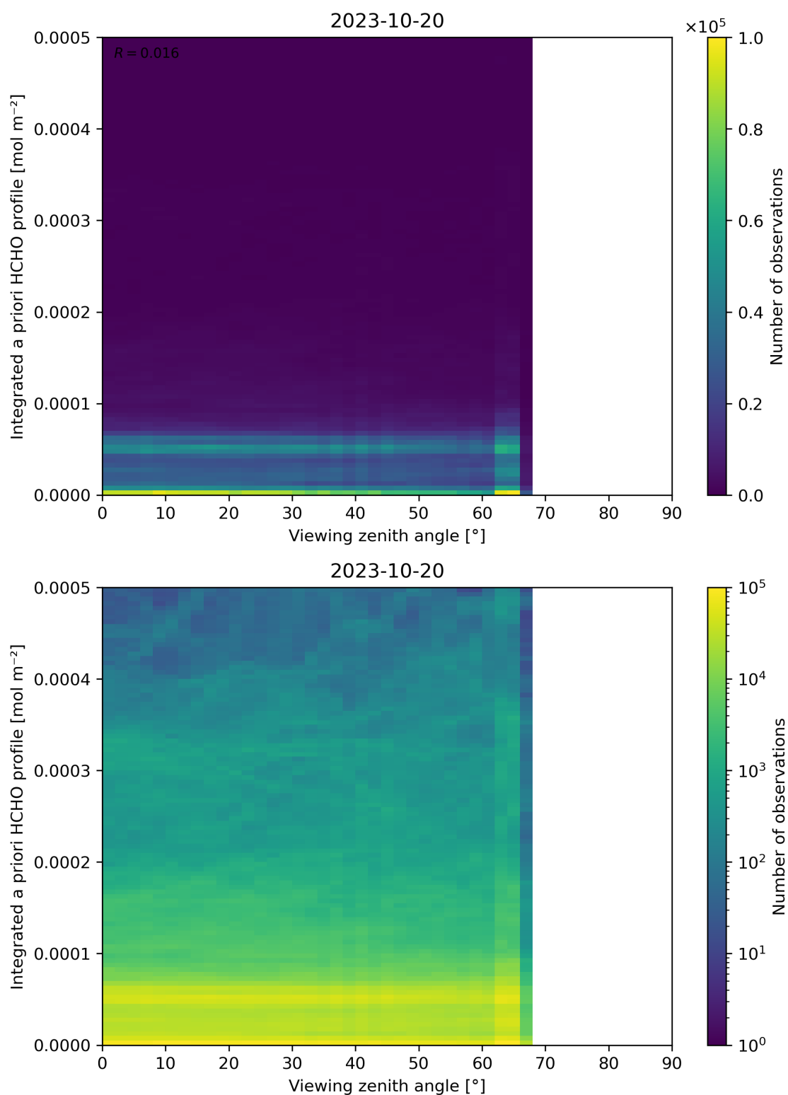
Figure 195: Scatter density plot of “Viewing zenith angle” against “Integrated a priori HCHO profile” for 2023-10-19 to 2023-10-21.
