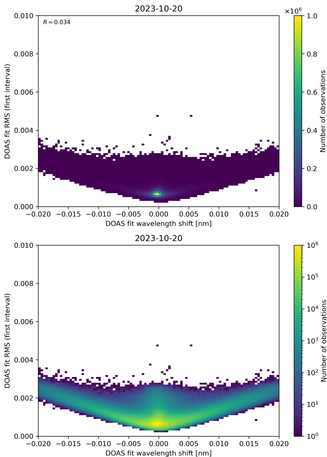
Figure 64: Scatter density plot of “DOAS fit wavelength shift” against “DOAS fit RMS (first interval)” for 2023-10-19 to 2023-10-21.
