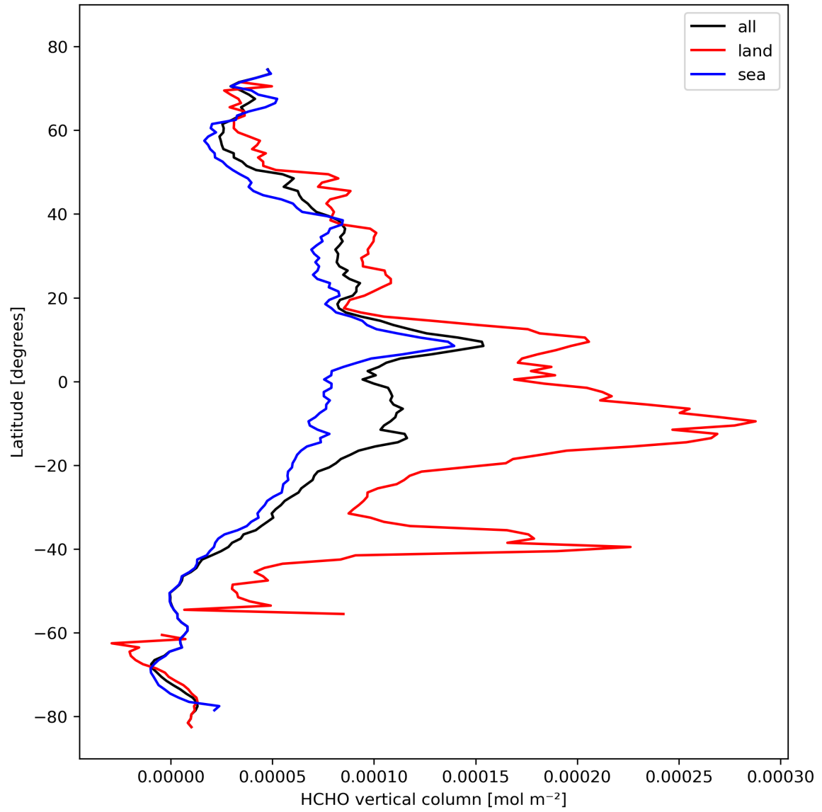
Figure 21: Zonal average of “HCHO vertical column” for 2023-10-19 to 2023-10-21.
