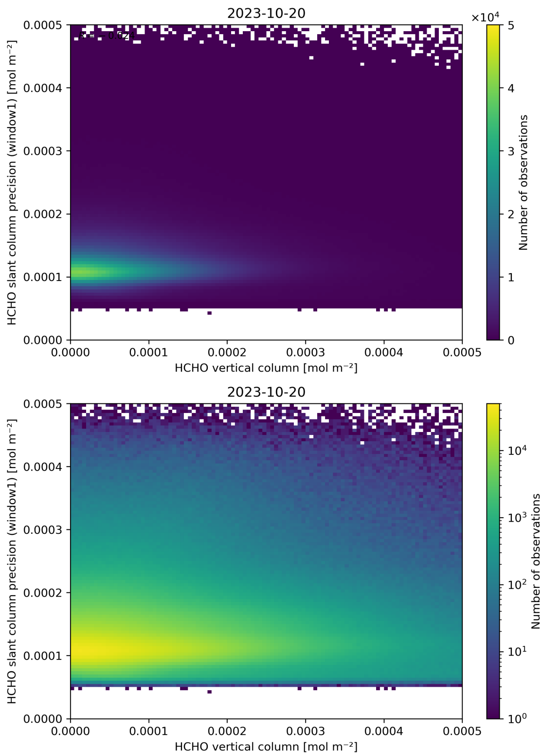
Figure 130: Scatter density plot of “HCHO vertical column” against “HCHO slant column precision (window1)” for 2023-10-19 to 2023-10-21.
