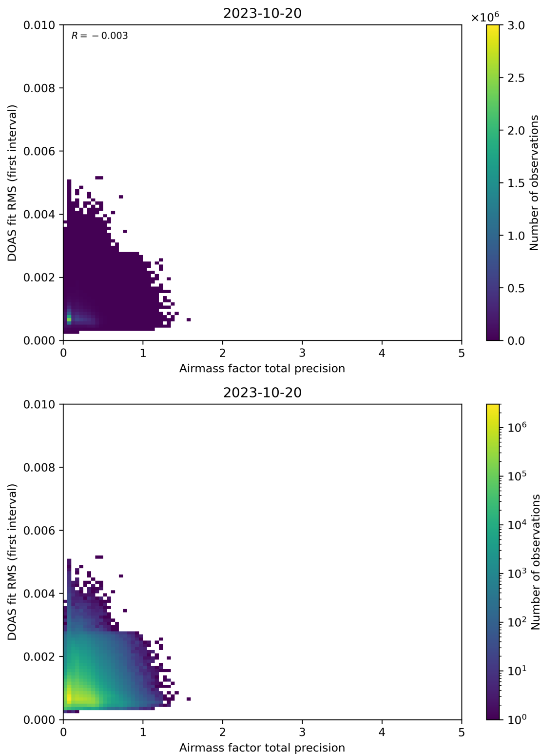
Figure 105: Scatter density plot of “Airmass factor total precision” against “DOAS fit RMS (first interval)” for 2023-10-19 to 2023-10-21.
