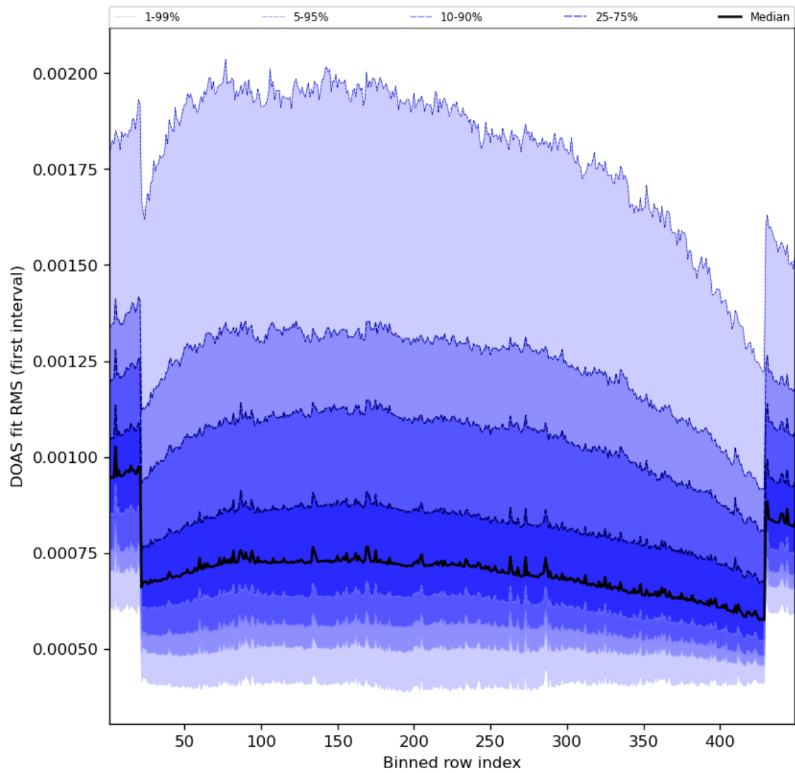
Figure 60: Along track statistics of “DOAS fit RMS (first interval)” for 2023-10-19 to 2023-10-21
