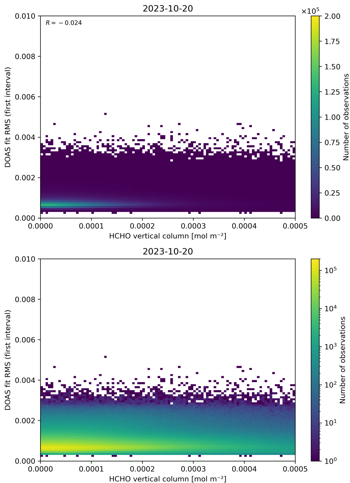
Figure 123: Scatter density plot of “HCHO vertical column” against “DOAS fit RMS (first interval)” for 2023-10-19 to 2023-10-21.
