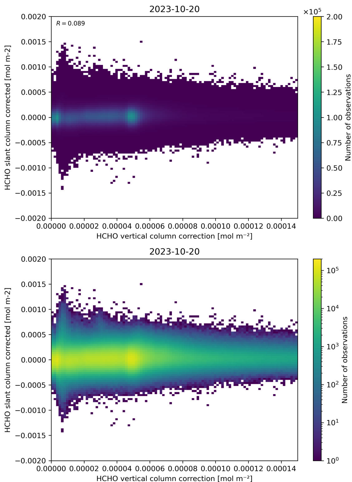
Figure 116: Scatter density plot of “HCHO vertical column correction” against “HCHO slant column corrected” for 2023-10-19 to 2023-10-21.
