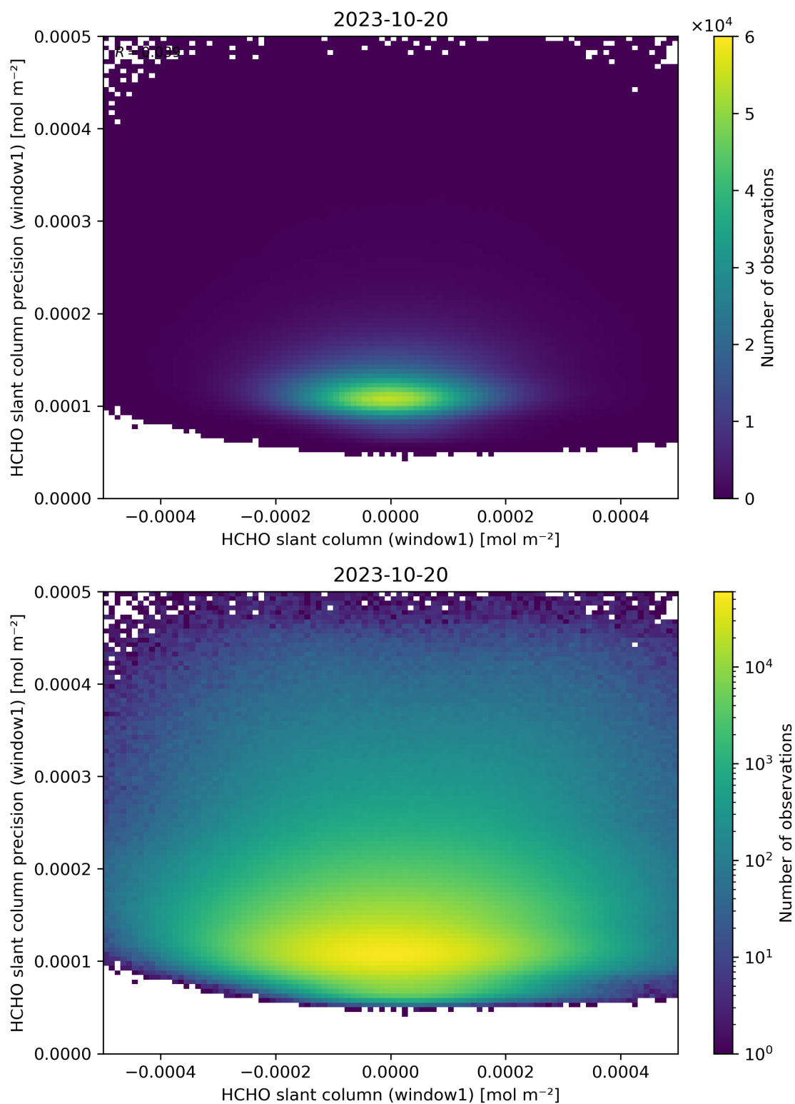
Figure 84: Scatter density plot of “HCHO slant column (window1)” against “HCHO slant column precision (window1)” for 2023-10-19 to 2023-10-21.
