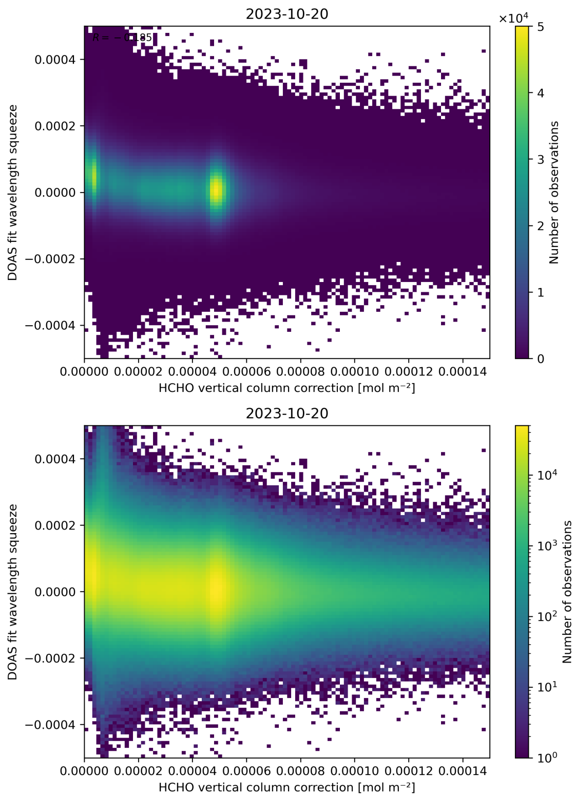
Figure 114: Scatter density plot of “HCHO vertical column correction” against “DOAS fit wavelength squeeze” for 2023-10-19 to 2023-10-21.
