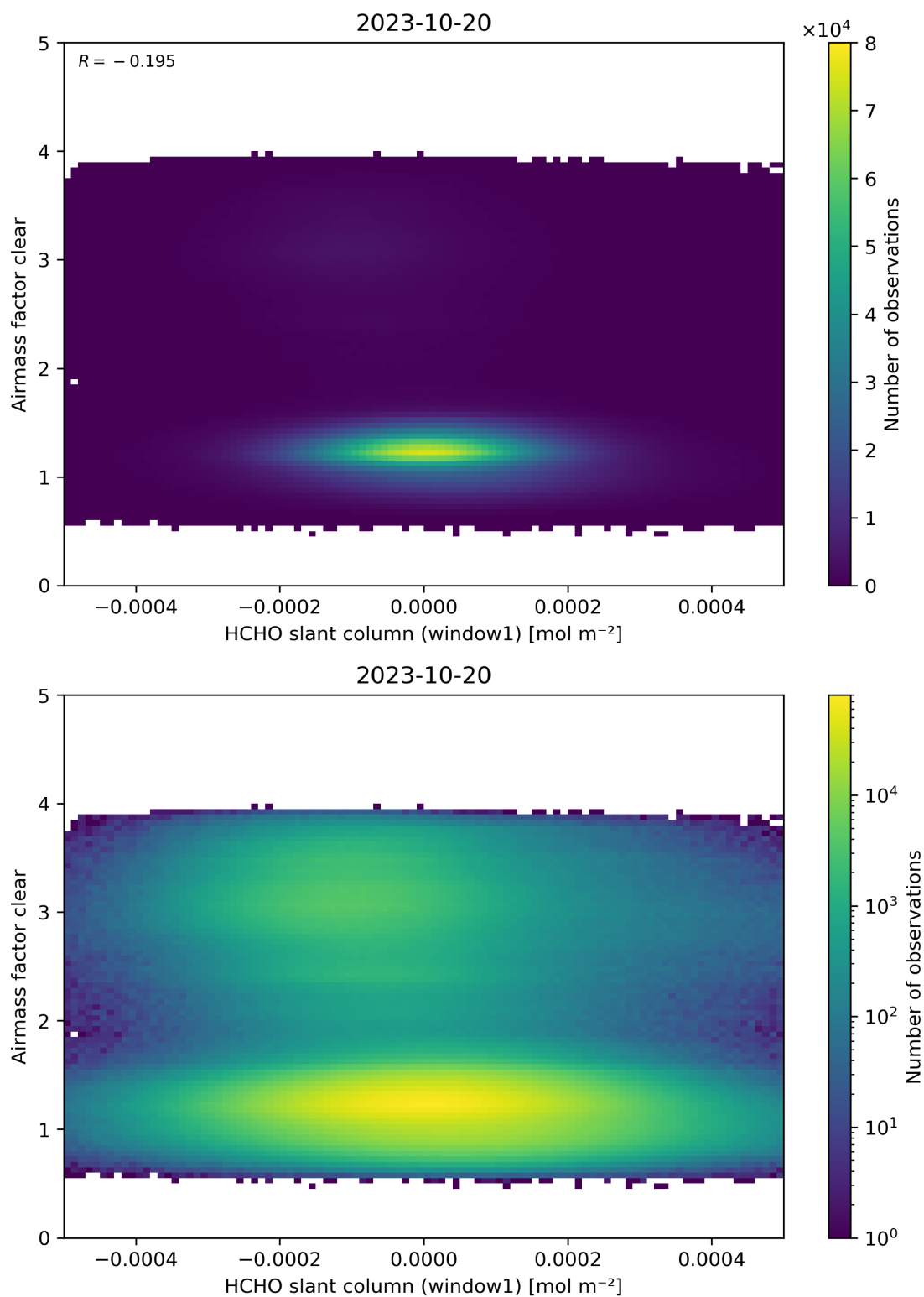
Figure 81: Scatter density plot of “HCHO slant column (window1)” against “Airmass factor clear” for 2023-10-19 to 2023-10-21.
