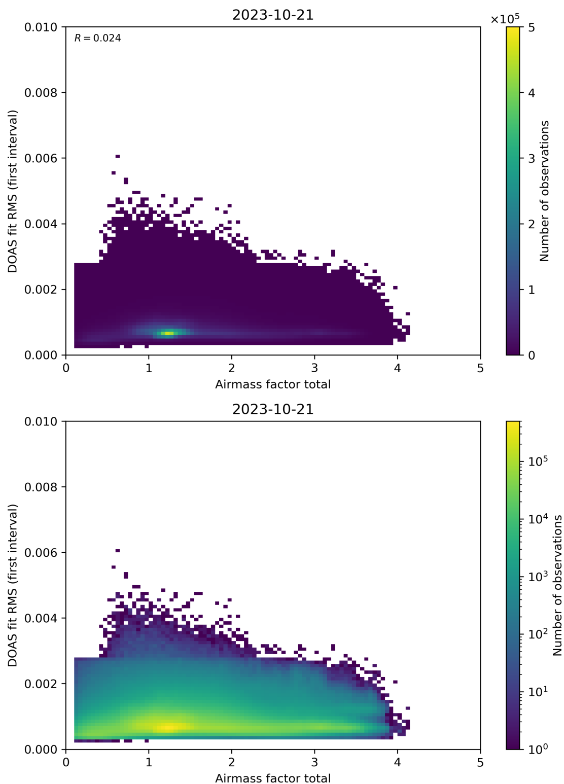
Figure 97: Scatter density plot of “Airmass factor total” against “DOAS fit RMS (first interval)” for 2023-10-20 to 2023-10-22.
