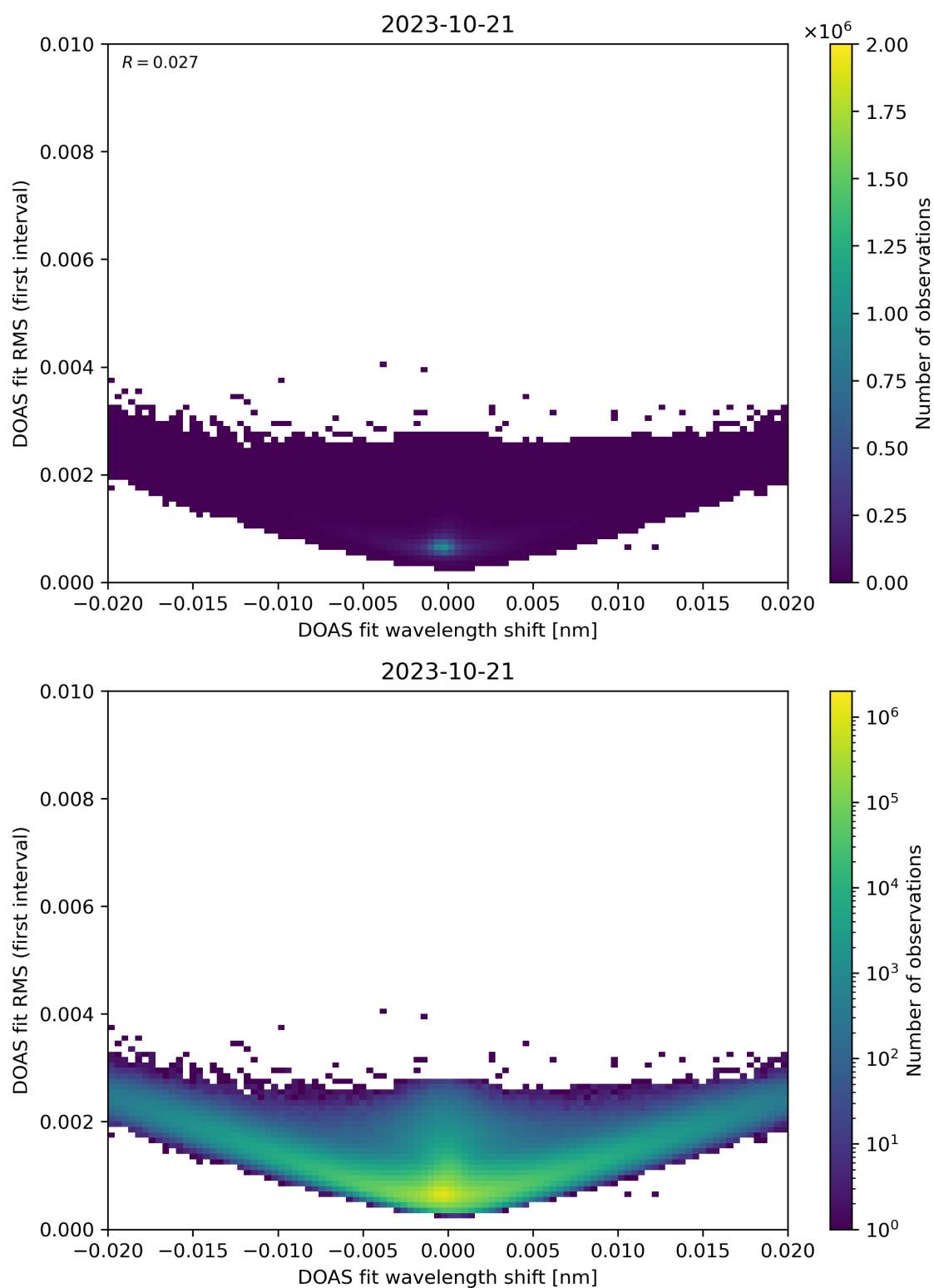
Figure 64: Scatter density plot of “DOAS fit wavelength shift” against “DOAS fit RMS (first interval)” for 2023-10-20 to 2023-10-22.
