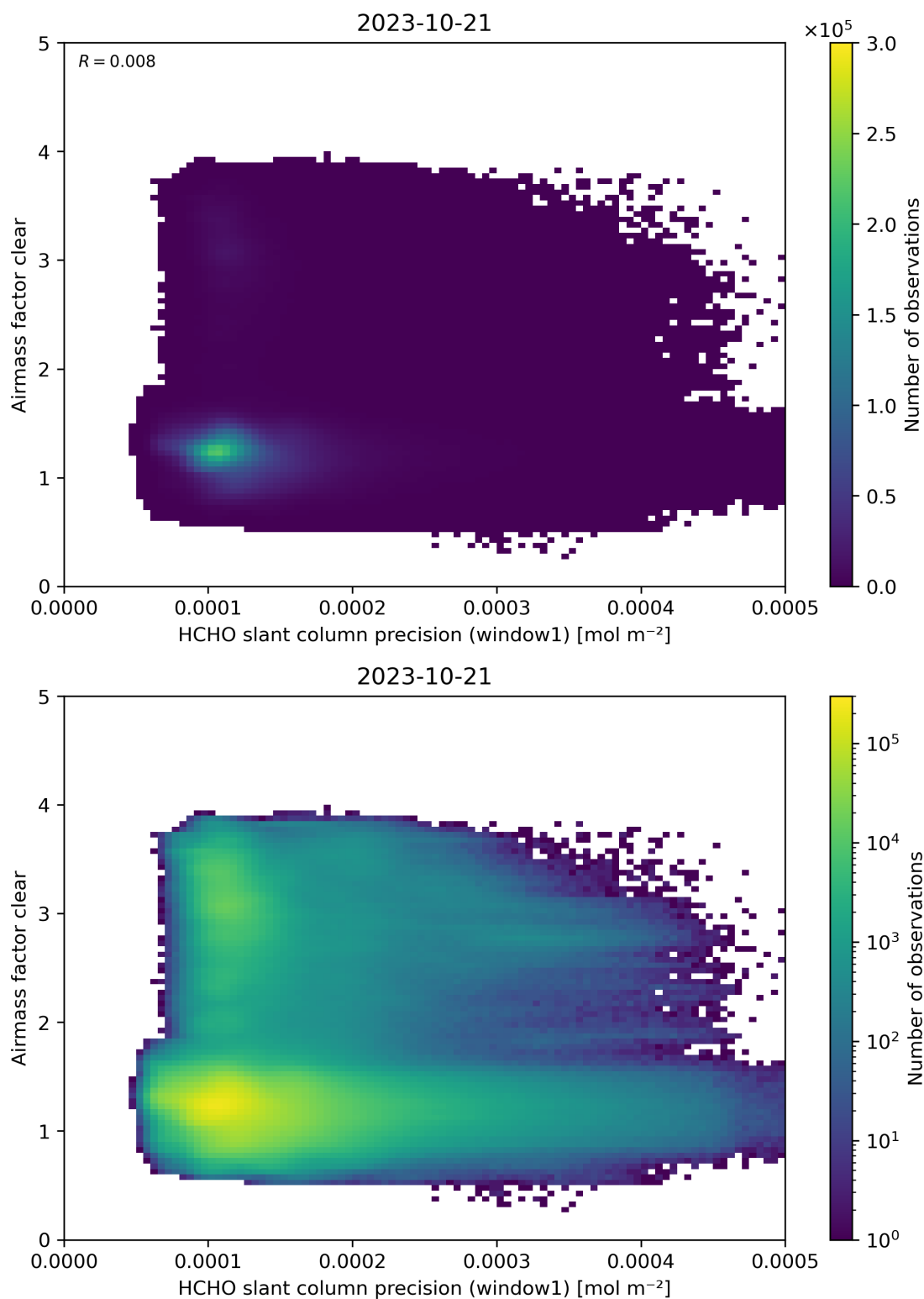
Figure 91: Scatter density plot of “HCHO slant column precision (window1)” against “Airmass factor clear” for 2023-10-20 to 2023-10-22.
