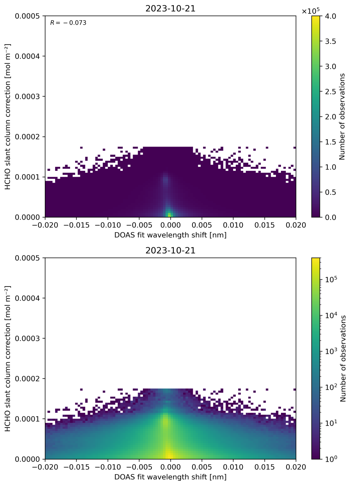
Figure 67: Scatter density plot of “DOAS fit wavelength shift” against “HCHO slant column correction” for 2023-10-20 to 2023-10-22.
