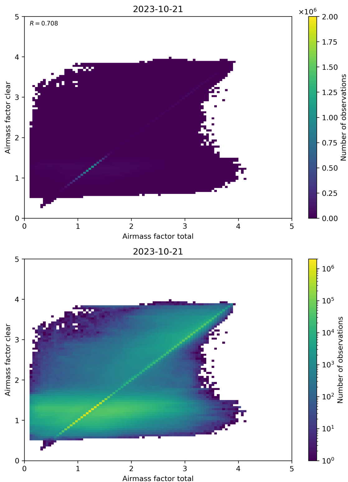
Figure 100: Scatter density plot of “Airmass factor total” against “Airmass factor clear” for 2023-10-20 to 2023-10-22.
