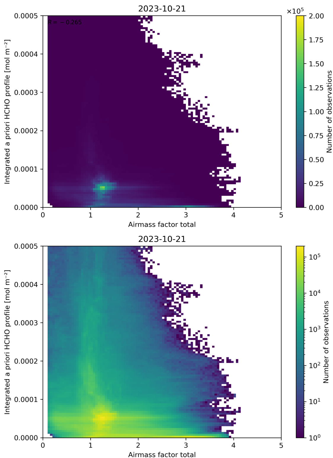
Figure 104: Scatter density plot of “Airmass factor total” against “Integrated a priori HCHO profile” for 2023-10-20 to 2023-10-22.
