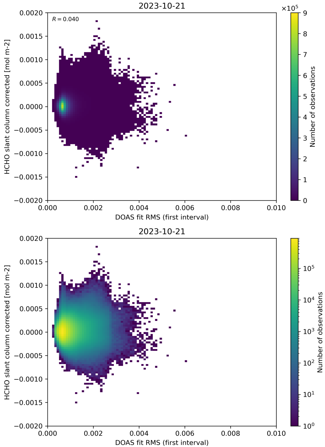
Figure 62: Scatter density plot of “DOAS fit RMS (first interval)” against “HCHO slant column corrected” for 2023-10-20 to 2023-10-22.
