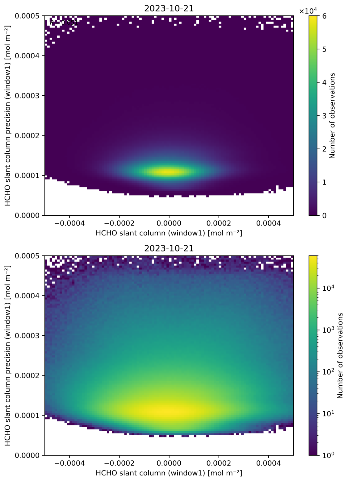
Figure 84: Scatter density plot of “HCHO slant column (window1)” against “HCHO slant column precision (window1)” for 2023-10-20 to 2023-10-22.
