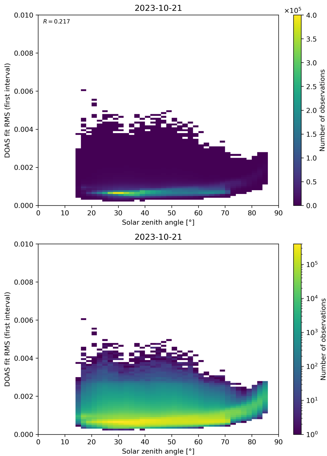
Figure 167: Scatter density plot of “Solar zenith angle” against “DOAS fit RMS (first interval)” for 2023-10-20 to 2023-10-22.
