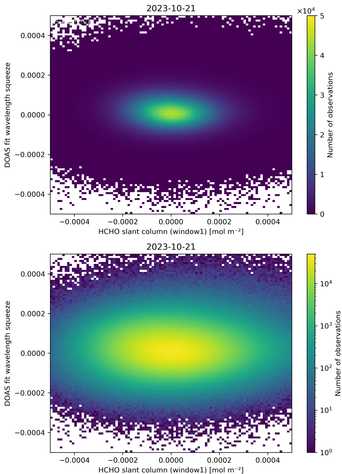
Figure 80: Scatter density plot of “HCHO slant column (window1)” against “DOAS fit wavelength squeeze” for 2023-10-20 to 2023-10-22.
