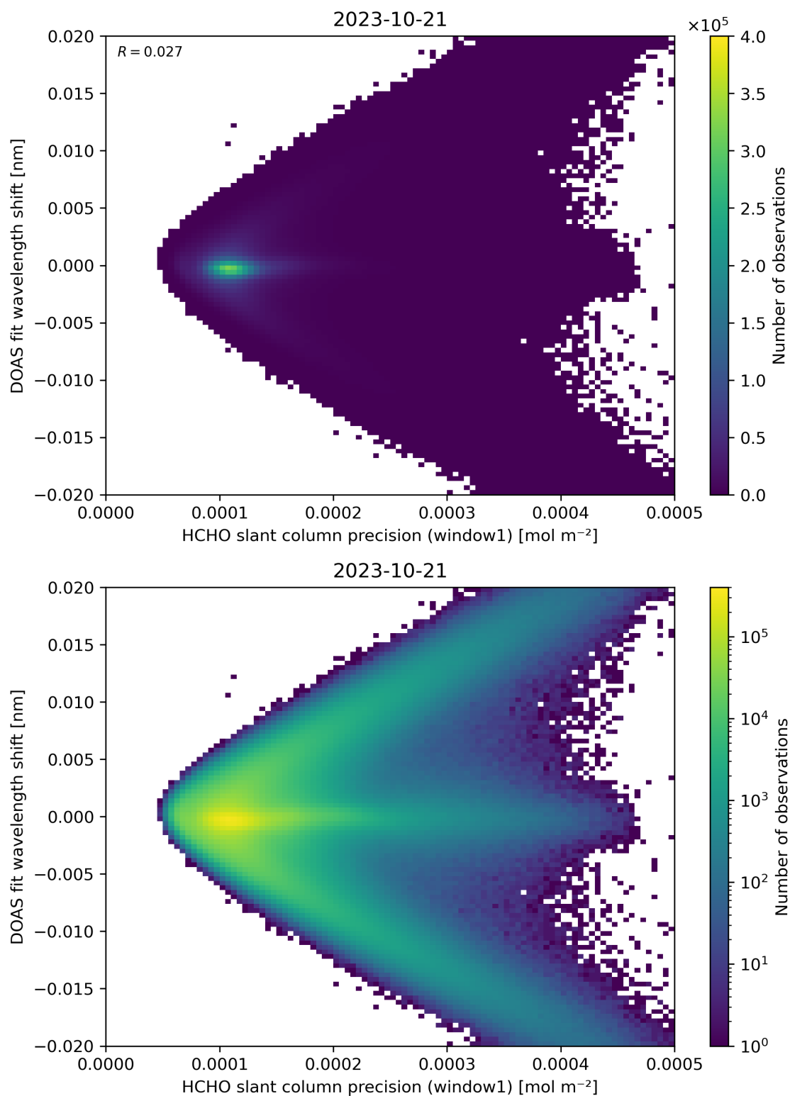
Figure 89: Scatter density plot of “HCHO slant column precision (window1)” against “DOAS fit wavelength shift” for 2023-10-20 to 2023-10-22.
