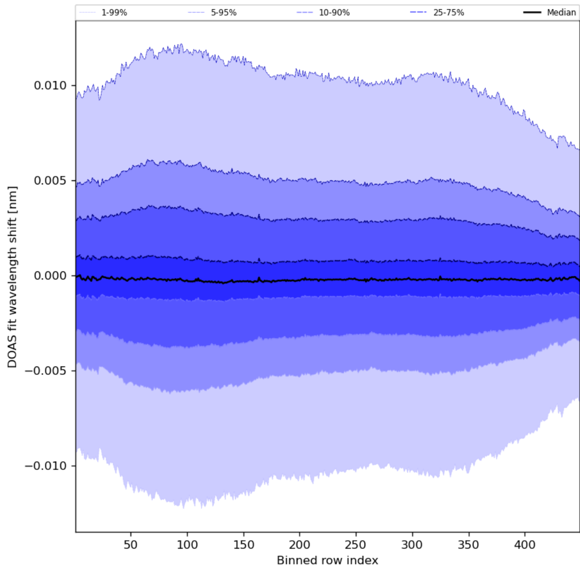
Figure 58: Along track statistics of “DOAS fit wavelength shift” for 2023-10-20 to 2023-10-22
