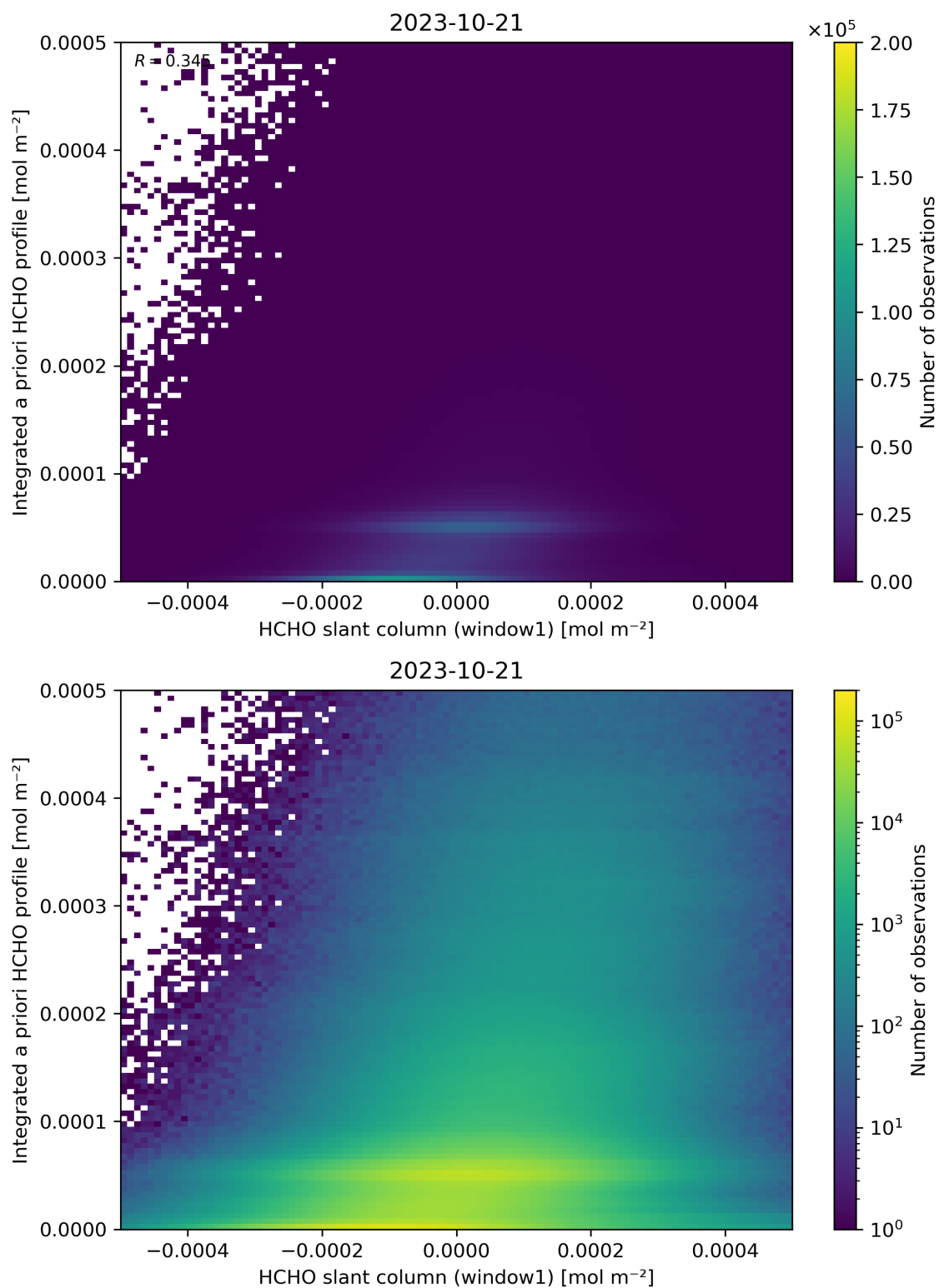
Figure 87: Scatter density plot of “HCHO slant column (window1)” against “Integrated a priori HCHO profile” for 2023-10-20 to 2023-10-22.
