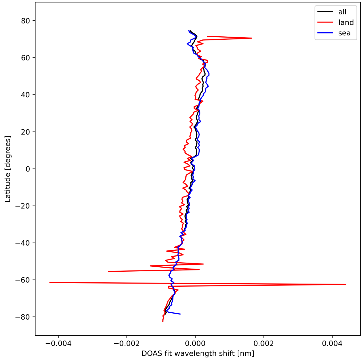
Figure 30: Zonal average of "DOAS fit wavelength shift" for 2023-10-20 to 2023-10-22.
