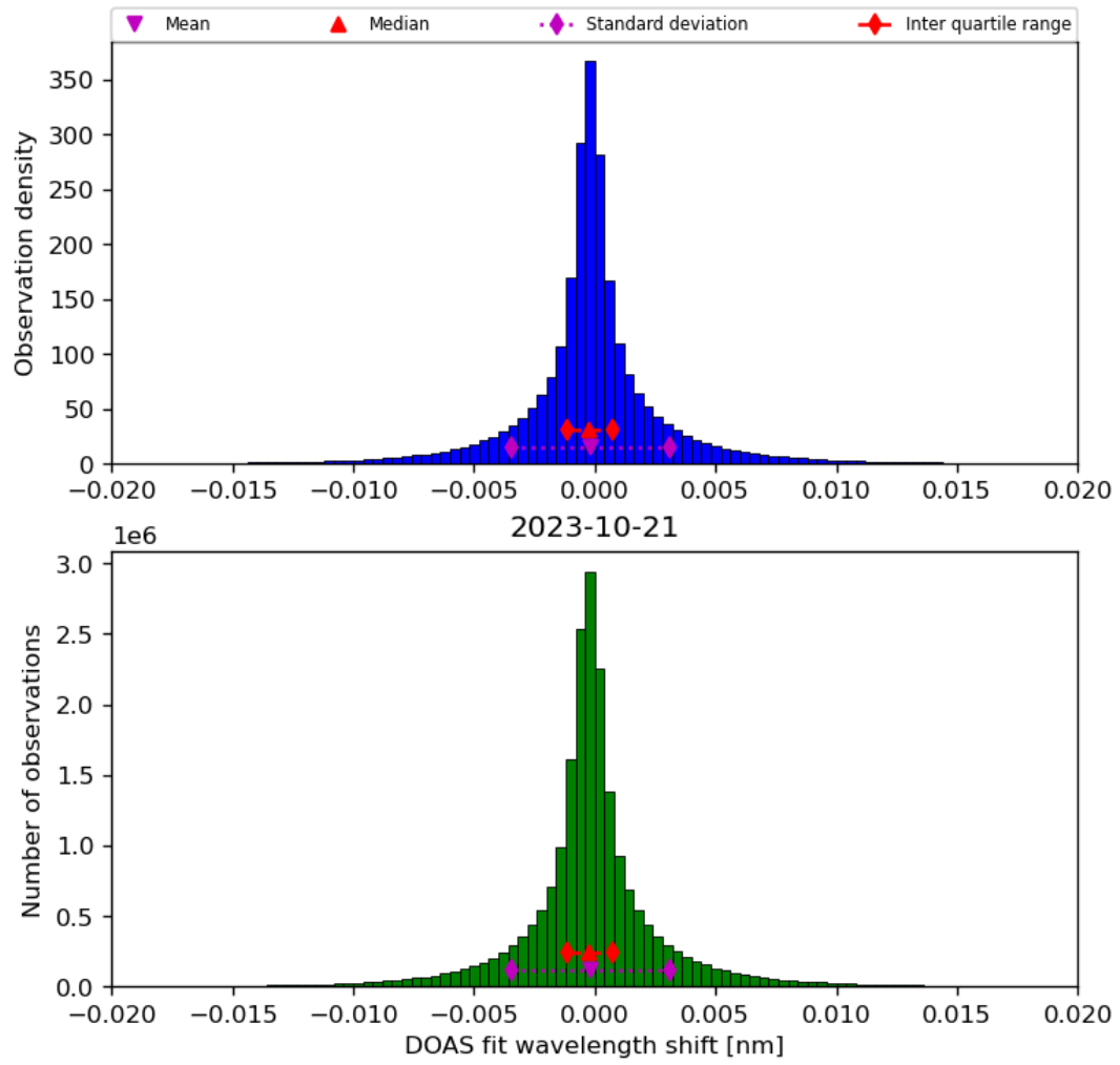
Figure 44: Histogram of “DOAS fit wavelength shift” for 2023-10-20 to 2023-10-22
