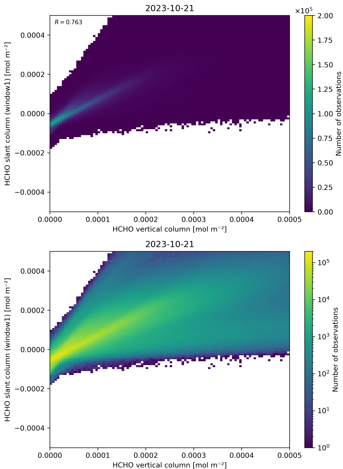
Figure 129: Scatter density plot of “HCHO vertical column” against “HCHO slant column (window1)” for 2023-10-20 to 2023-10-22.
