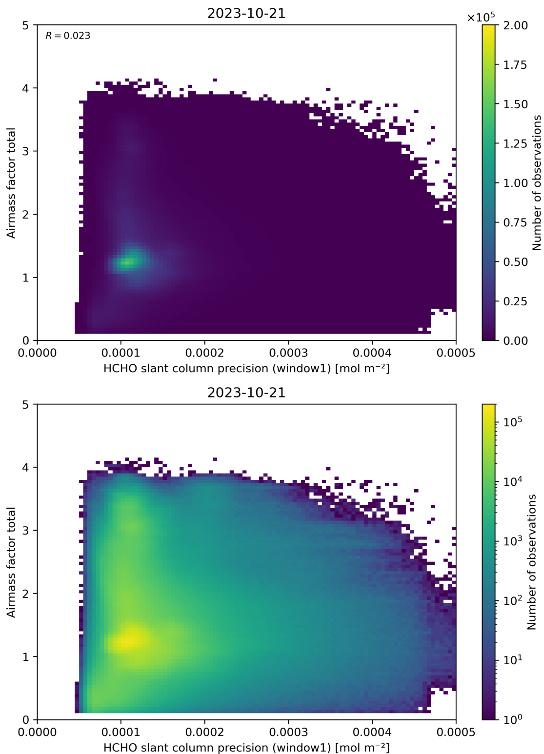
Figure 94: Scatter density plot of “HCHO slant column precision (window1)” against “Airmass factor total” for 2023-10-20 to 2023-10-22.
