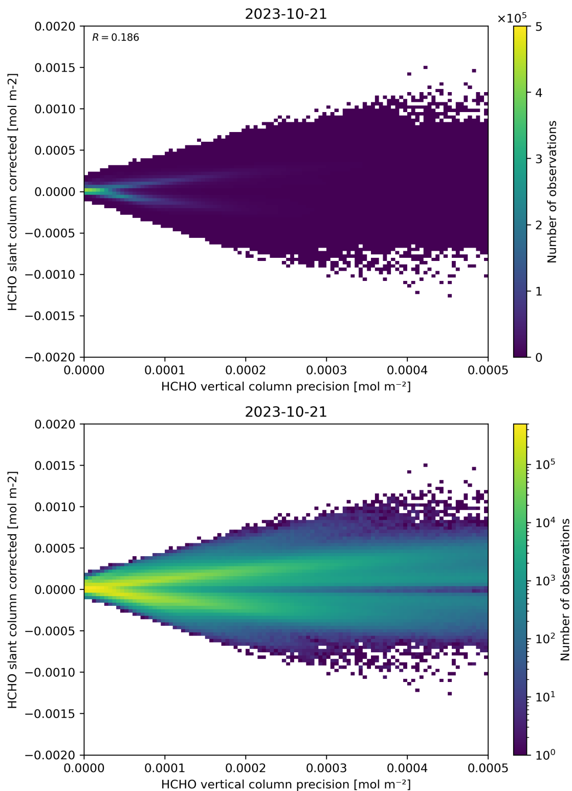
Figure 140: Scatter density plot of “HCHO vertical column precision” against “HCHO slant column corrected” for 2023-10-20 to 2023-10-22.
