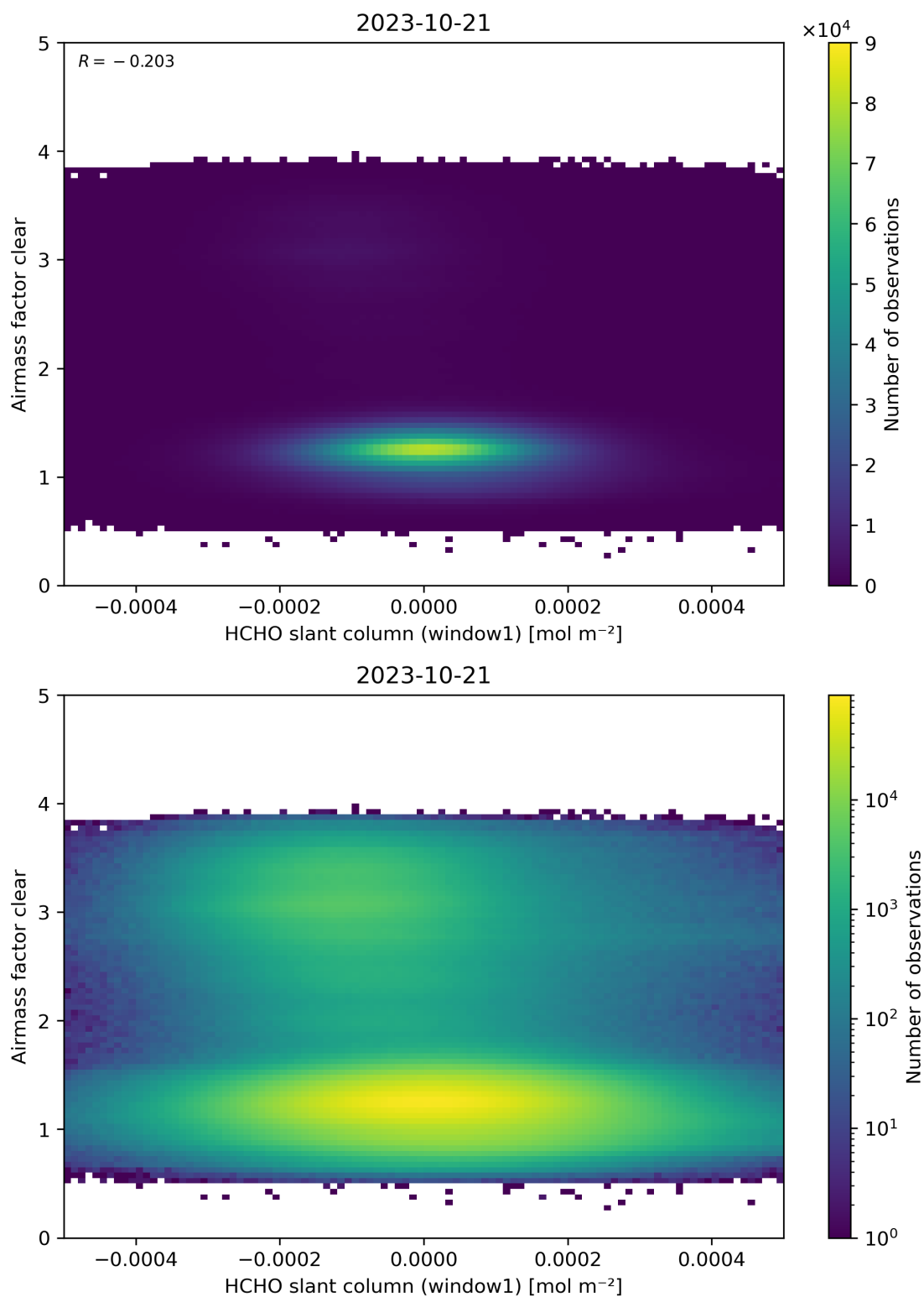
Figure 81: Scatter density plot of “HCHO slant column (window1)” against “Airmass factor clear” for 2023-10-20 to 2023-10-22.
