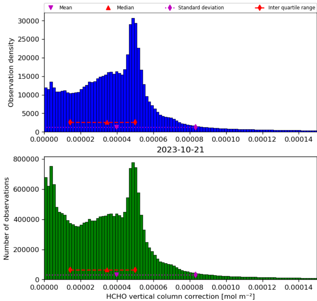
Figure 37: Histogram of “HCHO vertical column correction” for 2023-10-20 to 2023-10-22
