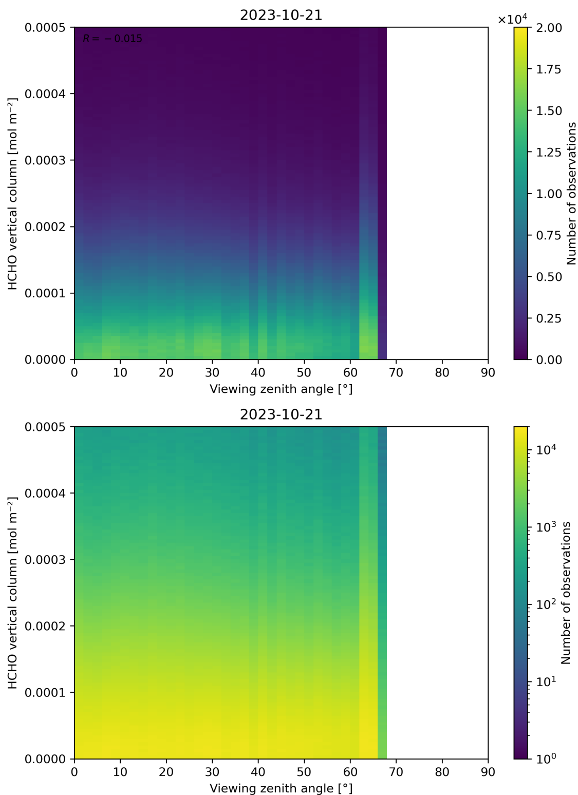
Figure 192: Scatter density plot of “Viewing zenith angle” against “HCHO vertical column” for 2023-10-20 to 2023-10-22.
