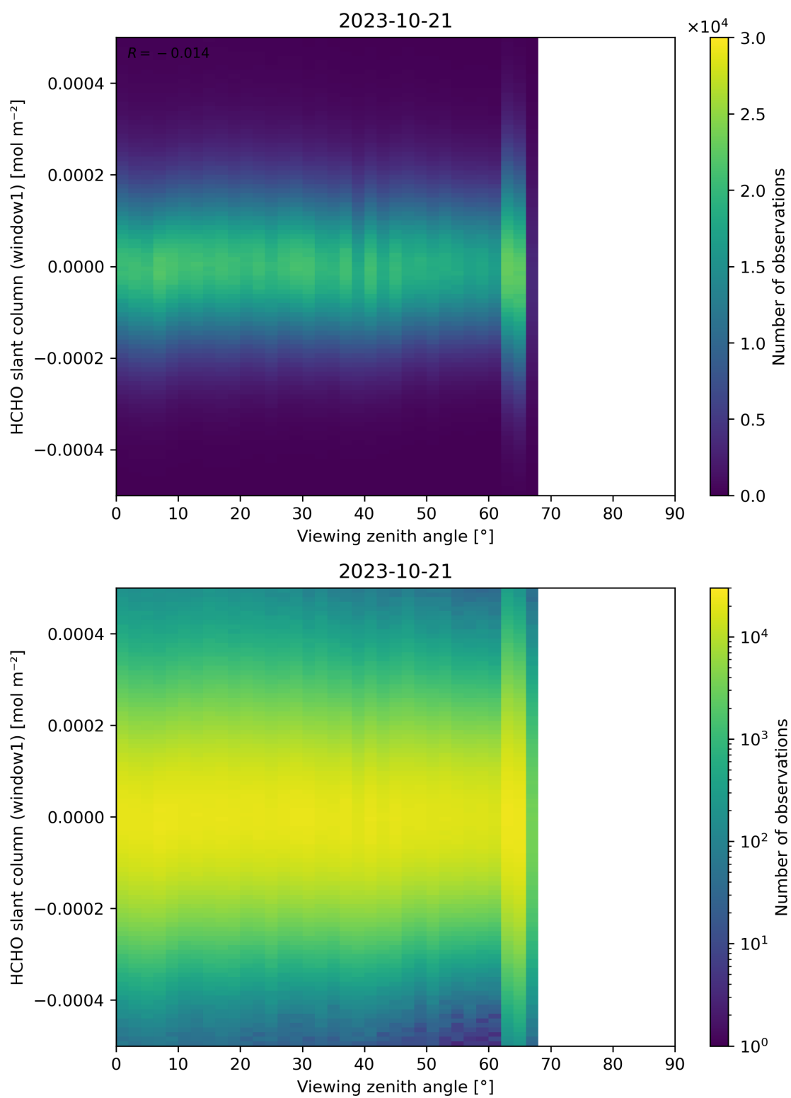
Figure 188: Scatter density plot of “Viewing zenith angle” against “HCHO slant column (window1)” for 2023-10-20 to 2023-10-22.
