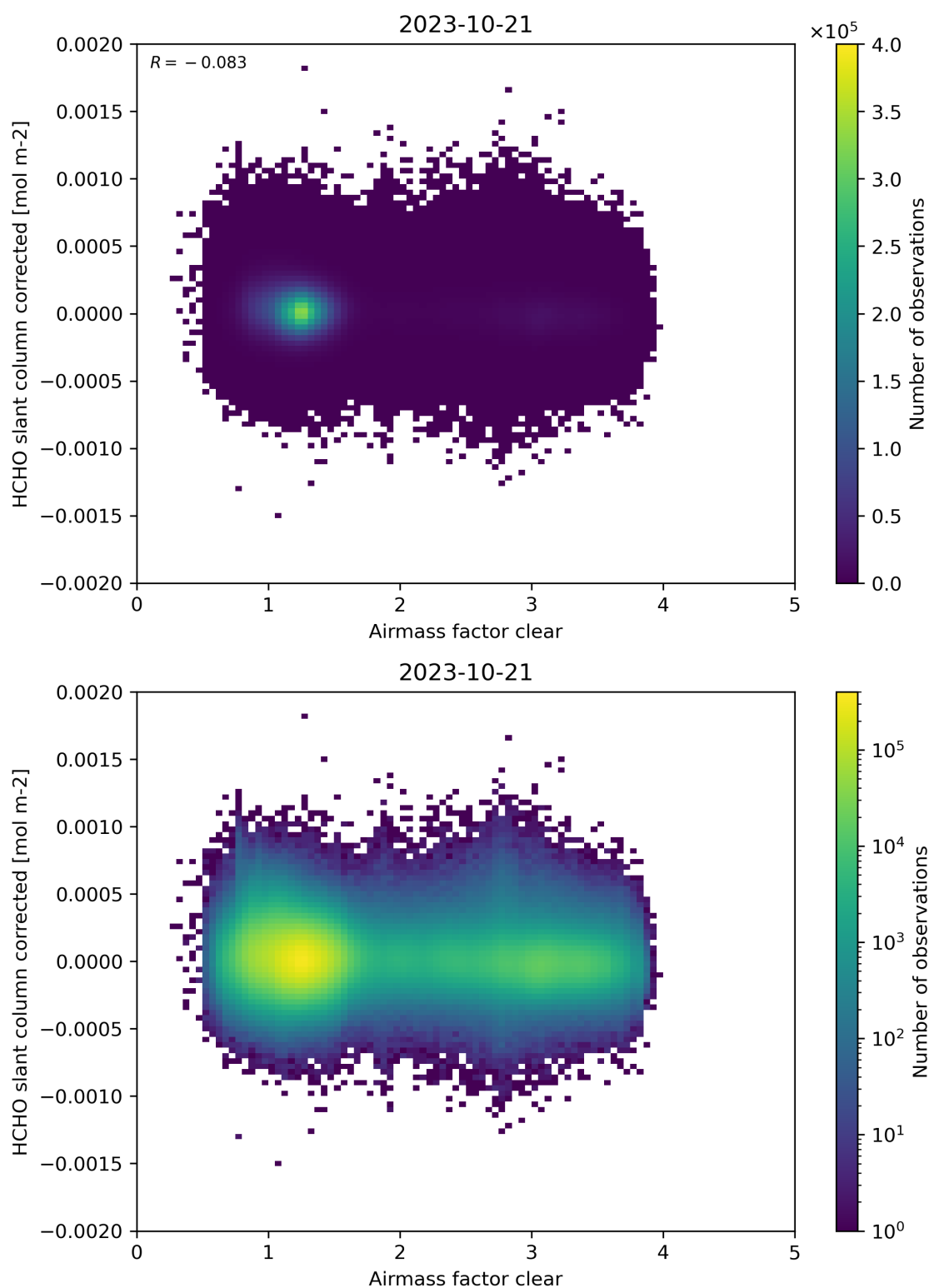
Figure 74: Scatter density plot of “Airmass factor clear” against “HCHO slant column corrected” for 2023-10-20 to 2023-10-22.
