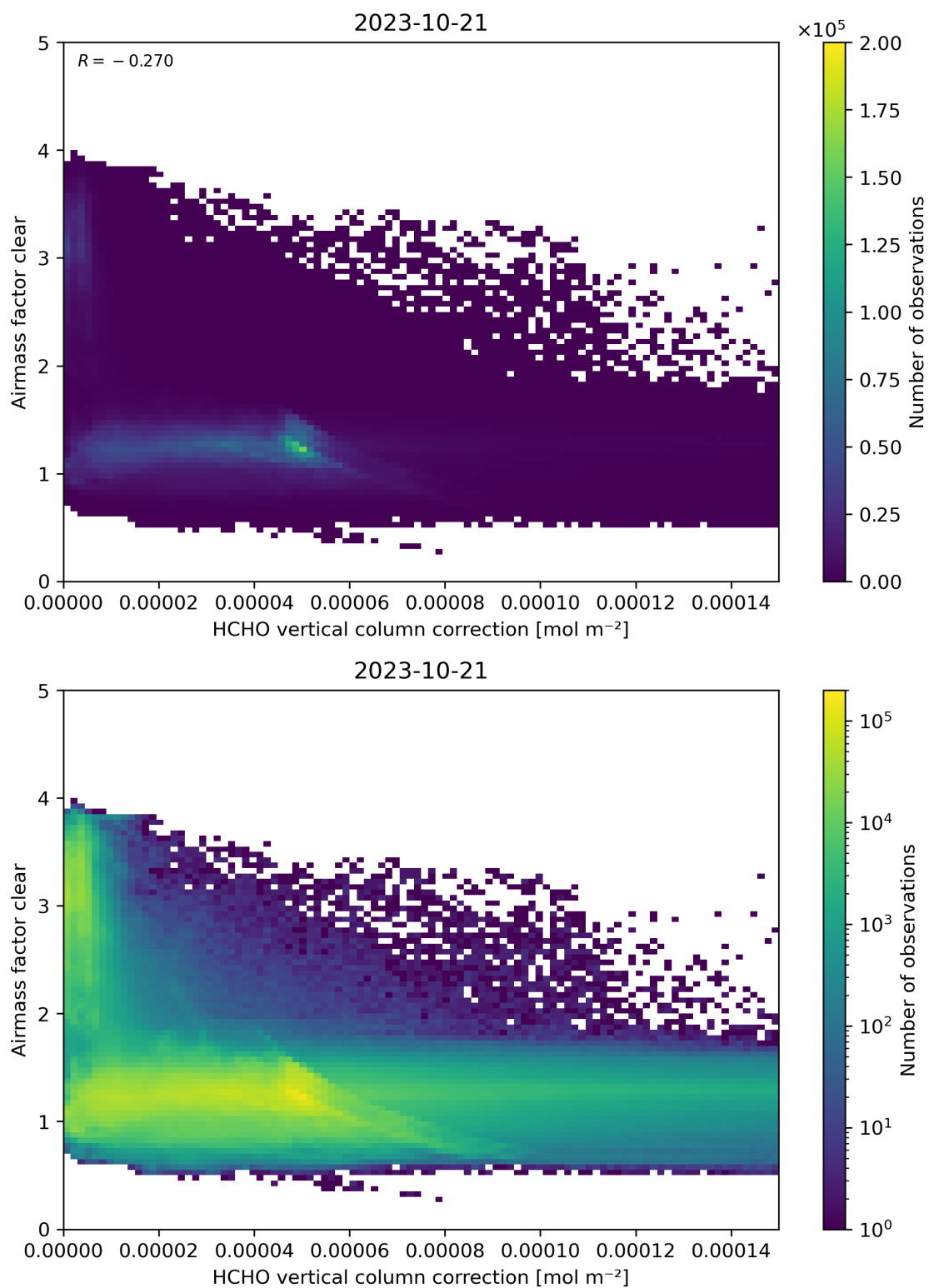
Figure 115: Scatter density plot of “HCHO vertical column correction” against “Airmass factor clear” for 2023-10-20 to 2023-10-22.
