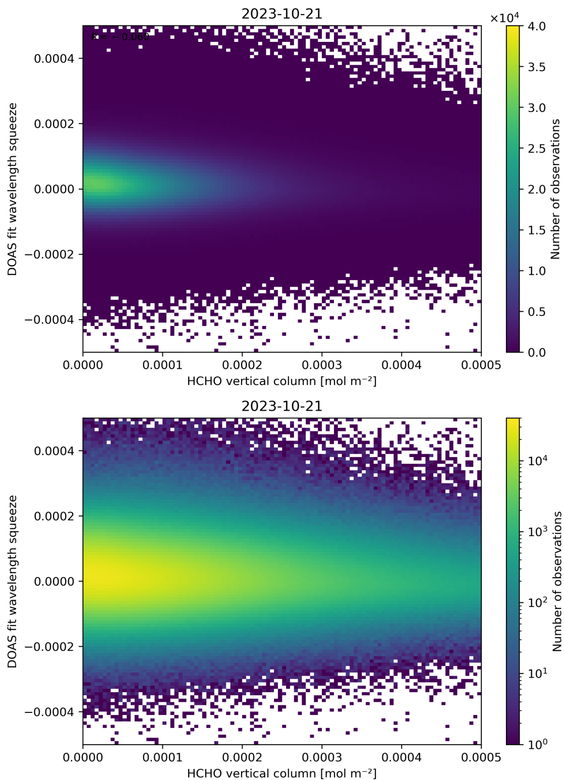
Figure 125: Scatter density plot of “HCHO vertical column” against “DOAS fit wavelength squeeze” for 2023-10-20 to 2023-10-22.
