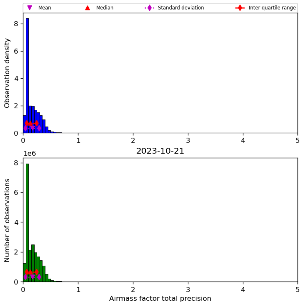
Figure 41: Histogram of “Airmass factor total precision” for 2023-10-20 to 2023-10-22
