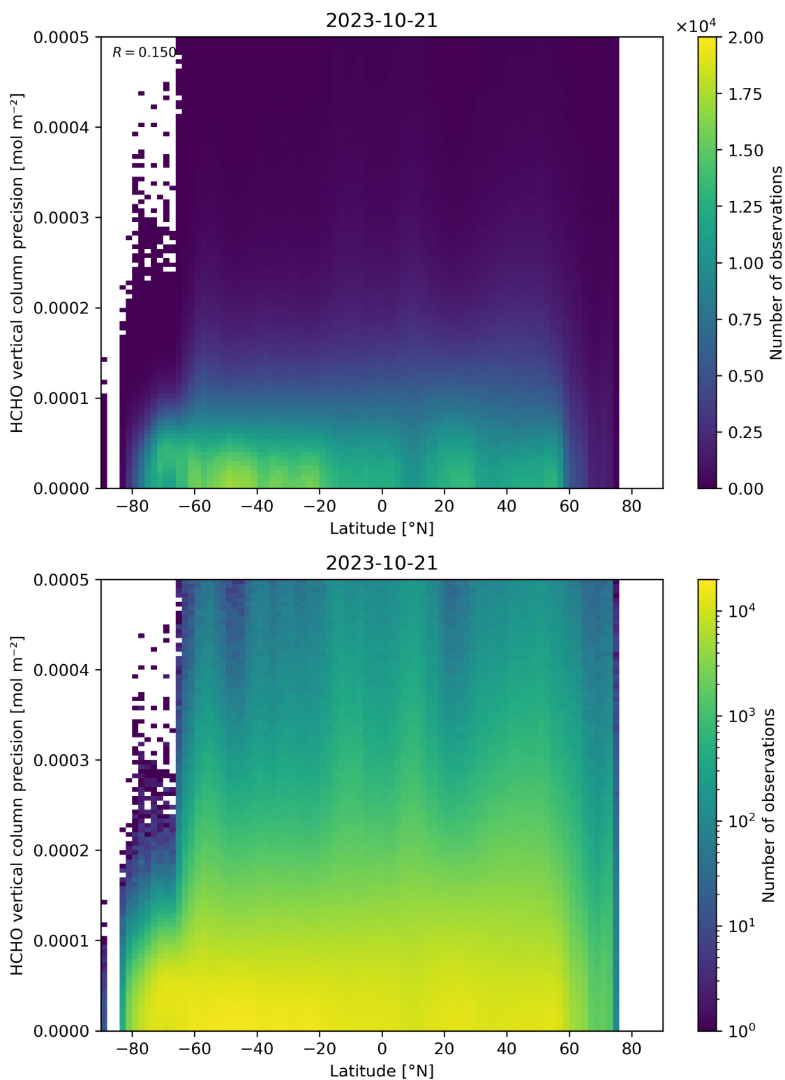
Figure 165: Scatter density plot of “Latitude” against “HCHO vertical column precision” for 2023-10-20 to 2023-10-22.
