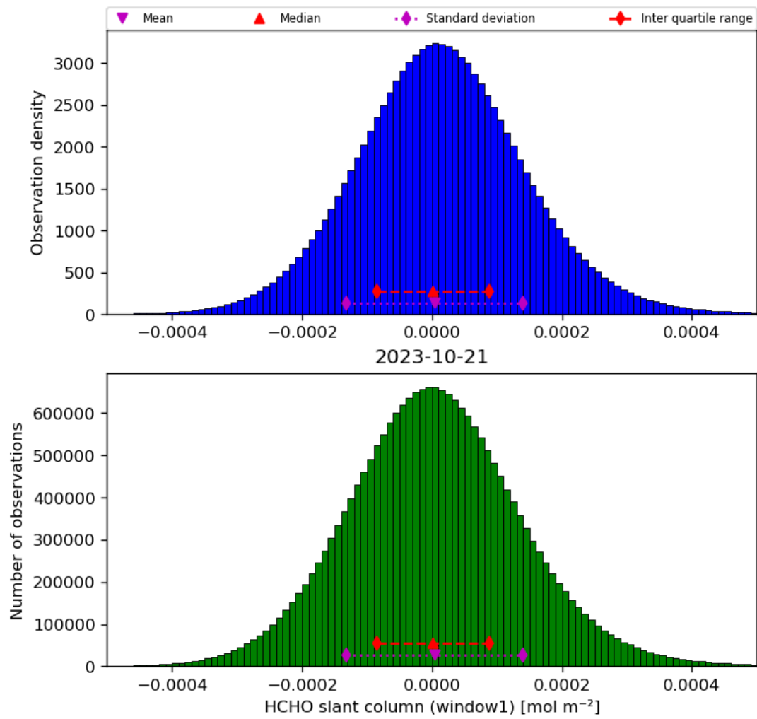
Figure 38: Histogram of “HCHO slant column (window1)” for 2023-10-20 to 2023-10-22
