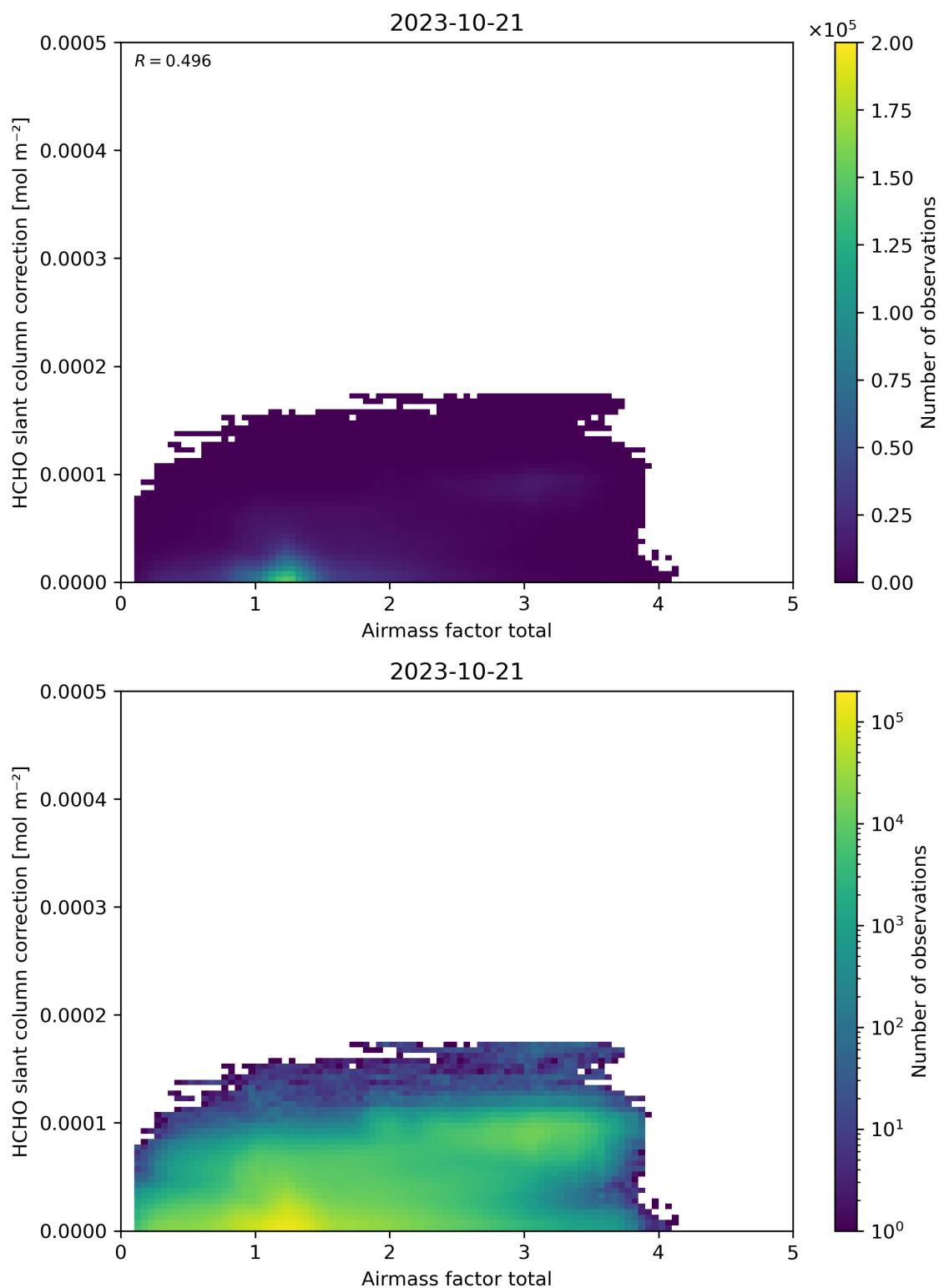
Figure 102: Scatter density plot of “Airmass factor total” against “HCHO slant column correction” for 2023-10-20 to 2023-10-22.
