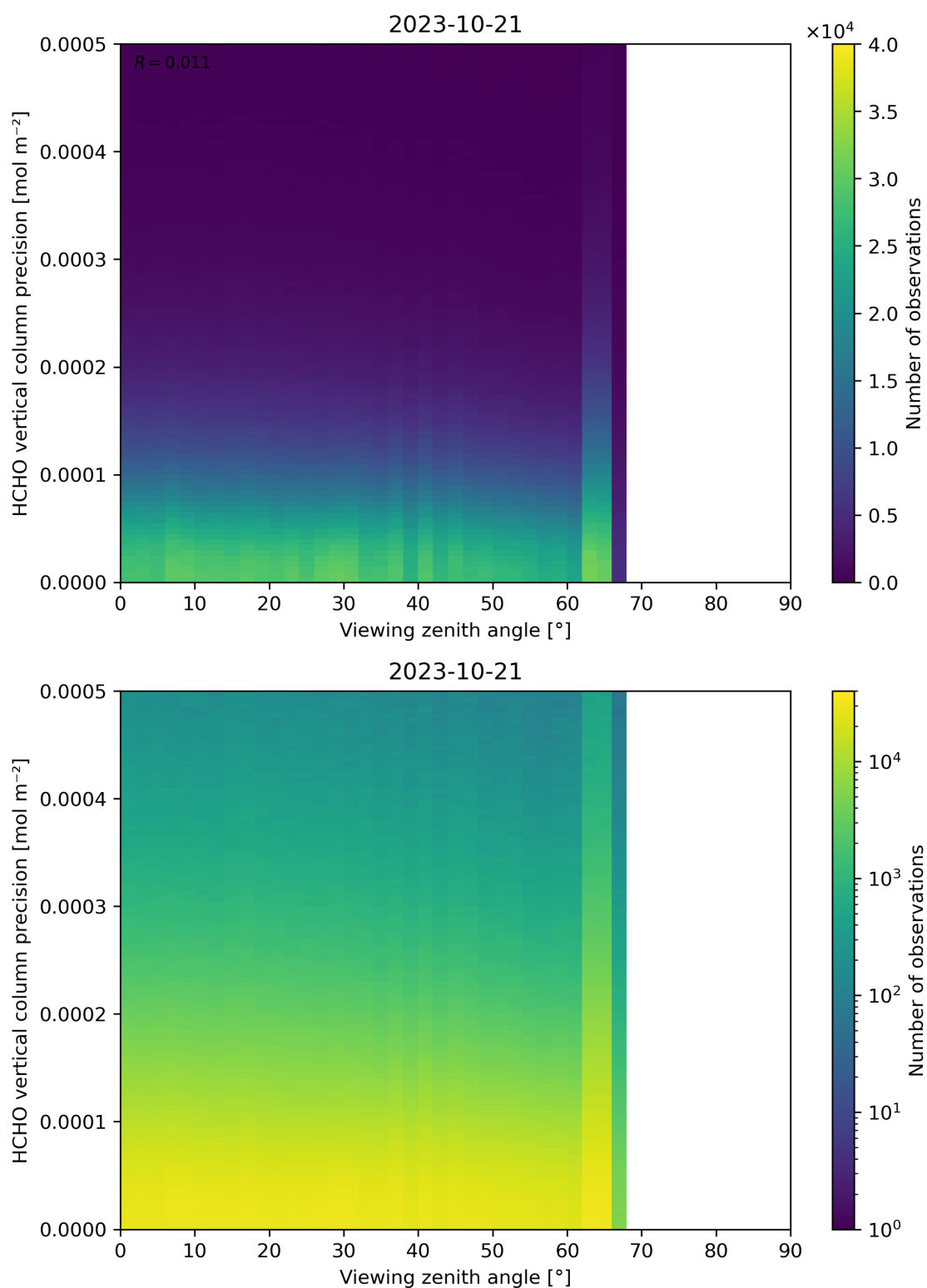
Figure 194: Scatter density plot of “Viewing zenith angle” against “HCHO vertical column precision” for 2023-10-20 to 2023-10-22.
