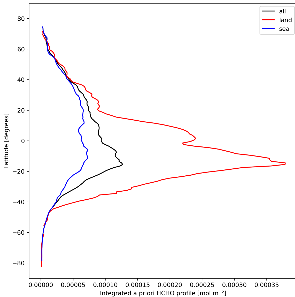
Figure 29: Zonal average of “Integrated a priori HCHO profile” for 2023-10-20 to 2023-10-22.
