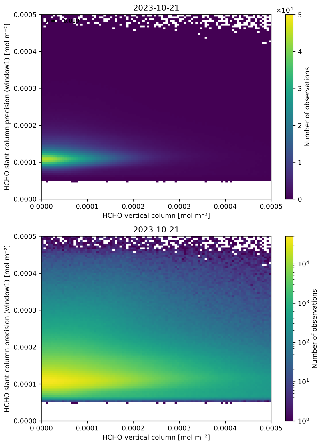
Figure 130: Scatter density plot of “HCHO vertical column” against “HCHO slant column precision (window1)” for 2023-10-20 to 2023-10-22.
