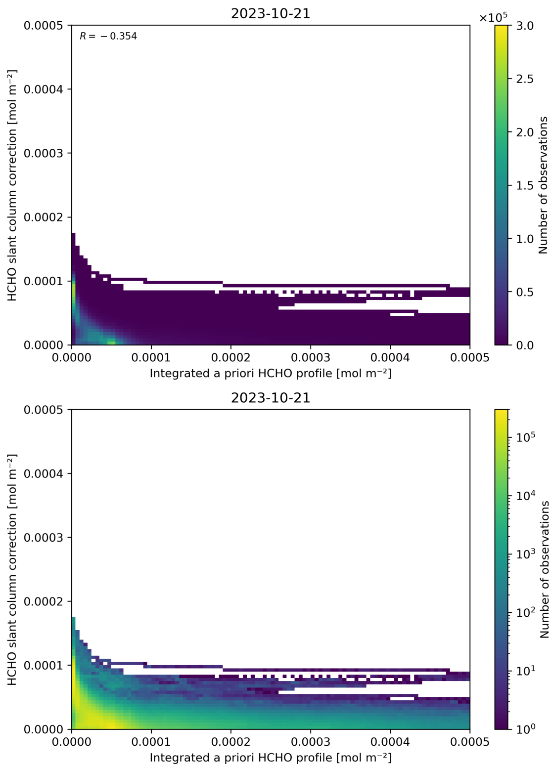
Figure 152: Scatter density plot of “Integrated a priori HCHO profile” against “HCHO slant column correction” for 2023-10-20 to 2023-10-22.
