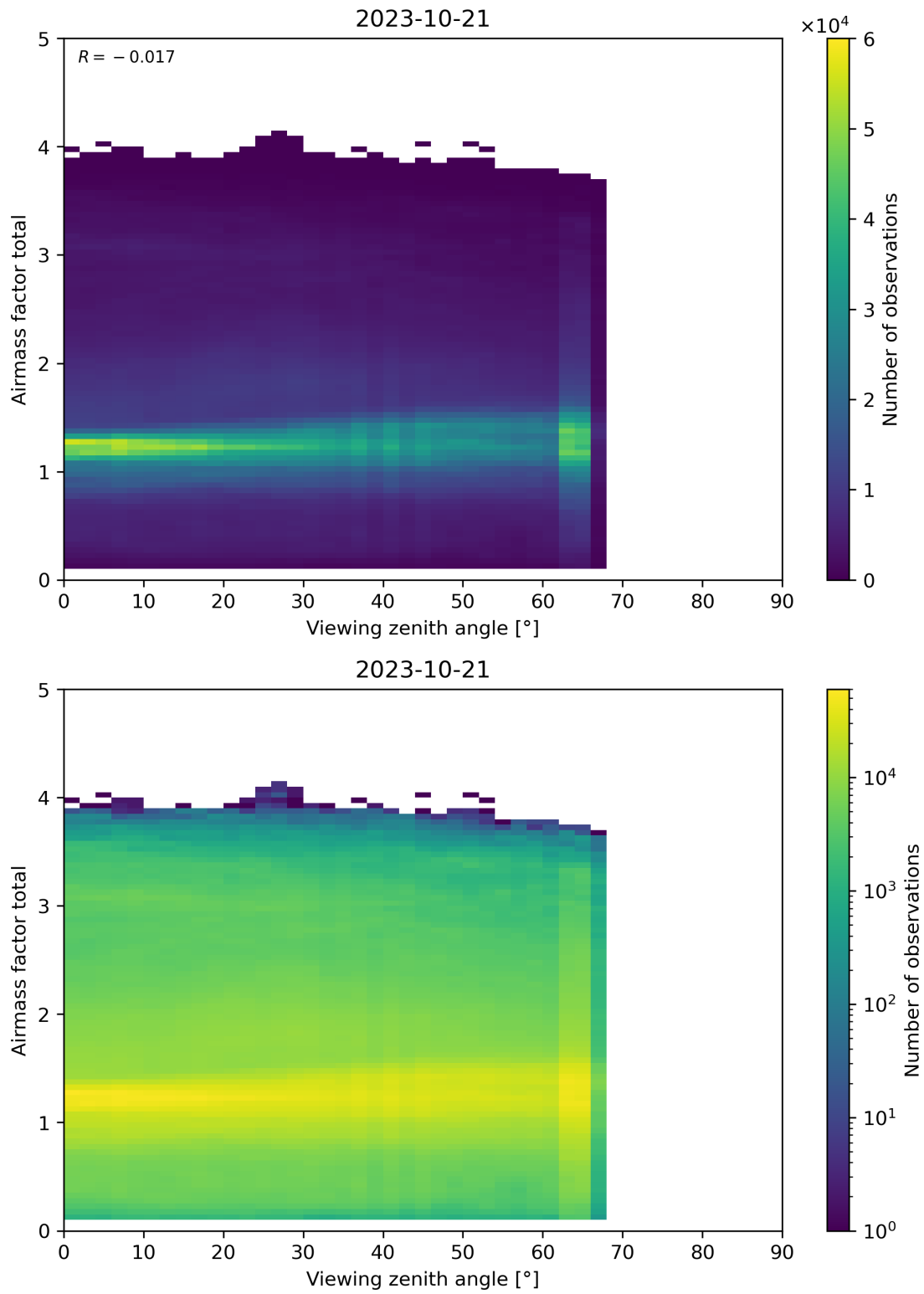
Figure 190: Scatter density plot of “Viewing zenith angle” against “Airmass factor total” for 2023-10-20 to 2023-10-22.
