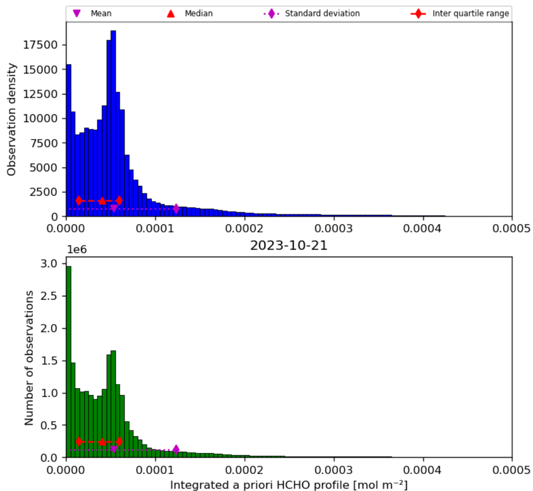
Figure 43: Histogram of “Integrated a priori HCHO profile” for 2023-10-20 to 2023-10-22
