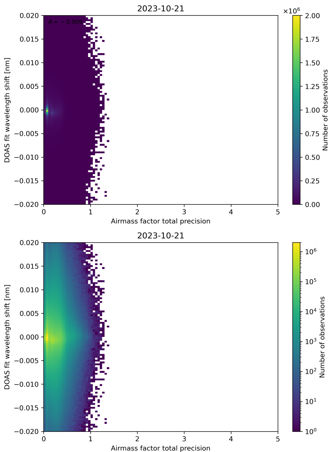
Figure 106: Scatter density plot of “Airmass factor total precision” against “DOAS fit wavelength shift” for 2023-10-20 to 2023-10-22.
