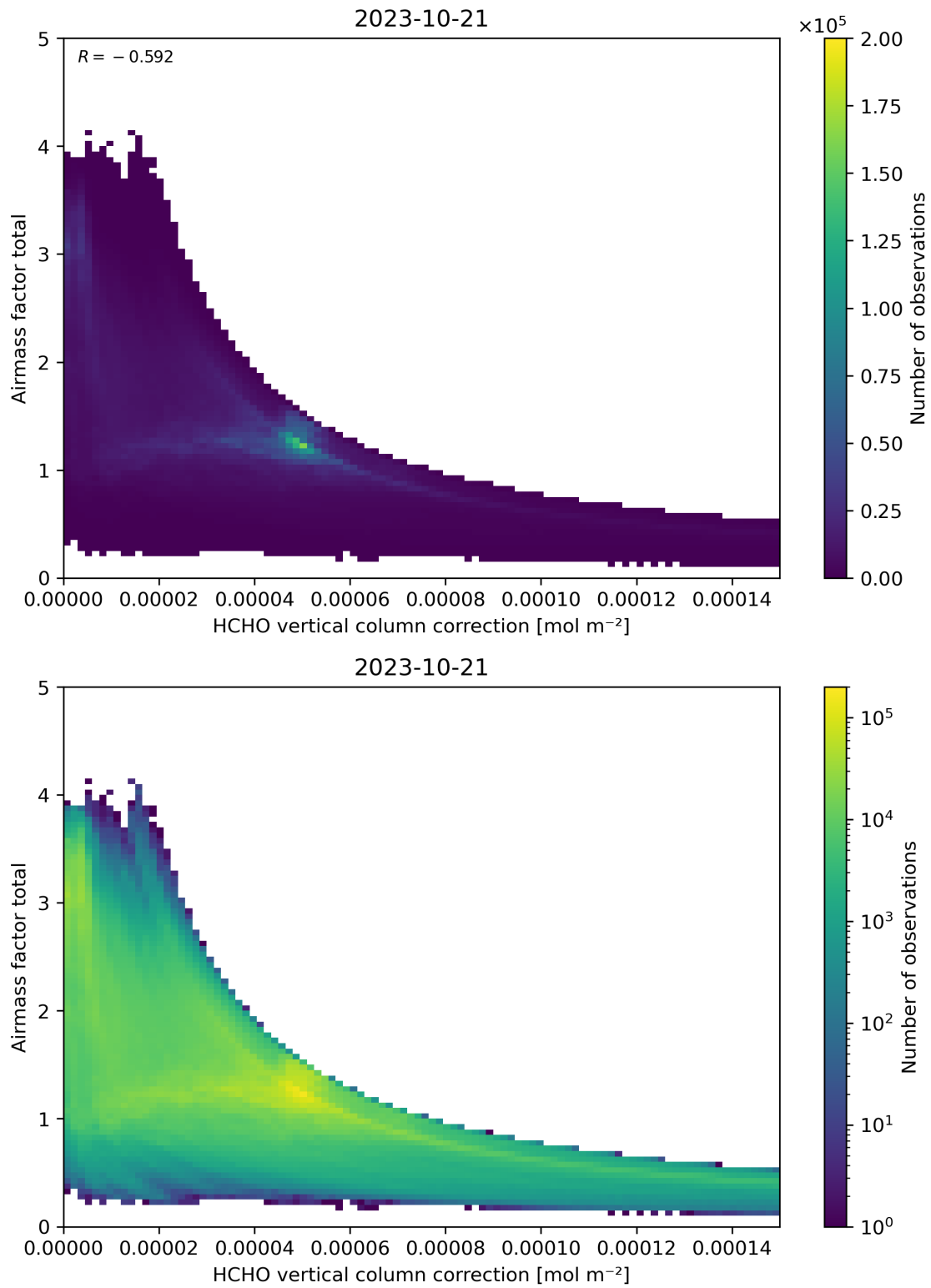
Figure 120: Scatter density plot of “HCHO vertical column correction” against “Airmass factor total” for 2023-10-20 to 2023-10-22.
