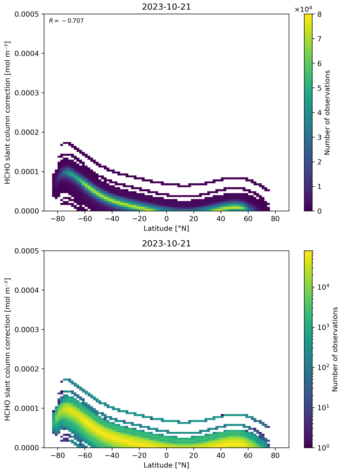
Figure 158: Scatter density plot of “Latitude” against “HCHO slant column correction” for 2023-10-20 to 2023-10-22.
