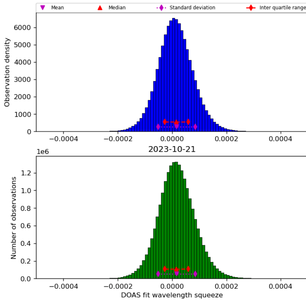
Figure 45: Histogram of “DOAS fit wavelength squeeze” for 2023-10-20 to 2023-10-22
