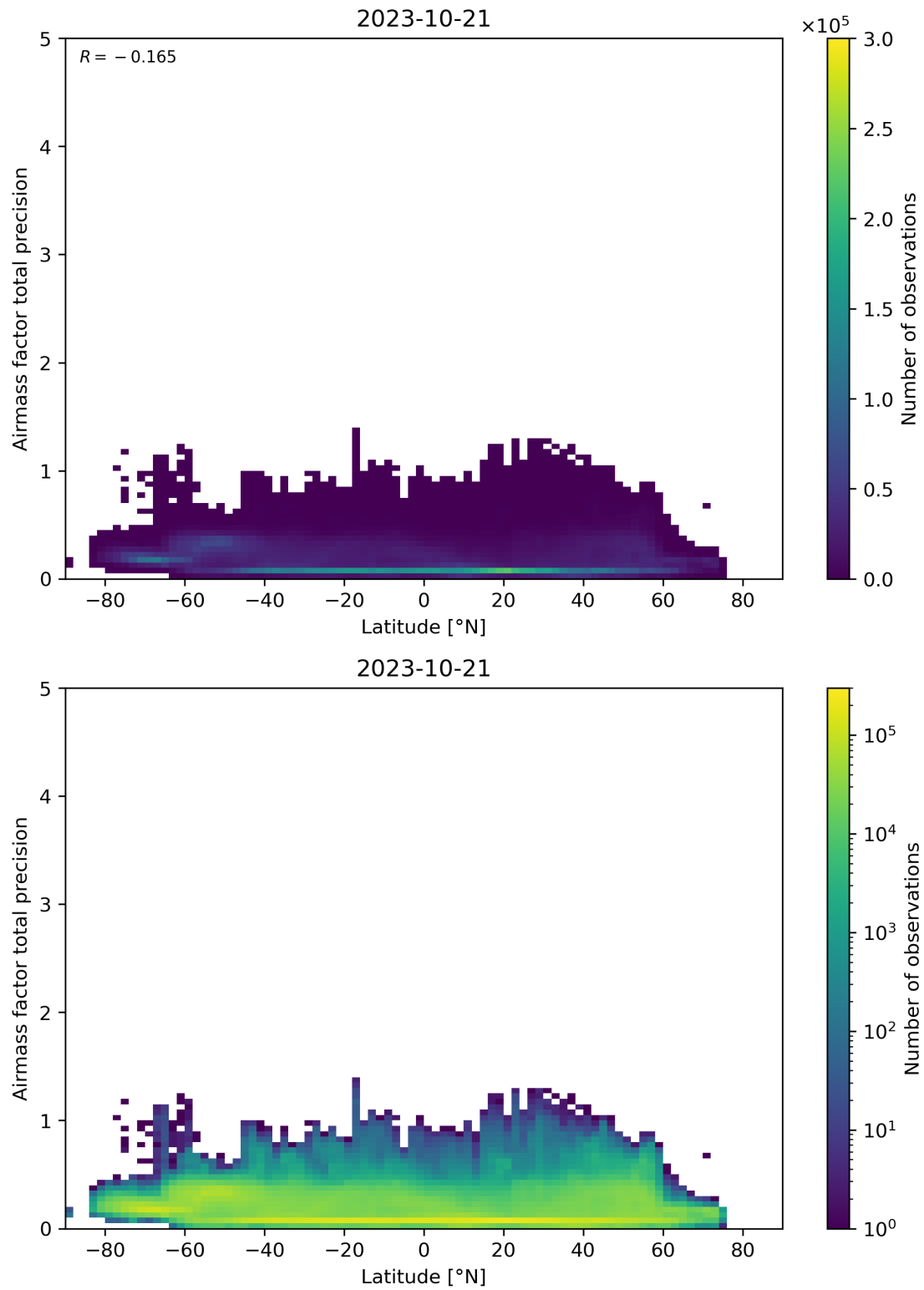
Figure 162: Scatter density plot of “Latitude” against “Airmass factor total precision” for 2023-10-20 to 2023-10-22.
