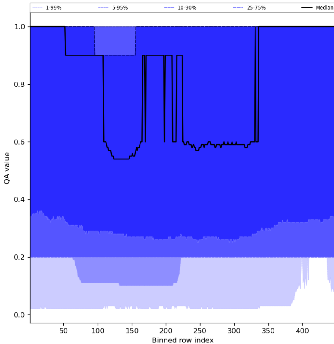
Figure 48: Along track statistics of “QA value” for 2023-10-20 to 2023-10-22
