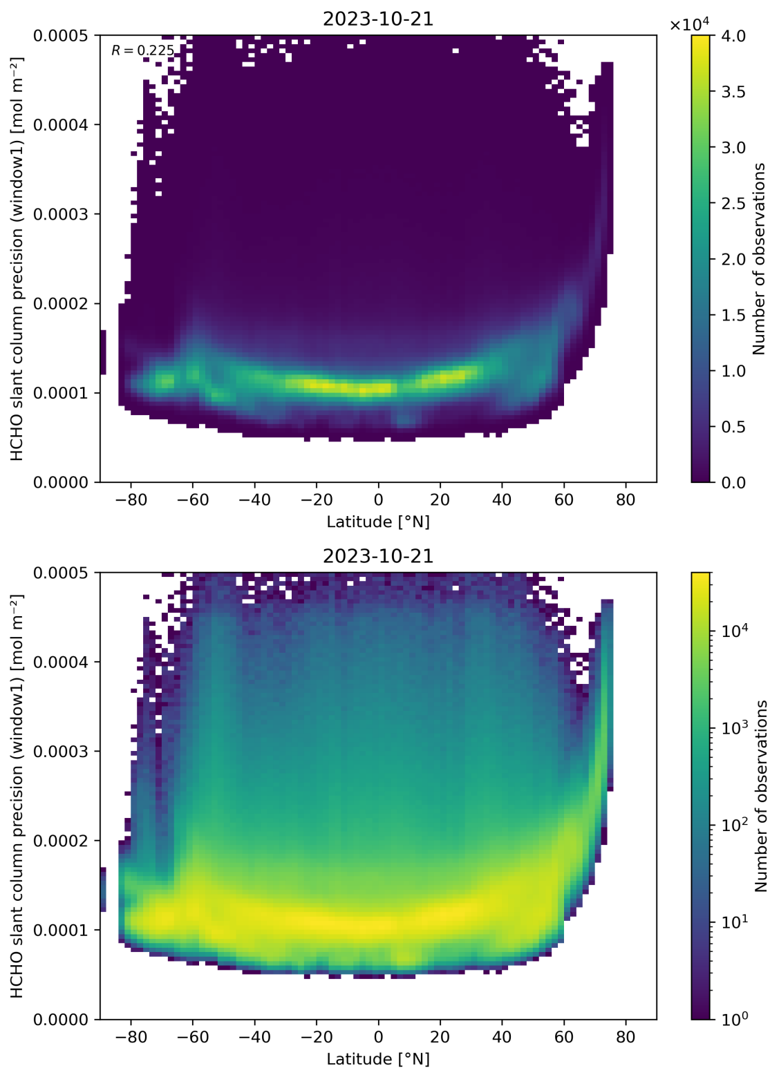
Figure 160: Scatter density plot of “Latitude” against “HCHO slant column precision (window1)” for 2023-10-20 to 2023-10-22.
