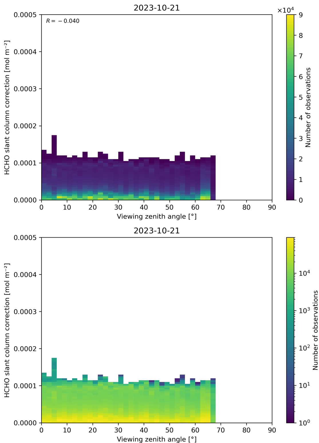
Figure 187: Scatter density plot of “Viewing zenith angle” against “HCHO slant column correction” for 2023-10-20 to 2023-10-22.
