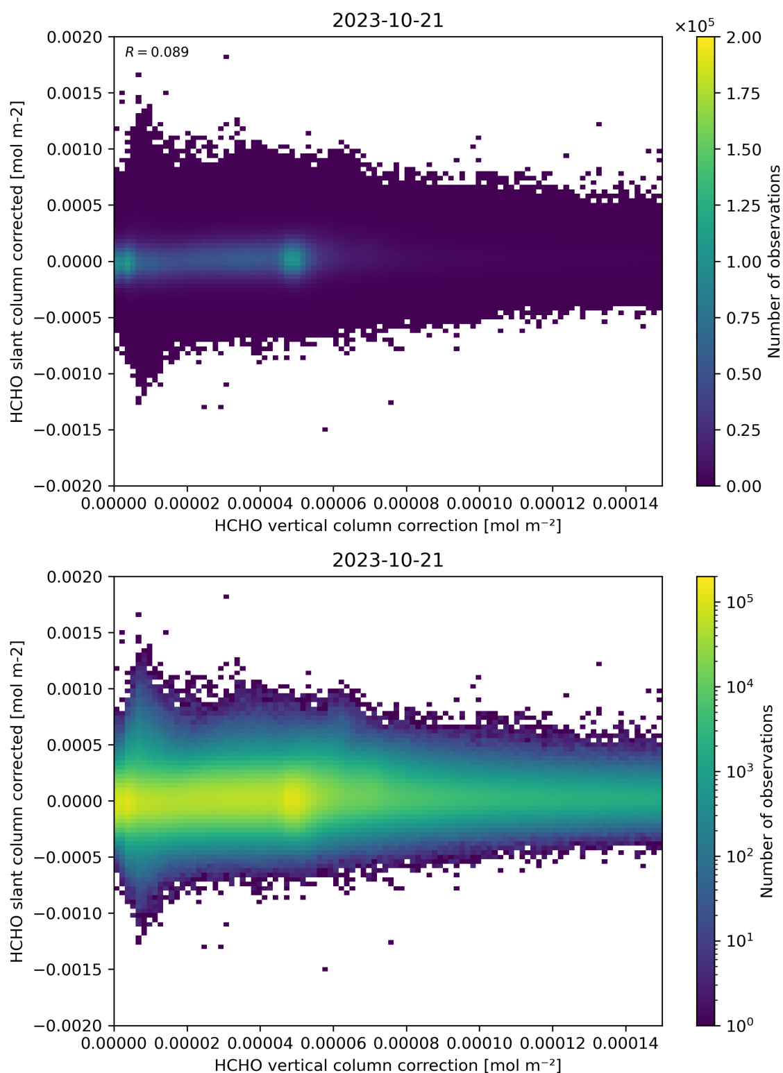
Figure 116: Scatter density plot of “HCHO vertical column correction” against “HCHO slant column corrected” for 2023-10-20 to 2023-10-22.
