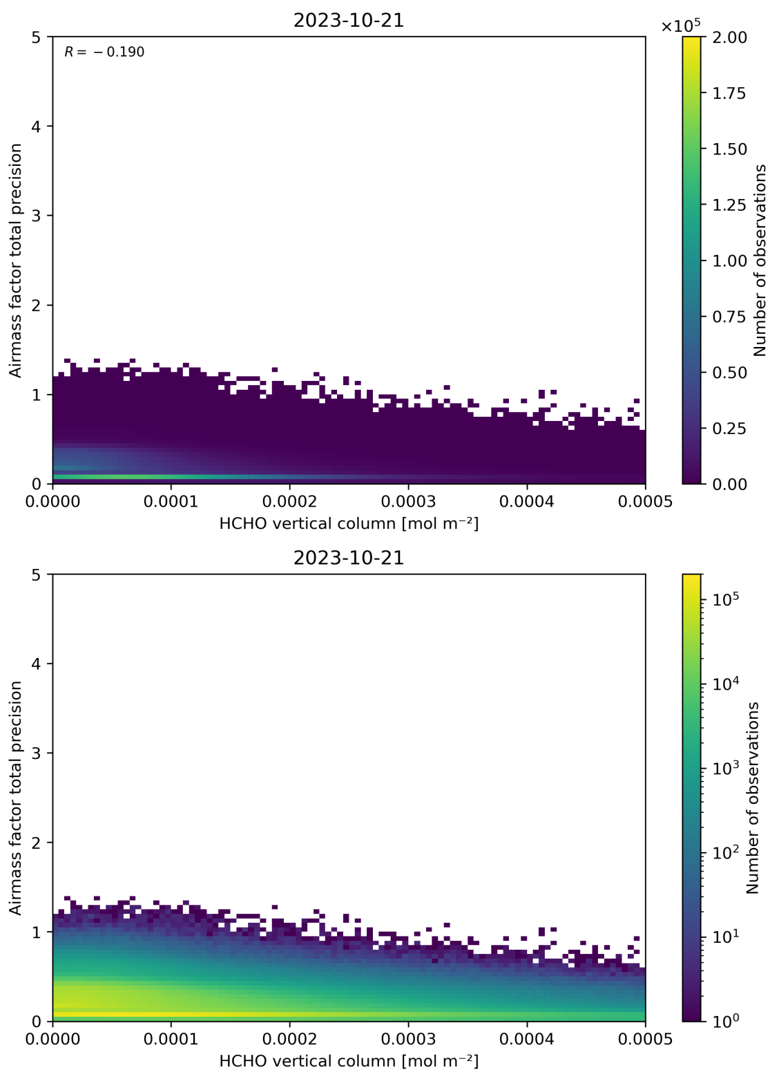
Figure 132: Scatter density plot of “HCHO vertical column” against “Airmass factor total precision” for 2023-10-20 to 2023-10-22.
