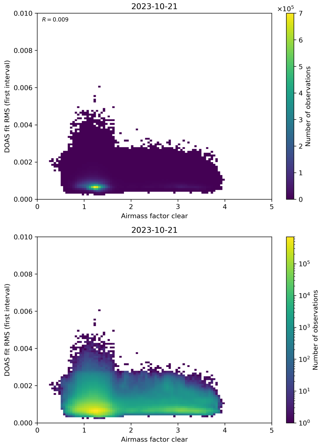
Figure 71: Scatter density plot of “Airmass factor clear” against “DOAS fit RMS (first interval)” for 2023-10-20 to 2023-10-22.
