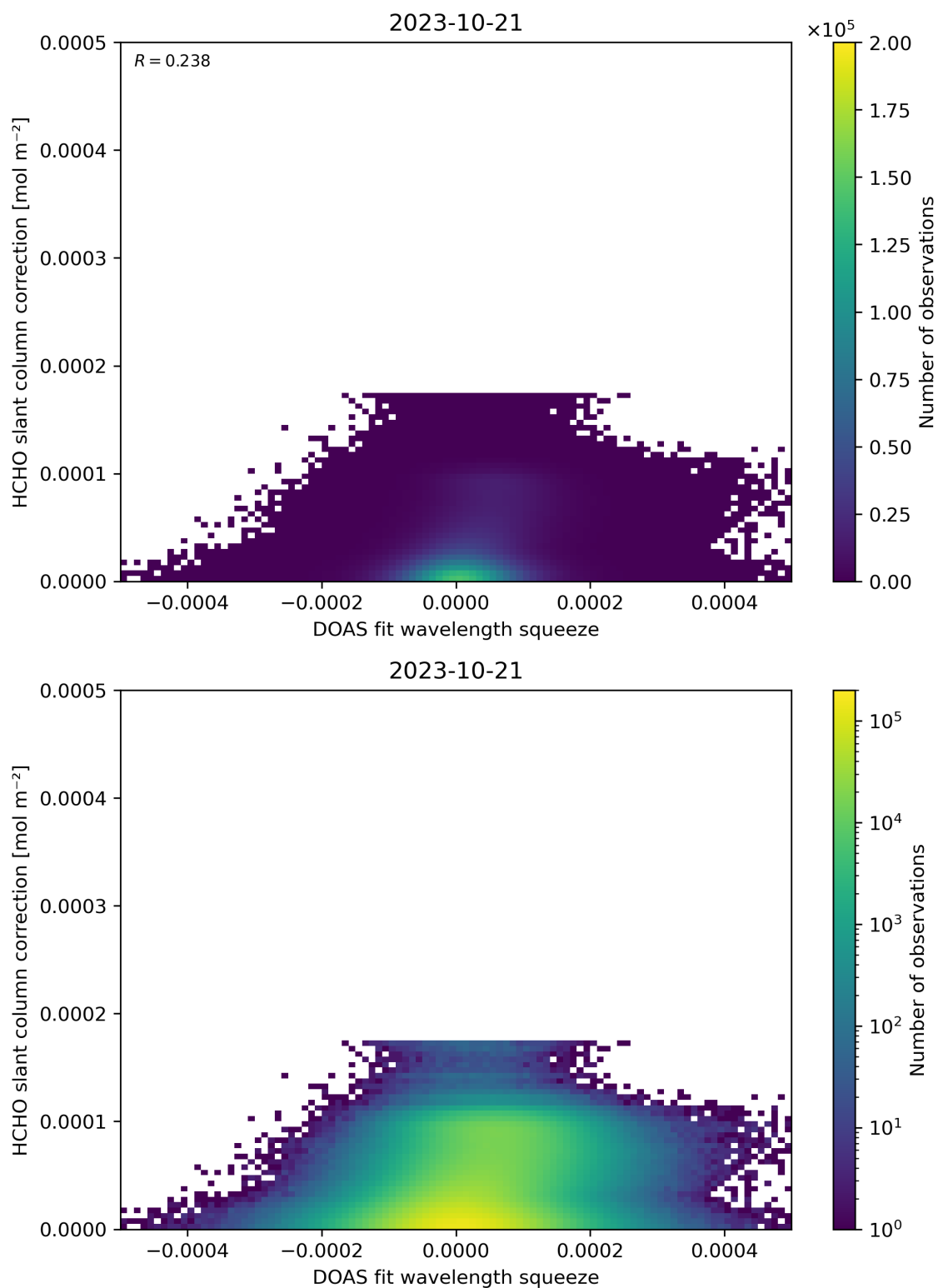
Figure 70: Scatter density plot of “DOAS fit wavelength squeeze” against “HCHO slant column correction” for 2023-10-20 to 2023-10-22.
