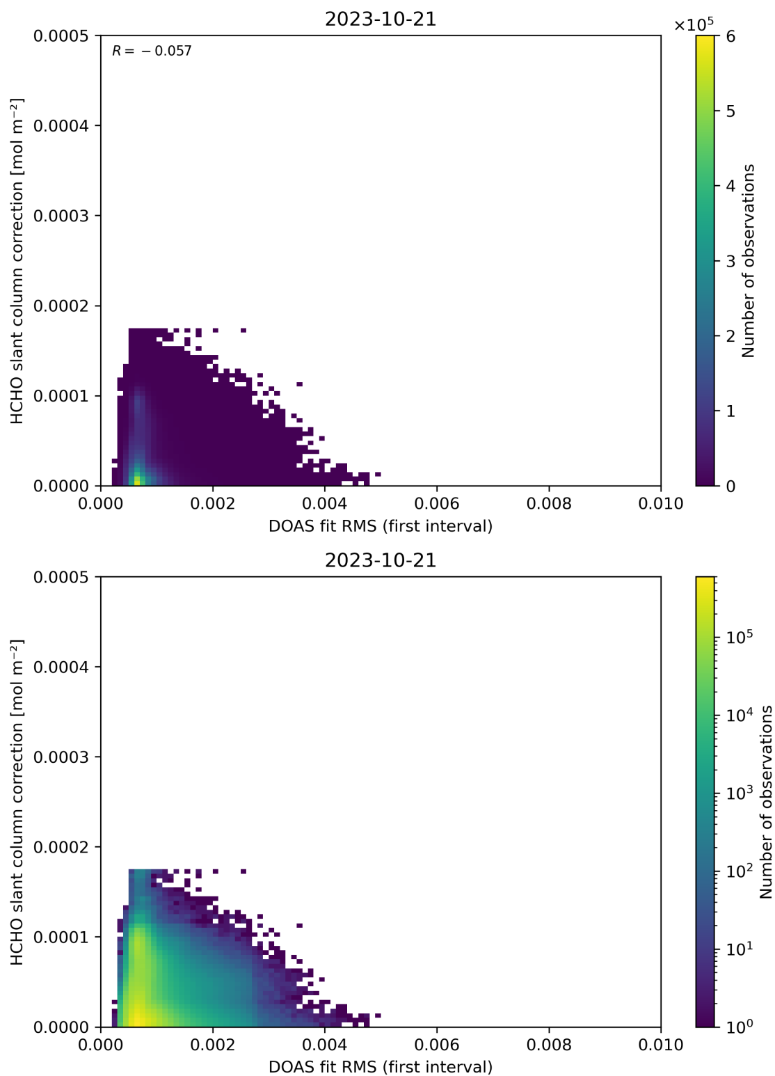
Figure 63: Scatter density plot of “DOAS fit RMS (first interval)” against “HCHO slant column correction” for 2023-10-20 to 2023-10-22.
