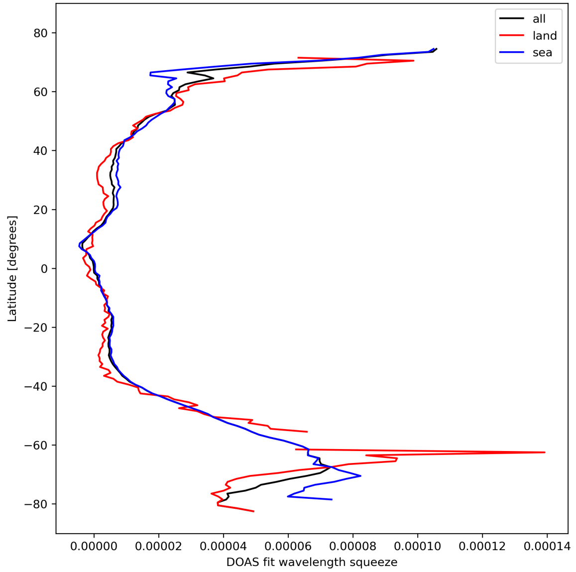
Figure 31: Zonal average of “DOAS fit wavelength squeeze” for 2023-10-20 to 2023-10-22.
