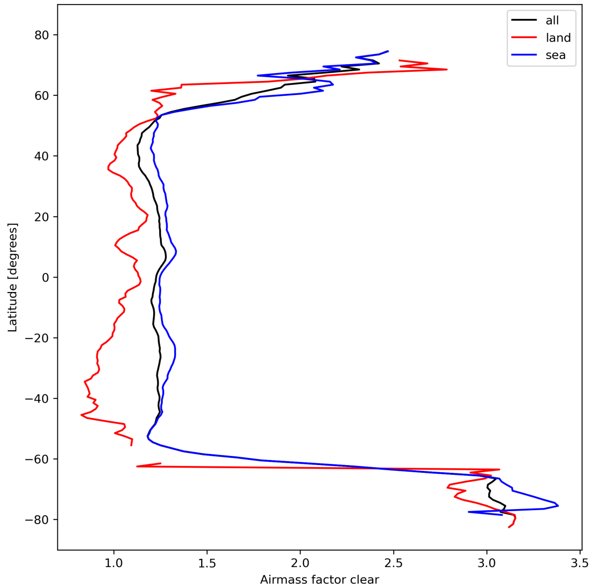
Figure 28: Zonal average of “Airmass factor clear” for 2023-10-20 to 2023-10-22.
