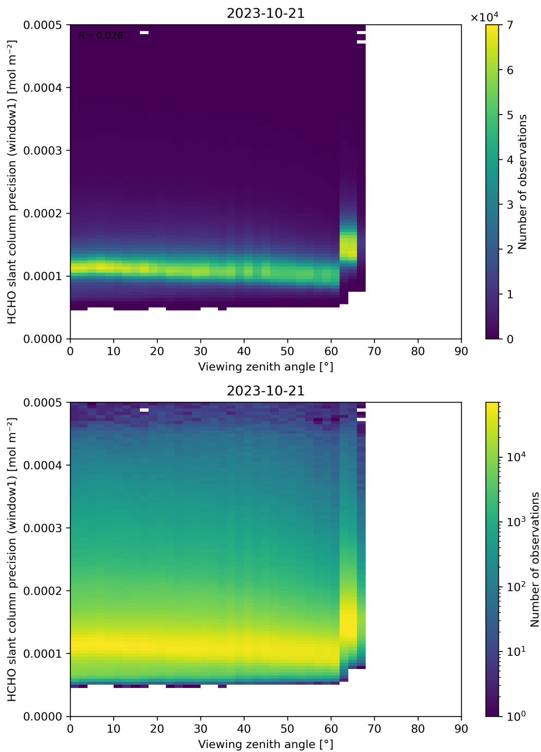
Figure 189: Scatter density plot of “Viewing zenith angle” against “HCHO slant column precision (window1)” for 2023-10-20 to 2023-10-22.
