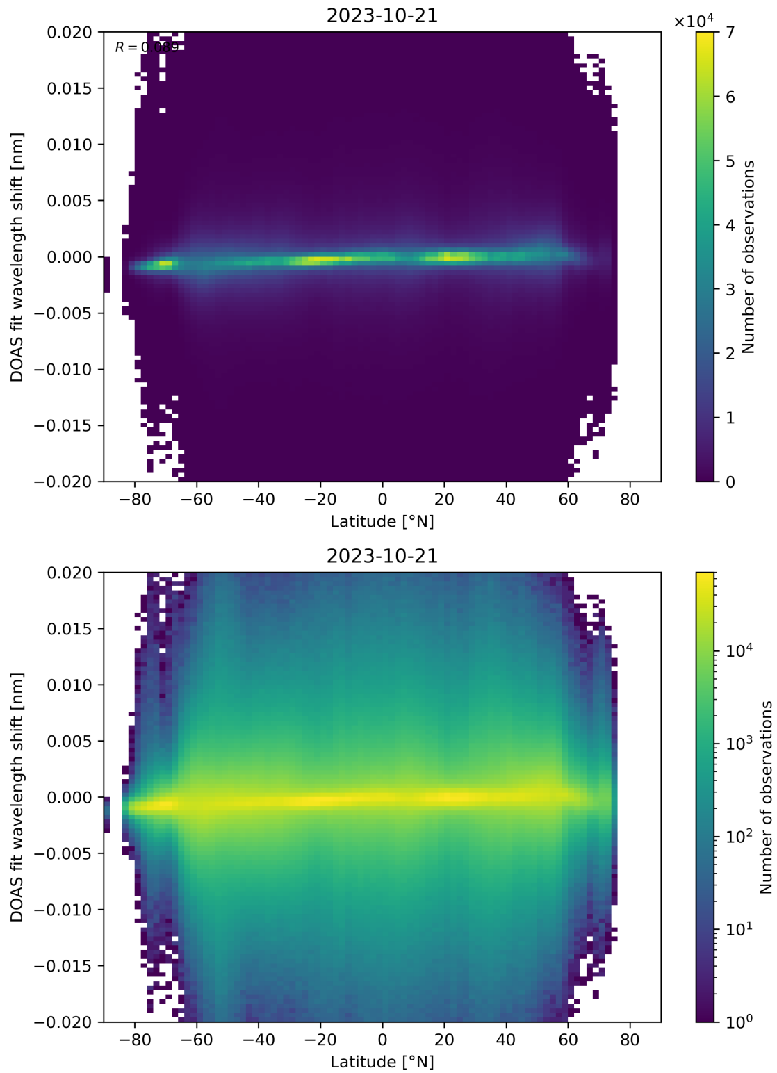
Figure 154: Scatter density plot of “Latitude” against “DOAS fit wavelength shift” for 2023-10-20 to 2023-10-22.
