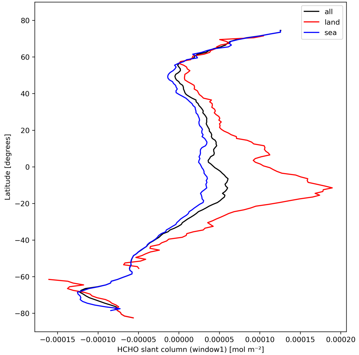
Figure 24: Zonal average of “HCHO slant column (window1)” for 2023-10-20 to 2023-10-22.
