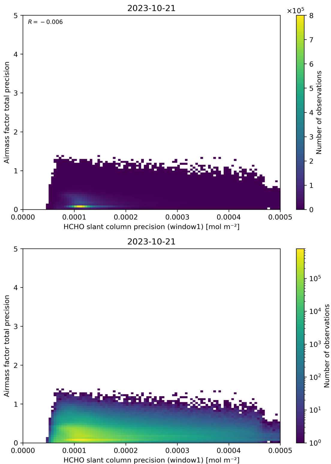
Figure 95: Scatter density plot of “HCHO slant column precision (window1)” against “Airmass factor total precision” for 2023-10-20 to 2023-10-22.
