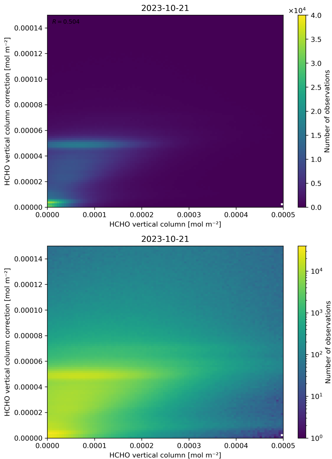
Figure 133: Scatter density plot of “HCHO vertical column” against “HCHO vertical column correction” for 2023-10-20 to 2023-10-22.
