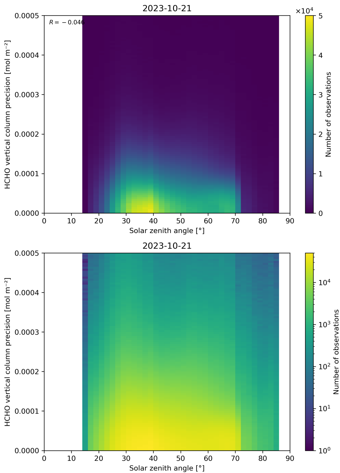
Figure 179: Scatter density plot of “Solar zenith angle” against “HCHO vertical column precision” for 2023-10-20 to 2023-10-22.
