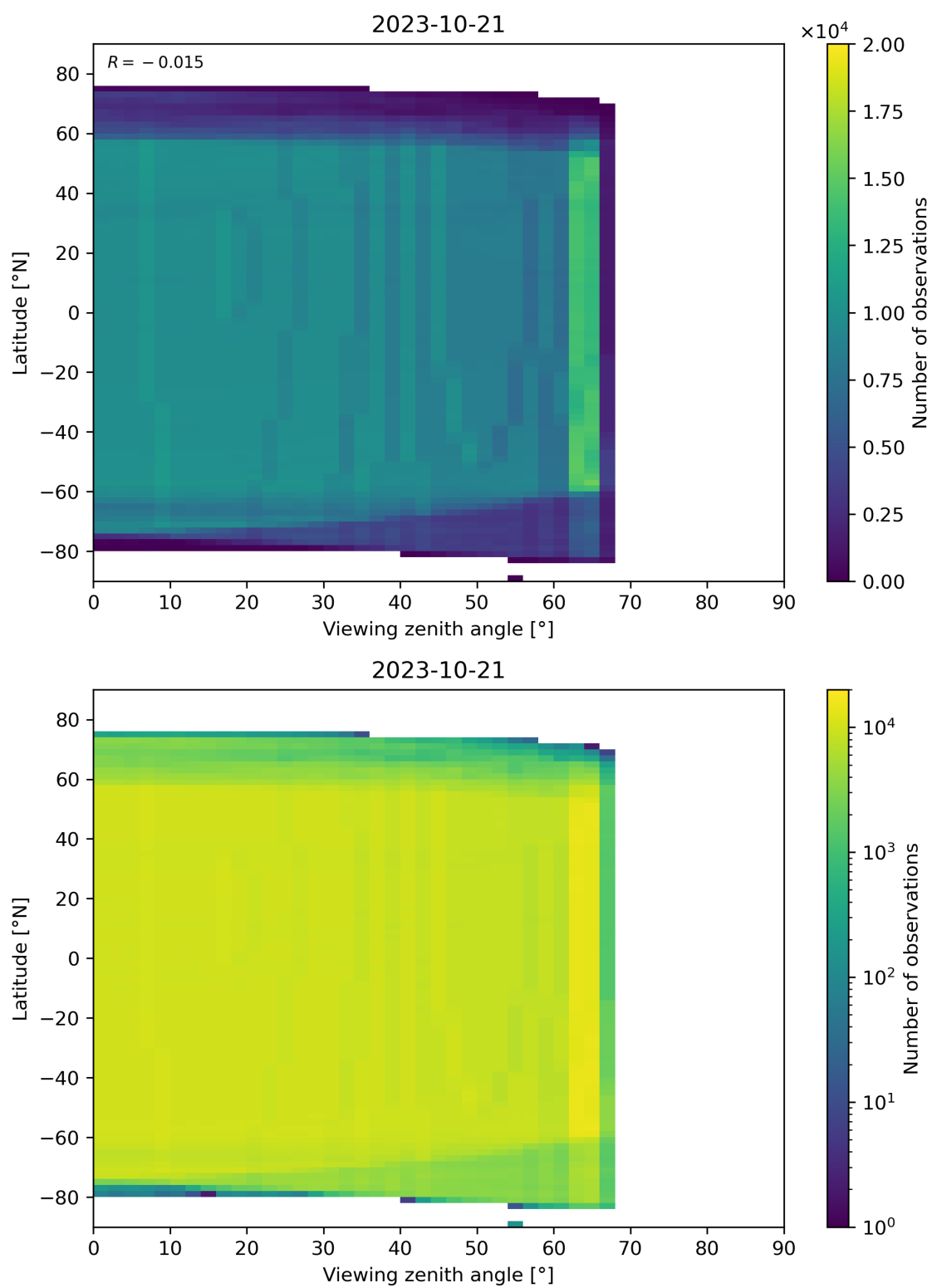
Figure 196: Scatter density plot of “Viewing zenith angle” against “Latitude” for 2023-10-20 to 2023-10-22.
