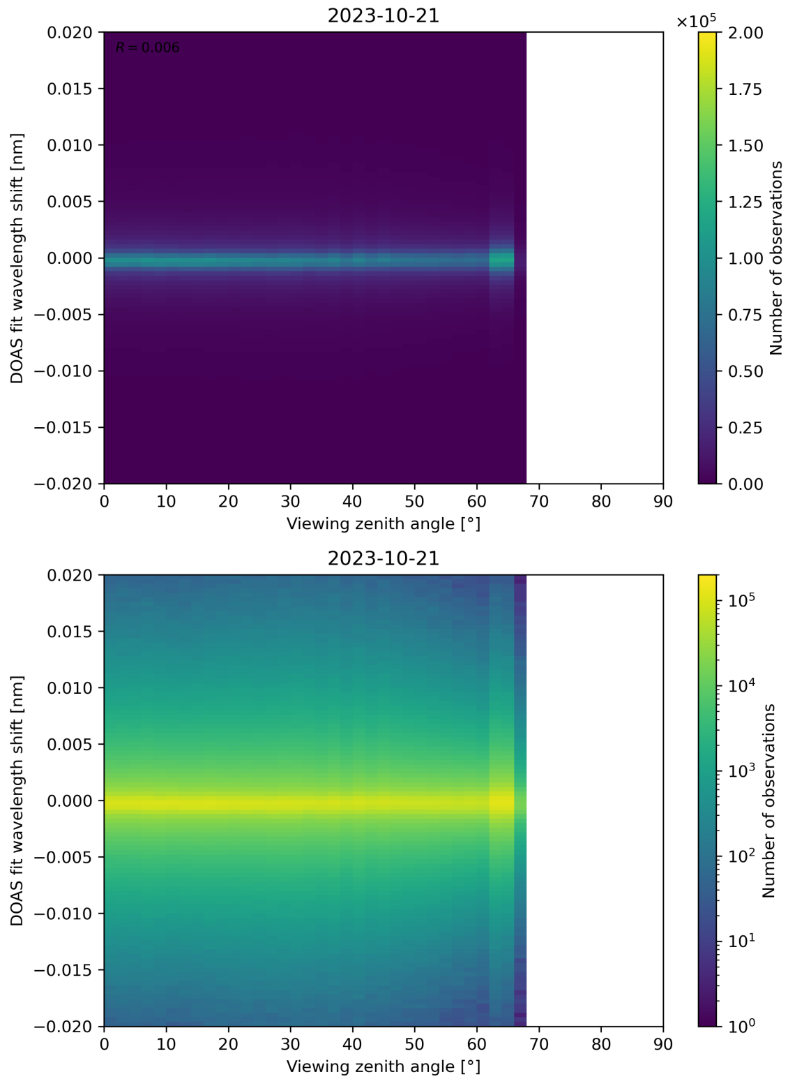
Figure 183: Scatter density plot of “Viewing zenith angle” against “DOAS fit wavelength shift” for 2023-10-20 to 2023-10-22.
