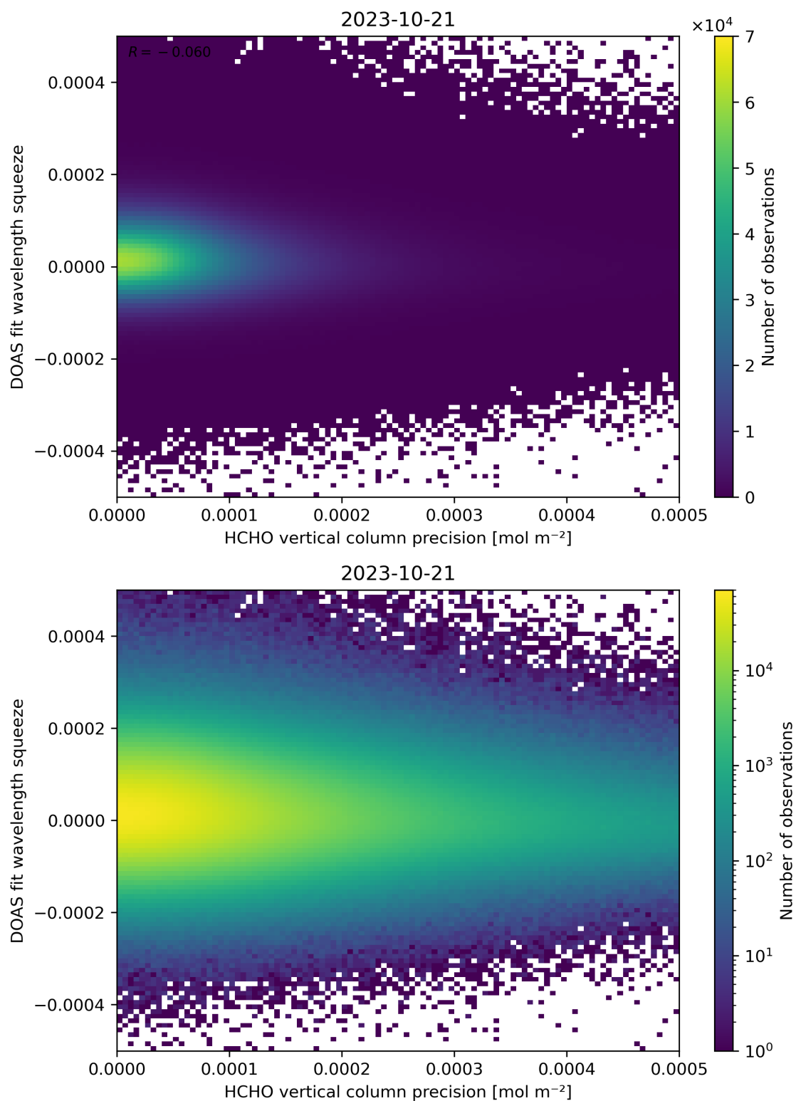
Figure 138: Scatter density plot of “HCHO vertical column precision” against “DOAS fit wavelength squeeze” for 2023-10-20 to 2023-10-22.
