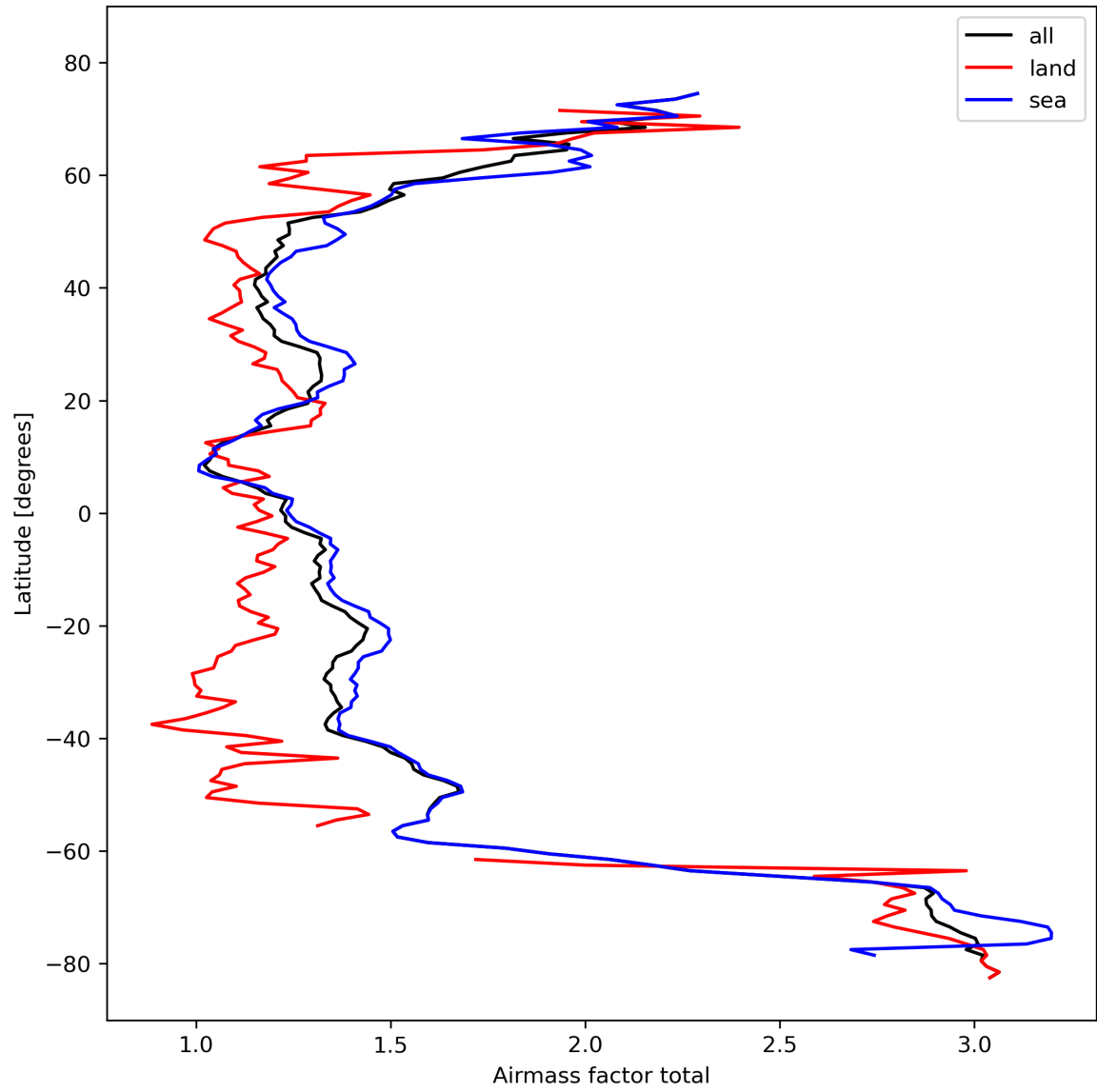
Figure 26: Zonal average of “Airmass factor total” for 2023-10-20 to 2023-10-22.
