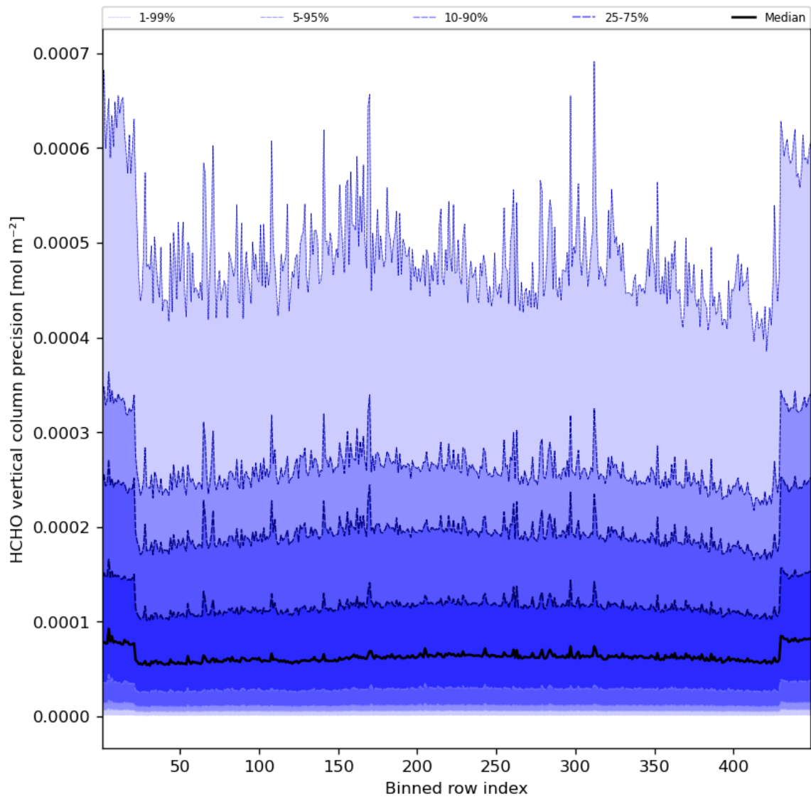
Figure 50: Along track statistics of “HCHO vertical column precision” for 2023-10-20 to 2023-10-22
