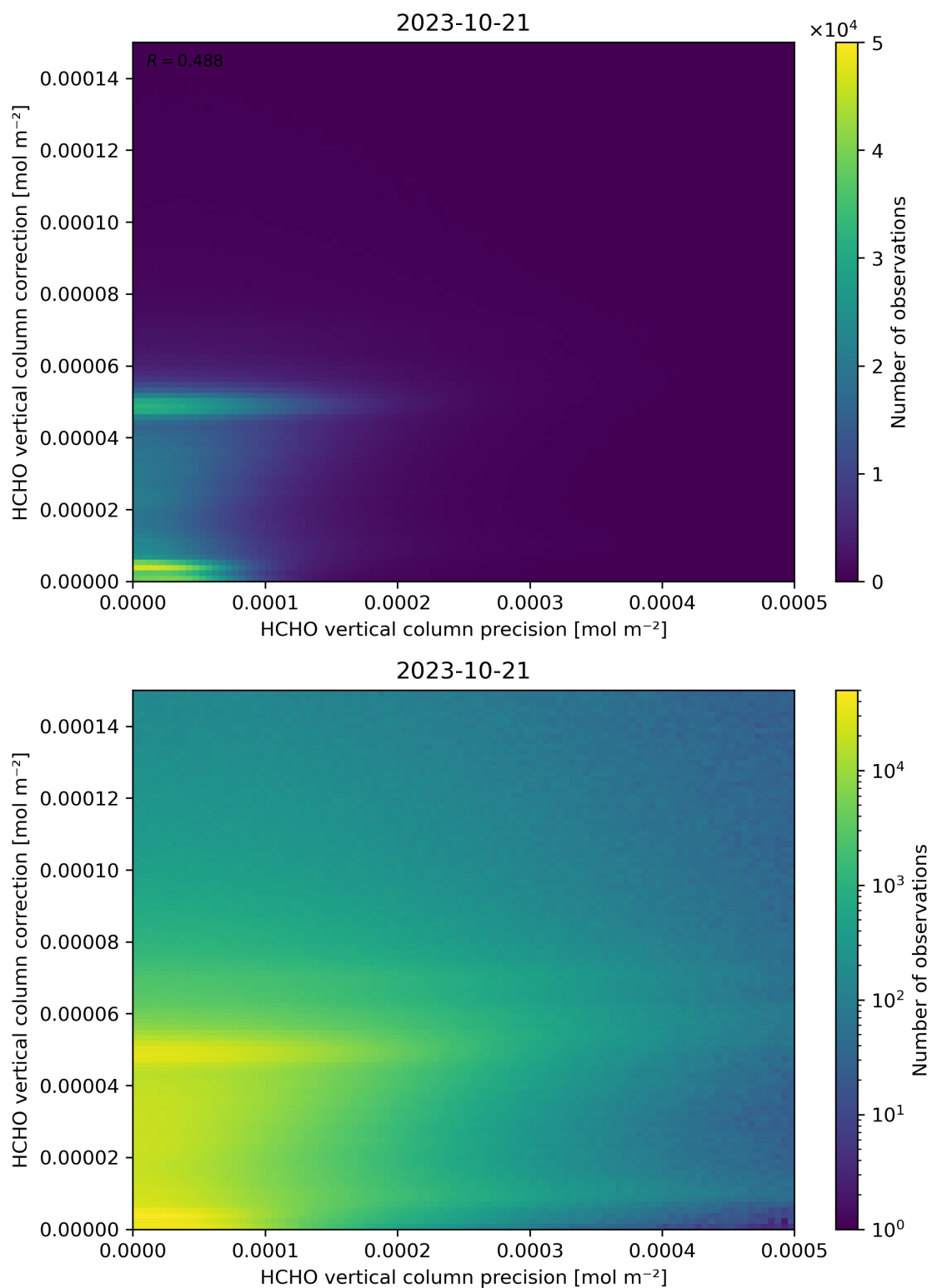
Figure 146: Scatter density plot of “HCHO vertical column precision” against “HCHO vertical column correction” for 2023-10-20 to 2023-10-22.
