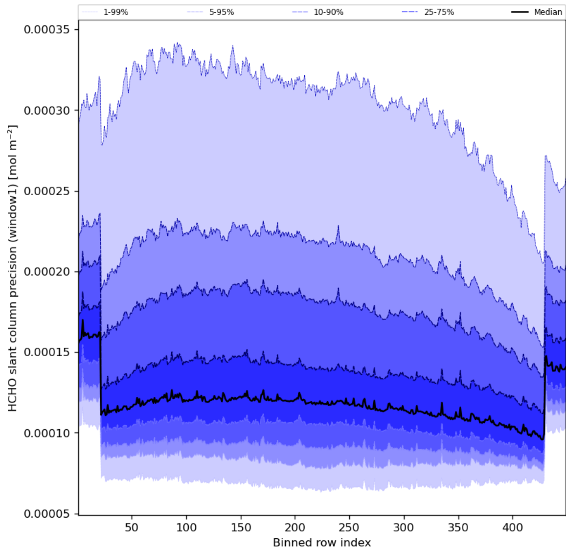
Figure 53: Along track statistics of “HCHO slant column precision (window1)” for 2023-10-20 to 2023-10-22
