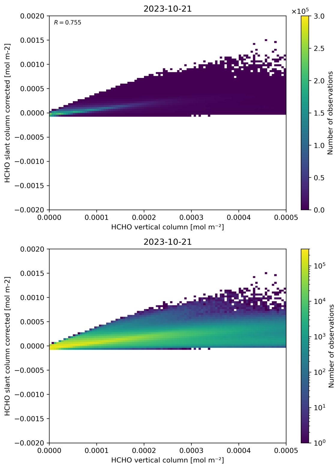
Figure 127: Scatter density plot of “HCHO vertical column” against “HCHO slant column corrected” for 2023-10-20 to 2023-10-22.
