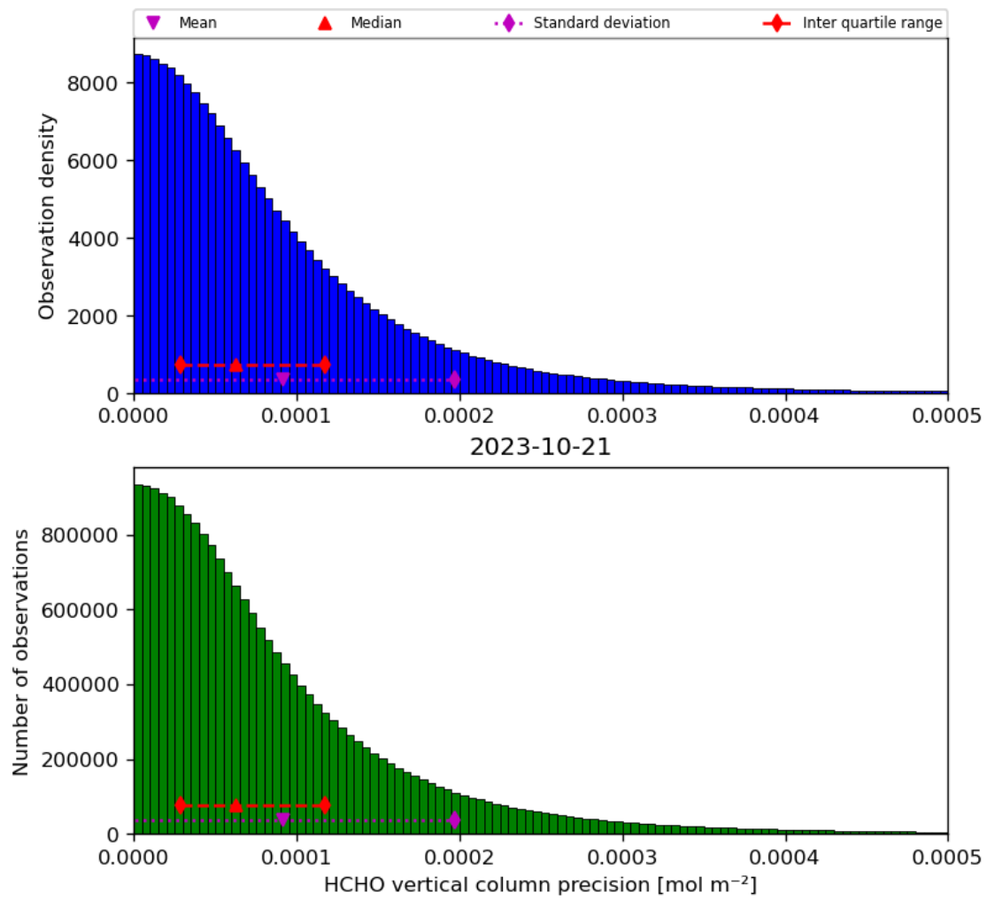
Figure 36: Histogram of “HCHO vertical column precision” for 2023-10-20 to 2023-10-22
