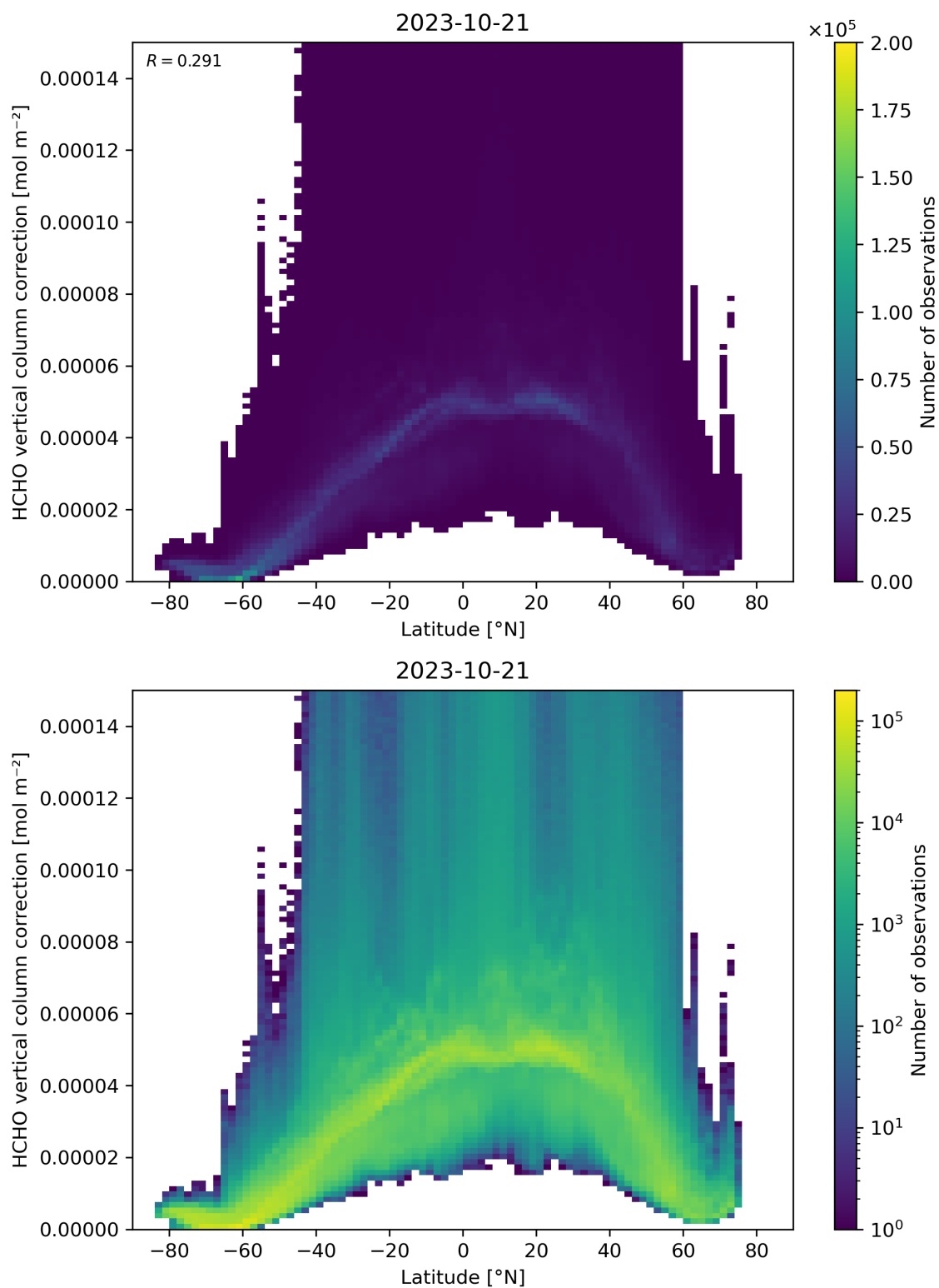
Figure 164: Scatter density plot of “Latitude” against “HCHO vertical column correction” for 2023-10-20 to 2023-10-22.
