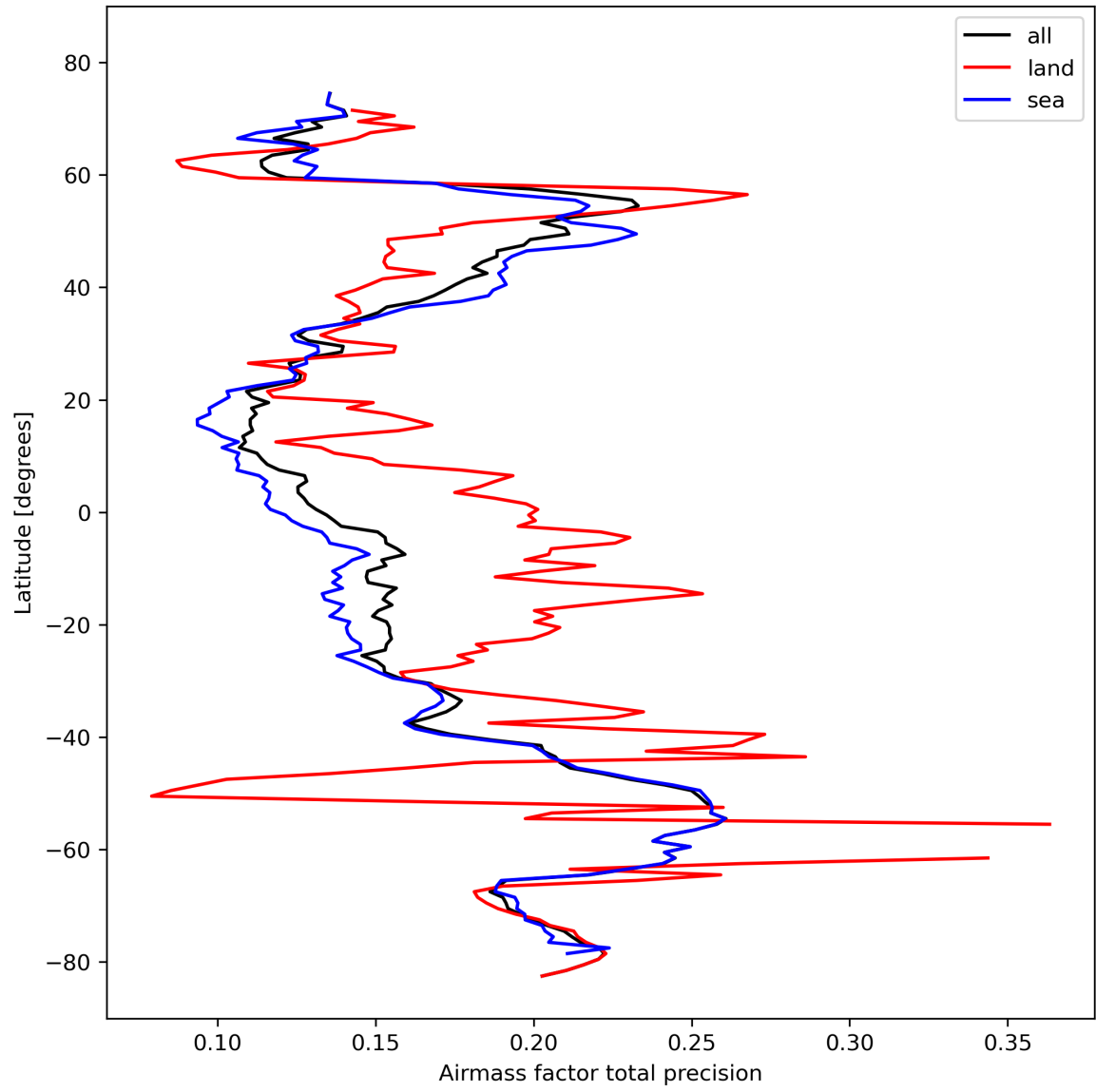
Figure 27: Zonal average of “Airmass factor total precision” for 2023-10-20 to 2023-10-22.
