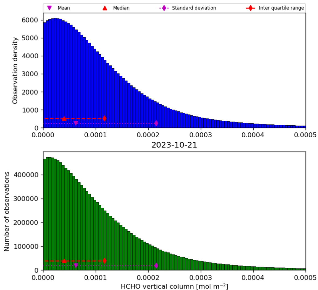
Figure 35: Histogram of “HCHO vertical column” for 2023-10-20 to 2023-10-22
