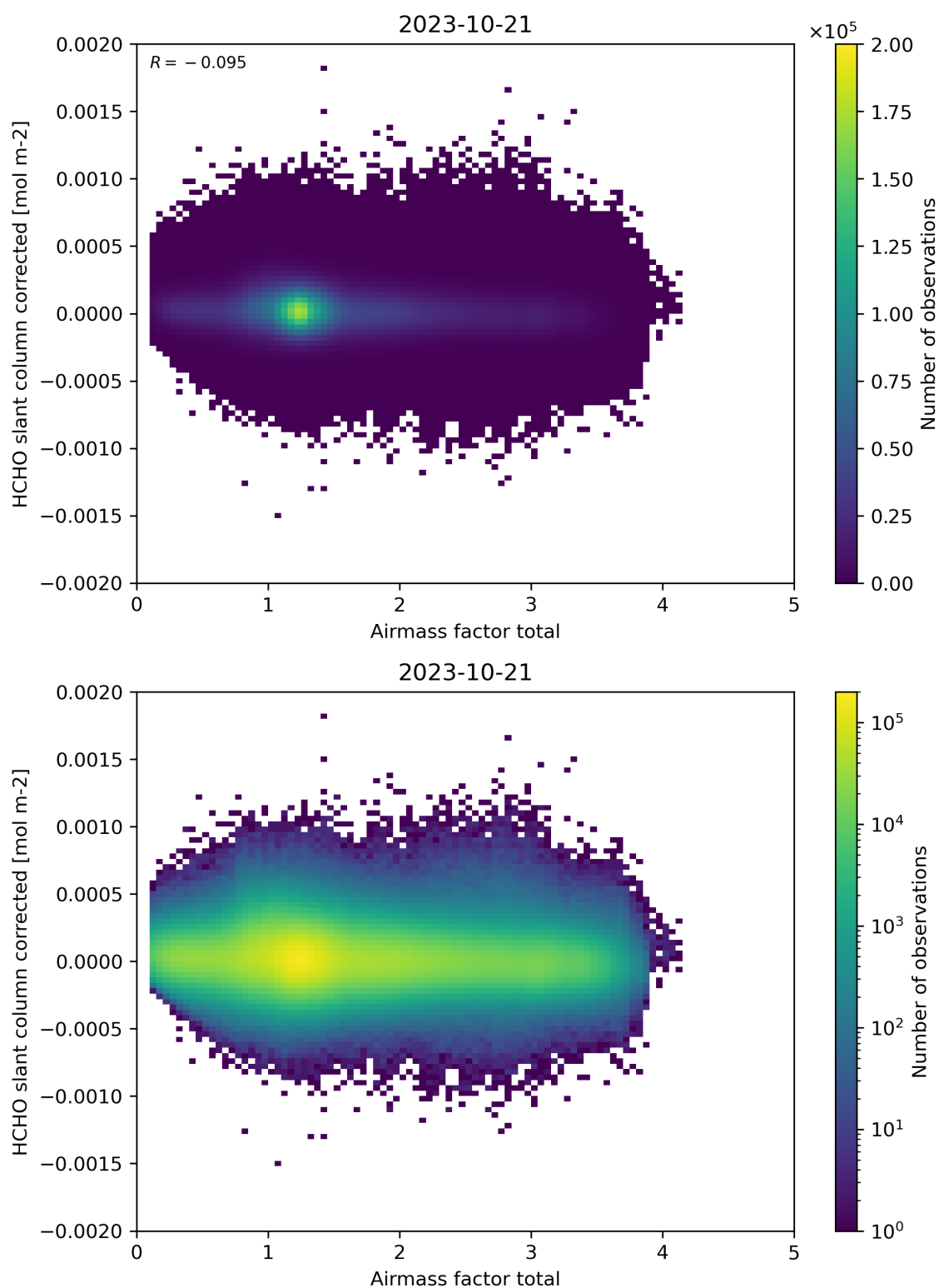
Figure 101: Scatter density plot of “Airmass factor total” against “HCHO slant column corrected” for 2023-10-20 to 2023-10-22.
