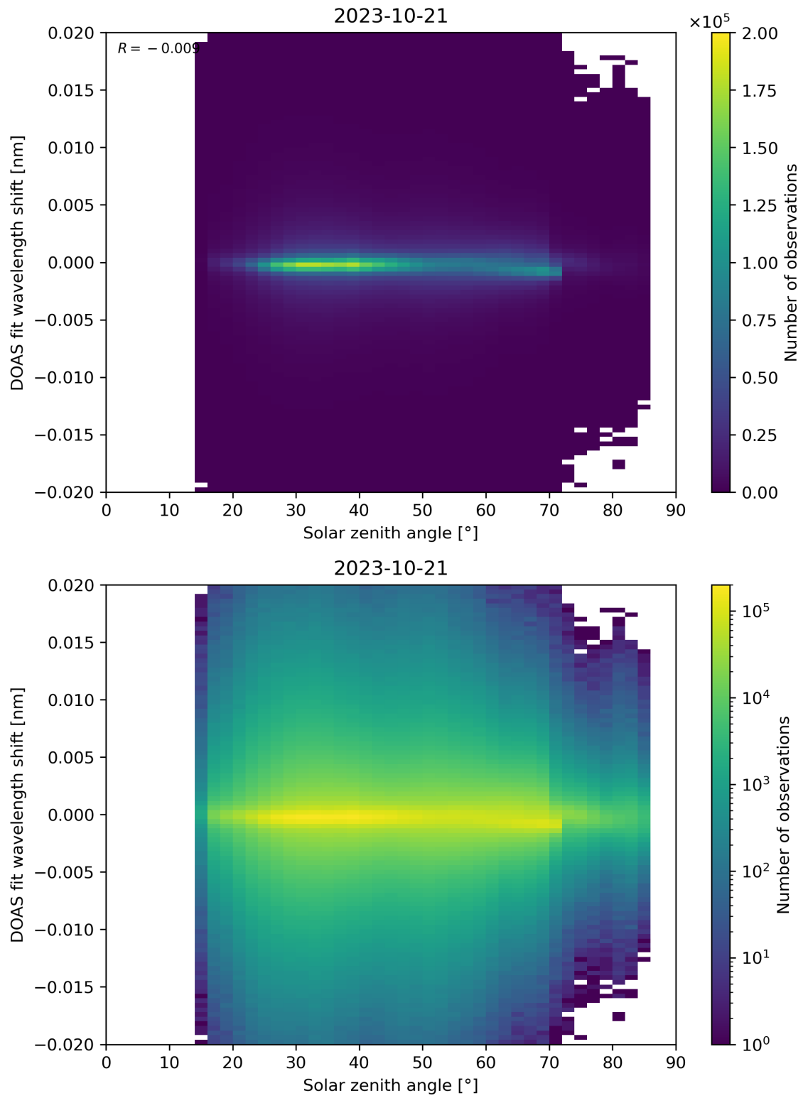
Figure 168: Scatter density plot of “Solar zenith angle” against “DOAS fit wavelength shift” for 2023-10-20 to 2023-10-22.
