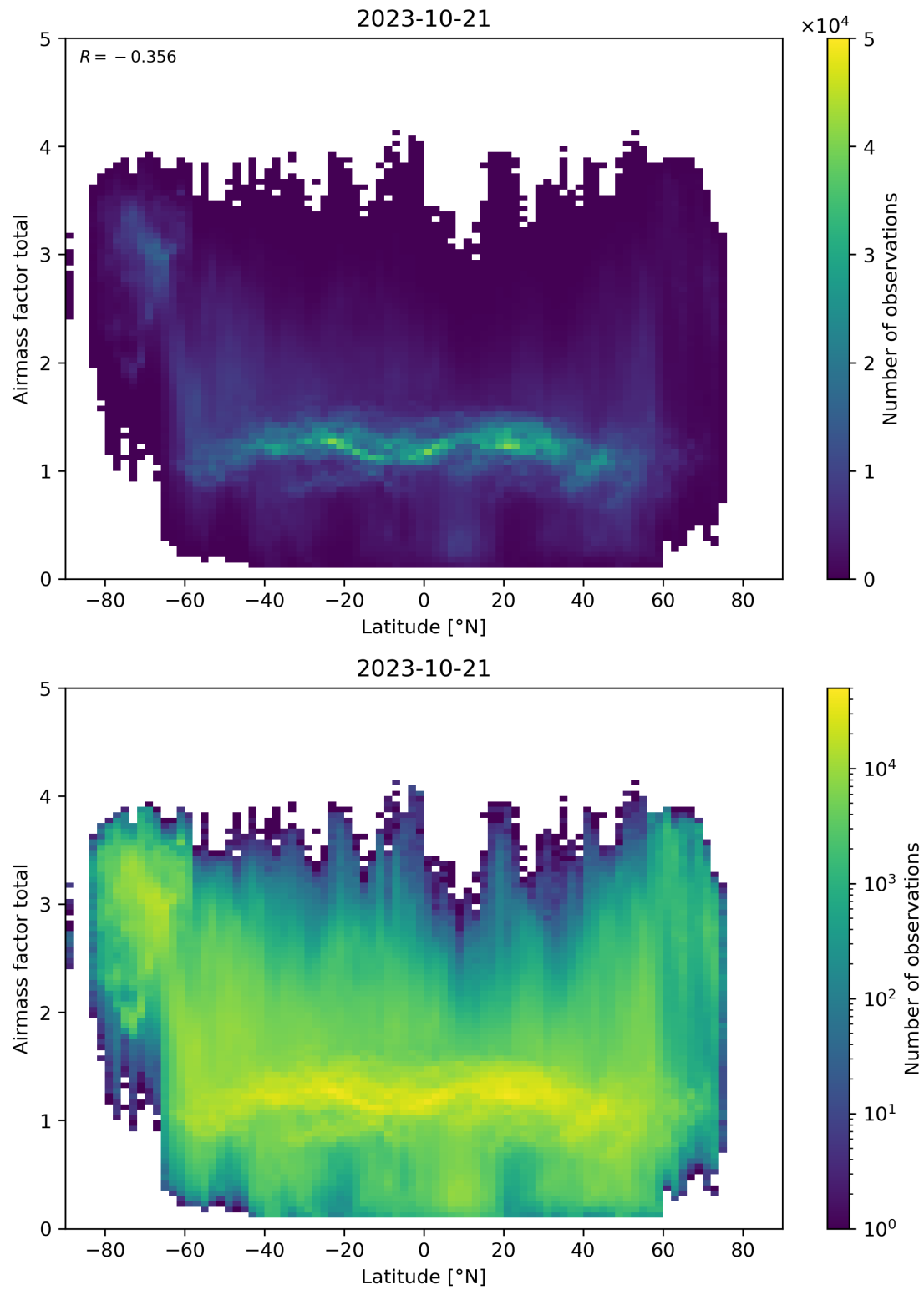
Figure 161: Scatter density plot of “Latitude” against “Airmass factor total” for 2023-10-20 to 2023-10-22.
