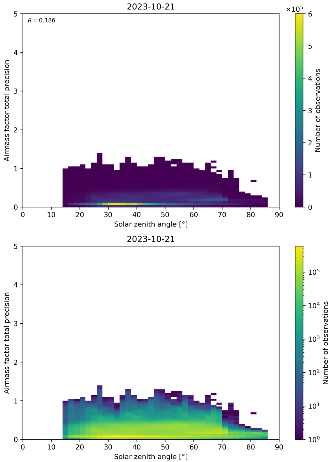
Figure 176: Scatter density plot of “Solar zenith angle” against “Airmass factor total precision” for 2023-10-20 to 2023-10-22.
