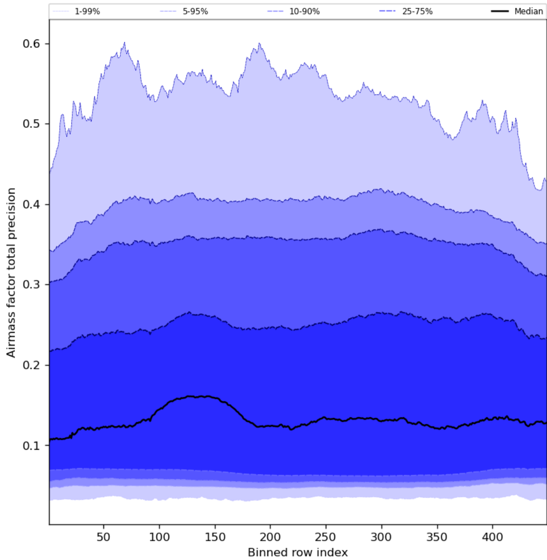
Figure 55: Along track statistics of “Airmass factor total precision” for 2023-10-20 to 2023-10-22
