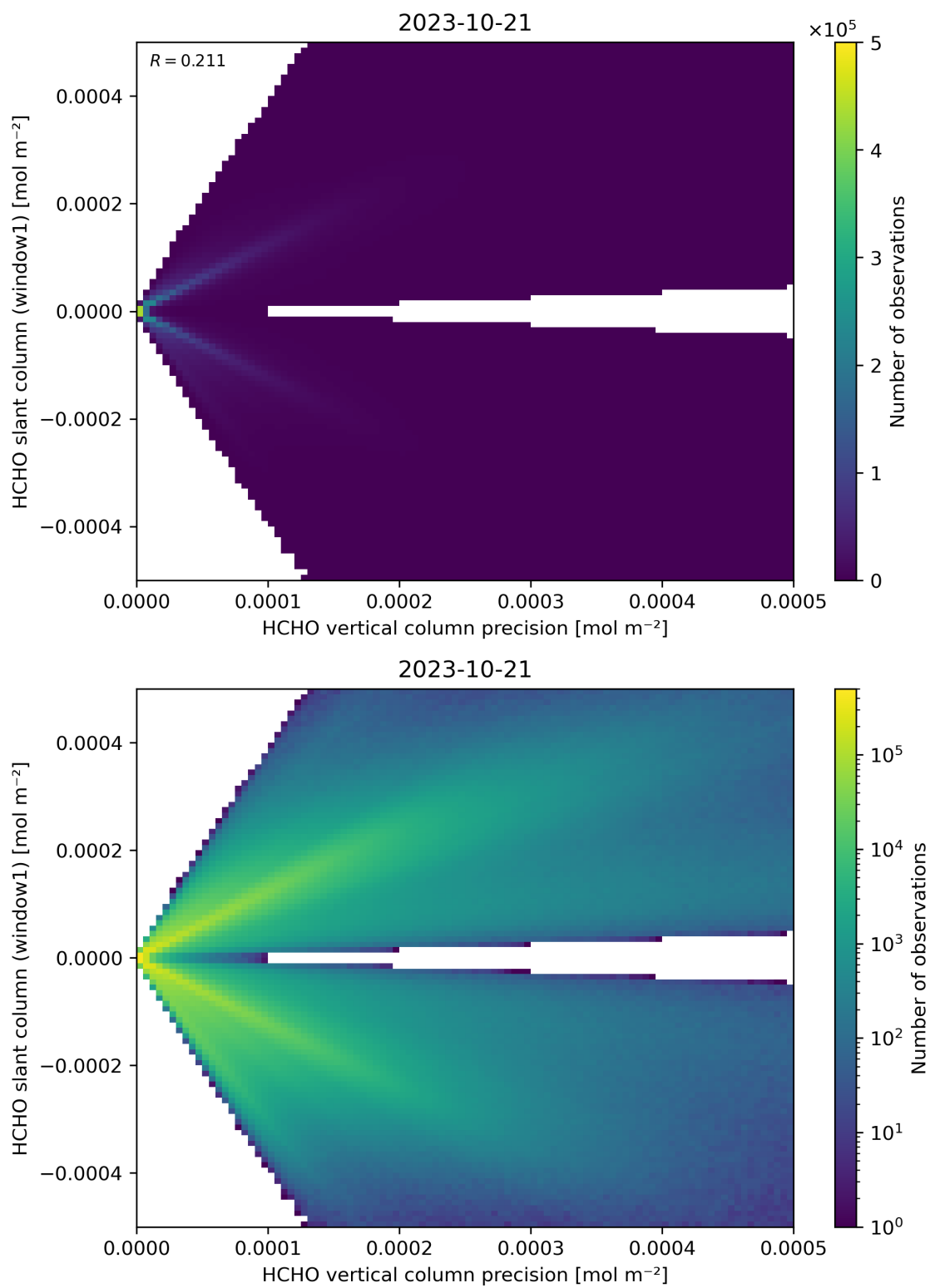
Figure 142: Scatter density plot of “HCHO vertical column precision” against “HCHO slant column (window1)” for 2023-10-20 to 2023-10-22.
