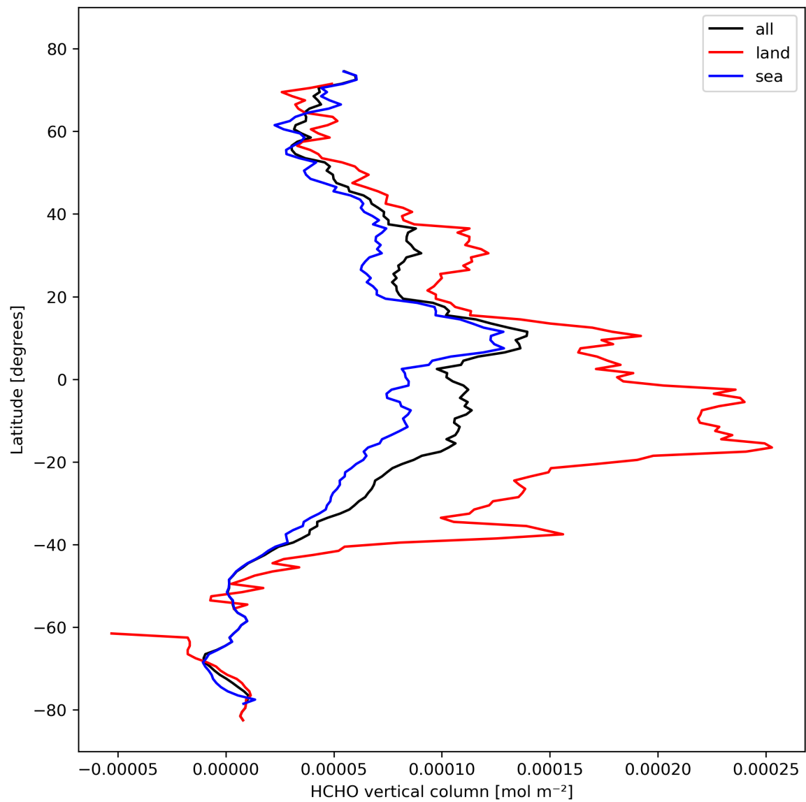
Figure 21: Zonal average of “HCHO vertical column” for 2023-10-20 to 2023-10-22.
