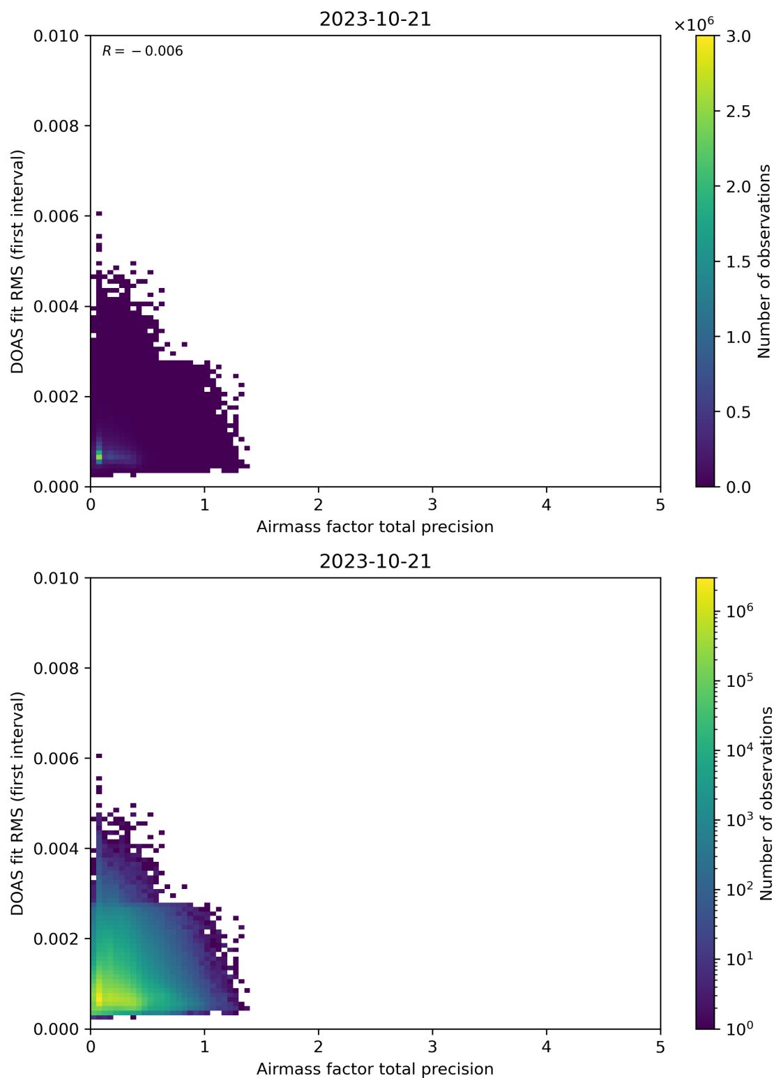
Figure 105: Scatter density plot of “Airmass factor total precision” against “DOAS fit RMS (first interval)” for 2023-10-20 to 2023-10-22.
