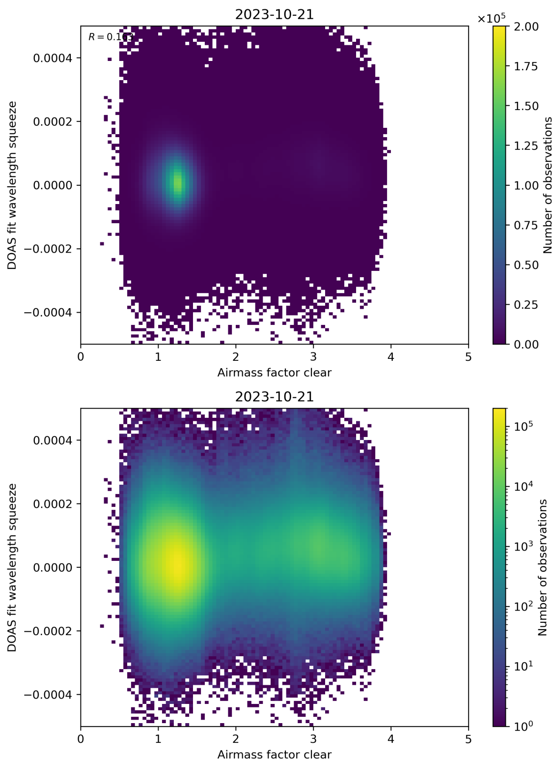
Figure 73: Scatter density plot of “Airmass factor clear” against “DOAS fit wavelength squeeze” for 2023-10-20 to 2023-10-22.
