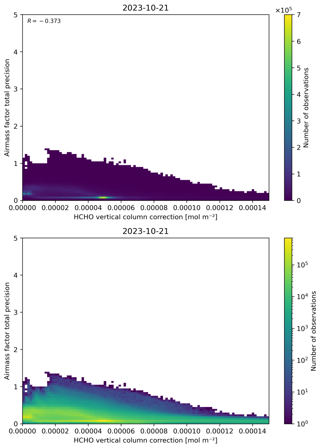
Figure 121: Scatter density plot of “HCHO vertical column correction” against “Airmass factor total precision” for 2023-10-20 to 2023-10-22.
