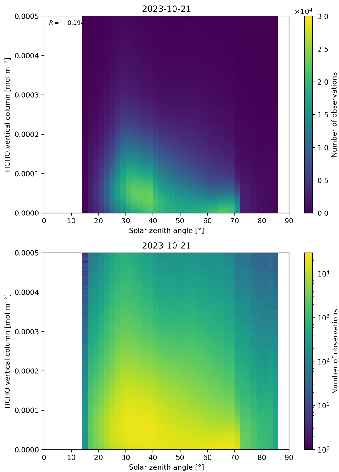
Figure 177: Scatter density plot of “Solar zenith angle” against “HCHO vertical column” for 2023-10-20 to 2023-10-22.
