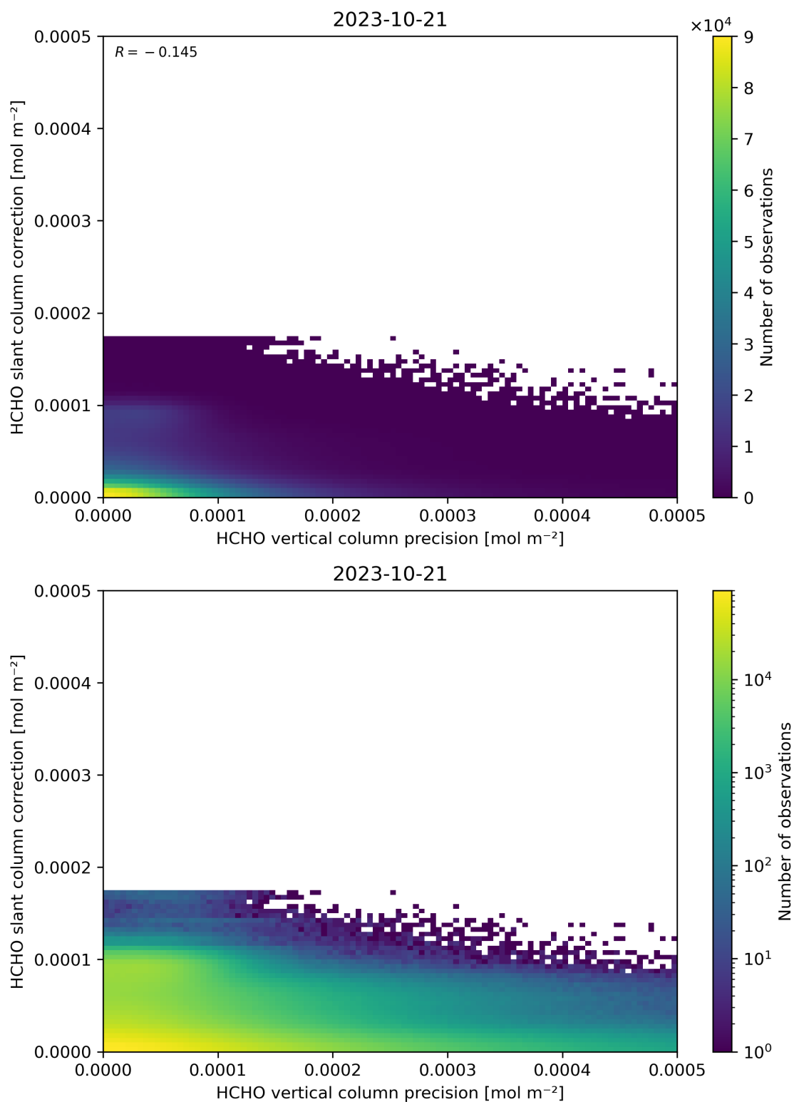
Figure 141: Scatter density plot of “HCHO vertical column precision” against “HCHO slant column correction” for 2023-10-20 to 2023-10-22.
