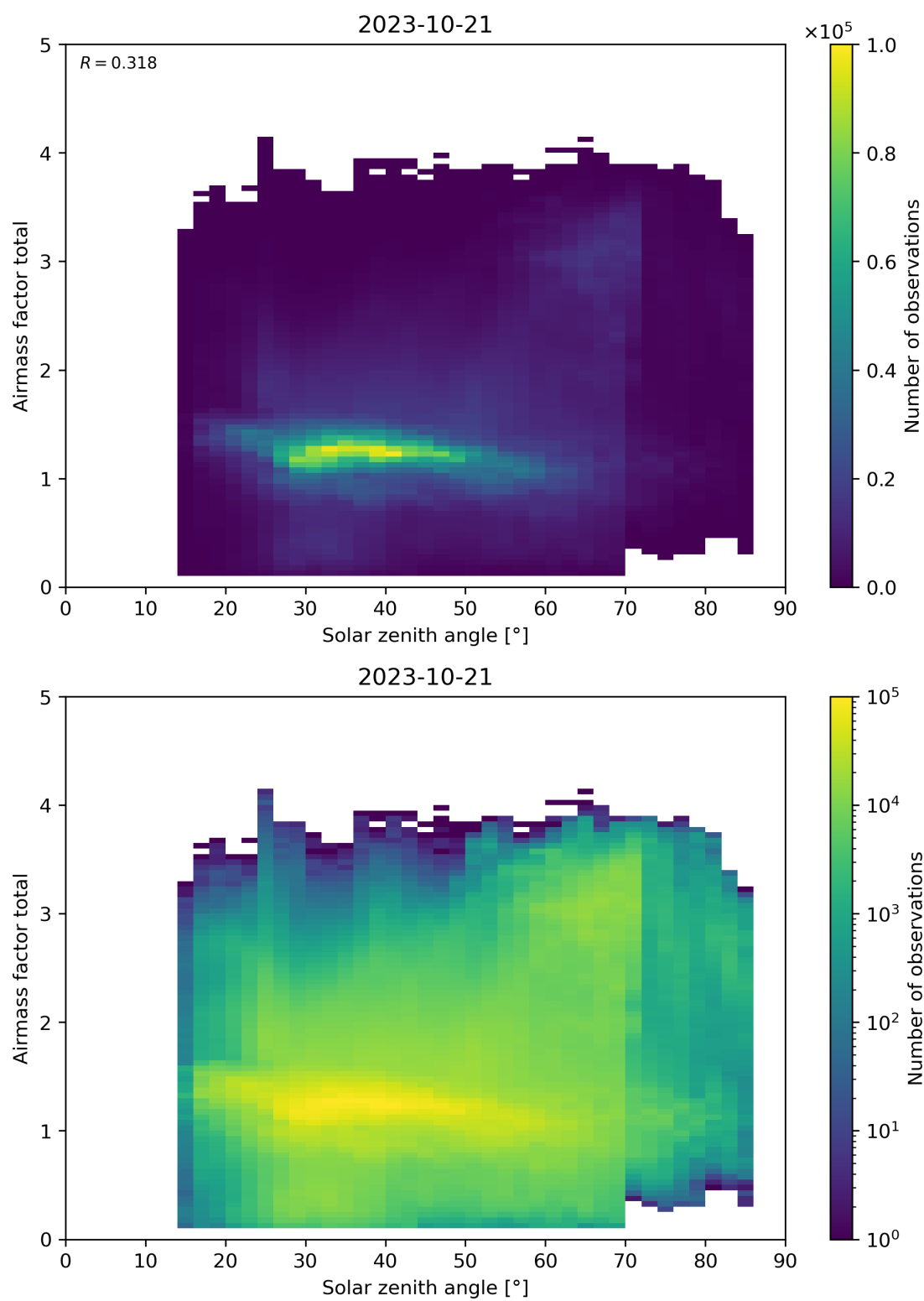
Figure 175: Scatter density plot of “Solar zenith angle” against “Airmass factor total” for 2023-10-20 to 2023-10-22.
