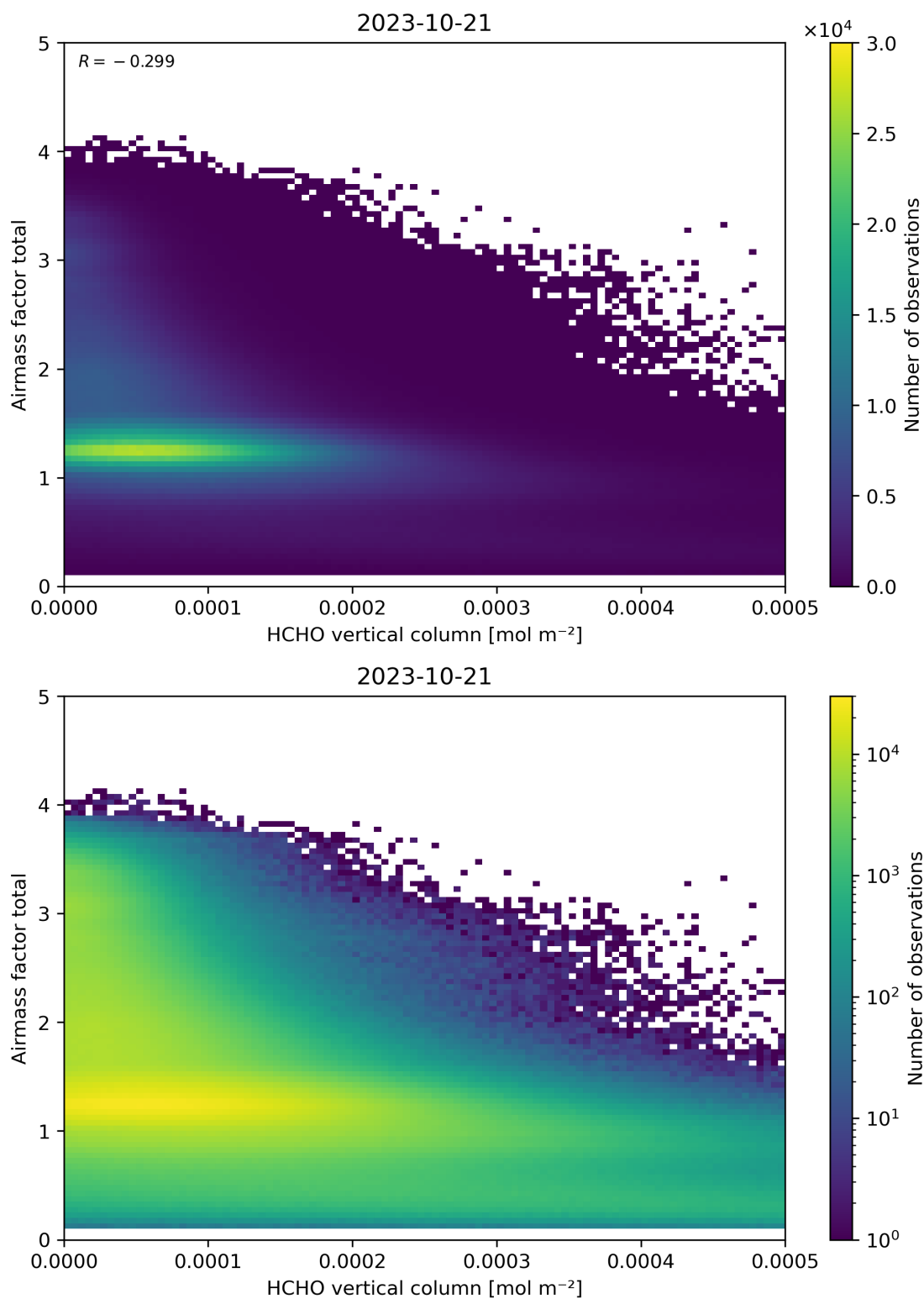
Figure 131: Scatter density plot of “HCHO vertical column” against “Airmass factor total” for 2023-10-20 to 2023-10-22.
