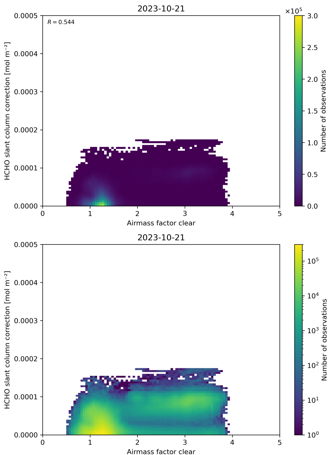
Figure 75: Scatter density plot of “Airmass factor clear” against “HCHO slant column correction” for 2023-10-20 to 2023-10-22.
