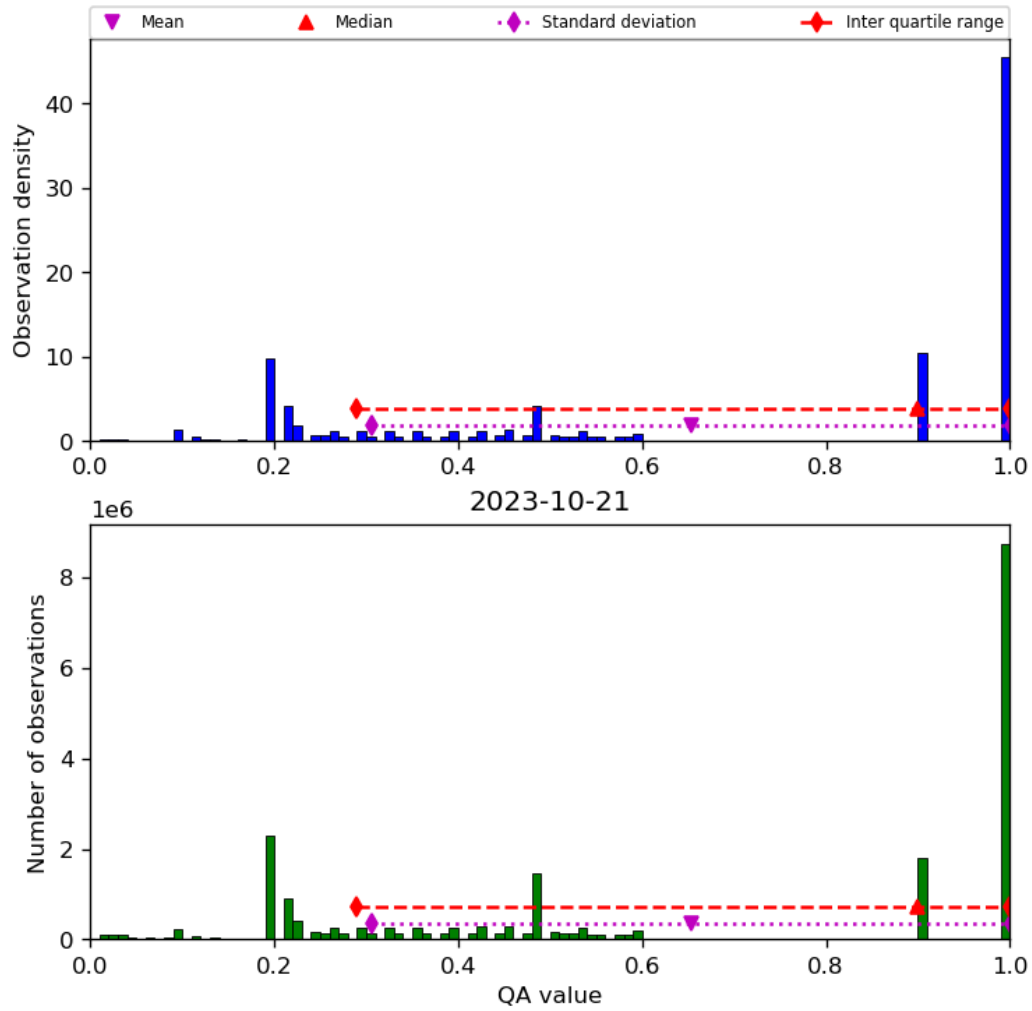
Figure 34: Histogram of “QA value” for 2023-10-20 to 2023-10-22
