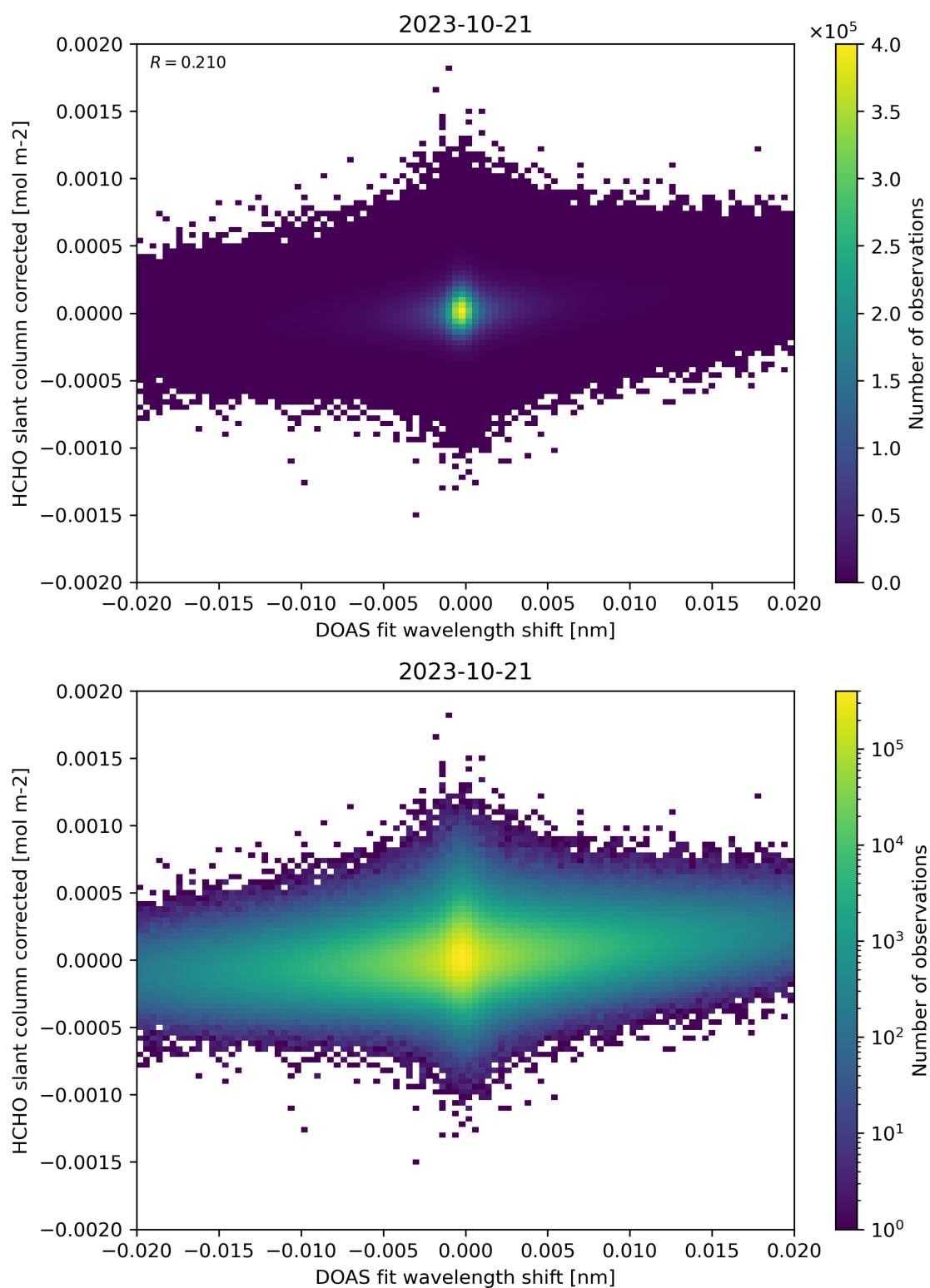
Figure 66: Scatter density plot of “DOAS fit wavelength shift” against “HCHO slant column corrected” for 2023-10-20 to 2023-10-22.
