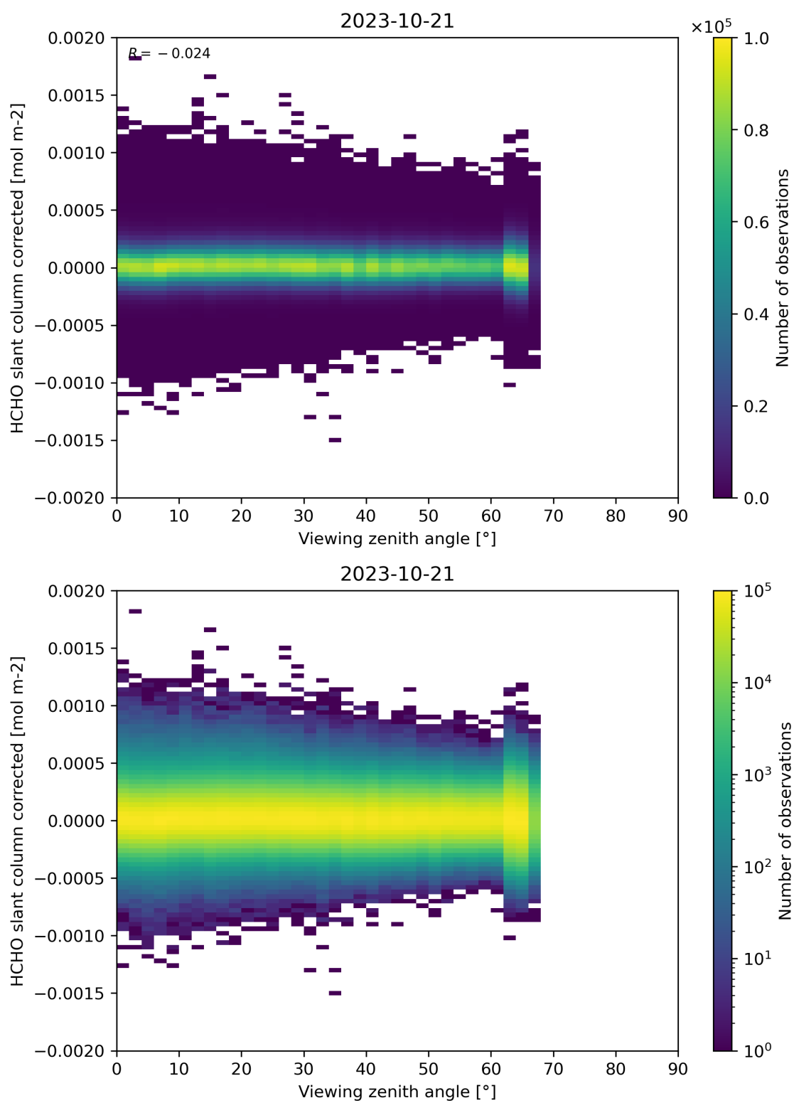
Figure 186: Scatter density plot of “Viewing zenith angle” against “HCHO slant column corrected” for 2023-10-20 to 2023-10-22.
