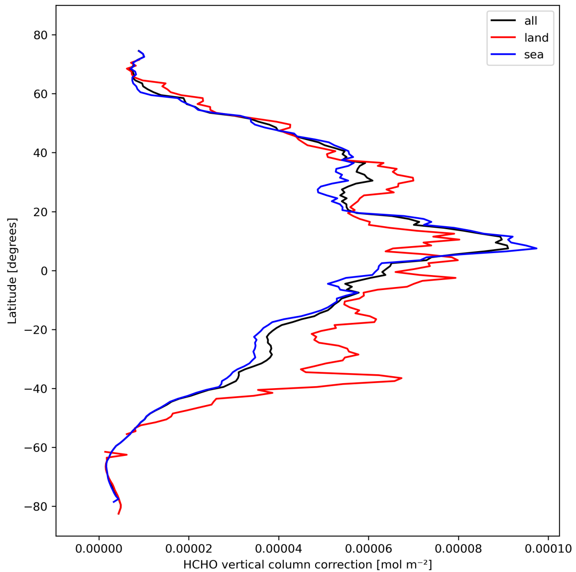
Figure 23: Zonal average of “HCHO vertical column correction” for 2023-10-20 to 2023-10-22.
