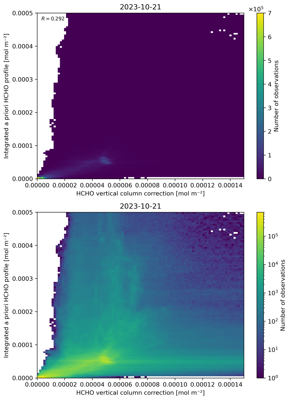
Figure 122: Scatter density plot of “HCHO vertical column correction” against “Integrated a priori HCHO profile” for 2023-10-20 to 2023-10-22.
