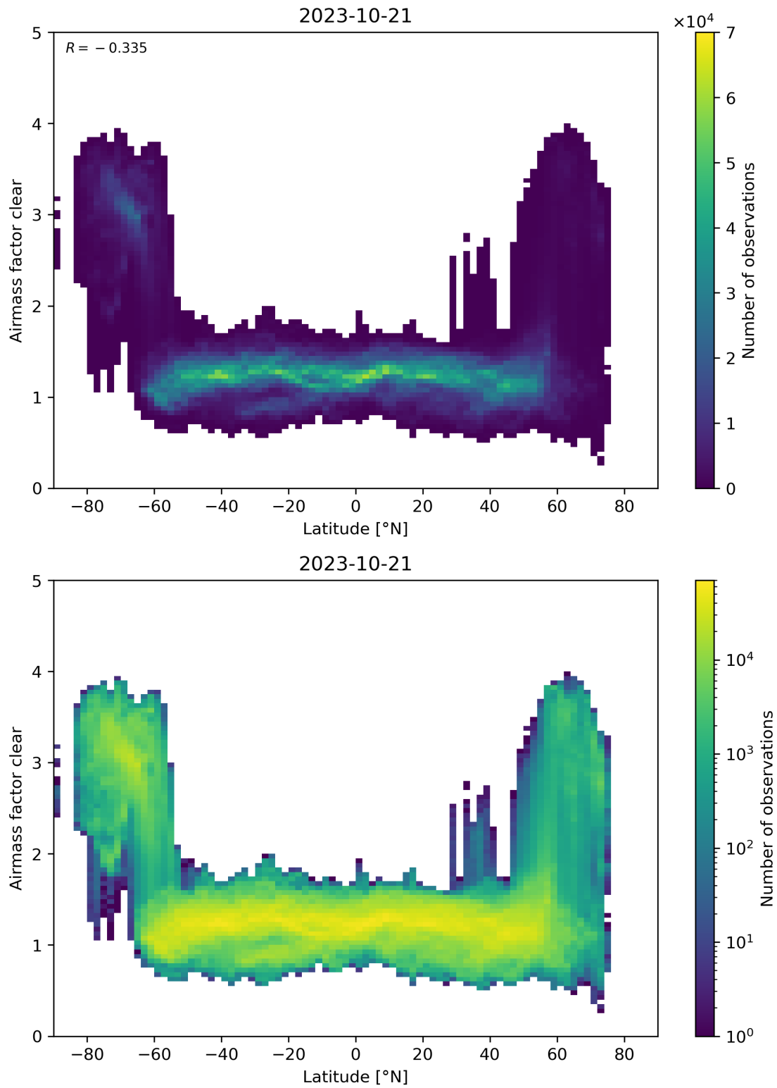
Figure 156: Scatter density plot of “Latitude” against “Airmass factor clear” for 2023-10-20 to 2023-10-22.
