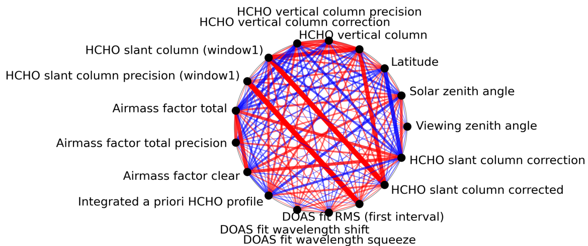
Figure 1: Map of correlation graph for 2023-10-20 to 2023-10-22.
