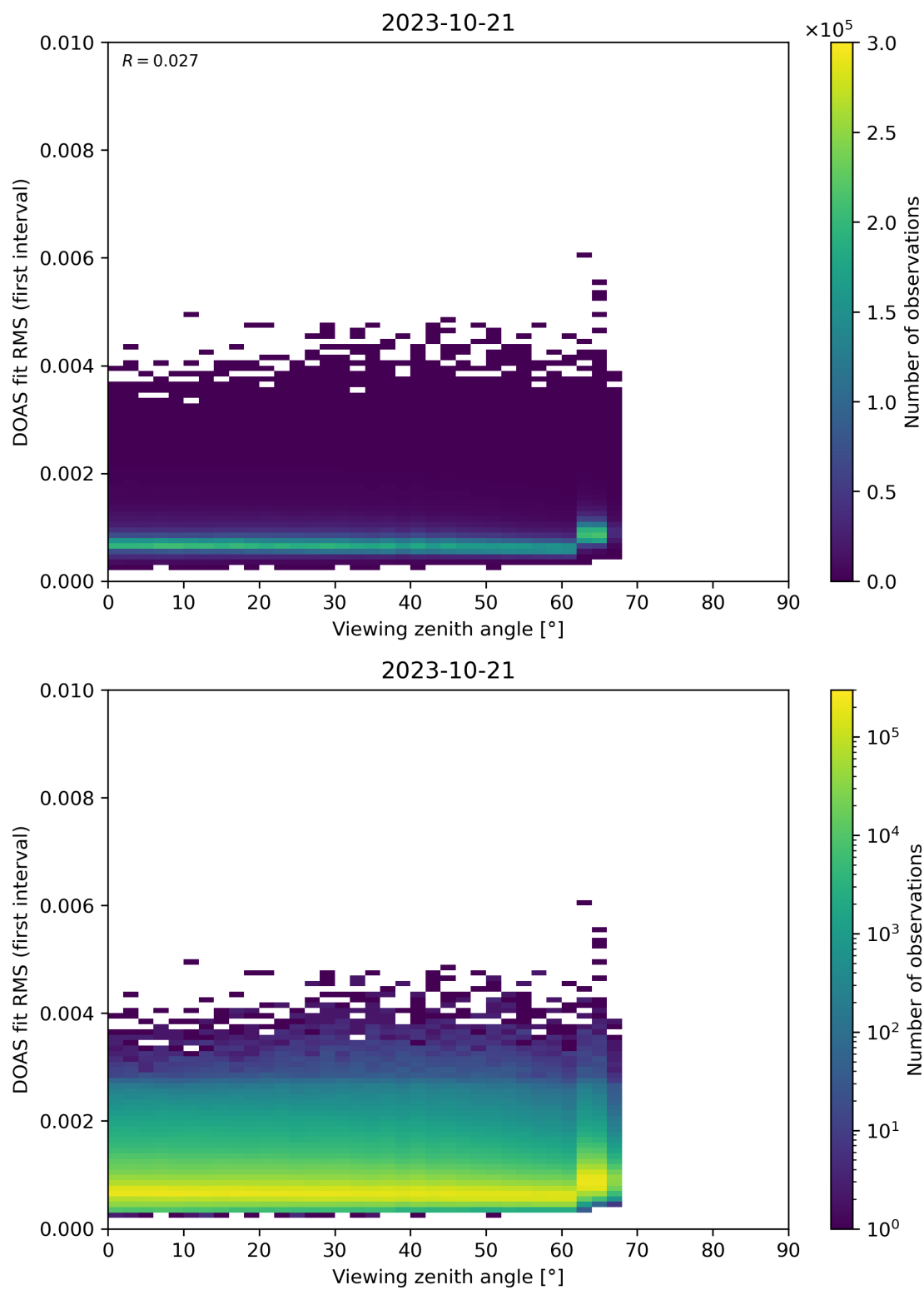
Figure 182: Scatter density plot of “Viewing zenith angle” against “DOAS fit RMS (first interval)” for 2023-10-20 to 2023-10-22.
