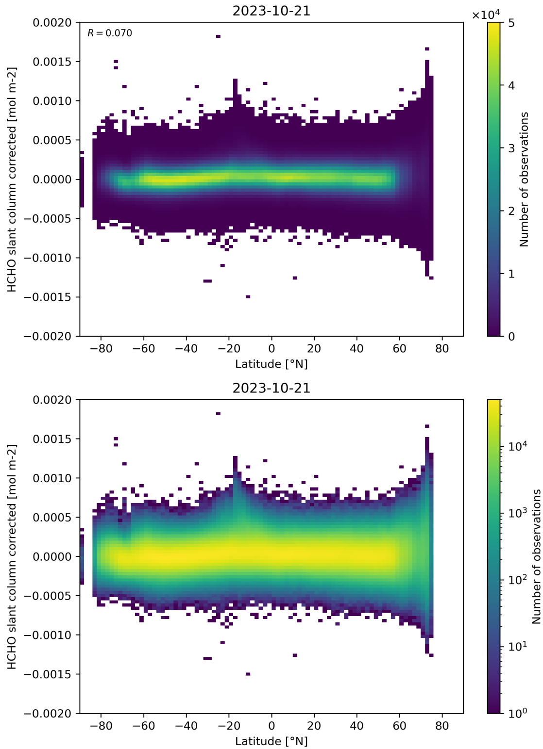
Figure 157: Scatter density plot of “Latitude” against “HCHO slant column corrected” for 2023-10-20 to 2023-10-22.
