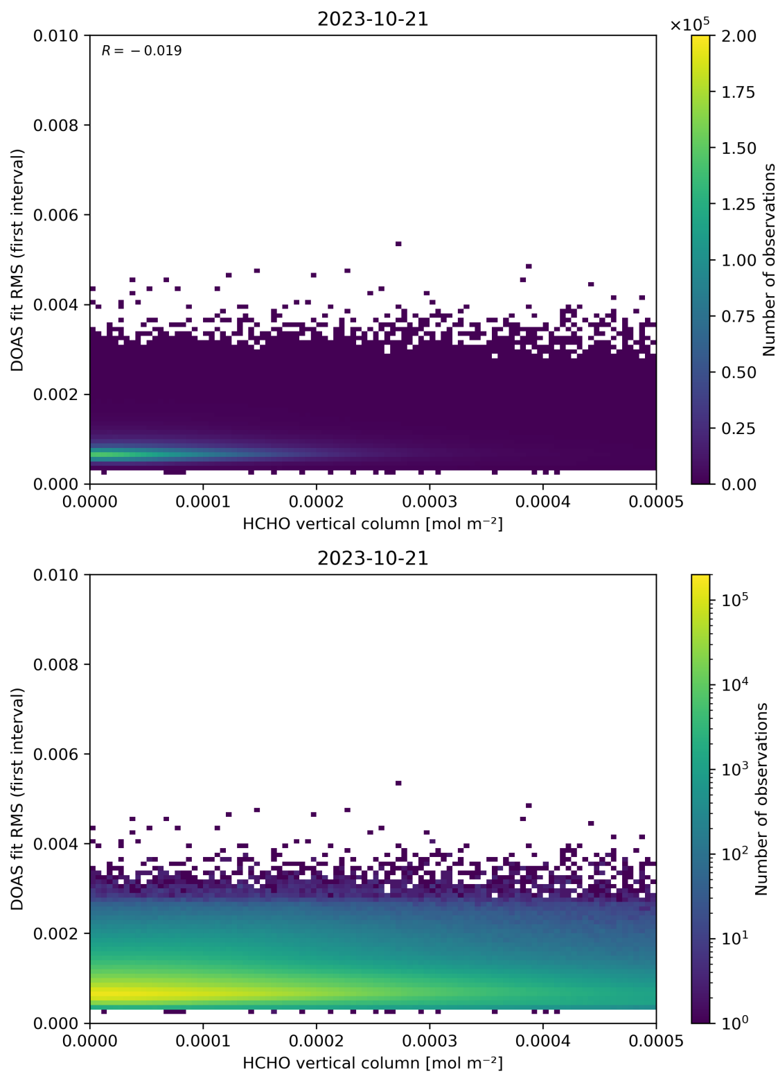
Figure 123: Scatter density plot of “HCHO vertical column” against “DOAS fit RMS (first interval)” for 2023-10-20 to 2023-10-22.
