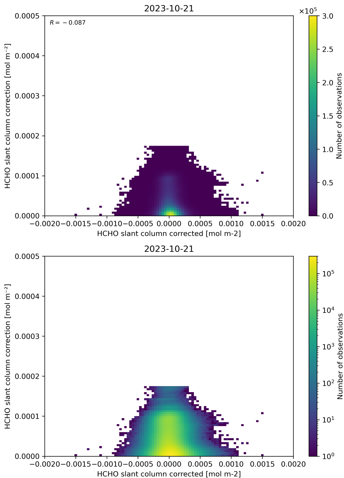
Figure 77: Scatter density plot of “HCHO slant column corrected” against “HCHO slant column correction” for 2023-10-20 to 2023-10-22.
