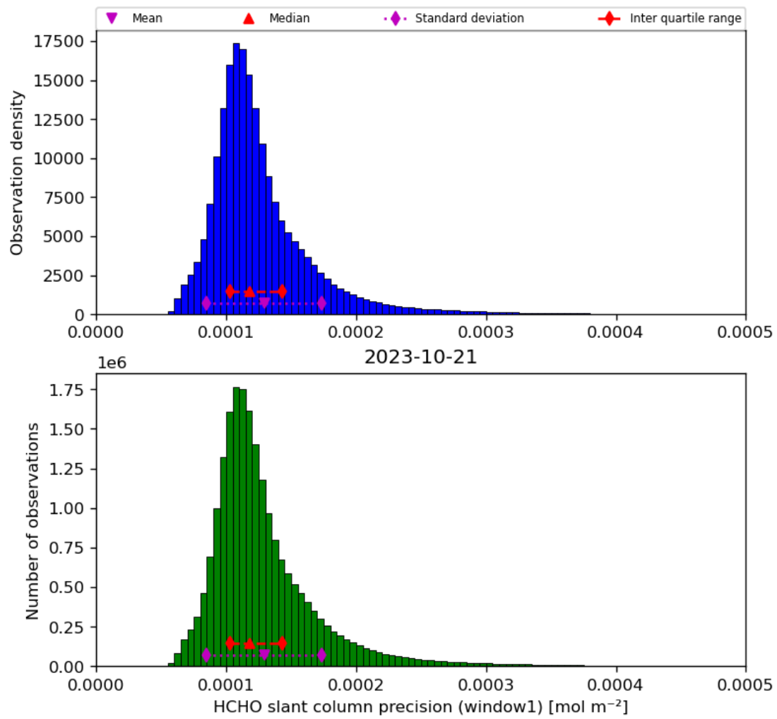
Figure 39: Histogram of “HCHO slant column precision (window1)” for 2023-10-20 to 2023-10-22
