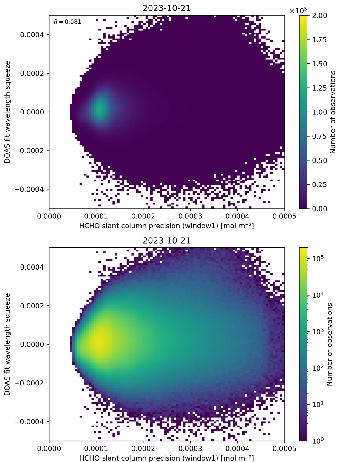
Figure 90: Scatter density plot of “HCHO slant column precision (window1)” against “DOAS fit wavelength squeeze” for 2023-10-20 to 2023-10-22.
