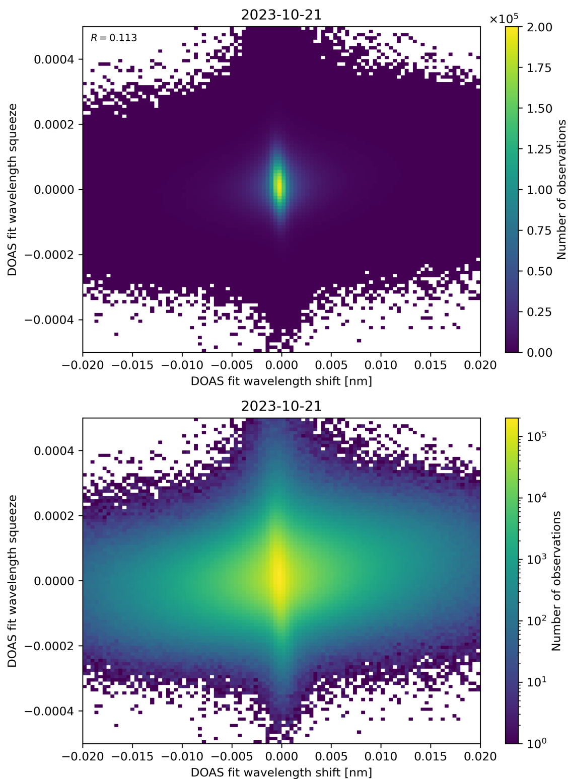
Figure 65: Scatter density plot of “DOAS fit wavelength shift” against “DOAS fit wavelength squeeze” for 2023-10-20 to 2023-10-22.
