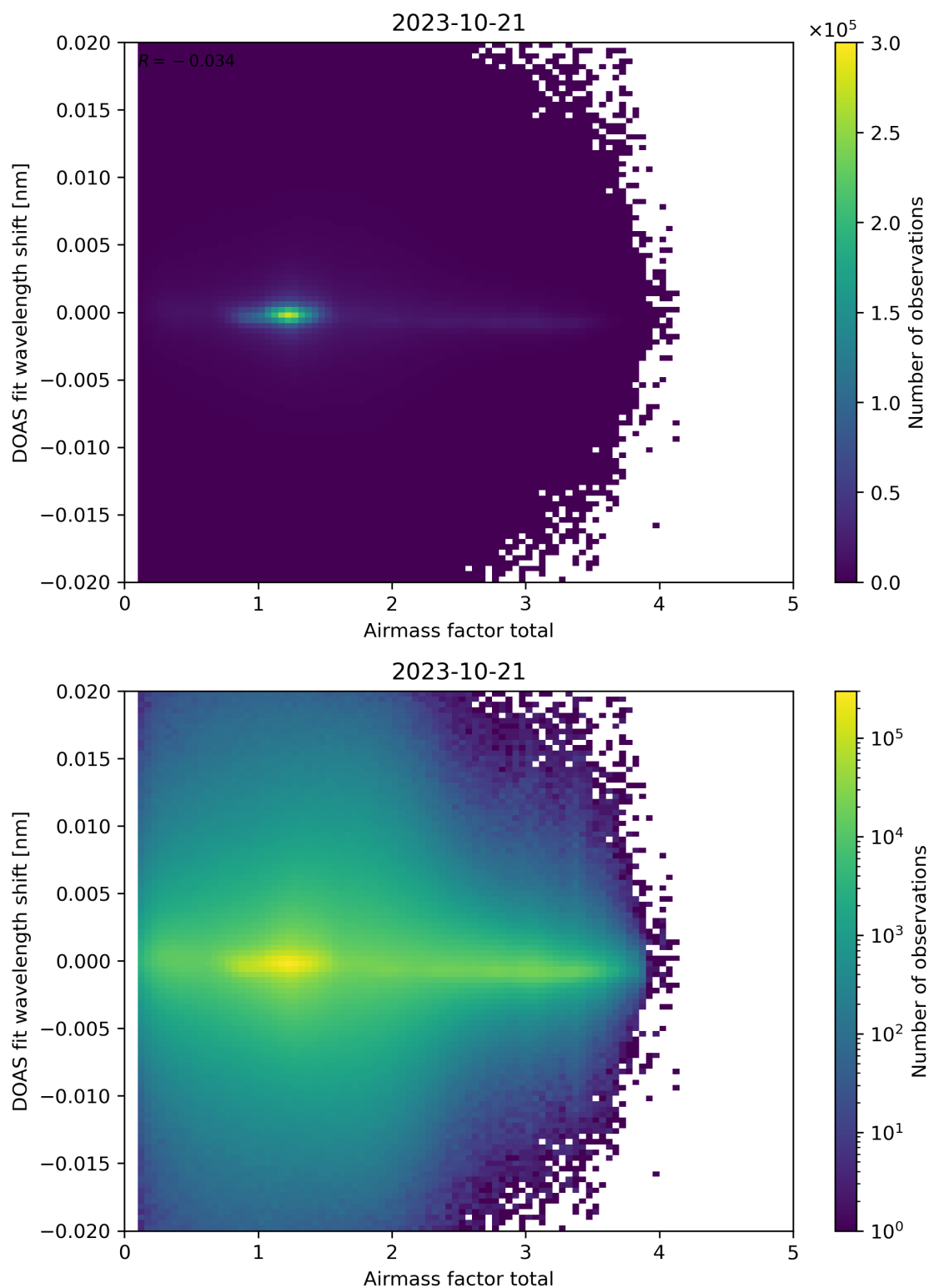
Figure 98: Scatter density plot of “Airmass factor total” against “DOAS fit wavelength shift” for 2023-10-20 to 2023-10-22.
