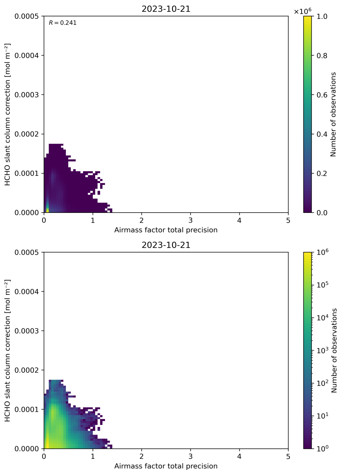
Figure 110: Scatter density plot of “Airmass factor total precision” against “HCHO slant column correction” for 2023-10-20 to 2023-10-22.
