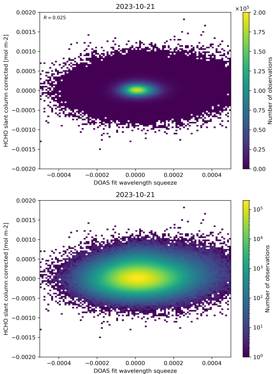
Figure 69: Scatter density plot of “DOAS fit wavelength squeeze” against “HCHO slant column corrected” for 2023-10-20 to 2023-10-22.
