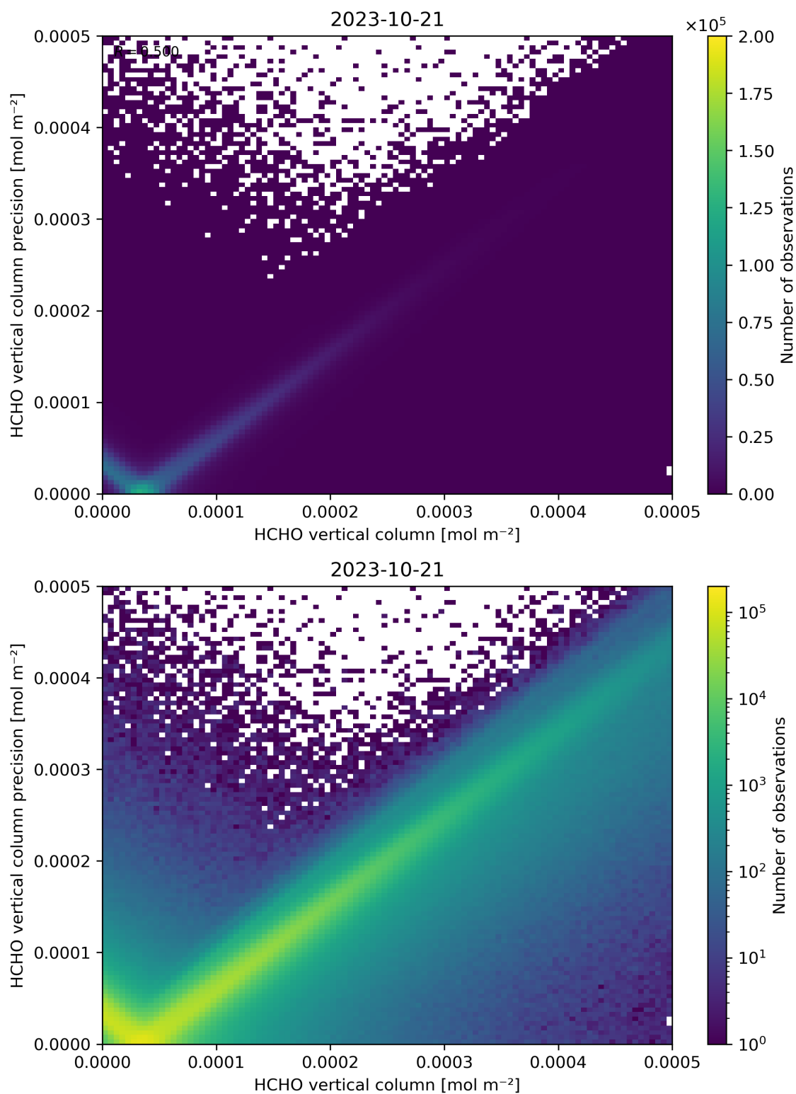
Figure 134: Scatter density plot of “HCHO vertical column” against “HCHO vertical column precision” for 2023-10-20 to 2023-10-22.
