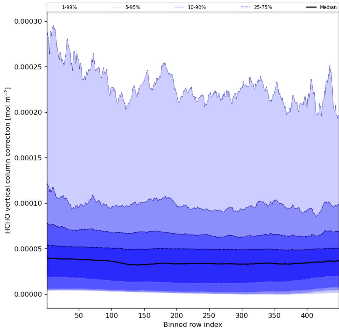
Figure 51: Along track statistics of “HCHO vertical column correction” for 2023-10-20 to 2023-10-22
