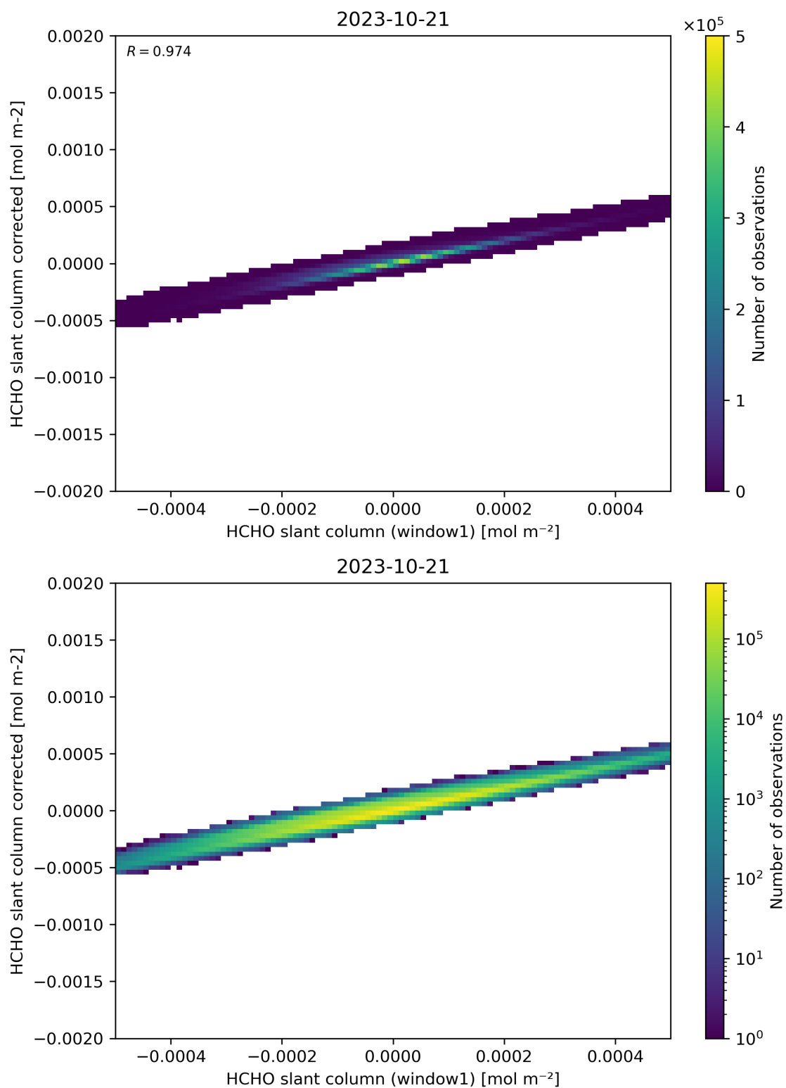
Figure 82: Scatter density plot of “HCHO slant column (window1)” against “HCHO slant column corrected” for 2023-10-20 to 2023-10-22.
