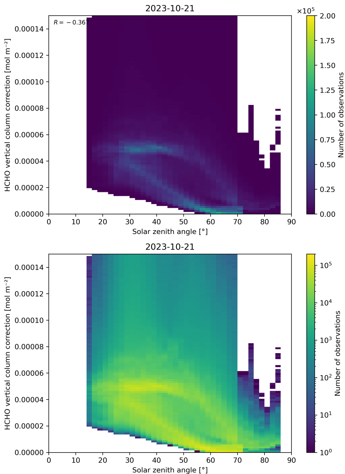
Figure 178: Scatter density plot of “Solar zenith angle” against “HCHO vertical column correction” for 2023-10-20 to 2023-10-22.
