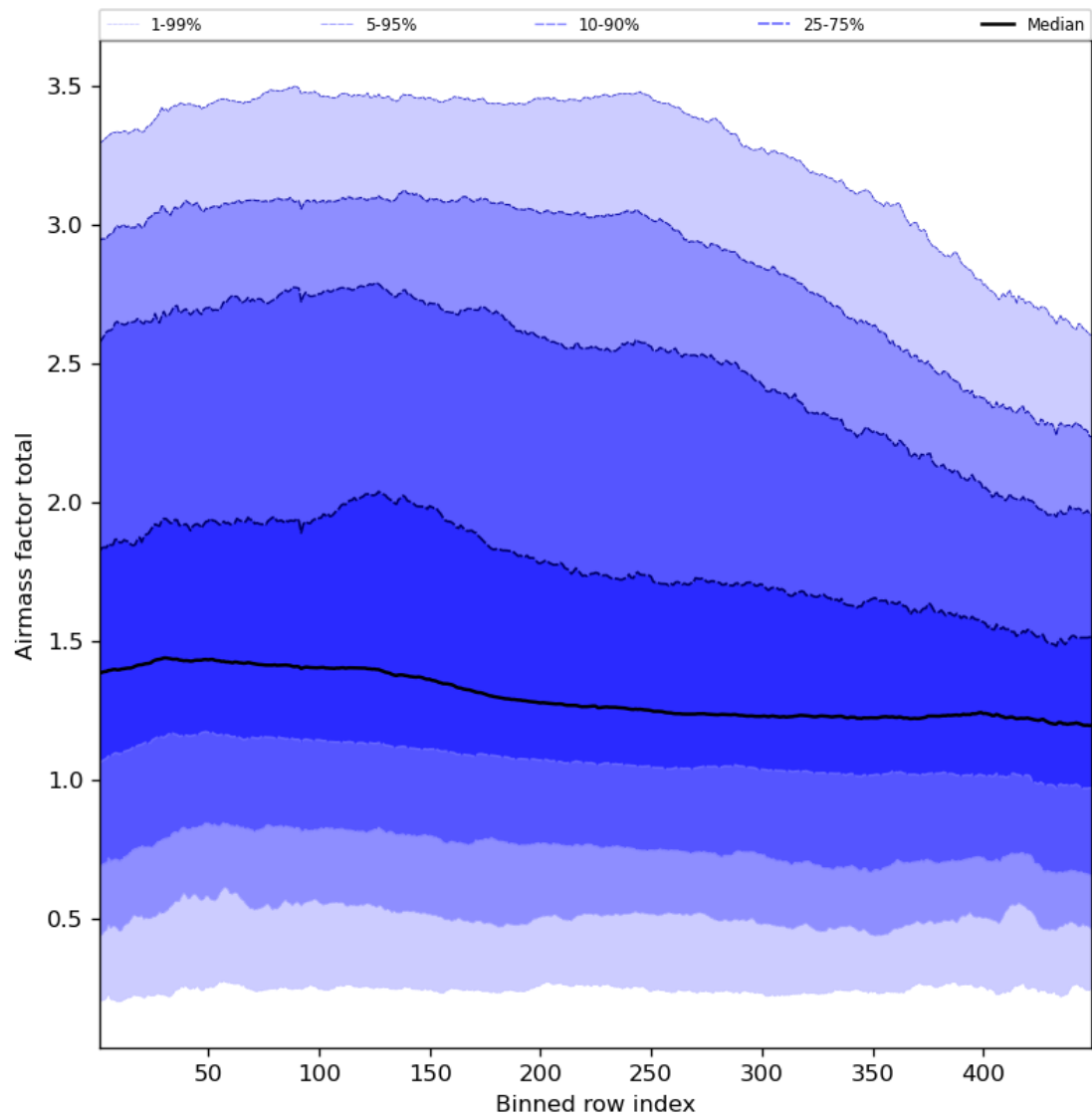
Figure 54: Along track statistics of “Airmass factor total” for 2023-10-20 to 2023-10-22
