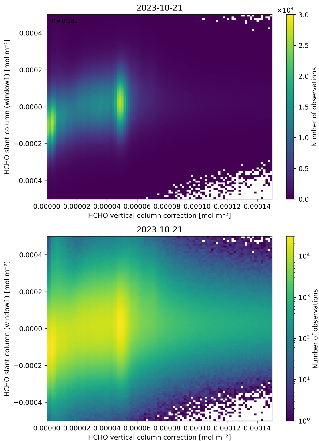
Figure 118: Scatter density plot of “HCHO vertical column correction” against “HCHO slant column (window1)” for 2023-10-20 to 2023-10-22.
