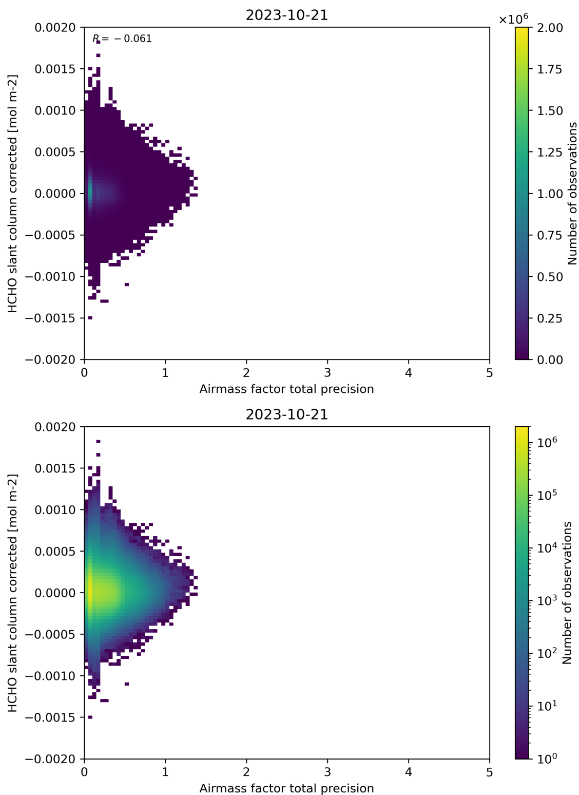
Figure 109: Scatter density plot of “Airmass factor total precision” against “HCHO slant column corrected” for 2023-10-20 to 2023-10-22.
