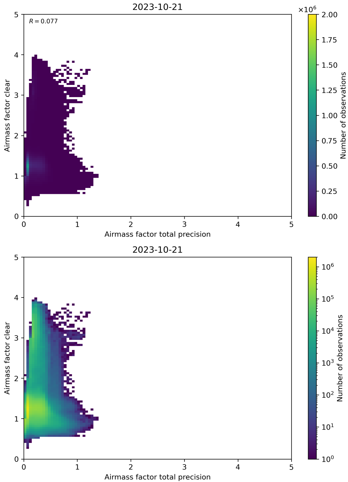
Figure 108: Scatter density plot of “Airmass factor total precision” against “Airmass factor clear” for 2023-10-20 to 2023-10-22.
