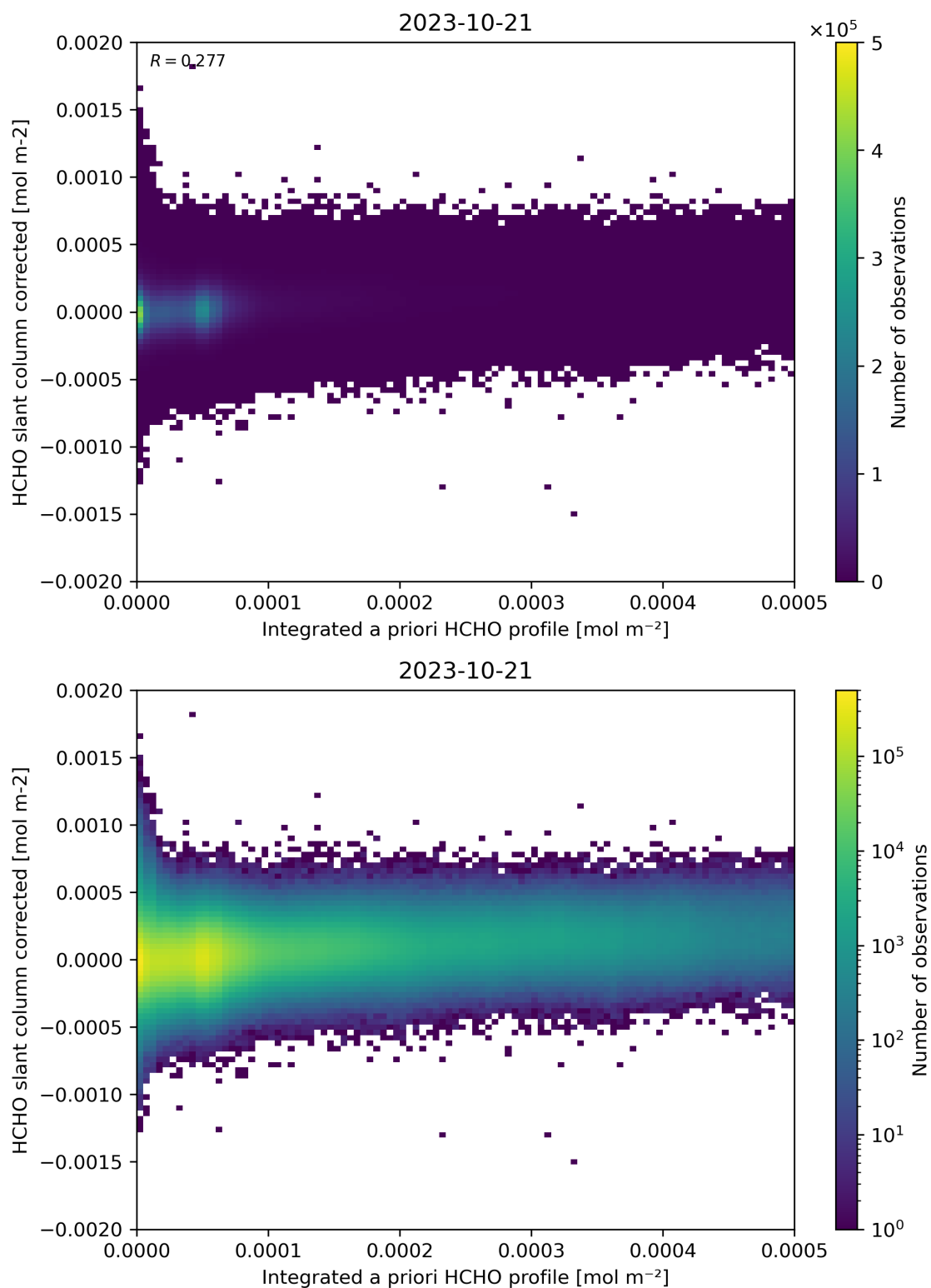
Figure 151: Scatter density plot of “Integrated a priori HCHO profile” against “HCHO slant column corrected” for 2023-10-20 to 2023-10-22.
