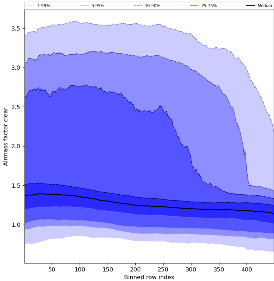
Figure 56: Along track statistics of “Airmass factor clear” for 2023-10-20 to 2023-10-22
