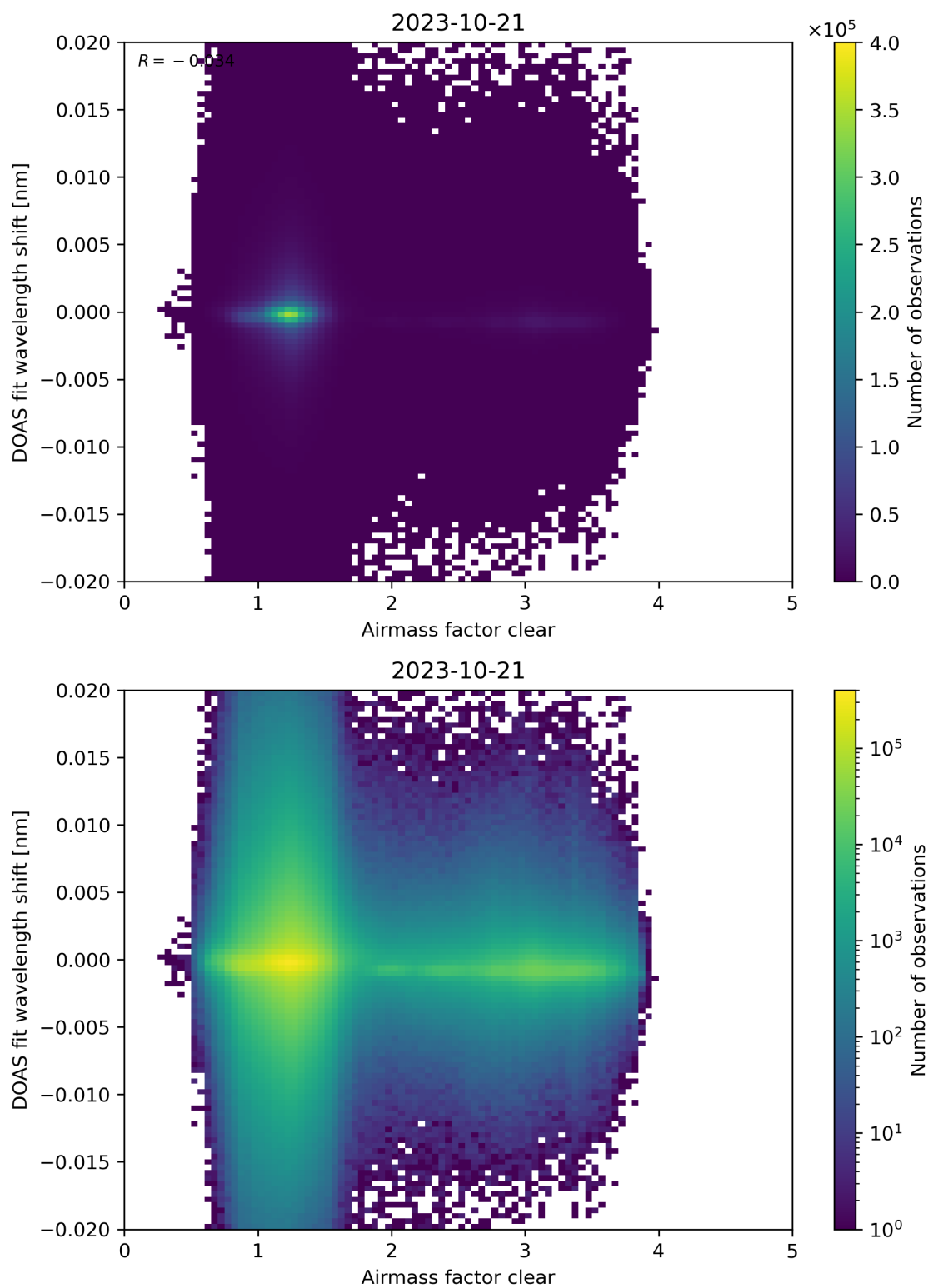
Figure 72: Scatter density plot of “Airmass factor clear” against “DOAS fit wavelength shift” for 2023-10-20 to 2023-10-22.
