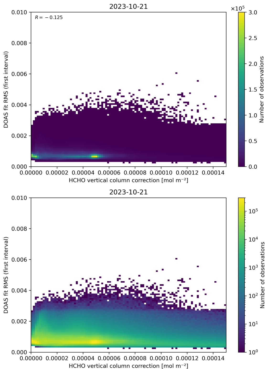
Figure 112: Scatter density plot of “HCHO vertical column correction” against “DOAS fit RMS (first interval)” for 2023-10-20 to 2023-10-22.
