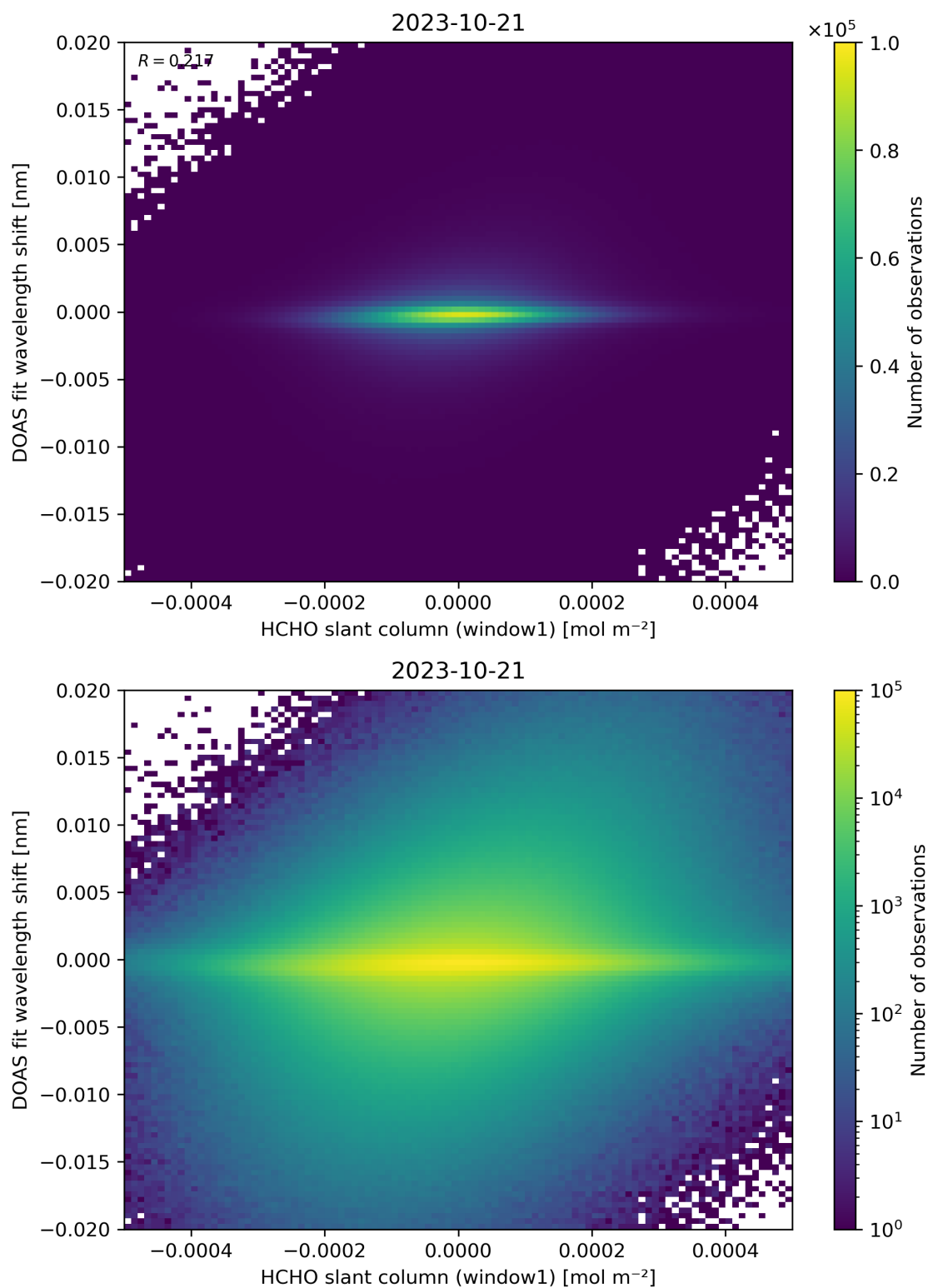
Figure 79: Scatter density plot of “HCHO slant column (window1)” against “DOAS fit wavelength shift” for 2023-10-20 to 2023-10-22.
