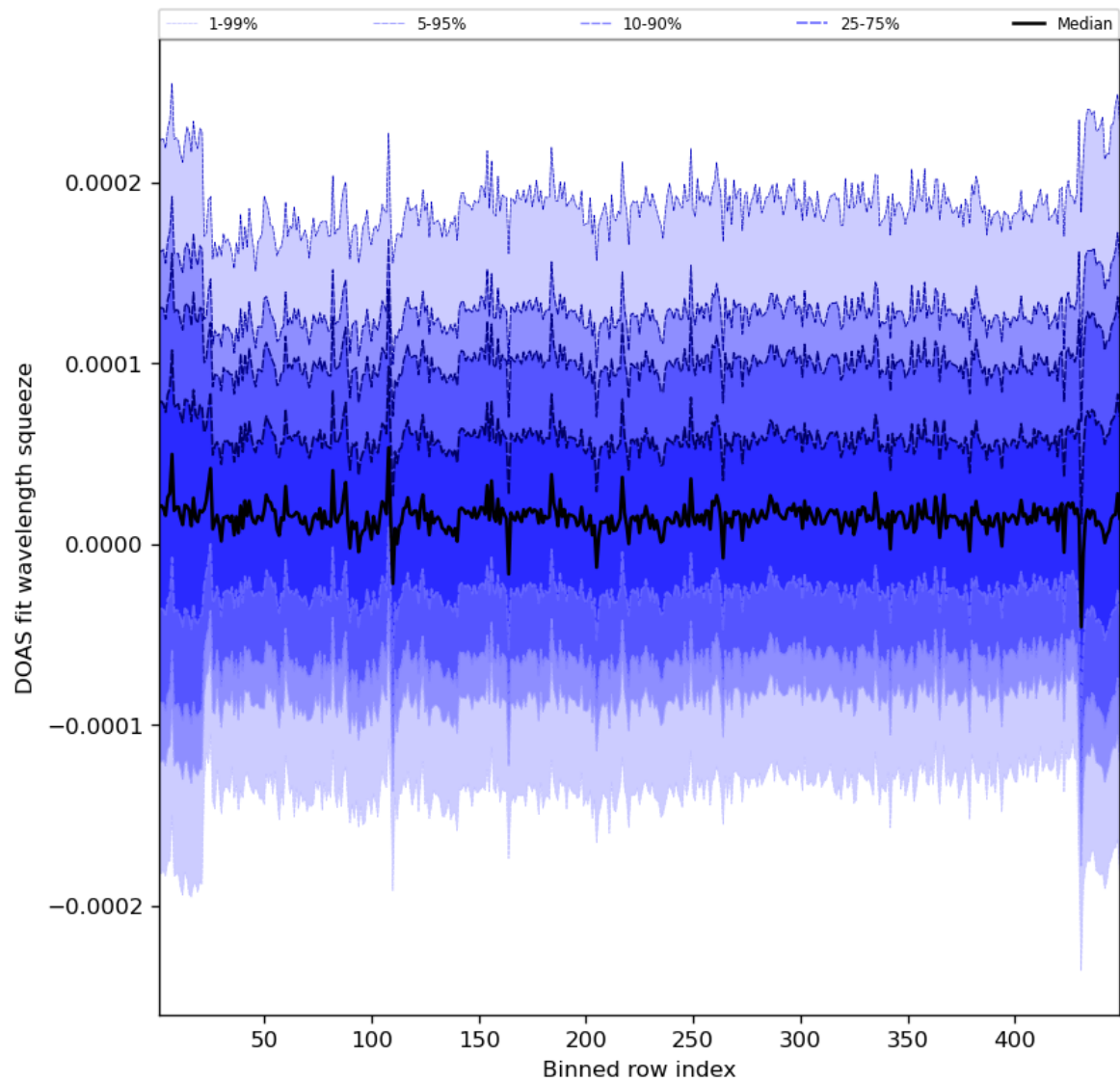
Figure 59: Along track statistics of “DOAS fit wavelength squeeze” for 2023-10-20 to 2023-10-22
