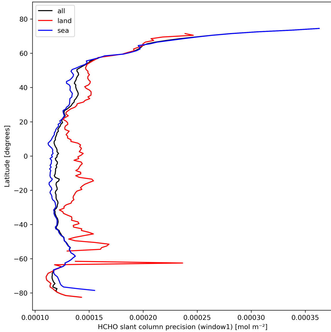
Figure 25: Zonal average of “HCHO slant column precision (window1)” for 2023-10-20 to 2023-10-22.
