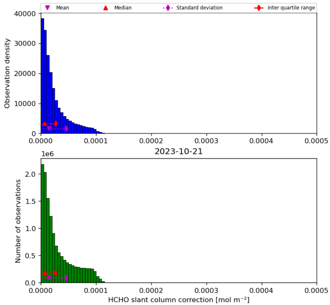
Figure 47: Histogram of “HCHO slant column correction” for 2023-10-20 to 2023-10-22
