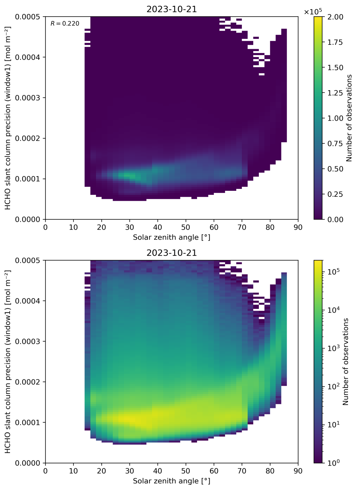
Figure 174: Scatter density plot of “Solar zenith angle” against “HCHO slant column precision (window1)” for 2023-10-20 to 2023-10-22.
