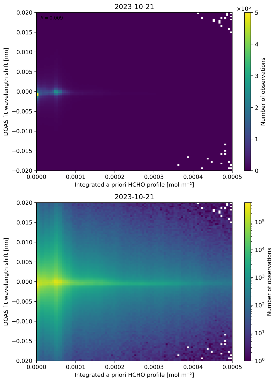
Figure 149: Scatter density plot of “Integrated a priori HCHO profile” against “DOAS fit wavelength shift” for 2023-10-20 to 2023-10-22.
