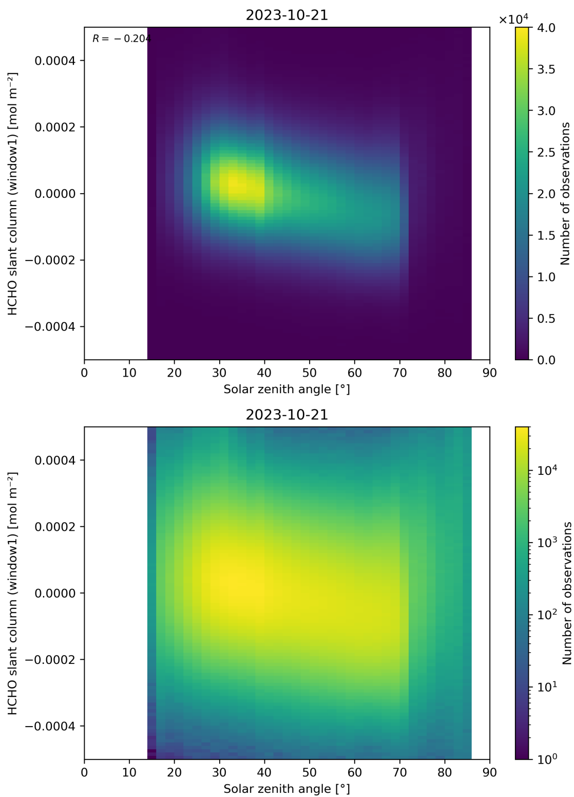
Figure 173: Scatter density plot of “Solar zenith angle” against “HCHO slant column (window1)” for 2023-10-20 to 2023-10-22.
