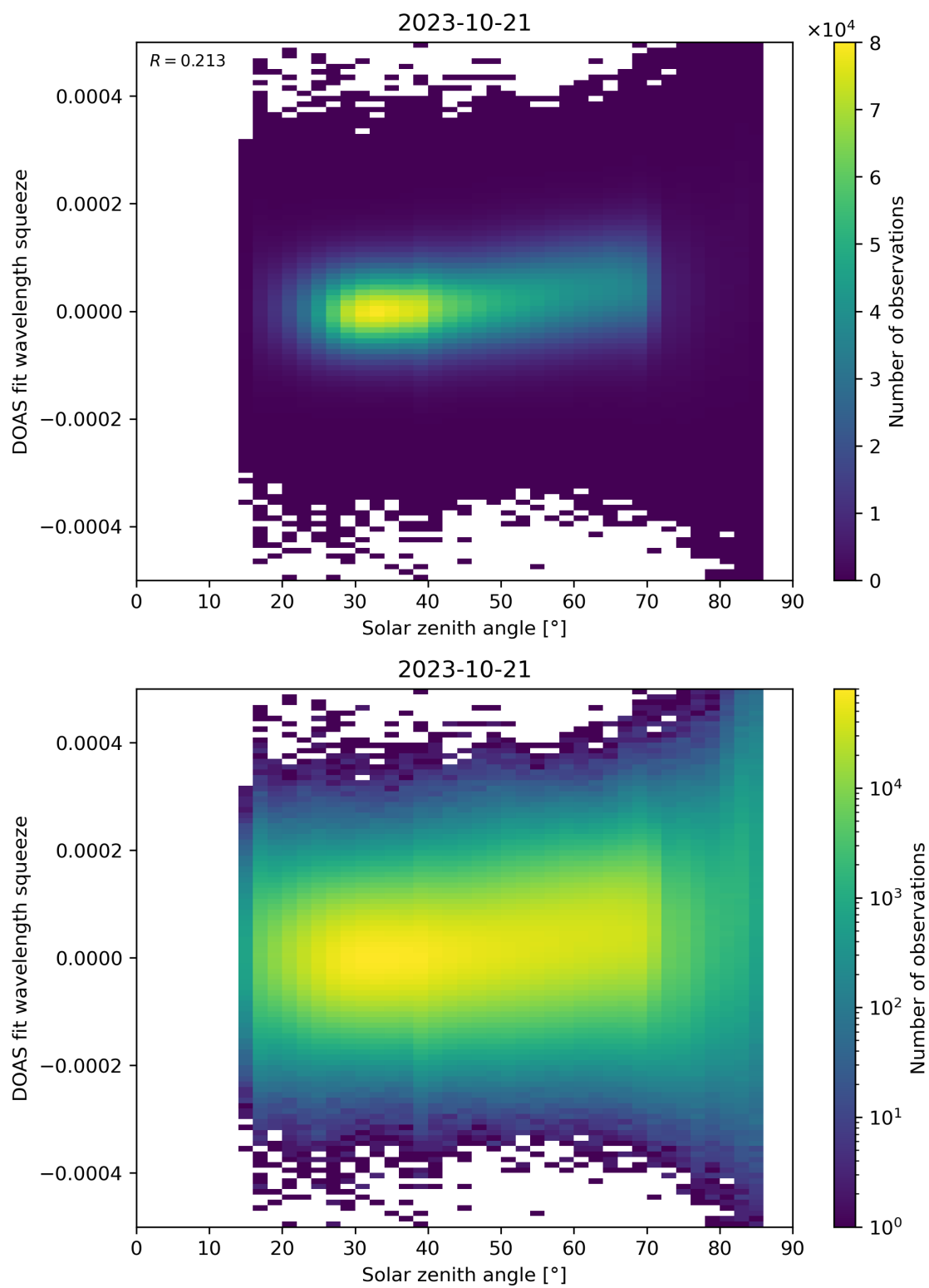
Figure 169: Scatter density plot of “Solar zenith angle” against “DOAS fit wavelength squeeze” for 2023-10-20 to 2023-10-22.
