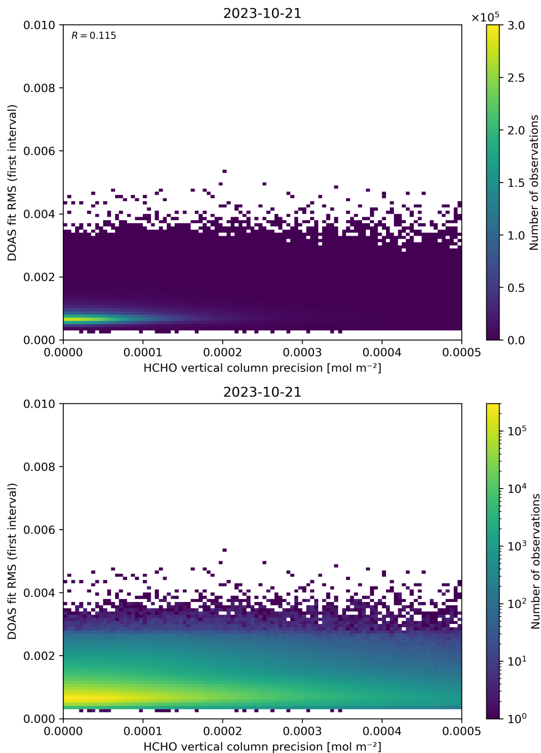
Figure 136: Scatter density plot of “HCHO vertical column precision” against “DOAS fit RMS (first interval)” for 2023-10-20 to 2023-10-22.
