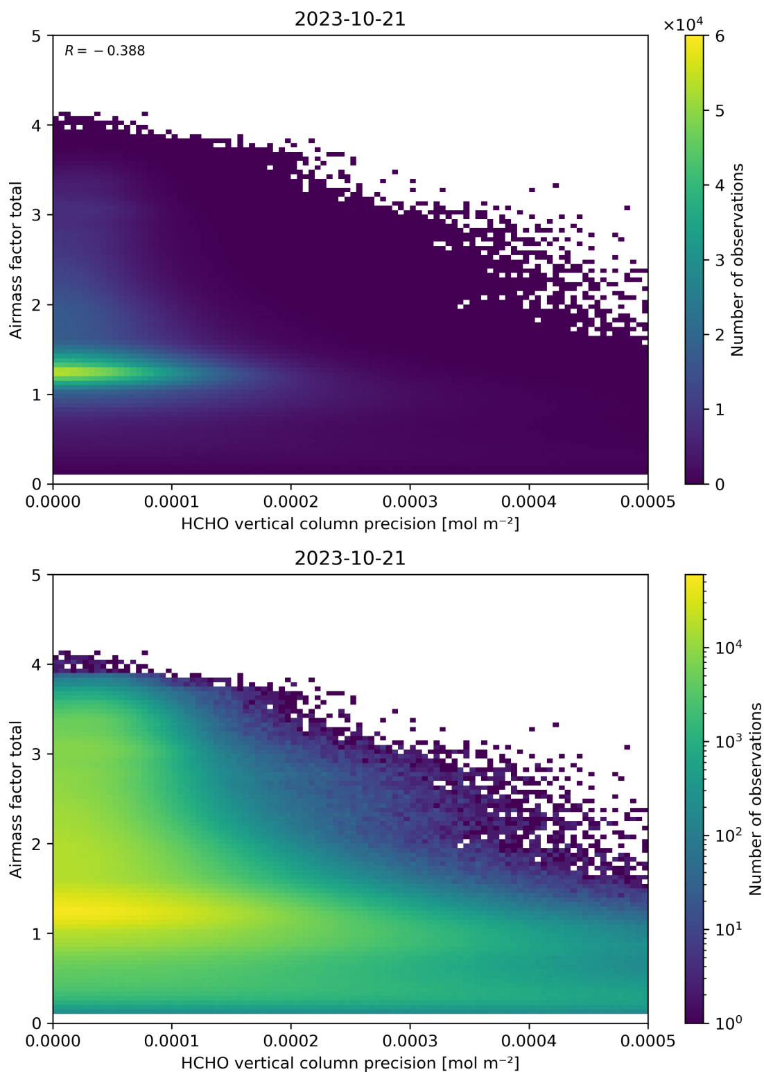
Figure 144: Scatter density plot of “HCHO vertical column precision” against “Airmass factor total” for 2023-10-20 to 2023-10-22.
