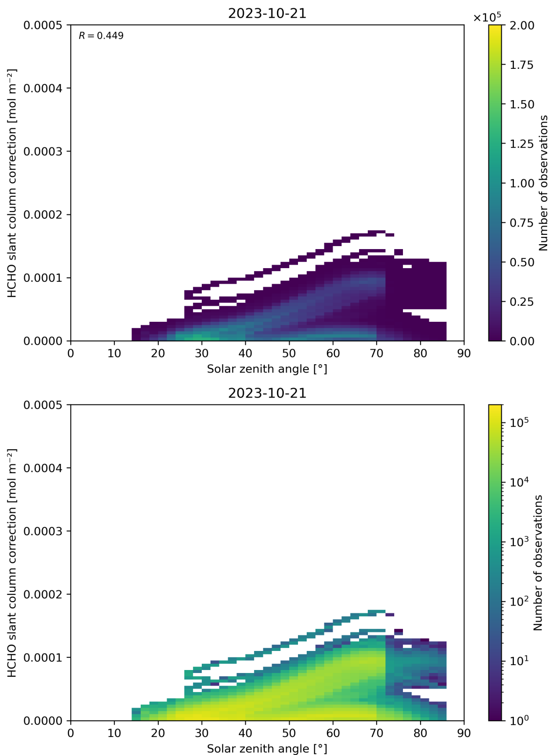
Figure 172: Scatter density plot of “Solar zenith angle” against “HCHO slant column correction” for 2023-10-20 to 2023-10-22.
