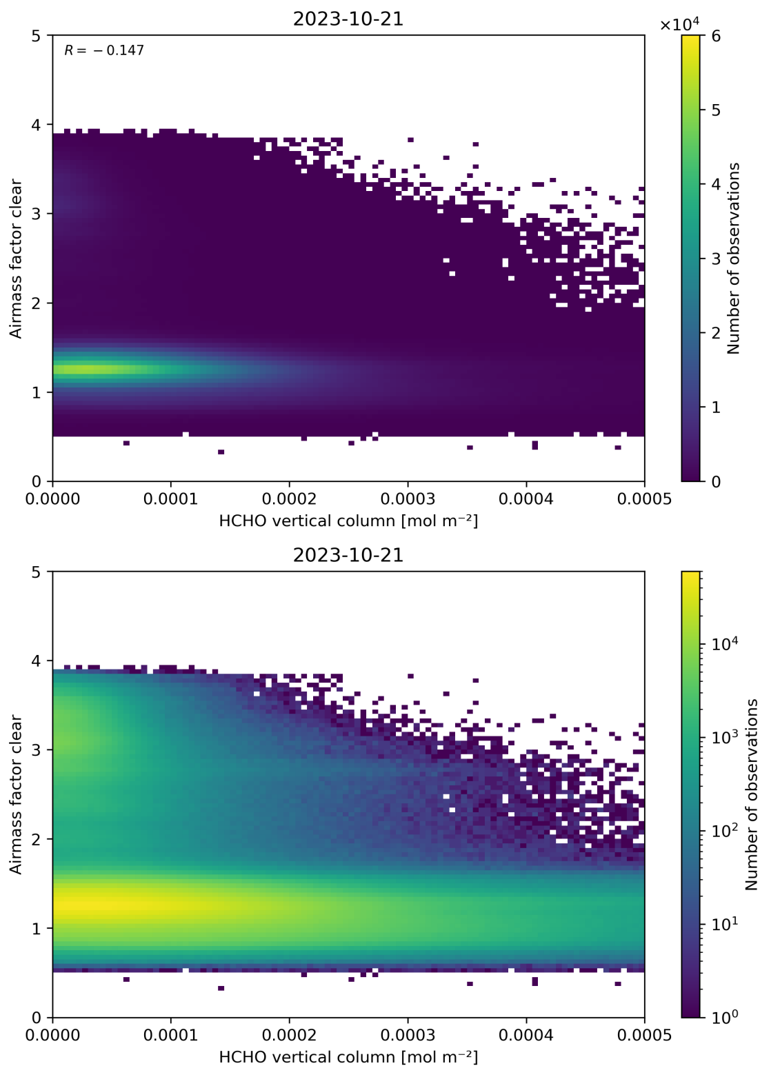
Figure 126: Scatter density plot of “HCHO vertical column” against “Airmass factor clear” for 2023-10-20 to 2023-10-22.
