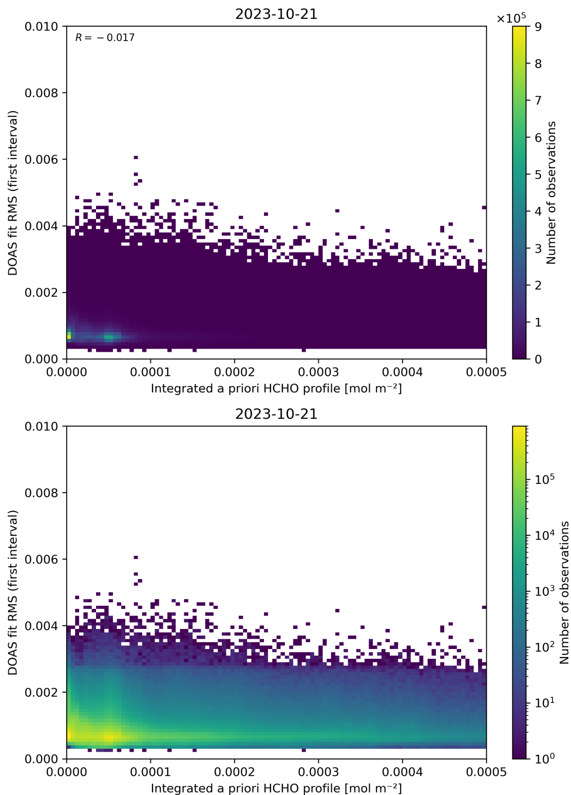
Figure 148: Scatter density plot of “Integrated a priori HCHO profile” against “DOAS fit RMS (first interval)” for 2023-10-20 to 2023-10-22.
