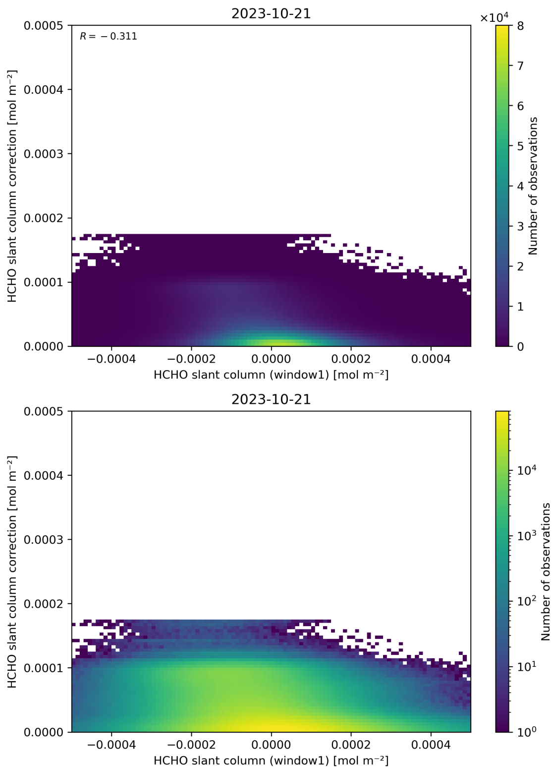
Figure 83: Scatter density plot of “HCHO slant column (window1)” against “HCHO slant column correction” for 2023-10-20 to 2023-10-22.
