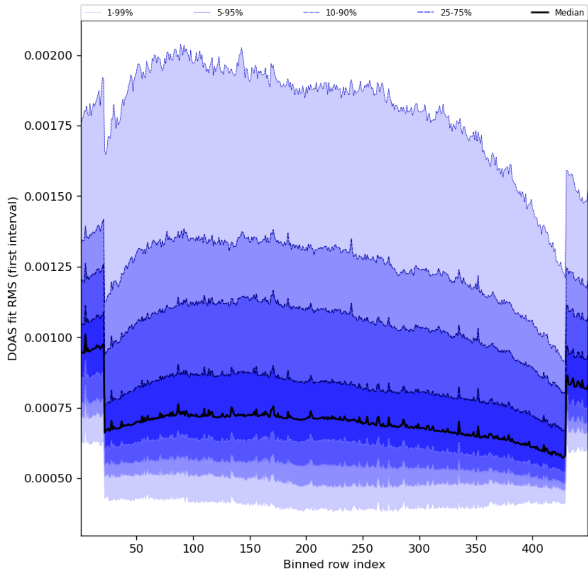
Figure 60: Along track statistics of “DOAS fit RMS (first interval)” for 2023-10-20 to 2023-10-22
