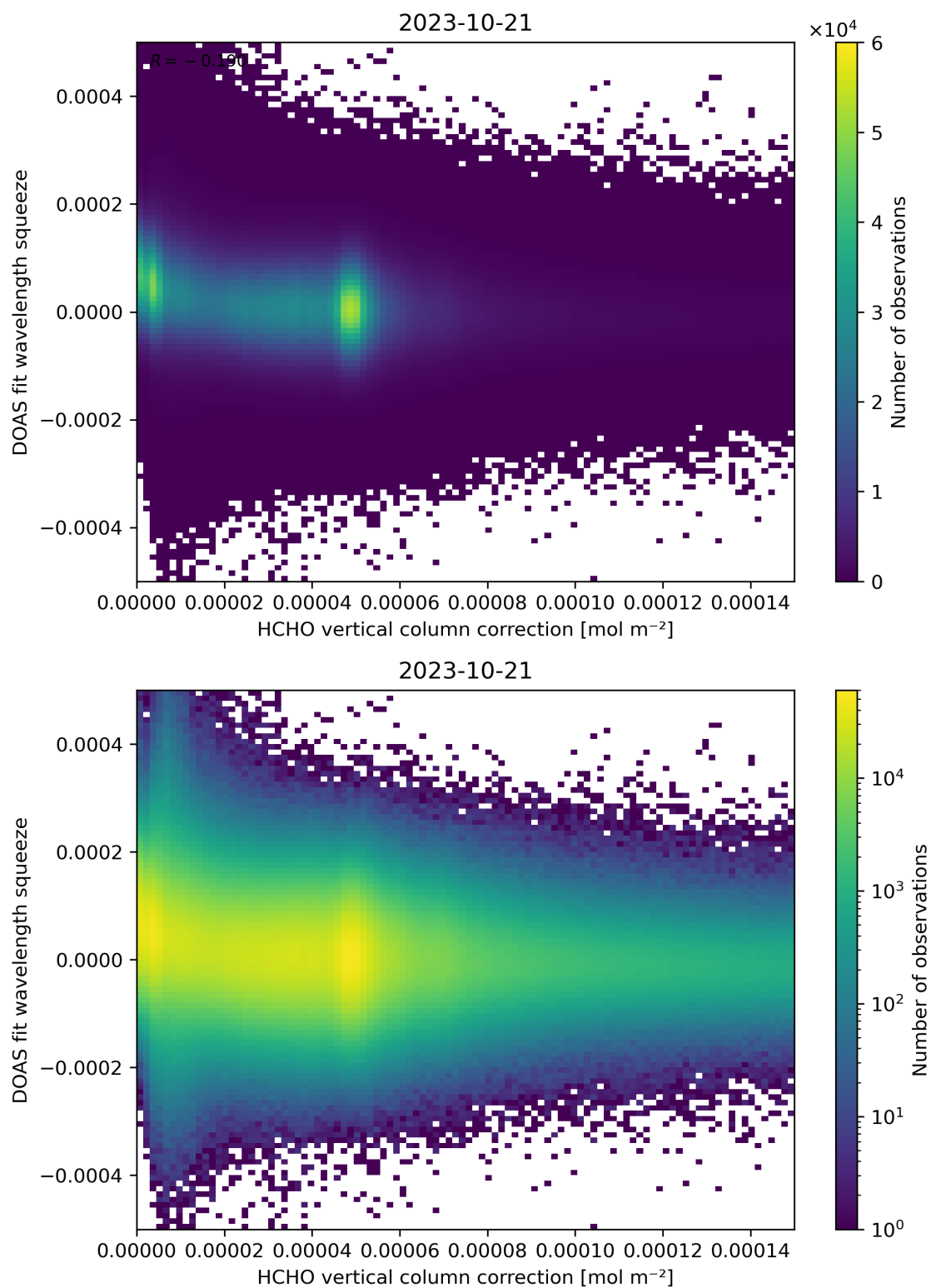
Figure 114: Scatter density plot of “HCHO vertical column correction” against “DOAS fit wavelength squeeze” for 2023-10-20 to 2023-10-22.
