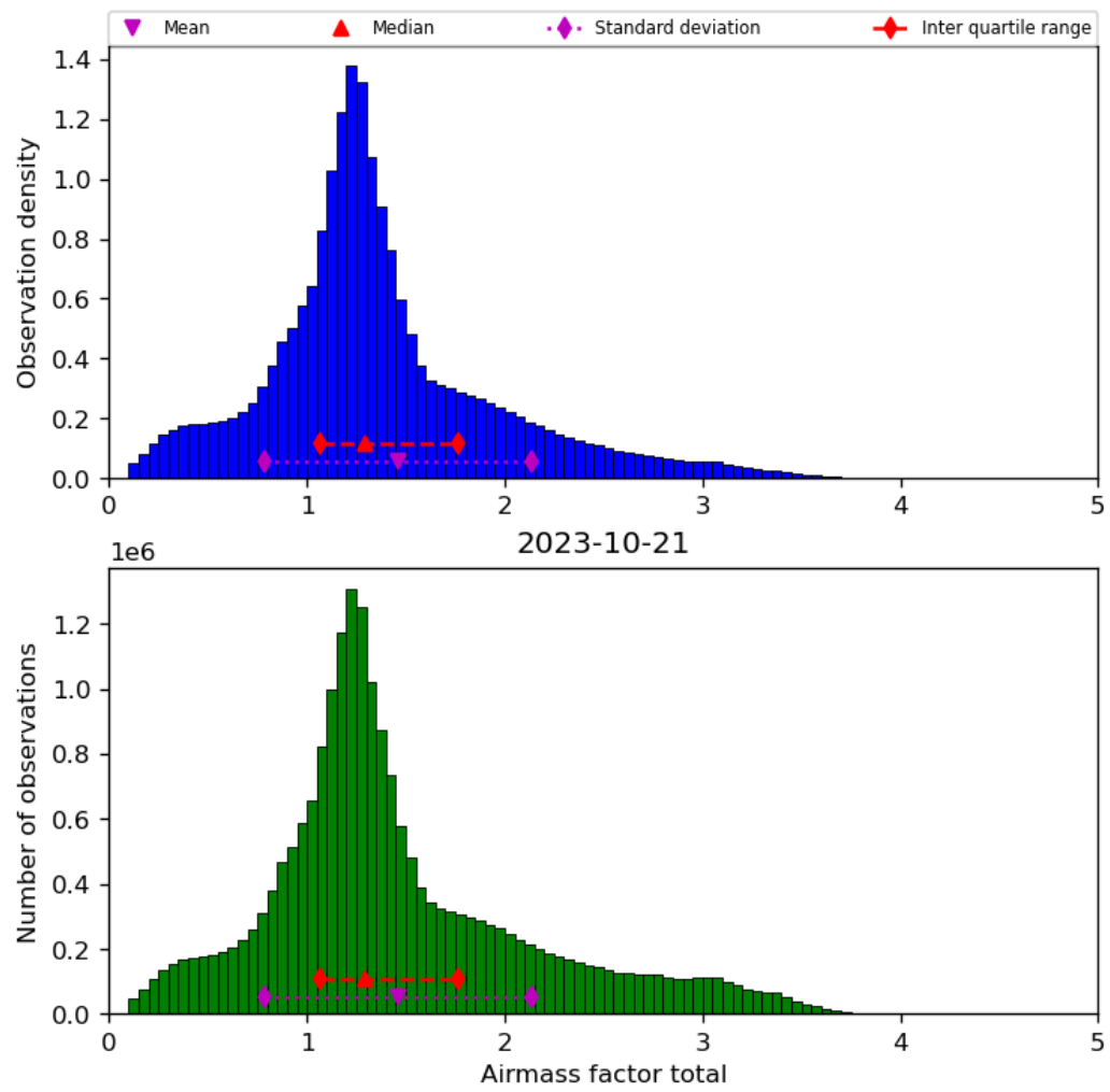
Figure 40: Histogram of “Airmass factor total” for 2023-10-20 to 2023-10-22
