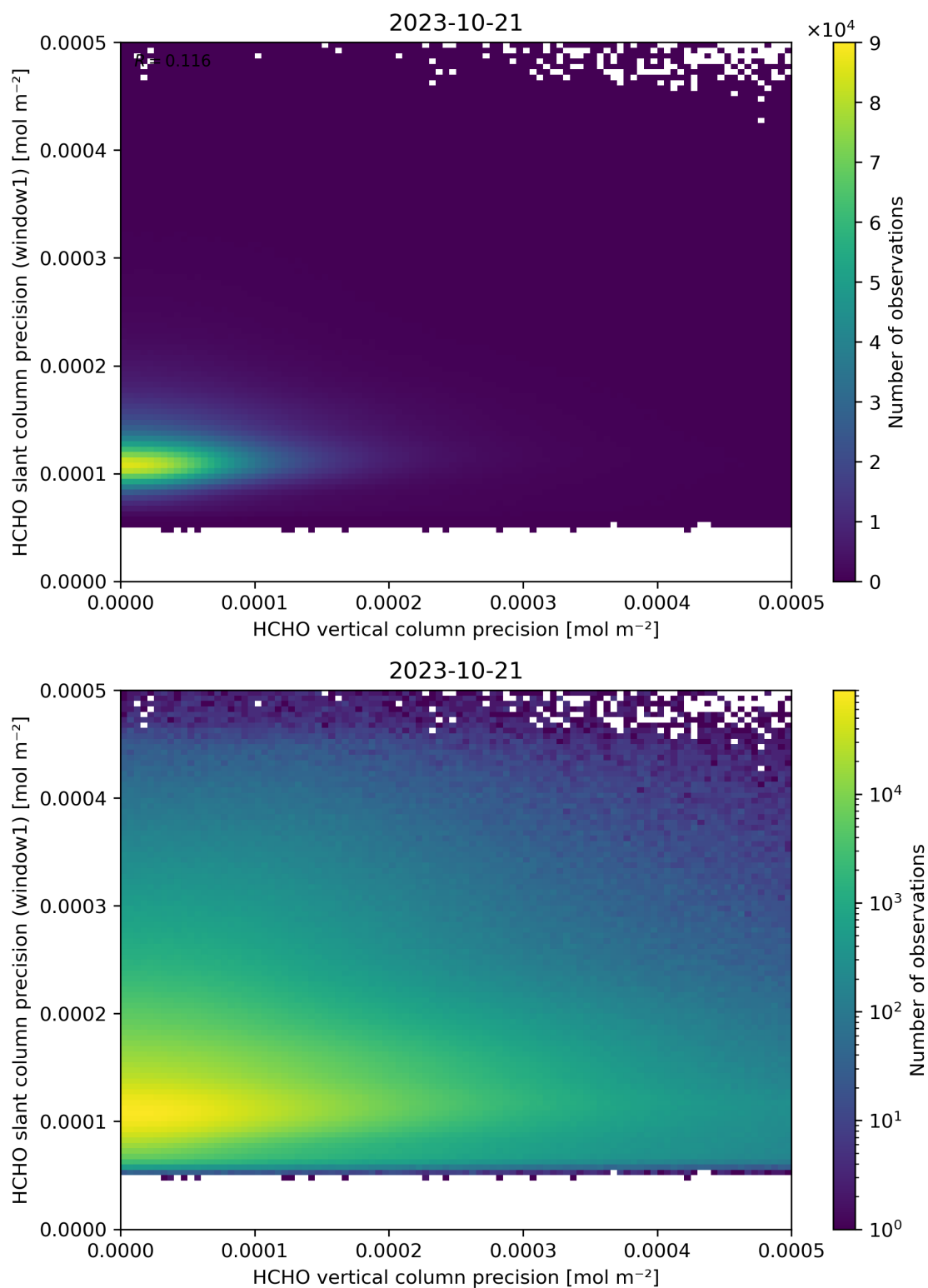
Figure 143: Scatter density plot of “HCHO vertical column precision” against “HCHO slant column precision (window1)” for 2023-10-20 to 2023-10-22.
