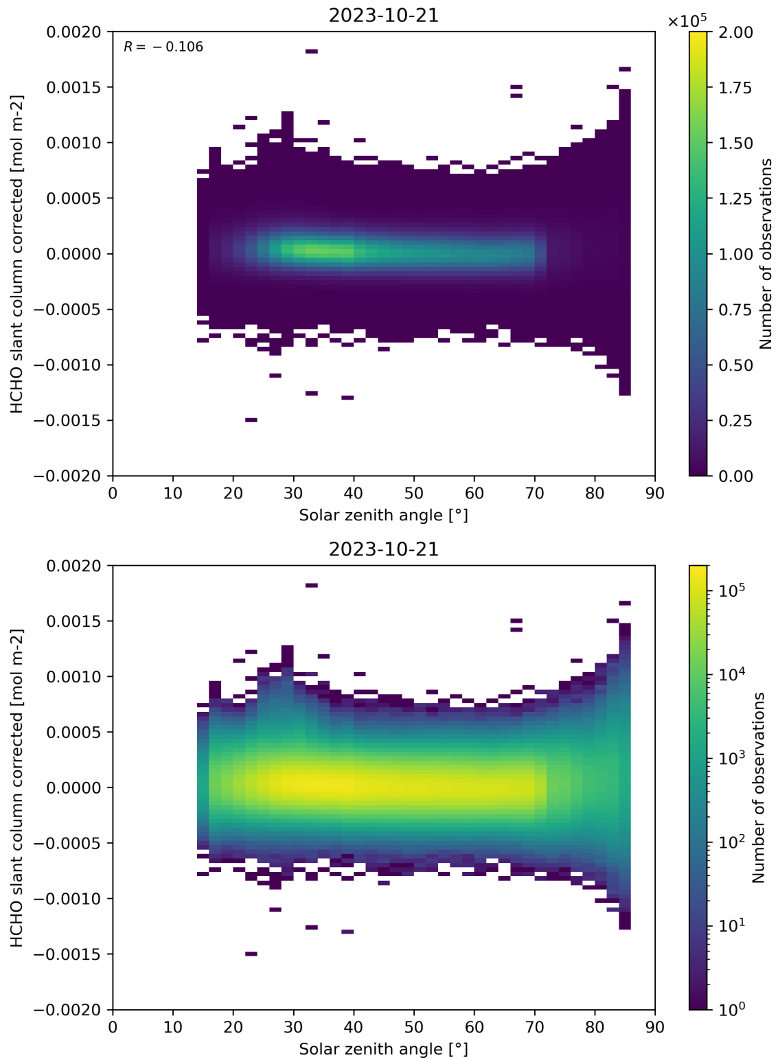
Figure 171: Scatter density plot of “Solar zenith angle” against “HCHO slant column corrected” for 2023-10-20 to 2023-10-22.
