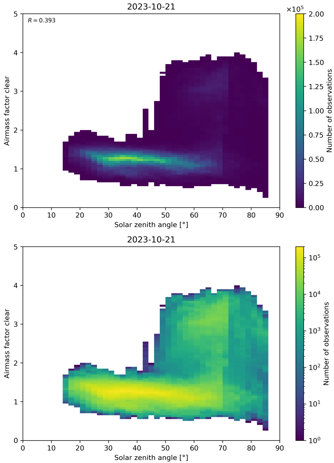
Figure 170: Scatter density plot of “Solar zenith angle” against “Airmass factor clear” for 2023-10-20 to 2023-10-22.
