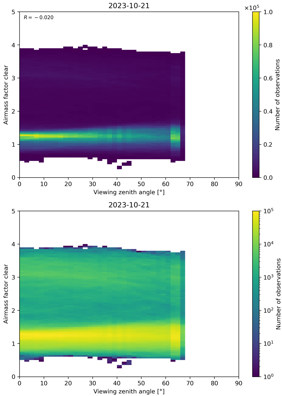
Figure 185: Scatter density plot of “Viewing zenith angle” against “Airmass factor clear” for 2023-10-20 to 2023-10-22.
