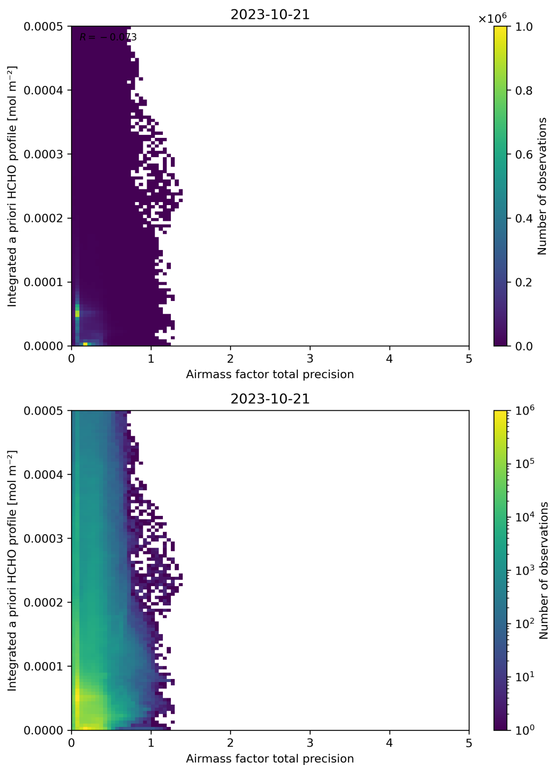
Figure 111: Scatter density plot of “Airmass factor total precision” against “Integrated a priori HCHO profile” for 2023-10-20 to 2023-10-22.
