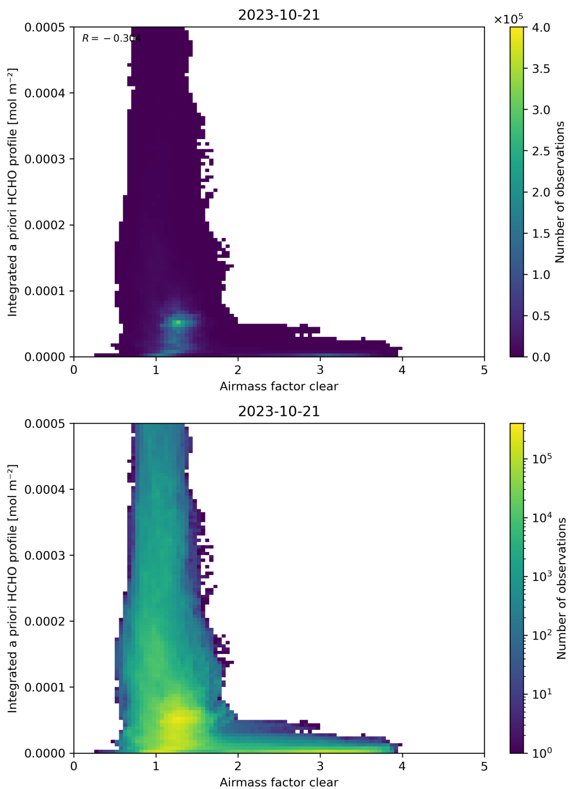
Figure 76: Scatter density plot of “Airmass factor clear” against “Integrated a priori HCHO profile” for 2023-10-20 to 2023-10-22.
