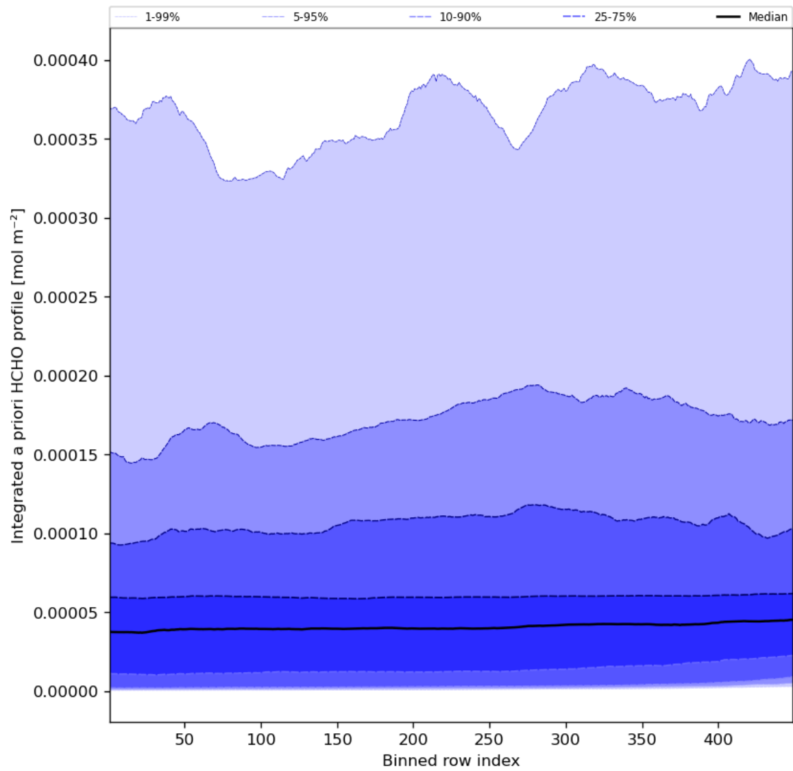
Figure 57: Along track statistics of “Integrated a priori HCHO profile” for 2023-10-20 to 2023-10-22
