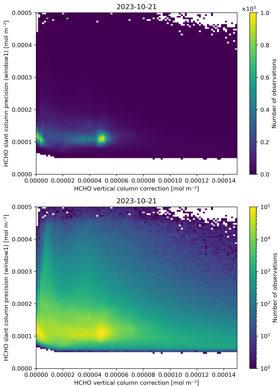
Figure 119: Scatter density plot of “HCHO vertical column correction” against “HCHO slant column precision (window1)” for 2023-10-20 to 2023-10-22.
