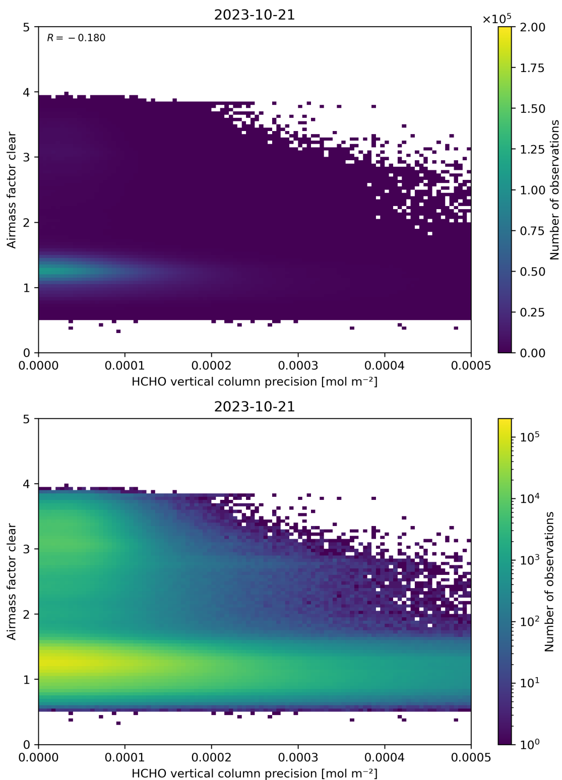
Figure 139: Scatter density plot of “HCHO vertical column precision” against “Airmass factor clear” for 2023-10-20 to 2023-10-22.
