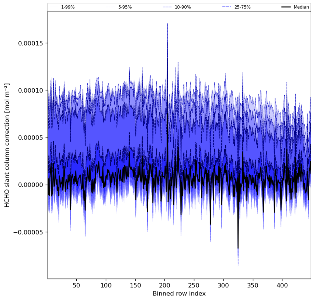
Figure 61: Along track statistics of “HCHO slant column correction” for 2023-10-20 to 2023-10-22
