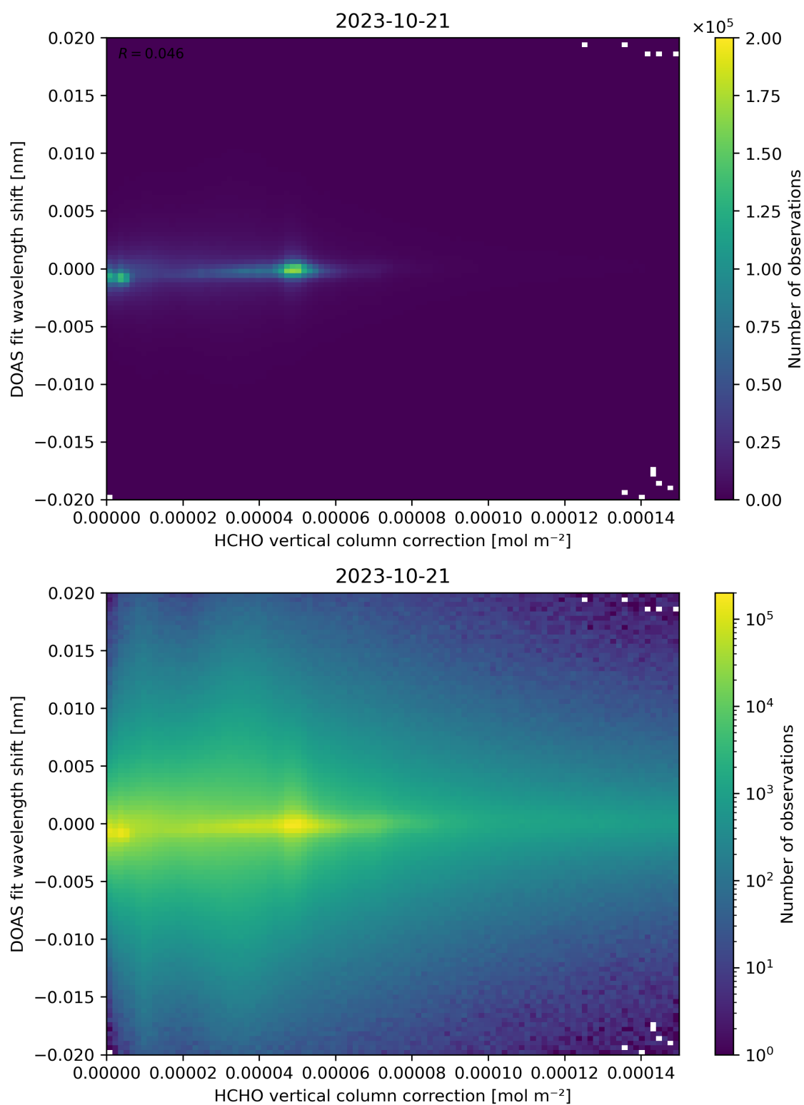
Figure 113: Scatter density plot of “HCHO vertical column correction” against “DOAS fit wavelength shift” for 2023-10-20 to 2023-10-22.
