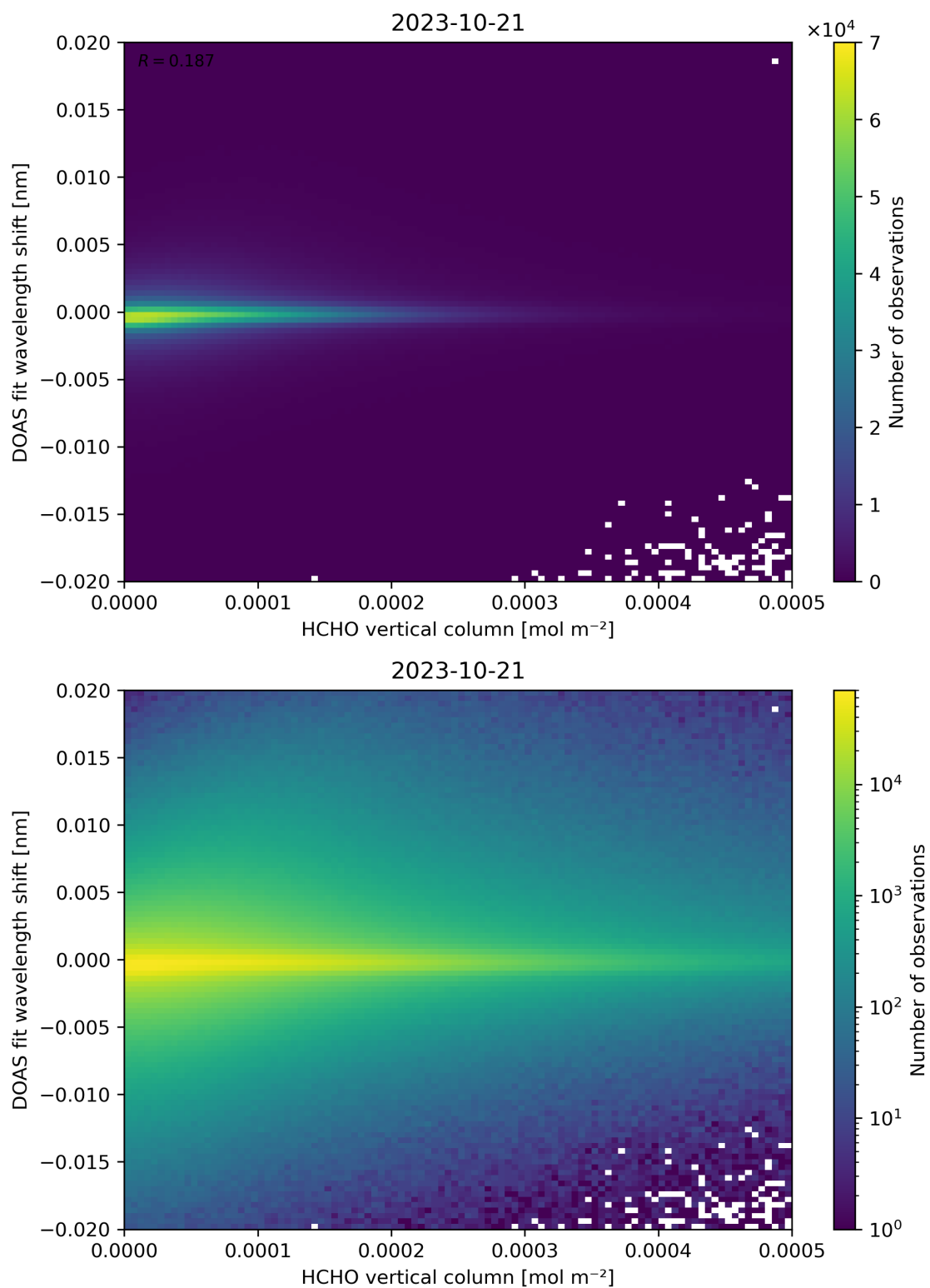
Figure 124: Scatter density plot of “HCHO vertical column” against “DOAS fit wavelength shift” for 2023-10-20 to 2023-10-22.
