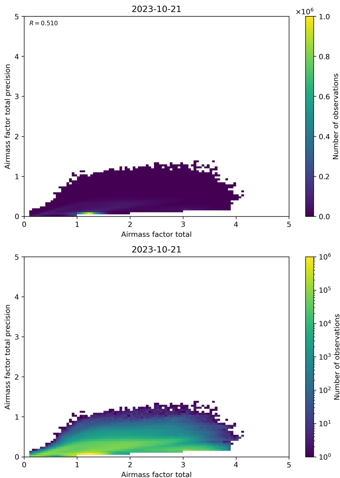
Figure 103: Scatter density plot of “Airmass factor total” against “Airmass factor total precision” for 2023-10-20 to 2023-10-22.
