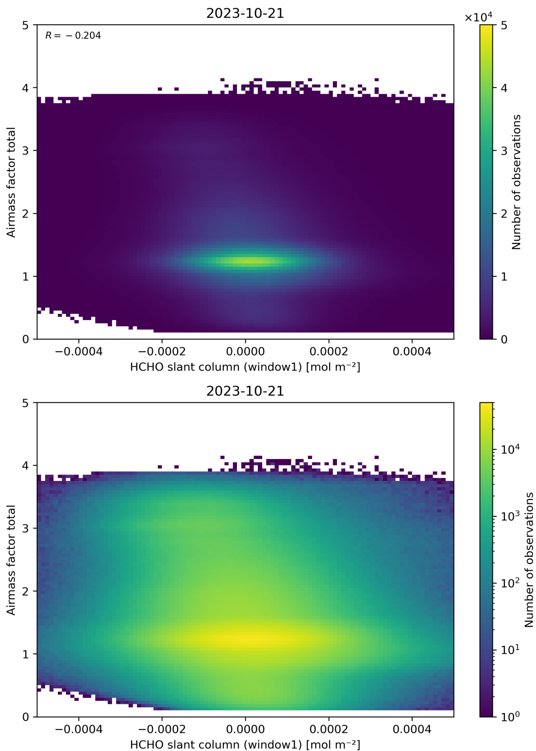
Figure 85: Scatter density plot of “HCHO slant column (window1)” against “Airmass factor total” for 2023-10-20 to 2023-10-22.
