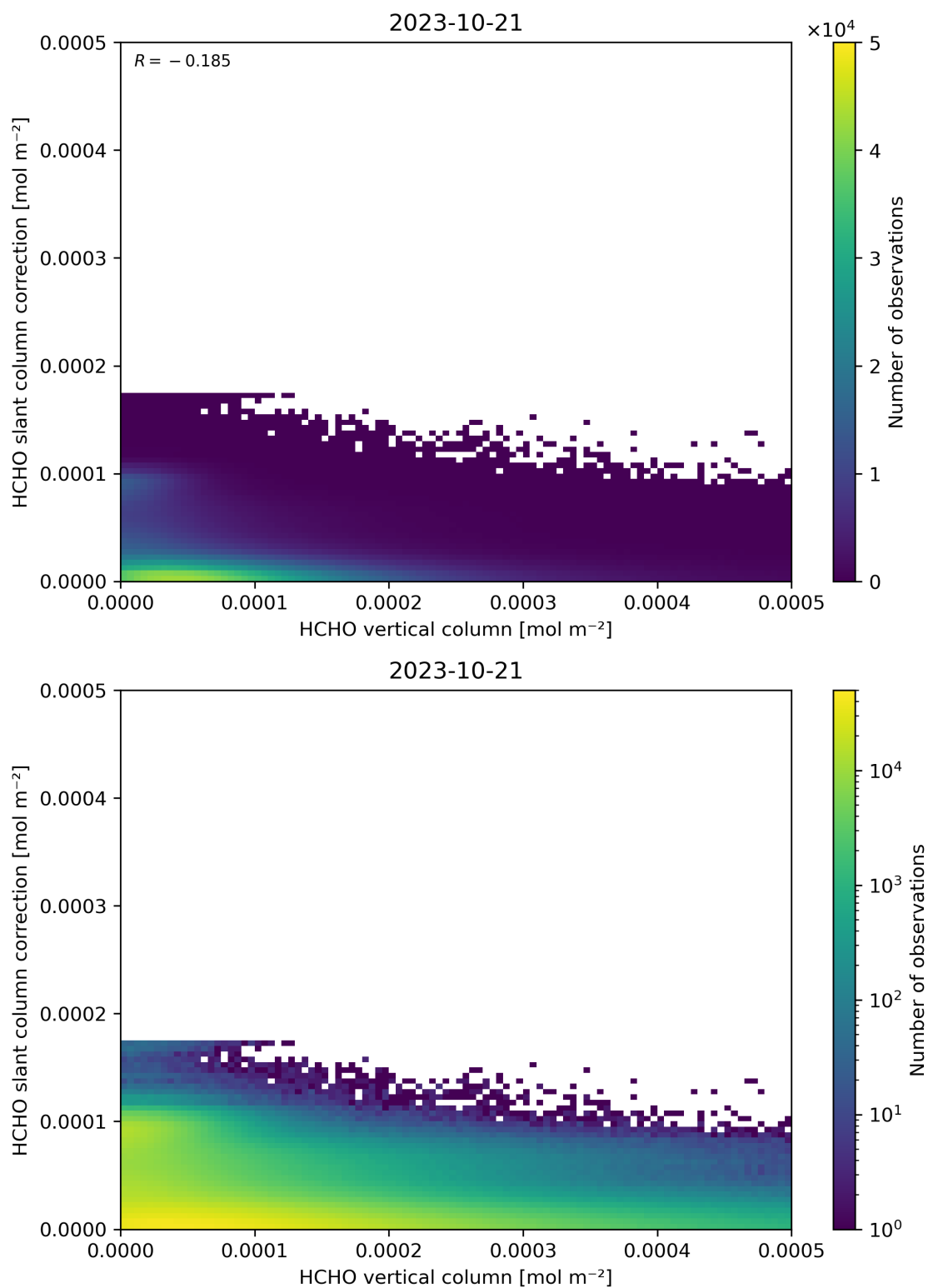
Figure 128: Scatter density plot of “HCHO vertical column” against “HCHO slant column correction” for 2023-10-20 to 2023-10-22.
