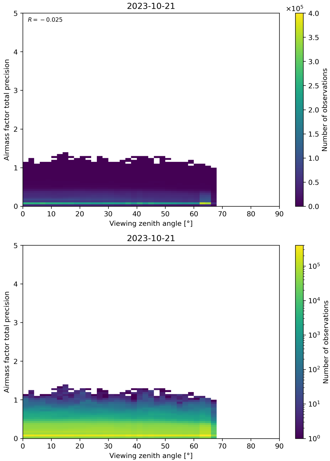
Figure 191: Scatter density plot of “Viewing zenith angle” against “Airmass factor total precision” for 2023-10-20 to 2023-10-22.
