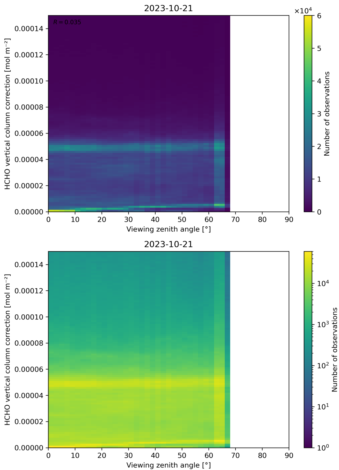
Figure 193: Scatter density plot of “Viewing zenith angle” against “HCHO vertical column correction” for 2023-10-20 to 2023-10-22.
