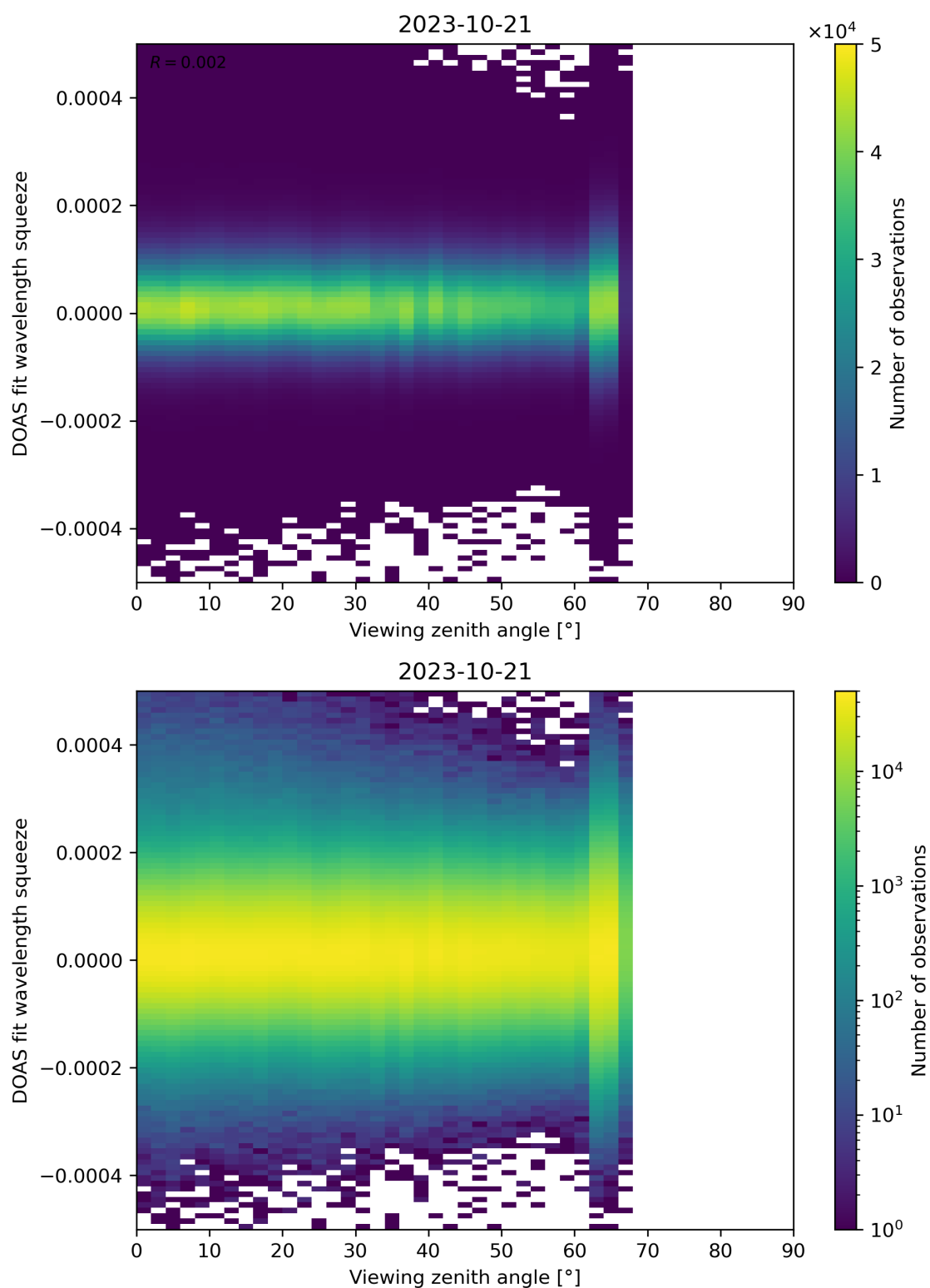
Figure 184: Scatter density plot of “Viewing zenith angle” against “DOAS fit wavelength squeeze” for 2023-10-20 to 2023-10-22.
