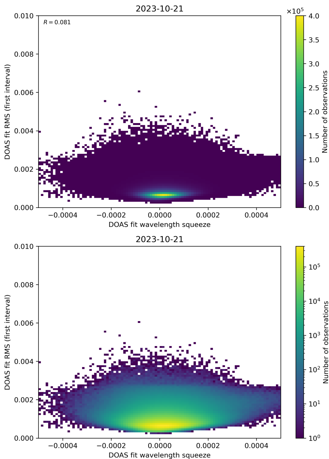
Figure 68: Scatter density plot of “DOAS fit wavelength squeeze” against “DOAS fit RMS (first interval)” for 2023-10-20 to 2023-10-22.
