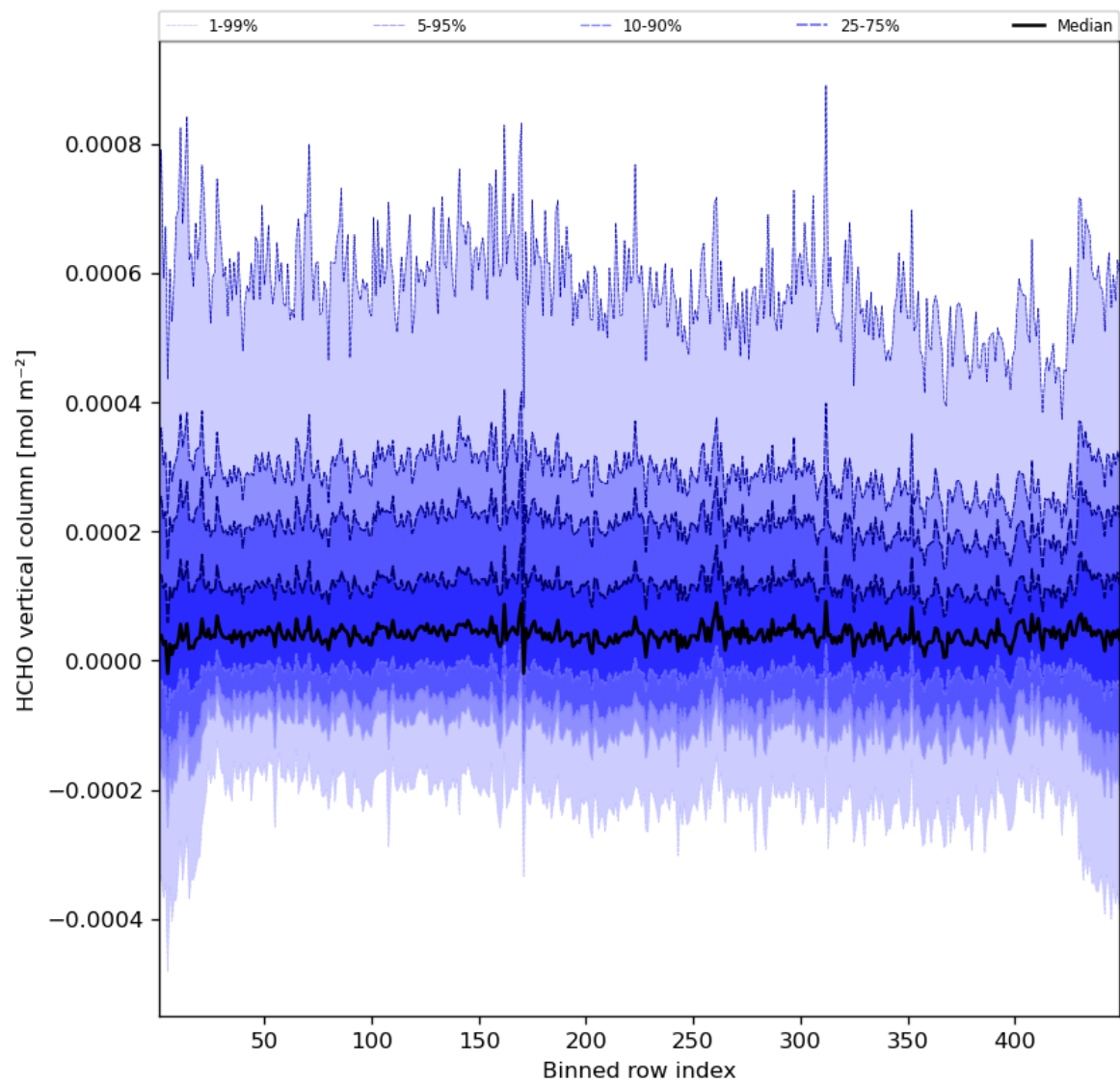
Figure 49: Along track statistics of “HCHO vertical column” for 2023-10-20 to 2023-10-22
