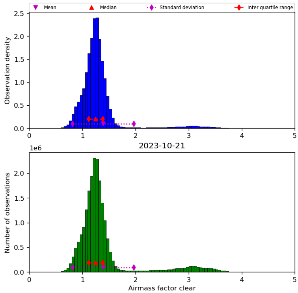
Figure 42: Histogram of “Airmass factor clear” for 2023-10-20 to 2023-10-22
