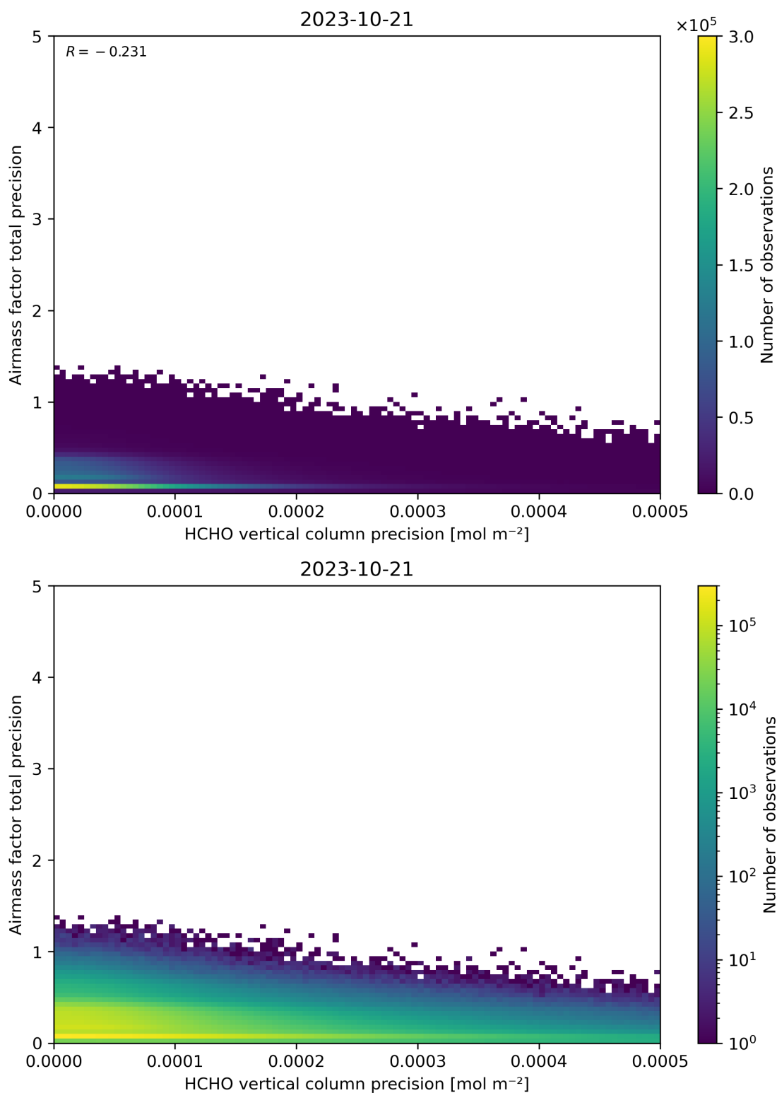
Figure 145: Scatter density plot of “HCHO vertical column precision” against “Airmass factor total precision” for 2023-10-20 to 2023-10-22.
