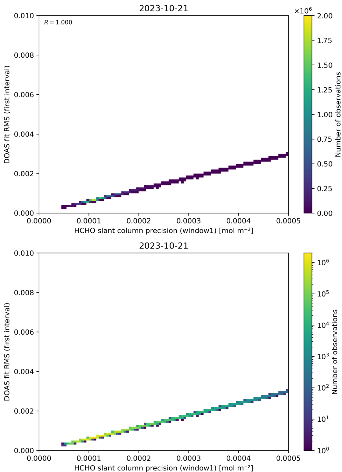
Figure 88: Scatter density plot of “HCHO slant column precision (window1)” against “DOAS fit RMS (first interval)” for 2023-10-20 to 2023-10-22.
