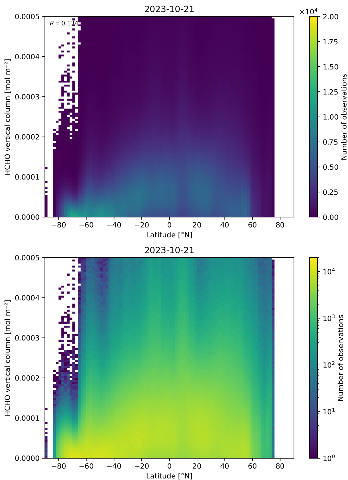
Figure 163: Scatter density plot of “Latitude” against “HCHO vertical column” for 2023-10-20 to 2023-10-22.
