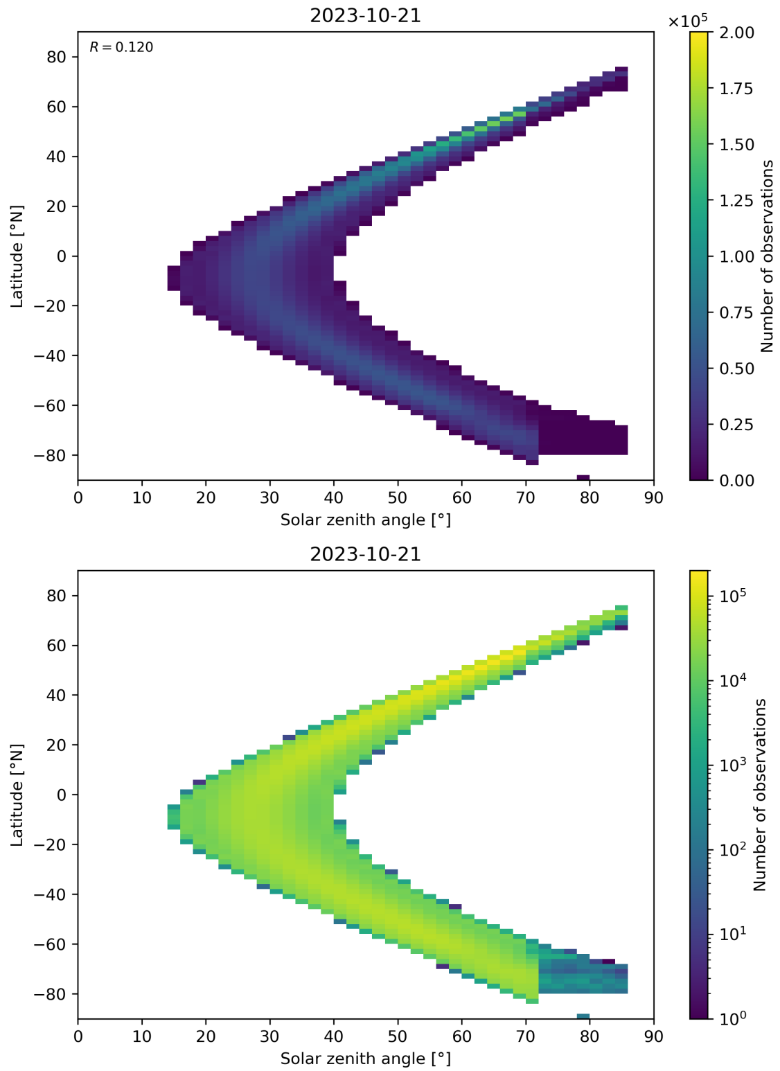
Figure 181: Scatter density plot of “Solar zenith angle” against “Latitude” for 2023-10-20 to 2023-10-22.
