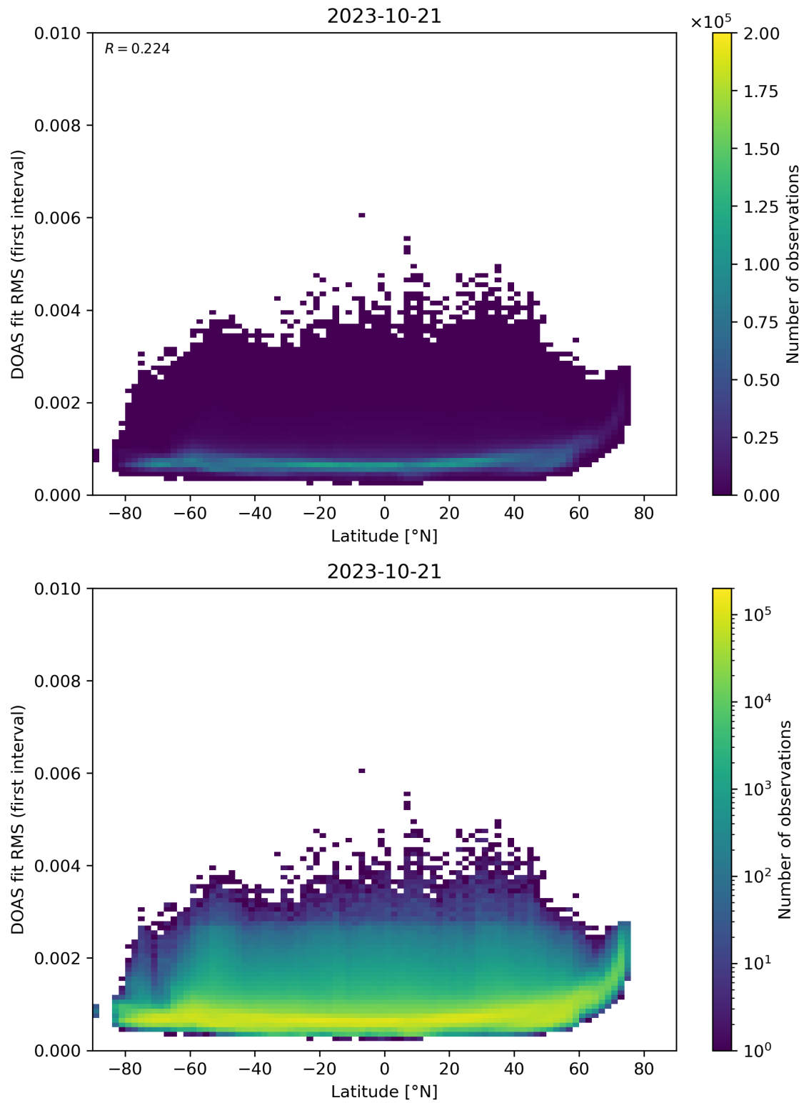
Figure 153: Scatter density plot of “Latitude” against “DOAS fit RMS (first interval)” for 2023-10-20 to 2023-10-22.
