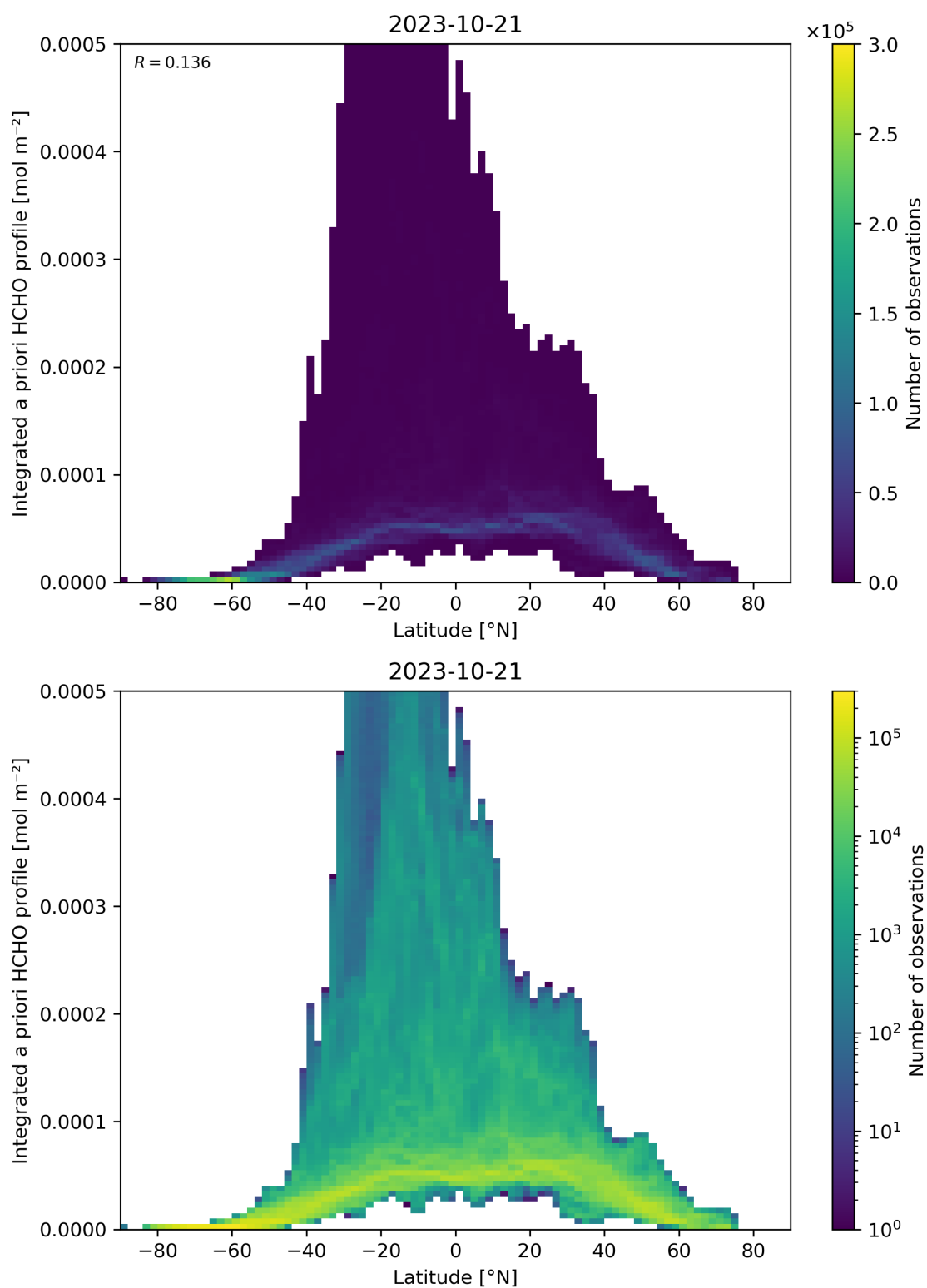
Figure 166: Scatter density plot of “Latitude” against “Integrated a priori HCHO profile” for 2023-10-20 to 2023-10-22.
