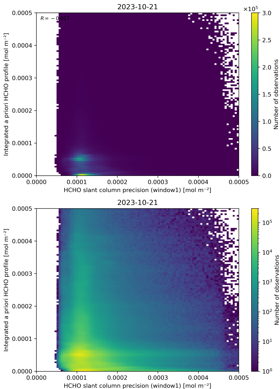
Figure 96: Scatter density plot of “HCHO slant column precision (window1)” against “Integrated a priori HCHO profile” for 2023-10-20 to 2023-10-22.
