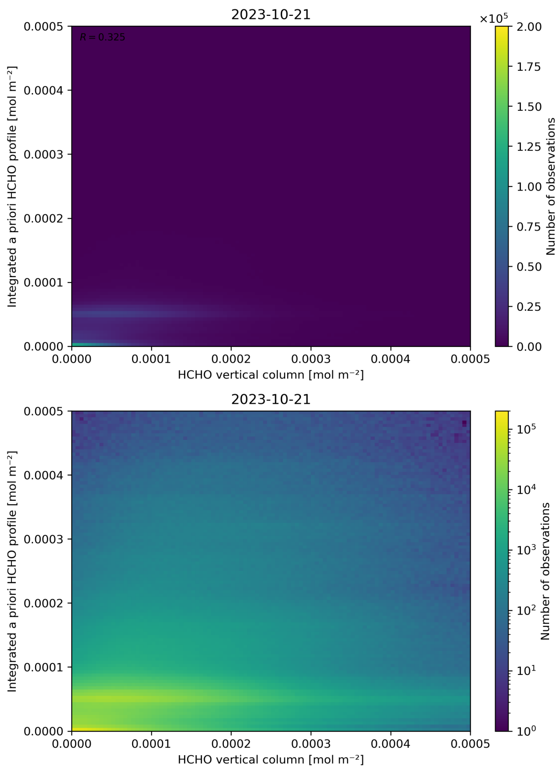
Figure 135: Scatter density plot of “HCHO vertical column” against “Integrated a priori HCHO profile” for 2023-10-20 to 2023-10-22.
