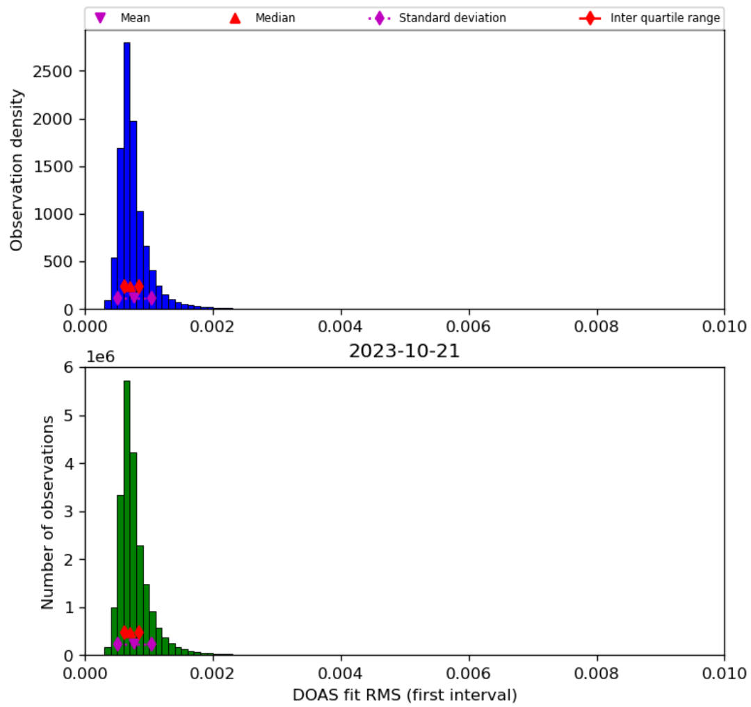
Figure 46: Histogram of “DOAS fit RMS (first interval)” for 2023-10-20 to 2023-10-22
