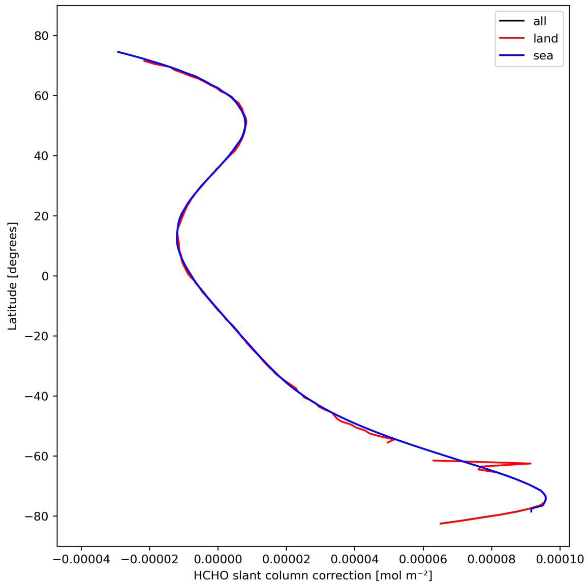
Figure 33: Zonal average of “HCHO slant column correction” for 2023-10-20 to 2023-10-22.
