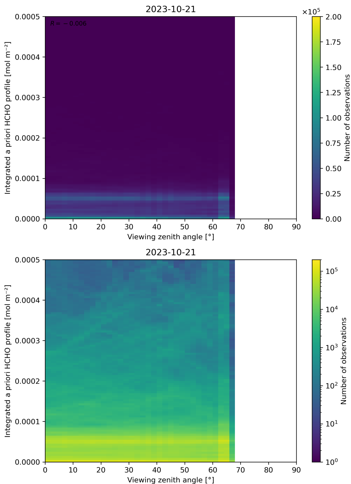
Figure 195: Scatter density plot of “Viewing zenith angle” against “Integrated a priori HCHO profile” for 2023-10-20 to 2023-10-22.
