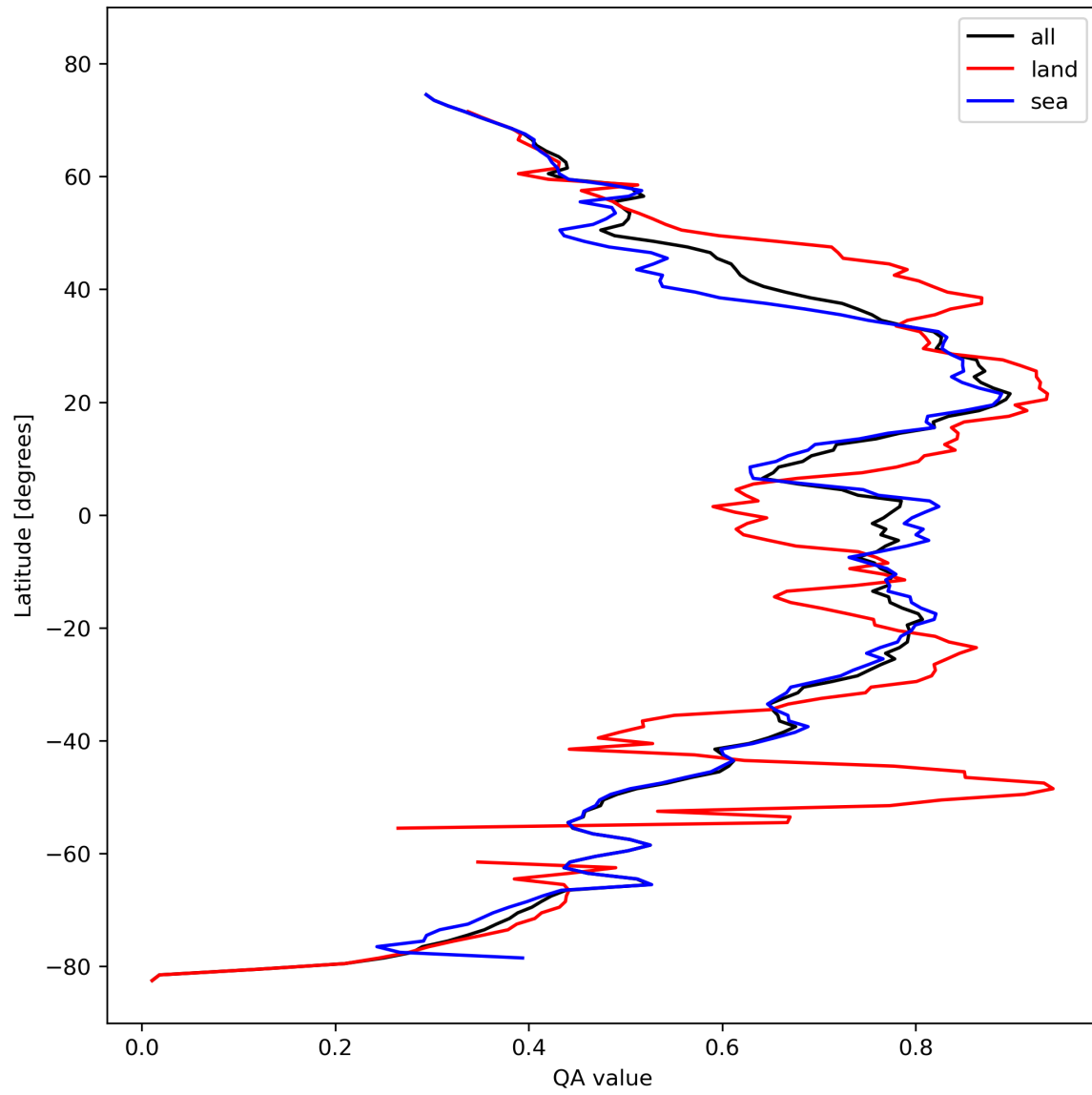
Figure 20: Zonal average of “QA value” for 2023-10-20 to 2023-10-22.
