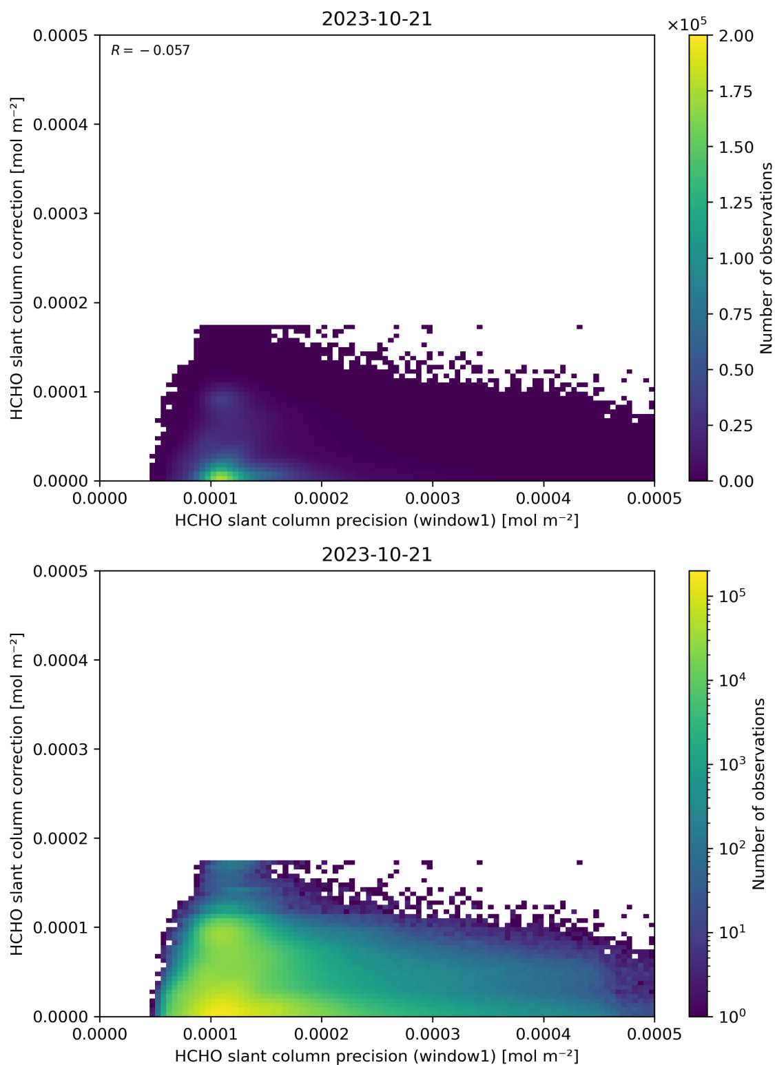
Figure 93: Scatter density plot of “HCHO slant column precision (window1)” against “HCHO slant column correction” for 2023-10-20 to 2023-10-22.
