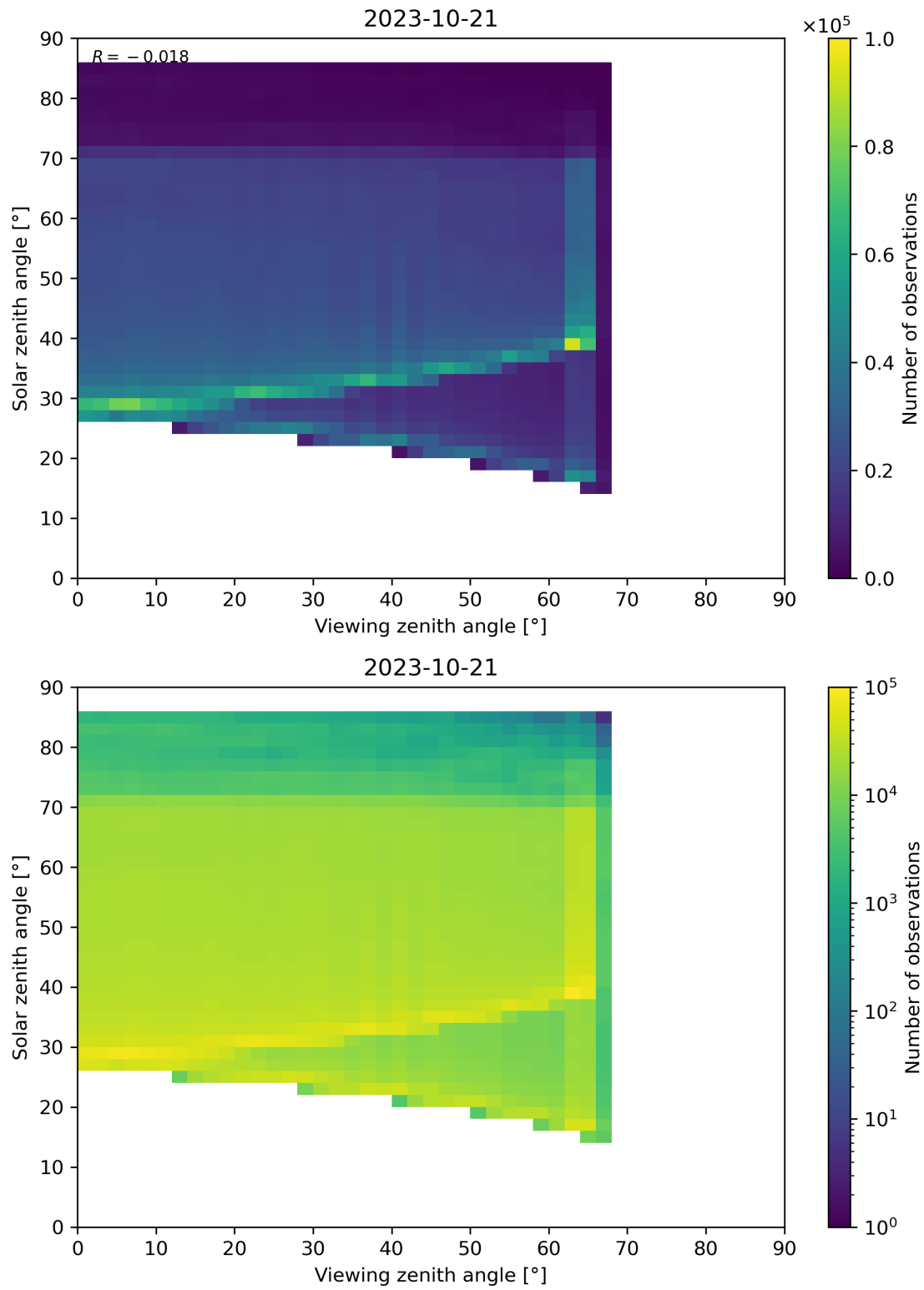
Figure 197: Scatter density plot of “Viewing zenith angle” against “Solar zenith angle” for 2023-10-20 to 2023-10-22.
