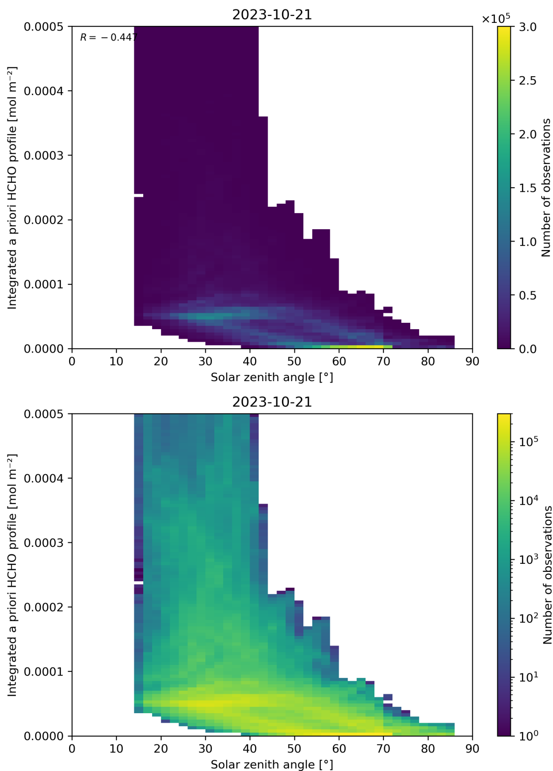
Figure 180: Scatter density plot of “Solar zenith angle” against “Integrated a priori HCHO profile” for 2023-10-20 to 2023-10-22.
