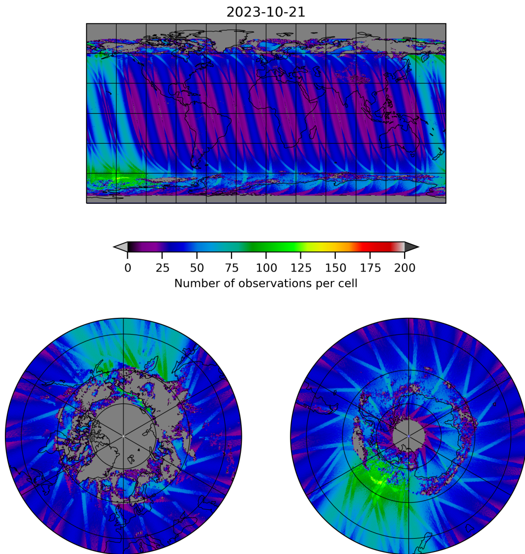
Figure 19: Map of the number of observations for 2023-10-20 to 2023-10-22
