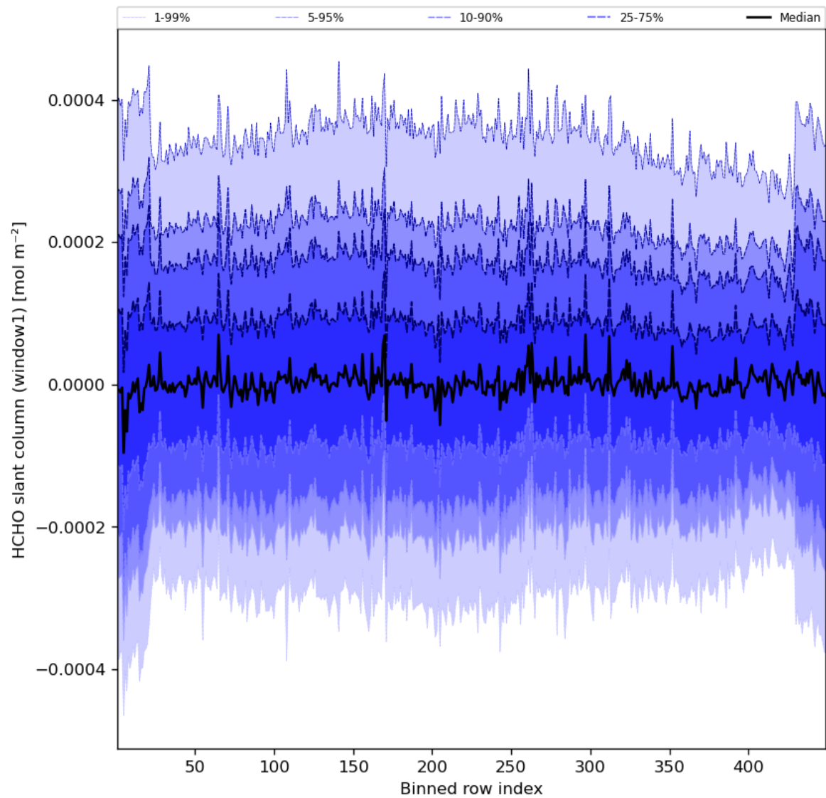
Figure 52: Along track statistics of “HCHO slant column (window1)” for 2023-10-20 to 2023-10-22
