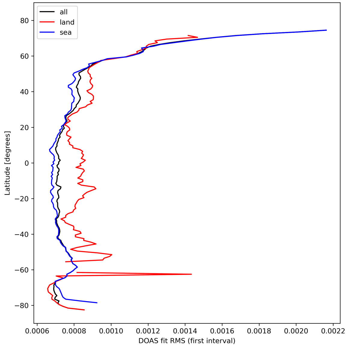
Figure 32: Zonal average of “DOAS fit RMS (first interval)” for 2023-10-20 to 2023-10-22.
