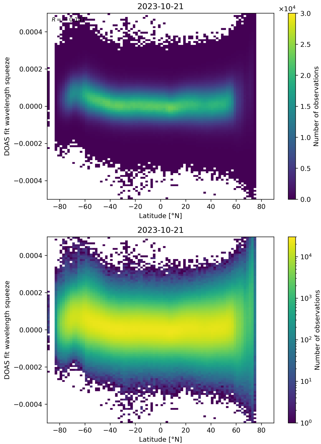
Figure 155: Scatter density plot of “Latitude” against “DOAS fit wavelength squeeze” for 2023-10-20 to 2023-10-22.
