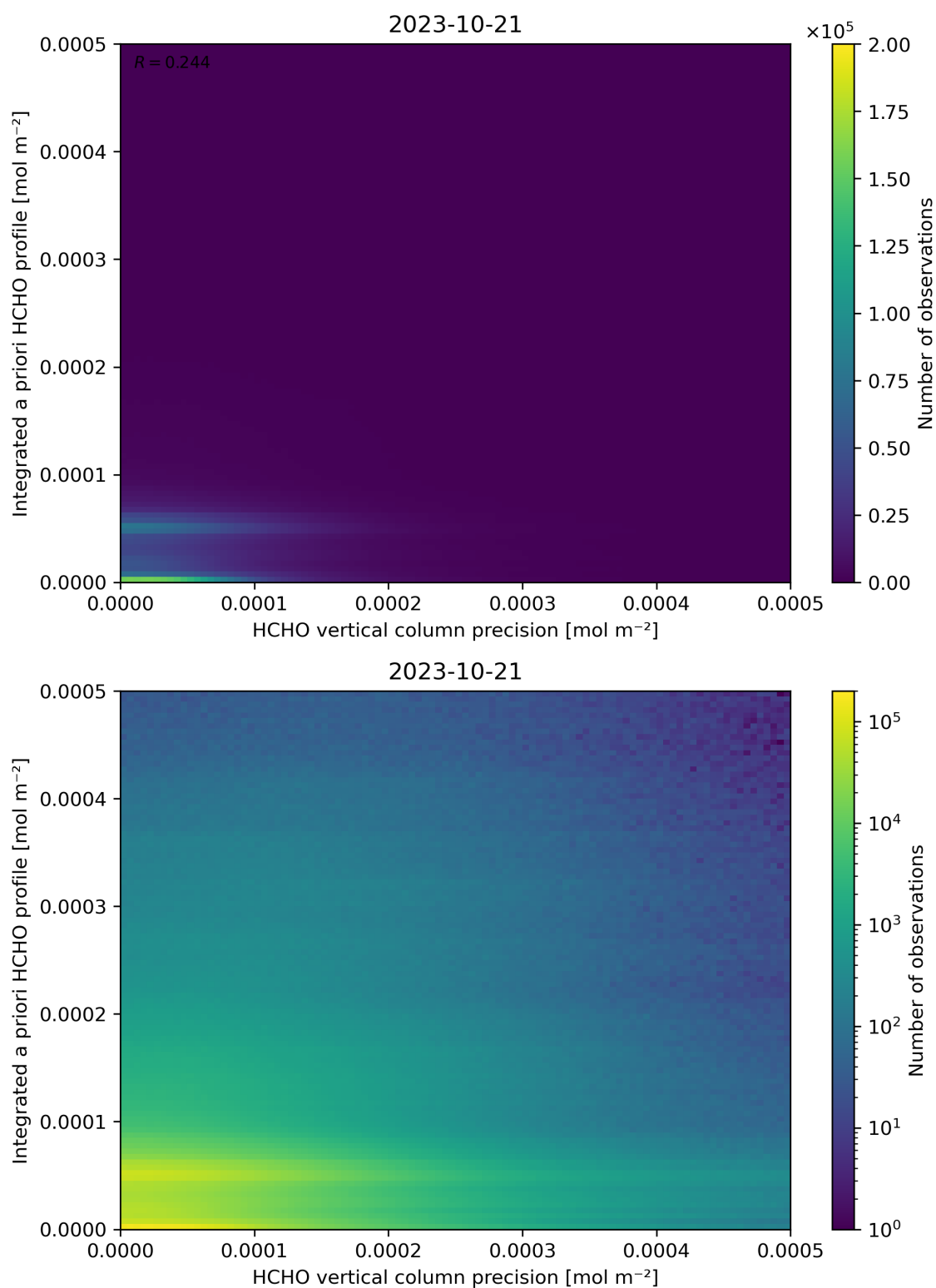
Figure 147: Scatter density plot of “HCHO vertical column precision” against “Integrated a priori HCHO profile” for 2023-10-20 to 2023-10-22.
