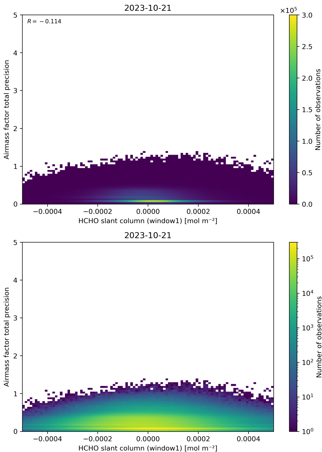
Figure 86: Scatter density plot of “HCHO slant column (window1)” against “Airmass factor total precision” for 2023-10-20 to 2023-10-22.
