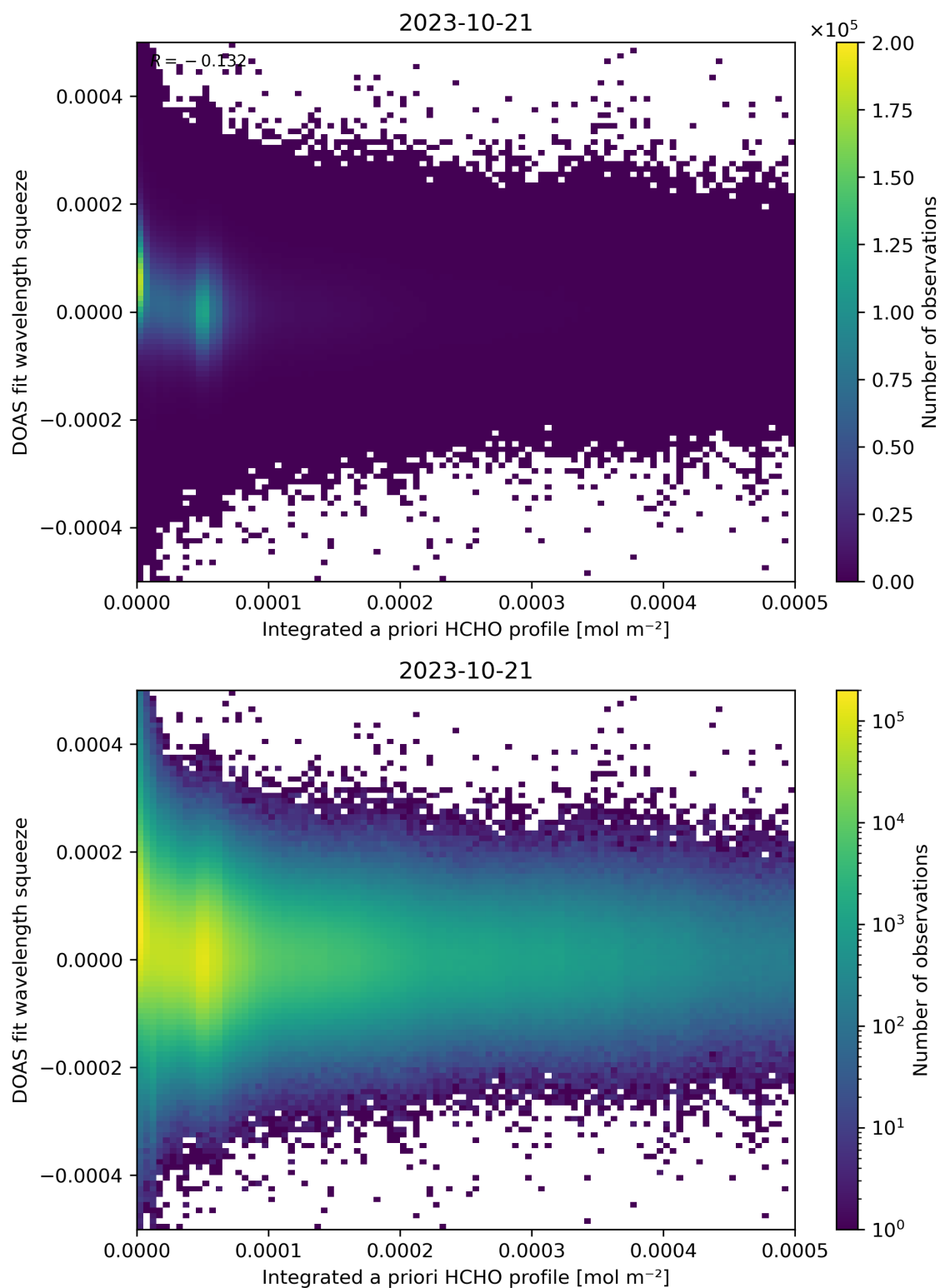
Figure 150: Scatter density plot of “Integrated a priori HCHO profile” against “DOAS fit wavelength squeeze” for 2023-10-20 to 2023-10-22.
