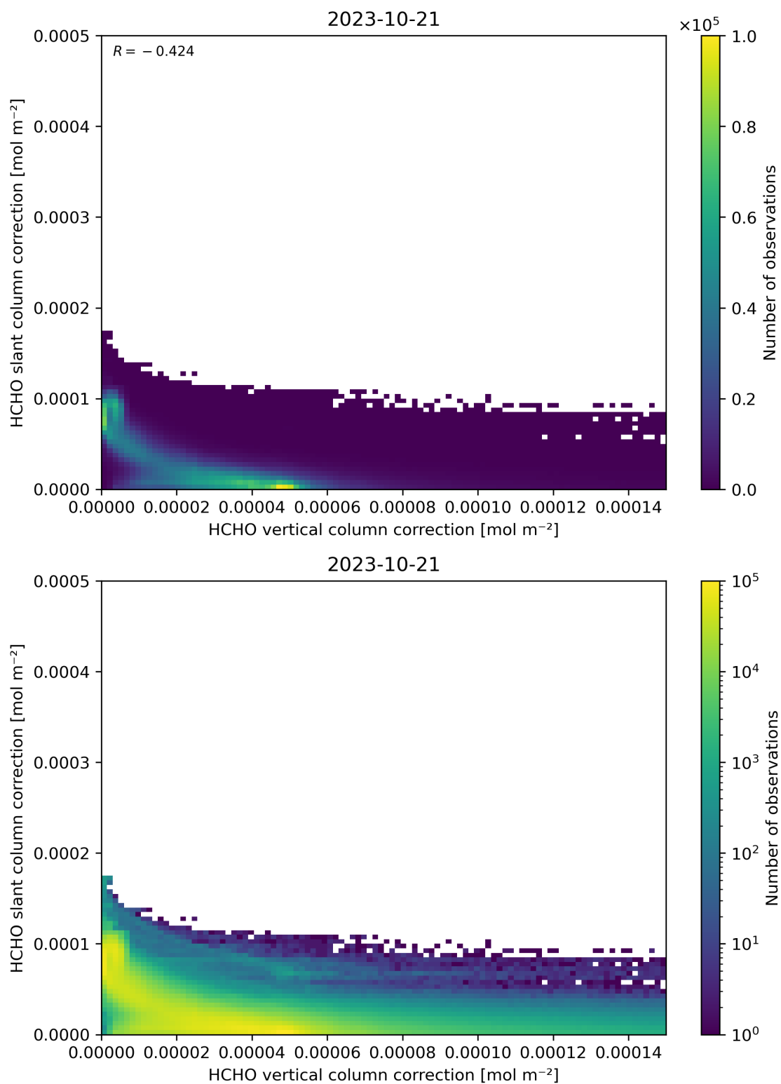
Figure 117: Scatter density plot of “HCHO vertical column correction” against “HCHO slant column correction” for 2023-10-20 to 2023-10-22.
