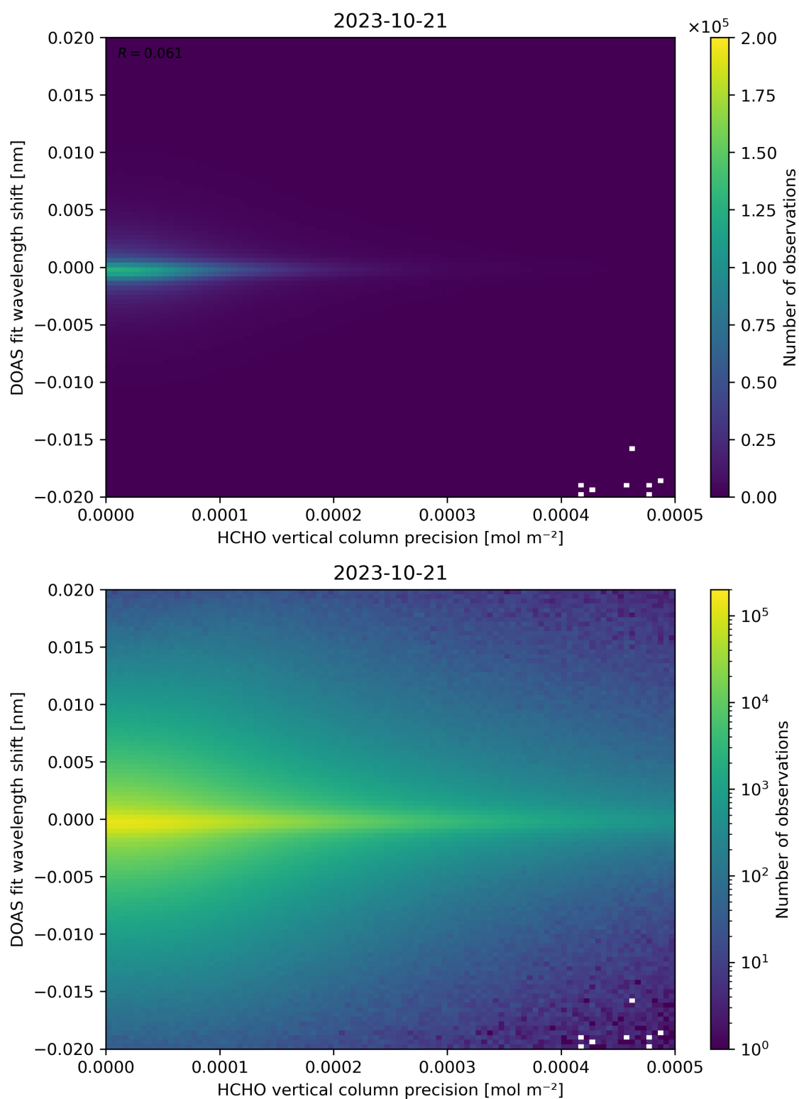
Figure 137: Scatter density plot of “HCHO vertical column precision” against “DOAS fit wavelength shift” for 2023-10-20 to 2023-10-22.
