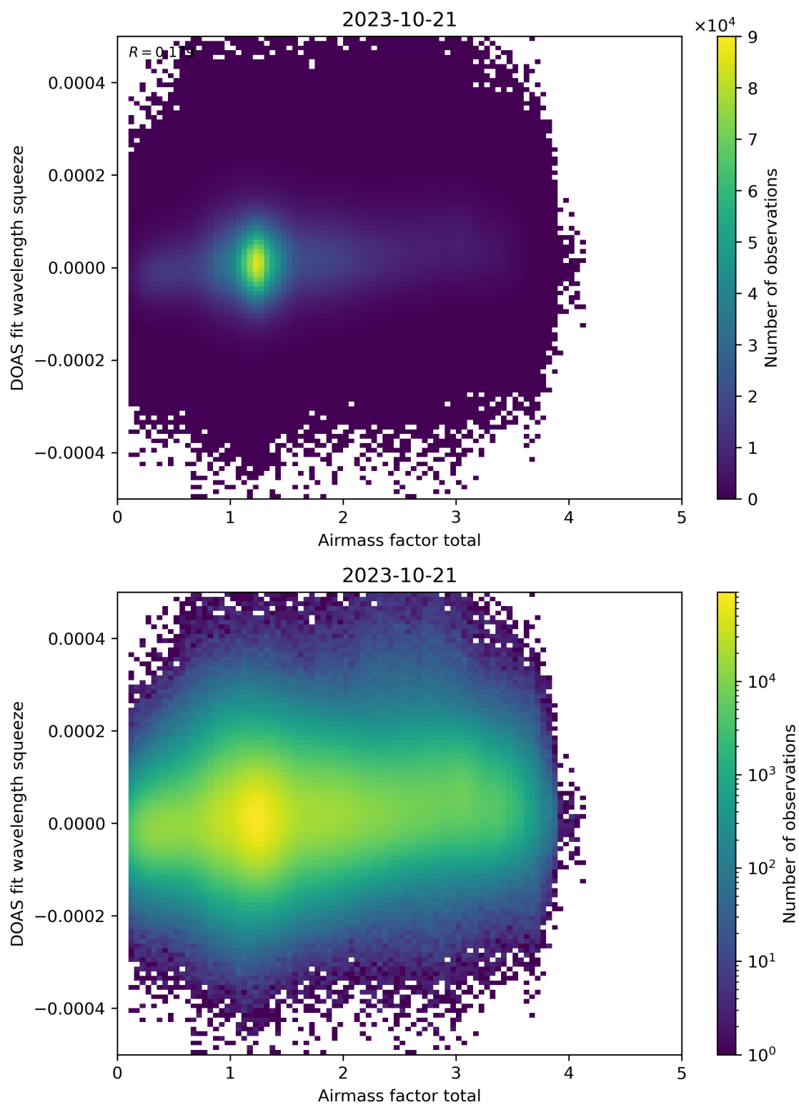
Figure 99: Scatter density plot of “Airmass factor total” against “DOAS fit wavelength squeeze” for 2023-10-20 to 2023-10-22.
