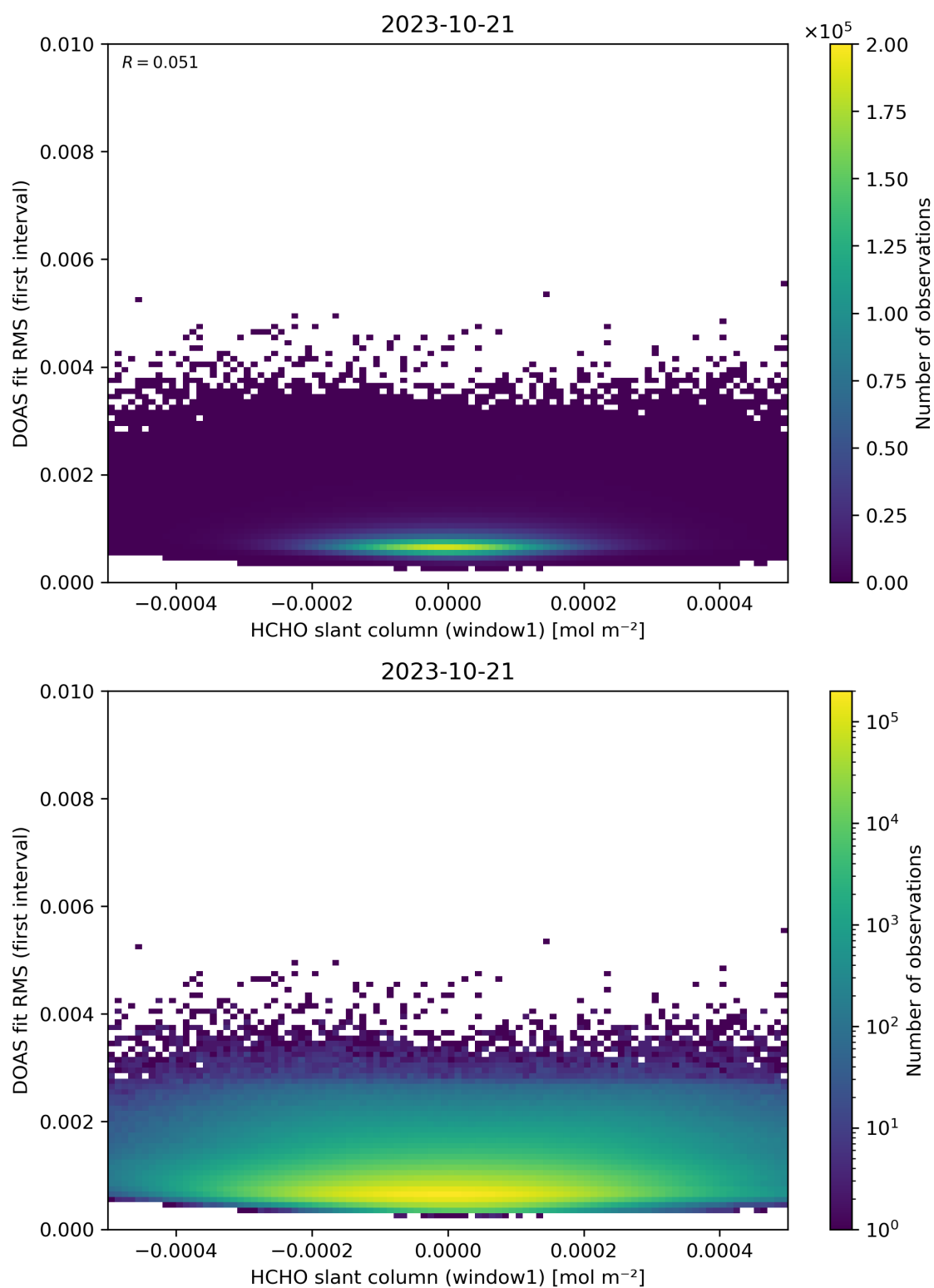
Figure 78: Scatter density plot of “HCHO slant column (window1)” against “DOAS fit RMS (first interval)” for 2023-10-20 to 2023-10-22.
