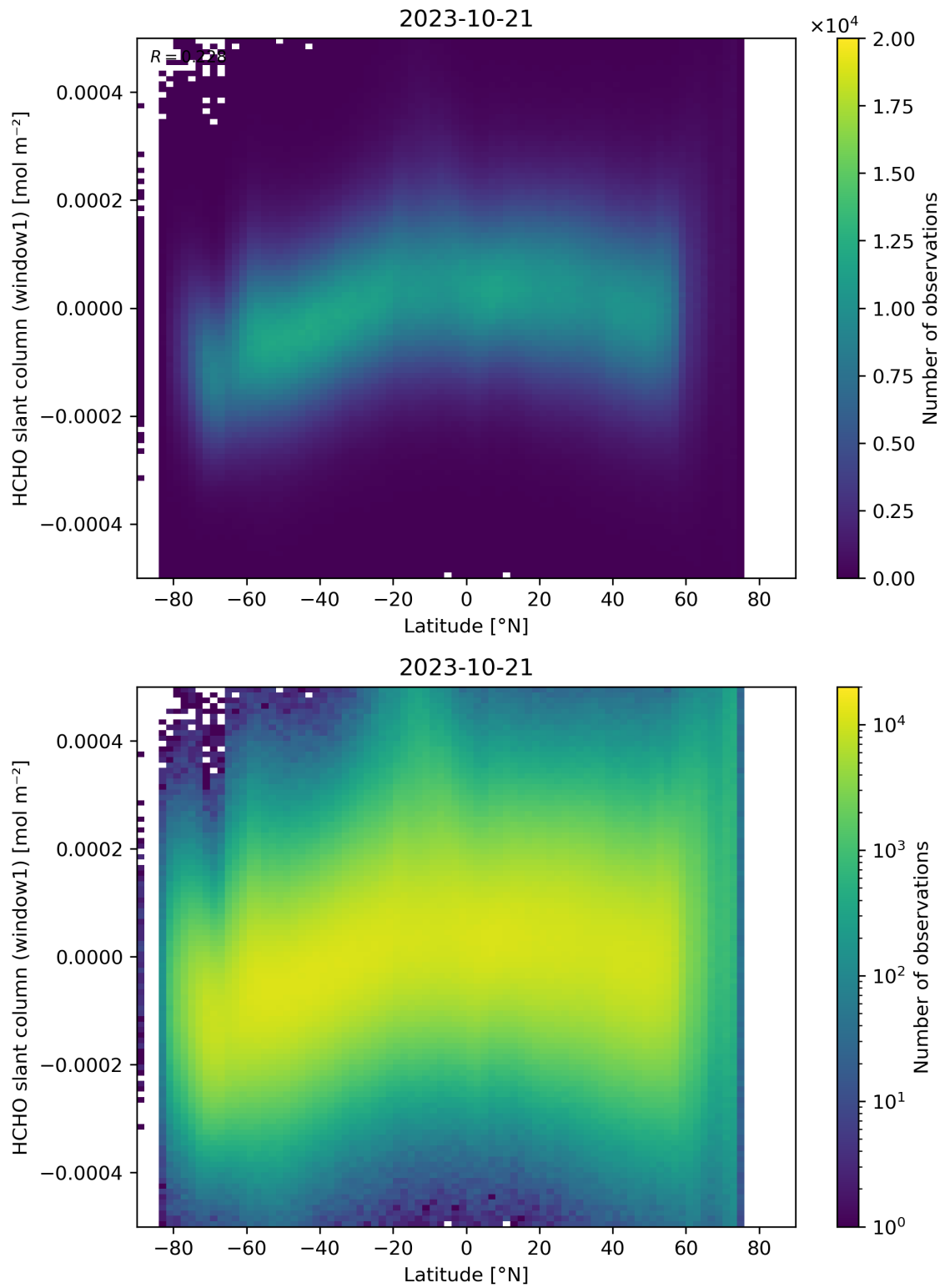
Figure 159: Scatter density plot of “Latitude” against “HCHO slant column (window1)” for 2023-10-20 to 2023-10-22.
