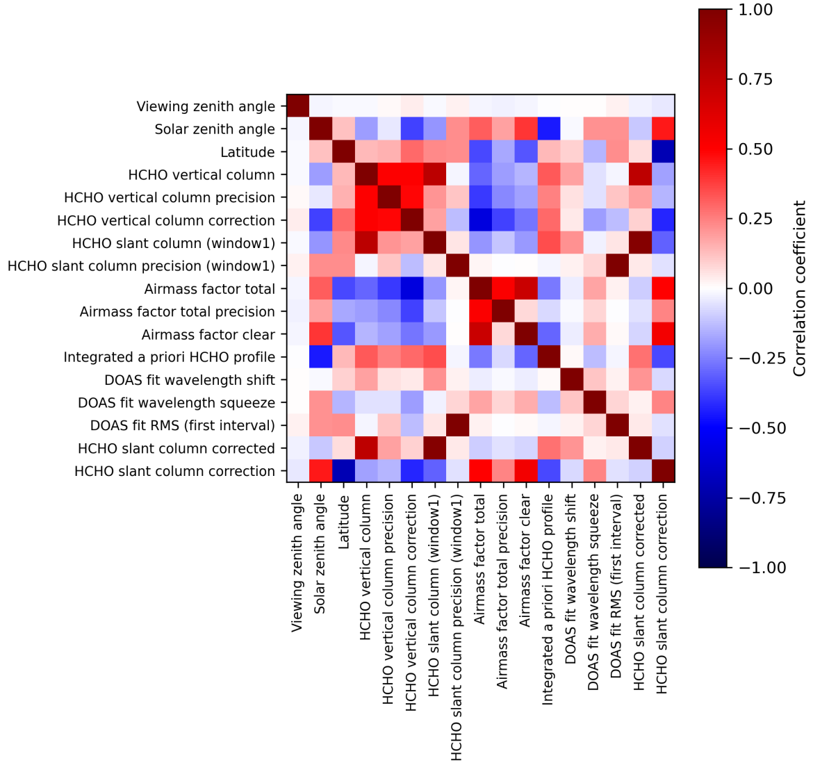
Figure 2: Map of correlation matrix for 2023-10-20 to 2023-10-22.
