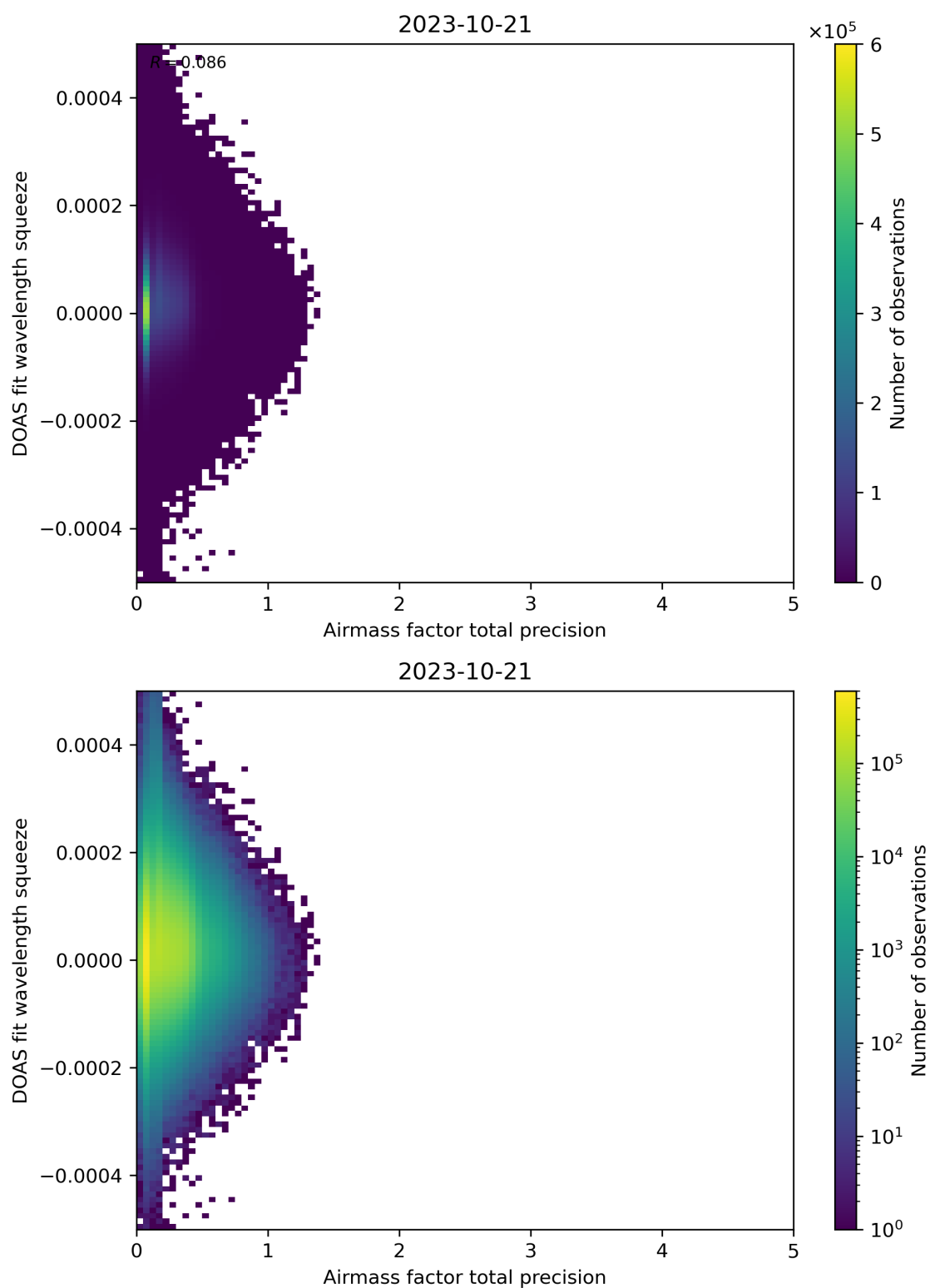
Figure 107: Scatter density plot of “Airmass factor total precision” against “DOAS fit wavelength squeeze” for 2023-10-20 to 2023-10-22.
