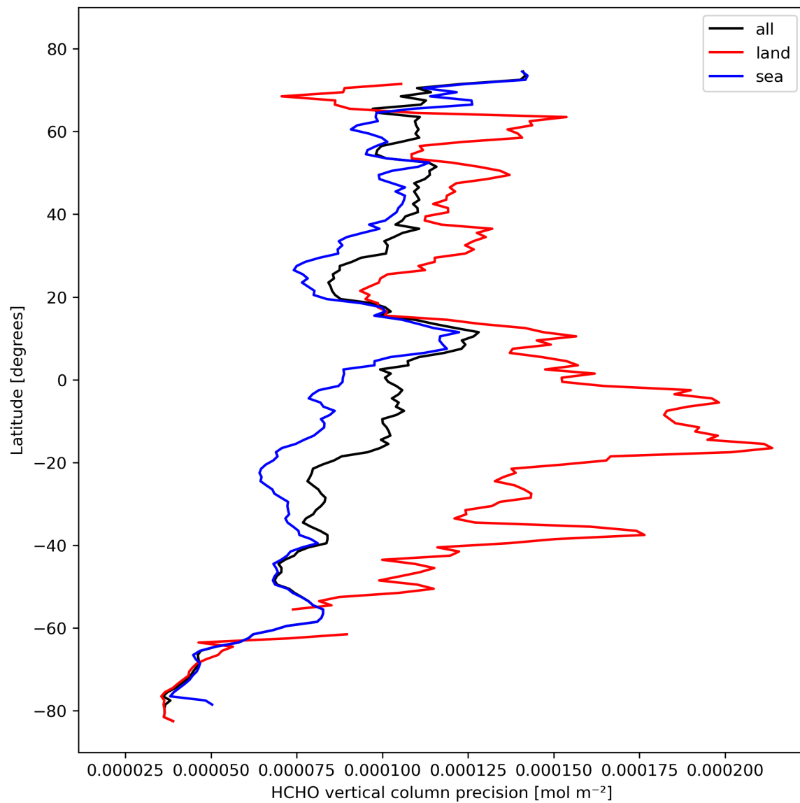
Figure 22: Zonal average of “HCHO vertical column precision” for 2023-10-20 to 2023-10-22.
