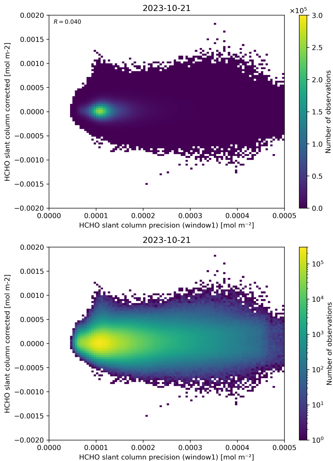
Figure 92: Scatter density plot of “HCHO slant column precision (window1)” against “HCHO slant column corrected” for 2023-10-20 to 2023-10-22.
