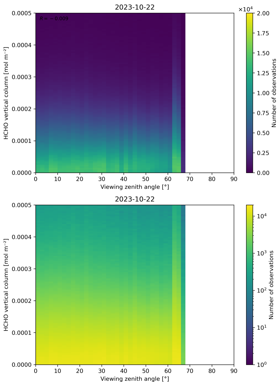
Figure 192: Scatter density plot of “Viewing zenith angle” against “HCHO vertical column” for 2023-10-22 to 2023-10-23.
