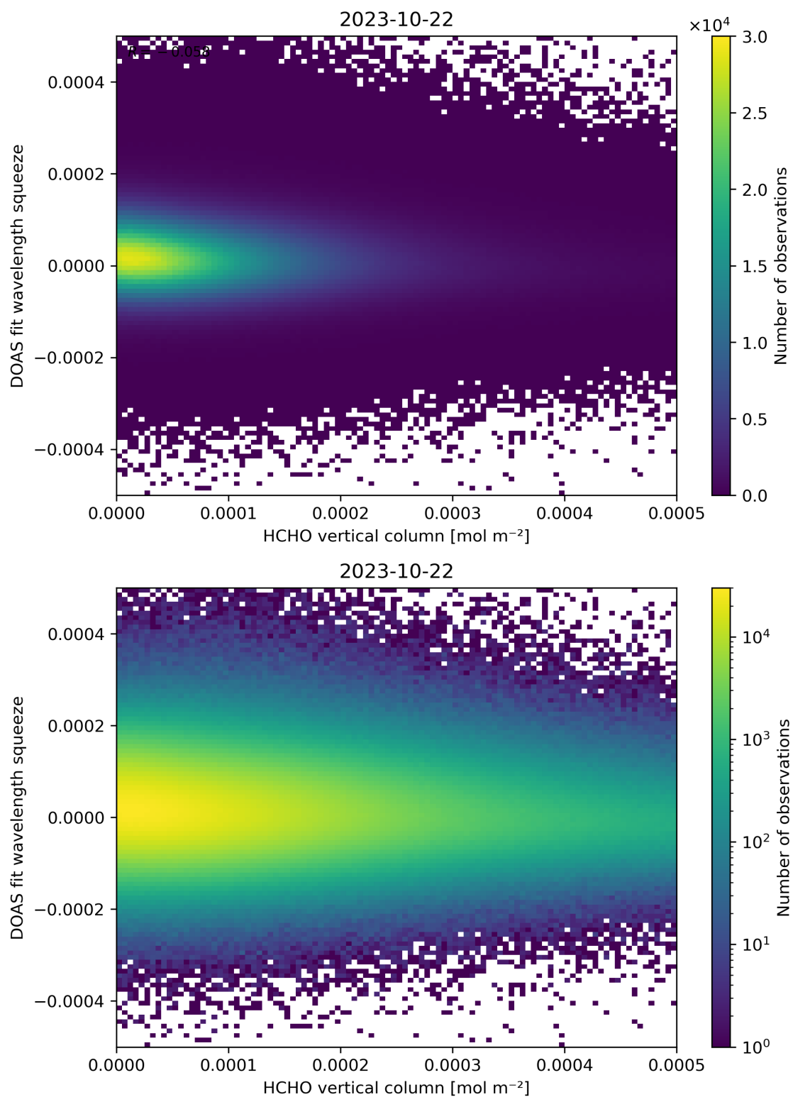
Figure 125: Scatter density plot of “HCHO vertical column” against “DOAS fit wavelength squeeze” for 2023-10-22 to 2023-10-23.
