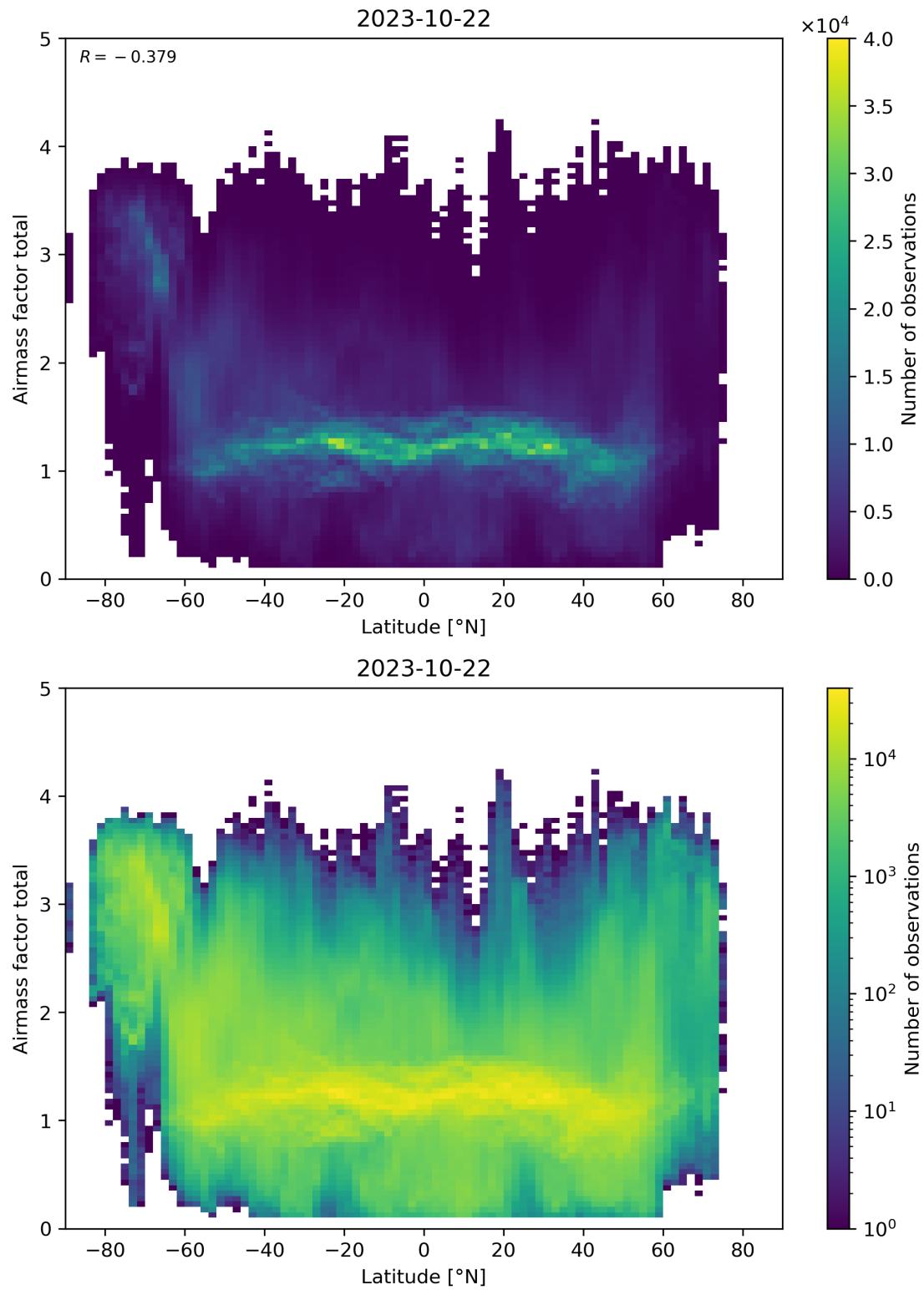
Figure 161: Scatter density plot of “Latitude” against “Airmass factor total” for 2023-10-22 to 2023-10-23.
