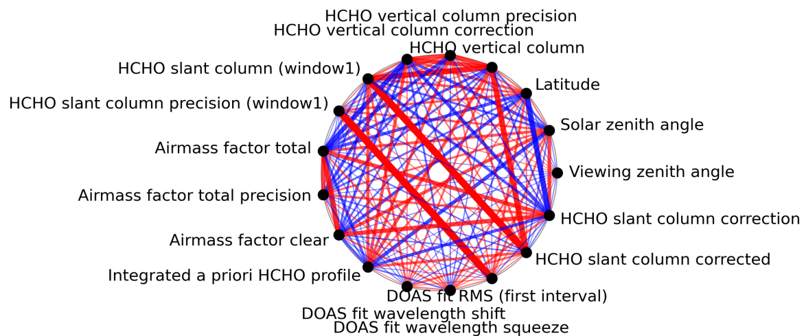
Figure 1: Map of correlation graph for 2023-10-22 to 2023-10-23.
