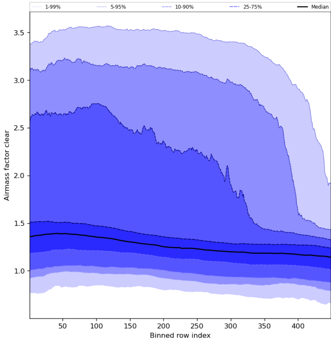
Figure 56: Along track statistics of “Airmass factor clear” for 2023-10-22 to 2023-10-23
