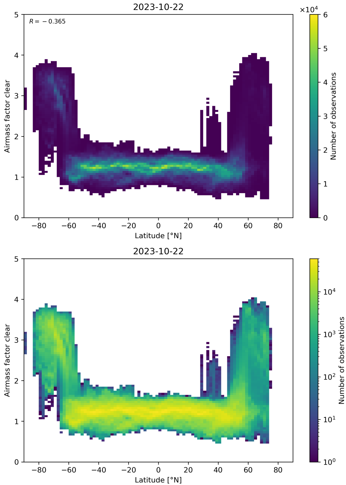
Figure 156: Scatter density plot of “Latitude” against “Airmass factor clear” for 2023-10-22 to 2023-10-23.
