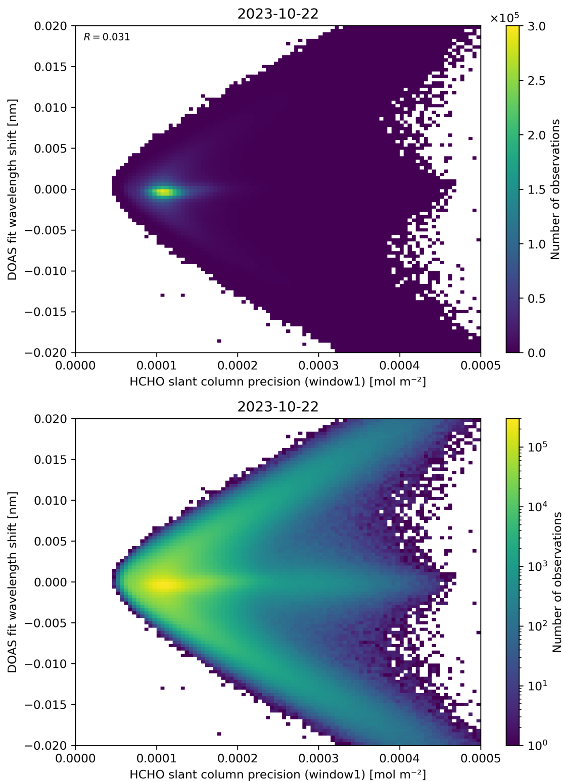
Figure 89: Scatter density plot of “HCHO slant column precision (window1)” against “DOAS fit wavelength shift” for 2023-10-22 to 2023-10-23.
