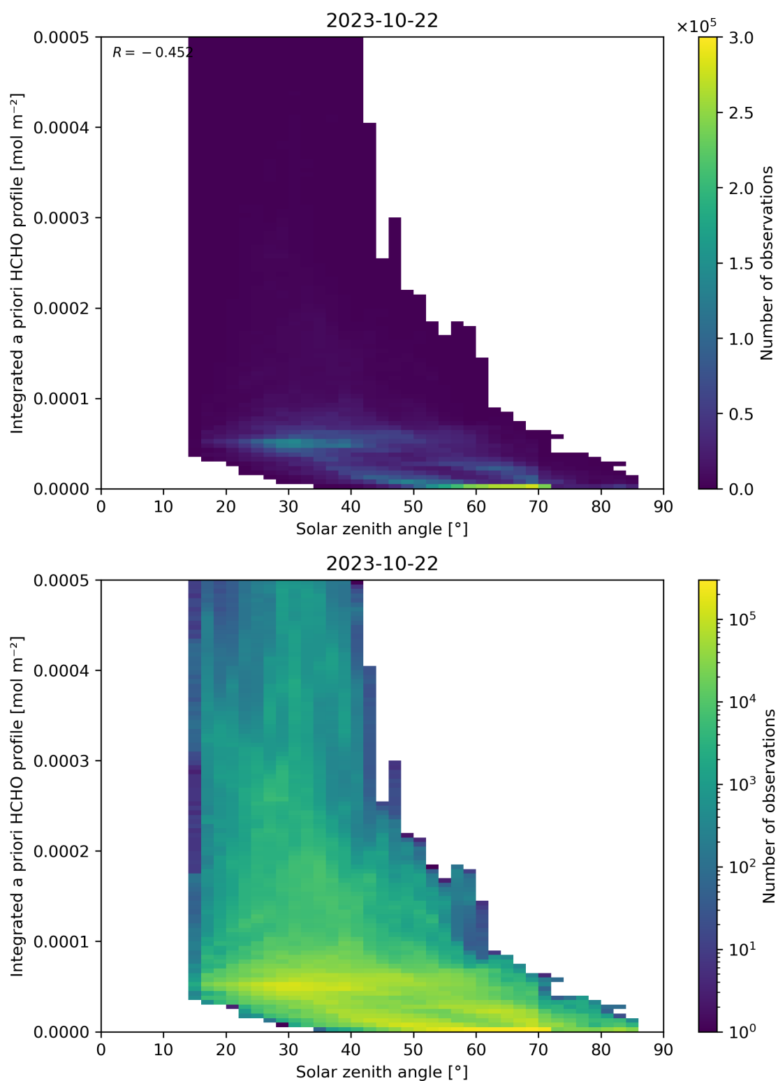
Figure 180: Scatter density plot of “Solar zenith angle” against “Integrated a priori HCHO profile” for 2023-10-22 to 2023-10-23.
