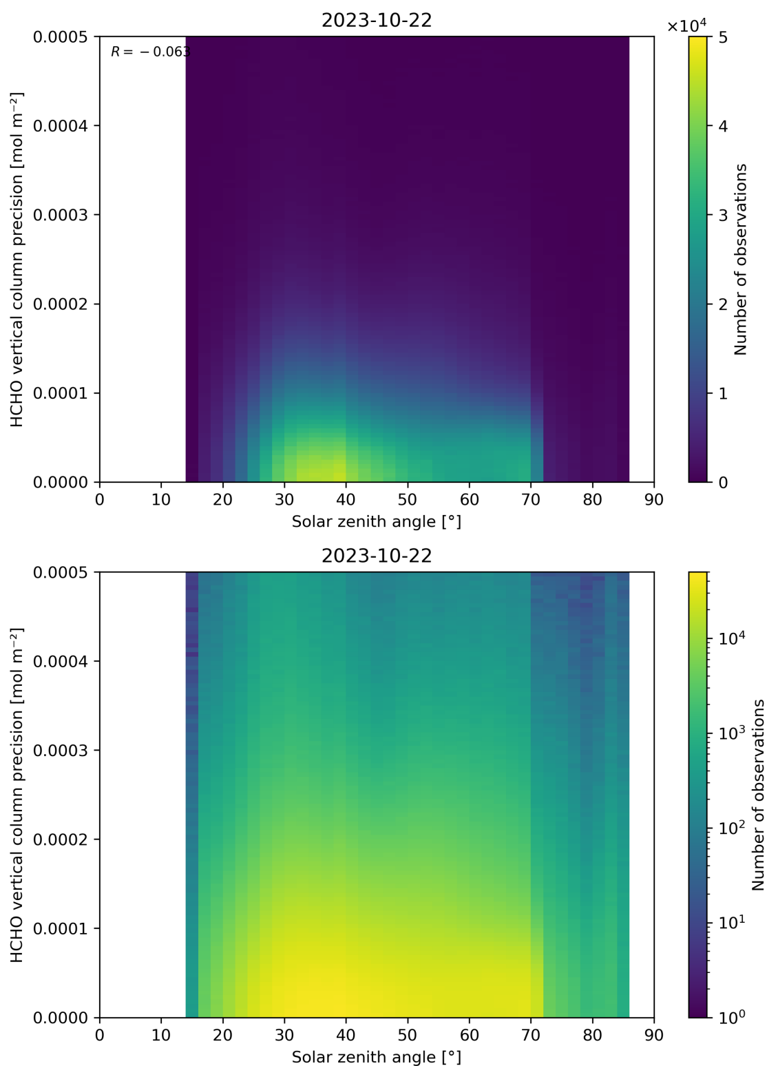
Figure 179: Scatter density plot of “Solar zenith angle” against “HCHO vertical column precision” for 2023-10-22 to 2023-10-23.
