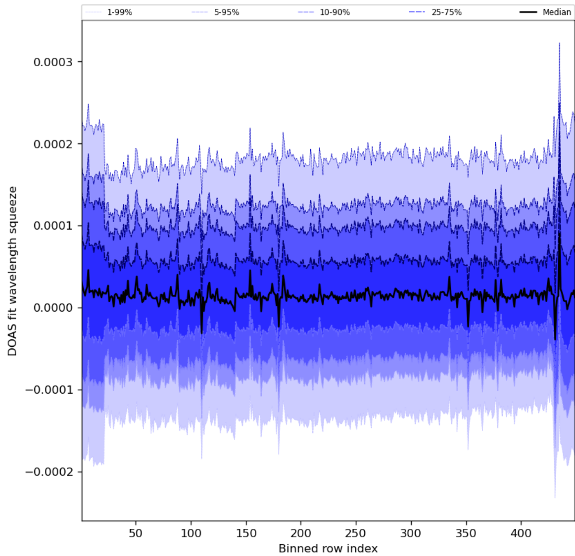
Figure 59: Along track statistics of “DOAS fit wavelength squeeze” for 2023-10-22 to 2023-10-23
