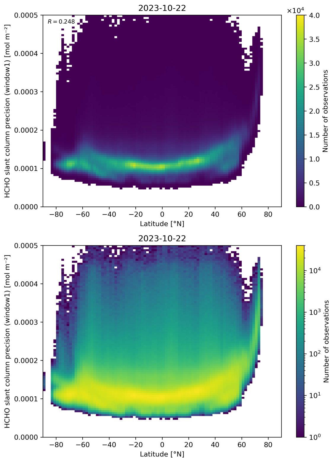
Figure 160: Scatter density plot of “Latitude” against “HCHO slant column precision (window1)” for 2023-10-22 to 2023-10-23.
