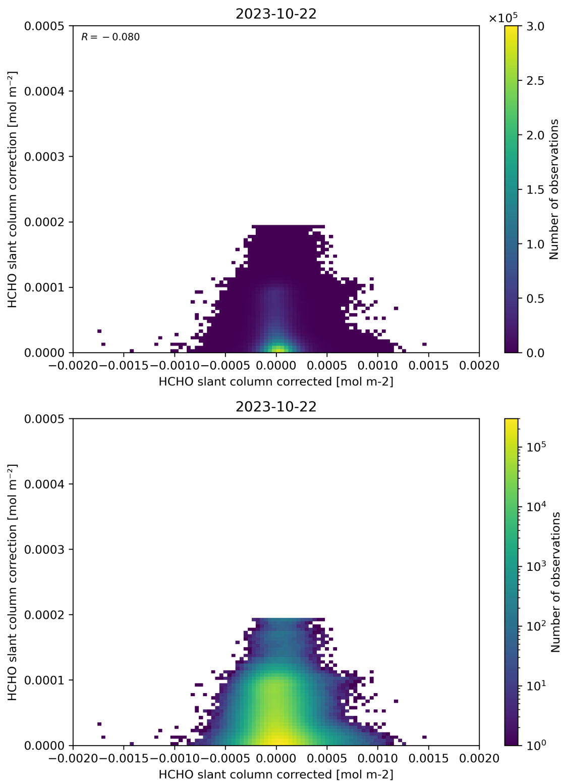
Figure 77: Scatter density plot of “HCHO slant column corrected” against “HCHO slant column correction” for 2023-10-22 to 2023-10-23.
