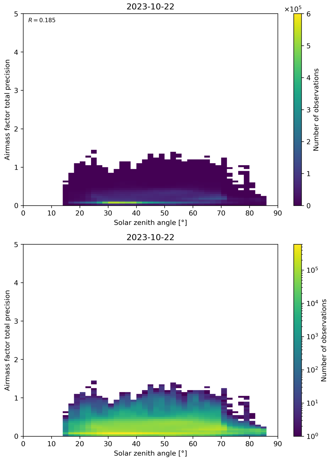
Figure 176: Scatter density plot of “Solar zenith angle” against “Airmass factor total precision” for 2023-10-22 to 2023-10-23.
