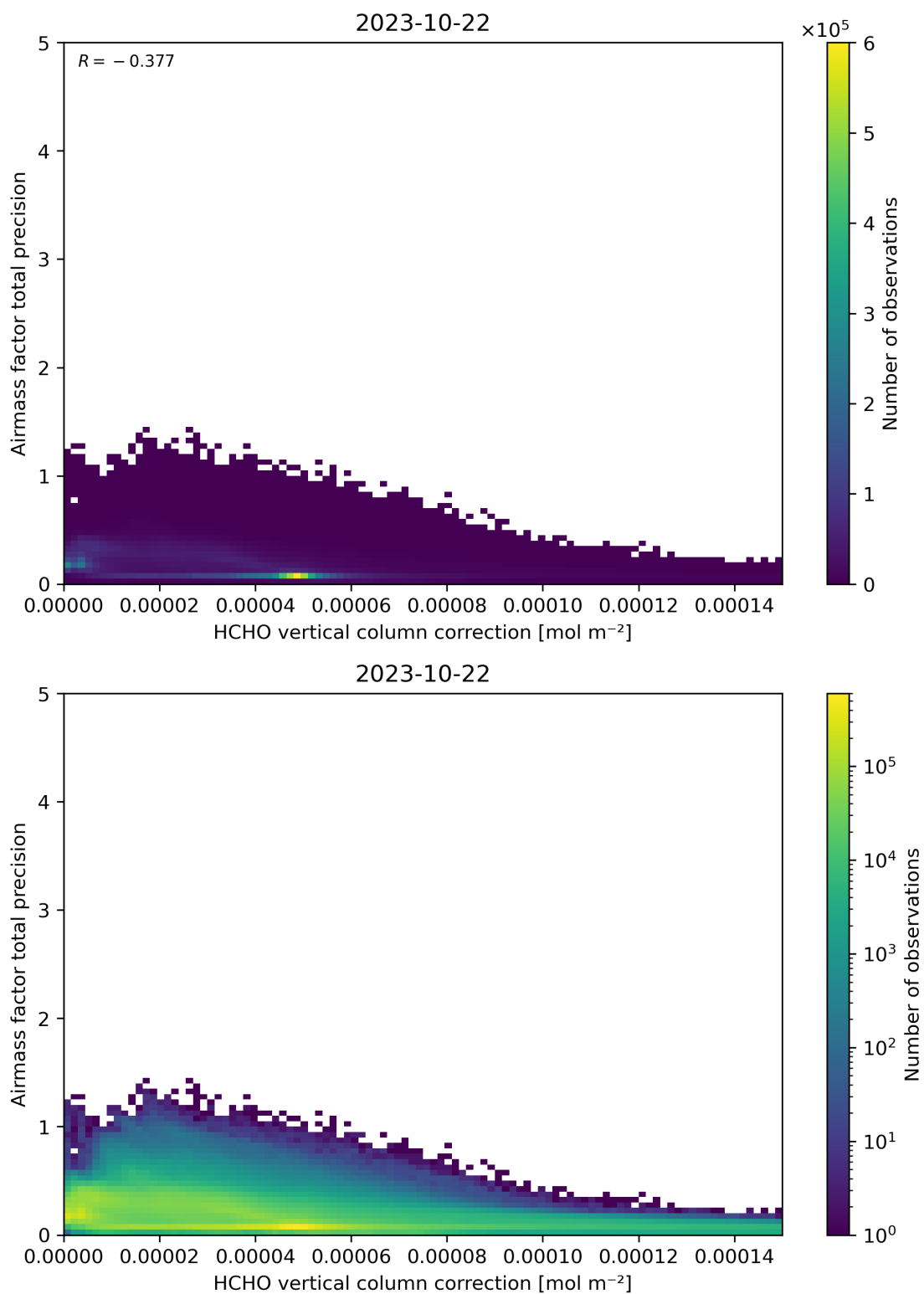
Figure 121: Scatter density plot of “HCHO vertical column correction” against “Airmass factor total precision” for 2023-10-22 to 2023-10-23.
