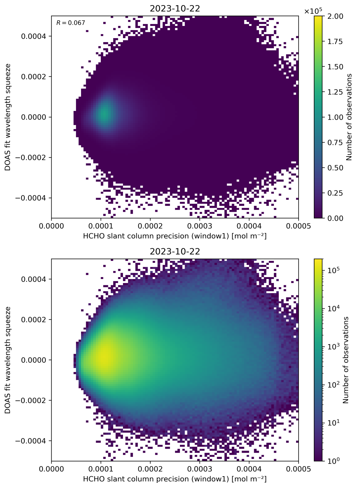
Figure 90: Scatter density plot of “HCHO slant column precision (window1)” against “DOAS fit wavelength squeeze” for 2023-10-22 to 2023-10-23.
