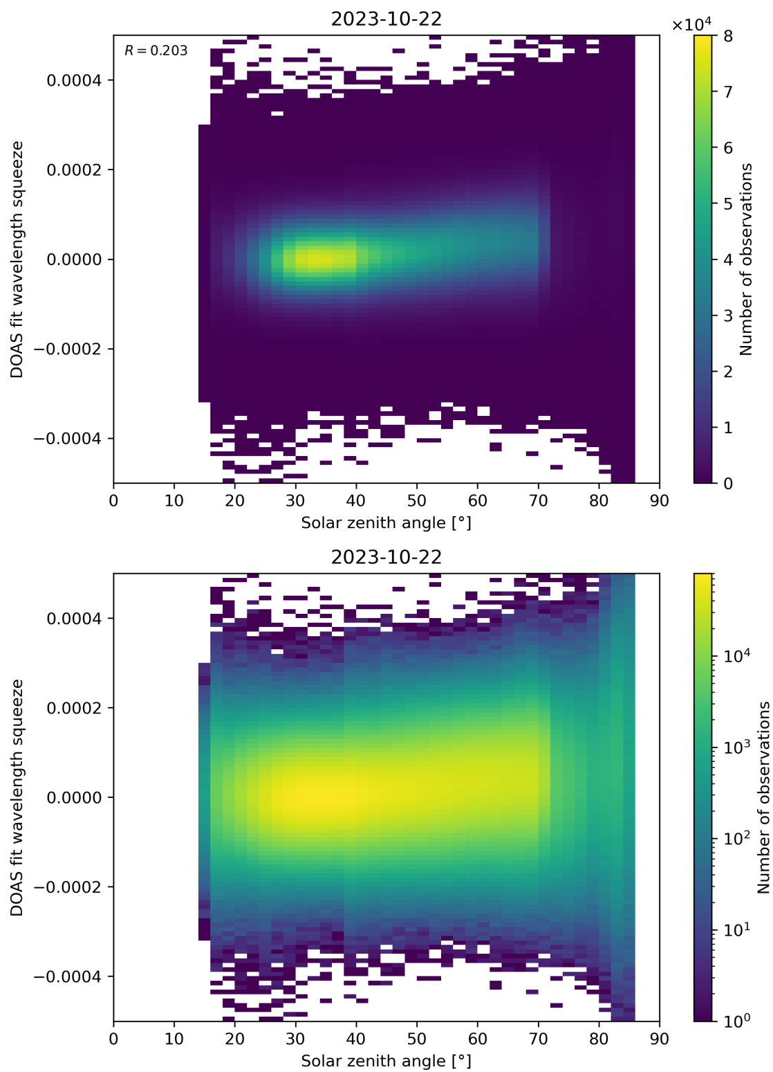
Figure 169: Scatter density plot of “Solar zenith angle” against “DOAS fit wavelength squeeze” for 2023-10-22 to 2023-10-23.
