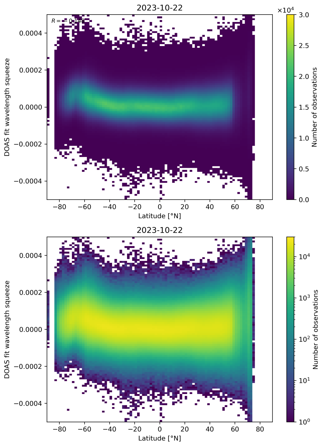
Figure 155: Scatter density plot of “Latitude” against “DOAS fit wavelength squeeze” for 2023-10-22 to 2023-10-23.
