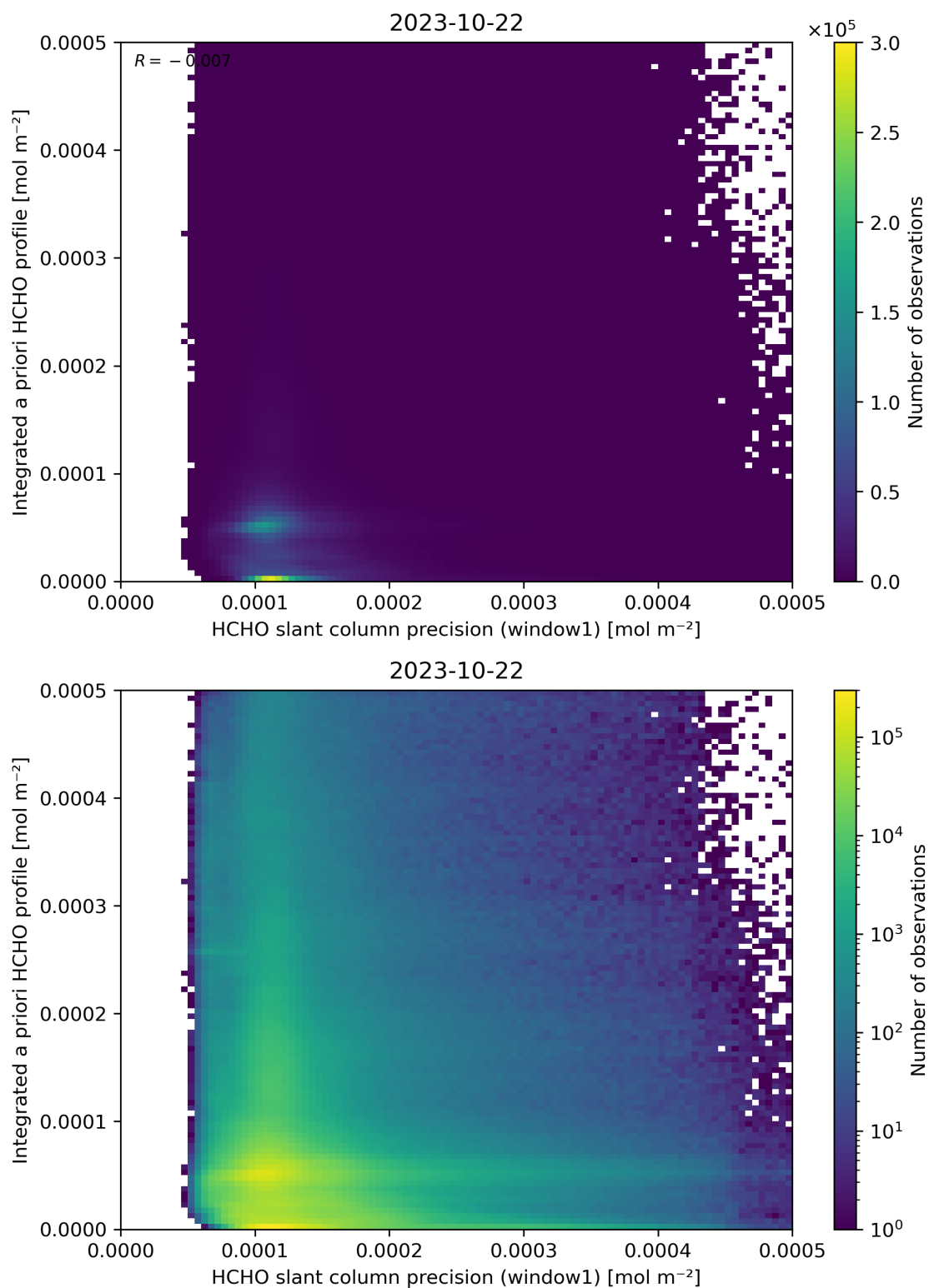
Figure 96: Scatter density plot of “HCHO slant column precision (window1)” against “Integrated a priori HCHO profile” for 2023-10-22 to 2023-10-23.
