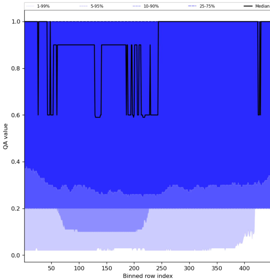
Figure 48: Along track statistics of “QA value” for 2023-10-22 to 2023-10-23
