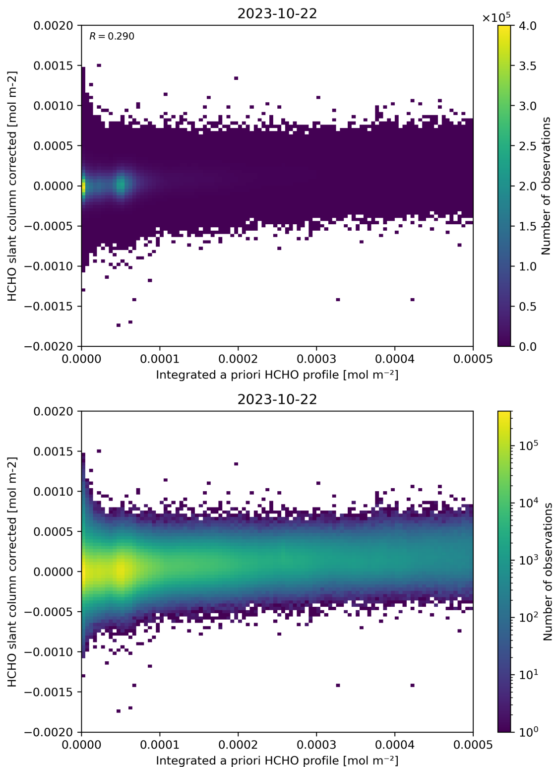
Figure 151: Scatter density plot of “Integrated a priori HCHO profile” against “HCHO slant column corrected” for 2023-10-22 to 2023-10-23.
