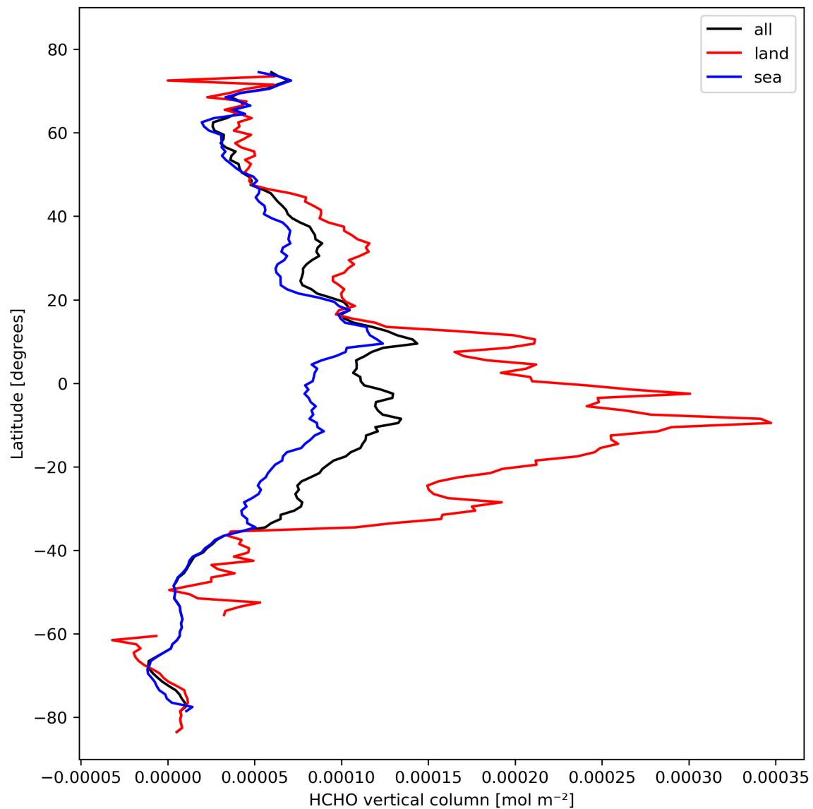
Figure 21: Zonal average of “HCHO vertical column” for 2023-10-22 to 2023-10-23.
