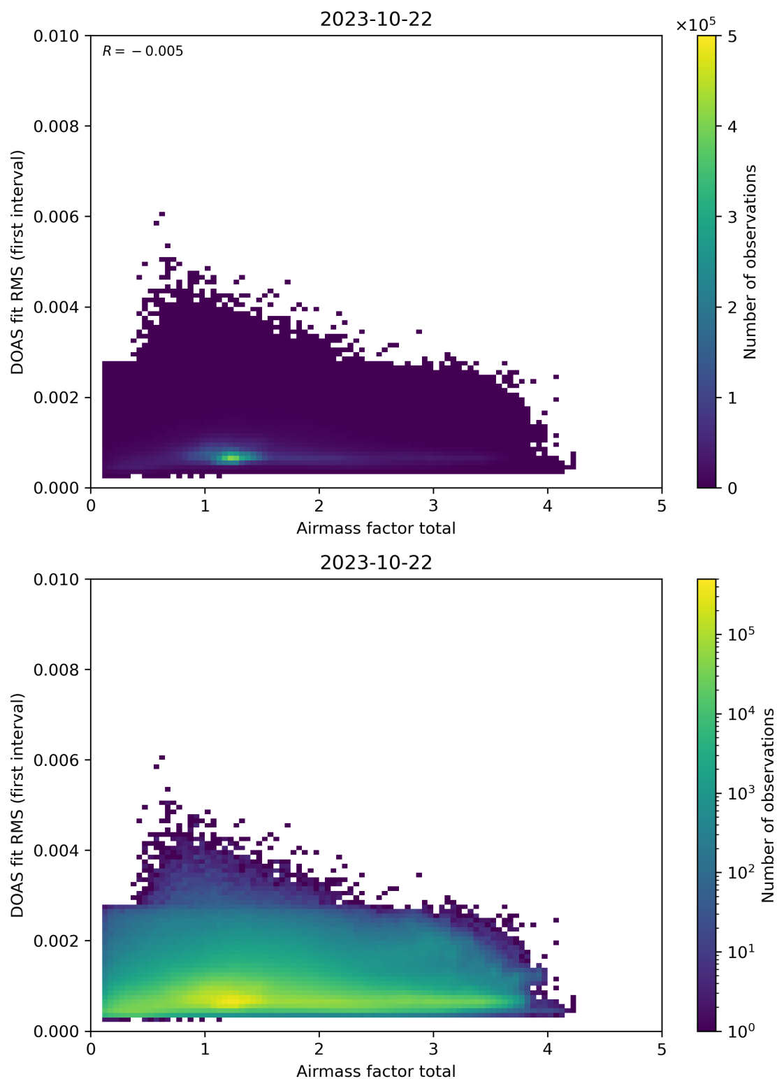
Figure 97: Scatter density plot of “Airmass factor total” against “DOAS fit RMS (first interval)” for 2023-10-22 to 2023-10-23.
