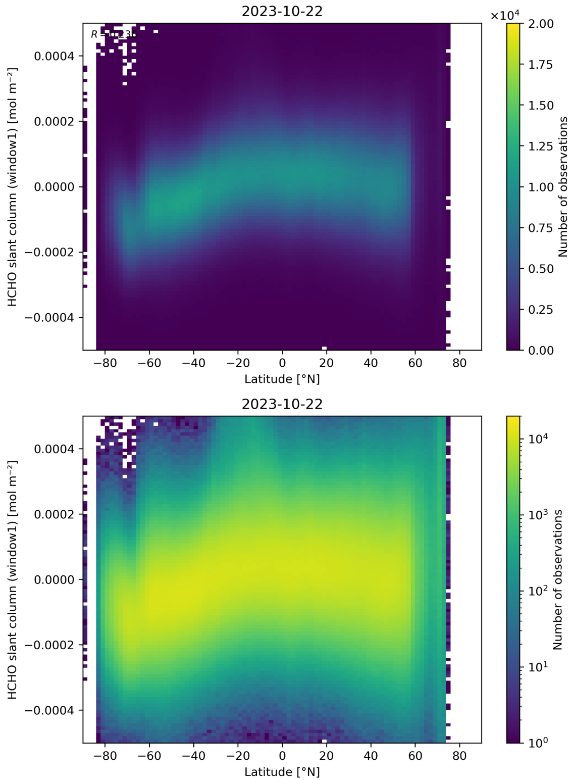
Figure 159: Scatter density plot of “Latitude” against “HCHO slant column (window1)” for 2023-10-22 to 2023-10-23.
