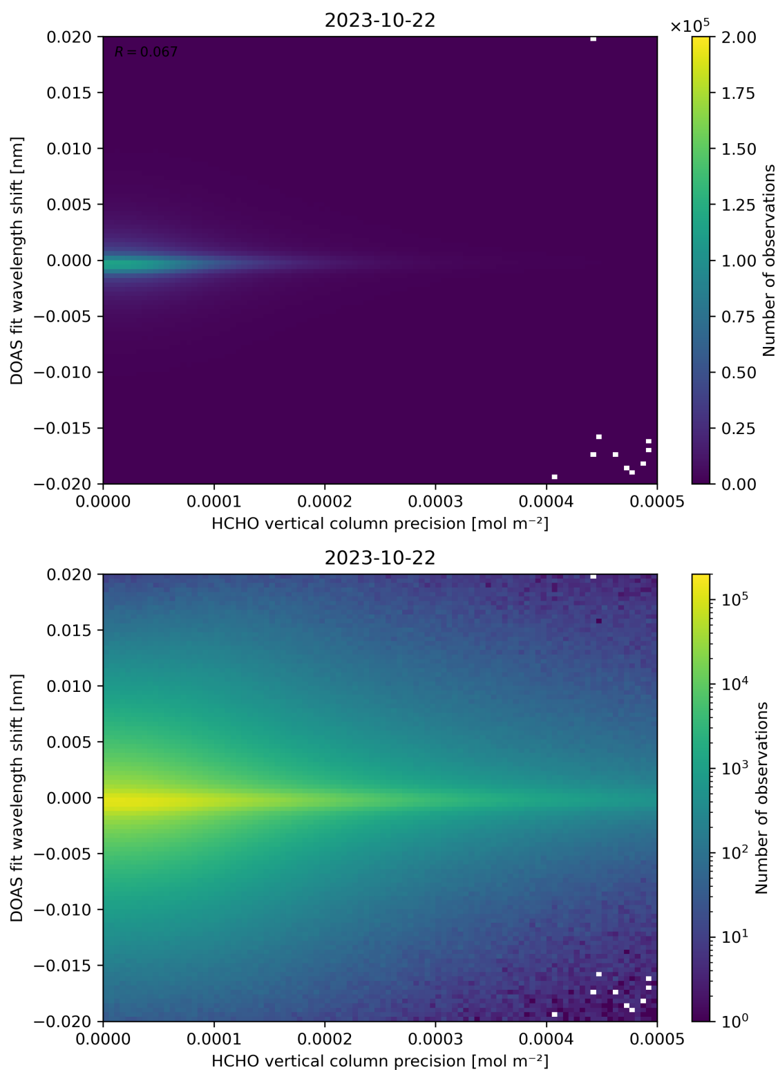
Figure 137: Scatter density plot of “HCHO vertical column precision” against “DOAS fit wavelength shift” for 2023-10-22 to 2023-10-23.
