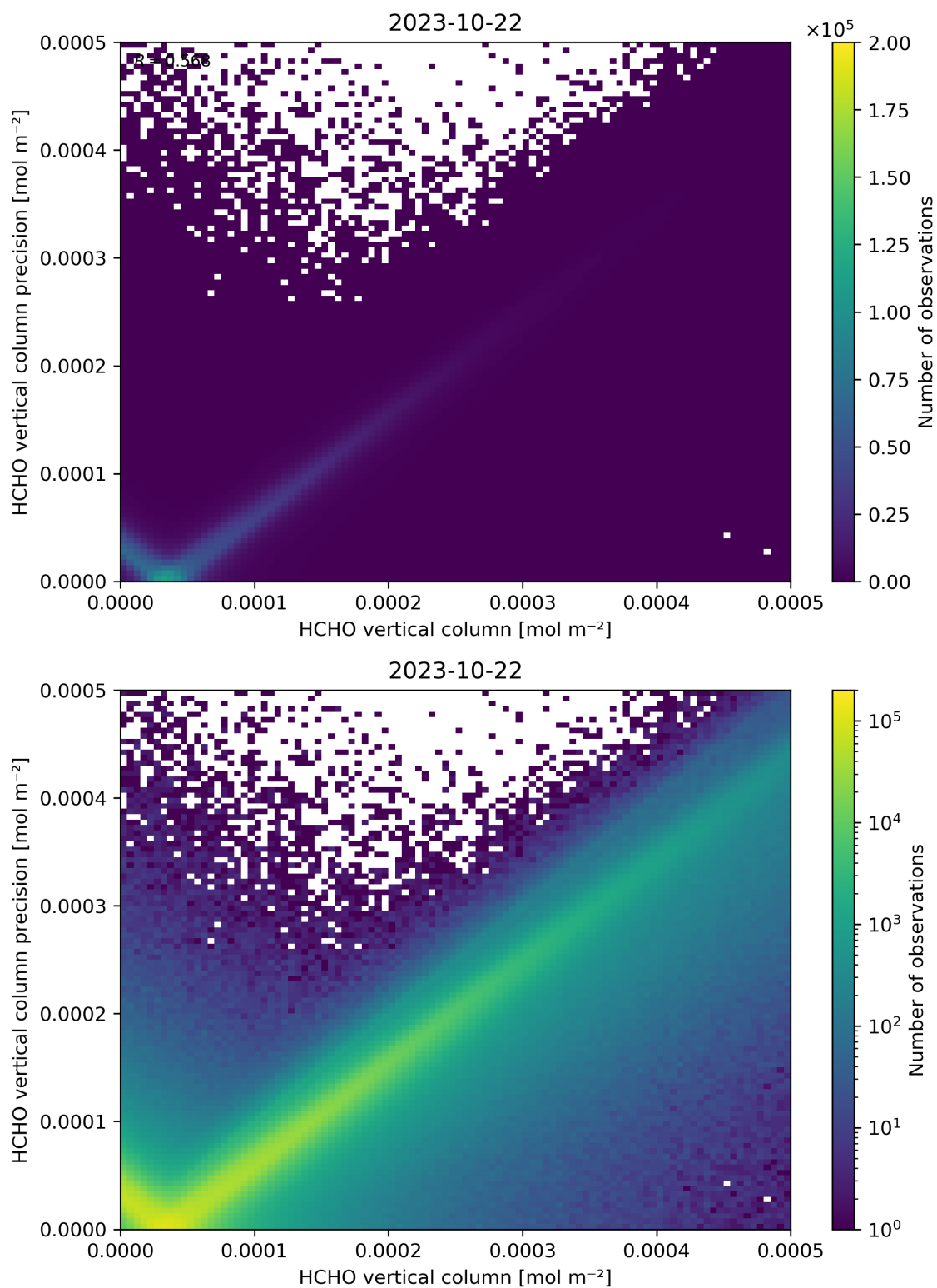
Figure 134: Scatter density plot of “HCHO vertical column” against “HCHO vertical column precision” for 2023-10-22 to 2023-10-23.
