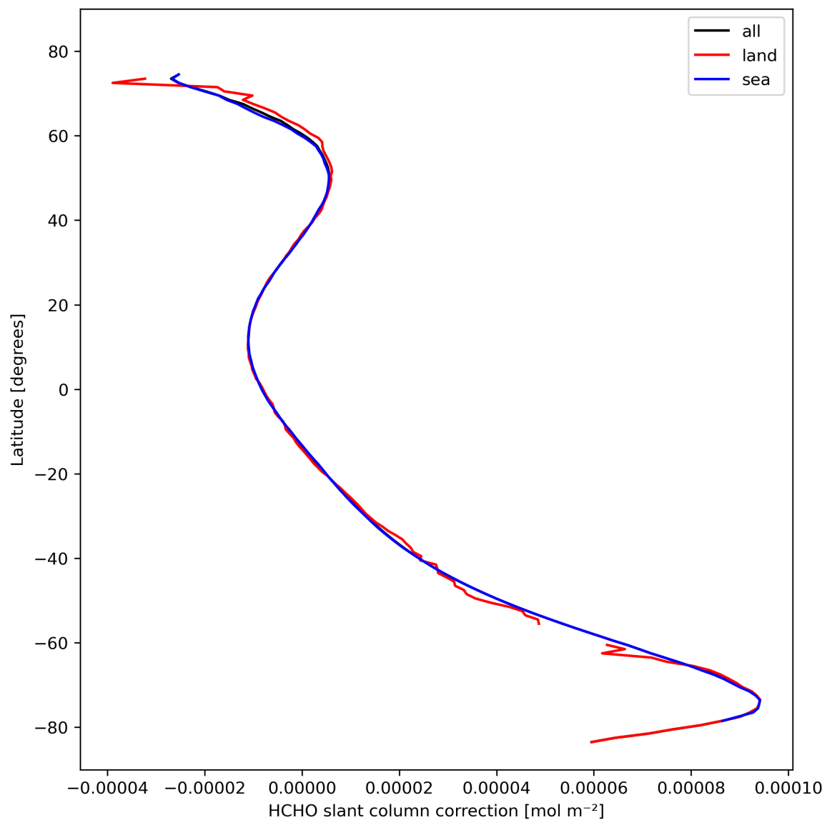
Figure 33: Zonal average of “HCHO slant column correction” for 2023-10-22 to 2023-10-23.
