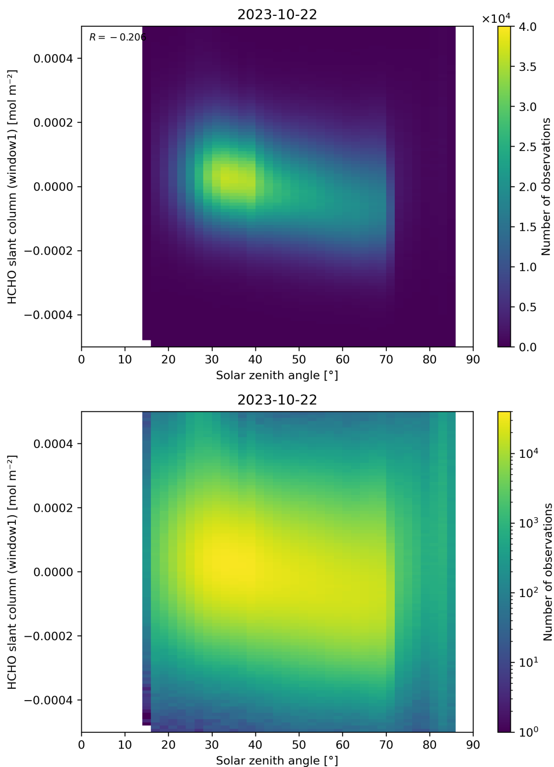
Figure 173: Scatter density plot of “Solar zenith angle” against “HCHO slant column (window1)” for 2023-10-22 to 2023-10-23.
