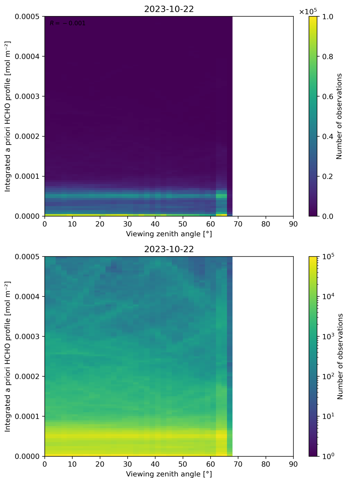
Figure 195: Scatter density plot of “Viewing zenith angle” against “Integrated a priori HCHO profile” for 2023-10-22 to 2023-10-23.
