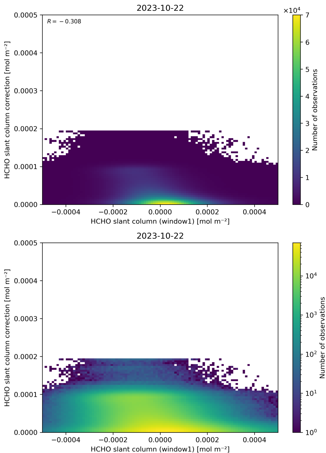
Figure 83: Scatter density plot of “HCHO slant column (window1)” against “HCHO slant column correction” for 2023-10-22 to 2023-10-23.
