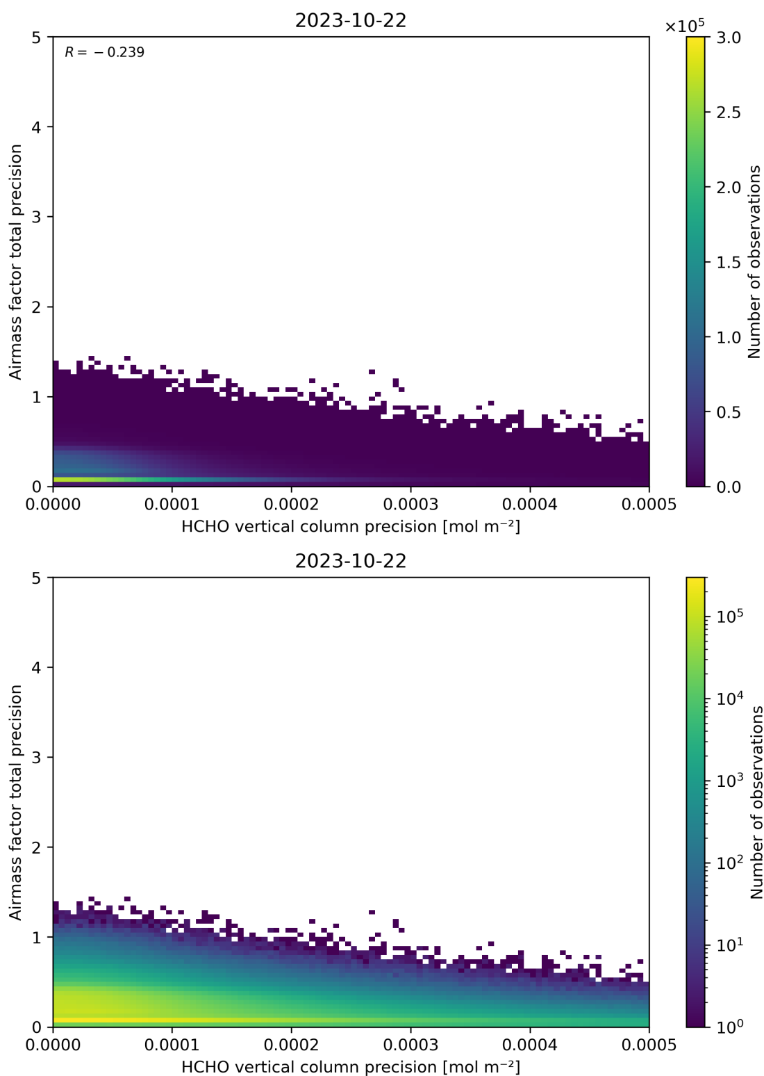
Figure 145: Scatter density plot of “HCHO vertical column precision” against “Airmass factor total precision” for 2023-10-22 to 2023-10-23.
