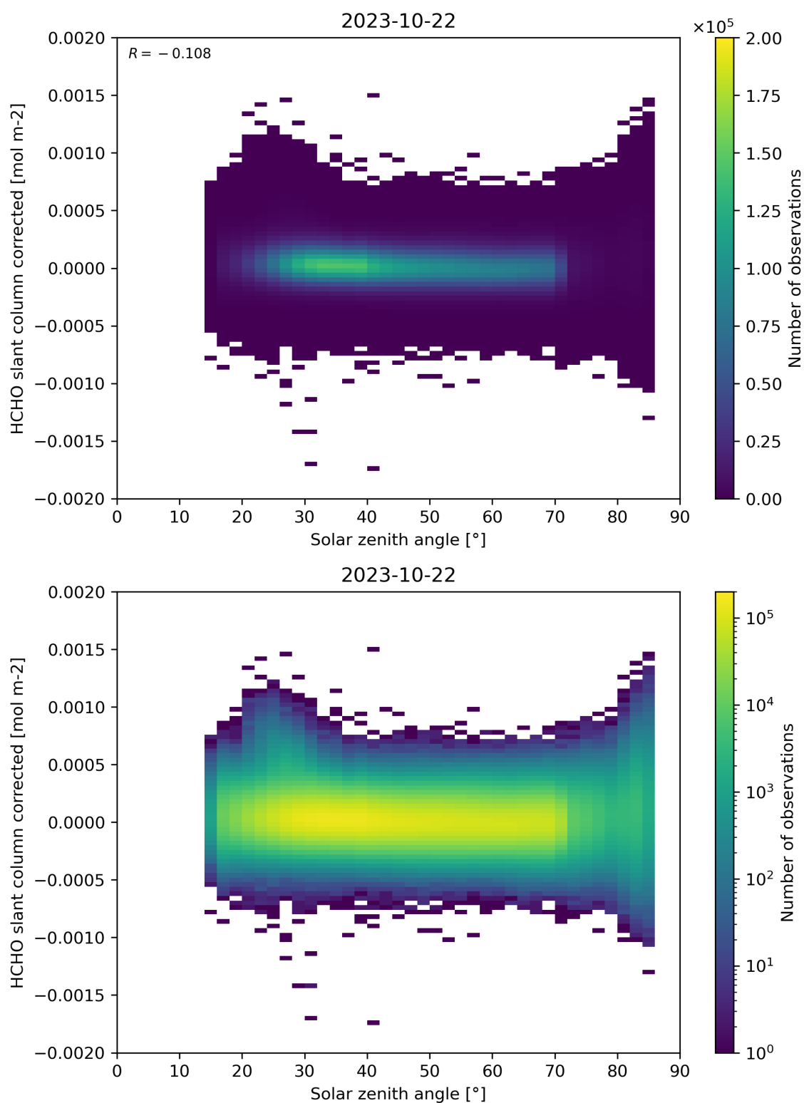
Figure 171: Scatter density plot of “Solar zenith angle” against “HCHO slant column corrected” for 2023-10-22 to 2023-10-23.
