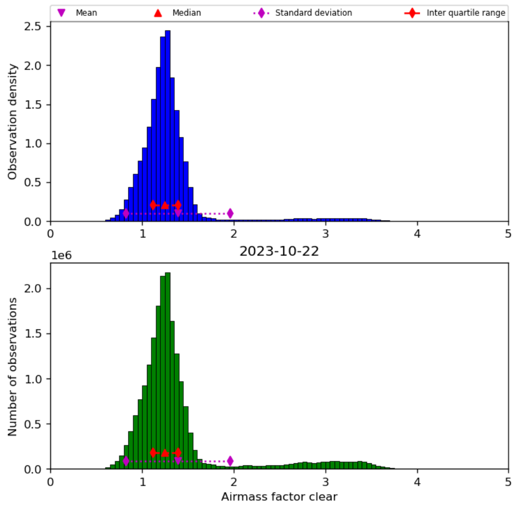
Figure 42: Histogram of “Airmass factor clear” for 2023-10-22 to 2023-10-23
