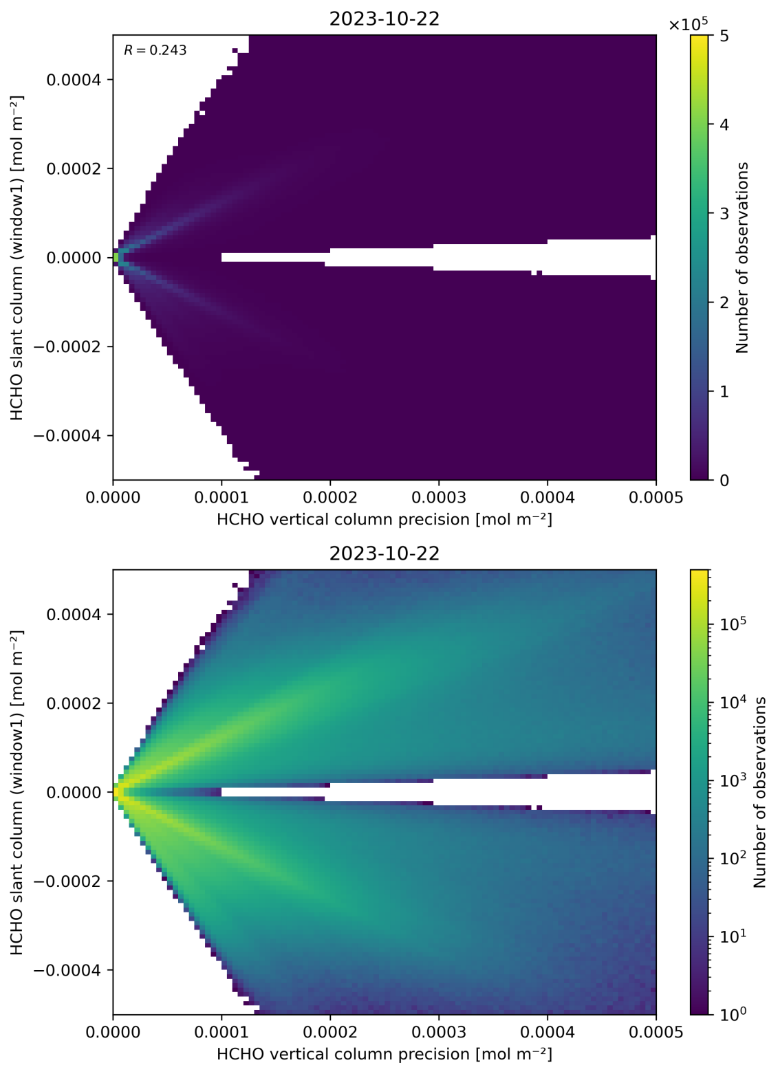
Figure 142: Scatter density plot of “HCHO vertical column precision” against “HCHO slant column (window1)” for 2023-10-22 to 2023-10-23.
