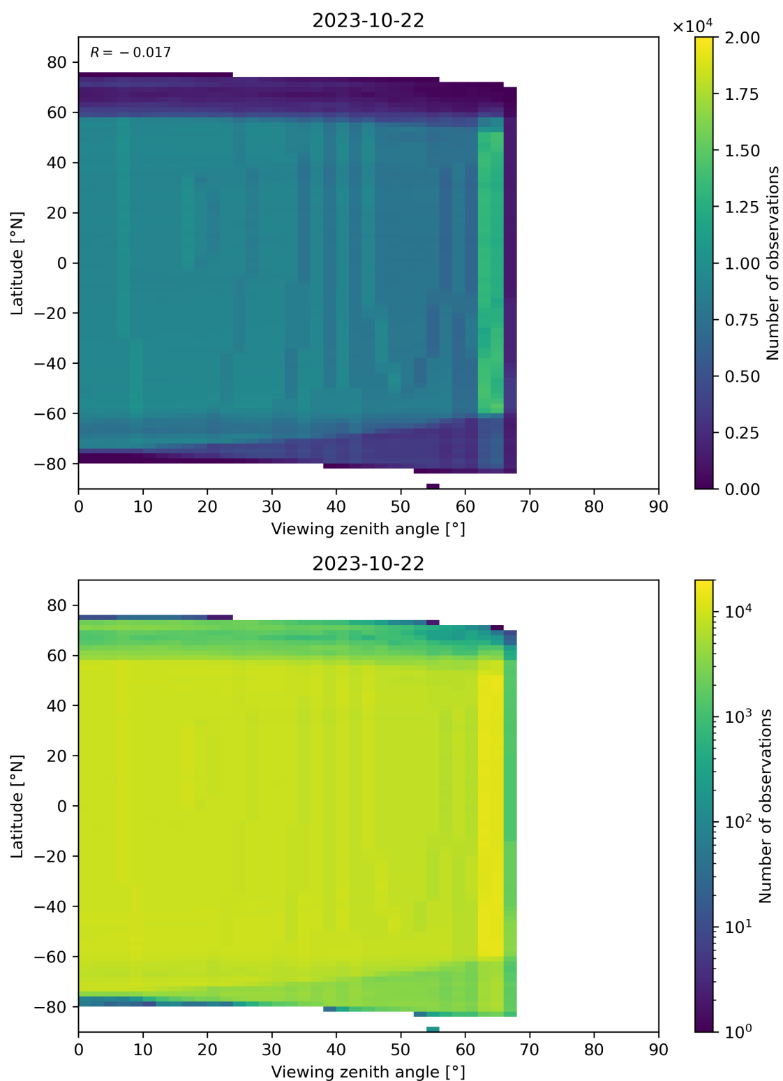
Figure 196: Scatter density plot of “Viewing zenith angle” against “Latitude” for 2023-10-22 to 2023-10-23.
