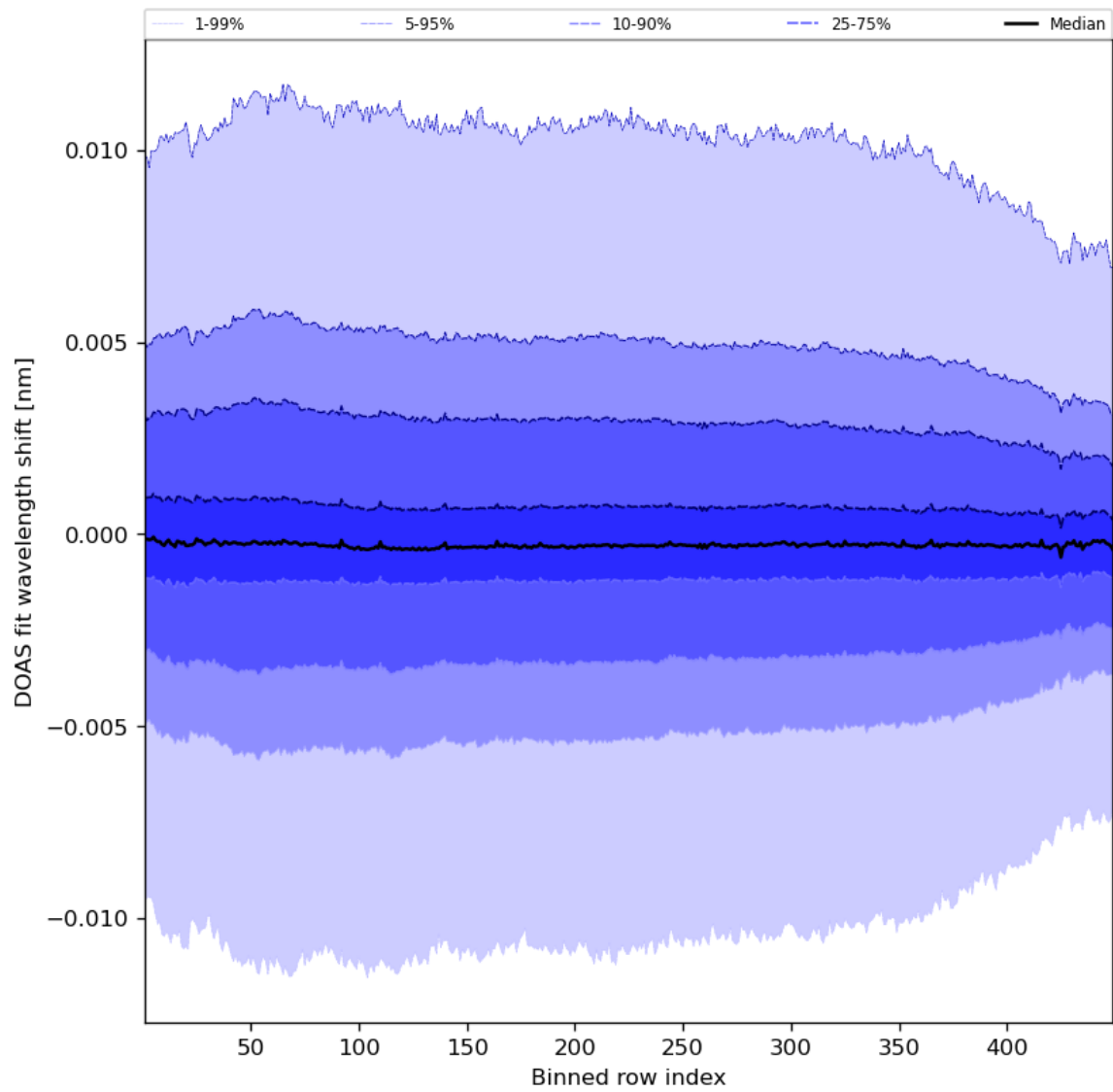
Figure 58: Along track statistics of “DOAS fit wavelength shift” for 2023-10-22 to 2023-10-23
