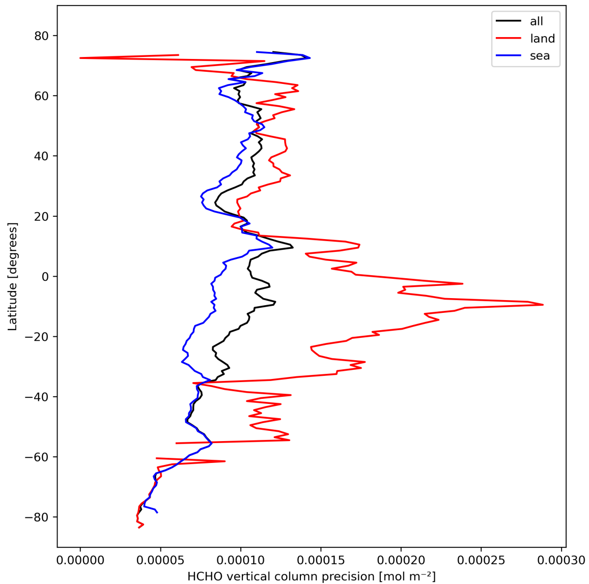
Figure 22: Zonal average of “HCHO vertical column precision” for 2023-10-22 to 2023-10-23.
