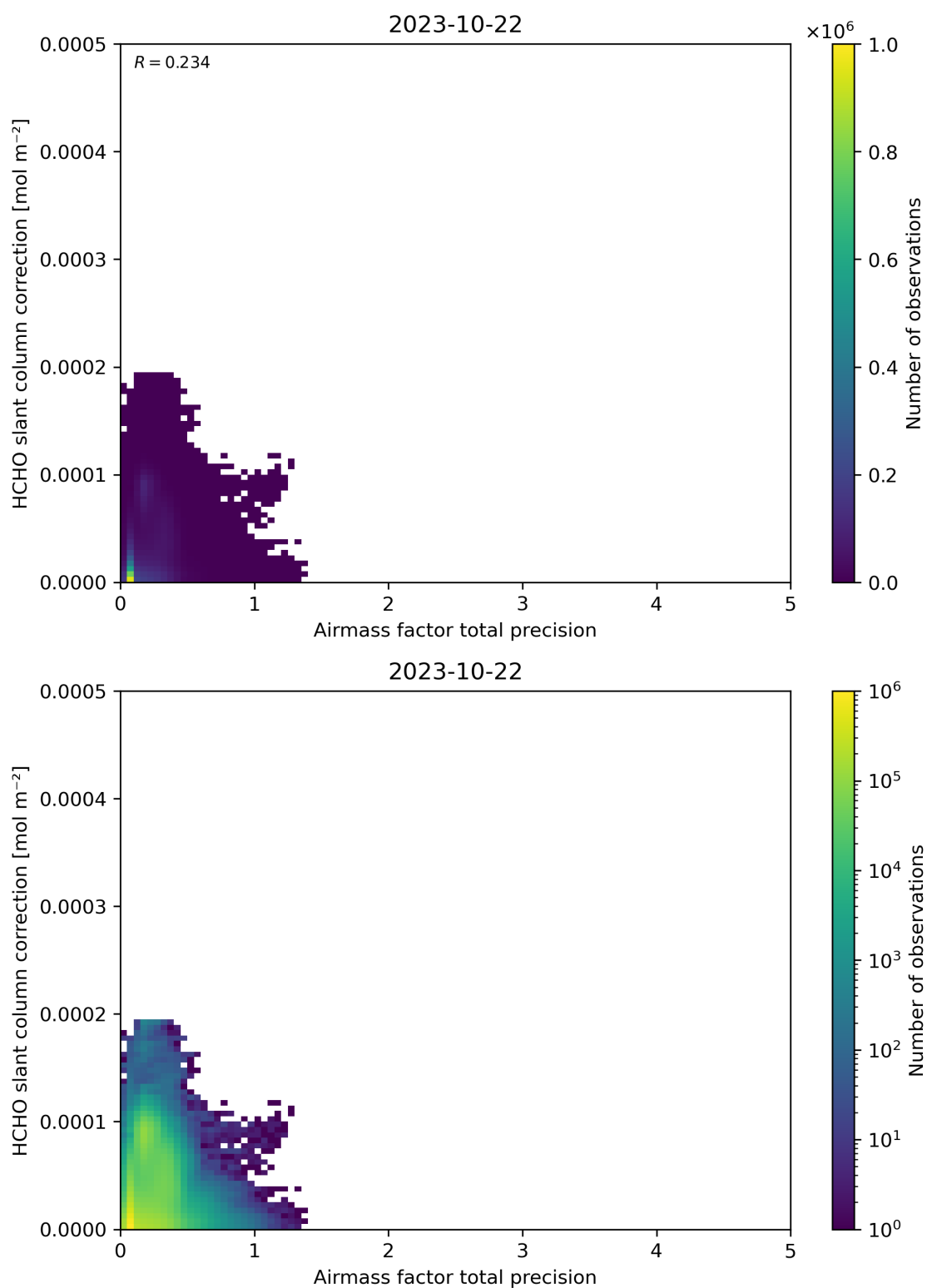
Figure 110: Scatter density plot of “Airmass factor total precision” against “HCHO slant column correction” for 2023-10-22 to 2023-10-23.
