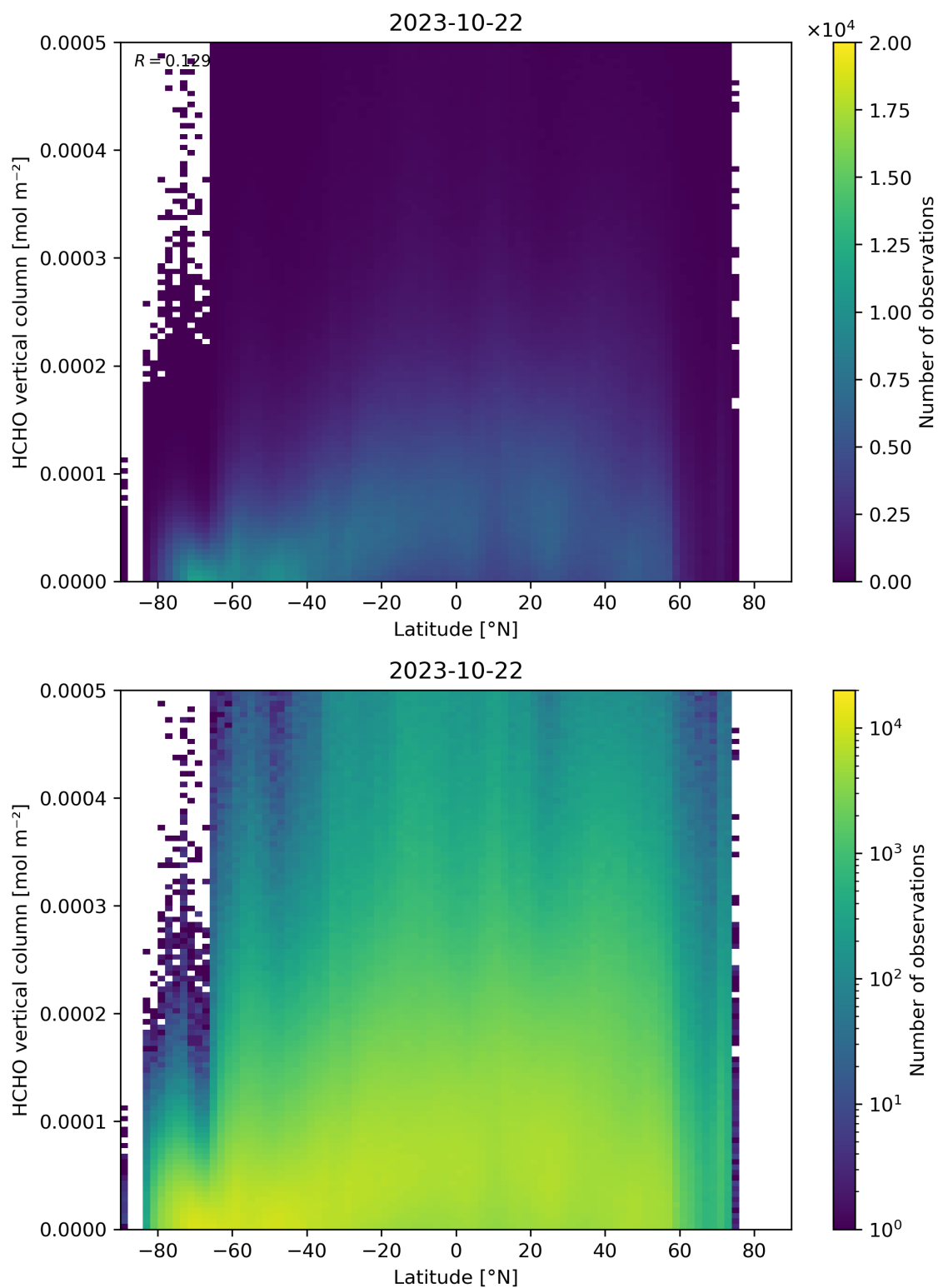
Figure 163: Scatter density plot of “Latitude” against “HCHO vertical column” for 2023-10-22 to 2023-10-23.
