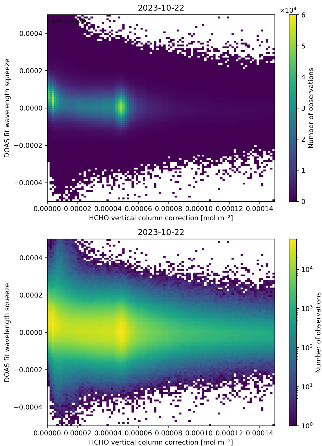
Figure 114: Scatter density plot of “HCHO vertical column correction” against “DOAS fit wavelength squeeze” for 2023-10-22 to 2023-10-23.
