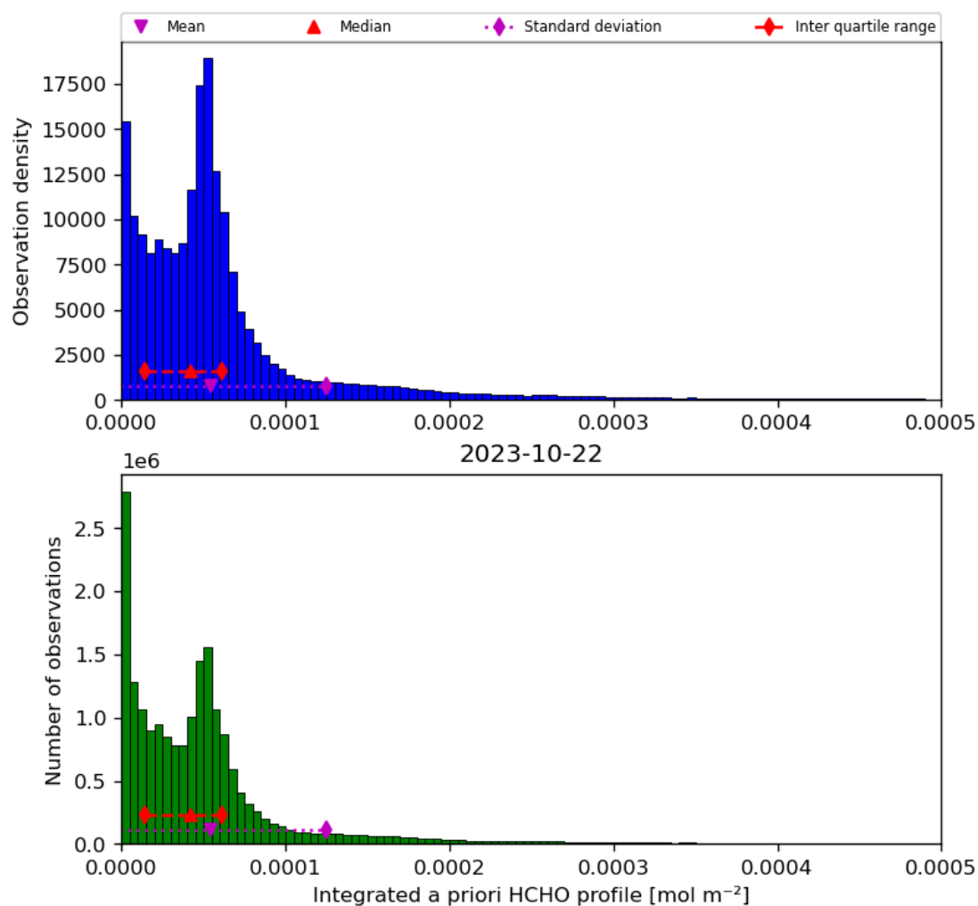
Figure 43: Histogram of “Integrated a priori HCHO profile” for 2023-10-22 to 2023-10-23
