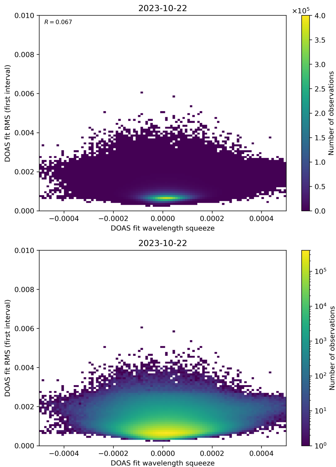
Figure 68: Scatter density plot of “DOAS fit wavelength squeeze” against “DOAS fit RMS (first interval)” for 2023-10-22 to 2023-10-23.
