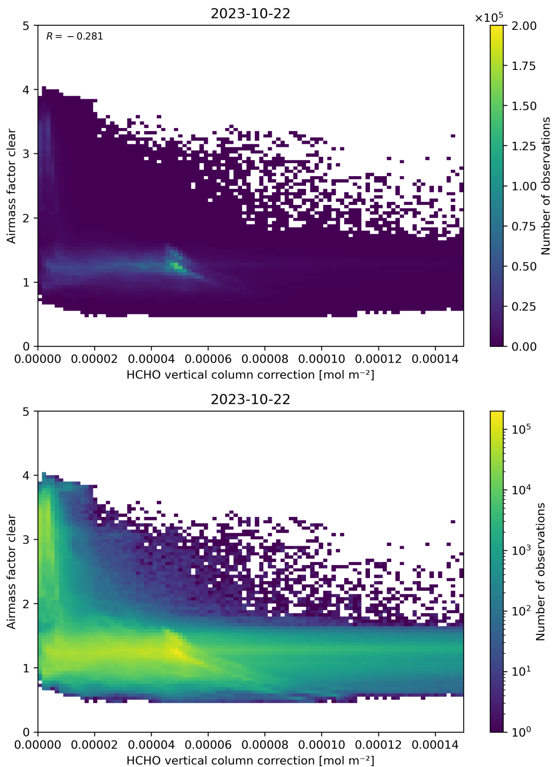
Figure 115: Scatter density plot of “HCHO vertical column correction” against “Airmass factor clear” for 2023-10-22 to 2023-10-23.
