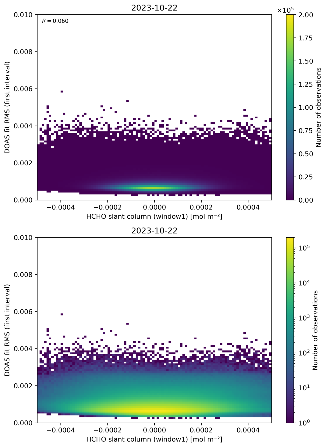
Figure 78: Scatter density plot of “HCHO slant column (window1)” against “DOAS fit RMS (first interval)” for 2023-10-22 to 2023-10-23.
