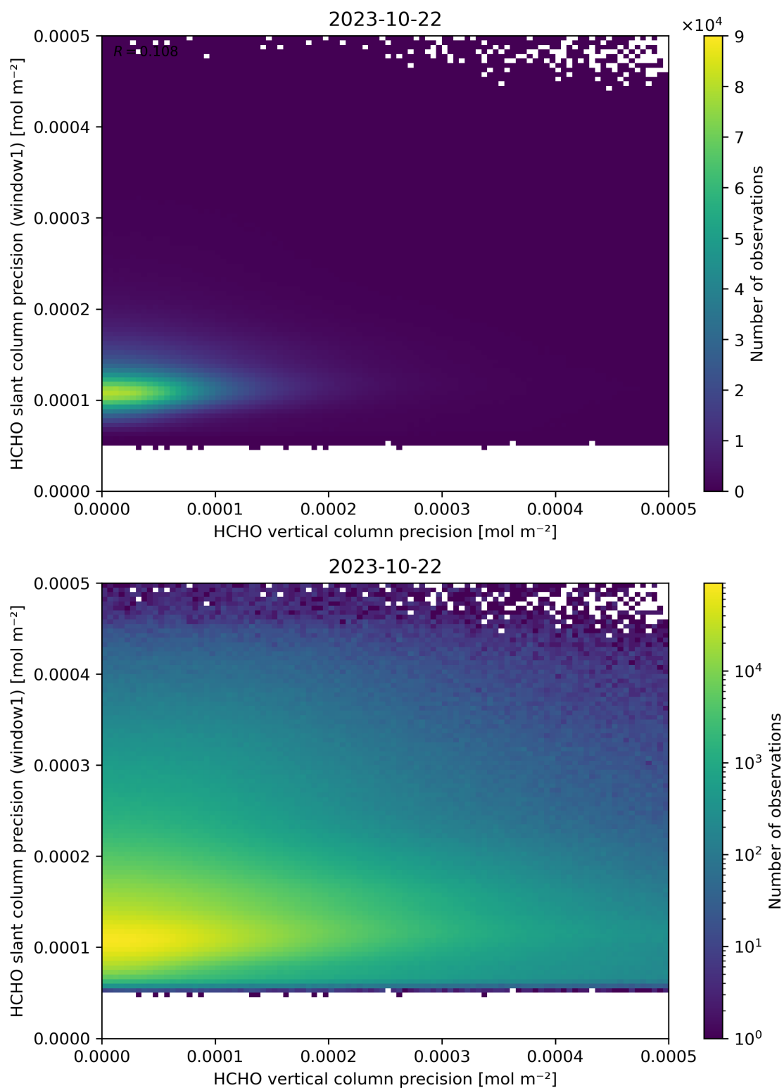
Figure 143: Scatter density plot of “HCHO vertical column precision” against “HCHO slant column precision (window1)” for 2023-10-22 to 2023-10-23.
