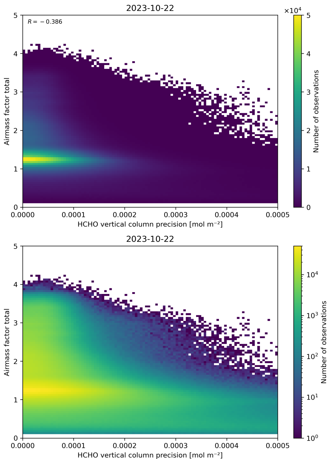
Figure 144: Scatter density plot of “HCHO vertical column precision” against “Airmass factor total” for 2023-10-22 to 2023-10-23.
