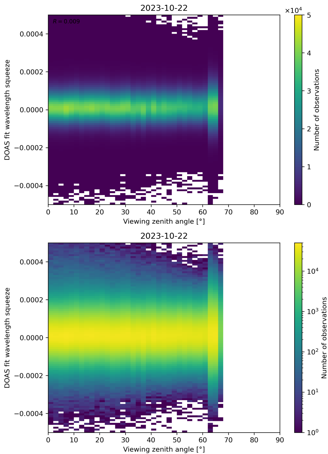
Figure 184: Scatter density plot of “Viewing zenith angle” against “DOAS fit wavelength squeeze” for 2023-10-22 to 2023-10-23.
