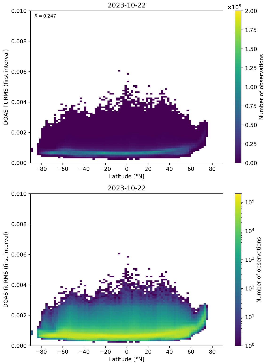
Figure 153: Scatter density plot of “Latitude” against “DOAS fit RMS (first interval)” for 2023-10-22 to 2023-10-23.
