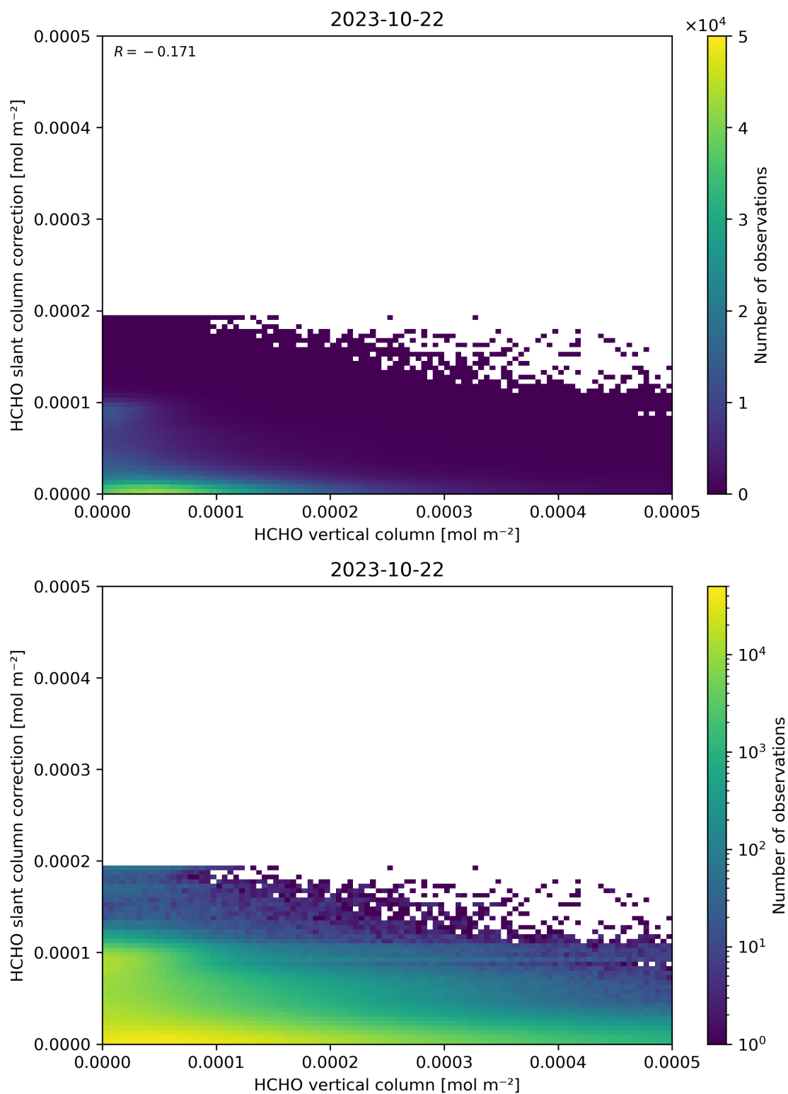
Figure 128: Scatter density plot of “HCHO vertical column” against “HCHO slant column correction” for 2023-10-22 to 2023-10-23.
