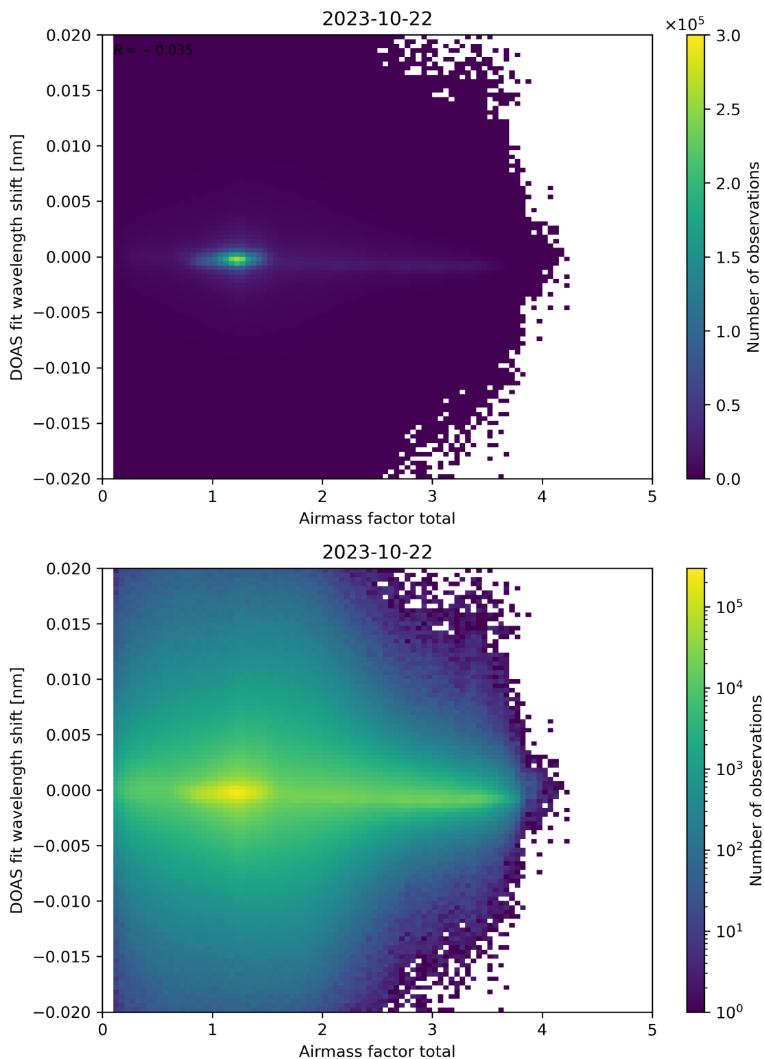
Figure 98: Scatter density plot of “Airmass factor total” against “DOAS fit wavelength shift” for 2023-10-22 to 2023-10-23.
