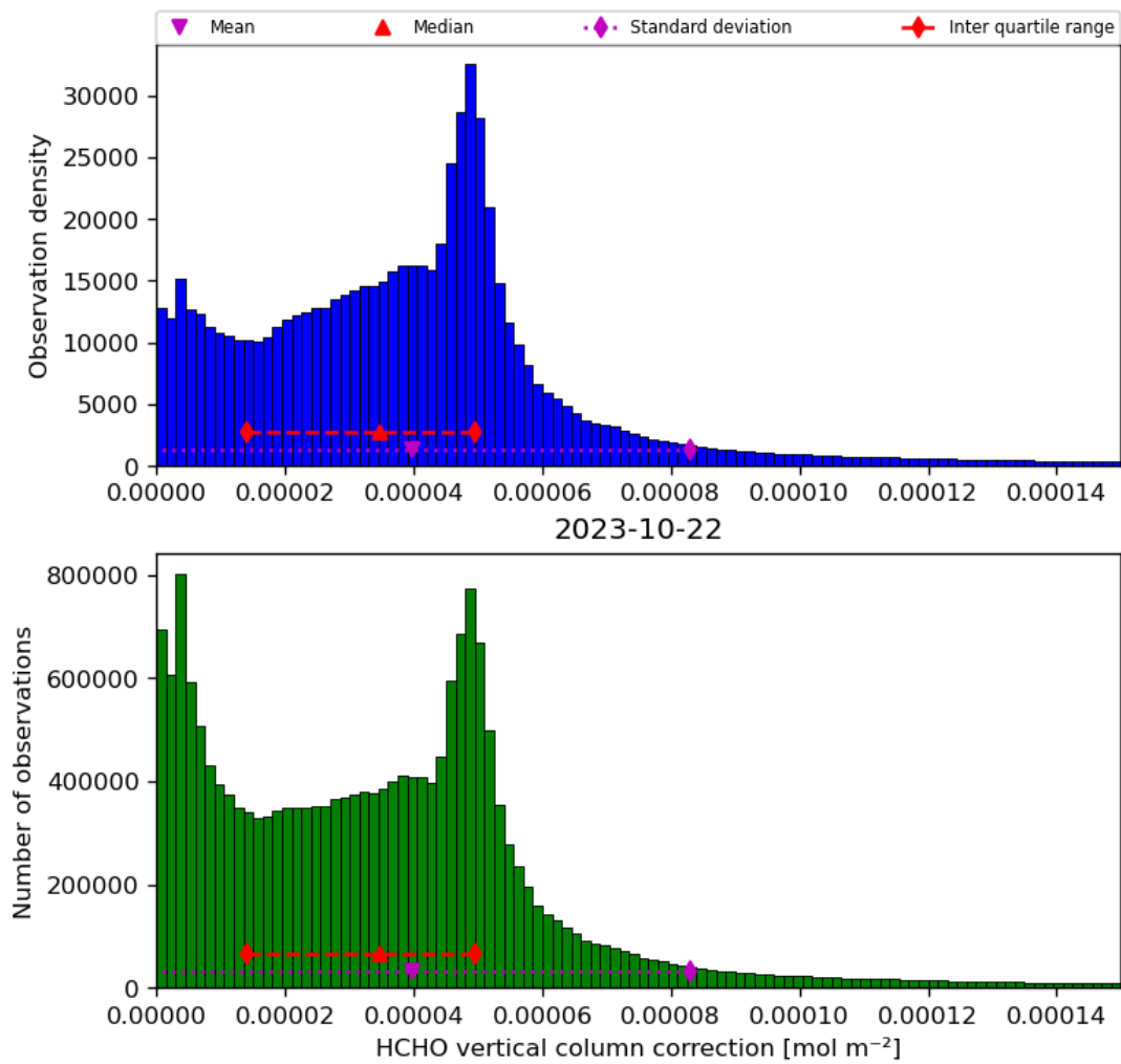
Figure 37: Histogram of “HCHO vertical column correction” for 2023-10-22 to 2023-10-23
