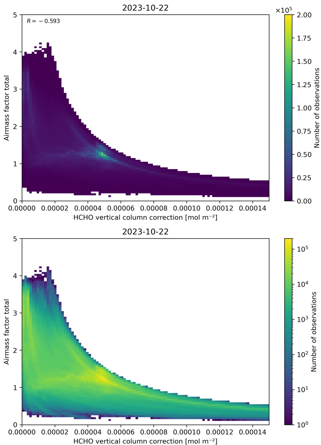
Figure 120: Scatter density plot of “HCHO vertical column correction” against “Airmass factor total” for 2023-10-22 to 2023-10-23.
