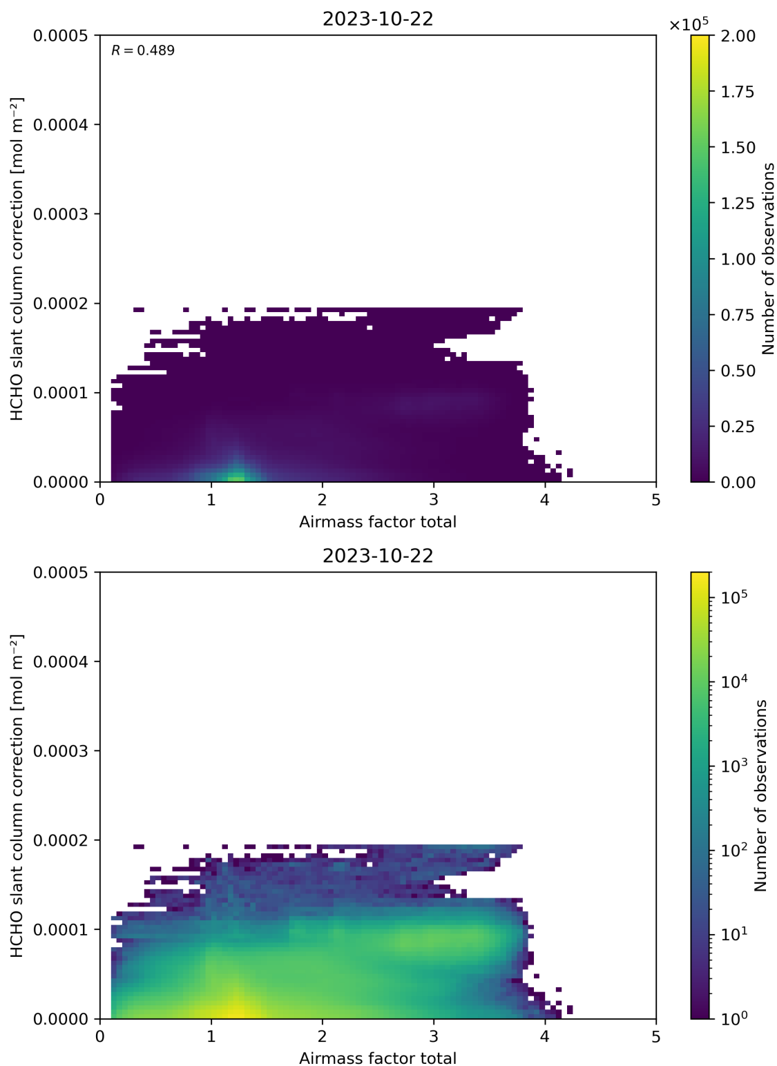
Figure 102: Scatter density plot of “Airmass factor total” against “HCHO slant column correction” for 2023-10-22 to 2023-10-23.
