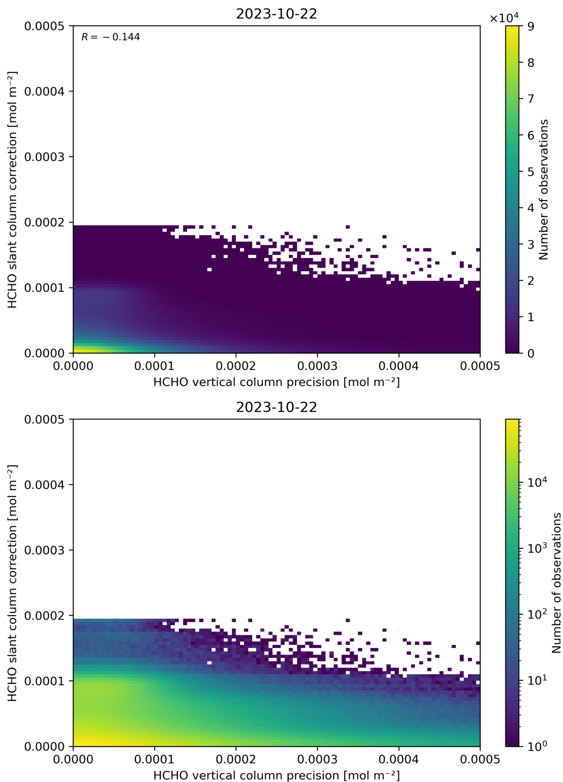
Figure 141: Scatter density plot of “HCHO vertical column precision” against “HCHO slant column correction” for 2023-10-22 to 2023-10-23.
