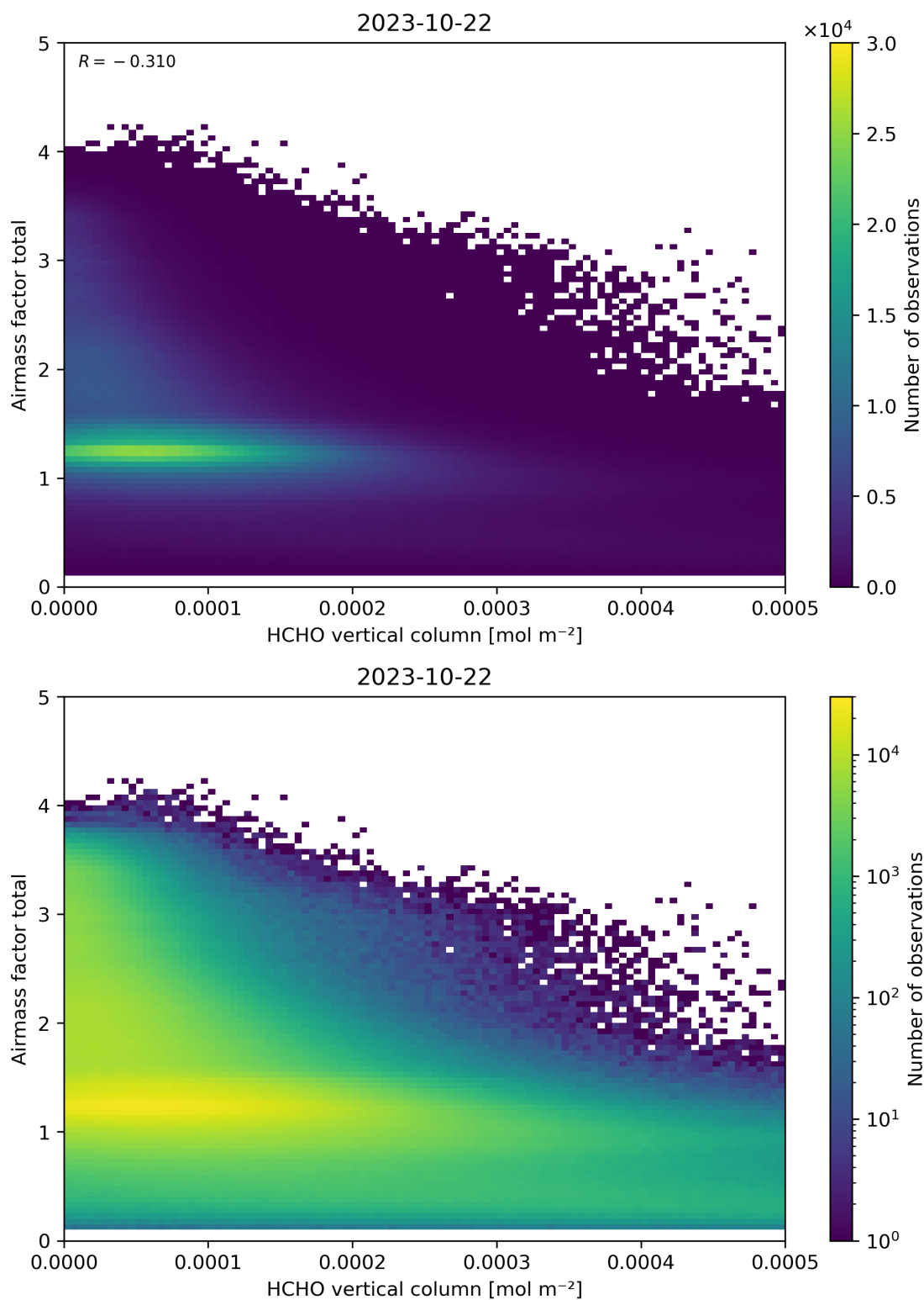
Figure 131: Scatter density plot of “HCHO vertical column” against “Airmass factor total” for 2023-10-22 to 2023-10-23.
