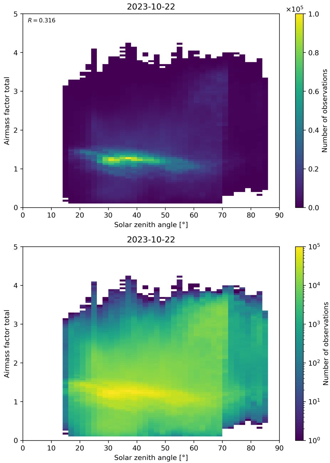
Figure 175: Scatter density plot of “Solar zenith angle” against “Airmass factor total” for 2023-10-22 to 2023-10-23.
