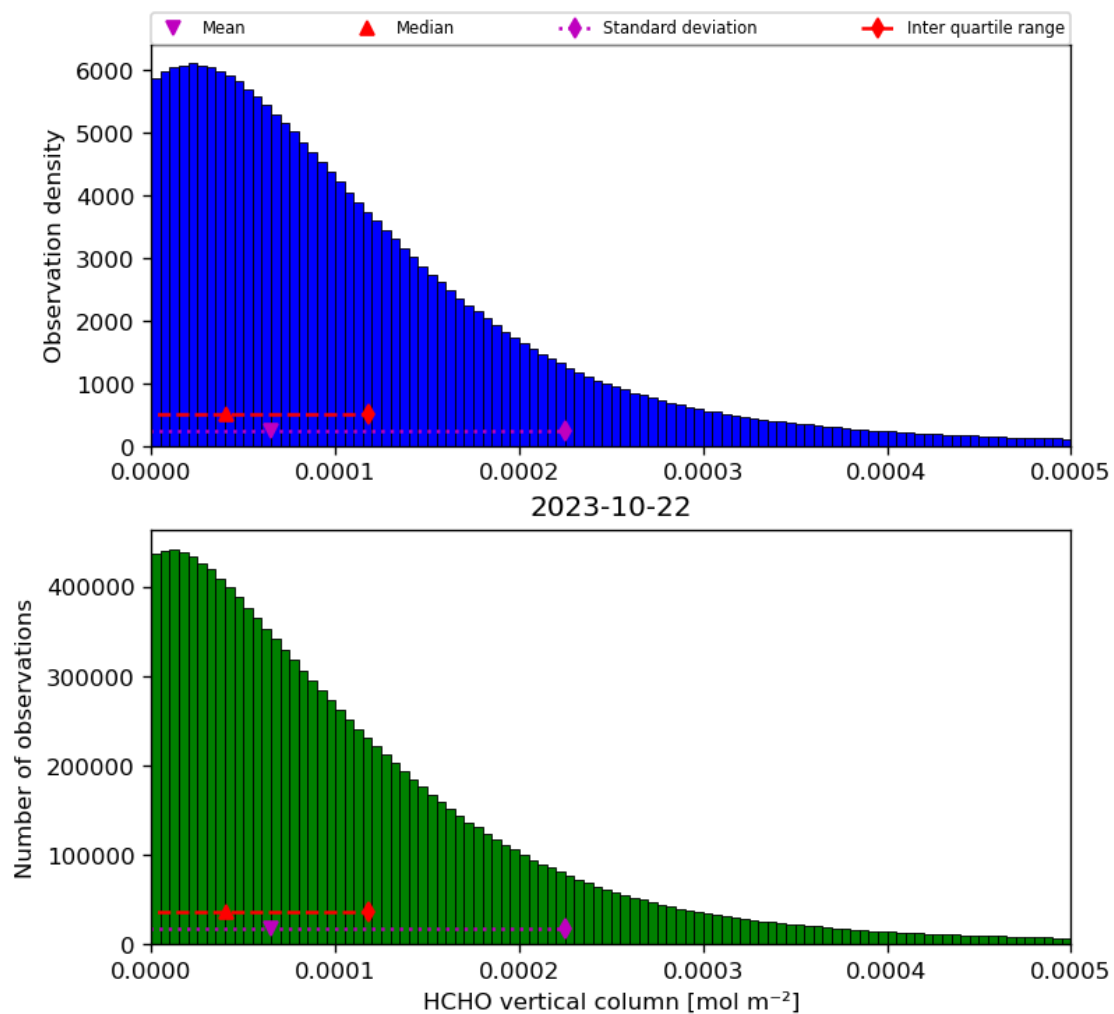
Figure 35: Histogram of “HCHO vertical column” for 2023-10-22 to 2023-10-23
