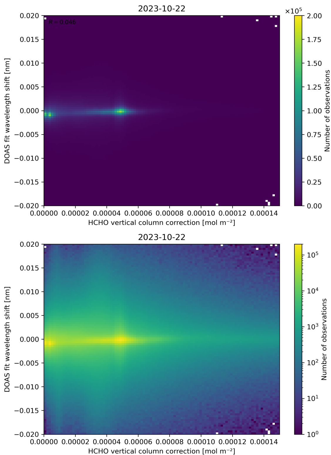
Figure 113: Scatter density plot of “HCHO vertical column correction” against “DOAS fit wavelength shift” for 2023-10-22 to 2023-10-23.
