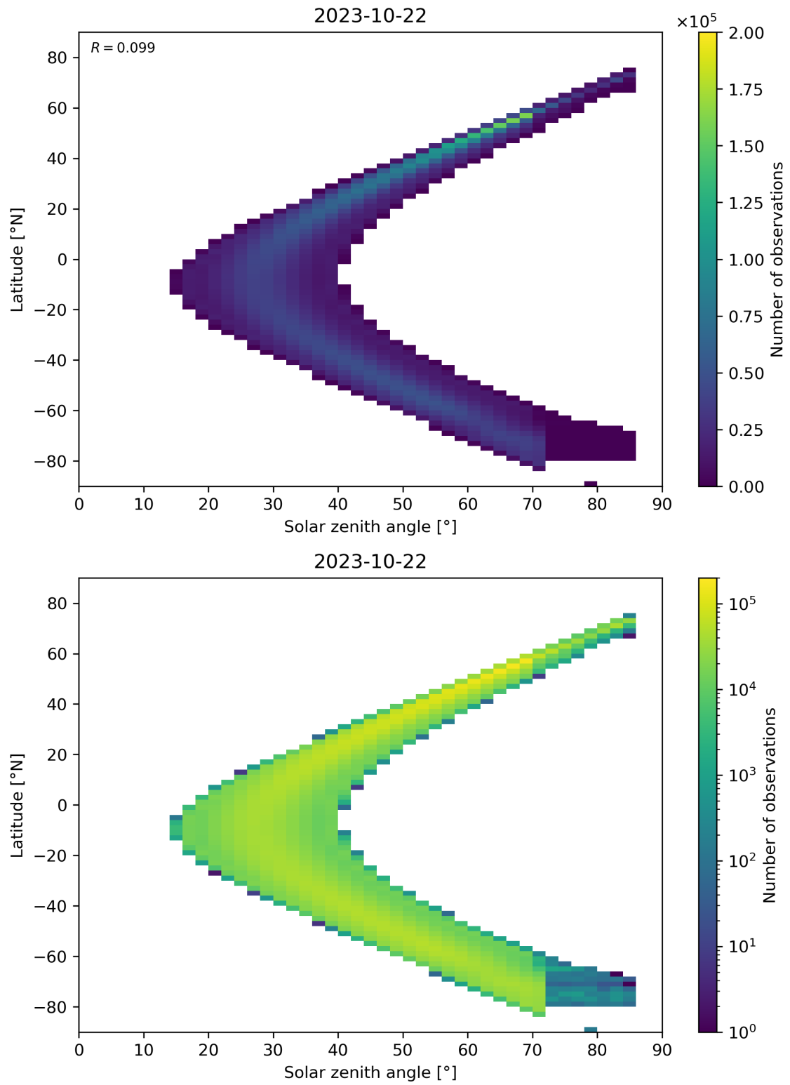
Figure 181: Scatter density plot of “Solar zenith angle” against “Latitude” for 2023-10-22 to 2023-10-23.
