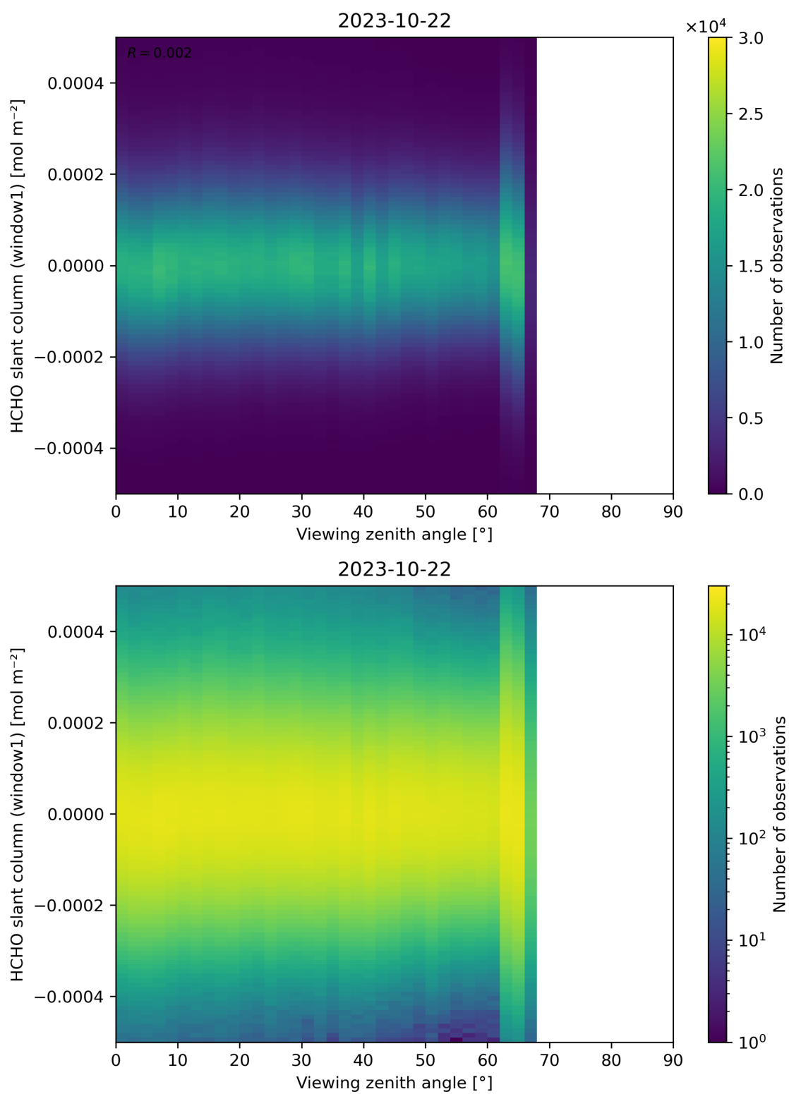
Figure 188: Scatter density plot of “Viewing zenith angle” against “HCHO slant column (window1)” for 2023-10-22 to 2023-10-23.
