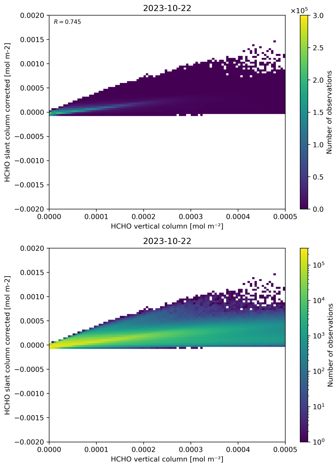
Figure 127: Scatter density plot of “HCHO vertical column” against “HCHO slant column corrected” for 2023-10-22 to 2023-10-23.
