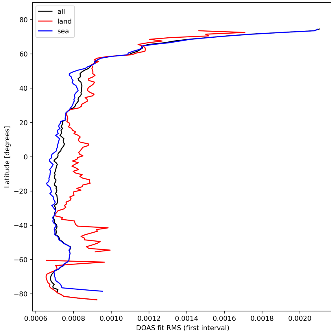
Figure 32: Zonal average of “DOAS fit RMS (first interval)” for 2023-10-22 to 2023-10-23.
