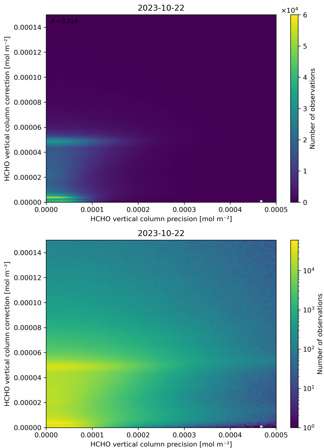
Figure 146: Scatter density plot of “HCHO vertical column precision” against “HCHO vertical column correction” for 2023-10-22 to 2023-10-23.
