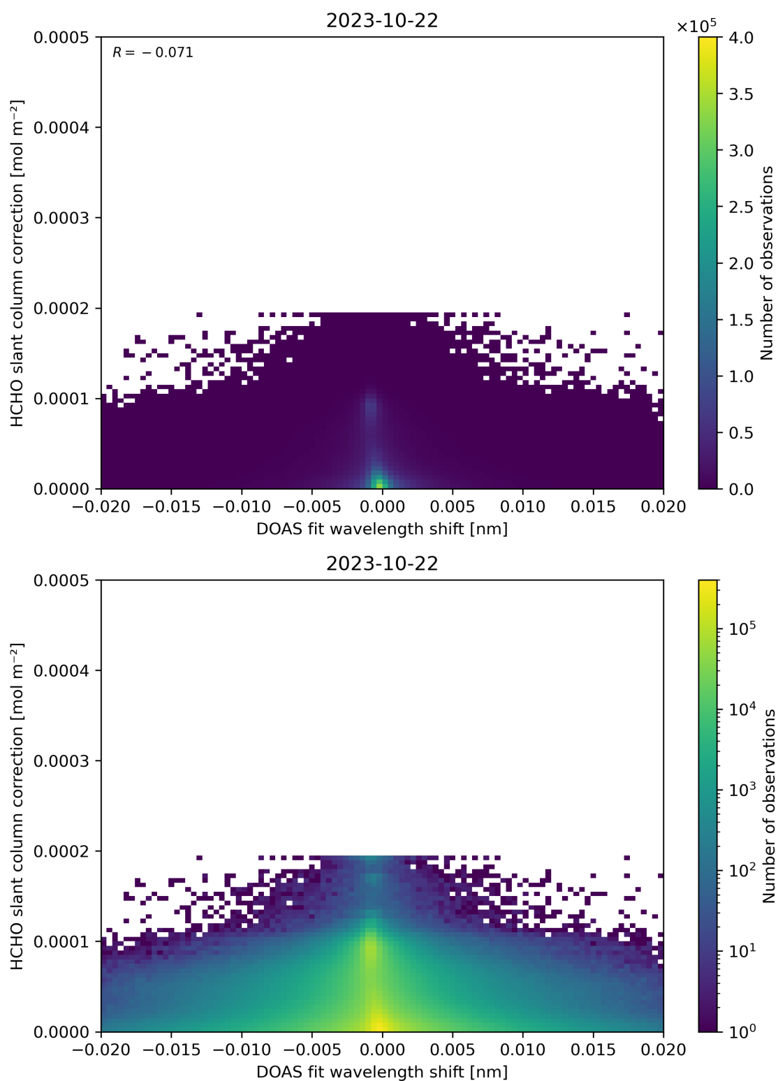
Figure 67: Scatter density plot of “DOAS fit wavelength shift” against “HCHO slant column correction” for 2023-10-22 to 2023-10-23.
