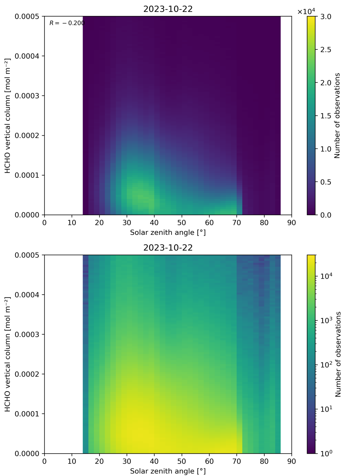
Figure 177: Scatter density plot of “Solar zenith angle” against “HCHO vertical column” for 2023-10-22 to 2023-10-23.
