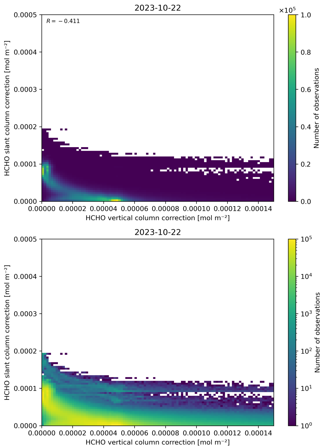
Figure 117: Scatter density plot of “HCHO vertical column correction” against “HCHO slant column correction” for 2023-10-22 to 2023-10-23.
