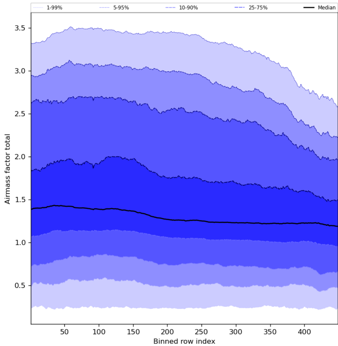
Figure 54: Along track statistics of “Airmass factor total” for 2023-10-22 to 2023-10-23
