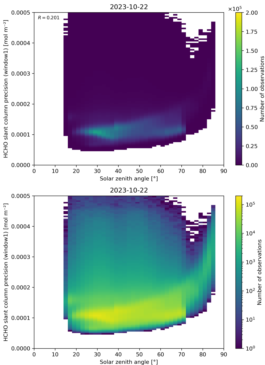
Figure 174: Scatter density plot of “Solar zenith angle” against “HCHO slant column precision (window1)” for 2023-10-22 to 2023-10-23.
