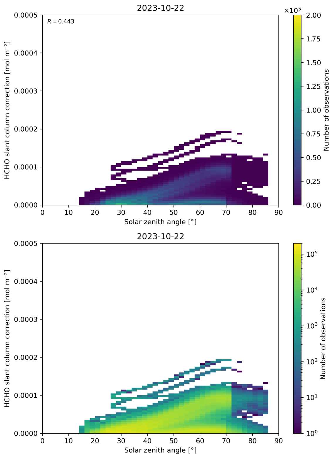
Figure 172: Scatter density plot of “Solar zenith angle” against “HCHO slant column correction” for 2023-10-22 to 2023-10-23.
