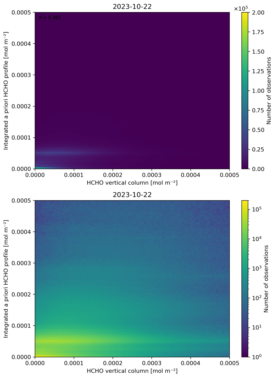
Figure 135: Scatter density plot of “HCHO vertical column” against “Integrated a priori HCHO profile” for 2023-10-22 to 2023-10-23.
