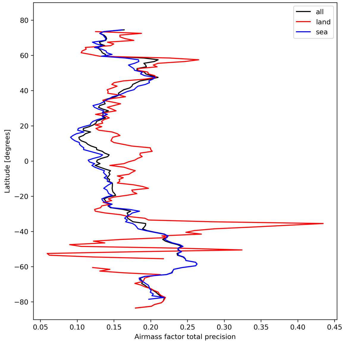
Figure 27: Zonal average of “Airmass factor total precision” for 2023-10-22 to 2023-10-23.
