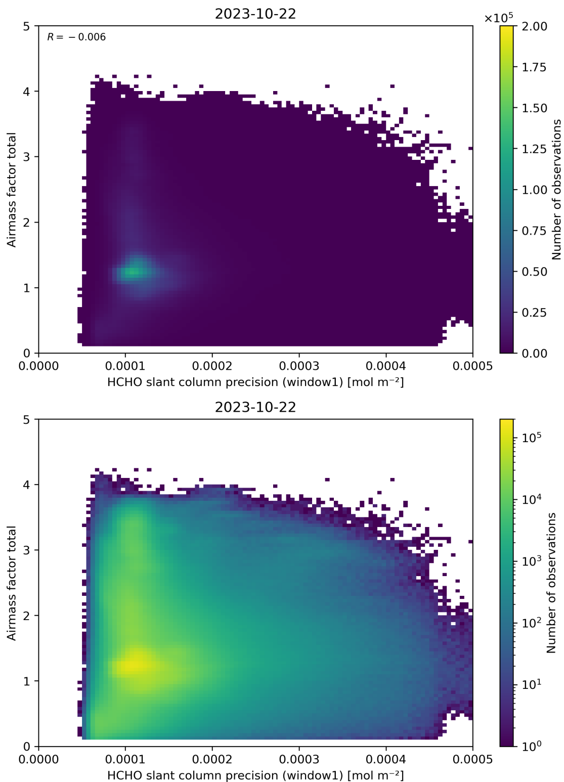
Figure 94: Scatter density plot of “HCHO slant column precision (window1)” against “Airmass factor total” for 2023-10-22 to 2023-10-23.
