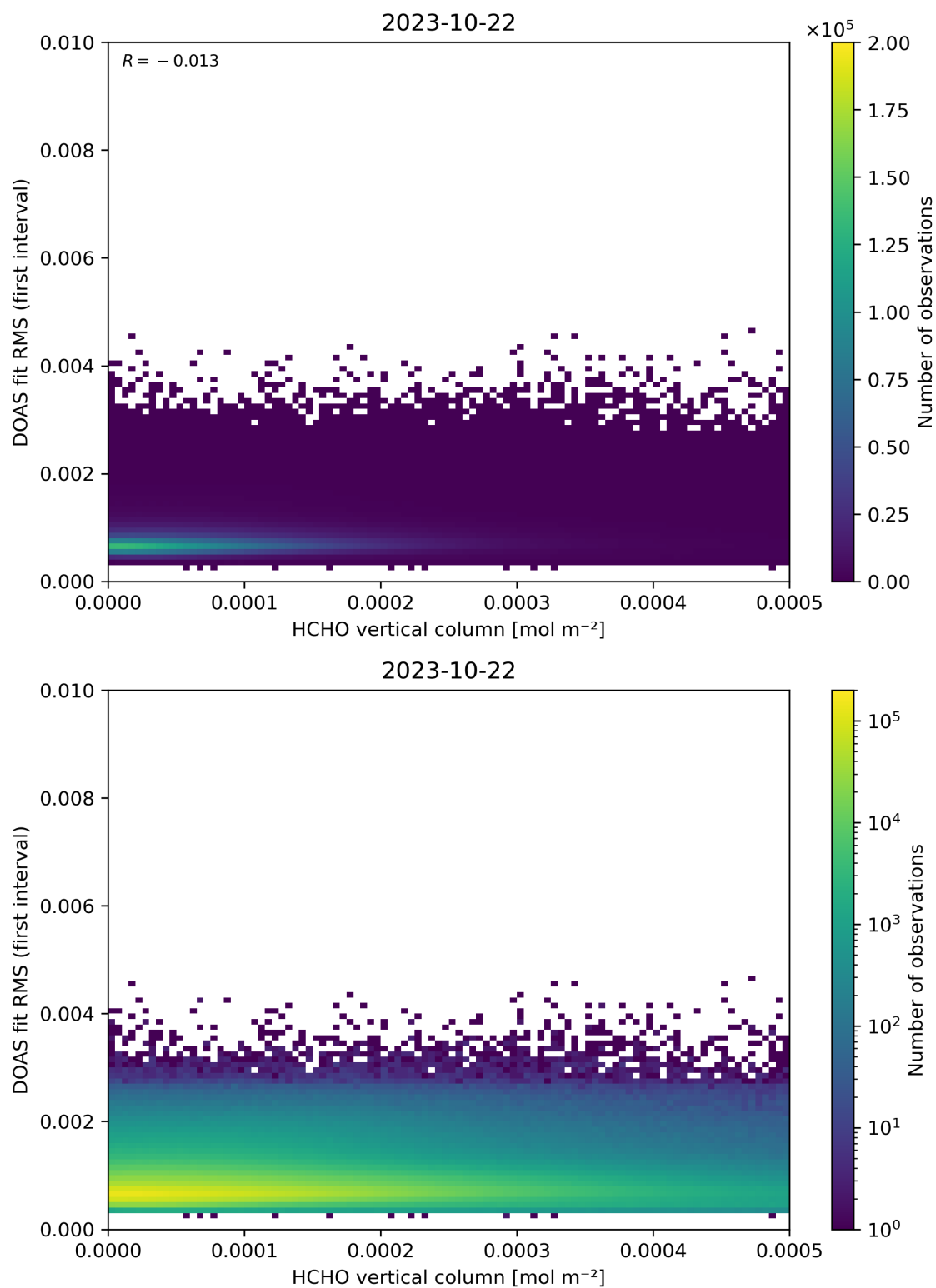
Figure 123: Scatter density plot of “HCHO vertical column” against “DOAS fit RMS (first interval)” for 2023-10-22 to 2023-10-23.
