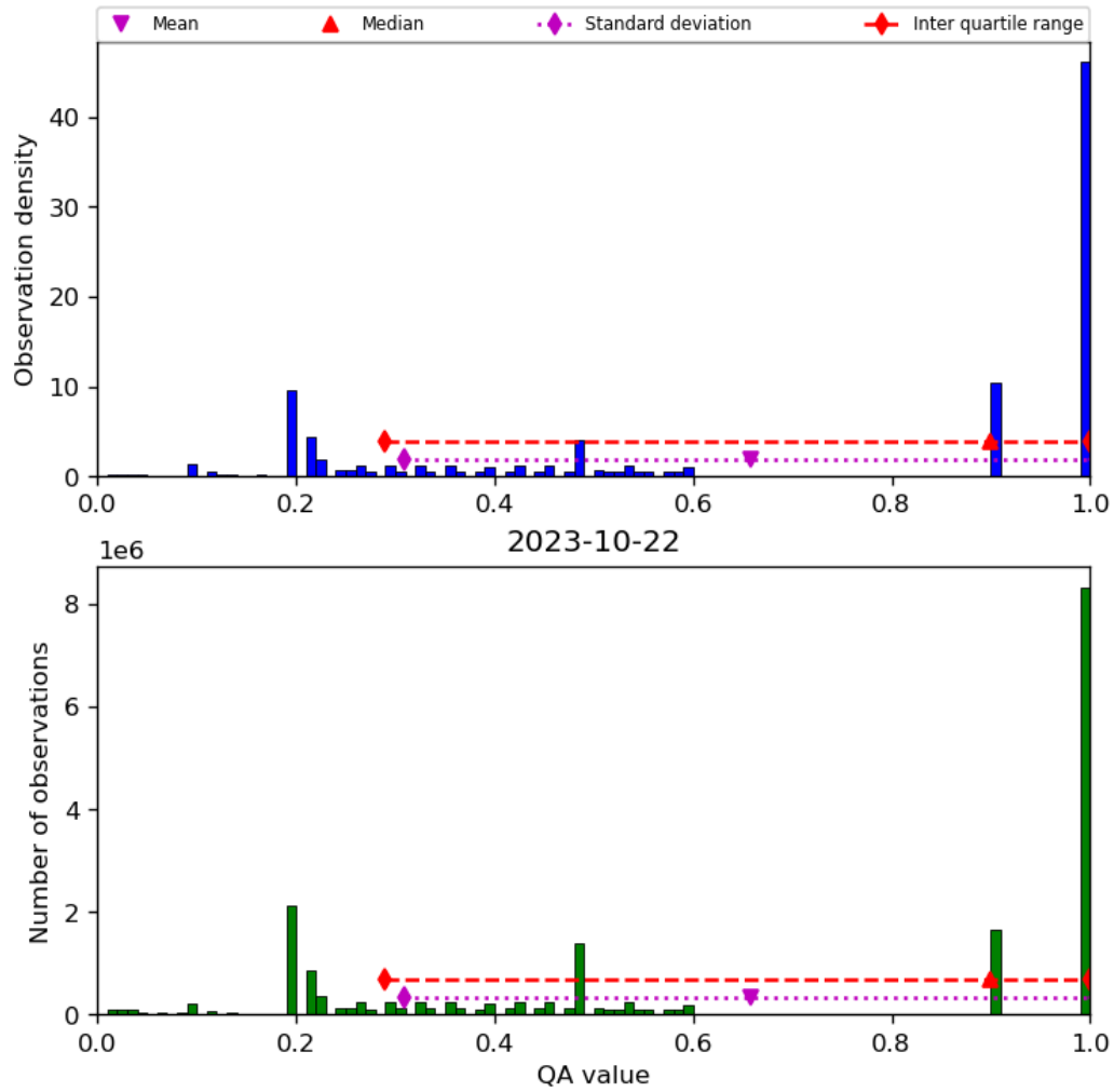
Figure 34: Histogram of “QA value” for 2023-10-22 to 2023-10-23
