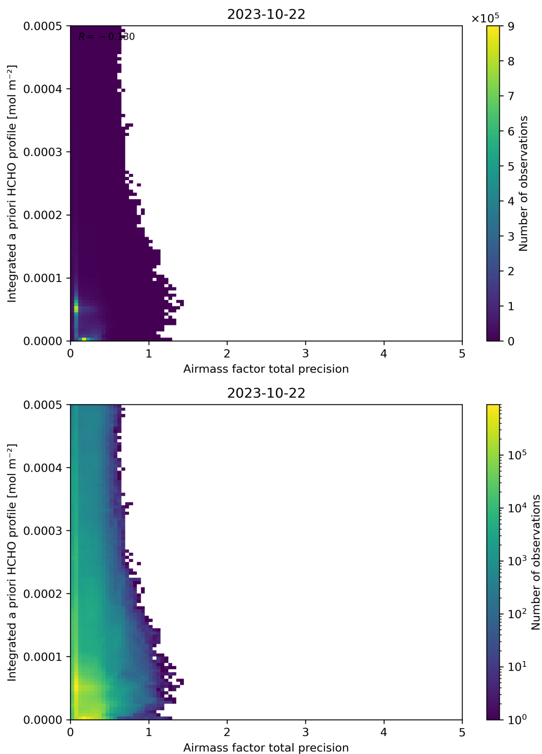
Figure 111: Scatter density plot of “Airmass factor total precision” against “Integrated a priori HCHO profile” for 2023-10-22 to 2023-10-23.
