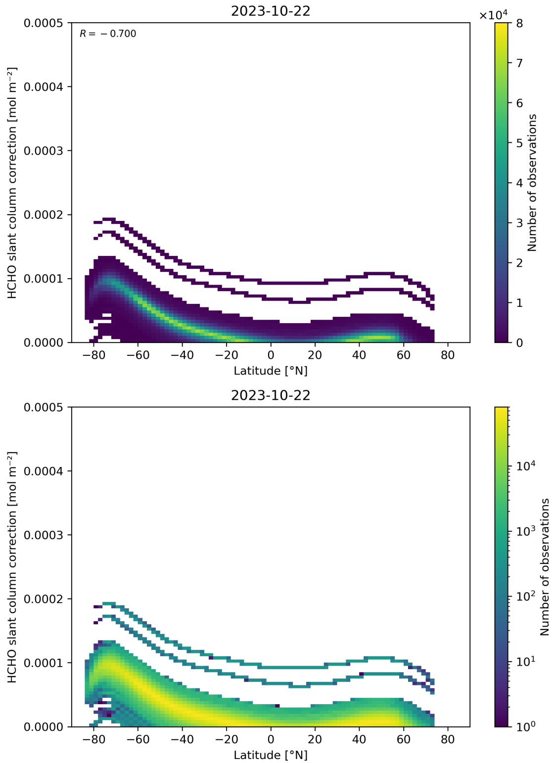
Figure 158: Scatter density plot of “Latitude” against “HCHO slant column correction” for 2023-10-22 to 2023-10-23.
