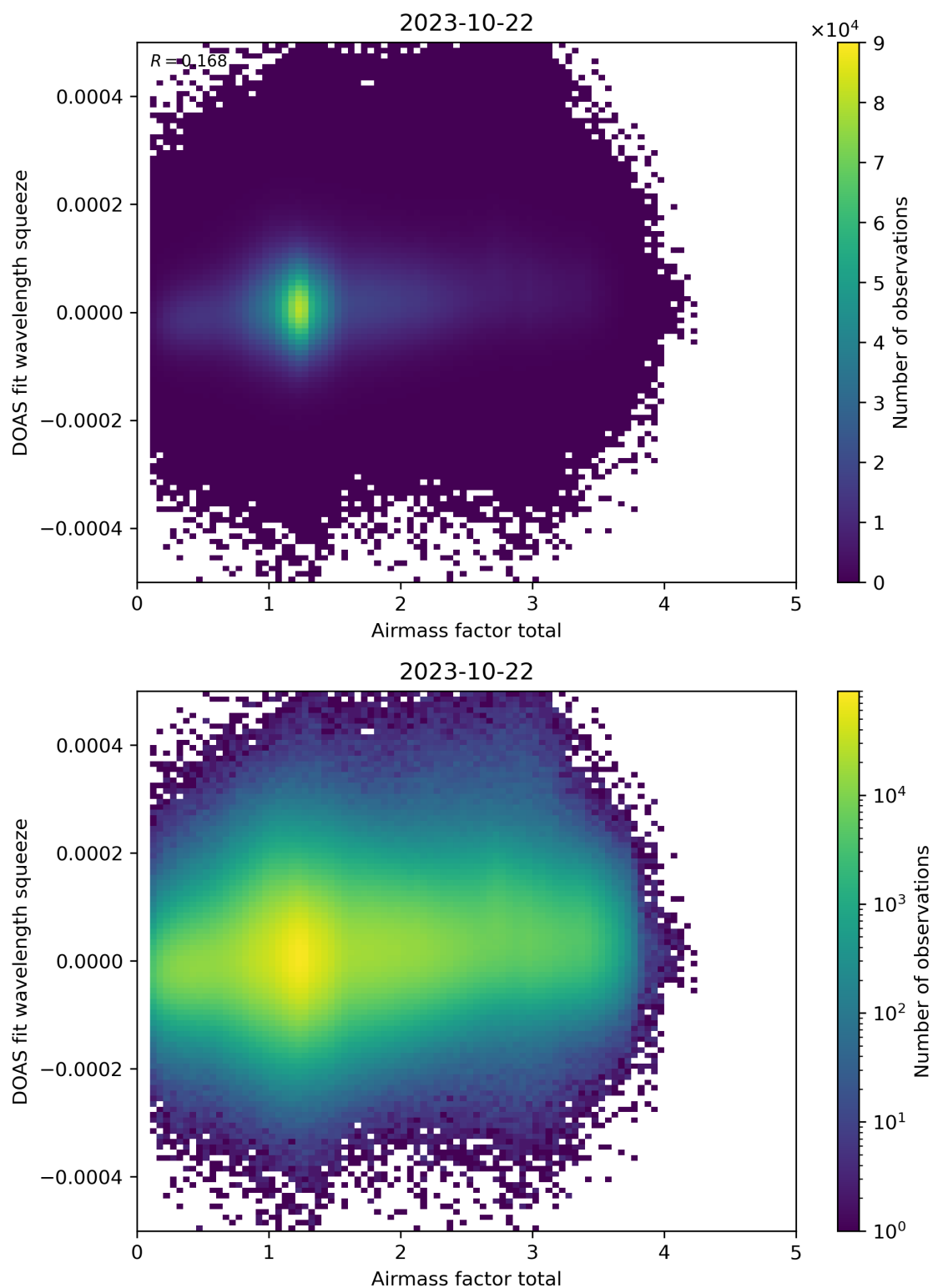
Figure 99: Scatter density plot of “Airmass factor total” against “DOAS fit wavelength squeeze” for 2023-10-22 to 2023-10-23.
