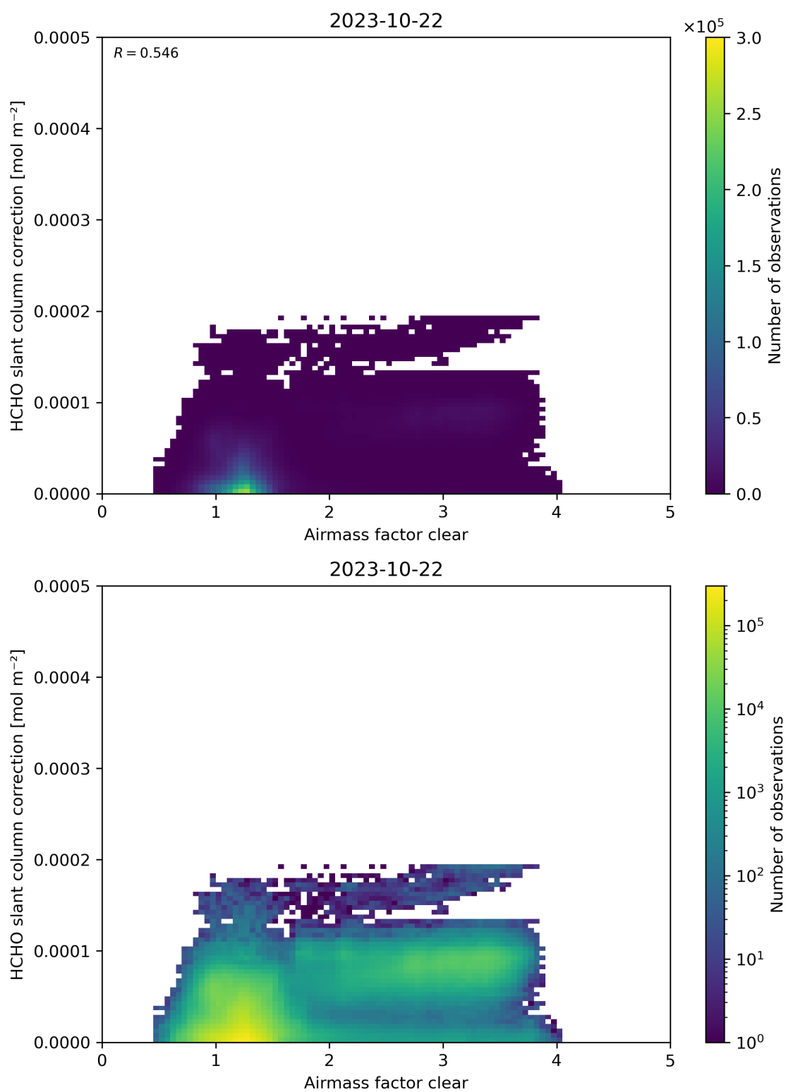
Figure 75: Scatter density plot of “Airmass factor clear” against “HCHO slant column correction” for 2023-10-22 to 2023-10-23.
