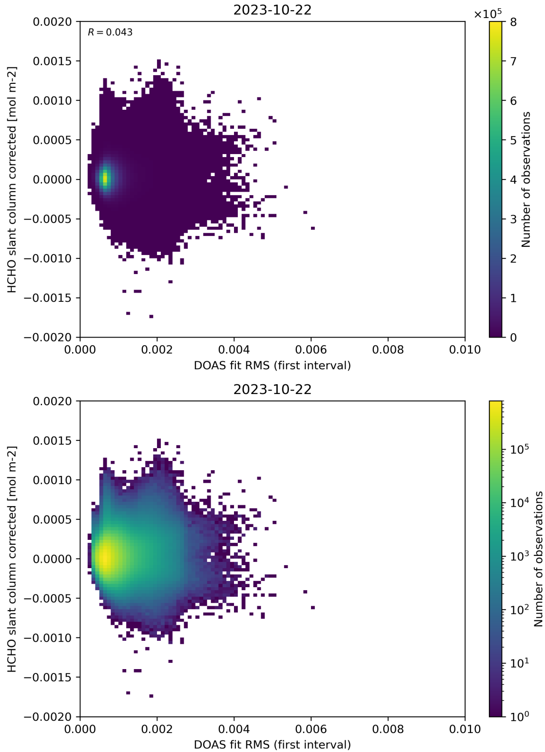
Figure 62: Scatter density plot of “DOAS fit RMS (first interval)” against “HCHO slant column corrected” for 2023-10-22 to 2023-10-23.
