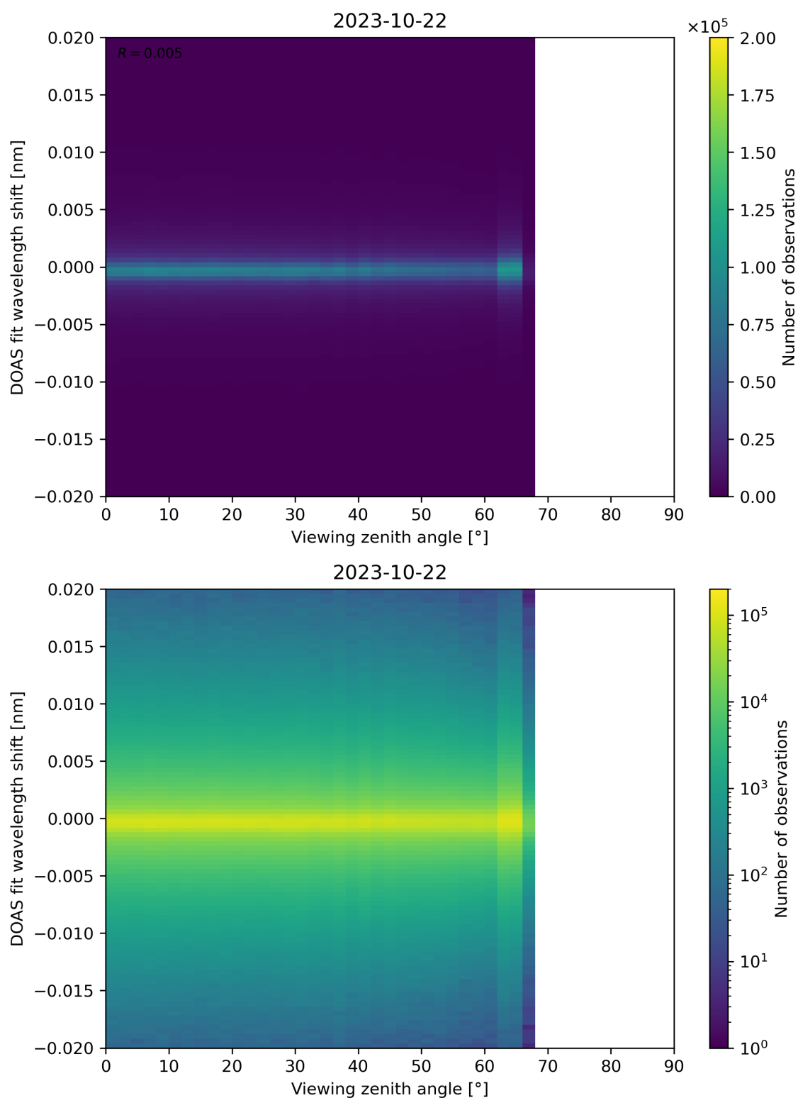
Figure 183: Scatter density plot of “Viewing zenith angle” against “DOAS fit wavelength shift” for 2023-10-22 to 2023-10-23.
