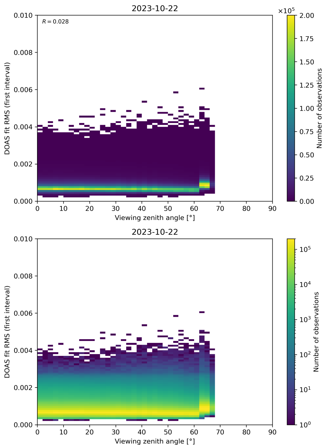
Figure 182: Scatter density plot of “Viewing zenith angle” against “DOAS fit RMS (first interval)” for 2023-10-22 to 2023-10-23.
