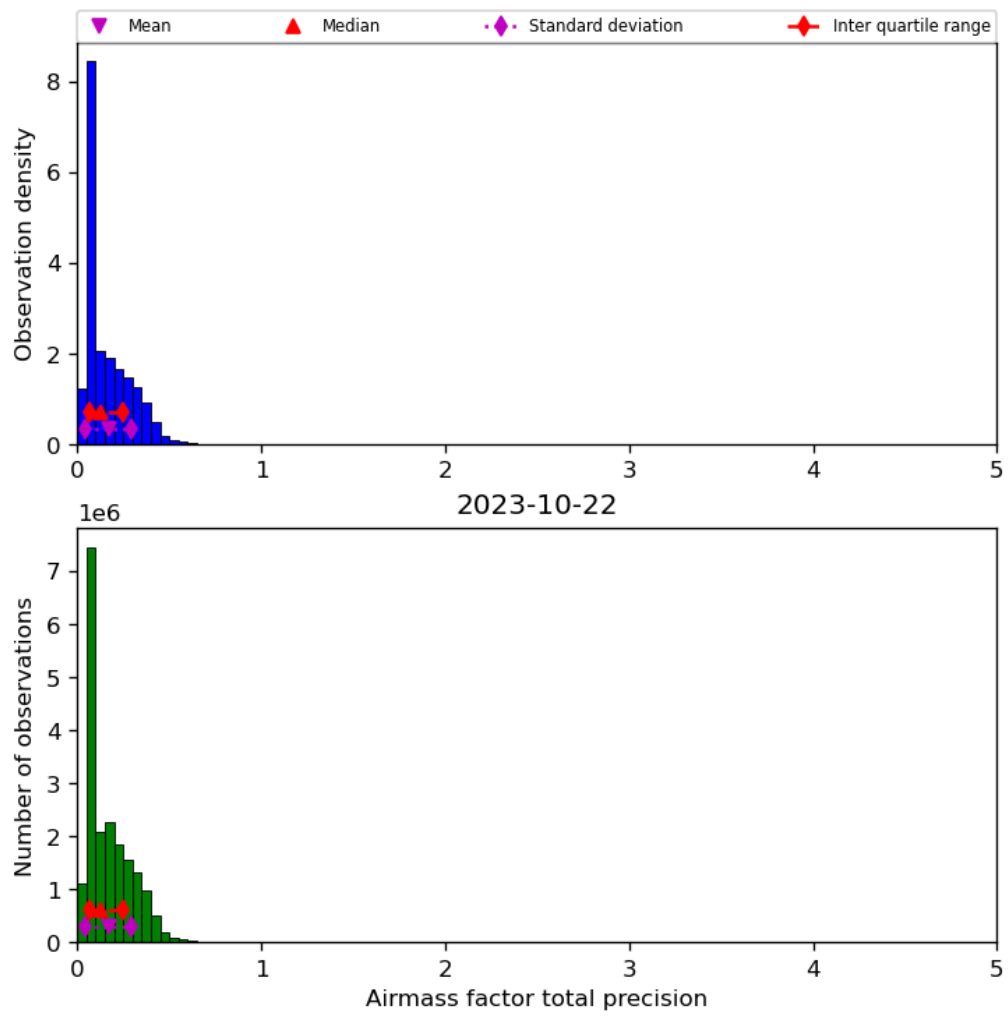
Figure 41: Histogram of “Airmass factor total precision” for 2023-10-22 to 2023-10-23
