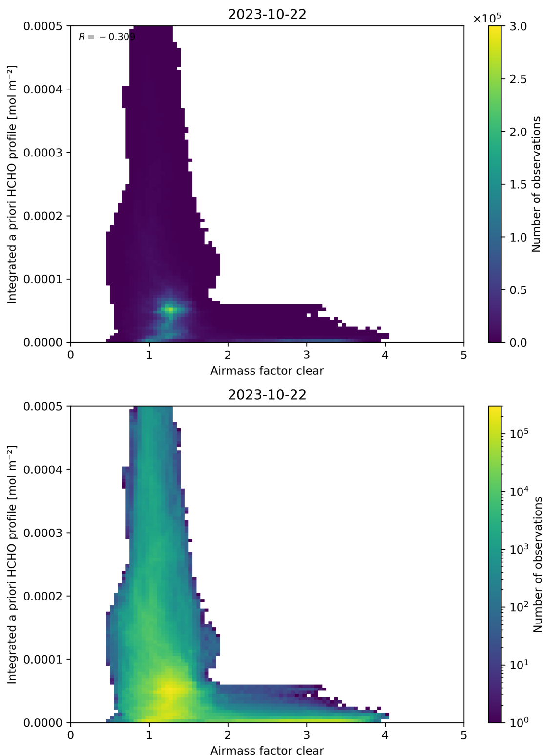
Figure 76: Scatter density plot of “Airmass factor clear” against “Integrated a priori HCHO profile” for 2023-10-22 to 2023-10-23.
