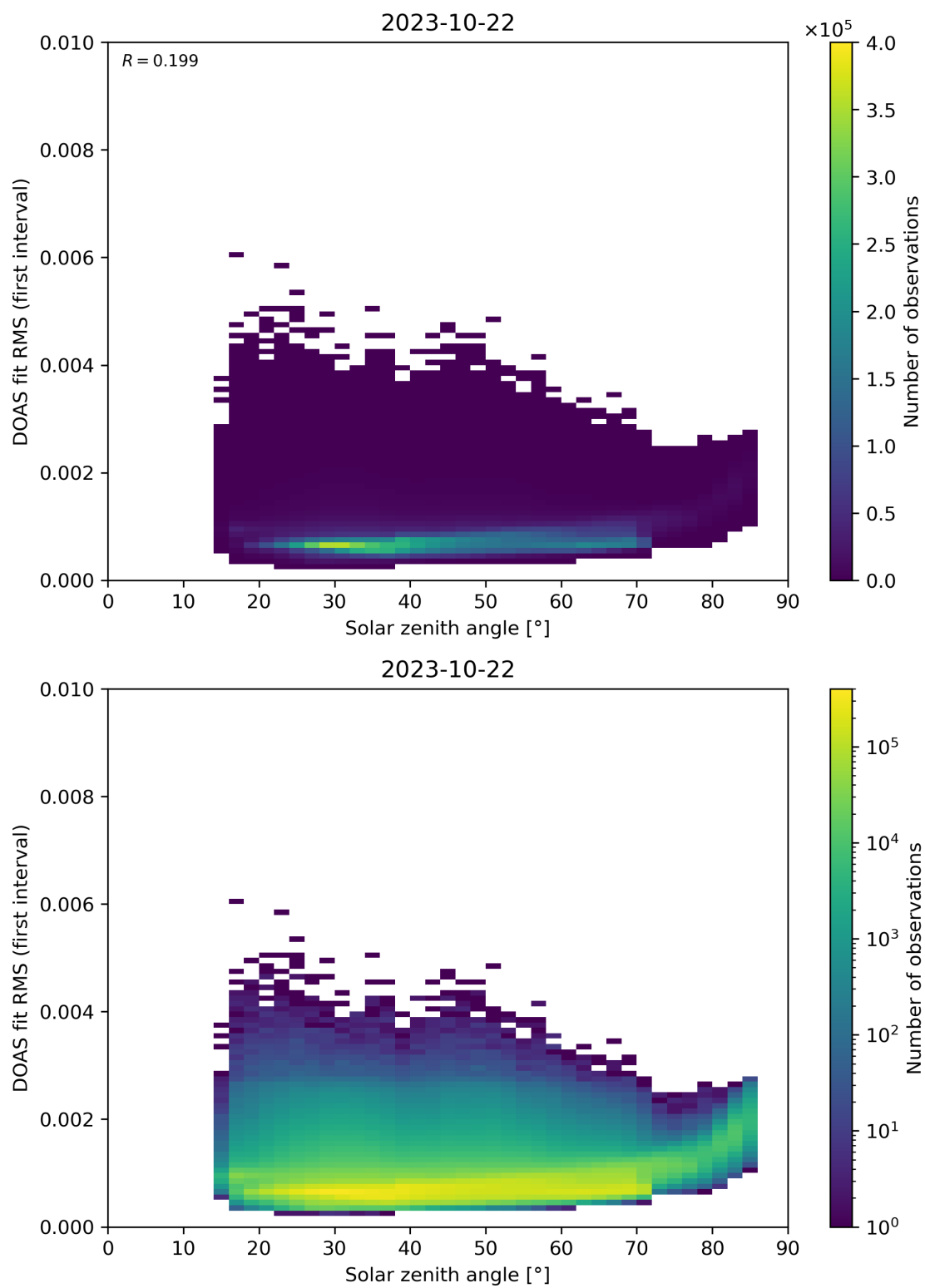
Figure 167: Scatter density plot of “Solar zenith angle” against “DOAS fit RMS (first interval)” for 2023-10-22 to 2023-10-23.
