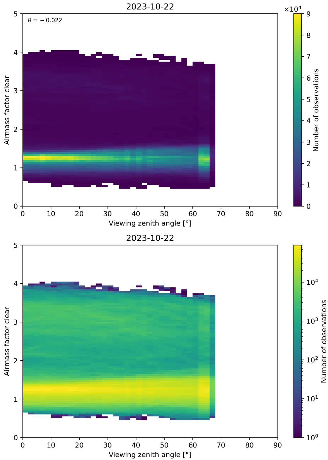
Figure 185: Scatter density plot of “Viewing zenith angle” against “Airmass factor clear” for 2023-10-22 to 2023-10-23.
