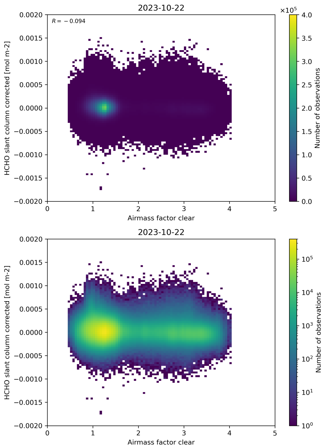
Figure 74: Scatter density plot of “Airmass factor clear” against “HCHO slant column corrected” for 2023-10-22 to 2023-10-23.
