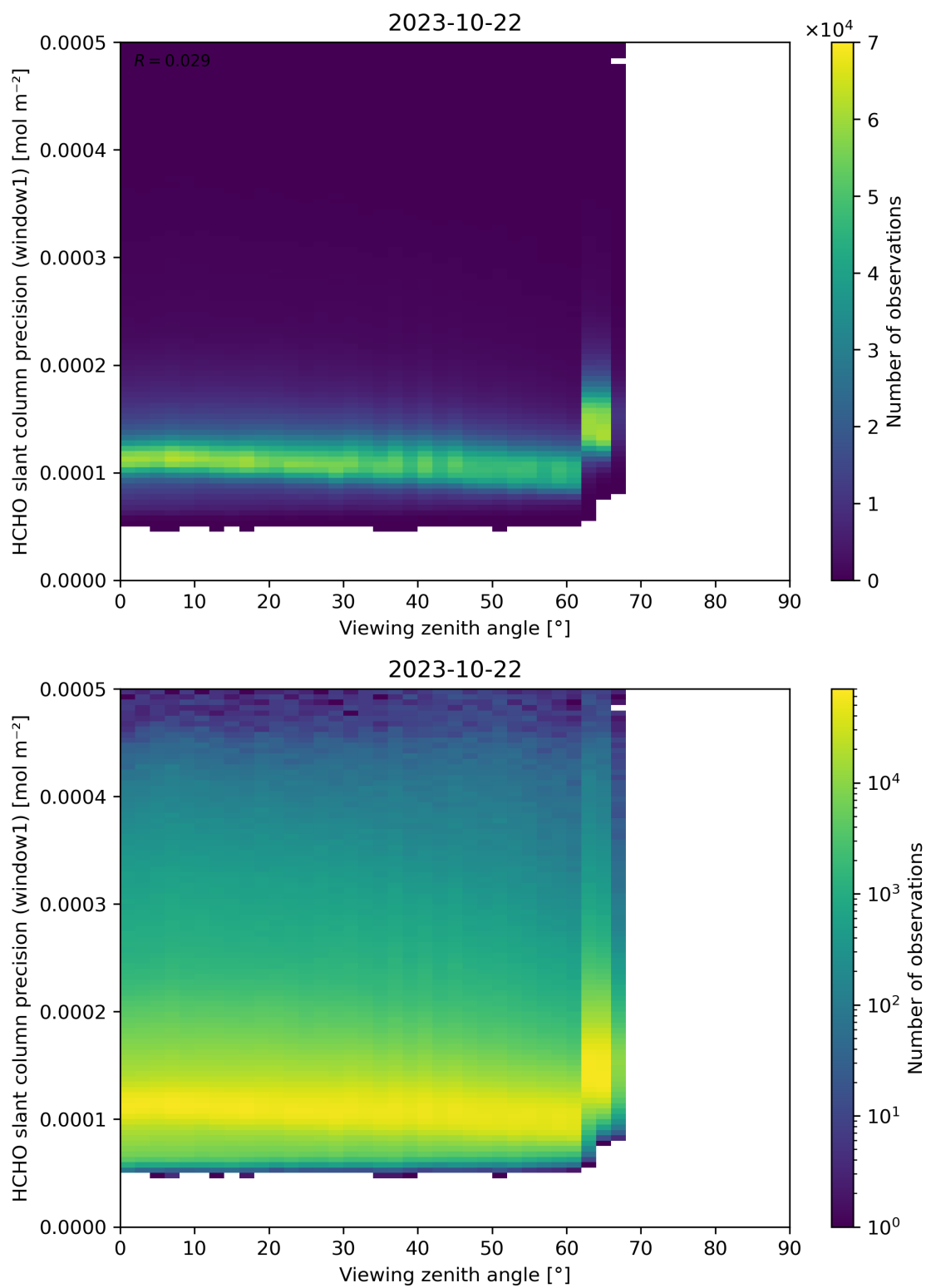
Figure 189: Scatter density plot of “Viewing zenith angle” against “HCHO slant column precision (window1)” for 2023-10-22 to 2023-10-23.
