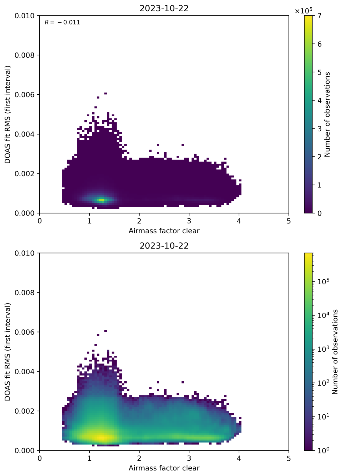
Figure 71: Scatter density plot of “Airmass factor clear” against “DOAS fit RMS (first interval)” for 2023-10-22 to 2023-10-23.
