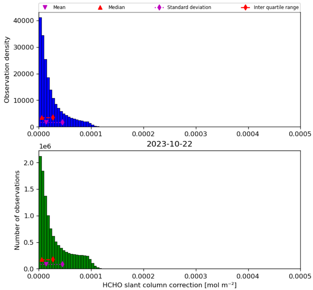
Figure 47: Histogram of “HCHO slant column correction” for 2023-10-22 to 2023-10-23
