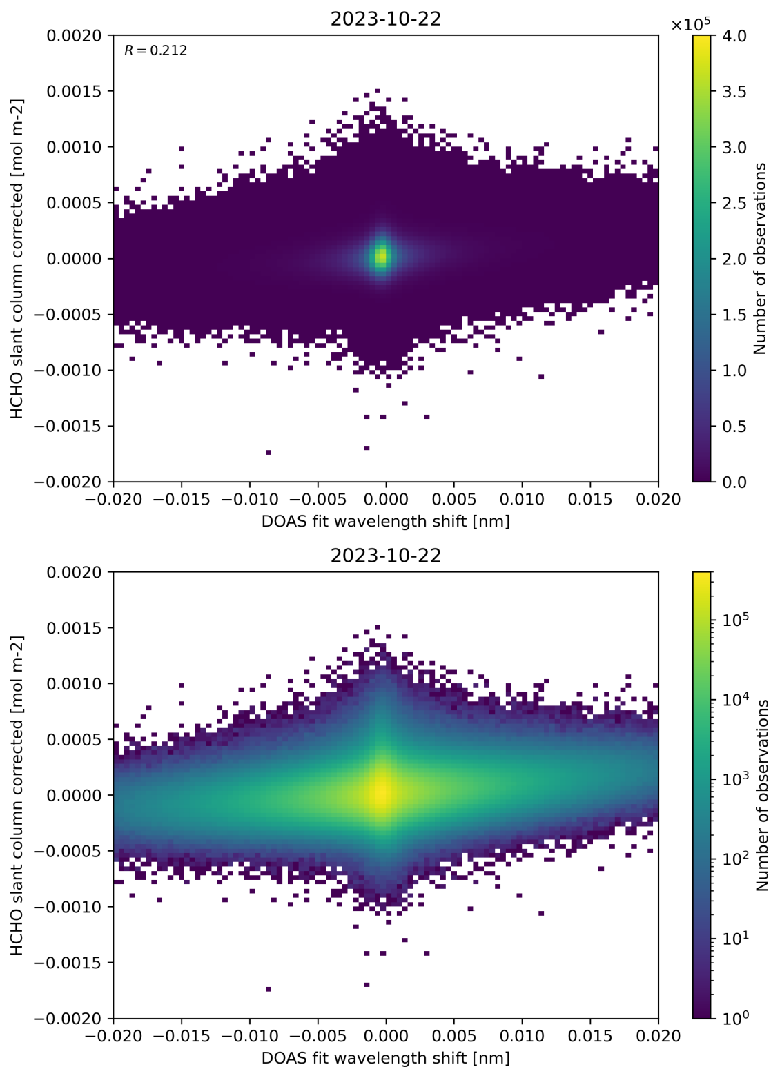
Figure 66: Scatter density plot of “DOAS fit wavelength shift” against “HCHO slant column corrected” for 2023-10-22 to 2023-10-23.
