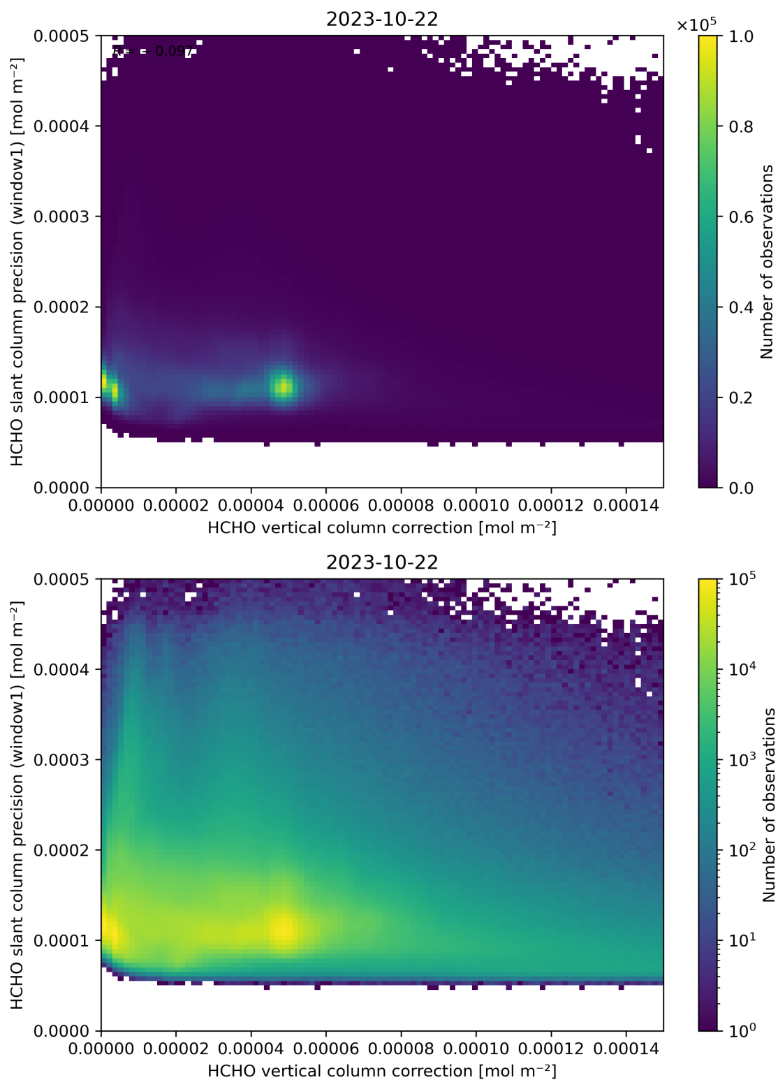
Figure 119: Scatter density plot of “HCHO vertical column correction” against “HCHO slant column precision (window1)” for 2023-10-22 to 2023-10-23.
