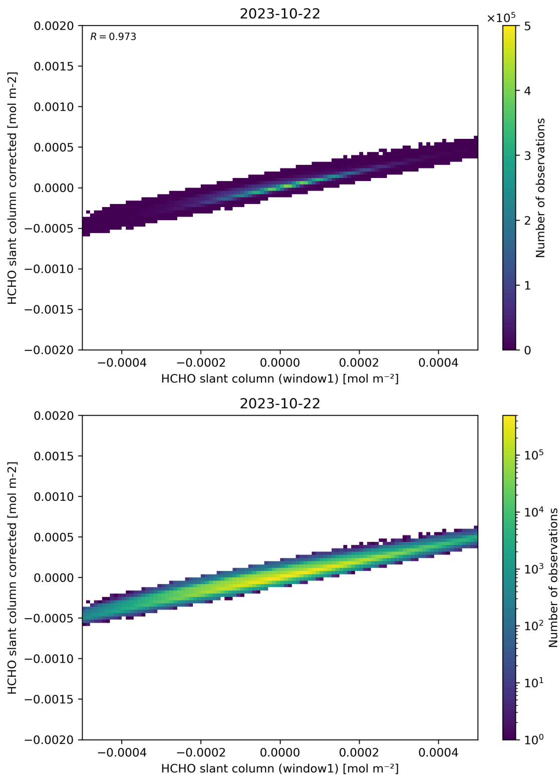
Figure 82: Scatter density plot of “HCHO slant column (window1)” against “HCHO slant column corrected” for 2023-10-22 to 2023-10-23.
