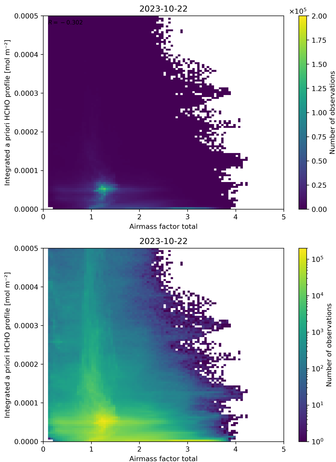
Figure 104: Scatter density plot of “Airmass factor total” against “Integrated a priori HCHO profile” for 2023-10-22 to 2023-10-23.
