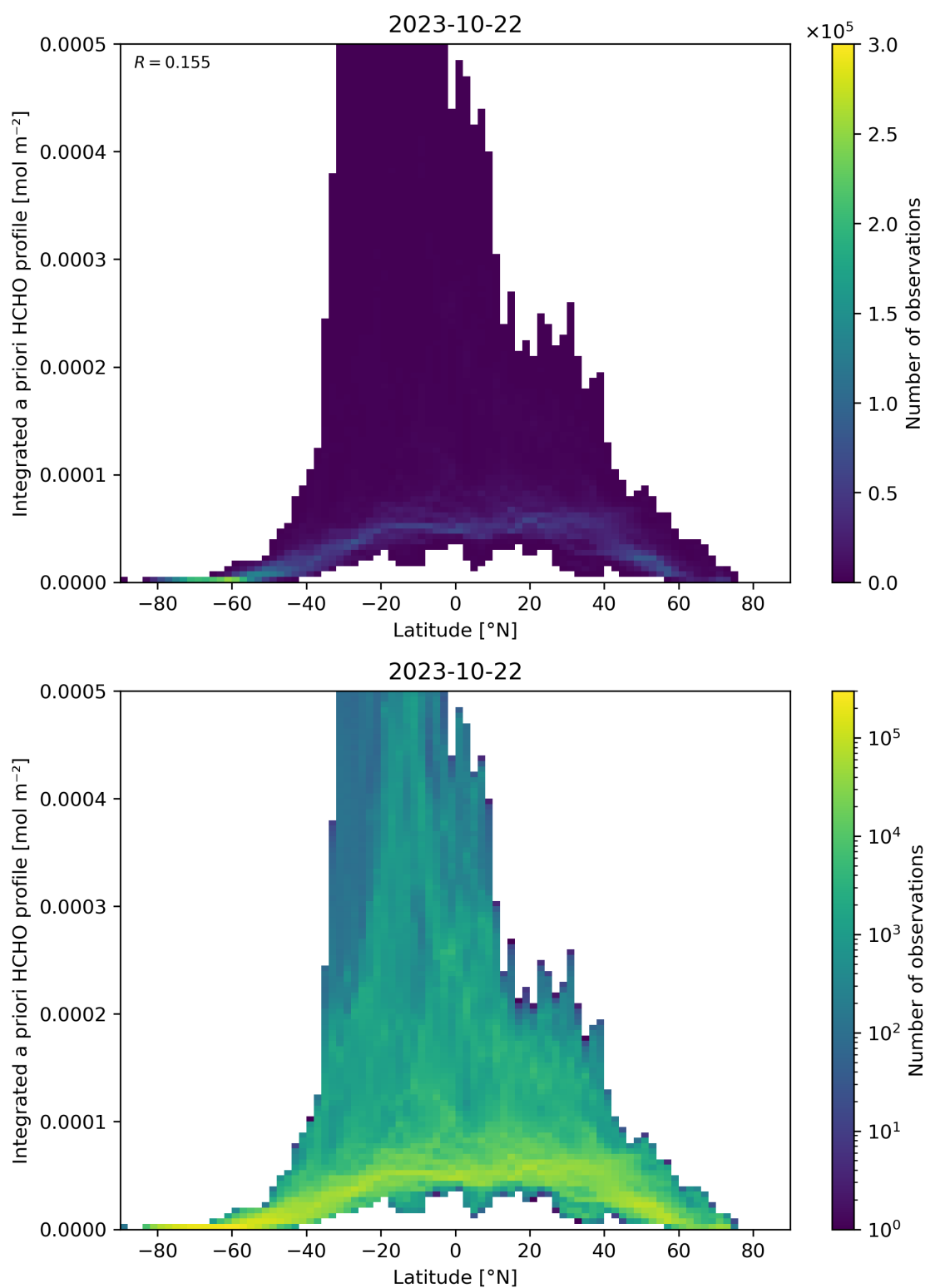
Figure 166: Scatter density plot of “Latitude” against “Integrated a priori HCHO profile” for 2023-10-22 to 2023-10-23.
