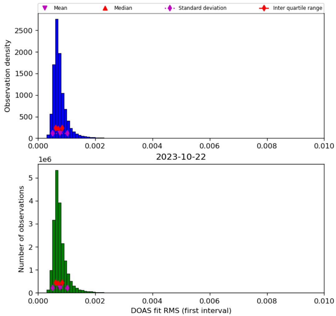
Figure 46: Histogram of “DOAS fit RMS (first interval)” for 2023-10-22 to 2023-10-23
