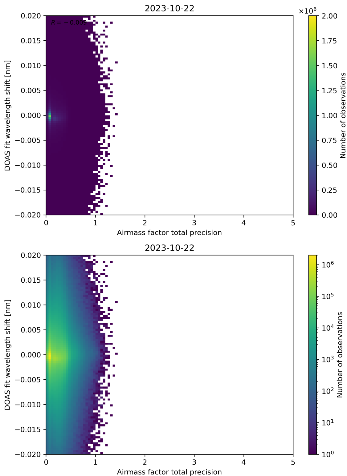
Figure 106: Scatter density plot of “Airmass factor total precision” against “DOAS fit wavelength shift” for 2023-10-22 to 2023-10-23.
