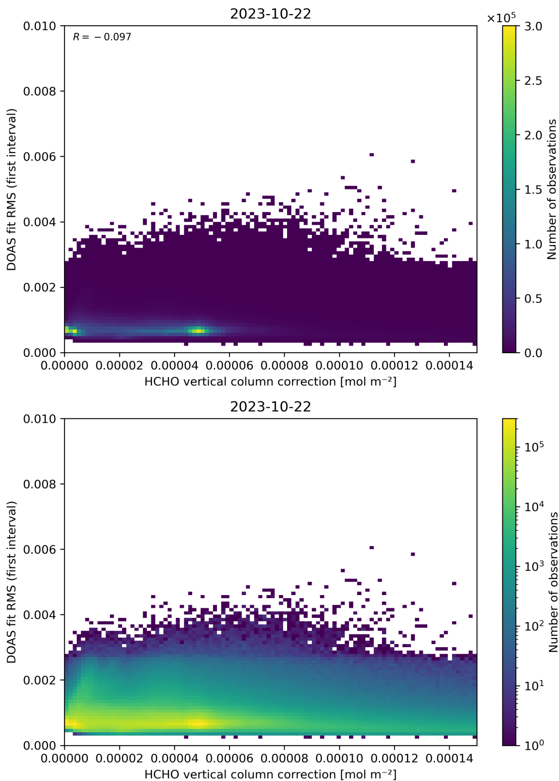
Figure 112: Scatter density plot of “HCHO vertical column correction” against “DOAS fit RMS (first interval)” for 2023-10-22 to 2023-10-23.
