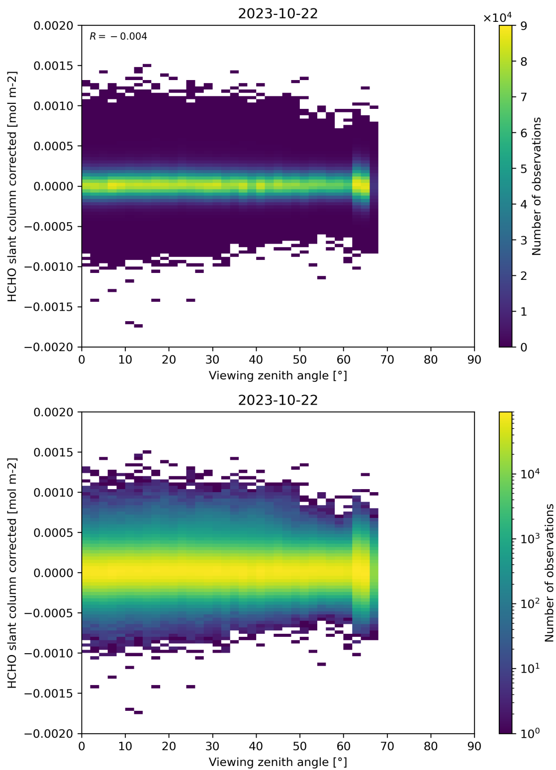
Figure 186: Scatter density plot of “Viewing zenith angle” against “HCHO slant column corrected” for 2023-10-22 to 2023-10-23.
