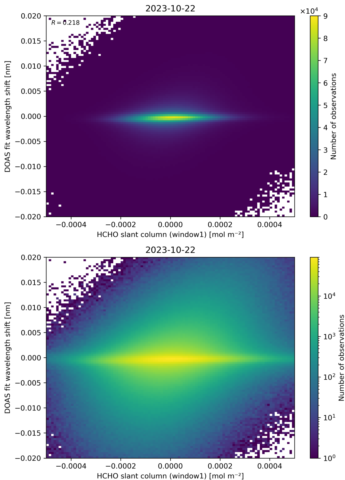
Figure 79: Scatter density plot of “HCHO slant column (window1)” against “DOAS fit wavelength shift” for 2023-10-22 to 2023-10-23.
