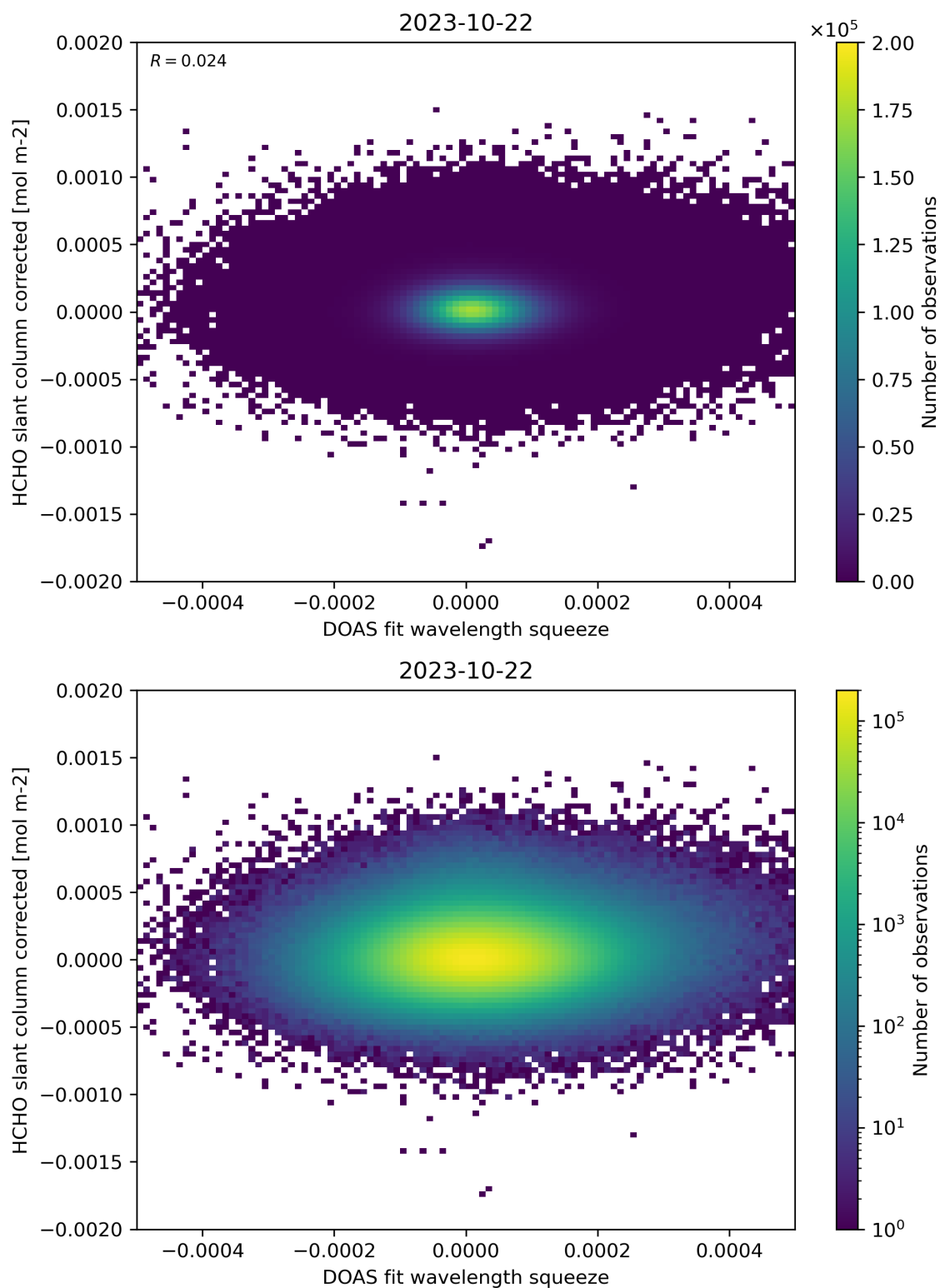
Figure 69: Scatter density plot of “DOAS fit wavelength squeeze” against “HCHO slant column corrected” for 2023-10-22 to 2023-10-23.
