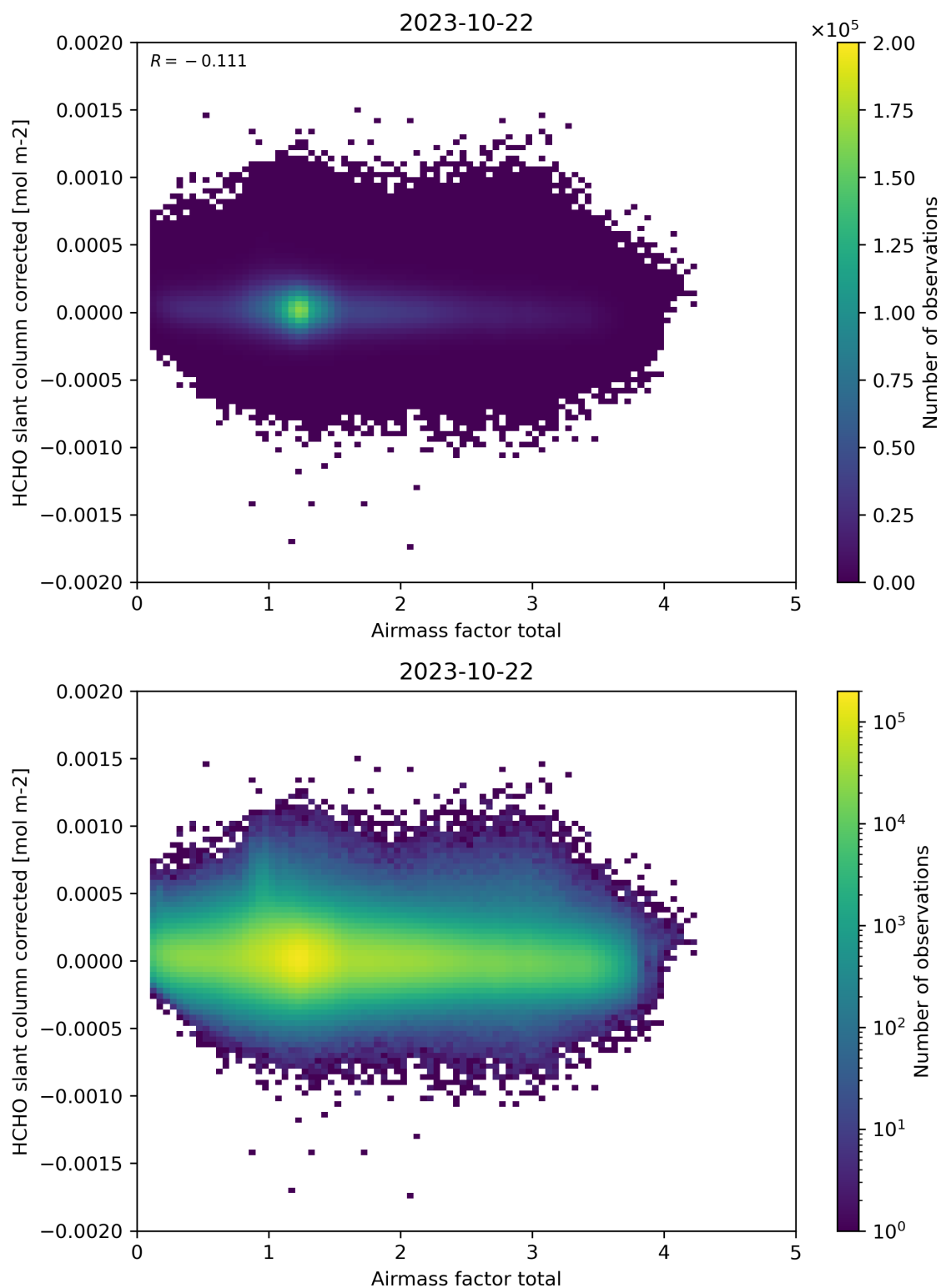
Figure 101: Scatter density plot of “Airmass factor total” against “HCHO slant column corrected” for 2023-10-22 to 2023-10-23.
