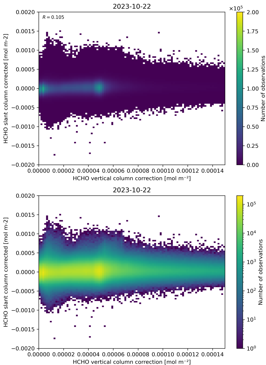
Figure 116: Scatter density plot of “HCHO vertical column correction” against “HCHO slant column corrected” for 2023-10-22 to 2023-10-23.
