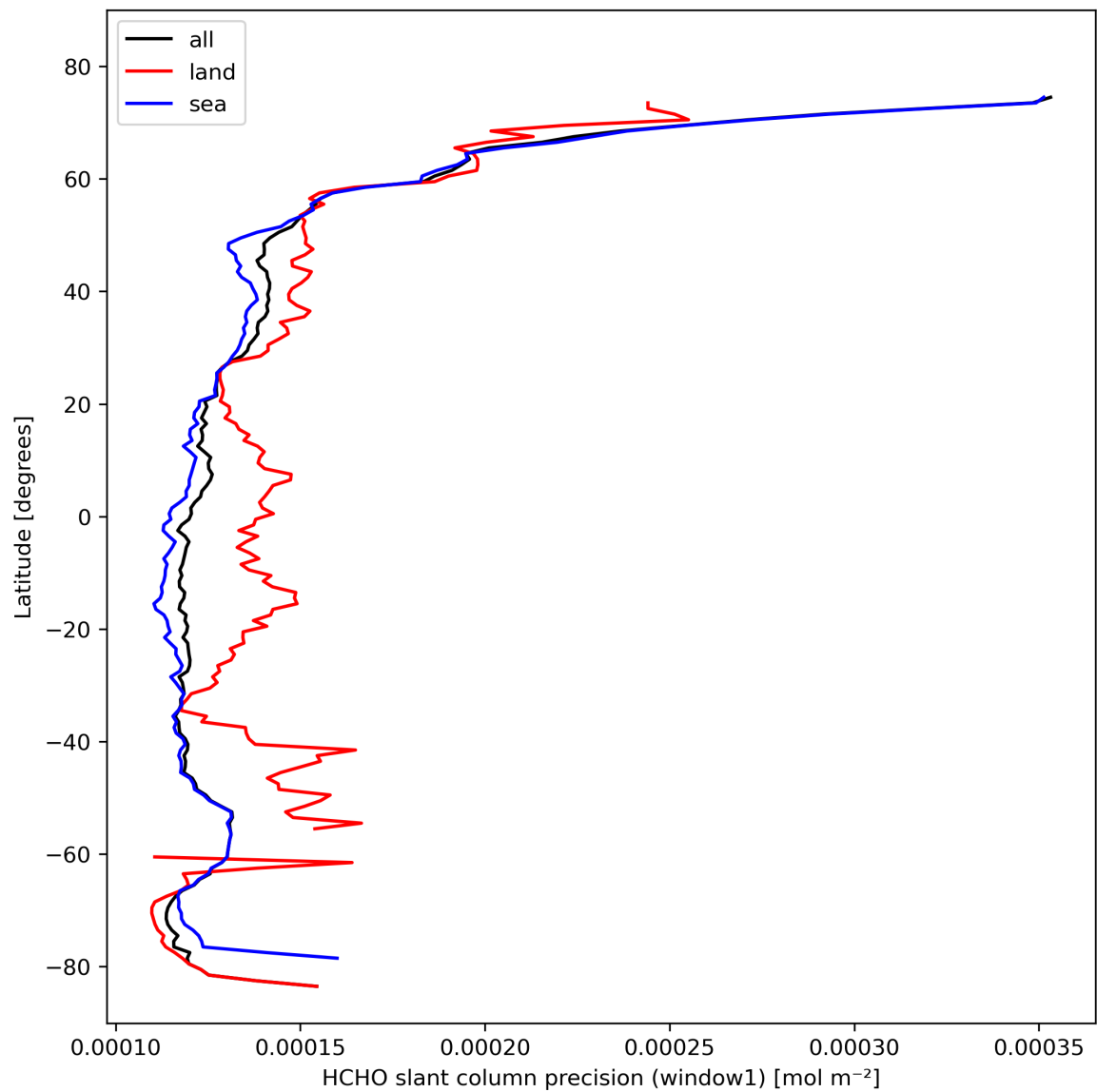
Figure 25: Zonal average of “HCHO slant column precision (window1)” for 2023-10-22 to 2023-10-23.
