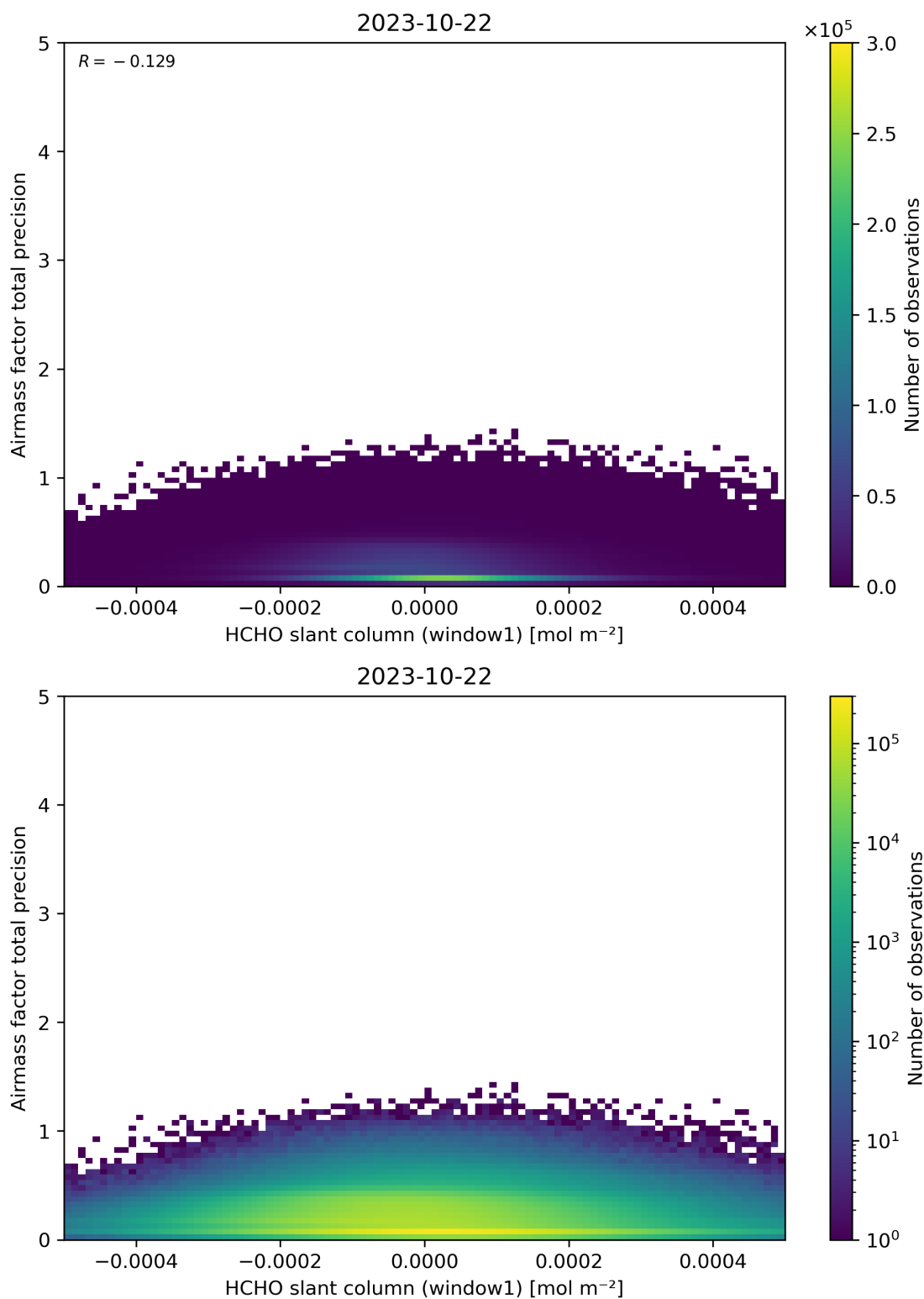
Figure 86: Scatter density plot of “HCHO slant column (window1)” against “Airmass factor total precision” for 2023-10-22 to 2023-10-23.
