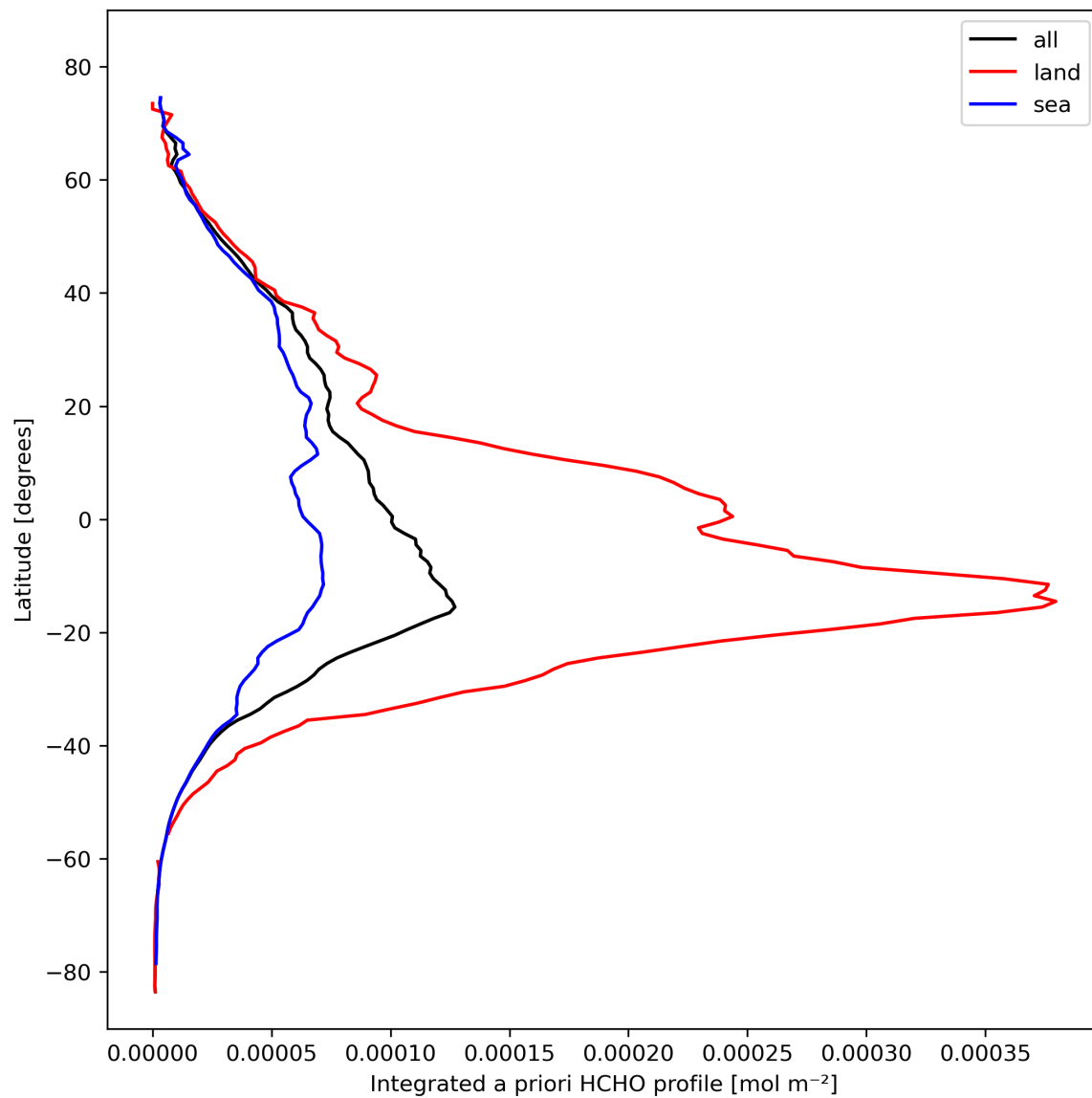
Figure 29: Zonal average of “Integrated a priori HCHO profile” for 2023-10-22 to 2023-10-23.
