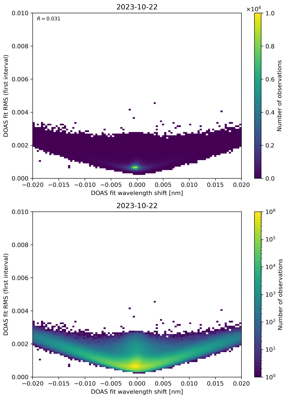
Figure 64: Scatter density plot of “DOAS fit wavelength shift” against “DOAS fit RMS (first interval)” for 2023-10-22 to 2023-10-23.
