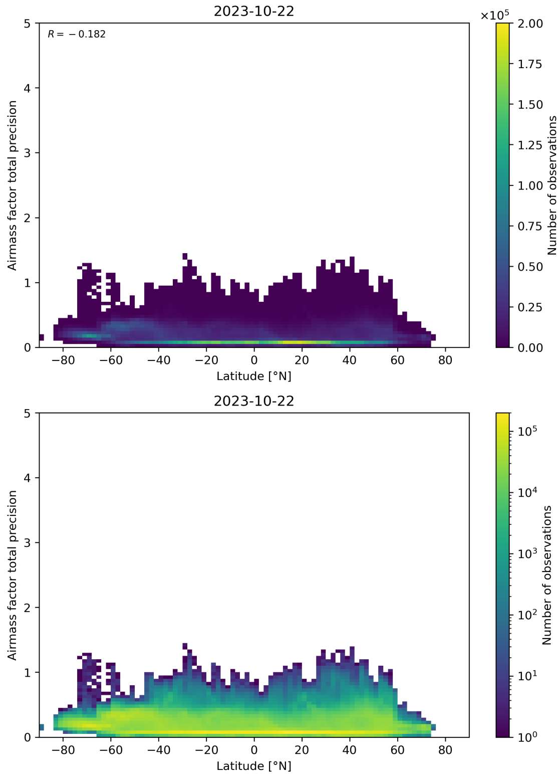
Figure 162: Scatter density plot of “Latitude” against “Airmass factor total precision” for 2023-10-22 to 2023-10-23.
