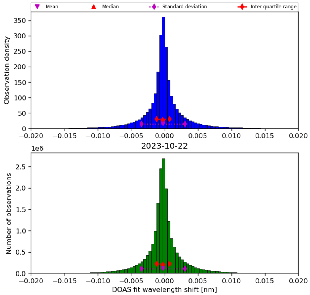
Figure 44: Histogram of “DOAS fit wavelength shift” for 2023-10-22 to 2023-10-23
