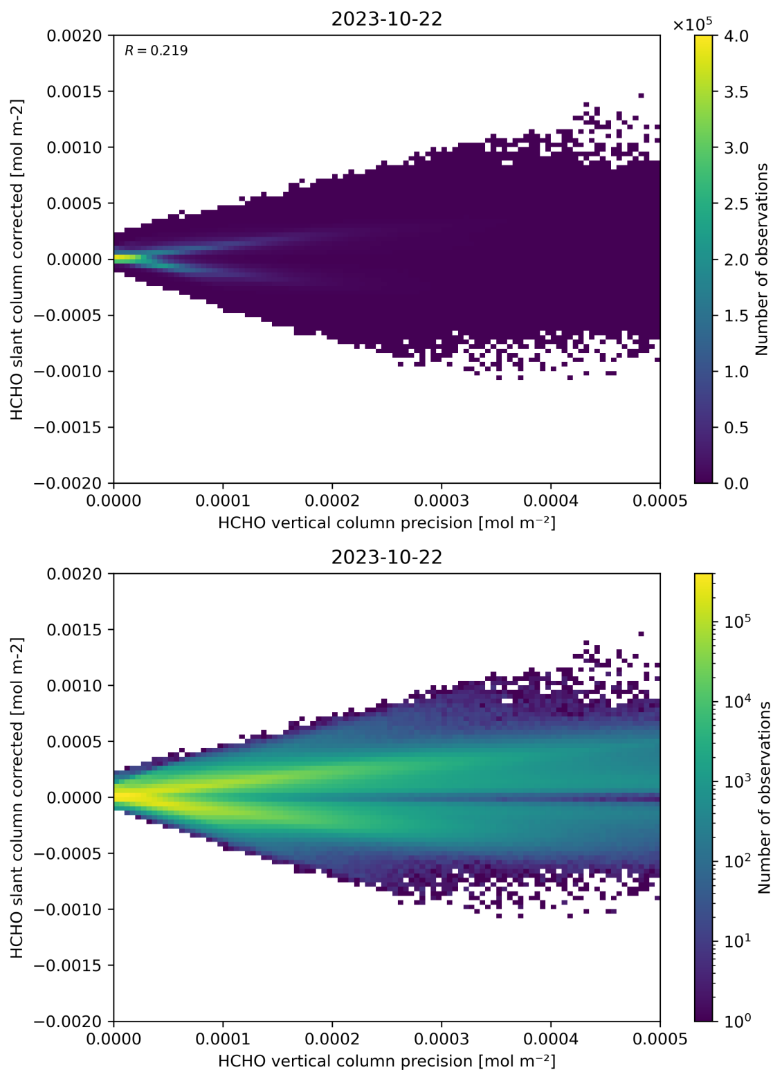
Figure 140: Scatter density plot of “HCHO vertical column precision” against “HCHO slant column corrected” for 2023-10-22 to 2023-10-23.
