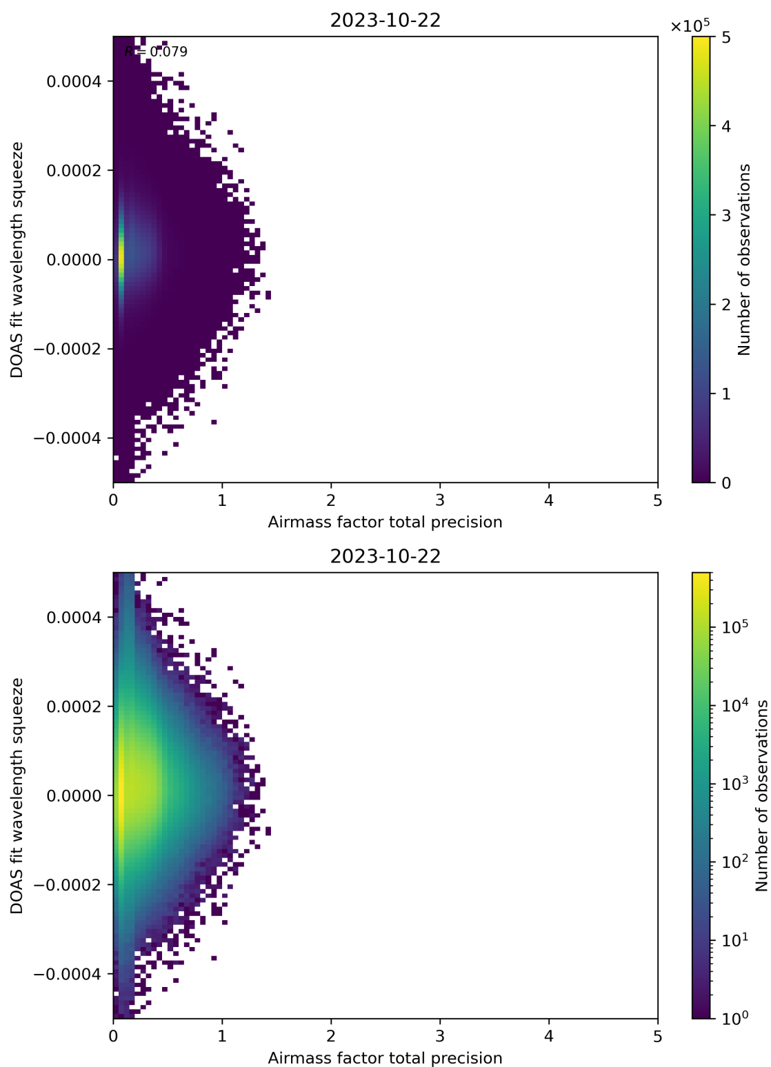
Figure 107: Scatter density plot of “Airmass factor total precision” against “DOAS fit wavelength squeeze” for 2023-10-22 to 2023-10-23.
