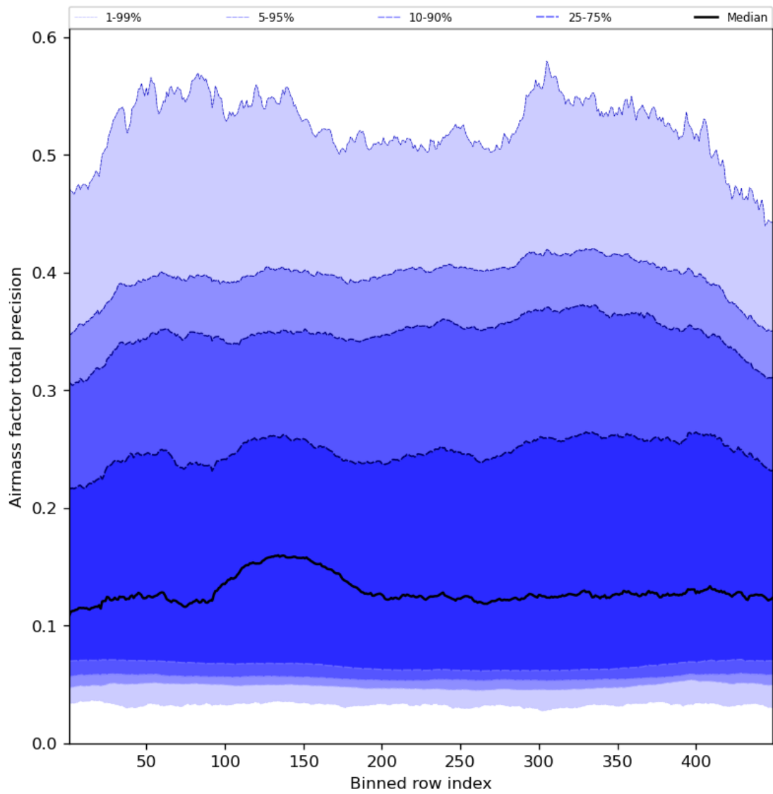
Figure 55: Along track statistics of “Airmass factor total precision” for 2023-10-22 to 2023-10-23
