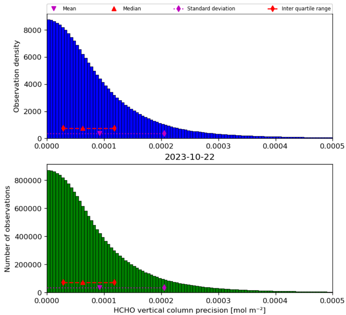
Figure 36: Histogram of “HCHO vertical column precision” for 2023-10-22 to 2023-10-23
