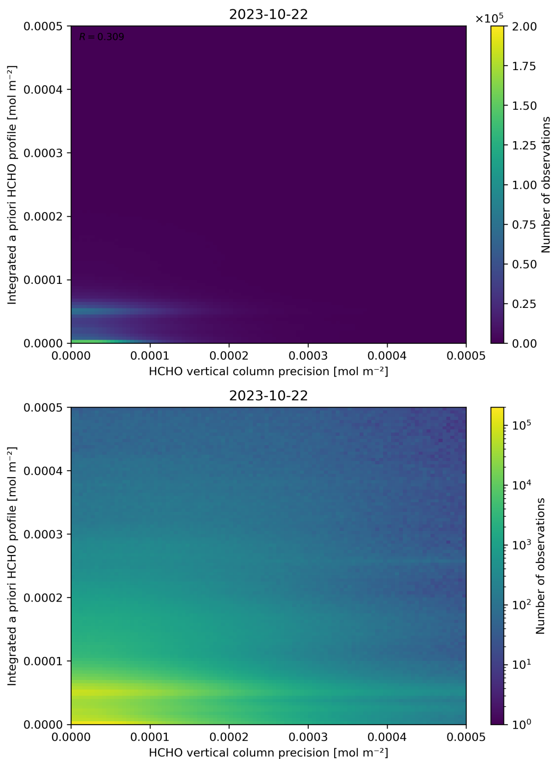
Figure 147: Scatter density plot of “HCHO vertical column precision” against “Integrated a priori HCHO profile” for 2023-10-22 to 2023-10-23.
