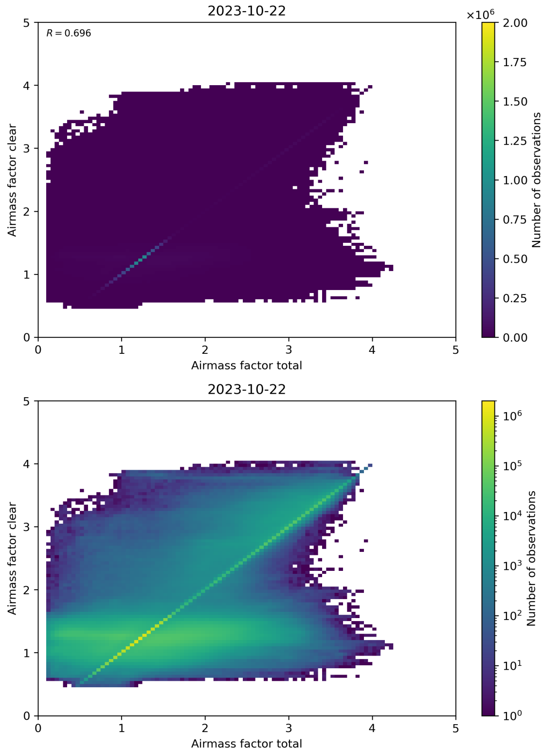
Figure 100: Scatter density plot of “Airmass factor total” against “Airmass factor clear” for 2023-10-22 to 2023-10-23.
