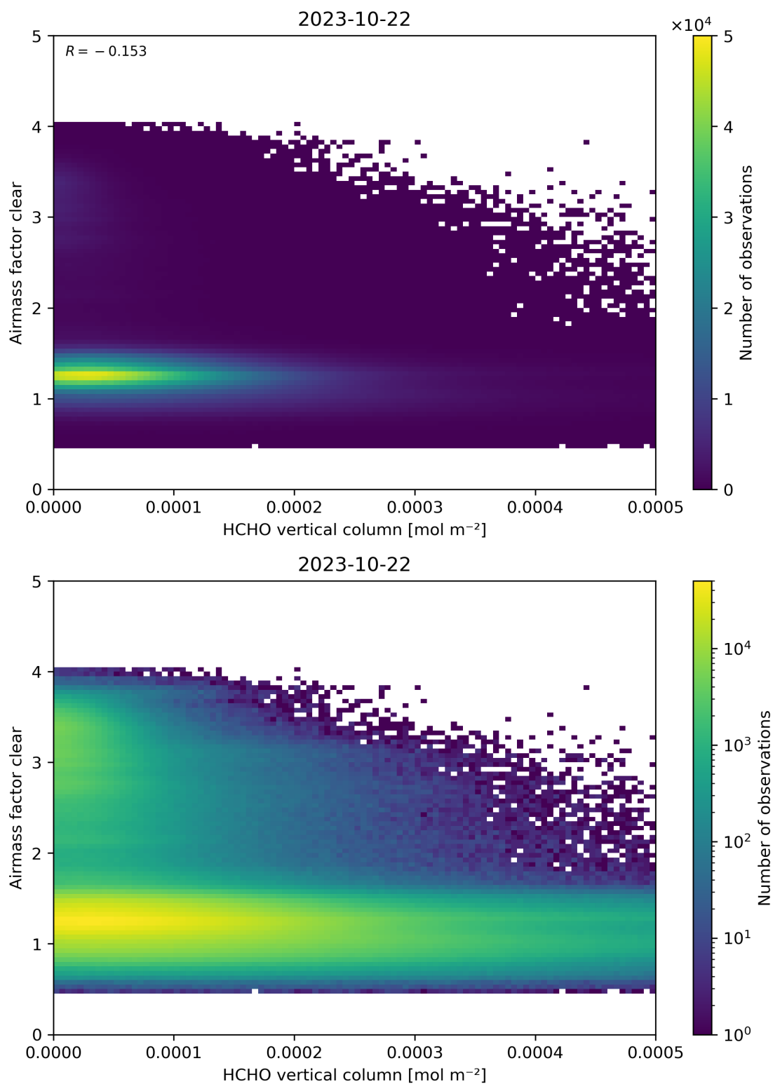
Figure 126: Scatter density plot of “HCHO vertical column” against “Airmass factor clear” for 2023-10-22 to 2023-10-23.
