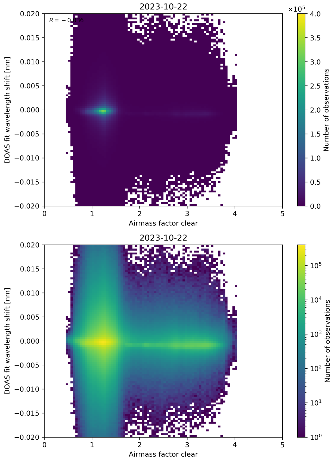
Figure 72: Scatter density plot of “Airmass factor clear” against “DOAS fit wavelength shift” for 2023-10-22 to 2023-10-23.
