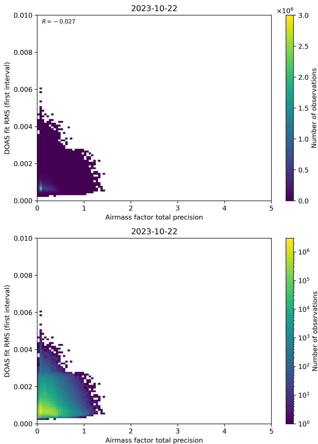
Figure 105: Scatter density plot of “Airmass factor total precision” against “DOAS fit RMS (first interval)” for 2023-10-22 to 2023-10-23.
