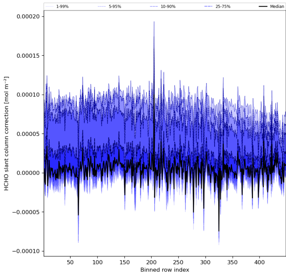
Figure 61: Along track statistics of “HCHO slant column correction” for 2023-10-22 to 2023-10-23
