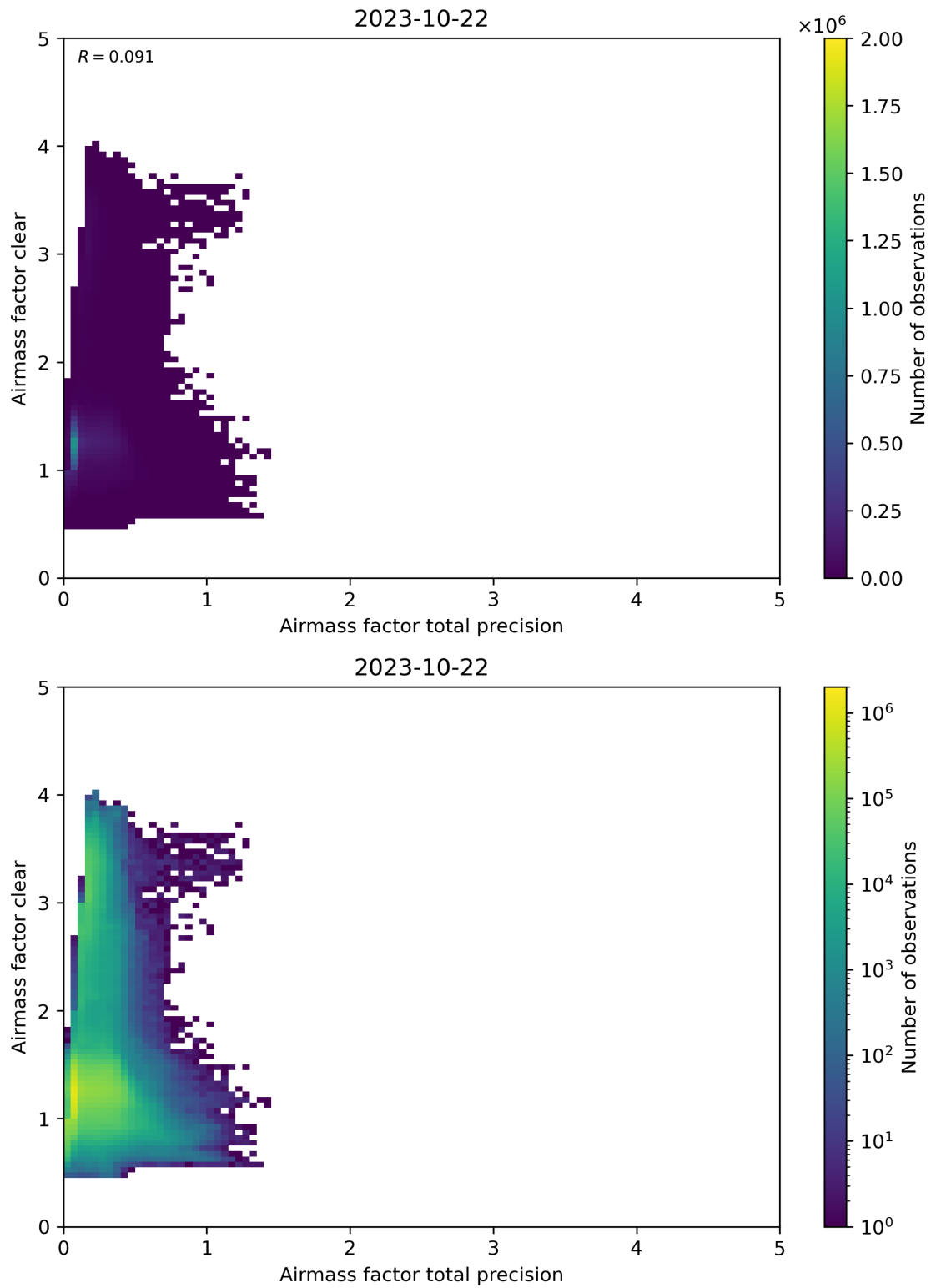
Figure 108: Scatter density plot of “Airmass factor total precision” against “Airmass factor clear” for 2023-10-22 to 2023-10-23.
