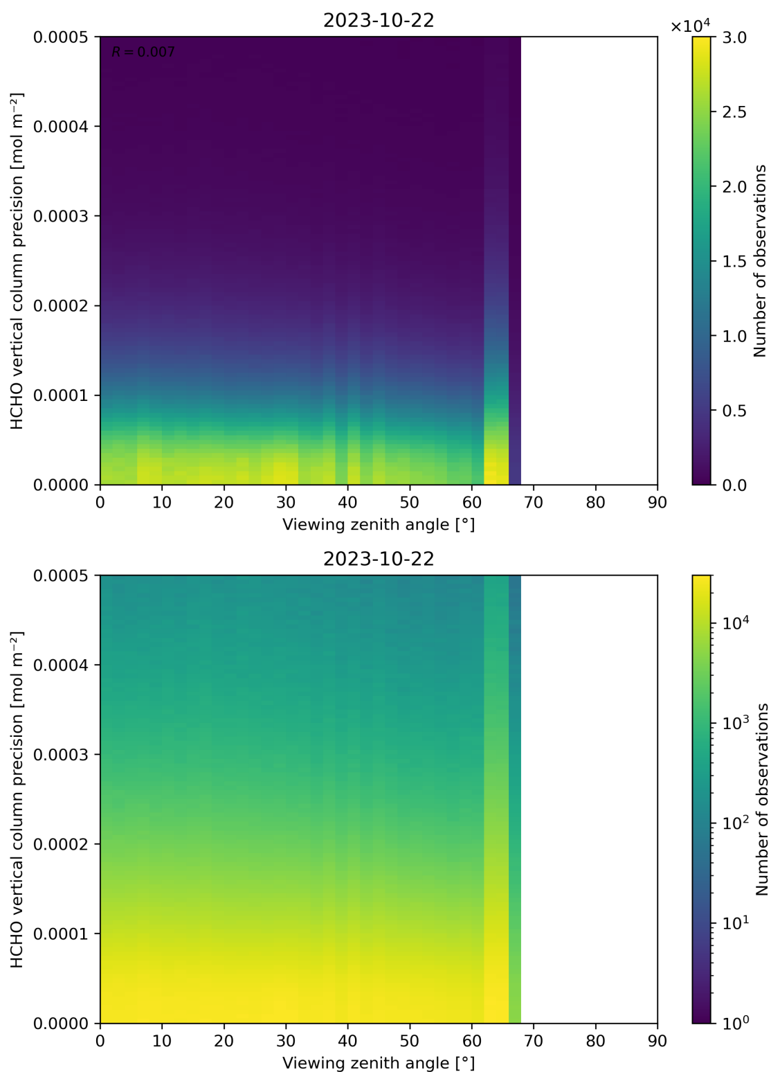
Figure 194: Scatter density plot of “Viewing zenith angle” against “HCHO vertical column precision” for 2023-10-22 to 2023-10-23.
