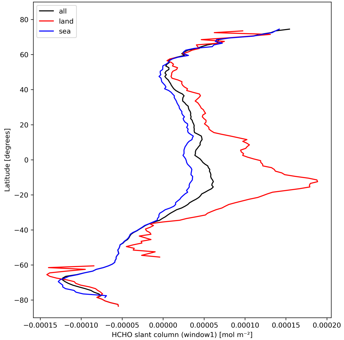
Figure 24: Zonal average of “HCHO slant column (window1)” for 2023-10-22 to 2023-10-23.
