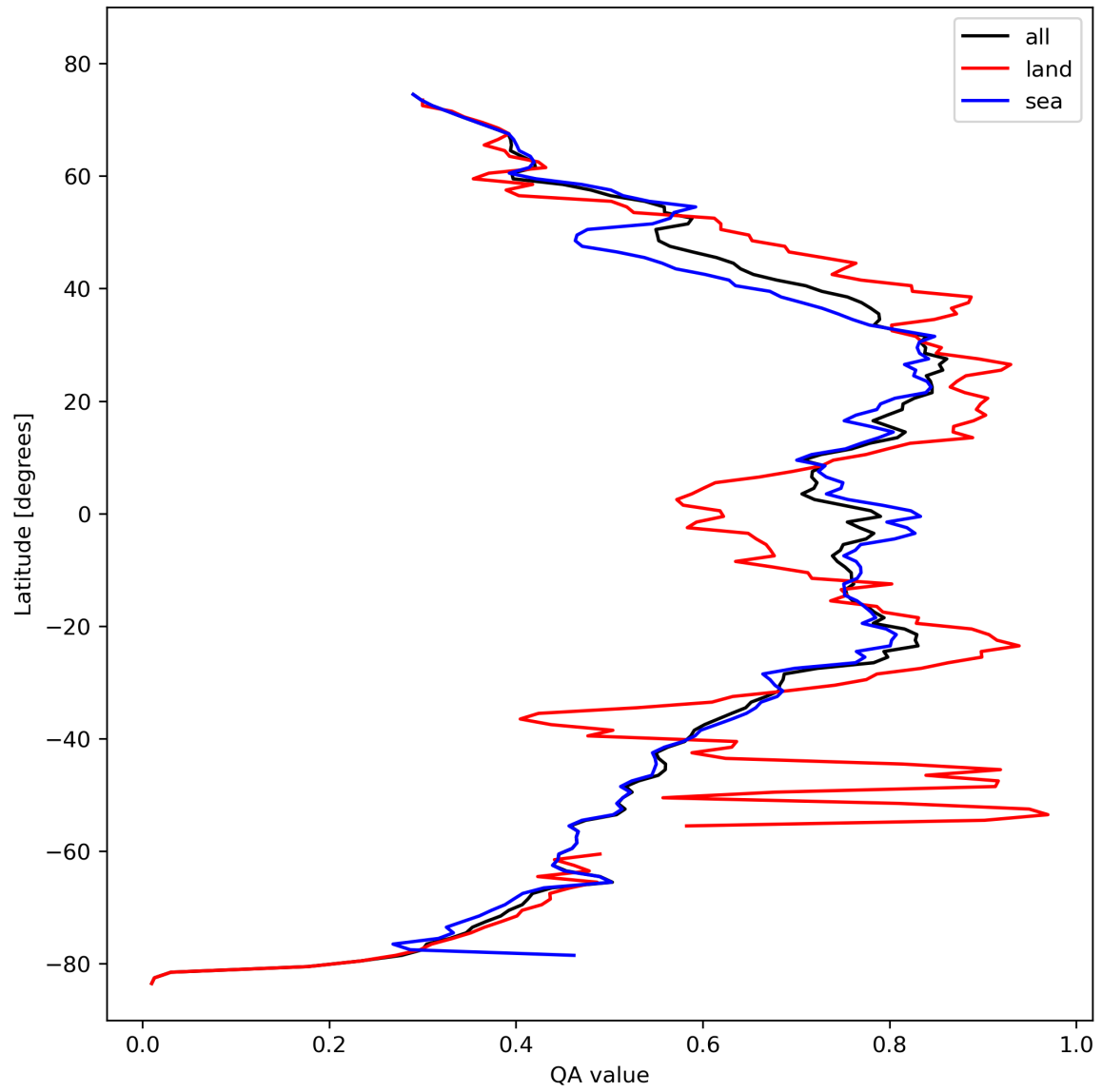
Figure 20: Zonal average of “QA value” for 2023-10-22 to 2023-10-23.
