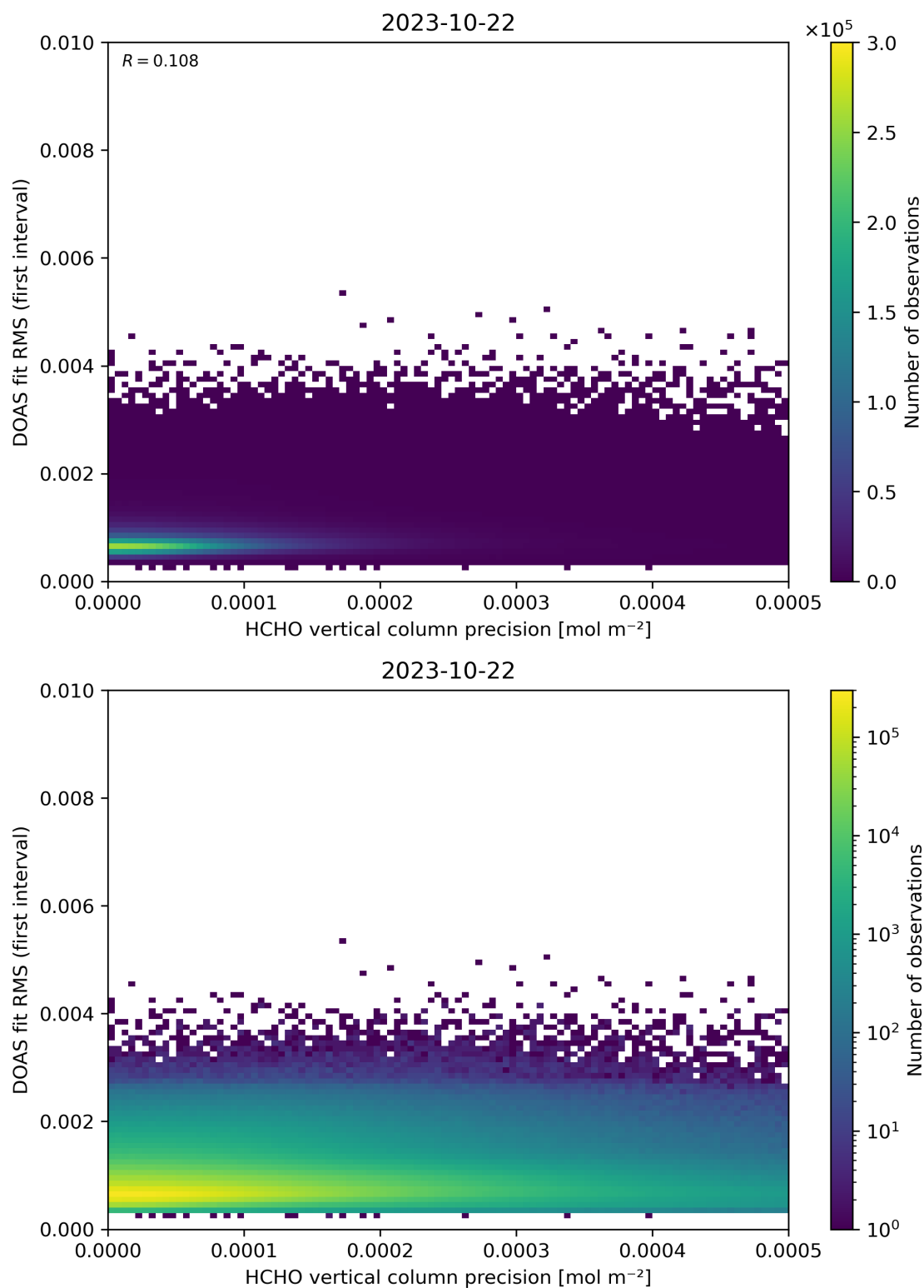
Figure 136: Scatter density plot of “HCHO vertical column precision” against “DOAS fit RMS (first interval)” for 2023-10-22 to 2023-10-23.
