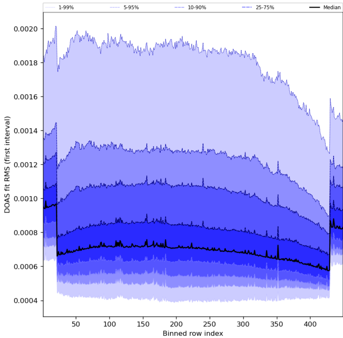
Figure 60: Along track statistics of “DOAS fit RMS (first interval)” for 2023-10-22 to 2023-10-23
