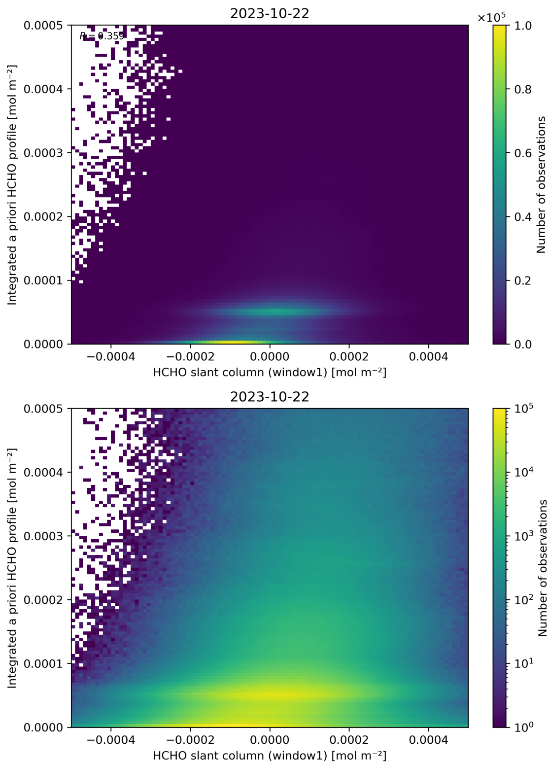
Figure 87: Scatter density plot of “HCHO slant column (window1)” against “Integrated a priori HCHO profile” for 2023-10-22 to 2023-10-23.
