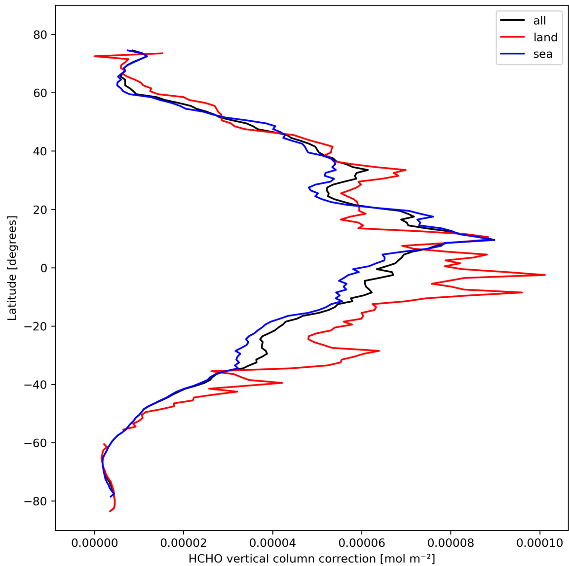
Figure 23: Zonal average of “HCHO vertical column correction” for 2023-10-22 to 2023-10-23.
