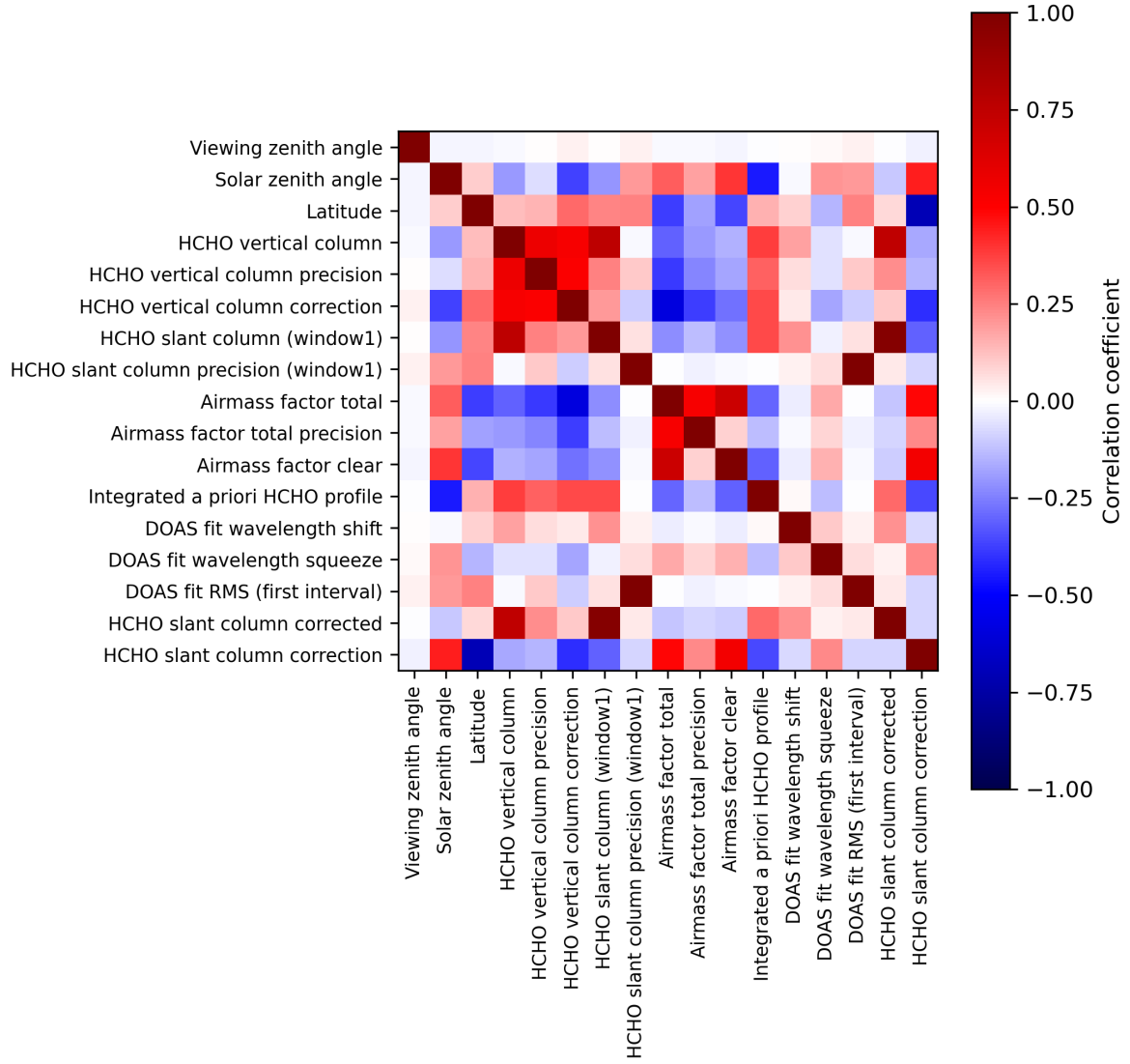
Figure 2: Map of correlation matrix for 2023-10-22 to 2023-10-23.
