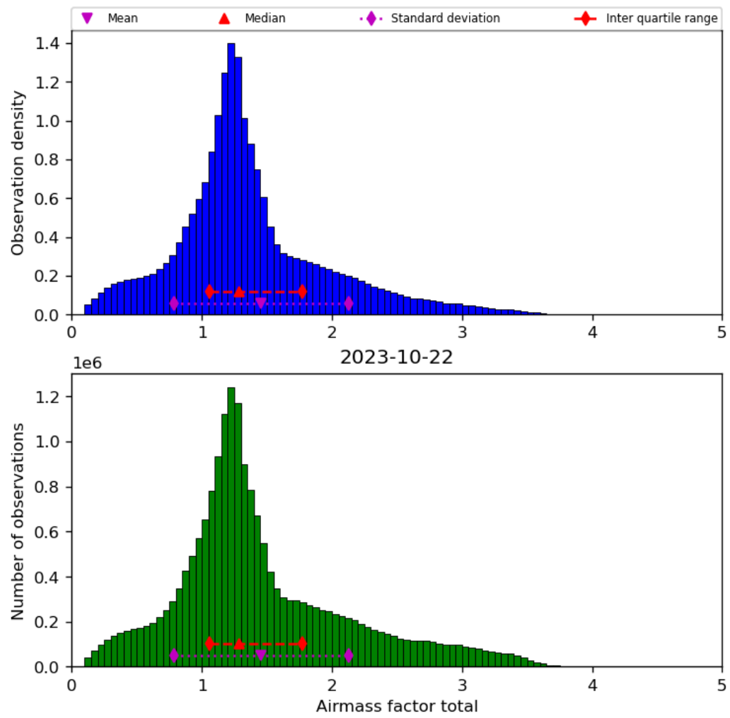
Figure 40: Histogram of “Airmass factor total” for 2023-10-22 to 2023-10-23
