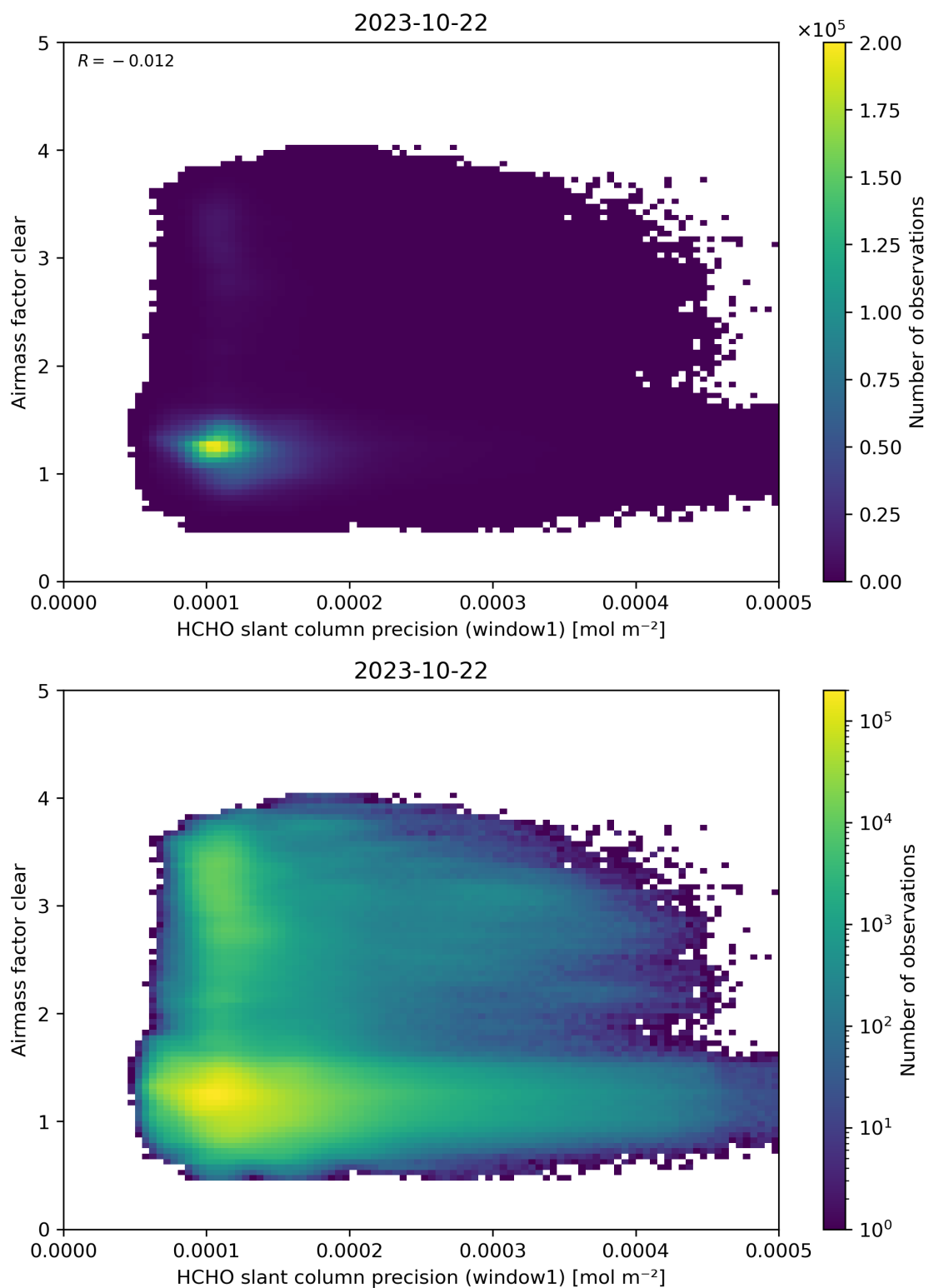
Figure 91: Scatter density plot of “HCHO slant column precision (window1)” against “Airmass factor clear” for 2023-10-22 to 2023-10-23.
