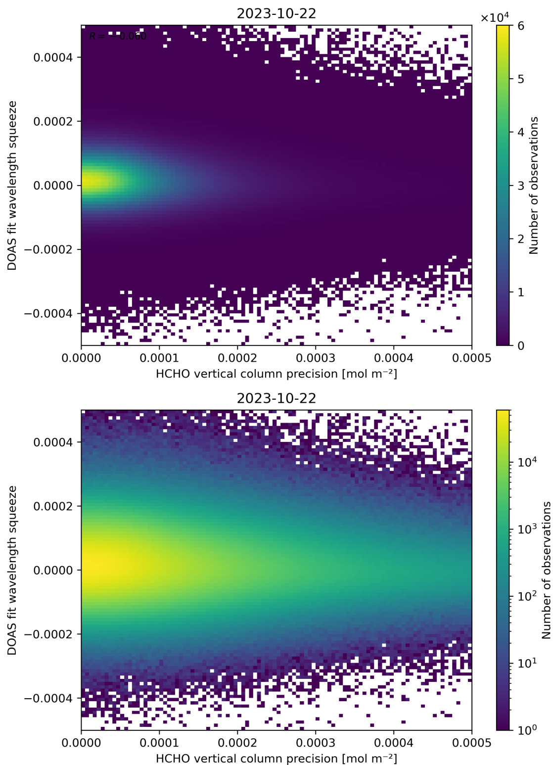
Figure 138: Scatter density plot of “HCHO vertical column precision” against “DOAS fit wavelength squeeze” for 2023-10-22 to 2023-10-23.
