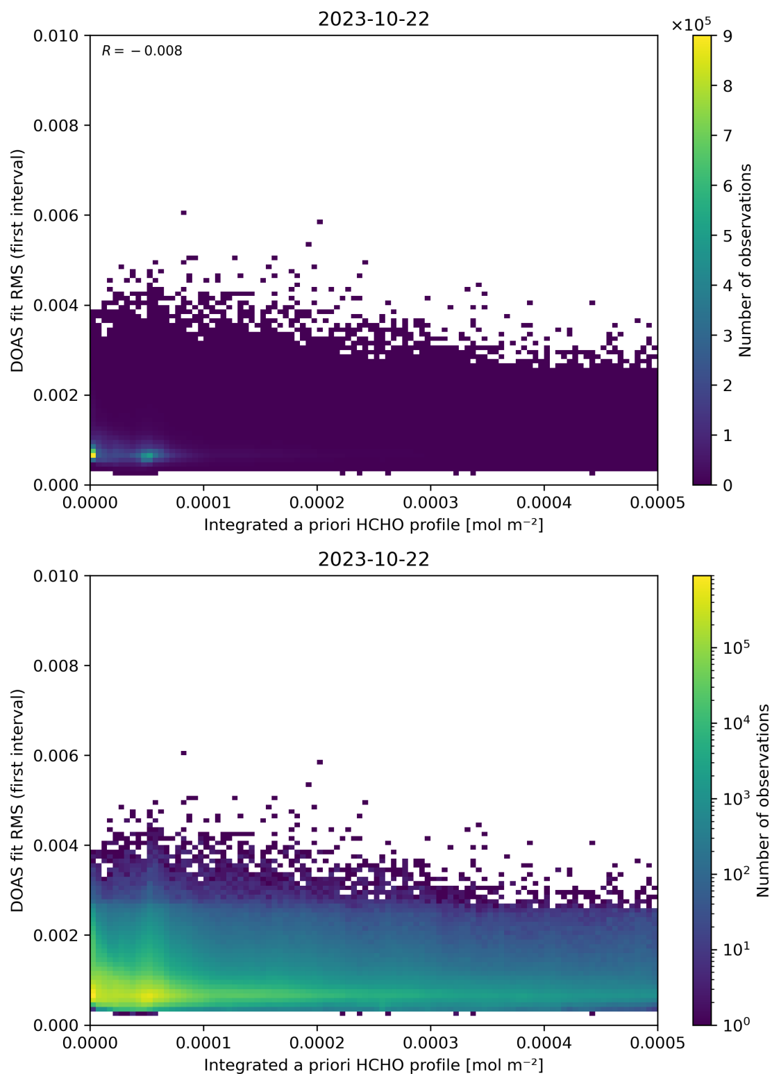
Figure 148: Scatter density plot of “Integrated a priori HCHO profile” against “DOAS fit RMS (first interval)” for 2023-10-22 to 2023-10-23.
