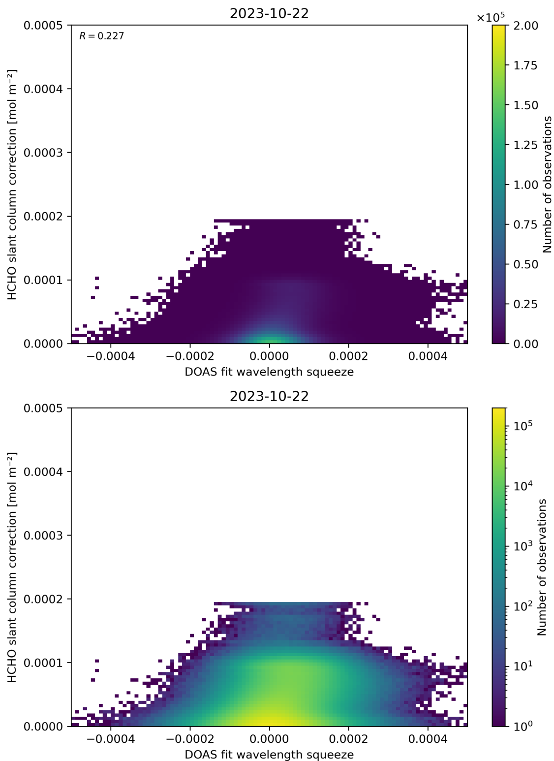
Figure 70: Scatter density plot of “DOAS fit wavelength squeeze” against “HCHO slant column correction” for 2023-10-22 to 2023-10-23.
