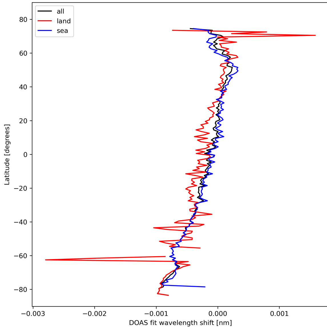
Figure 30: Zonal average of “DOAS fit wavelength shift” for 2023-10-22 to 2023-10-23.
