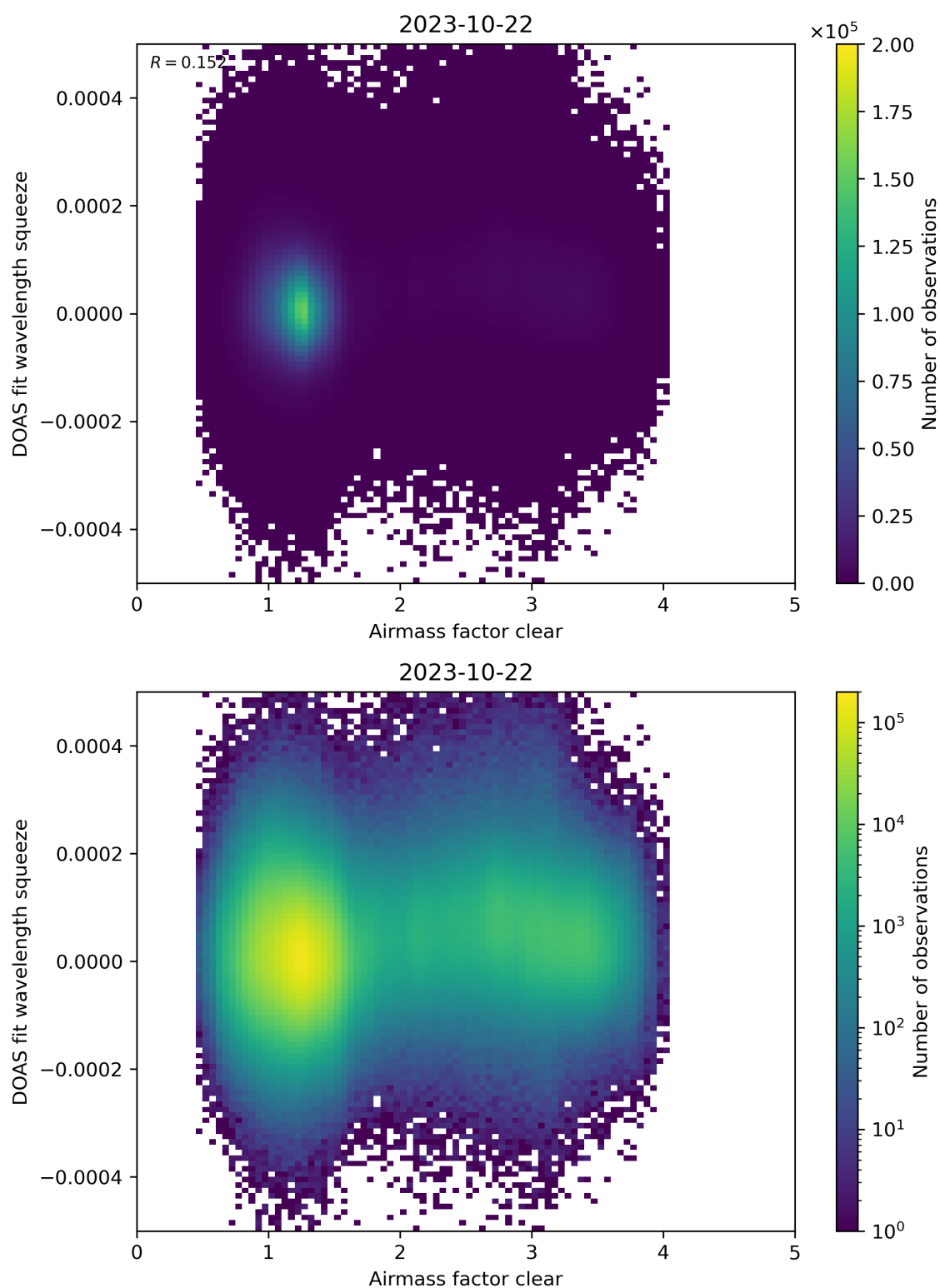
Figure 73: Scatter density plot of “Airmass factor clear” against “DOAS fit wavelength squeeze” for 2023-10-22 to 2023-10-23.
