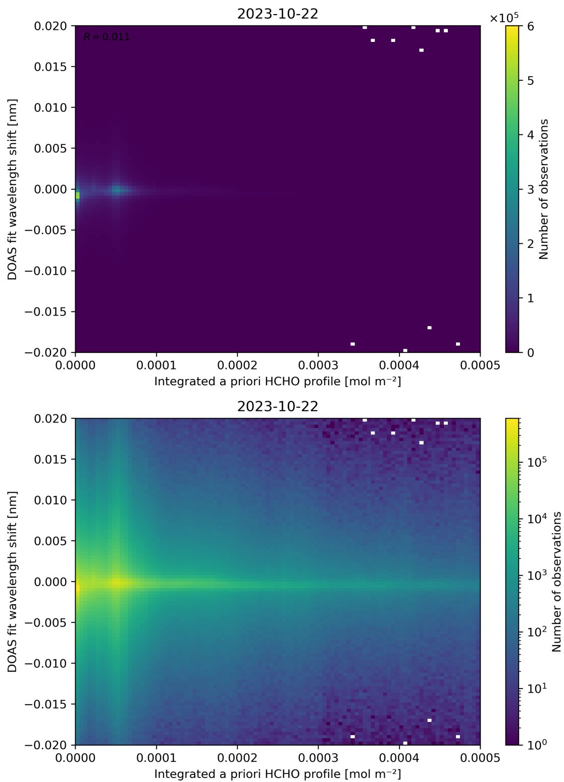
Figure 149: Scatter density plot of “Integrated a priori HCHO profile” against “DOAS fit wavelength shift” for 2023-10-22 to 2023-10-23.
