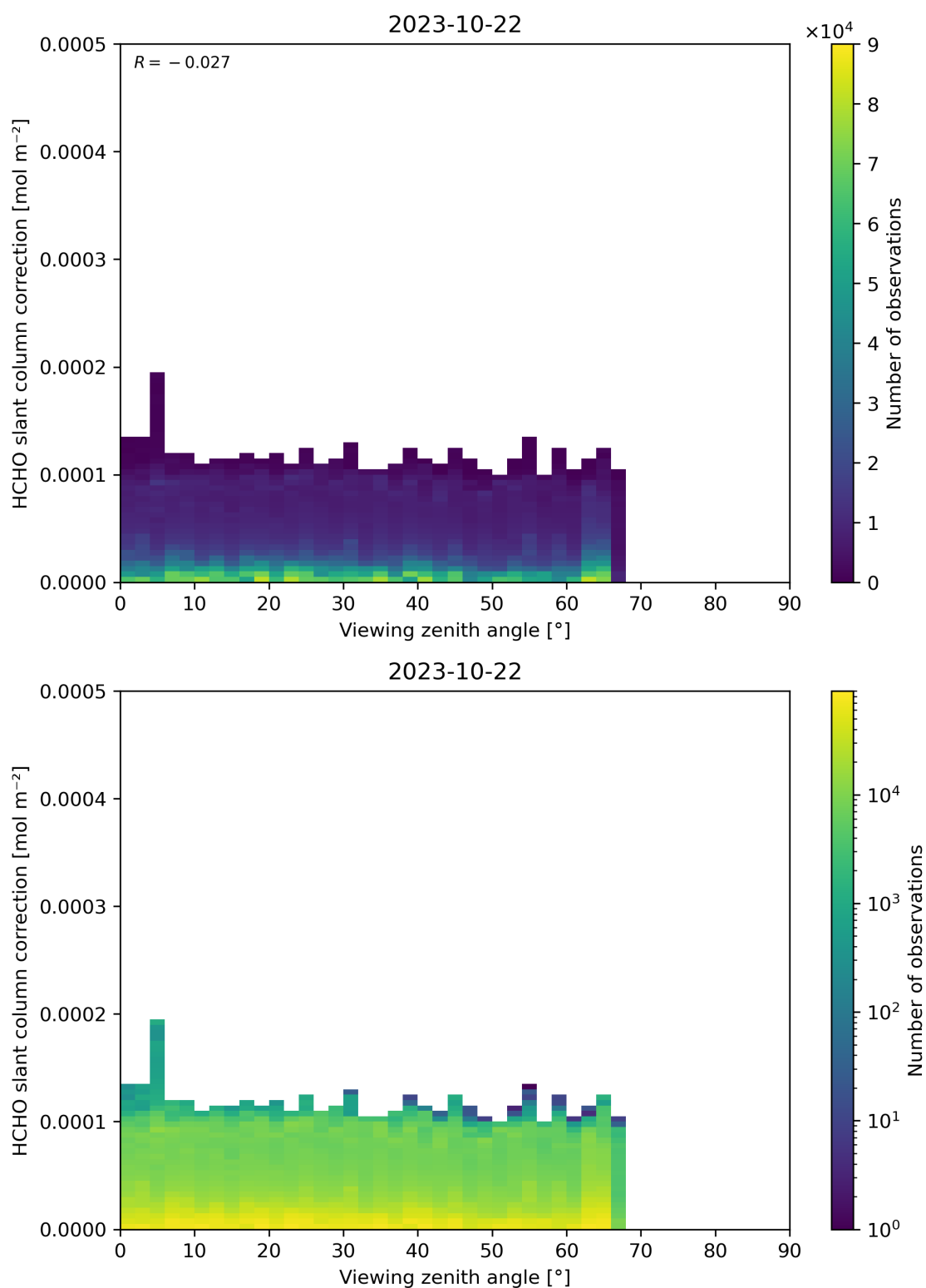
Figure 187: Scatter density plot of “Viewing zenith angle” against “HCHO slant column correction” for 2023-10-22 to 2023-10-23.
