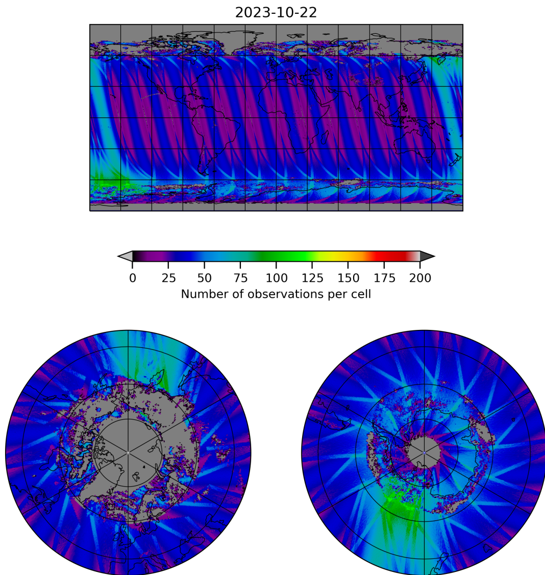
Figure 19: Map of the number of observations for 2023-10-22 to 2023-10-23
