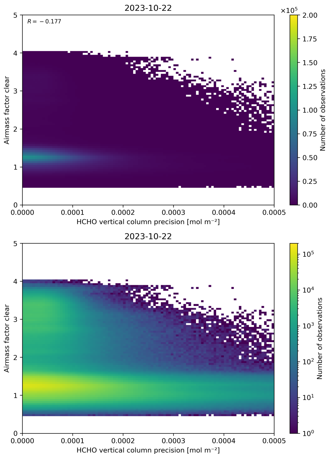
Figure 139: Scatter density plot of “HCHO vertical column precision” against “Airmass factor clear” for 2023-10-22 to 2023-10-23.
