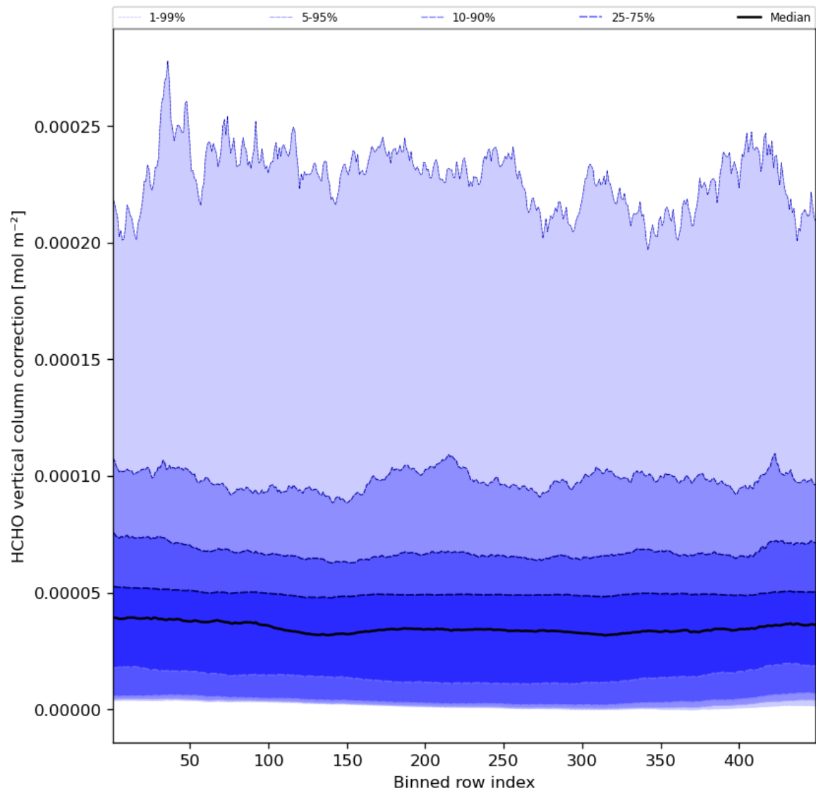
Figure 51: Along track statistics of “HCHO vertical column correction” for 2023-10-22 to 2023-10-23
