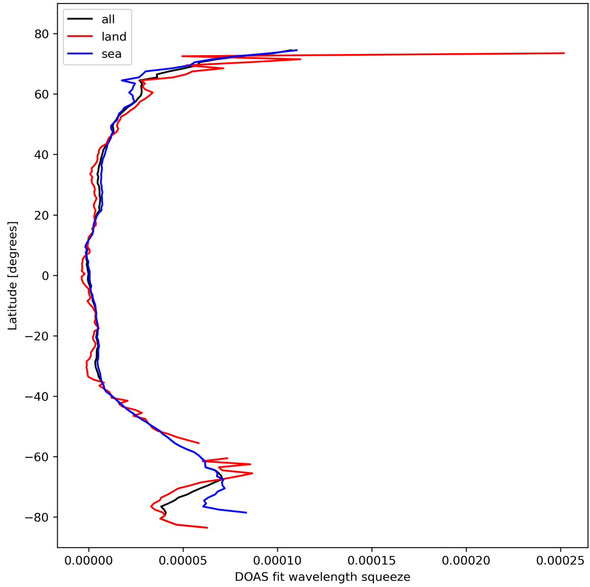
Figure 31: Zonal average of “DOAS fit wavelength squeeze” for 2023-10-22 to 2023-10-23.
