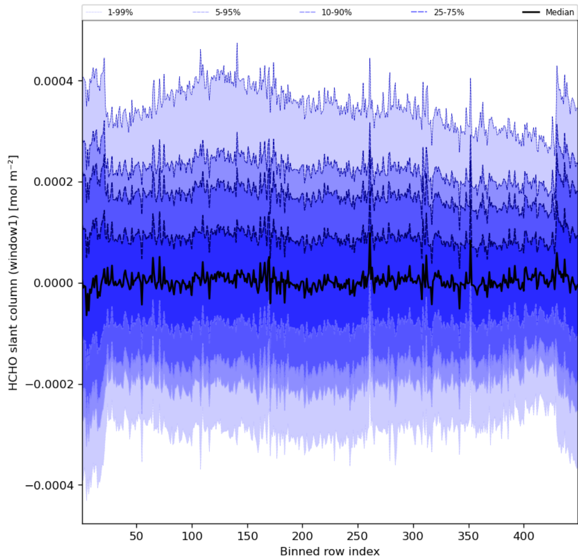
Figure 52: Along track statistics of “HCHO slant column (window1)” for 2023-10-22 to 2023-10-23
