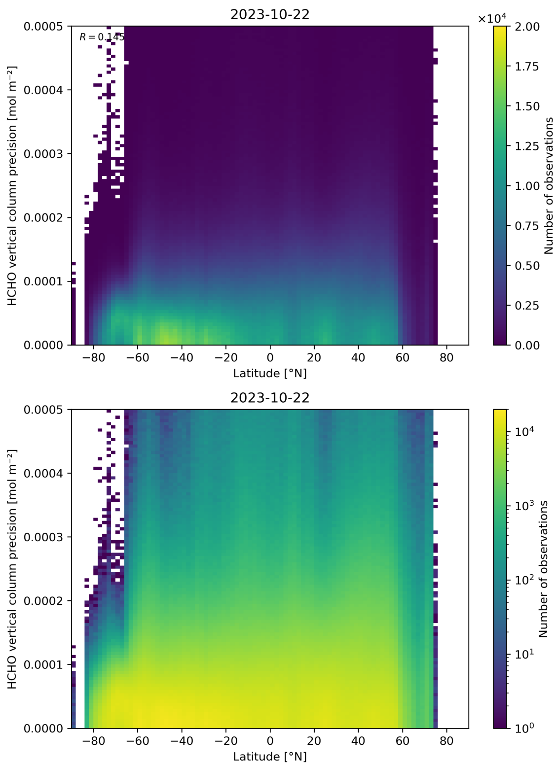
Figure 165: Scatter density plot of “Latitude” against “HCHO vertical column precision” for 2023-10-22 to 2023-10-23.
