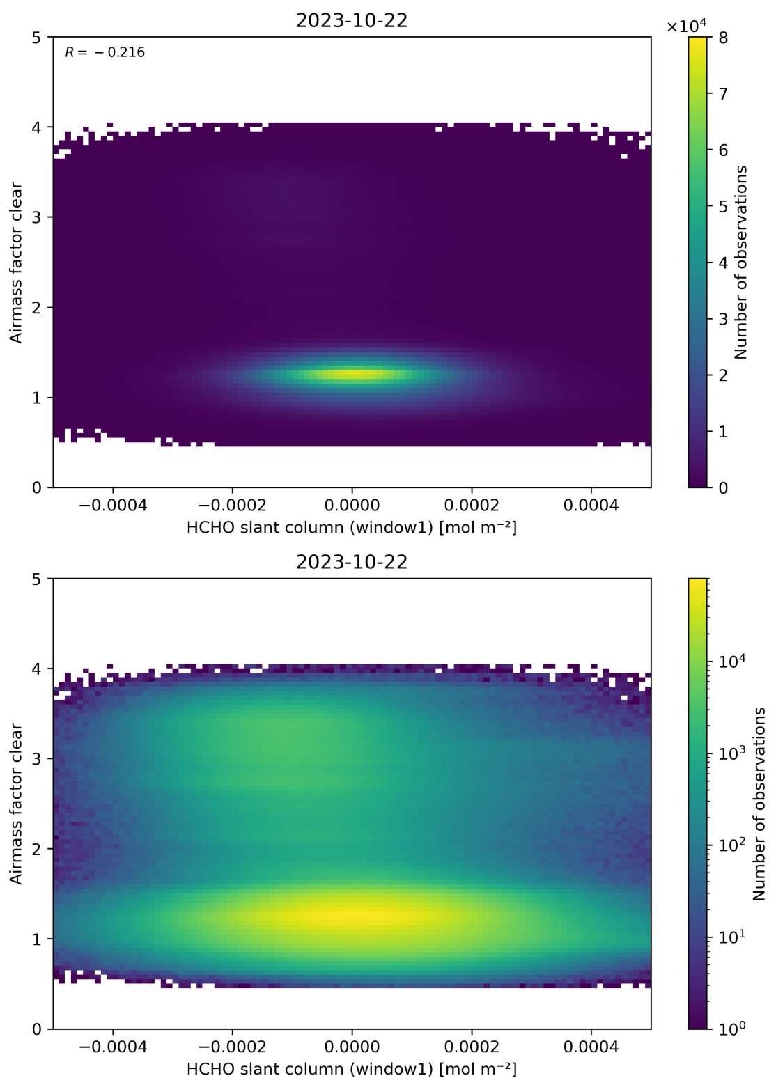
Figure 81: Scatter density plot of “HCHO slant column (window1)” against “Airmass factor clear” for 2023-10-22 to 2023-10-23.
