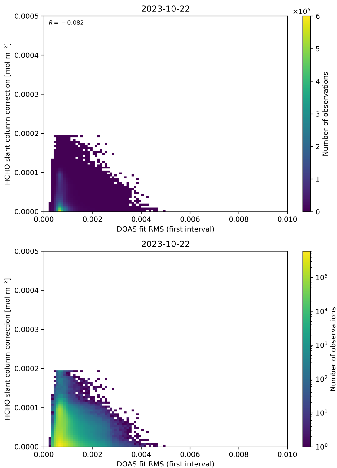
Figure 63: Scatter density plot of “DOAS fit RMS (first interval)” against “HCHO slant column correction” for 2023-10-22 to 2023-10-23.
