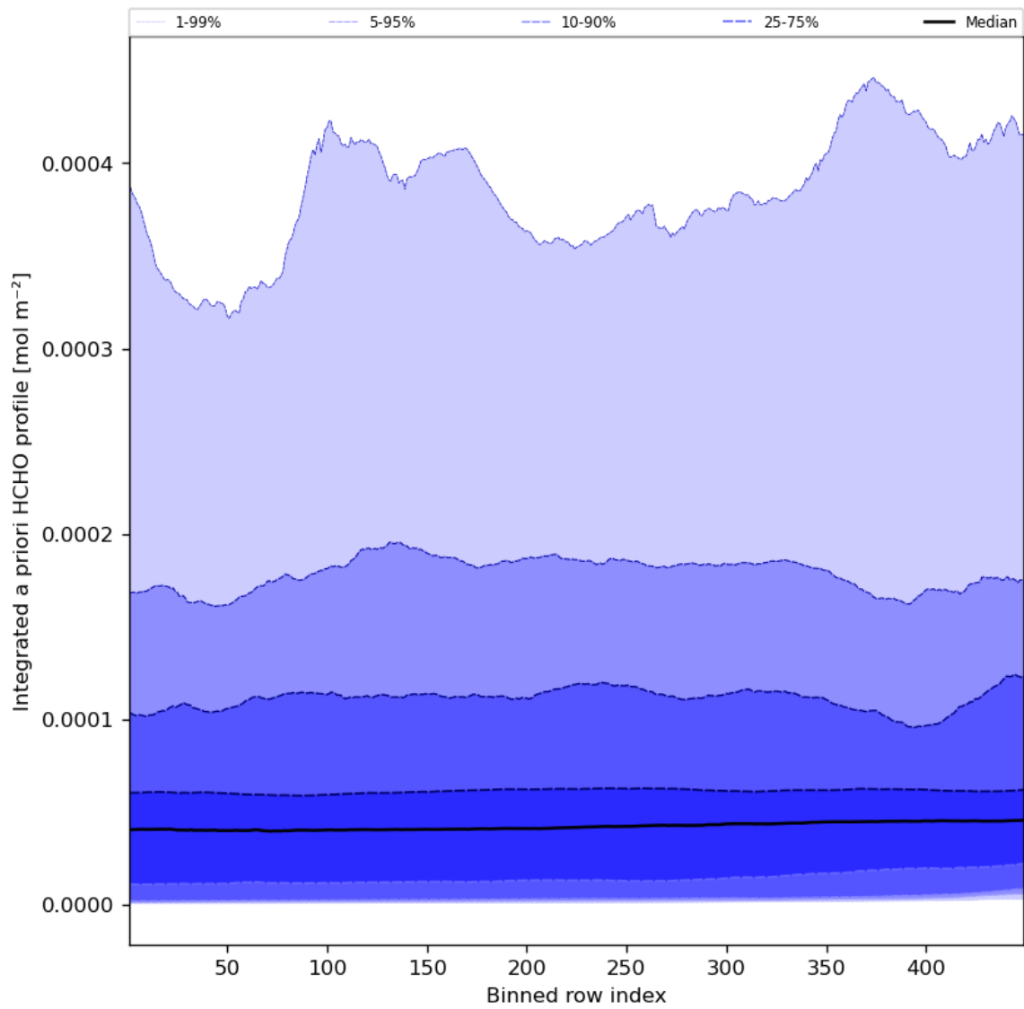
Figure 57: Along track statistics of “Integrated a priori HCHO profile” for 2023-10-22 to 2023-10-23
