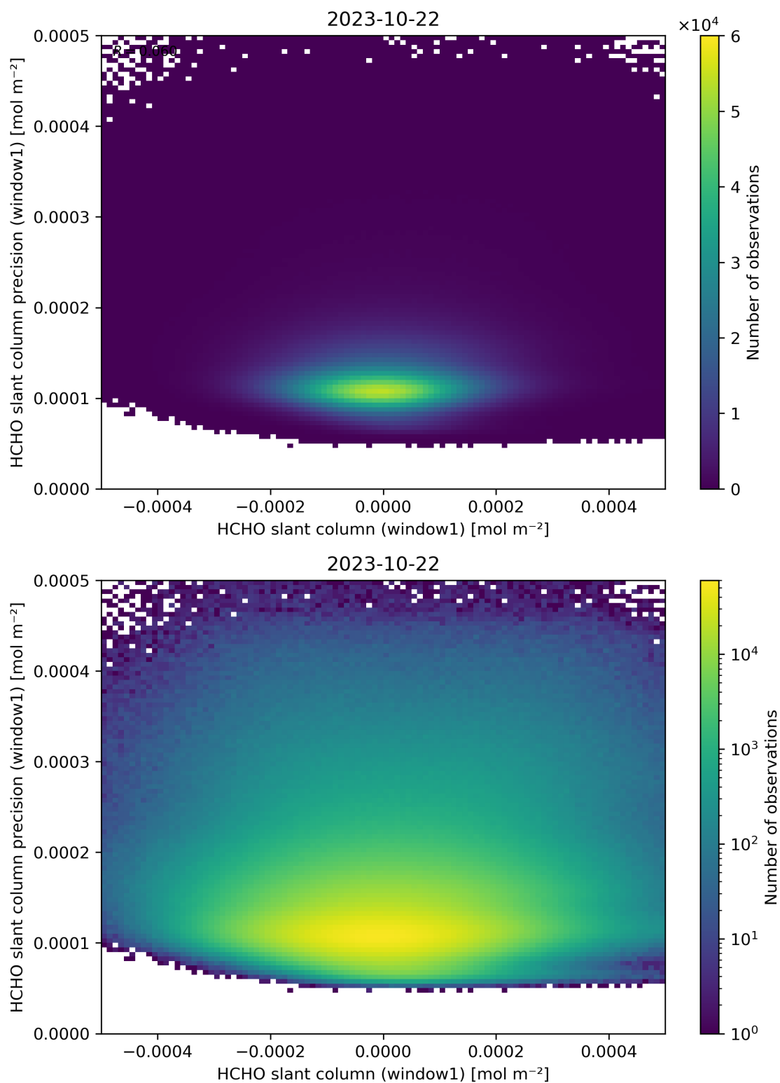
Figure 84: Scatter density plot of “HCHO slant column (window1)” against “HCHO slant column precision (window1)” for 2023-10-22 to 2023-10-23.
