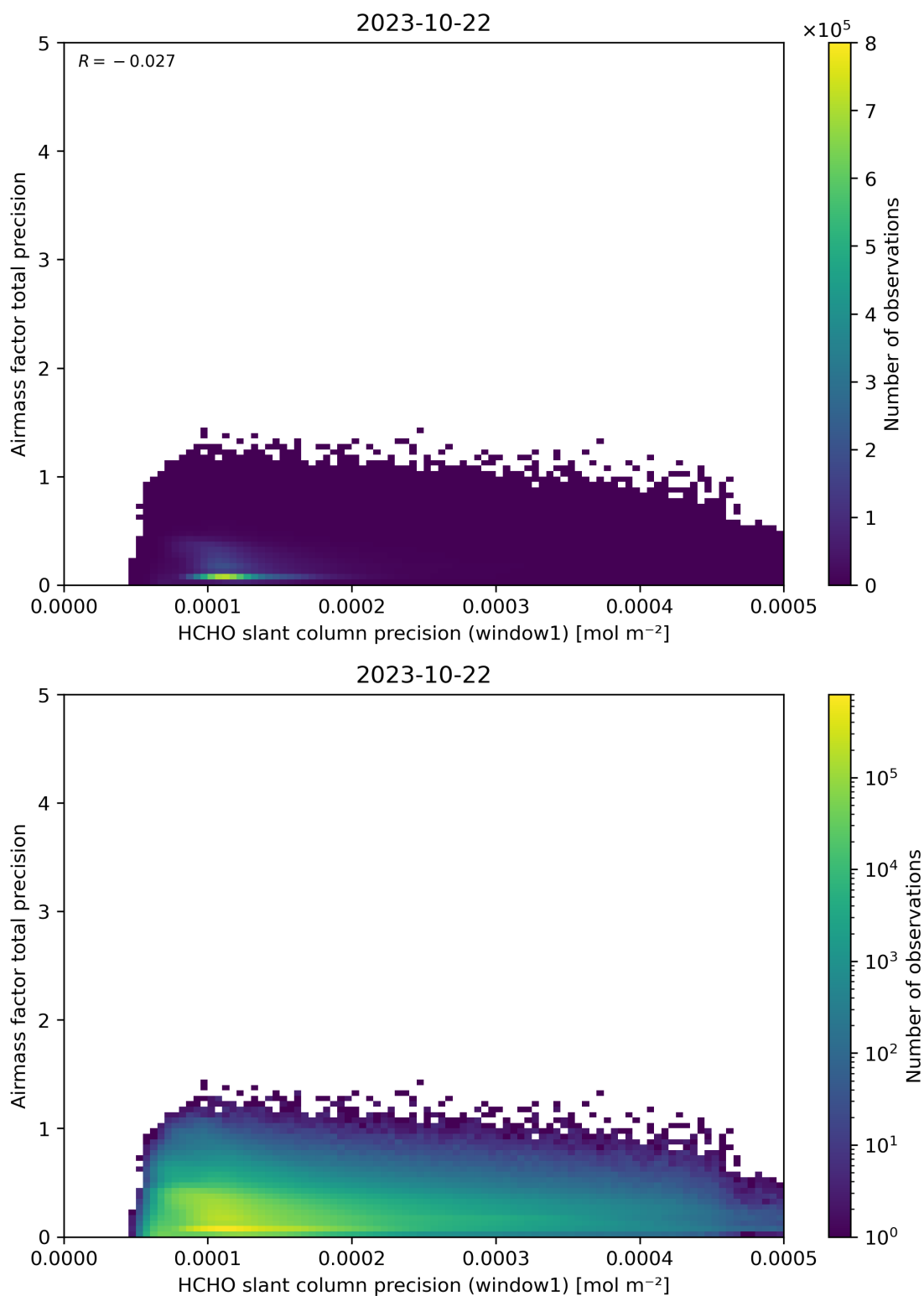
Figure 95: Scatter density plot of “HCHO slant column precision (window1)” against “Airmass factor total precision” for 2023-10-22 to 2023-10-23.
