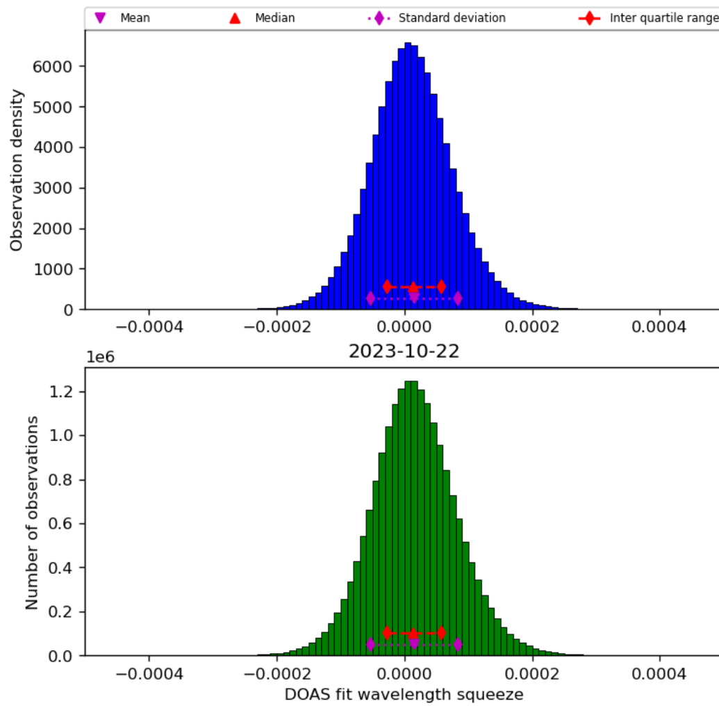
Figure 45: Histogram of “DOAS fit wavelength squeeze” for 2023-10-22 to 2023-10-23
