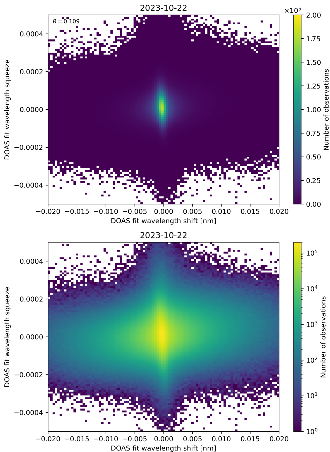
Figure 65: Scatter density plot of “DOAS fit wavelength shift” against “DOAS fit wavelength squeeze” for 2023-10-22 to 2023-10-23.
