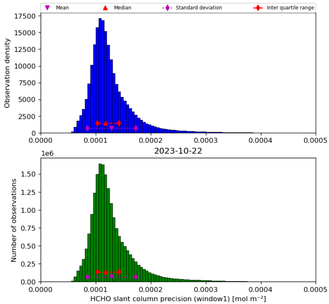
Figure 39: Histogram of “HCHO slant column precision (window1)” for 2023-10-22 to 2023-10-23
