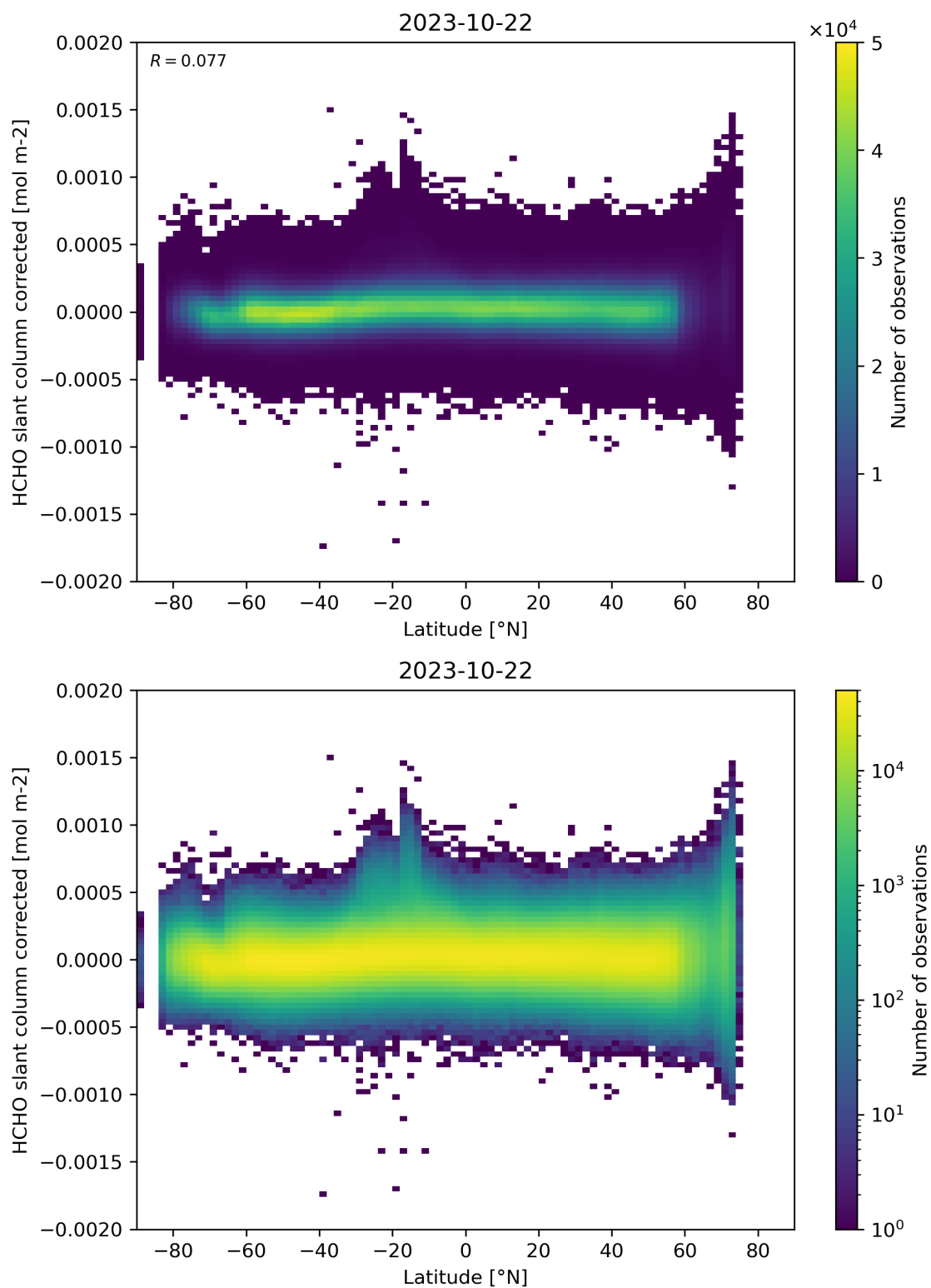
Figure 157: Scatter density plot of “Latitude” against “HCHO slant column corrected” for 2023-10-22 to 2023-10-23.
