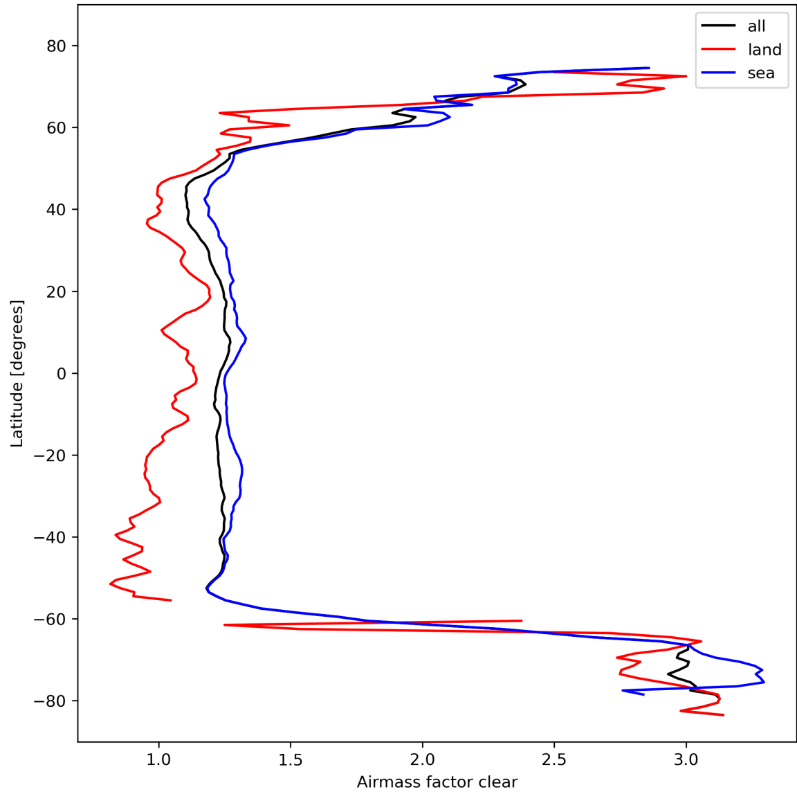
Figure 28: Zonal average of “Airmass factor clear” for 2023-10-22 to 2023-10-23.
