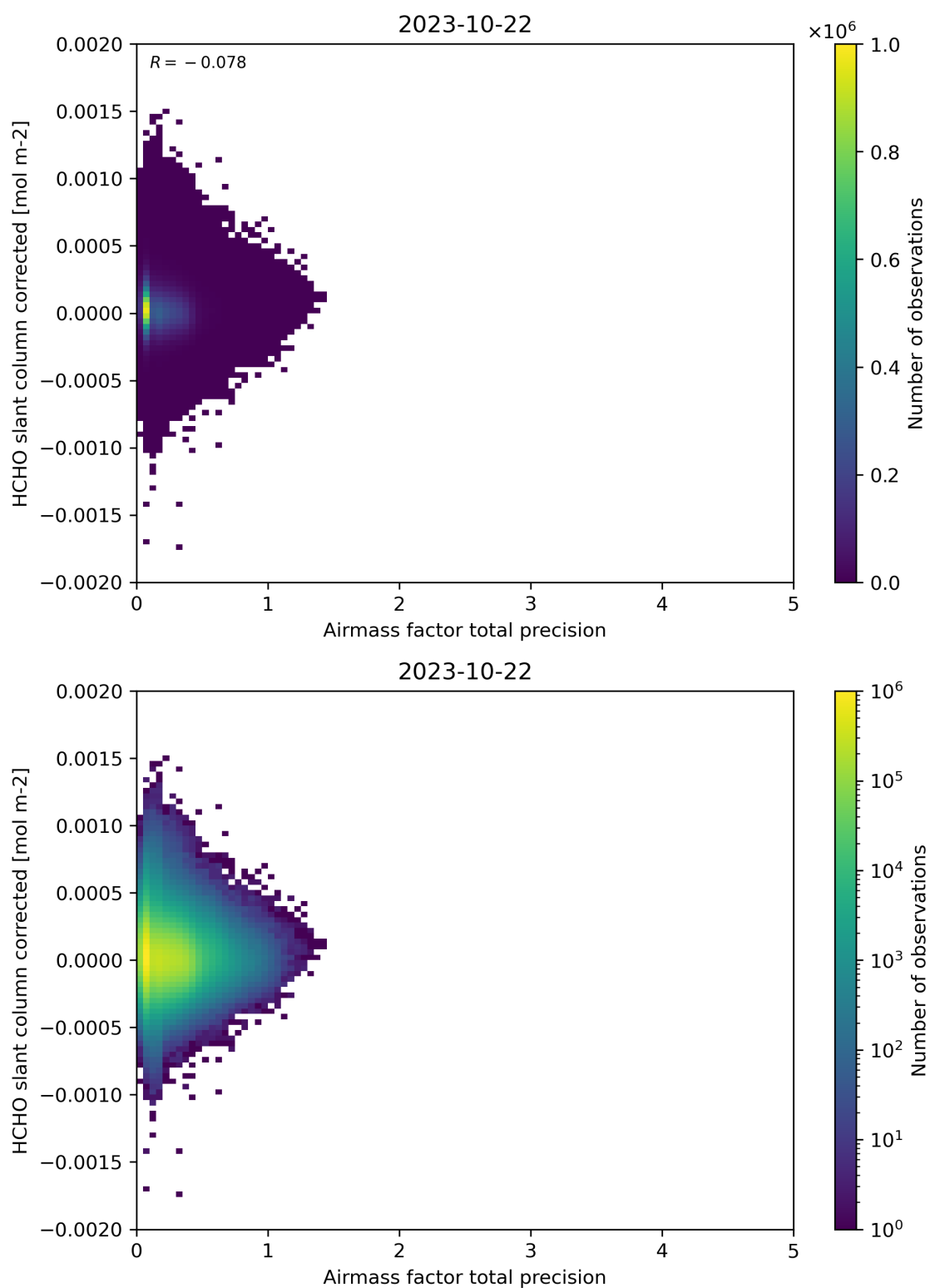
Figure 109: Scatter density plot of “Airmass factor total precision” against “HCHO slant column corrected” for 2023-10-22 to 2023-10-23.
