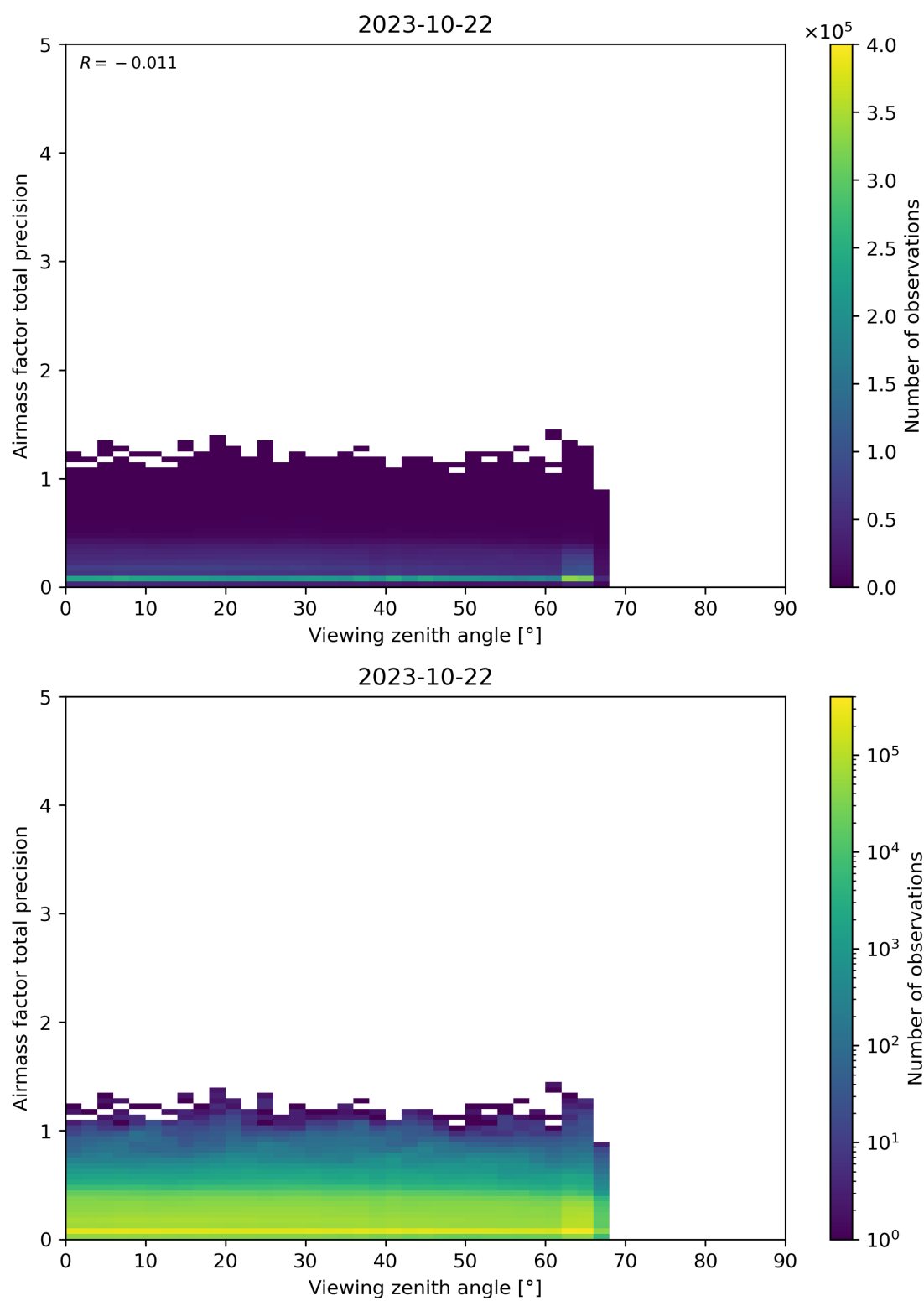
Figure 191: Scatter density plot of “Viewing zenith angle” against “Airmass factor total precision” for 2023-10-22 to 2023-10-23.
