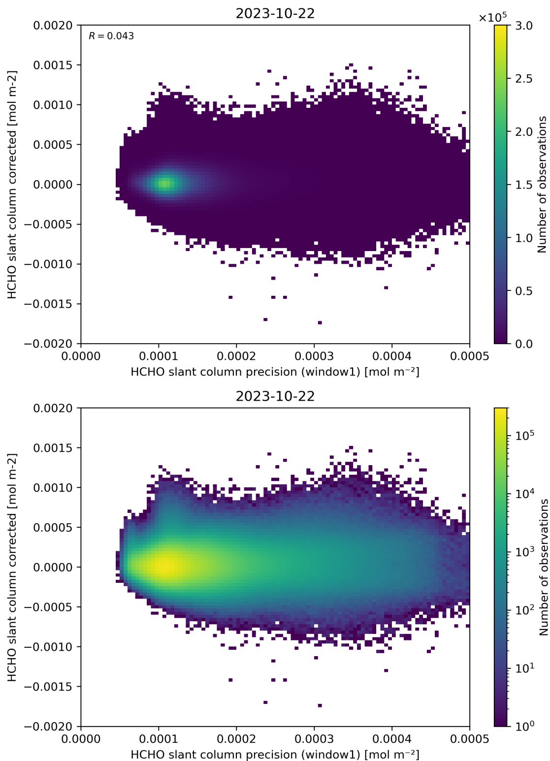
Figure 92: Scatter density plot of “HCHO slant column precision (window1)” against “HCHO slant column corrected” for 2023-10-22 to 2023-10-23.
