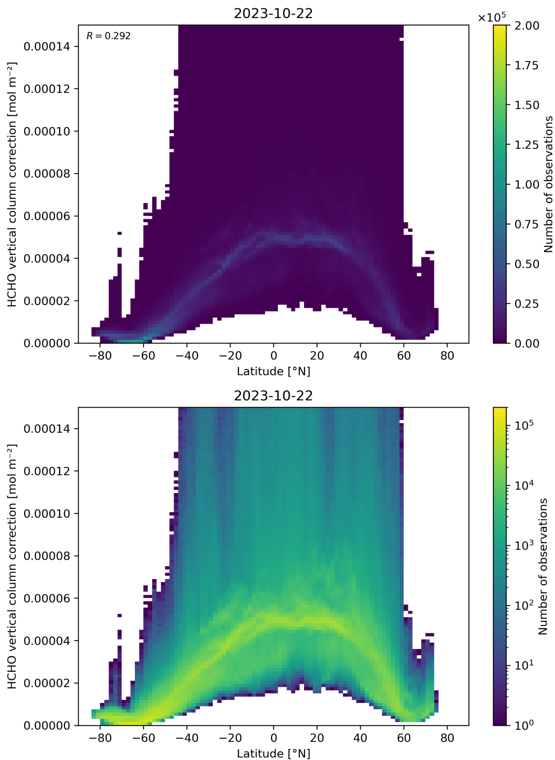
Figure 164: Scatter density plot of “Latitude” against “HCHO vertical column correction” for 2023-10-22 to 2023-10-23.
