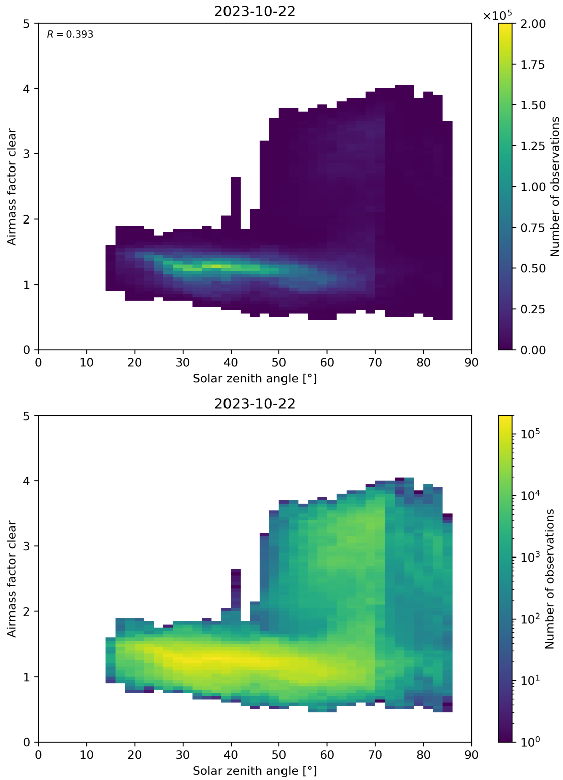
Figure 170: Scatter density plot of “Solar zenith angle” against “Airmass factor clear” for 2023-10-22 to 2023-10-23.
