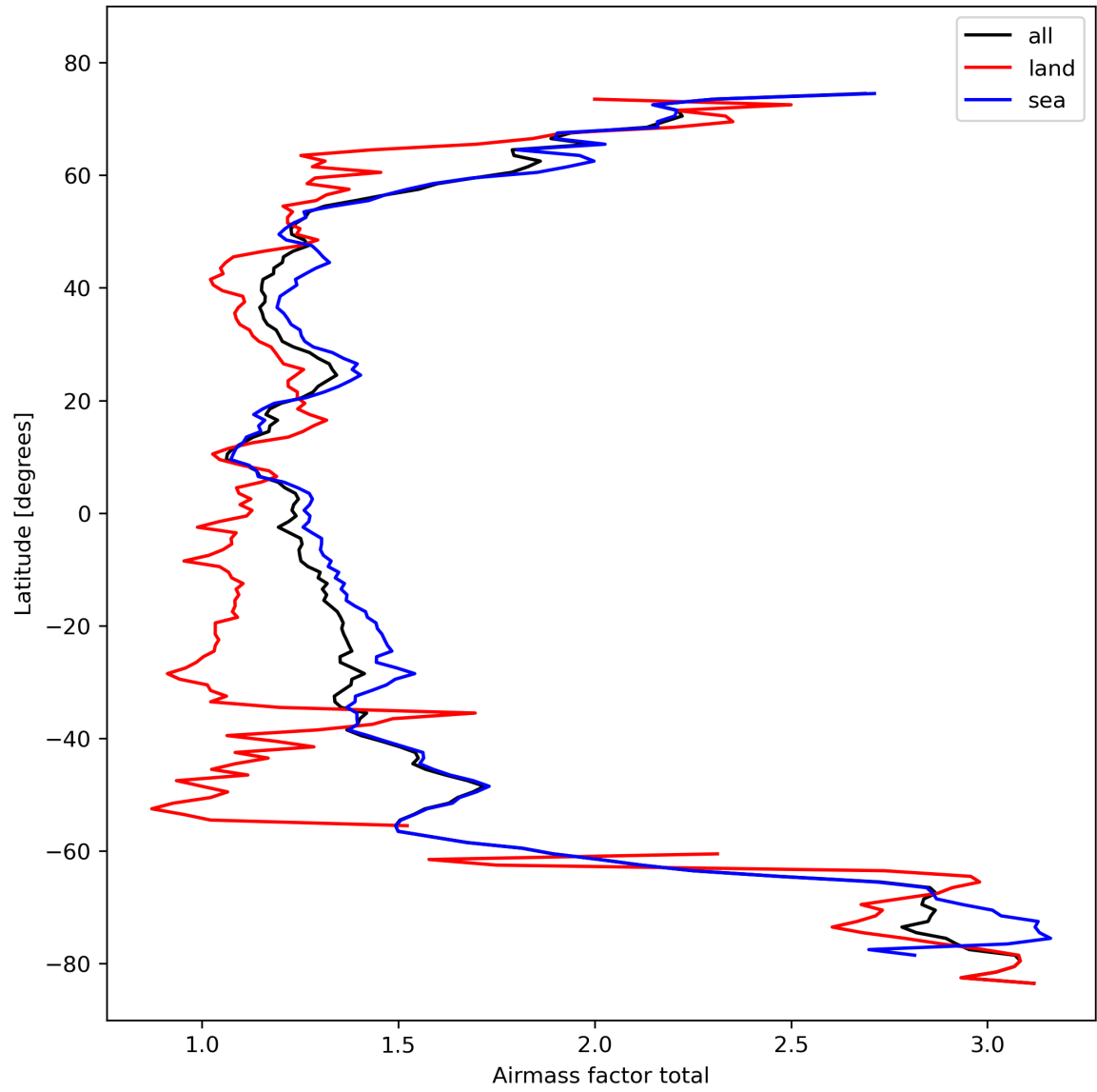
Figure 26: Zonal average of “Airmass factor total” for 2023-10-22 to 2023-10-23.
