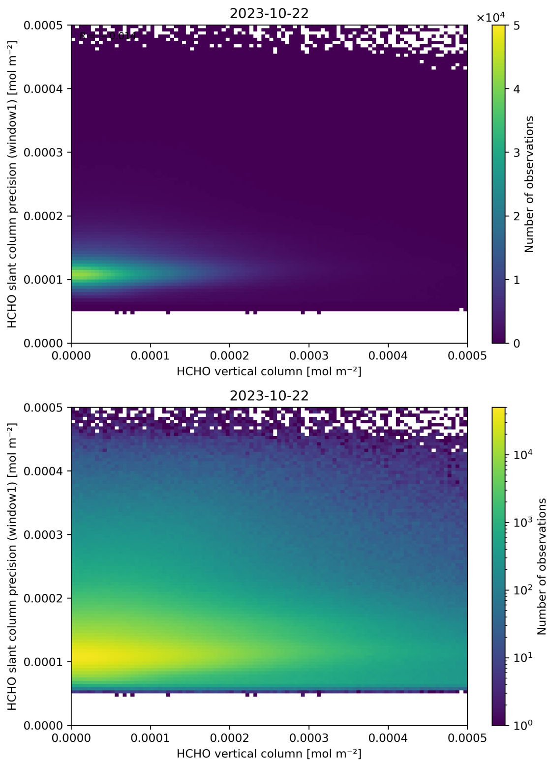
Figure 130: Scatter density plot of “HCHO vertical column” against “HCHO slant column precision (window1)” for 2023-10-22 to 2023-10-23.
