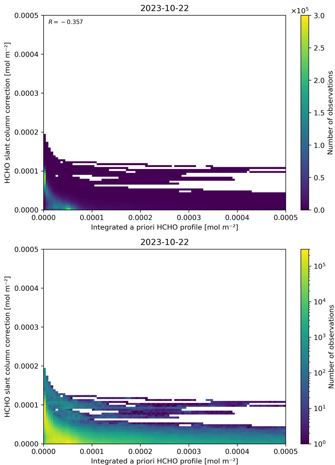
Figure 152: Scatter density plot of “Integrated a priori HCHO profile” against “HCHO slant column correction” for 2023-10-22 to 2023-10-23.
