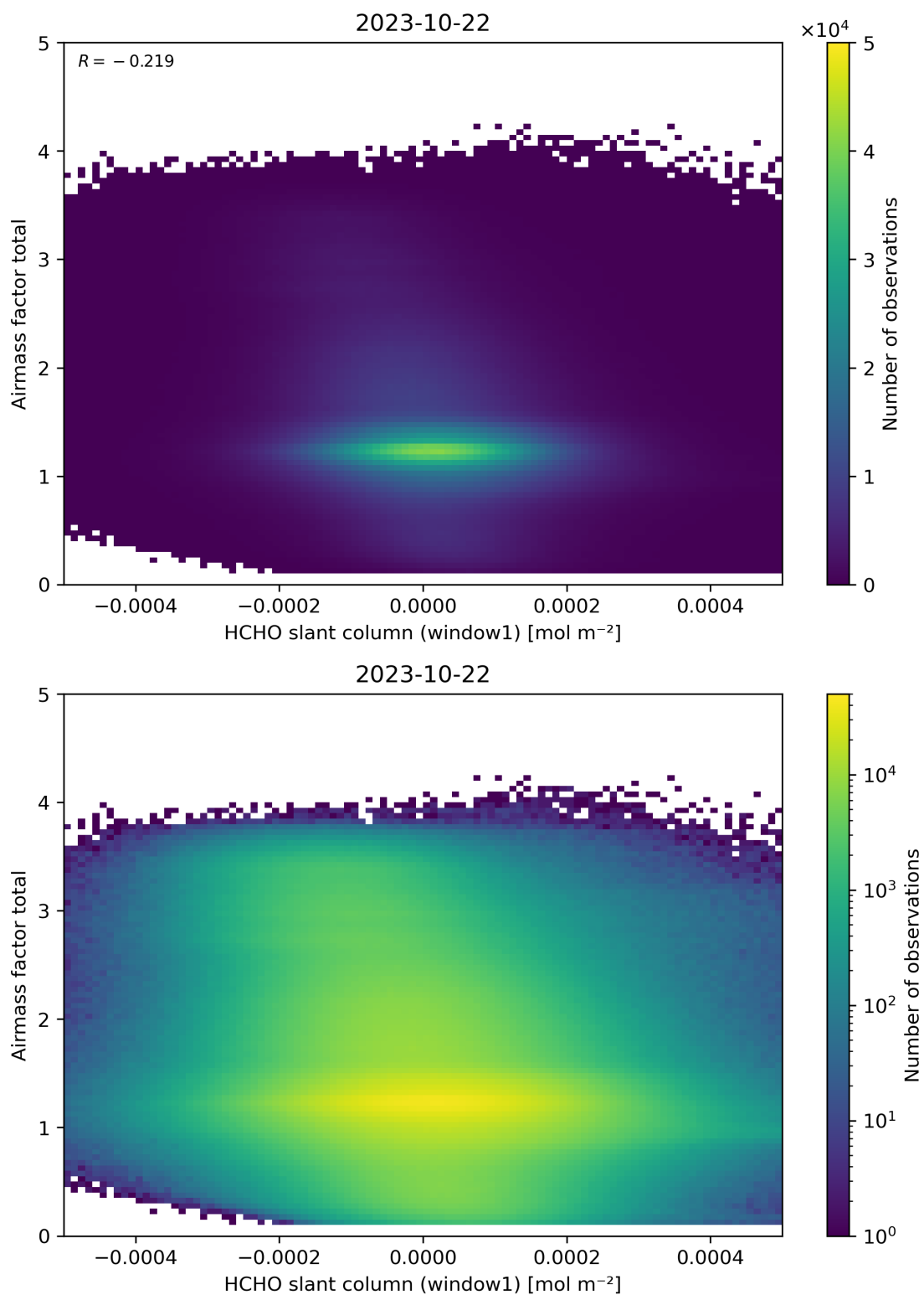
Figure 85: Scatter density plot of “HCHO slant column (window1)” against “Airmass factor total” for 2023-10-22 to 2023-10-23.
