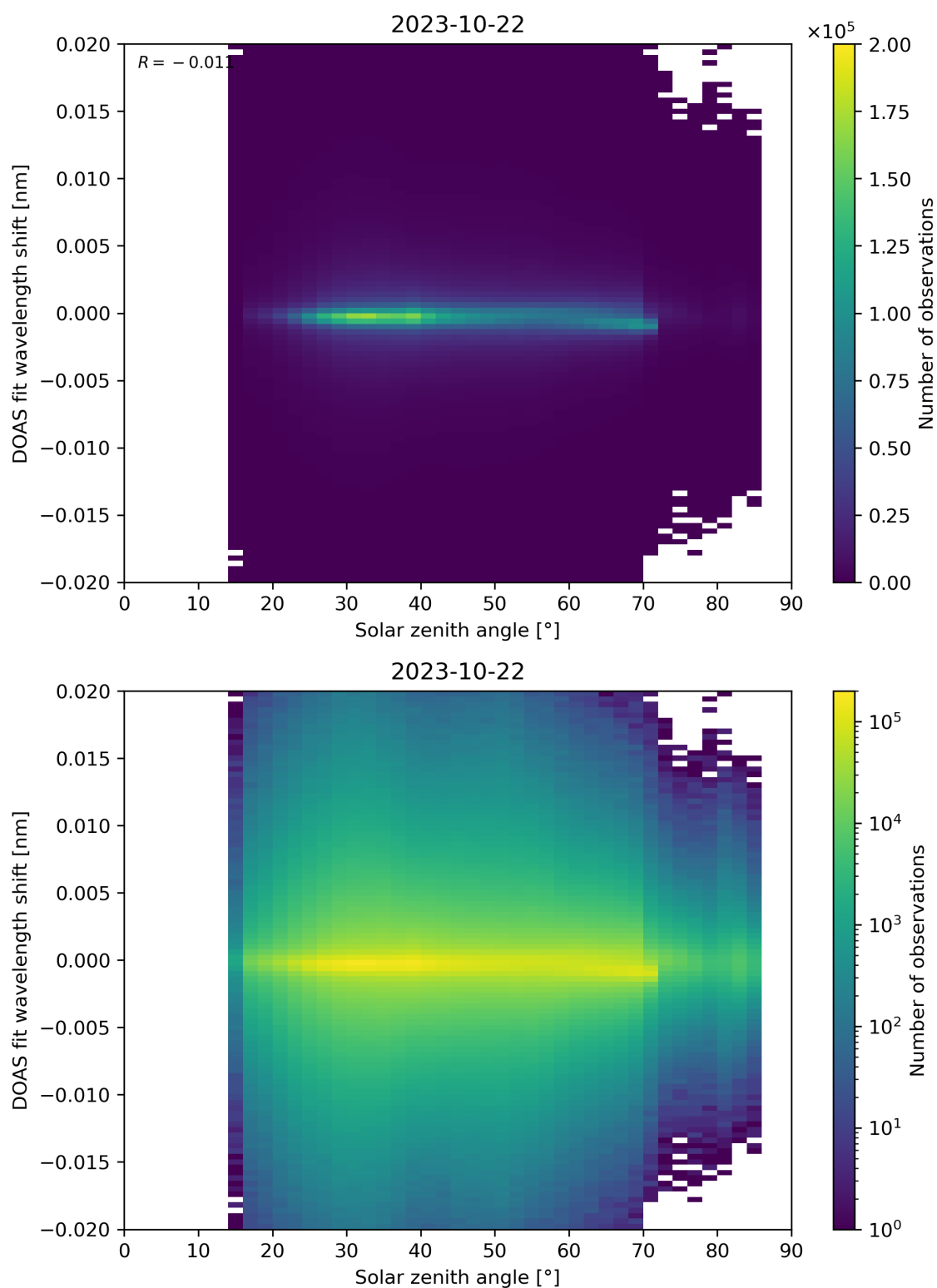
Figure 168: Scatter density plot of “Solar zenith angle” against “DOAS fit wavelength shift” for 2023-10-22 to 2023-10-23.
