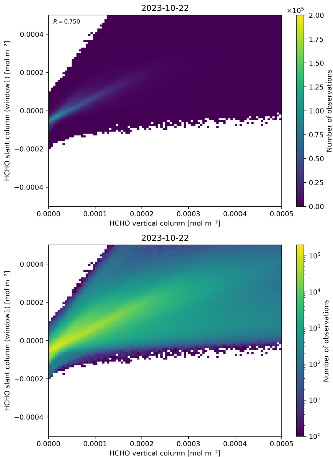
Figure 129: Scatter density plot of “HCHO vertical column” against “HCHO slant column (window1)” for 2023-10-22 to 2023-10-23.
