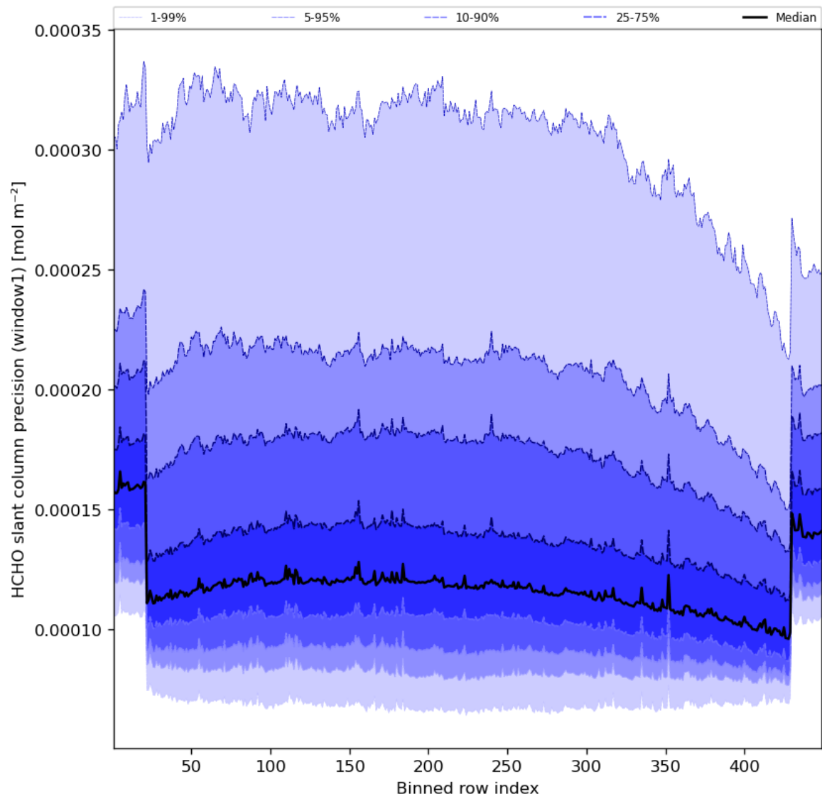
Figure 53: Along track statistics of “HCHO slant column precision (window1)” for 2023-10-22 to 2023-10-23
