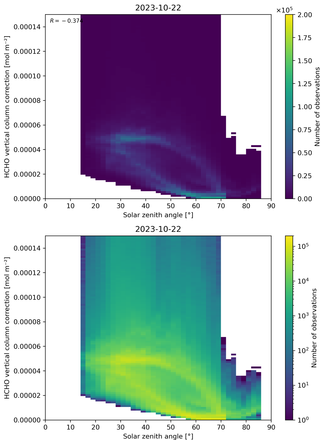
Figure 178: Scatter density plot of “Solar zenith angle” against “HCHO vertical column correction” for 2023-10-22 to 2023-10-23.
