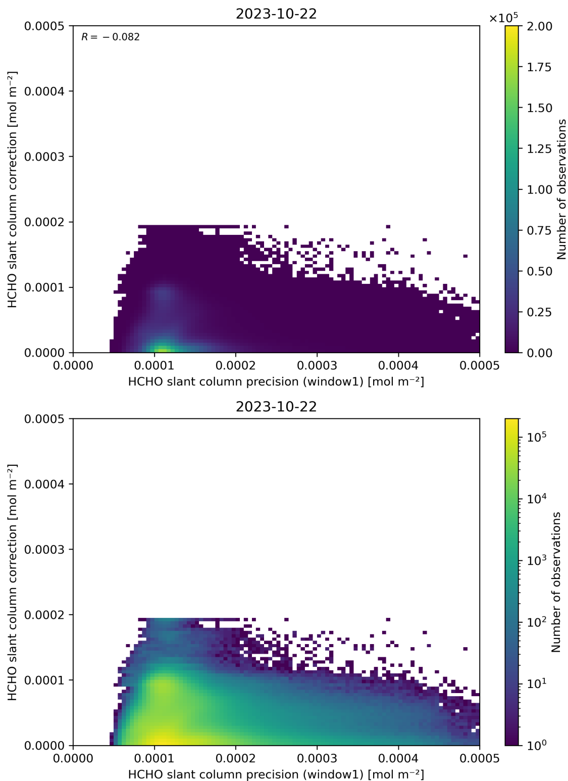
Figure 93: Scatter density plot of “HCHO slant column precision (window1)” against “HCHO slant column correction” for 2023-10-22 to 2023-10-23.
