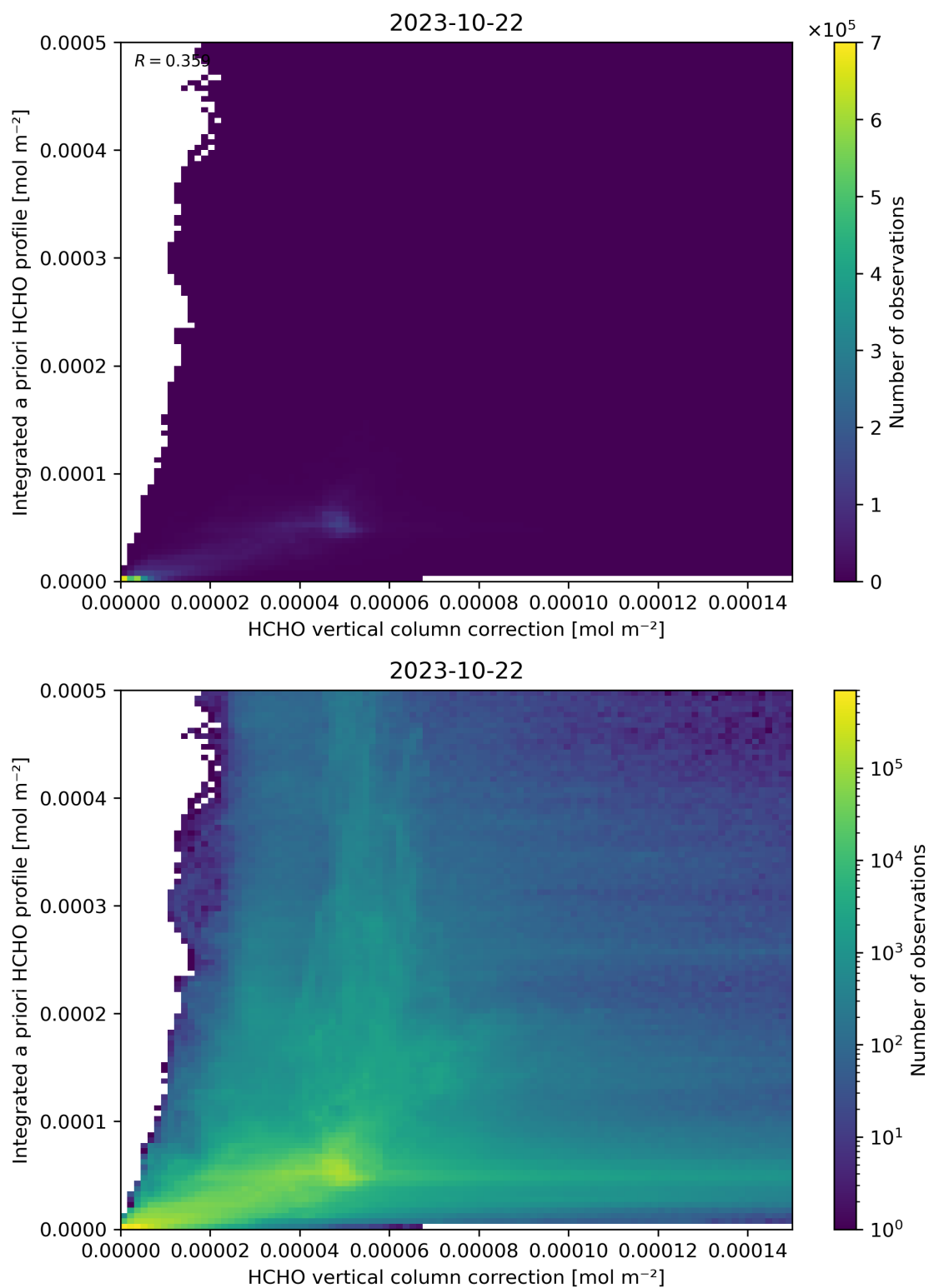
Figure 122: Scatter density plot of “HCHO vertical column correction” against “Integrated a priori HCHO profile” for 2023-10-22 to 2023-10-23.
