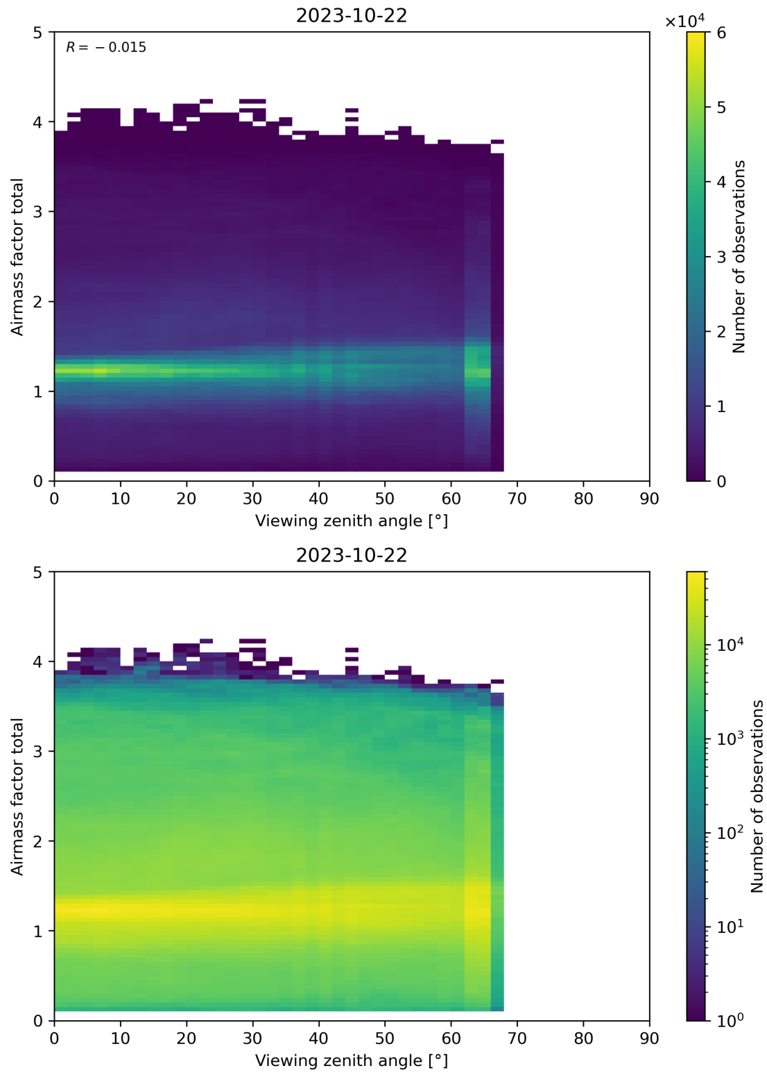
Figure 190: Scatter density plot of “Viewing zenith angle” against “Airmass factor total” for 2023-10-22 to 2023-10-23.
