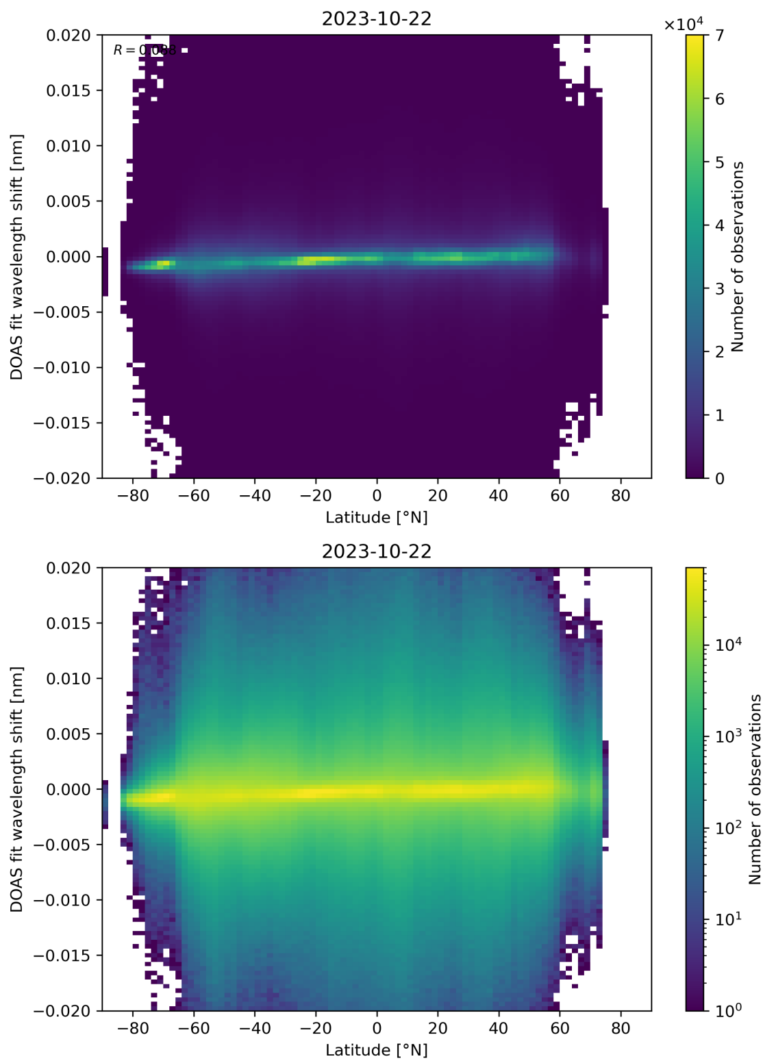
Figure 154: Scatter density plot of “Latitude” against “DOAS fit wavelength shift” for 2023-10-22 to 2023-10-23.
