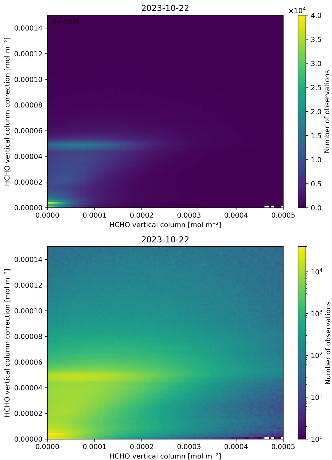
Figure 133: Scatter density plot of “HCHO vertical column” against “HCHO vertical column correction” for 2023-10-22 to 2023-10-23.
