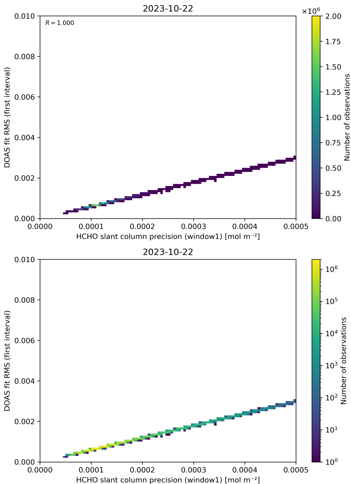
Figure 88: Scatter density plot of “HCHO slant column precision (window1)” against “DOAS fit RMS (first interval)” for 2023-10-22 to 2023-10-23.
