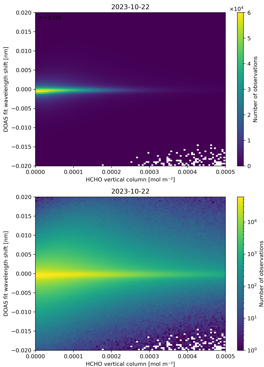
Figure 124: Scatter density plot of “HCHO vertical column” against “DOAS fit wavelength shift” for 2023-10-22 to 2023-10-23.
