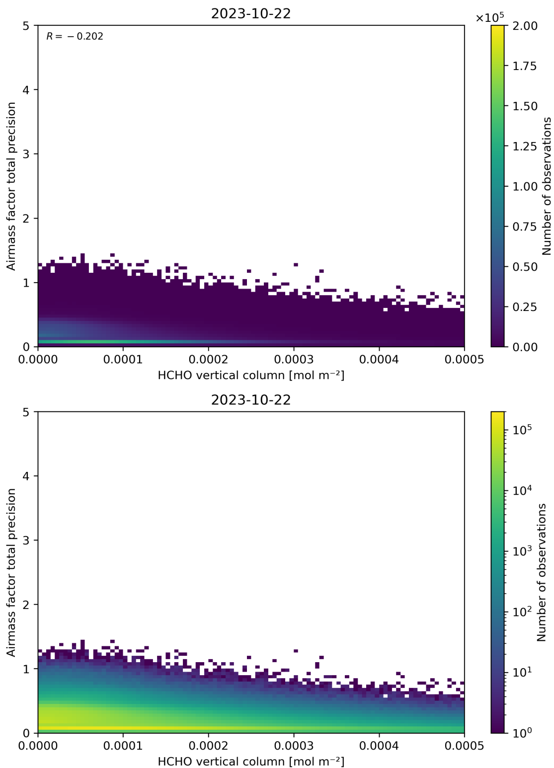
Figure 132: Scatter density plot of “HCHO vertical column” against “Airmass factor total precision” for 2023-10-22 to 2023-10-23.
