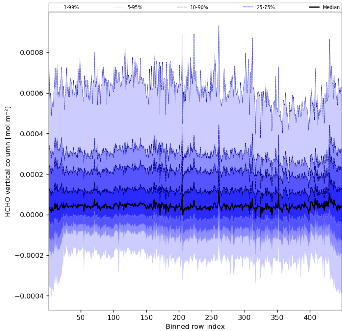
Figure 49: Along track statistics of “HCHO vertical column” for 2023-10-22 to 2023-10-23
