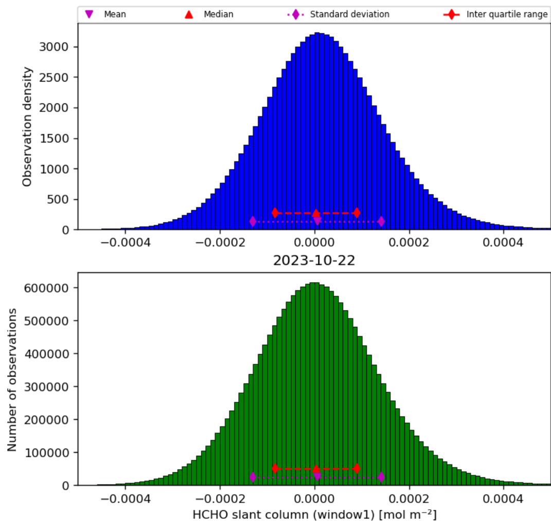
Figure 38: Histogram of “HCHO slant column (window1)” for 2023-10-22 to 2023-10-23
