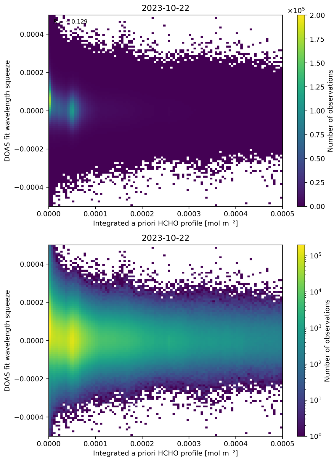
Figure 150: Scatter density plot of “Integrated a priori HCHO profile” against “DOAS fit wavelength squeeze” for 2023-10-22 to 2023-10-23.
