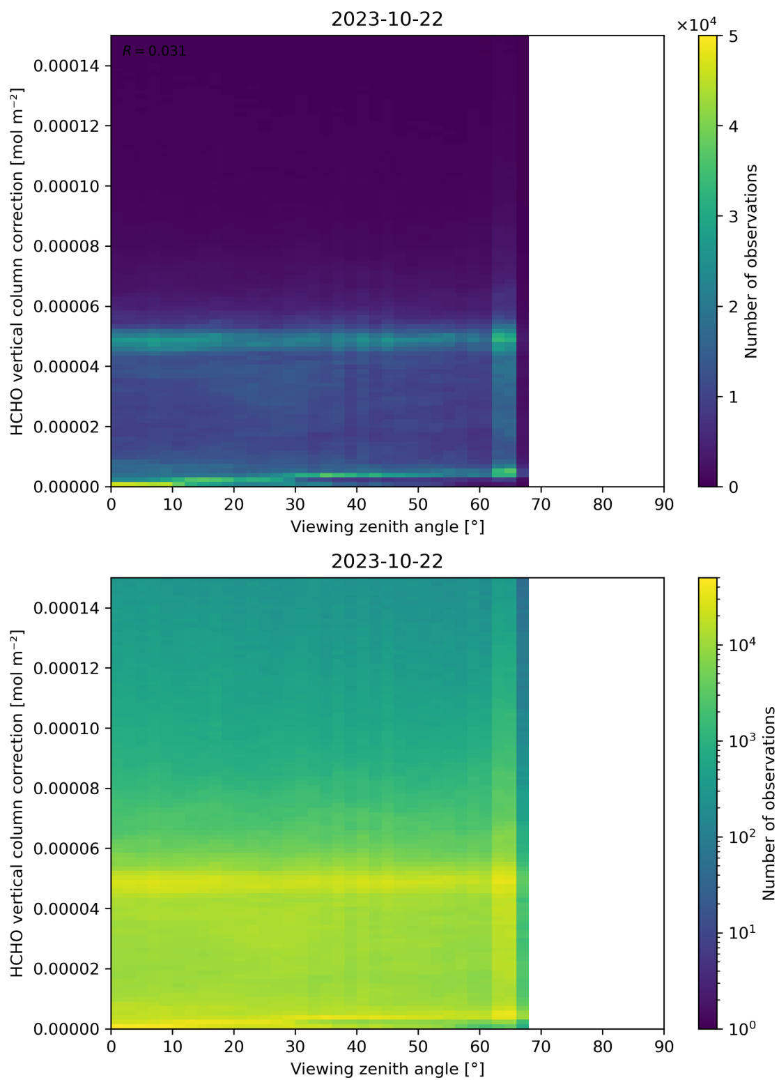
Figure 193: Scatter density plot of “Viewing zenith angle” against “HCHO vertical column correction” for 2023-10-22 to 2023-10-23.
