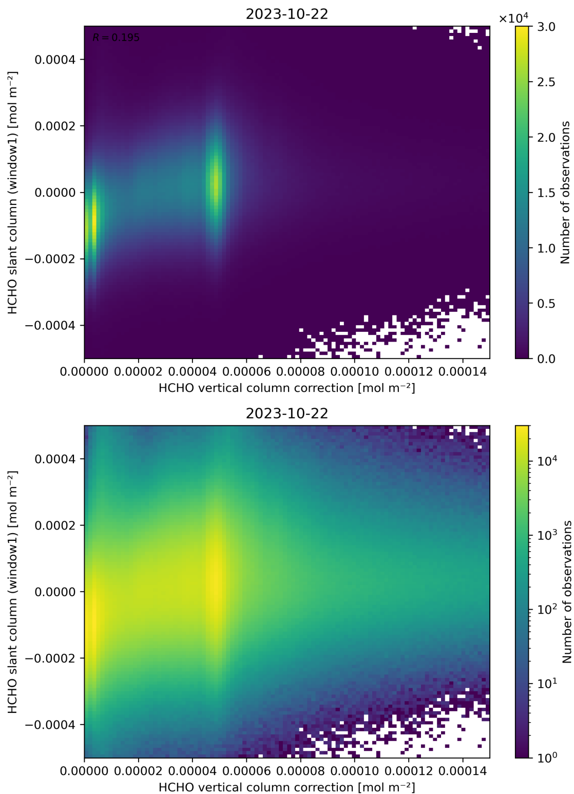
Figure 118: Scatter density plot of “HCHO vertical column correction” against “HCHO slant column (window1)” for 2023-10-22 to 2023-10-23.
