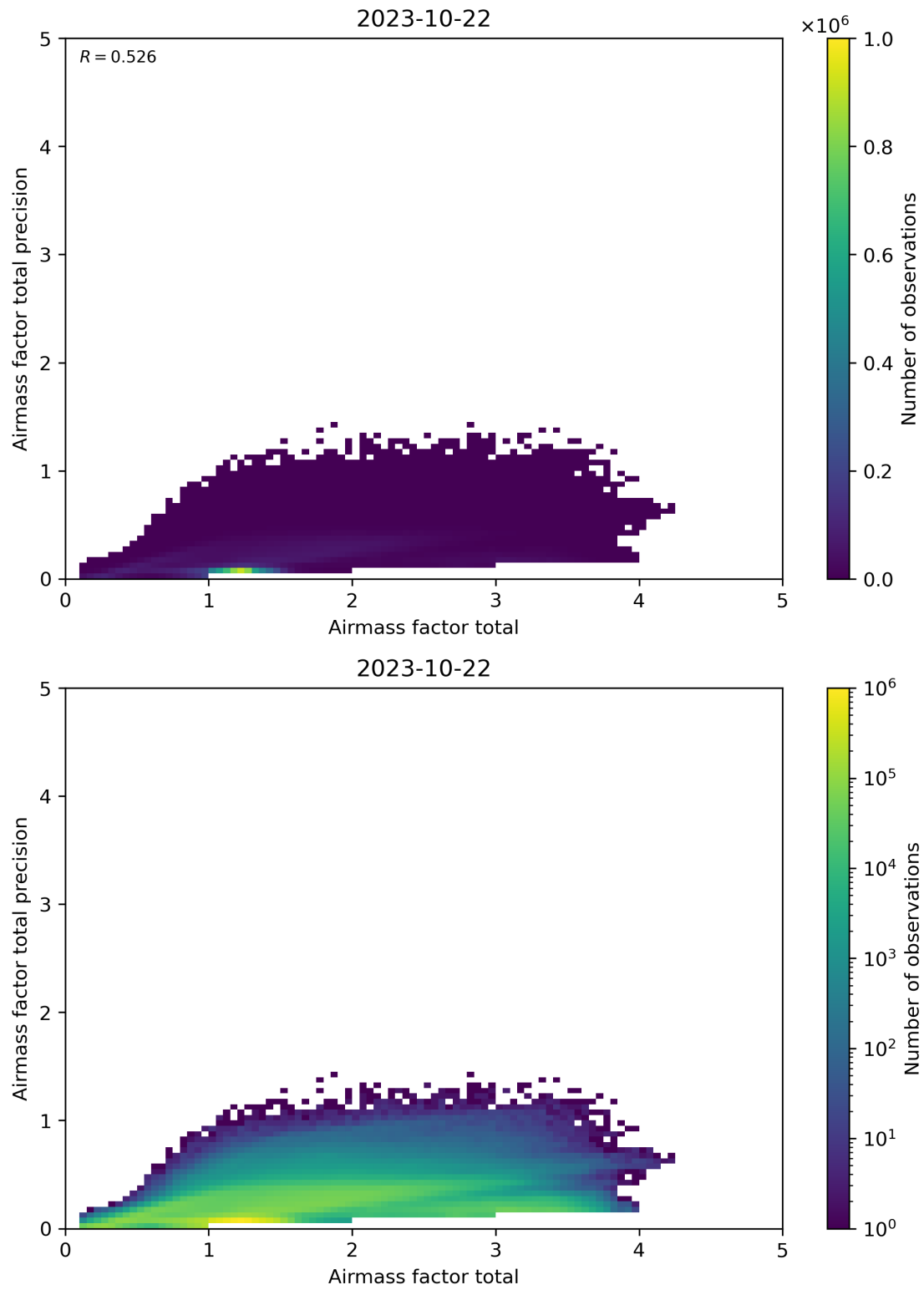
Figure 103: Scatter density plot of “Airmass factor total” against “Airmass factor total precision” for 2023-10-22 to 2023-10-23.
