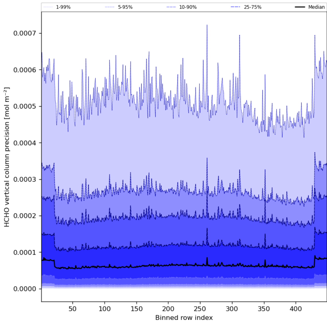
Figure 50: Along track statistics of “HCHO vertical column precision” for 2023-10-22 to 2023-10-23
