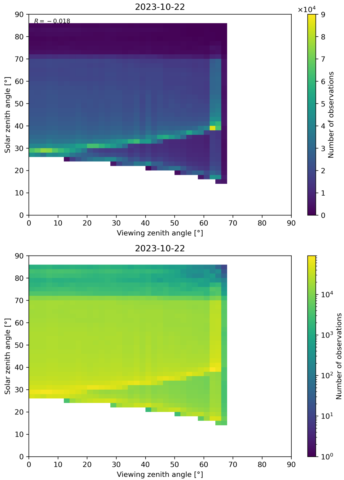
Figure 197: Scatter density plot of “Viewing zenith angle” against “Solar zenith angle” for 2023-10-22 to 2023-10-23.
