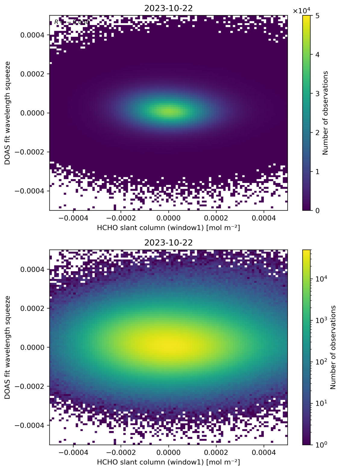
Figure 80: Scatter density plot of “HCHO slant column (window1)” against “DOAS fit wavelength squeeze” for 2023-10-22 to 2023-10-23.
