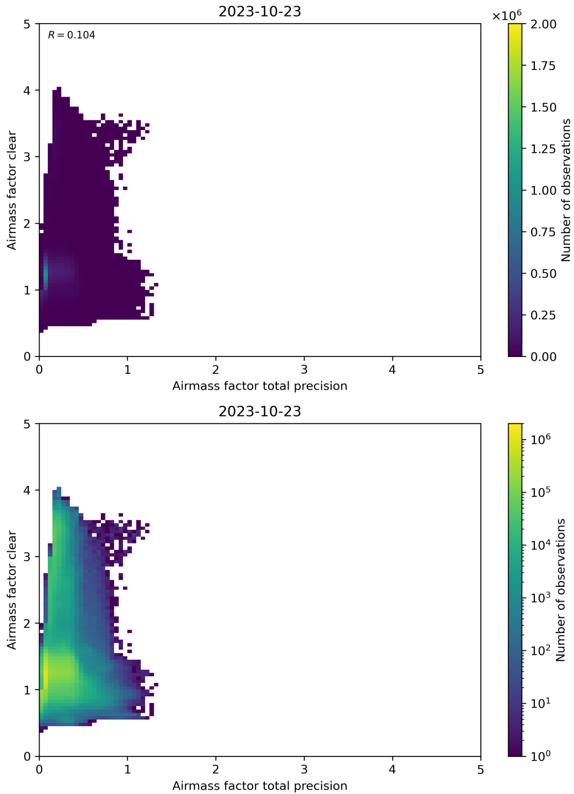
Figure 108: Scatter density plot of “Airmass factor total precision” against “Airmass factor clear” for 2023-10-22 to 2023-10-24.
