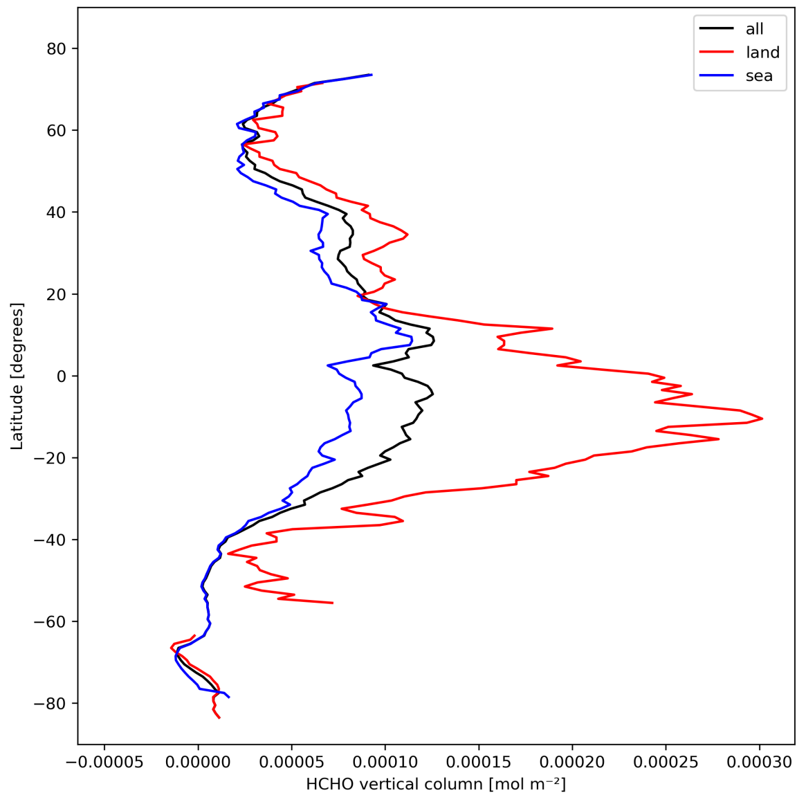
Figure 21: Zonal average of “HCHO vertical column” for 2023-10-22 to 2023-10-24.
