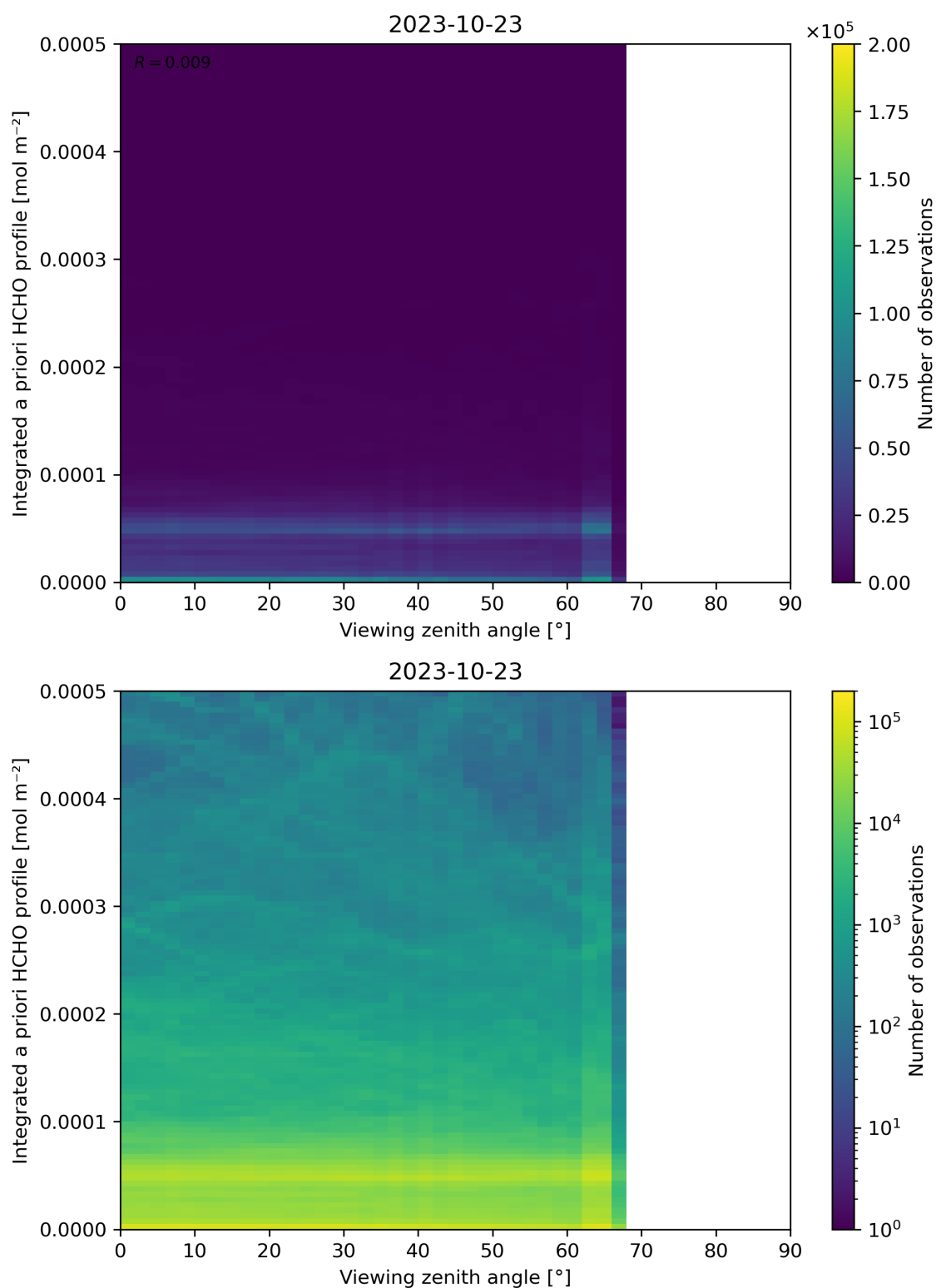
Figure 195: Scatter density plot of “Viewing zenith angle” against “Integrated a priori HCHO profile” for 2023-10-22 to 2023-10-24.
