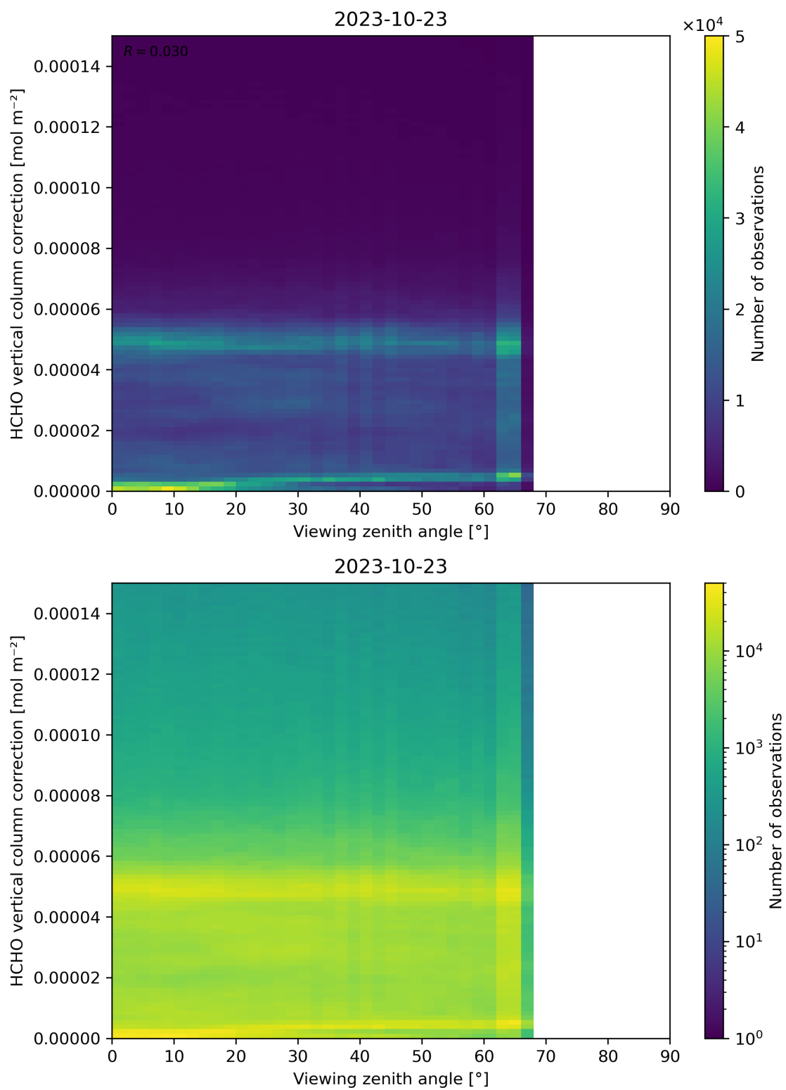
Figure 193: Scatter density plot of “Viewing zenith angle” against “HCHO vertical column correction” for 2023-10-22 to 2023-10-24.
