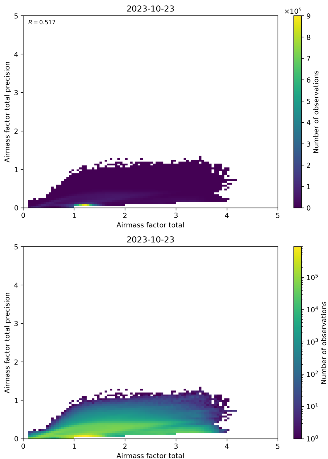
Figure 103: Scatter density plot of “Airmass factor total” against “Airmass factor total precision” for 2023-10-22 to 2023-10-24.
