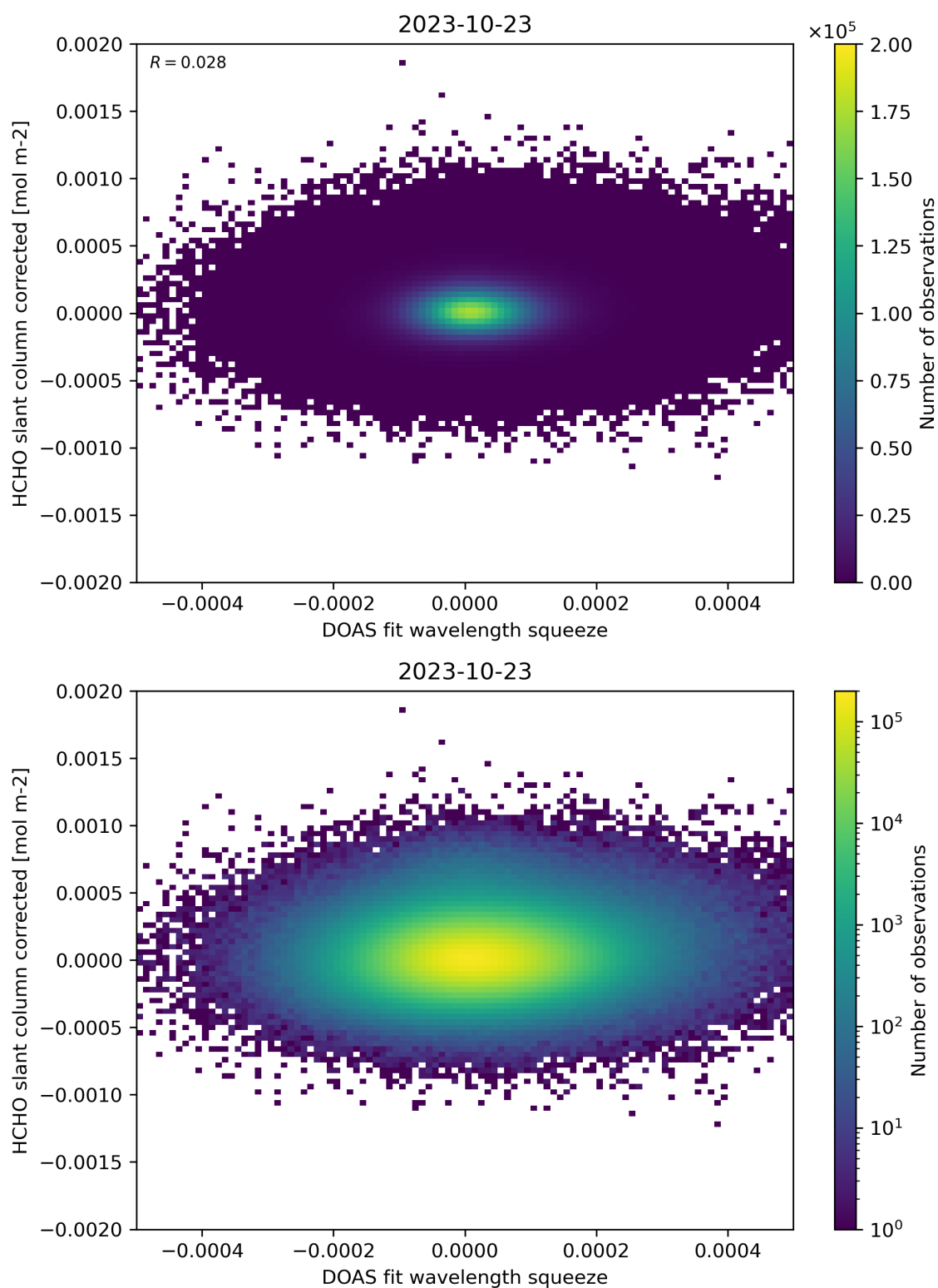
Figure 69: Scatter density plot of “DOAS fit wavelength squeeze” against “HCHO slant column corrected” for 2023-10-22 to 2023-10-24.
