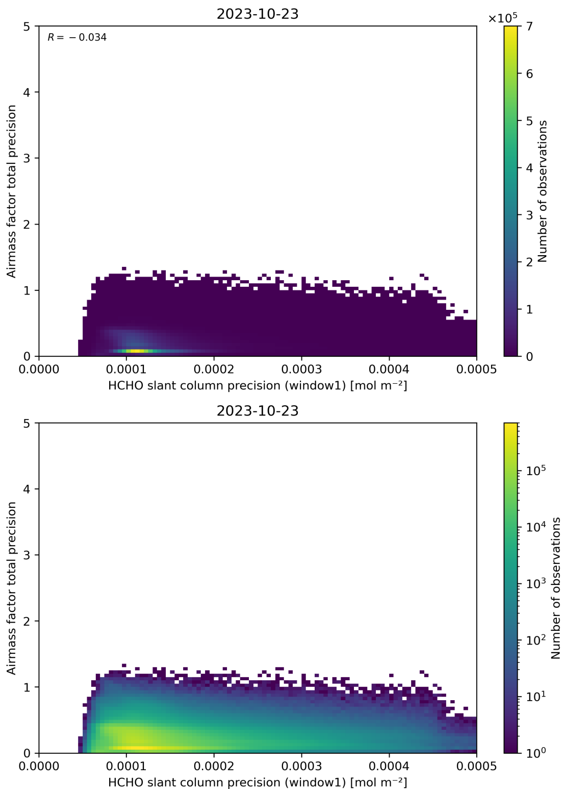
Figure 95: Scatter density plot of “HCHO slant column precision (window1)” against “Airmass factor total precision” for 2023-10-22 to 2023-10-24.
