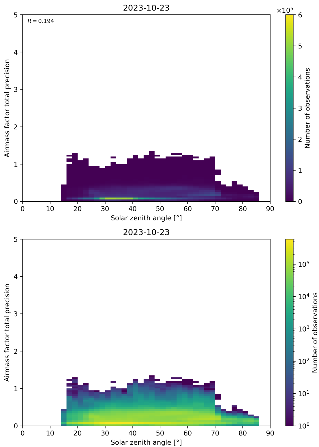
Figure 176: Scatter density plot of “Solar zenith angle” against “Airmass factor total precision” for 2023-10-22 to 2023-10-24.
