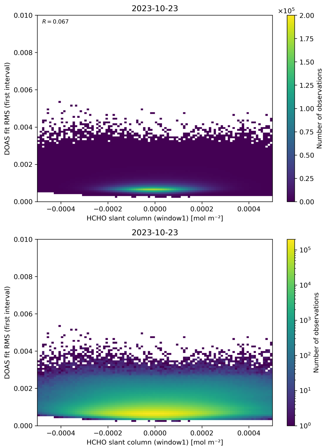
Figure 78: Scatter density plot of “HCHO slant column (window1)” against “DOAS fit RMS (first interval)” for 2023-10-22 to 2023-10-24.
