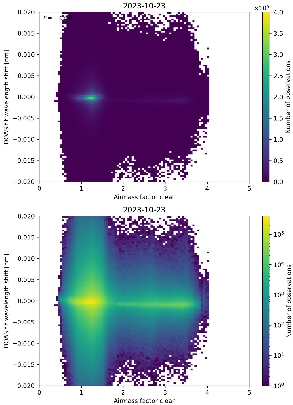
Figure 72: Scatter density plot of “Airmass factor clear” against “DOAS fit wavelength shift” for 2023-10-22 to 2023-10-24.
