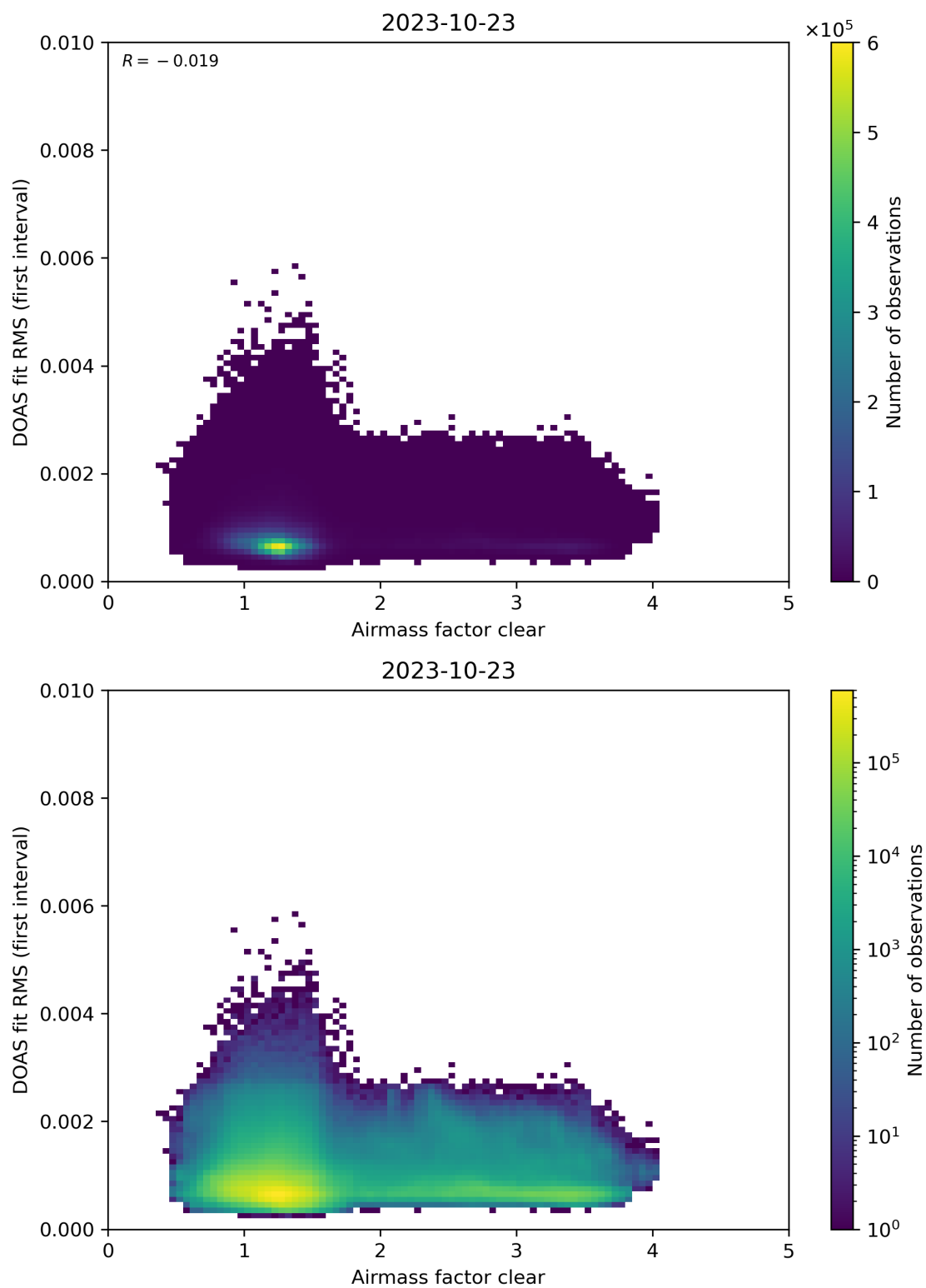
Figure 71: Scatter density plot of “Airmass factor clear” against “DOAS fit RMS (first interval)” for 2023-10-22 to 2023-10-24.
