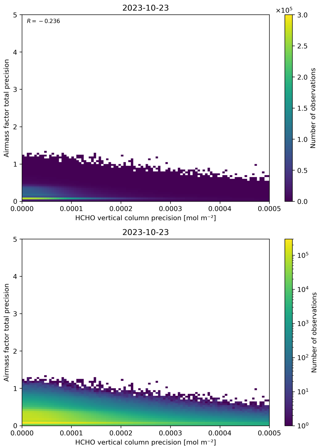
Figure 145: Scatter density plot of “HCHO vertical column precision” against “Airmass factor total precision” for 2023-10-22 to 2023-10-24.
