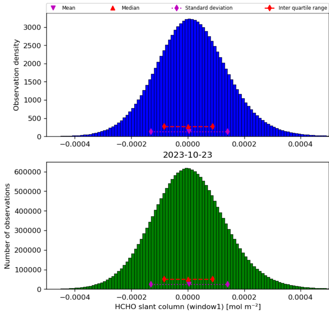
Figure 38: Histogram of “HCHO slant column (window1)” for 2023-10-22 to 2023-10-24
