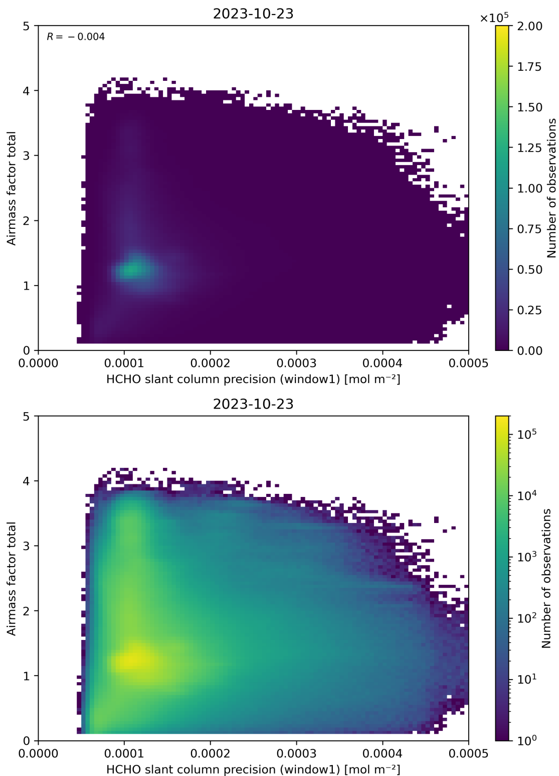
Figure 94: Scatter density plot of “HCHO slant column precision (window1)” against “Airmass factor total” for 2023-10-22 to 2023-10-24.
