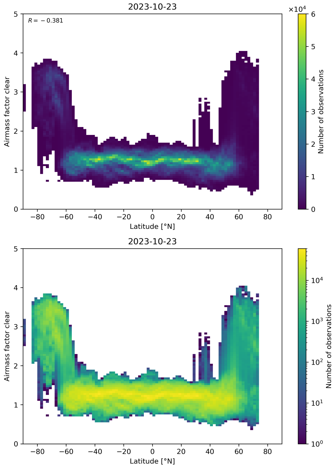
Figure 156: Scatter density plot of “Latitude” against “Airmass factor clear” for 2023-10-22 to 2023-10-24.
