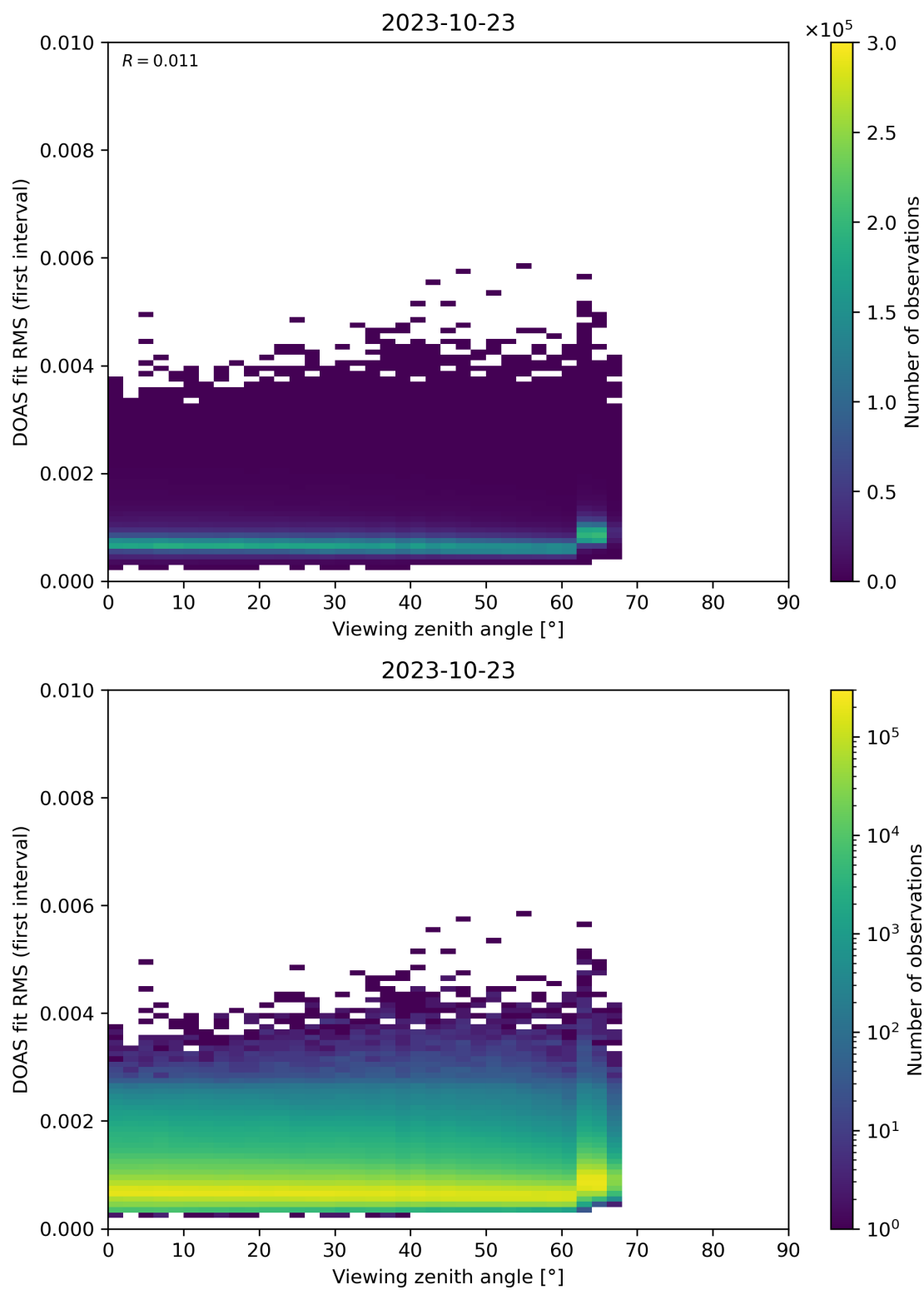
Figure 182: Scatter density plot of “Viewing zenith angle” against “DOAS fit RMS (first interval)” for 2023-10-22 to 2023-10-24.
