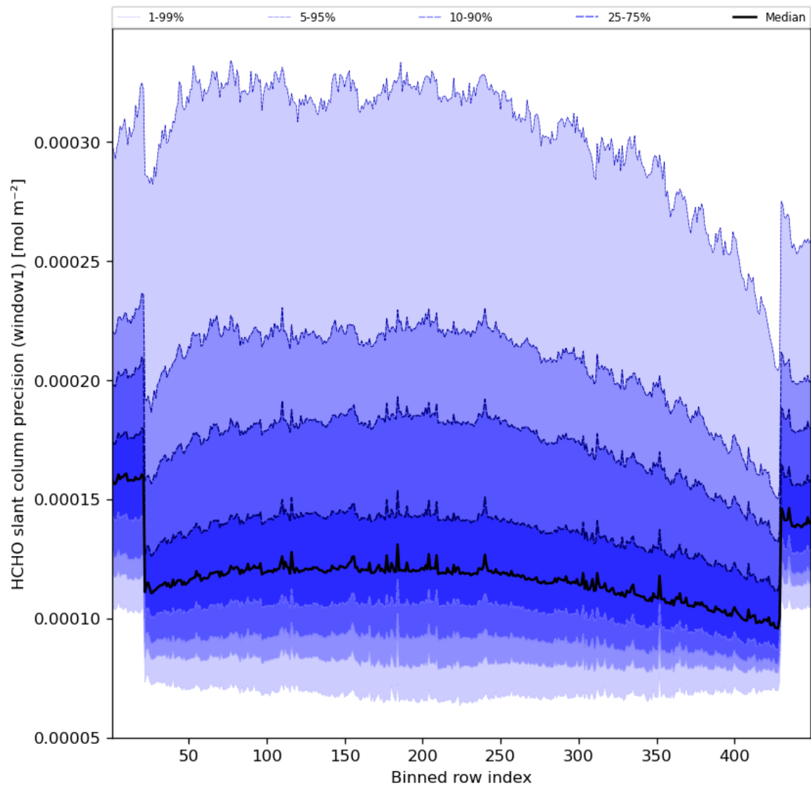
Figure 53: Along track statistics of "HCHO slant column precision (window1)" for 2023-10-22 to 2023-10-24
