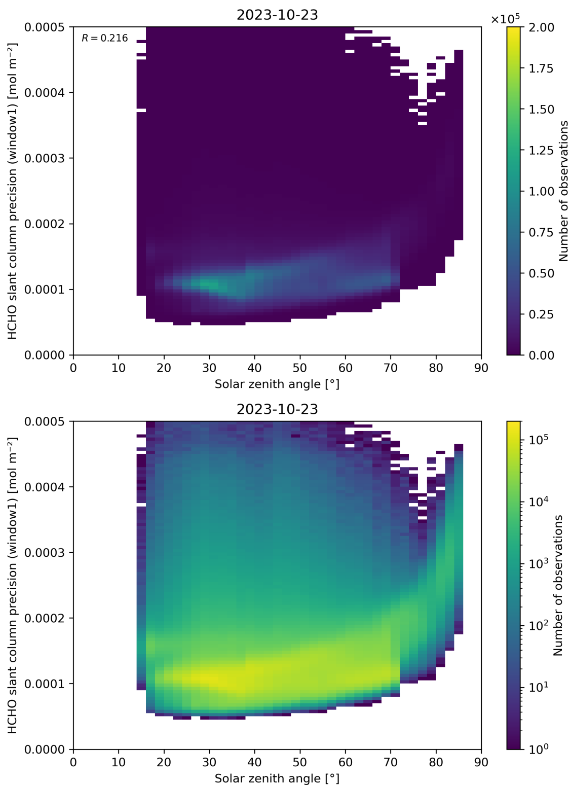
Figure 174: Scatter density plot of “Solar zenith angle” against “HCHO slant column precision (window1)” for 2023-10-22 to 2023-10-24.
