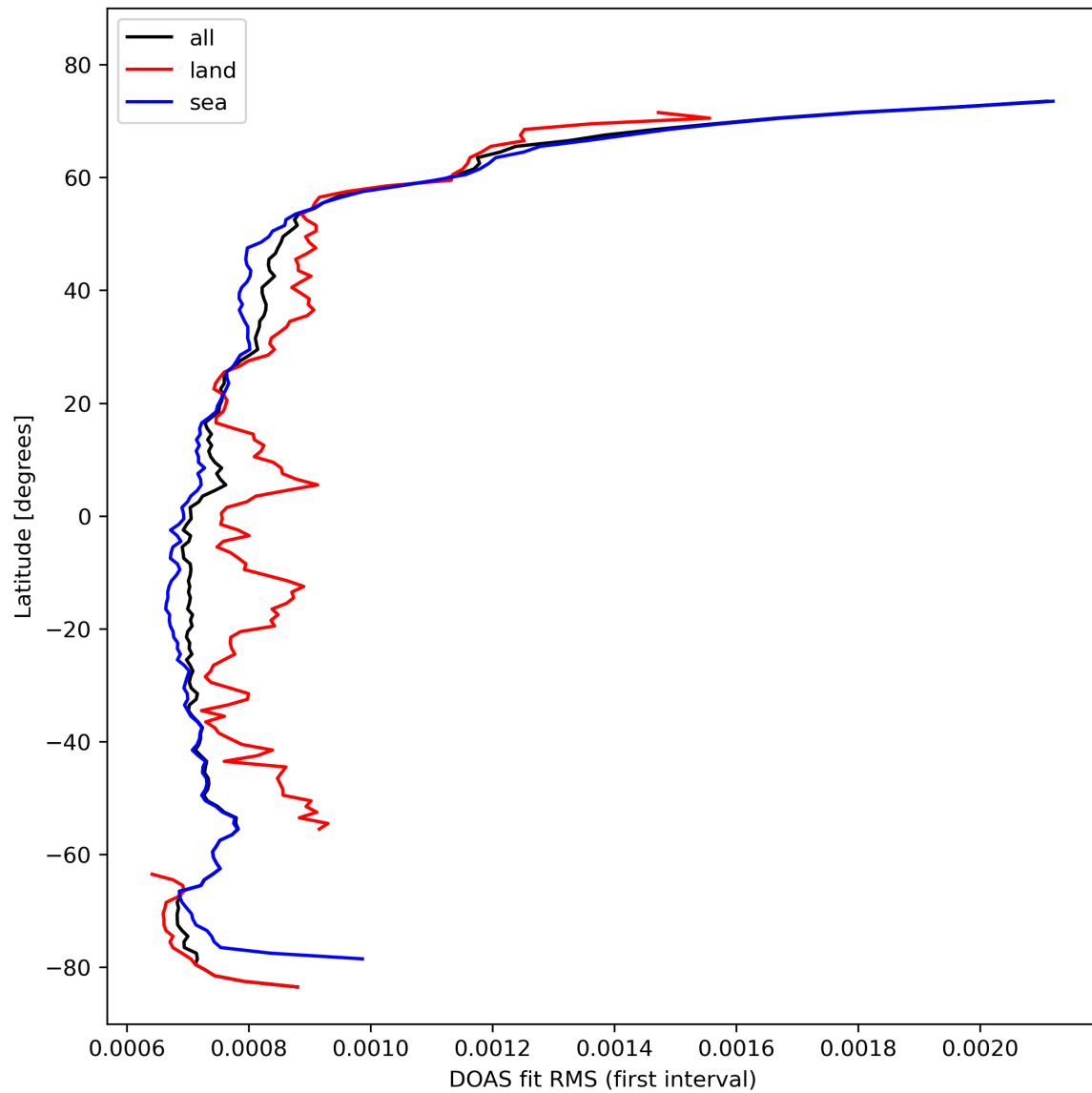
Figure 32: Zonal average of “DOAS fit RMS (first interval)” for 2023-10-22 to 2023-10-24.
