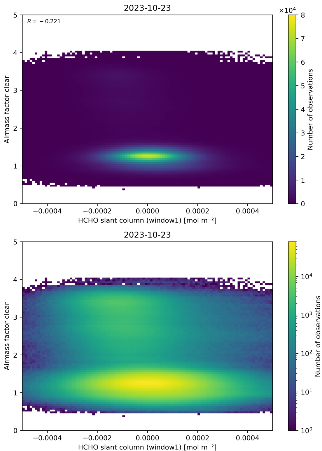
Figure 81: Scatter density plot of “HCHO slant column (window1)” against “Airmass factor clear” for 2023-10-22 to 2023-10-24.
