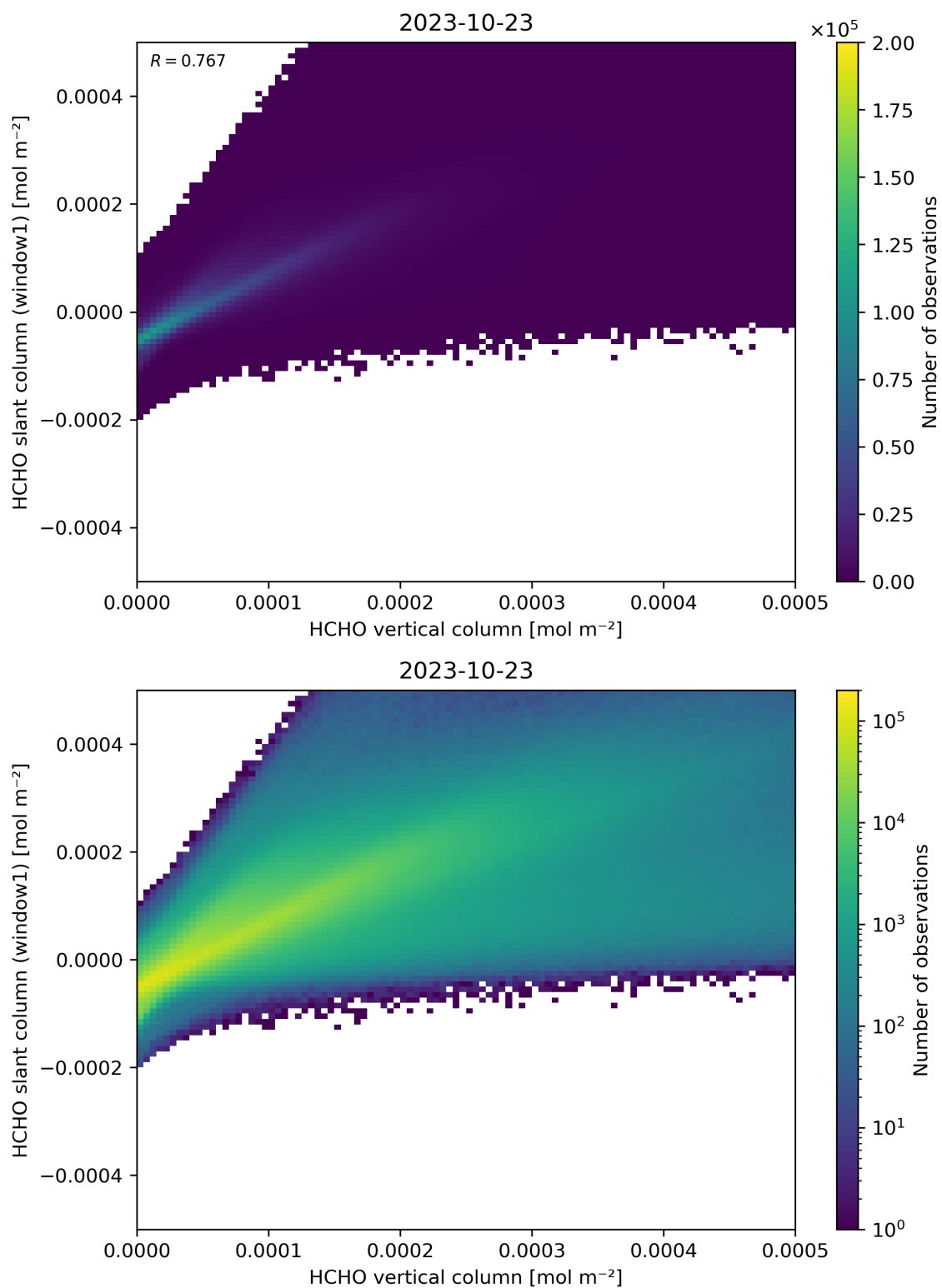
Figure 129: Scatter density plot of “HCHO vertical column” against “HCHO slant column (window1)” for 2023-10-22 to 2023-10-24.
