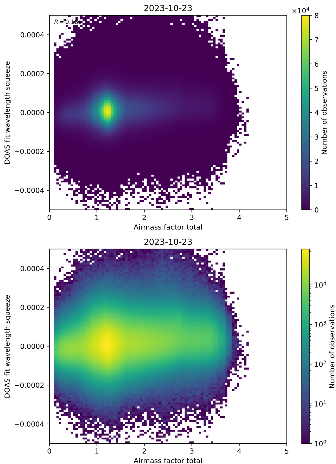
Figure 99: Scatter density plot of “Airmass factor total” against “DOAS fit wavelength squeeze” for 2023-10-22 to 2023-10-24.
