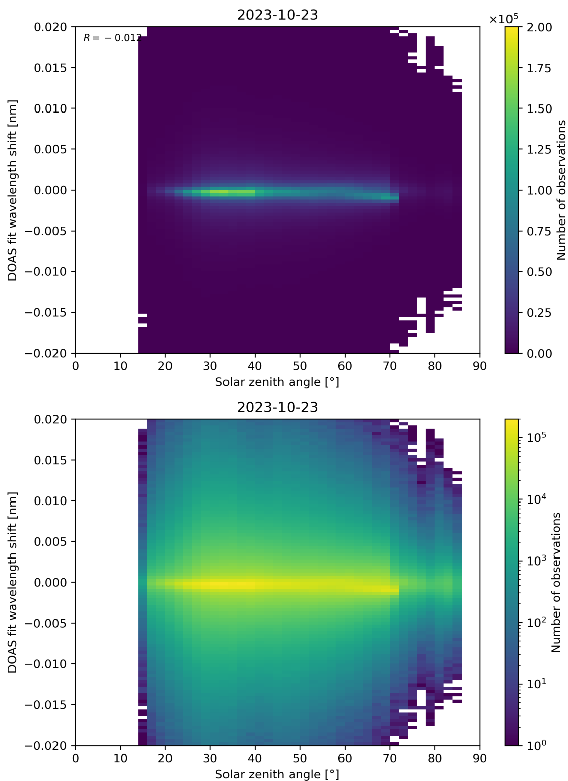
Figure 168: Scatter density plot of “Solar zenith angle” against “DOAS fit wavelength shift” for 2023-10-22 to 2023-10-24.
