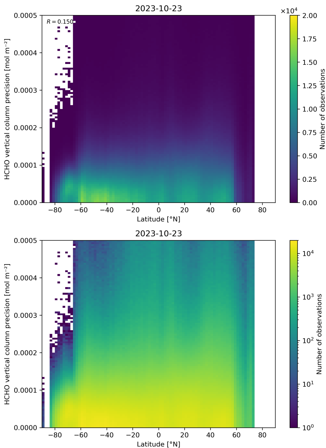
Figure 165: Scatter density plot of “Latitude” against “HCHO vertical column precision” for 2023-10-22 to 2023-10-24.
