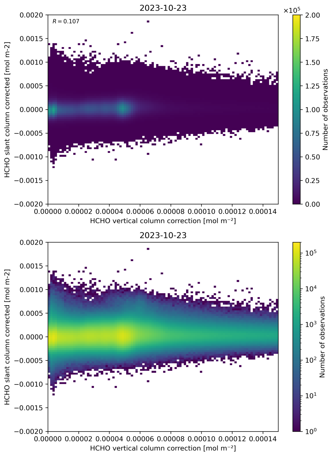
Figure 116: Scatter density plot of “HCHO vertical column correction” against “HCHO slant column corrected” for 2023-10-22 to 2023-10-24.
