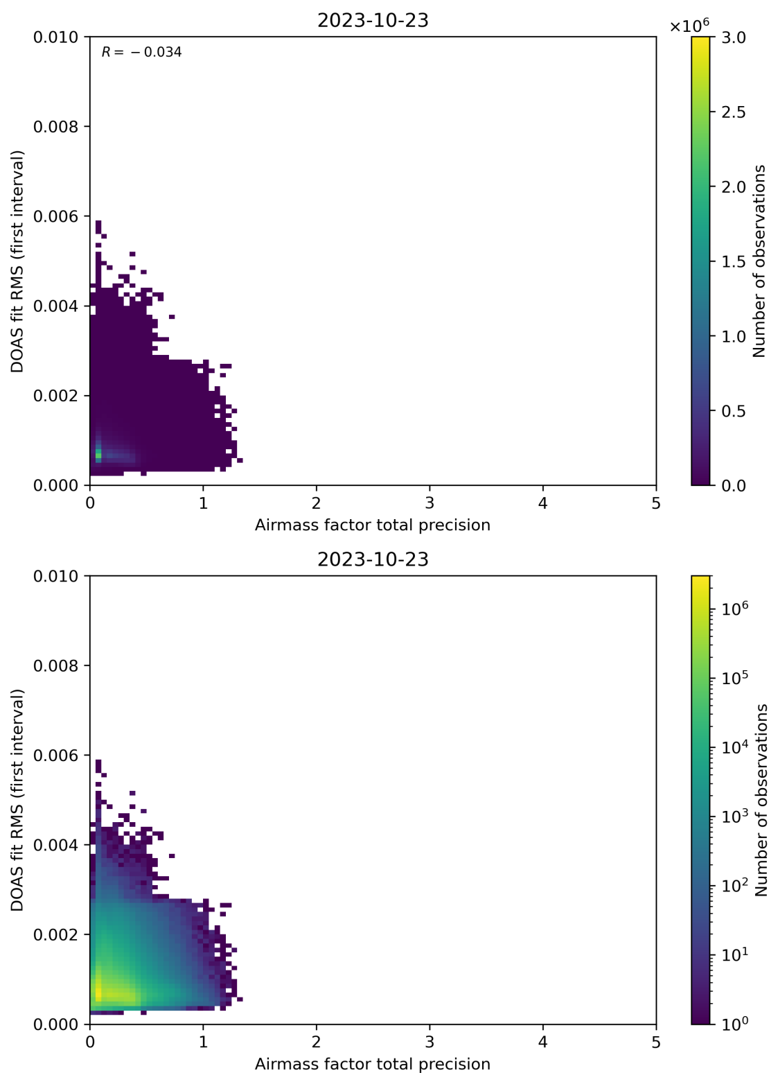
Figure 105: Scatter density plot of “Airmass factor total precision” against “DOAS fit RMS (first interval)” for 2023-10-22 to 2023-10-24.
