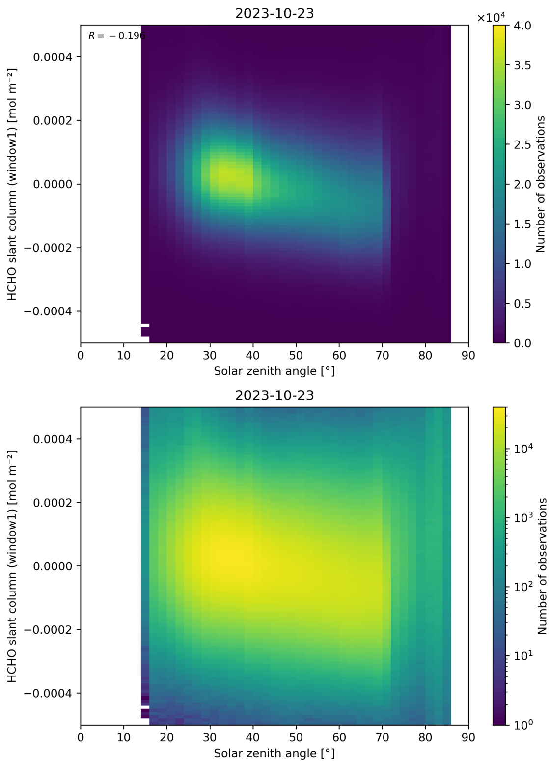
Figure 173: Scatter density plot of “Solar zenith angle” against “HCHO slant column (window1)” for 2023-10-22 to 2023-10-24.
