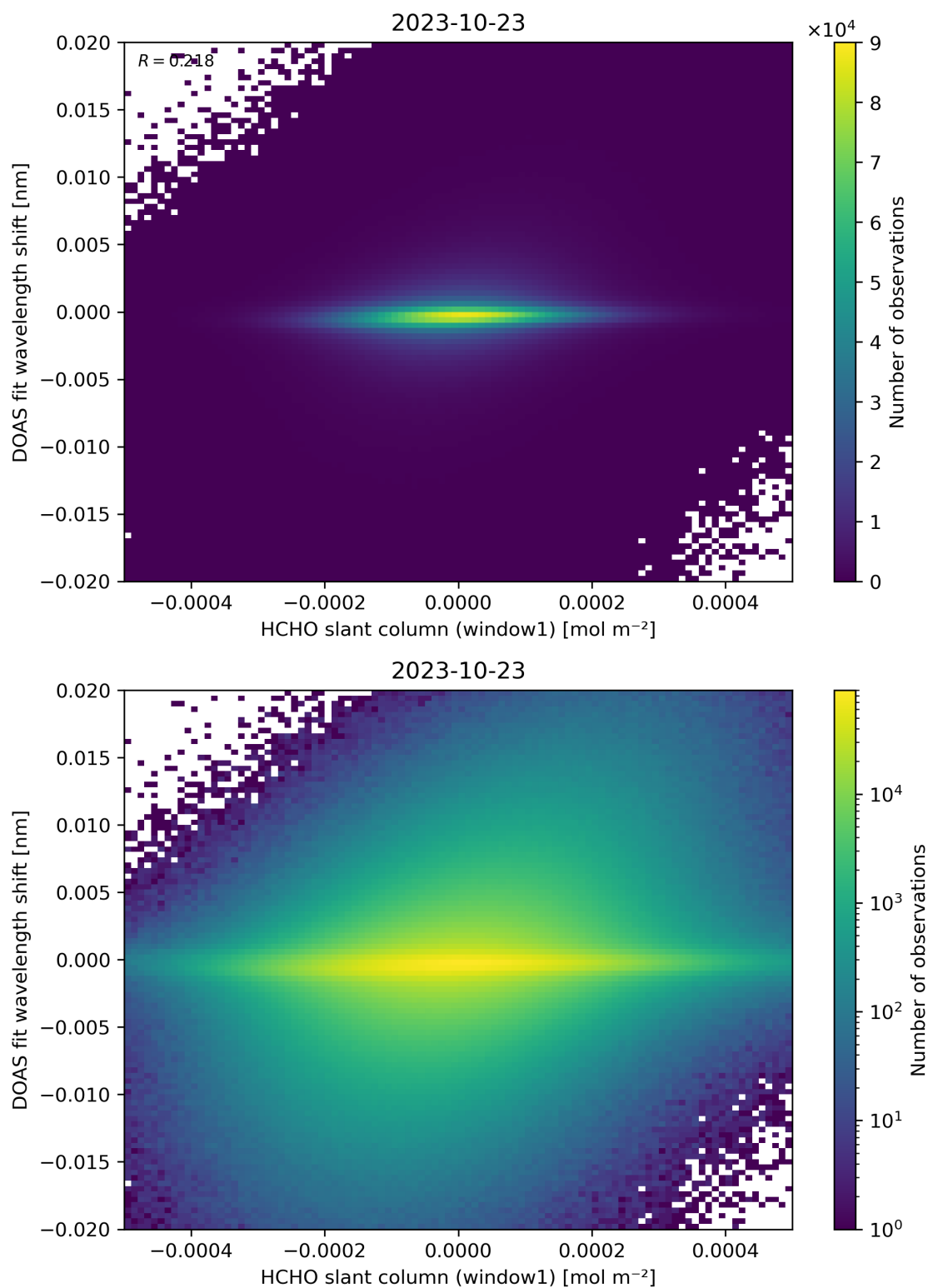
Figure 79: Scatter density plot of “HCHO slant column (window1)” against “DOAS fit wavelength shift” for 2023-10-22 to 2023-10-24.
