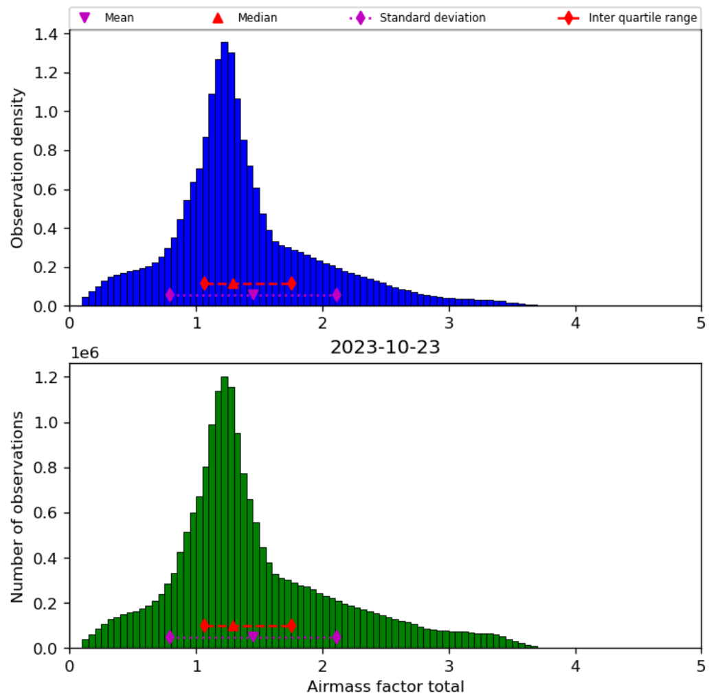
Figure 40: Histogram of “Airmass factor total” for 2023-10-22 to 2023-10-24
