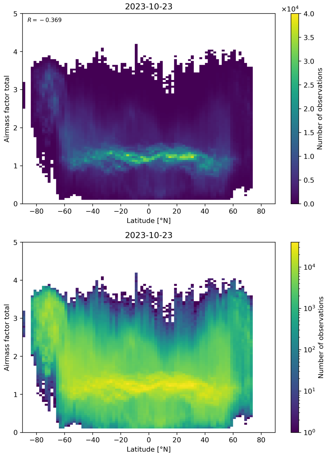
Figure 161: Scatter density plot of “Latitude” against “Airmass factor total” for 2023-10-22 to 2023-10-24.
