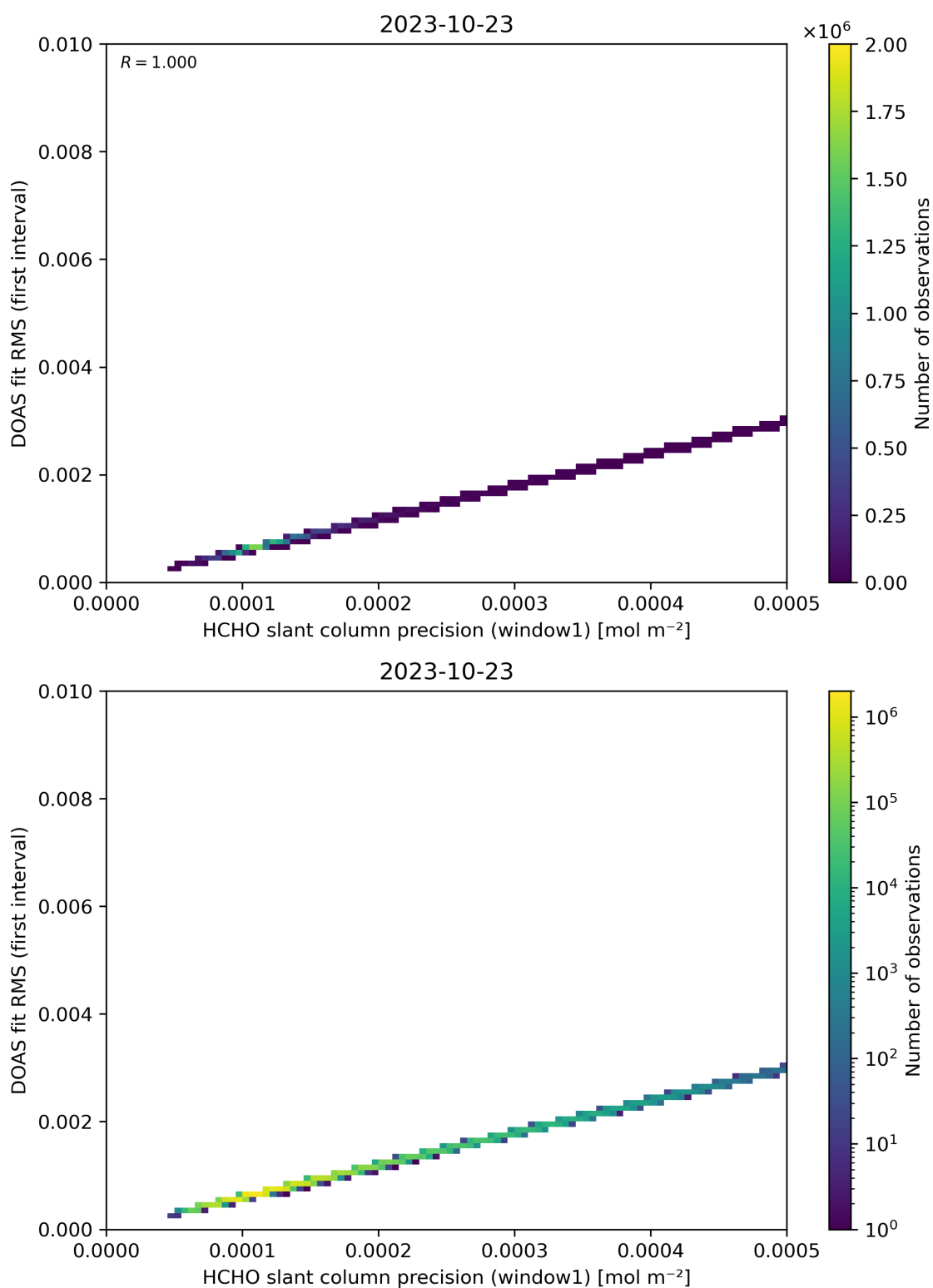
Figure 88: Scatter density plot of “HCHO slant column precision (window1)” against “DOAS fit RMS (first interval)” for 2023-10-22 to 2023-10-24.
