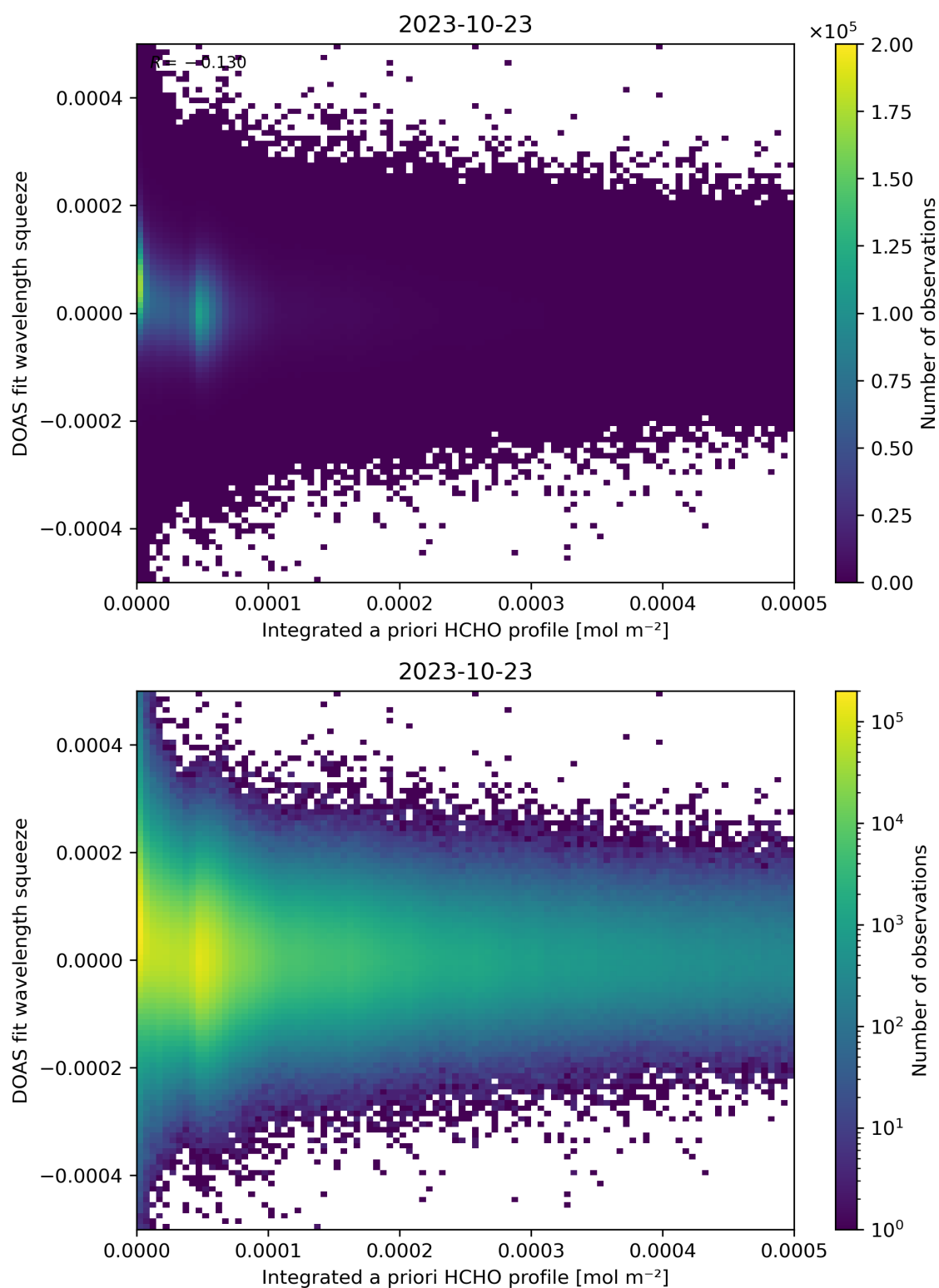
Figure 150: Scatter density plot of “Integrated a priori HCHO profile” against “DOAS fit wavelength squeeze” for 2023-10-22 to 2023-10-24.
