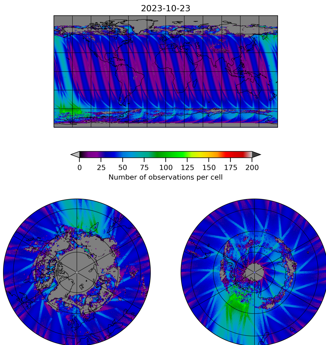
Figure 19: Map of the number of observations for 2023-10-22 to 2023-10-24
