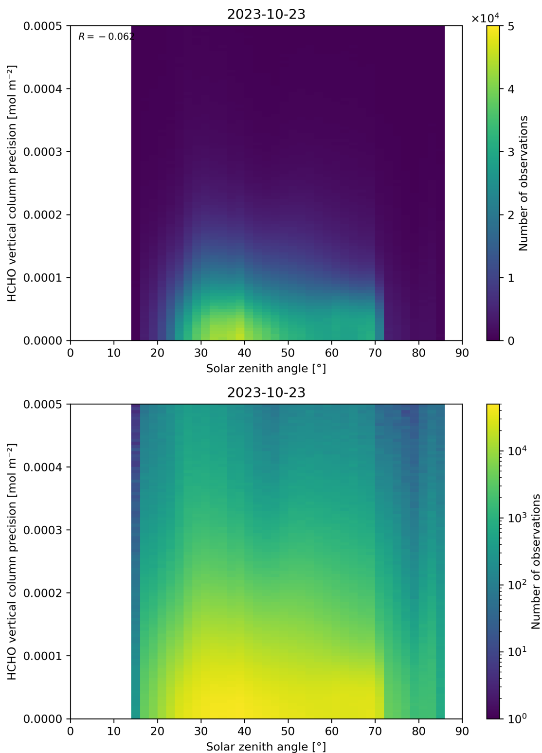
Figure 179: Scatter density plot of “Solar zenith angle” against “HCHO vertical column precision” for 2023-10-22 to 2023-10-24.
