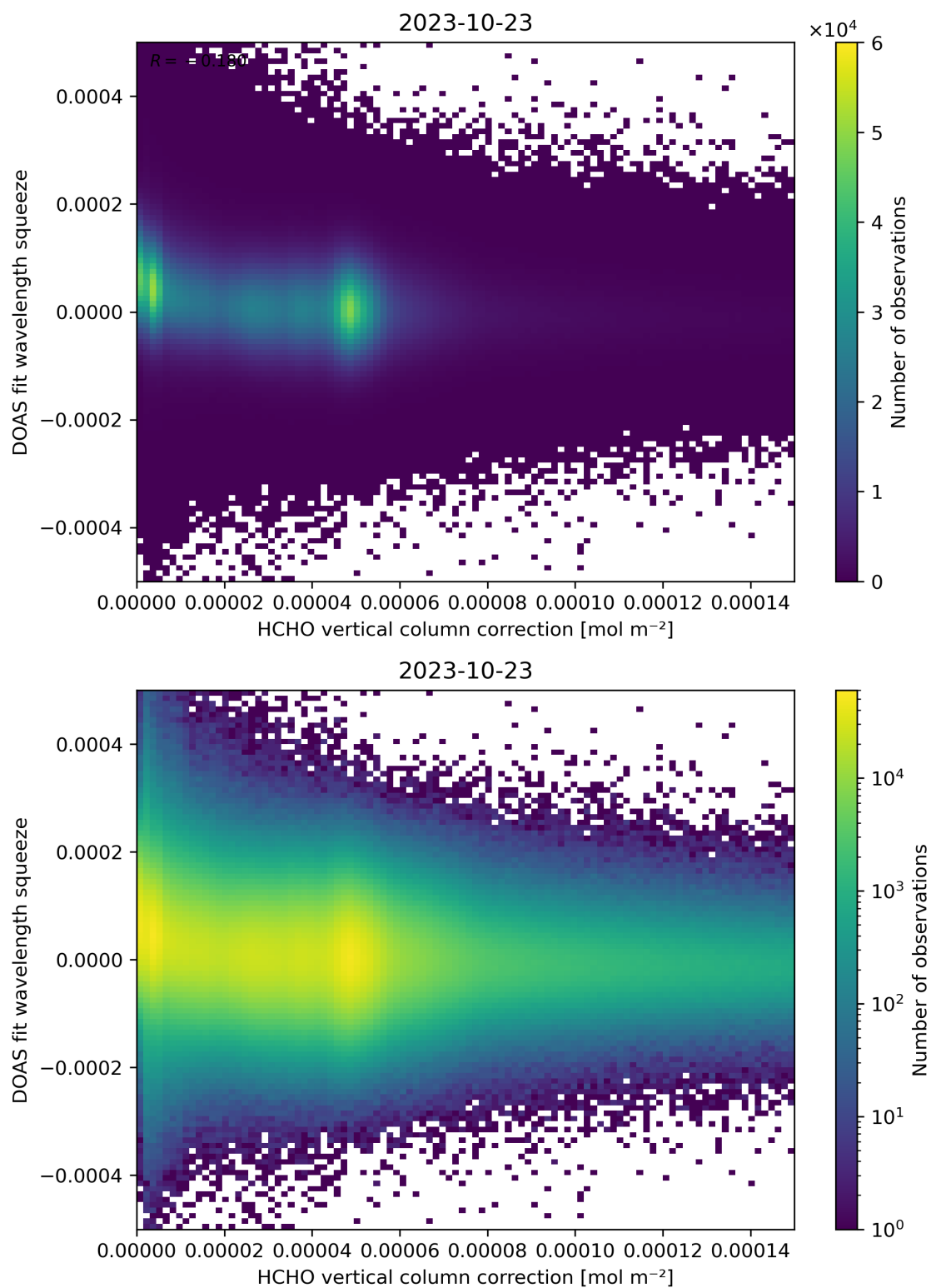
Figure 114: Scatter density plot of “HCHO vertical column correction” against “DOAS fit wavelength squeeze” for 2023-10-22 to 2023-10-24.
