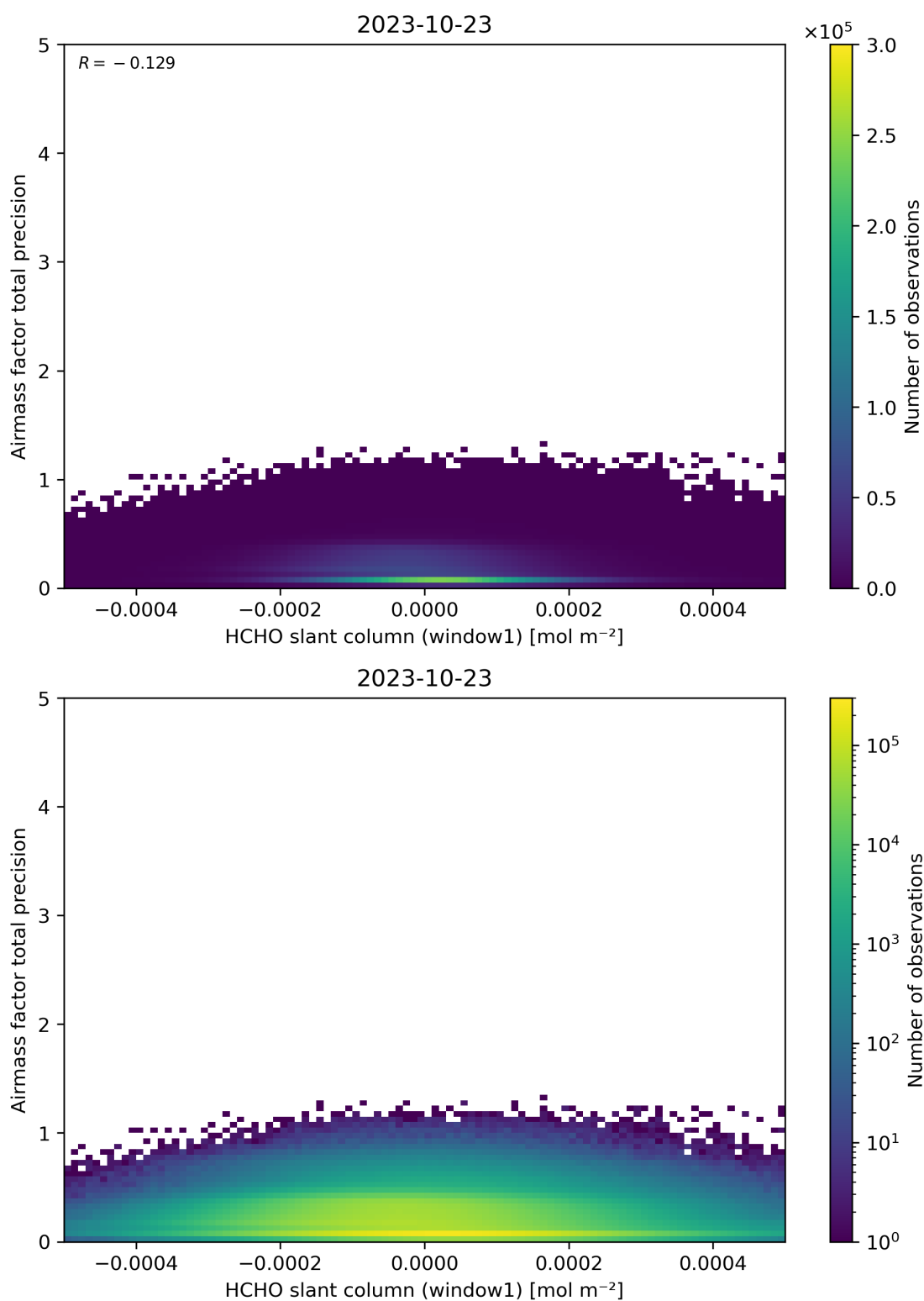
Figure 86: Scatter density plot of “HCHO slant column (window1)” against “Airmass factor total precision” for 2023-10-22 to 2023-10-24.
