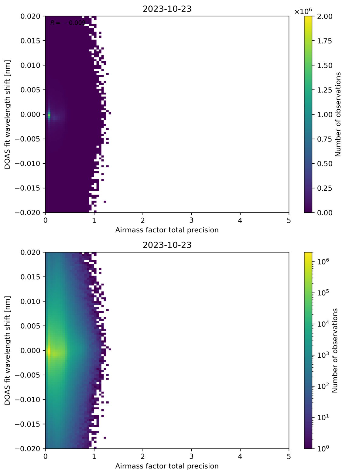
Figure 106: Scatter density plot of “Airmass factor total precision” against “DOAS fit wavelength shift” for 2023-10-22 to 2023-10-24.
