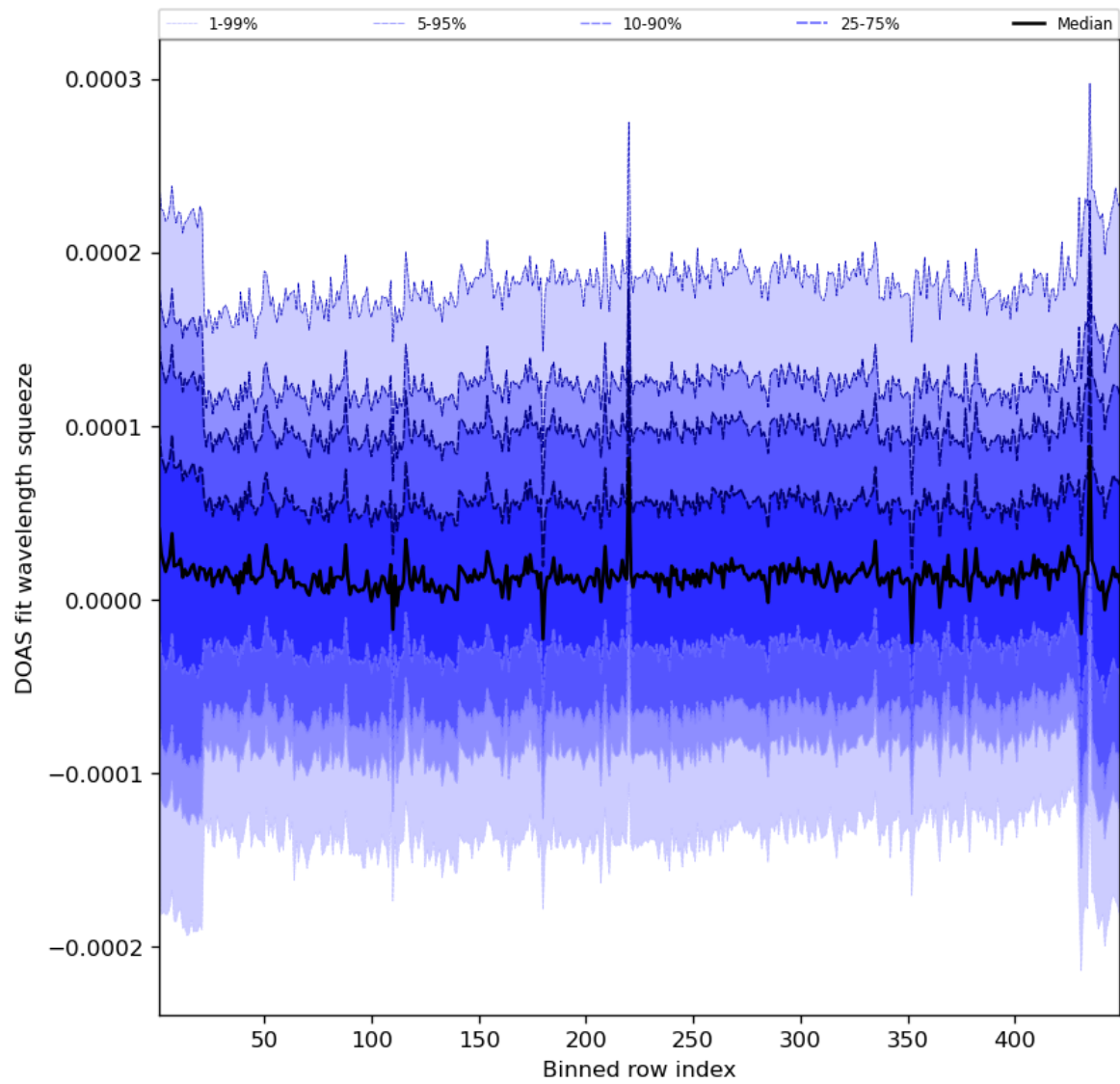
Figure 59: Along track statistics of “DOAS fit wavelength squeeze” for 2023-10-22 to 2023-10-24
