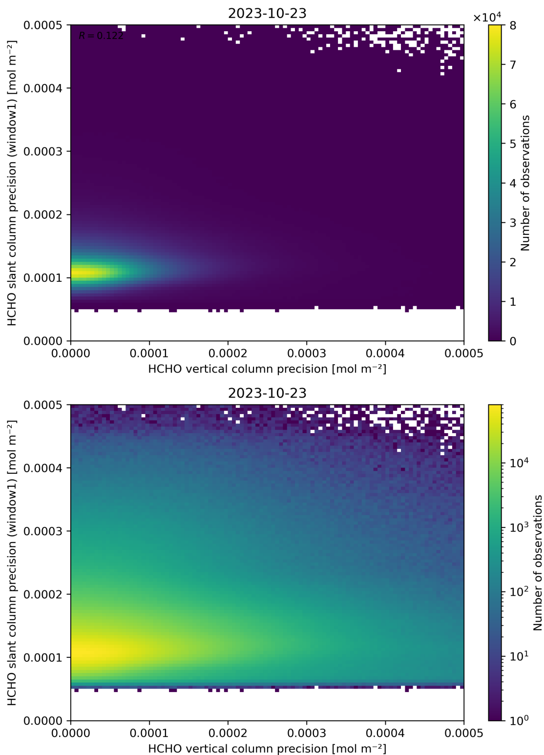
Figure 143: Scatter density plot of “HCHO vertical column precision” against “HCHO slant column precision (window1)” for 2023-10-22 to 2023-10-24.
