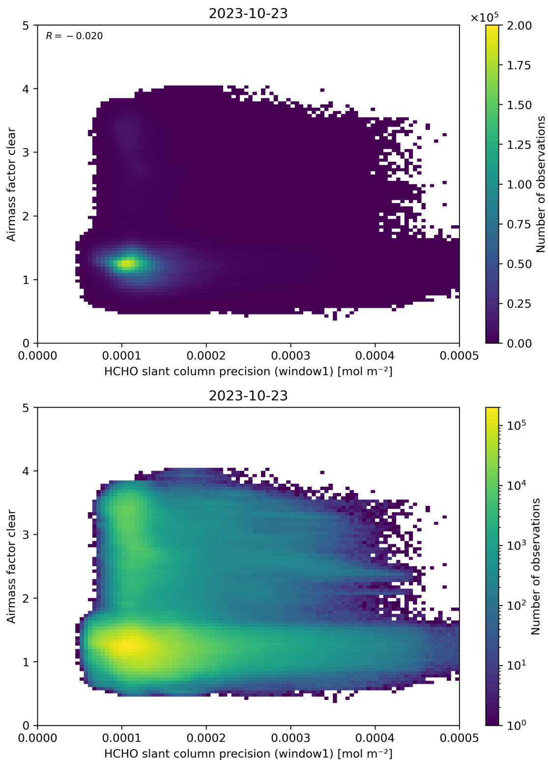
Figure 91: Scatter density plot of “HCHO slant column precision (window1)” against “Airmass factor clear” for 2023-10-22 to 2023-10-24.
