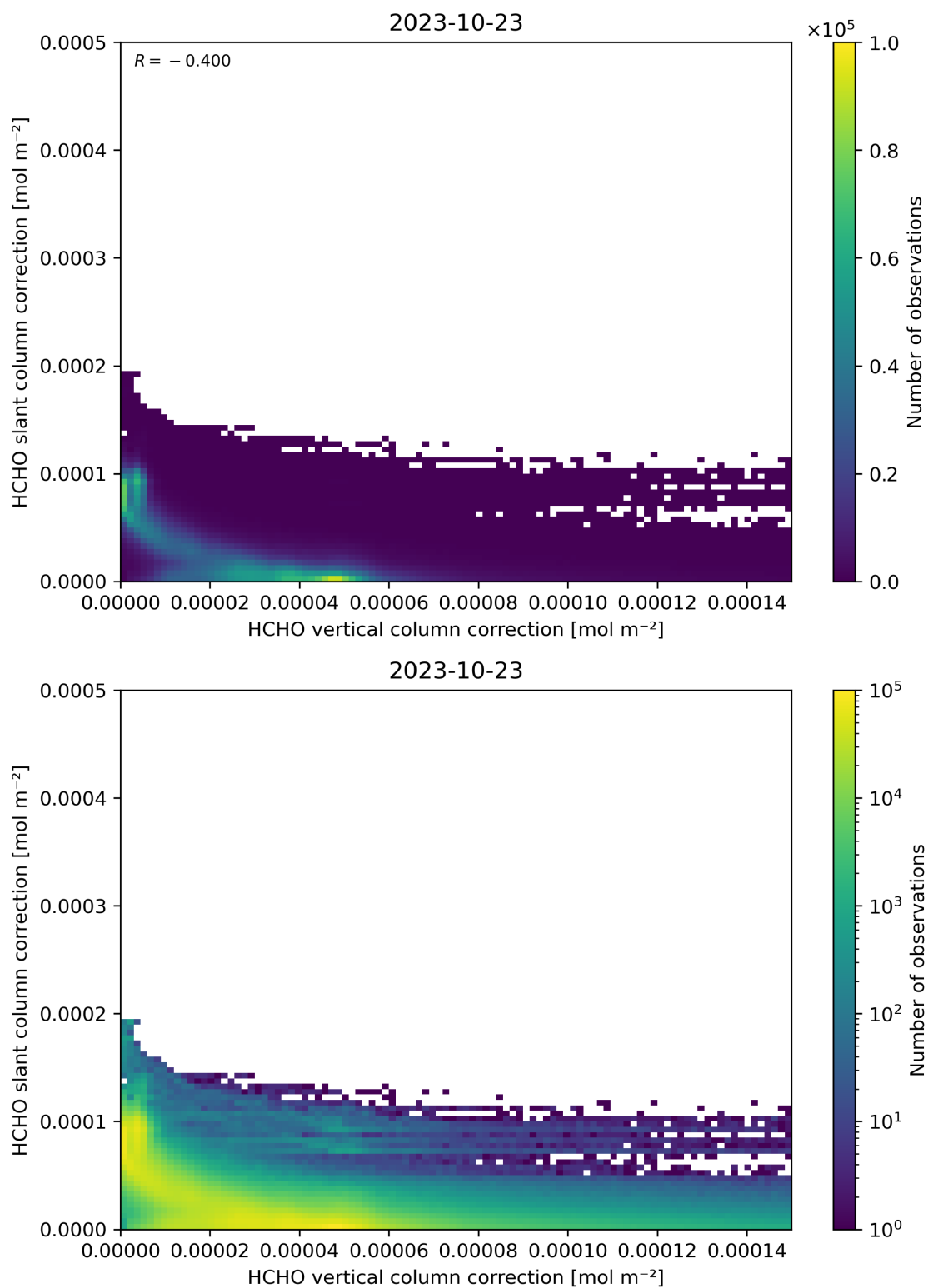
Figure 117: Scatter density plot of “HCHO vertical column correction” against “HCHO slant column correction” for 2023-10-22 to 2023-10-24.
