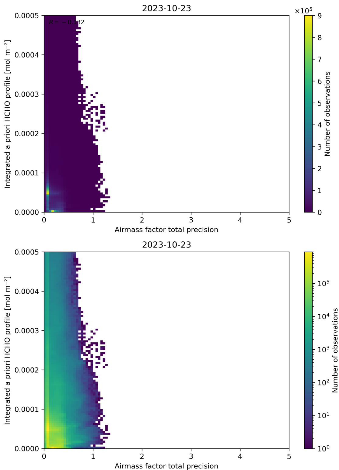
Figure 111: Scatter density plot of “Airmass factor total precision” against “Integrated a priori HCHO profile” for 2023-10-22 to 2023-10-24.
