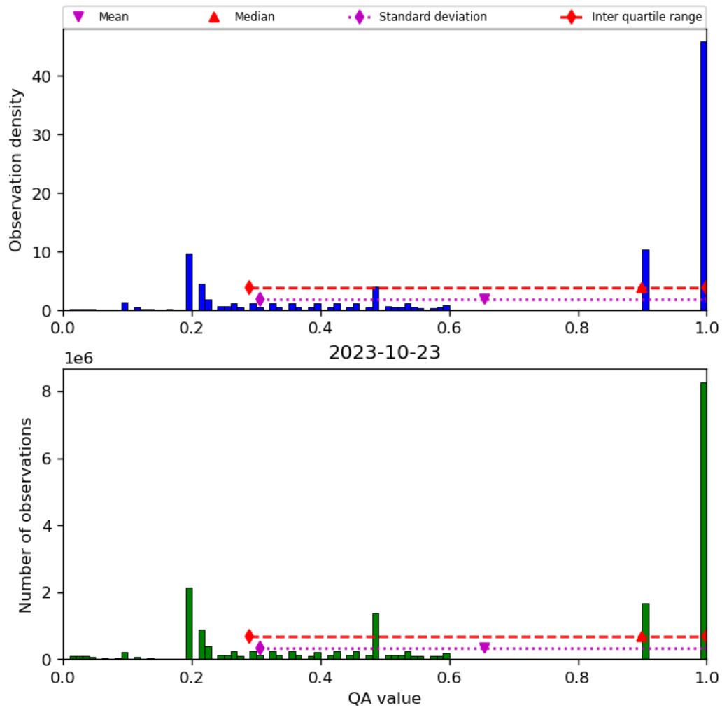
Figure 34: Histogram of “QA value” for 2023-10-22 to 2023-10-24
