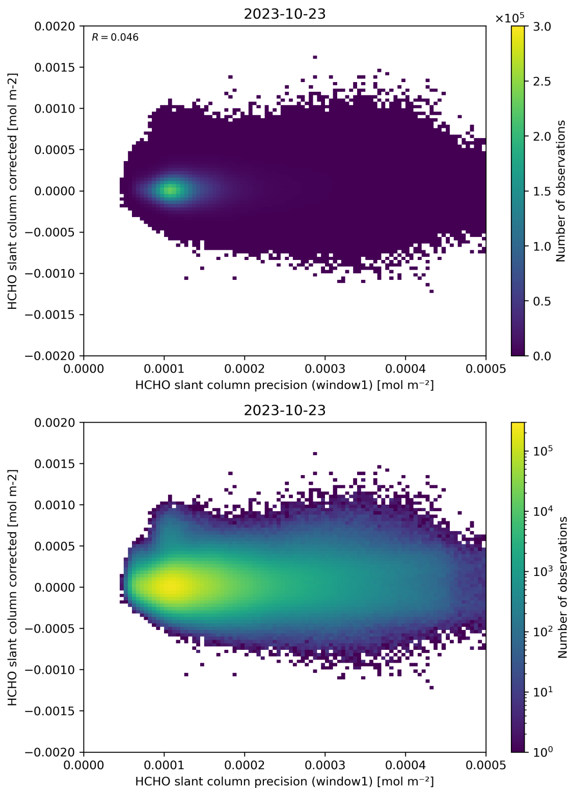
Figure 92: Scatter density plot of “HCHO slant column precision (window1)” against “HCHO slant column corrected” for 2023-10-22 to 2023-10-24.
