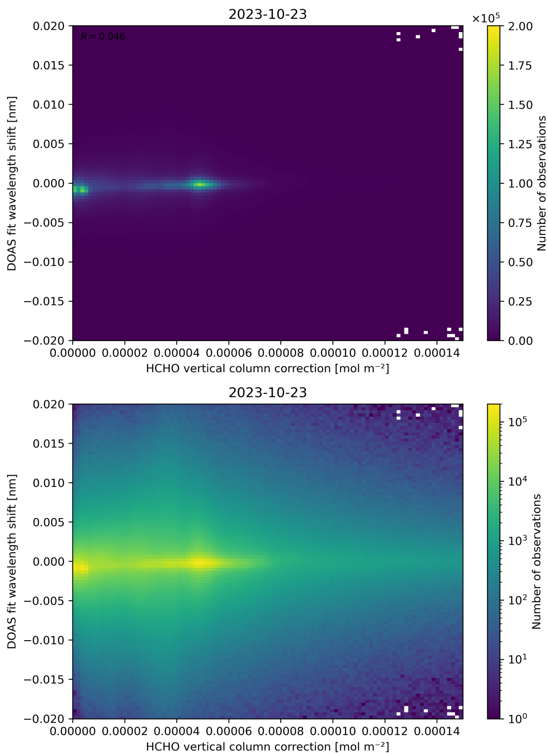
Figure 113: Scatter density plot of “HCHO vertical column correction” against “DOAS fit wavelength shift” for 2023-10-22 to 2023-10-24.
