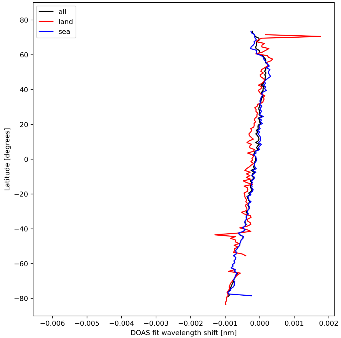
Figure 30: Zonal average of “DOAS fit wavelength shift” for 2023-10-22 to 2023-10-24.
