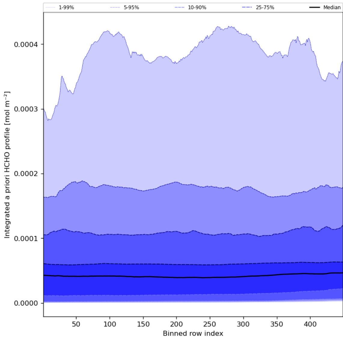
Figure 57: Along track statistics of “Integrated a priori HCHO profile” for 2023-10-22 to 2023-10-24
