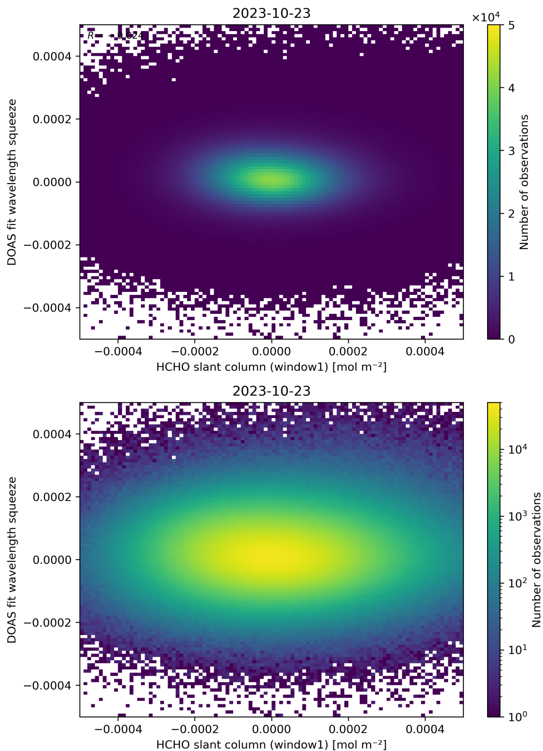
Figure 80: Scatter density plot of “HCHO slant column (window1)” against “DOAS fit wavelength squeeze” for 2023-10-22 to 2023-10-24.
