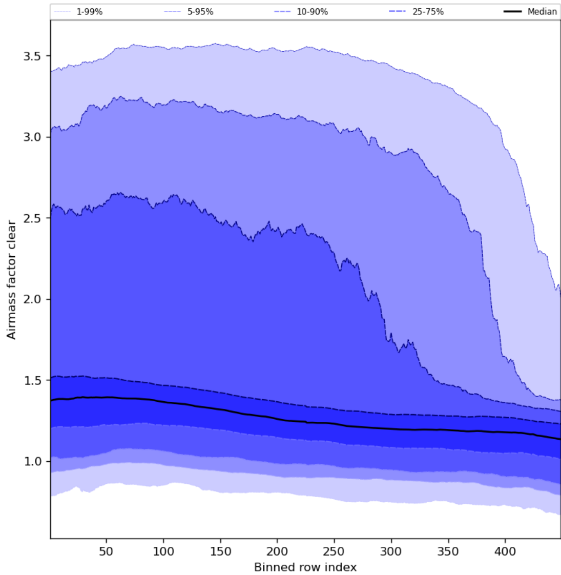
Figure 56: Along track statistics of “Airmass factor clear” for 2023-10-22 to 2023-10-24
