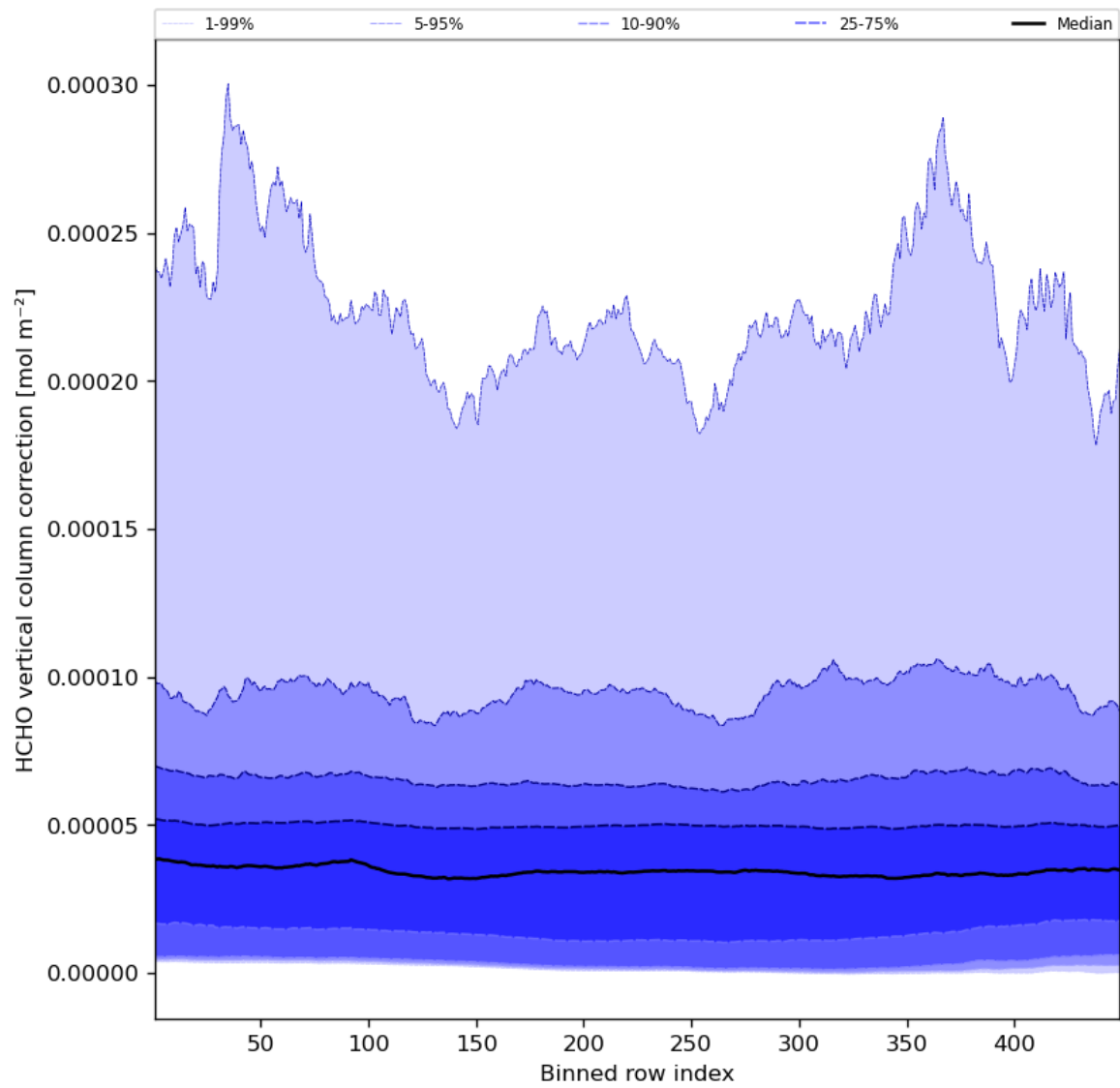
Figure 51: Along track statistics of “HCHO vertical column correction” for 2023-10-22 to 2023-10-24
