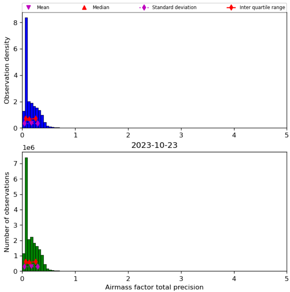
Figure 41: Histogram of “Airmass factor total precision” for 2023-10-22 to 2023-10-24
