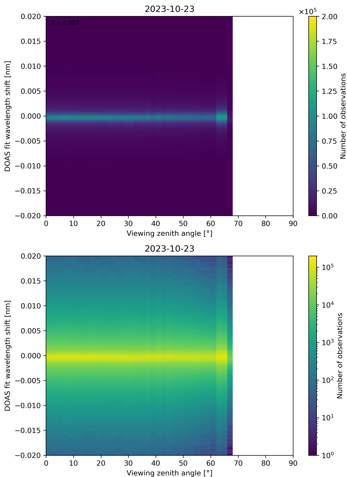
Figure 183: Scatter density plot of “Viewing zenith angle” against “DOAS fit wavelength shift” for 2023-10-22 to 2023-10-24.
