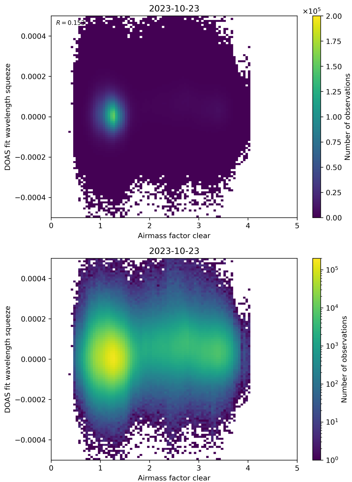
Figure 73: Scatter density plot of “Airmass factor clear” against “DOAS fit wavelength squeeze” for 2023-10-22 to 2023-10-24.
