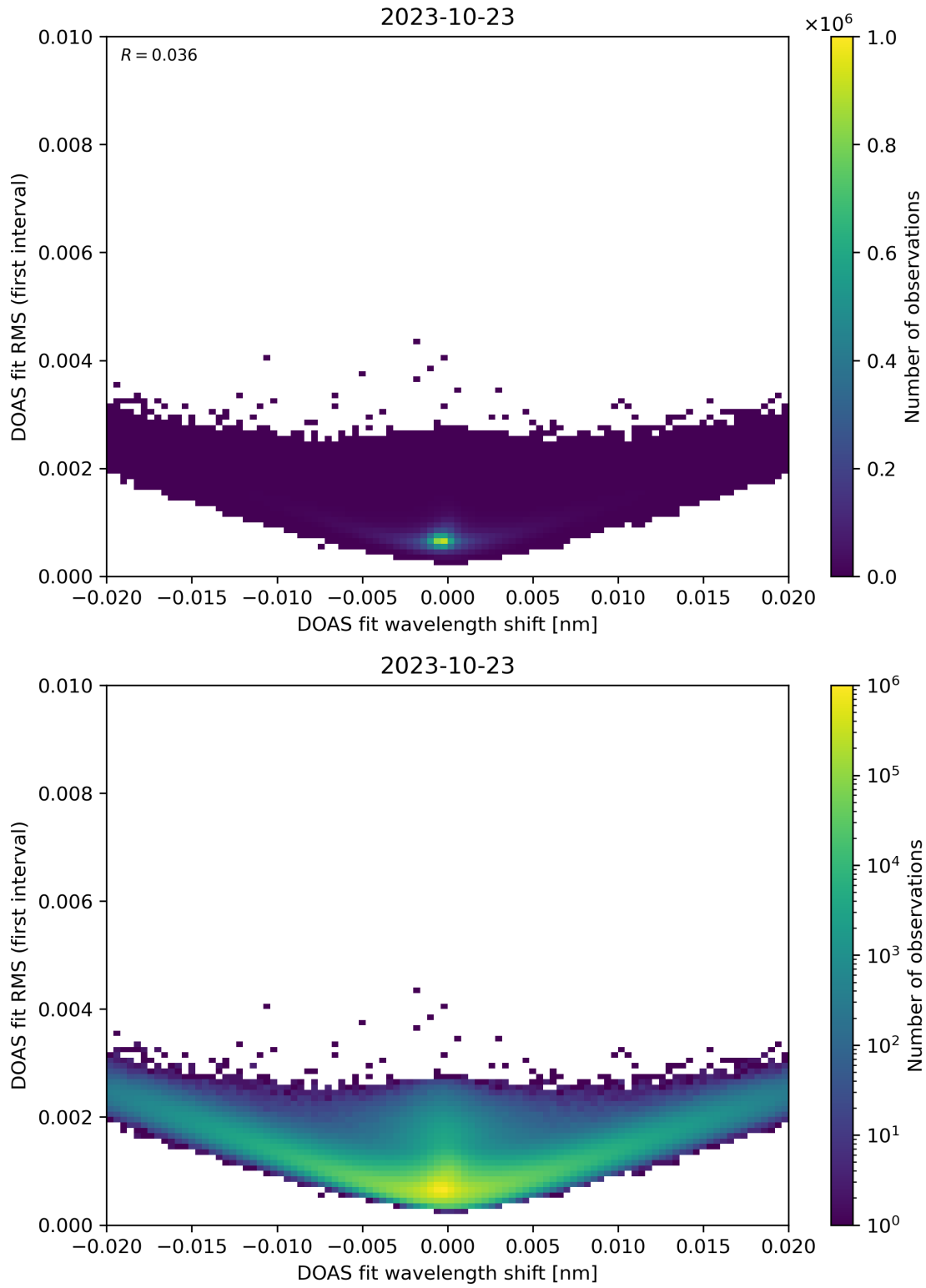
Figure 64: Scatter density plot of “DOAS fit wavelength shift” against “DOAS fit RMS (first interval)” for 2023-10-22 to 2023-10-24.
