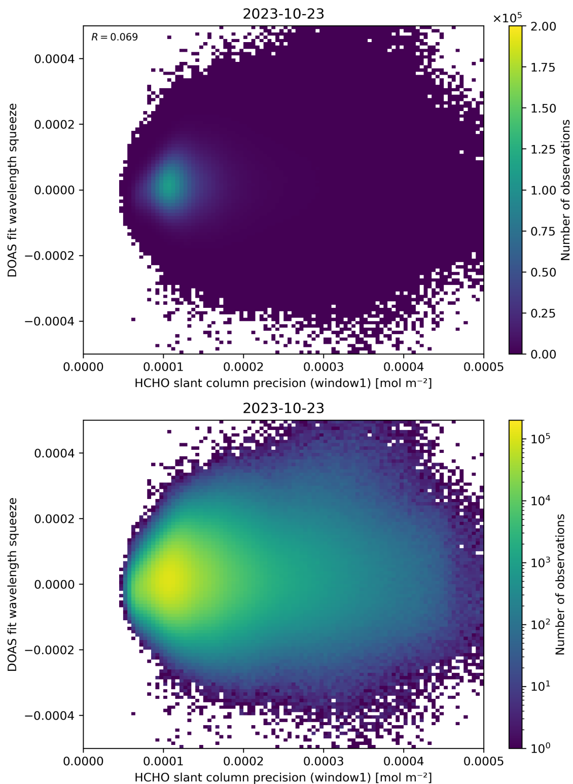
Figure 90: Scatter density plot of “HCHO slant column precision (window1)” against “DOAS fit wavelength squeeze” for 2023-10-22 to 2023-10-24.
