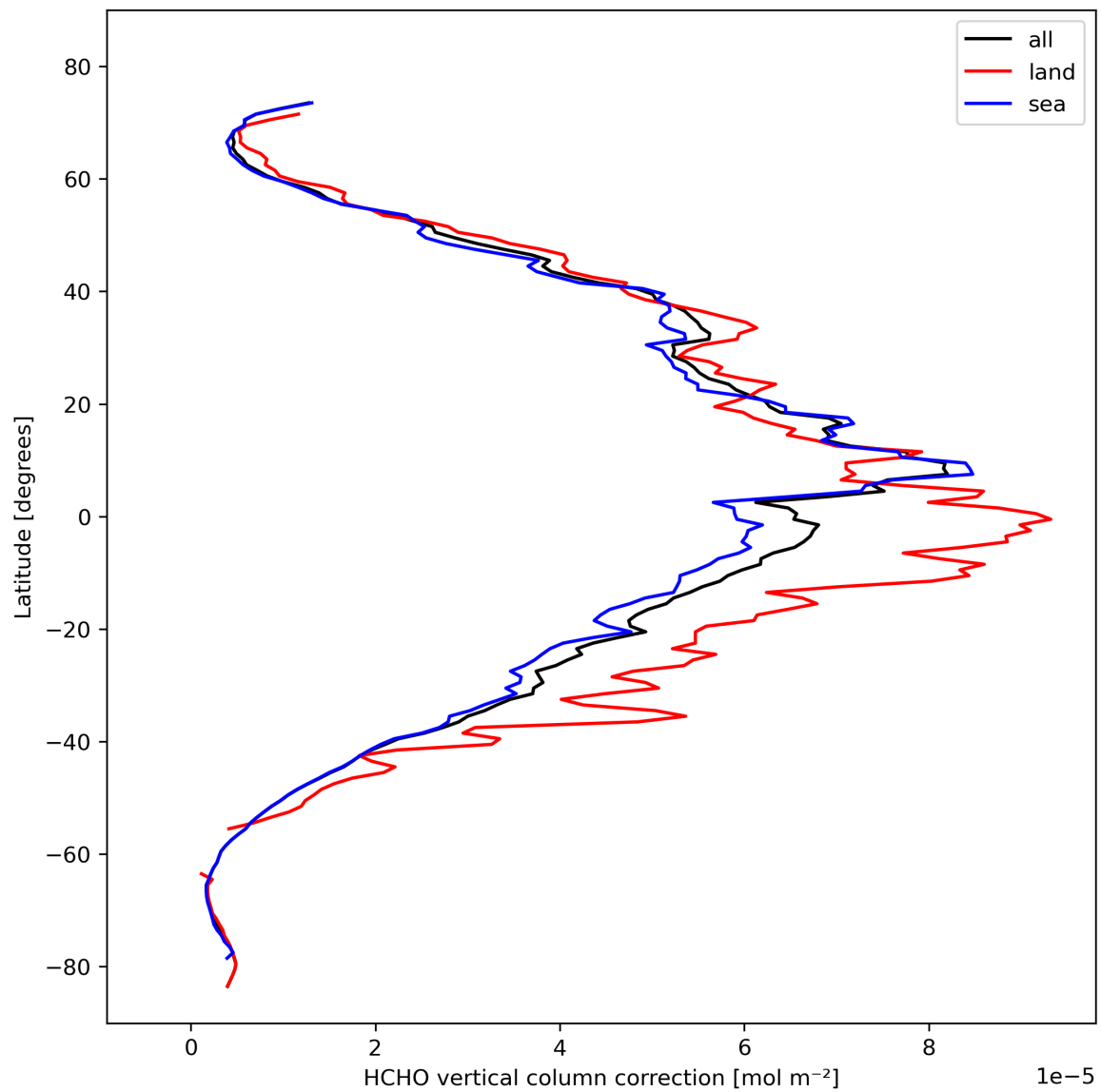
Figure 23: Zonal average of “HCHO vertical column correction” for 2023-10-22 to 2023-10-24.
