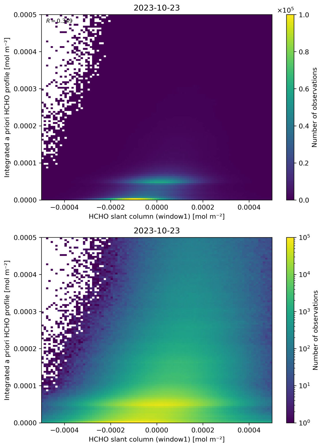
Figure 87: Scatter density plot of “HCHO slant column (window1)” against “Integrated a priori HCHO profile” for 2023-10-22 to 2023-10-24.
