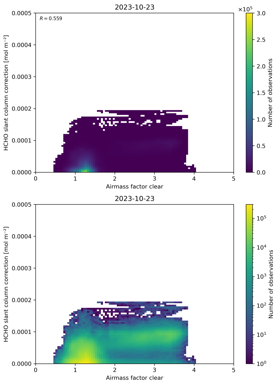
Figure 75: Scatter density plot of “Airmass factor clear” against “HCHO slant column correction” for 2023-10-22 to 2023-10-24.
