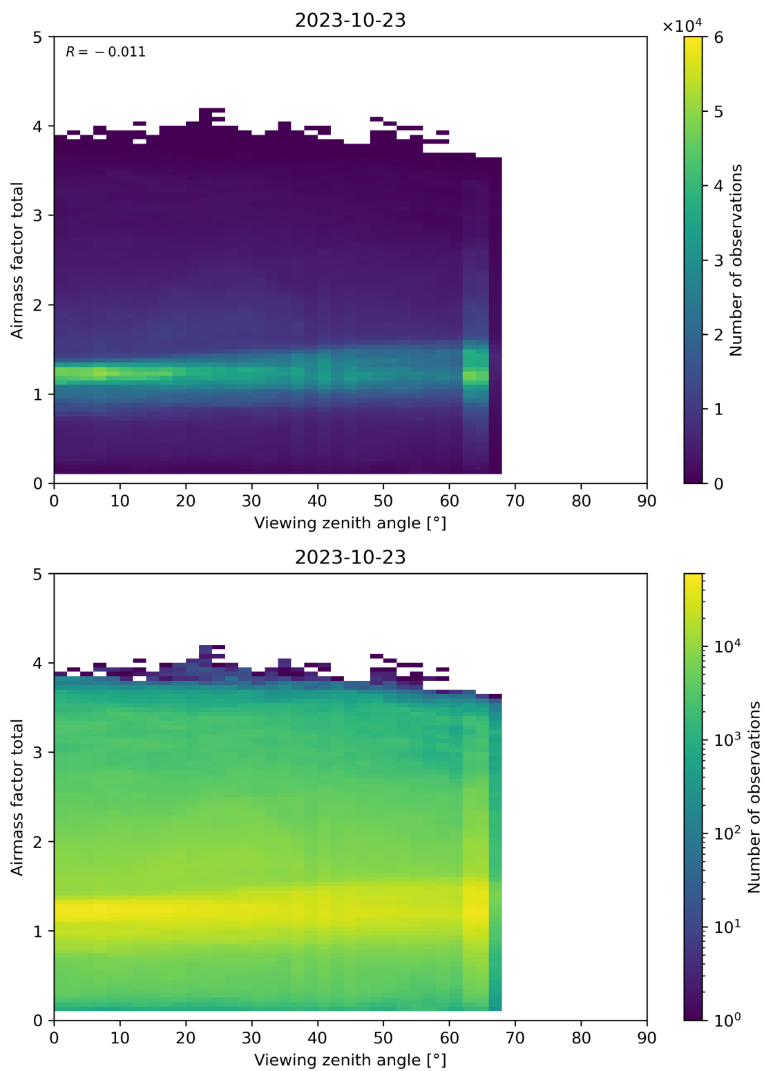
Figure 190: Scatter density plot of “Viewing zenith angle” against “Airmass factor total” for 2023-10-22 to 2023-10-24.
