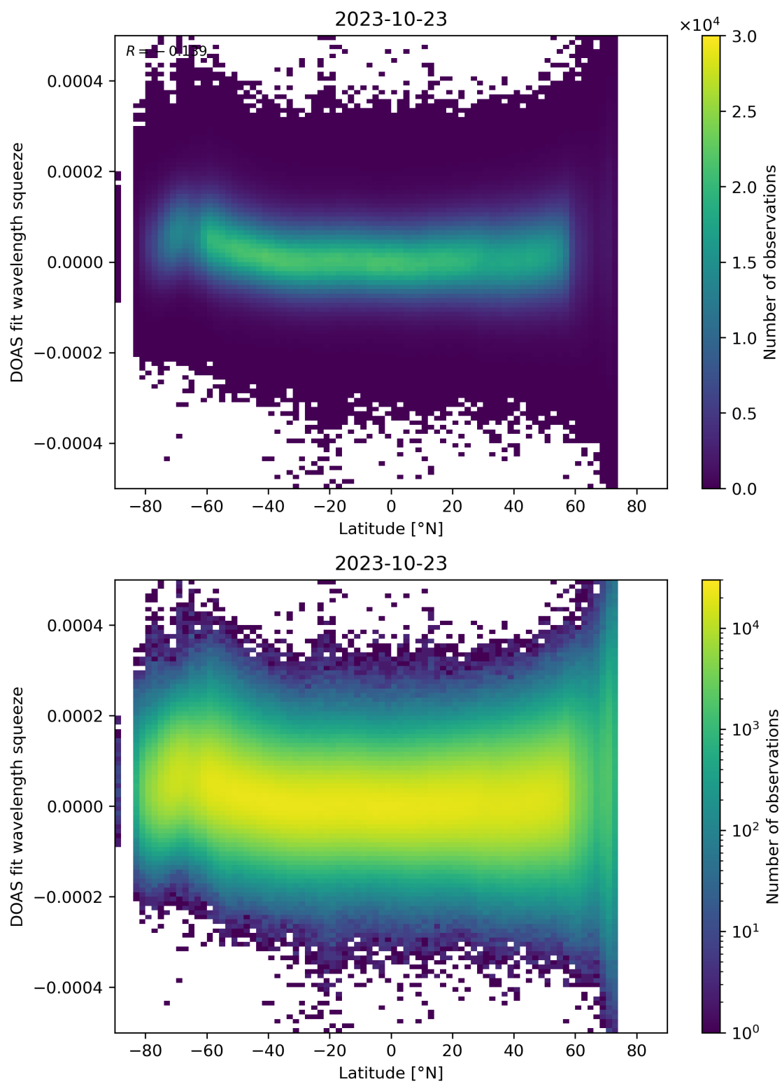
Figure 155: Scatter density plot of “Latitude” against “DOAS fit wavelength squeeze” for 2023-10-22 to 2023-10-24.
