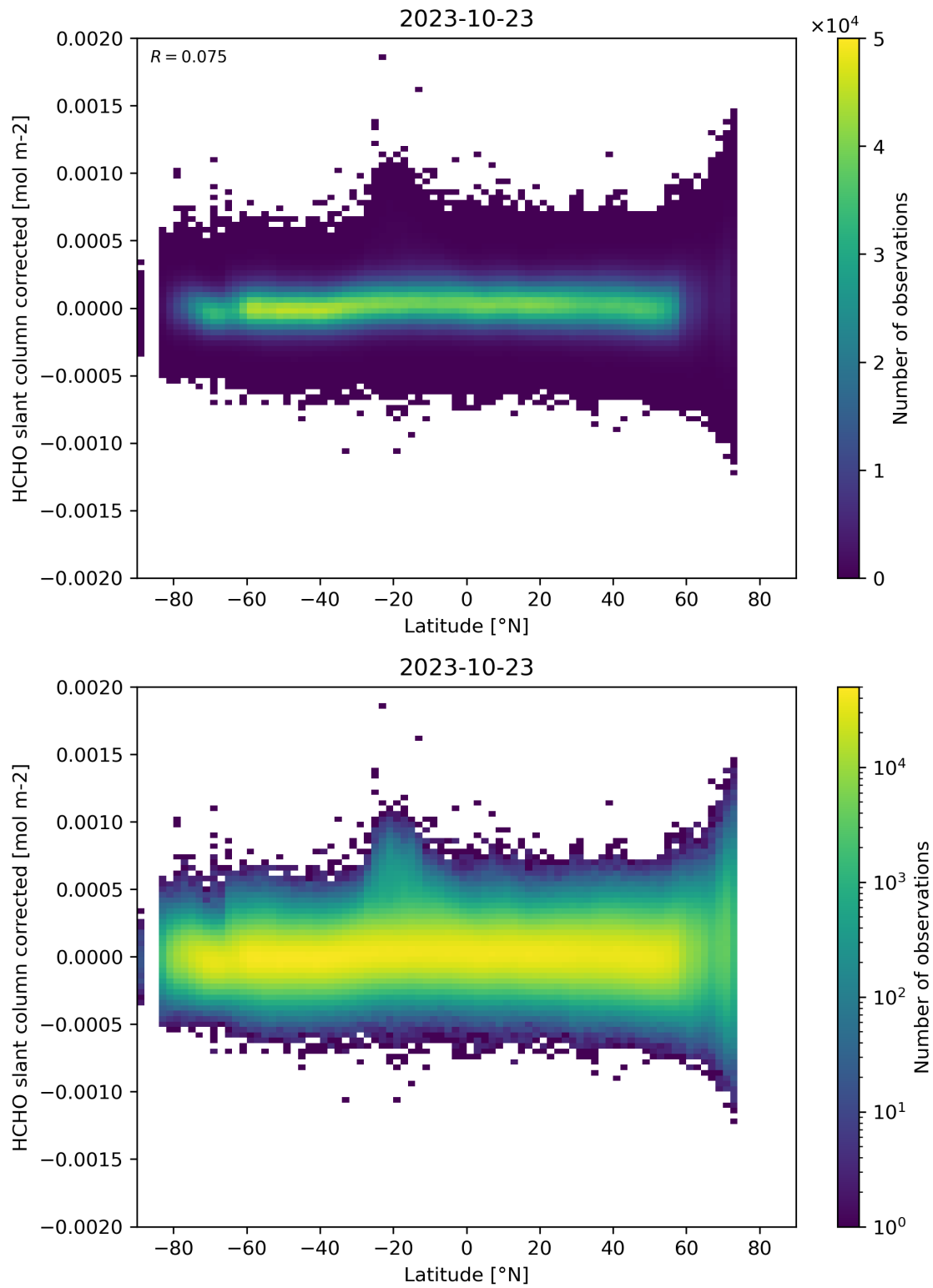
Figure 157: Scatter density plot of “Latitude” against “HCHO slant column corrected” for 2023-10-22 to 2023-10-24.
