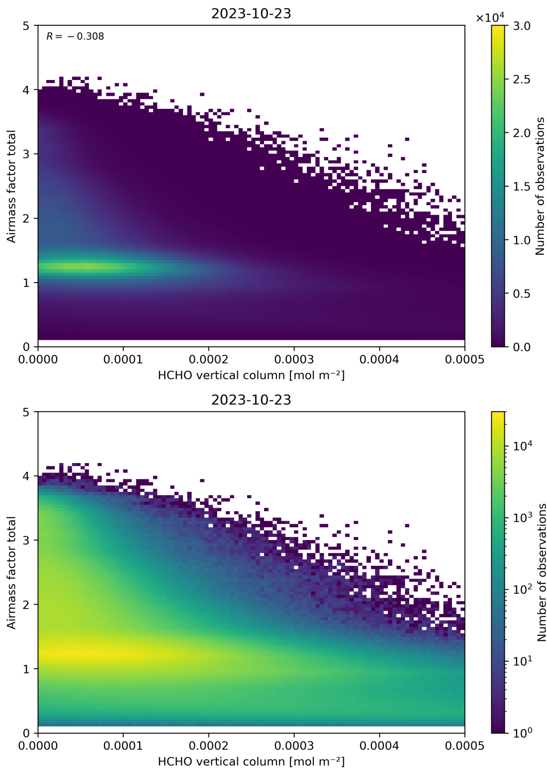
Figure 131: Scatter density plot of “HCHO vertical column” against “Airmass factor total” for 2023-10-22 to 2023-10-24.
