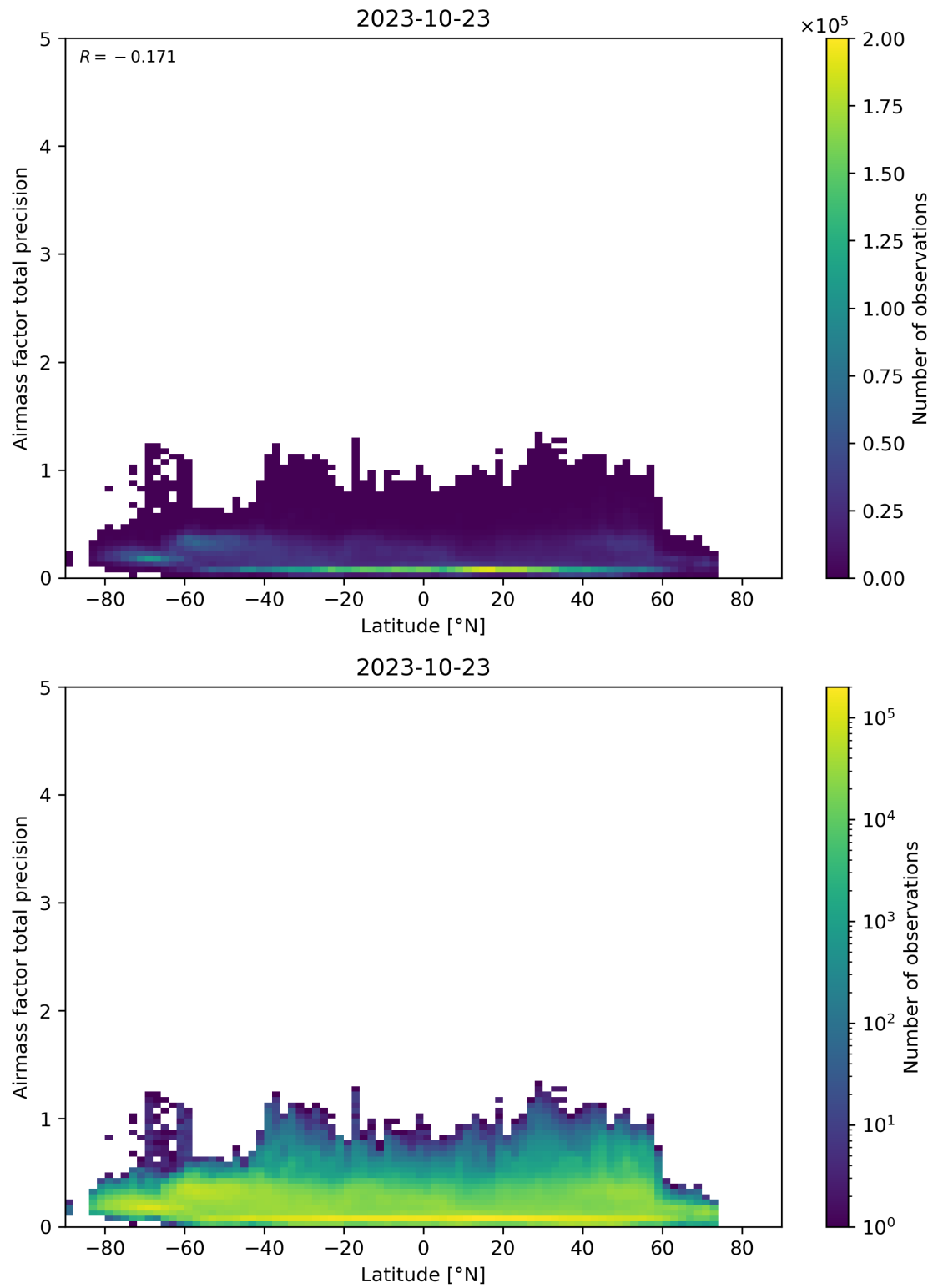
Figure 162: Scatter density plot of “Latitude” against “Airmass factor total precision” for 2023-10-22 to 2023-10-24.
