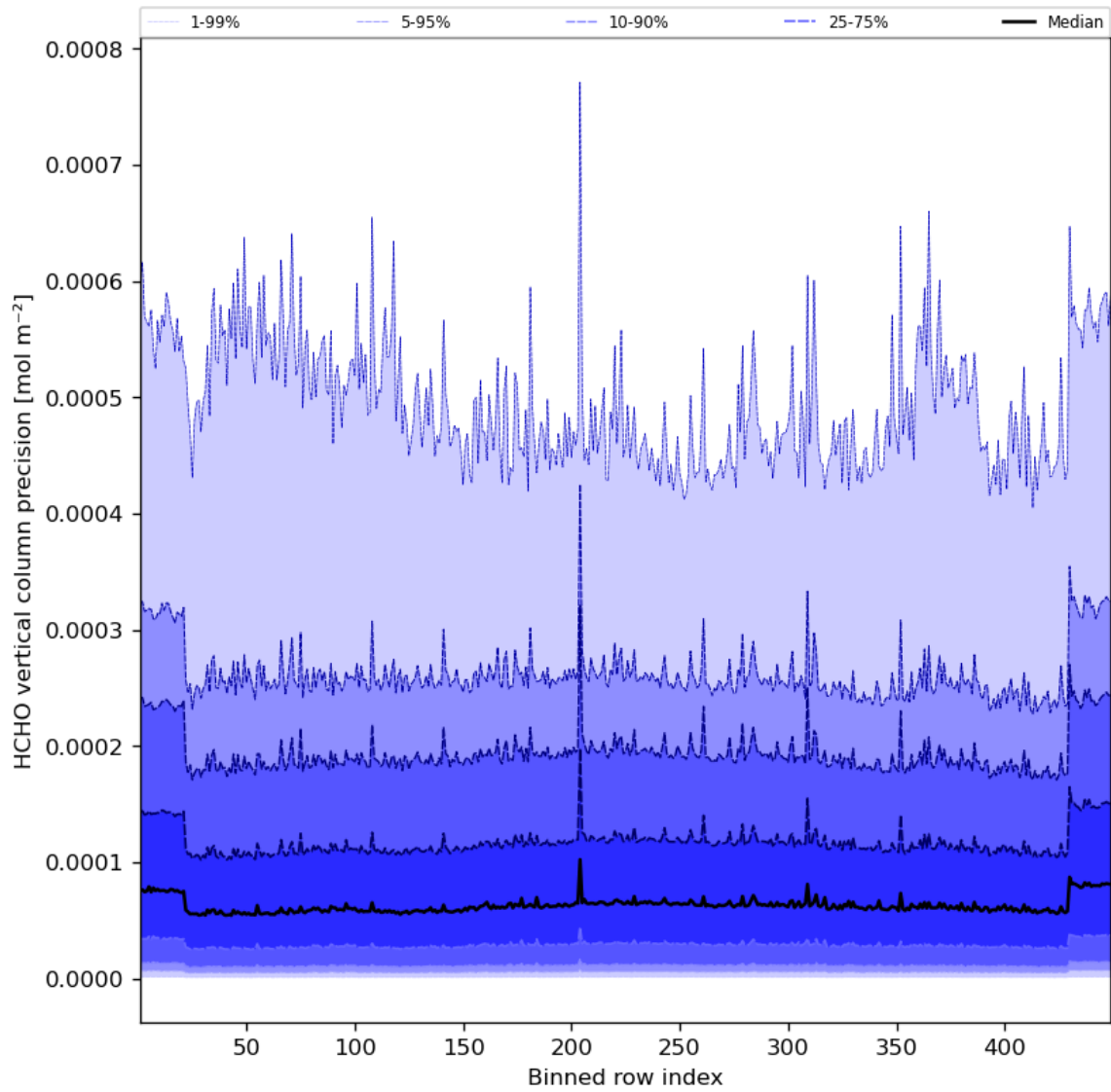
Figure 50: Along track statistics of “HCHO vertical column precision” for 2023-10-22 to 2023-10-24
