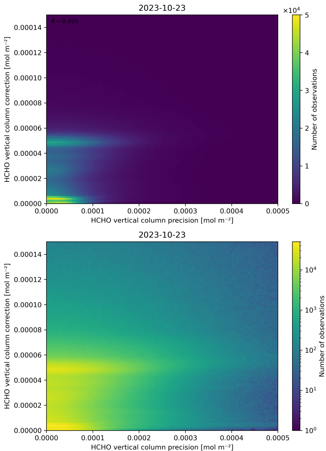
Figure 146: Scatter density plot of “HCHO vertical column precision” against “HCHO vertical column correction” for 2023-10-22 to 2023-10-24.
