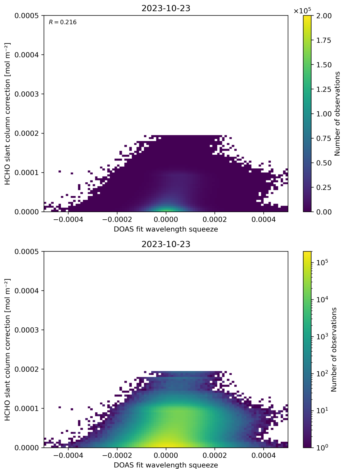
Figure 70: Scatter density plot of “DOAS fit wavelength squeeze” against “HCHO slant column correction” for 2023-10-22 to 2023-10-24.
