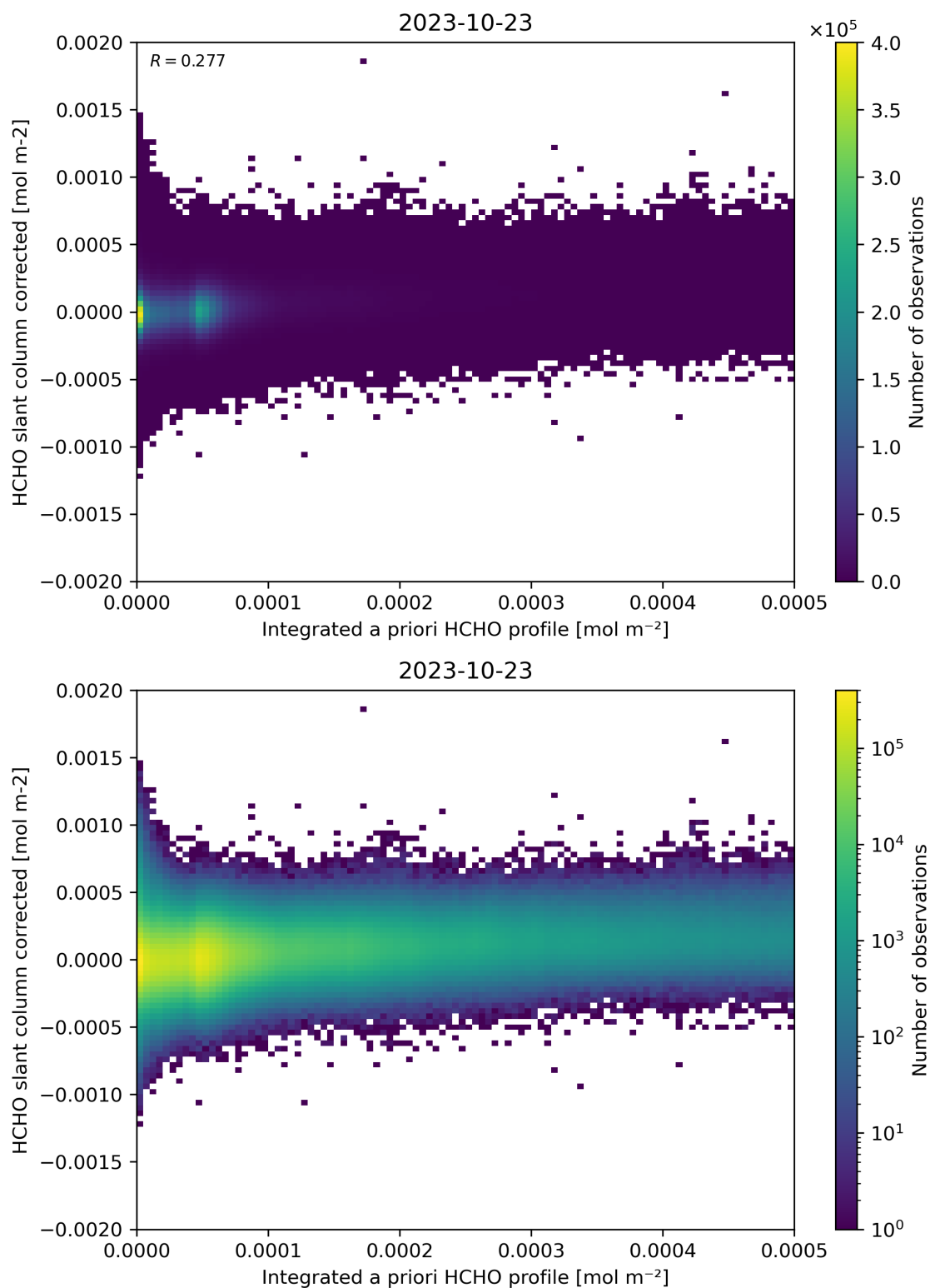
Figure 151: Scatter density plot of “Integrated a priori HCHO profile” against “HCHO slant column corrected” for 2023-10-22 to 2023-10-24.
