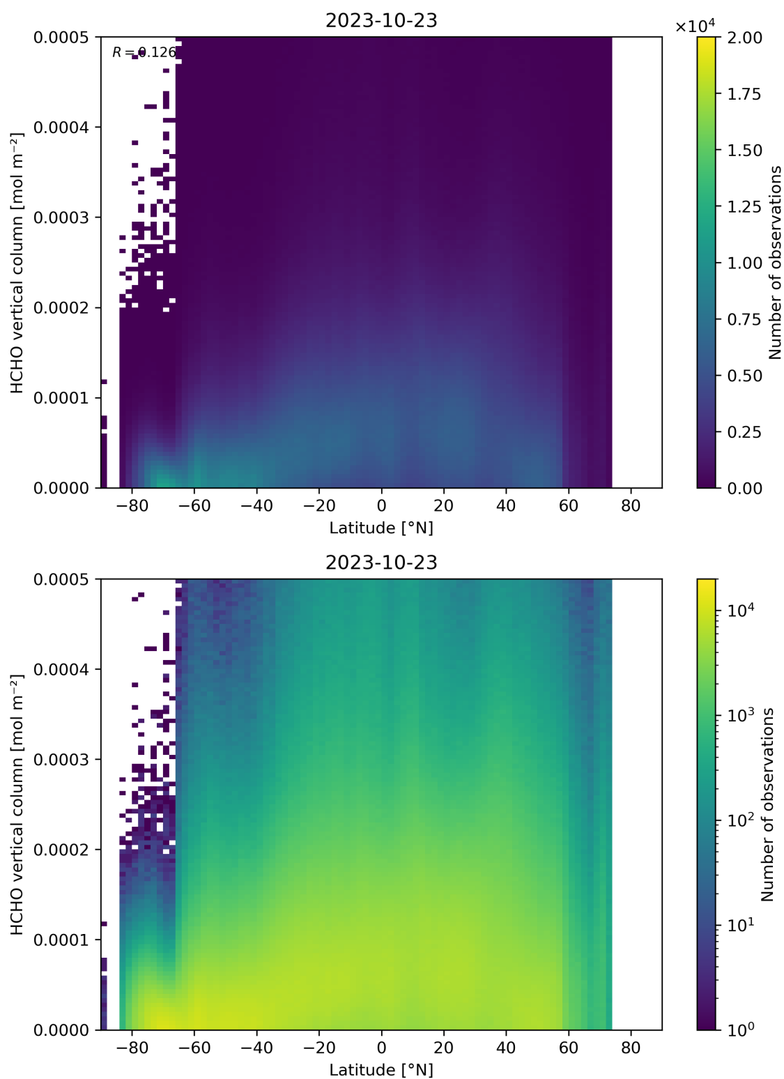
Figure 163: Scatter density plot of “Latitude” against “HCHO vertical column” for 2023-10-22 to 2023-10-24.
