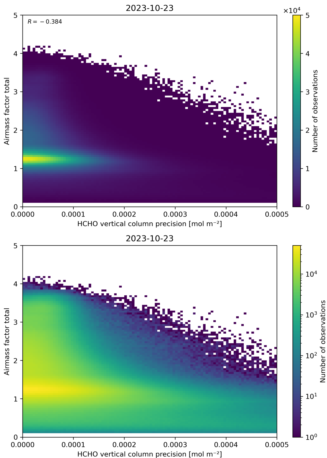
Figure 144: Scatter density plot of “HCHO vertical column precision” against “Airmass factor total” for 2023-10-22 to 2023-10-24.
