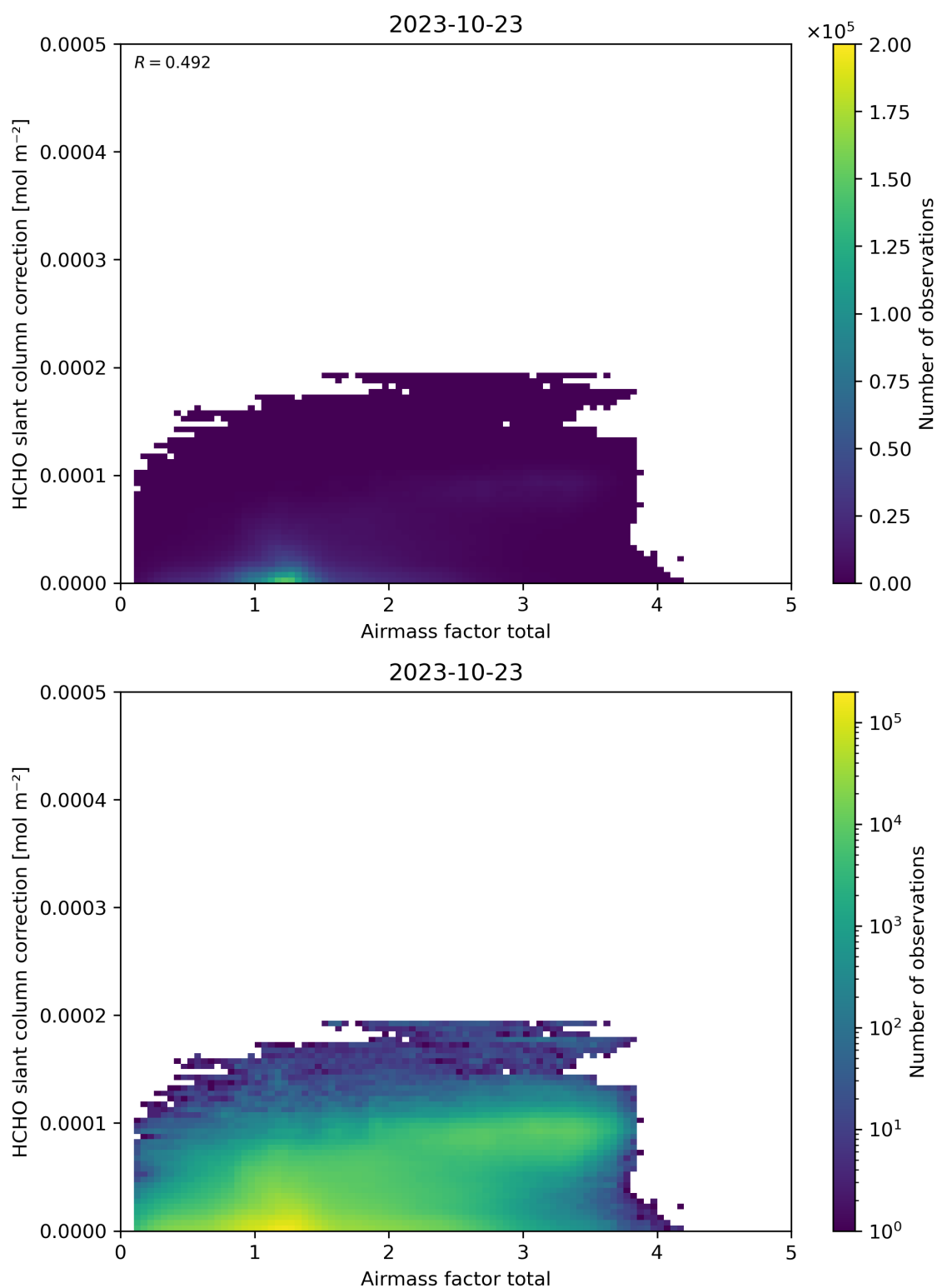
Figure 102: Scatter density plot of “Airmass factor total” against “HCHO slant column correction” for 2023-10-22 to 2023-10-24.
