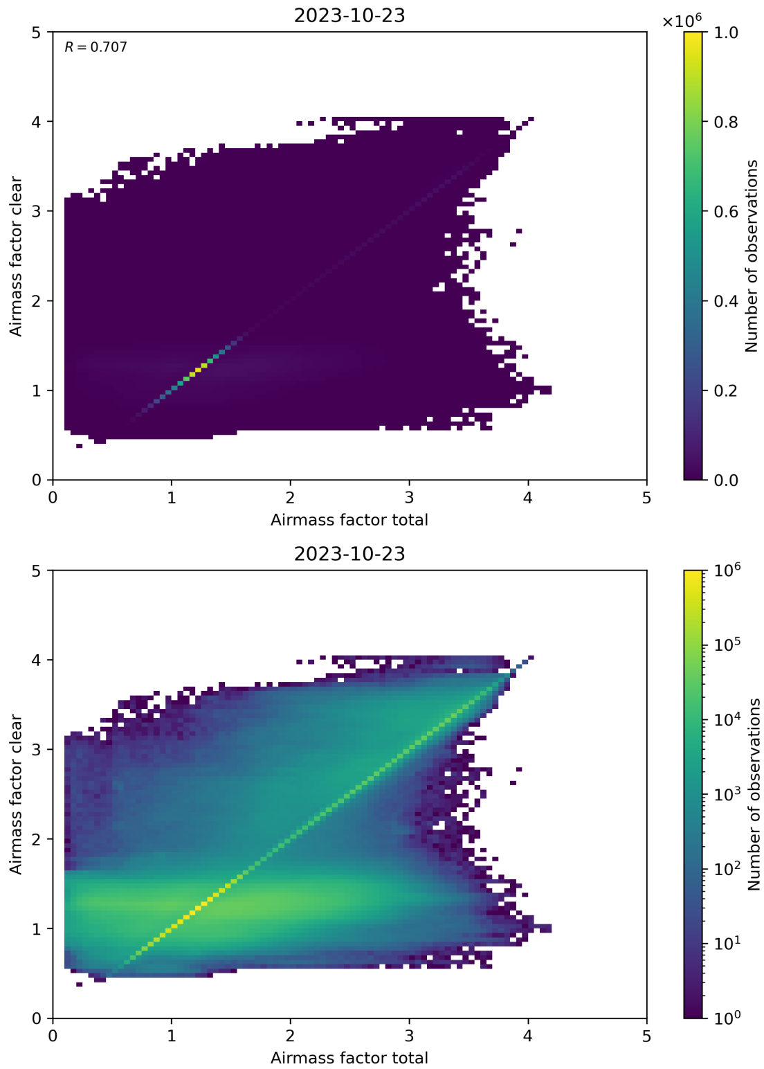
Figure 100: Scatter density plot of “Airmass factor total” against “Airmass factor clear” for 2023-10-22 to 2023-10-24.
