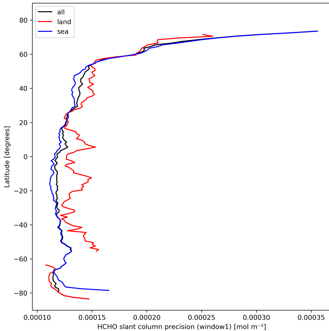
Figure 25: Zonal average of “HCHO slant column precision (window1)” for 2023-10-22 to 2023-10-24.
