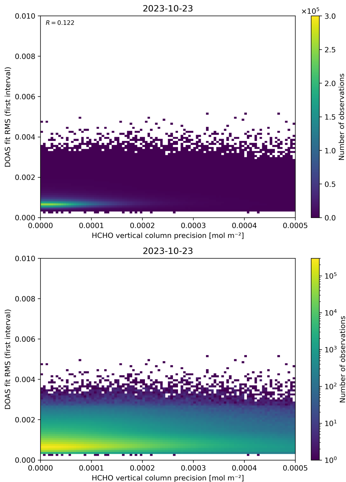
Figure 136: Scatter density plot of “HCHO vertical column precision” against “DOAS fit RMS (first interval)” for 2023-10-22 to 2023-10-24.
