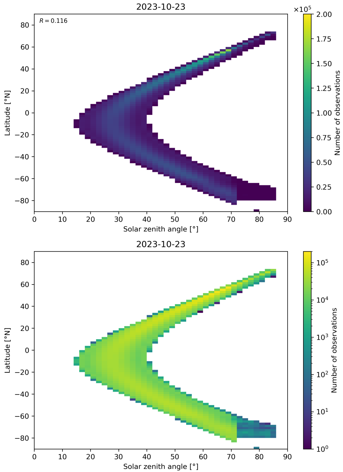
Figure 181: Scatter density plot of “Solar zenith angle” against “Latitude” for 2023-10-22 to 2023-10-24.
