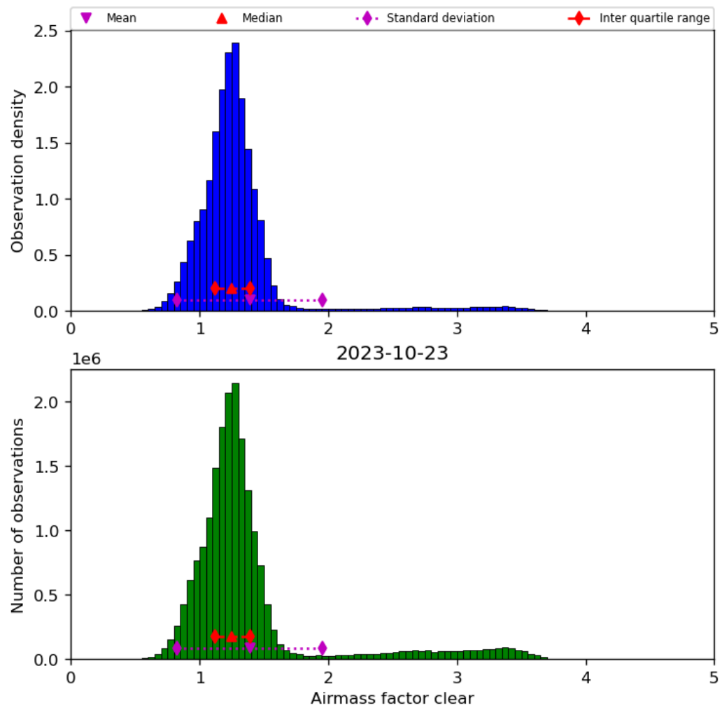
Figure 42: Histogram of “Airmass factor clear” for 2023-10-22 to 2023-10-24
