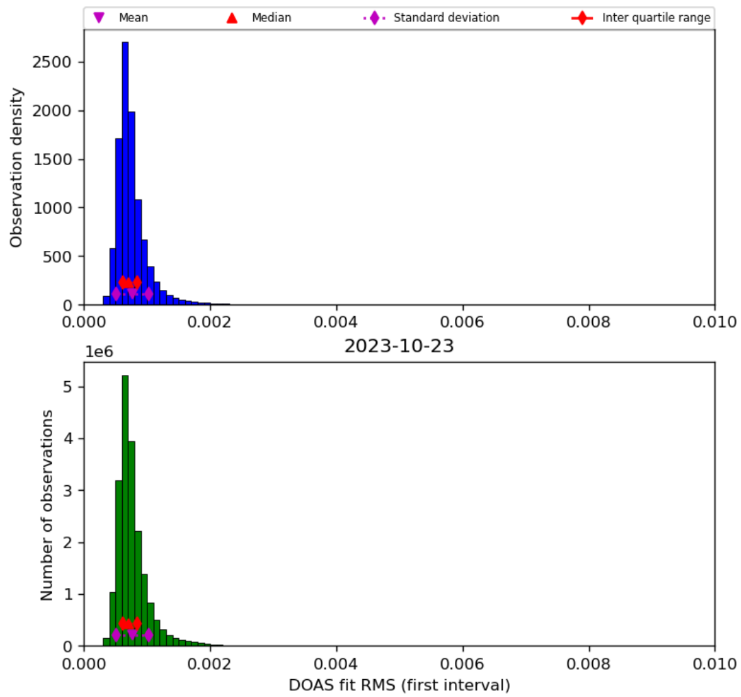
Figure 46: Histogram of “DOAS fit RMS (first interval)” for 2023-10-22 to 2023-10-24
