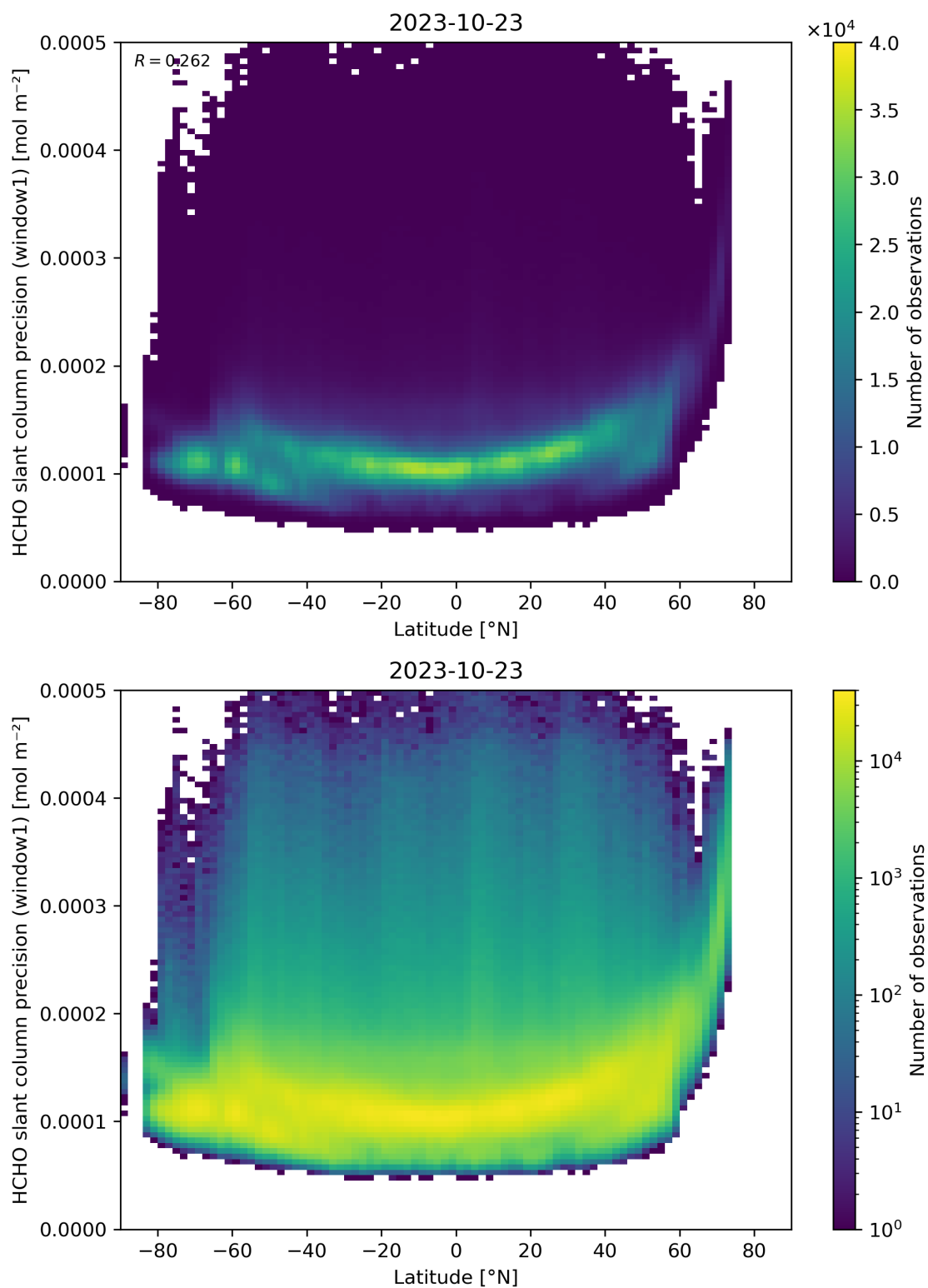
Figure 160: Scatter density plot of “Latitude” against “HCHO slant column precision (window1)” for 2023-10-22 to 2023-10-24.
