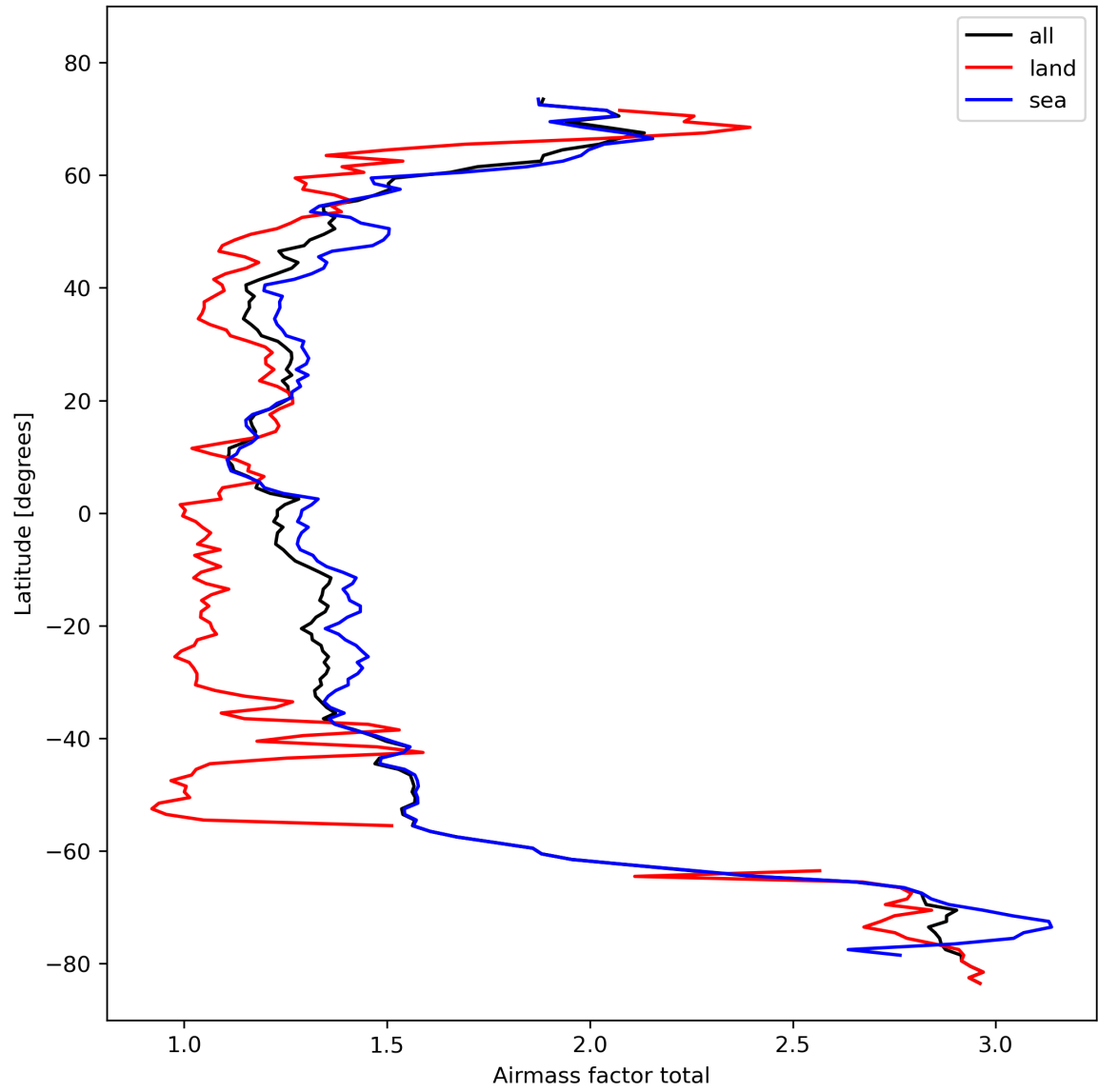
Figure 26: Zonal average of “Airmass factor total” for 2023-10-22 to 2023-10-24.
