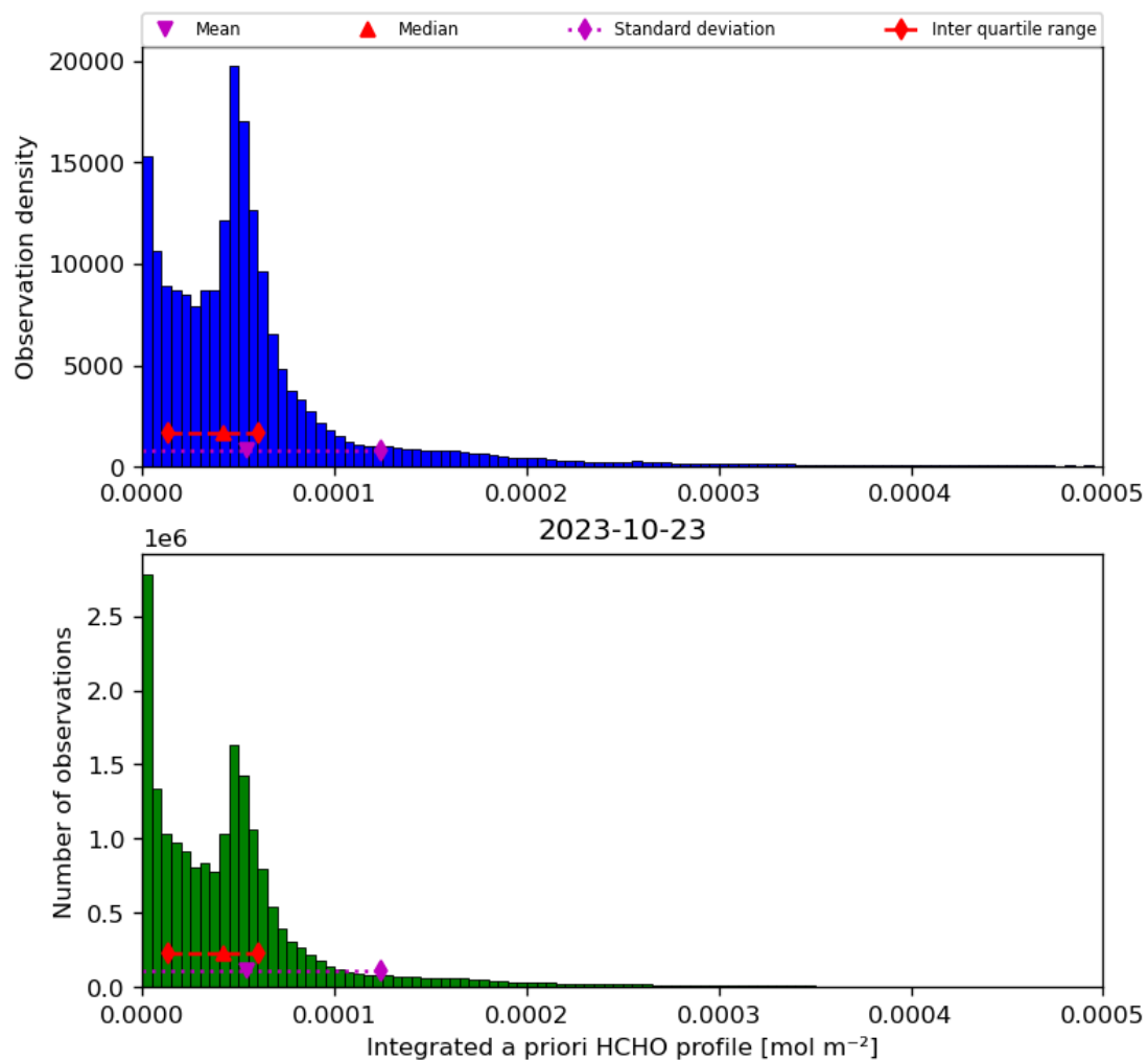
Figure 43: Histogram of “Integrated a priori HCHO profile” for 2023-10-22 to 2023-10-24
