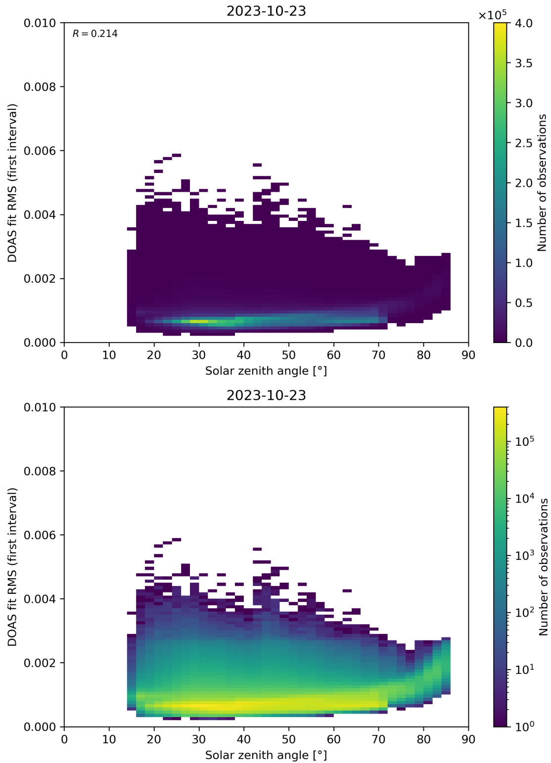
Figure 167: Scatter density plot of “Solar zenith angle” against “DOAS fit RMS (first interval)” for 2023-10-22 to 2023-10-24.
