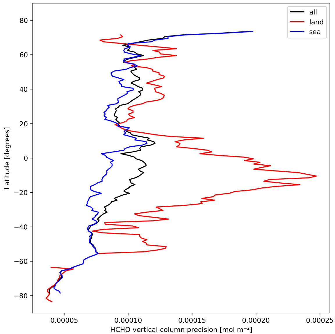
Figure 22: Zonal average of “HCHO vertical column precision” for 2023-10-22 to 2023-10-24.
