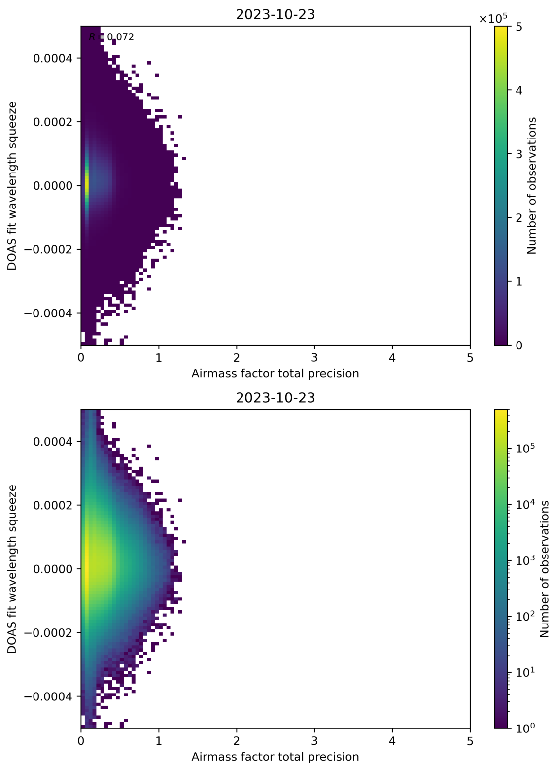
Figure 107: Scatter density plot of “Airmass factor total precision” against “DOAS fit wavelength squeeze” for 2023-10-22 to 2023-10-24.
