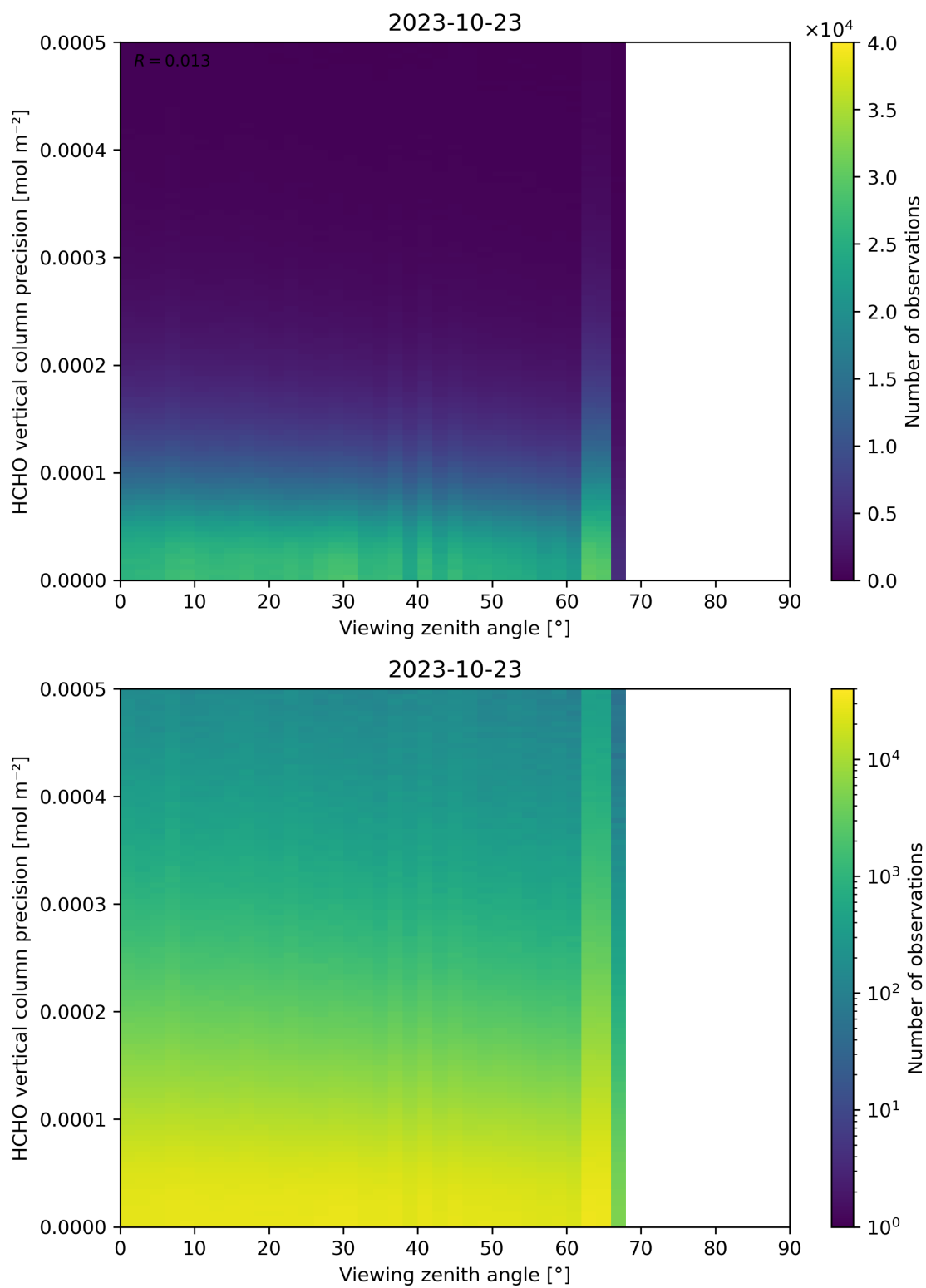
Figure 194: Scatter density plot of “Viewing zenith angle” against “HCHO vertical column precision” for 2023-10-22 to 2023-10-24.
