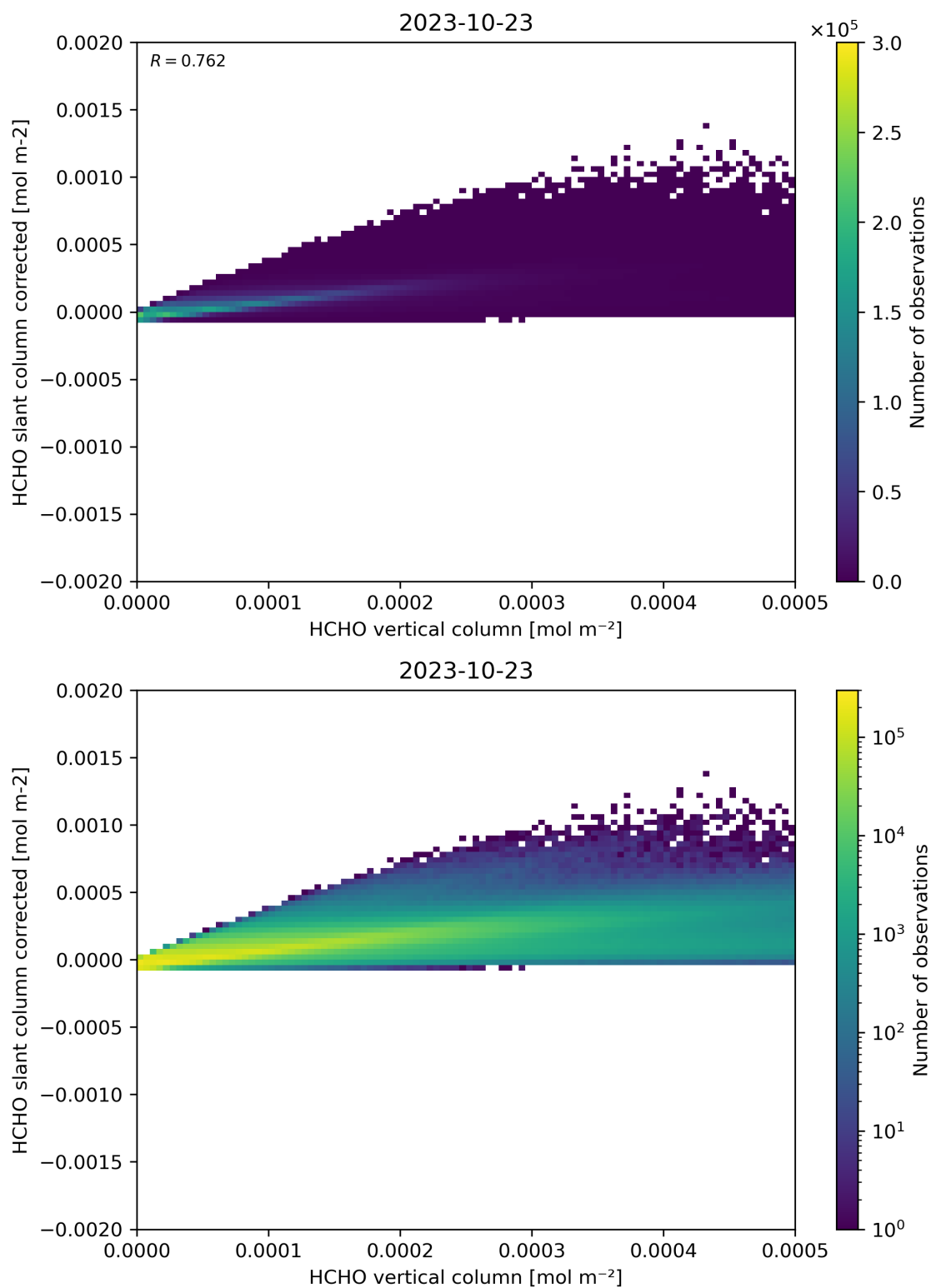
Figure 127: Scatter density plot of “HCHO vertical column” against “HCHO slant column corrected” for 2023-10-22 to 2023-10-24.
