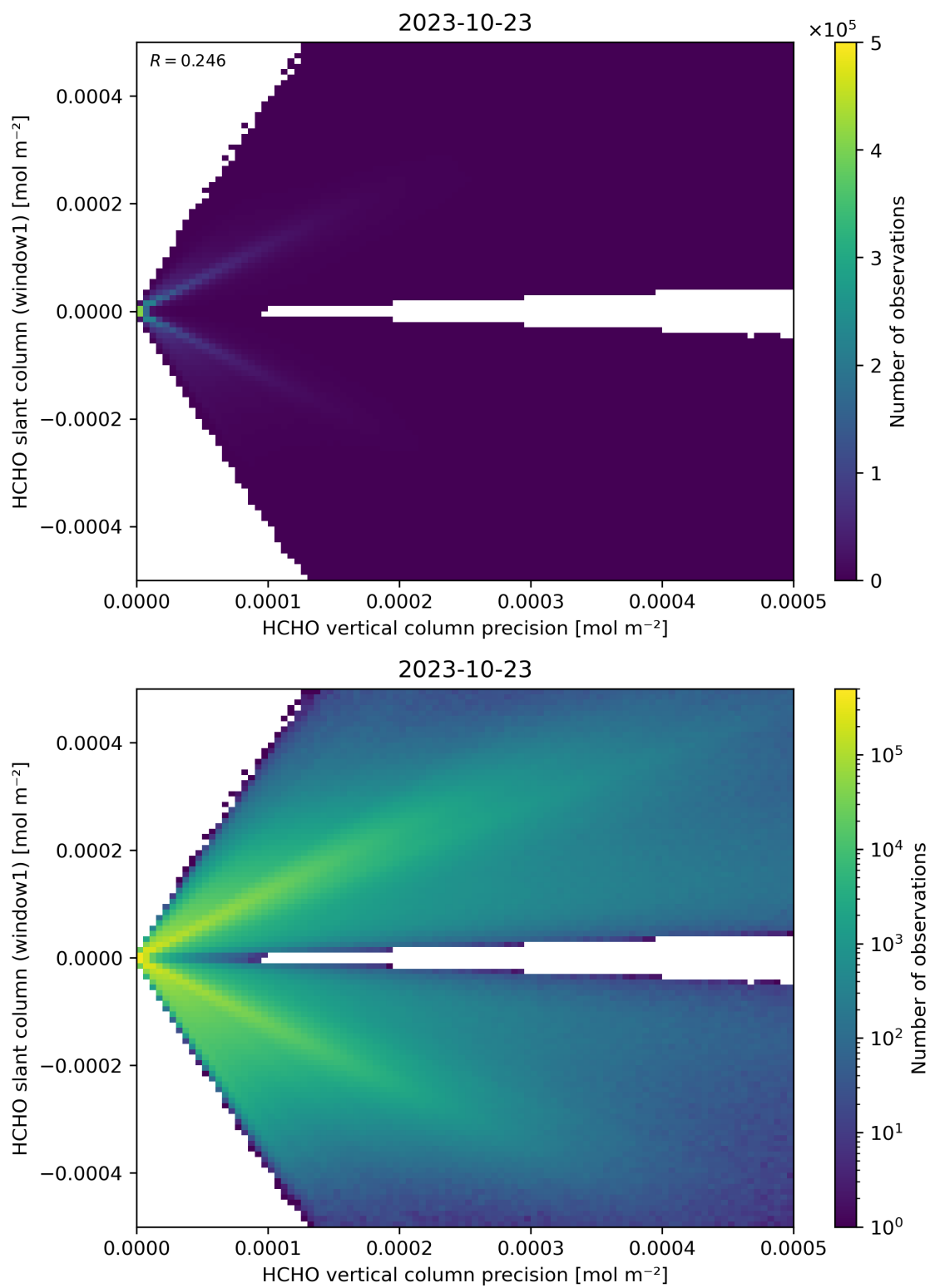
Figure 142: Scatter density plot of “HCHO vertical column precision” against “HCHO slant column (window1)” for 2023-10-22 to 2023-10-24.
