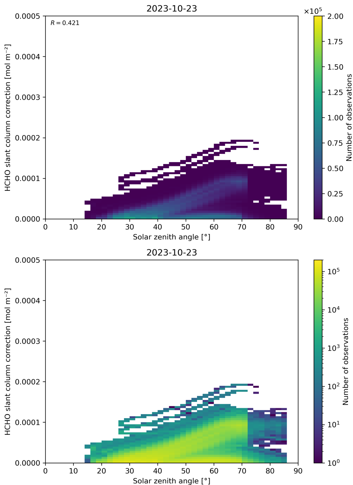
Figure 172: Scatter density plot of “Solar zenith angle” against “HCHO slant column correction” for 2023-10-22 to 2023-10-24.
