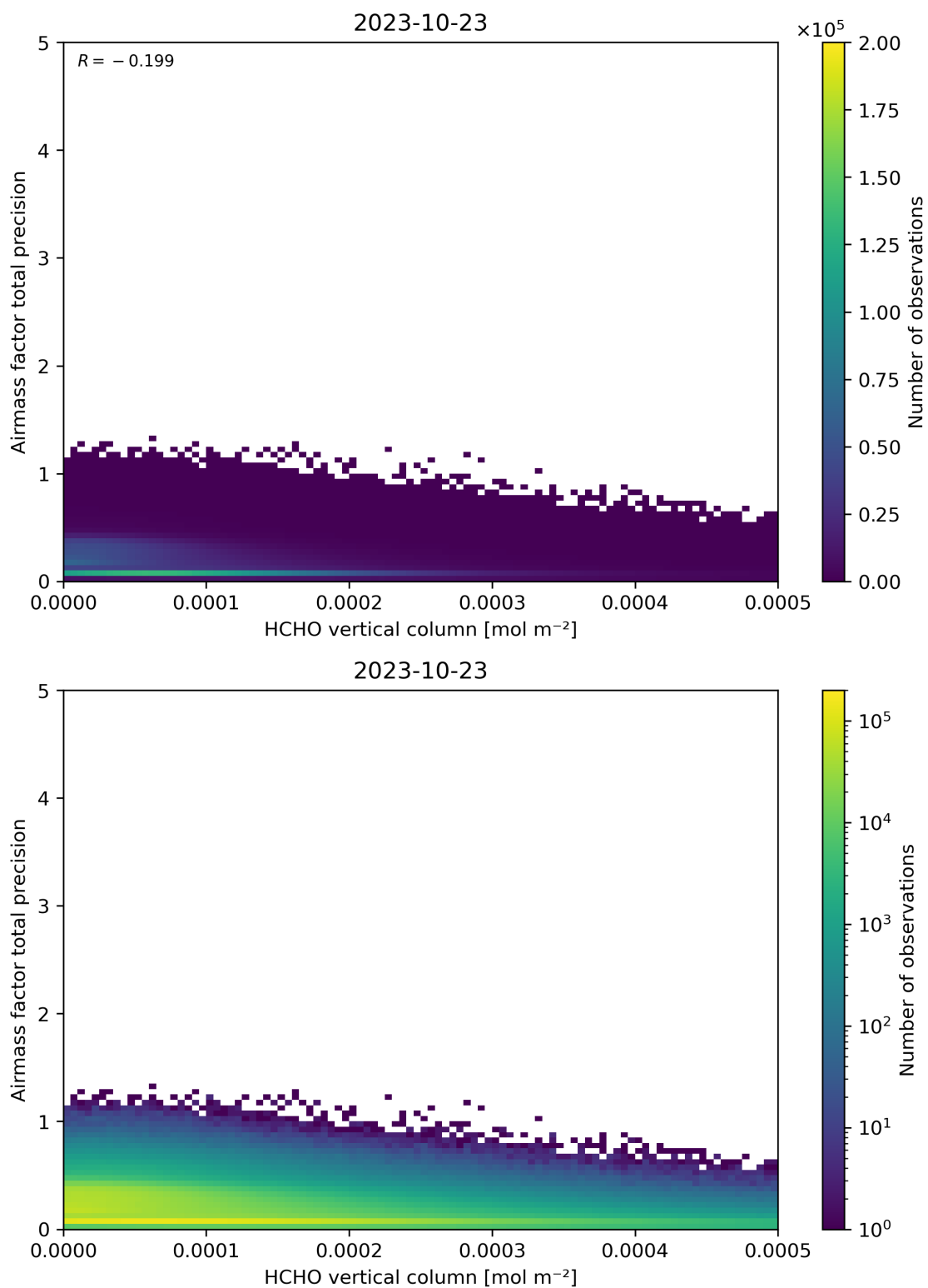
Figure 132: Scatter density plot of “HCHO vertical column” against “Airmass factor total precision” for 2023-10-22 to 2023-10-24.
