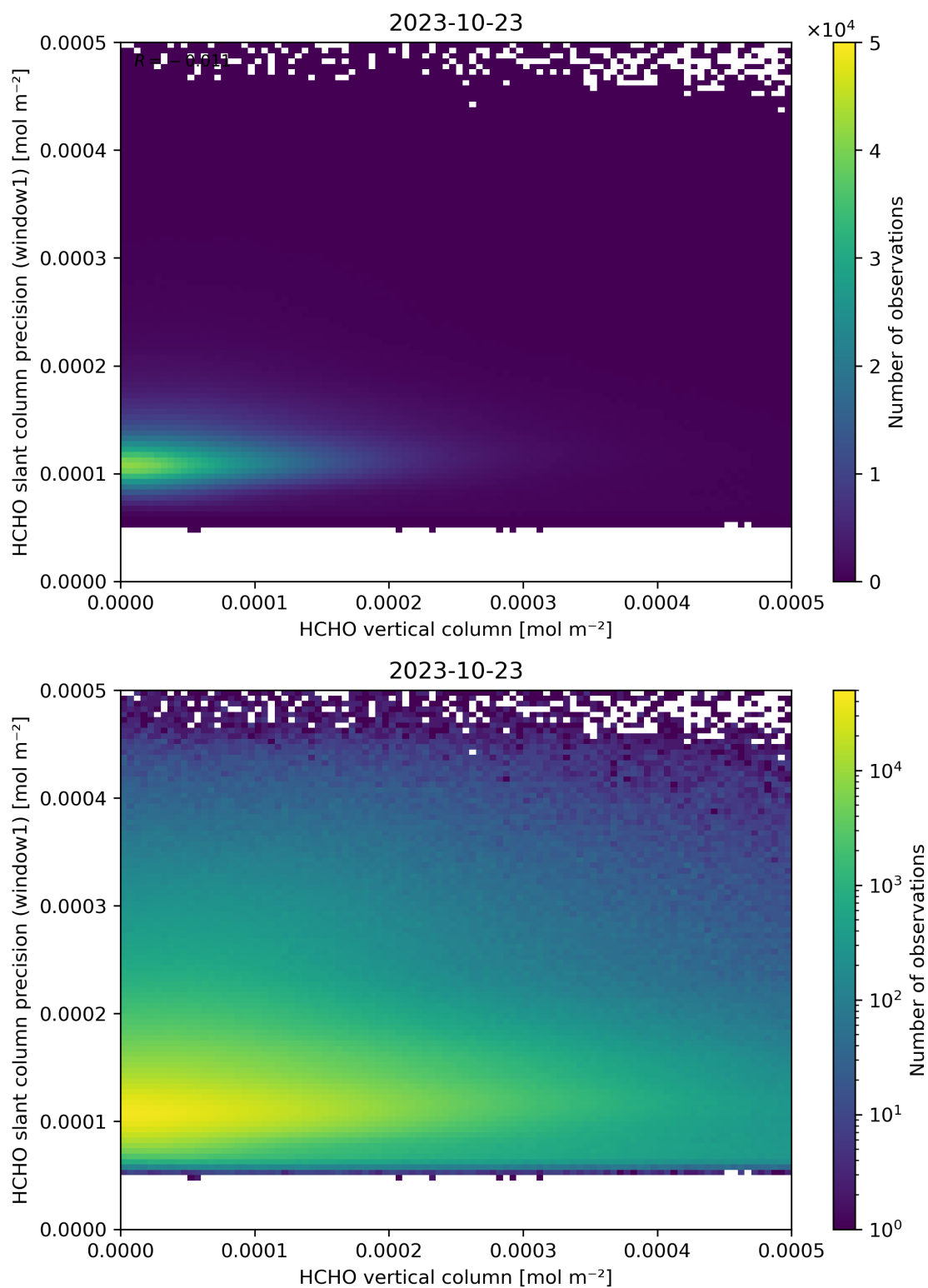
Figure 130: Scatter density plot of “HCHO vertical column” against “HCHO slant column precision (window1)” for 2023-10-22 to 2023-10-24.
