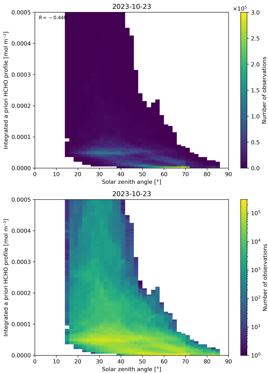
Figure 180: Scatter density plot of “Solar zenith angle” against “Integrated a priori HCHO profile” for 2023-10-22 to 2023-10-24.
