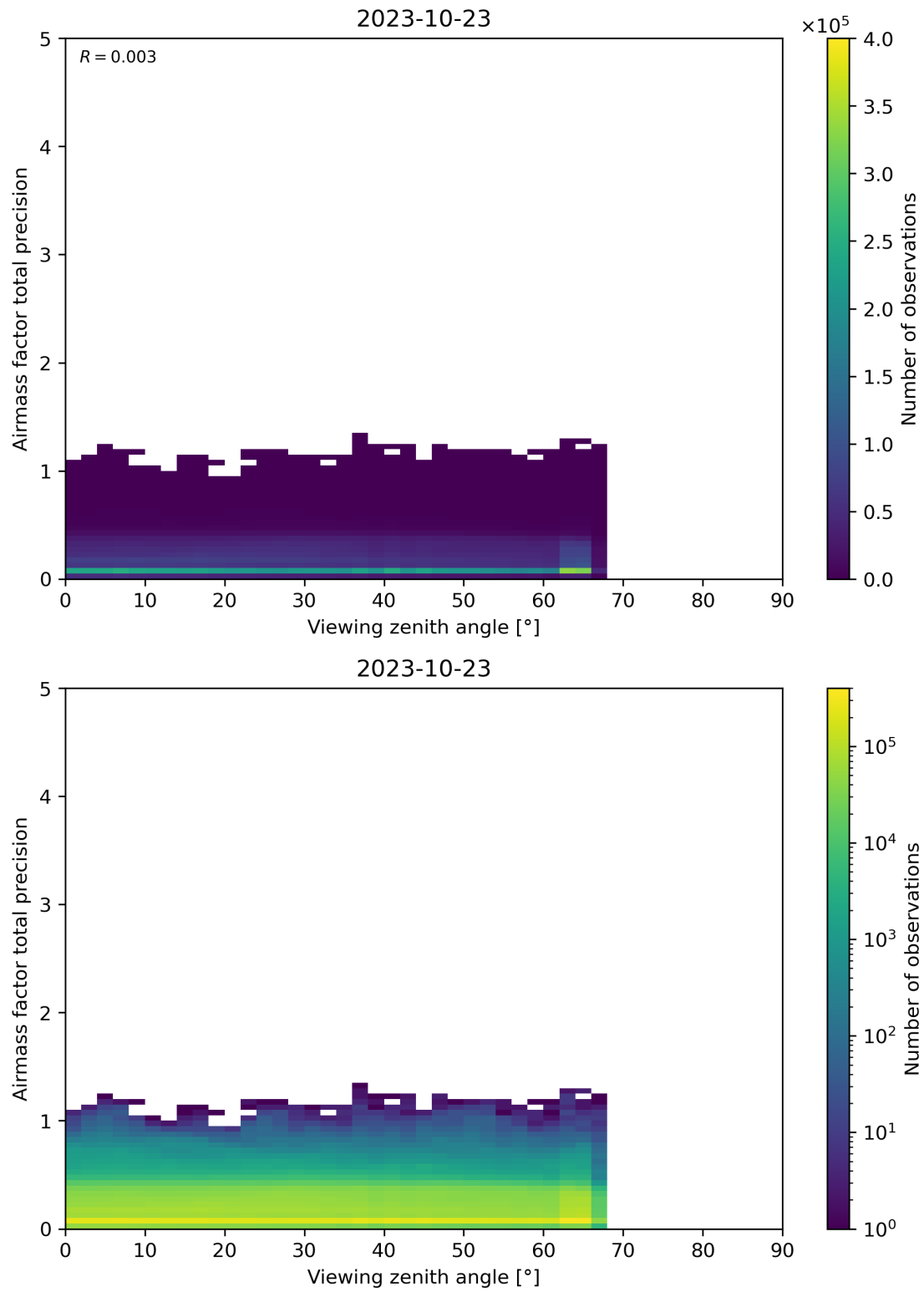
Figure 191: Scatter density plot of “Viewing zenith angle” against “Airmass factor total precision” for 2023-10-22 to 2023-10-24.
