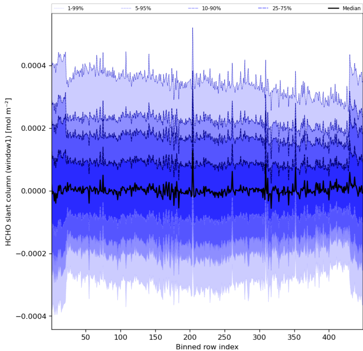
Figure 52: Along track statistics of “HCHO slant column (window1)” for 2023-10-22 to 2023-10-24
