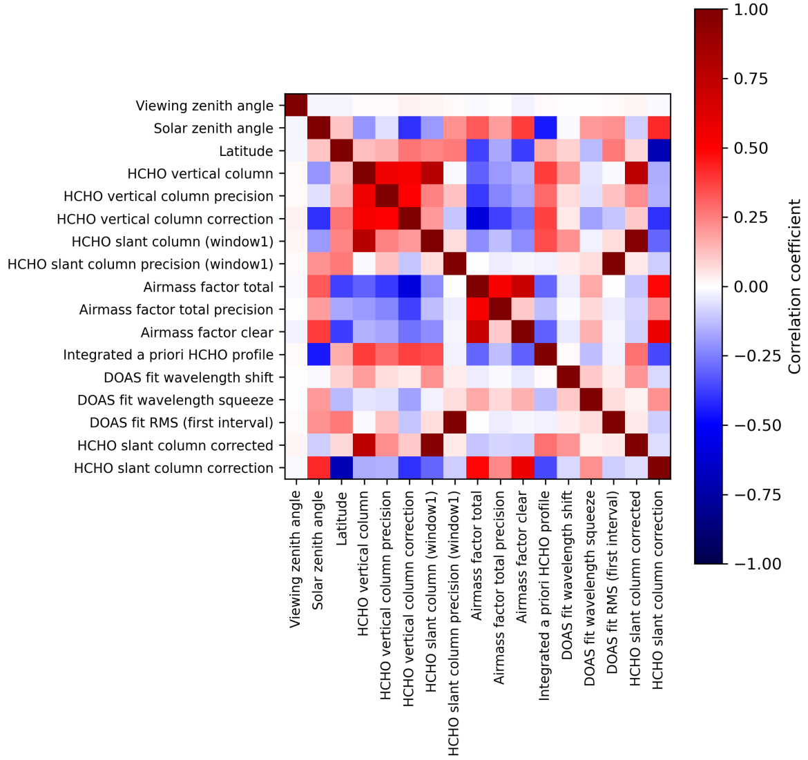
Figure 2: Map of correlation matrix for 2023-10-22 to 2023-10-24.
