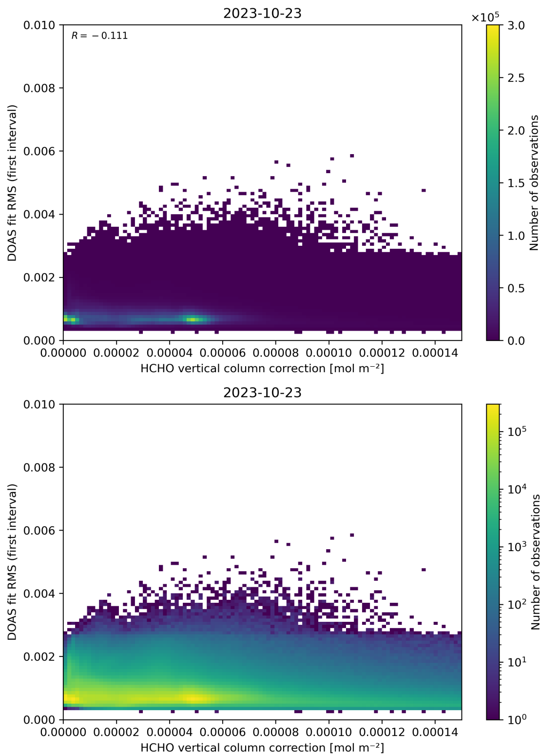
Figure 112: Scatter density plot of “HCHO vertical column correction” against “DOAS fit RMS (first interval)” for 2023-10-22 to 2023-10-24.
