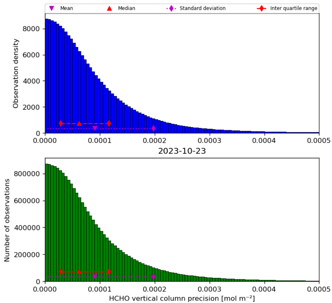
Figure 36: Histogram of “HCHO vertical column precision” for 2023-10-22 to 2023-10-24
