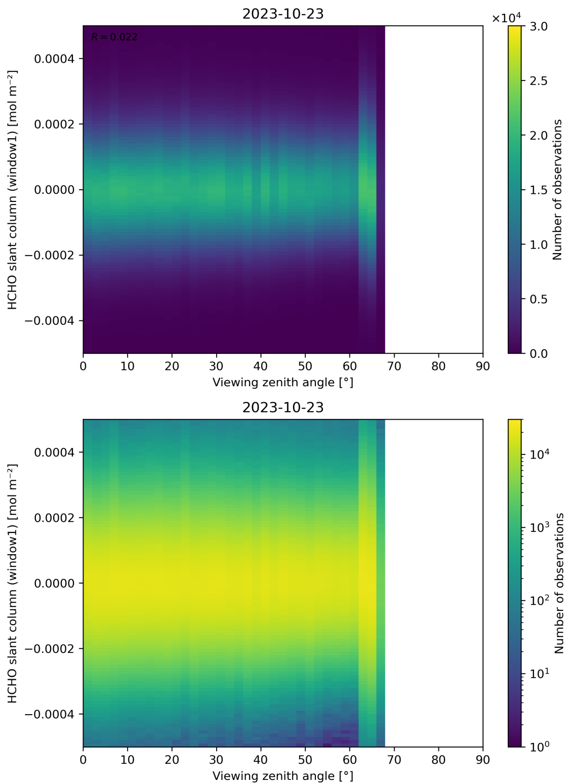
Figure 188: Scatter density plot of “Viewing zenith angle” against “HCHO slant column (window1)” for 2023-10-22 to 2023-10-24.
