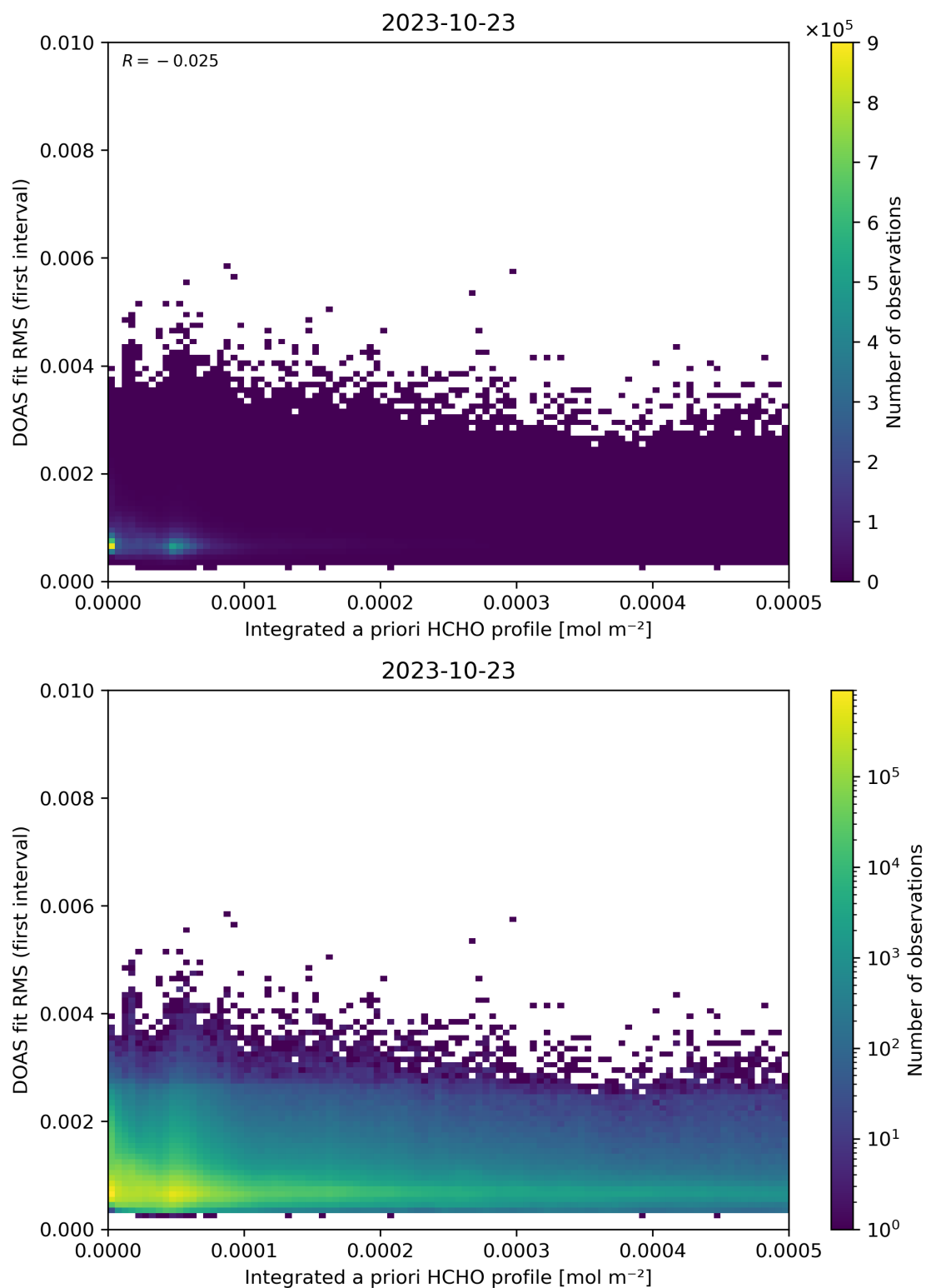
Figure 148: Scatter density plot of “Integrated a priori HCHO profile” against “DOAS fit RMS (first interval)” for 2023-10-22 to 2023-10-24.
