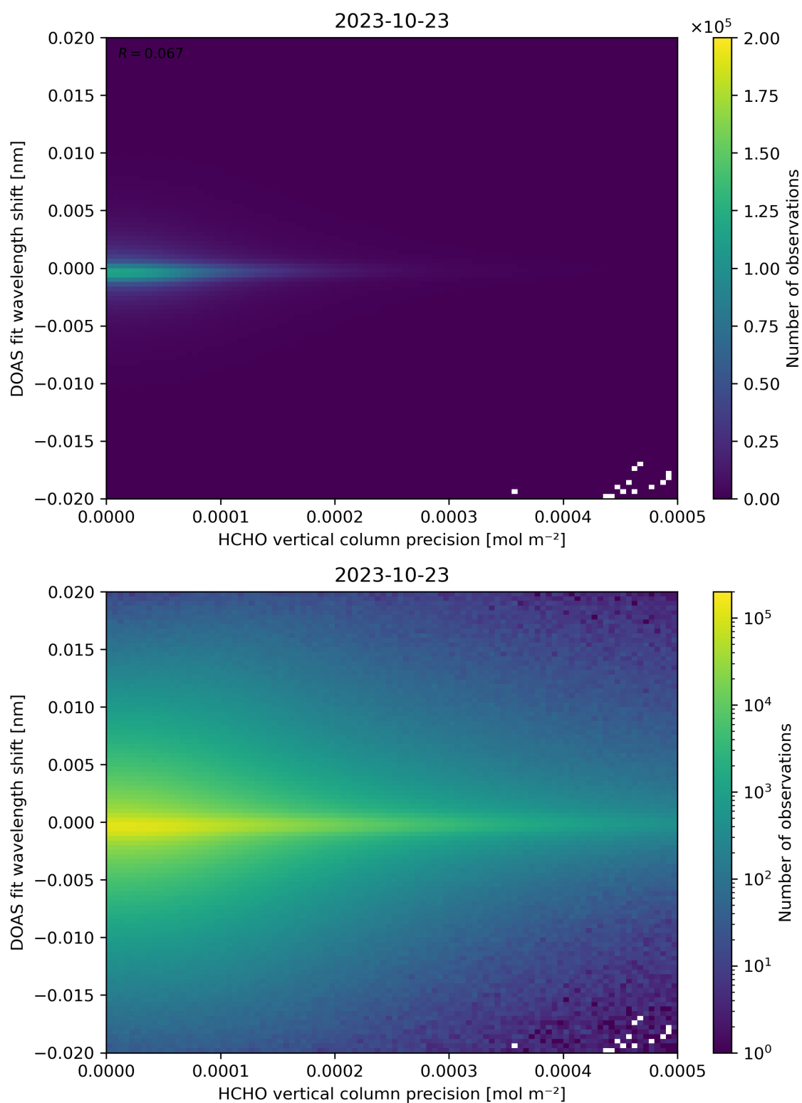
Figure 137: Scatter density plot of “HCHO vertical column precision” against “DOAS fit wavelength shift” for 2023-10-22 to 2023-10-24.
