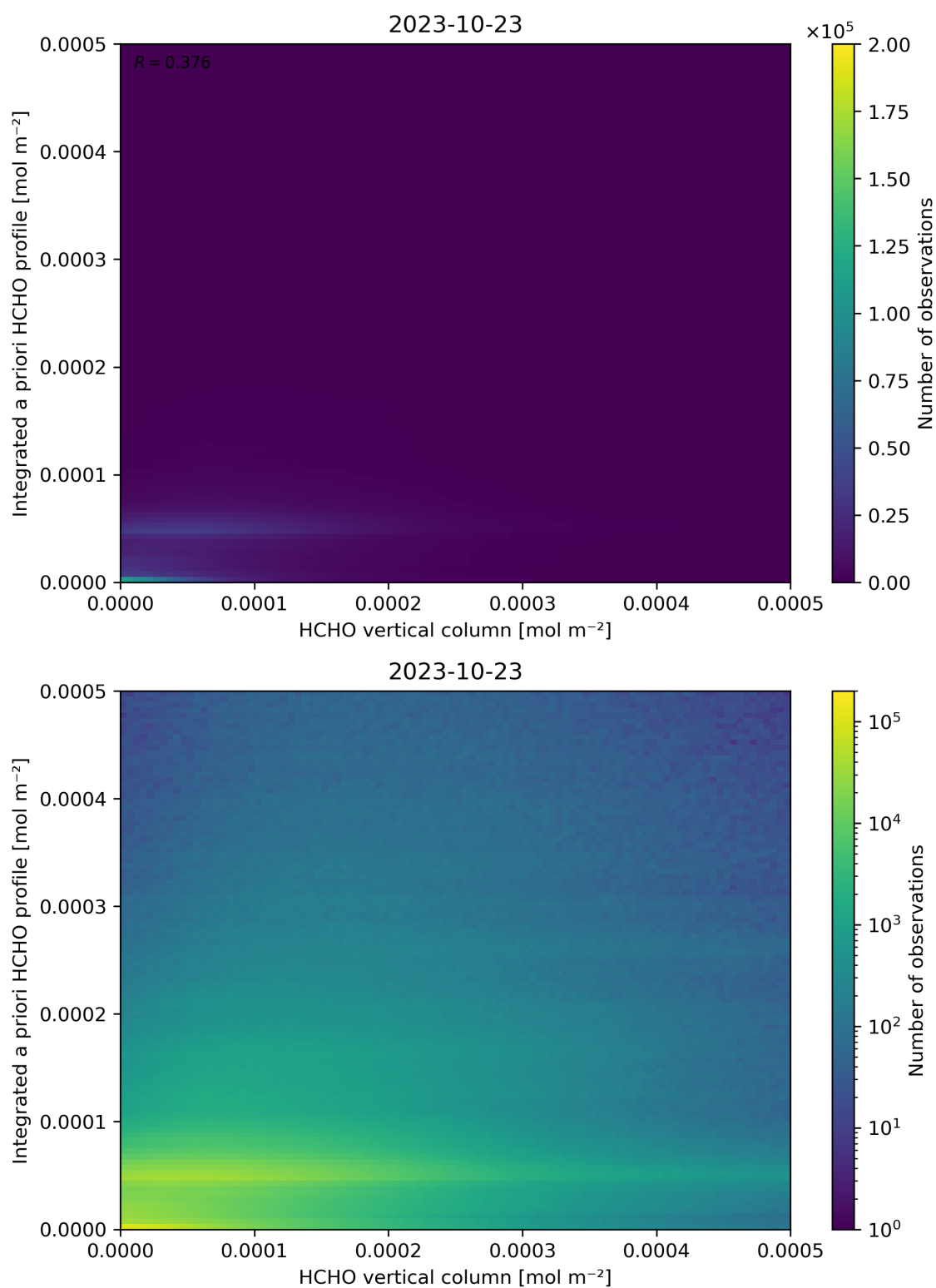
Figure 135: Scatter density plot of “HCHO vertical column” against “Integrated a priori HCHO profile” for 2023-10-22 to 2023-10-24.
