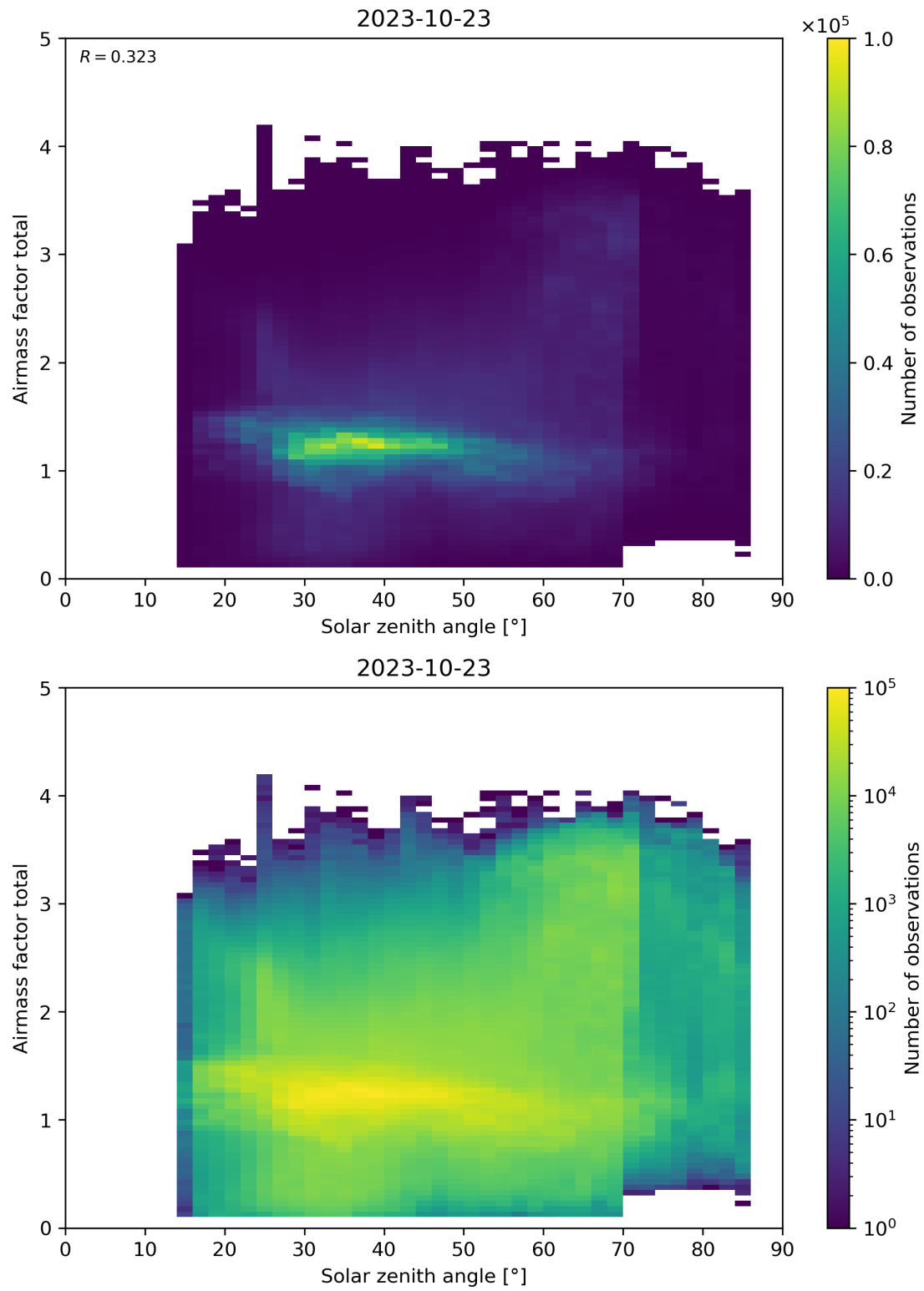
Figure 175: Scatter density plot of “Solar zenith angle” against “Airmass factor total” for 2023-10-22 to 2023-10-24.
