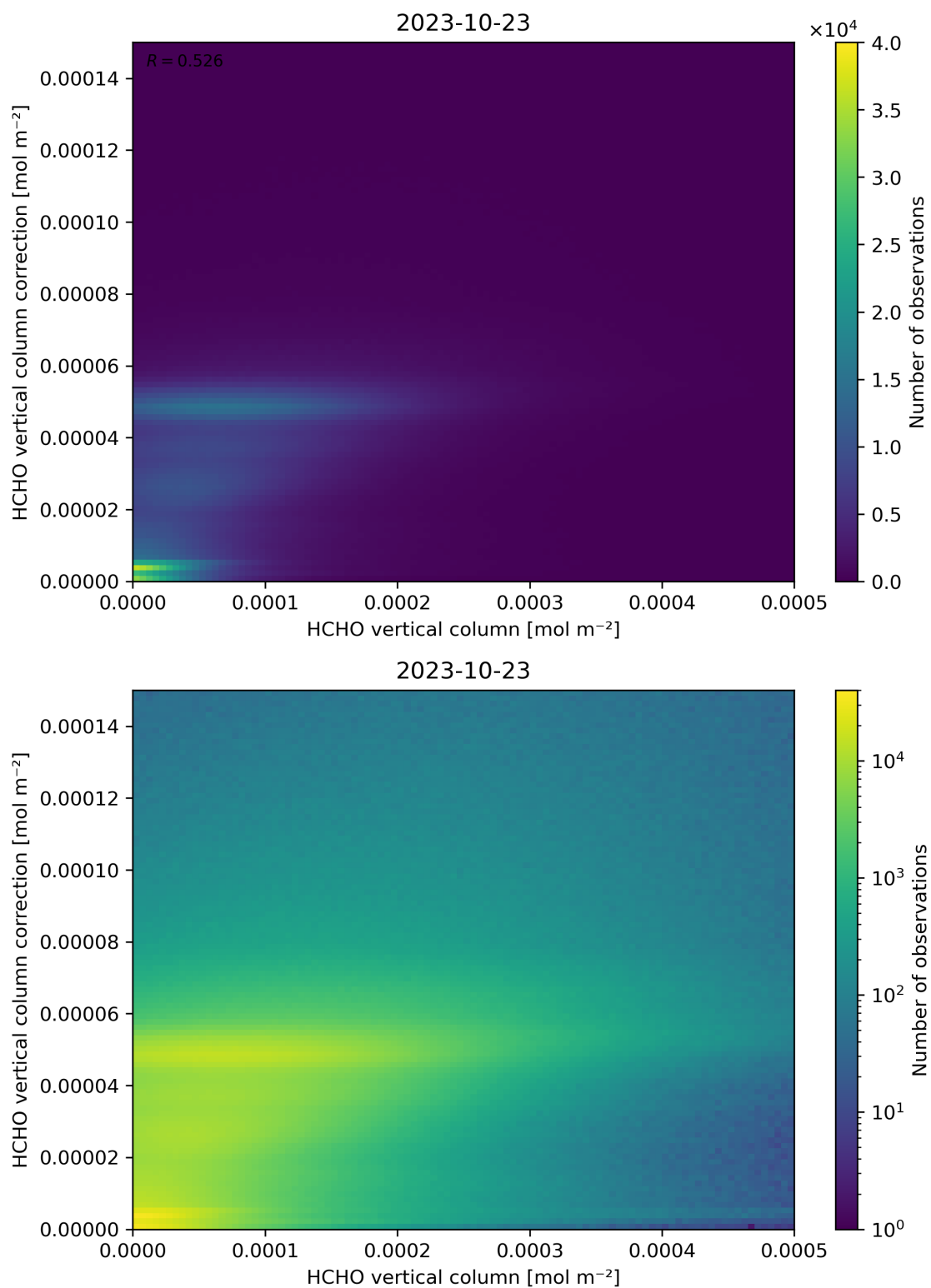
Figure 133: Scatter density plot of “HCHO vertical column” against “HCHO vertical column correction” for 2023-10-22 to 2023-10-24.
