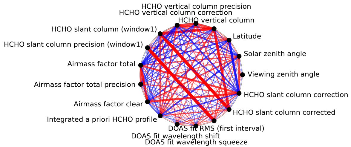
Figure 1: Map of correlation graph for 2023-10-22 to 2023-10-24.
