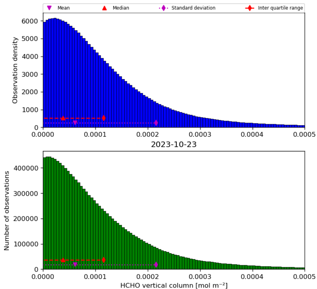
Figure 35: Histogram of “HCHO vertical column” for 2023-10-22 to 2023-10-24
