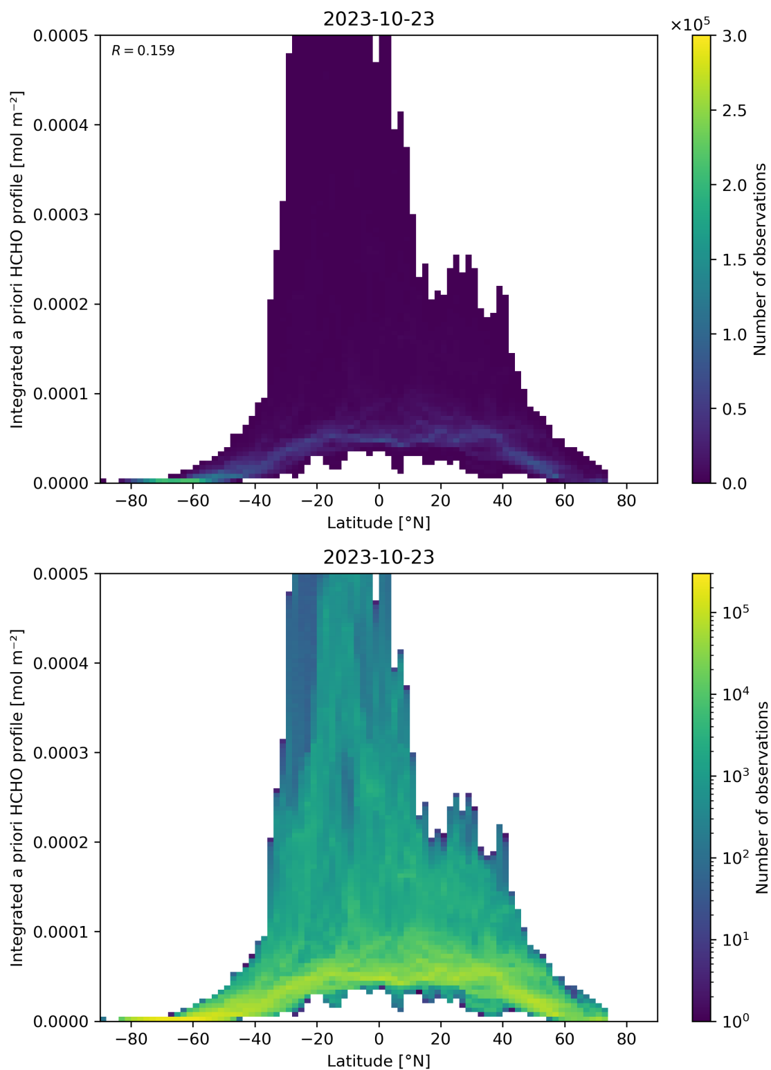
Figure 166: Scatter density plot of “Latitude” against “Integrated a priori HCHO profile” for 2023-10-22 to 2023-10-24.
