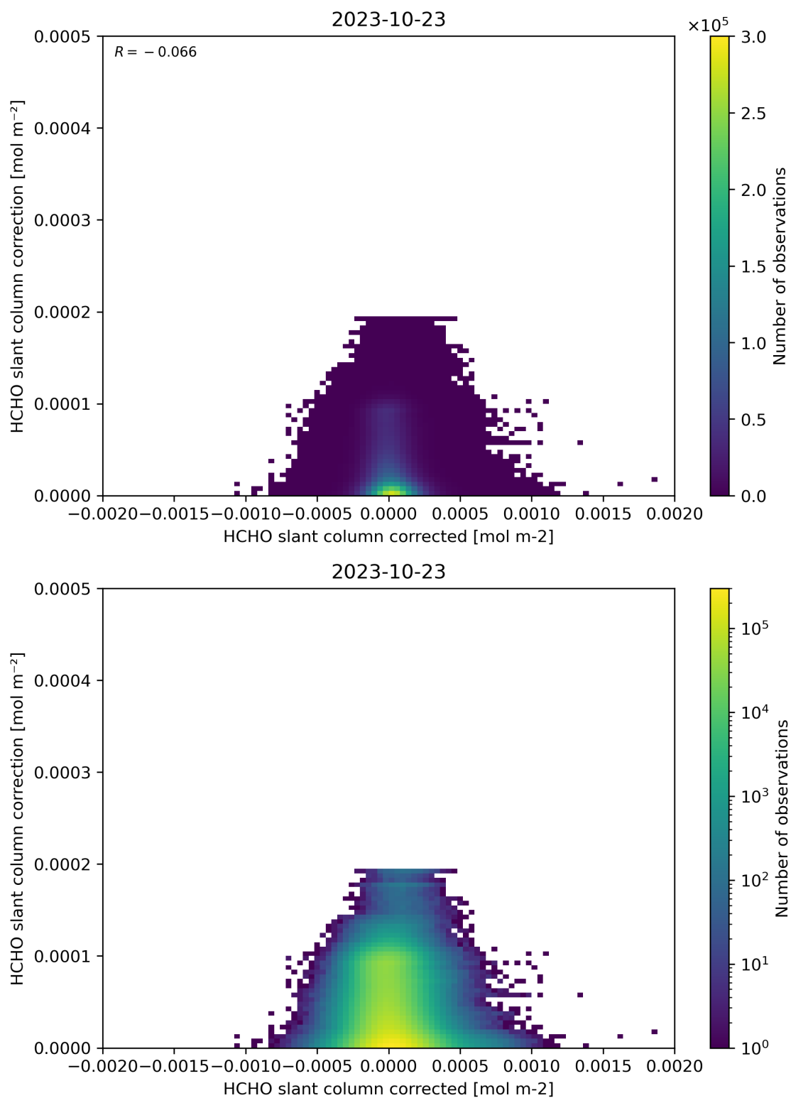
Figure 77: Scatter density plot of “HCHO slant column corrected” against “HCHO slant column correction” for 2023-10-22 to 2023-10-24.
