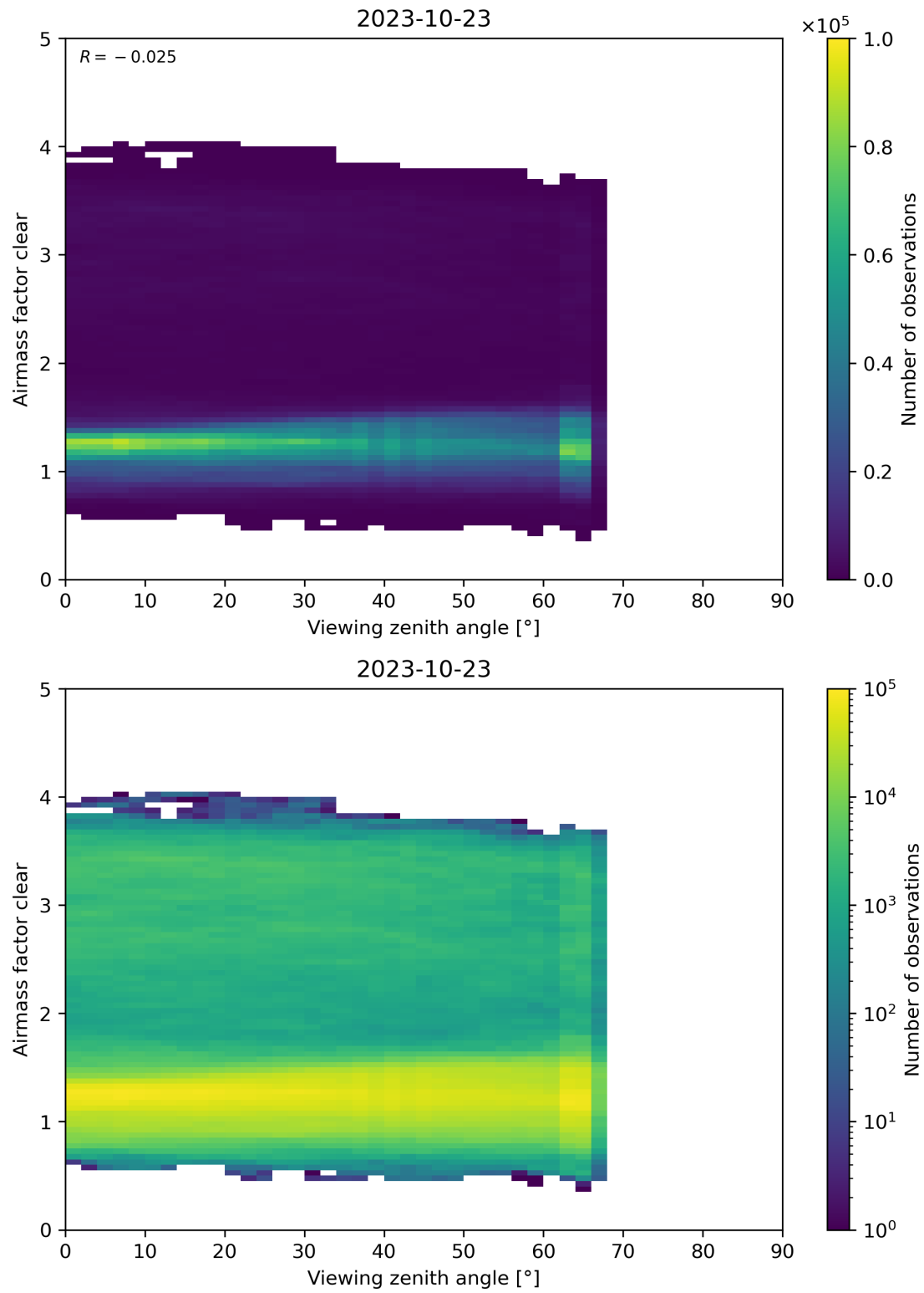
Figure 185: Scatter density plot of “Viewing zenith angle” against “Airmass factor clear” for 2023-10-22 to 2023-10-24.
