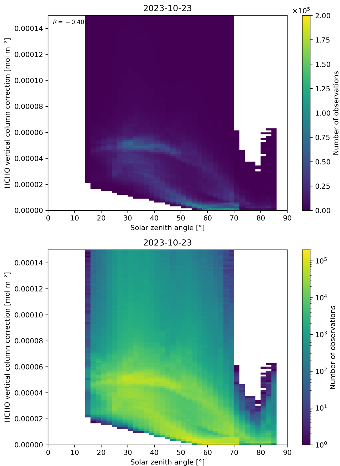
Figure 178: Scatter density plot of “Solar zenith angle” against “HCHO vertical column correction” for 2023-10-22 to 2023-10-24.
