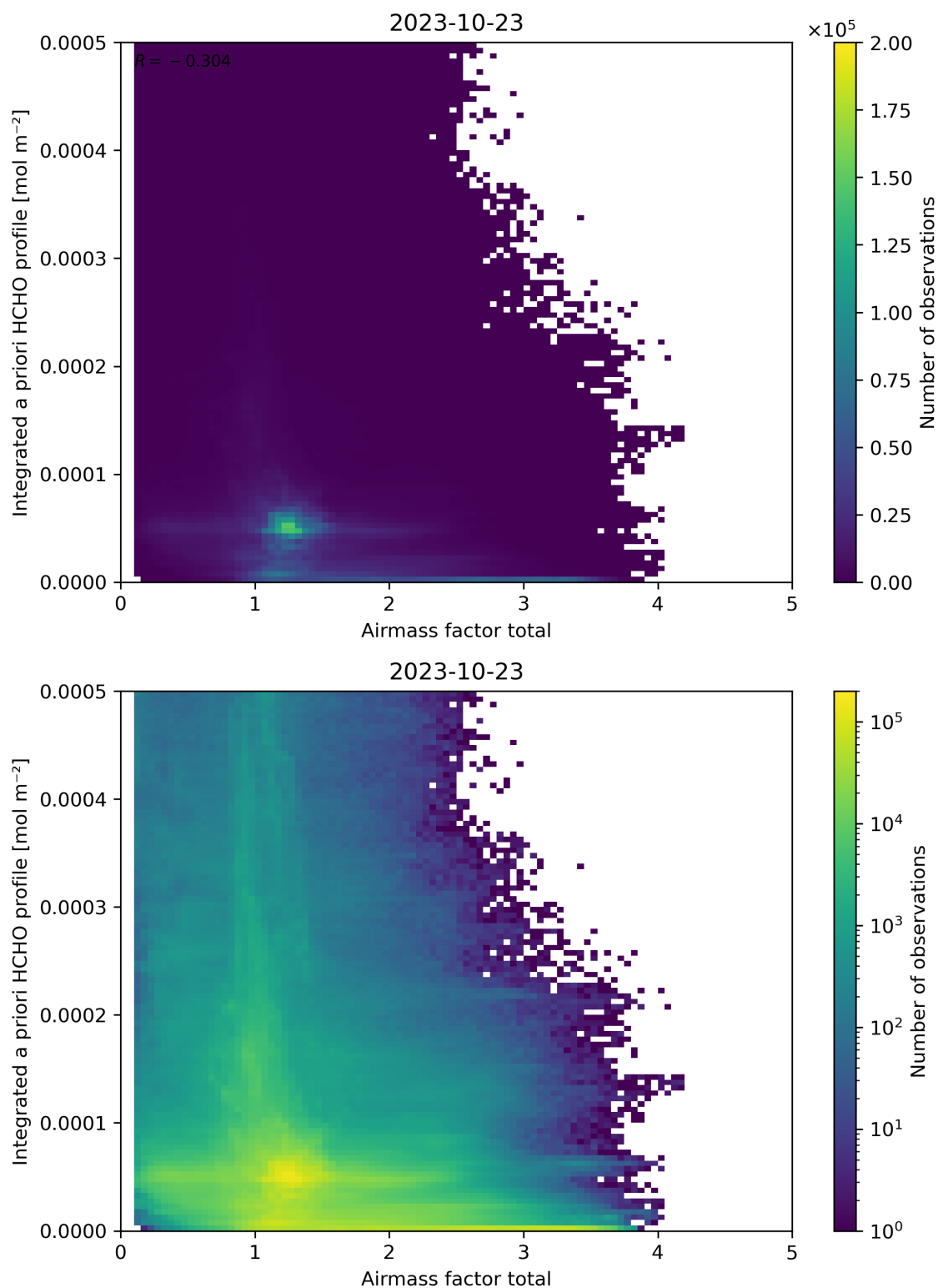
Figure 104: Scatter density plot of “Airmass factor total” against “Integrated a priori HCHO profile” for 2023-10-22 to 2023-10-24.
