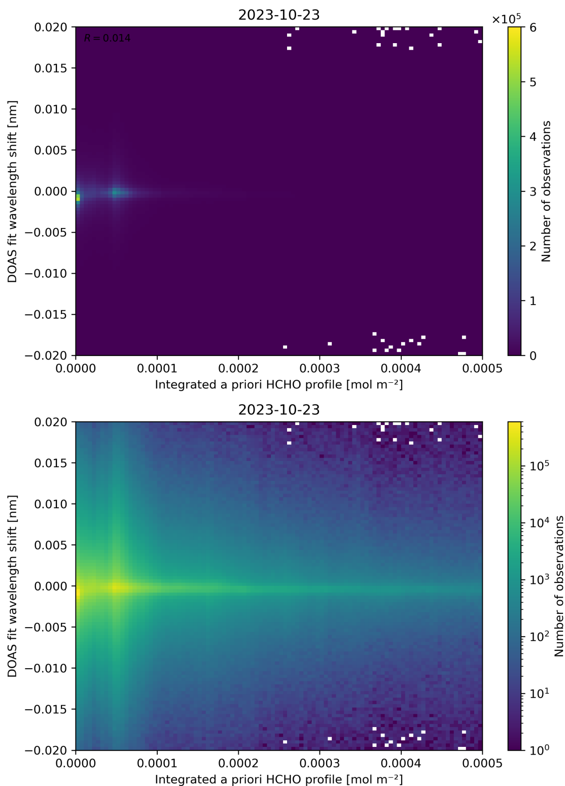
Figure 149: Scatter density plot of “Integrated a priori HCHO profile” against “DOAS fit wavelength shift” for 2023-10-22 to 2023-10-24.
