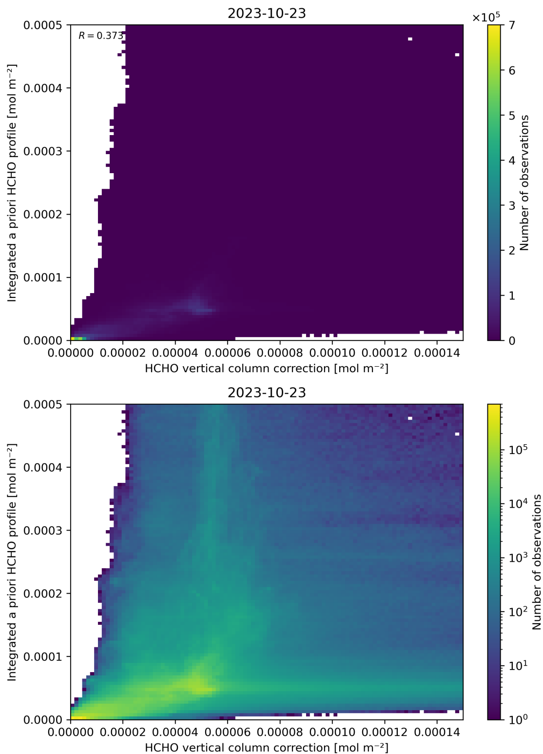
Figure 122: Scatter density plot of “HCHO vertical column correction” against “Integrated a priori HCHO profile” for 2023-10-22 to 2023-10-24.
