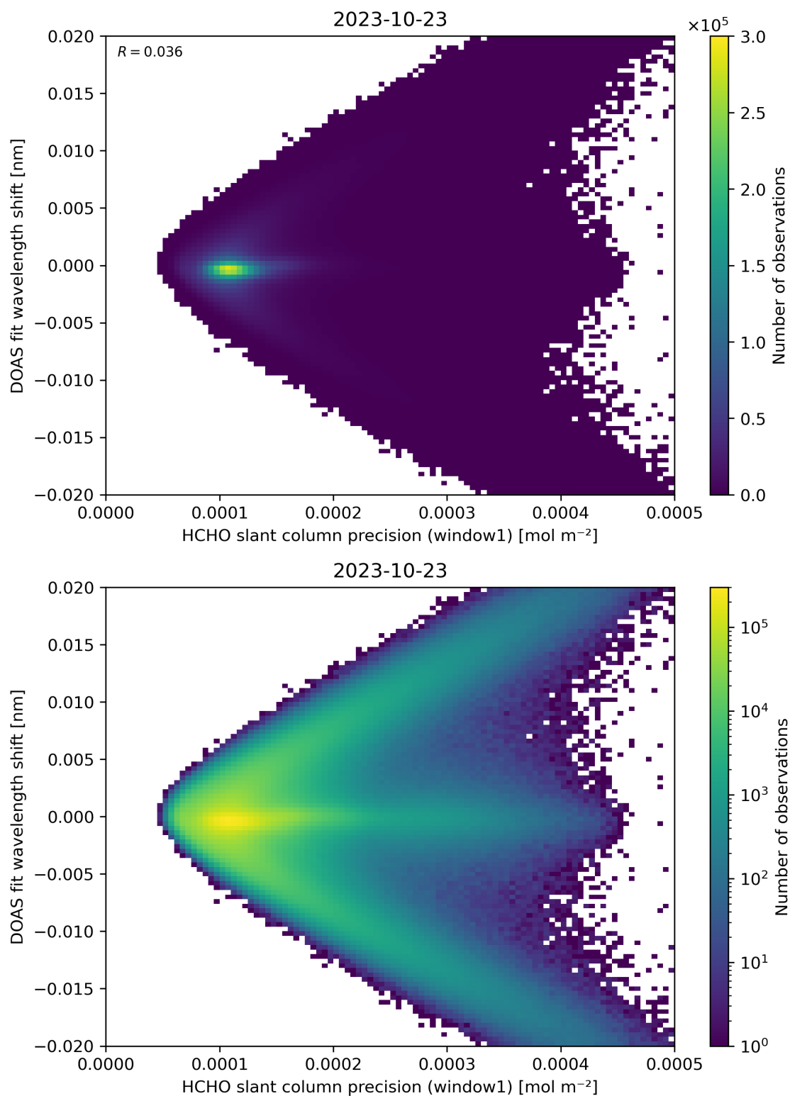
Figure 89: Scatter density plot of “HCHO slant column precision (window1)” against “DOAS fit wavelength shift” for 2023-10-22 to 2023-10-24.
