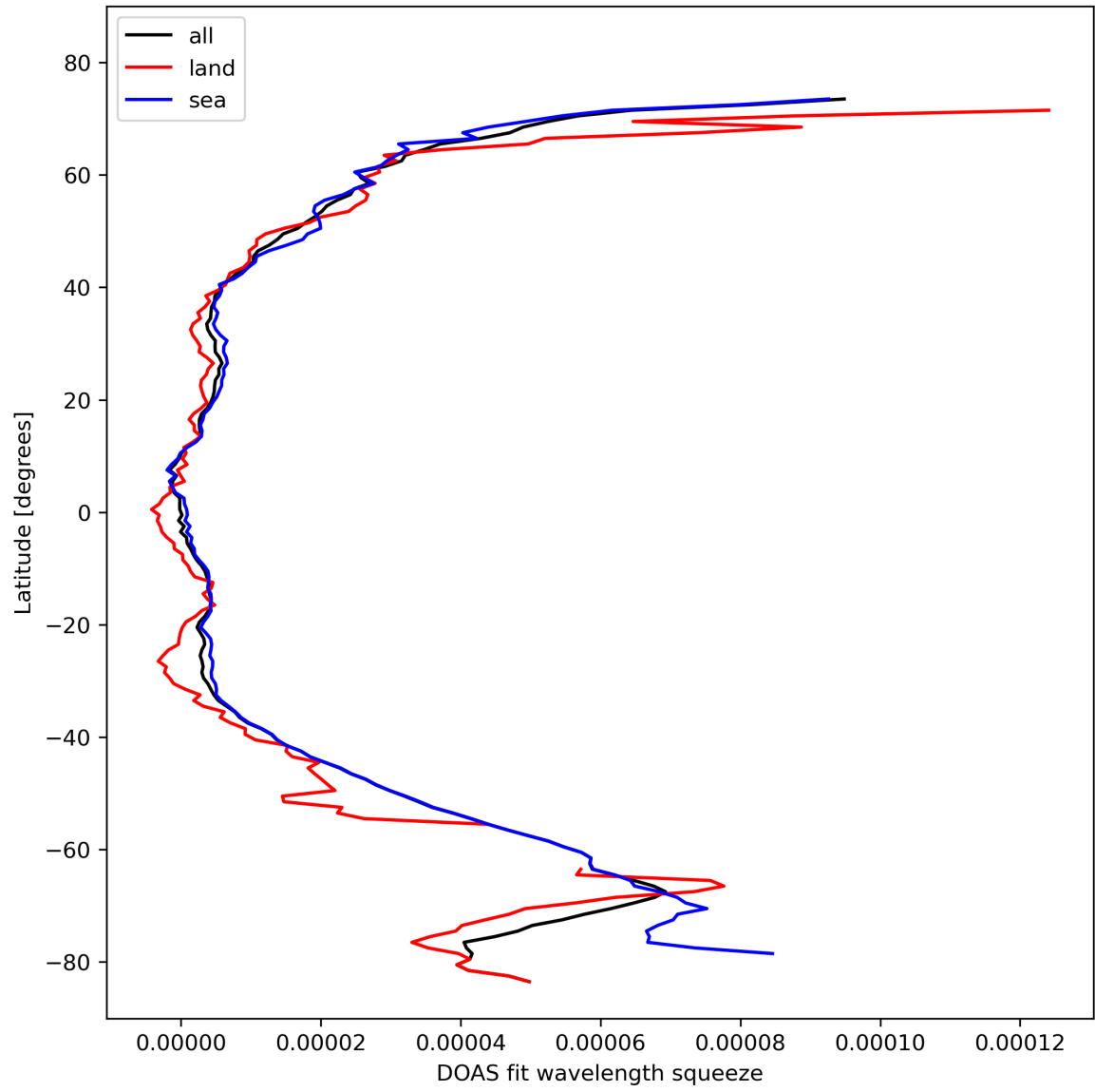
Figure 31: Zonal average of “DOAS fit wavelength squeeze” for 2023-10-22 to 2023-10-24.
