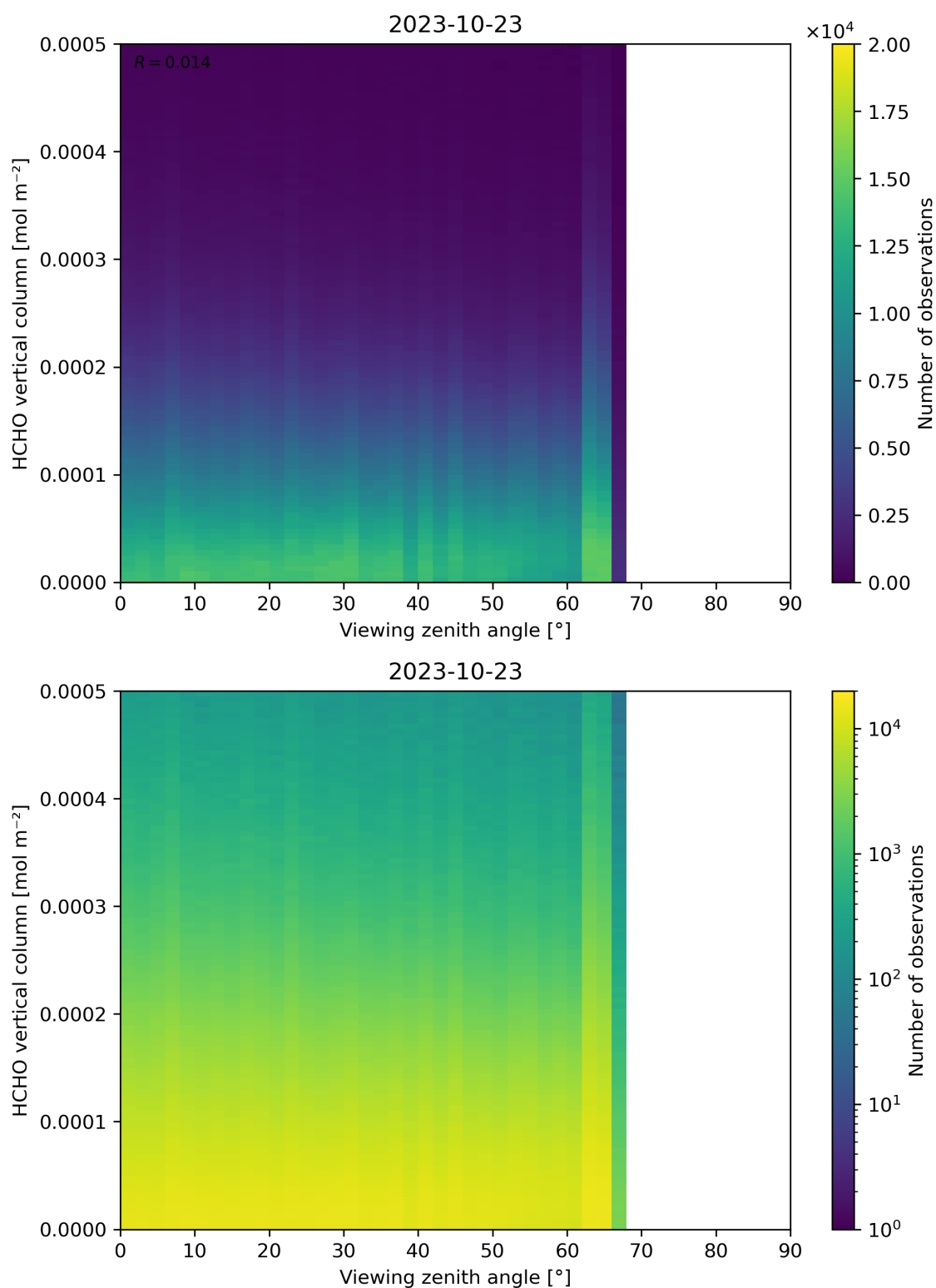
Figure 192: Scatter density plot of “Viewing zenith angle” against “HCHO vertical column” for 2023-10-22 to 2023-10-24.
