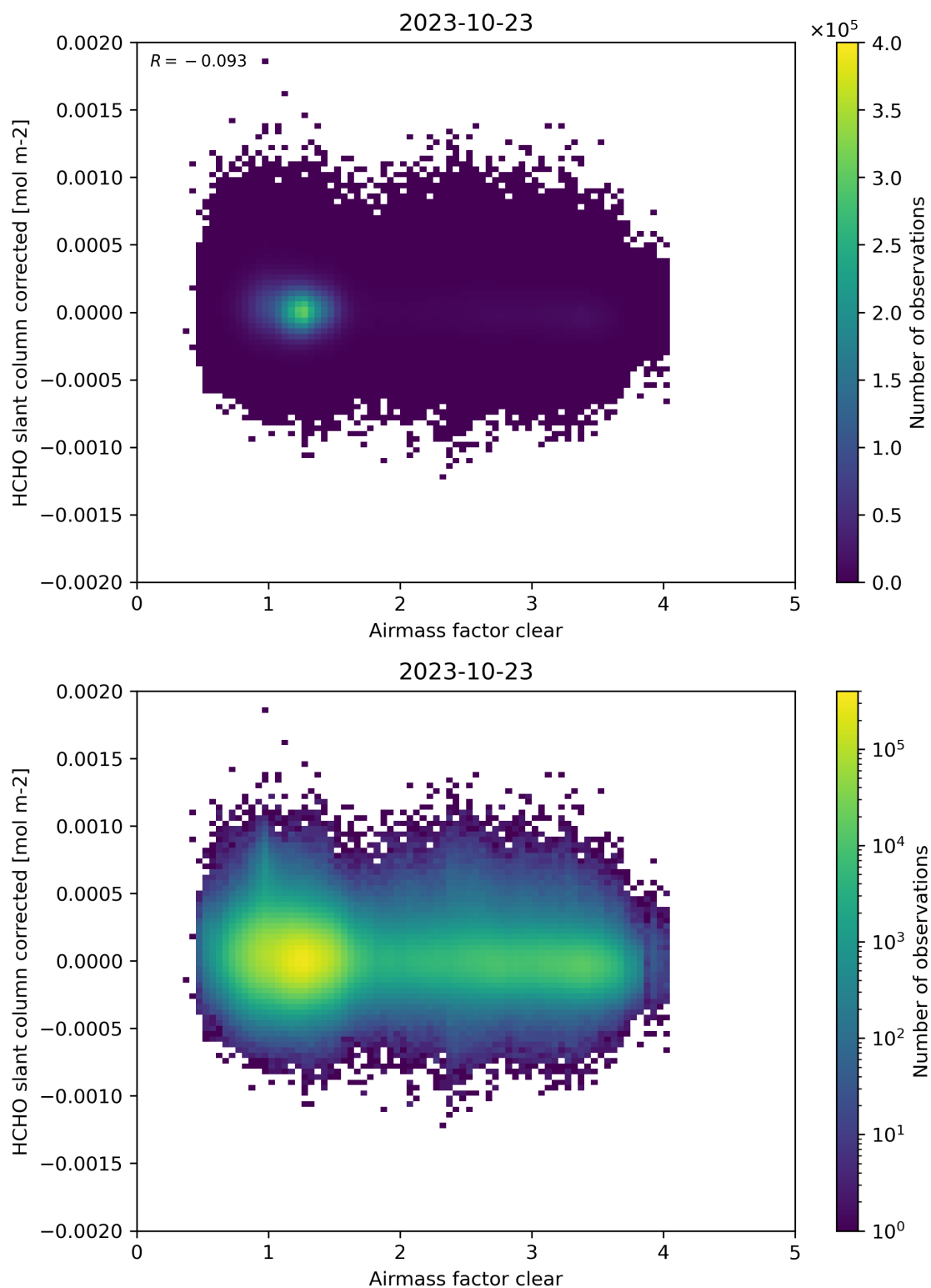
Figure 74: Scatter density plot of “Airmass factor clear” against “HCHO slant column corrected” for 2023-10-22 to 2023-10-24.
