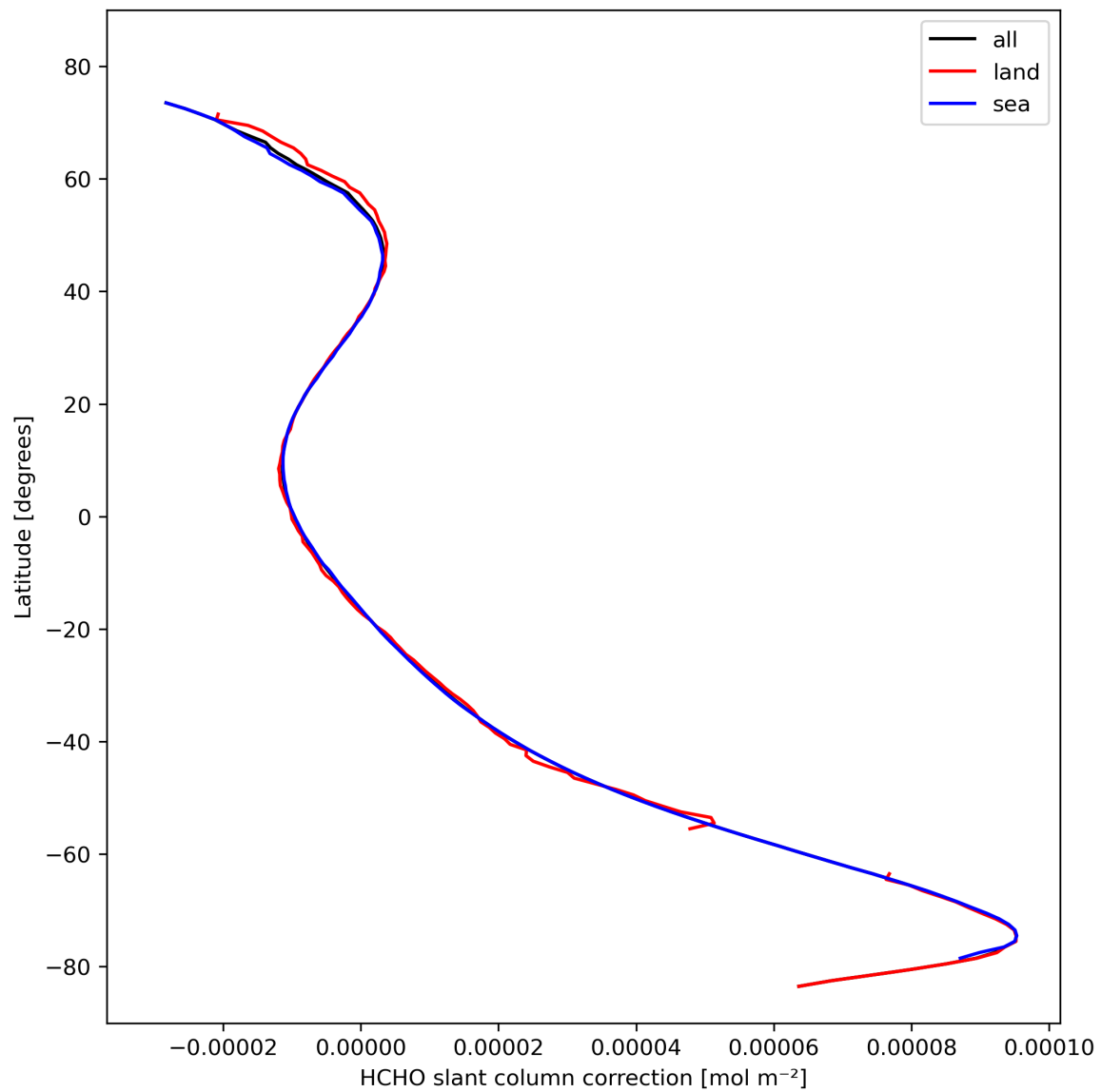
Figure 33: Zonal average of “HCHO slant column correction” for 2023-10-22 to 2023-10-24.
