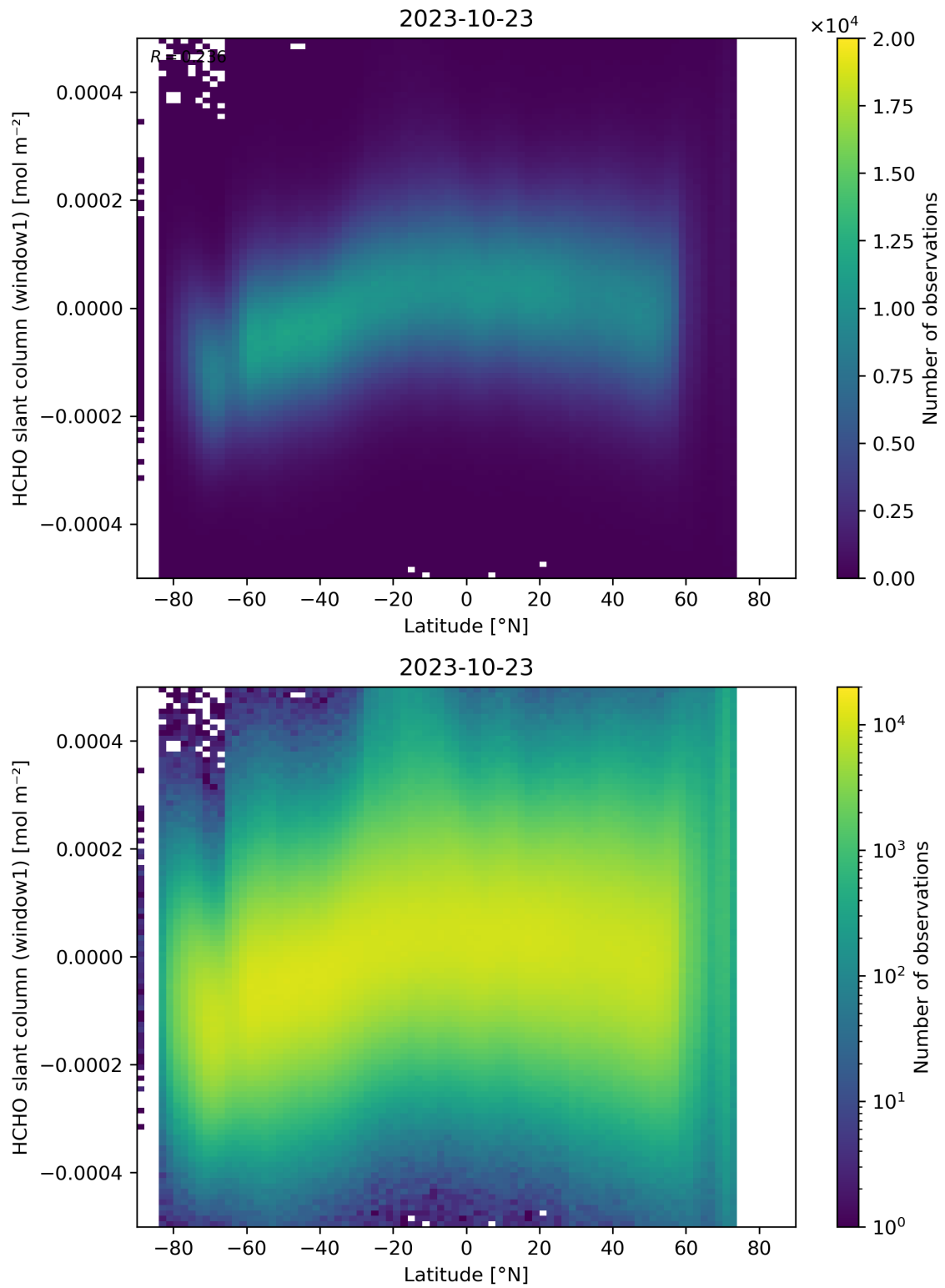
Figure 159: Scatter density plot of “Latitude” against “HCHO slant column (window1)” for 2023-10-22 to 2023-10-24.
