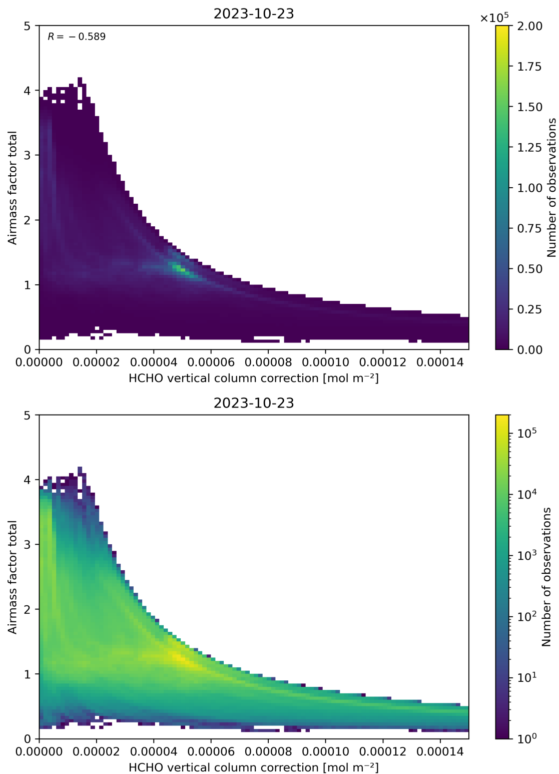
Figure 120: Scatter density plot of “HCHO vertical column correction” against “Airmass factor total” for 2023-10-22 to 2023-10-24.
