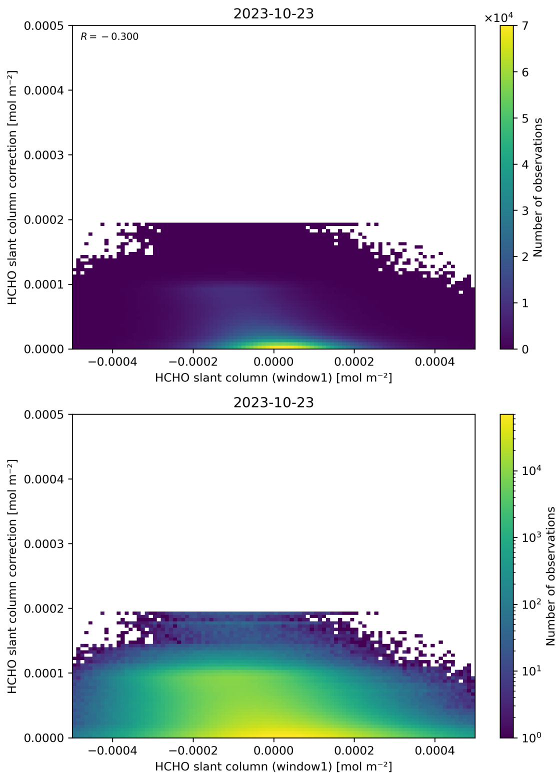
Figure 83: Scatter density plot of “HCHO slant column (window1)” against “HCHO slant column correction” for 2023-10-22 to 2023-10-24.
