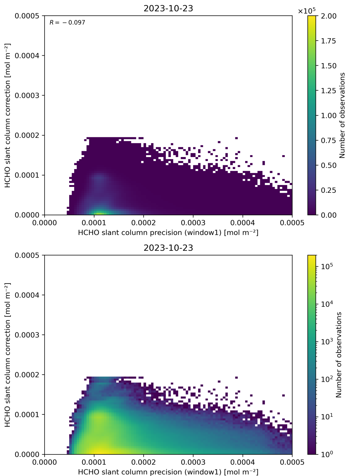
Figure 93: Scatter density plot of “HCHO slant column precision (window1)” against “HCHO slant column correction” for 2023-10-22 to 2023-10-24.
