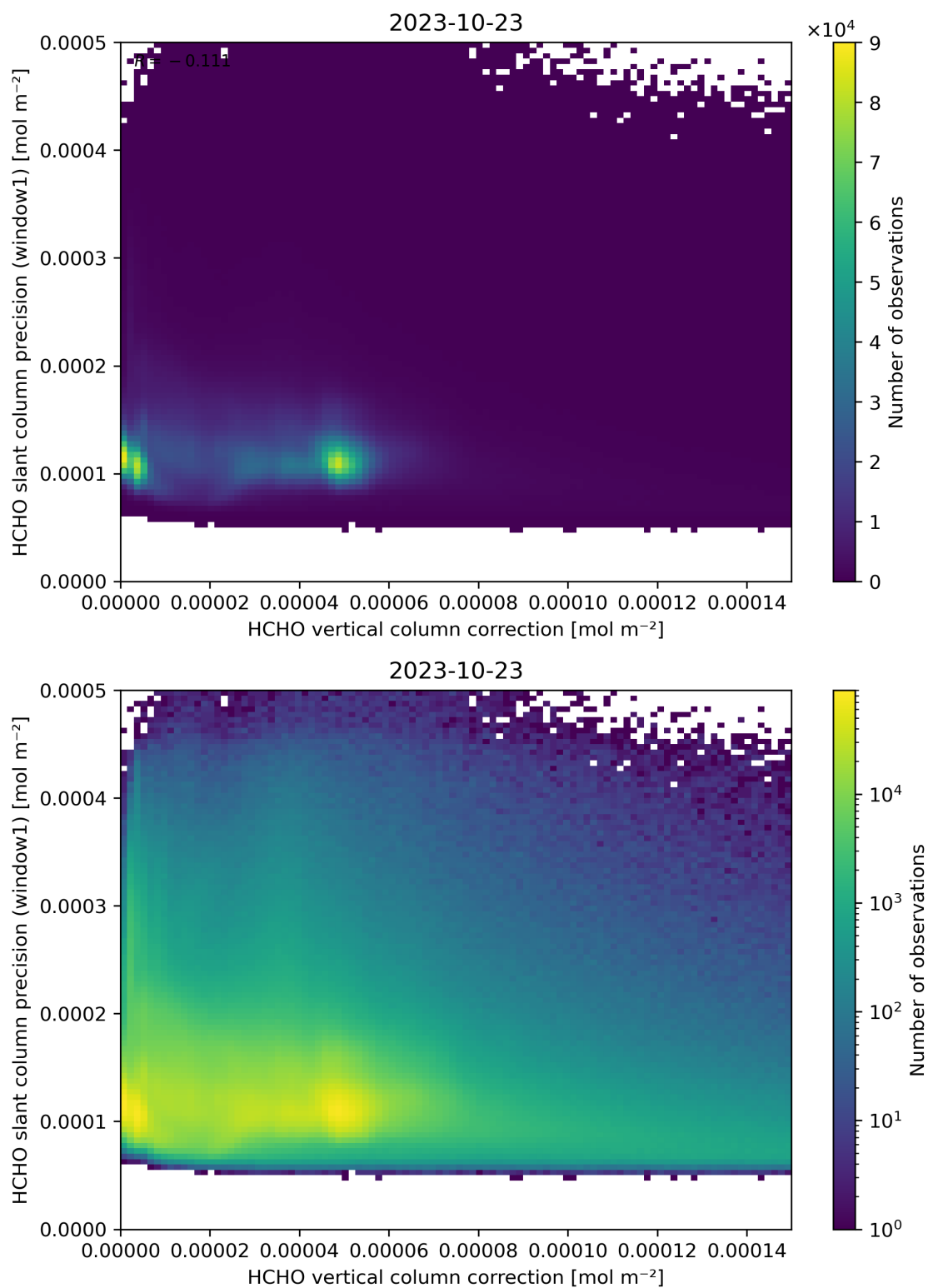
Figure 119: Scatter density plot of “HCHO vertical column correction” against “HCHO slant column precision (window1)” for 2023-10-22 to 2023-10-24.
