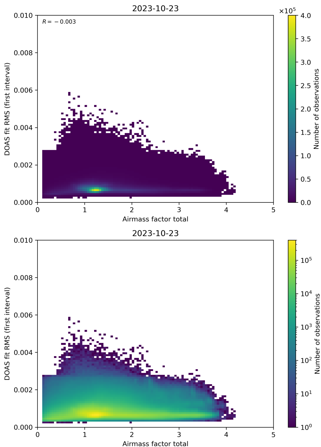
Figure 97: Scatter density plot of “Airmass factor total” against “DOAS fit RMS (first interval)” for 2023-10-22 to 2023-10-24.
