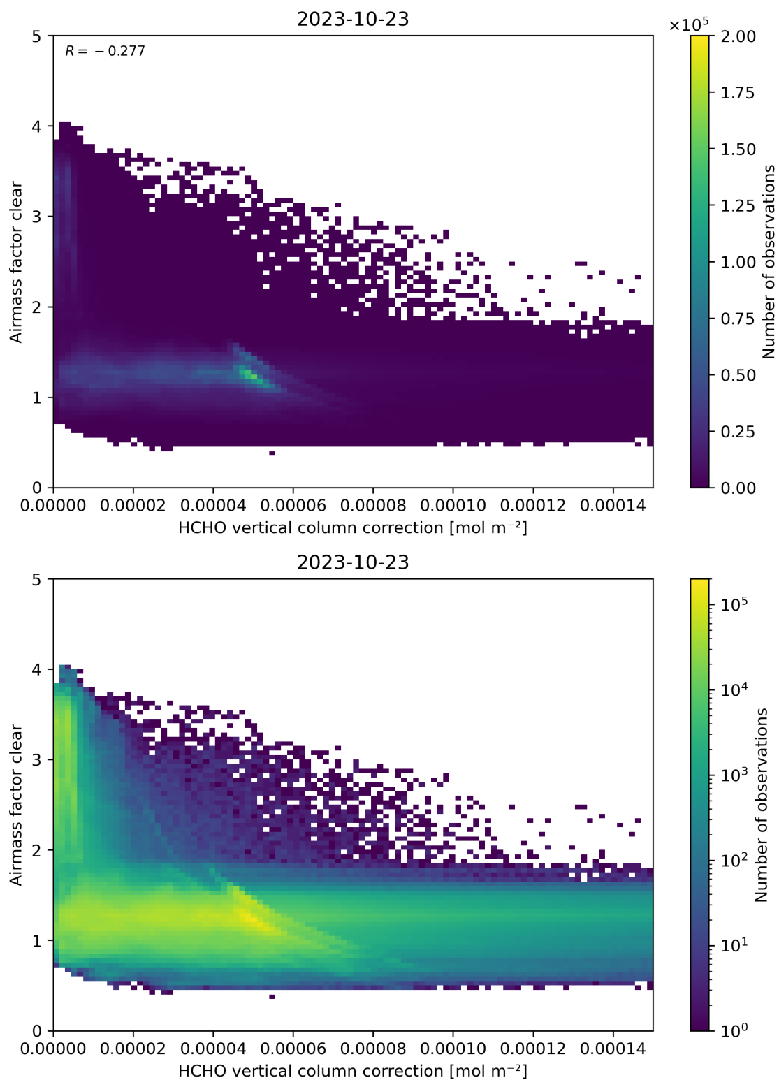
Figure 115: Scatter density plot of “HCHO vertical column correction” against “Airmass factor clear” for 2023-10-22 to 2023-10-24.
