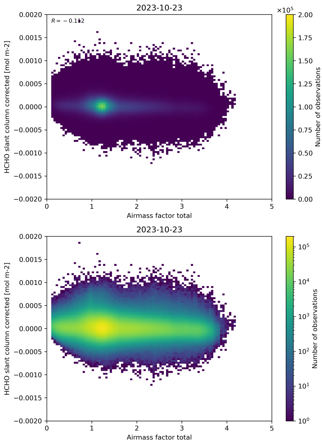
Figure 101: Scatter density plot of “Airmass factor total” against “HCHO slant column corrected” for 2023-10-22 to 2023-10-24.
