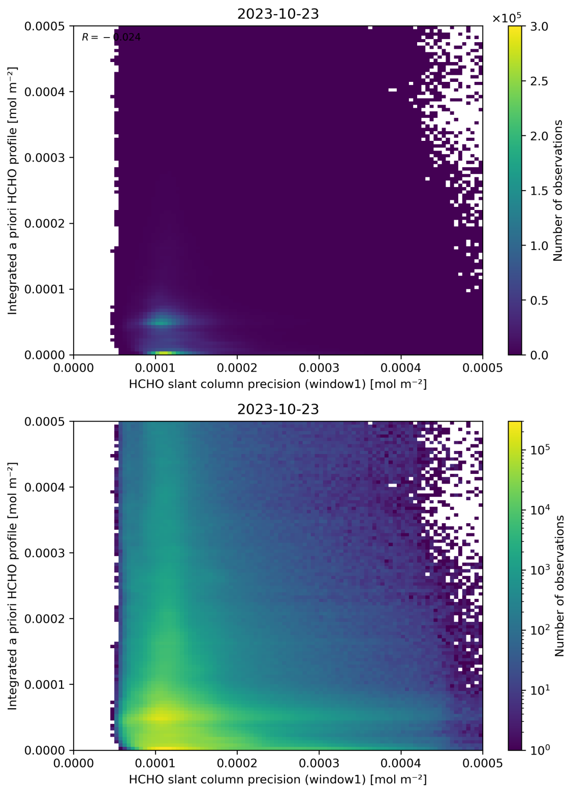
Figure 96: Scatter density plot of “HCHO slant column precision (window1)” against “Integrated a priori HCHO profile” for 2023-10-22 to 2023-10-24.
