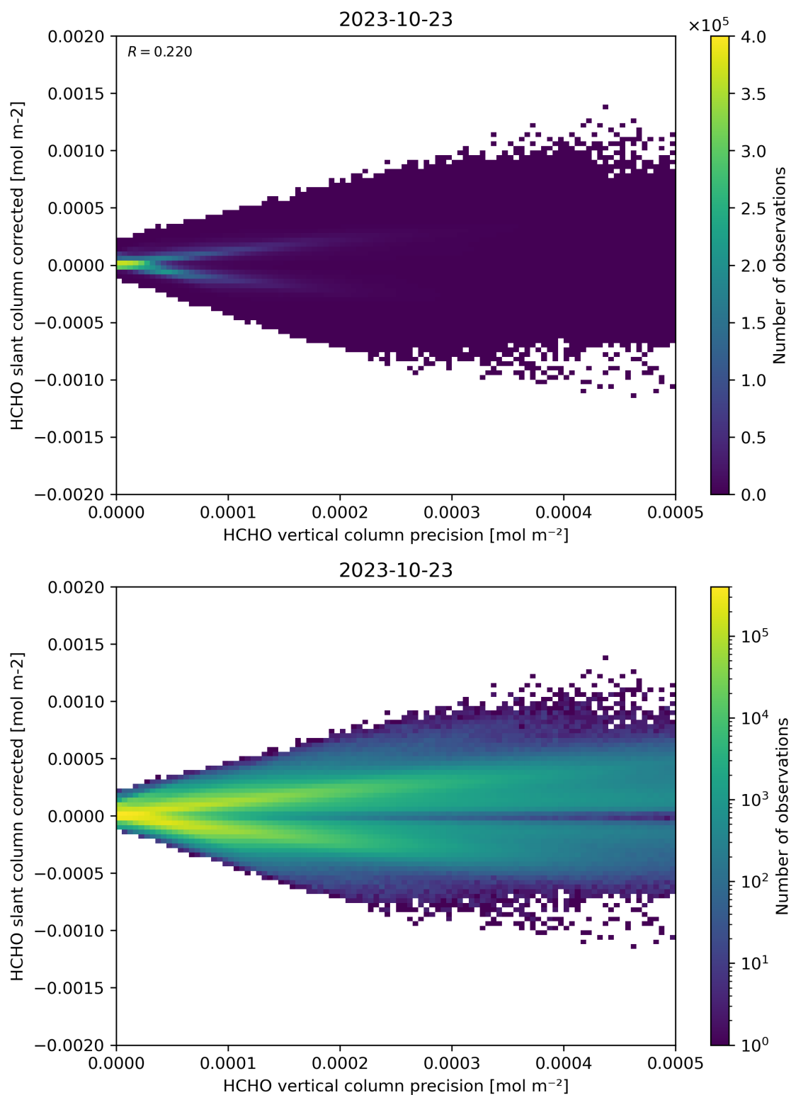
Figure 140: Scatter density plot of “HCHO vertical column precision” against “HCHO slant column corrected” for 2023-10-22 to 2023-10-24.
