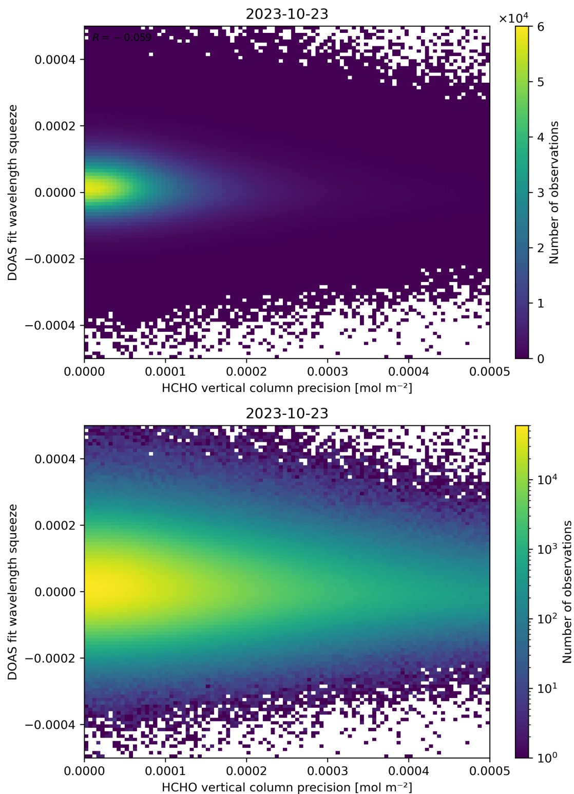
Figure 138: Scatter density plot of “HCHO vertical column precision” against “DOAS fit wavelength squeeze” for 2023-10-22 to 2023-10-24.
