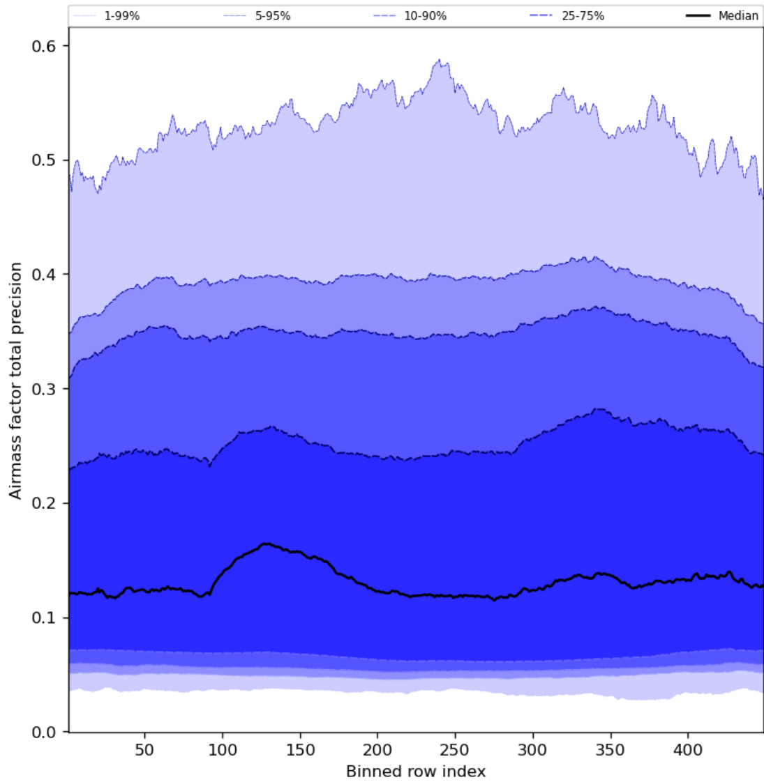
Figure 55: Along track statistics of “Airmass factor total precision” for 2023-10-22 to 2023-10-24
