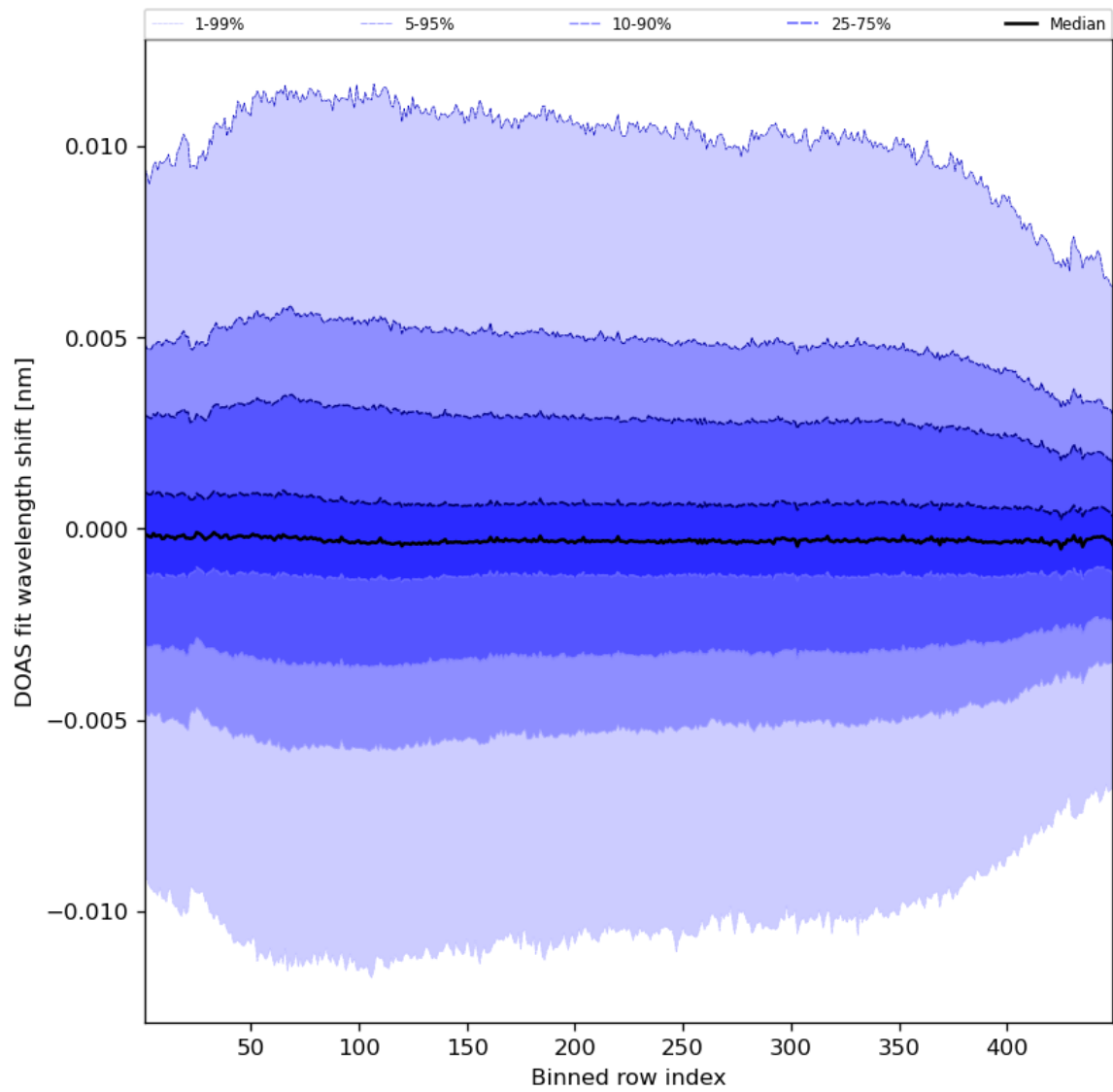
Figure 58: Along track statistics of “DOAS fit wavelength shift” for 2023-10-22 to 2023-10-24
