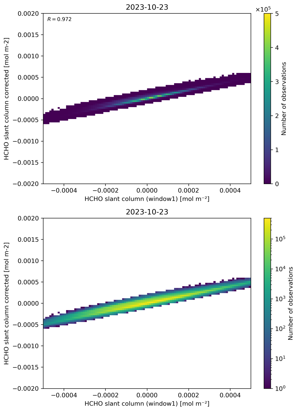
Figure 82: Scatter density plot of “HCHO slant column (window1)” against “HCHO slant column corrected” for 2023-10-22 to 2023-10-24.
