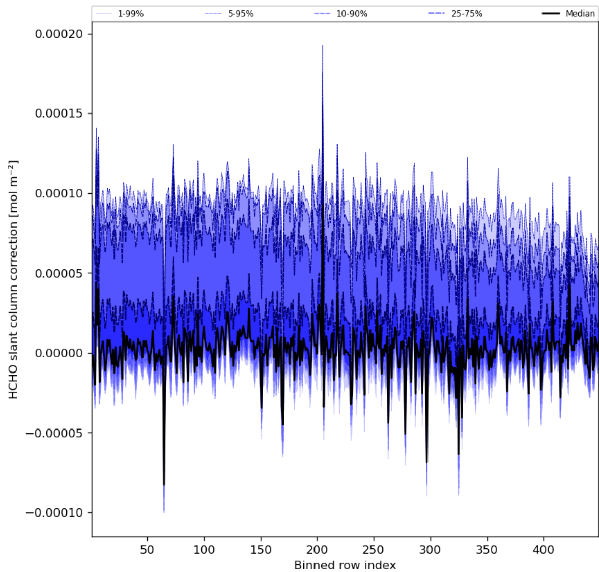
Figure 61: Along track statistics of “HCHO slant column correction” for 2023-10-22 to 2023-10-24
