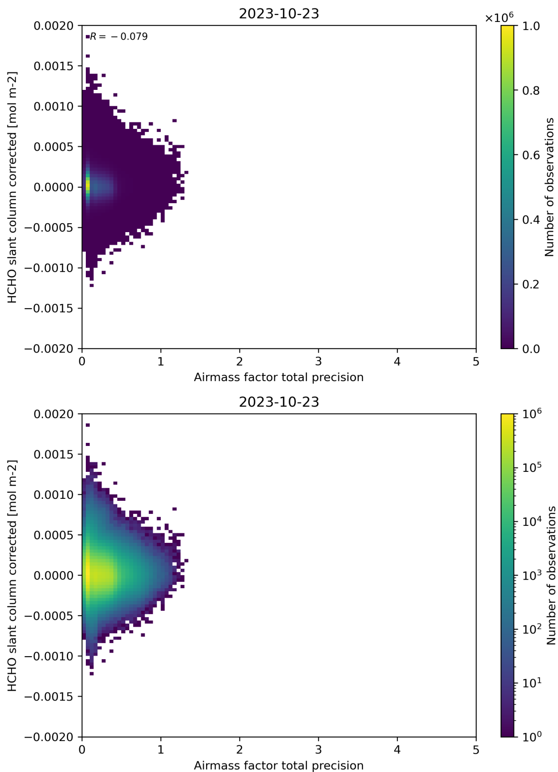
Figure 109: Scatter density plot of “Airmass factor total precision” against “HCHO slant column corrected” for 2023-10-22 to 2023-10-24.
