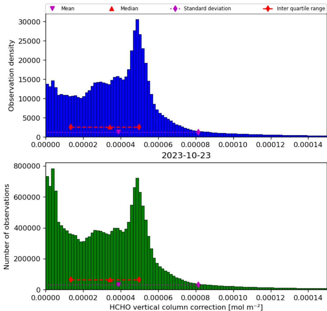
Figure 37: Histogram of “HCHO vertical column correction” for 2023-10-22 to 2023-10-24
