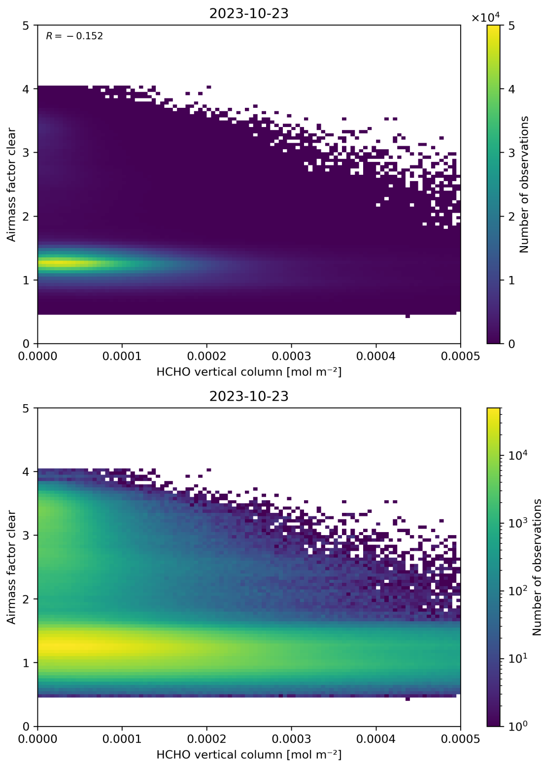
Figure 126: Scatter density plot of “HCHO vertical column” against “Airmass factor clear” for 2023-10-22 to 2023-10-24.
