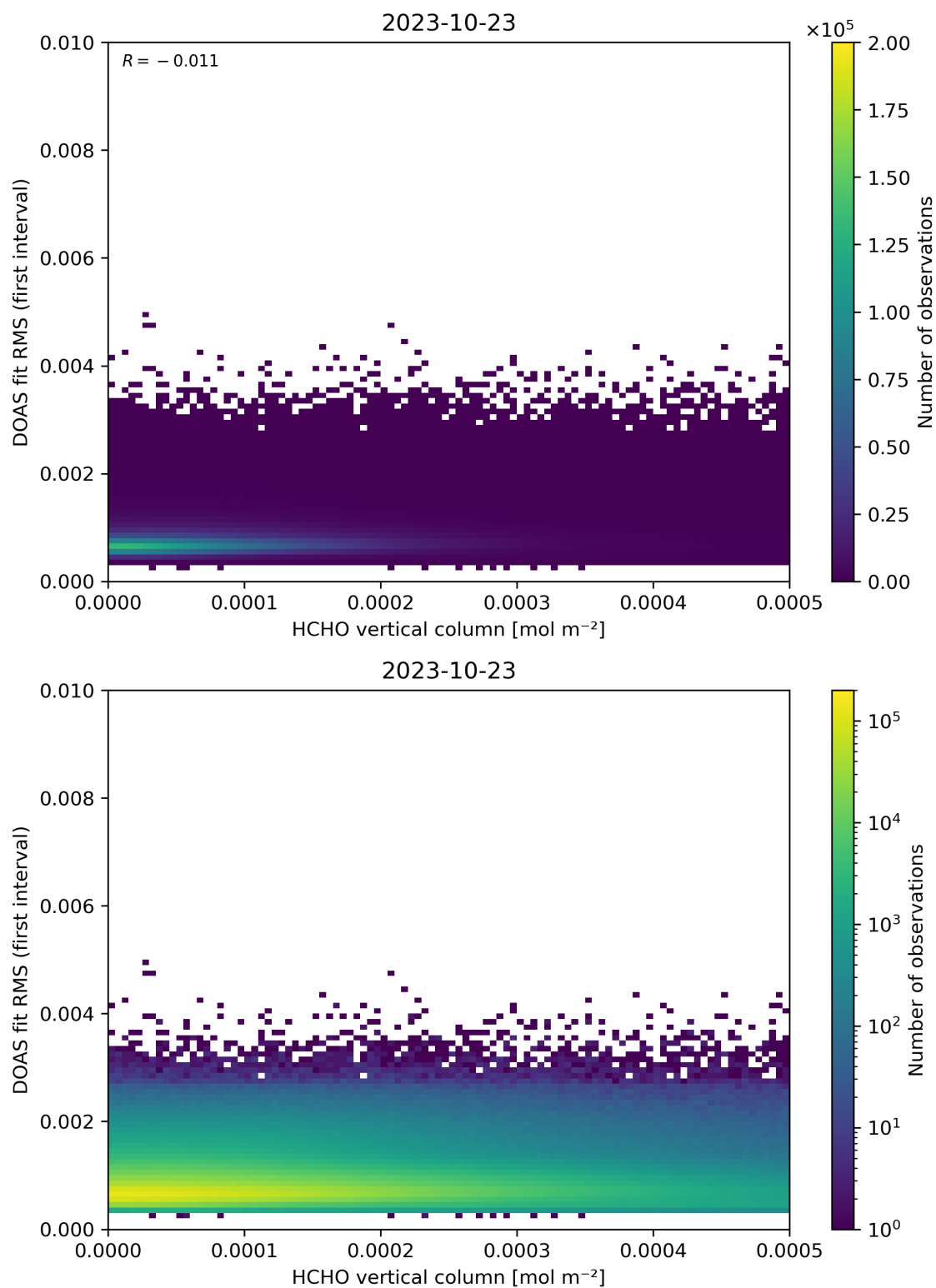
Figure 123: Scatter density plot of “HCHO vertical column” against “DOAS fit RMS (first interval)” for 2023-10-22 to 2023-10-24.
