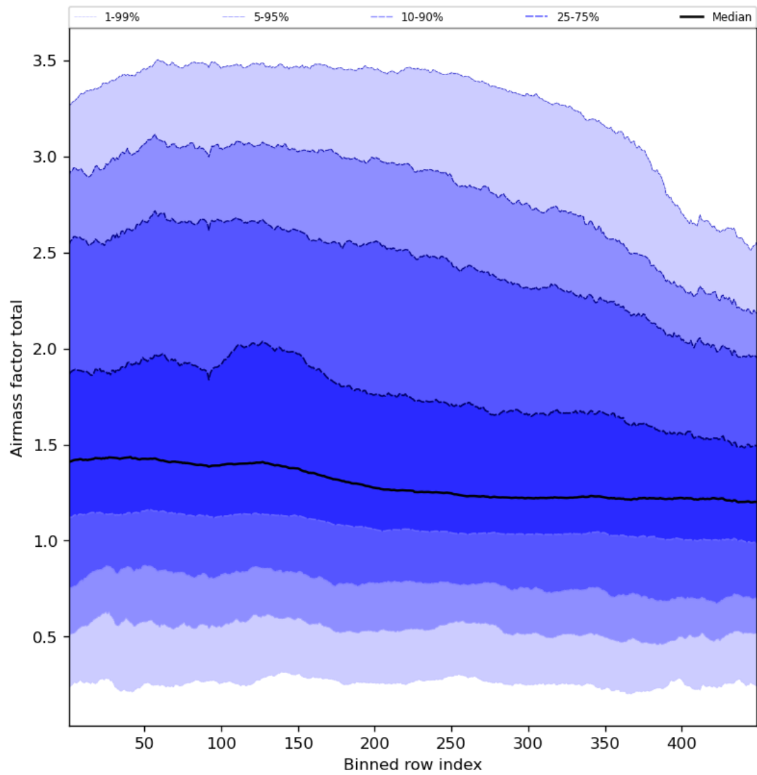
Figure 54: Along track statistics of “Airmass factor total” for 2023-10-22 to 2023-10-24
