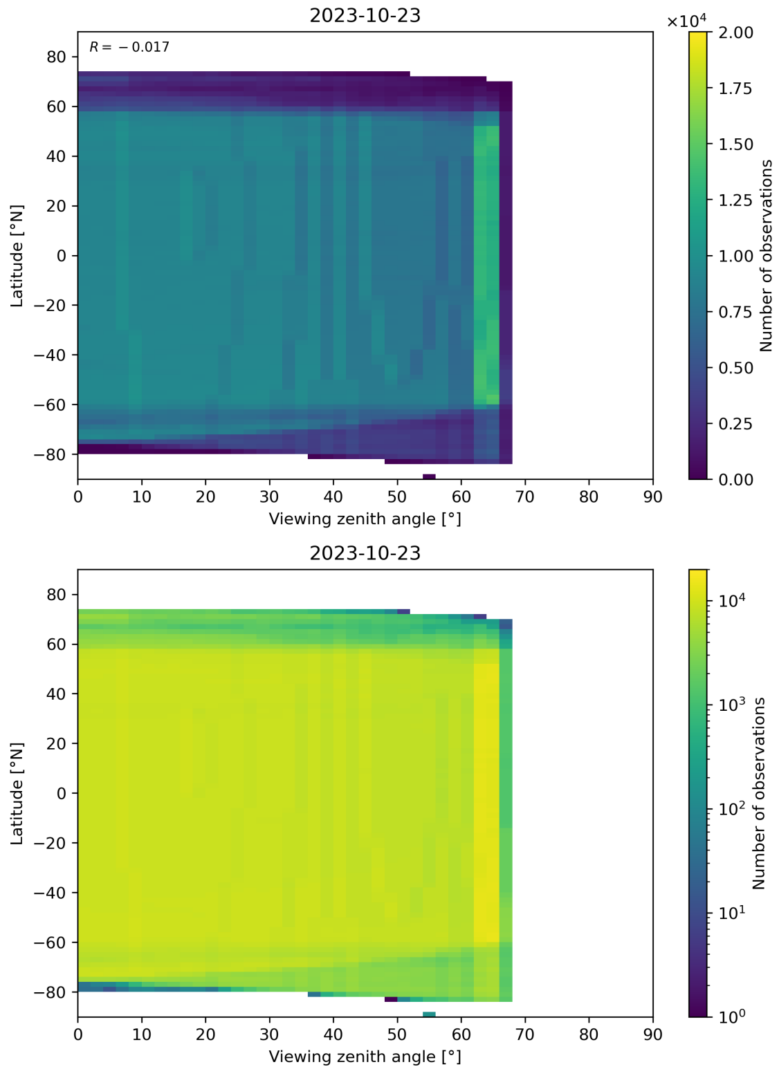
Figure 196: Scatter density plot of “Viewing zenith angle” against “Latitude” for 2023-10-22 to 2023-10-24.
