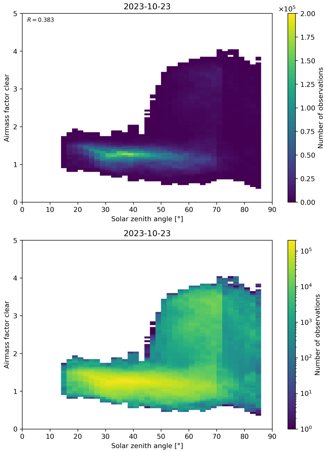
Figure 170: Scatter density plot of “Solar zenith angle” against “Airmass factor clear” for 2023-10-22 to 2023-10-24.
