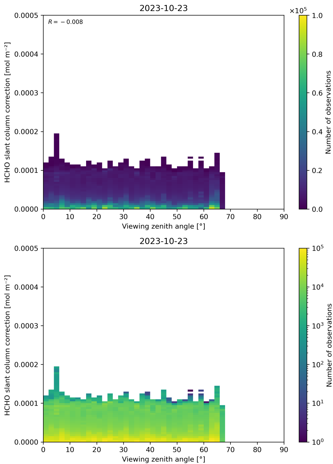
Figure 187: Scatter density plot of “Viewing zenith angle” against “HCHO slant column correction” for 2023-10-22 to 2023-10-24.
