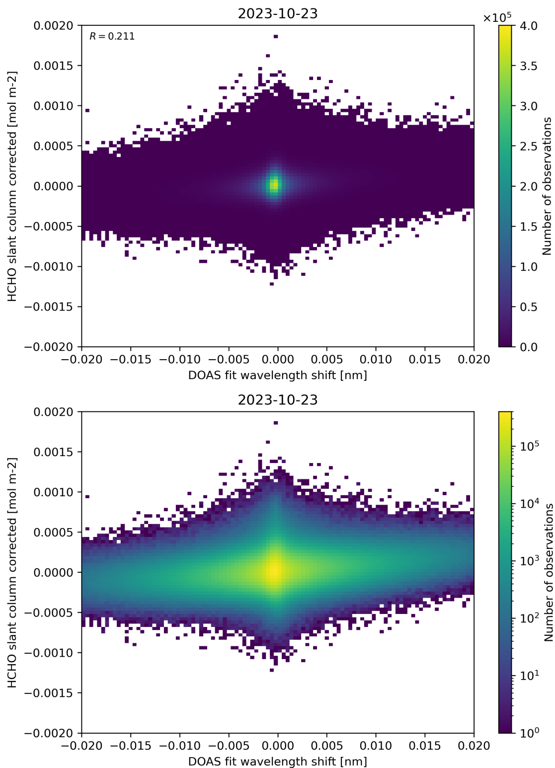
Figure 66: Scatter density plot of “DOAS fit wavelength shift” against “HCHO slant column corrected” for 2023-10-22 to 2023-10-24.
