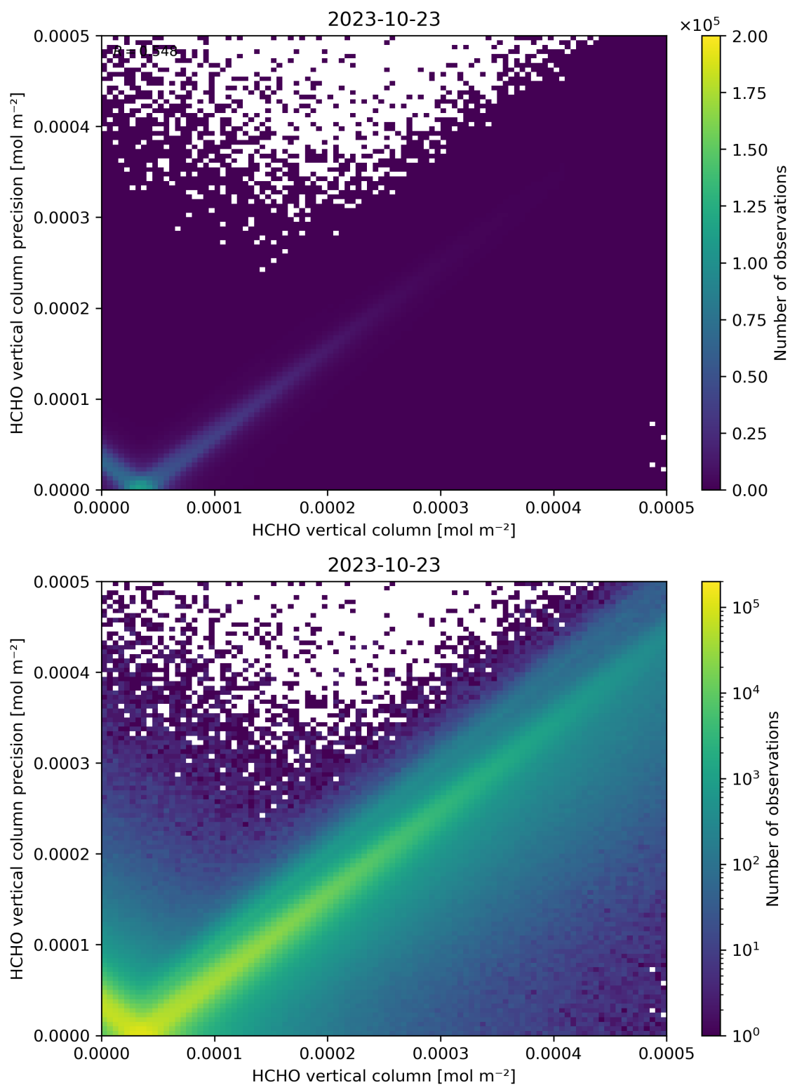
Figure 134: Scatter density plot of “HCHO vertical column” against “HCHO vertical column precision” for 2023-10-22 to 2023-10-24.
