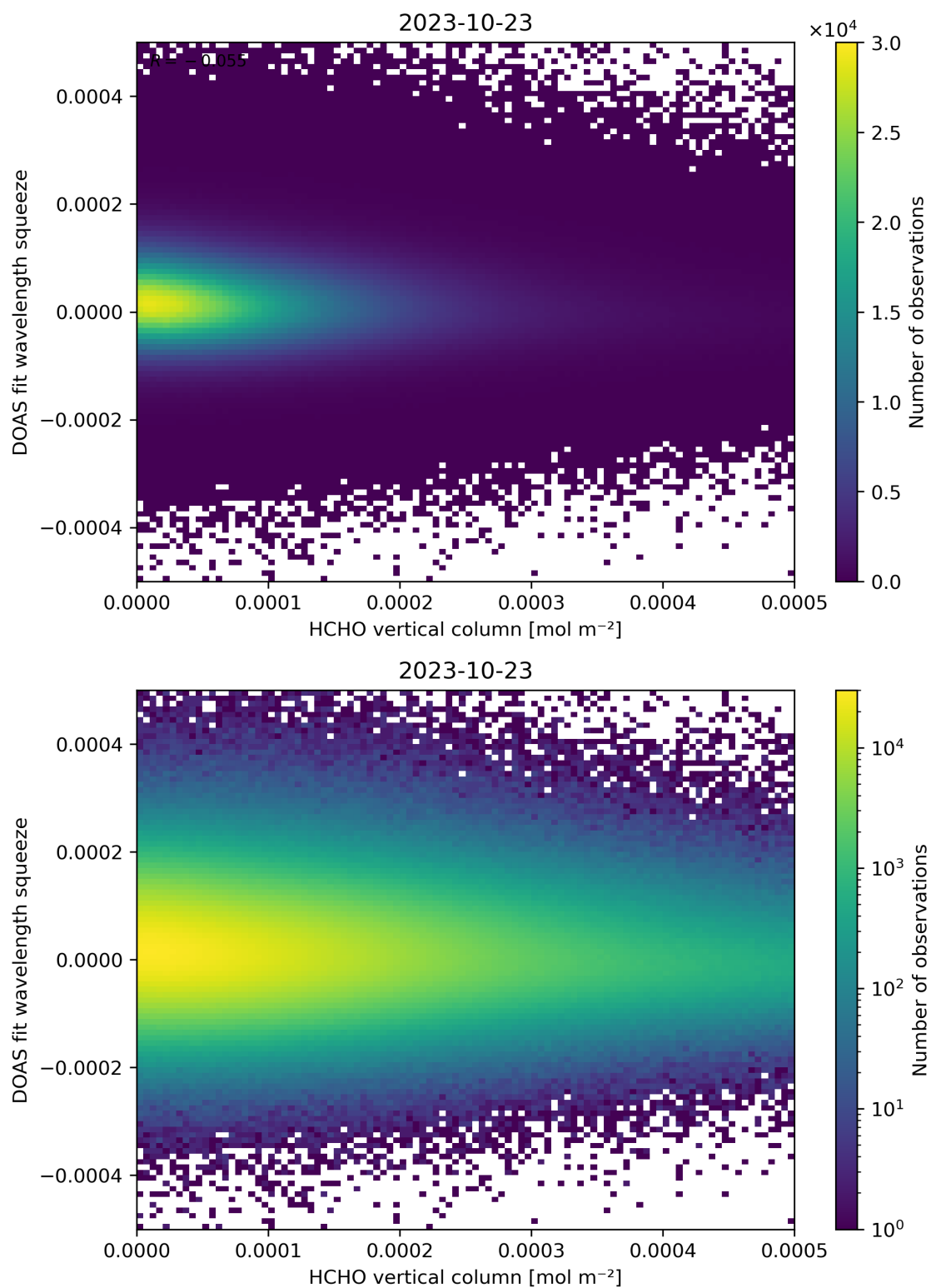
Figure 125: Scatter density plot of “HCHO vertical column” against “DOAS fit wavelength squeeze” for 2023-10-22 to 2023-10-24.
