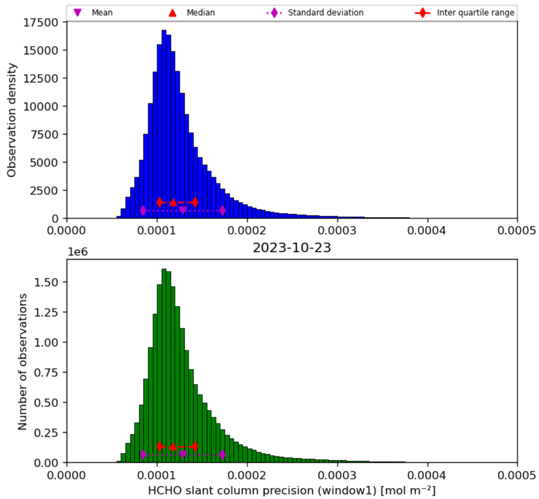
Figure 39: Histogram of “HCHO slant column precision (window1)” for 2023-10-22 to 2023-10-24
