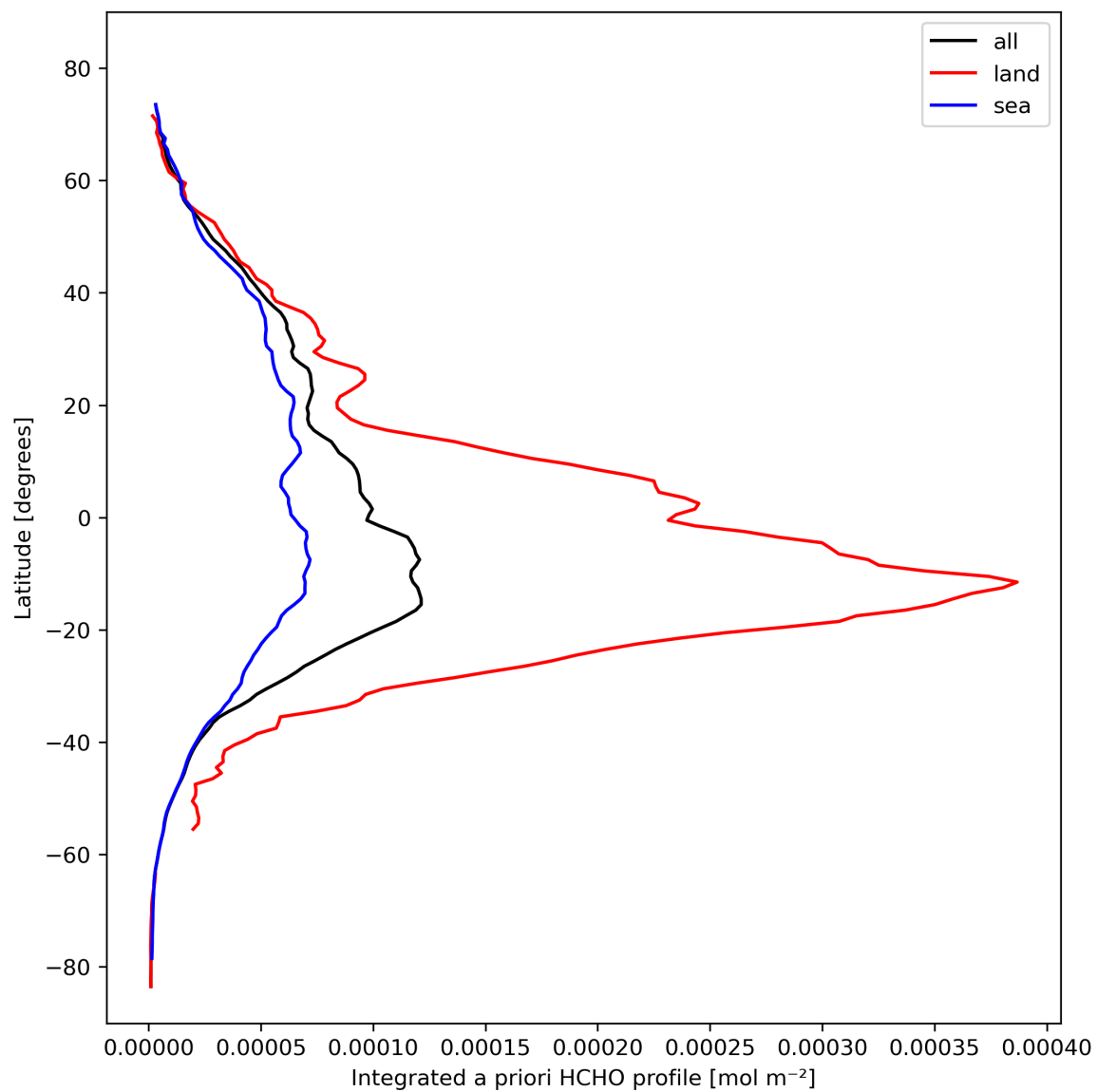
Figure 29: Zonal average of “Integrated a priori HCHO profile” for 2023-10-22 to 2023-10-24.
