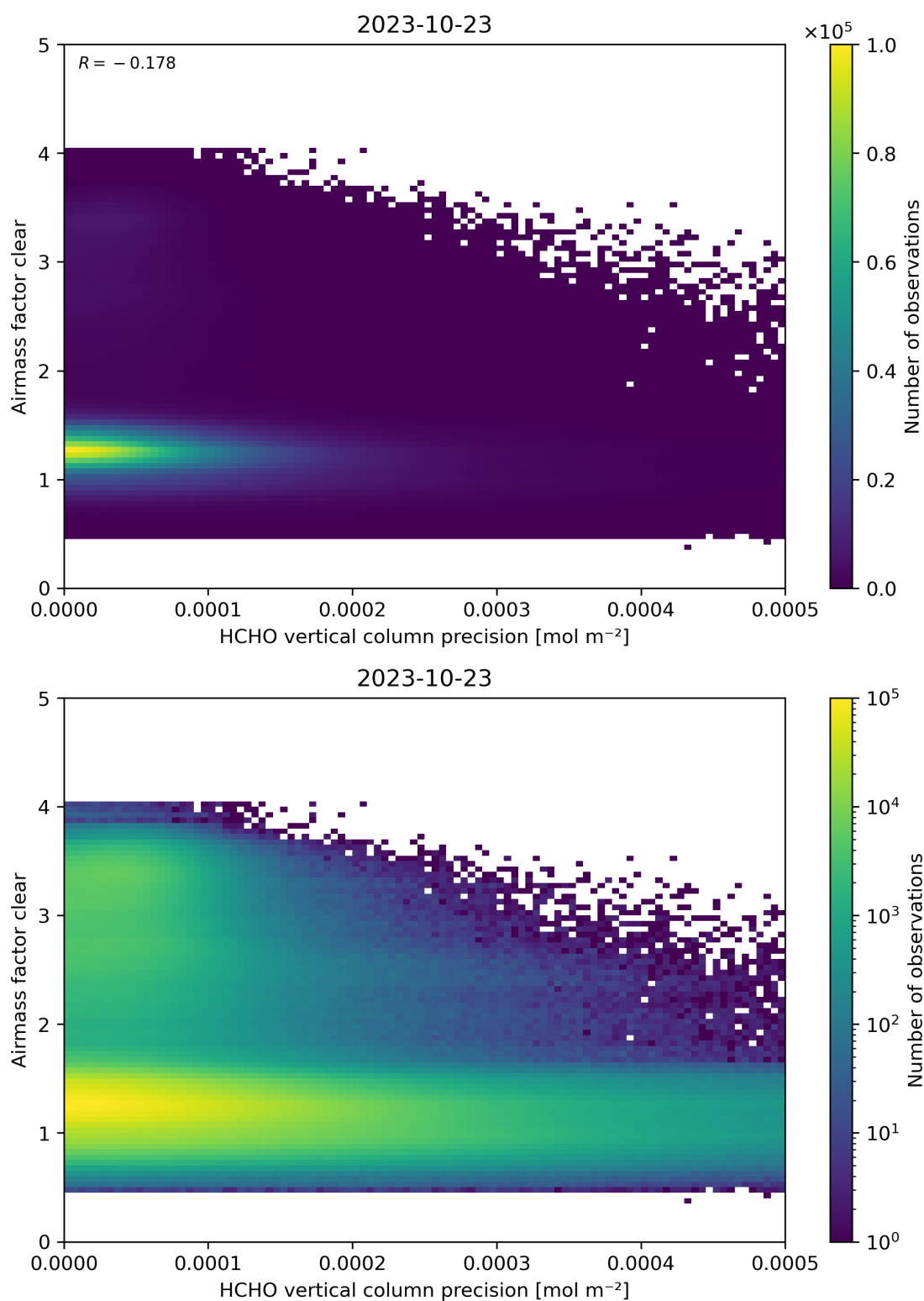
Figure 139: Scatter density plot of “HCHO vertical column precision” against “Airmass factor clear” for 2023-10-22 to 2023-10-24.
