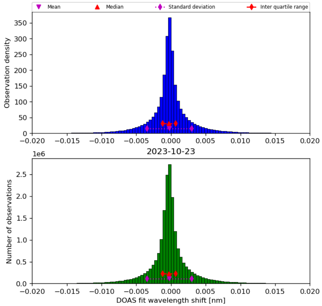
Figure 44: Histogram of “DOAS fit wavelength shift” for 2023-10-22 to 2023-10-24
