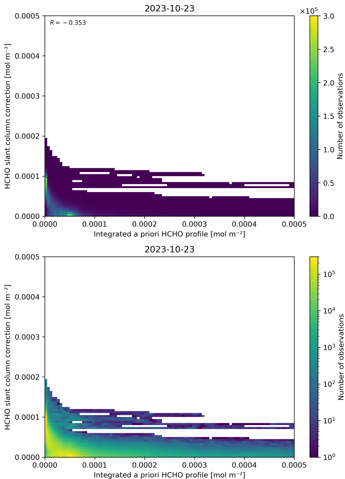
Figure 152: Scatter density plot of “Integrated a priori HCHO profile” against “HCHO slant column correction” for 2023-10-22 to 2023-10-24.
