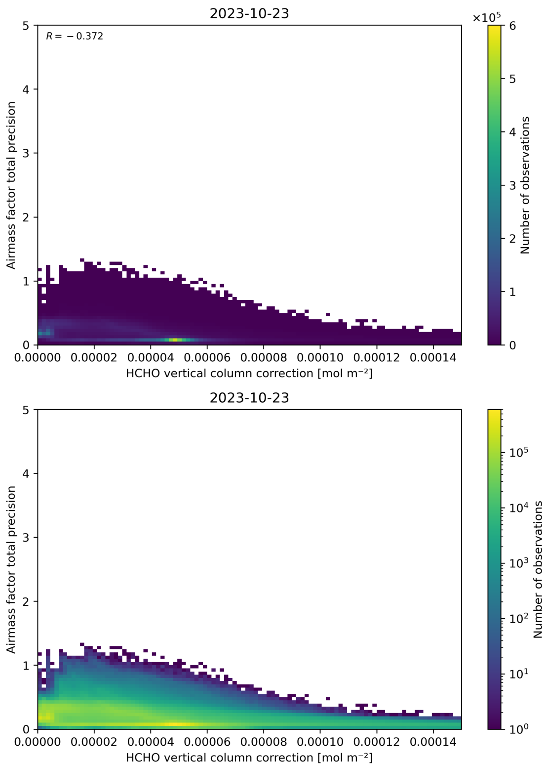
Figure 121: Scatter density plot of “HCHO vertical column correction” against “Airmass factor total precision” for 2023-10-22 to 2023-10-24.
