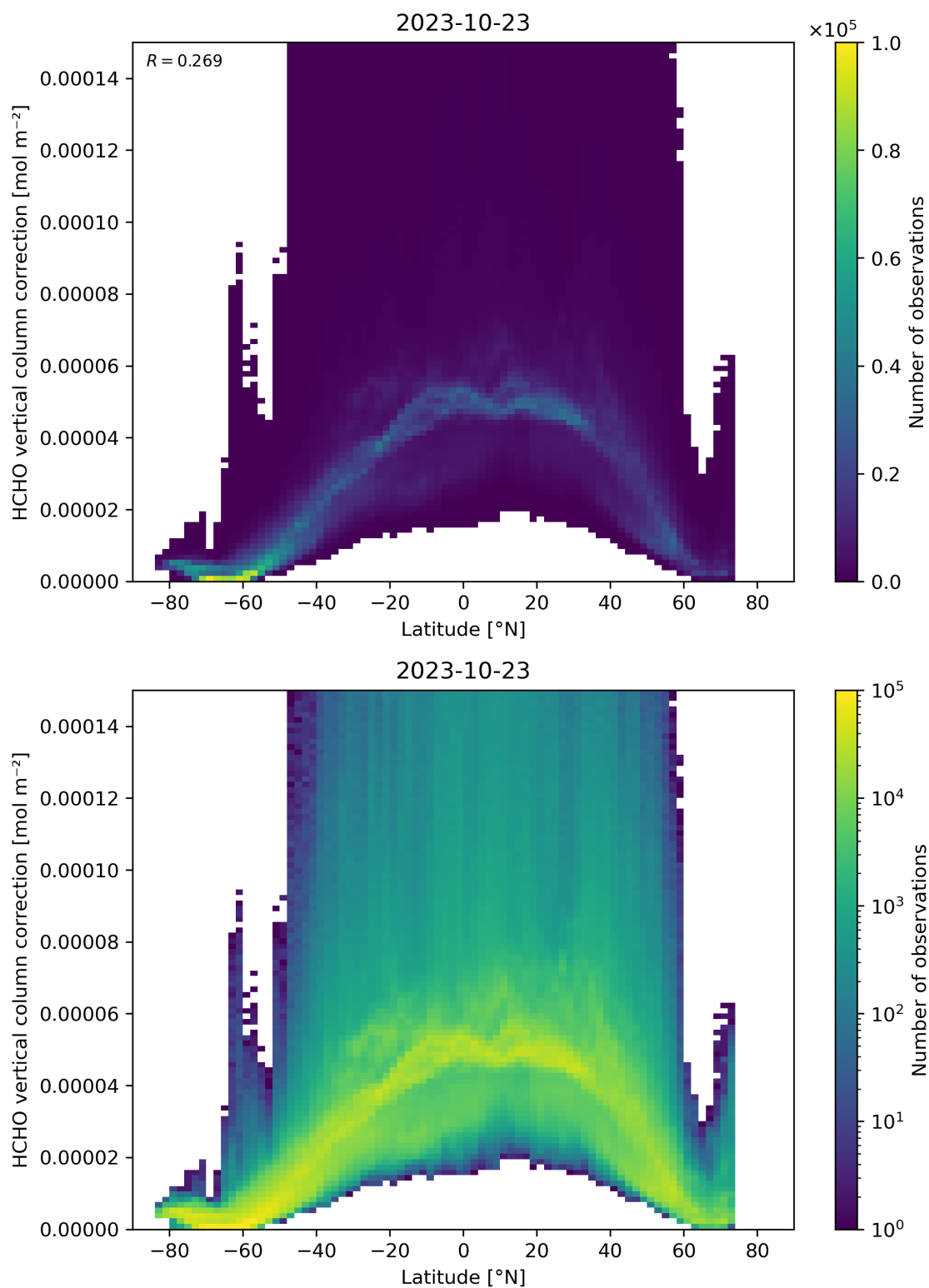
Figure 164: Scatter density plot of “Latitude” against “HCHO vertical column correction” for 2023-10-22 to 2023-10-24.
