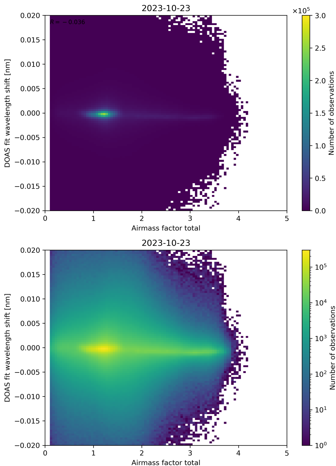
Figure 98: Scatter density plot of “Airmass factor total” against “DOAS fit wavelength shift” for 2023-10-22 to 2023-10-24.
