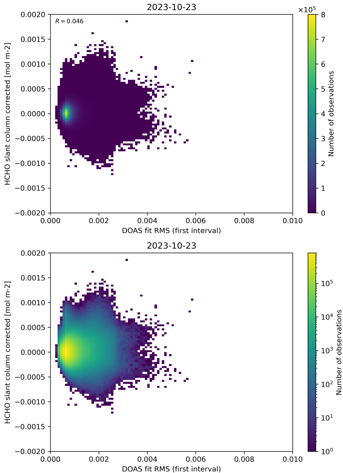
Figure 62: Scatter density plot of “DOAS fit RMS (first interval)” against “HCHO slant column corrected” for 2023-10-22 to 2023-10-24.
