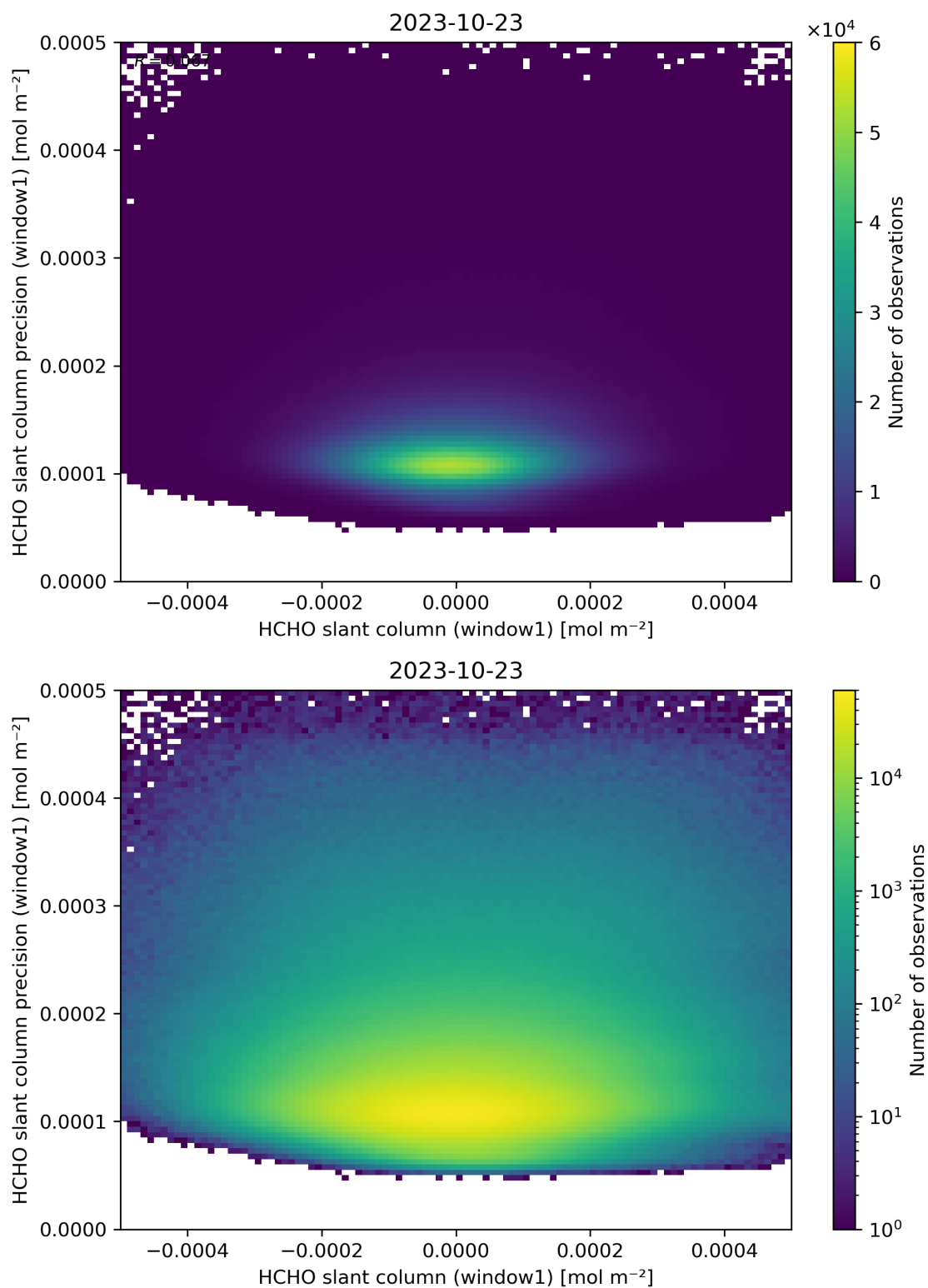
Figure 84: Scatter density plot of “HCHO slant column (window1)” against “HCHO slant column precision (window1)” for 2023-10-22 to 2023-10-24.
