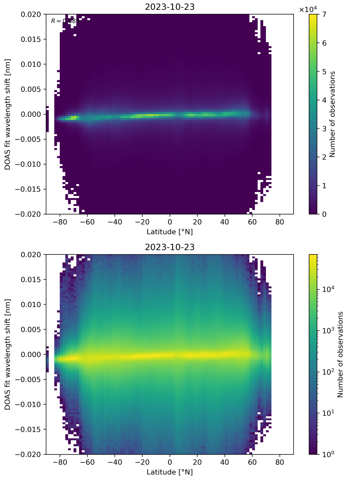
Figure 154: Scatter density plot of “Latitude” against “DOAS fit wavelength shift” for 2023-10-22 to 2023-10-24.
