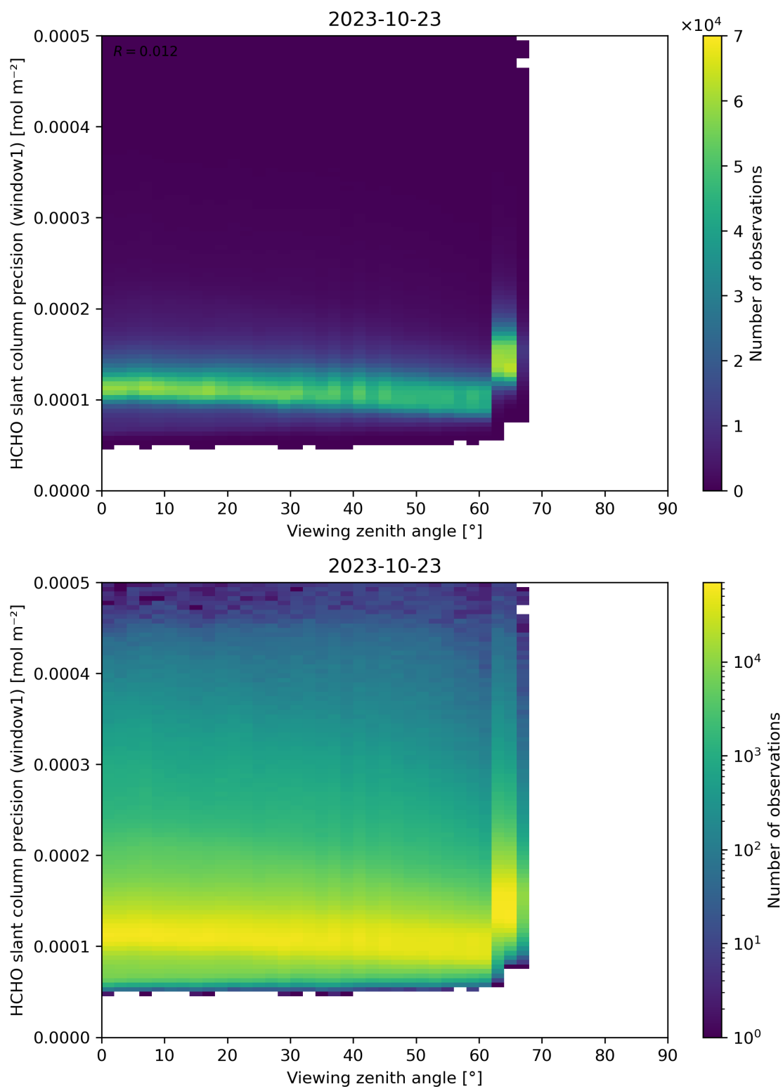
Figure 189: Scatter density plot of “Viewing zenith angle” against “HCHO slant column precision (window1)” for 2023-10-22 to 2023-10-24.
