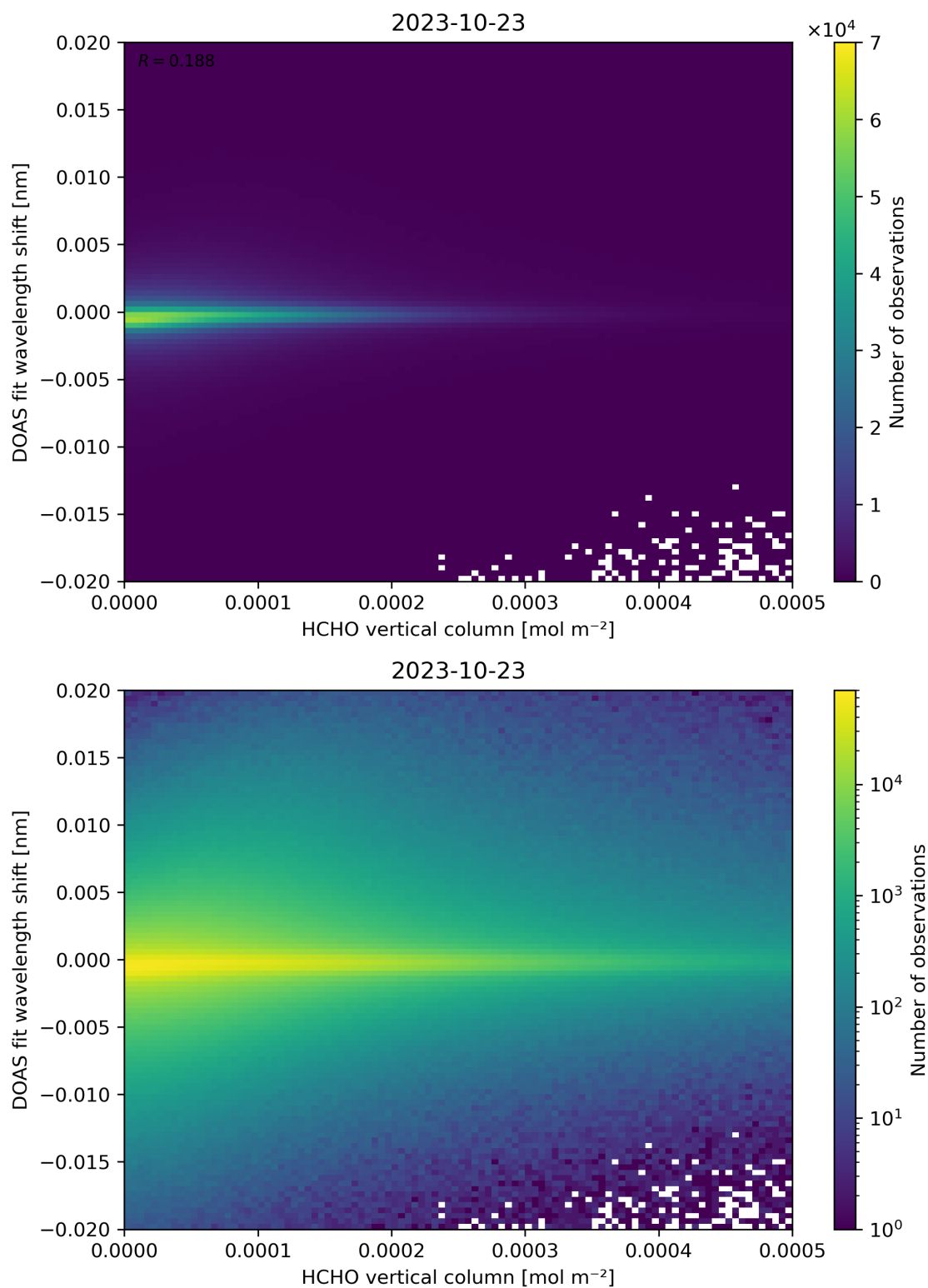
Figure 124: Scatter density plot of “HCHO vertical column” against “DOAS fit wavelength shift” for 2023-10-22 to 2023-10-24.
