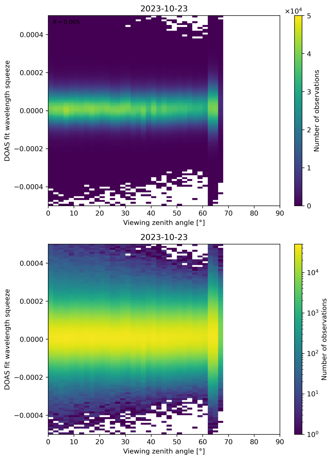
Figure 184: Scatter density plot of “Viewing zenith angle” against “DOAS fit wavelength squeeze” for 2023-10-22 to 2023-10-24.
