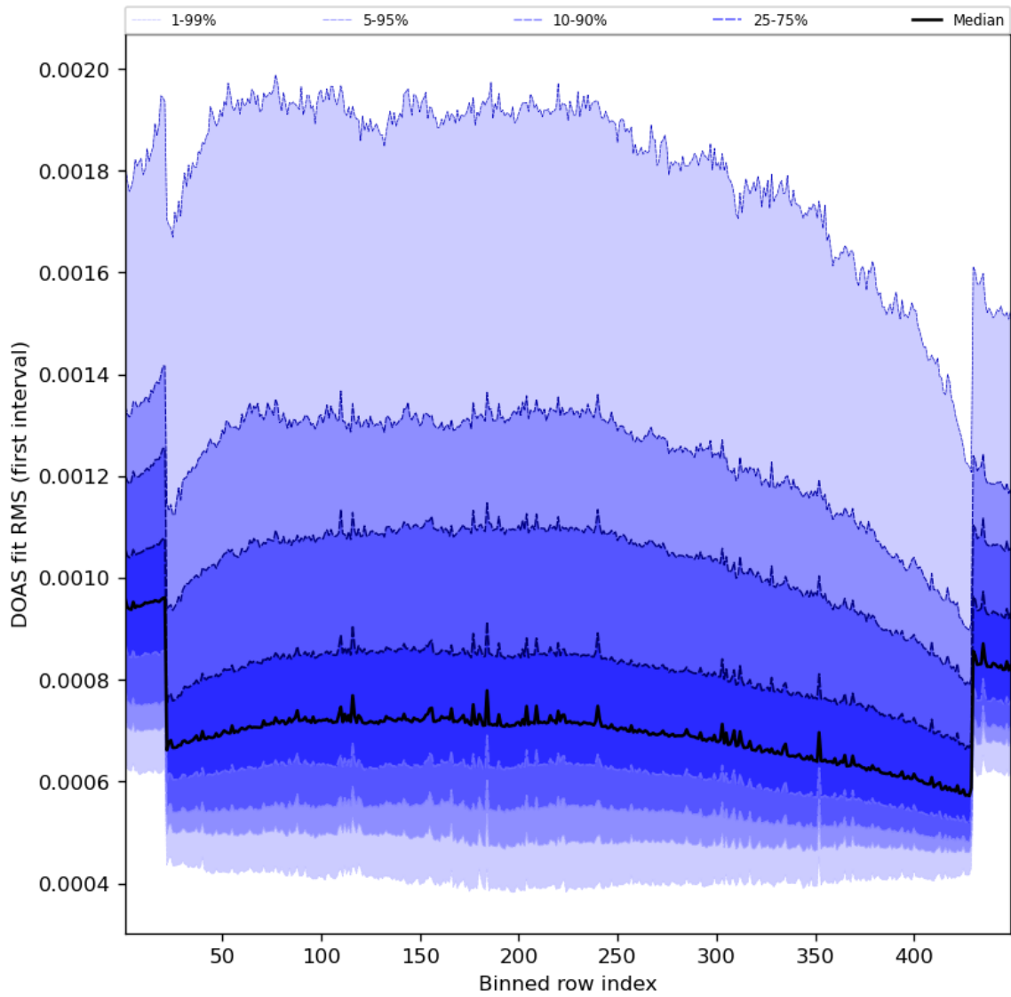
Figure 60: Along track statistics of “DOAS fit RMS (first interval)” for 2023-10-22 to 2023-10-24
