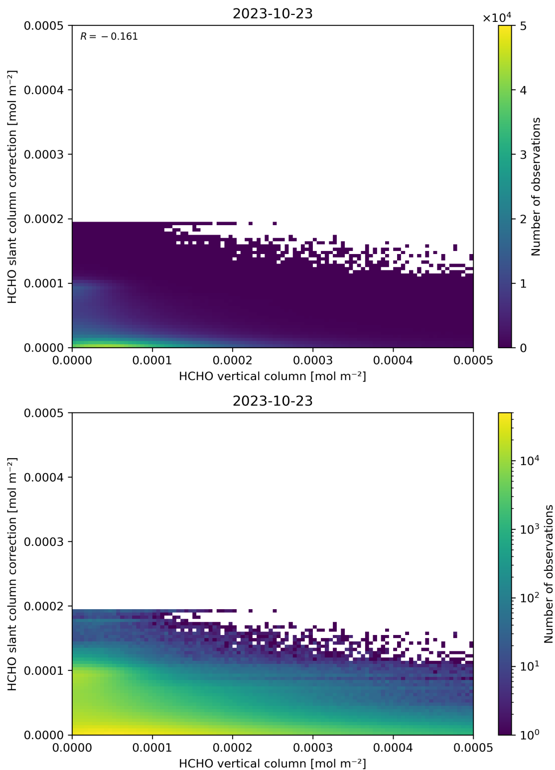
Figure 128: Scatter density plot of “HCHO vertical column” against “HCHO slant column correction” for 2023-10-22 to 2023-10-24.
