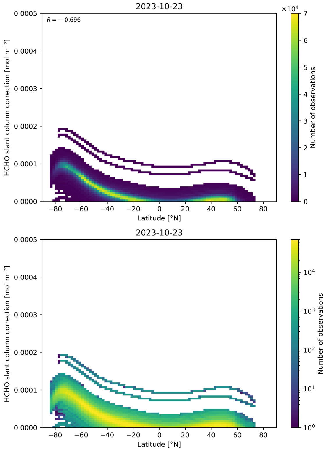
Figure 158: Scatter density plot of “Latitude” against “HCHO slant column correction” for 2023-10-22 to 2023-10-24.
