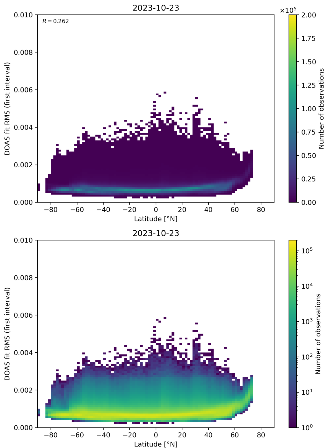
Figure 153: Scatter density plot of “Latitude” against “DOAS fit RMS (first interval)” for 2023-10-22 to 2023-10-24.
