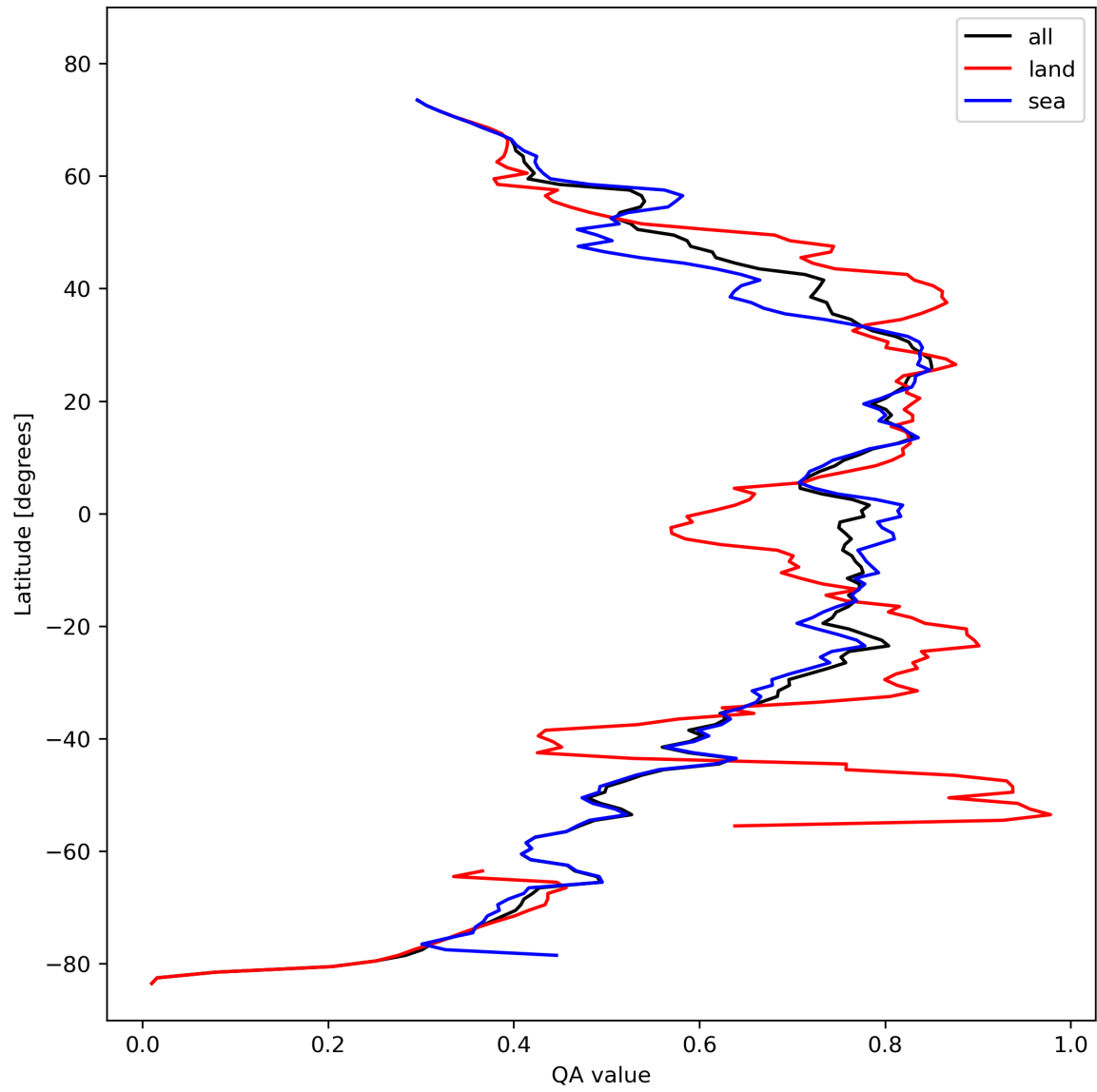
Figure 20: Zonal average of “QA value” for 2023-10-22 to 2023-10-24.
