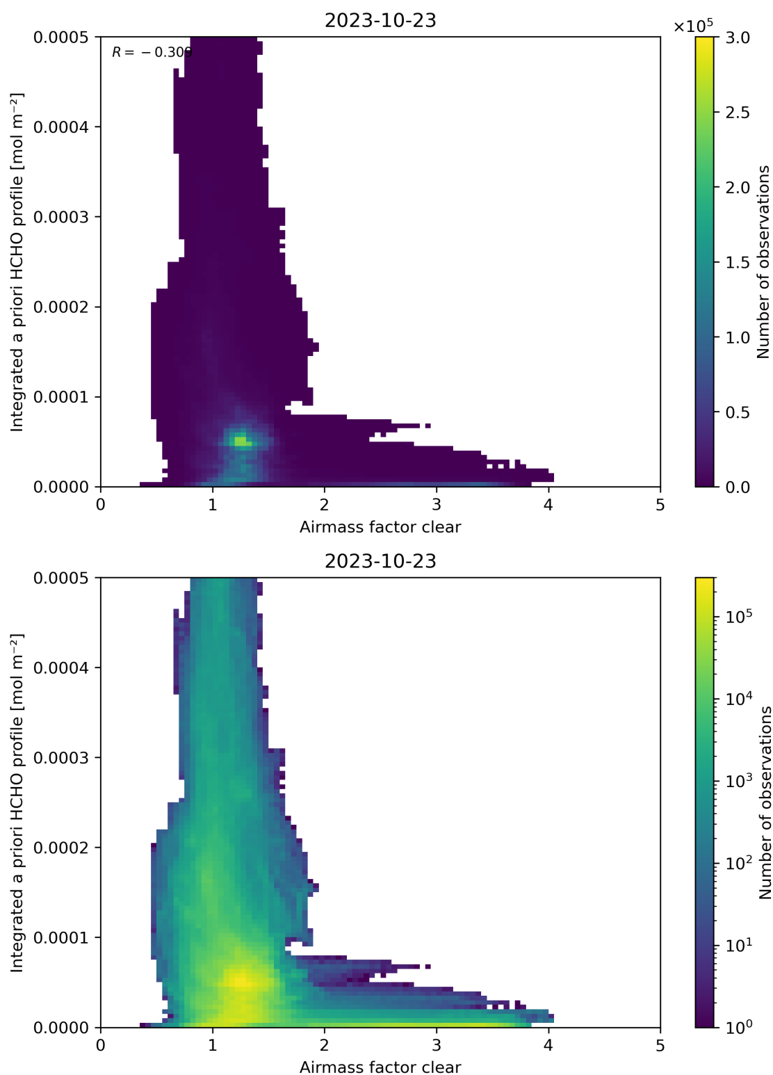
Figure 76: Scatter density plot of “Airmass factor clear” against “Integrated a priori HCHO profile” for 2023-10-22 to 2023-10-24.
