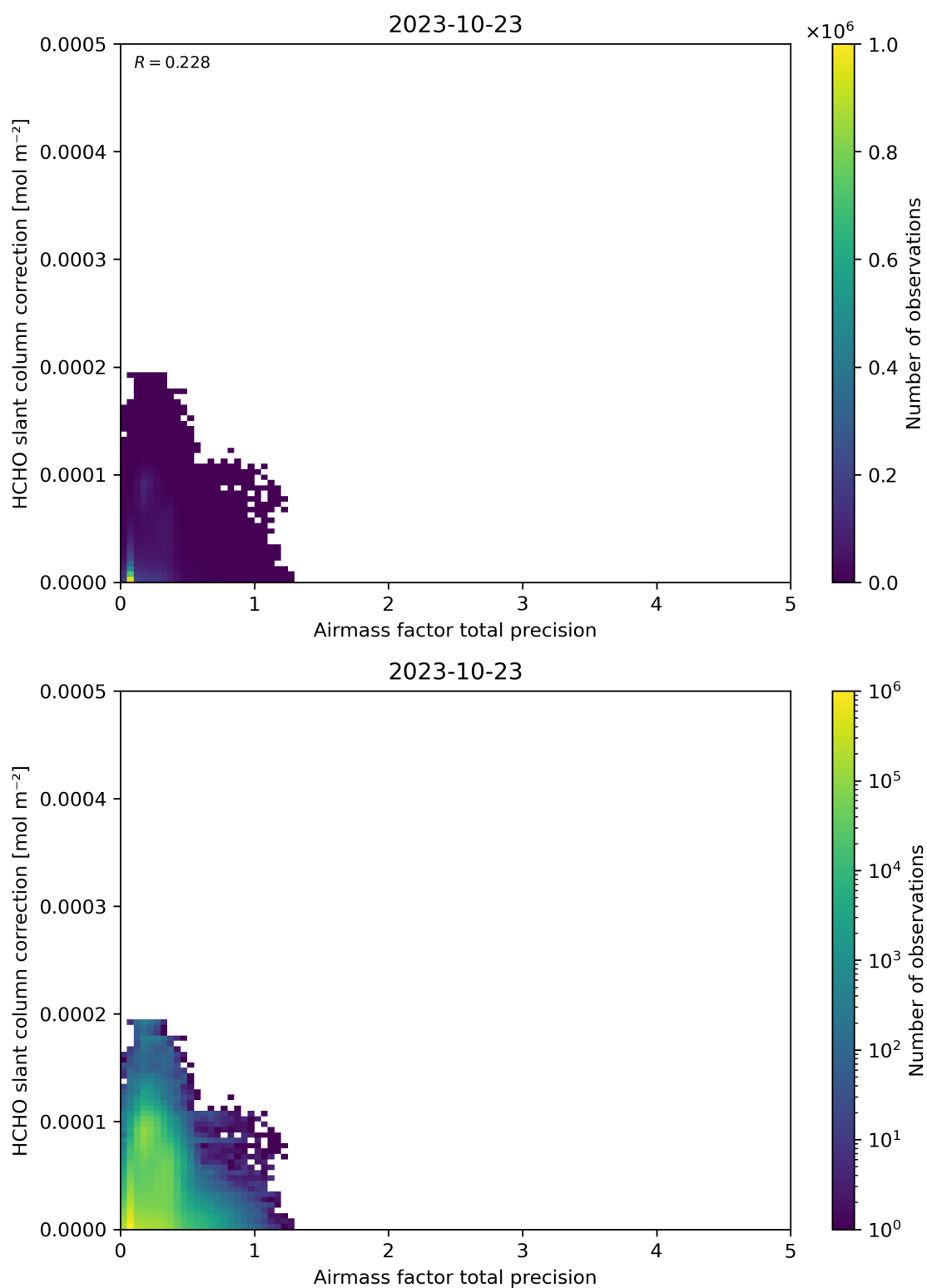
Figure 110: Scatter density plot of “Airmass factor total precision” against “HCHO slant column correction” for 2023-10-22 to 2023-10-24.
