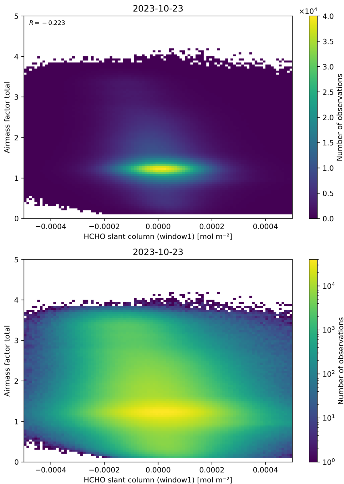
Figure 85: Scatter density plot of “HCHO slant column (window1)” against “Airmass factor total” for 2023-10-22 to 2023-10-24.
