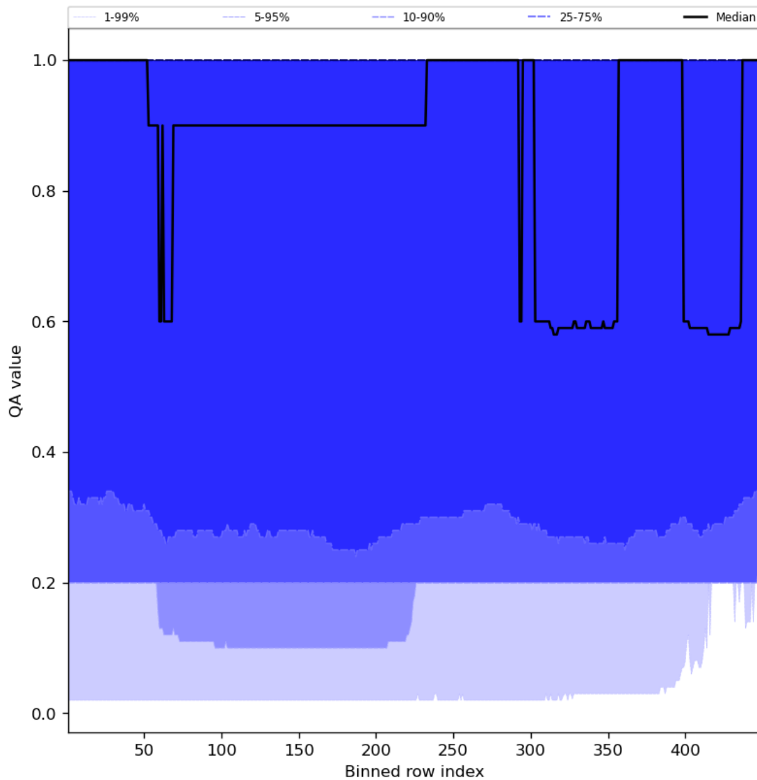
Figure 48: Along track statistics of “QA value” for 2023-10-22 to 2023-10-24
