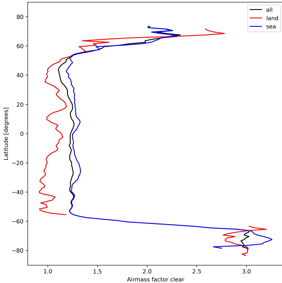
Figure 28: Zonal average of “Airmass factor clear” for 2023-10-22 to 2023-10-24.
