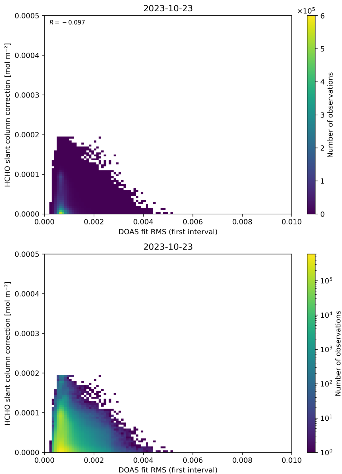
Figure 63: Scatter density plot of “DOAS fit RMS (first interval)” against “HCHO slant column correction” for 2023-10-22 to 2023-10-24.
