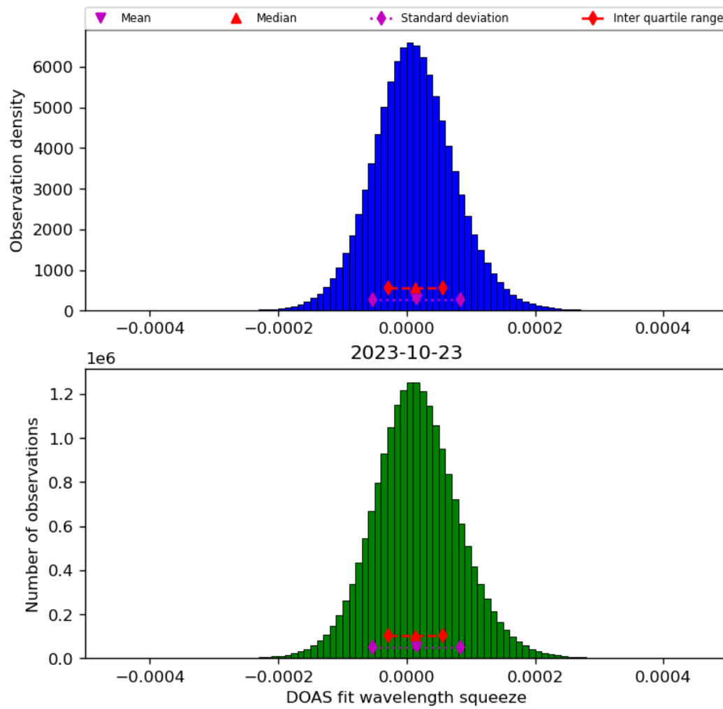
Figure 45: Histogram of “DOAS fit wavelength squeeze” for 2023-10-22 to 2023-10-24
