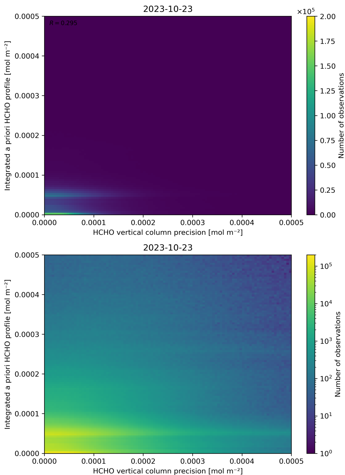
Figure 147: Scatter density plot of “HCHO vertical column precision” against “Integrated a priori HCHO profile” for 2023-10-22 to 2023-10-24.
