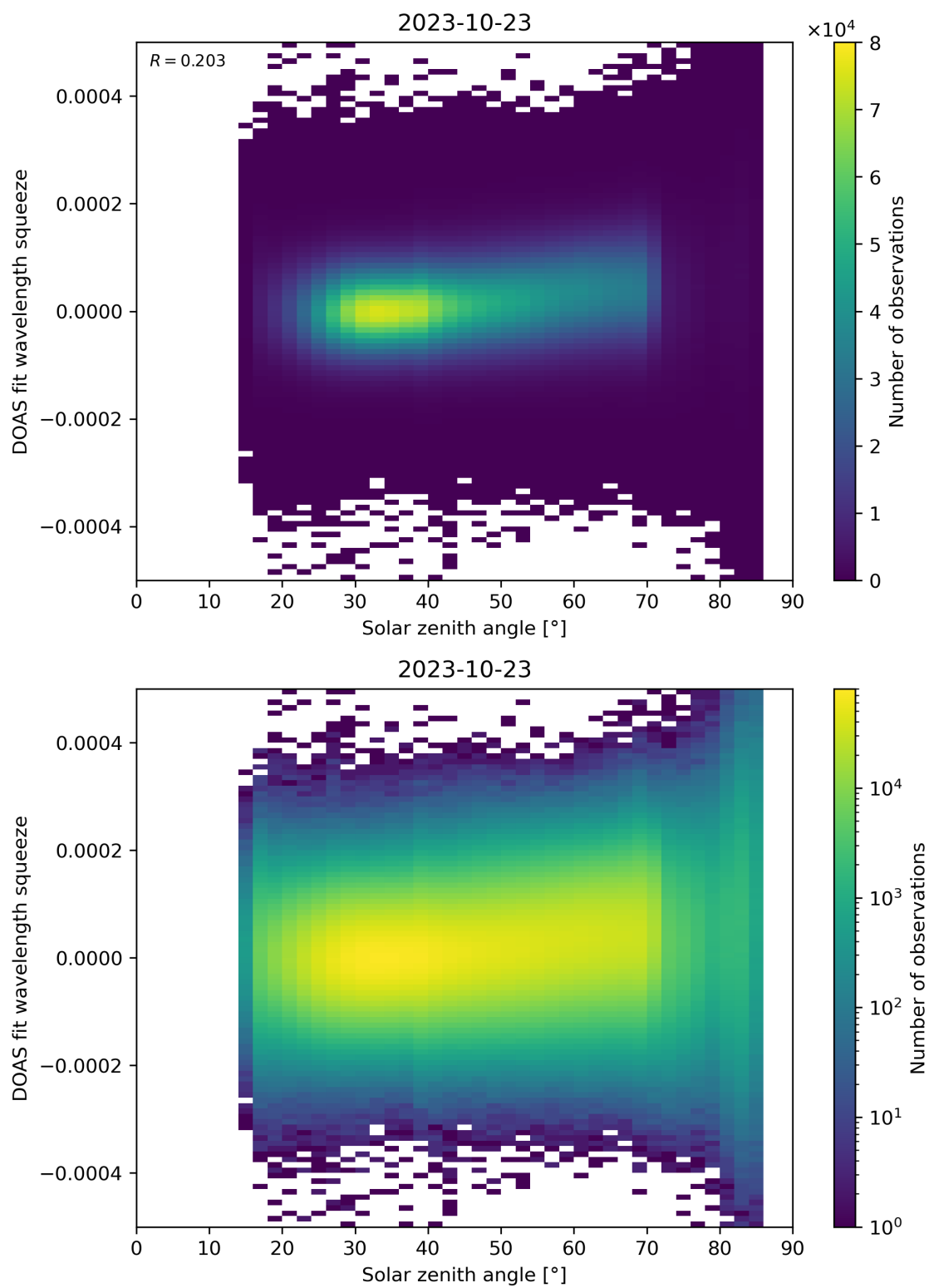
Figure 169: Scatter density plot of “Solar zenith angle” against “DOAS fit wavelength squeeze” for 2023-10-22 to 2023-10-24.
