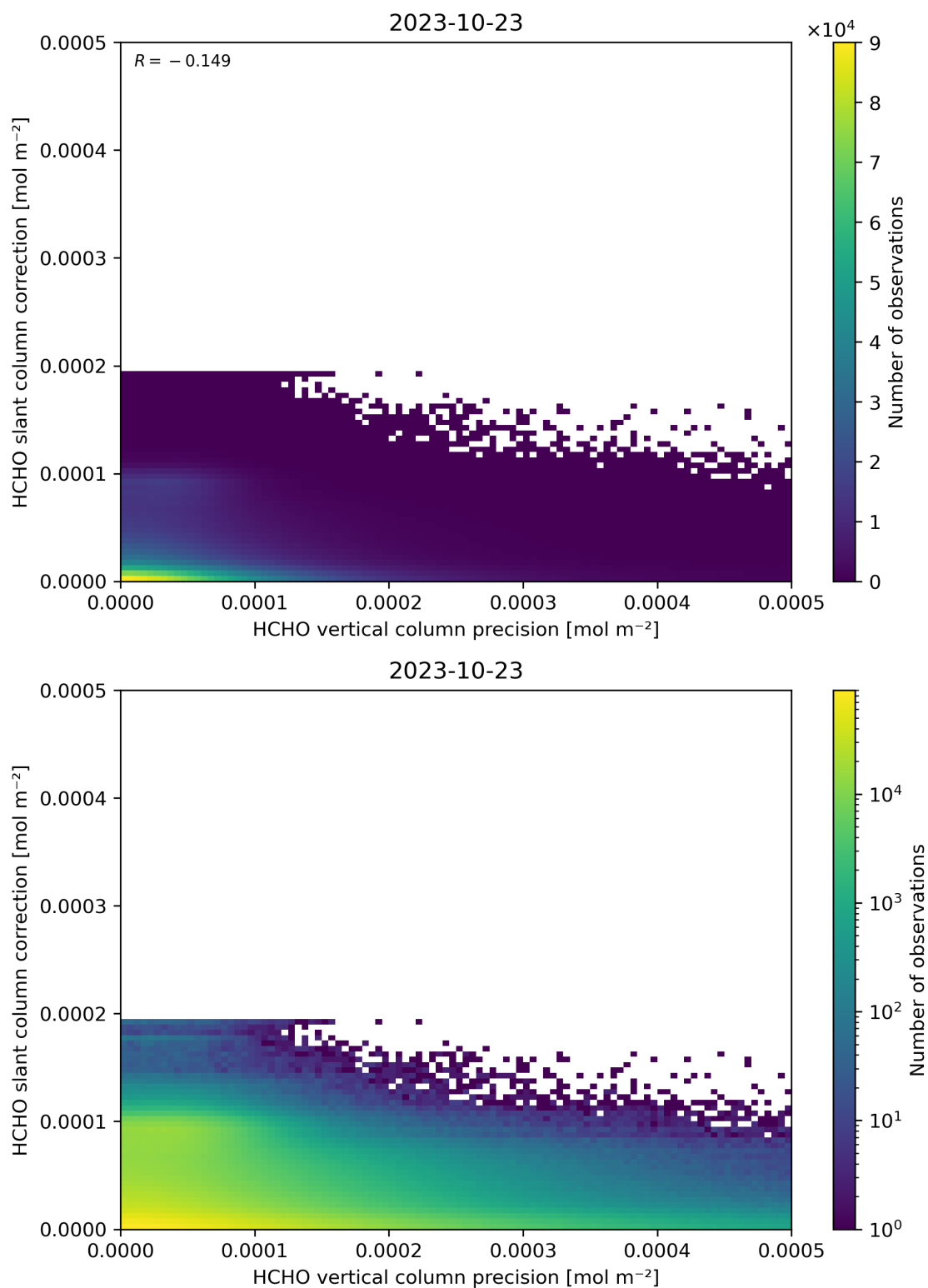
Figure 141: Scatter density plot of “HCHO vertical column precision” against “HCHO slant column correction” for 2023-10-22 to 2023-10-24.
