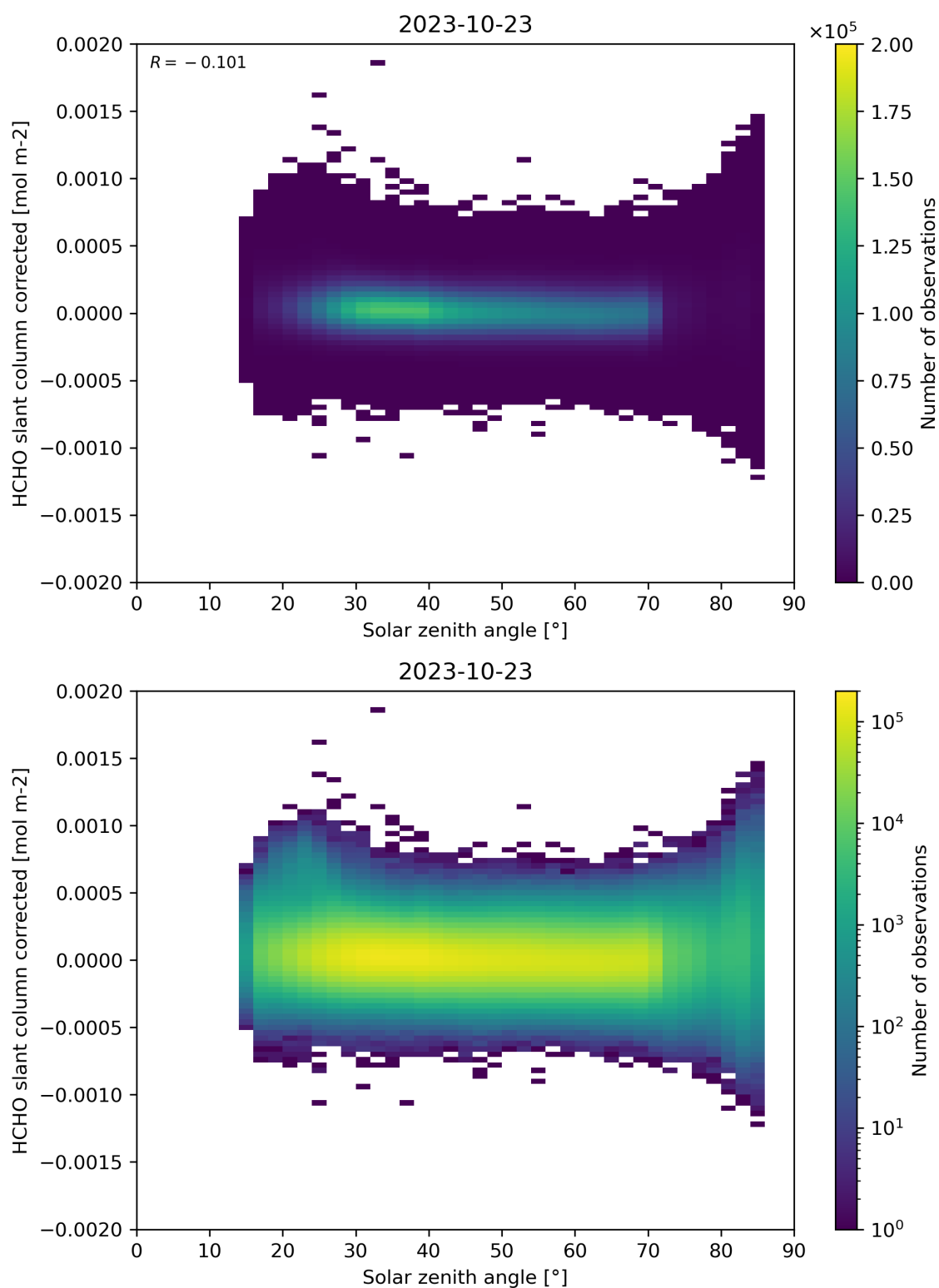
Figure 171: Scatter density plot of “Solar zenith angle” against “HCHO slant column corrected” for 2023-10-22 to 2023-10-24.
