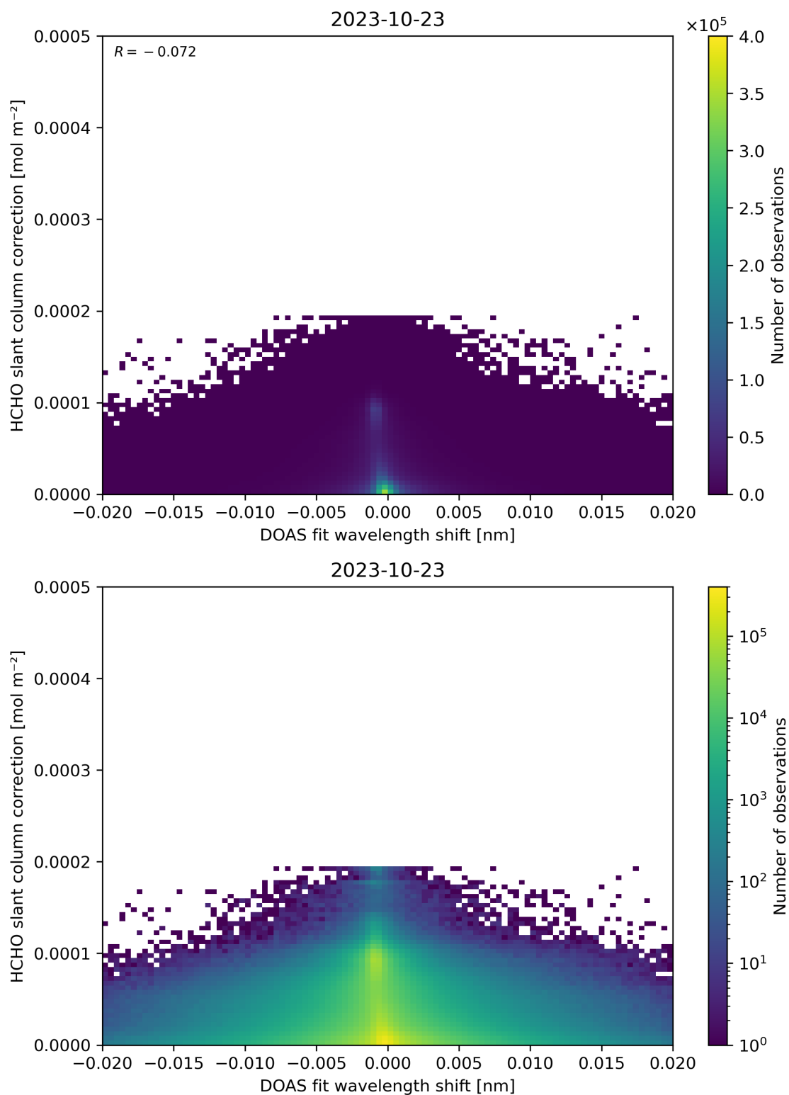
Figure 67: Scatter density plot of “DOAS fit wavelength shift” against “HCHO slant column correction” for 2023-10-22 to 2023-10-24.
