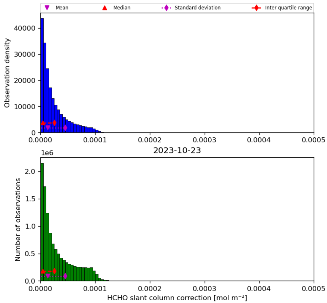
Figure 47: Histogram of “HCHO slant column correction” for 2023-10-22 to 2023-10-24
