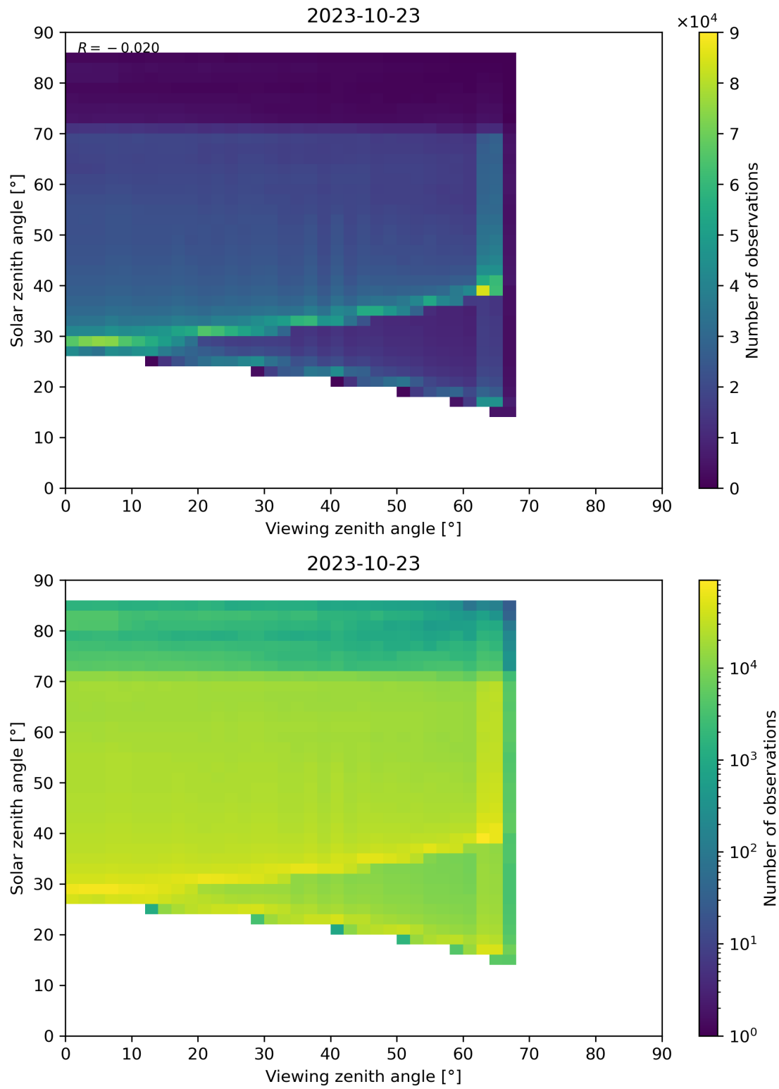
Figure 197: Scatter density plot of “Viewing zenith angle” against “Solar zenith angle” for 2023-10-22 to 2023-10-24.
