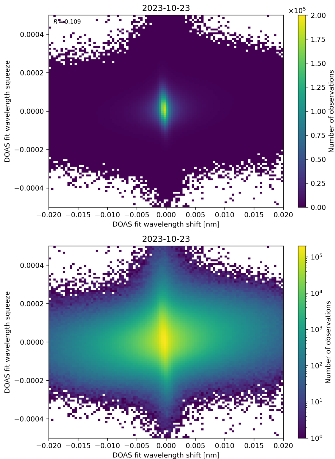
Figure 65: Scatter density plot of “DOAS fit wavelength shift” against “DOAS fit wavelength squeeze” for 2023-10-22 to 2023-10-24.
