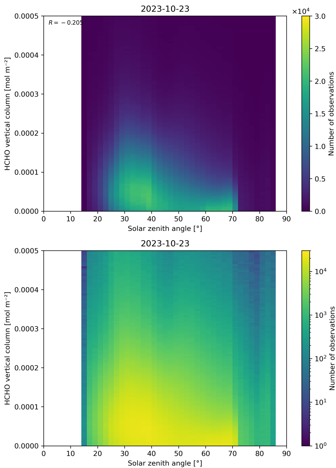
Figure 177: Scatter density plot of “Solar zenith angle” against “HCHO vertical column” for 2023-10-22 to 2023-10-24.
