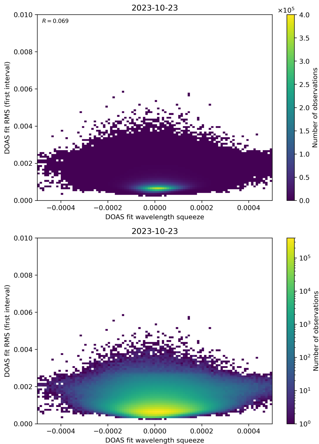
Figure 68: Scatter density plot of “DOAS fit wavelength squeeze” against “DOAS fit RMS (first interval)” for 2023-10-22 to 2023-10-24.
