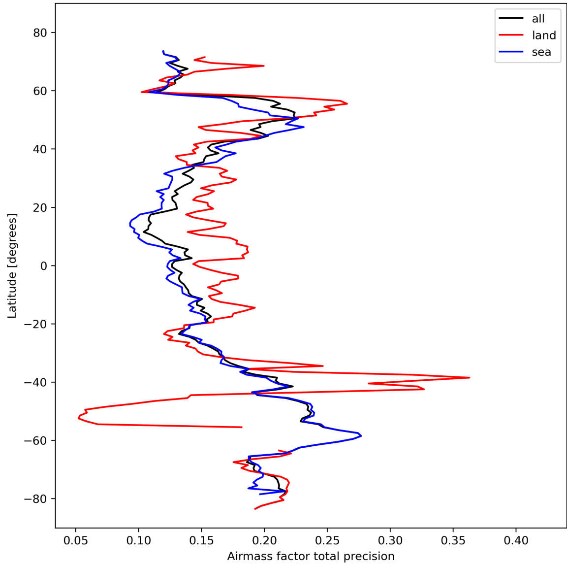
Figure 27: Zonal average of “Airmass factor total precision” for 2023-10-22 to 2023-10-24.
