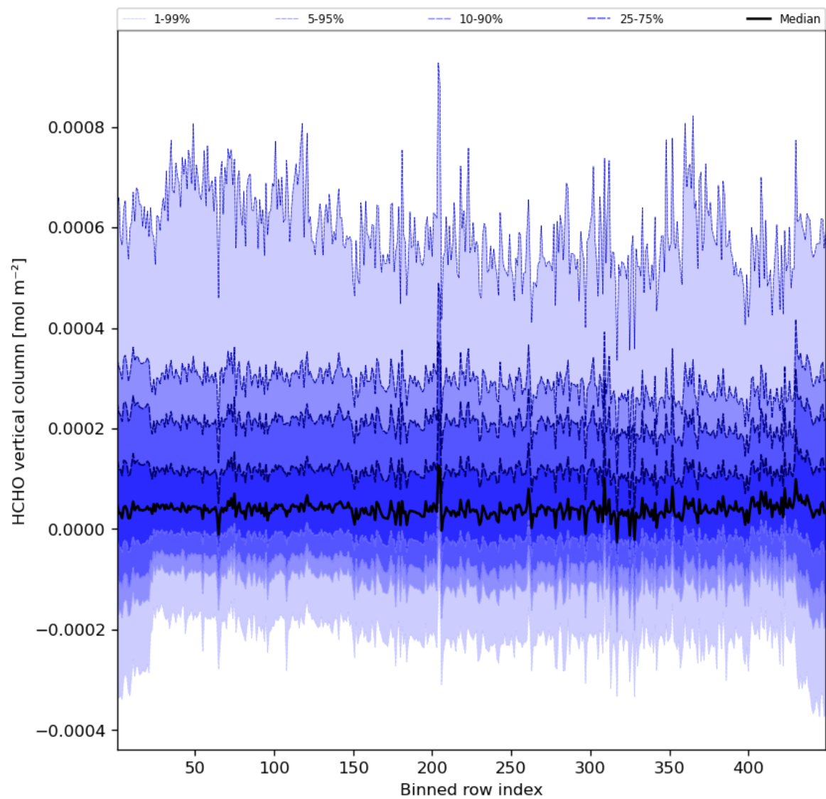
Figure 49: Along track statistics of “HCHO vertical column” for 2023-10-22 to 2023-10-24
