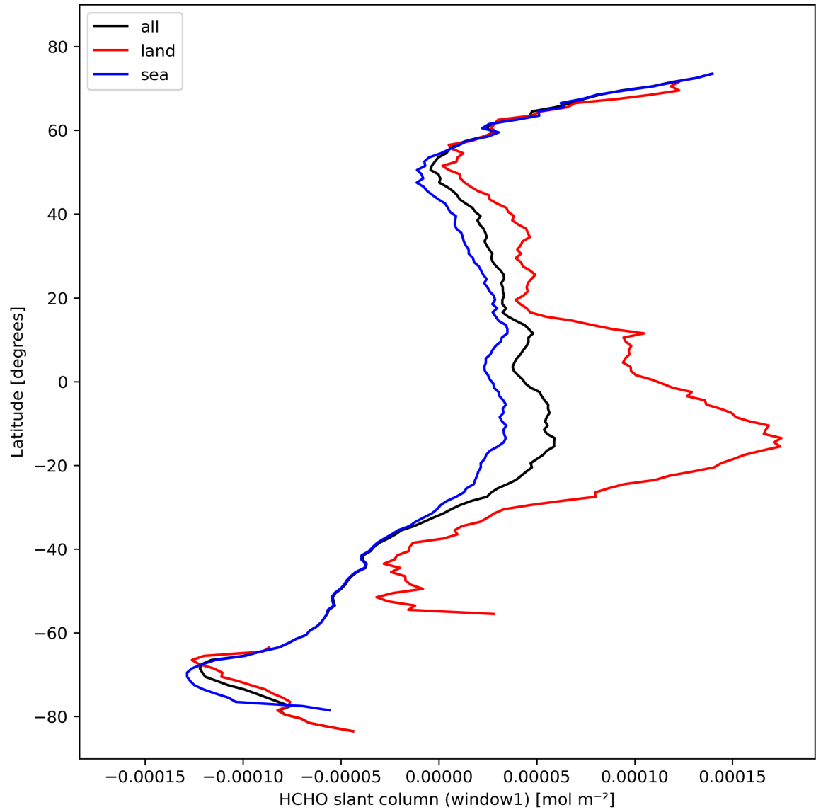
Figure 24: Zonal average of “HCHO slant column (window1)” for 2023-10-22 to 2023-10-24.
