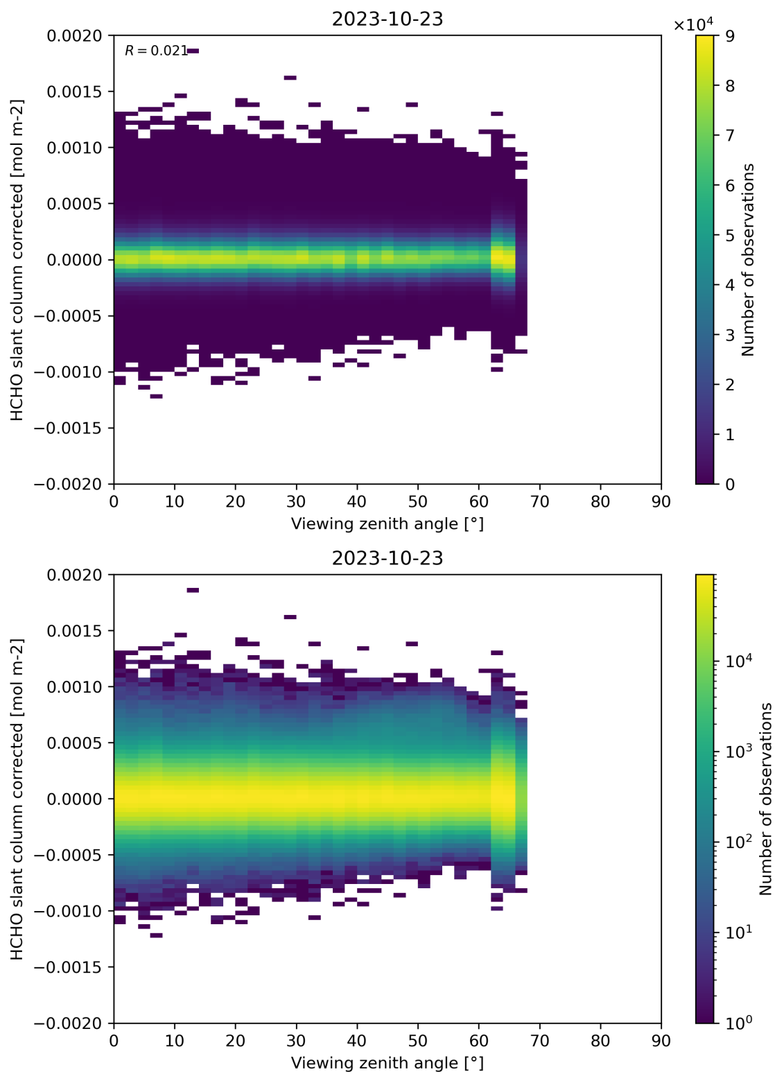
Figure 186: Scatter density plot of “Viewing zenith angle” against “HCHO slant column corrected” for 2023-10-22 to 2023-10-24.
