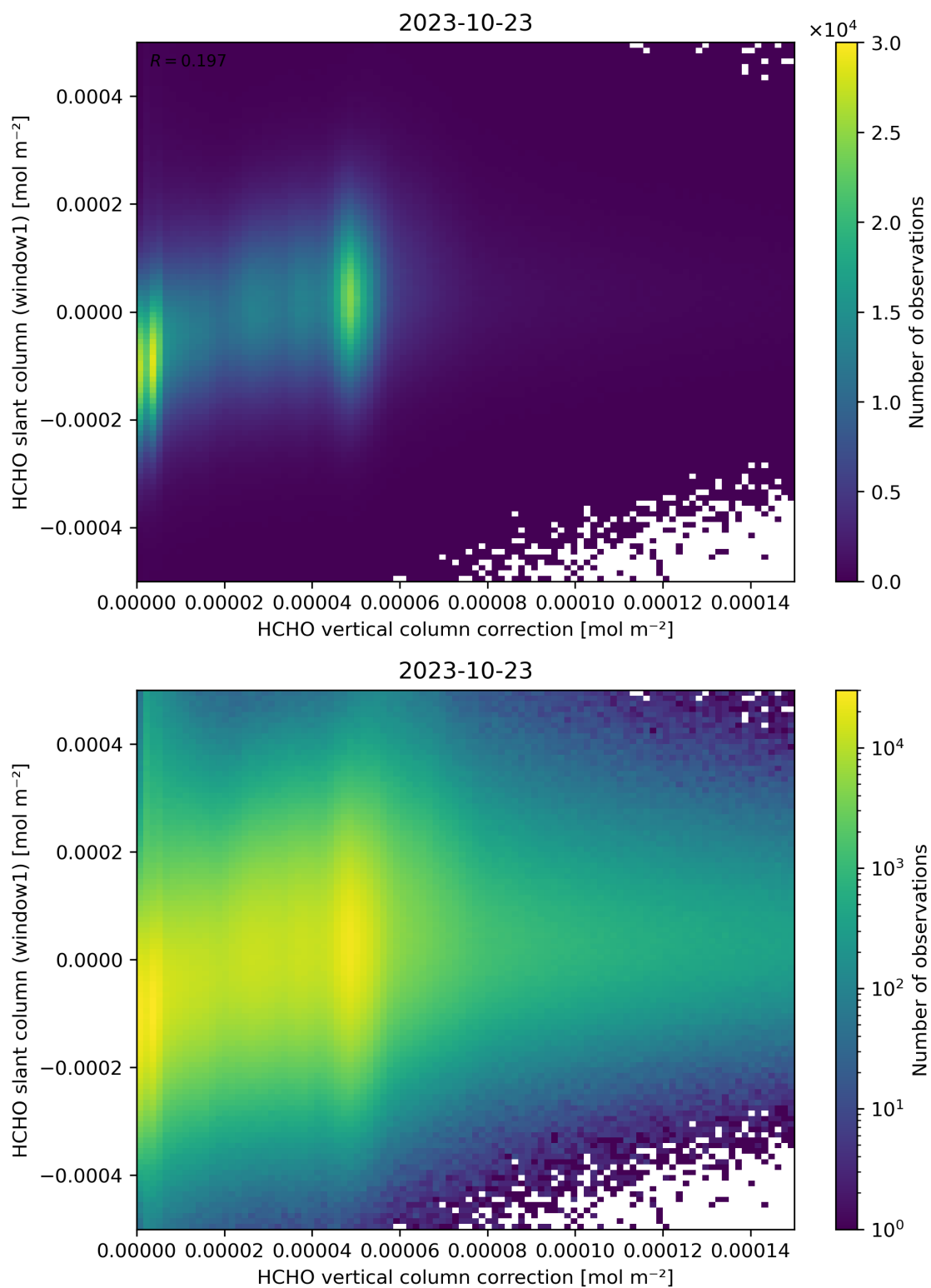
Figure 118: Scatter density plot of “HCHO vertical column correction” against “HCHO slant column (window1)” for 2023-10-22 to 2023-10-24.
