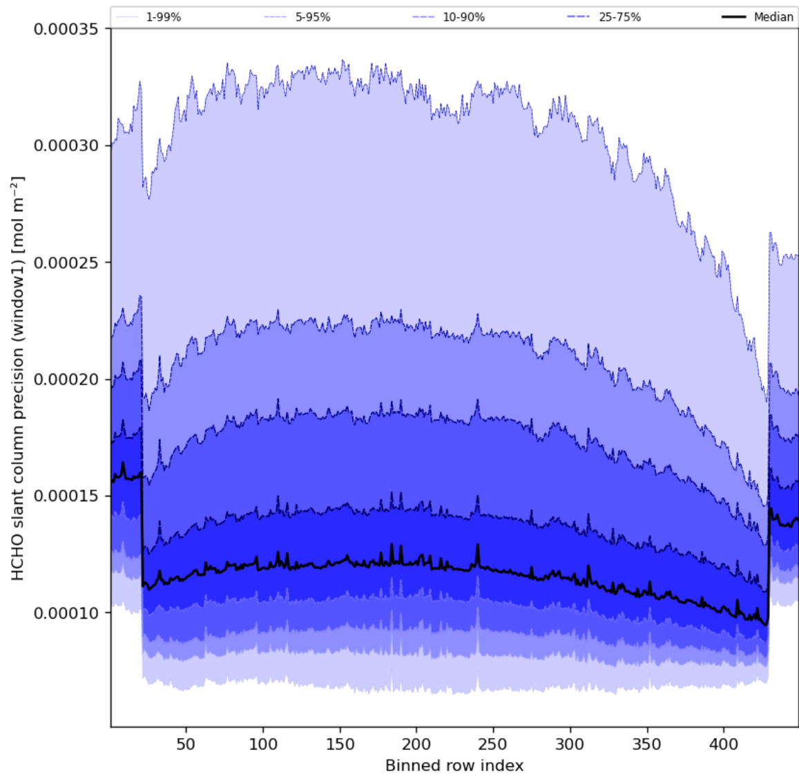
Figure 53: Along track statistics of “HCHO slant column precision (window1)” for 2023-10-23 to 2023-10-25
