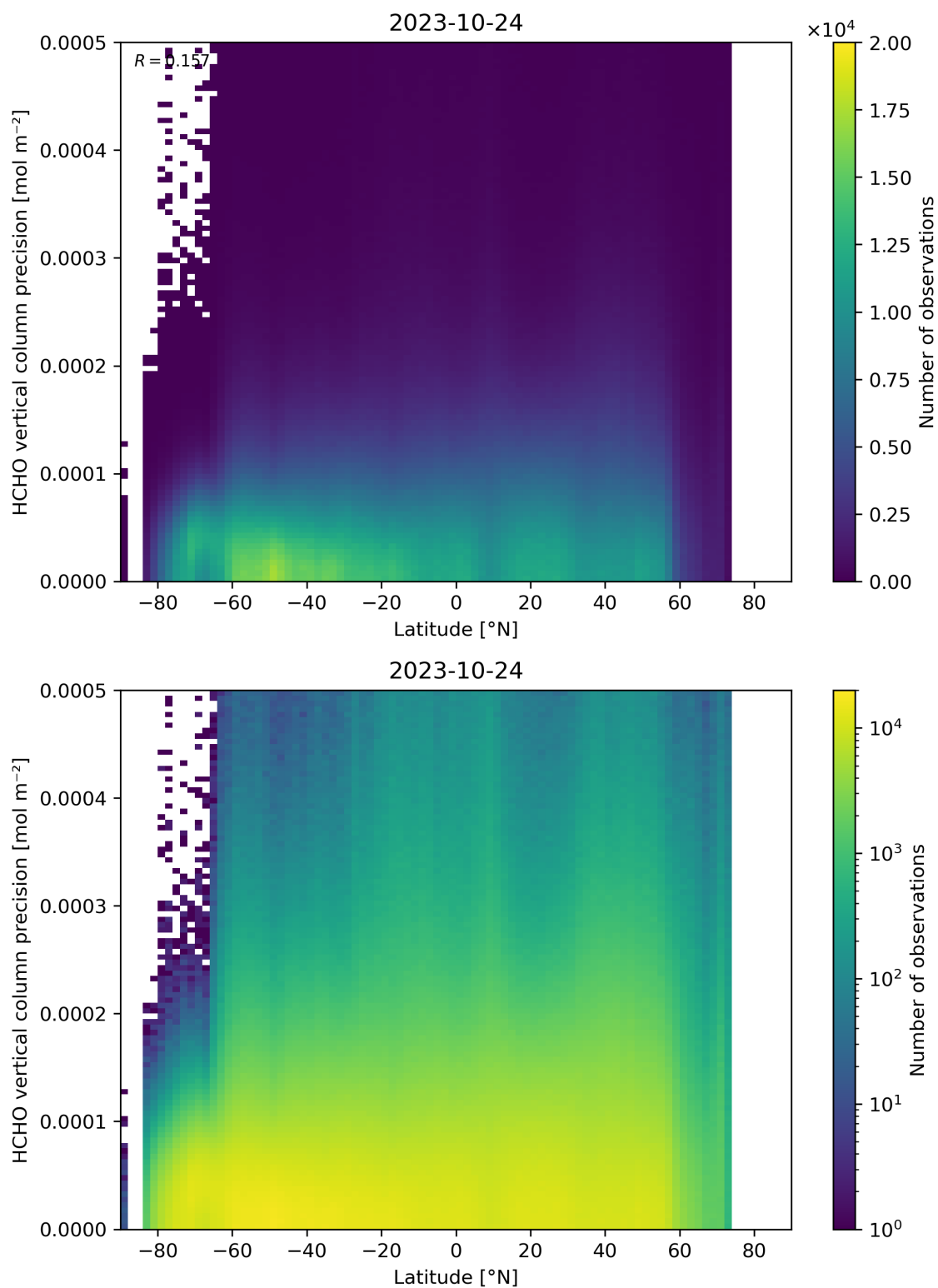
Figure 165: Scatter density plot of “Latitude” against “HCHO vertical column precision” for 2023-10-23 to 2023-10-25.
