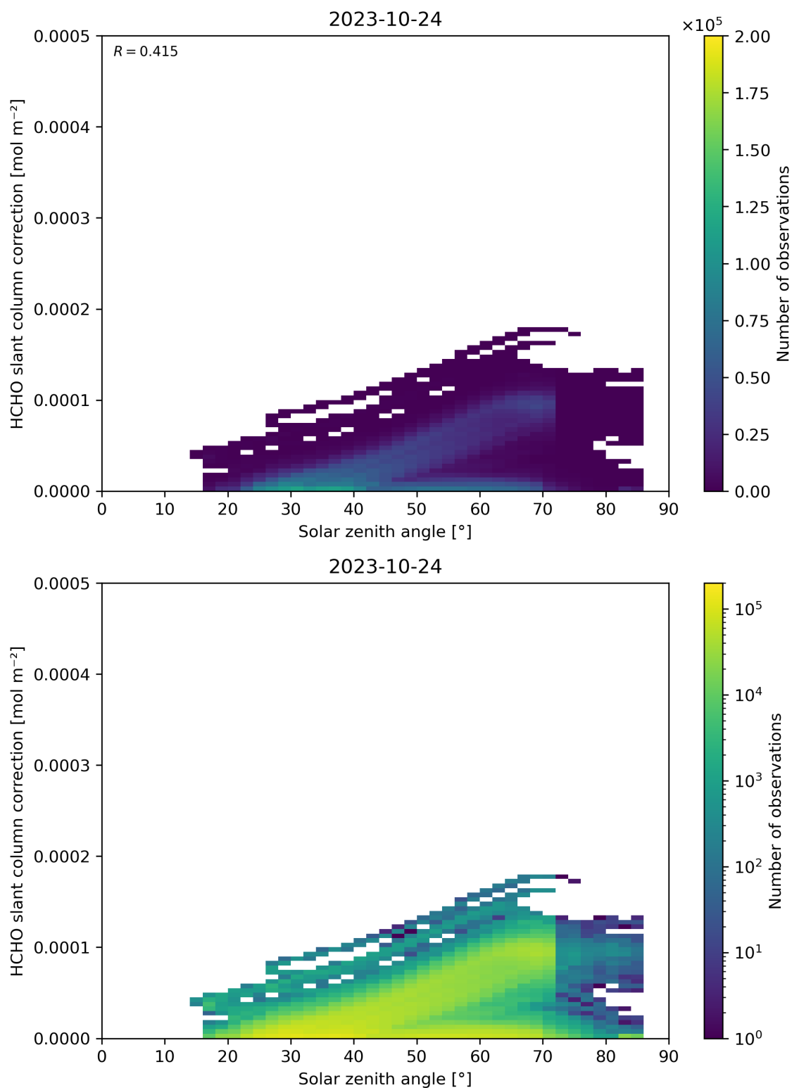
Figure 172: Scatter density plot of “Solar zenith angle” against “HCHO slant column correction” for 2023-10-23 to 2023-10-25.
