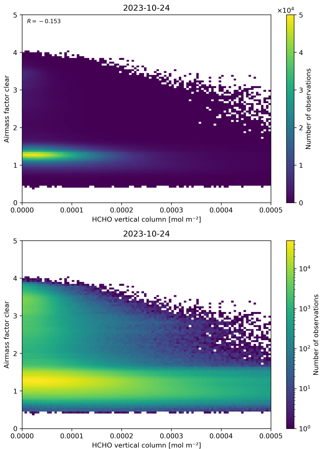
Figure 126: Scatter density plot of “HCHO vertical column” against “Airmass factor clear” for 2023-10-23 to 2023-10-25.
