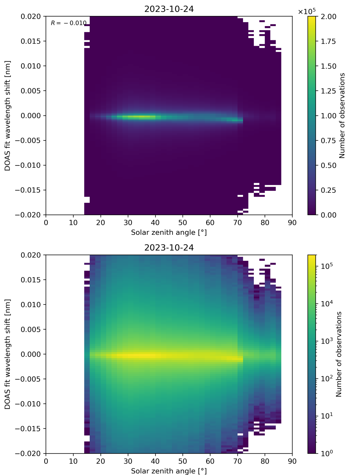
Figure 168: Scatter density plot of “Solar zenith angle” against “DOAS fit wavelength shift” for 2023-10-23 to 2023-10-25.
