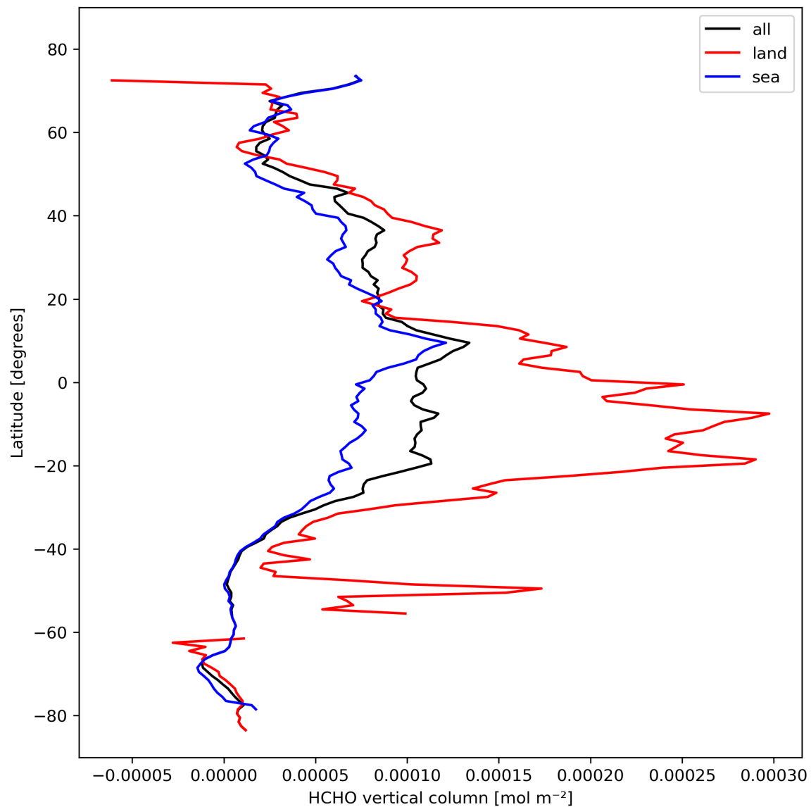
Figure 21: Zonal average of “HCHO vertical column” for 2023-10-23 to 2023-10-25.
