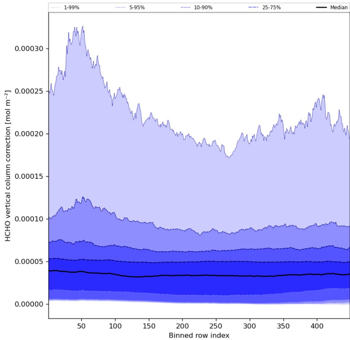
Figure 51: Along track statistics of “HCHO vertical column correction” for 2023-10-23 to 2023-10-25
