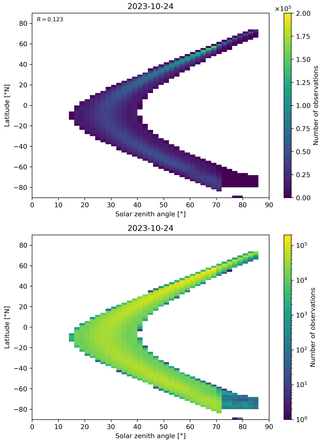
Figure 181: Scatter density plot of “Solar zenith angle” against “Latitude” for 2023-10-23 to 2023-10-25.
