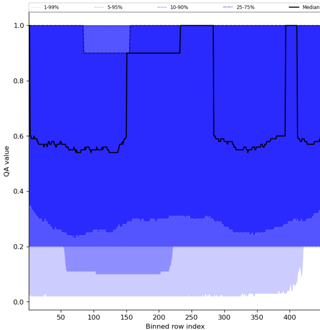
Figure 48: Along track statistics of “QA value” for 2023-10-23 to 2023-10-25
