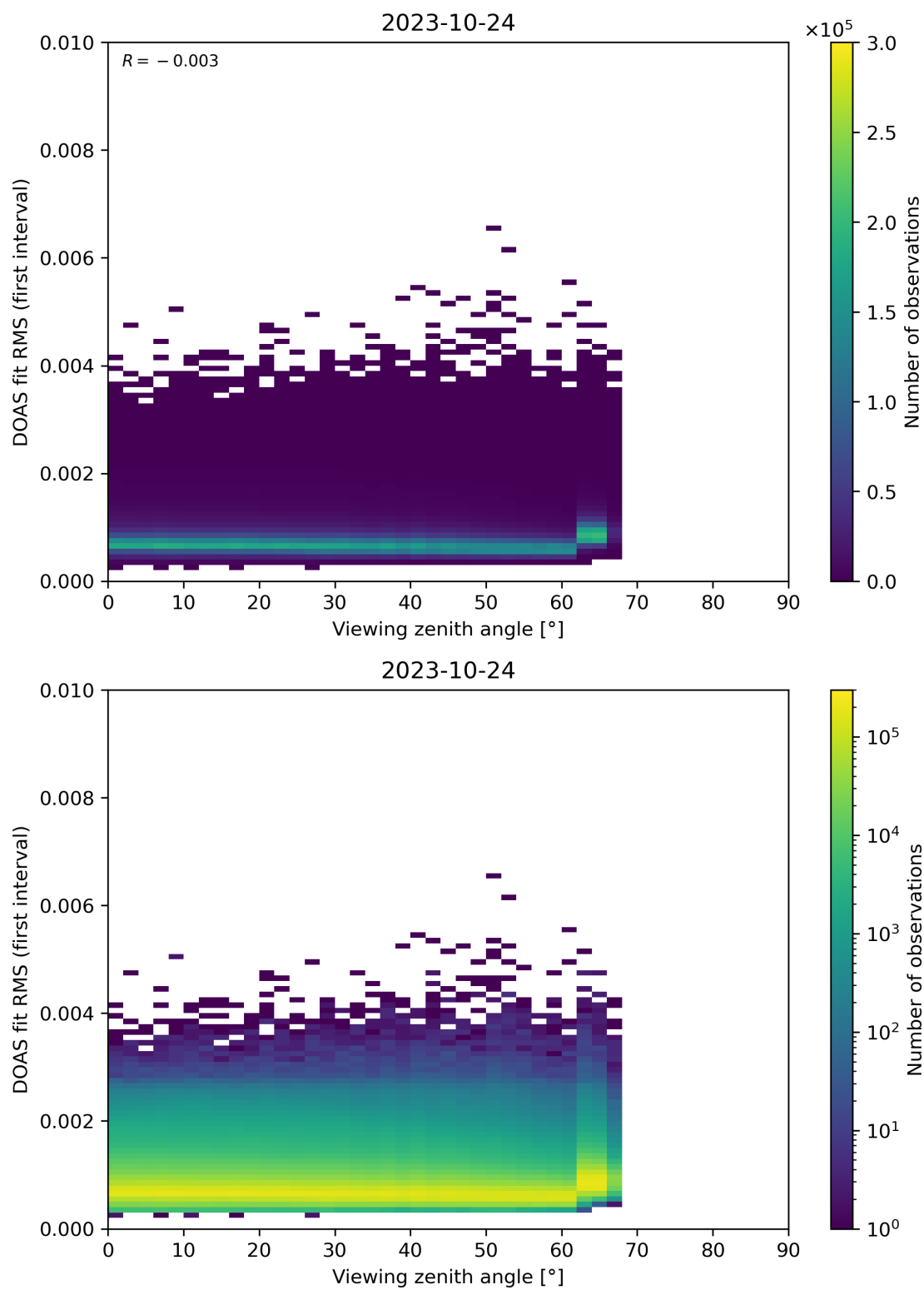
Figure 182: Scatter density plot of “Viewing zenith angle” against “DOAS fit RMS (first interval)” for 2023-10-23 to 2023-10-25.
