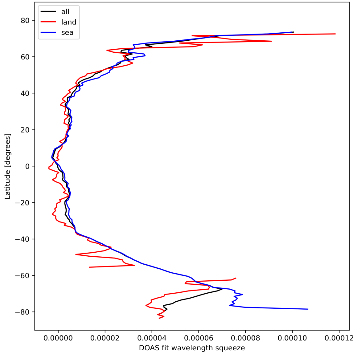
Figure 31: Zonal average of “DOAS fit wavelength squeeze” for 2023-10-23 to 2023-10-25.
