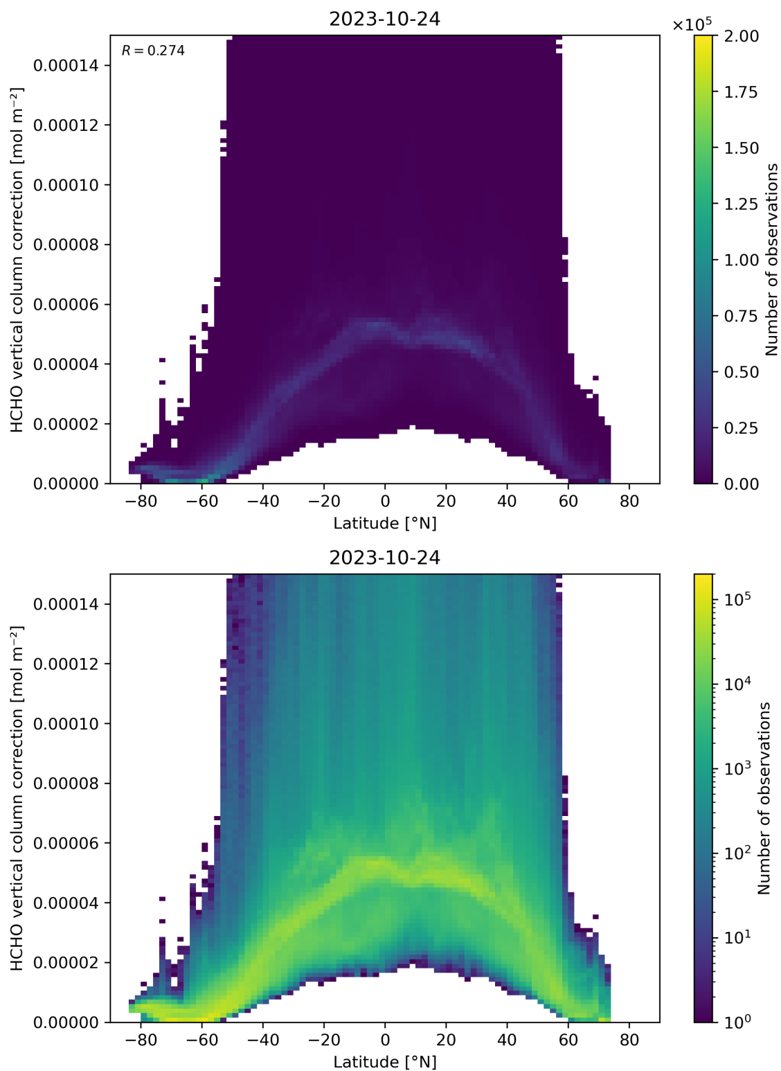
Figure 164: Scatter density plot of “Latitude” against “HCHO vertical column correction” for 2023-10-23 to 2023-10-25.
