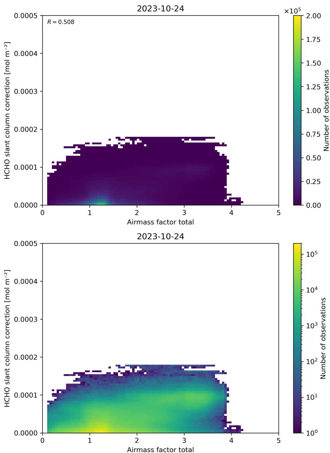
Figure 102: Scatter density plot of “Airmass factor total” against “HCHO slant column correction” for 2023-10-23 to 2023-10-25.
