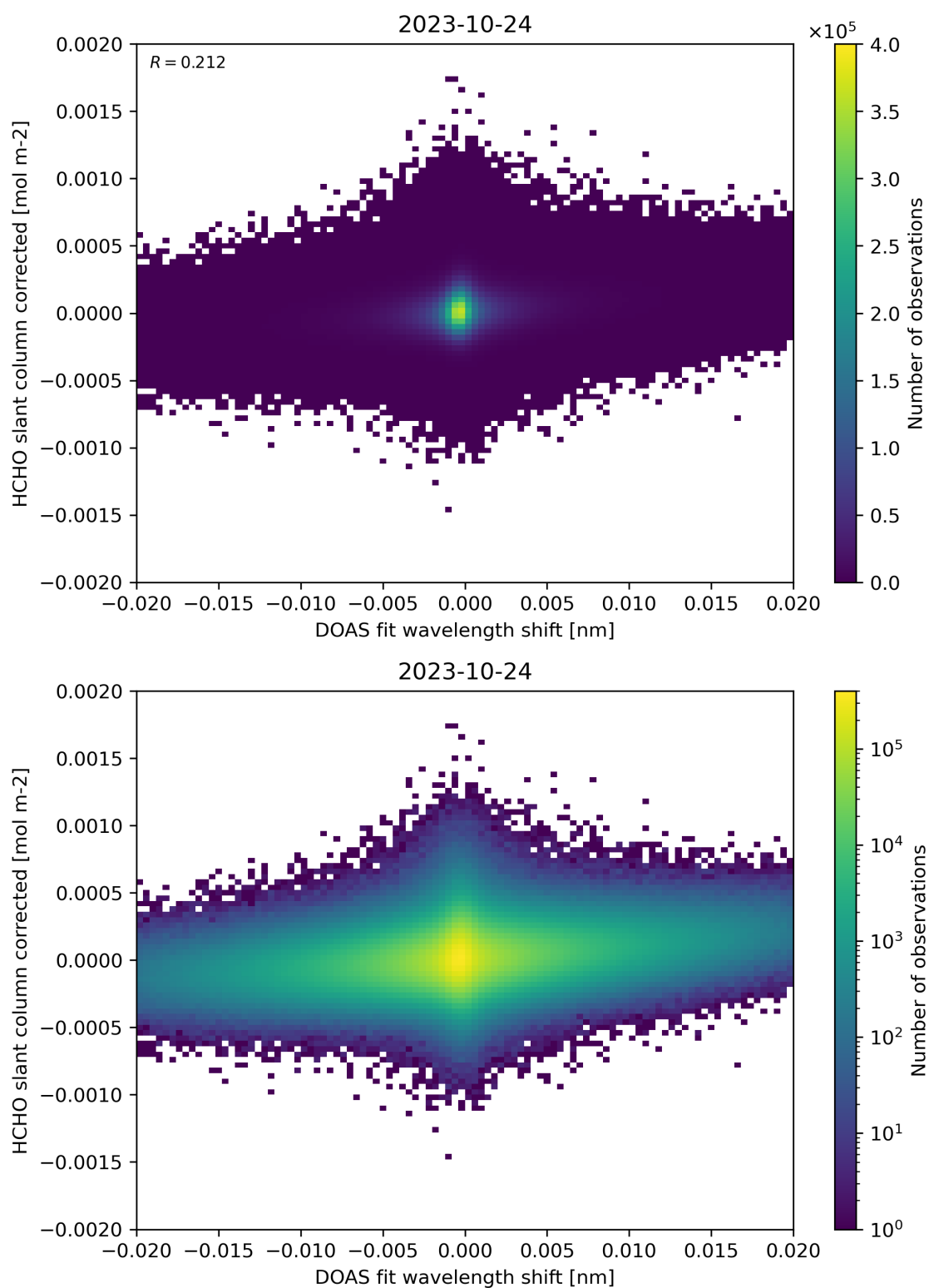
Figure 66: Scatter density plot of “DOAS fit wavelength shift” against “HCHO slant column corrected” for 2023-10-23 to 2023-10-25.
