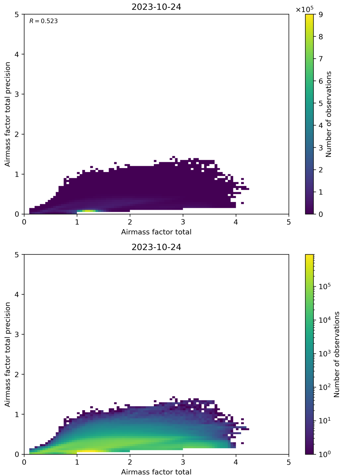
Figure 103: Scatter density plot of “Airmass factor total” against “Airmass factor total precision” for 2023-10-23 to 2023-10-25.
