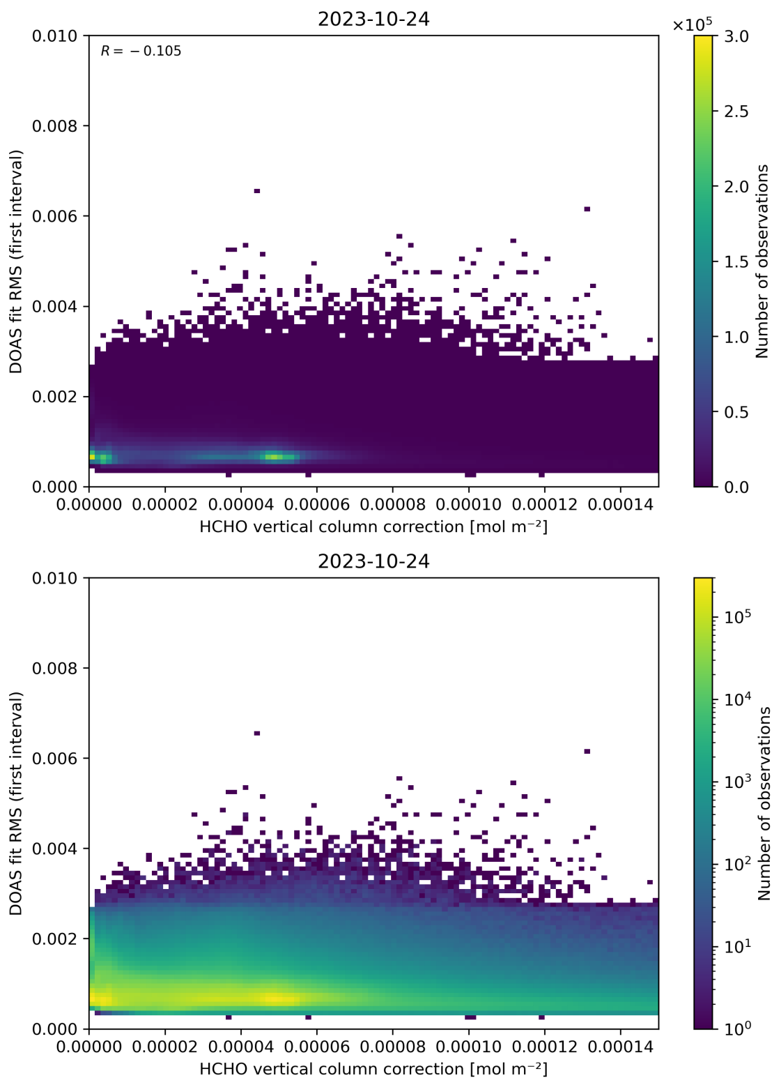
Figure 112: Scatter density plot of “HCHO vertical column correction” against “DOAS fit RMS (first interval)” for 2023-10-23 to 2023-10-25.
