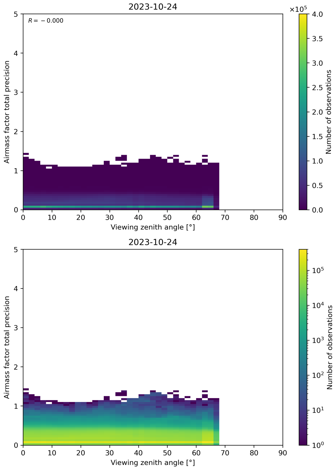
Figure 191: Scatter density plot of “Viewing zenith angle” against “Airmass factor total precision” for 2023-10-23 to 2023-10-25.
