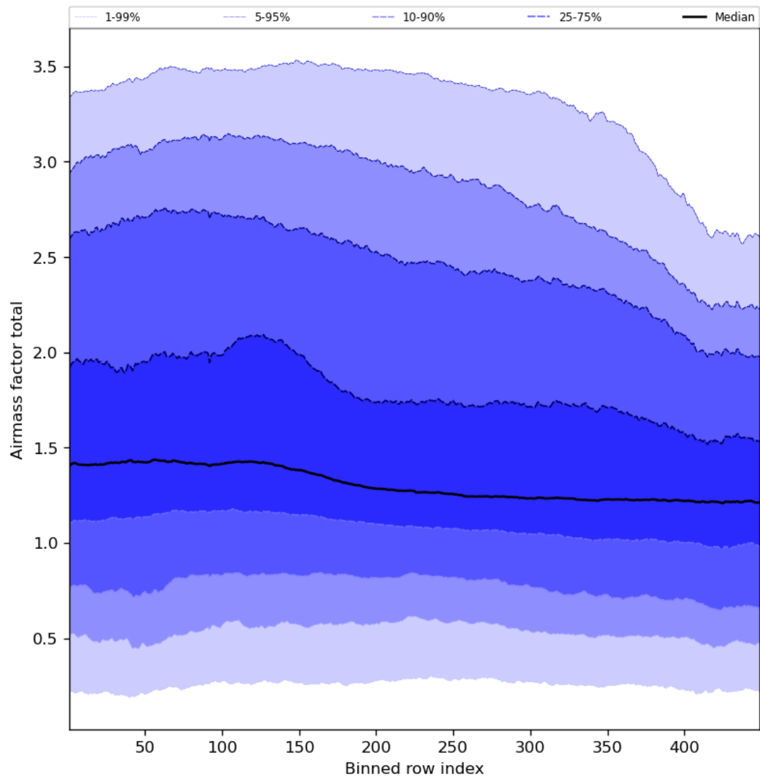
Figure 54: Along track statistics of “Airmass factor total” for 2023-10-23 to 2023-10-25
