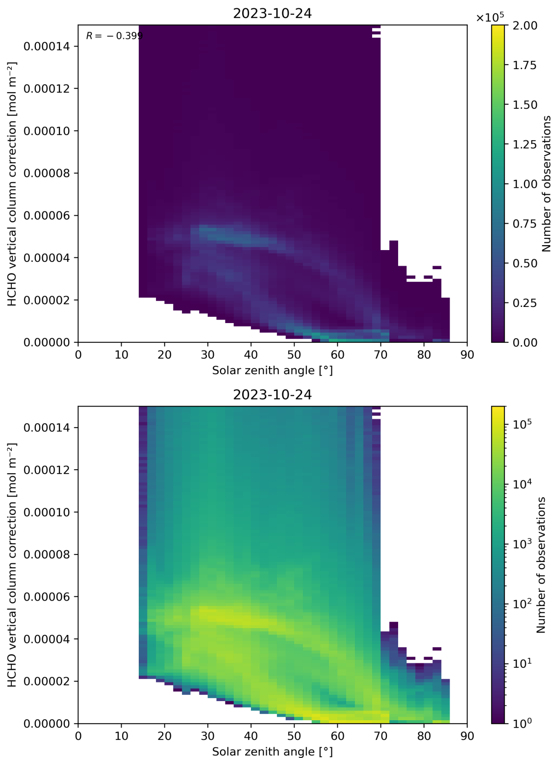
Figure 178: Scatter density plot of “Solar zenith angle” against “HCHO vertical column correction” for 2023-10-23 to 2023-10-25.
