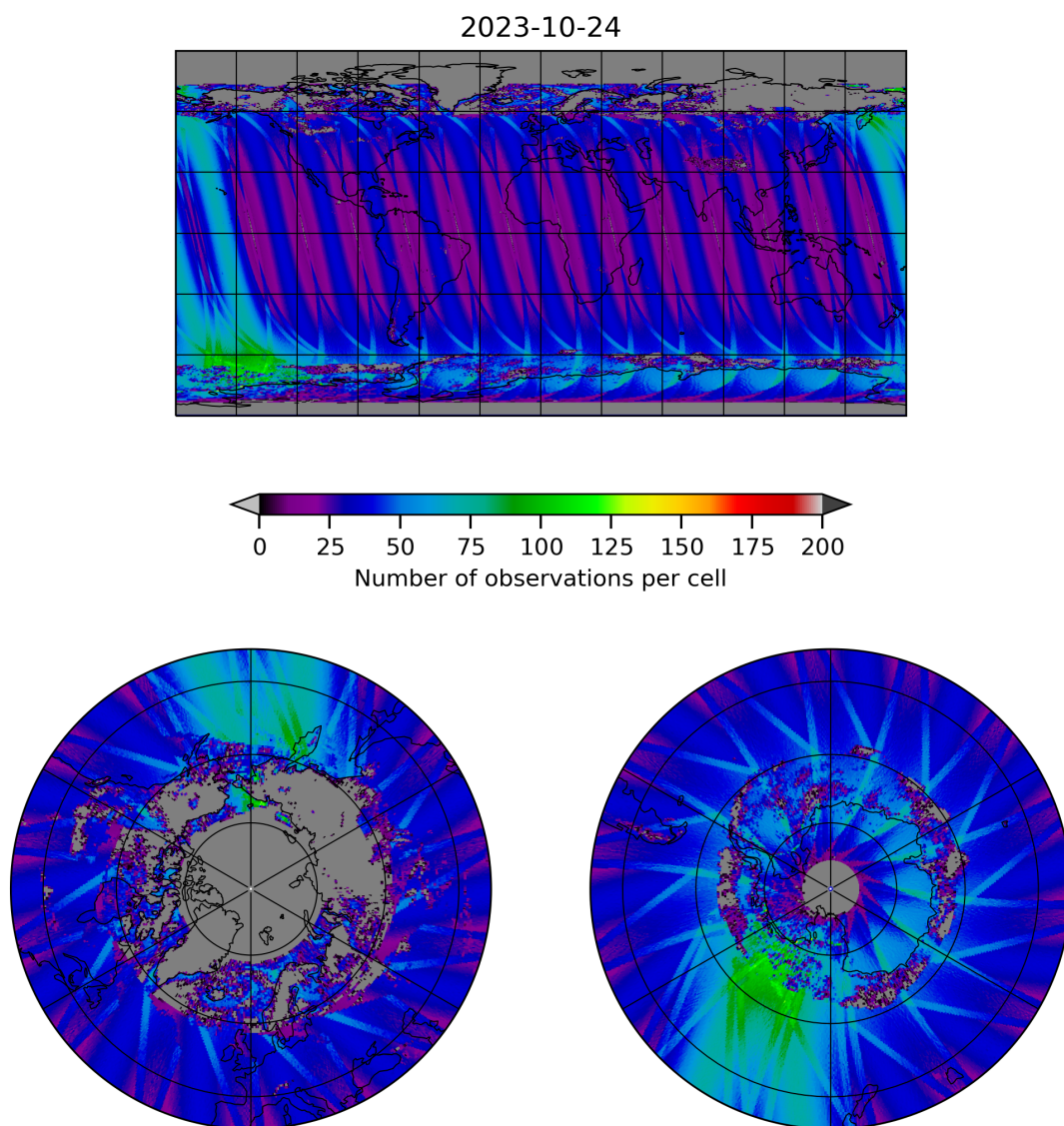
Figure 19: Map of the number of observations for 2023-10-23 to 2023-10-25
