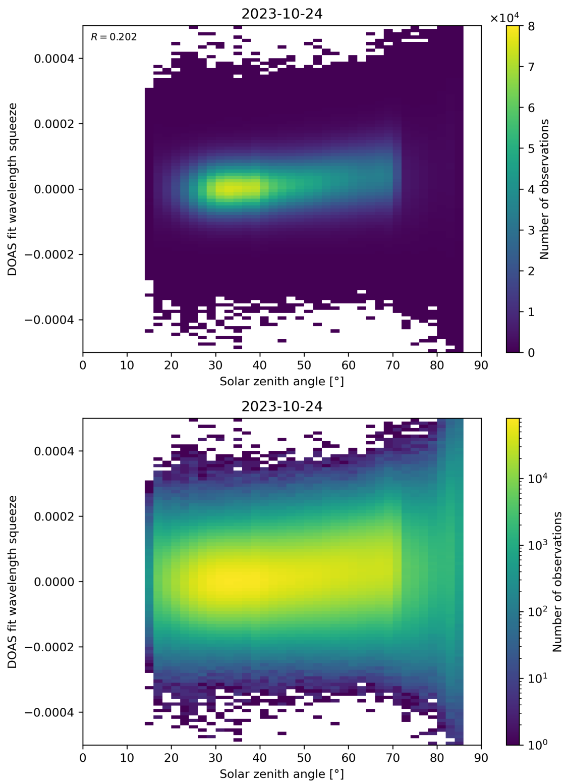
Figure 169: Scatter density plot of “Solar zenith angle” against “DOAS fit wavelength squeeze” for 2023-10-23 to 2023-10-25.
