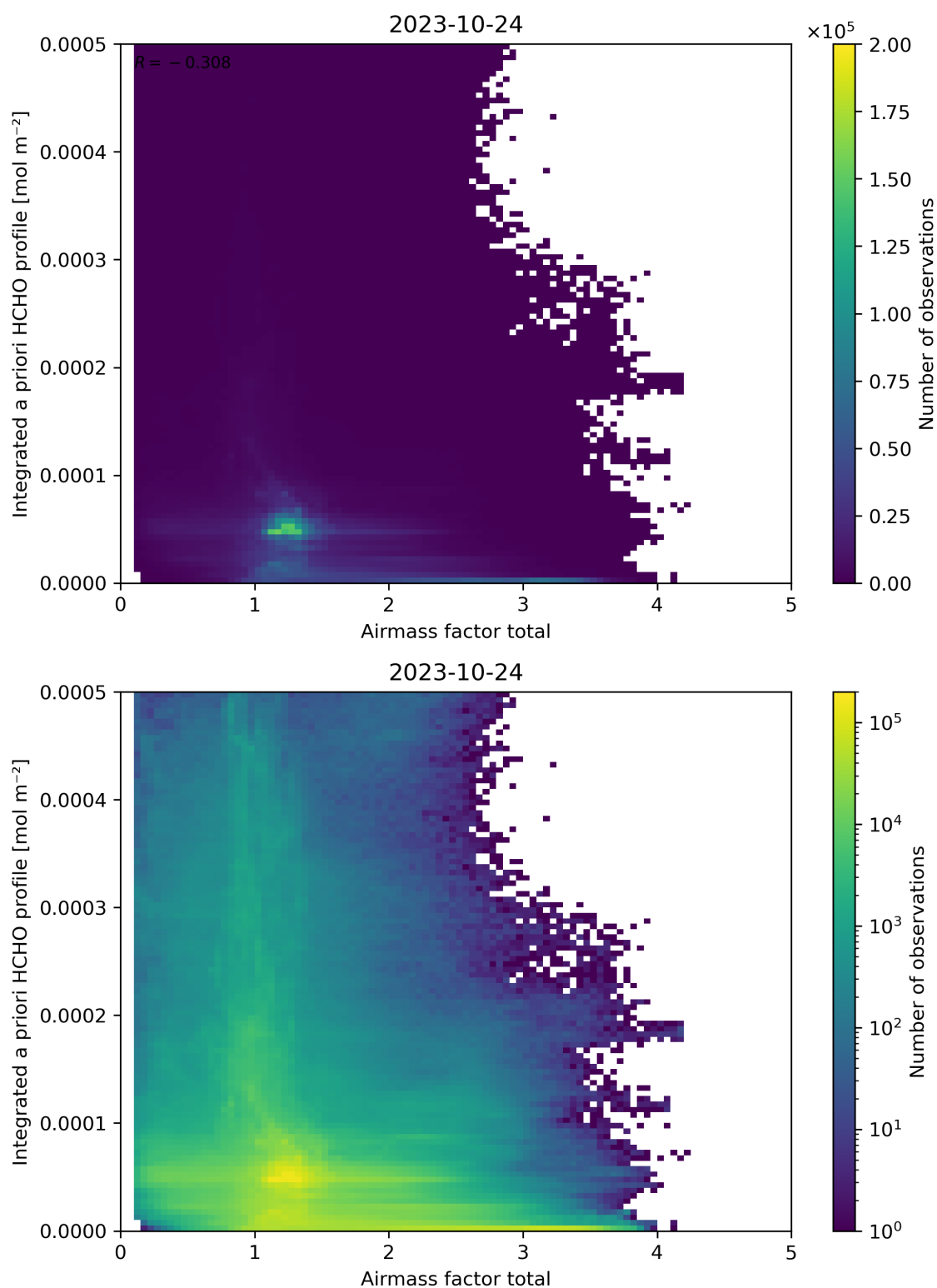
Figure 104: Scatter density plot of “Airmass factor total” against “Integrated a priori HCHO profile” for 2023-10-23 to 2023-10-25.
