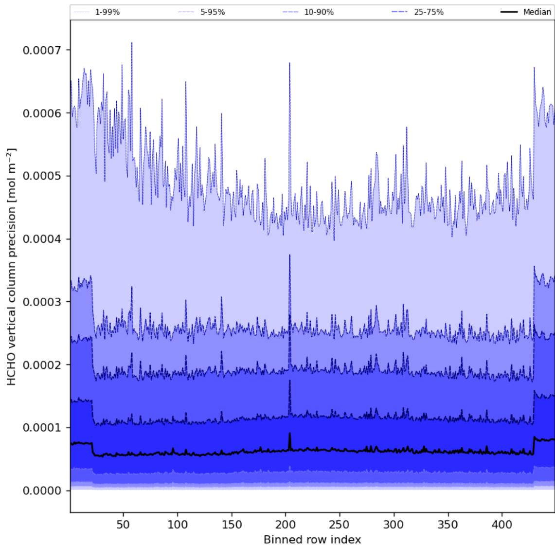
Figure 50: Along track statistics of “HCHO vertical column precision” for 2023-10-23 to 2023-10-25
