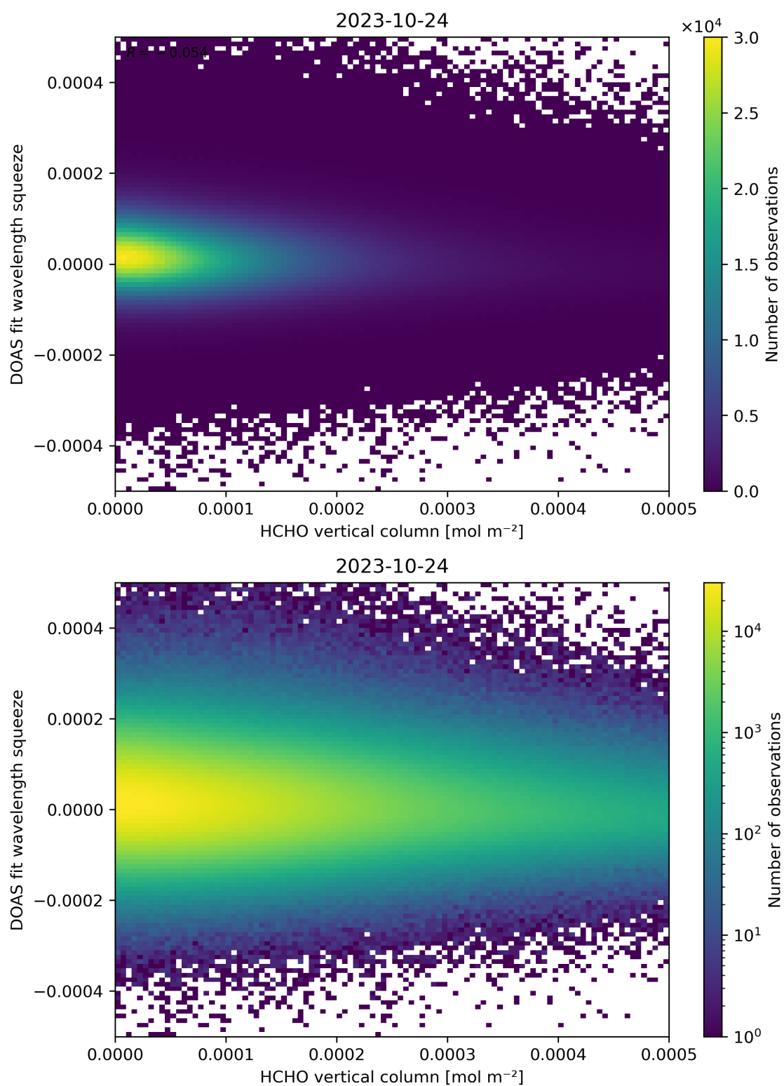
Figure 125: Scatter density plot of “HCHO vertical column” against “DOAS fit wavelength squeeze” for 2023-10-23 to 2023-10-25.
