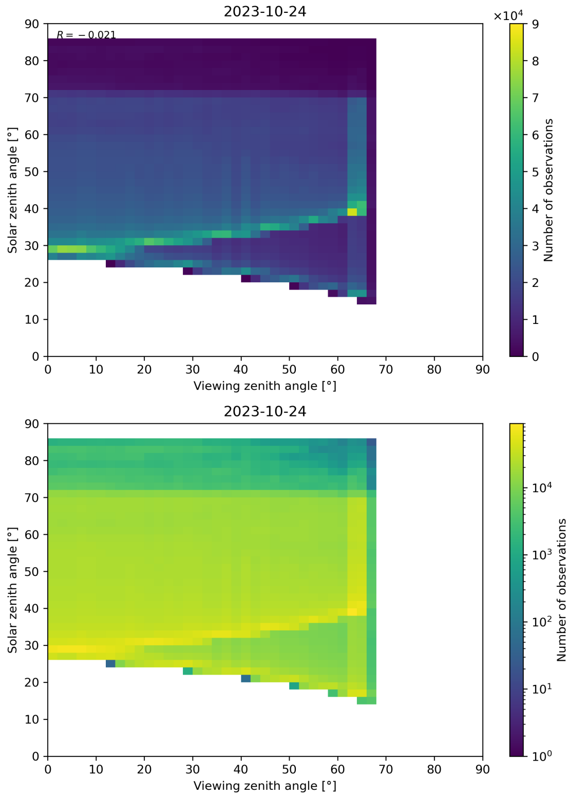
Figure 197: Scatter density plot of “Viewing zenith angle” against “Solar zenith angle” for 2023-10-23 to 2023-10-25.
