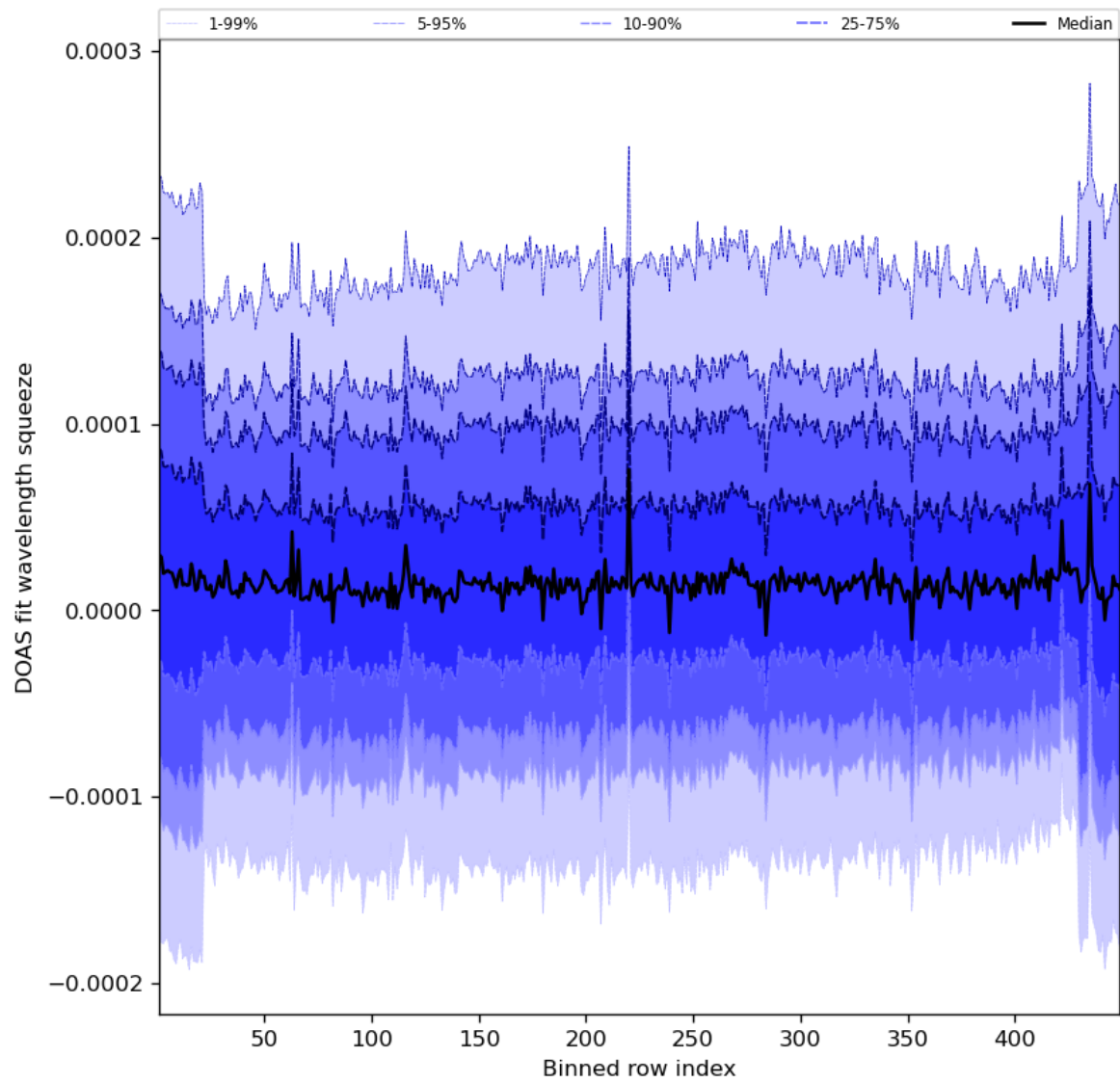
Figure 59: Along track statistics of “DOAS fit wavelength squeeze” for 2023-10-23 to 2023-10-25
