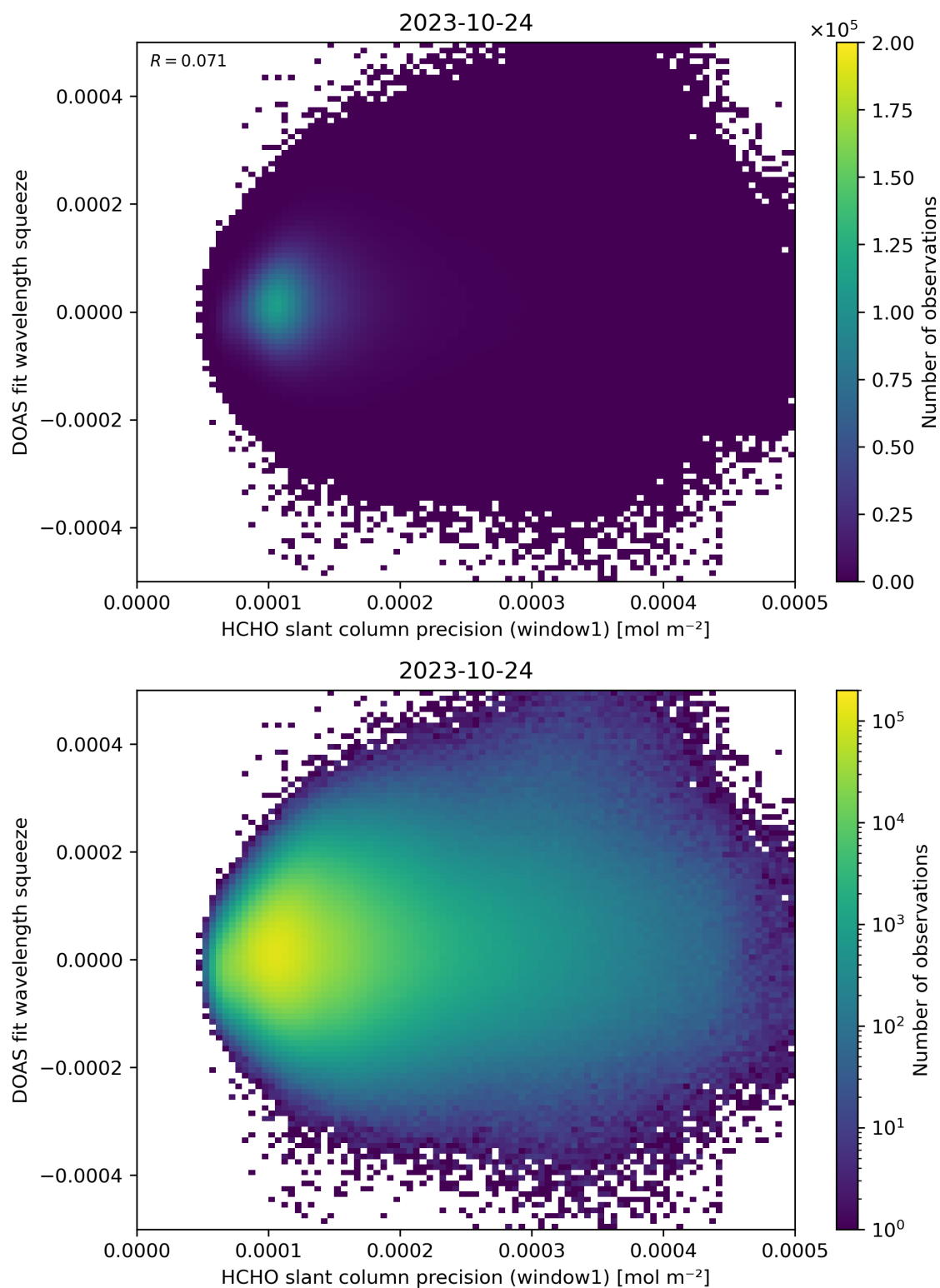
Figure 90: Scatter density plot of “HCHO slant column precision (window1)” against “DOAS fit wavelength squeeze” for 2023-10-23 to 2023-10-25.
