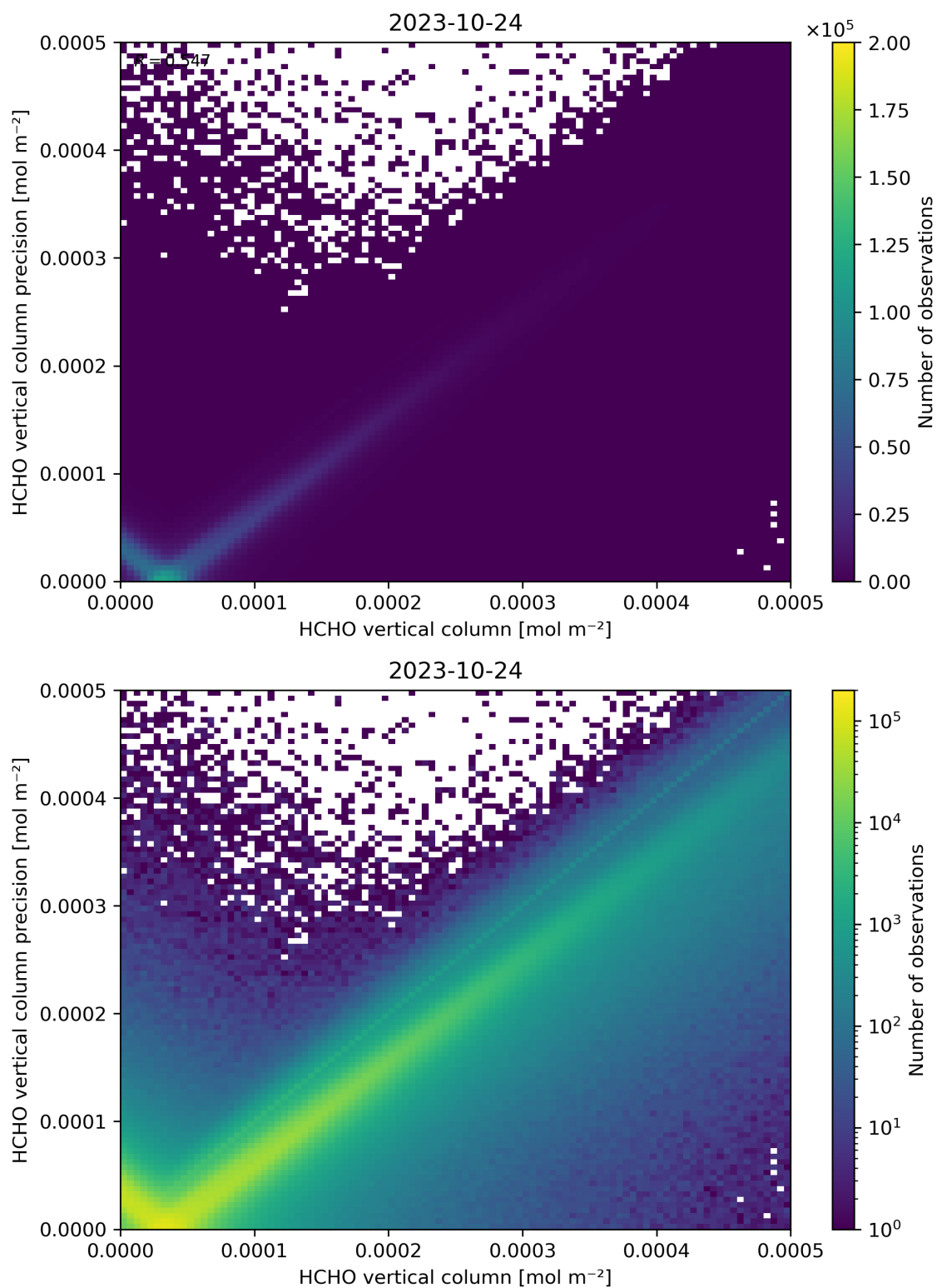
Figure 134: Scatter density plot of “HCHO vertical column” against “HCHO vertical column precision” for 2023-10-23 to 2023-10-25.
