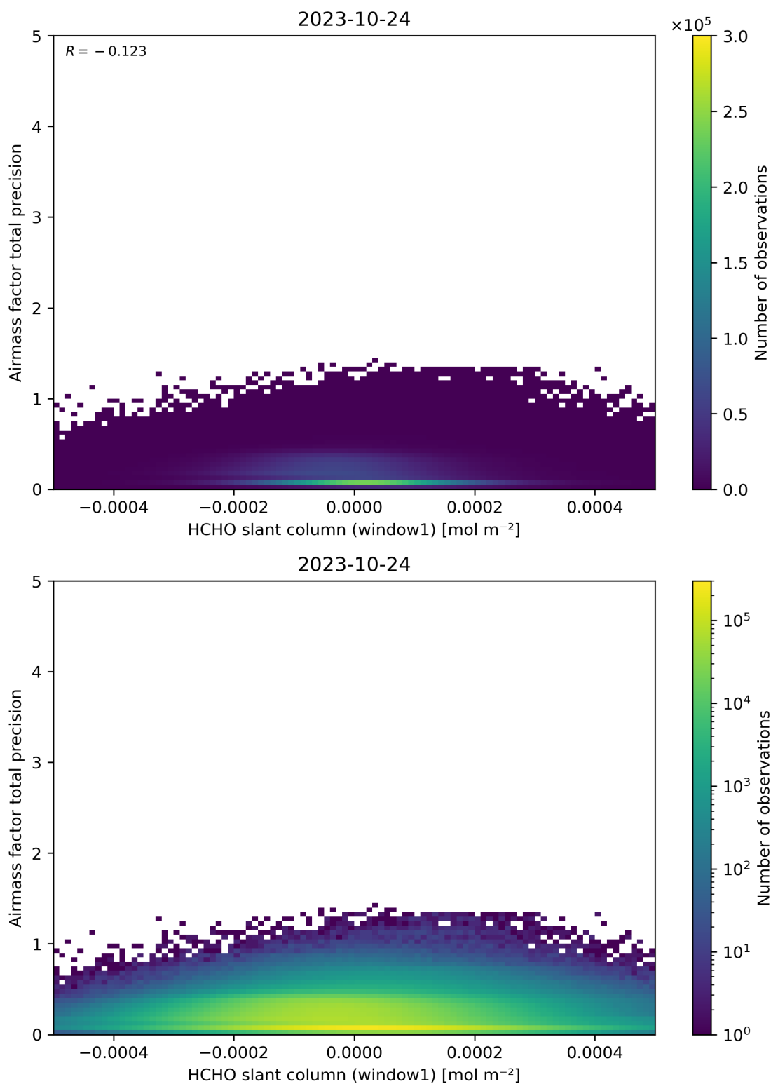
Figure 86: Scatter density plot of “HCHO slant column (window1)” against “Airmass factor total precision” for 2023-10-23 to 2023-10-25.
