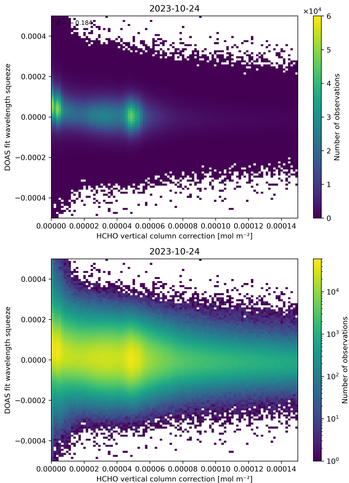
Figure 114: Scatter density plot of “HCHO vertical column correction” against “DOAS fit wavelength squeeze” for 2023-10-23 to 2023-10-25.
