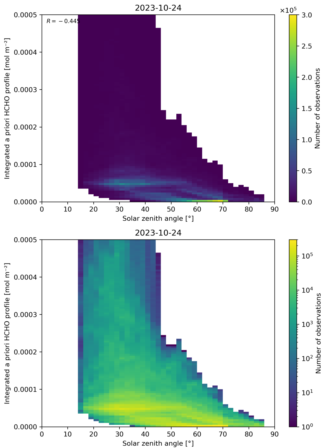
Figure 180: Scatter density plot of “Solar zenith angle” against “Integrated a priori HCHO profile” for 2023-10-23 to 2023-10-25.
