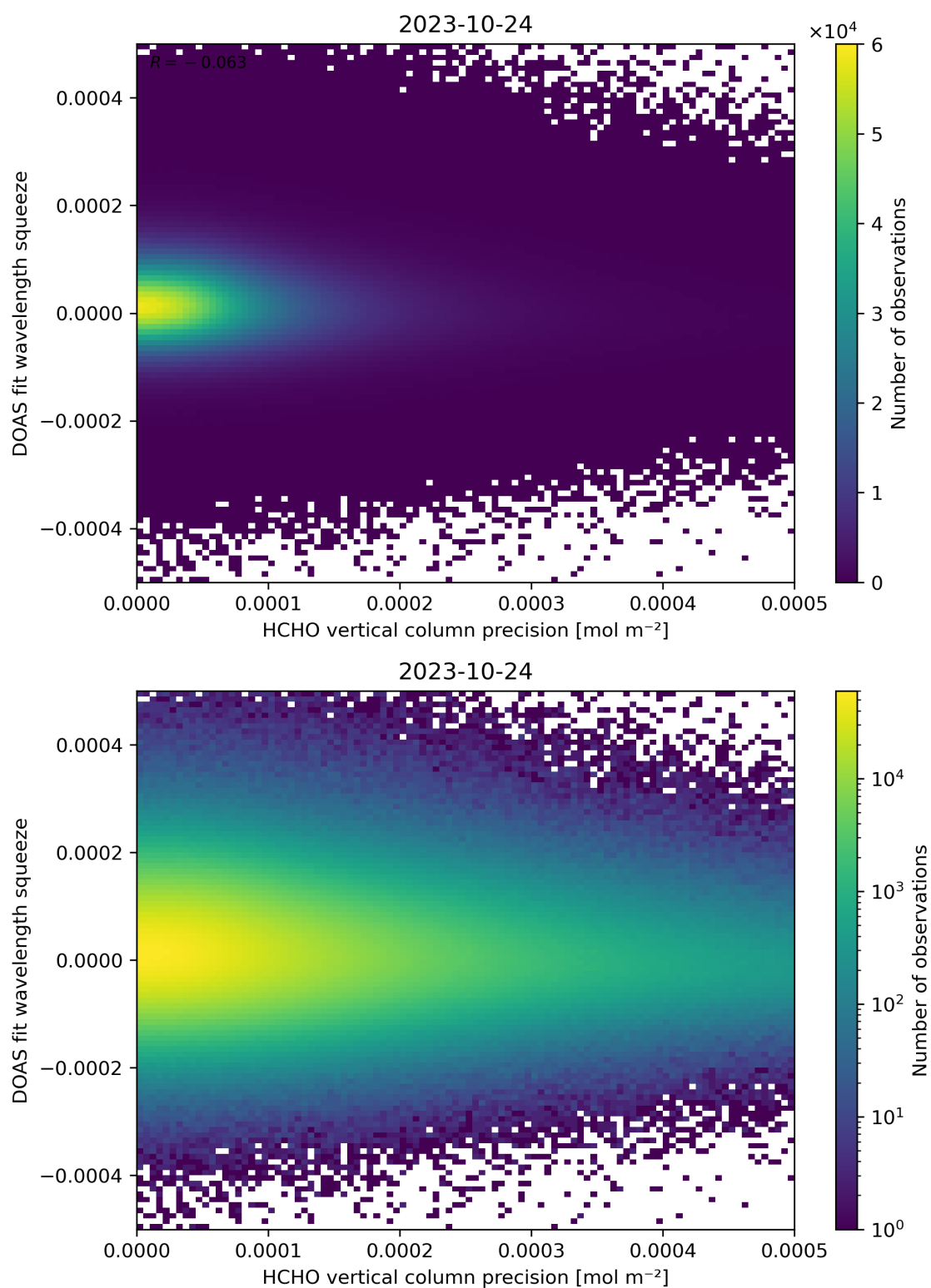
Figure 138: Scatter density plot of “HCHO vertical column precision” against “DOAS fit wavelength squeeze” for 2023-10-23 to 2023-10-25.
