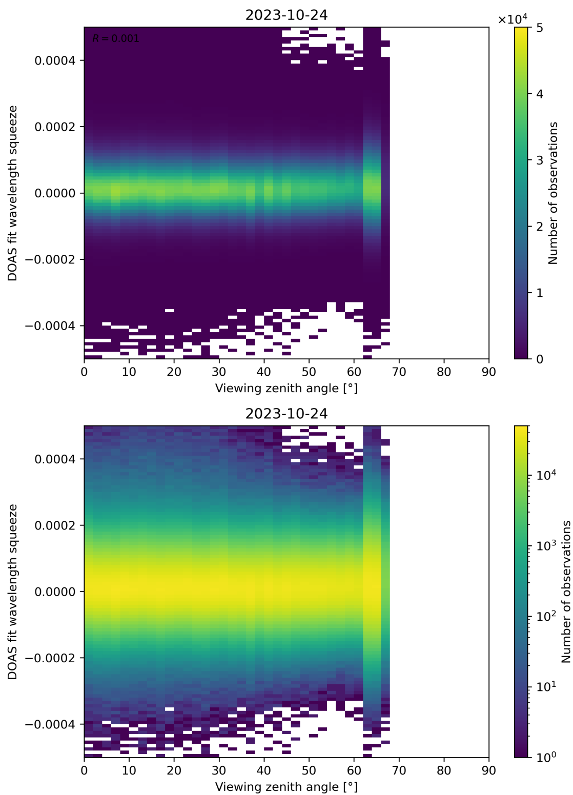
Figure 184: Scatter density plot of “Viewing zenith angle” against “DOAS fit wavelength squeeze” for 2023-10-23 to 2023-10-25.
