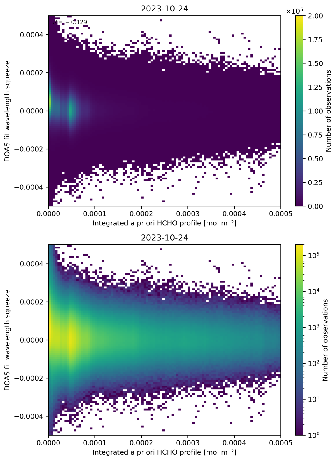
Figure 150: Scatter density plot of “Integrated a priori HCHO profile” against “DOAS fit wavelength squeeze” for 2023-10-23 to 2023-10-25.
