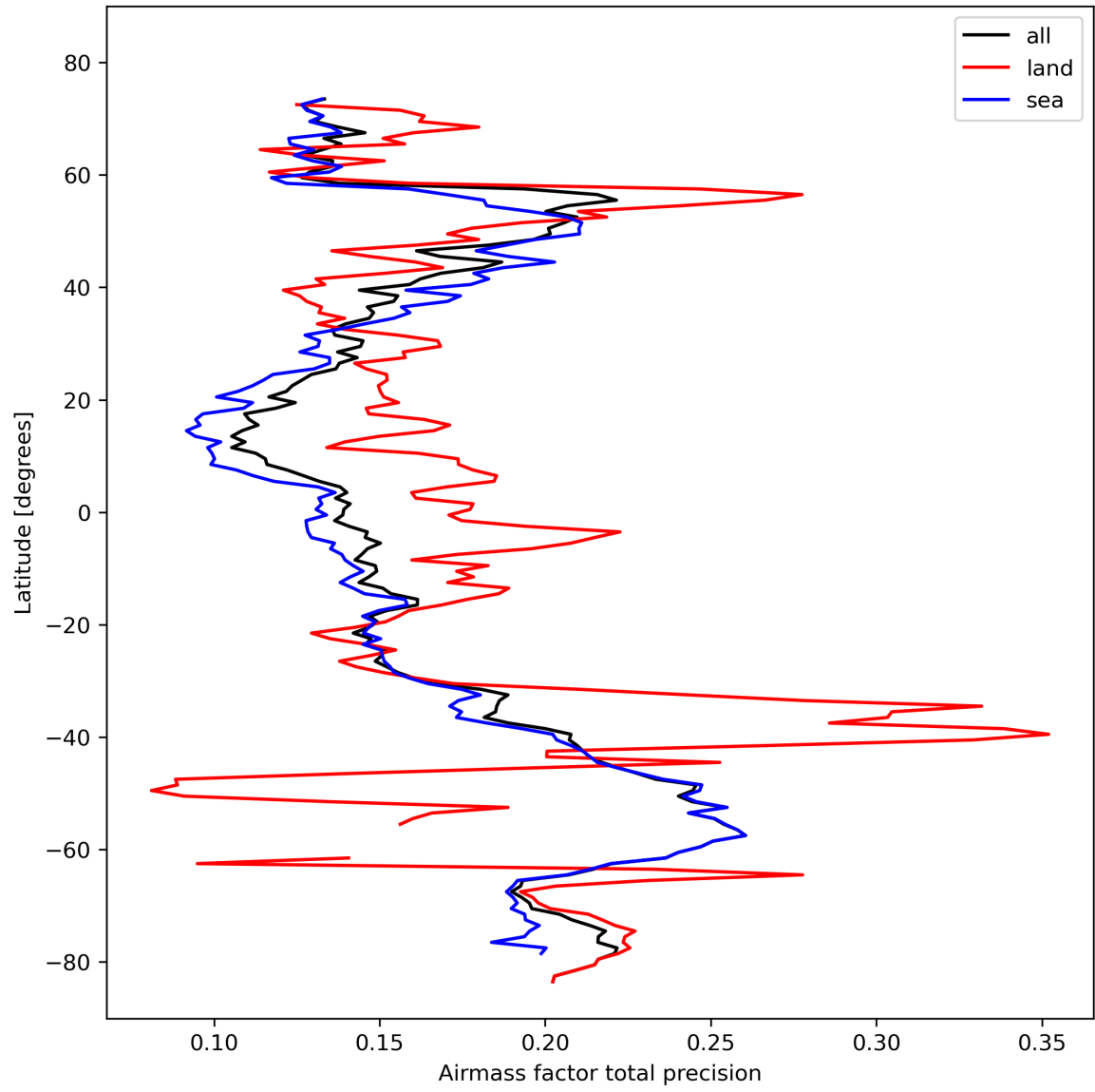
Figure 27: Zonal average of “Airmass factor total precision” for 2023-10-23 to 2023-10-25.
