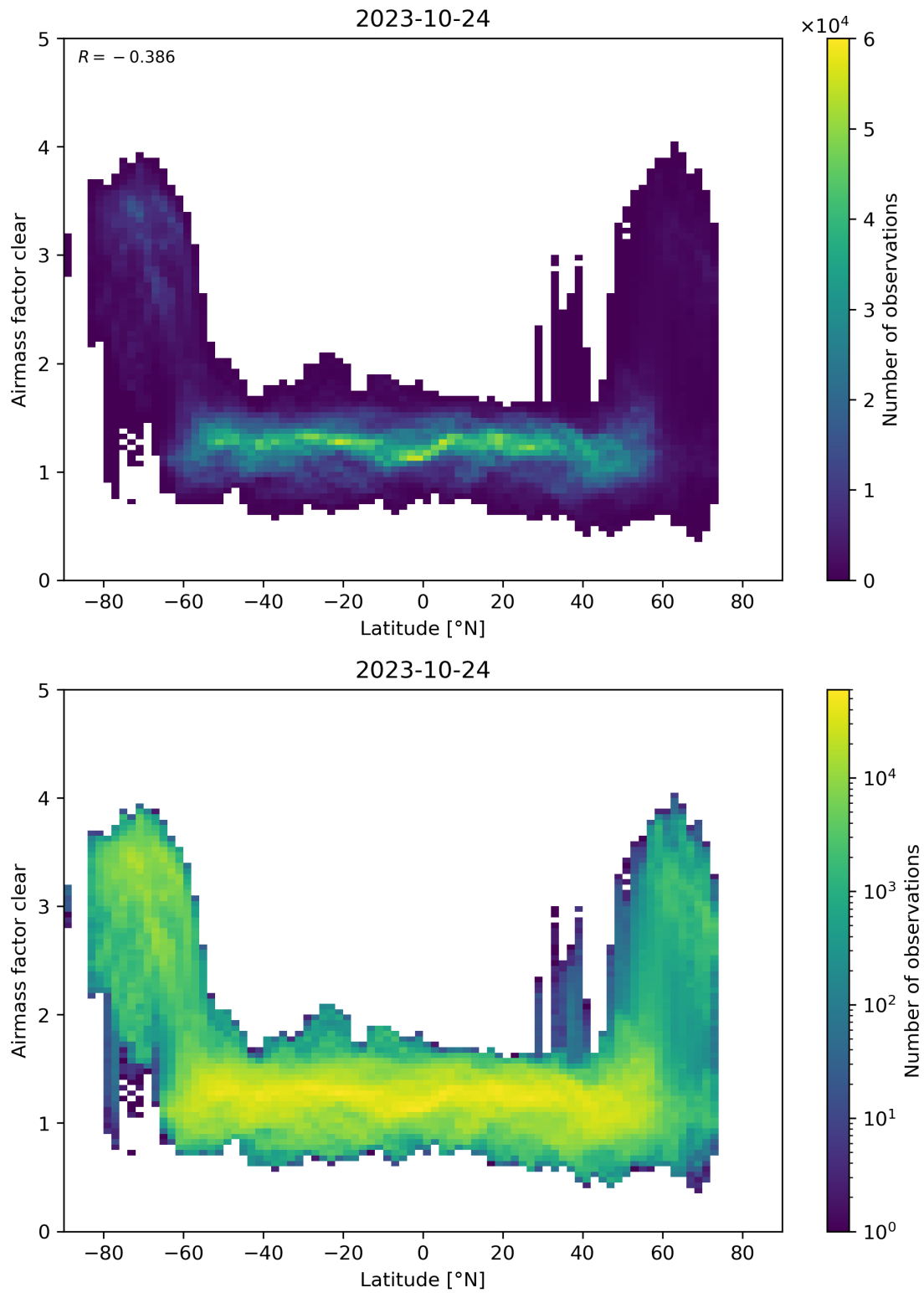
Figure 156: Scatter density plot of “Latitude” against “Airmass factor clear” for 2023-10-23 to 2023-10-25.
