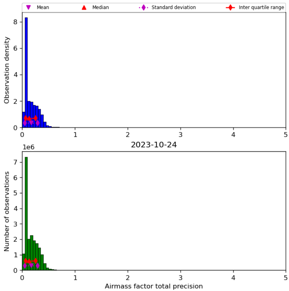
Figure 41: Histogram of “Airmass factor total precision” for 2023-10-23 to 2023-10-25
