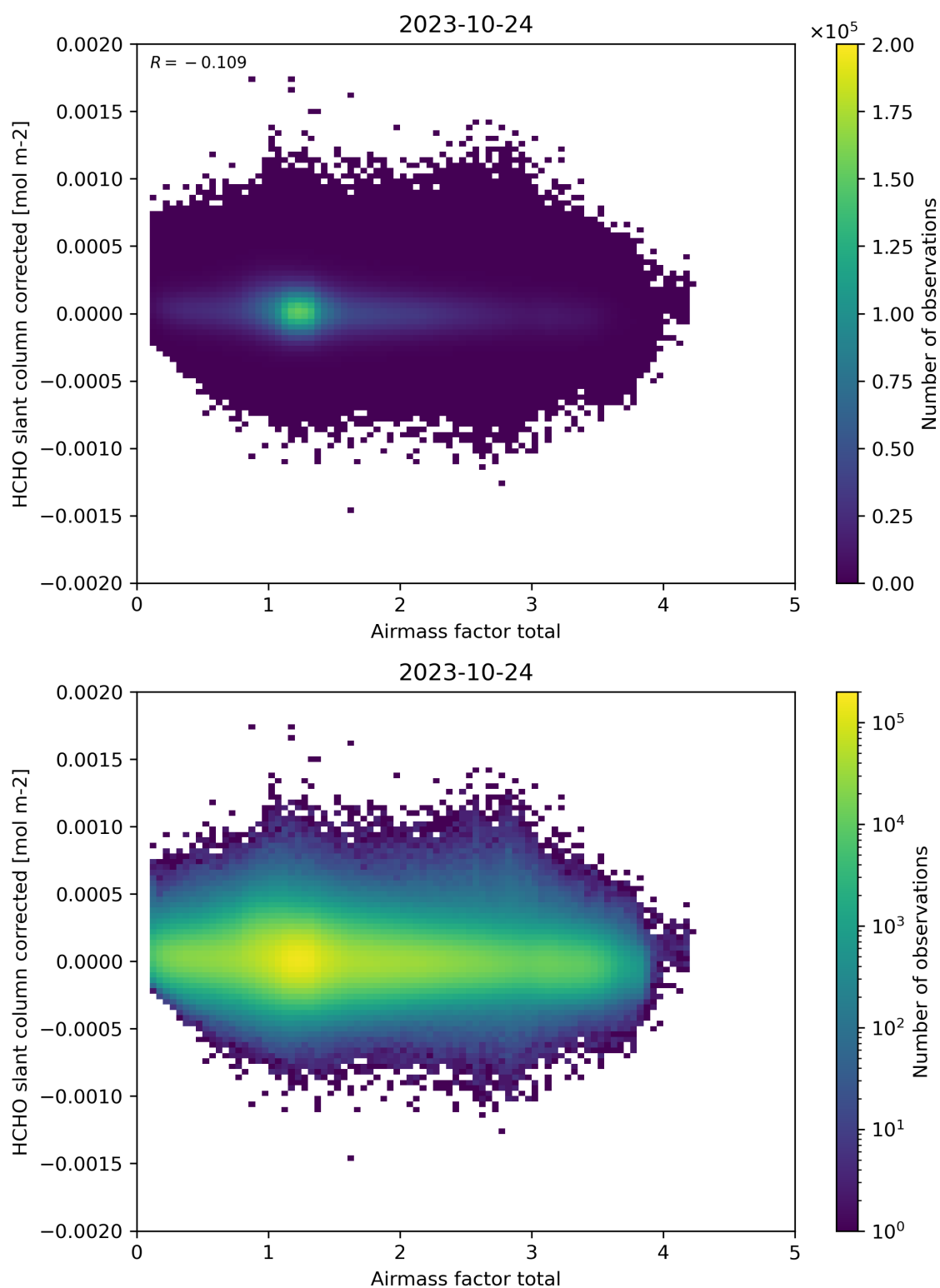
Figure 101: Scatter density plot of “Airmass factor total” against “HCHO slant column corrected” for 2023-10-23 to 2023-10-25.
