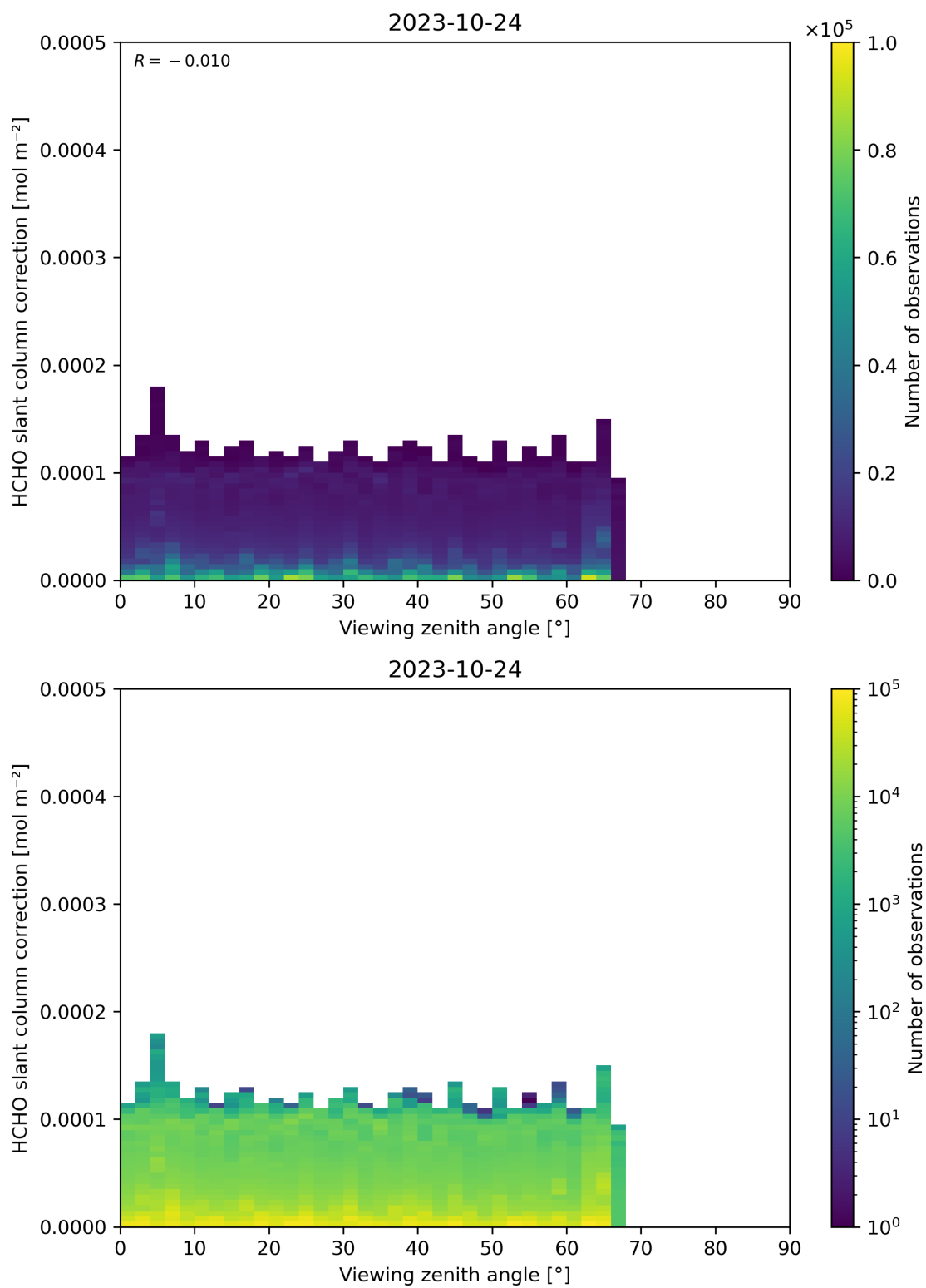
Figure 187: Scatter density plot of “Viewing zenith angle” against “HCHO slant column correction” for 2023-10-23 to 2023-10-25.
