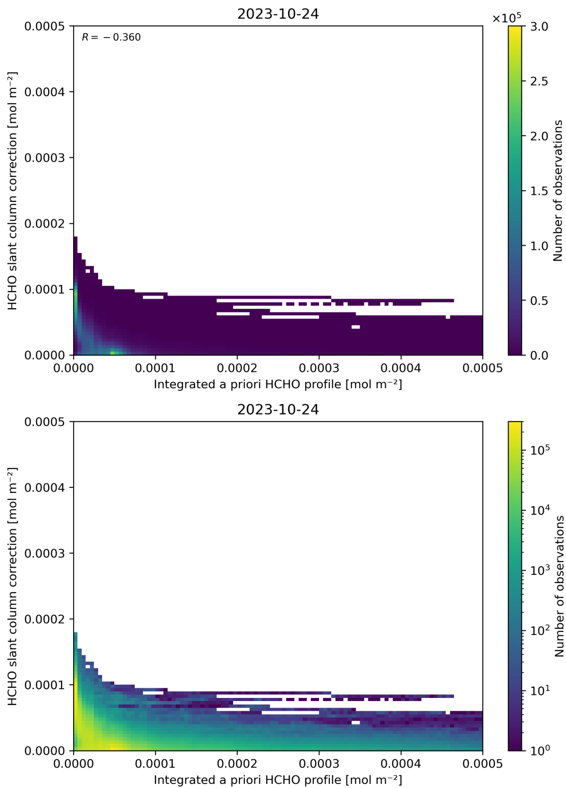
Figure 152: Scatter density plot of “Integrated a priori HCHO profile” against “HCHO slant column correction” for 2023-10-23 to 2023-10-25.
