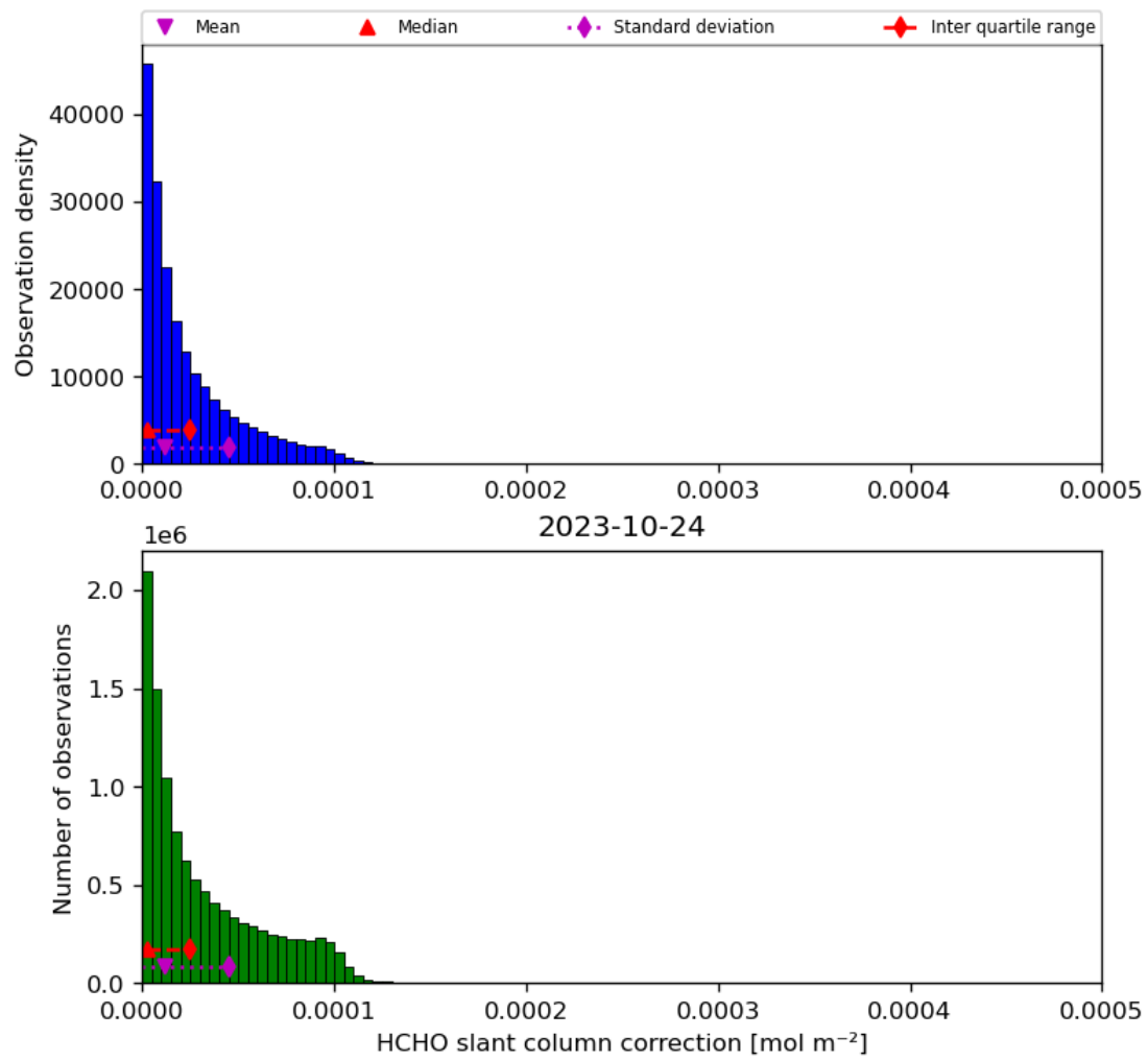
Figure 47: Histogram of “HCHO slant column correction” for 2023-10-23 to 2023-10-25
