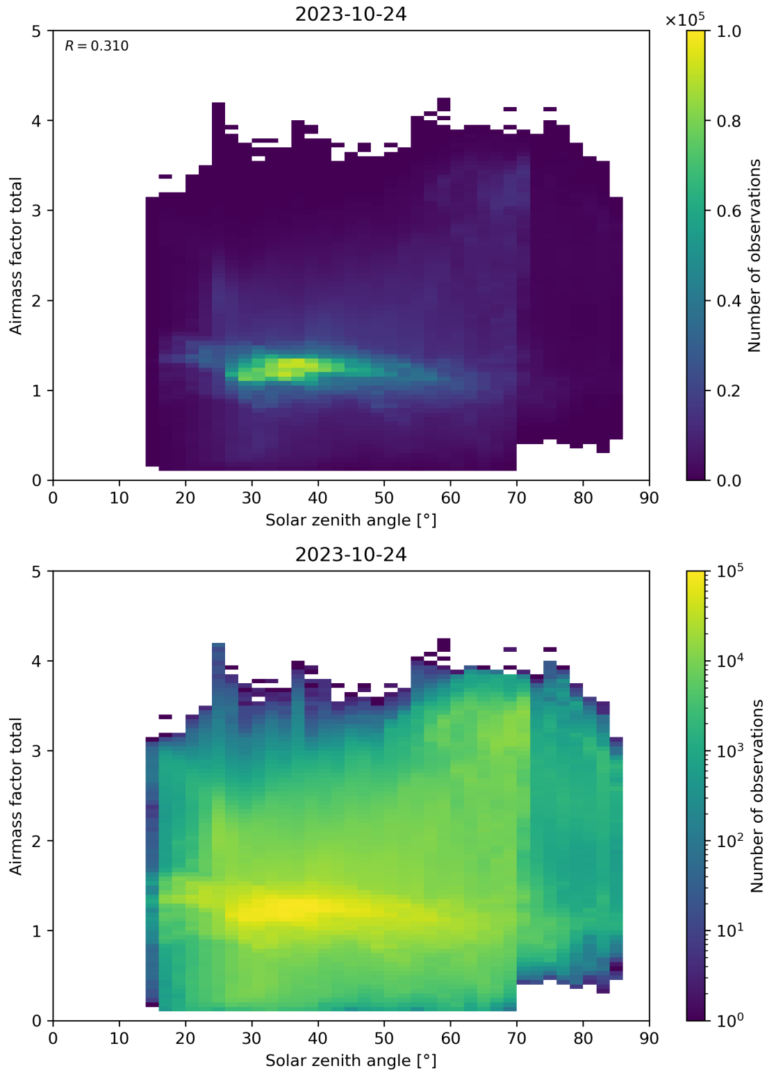
Figure 175: Scatter density plot of “Solar zenith angle” against “Airmass factor total” for 2023-10-23 to 2023-10-25.
