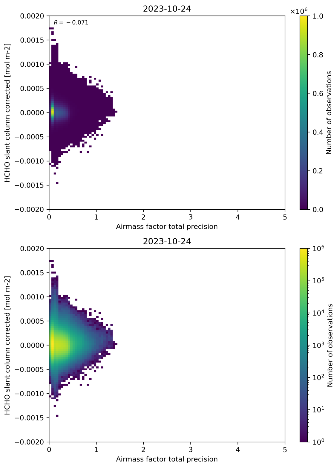
Figure 109: Scatter density plot of “Airmass factor total precision” against “HCHO slant column corrected” for 2023-10-23 to 2023-10-25.
