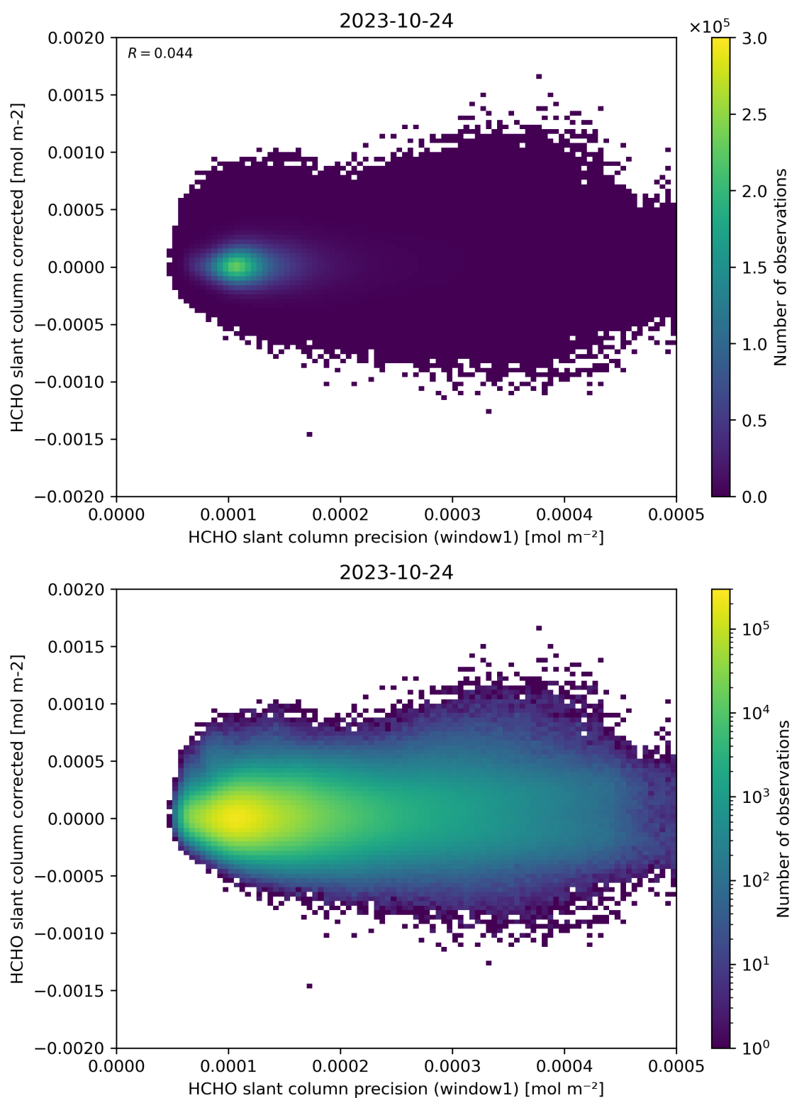
Figure 92: Scatter density plot of “HCHO slant column precision (window1)” against “HCHO slant column corrected” for 2023-10-23 to 2023-10-25.
