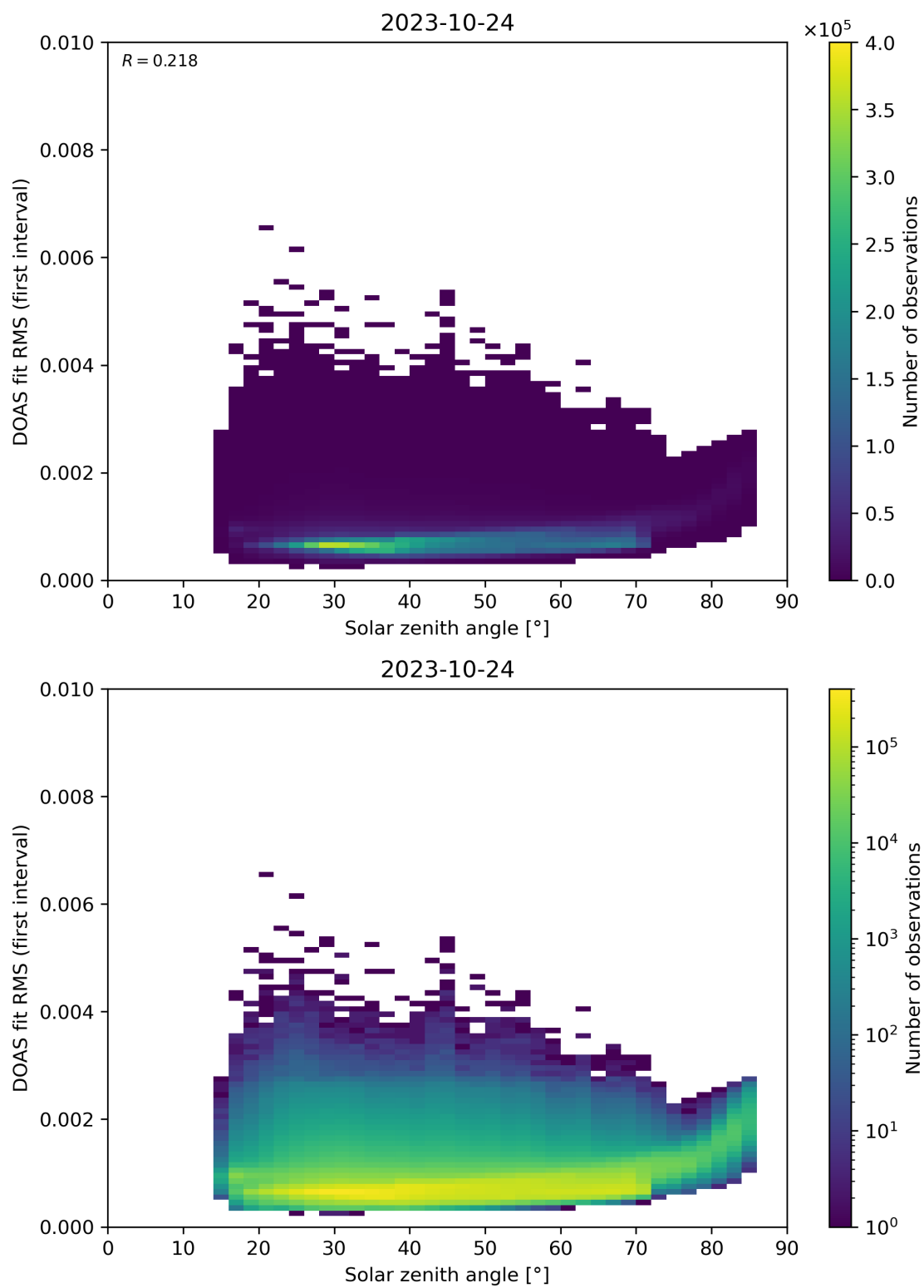
Figure 167: Scatter density plot of “Solar zenith angle” against “DOAS fit RMS (first interval)” for 2023-10-23 to 2023-10-25.
