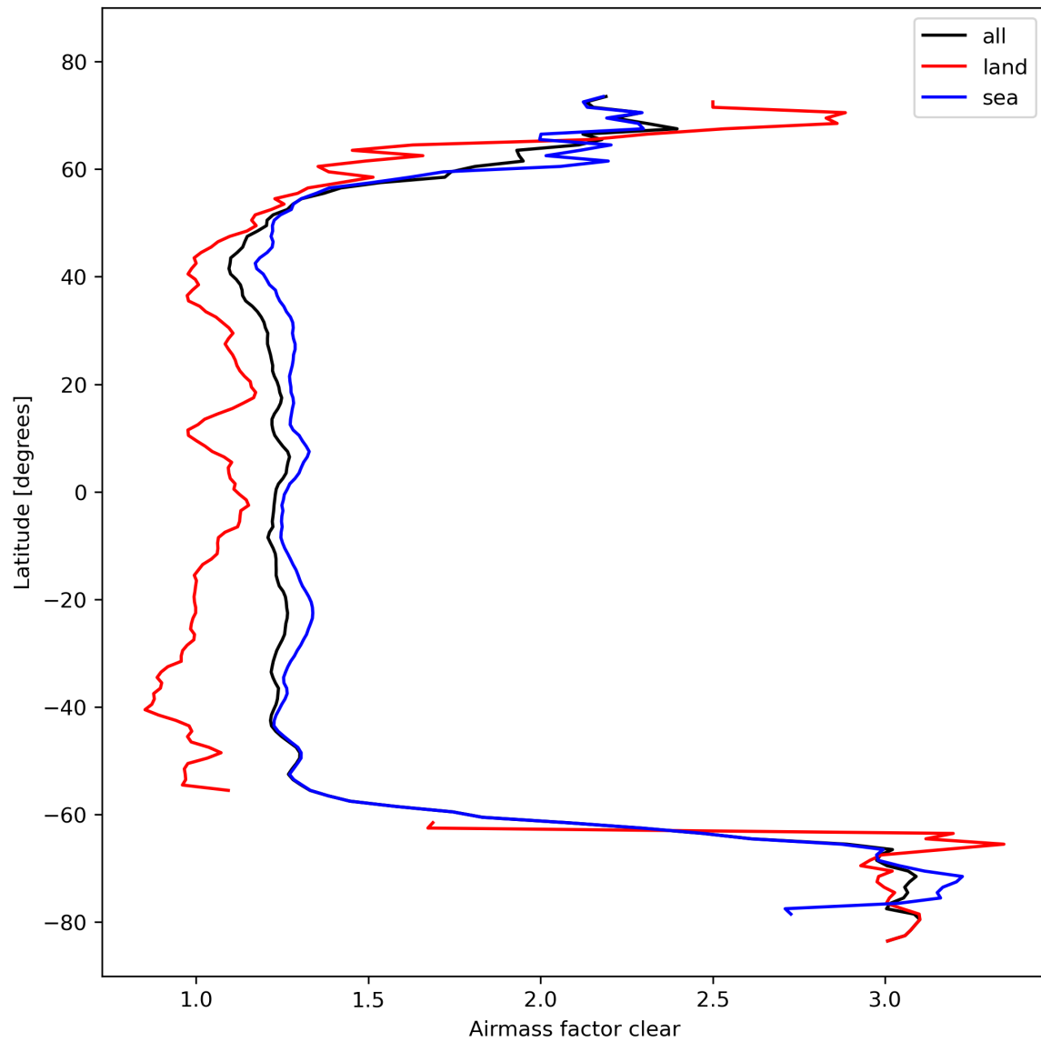
Figure 28: Zonal average of “Airmass factor clear” for 2023-10-23 to 2023-10-25.
