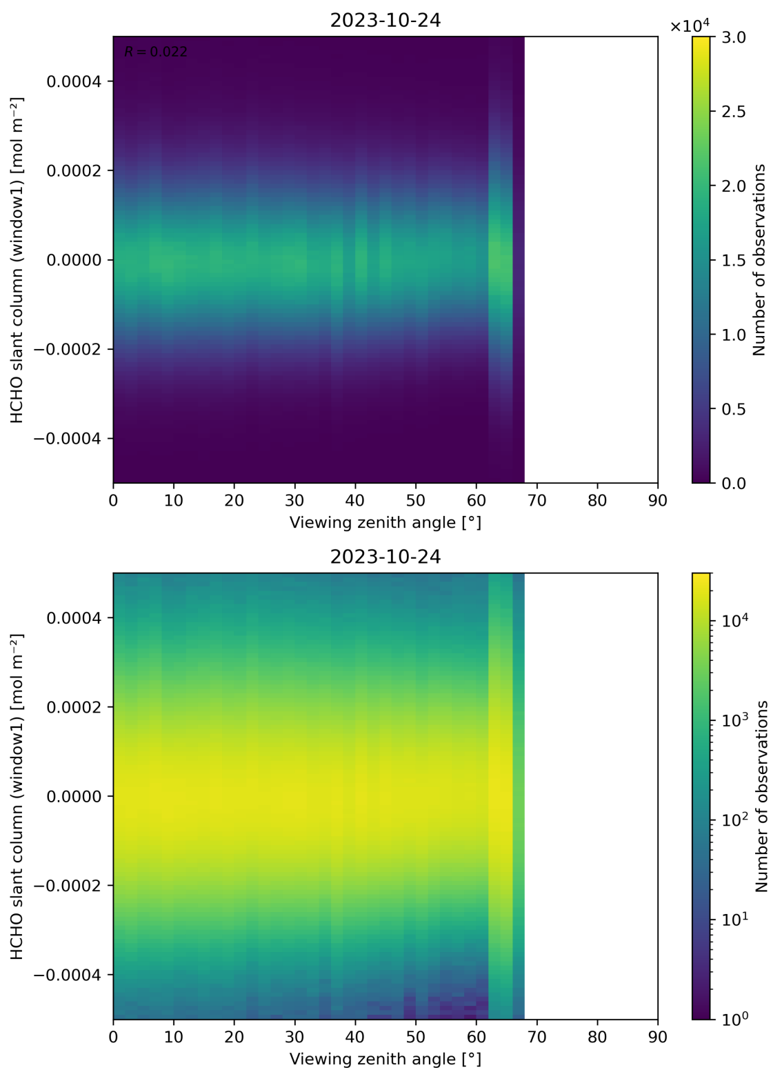
Figure 188: Scatter density plot of “Viewing zenith angle” against “HCHO slant column (window1)” for 2023-10-23 to 2023-10-25.
