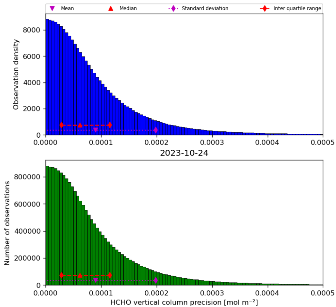
Figure 36: Histogram of “HCHO vertical column precision” for 2023-10-23 to 2023-10-25
