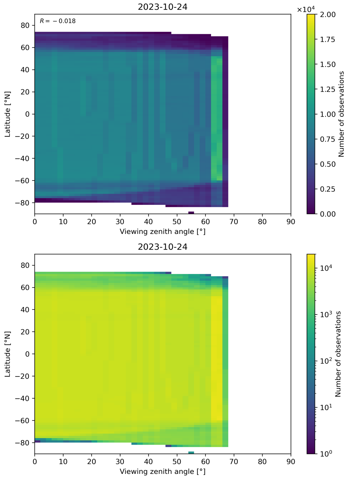
Figure 196: Scatter density plot of “Viewing zenith angle” against “Latitude” for 2023-10-23 to 2023-10-25.
