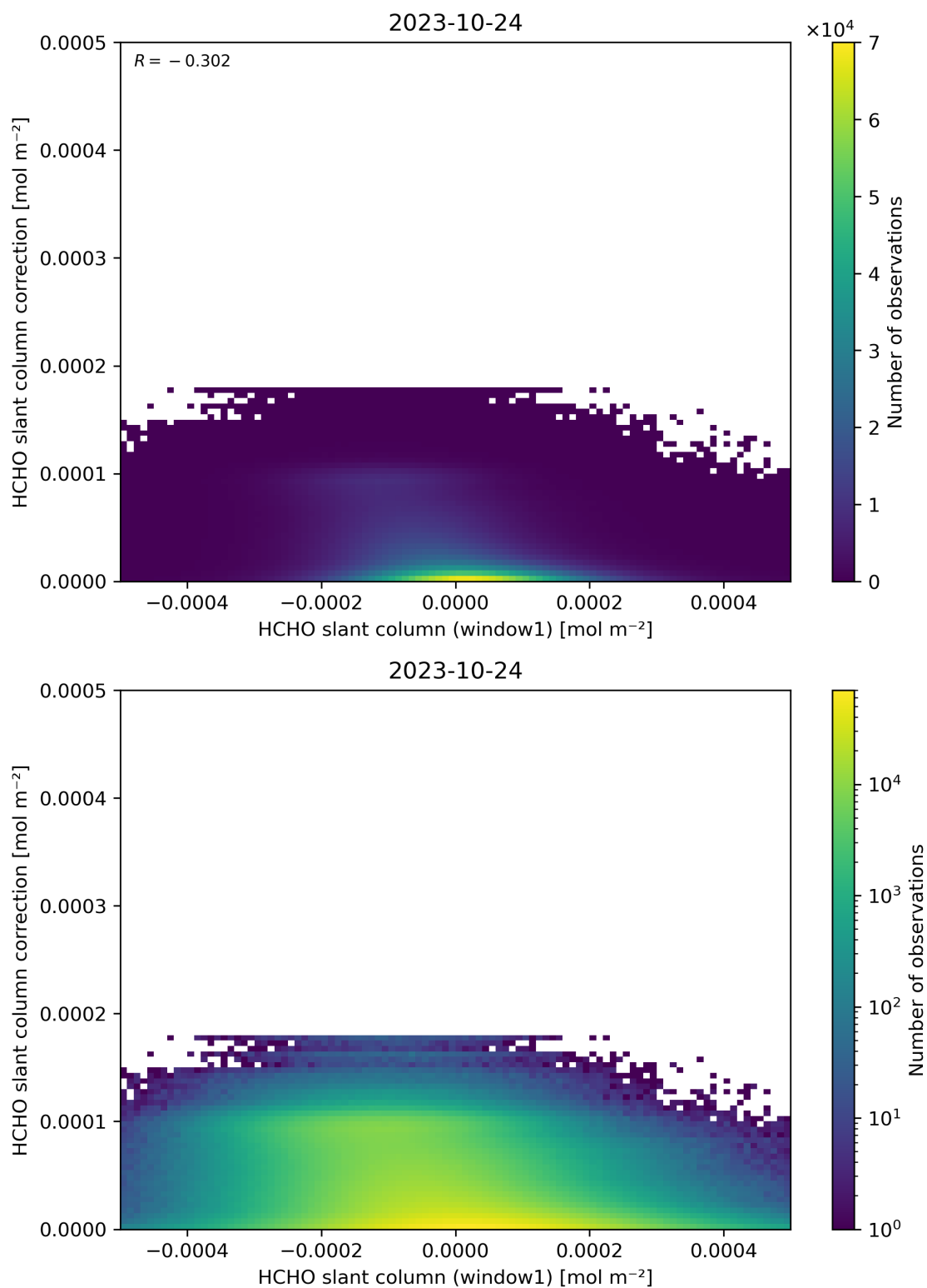
Figure 83: Scatter density plot of “HCHO slant column (window1)” against “HCHO slant column correction” for 2023-10-23 to 2023-10-25.
