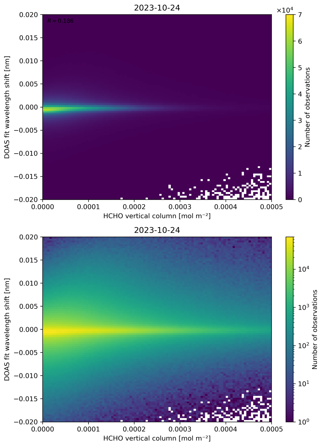
Figure 124: Scatter density plot of “HCHO vertical column” against “DOAS fit wavelength shift” for 2023-10-23 to 2023-10-25.
