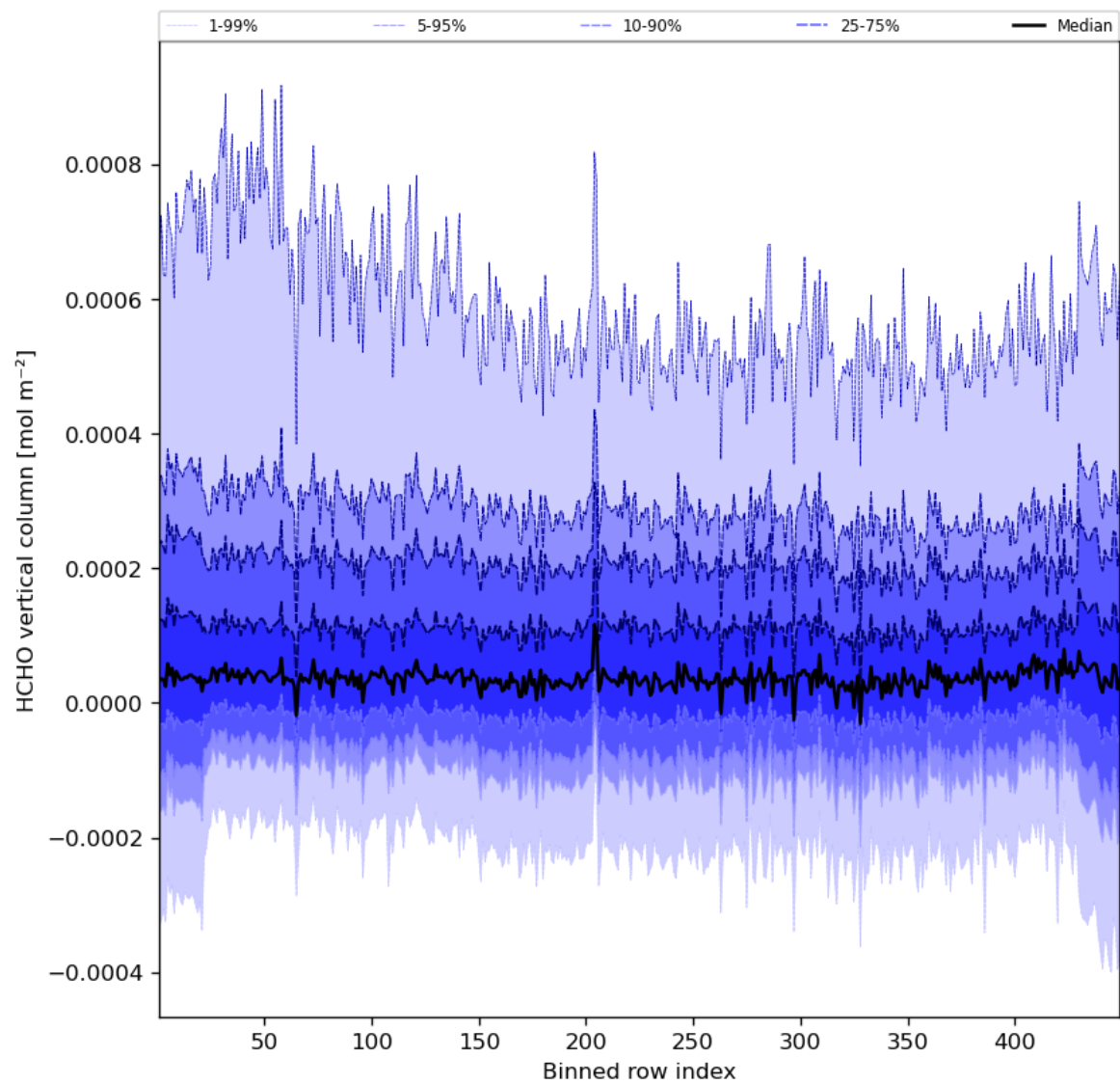
Figure 49: Along track statistics of “HCHO vertical column” for 2023-10-23 to 2023-10-25
