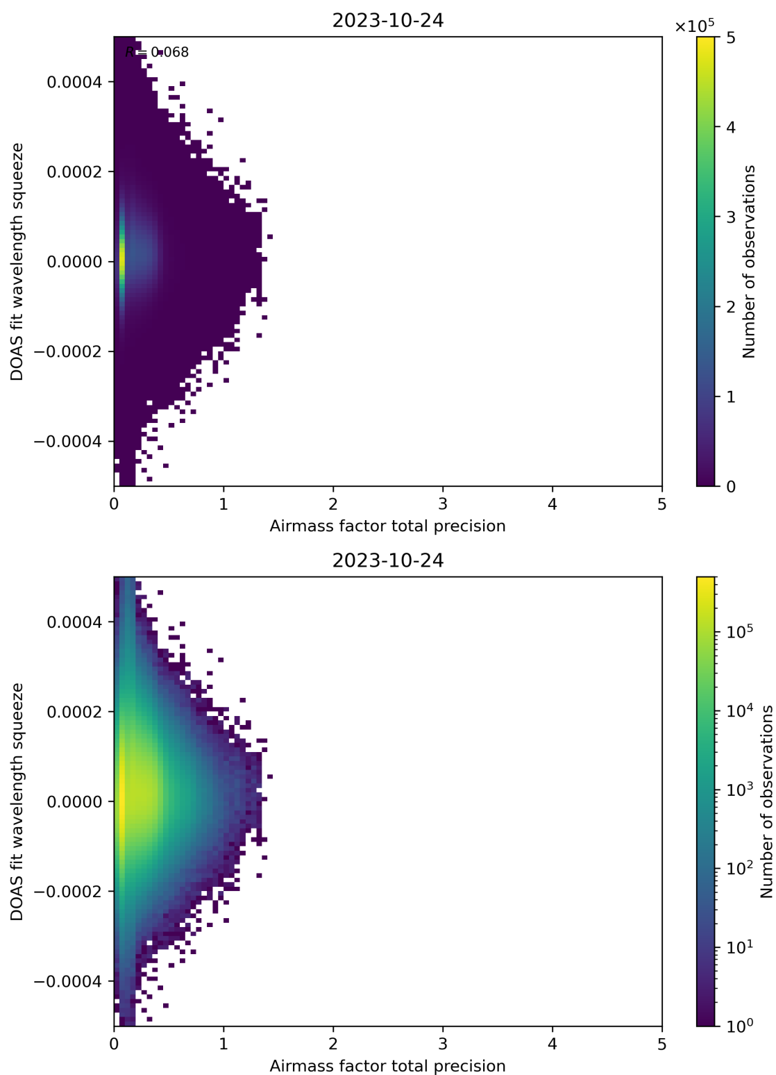
Figure 107: Scatter density plot of “Airmass factor total precision” against “DOAS fit wavelength squeeze” for 2023-10-23 to 2023-10-25.
