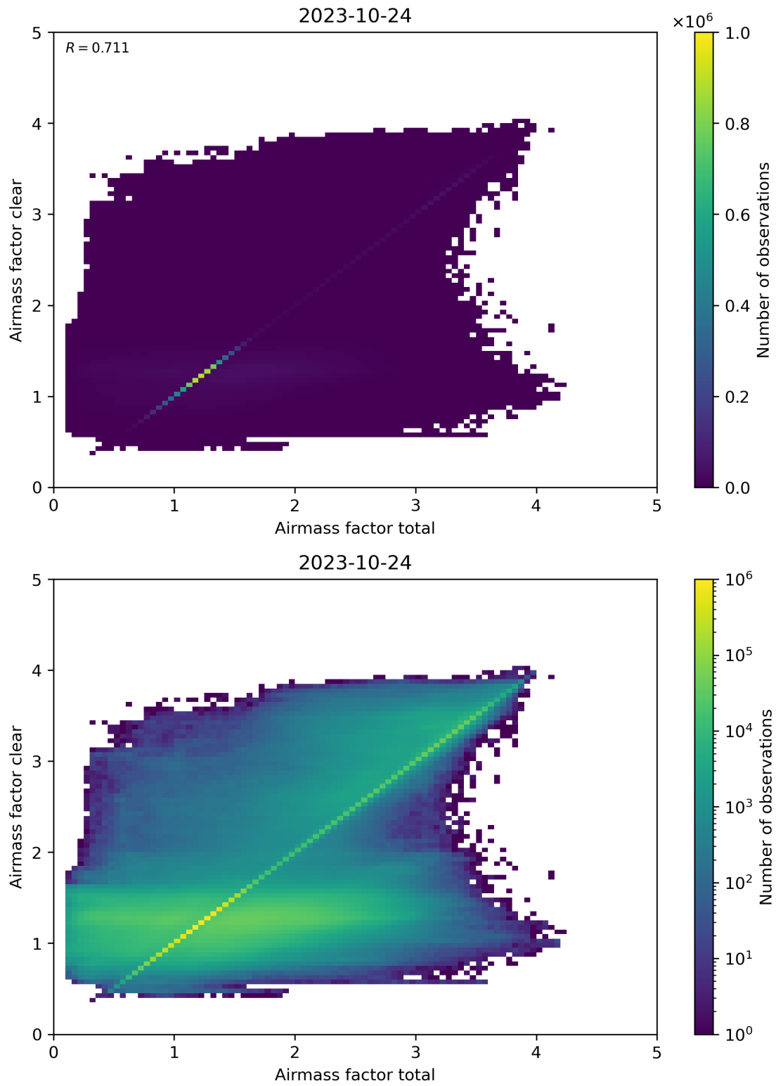
Figure 100: Scatter density plot of “Airmass factor total” against “Airmass factor clear” for 2023-10-23 to 2023-10-25.
