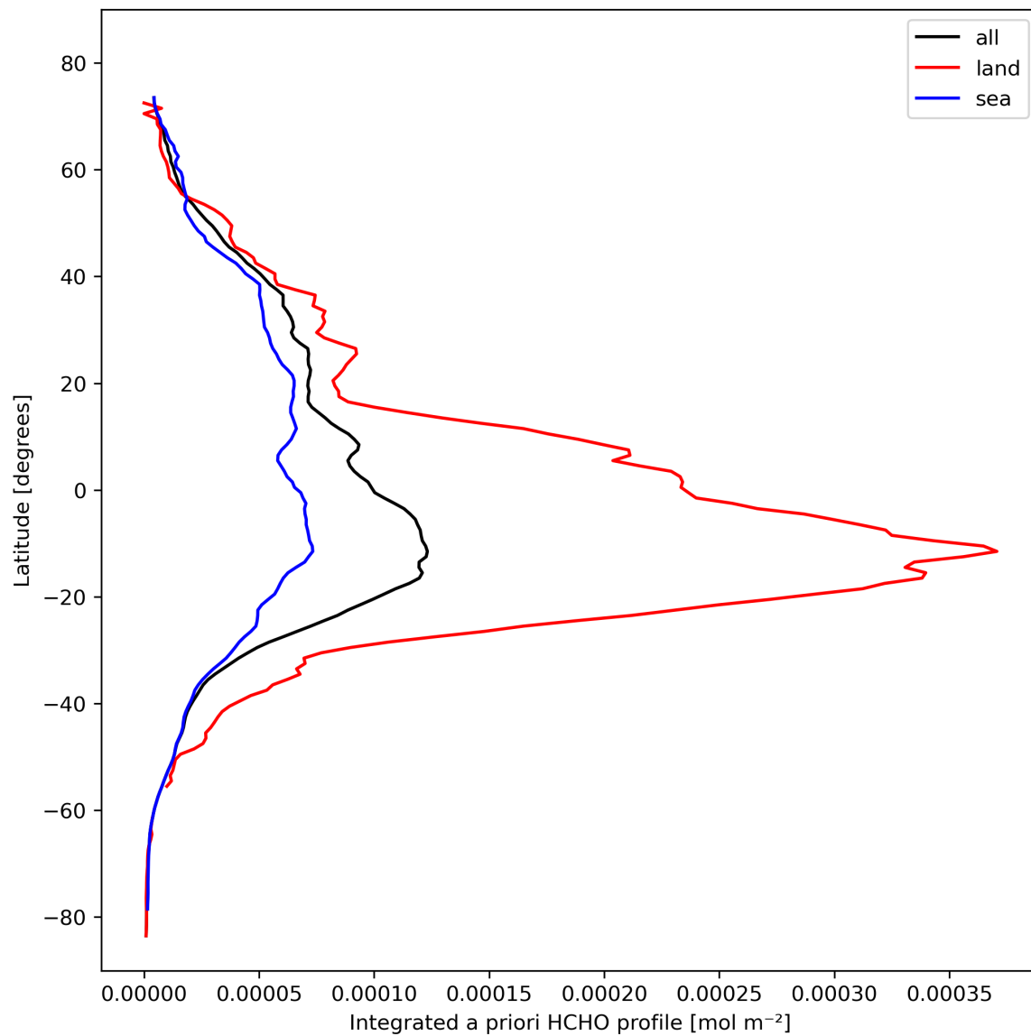
Figure 29: Zonal average of “Integrated a priori HCHO profile” for 2023-10-23 to 2023-10-25.
