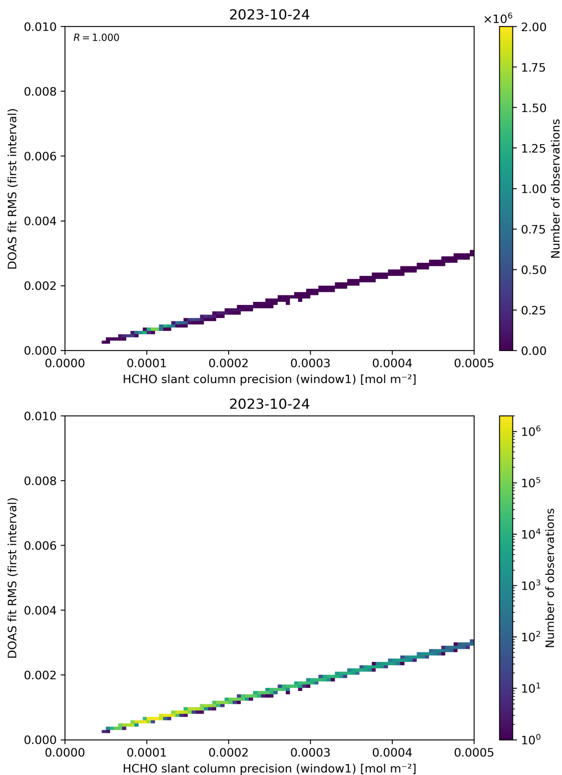
Figure 88: Scatter density plot of “HCHO slant column precision (window1)” against “DOAS fit RMS (first interval)” for 2023-10-23 to 2023-10-25.
