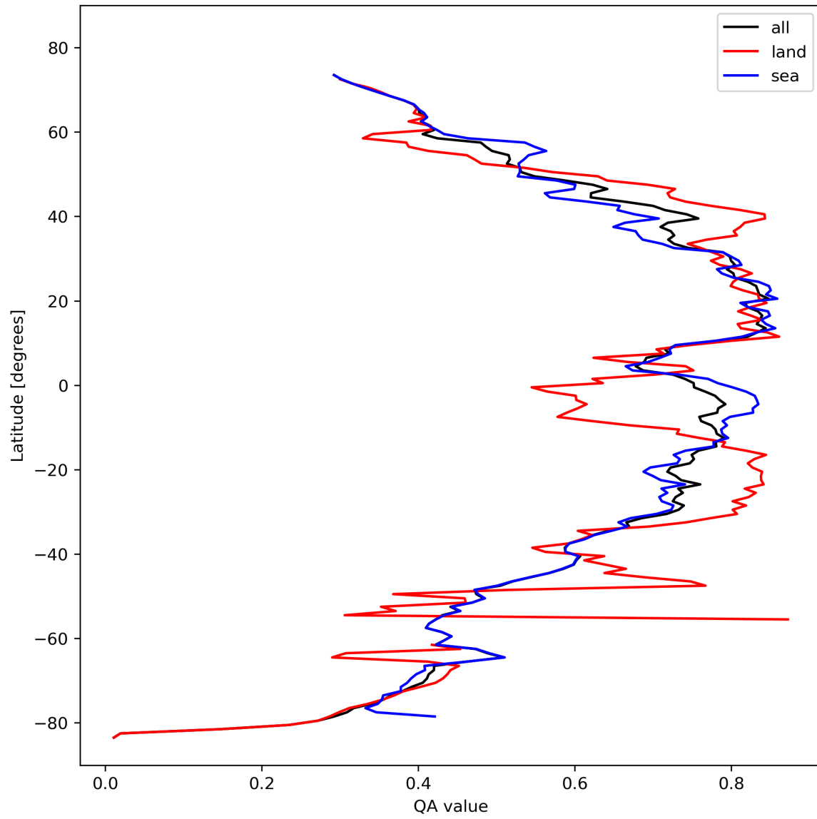
Figure 20: Zonal average of “QA value” for 2023-10-23 to 2023-10-25.
