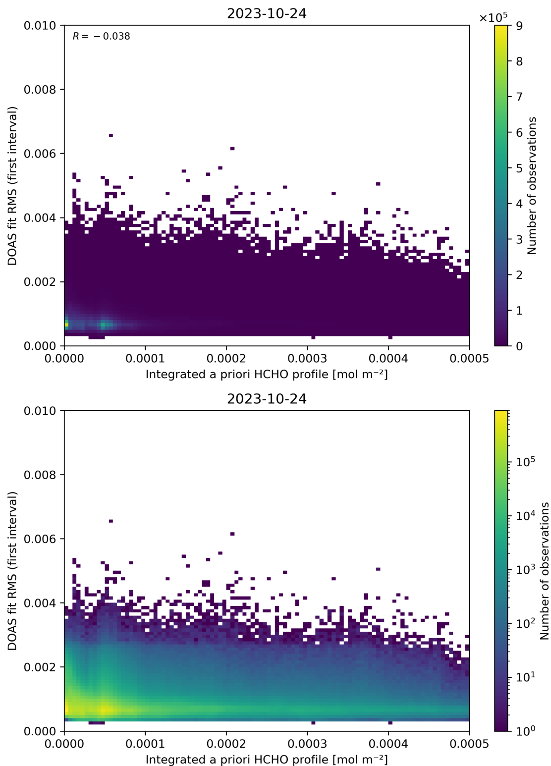
Figure 148: Scatter density plot of “Integrated a priori HCHO profile” against “DOAS fit RMS (first interval)” for 2023-10-23 to 2023-10-25.
