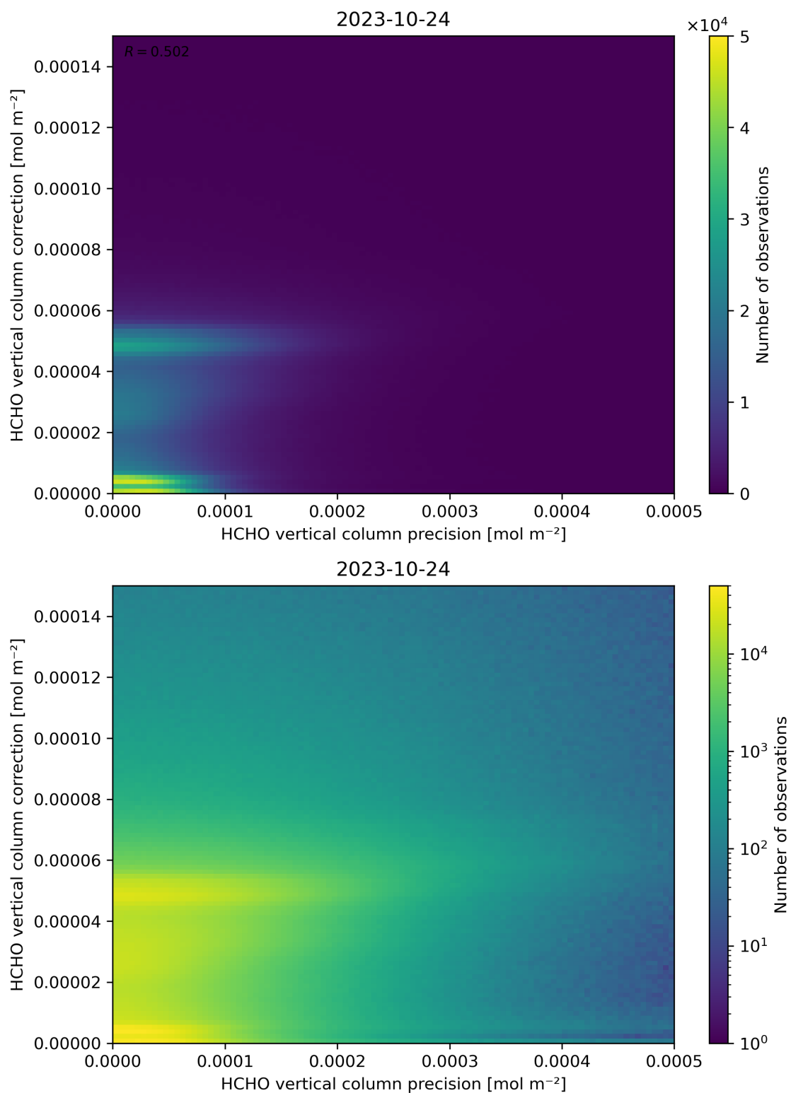
Figure 146: Scatter density plot of “HCHO vertical column precision” against “HCHO vertical column correction” for 2023-10-23 to 2023-10-25.
