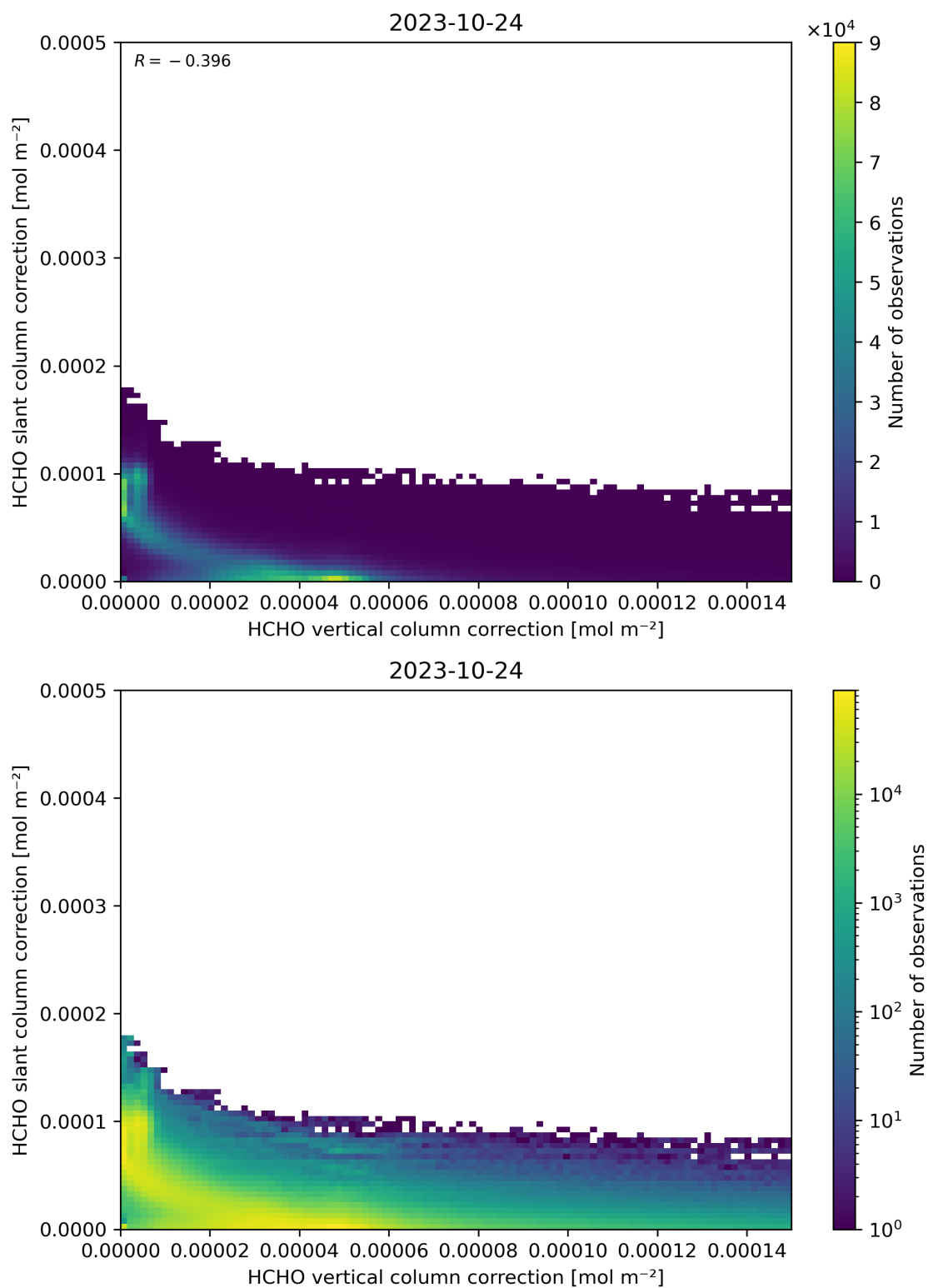
Figure 117: Scatter density plot of “HCHO vertical column correction” against “HCHO slant column correction” for 2023-10-23 to 2023-10-25.
