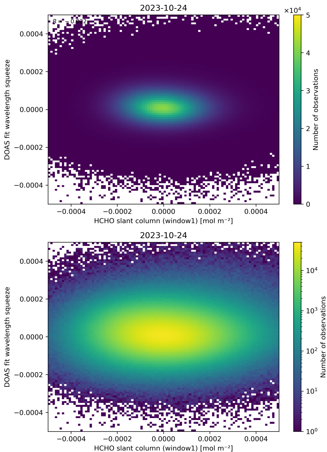
Figure 80: Scatter density plot of “HCHO slant column (window1)” against “DOAS fit wavelength squeeze” for 2023-10-23 to 2023-10-25.
