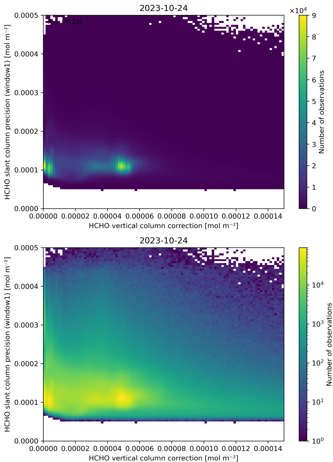
Figure 119: Scatter density plot of “HCHO vertical column correction” against “HCHO slant column precision (window1)” for 2023-10-23 to 2023-10-25.
