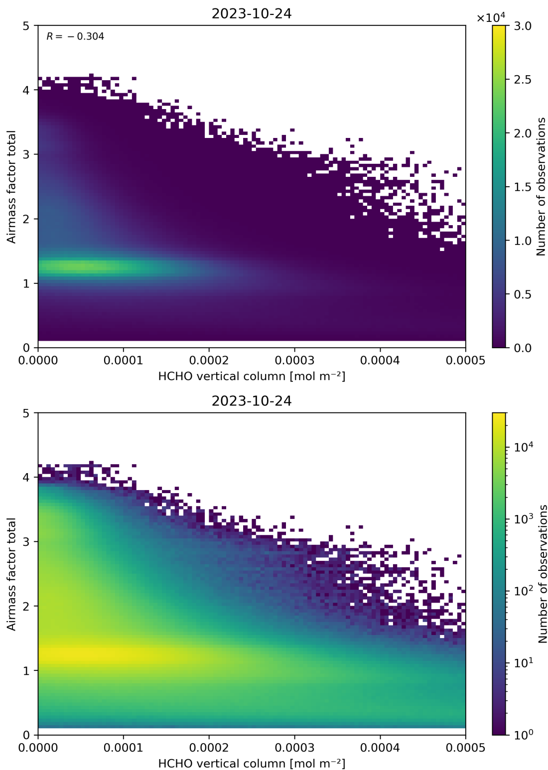
Figure 131: Scatter density plot of “HCHO vertical column” against “Airmass factor total” for 2023-10-23 to 2023-10-25.
