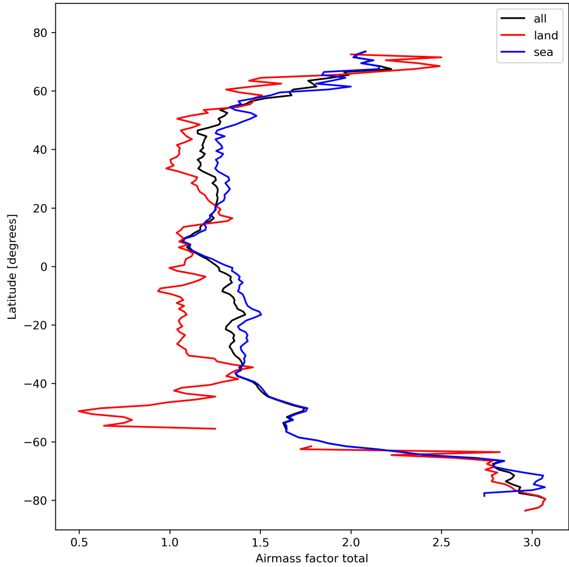
Figure 26: Zonal average of “Airmass factor total” for 2023-10-23 to 2023-10-25.
