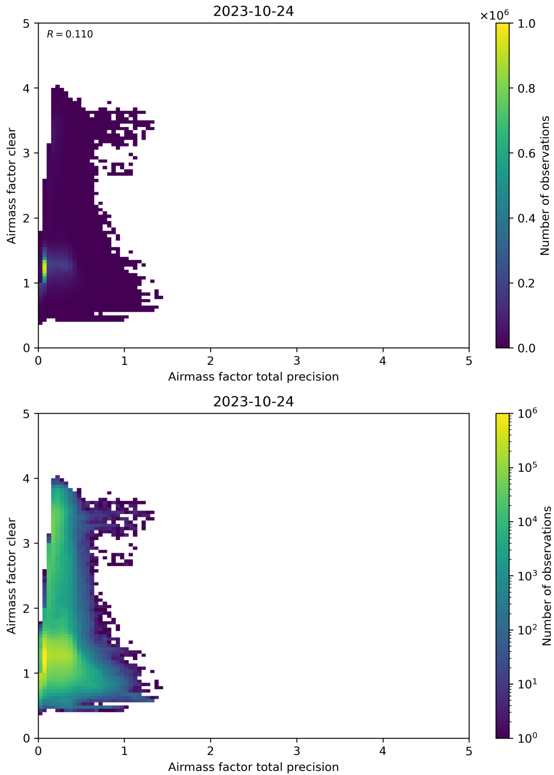
Figure 108: Scatter density plot of “Airmass factor total precision” against “Airmass factor clear” for 2023-10-23 to 2023-10-25.
