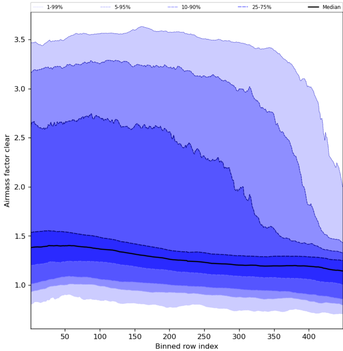
Figure 56: Along track statistics of “Airmass factor clear” for 2023-10-23 to 2023-10-25
