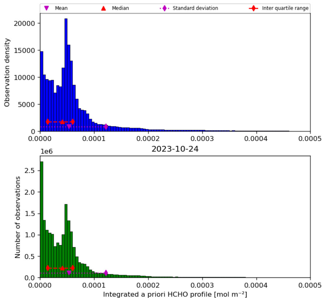
Figure 43: Histogram of “Integrated a priori HCHO profile” for 2023-10-23 to 2023-10-25
