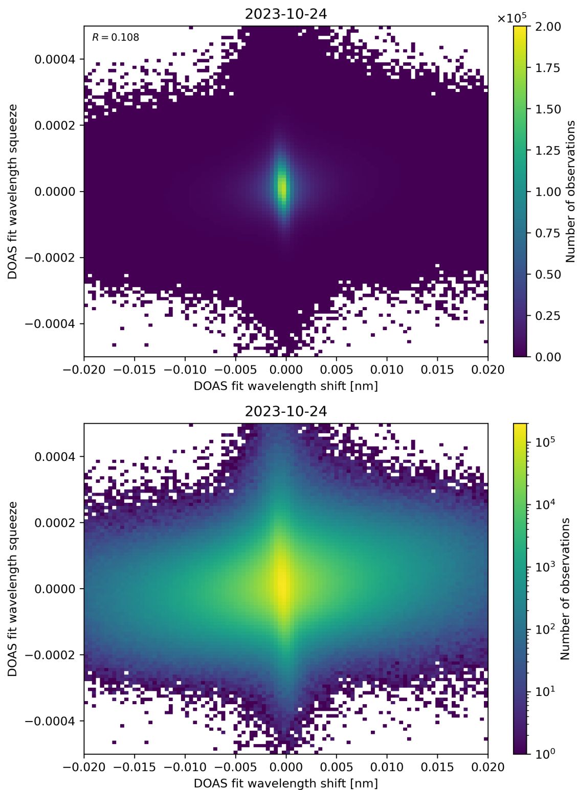
Figure 65: Scatter density plot of “DOAS fit wavelength shift” against “DOAS fit wavelength squeeze” for 2023-10-23 to 2023-10-25.
