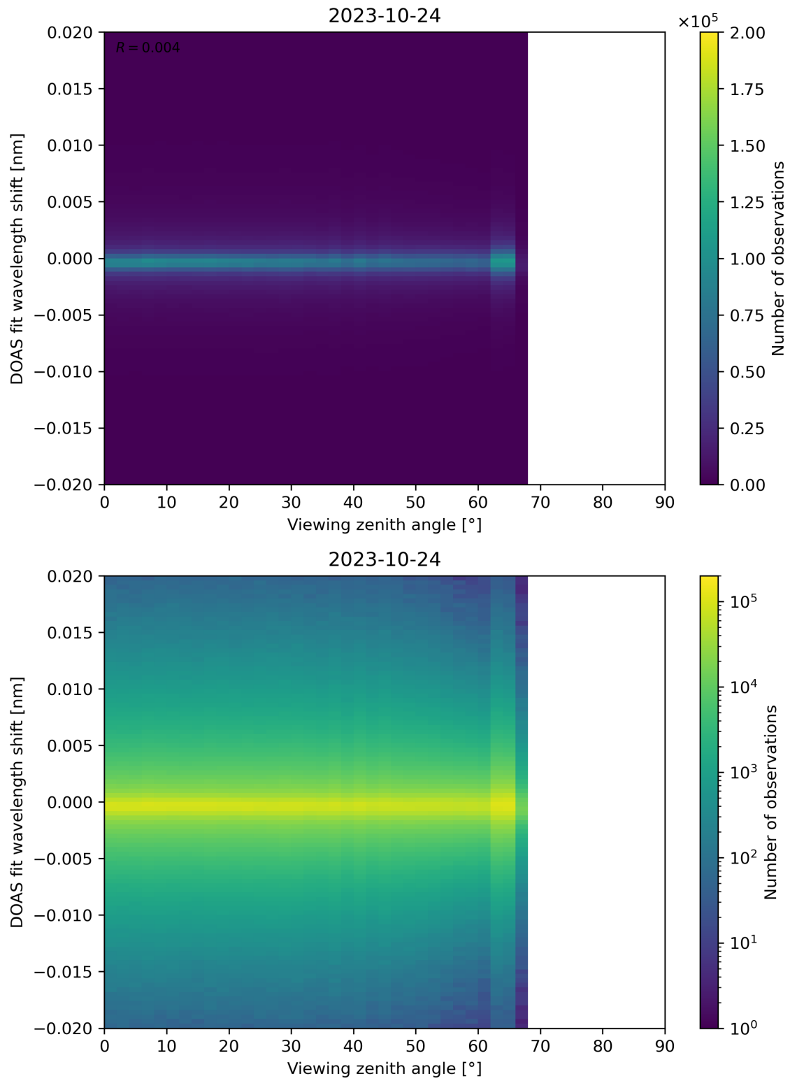
Figure 183: Scatter density plot of “Viewing zenith angle” against “DOAS fit wavelength shift” for 2023-10-23 to 2023-10-25.
