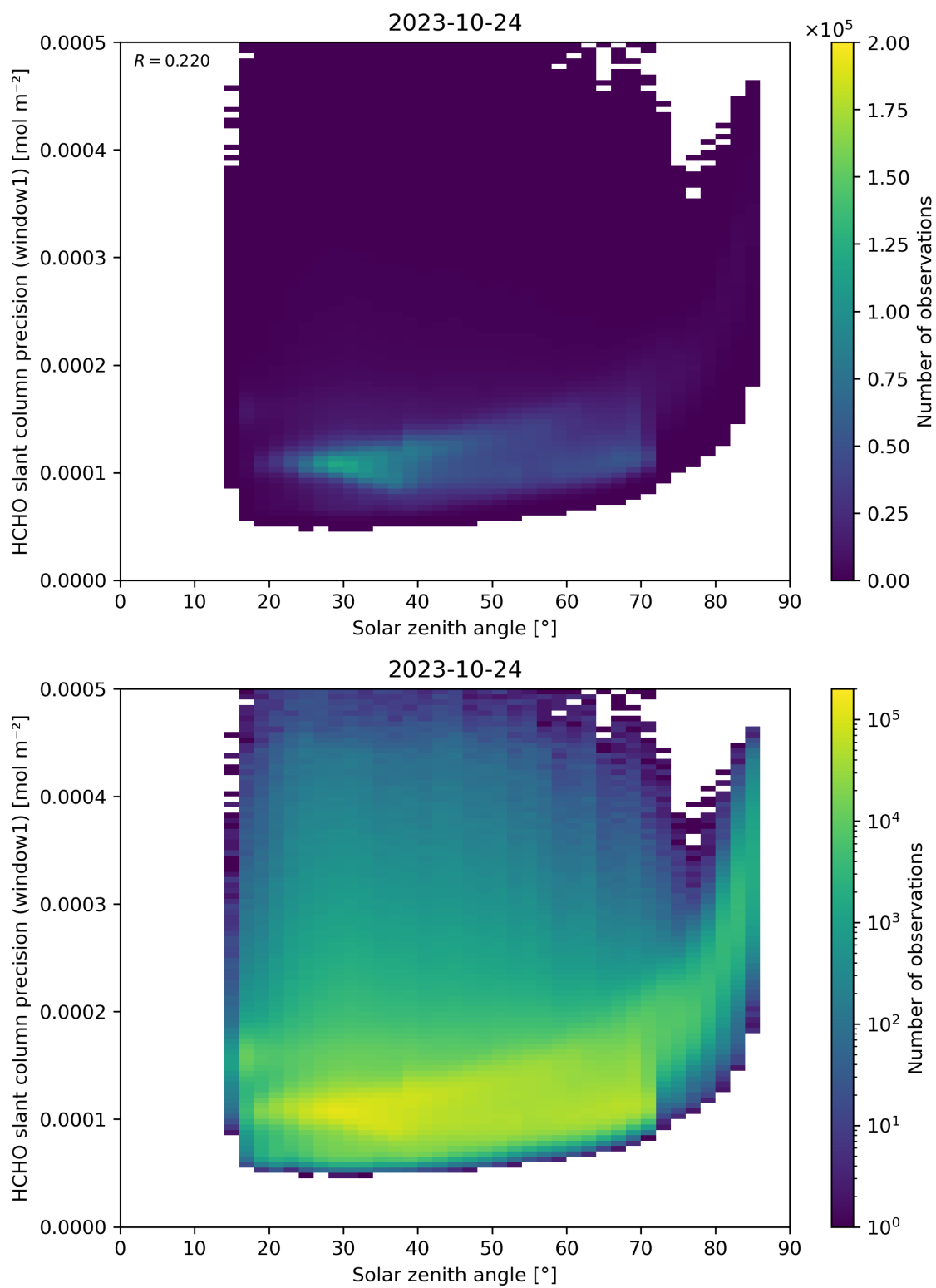
Figure 174: Scatter density plot of “Solar zenith angle” against “HCHO slant column precision (window1)” for 2023-10-23 to 2023-10-25.
