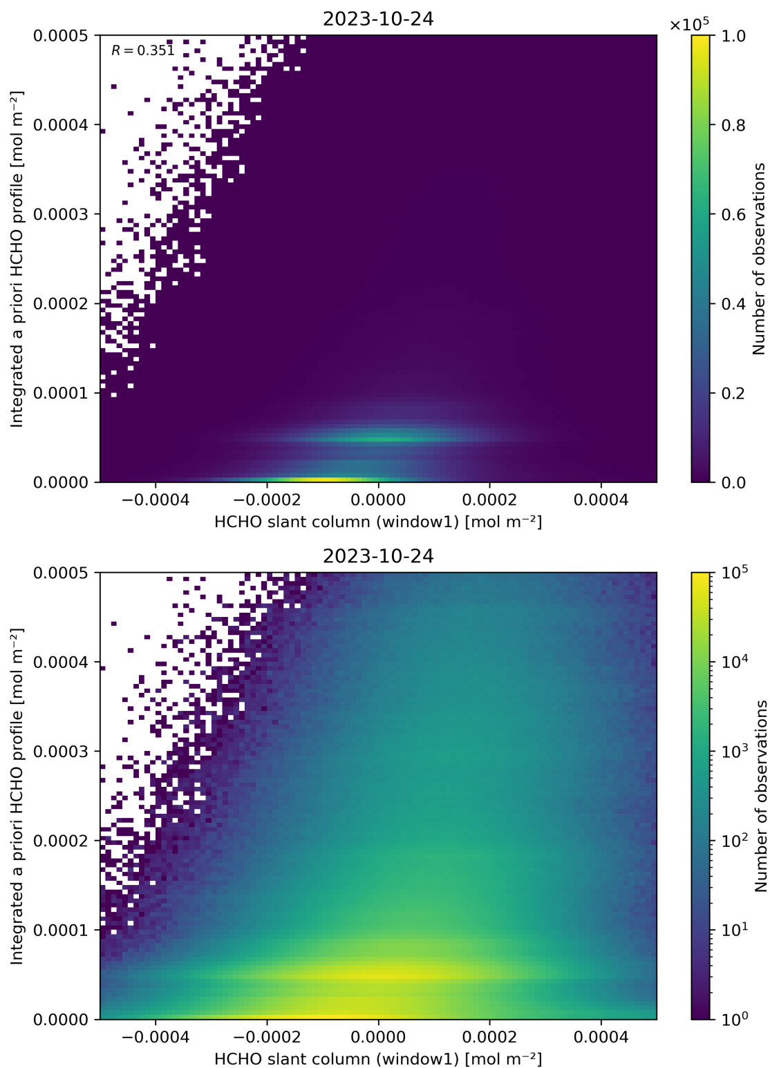
Figure 87: Scatter density plot of “HCHO slant column (window1)” against “Integrated a priori HCHO profile” for 2023-10-23 to 2023-10-25.
