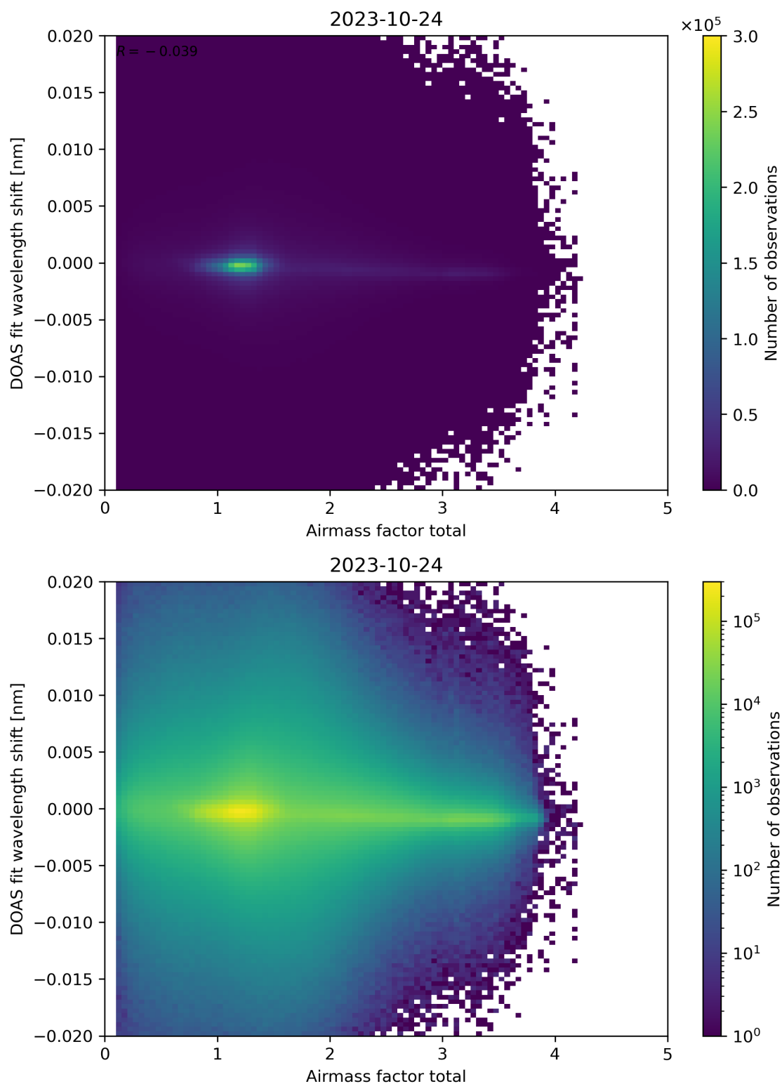
Figure 98: Scatter density plot of “Airmass factor total” against “DOAS fit wavelength shift” for 2023-10-23 to 2023-10-25.
