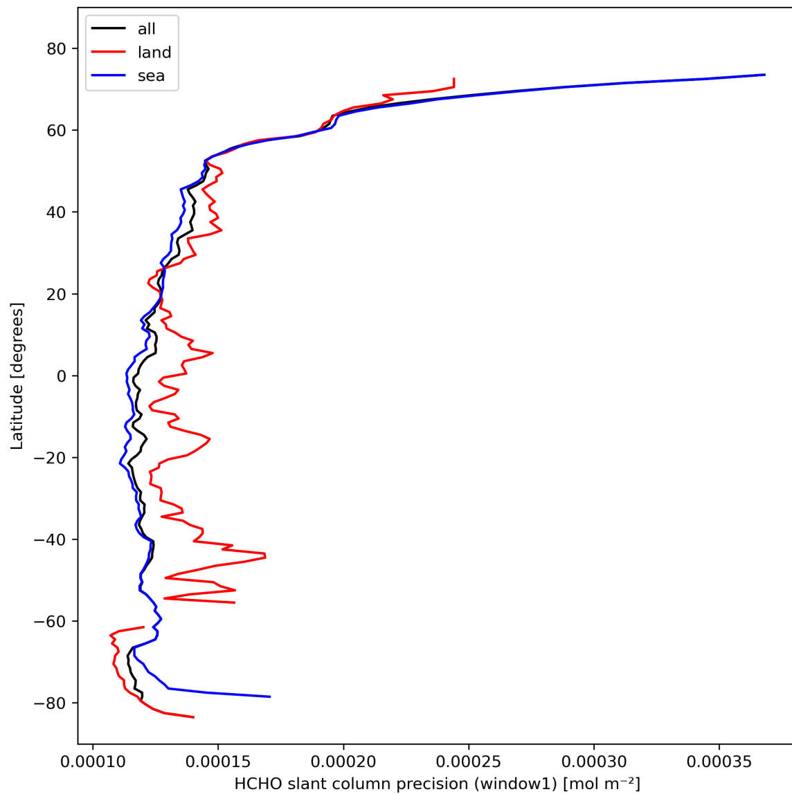
Figure 25: Zonal average of “HCHO slant column precision (window1)” for 2023-10-23 to 2023-10-25.
