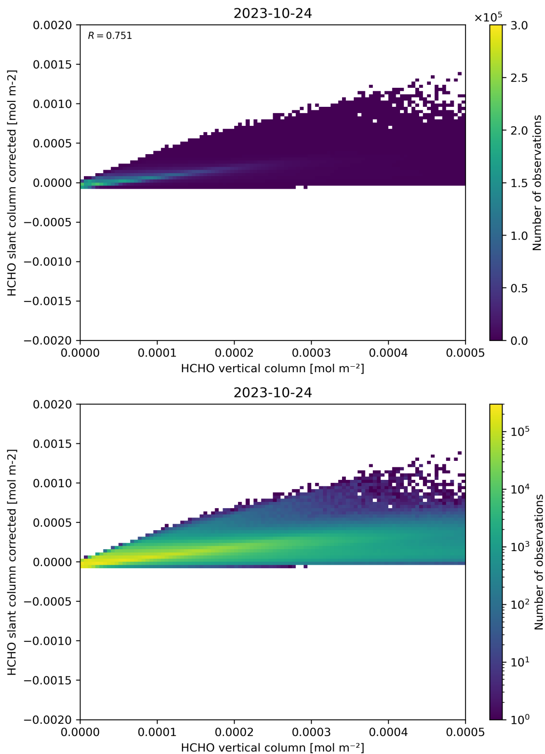
Figure 127: Scatter density plot of “HCHO vertical column” against “HCHO slant column corrected” for 2023-10-23 to 2023-10-25.
