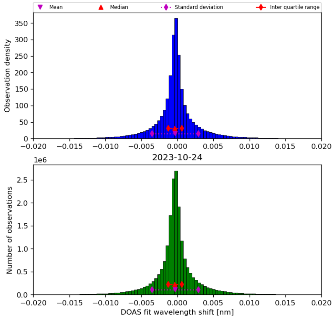
Figure 44: Histogram of “DOAS fit wavelength shift” for 2023-10-23 to 2023-10-25
