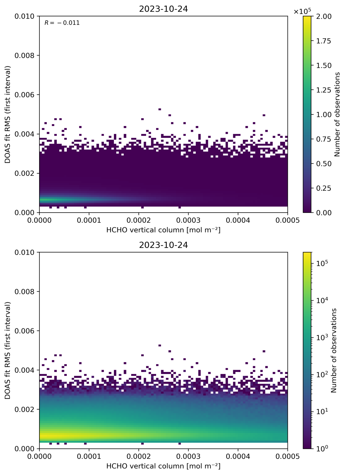
Figure 123: Scatter density plot of “HCHO vertical column” against “DOAS fit RMS (first interval)” for 2023-10-23 to 2023-10-25.
