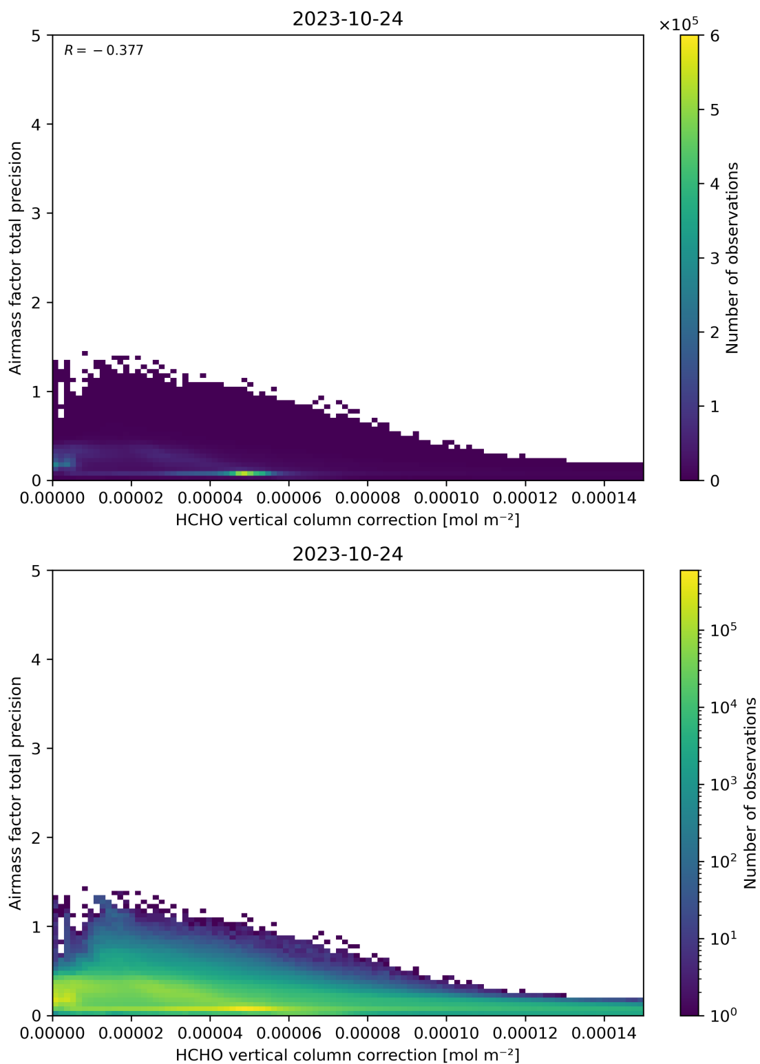
Figure 121: Scatter density plot of “HCHO vertical column correction” against “Airmass factor total precision” for 2023-10-23 to 2023-10-25.
