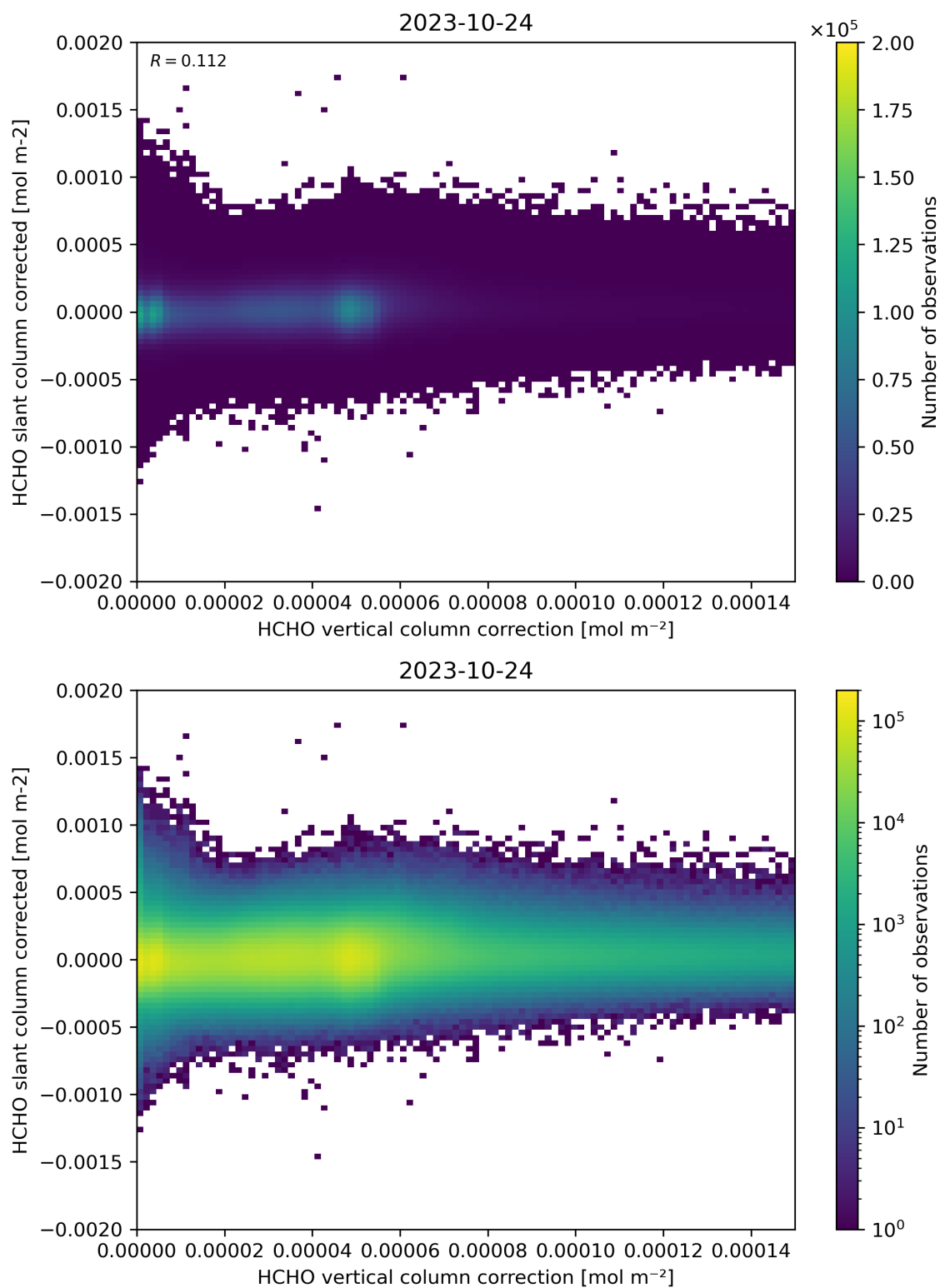
Figure 116: Scatter density plot of “HCHO vertical column correction” against “HCHO slant column corrected” for 2023-10-23 to 2023-10-25.
