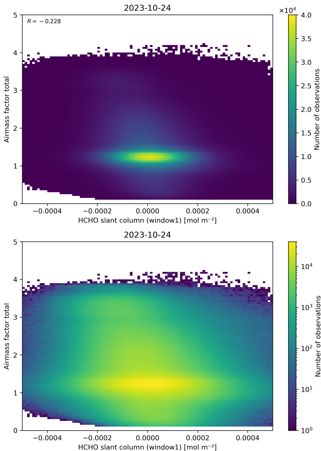
Figure 85: Scatter density plot of “HCHO slant column (window1)” against “Airmass factor total” for 2023-10-23 to 2023-10-25.
