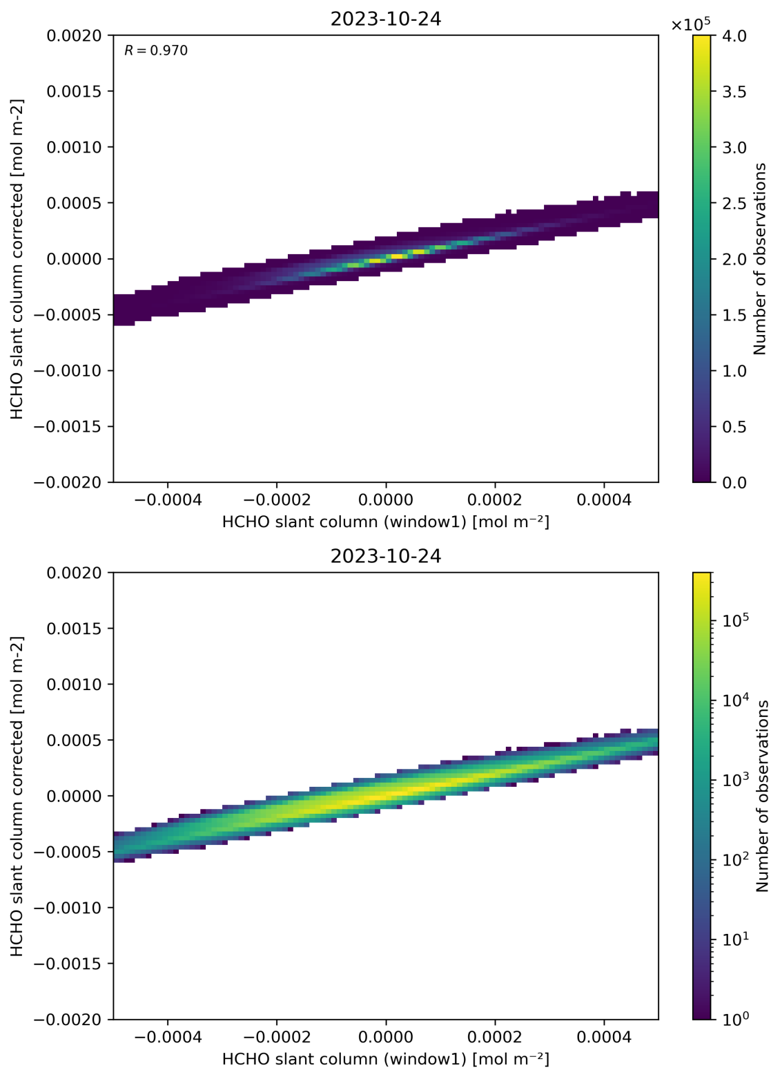
Figure 82: Scatter density plot of “HCHO slant column (window1)” against “HCHO slant column corrected” for 2023-10-23 to 2023-10-25.
