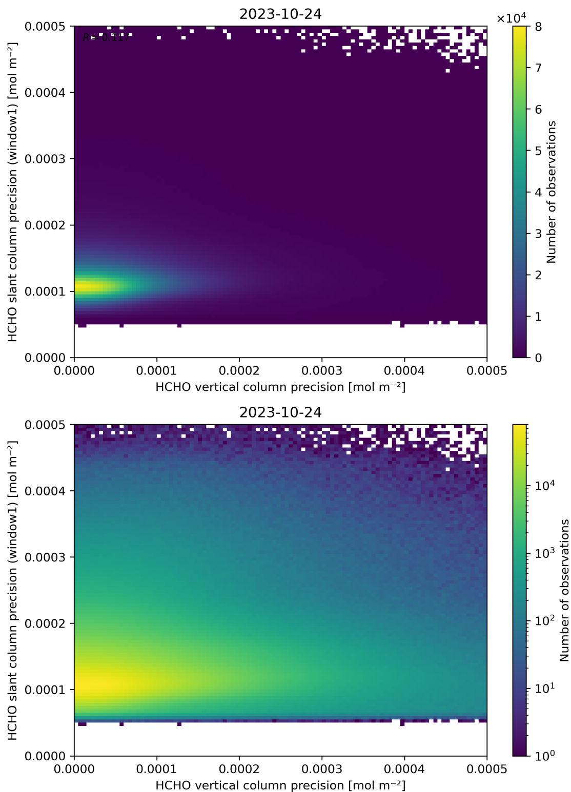
Figure 143: Scatter density plot of “HCHO vertical column precision” against “HCHO slant column precision (window1)” for 2023-10-23 to 2023-10-25.
