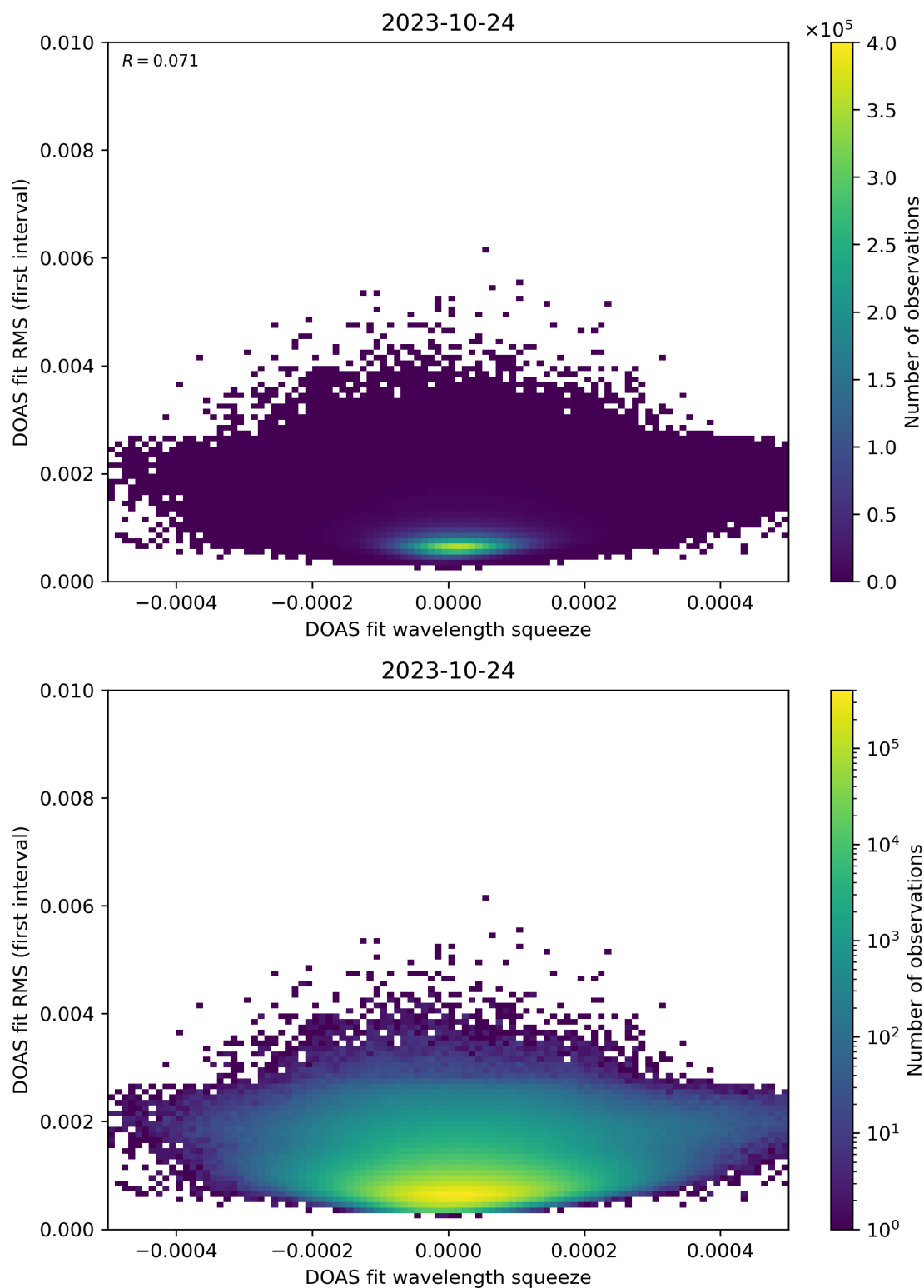
Figure 68: Scatter density plot of “DOAS fit wavelength squeeze” against “DOAS fit RMS (first interval)” for 2023-10-23 to 2023-10-25.
