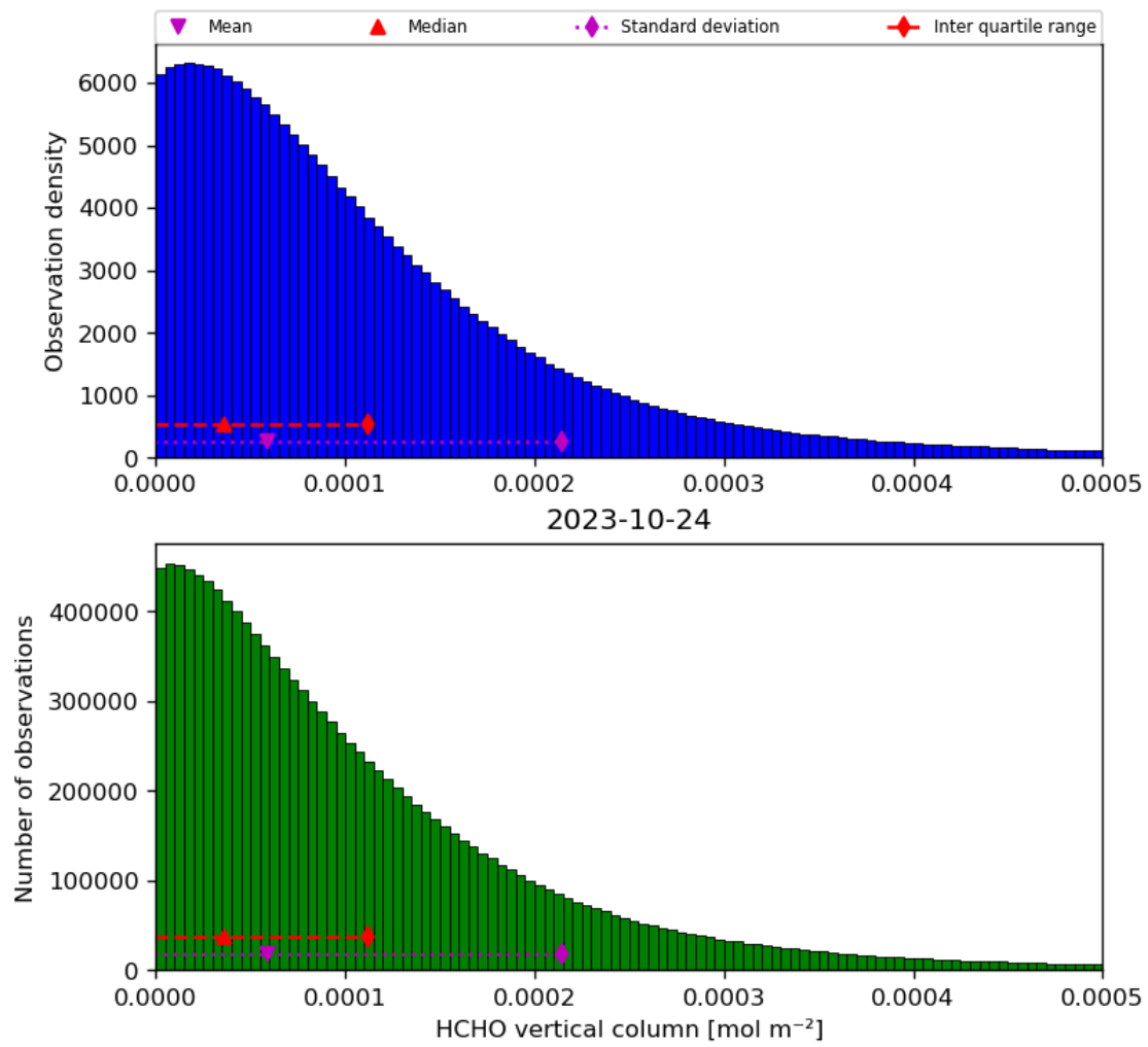
Figure 35: Histogram of “HCHO vertical column” for 2023-10-23 to 2023-10-25
