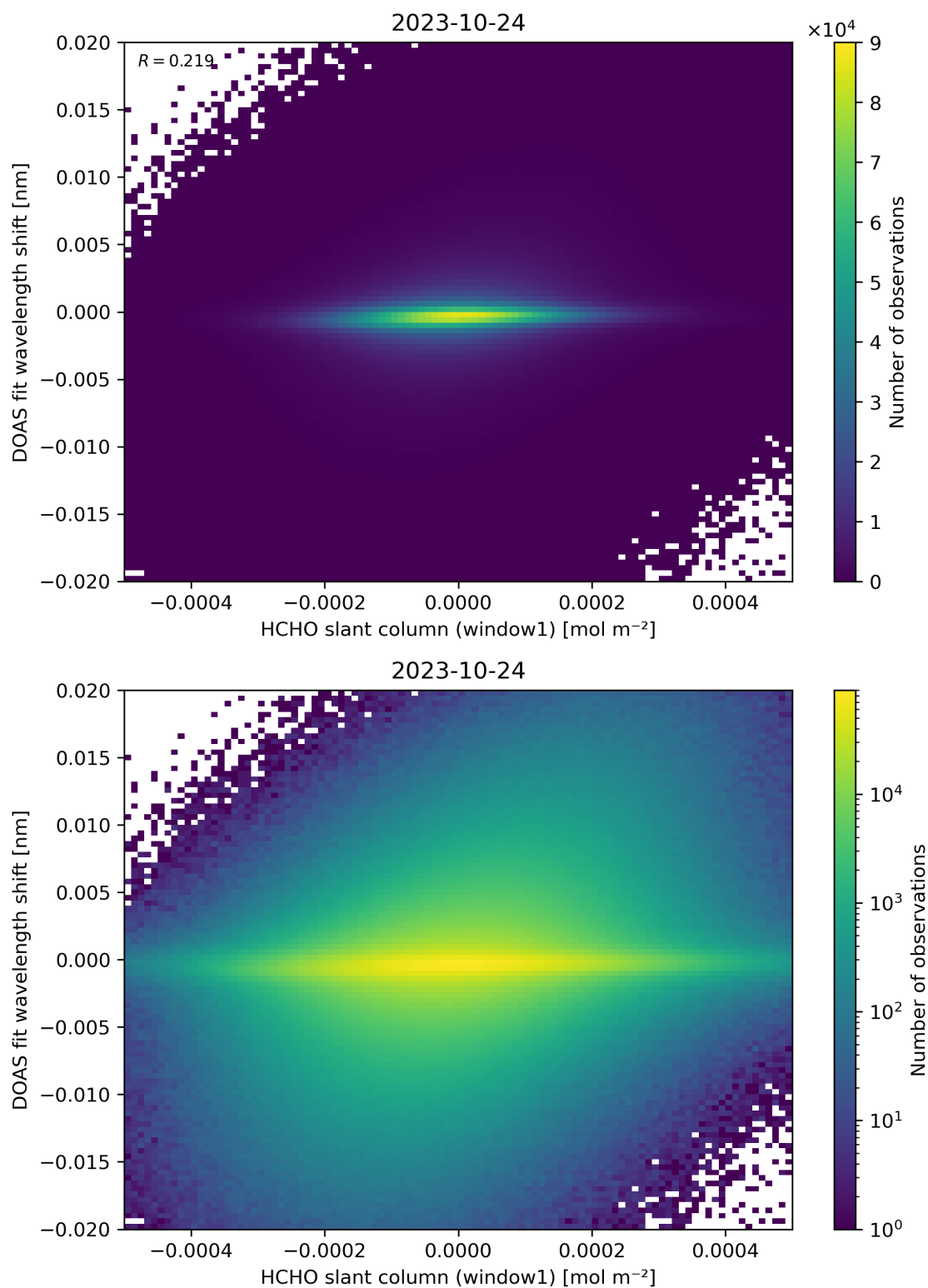
Figure 79: Scatter density plot of “HCHO slant column (window1)” against “DOAS fit wavelength shift” for 2023-10-23 to 2023-10-25.
