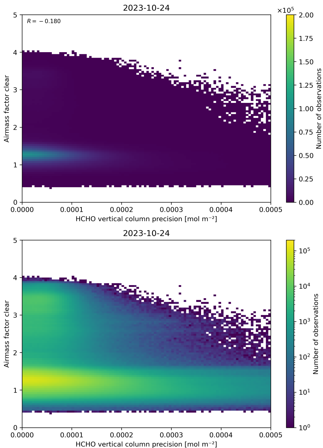
Figure 139: Scatter density plot of “HCHO vertical column precision” against “Airmass factor clear” for 2023-10-23 to 2023-10-25.
