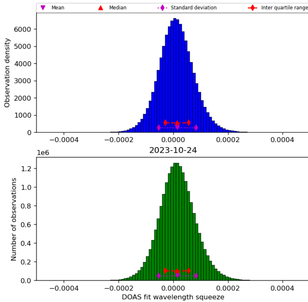
Figure 45: Histogram of “DOAS fit wavelength squeeze” for 2023-10-23 to 2023-10-25
