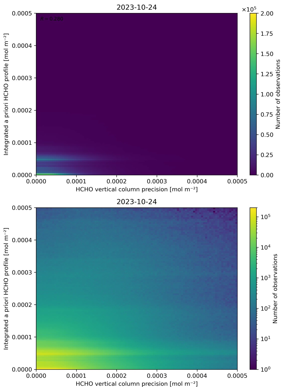
Figure 147: Scatter density plot of “HCHO vertical column precision” against “Integrated a priori HCHO profile” for 2023-10-23 to 2023-10-25.
