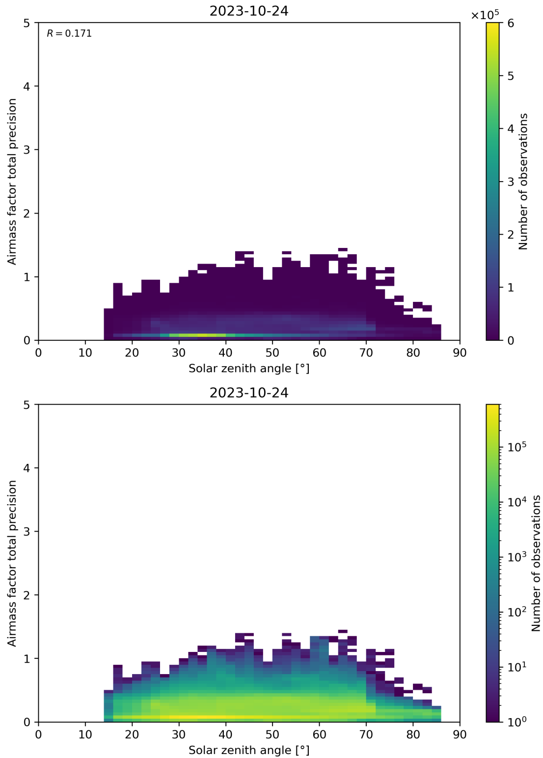
Figure 176: Scatter density plot of “Solar zenith angle” against “Airmass factor total precision” for 2023-10-23 to 2023-10-25.
