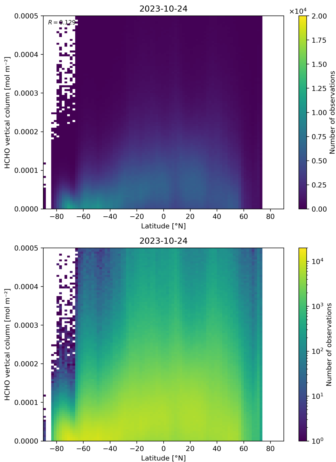
Figure 163: Scatter density plot of “Latitude” against “HCHO vertical column” for 2023-10-23 to 2023-10-25.
