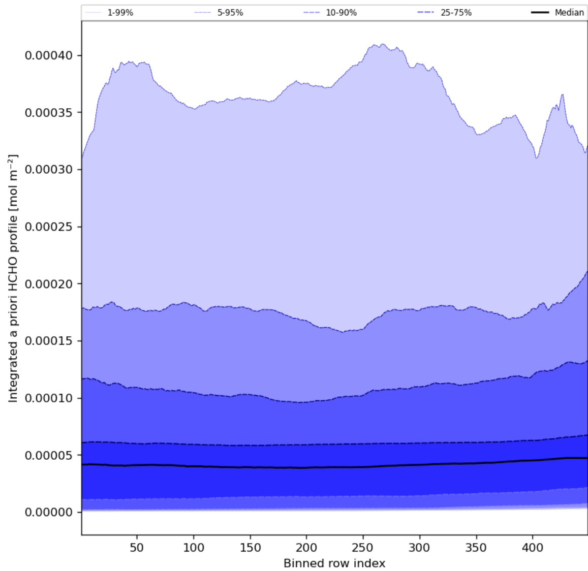
Figure 57: Along track statistics of "Integrated a priori HCHO profile" for 2023-10-23 to 2023-10-25
