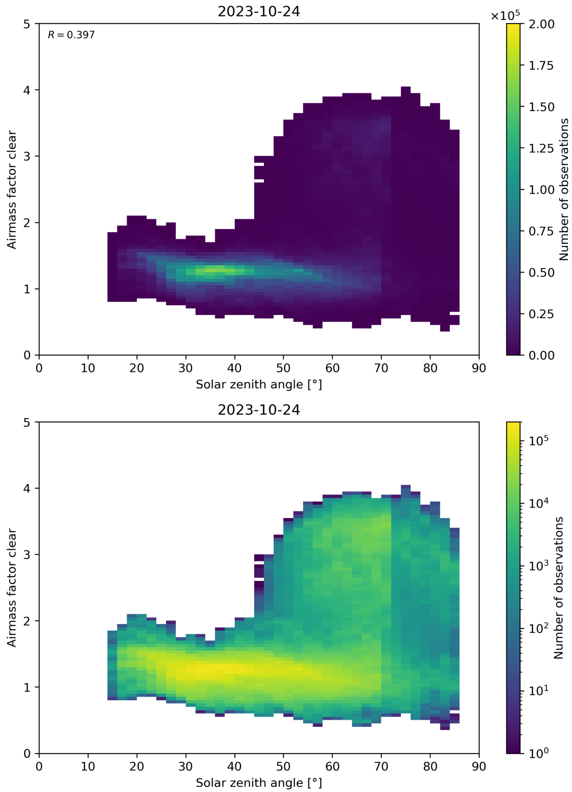
Figure 170: Scatter density plot of “Solar zenith angle” against “Airmass factor clear” for 2023-10-23 to 2023-10-25.
