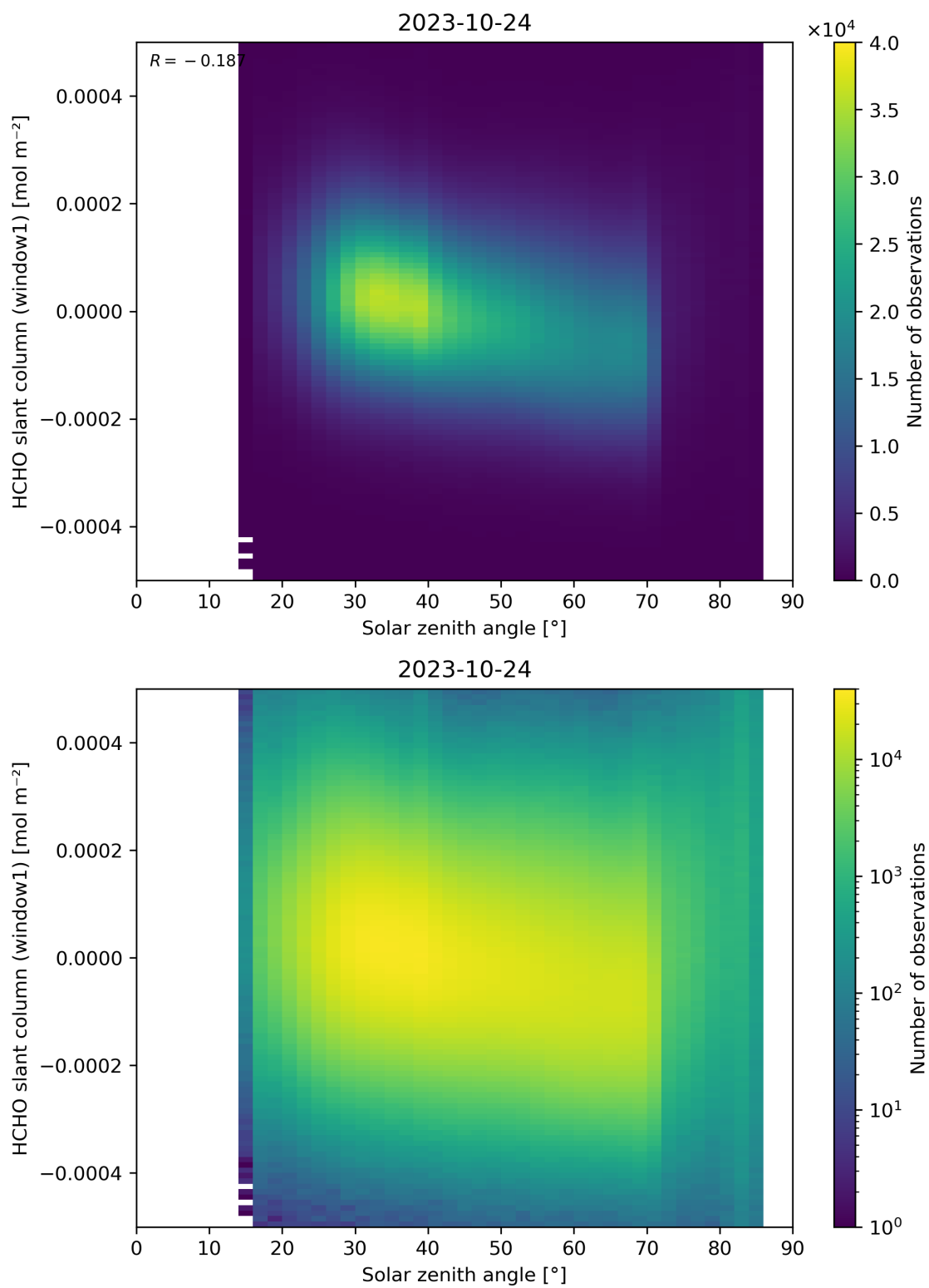
Figure 173: Scatter density plot of “Solar zenith angle” against “HCHO slant column (window1)” for 2023-10-23 to 2023-10-25.
