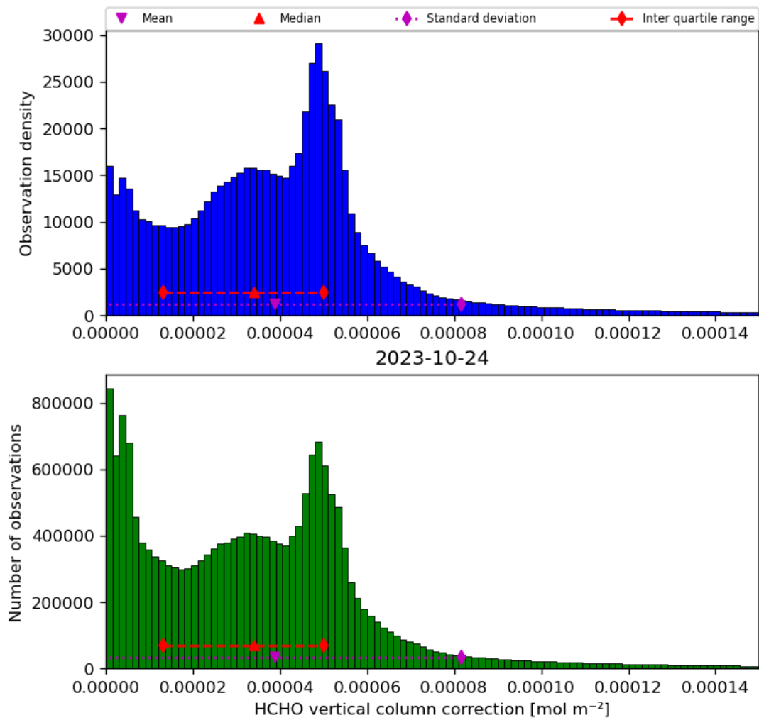
Figure 37: Histogram of “HCHO vertical column correction” for 2023-10-23 to 2023-10-25
