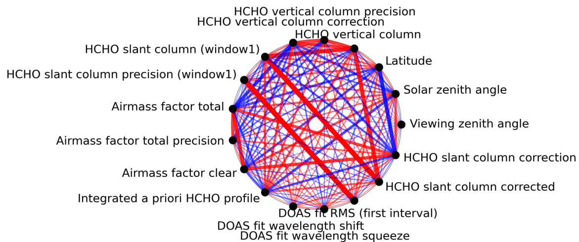
Figure 1: Map of correlation graph for 2023-10-23 to 2023-10-25.
