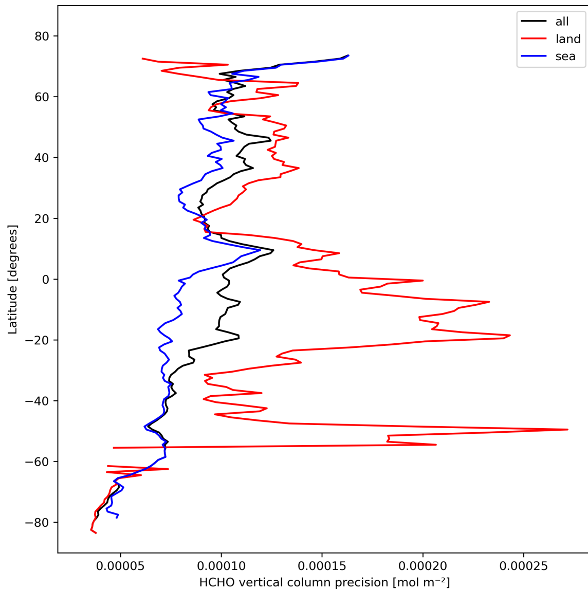
Figure 22: Zonal average of “HCHO vertical column precision” for 2023-10-23 to 2023-10-25.
