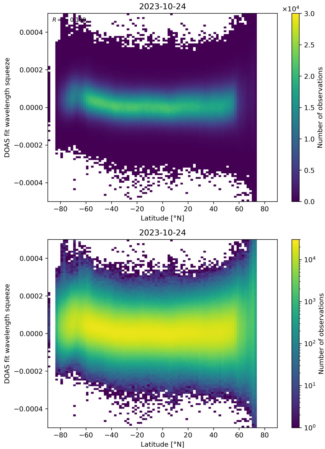
Figure 155: Scatter density plot of “Latitude” against “DOAS fit wavelength squeeze” for 2023-10-23 to 2023-10-25.
