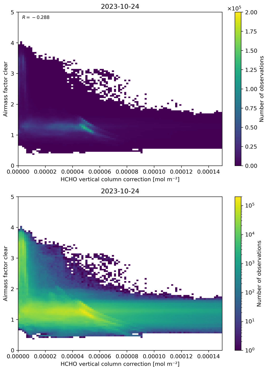
Figure 115: Scatter density plot of “HCHO vertical column correction” against “Airmass factor clear” for 2023-10-23 to 2023-10-25.
