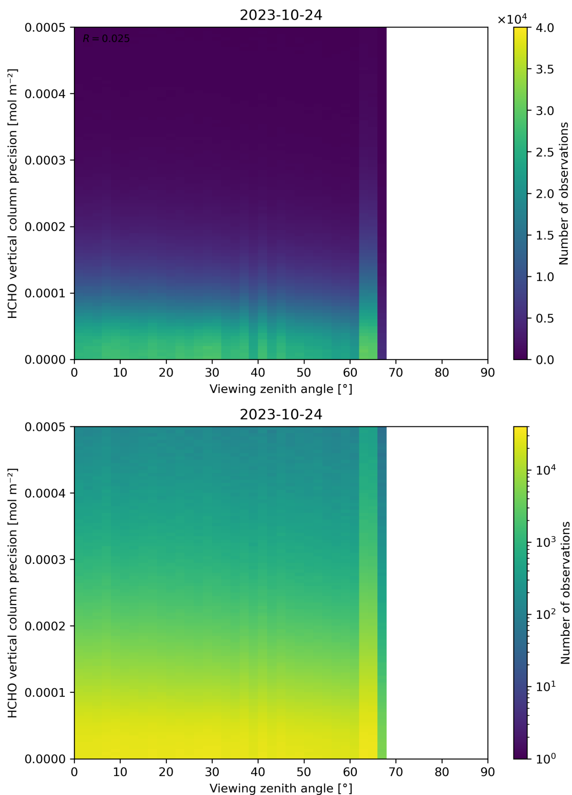
Figure 194: Scatter density plot of “Viewing zenith angle” against “HCHO vertical column precision” for 2023-10-23 to 2023-10-25.
