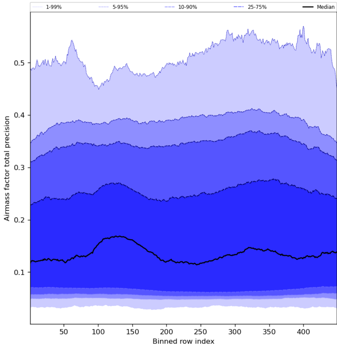
Figure 55: Along track statistics of “Airmass factor total precision” for 2023-10-23 to 2023-10-25
