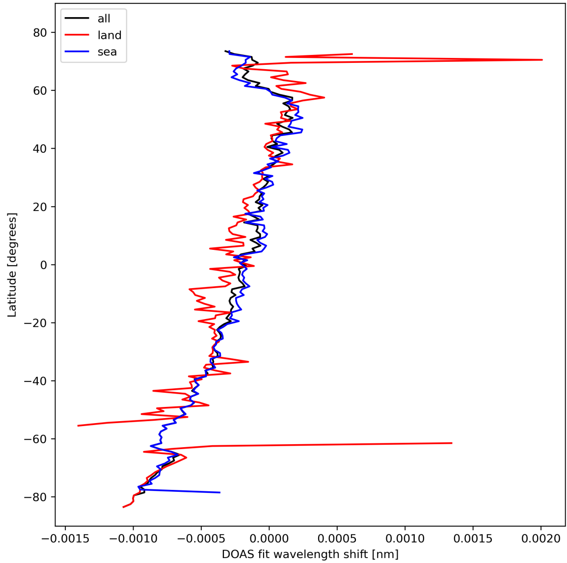
Figure 30: Zonal average of “DOAS fit wavelength shift” for 2023-10-23 to 2023-10-25.
