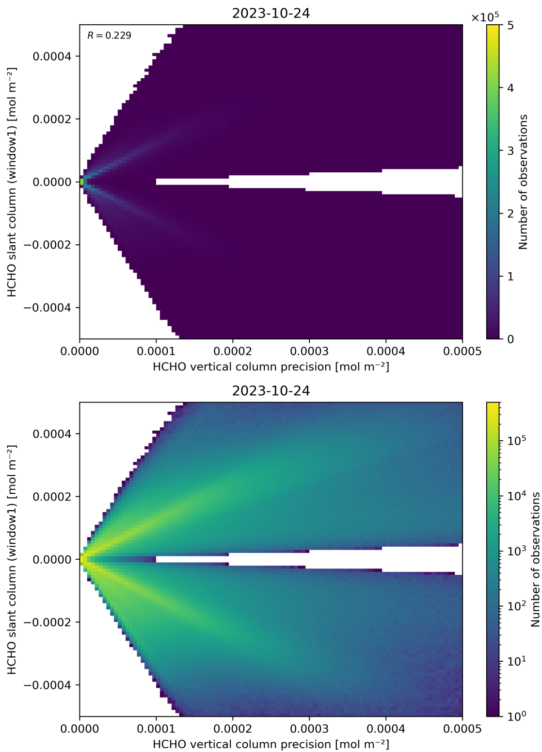
Figure 142: Scatter density plot of “HCHO vertical column precision” against “HCHO slant column (window1)” for 2023-10-23 to 2023-10-25.
