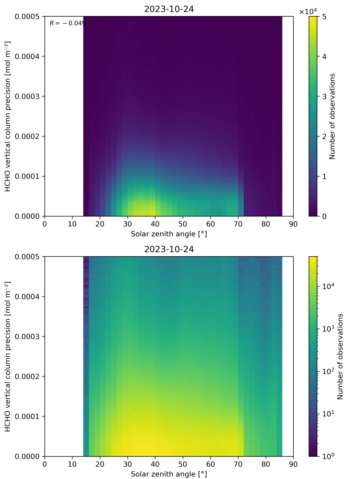
Figure 179: Scatter density plot of “Solar zenith angle” against “HCHO vertical column precision” for 2023-10-23 to 2023-10-25.
