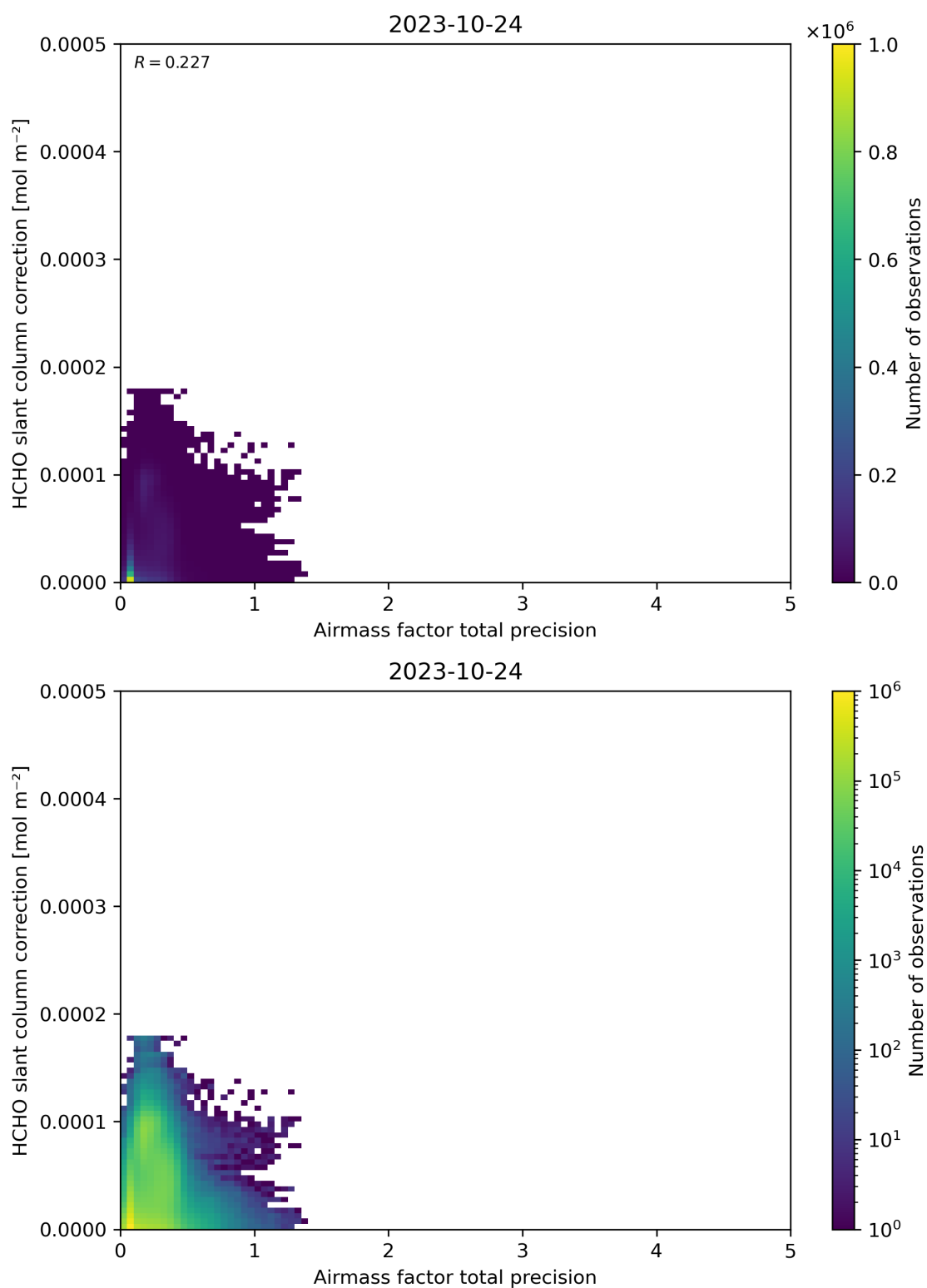
Figure 110: Scatter density plot of “Airmass factor total precision” against “HCHO slant column correction” for 2023-10-23 to 2023-10-25.
