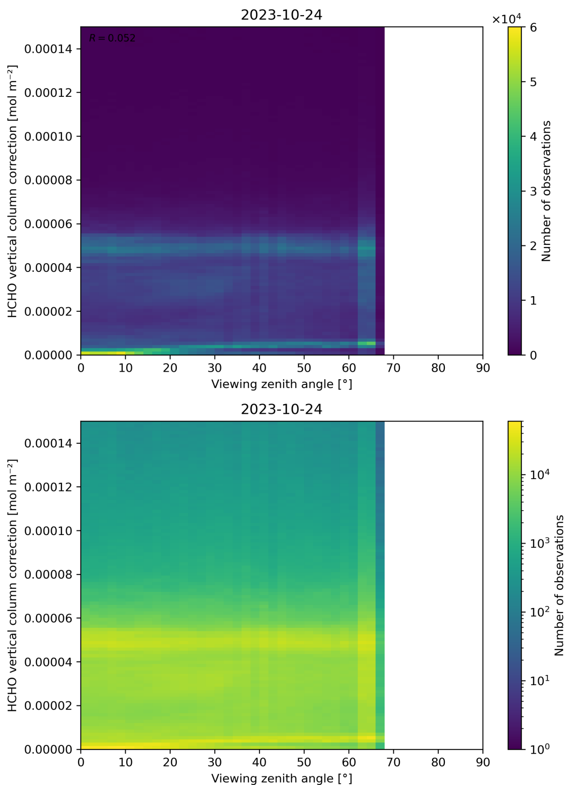
Figure 193: Scatter density plot of “Viewing zenith angle” against “HCHO vertical column correction” for 2023-10-23 to 2023-10-25.
