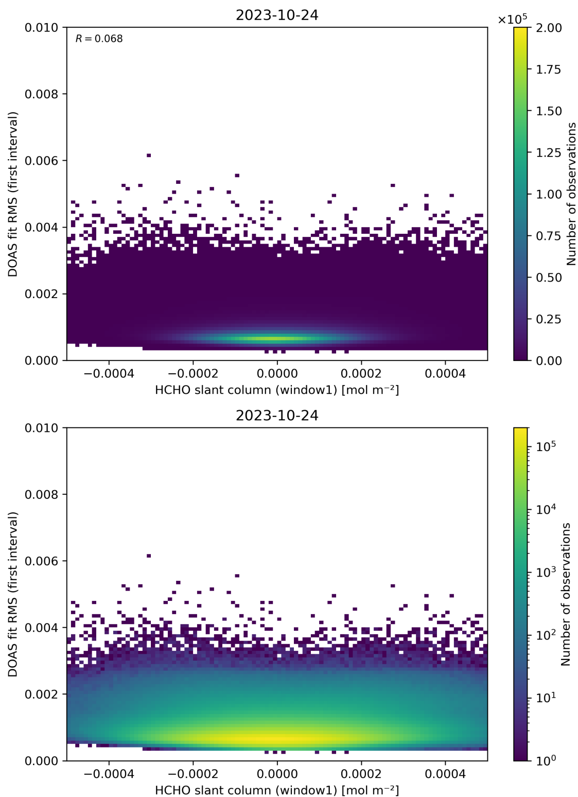
Figure 78: Scatter density plot of “HCHO slant column (window1)” against “DOAS fit RMS (first interval)” for 2023-10-23 to 2023-10-25.
