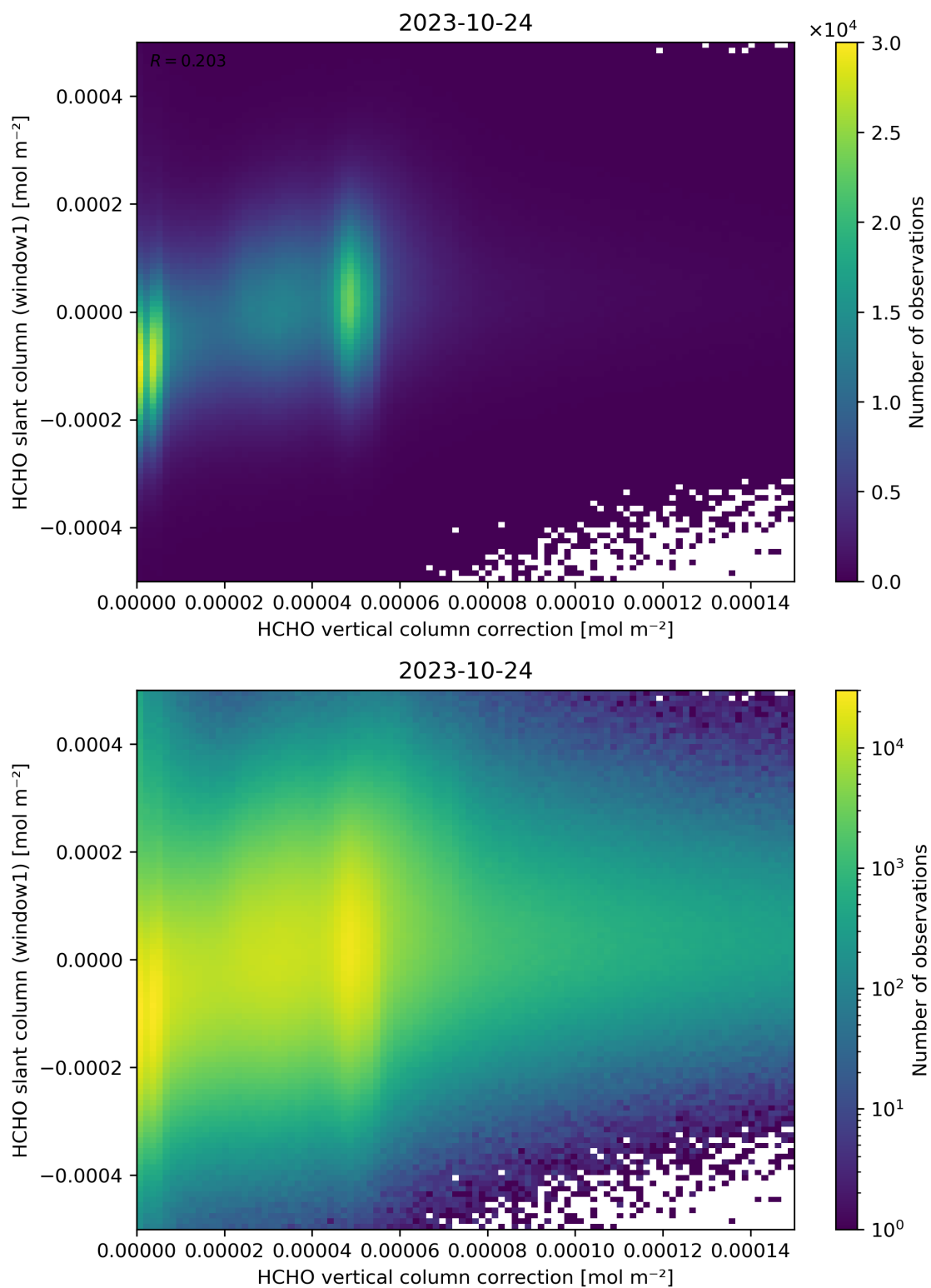
Figure 118: Scatter density plot of “HCHO vertical column correction” against “HCHO slant column (window1)” for 2023-10-23 to 2023-10-25.
