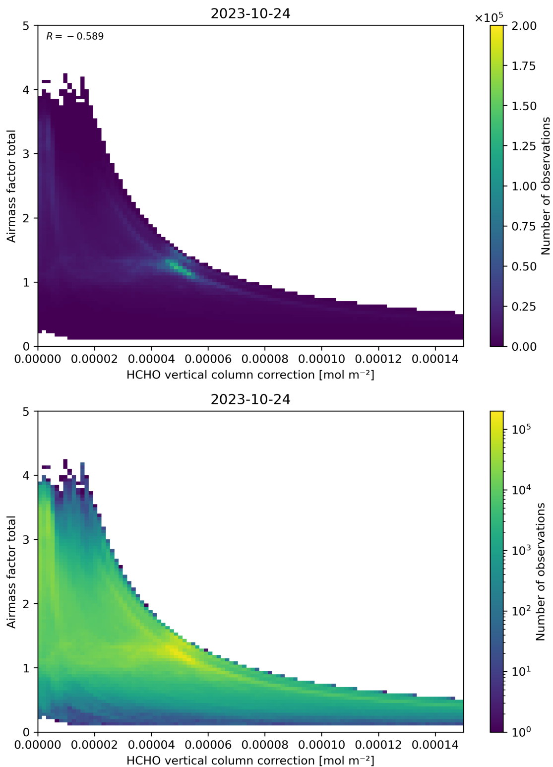
Figure 120: Scatter density plot of “HCHO vertical column correction” against “Airmass factor total” for 2023-10-23 to 2023-10-25.
