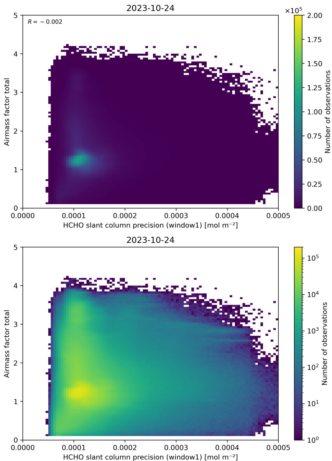
Figure 94: Scatter density plot of “HCHO slant column precision (window1)” against “Airmass factor total” for 2023-10-23 to 2023-10-25.
