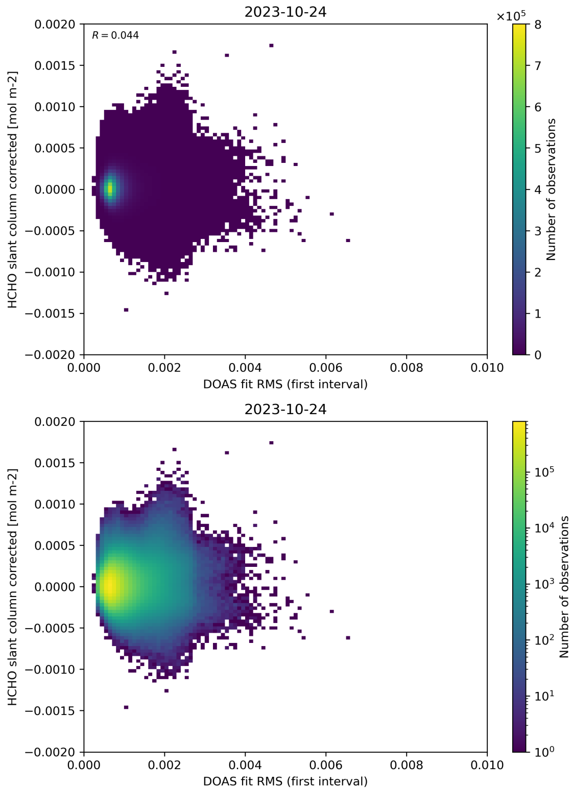
Figure 62: Scatter density plot of “DOAS fit RMS (first interval)” against “HCHO slant column corrected” for 2023-10-23 to 2023-10-25.
