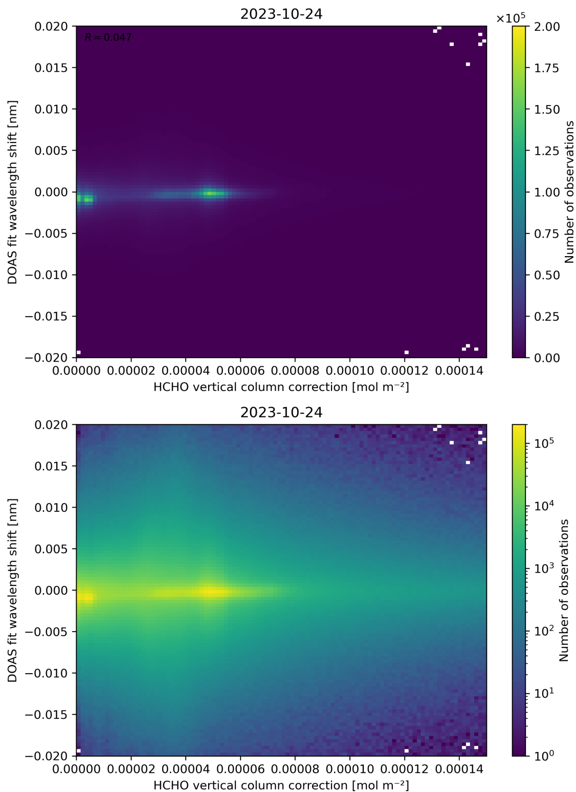
Figure 113: Scatter density plot of “HCHO vertical column correction” against “DOAS fit wavelength shift” for 2023-10-23 to 2023-10-25.
