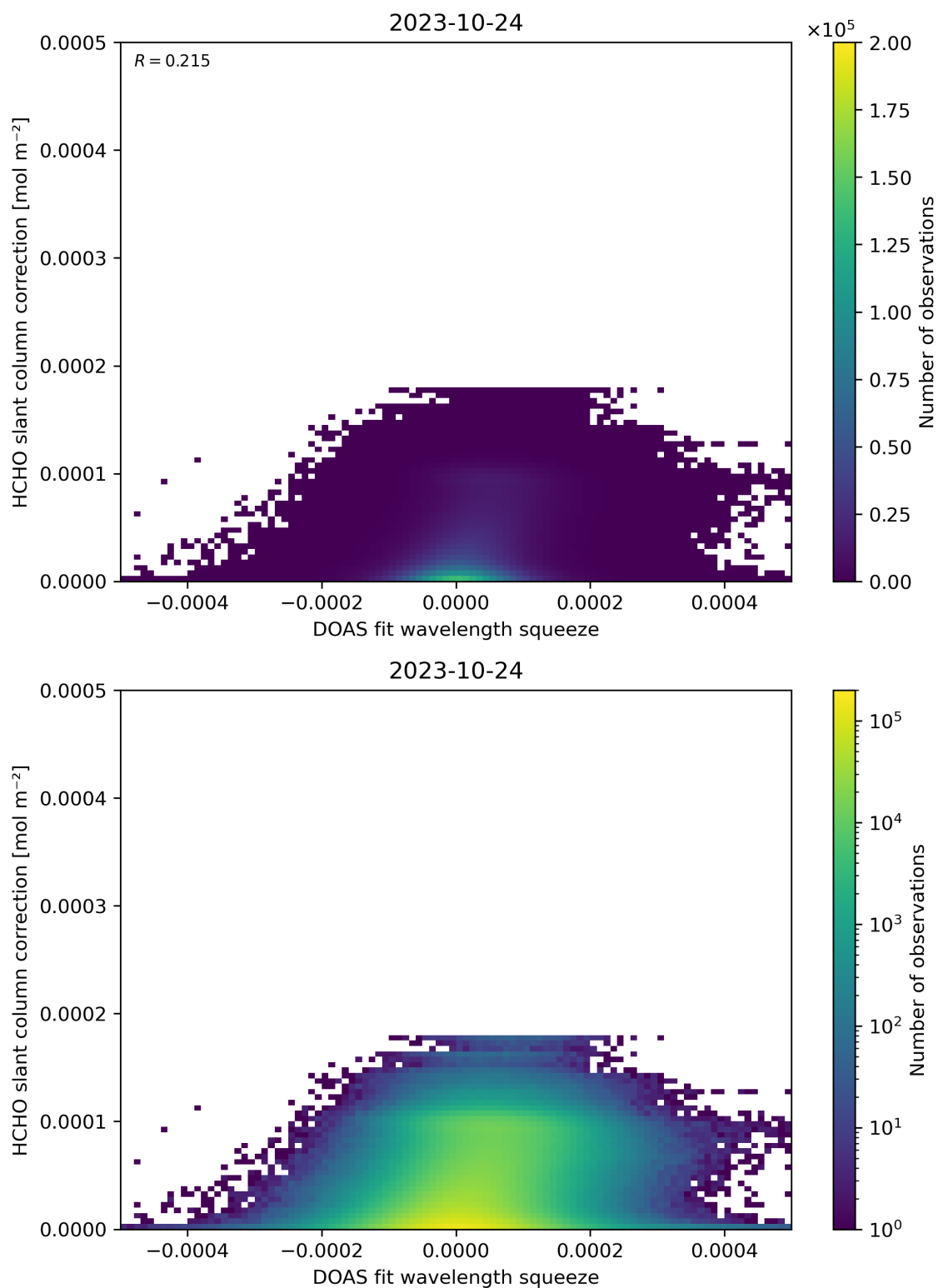
Figure 70: Scatter density plot of “DOAS fit wavelength squeeze” against “HCHO slant column correction” for 2023-10-23 to 2023-10-25.
