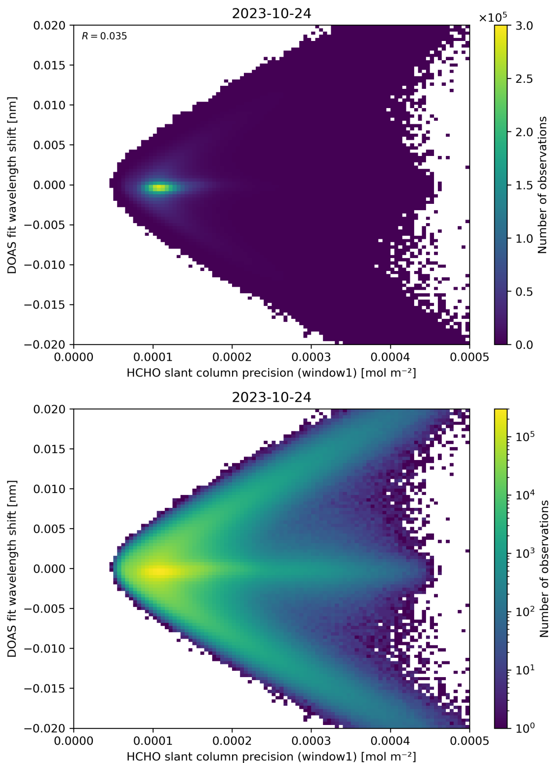
Figure 89: Scatter density plot of “HCHO slant column precision (window1)” against “DOAS fit wavelength shift” for 2023-10-23 to 2023-10-25.
