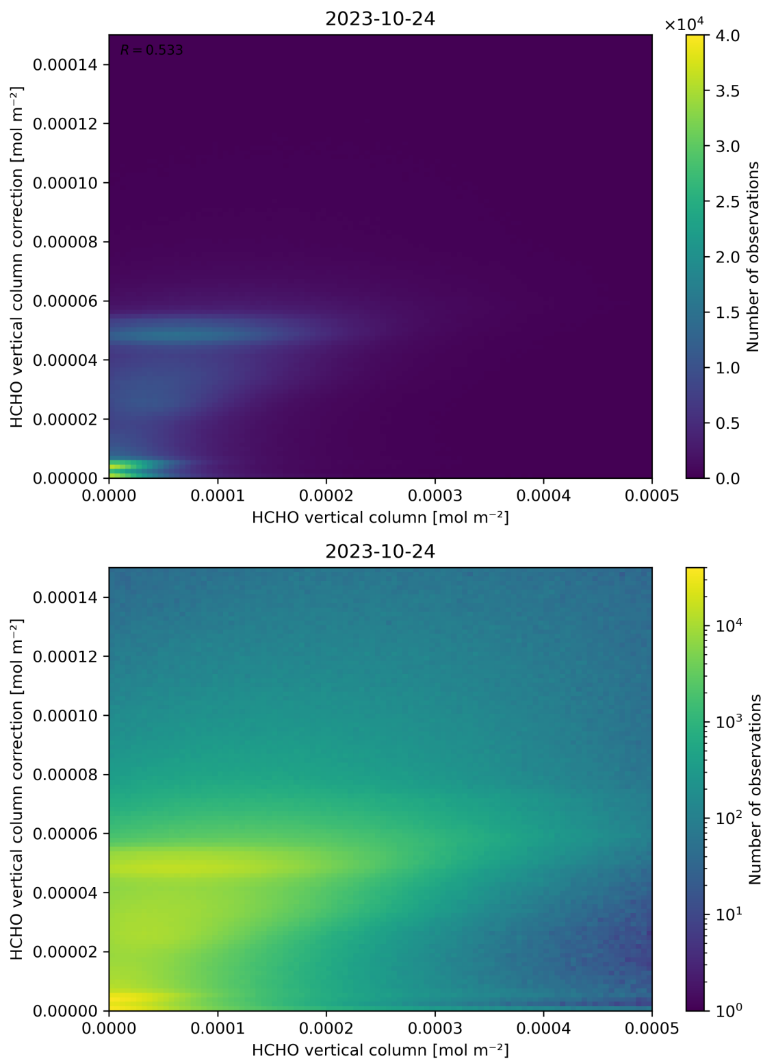
Figure 133: Scatter density plot of “HCHO vertical column” against “HCHO vertical column correction” for 2023-10-23 to 2023-10-25.
