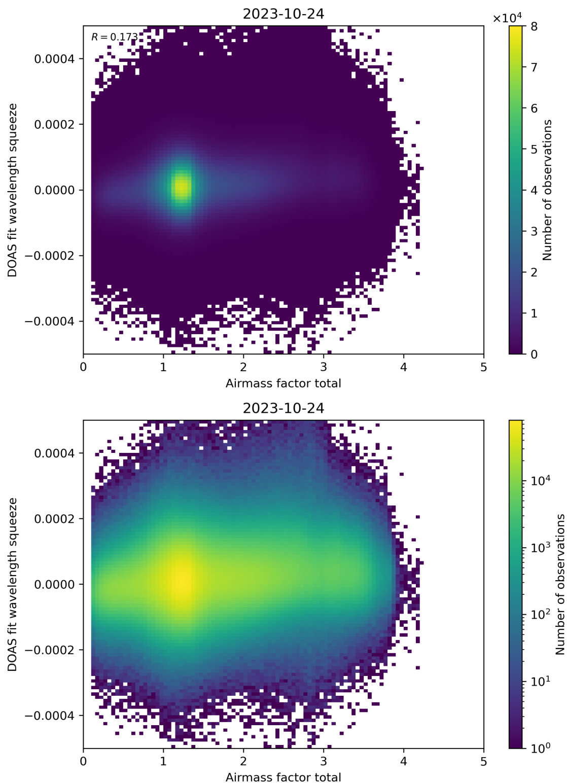
Figure 99: Scatter density plot of “Airmass factor total” against “DOAS fit wavelength squeeze” for 2023-10-23 to 2023-10-25.
