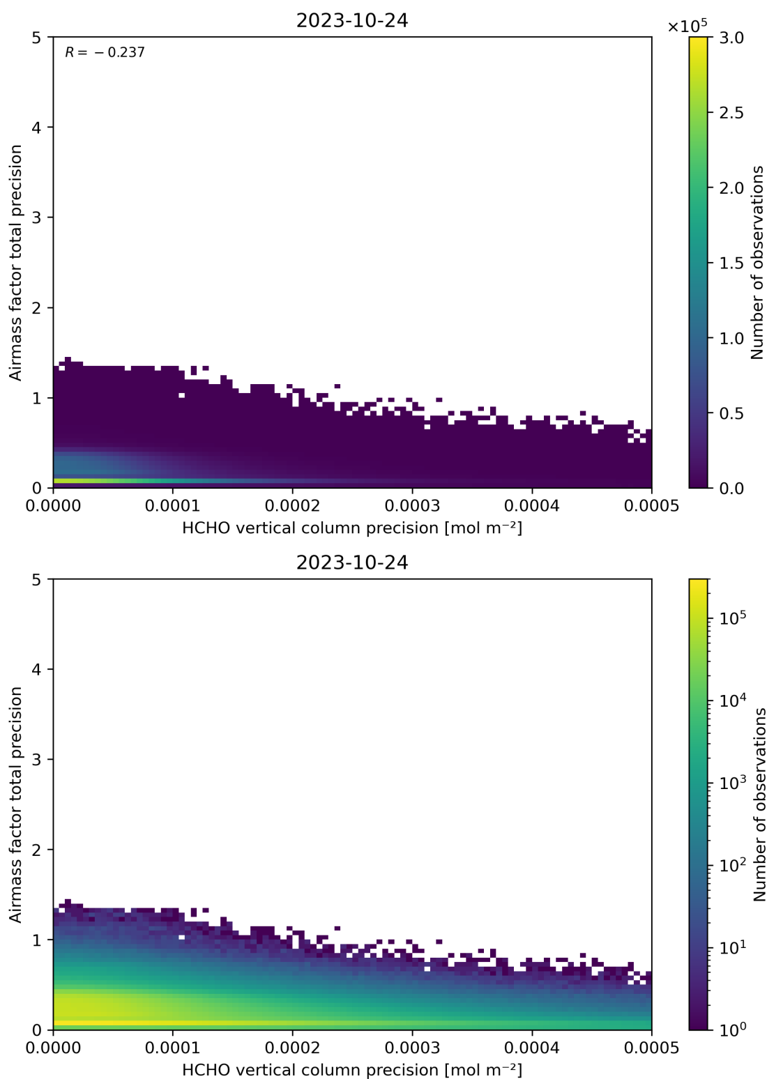
Figure 145: Scatter density plot of “HCHO vertical column precision” against “Airmass factor total precision” for 2023-10-23 to 2023-10-25.
