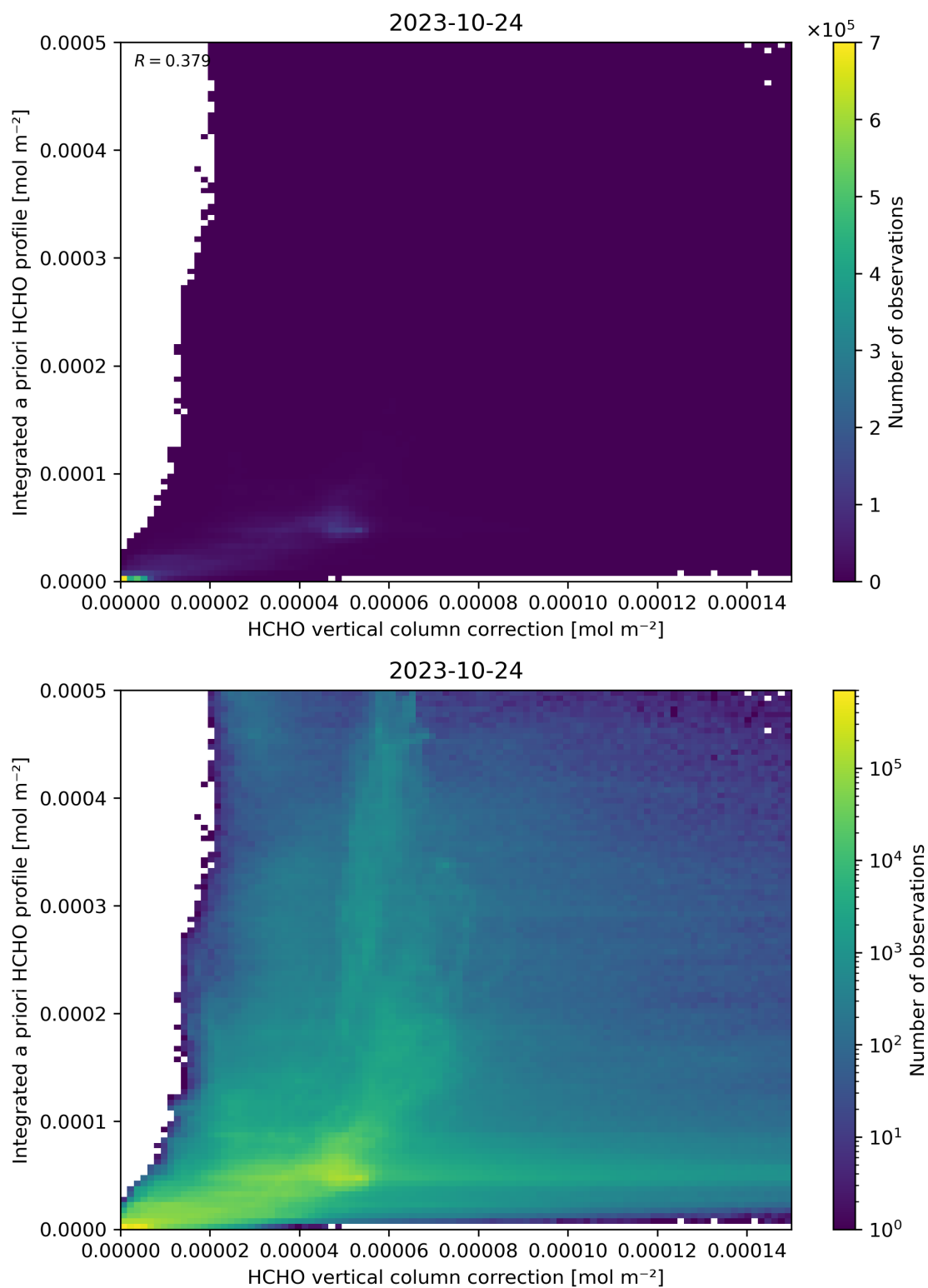
Figure 122: Scatter density plot of “HCHO vertical column correction” against “Integrated a priori HCHO profile” for 2023-10-23 to 2023-10-25.
