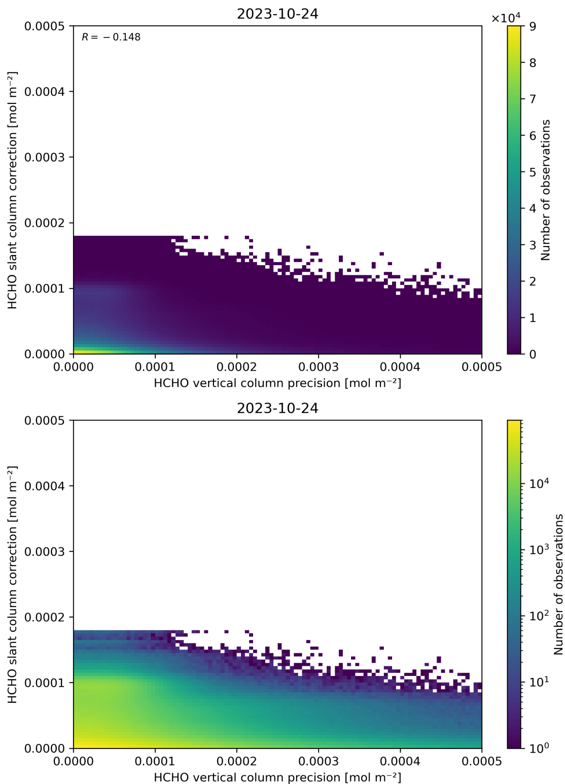
Figure 141: Scatter density plot of “HCHO vertical column precision” against “HCHO slant column correction” for 2023-10-23 to 2023-10-25.
