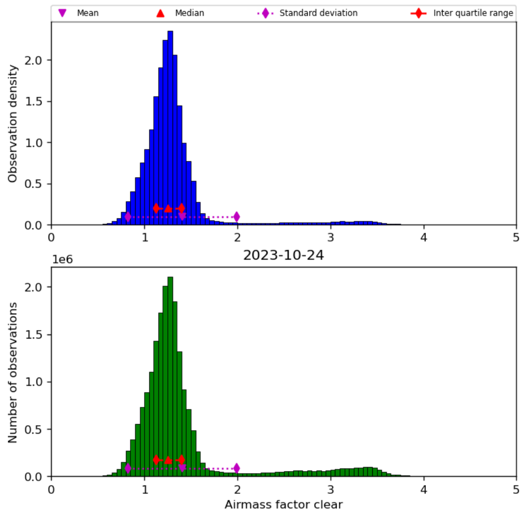
Figure 42: Histogram of “Airmass factor clear” for 2023-10-23 to 2023-10-25
