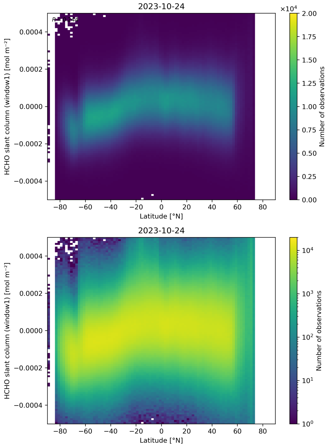
Figure 159: Scatter density plot of “Latitude” against “HCHO slant column (window1)” for 2023-10-23 to 2023-10-25.
