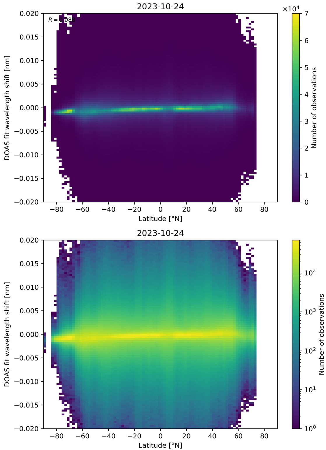
Figure 154: Scatter density plot of “Latitude” against “DOAS fit wavelength shift” for 2023-10-23 to 2023-10-25.
