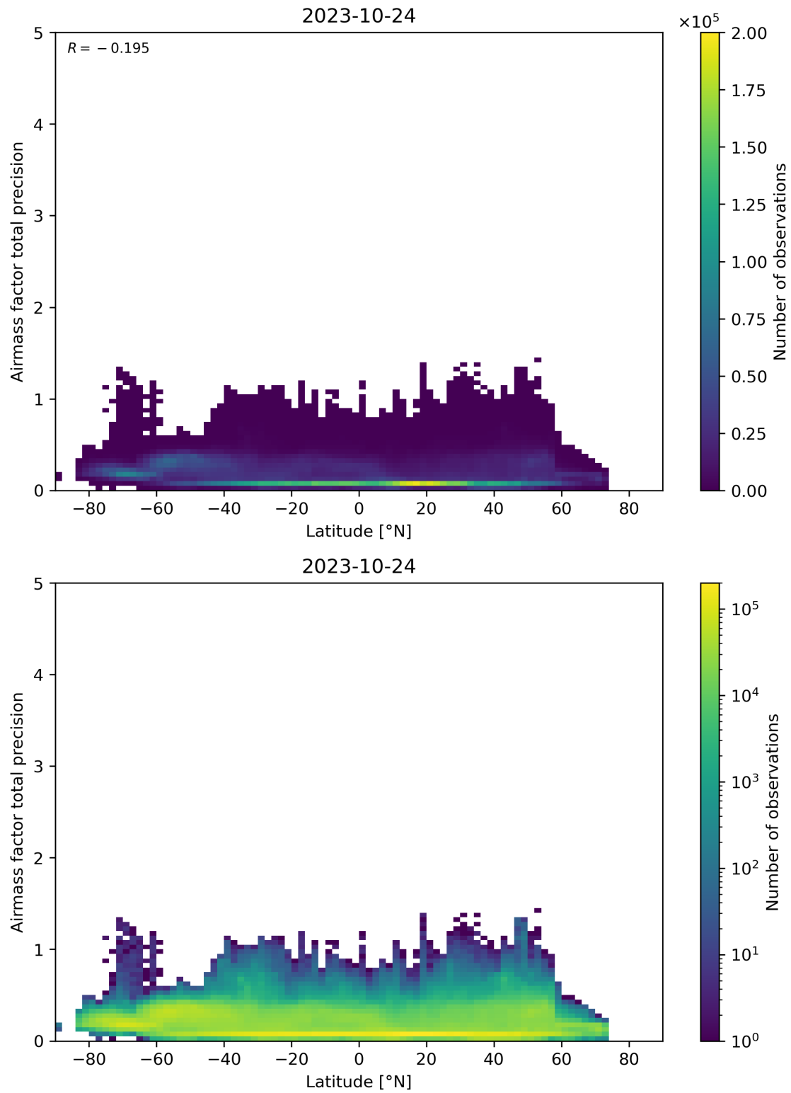
Figure 162: Scatter density plot of “Latitude” against “Airmass factor total precision” for 2023-10-23 to 2023-10-25.
