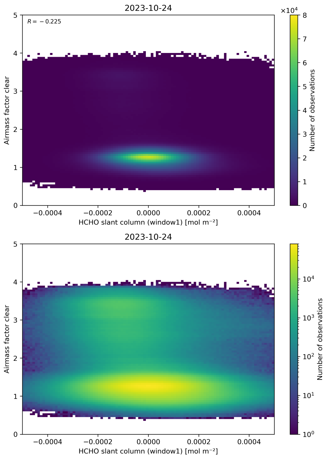
Figure 81: Scatter density plot of “HCHO slant column (window1)” against “Airmass factor clear” for 2023-10-23 to 2023-10-25.
