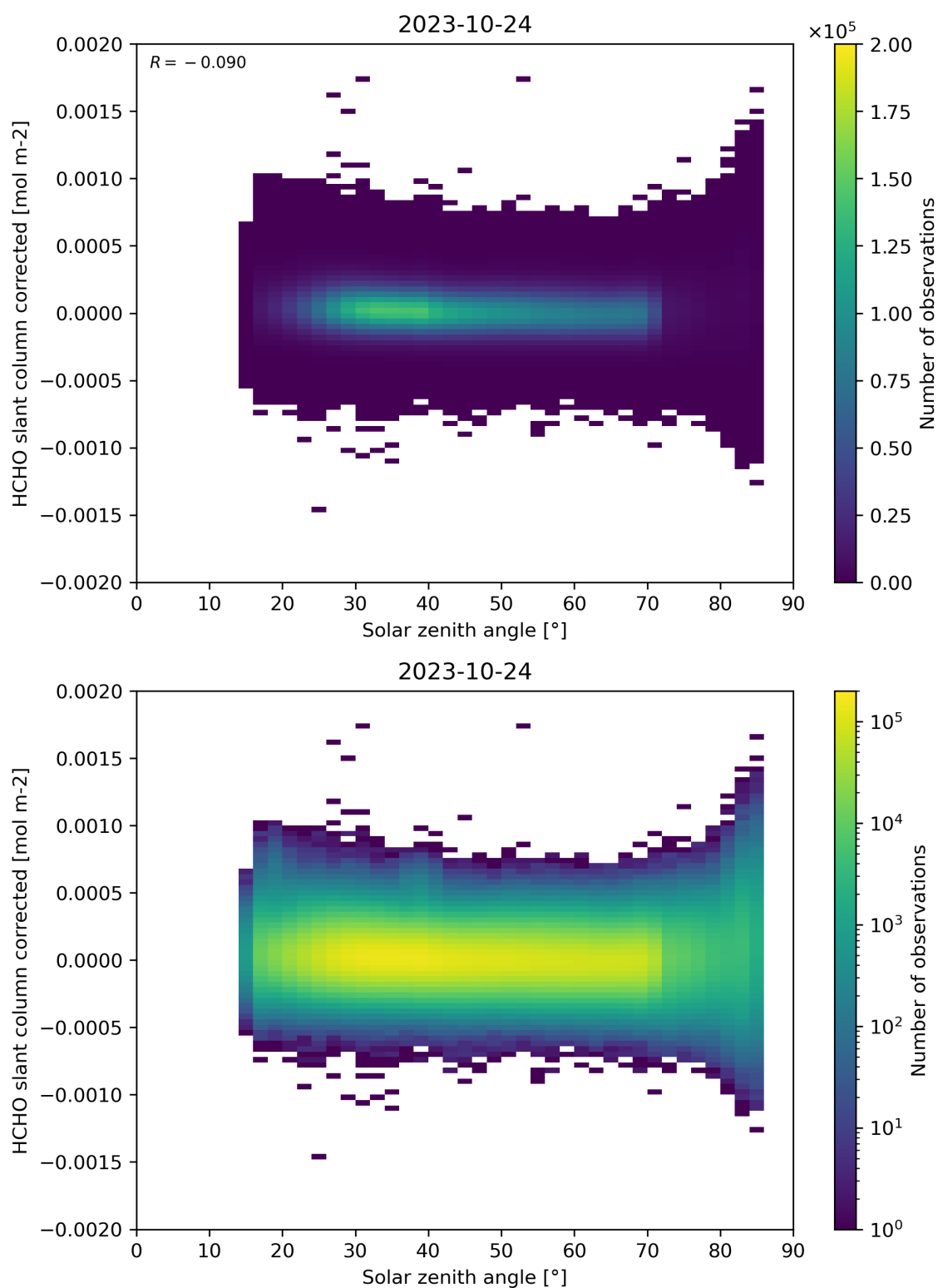
Figure 171: Scatter density plot of “Solar zenith angle” against “HCHO slant column corrected” for 2023-10-23 to 2023-10-25.
