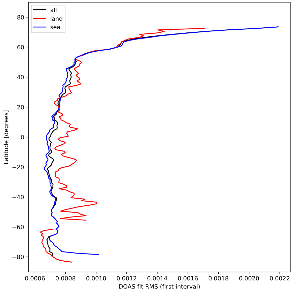
Figure 32: Zonal average of “DOAS fit RMS (first interval)” for 2023-10-23 to 2023-10-25.
