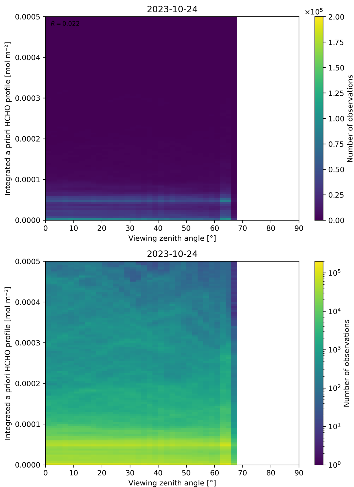
Figure 195: Scatter density plot of “Viewing zenith angle” against “Integrated a priori HCHO profile” for 2023-10-23 to 2023-10-25.
