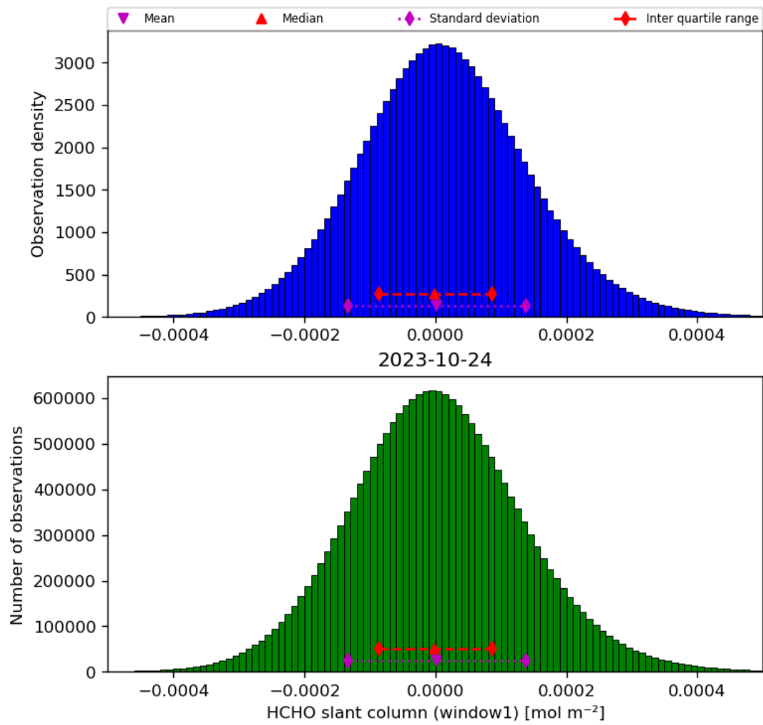
Figure 38: Histogram of “HCHO slant column (window1)” for 2023-10-23 to 2023-10-25
