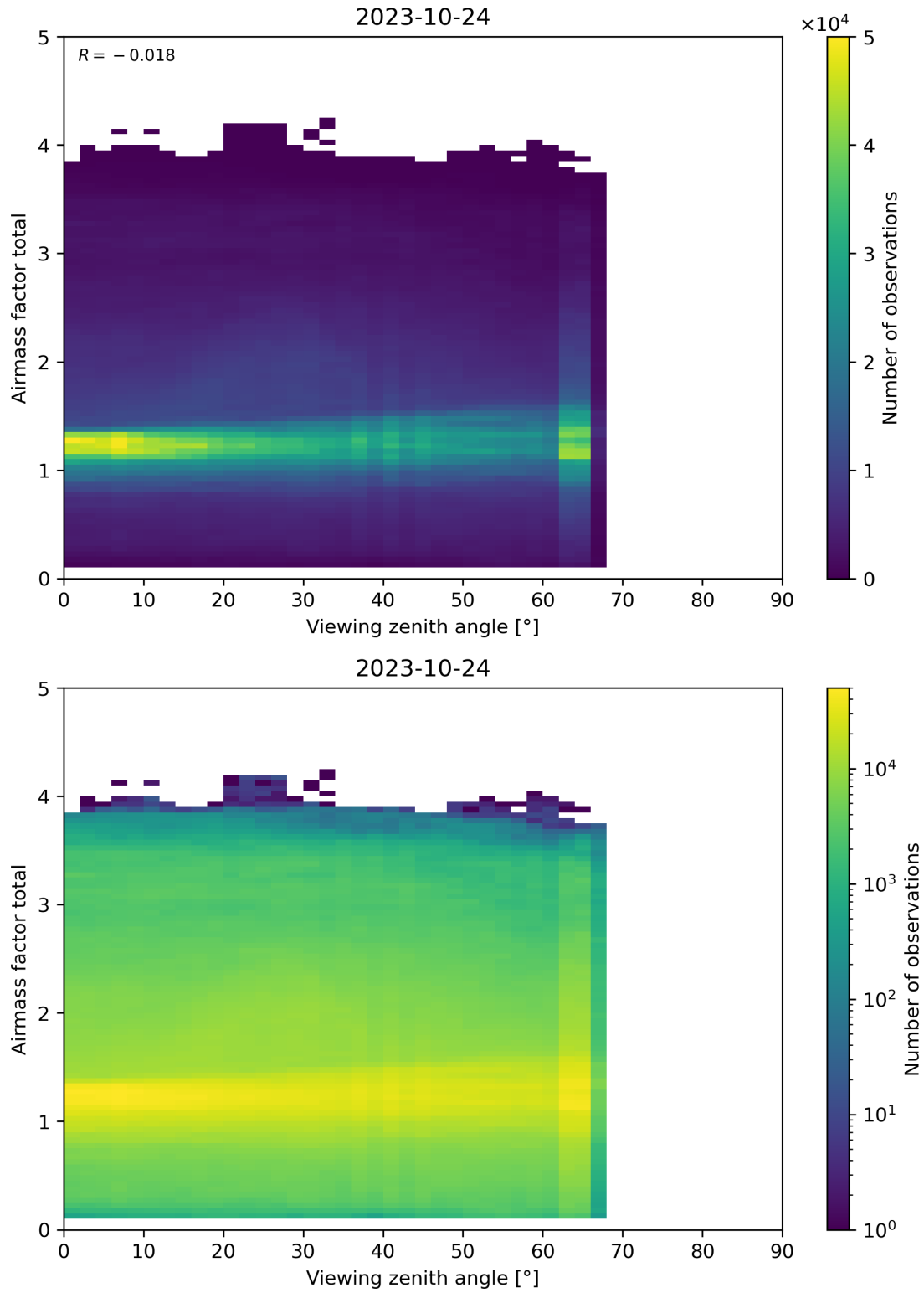
Figure 190: Scatter density plot of “Viewing zenith angle” against “Airmass factor total” for 2023-10-23 to 2023-10-25.
