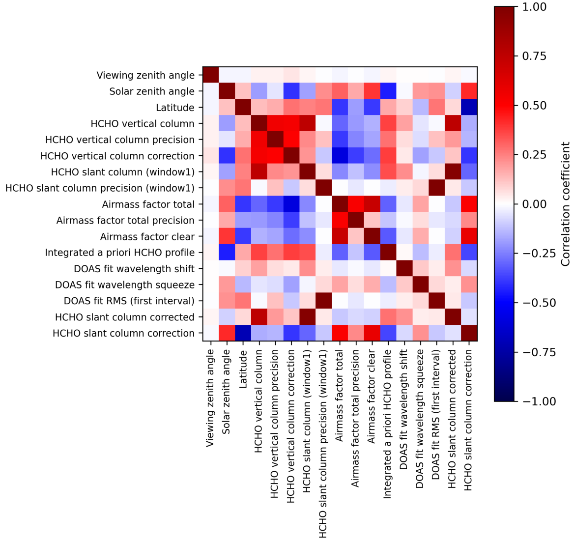
Figure 2: Map of correlation matrix for 2023-10-23 to 2023-10-25.
