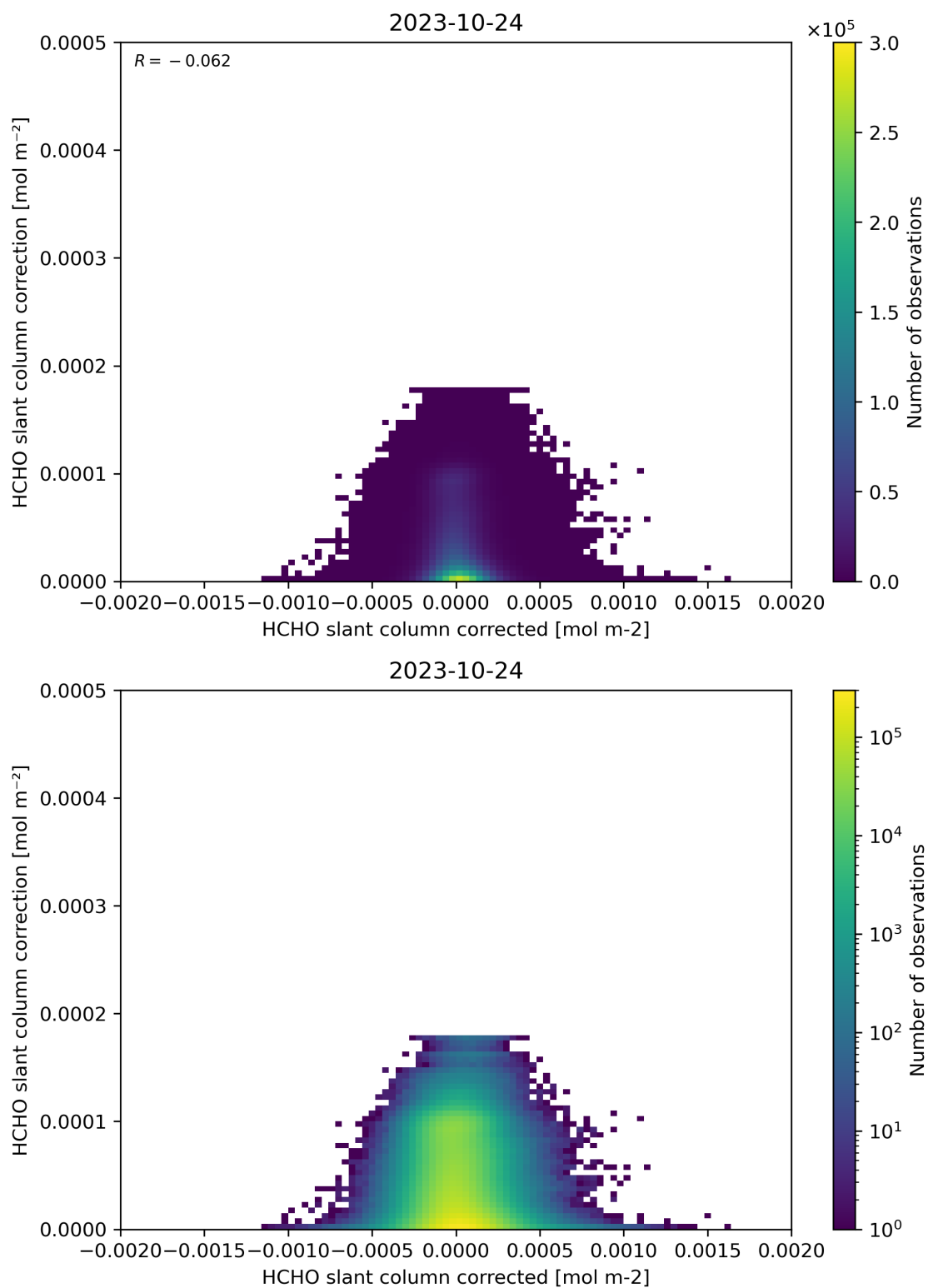
Figure 77: Scatter density plot of “HCHO slant column corrected” against “HCHO slant column correction” for 2023-10-23 to 2023-10-25.
