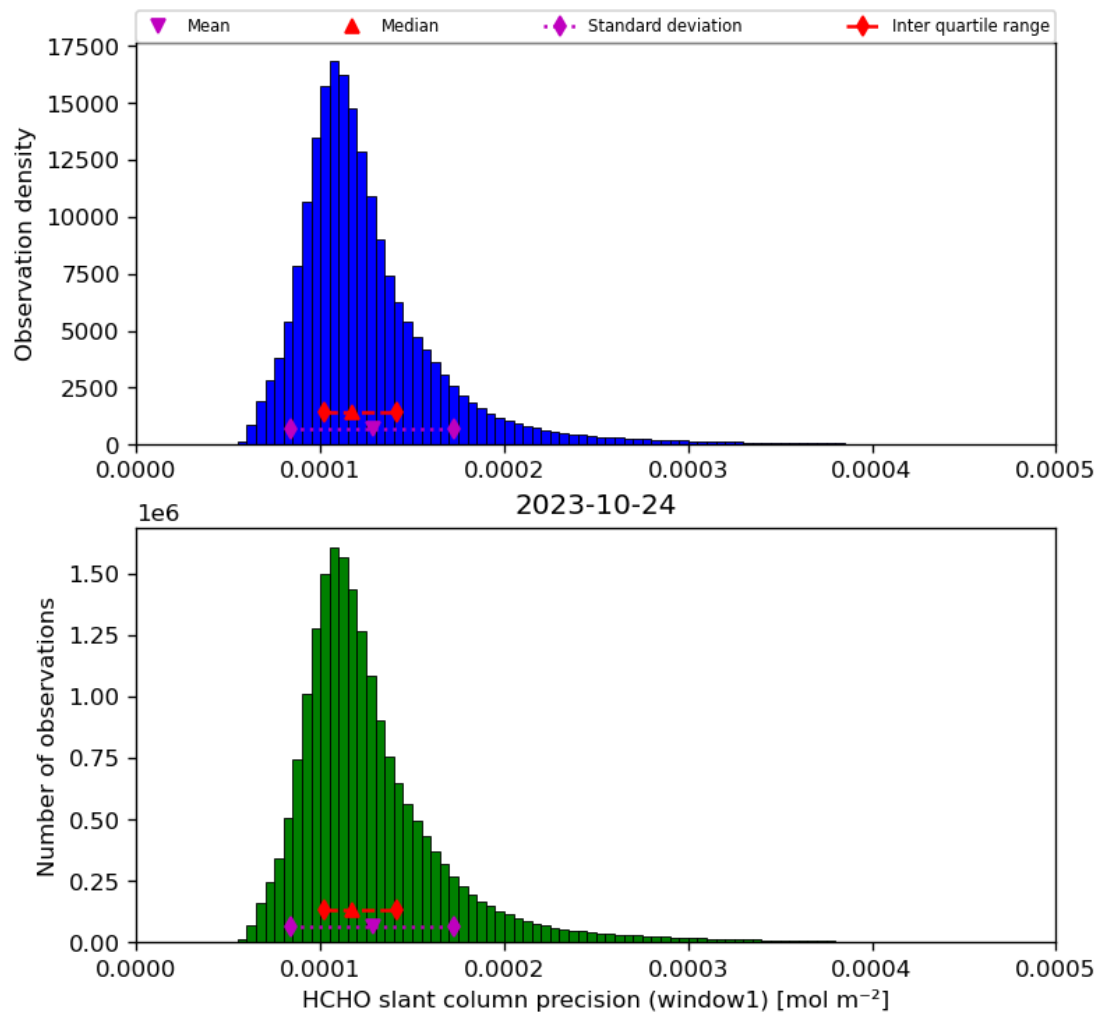
Figure 39: Histogram of “HCHO slant column precision (window1)” for 2023-10-23 to 2023-10-25
