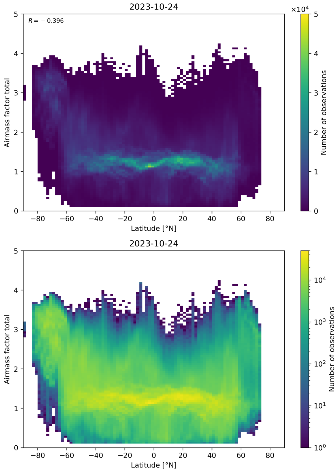
Figure 161: Scatter density plot of “Latitude” against “Airmass factor total” for 2023-10-23 to 2023-10-25.
