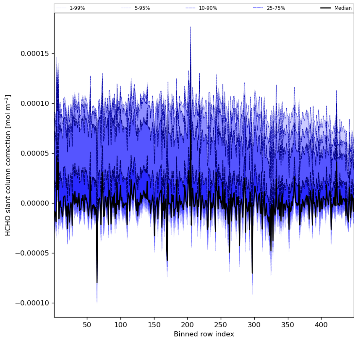
Figure 61: Along track statistics of “HCHO slant column correction” for 2023-10-23 to 2023-10-25
