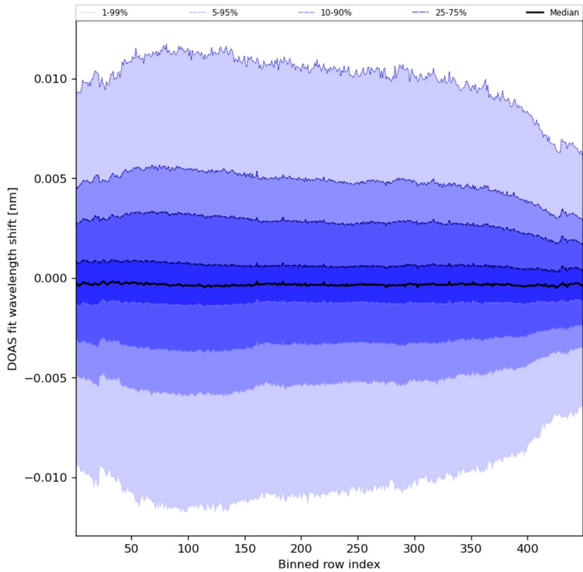
Figure 58: Along track statistics of “DOAS fit wavelength shift” for 2023-10-23 to 2023-10-25
