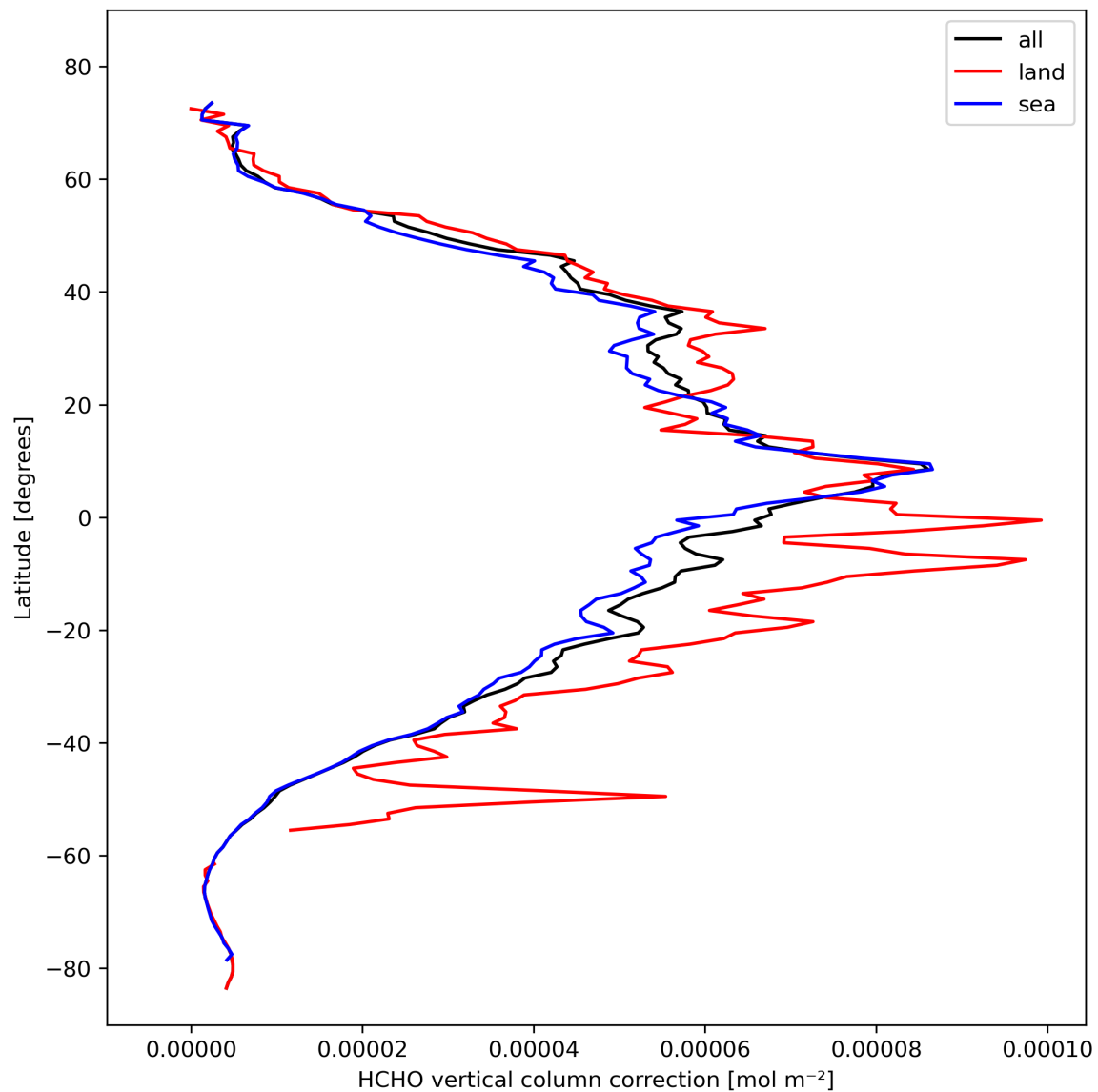
Figure 23: Zonal average of “HCHO vertical column correction” for 2023-10-23 to 2023-10-25.
