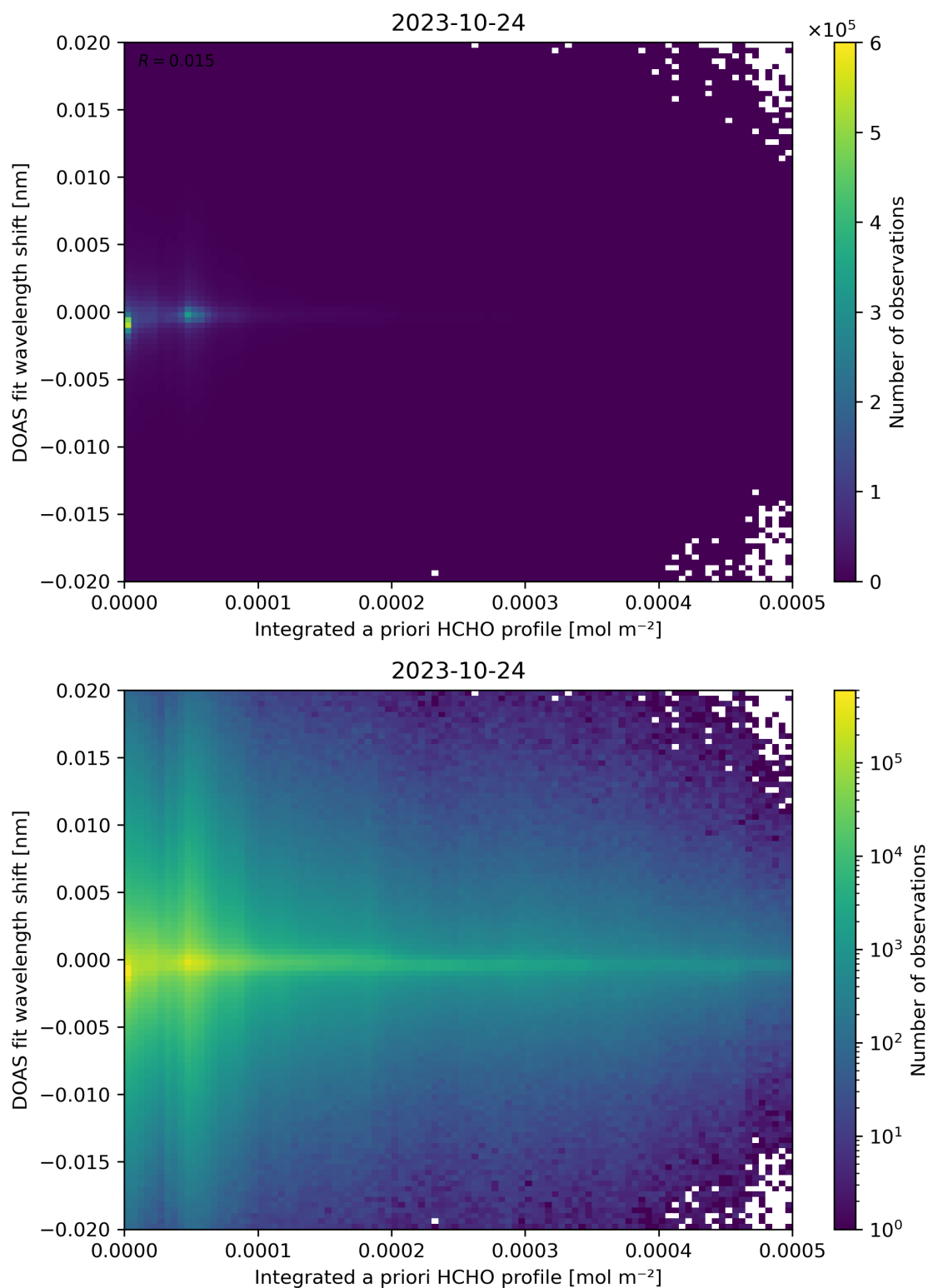
Figure 149: Scatter density plot of “Integrated a priori HCHO profile” against “DOAS fit wavelength shift” for 2023-10-23 to 2023-10-25.
