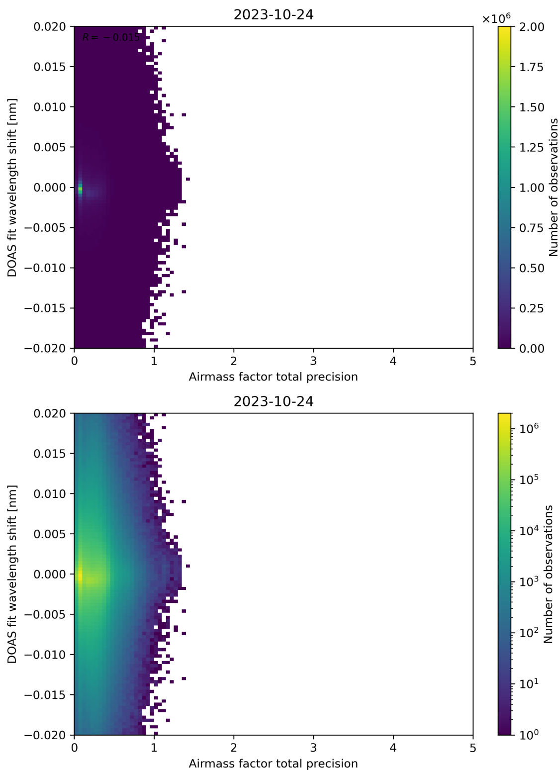
Figure 106: Scatter density plot of “Airmass factor total precision” against “DOAS fit wavelength shift” for 2023-10-23 to 2023-10-25.
