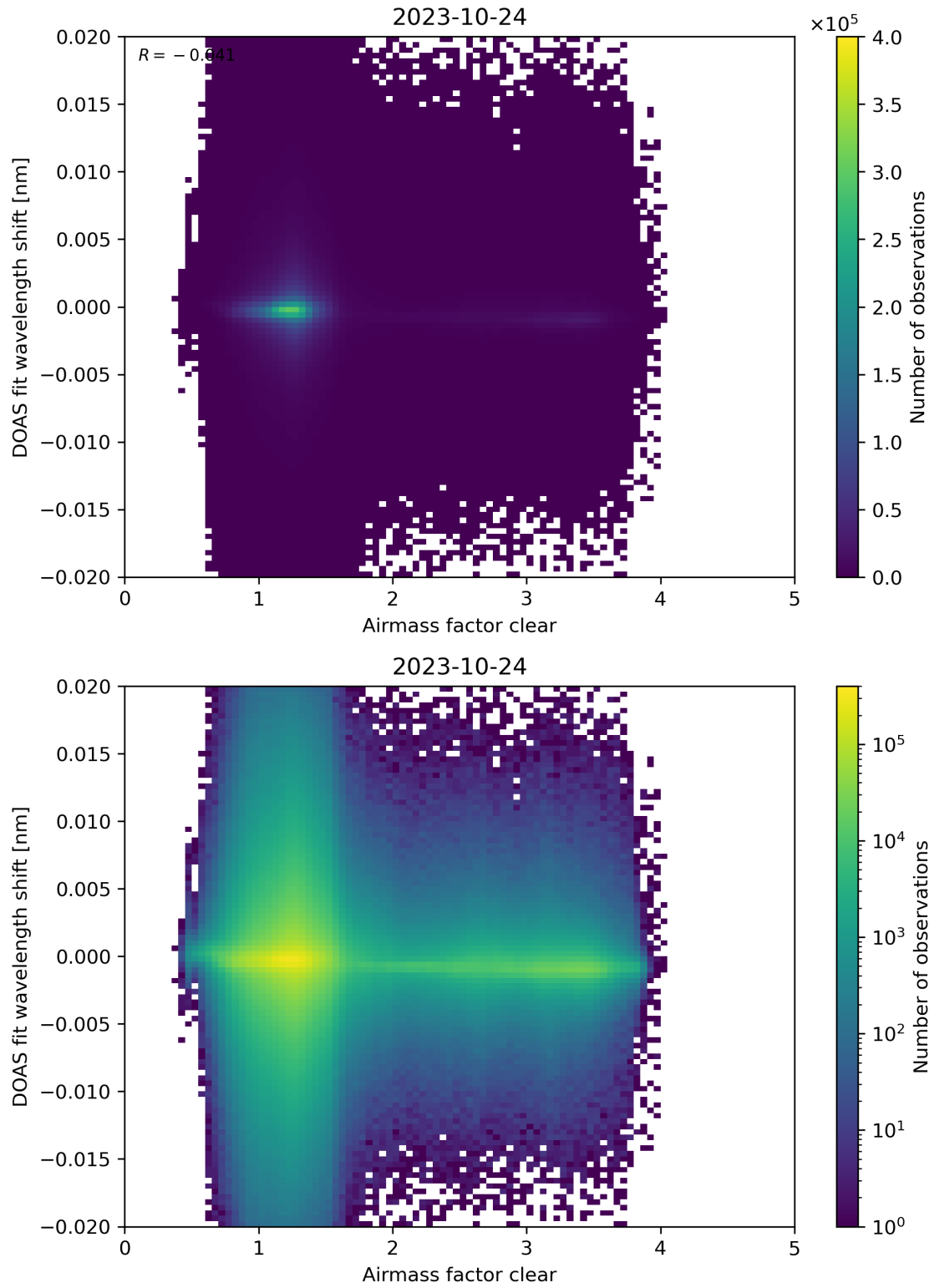
Figure 72: Scatter density plot of “Airmass factor clear” against “DOAS fit wavelength shift” for 2023-10-23 to 2023-10-25.
