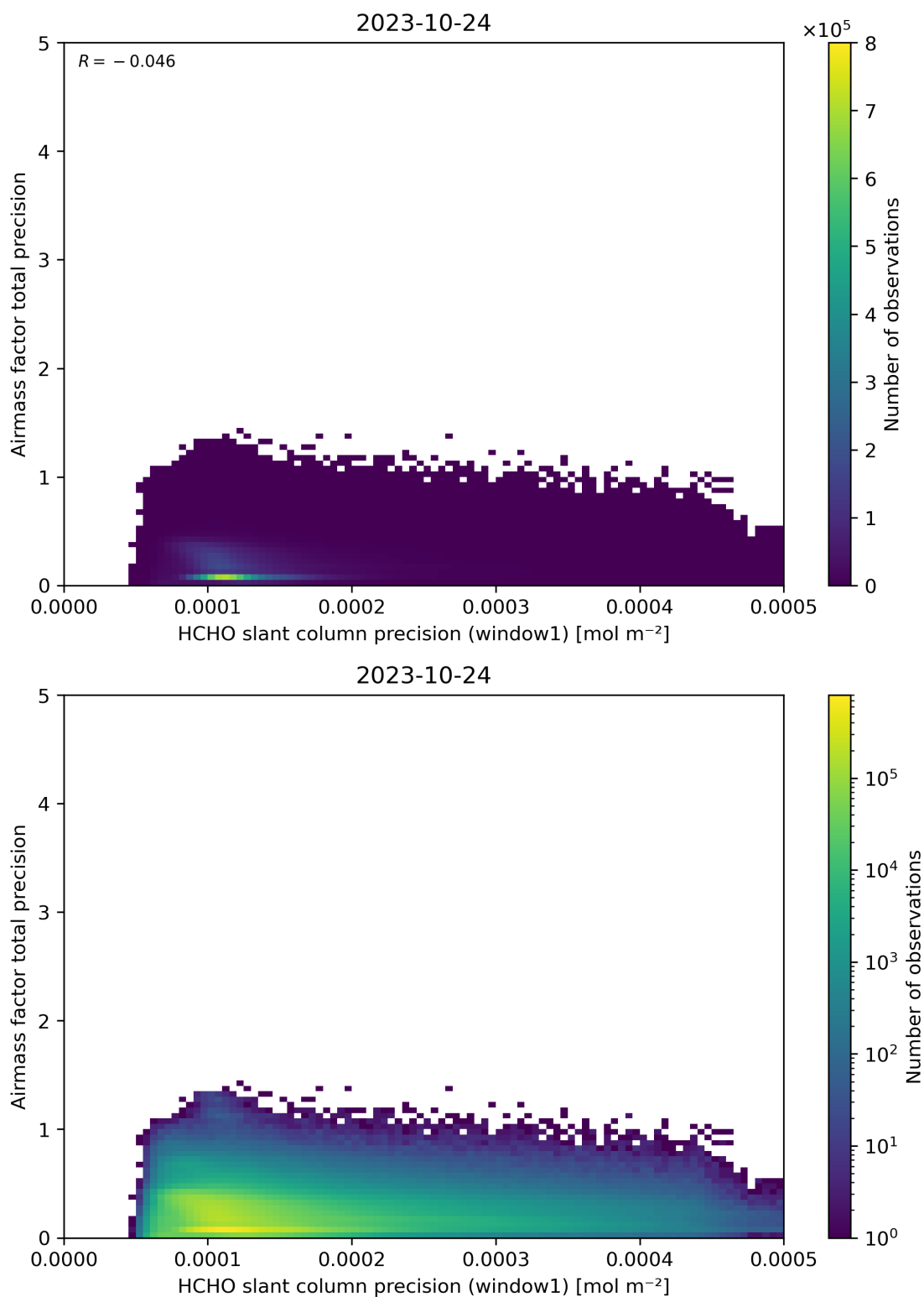
Figure 95: Scatter density plot of “HCHO slant column precision (window1)” against “Airmass factor total precision” for 2023-10-23 to 2023-10-25.
