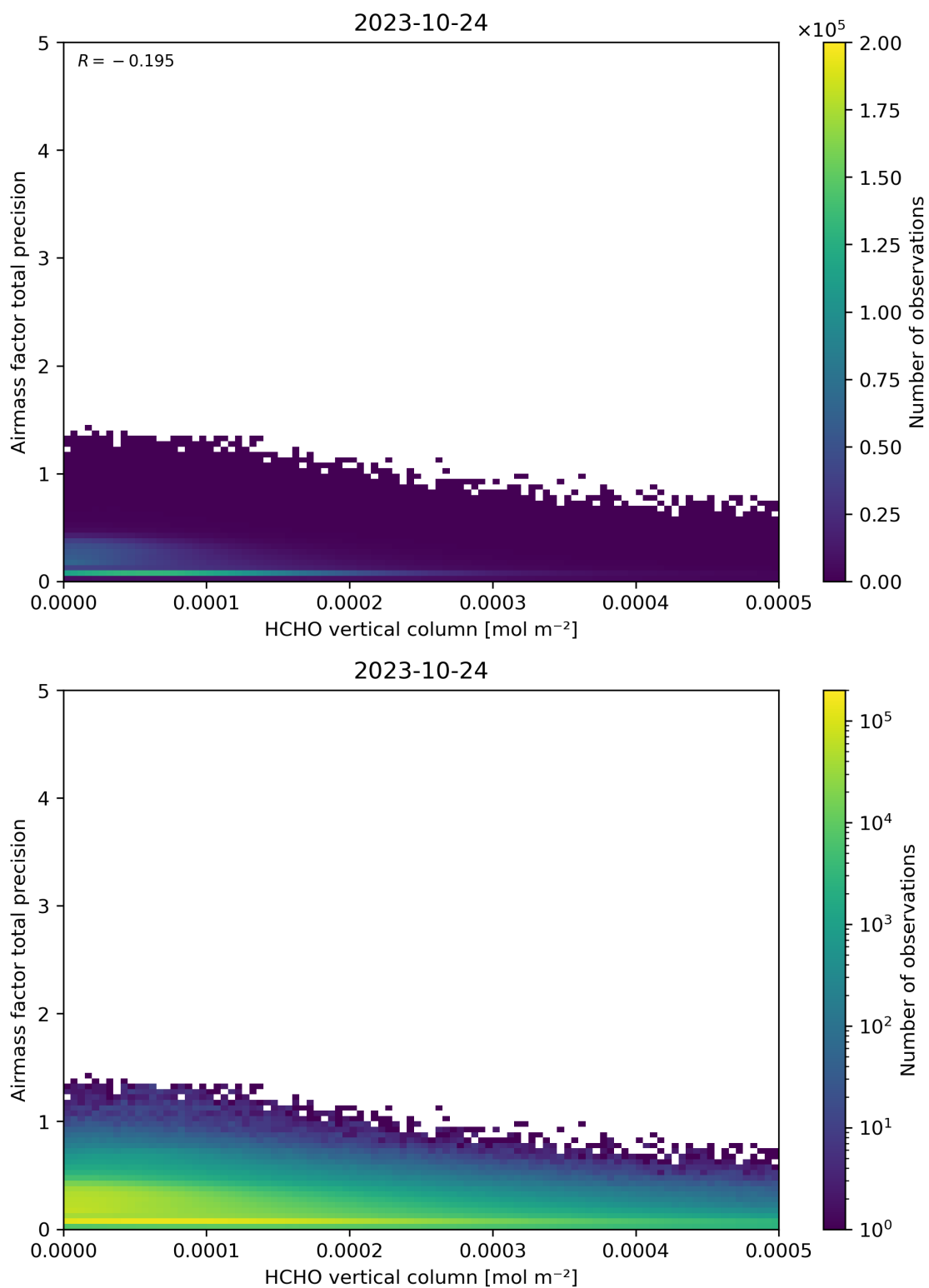
Figure 132: Scatter density plot of “HCHO vertical column” against “Airmass factor total precision” for 2023-10-23 to 2023-10-25.
