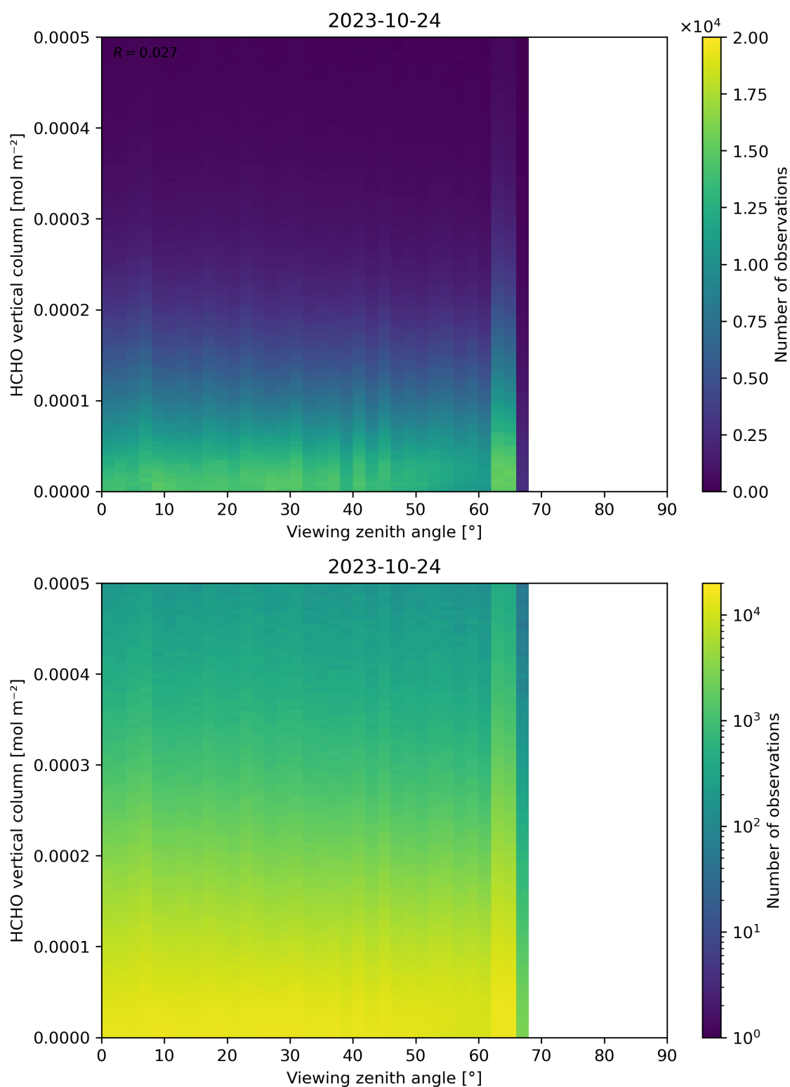
Figure 192: Scatter density plot of “Viewing zenith angle” against “HCHO vertical column” for 2023-10-23 to 2023-10-25.
