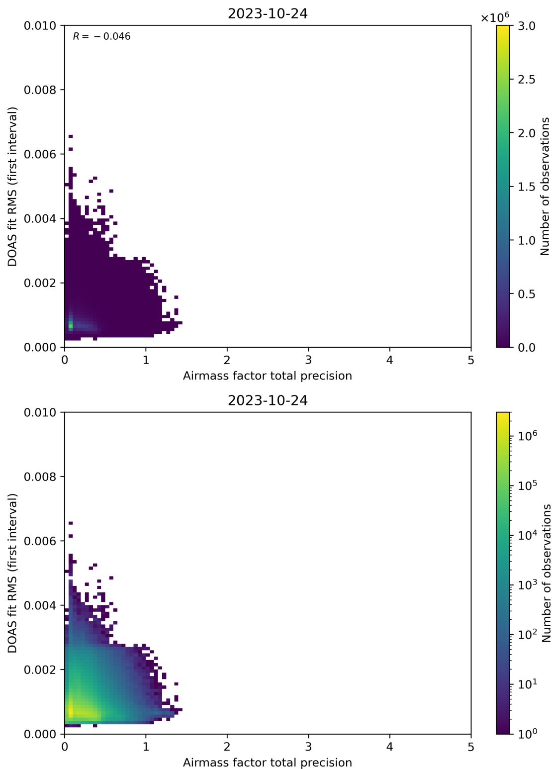
Figure 105: Scatter density plot of “Airmass factor total precision” against “DOAS fit RMS (first interval)” for 2023-10-23 to 2023-10-25.
