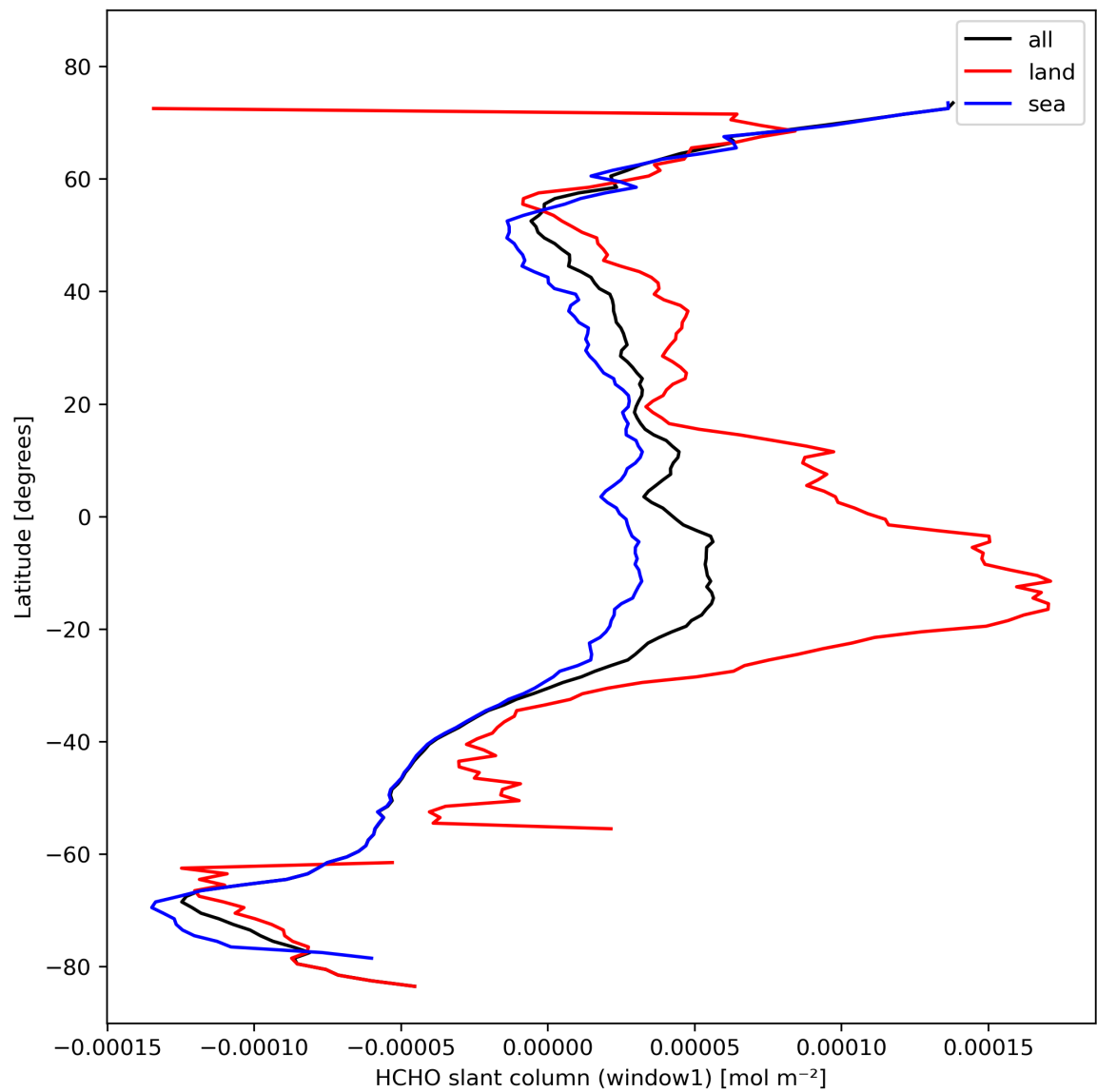
Figure 24: Zonal average of “HCHO slant column (window1)” for 2023-10-23 to 2023-10-25.
