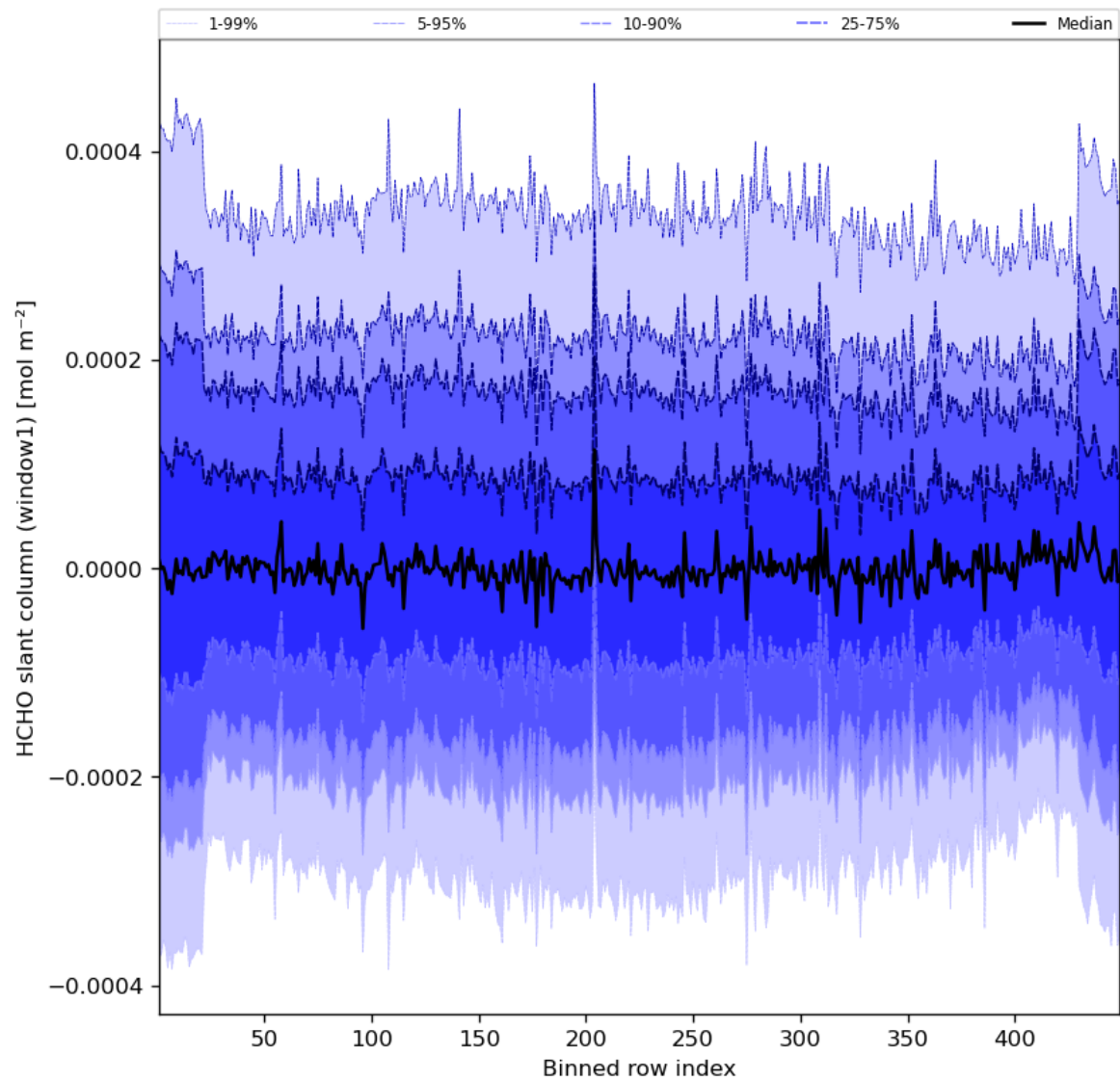
Figure 52: Along track statistics of “HCHO slant column (window1)” for 2023-10-23 to 2023-10-25
