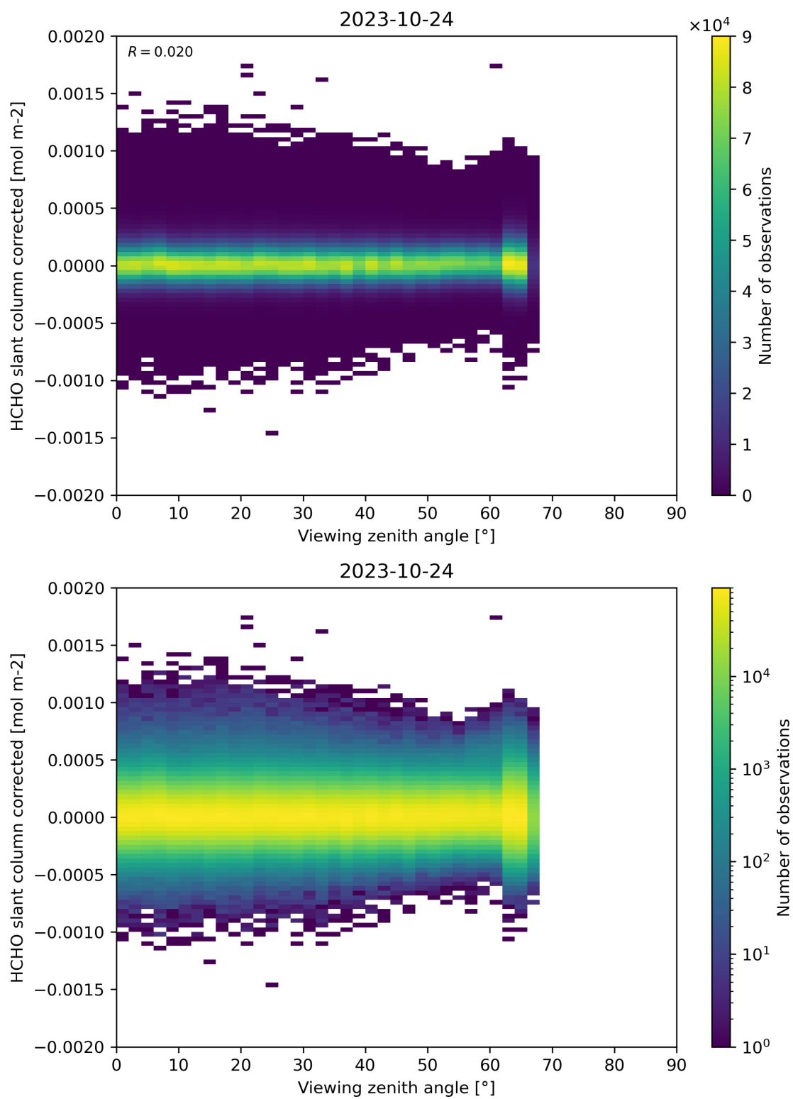
Figure 186: Scatter density plot of “Viewing zenith angle” against “HCHO slant column corrected” for 2023-10-23 to 2023-10-25.
