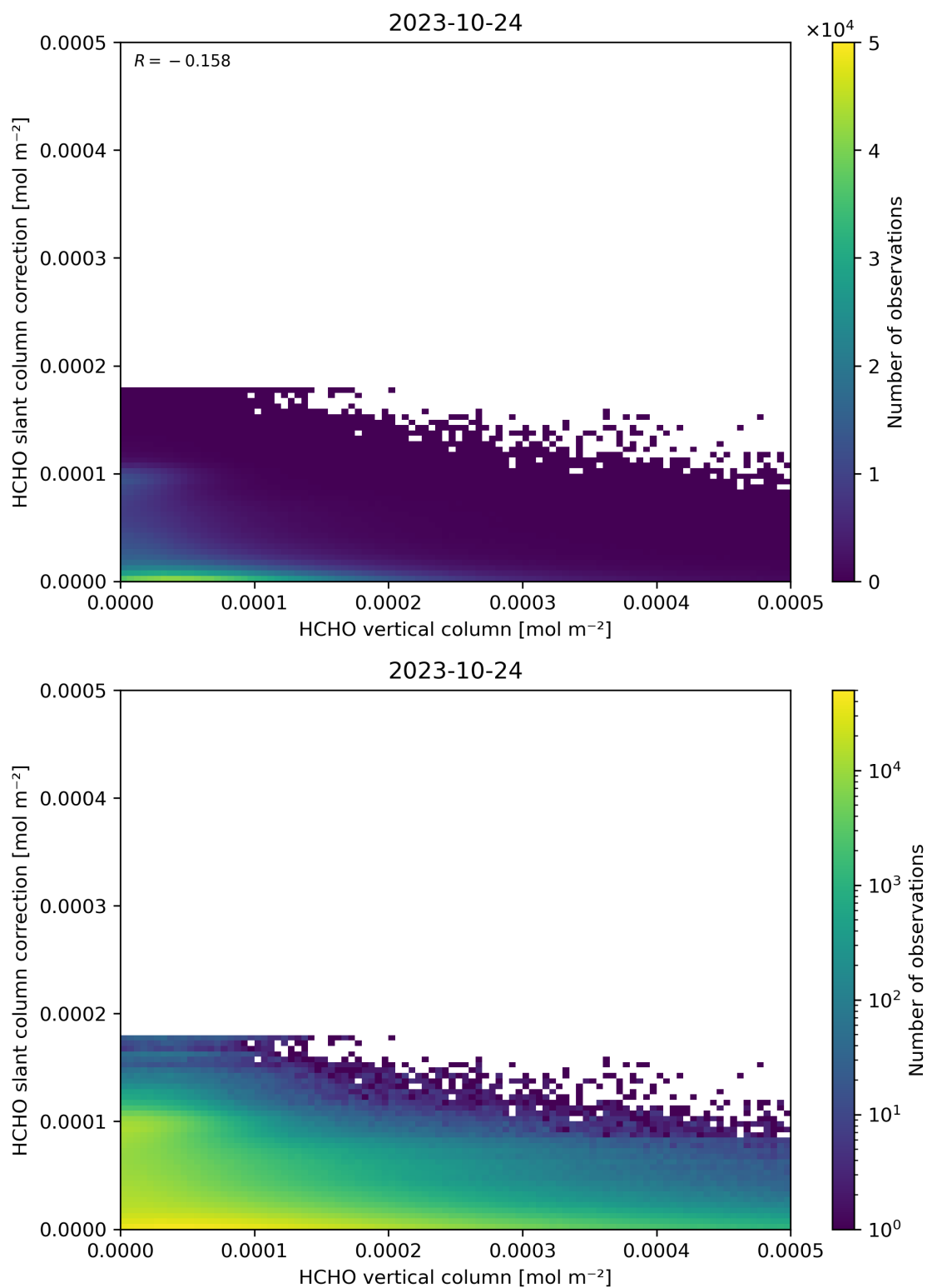
Figure 128: Scatter density plot of “HCHO vertical column” against “HCHO slant column correction” for 2023-10-23 to 2023-10-25.
