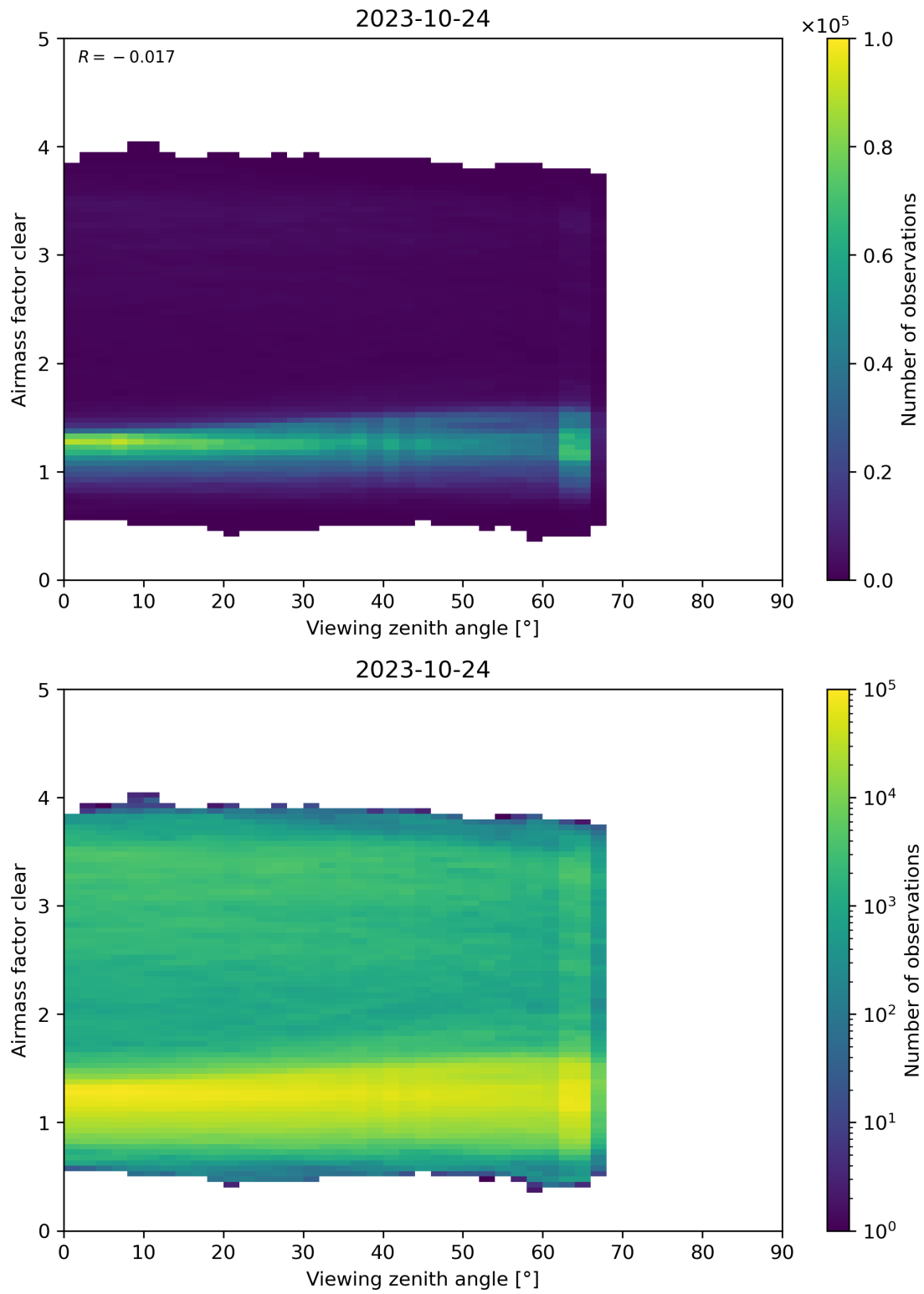
Figure 185: Scatter density plot of “Viewing zenith angle” against “Airmass factor clear” for 2023-10-23 to 2023-10-25.
