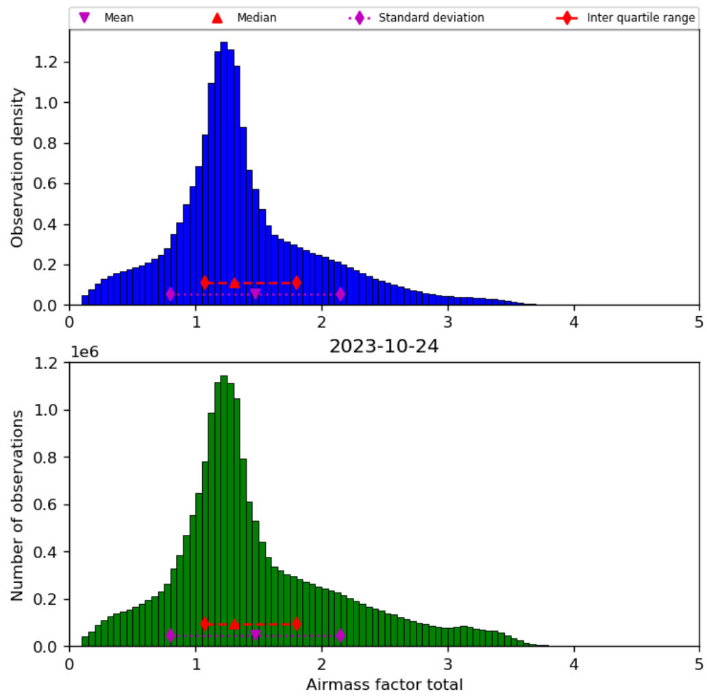
Figure 40: Histogram of “Airmass factor total” for 2023-10-23 to 2023-10-25
