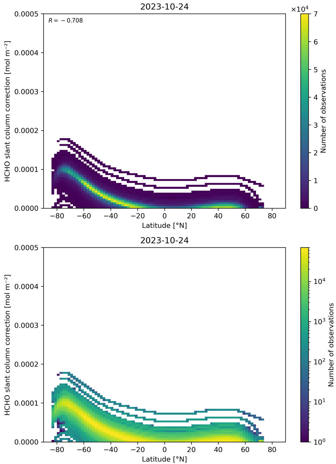
Figure 158: Scatter density plot of “Latitude” against “HCHO slant column correction” for 2023-10-23 to 2023-10-25.
