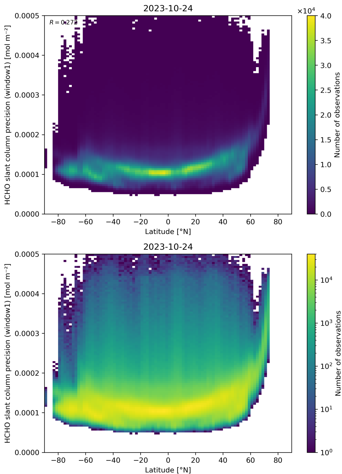
Figure 160: Scatter density plot of “Latitude” against “HCHO slant column precision (window1)” for 2023-10-23 to 2023-10-25.
