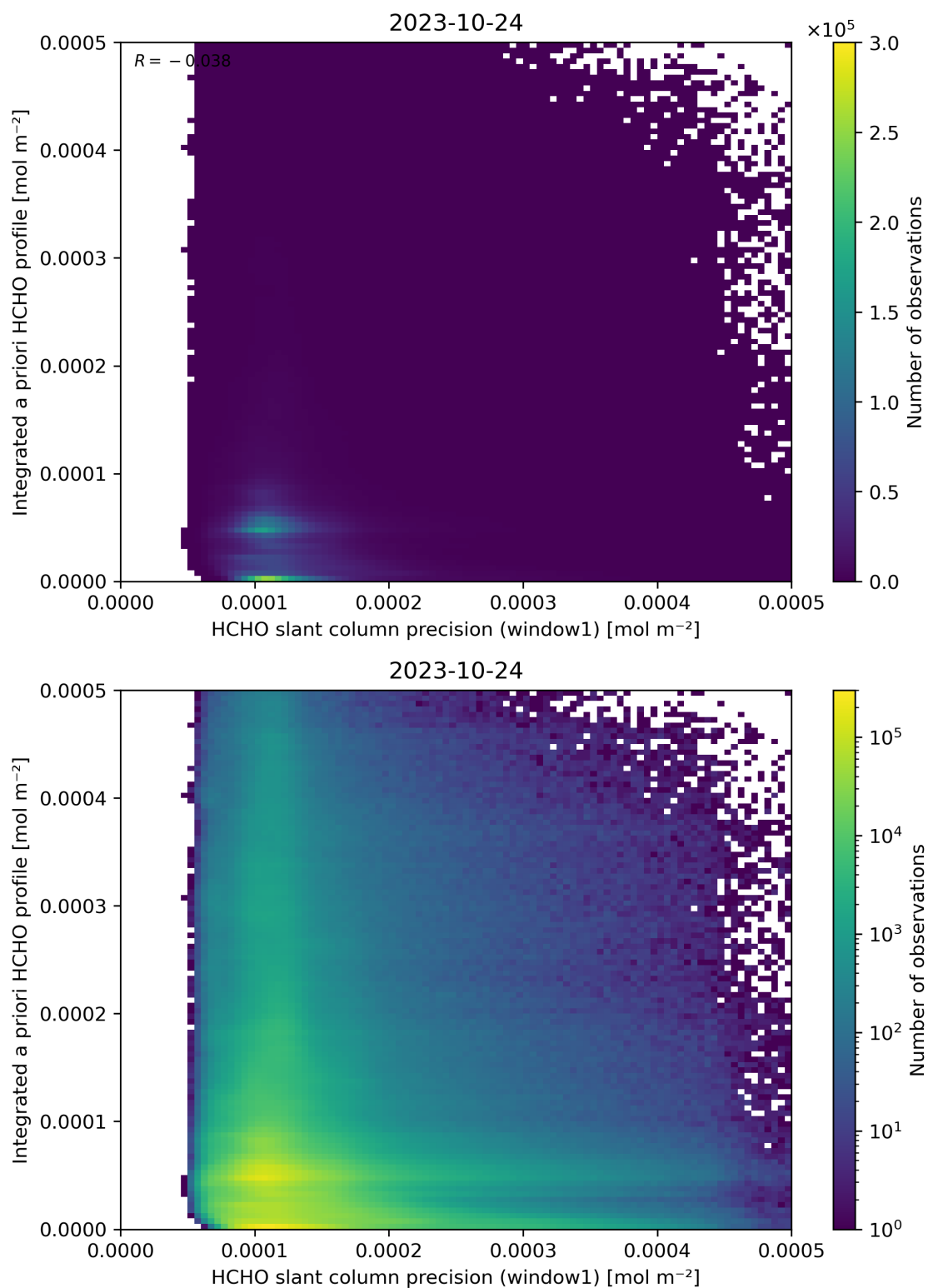
Figure 96: Scatter density plot of “HCHO slant column precision (window1)” against “Integrated a priori HCHO profile” for 2023-10-23 to 2023-10-25.
