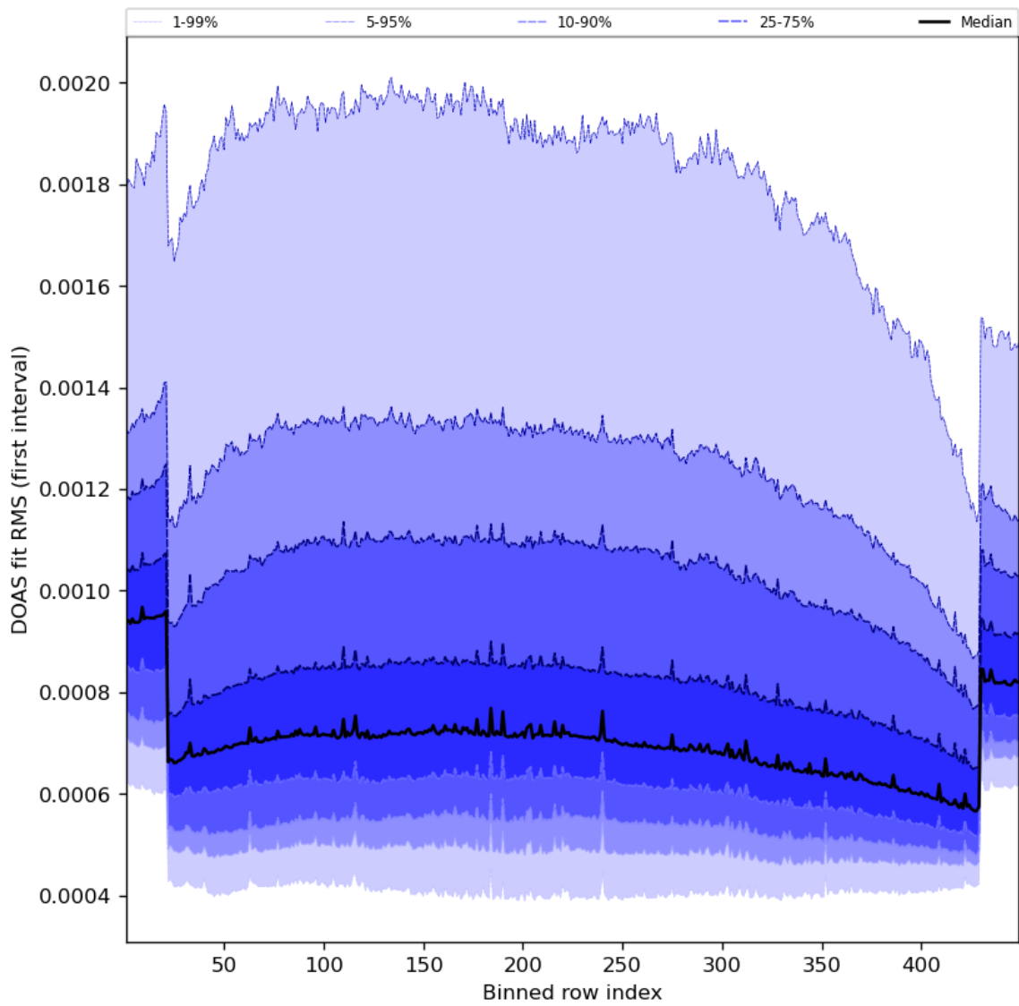
Figure 60: Along track statistics of “DOAS fit RMS (first interval)” for 2023-10-23 to 2023-10-25
