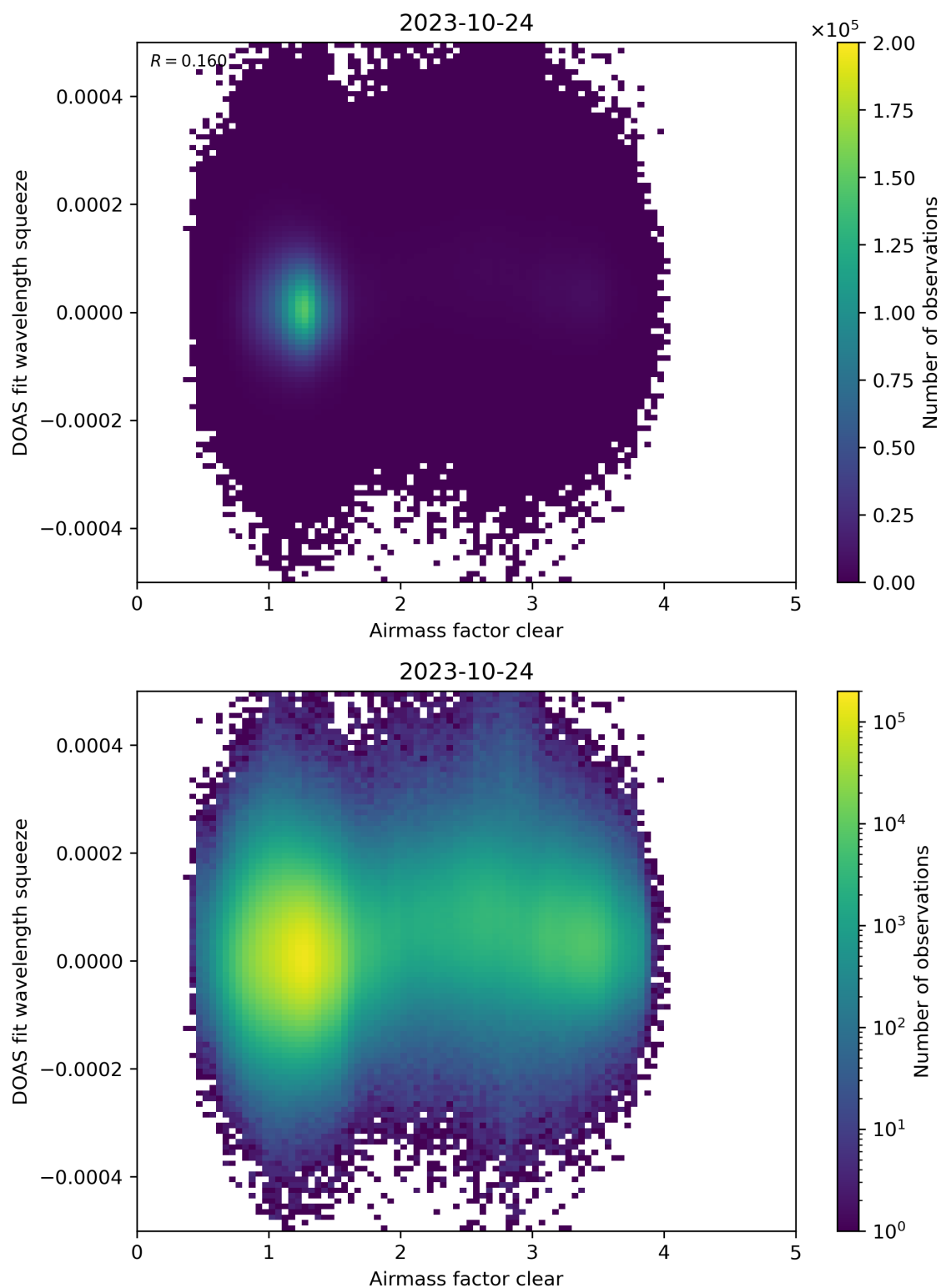
Figure 73: Scatter density plot of “Airmass factor clear” against “DOAS fit wavelength squeeze” for 2023-10-23 to 2023-10-25.
