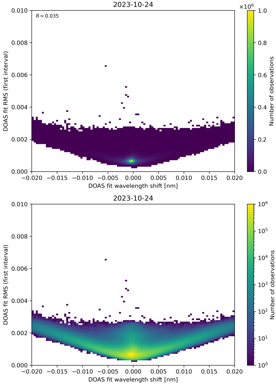
Figure 64: Scatter density plot of “DOAS fit wavelength shift” against “DOAS fit RMS (first interval)” for 2023-10-23 to 2023-10-25.
