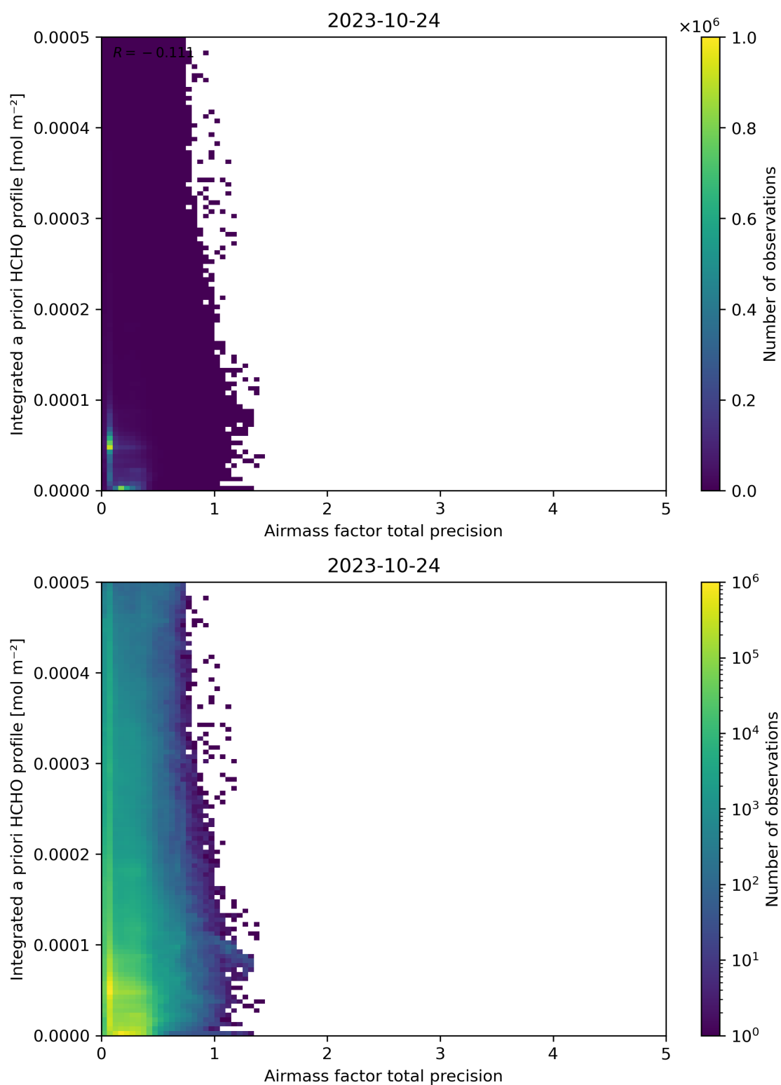
Figure 111: Scatter density plot of “Airmass factor total precision” against “Integrated a priori HCHO profile” for 2023-10-23 to 2023-10-25.
