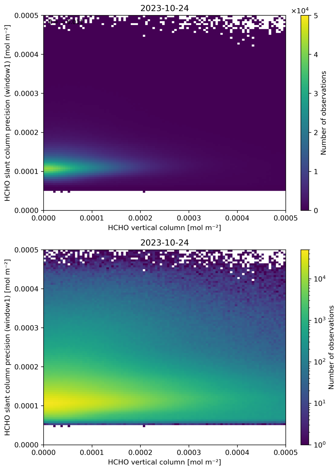
Figure 130: Scatter density plot of “HCHO vertical column” against “HCHO slant column precision (window1)” for 2023-10-23 to 2023-10-25.
