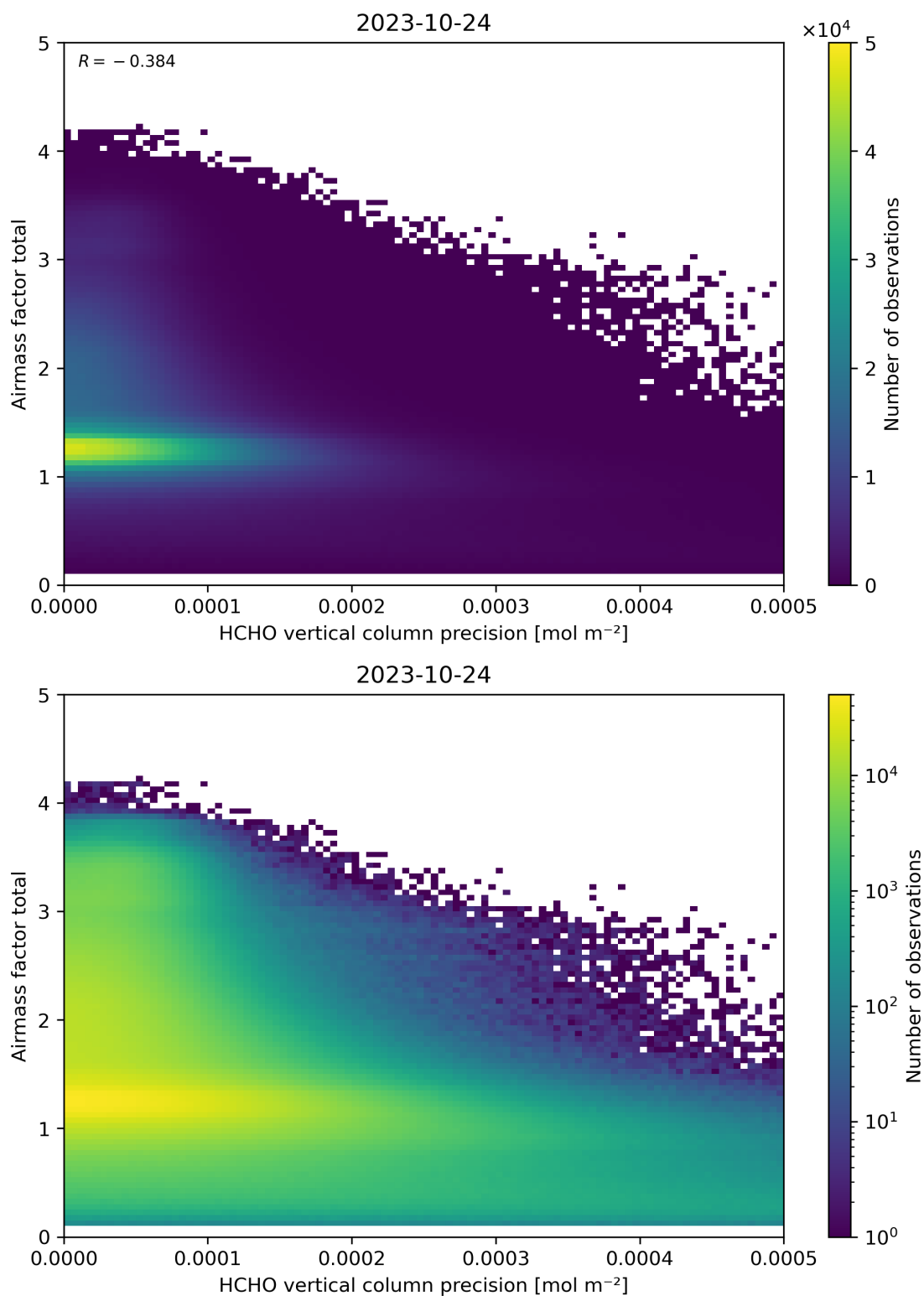
Figure 144: Scatter density plot of “HCHO vertical column precision” against “Airmass factor total” for 2023-10-23 to 2023-10-25.
