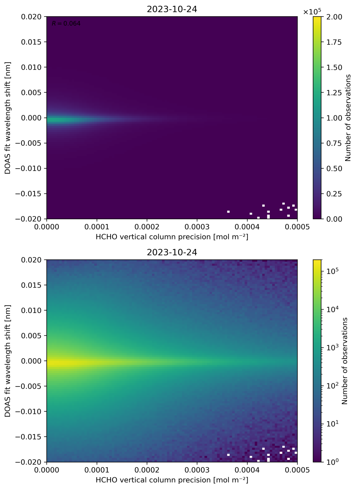
Figure 137: Scatter density plot of “HCHO vertical column precision” against “DOAS fit wavelength shift” for 2023-10-23 to 2023-10-25.
