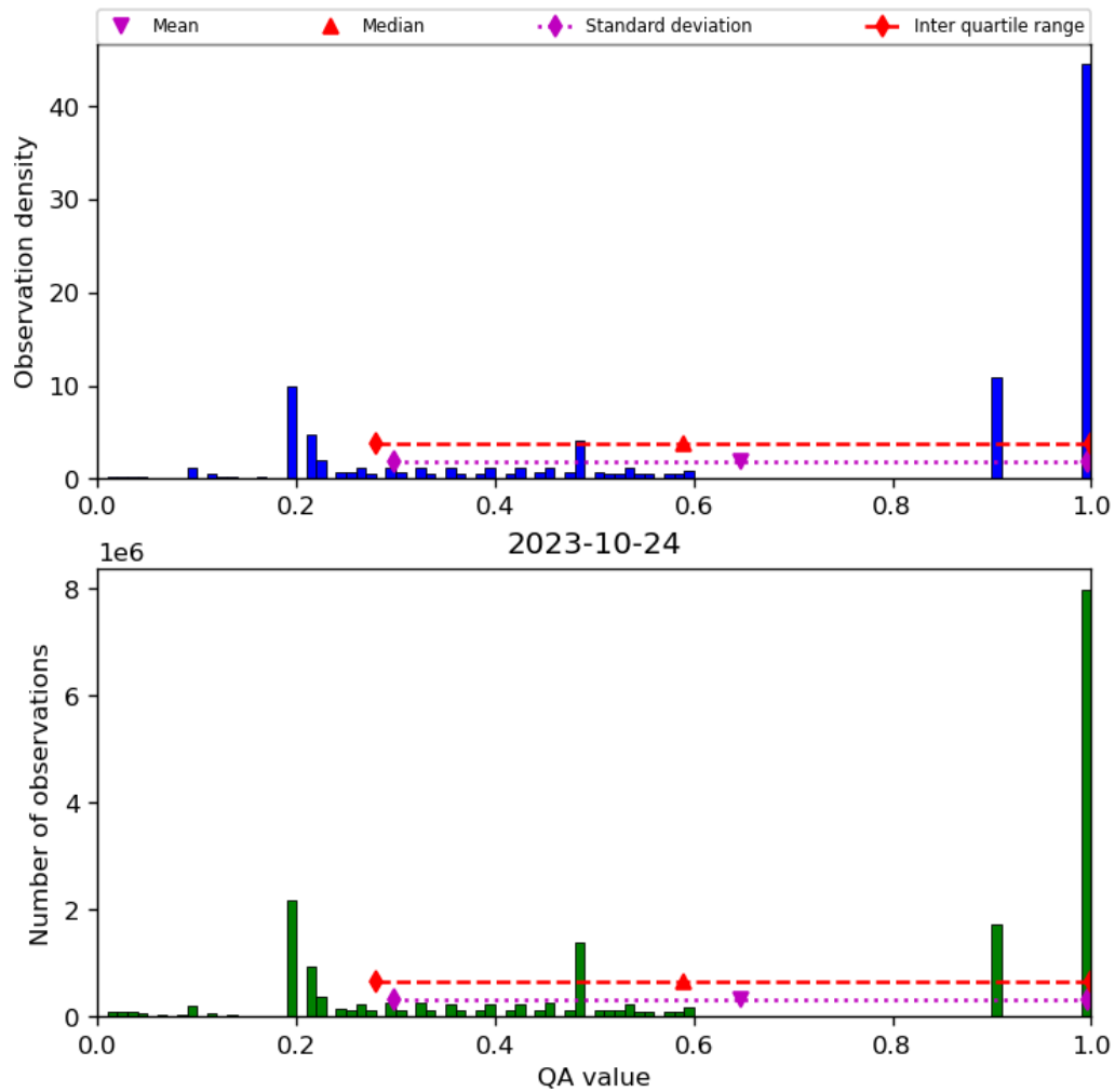
Figure 34: Histogram of “QA value” for 2023-10-23 to 2023-10-25
