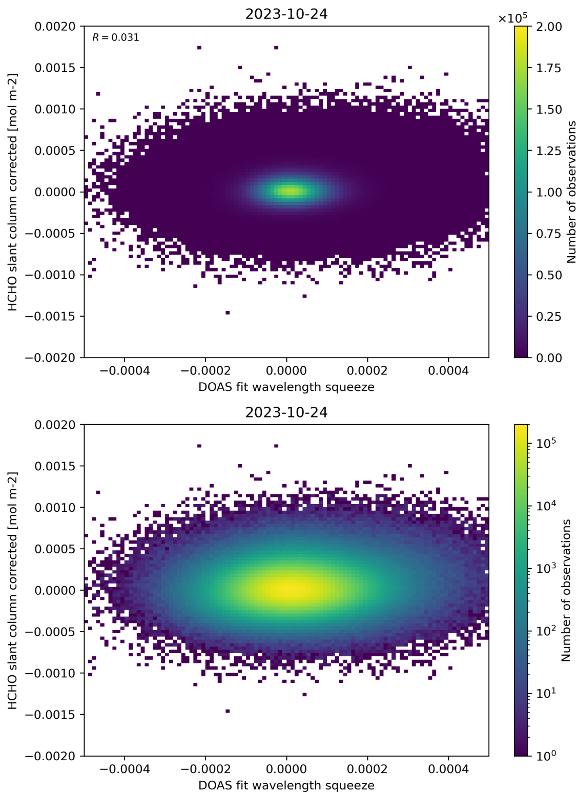
Figure 69: Scatter density plot of “DOAS fit wavelength squeeze” against “HCHO slant column corrected” for 2023-10-23 to 2023-10-25.
