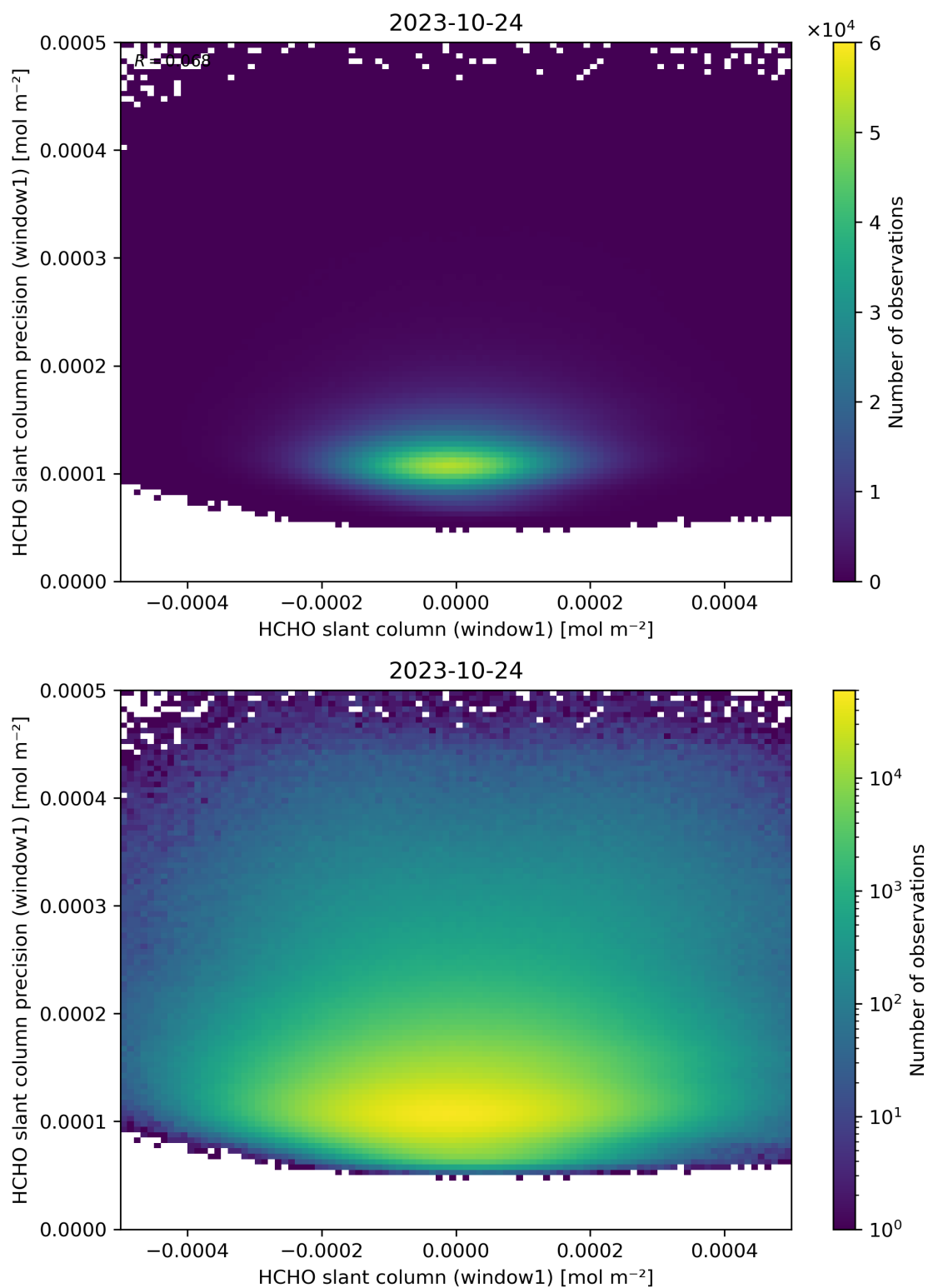
Figure 84: Scatter density plot of “HCHO slant column (window1)” against “HCHO slant column precision (window1)” for 2023-10-23 to 2023-10-25.
