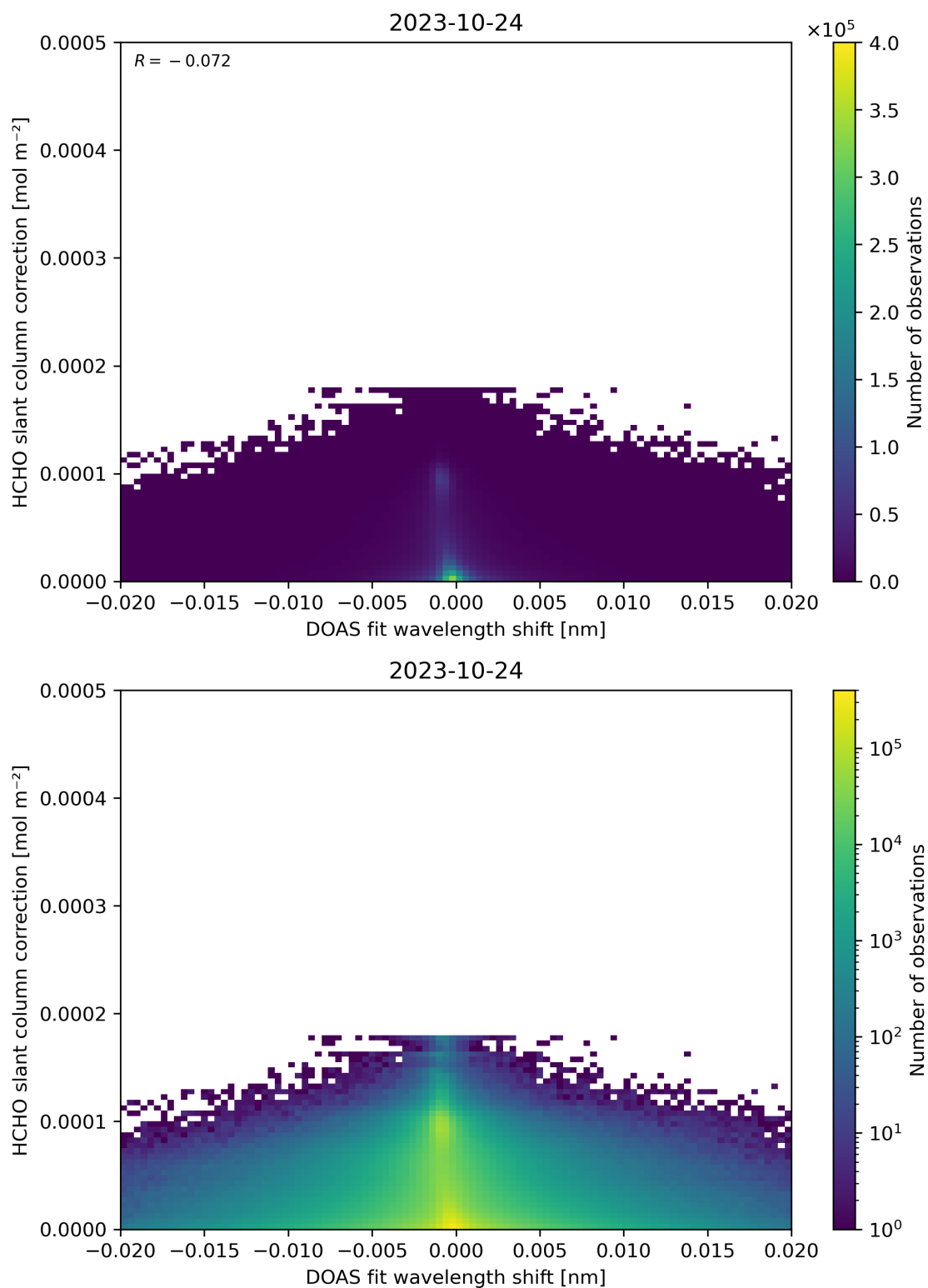
Figure 67: Scatter density plot of “DOAS fit wavelength shift” against “HCHO slant column correction” for 2023-10-23 to 2023-10-25.
