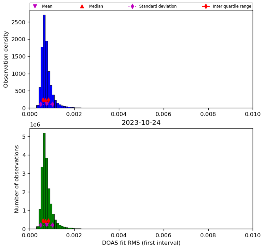
Figure 46: Histogram of “DOAS fit RMS (first interval)” for 2023-10-23 to 2023-10-25
