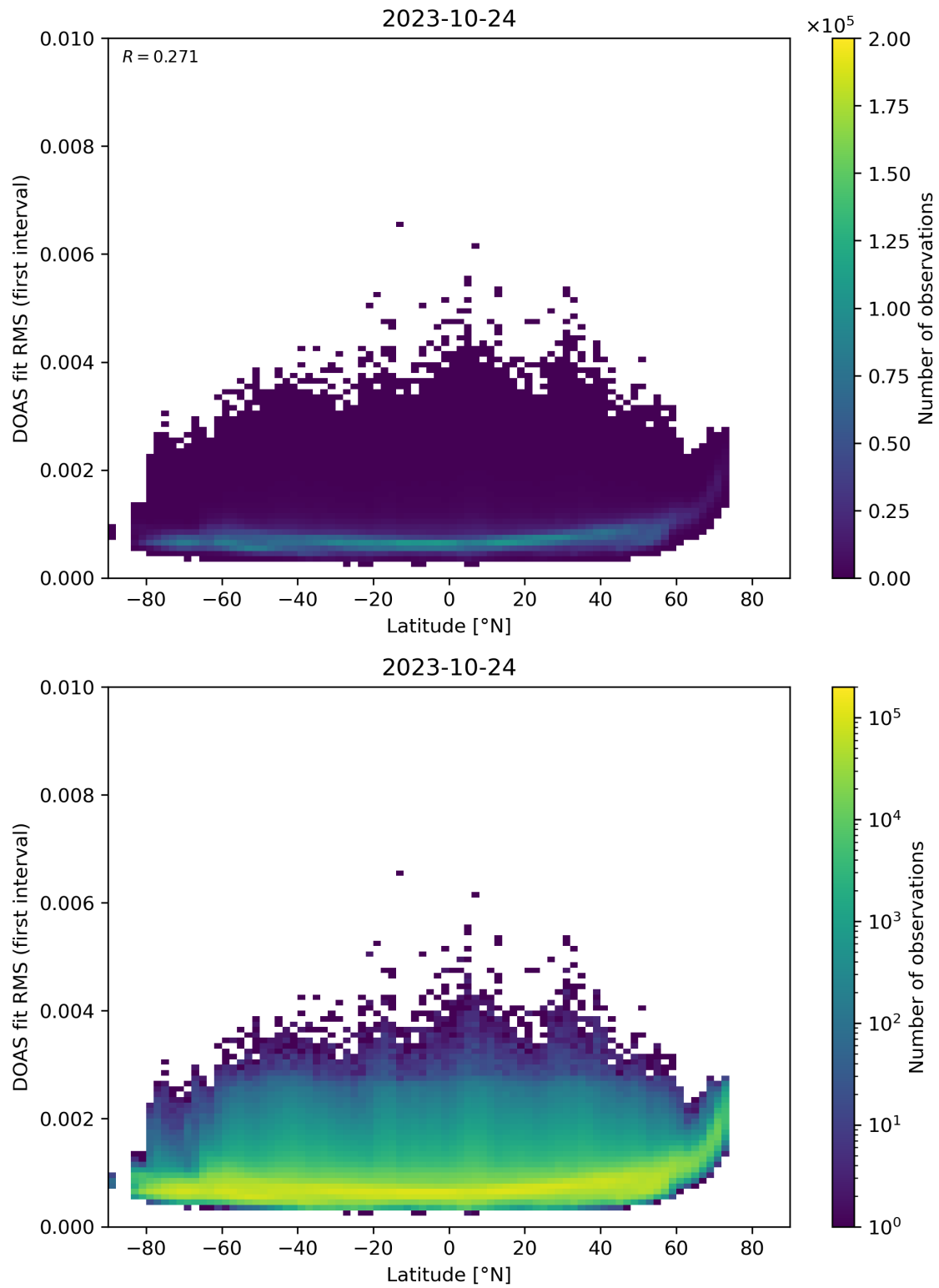
Figure 153: Scatter density plot of “Latitude” against “DOAS fit RMS (first interval)” for 2023-10-23 to 2023-10-25.
