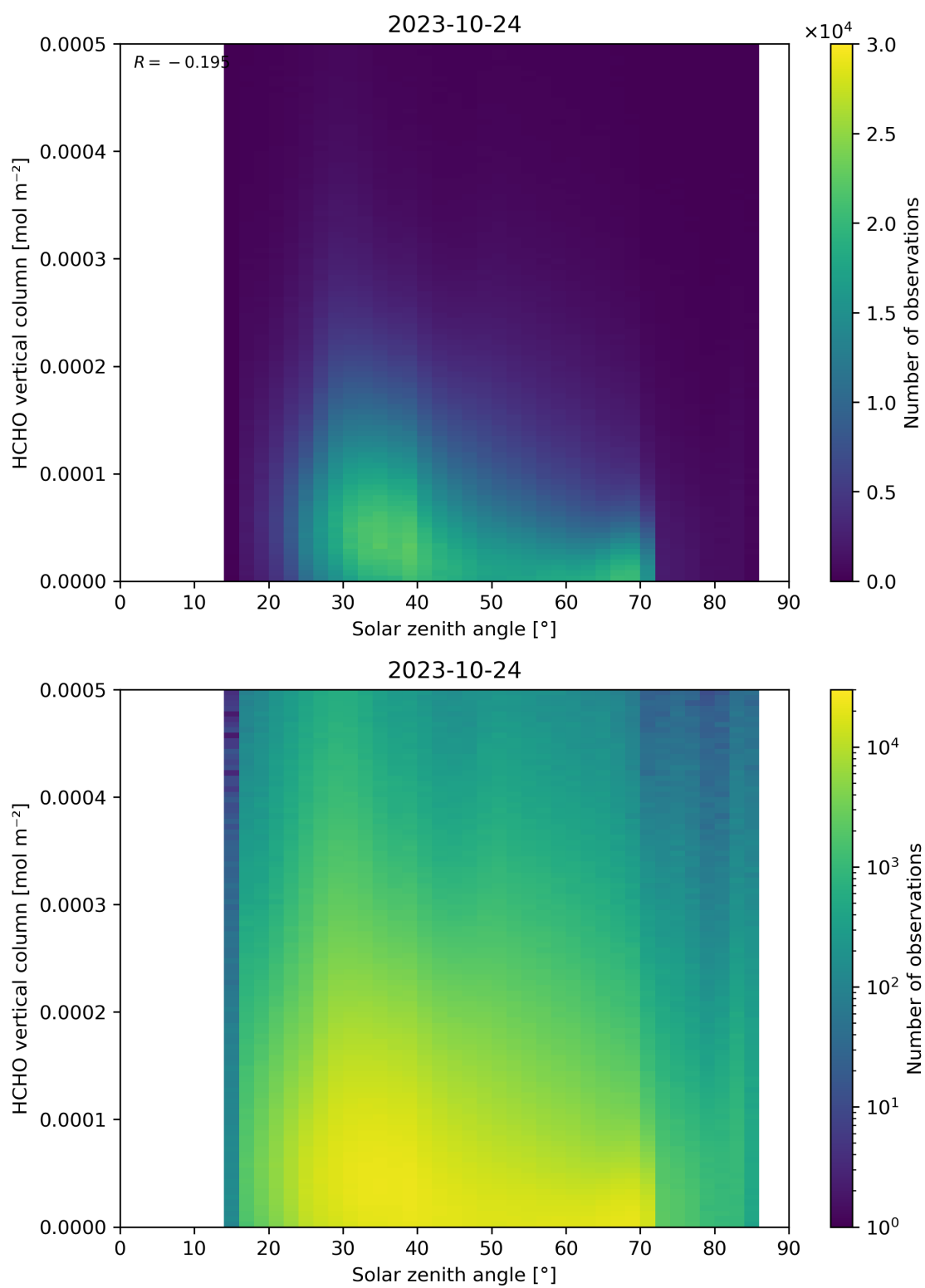
Figure 177: Scatter density plot of “Solar zenith angle” against “HCHO vertical column” for 2023-10-23 to 2023-10-25.
