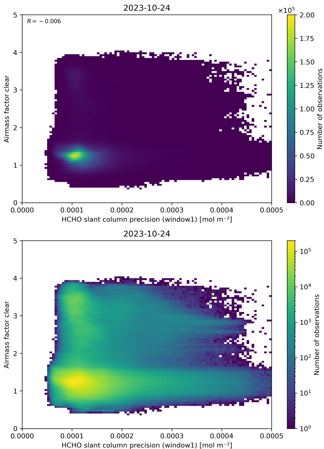
Figure 91: Scatter density plot of “HCHO slant column precision (window1)” against “Airmass factor clear” for 2023-10-23 to 2023-10-25.
