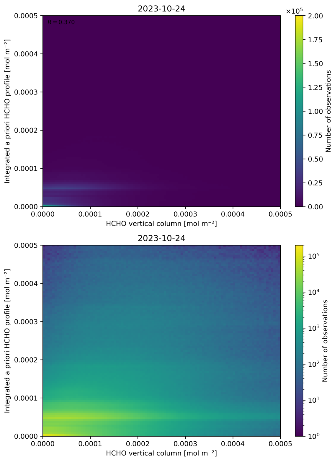
Figure 135: Scatter density plot of “HCHO vertical column” against “Integrated a priori HCHO profile” for 2023-10-23 to 2023-10-25.
