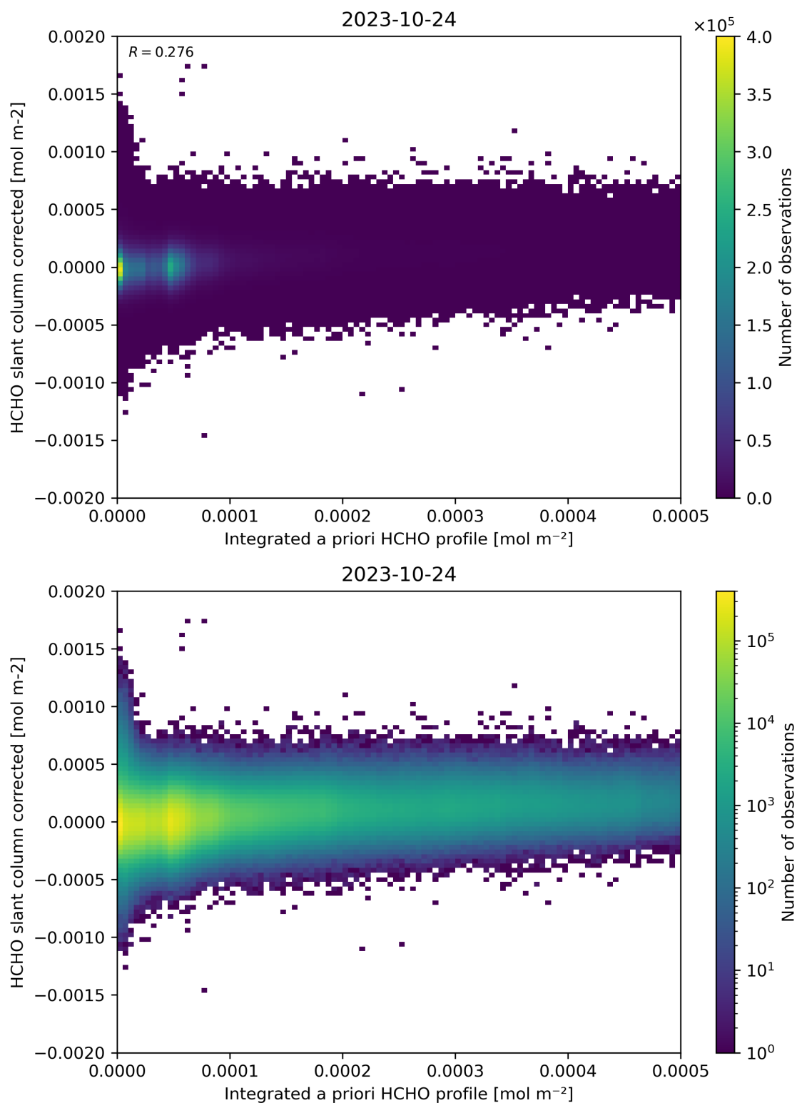
Figure 151: Scatter density plot of “Integrated a priori HCHO profile” against “HCHO slant column corrected” for 2023-10-23 to 2023-10-25.
