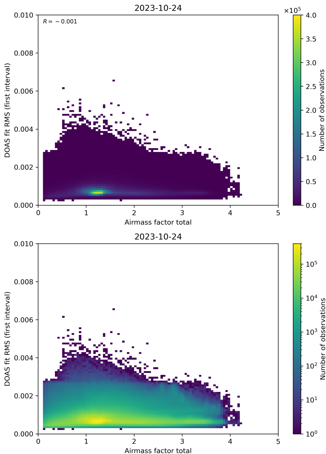
Figure 97: Scatter density plot of “Airmass factor total” against “DOAS fit RMS (first interval)” for 2023-10-23 to 2023-10-25.
