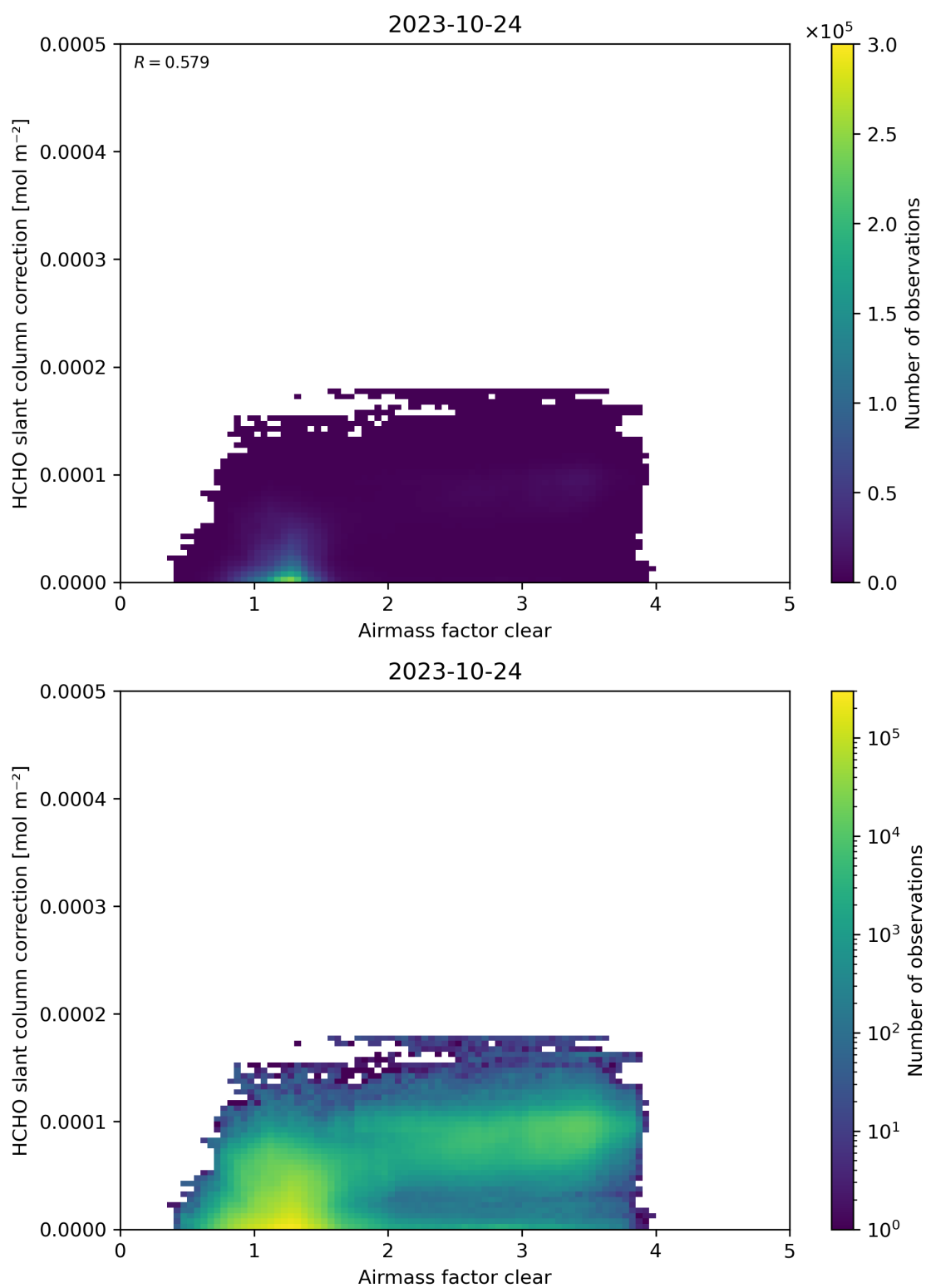
Figure 75: Scatter density plot of “Airmass factor clear” against “HCHO slant column correction” for 2023-10-23 to 2023-10-25.
