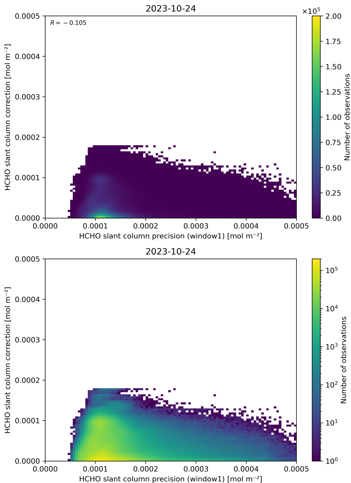
Figure 93: Scatter density plot of “HCHO slant column precision (window1)” against “HCHO slant column correction” for 2023-10-23 to 2023-10-25.
