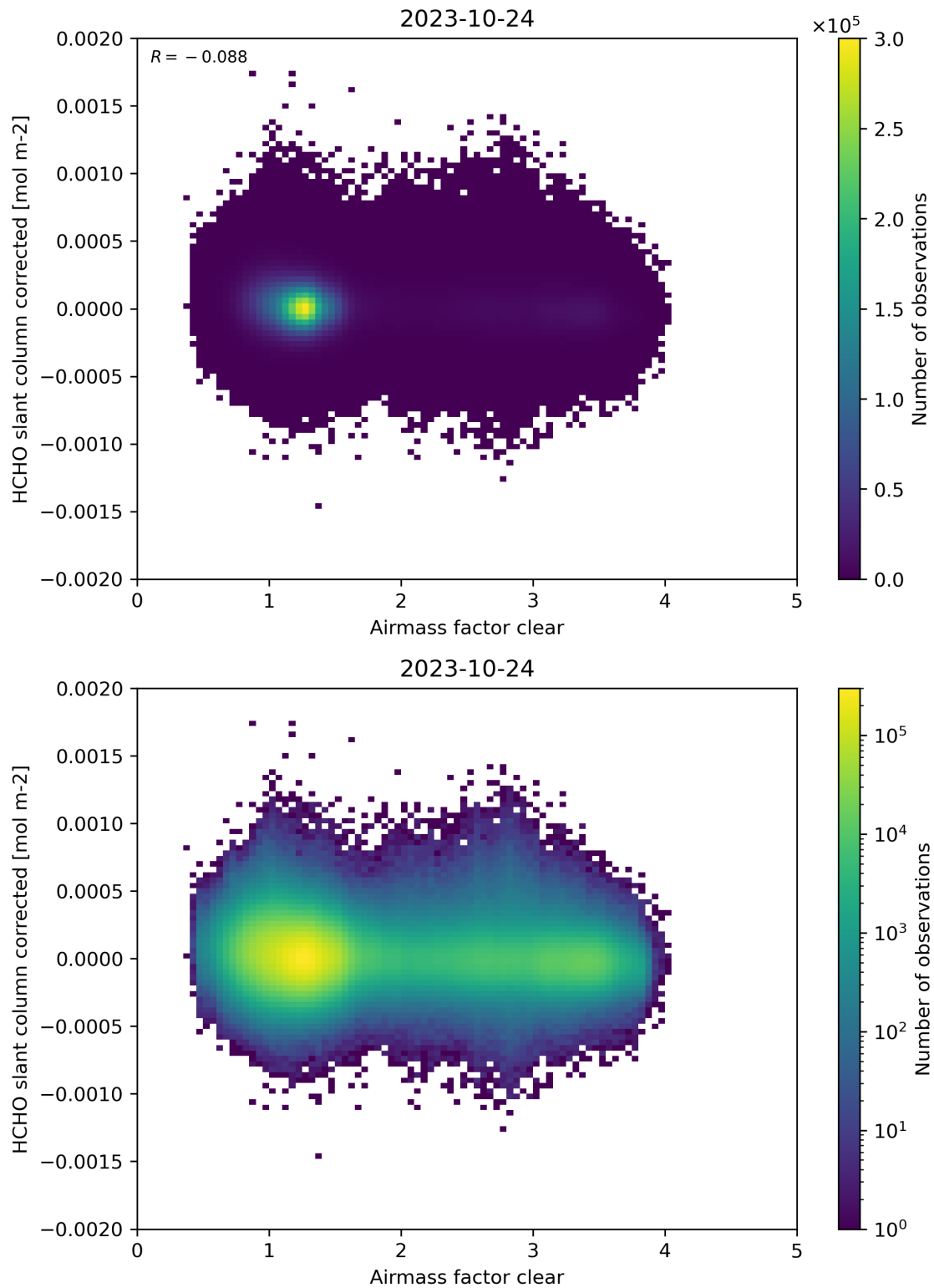
Figure 74: Scatter density plot of “Airmass factor clear” against “HCHO slant column corrected” for 2023-10-23 to 2023-10-25.
