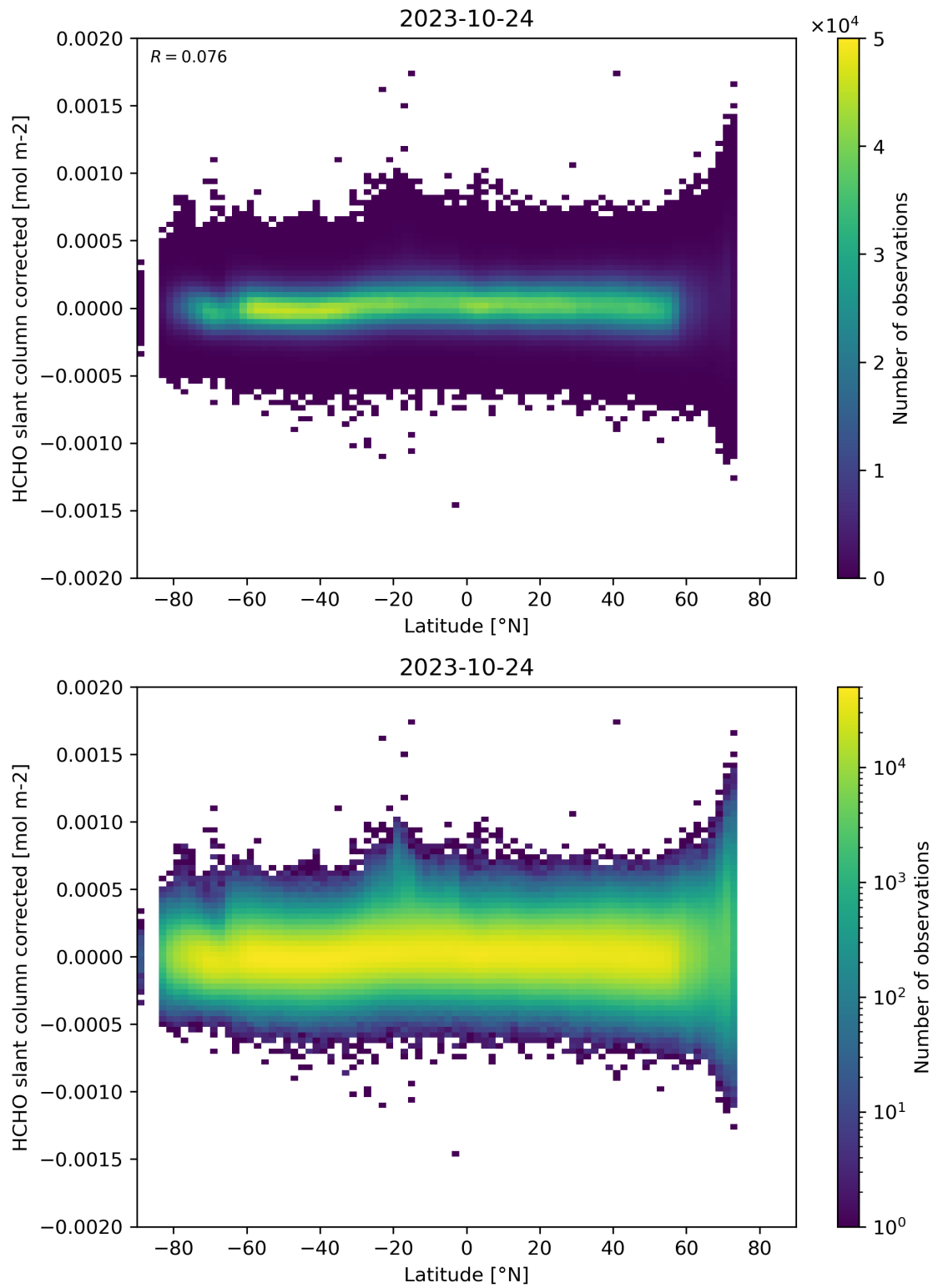
Figure 157: Scatter density plot of “Latitude” against “HCHO slant column corrected” for 2023-10-23 to 2023-10-25.
