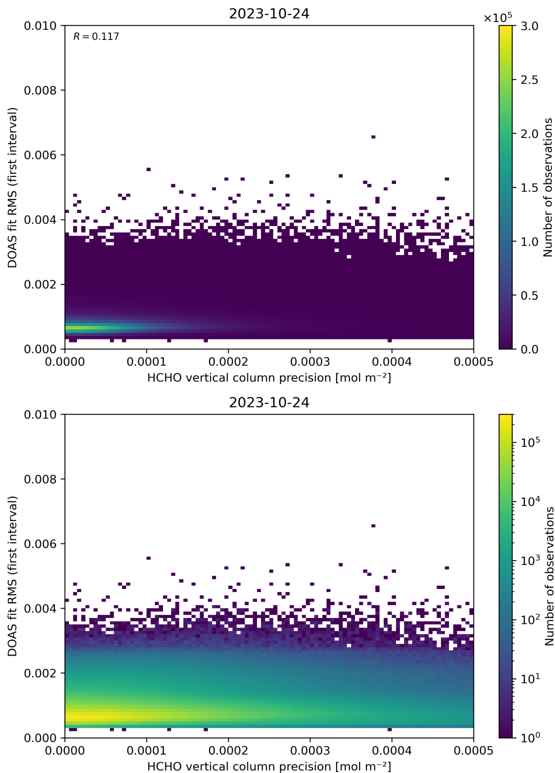
Figure 136: Scatter density plot of “HCHO vertical column precision” against “DOAS fit RMS (first interval)” for 2023-10-23 to 2023-10-25.
