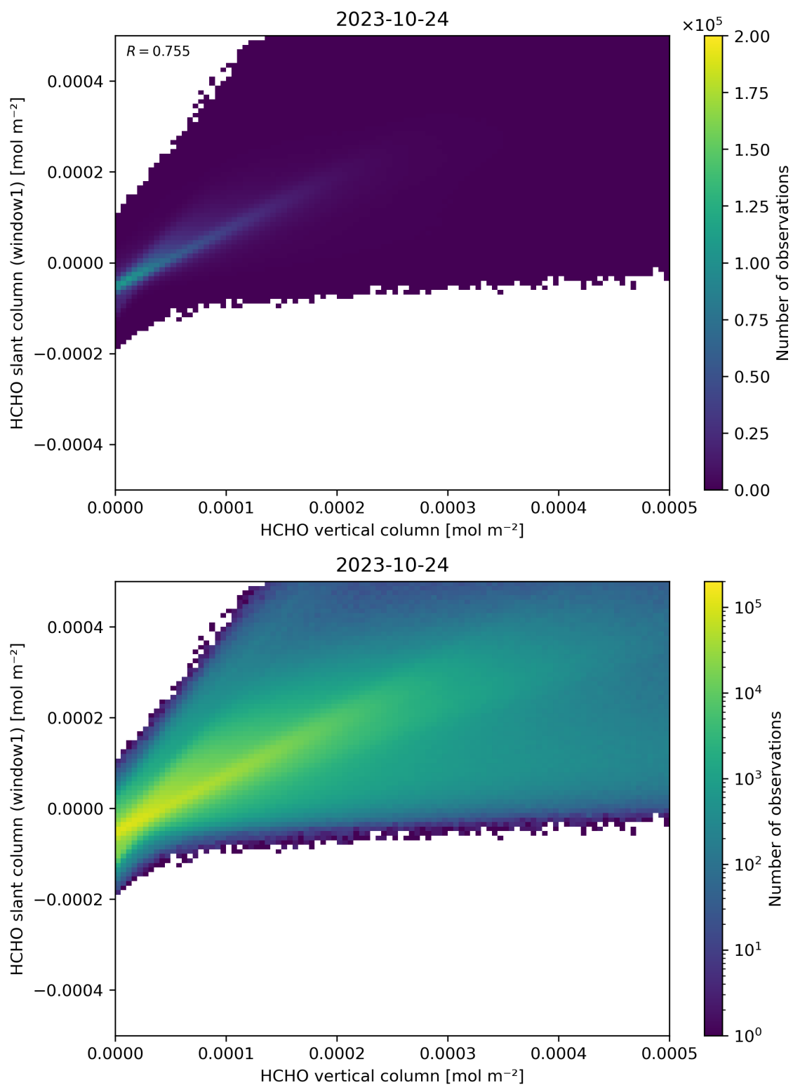
Figure 129: Scatter density plot of “HCHO vertical column” against “HCHO slant column (window1)” for 2023-10-23 to 2023-10-25.
