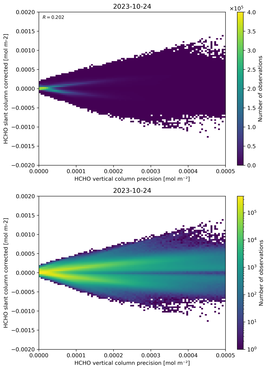
Figure 140: Scatter density plot of “HCHO vertical column precision” against “HCHO slant column corrected” for 2023-10-23 to 2023-10-25.
