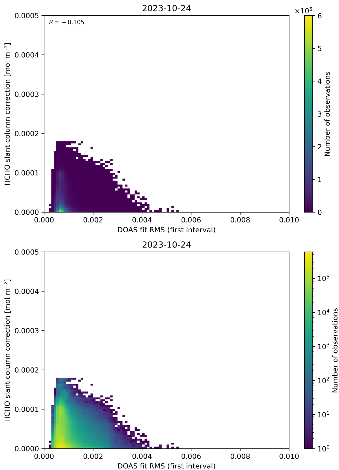
Figure 63: Scatter density plot of “DOAS fit RMS (first interval)” against “HCHO slant column correction” for 2023-10-23 to 2023-10-25.
