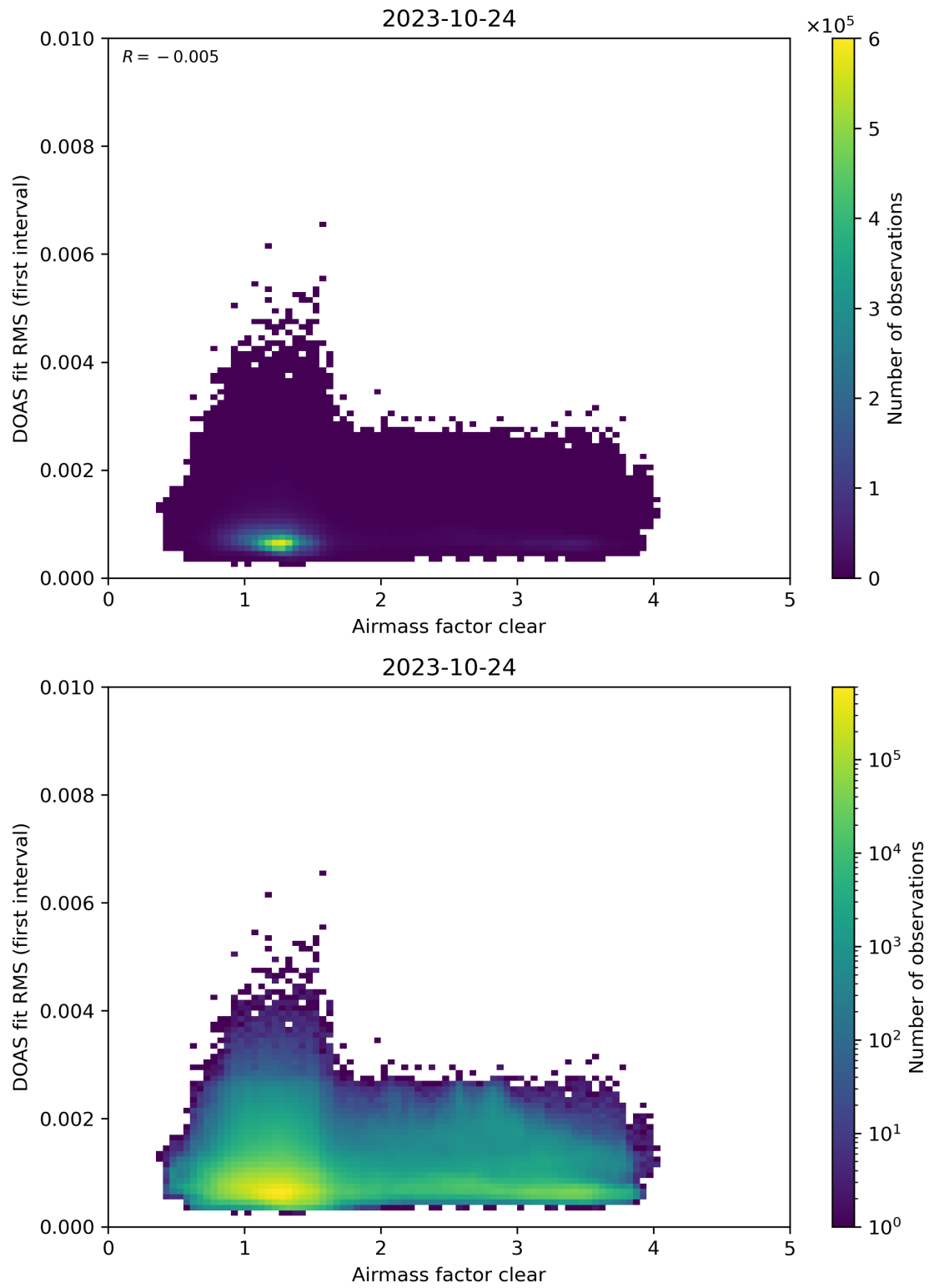
Figure 71: Scatter density plot of “Airmass factor clear” against “DOAS fit RMS (first interval)” for 2023-10-23 to 2023-10-25.
