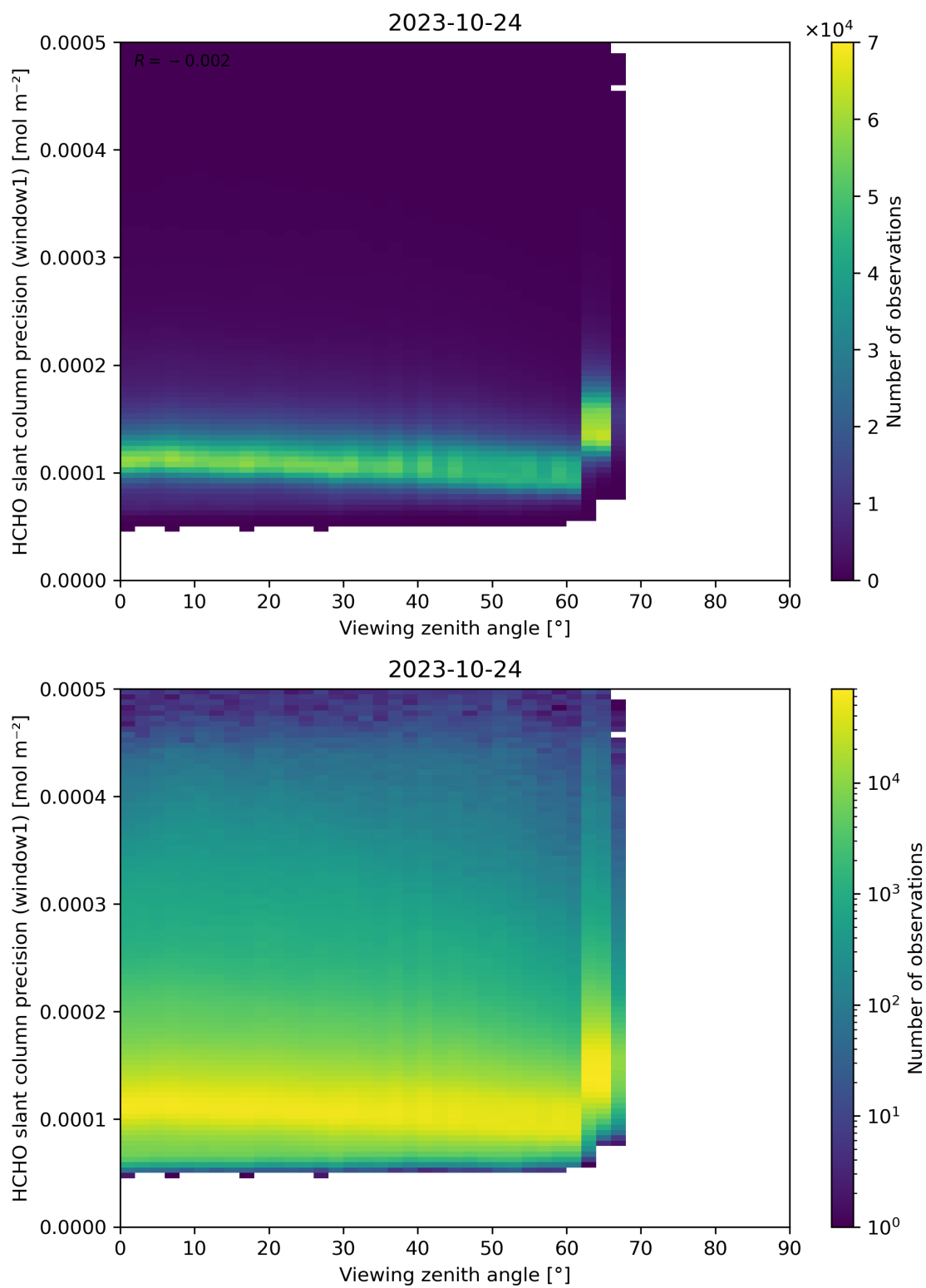
Figure 189: Scatter density plot of “Viewing zenith angle” against “HCHO slant column precision (window1)” for 2023-10-23 to 2023-10-25.
