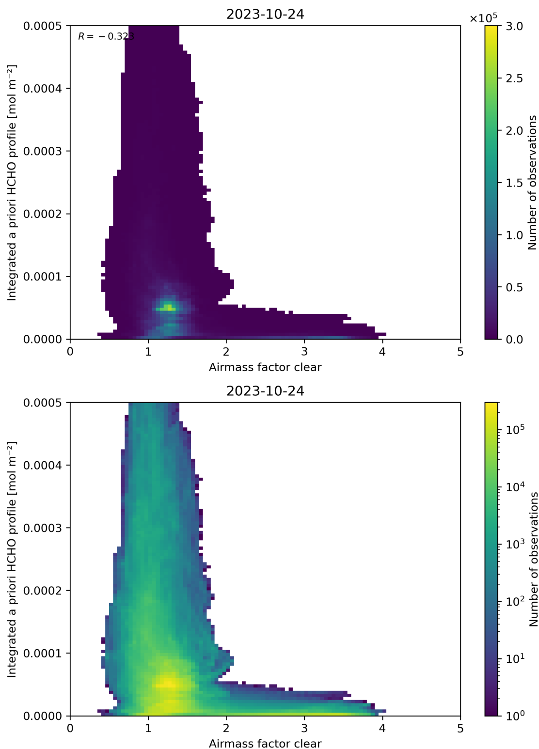
Figure 76: Scatter density plot of “Airmass factor clear” against “Integrated a priori HCHO profile” for 2023-10-23 to 2023-10-25.
