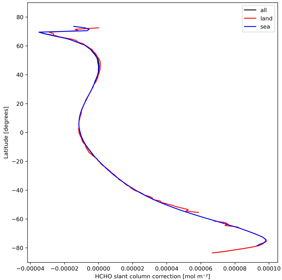
Figure 33: Zonal average of “HCHO slant column correction” for 2023-10-23 to 2023-10-25.
