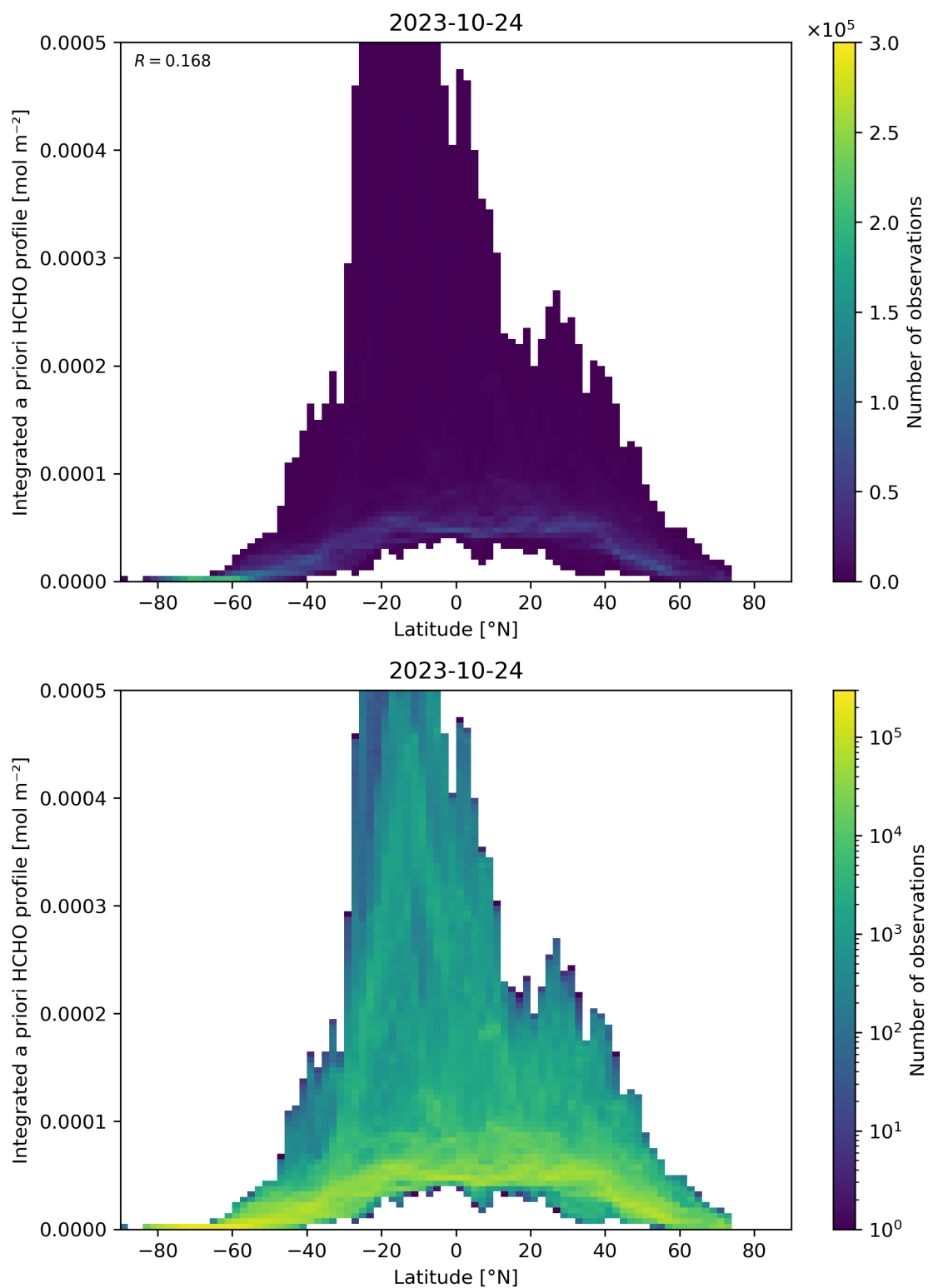
Figure 166: Scatter density plot of “Latitude” against “Integrated a priori HCHO profile” for 2023-10-23 to 2023-10-25.
