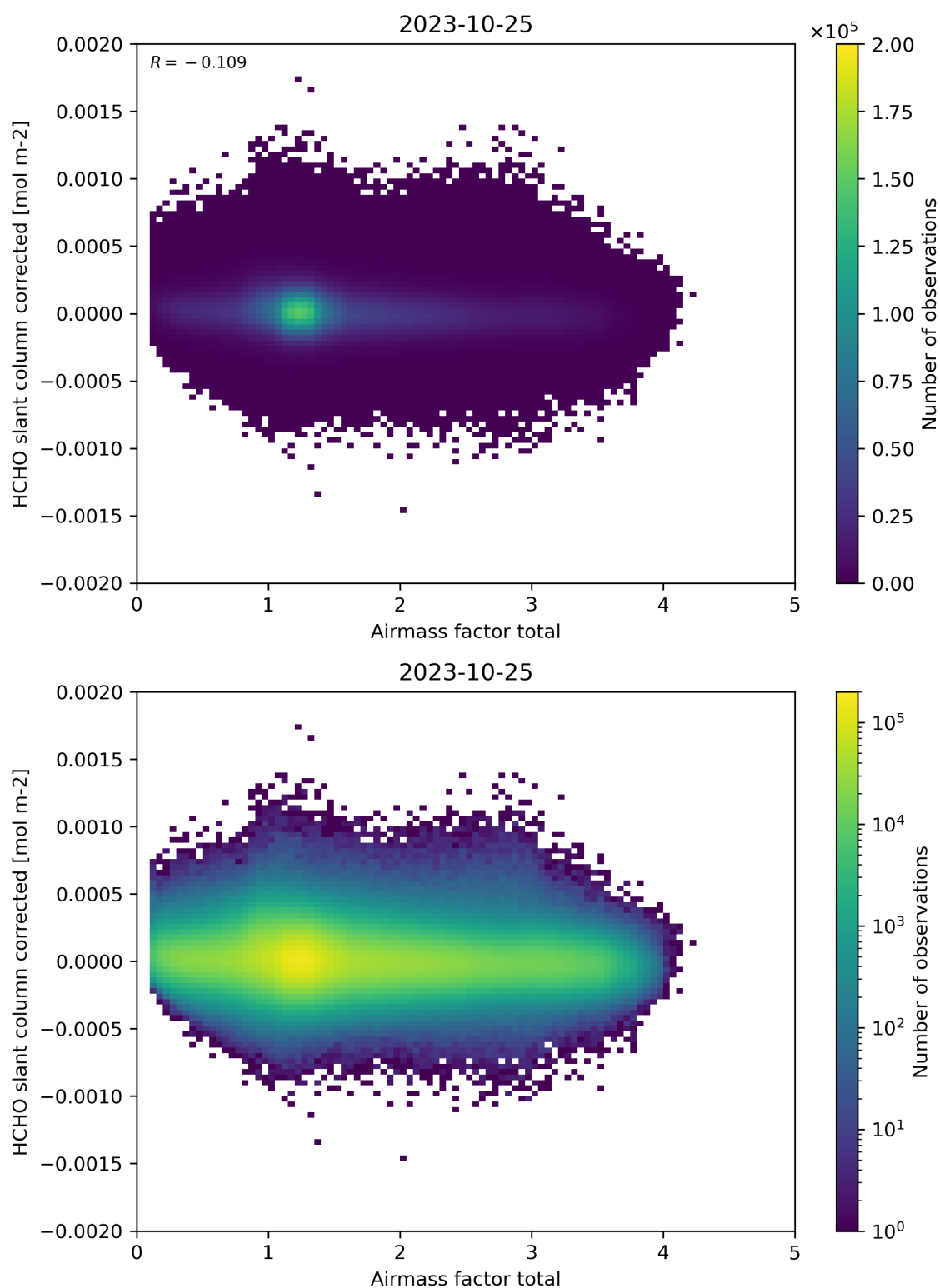
Figure 101: Scatter density plot of “Airmass factor total” against “HCHO slant column corrected” for 2023-10-24 to 2023-10-26.
