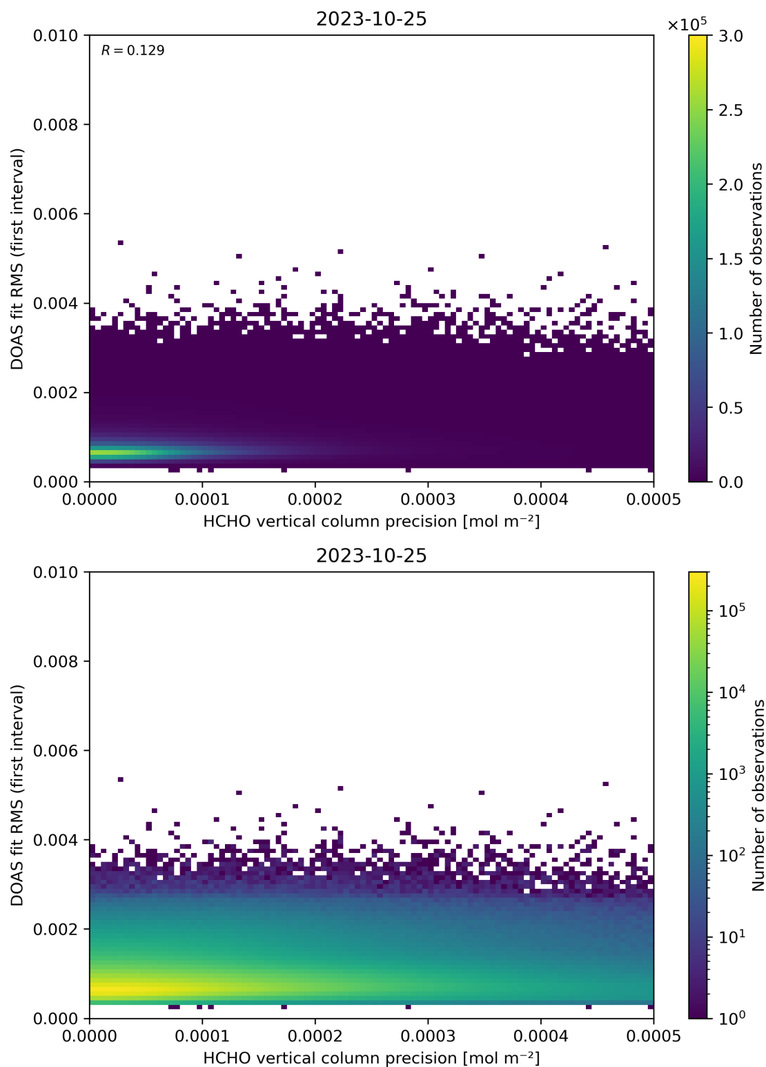
Figure 136: Scatter density plot of “HCHO vertical column precision” against “DOAS fit RMS (first interval)” for 2023-10-24 to 2023-10-26.
