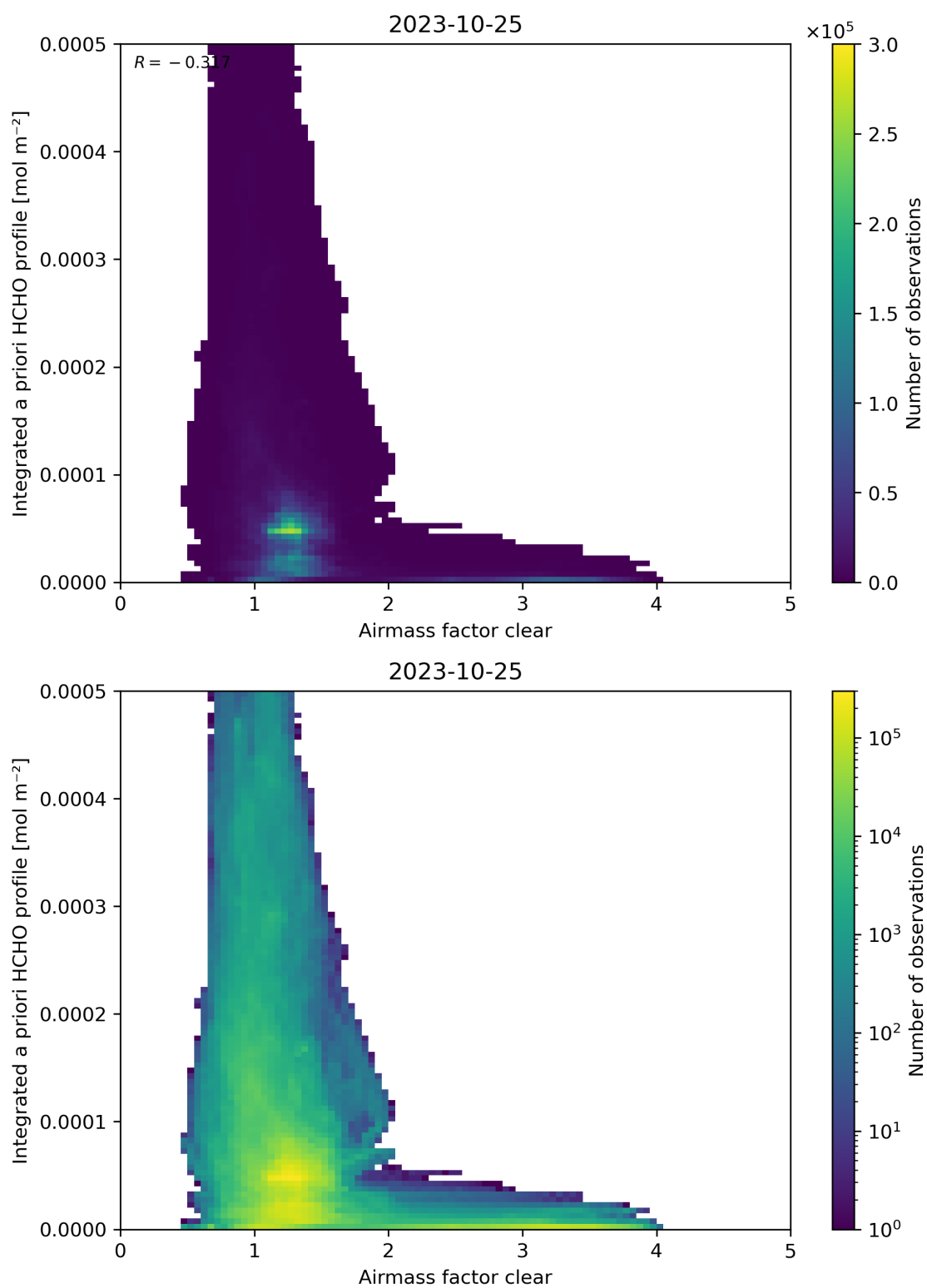
Figure 76: Scatter density plot of “Airmass factor clear” against “Integrated a priori HCHO profile” for 2023-10-24 to 2023-10-26.
