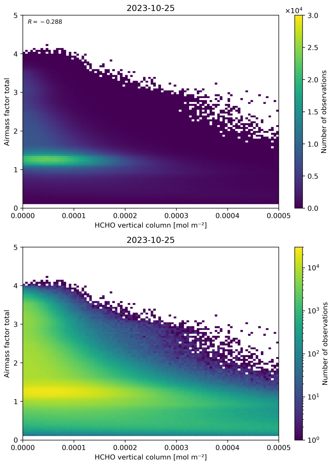
Figure 131: Scatter density plot of “HCHO vertical column” against “Airmass factor total” for 2023-10-24 to 2023-10-26.
