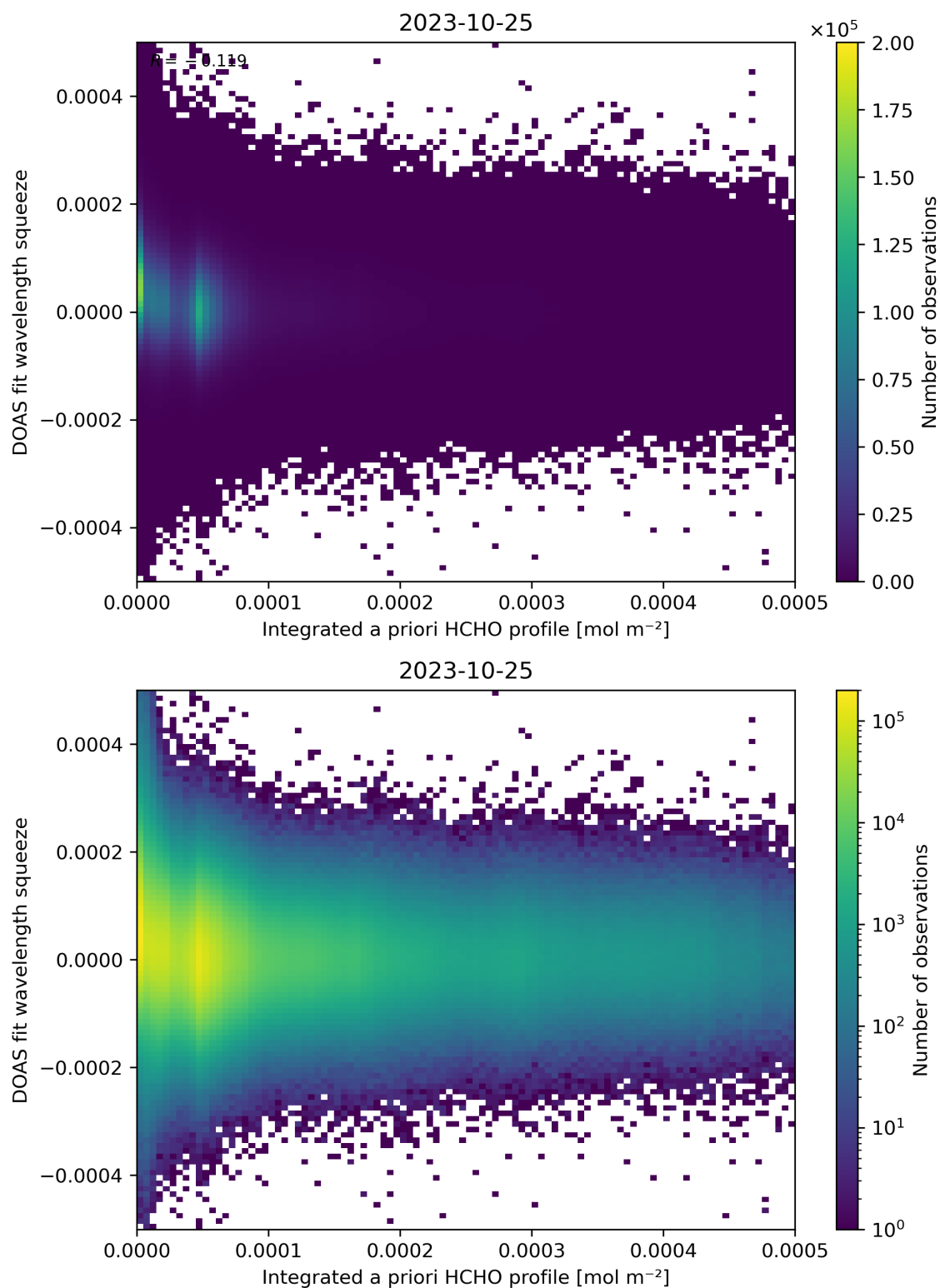
Figure 150: Scatter density plot of “Integrated a priori HCHO profile” against “DOAS fit wavelength squeeze” for 2023-10-24 to 2023-10-26.
