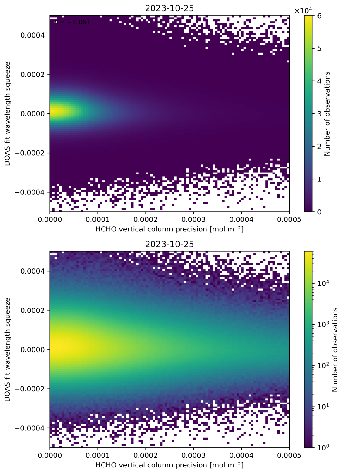
Figure 138: Scatter density plot of “HCHO vertical column precision” against “DOAS fit wavelength squeeze” for 2023-10-24 to 2023-10-26.
