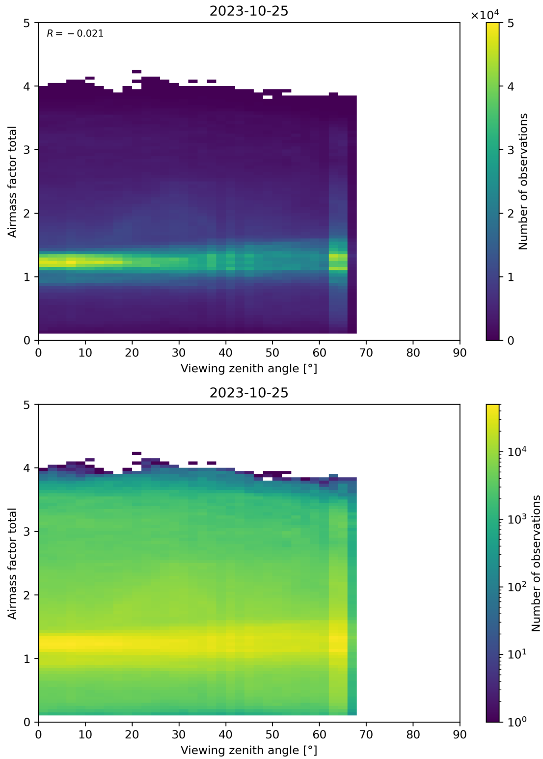
Figure 190: Scatter density plot of “Viewing zenith angle” against “Airmass factor total” for 2023-10-24 to 2023-10-26.
