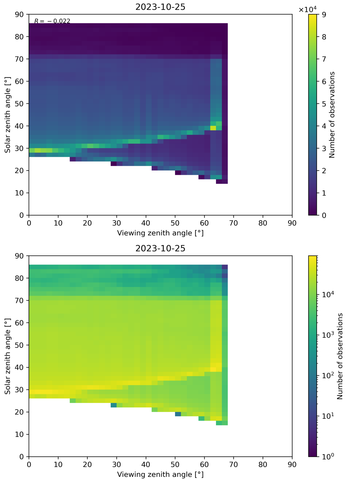
Figure 197: Scatter density plot of “Viewing zenith angle” against “Solar zenith angle” for 2023-10-24 to 2023-10-26.
