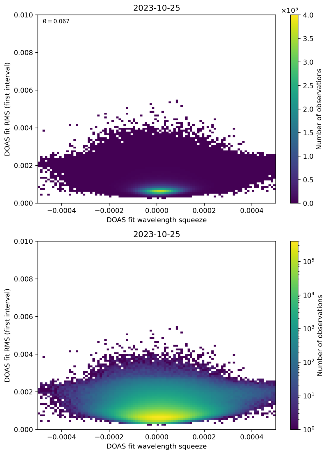
Figure 68: Scatter density plot of “DOAS fit wavelength squeeze” against “DOAS fit RMS (first interval)” for 2023-10-24 to 2023-10-26.
