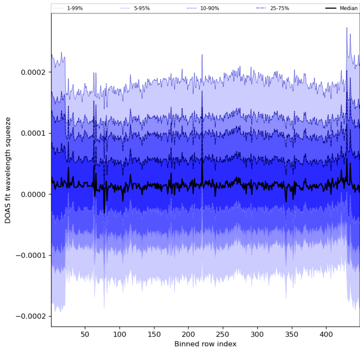
Figure 59: Along track statistics of “DOAS fit wavelength squeeze” for 2023-10-24 to 2023-10-26
