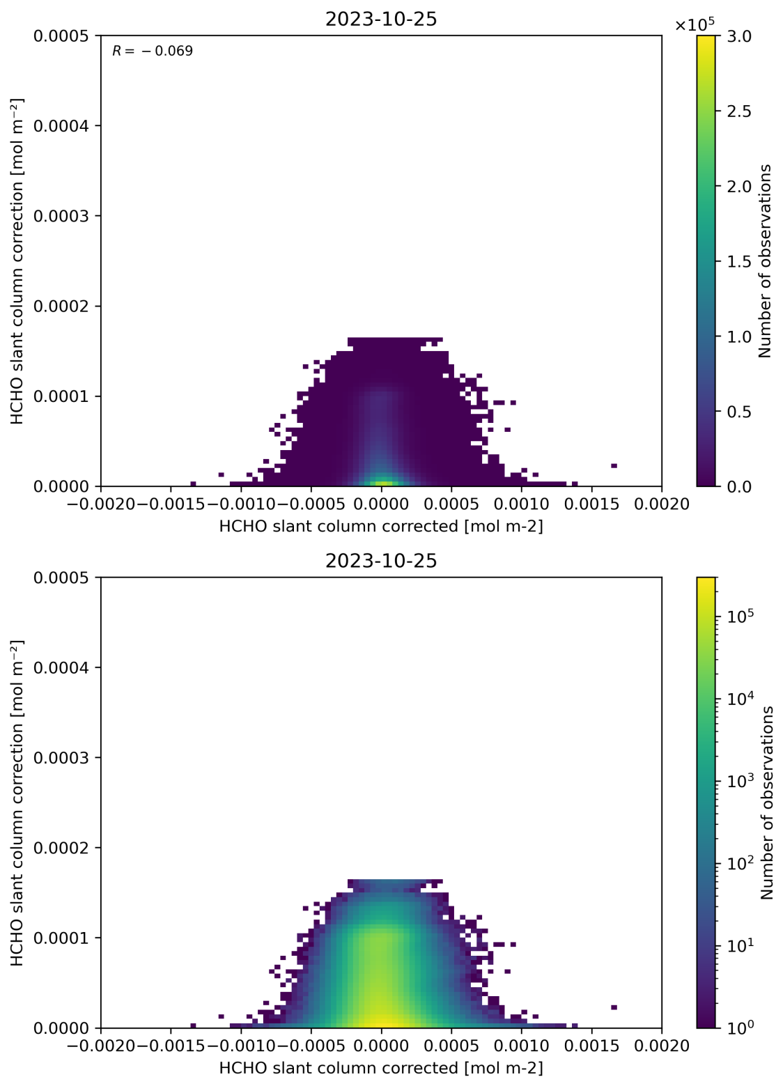
Figure 77: Scatter density plot of “HCHO slant column corrected” against “HCHO slant column correction” for 2023-10-24 to 2023-10-26.
