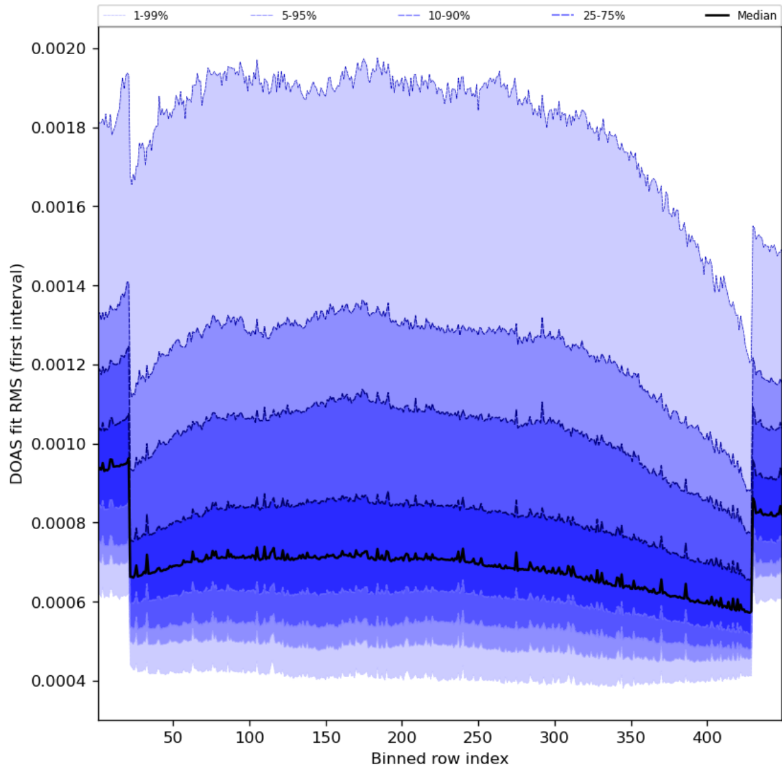
Figure 60: Along track statistics of “DOAS fit RMS (first interval)” for 2023-10-24 to 2023-10-26
