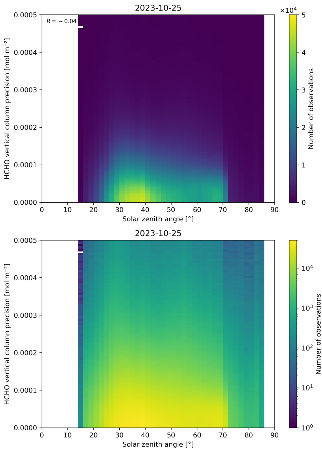
Figure 179: Scatter density plot of “Solar zenith angle” against “HCHO vertical column precision” for 2023-10-24 to 2023-10-26.
