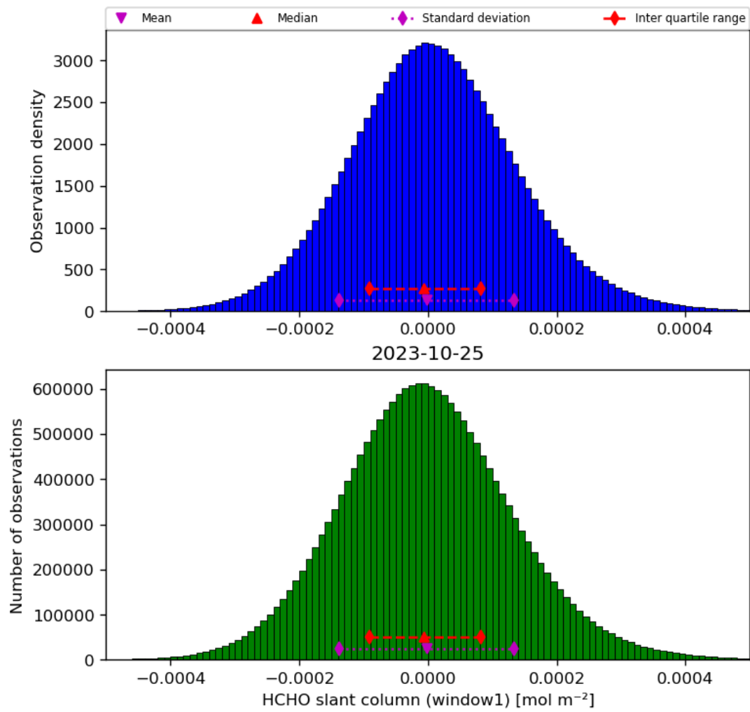
Figure 38: Histogram of “HCHO slant column (window1)” for 2023-10-24 to 2023-10-26
