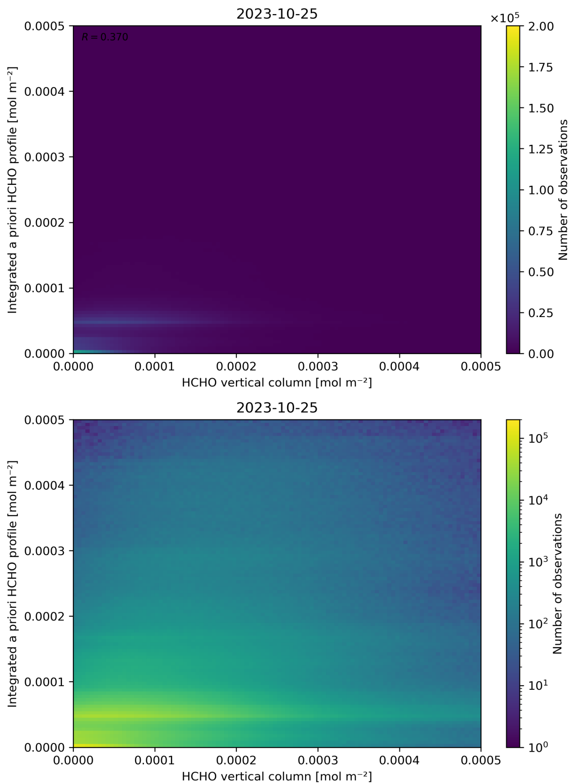
Figure 135: Scatter density plot of “HCHO vertical column” against “Integrated a priori HCHO profile” for 2023-10-24 to 2023-10-26.
