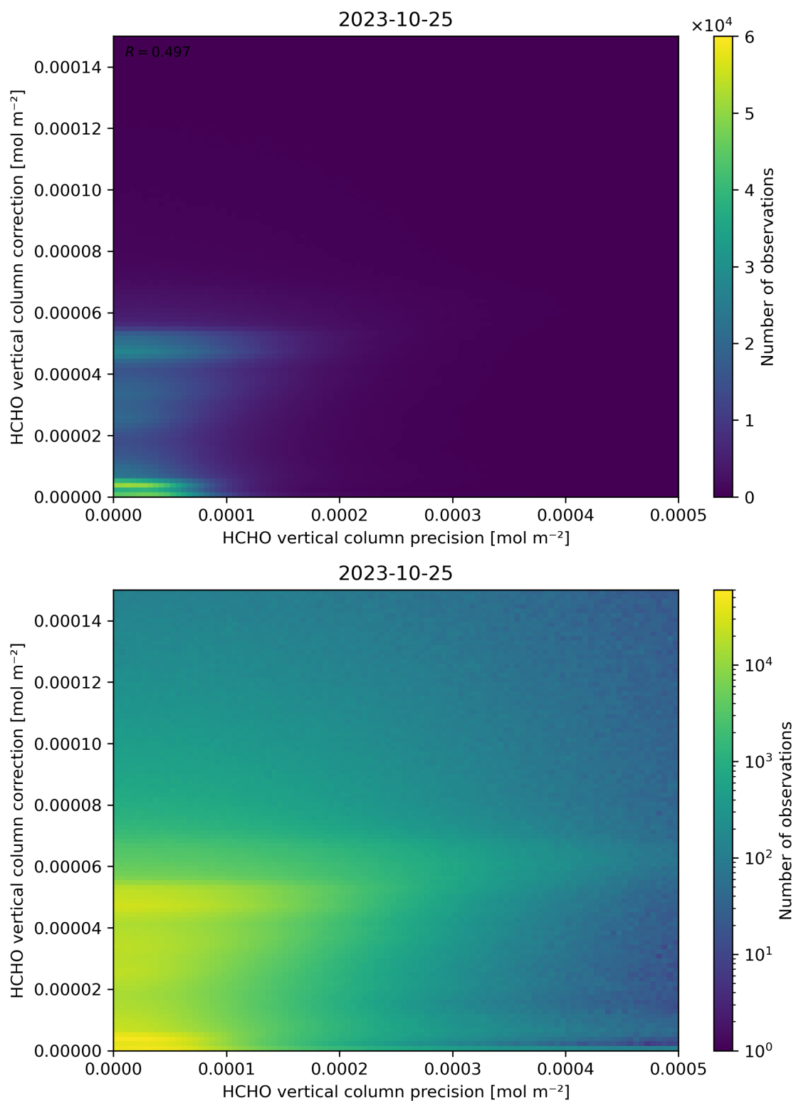
Figure 146: Scatter density plot of “HCHO vertical column precision” against “HCHO vertical column correction” for 2023-10-24 to 2023-10-26.
