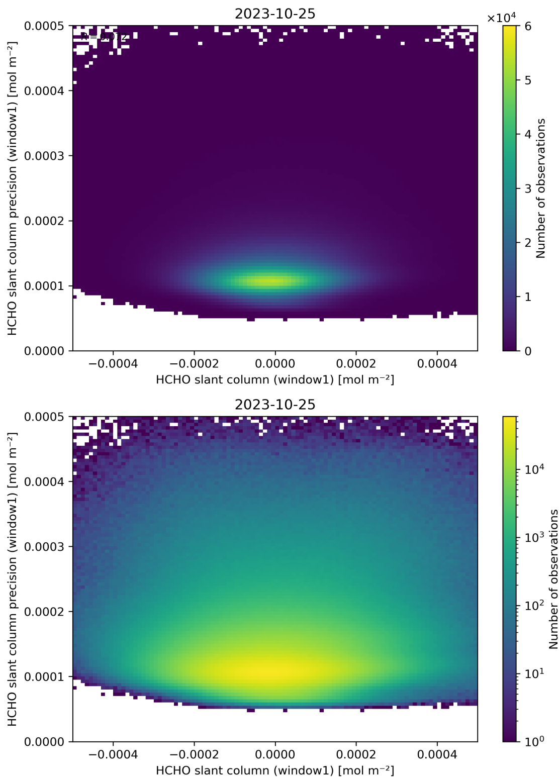
Figure 84: Scatter density plot of “HCHO slant column (window1)” against “HCHO slant column precision (window1)” for 2023-10-24 to 2023-10-26.
