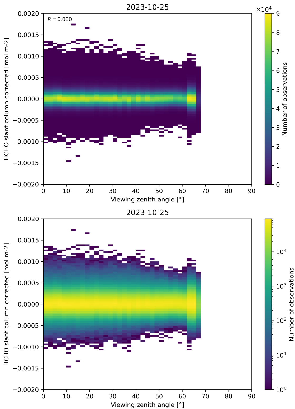
Figure 186: Scatter density plot of “Viewing zenith angle” against “HCHO slant column corrected” for 2023-10-24 to 2023-10-26.
