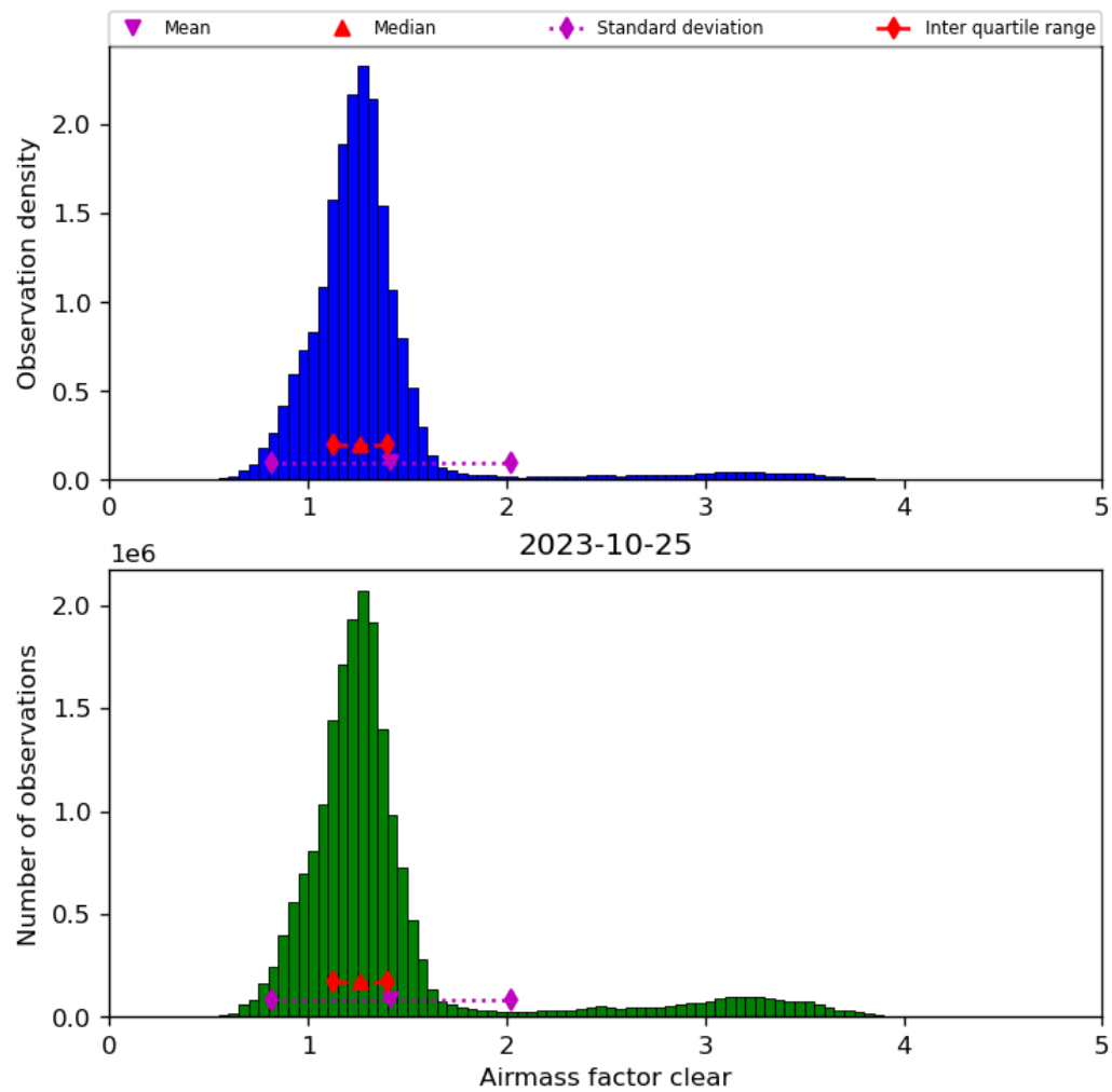
Figure 42: Histogram of “Airmass factor clear” for 2023-10-24 to 2023-10-26
