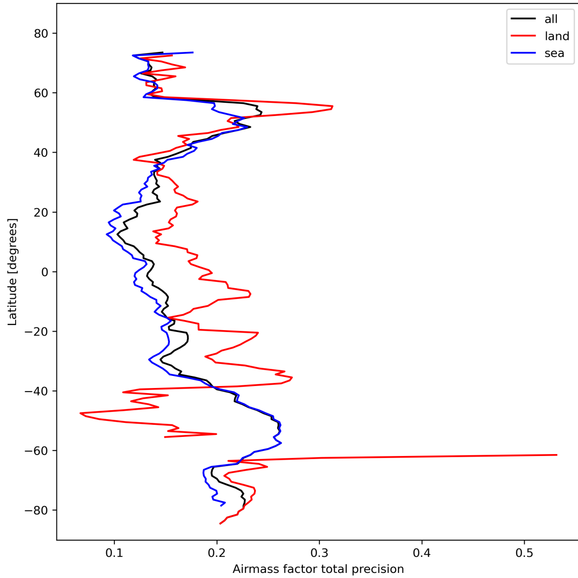
Figure 27: Zonal average of “Airmass factor total precision” for 2023-10-24 to 2023-10-26.
