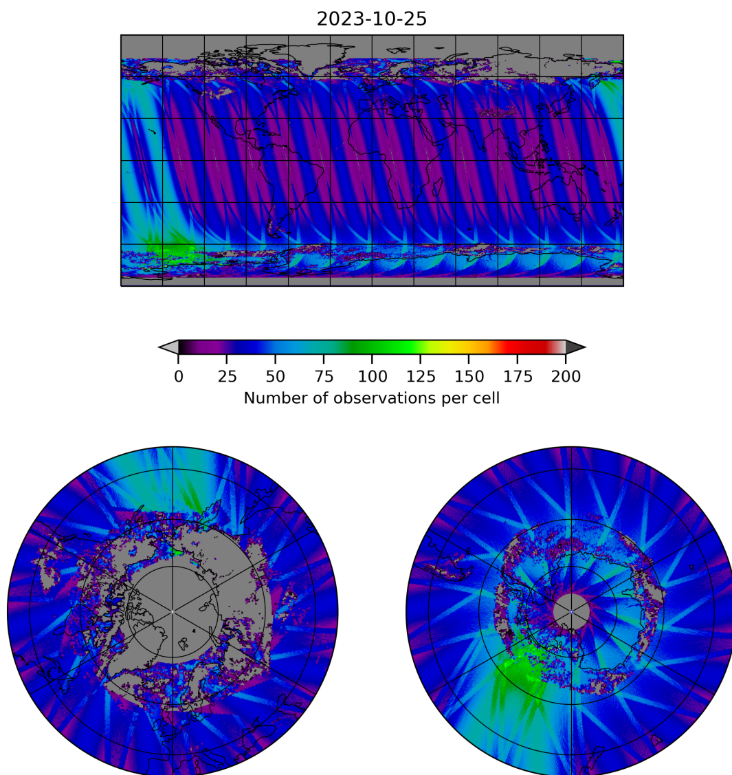
Figure 19: Map of the number of observations for 2023-10-24 to 2023-10-26
