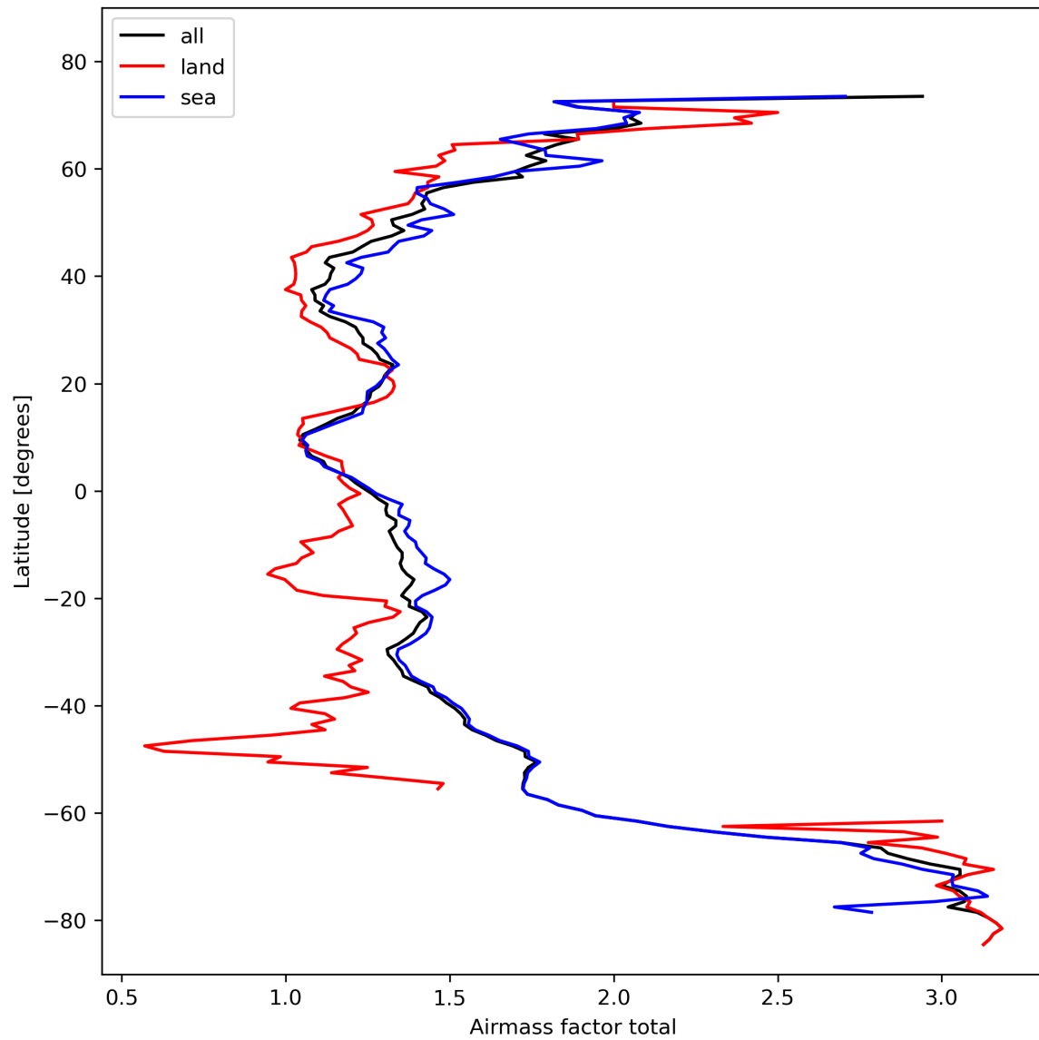
Figure 26: Zonal average of “Airmass factor total” for 2023-10-24 to 2023-10-26.
