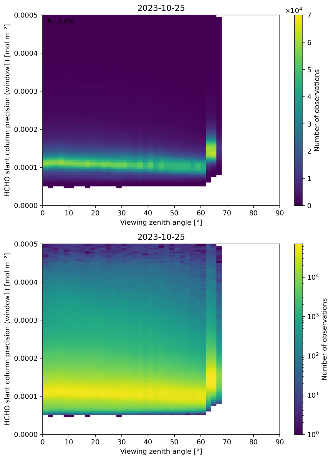
Figure 189: Scatter density plot of “Viewing zenith angle” against “HCHO slant column precision (window1)” for 2023-10-24 to 2023-10-26.
