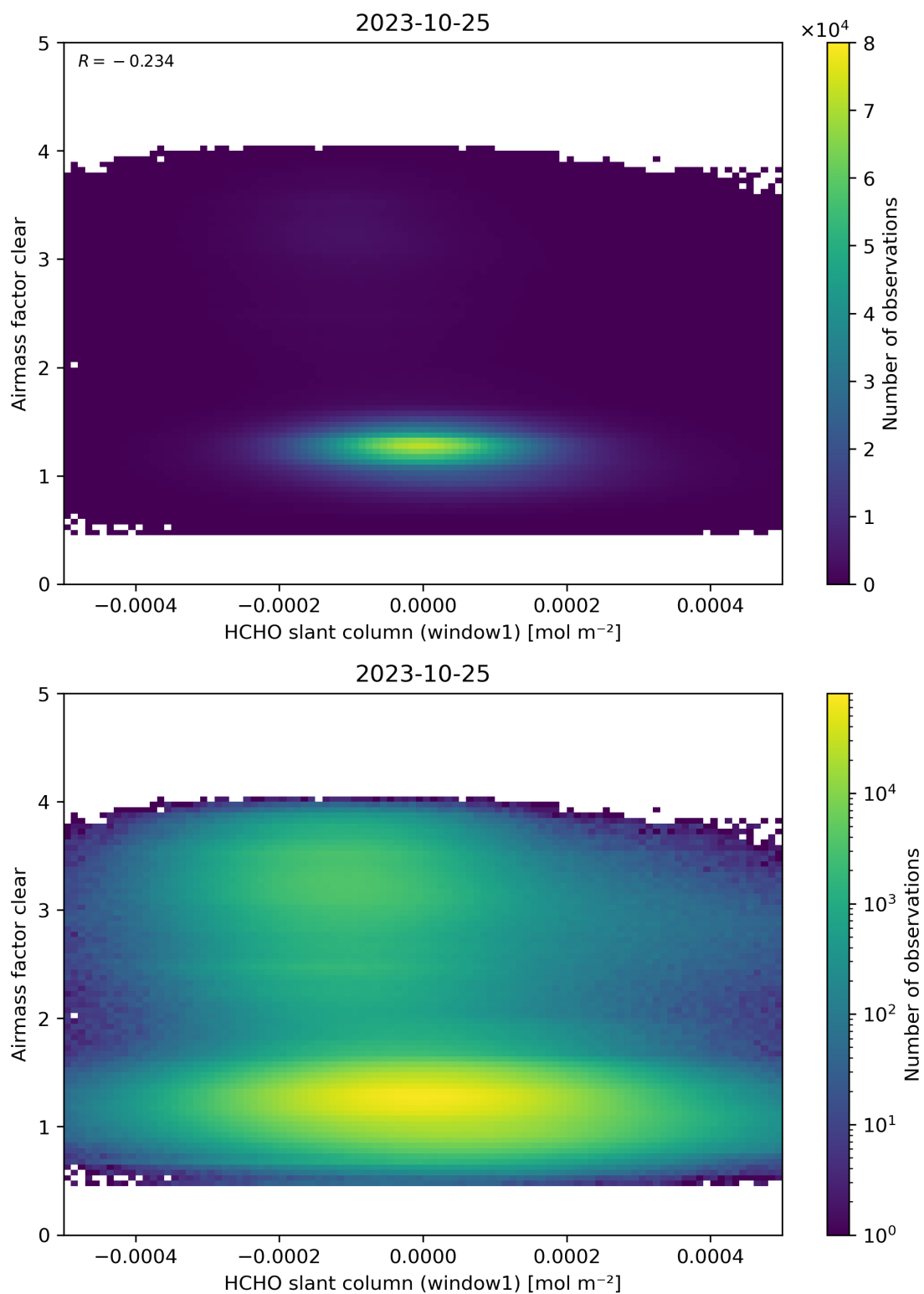
Figure 81: Scatter density plot of “HCHO slant column (window1)” against “Airmass factor clear” for 2023-10-24 to 2023-10-26.
