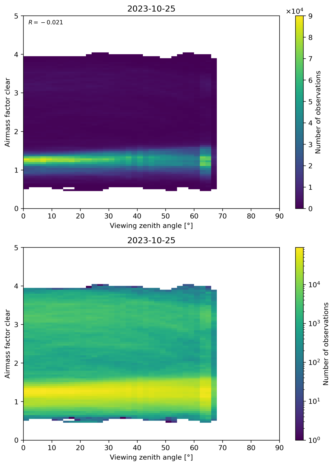
Figure 185: Scatter density plot of “Viewing zenith angle” against “Airmass factor clear” for 2023-10-24 to 2023-10-26.
