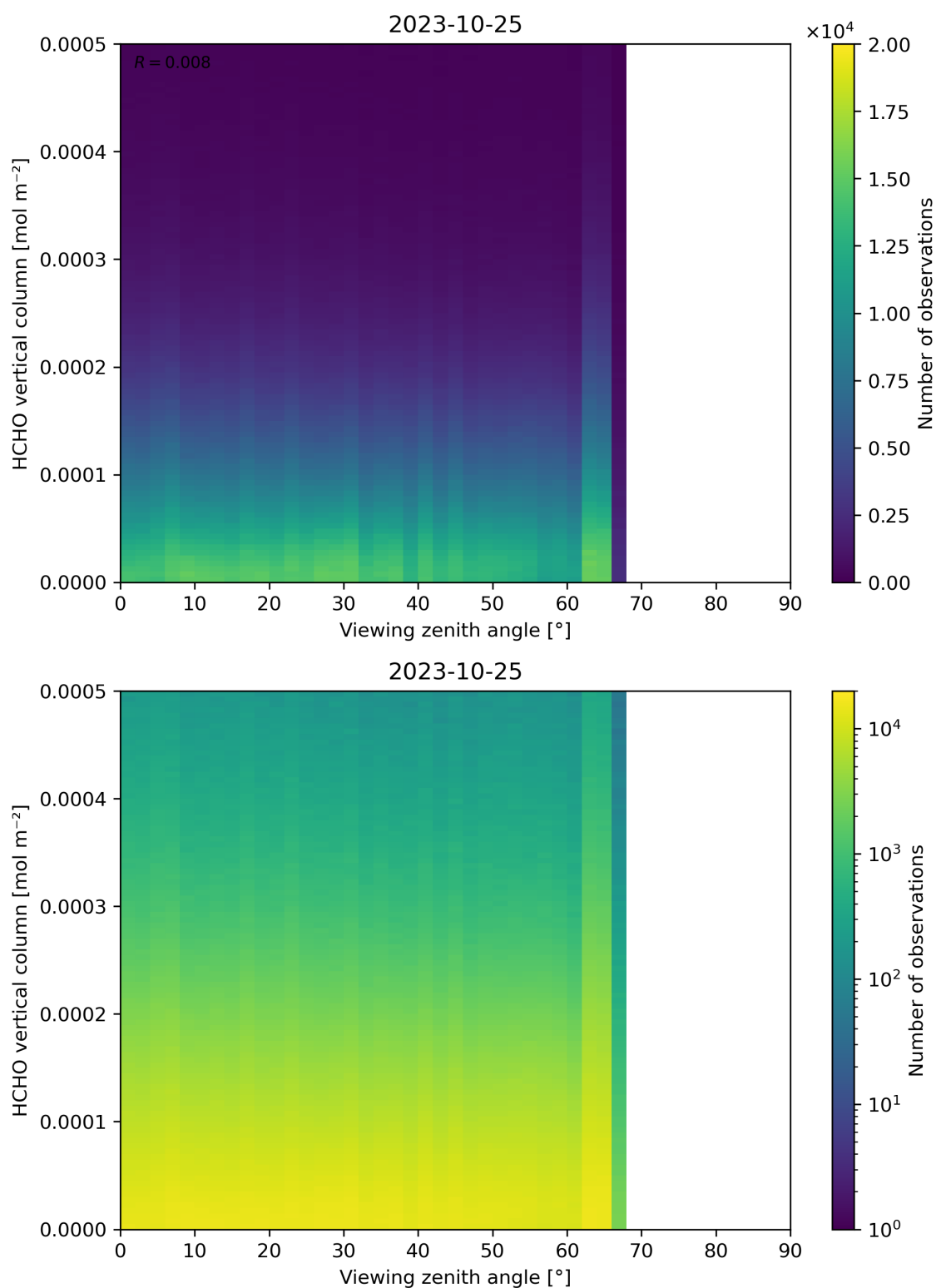
Figure 192: Scatter density plot of “Viewing zenith angle” against “HCHO vertical column” for 2023-10-24 to 2023-10-26.
