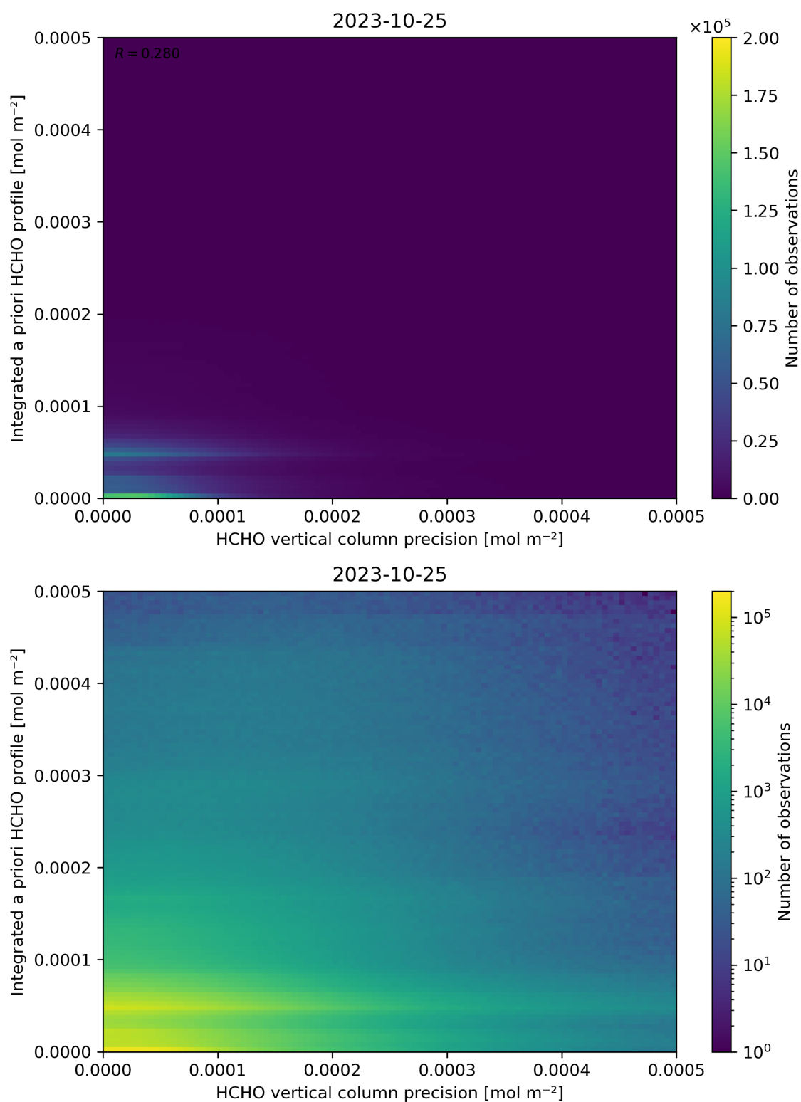
Figure 147: Scatter density plot of “HCHO vertical column precision” against “Integrated a priori HCHO profile” for 2023-10-24 to 2023-10-26.
