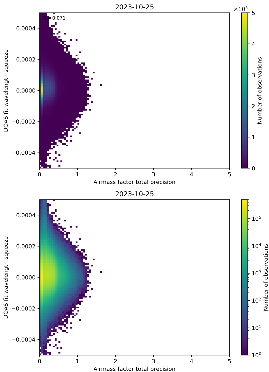
Figure 107: Scatter density plot of “Airmass factor total precision” against “DOAS fit wavelength squeeze” for 2023-10-24 to 2023-10-26.
