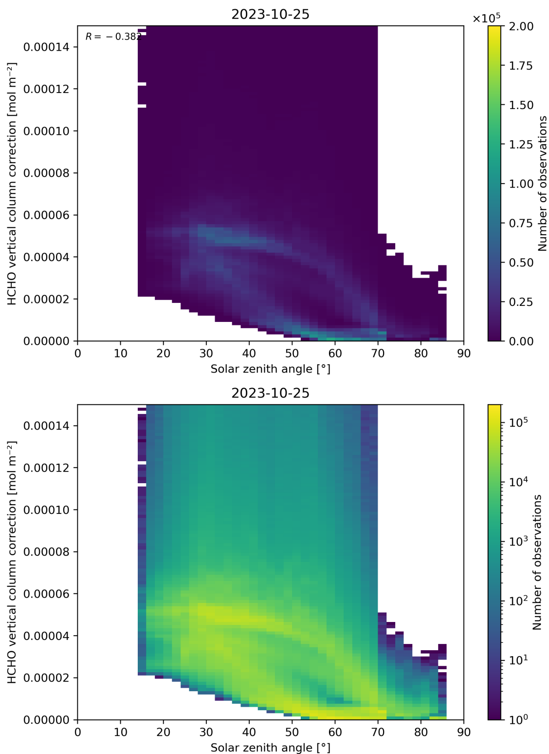
Figure 178: Scatter density plot of “Solar zenith angle” against “HCHO vertical column correction” for 2023-10-24 to 2023-10-26.
