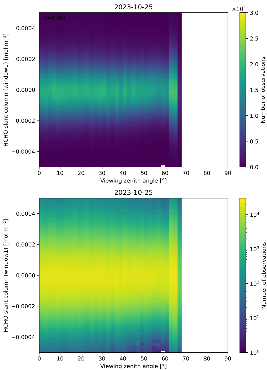
Figure 188: Scatter density plot of “Viewing zenith angle” against “HCHO slant column (window1)” for 2023-10-24 to 2023-10-26.
