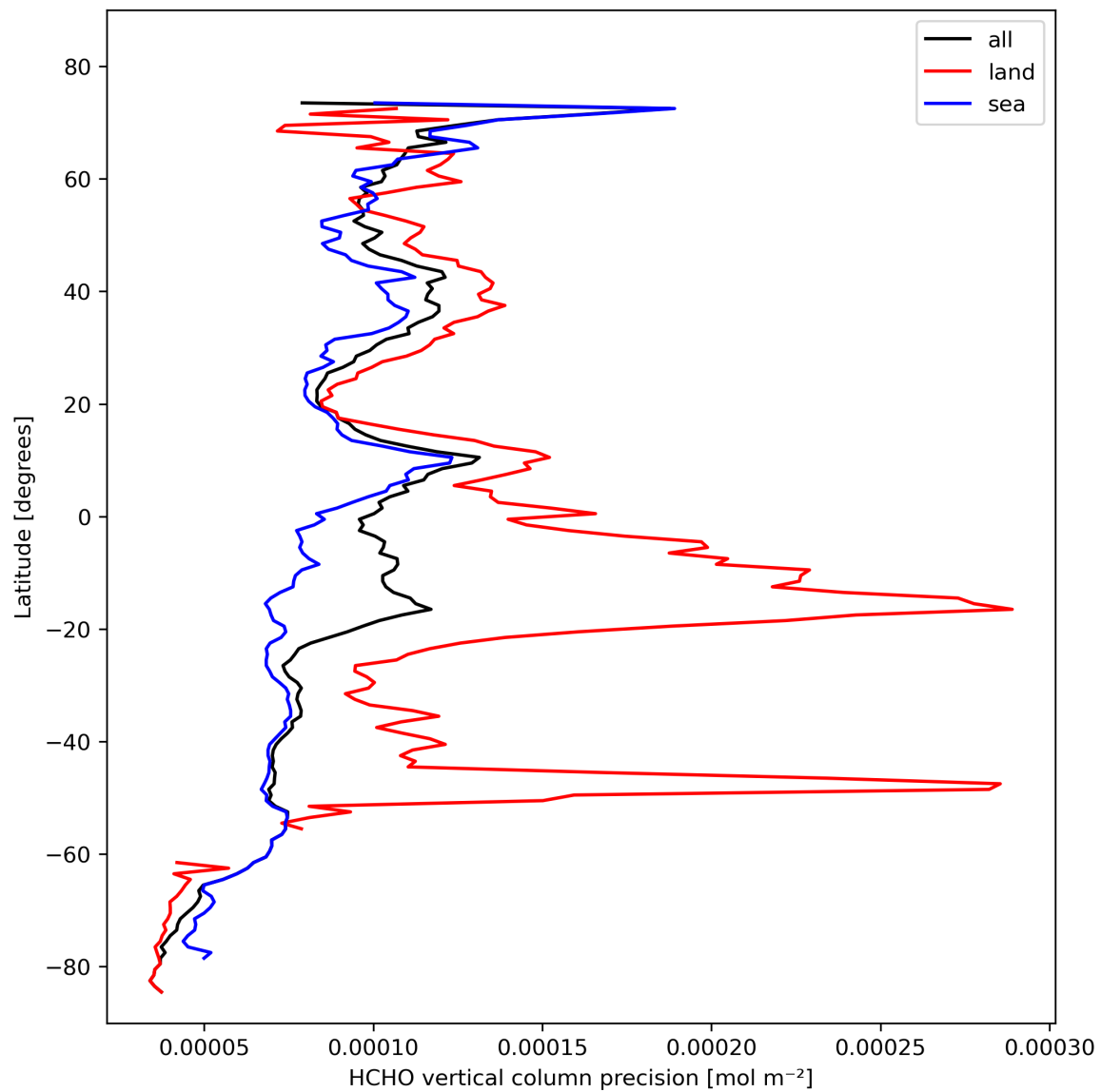
Figure 22: Zonal average of “HCHO vertical column precision” for 2023-10-24 to 2023-10-26.
