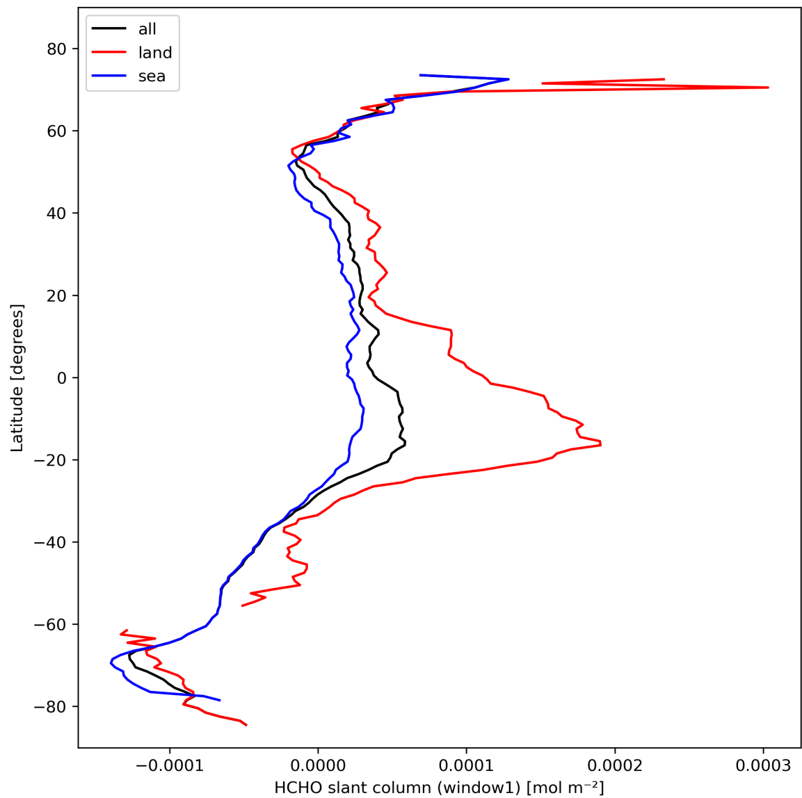
Figure 24: Zonal average of “HCHO slant column (window1)” for 2023-10-24 to 2023-10-26.
