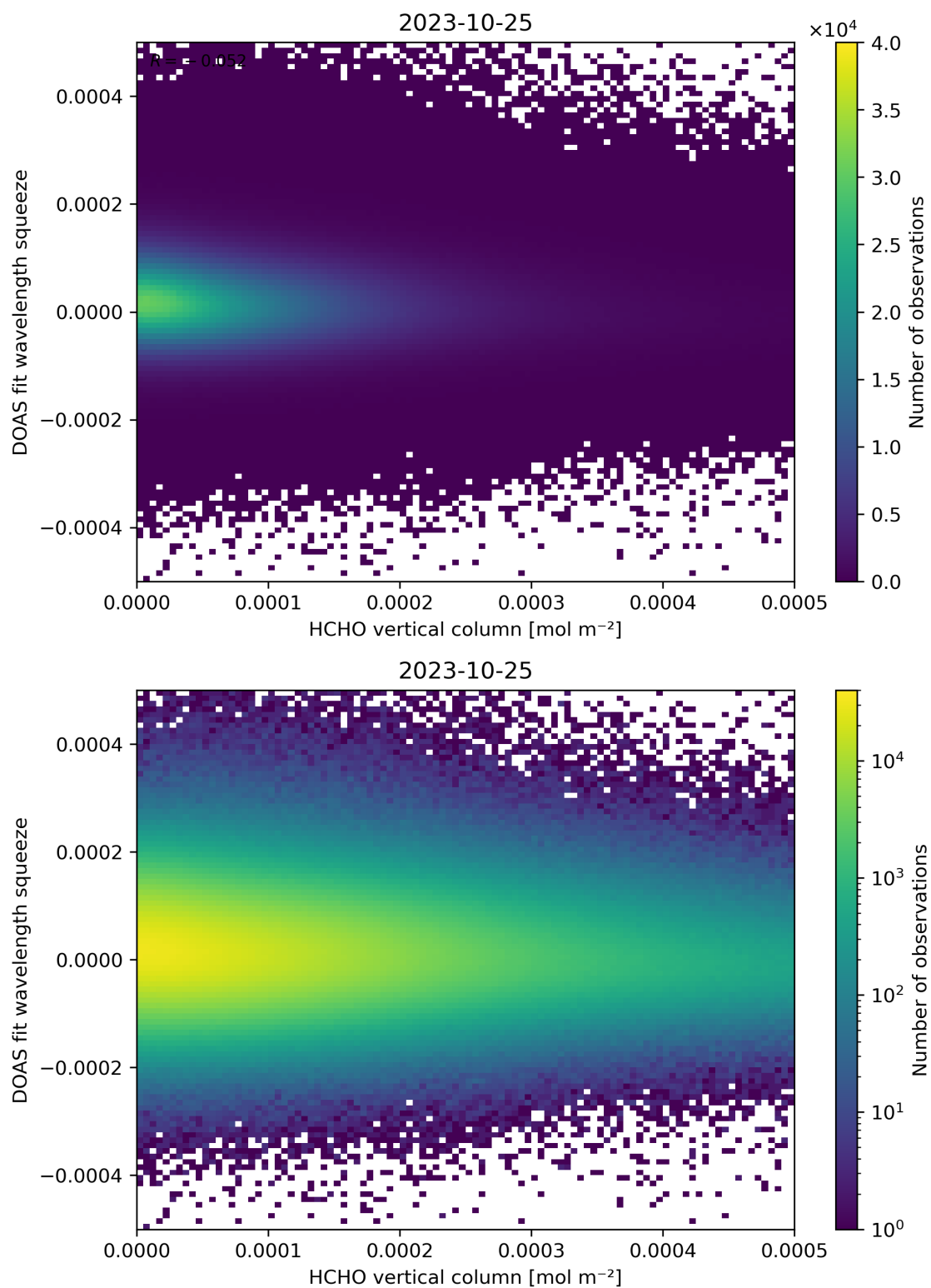
Figure 125: Scatter density plot of “HCHO vertical column” against “DOAS fit wavelength squeeze” for 2023-10-24 to 2023-10-26.
