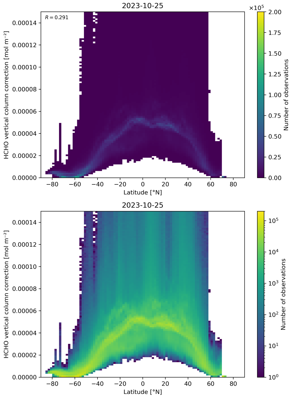
Figure 164: Scatter density plot of “Latitude” against “HCHO vertical column correction” for 2023-10-24 to 2023-10-26.
