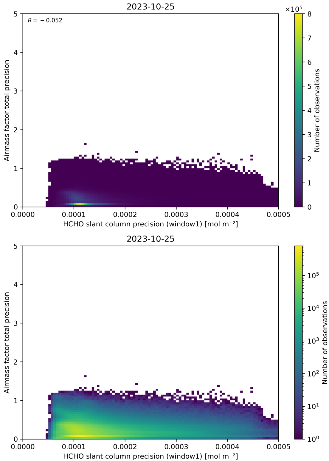
Figure 95: Scatter density plot of “HCHO slant column precision (window1)” against “Airmass factor total precision” for 2023-10-24 to 2023-10-26.
