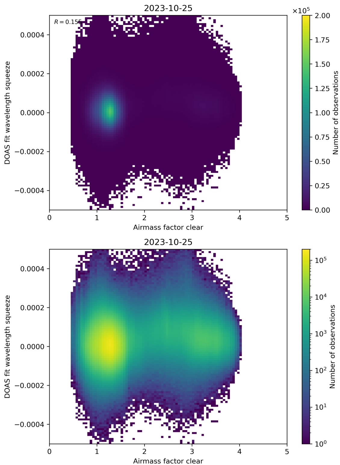
Figure 73: Scatter density plot of “Airmass factor clear” against “DOAS fit wavelength squeeze” for 2023-10-24 to 2023-10-26.
