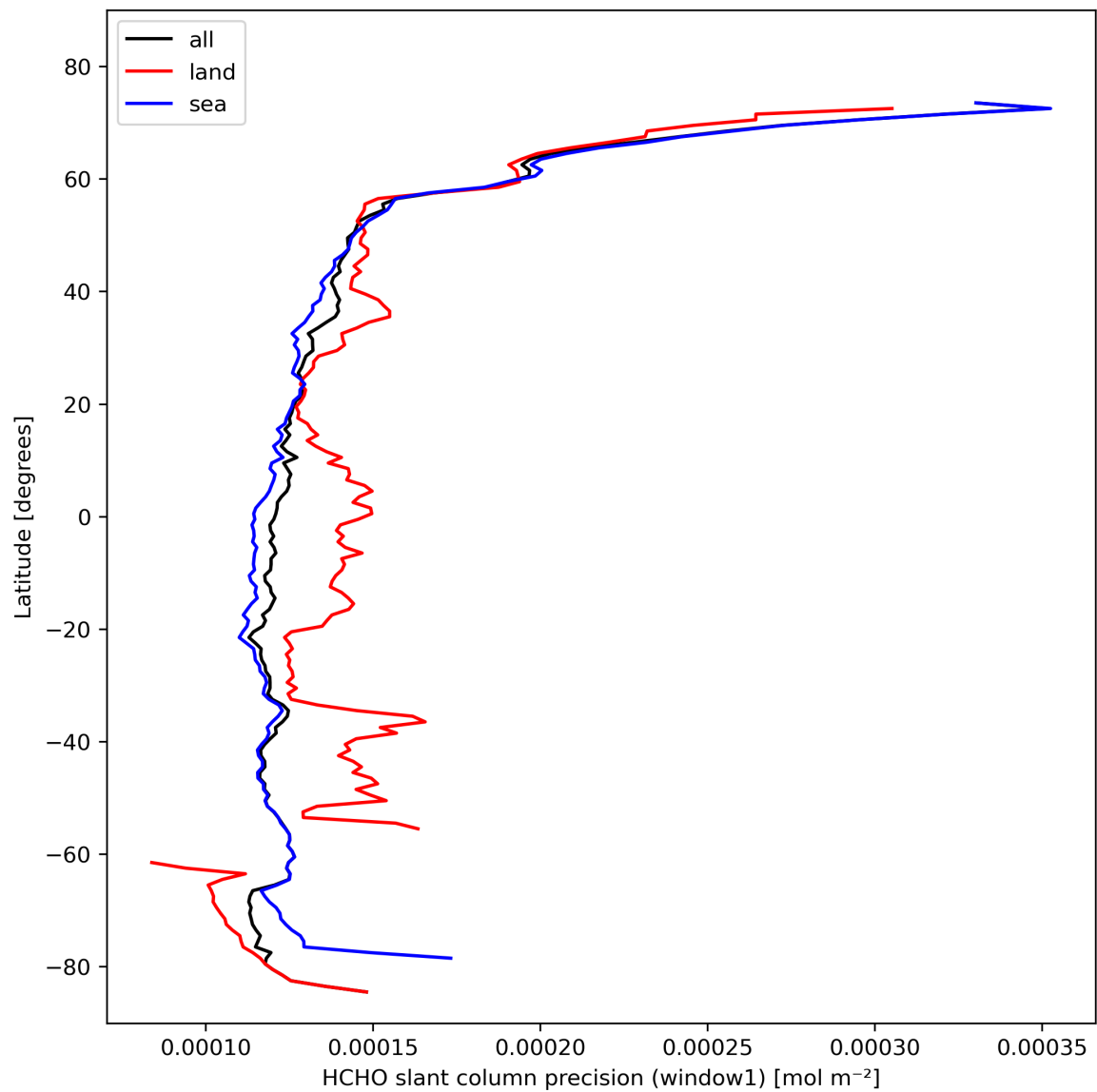
Figure 25: Zonal average of “HCHO slant column precision (window1)” for 2023-10-24 to 2023-10-26.
