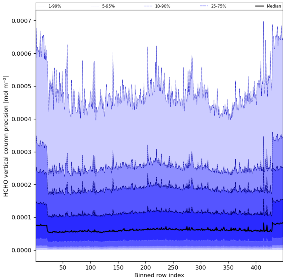
Figure 50: Along track statistics of “HCHO vertical column precision” for 2023-10-24 to 2023-10-26
