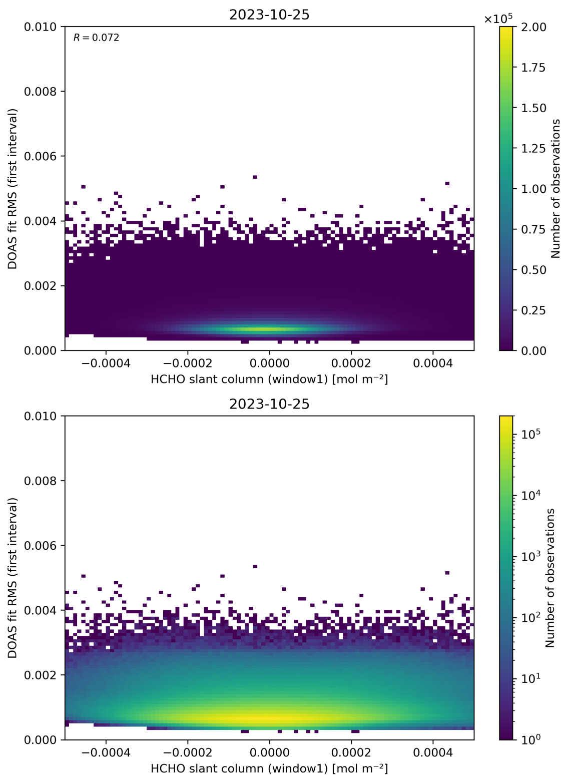
Figure 78: Scatter density plot of “HCHO slant column (window1)” against “DOAS fit RMS (first interval)” for 2023-10-24 to 2023-10-26.
