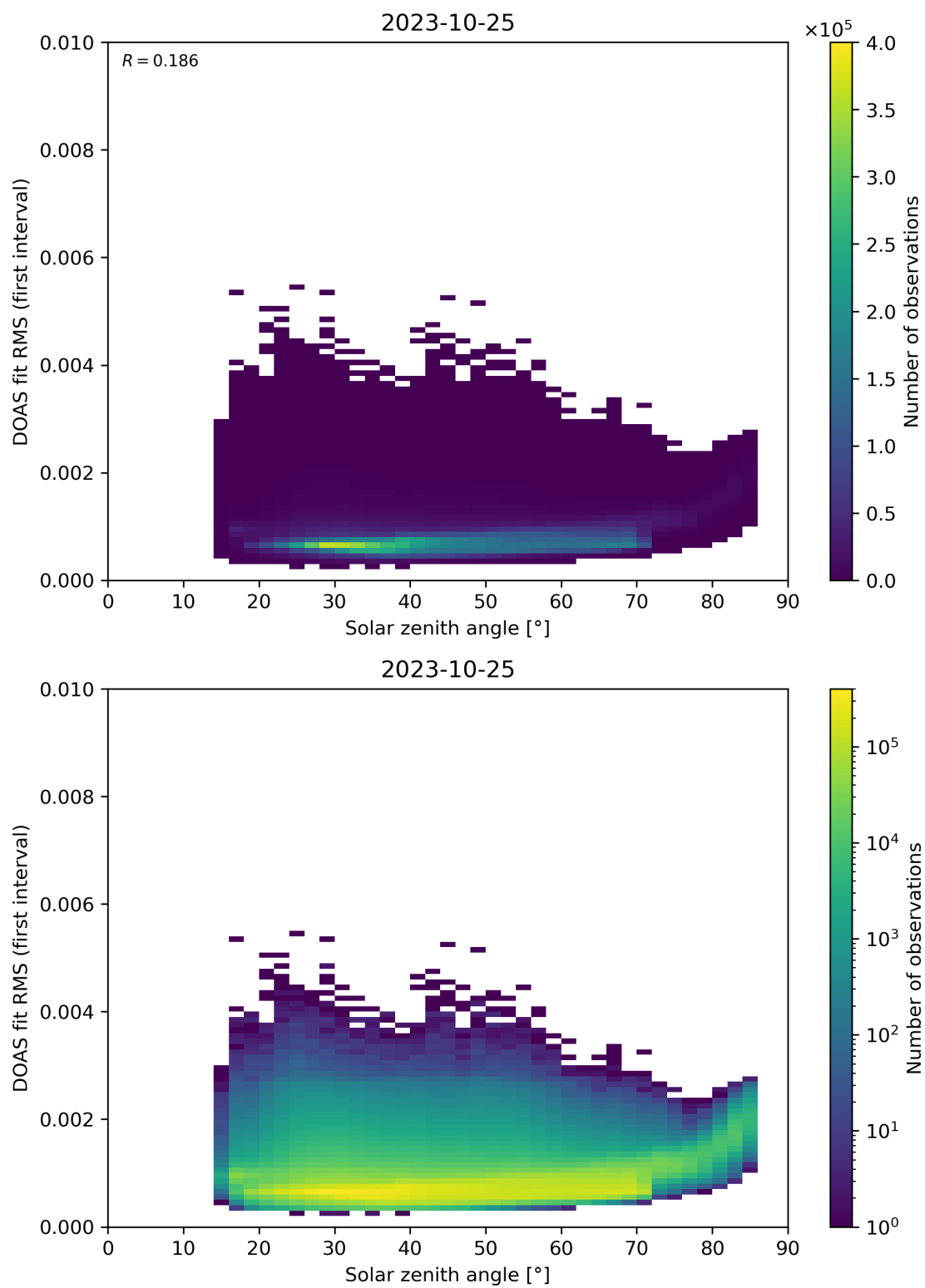
Figure 167: Scatter density plot of “Solar zenith angle” against “DOAS fit RMS (first interval)” for 2023-10-24 to 2023-10-26.
