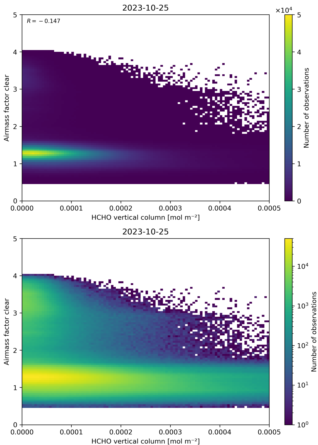
Figure 126: Scatter density plot of “HCHO vertical column” against “Airmass factor clear” for 2023-10-24 to 2023-10-26.
