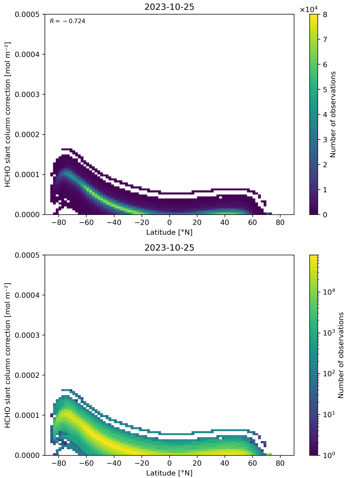
Figure 158: Scatter density plot of “Latitude” against “HCHO slant column correction” for 2023-10-24 to 2023-10-26.
