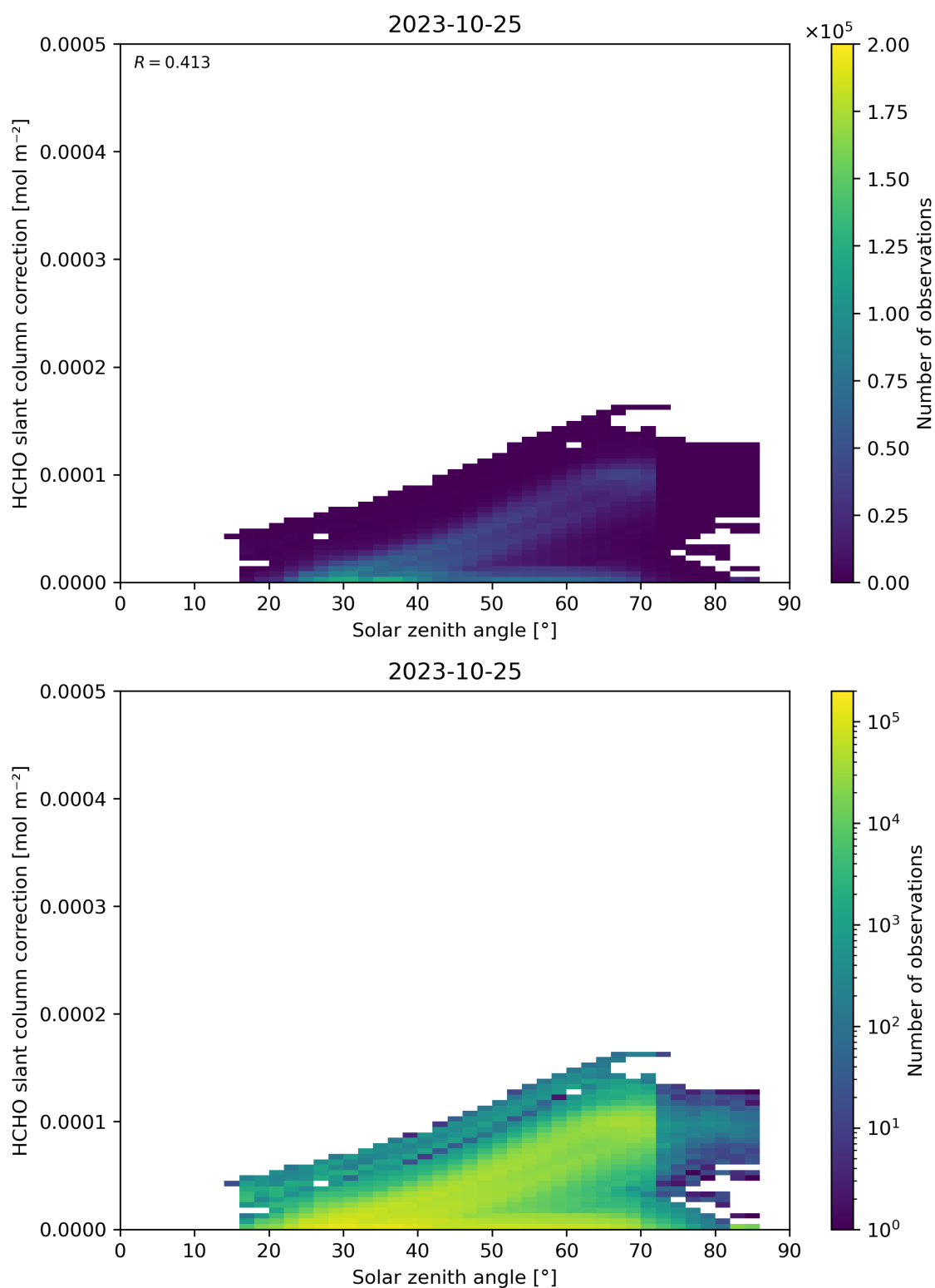
Figure 172: Scatter density plot of “Solar zenith angle” against “HCHO slant column correction” for 2023-10-24 to 2023-10-26.
