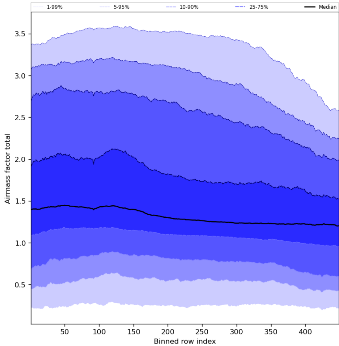
Figure 54: Along track statistics of “Airmass factor total” for 2023-10-24 to 2023-10-26
