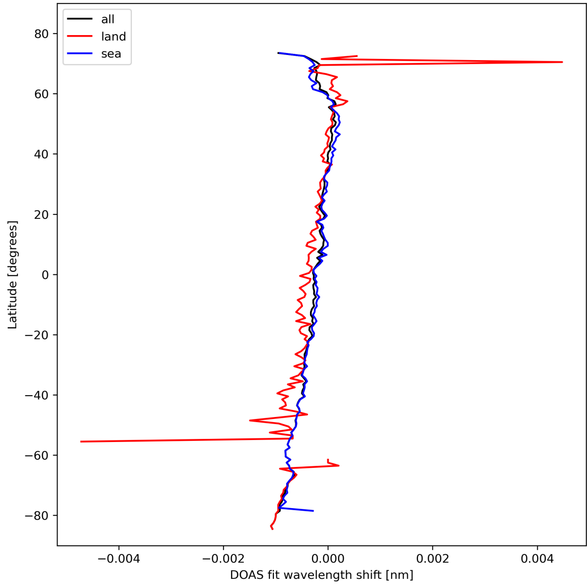
Figure 30: Zonal average of “DOAS fit wavelength shift” for 2023-10-24 to 2023-10-26.
