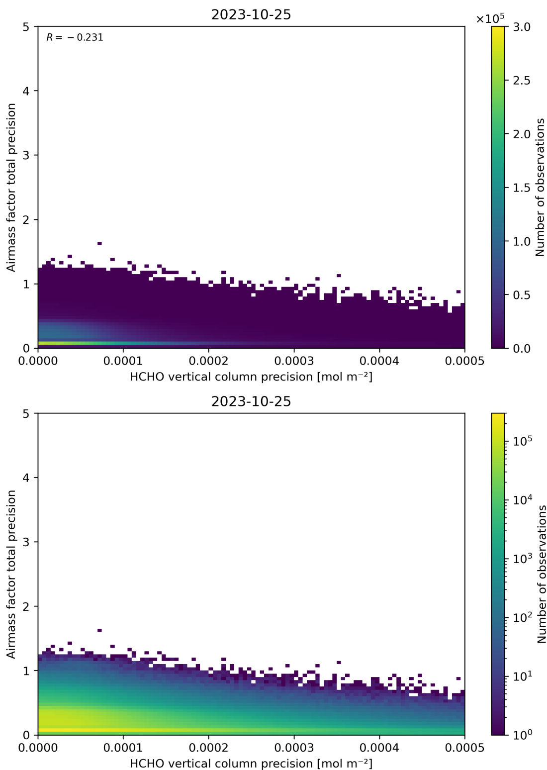
Figure 145: Scatter density plot of “HCHO vertical column precision” against “Airmass factor total precision” for 2023-10-24 to 2023-10-26.
