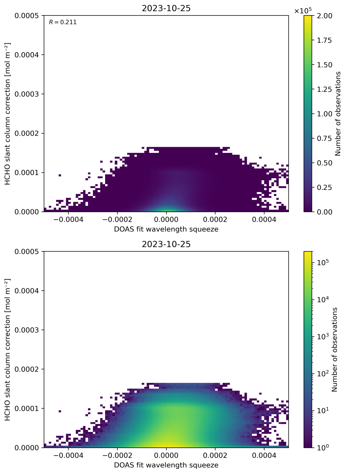
Figure 70: Scatter density plot of “DOAS fit wavelength squeeze” against “HCHO slant column correction” for 2023-10-24 to 2023-10-26.
