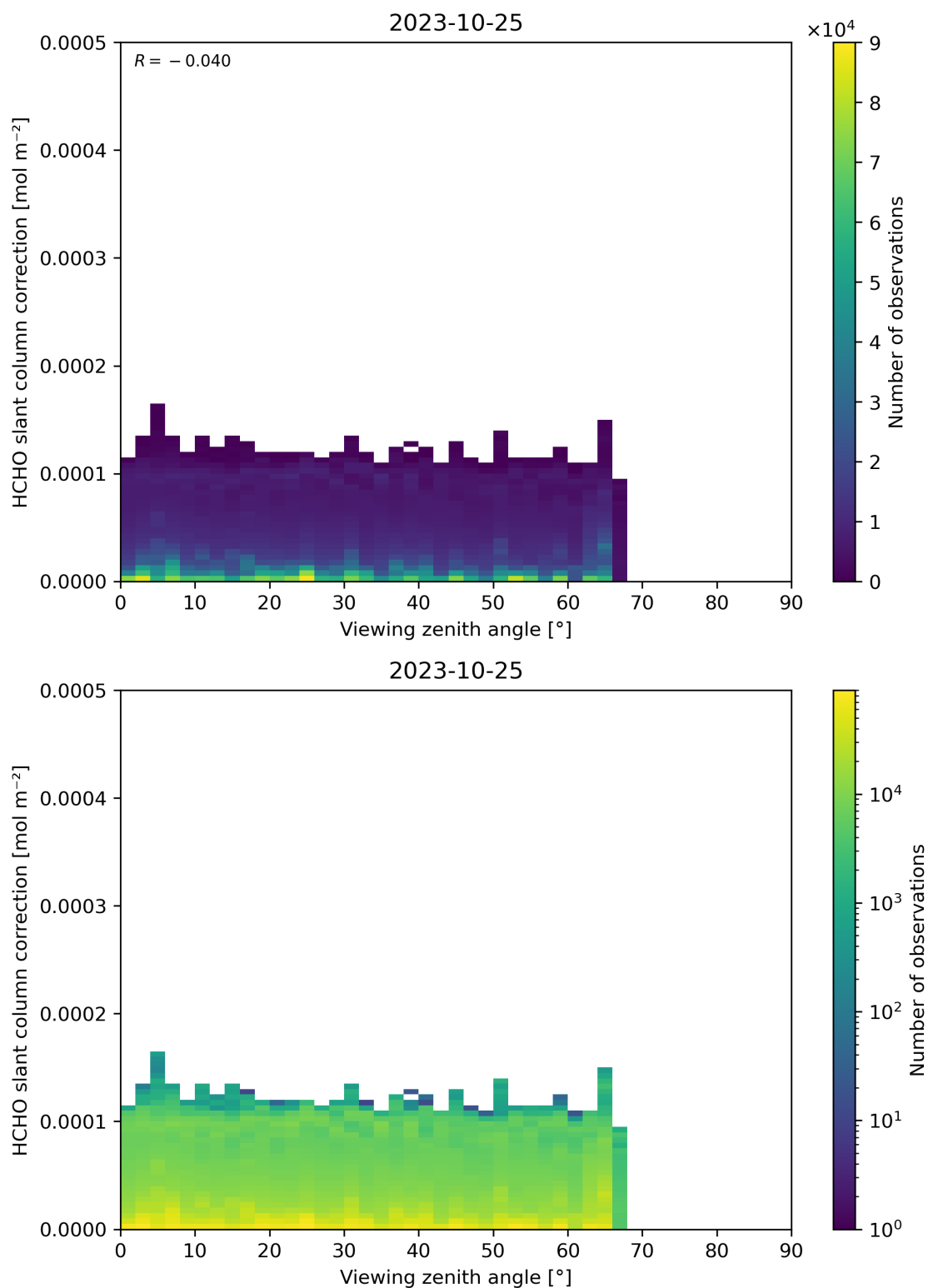
Figure 187: Scatter density plot of “Viewing zenith angle” against “HCHO slant column correction” for 2023-10-24 to 2023-10-26.
