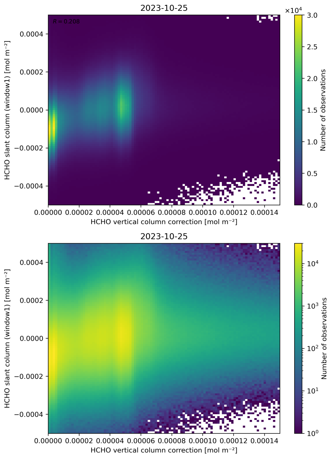
Figure 118: Scatter density plot of “HCHO vertical column correction” against “HCHO slant column (window1)” for 2023-10-24 to 2023-10-26.
