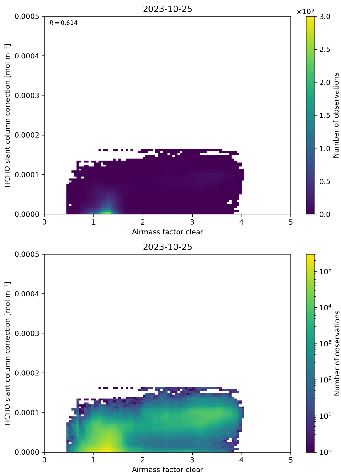
Figure 75: Scatter density plot of “Airmass factor clear” against “HCHO slant column correction” for 2023-10-24 to 2023-10-26.
