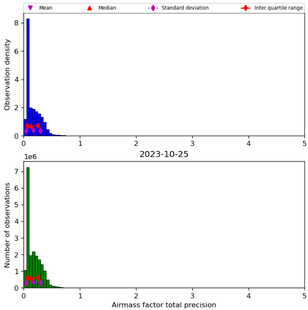
Figure 41: Histogram of “Airmass factor total precision” for 2023-10-24 to 2023-10-26
