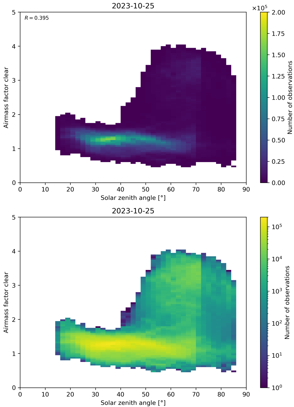
Figure 170: Scatter density plot of “Solar zenith angle” against “Airmass factor clear” for 2023-10-24 to 2023-10-26.
