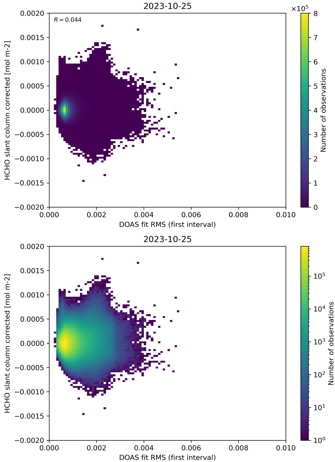
Figure 62: Scatter density plot of “DOAS fit RMS (first interval)” against “HCHO slant column corrected” for 2023-10-24 to 2023-10-26.
