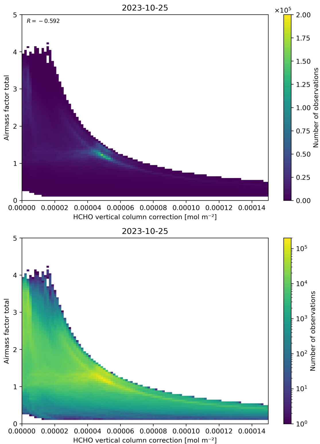
Figure 120: Scatter density plot of “HCHO vertical column correction” against “Airmass factor total” for 2023-10-24 to 2023-10-26.
