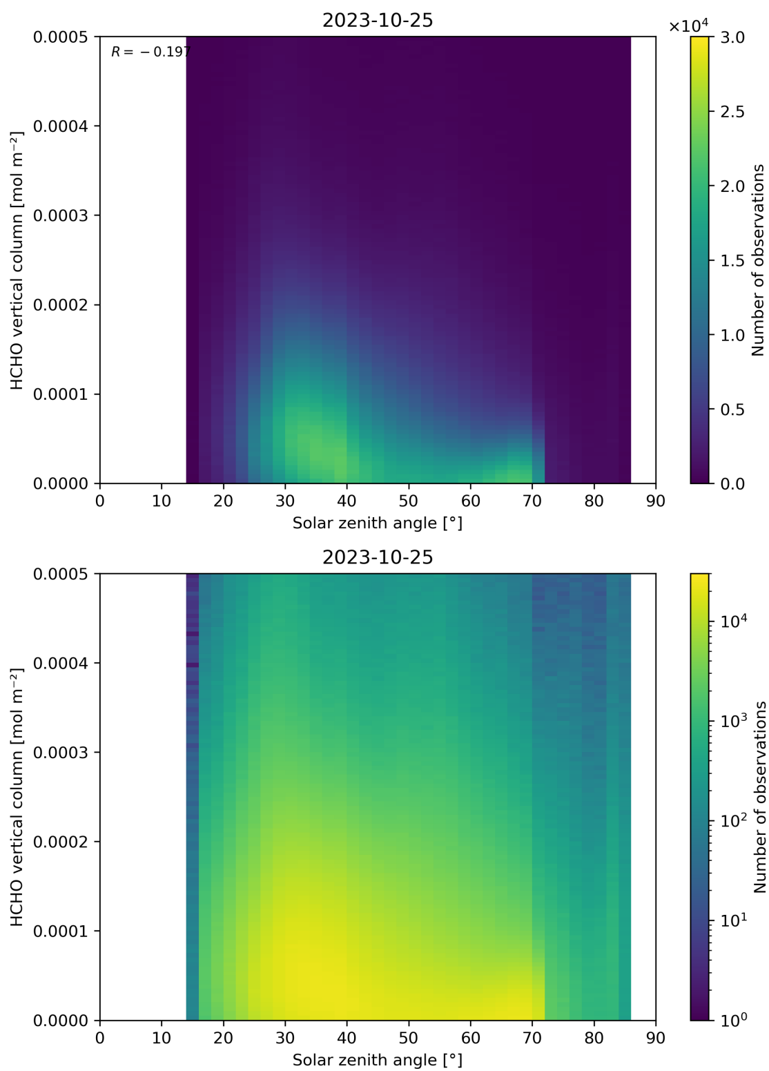
Figure 177: Scatter density plot of “Solar zenith angle” against “HCHO vertical column” for 2023-10-24 to 2023-10-26.
