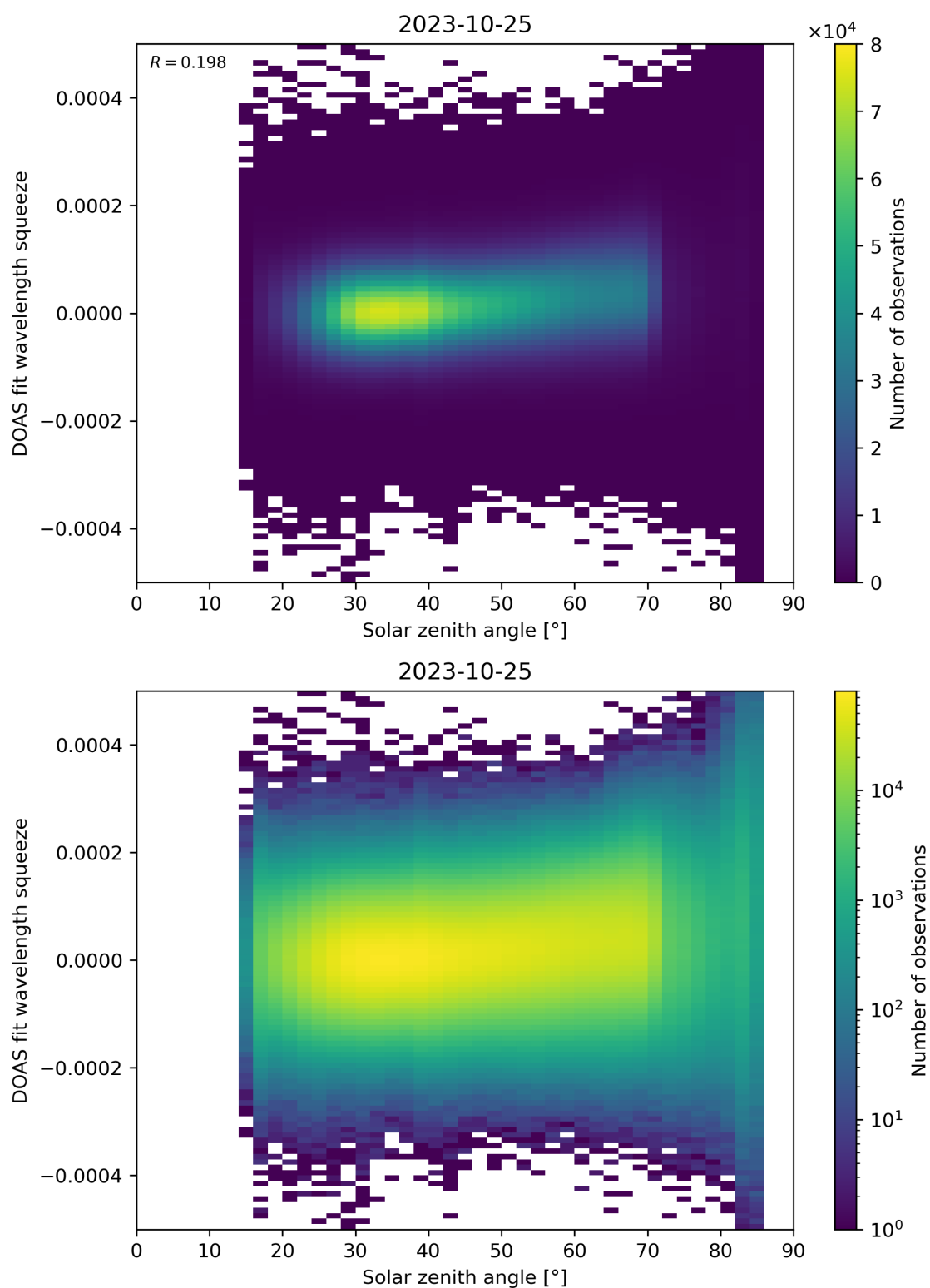
Figure 169: Scatter density plot of “Solar zenith angle” against “DOAS fit wavelength squeeze” for 2023-10-24 to 2023-10-26.
