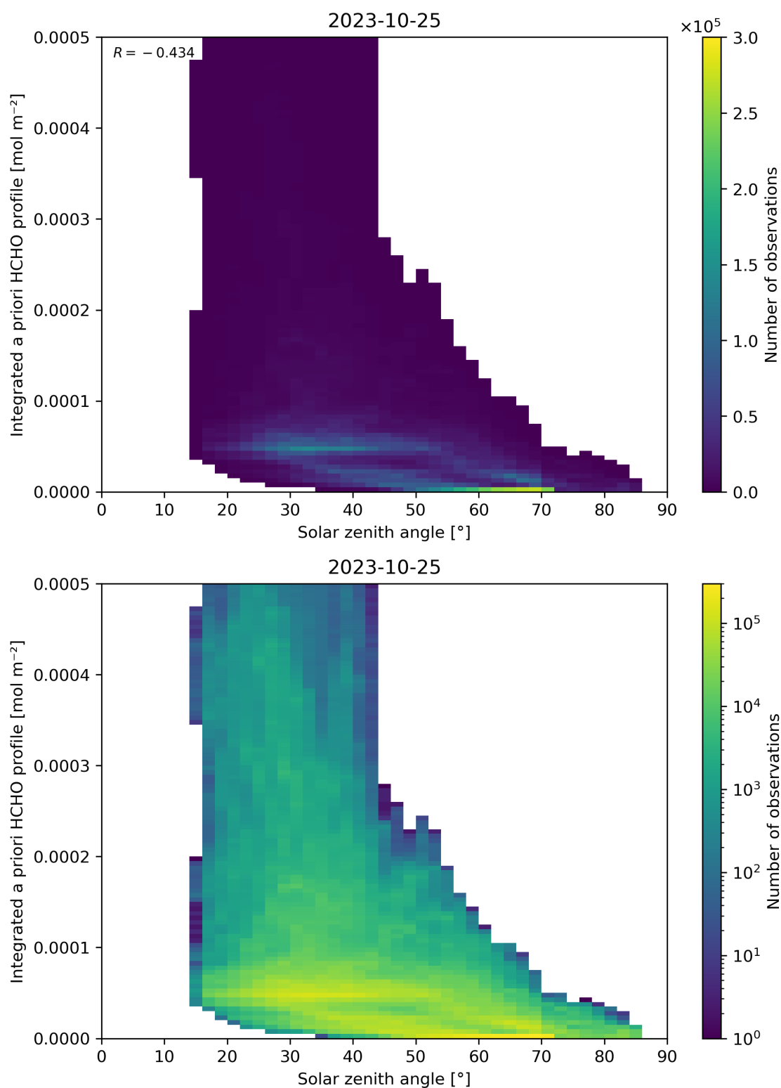
Figure 180: Scatter density plot of “Solar zenith angle” against “Integrated a priori HCHO profile” for 2023-10-24 to 2023-10-26.
