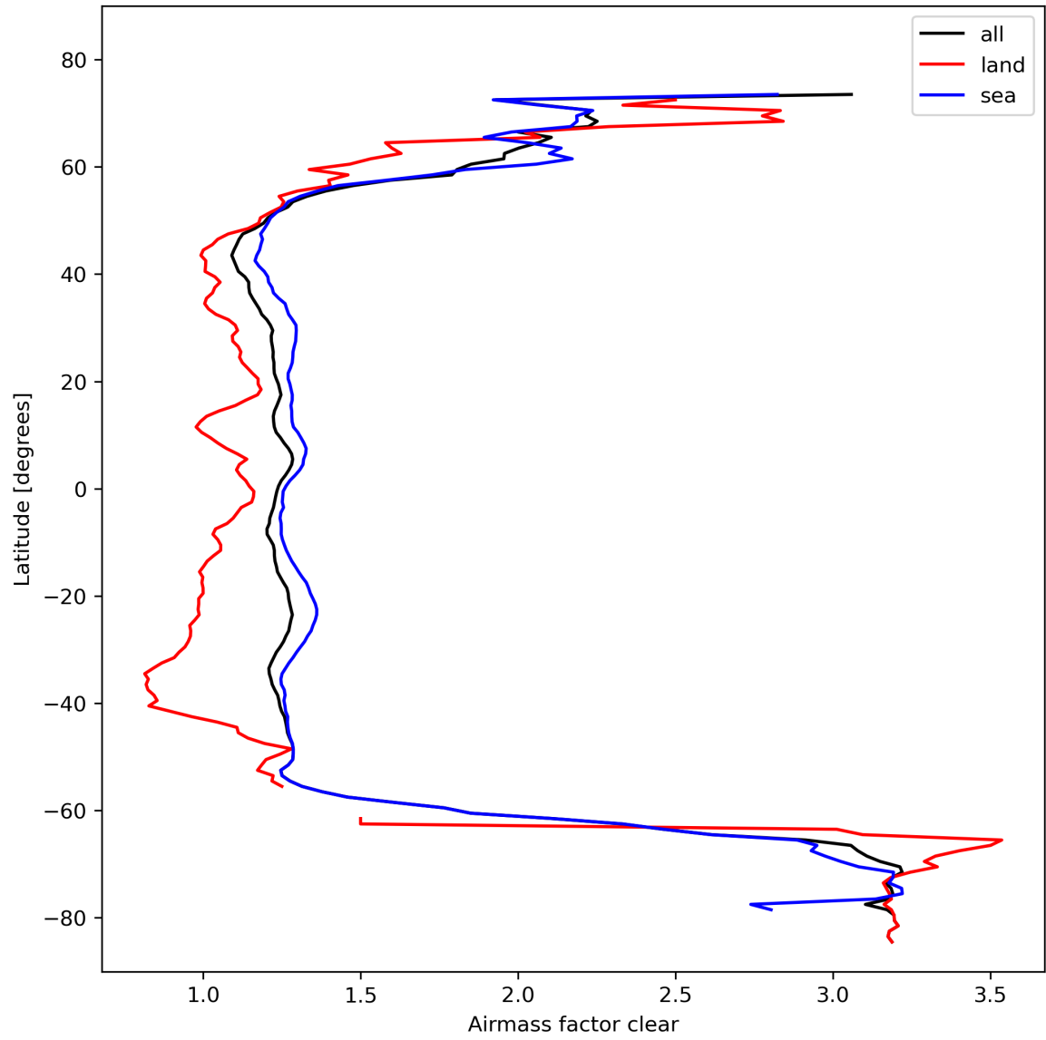
Figure 28: Zonal average of “Airmass factor clear” for 2023-10-24 to 2023-10-26.
