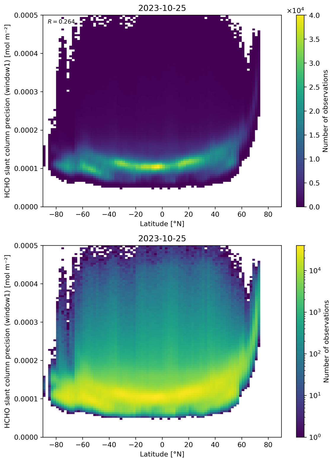
Figure 160: Scatter density plot of “Latitude” against “HCHO slant column precision (window1)” for 2023-10-24 to 2023-10-26.
