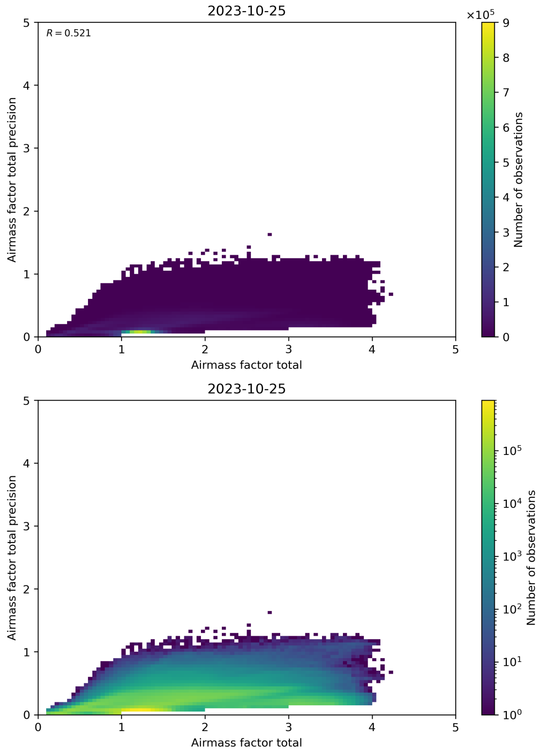
Figure 103: Scatter density plot of “Airmass factor total” against “Airmass factor total precision” for 2023-10-24 to 2023-10-26.
