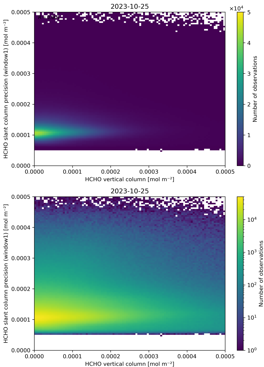
Figure 130: Scatter density plot of “HCHO vertical column” against “HCHO slant column precision (window1)” for 2023-10-24 to 2023-10-26.
