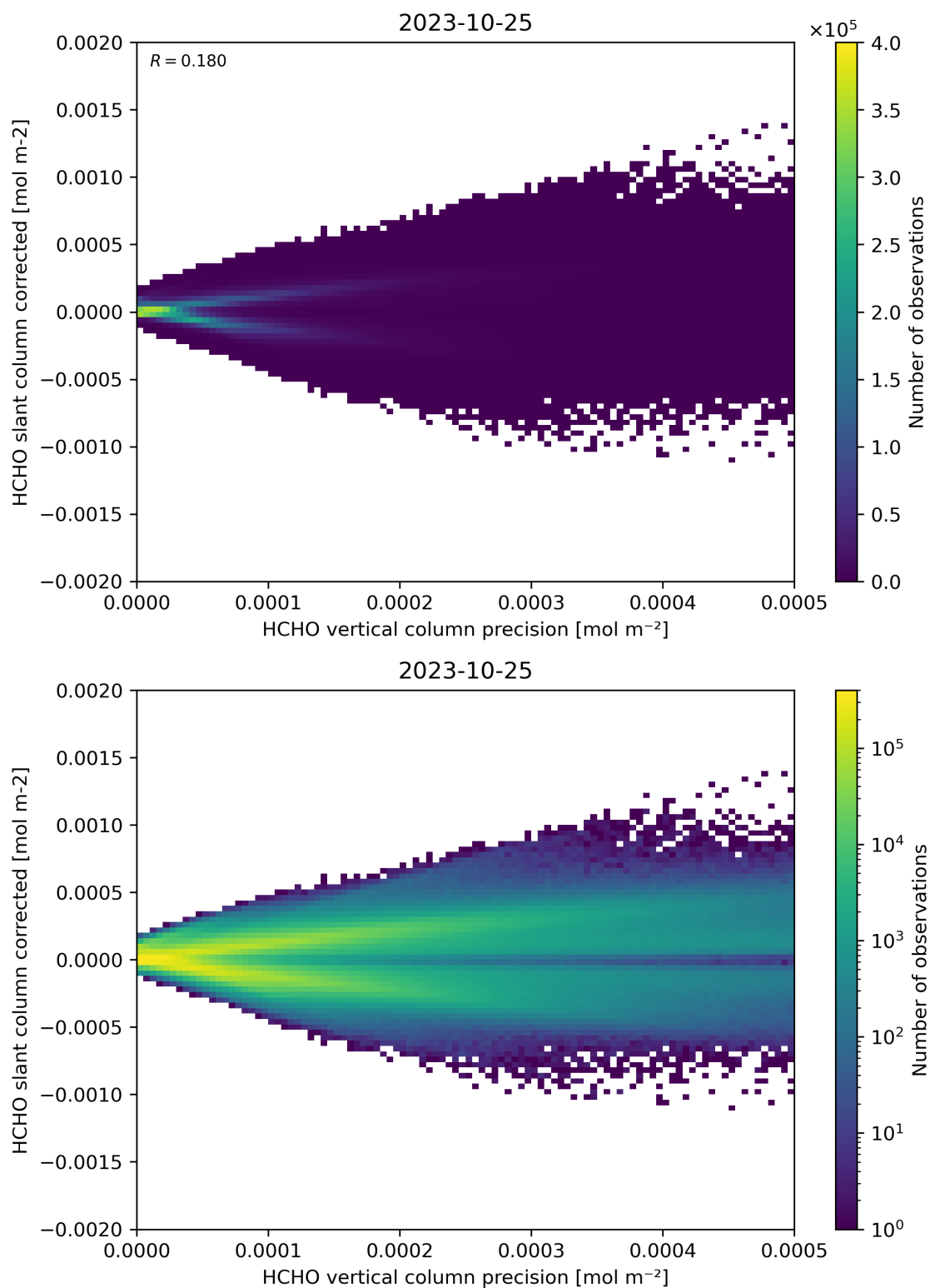
Figure 140: Scatter density plot of “HCHO vertical column precision” against “HCHO slant column corrected” for 2023-10-24 to 2023-10-26.
