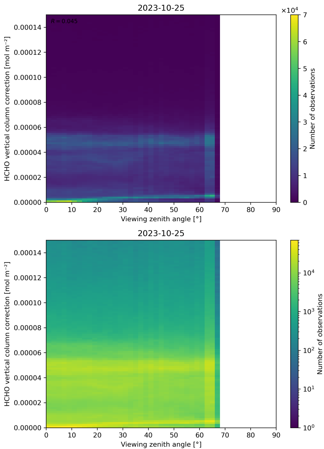
Figure 193: Scatter density plot of “Viewing zenith angle” against “HCHO vertical column correction” for 2023-10-24 to 2023-10-26.
