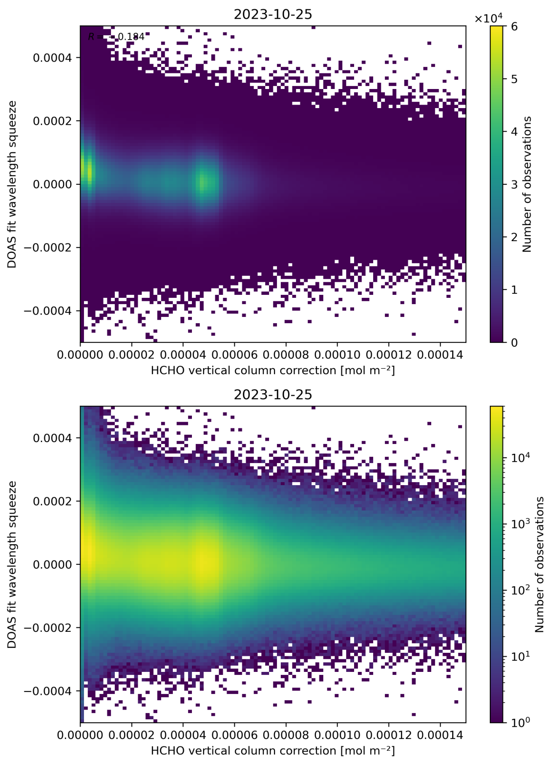
Figure 114: Scatter density plot of “HCHO vertical column correction” against “DOAS fit wavelength squeeze” for 2023-10-24 to 2023-10-26.
