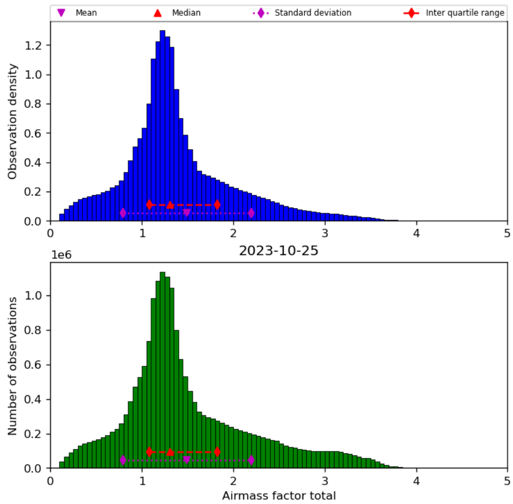
Figure 40: Histogram of “Airmass factor total” for 2023-10-24 to 2023-10-26
