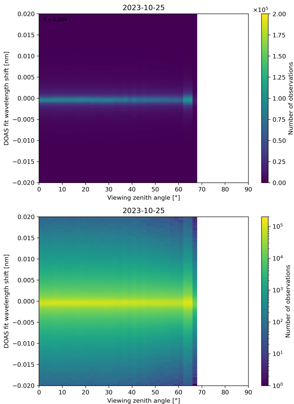
Figure 183: Scatter density plot of “Viewing zenith angle” against “DOAS fit wavelength shift” for 2023-10-24 to 2023-10-26.
