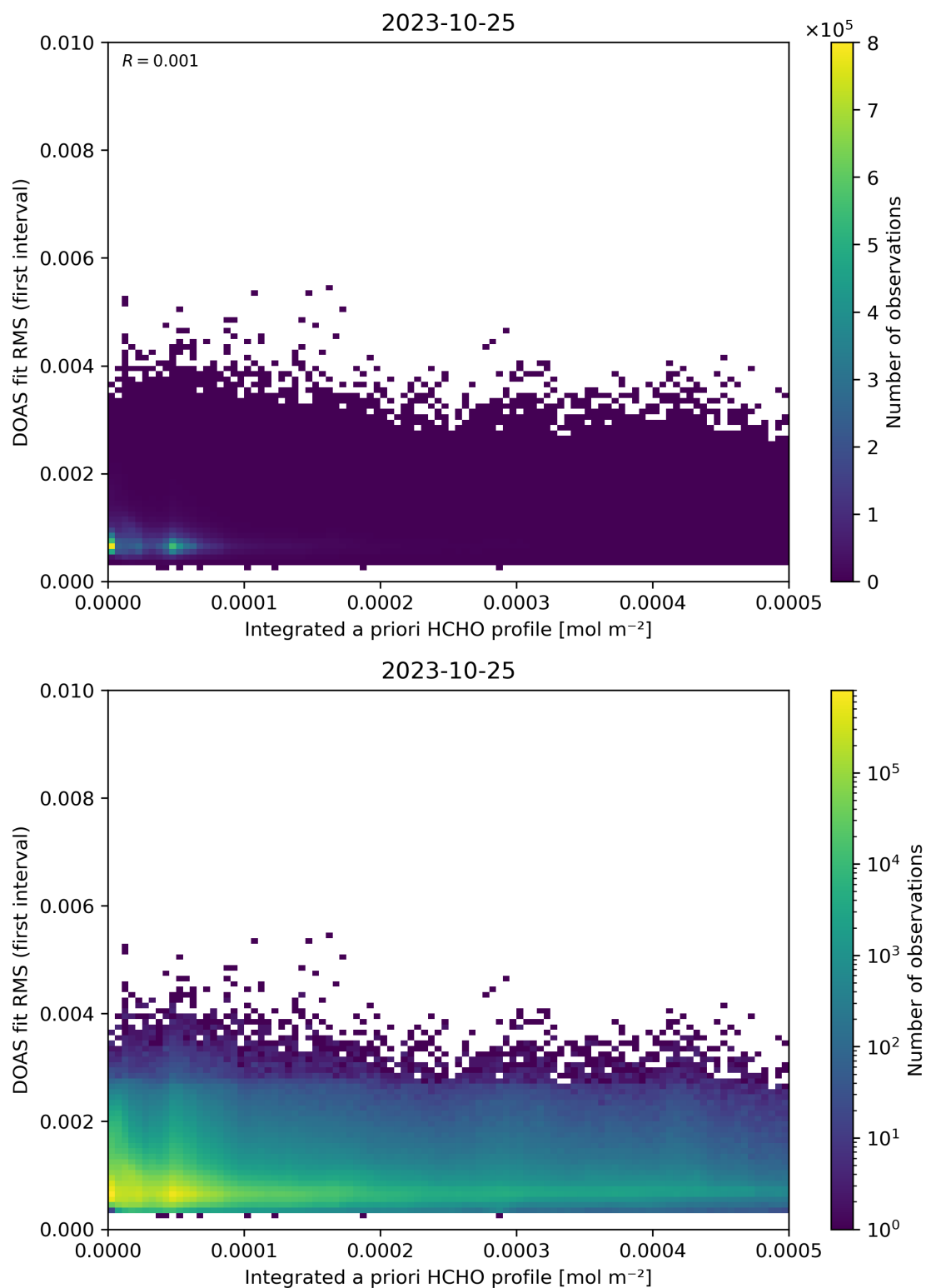
Figure 148: Scatter density plot of “Integrated a priori HCHO profile” against “DOAS fit RMS (first interval)” for 2023-10-24 to 2023-10-26.
