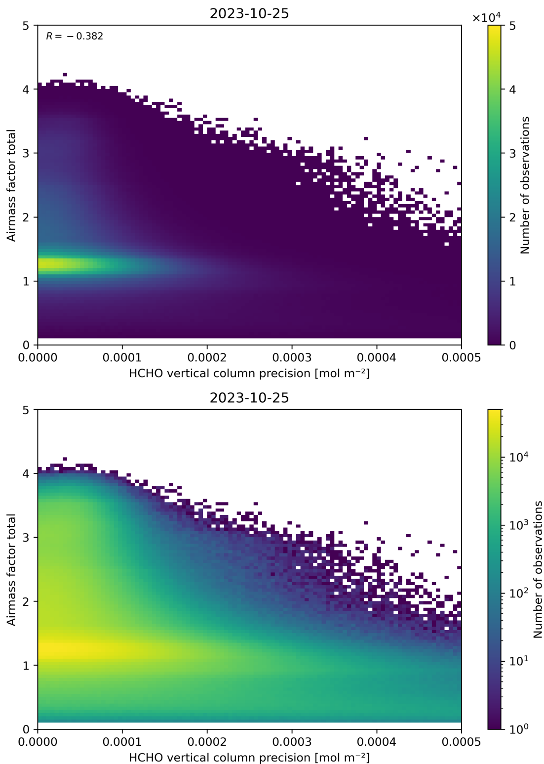
Figure 144: Scatter density plot of “HCHO vertical column precision” against “Airmass factor total” for 2023-10-24 to 2023-10-26.
