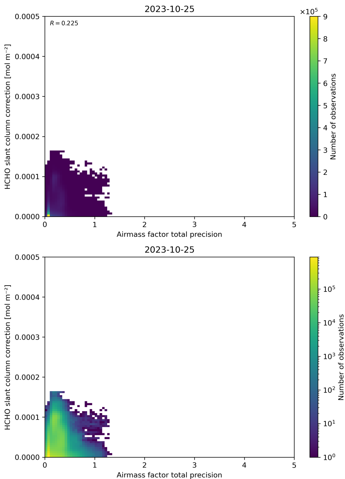
Figure 110: Scatter density plot of “Airmass factor total precision” against “HCHO slant column correction” for 2023-10-24 to 2023-10-26.
