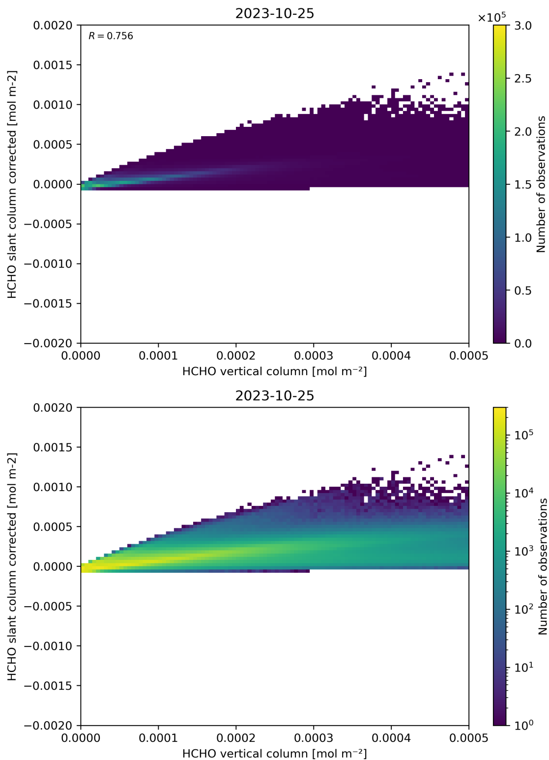
Figure 127: Scatter density plot of “HCHO vertical column” against “HCHO slant column corrected” for 2023-10-24 to 2023-10-26.
