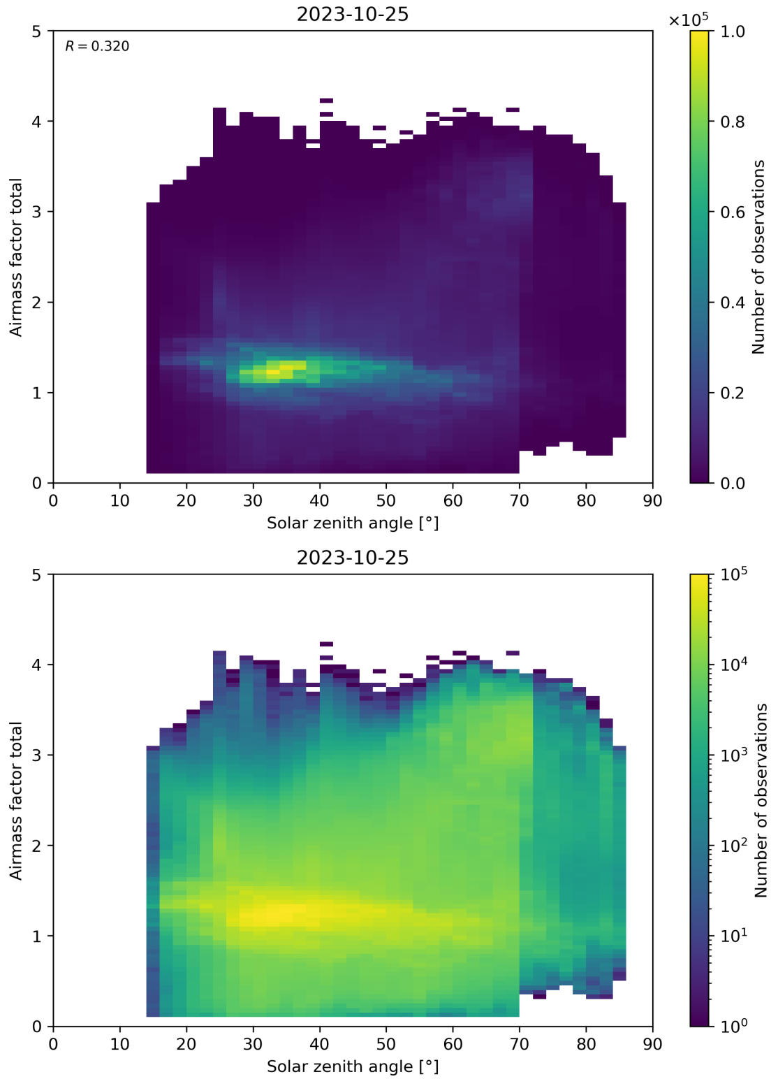
Figure 175: Scatter density plot of “Solar zenith angle” against “Airmass factor total” for 2023-10-24 to 2023-10-26.
