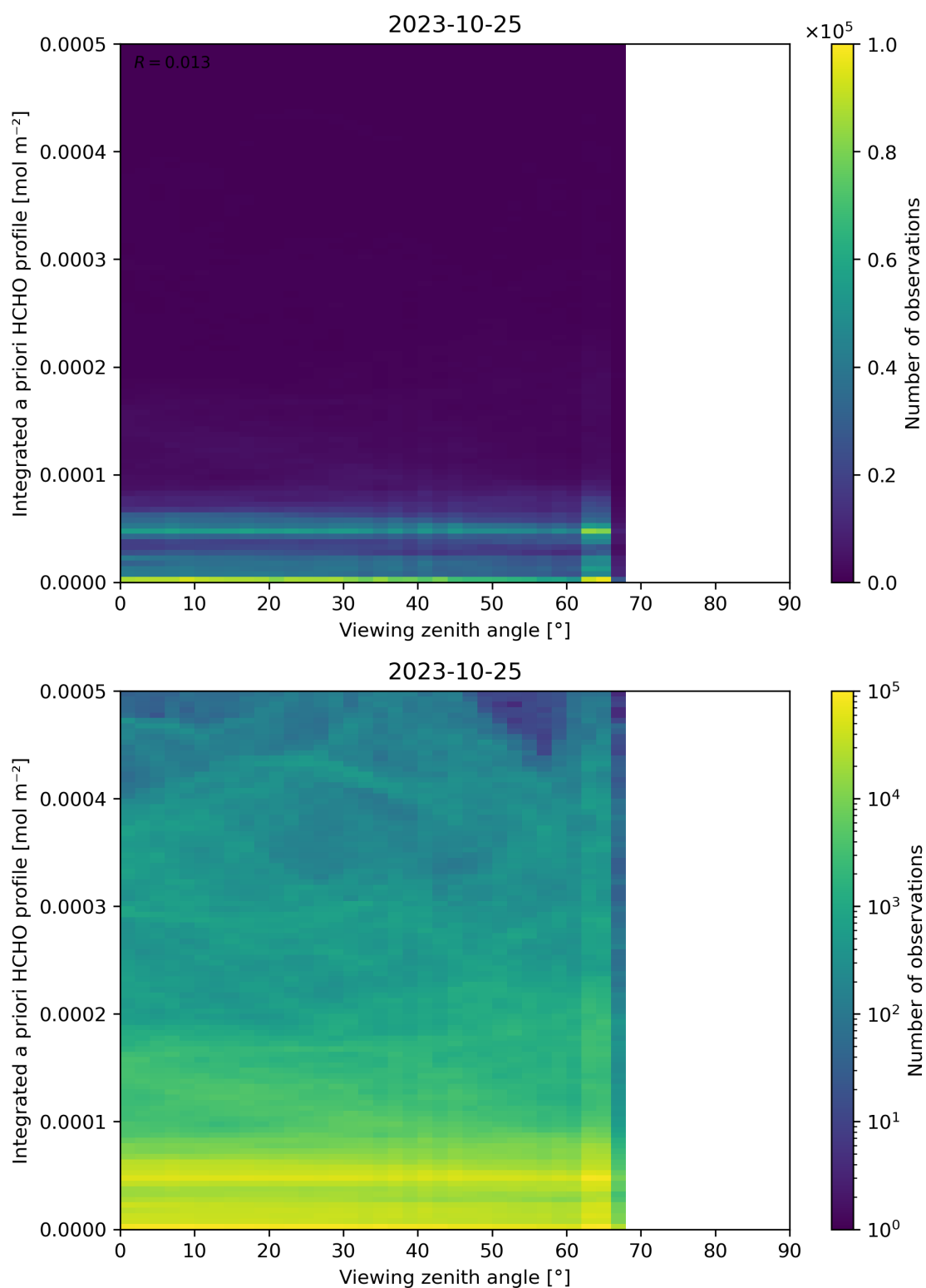
Figure 195: Scatter density plot of “Viewing zenith angle” against “Integrated a priori HCHO profile” for 2023-10-24 to 2023-10-26.
