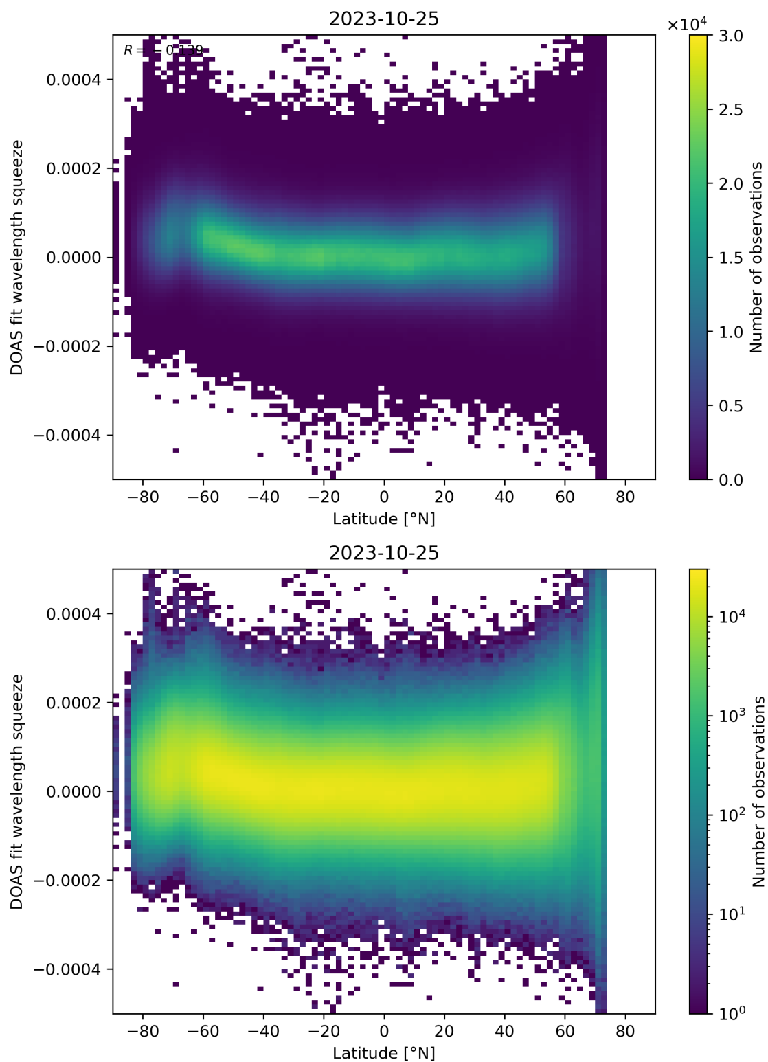
Figure 155: Scatter density plot of “Latitude” against “DOAS fit wavelength squeeze” for 2023-10-24 to 2023-10-26.
