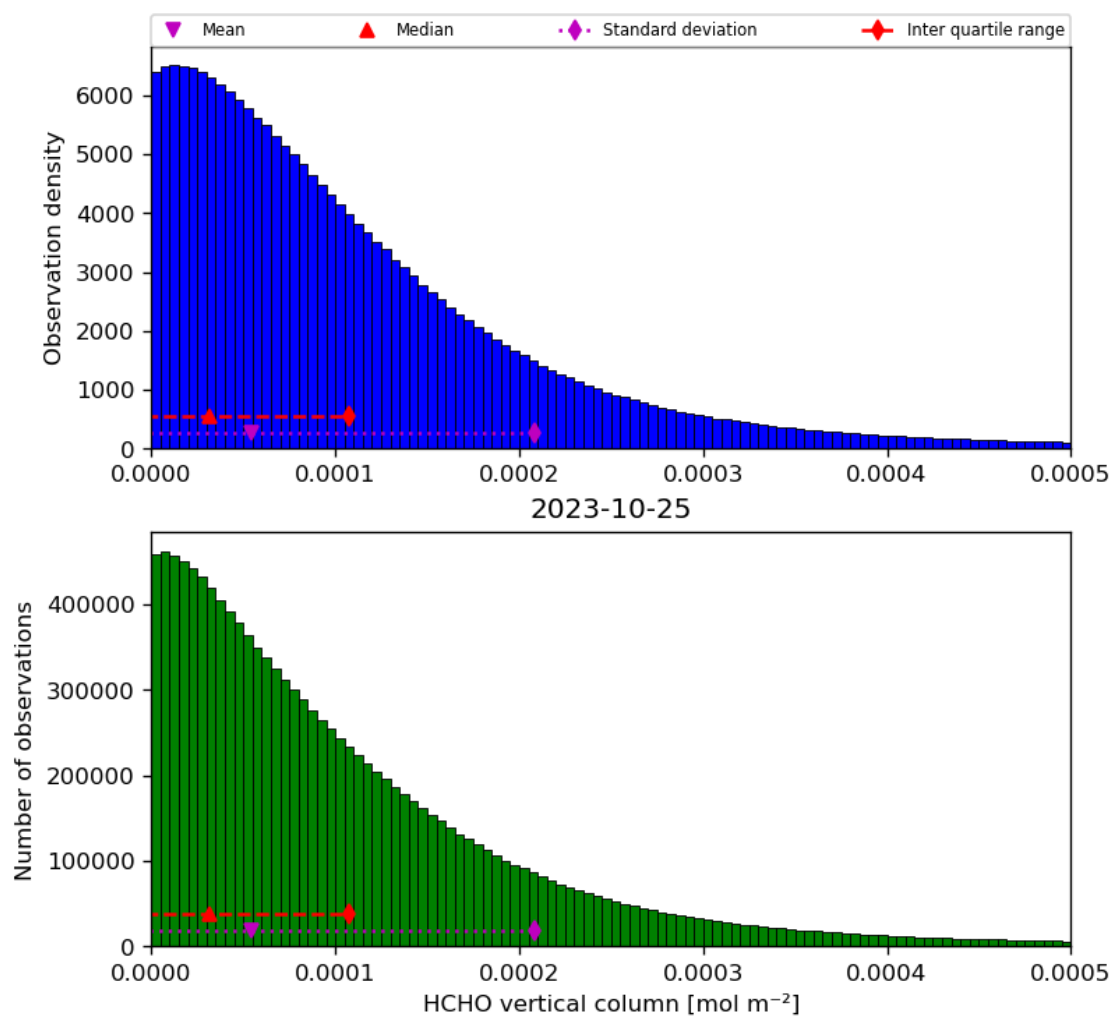
Figure 35: Histogram of “HCHO vertical column” for 2023-10-24 to 2023-10-26
