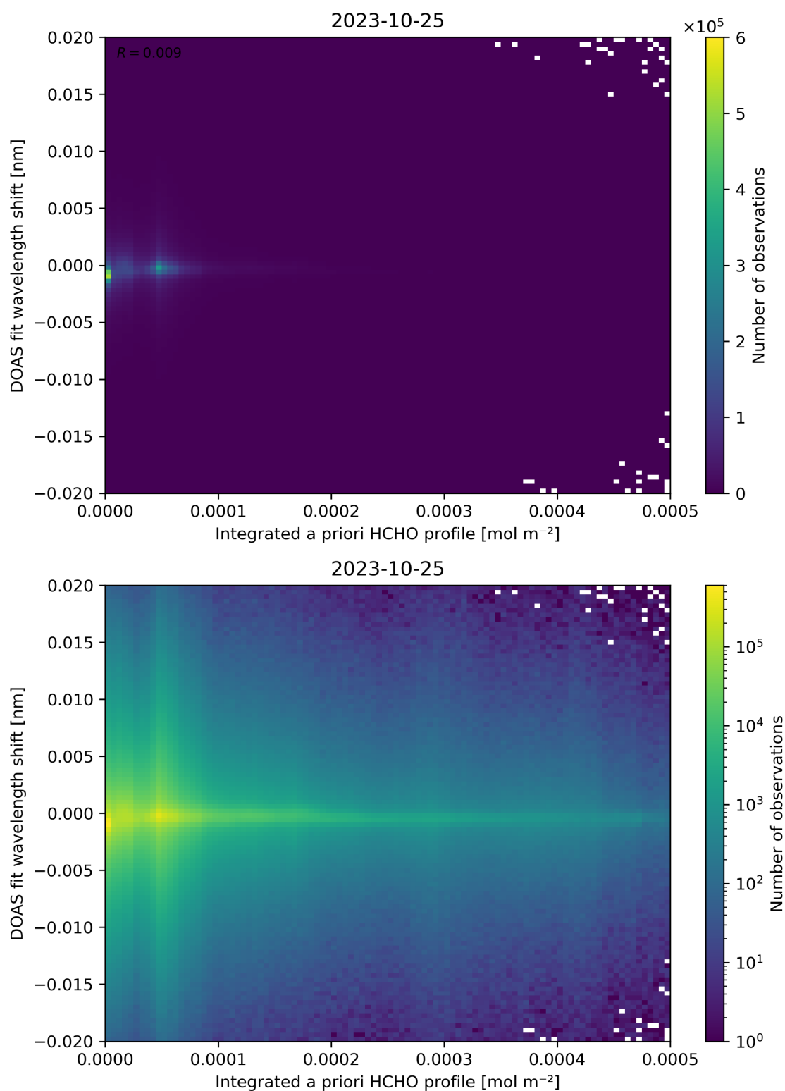
Figure 149: Scatter density plot of “Integrated a priori HCHO profile” against “DOAS fit wavelength shift” for 2023-10-24 to 2023-10-26.
