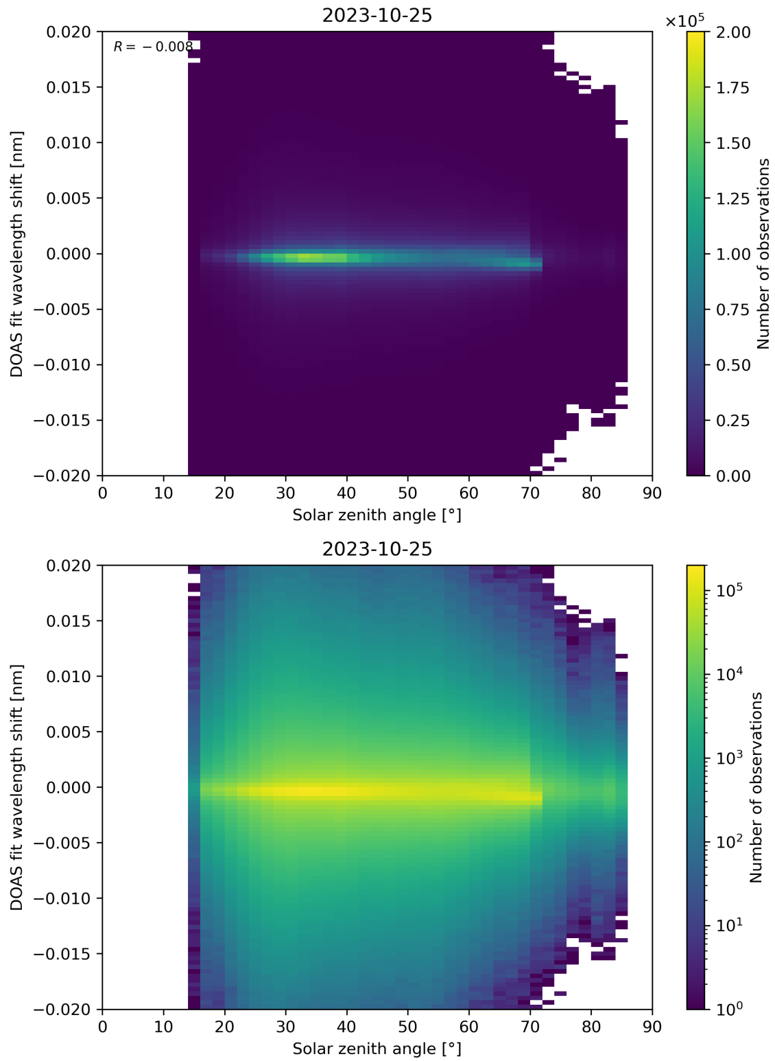
Figure 168: Scatter density plot of “Solar zenith angle” against “DOAS fit wavelength shift” for 2023-10-24 to 2023-10-26.
