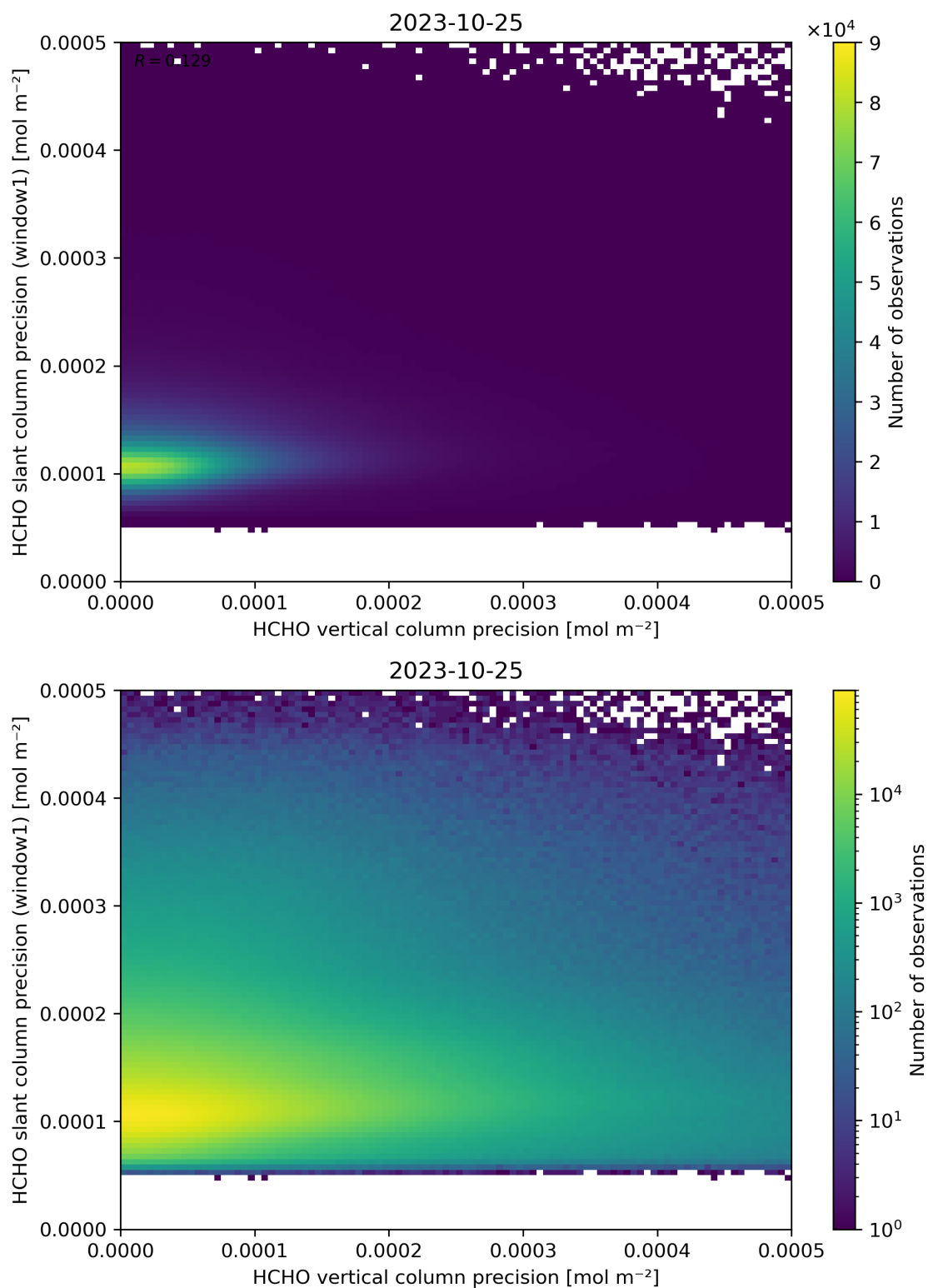
Figure 143: Scatter density plot of “HCHO vertical column precision” against “HCHO slant column precision (window1)” for 2023-10-24 to 2023-10-26.
