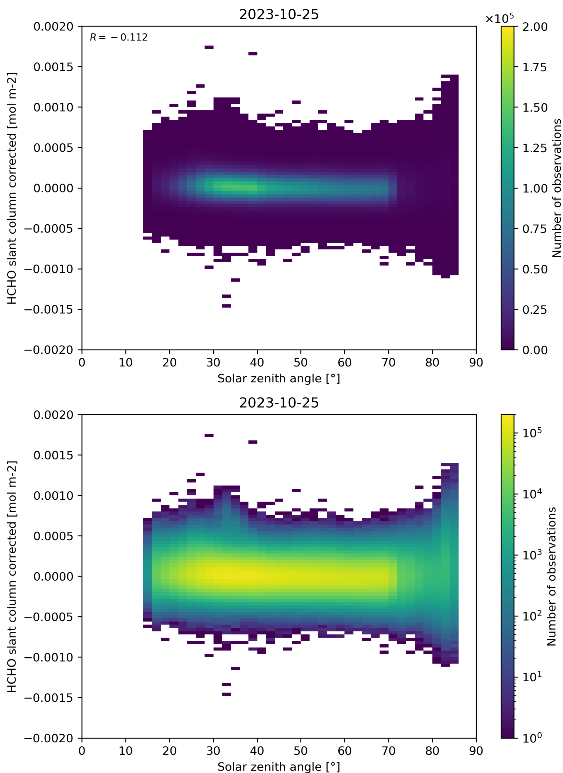
Figure 171: Scatter density plot of “Solar zenith angle” against “HCHO slant column corrected” for 2023-10-24 to 2023-10-26.
