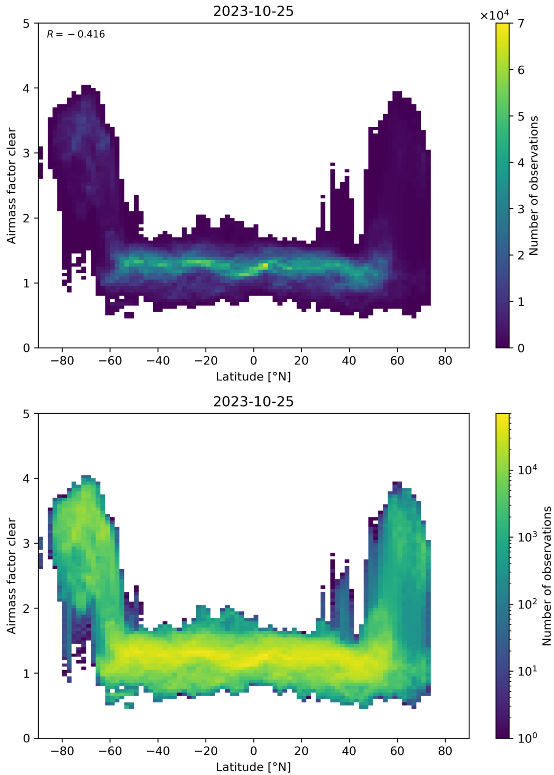
Figure 156: Scatter density plot of “Latitude” against “Airmass factor clear” for 2023-10-24 to 2023-10-26.
