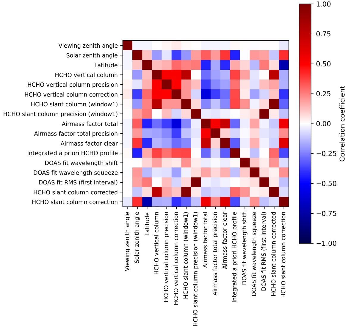
Figure 2: Map of correlation matrix for 2023-10-24 to 2023-10-26.
