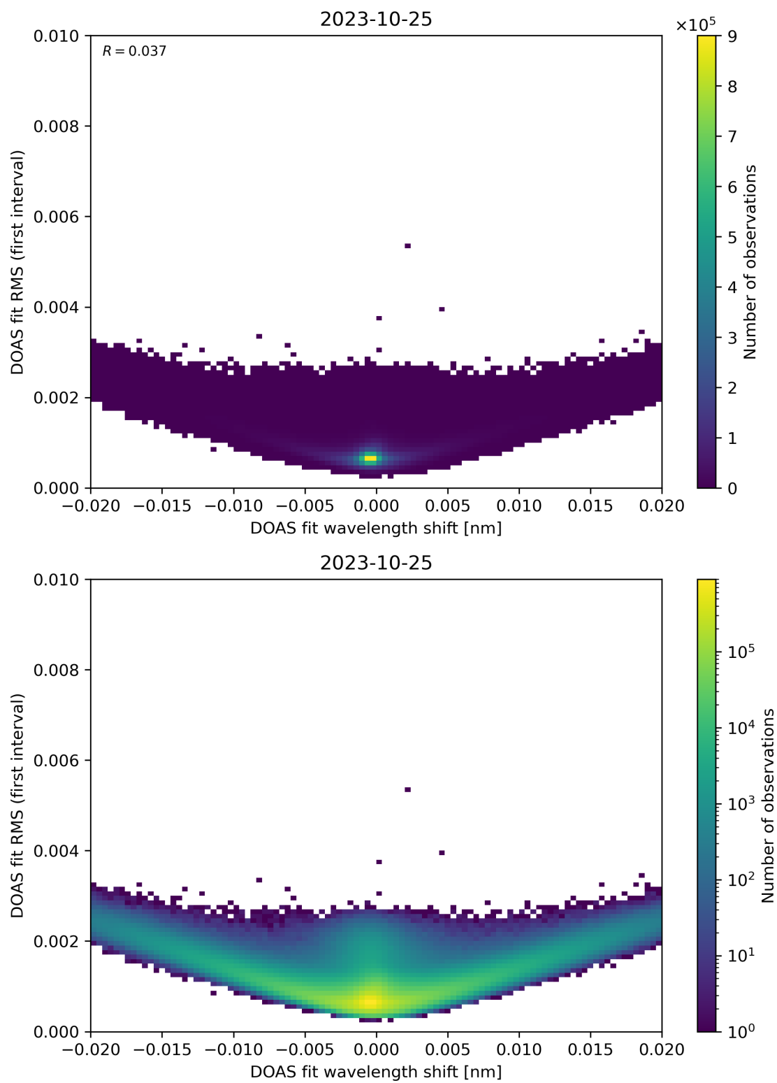
Figure 64: Scatter density plot of “DOAS fit wavelength shift” against “DOAS fit RMS (first interval)” for 2023-10-24 to 2023-10-26.
