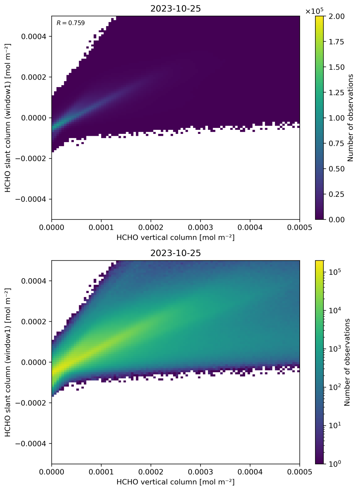
Figure 129: Scatter density plot of “HCHO vertical column” against “HCHO slant column (window1)” for 2023-10-24 to 2023-10-26.
