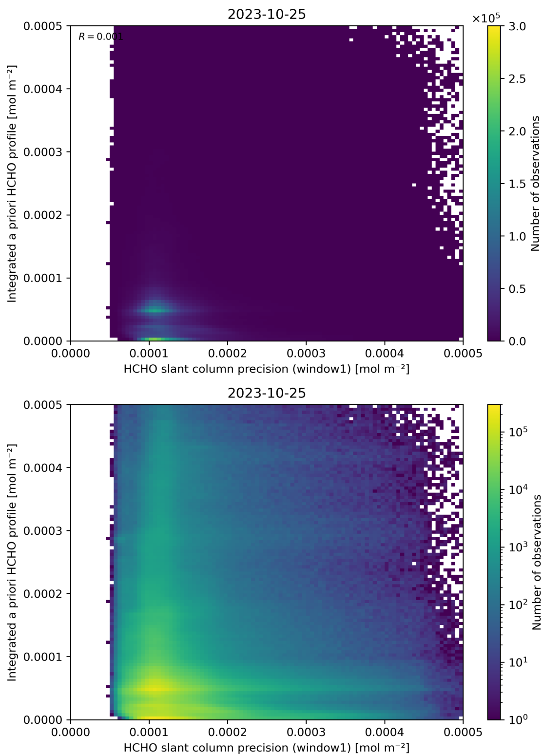
Figure 96: Scatter density plot of “HCHO slant column precision (window1)” against “Integrated a priori HCHO profile” for 2023-10-24 to 2023-10-26.
