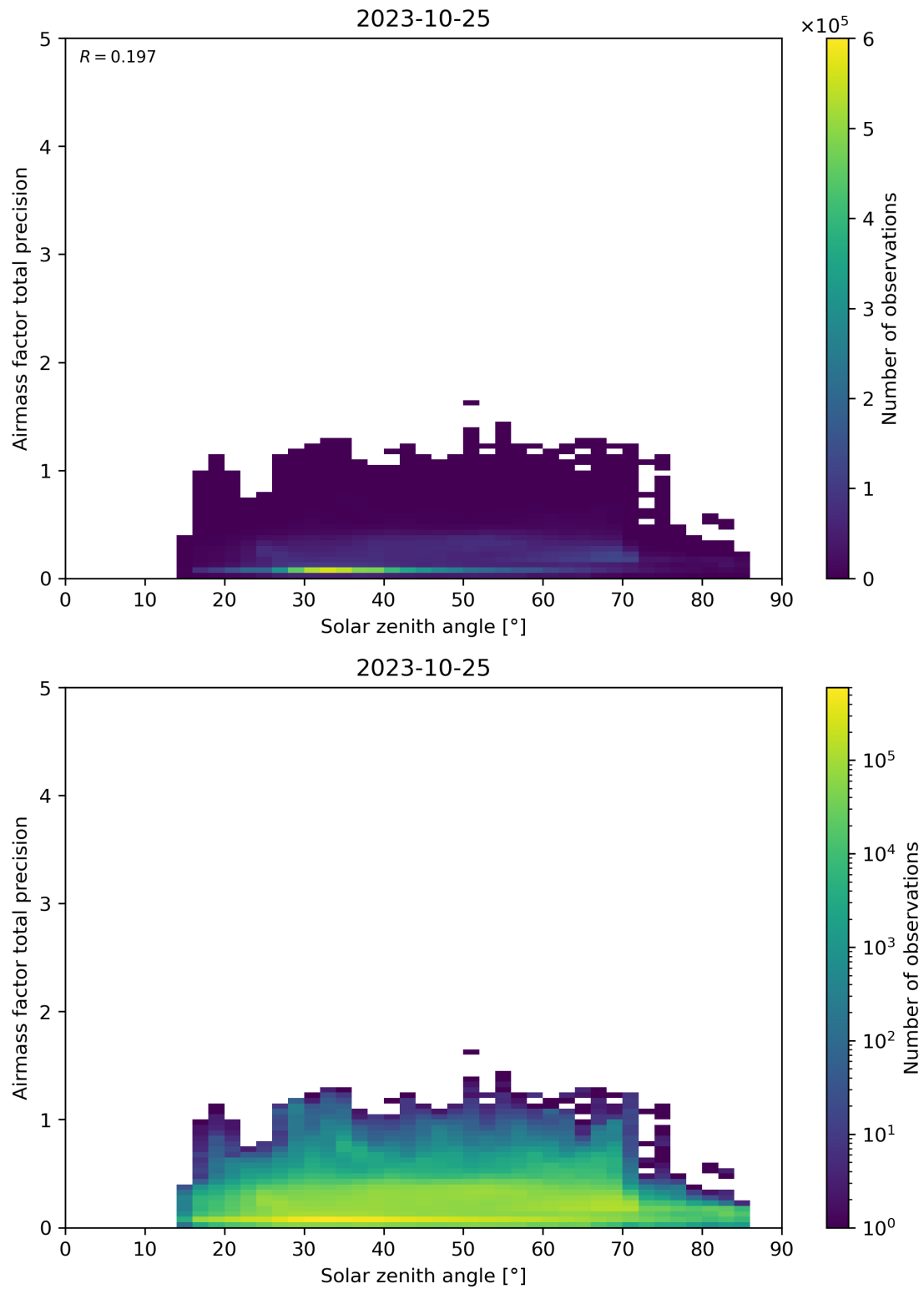
Figure 176: Scatter density plot of “Solar zenith angle” against “Airmass factor total precision” for 2023-10-24 to 2023-10-26.
