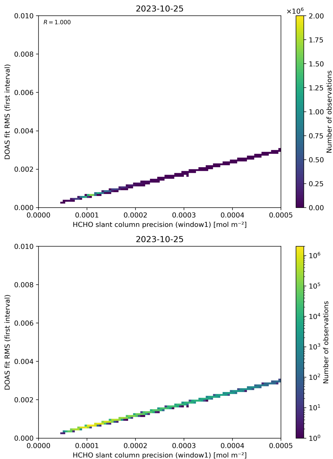
Figure 88: Scatter density plot of “HCHO slant column precision (window1)” against “DOAS fit RMS (first interval)” for 2023-10-24 to 2023-10-26.
