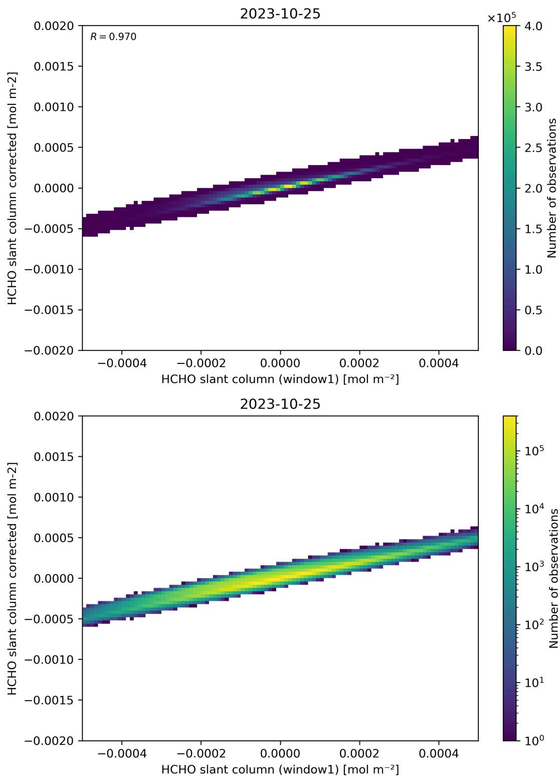
Figure 82: Scatter density plot of “HCHO slant column (window1)” against “HCHO slant column corrected” for 2023-10-24 to 2023-10-26.
