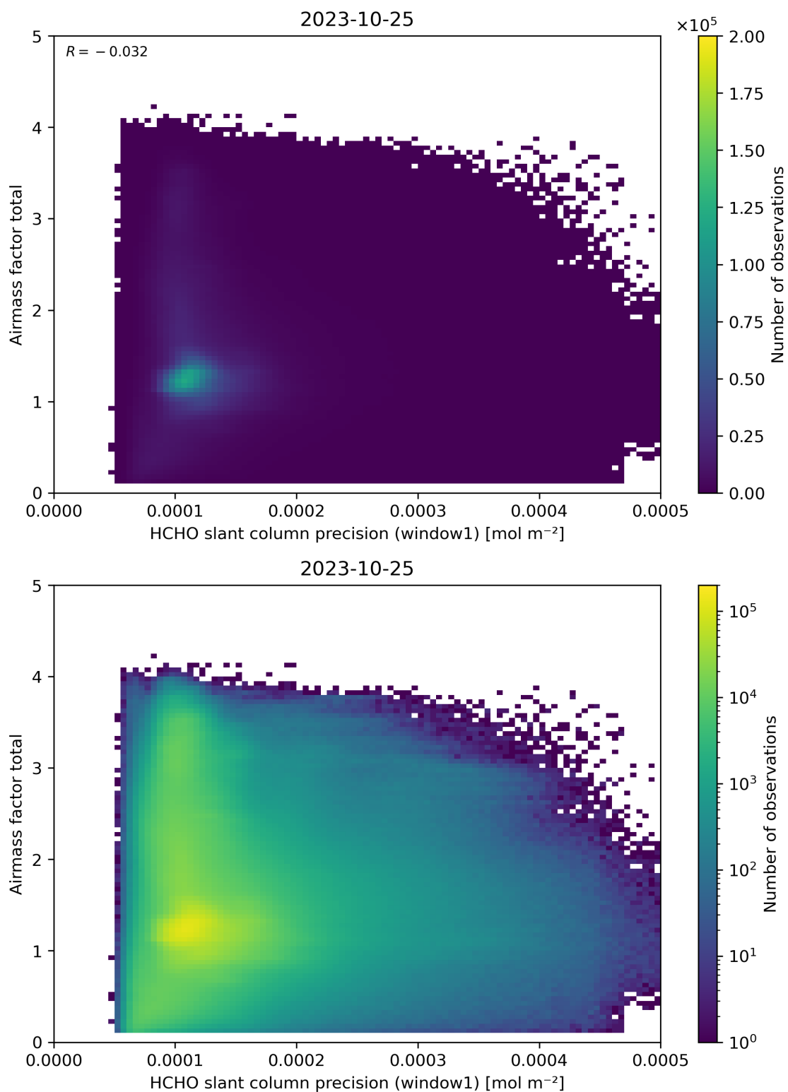
Figure 94: Scatter density plot of “HCHO slant column precision (window1)” against “Airmass factor total” for 2023-10-24 to 2023-10-26.
