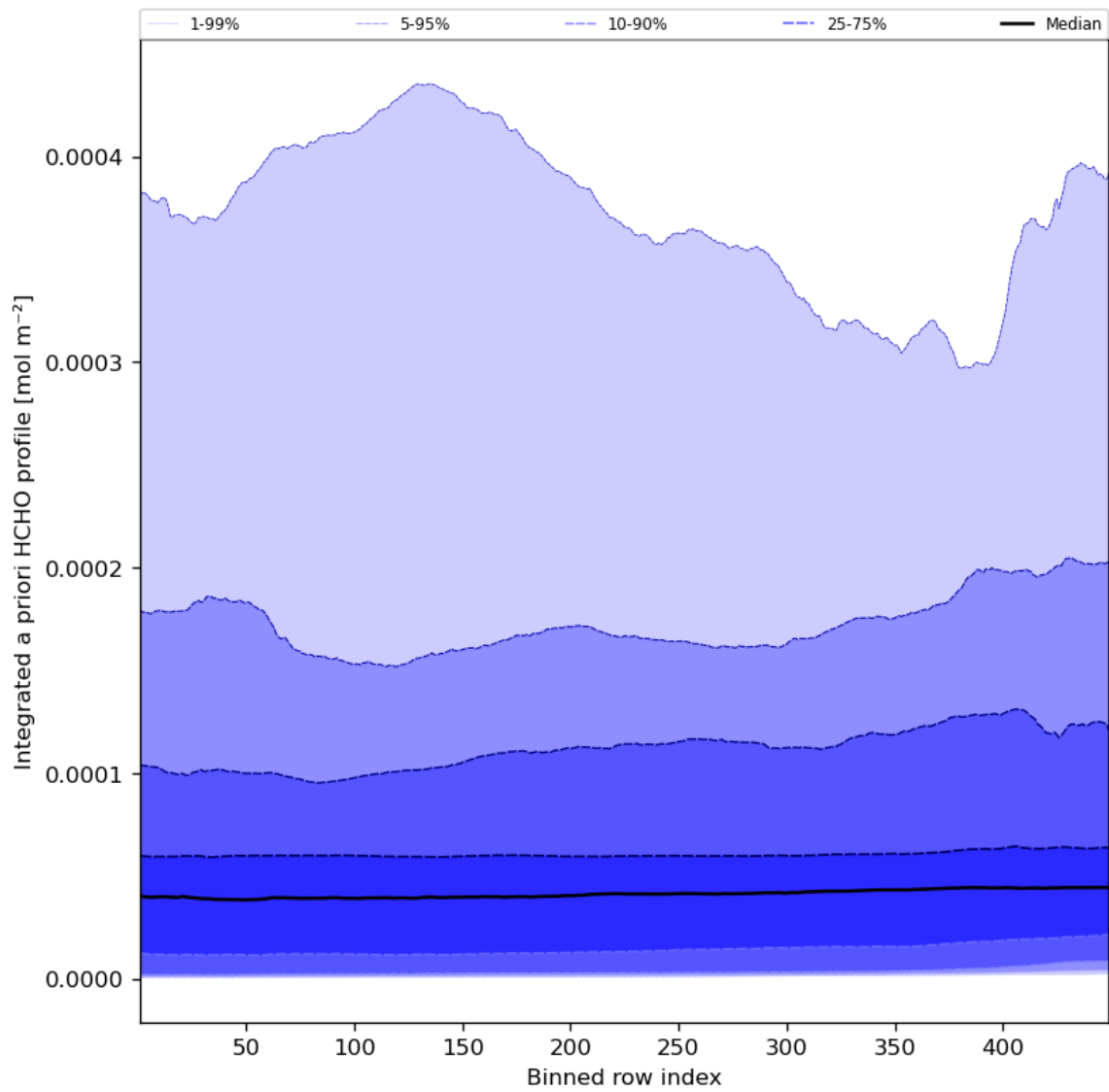
Figure 57: Along track statistics of “Integrated a priori HCHO profile” for 2023-10-24 to 2023-10-26
