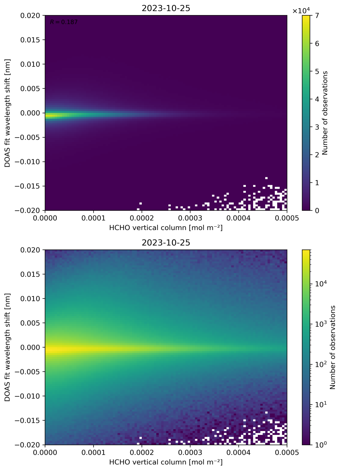
Figure 124: Scatter density plot of “HCHO vertical column” against “DOAS fit wavelength shift” for 2023-10-24 to 2023-10-26.
