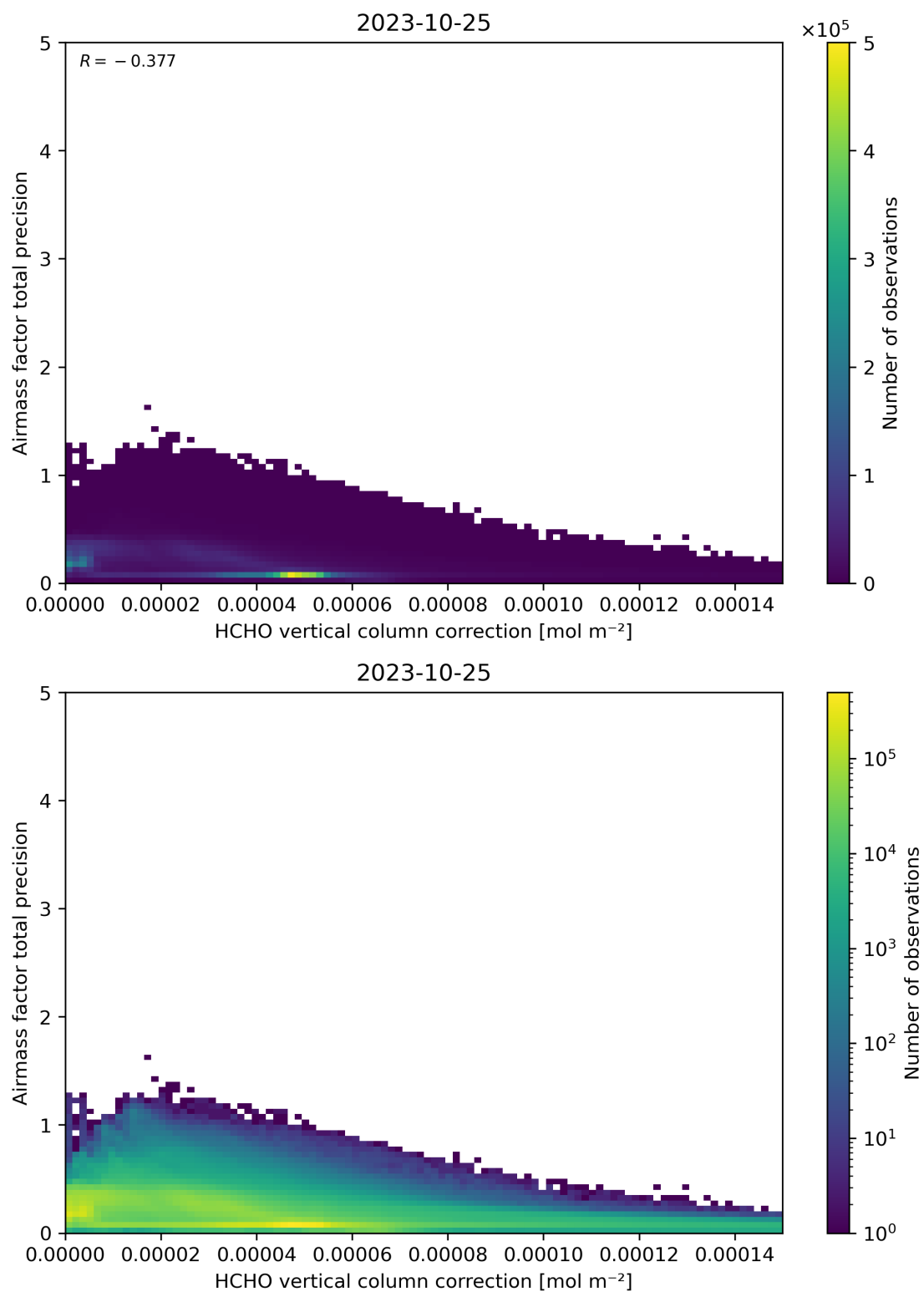
Figure 121: Scatter density plot of “HCHO vertical column correction” against “Airmass factor total precision” for 2023-10-24 to 2023-10-26.
