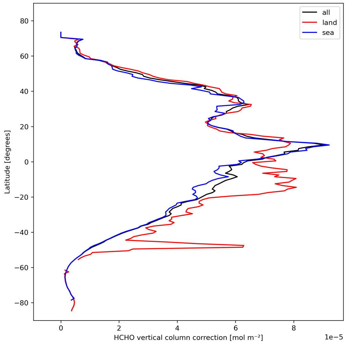
Figure 23: Zonal average of “HCHO vertical column correction” for 2023-10-24 to 2023-10-26.
