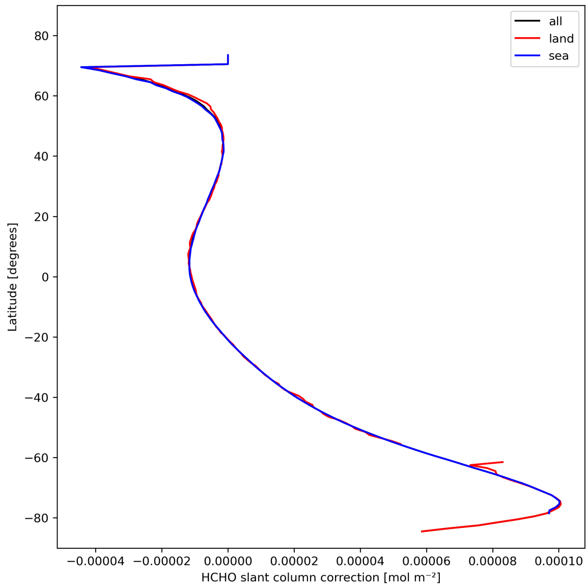
Figure 33: Zonal average of “HCHO slant column correction” for 2023-10-24 to 2023-10-26.
