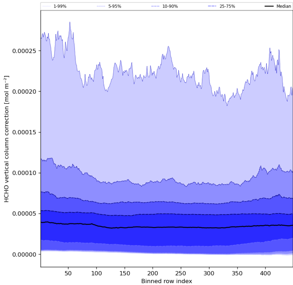
Figure 51: Along track statistics of “HCHO vertical column correction” for 2023-10-24 to 2023-10-26
