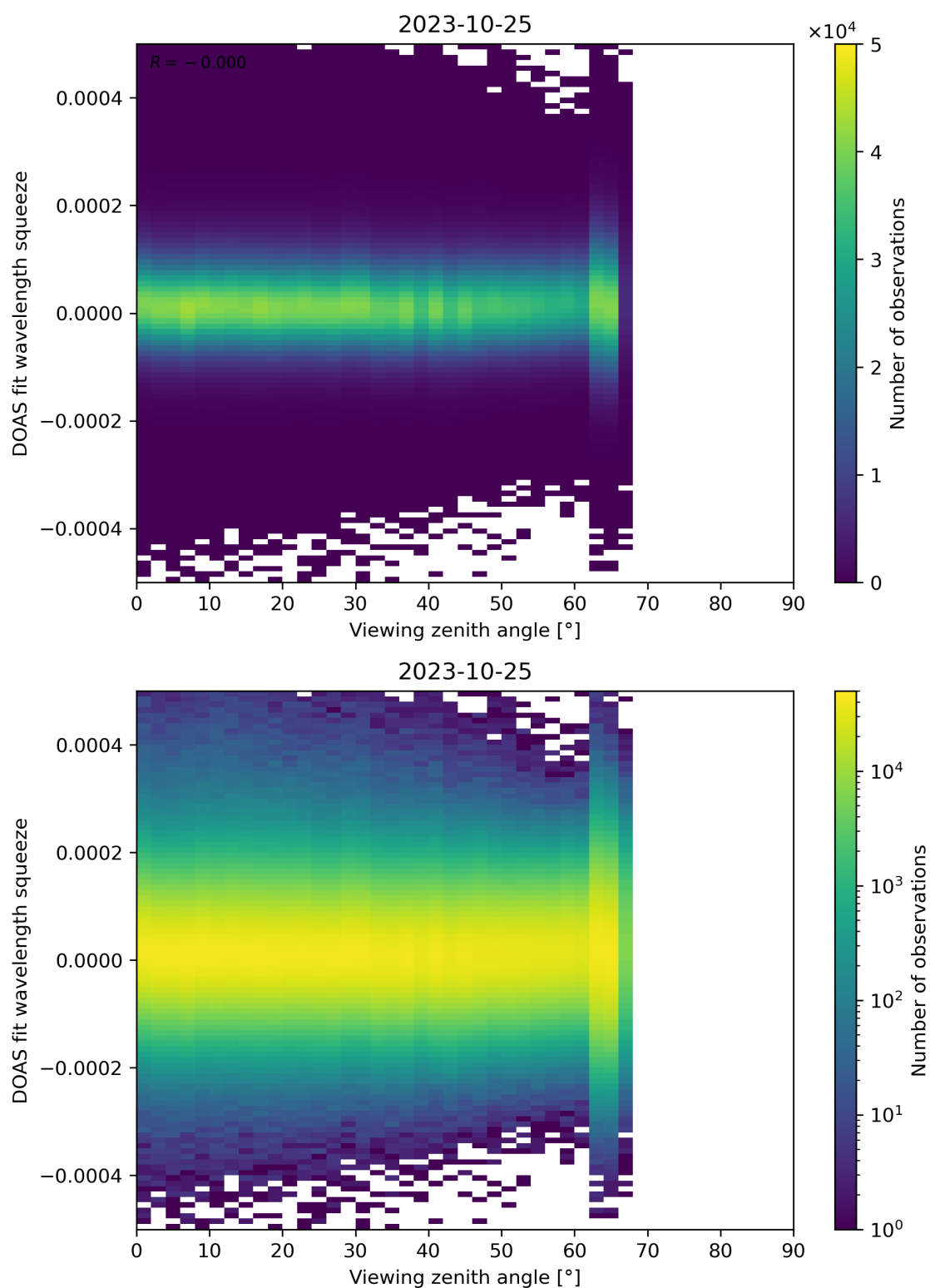
Figure 184: Scatter density plot of “Viewing zenith angle” against “DOAS fit wavelength squeeze” for 2023-10-24 to 2023-10-26.
