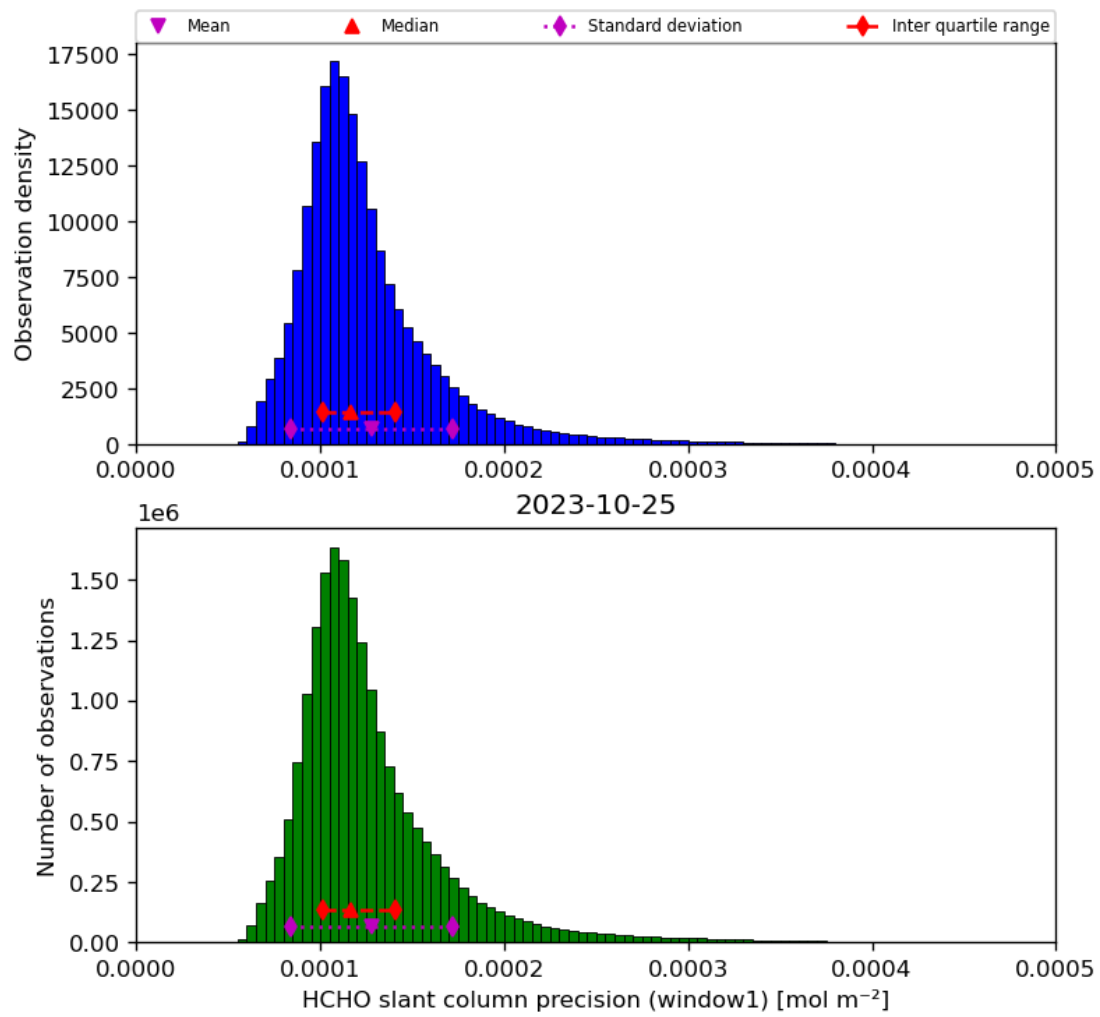
Figure 39: Histogram of “HCHO slant column precision (window1)” for 2023-10-24 to 2023-10-26
