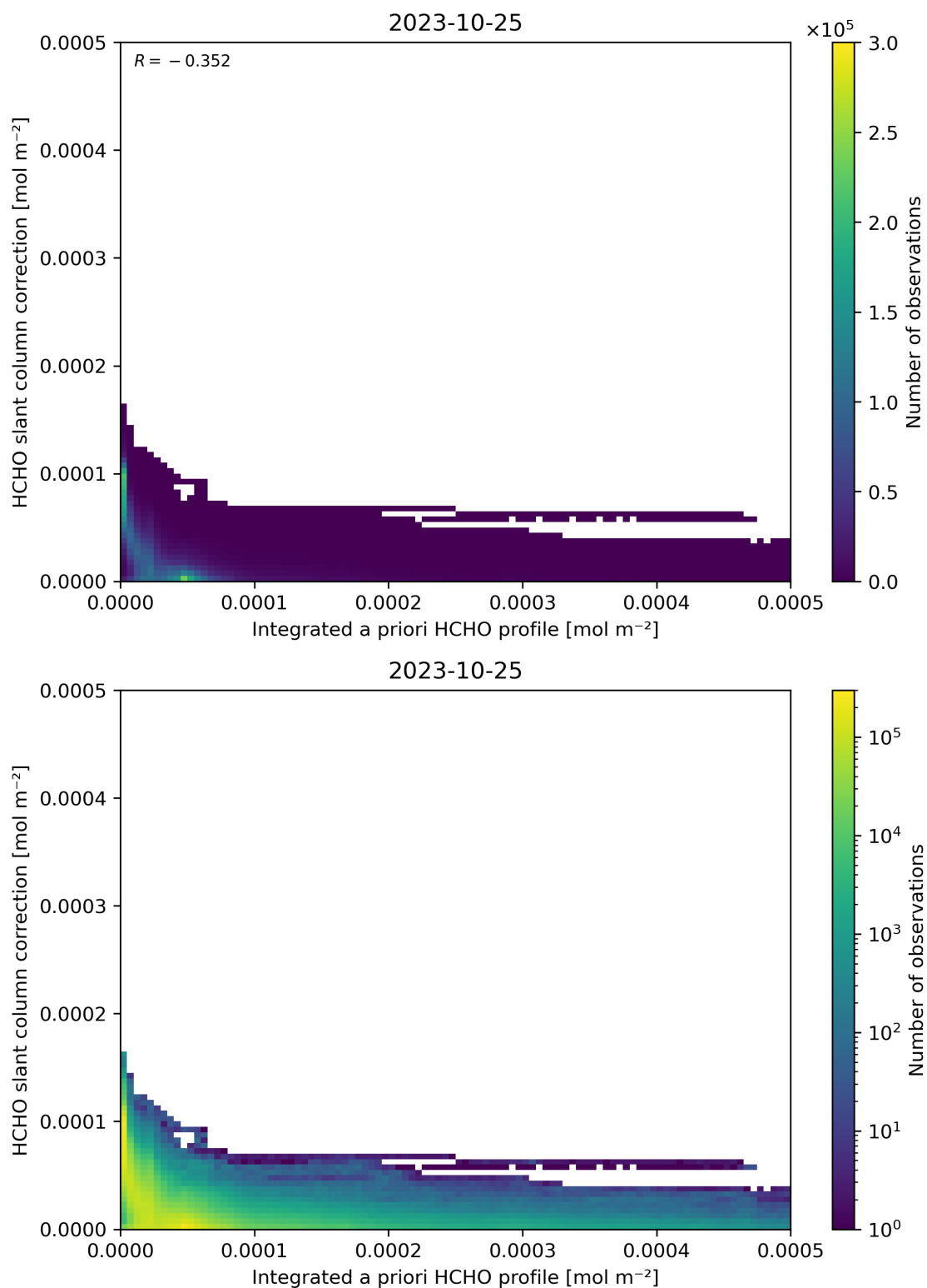
Figure 152: Scatter density plot of “Integrated a priori HCHO profile” against “HCHO slant column correction” for 2023-10-24 to 2023-10-26.
