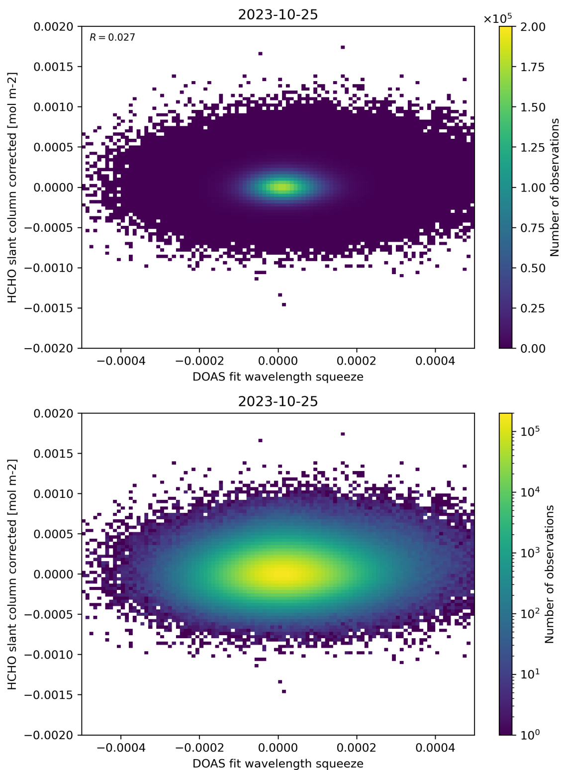
Figure 69: Scatter density plot of “DOAS fit wavelength squeeze” against “HCHO slant column corrected” for 2023-10-24 to 2023-10-26.
