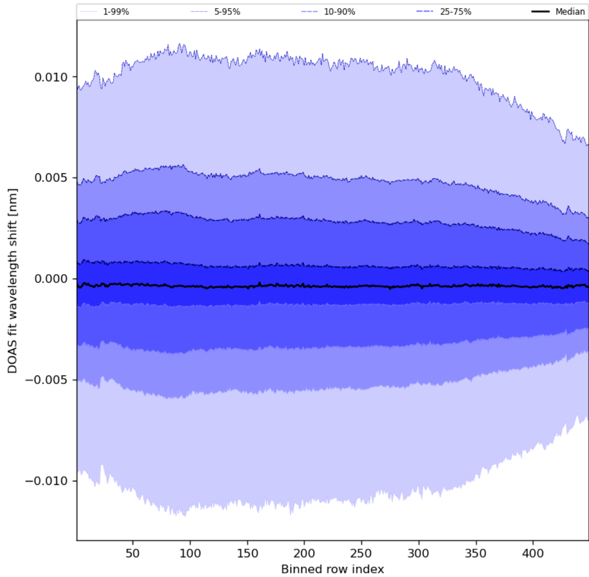
Figure 58: Along track statistics of “DOAS fit wavelength shift” for 2023-10-24 to 2023-10-26
