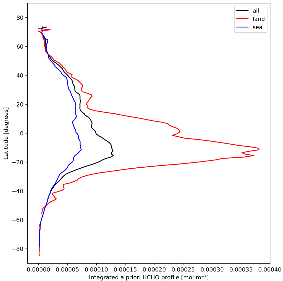
Figure 29: Zonal average of “Integrated a priori HCHO profile” for 2023-10-24 to 2023-10-26.
