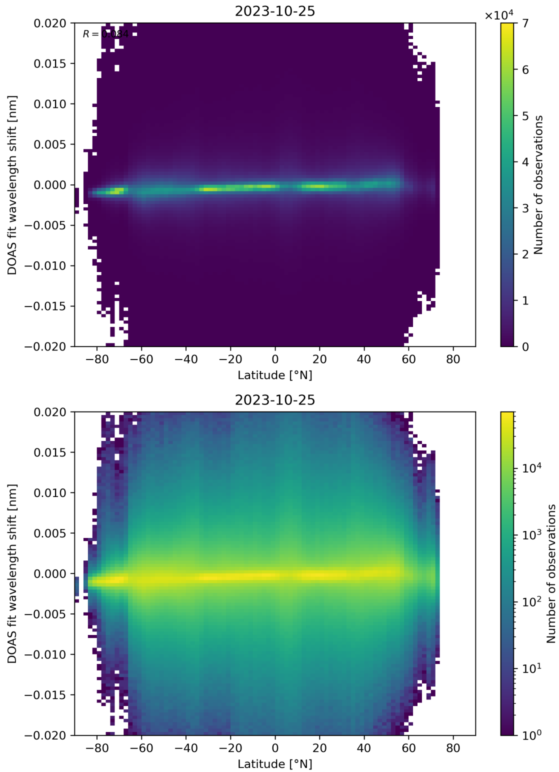
Figure 154: Scatter density plot of “Latitude” against “DOAS fit wavelength shift” for 2023-10-24 to 2023-10-26.
