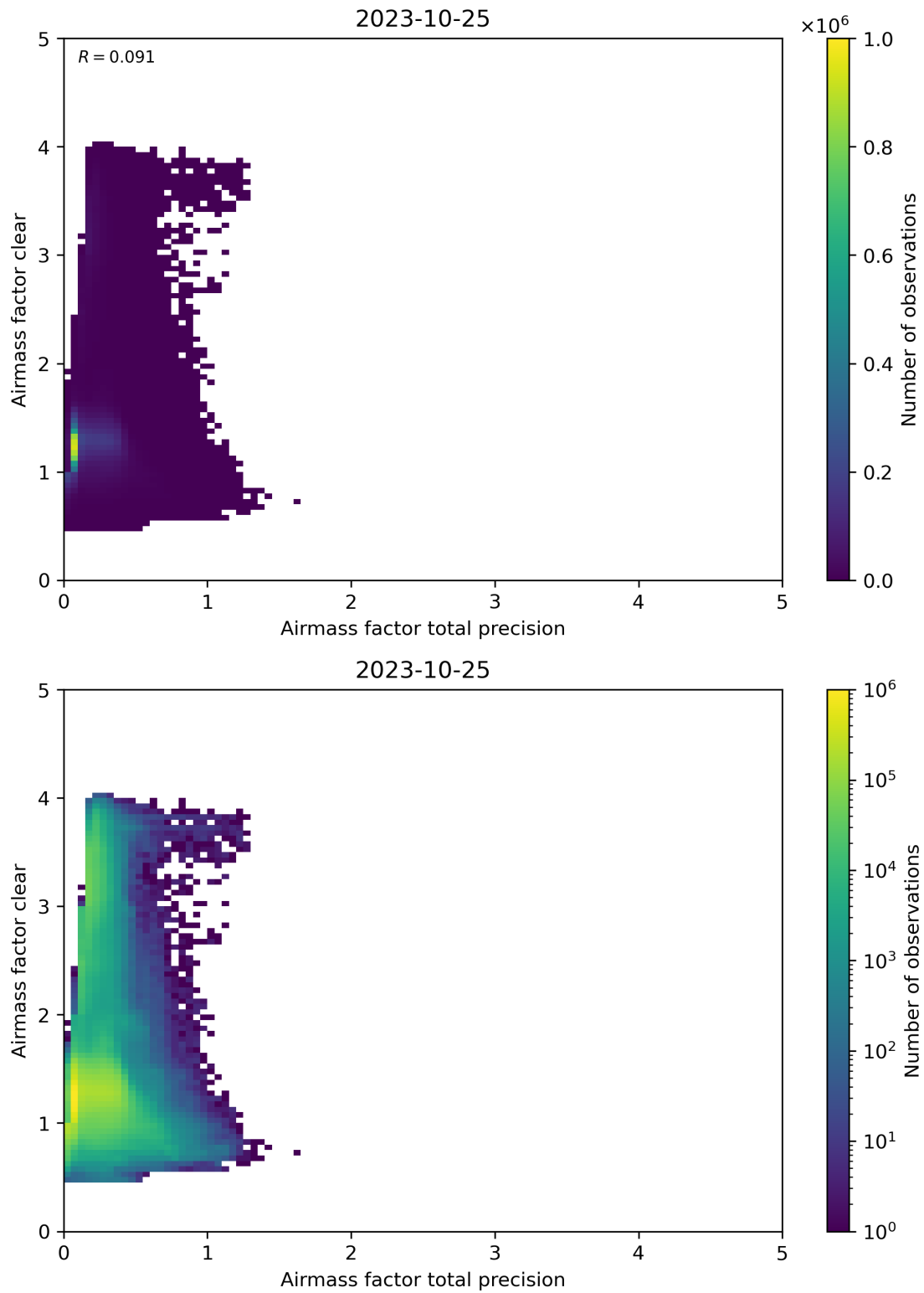
Figure 108: Scatter density plot of “Airmass factor total precision” against “Airmass factor clear” for 2023-10-24 to 2023-10-26.
