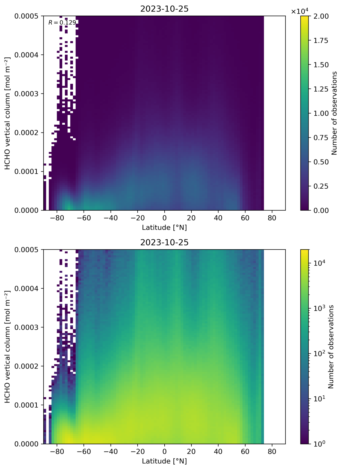
Figure 163: Scatter density plot of “Latitude” against “HCHO vertical column” for 2023-10-24 to 2023-10-26.
