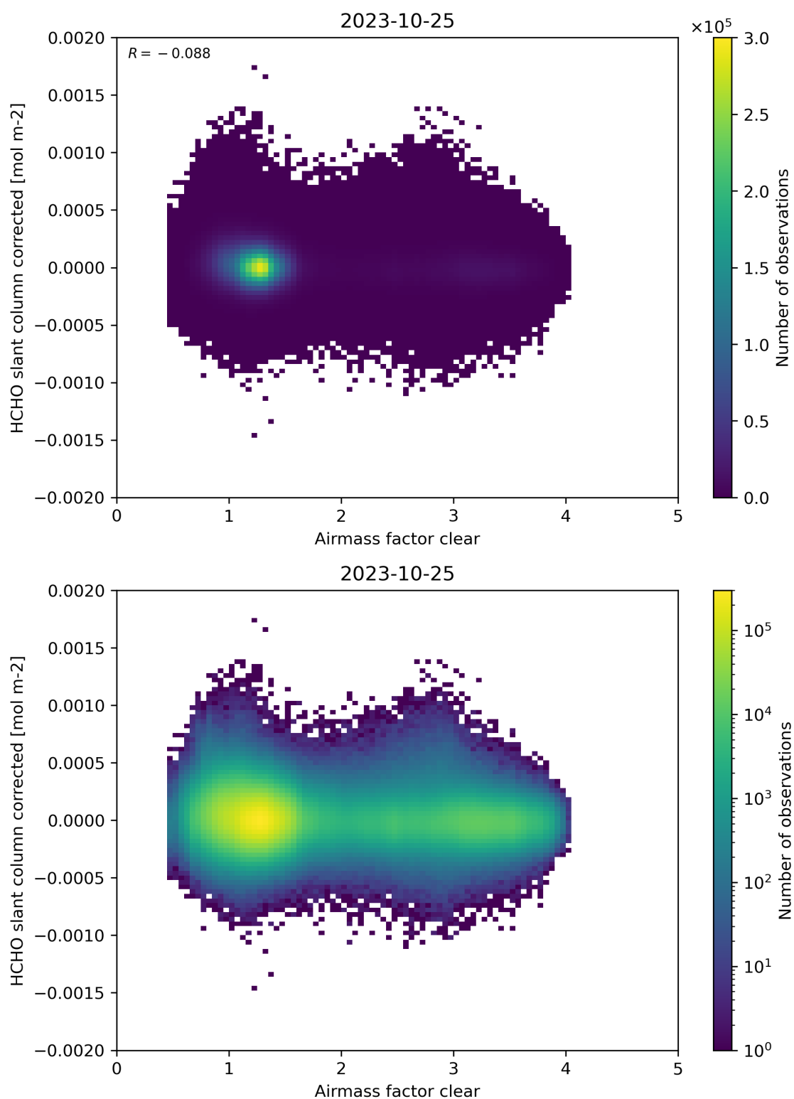
Figure 74: Scatter density plot of “Airmass factor clear” against “HCHO slant column corrected” for 2023-10-24 to 2023-10-26.
