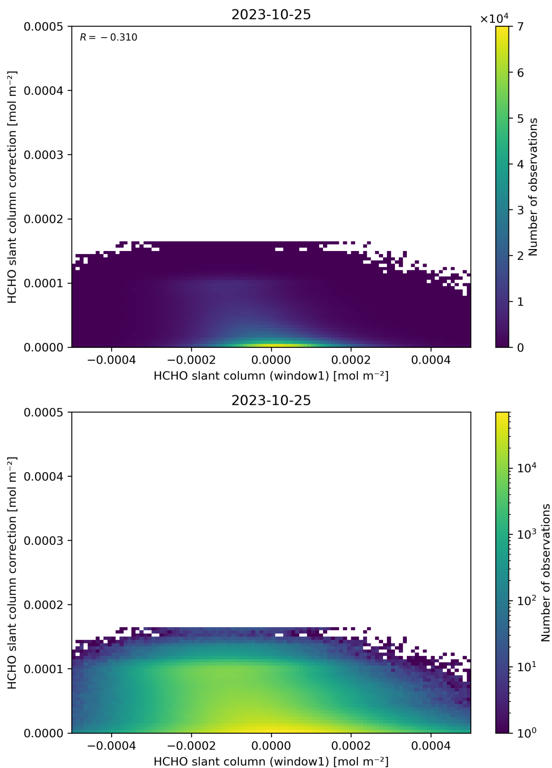
Figure 83: Scatter density plot of “HCHO slant column (window1)” against “HCHO slant column correction” for 2023-10-24 to 2023-10-26.
