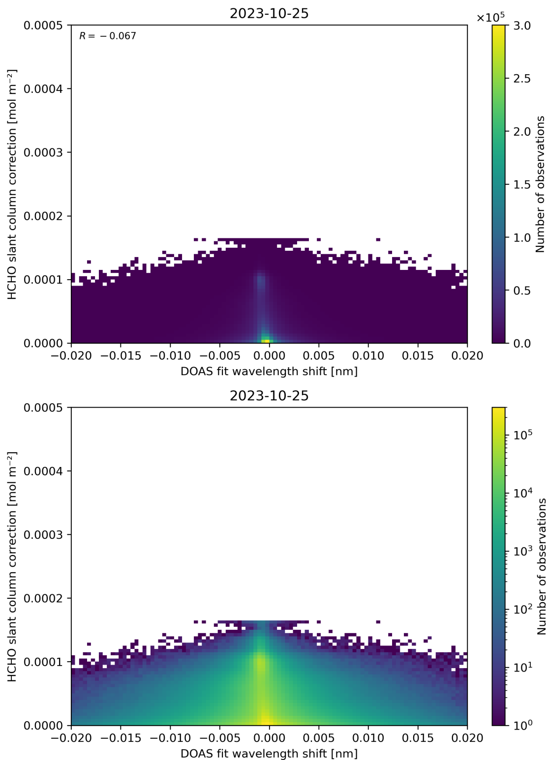
Figure 67: Scatter density plot of “DOAS fit wavelength shift” against “HCHO slant column correction” for 2023-10-24 to 2023-10-26.
