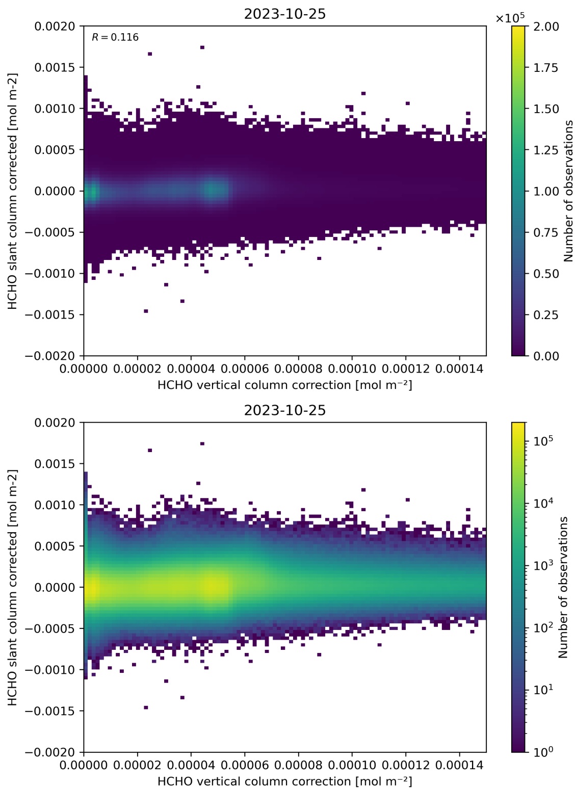
Figure 116: Scatter density plot of “HCHO vertical column correction” against “HCHO slant column corrected” for 2023-10-24 to 2023-10-26.
