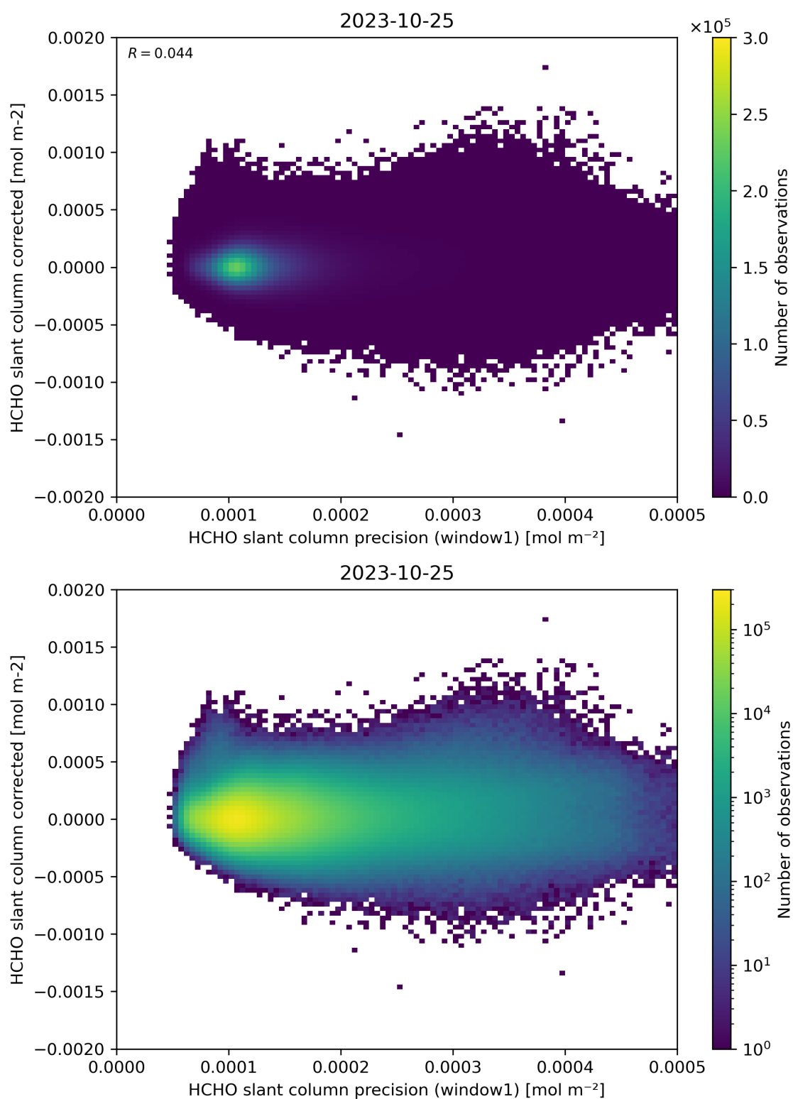
Figure 92: Scatter density plot of “HCHO slant column precision (window1)” against “HCHO slant column corrected” for 2023-10-24 to 2023-10-26.
