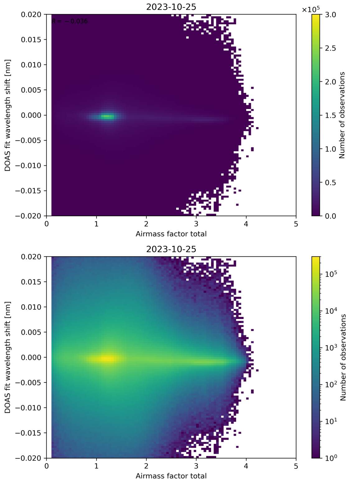
Figure 98: Scatter density plot of “Airmass factor total” against “DOAS fit wavelength shift” for 2023-10-24 to 2023-10-26.
