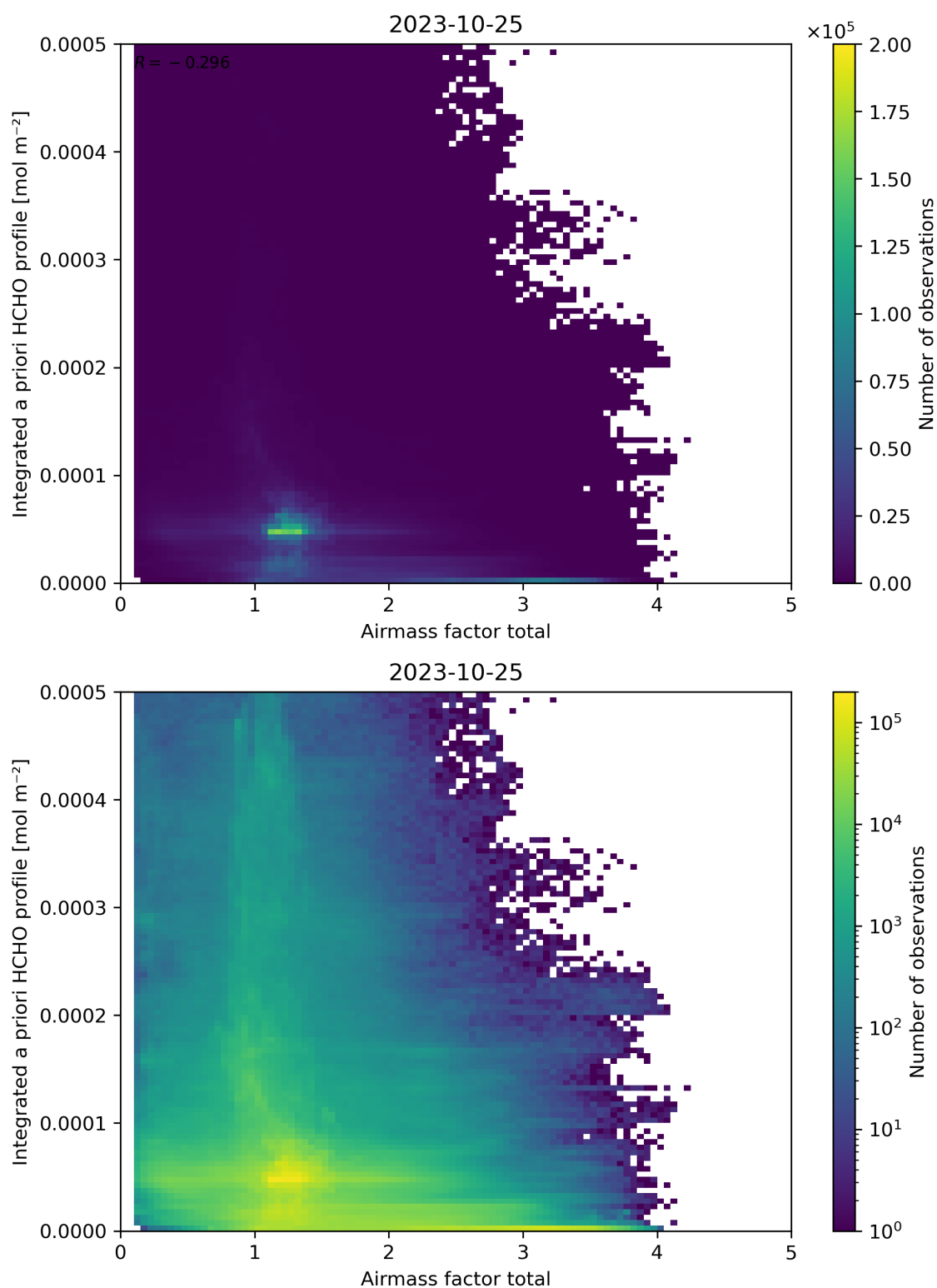
Figure 104: Scatter density plot of “Airmass factor total” against “Integrated a priori HCHO profile” for 2023-10-24 to 2023-10-26.
