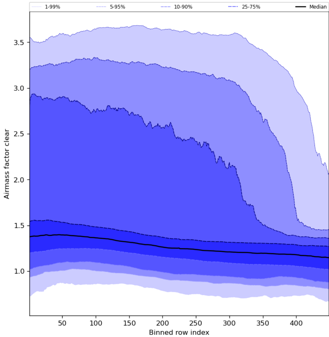
Figure 56: Along track statistics of “Airmass factor clear” for 2023-10-24 to 2023-10-26
