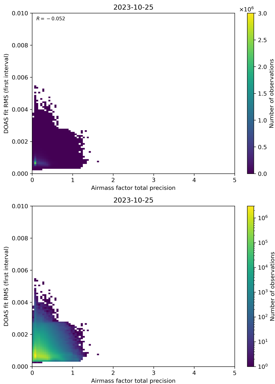
Figure 105: Scatter density plot of “Airmass factor total precision” against “DOAS fit RMS (first interval)” for 2023-10-24 to 2023-10-26.
