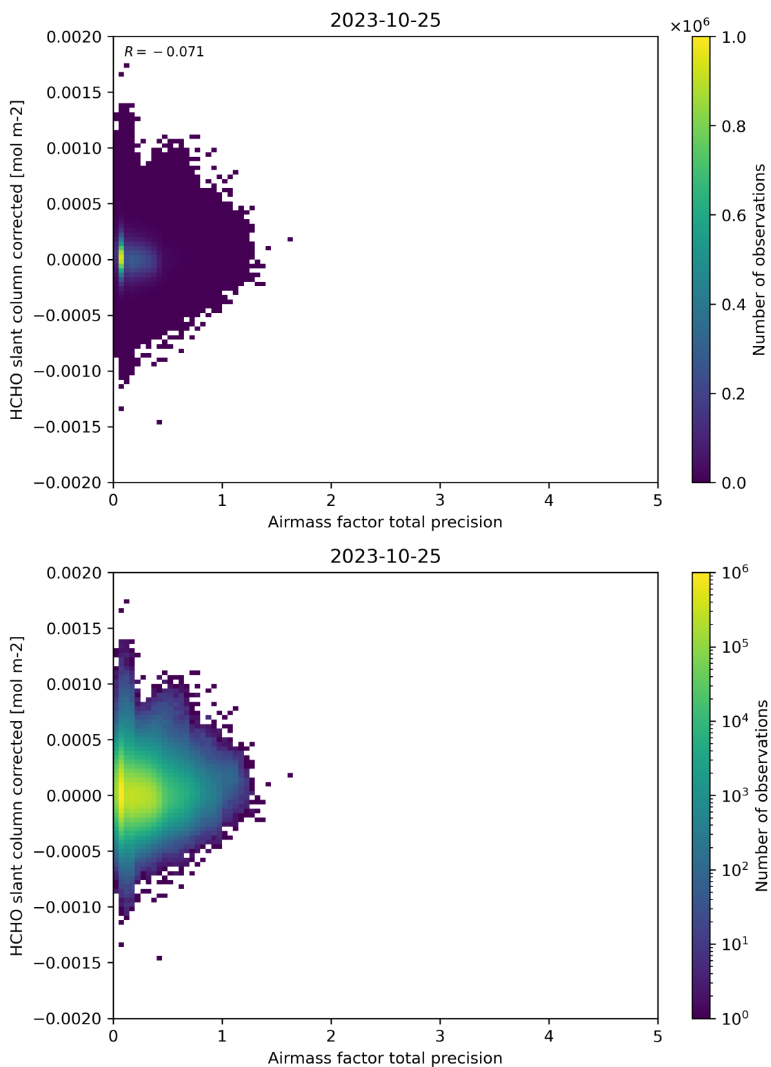
Figure 109: Scatter density plot of “Airmass factor total precision” against “HCHO slant column corrected” for 2023-10-24 to 2023-10-26.
