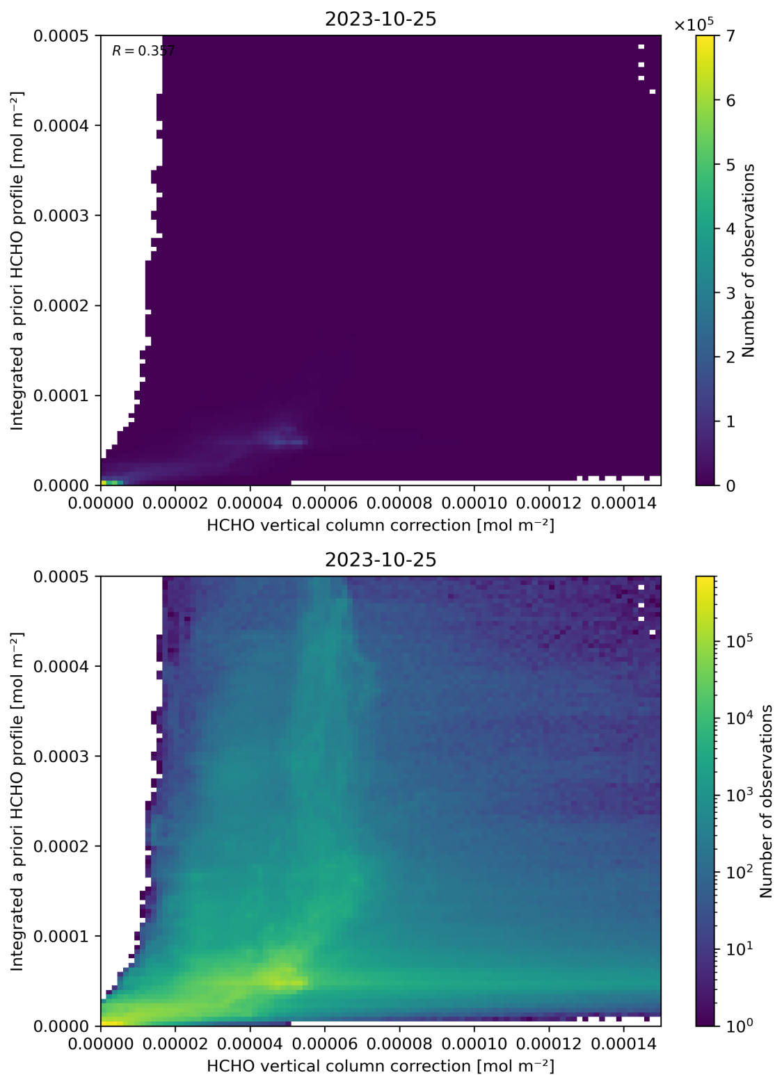
Figure 122: Scatter density plot of “HCHO vertical column correction” against “Integrated a priori HCHO profile” for 2023-10-24 to 2023-10-26.
