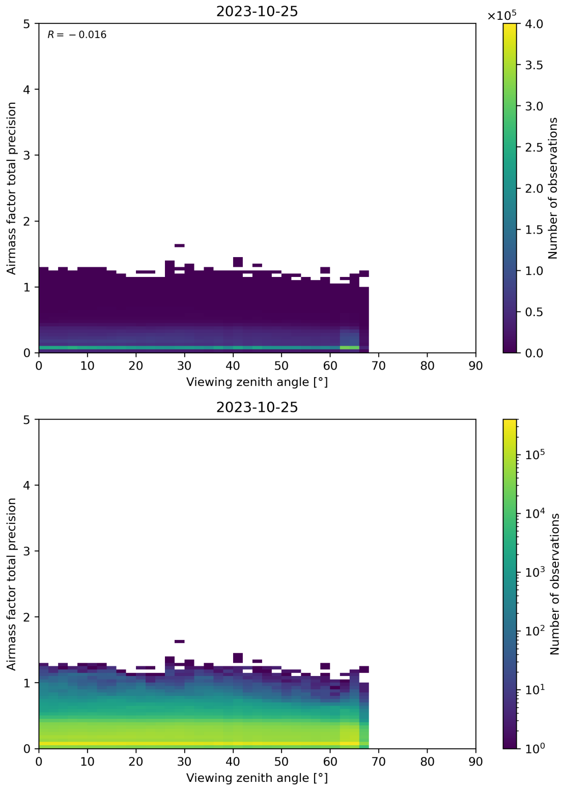
Figure 191: Scatter density plot of “Viewing zenith angle” against “Airmass factor total precision” for 2023-10-24 to 2023-10-26.
