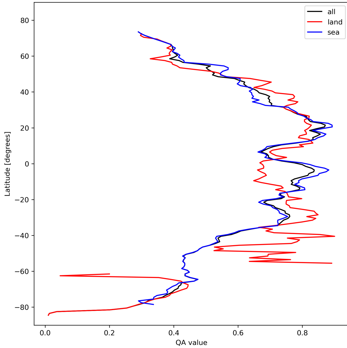
Figure 20: Zonal average of "QA value" for 2023-10-24 to 2023-10-26.
