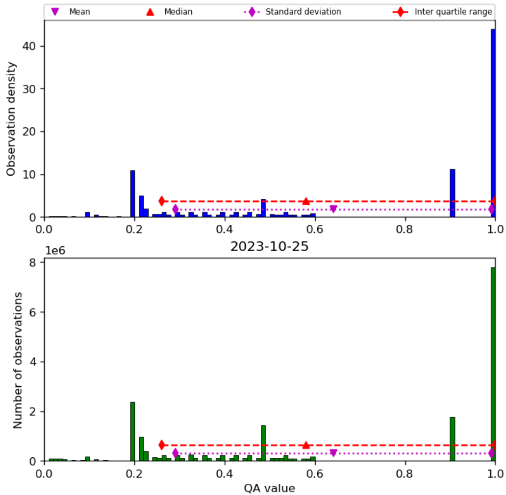
Figure 34: Histogram of “QA value” for 2023-10-24 to 2023-10-26
