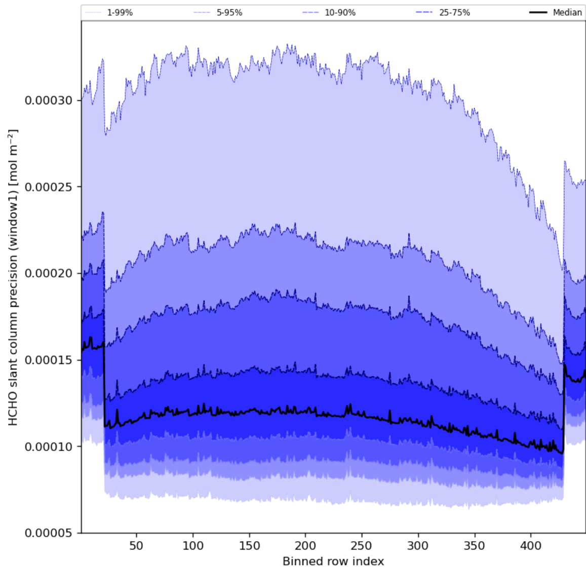
Figure 53: Along track statistics of “HCHO slant column precision (window1)” for 2023-10-24 to 2023-10-26
