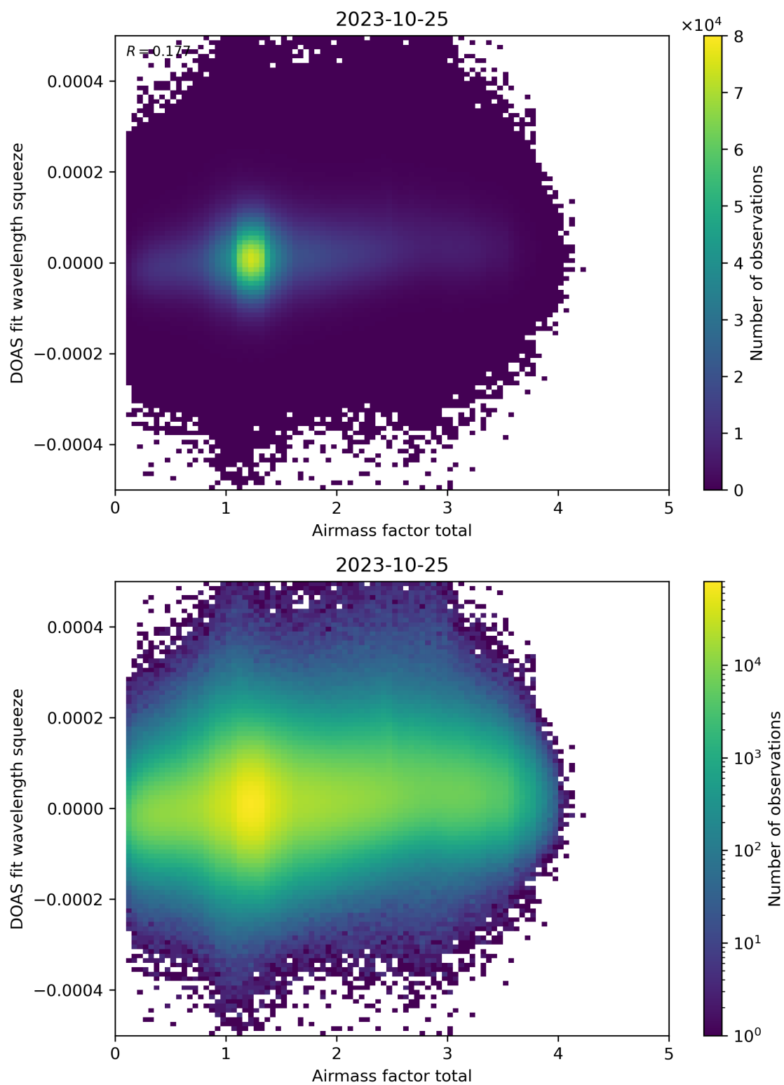
Figure 99: Scatter density plot of “Airmass factor total” against “DOAS fit wavelength squeeze” for 2023-10-24 to 2023-10-26.
