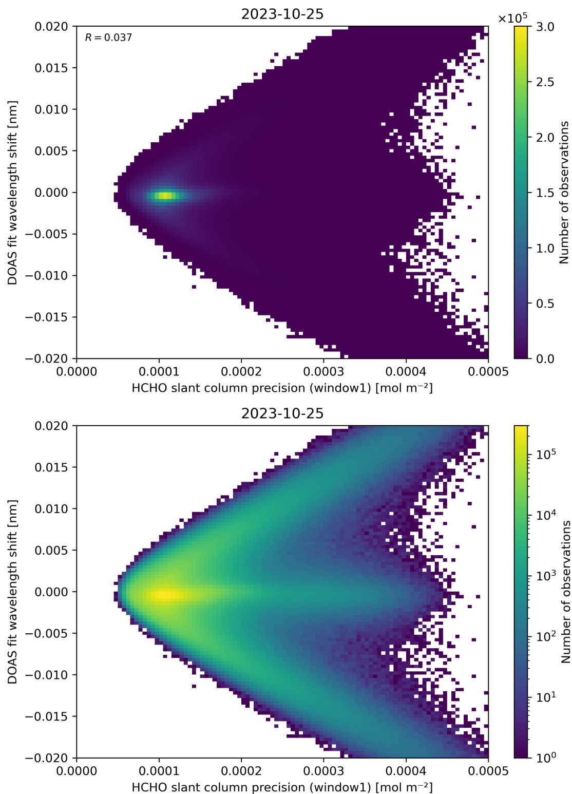
Figure 89: Scatter density plot of “HCHO slant column precision (window1)” against “DOAS fit wavelength shift” for 2023-10-24 to 2023-10-26.
