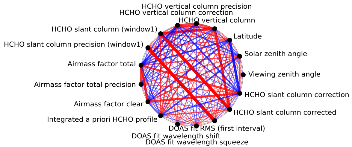
Figure 1: Map of correlation graph for 2023-10-24 to 2023-10-26.
