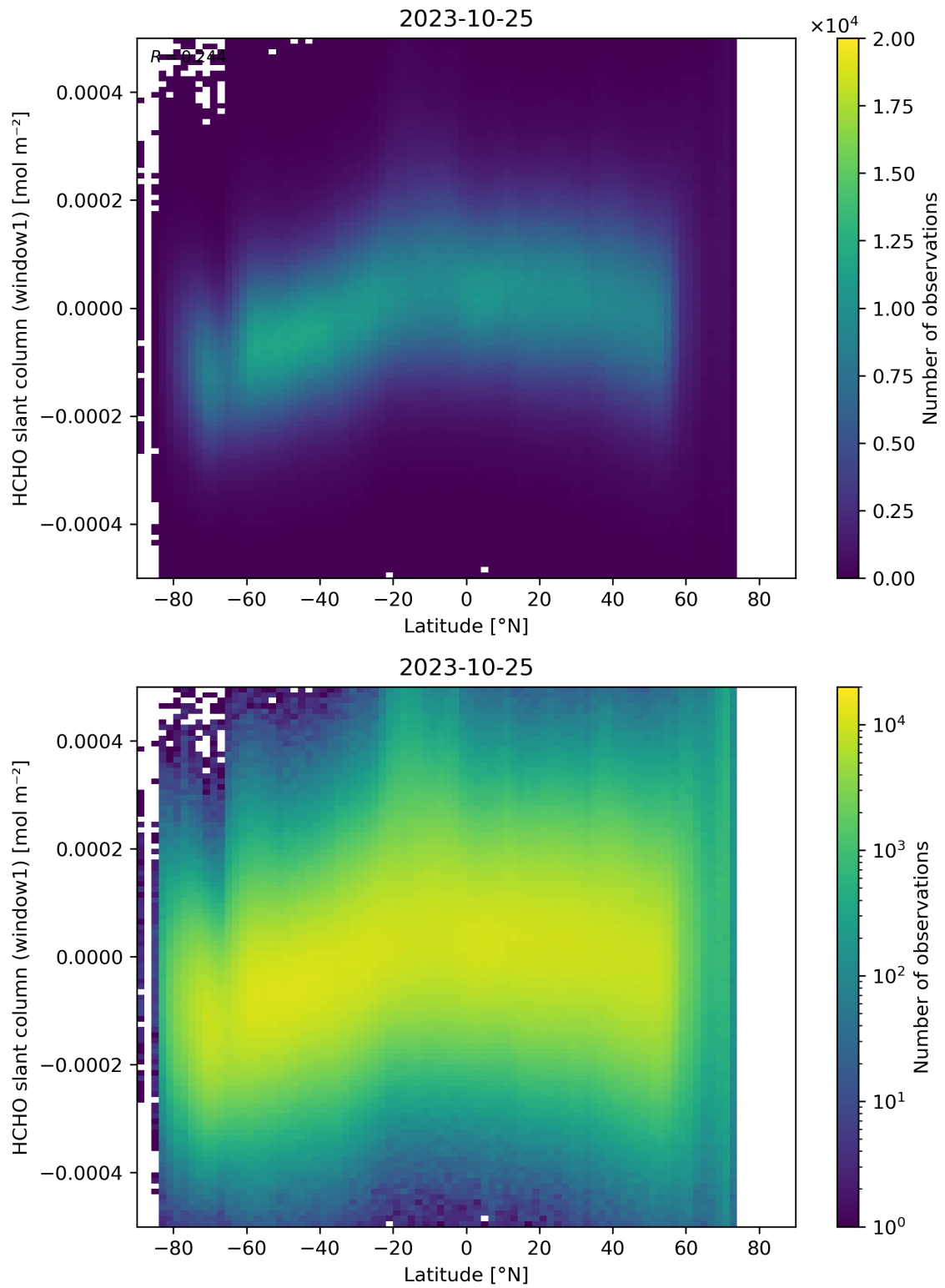
Figure 159: Scatter density plot of “Latitude” against “HCHO slant column (window1)” for 2023-10-24 to 2023-10-26.
