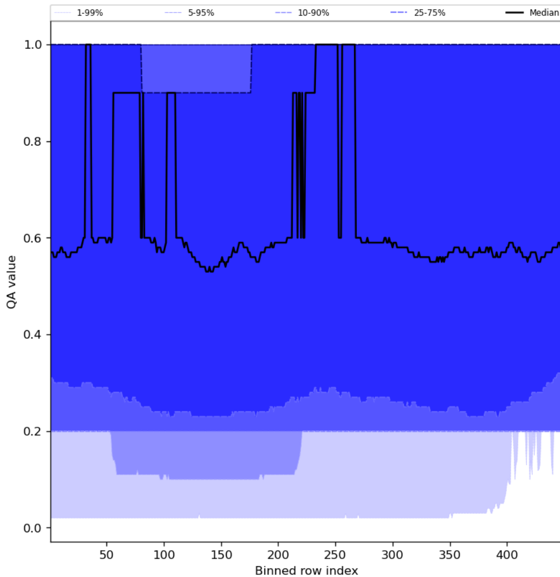
Figure 48: Along track statistics of “QA value” for 2023-10-24 to 2023-10-26
