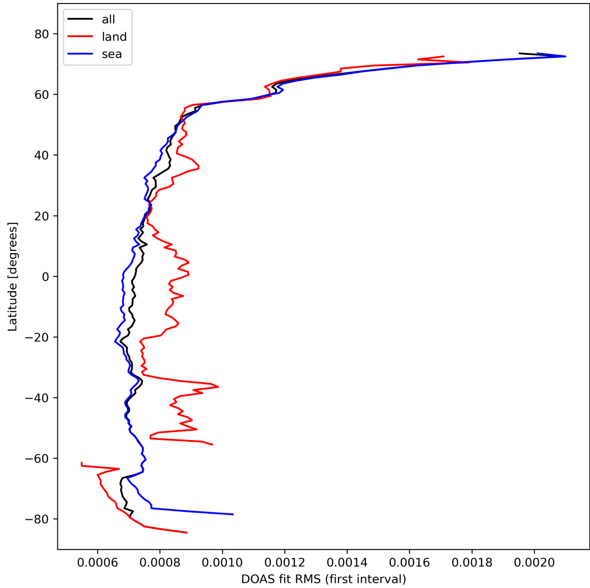
Figure 32: Zonal average of “DOAS fit RMS (first interval)” for 2023-10-24 to 2023-10-26.
