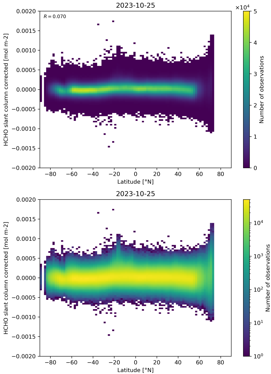
Figure 157: Scatter density plot of “Latitude” against “HCHO slant column corrected” for 2023-10-24 to 2023-10-26.
