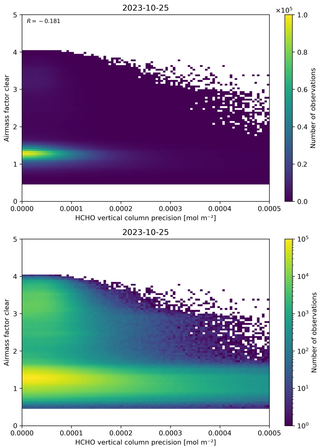
Figure 139: Scatter density plot of “HCHO vertical column precision” against “Airmass factor clear” for 2023-10-24 to 2023-10-26.
