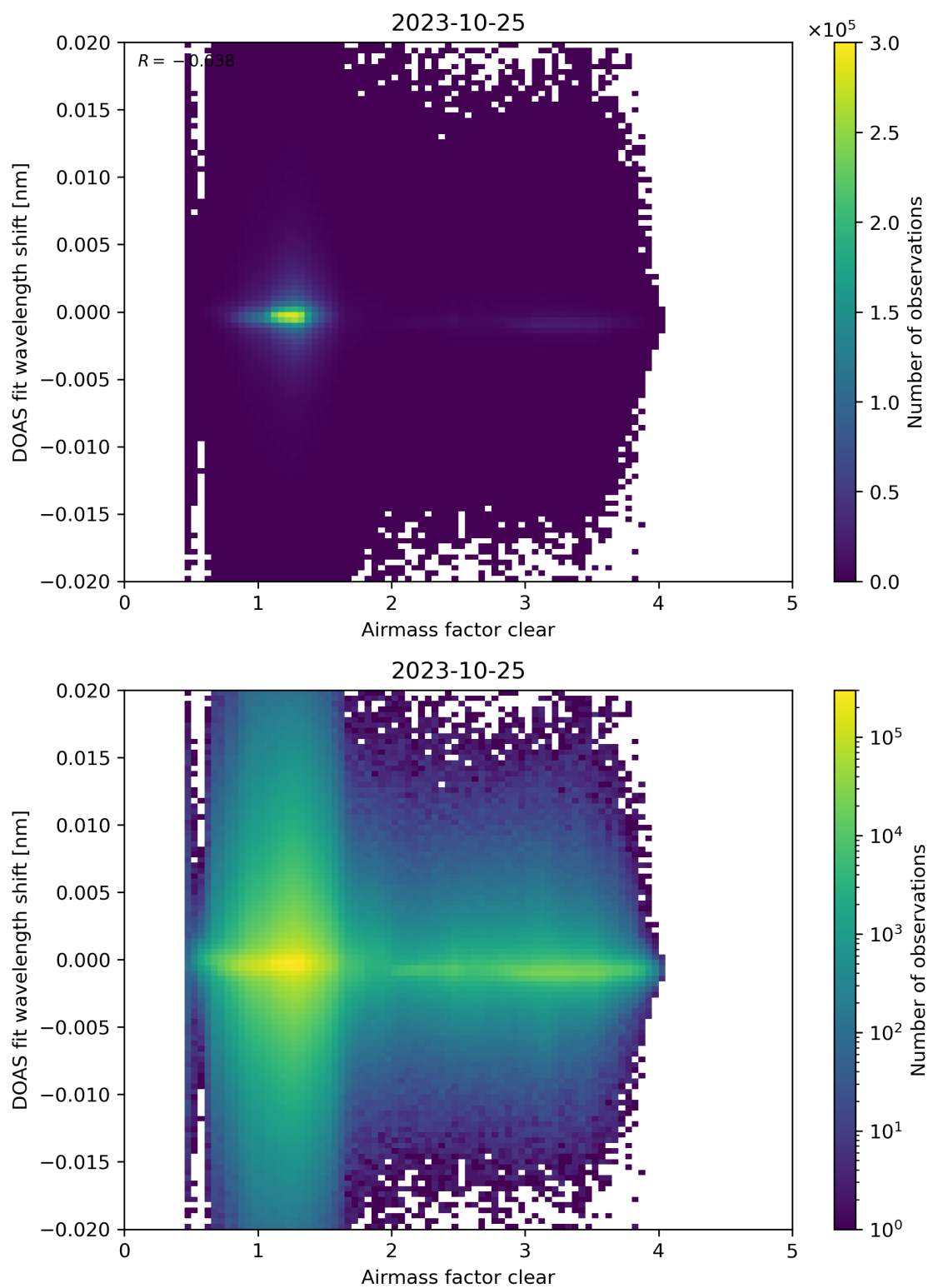
Figure 72: Scatter density plot of “Airmass factor clear” against “DOAS fit wavelength shift” for 2023-10-24 to 2023-10-26.
