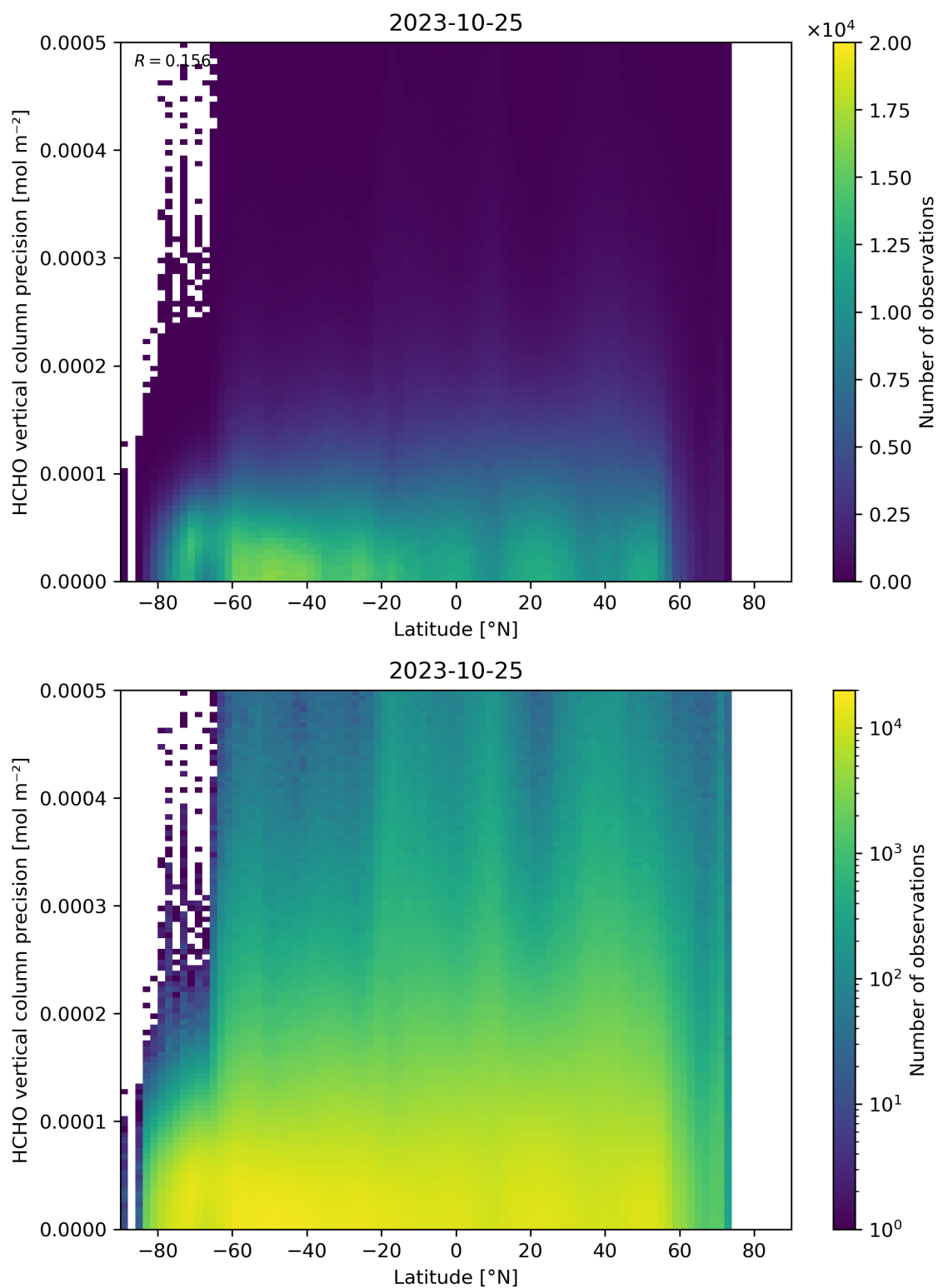
Figure 165: Scatter density plot of “Latitude” against “HCHO vertical column precision” for 2023-10-24 to 2023-10-26.
