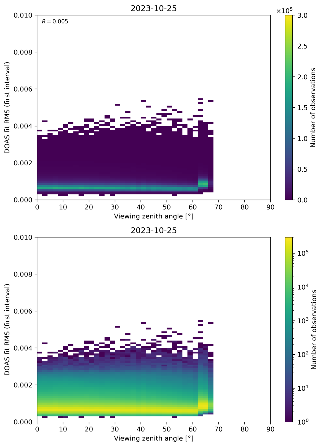
Figure 182: Scatter density plot of “Viewing zenith angle” against “DOAS fit RMS (first interval)” for 2023-10-24 to 2023-10-26.
