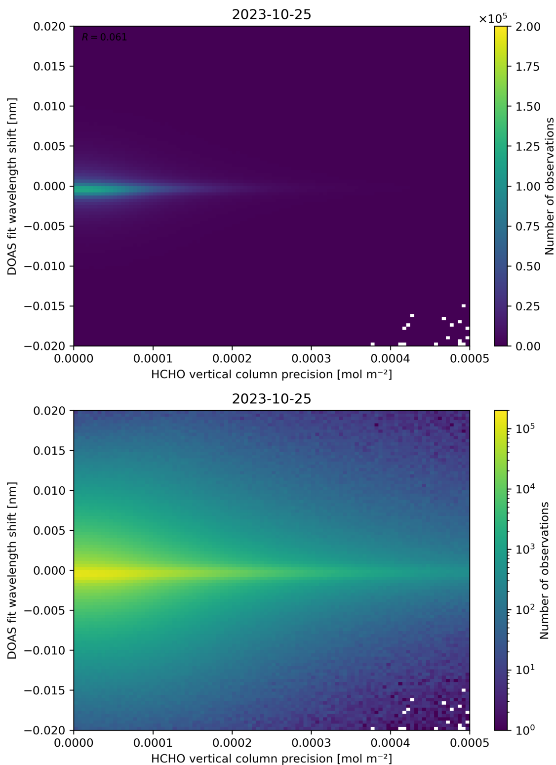
Figure 137: Scatter density plot of “HCHO vertical column precision” against “DOAS fit wavelength shift” for 2023-10-24 to 2023-10-26.
