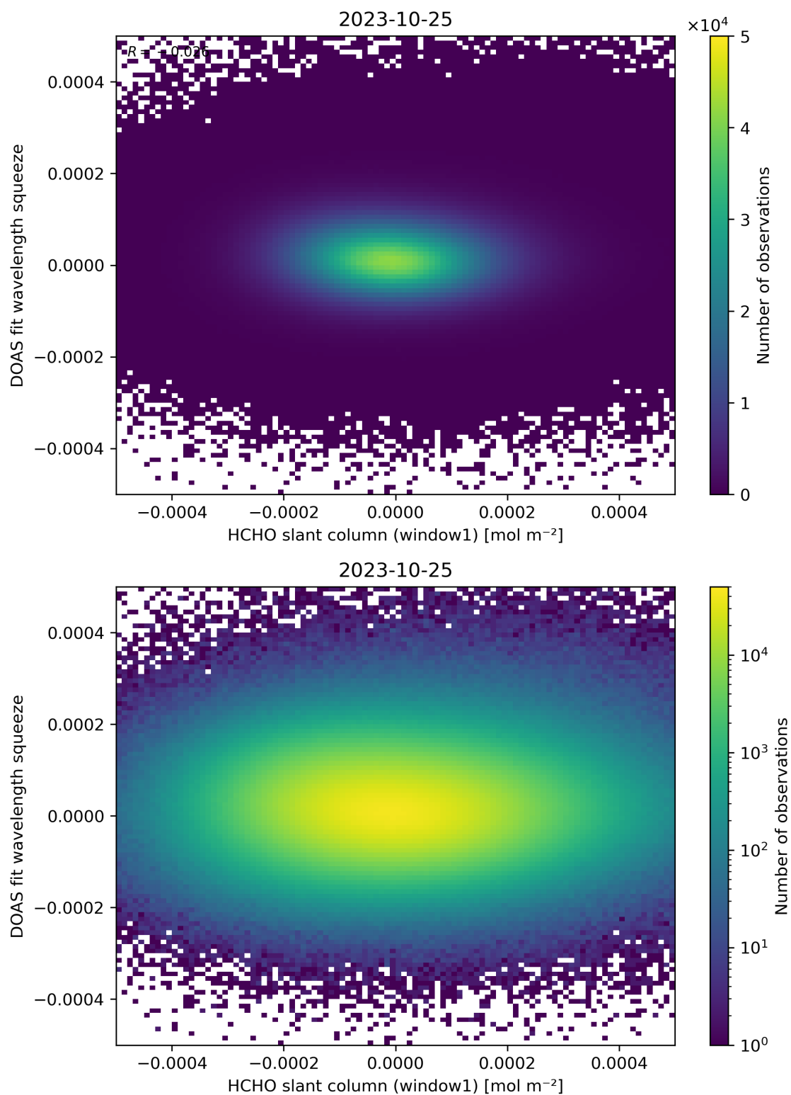
Figure 80: Scatter density plot of “HCHO slant column (window1)” against “DOAS fit wavelength squeeze” for 2023-10-24 to 2023-10-26.
