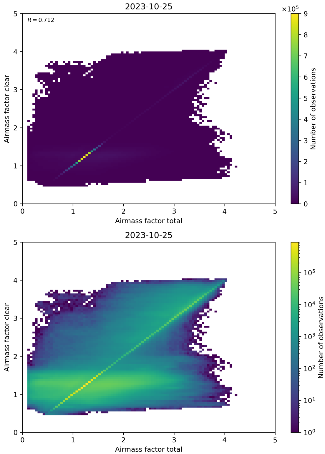
Figure 100: Scatter density plot of “Airmass factor total” against “Airmass factor clear” for 2023-10-24 to 2023-10-26.
