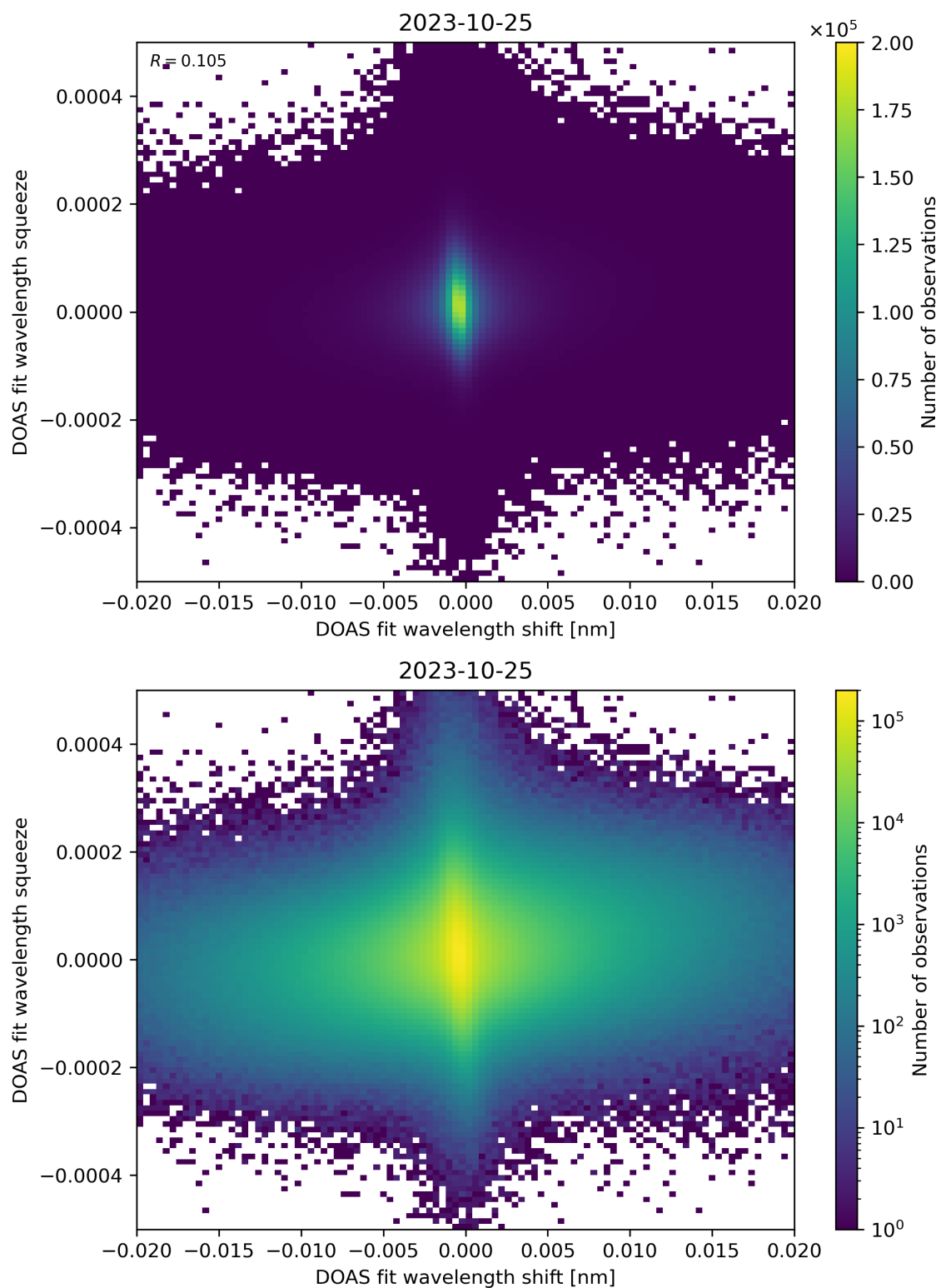
Figure 65: Scatter density plot of “DOAS fit wavelength shift” against “DOAS fit wavelength squeeze” for 2023-10-24 to 2023-10-26.
