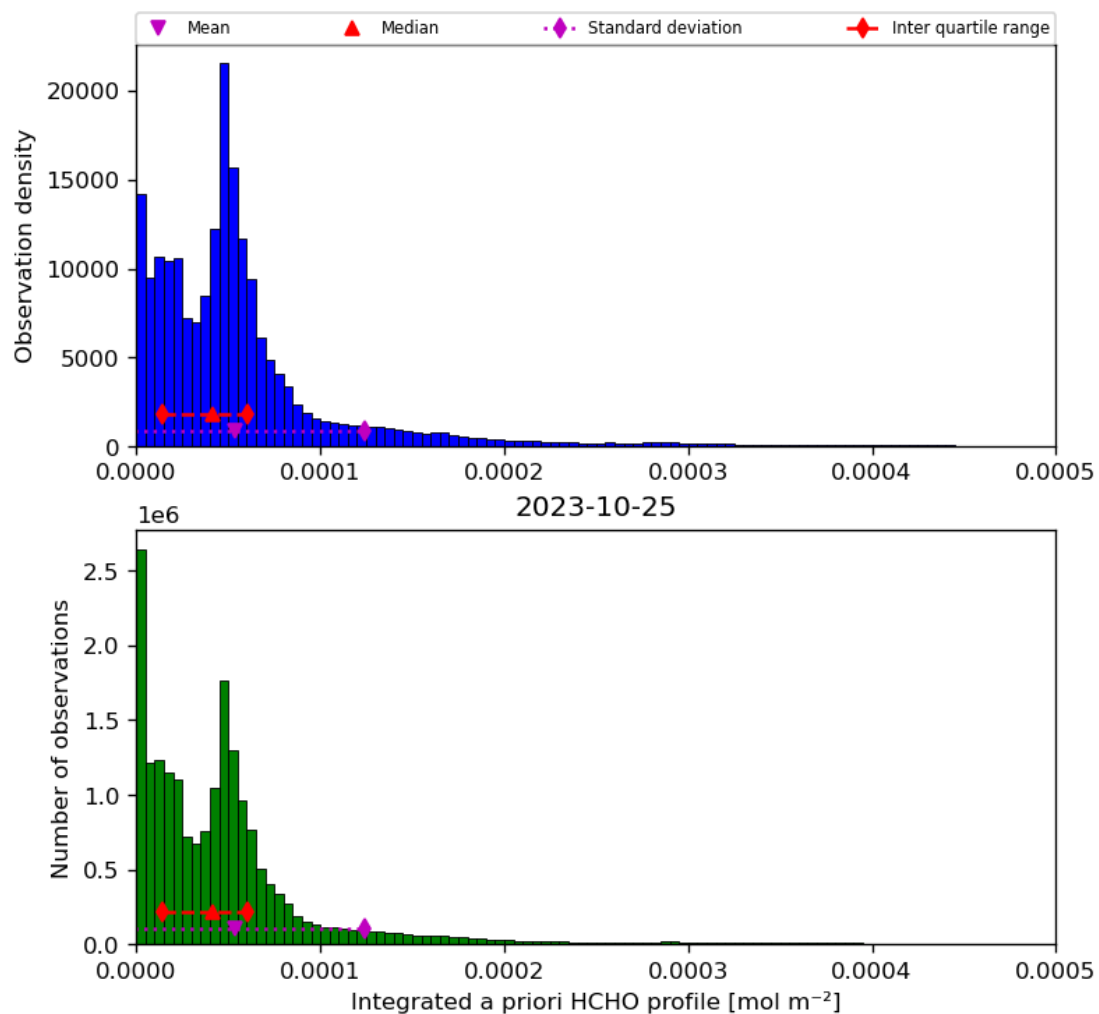
Figure 43: Histogram of “Integrated a priori HCHO profile” for 2023-10-24 to 2023-10-26
