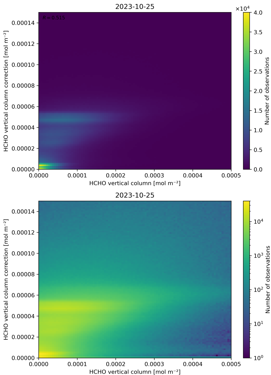
Figure 133: Scatter density plot of “HCHO vertical column” against “HCHO vertical column correction” for 2023-10-24 to 2023-10-26.
