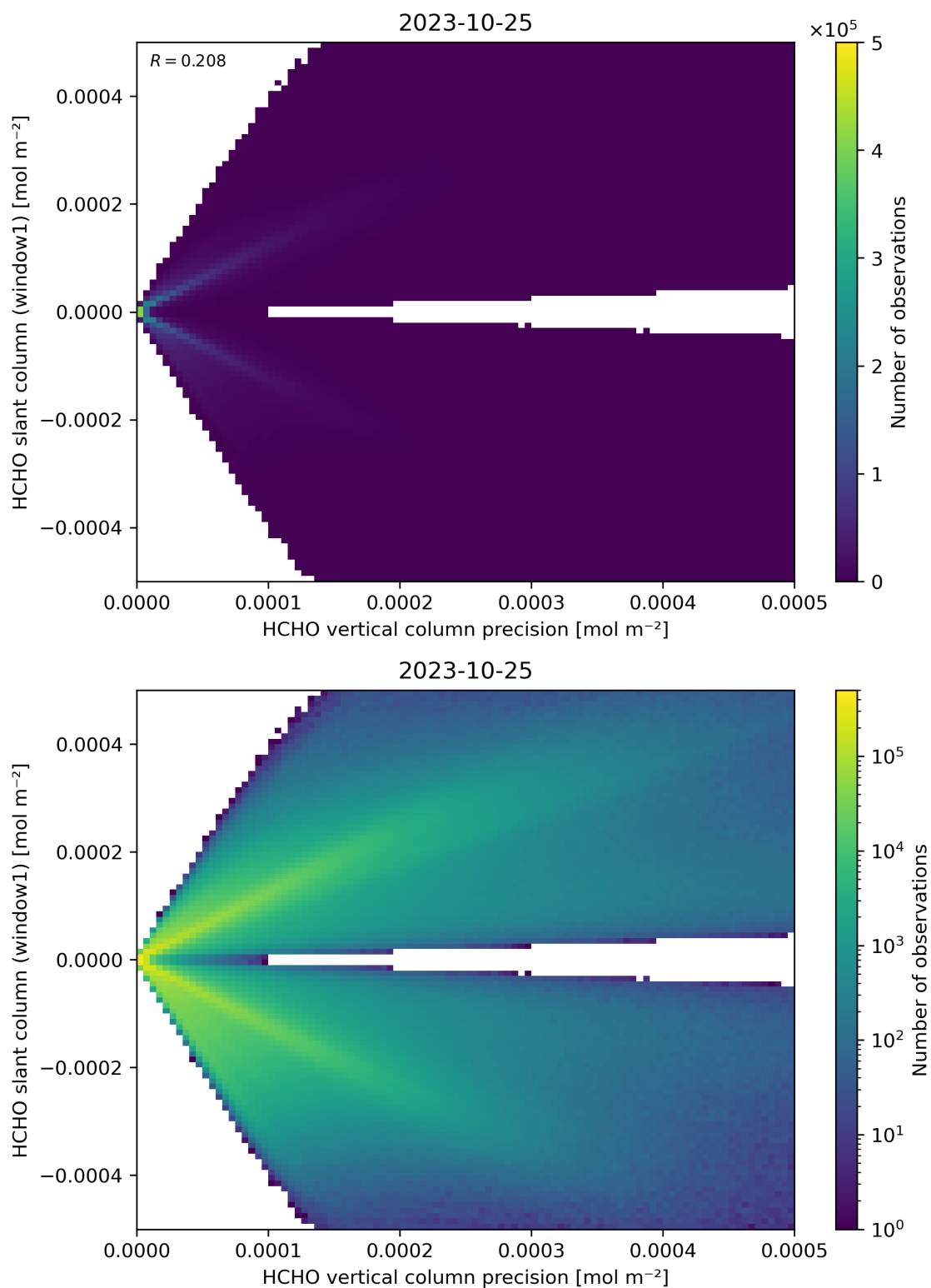
Figure 142: Scatter density plot of “HCHO vertical column precision” against “HCHO slant column (window1)” for 2023-10-24 to 2023-10-26.
