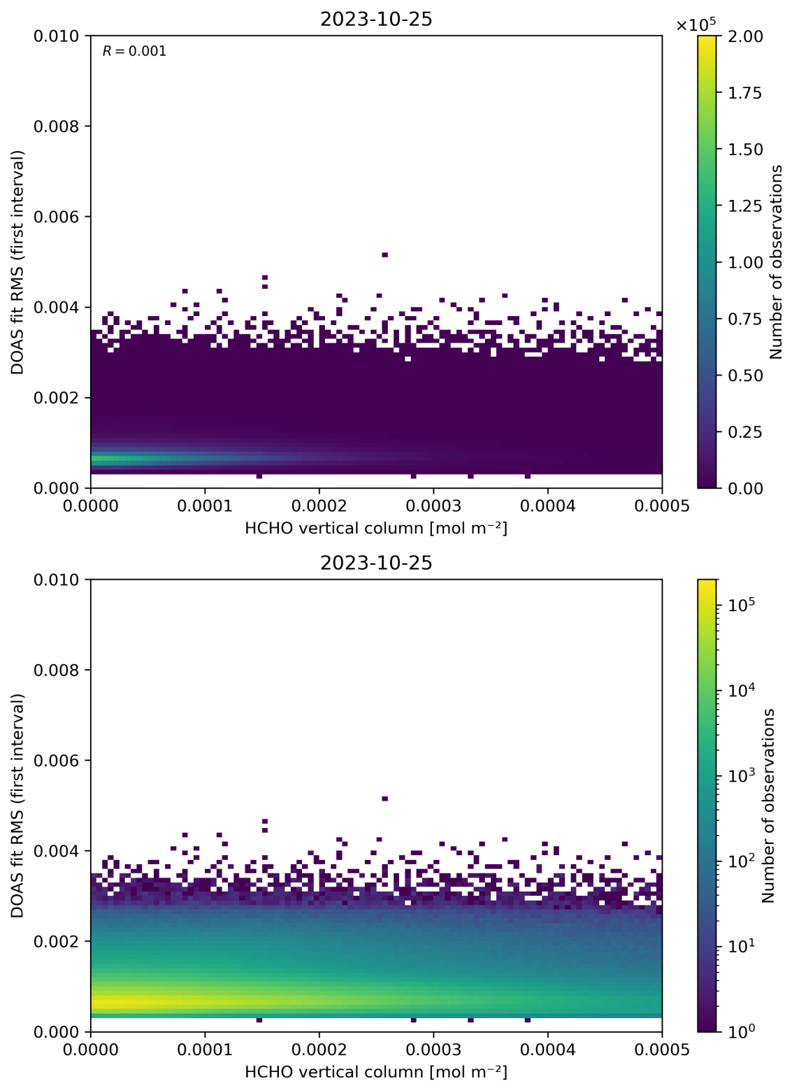
Figure 123: Scatter density plot of “HCHO vertical column” against “DOAS fit RMS (first interval)” for 2023-10-24 to 2023-10-26.
