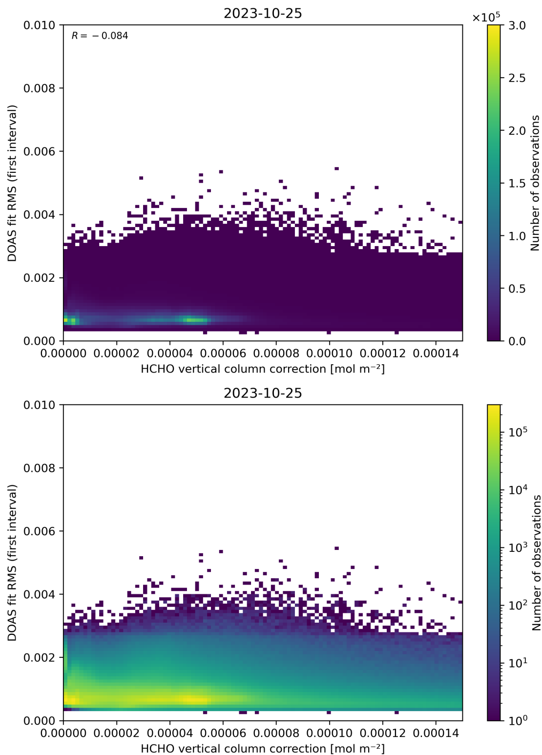
Figure 112: Scatter density plot of “HCHO vertical column correction” against “DOAS fit RMS (first interval)” for 2023-10-24 to 2023-10-26.
