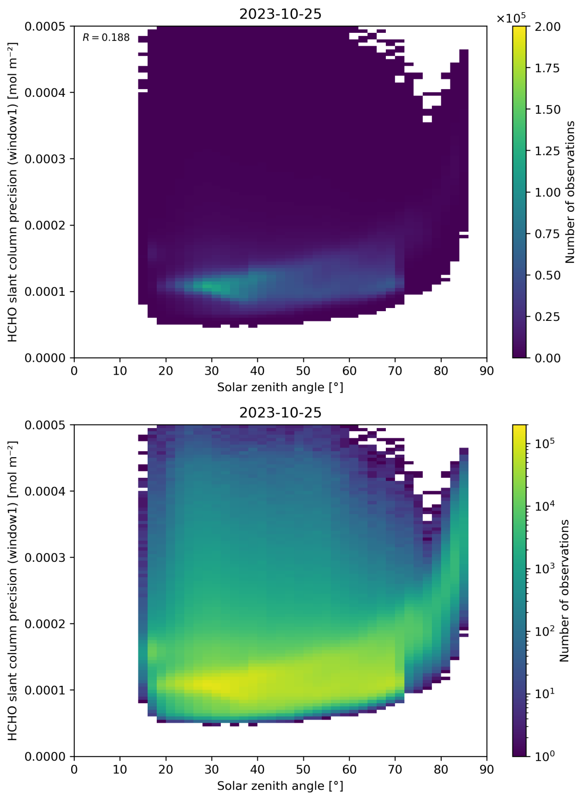
Figure 174: Scatter density plot of “Solar zenith angle” against “HCHO slant column precision (window1)” for 2023-10-24 to 2023-10-26.
