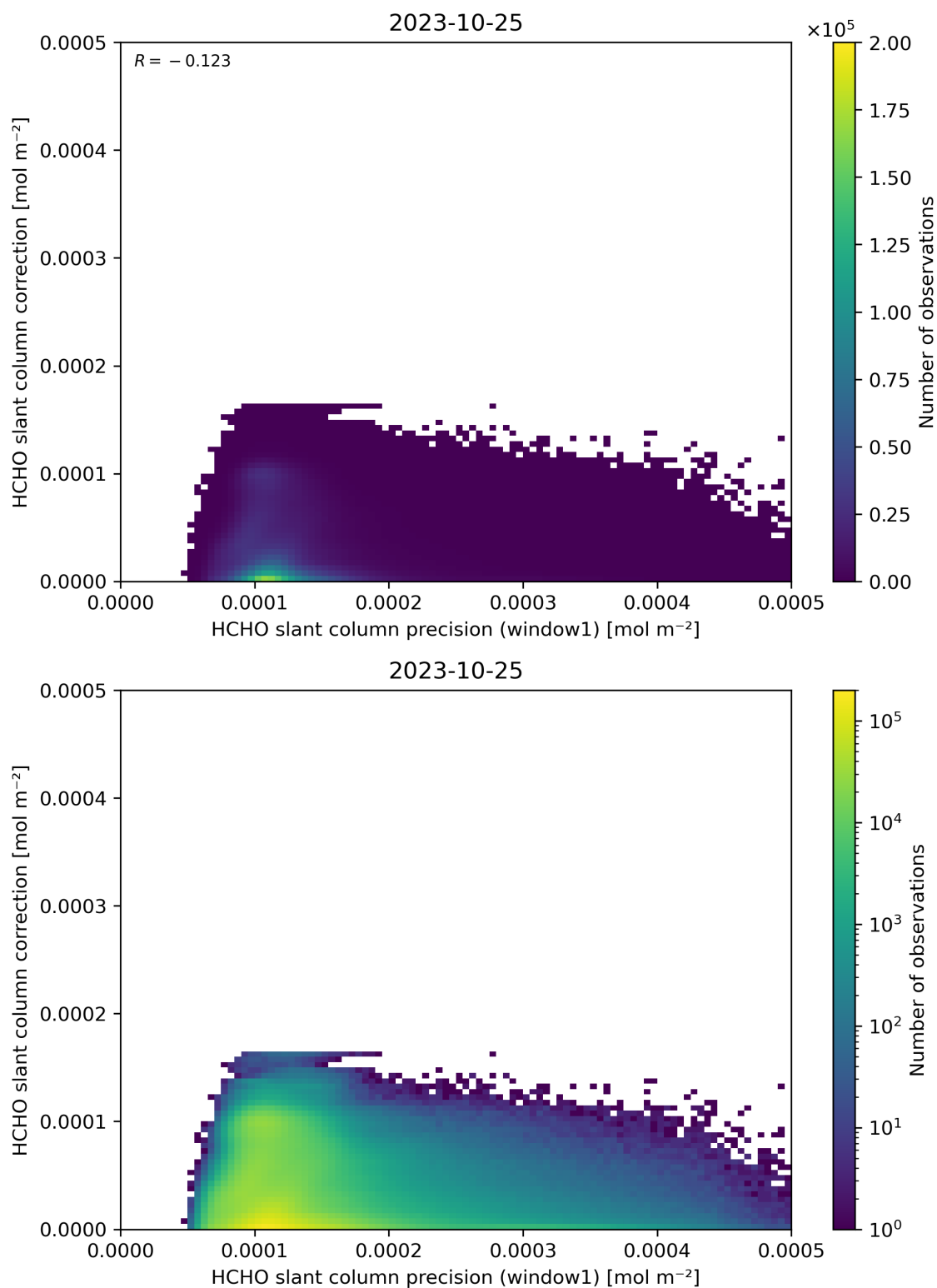
Figure 93: Scatter density plot of “HCHO slant column precision (window1)” against “HCHO slant column correction” for 2023-10-24 to 2023-10-26.
