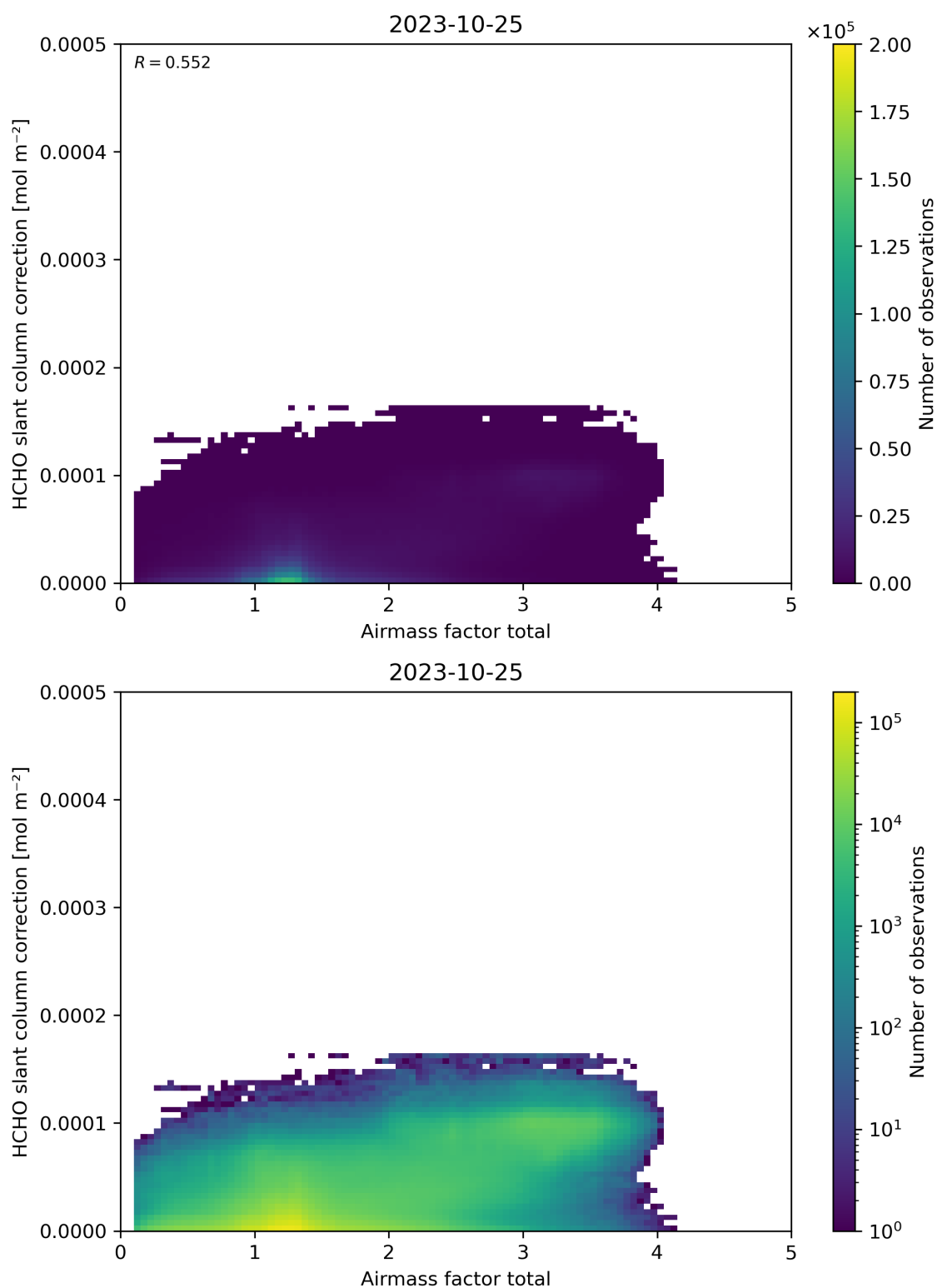
Figure 102: Scatter density plot of “Airmass factor total” against “HCHO slant column correction” for 2023-10-24 to 2023-10-26.
