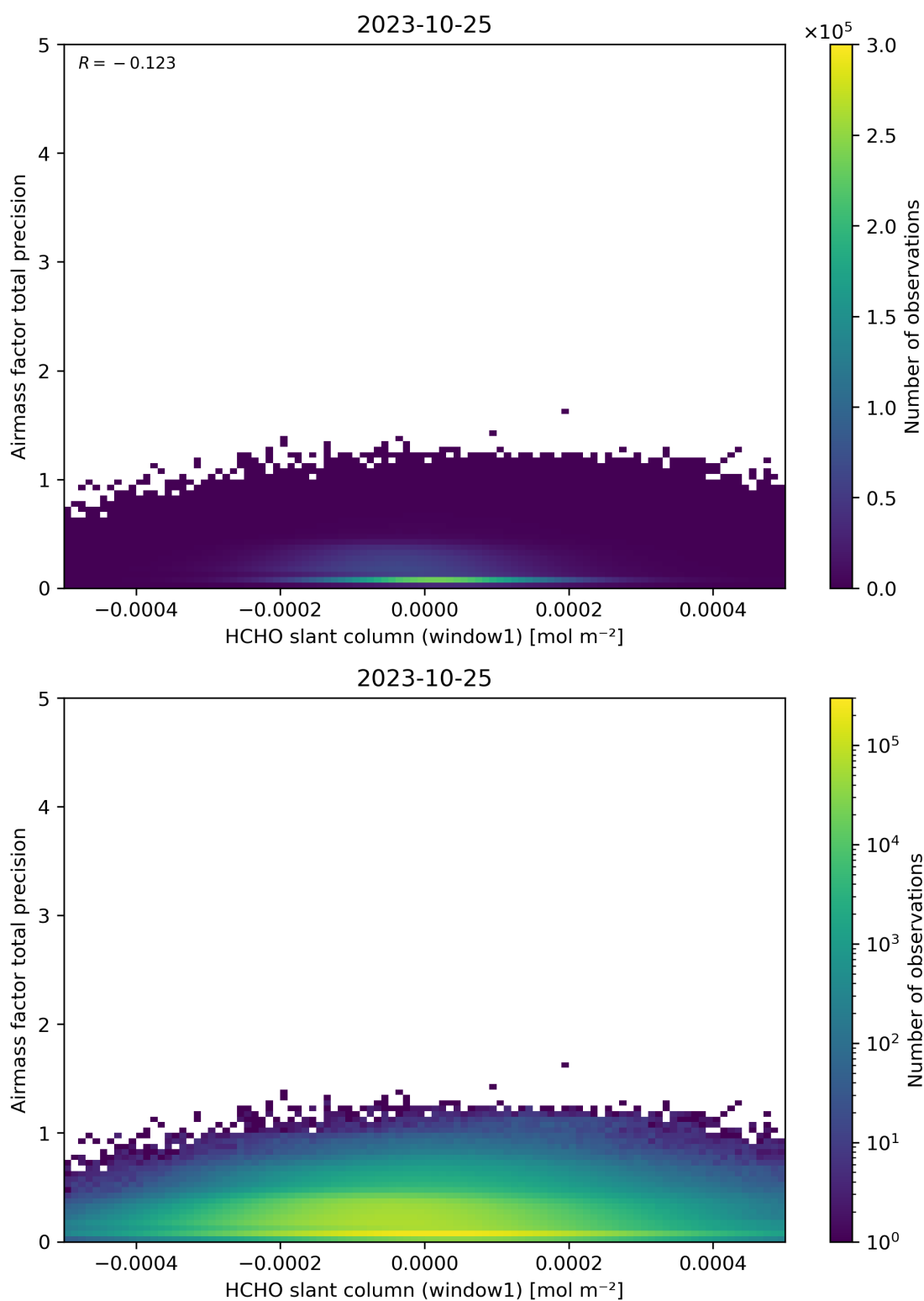
Figure 86: Scatter density plot of “HCHO slant column (window1)” against “Airmass factor total precision” for 2023-10-24 to 2023-10-26.
