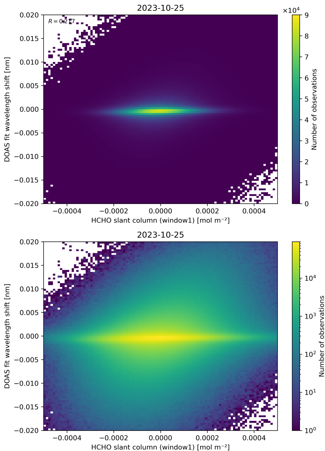
Figure 79: Scatter density plot of “HCHO slant column (window1)” against “DOAS fit wavelength shift” for 2023-10-24 to 2023-10-26.
