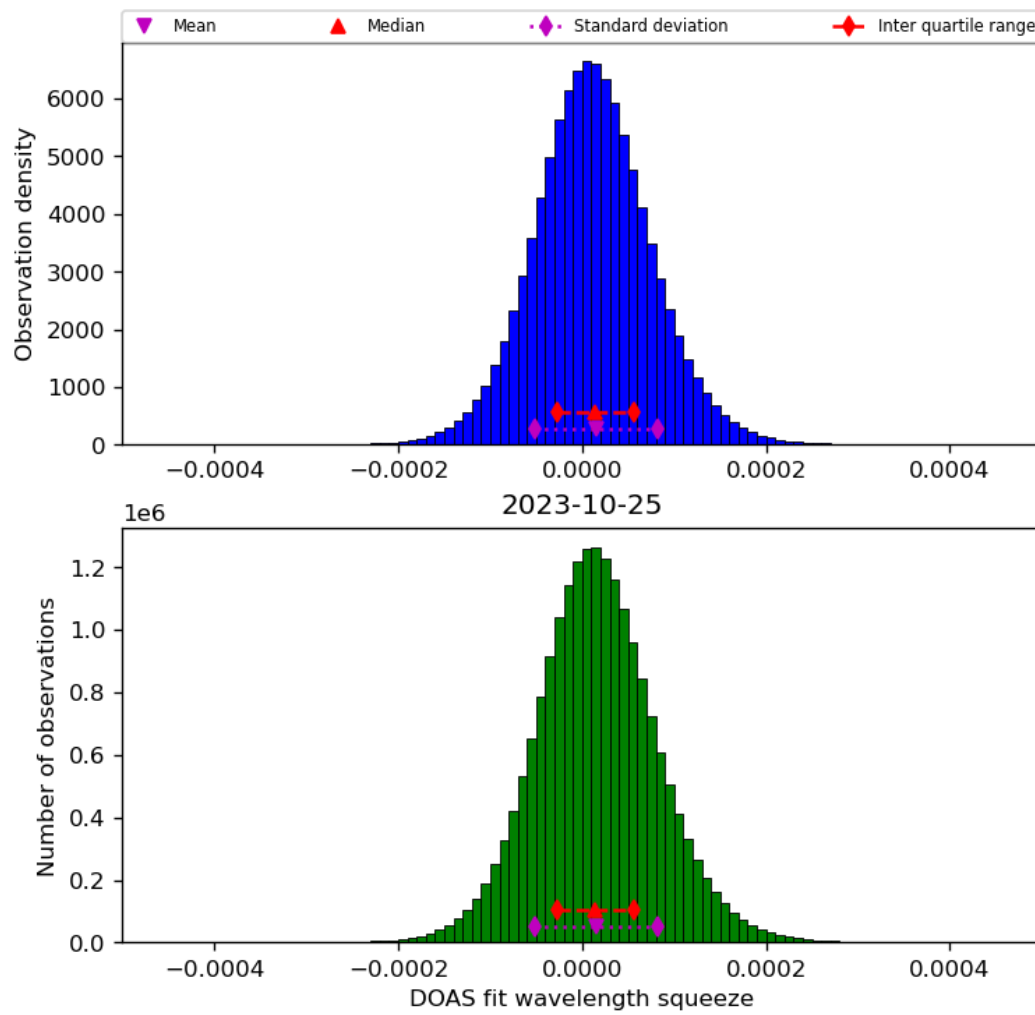
Figure 45: Histogram of “DOAS fit wavelength squeeze” for 2023-10-24 to 2023-10-26
