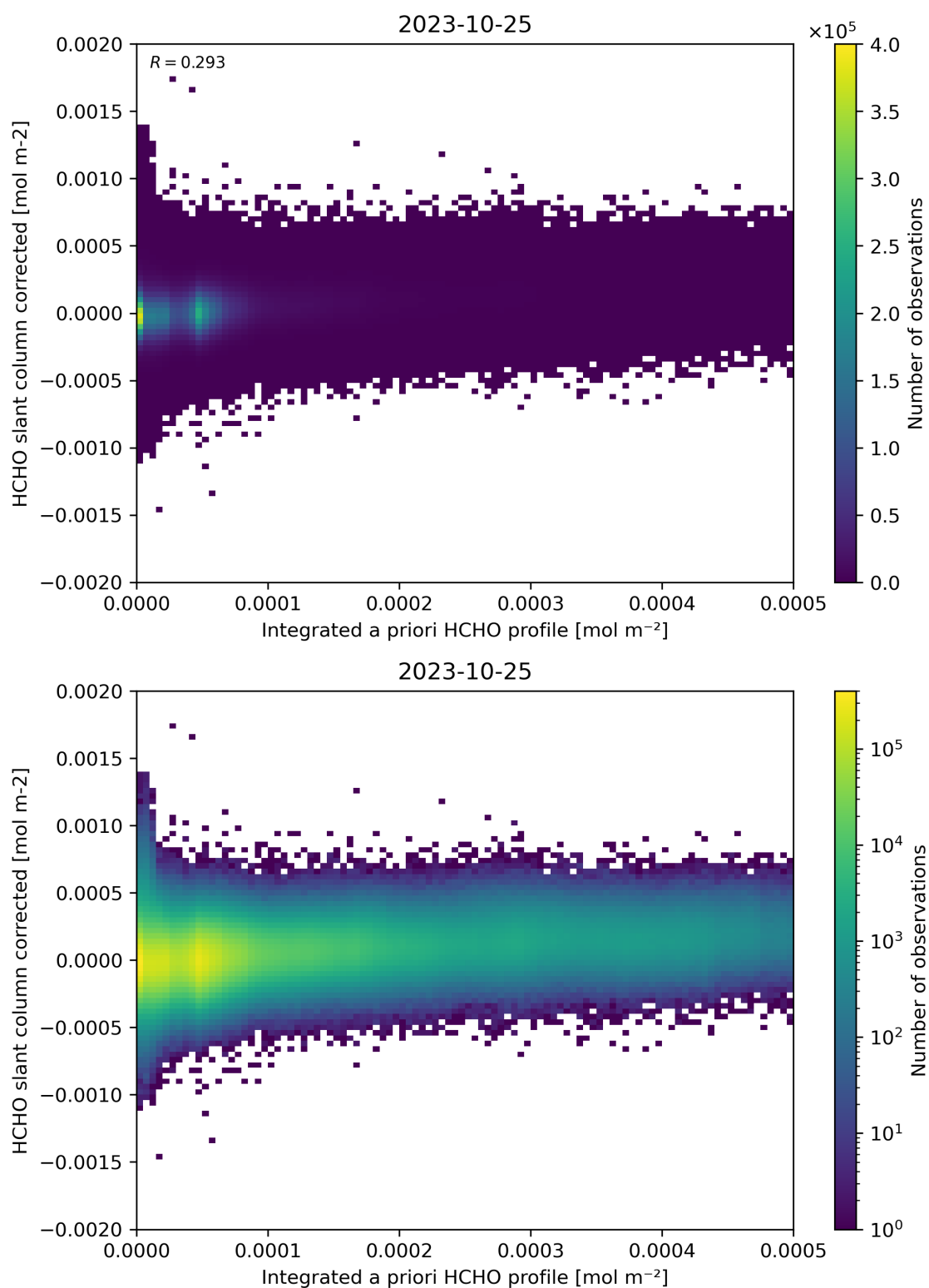
Figure 151: Scatter density plot of “Integrated a priori HCHO profile” against “HCHO slant column corrected” for 2023-10-24 to 2023-10-26.
