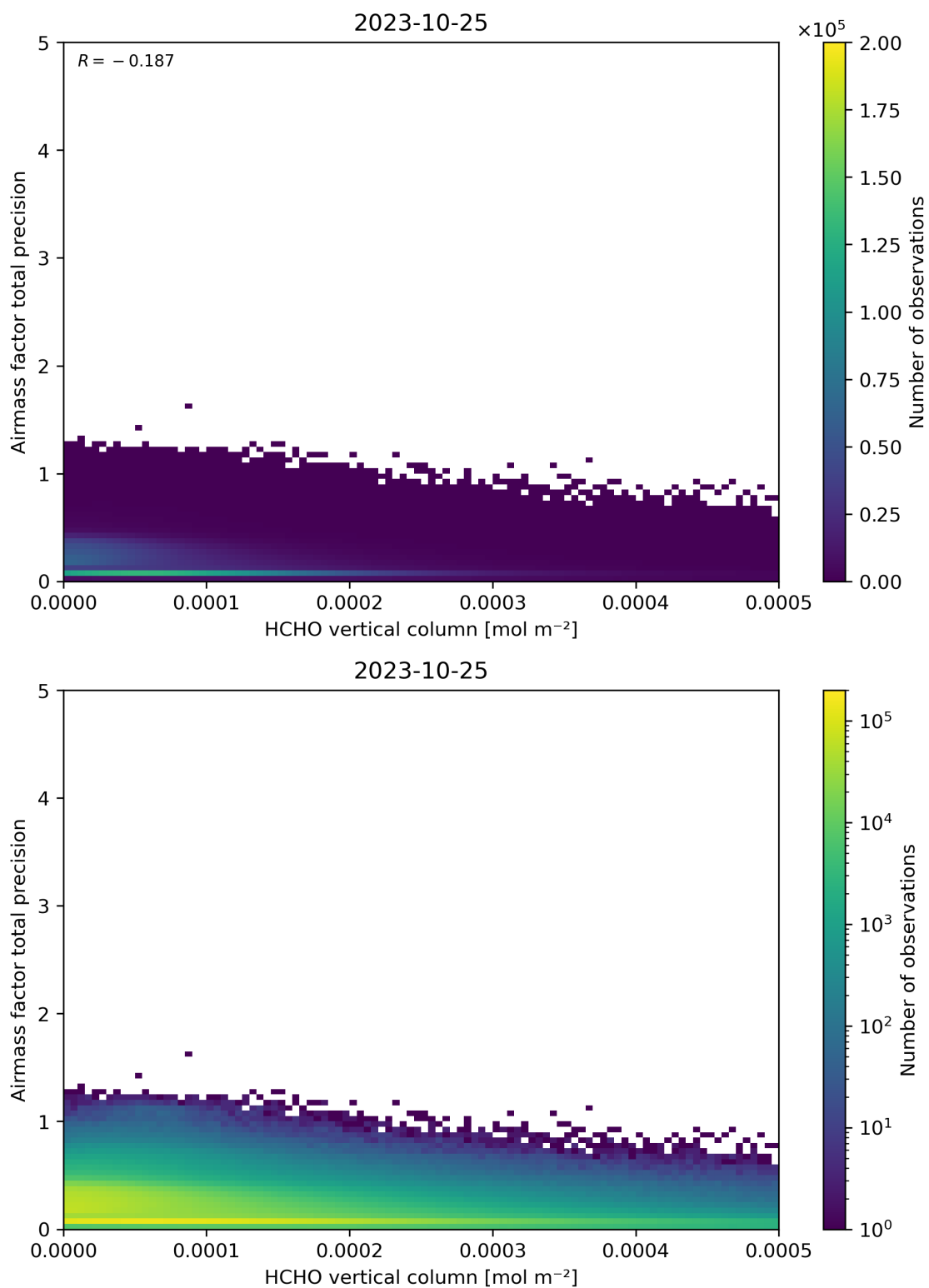
Figure 132: Scatter density plot of “HCHO vertical column” against “Airmass factor total precision” for 2023-10-24 to 2023-10-26.
