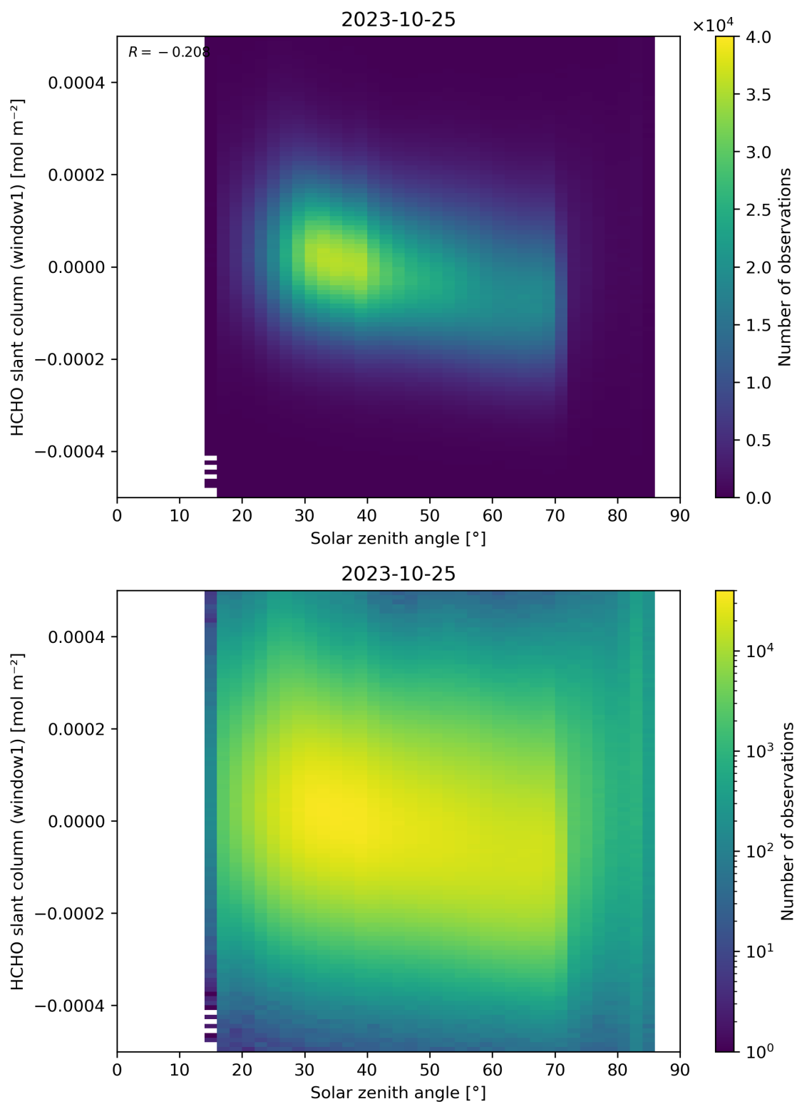
Figure 173: Scatter density plot of “Solar zenith angle” against “HCHO slant column (window1)” for 2023-10-24 to 2023-10-26.
