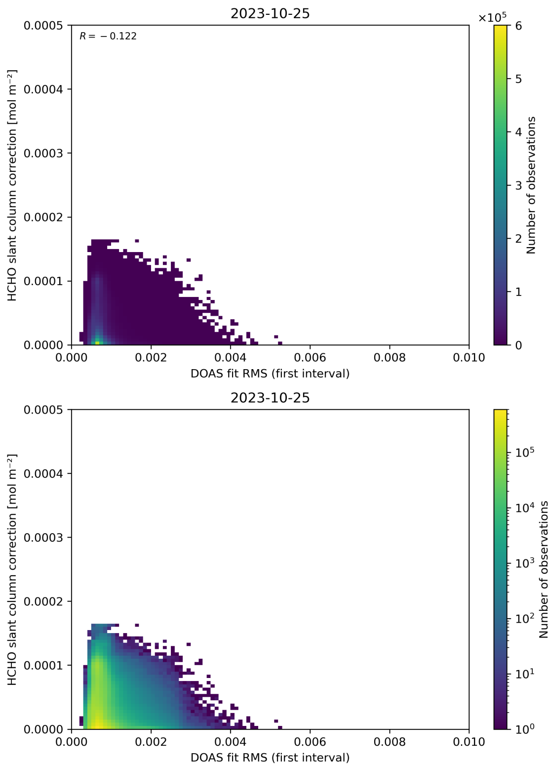
Figure 63: Scatter density plot of “DOAS fit RMS (first interval)” against “HCHO slant column correction” for 2023-10-24 to 2023-10-26.
