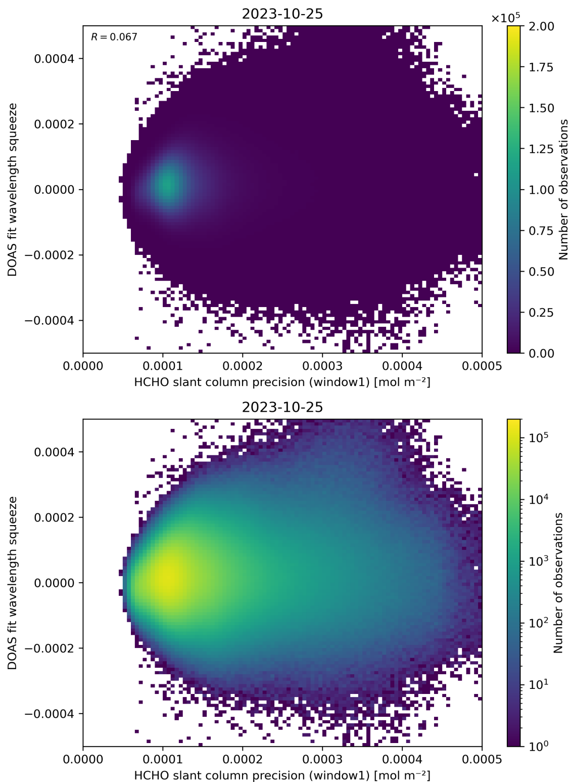
Figure 90: Scatter density plot of “HCHO slant column precision (window1)” against “DOAS fit wavelength squeeze” for 2023-10-24 to 2023-10-26.
