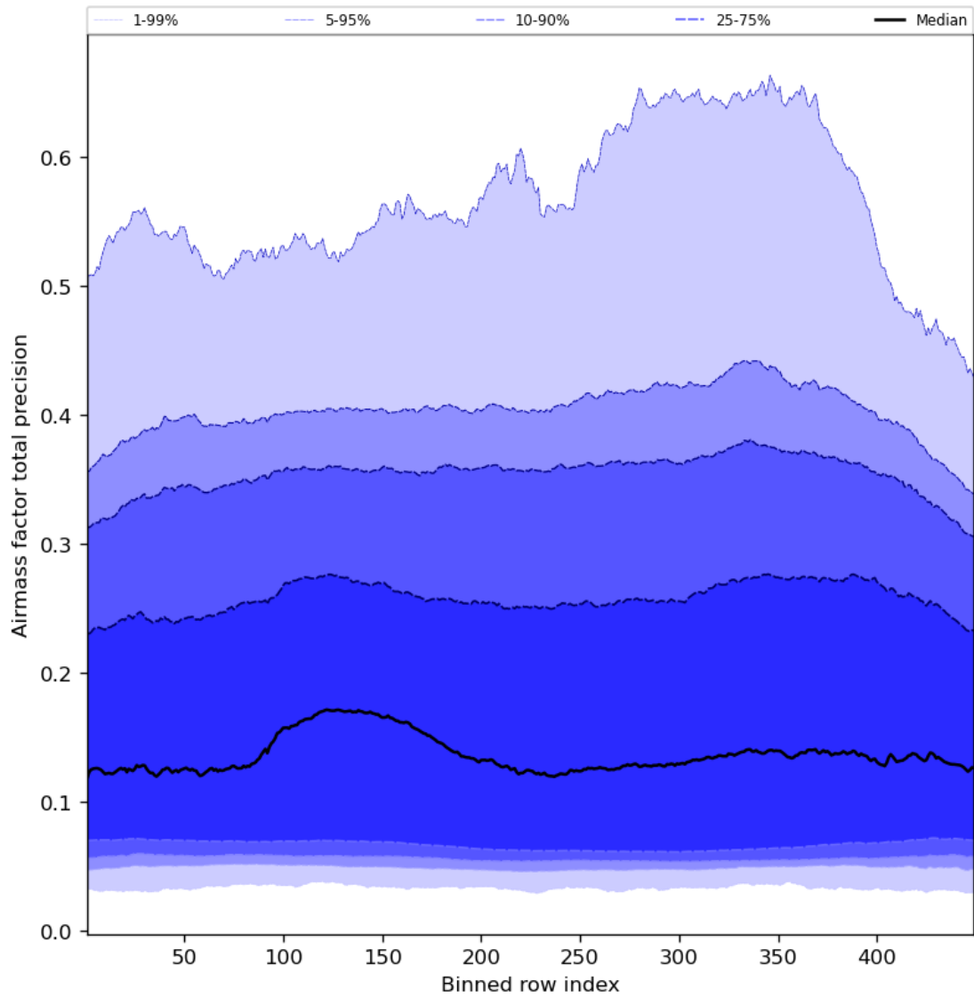
Figure 55: Along track statistics of “Airmass factor total precision” for 2023-10-24 to 2023-10-26
