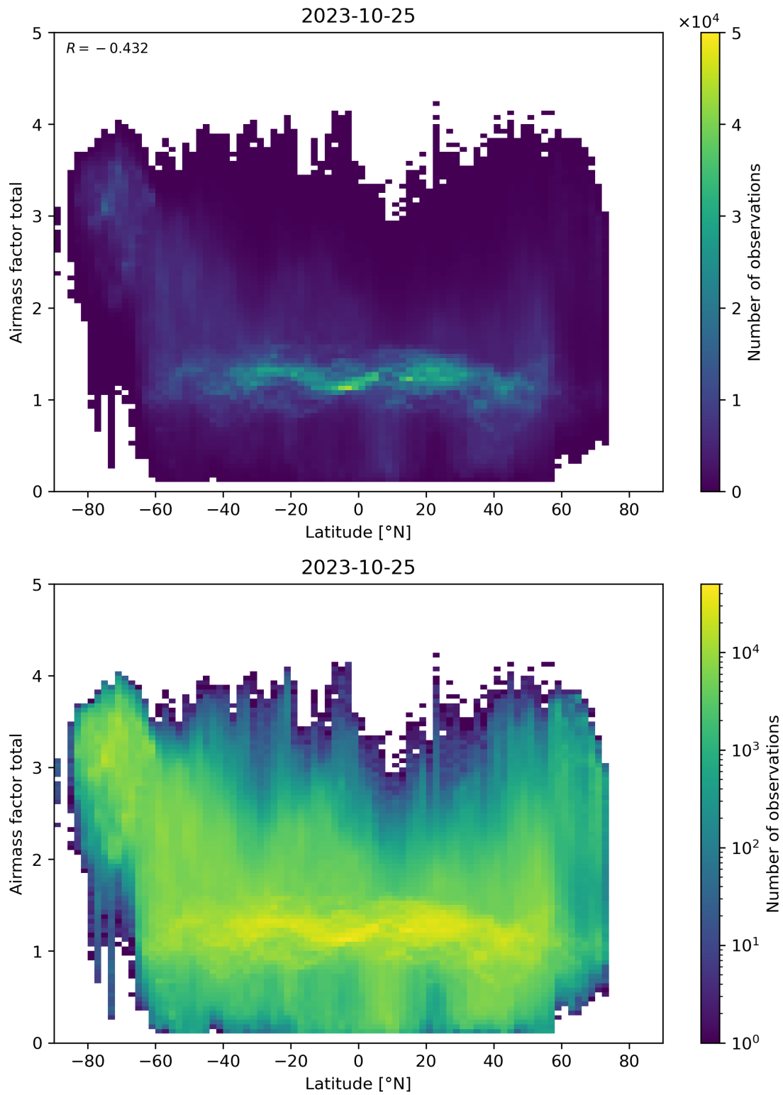
Figure 161: Scatter density plot of “Latitude” against “Airmass factor total” for 2023-10-24 to 2023-10-26.
