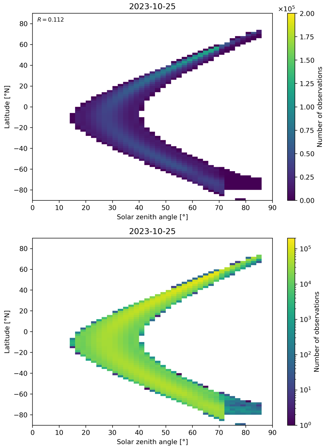
Figure 181: Scatter density plot of “Solar zenith angle” against “Latitude” for 2023-10-24 to 2023-10-26.
