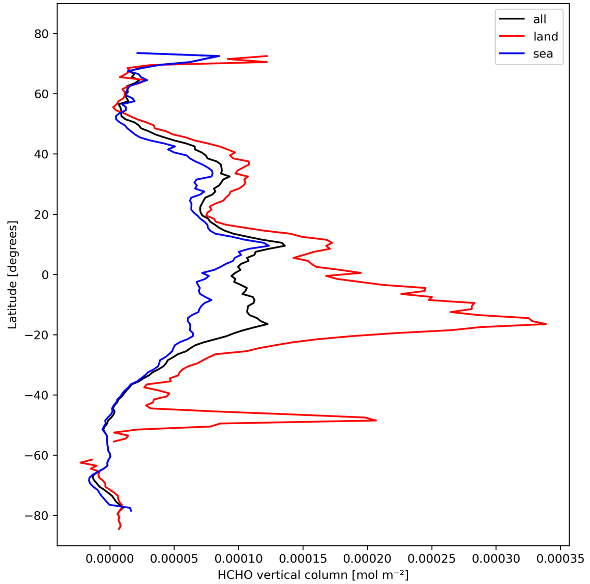
Figure 21: Zonal average of “HCHO vertical column” for 2023-10-24 to 2023-10-26.
