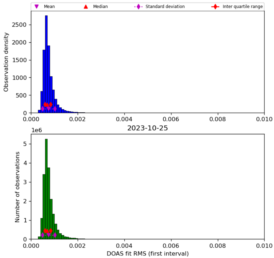
Figure 46: Histogram of “DOAS fit RMS (first interval)” for 2023-10-24 to 2023-10-26
