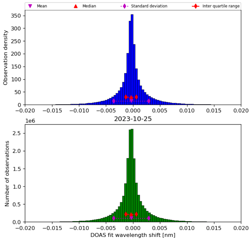
Figure 44: Histogram of “DOAS fit wavelength shift” for 2023-10-24 to 2023-10-26
