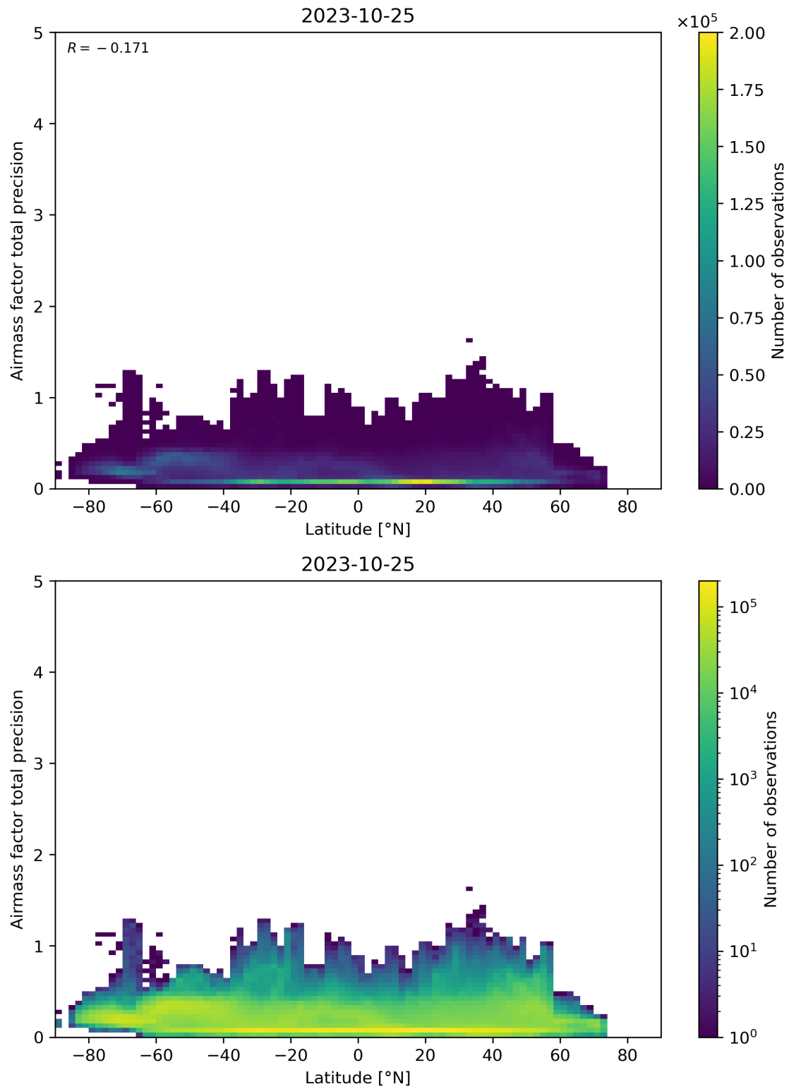
Figure 162: Scatter density plot of “Latitude” against “Airmass factor total precision” for 2023-10-24 to 2023-10-26.
