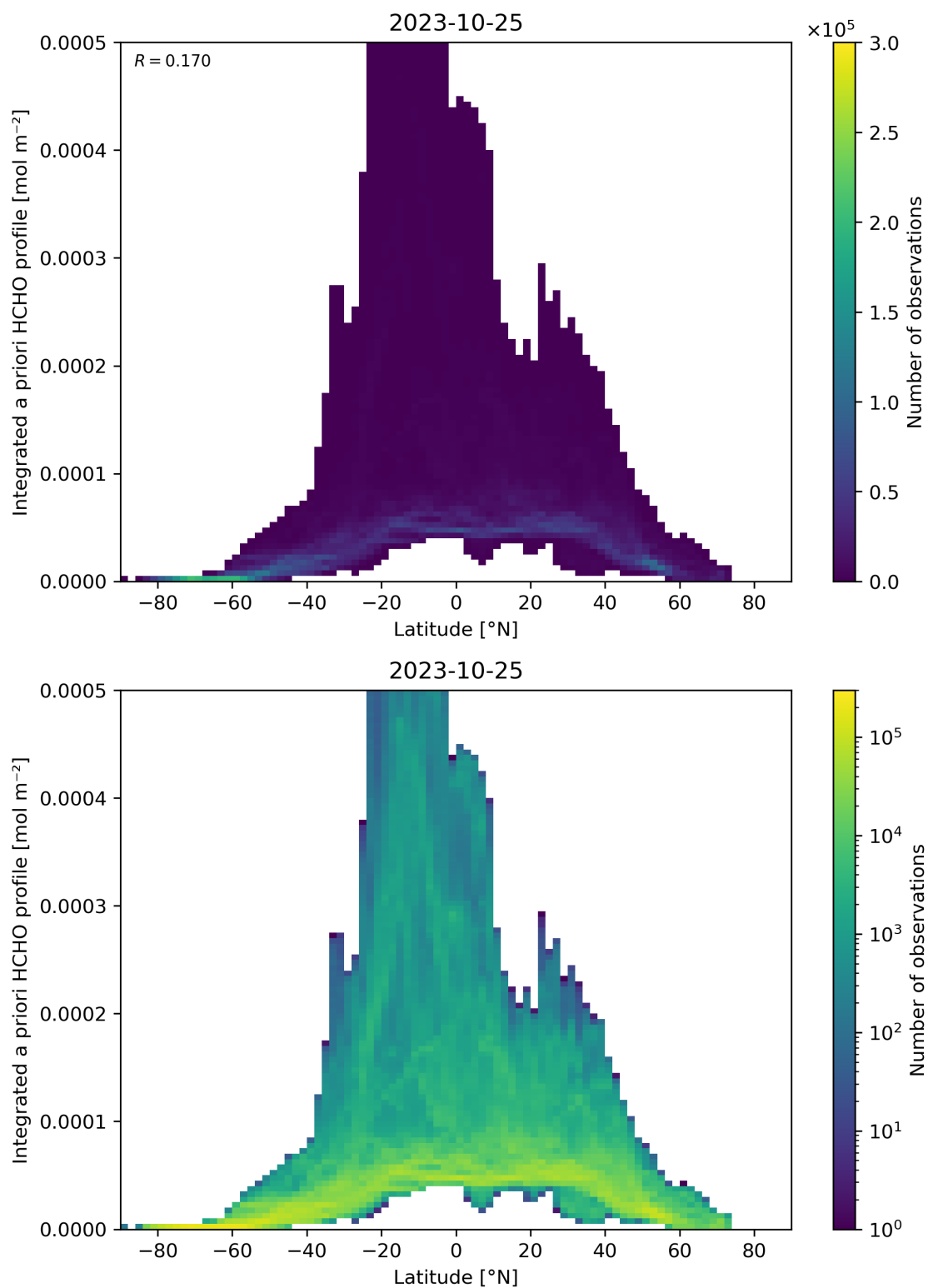
Figure 166: Scatter density plot of “Latitude” against “Integrated a priori HCHO profile” for 2023-10-24 to 2023-10-26.
