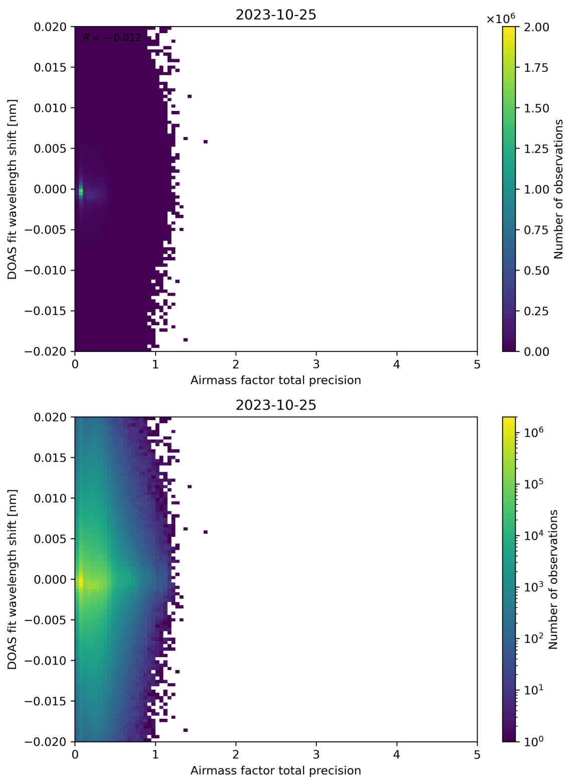
Figure 106: Scatter density plot of “Airmass factor total precision” against “DOAS fit wavelength shift” for 2023-10-24 to 2023-10-26.
