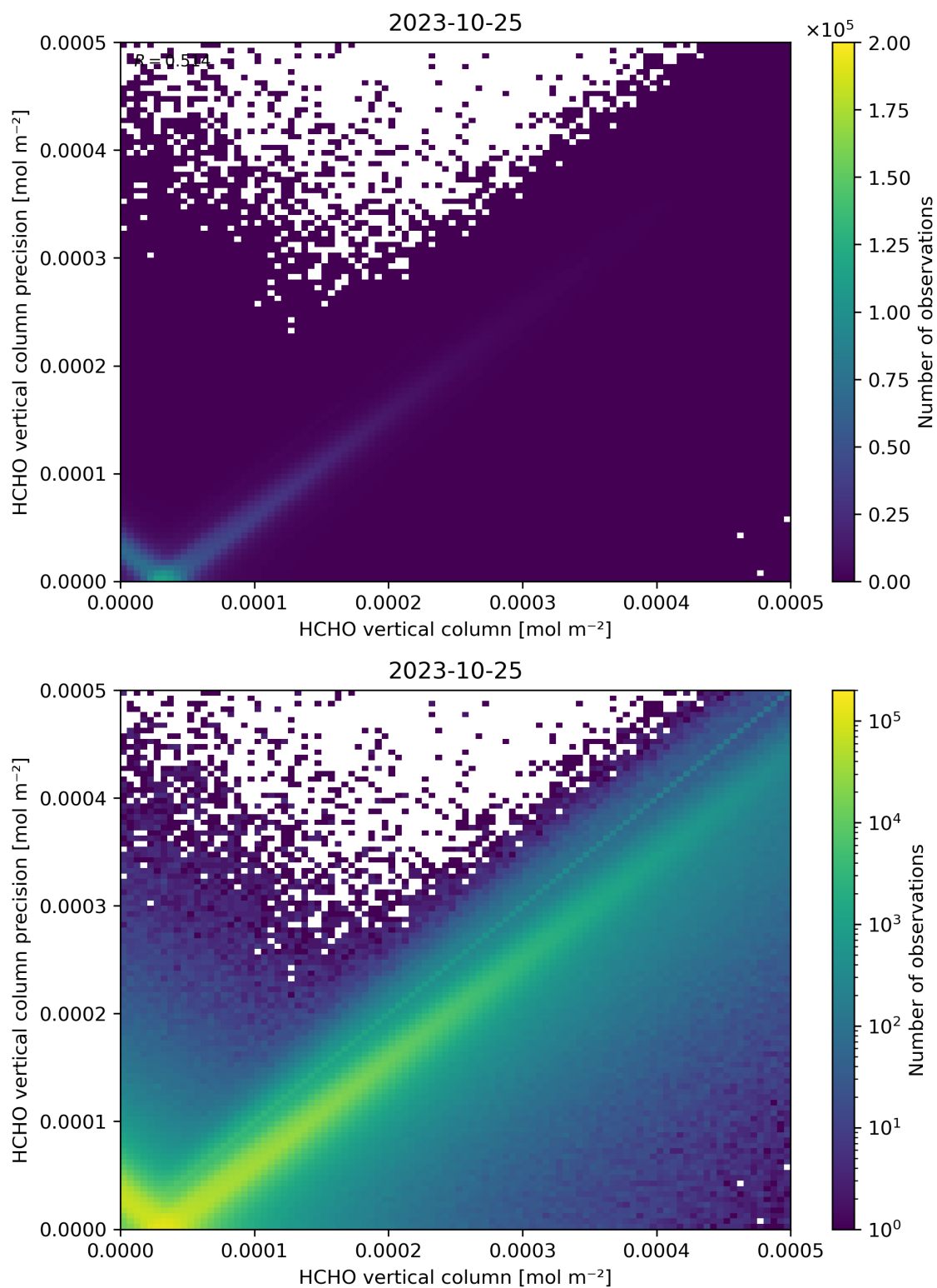
Figure 134: Scatter density plot of “HCHO vertical column” against “HCHO vertical column precision” for 2023-10-24 to 2023-10-26.
