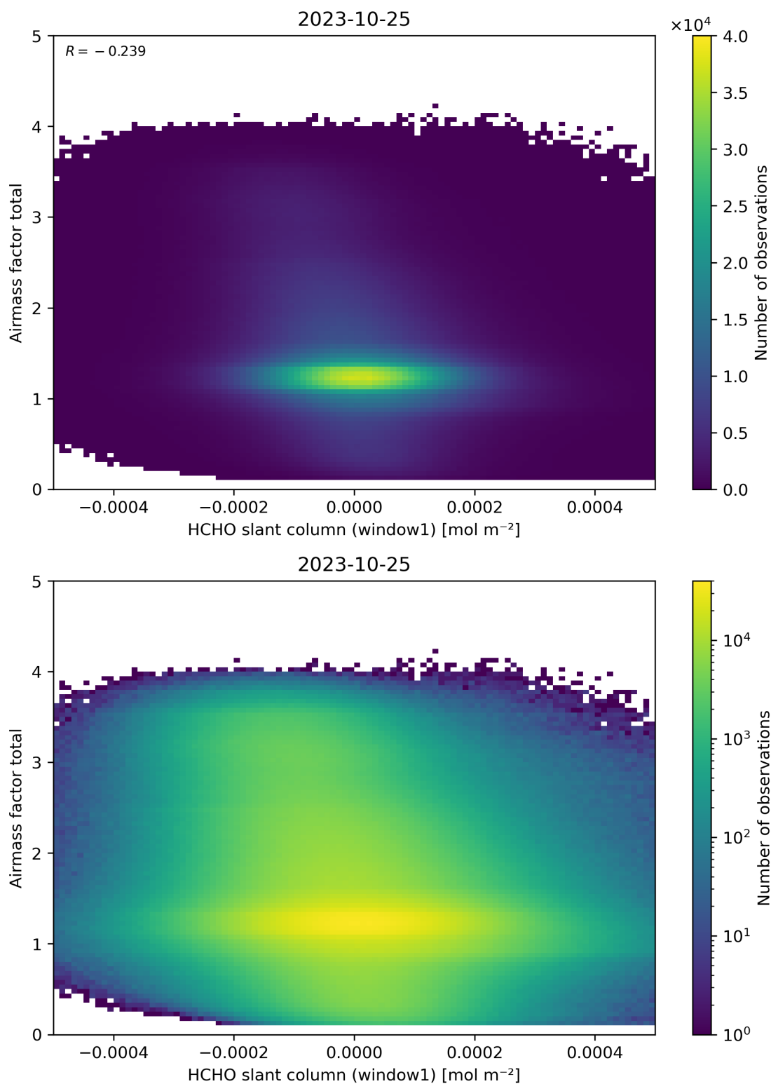
Figure 85: Scatter density plot of “HCHO slant column (window1)” against “Airmass factor total” for 2023-10-24 to 2023-10-26.
