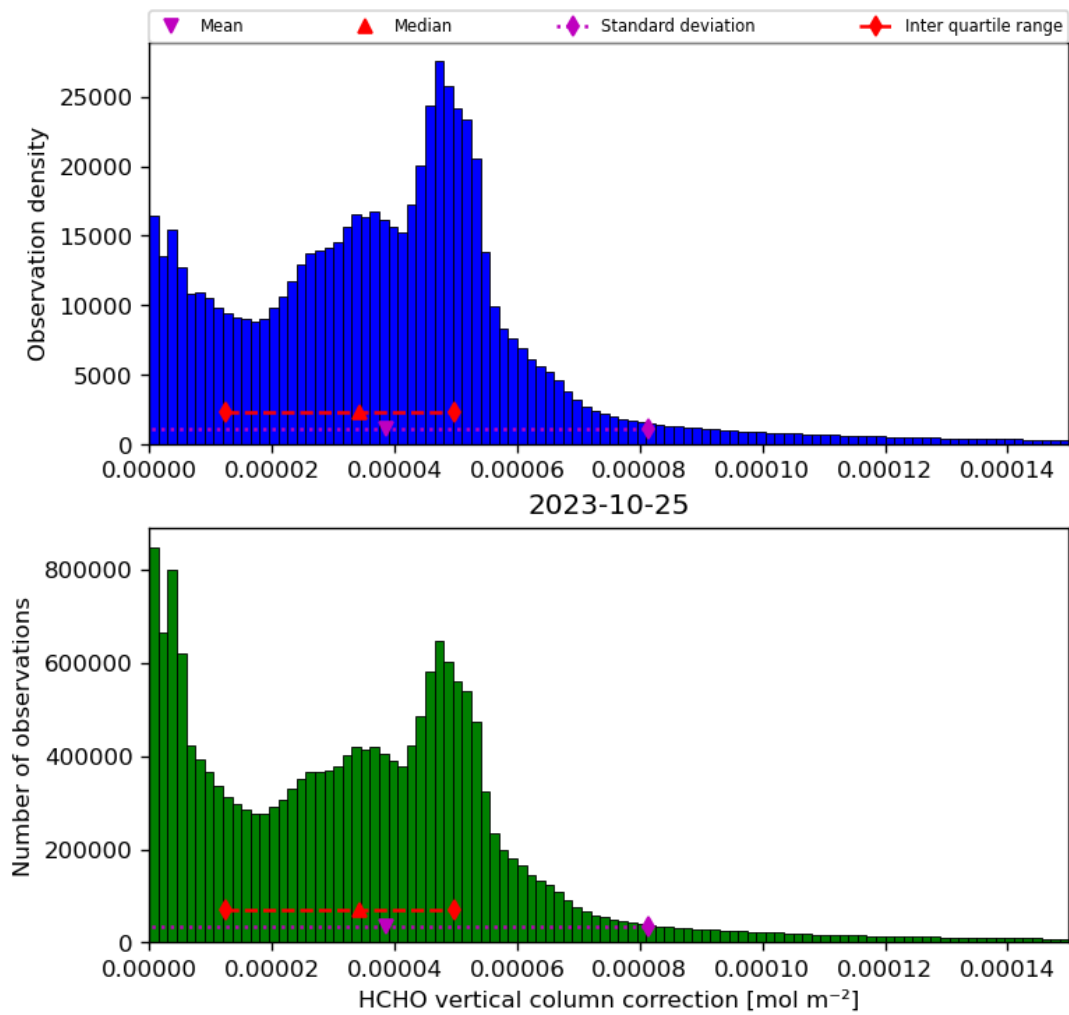
Figure 37: Histogram of “HCHO vertical column correction” for 2023-10-24 to 2023-10-26
