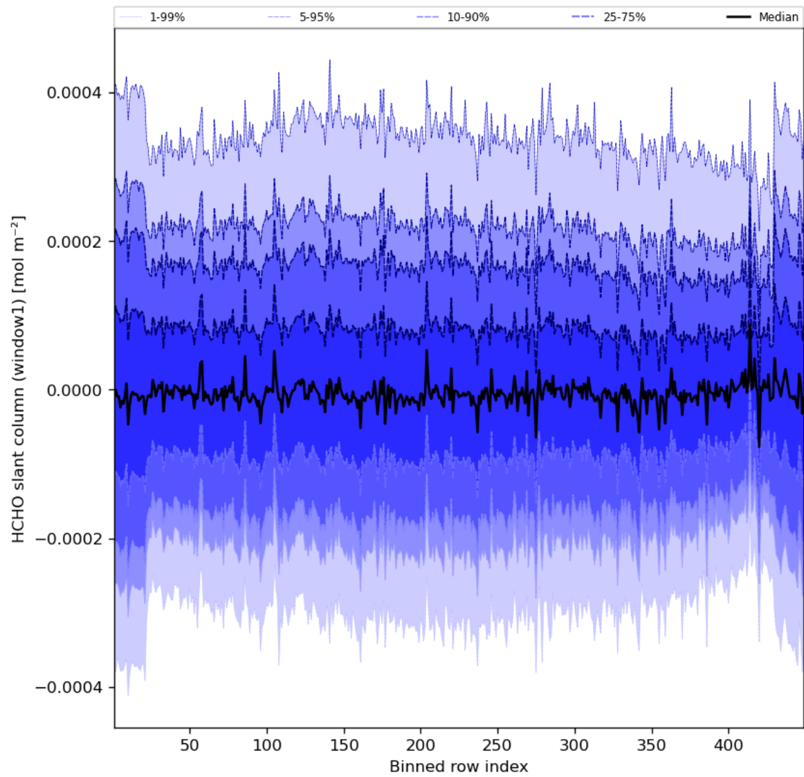
Figure 52: Along track statistics of “HCHO slant column (window1)” for 2023-10-24 to 2023-10-26
