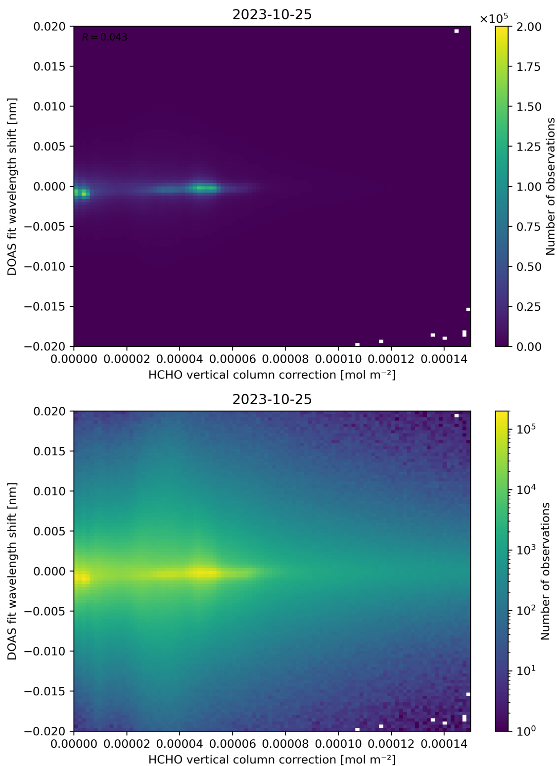
Figure 113: Scatter density plot of “HCHO vertical column correction” against “DOAS fit wavelength shift” for 2023-10-24 to 2023-10-26.
