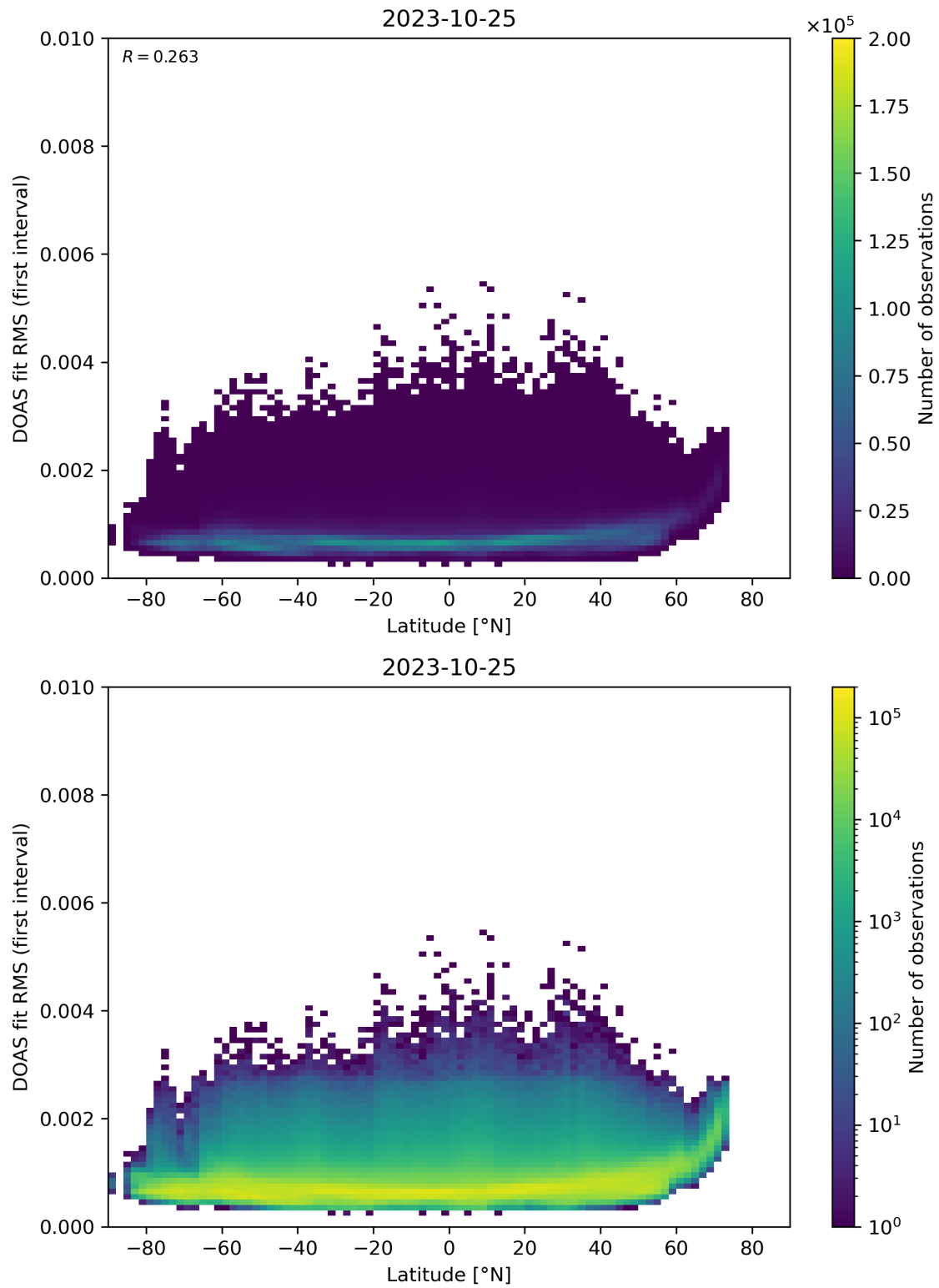
Figure 153: Scatter density plot of “Latitude” against “DOAS fit RMS (first interval)” for 2023-10-24 to 2023-10-26.
