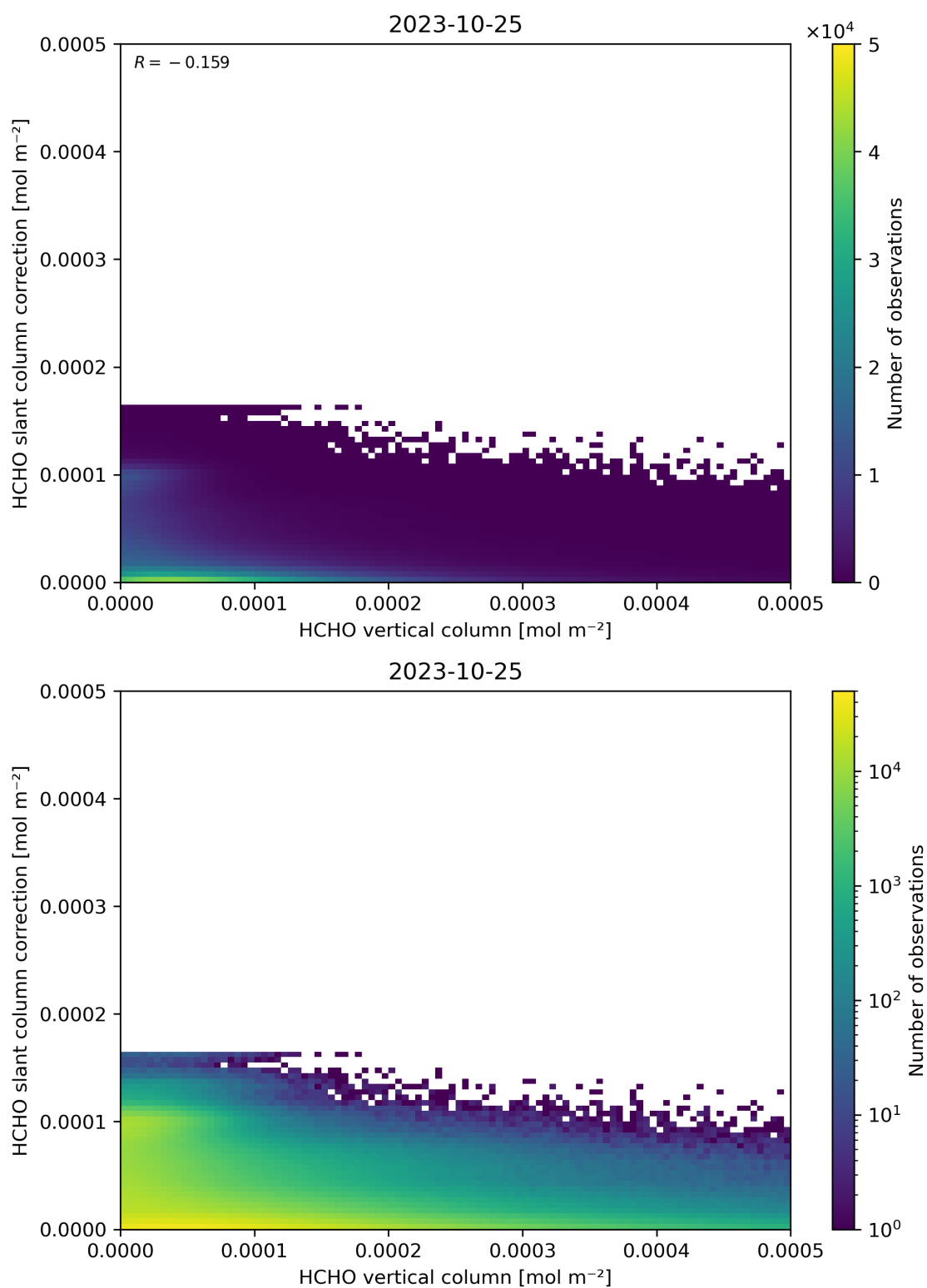
Figure 128: Scatter density plot of “HCHO vertical column” against “HCHO slant column correction” for 2023-10-24 to 2023-10-26.
