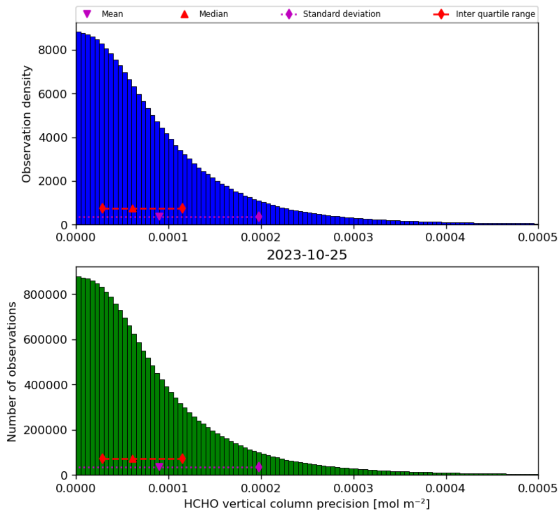
Figure 36: Histogram of “HCHO vertical column precision” for 2023-10-24 to 2023-10-26
