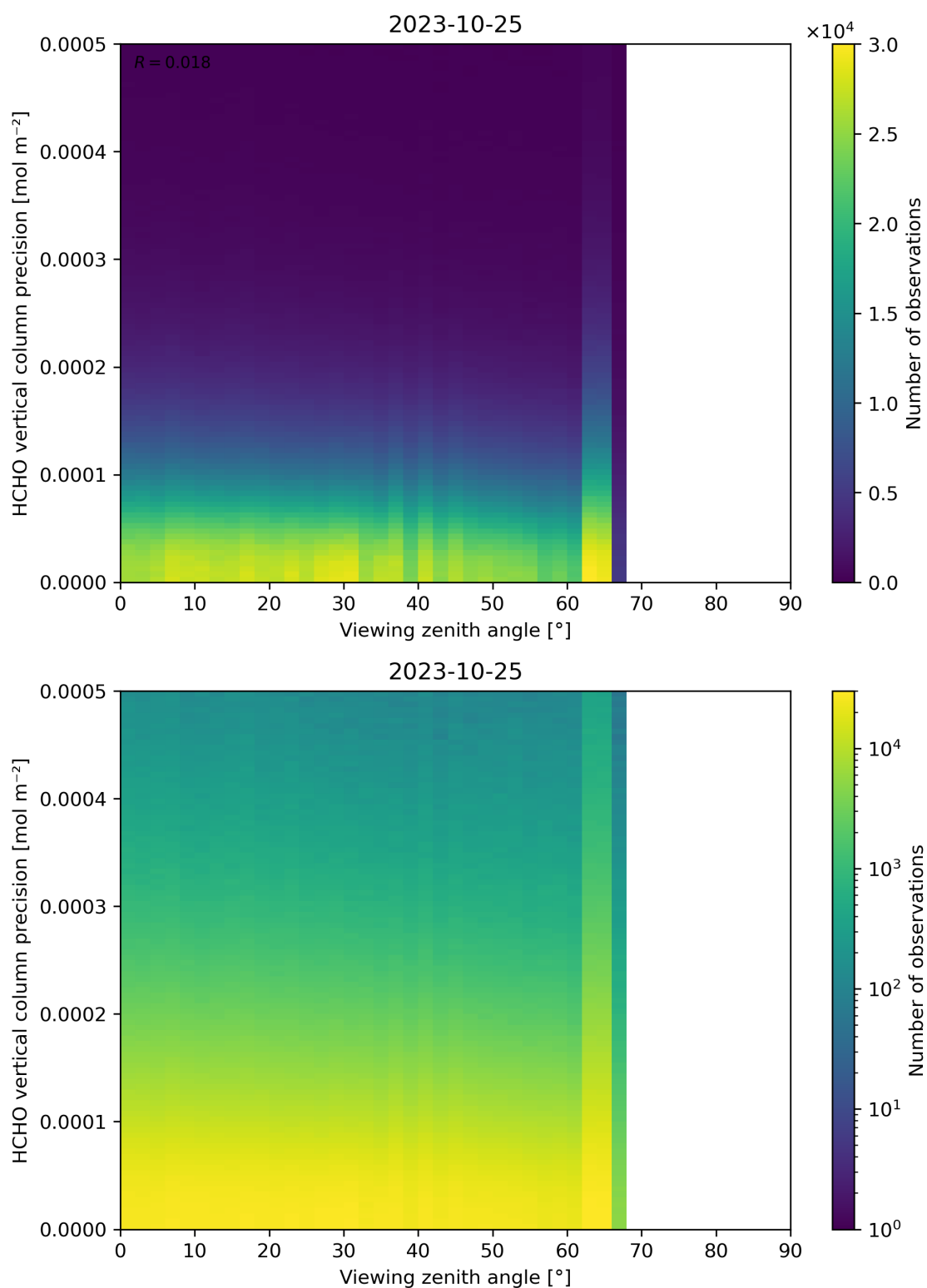
Figure 194: Scatter density plot of “Viewing zenith angle” against “HCHO vertical column precision” for 2023-10-24 to 2023-10-26.
