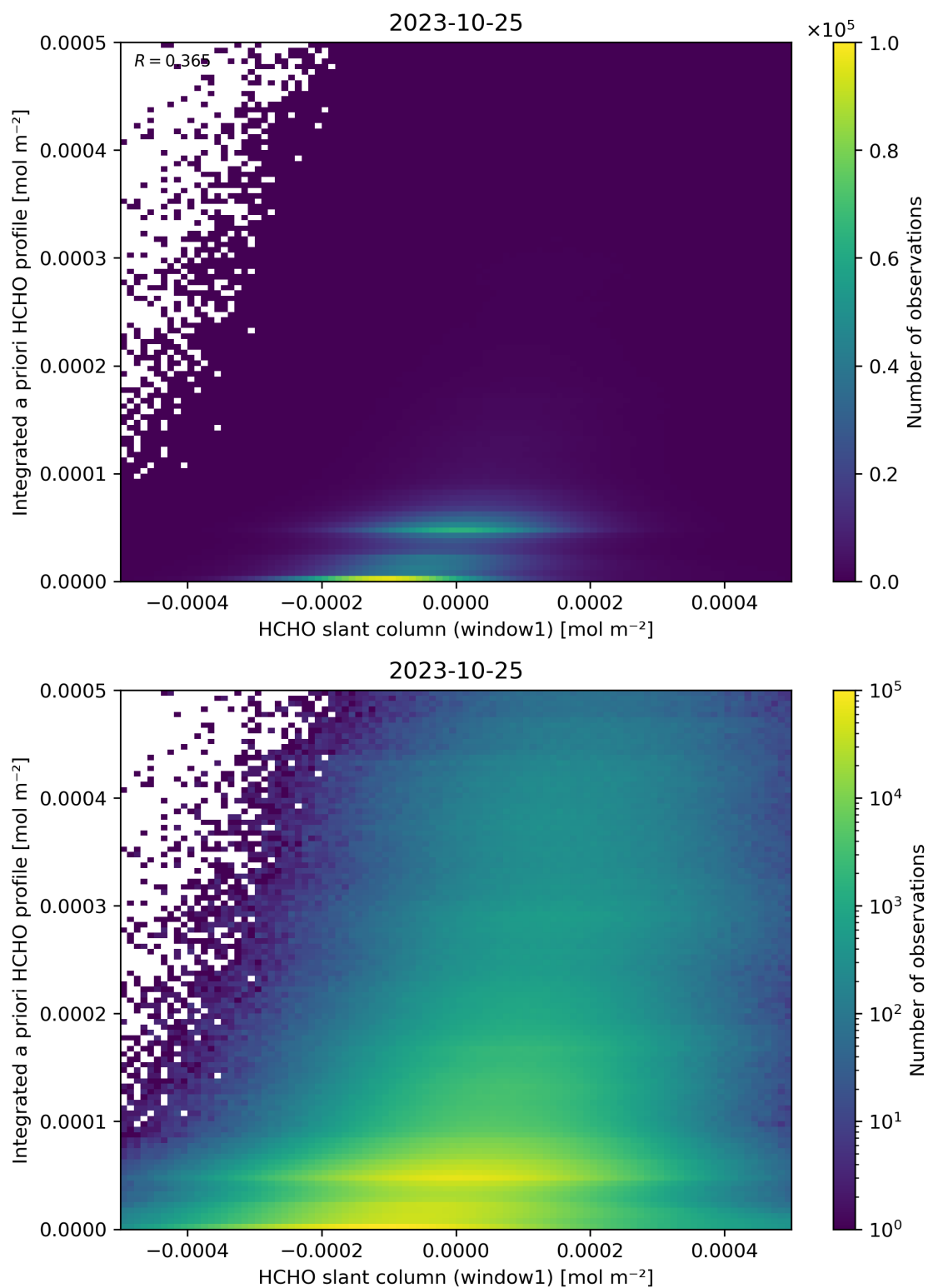
Figure 87: Scatter density plot of “HCHO slant column (window1)” against “Integrated a priori HCHO profile” for 2023-10-24 to 2023-10-26.
