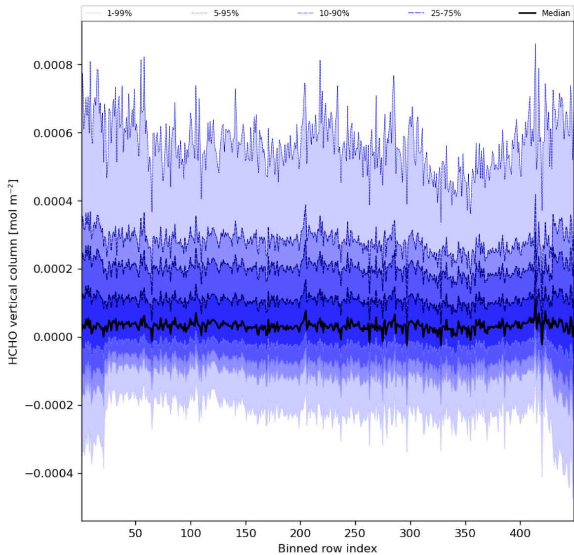
Figure 49: Along track statistics of “HCHO vertical column” for 2023-10-24 to 2023-10-26
