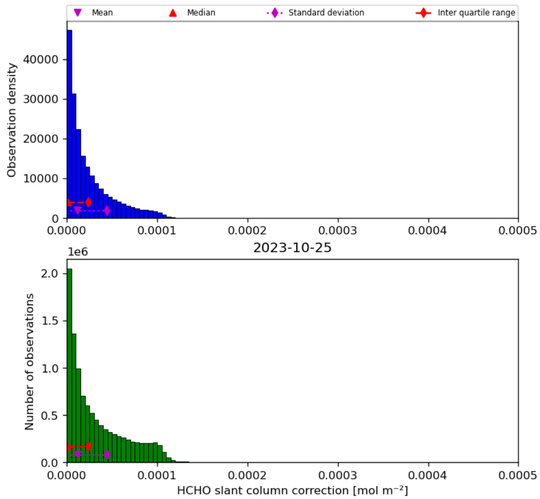
Figure 47: Histogram of “HCHO slant column correction” for 2023-10-24 to 2023-10-26
