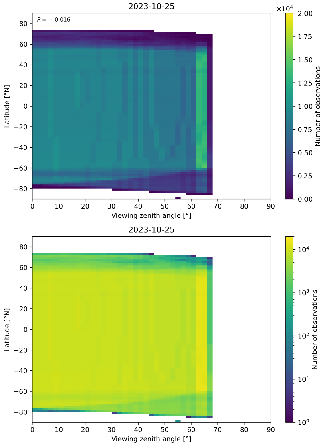
Figure 196: Scatter density plot of “Viewing zenith angle” against “Latitude” for 2023-10-24 to 2023-10-26.
