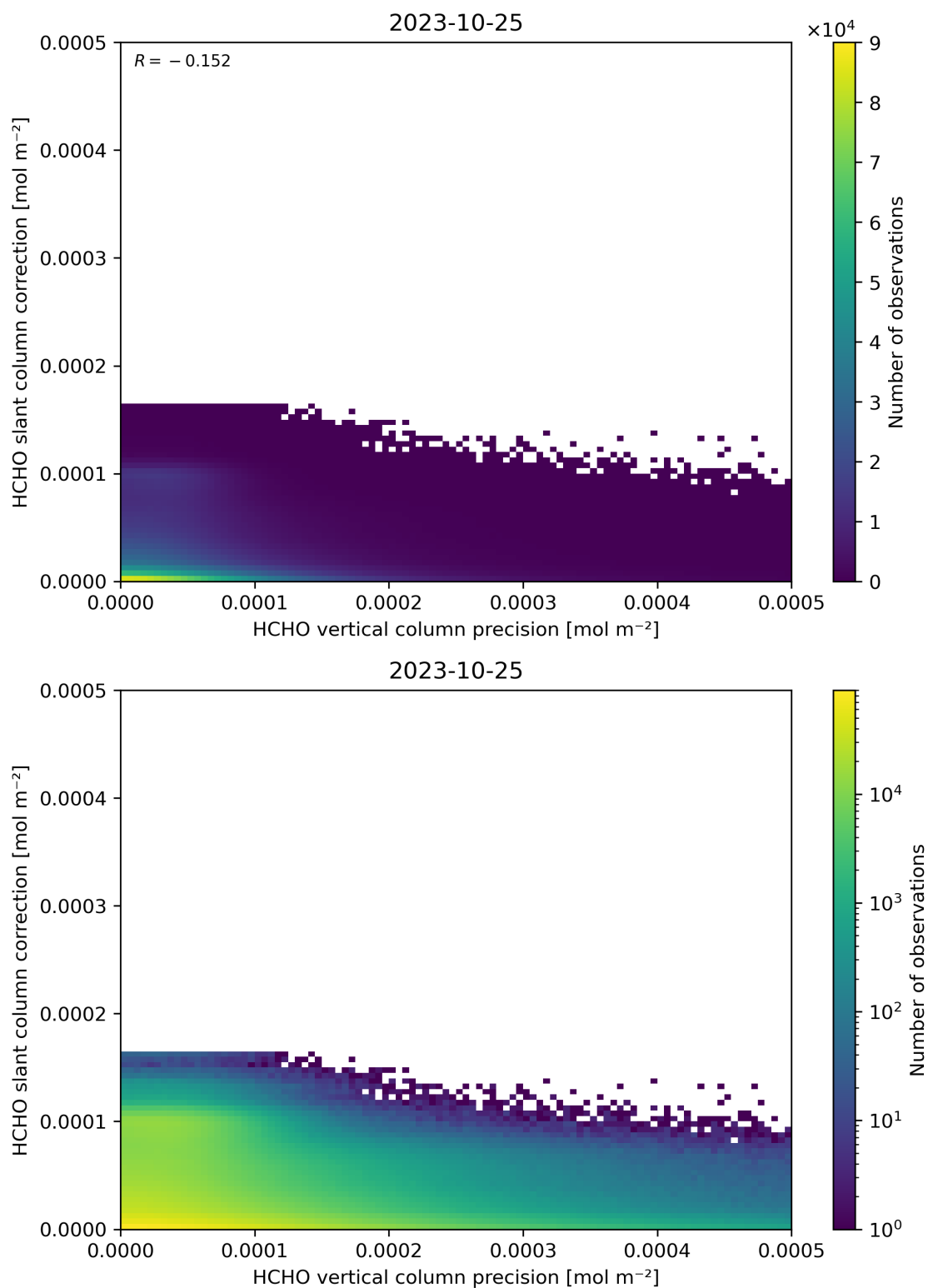
Figure 141: Scatter density plot of “HCHO vertical column precision” against “HCHO slant column correction” for 2023-10-24 to 2023-10-26.
