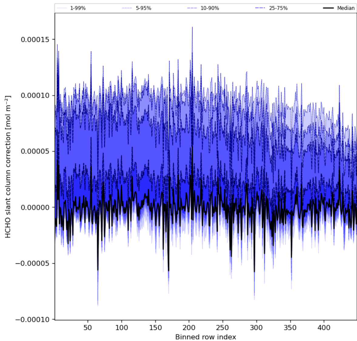
Figure 61: Along track statistics of “HCHO slant column correction” for 2023-10-24 to 2023-10-26
