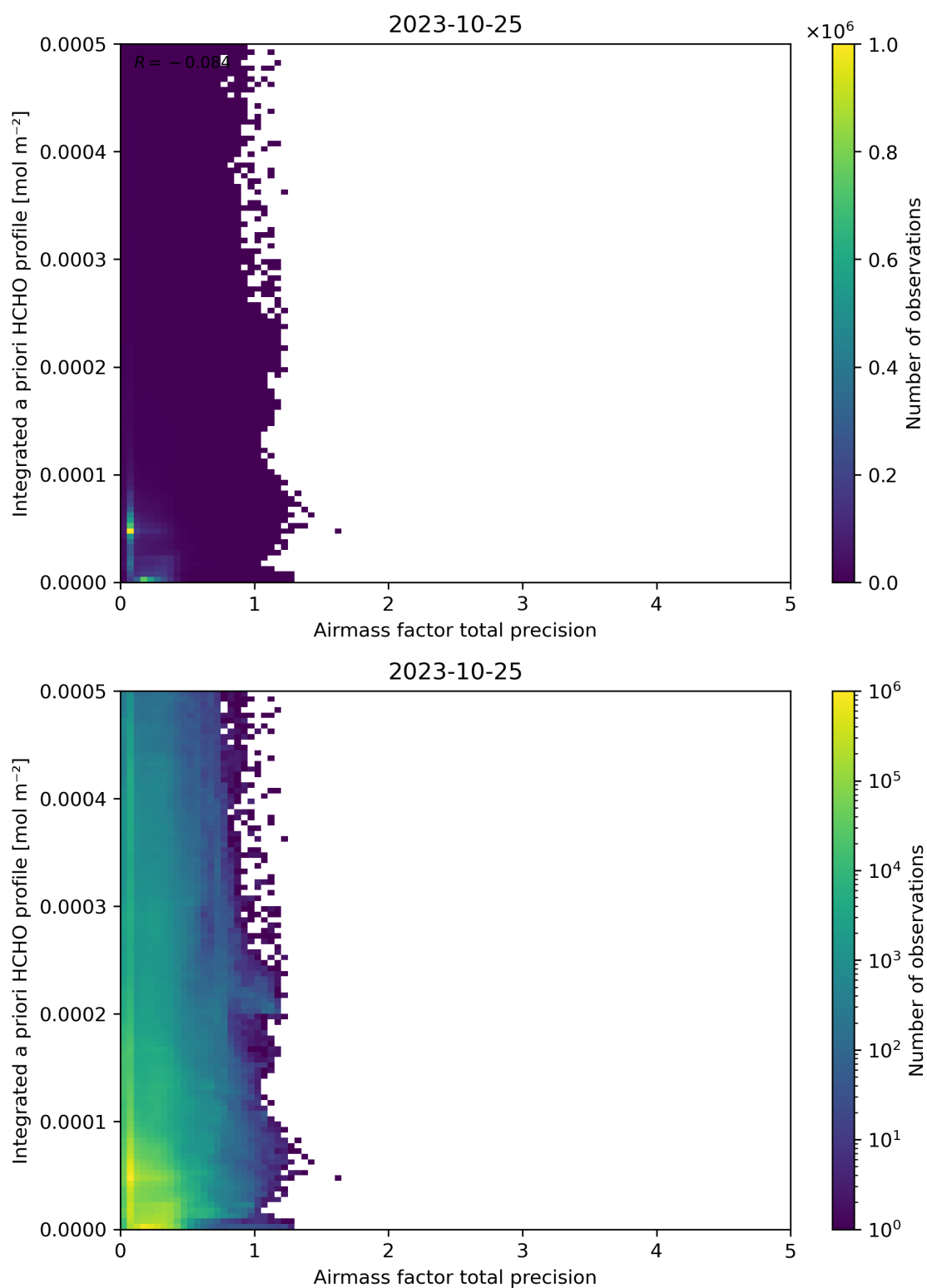
Figure 111: Scatter density plot of “Airmass factor total precision” against “Integrated a priori HCHO profile” for 2023-10-24 to 2023-10-26.
