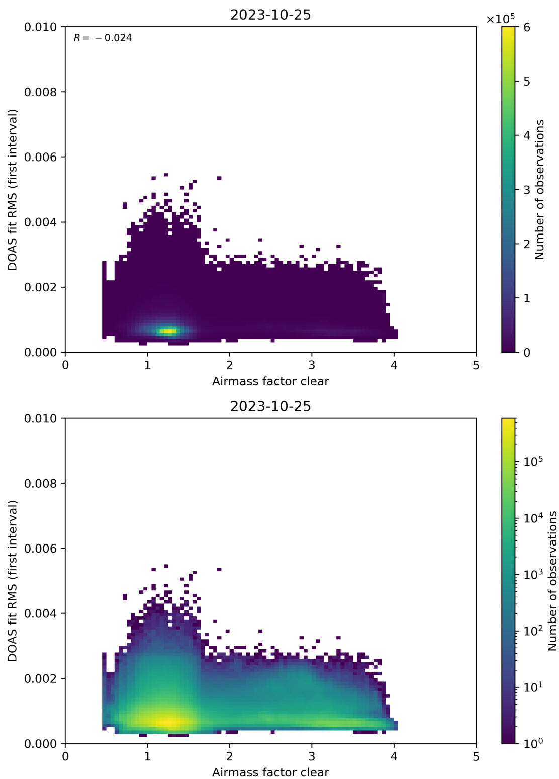
Figure 71: Scatter density plot of “Airmass factor clear” against “DOAS fit RMS (first interval)” for 2023-10-24 to 2023-10-26.
