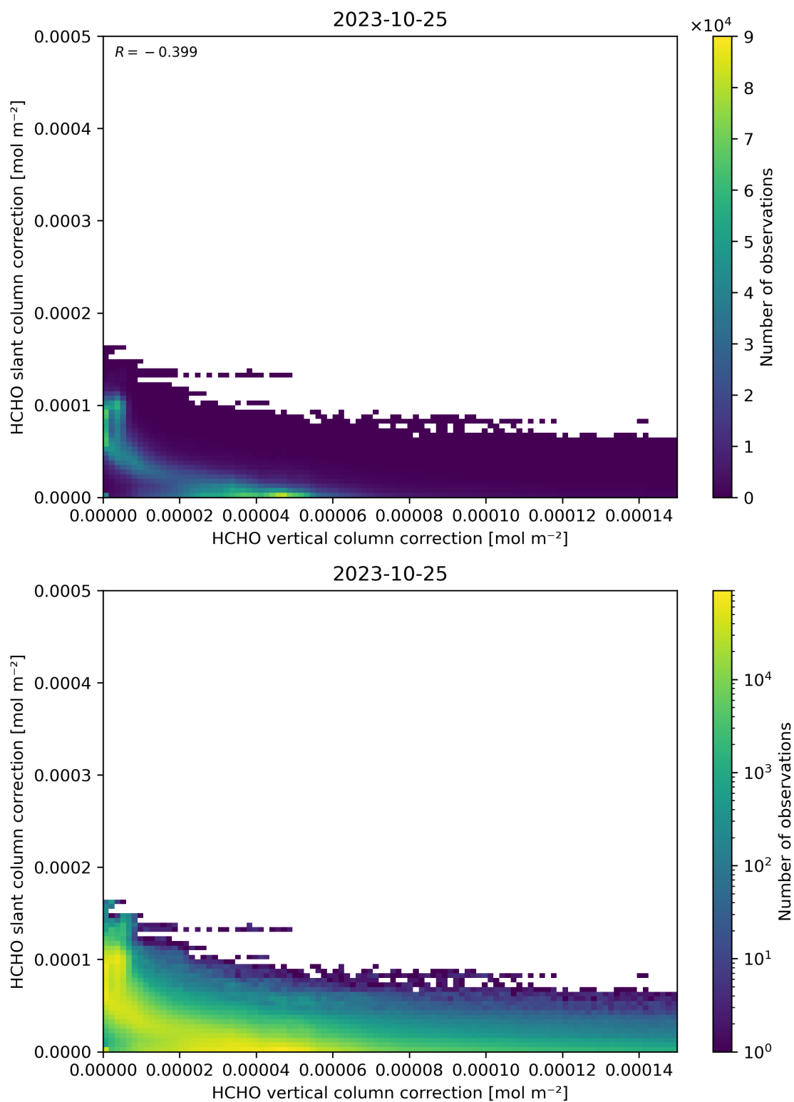
Figure 117: Scatter density plot of “HCHO vertical column correction” against “HCHO slant column correction” for 2023-10-24 to 2023-10-26.
