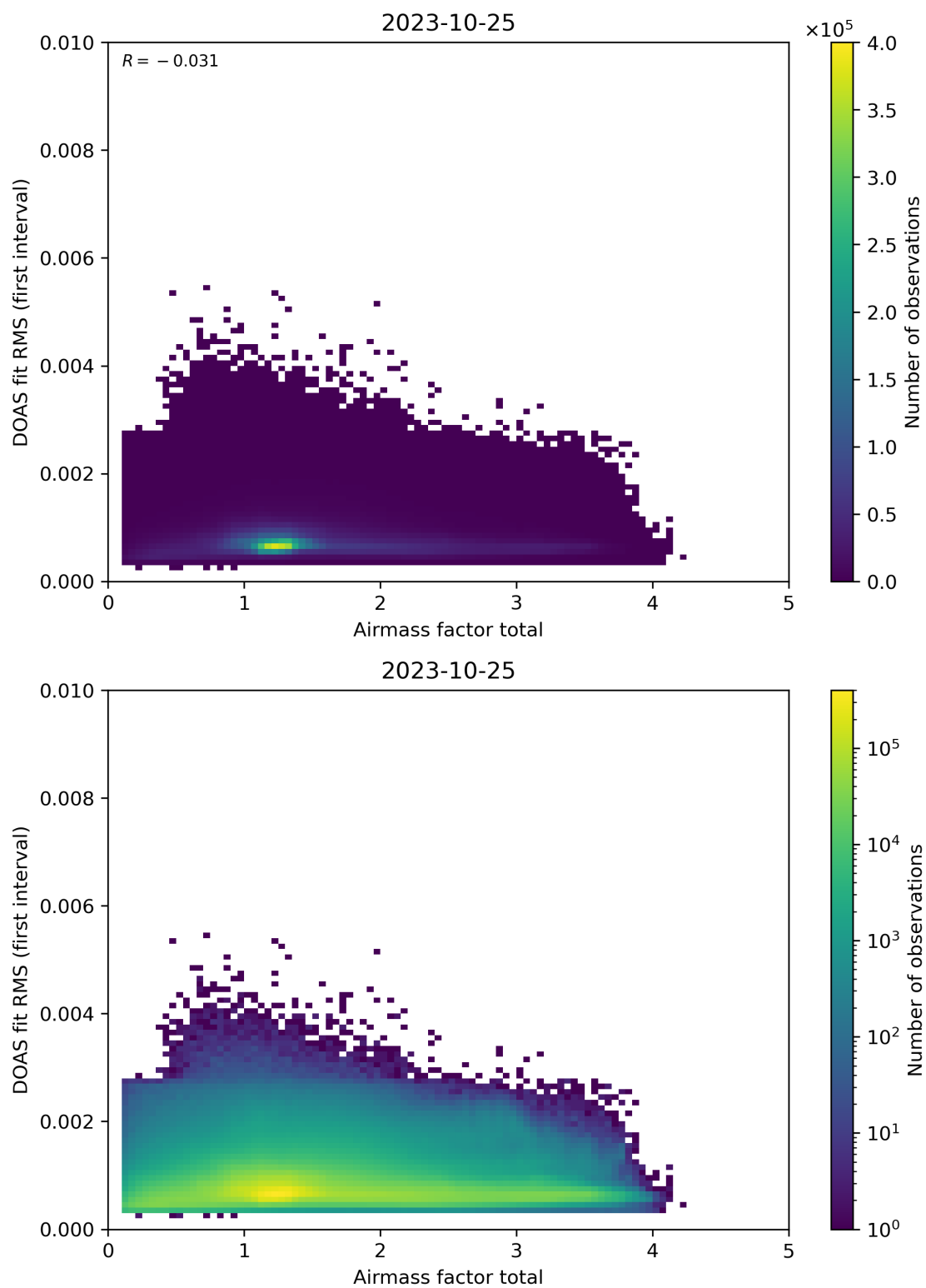
Figure 97: Scatter density plot of “Airmass factor total” against “DOAS fit RMS (first interval)” for 2023-10-24 to 2023-10-26.
