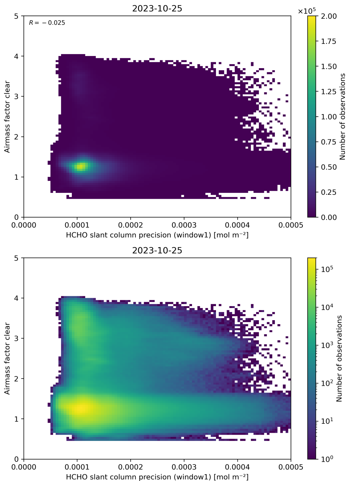
Figure 91: Scatter density plot of “HCHO slant column precision (window1)” against “Airmass factor clear” for 2023-10-24 to 2023-10-26.
