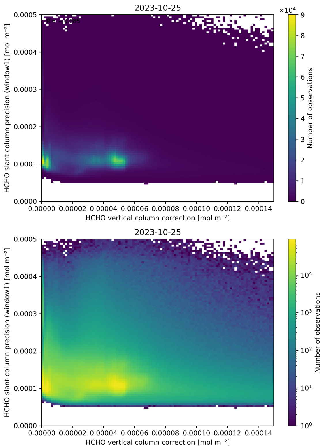
Figure 119: Scatter density plot of “HCHO vertical column correction” against “HCHO slant column precision (window1)” for 2023-10-24 to 2023-10-26.
