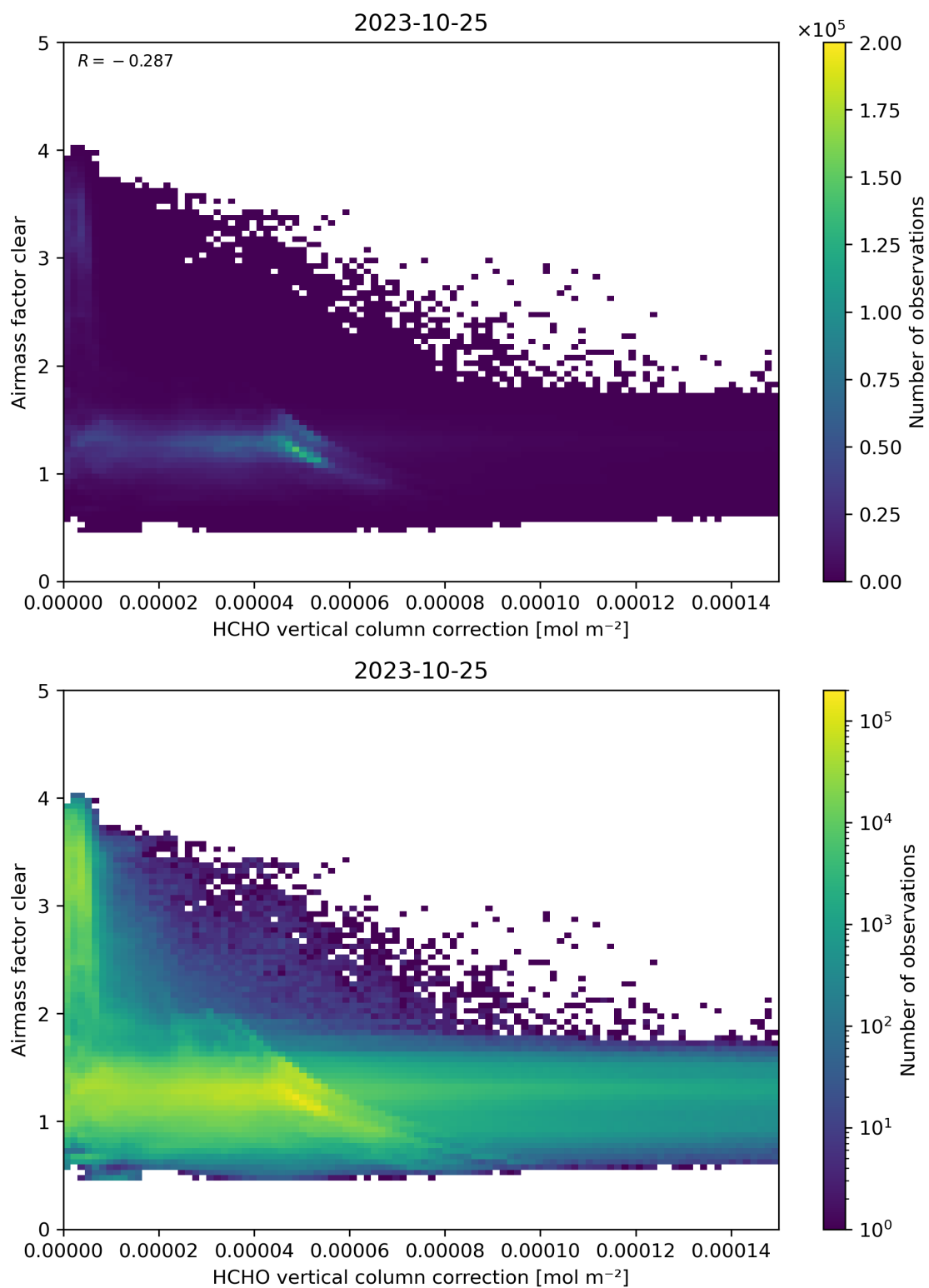
Figure 115: Scatter density plot of “HCHO vertical column correction” against “Airmass factor clear” for 2023-10-24 to 2023-10-26.
