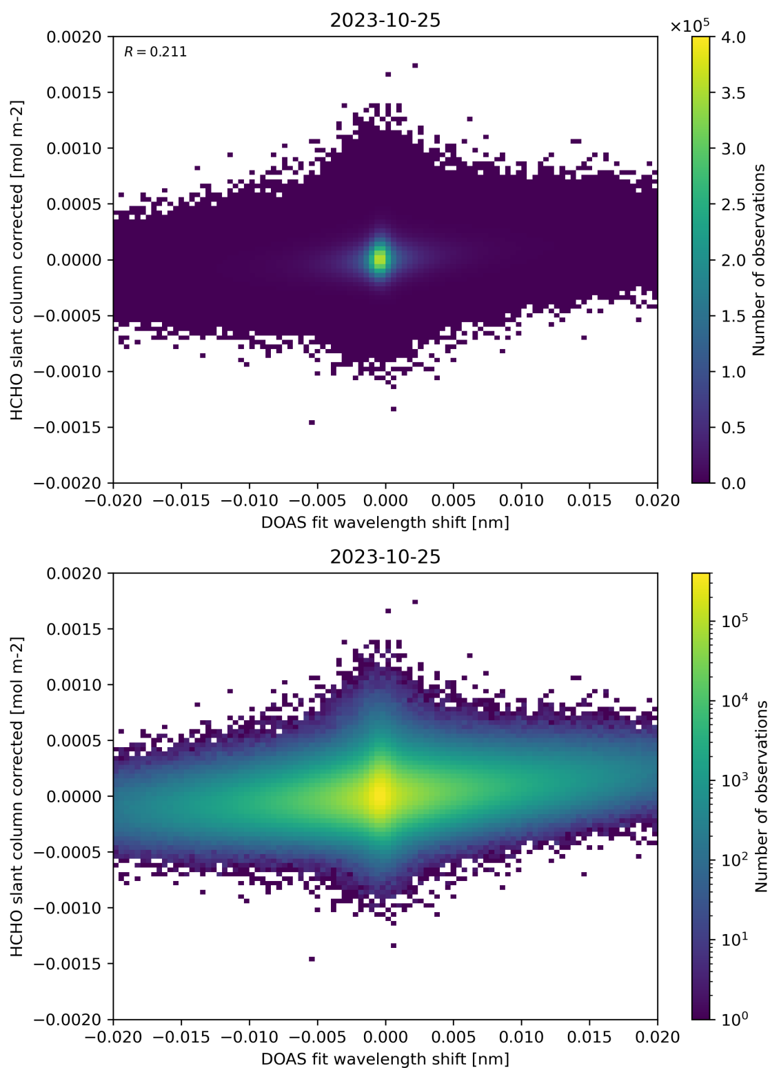
Figure 66: Scatter density plot of “DOAS fit wavelength shift” against “HCHO slant column corrected” for 2023-10-24 to 2023-10-26.
