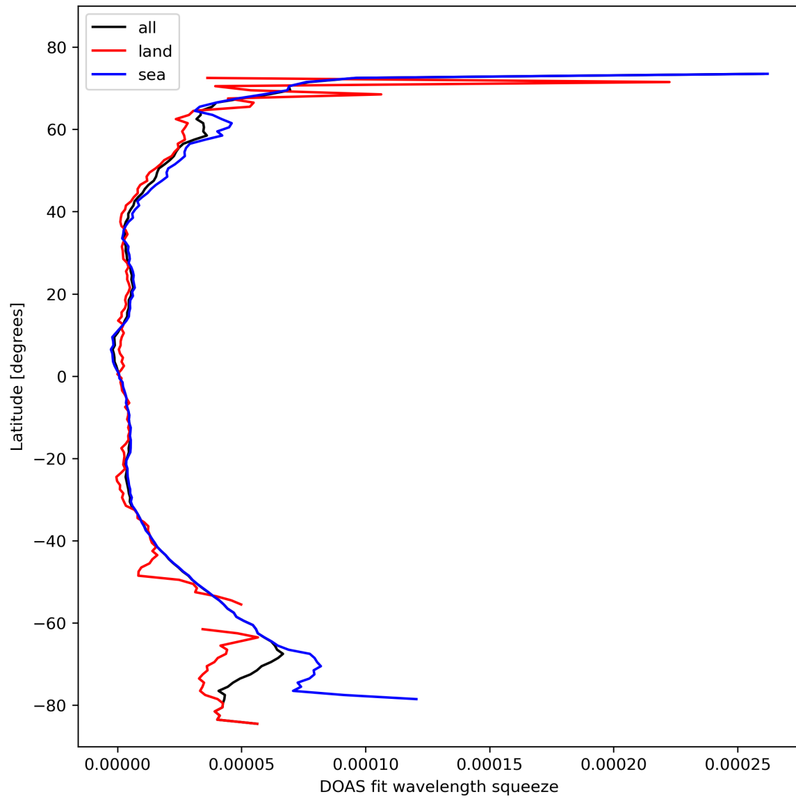
Figure 31: Zonal average of “DOAS fit wavelength squeeze” for 2023-10-24 to 2023-10-26.
