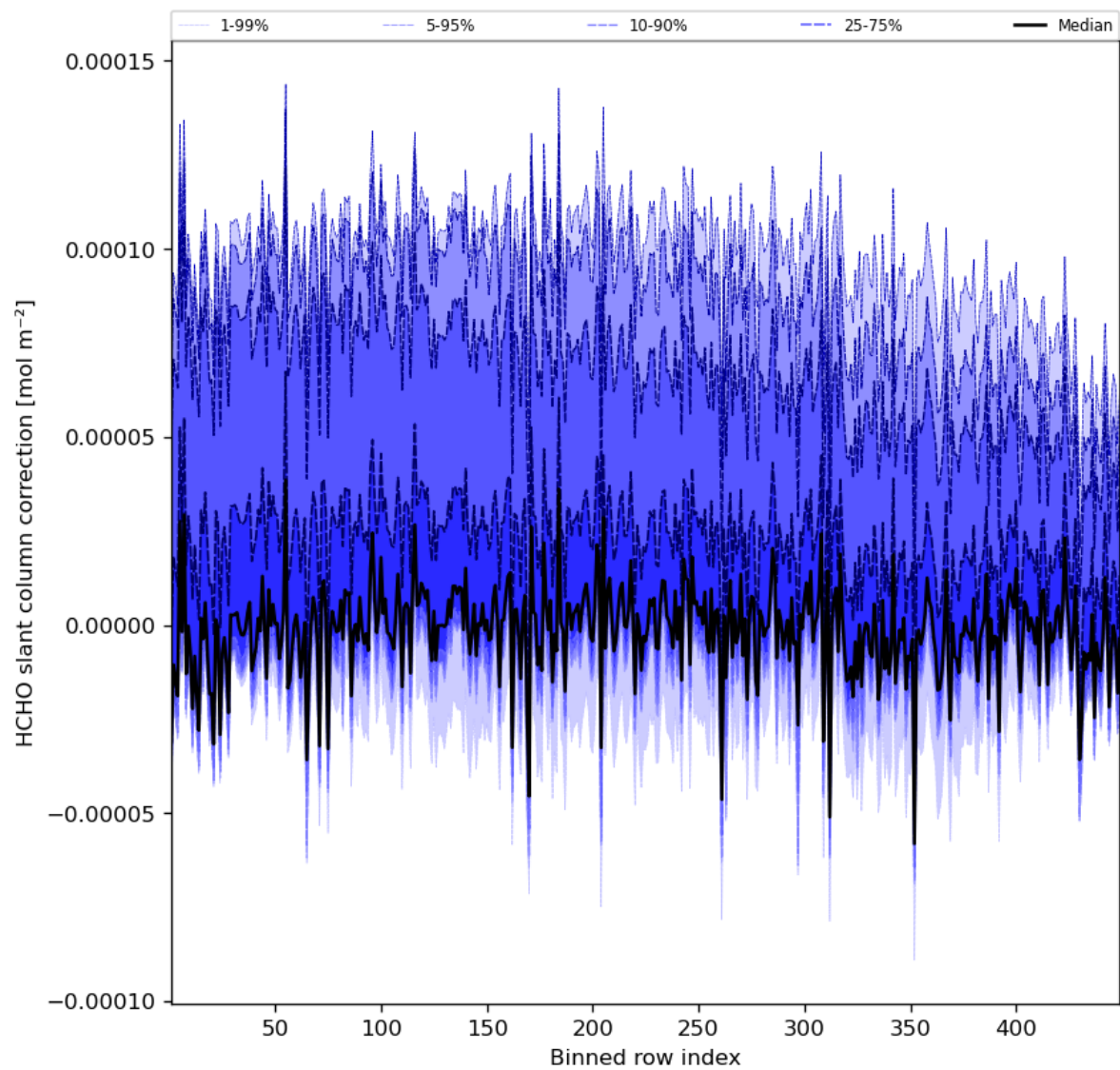
Figure 61: Along track statistics of “HCHO slant column correction” for 2023-10-25 to 2023-10-27
