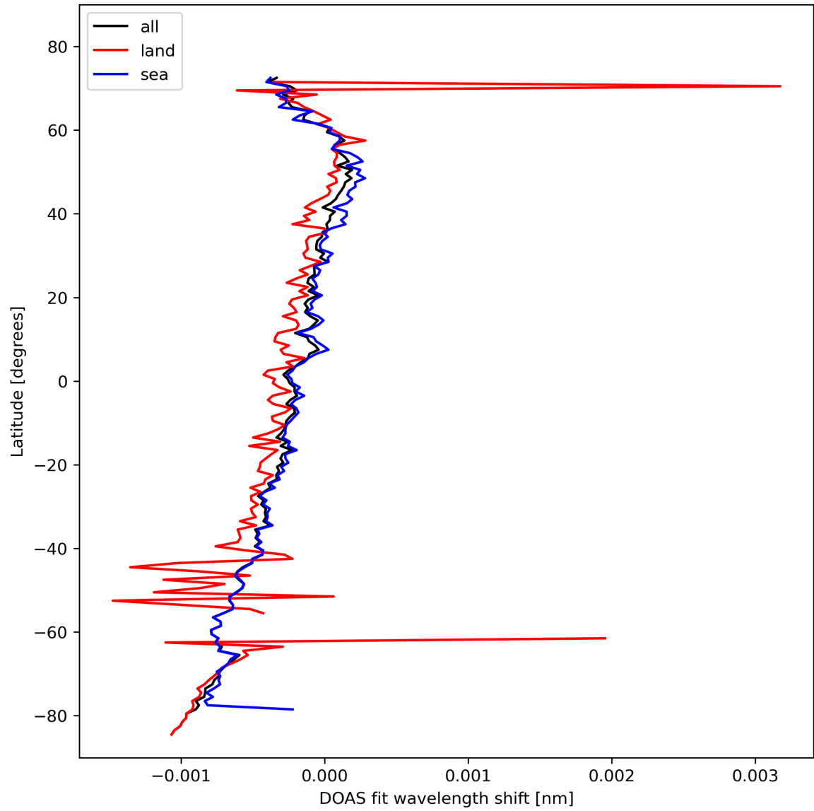
Figure 30: Zonal average of “DOAS fit wavelength shift” for 2023-10-25 to 2023-10-27.
