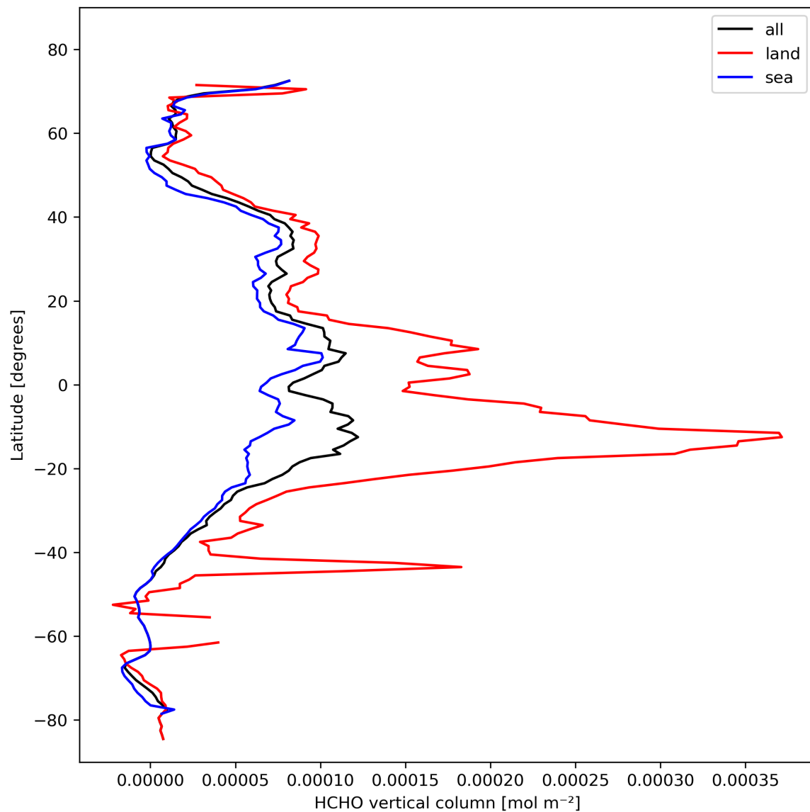
Figure 21: Zonal average of “HCHO vertical column” for 2023-10-25 to 2023-10-27.
