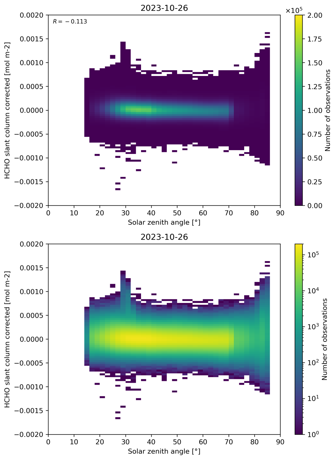
Figure 171: Scatter density plot of “Solar zenith angle” against “HCHO slant column corrected” for 2023-10-25 to 2023-10-27.
