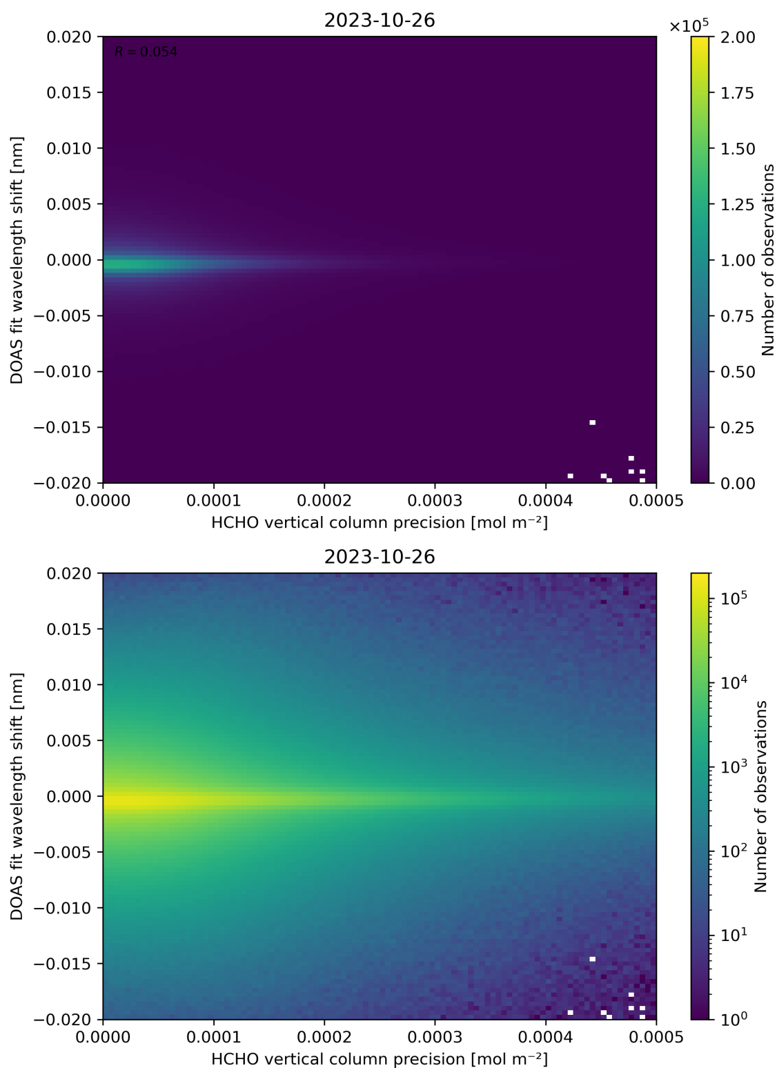
Figure 137: Scatter density plot of “HCHO vertical column precision” against “DOAS fit wavelength shift” for 2023-10-25 to 2023-10-27.
