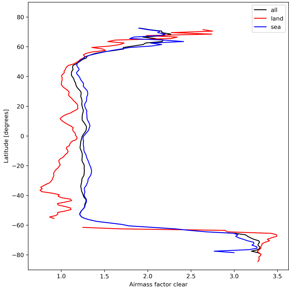
Figure 28: Zonal average of “Airmass factor clear” for 2023-10-25 to 2023-10-27.
