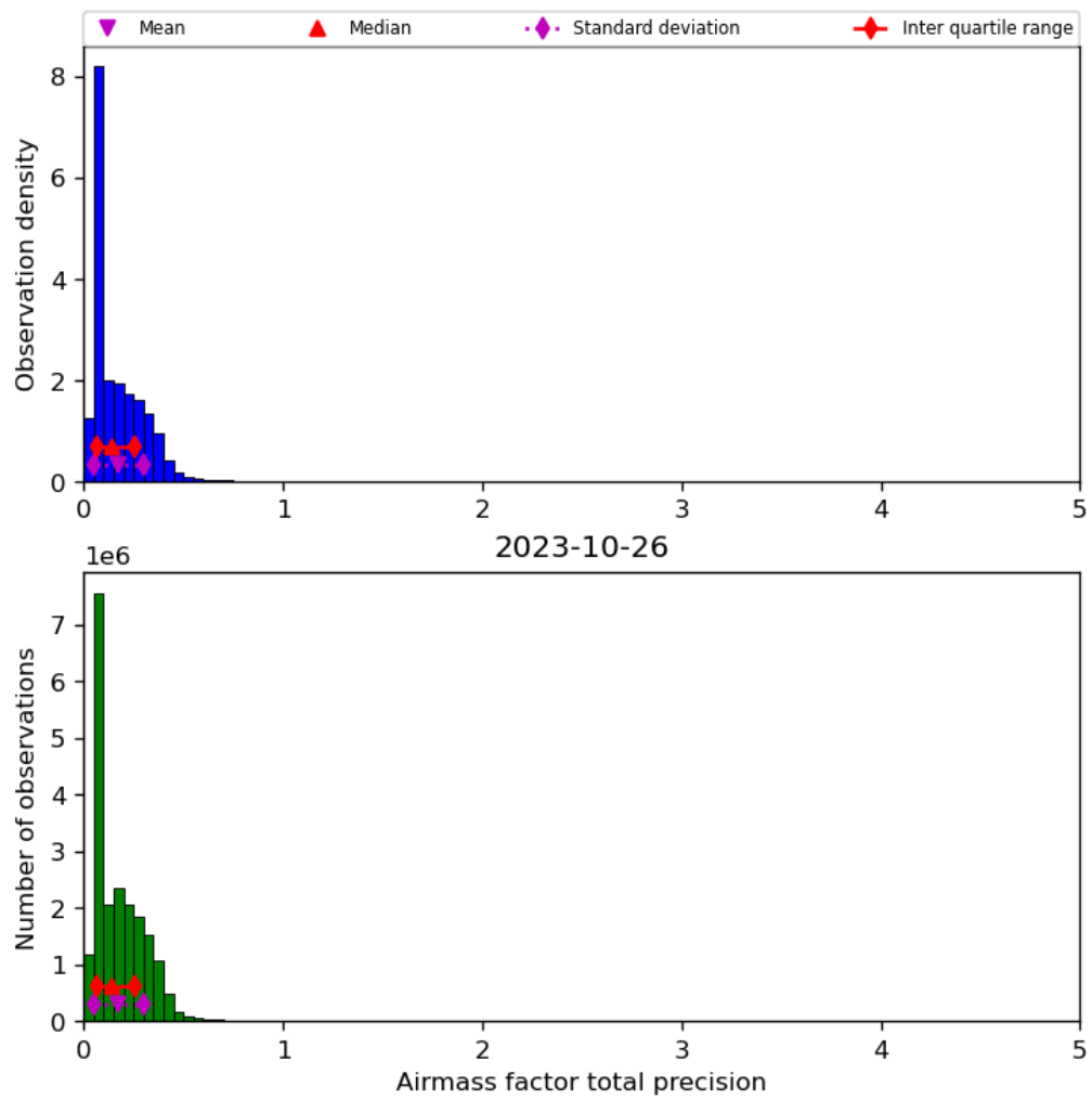
Figure 41: Histogram of “Airmass factor total precision” for 2023-10-25 to 2023-10-27
