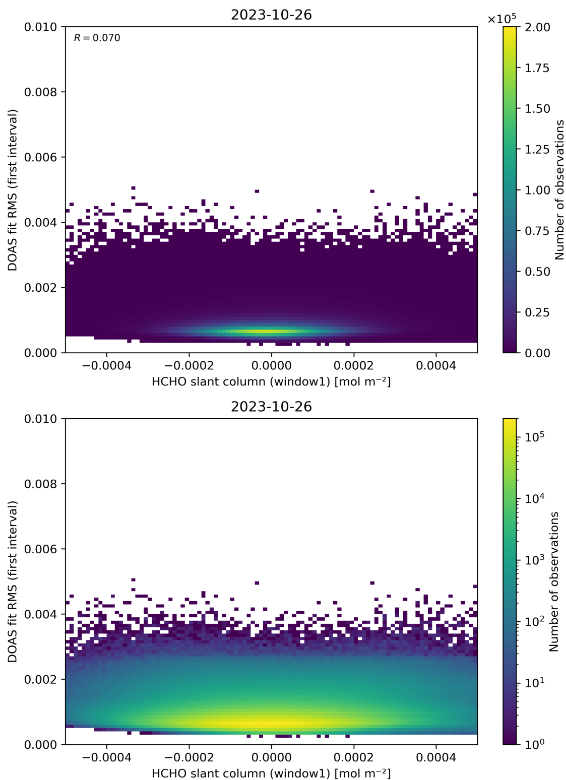
Figure 78: Scatter density plot of “HCHO slant column (window1)” against “DOAS fit RMS (first interval)” for 2023-10-25 to 2023-10-27.
