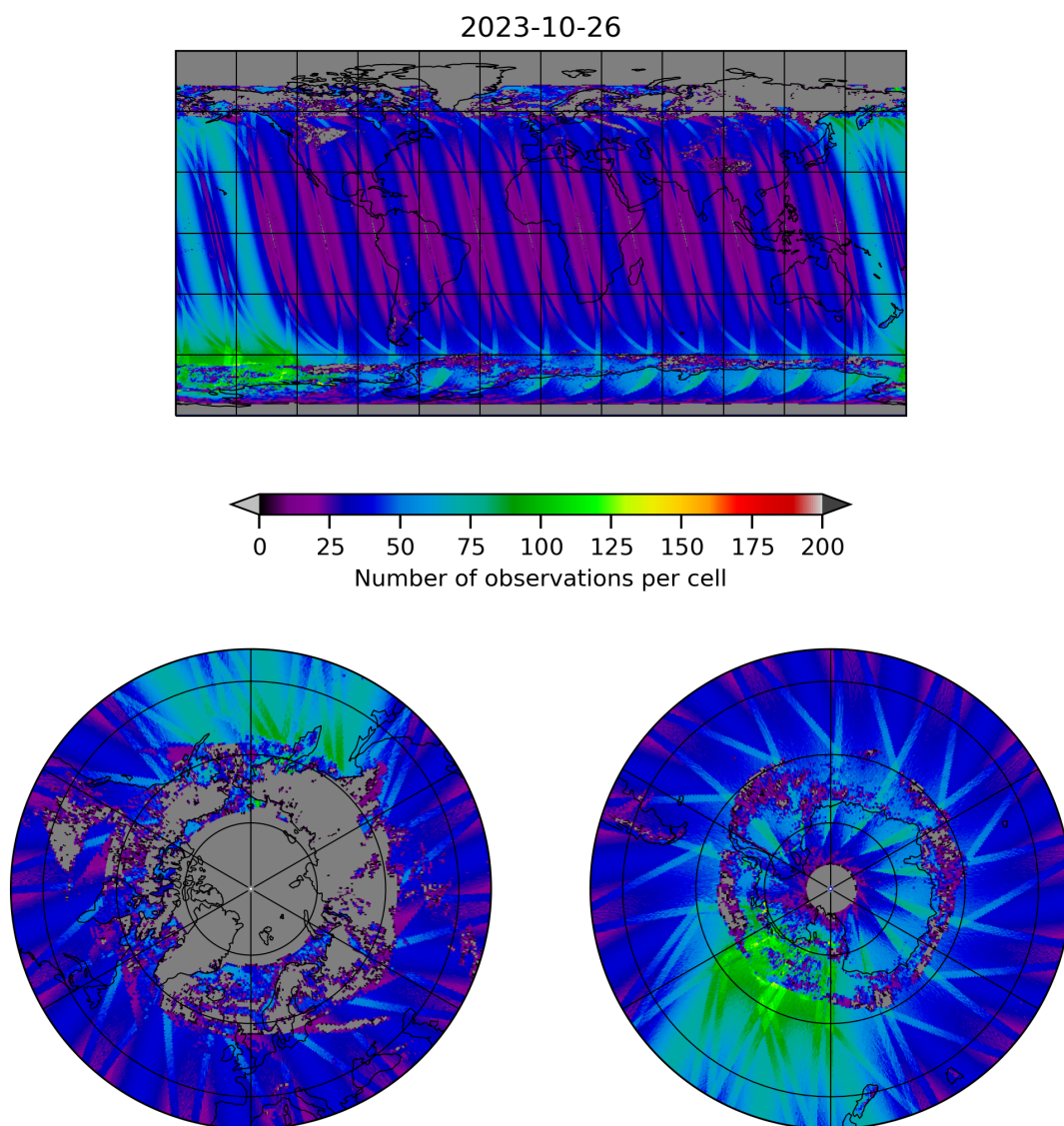
Figure 19: Map of the number of observations for 2023-10-25 to 2023-10-27
