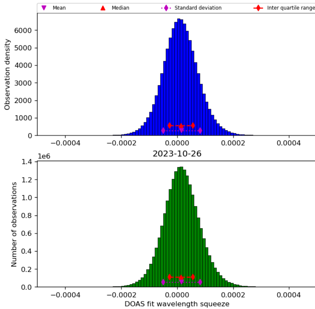
Figure 45: Histogram of “DOAS fit wavelength squeeze” for 2023-10-25 to 2023-10-27
