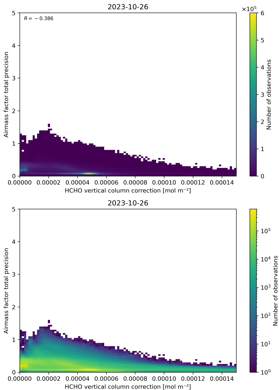
Figure 121: Scatter density plot of “HCHO vertical column correction” against “Airmass factor total precision” for 2023-10-25 to 2023-10-27.
