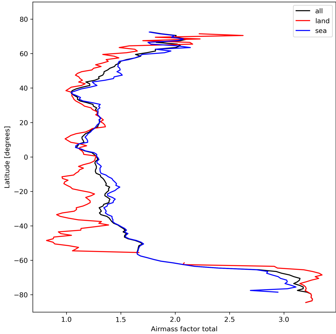
Figure 26: Zonal average of “Airmass factor total” for 2023-10-25 to 2023-10-27.
