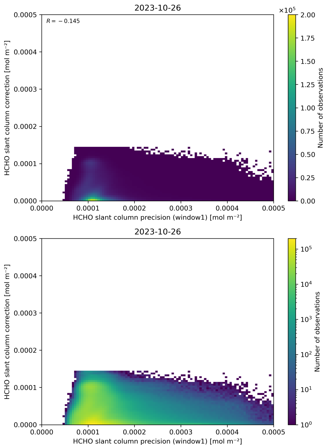
Figure 93: Scatter density plot of “HCHO slant column precision (window1)” against “HCHO slant column correction” for 2023-10-25 to 2023-10-27.
