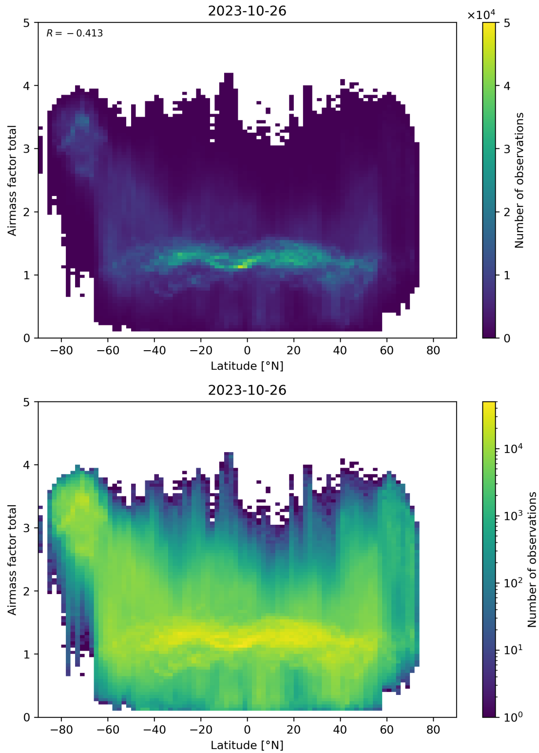
Figure 161: Scatter density plot of “Latitude” against “Airmass factor total” for 2023-10-25 to 2023-10-27.
