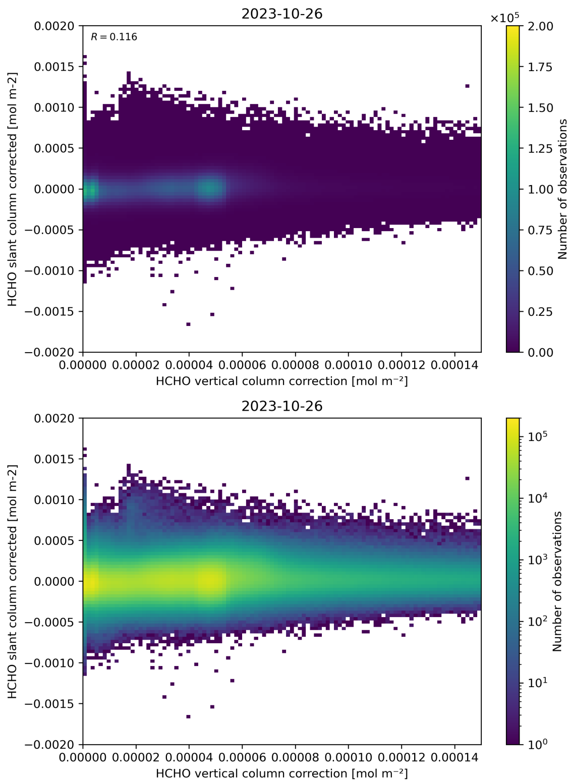
Figure 116: Scatter density plot of “HCHO vertical column correction” against “HCHO slant column corrected” for 2023-10-25 to 2023-10-27.
