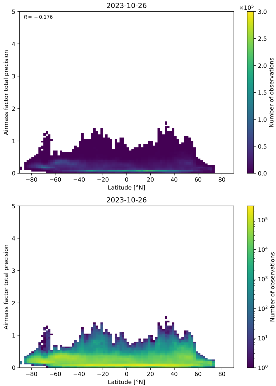
Figure 162: Scatter density plot of “Latitude” against “Airmass factor total precision” for 2023-10-25 to 2023-10-27.
