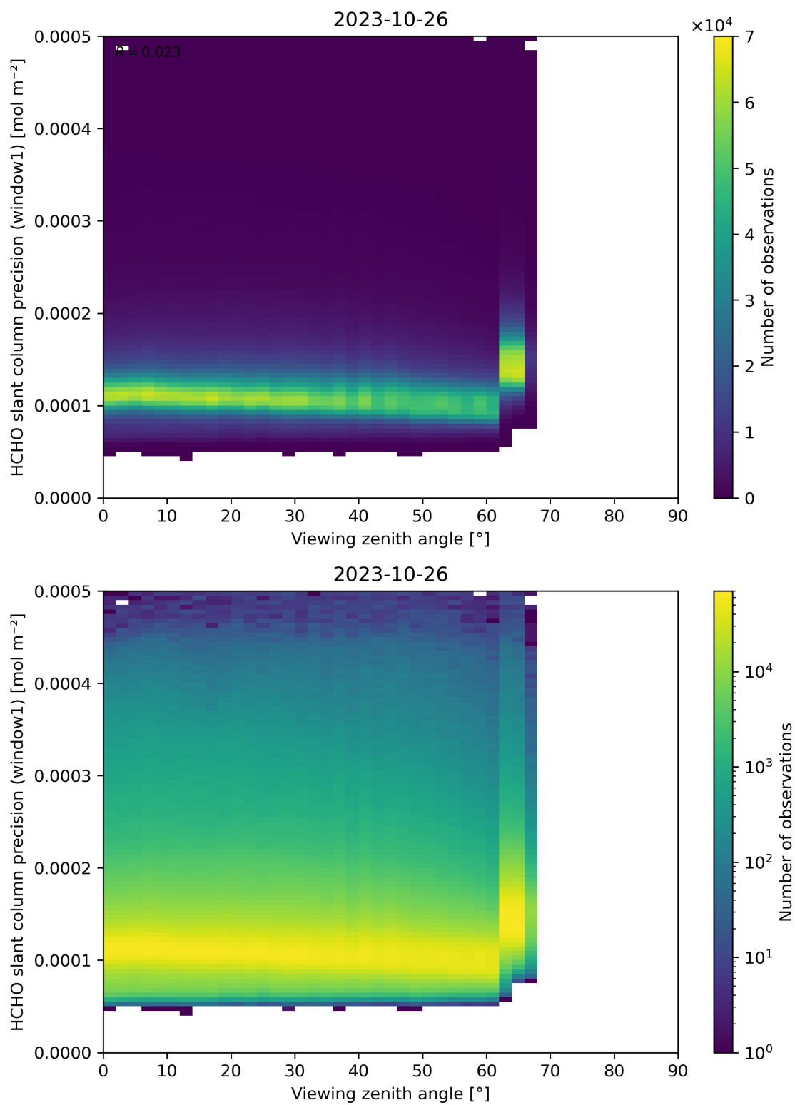
Figure 189: Scatter density plot of “Viewing zenith angle” against “HCHO slant column precision (window1)” for 2023-10-25 to 2023-10-27.
