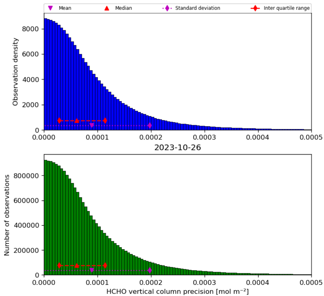
Figure 36: Histogram of “HCHO vertical column precision” for 2023-10-25 to 2023-10-27
