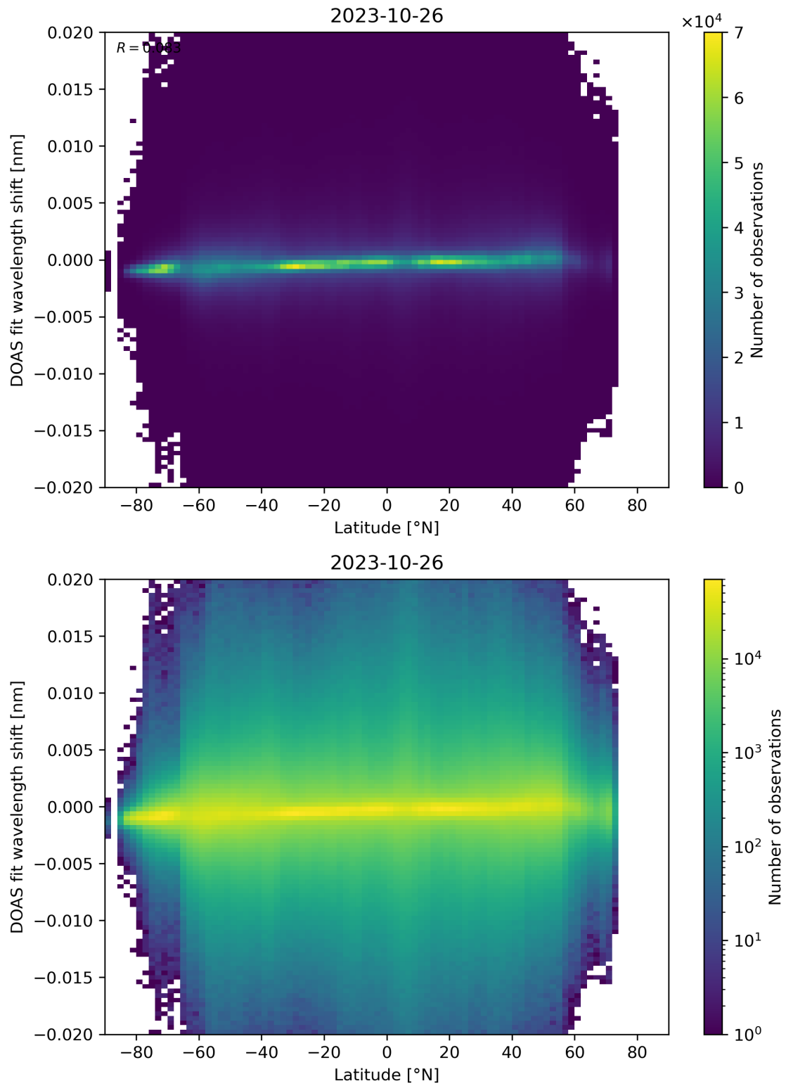
Figure 154: Scatter density plot of “Latitude” against “DOAS fit wavelength shift” for 2023-10-25 to 2023-10-27.
