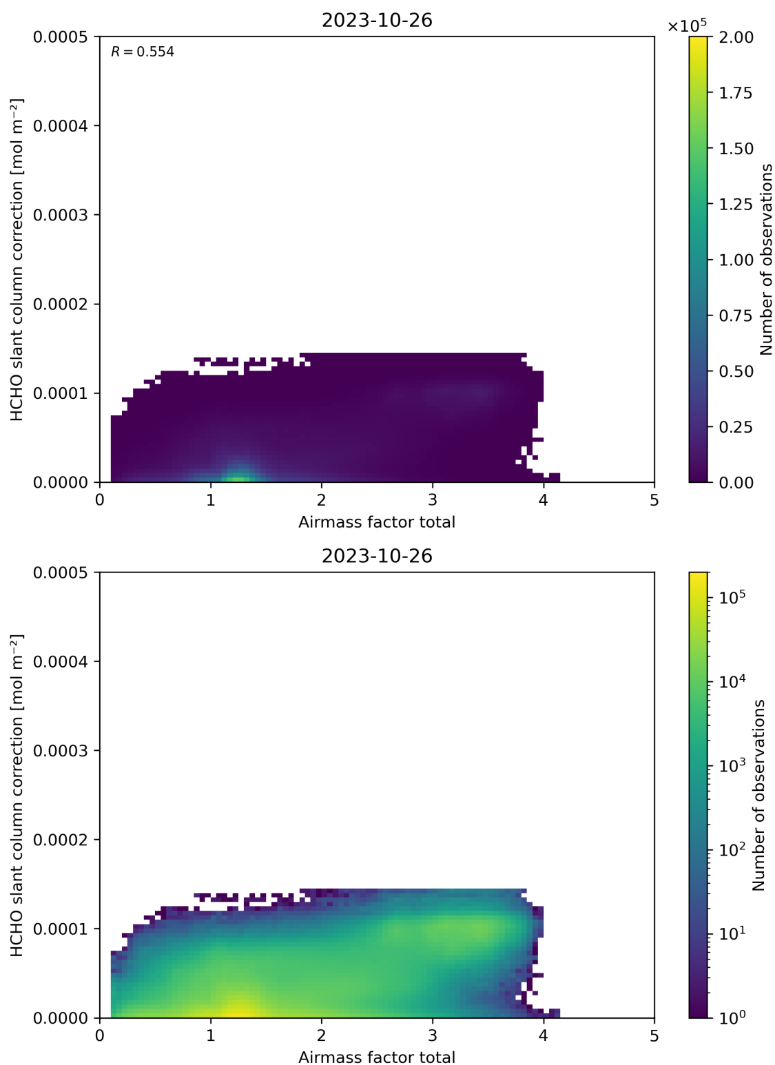
Figure 102: Scatter density plot of “Airmass factor total” against “HCHO slant column correction” for 2023-10-25 to 2023-10-27.
