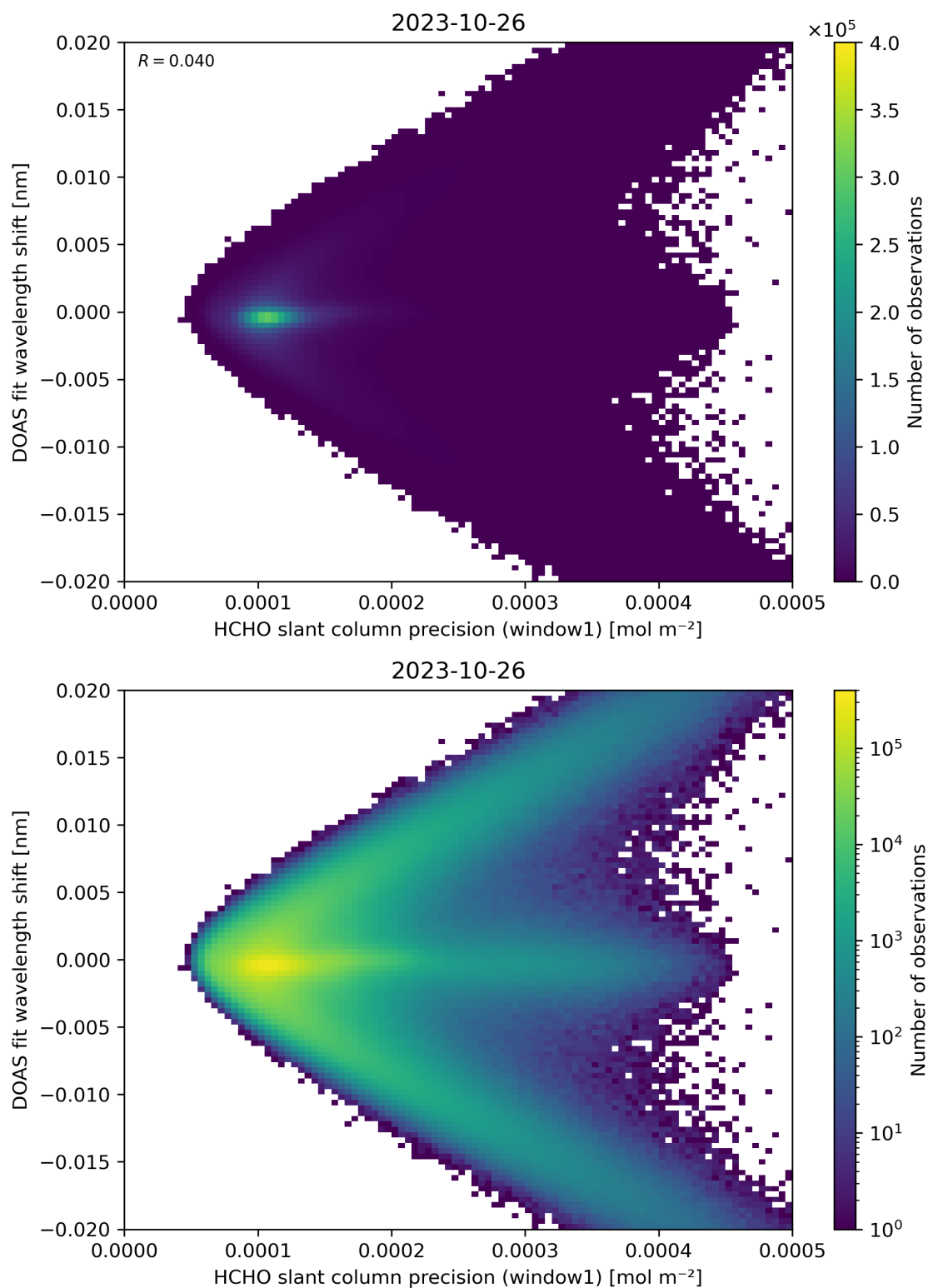
Figure 89: Scatter density plot of “HCHO slant column precision (window1)” against “DOAS fit wavelength shift” for 2023-10-25 to 2023-10-27.
