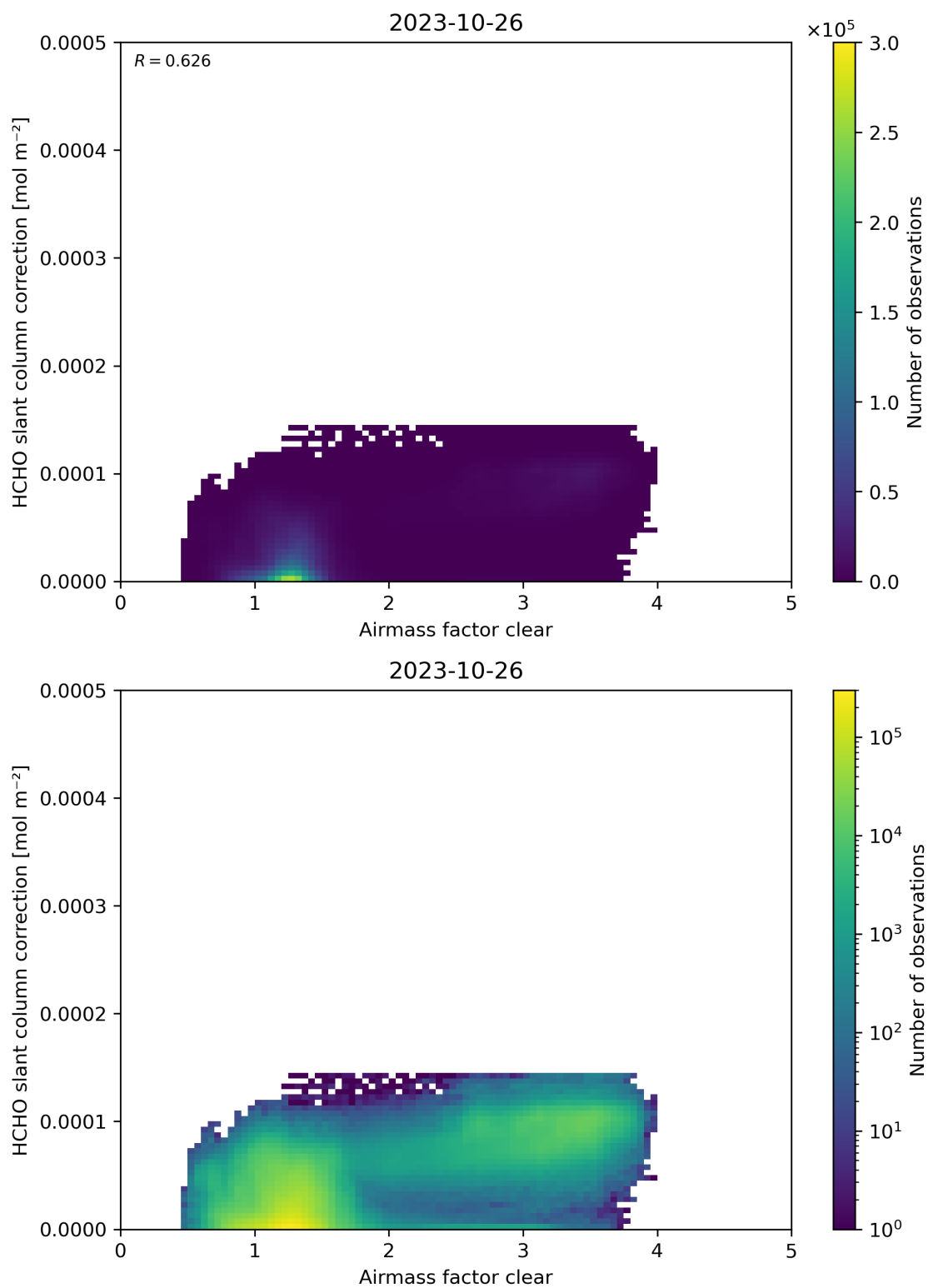
Figure 75: Scatter density plot of “Airmass factor clear” against “HCHO slant column correction” for 2023-10-25 to 2023-10-27.
