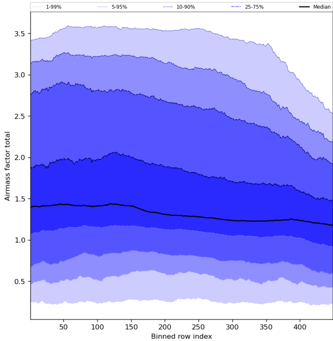
Figure 54: Along track statistics of “Airmass factor total” for 2023-10-25 to 2023-10-27
