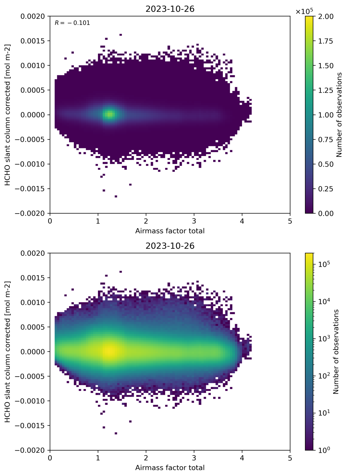
Figure 101: Scatter density plot of “Airmass factor total” against “HCHO slant column corrected” for 2023-10-25 to 2023-10-27.
