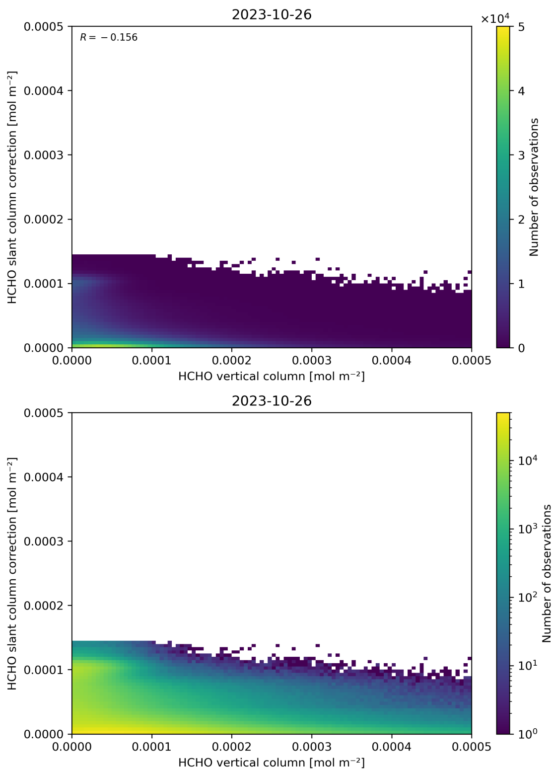
Figure 128: Scatter density plot of “HCHO vertical column” against “HCHO slant column correction” for 2023-10-25 to 2023-10-27.
