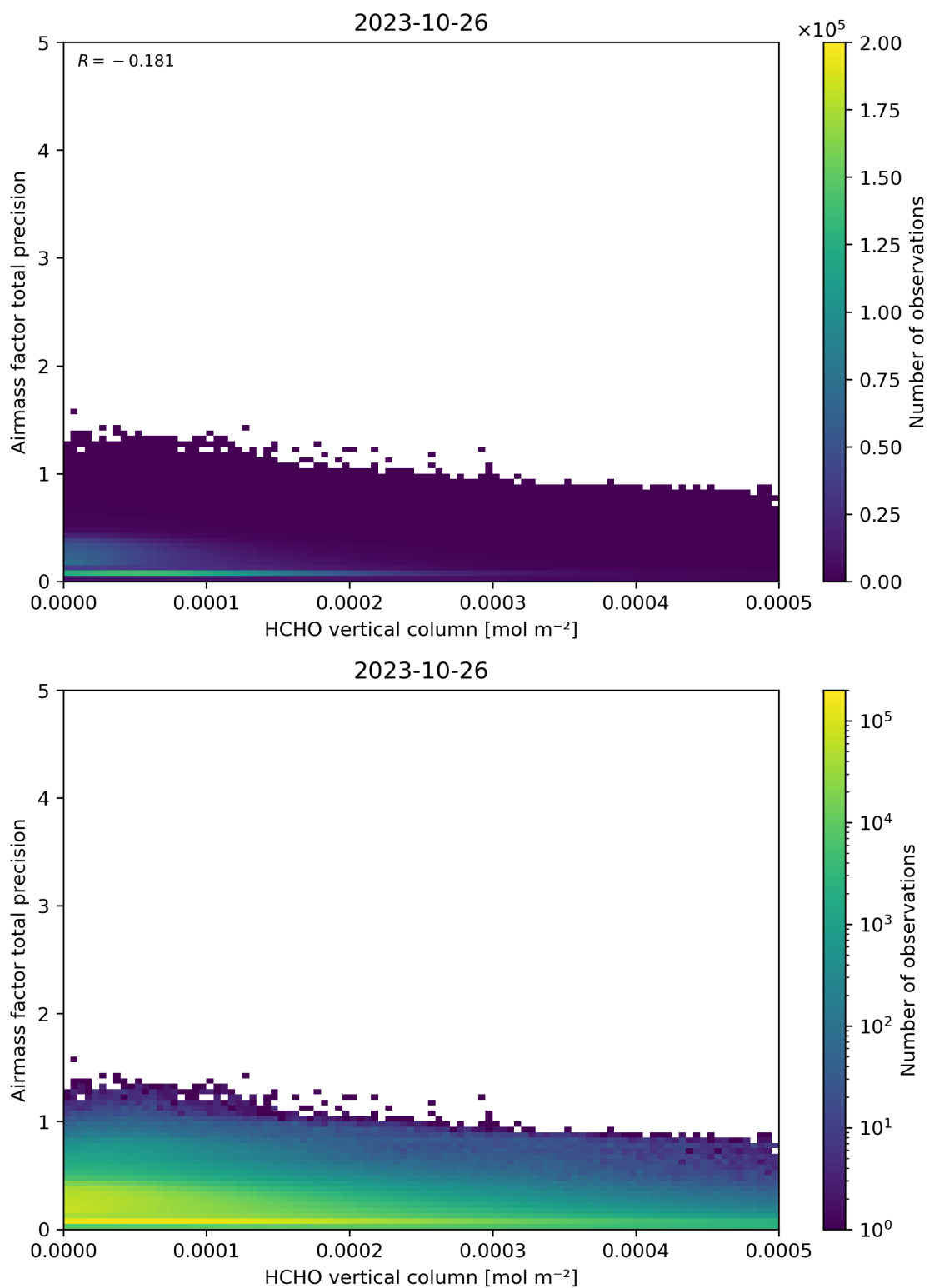
Figure 132: Scatter density plot of “HCHO vertical column” against “Airmass factor total precision” for 2023-10-25 to 2023-10-27.
