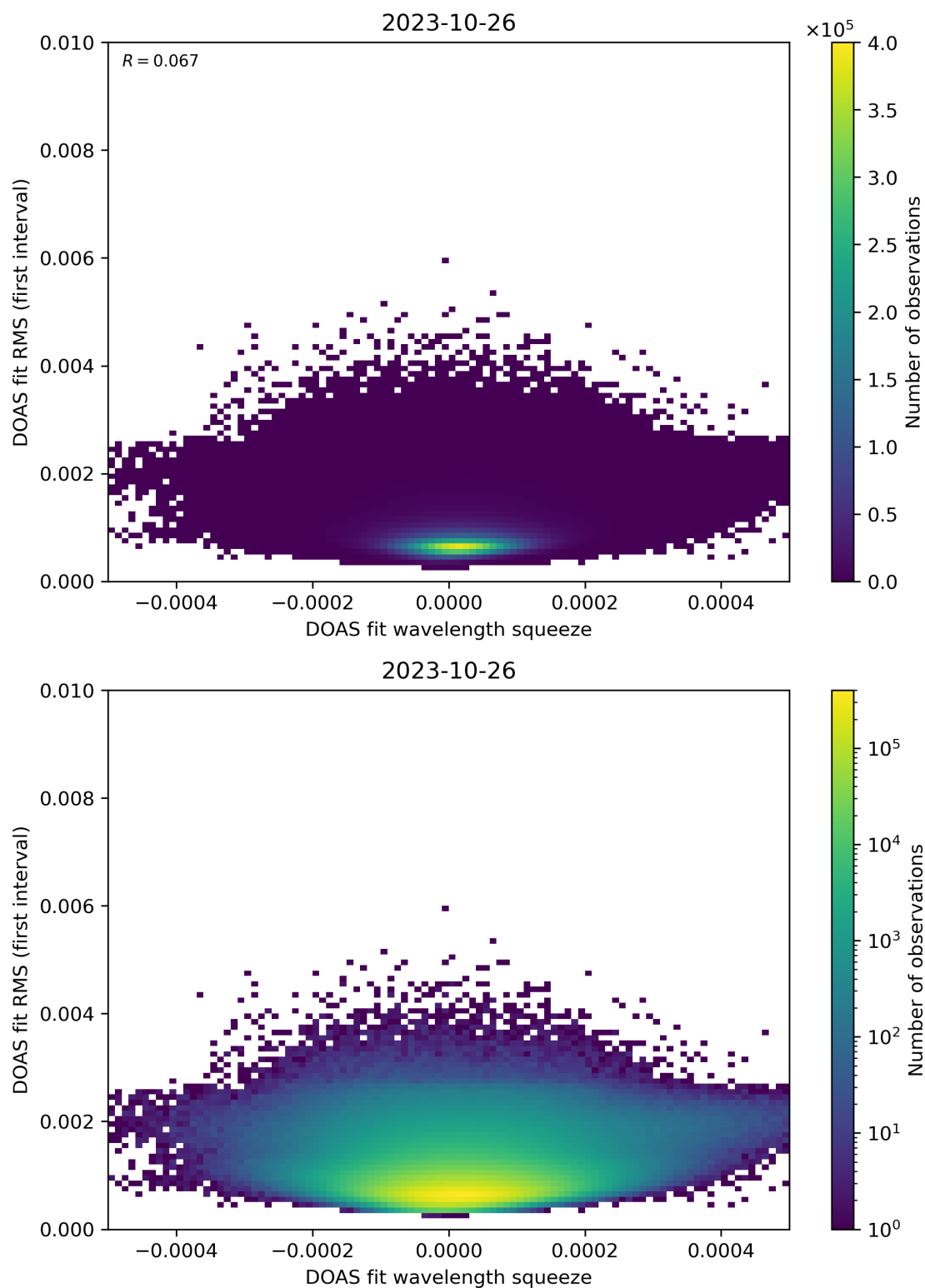
Figure 68: Scatter density plot of “DOAS fit wavelength squeeze” against “DOAS fit RMS (first interval)” for 2023-10-25 to 2023-10-27.
