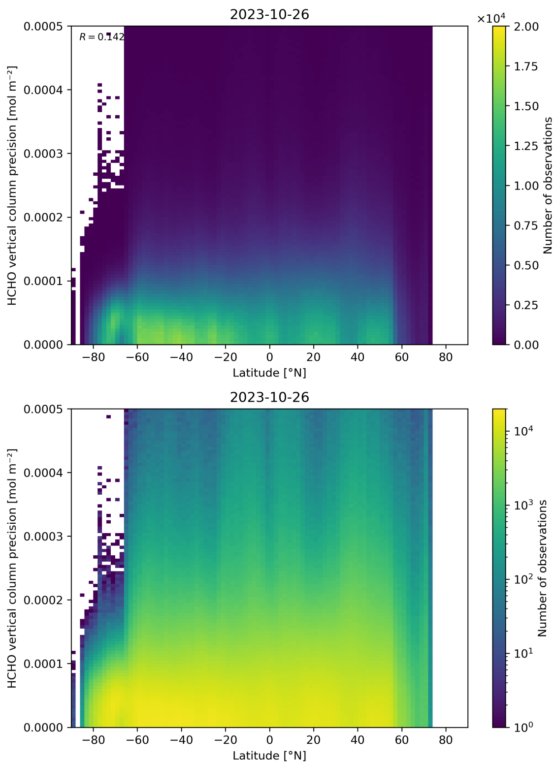
Figure 165: Scatter density plot of “Latitude” against “HCHO vertical column precision” for 2023-10-25 to 2023-10-27.
