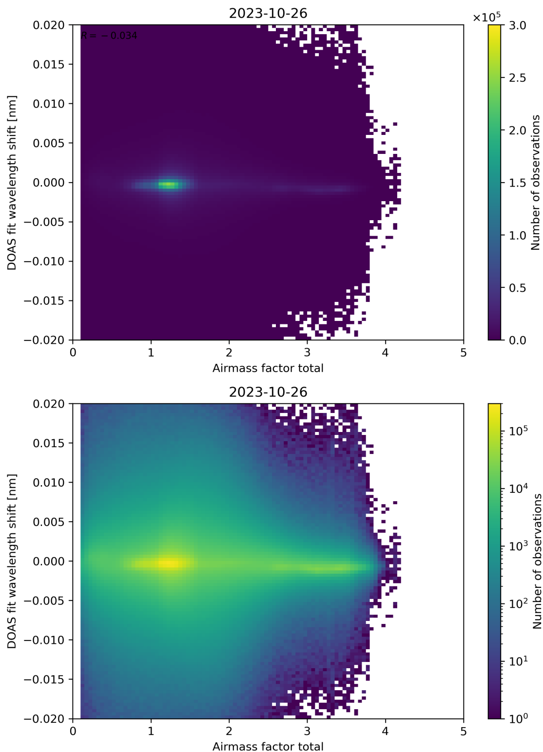
Figure 98: Scatter density plot of “Airmass factor total” against “DOAS fit wavelength shift” for 2023-10-25 to 2023-10-27.
