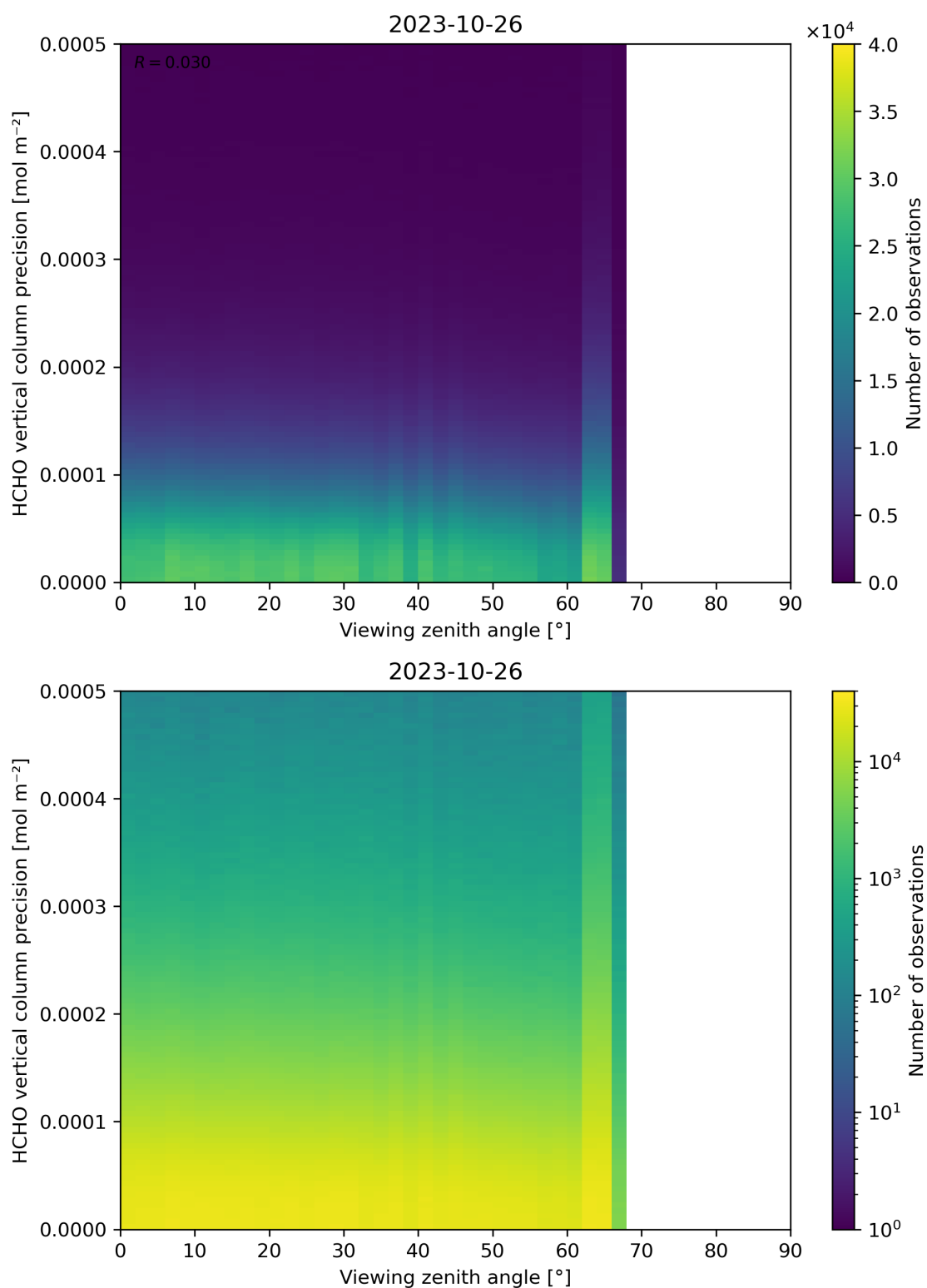
Figure 194: Scatter density plot of “Viewing zenith angle” against “HCHO vertical column precision” for 2023-10-25 to 2023-10-27.
