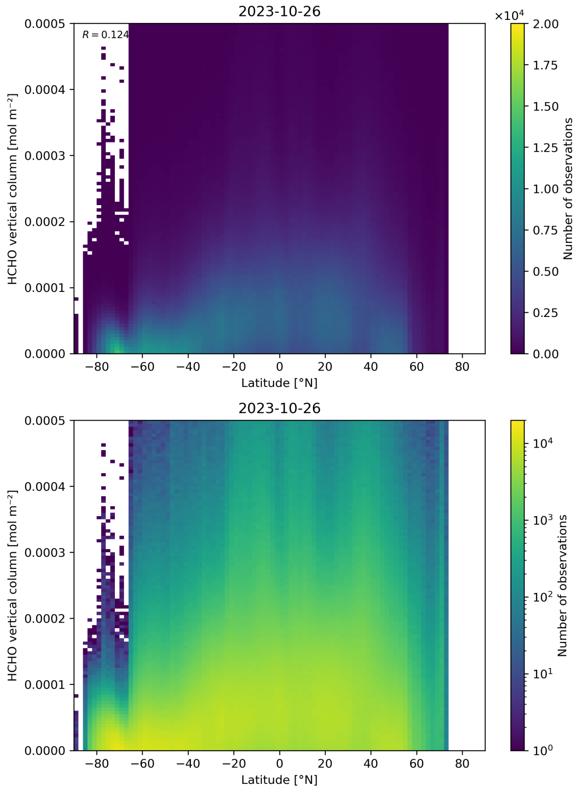
Figure 163: Scatter density plot of “Latitude” against “HCHO vertical column” for 2023-10-25 to 2023-10-27.
