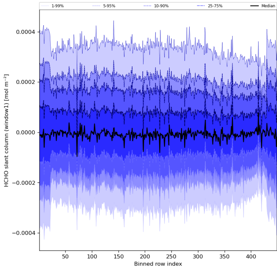
Figure 52: Along track statistics of "HCHO slant column (window1)" for 2023-10-25 to 2023-10-27
