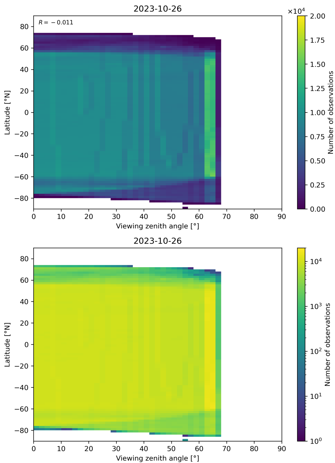
Figure 196: Scatter density plot of “Viewing zenith angle” against “Latitude” for 2023-10-25 to 2023-10-27.
