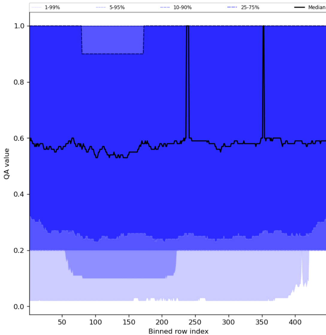
Figure 48: Along track statistics of “QA value” for 2023-10-25 to 2023-10-27
