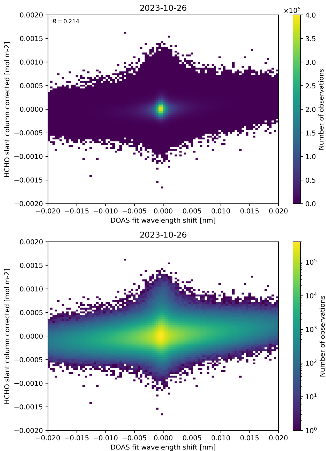
Figure 66: Scatter density plot of “DOAS fit wavelength shift” against “HCHO slant column corrected” for 2023-10-25 to 2023-10-27.
