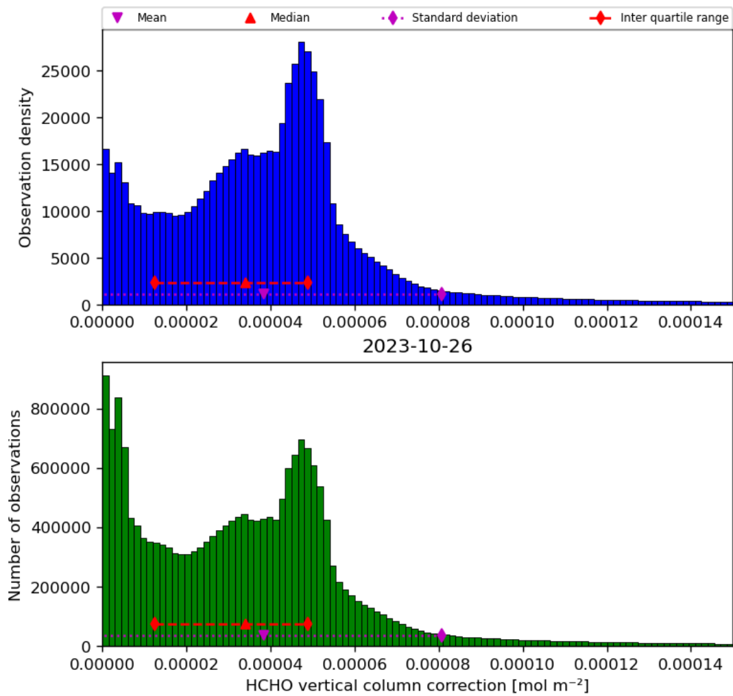
Figure 37: Histogram of “HCHO vertical column correction” for 2023-10-25 to 2023-10-27
