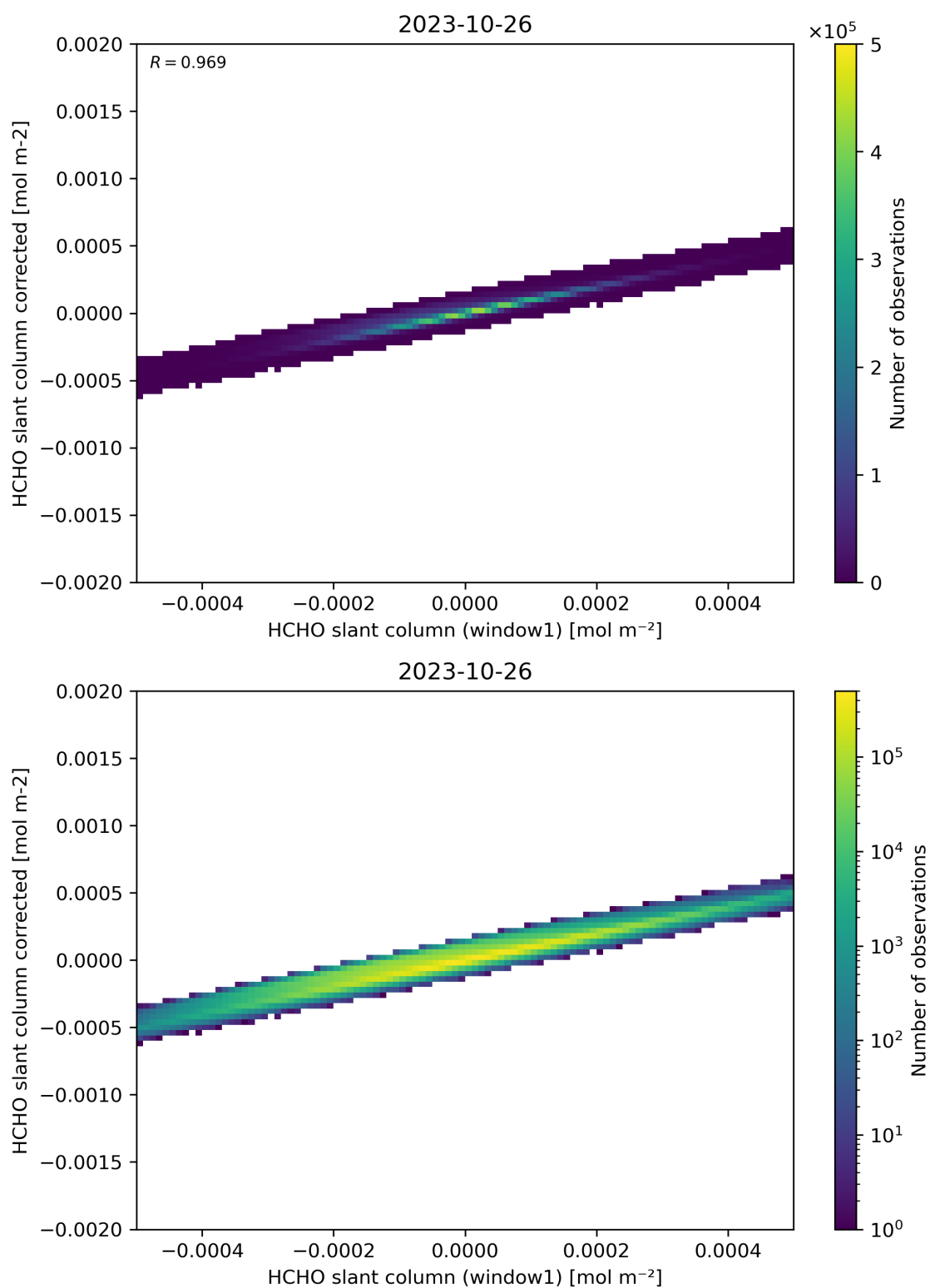
Figure 82: Scatter density plot of “HCHO slant column (window1)” against “HCHO slant column corrected” for 2023-10-25 to 2023-10-27.
