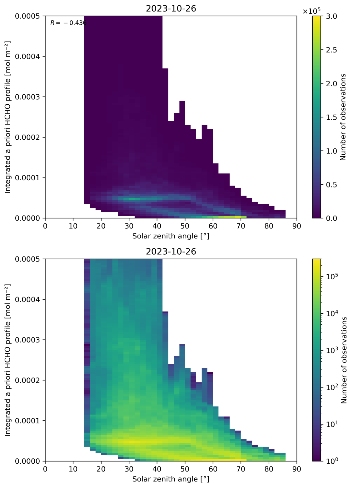
Figure 180: Scatter density plot of “Solar zenith angle” against “Integrated a priori HCHO profile” for 2023-10-25 to 2023-10-27.
