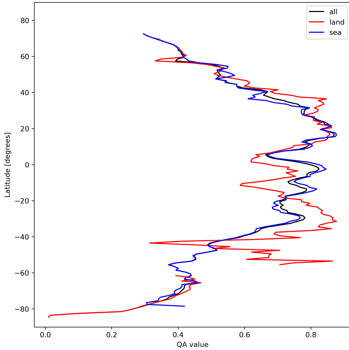
Figure 20: Zonal average of “QA value” for 2023-10-25 to 2023-10-27.
