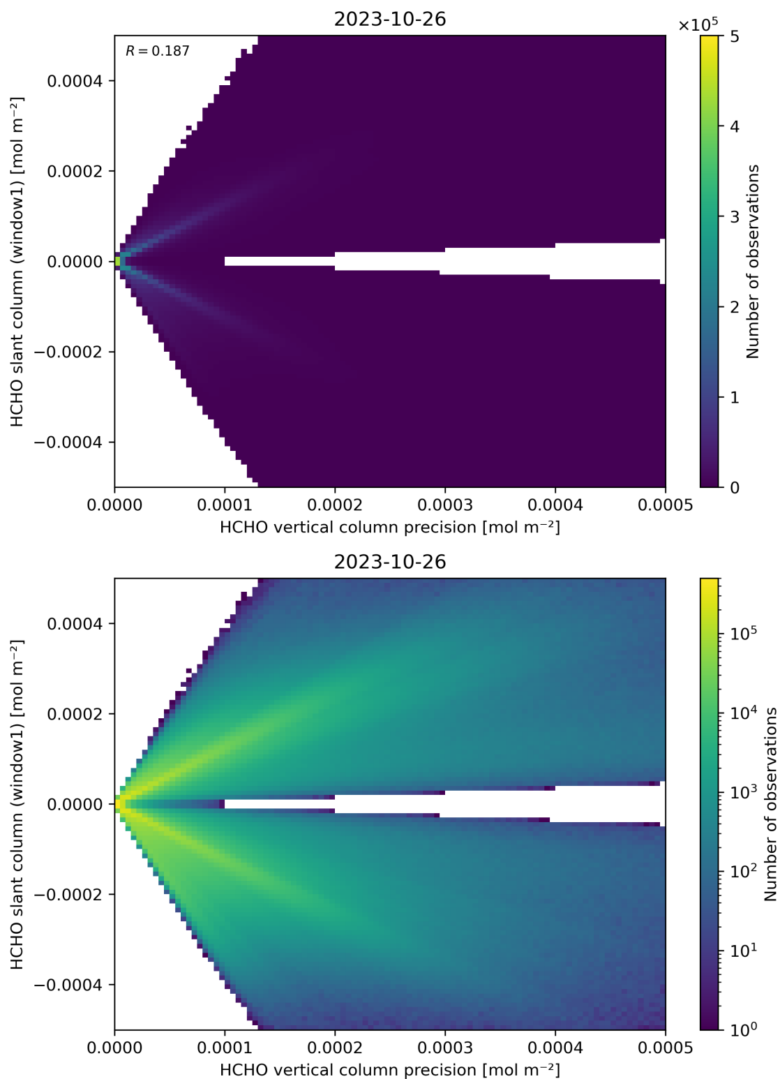
Figure 142: Scatter density plot of “HCHO vertical column precision” against “HCHO slant column (window1)” for 2023-10-25 to 2023-10-27.
