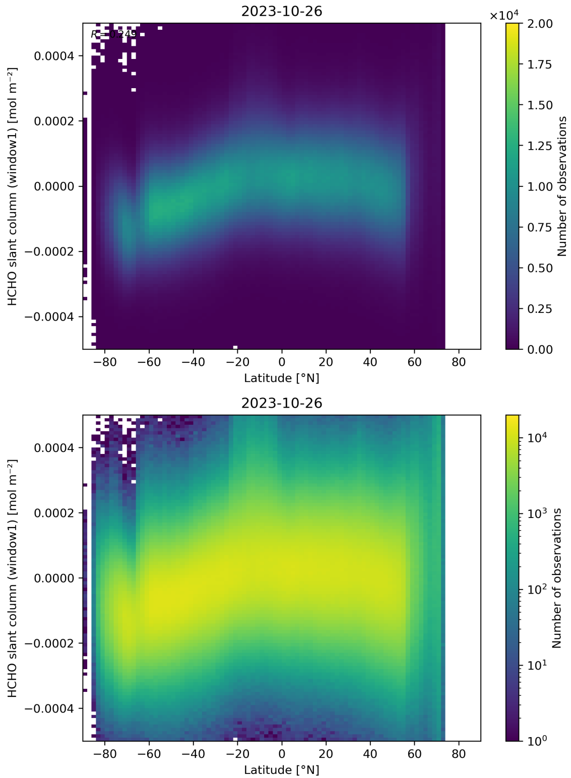
Figure 159: Scatter density plot of “Latitude” against “HCHO slant column (window1)” for 2023-10-25 to 2023-10-27.
