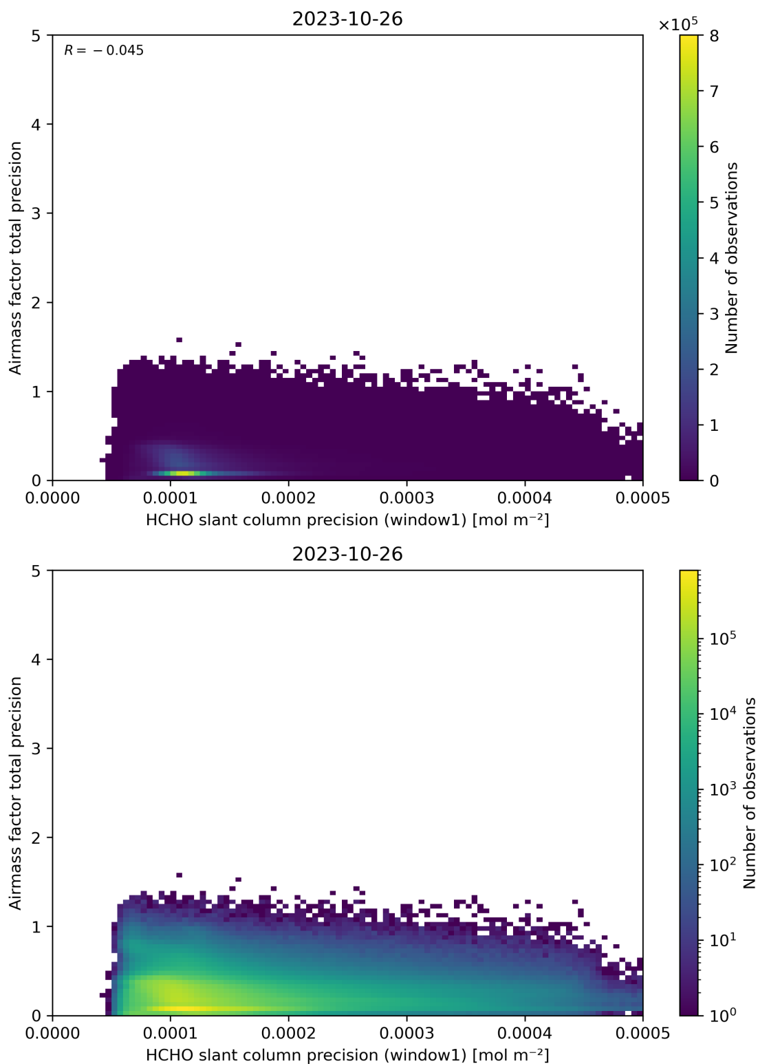
Figure 95: Scatter density plot of “HCHO slant column precision (window1)” against “Airmass factor total precision” for 2023-10-25 to 2023-10-27.
