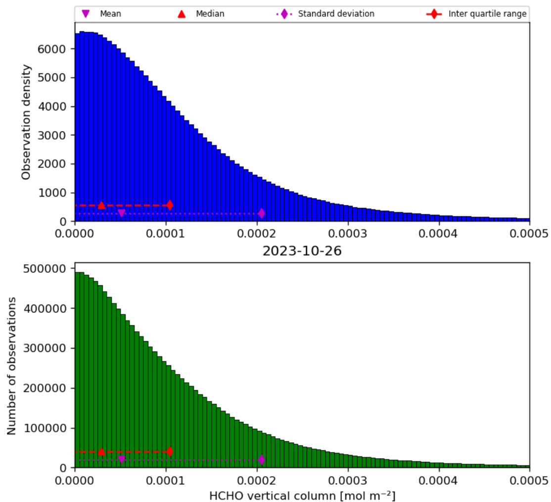
Figure 35: Histogram of “HCHO vertical column” for 2023-10-25 to 2023-10-27
