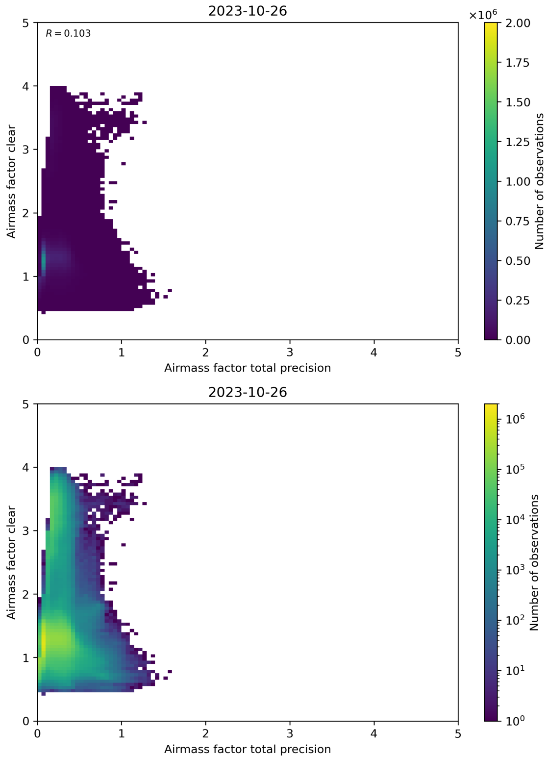
Figure 108: Scatter density plot of “Airmass factor total precision” against “Airmass factor clear” for 2023-10-25 to 2023-10-27.
