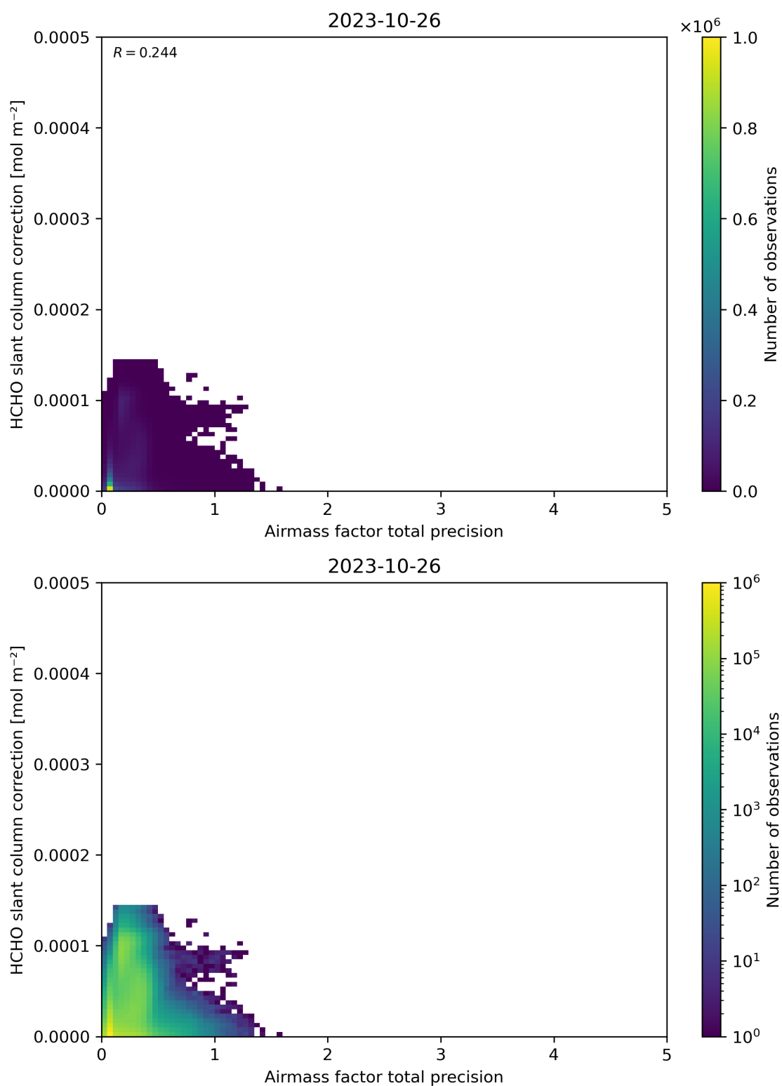
Figure 110: Scatter density plot of “Airmass factor total precision” against “HCHO slant column correction” for 2023-10-25 to 2023-10-27.
