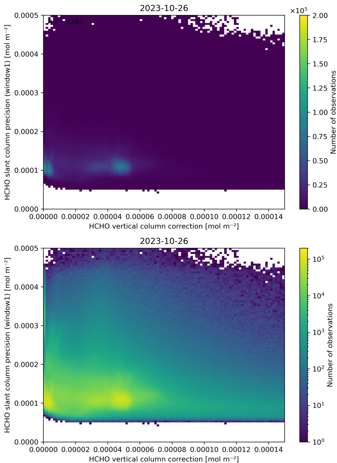
Figure 119: Scatter density plot of “HCHO vertical column correction” against “HCHO slant column precision (window1)” for 2023-10-25 to 2023-10-27.
