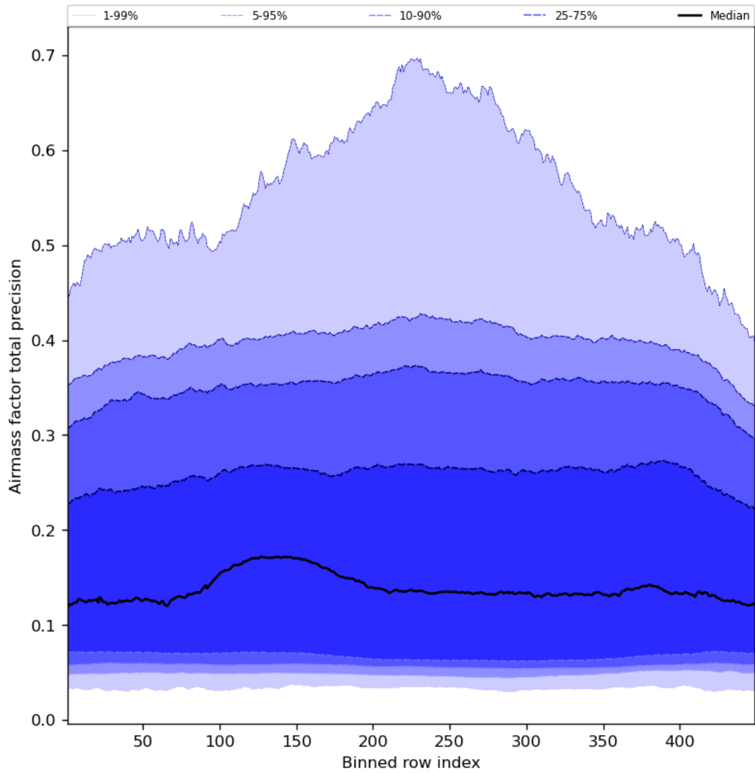
Figure 55: Along track statistics of “Airmass factor total precision” for 2023-10-25 to 2023-10-27
