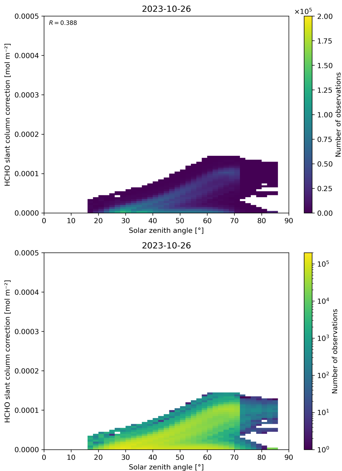
Figure 172: Scatter density plot of “Solar zenith angle” against “HCHO slant column correction” for 2023-10-25 to 2023-10-27.
