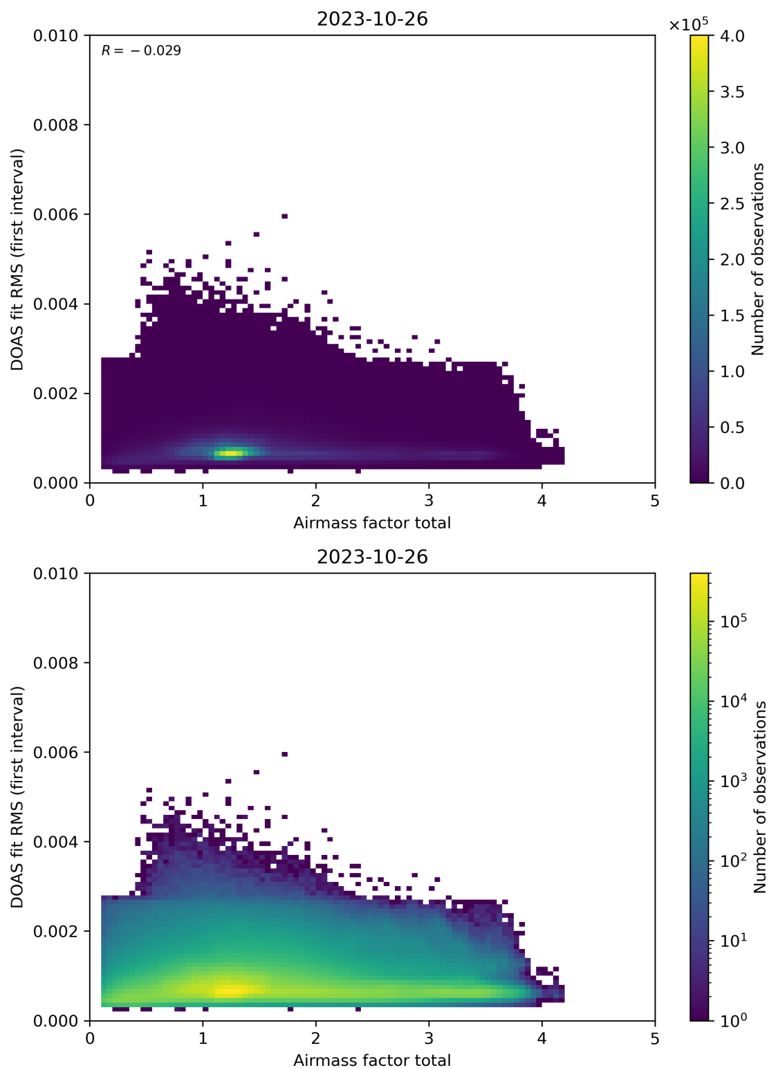
Figure 97: Scatter density plot of “Airmass factor total” against “DOAS fit RMS (first interval)” for 2023-10-25 to 2023-10-27.
