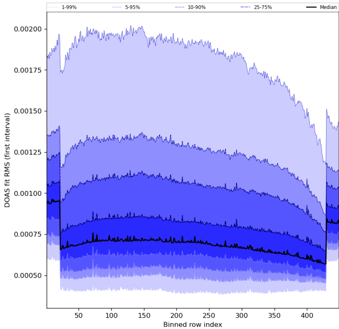
Figure 60: Along track statistics of “DOAS fit RMS (first interval)” for 2023-10-25 to 2023-10-27
