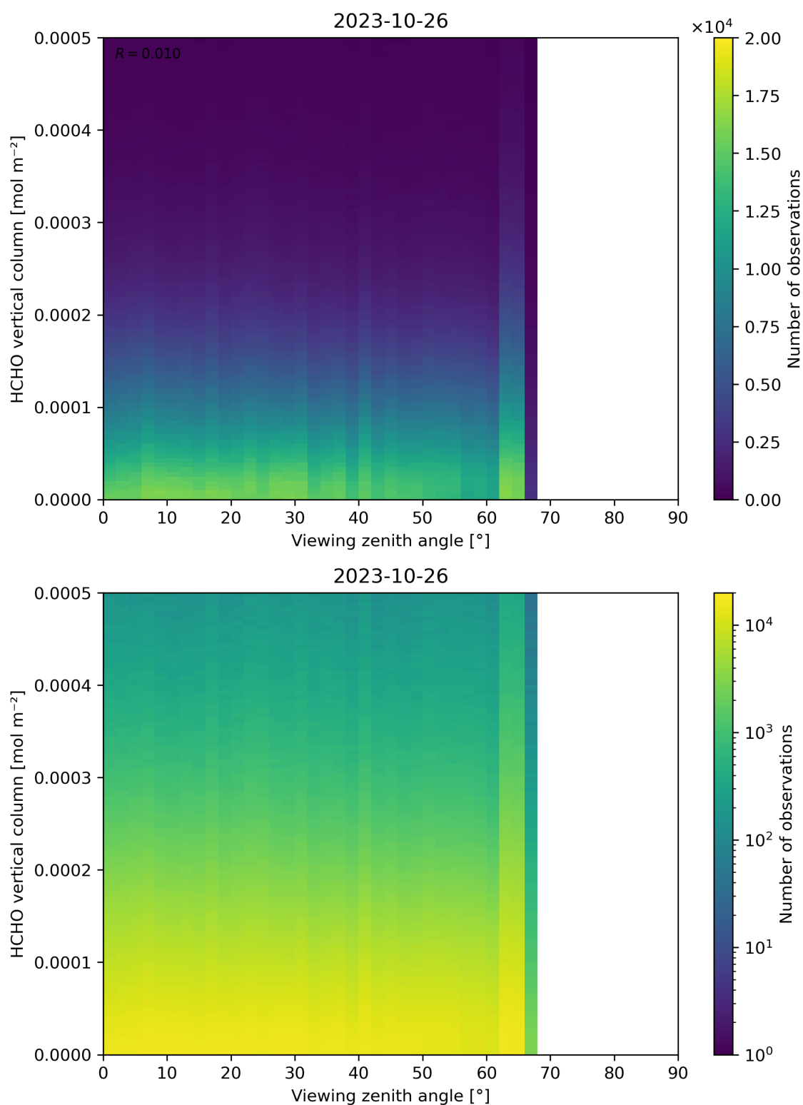
Figure 192: Scatter density plot of “Viewing zenith angle” against “HCHO vertical column” for 2023-10-25 to 2023-10-27.
