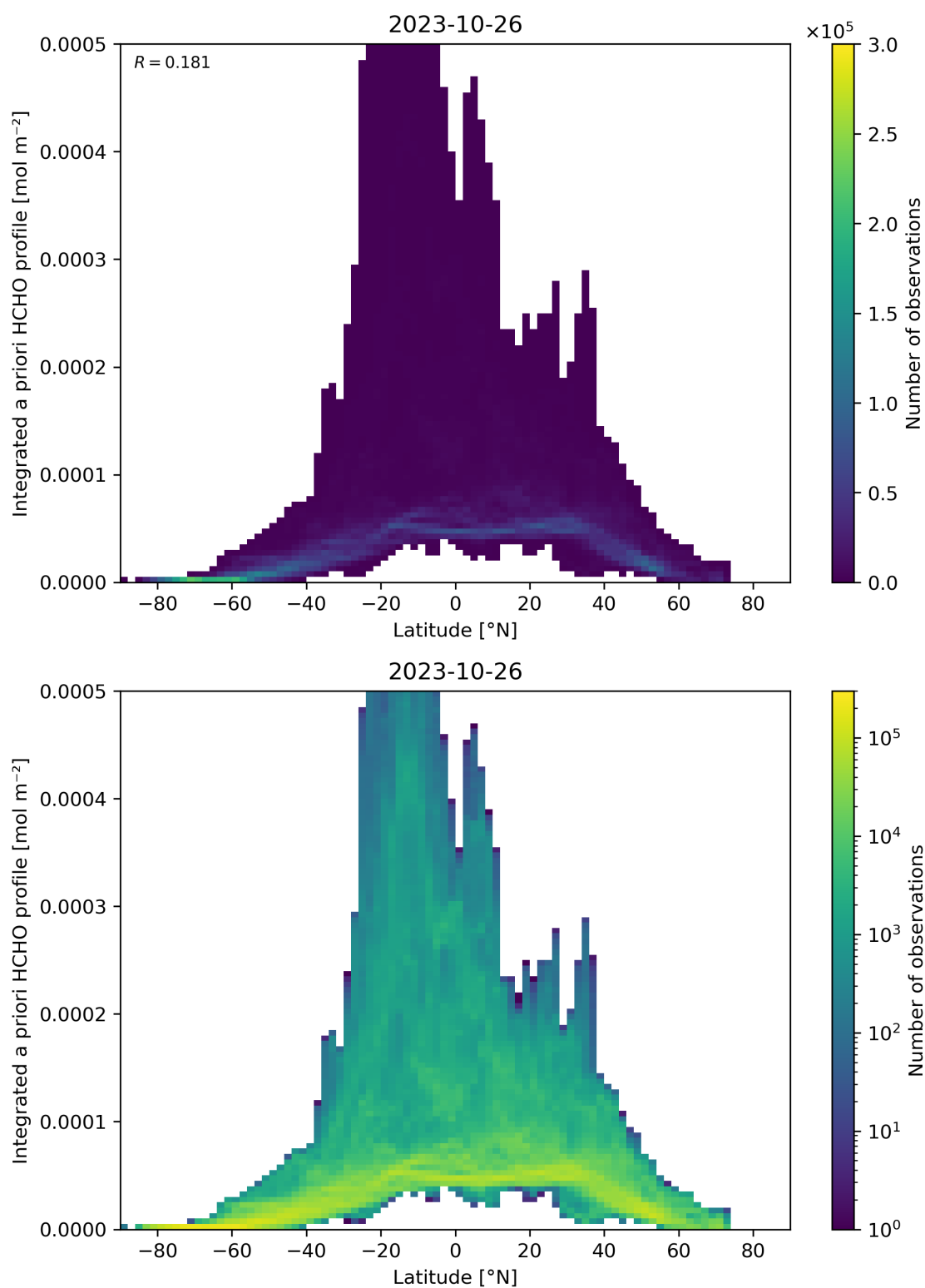
Figure 166: Scatter density plot of “Latitude” against “Integrated a priori HCHO profile” for 2023-10-25 to 2023-10-27.
