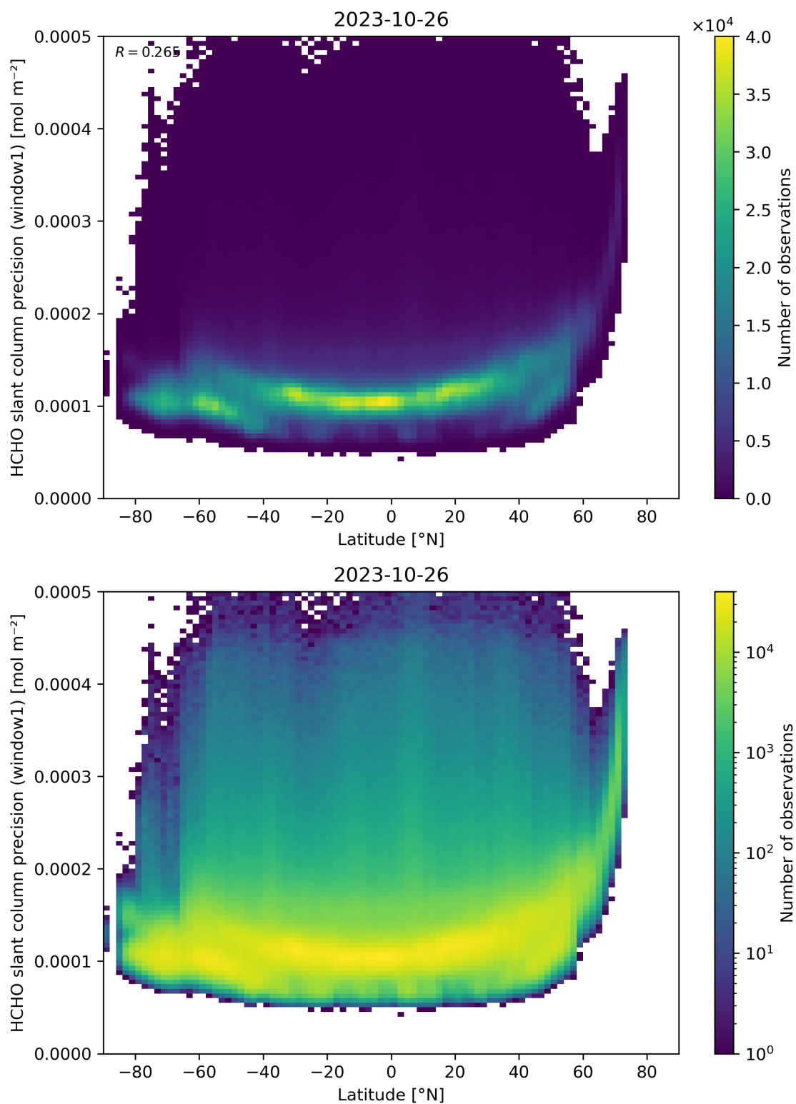
Figure 160: Scatter density plot of “Latitude” against “HCHO slant column precision (window1)” for 2023-10-25 to 2023-10-27.
