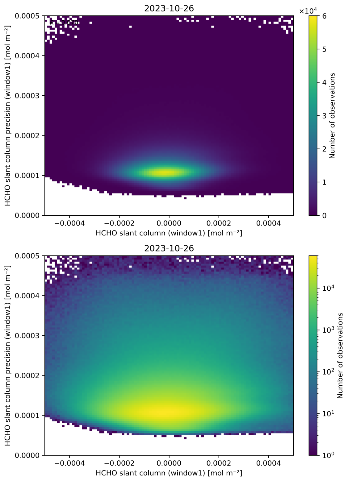
Figure 84: Scatter density plot of “HCHO slant column (window1)” against “HCHO slant column precision (window1)” for 2023-10-25 to 2023-10-27.
