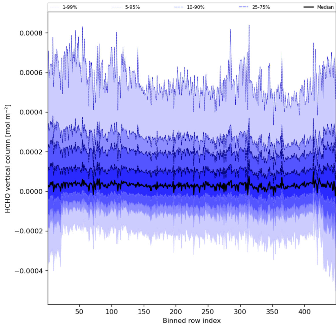
Figure 49: Along track statistics of “HCHO vertical column” for 2023-10-25 to 2023-10-27
