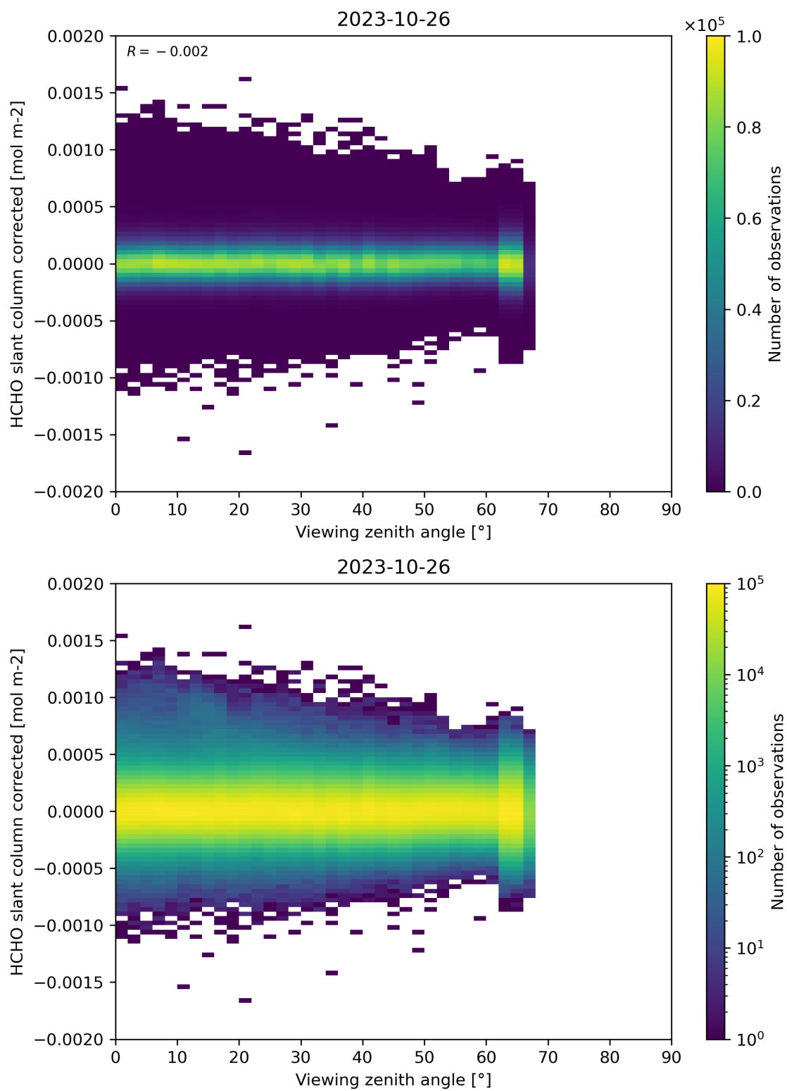
Figure 186: Scatter density plot of “Viewing zenith angle” against “HCHO slant column corrected” for 2023-10-25 to 2023-10-27.
