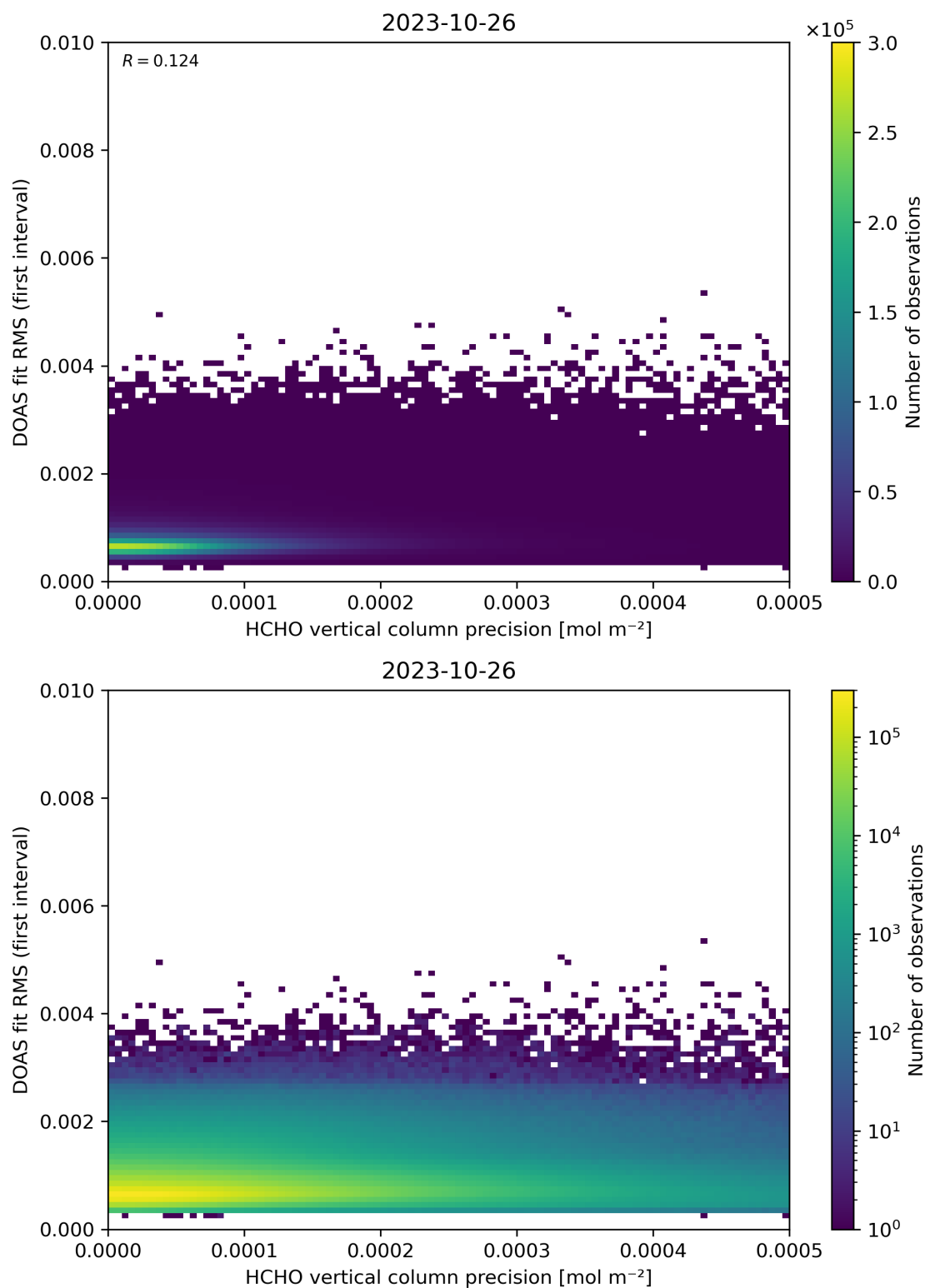
Figure 136: Scatter density plot of “HCHO vertical column precision” against “DOAS fit RMS (first interval)” for 2023-10-25 to 2023-10-27.
