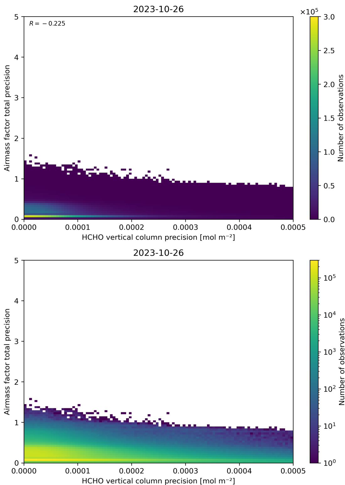
Figure 145: Scatter density plot of “HCHO vertical column precision” against “Air mass factor total precision” for 2023-10-25 to 2023-10-27.
