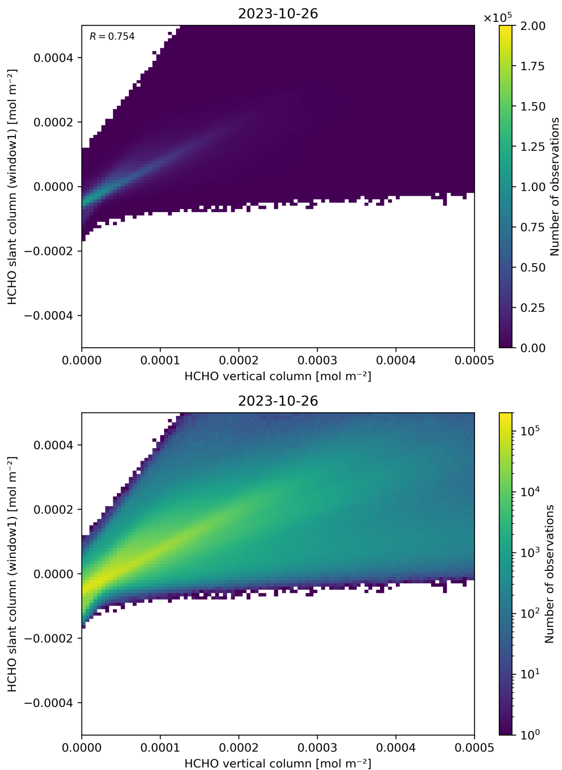
Figure 129: Scatter density plot of “HCHO vertical column” against “HCHO slant column (window1)” for 2023-10-25 to 2023-10-27.
