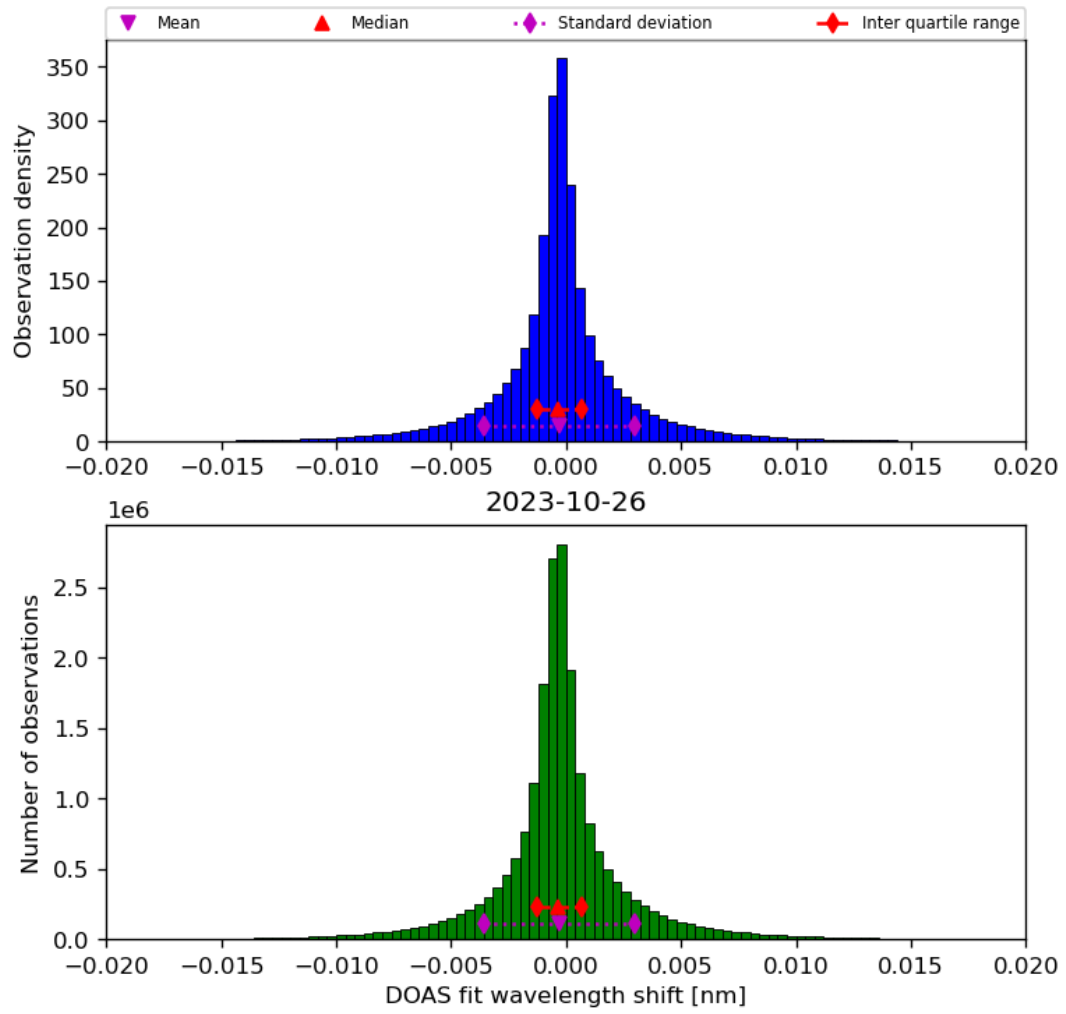
Figure 44: Histogram of “DOAS fit wavelength shift” for 2023-10-25 to 2023-10-27
