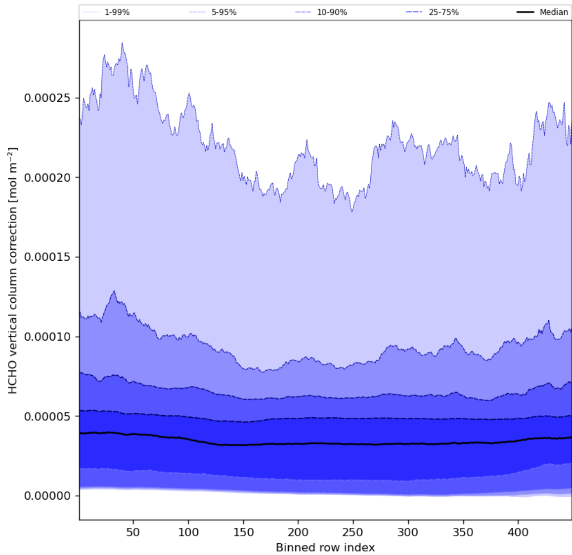
Figure 51: Along track statistics of “HCHO vertical column correction” for 2023-10-25 to 2023-10-27
