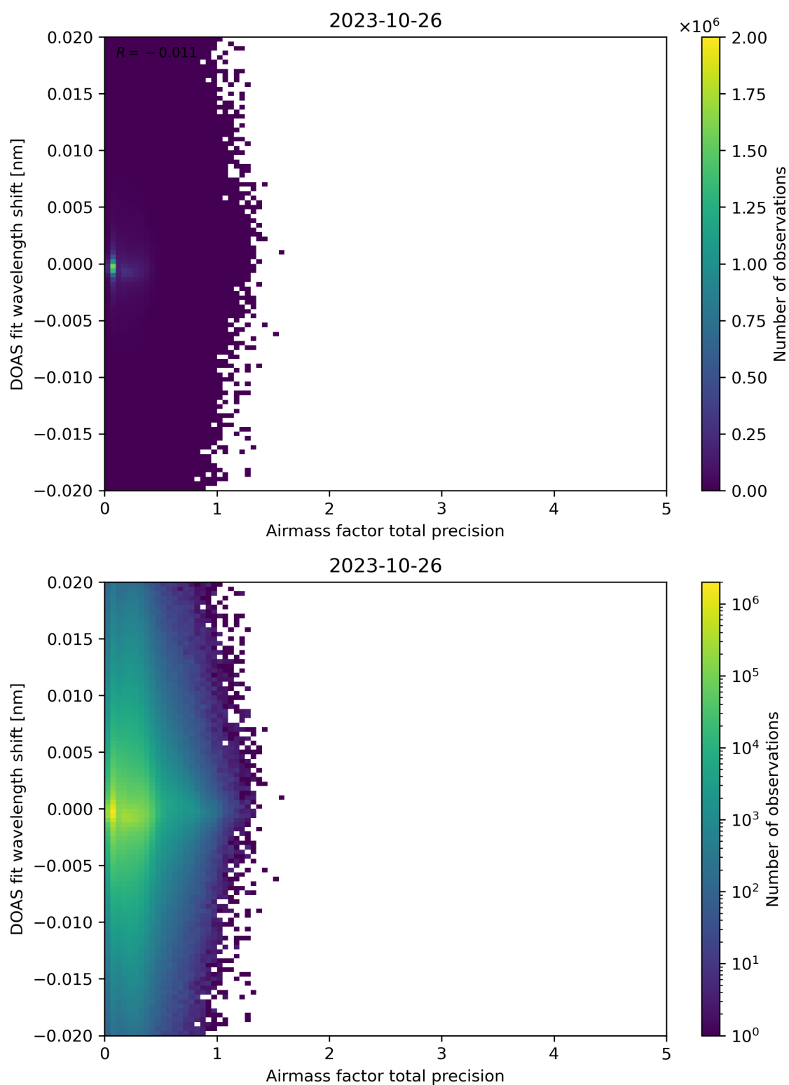
Figure 106: Scatter density plot of “Airmass factor total precision” against “DOAS fit wavelength shift” for 2023-10-25 to 2023-10-27.
