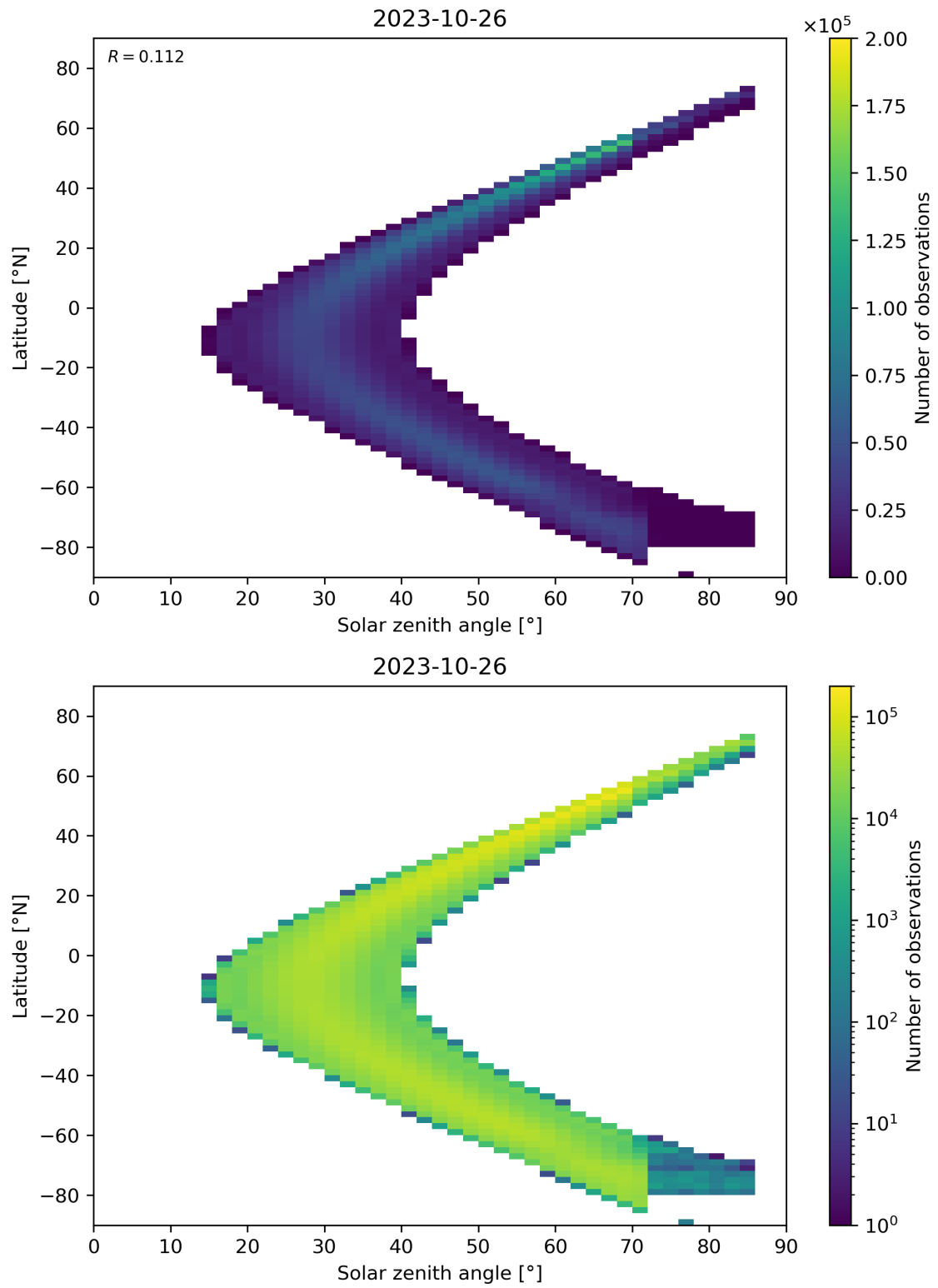
Figure 181: Scatter density plot of “Solar zenith angle” against “Latitude” for 2023-10-25 to 2023-10-27.
