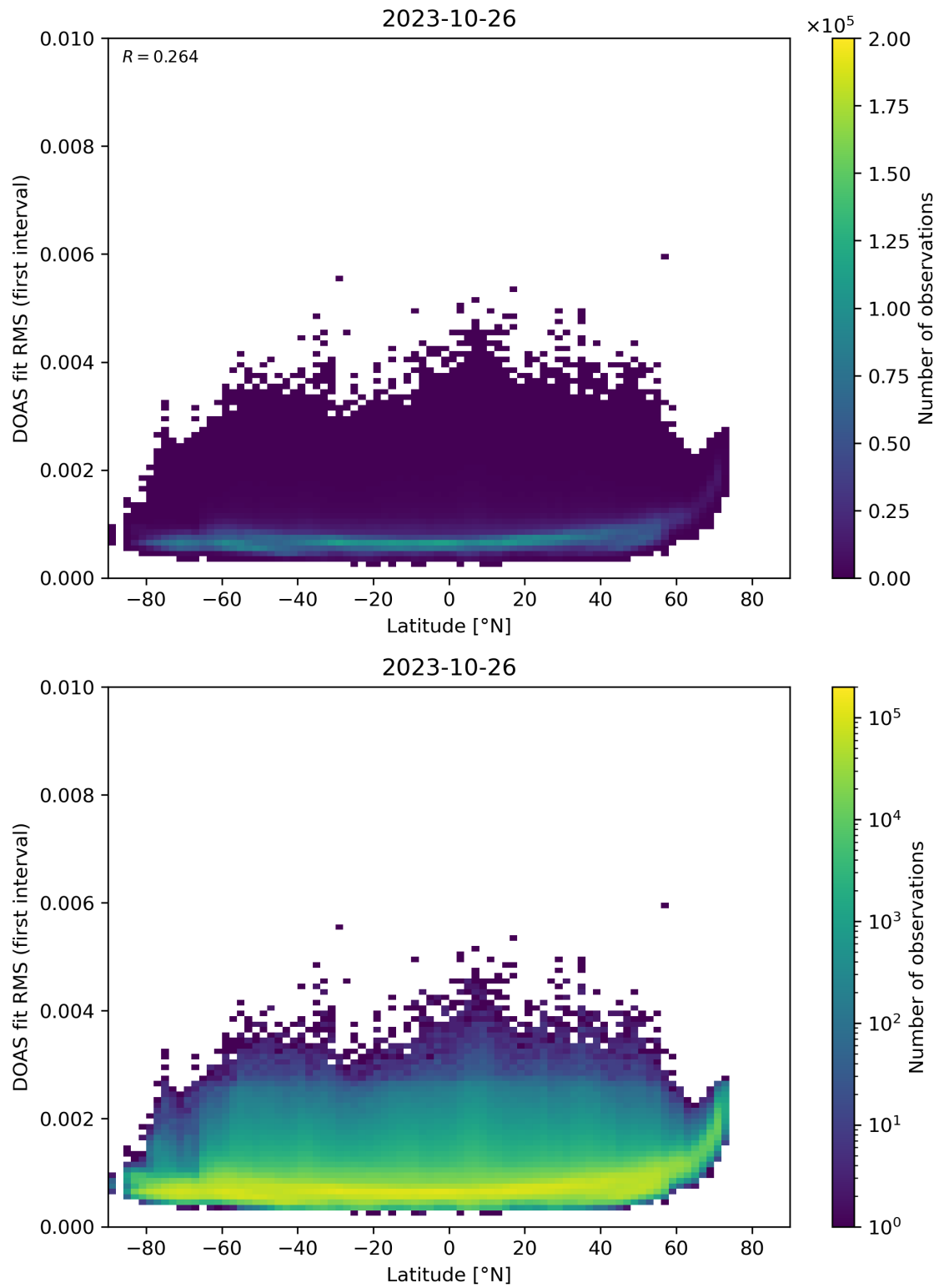
Figure 153: Scatter density plot of “Latitude” against “DOAS fit RMS (first interval)” for 2023-10-25 to 2023-10-27.
