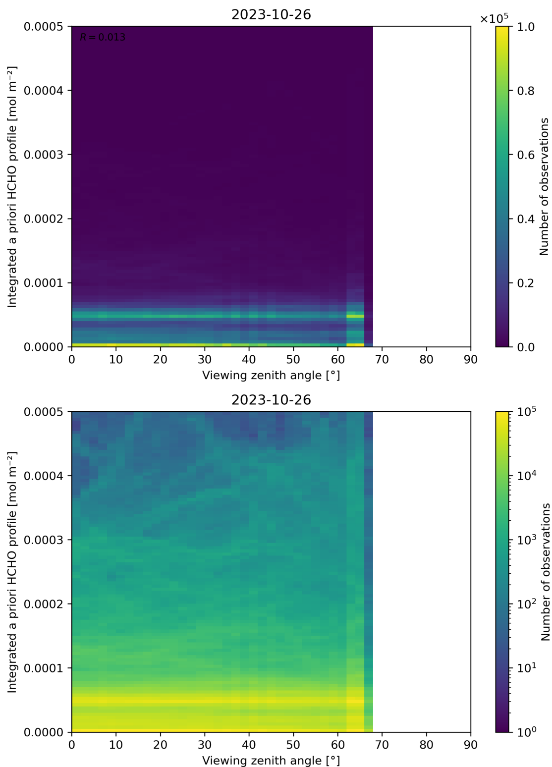
Figure 195: Scatter density plot of “Viewing zenith angle” against “Integrated a priori HCHO profile” for 2023-10-25 to 2023-10-27.
