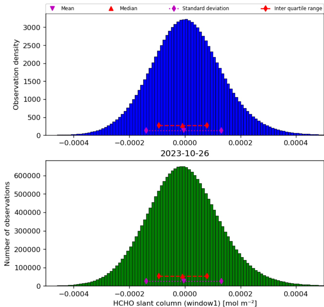
Figure 38: Histogram of “HCHO slant column (window1)” for 2023-10-25 to 2023-10-27
