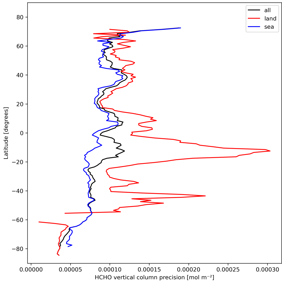
Figure 22: Zonal average of “HCHO vertical column precision” for 2023-10-25 to 2023-10-27.
