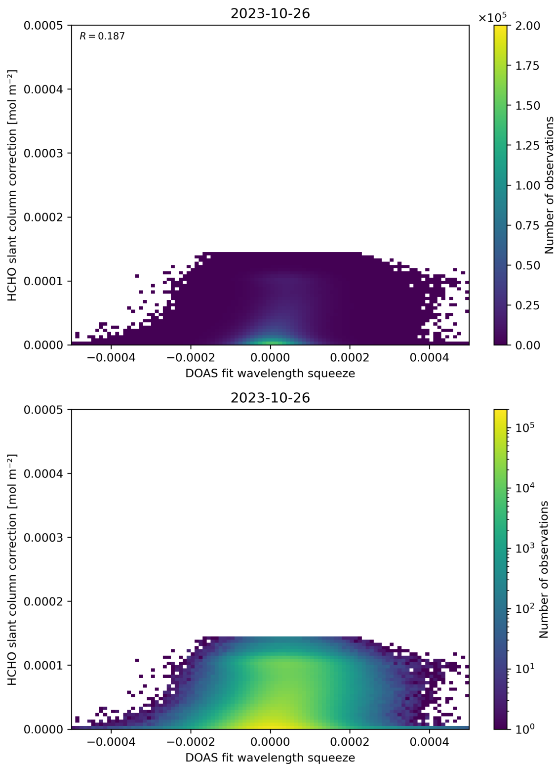
Figure 70: Scatter density plot of “DOAS fit wavelength squeeze” against “HCHO slant column correction” for 2023-10-25 to 2023-10-27.
