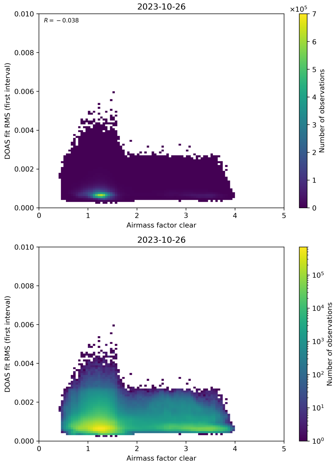
Figure 71: Scatter density plot of “Airmass factor clear” against “DOAS fit RMS (first interval)” for 2023-10-25 to 2023-10-27.
