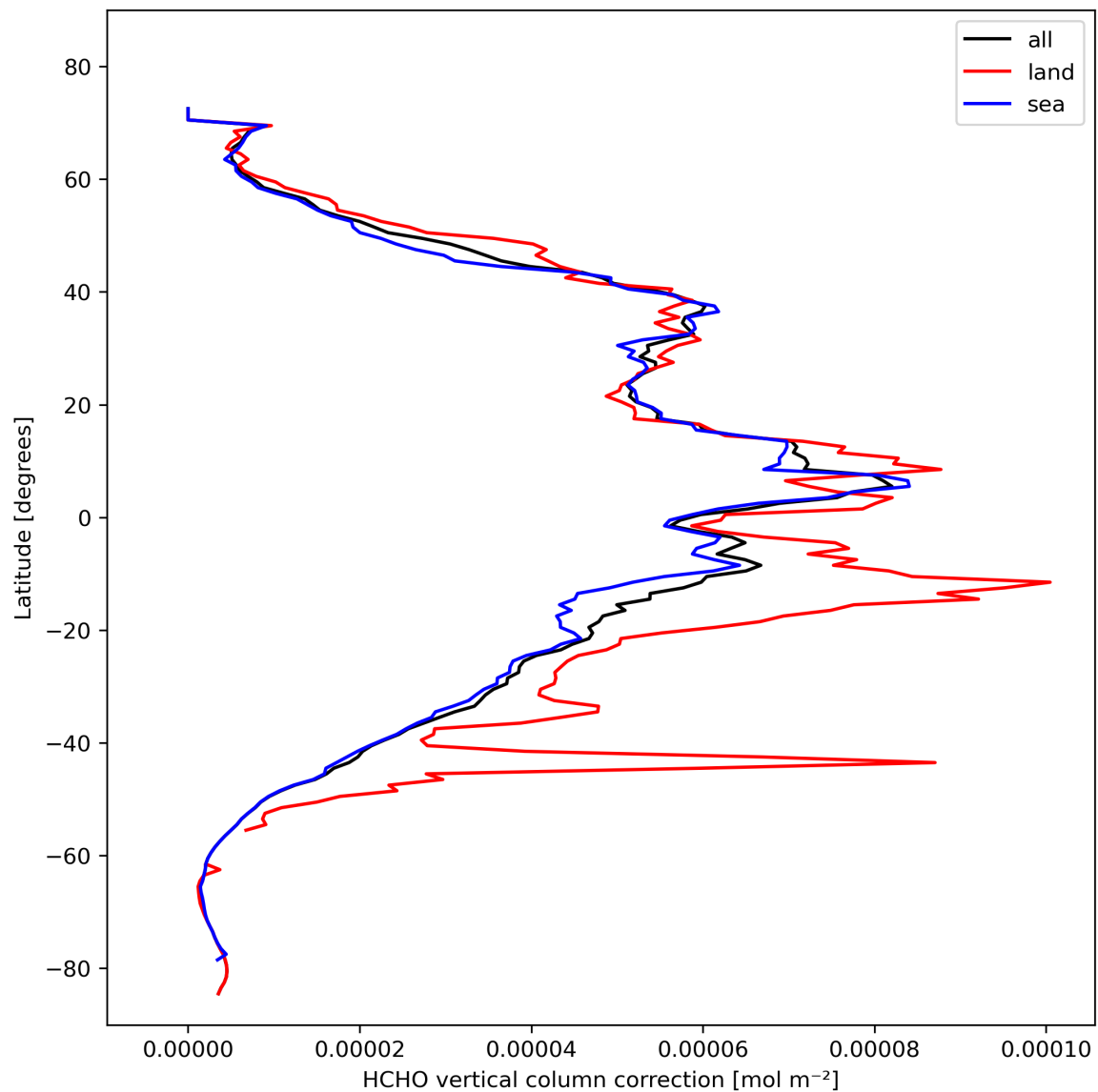
Figure 23: Zonal average of “HCHO vertical column correction” for 2023-10-25 to 2023-10-27.
