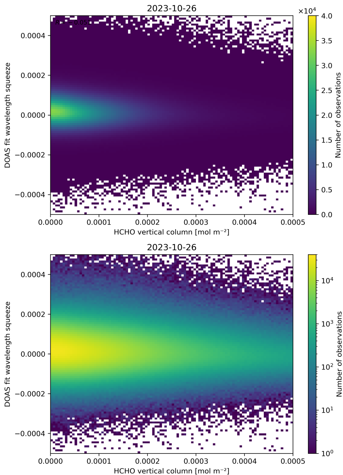
Figure 125: Scatter density plot of “HCHO vertical column” against “DOAS fit wavelength squeeze” for 2023-10-25 to 2023-10-27.
