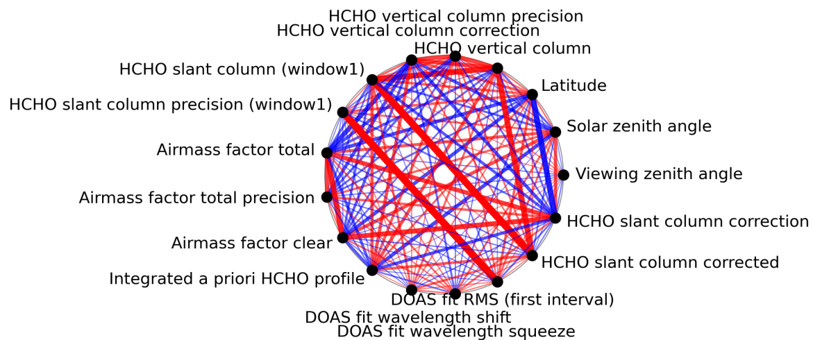
Figure 1: Map of correlation graph for 2023-10-25 to 2023-10-27.
