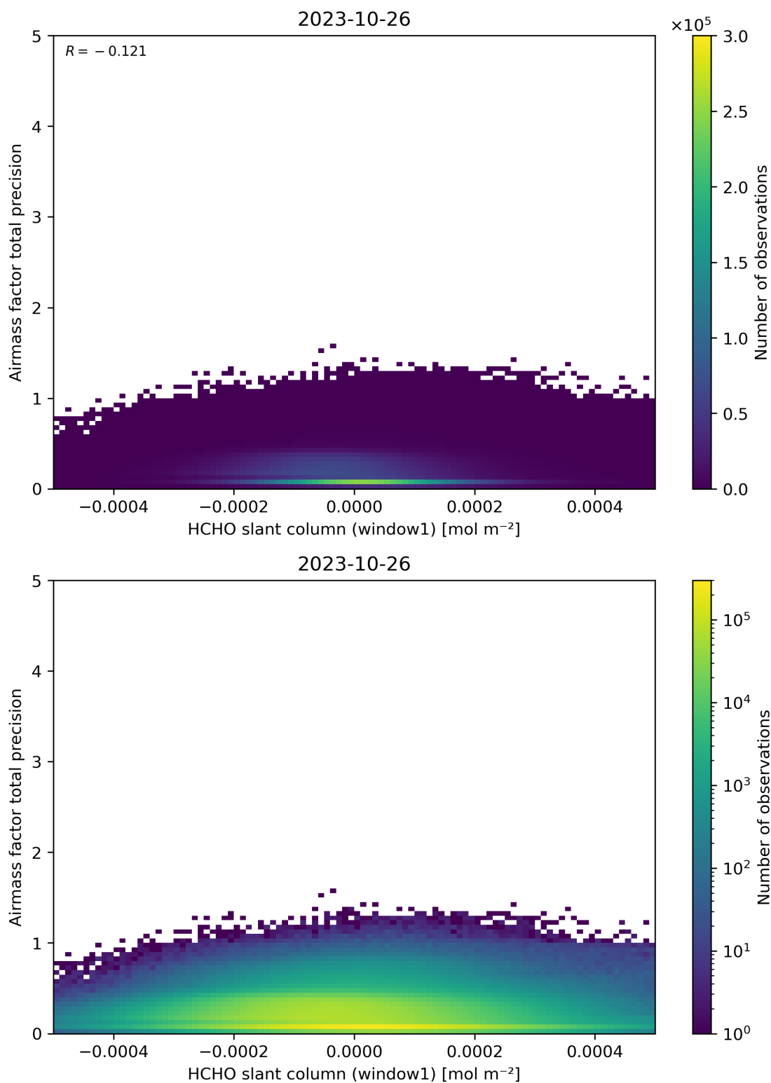
Figure 86: Scatter density plot of “HCHO slant column (window1)” against “Airmass factor total precision” for 2023-10-25 to 2023-10-27.
