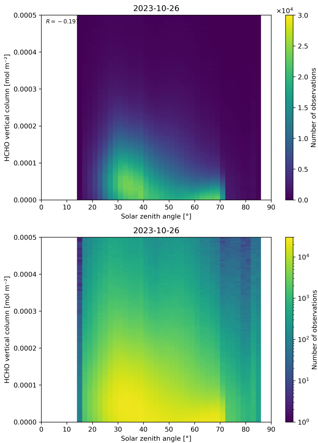
Figure 177: Scatter density plot of “Solar zenith angle” against “HCHO vertical column” for 2023-10-25 to 2023-10-27.
