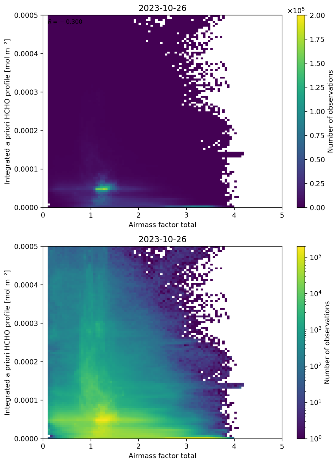
Figure 104: Scatter density plot of “Airmass factor total” against “Integrated a priori HCHO profile” for 2023-10-25 to 2023-10-27.
