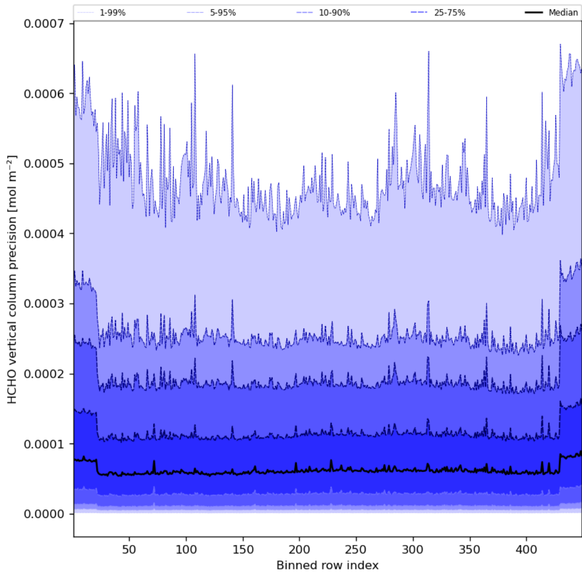
Figure 50: Along track statistics of “HCHO vertical column precision” for 2023-10-25 to 2023-10-27
