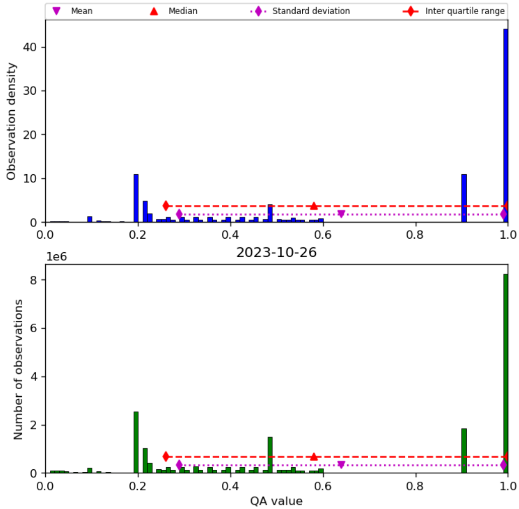
Figure 34: Histogram of “QA value” for 2023-10-25 to 2023-10-27
