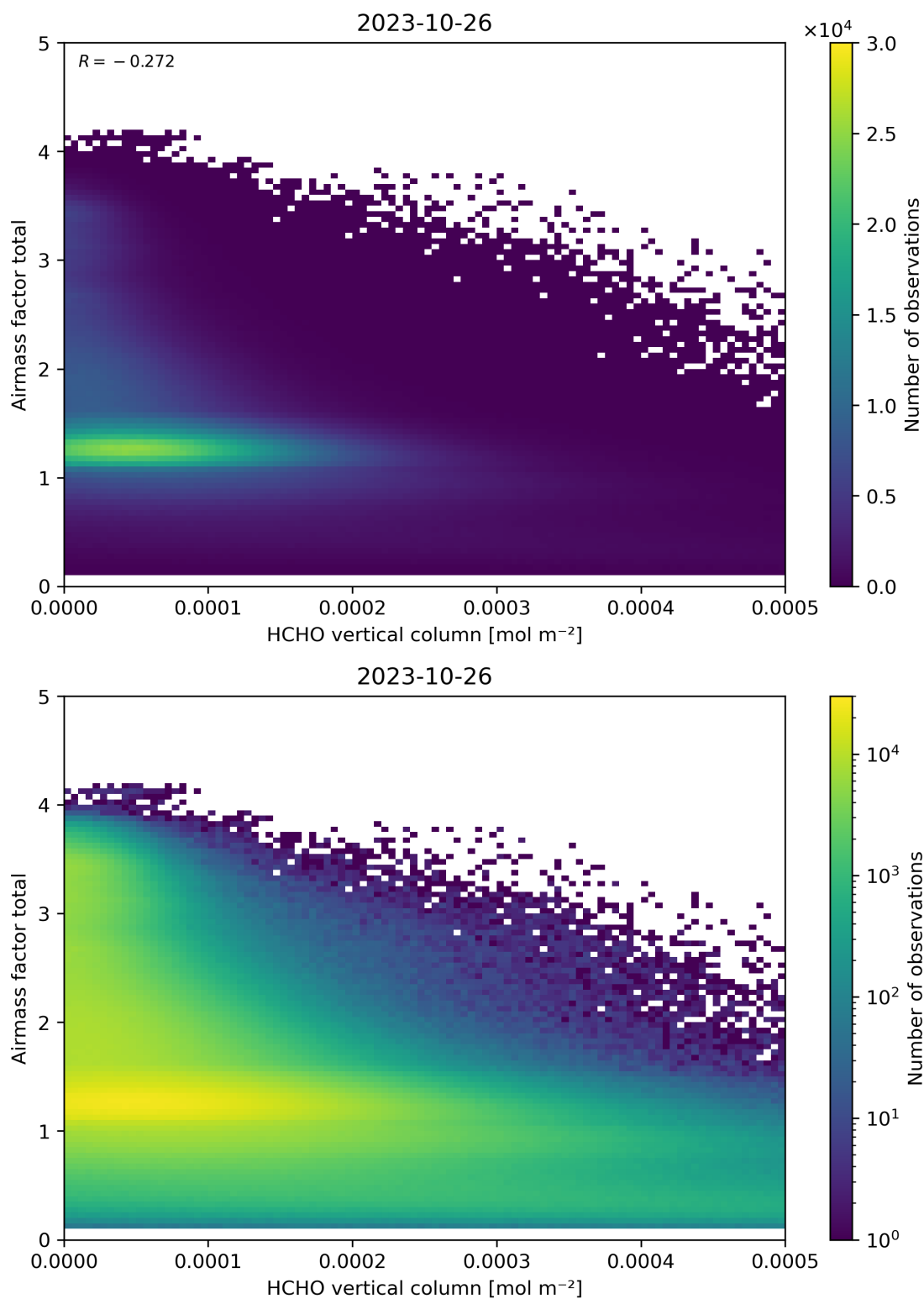
Figure 131: Scatter density plot of “HCHO vertical column” against “Airmass factor total” for 2023-10-25 to 2023-10-27.
