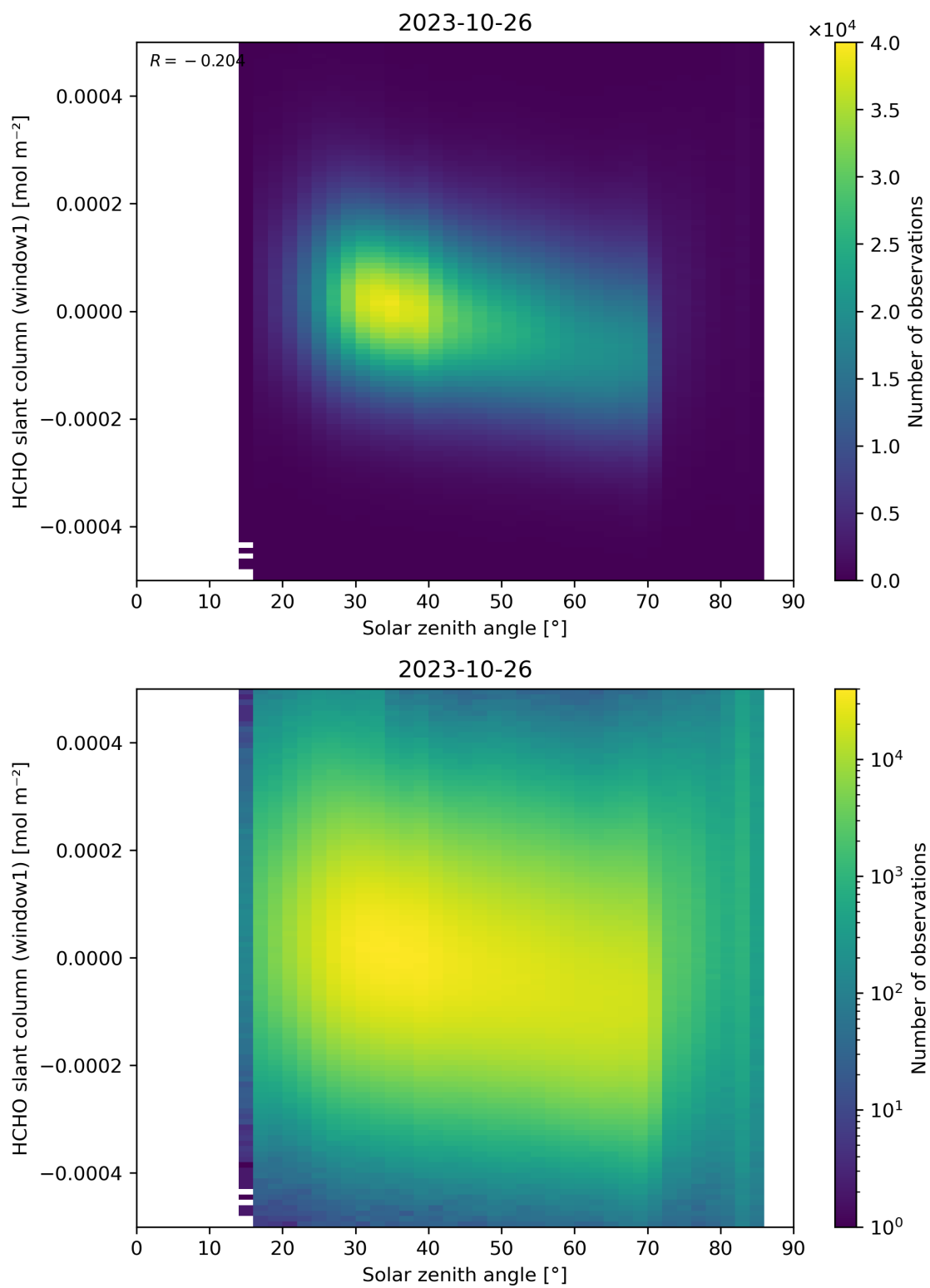
Figure 173: Scatter density plot of “Solar zenith angle” against “HCHO slant column (window1)” for 2023-10-25 to 2023-10-27.
