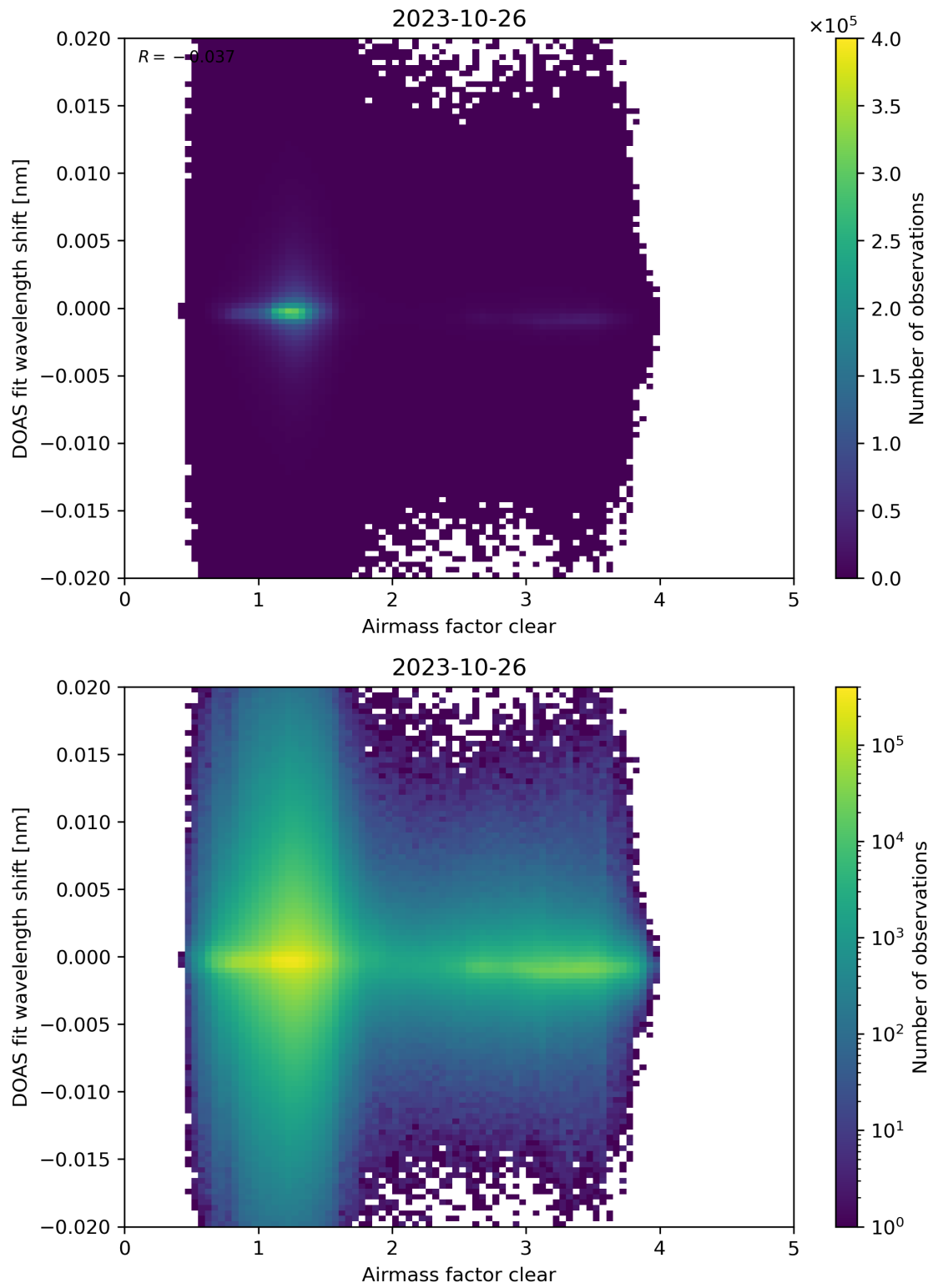
Figure 72: Scatter density plot of “Airmass factor clear” against “DOAS fit wavelength shift” for 2023-10-25 to 2023-10-27.
