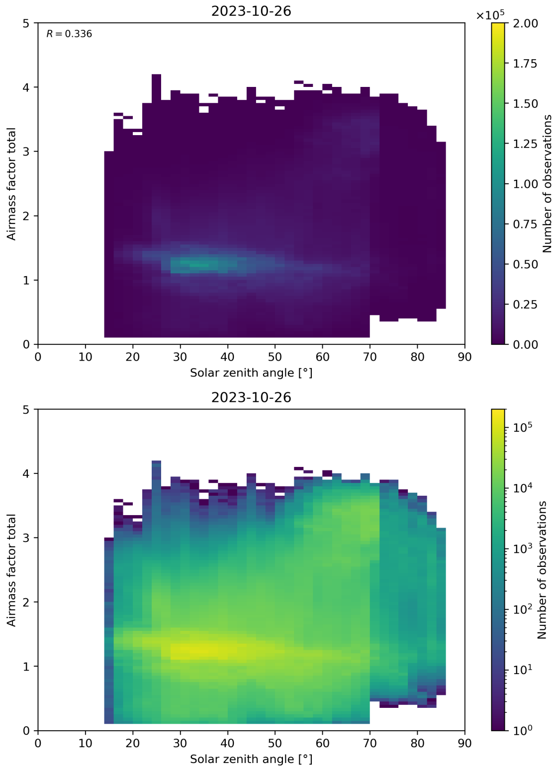
Figure 175: Scatter density plot of “Solar zenith angle” against “Airmass factor total” for 2023-10-25 to 2023-10-27.
