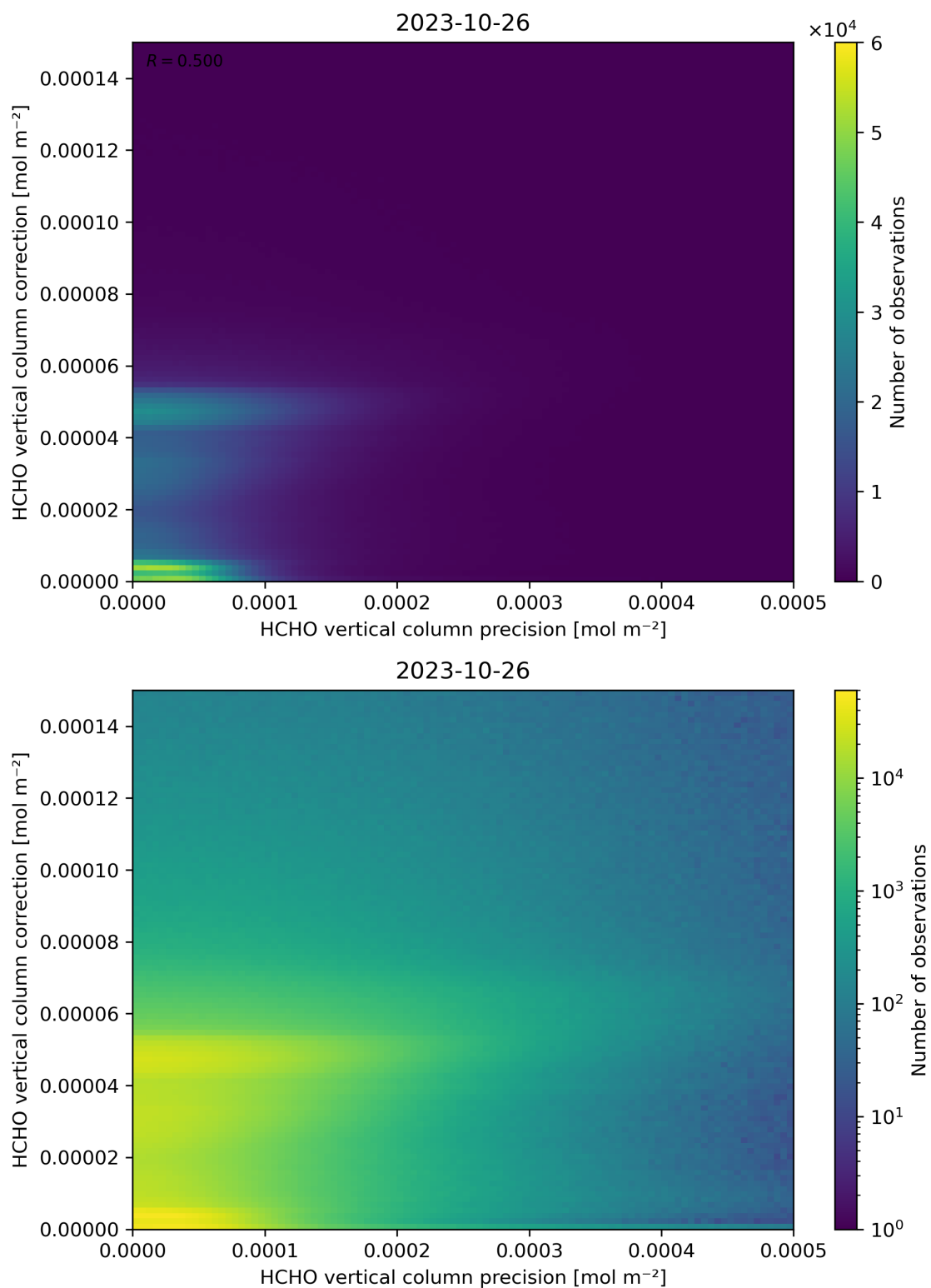
Figure 146: Scatter density plot of “HCHO vertical column precision” against “HCHO vertical column correction” for 2023-10-25 to 2023-10-27.
