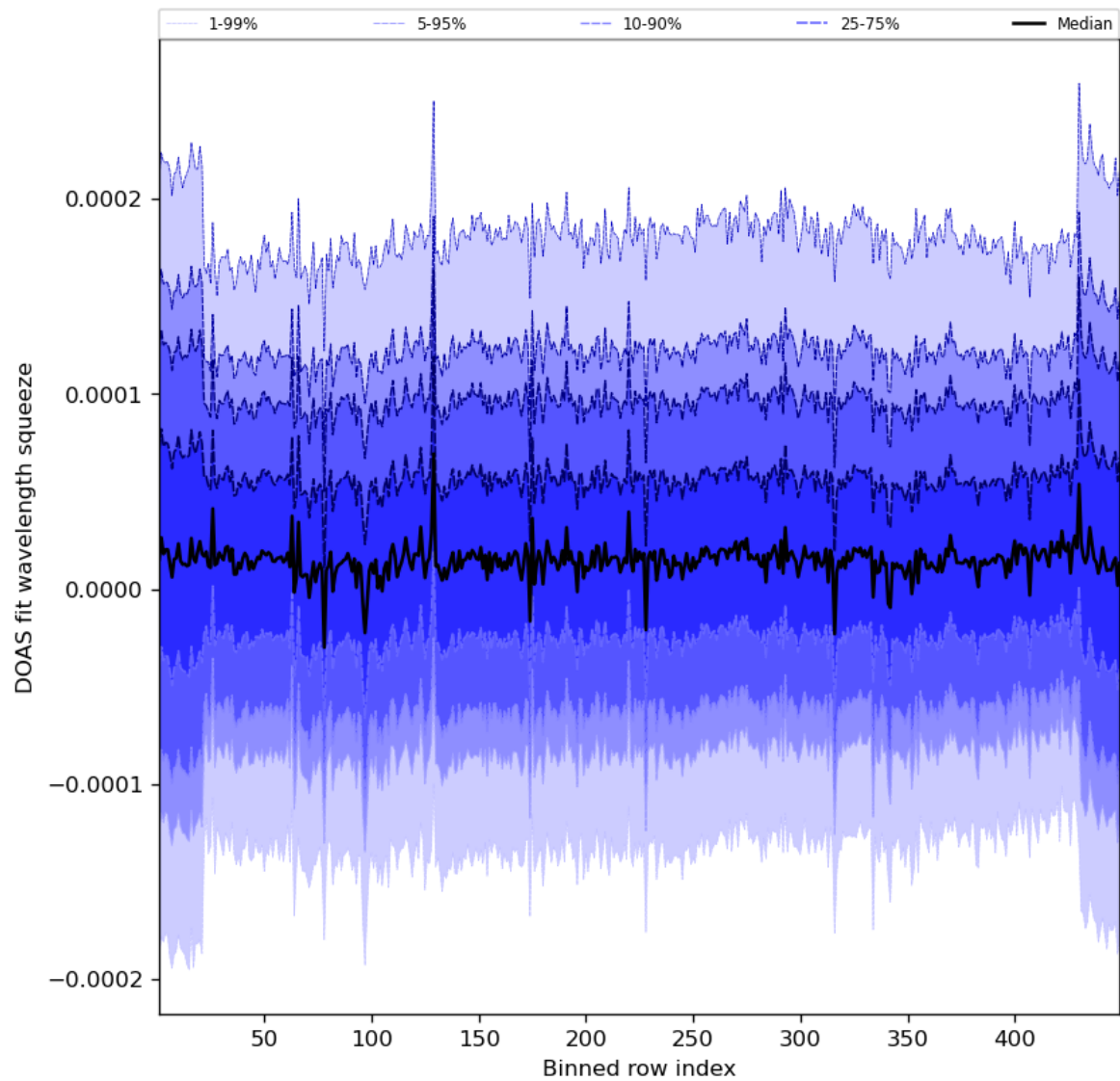
Figure 59: Along track statistics of “DOAS fit wavelength squeeze” for 2023-10-25 to 2023-10-27
