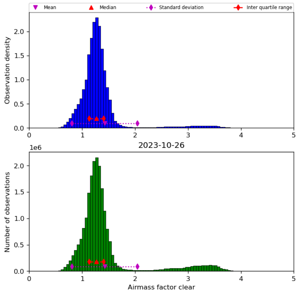
Figure 42: Histogram of “Airmass factor clear” for 2023-10-25 to 2023-10-27
