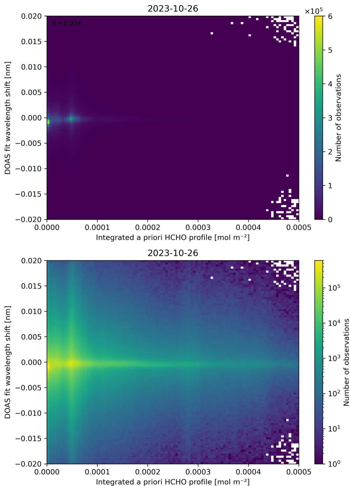
Figure 149: Scatter density plot of “Integrated a priori HCHO profile” against “DOAS fit wavelength shift” for 2023-10-25 to 2023-10-27.
