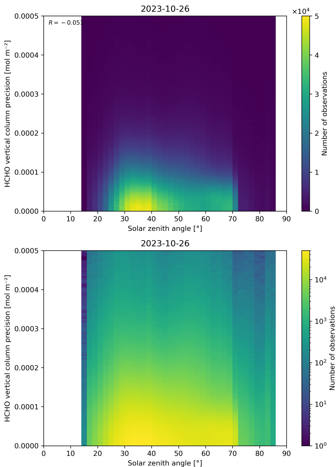
Figure 179: Scatter density plot of “Solar zenith angle” against “HCHO vertical column precision” for 2023-10-25 to 2023-10-27.
