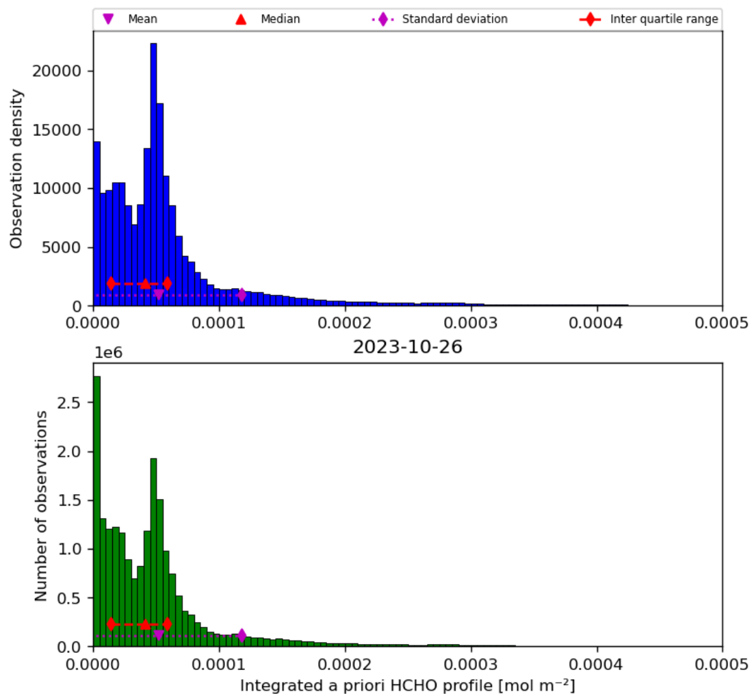
Figure 43: Histogram of “Integrated a priori HCHO profile” for 2023-10-25 to 2023-10-27
