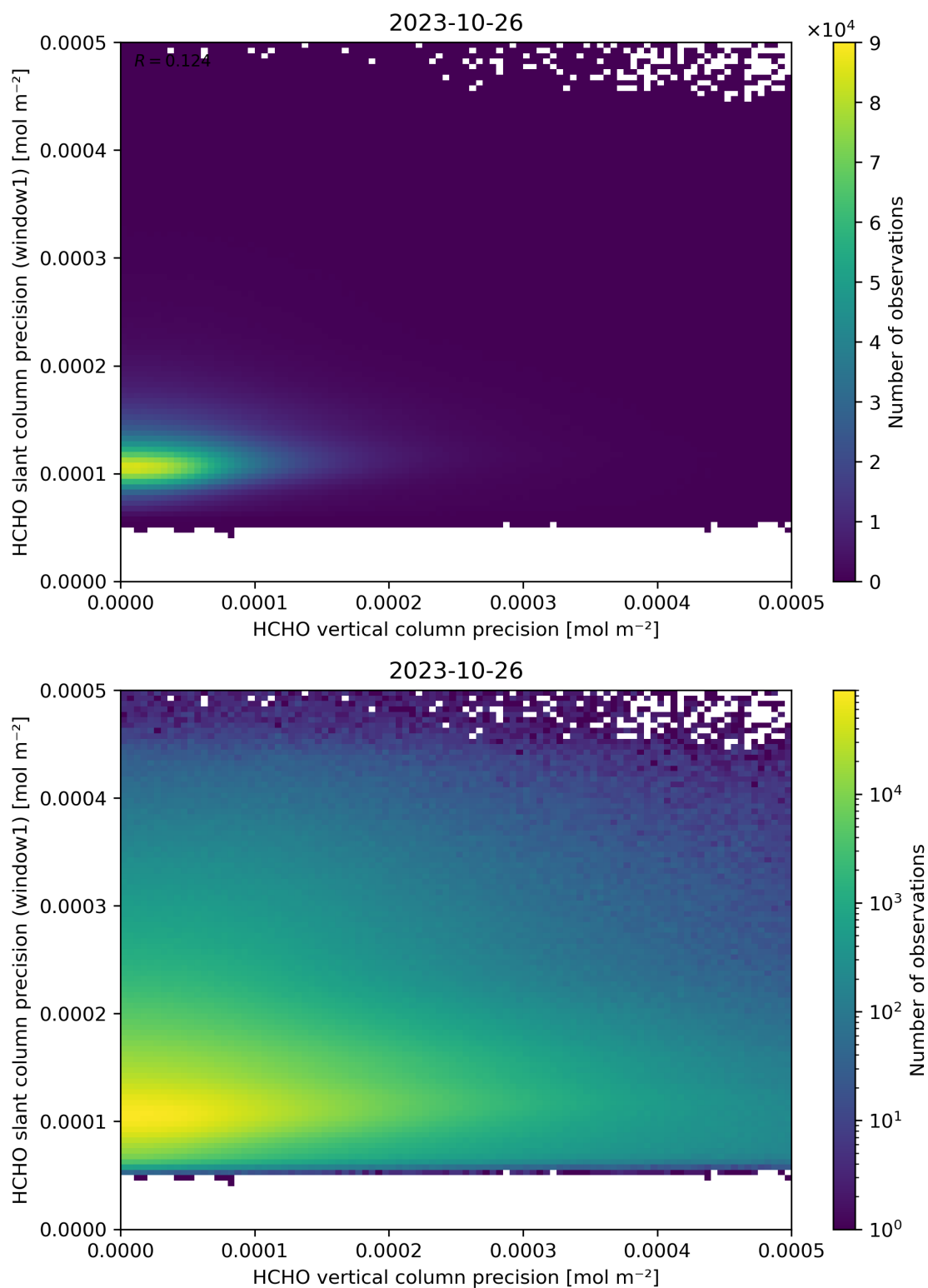
Figure 143: Scatter density plot of “HCHO vertical column precision” against “HCHO slant column precision (window1)” for 2023-10-25 to 2023-10-27.
