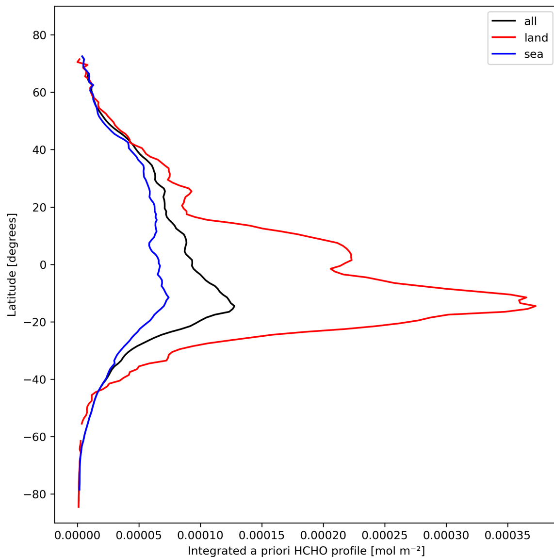
Figure 29: Zonal average of “Integrated a priori HCHO profile” for 2023-10-25 to 2023-10-27.
