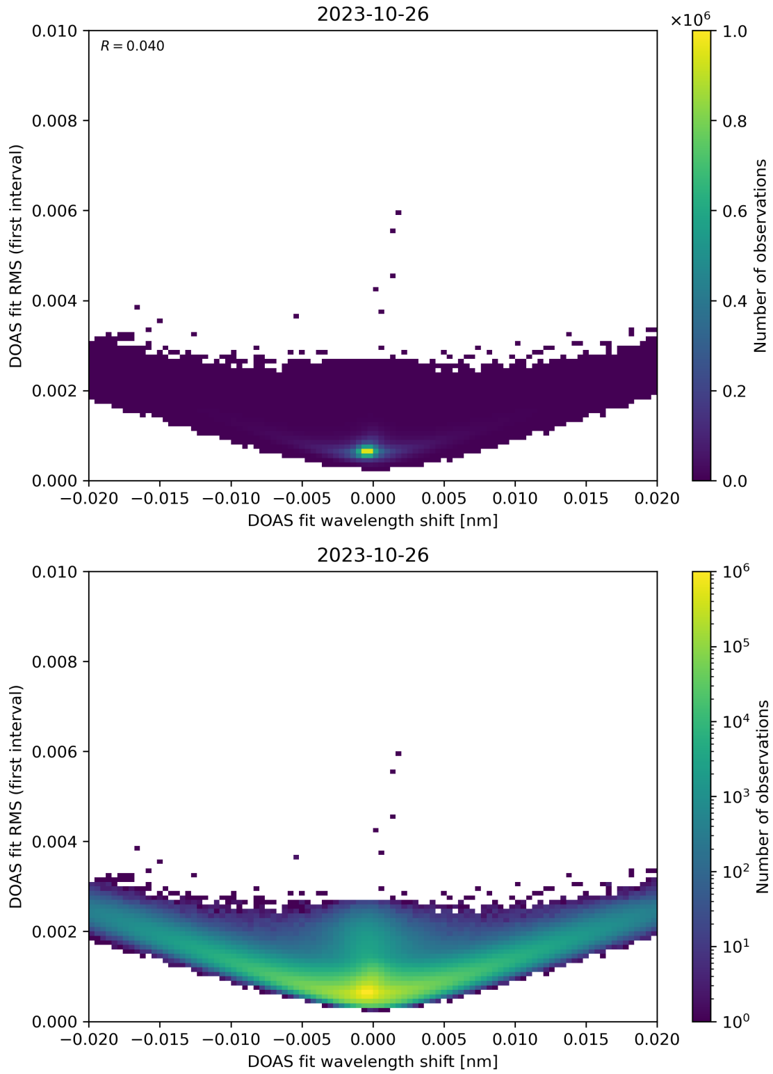
Figure 64: Scatter density plot of “DOAS fit wavelength shift” against “DOAS fit RMS (first interval)” for 2023-10-25 to 2023-10-27.
