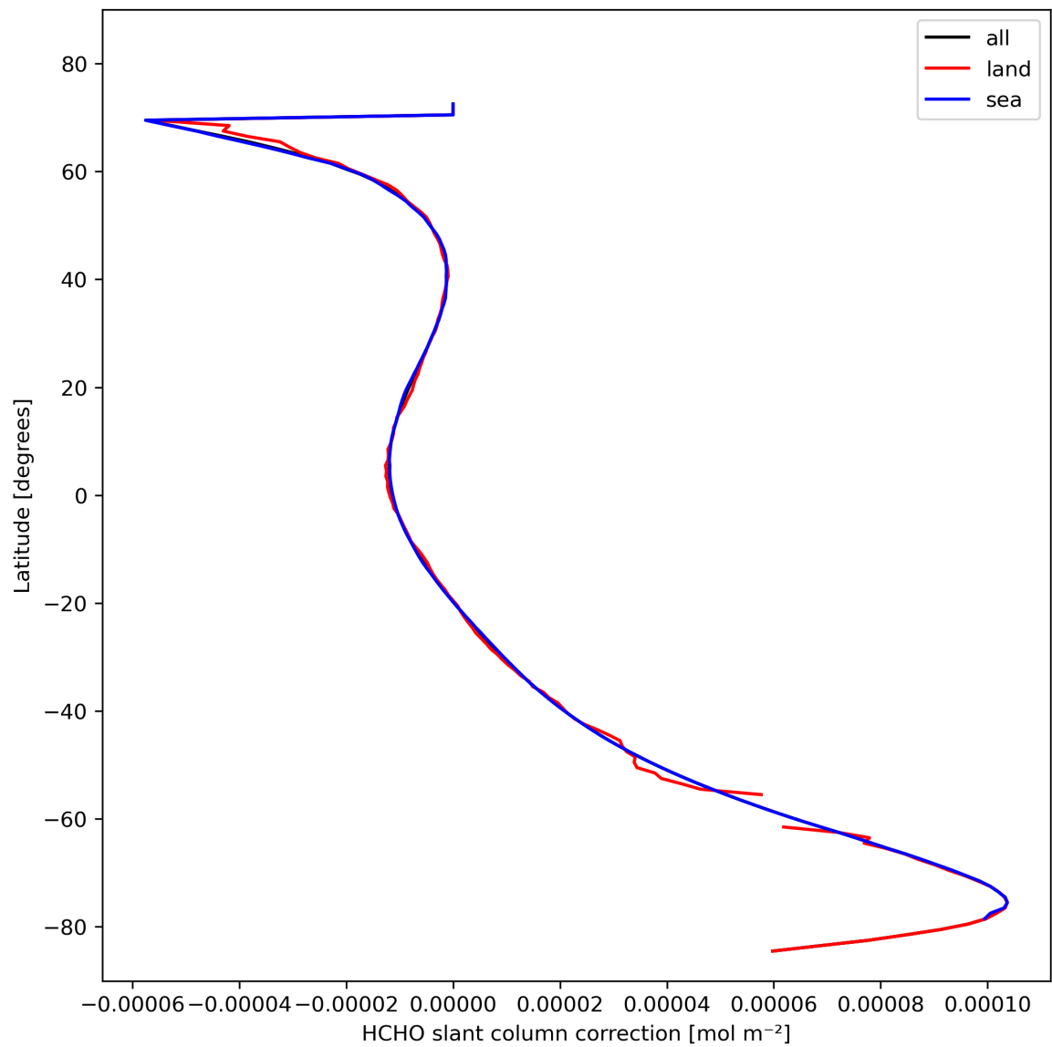
Figure 33: Zonal average of “HCHO slant column correction” for 2023-10-25 to 2023-10-27.
