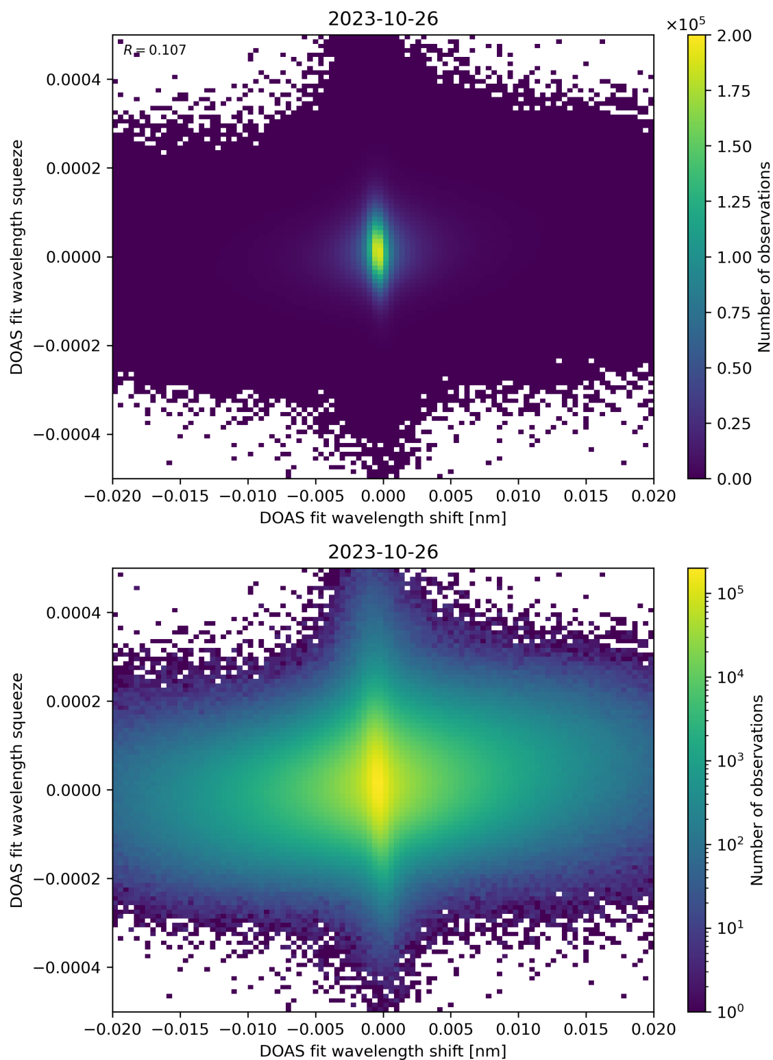
Figure 65: Scatter density plot of “DOAS fit wavelength shift” against “DOAS fit wavelength squeeze” for 2023-10-25 to 2023-10-27.
