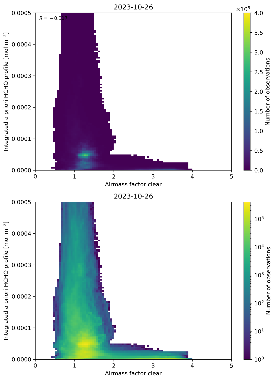
Figure 76: Scatter density plot of “Airmass factor clear” against “Integrated a priori HCHO profile” for 2023-10-25 to 2023-10-27.
