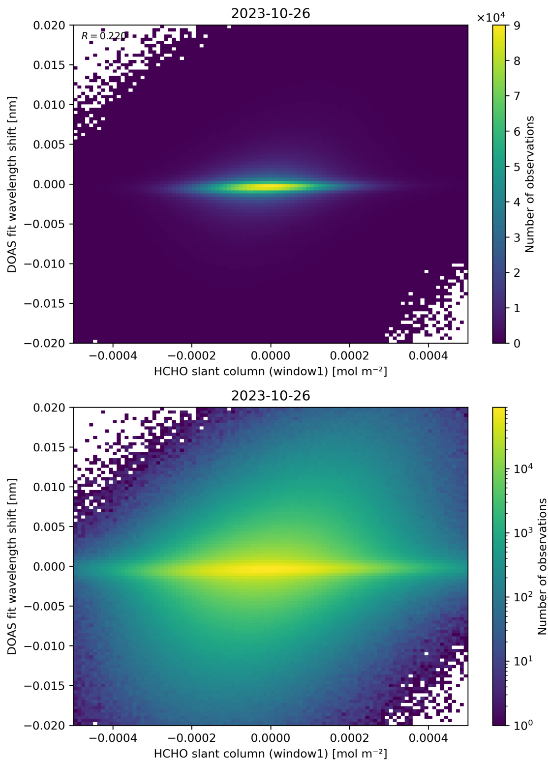
Figure 79: Scatter density plot of “HCHO slant column (window1)” against “DOAS fit wavelength shift” for 2023-10-25 to 2023-10-27.
