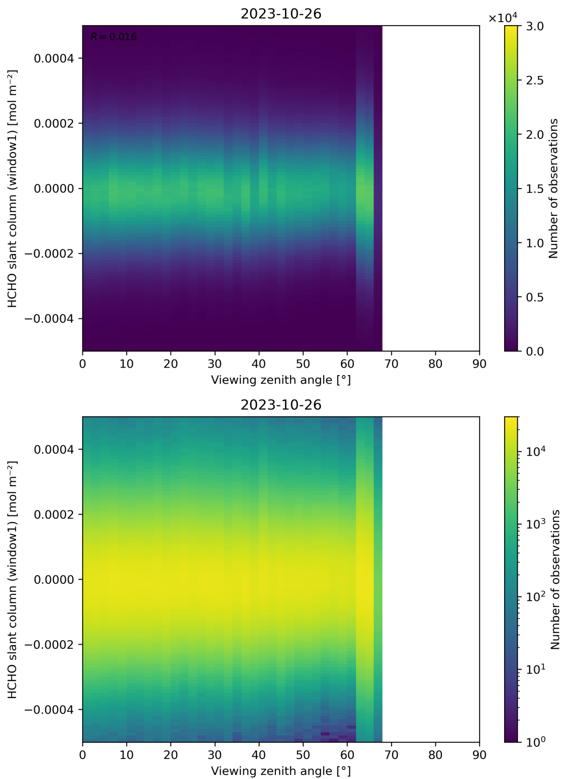
Figure 188: Scatter density plot of “Viewing zenith angle” against “HCHO slant column (window1)” for 2023-10-25 to 2023-10-27.
