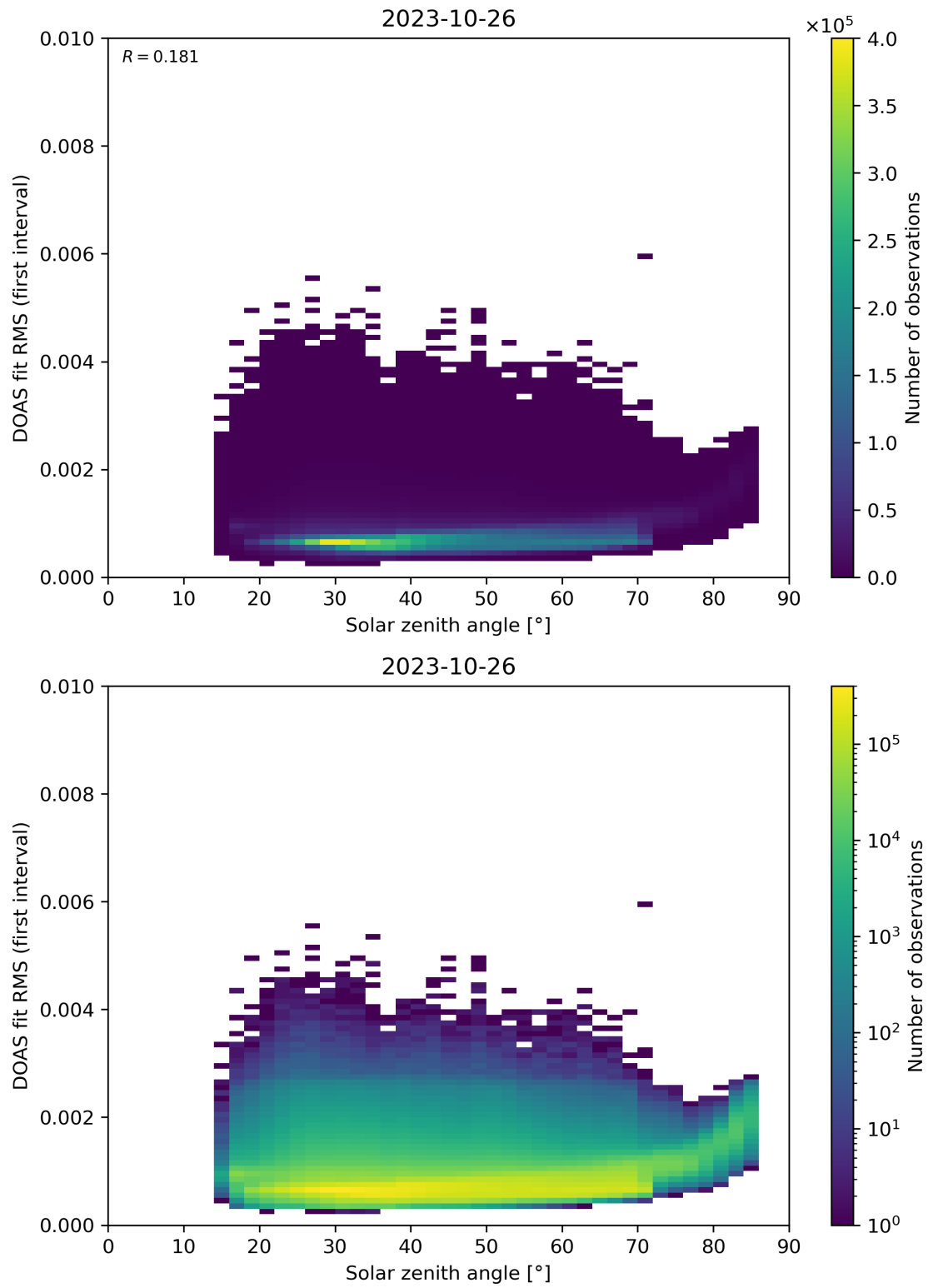
Figure 167: Scatter density plot of “Solar zenith angle” against “DOAS fit RMS (first interval)” for 2023-10-25 to 2023-10-27.
