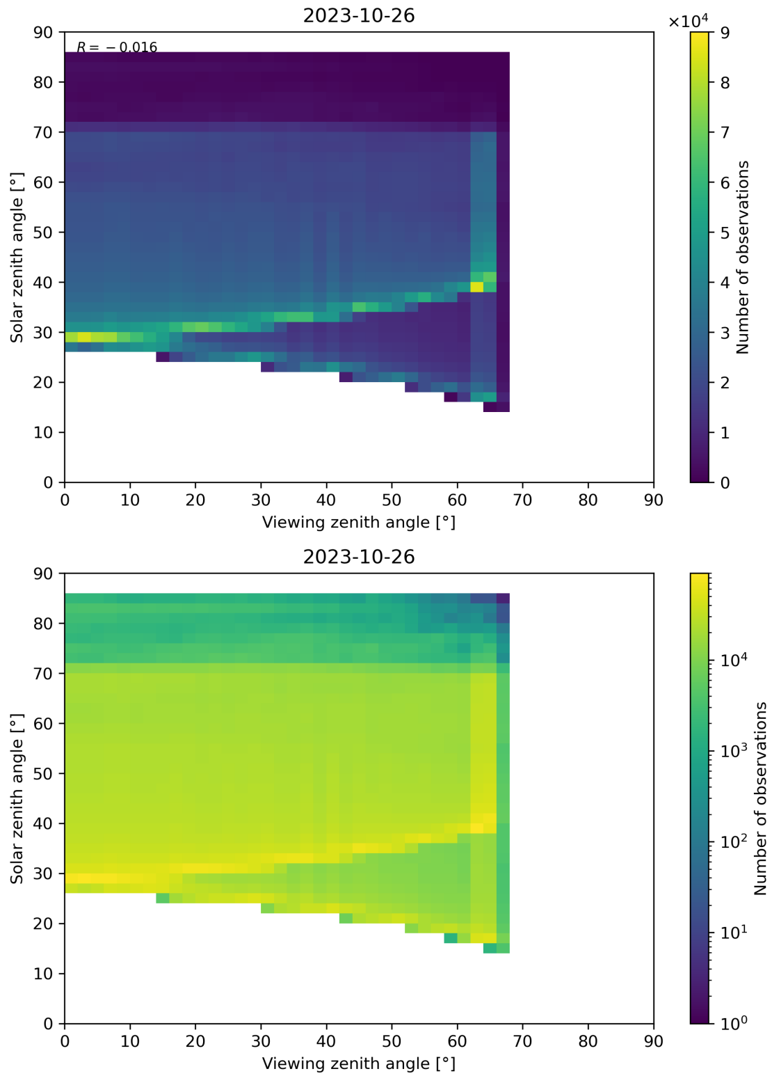
Figure 197: Scatter density plot of “Viewing zenith angle” against “Solar zenith angle” for 2023-10-25 to 2023-10-27.
