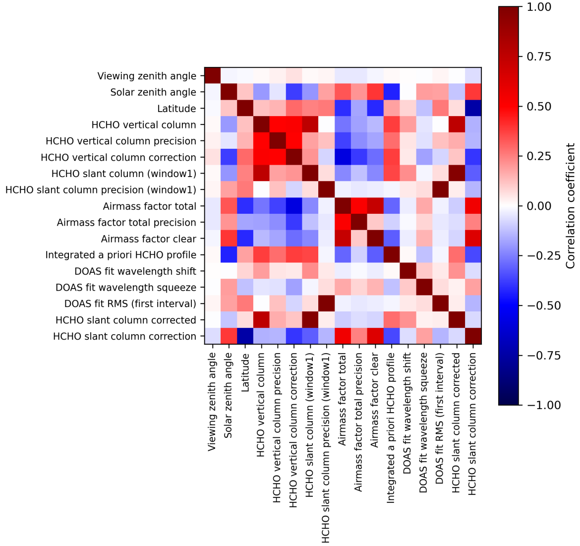
Figure 2: Map of correlation matrix for 2023-10-25 to 2023-10-27.
