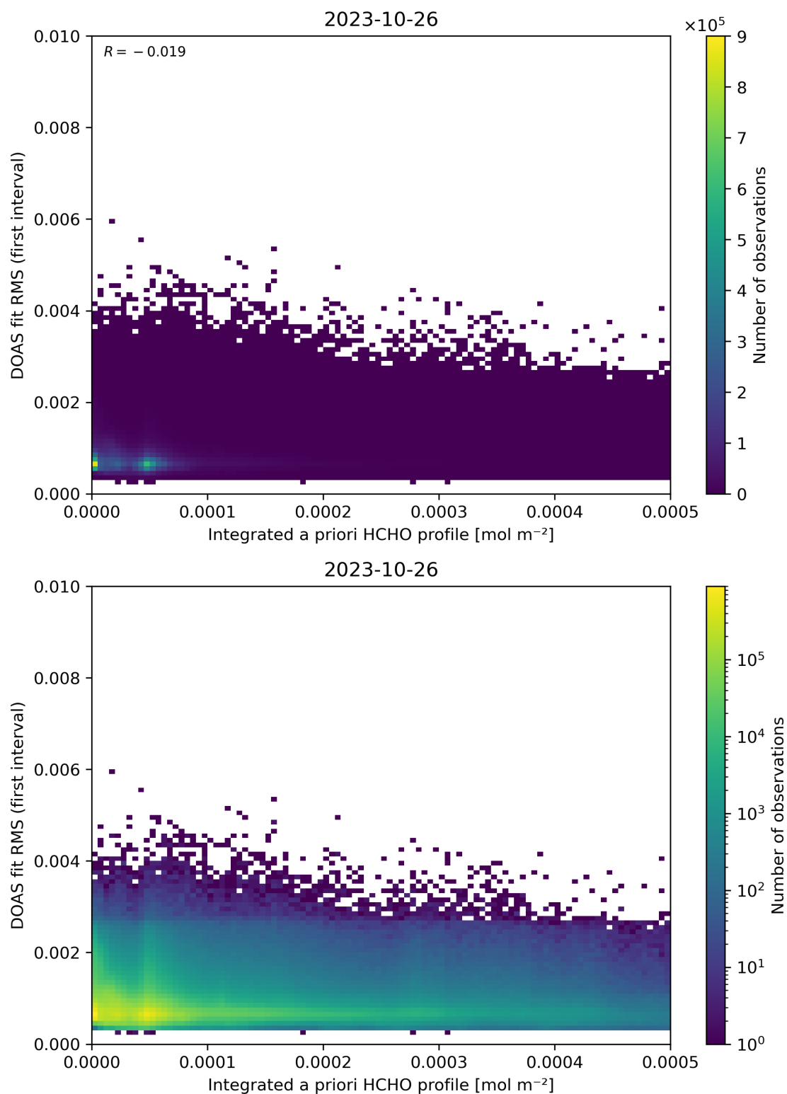
Figure 148: Scatter density plot of “Integrated a priori HCHO profile” against “DOAS fit RMS (first interval)” for 2023-10-25 to 2023-10-27.
