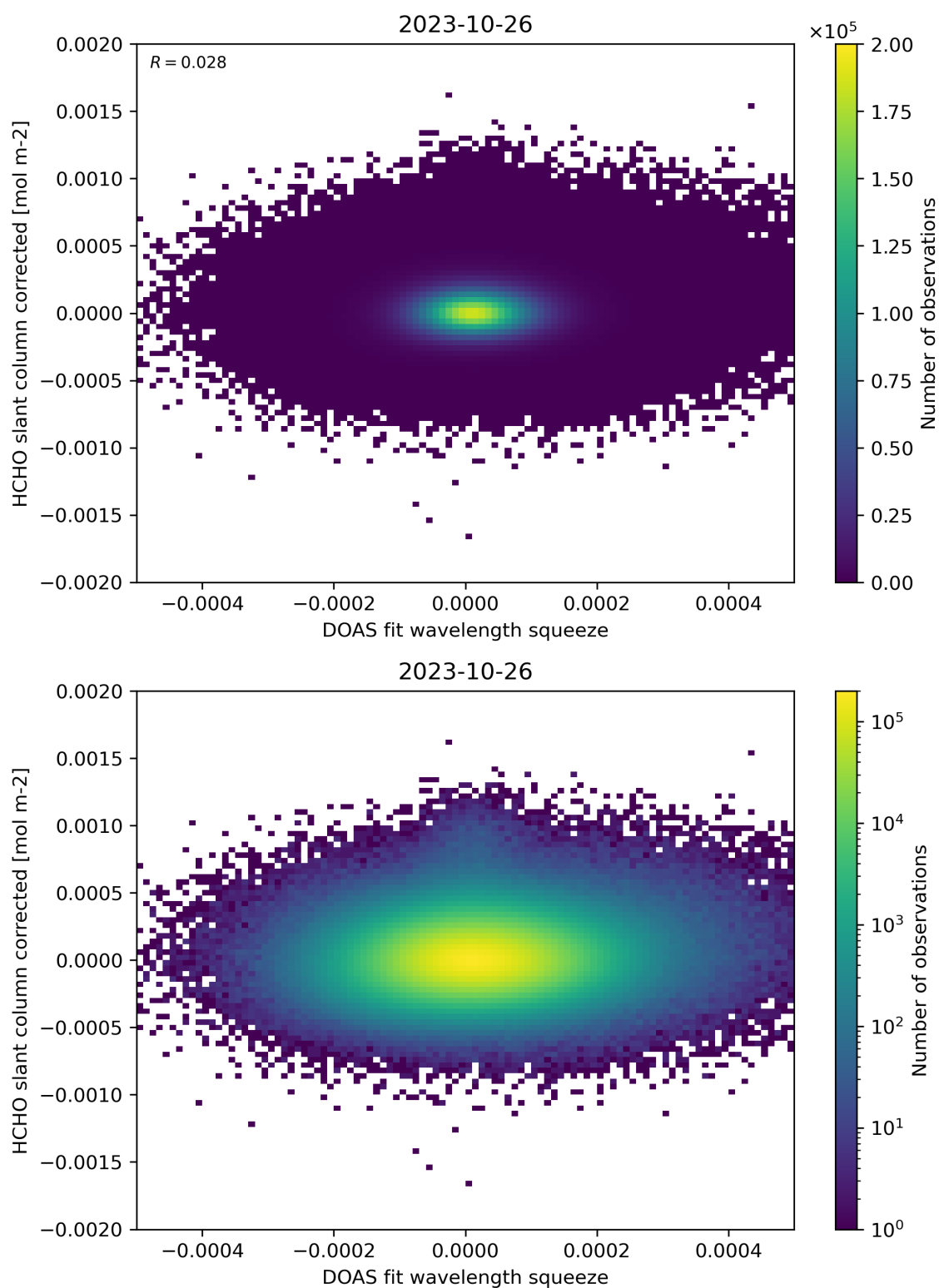
Figure 69: Scatter density plot of “DOAS fit wavelength squeeze” against “HCHO slant column corrected” for 2023-10-25 to 2023-10-27.
