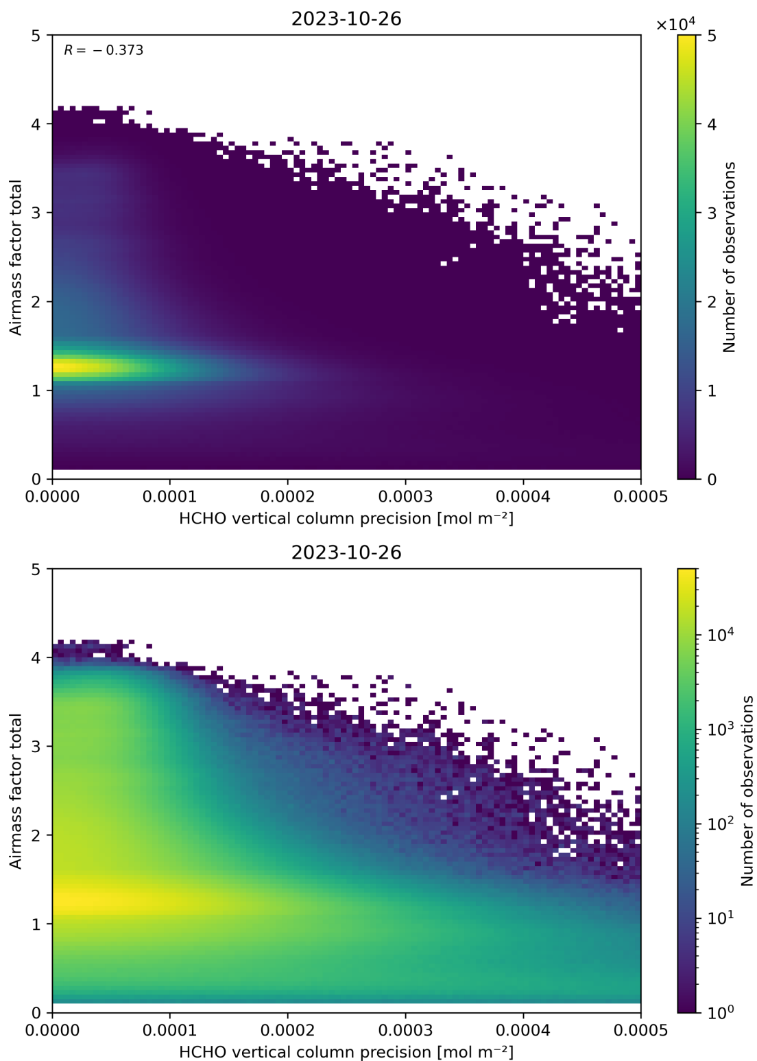
Figure 144: Scatter density plot of “HCHO vertical column precision” against “Airmass factor total” for 2023-10-25 to 2023-10-27.
