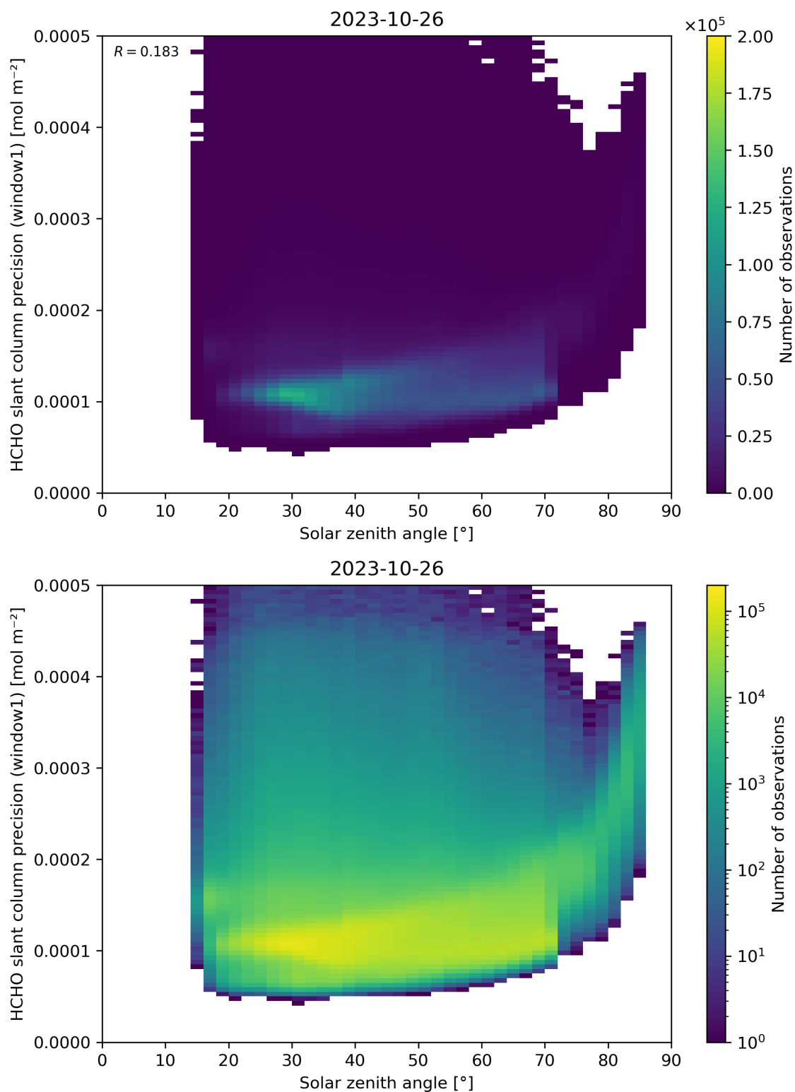
Figure 174: Scatter density plot of “Solar zenith angle” against “HCHO slant column precision (window1)” for 2023-10-25 to 2023-10-27.
