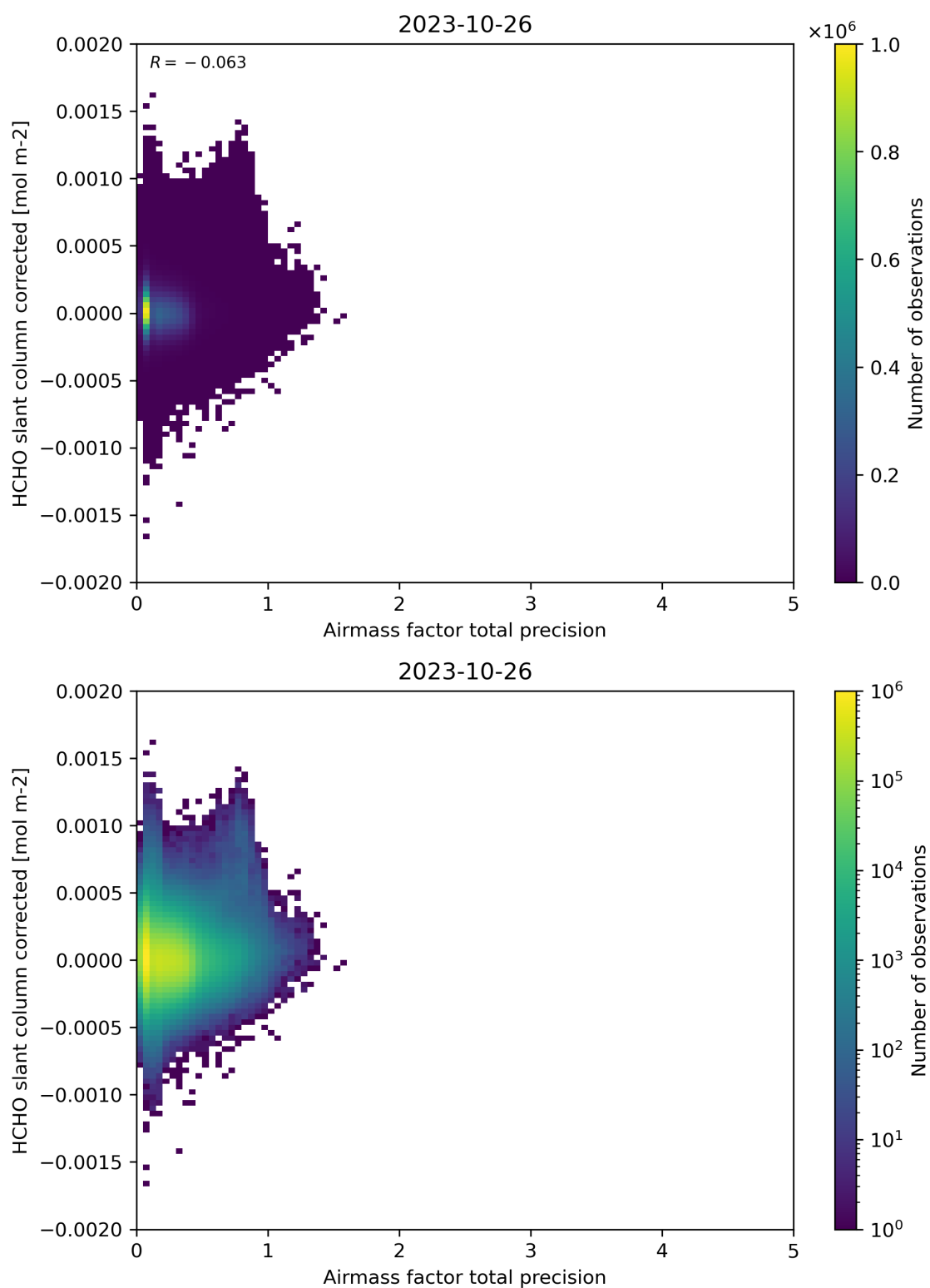
Figure 109: Scatter density plot of “Airmass factor total precision” against “HCHO slant column corrected” for 2023-10-25 to 2023-10-27.
