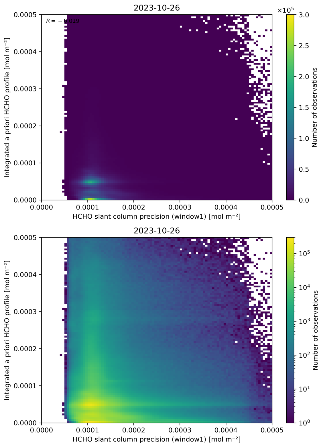
Figure 96: Scatter density plot of “HCHO slant column precision (window1)” against “Integrated a priori HCHO profile” for 2023-10-25 to 2023-10-27.
