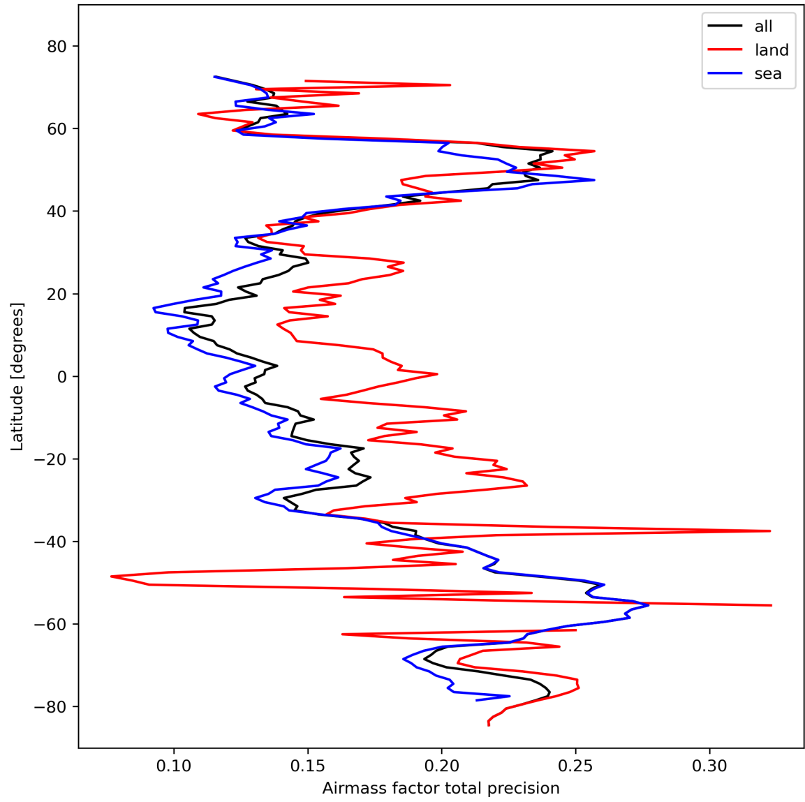
Figure 27: Zonal average of “Airmass factor total precision” for 2023-10-25 to 2023-10-27.
