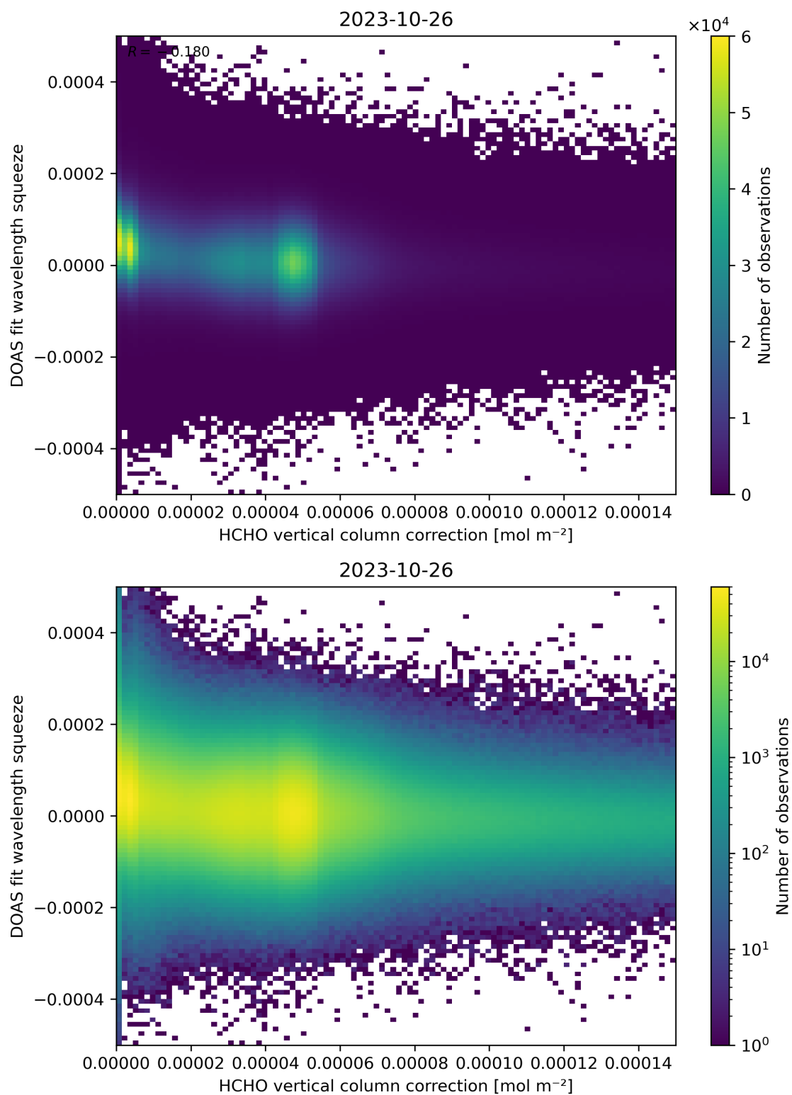
Figure 114: Scatter density plot of “HCHO vertical column correction” against “DOAS fit wavelength squeeze” for 2023-10-25 to 2023-10-27.
