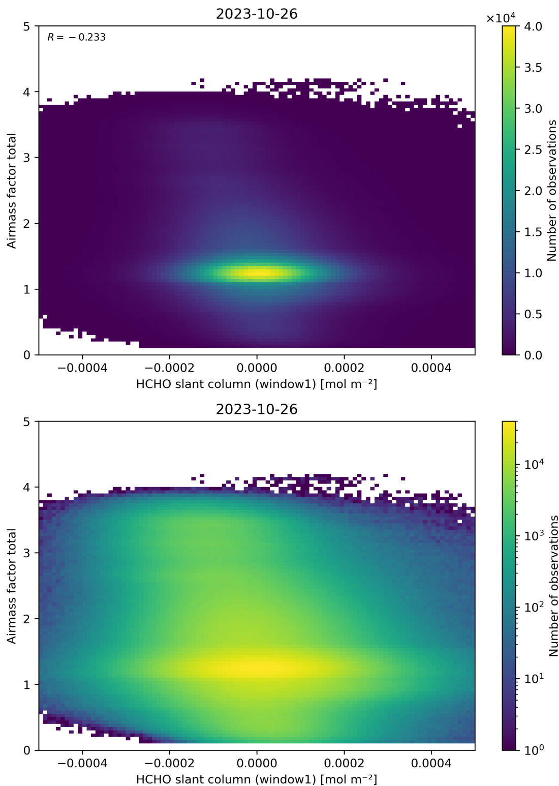
Figure 85: Scatter density plot of “HCHO slant column (window1)” against “Airmass factor total” for 2023-10-25 to 2023-10-27.
