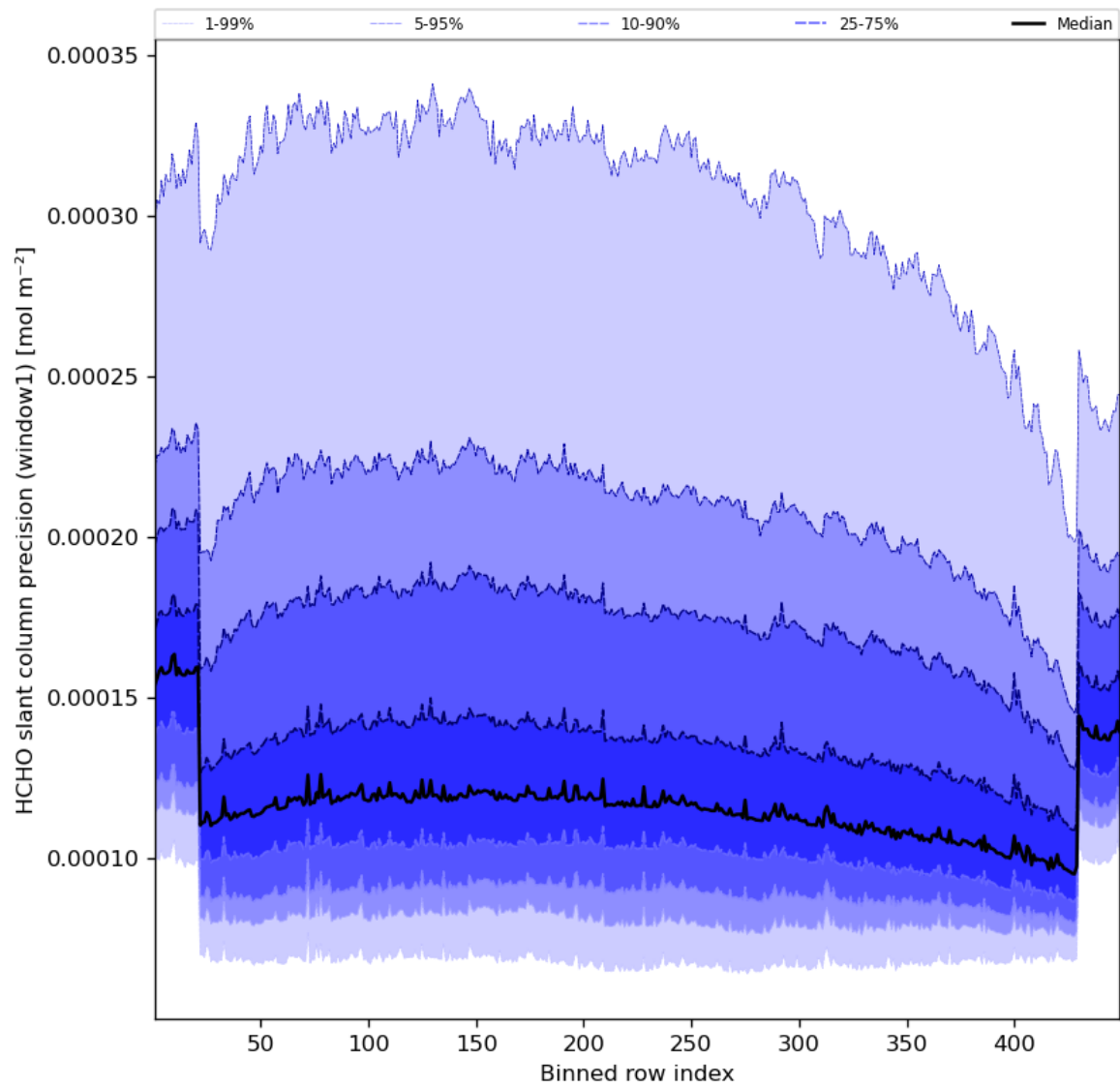
Figure 53: Along track statistics of “HCHO slant column precision (window1)” for 2023-10-25 to 2023-10-27
