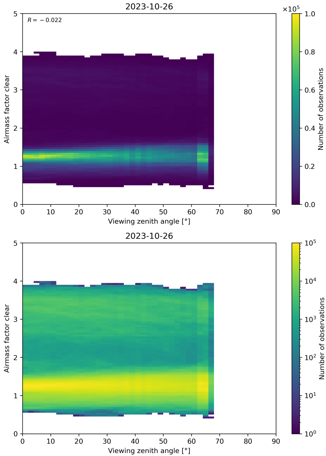
Figure 185: Scatter density plot of “Viewing zenith angle” against “Airmass factor clear” for 2023-10-25 to 2023-10-27.
