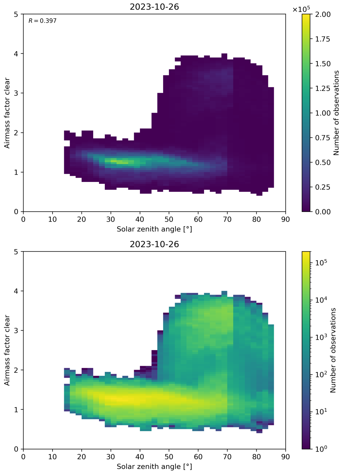
Figure 170: Scatter density plot of “Solar zenith angle” against “Airmass factor clear” for 2023-10-25 to 2023-10-27.
