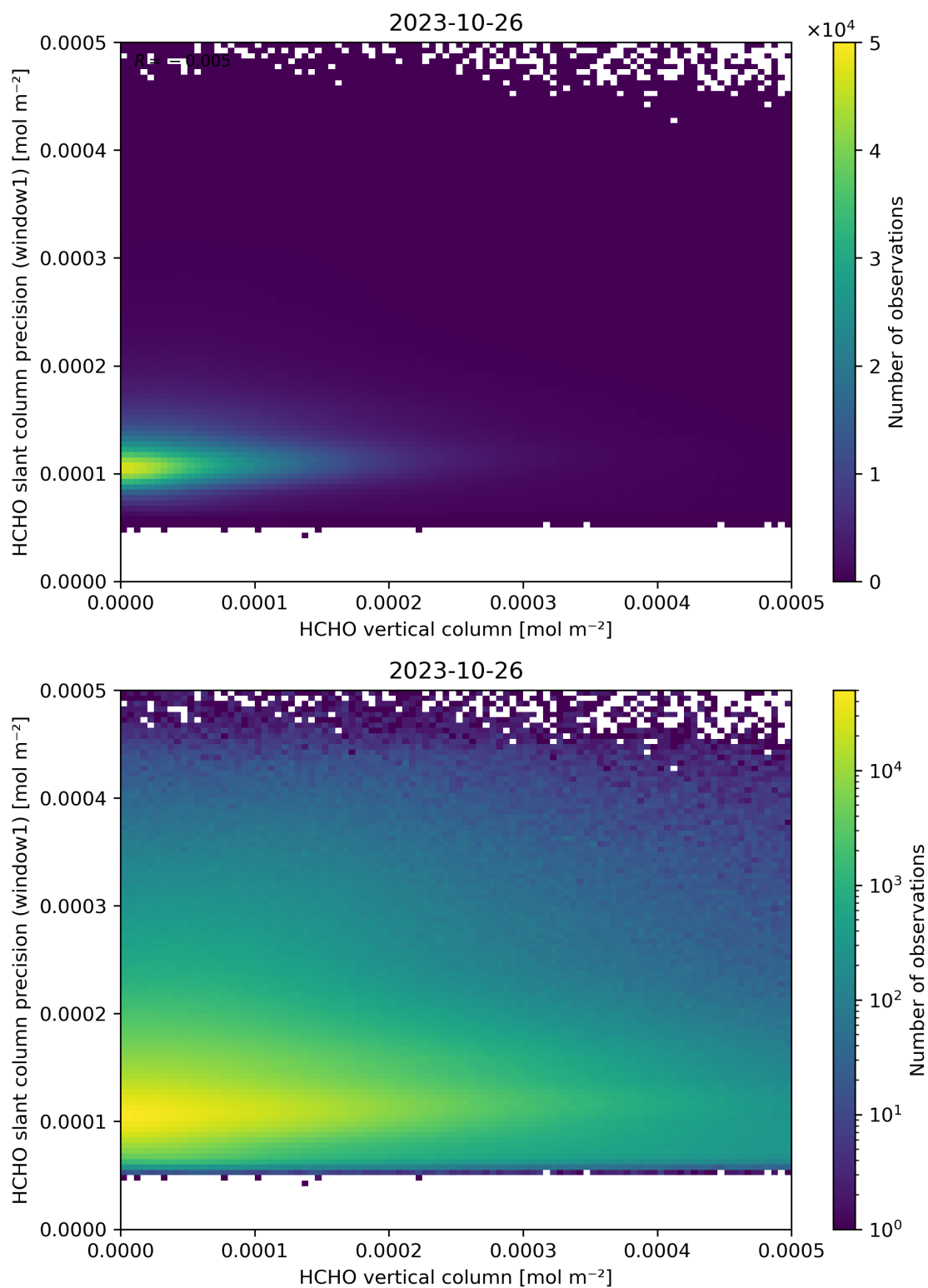
Figure 130: Scatter density plot of “HCHO vertical column” against “HCHO slant column precision (window1)” for 2023-10-25 to 2023-10-27.
