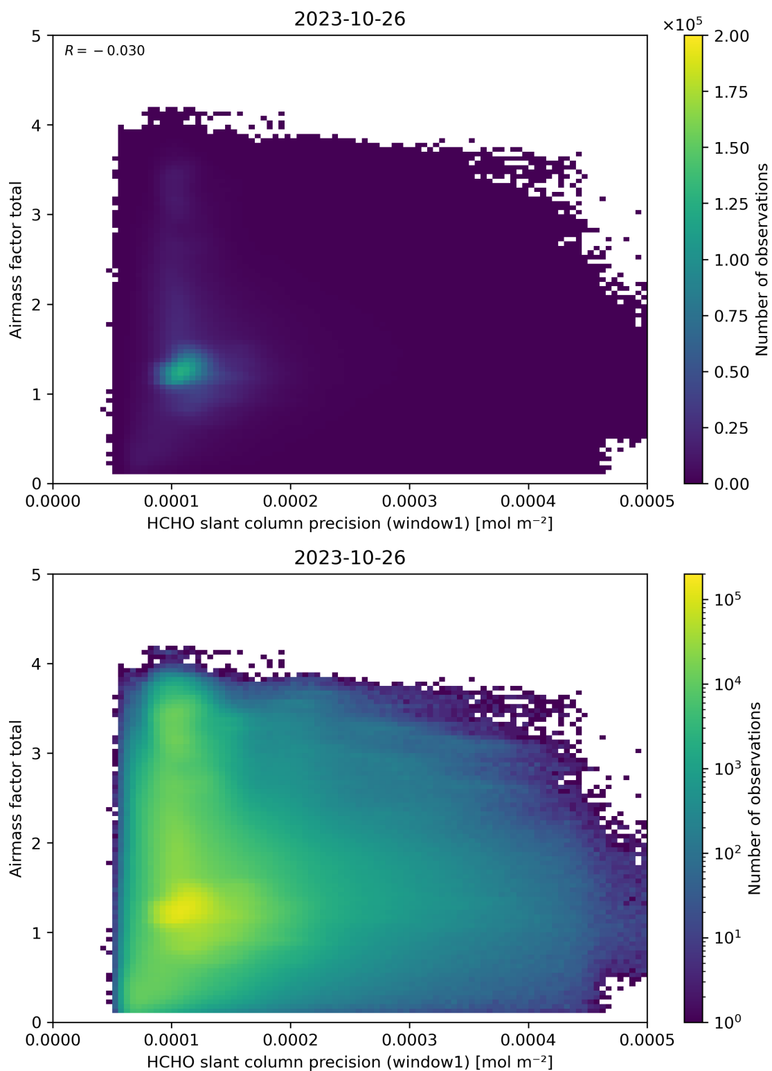
Figure 94: Scatter density plot of “HCHO slant column precision (window1)” against “Airmass factor total” for 2023-10-25 to 2023-10-27.
