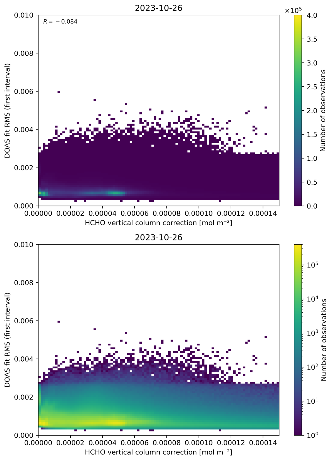
Figure 112: Scatter density plot of “HCHO vertical column correction” against “DOAS fit RMS (first interval)” for 2023-10-25 to 2023-10-27.
