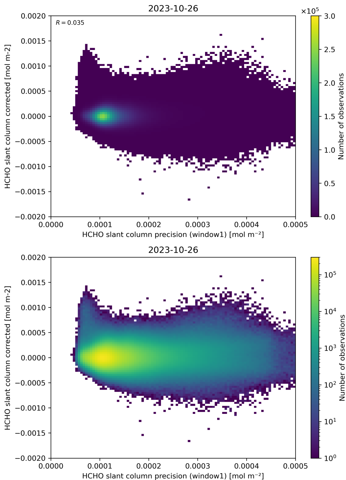
Figure 92: Scatter density plot of “HCHO slant column precision (window1)” against “HCHO slant column corrected” for 2023-10-25 to 2023-10-27.
