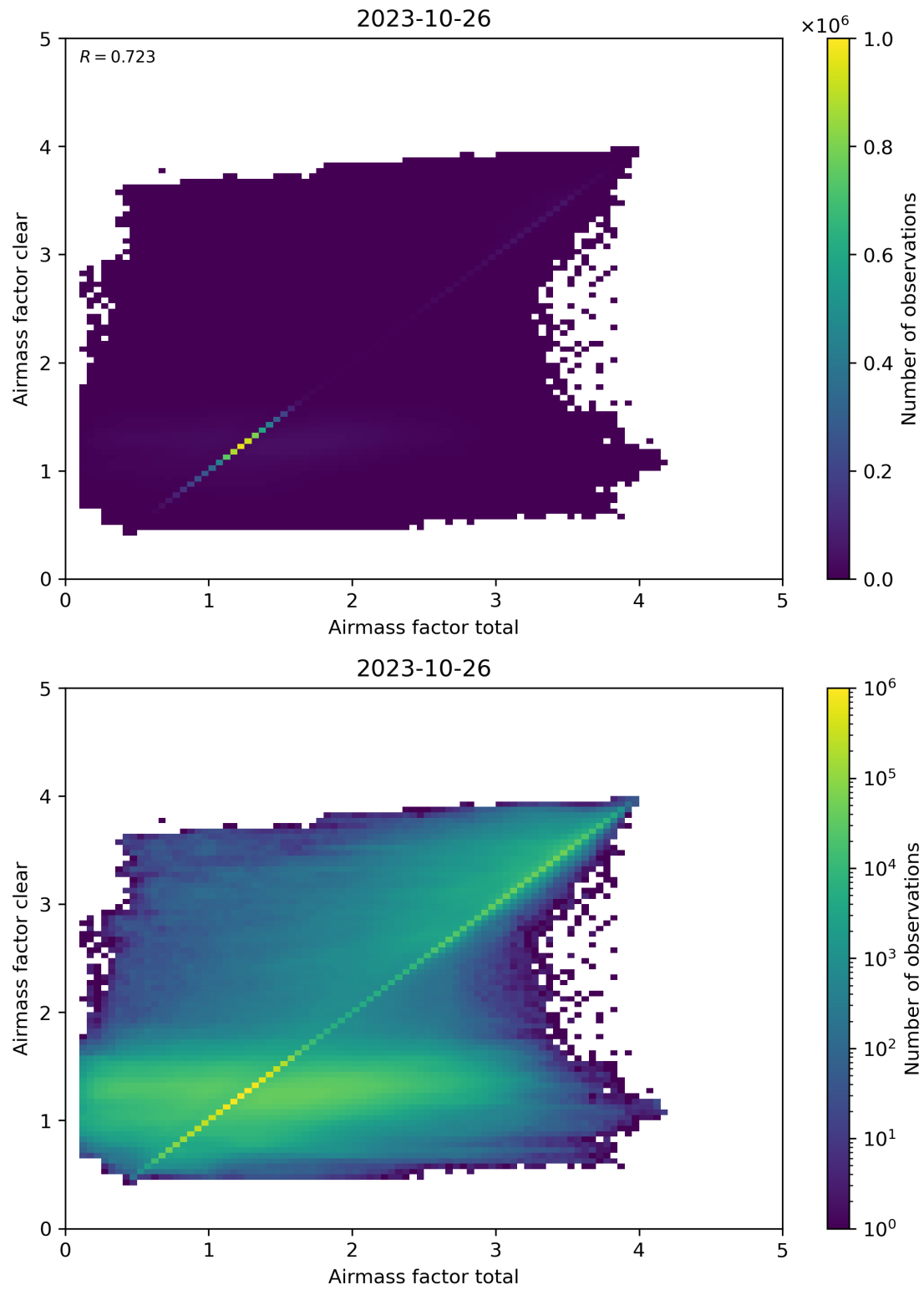
Figure 100: Scatter density plot of “Airmass factor total” against “Airmass factor clear” for 2023-10-25 to 2023-10-27.
