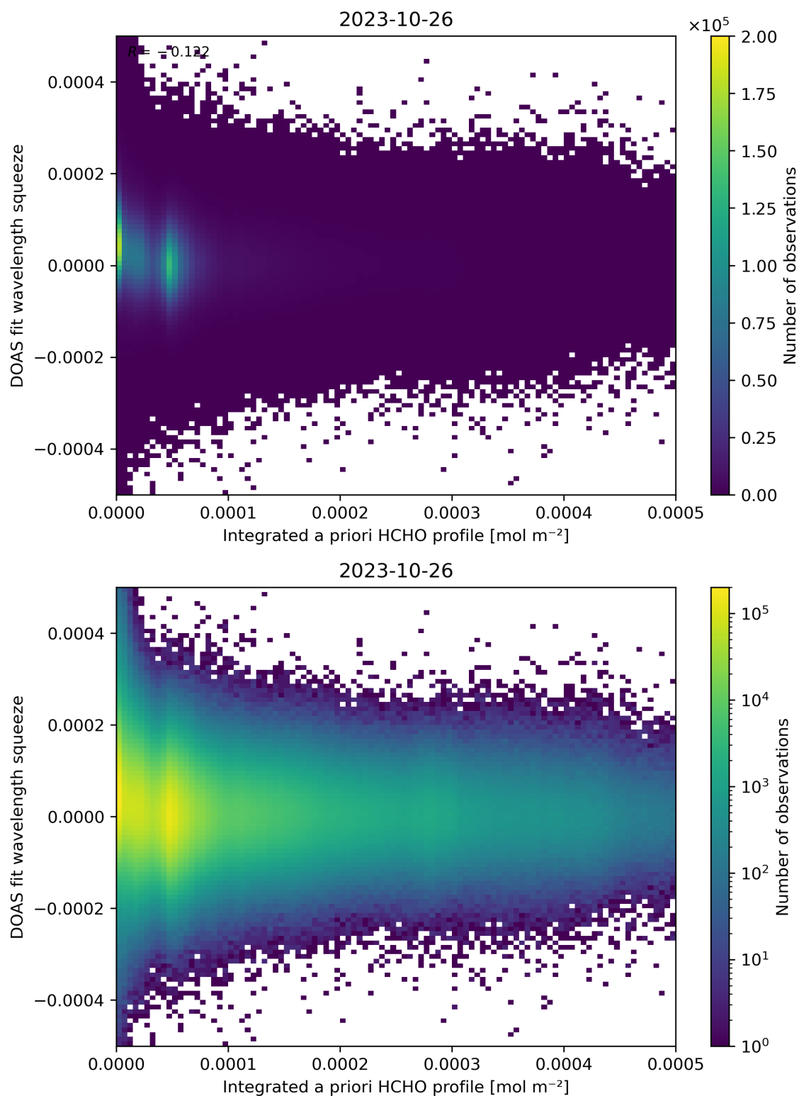
Figure 150: Scatter density plot of “Integrated a priori HCHO profile” against “DOAS fit wavelength squeeze” for 2023-10-25 to 2023-10-27.
