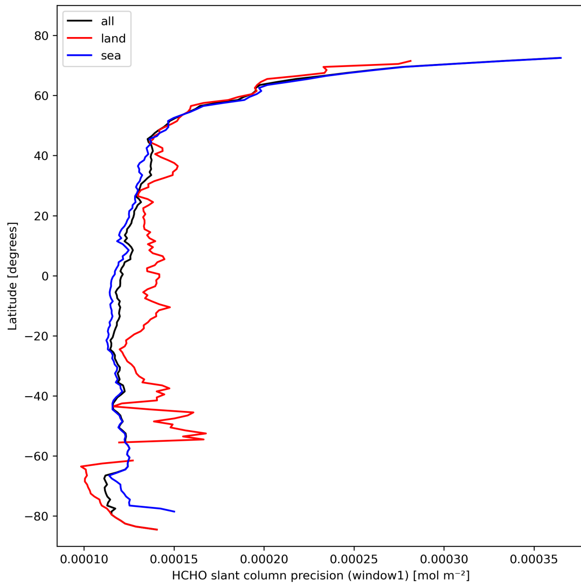
Figure 25: Zonal average of “HCHO slant column precision (window1)” for 2023-10-25 to 2023-10-27.
