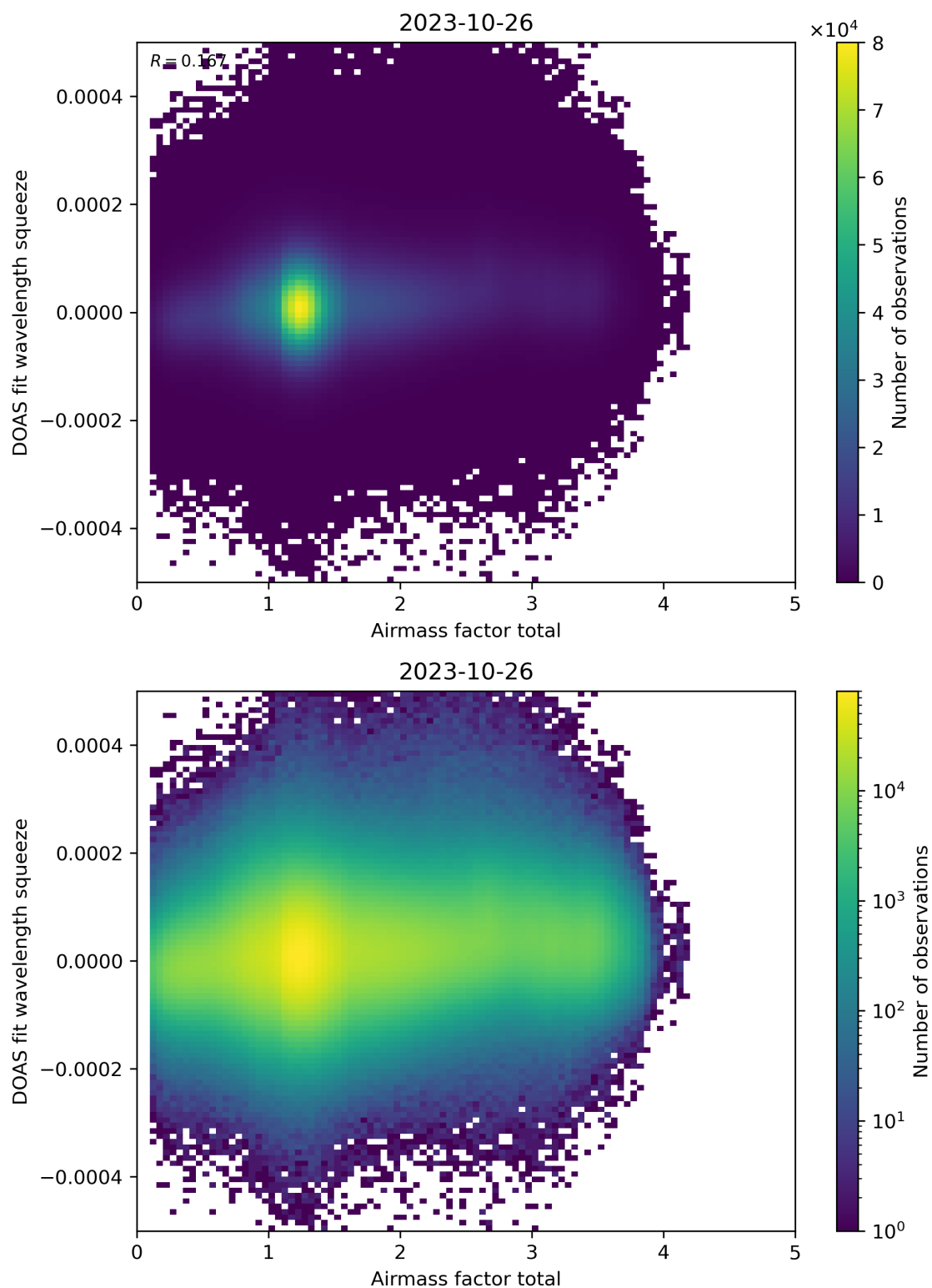
Figure 99: Scatter density plot of “Airmass factor total” against “DOAS fit wavelength squeeze” for 2023-10-25 to 2023-10-27.
