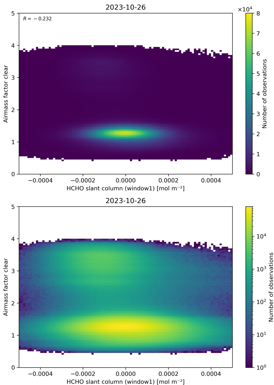
Figure 81: Scatter density plot of “HCHO slant column (window1)” against “Airmass factor clear” for 2023-10-25 to 2023-10-27.
