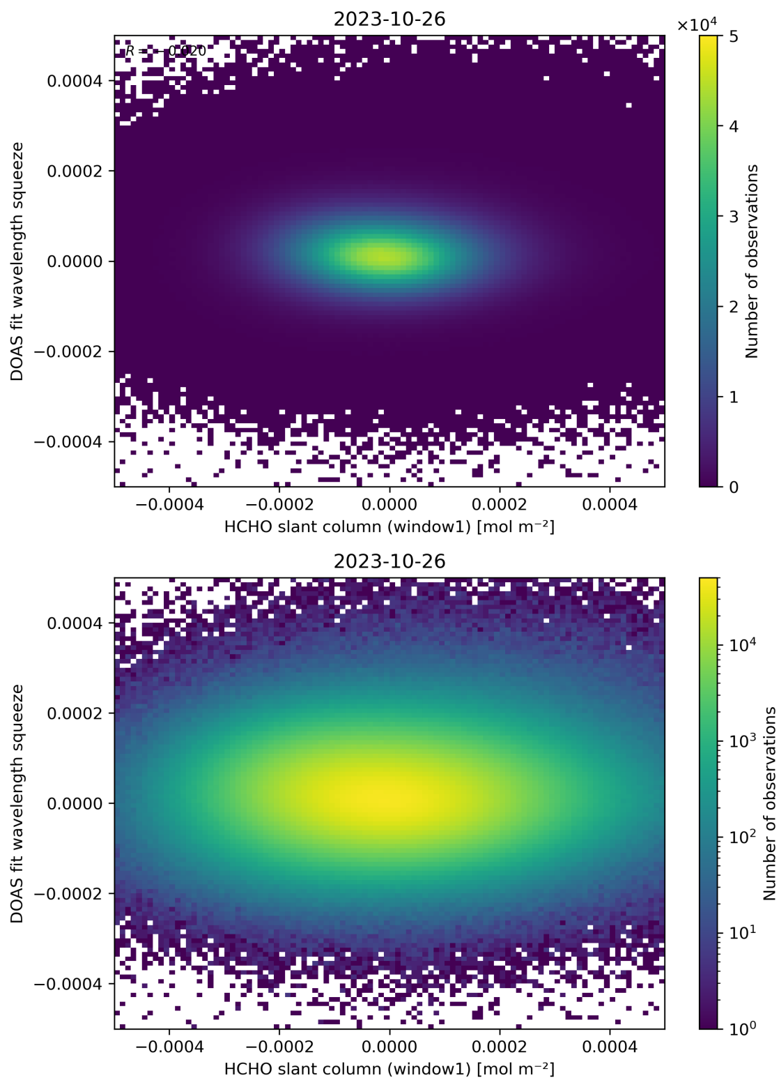
Figure 80: Scatter density plot of “HCHO slant column (window1)” against “DOAS fit wavelength squeeze” for 2023-10-25 to 2023-10-27.
