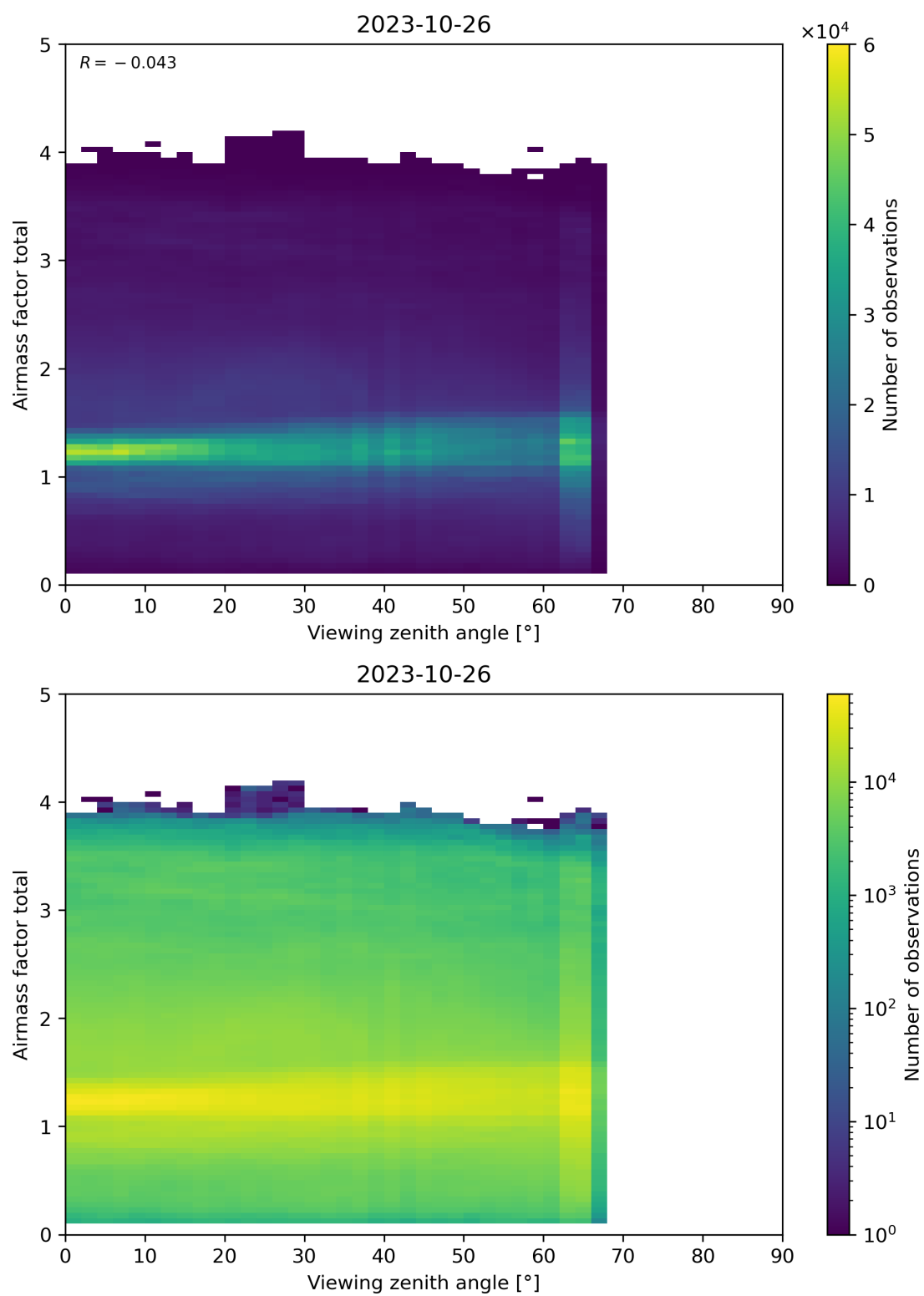
Figure 190: Scatter density plot of “Viewing zenith angle” against “Airmass factor total” for 2023-10-25 to 2023-10-27.
