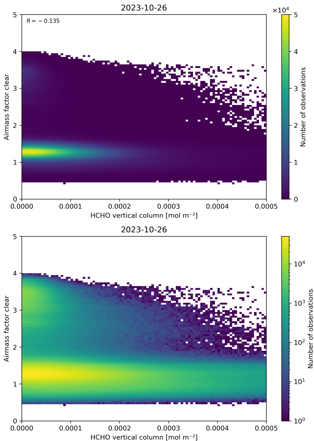
Figure 126: Scatter density plot of “HCHO vertical column” against “Airmass factor clear” for 2023-10-25 to 2023-10-27.
