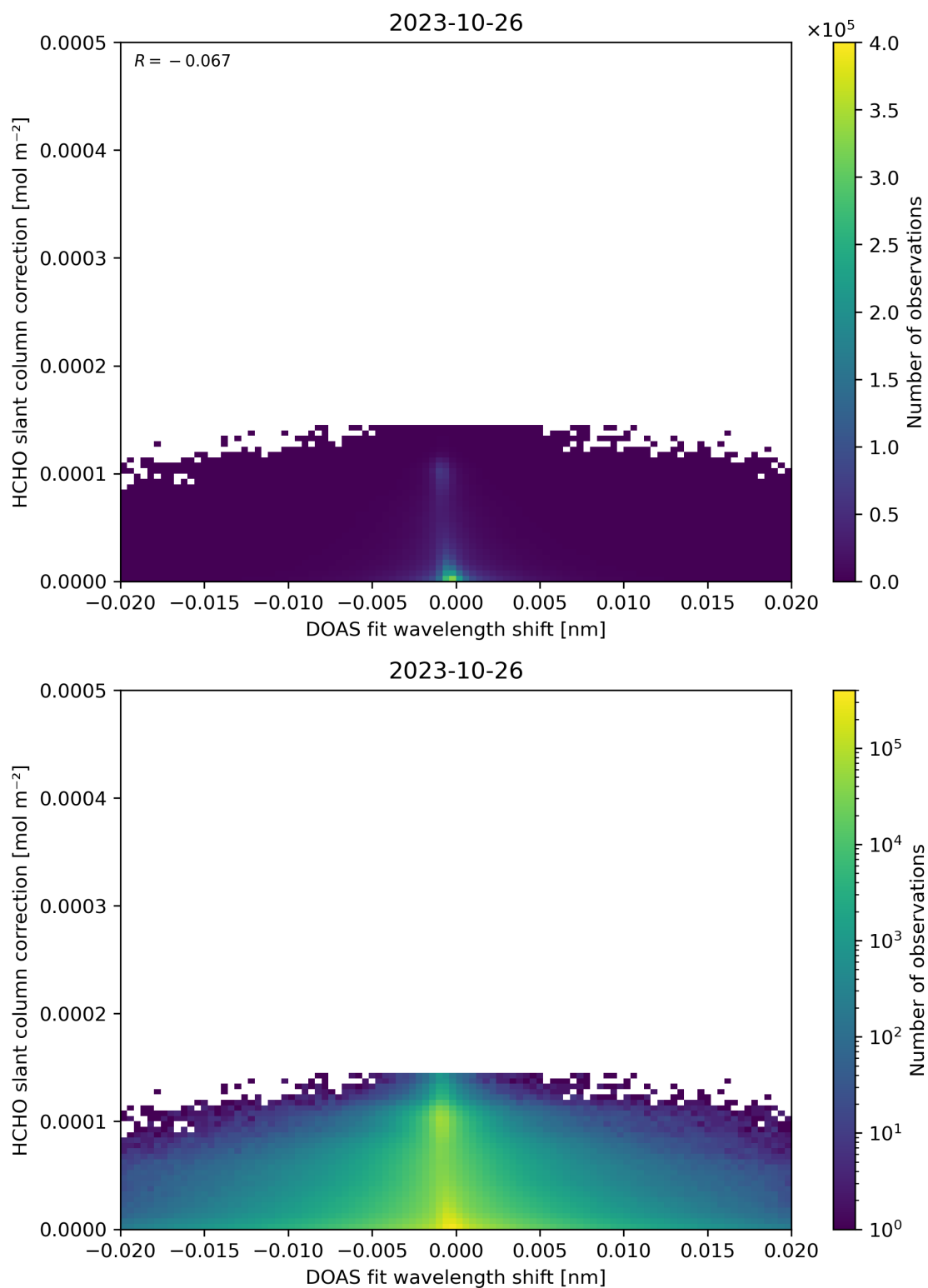
Figure 67: Scatter density plot of “DOAS fit wavelength shift” against “HCHO slant column correction” for 2023-10-25 to 2023-10-27.
