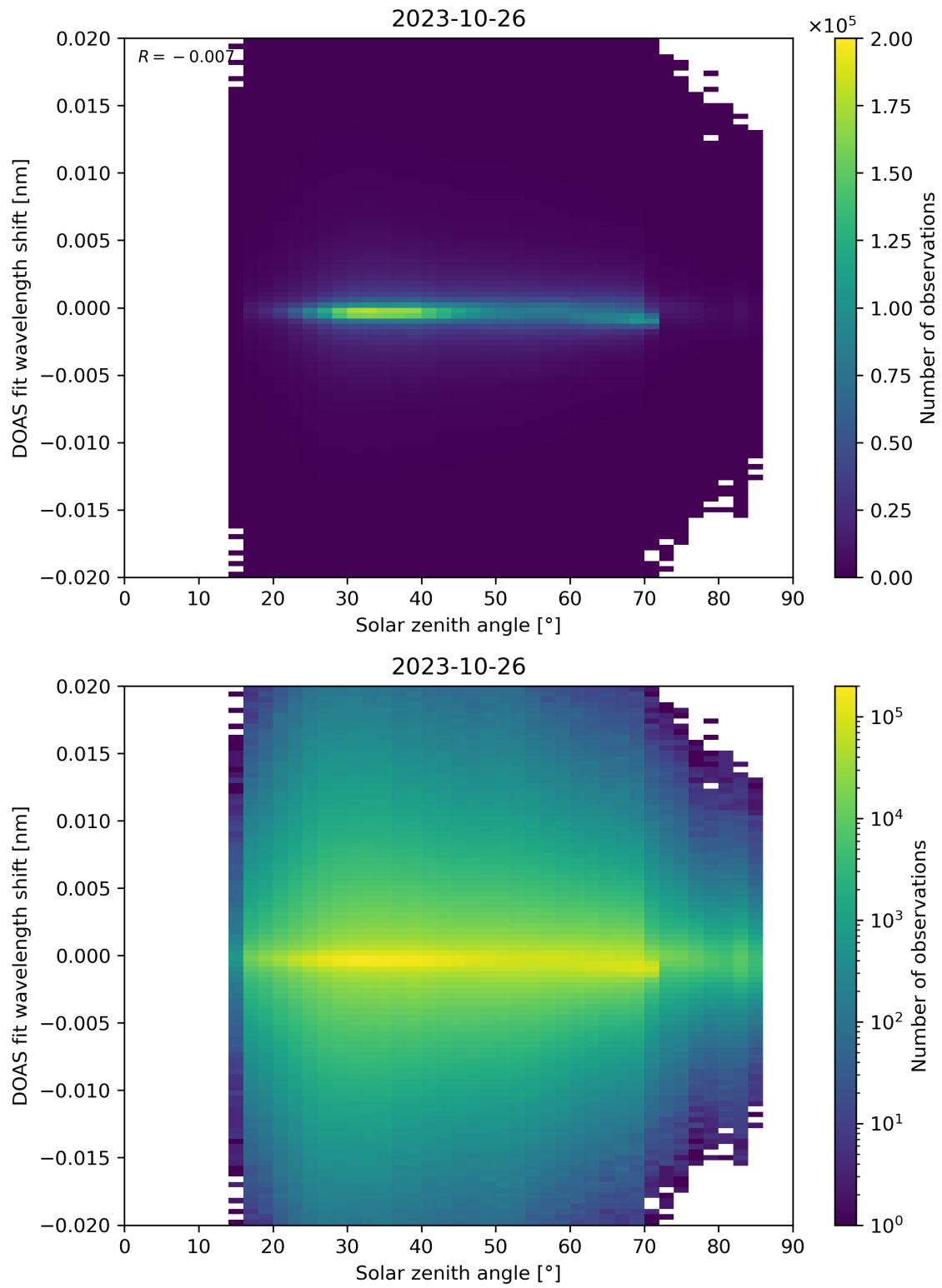
Figure 168: Scatter density plot of “Solar zenith angle” against “DOAS fit wavelength shift” for 2023-10-25 to 2023-10-27.
