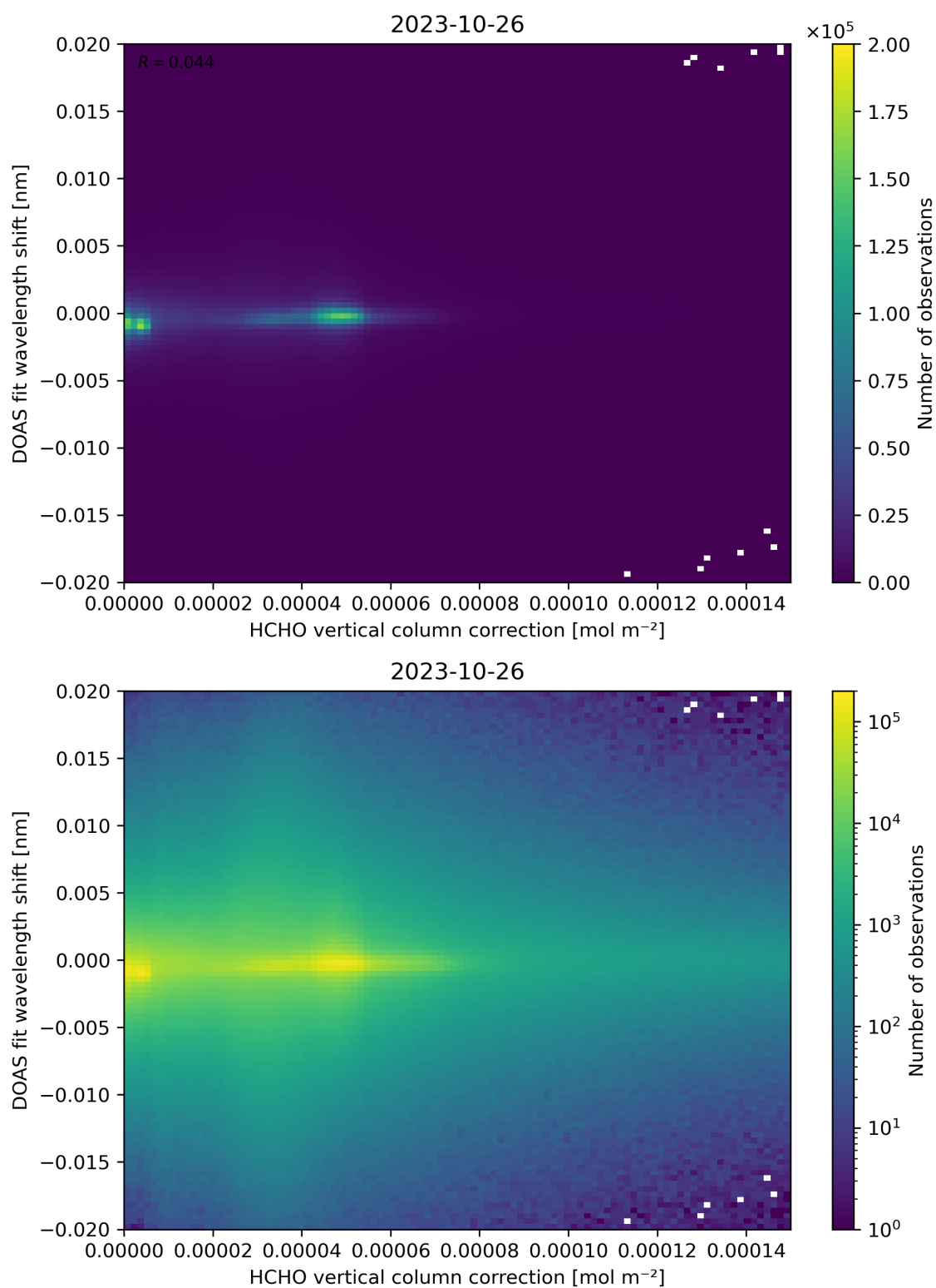
Figure 113: Scatter density plot of “HCHO vertical column correction” against “DOAS fit wavelength shift” for 2023-10-25 to 2023-10-27.
