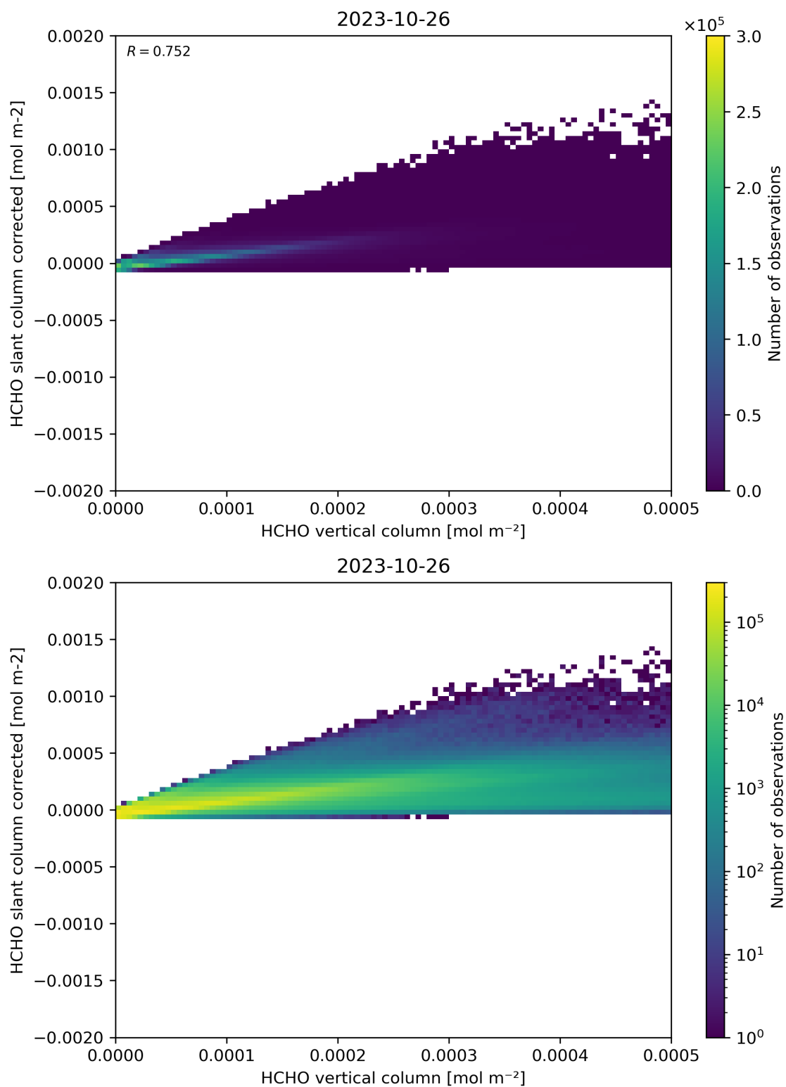
Figure 127: Scatter density plot of “HCHO vertical column” against “HCHO slant column corrected” for 2023-10-25 to 2023-10-27.
