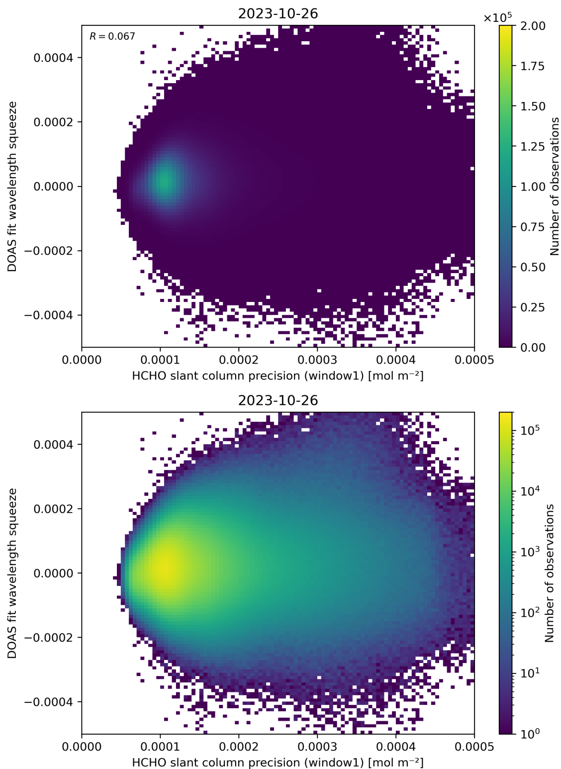
Figure 90: Scatter density plot of “HCHO slant column precision (window1)” against “DOAS fit wavelength squeeze” for 2023-10-25 to 2023-10-27.
