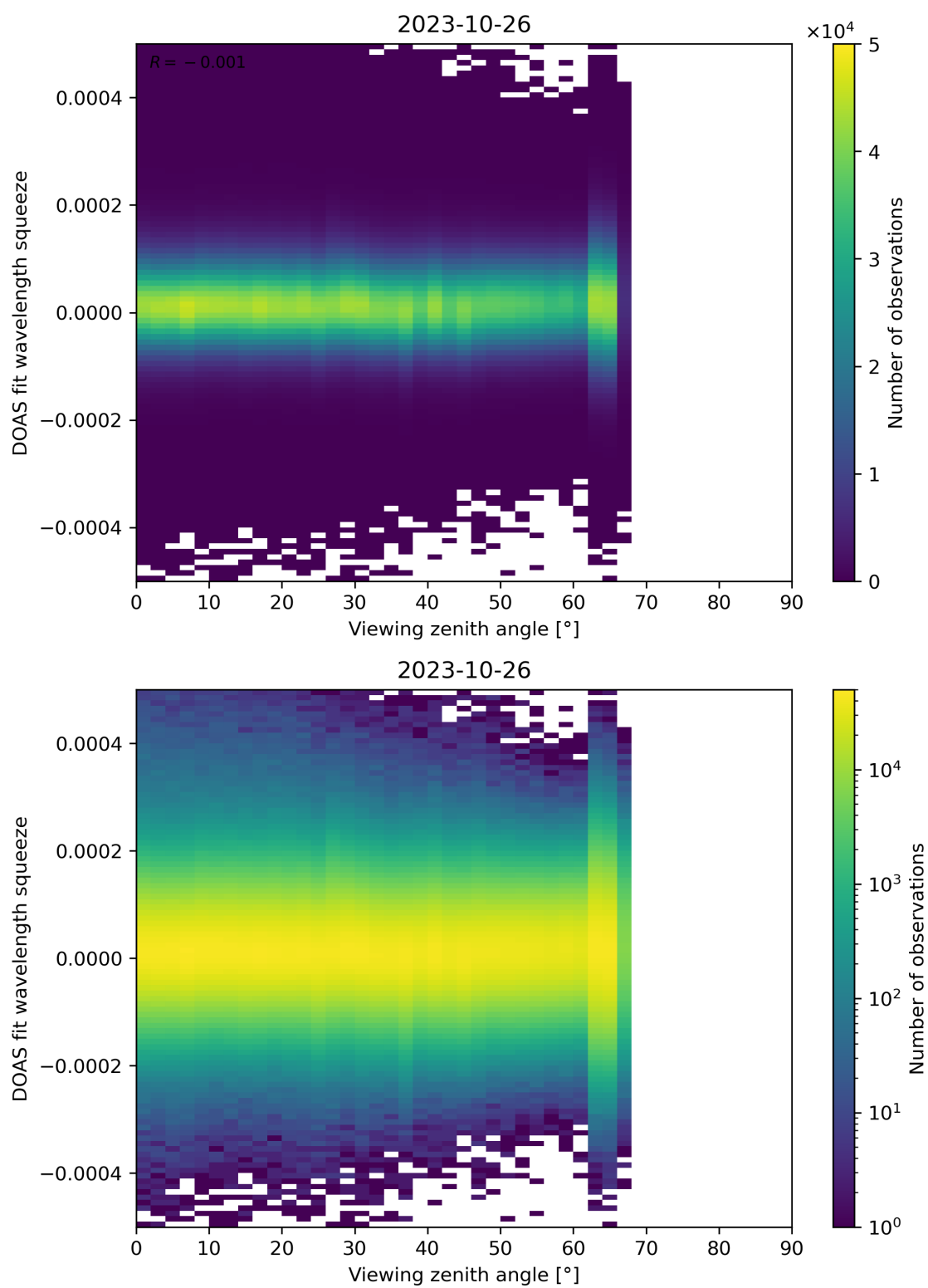
Figure 184: Scatter density plot of “Viewing zenith angle” against “DOAS fit wavelength squeeze” for 2023-10-25 to 2023-10-27.
