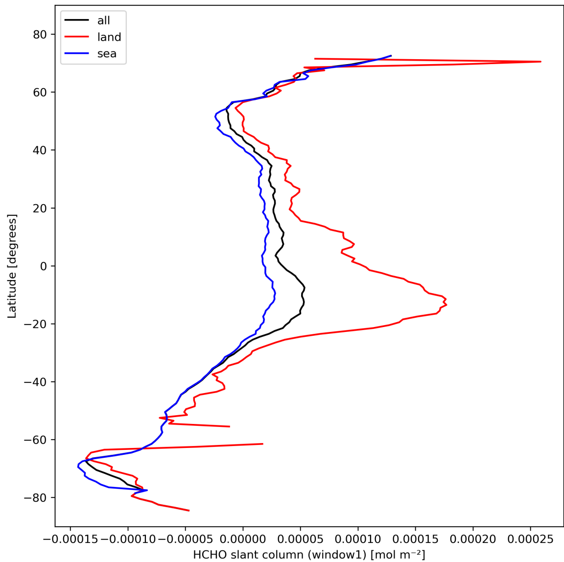
Figure 24: Zonal average of “HCHO slant column (window1)” for 2023-10-25 to 2023-10-27.
