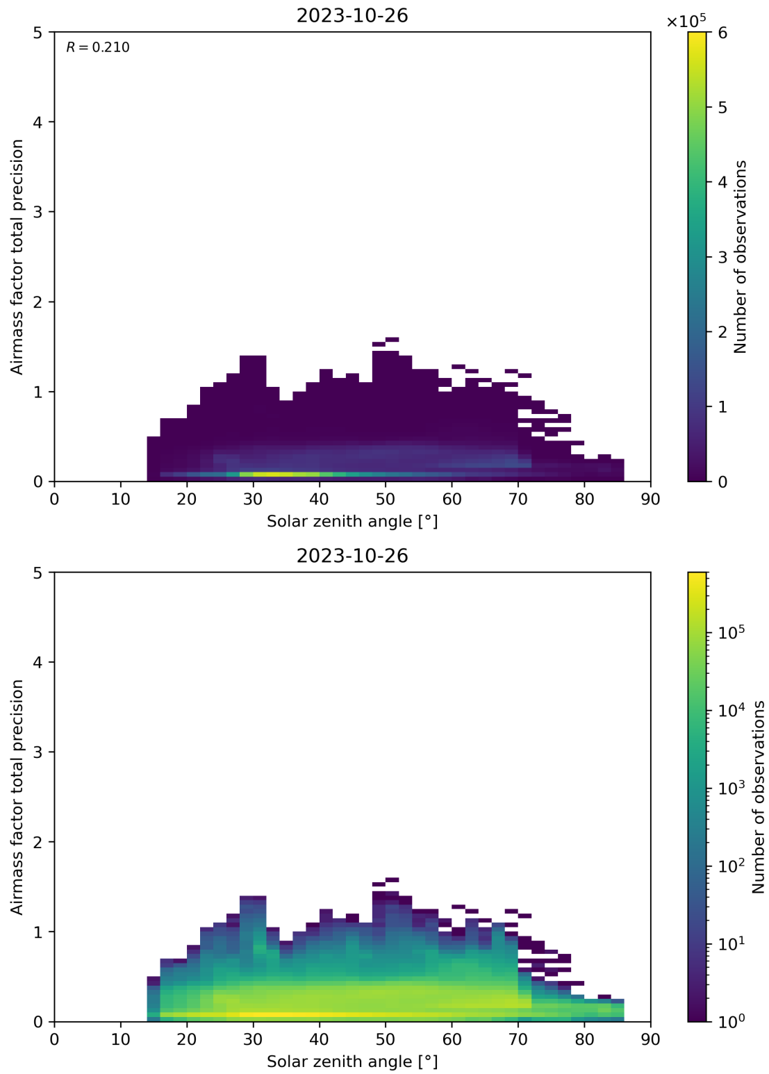
Figure 176: Scatter density plot of “Solar zenith angle” against “Airmass factor total precision” for 2023-10-25 to 2023-10-27.
