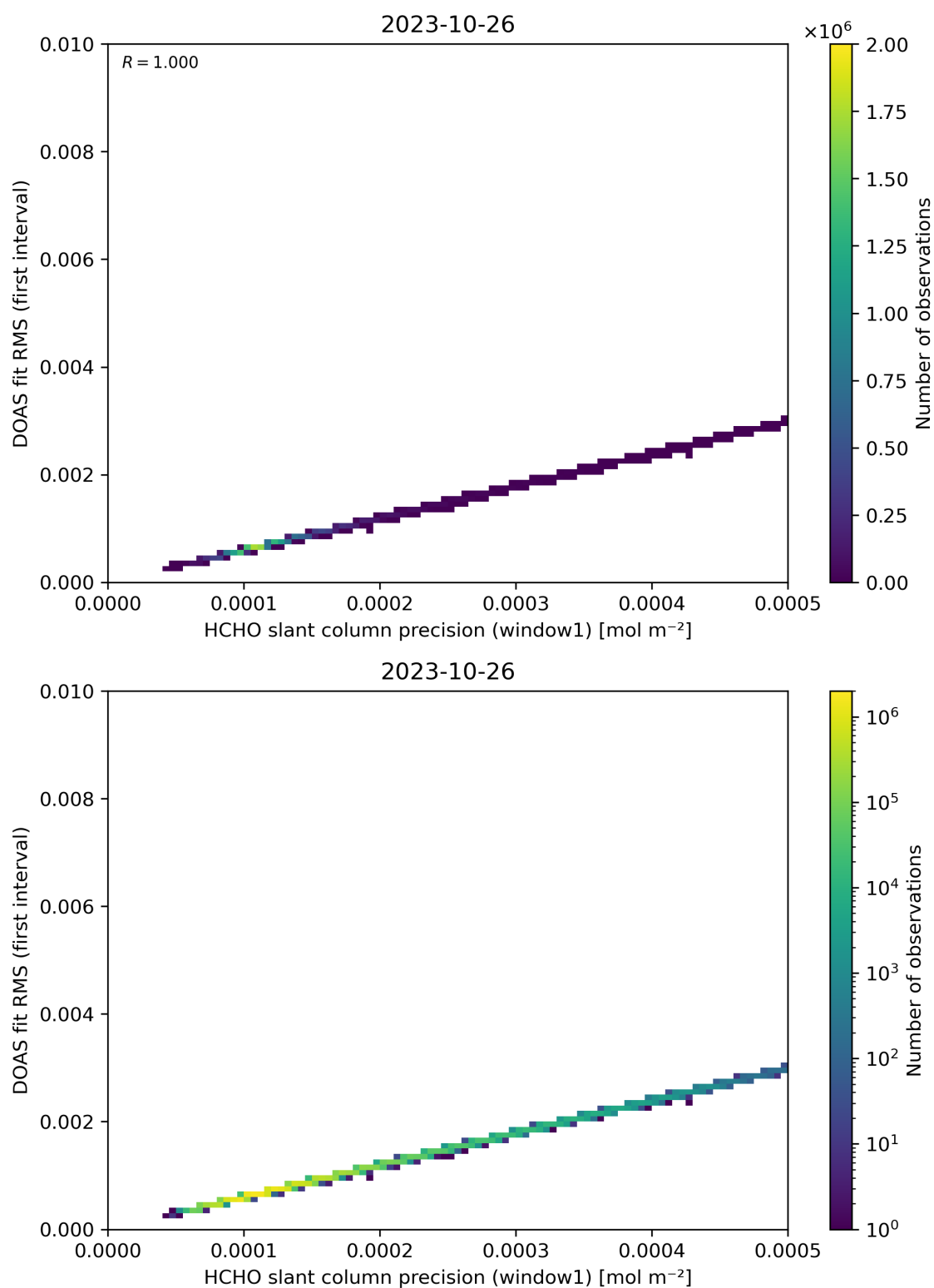
Figure 88: Scatter density plot of “HCHO slant column precision (window1)” against “DOAS fit RMS (first interval)” for 2023-10-25 to 2023-10-27.
