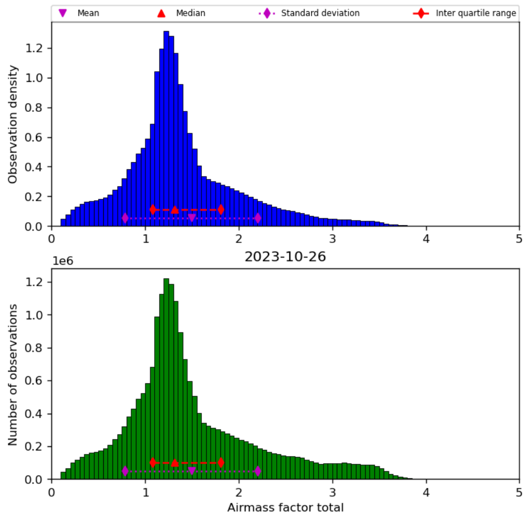
Figure 40: Histogram of “Airmass factor total” for 2023-10-25 to 2023-10-27
