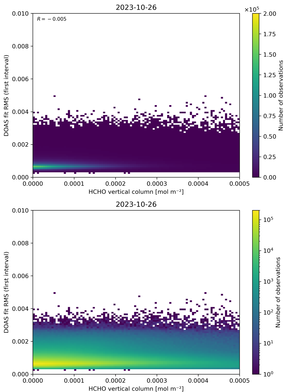
Figure 123: Scatter density plot of “HCHO vertical column” against “DOAS fit RMS (first interval)” for 2023-10-25 to 2023-10-27.
