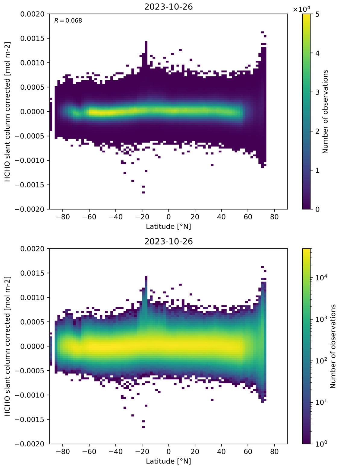
Figure 157: Scatter density plot of “Latitude” against “HCHO slant column corrected” for 2023-10-25 to 2023-10-27.
