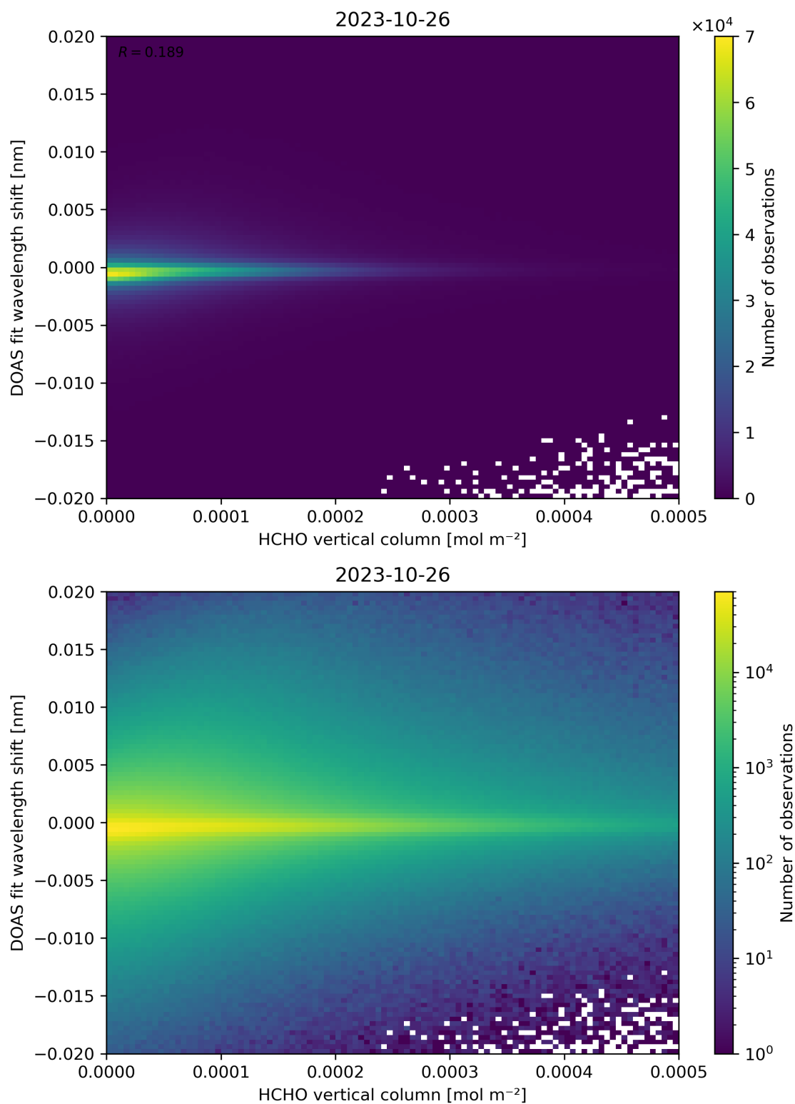
Figure 124: Scatter density plot of “HCHO vertical column” against “DOAS fit wavelength shift” for 2023-10-25 to 2023-10-27.
