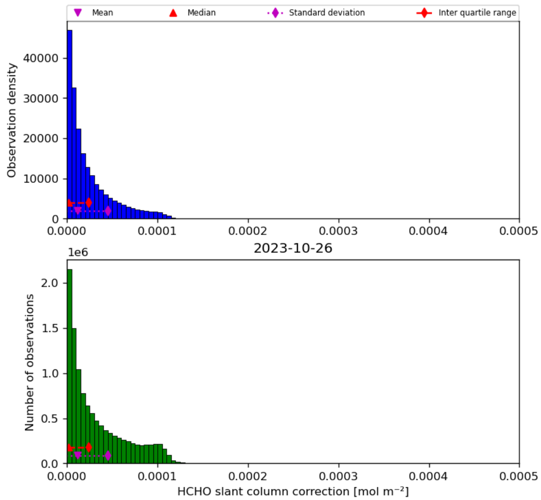
Figure 47: Histogram of “HCHO slant column correction” for 2023-10-25 to 2023-10-27
