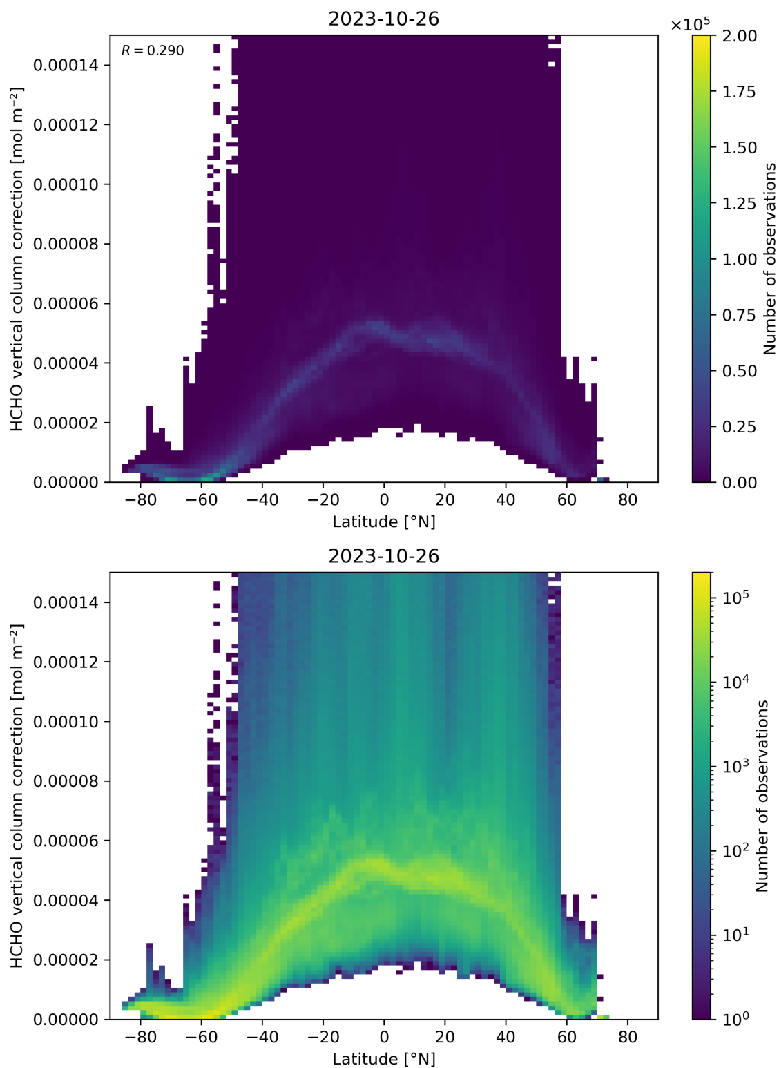
Figure 164: Scatter density plot of “Latitude” against “HCHO vertical column correction” for 2023-10-25 to 2023-10-27.
