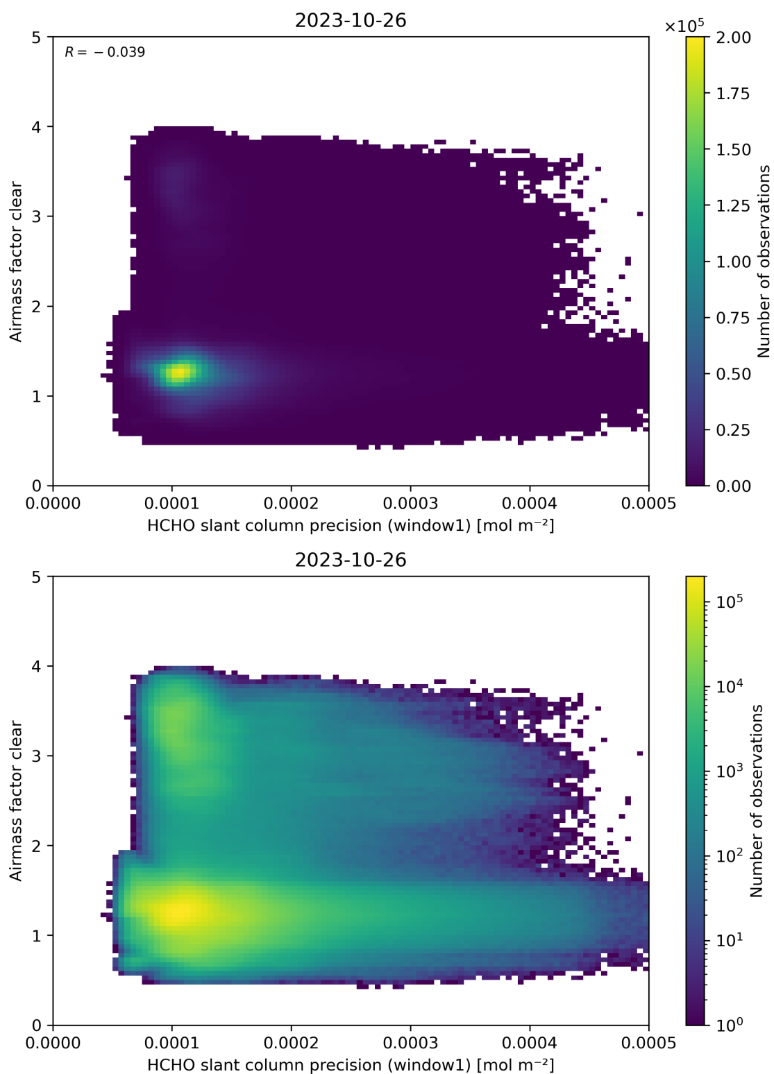
Figure 91: Scatter density plot of “HCHO slant column precision (window1)” against “Airmass factor clear” for 2023-10-25 to 2023-10-27.
