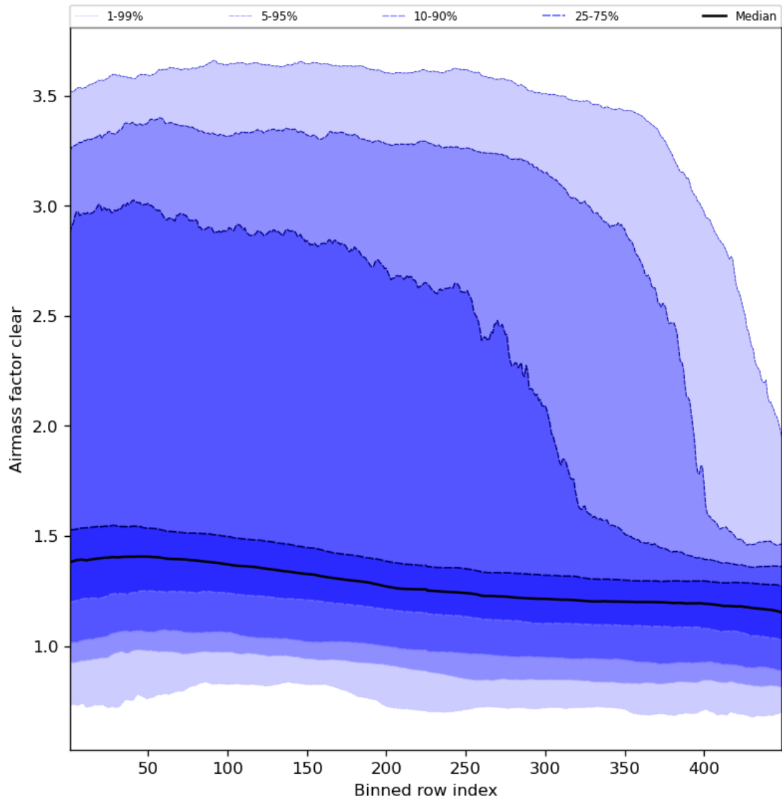
Figure 56: Along track statistics of “Airmass factor clear” for 2023-10-25 to 2023-10-27
