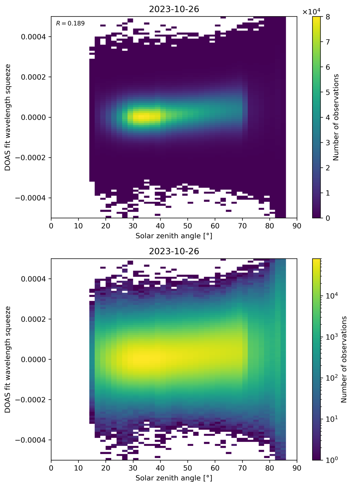
Figure 169: Scatter density plot of “Solar zenith angle” against “DOAS fit wavelength squeeze” for 2023-10-25 to 2023-10-27.
