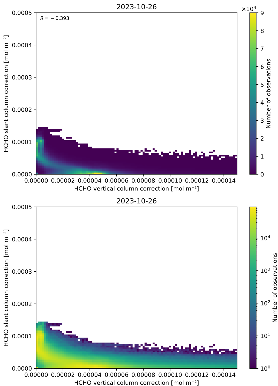
Figure 117: Scatter density plot of “HCHO vertical column correction” against “HCHO slant column correction” for 2023-10-25 to 2023-10-27.
