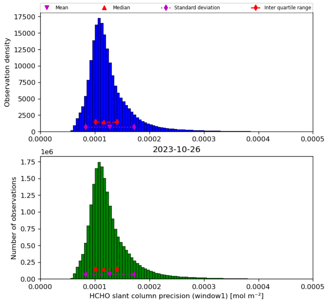
Figure 39: Histogram of “HCHO slant column precision (window1)” for 2023-10-25 to 2023-10-27
