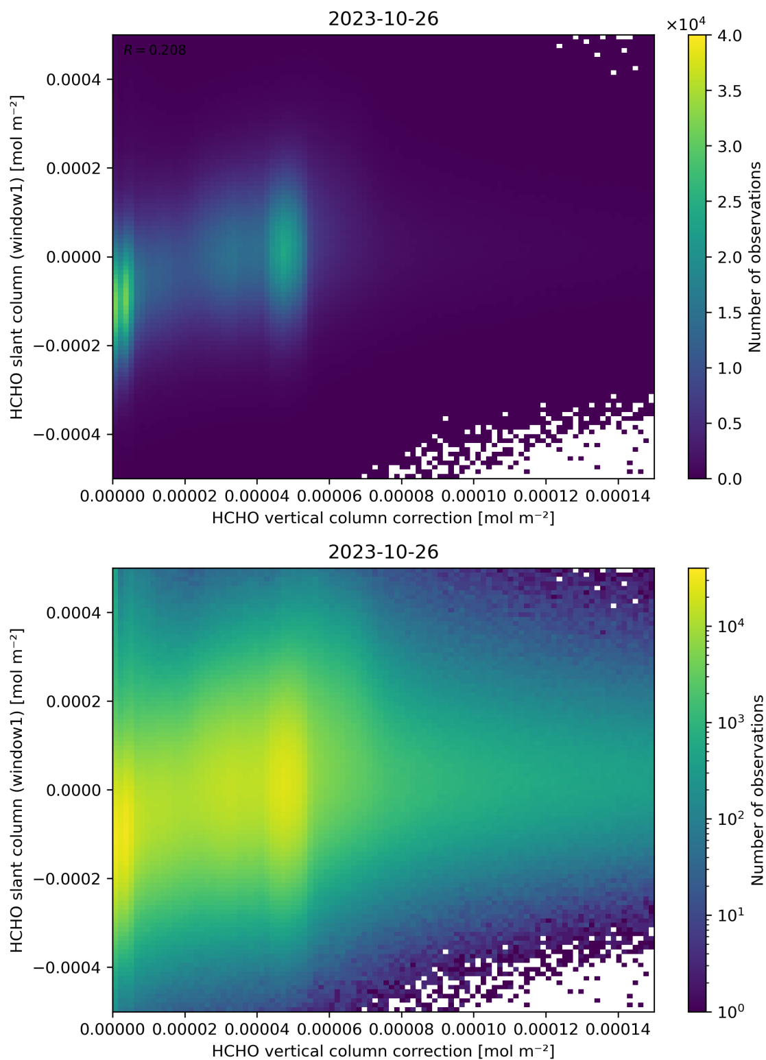
Figure 118: Scatter density plot of “HCHO vertical column correction” against “HCHO slant column (window1)” for 2023-10-25 to 2023-10-27.
