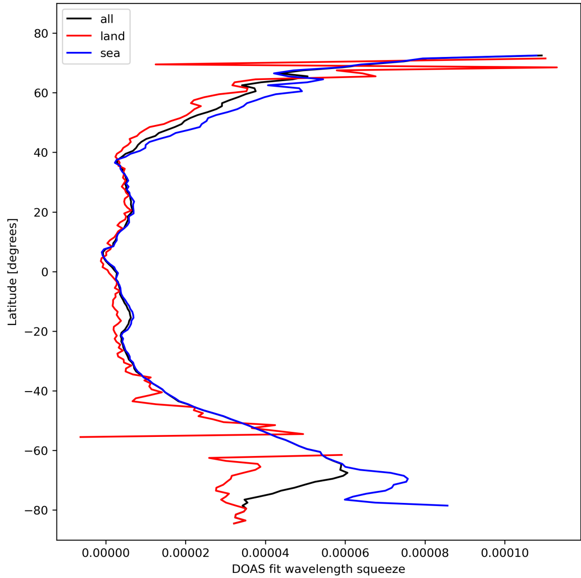
Figure 31: Zonal average of “DOAS fit wavelength squeeze” for 2023-10-25 to 2023-10-27.
