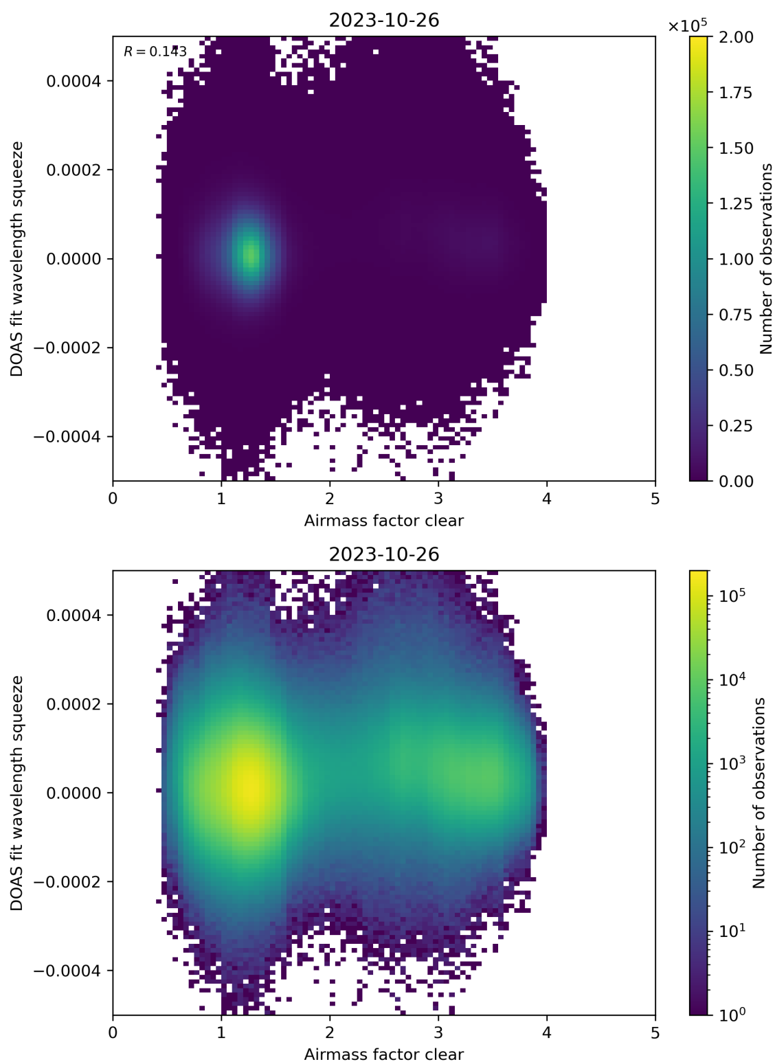
Figure 73: Scatter density plot of “Airmass factor clear” against “DOAS fit wavelength squeeze” for 2023-10-25 to 2023-10-27.
