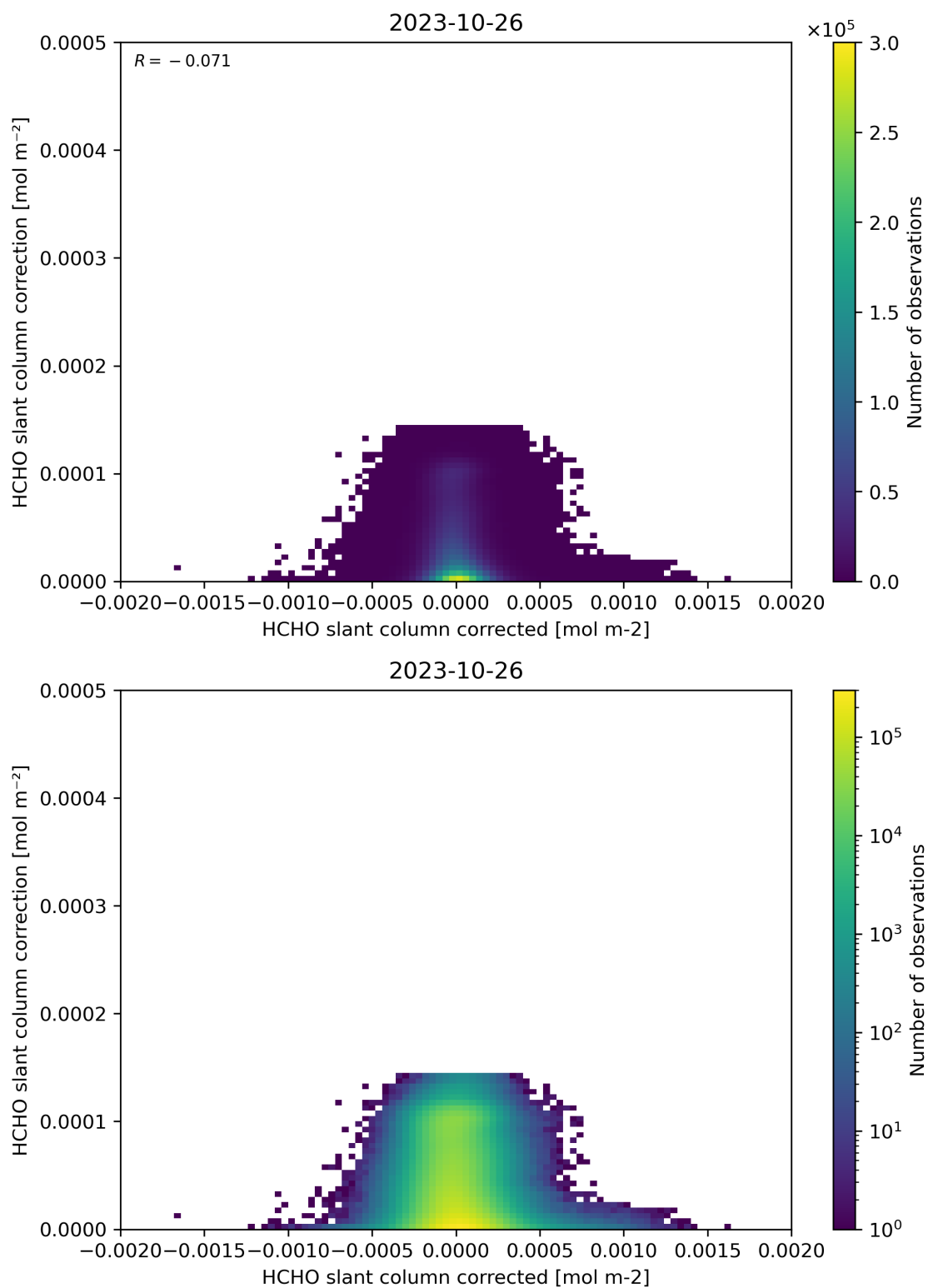
Figure 77: Scatter density plot of “HCHO slant column corrected” against “HCHO slant column correction” for 2023-10-25 to 2023-10-27.
