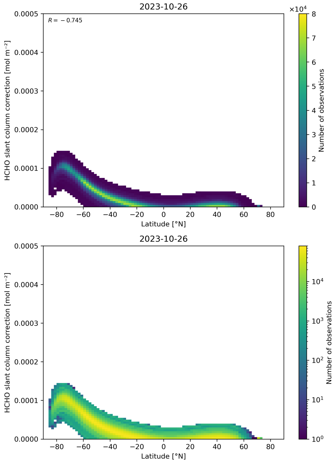
Figure 158: Scatter density plot of “Latitude” against “HCHO slant column correction” for 2023-10-25 to 2023-10-27.
