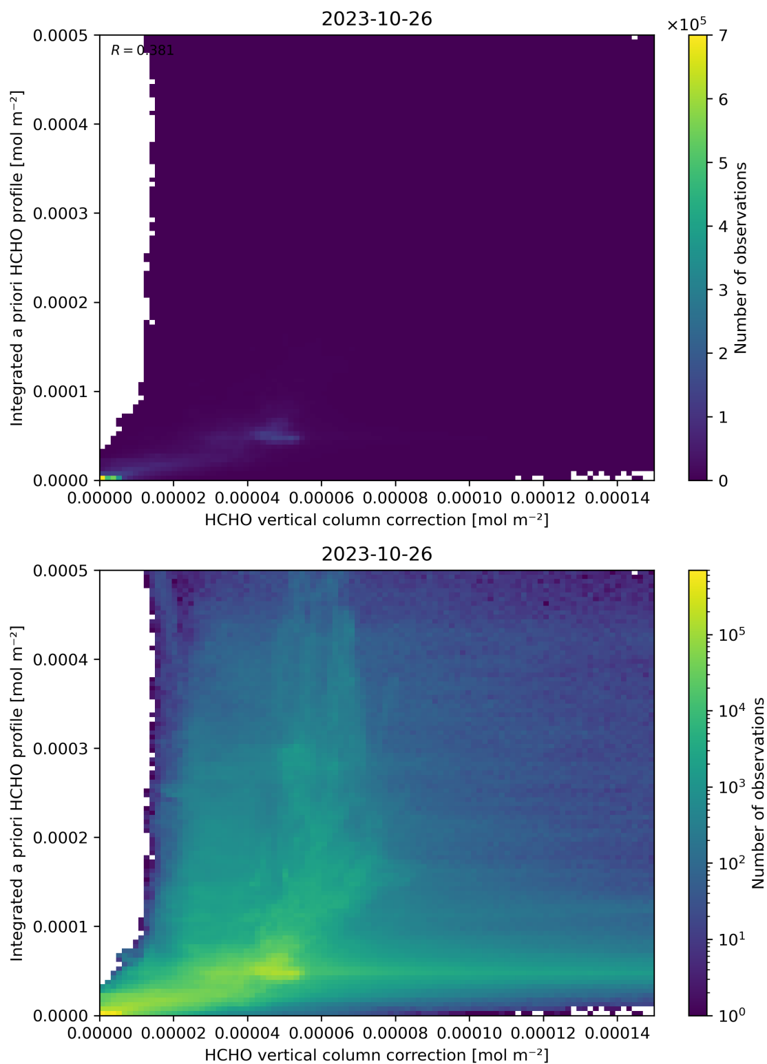
Figure 122: Scatter density plot of “HCHO vertical column correction” against “Integrated a priori HCHO profile” for 2023-10-25 to 2023-10-27.
