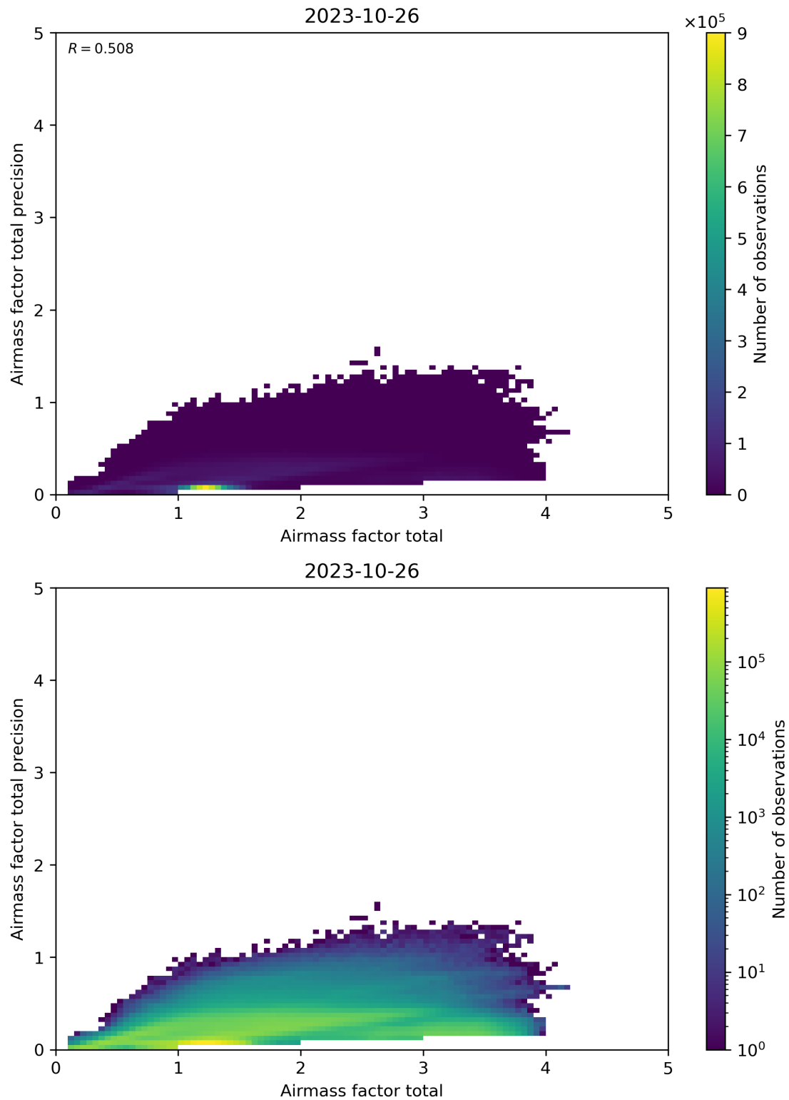
Figure 103: Scatter density plot of “Airmass factor total” against “Airmass factor total precision” for 2023-10-25 to 2023-10-27.
