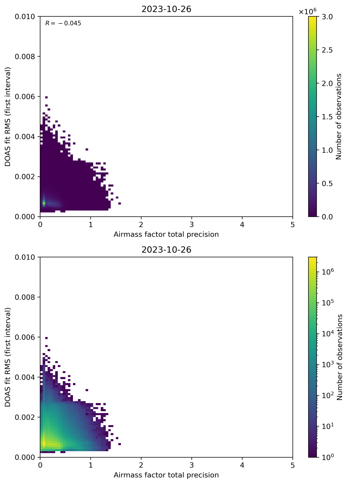
Figure 105: Scatter density plot of “Airmass factor total precision” against “DOAS fit RMS (first interval)” for 2023-10-25 to 2023-10-27.
