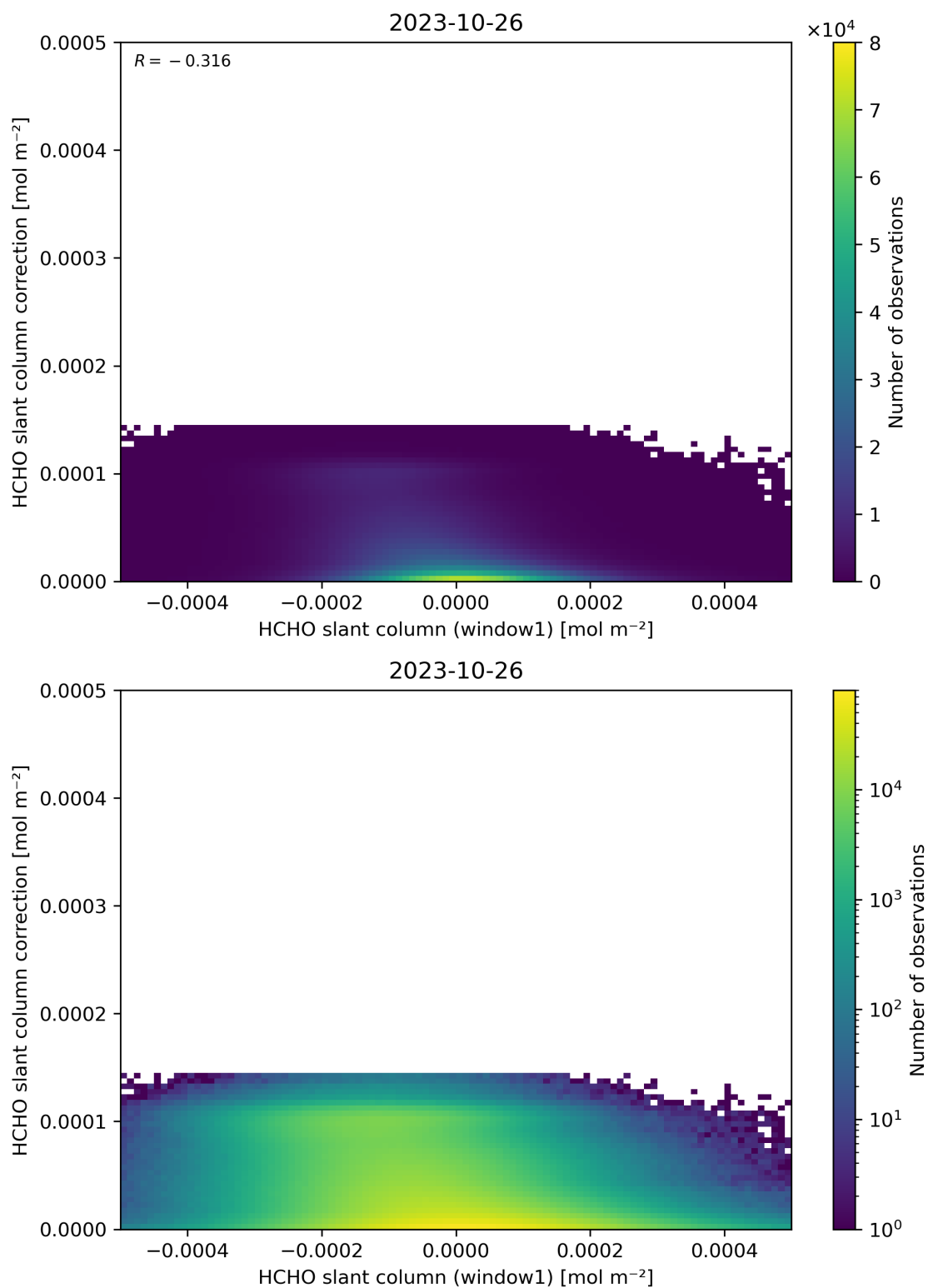
Figure 83: Scatter density plot of “HCHO slant column (window1)” against “HCHO slant column correction” for 2023-10-25 to 2023-10-27.
