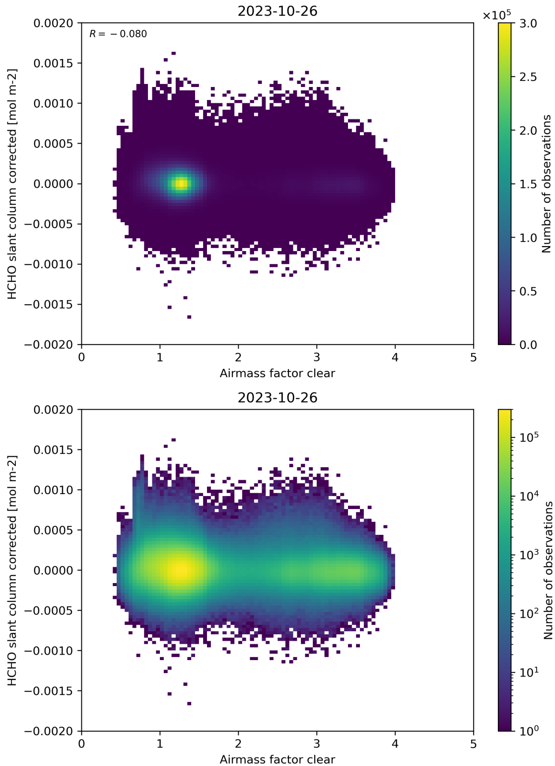
Figure 74: Scatter density plot of “Airmass factor clear” against “HCHO slant column corrected” for 2023-10-25 to 2023-10-27.
