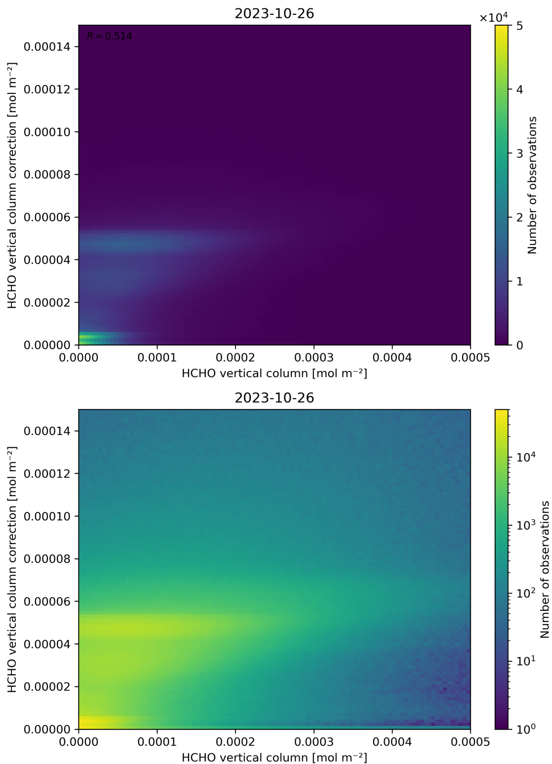
Figure 133: Scatter density plot of “HCHO vertical column” against “HCHO vertical column correction” for 2023-10-25 to 2023-10-27.
