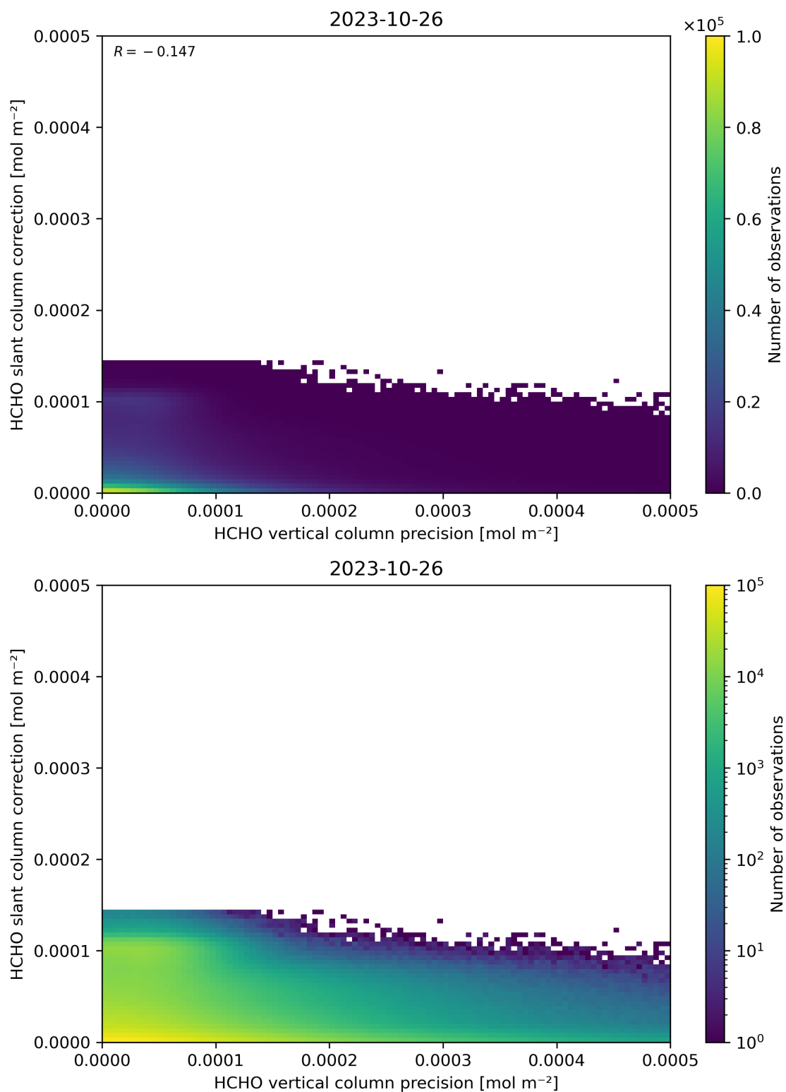
Figure 141: Scatter density plot of “HCHO vertical column precision” against “HCHO slant column correction” for 2023-10-25 to 2023-10-27.
