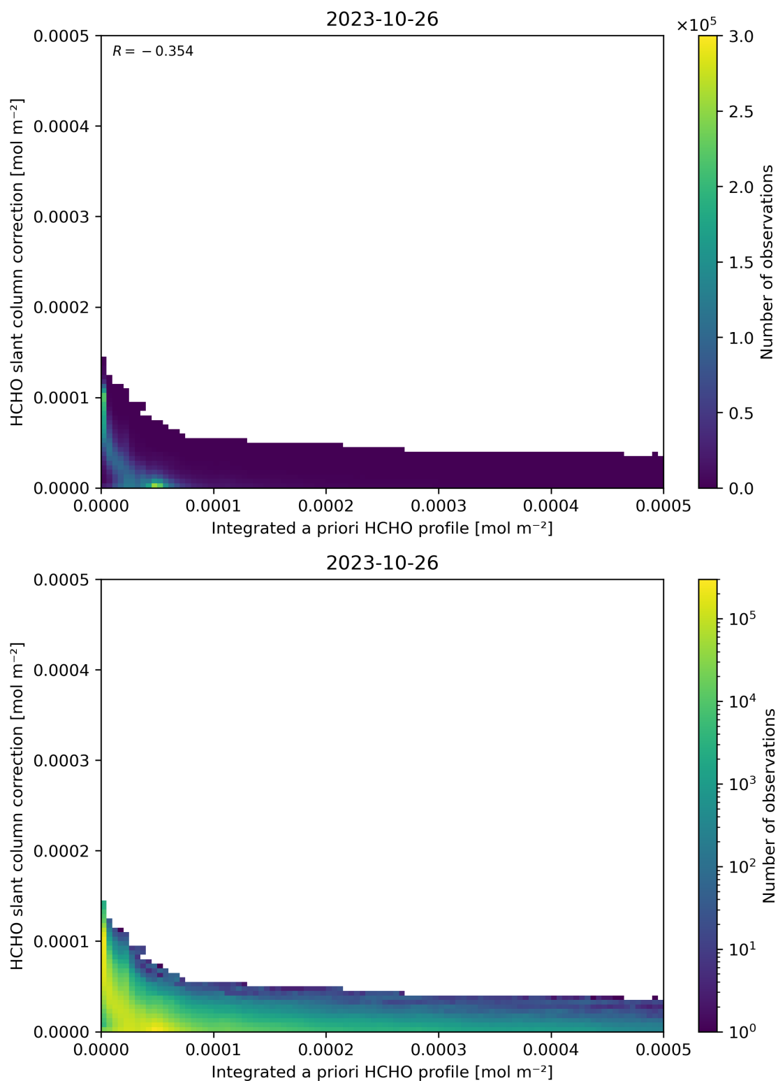
Figure 152: Scatter density plot of “Integrated a priori HCHO profile” against “HCHO slant column correction” for 2023-10-25 to 2023-10-27.
