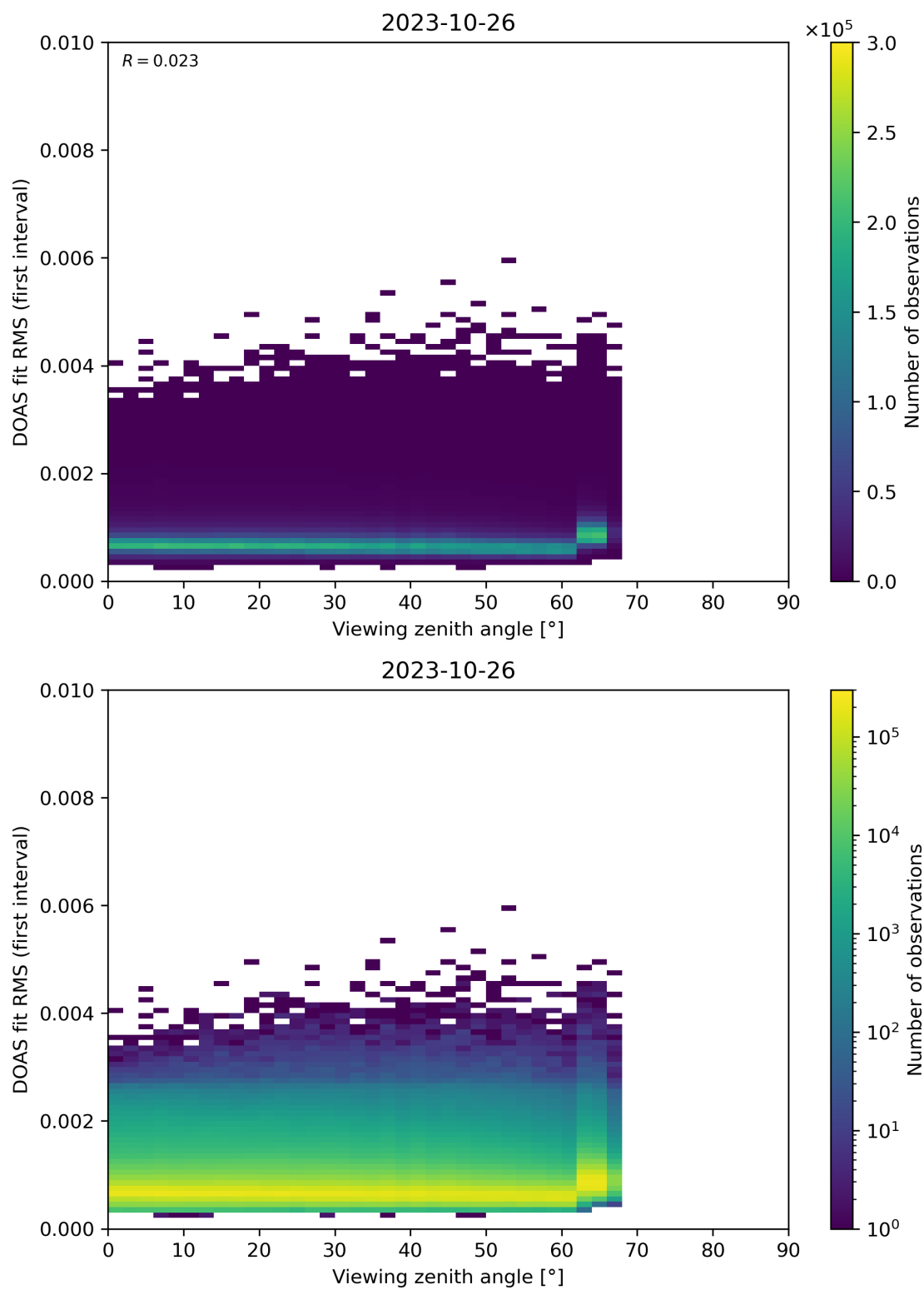
Figure 182: Scatter density plot of “Viewing zenith angle” against “DOAS fit RMS (first interval)” for 2023-10-25 to 2023-10-27.
