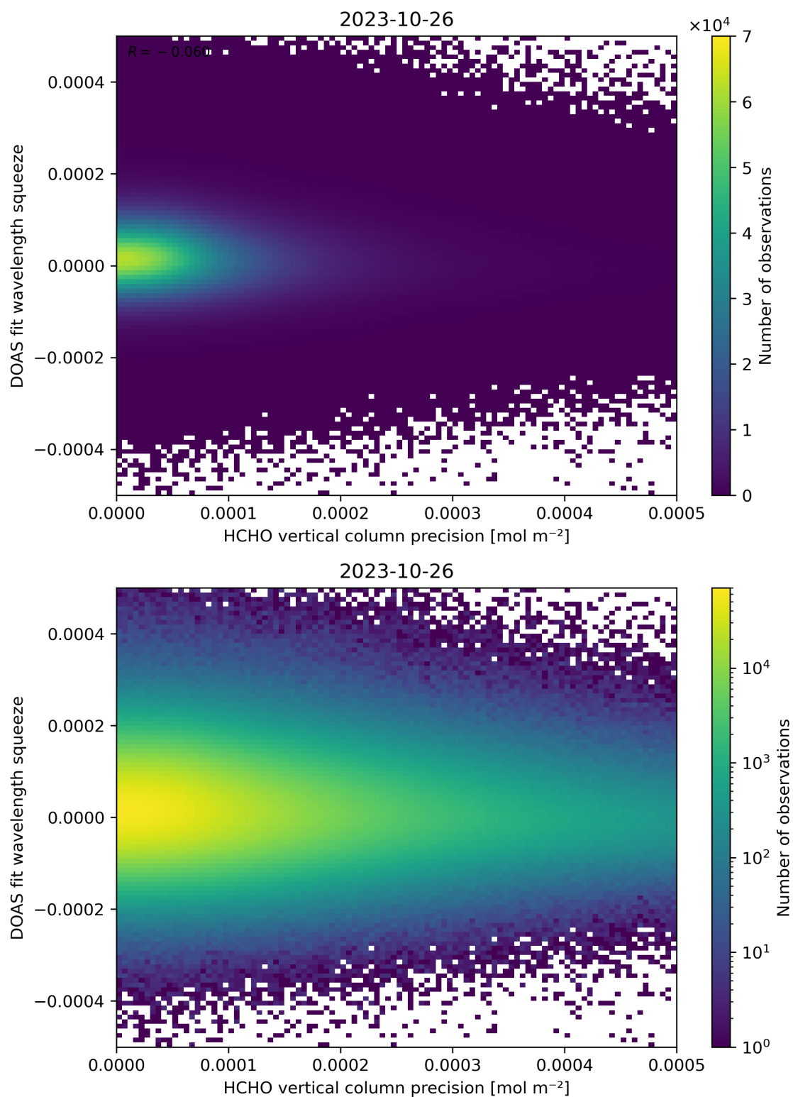
Figure 138: Scatter density plot of “HCHO vertical column precision” against “DOAS fit wavelength squeeze” for 2023-10-25 to 2023-10-27.
