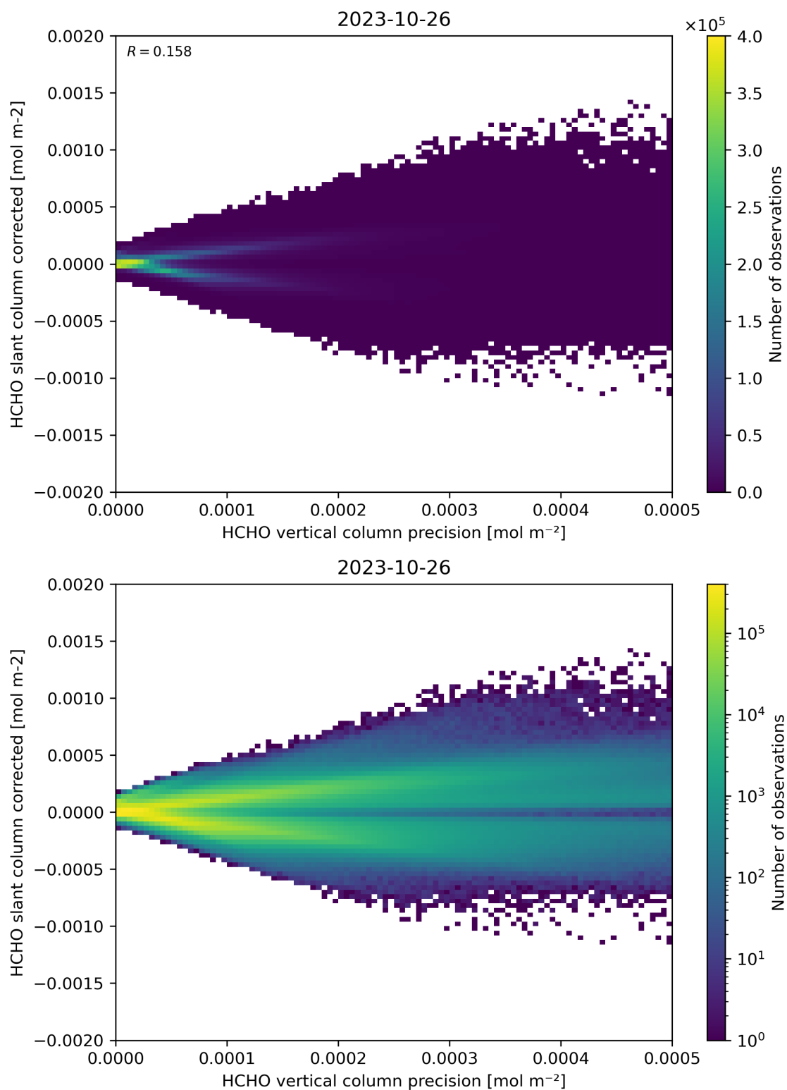
Figure 140: Scatter density plot of “HCHO vertical column precision” against “HCHO slant column corrected” for 2023-10-25 to 2023-10-27.
