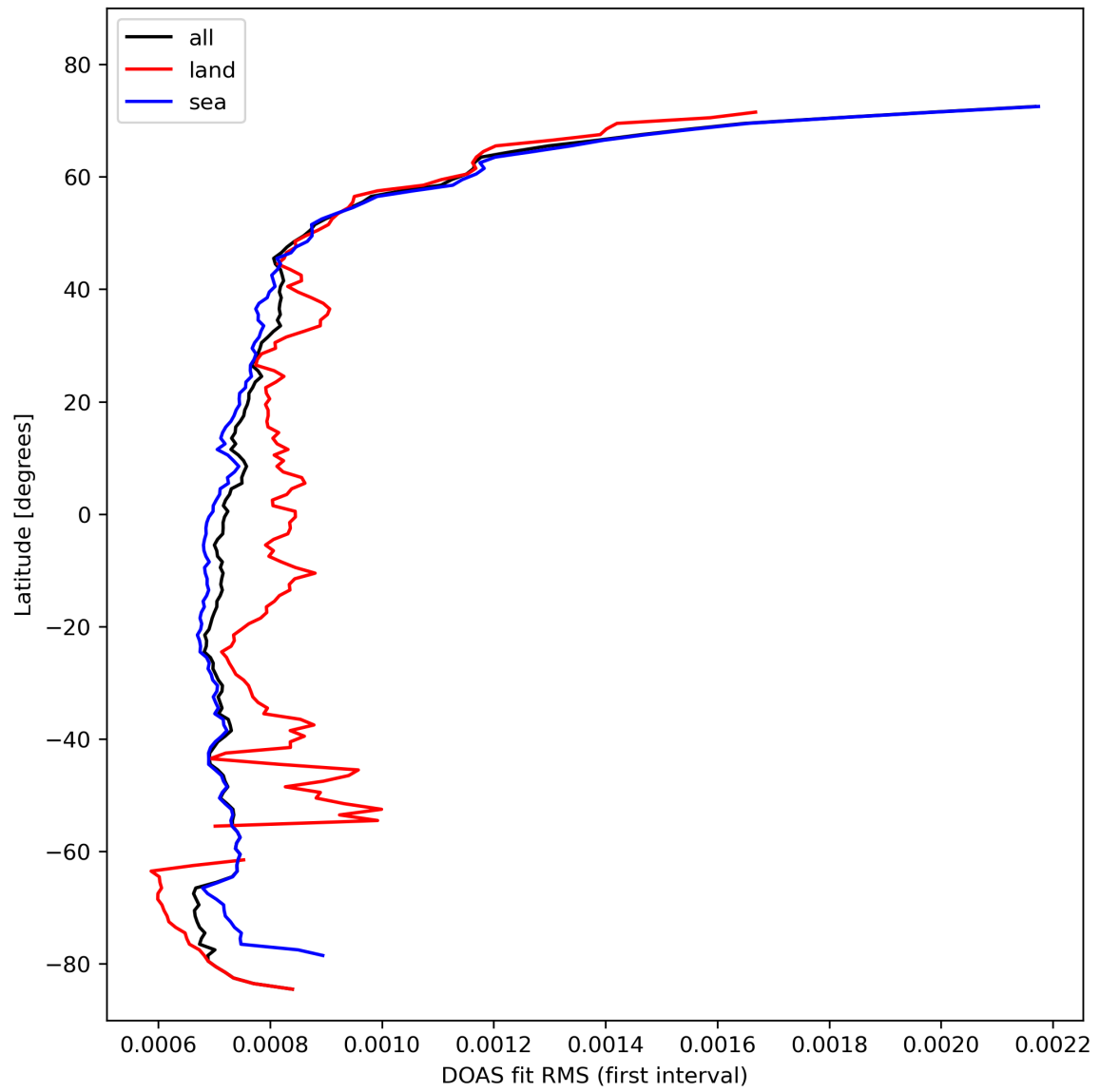
Figure 32: Zonal average of “DOAS fit RMS (first interval)” for 2023-10-25 to 2023-10-27.
