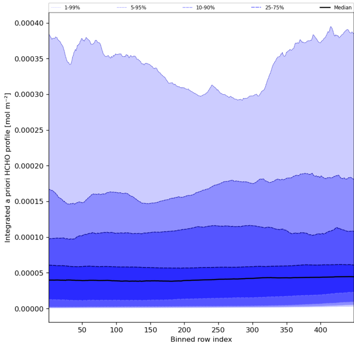
Figure 57: Along track statistics of “Integrated a priori HCHO profile” for 2023-10-25 to 2023-10-27
