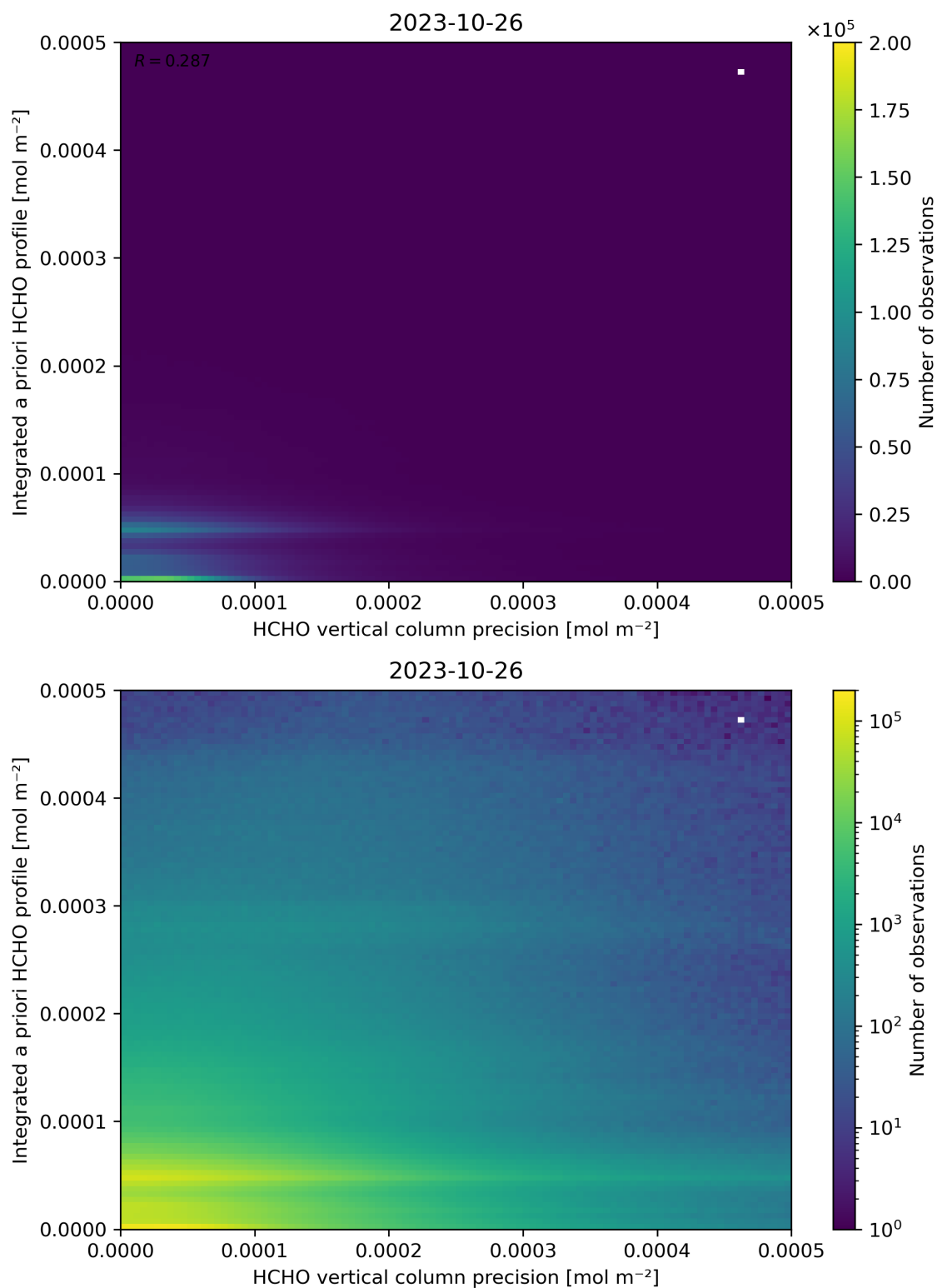
Figure 147: Scatter density plot of “HCHO vertical column precision” against “Integrated a priori HCHO profile” for 2023-10-25 to 2023-10-27.
