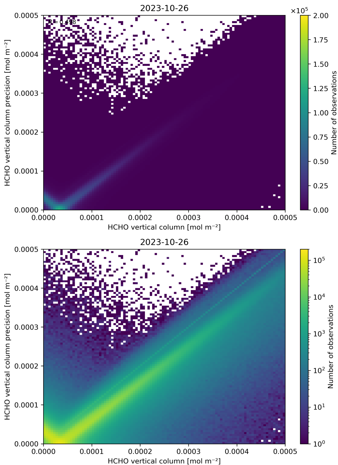
Figure 134: Scatter density plot of “HCHO vertical column” against “HCHO vertical column precision” for 2023-10-25 to 2023-10-27.
