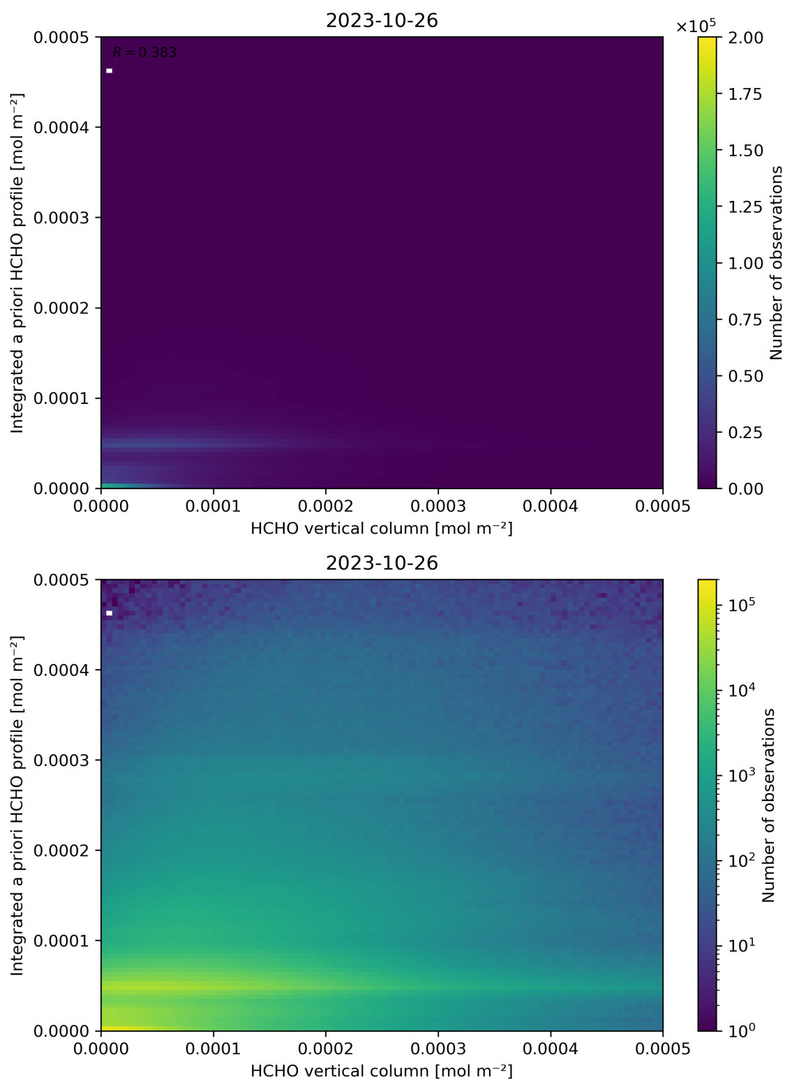
Figure 135: Scatter density plot of “HCHO vertical column” against “Integrated a priori HCHO profile” for 2023-10-25 to 2023-10-27.
