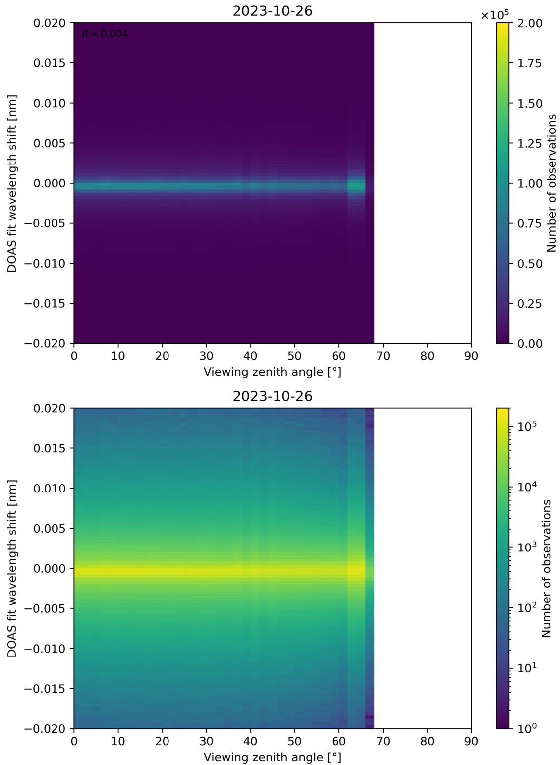
Figure 183: Scatter density plot of “Viewing zenith angle” against “DOAS fit wavelength shift” for 2023-10-25 to 2023-10-27.
