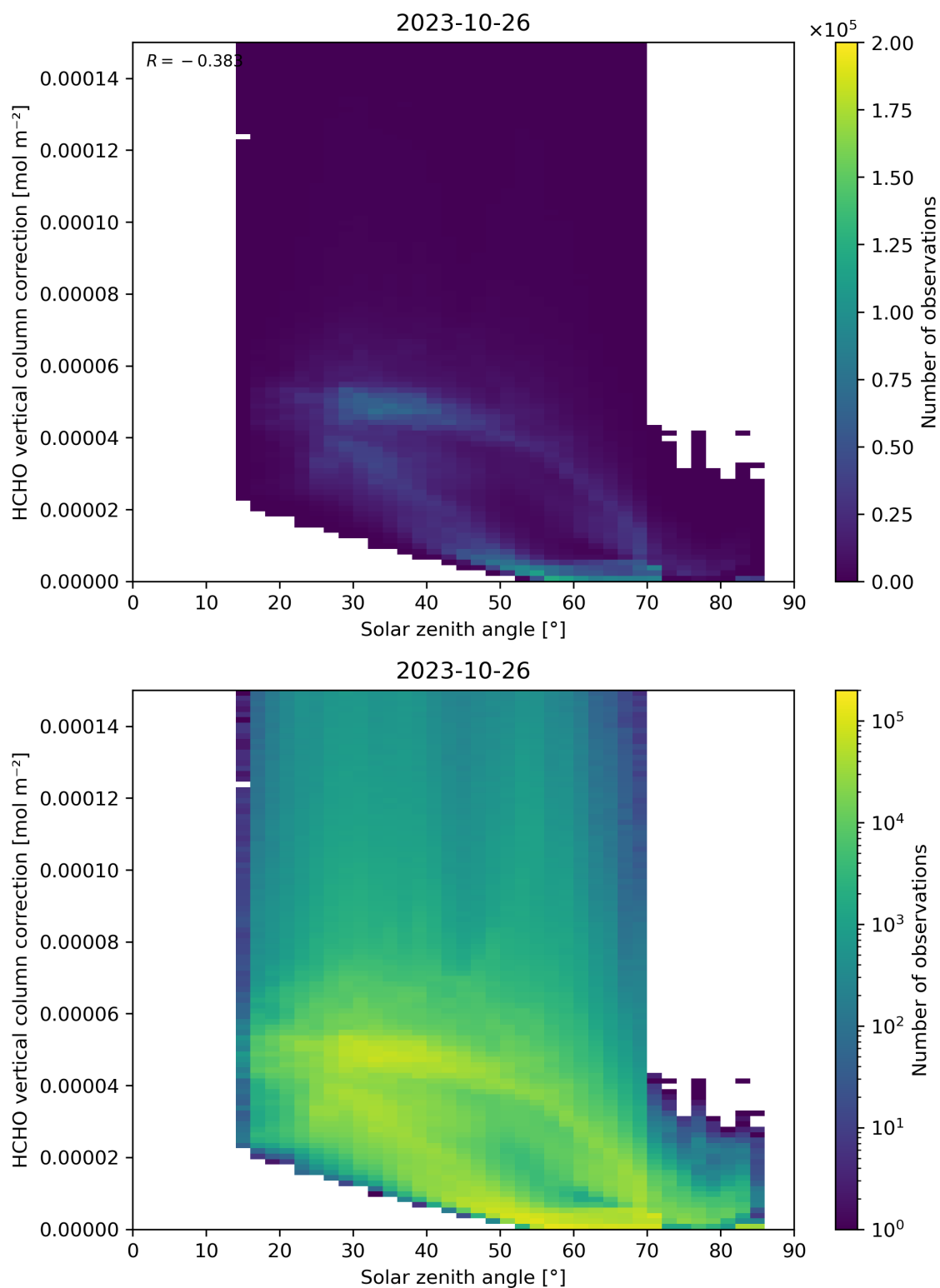
Figure 178: Scatter density plot of “Solar zenith angle” against “HCHO vertical column correction” for 2023-10-25 to 2023-10-27.
