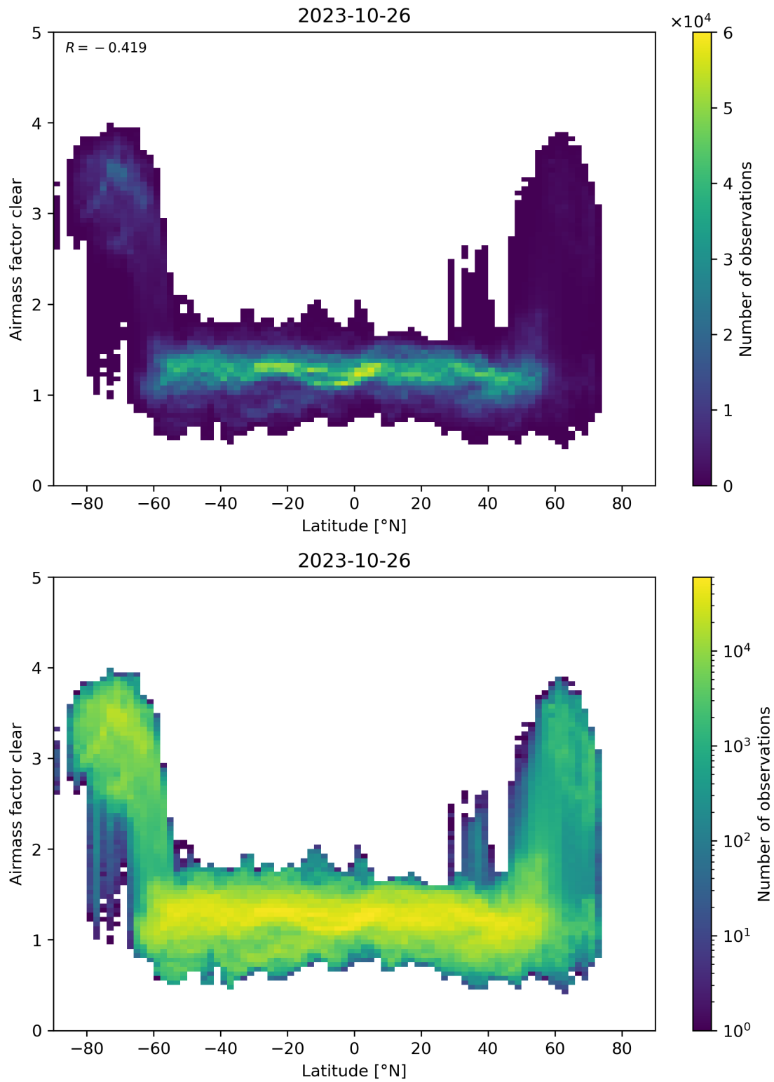
Figure 156: Scatter density plot of “Latitude” against “Airmass factor clear” for 2023-10-25 to 2023-10-27.
