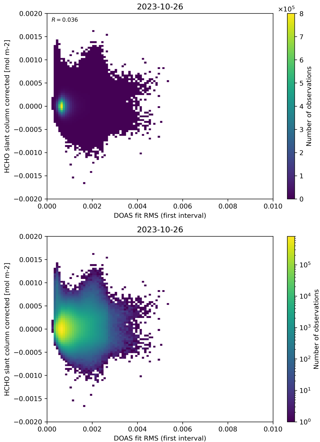
Figure 62: Scatter density plot of “DOAS fit RMS (first interval)” against “HCHO slant column corrected” for 2023-10-25 to 2023-10-27.
