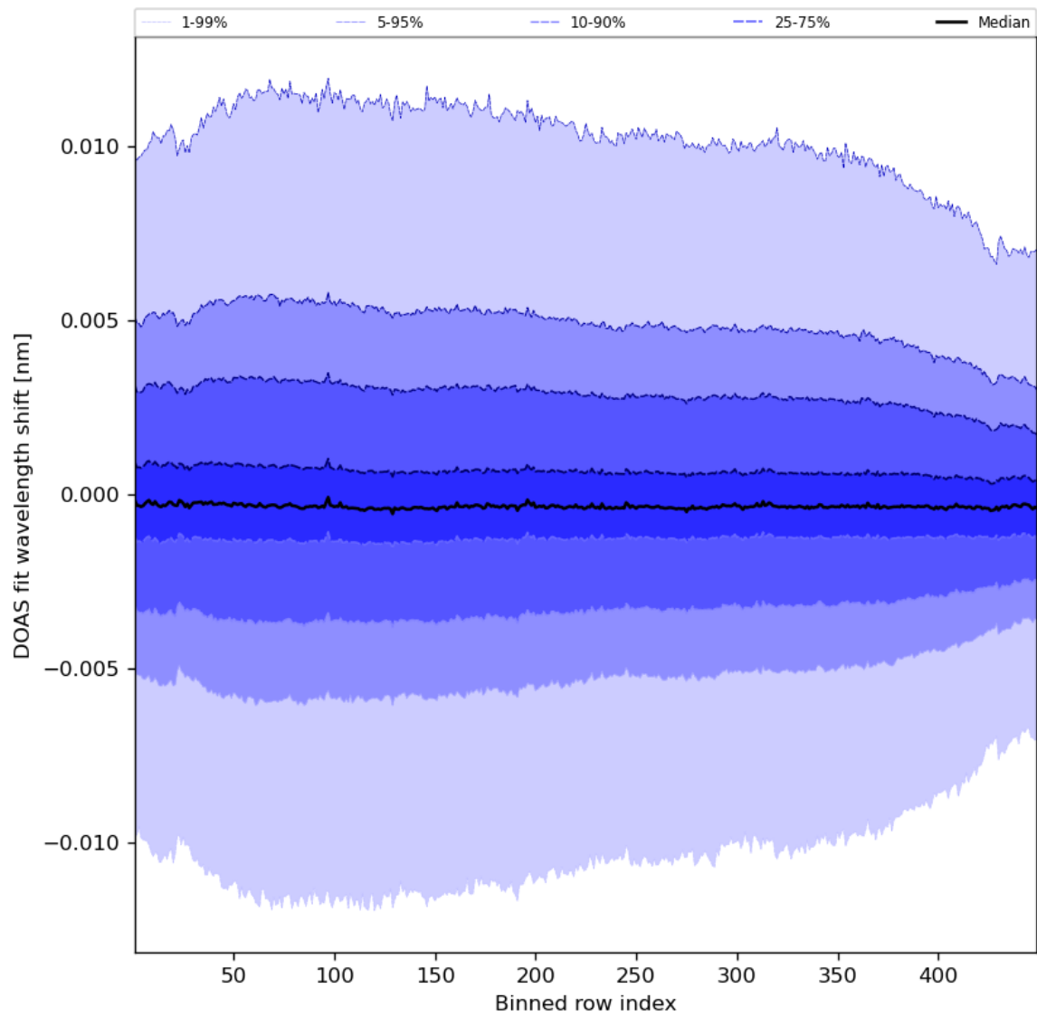
Figure 58: Along track statistics of “DOAS fit wavelength shift” for 2023-10-25 to 2023-10-27
