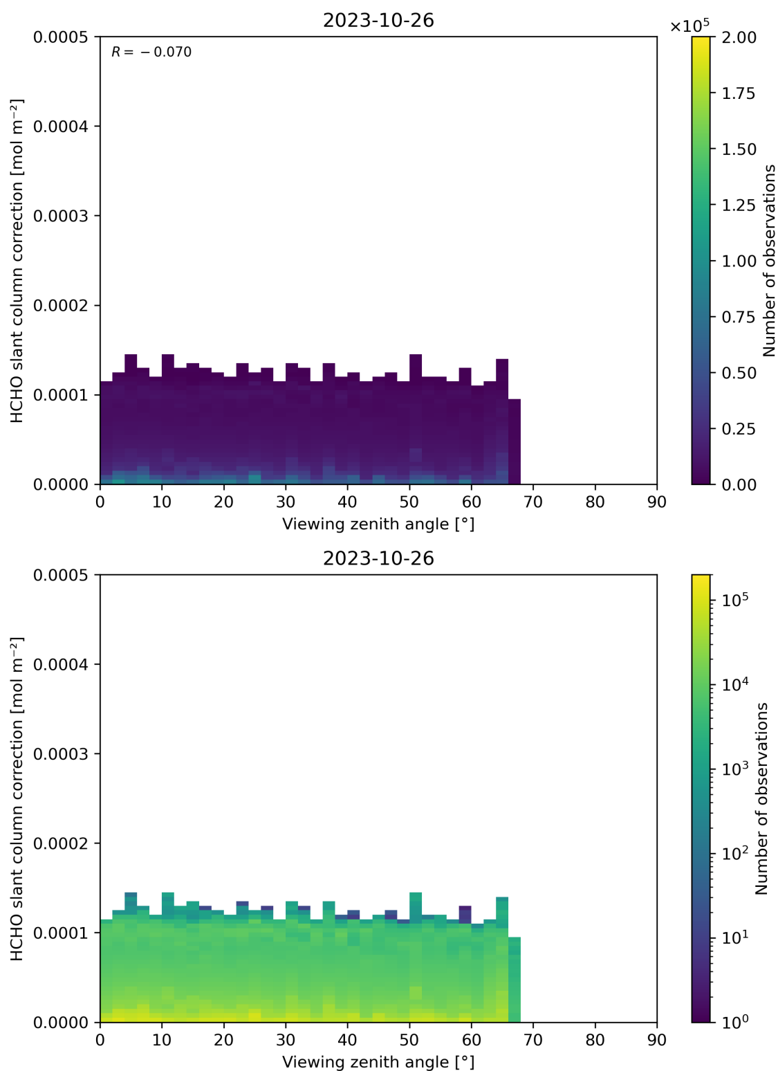
Figure 187: Scatter density plot of “Viewing zenith angle” against “HCHO slant column correction” for 2023-10-25 to 2023-10-27.
