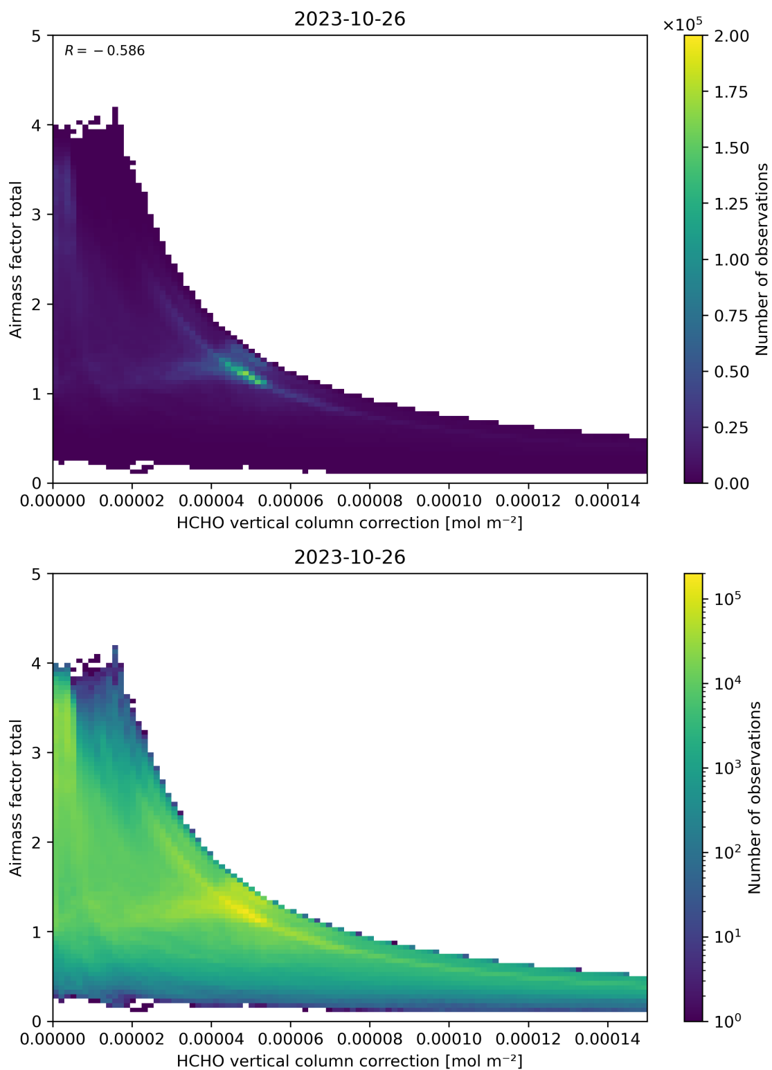
Figure 120: Scatter density plot of “HCHO vertical column correction” against “Airmass factor total” for 2023-10-25 to 2023-10-27.
