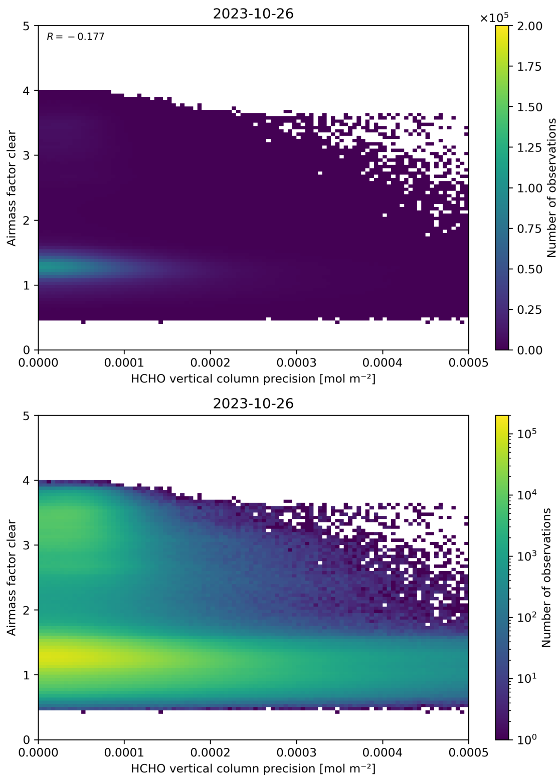
Figure 139: Scatter density plot of “HCHO vertical column precision” against “Airmass factor clear” for 2023-10-25 to 2023-10-27.
