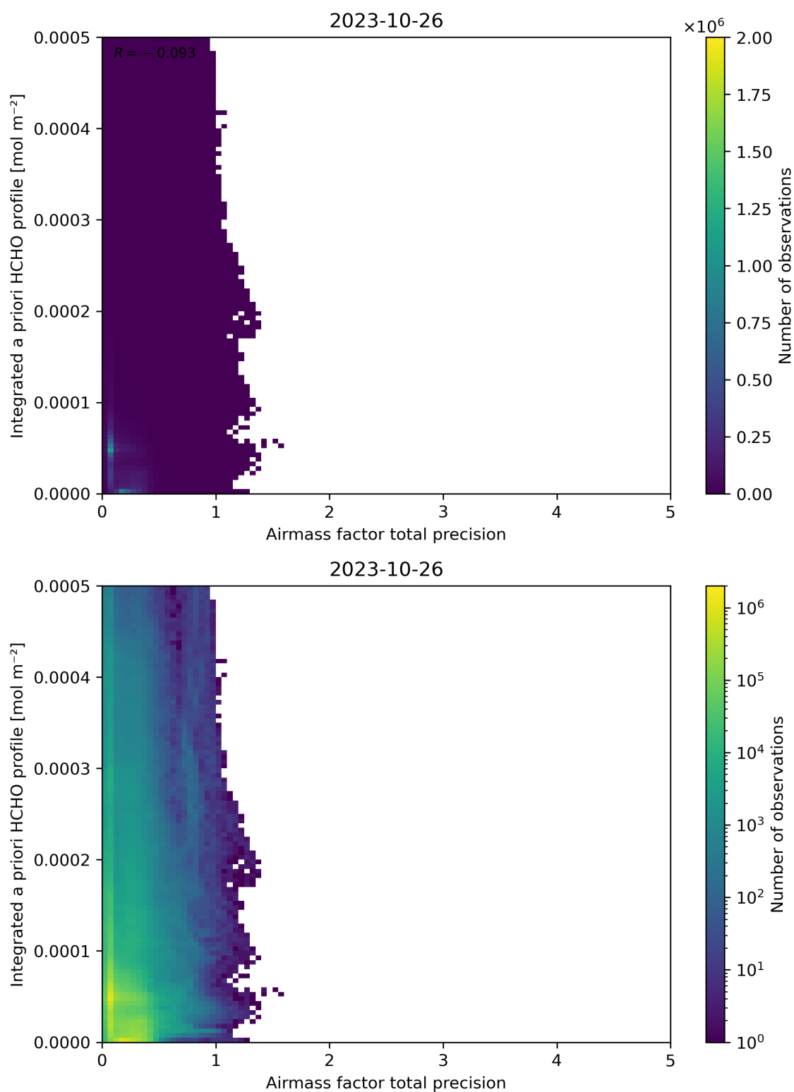
Figure 111: Scatter density plot of “Airmass factor total precision” against “Integrated a priori HCHO profile” for 2023-10-25 to 2023-10-27.
