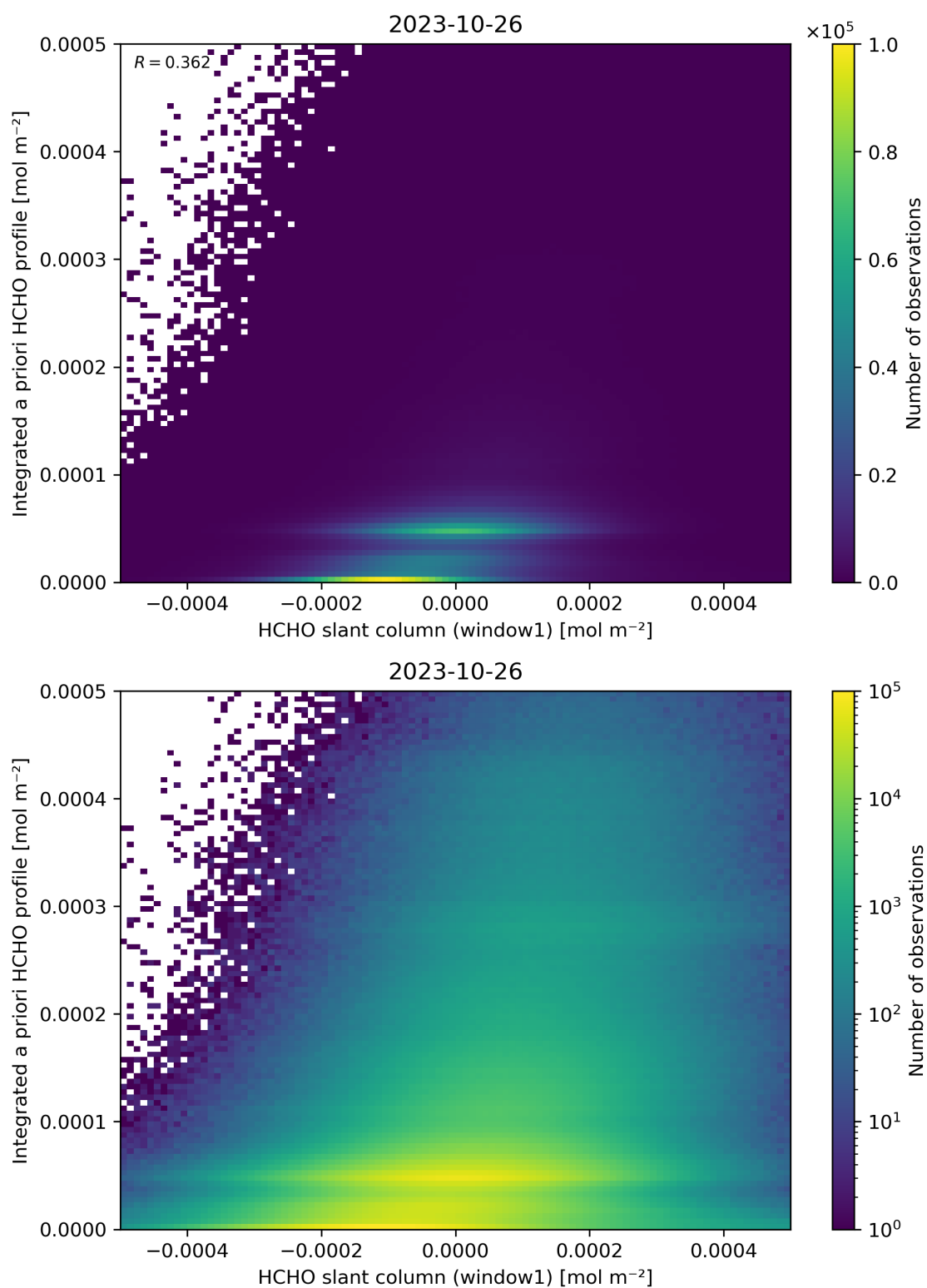
Figure 87: Scatter density plot of “HCHO slant column (window1)” against “Integrated a priori HCHO profile” for 2023-10-25 to 2023-10-27.
