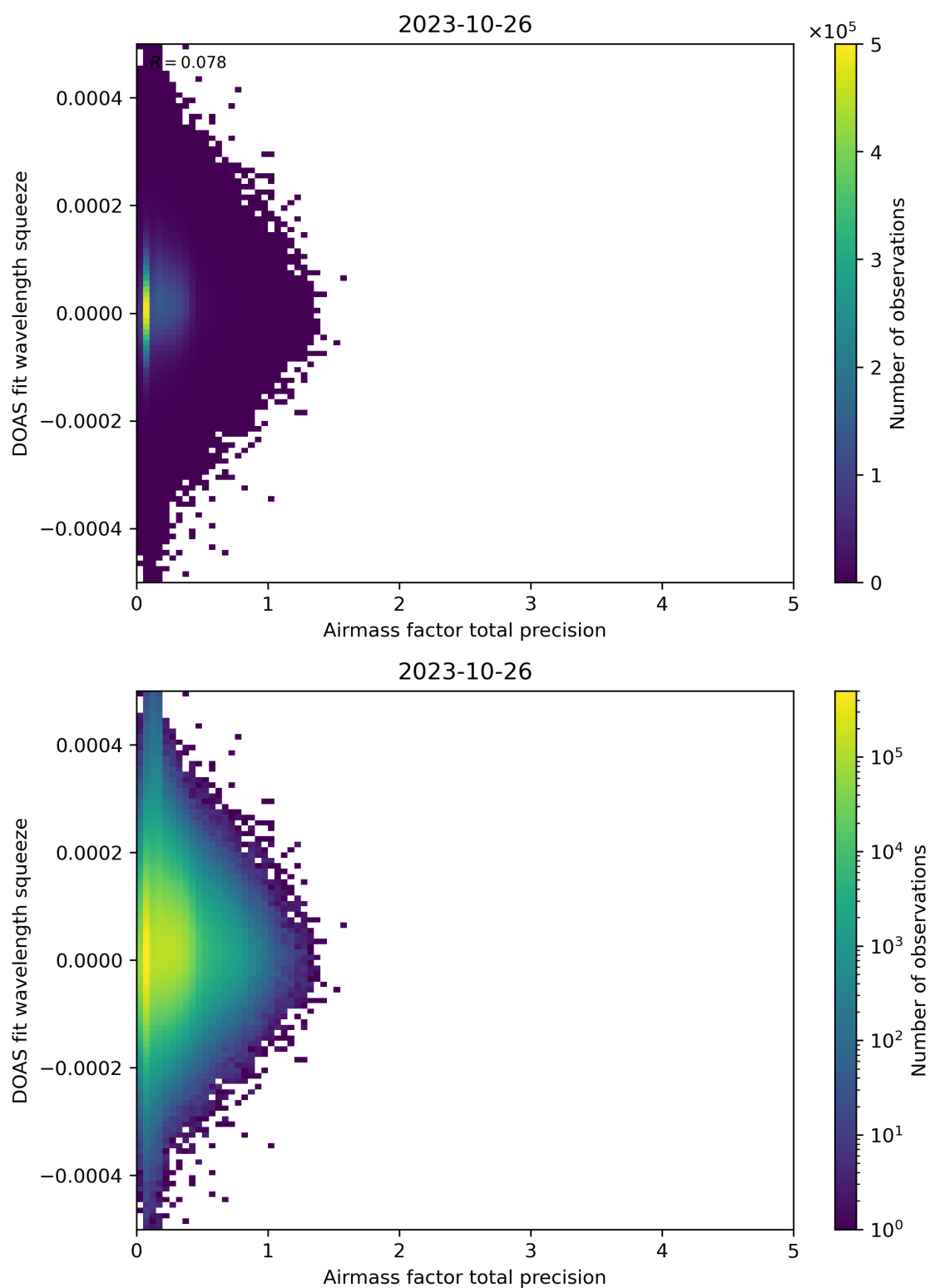
Figure 107: Scatter density plot of “Airmass factor total precision” against “DOAS fit wavelength squeeze” for 2023-10-25 to 2023-10-27.
