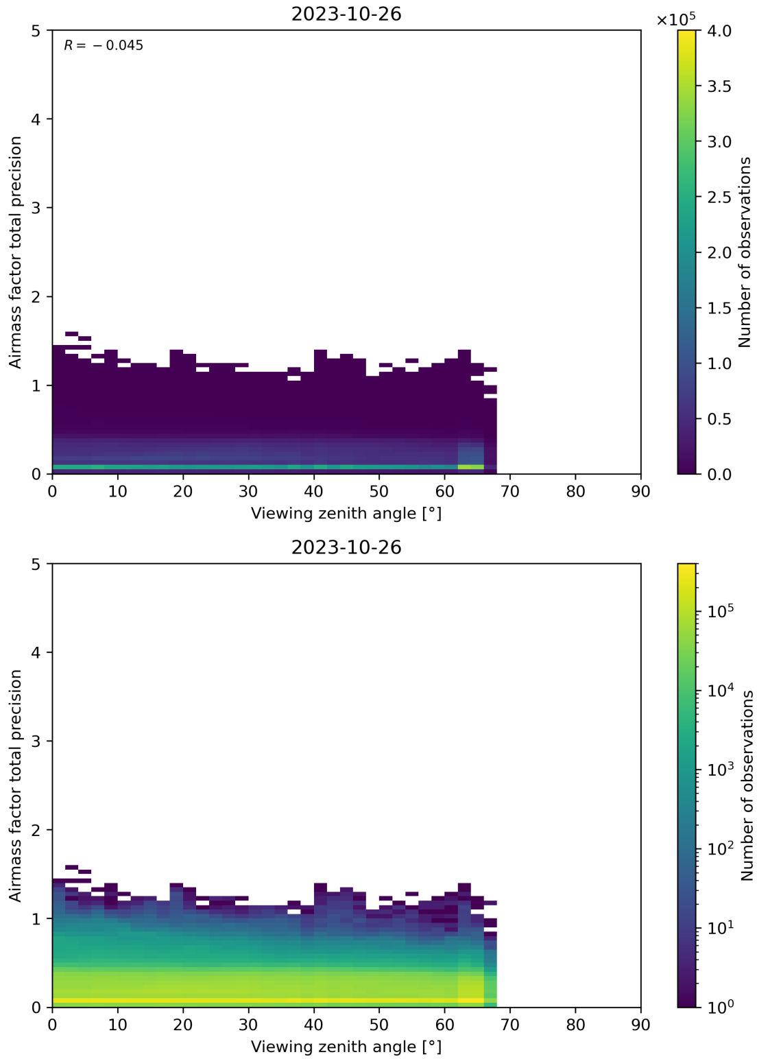
Figure 191: Scatter density plot of “Viewing zenith angle” against “Airmass factor total precision” for 2023-10-25 to 2023-10-27.
