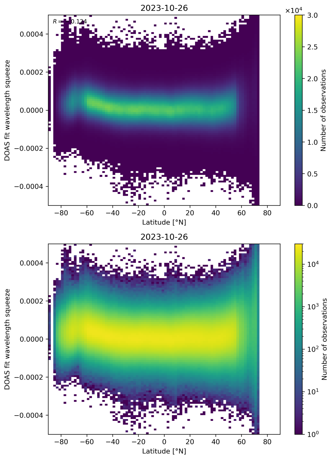
Figure 155: Scatter density plot of “Latitude” against “DOAS fit wavelength squeeze” for 2023-10-25 to 2023-10-27.
