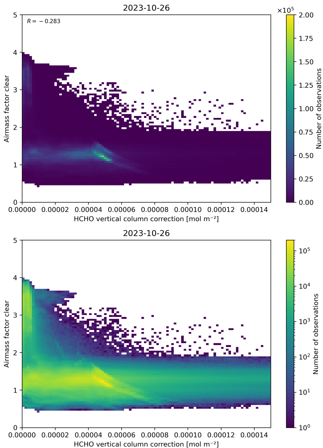
Figure 115: Scatter density plot of “HCHO vertical column correction” against “Airmass factor clear” for 2023-10-25 to 2023-10-27.
