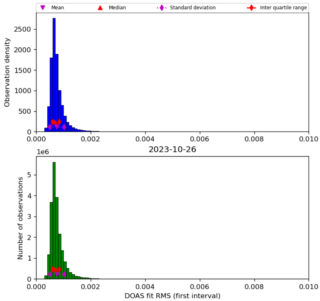
Figure 46: Histogram of “DOAS fit RMS (first interval)” for 2023-10-25 to 2023-10-27
