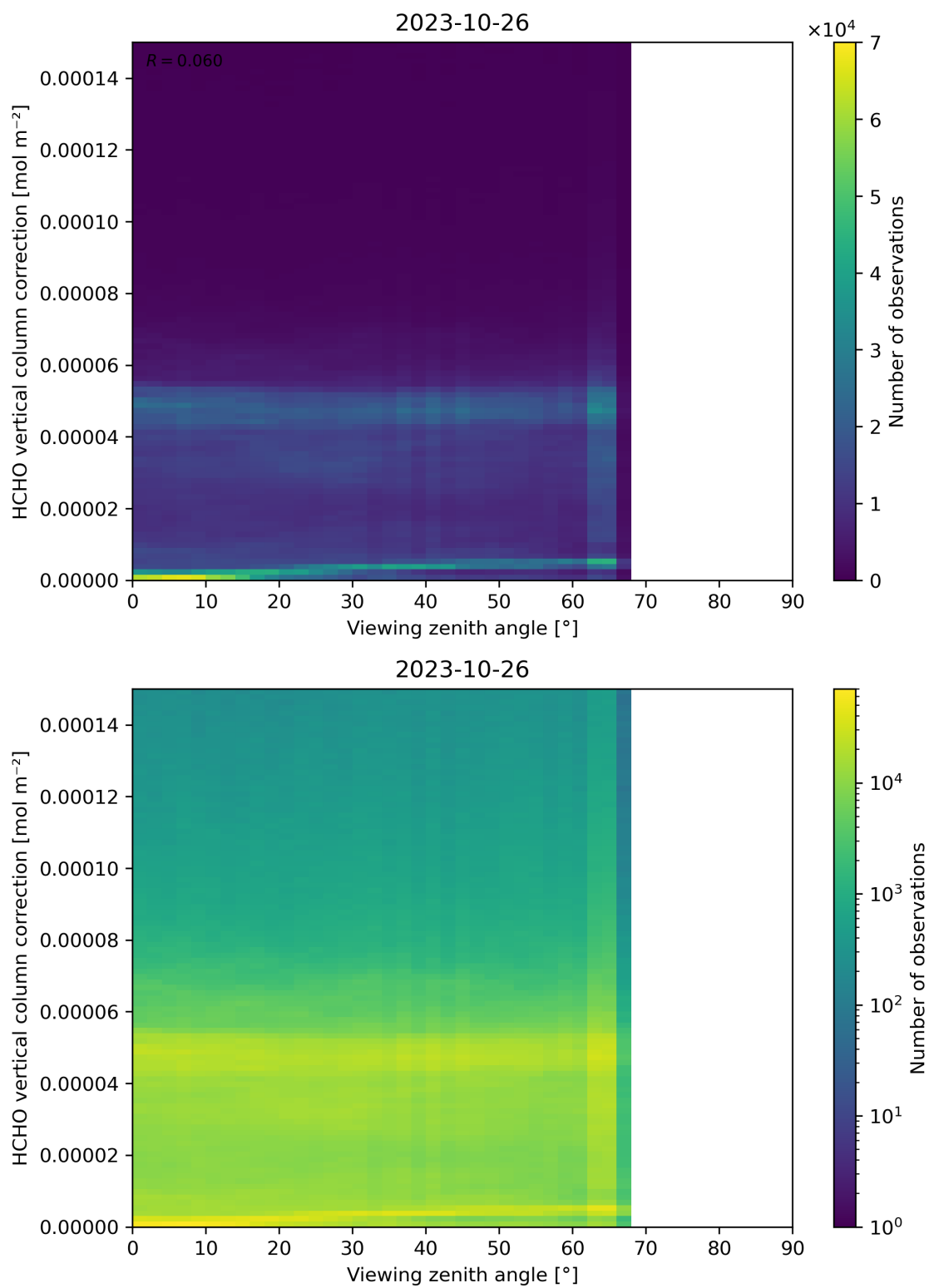
Figure 193: Scatter density plot of “Viewing zenith angle” against “HCHO vertical column correction” for 2023-10-25 to 2023-10-27.
