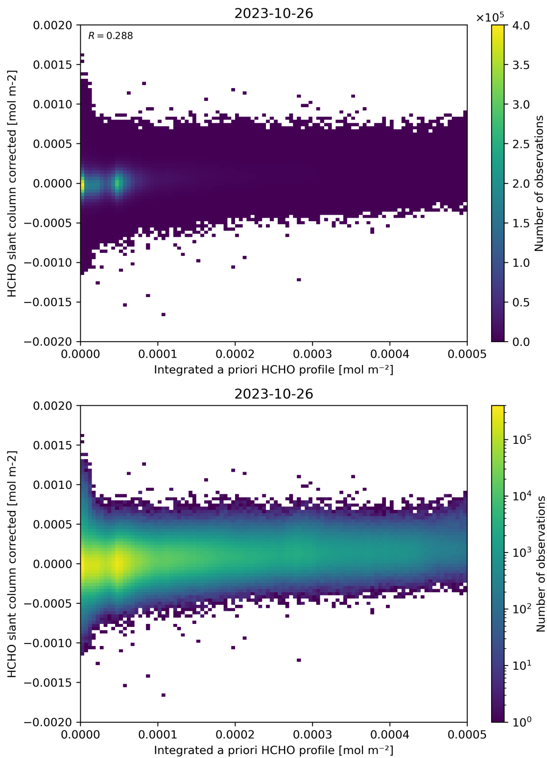
Figure 151: Scatter density plot of “Integrated a priori HCHO profile” against “HCHO slant column corrected” for 2023-10-25 to 2023-10-27.
