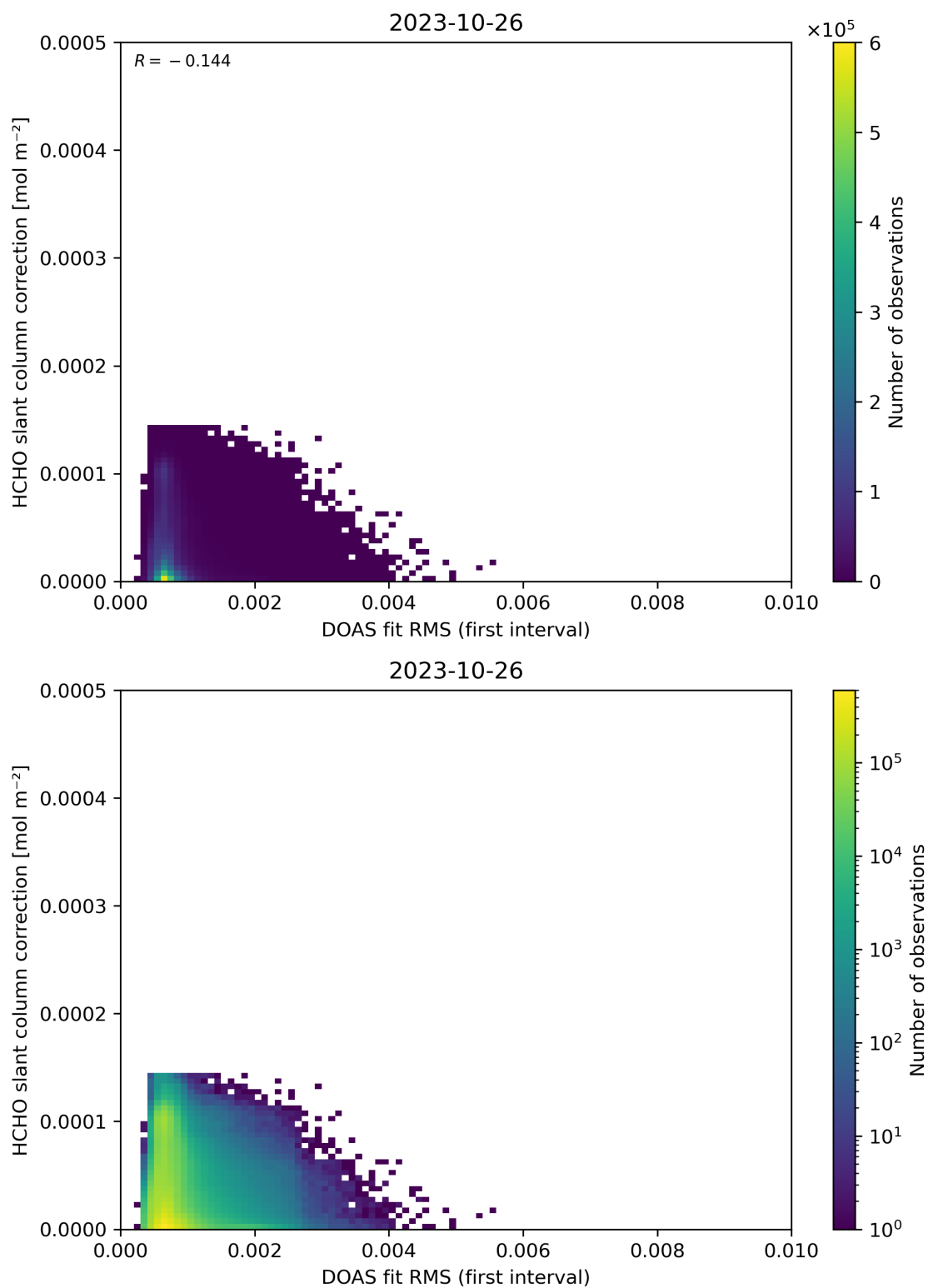
Figure 63: Scatter density plot of “DOAS fit RMS (first interval)” against “HCHO slant column correction” for 2023-10-25 to 2023-10-27.
