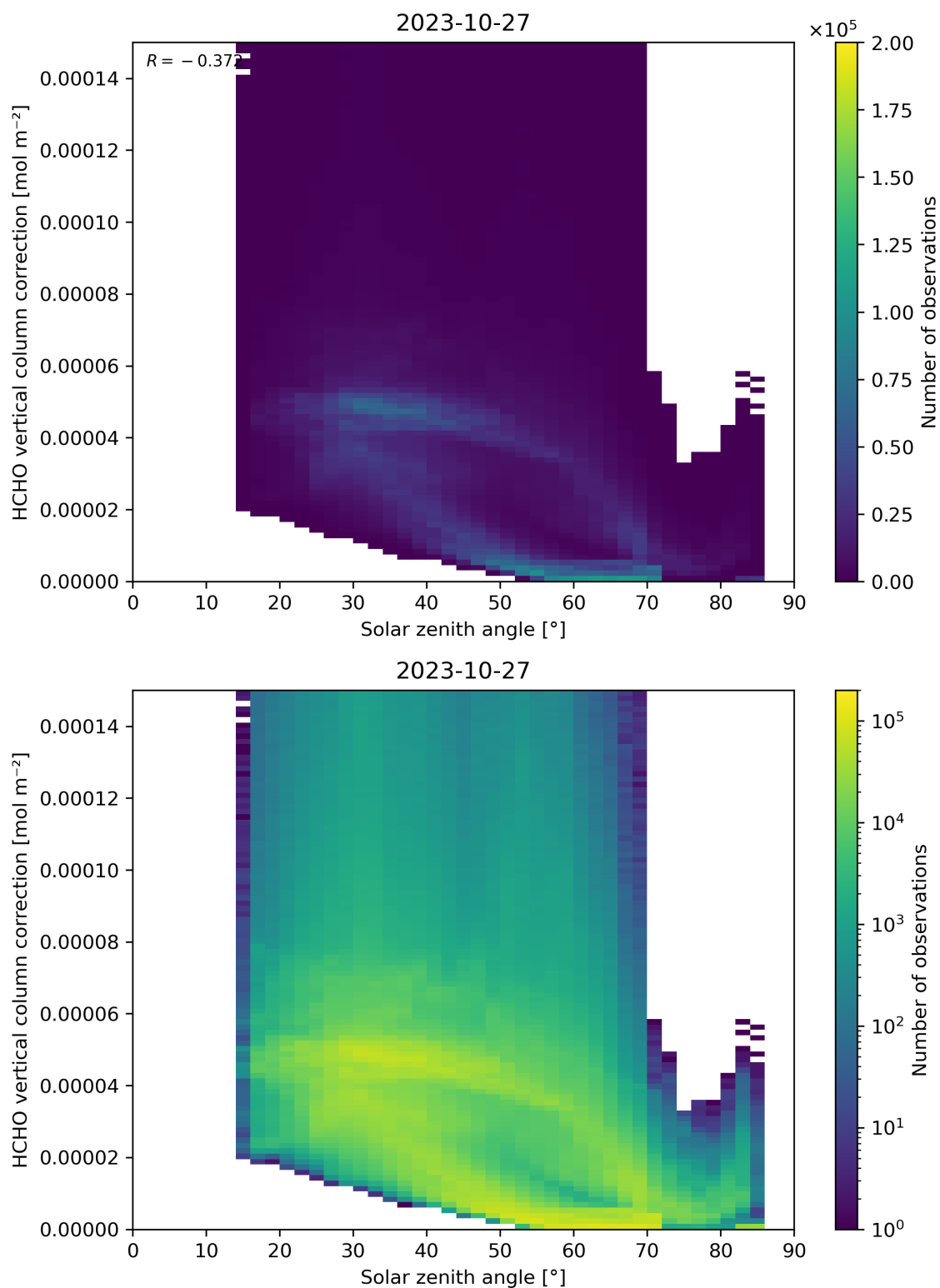
Figure 178: Scatter density plot of “Solar zenith angle” against “HCHO vertical column correction” for 2023-10-27 to 2023-10-28.
