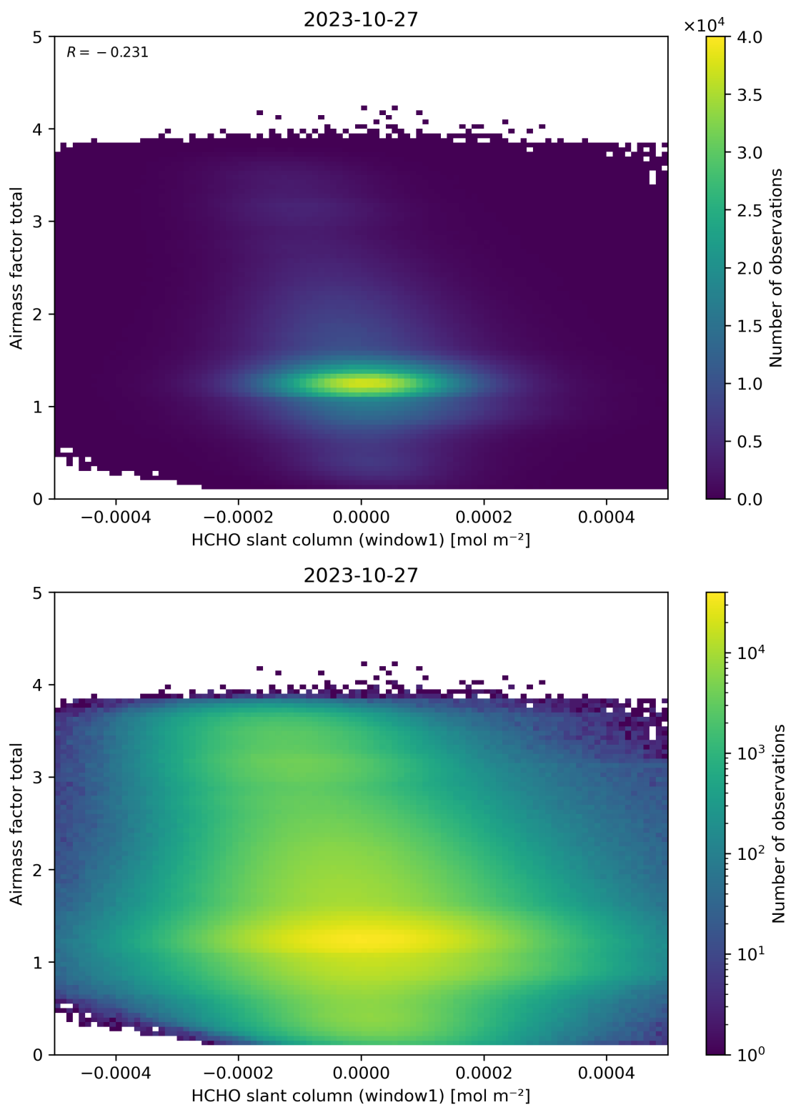
Figure 85: Scatter density plot of “HCHO slant column (window1)” against “Airmass factor total” for 2023-10-27 to 2023-10-28.
