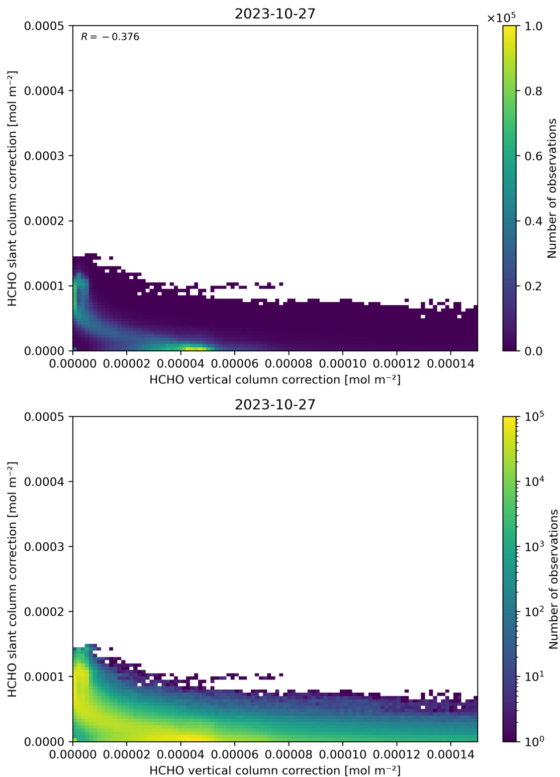
Figure 117: Scatter density plot of “HCHO vertical column correction” against “HCHO slant column correction” for 2023-10-27 to 2023-10-28.
