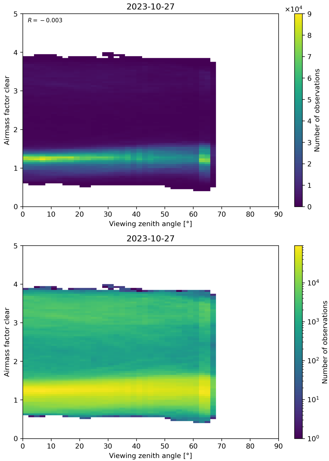
Figure 185: Scatter density plot of “Viewing zenith angle” against “Airmass factor clear” for 2023-10-27 to 2023-10-28.
