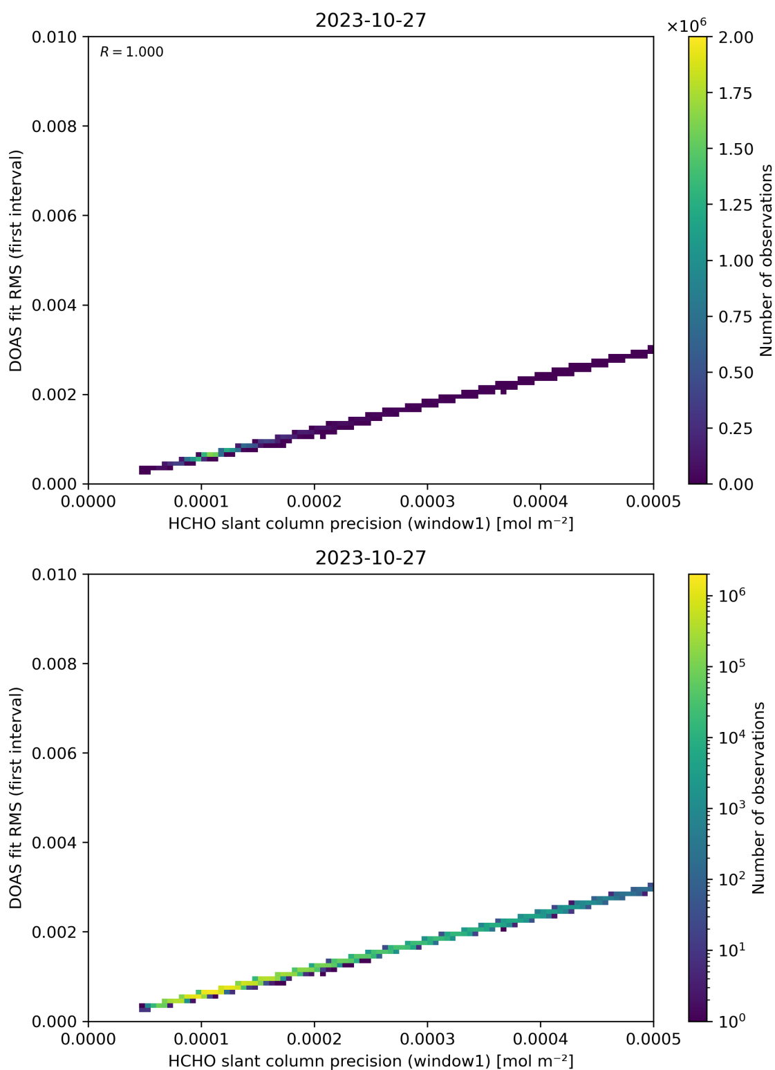
Figure 88: Scatter density plot of “HCHO slant column precision (window1)” against “DOAS fit RMS (first interval)” for 2023-10-27 to 2023-10-28.
