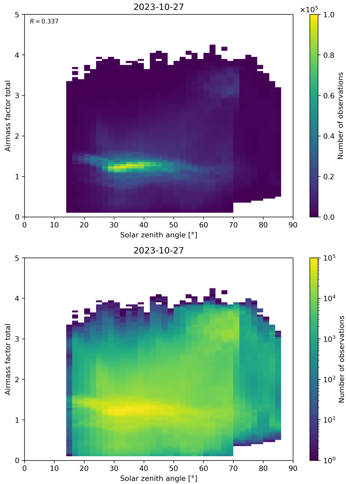
Figure 175: Scatter density plot of “Solar zenith angle” against “Airmass factor total” for 2023-10-27 to 2023-10-28.
