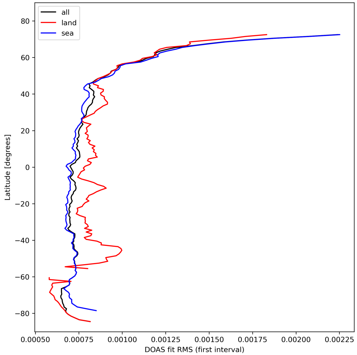
Figure 32: Zonal average of “DOAS fit RMS (first interval)” for 2023-10-27 to 2023-10-28.
