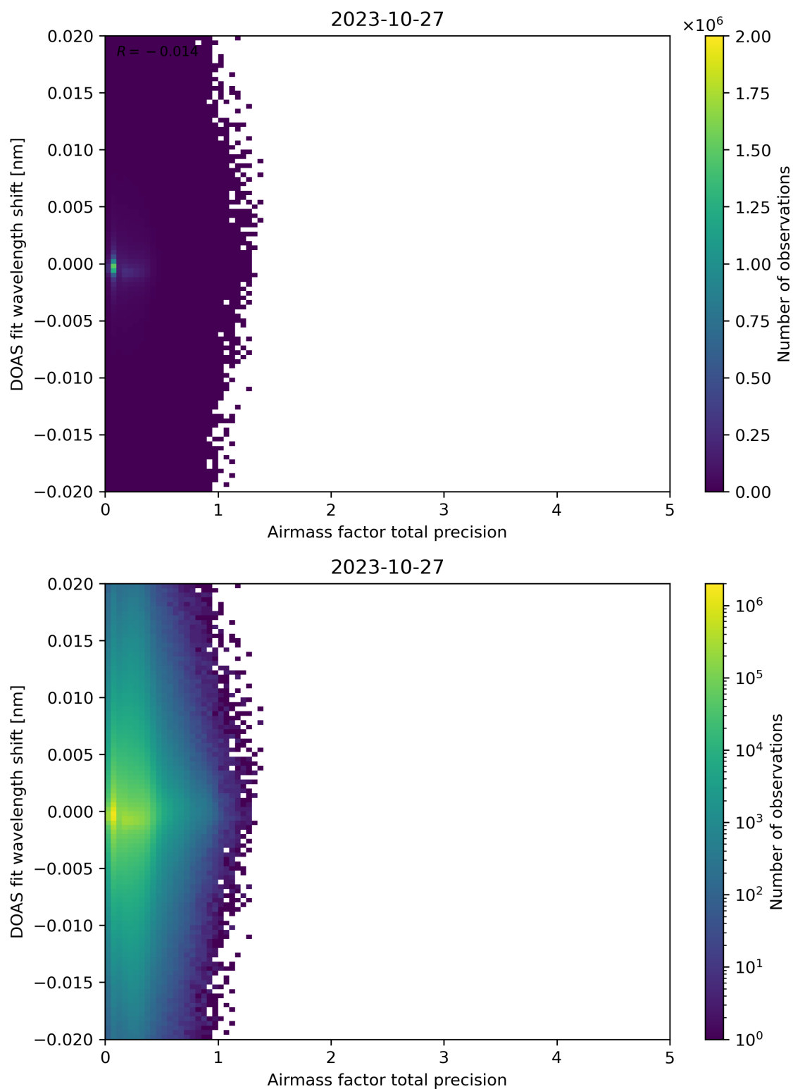
Figure 106: Scatter density plot of “Airmass factor total precision” against “DOAS fit wavelength shift” for 2023-10-27 to 2023-10-28.
