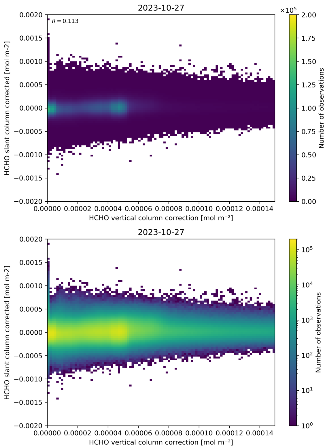
Figure 116: Scatter density plot of “HCHO vertical column correction” against “HCHO slant column corrected” for 2023-10-27 to 2023-10-28.
