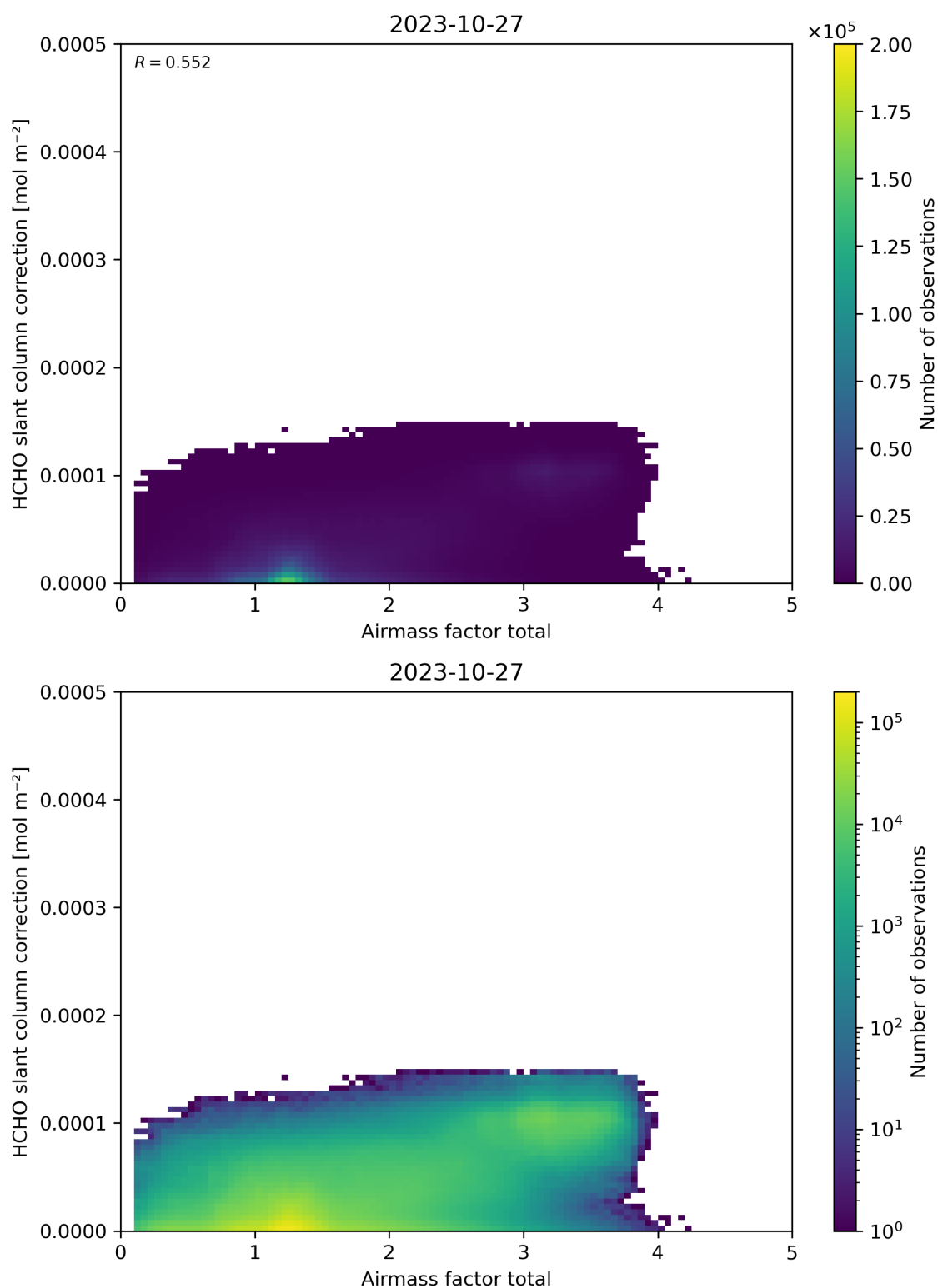
Figure 102: Scatter density plot of “Airmass factor total” against “HCHO slant column correction” for 2023-10-27 to 2023-10-28.
