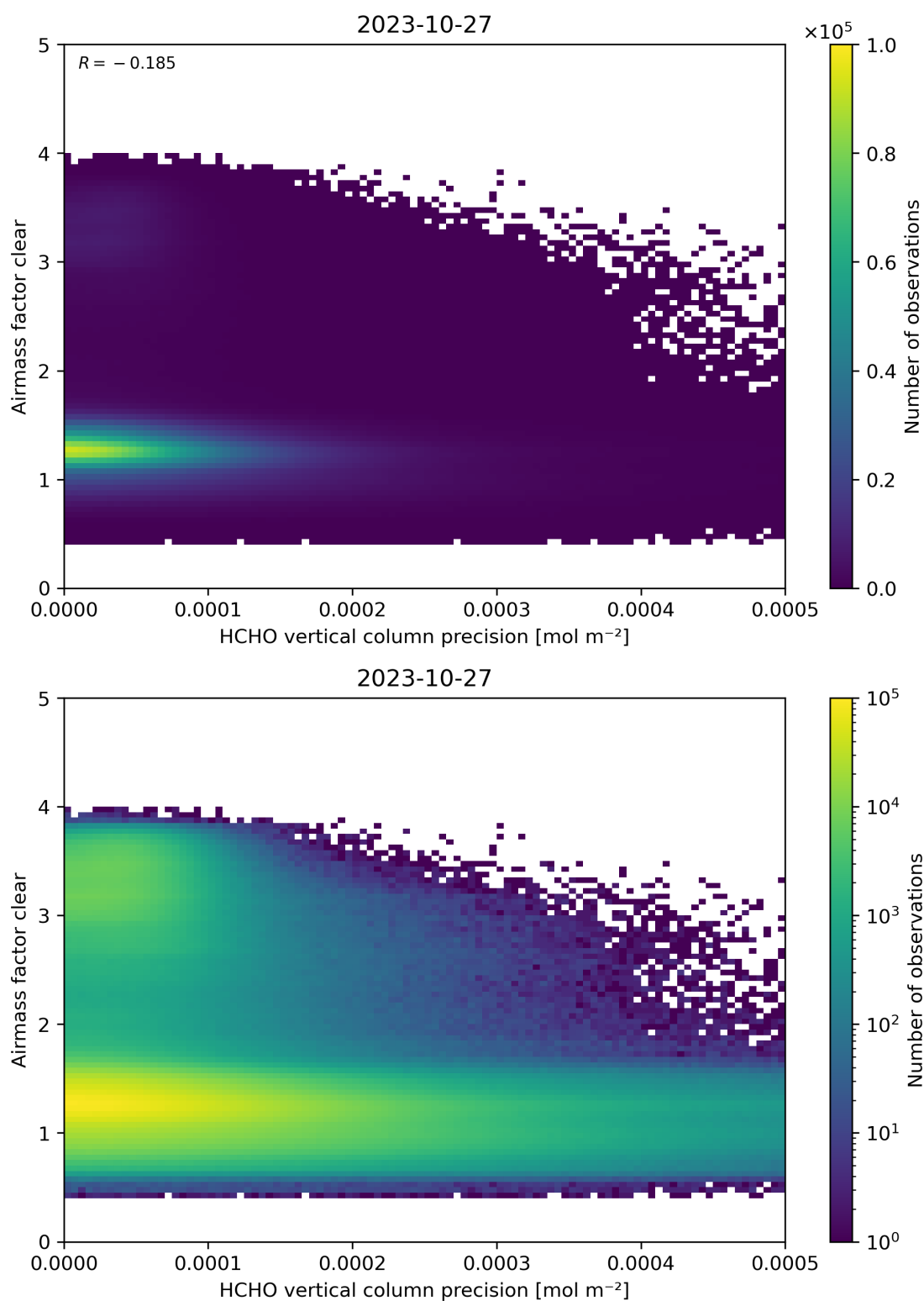
Figure 139: Scatter density plot of “HCHO vertical column precision” against “Airmass factor clear” for 2023-10-27 to 2023-10-28.
