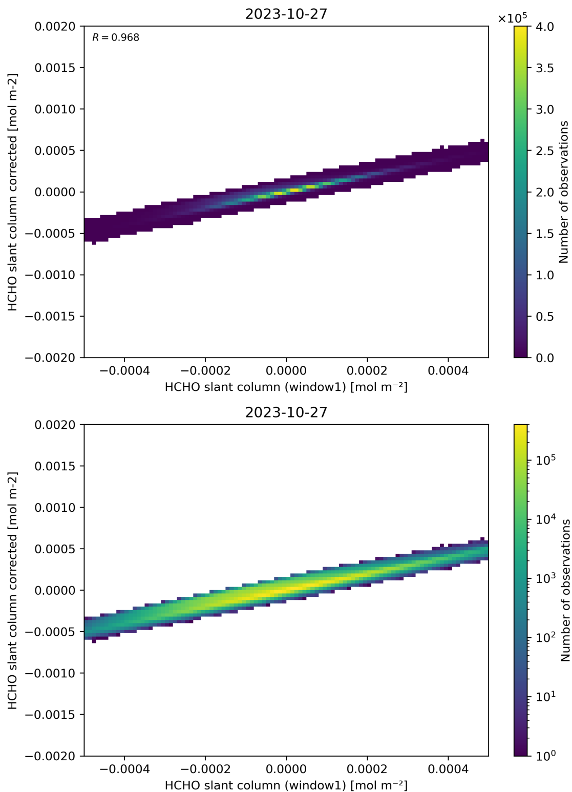
Figure 82: Scatter density plot of “HCHO slant column (window1)” against “HCHO slant column corrected” for 2023-10-27 to 2023-10-28.
