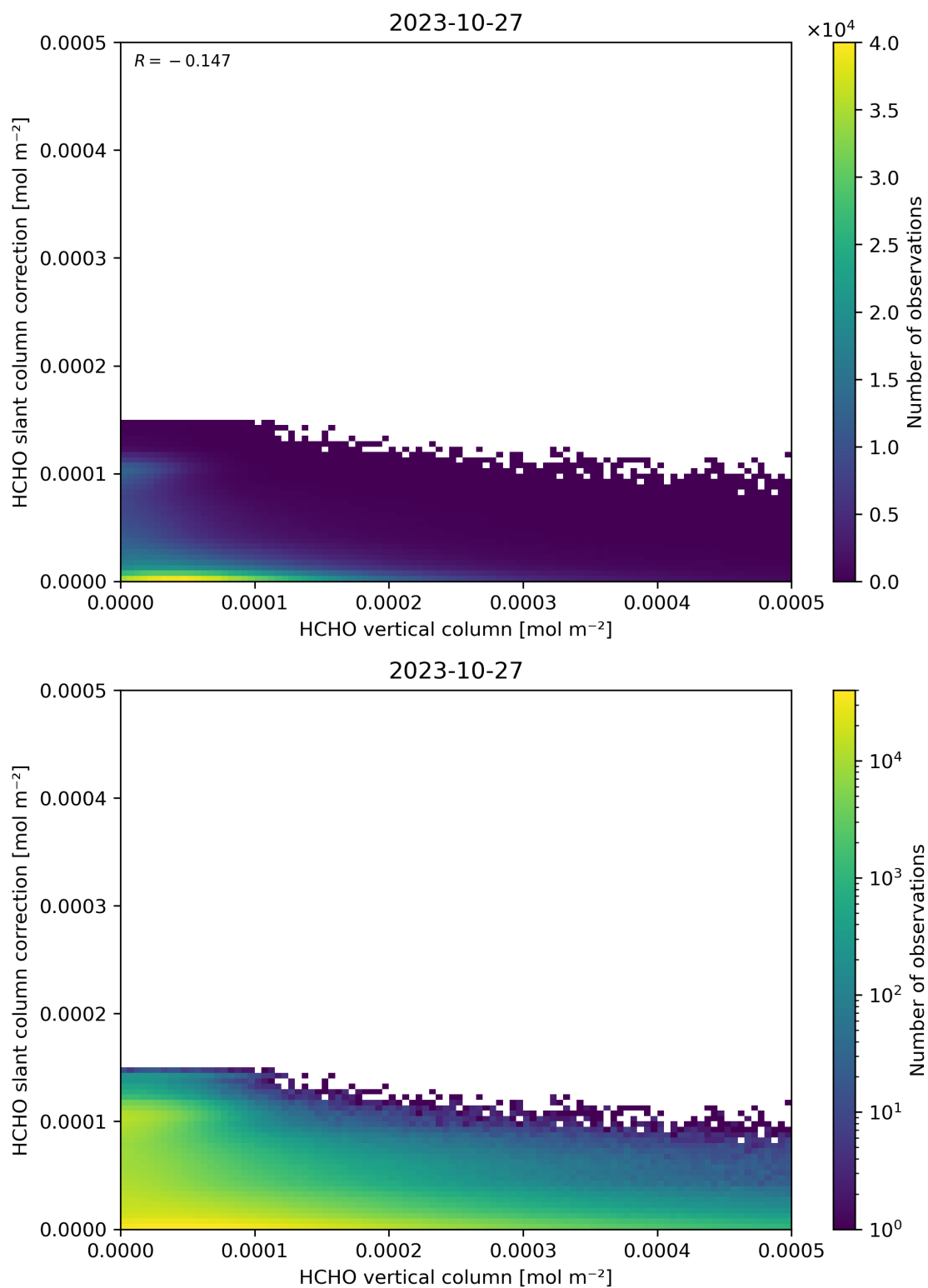
Figure 128: Scatter density plot of “HCHO vertical column” against “HCHO slant column correction” for 2023-10-27 to 2023-10-28.
