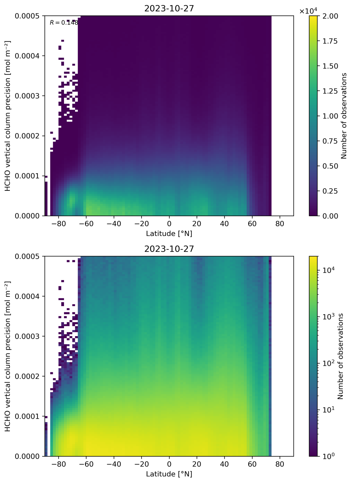
Figure 165: Scatter density plot of “Latitude” against “HCHO vertical column precision” for 2023-10-27 to 2023-10-28.
