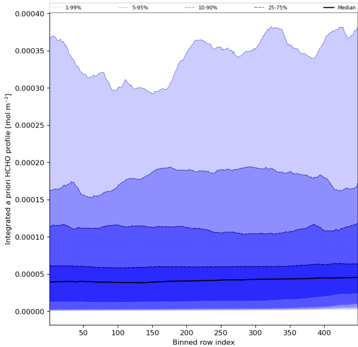
Figure 57: Along track statistics of "Integrated a priori HCHO profile" for 2023-10-27 to 2023-10-28
