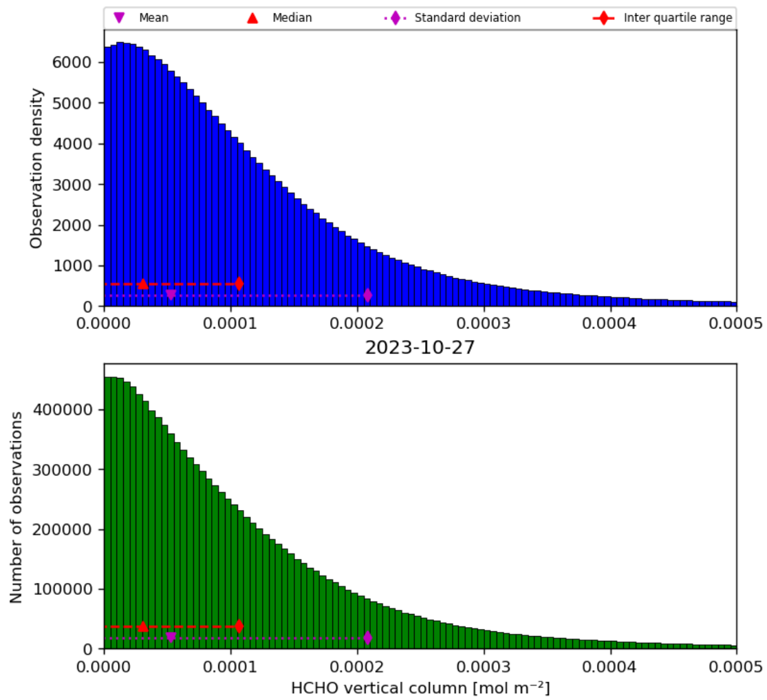
Figure 35: Histogram of “HCHO vertical column” for 2023-10-27 to 2023-10-28
