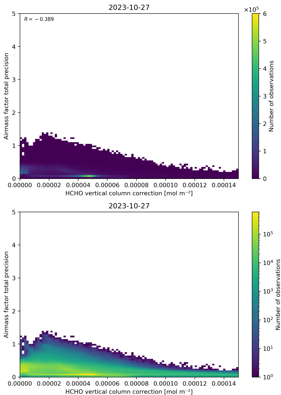
Figure 121: Scatter density plot of “HCHO vertical column correction” against “Airmass factor total precision” for 2023-10-27 to 2023-10-28.
