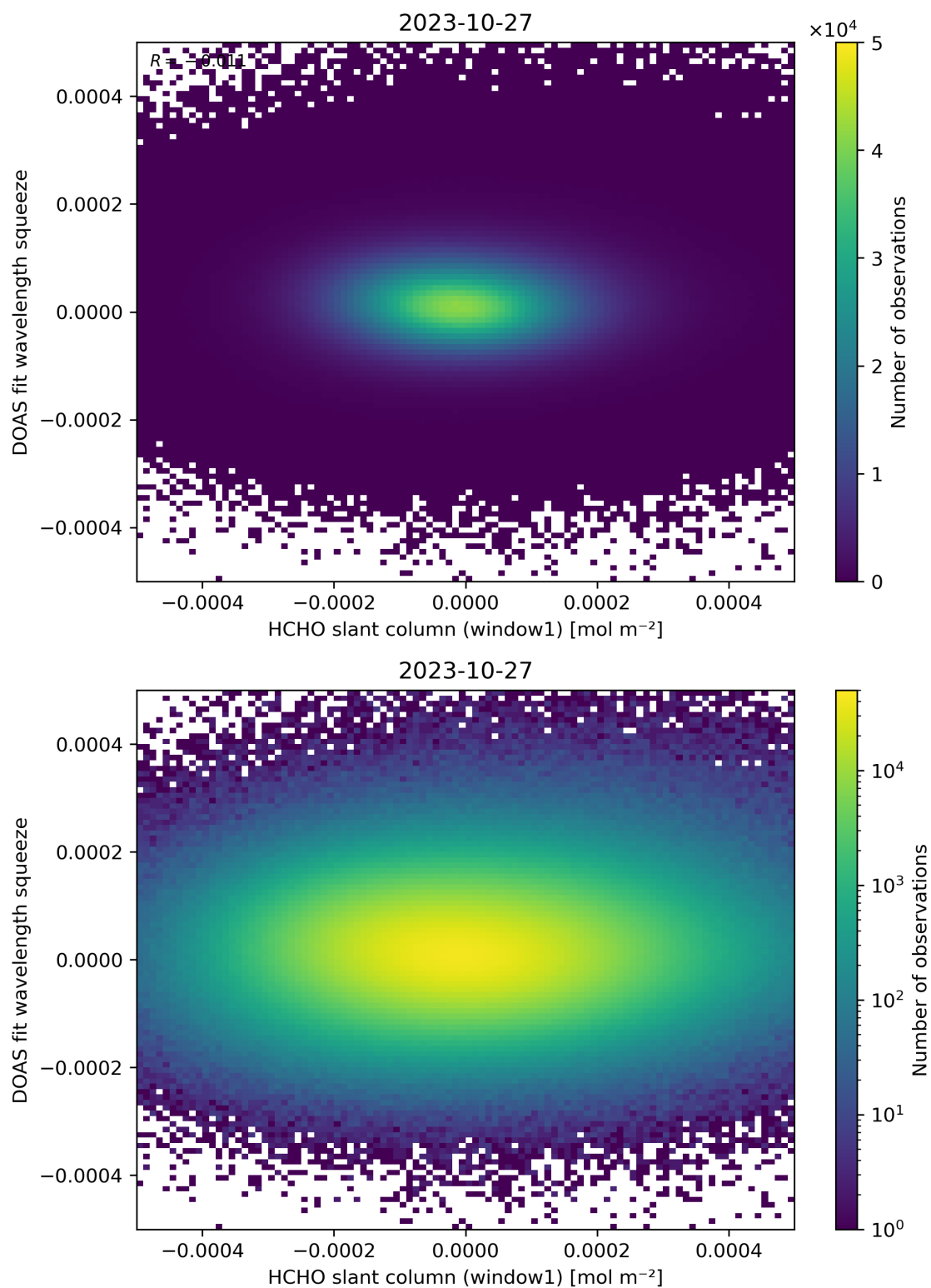
Figure 80: Scatter density plot of “HCHO slant column (window1)” against “DOAS fit wavelength squeeze” for 2023-10-27 to 2023-10-28.
