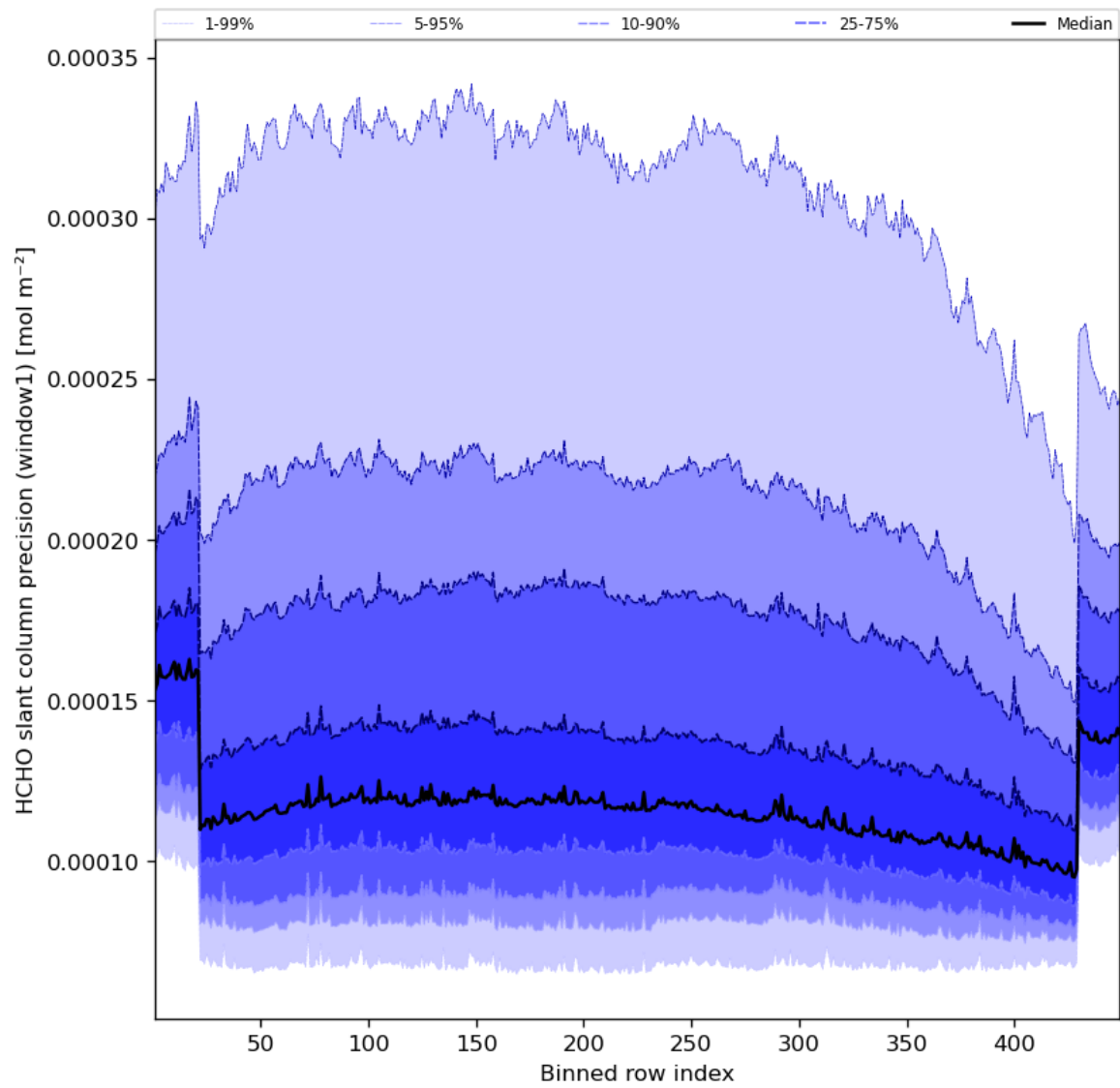
Figure 53: Along track statistics of “HCHO slant column precision (window1)” for 2023-10-27 to 2023-10-28
