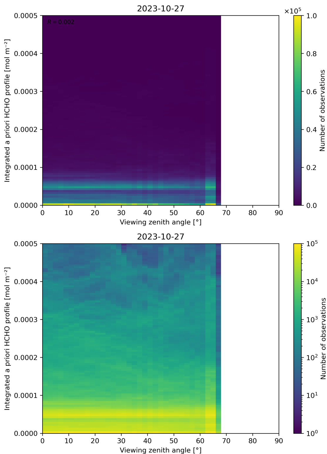
Figure 195: Scatter density plot of “Viewing zenith angle” against “Integrated a priori HCHO profile” for 2023-10-27 to 2023-10-28.
