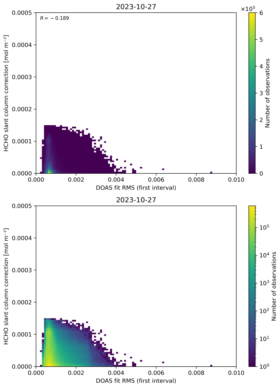
Figure 63: Scatter density plot of “DOAS fit RMS (first interval)” against “HCHO slant column correction” for 2023-10-27 to 2023-10-28.
