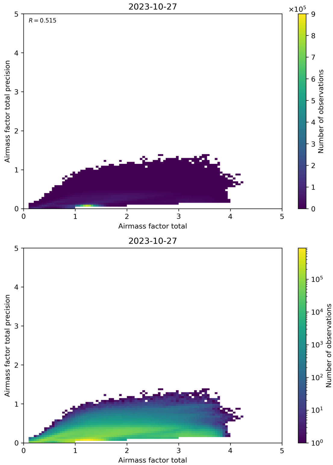
Figure 103: Scatter density plot of “Airmass factor total” against “Airmass factor total precision” for 2023-10-27 to 2023-10-28.
