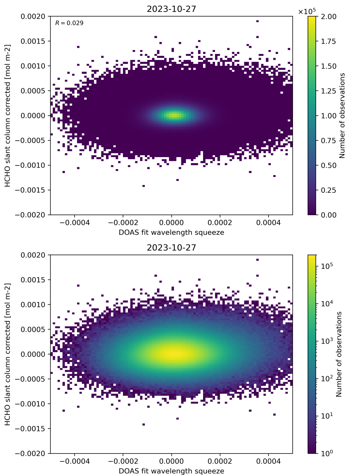
Figure 69: Scatter density plot of “DOAS fit wavelength squeeze” against “HCHO slant column corrected” for 2023-10-27 to 2023-10-28.
