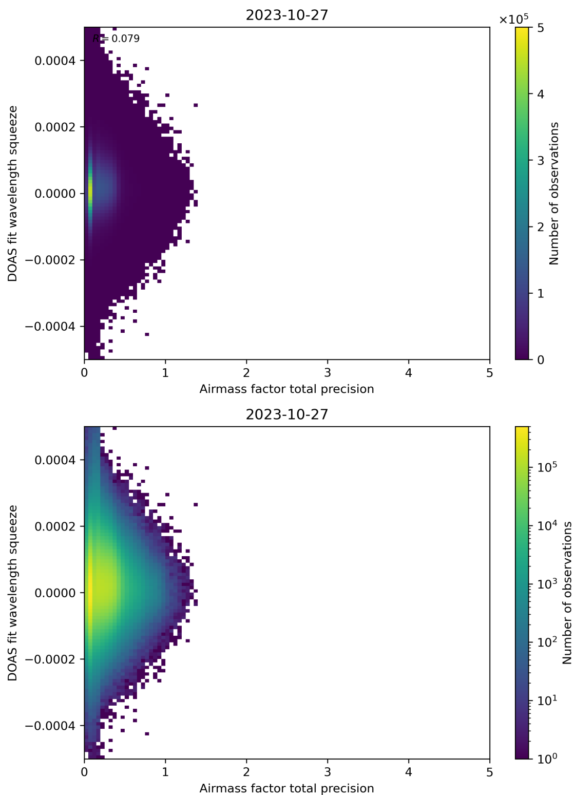
Figure 107: Scatter density plot of “Airmass factor total precision” against “DOAS fit wavelength squeeze” for 2023-10-27 to 2023-10-28.
