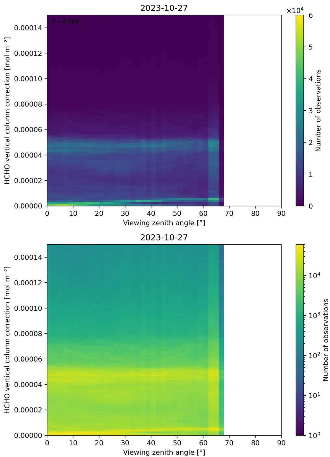
Figure 193: Scatter density plot of “Viewing zenith angle” against “HCHO vertical column correction” for 2023-10-27 to 2023-10-28.
