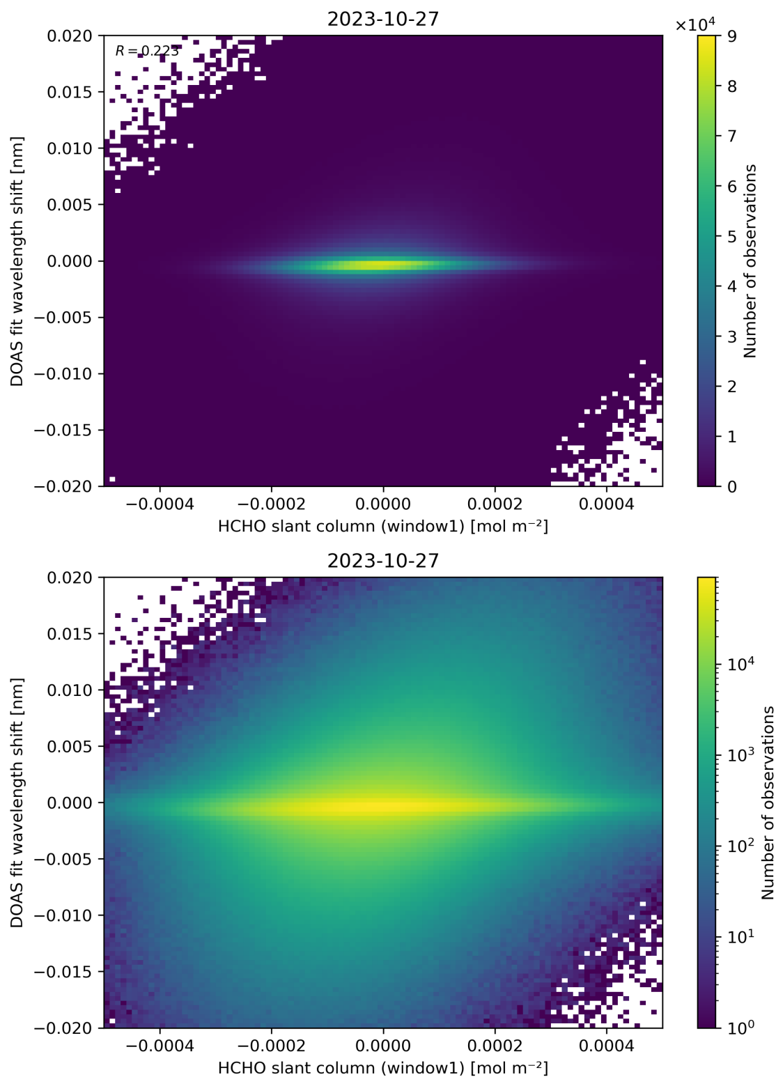
Figure 79: Scatter density plot of “HCHO slant column (window1)” against “DOAS fit wavelength shift” for 2023-10-27 to 2023-10-28.
