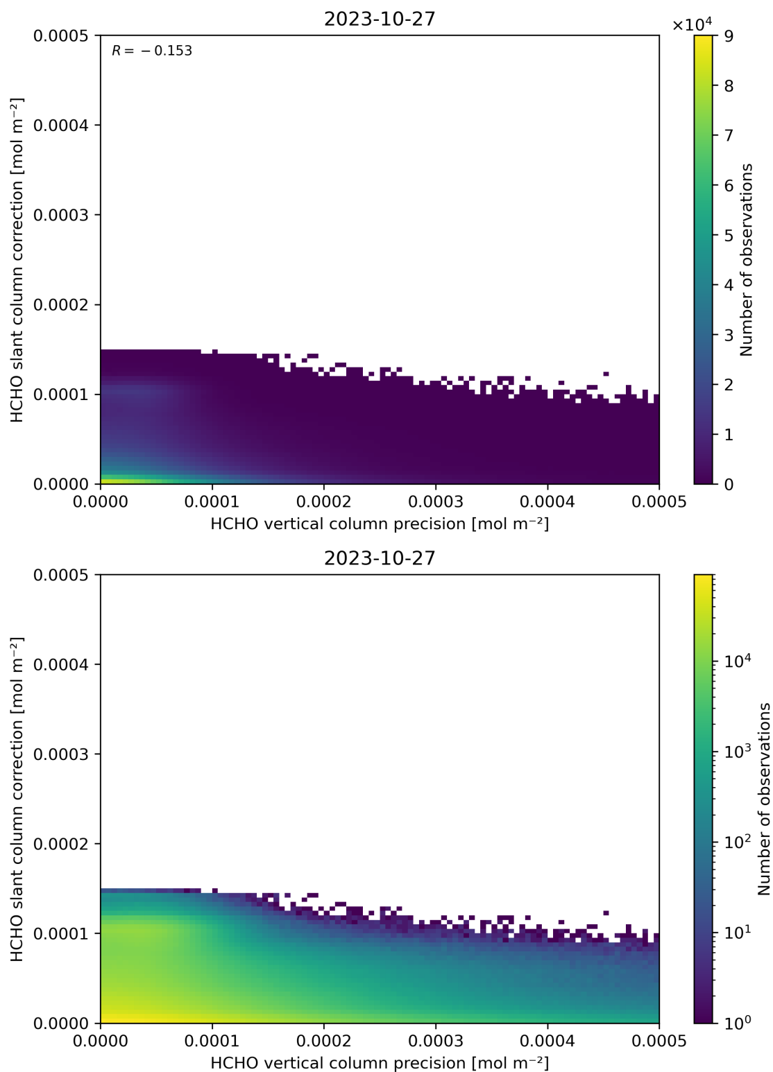
Figure 141: Scatter density plot of “HCHO vertical column precision” against “HCHO slant column correction” for 2023-10-27 to 2023-10-28.
