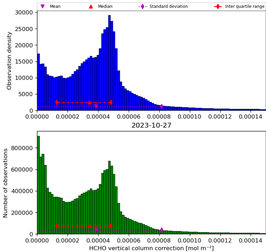
Figure 37: Histogram of “HCHO vertical column correction” for 2023-10-27 to 2023-10-28
