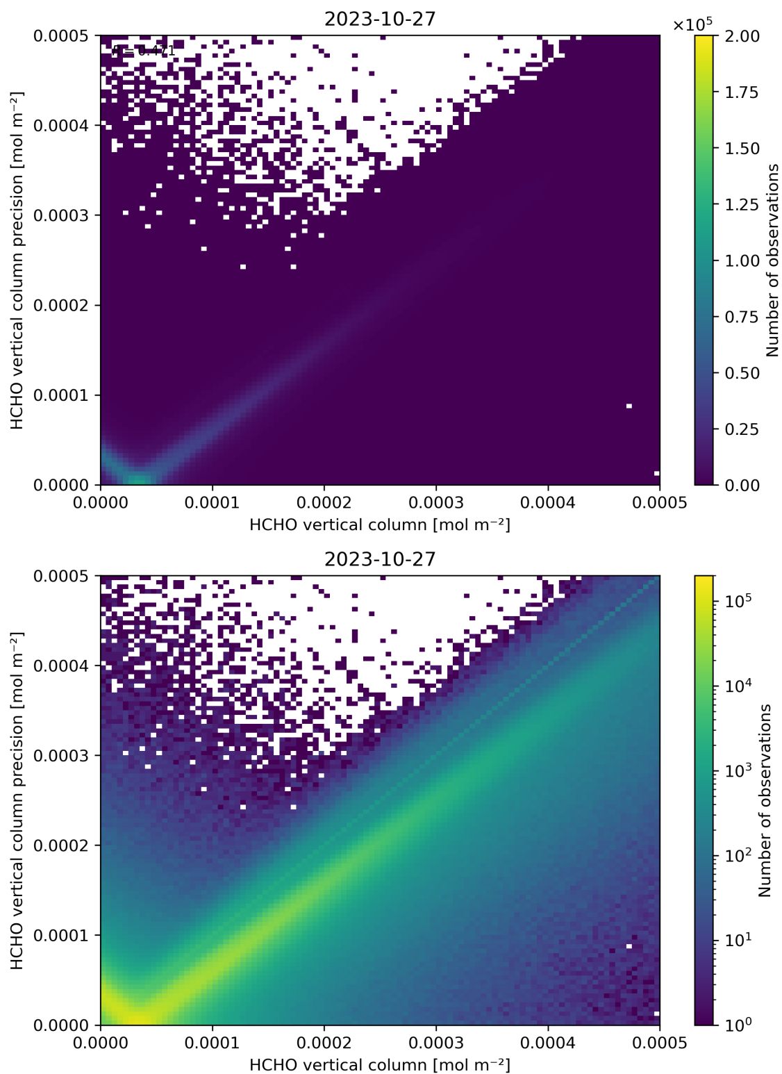
Figure 134: Scatter density plot of “HCHO vertical column” against “HCHO vertical column precision” for 2023-10-27 to 2023-10-28.
