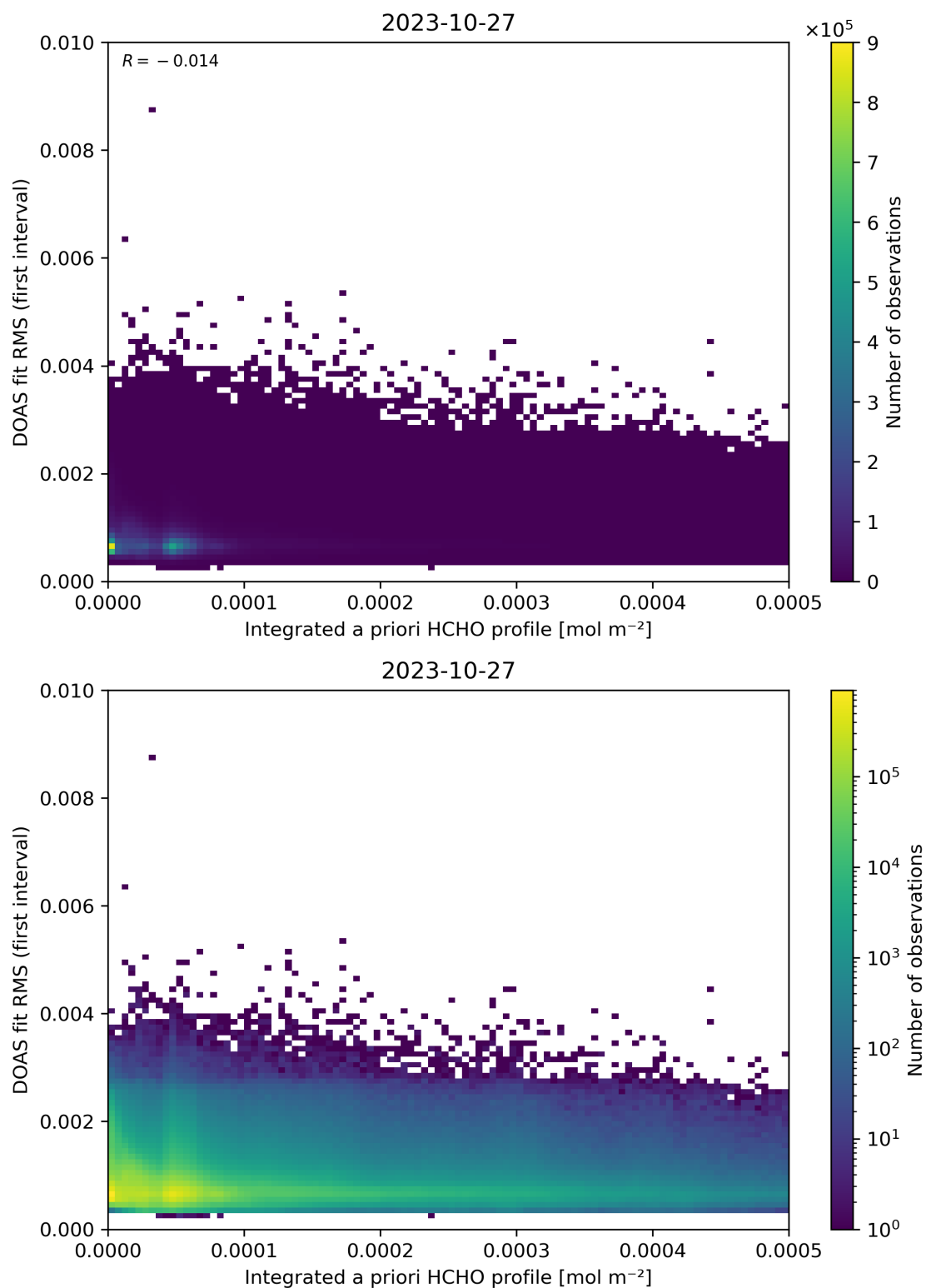
Figure 148: Scatter density plot of “Integrated a priori HCHO profile” against “DOAS fit RMS (first interval)” for 2023-10-27 to 2023-10-28.
