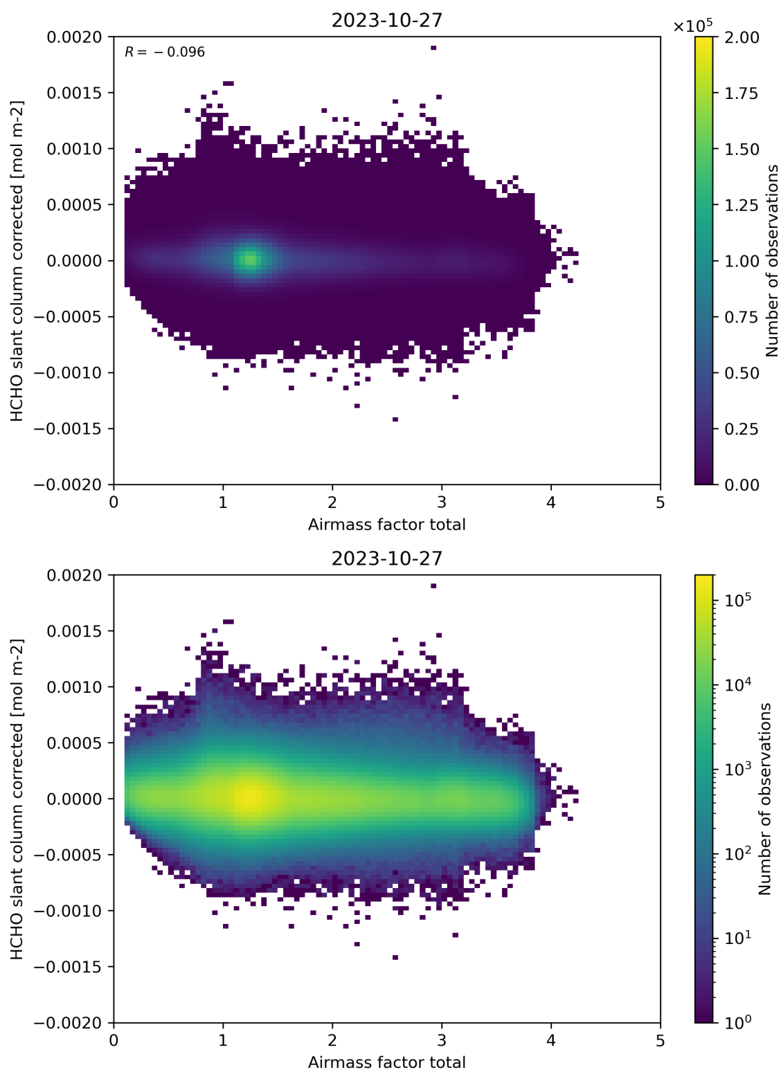
Figure 101: Scatter density plot of “Airmass factor total” against “HCHO slant column corrected” for 2023-10-27 to 2023-10-28.
