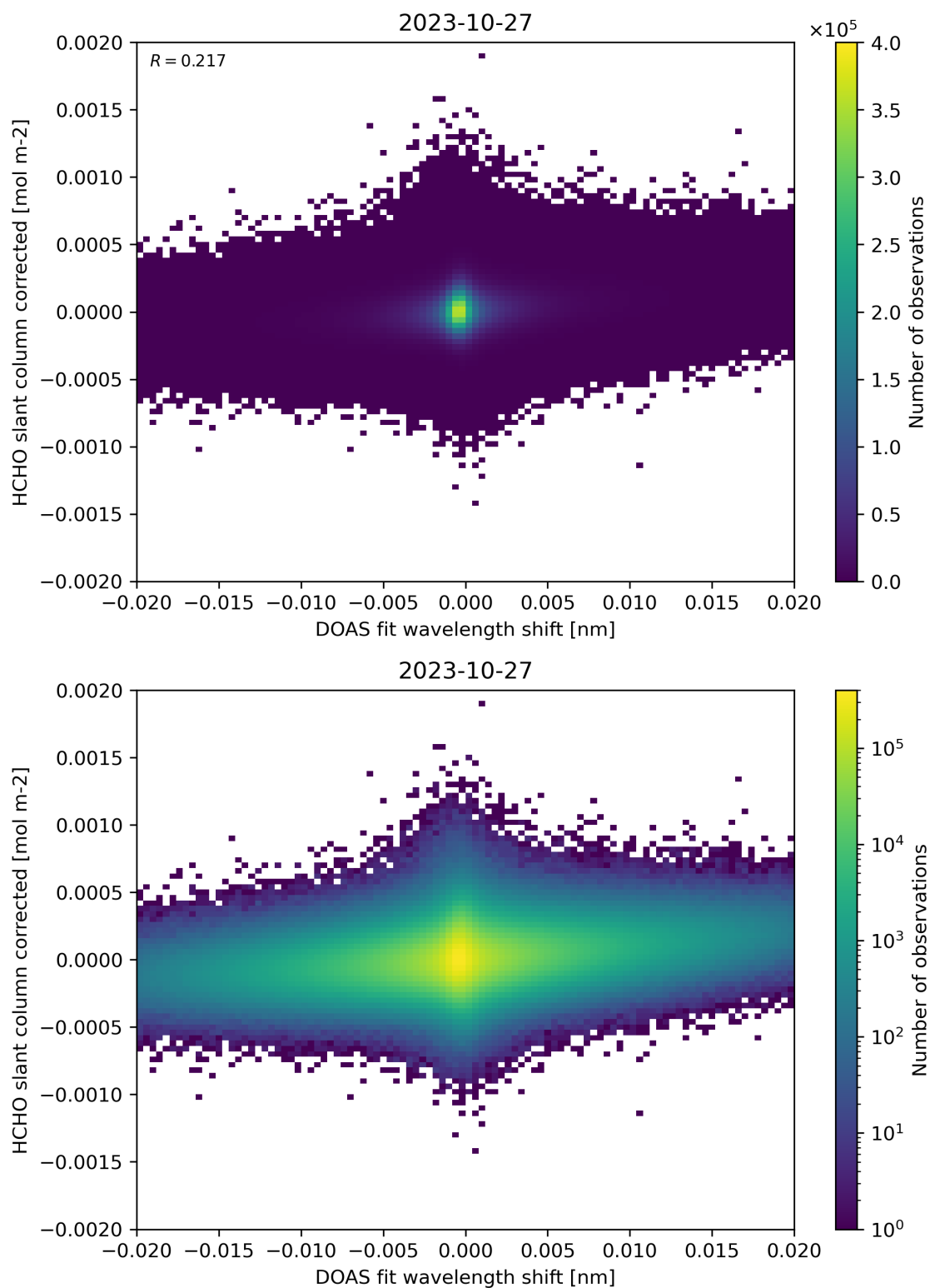
Figure 66: Scatter density plot of “DOAS fit wavelength shift” against “HCHO slant column corrected” for 2023-10-27 to 2023-10-28.
