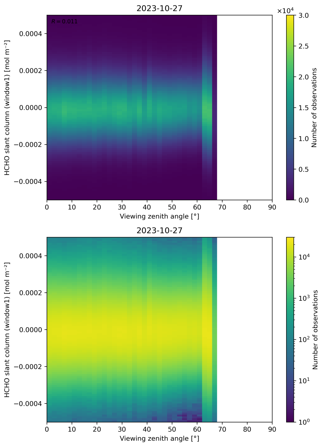
Figure 188: Scatter density plot of “Viewing zenith angle” against “HCHO slant column (window1)” for 2023-10-27 to 2023-10-28.
