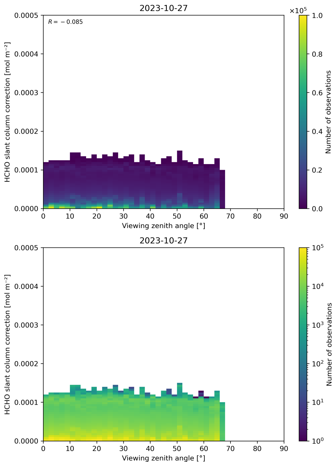
Figure 187: Scatter density plot of “Viewing zenith angle” against “HCHO slant column correction” for 2023-10-27 to 2023-10-28.
