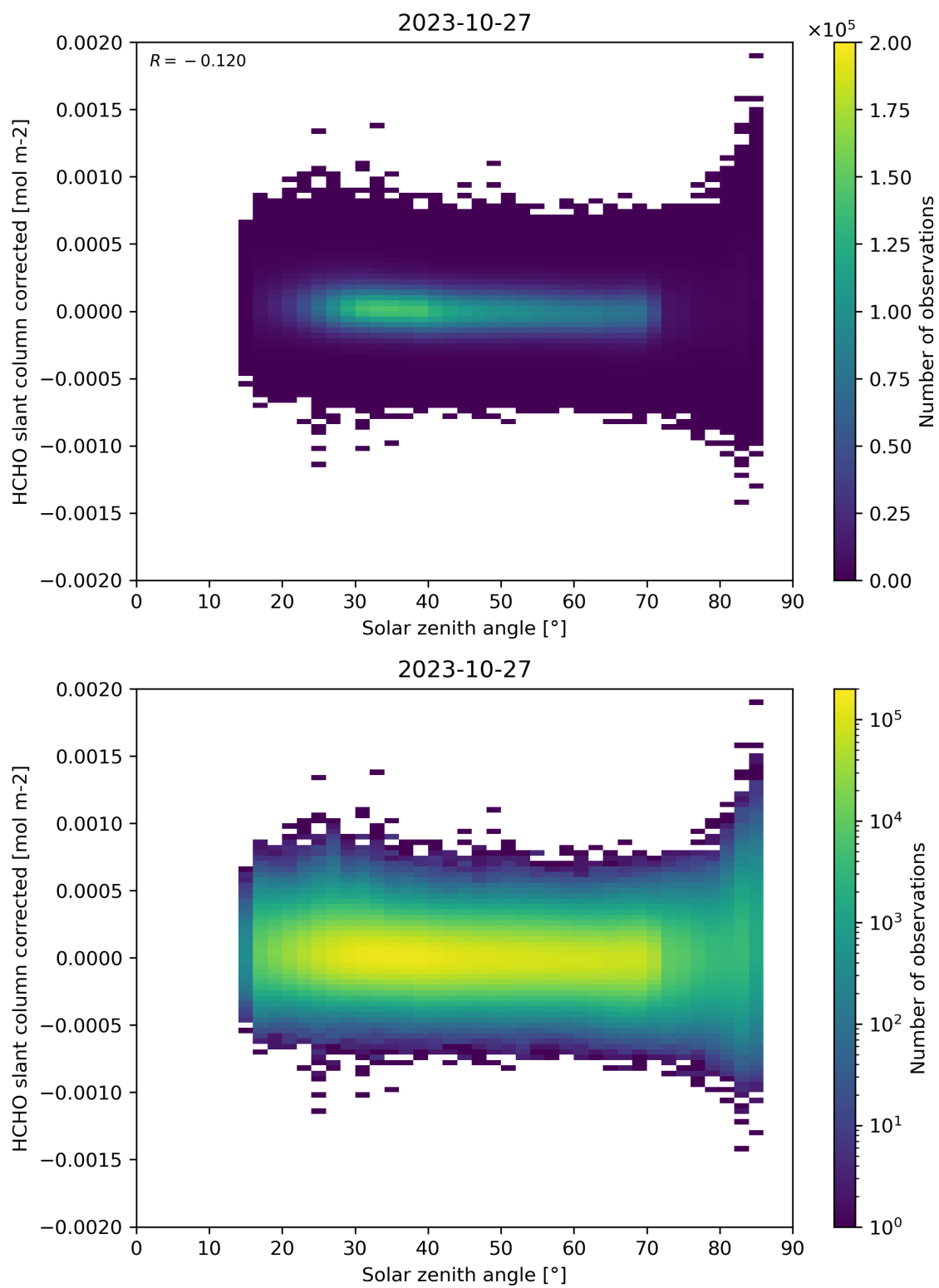
Figure 171: Scatter density plot of “Solar zenith angle” against “HCHO slant column corrected” for 2023-10-27 to 2023-10-28.
