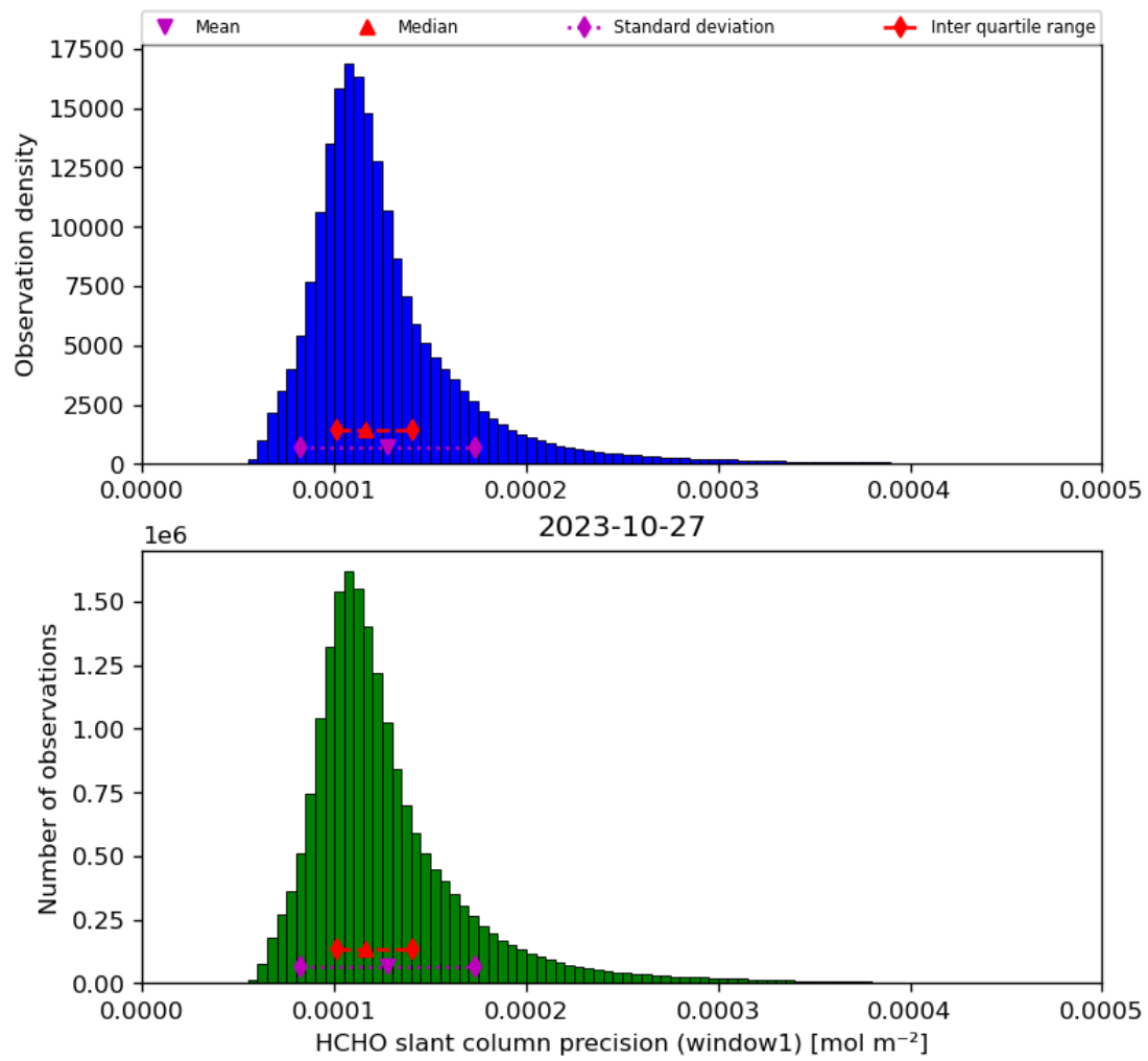
Figure 39: Histogram of “HCHO slant column precision (window1)” for 2023-10-27 to 2023-10-28
