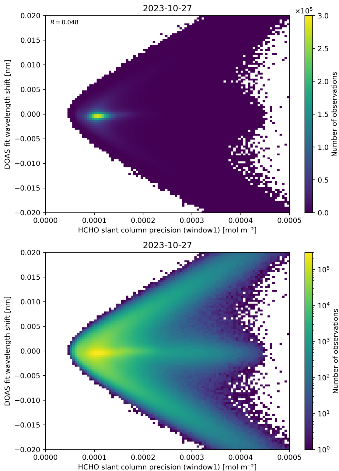
Figure 89: Scatter density plot of “HCHO slant column precision (window1)” against “DOAS fit wavelength shift” for 2023-10-27 to 2023-10-28.
