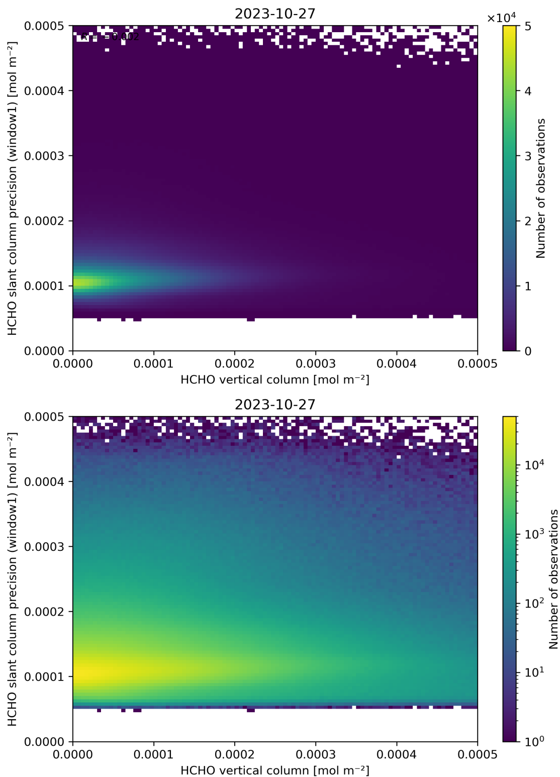
Figure 130: Scatter density plot of “HCHO vertical column” against “HCHO slant column precision (window1)” for 2023-10-27 to 2023-10-28.
