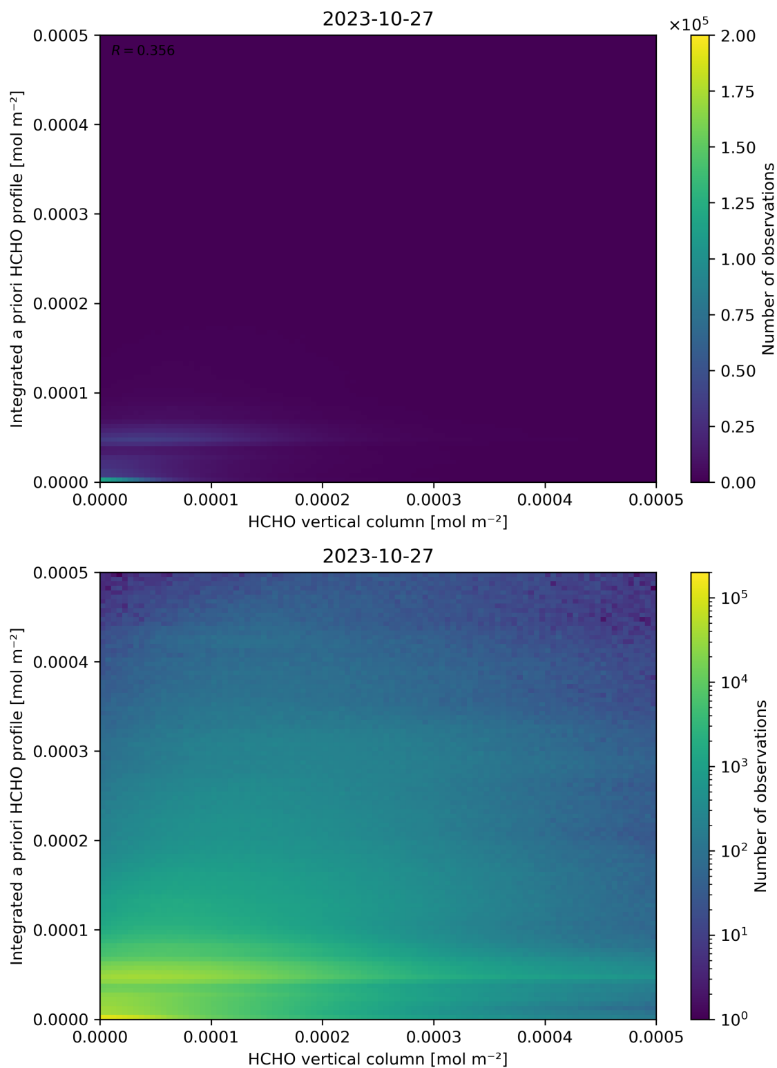
Figure 135: Scatter density plot of “HCHO vertical column” against “Integrated a priori HCHO profile” for 2023-10-27 to 2023-10-28.
