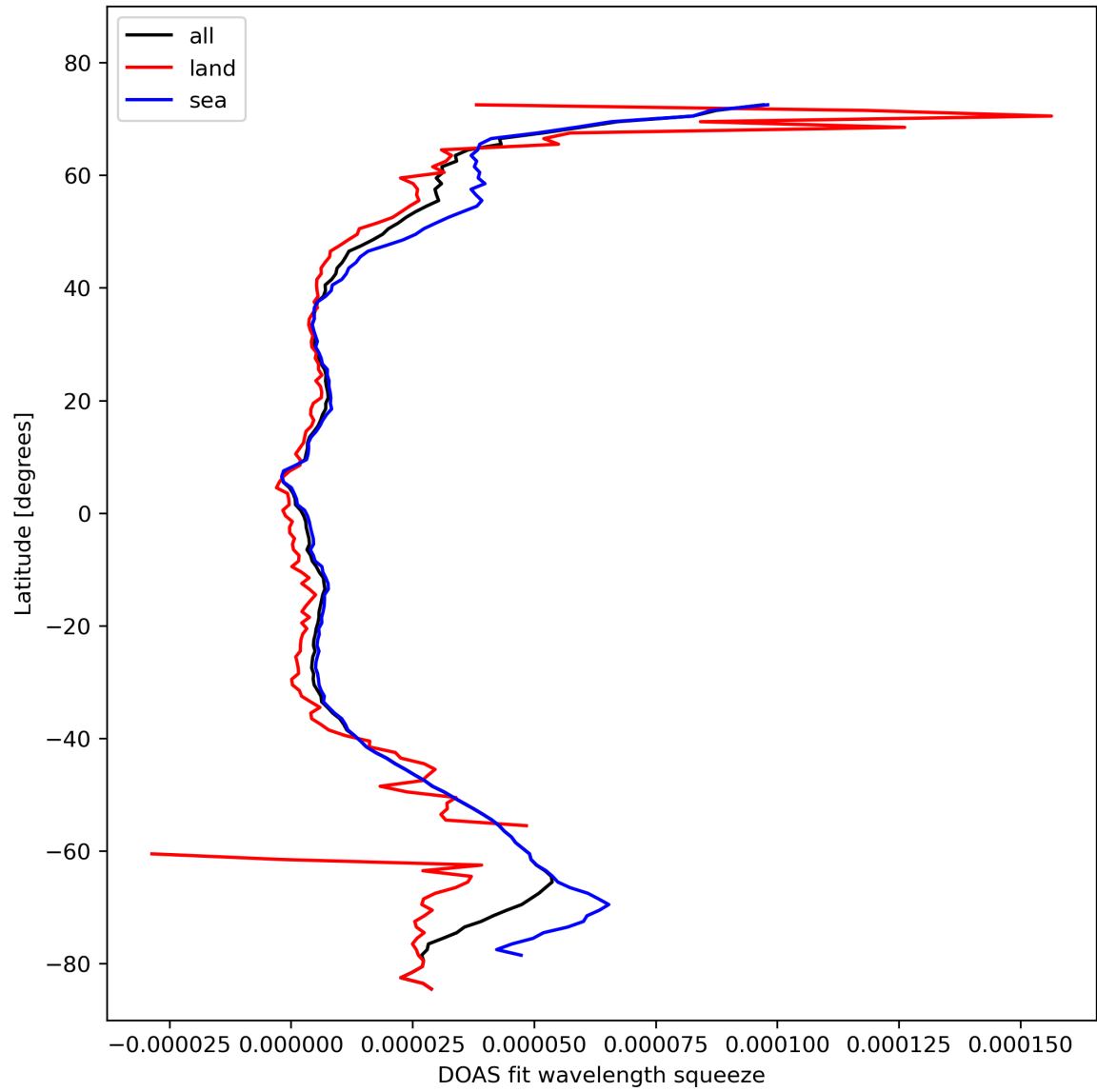
Figure 31: Zonal average of “DOAS fit wavelength squeeze” for 2023-10-27 to 2023-10-28.
