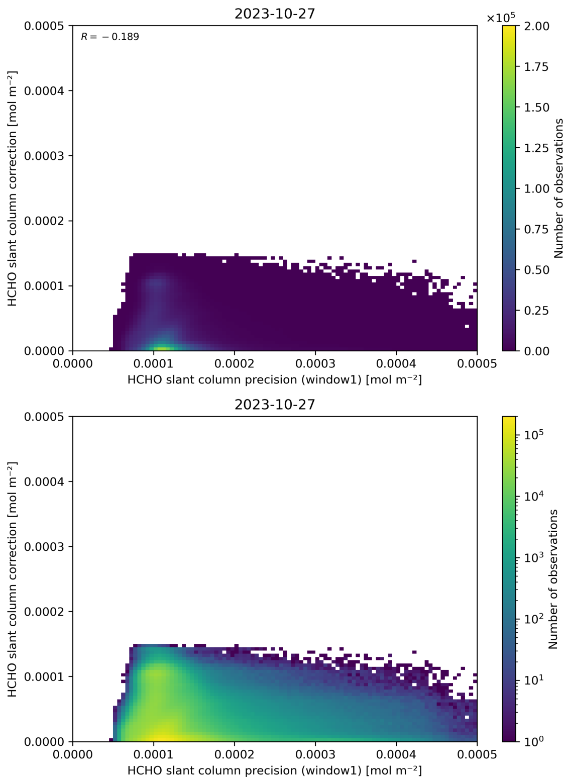
Figure 93: Scatter density plot of “HCHO slant column precision (window1)” against “HCHO slant column correction” for 2023-10-27 to 2023-10-28.
