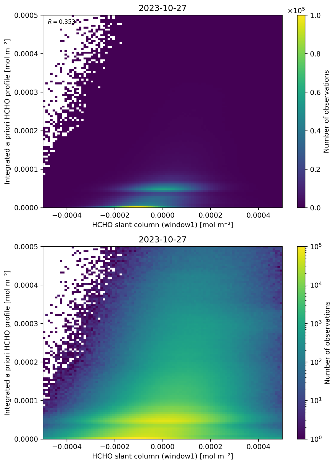
Figure 87: Scatter density plot of “HCHO slant column (window1)” against “Integrated a priori HCHO profile” for 2023-10-27 to 2023-10-28.
