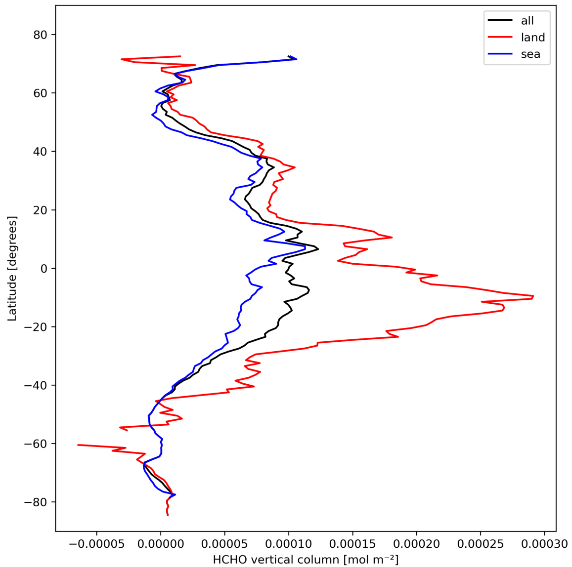
Figure 21: Zonal average of “HCHO vertical column” for 2023-10-27 to 2023-10-28.
