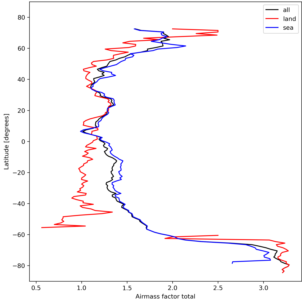
Figure 26: Zonal average of “Airmass factor total” for 2023-10-27 to 2023-10-28.
