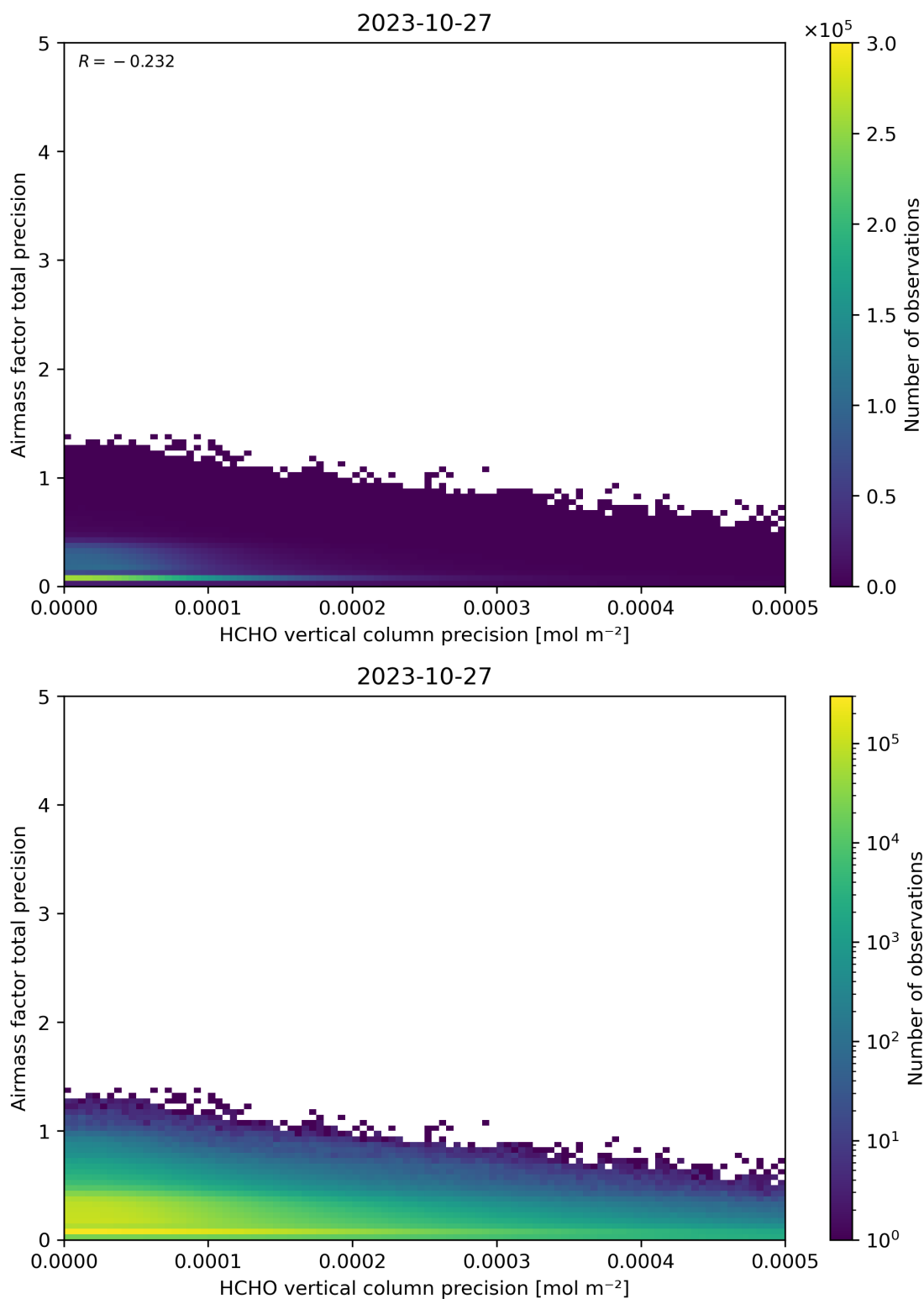
Figure 145: Scatter density plot of “HCHO vertical column precision” against “Airmass factor total precision” for 2023-10-27 to 2023-10-28.
