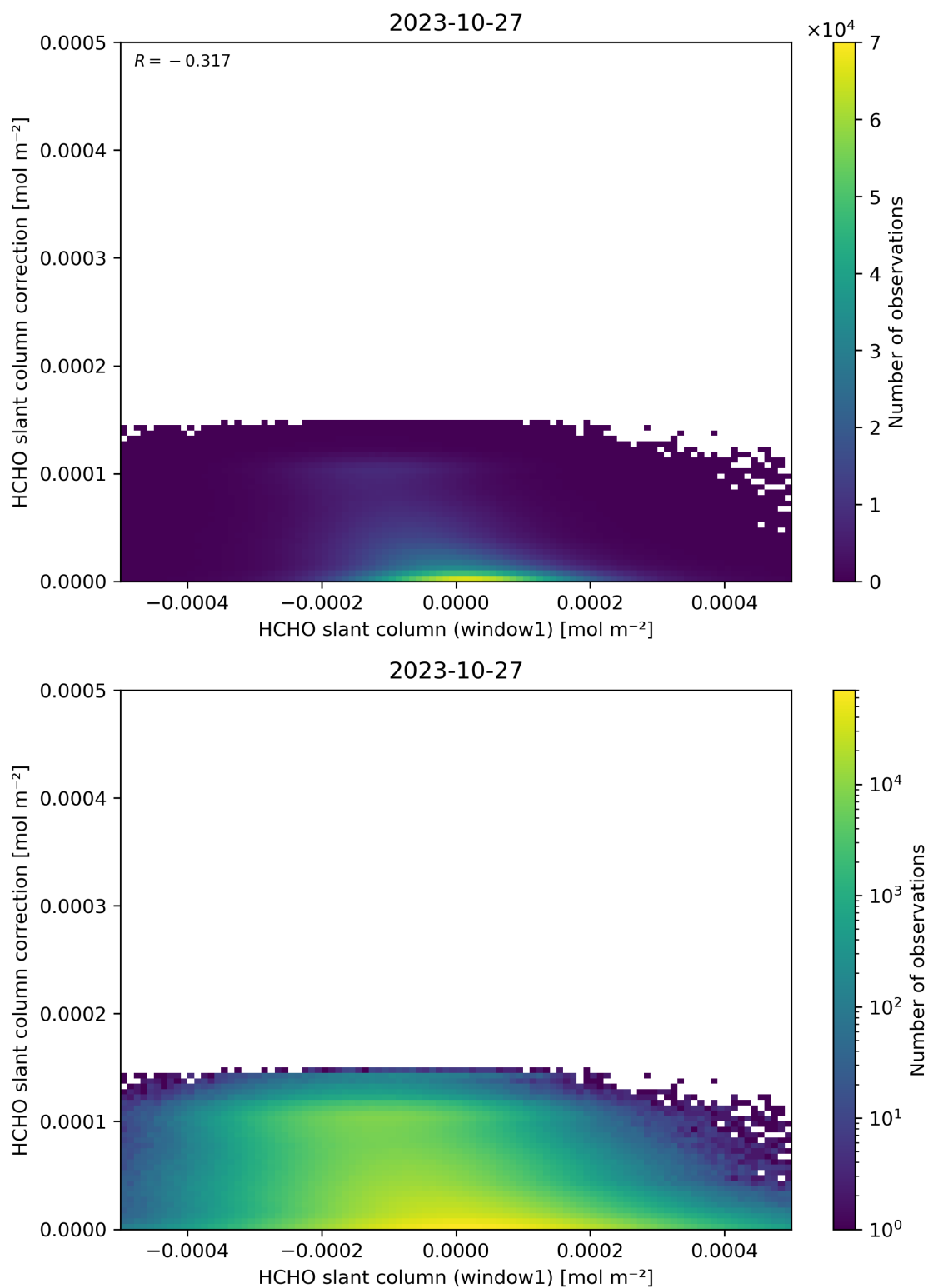
Figure 83: Scatter density plot of “HCHO slant column (window1)” against “HCHO slant column correction” for 2023-10-27 to 2023-10-28.
