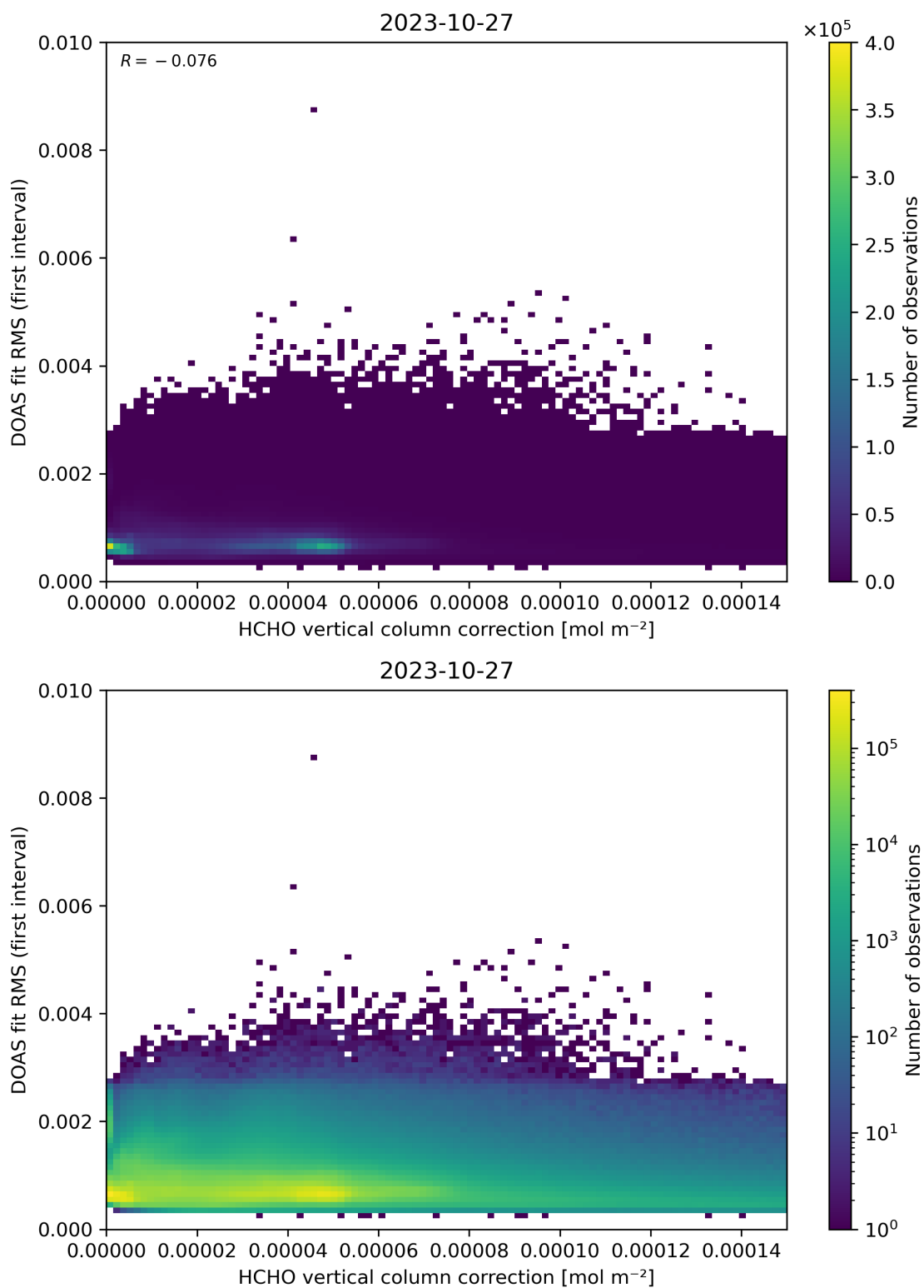
Figure 112: Scatter density plot of “HCHO vertical column correction” against “DOAS fit RMS (first interval)” for 2023-10-27 to 2023-10-28.
