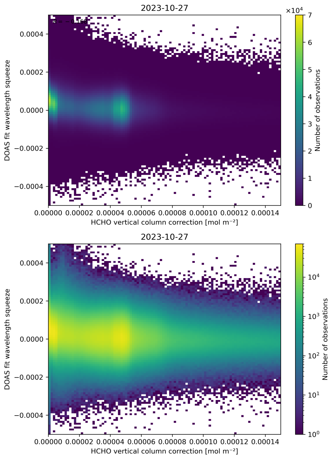
Figure 114: Scatter density plot of “HCHO vertical column correction” against “DOAS fit wavelength squeeze” for 2023-10-27 to 2023-10-28.
