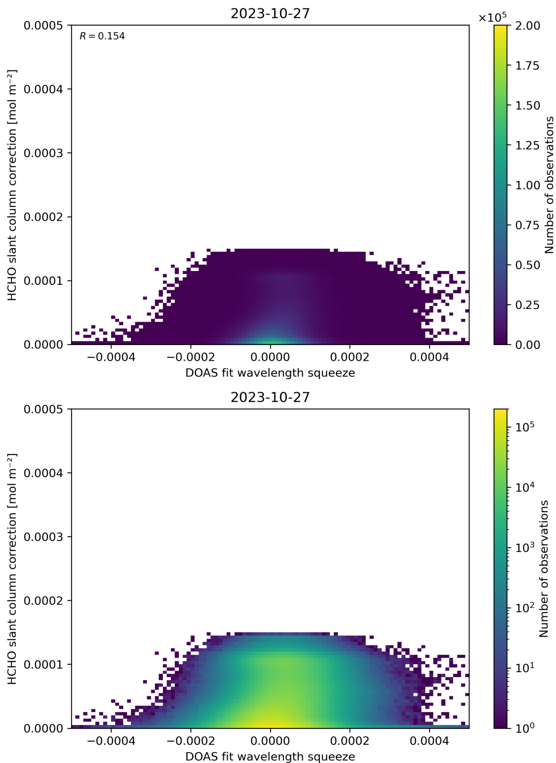
Figure 70: Scatter density plot of “DOAS fit wavelength squeeze” against “HCHO slant column correction” for 2023-10-27 to 2023-10-28.
