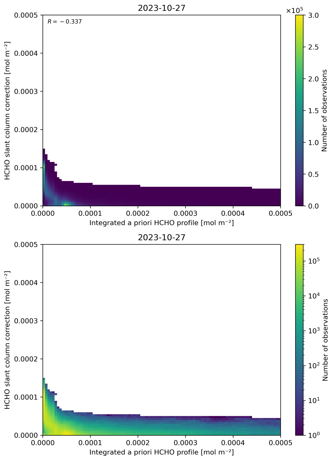
Figure 152: Scatter density plot of “Integrated a priori HCHO profile” against “HCHO slant column correction” for 2023-10-27 to 2023-10-28.
