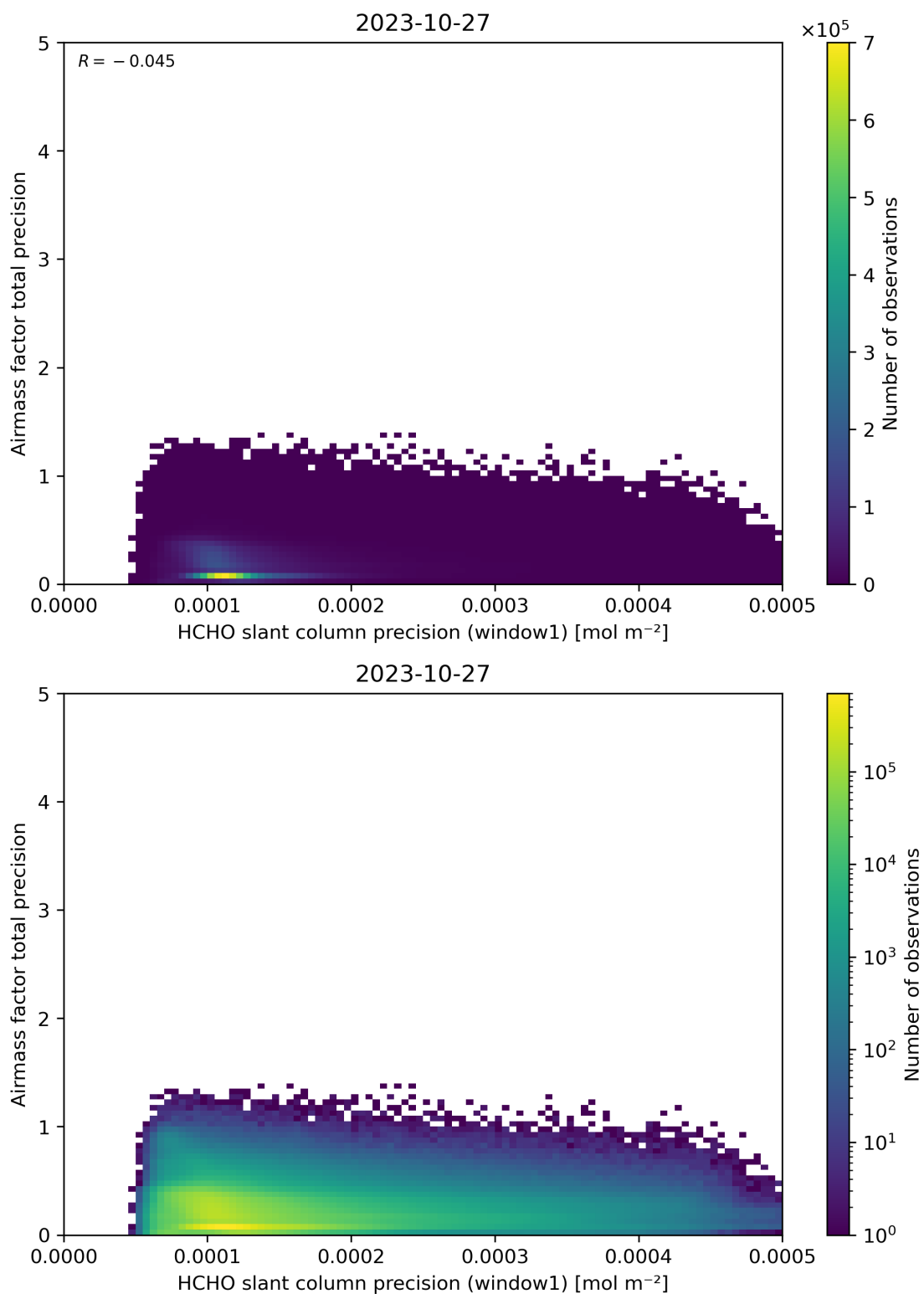
Figure 95: Scatter density plot of “HCHO slant column precision (window1)” against “Airmass factor total precision” for 2023-10-27 to 2023-10-28.
