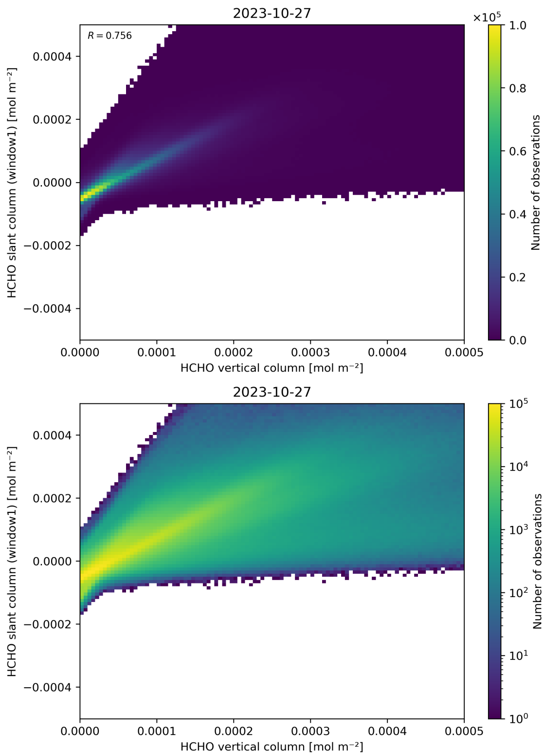
Figure 129: Scatter density plot of “HCHO vertical column” against “HCHO slant column (window1)” for 2023-10-27 to 2023-10-28.
