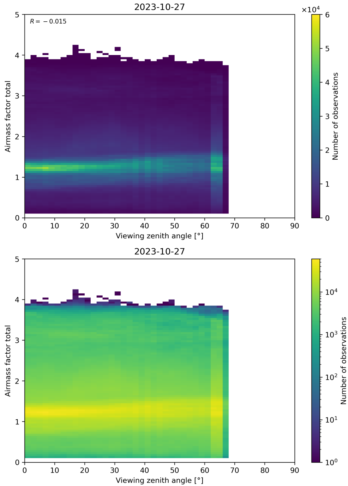
Figure 190: Scatter density plot of “Viewing zenith angle” against “Airmass factor total” for 2023-10-27 to 2023-10-28.
