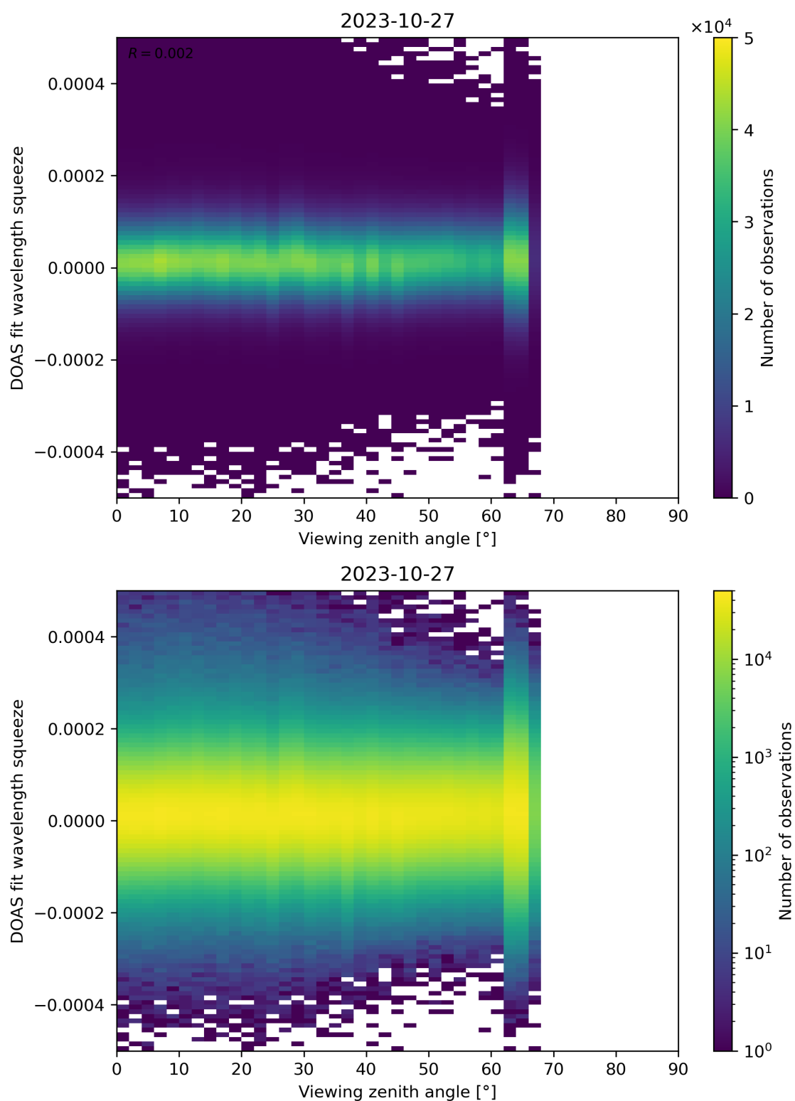
Figure 184: Scatter density plot of “Viewing zenith angle” against “DOAS fit wavelength squeeze” for 2023-10-27 to 2023-10-28.
