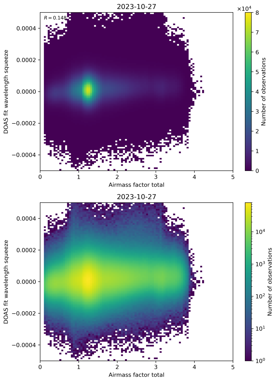
Figure 99: Scatter density plot of “Airmass factor total” against “DOAS fit wavelength squeeze” for 2023-10-27 to 2023-10-28.
