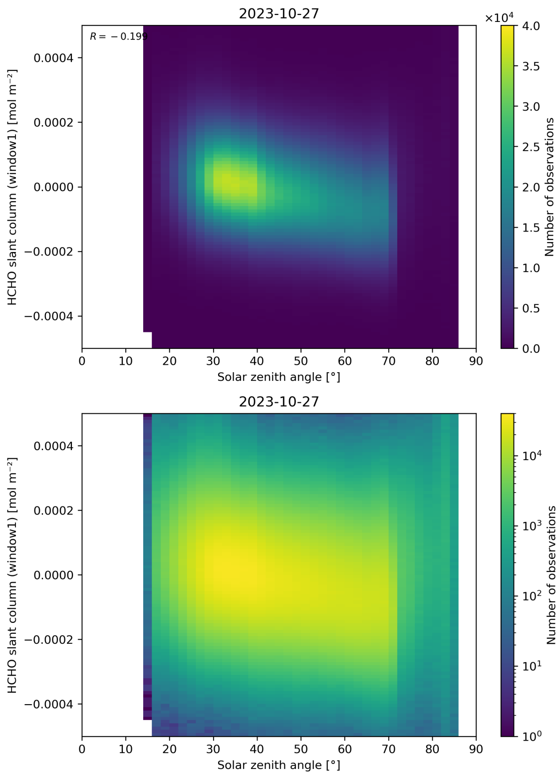
Figure 173: Scatter density plot of “Solar zenith angle” against “HCHO slant column (window1)” for 2023-10-27 to 2023-10-28.
