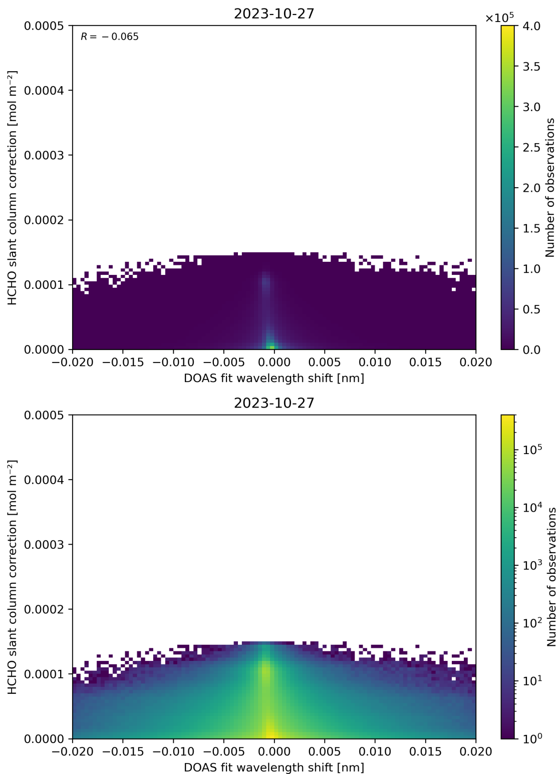
Figure 67: Scatter density plot of “DOAS fit wavelength shift” against “HCHO slant column correction” for 2023-10-27 to 2023-10-28.
