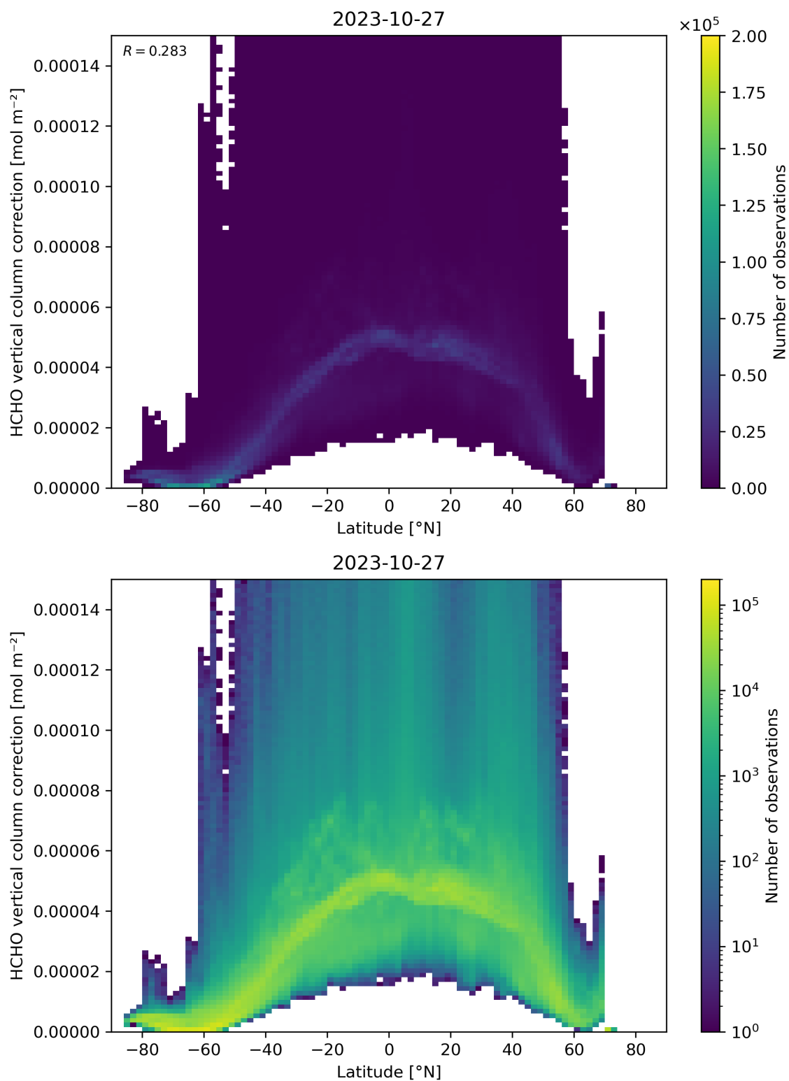
Figure 164: Scatter density plot of “Latitude” against “HCHO vertical column correction” for 2023-10-27 to 2023-10-28.
