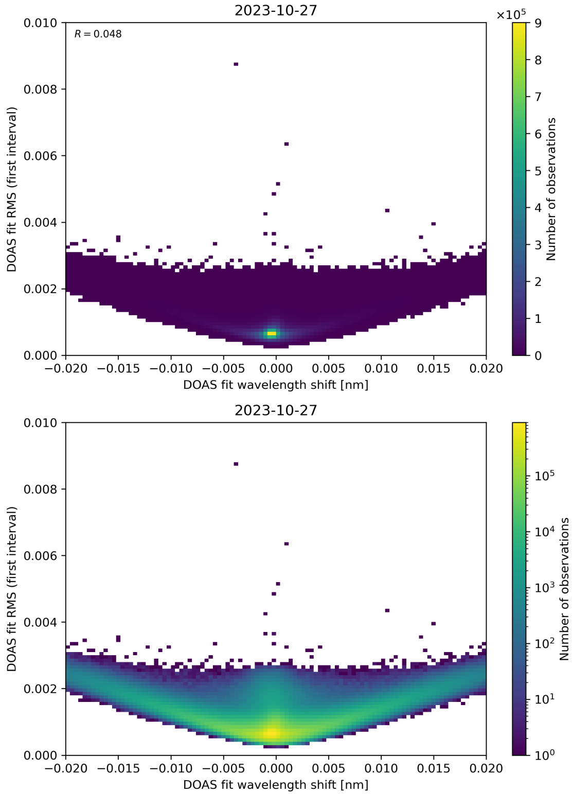
Figure 64: Scatter density plot of “DOAS fit wavelength shift” against “DOAS fit RMS (first interval)” for 2023-10-27 to 2023-10-28.
