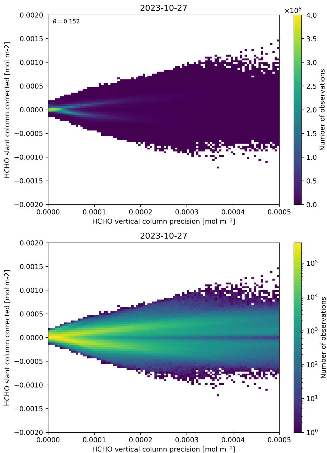
Figure 140: Scatter density plot of “HCHO vertical column precision” against “HCHO slant column corrected” for 2023-10-27 to 2023-10-28.
