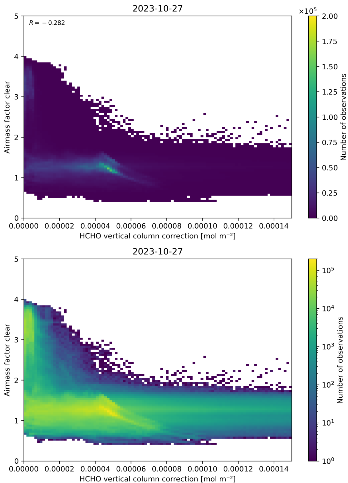
Figure 115: Scatter density plot of “HCHO vertical column correction” against “Airmass factor clear” for 2023-10-27 to 2023-10-28.
