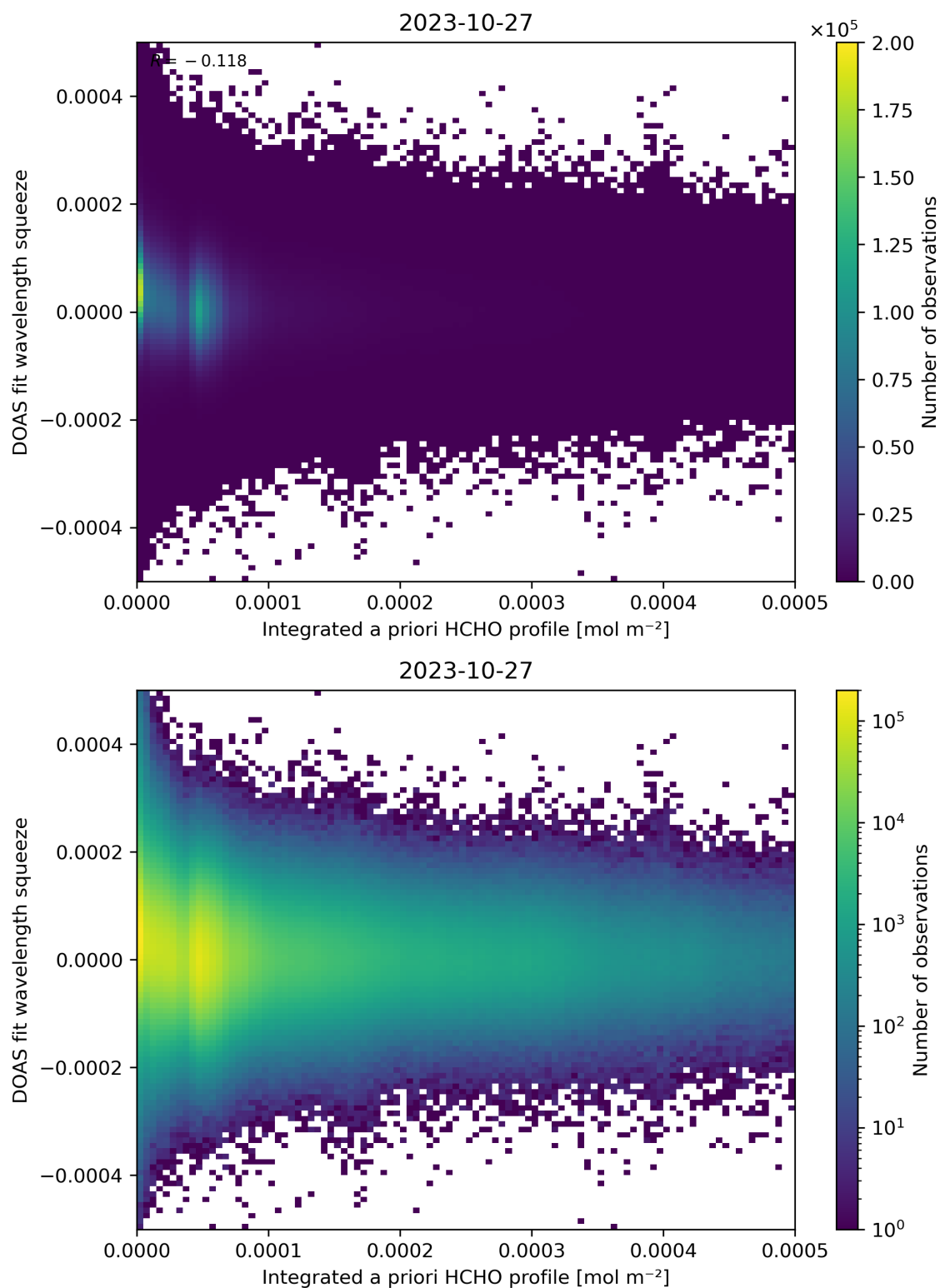
Figure 150: Scatter density plot of “Integrated a priori HCHO profile” against “DOAS fit wavelength squeeze” for 2023-10-27 to 2023-10-28.
