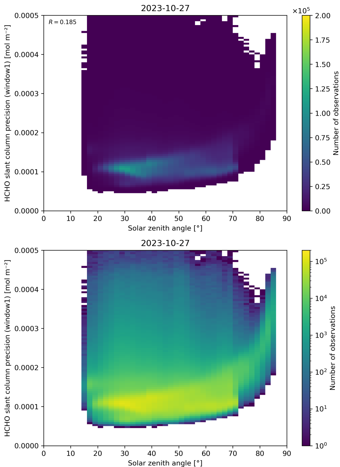
Figure 174: Scatter density plot of “Solar zenith angle” against “HCHO slant column precision (window1)” for 2023-10-27 to 2023-10-28.
