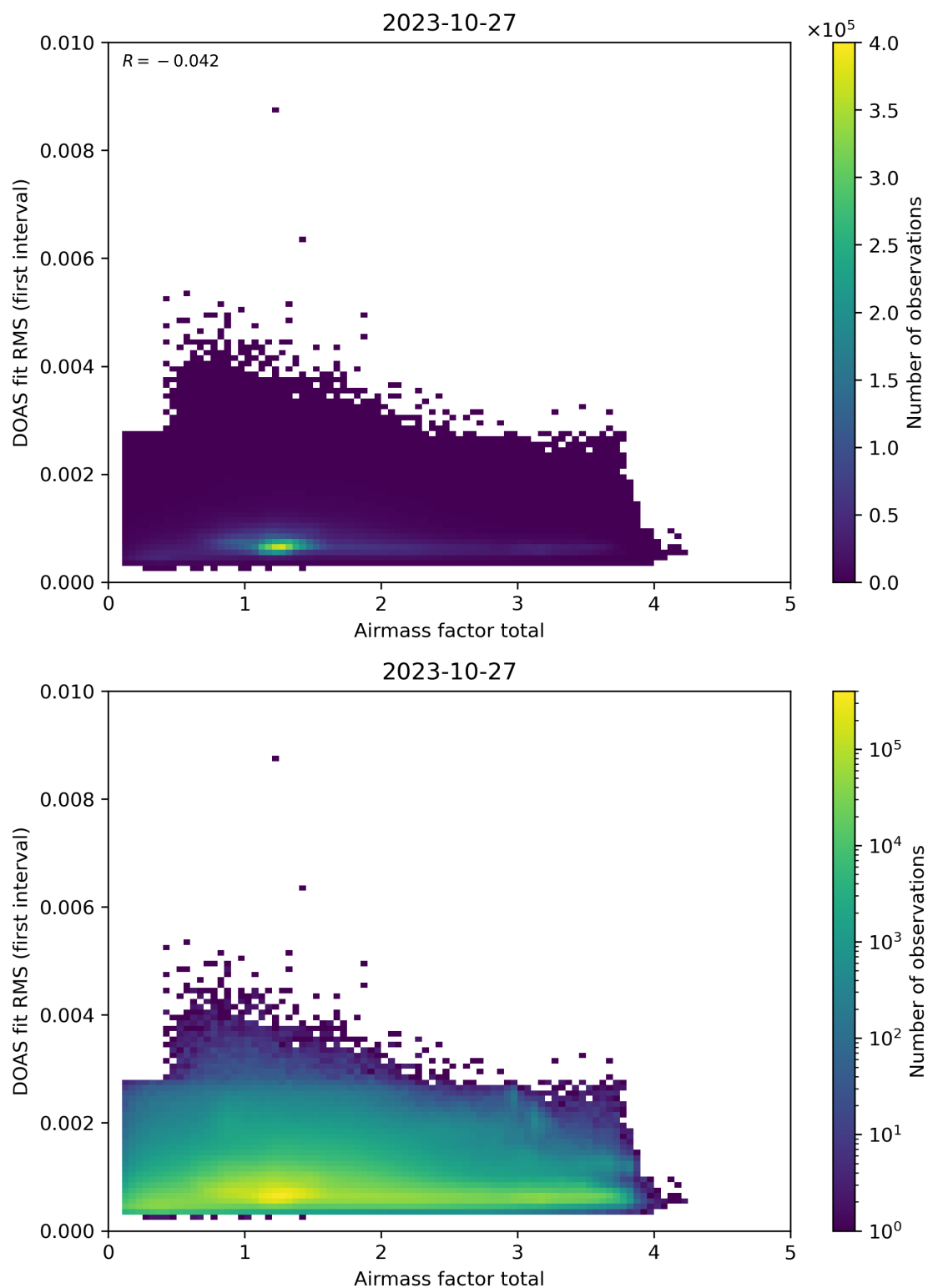
Figure 97: Scatter density plot of “Airmass factor total” against “DOAS fit RMS (first interval)” for 2023-10-27 to 2023-10-28.
