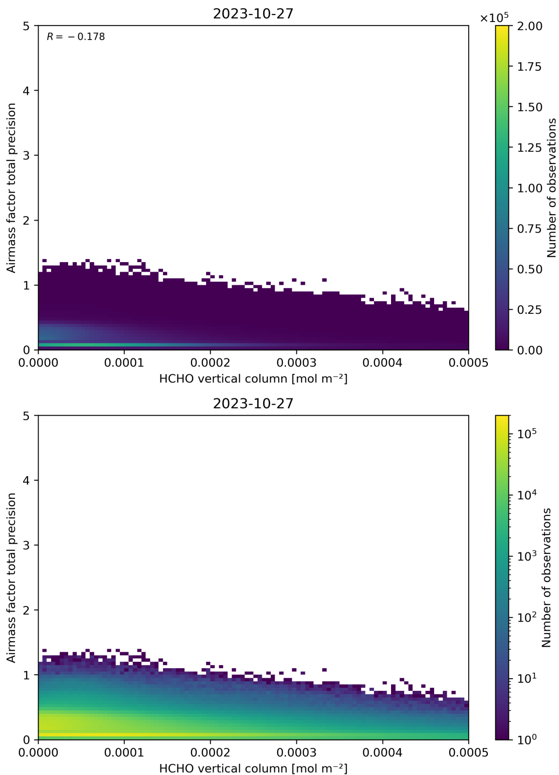
Figure 132: Scatter density plot of “HCHO vertical column” against “Airmass factor total precision” for 2023-10-27 to 2023-10-28.
