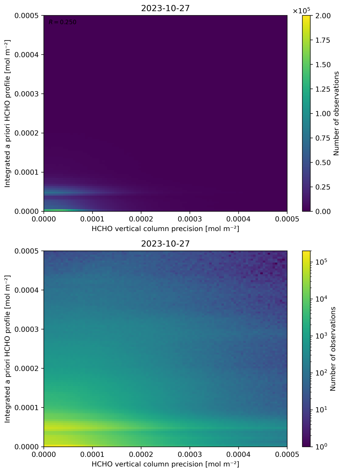
Figure 147: Scatter density plot of “HCHO vertical column precision” against “Integrated a priori HCHO profile” for 2023-10-27 to 2023-10-28.
