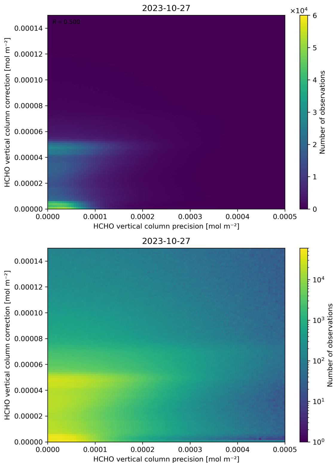
Figure 146: Scatter density plot of “HCHO vertical column precision” against “HCHO vertical column correction” for 2023-10-27 to 2023-10-28.
