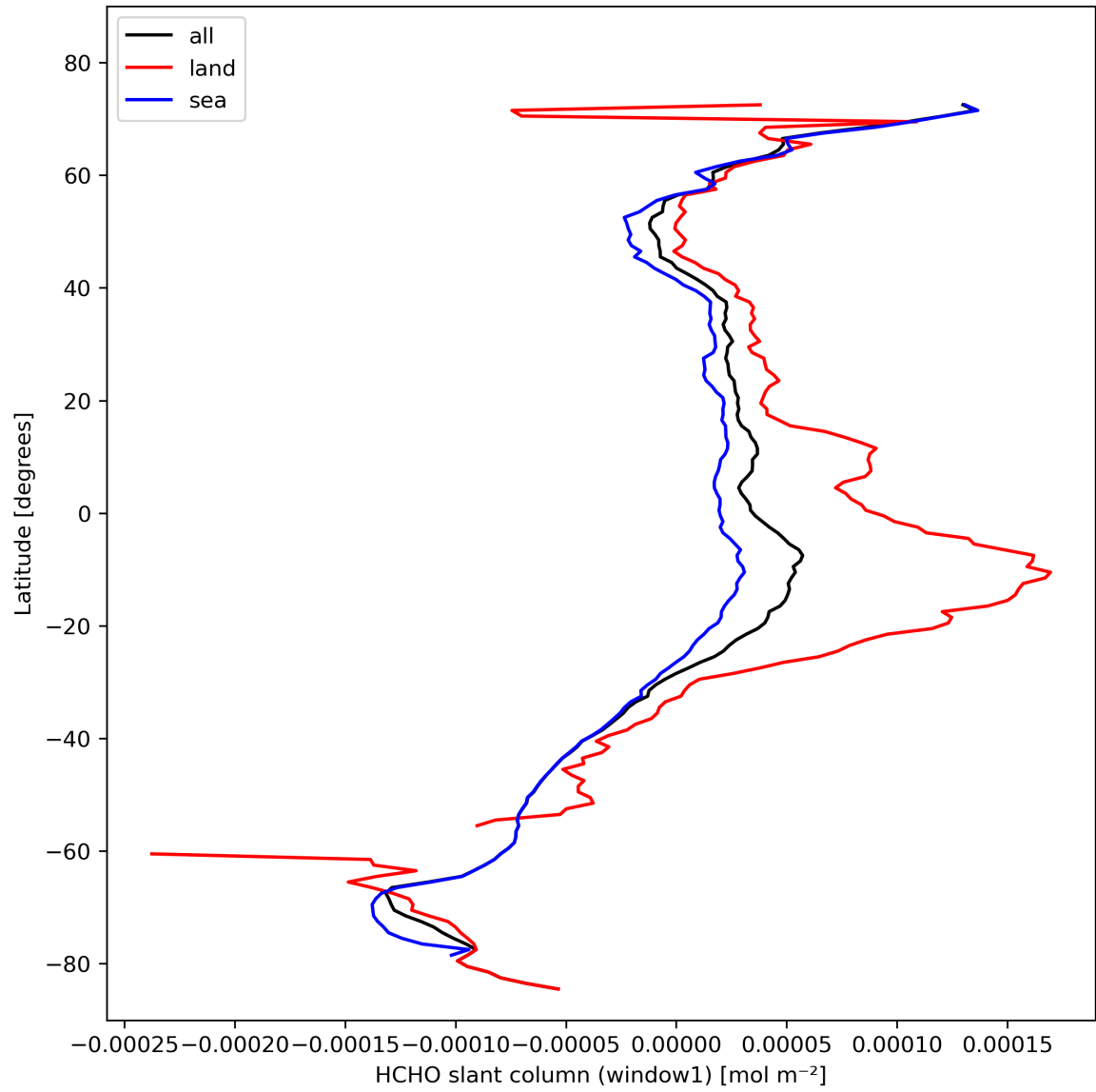
Figure 24: Zonal average of “HCHO slant column (window1)” for 2023-10-27 to 2023-10-28.
