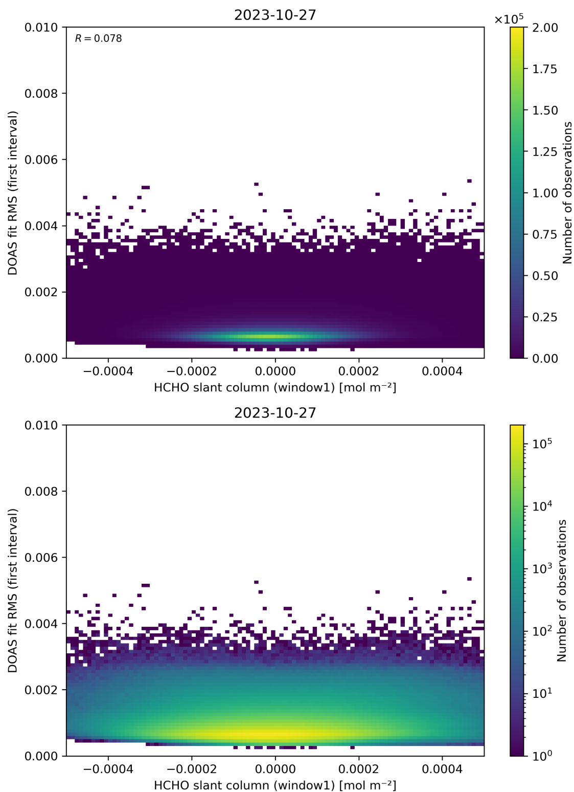
Figure 78: Scatter density plot of “HCHO slant column (window1)” against “DOAS fit RMS (first interval)” for 2023-10-27 to 2023-10-28.
