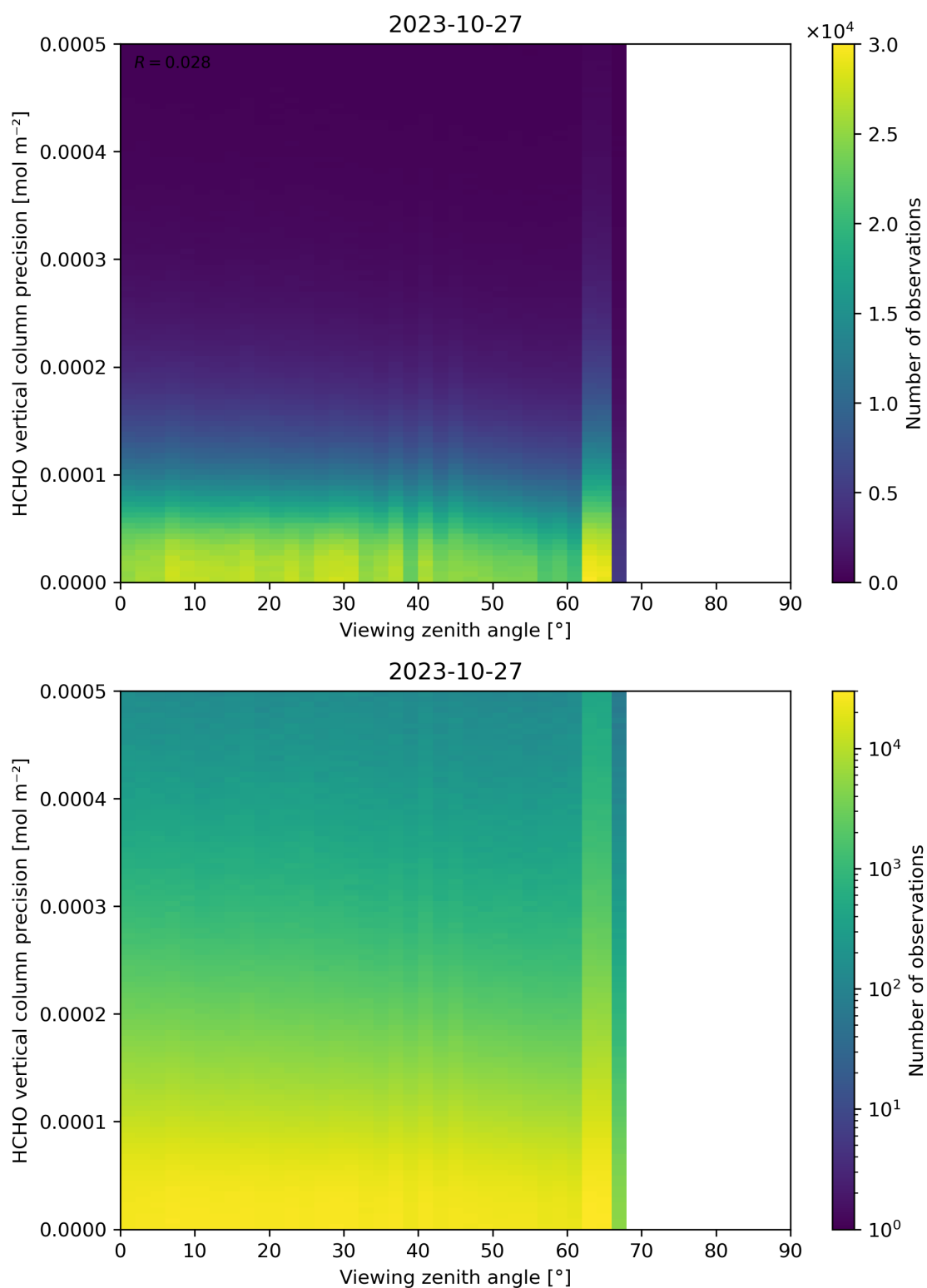
Figure 194: Scatter density plot of “Viewing zenith angle” against “HCHO vertical column precision” for 2023-10-27 to 2023-10-28.
