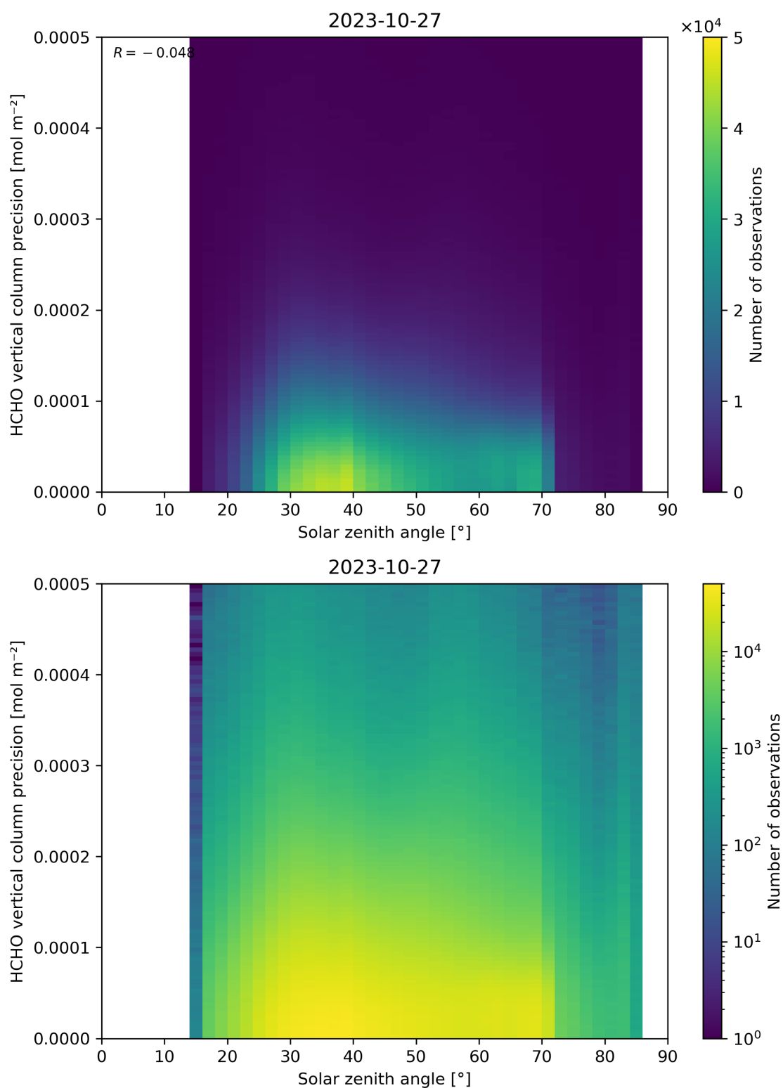
Figure 179: Scatter density plot of “Solar zenith angle” against “HCHO vertical column precision” for 2023-10-27 to 2023-10-28.
