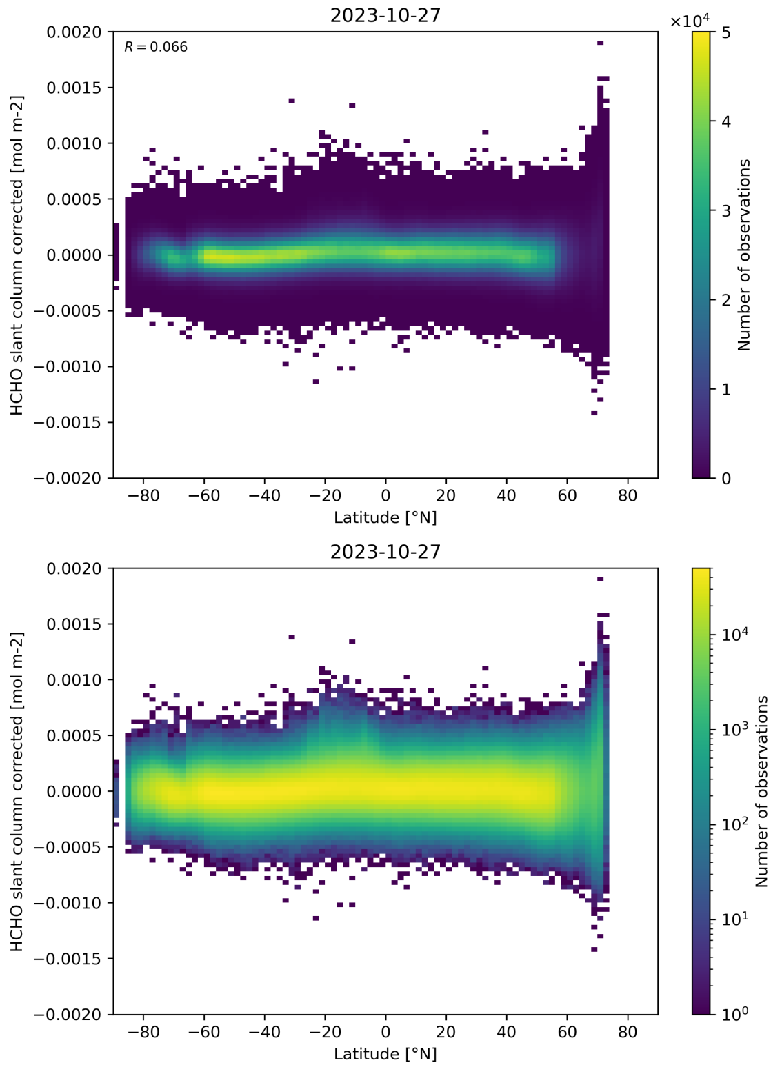
Figure 157: Scatter density plot of “Latitude” against “HCHO slant column corrected” for 2023-10-27 to 2023-10-28.
