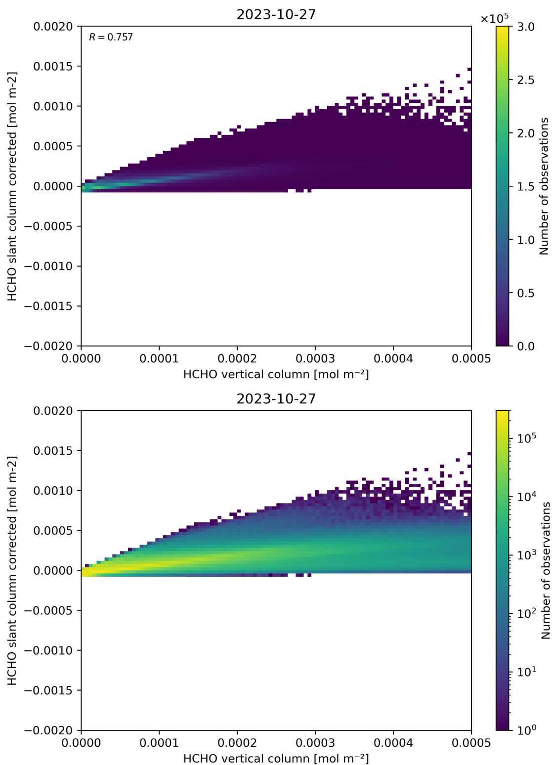
Figure 127: Scatter density plot of “HCHO vertical column” against “HCHO slant column corrected” for 2023-10-27 to 2023-10-28.
