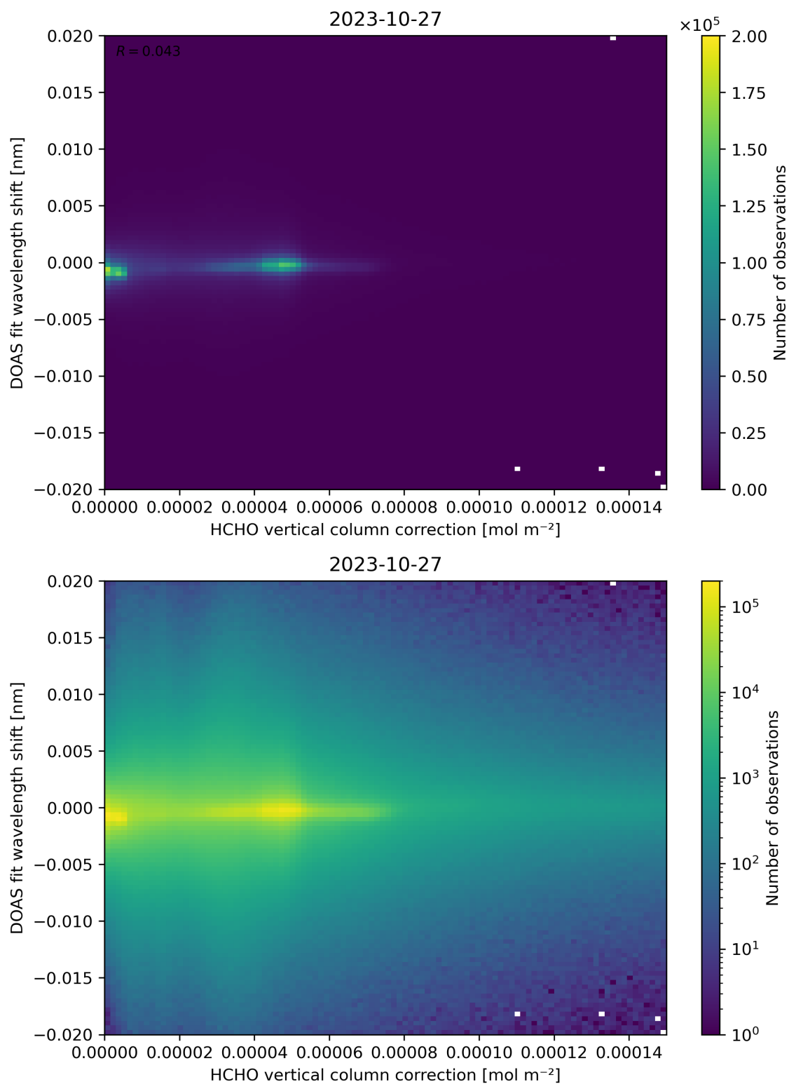
Figure 113: Scatter density plot of “HCHO vertical column correction” against “DOAS fit wavelength shift” for 2023-10-27 to 2023-10-28.
