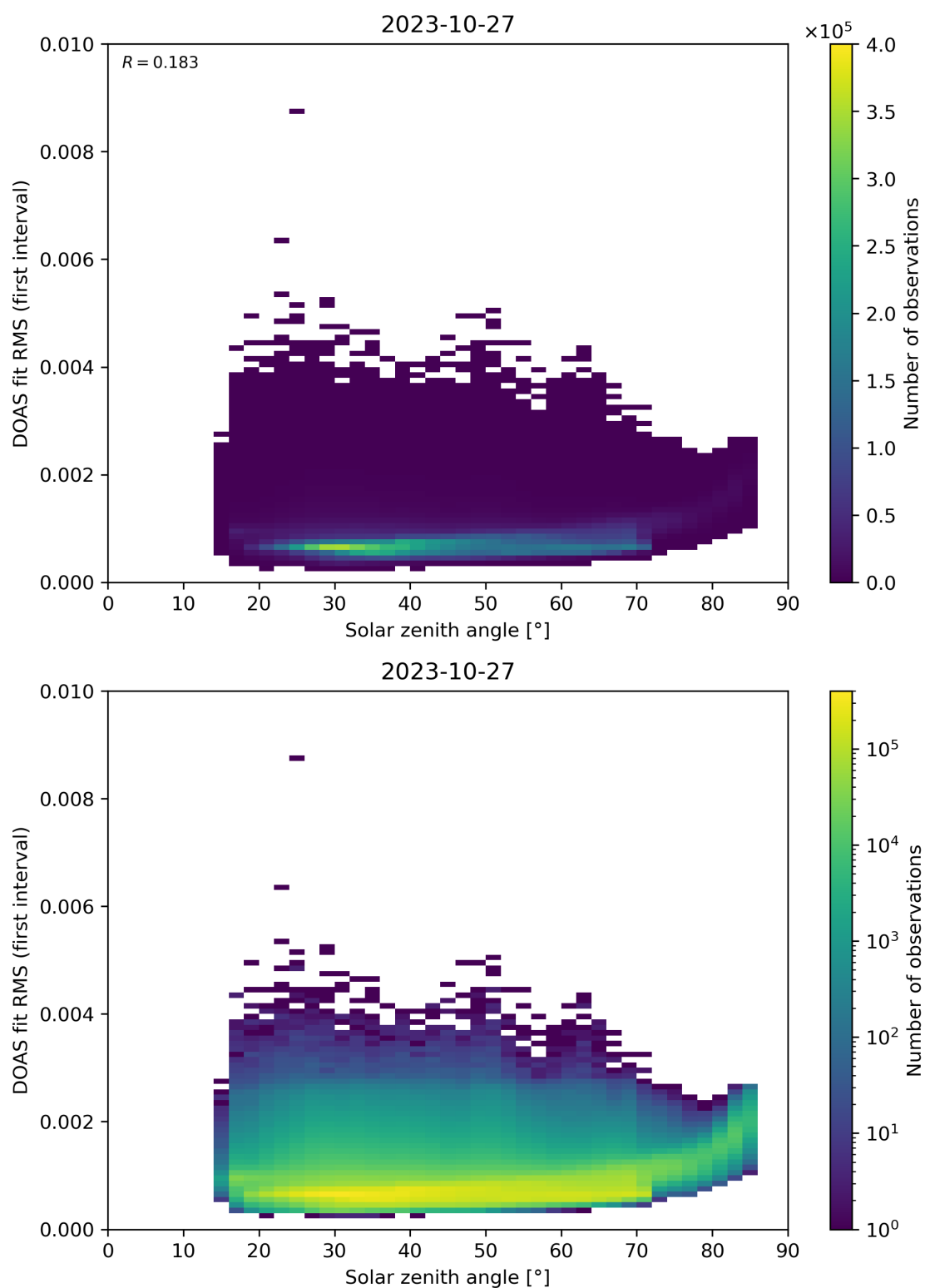
Figure 167: Scatter density plot of “Solar zenith angle” against “DOAS fit RMS (first interval)” for 2023-10-27 to 2023-10-28.
