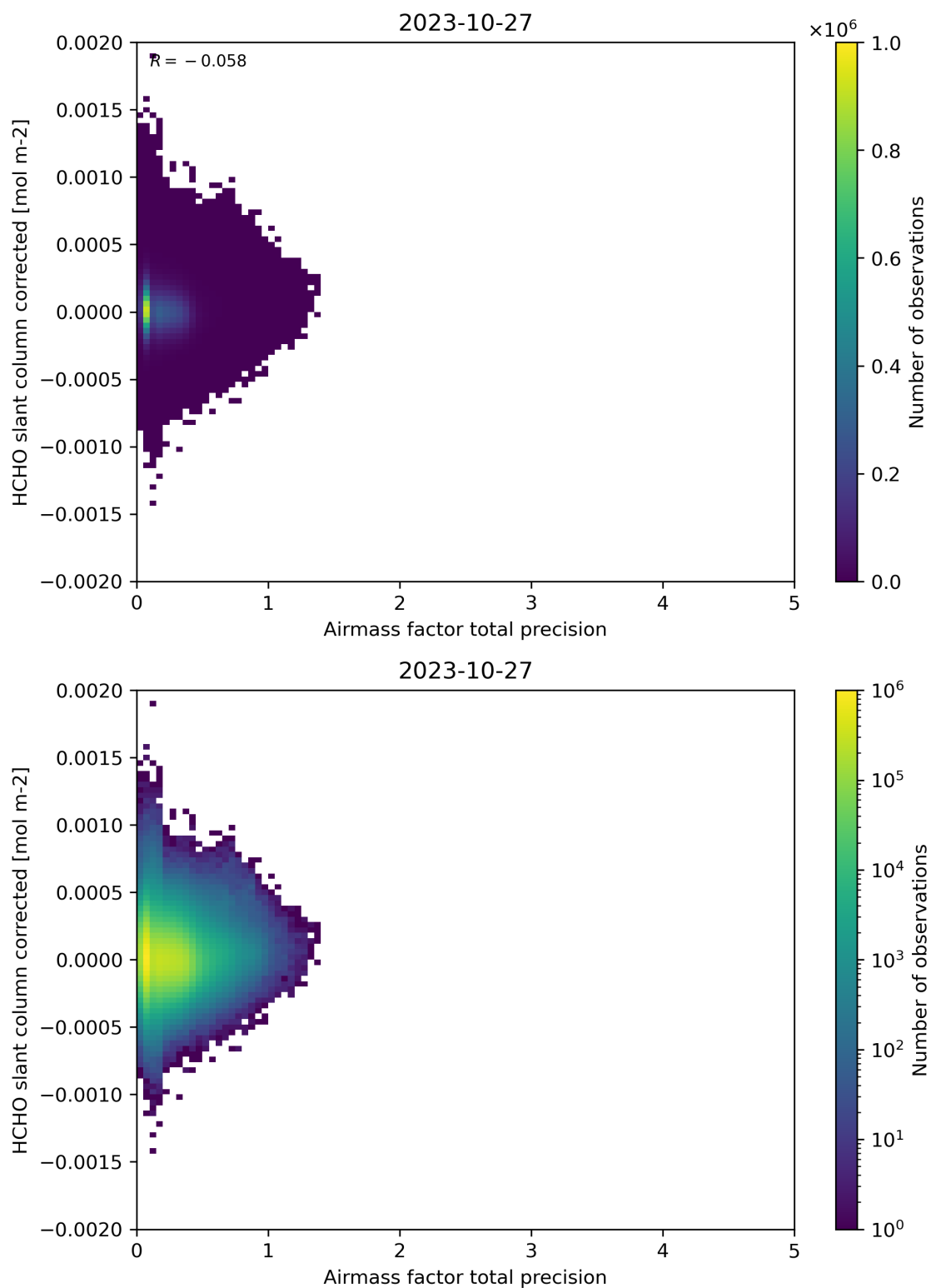
Figure 109: Scatter density plot of “Airmass factor total precision” against “HCHO slant column corrected” for 2023-10-27 to 2023-10-28.
