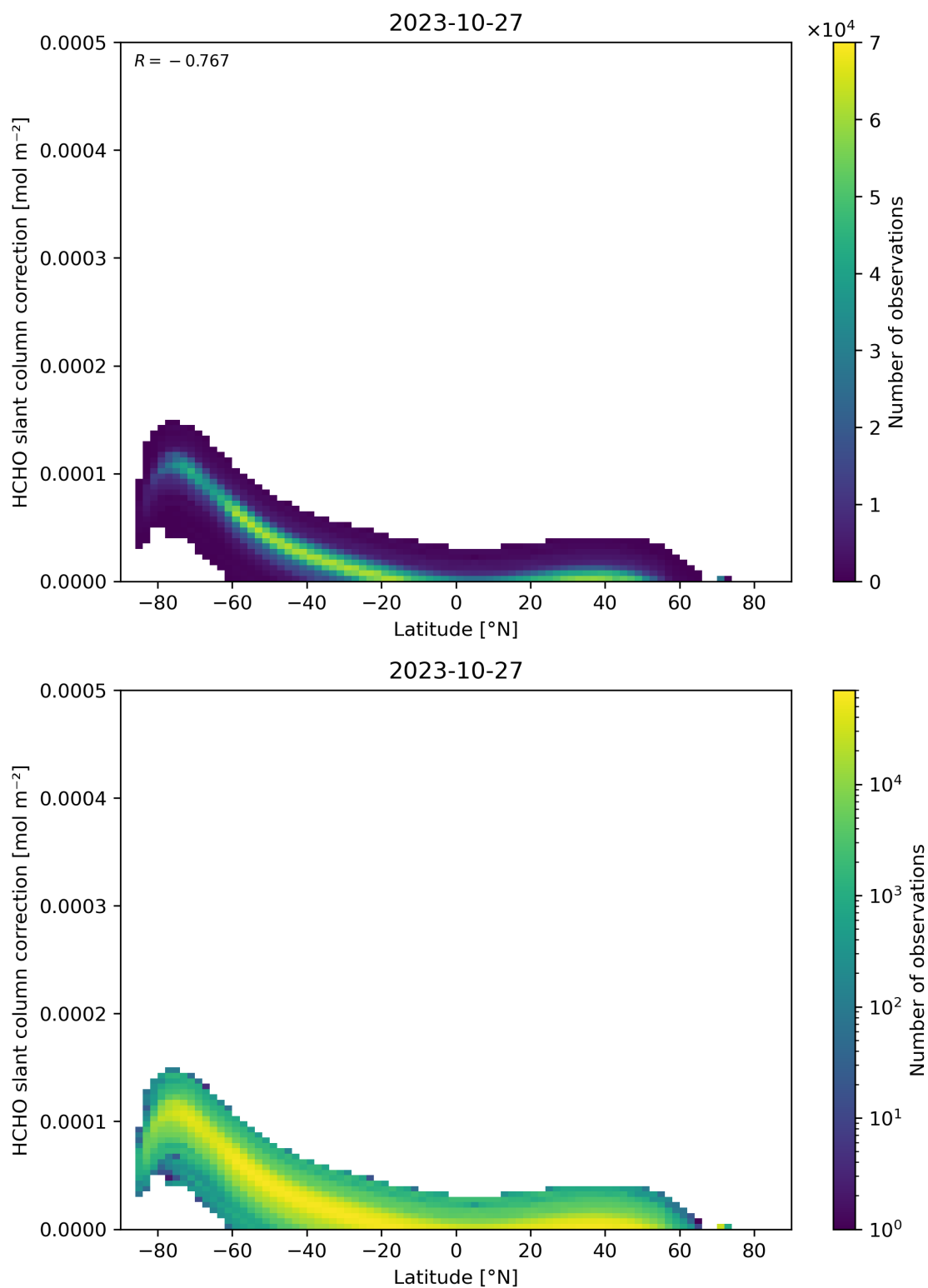
Figure 158: Scatter density plot of “Latitude” against “HCHO slant column correction” for 2023-10-27 to 2023-10-28.
