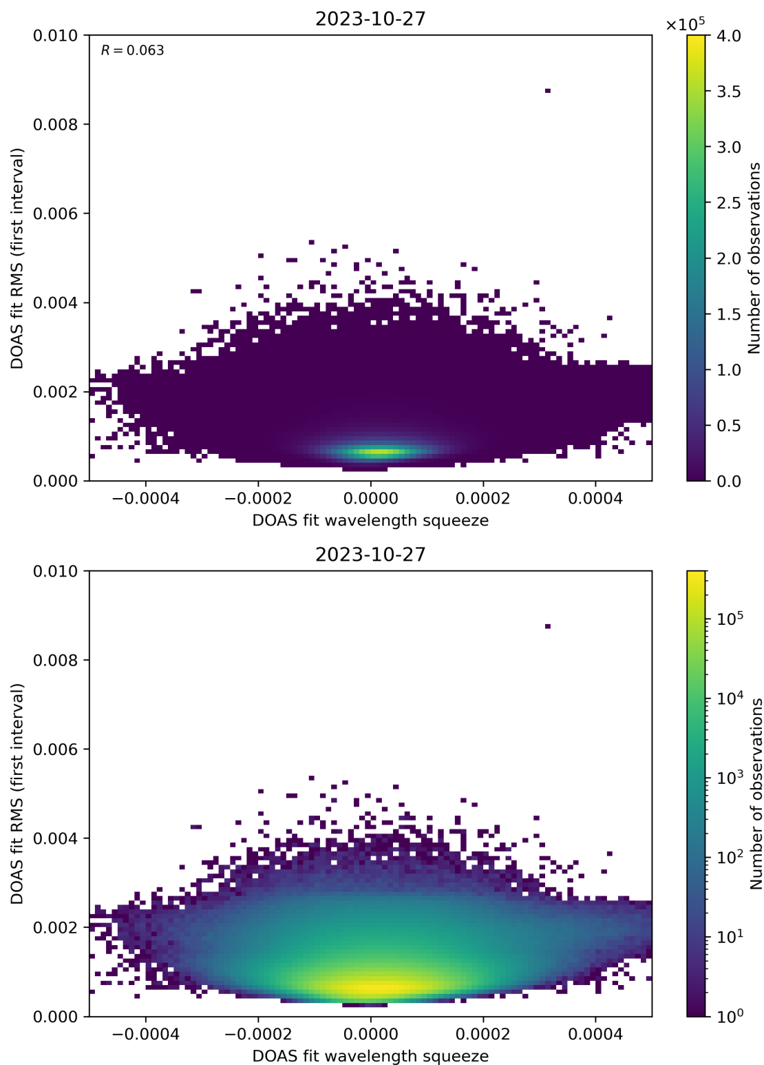
Figure 68: Scatter density plot of “DOAS fit wavelength squeeze” against “DOAS fit RMS (first interval)” for 2023-10-27 to 2023-10-28.
