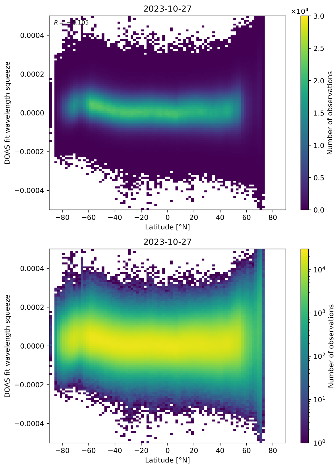
Figure 155: Scatter density plot of “Latitude” against “DOAS fit wavelength squeeze” for 2023-10-27 to 2023-10-28.
