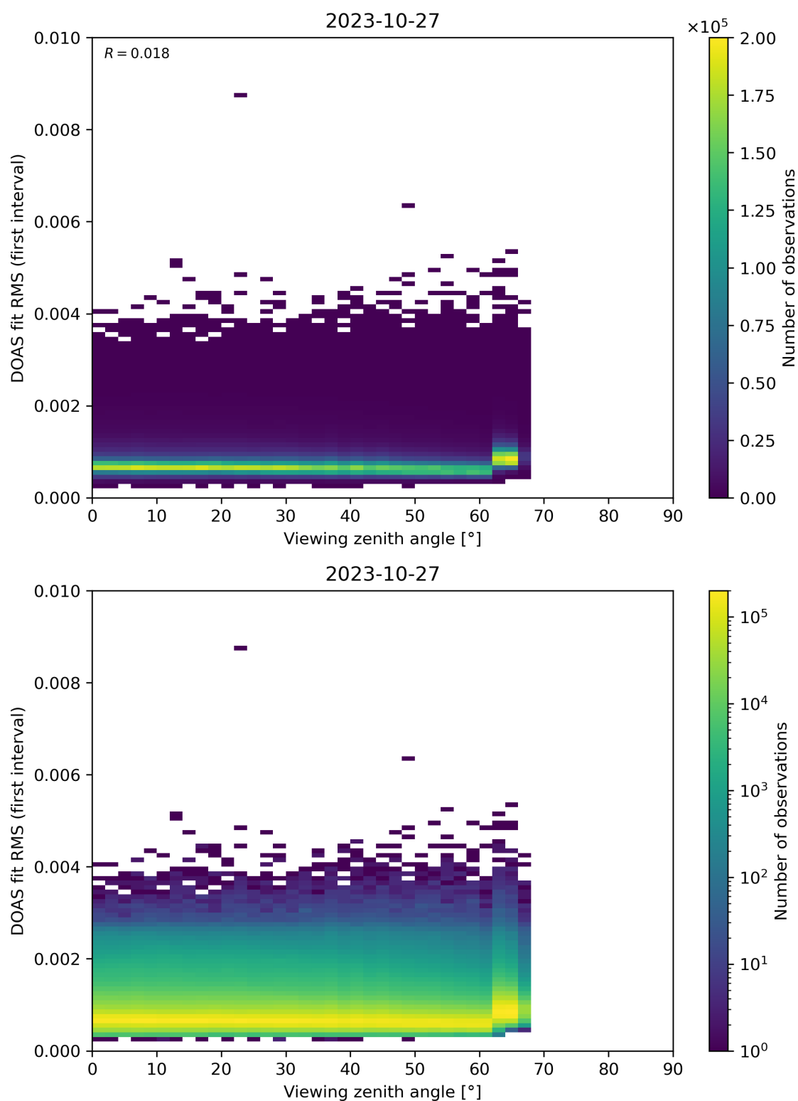
Figure 182: Scatter density plot of “Viewing zenith angle” against “DOAS fit RMS (first interval)” for 2023-10-27 to 2023-10-28.
