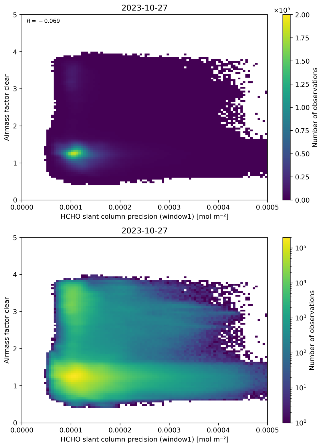
Figure 91: Scatter density plot of “HCHO slant column precision (window1)” against “Airmass factor clear” for 2023-10-27 to 2023-10-28.
