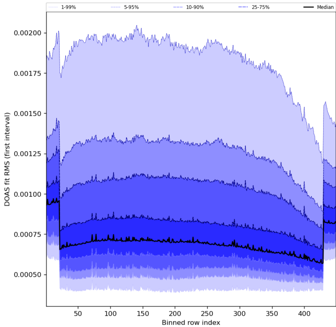
Figure 60: Along track statistics of “DOAS fit RMS (first interval)” for 2023-10-27 to 2023-10-28
