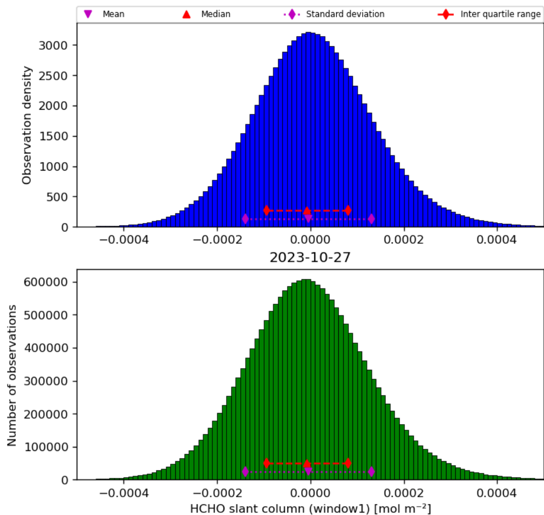
Figure 38: Histogram of “HCHO slant column (window1)” for 2023-10-27 to 2023-10-28
