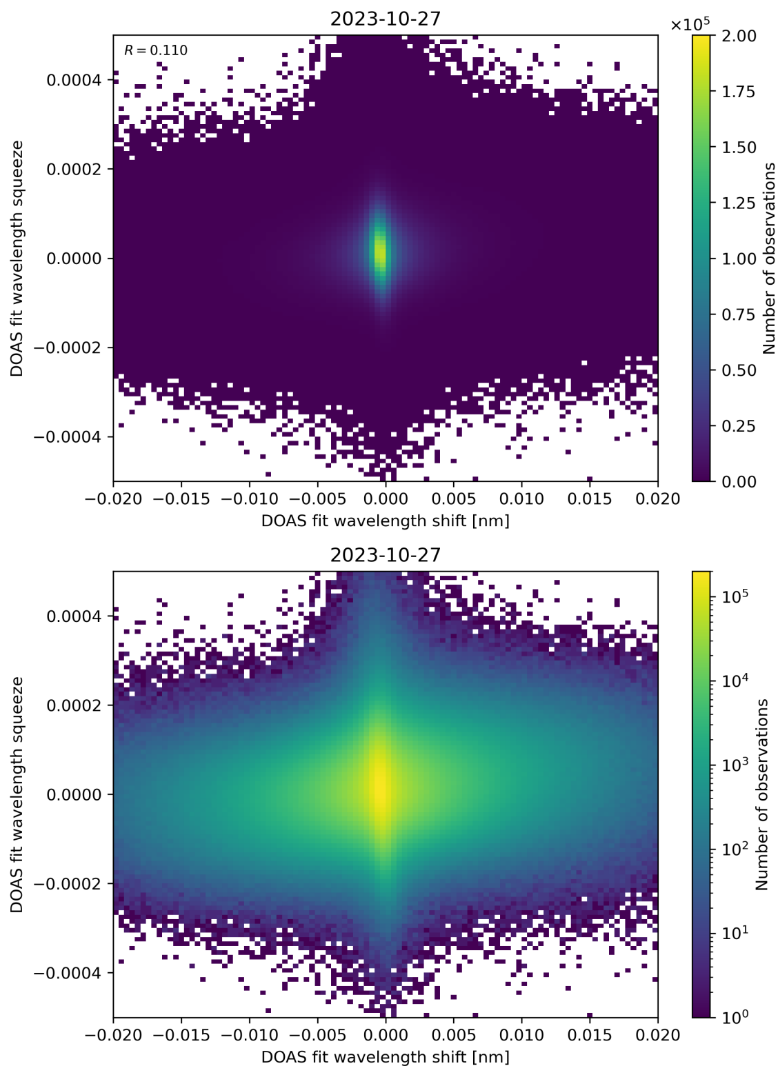
Figure 65: Scatter density plot of “DOAS fit wavelength shift” against “DOAS fit wavelength squeeze” for 2023-10-27 to 2023-10-28.
