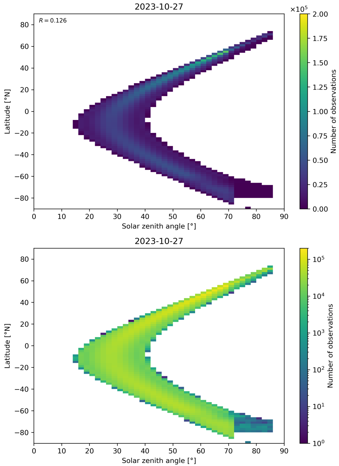
Figure 181: Scatter density plot of “Solar zenith angle” against “Latitude” for 2023-10-27 to 2023-10-28.
