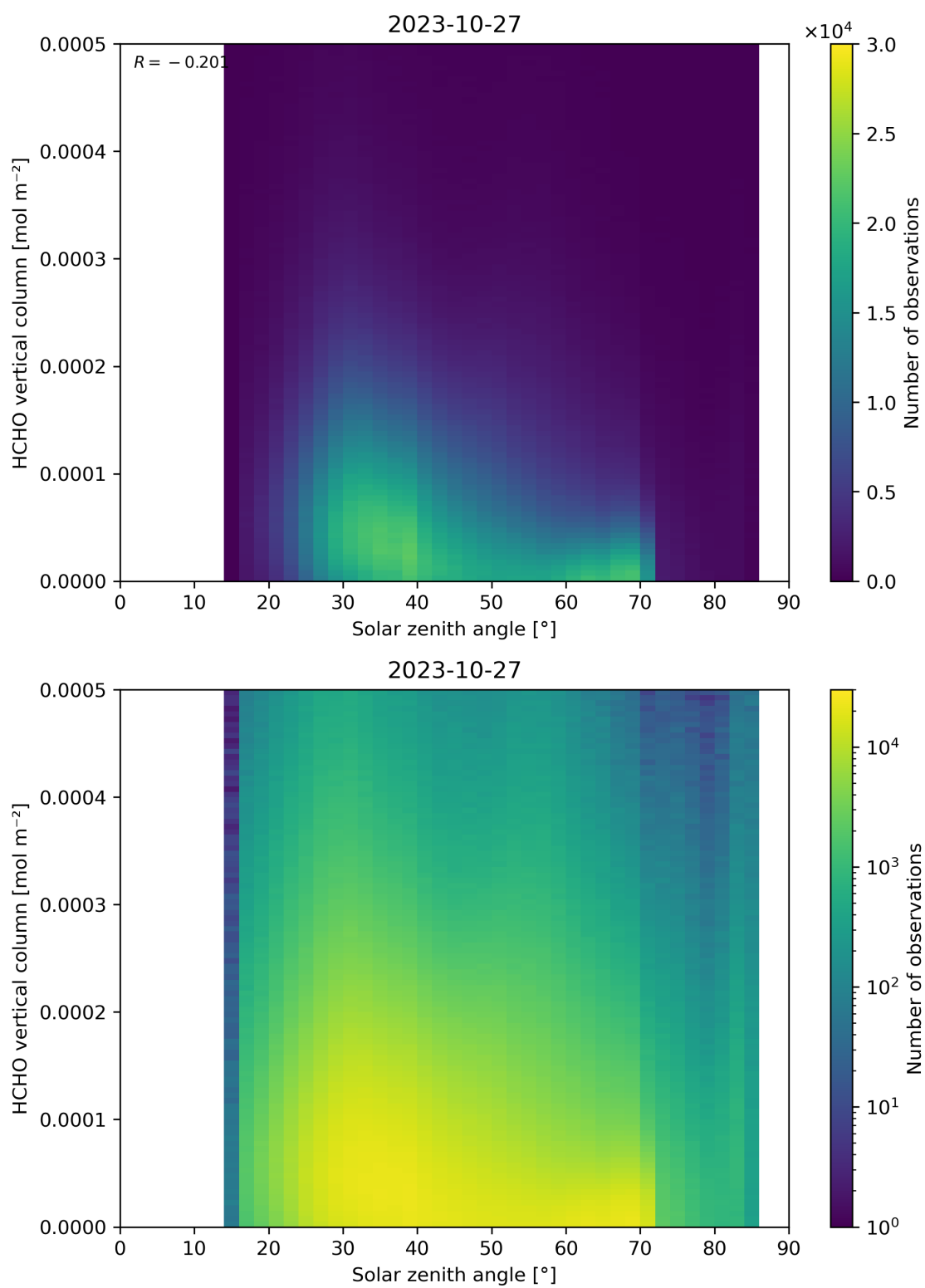
Figure 177: Scatter density plot of “Solar zenith angle” against “HCHO vertical column” for 2023-10-27 to 2023-10-28.
