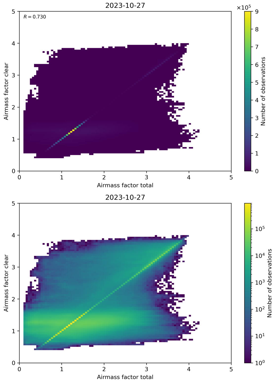
Figure 100: Scatter density plot of “Airmass factor total” against “Airmass factor clear” for 2023-10-27 to 2023-10-28.
