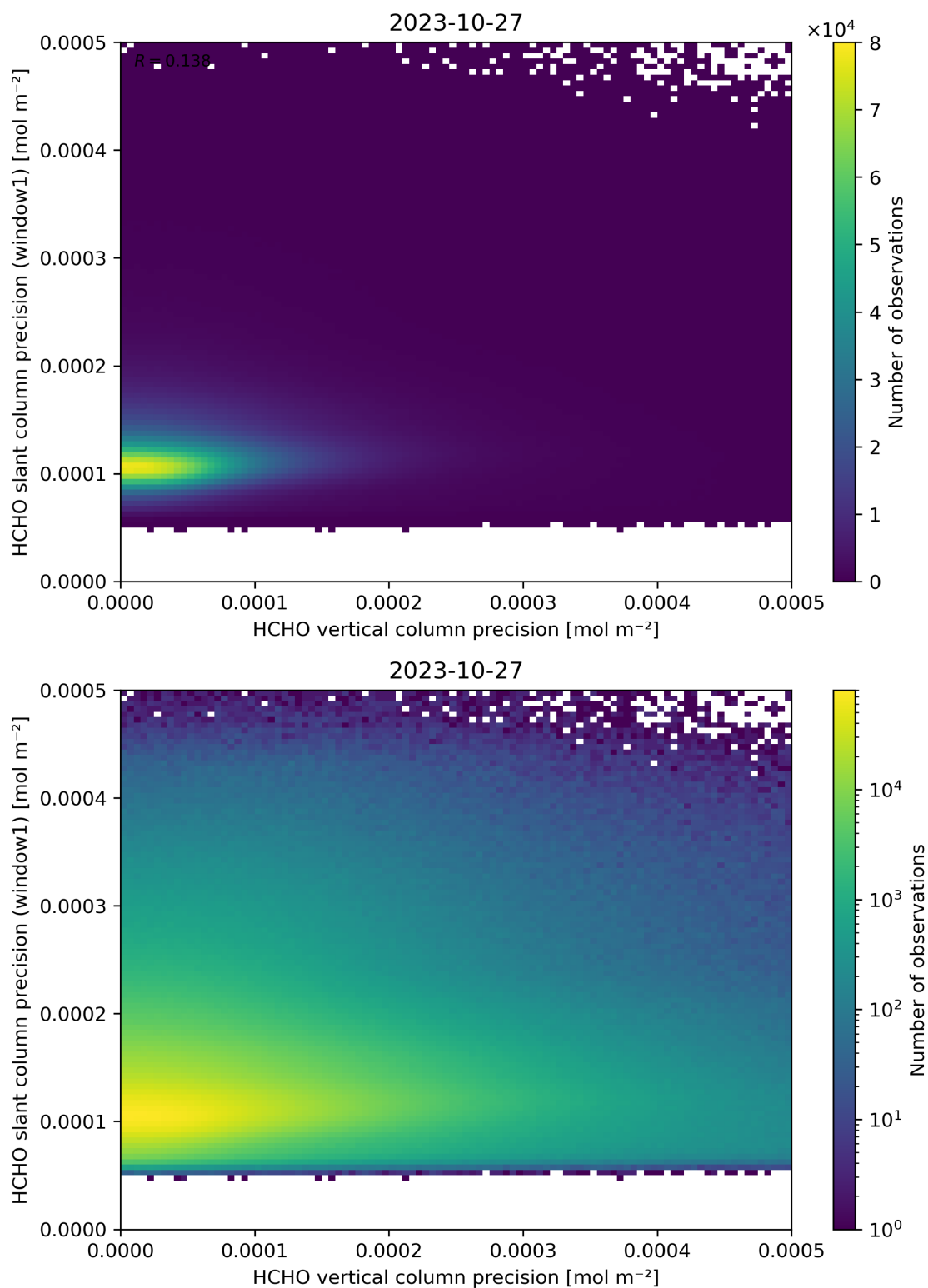
Figure 143: Scatter density plot of “HCHO vertical column precision” against “HCHO slant column precision (window1)” for 2023-10-27 to 2023-10-28.
