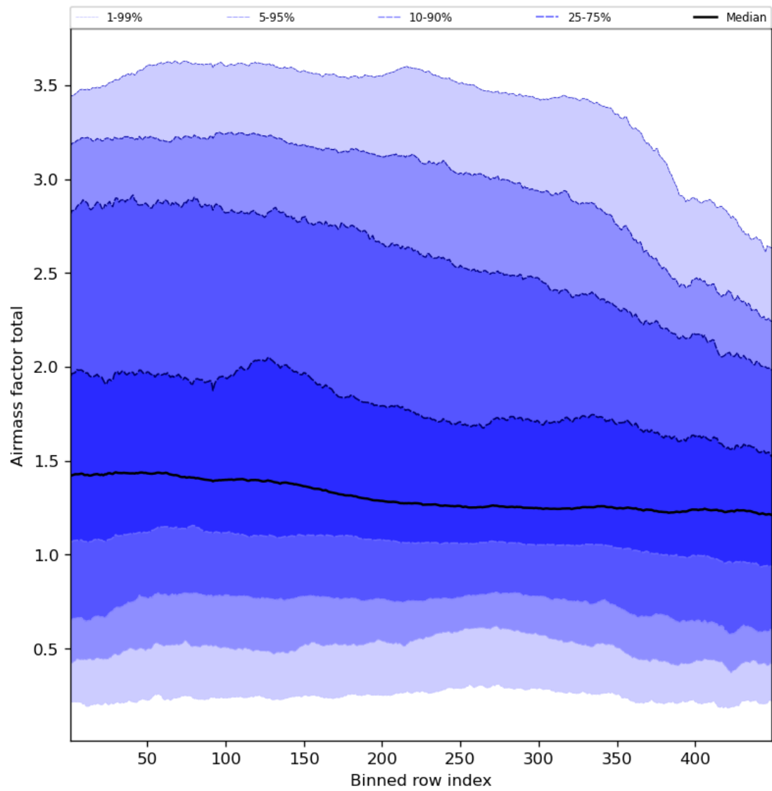
Figure 54: Along track statistics of “Airmass factor total” for 2023-10-27 to 2023-10-28
