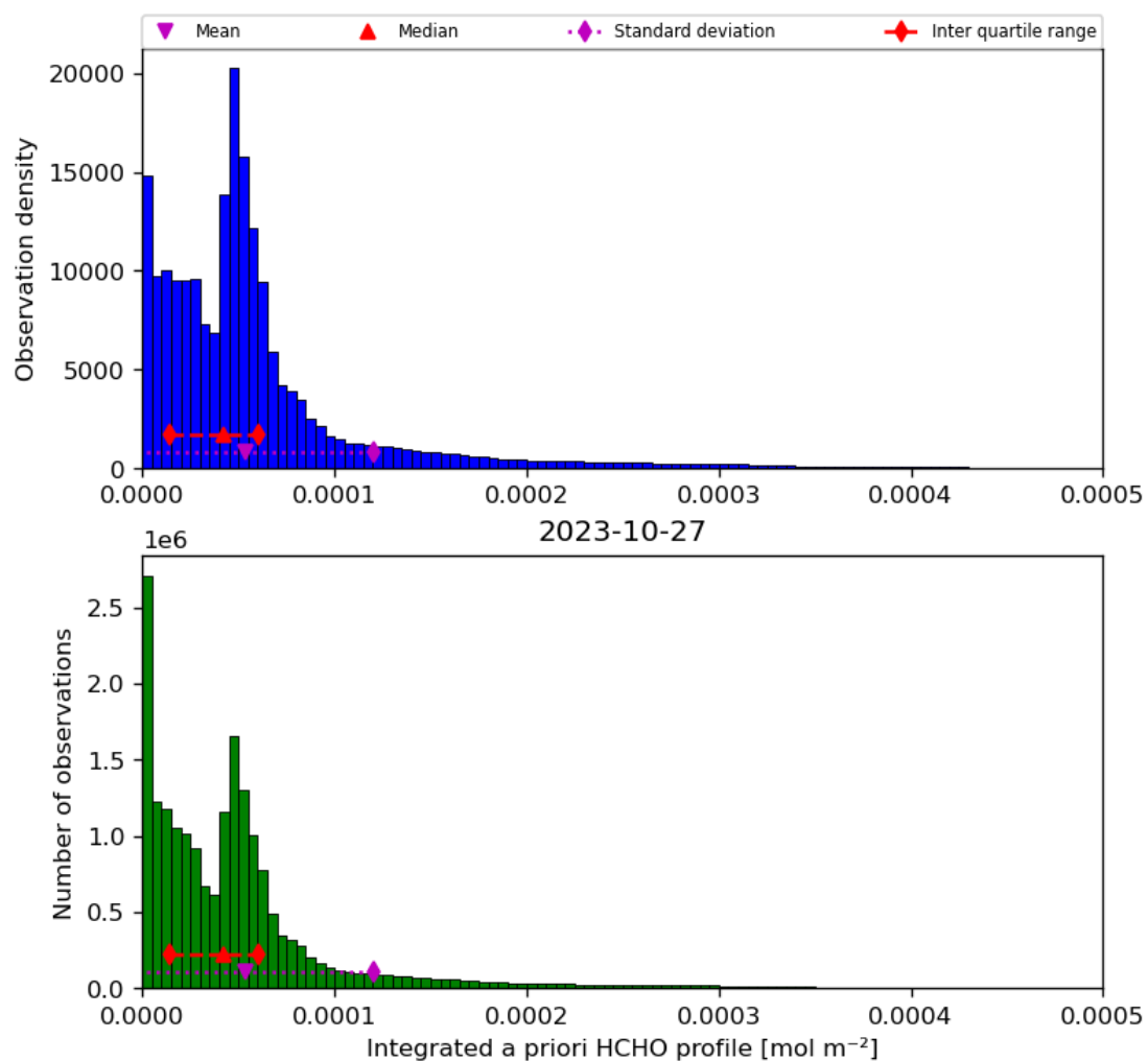
Figure 43: Histogram of “Integrated a priori HCHO profile” for 2023-10-27 to 2023-10-28
