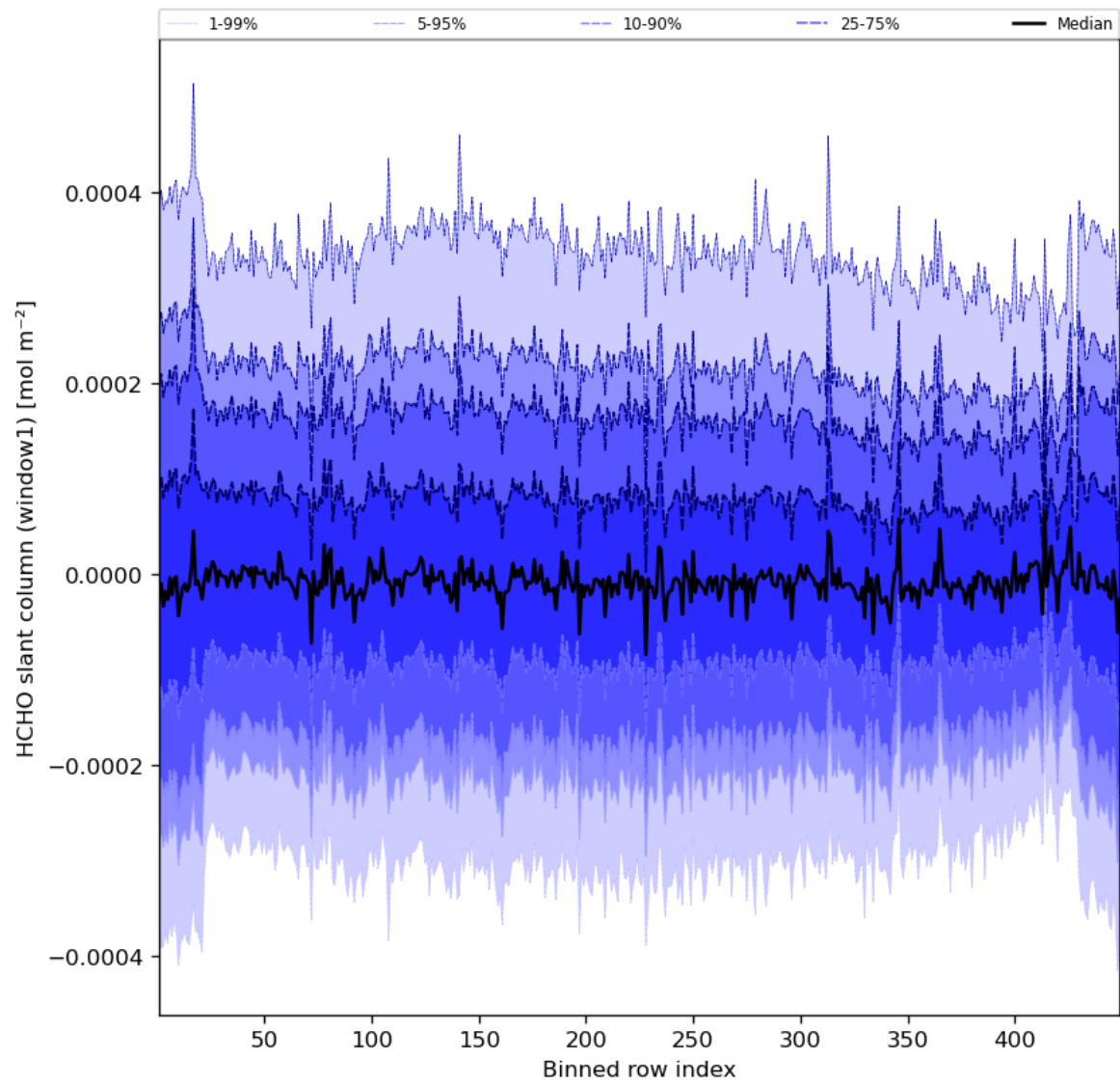
Figure 52: Along track statistics of “HCHO slant column (window1)” for 2023-10-27 to 2023-10-28
