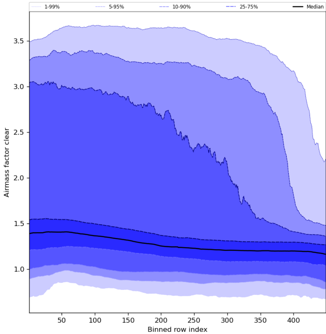
Figure 56: Along track statistics of “Airmass factor clear” for 2023-10-27 to 2023-10-28
