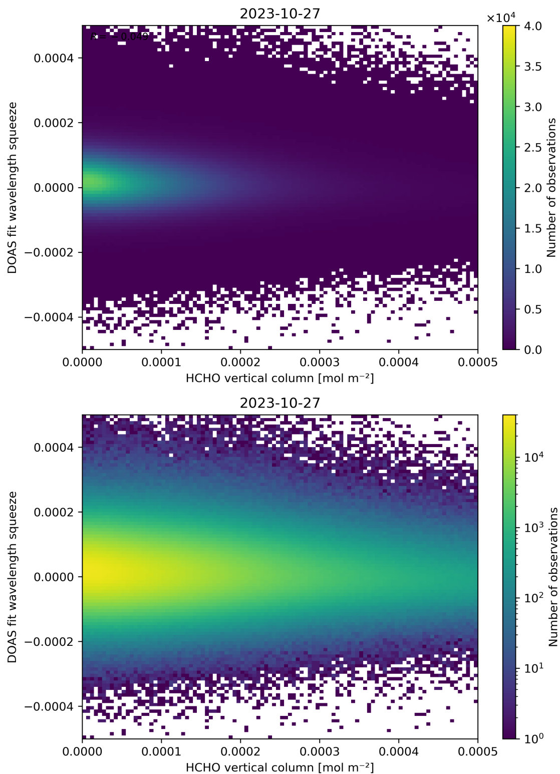
Figure 125: Scatter density plot of “HCHO vertical column” against “DOAS fit wavelength squeeze” for 2023-10-27 to 2023-10-28.
