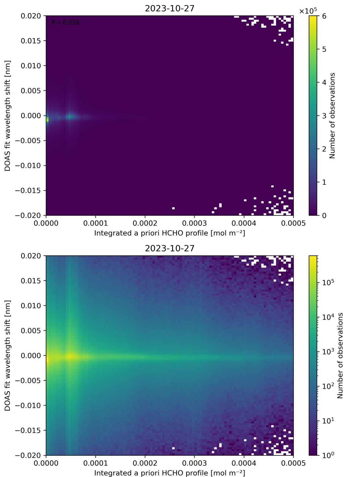
Figure 149: Scatter density plot of “Integrated a priori HCHO profile” against “DOAS fit wavelength shift” for 2023-10-27 to 2023-10-28.
