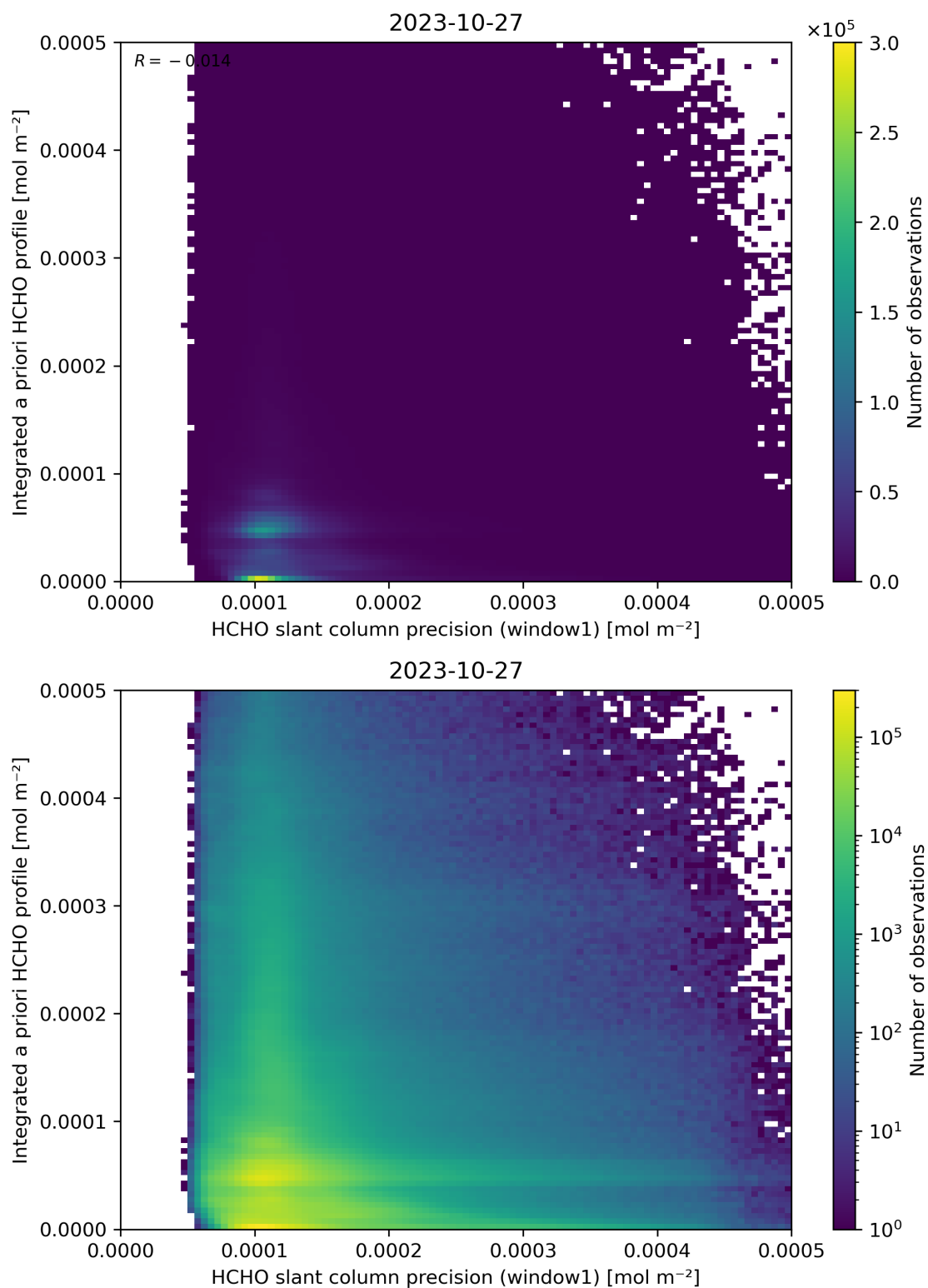
Figure 96: Scatter density plot of “HCHO slant column precision (window1)” against “Integrated a priori HCHO profile” for 2023-10-27 to 2023-10-28.
