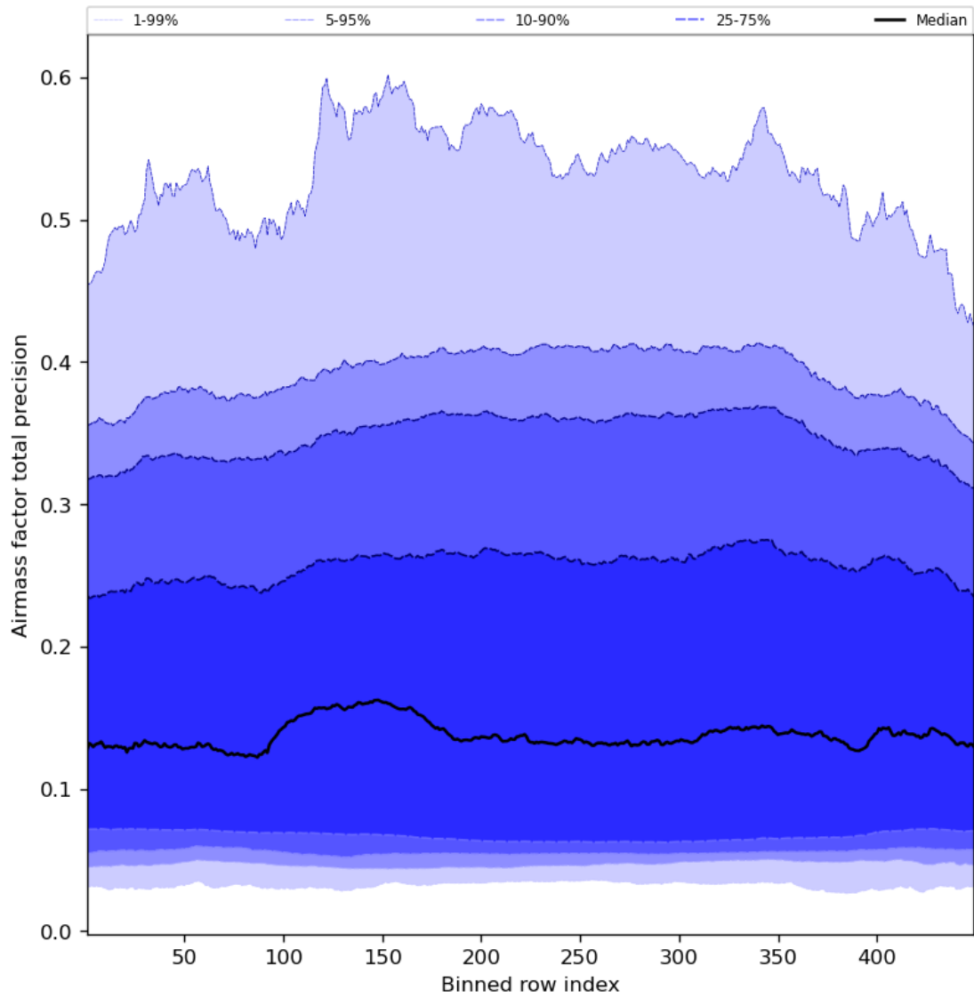
Figure 55: Along track statistics of “Airmass factor total precision” for 2023-10-27 to 2023-10-28
