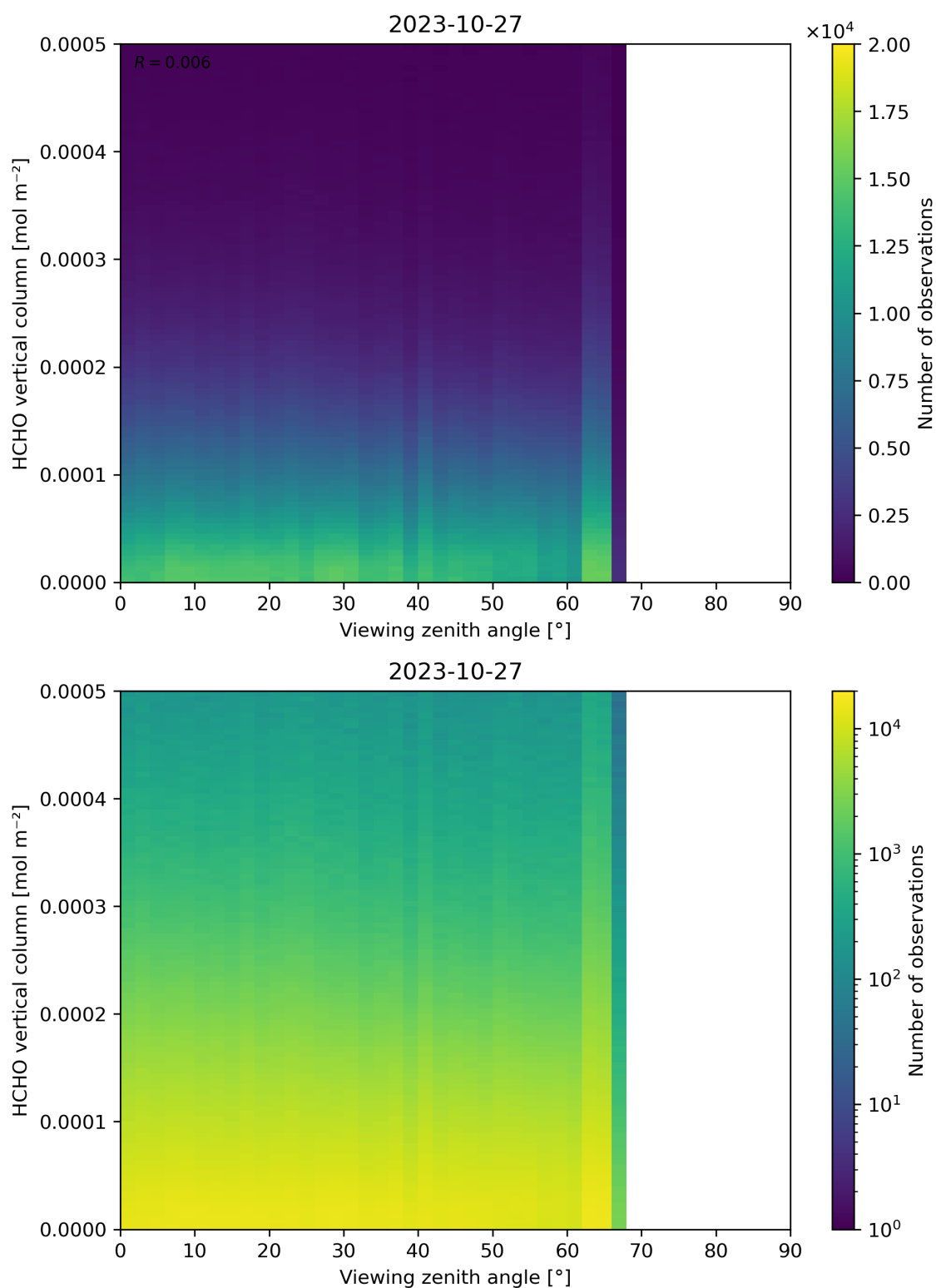
Figure 192: Scatter density plot of “Viewing zenith angle” against “HCHO vertical column” for 2023-10-27 to 2023-10-28.
