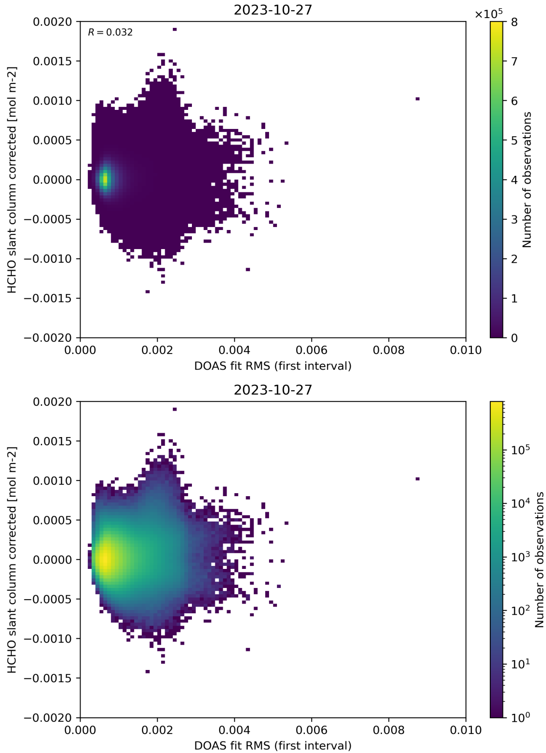
Figure 62: Scatter density plot of “DOAS fit RMS (first interval)” against “HCHO slant column corrected” for 2023-10-27 to 2023-10-28.
