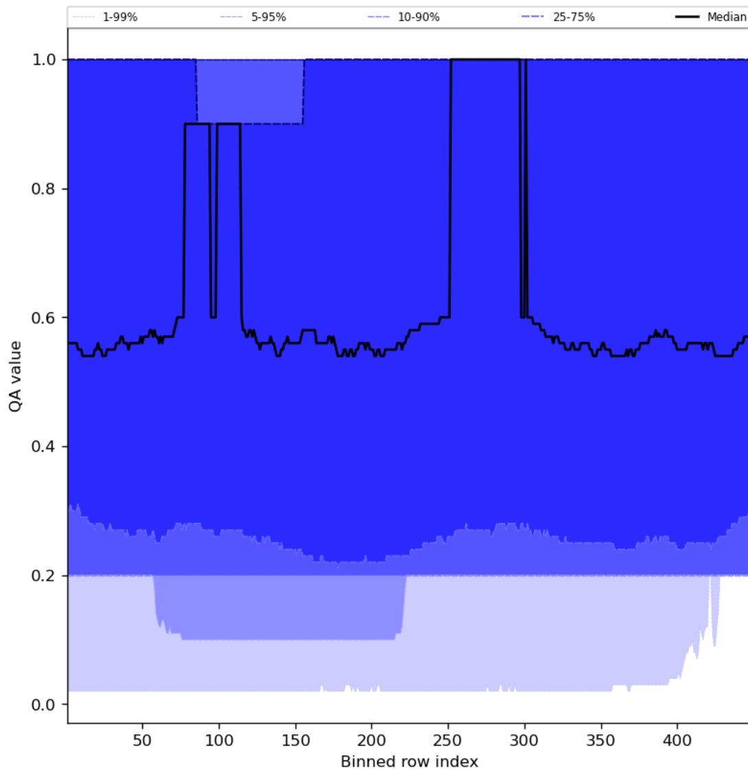
Figure 48: Along track statistics of “QA value” for 2023-10-27 to 2023-10-28
