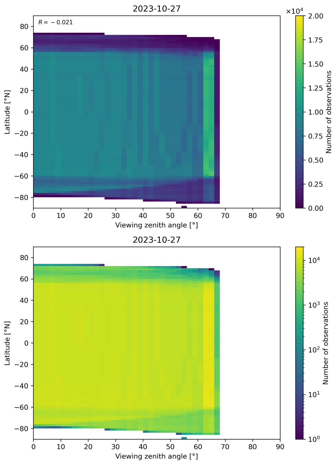
Figure 196: Scatter density plot of “Viewing zenith angle” against “Latitude” for 2023-10-27 to 2023-10-28.
