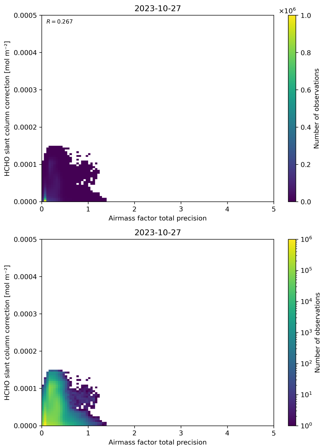
Figure 110: Scatter density plot of “Airmass factor total precision” against “HCHO slant column correction” for 2023-10-27 to 2023-10-28.
