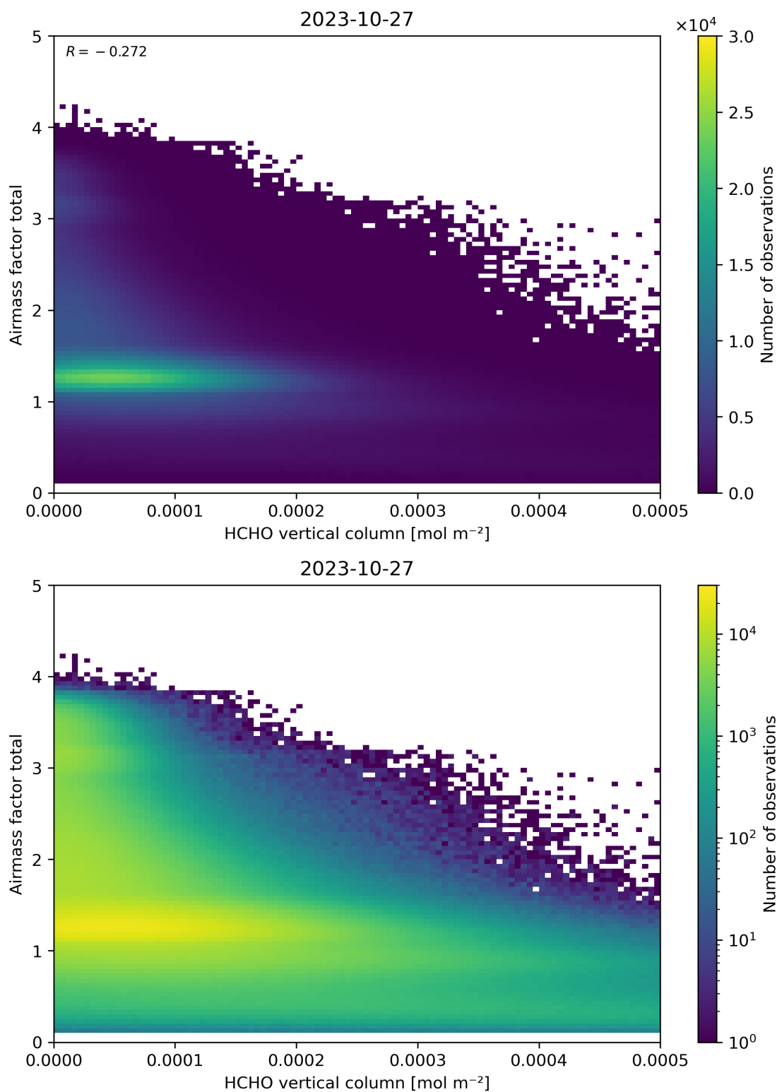
Figure 131: Scatter density plot of “HCHO vertical column” against “Airmass factor total” for 2023-10-27 to 2023-10-28.
