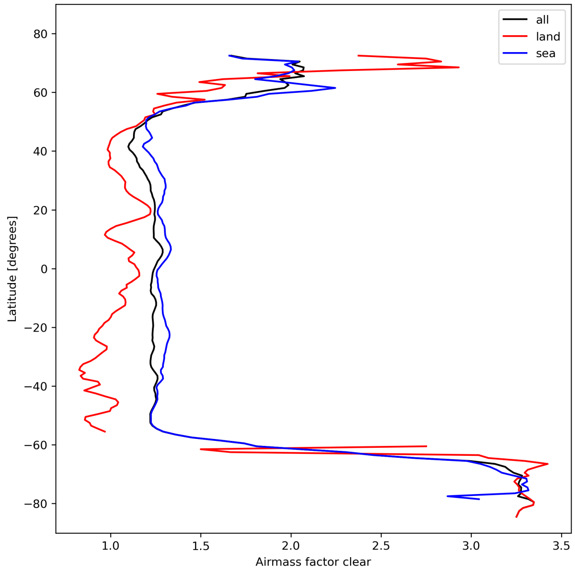
Figure 28: Zonal average of “Airmass factor clear” for 2023-10-27 to 2023-10-28.
