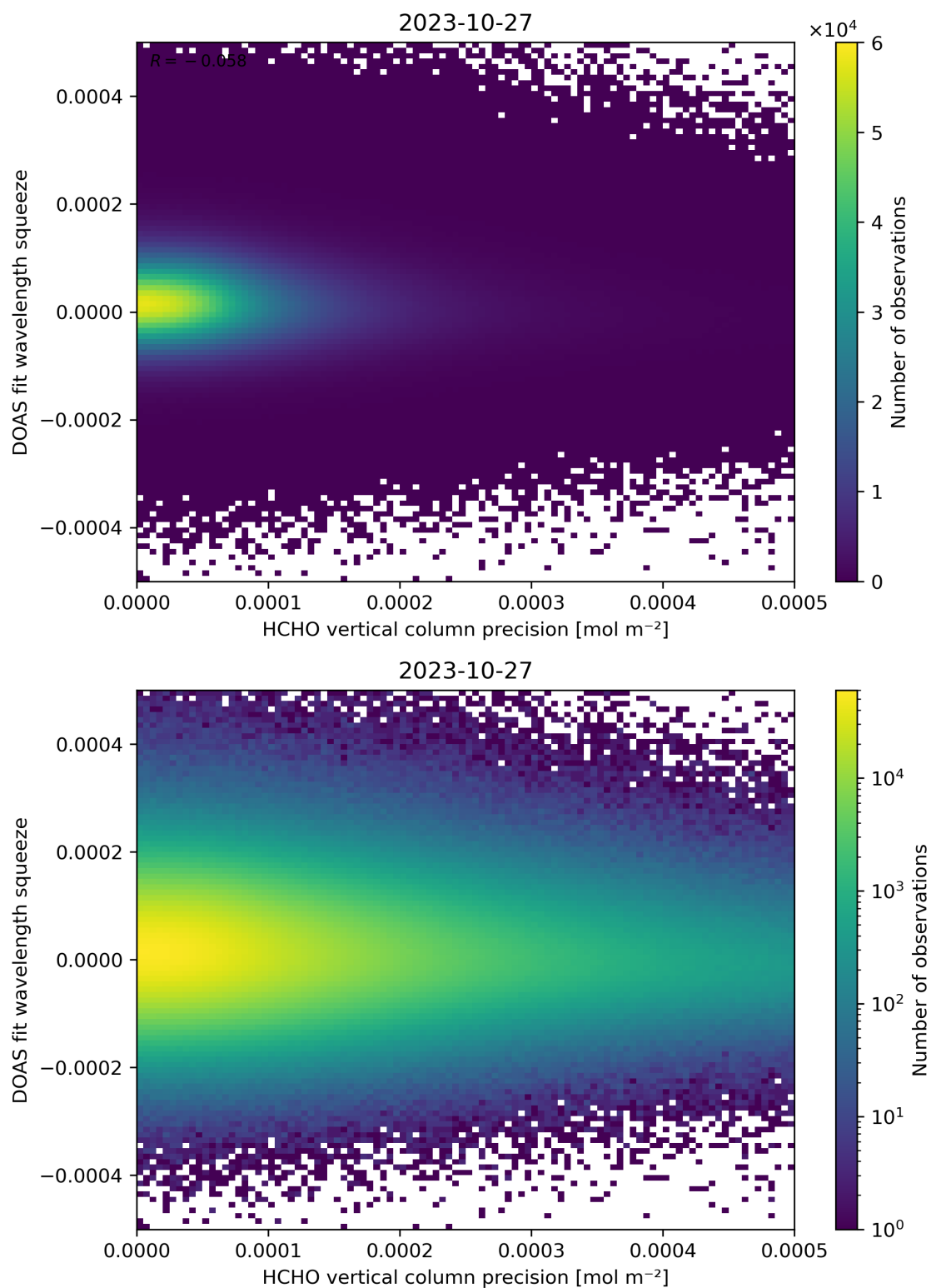
Figure 138: Scatter density plot of “HCHO vertical column precision” against “DOAS fit wavelength squeeze” for 2023-10-27 to 2023-10-28.
