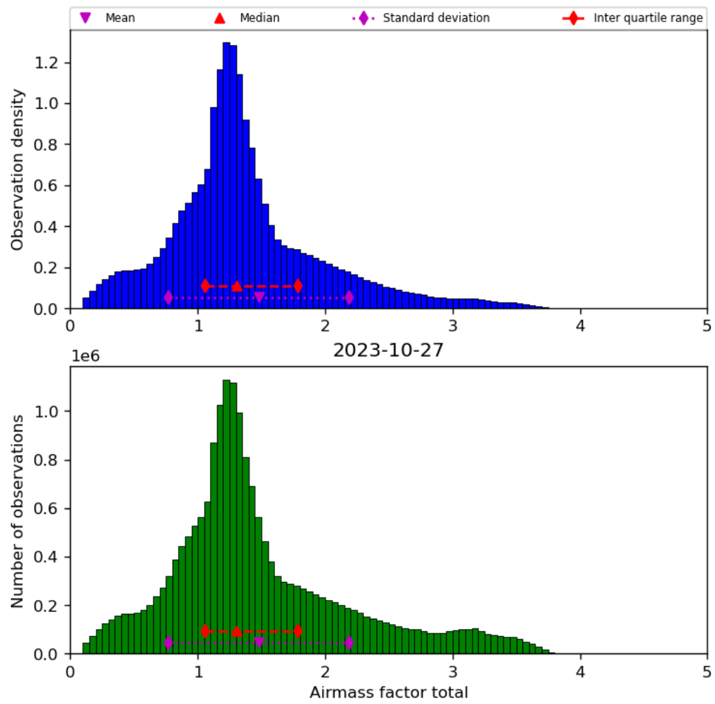
Figure 40: Histogram of “Airmass factor total” for 2023-10-27 to 2023-10-28
