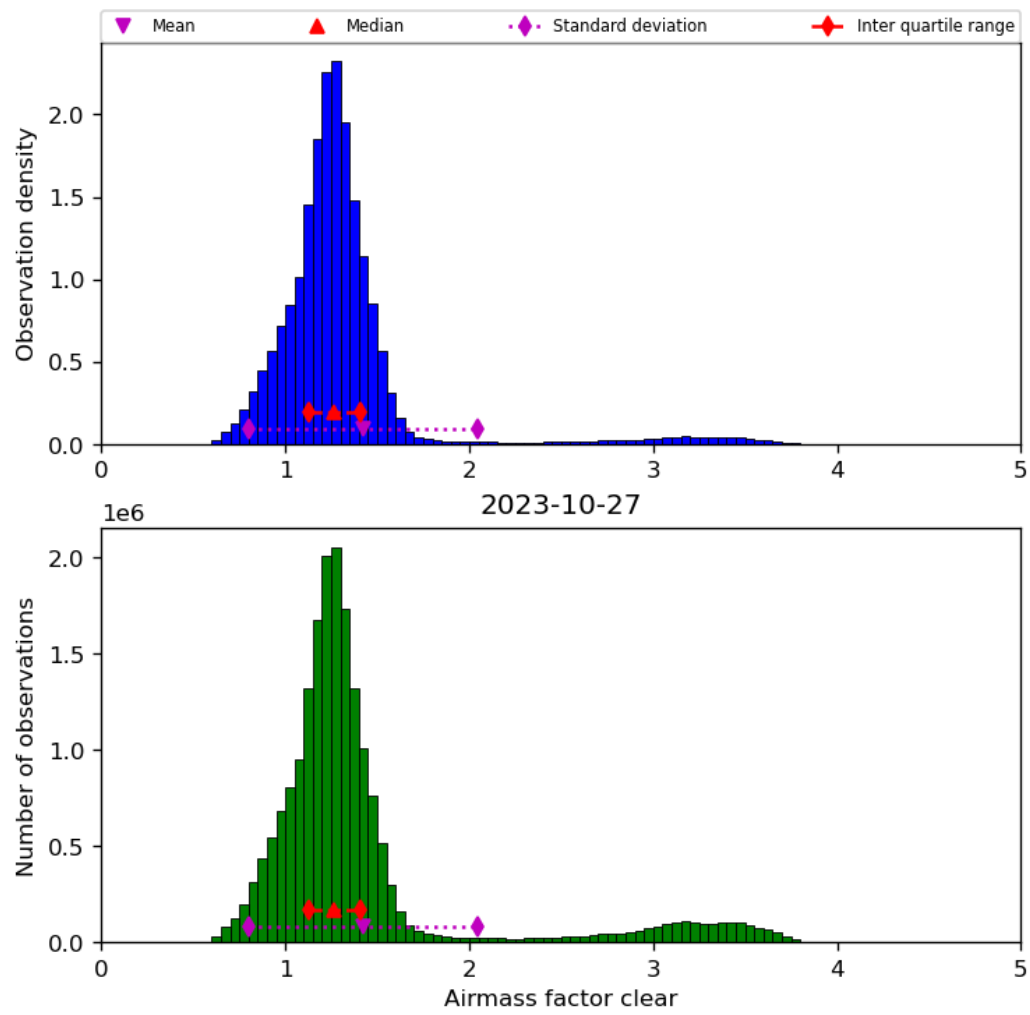
Figure 42: Histogram of “Airmass factor clear” for 2023-10-27 to 2023-10-28
