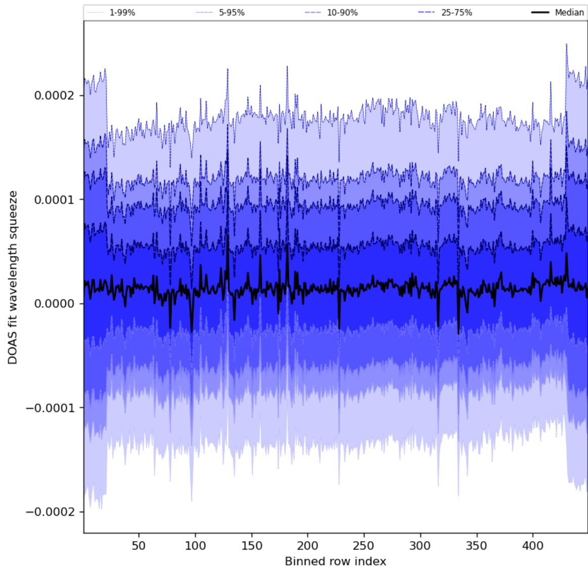
Figure 59: Along track statistics of “DOAS fit wavelength squeeze” for 2023-10-27 to 2023-10-28
