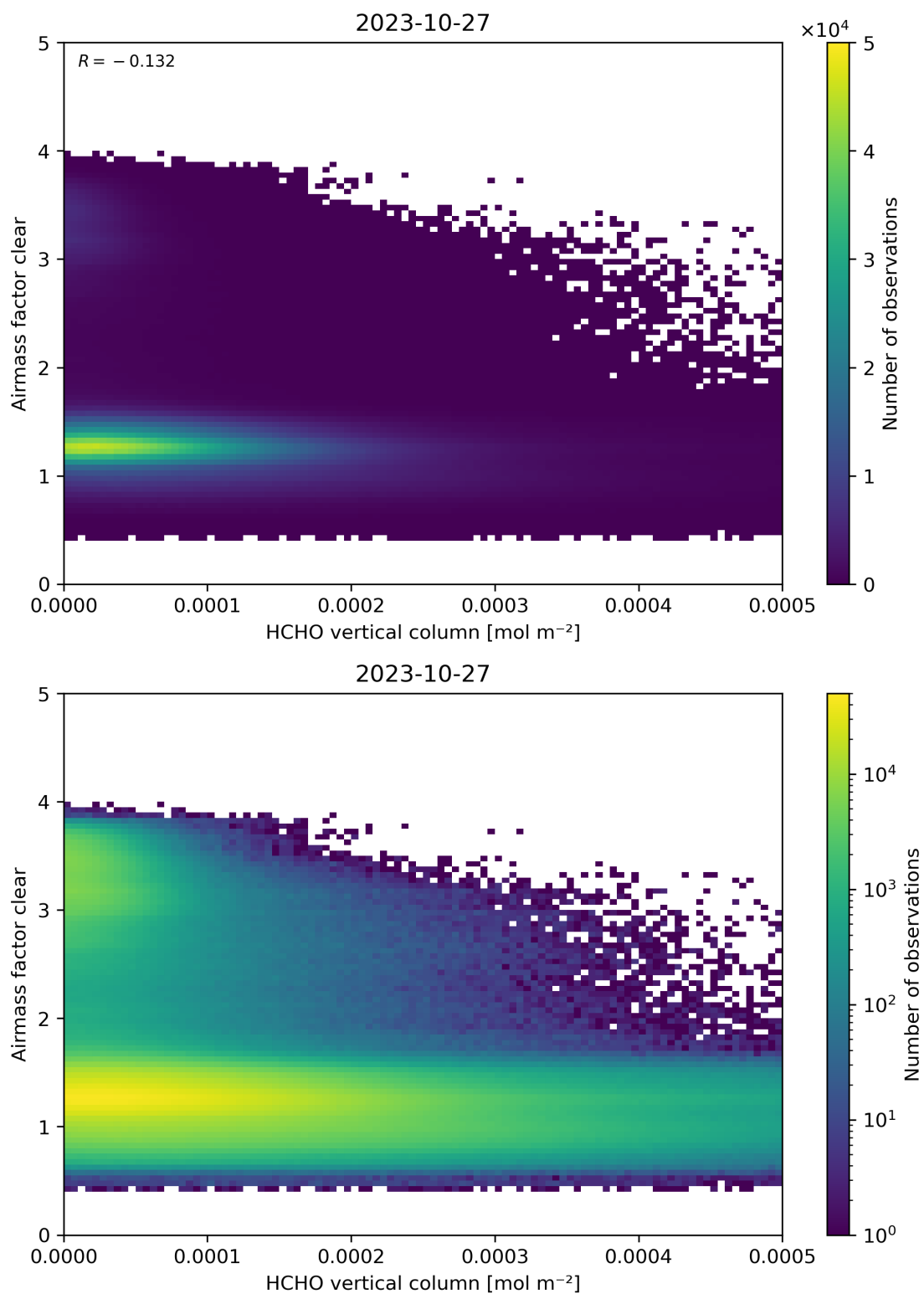
Figure 126: Scatter density plot of “HCHO vertical column” against “Airmass factor clear” for 2023-10-27 to 2023-10-28.
