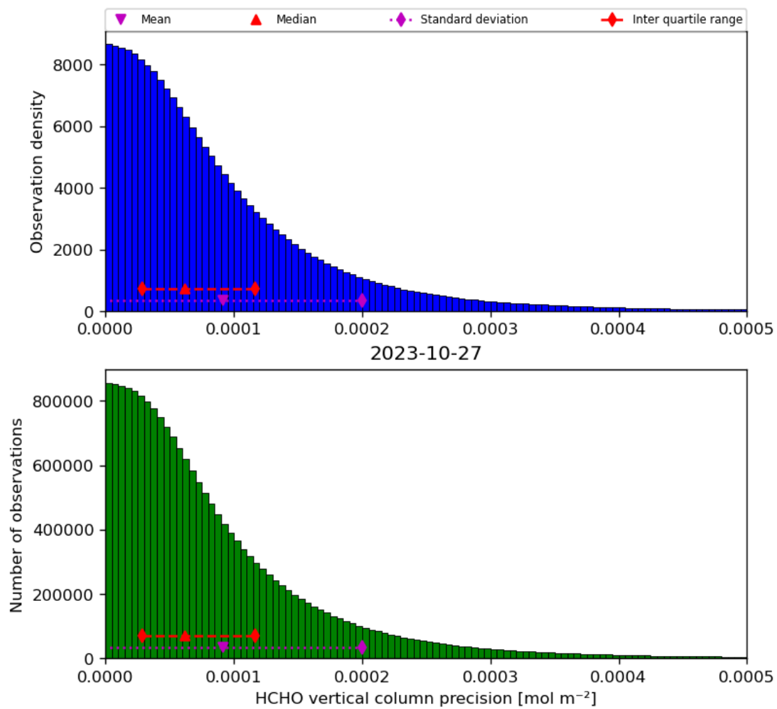
Figure 36: Histogram of “HCHO vertical column precision” for 2023-10-27 to 2023-10-28
