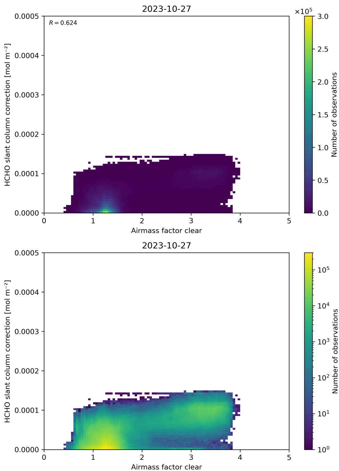
Figure 75: Scatter density plot of “Airmass factor clear” against “HCHO slant column correction” for 2023-10-27 to 2023-10-28.
