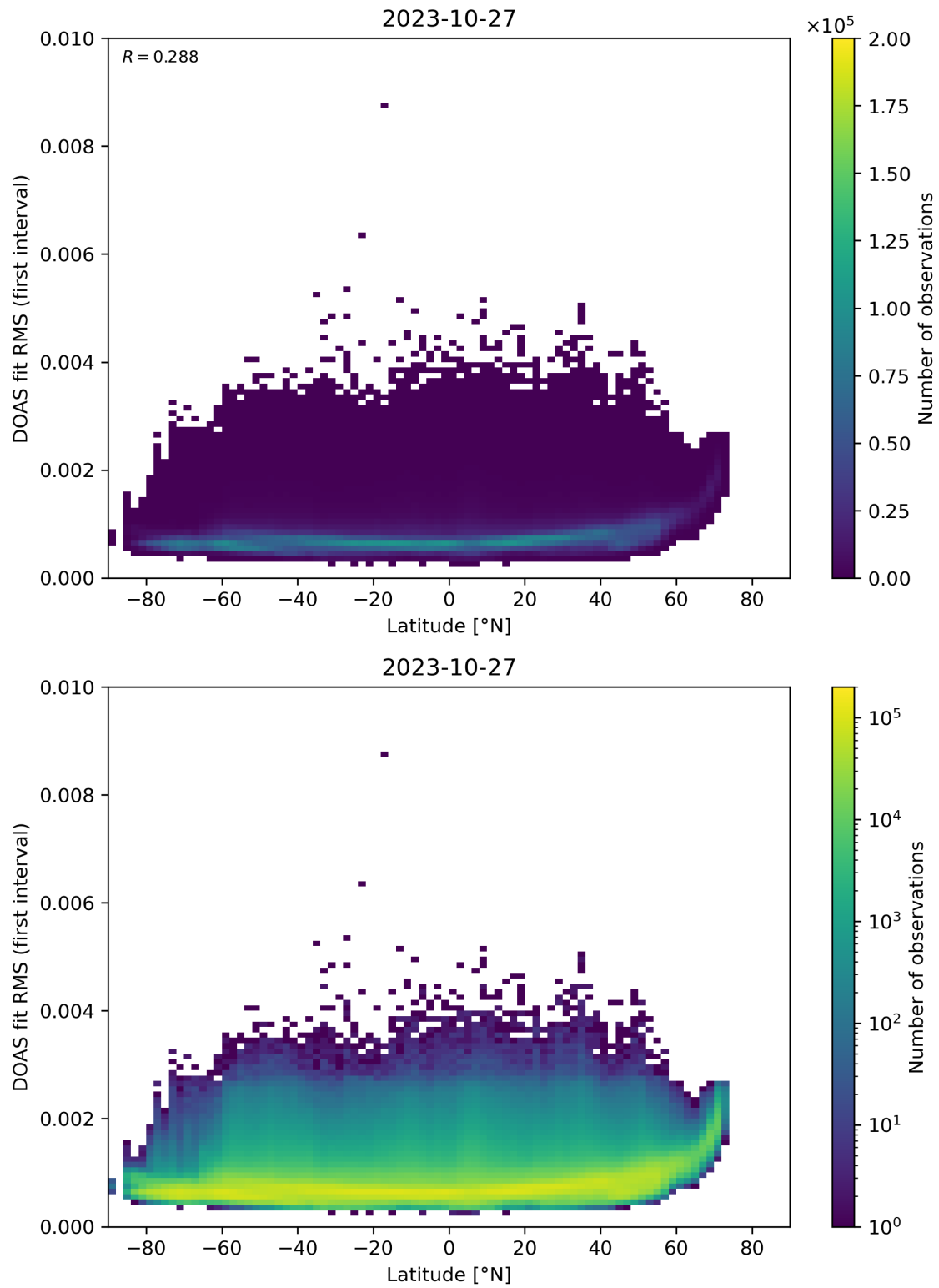
Figure 153: Scatter density plot of “Latitude” against “DOAS fit RMS (first interval)” for 2023-10-27 to 2023-10-28.
