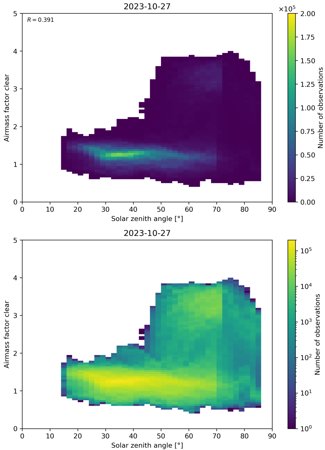
Figure 170: Scatter density plot of “Solar zenith angle” against “Airmass factor clear” for 2023-10-27 to 2023-10-28.
