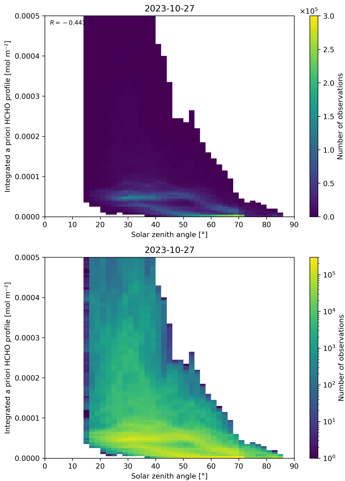
Figure 180: Scatter density plot of “Solar zenith angle” against “Integrated a priori HCHO profile” for 2023-10-27 to 2023-10-28.
