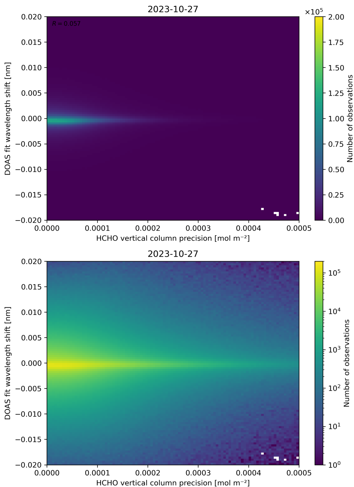
Figure 137: Scatter density plot of “HCHO vertical column precision” against “DOAS fit wavelength shift” for 2023-10-27 to 2023-10-28.
