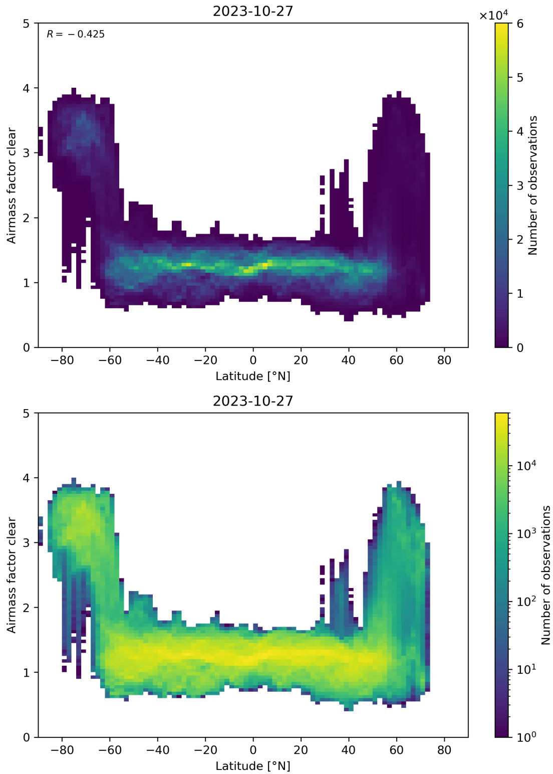
Figure 156: Scatter density plot of “Latitude” against “Airmass factor clear” for 2023-10-27 to 2023-10-28.
