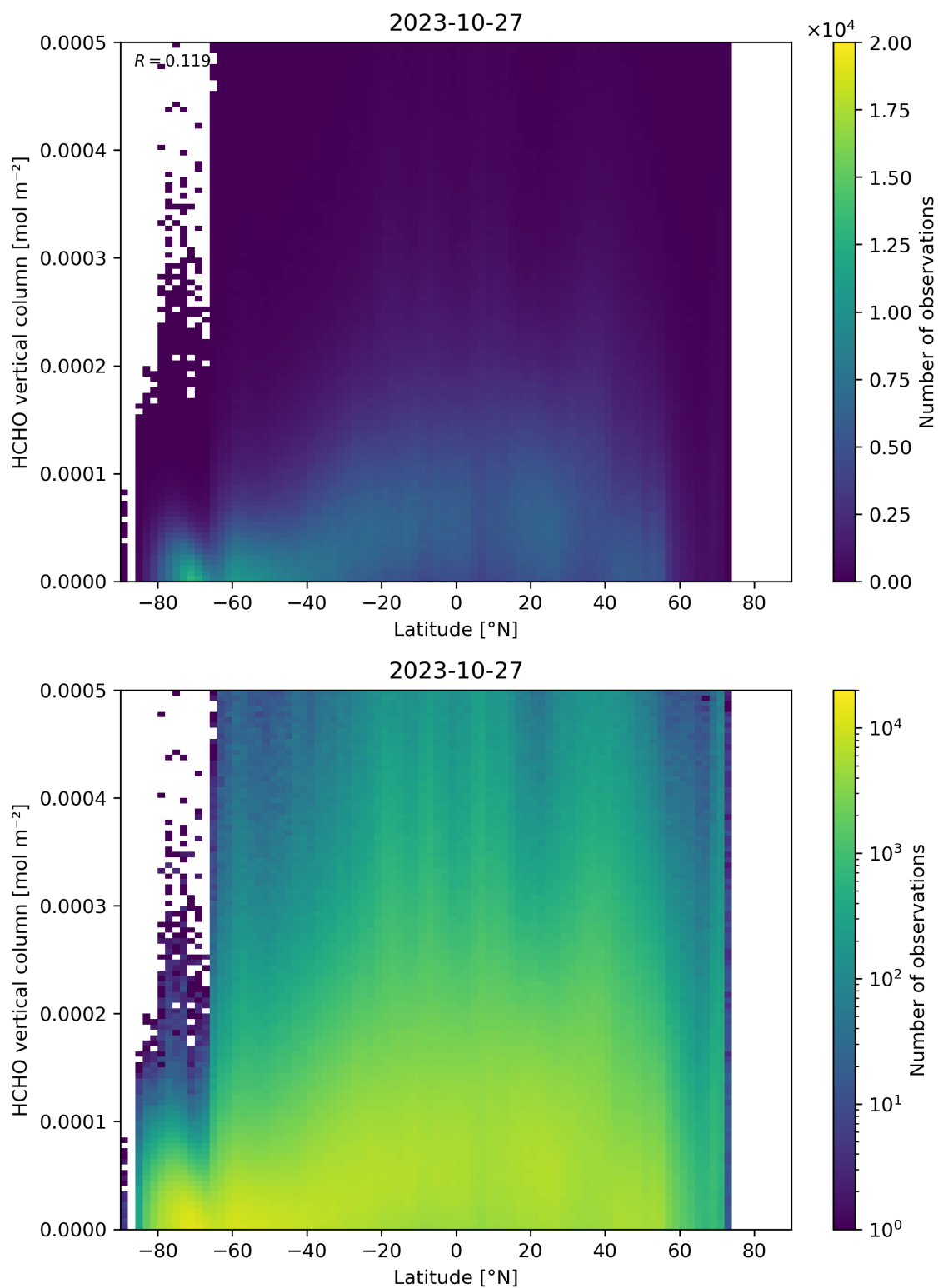
Figure 163: Scatter density plot of “Latitude” against “HCHO vertical column” for 2023-10-27 to 2023-10-28.
