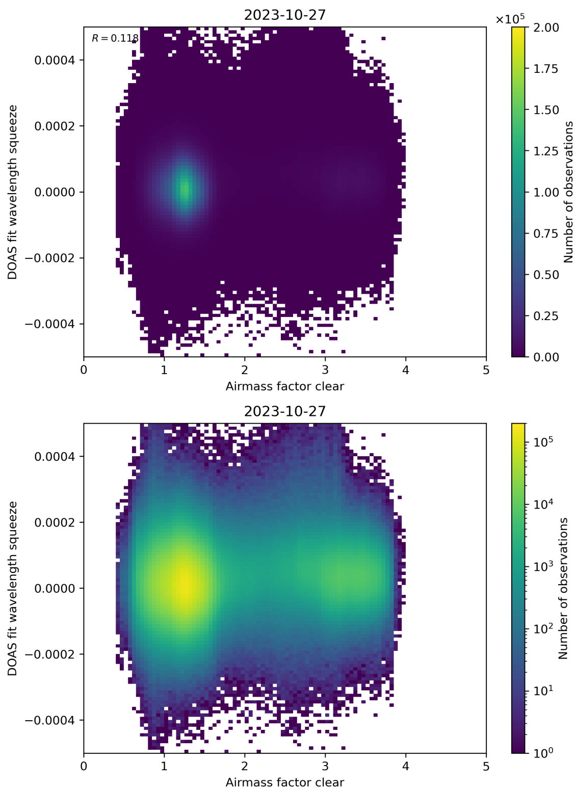
Figure 73: Scatter density plot of “Airmass factor clear” against “DOAS fit wavelength squeeze” for 2023-10-27 to 2023-10-28.
