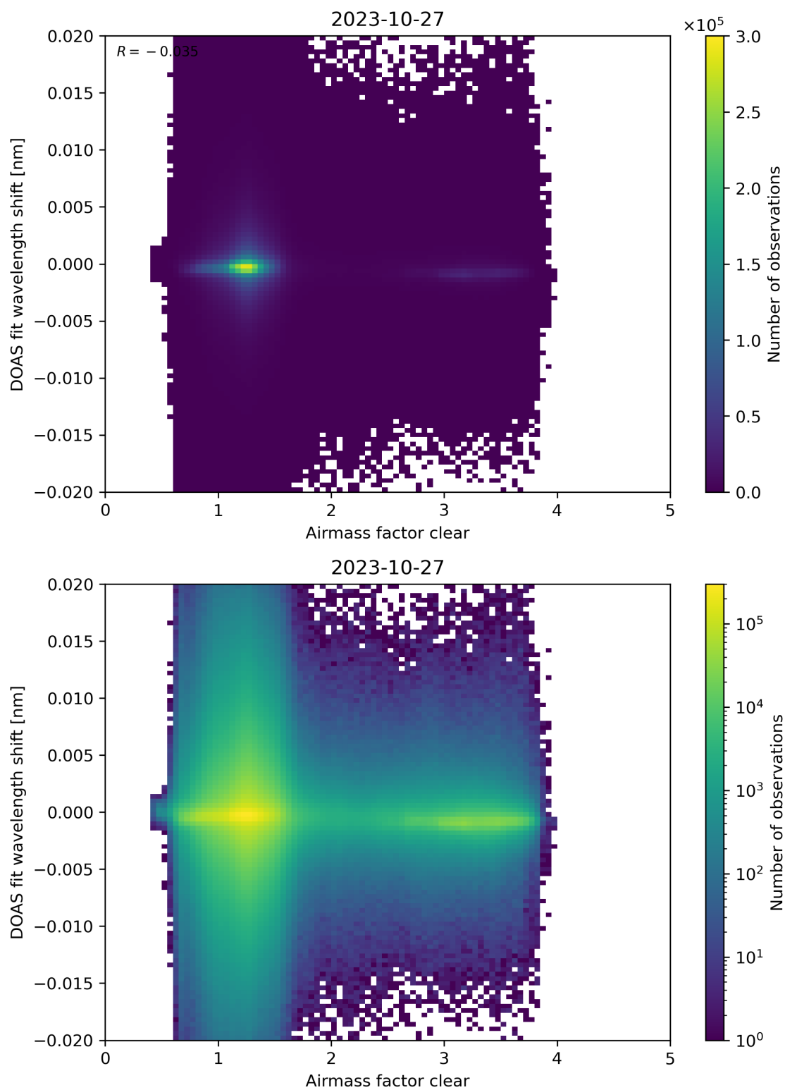
Figure 72: Scatter density plot of “Airmass factor clear” against “DOAS fit wavelength shift” for 2023-10-27 to 2023-10-28.
