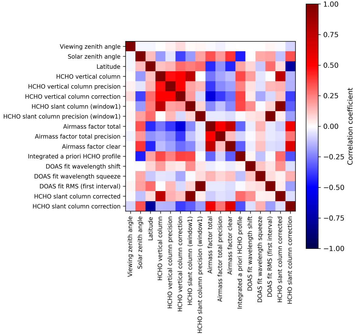
Figure 2: Map of correlation matrix for 2023-10-27 to 2023-10-28.
