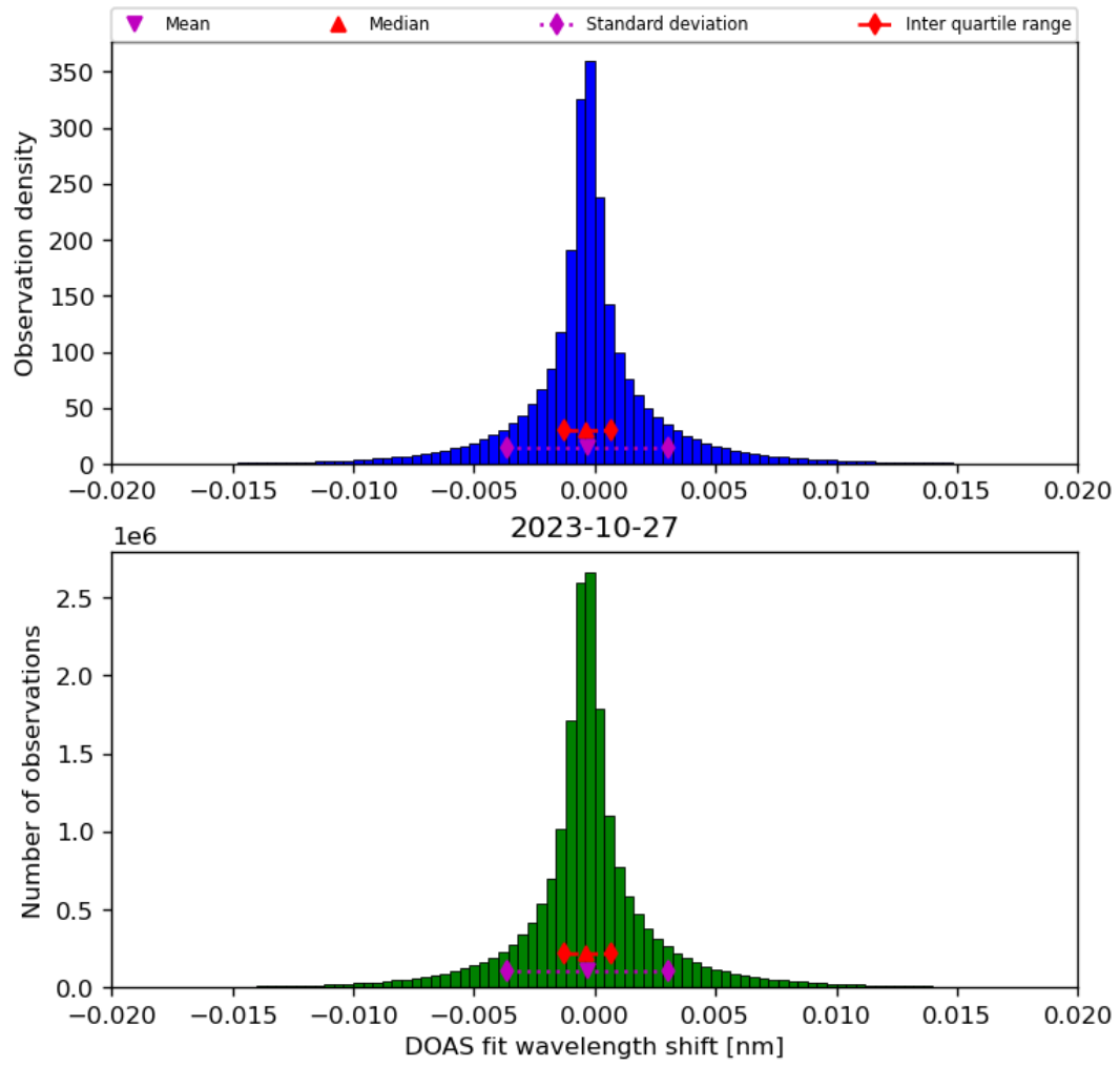
Figure 44: Histogram of “DOAS fit wavelength shift” for 2023-10-27 to 2023-10-28
