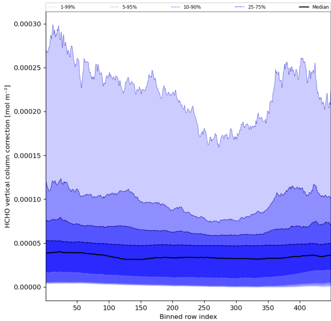
Figure 51: Along track statistics of “HCHO vertical column correction” for 2023-10-27 to 2023-10-28
