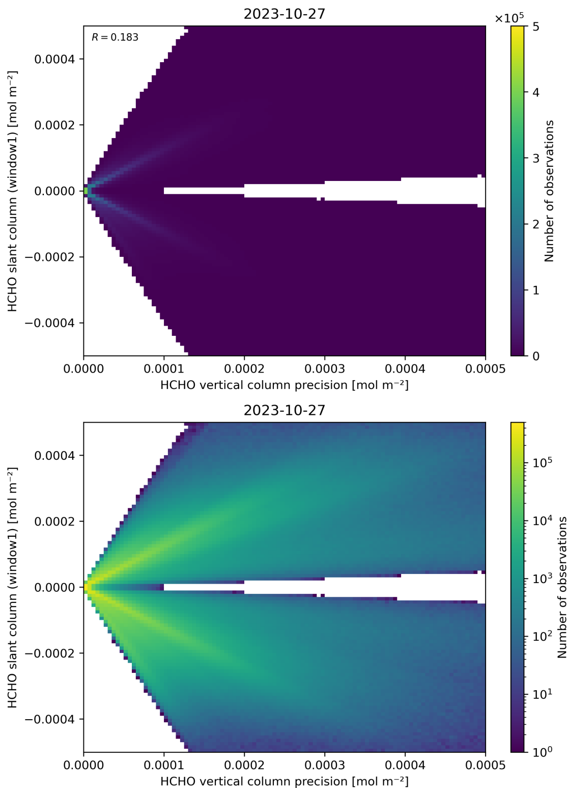
Figure 142: Scatter density plot of “HCHO vertical column precision” against “HCHO slant column (window1)” for 2023-10-27 to 2023-10-28.
