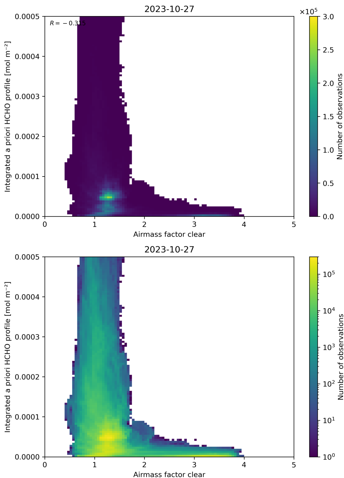
Figure 76: Scatter density plot of “Airmass factor clear” against “Integrated a priori HCHO profile” for 2023-10-27 to 2023-10-28.
