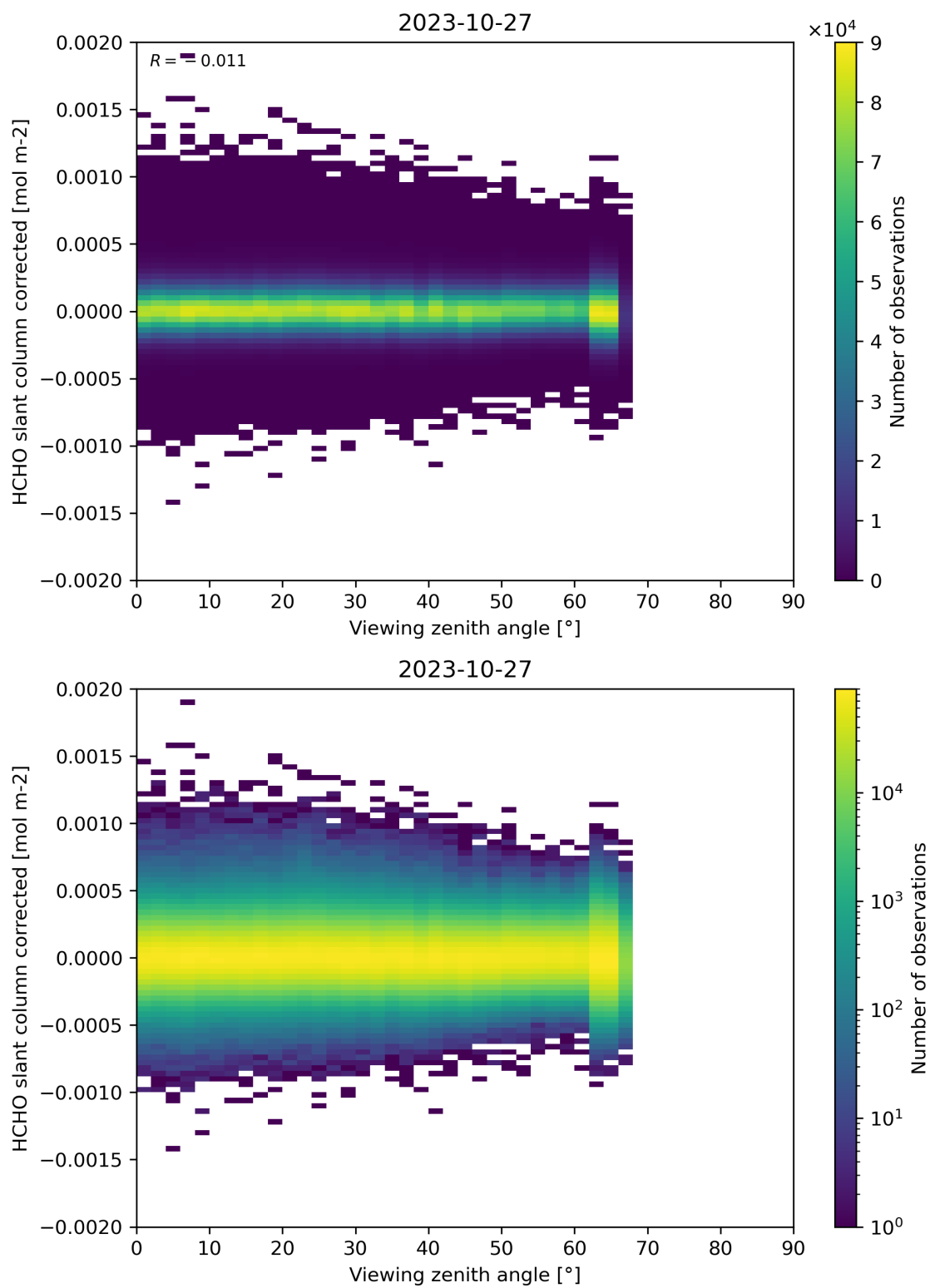
Figure 186: Scatter density plot of “Viewing zenith angle” against “HCHO slant column corrected” for 2023-10-27 to 2023-10-28.
