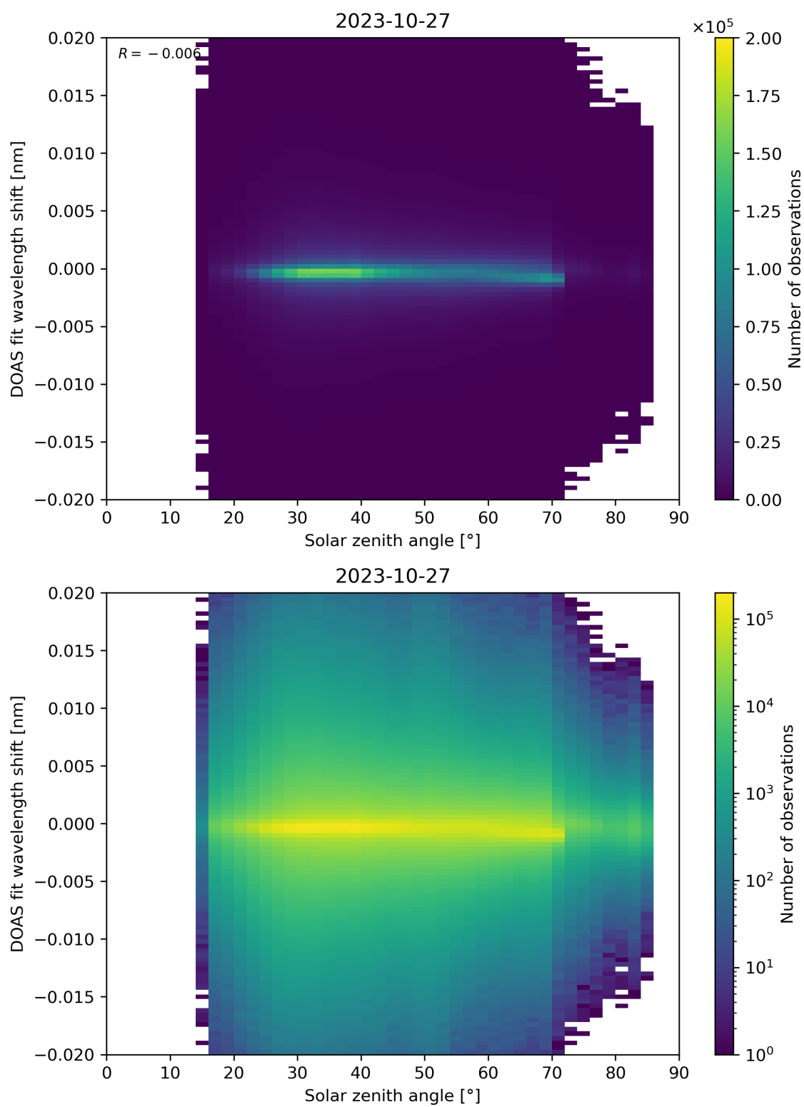
Figure 168: Scatter density plot of “Solar zenith angle” against “DOAS fit wavelength shift” for 2023-10-27 to 2023-10-28.
