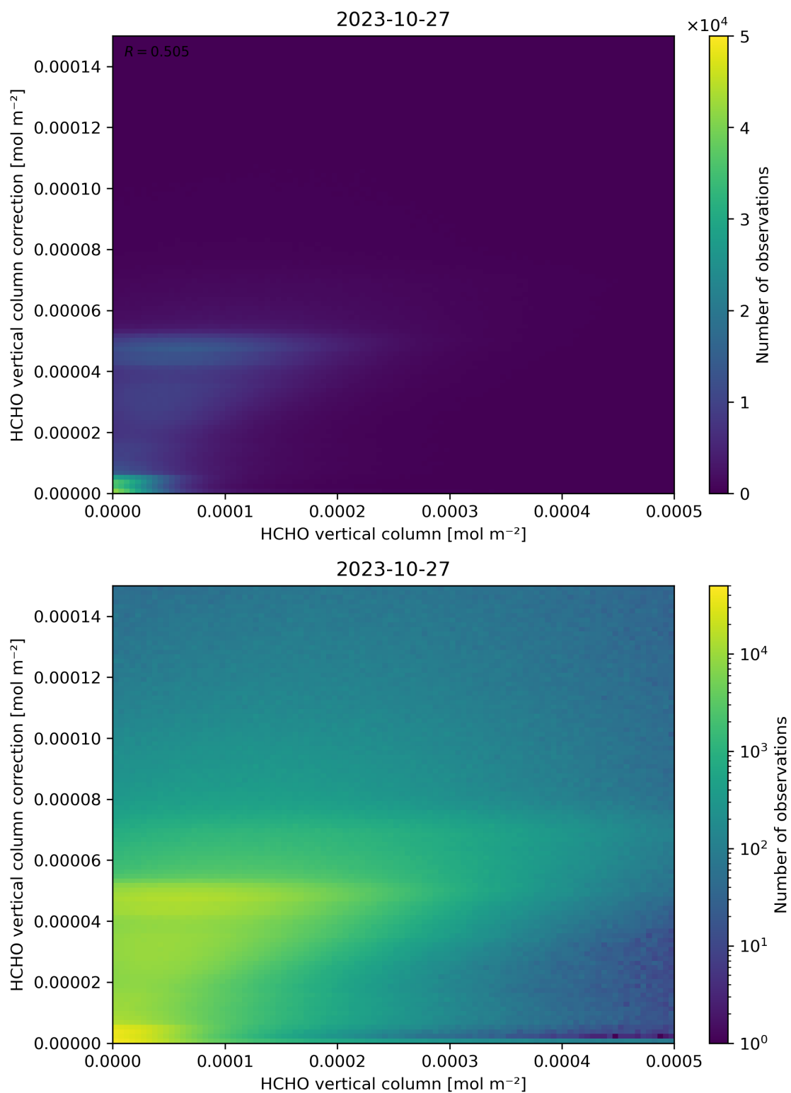
Figure 133: Scatter density plot of “HCHO vertical column” against “HCHO vertical column correction” for 2023-10-27 to 2023-10-28.
