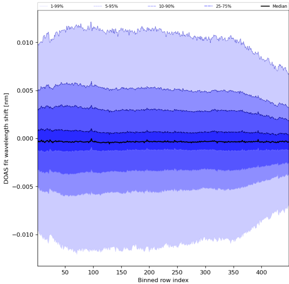
Figure 58: Along track statistics of “DOAS fit wavelength shift” for 2023-10-27 to 2023-10-28
