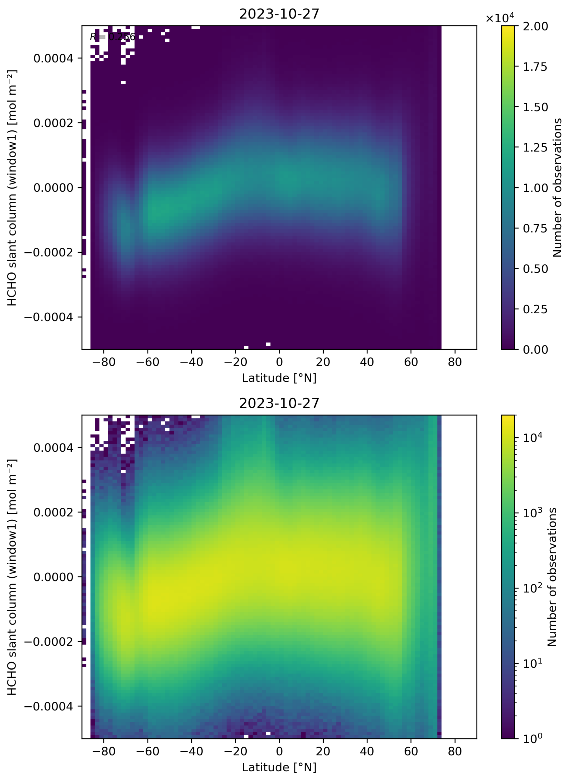
Figure 159: Scatter density plot of “Latitude” against “HCHO slant column (window1)” for 2023-10-27 to 2023-10-28.
