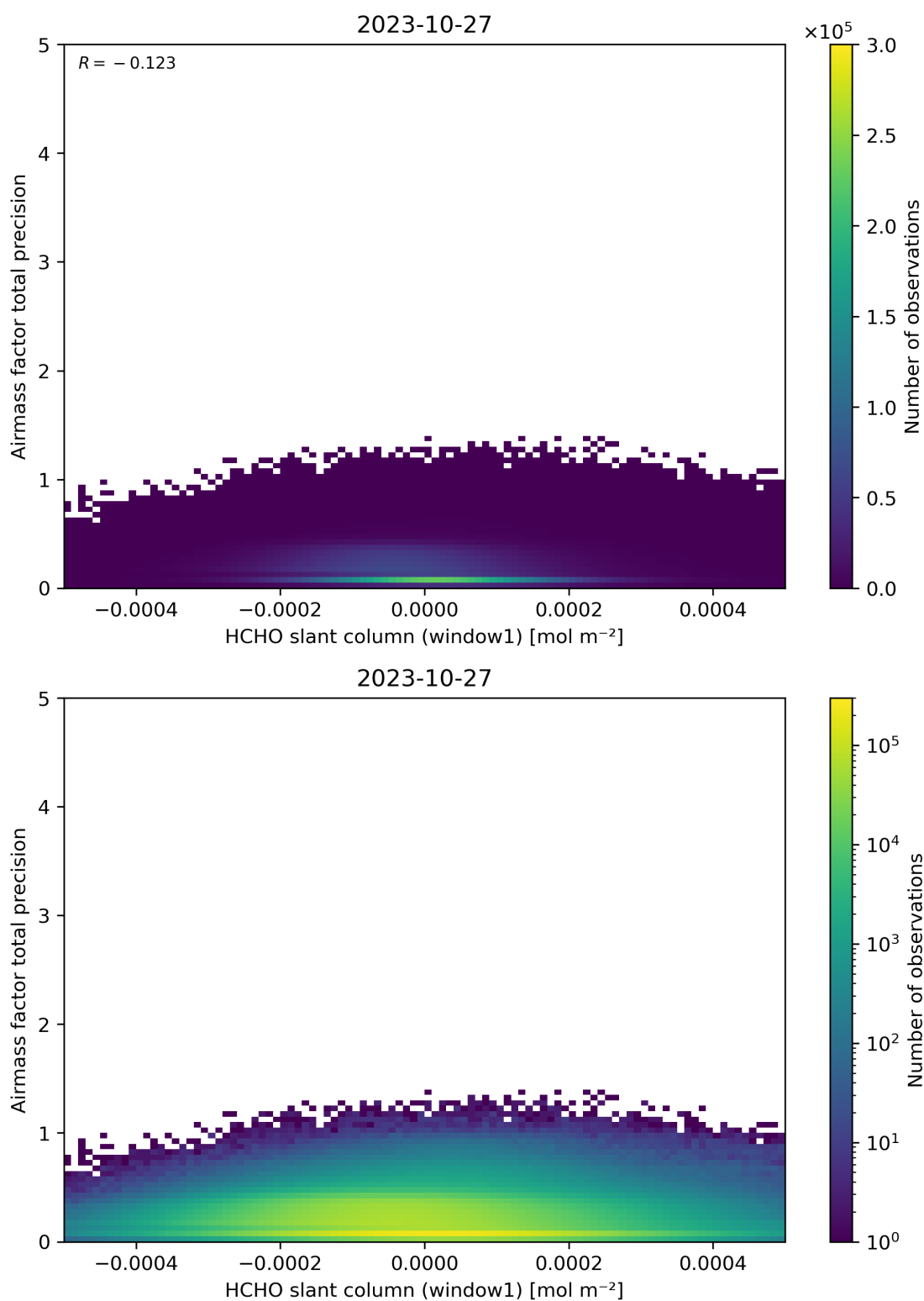
Figure 86: Scatter density plot of “HCHO slant column (window1)” against “Airmass factor total precision” for 2023-10-27 to 2023-10-28.
