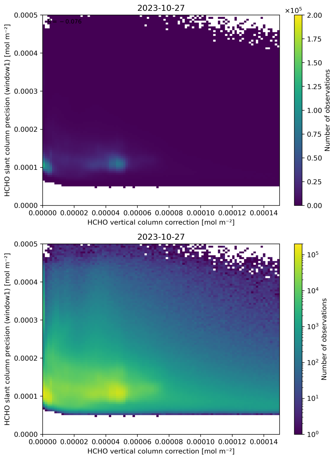
Figure 119: Scatter density plot of “HCHO vertical column correction” against “HCHO slant column precision (window1)” for 2023-10-27 to 2023-10-28.
