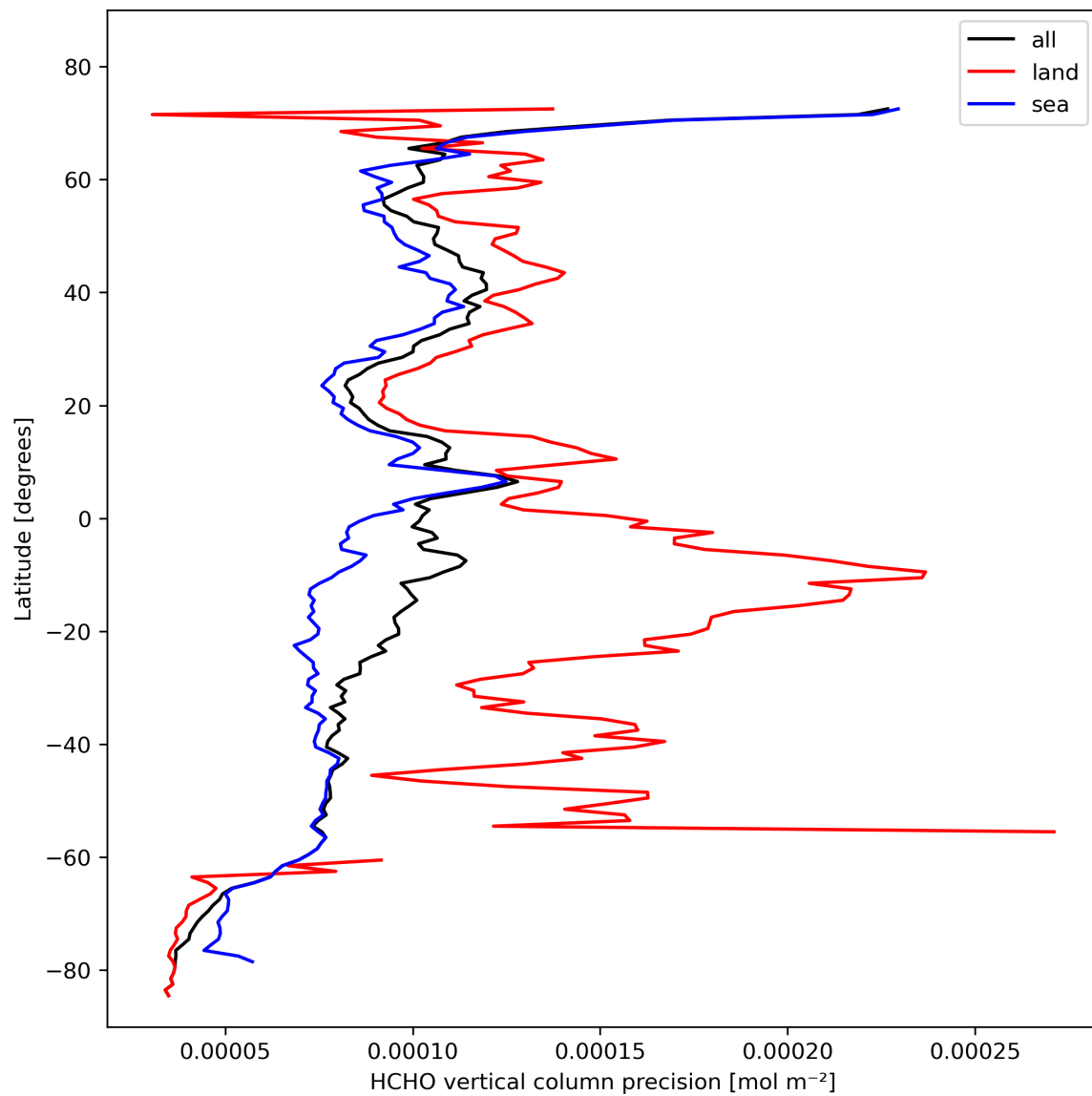
Figure 22: Zonal average of “HCHO vertical column precision” for 2023-10-27 to 2023-10-28.
