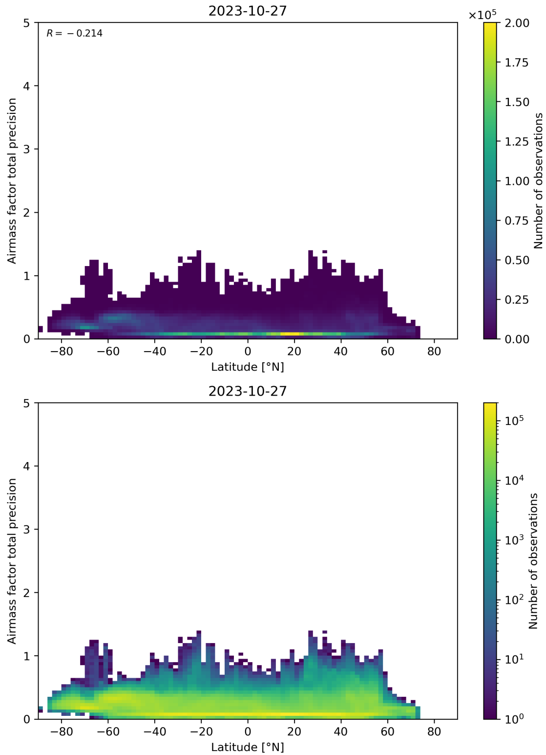
Figure 162: Scatter density plot of “Latitude” against “Airmass factor total precision” for 2023-10-27 to 2023-10-28.
