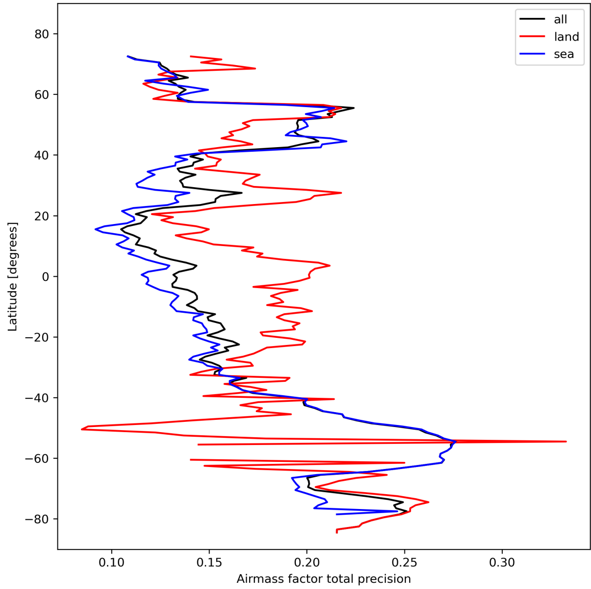
Figure 27: Zonal average of “Airmass factor total precision” for 2023-10-27 to 2023-10-28.
