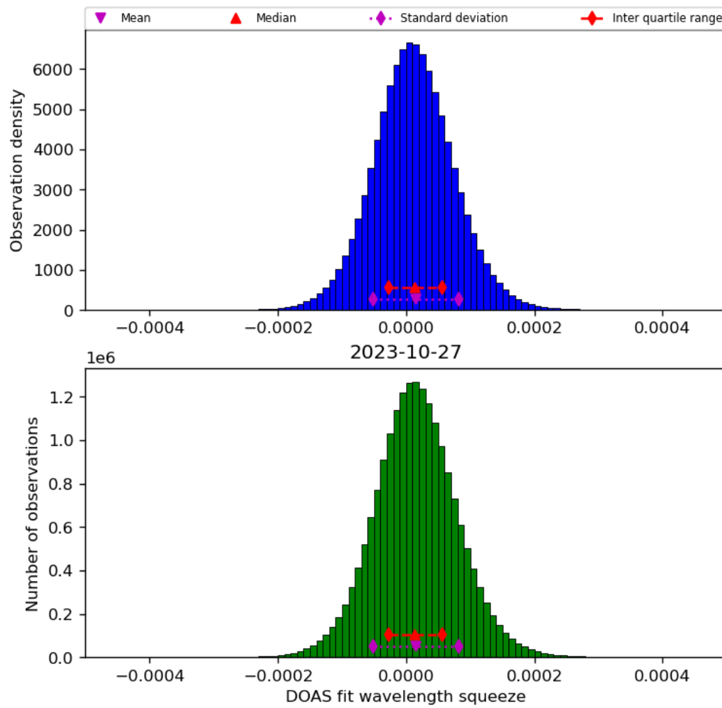
Figure 45: Histogram of “DOAS fit wavelength squeeze” for 2023-10-27 to 2023-10-28
