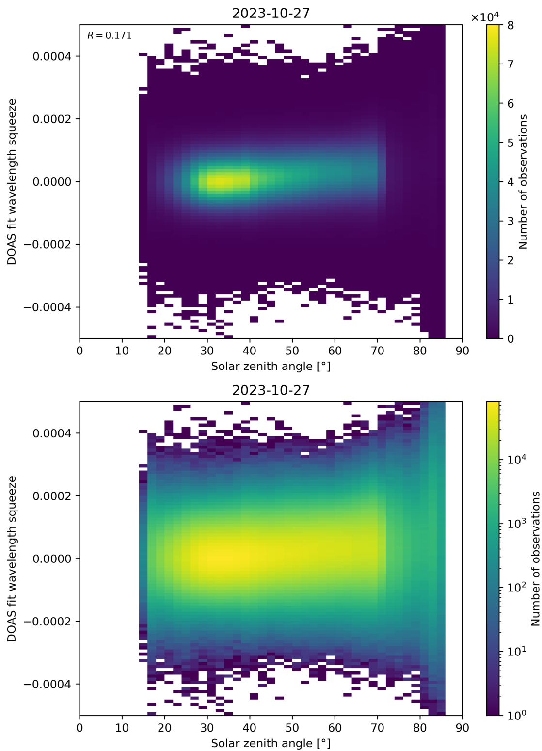
Figure 169: Scatter density plot of “Solar zenith angle” against “DOAS fit wavelength squeeze” for 2023-10-27 to 2023-10-28.
