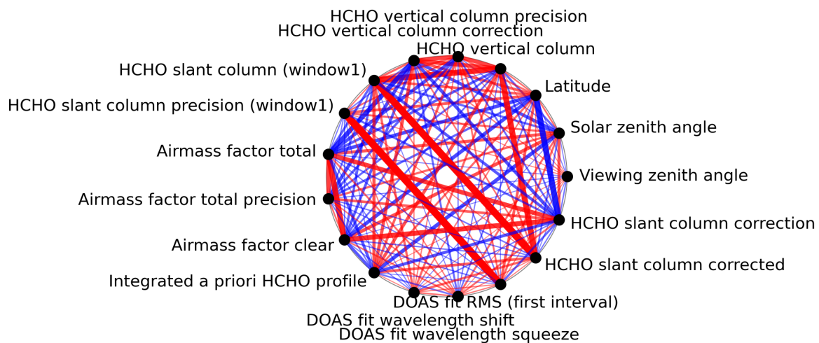
Figure 1: Map of correlation graph for 2023-10-27 to 2023-10-28.
