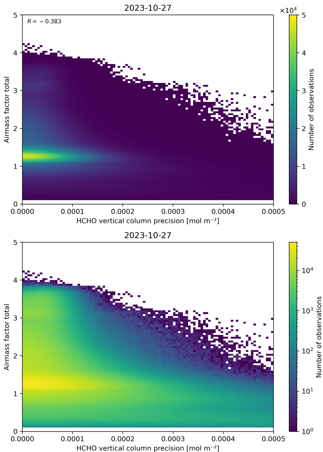
Figure 144: Scatter density plot of “HCHO vertical column precision” against “Airmass factor total” for 2023-10-27 to 2023-10-28.
