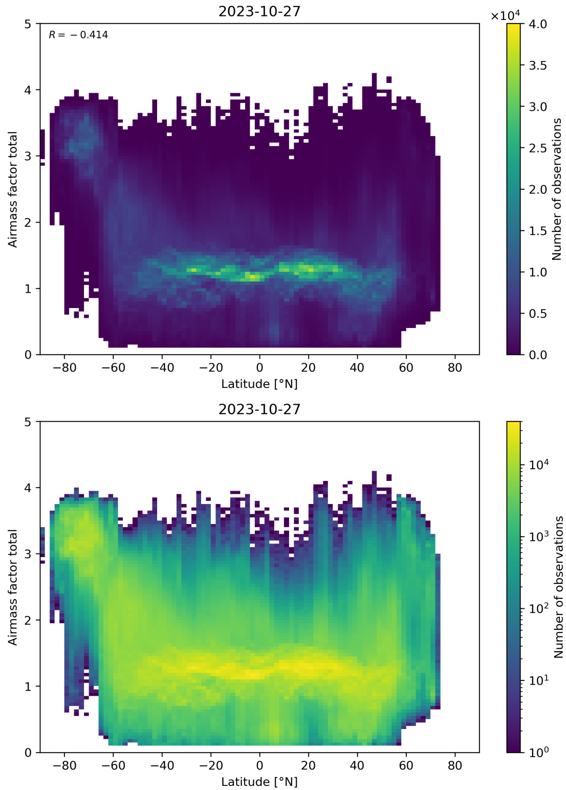
Figure 161: Scatter density plot of “Latitude” against “Airmass factor total” for 2023-10-27 to 2023-10-28.
