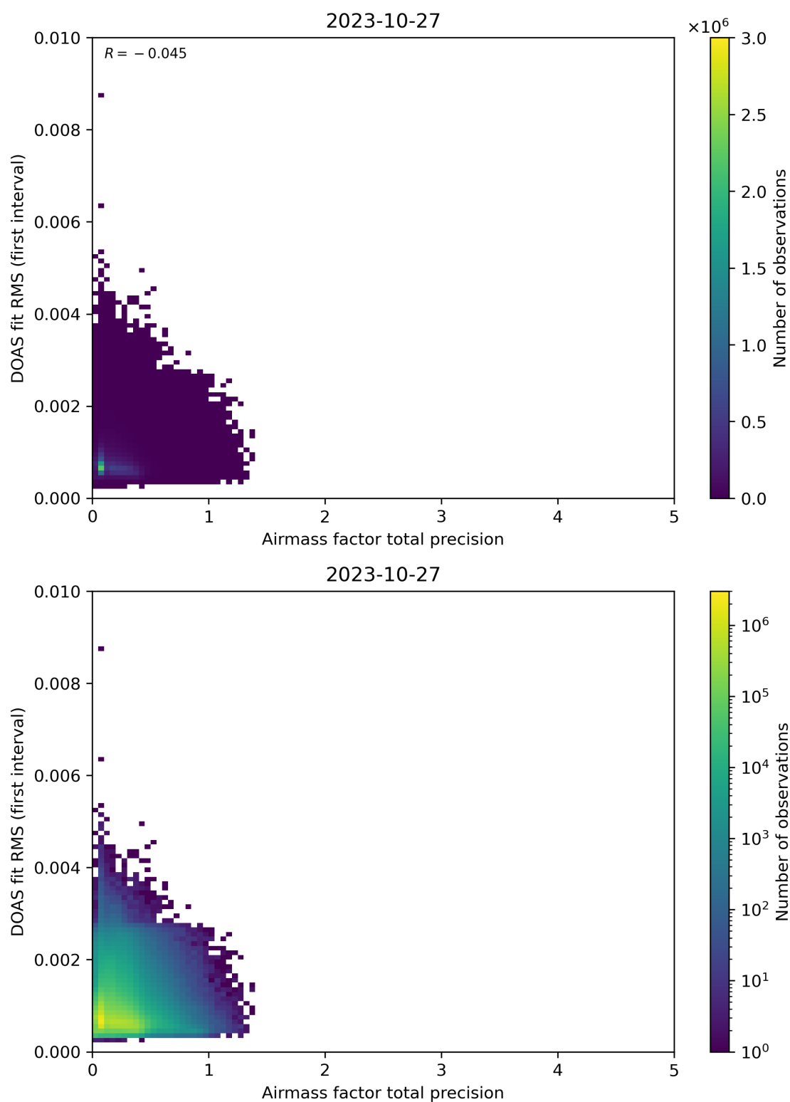
Figure 105: Scatter density plot of “Airmass factor total precision” against “DOAS fit RMS (first interval)” for 2023-10-27 to 2023-10-28.
