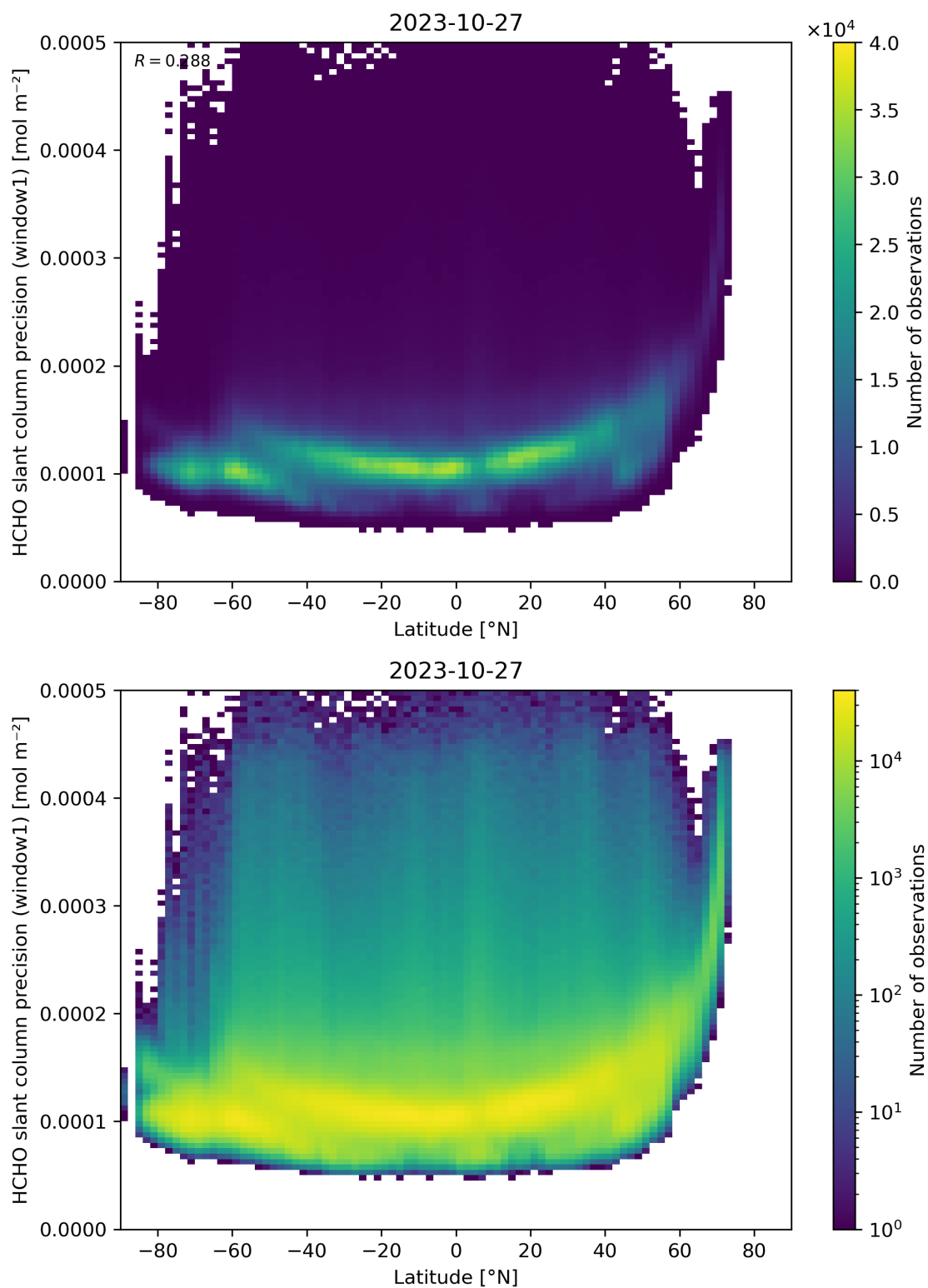
Figure 160: Scatter density plot of “Latitude” against “HCHO slant column precision (window1)” for 2023-10-27 to 2023-10-28.
