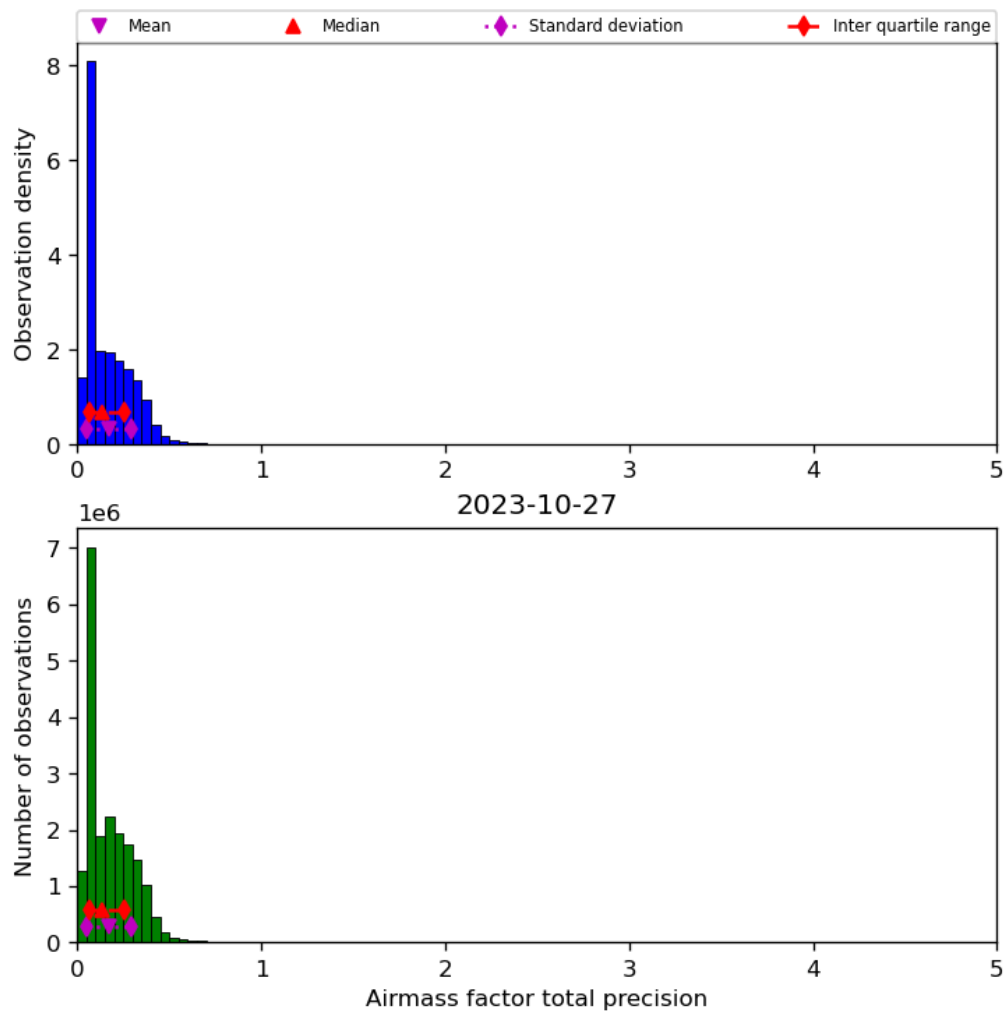
Figure 41: Histogram of “Airmass factor total precision” for 2023-10-27 to 2023-10-28
