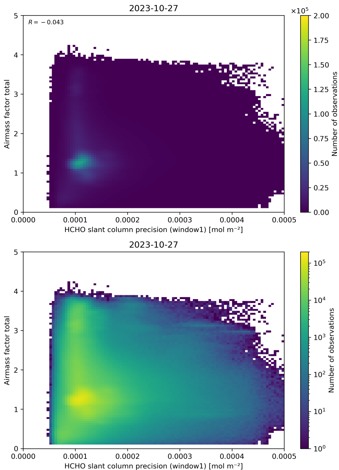
Figure 94: Scatter density plot of “HCHO slant column precision (window1)” against “Airmass factor total” for 2023-10-27 to 2023-10-28.
