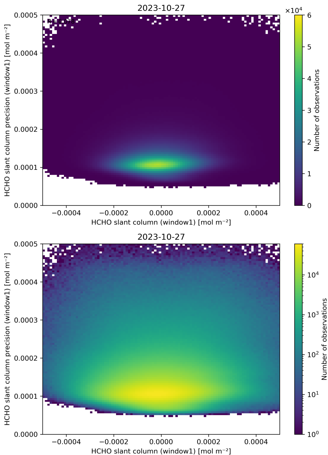
Figure 84: Scatter density plot of “HCHO slant column (window1)” against “HCHO slant column precision (window1)” for 2023-10-27 to 2023-10-28.
