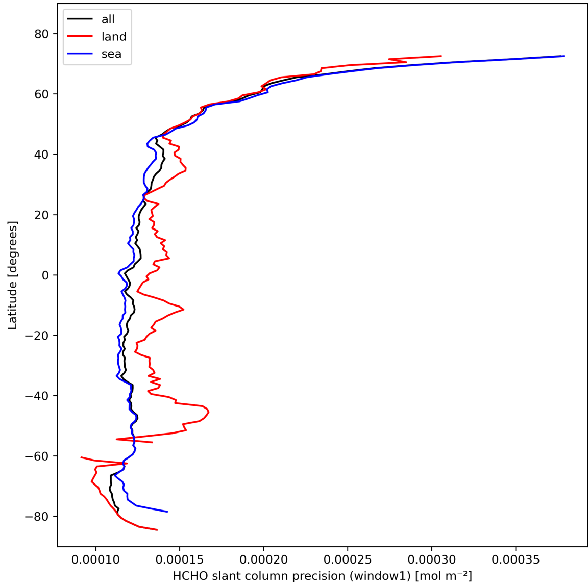
Figure 25: Zonal average of “HCHO slant column precision (window1)” for 2023-10-27 to 2023-10-28.
