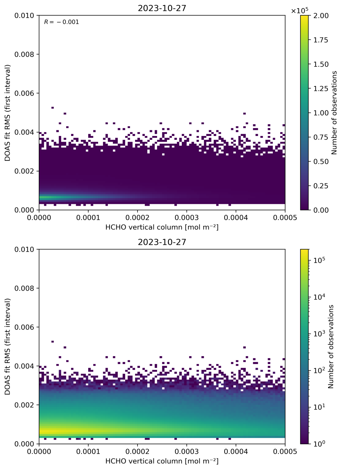
Figure 123: Scatter density plot of “HCHO vertical column” against “DOAS fit RMS (first interval)” for 2023-10-27 to 2023-10-28.
