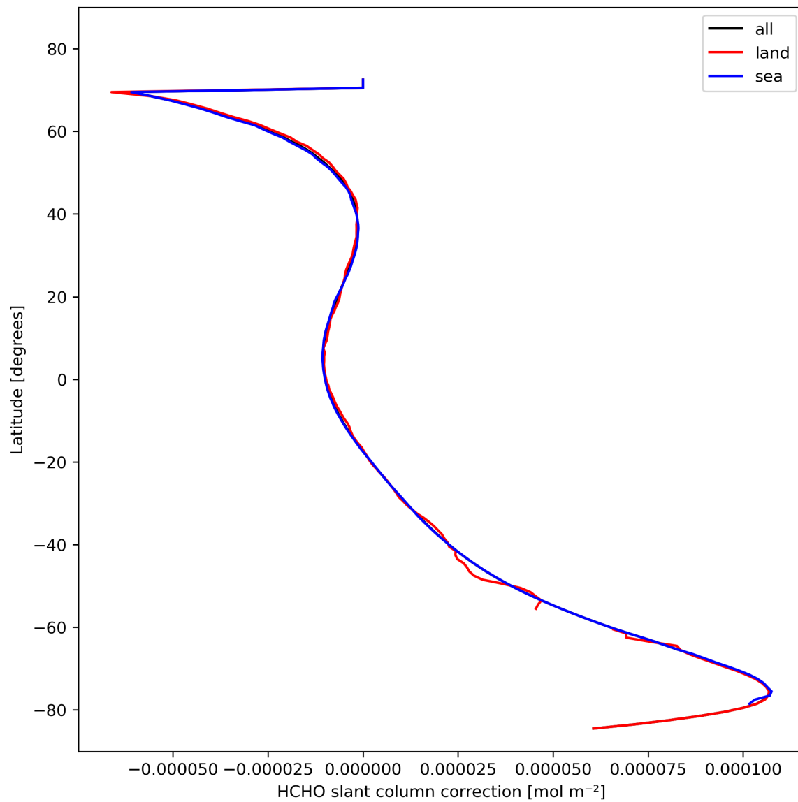
Figure 33: Zonal average of “HCHO slant column correction” for 2023-10-27 to 2023-10-28.
