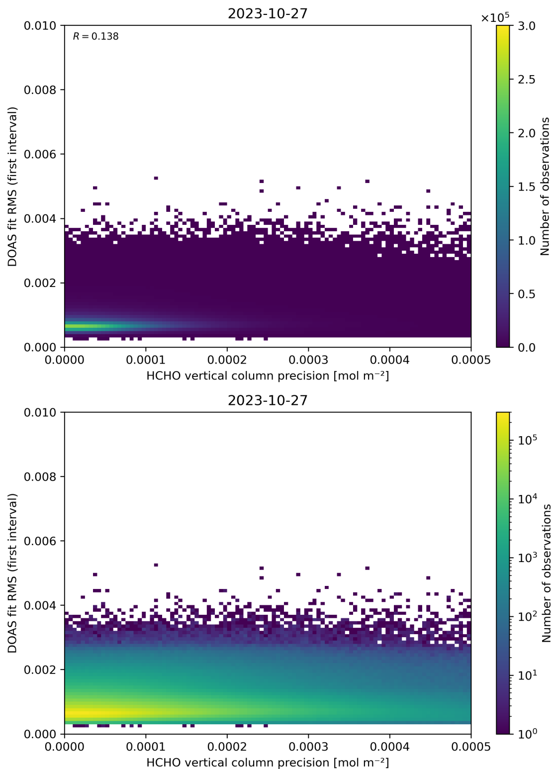
Figure 136: Scatter density plot of “HCHO vertical column precision” against “DOAS fit RMS (first interval)” for 2023-10-27 to 2023-10-28.
