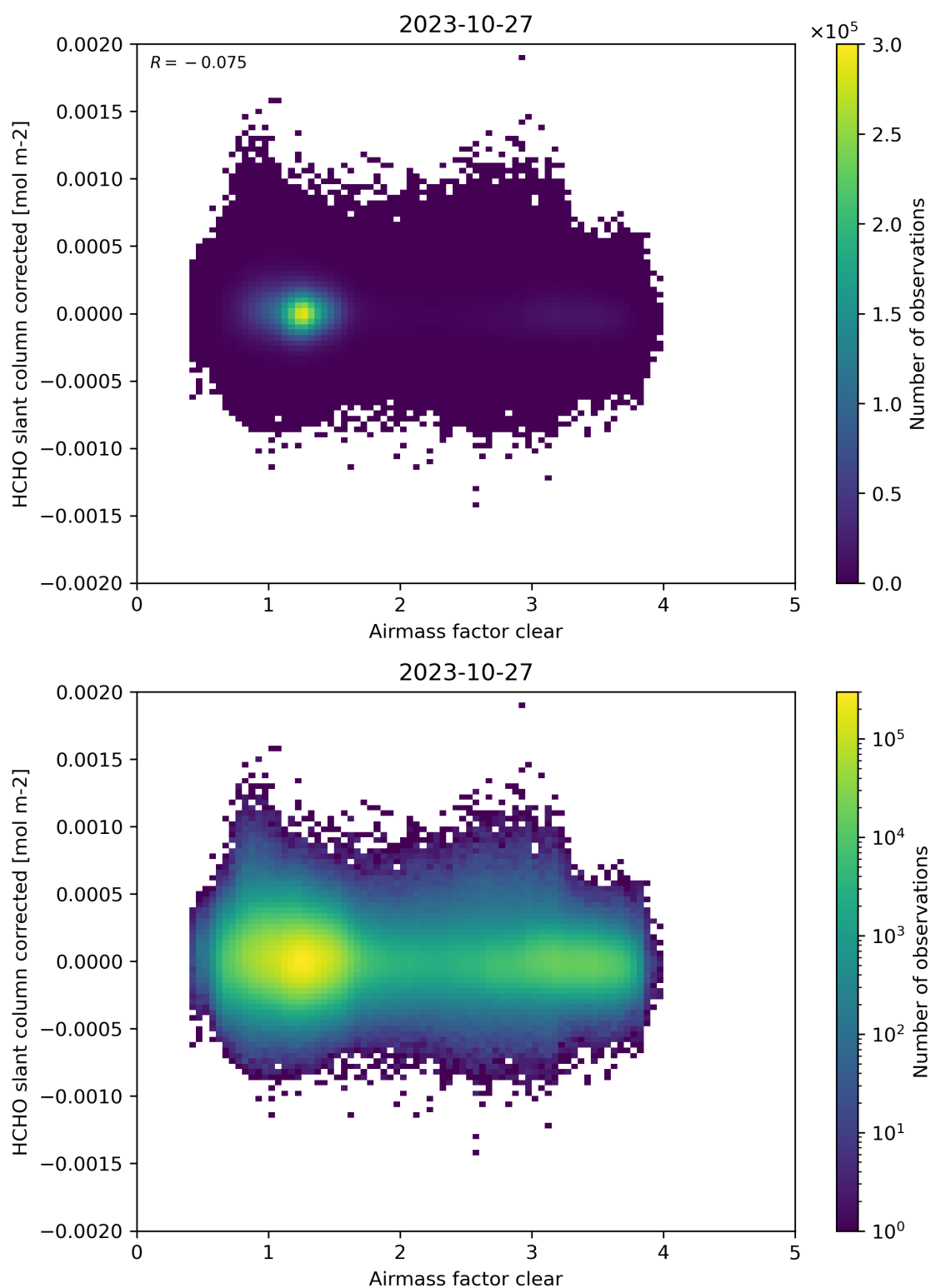
Figure 74: Scatter density plot of “Airmass factor clear” against “HCHO slant column corrected” for 2023-10-27 to 2023-10-28.
