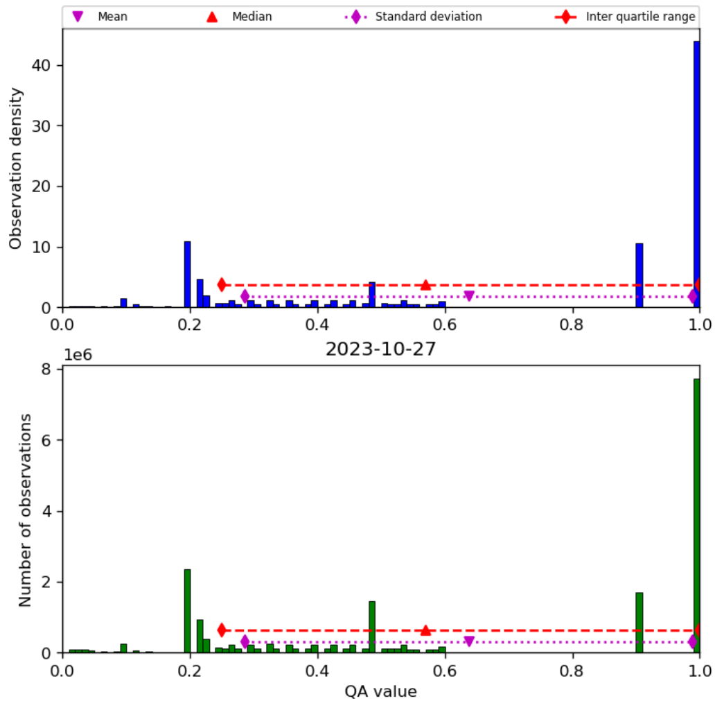
Figure 34: Histogram of “QA value” for 2023-10-27 to 2023-10-28
