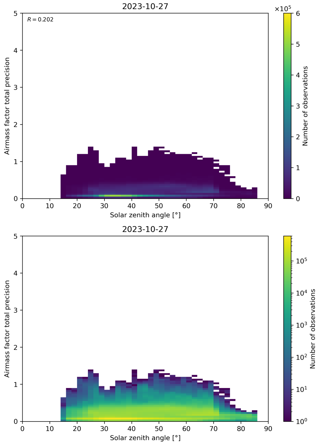
Figure 176: Scatter density plot of “Solar zenith angle” against “Airmass factor total precision” for 2023-10-27 to 2023-10-28.
