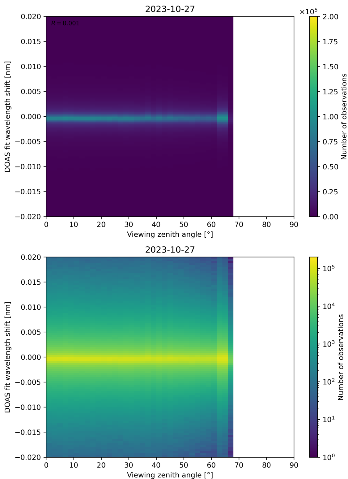
Figure 183: Scatter density plot of “Viewing zenith angle” against “DOAS fit wavelength shift” for 2023-10-27 to 2023-10-28.
