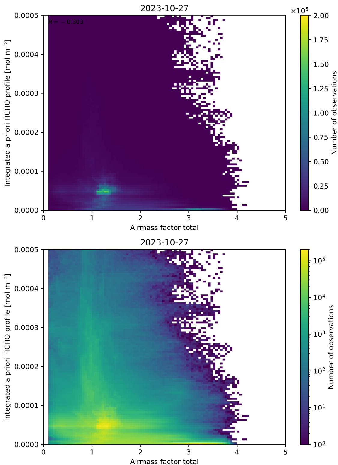
Figure 104: Scatter density plot of “Airmass factor total” against “Integrated a priori HCHO profile” for 2023-10-27 to 2023-10-28.
