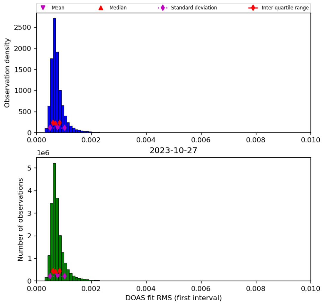
Figure 46: Histogram of “DOAS fit RMS (first interval)” for 2023-10-27 to 2023-10-28
