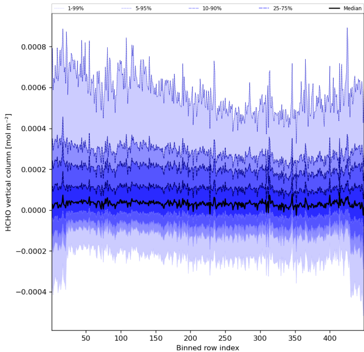
Figure 49: Along track statistics of “HCHO vertical column” for 2023-10-27 to 2023-10-28
