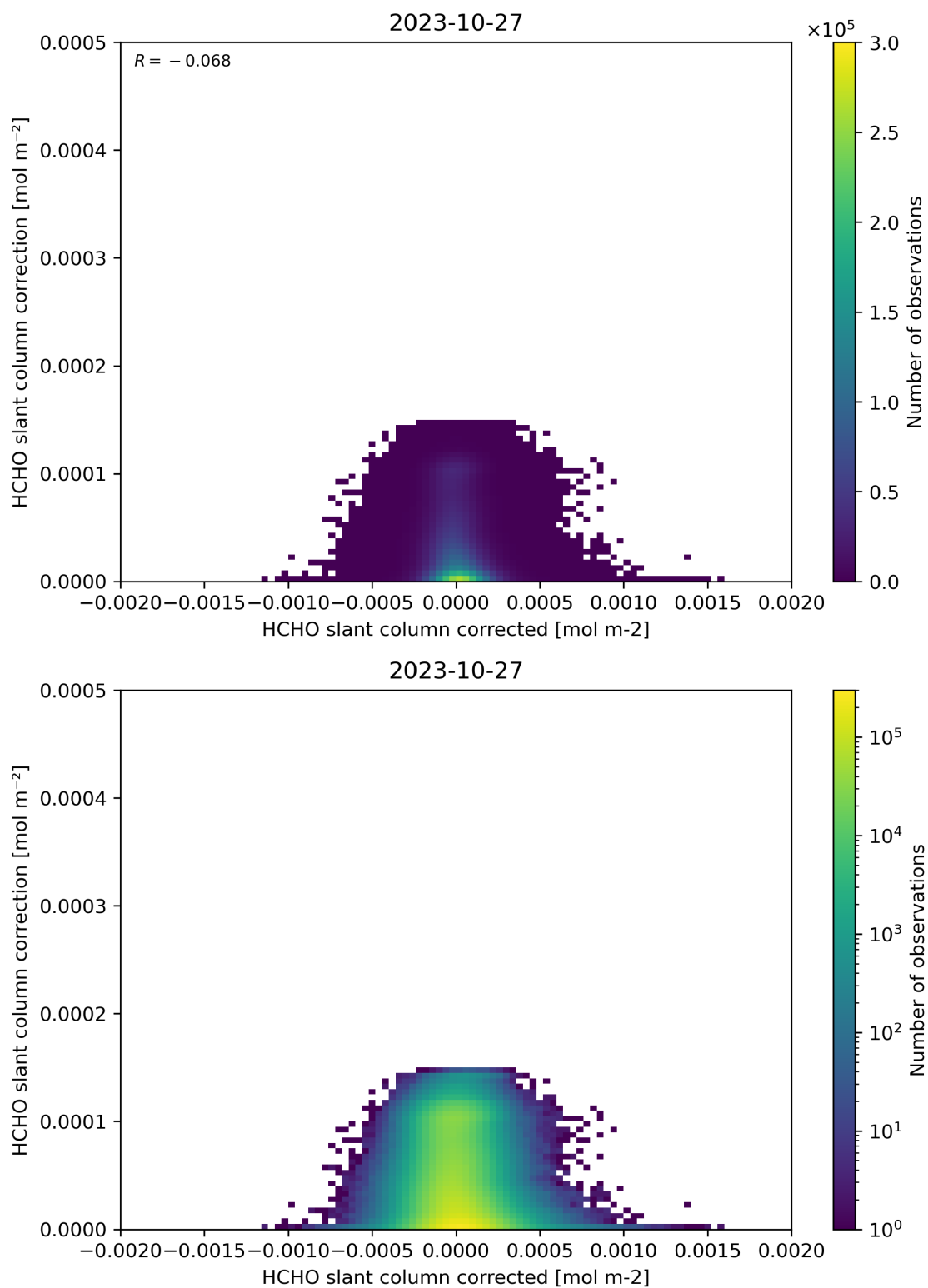
Figure 77: Scatter density plot of “HCHO slant column corrected” against “HCHO slant column correction” for 2023-10-27 to 2023-10-28.
