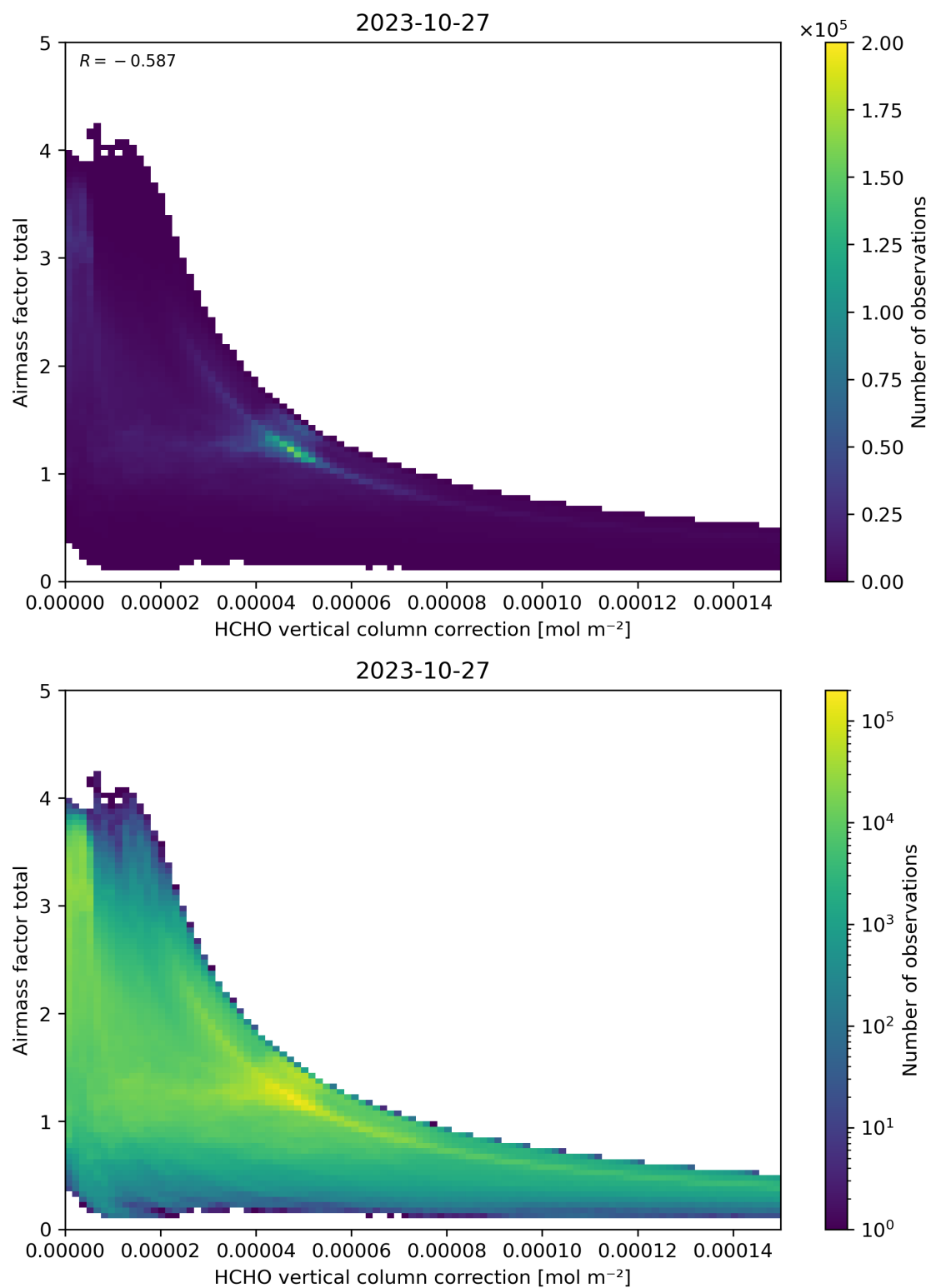
Figure 120: Scatter density plot of “HCHO vertical column correction” against “Airmass factor total” for 2023-10-27 to 2023-10-28.
