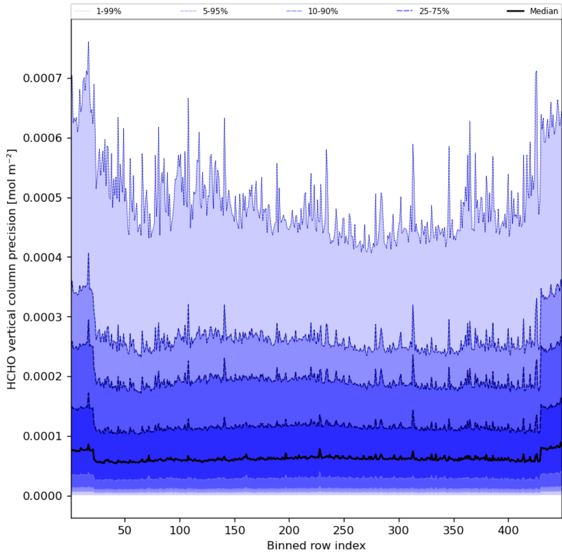
Figure 50: Along track statistics of “HCHO vertical column precision” for 2023-10-27 to 2023-10-28
