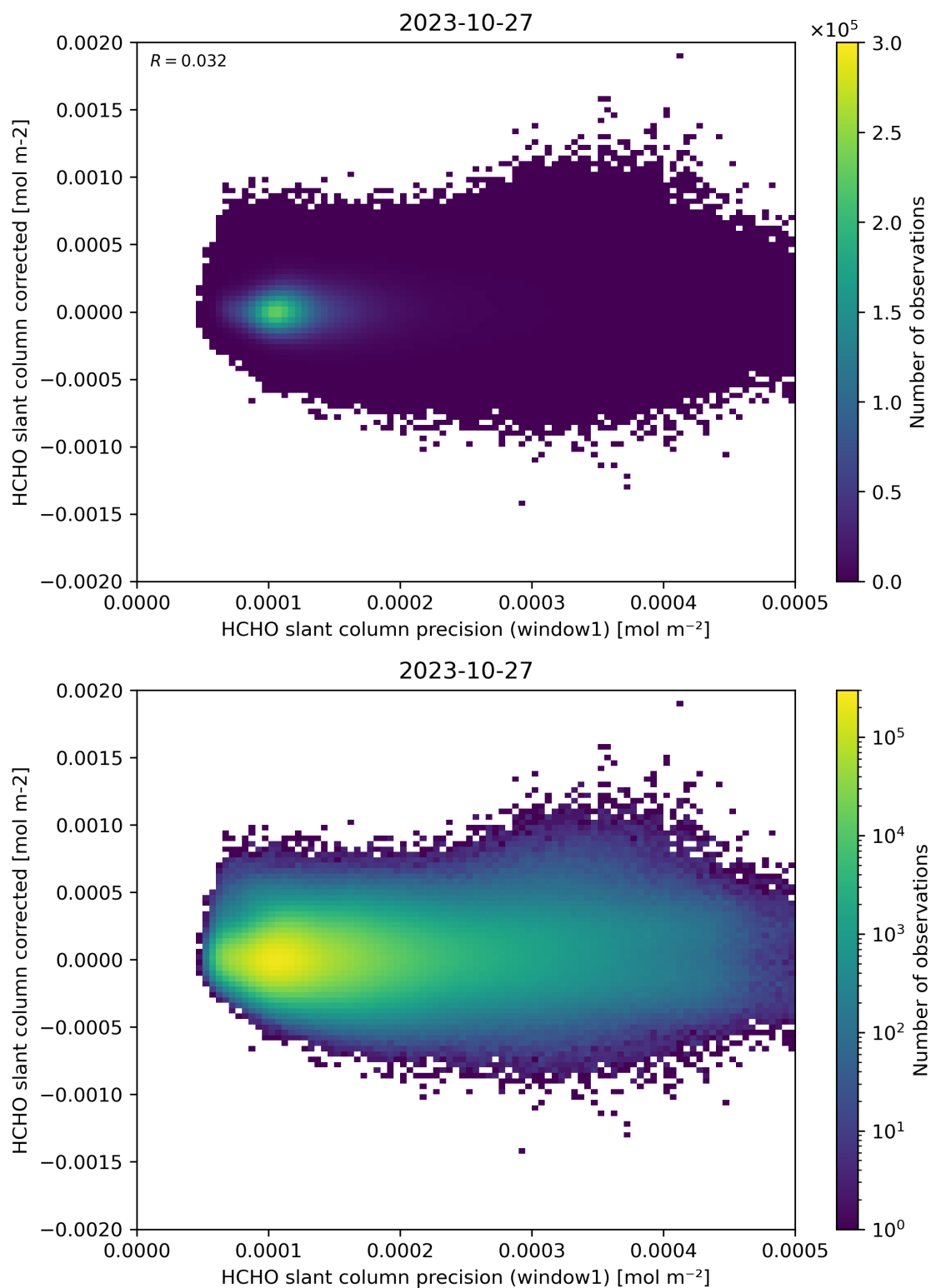
Figure 92: Scatter density plot of “HCHO slant column precision (window1)” against “HCHO slant column corrected” for 2023-10-27 to 2023-10-28.
