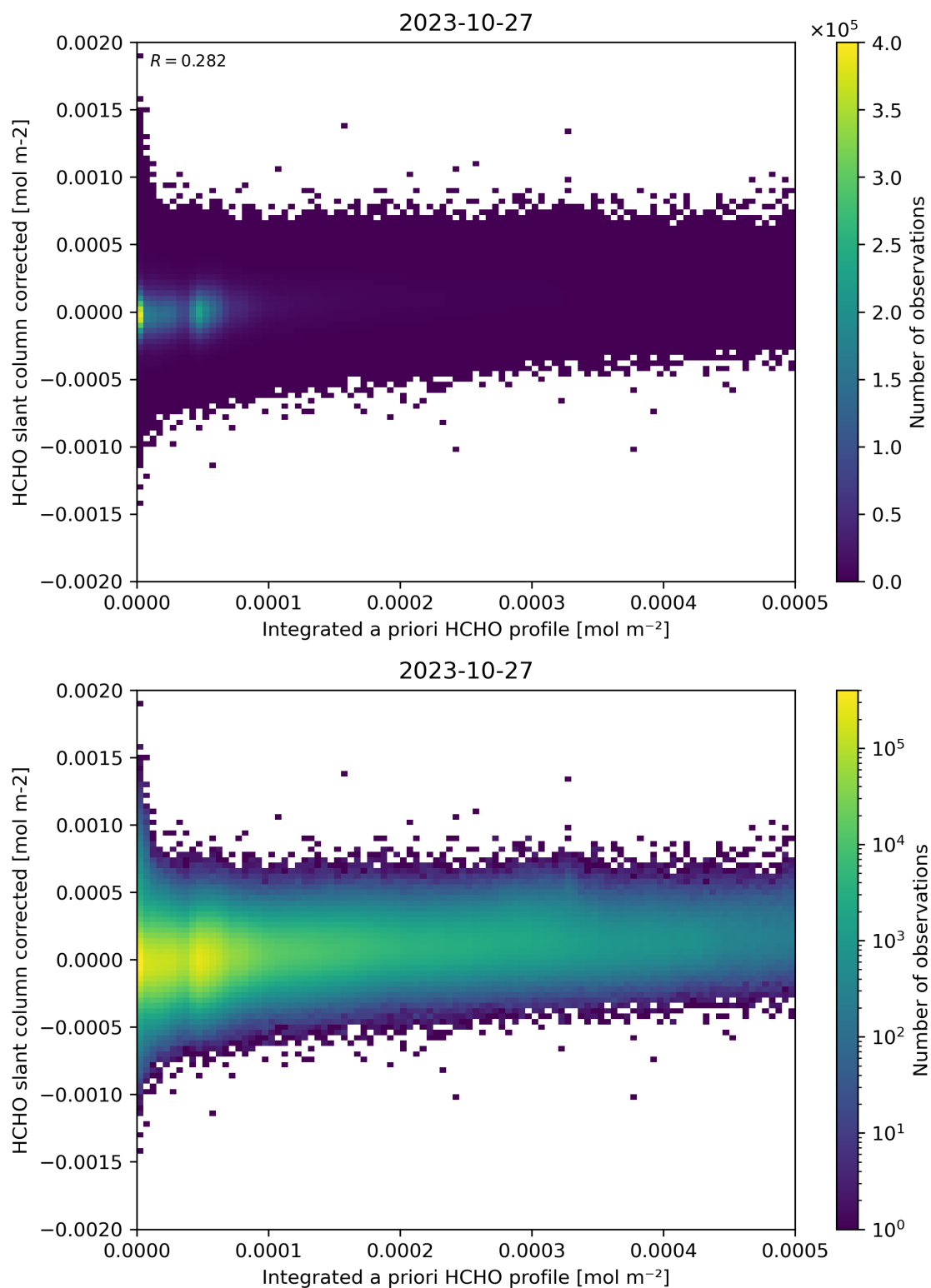
Figure 151: Scatter density plot of “Integrated a priori HCHO profile” against “HCHO slant column corrected” for 2023-10-27 to 2023-10-28.
