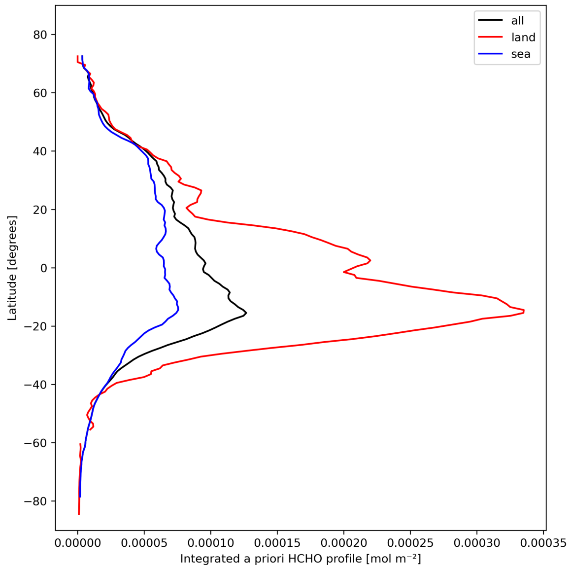
Figure 29: Zonal average of “Integrated a priori HCHO profile” for 2023-10-27 to 2023-10-28.
