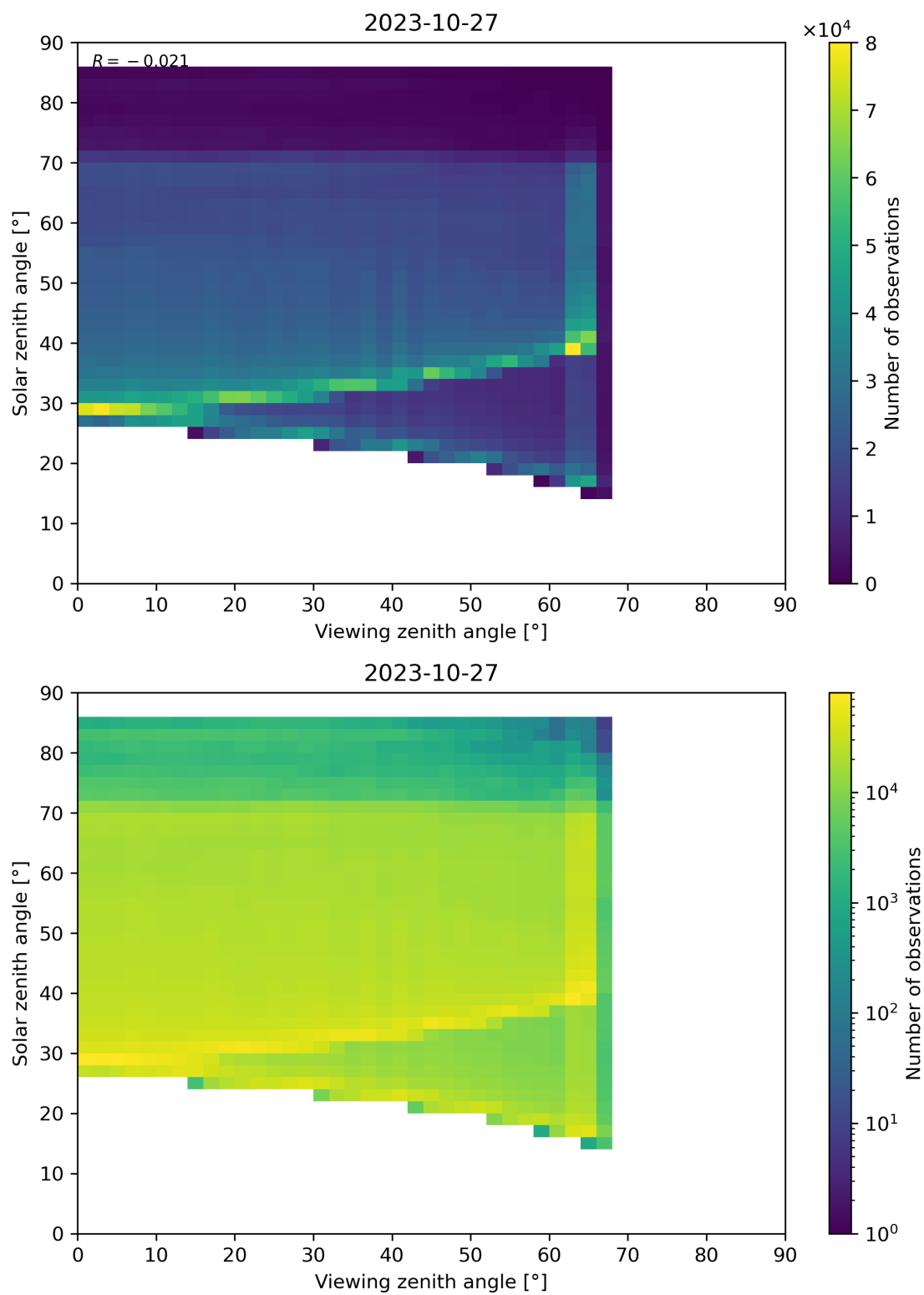
Figure 197: Scatter density plot of “Viewing zenith angle” against “Solar zenith angle” for 2023-10-27 to 2023-10-28.
