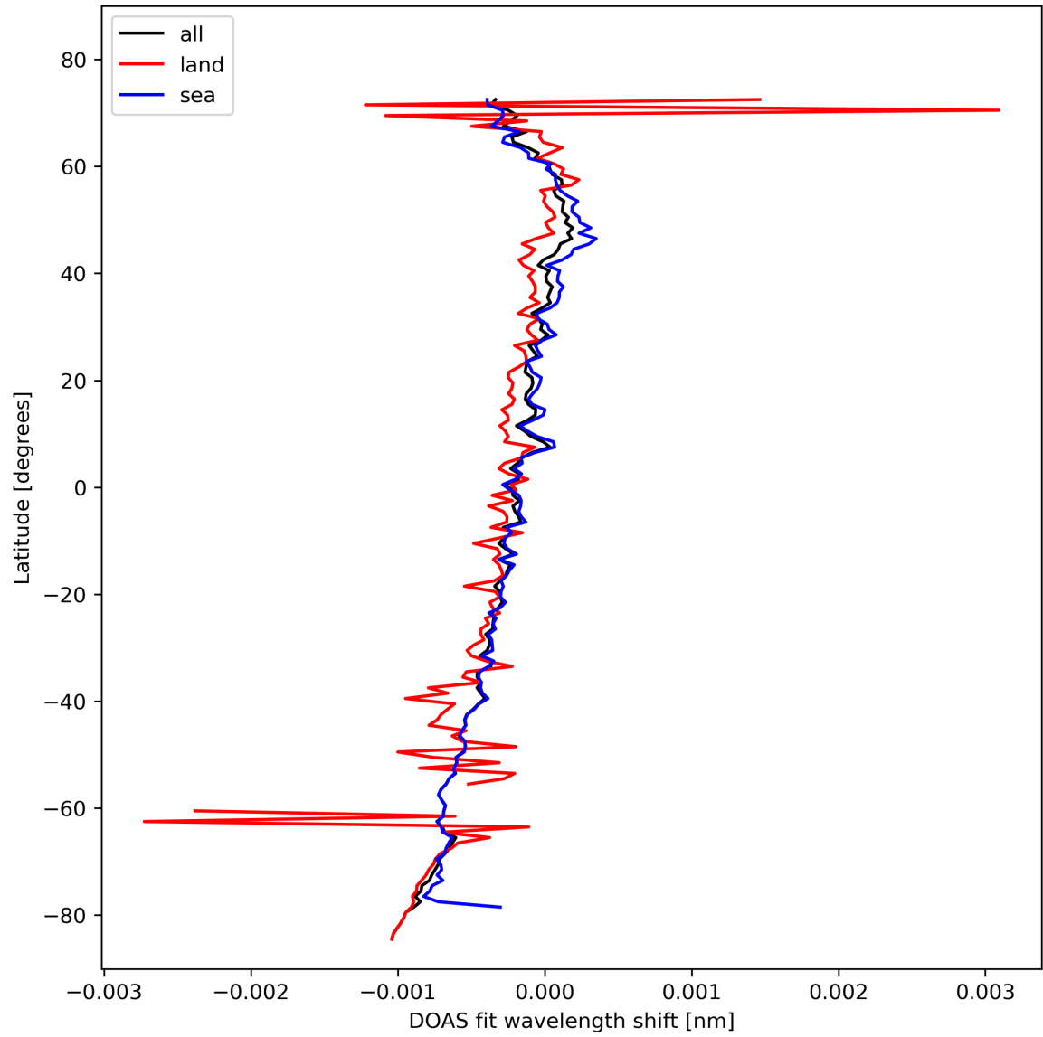
Figure 30: Zonal average of "DOAS fit wavelength shift" for 2023-10-27 to 2023-10-28.
