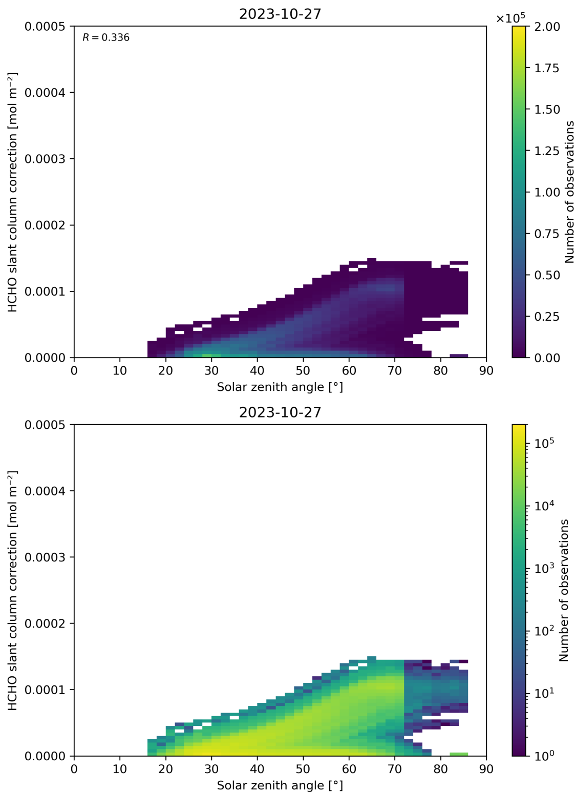
Figure 172: Scatter density plot of “Solar zenith angle” against “HCHO slant column correction” for 2023-10-27 to 2023-10-28.
