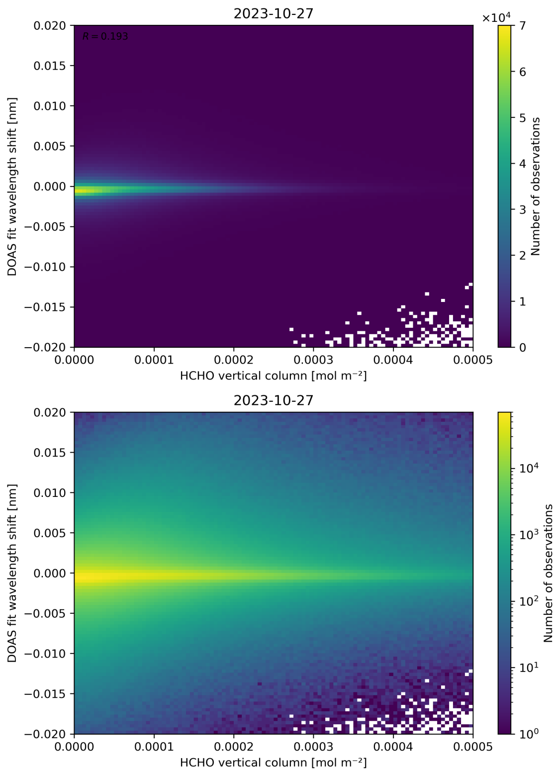
Figure 124: Scatter density plot of “HCHO vertical column” against “DOAS fit wavelength shift” for 2023-10-27 to 2023-10-28.
