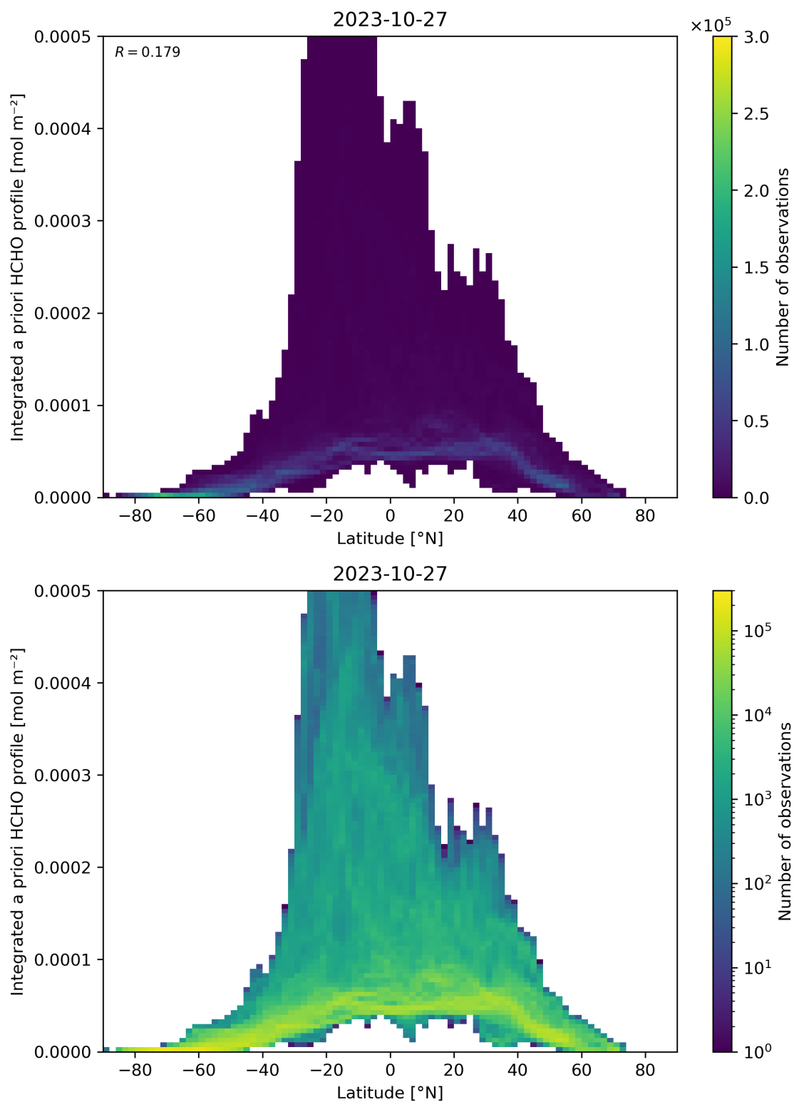
Figure 166: Scatter density plot of “Latitude” against “Integrated a priori HCHO profile” for 2023-10-27 to 2023-10-28.
