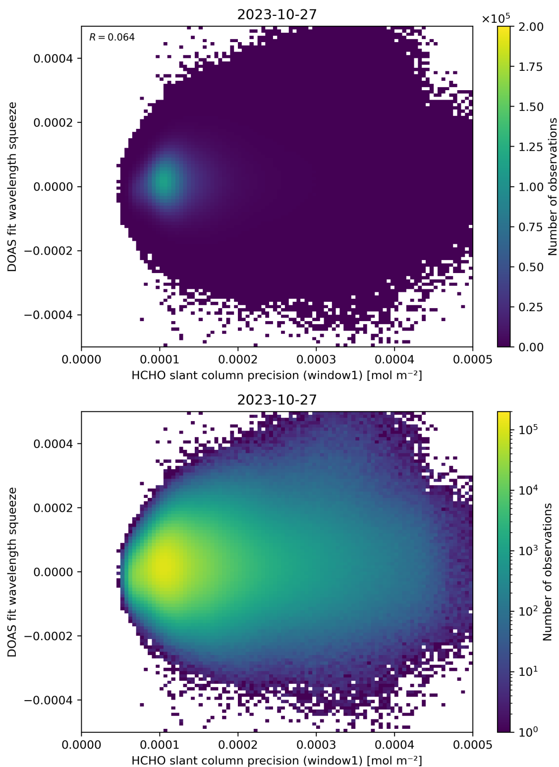
Figure 90: Scatter density plot of “HCHO slant column precision (window1)” against “DOAS fit wavelength squeeze” for 2023-10-27 to 2023-10-28.
