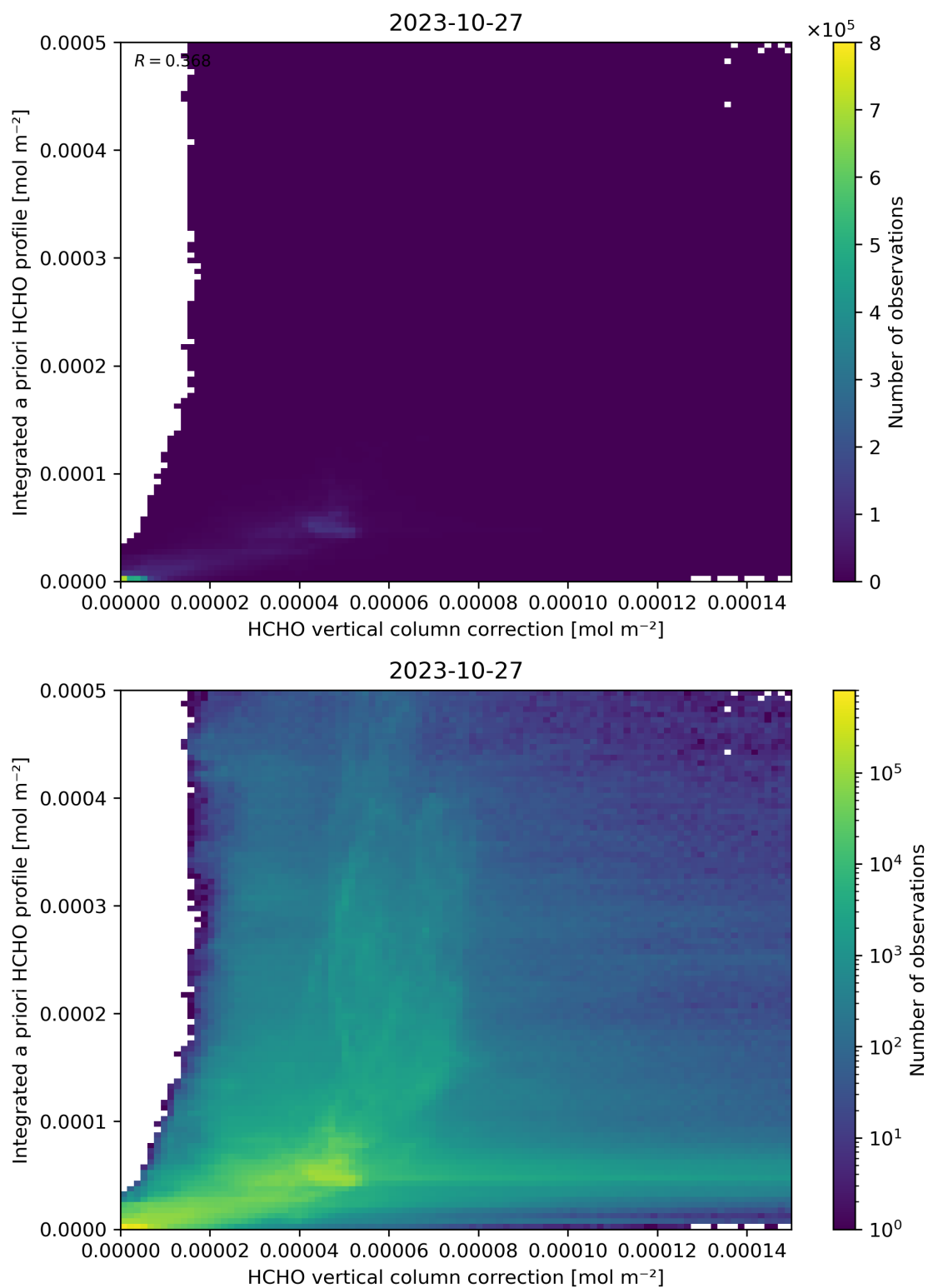
Figure 122: Scatter density plot of “HCHO vertical column correction” against “Integrated a priori HCHO profile” for 2023-10-27 to 2023-10-28.
