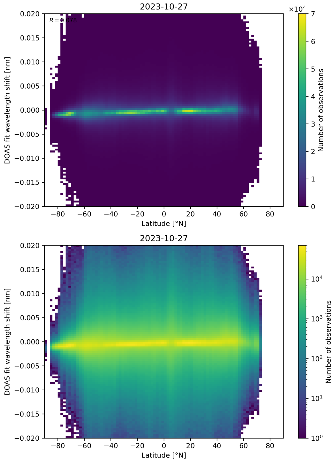
Figure 154: Scatter density plot of “Latitude” against “DOAS fit wavelength shift” for 2023-10-27 to 2023-10-28.
