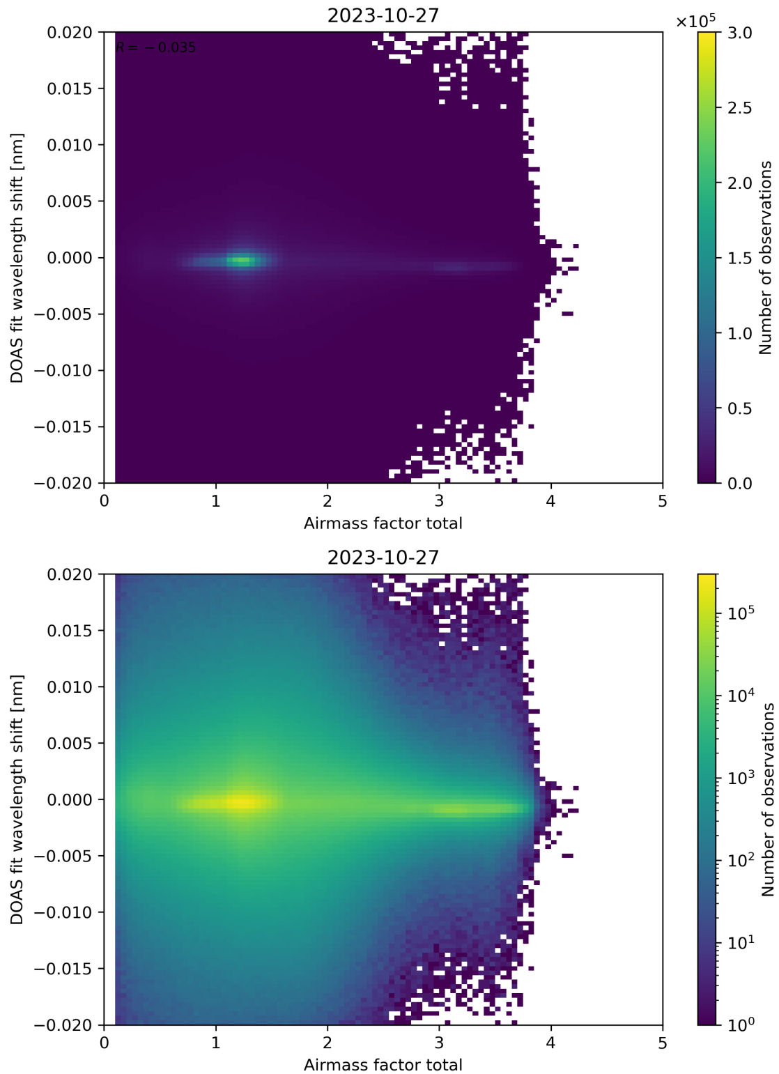
Figure 98: Scatter density plot of “Airmass factor total” against “DOAS fit wavelength shift” for 2023-10-27 to 2023-10-28.
