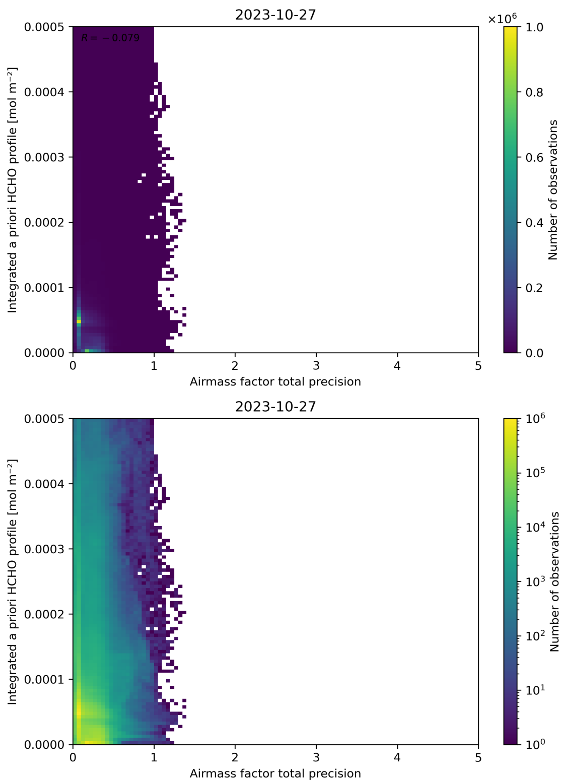
Figure 111: Scatter density plot of “Airmass factor total precision” against “Integrated a priori HCHO profile” for 2023-10-27 to 2023-10-28.
