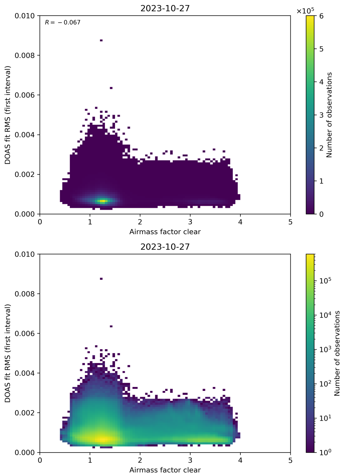
Figure 71: Scatter density plot of “Airmass factor clear” against “DOAS fit RMS (first interval)” for 2023-10-27 to 2023-10-28.
