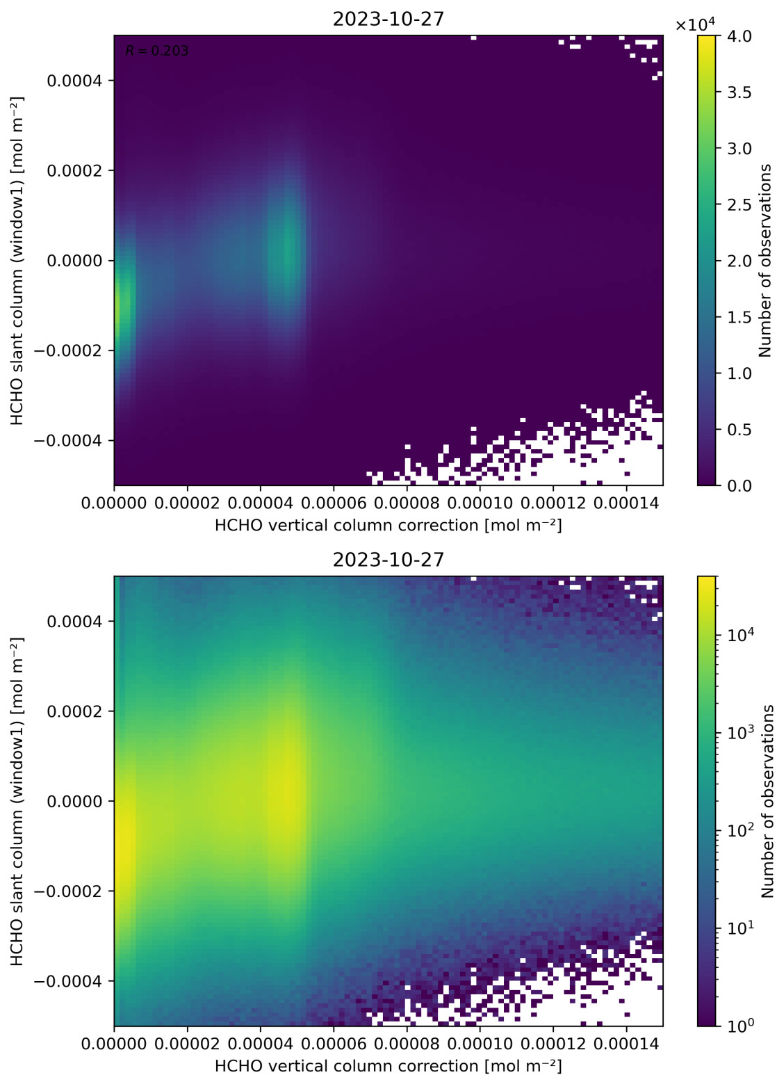
Figure 118: Scatter density plot of “HCHO vertical column correction” against “HCHO slant column (window1)” for 2023-10-27 to 2023-10-28.
