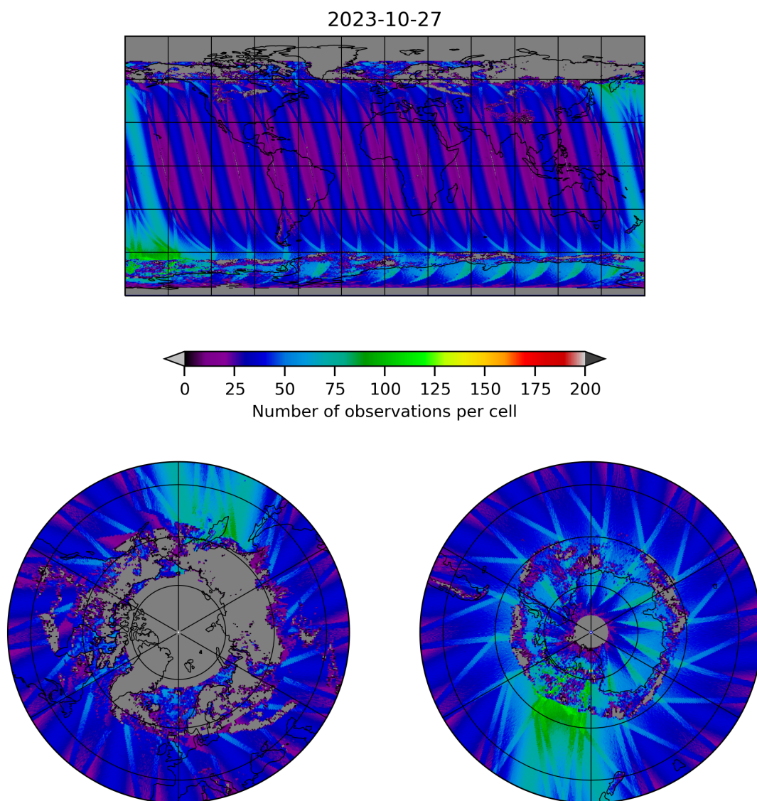
Figure 19: Map of the number of observations for 2023-10-27 to 2023-10-28
