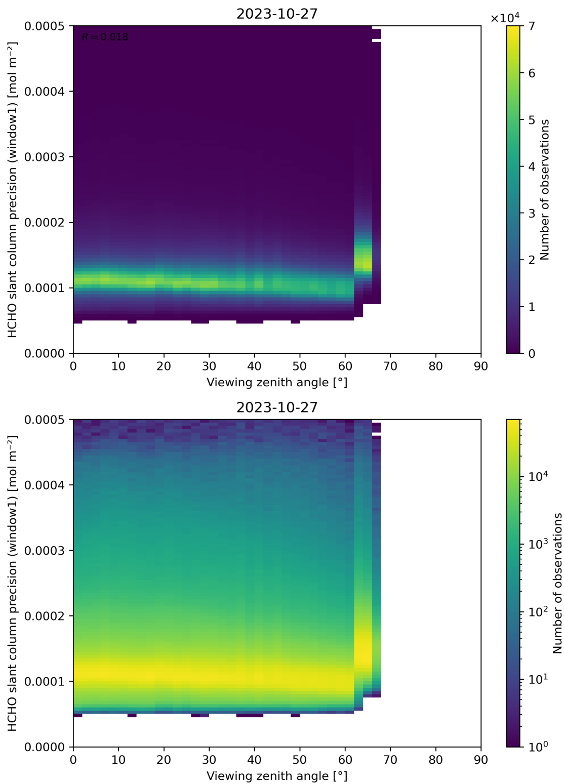
Figure 189: Scatter density plot of “Viewing zenith angle” against “HCHO slant column precision (window1)” for 2023-10-27 to 2023-10-28.
