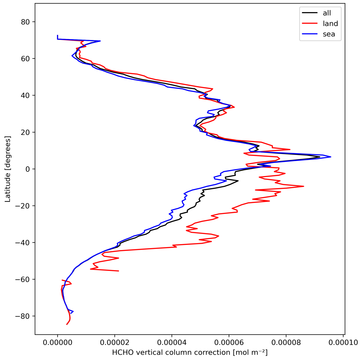
Figure 23: Zonal average of “HCHO vertical column correction” for 2023-10-27 to 2023-10-28.
