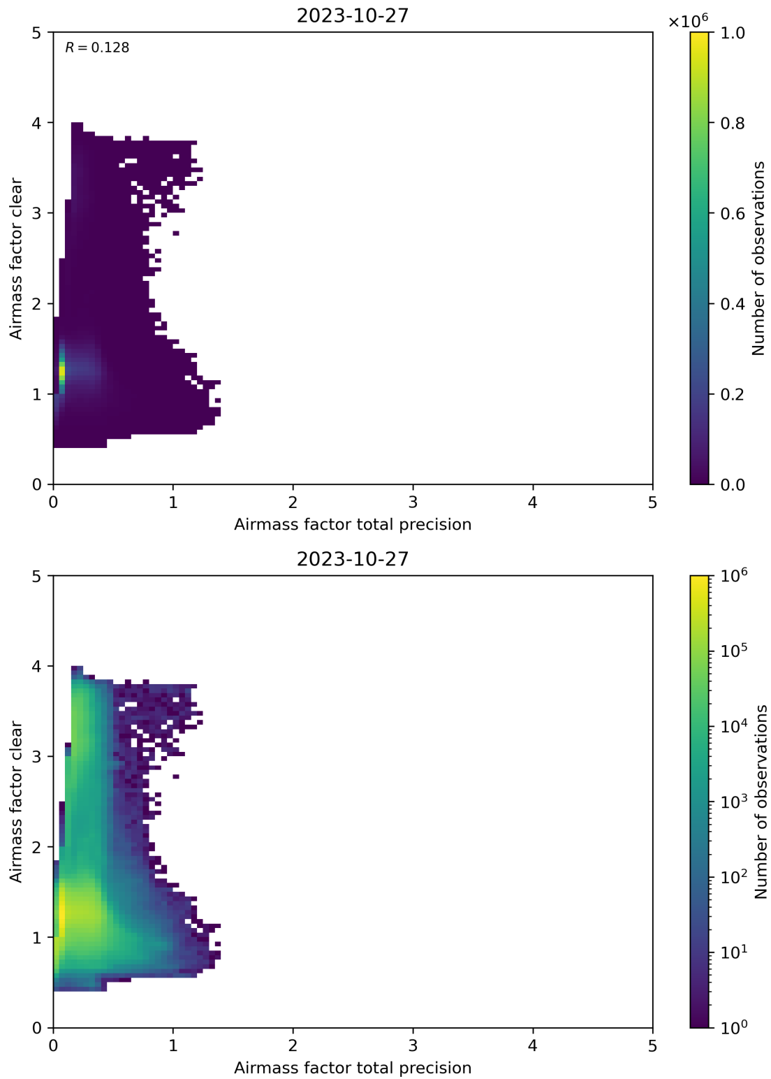
Figure 108: Scatter density plot of “Airmass factor total precision” against “Airmass factor clear” for 2023-10-27 to 2023-10-28.
