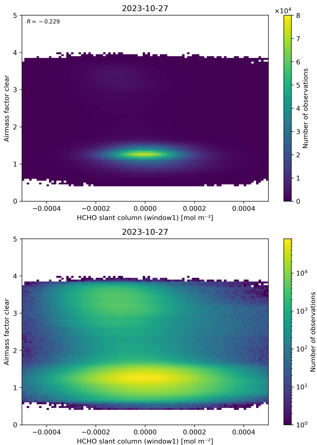
Figure 81: Scatter density plot of “HCHO slant column (window1)” against “Airmass factor clear” for 2023-10-27 to 2023-10-28.
