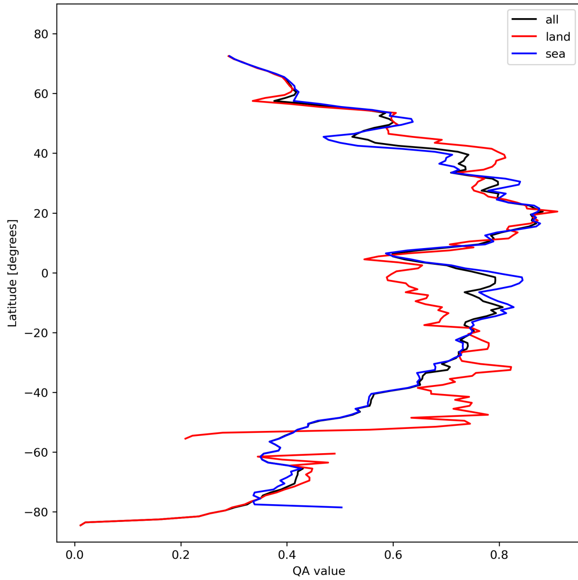
Figure 20: Zonal average of “QA value” for 2023-10-27 to 2023-10-28.
