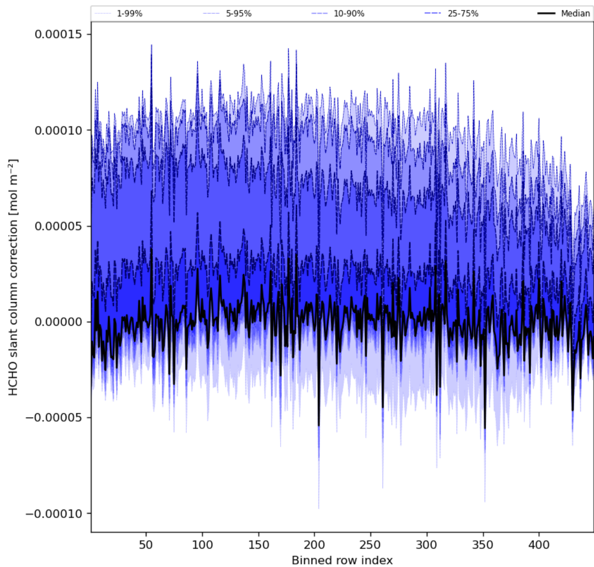
Figure 61: Along track statistics of “HCHO slant column correction” for 2023-10-27 to 2023-10-28
