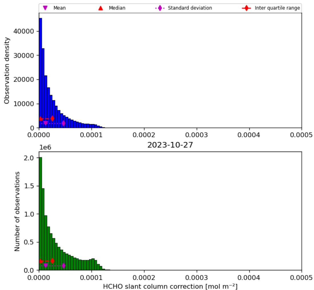
Figure 47: Histogram of “HCHO slant column correction” for 2023-10-27 to 2023-10-28
