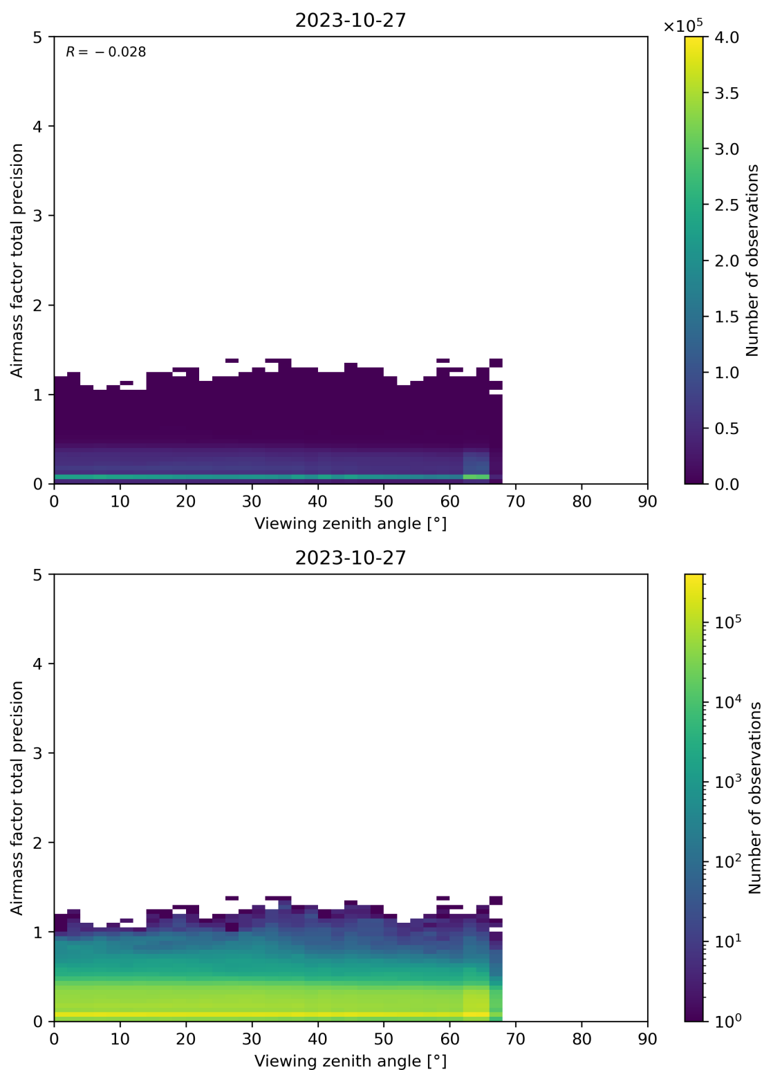
Figure 191: Scatter density plot of “Viewing zenith angle” against “Airmass factor total precision” for 2023-10-27 to 2023-10-28.
