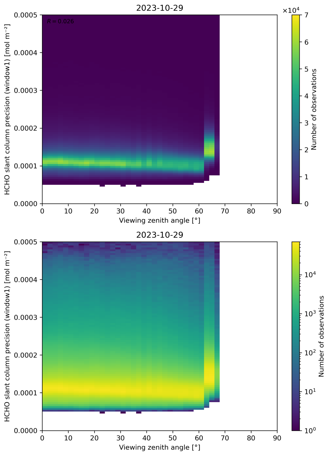
Figure 189: Scatter density plot of “Viewing zenith angle” against “HCHO slant column precision (window1)” for 2023-10-28 to 2023-10-30.
