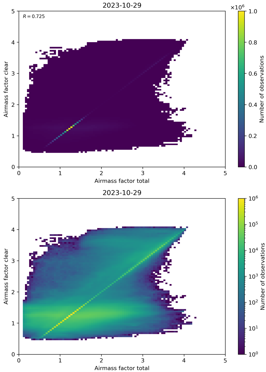
Figure 100: Scatter density plot of “Airmass factor total” against “Airmass factor clear” for 2023-10-28 to 2023-10-30.
