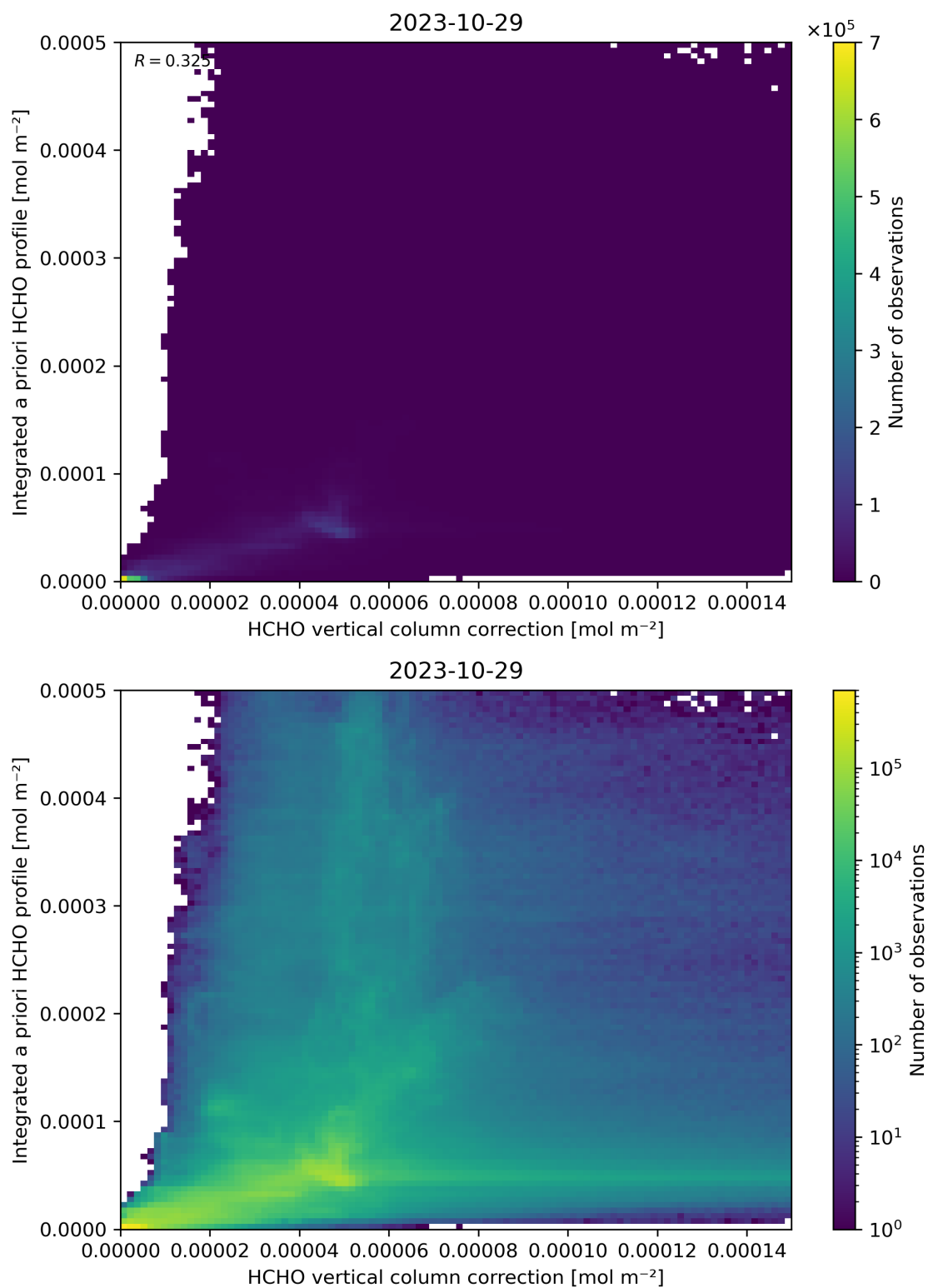
Figure 122: Scatter density plot of “HCHO vertical column correction” against “Integrated a priori HCHO profile” for 2023-10-28 to 2023-10-30.
