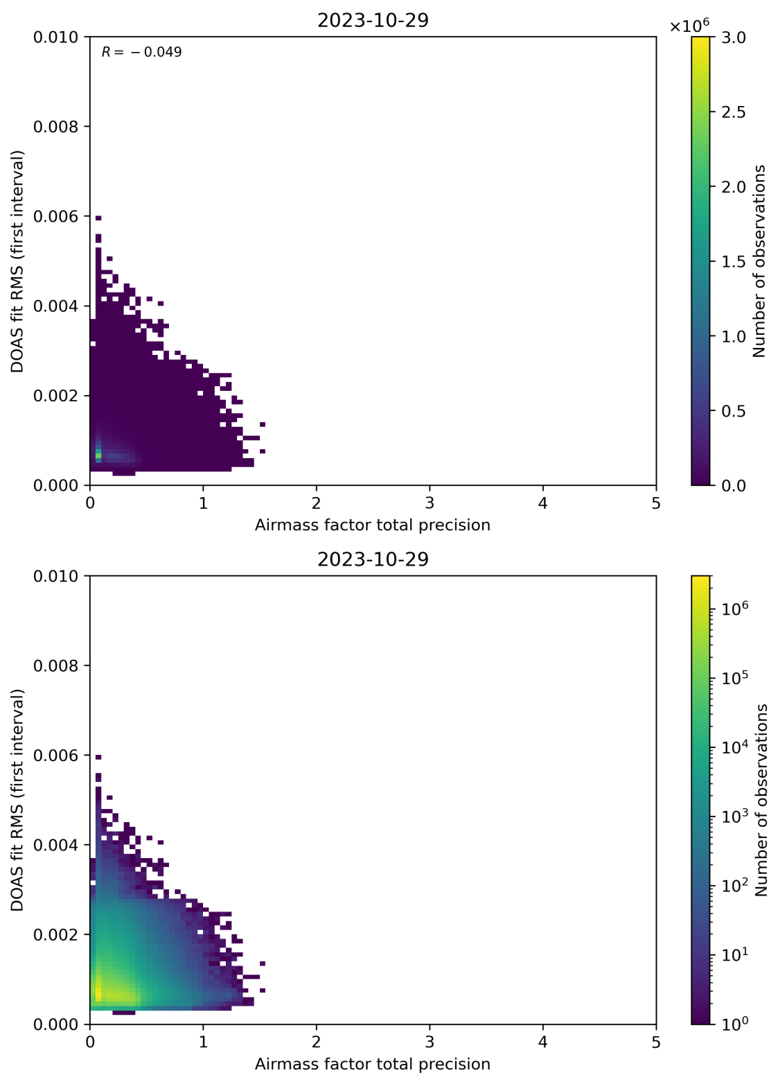
Figure 105: Scatter density plot of “Airmass factor total precision” against “DOAS fit RMS (first interval)” for 2023-10-28 to 2023-10-30.
