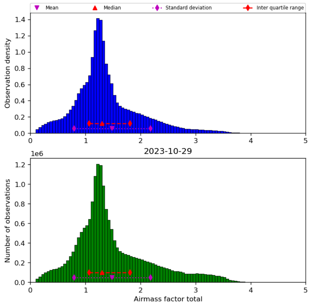
Figure 40: Histogram of “Airmass factor total” for 2023-10-28 to 2023-10-30
