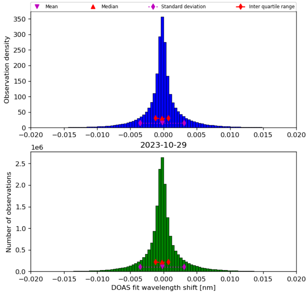
Figure 44: Histogram of “DOAS fit wavelength shift” for 2023-10-28 to 2023-10-30
