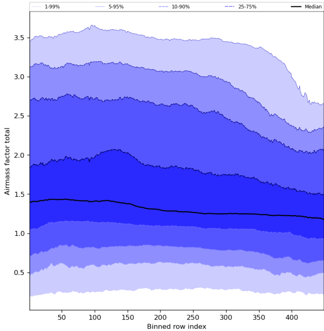
Figure 54: Along track statistics of “Airmass factor total” for 2023-10-28 to 2023-10-30
