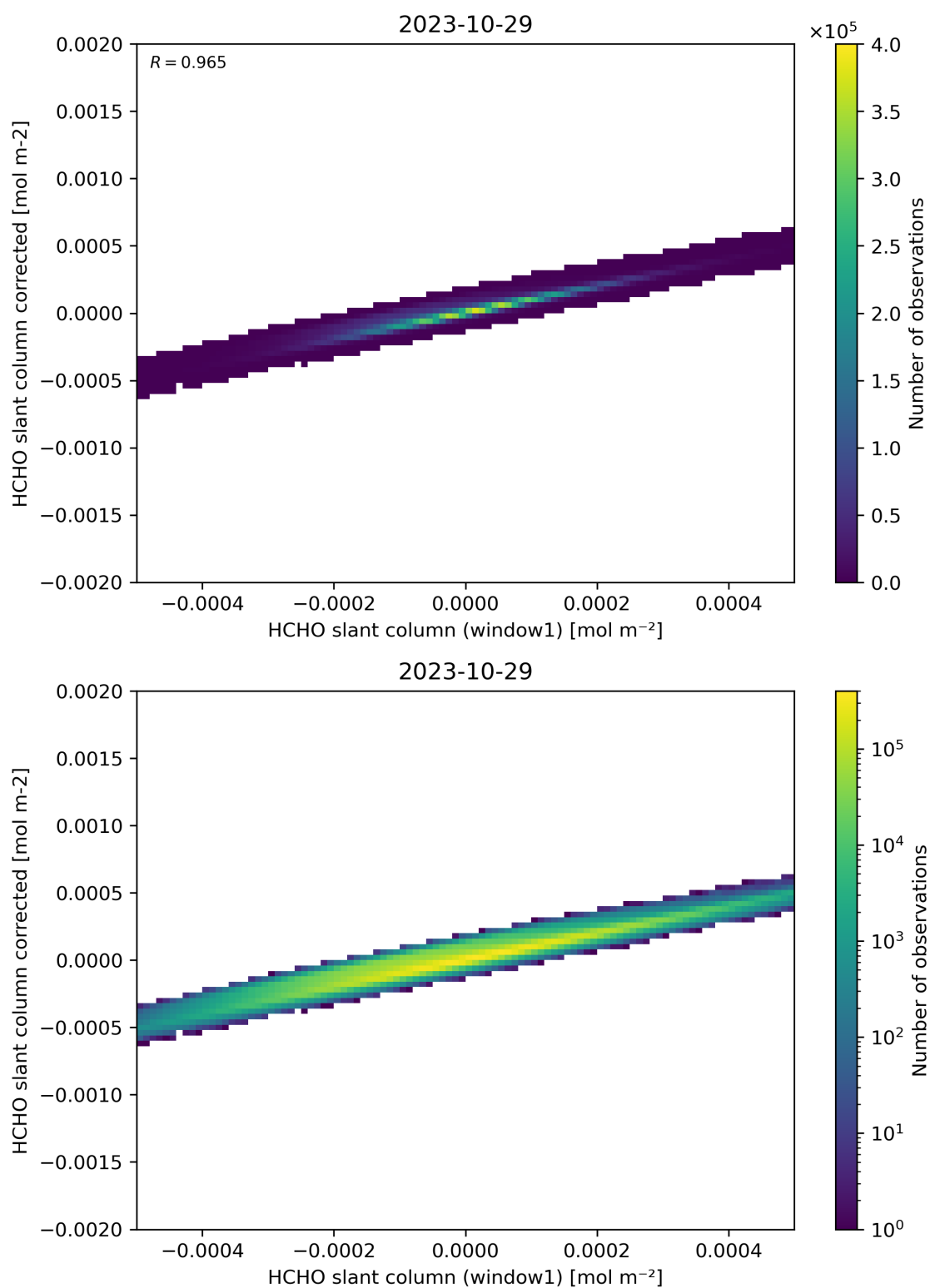
Figure 82: Scatter density plot of “HCHO slant column (window1)” against “HCHO slant column corrected” for 2023-10-28 to 2023-10-30.
