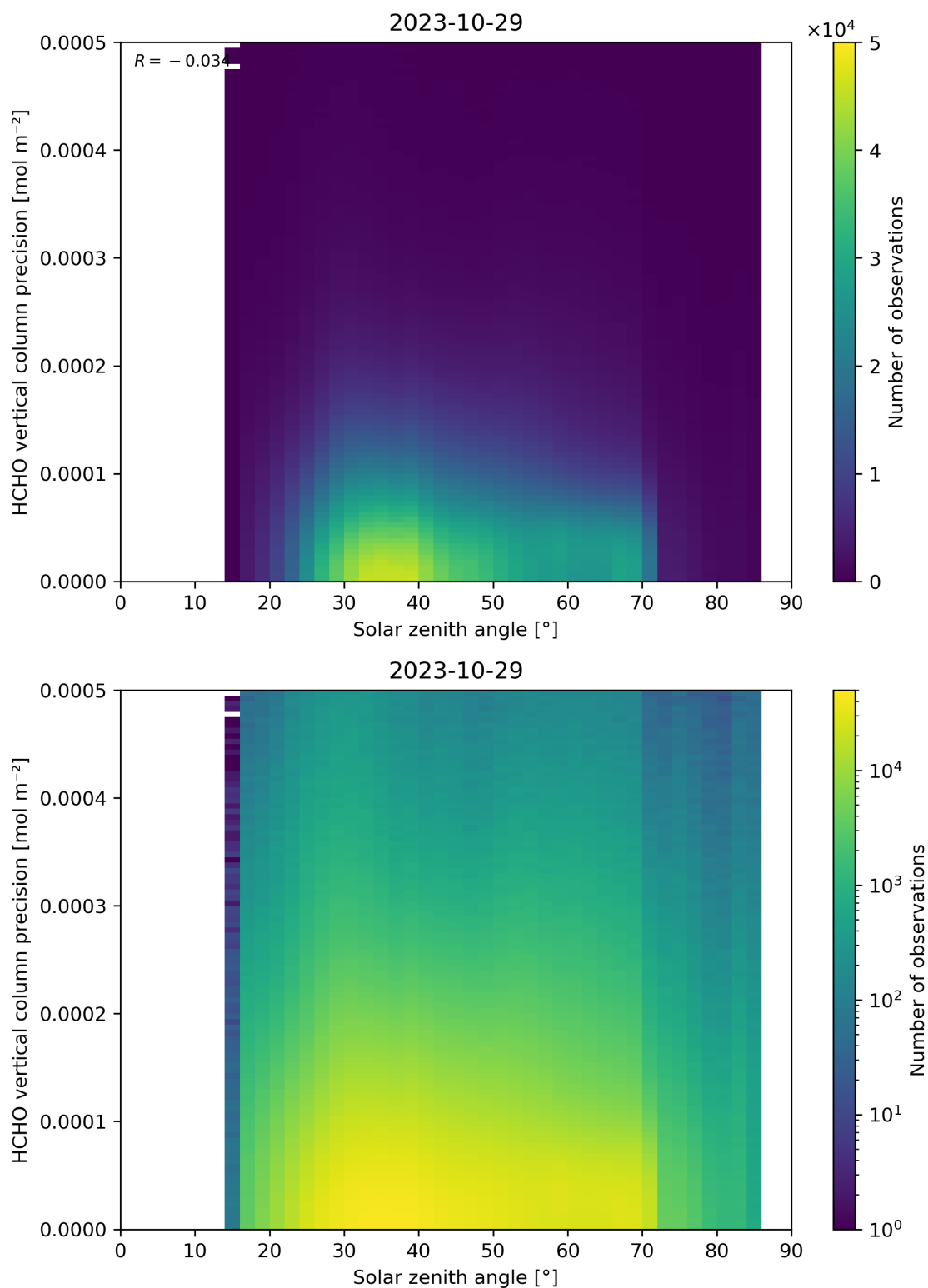
Figure 179: Scatter density plot of “Solar zenith angle” against “HCHO vertical column precision” for 2023-10-28 to 2023-10-30.
