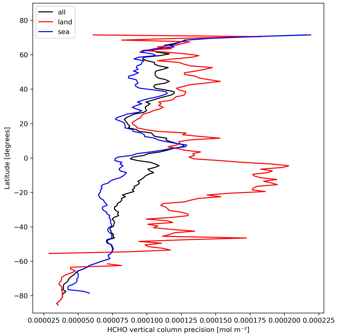
Figure 22: Zonal average of “HCHO vertical column precision” for 2023-10-28 to 2023-10-30.
