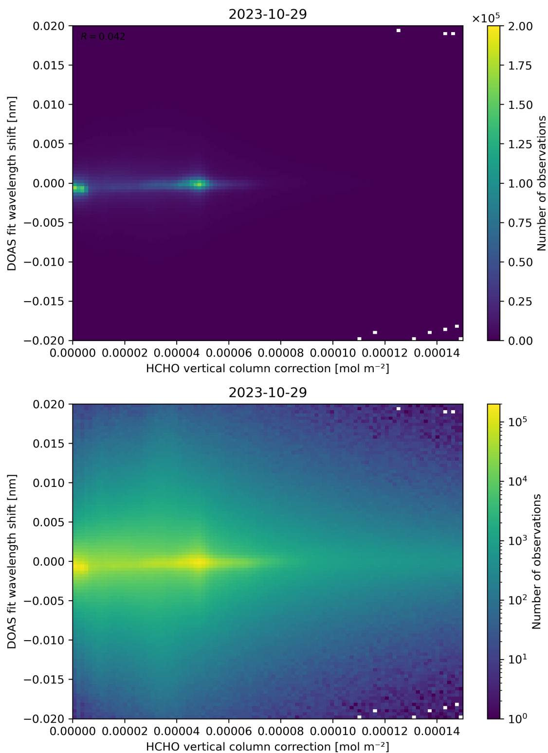
Figure 113: Scatter density plot of “HCHO vertical column correction” against “DOAS fit wavelength shift” for 2023-10-28 to 2023-10-30.
