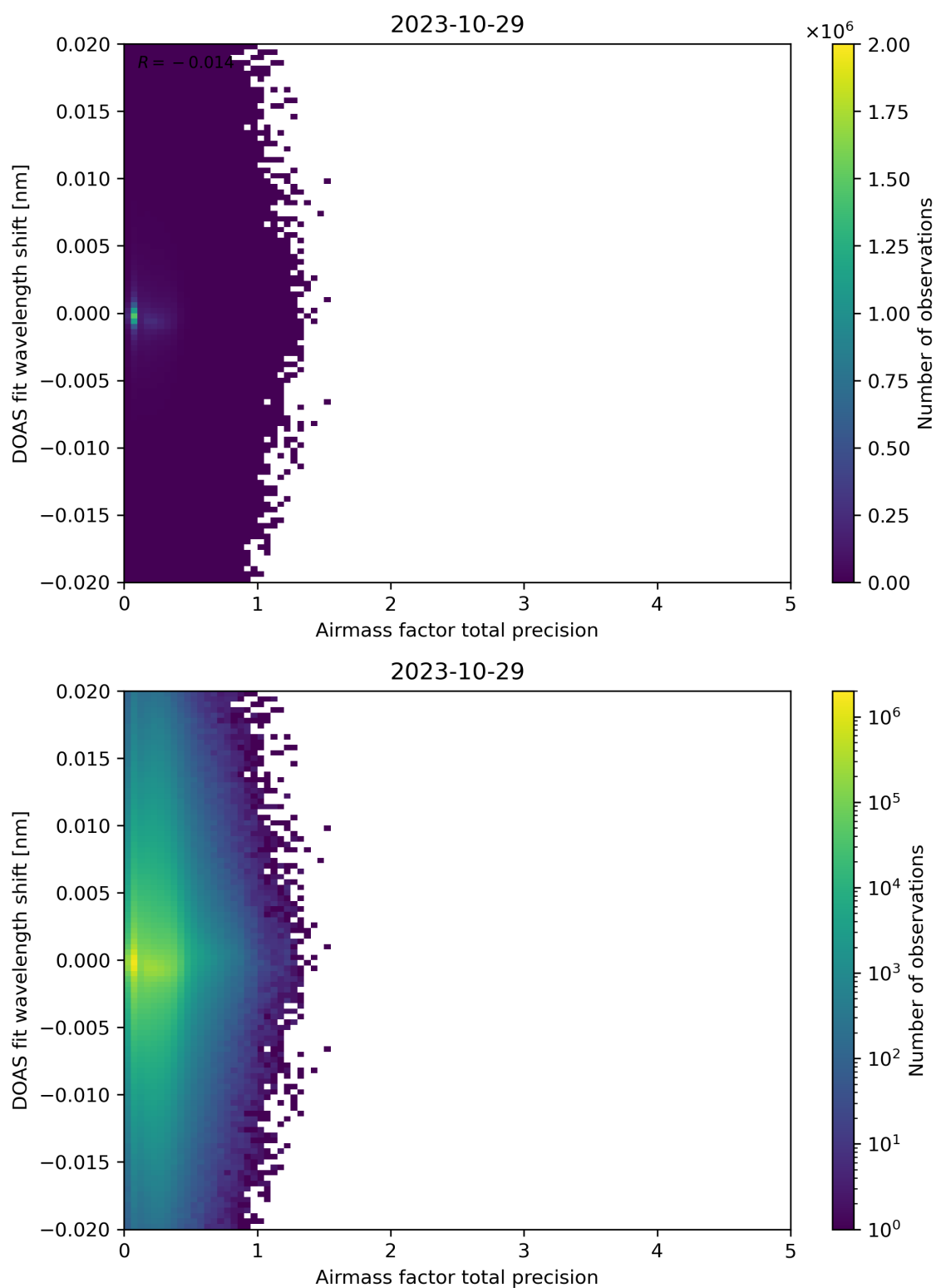
Figure 106: Scatter density plot of “Airmass factor total precision” against “DOAS fit wavelength shift” for 2023-10-28 to 2023-10-30.
