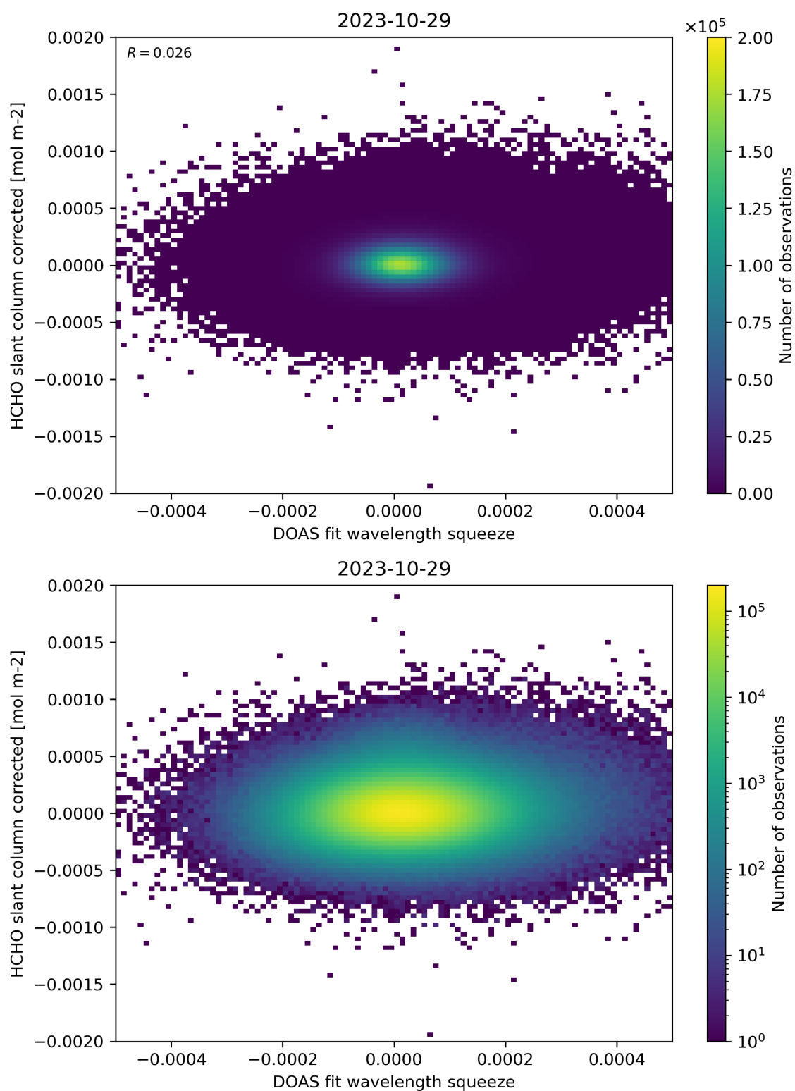
Figure 69: Scatter density plot of “DOAS fit wavelength squeeze” against “HCHO slant column corrected” for 2023-10-28 to 2023-10-30.
