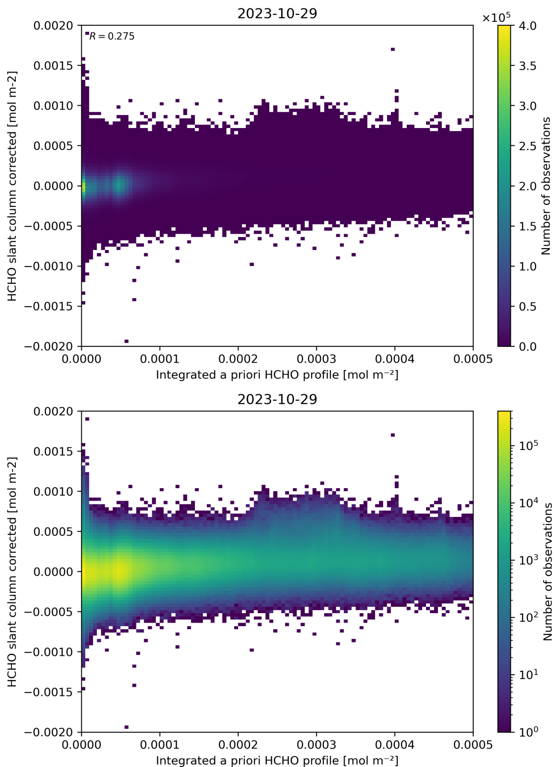
Figure 151: Scatter density plot of “Integrated a priori HCHO profile” against “HCHO slant column corrected” for 2023-10-28 to 2023-10-30.
