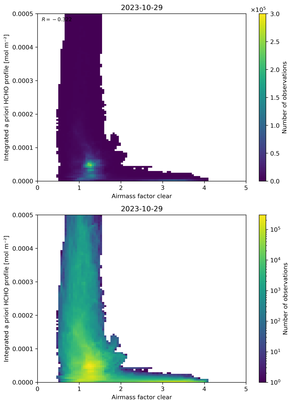
Figure 76: Scatter density plot of “Airmass factor clear” against “Integrated a priori HCHO profile” for 2023-10-28 to 2023-10-30.
