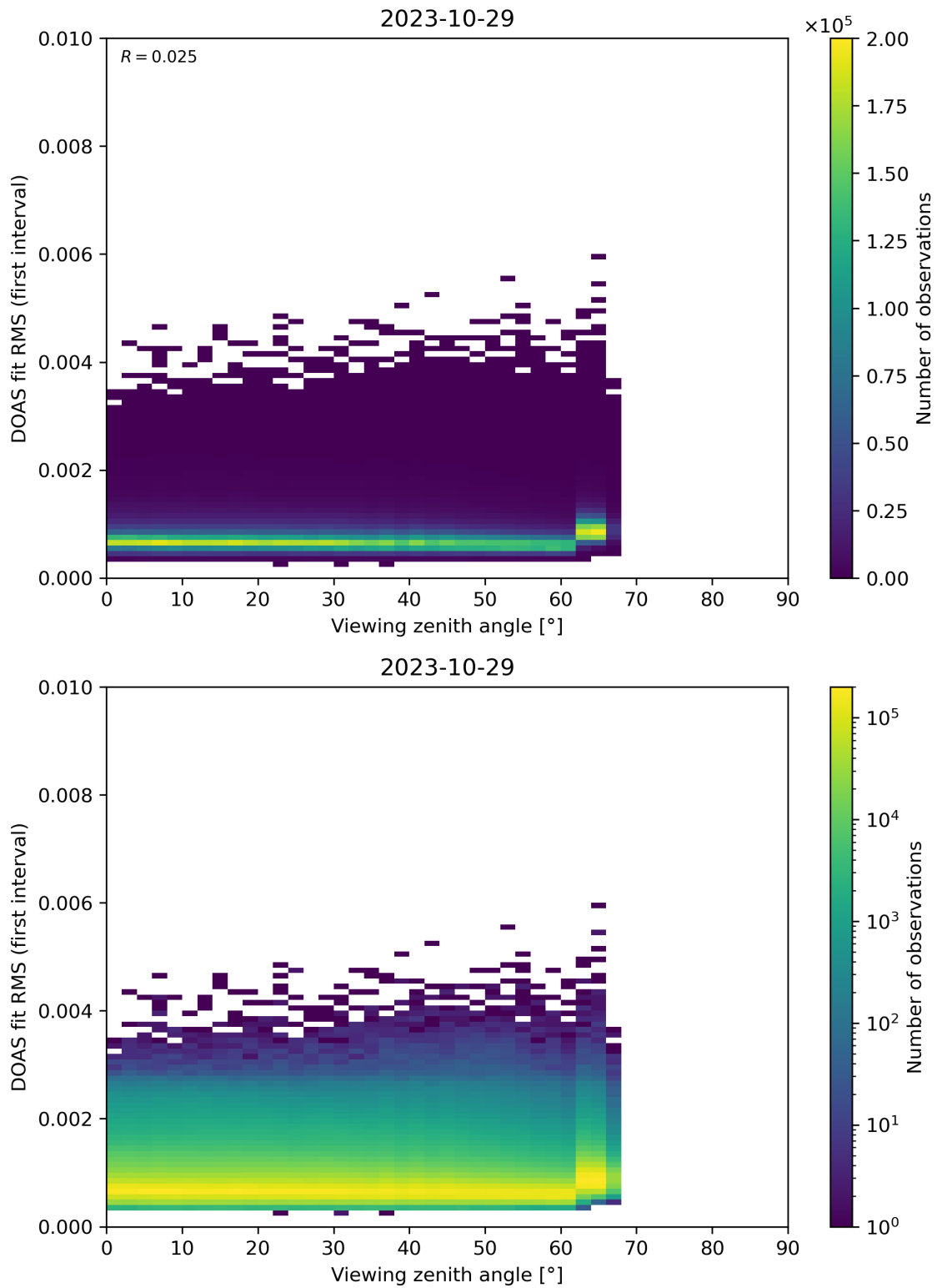
Figure 182: Scatter density plot of “Viewing zenith angle” against “DOAS fit RMS (first interval)” for 2023-10-28 to 2023-10-30.
