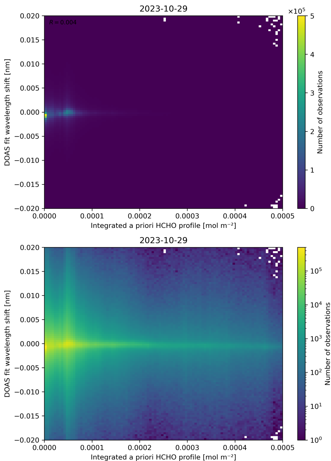
Figure 149: Scatter density plot of “Integrated a priori HCHO profile” against “DOAS fit wavelength shift” for 2023-10-28 to 2023-10-30.
