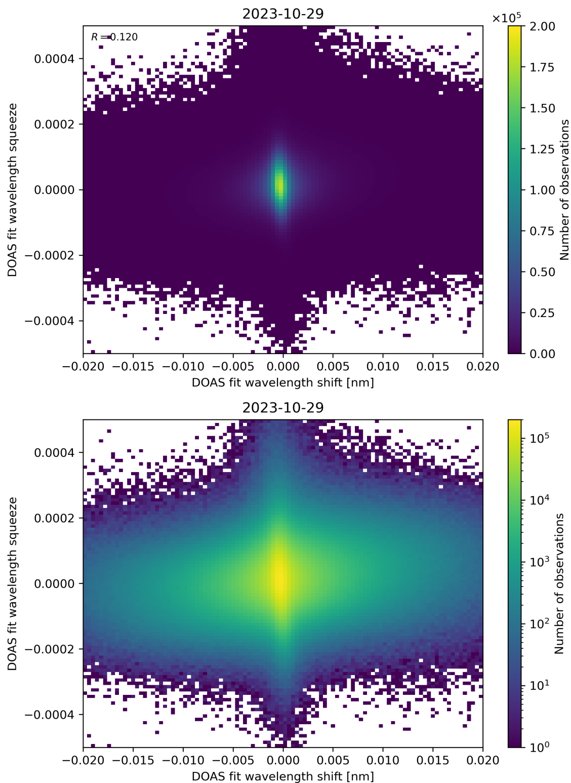
Figure 65: Scatter density plot of “DOAS fit wavelength shift” against “DOAS fit wavelength squeeze” for 2023-10-28 to 2023-10-30.
