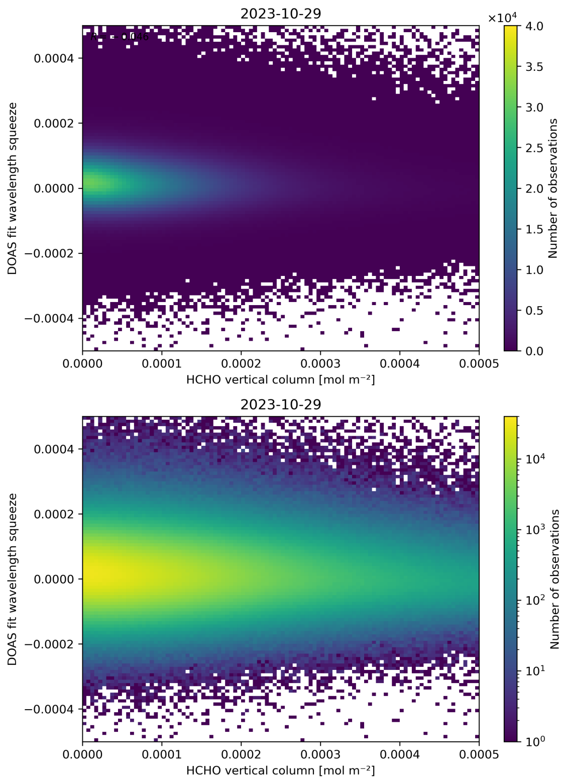
Figure 125: Scatter density plot of “HCHO vertical column” against “DOAS fit wavelength squeeze” for 2023-10-28 to 2023-10-30.
