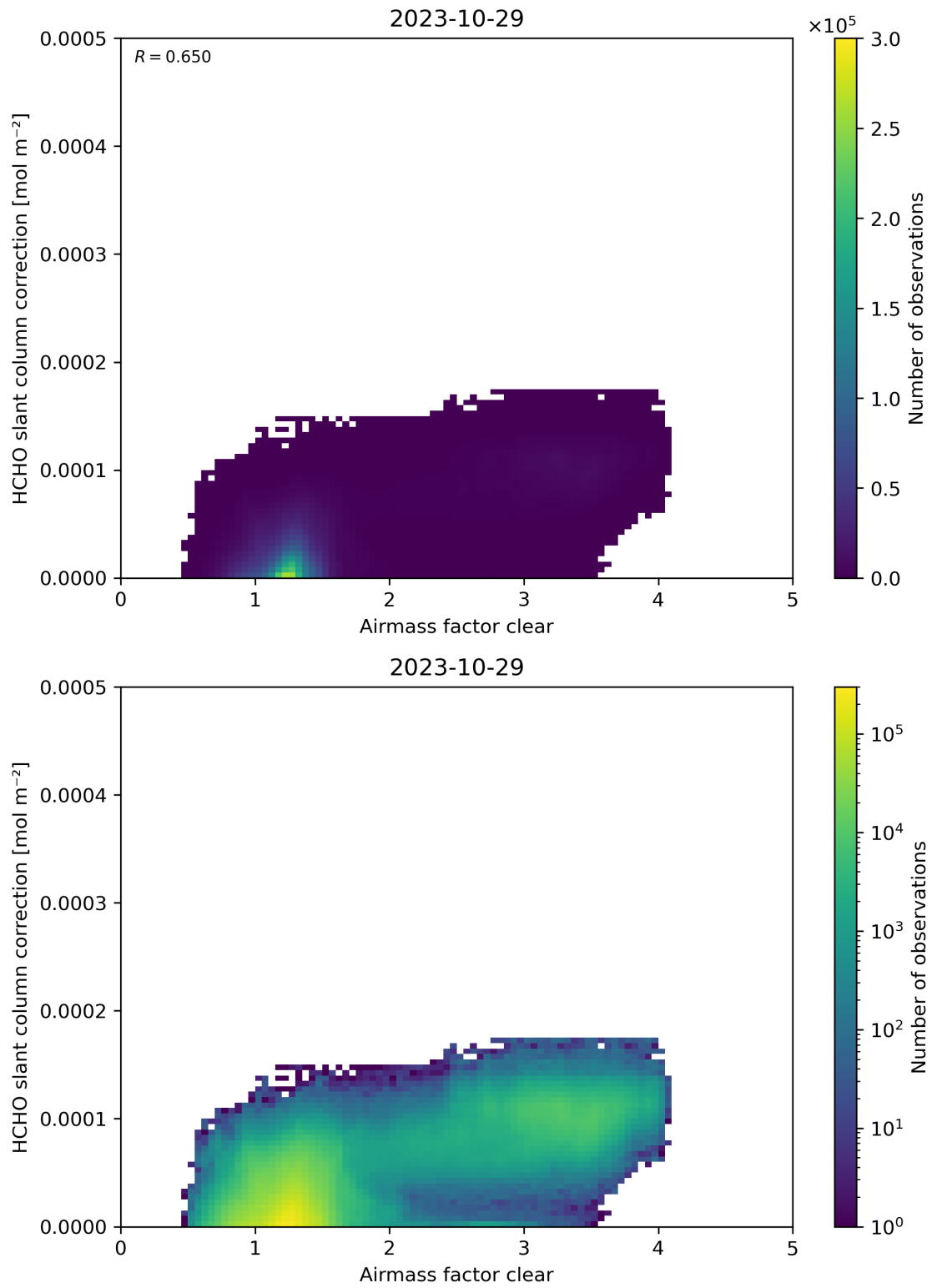
Figure 75: Scatter density plot of “Airmass factor clear” against “HCHO slant column correction” for 2023-10-28 to 2023-10-30.
