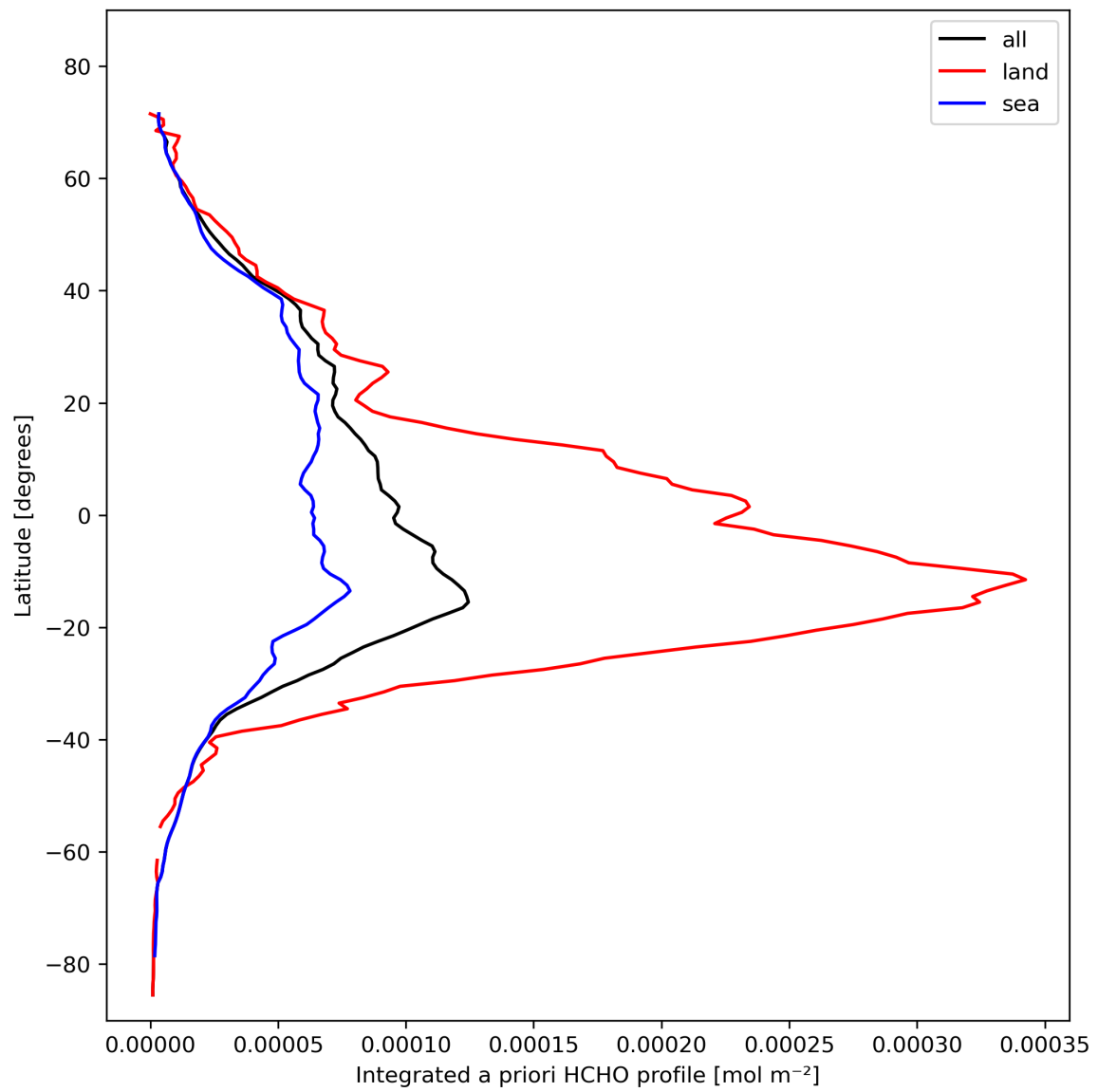
Figure 29: Zonal average of “Integrated a priori HCHO profile” for 2023-10-28 to 2023-10-30.
