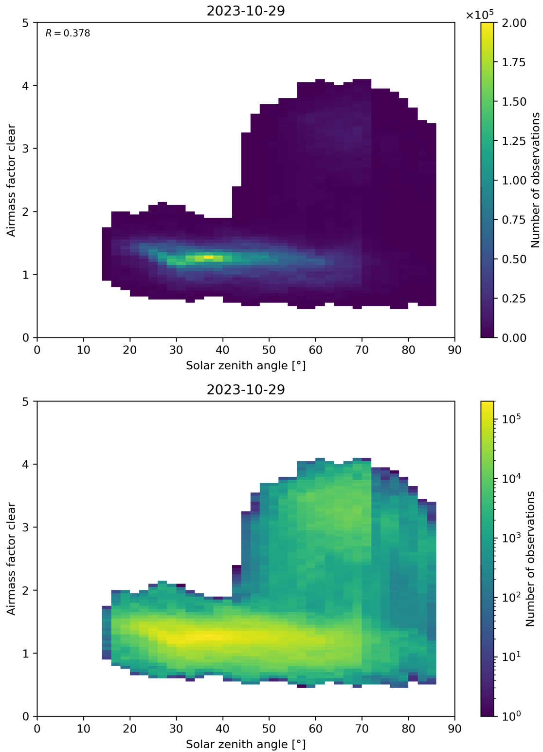
Figure 170: Scatter density plot of “Solar zenith angle” against “Airmass factor clear” for 2023-10-28 to 2023-10-30.
