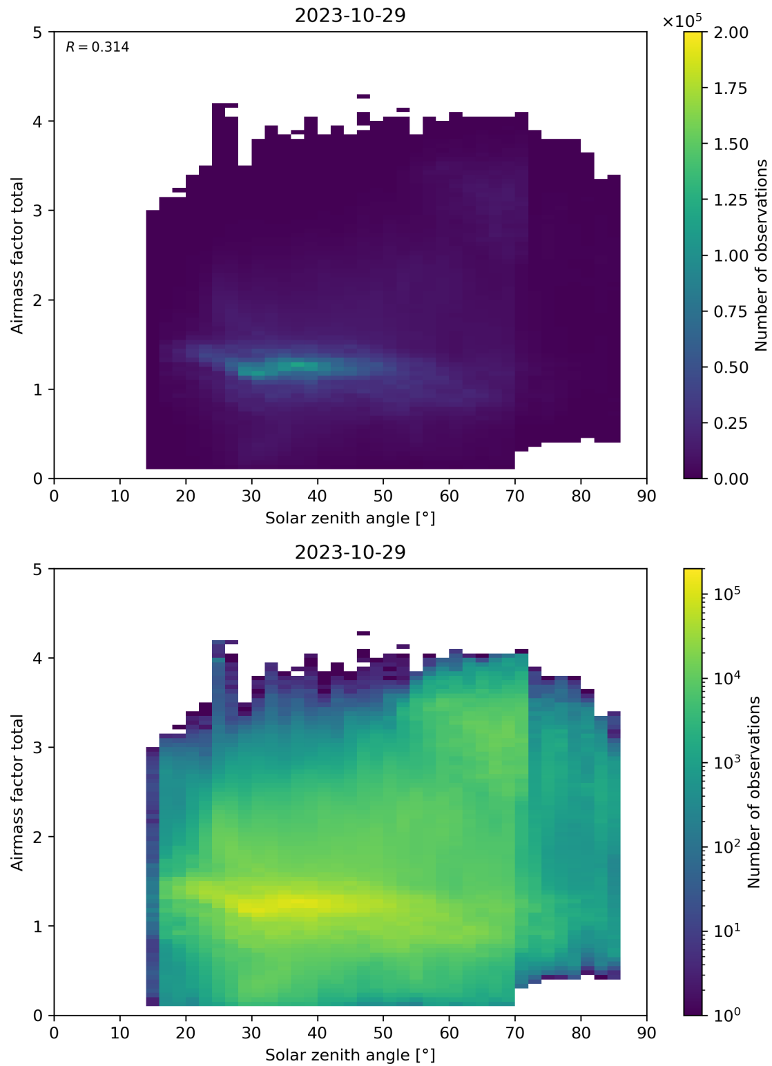
Figure 175: Scatter density plot of “Solar zenith angle” against “Airmass factor total” for 2023-10-28 to 2023-10-30.
