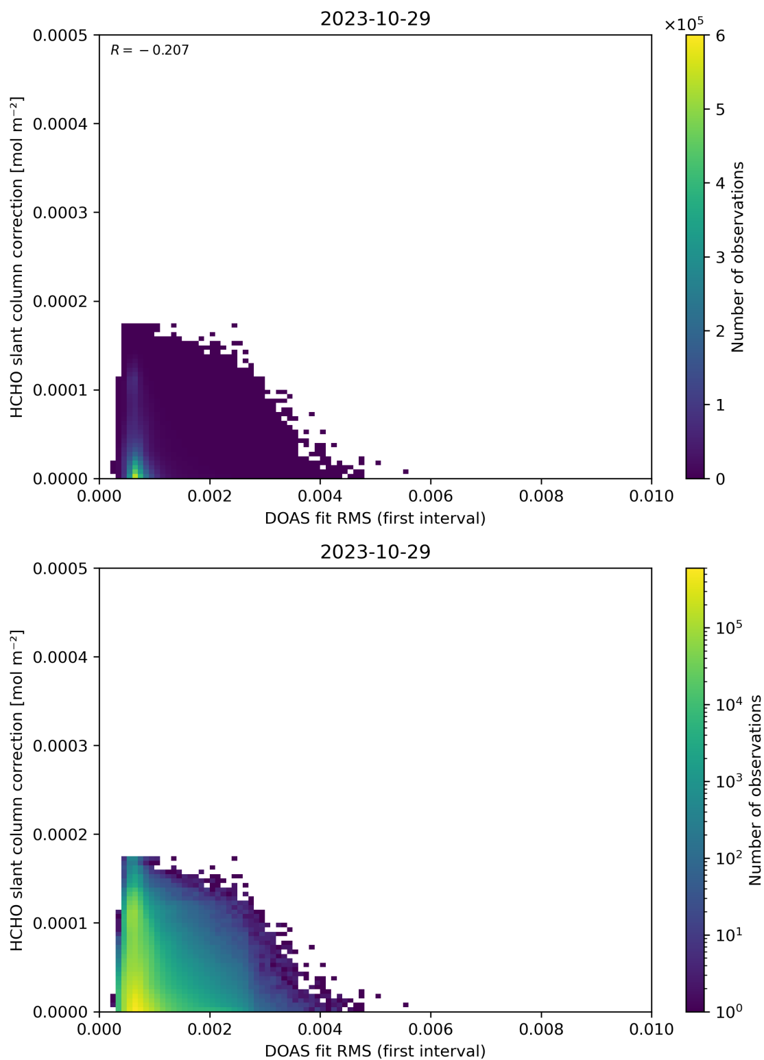
Figure 63: Scatter density plot of “DOAS fit RMS (first interval)” against “HCHO slant column correction” for 2023-10-28 to 2023-10-30.
