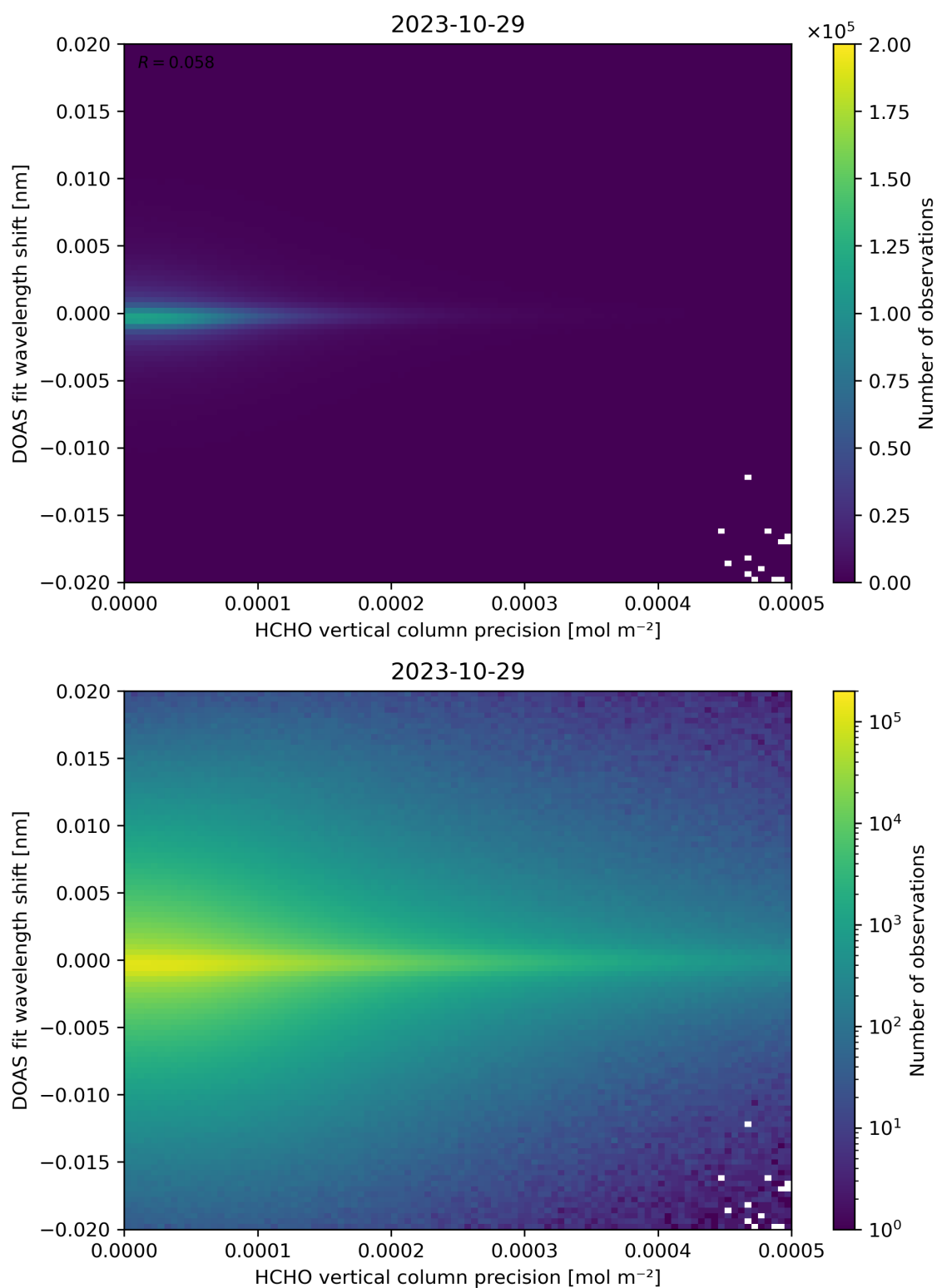
Figure 137: Scatter density plot of “HCHO vertical column precision” against “DOAS fit wavelength shift” for 2023-10-28 to 2023-10-30.
