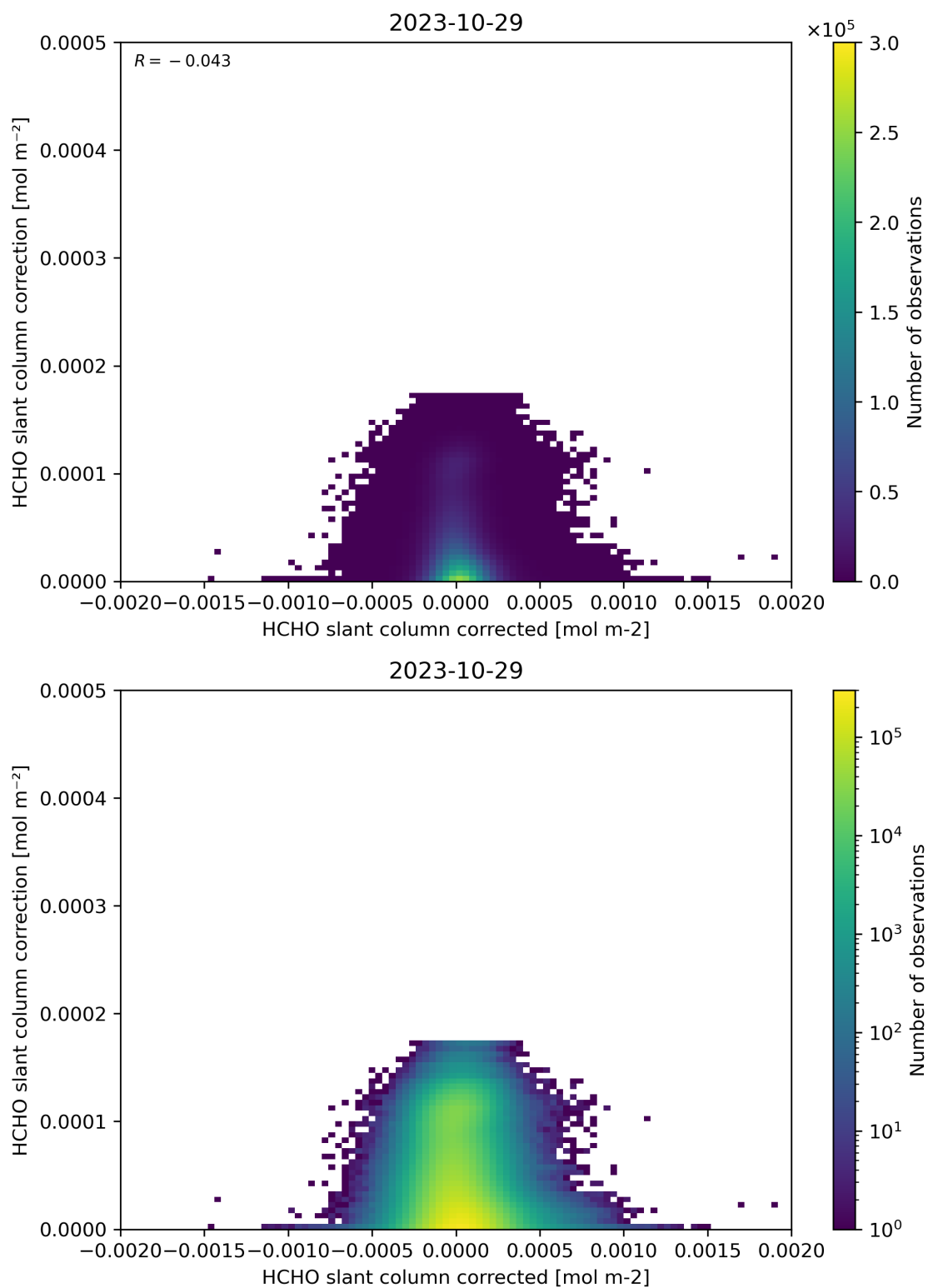
Figure 77: Scatter density plot of “HCHO slant column corrected” against “HCHO slant column correction” for 2023-10-28 to 2023-10-30.
