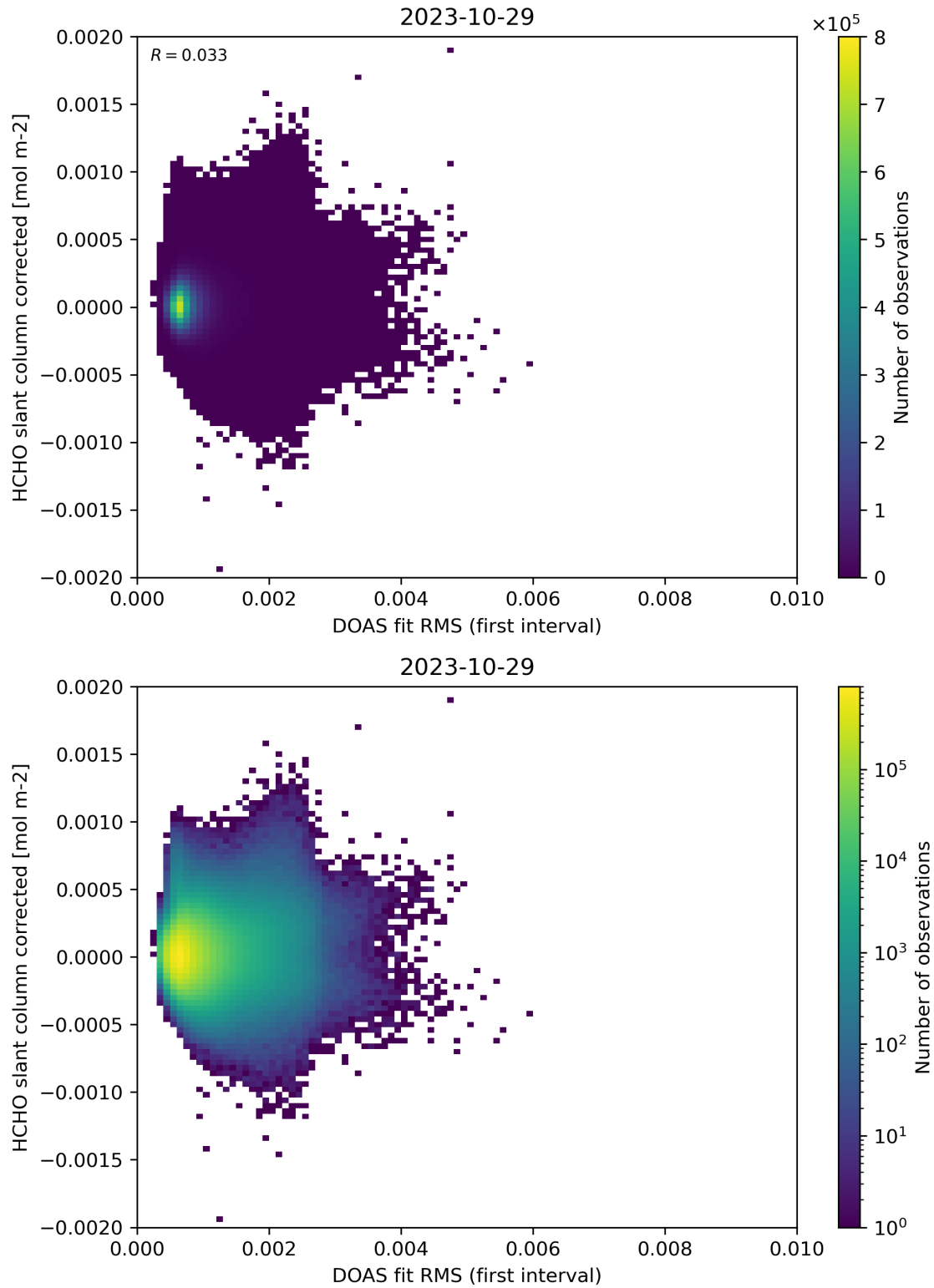
Figure 62: Scatter density plot of “DOAS fit RMS (first interval)” against “HCHO slant column corrected” for 2023-10-28 to 2023-10-30.
