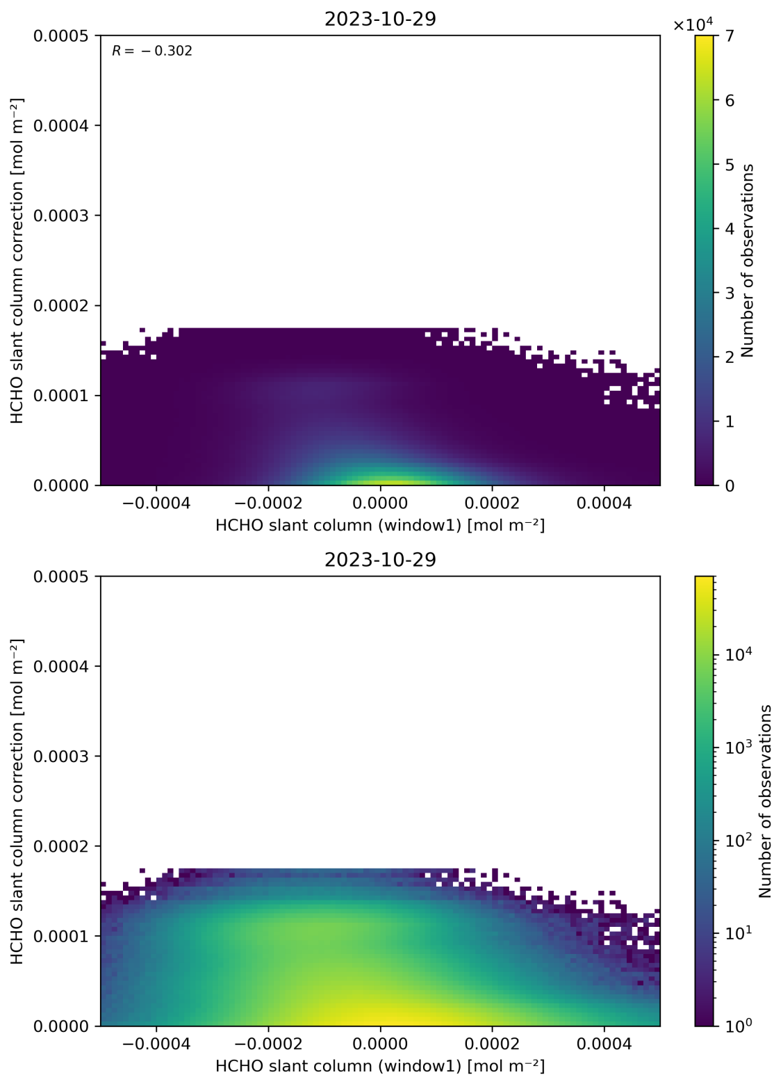
Figure 83: Scatter density plot of “HCHO slant column (window1)” against “HCHO slant column correction” for 2023-10-28 to 2023-10-30.
