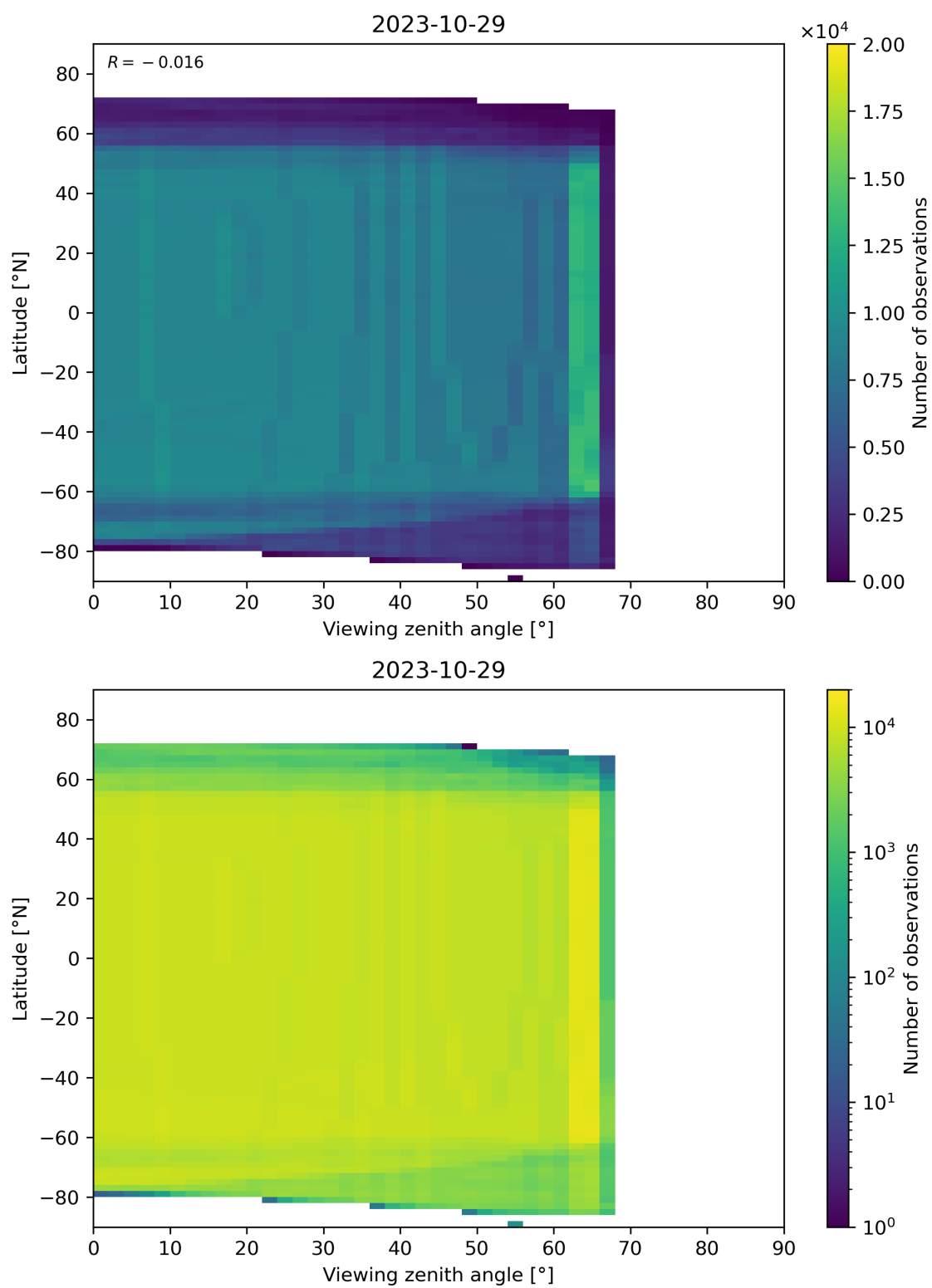
Figure 196: Scatter density plot of “Viewing zenith angle” against “Latitude” for 2023-10-28 to 2023-10-30.
