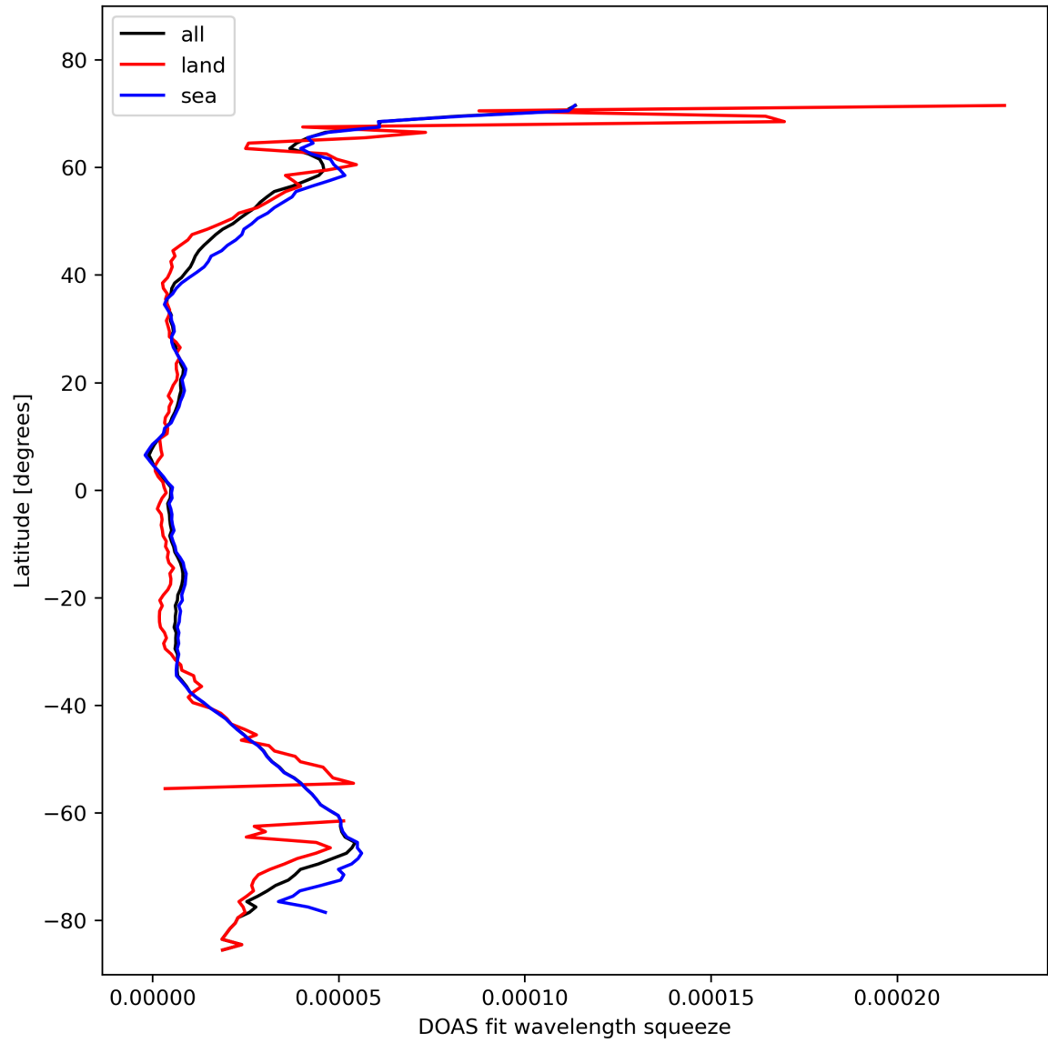
Figure 31: Zonal average of “DOAS fit wavelength squeeze” for 2023-10-28 to 2023-10-30.
