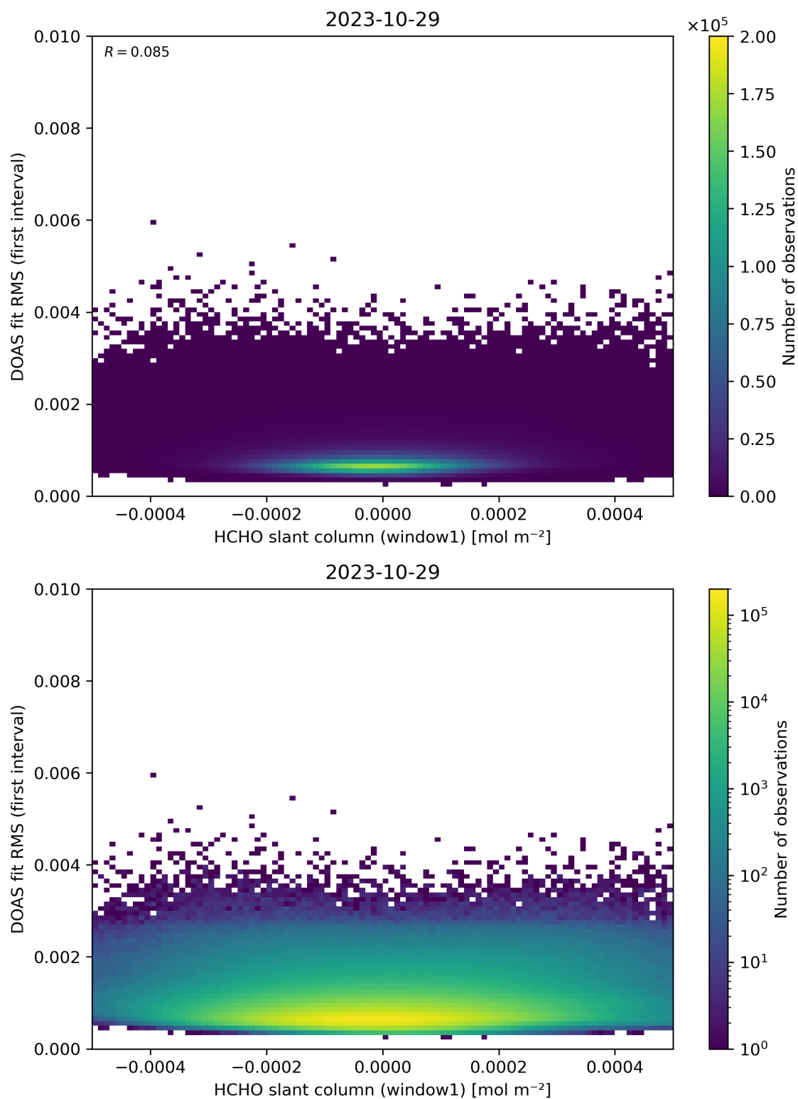
Figure 78: Scatter density plot of “HCHO slant column (window1)” against “DOAS fit RMS (first interval)” for 2023-10-28 to 2023-10-30.
