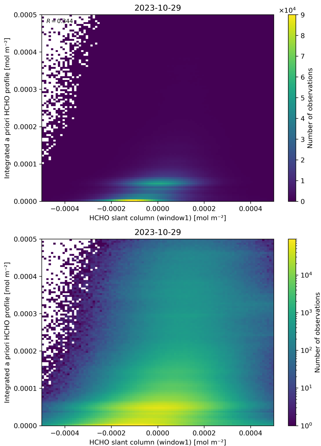
Figure 87: Scatter density plot of “HCHO slant column (window1)” against “Integrated a priori HCHO profile” for 2023-10-28 to 2023-10-30.
