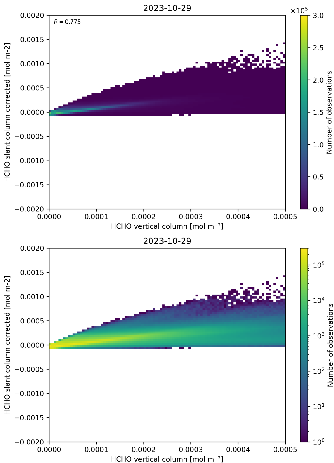
Figure 127: Scatter density plot of “HCHO vertical column” against “HCHO slant column corrected” for 2023-10-28 to 2023-10-30.
