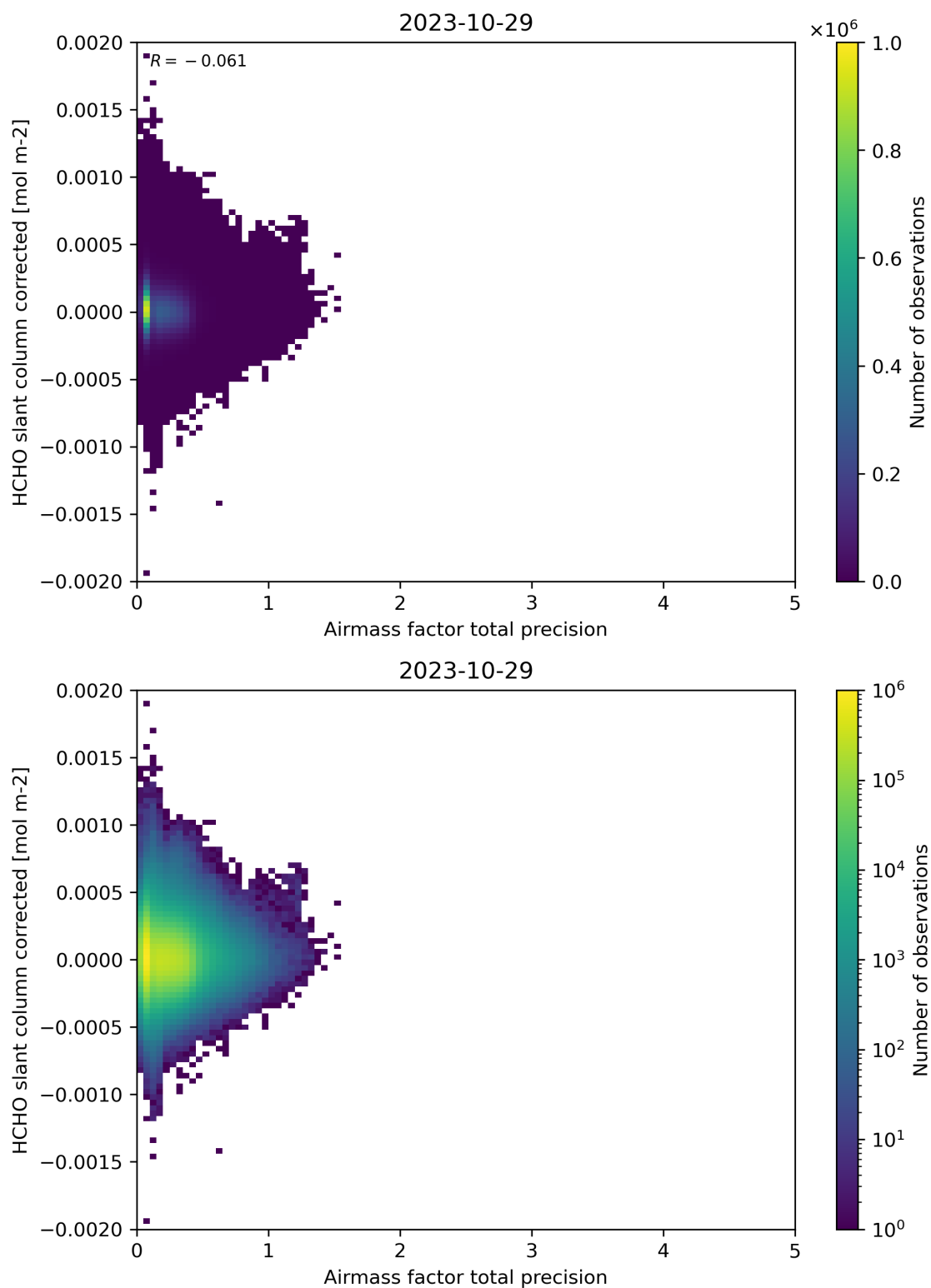
Figure 109: Scatter density plot of “Airmass factor total precision” against “HCHO slant column corrected” for 2023-10-28 to 2023-10-30.
