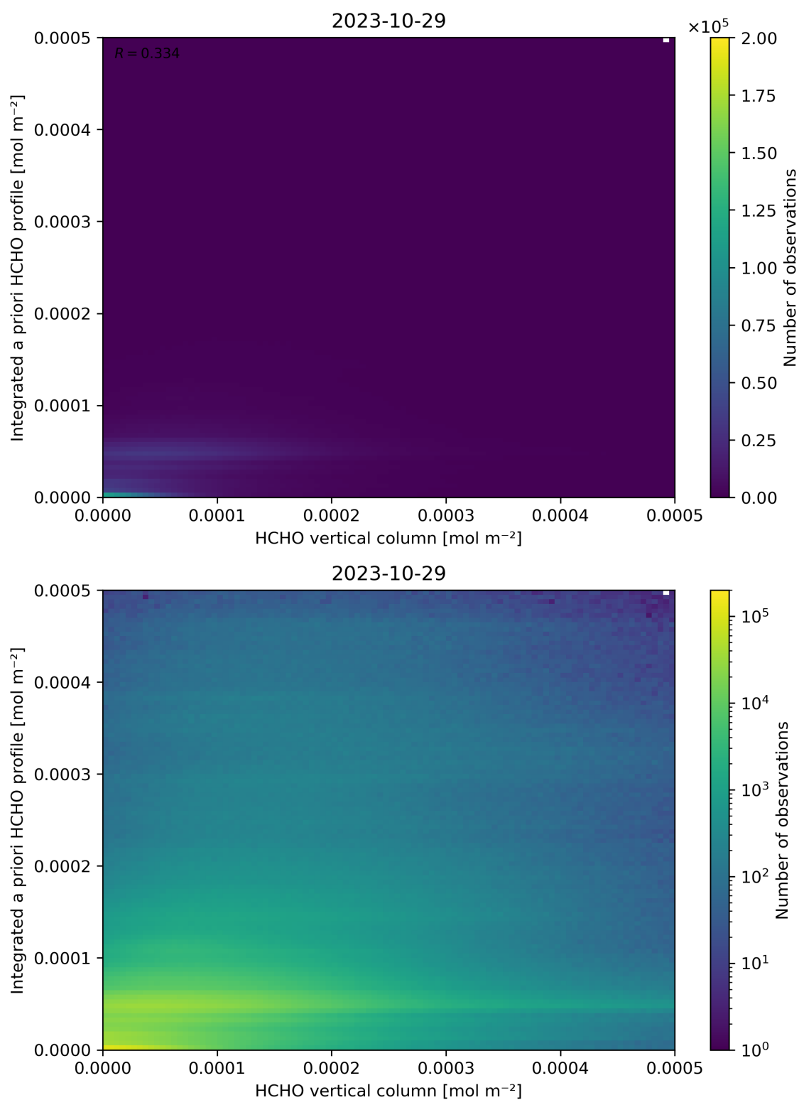
Figure 135: Scatter density plot of “HCHO vertical column” against “Integrated a priori HCHO profile” for 2023-10-28 to 2023-10-30.
