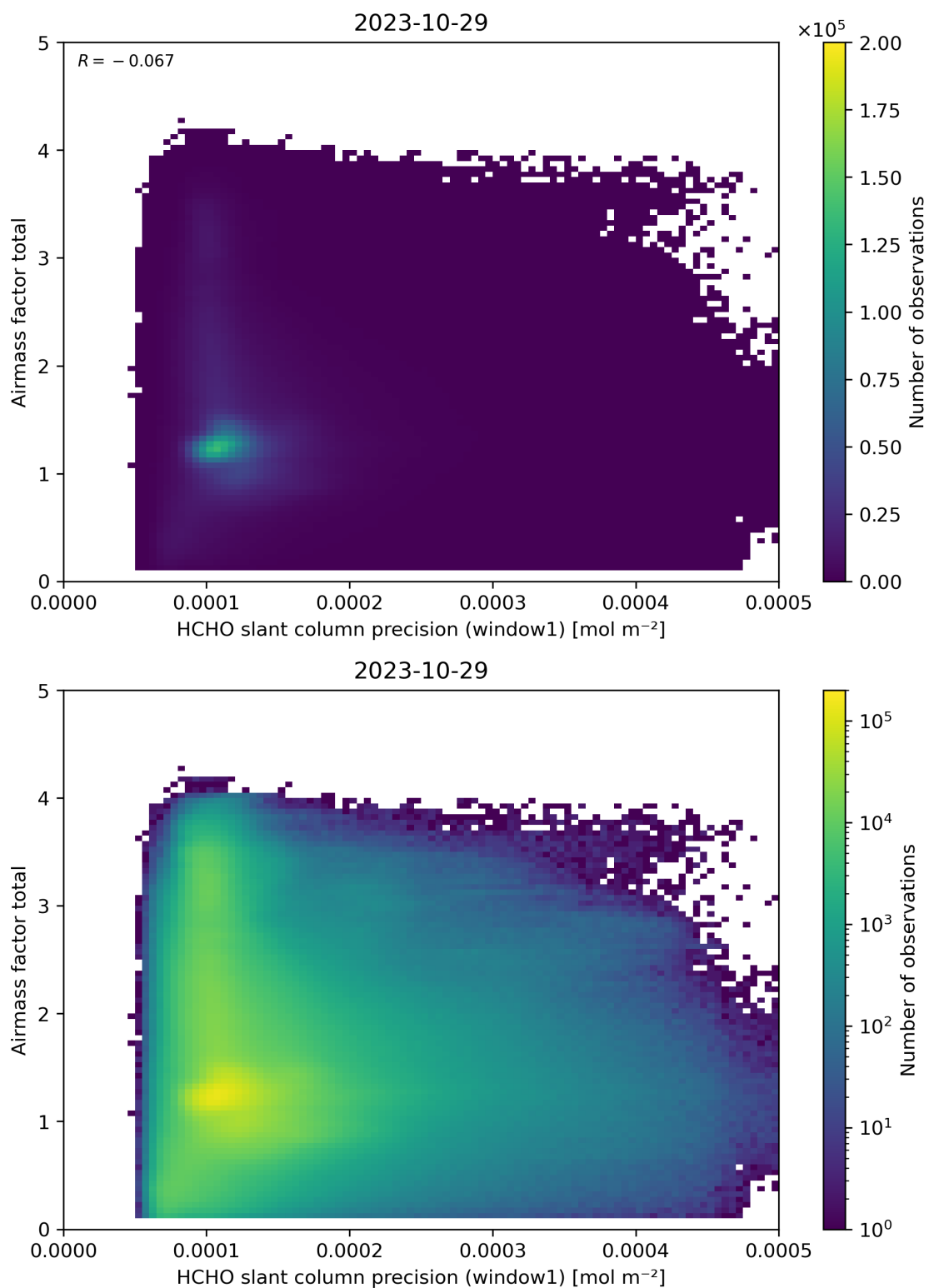
Figure 94: Scatter density plot of “HCHO slant column precision (window1)” against “Airmass factor total” for 2023-10-28 to 2023-10-30.
