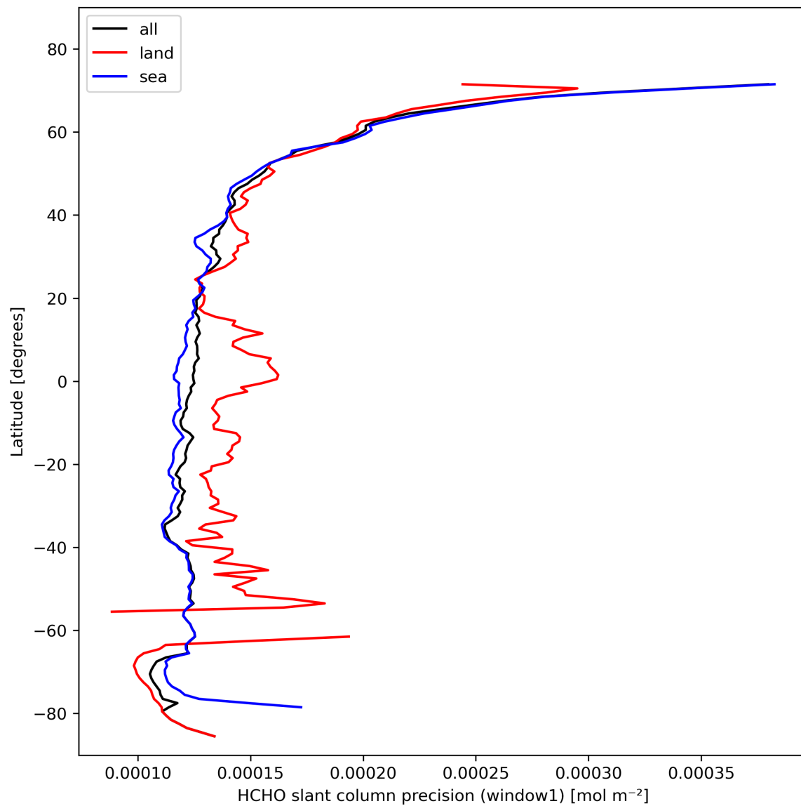
Figure 25: Zonal average of “HCHO slant column precision (window1)” for 2023-10-28 to 2023-10-30.
