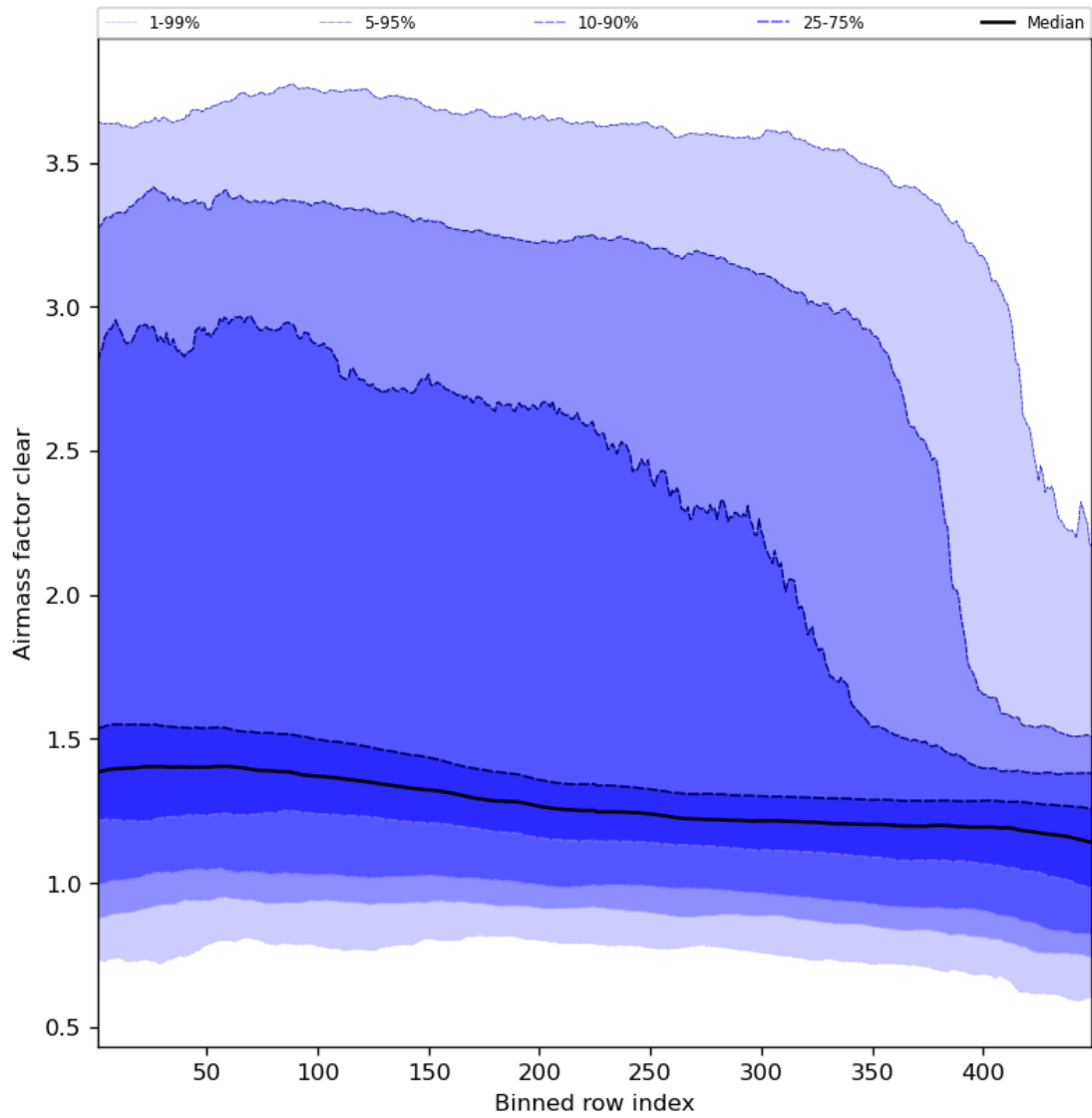
Figure 56: Along track statistics of “Airmass factor clear” for 2023-10-28 to 2023-10-30
