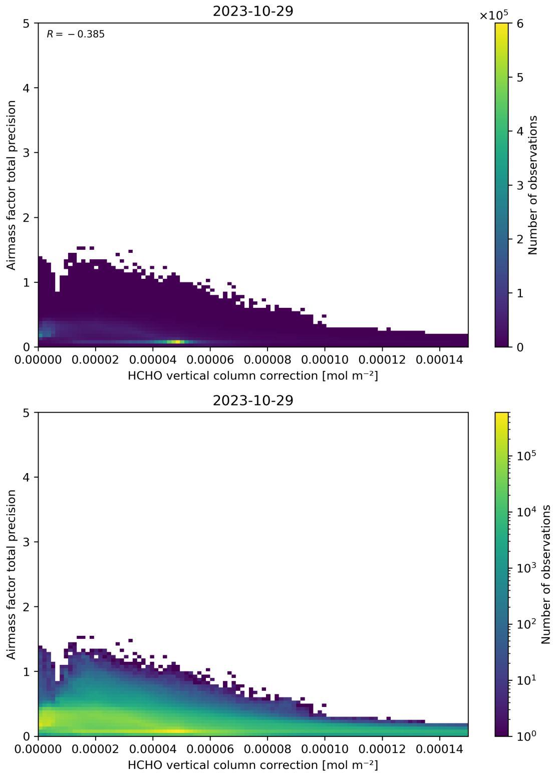
Figure 121: Scatter density plot of “HCHO vertical column correction” against “Airmass factor total precision” for 2023-10-28 to 2023-10-30.
