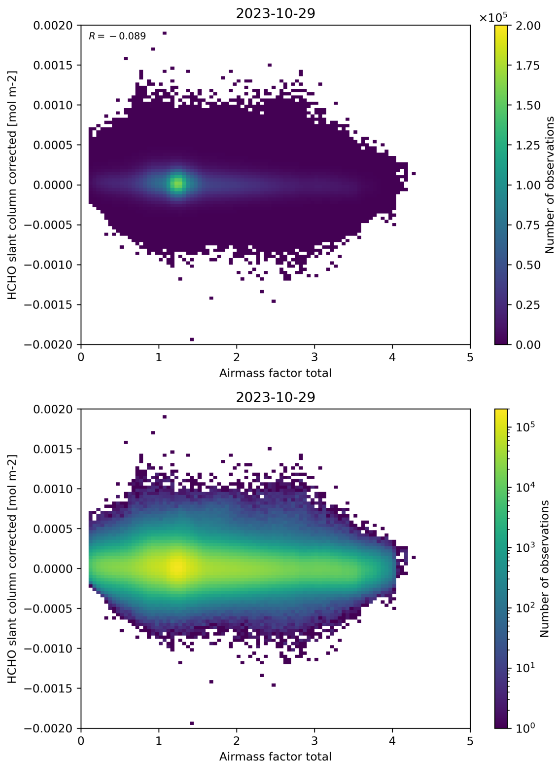
Figure 101: Scatter density plot of “Airmass factor total” against “HCHO slant column corrected” for 2023-10-28 to 2023-10-30.
