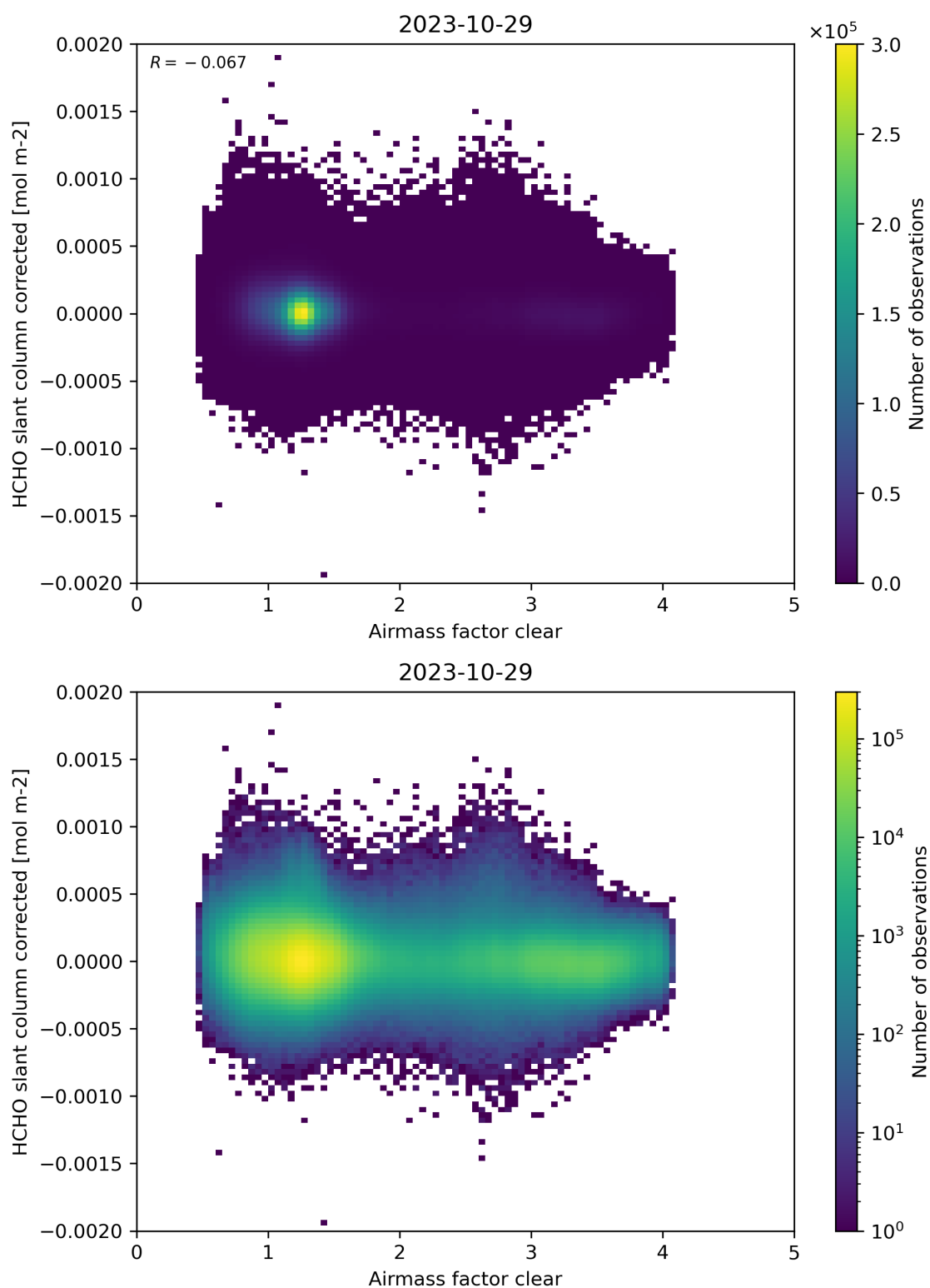
Figure 74: Scatter density plot of “Airmass factor clear” against “HCHO slant column corrected” for 2023-10-28 to 2023-10-30.
