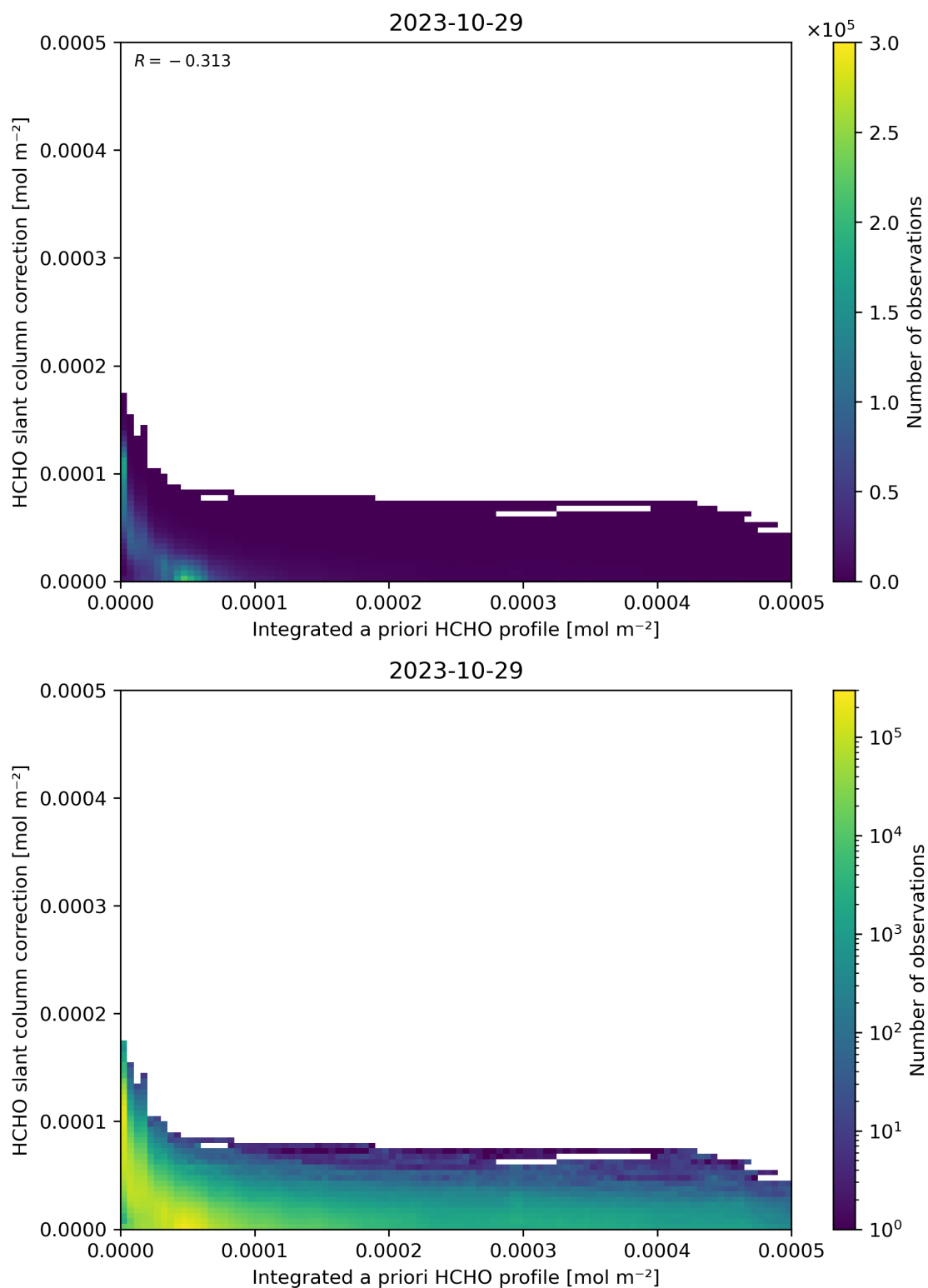
Figure 152: Scatter density plot of “Integrated a priori HCHO profile” against “HCHO slant column correction” for 2023-10-28 to 2023-10-30.
