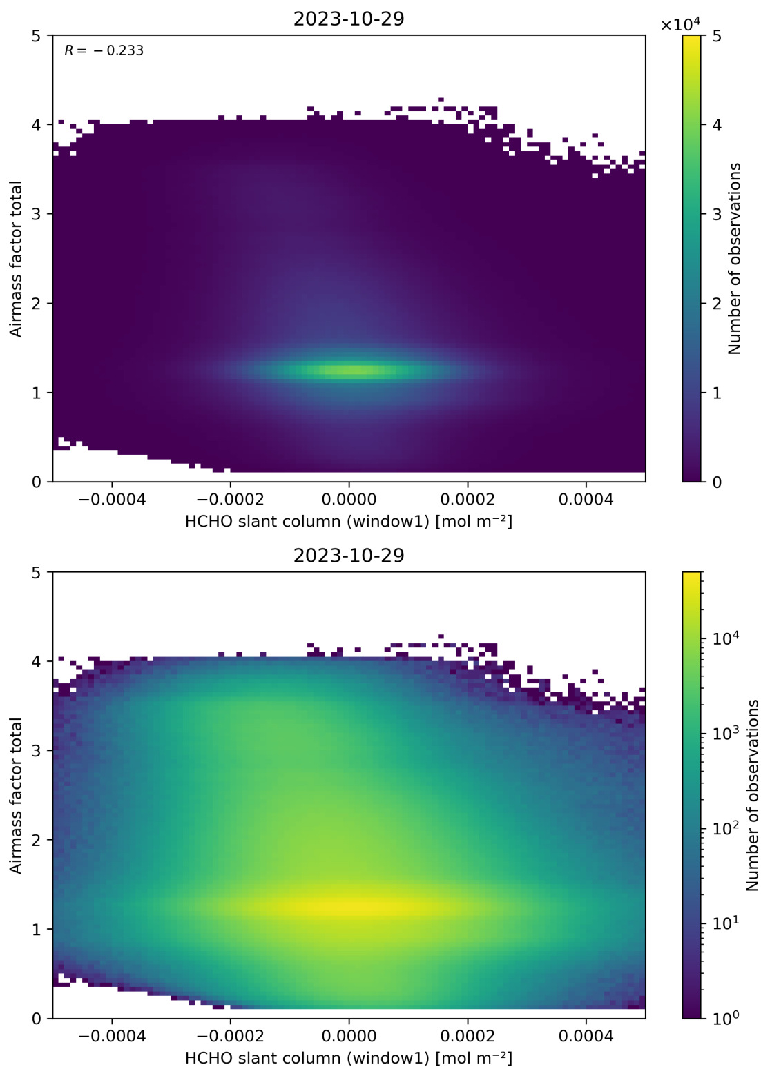
Figure 85: Scatter density plot of “HCHO slant column (window1)” against “Airmass factor total” for 2023-10-28 to 2023-10-30.
