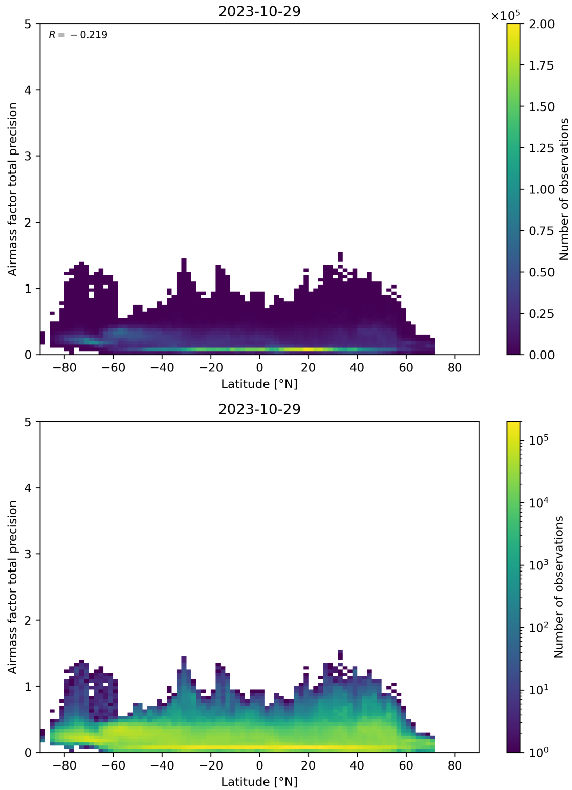
Figure 162: Scatter density plot of “Latitude” against “Airmass factor total precision” for 2023-10-28 to 2023-10-30.
