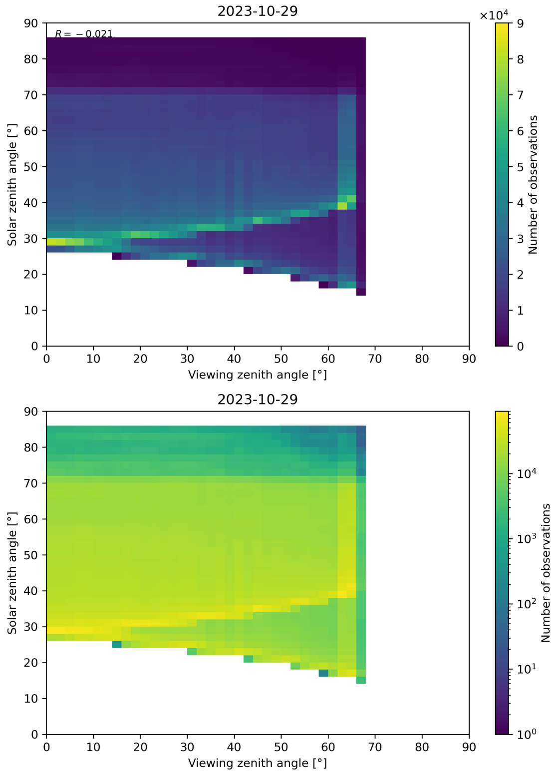
Figure 197: Scatter density plot of “Viewing zenith angle” against “Solar zenith angle” for 2023-10-28 to 2023-10-30.
