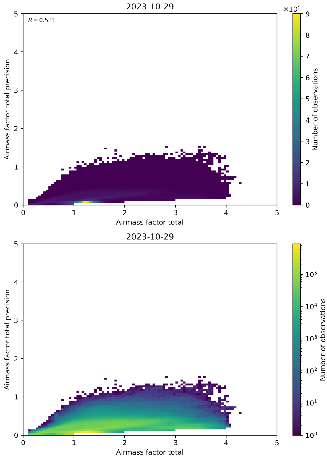
Figure 103: Scatter density plot of “Airmass factor total” against “Airmass factor total precision” for 2023-10-28 to 2023-10-30.
