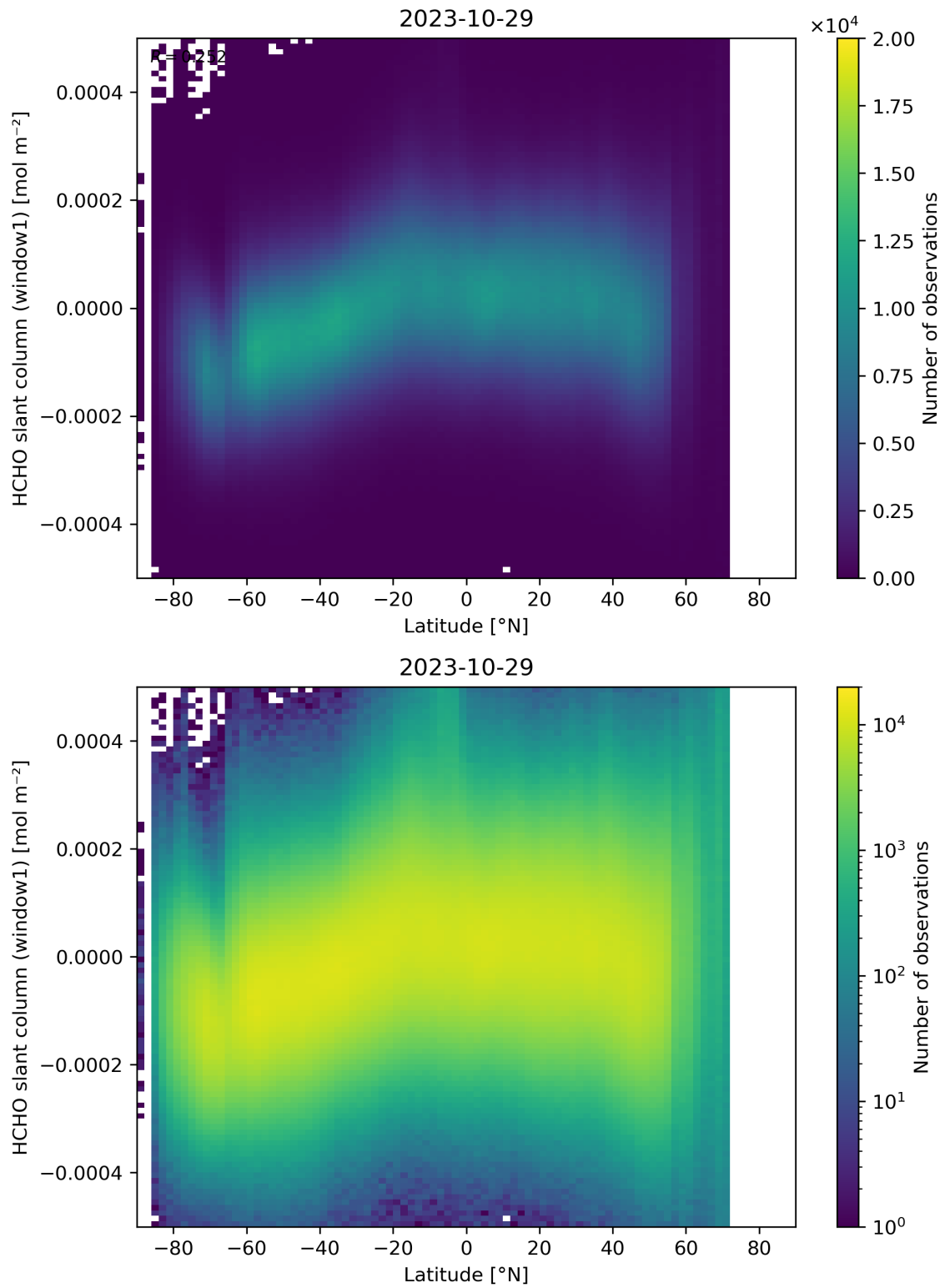
Figure 159: Scatter density plot of “Latitude” against “HCHO slant column (window1)” for 2023-10-28 to 2023-10-30.
