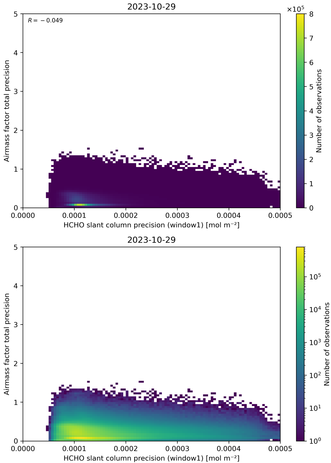
Figure 95: Scatter density plot of “HCHO slant column precision (window1)” against “Airmass factor total precision” for 2023-10-28 to 2023-10-30.
