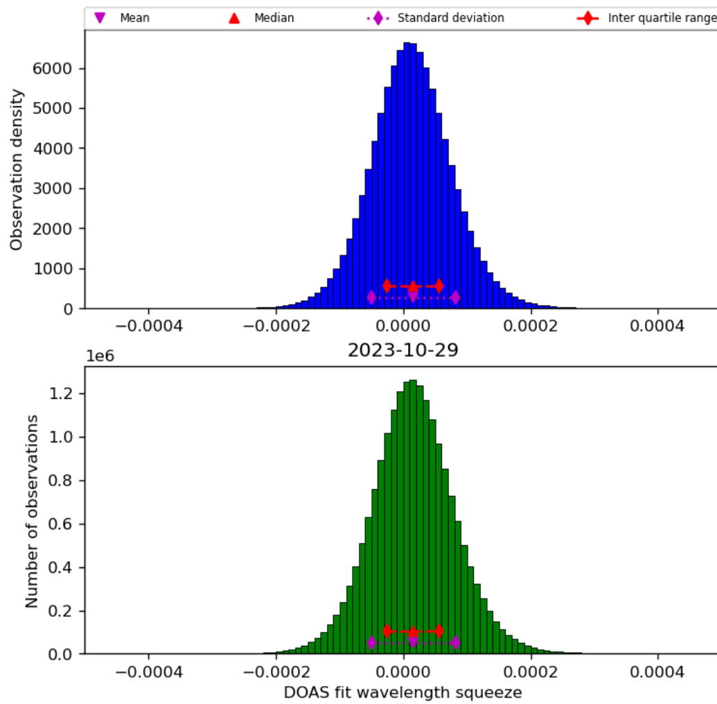
Figure 45: Histogram of “DOAS fit wavelength squeeze” for 2023-10-28 to 2023-10-30
