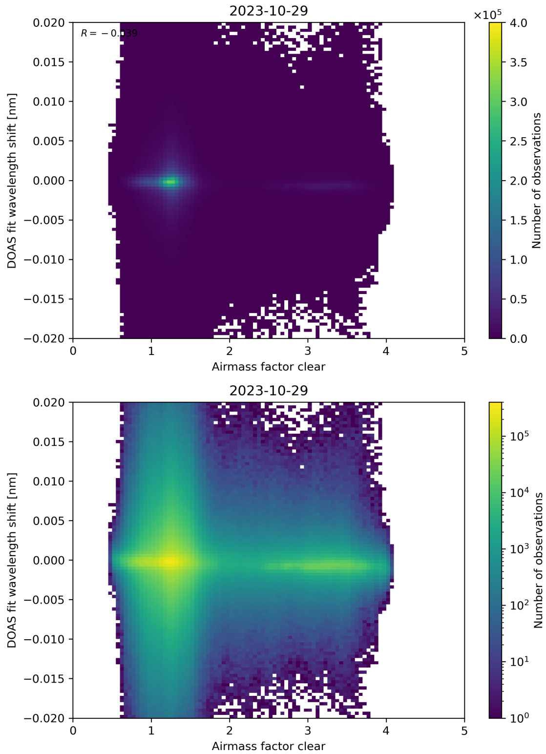
Figure 72: Scatter density plot of “Airmass factor clear” against “DOAS fit wavelength shift” for 2023-10-28 to 2023-10-30.
