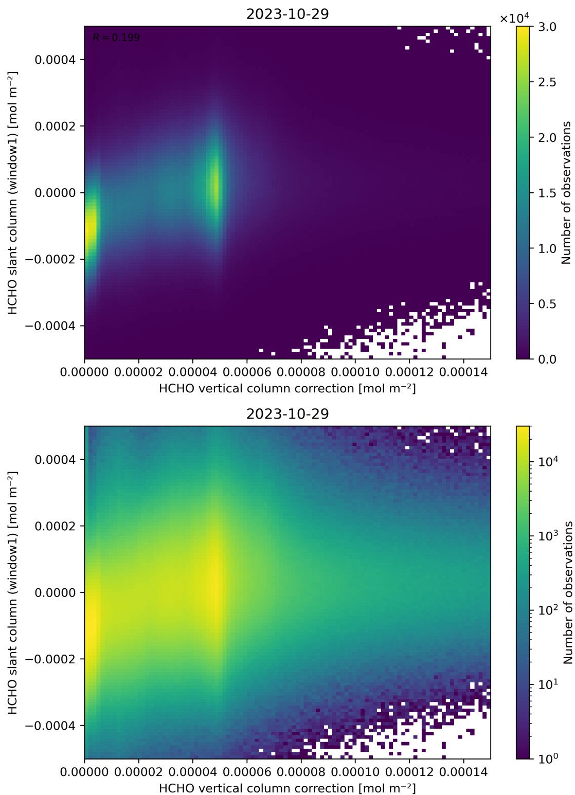
Figure 118: Scatter density plot of “HCHO vertical column correction” against “HCHO slant column (window1)” for 2023-10-28 to 2023-10-30.
