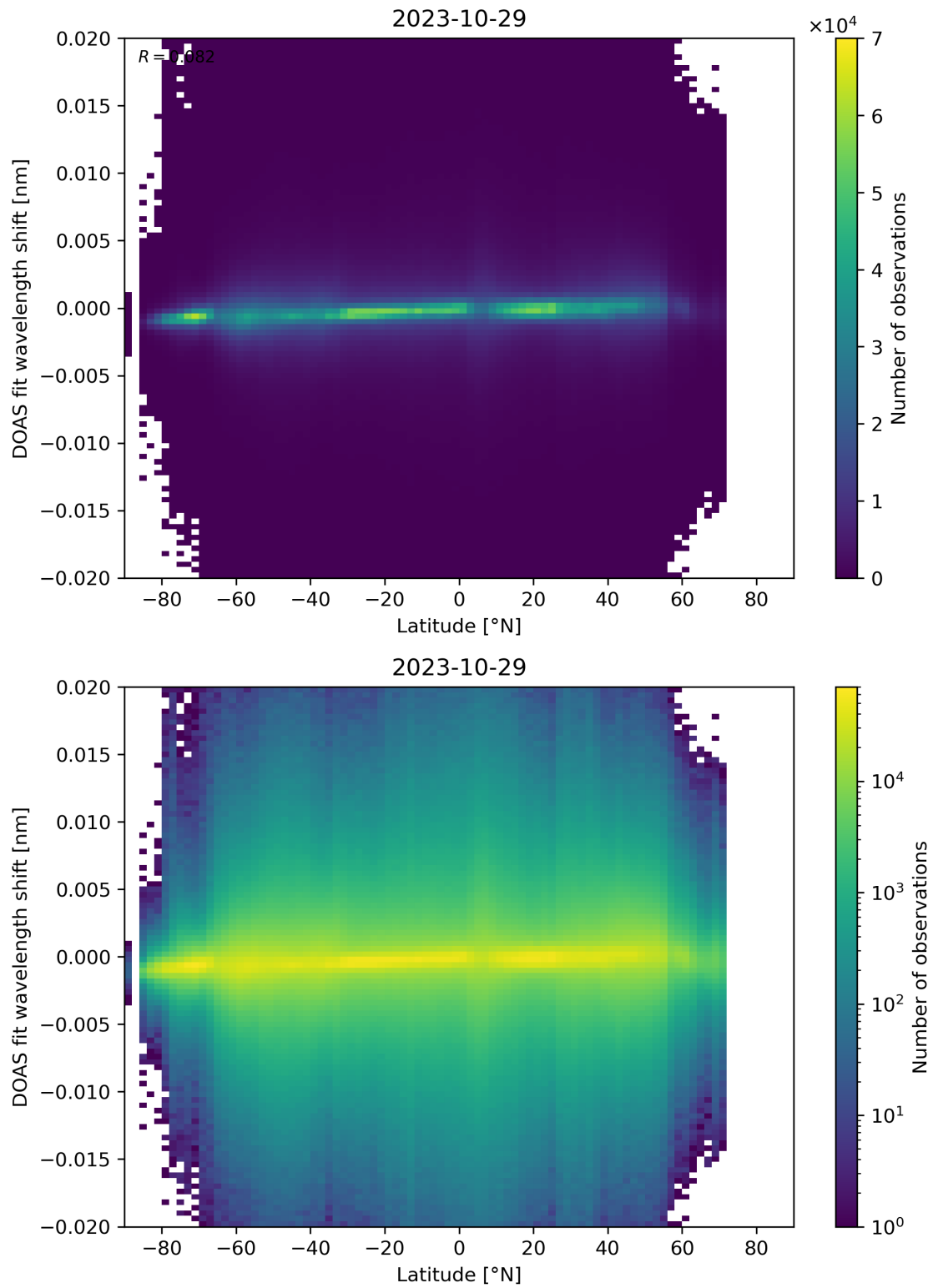
Figure 154: Scatter density plot of “Latitude” against “DOAS fit wavelength shift” for 2023-10-28 to 2023-10-30.
