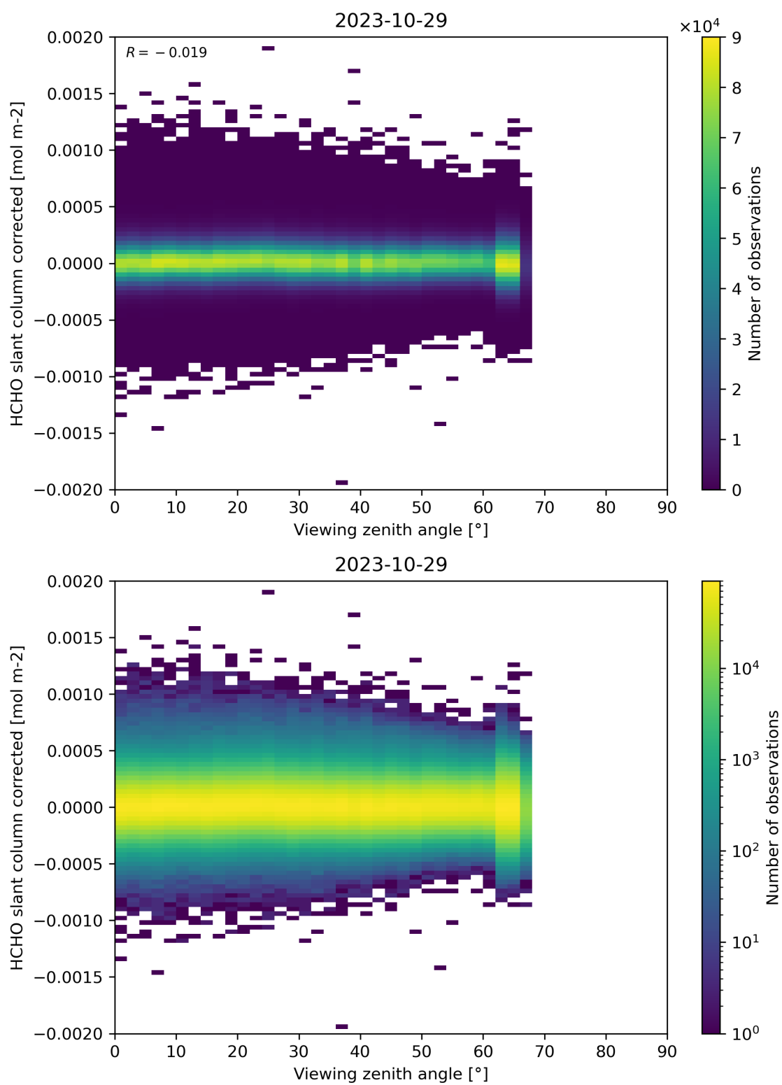
Figure 186: Scatter density plot of “Viewing zenith angle” against “HCHO slant column corrected” for 2023-10-28 to 2023-10-30.
