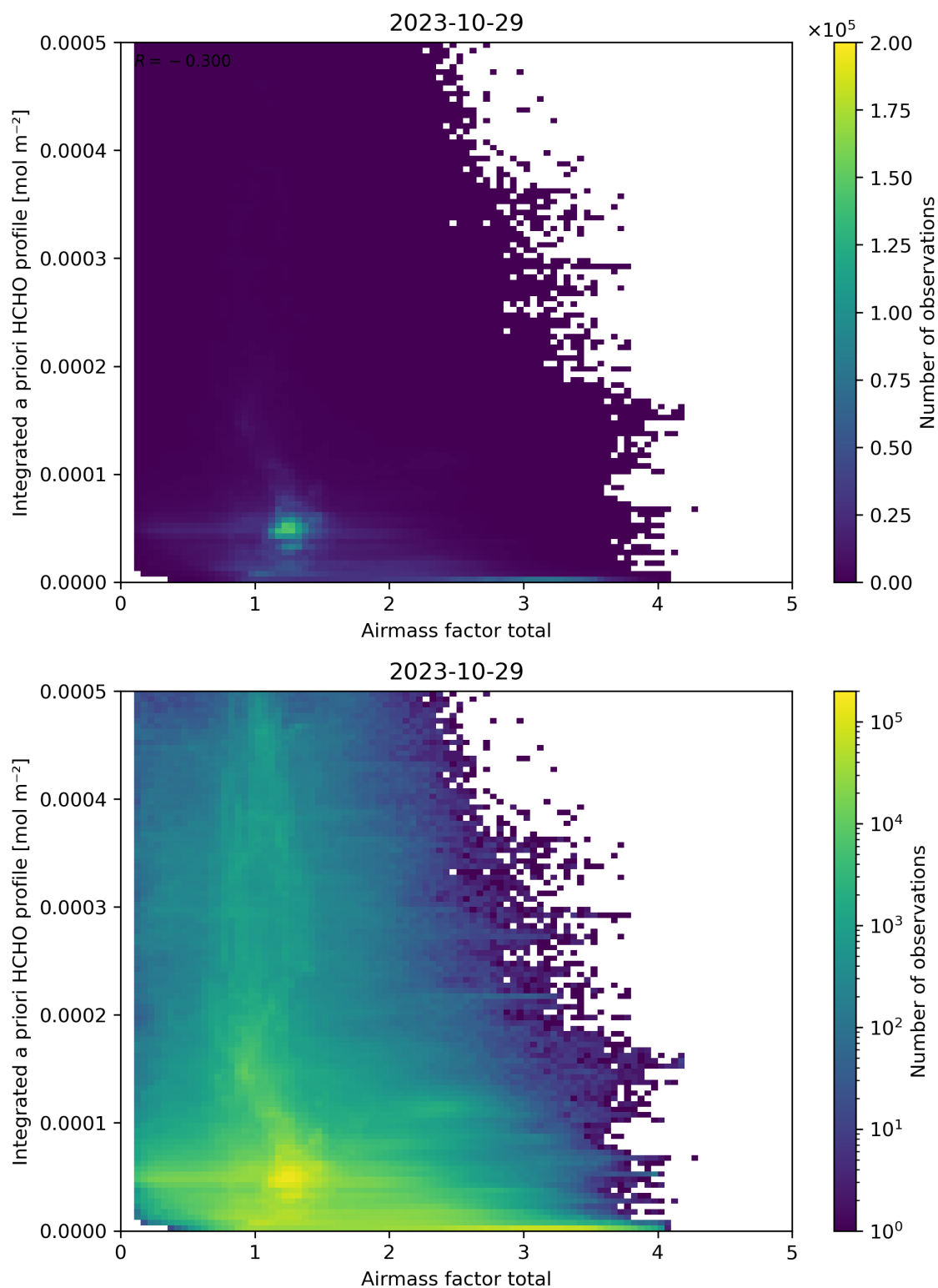
Figure 104: Scatter density plot of “Airmass factor total” against “Integrated a priori HCHO profile” for 2023-10-28 to 2023-10-30.
