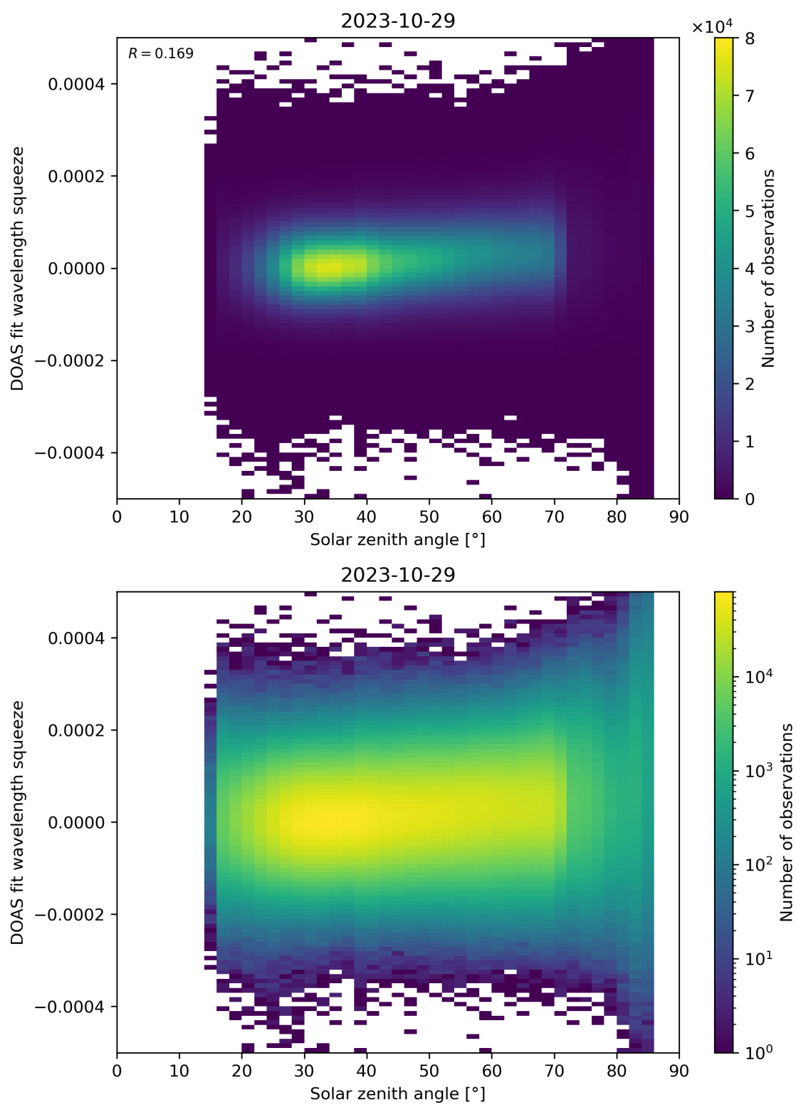
Figure 169: Scatter density plot of “Solar zenith angle” against “DOAS fit wavelength squeeze” for 2023-10-28 to 2023-10-30.
