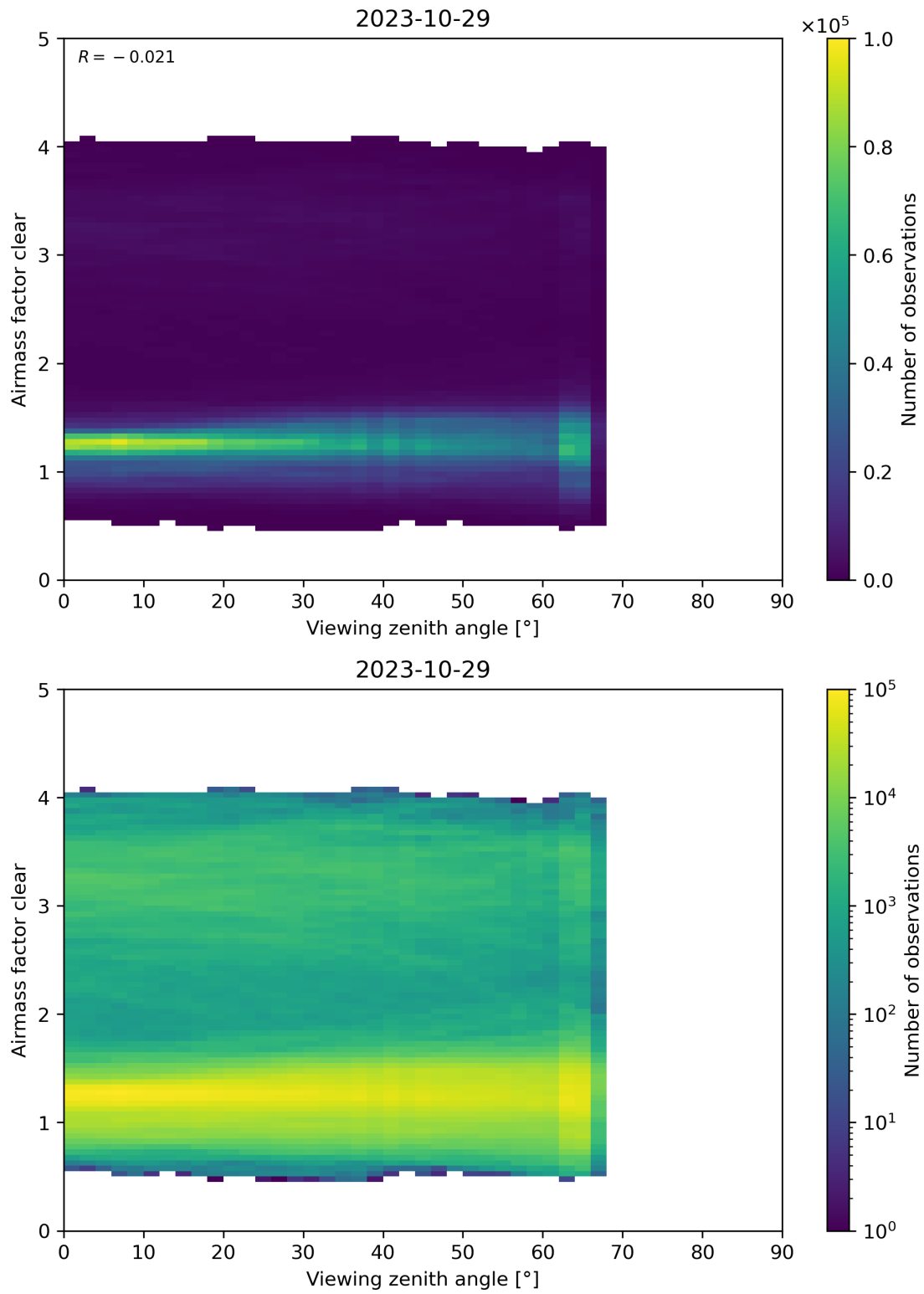
Figure 185: Scatter density plot of “Viewing zenith angle” against “Airmass factor clear” for 2023-10-28 to 2023-10-30.
