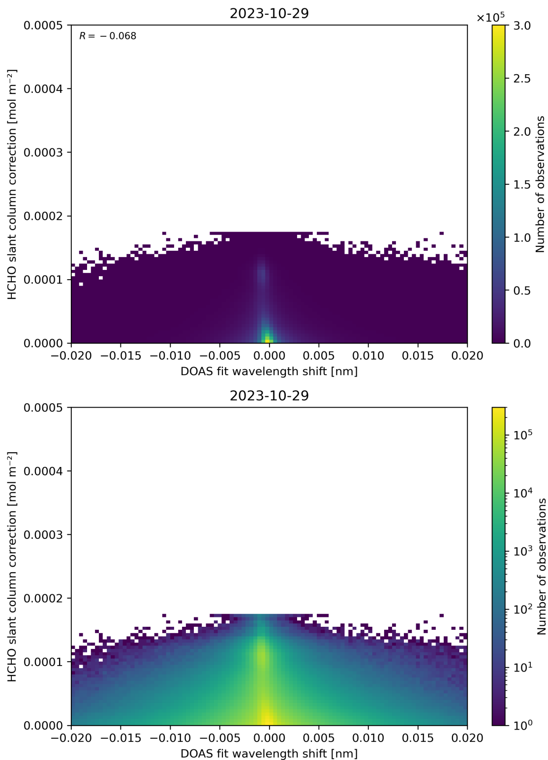
Figure 67: Scatter density plot of “DOAS fit wavelength shift” against “HCHO slant column correction” for 2023-10-28 to 2023-10-30.
