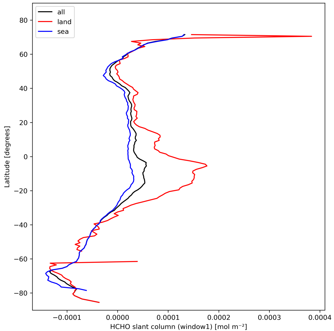
Figure 24: Zonal average of “HCHO slant column (window1)” for 2023-10-28 to 2023-10-30.
