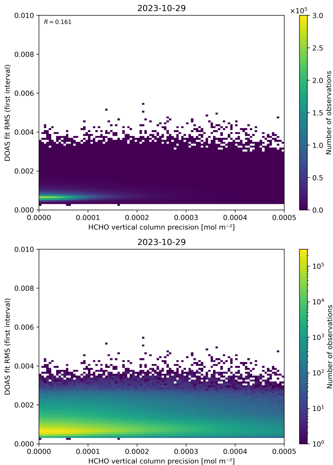
Figure 136: Scatter density plot of “HCHO vertical column precision” against “DOAS fit RMS (first interval)” for 2023-10-28 to 2023-10-30.
