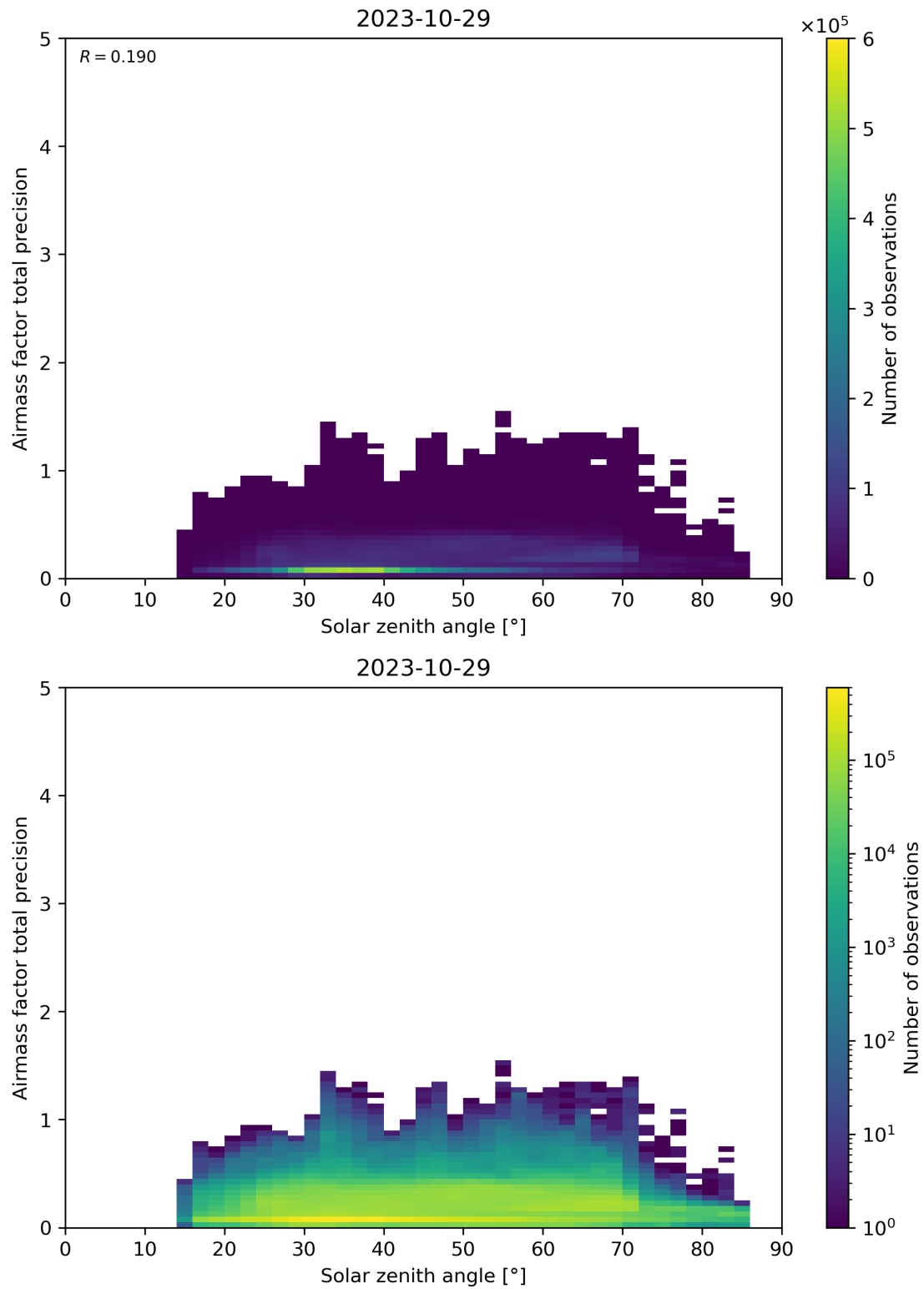
Figure 176: Scatter density plot of “Solar zenith angle” against “Airmass factor total precision” for 2023-10-28 to 2023-10-30.
