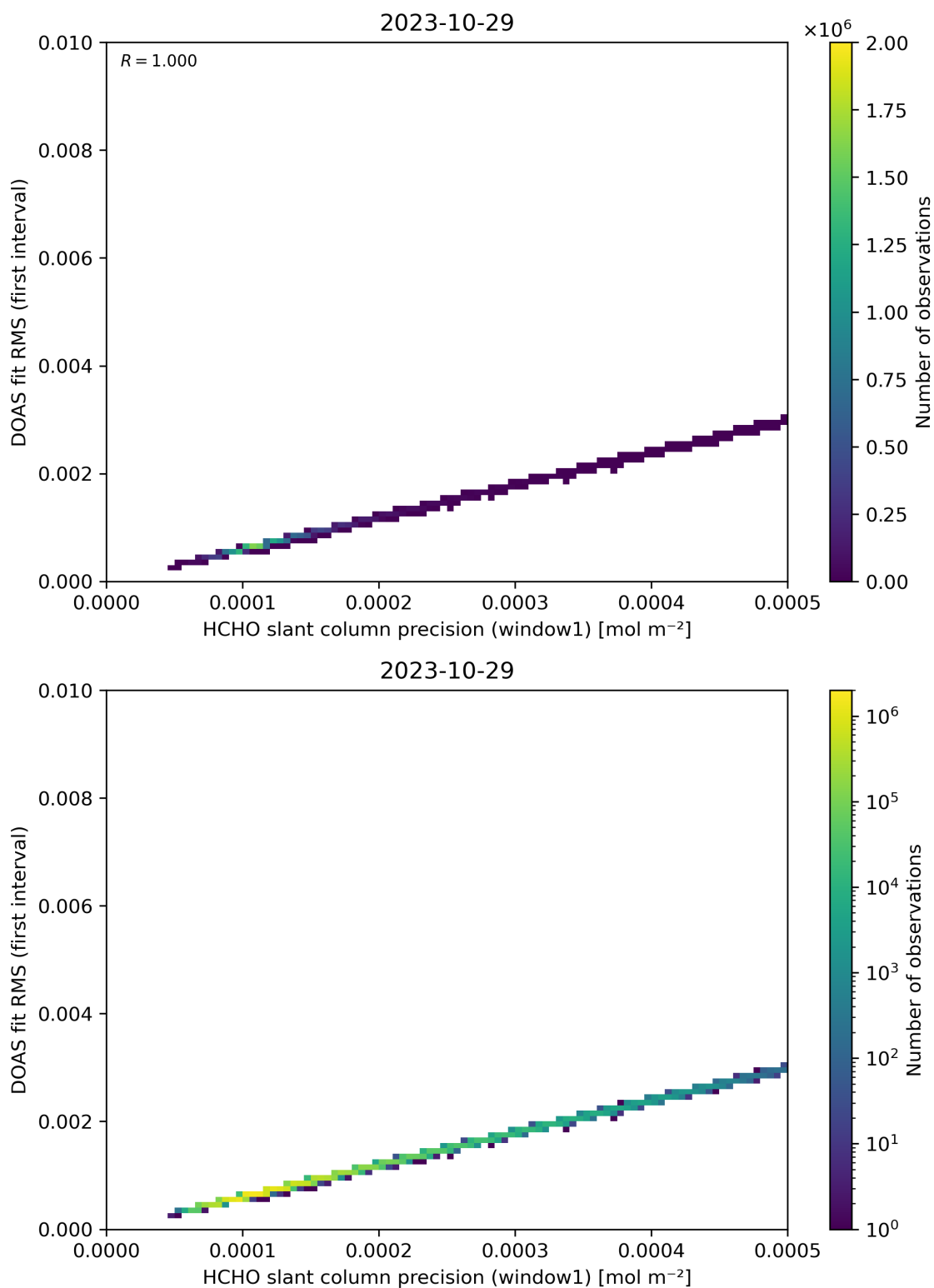
Figure 88: Scatter density plot of “HCHO slant column precision (window1)” against “DOAS fit RMS (first interval)” for 2023-10-28 to 2023-10-30.
