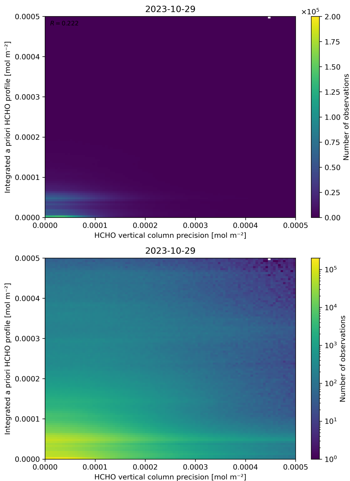
Figure 147: Scatter density plot of “HCHO vertical column precision” against “Integrated a priori HCHO profile” for 2023-10-28 to 2023-10-30.
