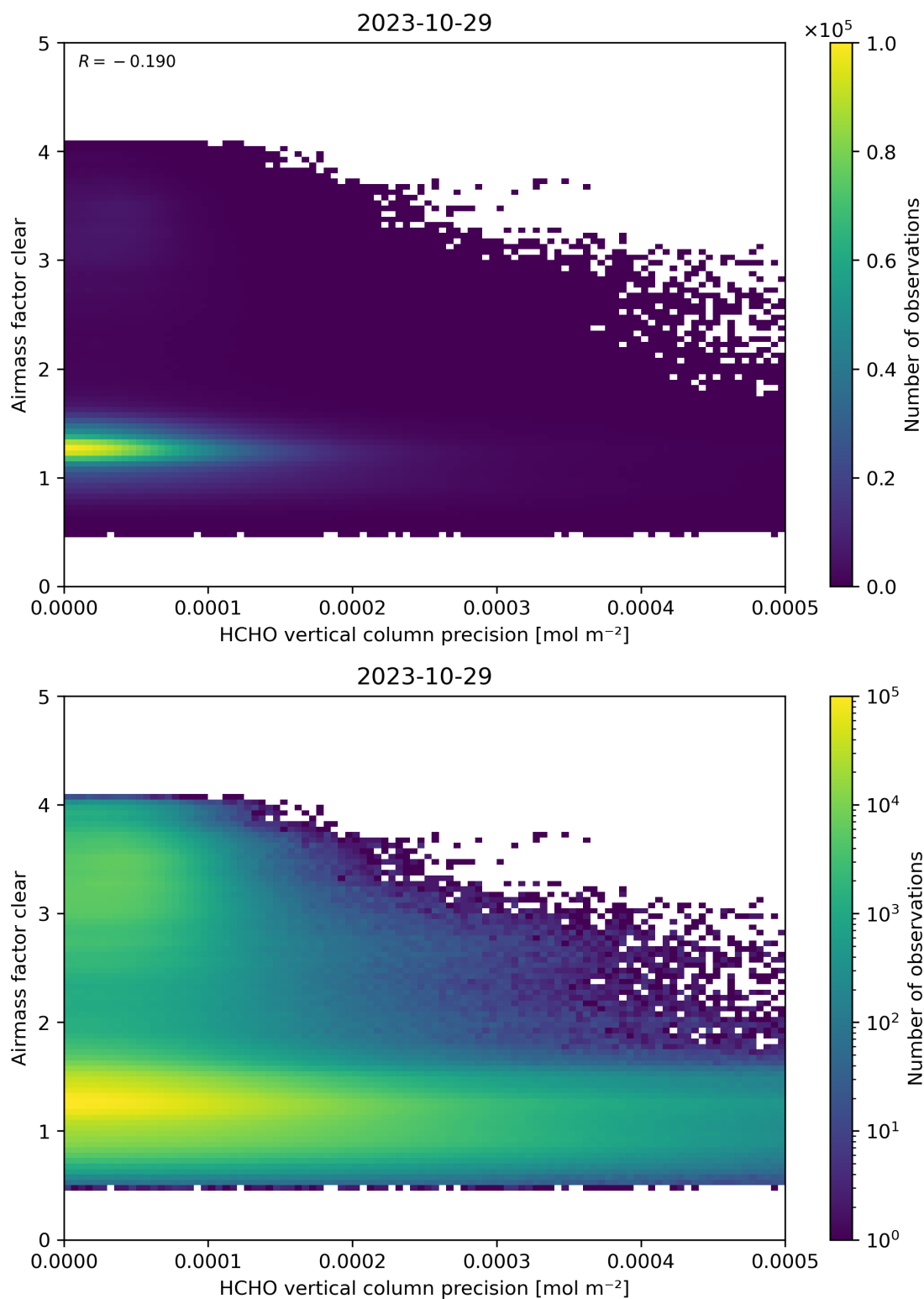
Figure 139: Scatter density plot of “HCHO vertical column precision” against “Airmass factor clear” for 2023-10-28 to 2023-10-30.
