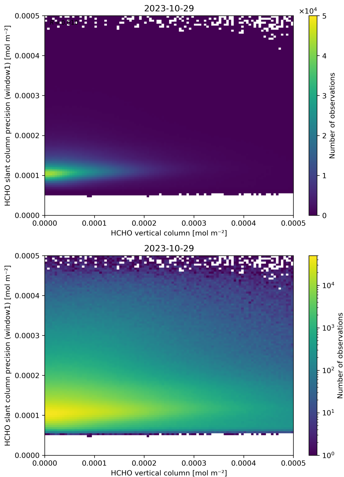
Figure 130: Scatter density plot of “HCHO vertical column” against “HCHO slant column precision (window1)” for 2023-10-28 to 2023-10-30.
