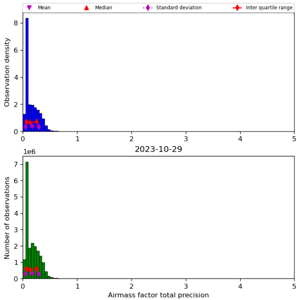
Figure 41: Histogram of “Airmass factor total precision” for 2023-10-28 to 2023-10-30
