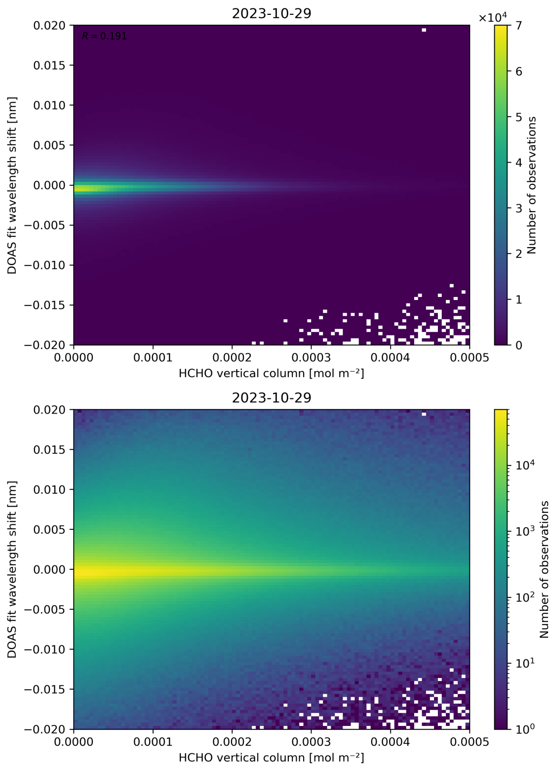
Figure 124: Scatter density plot of “HCHO vertical column” against “DOAS fit wavelength shift” for 2023-10-28 to 2023-10-30.
