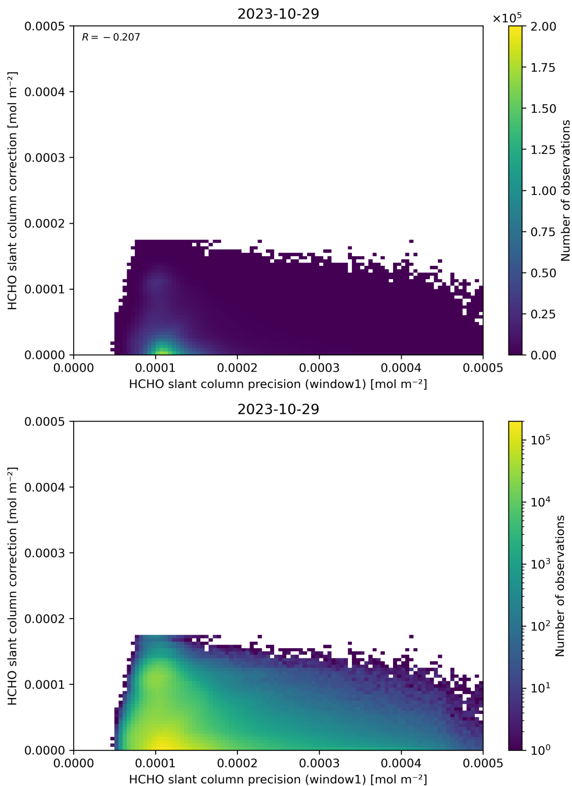
Figure 93: Scatter density plot of “HCHO slant column precision (window1)” against “HCHO slant column correction” for 2023-10-28 to 2023-10-30.
