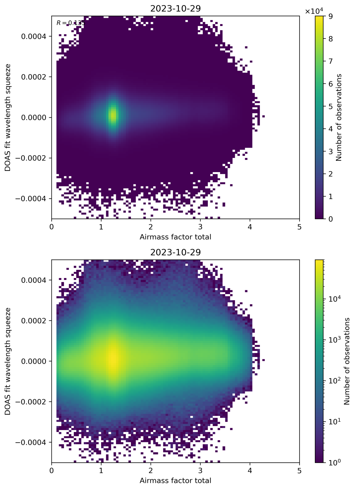
Figure 99: Scatter density plot of “Airmass factor total” against “DOAS fit wavelength squeeze” for 2023-10-28 to 2023-10-30.
