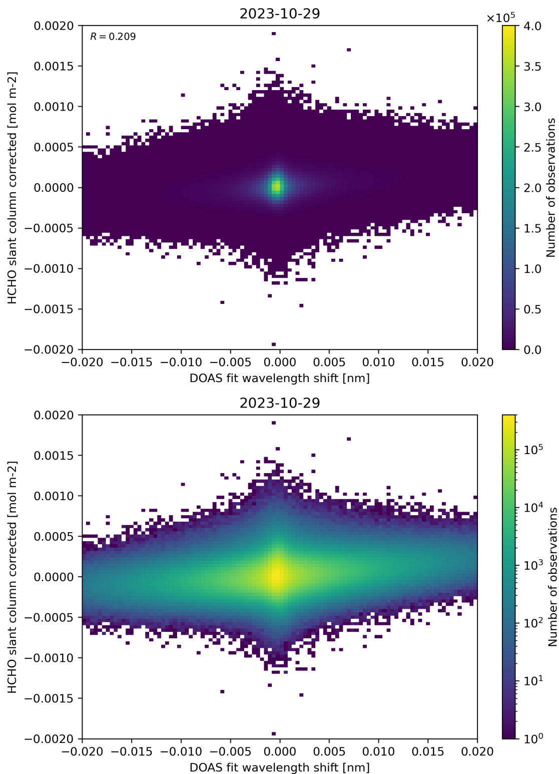
Figure 66: Scatter density plot of “DOAS fit wavelength shift” against “HCHO slant column corrected” for 2023-10-28 to 2023-10-30.
