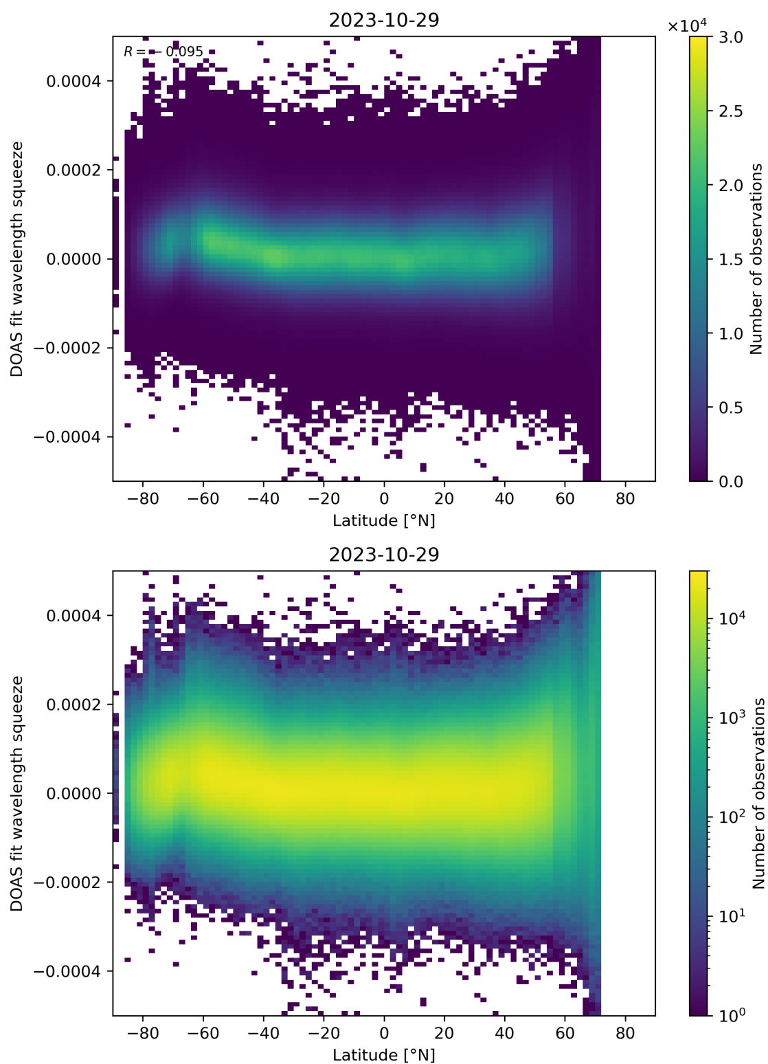
Figure 155: Scatter density plot of “Latitude” against “DOAS fit wavelength squeeze” for 2023-10-28 to 2023-10-30.
