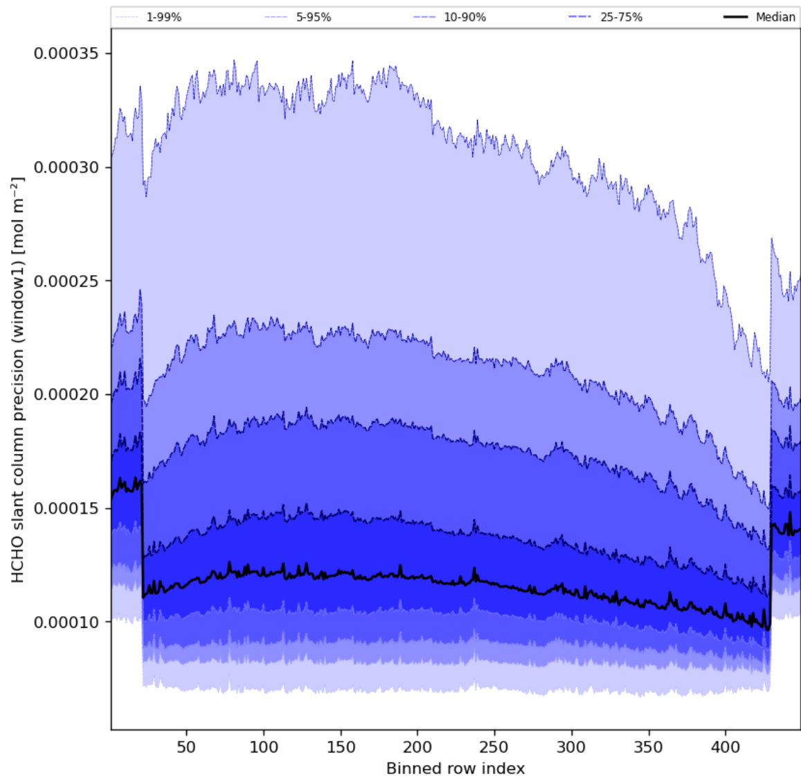
Figure 53: Along track statistics of “HCHO slant column precision (window1)” for 2023-10-28 to 2023-10-30
