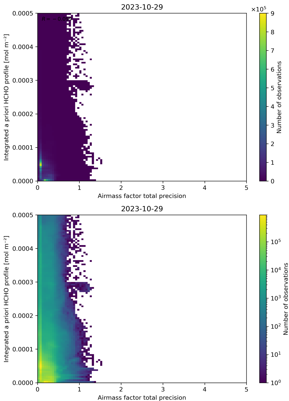
Figure 111: Scatter density plot of “Airmass factor total precision” against “Integrated a priori HCHO profile” for 2023-10-28 to 2023-10-30.
