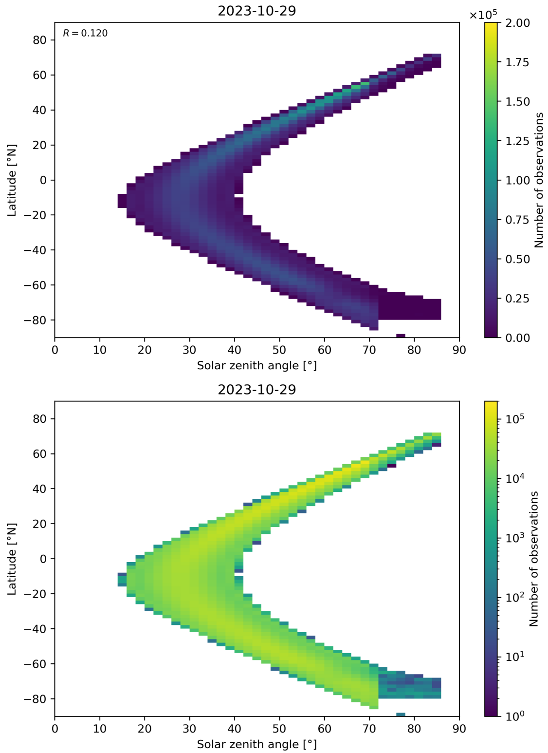
Figure 181: Scatter density plot of “Solar zenith angle” against “Latitude” for 2023-10-28 to 2023-10-30.
