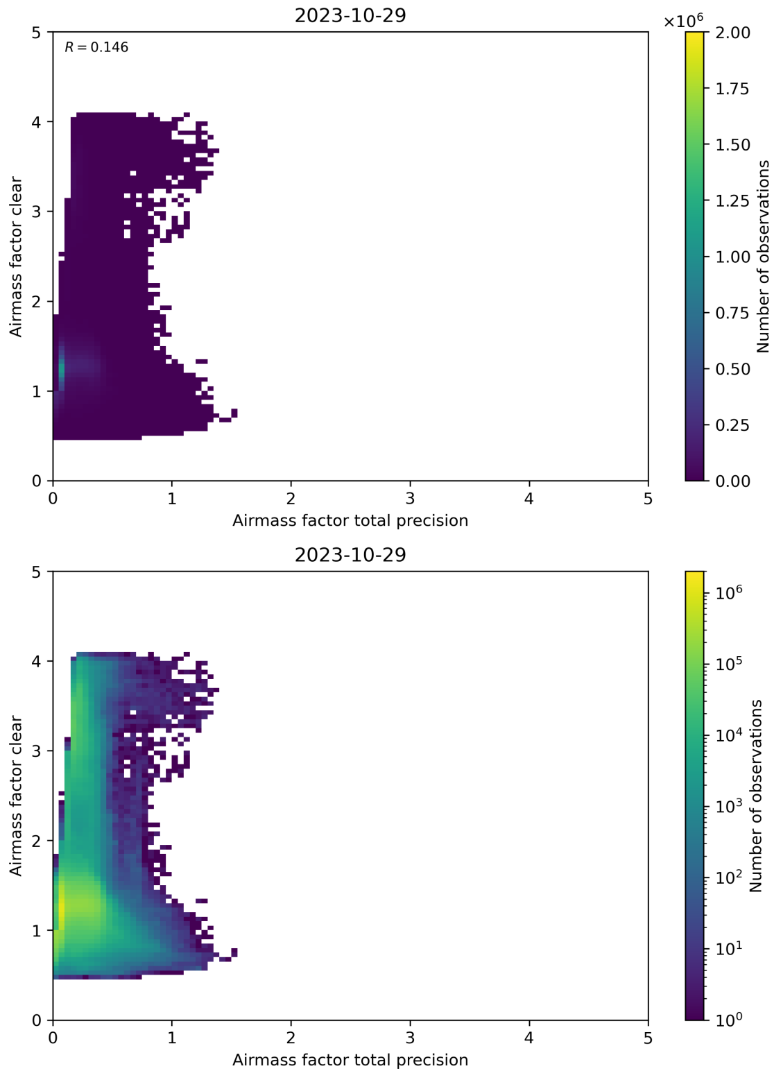
Figure 108: Scatter density plot of “Airmass factor total precision” against “Airmass factor clear” for 2023-10-28 to 2023-10-30.
