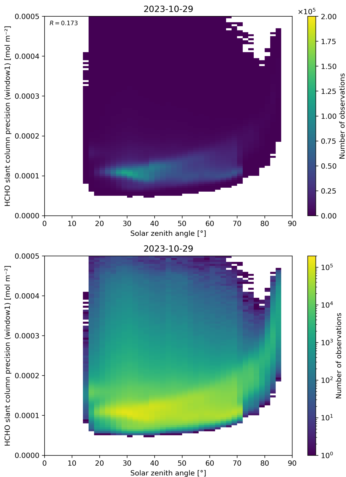
Figure 174: Scatter density plot of “Solar zenith angle” against “HCHO slant column precision (window1)” for 2023-10-28 to 2023-10-30.
