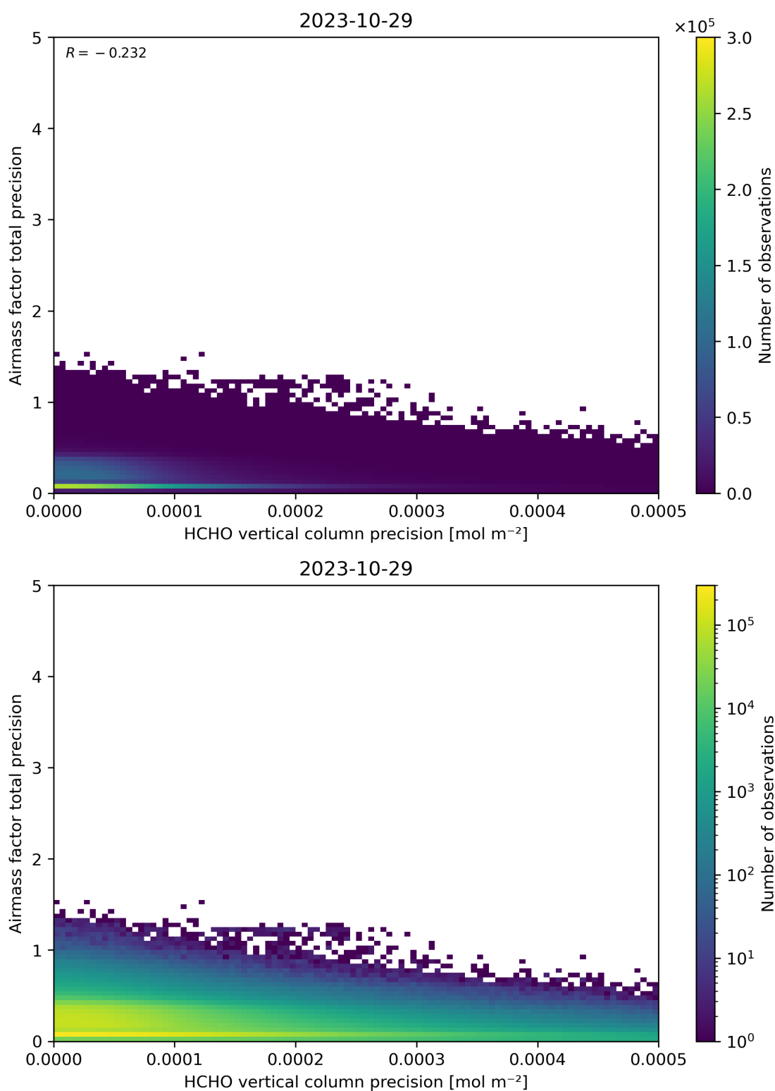
Figure 145: Scatter density plot of “HCHO vertical column precision” against “Airmass factor total precision” for 2023-10-28 to 2023-10-30.
