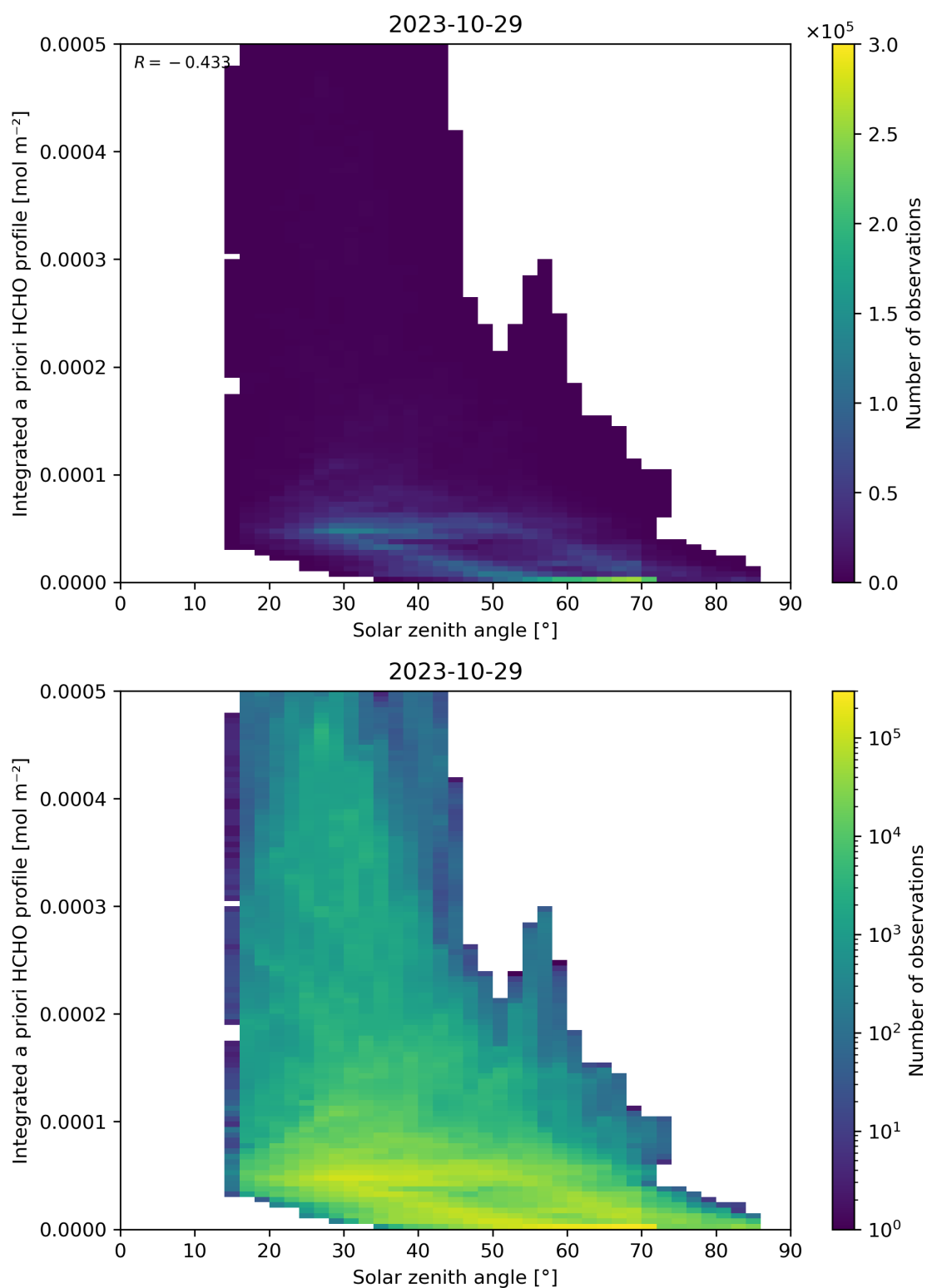
Figure 180: Scatter density plot of “Solar zenith angle” against “Integrated a priori HCHO profile” for 2023-10-28 to 2023-10-30.
