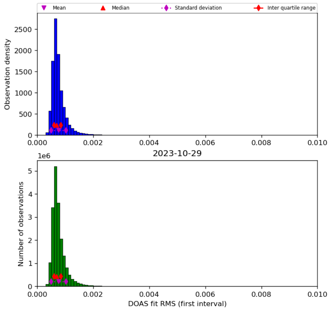
Figure 46: Histogram of “DOAS fit RMS (first interval)” for 2023-10-28 to 2023-10-30
