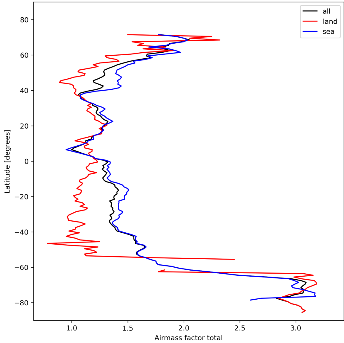
Figure 26: Zonal average of “Airmass factor total” for 2023-10-28 to 2023-10-30.
