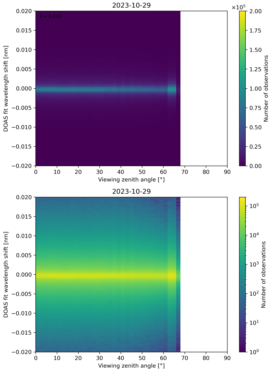
Figure 183: Scatter density plot of “Viewing zenith angle” against “DOAS fit wavelength shift” for 2023-10-28 to 2023-10-30.
