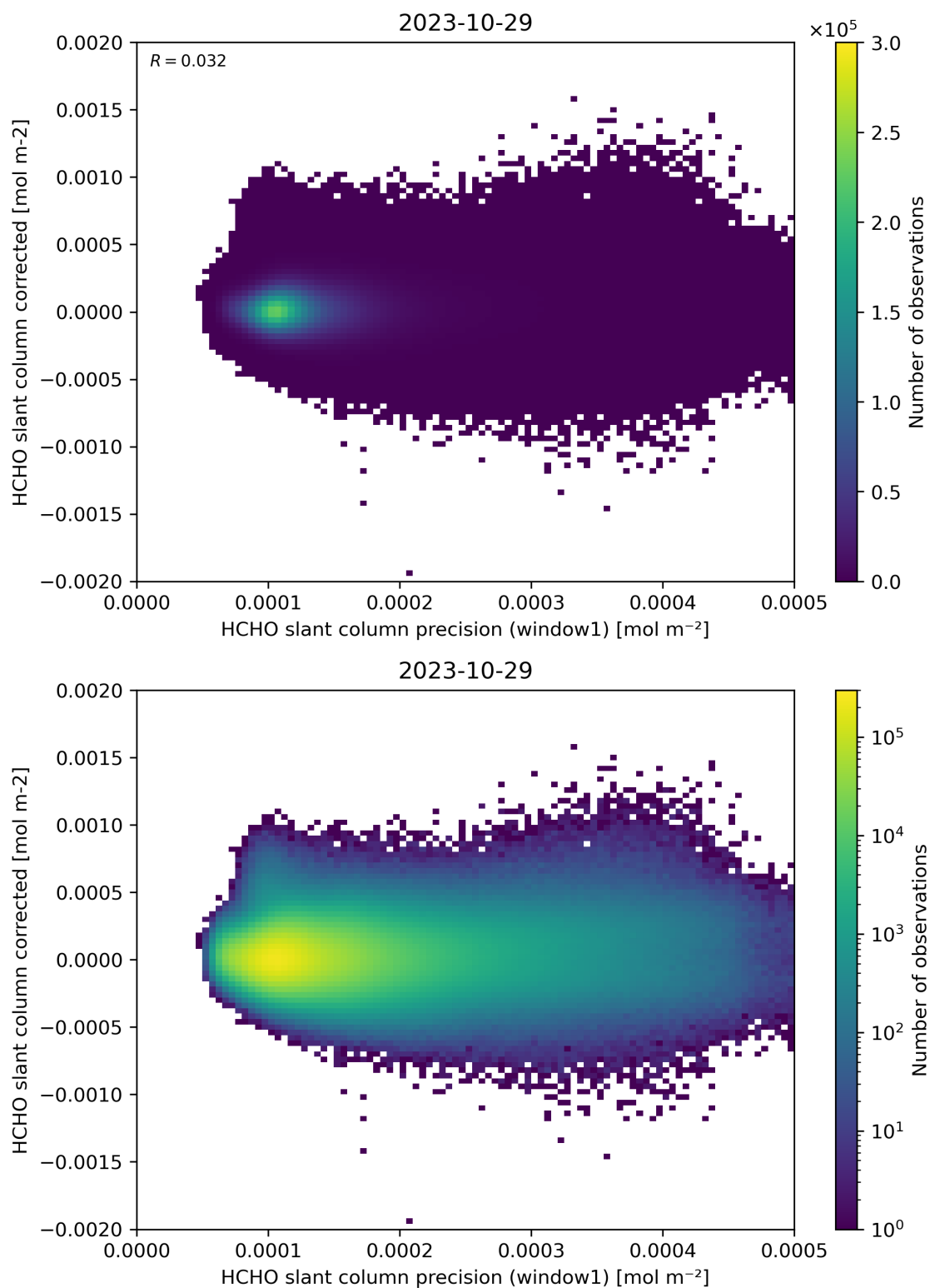
Figure 92: Scatter density plot of “HCHO slant column precision (window1)” against “HCHO slant column corrected” for 2023-10-28 to 2023-10-30.
