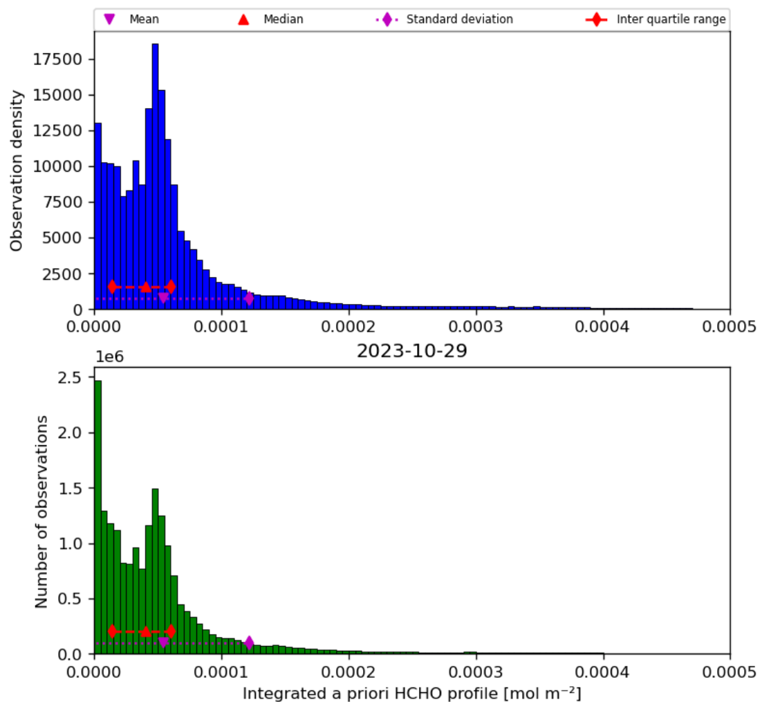
Figure 43: Histogram of “Integrated a priori HCHO profile” for 2023-10-28 to 2023-10-30
