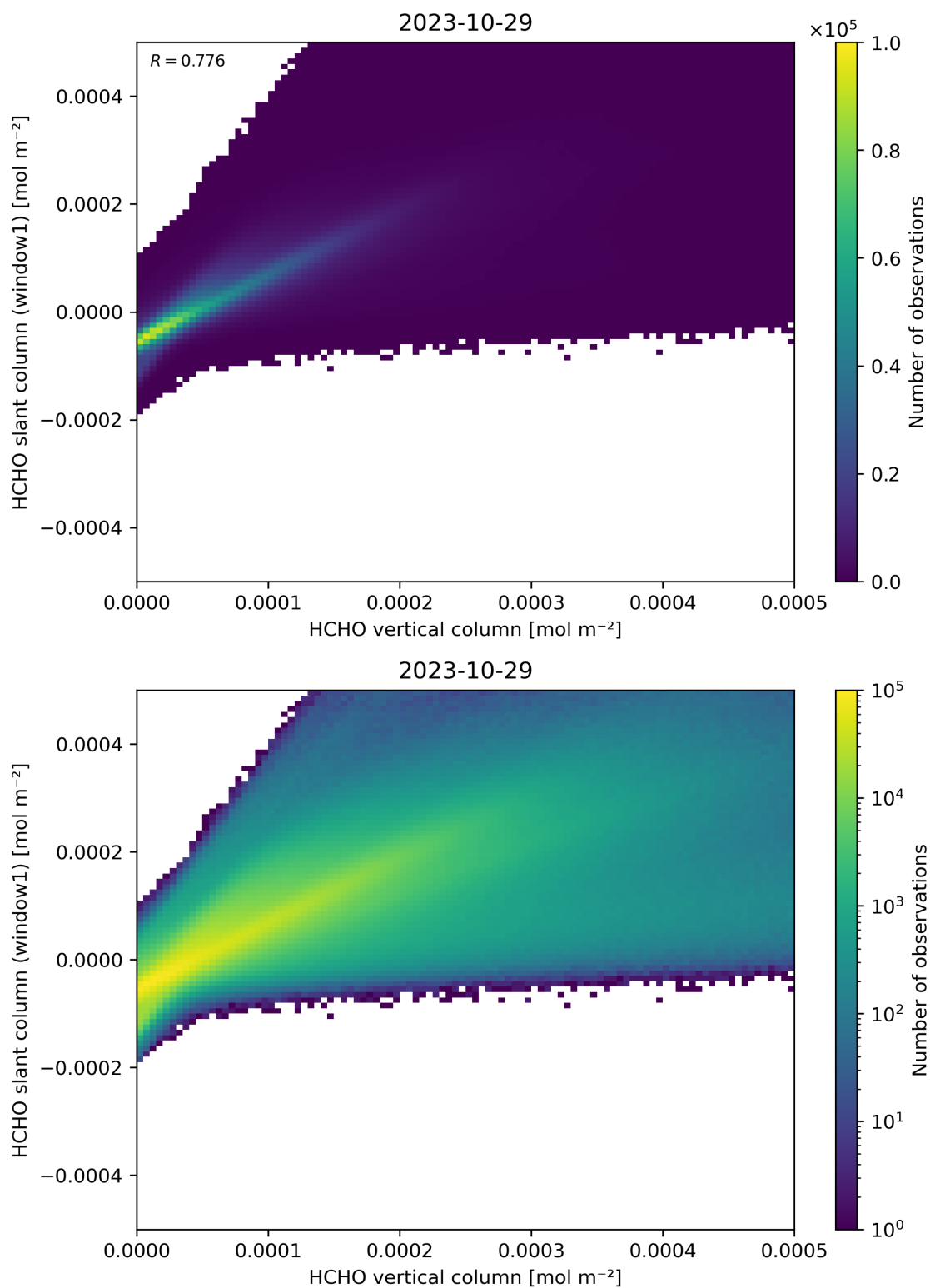
Figure 129: Scatter density plot of “HCHO vertical column” against “HCHO slant column (window1)” for 2023-10-28 to 2023-10-30.
