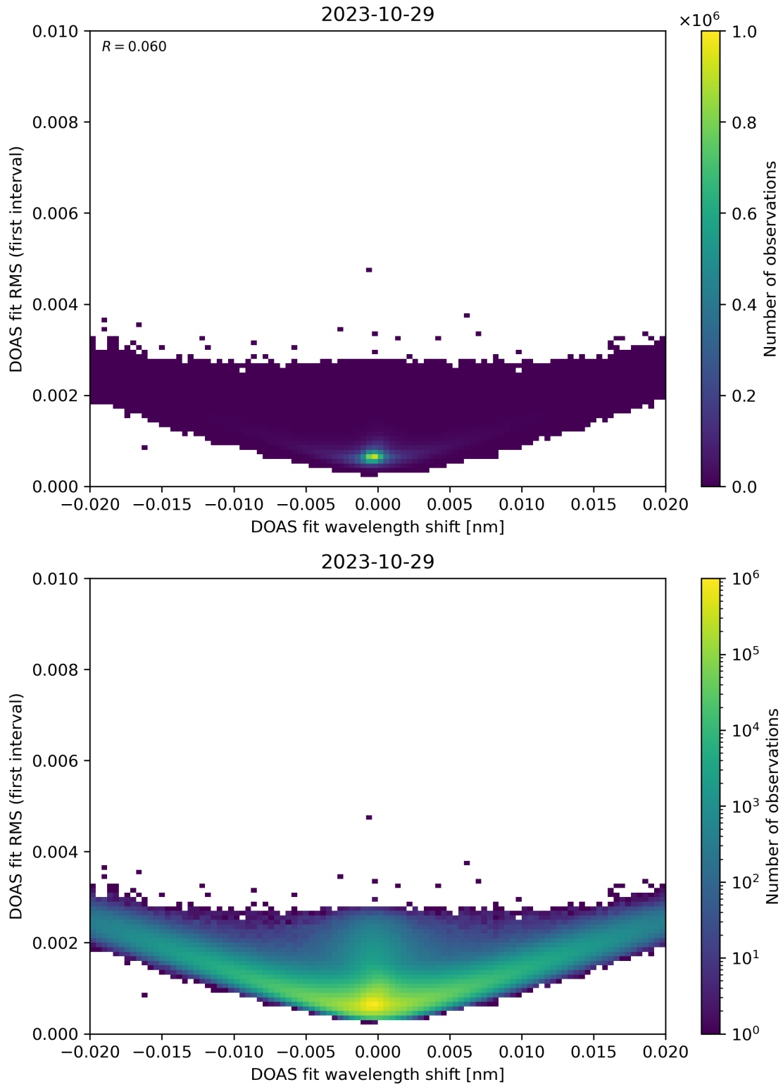
Figure 64: Scatter density plot of “DOAS fit wavelength shift” against “DOAS fit RMS (first interval)” for 2023-10-28 to 2023-10-30.
