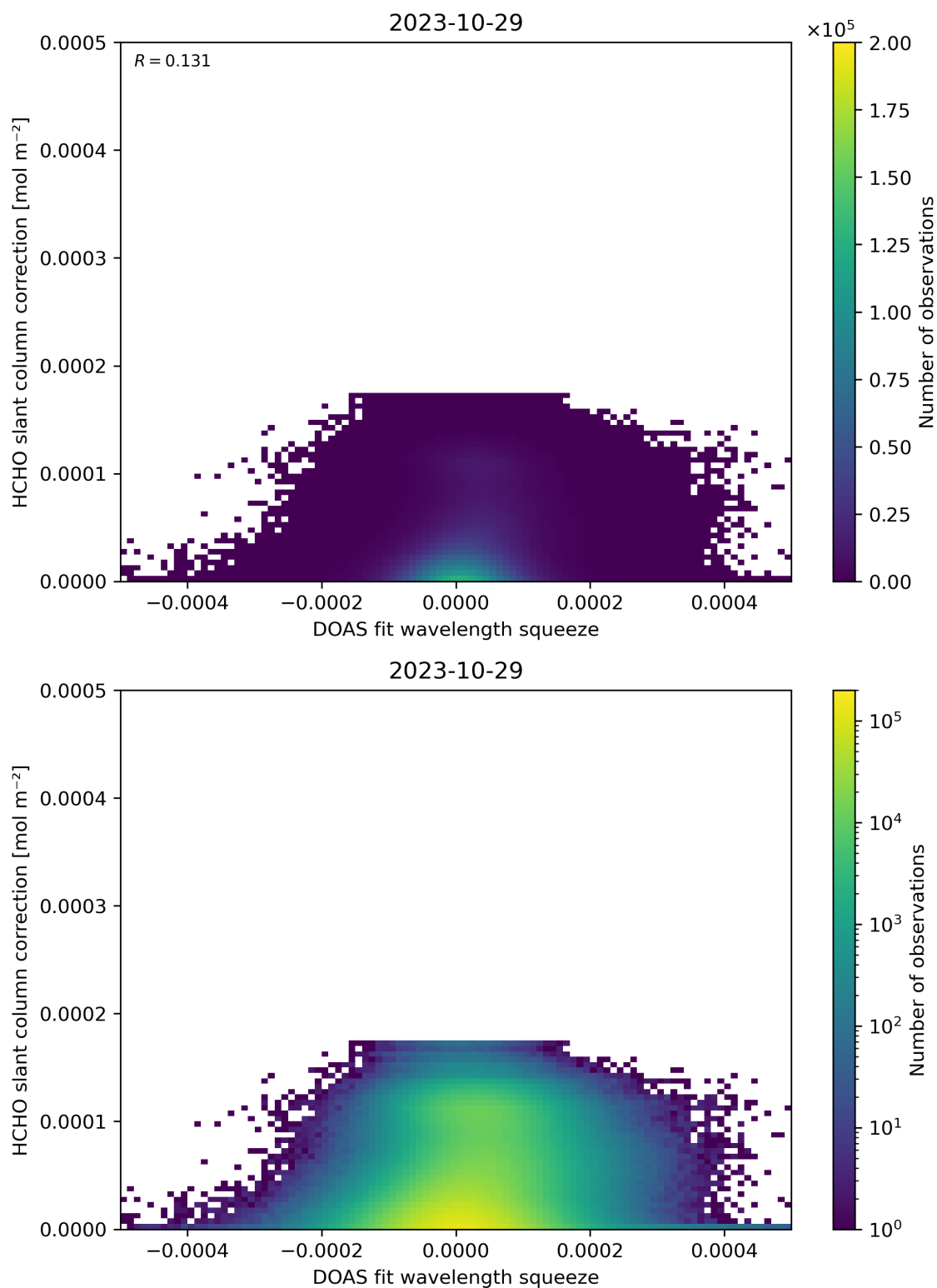
Figure 70: Scatter density plot of “DOAS fit wavelength squeeze” against “HCHO slant column correction” for 2023-10-28 to 2023-10-30.
