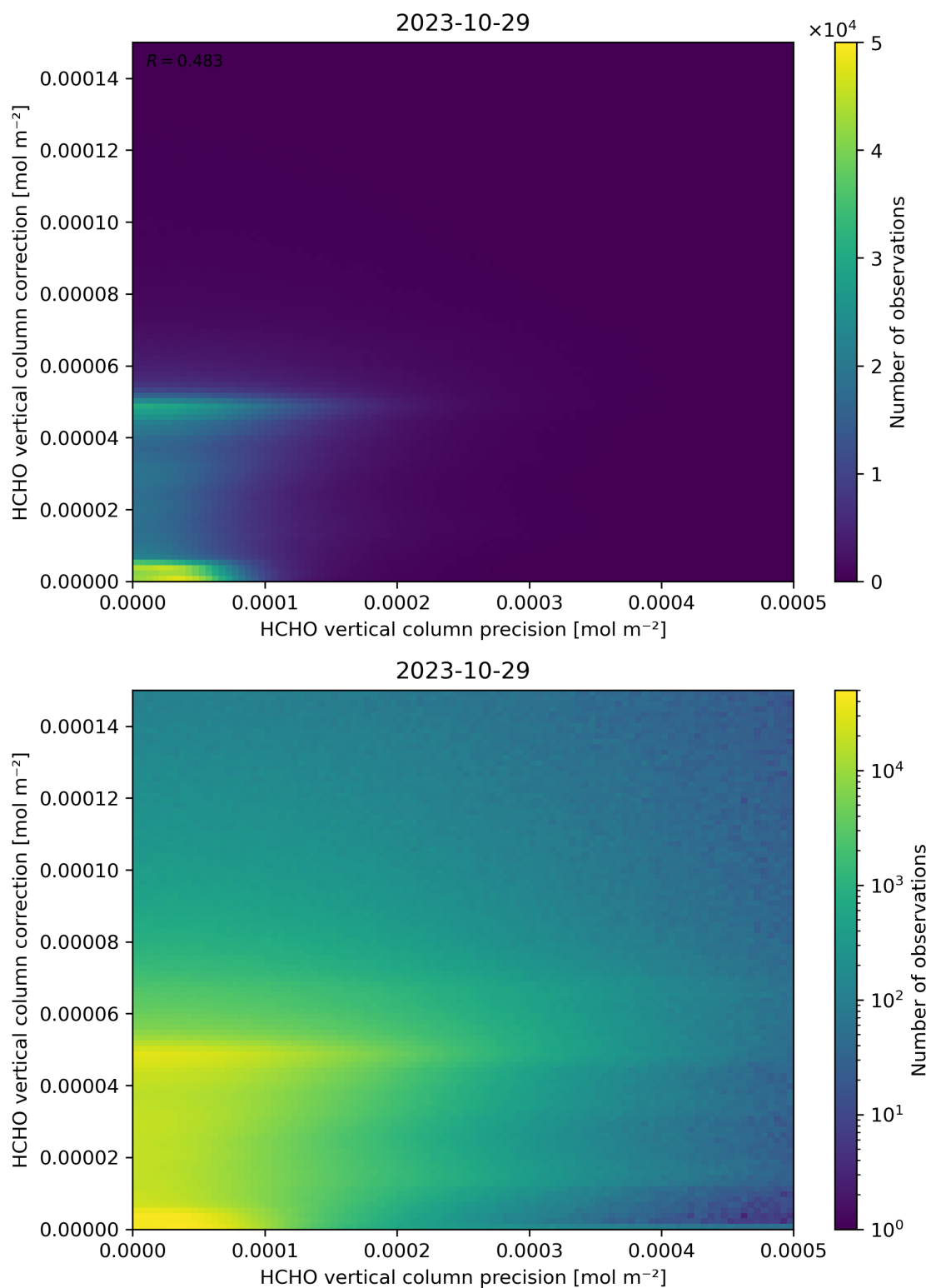
Figure 146: Scatter density plot of “HCHO vertical column precision” against “HCHO vertical column correction” for 2023-10-28 to 2023-10-30.
