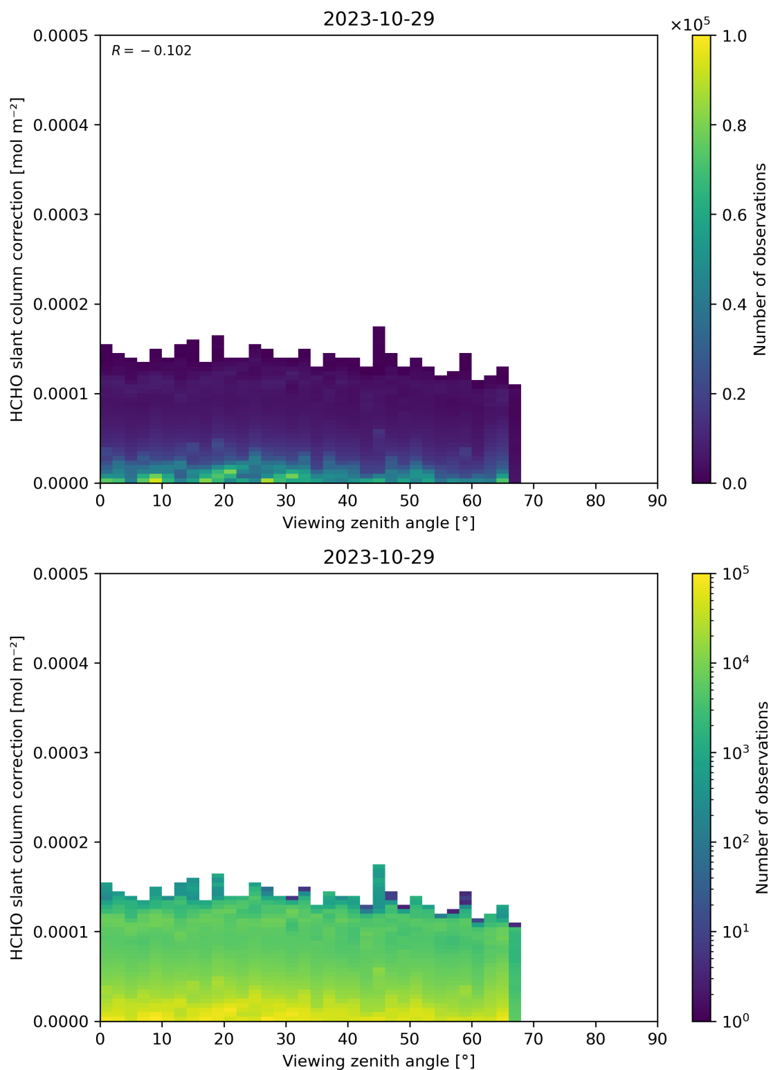
Figure 187: Scatter density plot of “Viewing zenith angle” against “HCHO slant column correction” for 2023-10-28 to 2023-10-30.
