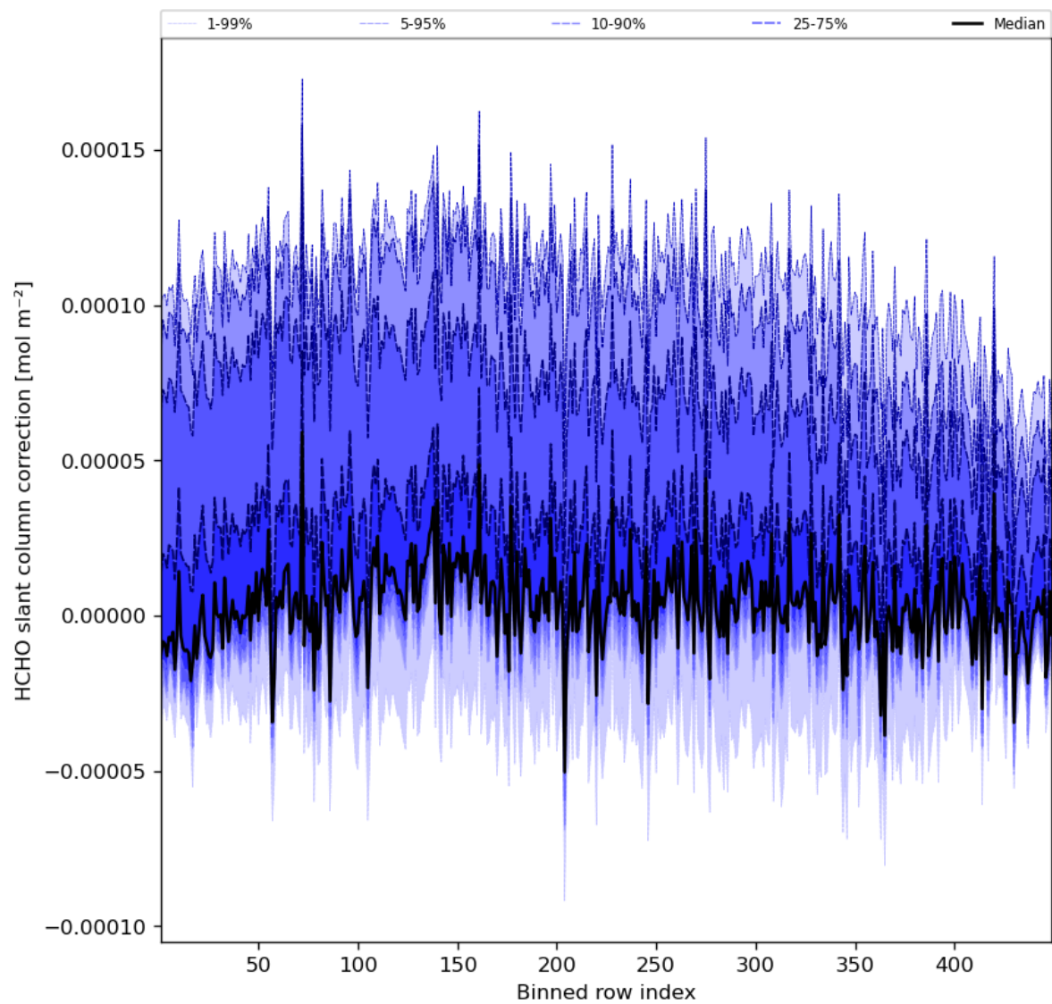
Figure 61: Along track statistics of “HCHO slant column correction” for 2023-10-28 to 2023-10-30
