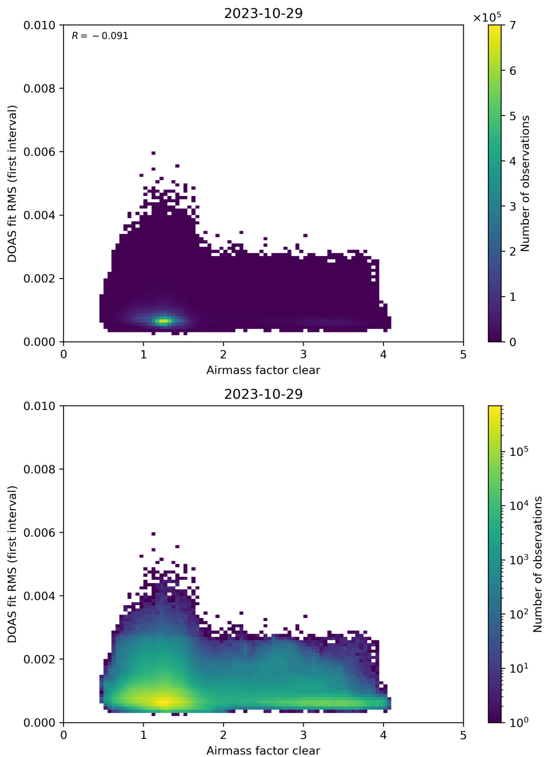
Figure 71: Scatter density plot of “Airmass factor clear” against “DOAS fit RMS (first interval)” for 2023-10-28 to 2023-10-30.
