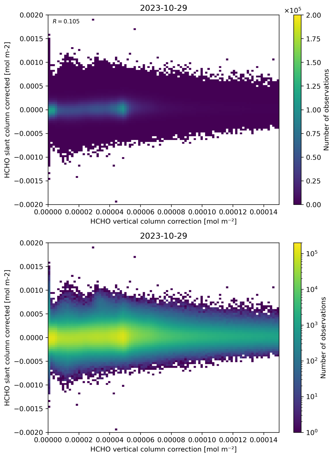
Figure 116: Scatter density plot of “HCHO vertical column correction” against “HCHO slant column corrected” for 2023-10-28 to 2023-10-30.
