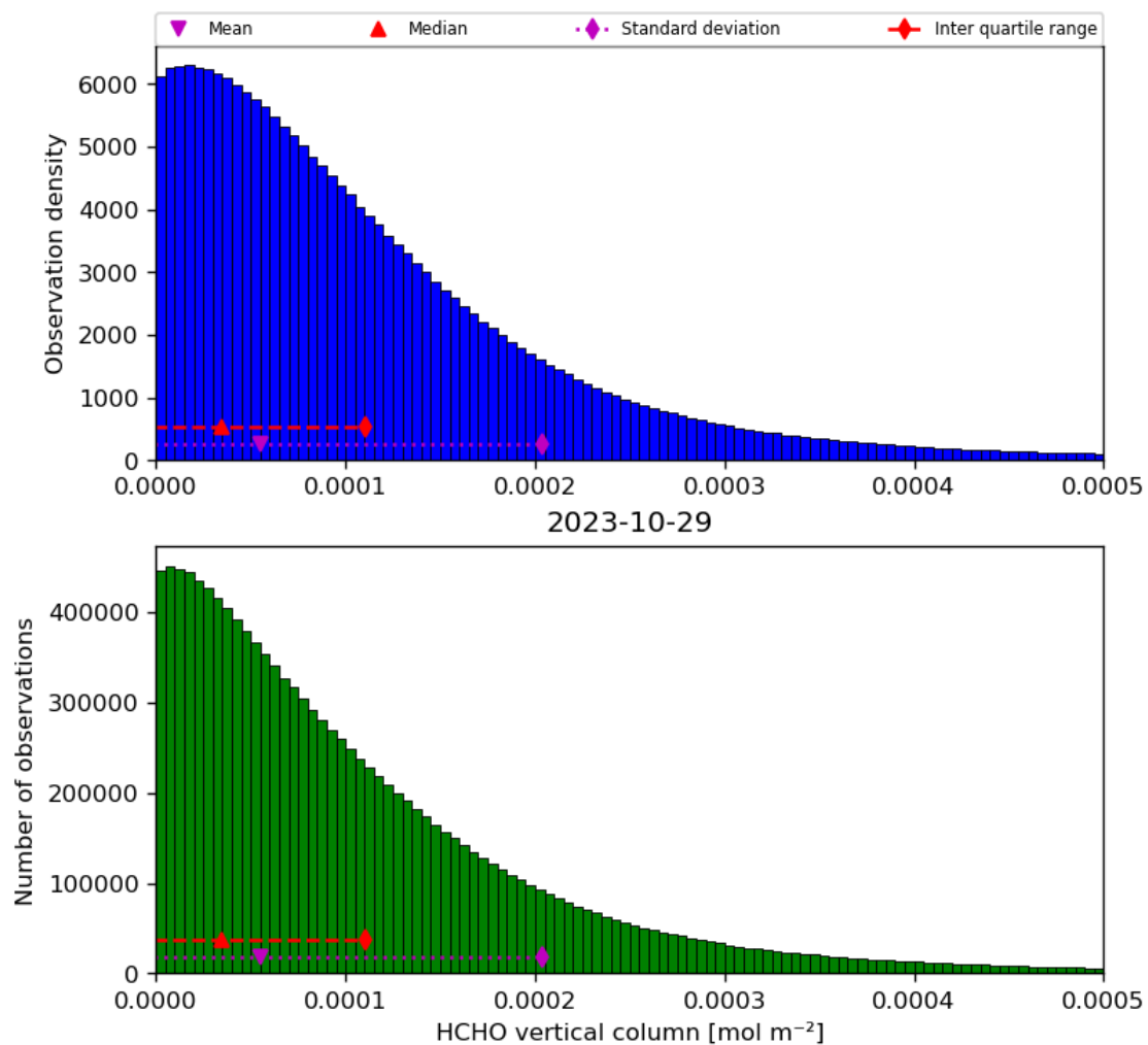
Figure 35: Histogram of “HCHO vertical column” for 2023-10-28 to 2023-10-30
