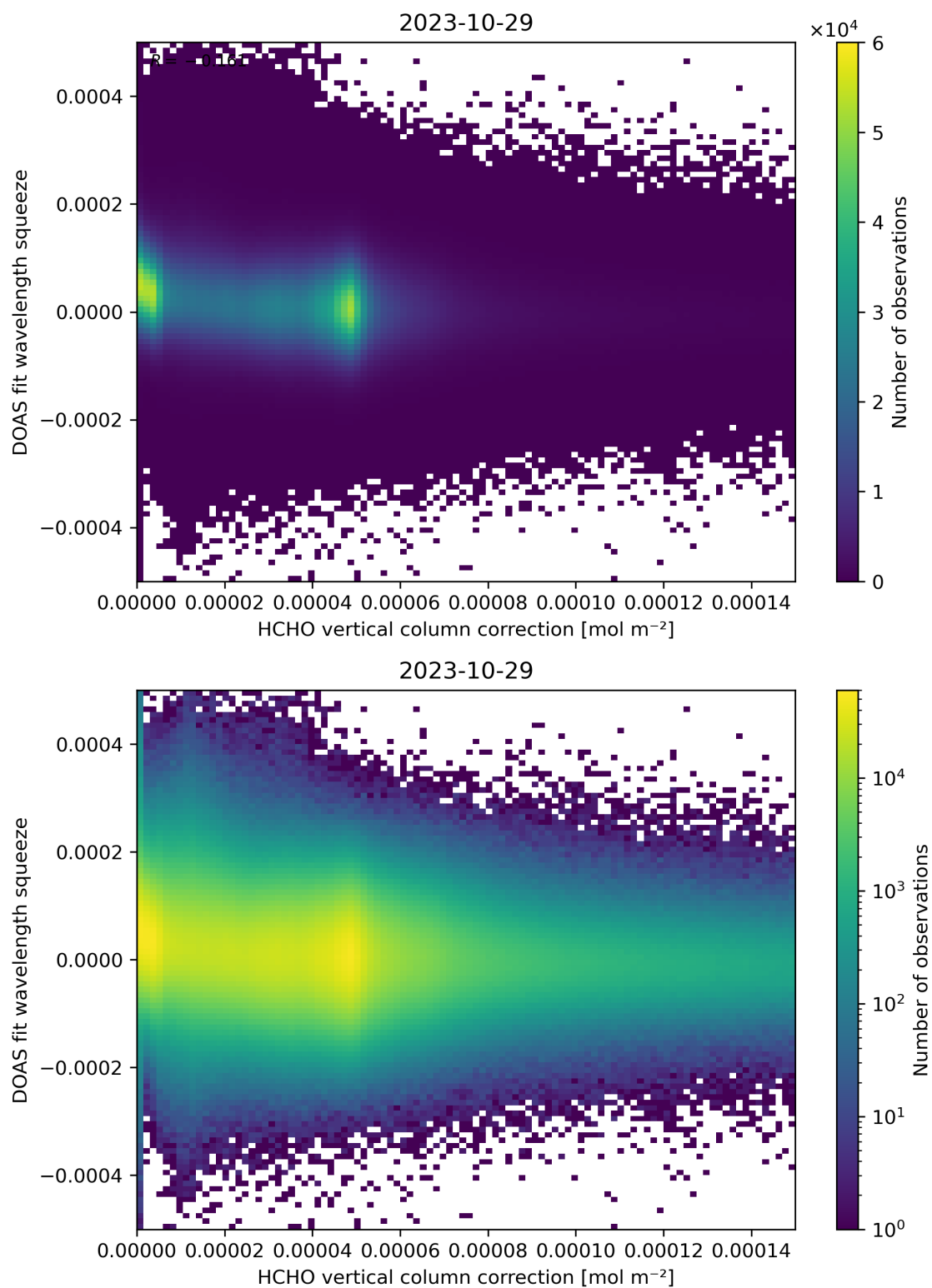
Figure 114: Scatter density plot of “HCHO vertical column correction” against “DOAS fit wavelength squeeze” for 2023-10-28 to 2023-10-30.
