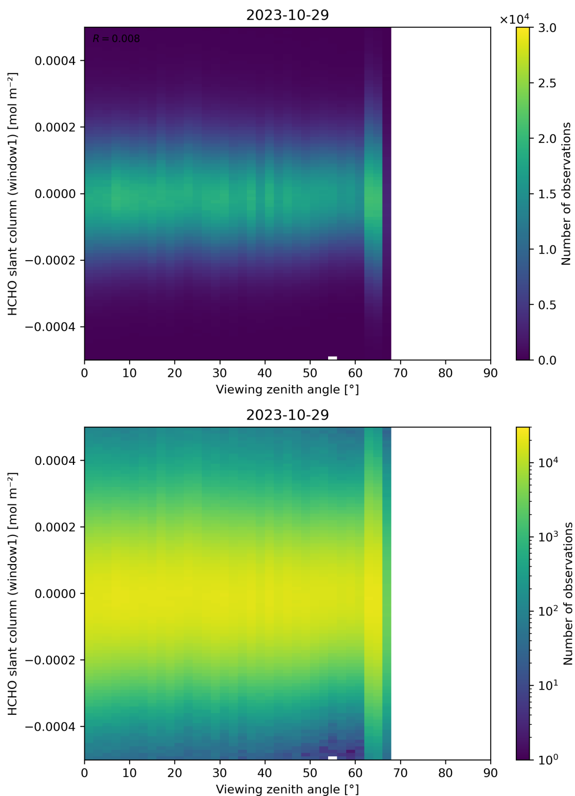
Figure 188: Scatter density plot of “Viewing zenith angle” against “HCHO slant column (window1)” for 2023-10-28 to 2023-10-30.
