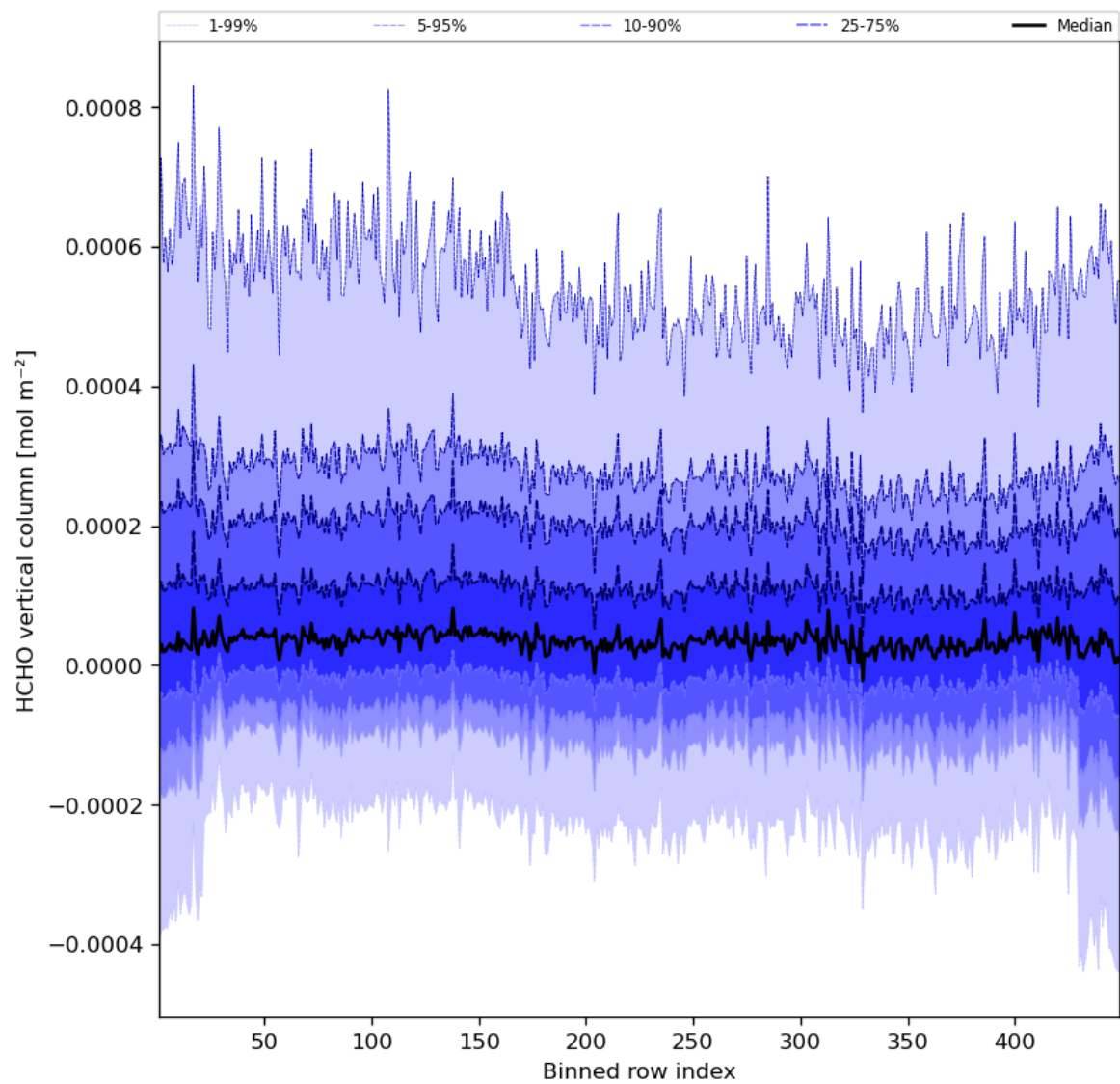
Figure 49: Along track statistics of “HCHO vertical column” for 2023-10-28 to 2023-10-30
