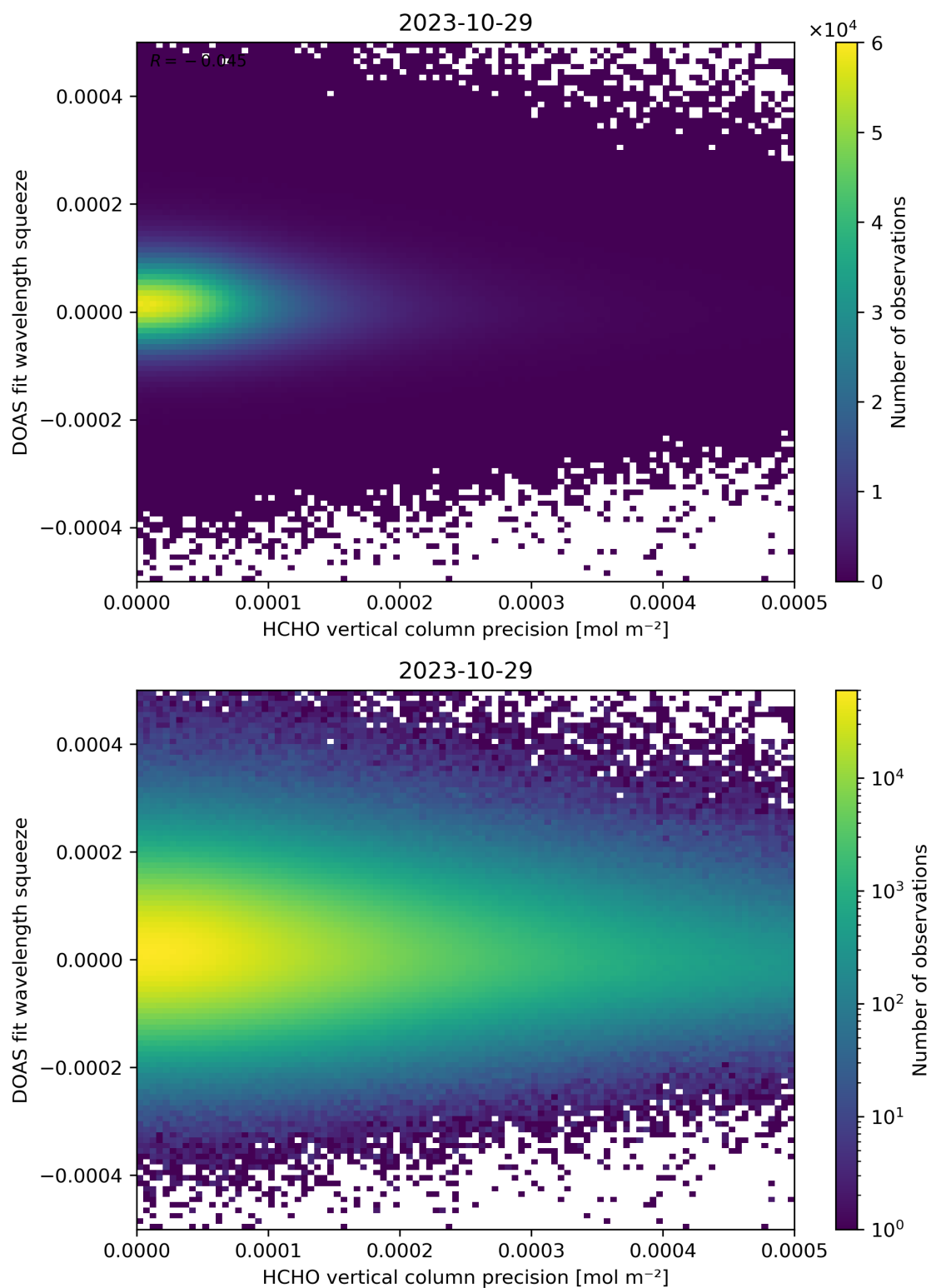
Figure 138: Scatter density plot of “HCHO vertical column precision” against “DOAS fit wavelength squeeze” for 2023-10-28 to 2023-10-30.
