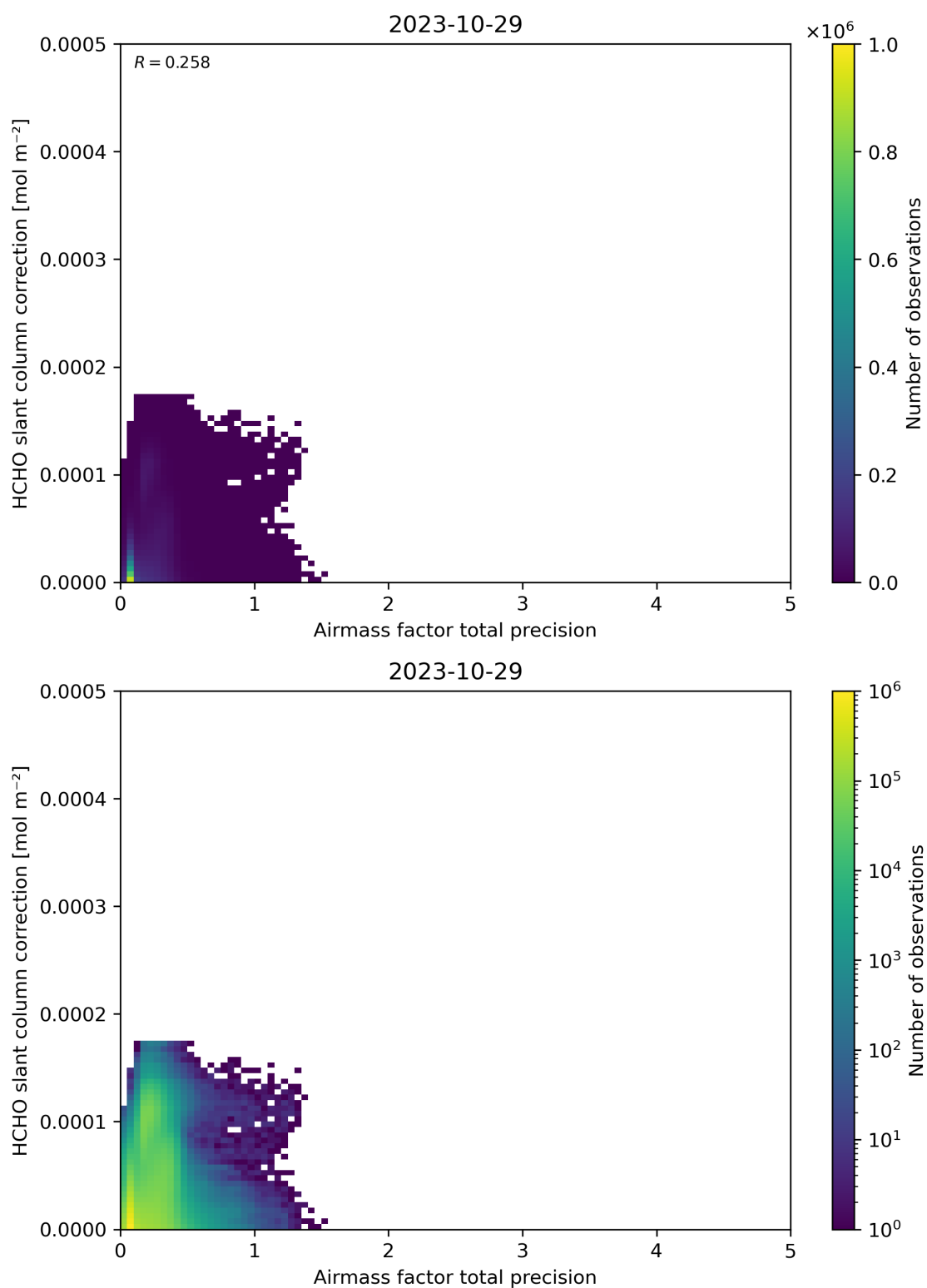
Figure 110: Scatter density plot of “Airmass factor total precision” against “HCHO slant column correction” for 2023-10-28 to 2023-10-30.
