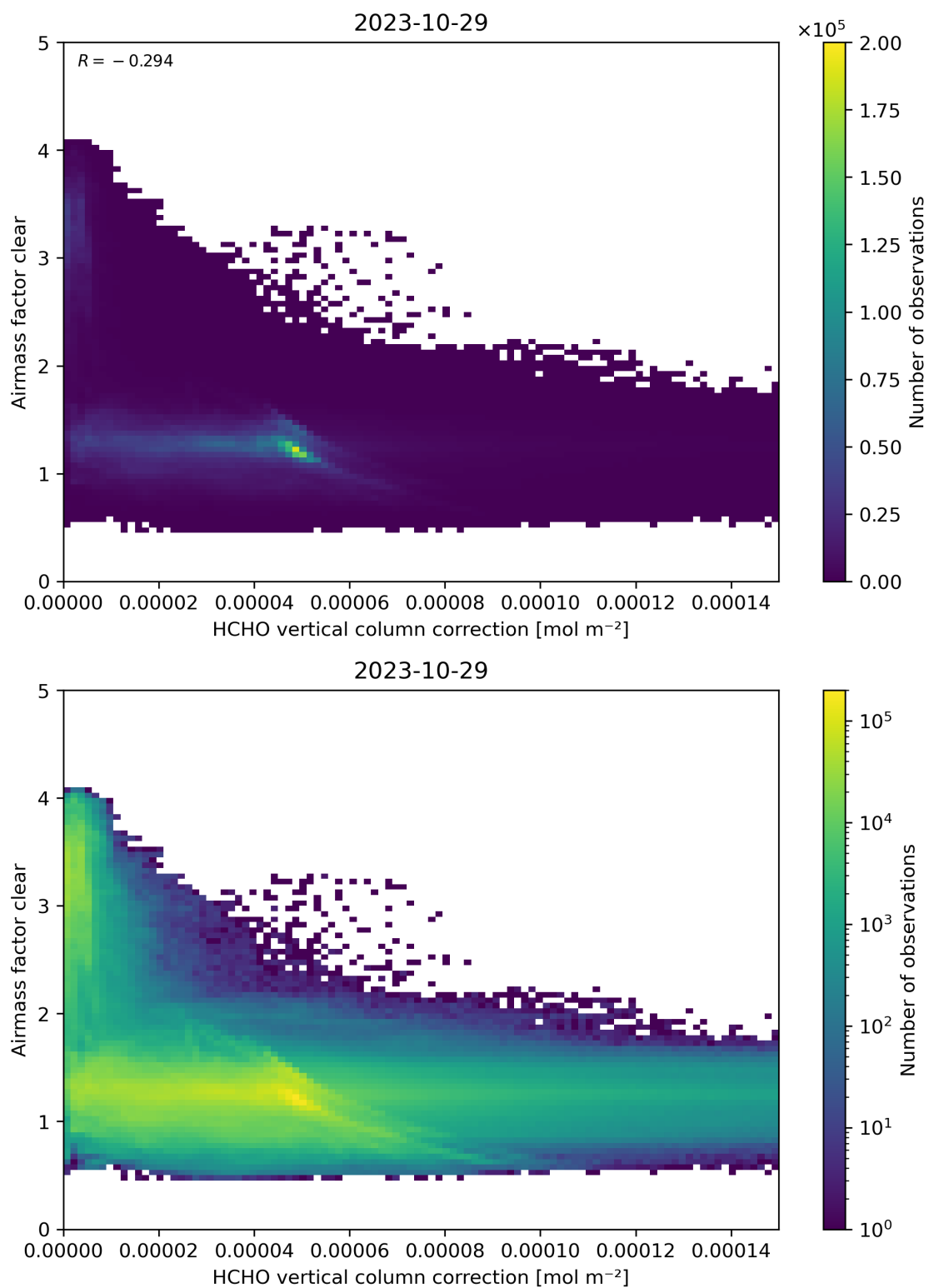
Figure 115: Scatter density plot of “HCHO vertical column correction” against “Airmass factor clear” for 2023-10-28 to 2023-10-30.
