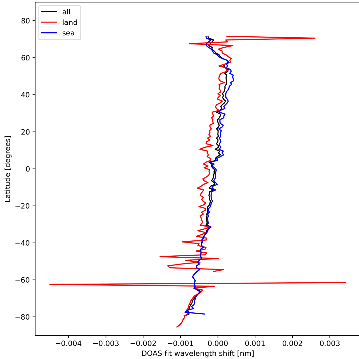
Figure 30: Zonal average of "DOAS fit wavelength shift" for 2023-10-28 to 2023-10-30.
