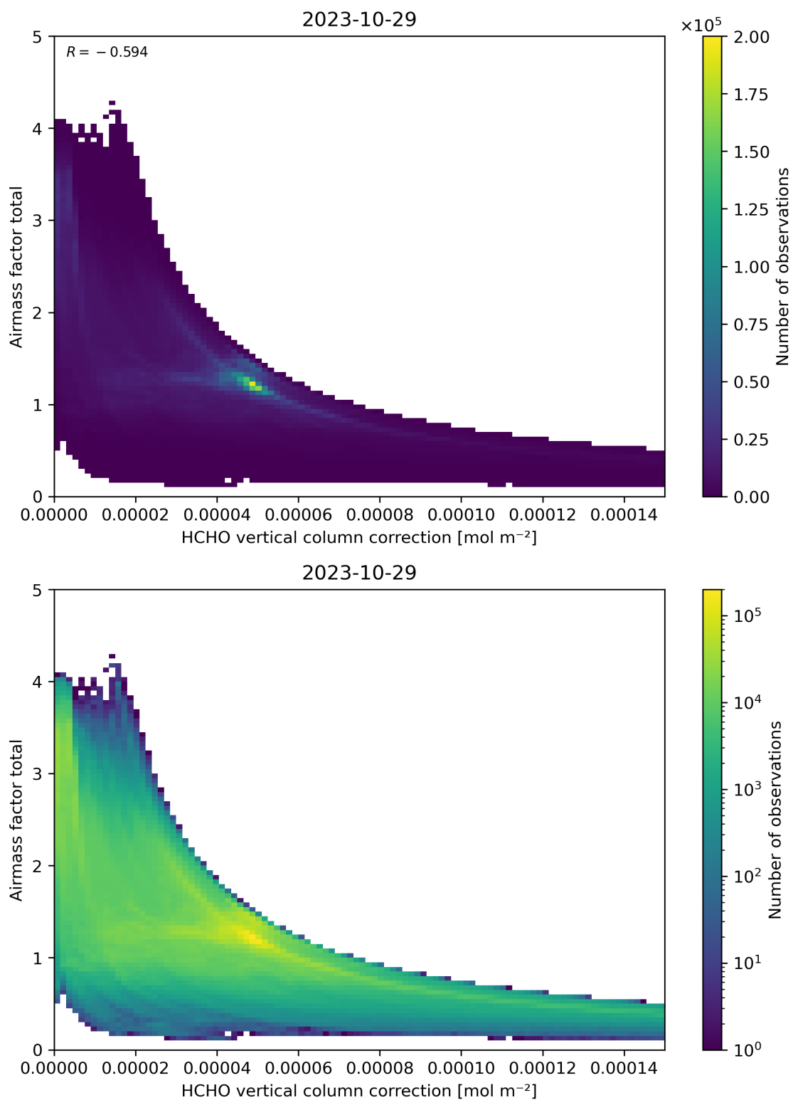
Figure 120: Scatter density plot of “HCHO vertical column correction” against “Airmass factor total” for 2023-10-28 to 2023-10-30.
