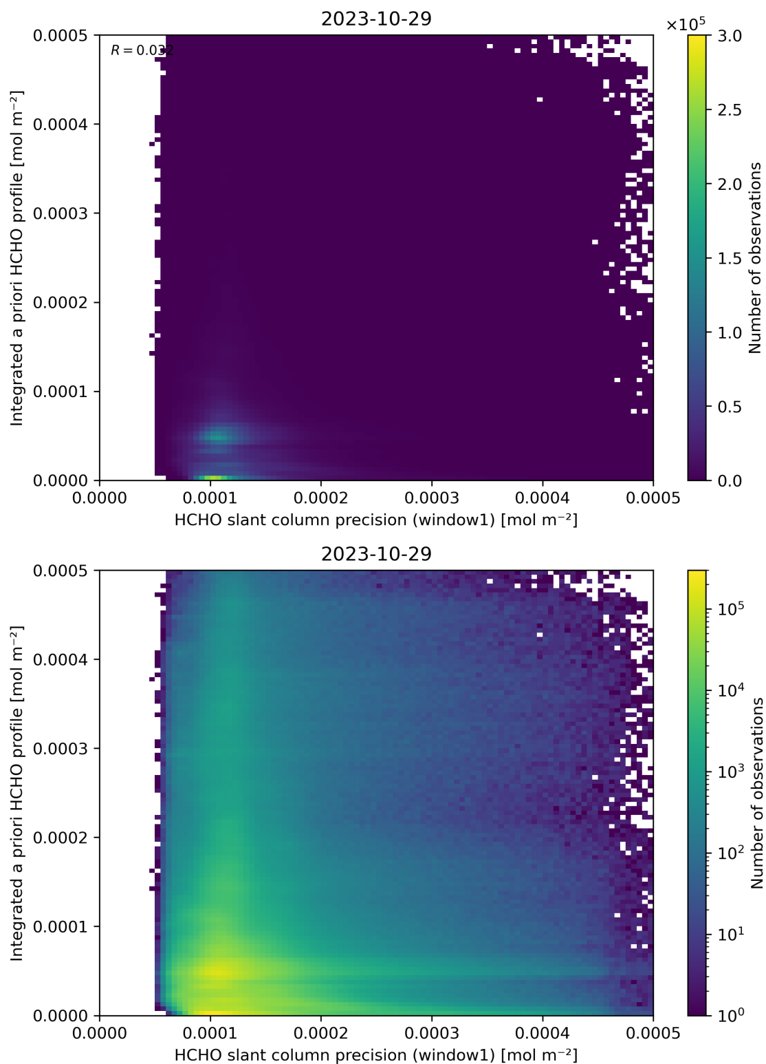
Figure 96: Scatter density plot of “HCHO slant column precision (window1)” against “Integrated a priori HCHO profile” for 2023-10-28 to 2023-10-30.
