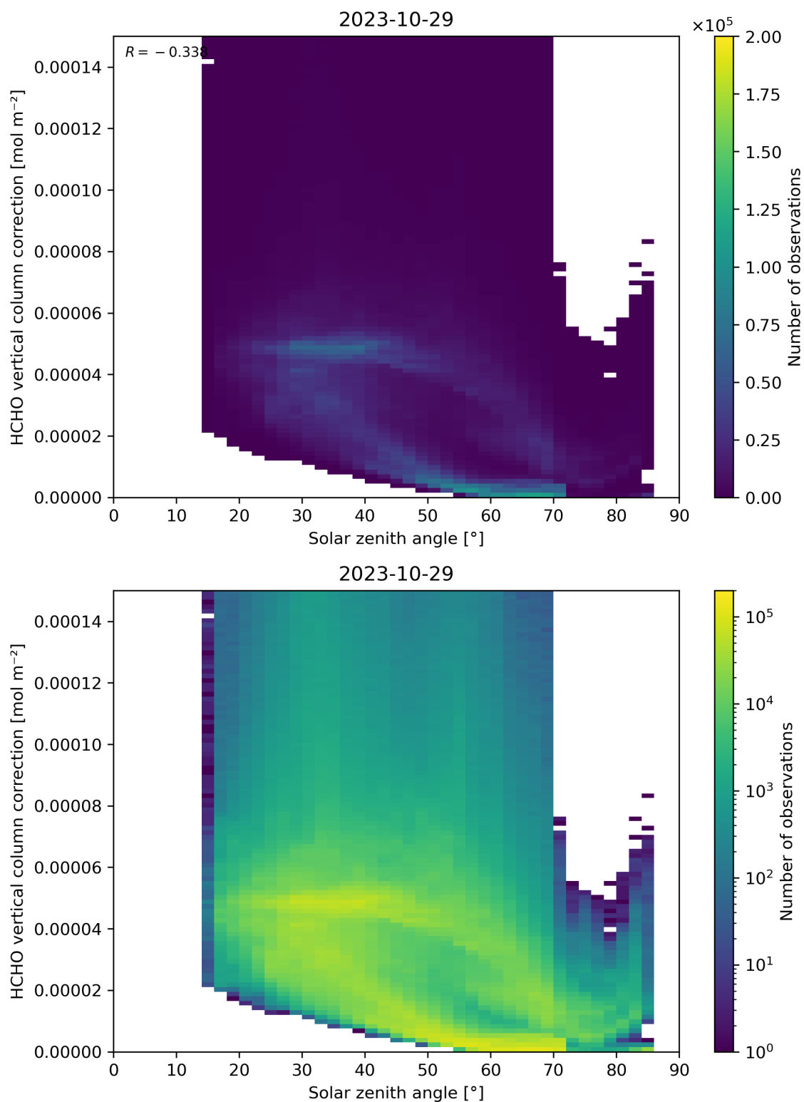
Figure 178: Scatter density plot of “Solar zenith angle” against “HCHO vertical column correction” for 2023-10-28 to 2023-10-30.
