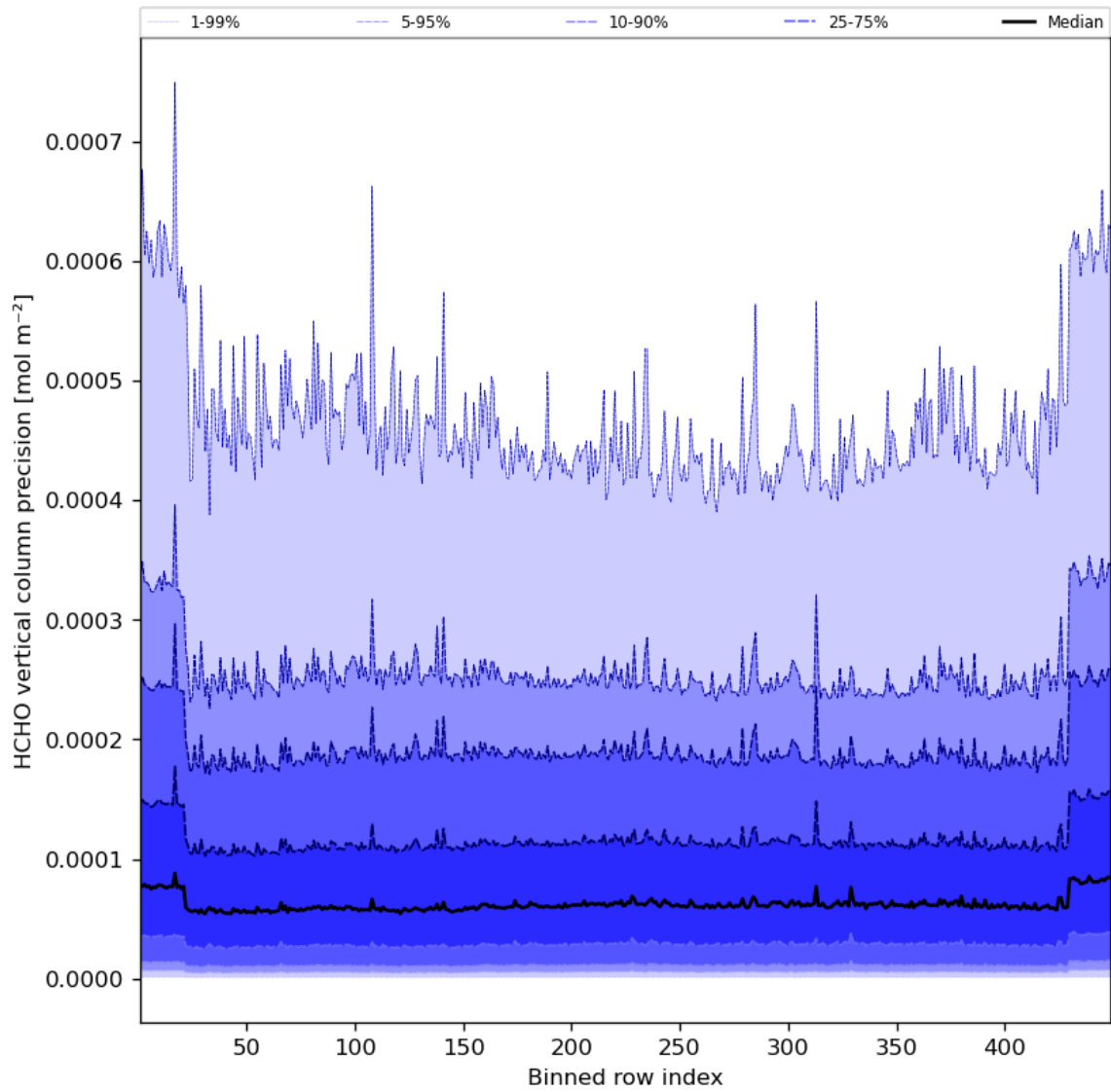
Figure 50: Along track statistics of “HCHO vertical column precision” for 2023-10-28 to 2023-10-30
