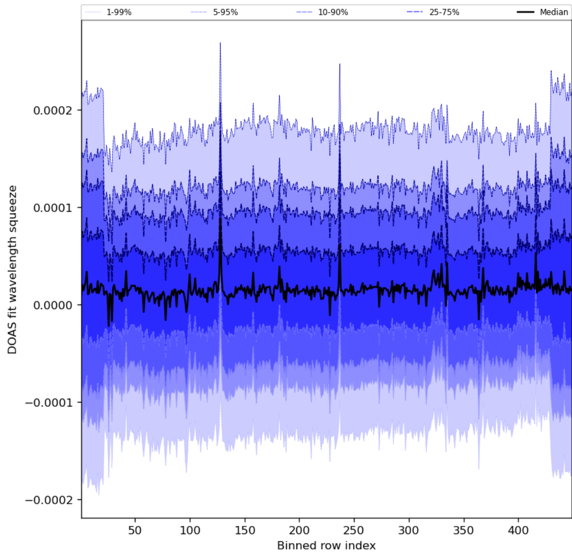
Figure 59: Along track statistics of “DOAS fit wavelength squeeze” for 2023-10-28 to 2023-10-30
