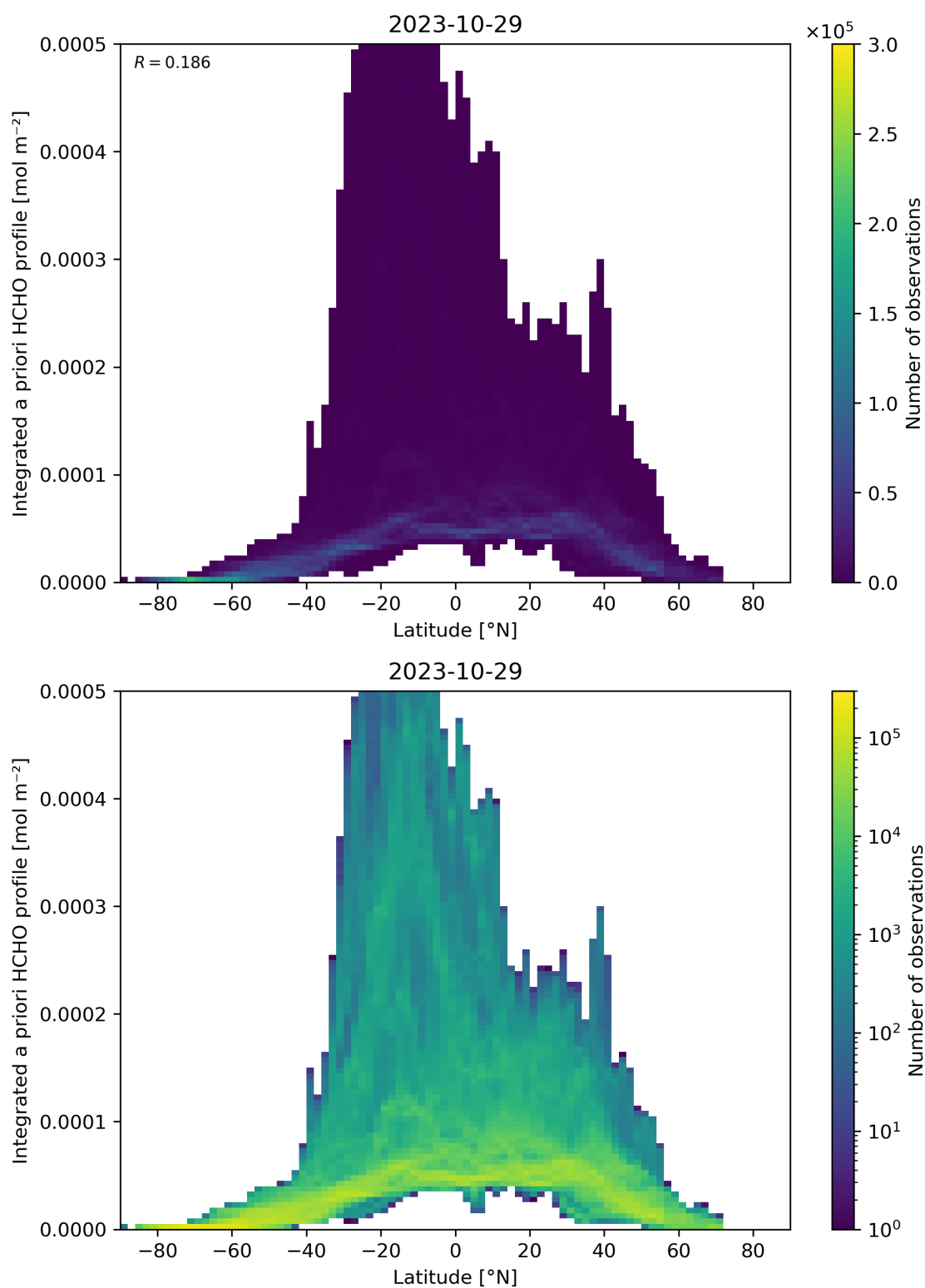
Figure 166: Scatter density plot of “Latitude” against “Integrated a priori HCHO profile” for 2023-10-28 to 2023-10-30.
