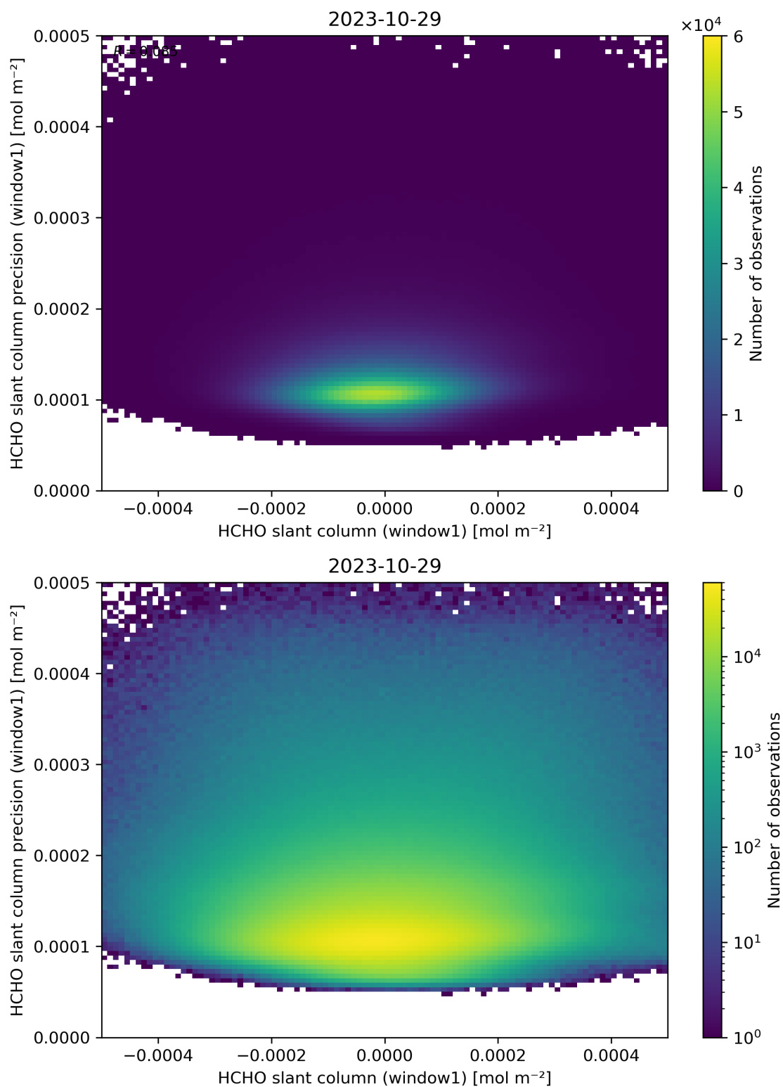
Figure 84: Scatter density plot of “HCHO slant column (window1)” against “HCHO slant column precision (window1)” for 2023-10-28 to 2023-10-30.
