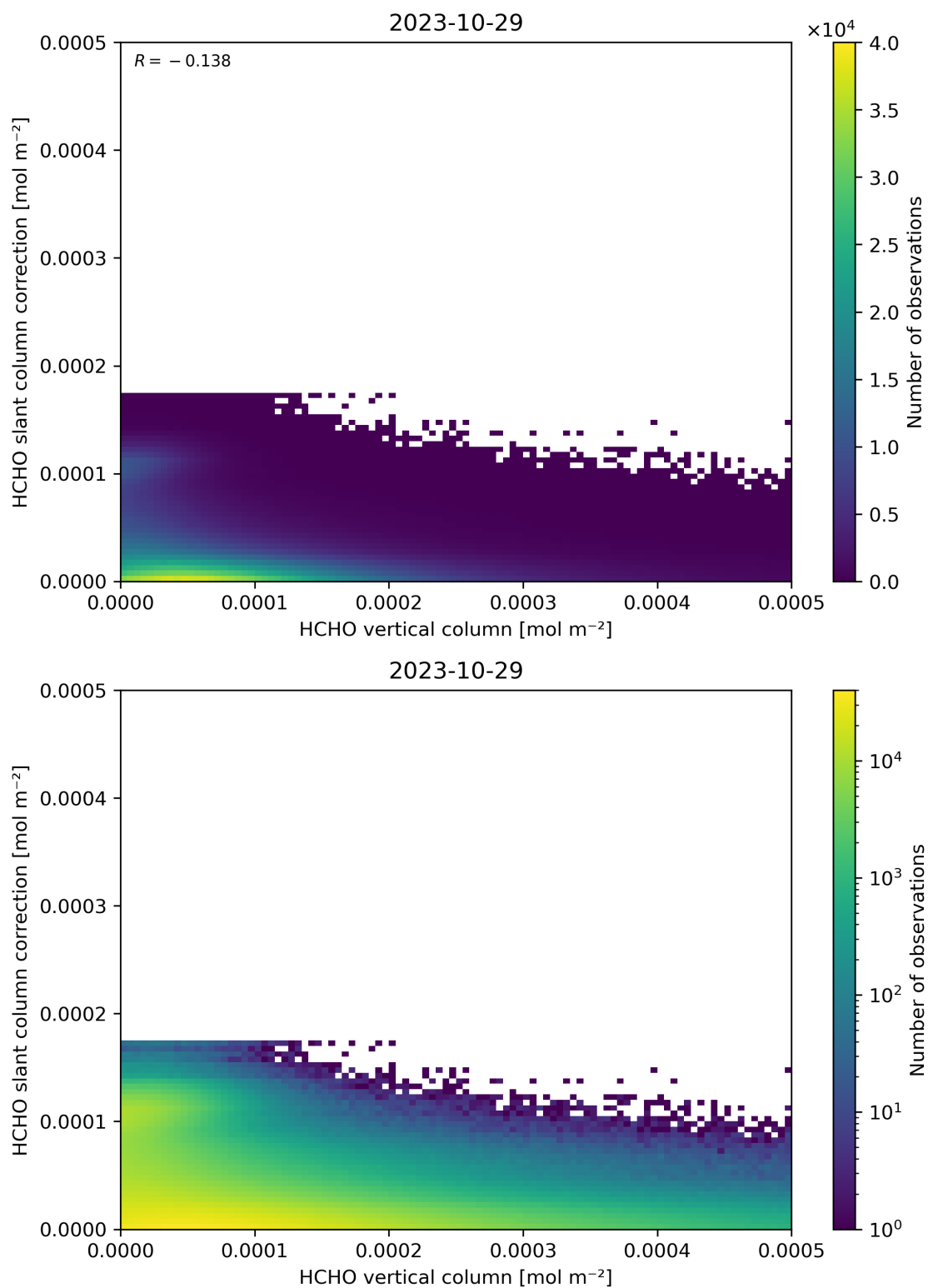
Figure 128: Scatter density plot of “HCHO vertical column” against “HCHO slant column correction” for 2023-10-28 to 2023-10-30.
