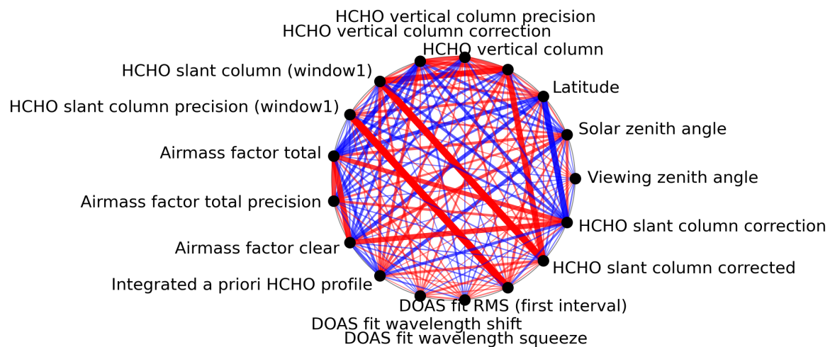
Figure 1: Map of correlation graph for 2023-10-28 to 2023-10-30.
