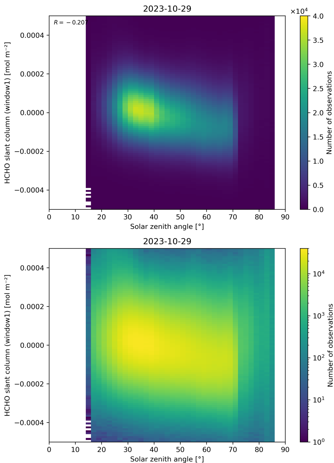
Figure 173: Scatter density plot of “Solar zenith angle” against “HCHO slant column (window1)” for 2023-10-28 to 2023-10-30.
