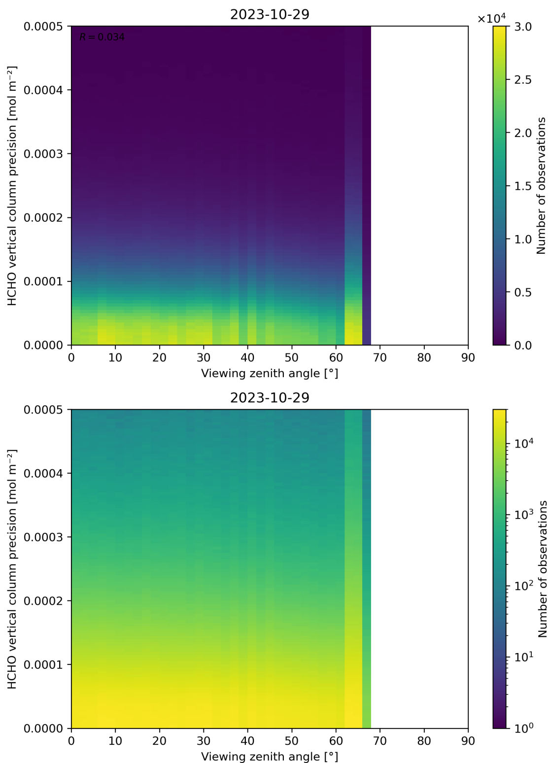
Figure 194: Scatter density plot of “Viewing zenith angle” against “HCHO vertical column precision” for 2023-10-28 to 2023-10-30.
