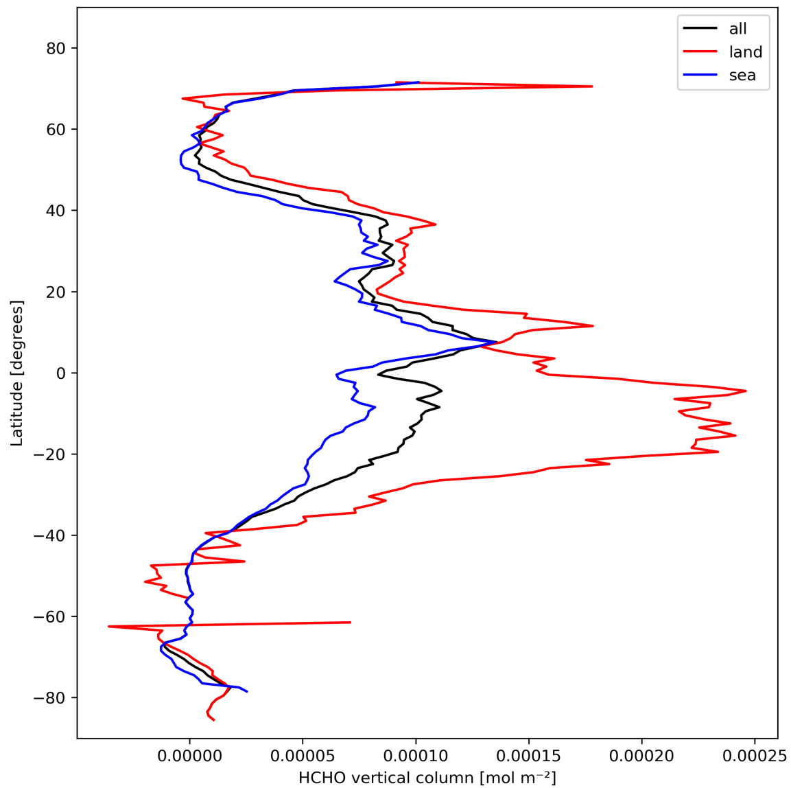
Figure 21: Zonal average of “HCHO vertical column” for 2023-10-28 to 2023-10-30.
