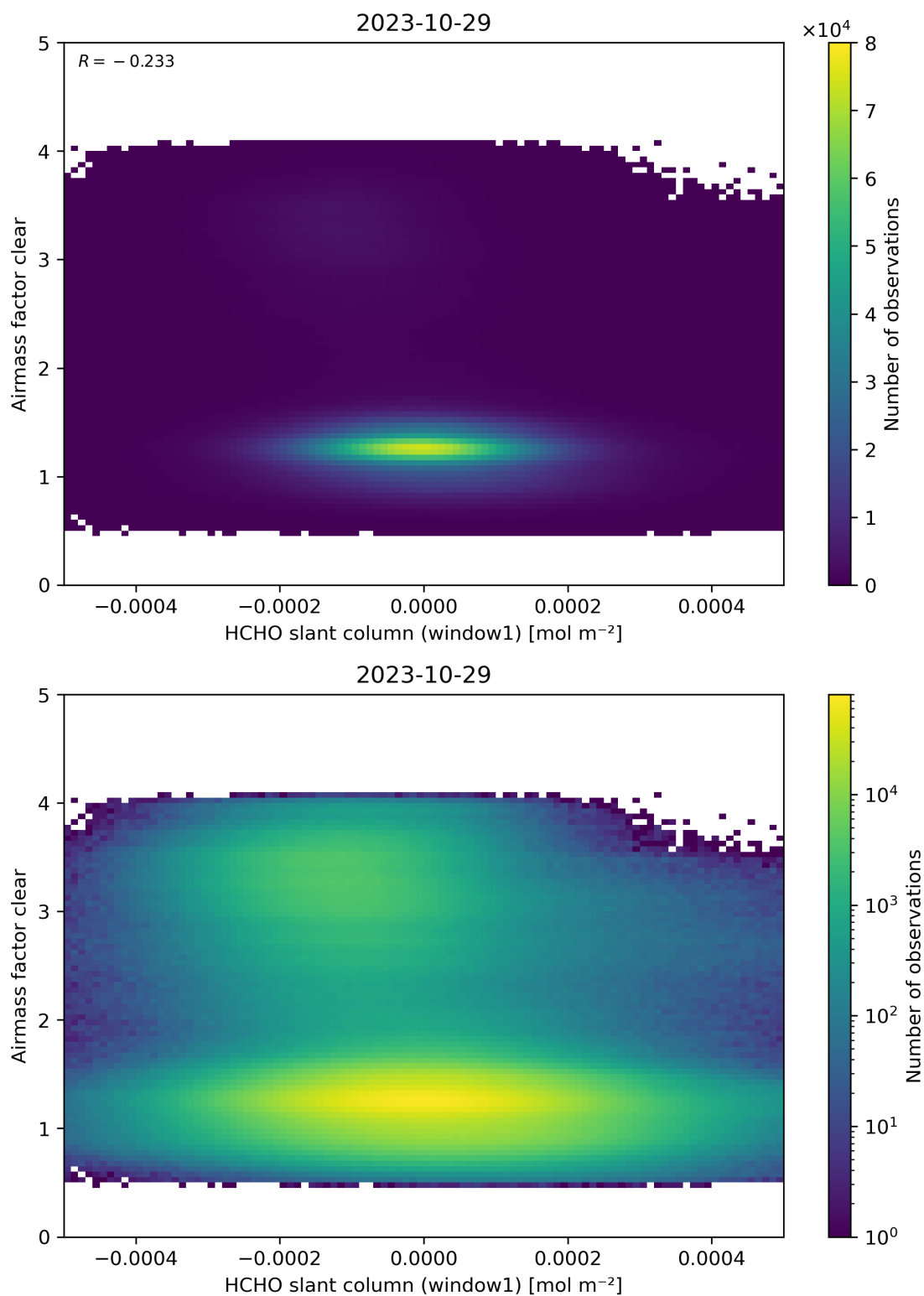
Figure 81: Scatter density plot of “HCHO slant column (window1)” against “Airmass factor clear” for 2023-10-28 to 2023-10-30.
