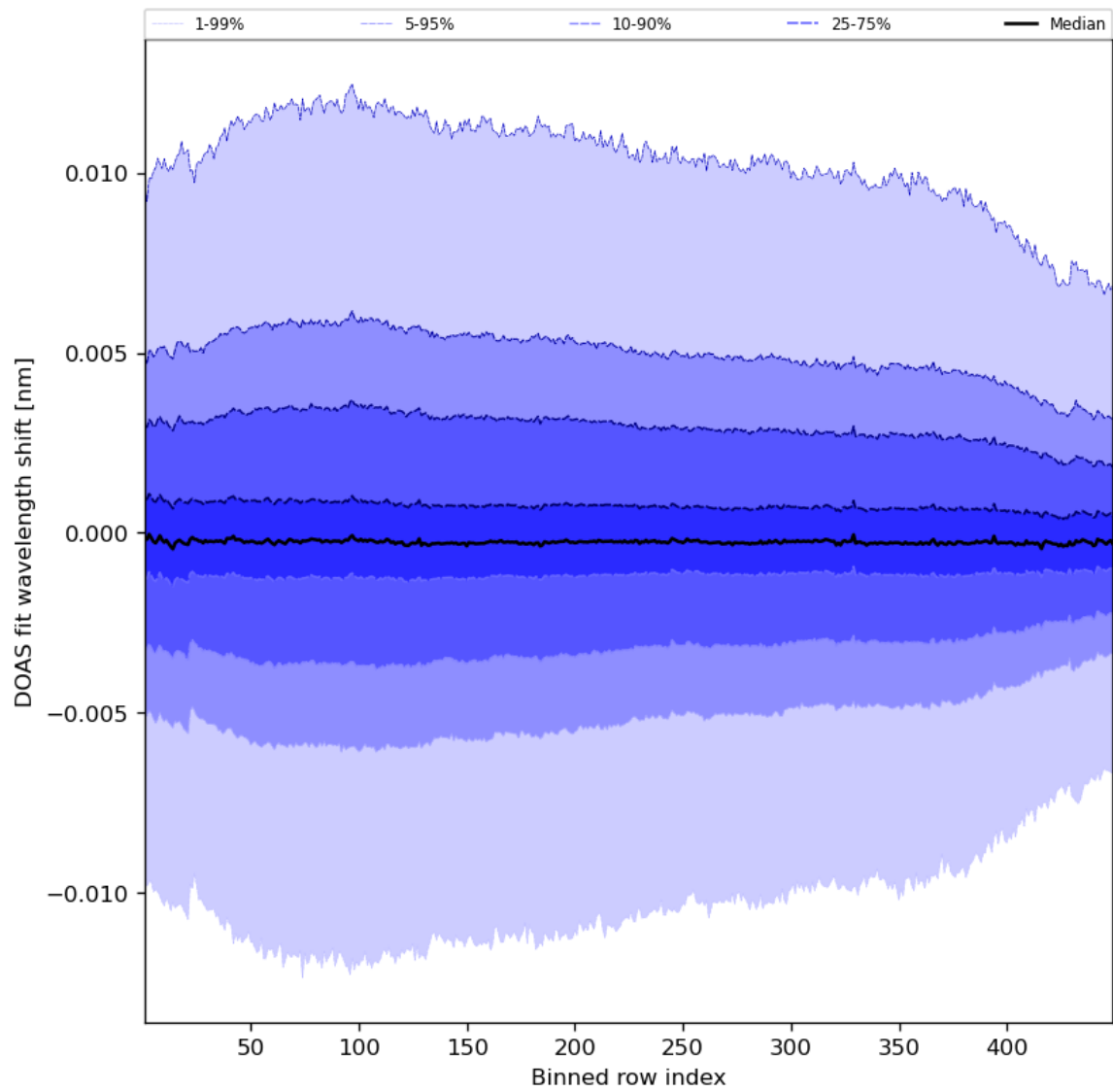
Figure 58: Along track statistics of “DOAS fit wavelength shift” for 2023-10-28 to 2023-10-30
