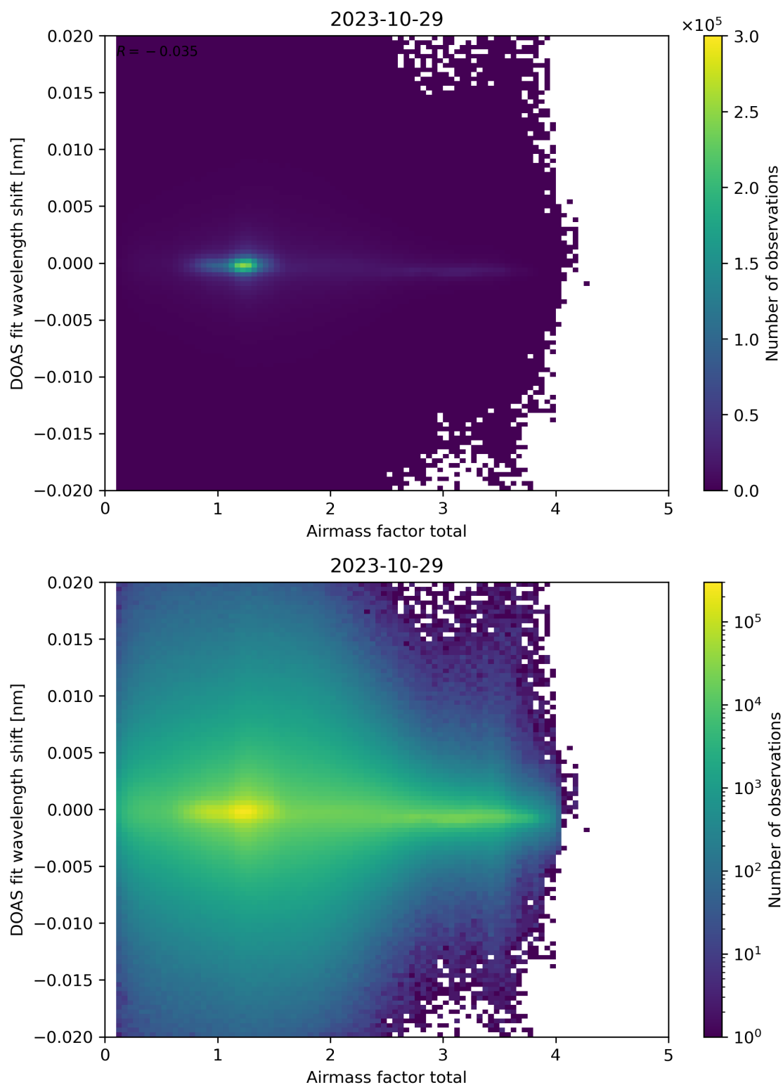
Figure 98: Scatter density plot of “Airmass factor total” against “DOAS fit wavelength shift” for 2023-10-28 to 2023-10-30.
