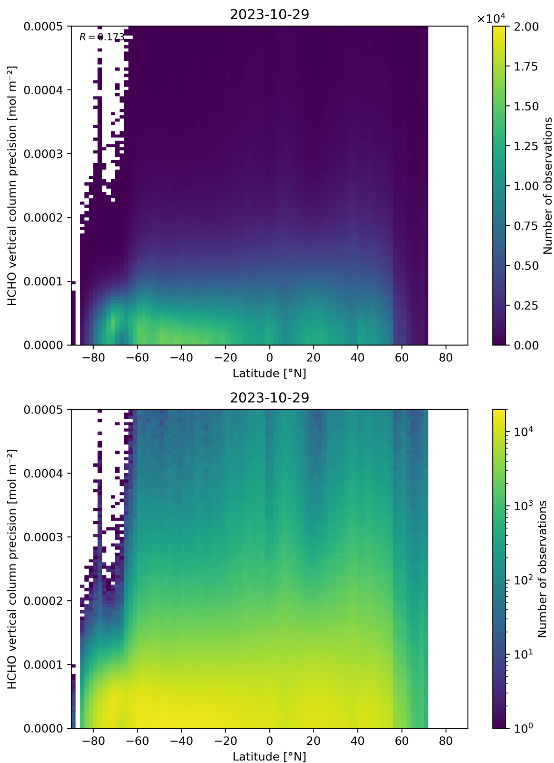
Figure 165: Scatter density plot of “Latitude” against “HCHO vertical column precision” for 2023-10-28 to 2023-10-30.
