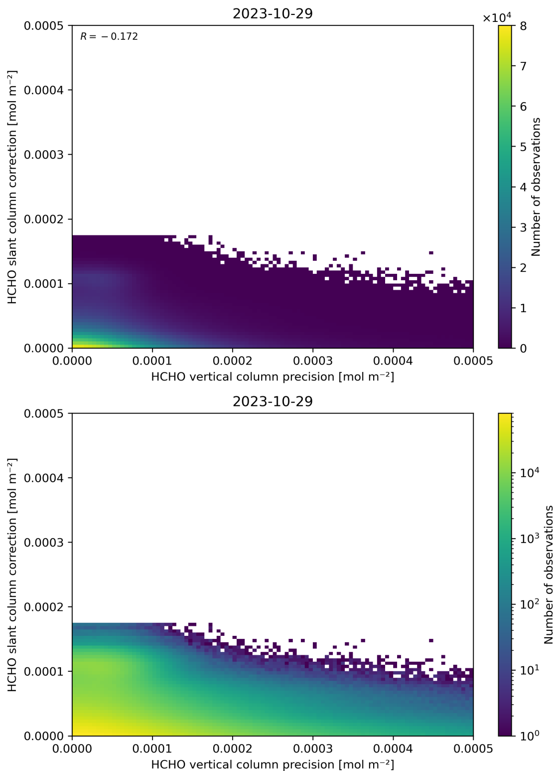
Figure 141: Scatter density plot of “HCHO vertical column precision” against “HCHO slant column correction” for 2023-10-28 to 2023-10-30.
