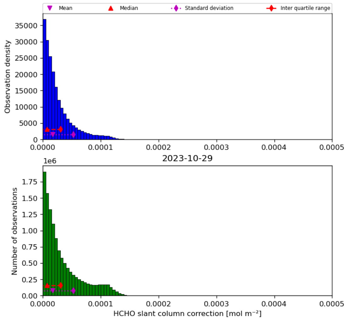
Figure 47: Histogram of “HCHO slant column correction” for 2023-10-28 to 2023-10-30
