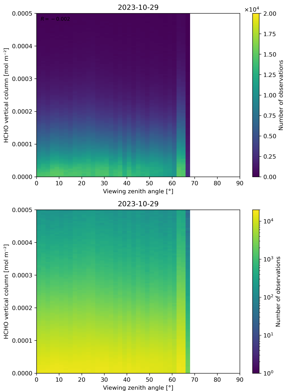
Figure 192: Scatter density plot of “Viewing zenith angle” against “HCHO vertical column” for 2023-10-28 to 2023-10-30.
