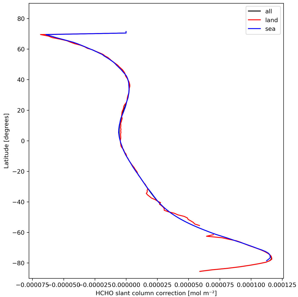
Figure 33: Zonal average of “HCHO slant column correction” for 2023-10-28 to 2023-10-30.
