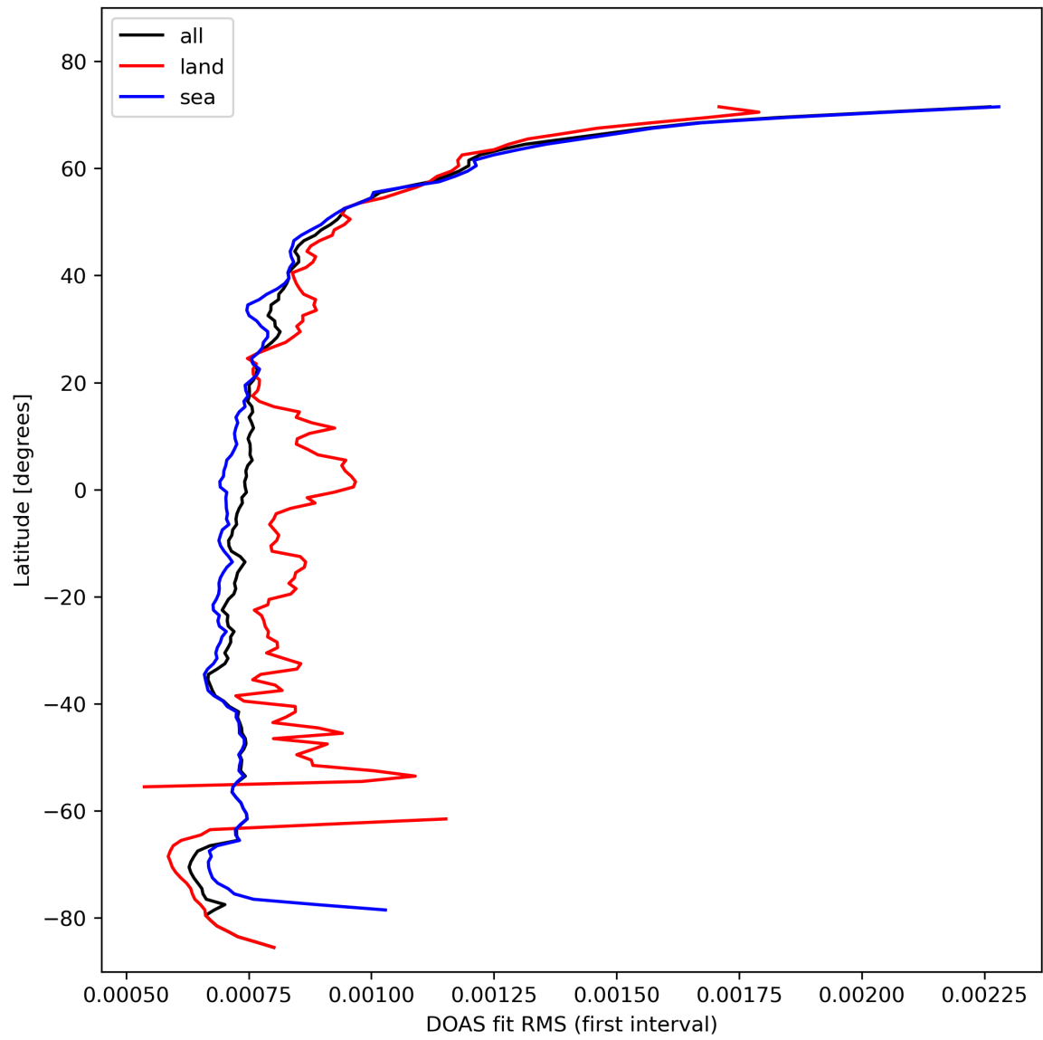
Figure 32: Zonal average of “DOAS fit RMS (first interval)” for 2023-10-28 to 2023-10-30.
