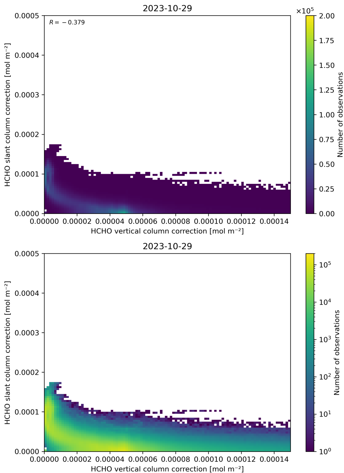
Figure 117: Scatter density plot of “HCHO vertical column correction” against “HCHO slant column correction” for 2023-10-28 to 2023-10-30.
