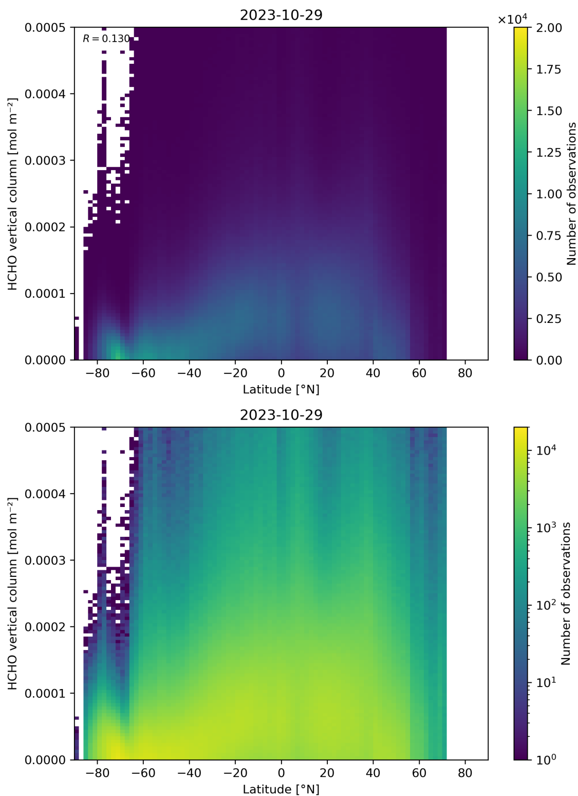
Figure 163: Scatter density plot of “Latitude” against “HCHO vertical column” for 2023-10-28 to 2023-10-30.
