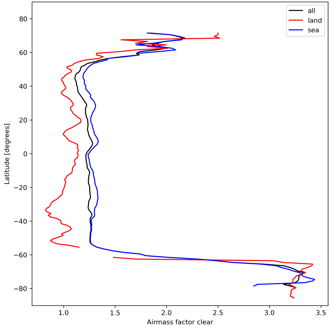
Figure 28: Zonal average of “Airmass factor clear” for 2023-10-28 to 2023-10-30.
