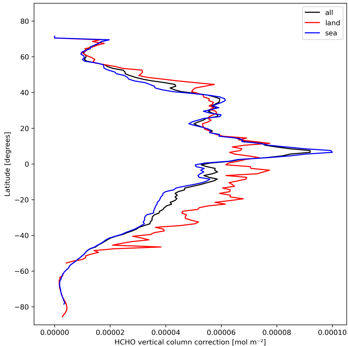
Figure 23: Zonal average of “HCHO vertical column correction” for 2023-10-28 to 2023-10-30.
