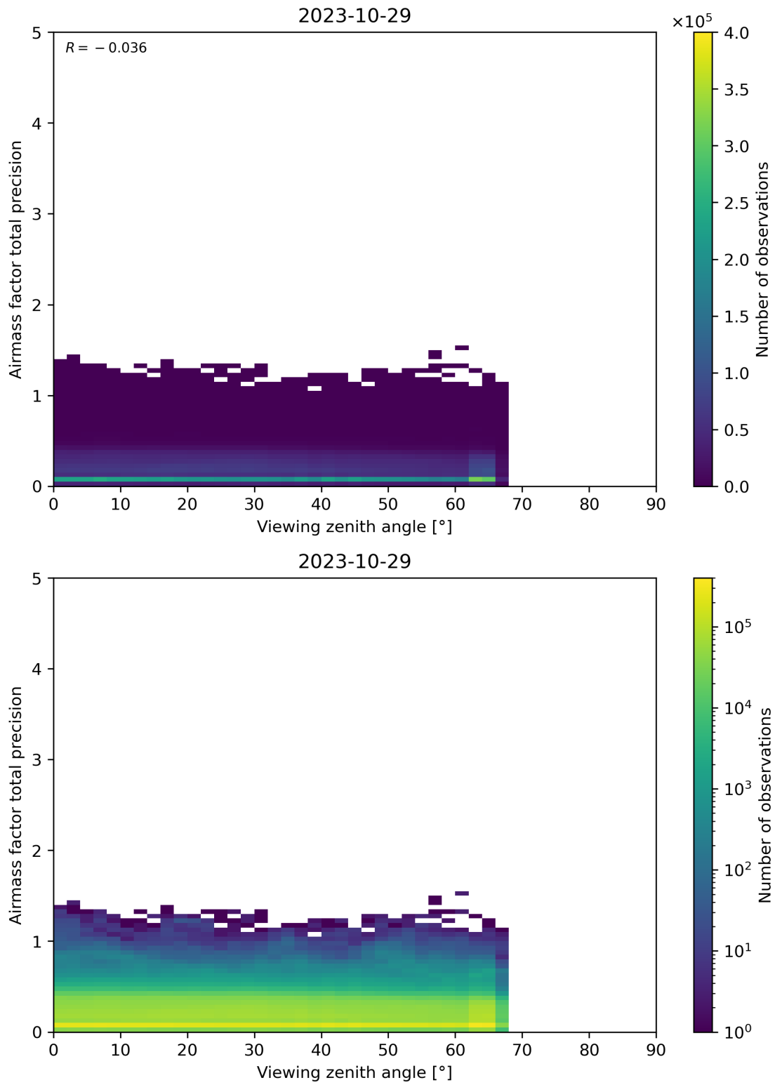
Figure 191: Scatter density plot of “Viewing zenith angle” against “Airmass factor total precision” for 2023-10-28 to 2023-10-30.
