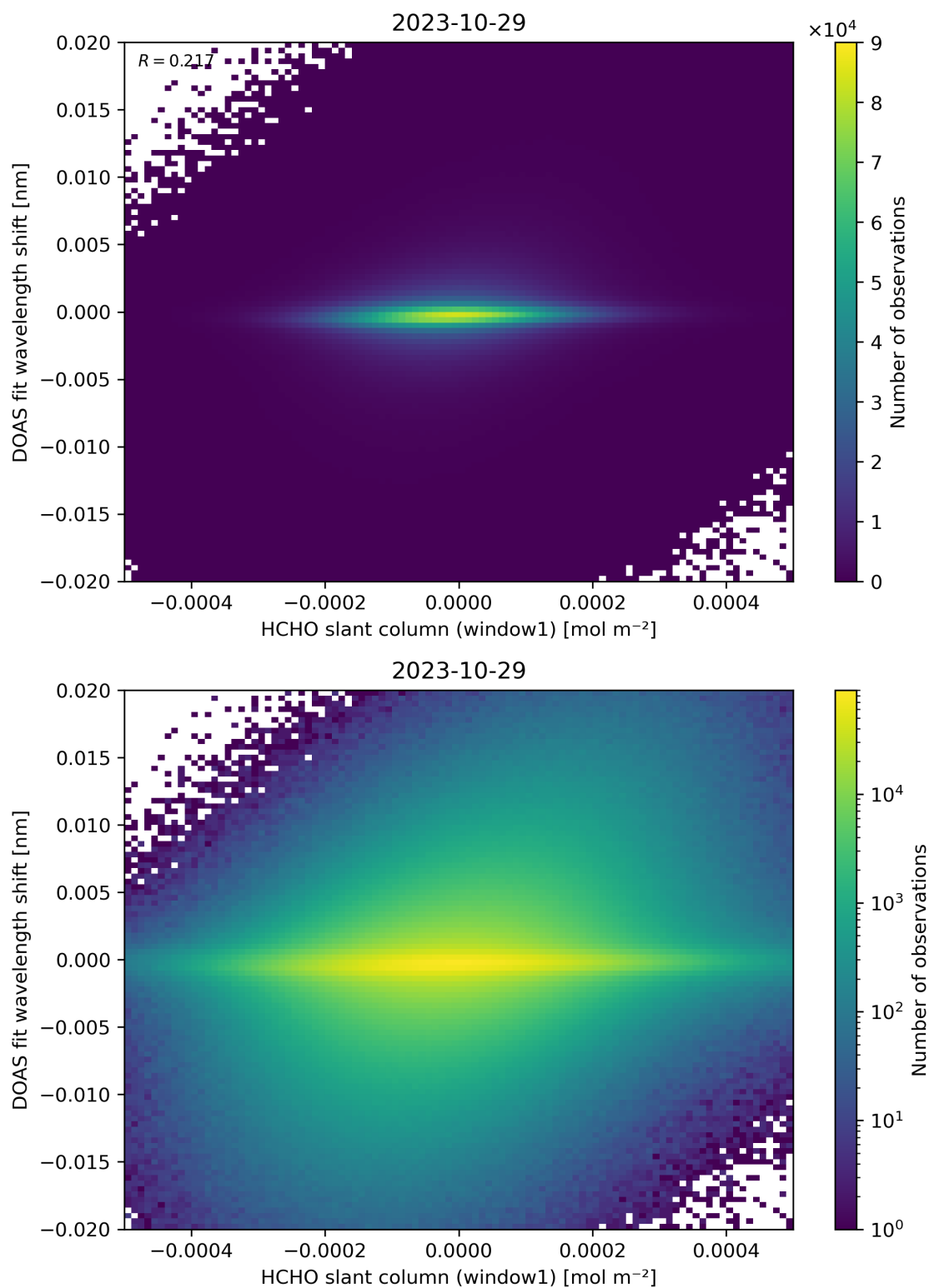
Figure 79: Scatter density plot of “HCHO slant column (window1)” against “DOAS fit wavelength shift” for 2023-10-28 to 2023-10-30.
