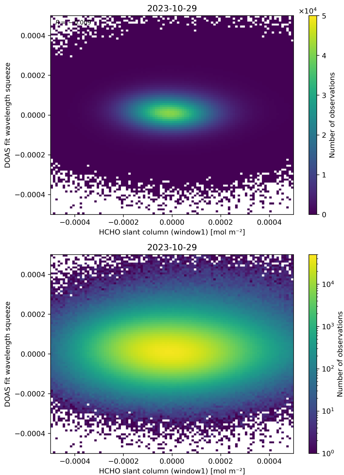
Figure 80: Scatter density plot of “HCHO slant column (window1)” against “DOAS fit wavelength squeeze” for 2023-10-28 to 2023-10-30.
