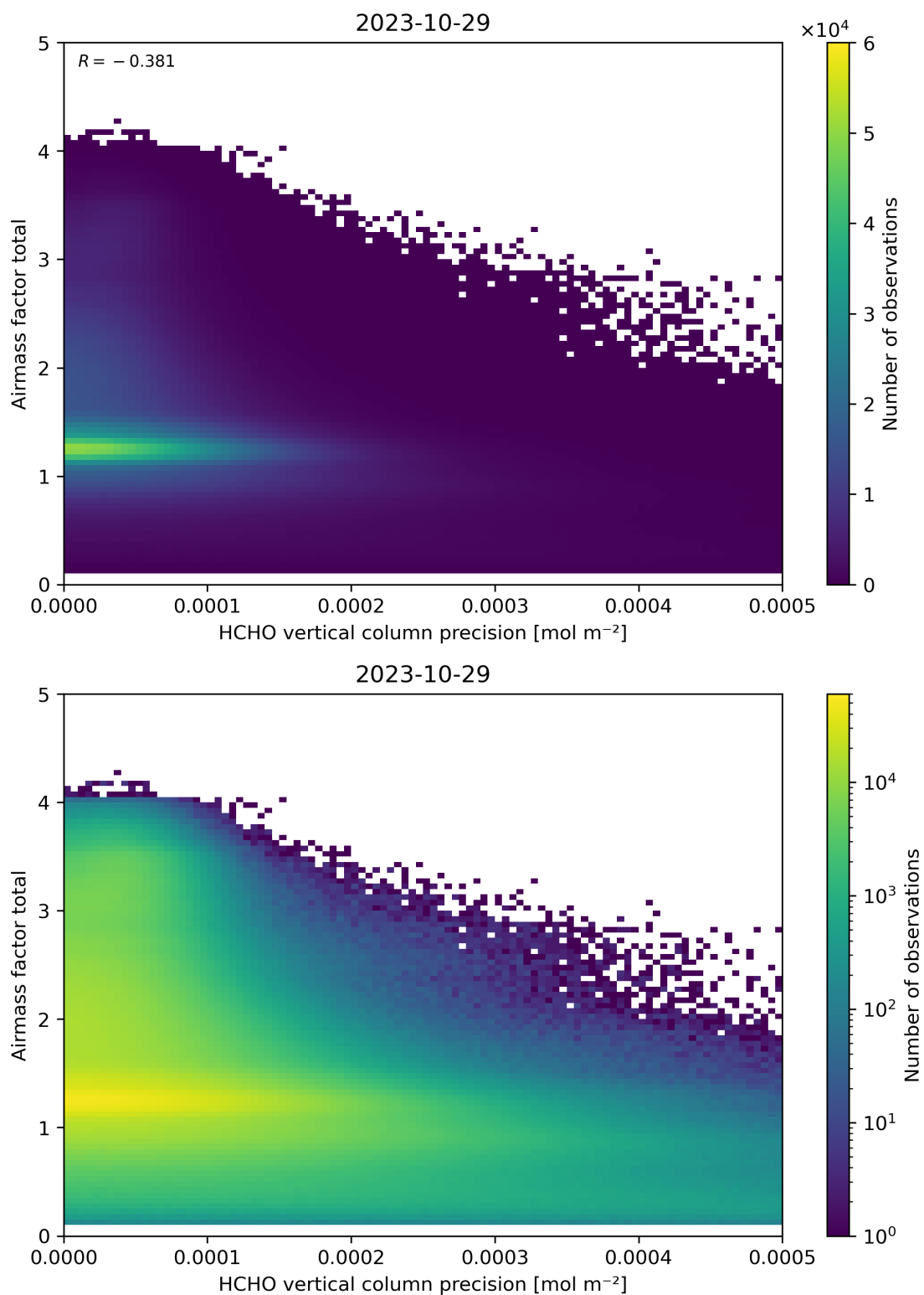
Figure 144: Scatter density plot of “HCHO vertical column precision” against “Airmass factor total” for 2023-10-28 to 2023-10-30.
