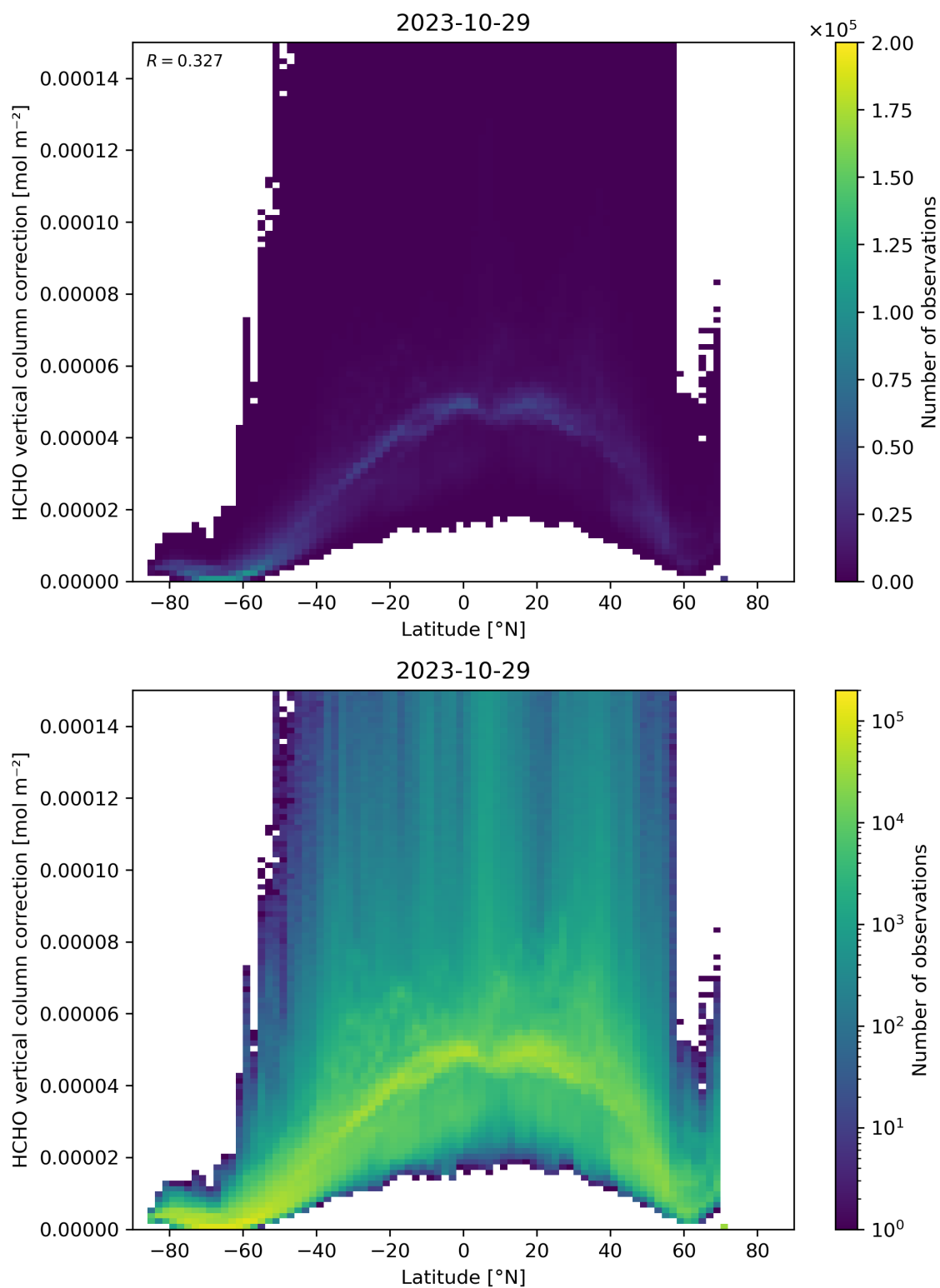
Figure 164: Scatter density plot of “Latitude” against “HCHO vertical column correction” for 2023-10-28 to 2023-10-30.
