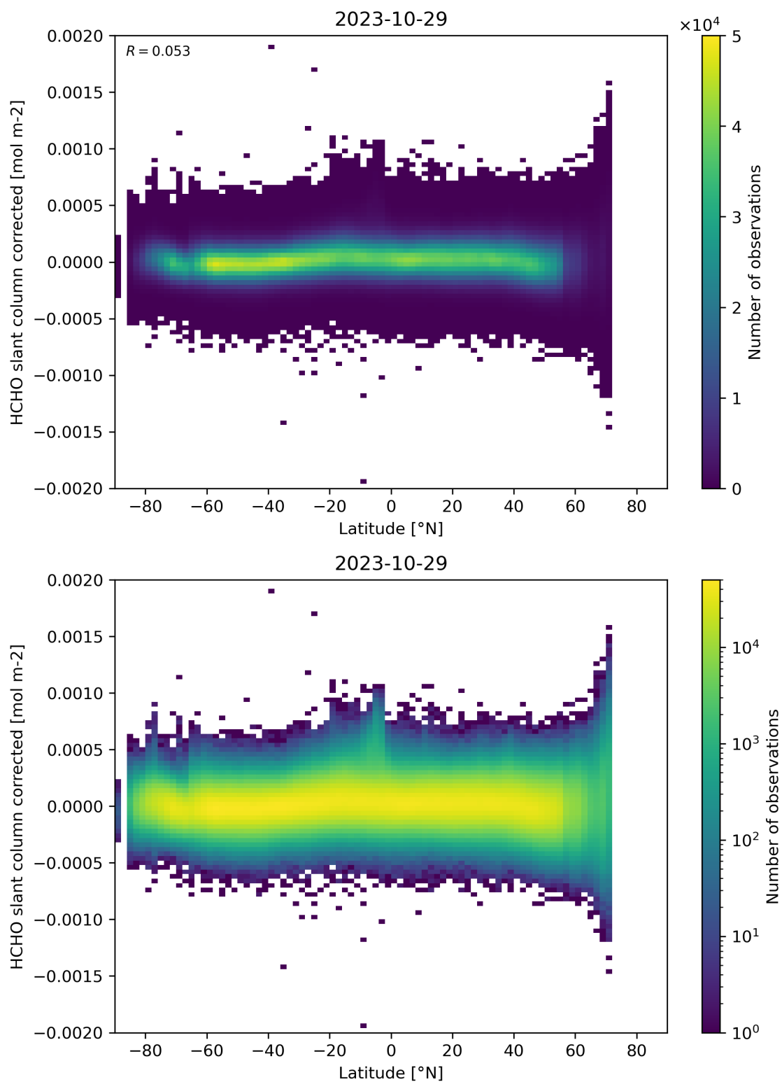
Figure 157: Scatter density plot of “Latitude” against “HCHO slant column corrected” for 2023-10-28 to 2023-10-30.
