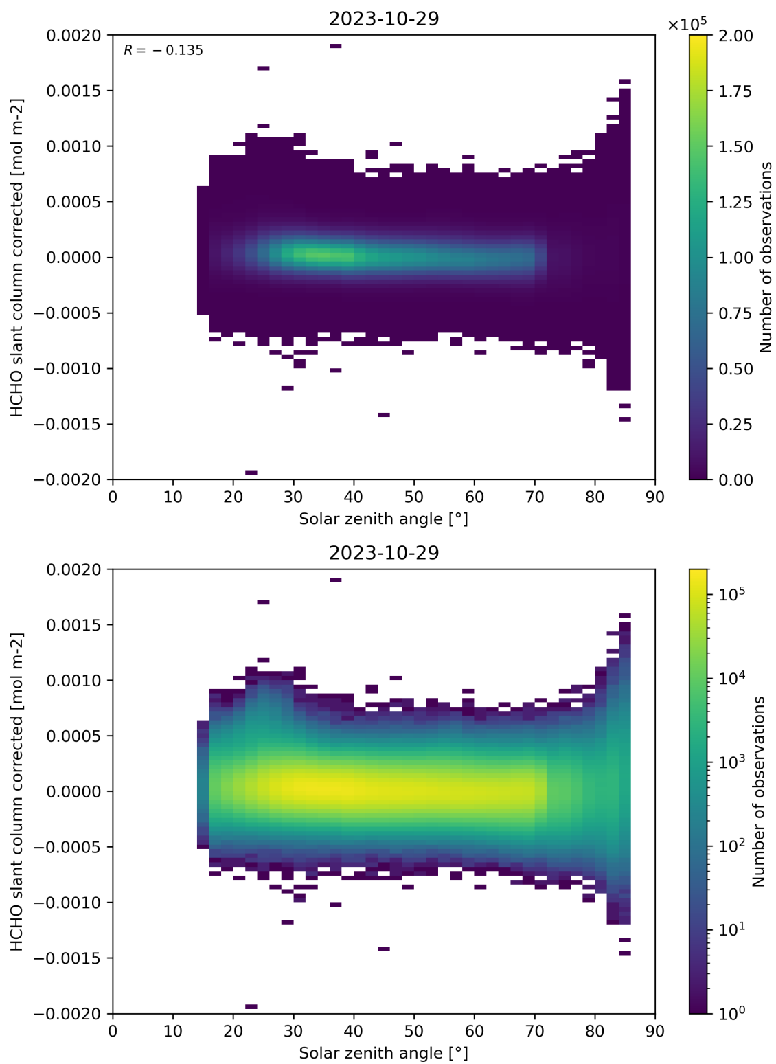
Figure 171: Scatter density plot of “Solar zenith angle” against “HCHO slant column corrected” for 2023-10-28 to 2023-10-30.
