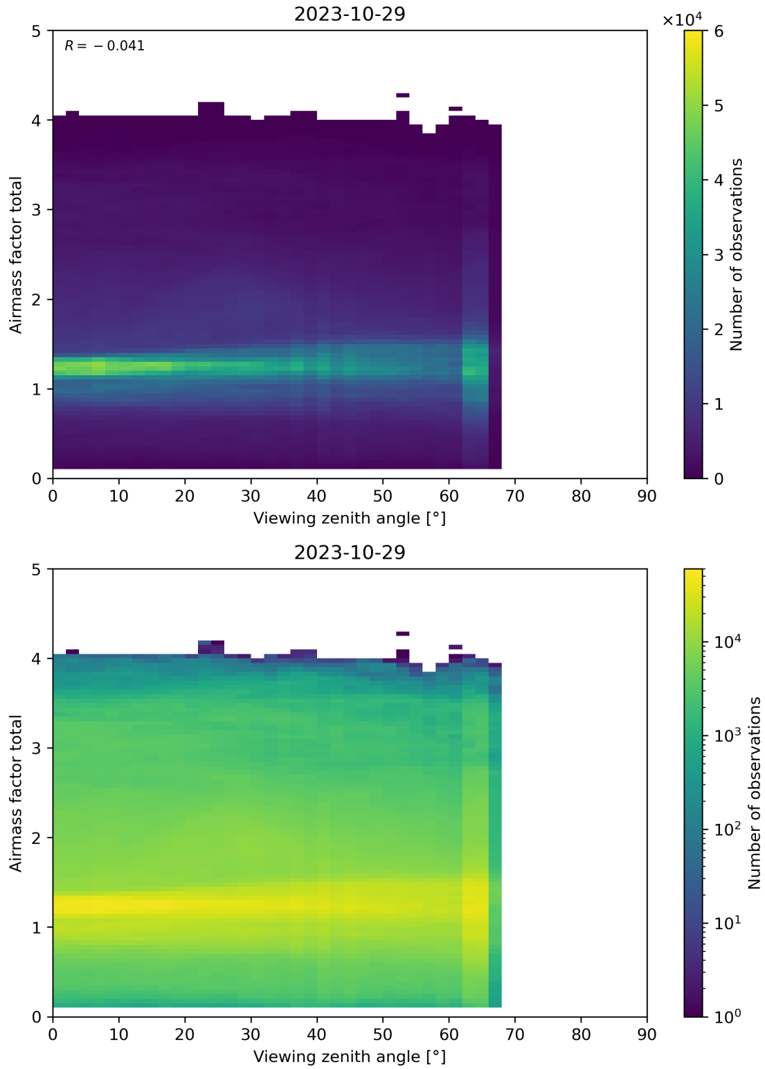
Figure 190: Scatter density plot of “Viewing zenith angle” against “Airmass factor total” for 2023-10-28 to 2023-10-30.
