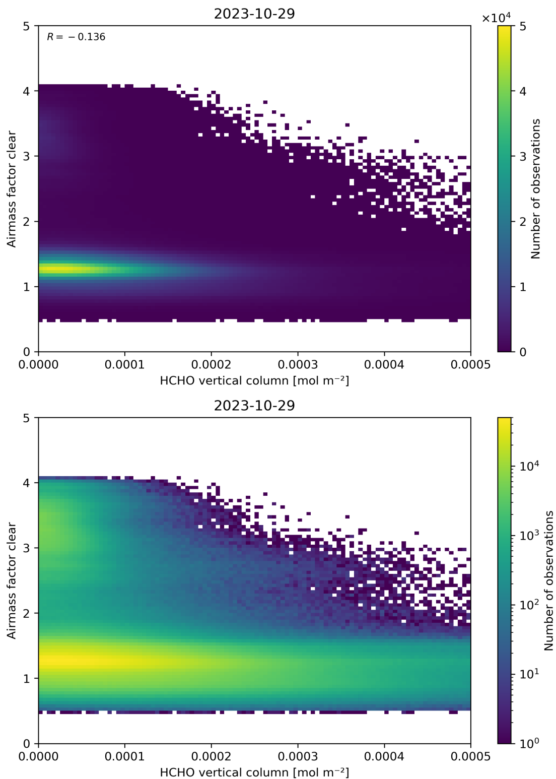
Figure 126: Scatter density plot of “HCHO vertical column” against “Airmass factor clear” for 2023-10-28 to 2023-10-30.
