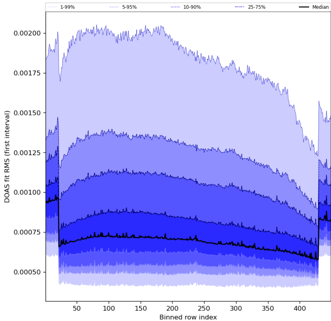
Figure 60: Along track statistics of “DOAS fit RMS (first interval)” for 2023-10-28 to 2023-10-30
