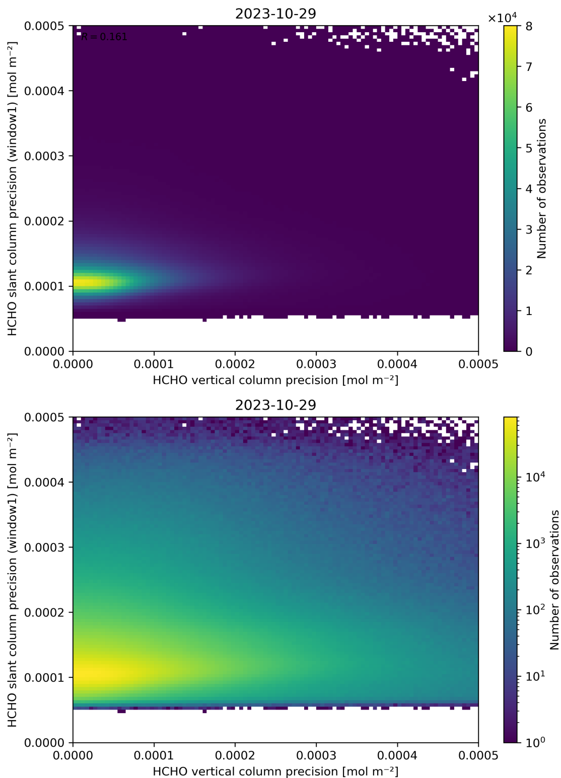
Figure 143: Scatter density plot of “HCHO vertical column precision” against “HCHO slant column precision (window1)” for 2023-10-28 to 2023-10-30.
