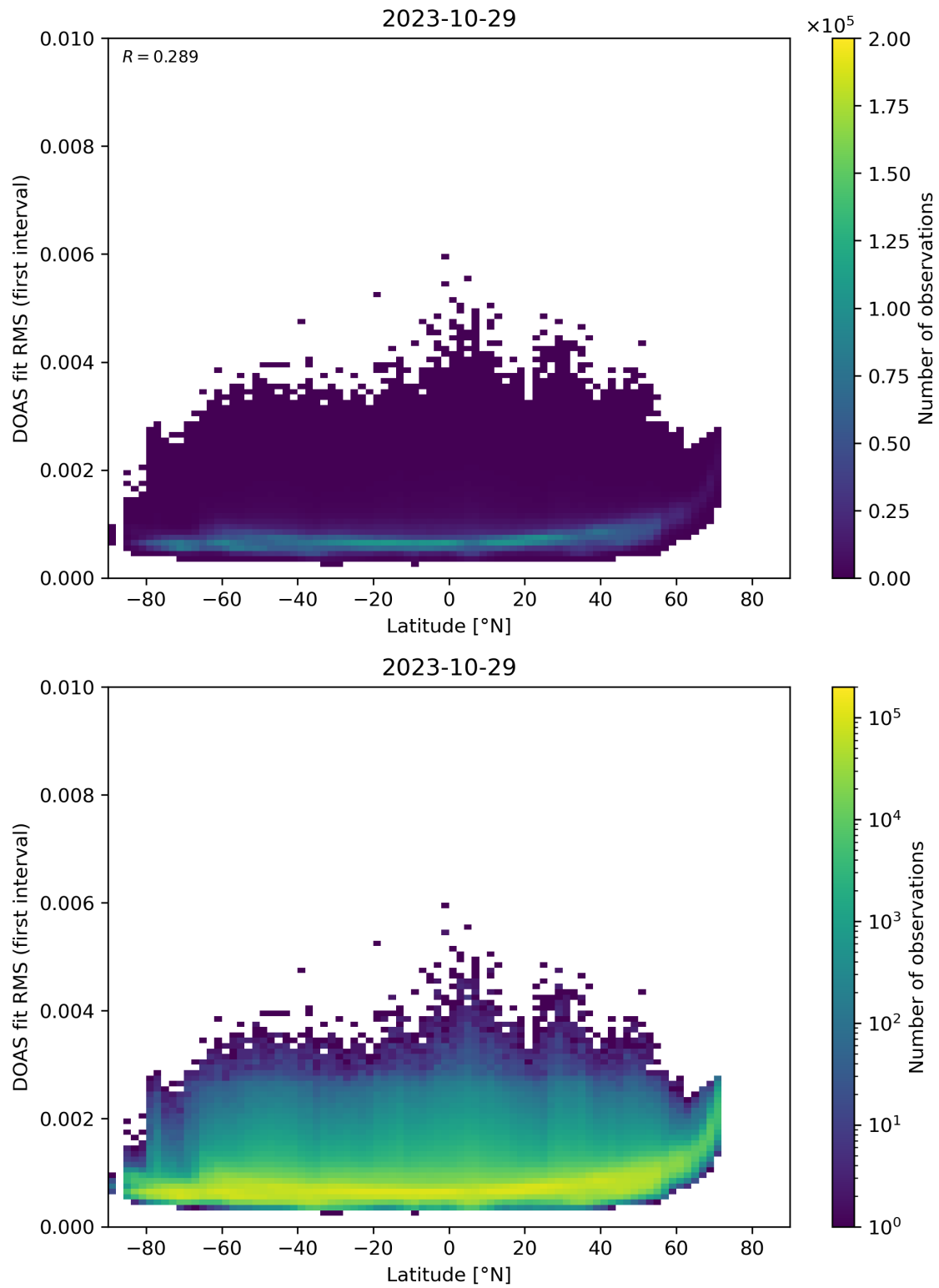
Figure 153: Scatter density plot of “Latitude” against “DOAS fit RMS (first interval)” for 2023-10-28 to 2023-10-30.
