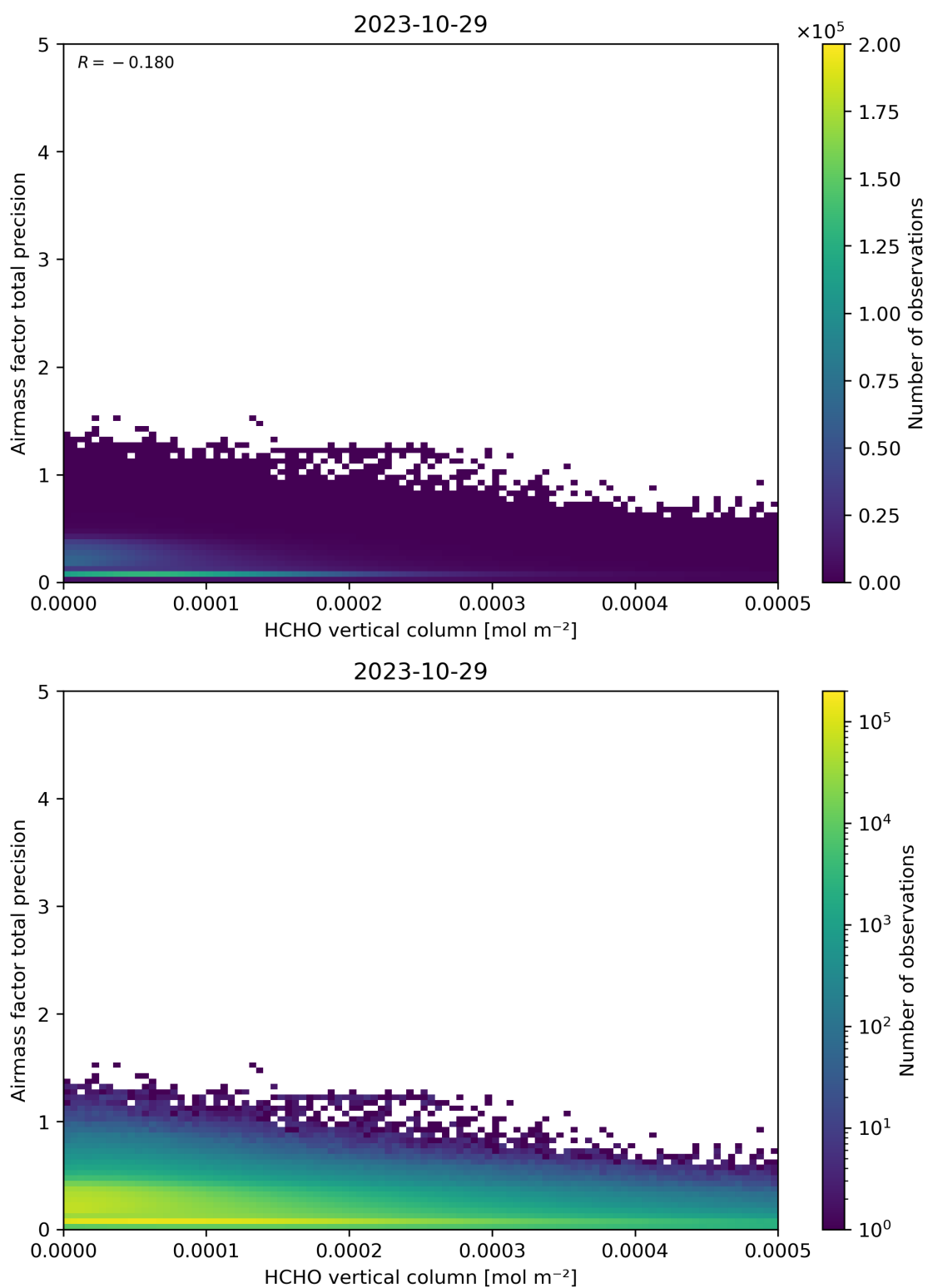
Figure 132: Scatter density plot of “HCHO vertical column” against “Airmass factor total precision” for 2023-10-28 to 2023-10-30.
