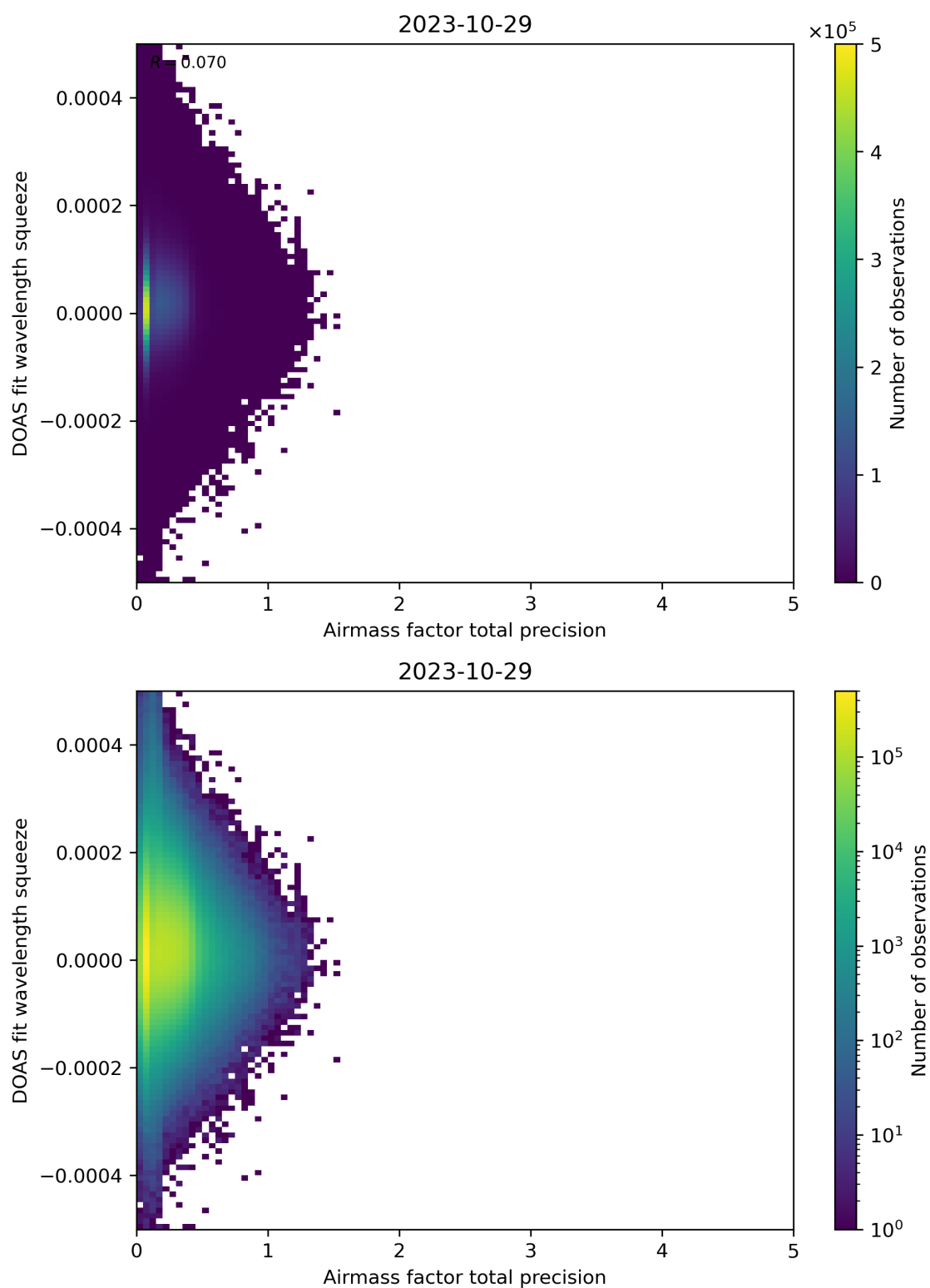
Figure 107: Scatter density plot of “Airmass factor total precision” against “DOAS fit wavelength squeeze” for 2023-10-28 to 2023-10-30.
