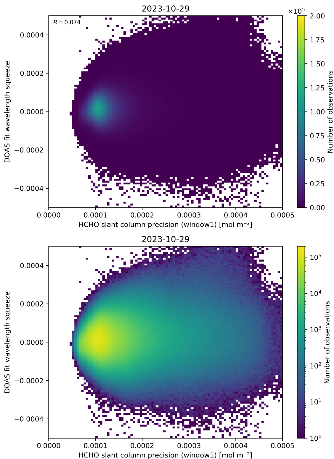
Figure 90: Scatter density plot of “HCHO slant column precision (window1)” against “DOAS fit wavelength squeeze” for 2023-10-28 to 2023-10-30.
