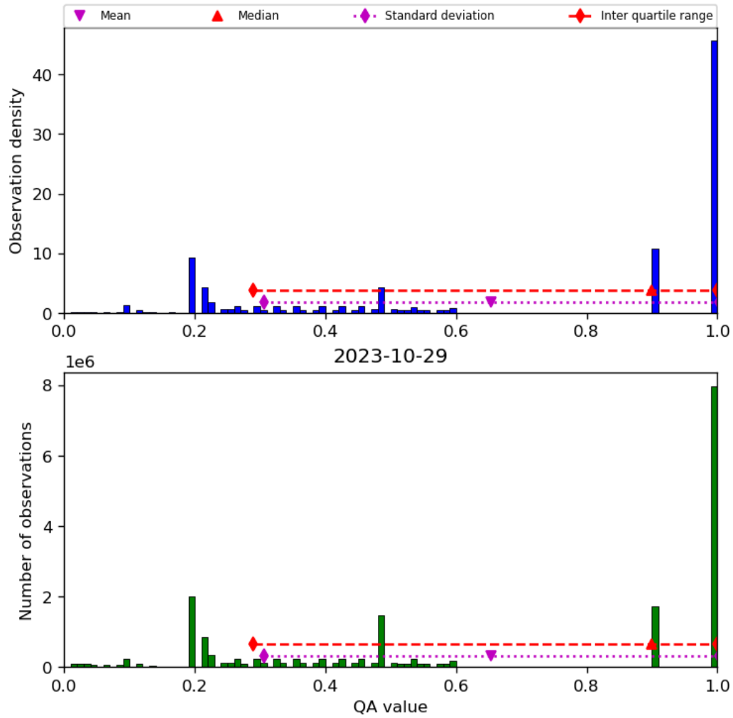
Figure 34: Histogram of “QA value” for 2023-10-28 to 2023-10-30
