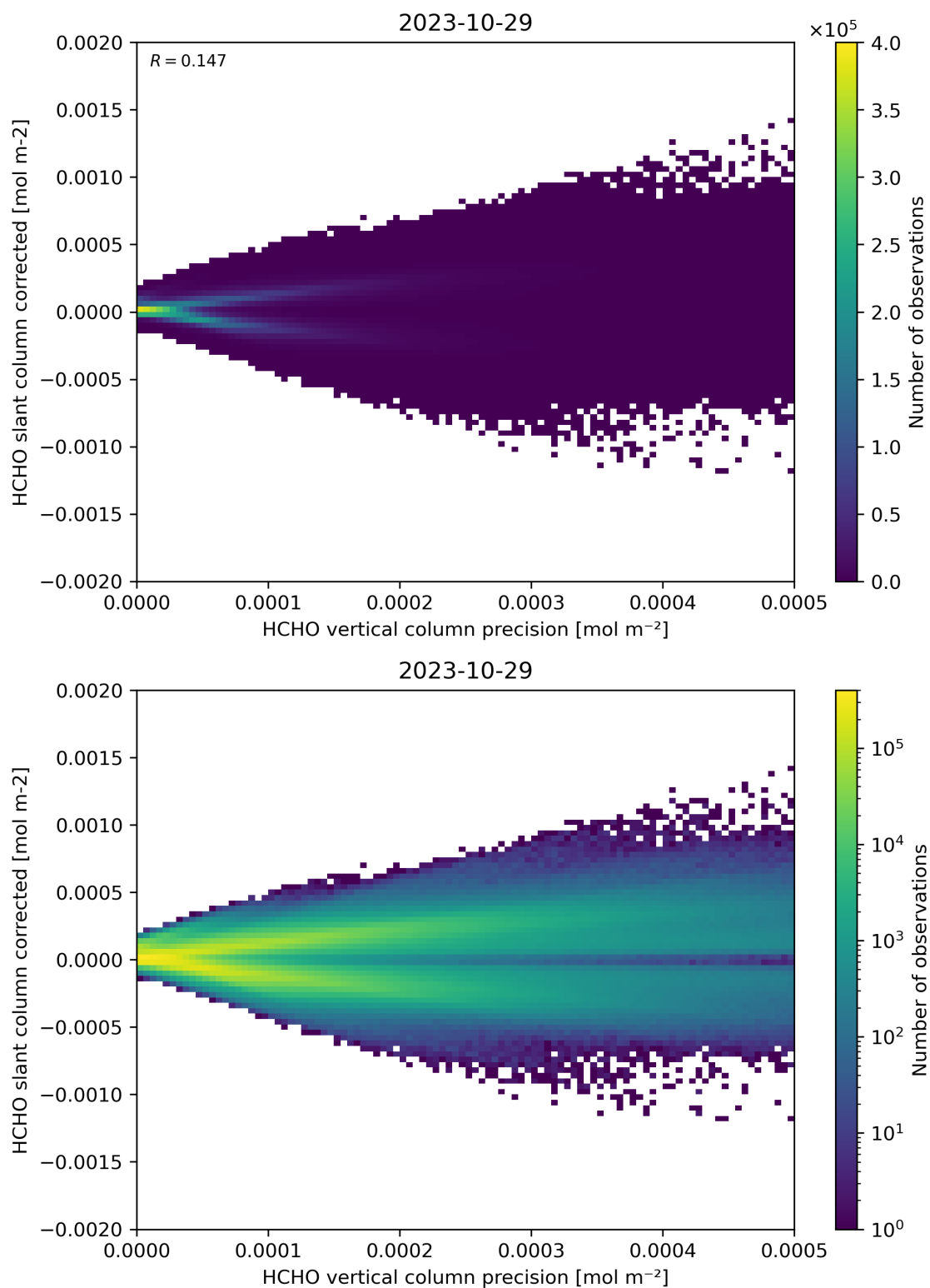
Figure 140: Scatter density plot of “HCHO vertical column precision” against “HCHO slant column corrected” for 2023-10-28 to 2023-10-30.
