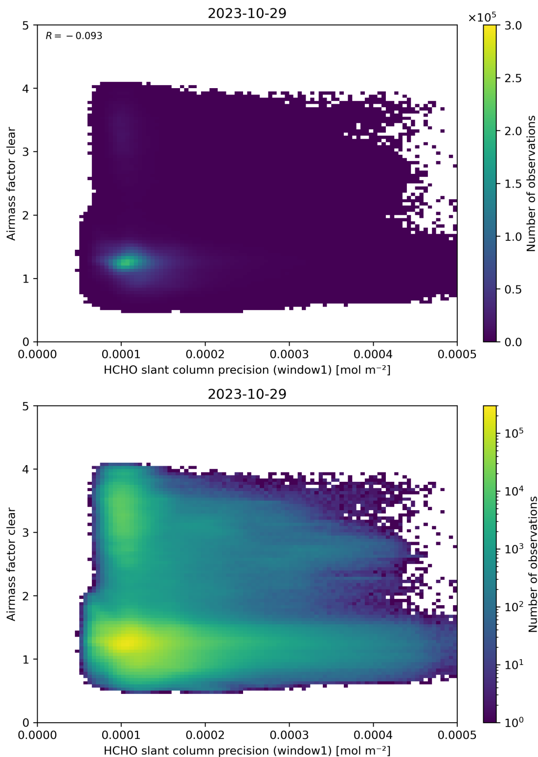
Figure 91: Scatter density plot of “HCHO slant column precision (window1)” against “Airmass factor clear” for 2023-10-28 to 2023-10-30.
