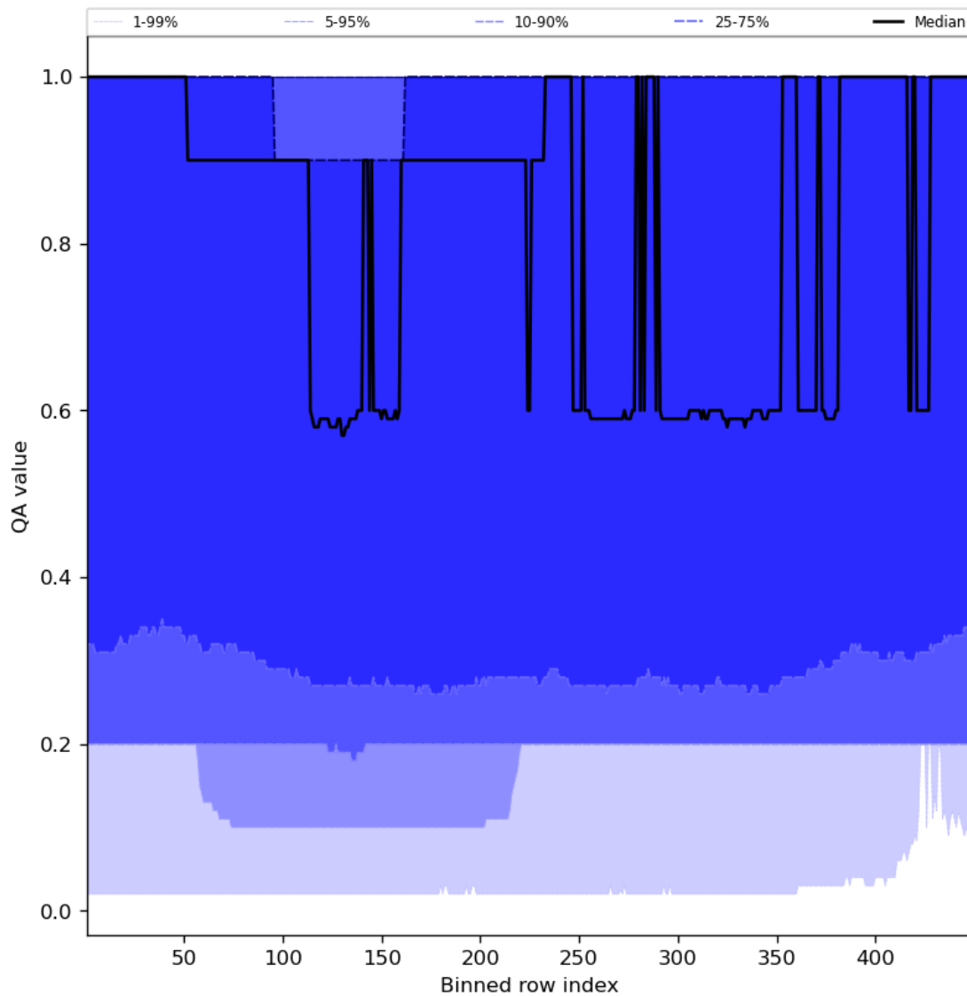
Figure 48: Along track statistics of “QA value” for 2023-10-28 to 2023-10-30
