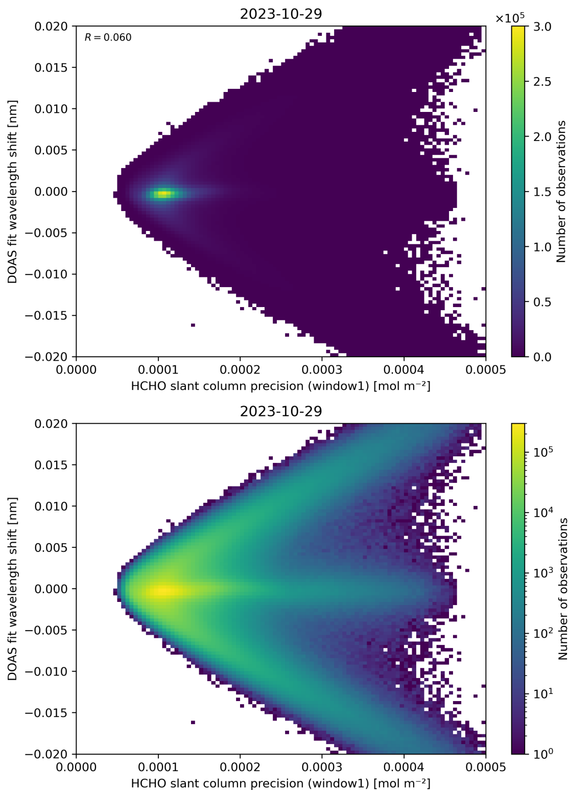
Figure 89: Scatter density plot of “HCHO slant column precision (window1)” against “DOAS fit wavelength shift” for 2023-10-28 to 2023-10-30.
