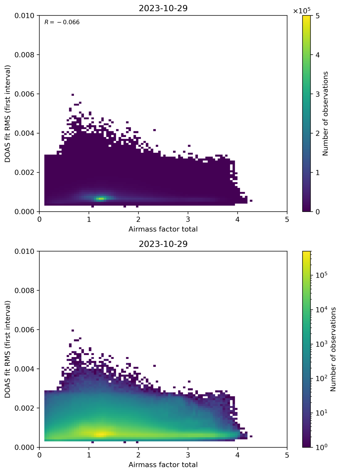
Figure 97: Scatter density plot of “Airmass factor total” against “DOAS fit RMS (first interval)” for 2023-10-28 to 2023-10-30.
