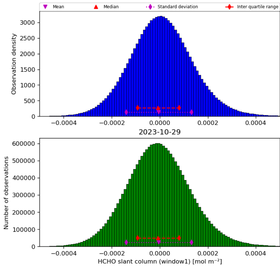
Figure 38: Histogram of “HCHO slant column (window1)” for 2023-10-28 to 2023-10-30
