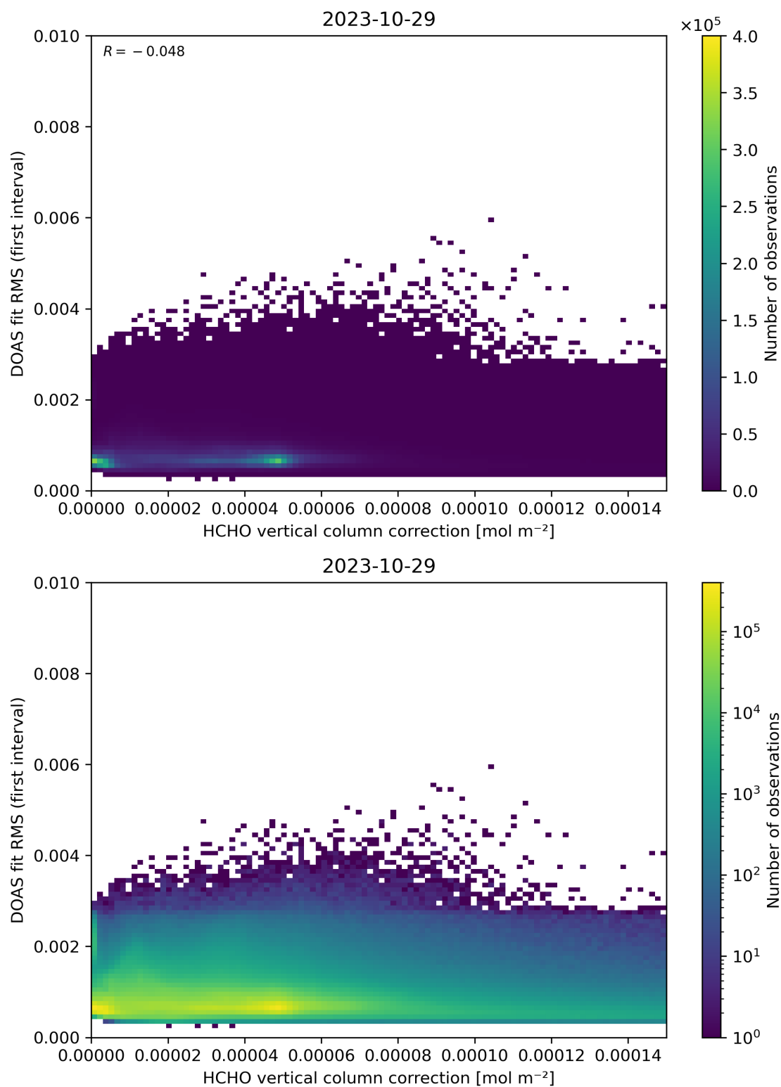
Figure 112: Scatter density plot of “HCHO vertical column correction” against “DOAS fit RMS (first interval)” for 2023-10-28 to 2023-10-30.
