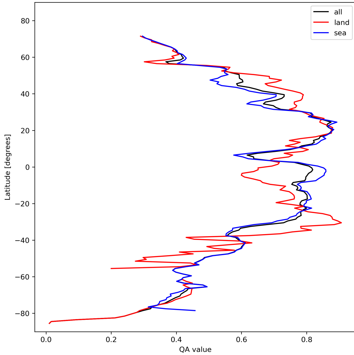
Figure 20: Zonal average of “QA value” for 2023-10-28 to 2023-10-30.
