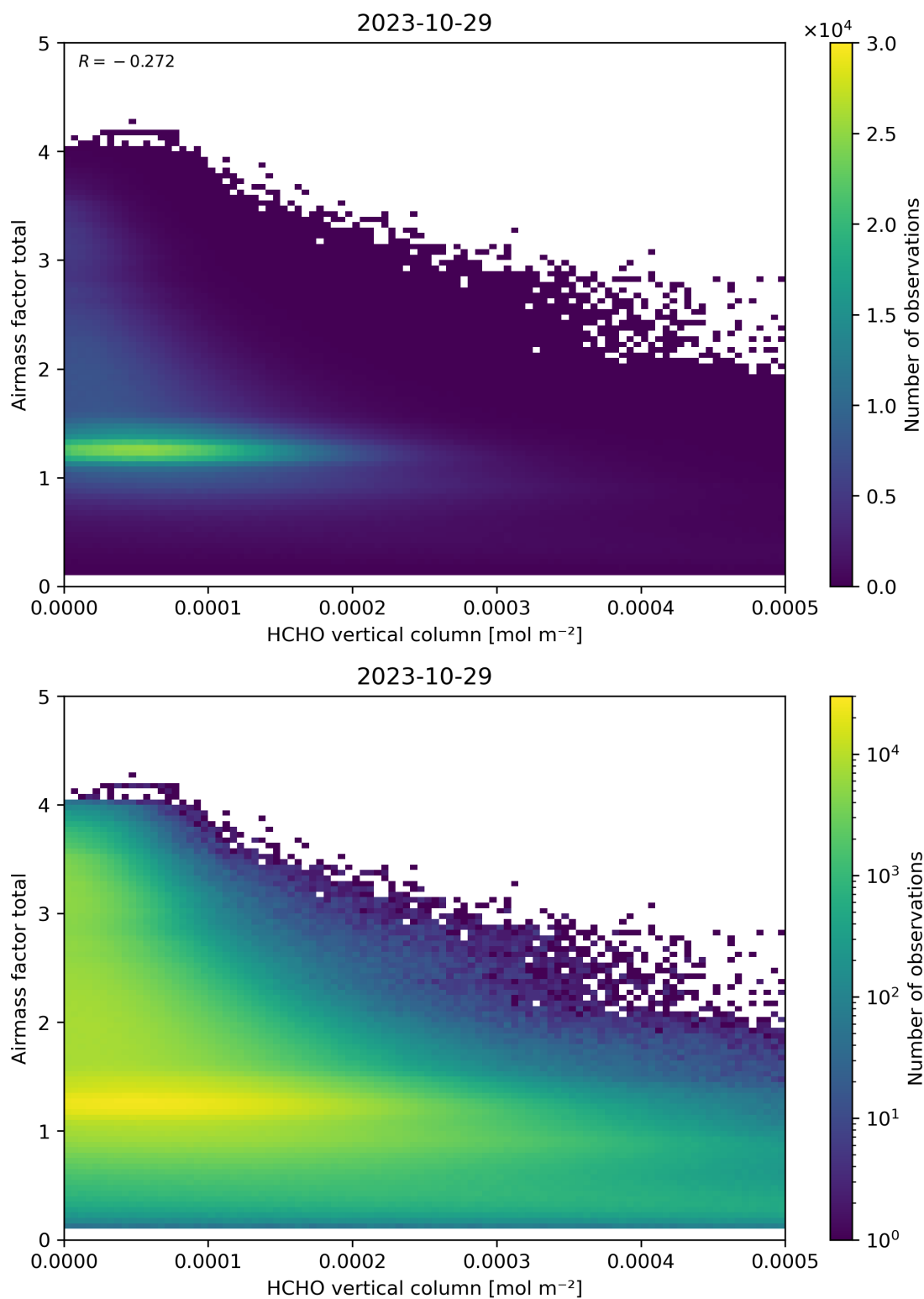
Figure 131: Scatter density plot of “HCHO vertical column” against “Airmass factor total” for 2023-10-28 to 2023-10-30.
