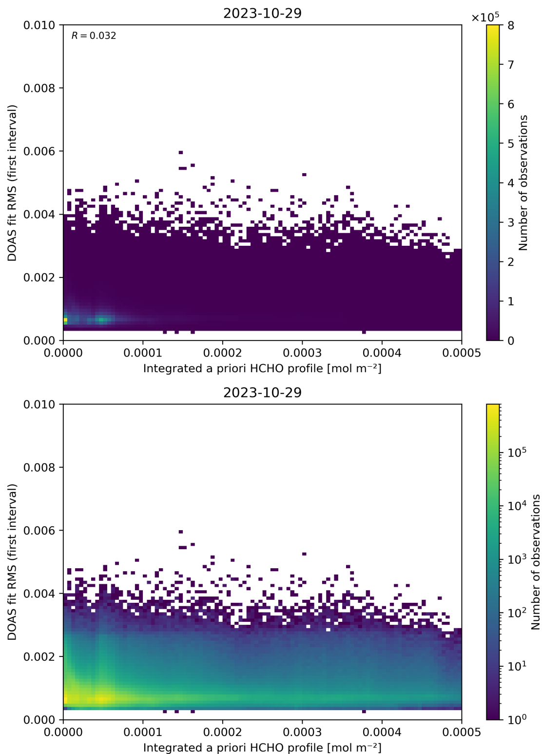
Figure 148: Scatter density plot of “Integrated a priori HCHO profile” against “DOAS fit RMS (first interval)” for 2023-10-28 to 2023-10-30.
