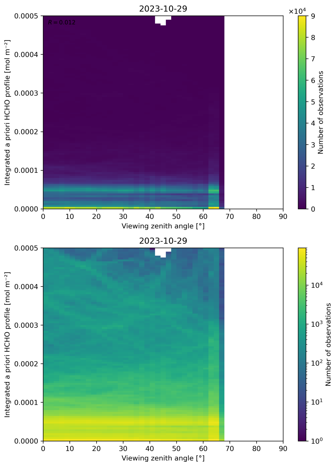
Figure 195: Scatter density plot of “Viewing zenith angle” against “Integrated a priori HCHO profile” for 2023-10-28 to 2023-10-30.
