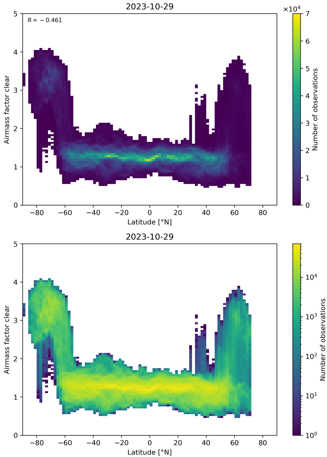
Figure 156: Scatter density plot of “Latitude” against “Airmass factor clear” for 2023-10-28 to 2023-10-30.
