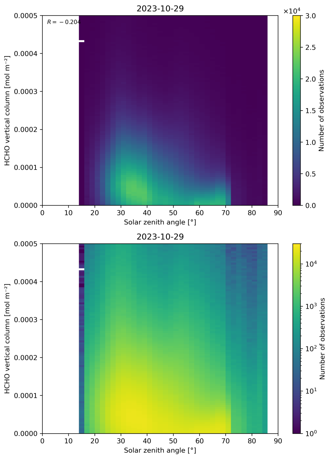
Figure 177: Scatter density plot of “Solar zenith angle” against “HCHO vertical column” for 2023-10-28 to 2023-10-30.
