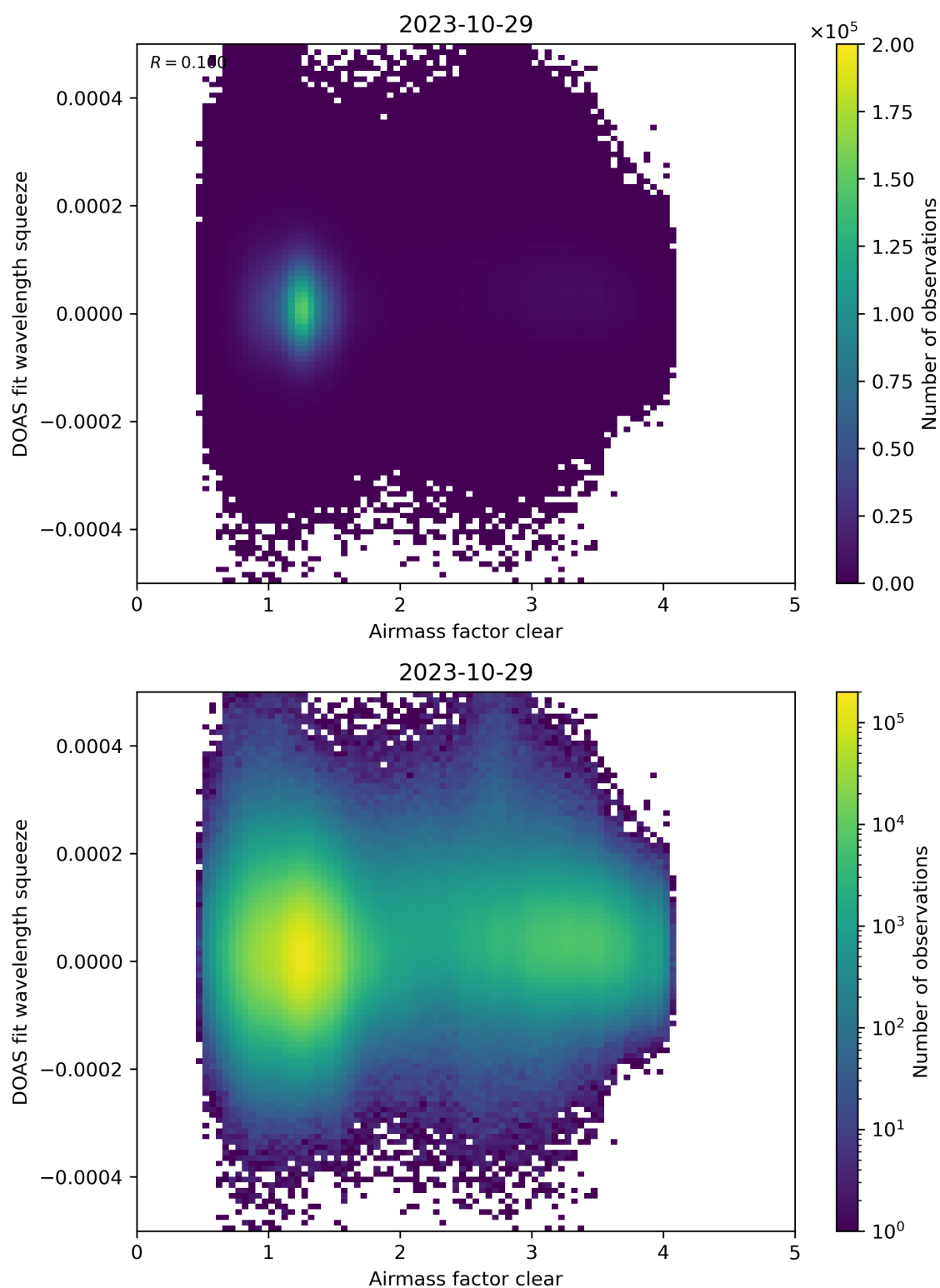
Figure 73: Scatter density plot of “Airmass factor clear” against “DOAS fit wavelength squeeze” for 2023-10-28 to 2023-10-30.
