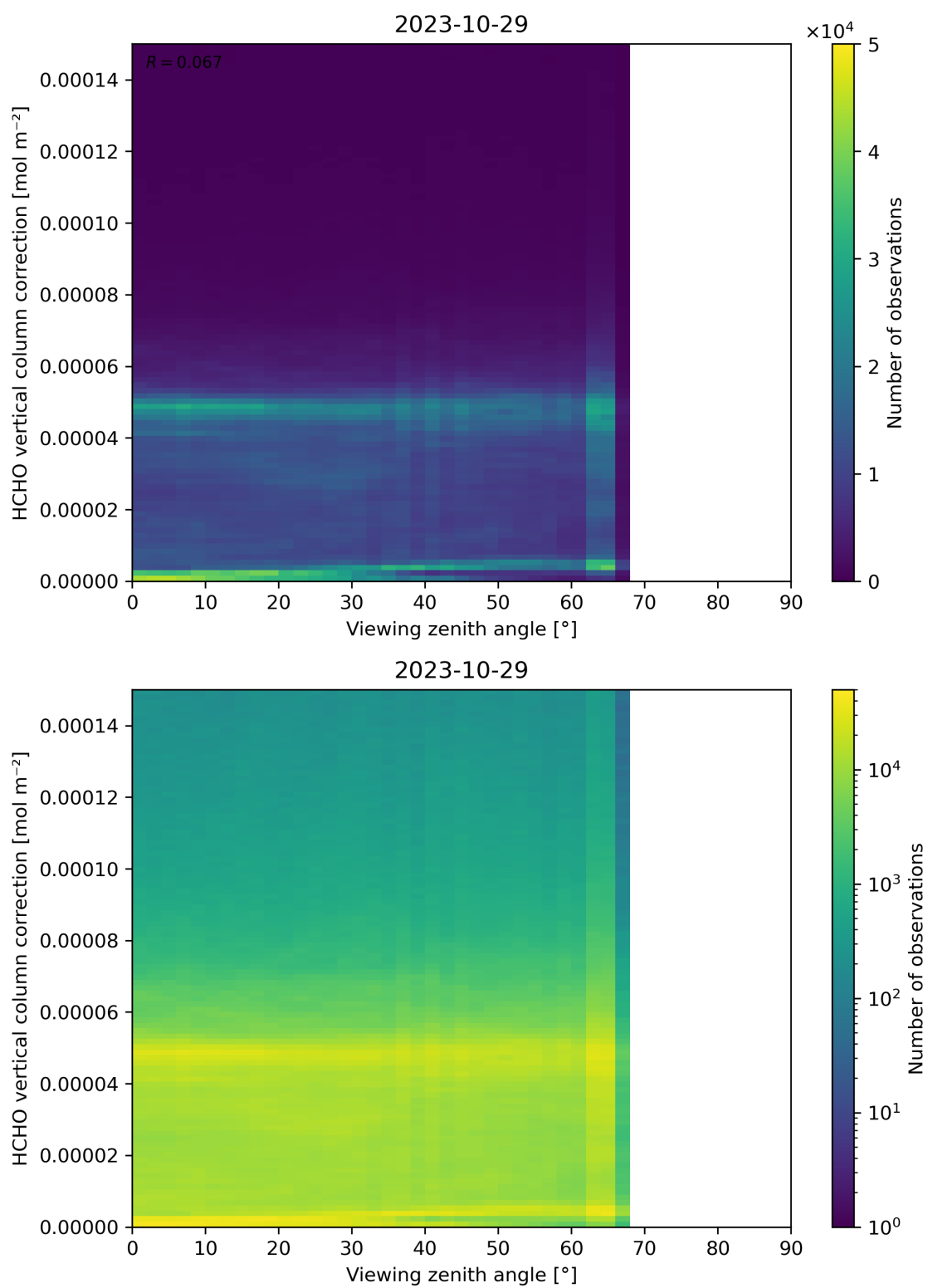
Figure 193: Scatter density plot of “Viewing zenith angle” against “HCHO vertical column correction” for 2023-10-28 to 2023-10-30.
