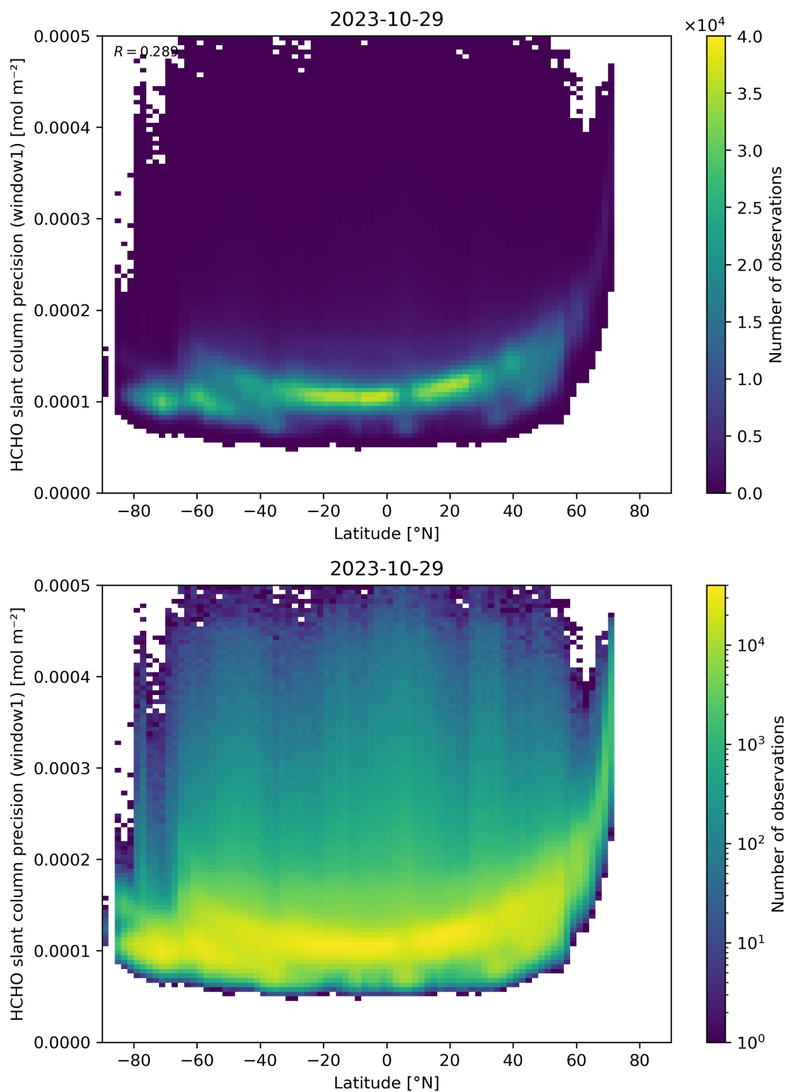
Figure 160: Scatter density plot of “Latitude” against “HCHO slant column precision (window1)” for 2023-10-28 to 2023-10-30.
