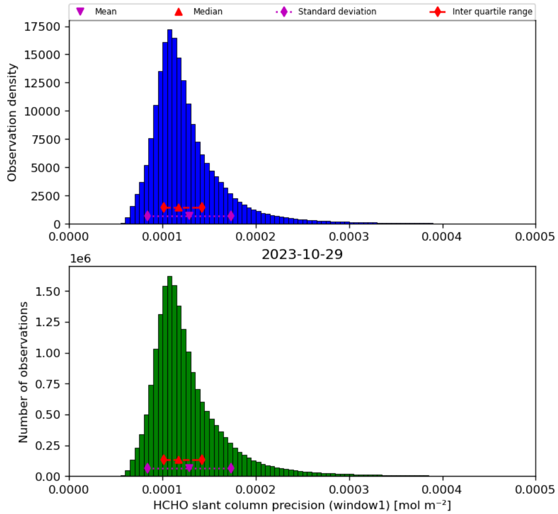
Figure 39: Histogram of “HCHO slant column precision (window1)” for 2023-10-28 to 2023-10-30
