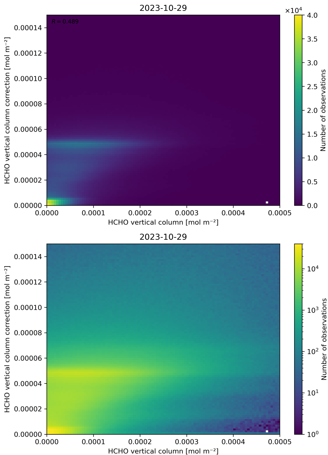
Figure 133: Scatter density plot of “HCHO vertical column” against “HCHO vertical column correction” for 2023-10-28 to 2023-10-30.
