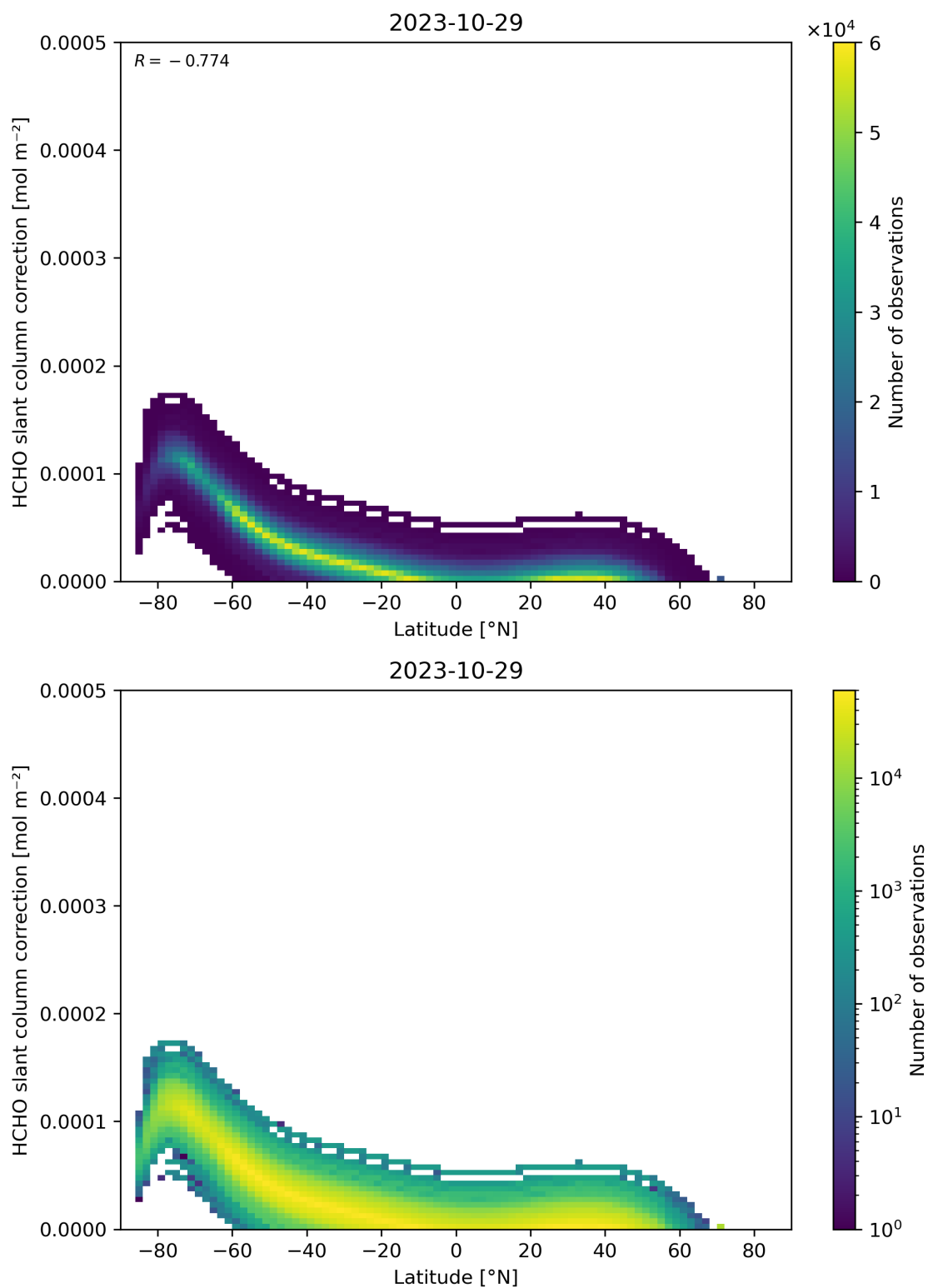
Figure 158: Scatter density plot of “Latitude” against “HCHO slant column correction” for 2023-10-28 to 2023-10-30.
