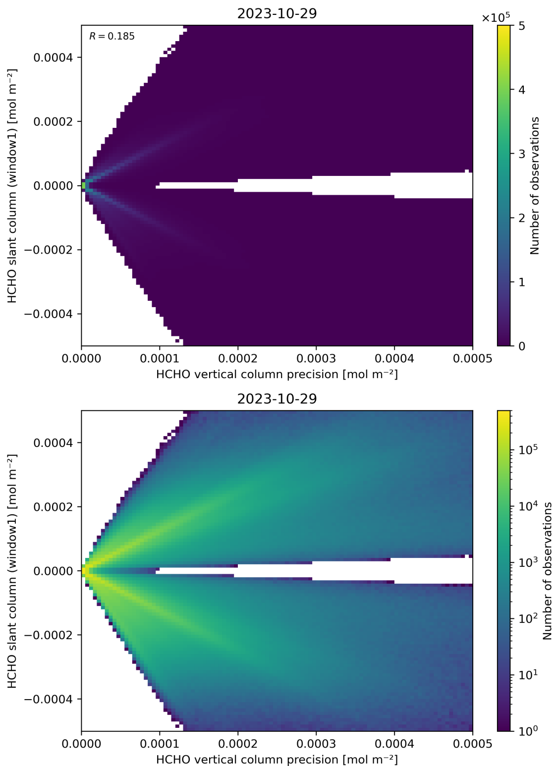
Figure 142: Scatter density plot of “HCHO vertical column precision” against “HCHO slant column (window1)” for 2023-10-28 to 2023-10-30.
