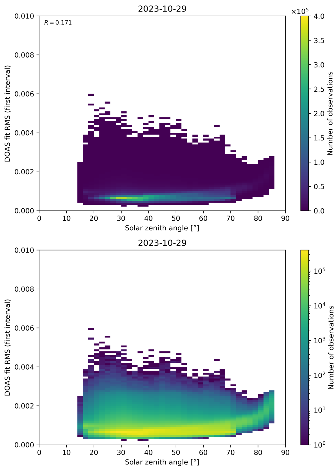
Figure 167: Scatter density plot of “Solar zenith angle” against “DOAS fit RMS (first interval)” for 2023-10-28 to 2023-10-30.
