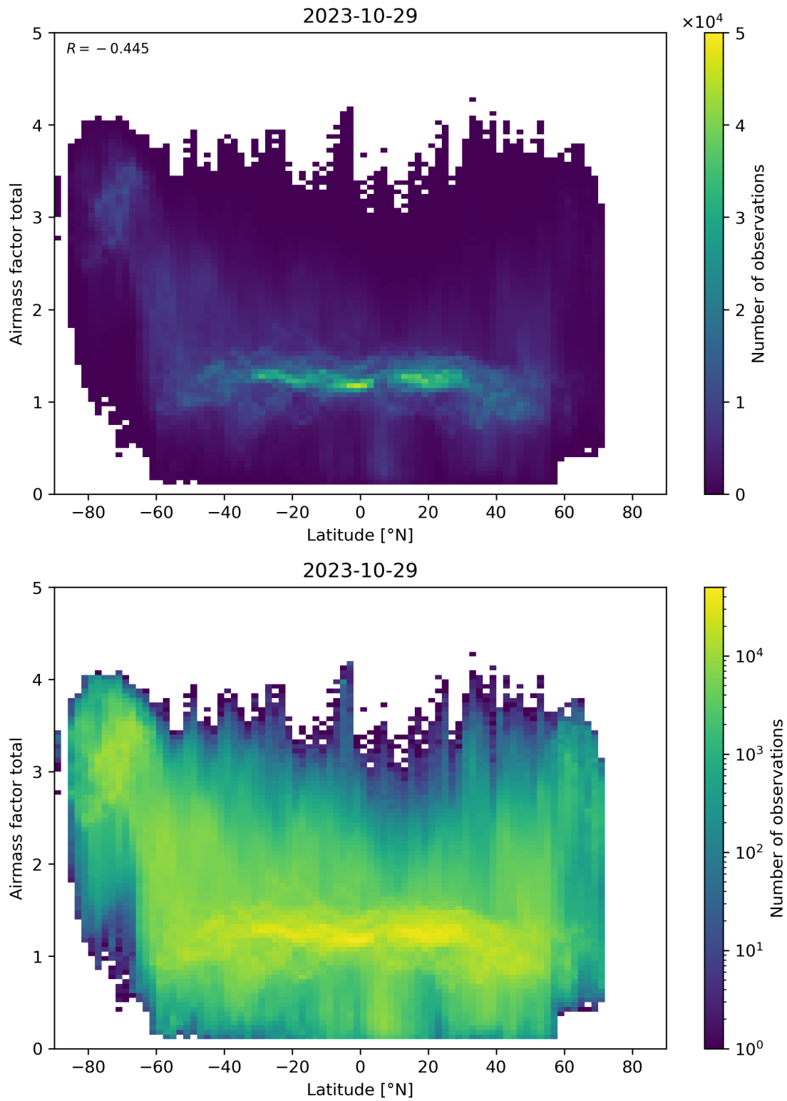
Figure 161: Scatter density plot of “Latitude” against “Airmass factor total” for 2023-10-28 to 2023-10-30.
