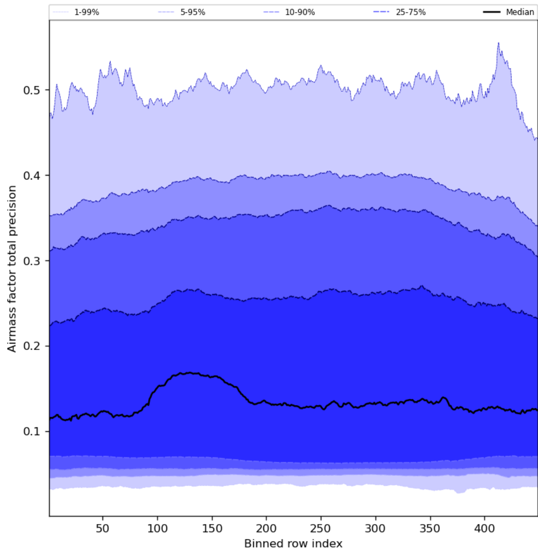
Figure 55: Along track statistics of “Airmass factor total precision” for 2023-10-28 to 2023-10-30
