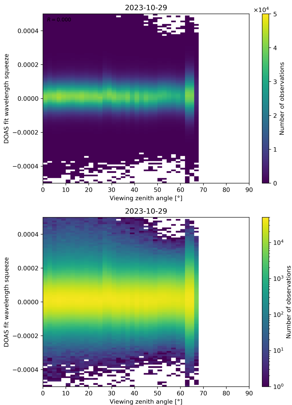
Figure 184: Scatter density plot of “Viewing zenith angle” against “DOAS fit wavelength squeeze” for 2023-10-28 to 2023-10-30.
