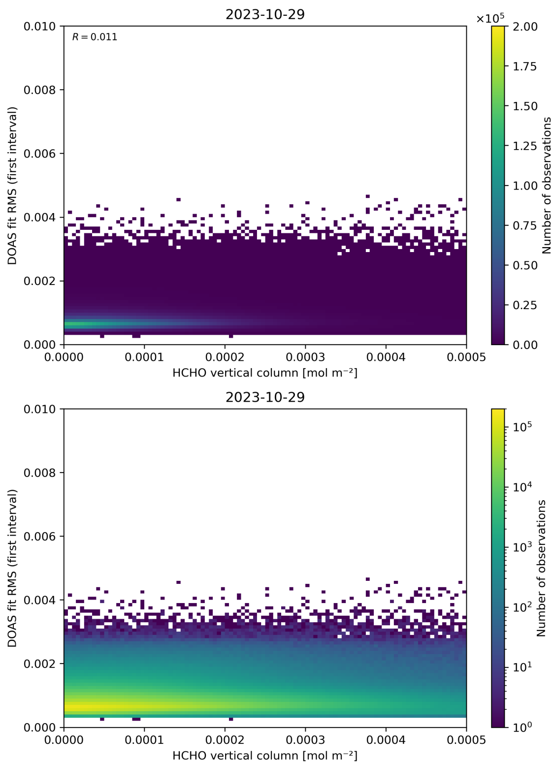
Figure 123: Scatter density plot of “HCHO vertical column” against “DOAS fit RMS (first interval)” for 2023-10-28 to 2023-10-30.
