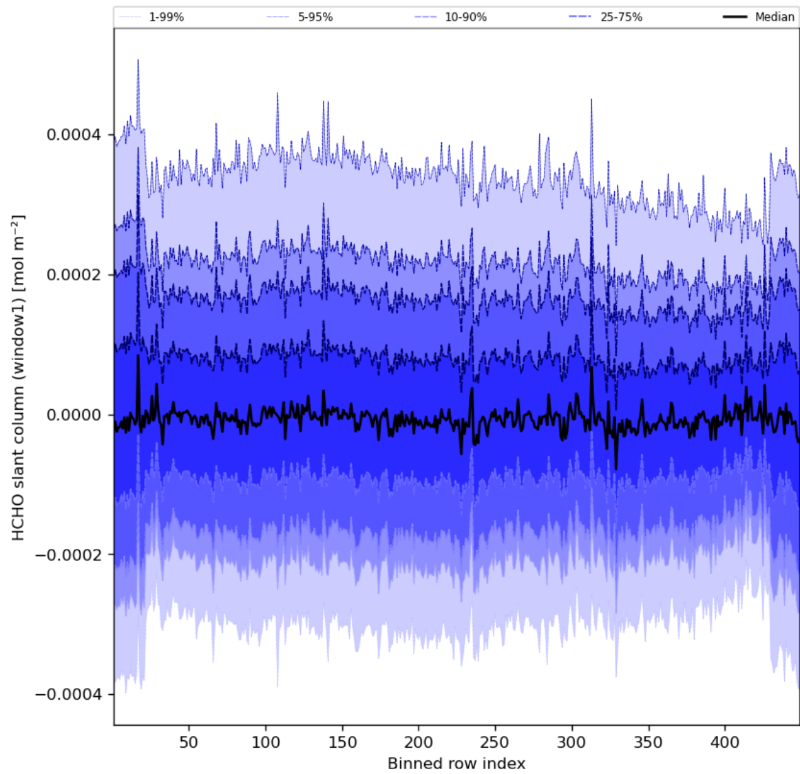
Figure 52: Along track statistics of “HCHO slant column (window1)” for 2023-10-28 to 2023-10-30
