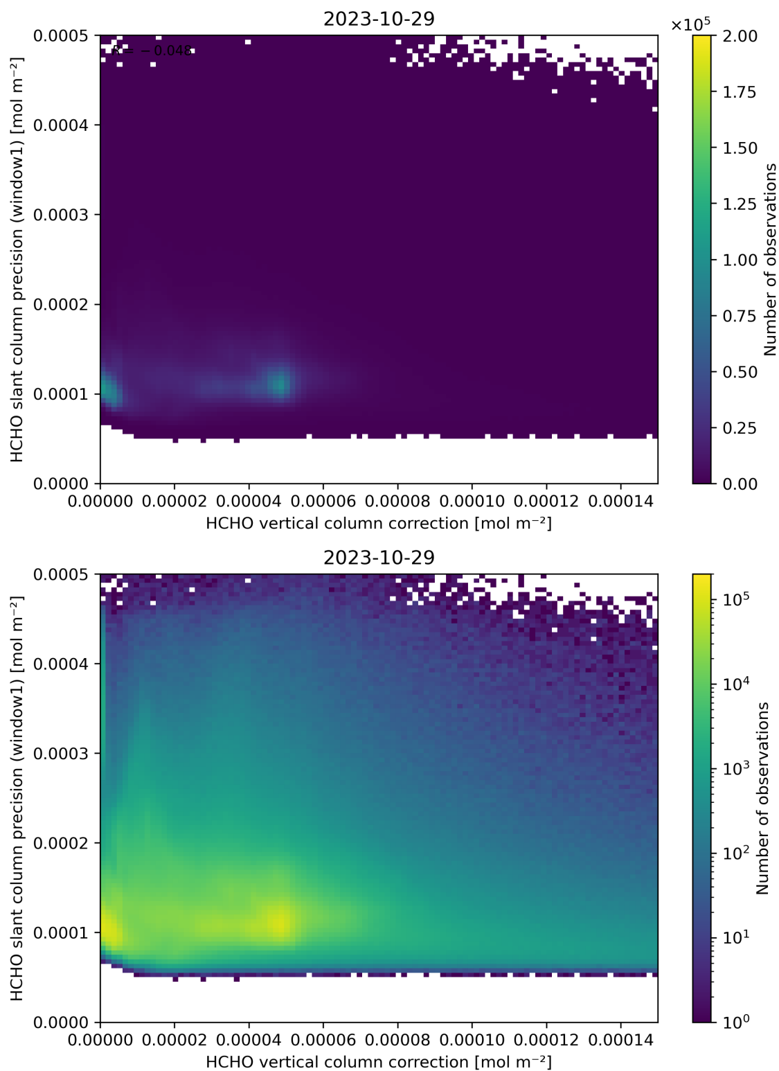
Figure 119: Scatter density plot of “HCHO vertical column correction” against “HCHO slant column precision (window1)” for 2023-10-28 to 2023-10-30.
