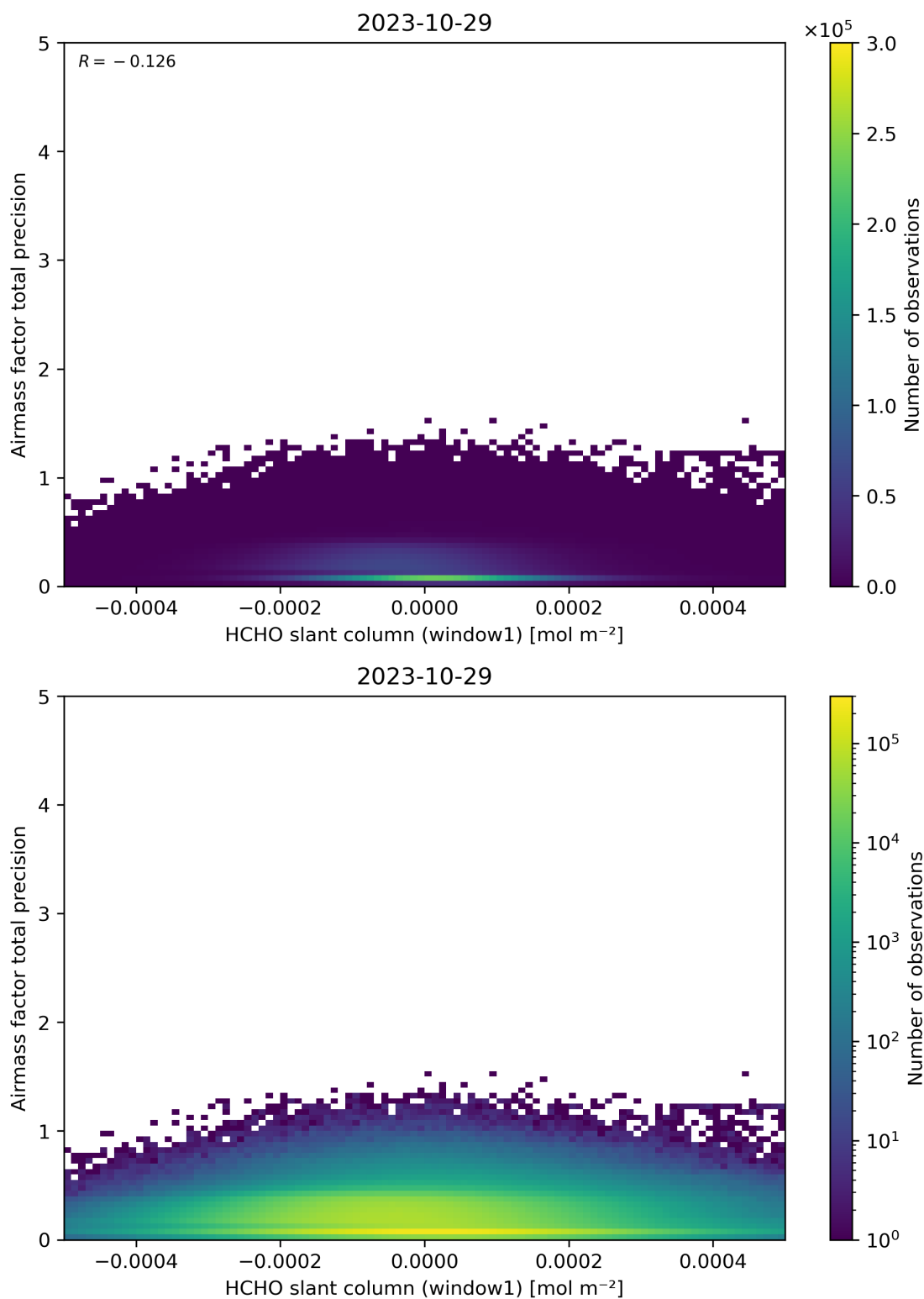
Figure 86: Scatter density plot of “HCHO slant column (window1)” against “Airmass factor total precision” for 2023-10-28 to 2023-10-30.
