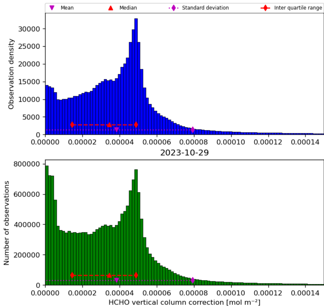
Figure 37: Histogram of “HCHO vertical column correction” for 2023-10-28 to 2023-10-30
