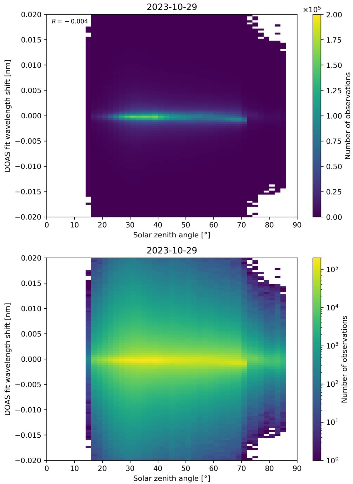
Figure 168: Scatter density plot of “Solar zenith angle” against “DOAS fit wavelength shift” for 2023-10-28 to 2023-10-30.
