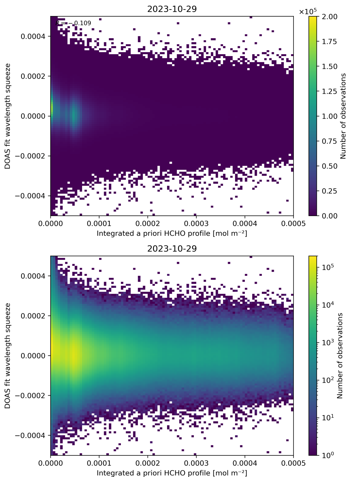
Figure 150: Scatter density plot of “Integrated a priori HCHO profile” against “DOAS fit wavelength squeeze” for 2023-10-28 to 2023-10-30.
