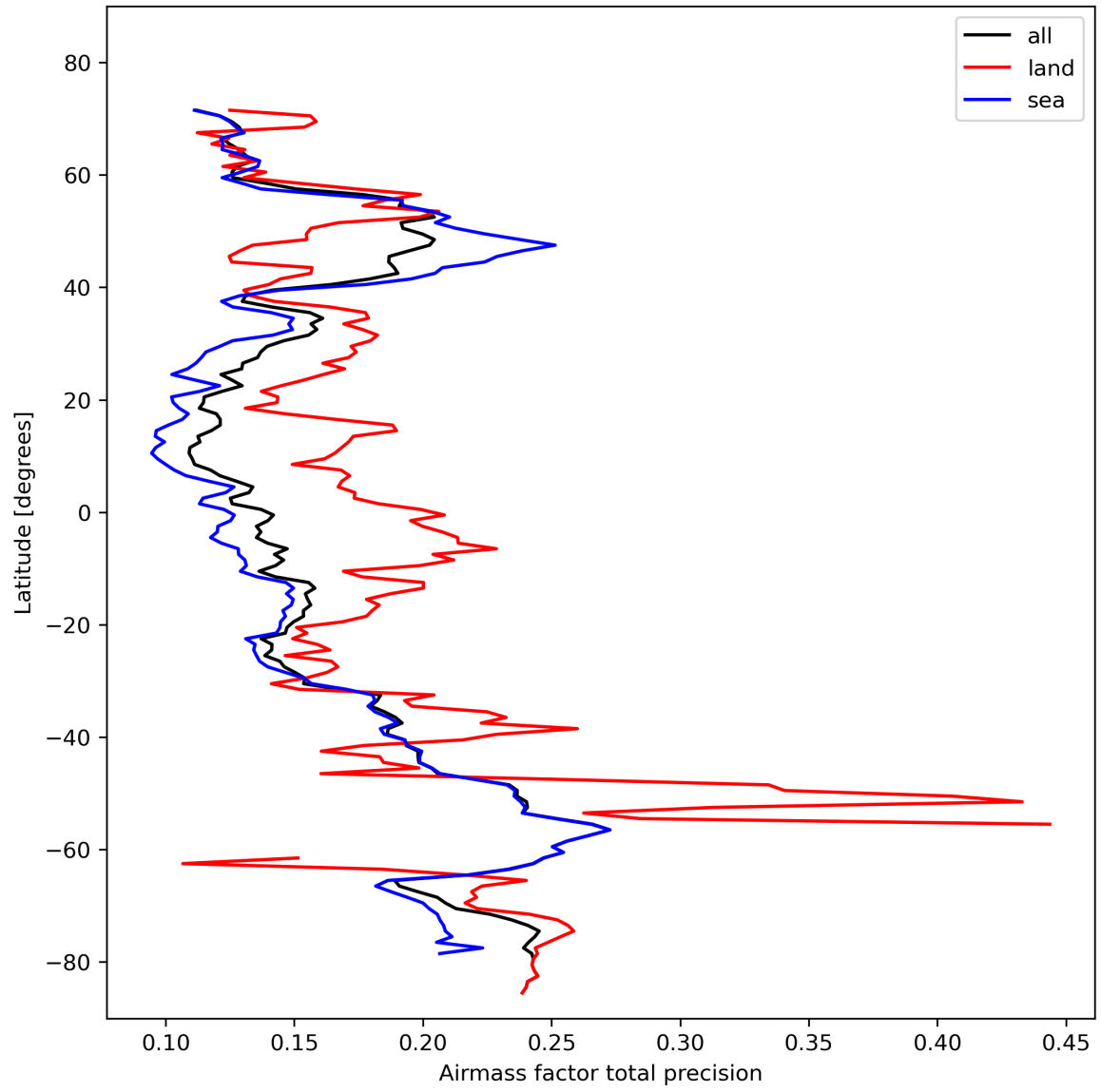
Figure 27: Zonal average of “Airmass factor total precision” for 2023-10-28 to 2023-10-30.
