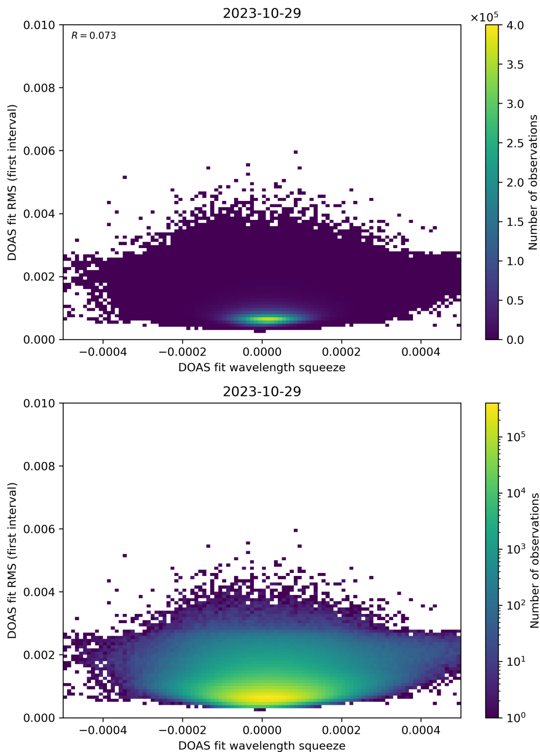
Figure 68: Scatter density plot of “DOAS fit wavelength squeeze” against “DOAS fit RMS (first interval)” for 2023-10-28 to 2023-10-30.
