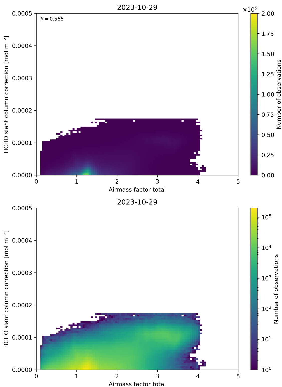
Figure 102: Scatter density plot of “Airmass factor total” against “HCHO slant column correction” for 2023-10-28 to 2023-10-30.
