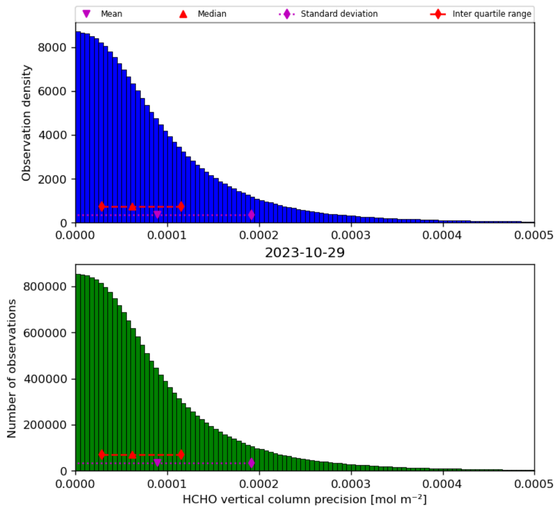
Figure 36: Histogram of “HCHO vertical column precision” for 2023-10-28 to 2023-10-30
