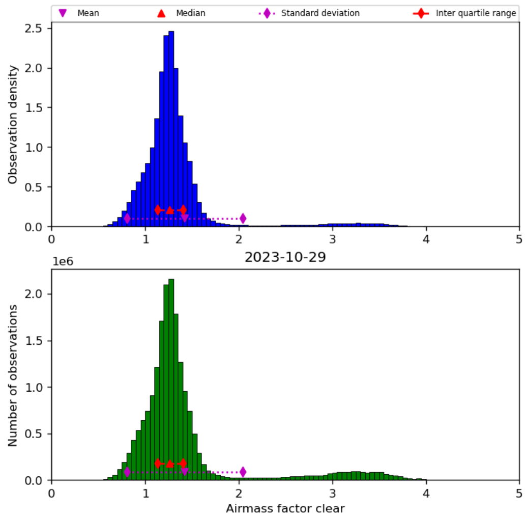
Figure 42: Histogram of "Airmass factor clear" for 2023-10-28 to 2023-10-30
