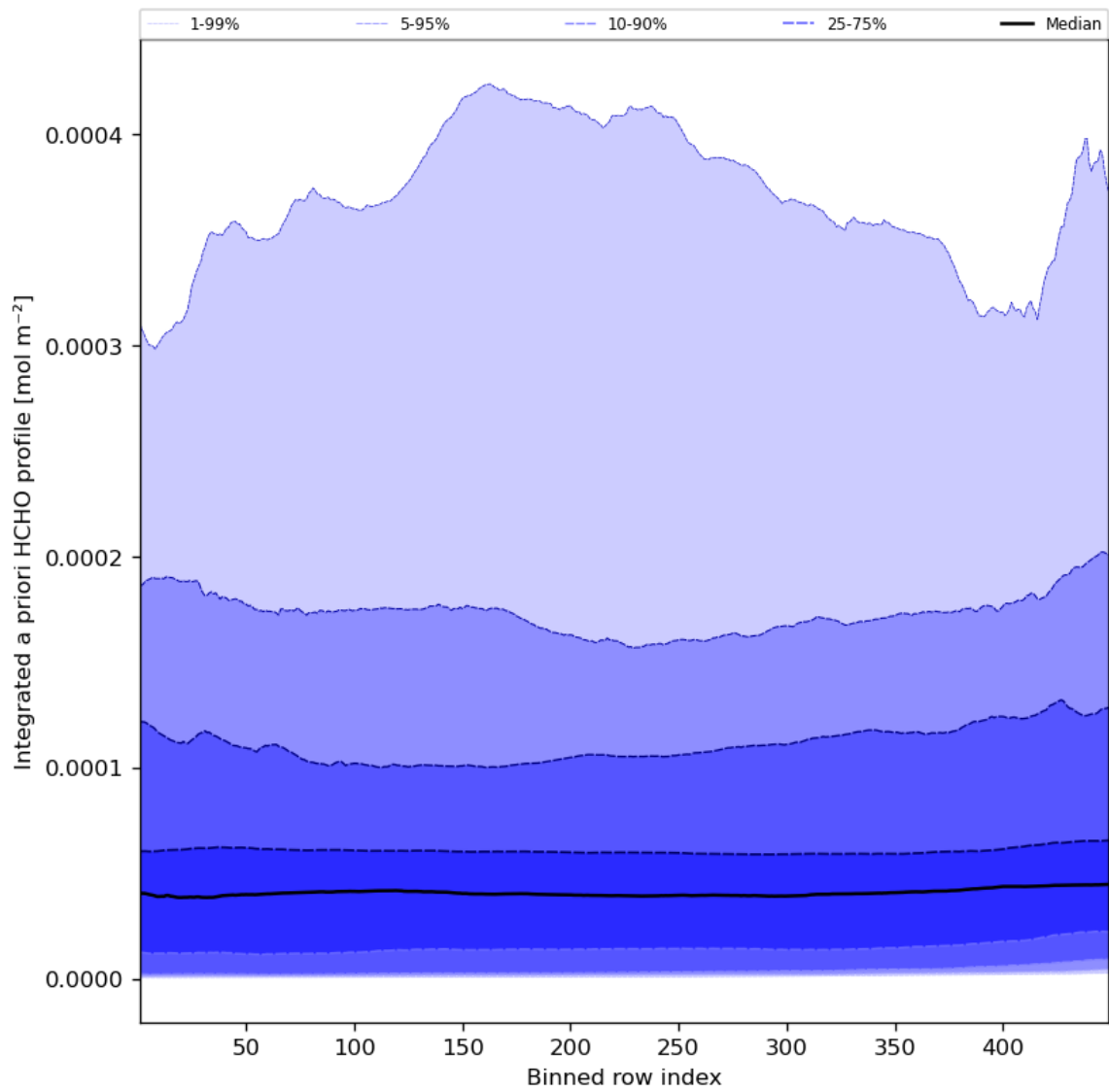
Figure 57: Along track statistics of “Integrated a priori HCHO profile” for 2023-10-28 to 2023-10-30
