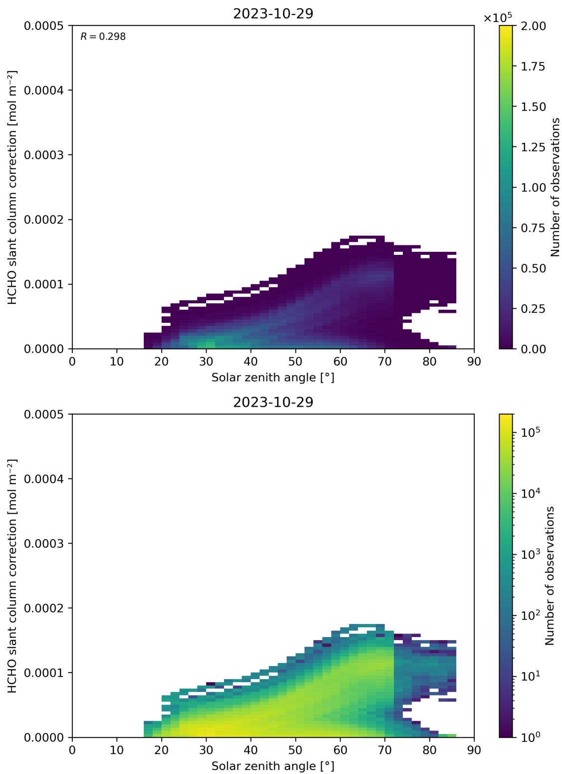
Figure 172: Scatter density plot of “Solar zenith angle” against “HCHO slant column correction” for 2023-10-28 to 2023-10-30.
