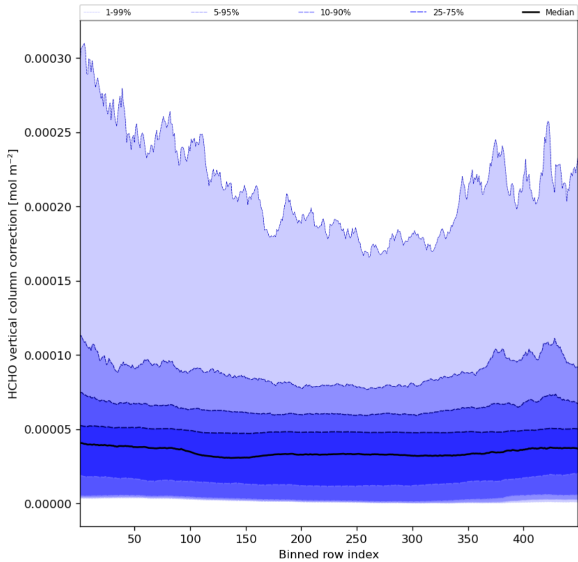
Figure 51: Along track statistics of “HCHO vertical column correction” for 2023-10-28 to 2023-10-30
