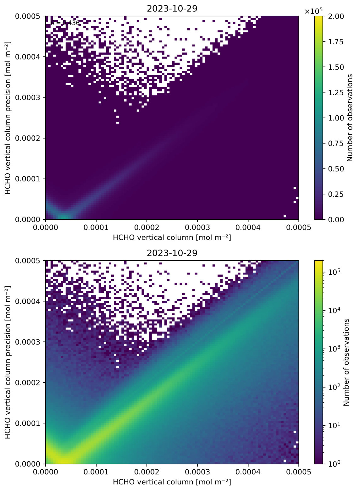
Figure 134: Scatter density plot of “HCHO vertical column” against “HCHO vertical column precision” for 2023-10-28 to 2023-10-30.
