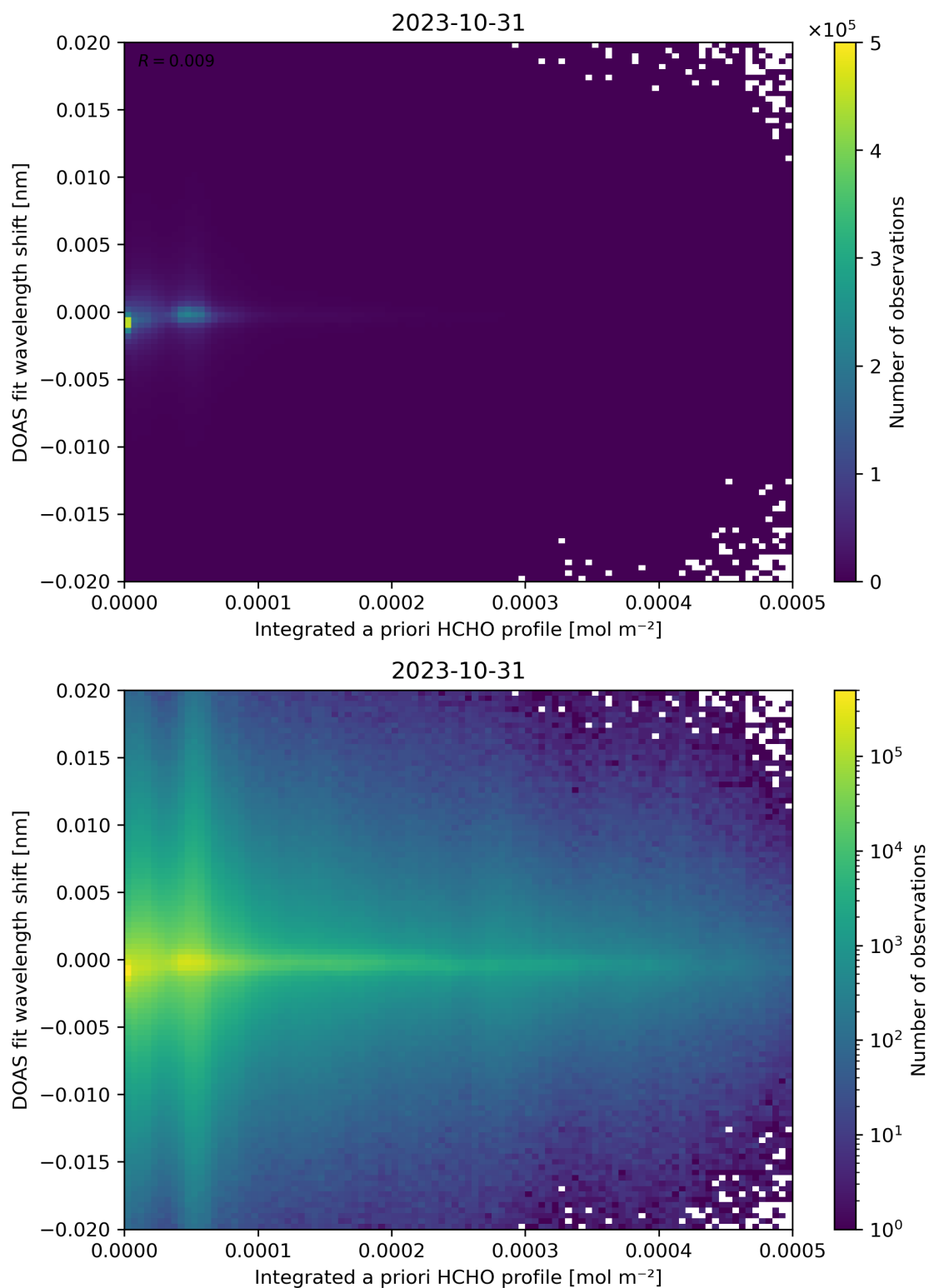
Figure 149: Scatter density plot of “Integrated a priori HCHO profile” against “DOAS fit wavelength shift” for 2023-10-30 to 2023-11-01.
