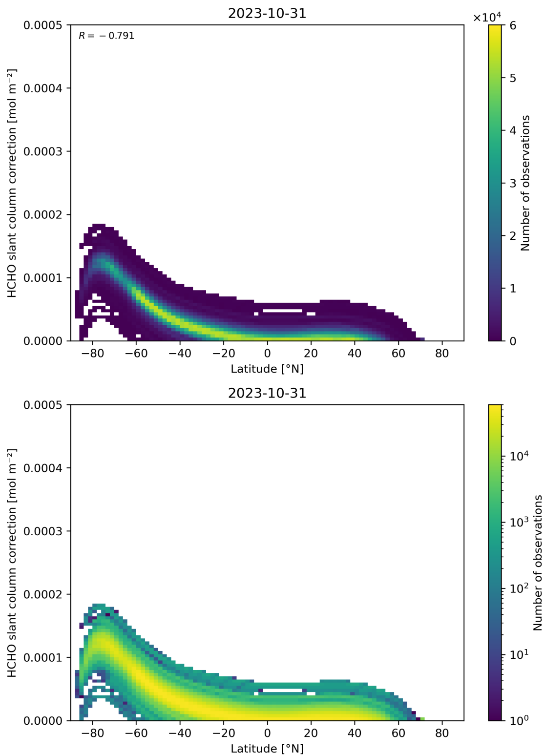
Figure 158: Scatter density plot of “Latitude” against “HCHO slant column correction” for 2023-10-30 to 2023-11-01.
