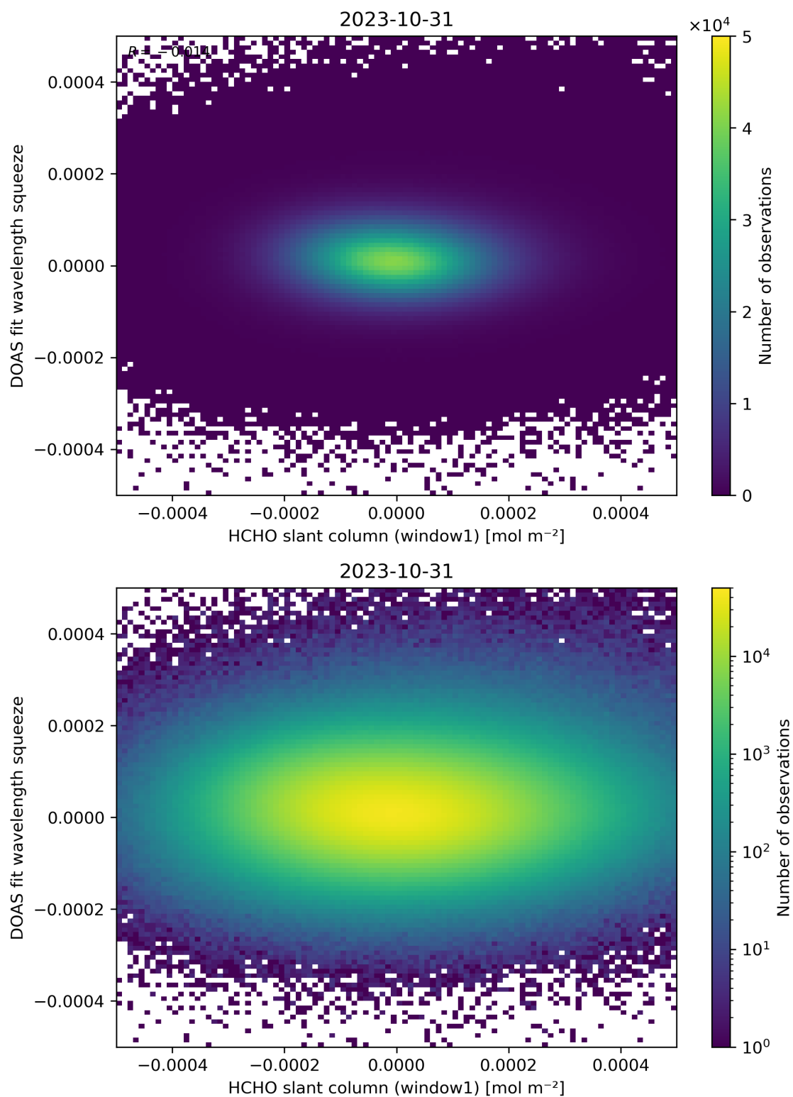
Figure 80: Scatter density plot of “HCHO slant column (window1)” against “DOAS fit wavelength squeeze” for 2023-10-30 to 2023-11-01.
