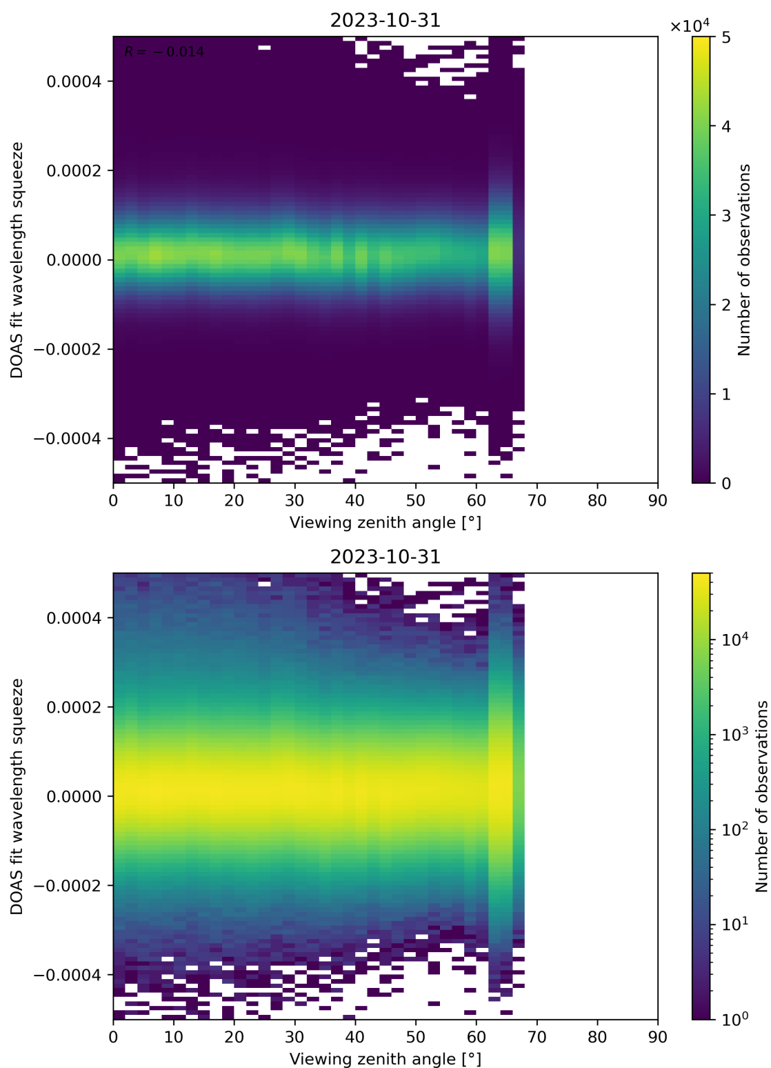
Figure 184: Scatter density plot of “Viewing zenith angle” against “DOAS fit wavelength squeeze” for 2023-10-30 to 2023-11-01.
