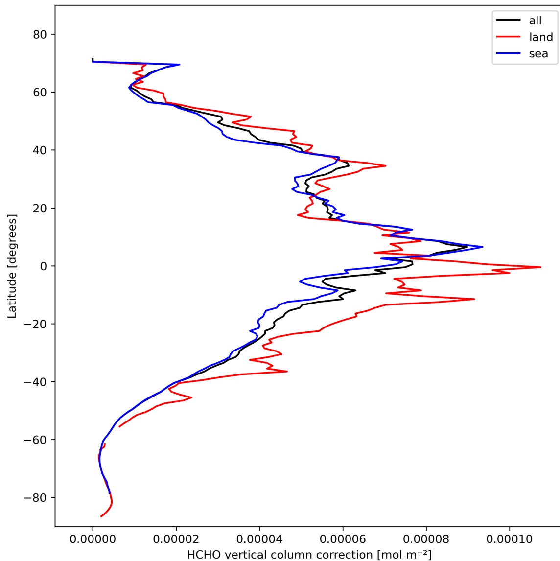
Figure 23: Zonal average of “HCHO vertical column correction” for 2023-10-30 to 2023-11-01.
