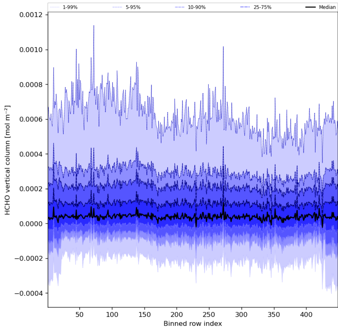
Figure 49: Along track statistics of “HCHO vertical column” for 2023-10-30 to 2023-11-01
