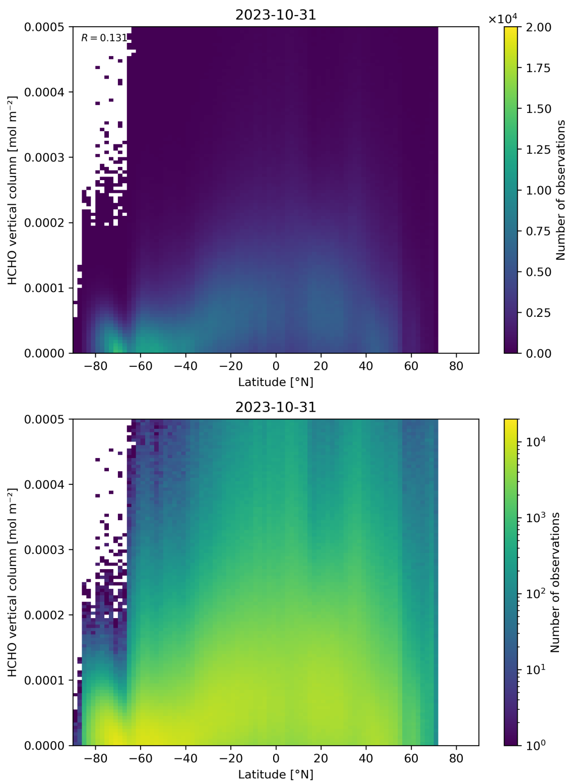
Figure 163: Scatter density plot of “Latitude” against “HCHO vertical column” for 2023-10-30 to 2023-11-01.
