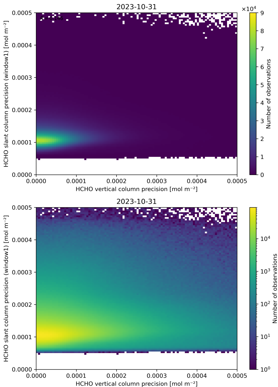
Figure 143: Scatter density plot of “HCHO vertical column precision” against “HCHO slant column precision (window1)” for 2023-10-30 to 2023-11-01.
