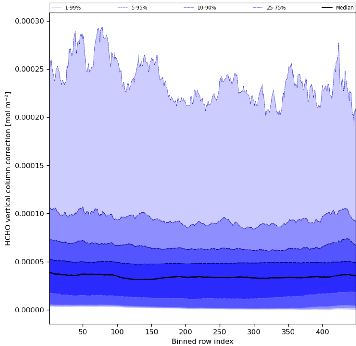
Figure 51: Along track statistics of “HCHO vertical column correction” for 2023-10-30 to 2023-11-01
