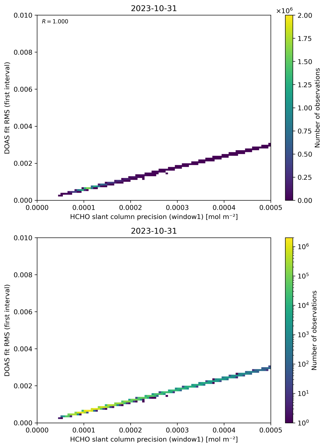
Figure 88: Scatter density plot of “HCHO slant column precision (window1)” against “DOAS fit RMS (first interval)” for 2023-10-30 to 2023-11-01.
