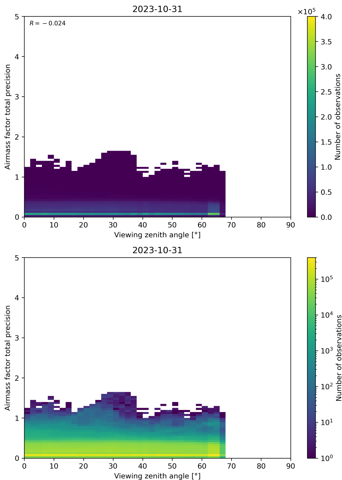
Figure 191: Scatter density plot of “Viewing zenith angle” against “Airmass factor total precision” for 2023-10-30 to 2023-11-01.
