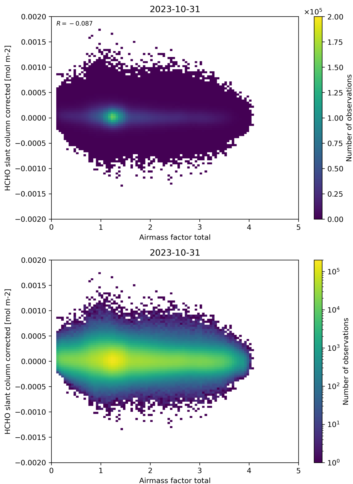
Figure 101: Scatter density plot of “Airmass factor total” against “HCHO slant column corrected” for 2023-10-30 to 2023-11-01.
