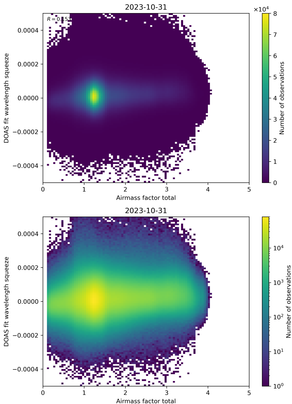
Figure 99: Scatter density plot of “Airmass factor total” against “DOAS fit wavelength squeeze” for 2023-10-30 to 2023-11-01.
