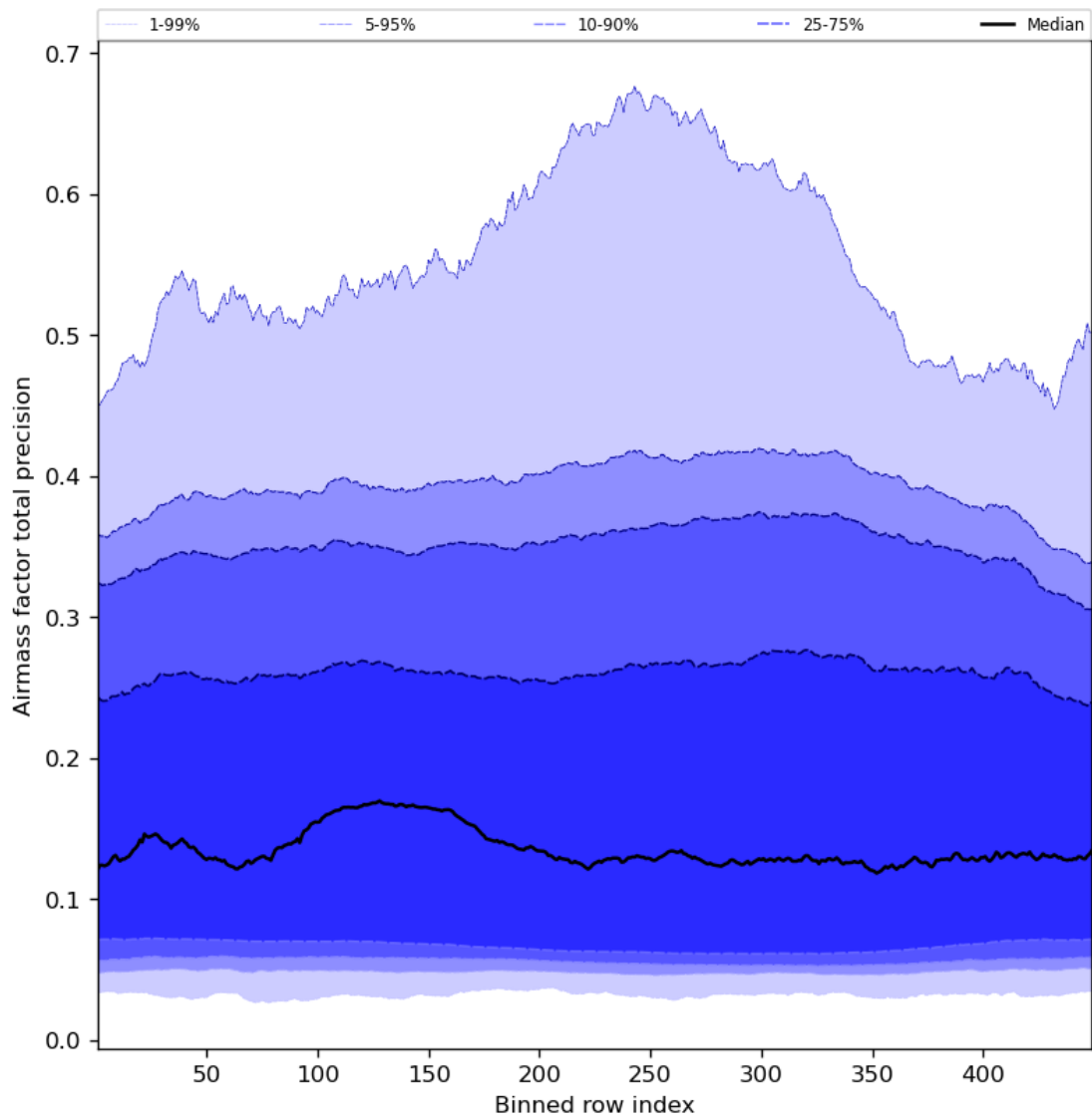
Figure 55: Along track statistics of “Airmass factor total precision” for 2023-10-30 to 2023-11-01
