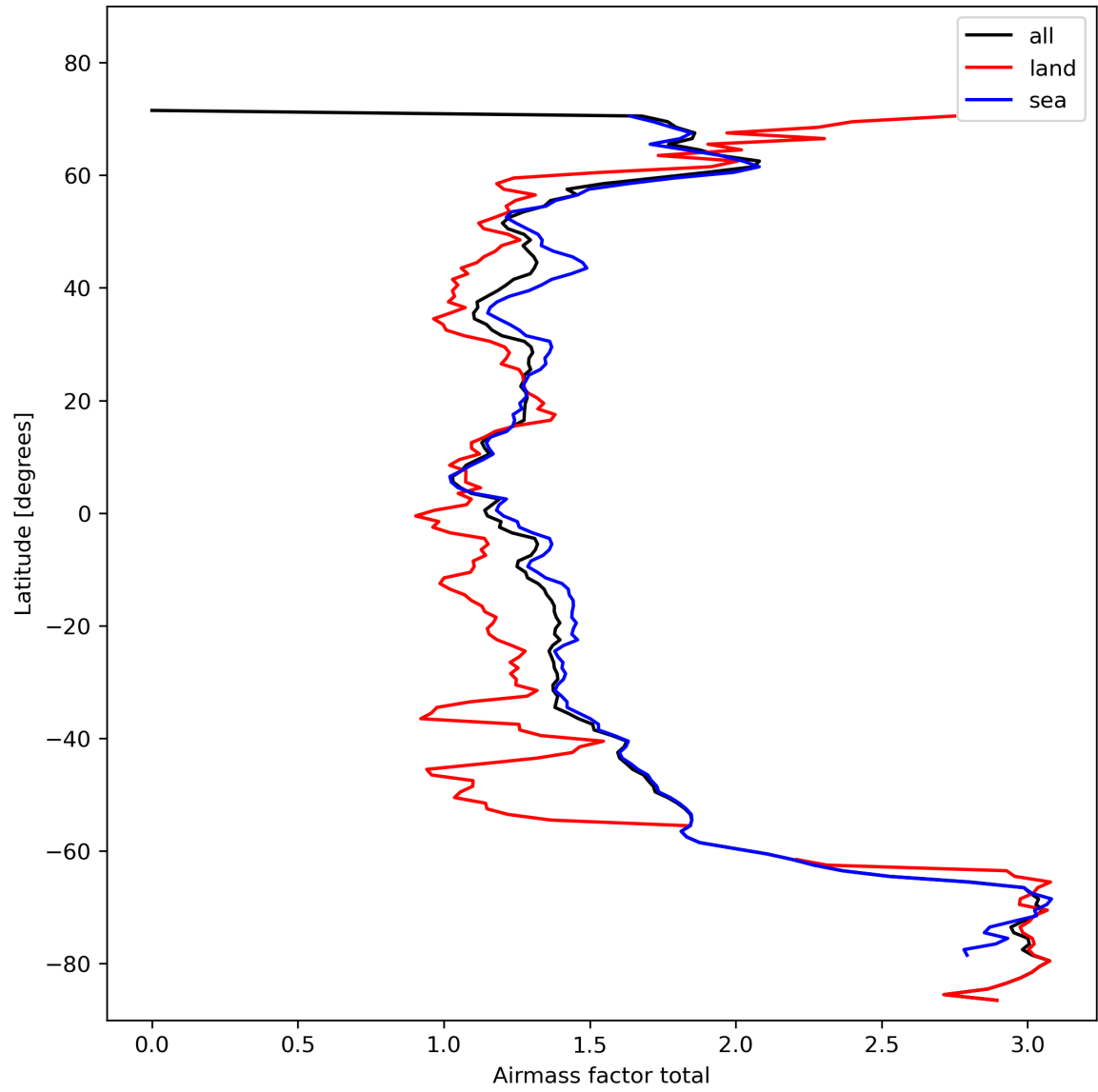
Figure 26: Zonal average of “Airmass factor total” for 2023-10-30 to 2023-11-01.
