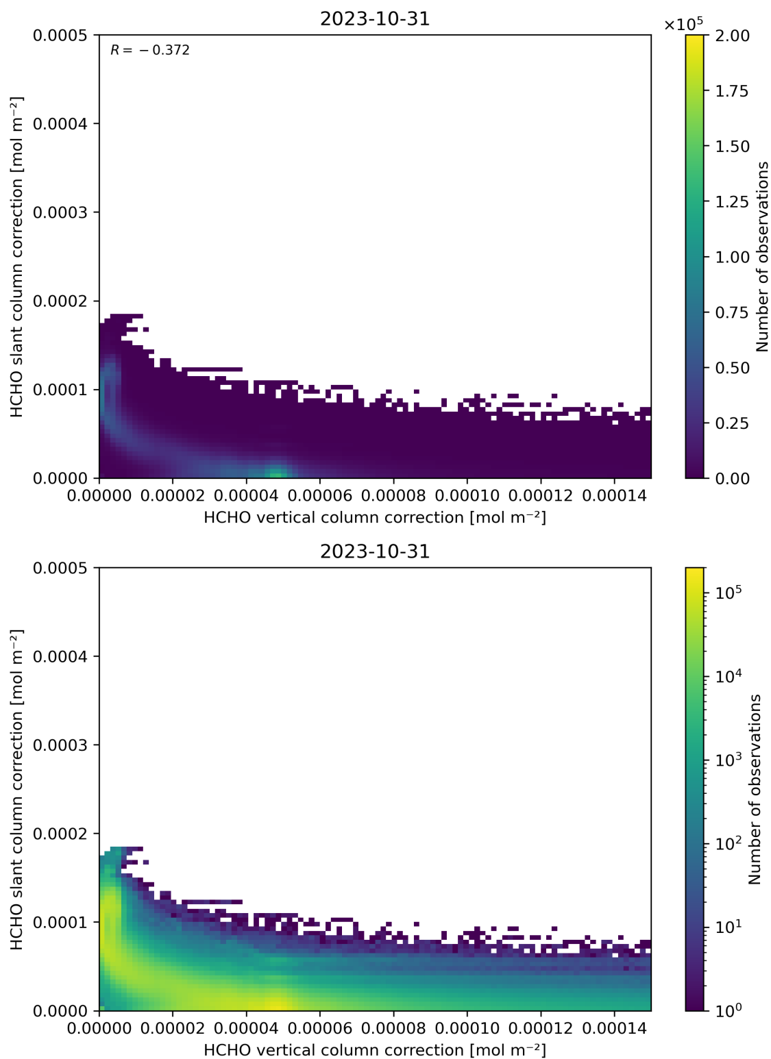
Figure 117: Scatter density plot of “HCHO vertical column correction” against “HCHO slant column correction” for 2023-10-30 to 2023-11-01.
