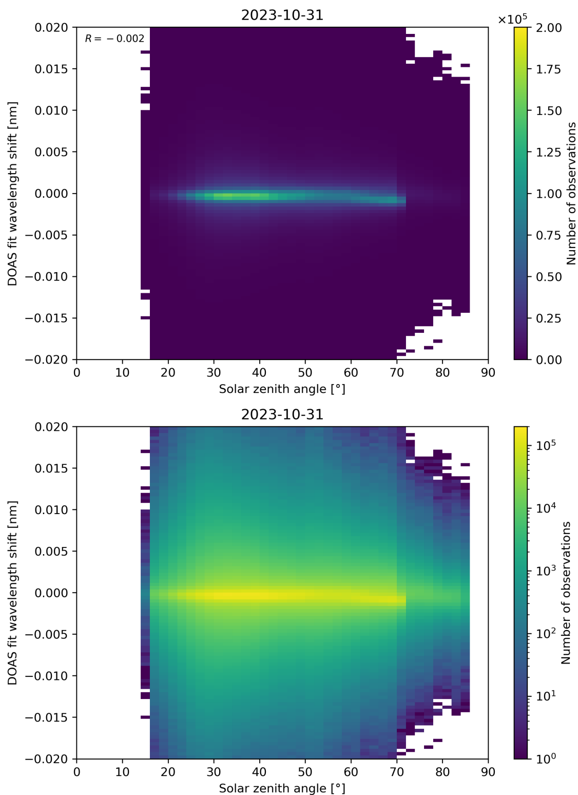
Figure 168: Scatter density plot of “Solar zenith angle” against “DOAS fit wavelength shift” for 2023-10-30 to 2023-11-01.
