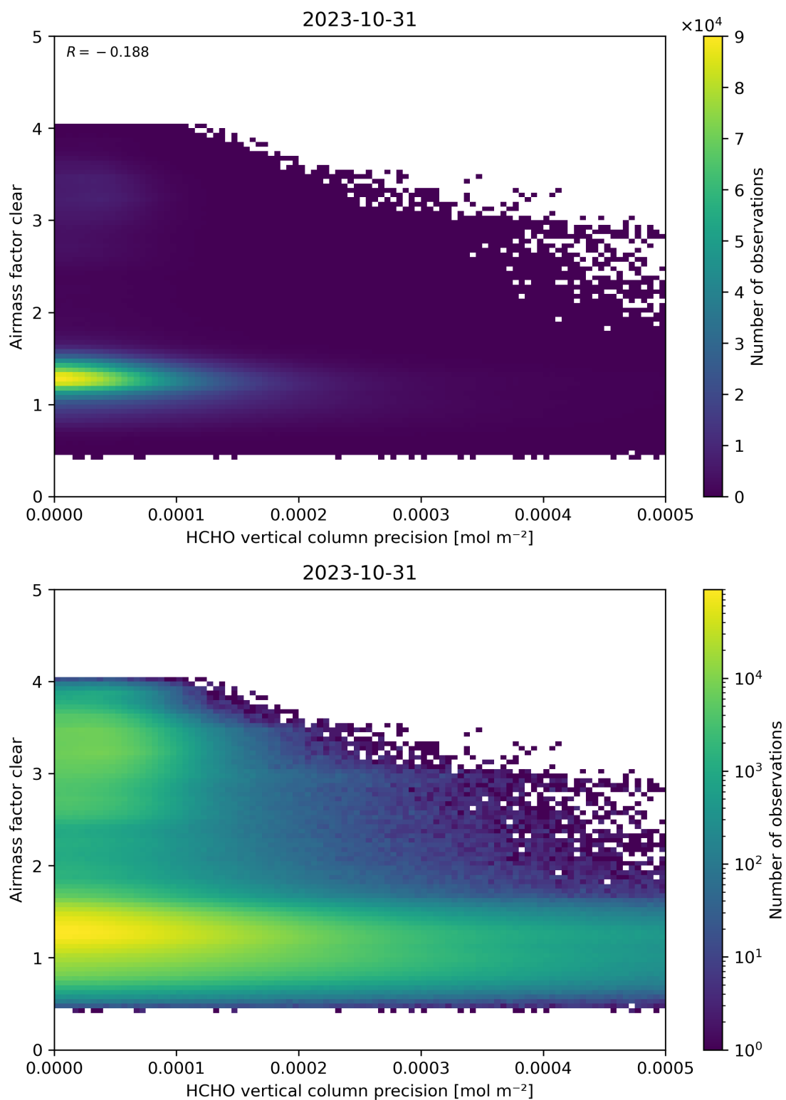
Figure 139: Scatter density plot of “HCHO vertical column precision” against “Airmass factor clear” for 2023-10-30 to 2023-11-01.
