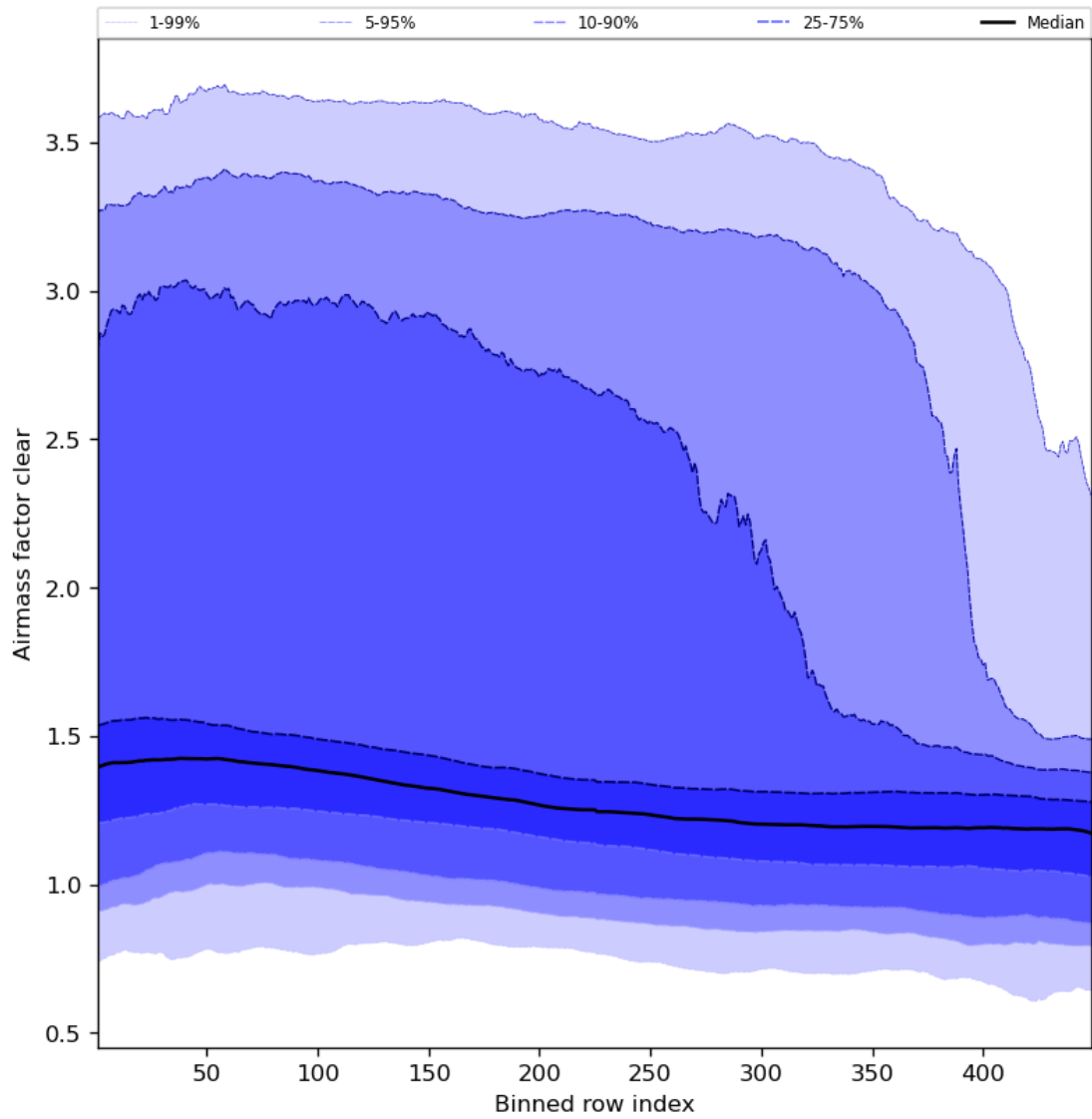
Figure 56: Along track statistics of “Airmass factor clear” for 2023-10-30 to 2023-11-01
