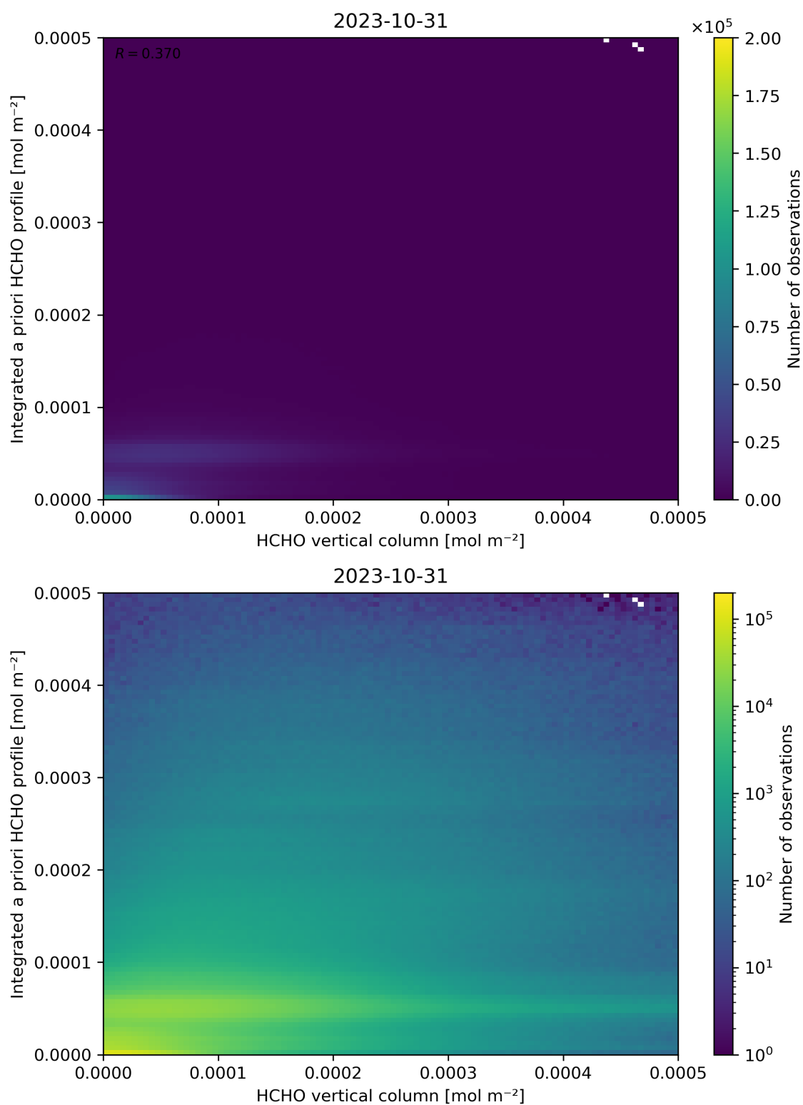
Figure 135: Scatter density plot of “HCHO vertical column” against “Integrated a priori HCHO profile” for 2023-10-30 to 2023-11-01.
