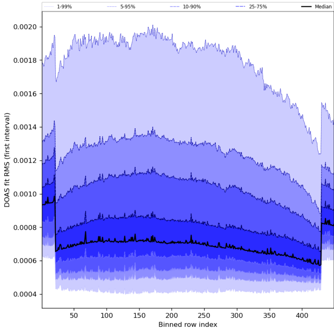
Figure 60: Along track statistics of “DOAS fit RMS (first interval)” for 2023-10-30 to 2023-11-01
