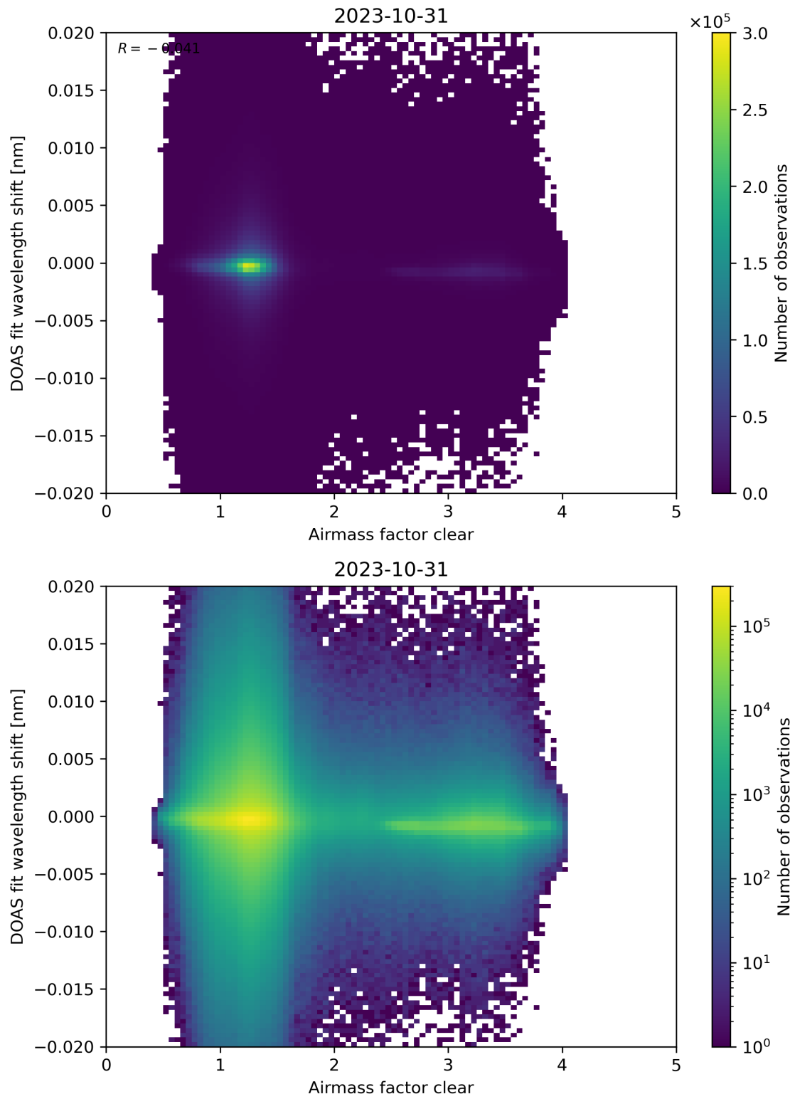
Figure 72: Scatter density plot of “Airmass factor clear” against “DOAS fit wavelength shift” for 2023-10-30 to 2023-11-01.
