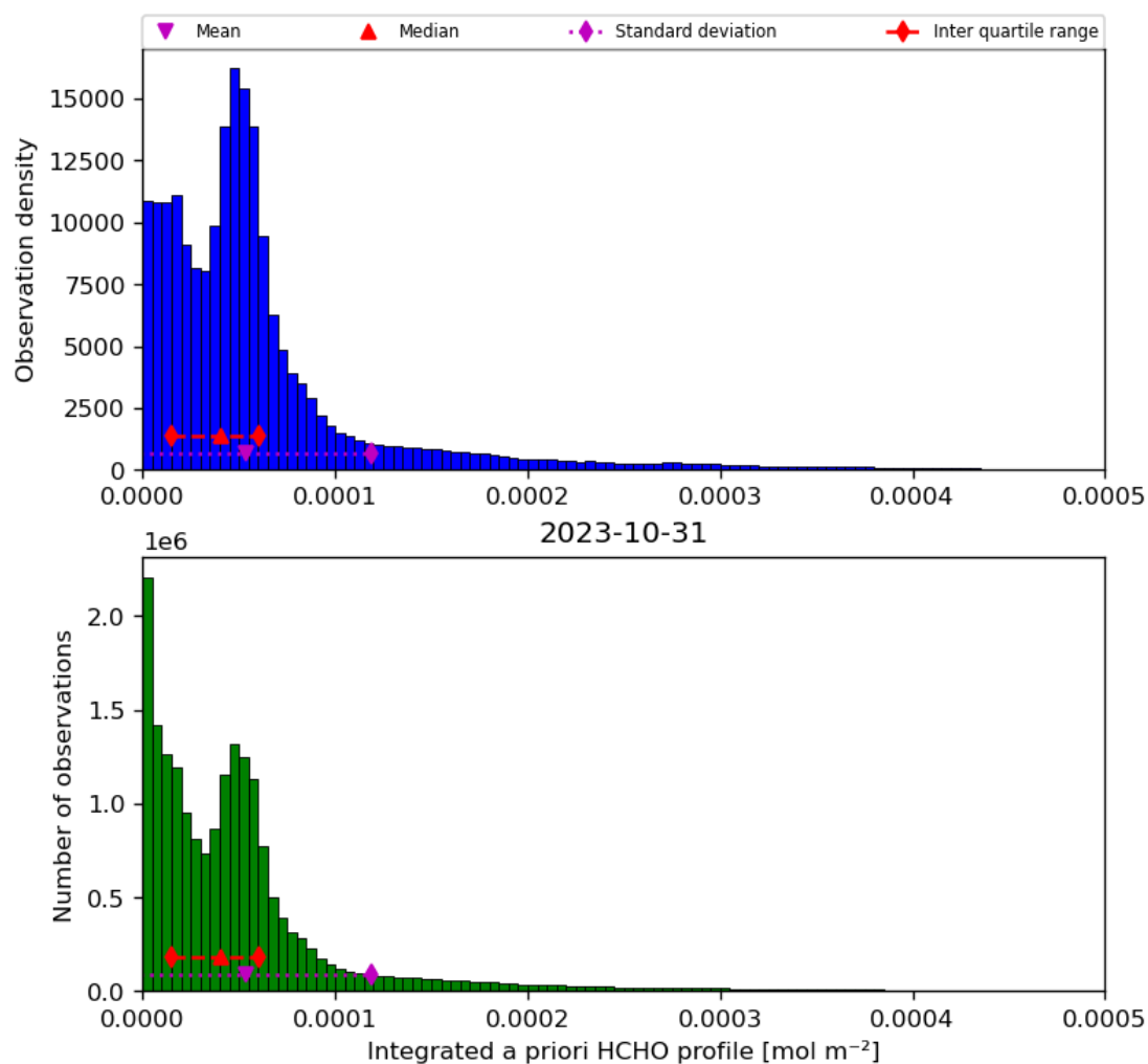
Figure 43: Histogram of “Integrated a priori HCHO profile” for 2023-10-30 to 2023-11-01
