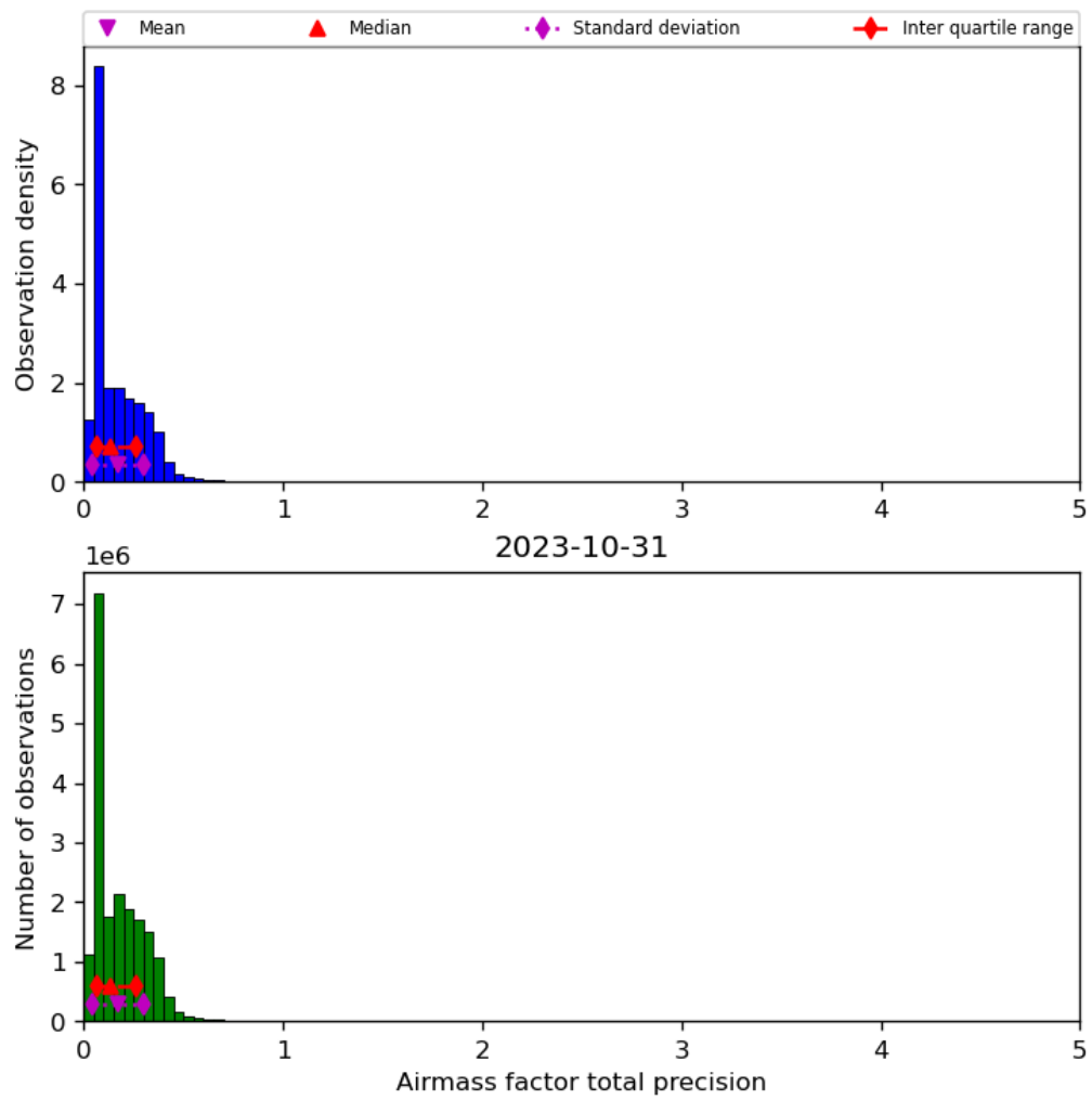
Figure 41: Histogram of “Airmass factor total precision” for 2023-10-30 to 2023-11-01
