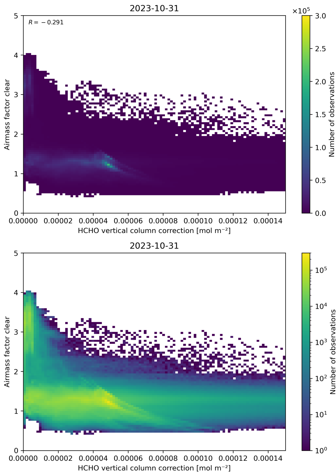
Figure 115: Scatter density plot of “HCHO vertical column correction” against “Airmass factor clear” for 2023-10-30 to 2023-11-01.
