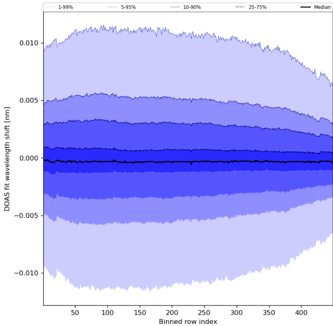
Figure 58: Along track statistics of “DOAS fit wavelength shift” for 2023-10-30 to 2023-11-01
