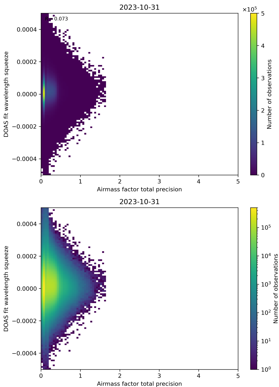
Figure 107: Scatter density plot of “Airmass factor total precision” against “DOAS fit wavelength squeeze” for 2023-10-30 to 2023-11-01.
