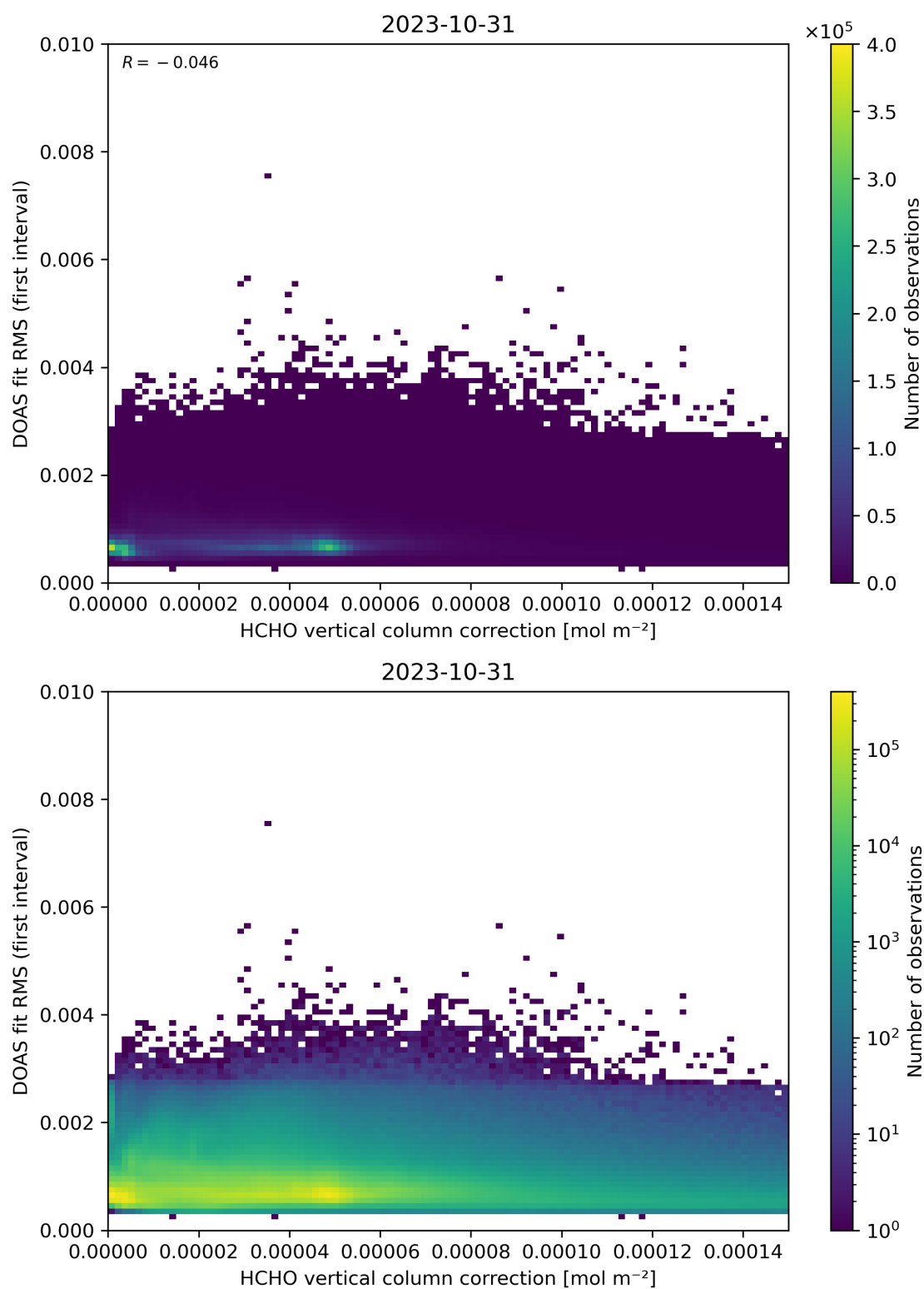
Figure 112: Scatter density plot of “HCHO vertical column correction” against “DOAS fit RMS (first interval)” for 2023-10-30 to 2023-11-01.
