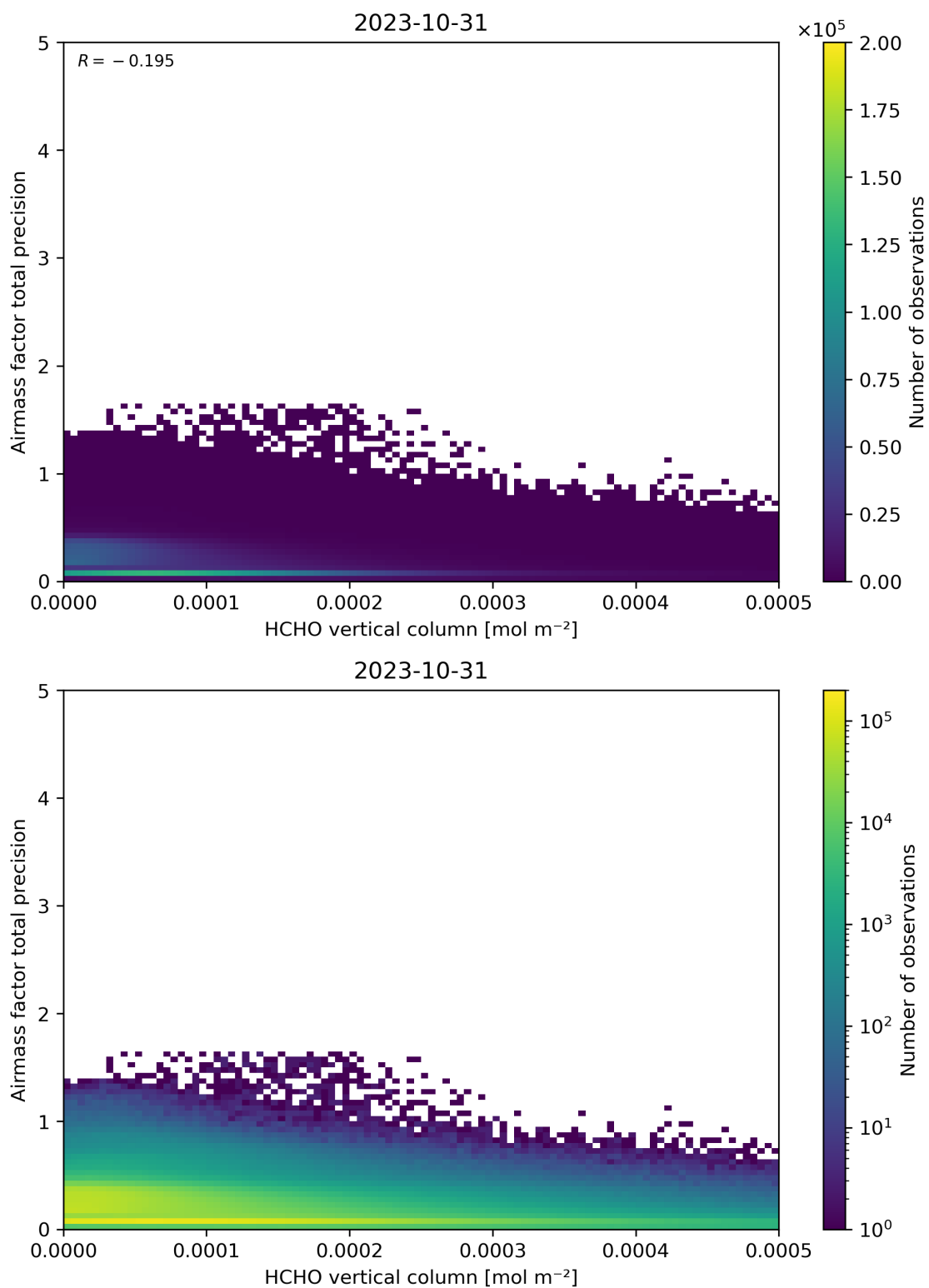
Figure 132: Scatter density plot of “HCHO vertical column” against “Airmass factor total precision” for 2023-10-30 to 2023-11-01.
