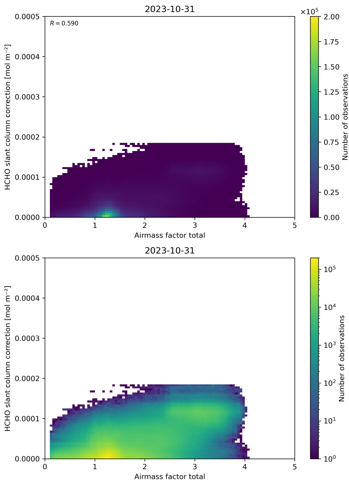
Figure 102: Scatter density plot of “Airmass factor total” against “HCHO slant column correction” for 2023-10-30 to 2023-11-01.
