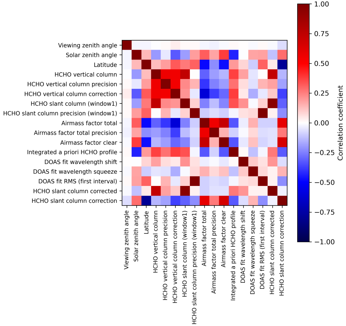
Figure 2: Map of correlation matrix for 2023-10-30 to 2023-11-01.
