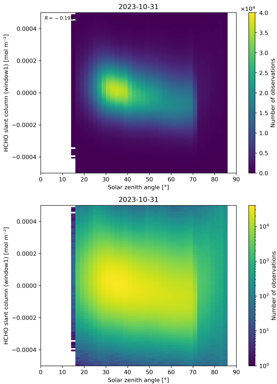
Figure 173: Scatter density plot of “Solar zenith angle” against “HCHO slant column (window1)” for 2023-10-30 to 2023-11-01.
