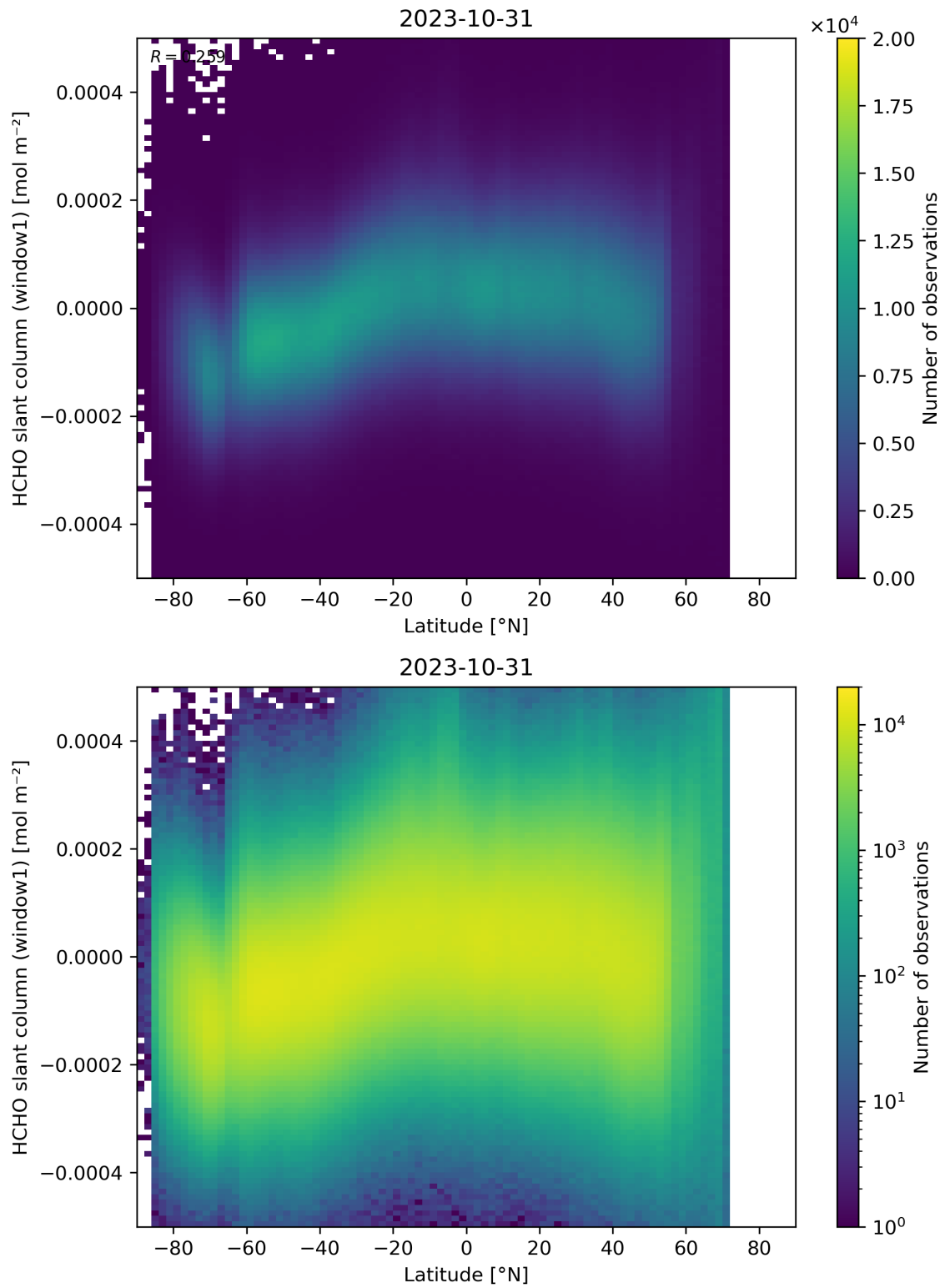
Figure 159: Scatter density plot of “Latitude” against “HCHO slant column (window1)” for 2023-10-30 to 2023-11-01.
