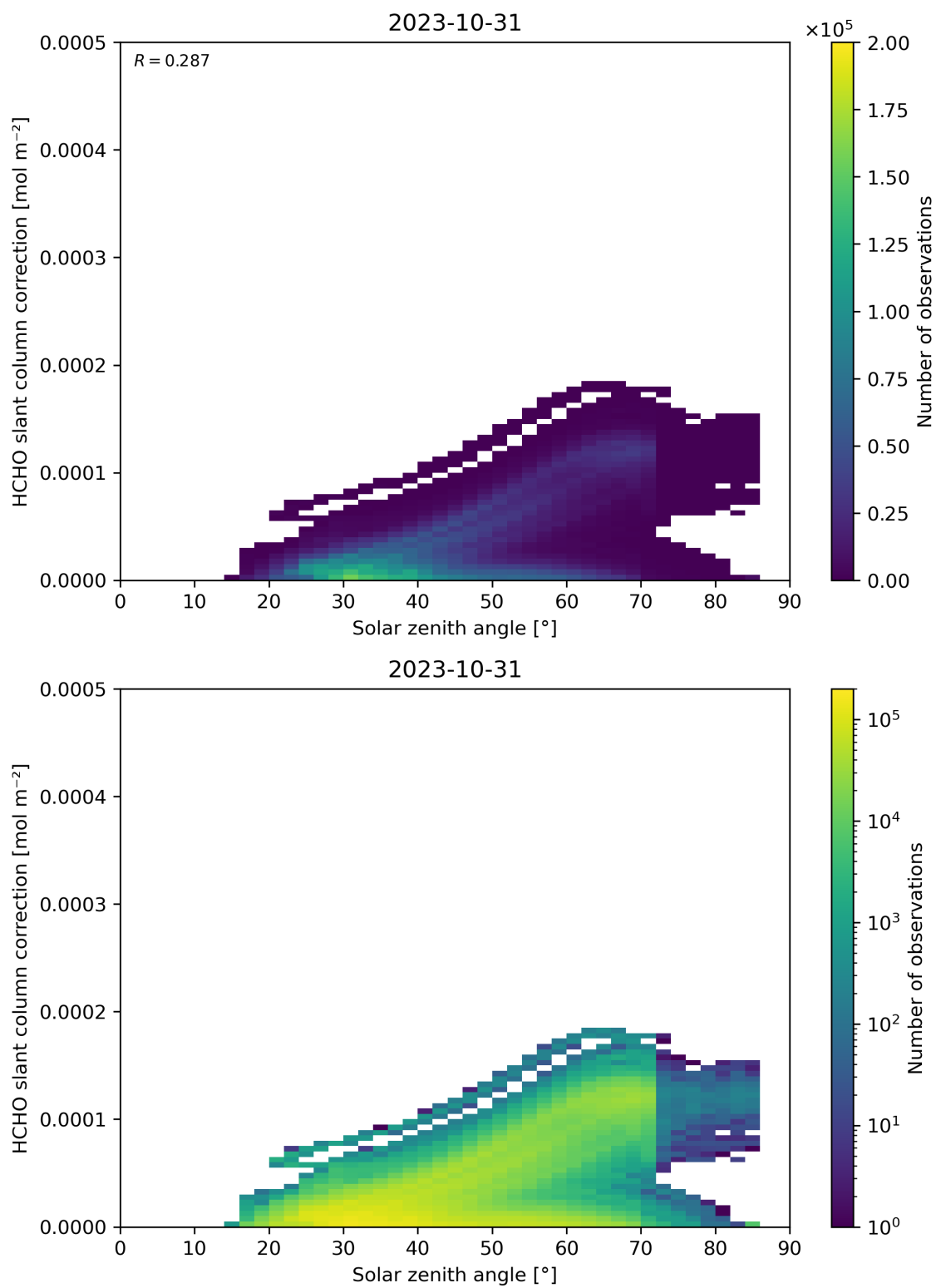
Figure 172: Scatter density plot of “Solar zenith angle” against “HCHO slant column correction” for 2023-10-30 to 2023-11-01.
