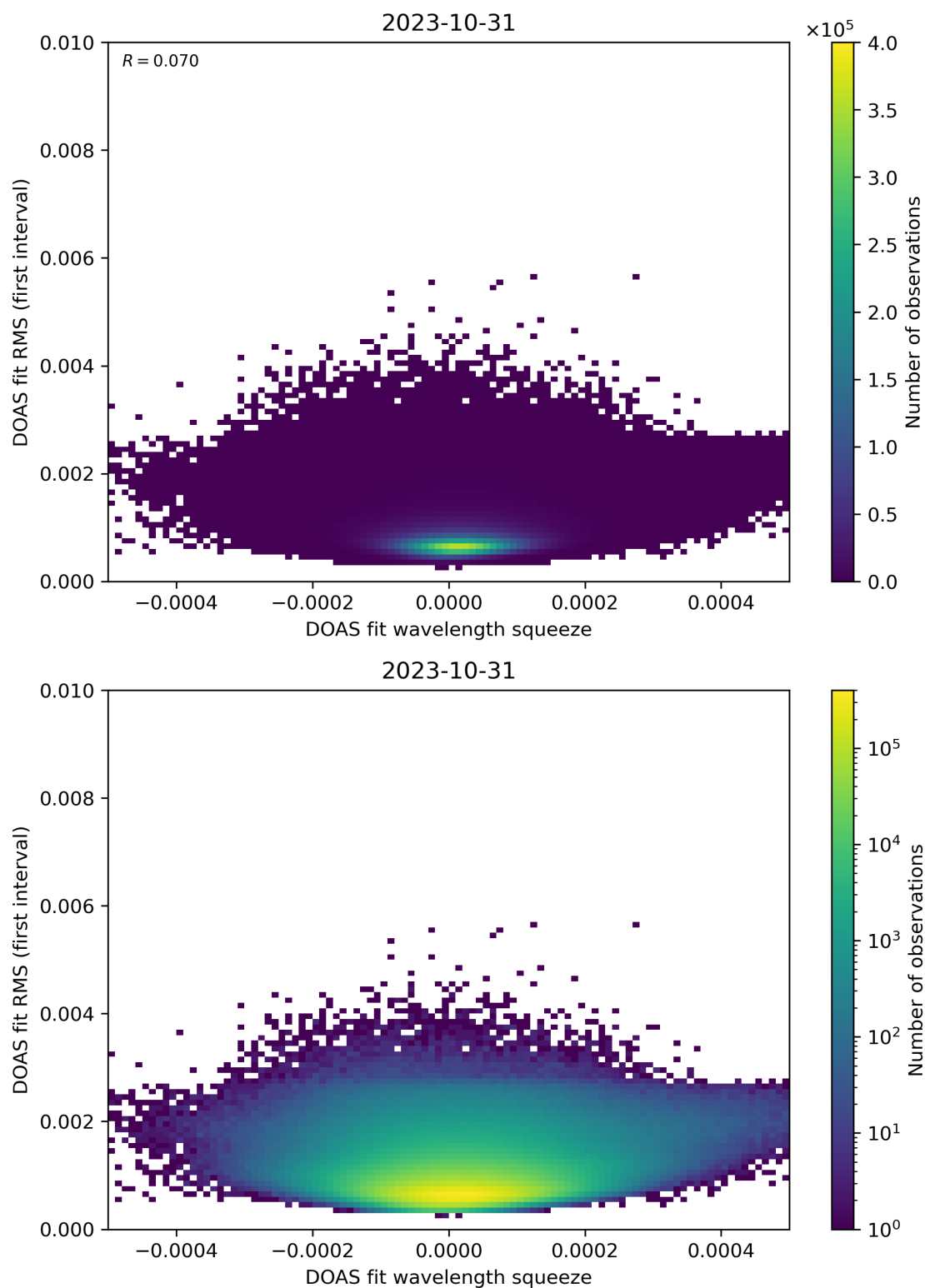
Figure 68: Scatter density plot of “DOAS fit wavelength squeeze” against “DOAS fit RMS (first interval)” for 2023-10-30 to 2023-11-01.
