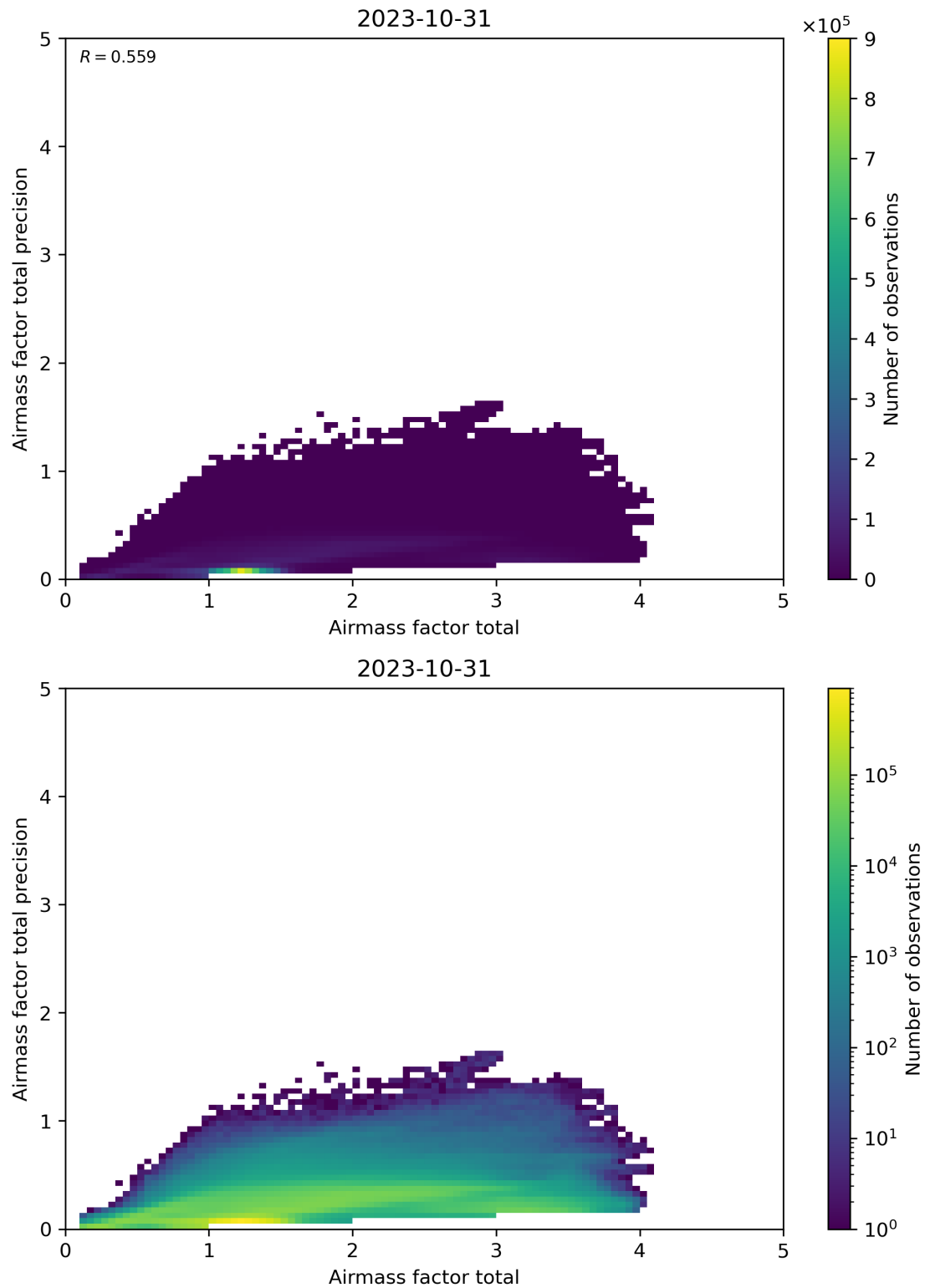
Figure 103: Scatter density plot of “Airmass factor total” against “Airmass factor total precision” for 2023-10-30 to 2023-11-01.
