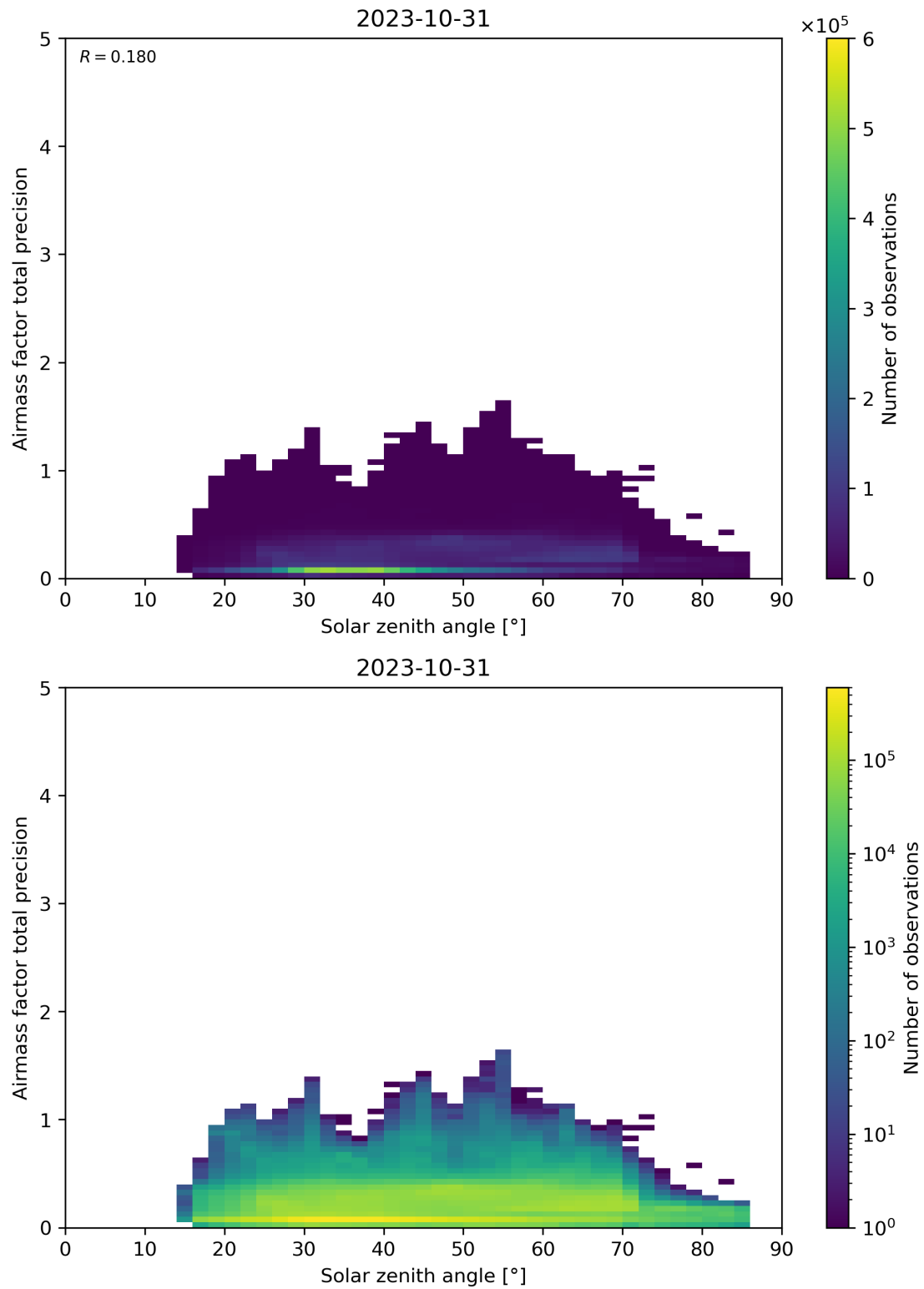
Figure 176: Scatter density plot of “Solar zenith angle” against “Airmass factor total precision” for 2023-10-30 to 2023-11-01.
