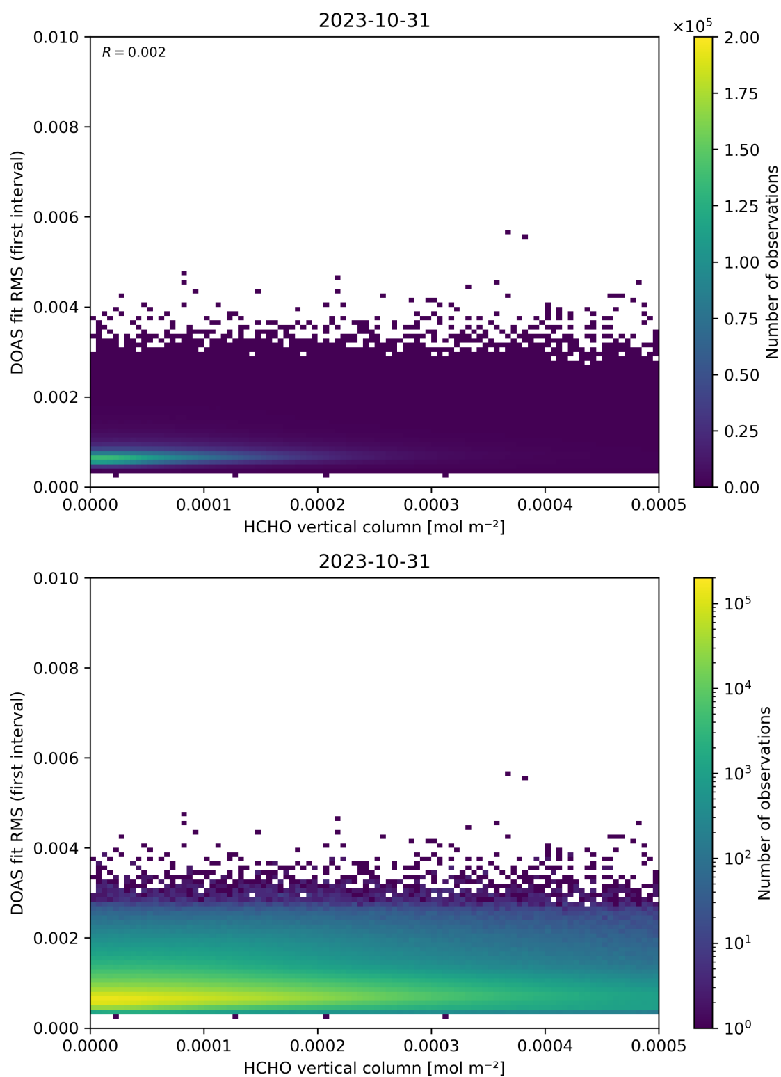
Figure 123: Scatter density plot of “HCHO vertical column” against “DOAS fit RMS (first interval)” for 2023-10-30 to 2023-11-01.
