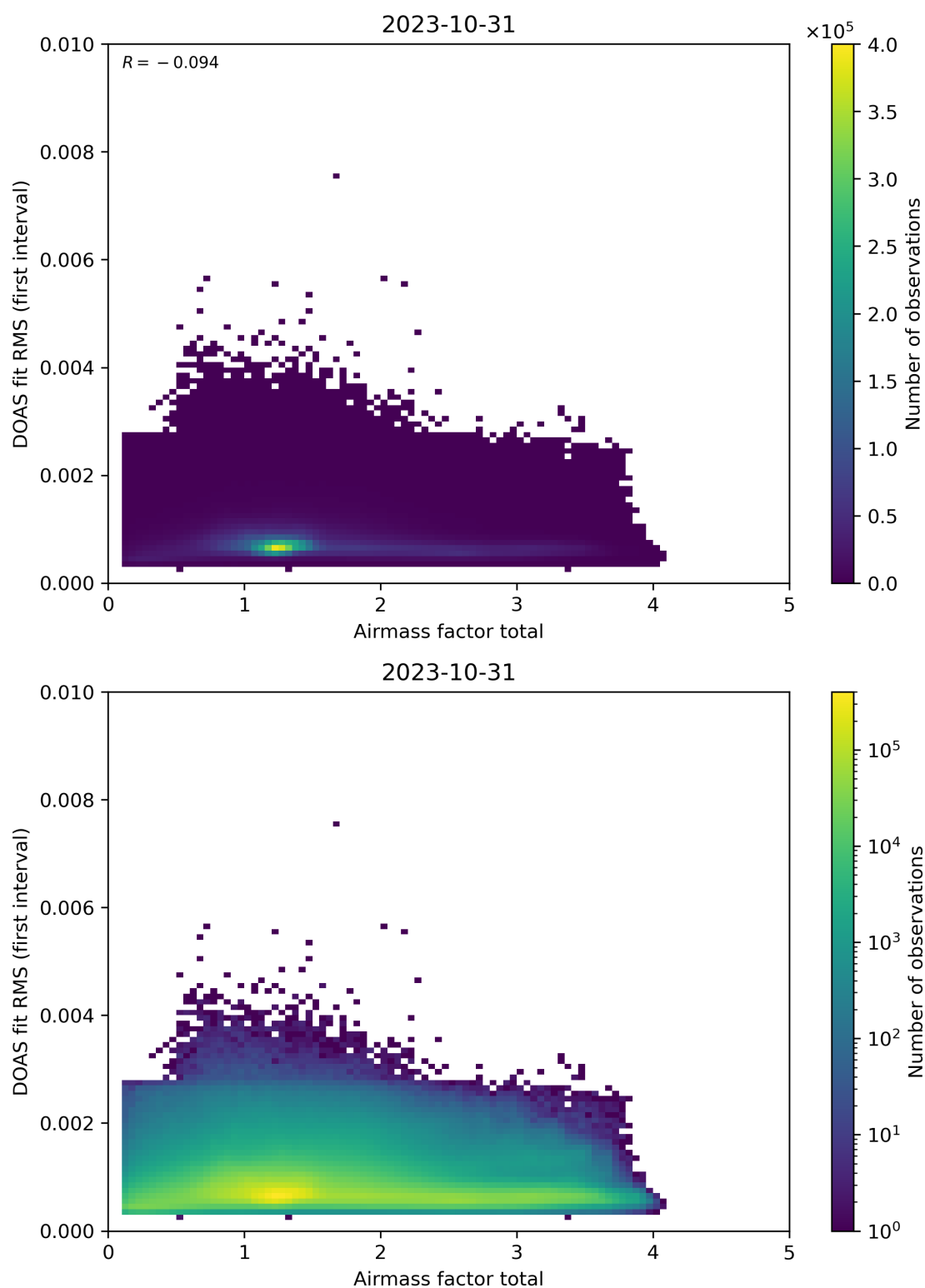
Figure 97: Scatter density plot of “Airmass factor total” against “DOAS fit RMS (first interval)” for 2023-10-30 to 2023-11-01.
