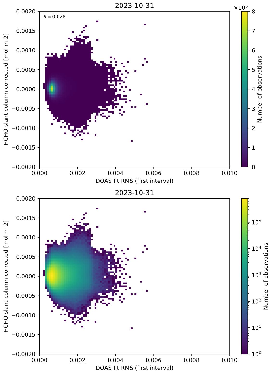
Figure 62: Scatter density plot of “DOAS fit RMS (first interval)” against “HCHO slant column corrected” for 2023-10-30 to 2023-11-01.
