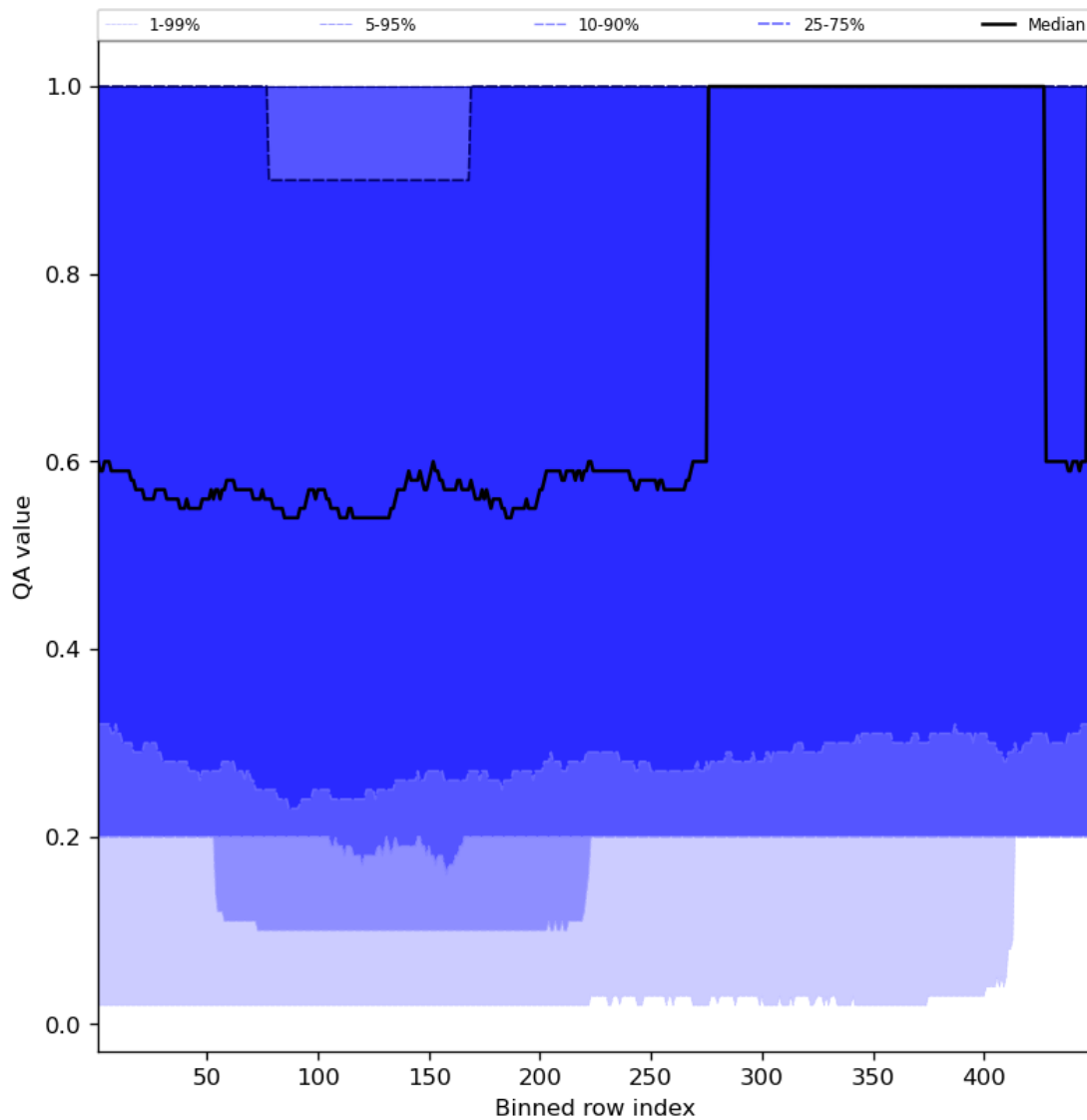
Figure 48: Along track statistics of “QA value” for 2023-10-30 to 2023-11-01
