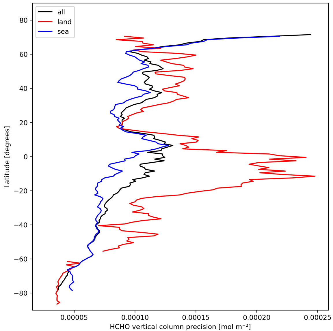
Figure 22: Zonal average of “HCHO vertical column precision” for 2023-10-30 to 2023-11-01.
