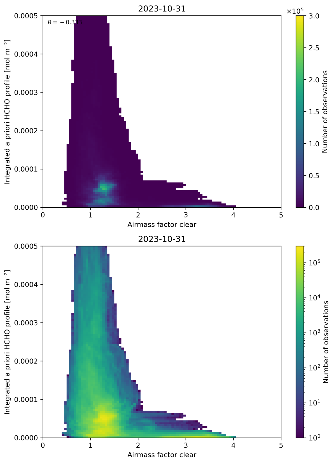
Figure 76: Scatter density plot of “Airmass factor clear” against “Integrated a priori HCHO profile” for 2023-10-30 to 2023-11-01.
