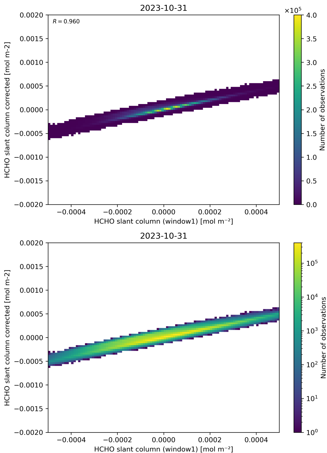
Figure 82: Scatter density plot of “HCHO slant column (window1)” against “HCHO slant column corrected” for 2023-10-30 to 2023-11-01.
