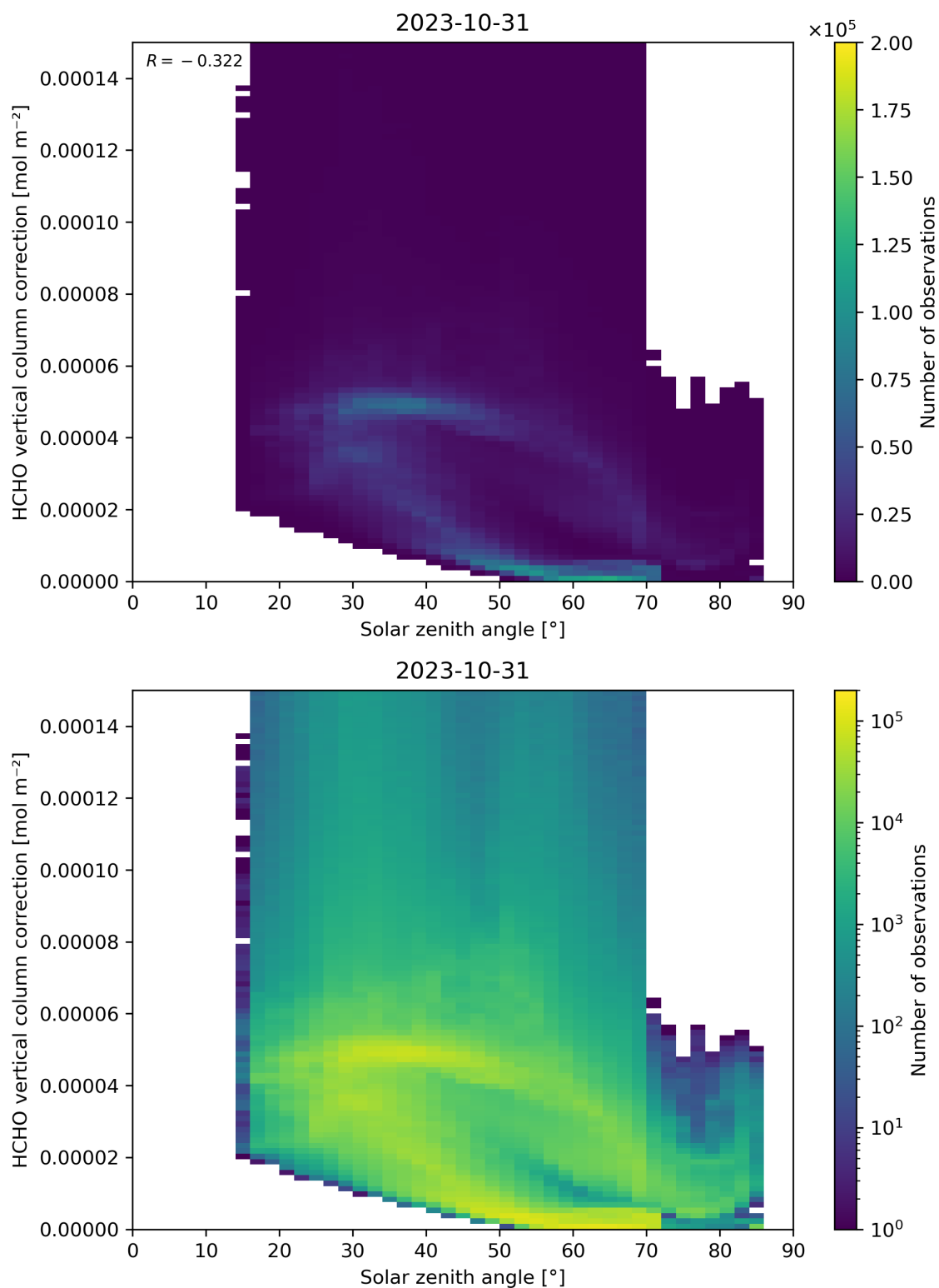
Figure 178: Scatter density plot of “Solar zenith angle” against “HCHO vertical column correction” for 2023-10-30 to 2023-11-01.
