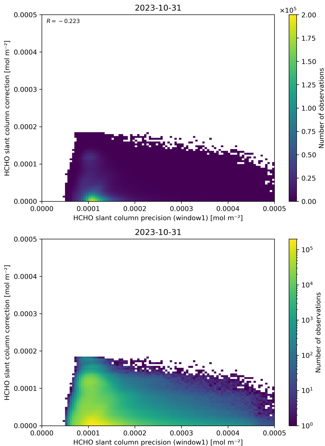
Figure 93: Scatter density plot of “HCHO slant column precision (window1)” against “HCHO slant column correction” for 2023-10-30 to 2023-11-01.
