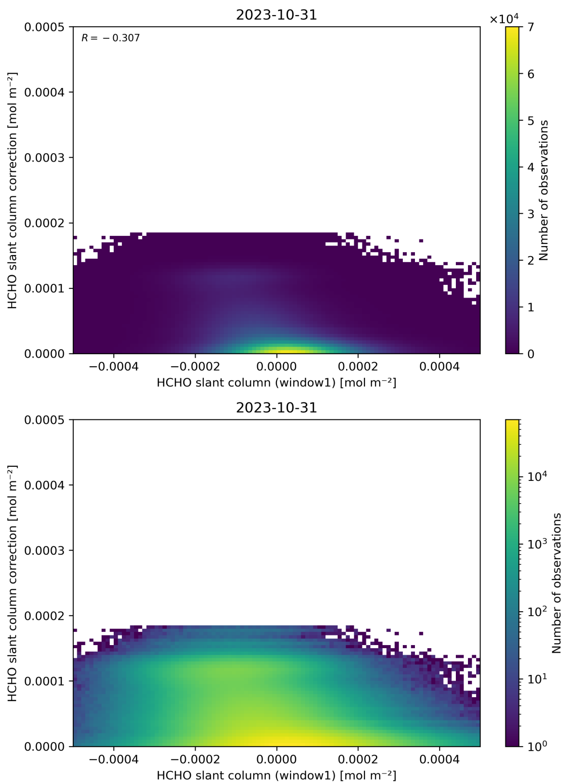
Figure 83: Scatter density plot of “HCHO slant column (window1)” against “HCHO slant column correction” for 2023-10-30 to 2023-11-01.
