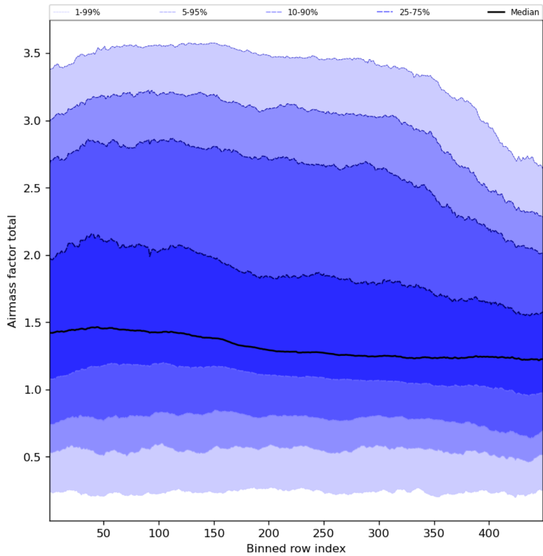
Figure 54: Along track statistics of “Airmass factor total” for 2023-10-30 to 2023-11-01
