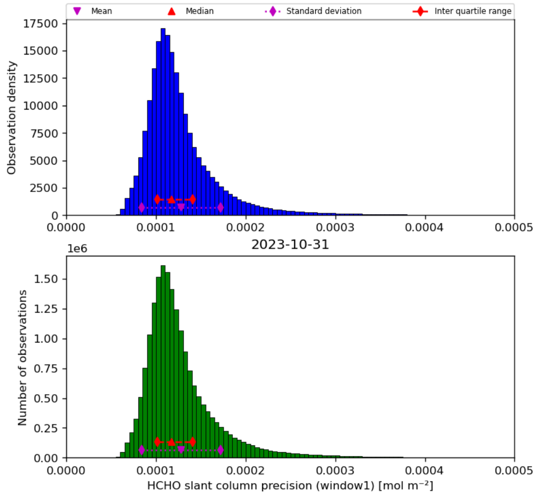
Figure 39: Histogram of “HCHO slant column precision (window1)” for 2023-10-30 to 2023-11-01
