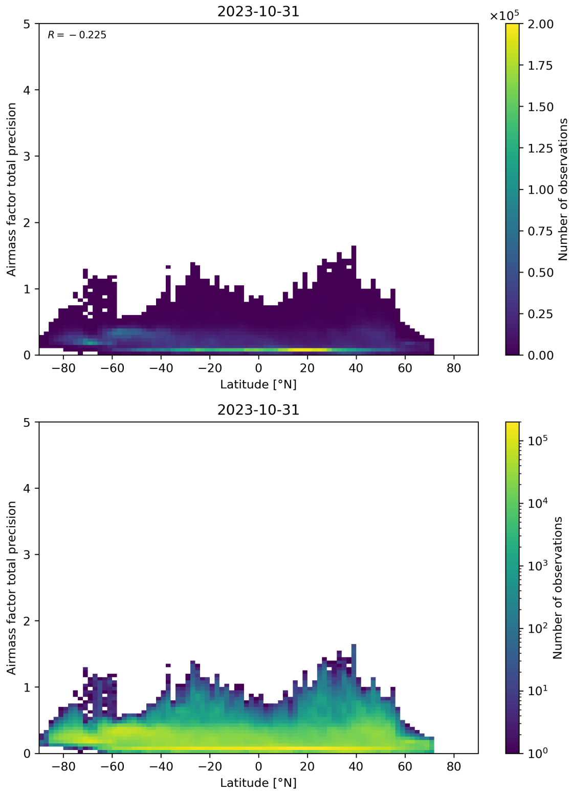
Figure 162: Scatter density plot of “Latitude” against “Airmass factor total precision” for 2023-10-30 to 2023-11-01.
