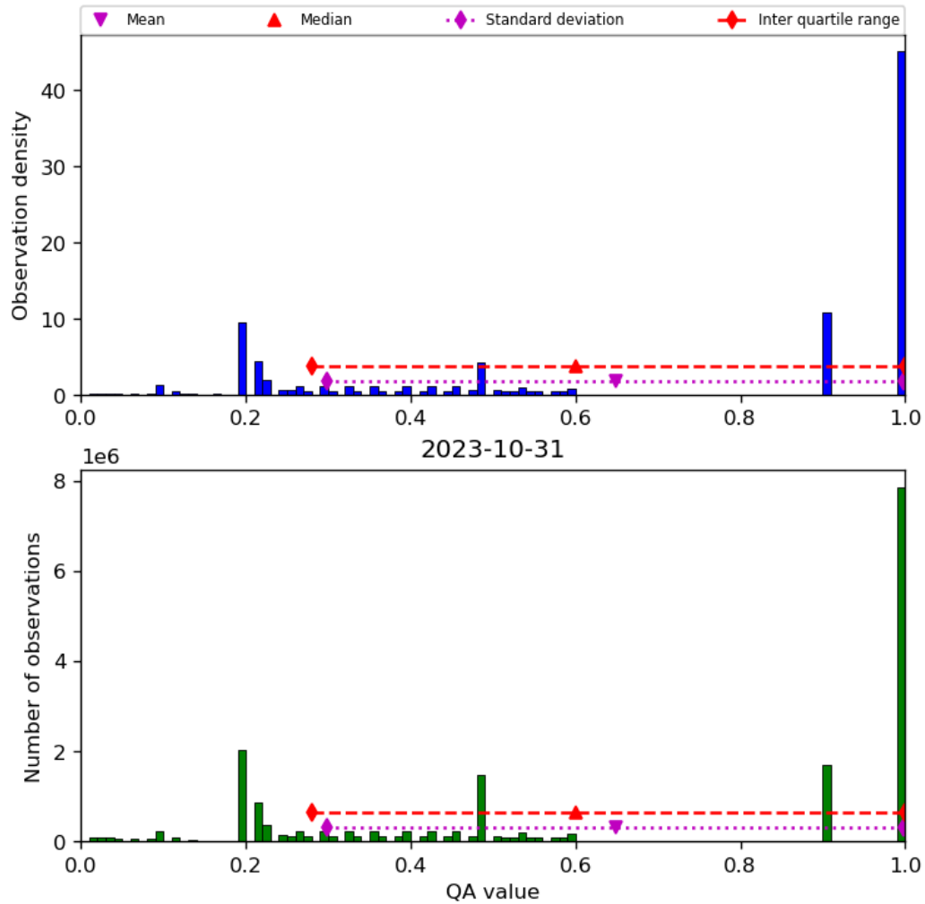
Figure 34: Histogram of “QA value” for 2023-10-30 to 2023-11-01
