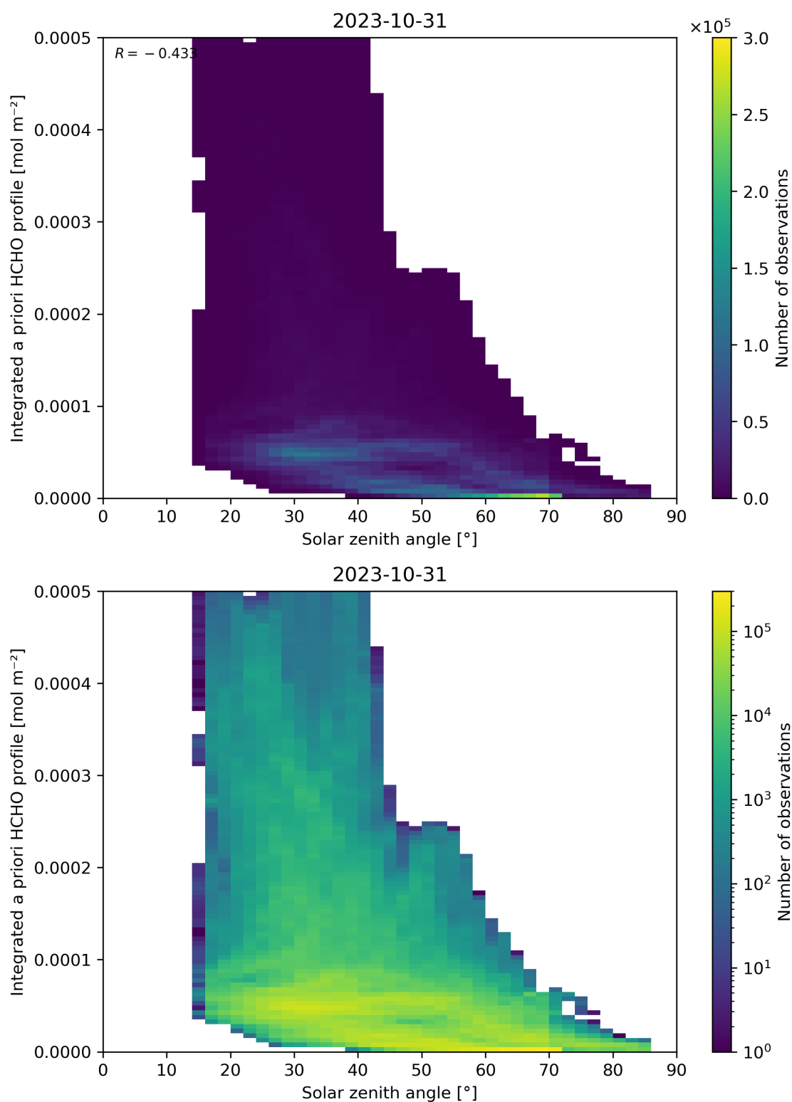
Figure 180: Scatter density plot of “Solar zenith angle” against “Integrated a priori HCHO profile” for 2023-10-30 to 2023-11-01.
