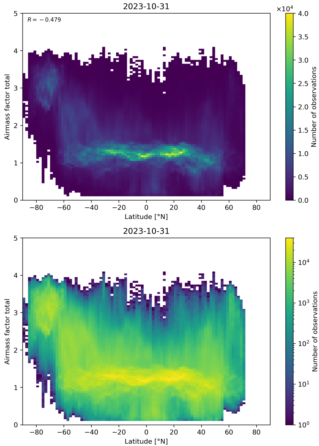
Figure 161: Scatter density plot of “Latitude” against “Airmass factor total” for 2023-10-30 to 2023-11-01.
