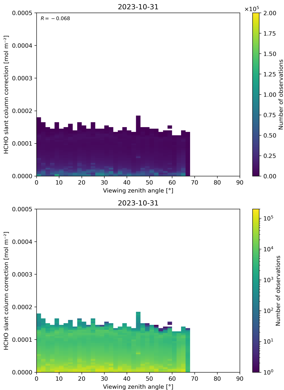
Figure 187: Scatter density plot of “Viewing zenith angle” against “HCHO slant column correction” for 2023-10-30 to 2023-11-01.
