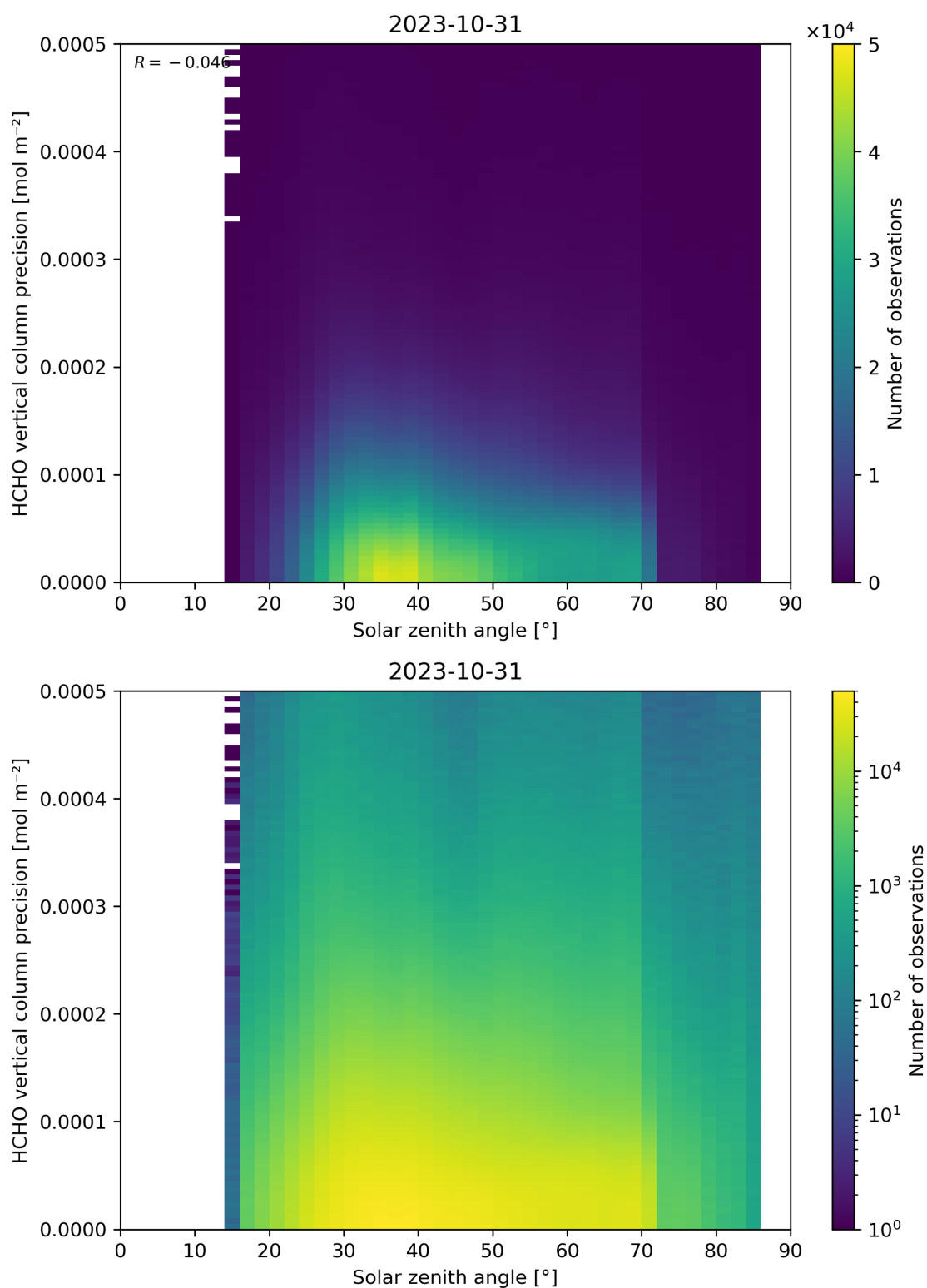
Figure 179: Scatter density plot of “Solar zenith angle” against “HCHO vertical column precision” for 2023-10-30 to 2023-11-01.
