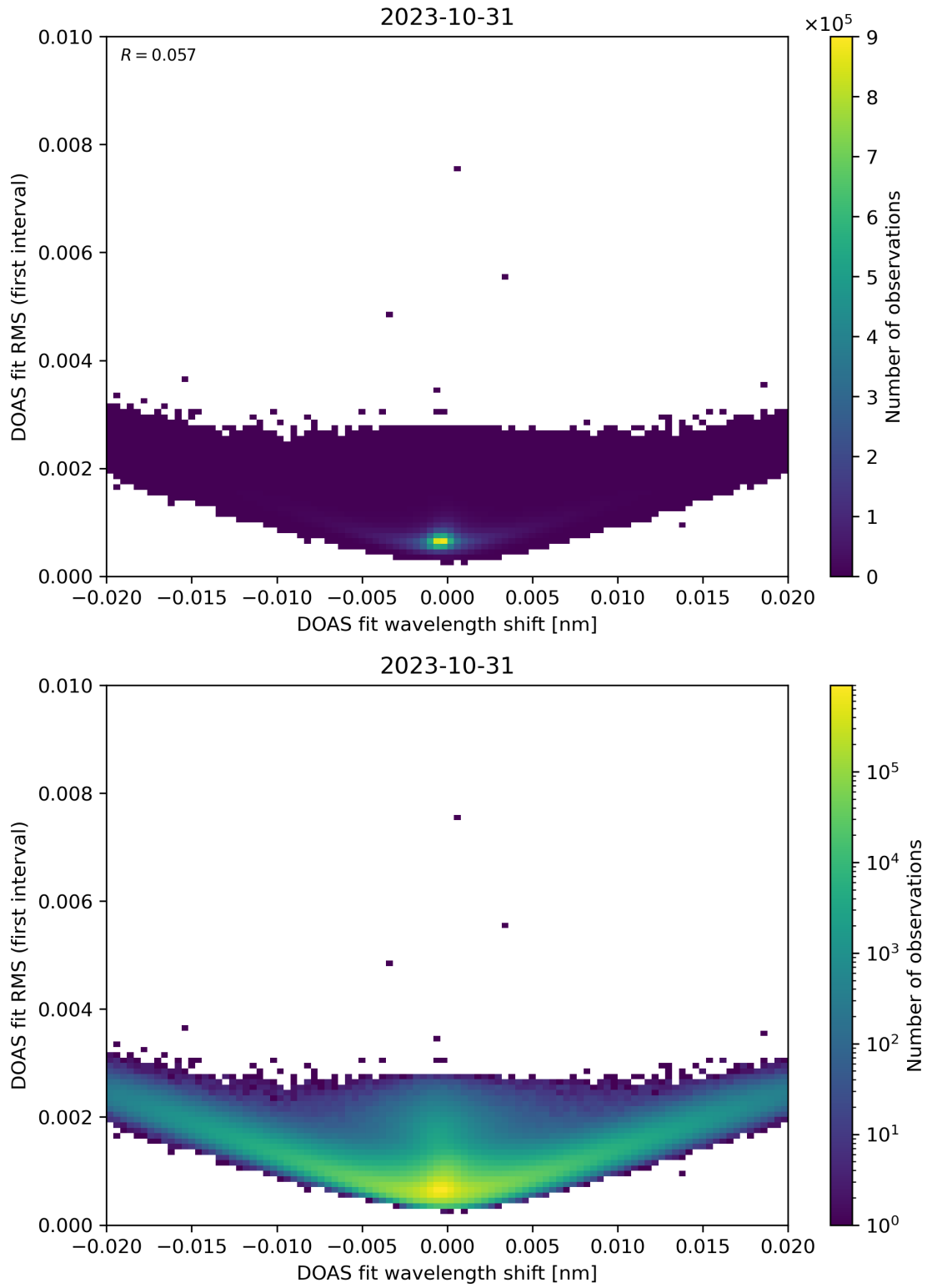
Figure 64: Scatter density plot of “DOAS fit wavelength shift” against “DOAS fit RMS (first interval)” for 2023-10-30 to 2023-11-01.
