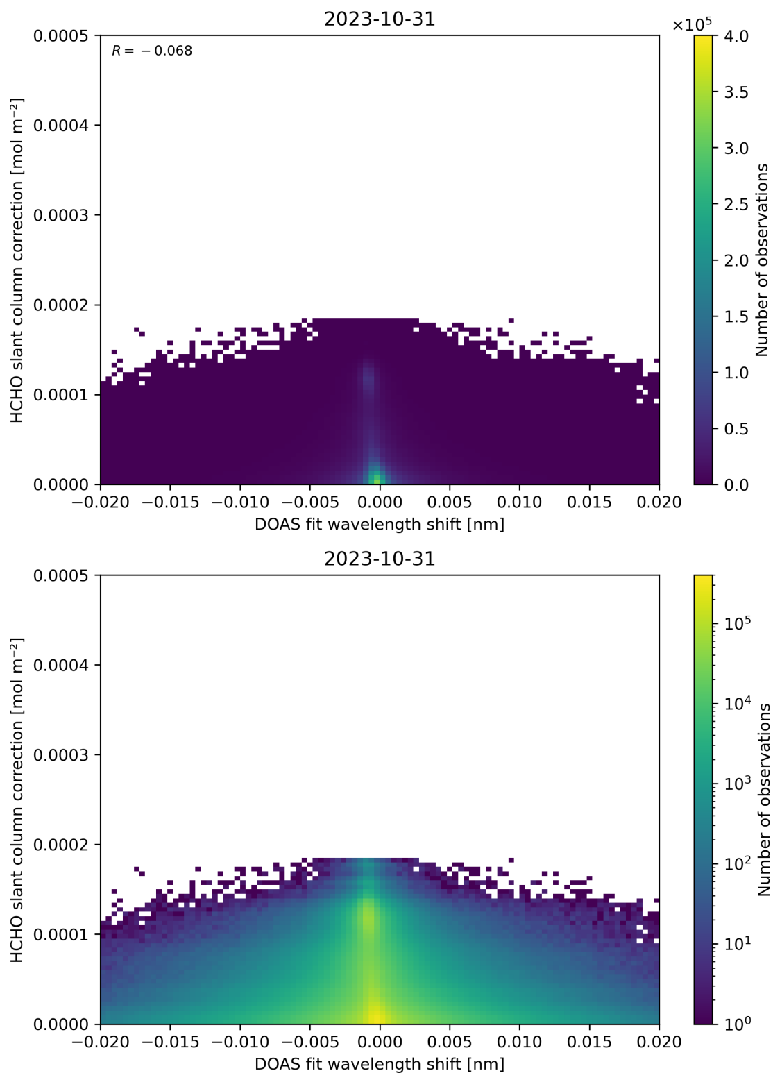
Figure 67: Scatter density plot of “DOAS fit wavelength shift” against “HCHO slant column correction” for 2023-10-30 to 2023-11-01.
