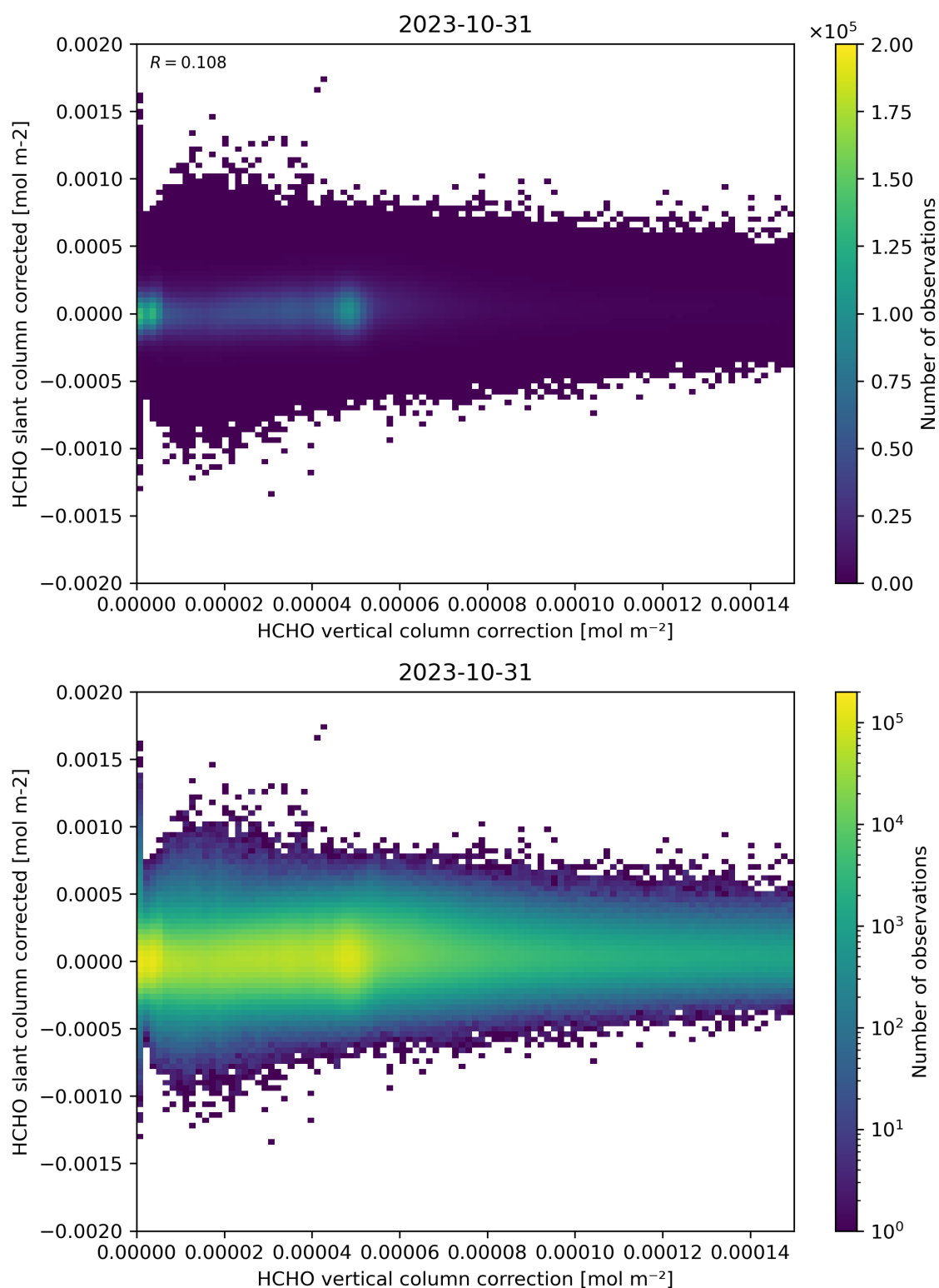
Figure 116: Scatter density plot of “HCHO vertical column correction” against “HCHO slant column corrected” for 2023-10-30 to 2023-11-01.
