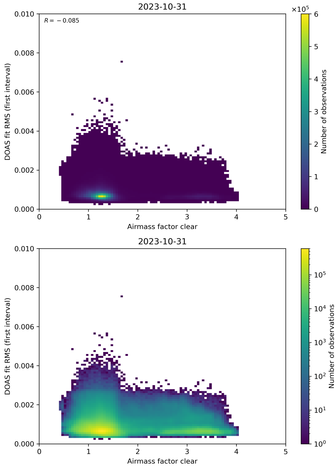
Figure 71: Scatter density plot of “Airmass factor clear” against “DOAS fit RMS (first interval)” for 2023-10-30 to 2023-11-01.
