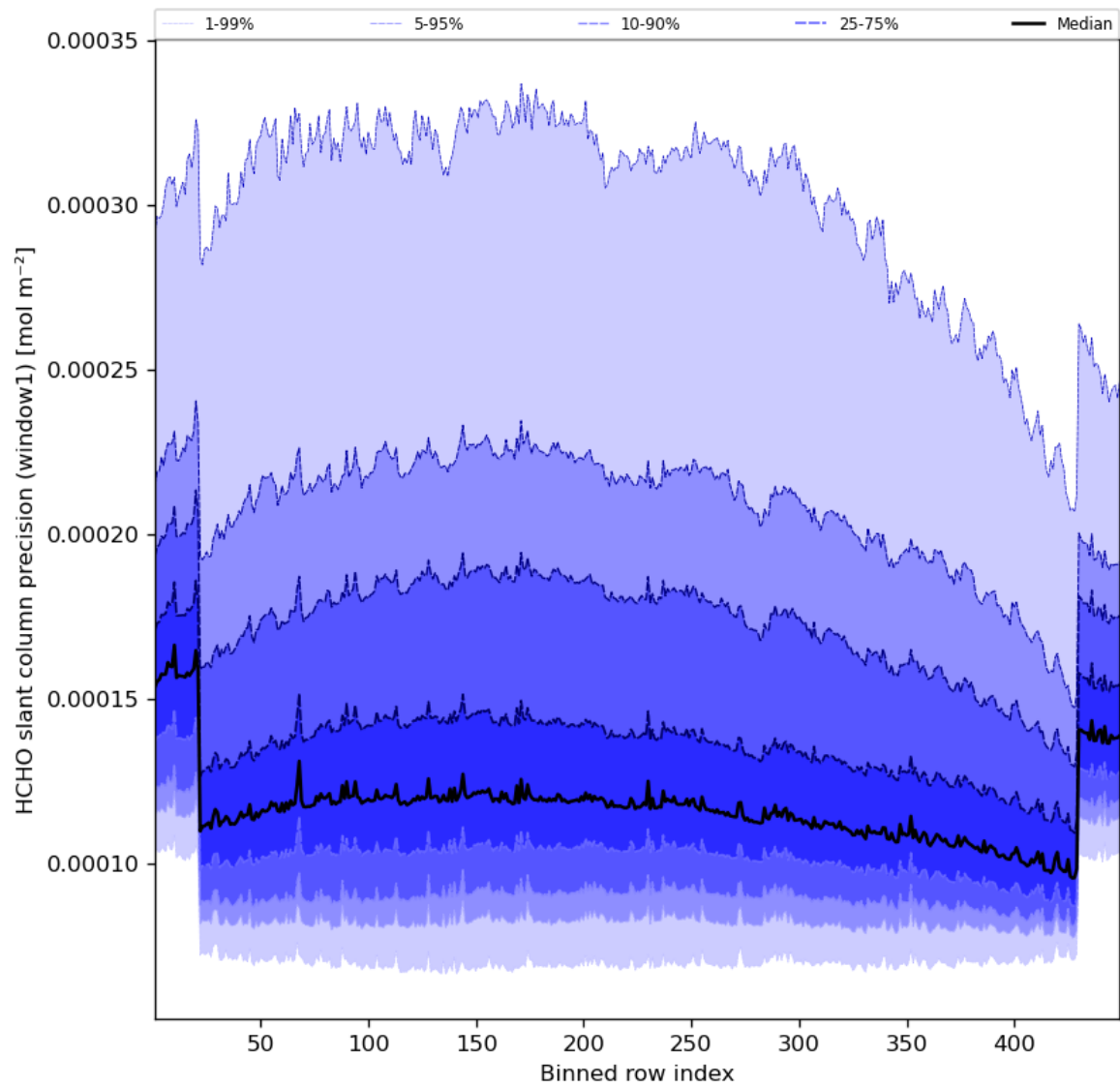
Figure 53: Along track statistics of “HCHO slant column precision (window1)” for 2023-10-30 to 2023-11-01
