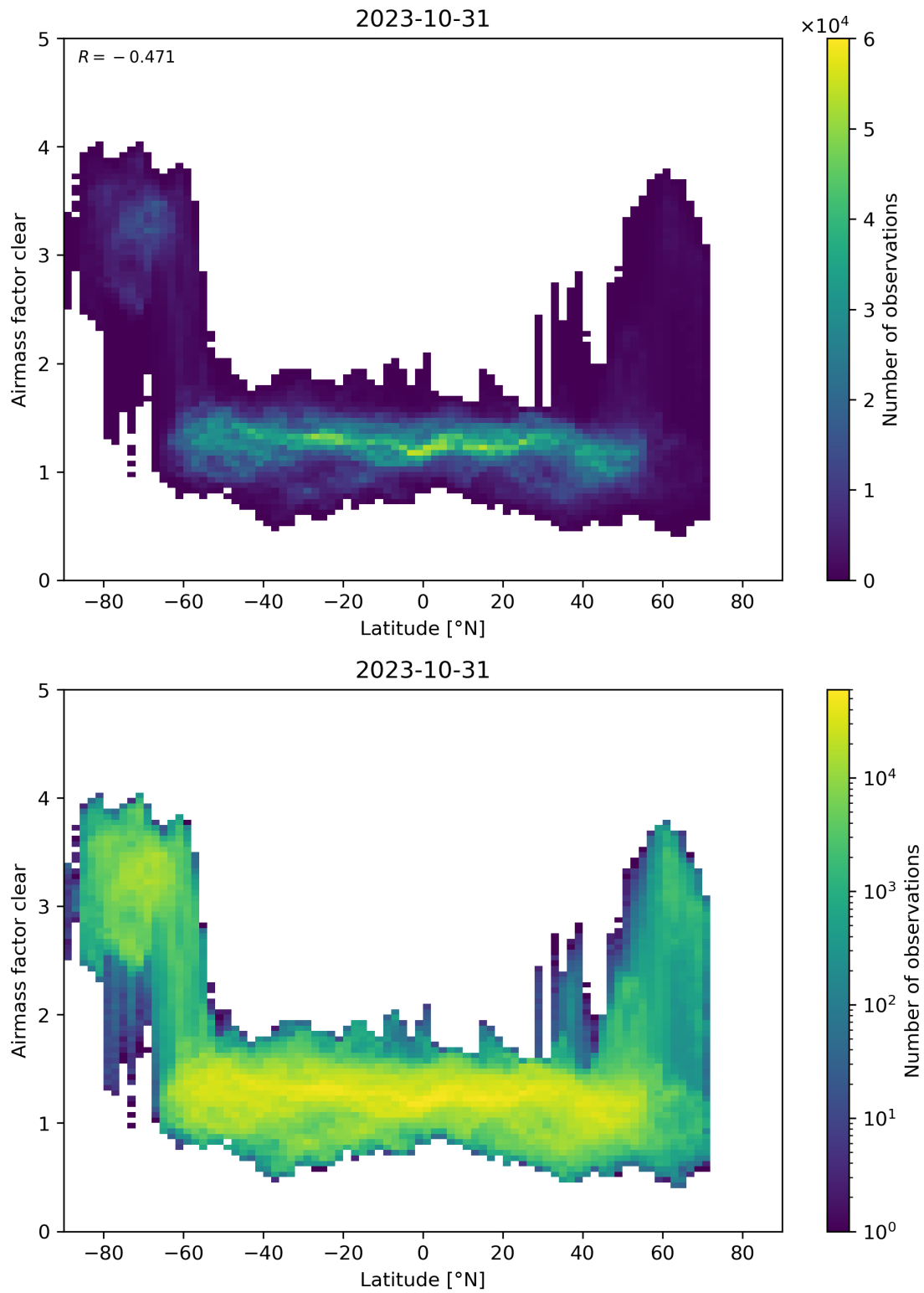
Figure 156: Scatter density plot of “Latitude” against “Airmass factor clear” for 2023-10-30 to 2023-11-01.
