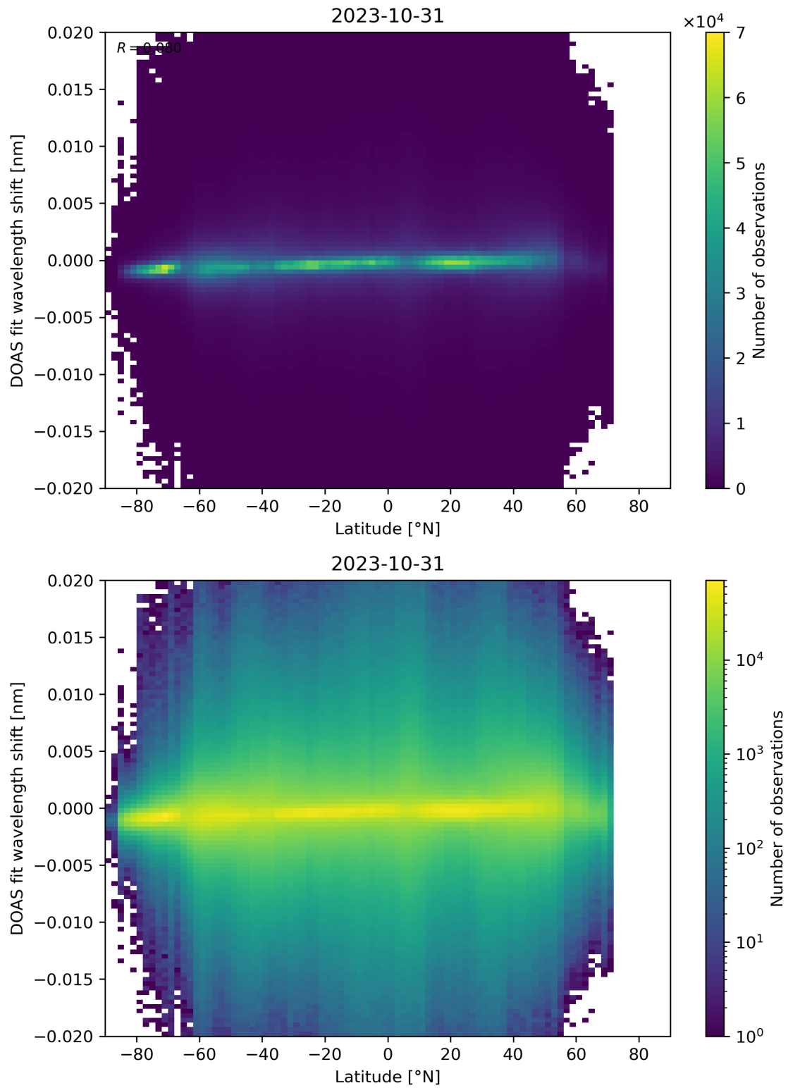
Figure 154: Scatter density plot of “Latitude” against “DOAS fit wavelength shift” for 2023-10-30 to 2023-11-01.
