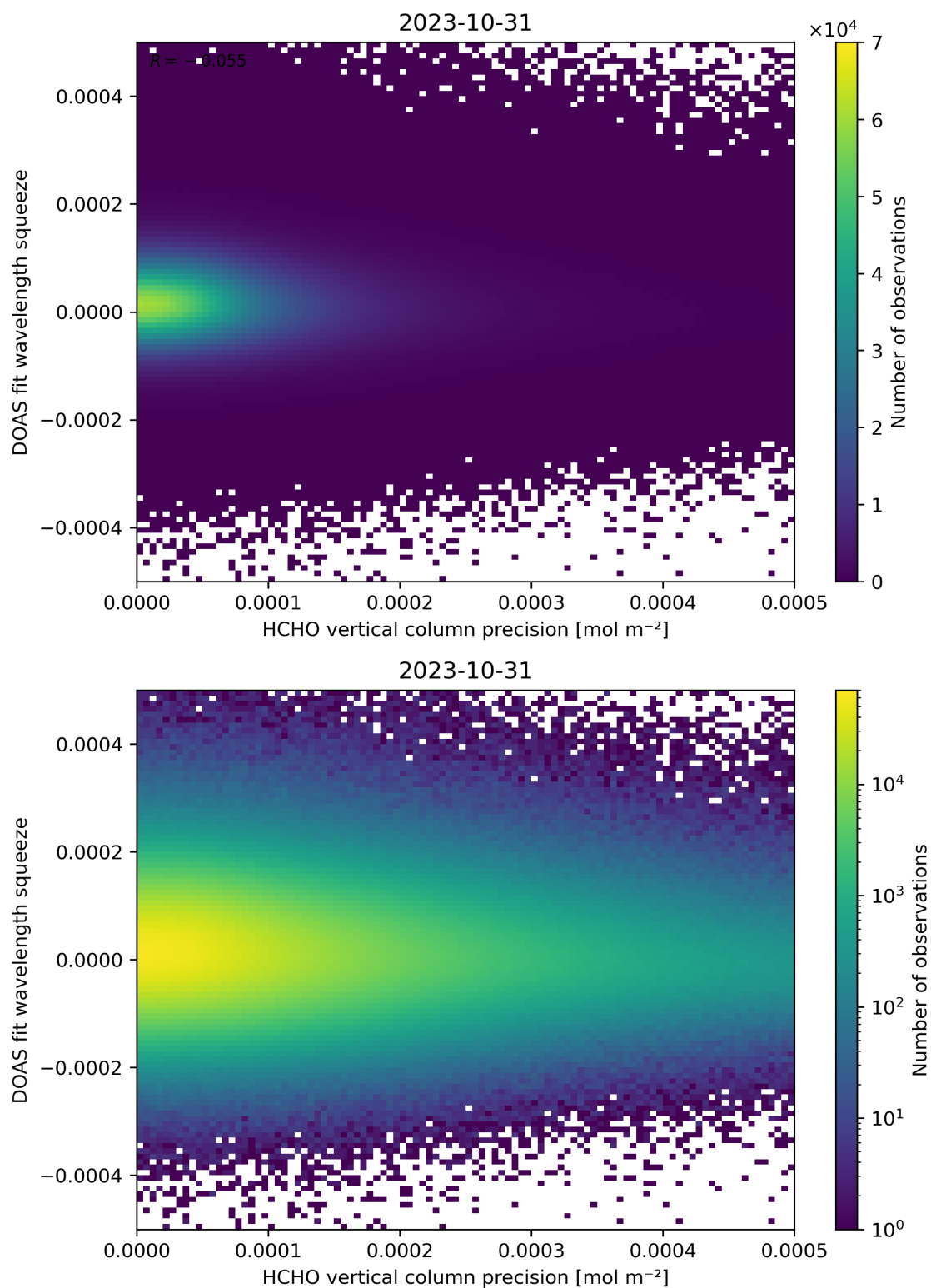
Figure 138: Scatter density plot of “HCHO vertical column precision” against “DOAS fit wavelength squeeze” for 2023-10-30 to 2023-11-01.
