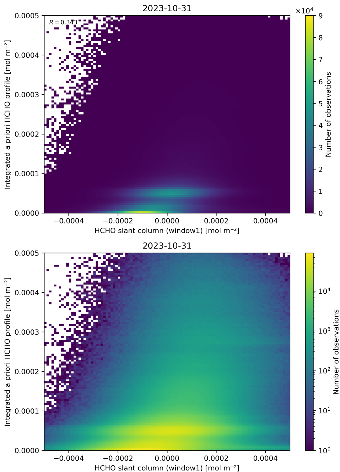
Figure 87: Scatter density plot of “HCHO slant column (window1)” against “Integrated a priori HCHO profile” for 2023-10-30 to 2023-11-01.
