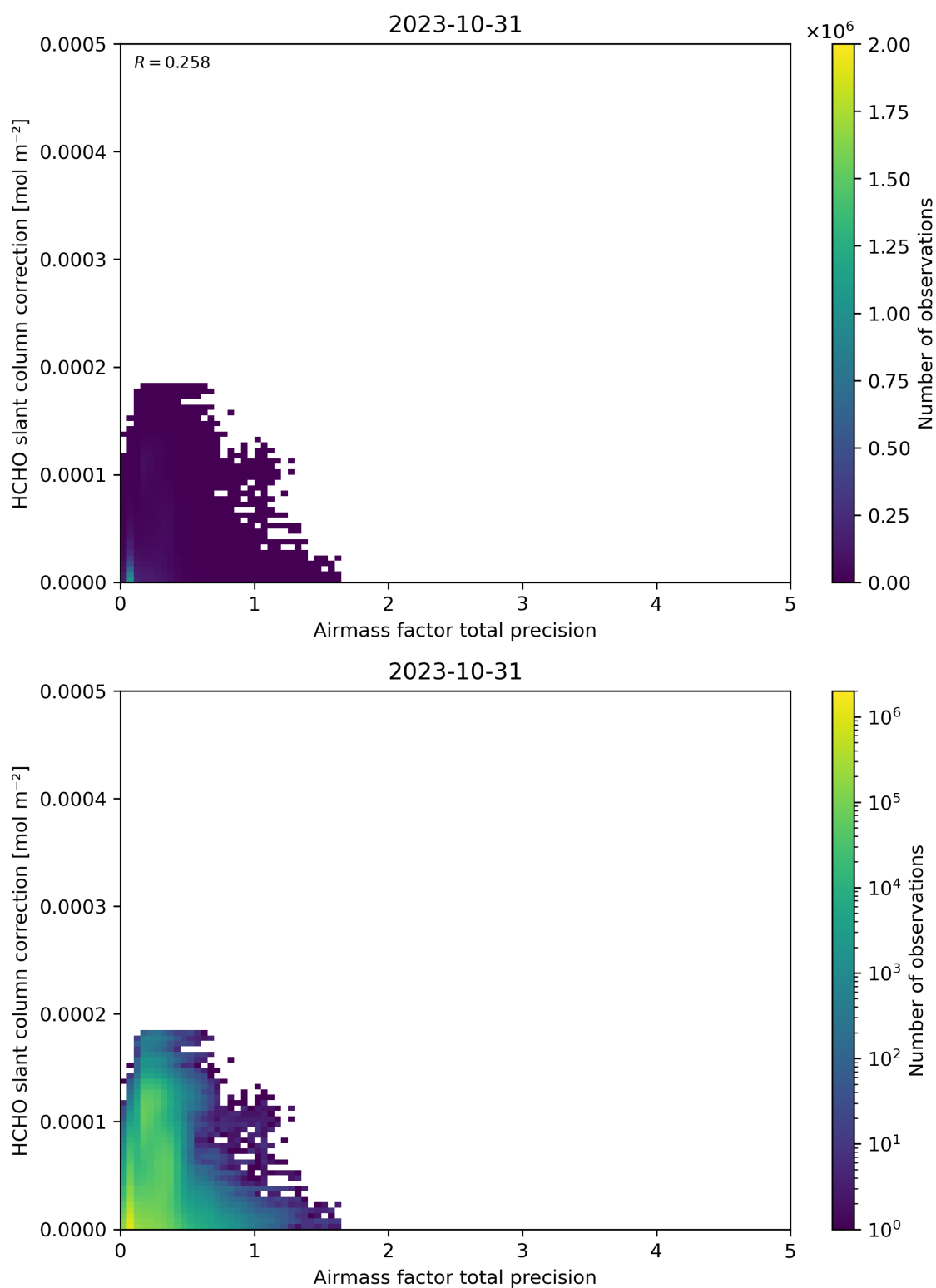
Figure 110: Scatter density plot of “Airmass factor total precision” against “HCHO slant column correction” for 2023-10-30 to 2023-11-01.
