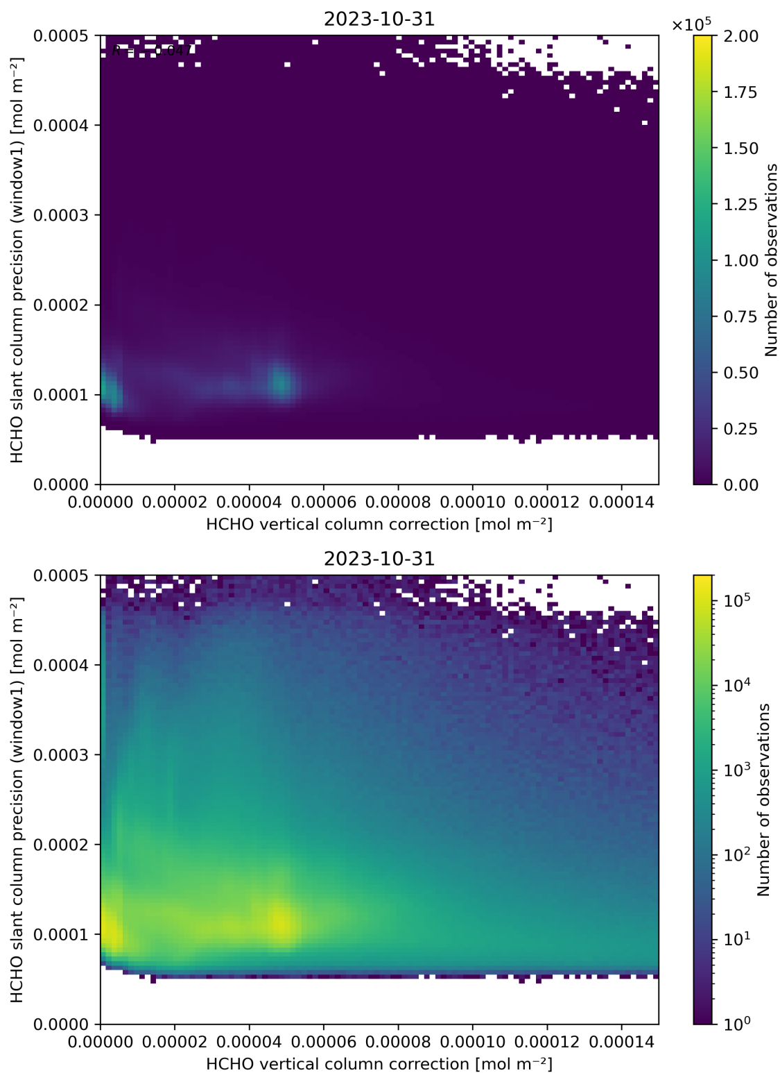
Figure 119: Scatter density plot of “HCHO vertical column correction” against “HCHO slant column precision (window1)” for 2023-10-30 to 2023-11-01.
