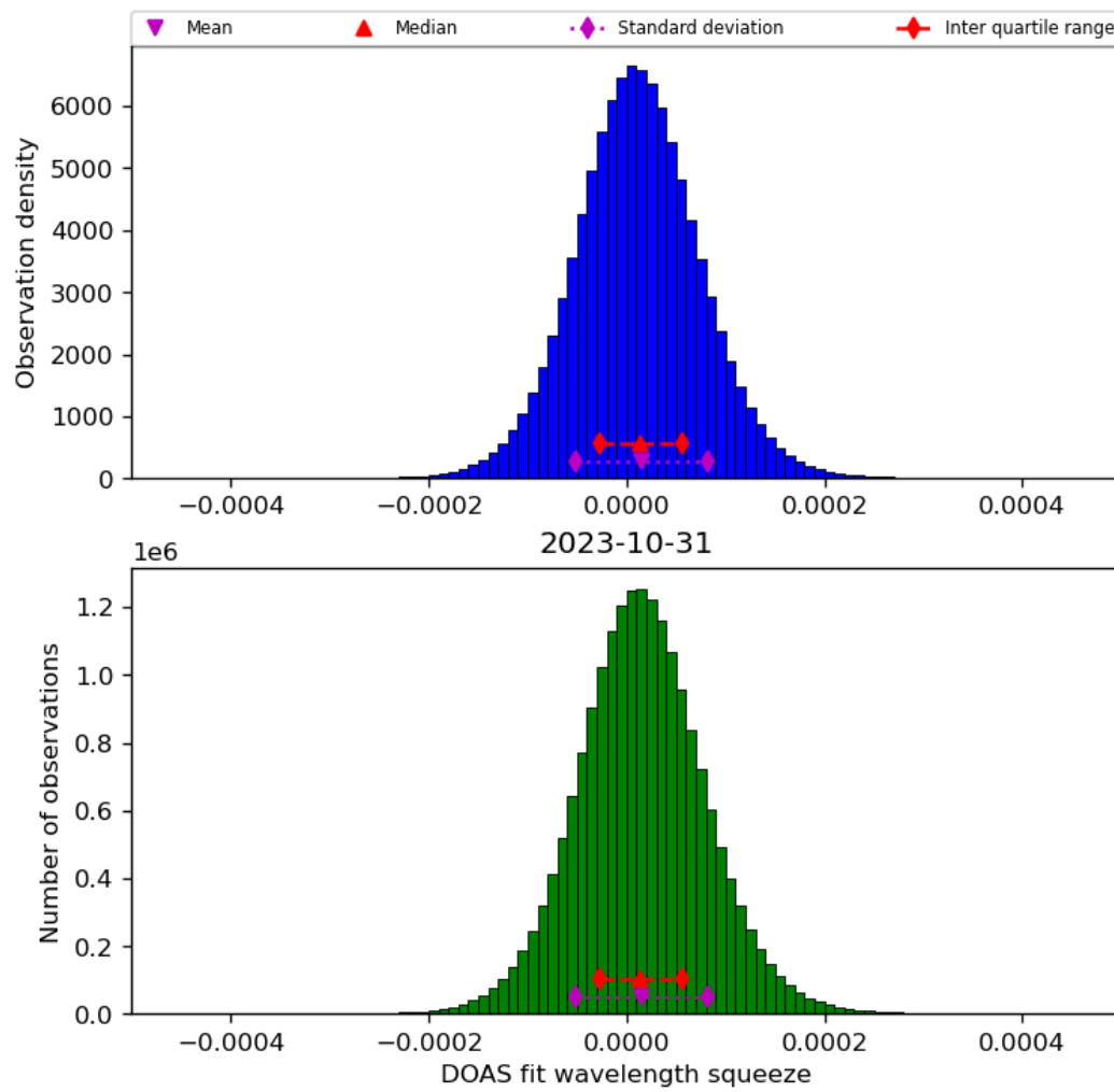
Figure 45: Histogram of “DOAS fit wavelength squeeze” for 2023-10-30 to 2023-11-01
