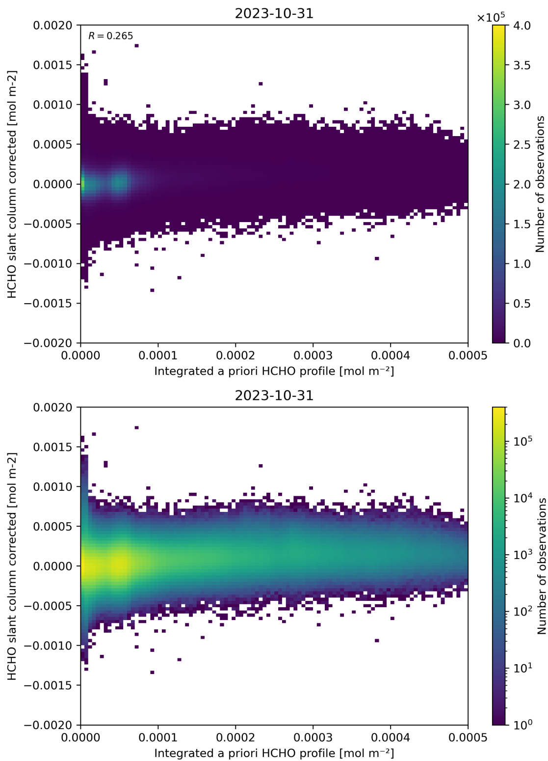
Figure 151: Scatter density plot of “Integrated a priori HCHO profile” against “HCHO slant column corrected” for 2023-10-30 to 2023-11-01.
