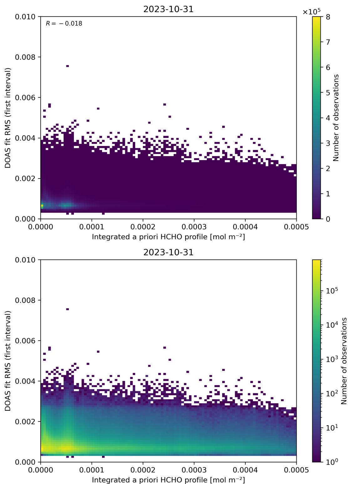
Figure 148: Scatter density plot of “Integrated a priori HCHO profile” against “DOAS fit RMS (first interval)” for 2023-10-30 to 2023-11-01.
