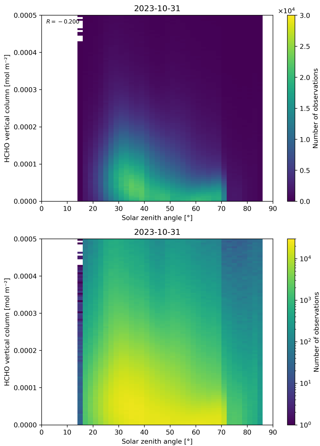
Figure 177: Scatter density plot of “Solar zenith angle” against “HCHO vertical column” for 2023-10-30 to 2023-11-01.
