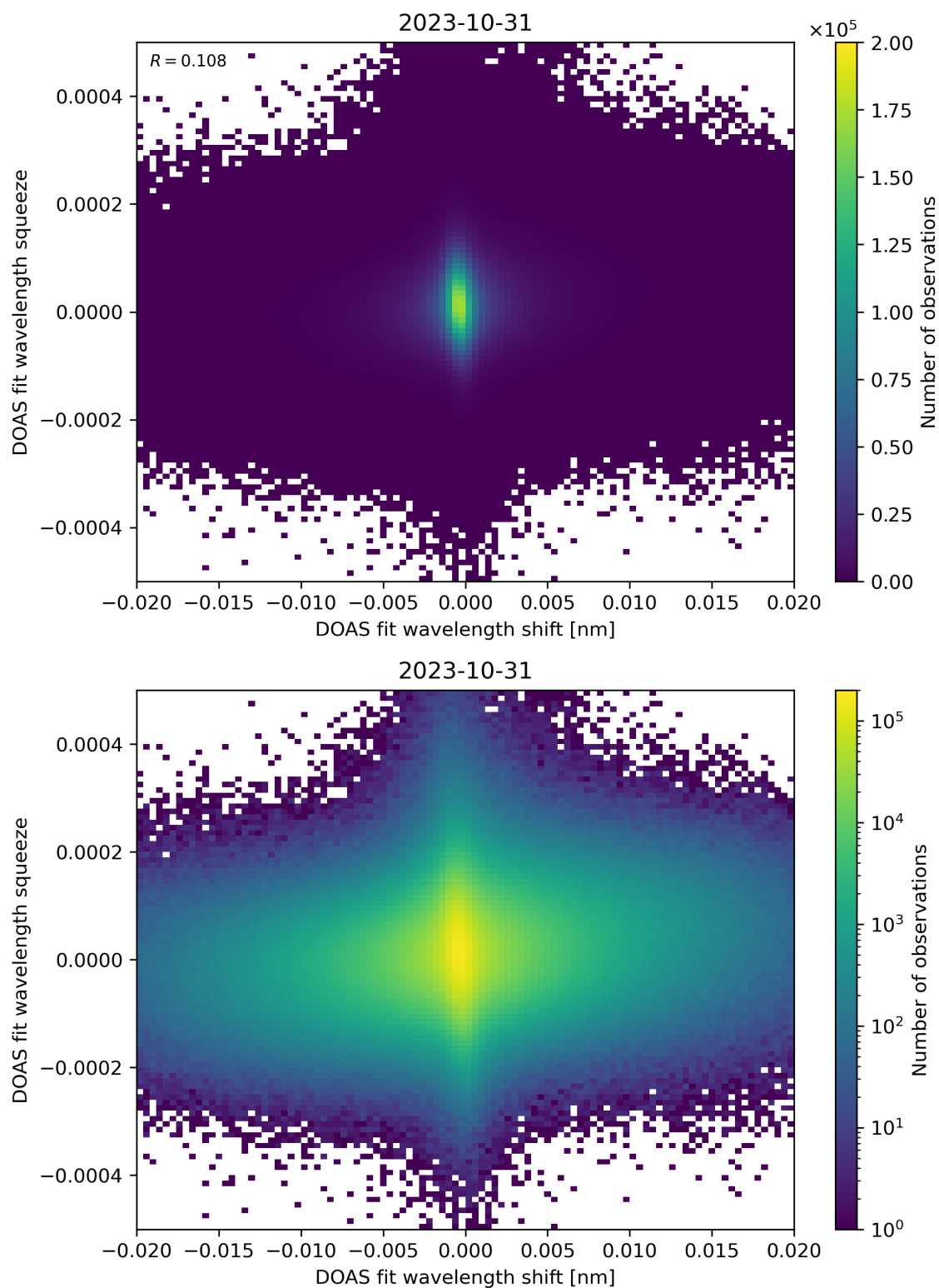
Figure 65: Scatter density plot of “DOAS fit wavelength shift” against “DOAS fit wavelength squeeze” for 2023-10-30 to 2023-11-01.
