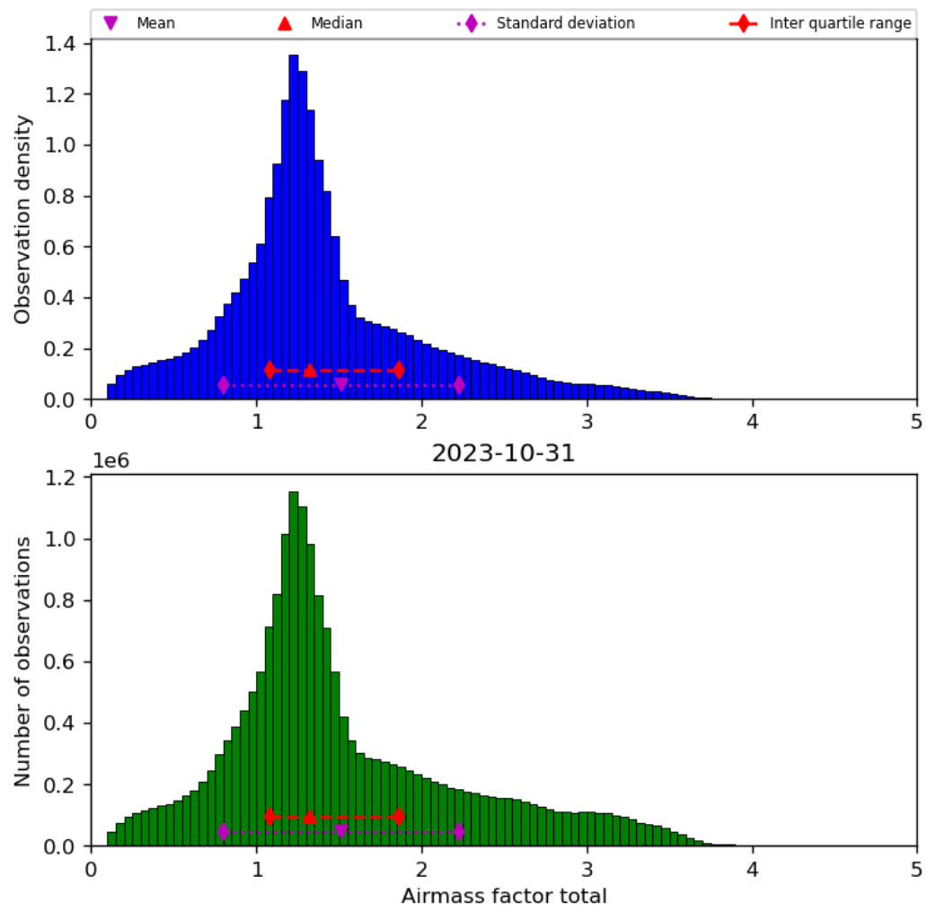
Figure 40: Histogram of “Airmass factor total” for 2023-10-30 to 2023-11-01
