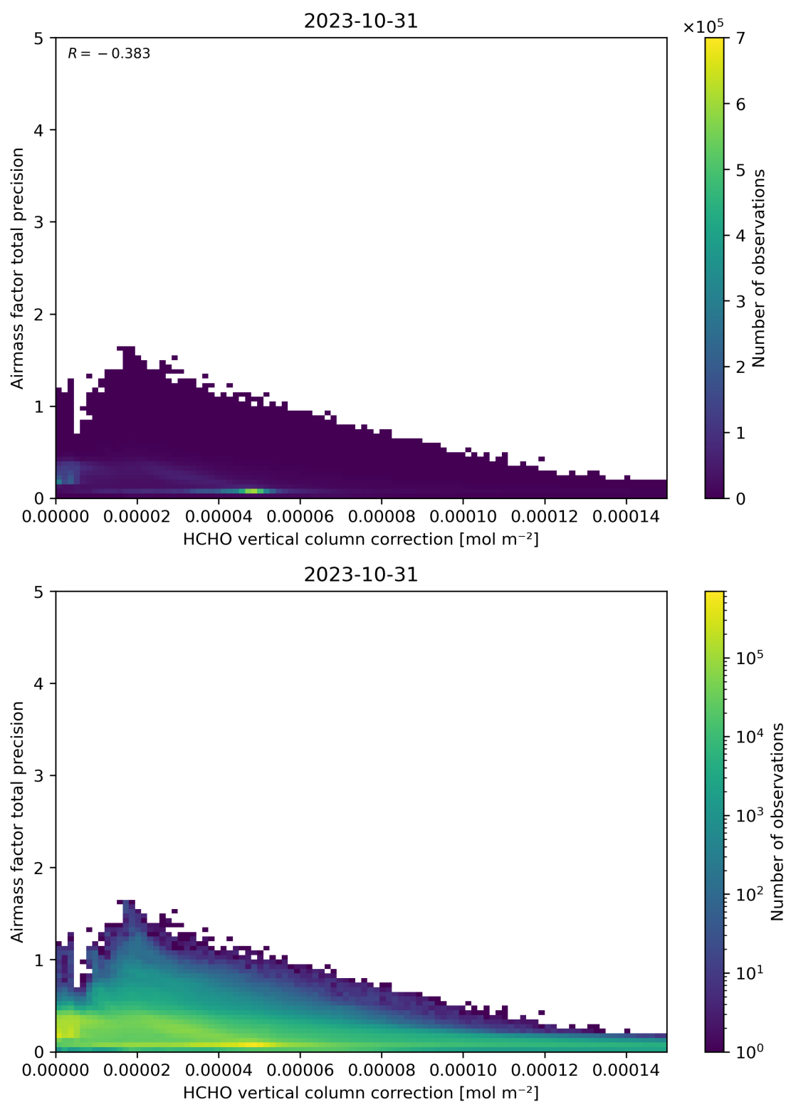
Figure 121: Scatter density plot of “HCHO vertical column correction” against “Airmass factor total precision” for 2023-10-30 to 2023-11-01.
