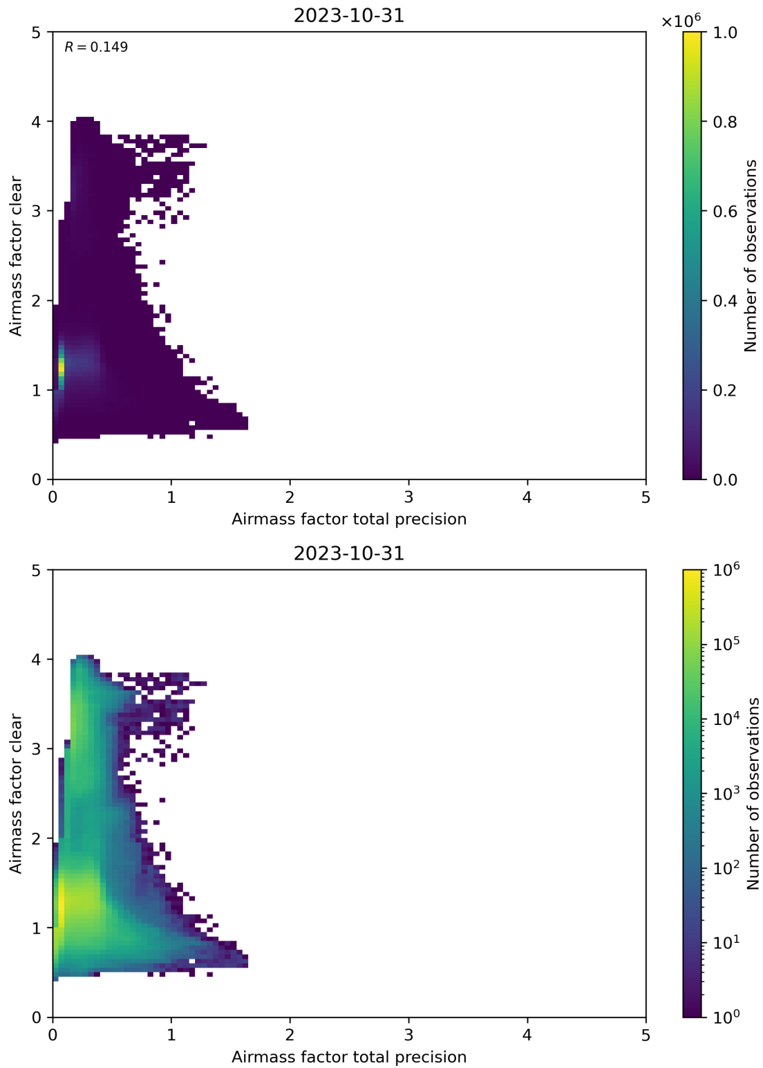
Figure 108: Scatter density plot of “Airmass factor total precision” against “Airmass factor clear” for 2023-10-30 to 2023-11-01.
