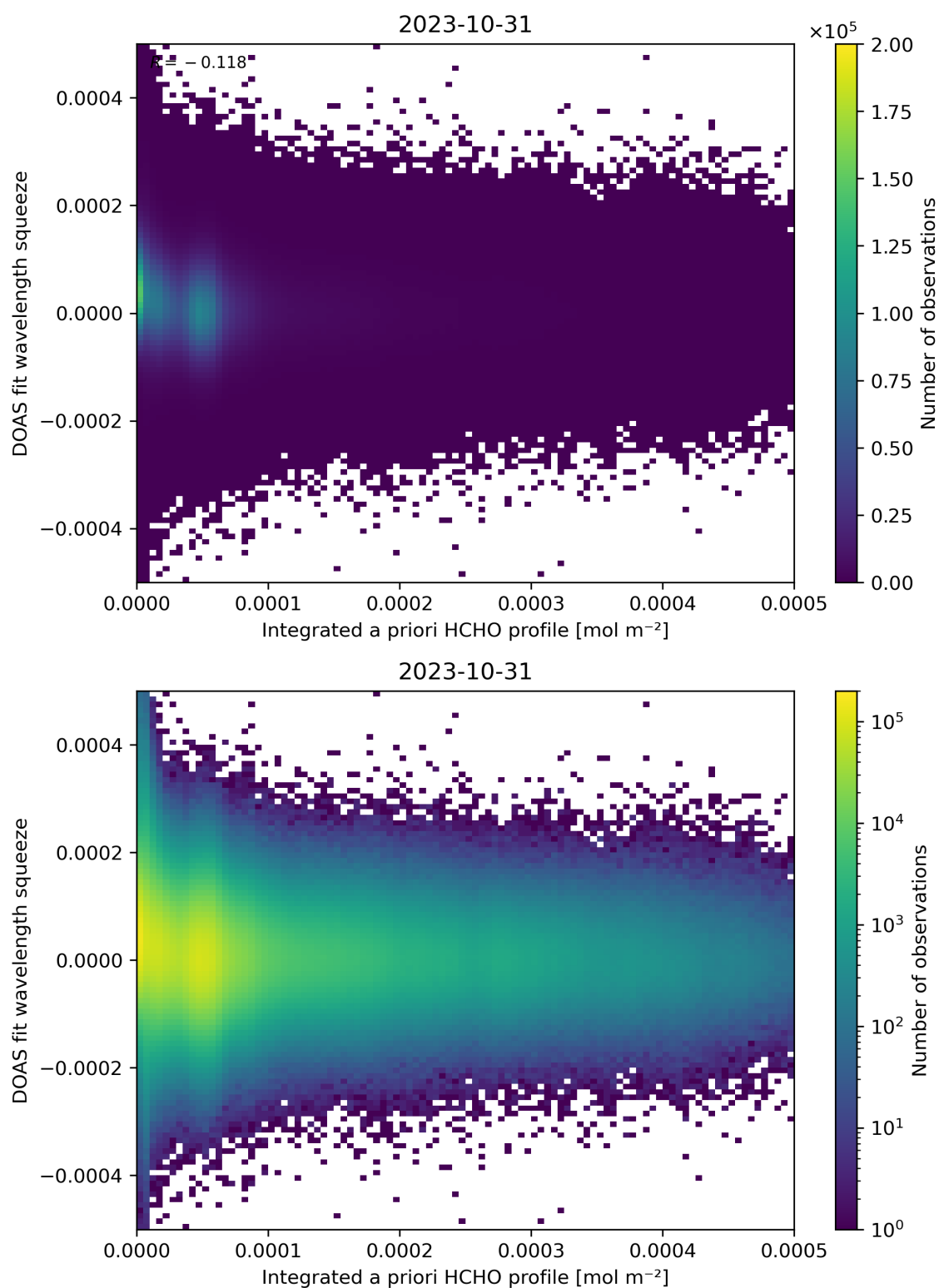
Figure 150: Scatter density plot of “Integrated a priori HCHO profile” against “DOAS fit wavelength squeeze” for 2023-10-30 to 2023-11-01.
