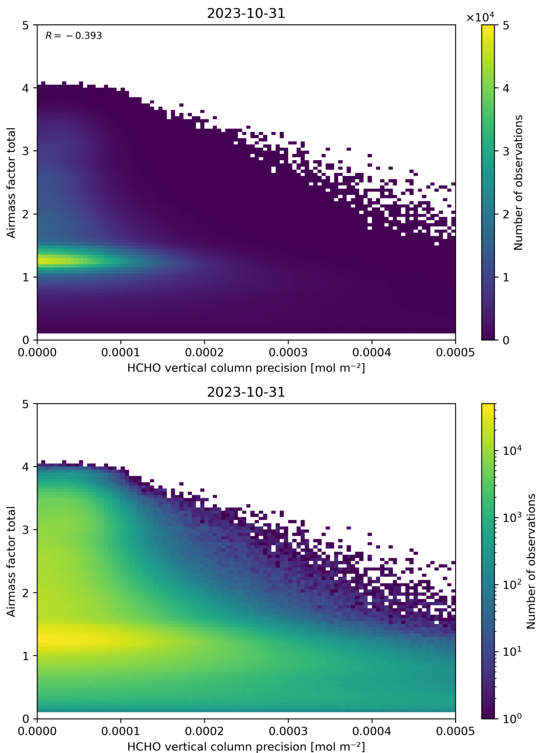
Figure 144: Scatter density plot of “HCHO vertical column precision” against “Airmass factor total” for 2023-10-30 to 2023-11-01.
