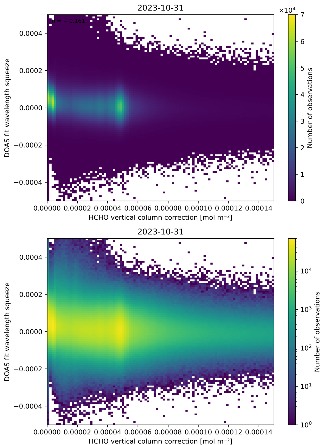
Figure 114: Scatter density plot of “HCHO vertical column correction” against “DOAS fit wavelength squeeze” for 2023-10-30 to 2023-11-01.
