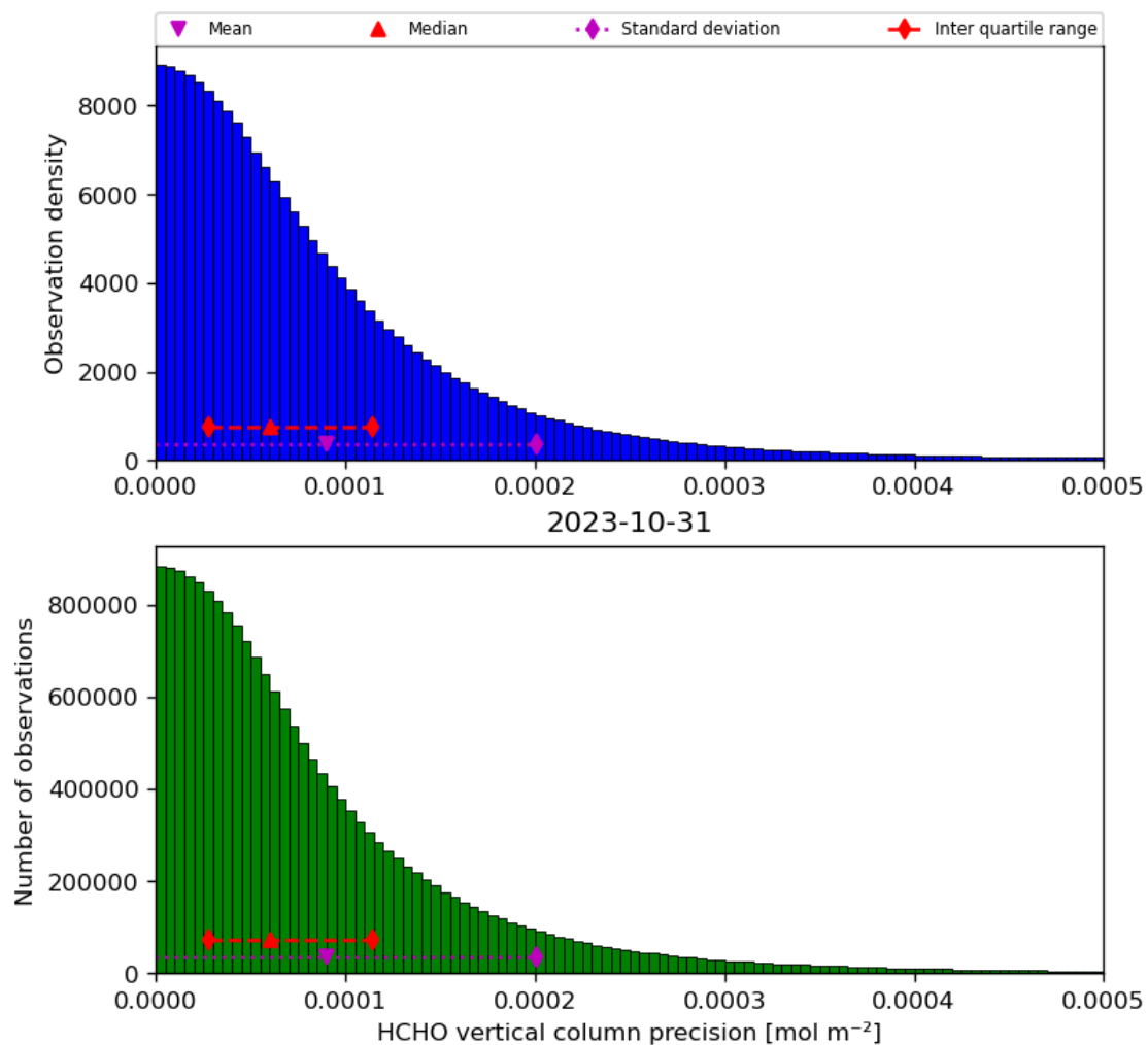
Figure 36: Histogram of “HCHO vertical column precision” for 2023-10-30 to 2023-11-01
