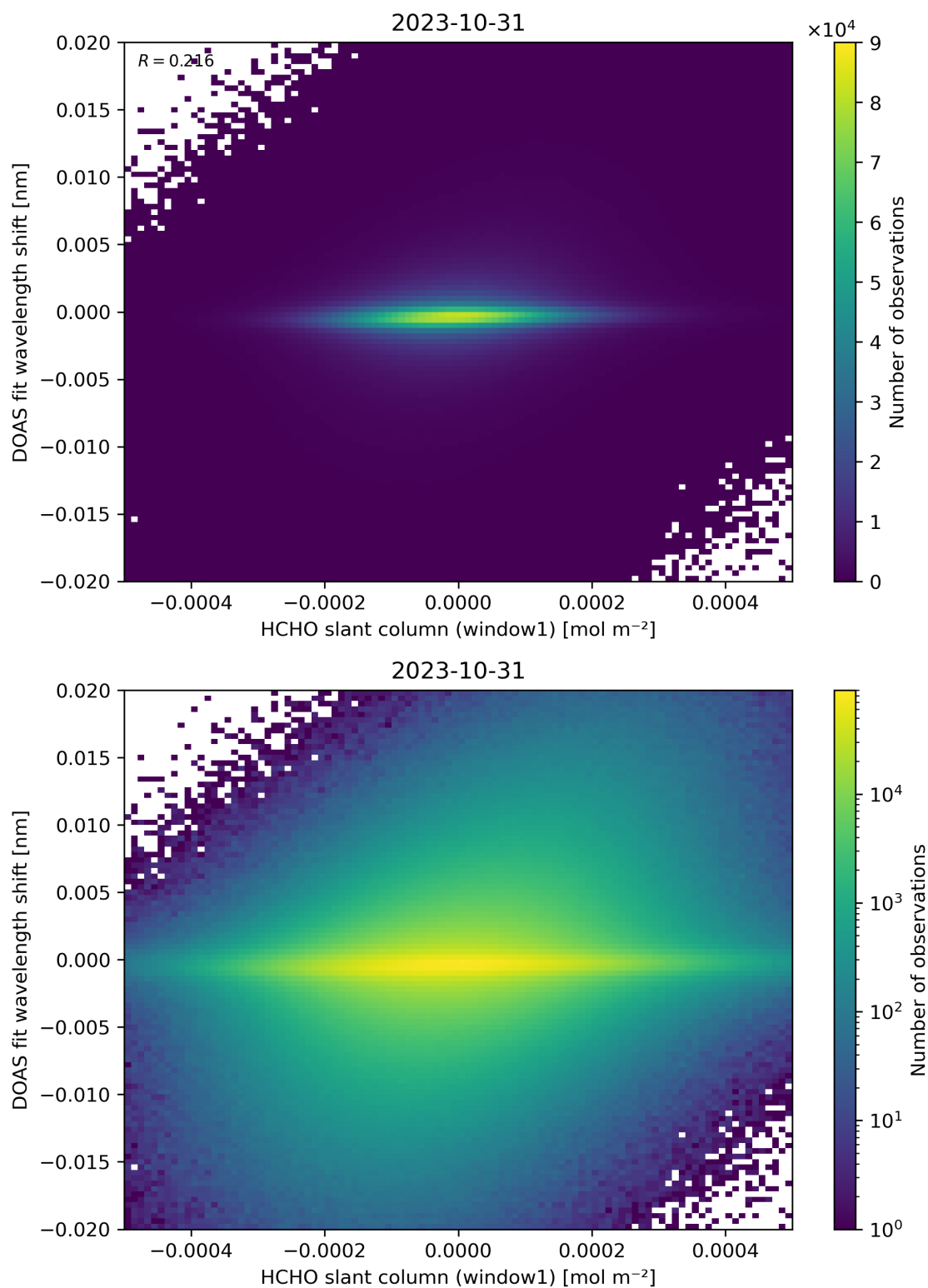
Figure 79: Scatter density plot of “HCHO slant column (window1)” against “DOAS fit wavelength shift” for 2023-10-30 to 2023-11-01.
