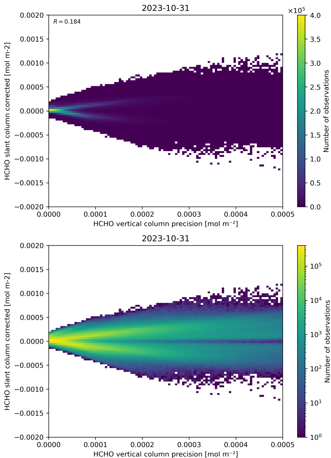
Figure 140: Scatter density plot of “HCHO vertical column precision” against “HCHO slant column corrected” for 2023-10-30 to 2023-11-01.
