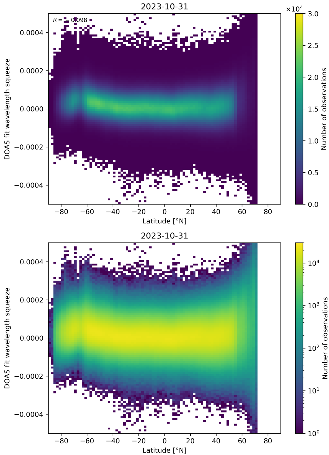
Figure 155: Scatter density plot of “Latitude” against “DOAS fit wavelength squeeze” for 2023-10-30 to 2023-11-01.
