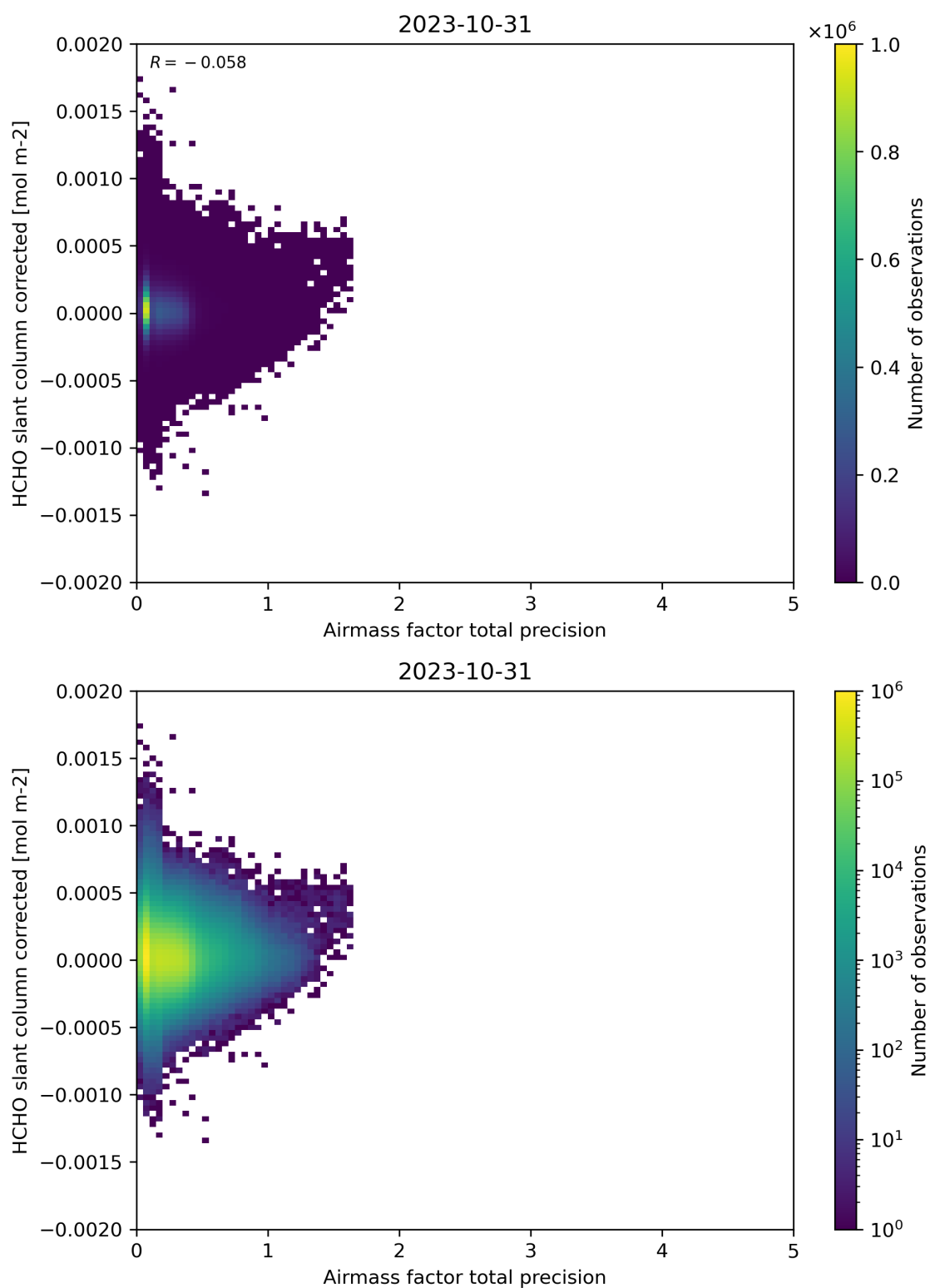
Figure 109: Scatter density plot of “Airmass factor total precision” against “HCHO slant column corrected” for 2023-10-30 to 2023-11-01.
