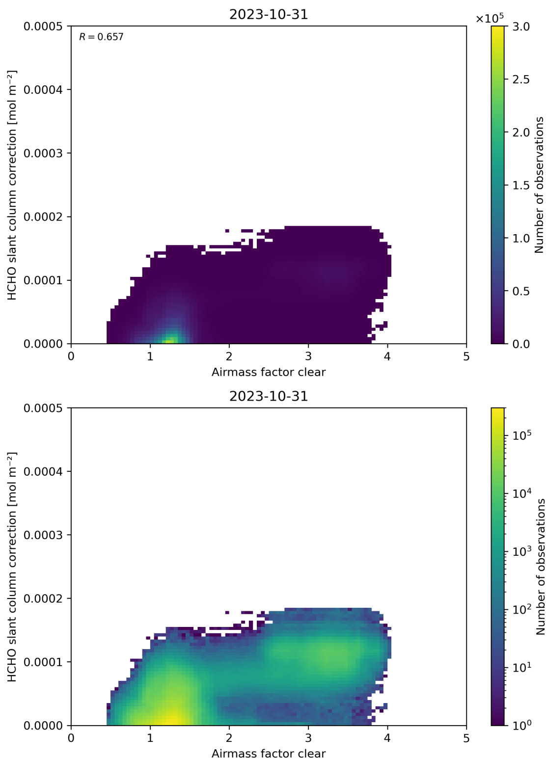
Figure 75: Scatter density plot of “Airmass factor clear” against “HCHO slant column correction” for 2023-10-30 to 2023-11-01.
