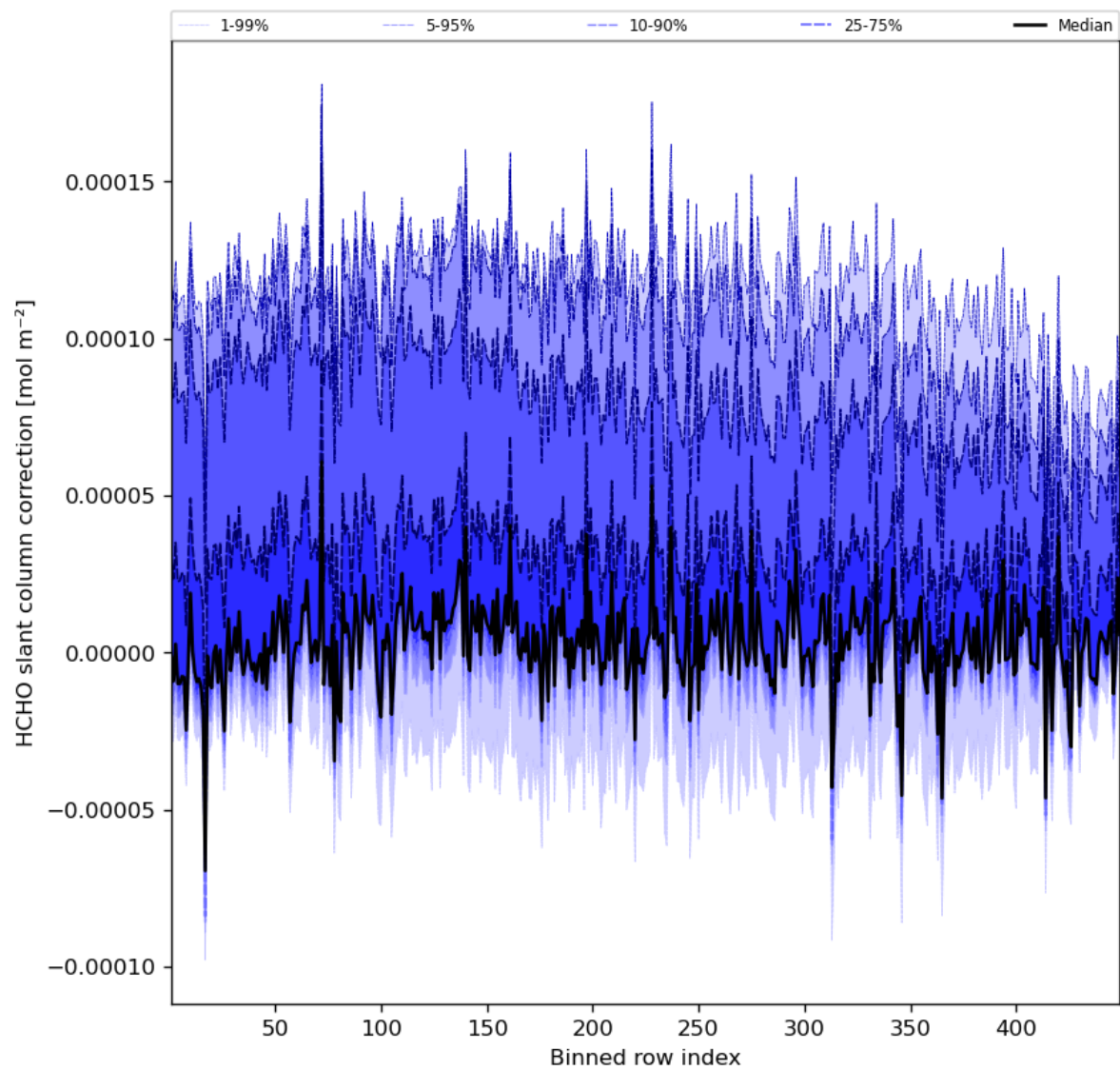
Figure 61: Along track statistics of “HCHO slant column correction” for 2023-10-30 to 2023-11-01
