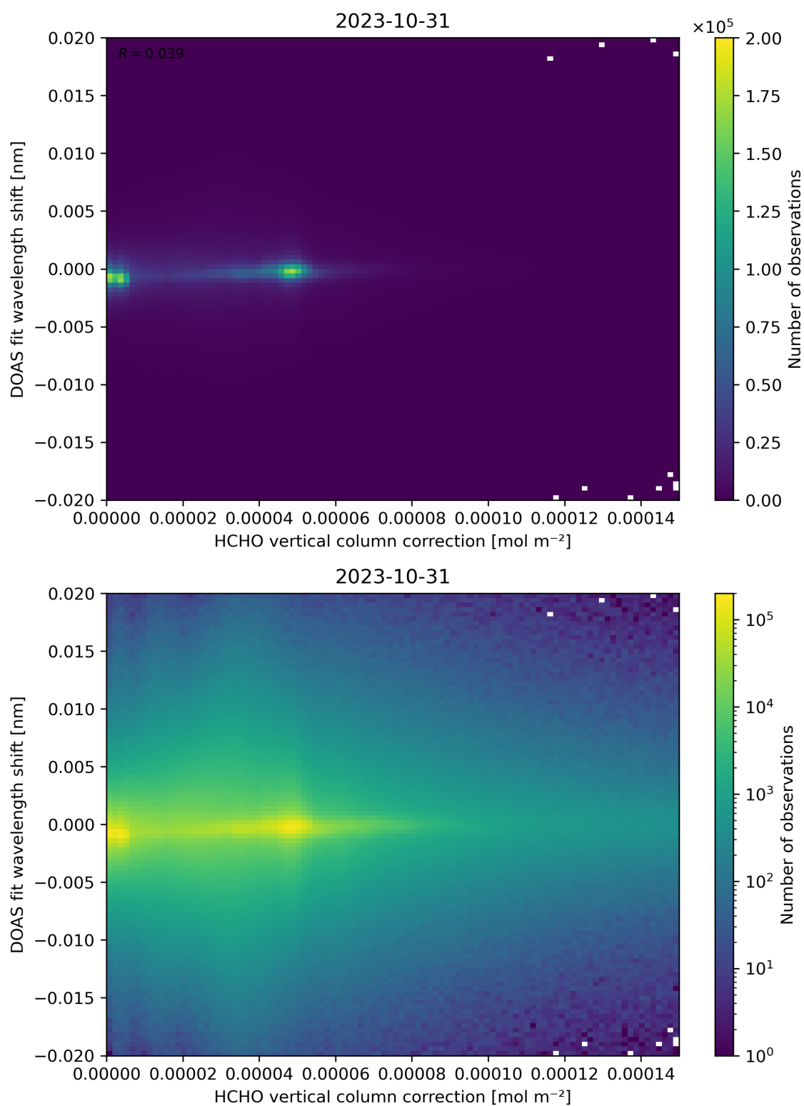
Figure 113: Scatter density plot of “HCHO vertical column correction” against “DOAS fit wavelength shift” for 2023-10-30 to 2023-11-01.
