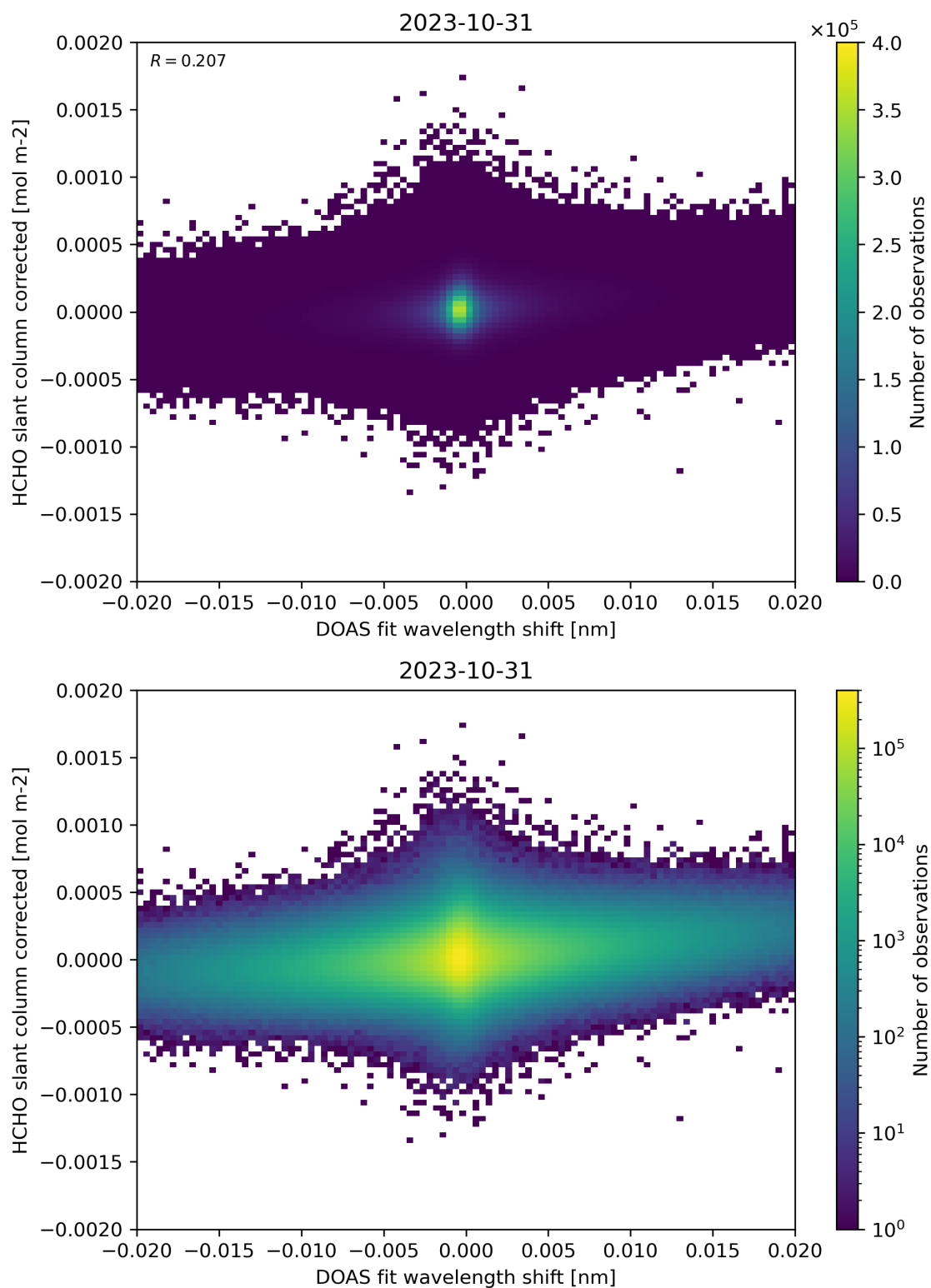
Figure 66: Scatter density plot of “DOAS fit wavelength shift” against “HCHO slant column corrected” for 2023-10-30 to 2023-11-01.
