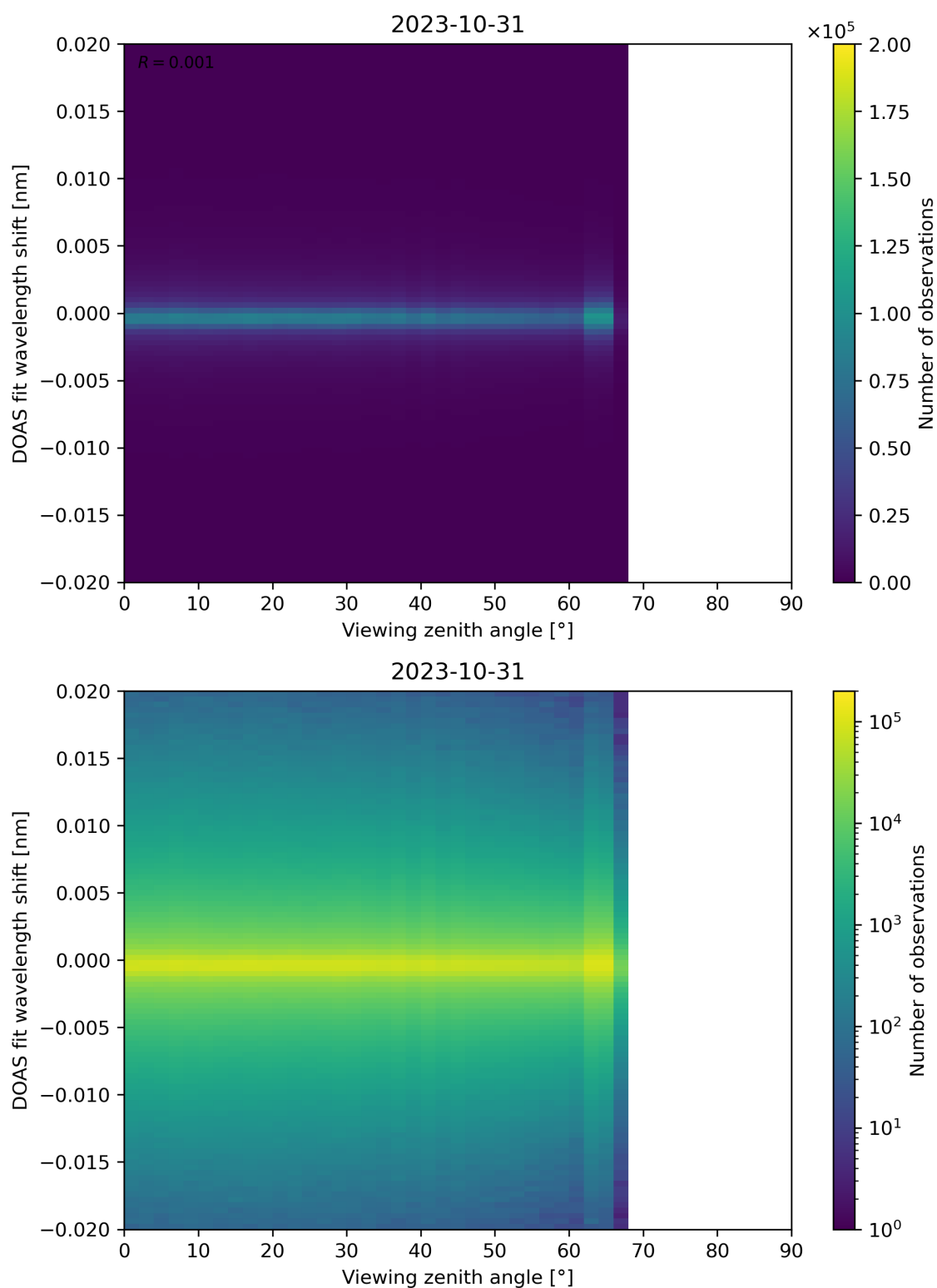
Figure 183: Scatter density plot of “Viewing zenith angle” against “DOAS fit wavelength shift” for 2023-10-30 to 2023-11-01.
