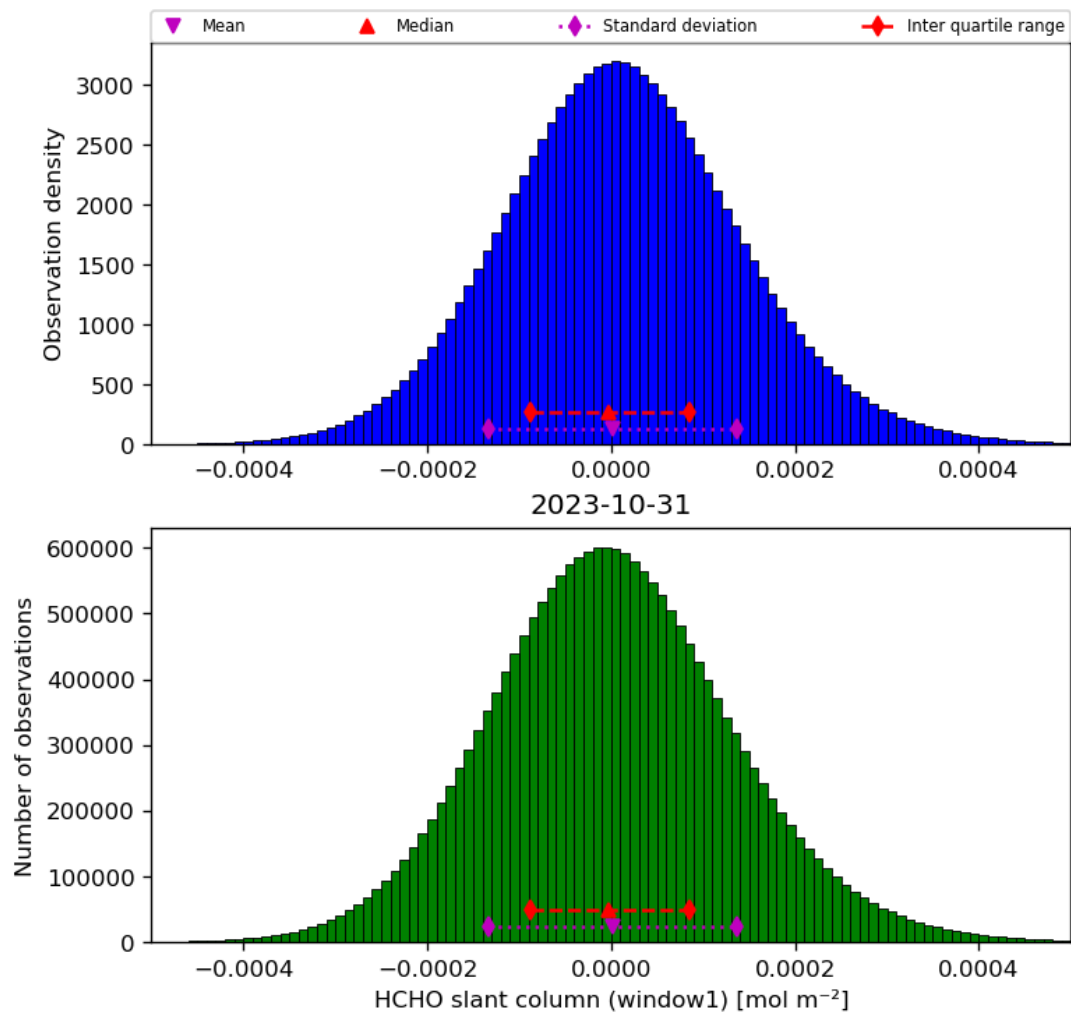
Figure 38: Histogram of “HCHO slant column (window1)” for 2023-10-30 to 2023-11-01
