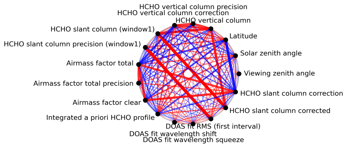
Figure 1: Map of correlation graph for 2023-10-30 to 2023-11-01.
