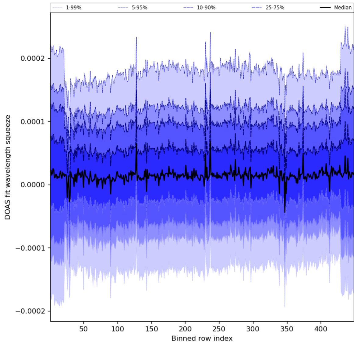
Figure 59: Along track statistics of “DOAS fit wavelength squeeze” for 2023-10-30 to 2023-11-01
