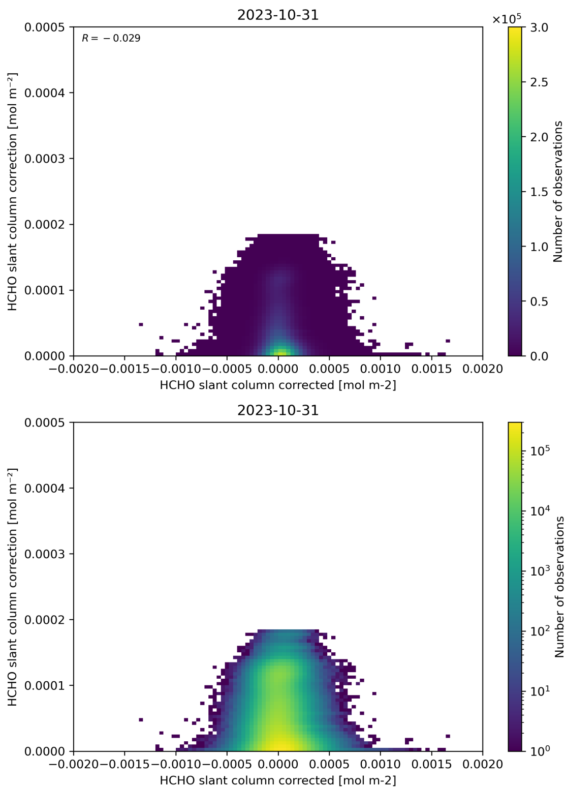
Figure 77: Scatter density plot of “HCHO slant column corrected” against “HCHO slant column correction” for 2023-10-30 to 2023-11-01.
