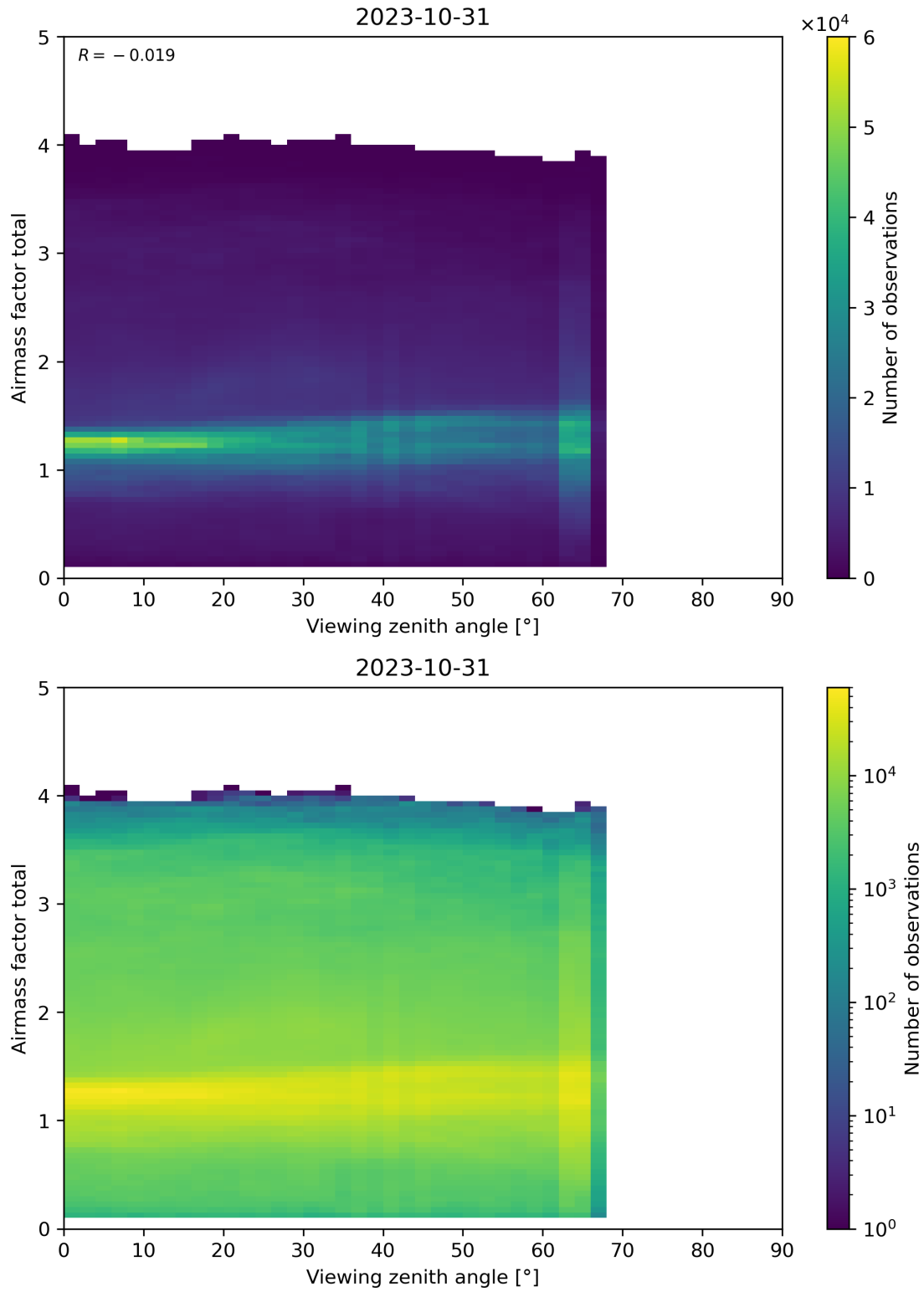
Figure 190: Scatter density plot of “Viewing zenith angle” against “Airmass factor total” for 2023-10-30 to 2023-11-01.
