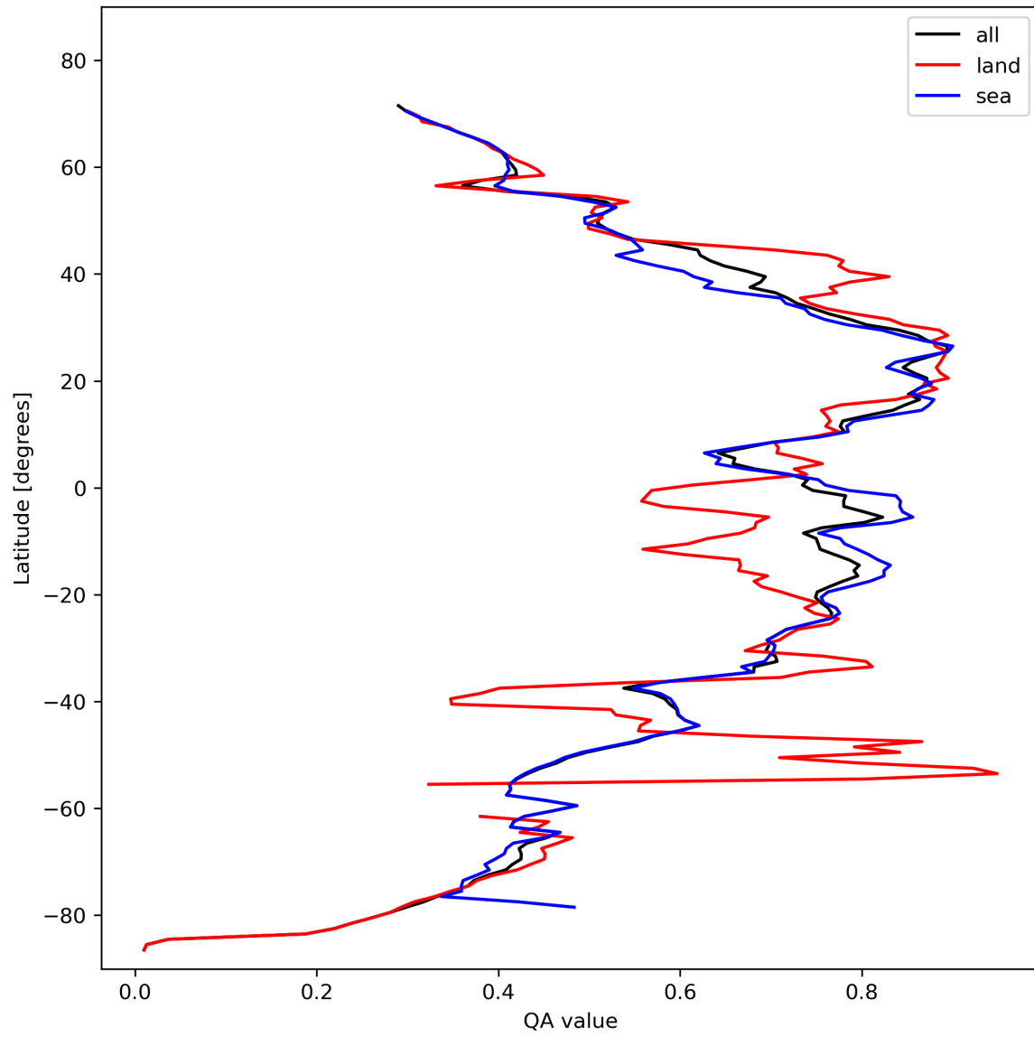
Figure 20: Zonal average of “QA value” for 2023-10-30 to 2023-11-01.
