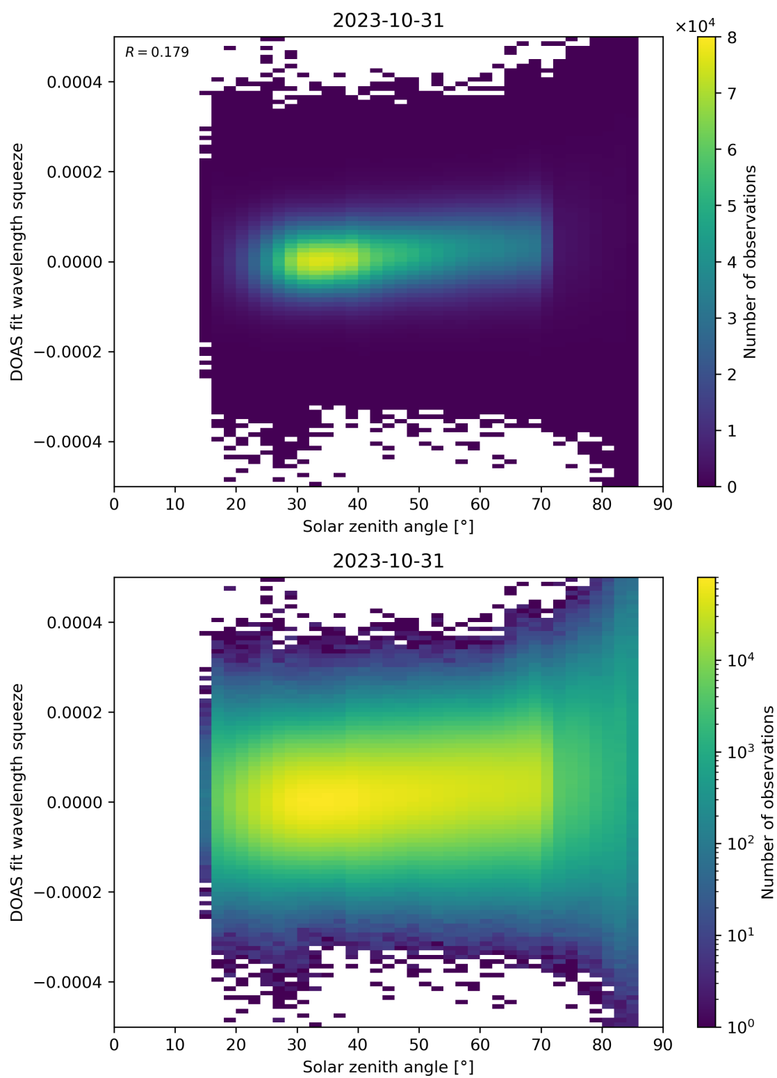
Figure 169: Scatter density plot of “Solar zenith angle” against “DOAS fit wavelength squeeze” for 2023-10-30 to 2023-11-01.
