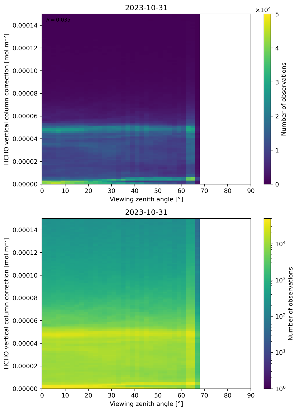
Figure 193: Scatter density plot of “Viewing zenith angle” against “HCHO vertical column correction” for 2023-10-30 to 2023-11-01.
