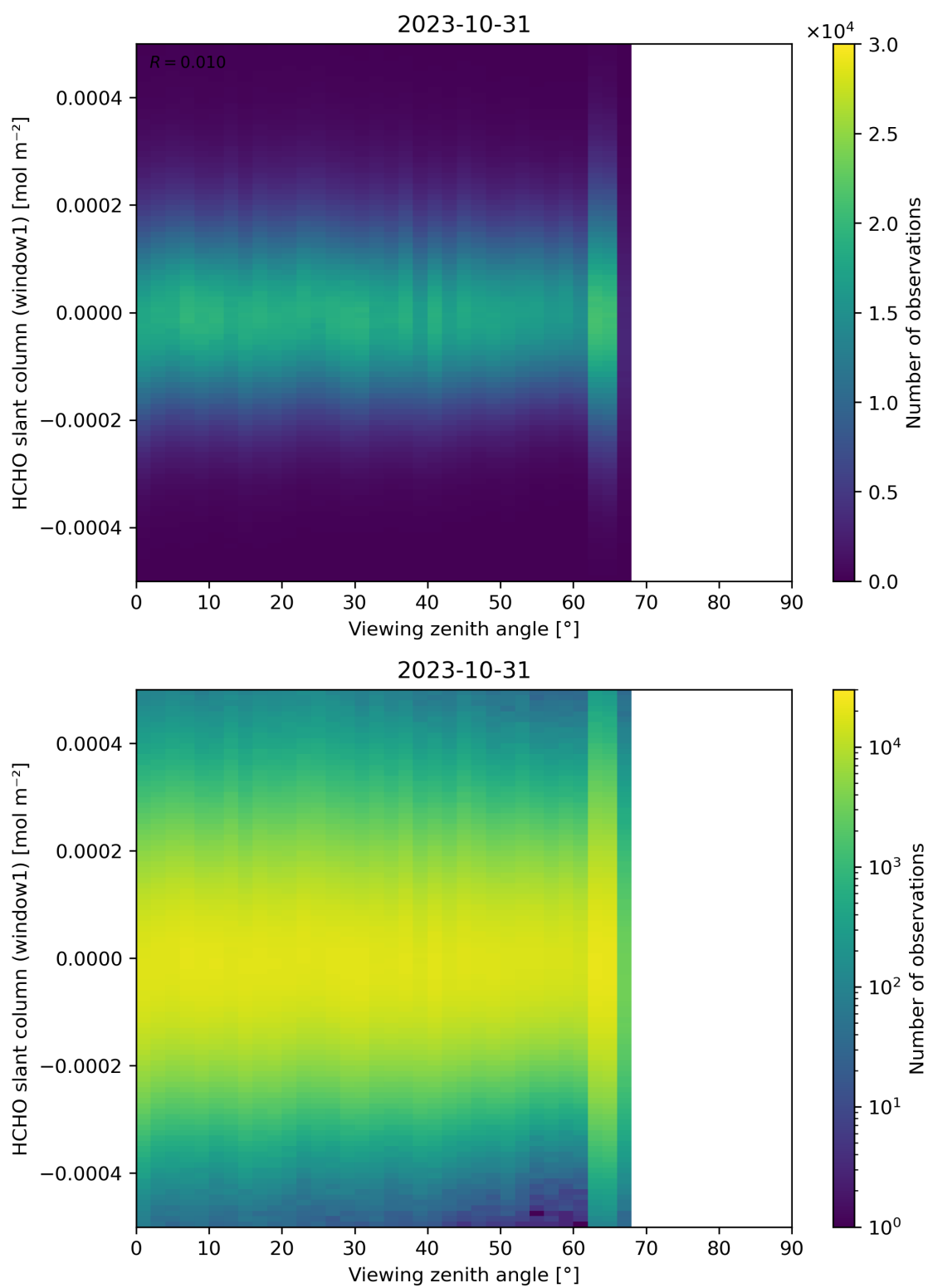
Figure 188: Scatter density plot of “Viewing zenith angle” against “HCHO slant column (window1)” for 2023-10-30 to 2023-11-01.
