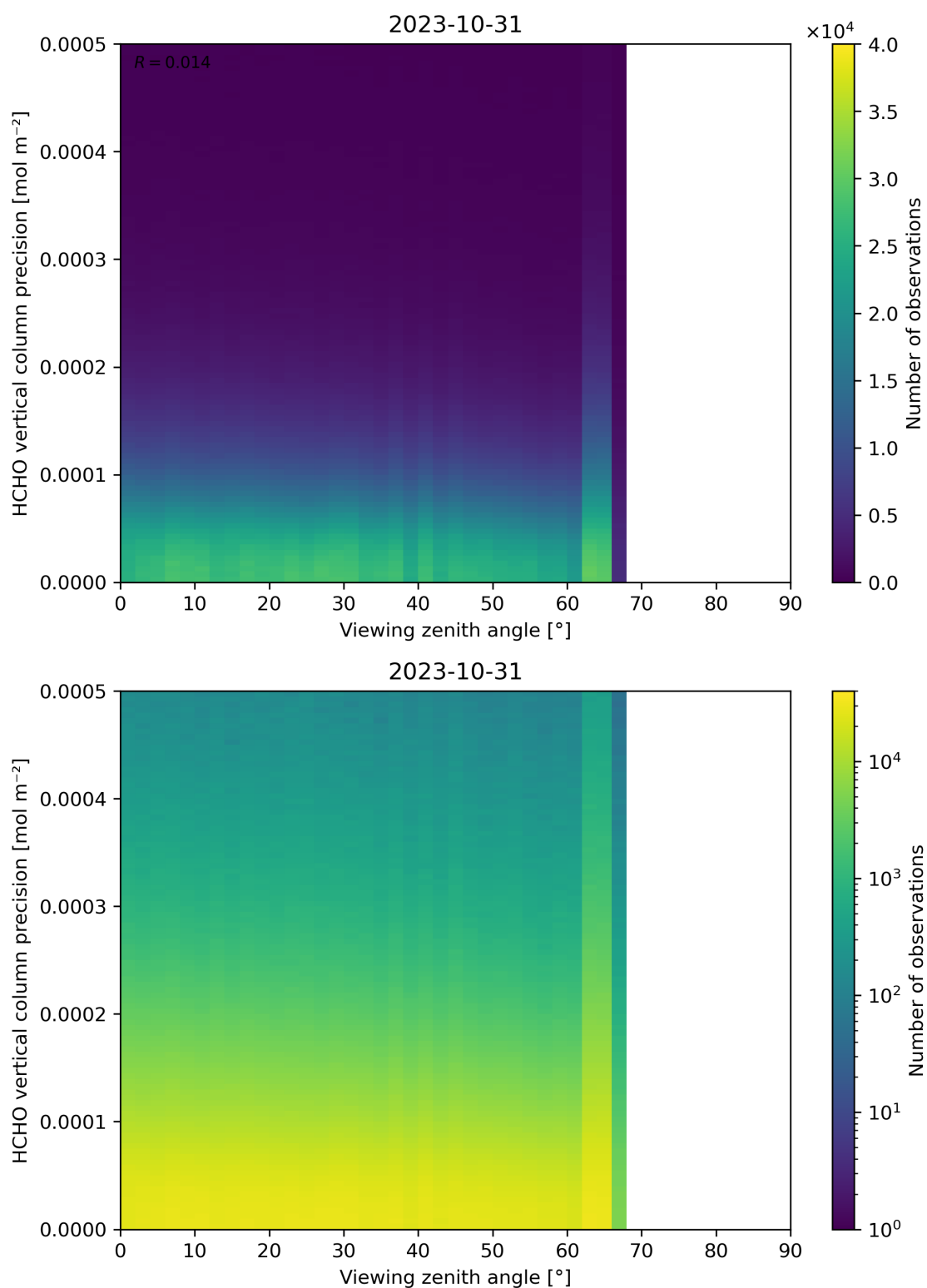
Figure 194: Scatter density plot of “Viewing zenith angle” against “HCHO vertical column precision” for 2023-10-30 to 2023-11-01.
