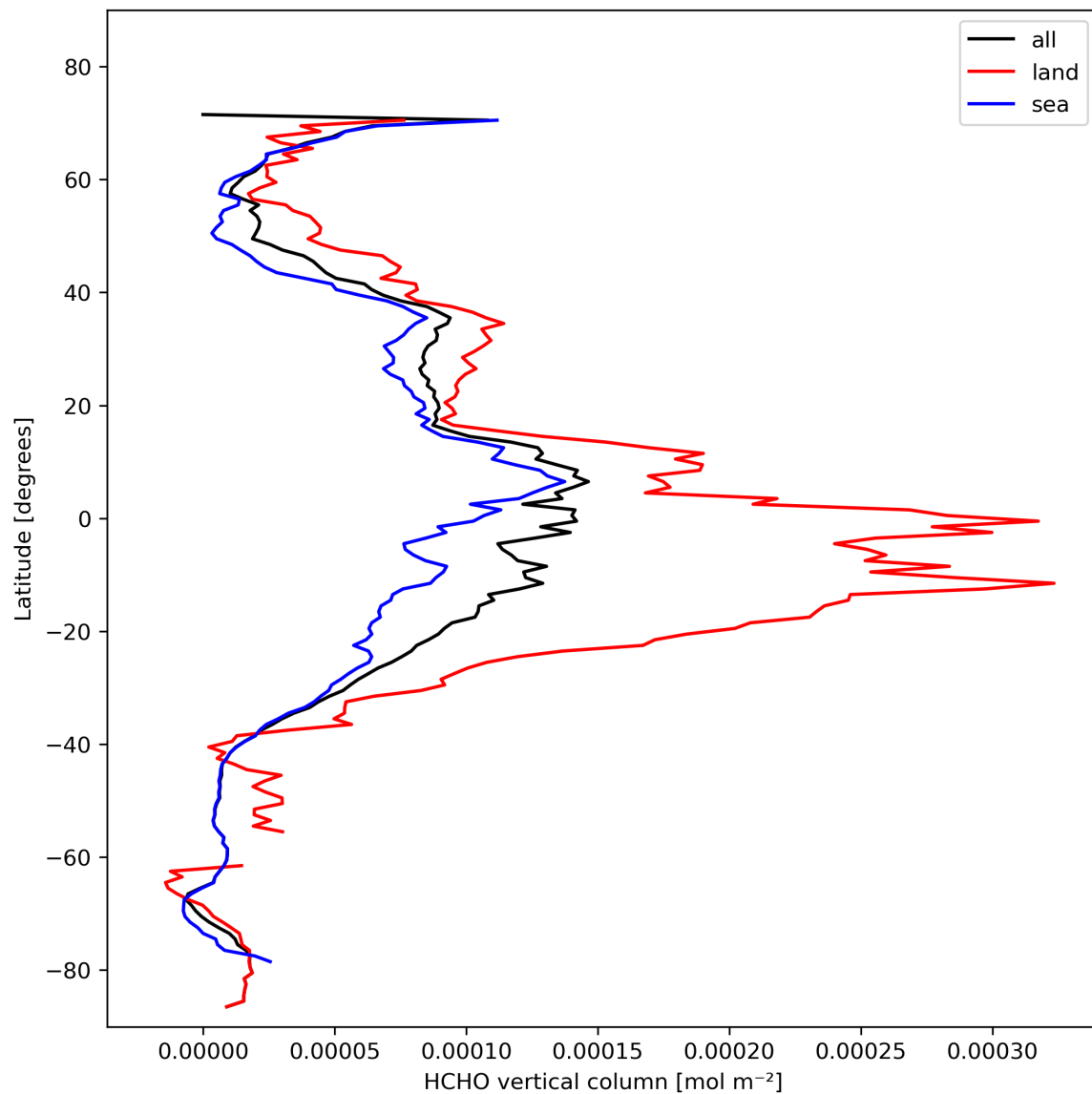
Figure 21: Zonal average of “HCHO vertical column” for 2023-10-30 to 2023-11-01.
