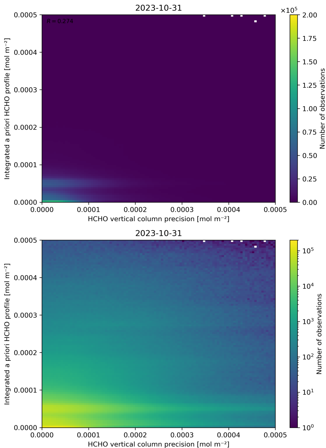
Figure 147: Scatter density plot of “HCHO vertical column precision” against “Integrated a priori HCHO profile” for 2023-10-30 to 2023-11-01.
