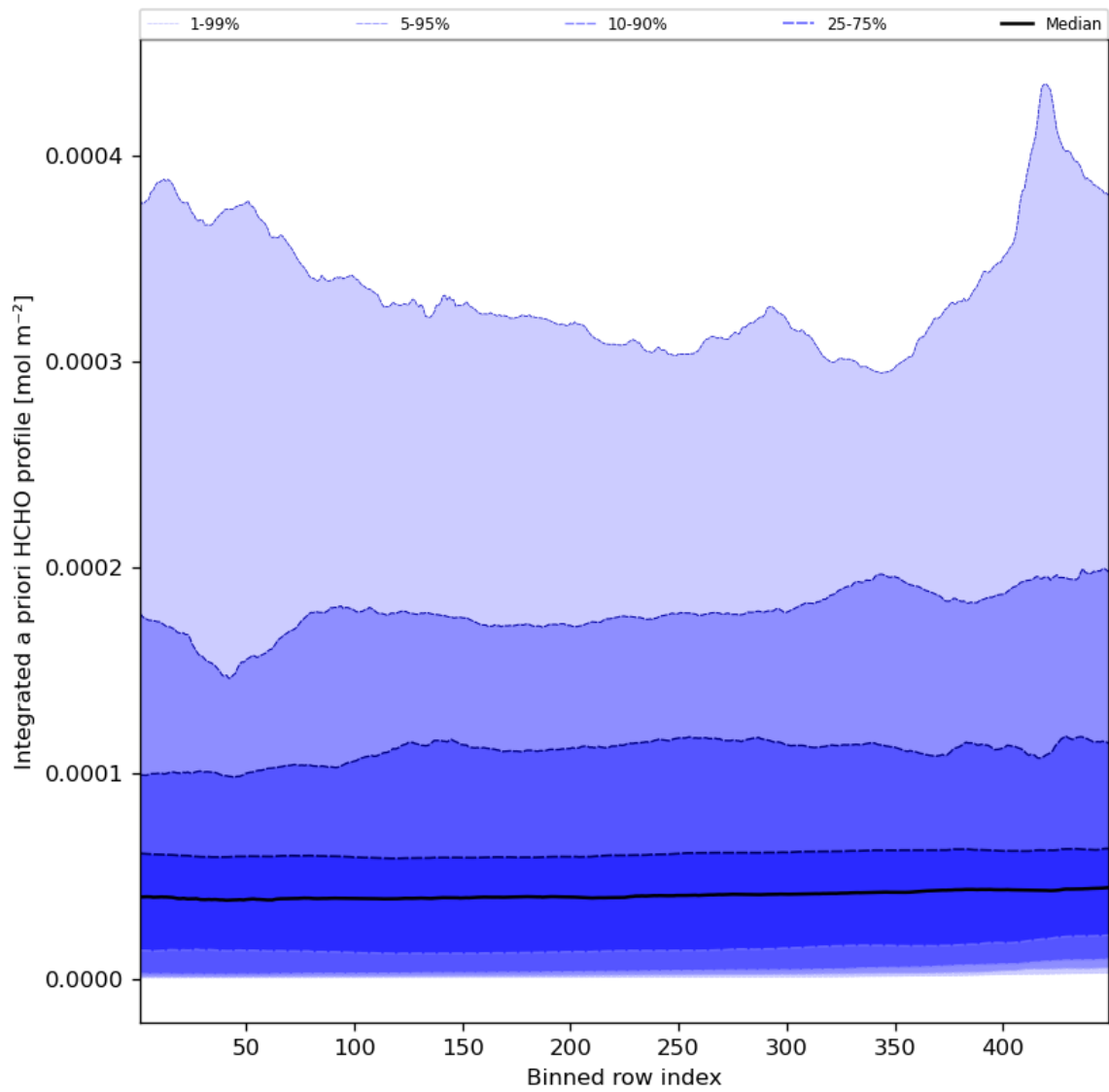
Figure 57: Along track statistics of “Integrated a priori HCHO profile” for 2023-10-30 to 2023-11-01
