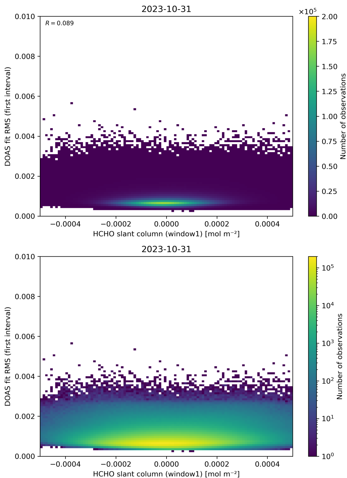
Figure 78: Scatter density plot of “HCHO slant column (window1)” against “DOAS fit RMS (first interval)” for 2023-10-30 to 2023-11-01.
