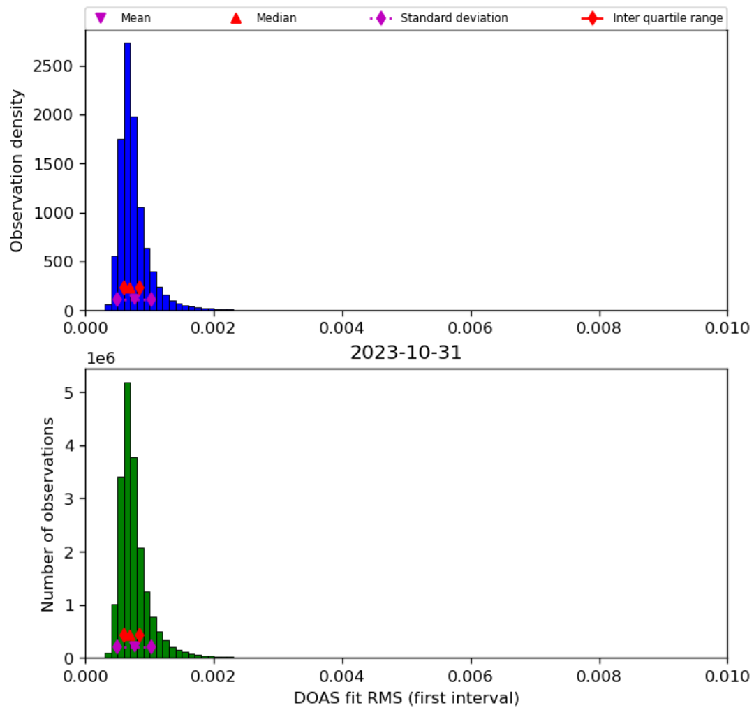
Figure 46: Histogram of “DOAS fit RMS (first interval)” for 2023-10-30 to 2023-11-01
