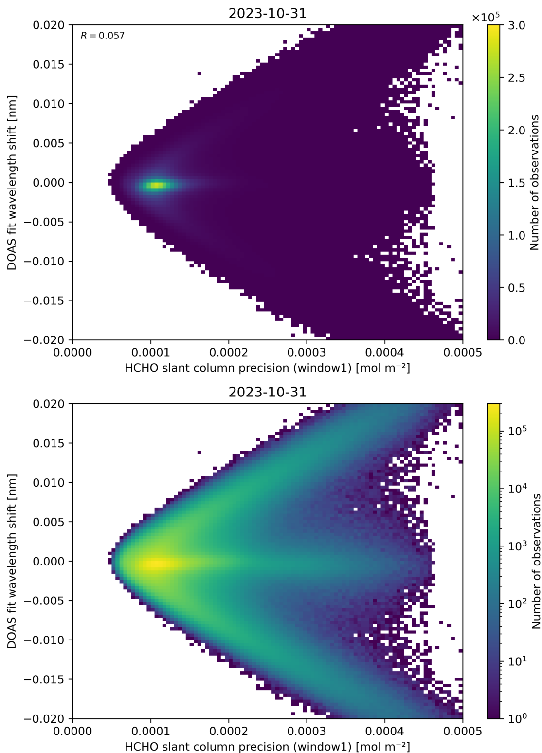
Figure 89: Scatter density plot of “HCHO slant column precision (window1)” against “DOAS fit wavelength shift” for 2023-10-30 to 2023-11-01.
