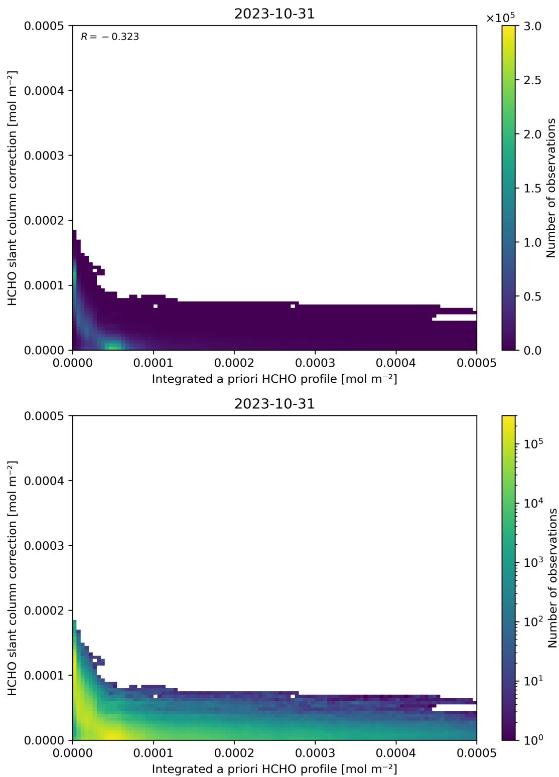
Figure 152: Scatter density plot of “Integrated a priori HCHO profile” against “HCHO slant column correction” for 2023-10-30 to 2023-11-01.
