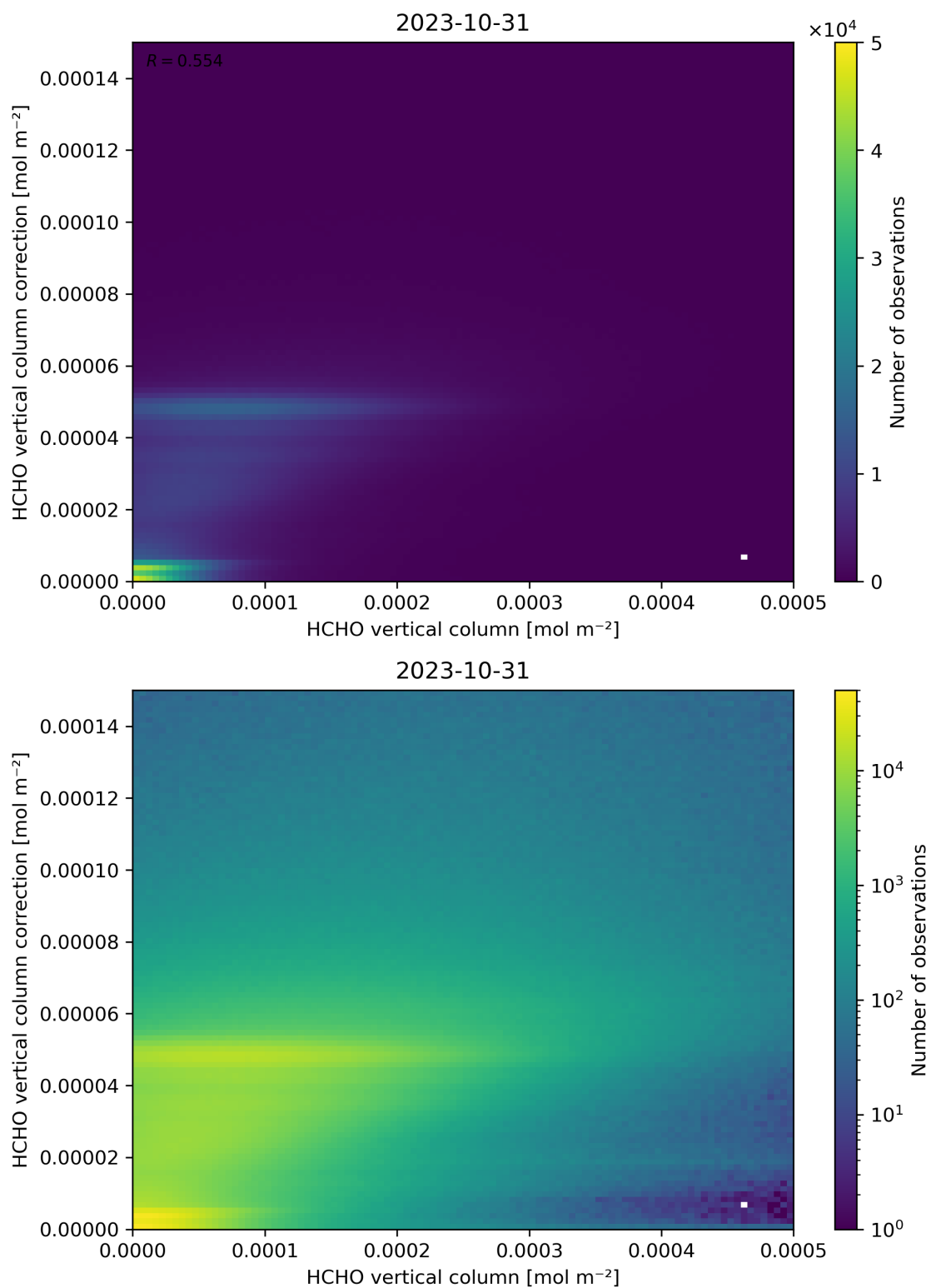
Figure 133: Scatter density plot of “HCHO vertical column” against “HCHO vertical column correction” for 2023-10-30 to 2023-11-01.
