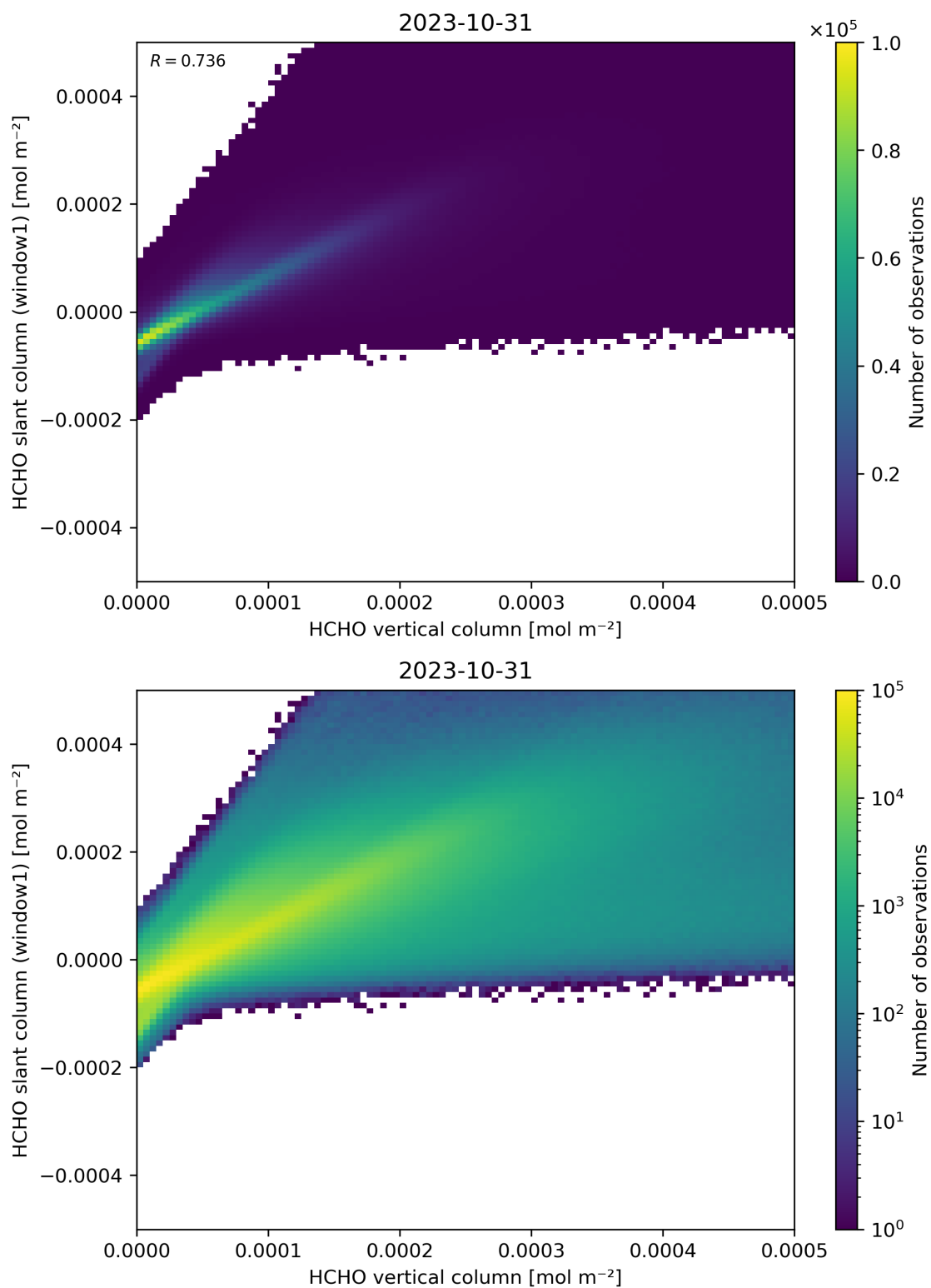
Figure 129: Scatter density plot of “HCHO vertical column” against “HCHO slant column (window1)” for 2023-10-30 to 2023-11-01.
