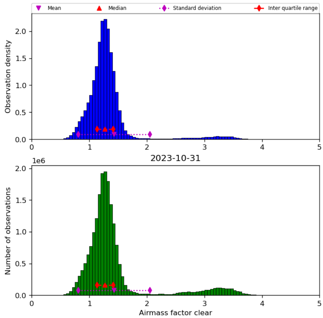
Figure 42: Histogram of “Airmass factor clear” for 2023-10-30 to 2023-11-01
