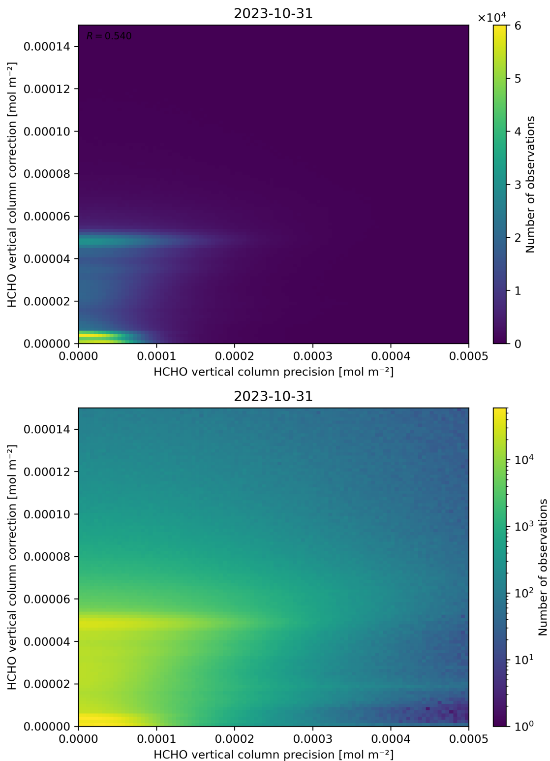
Figure 146: Scatter density plot of “HCHO vertical column precision” against “HCHO vertical column correction” for 2023-10-30 to 2023-11-01.
