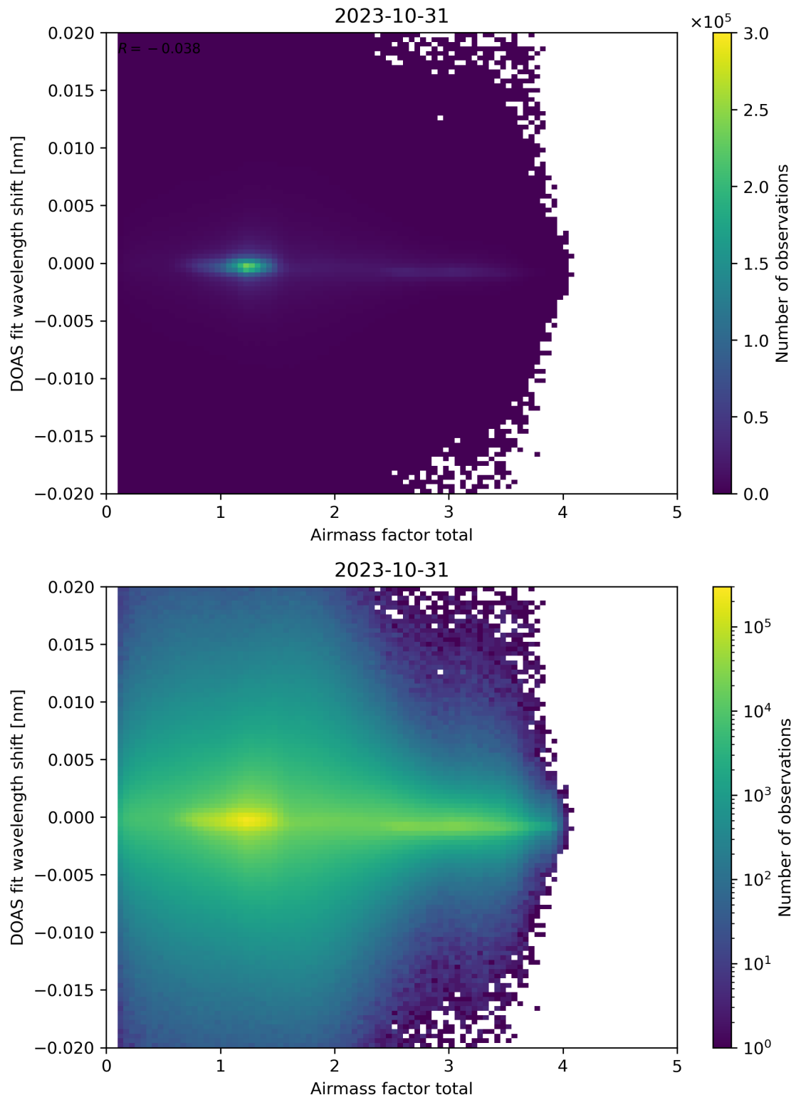
Figure 98: Scatter density plot of “Airmass factor total” against “DOAS fit wavelength shift” for 2023-10-30 to 2023-11-01.
