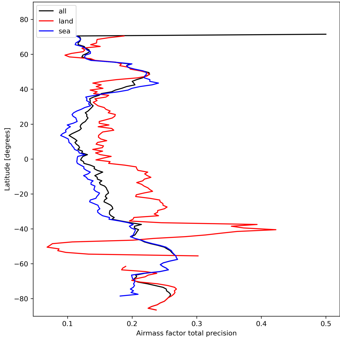
Figure 27: Zonal average of “Airmass factor total precision” for 2023-10-30 to 2023-11-01.
