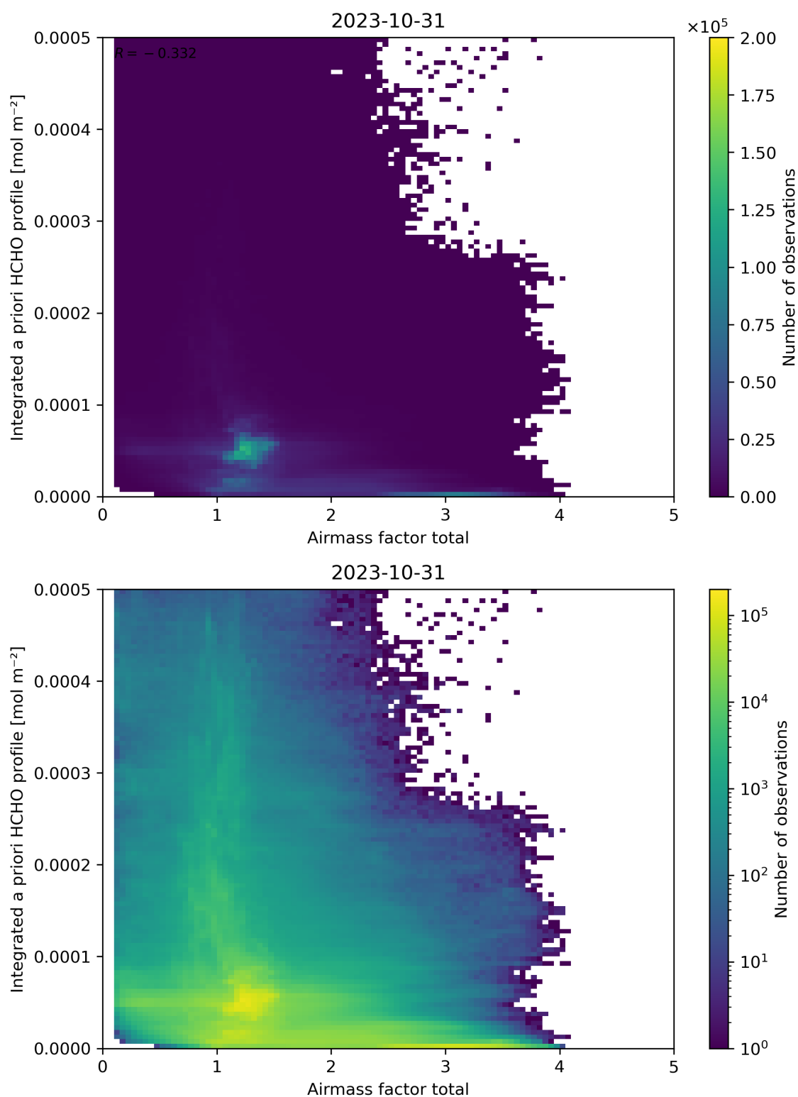
Figure 104: Scatter density plot of “Airmass factor total” against “Integrated a priori HCHO profile” for 2023-10-30 to 2023-11-01.
