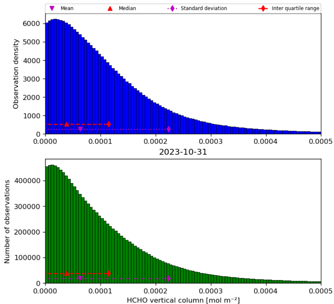
Figure 35: Histogram of “HCHO vertical column” for 2023-10-30 to 2023-11-01
