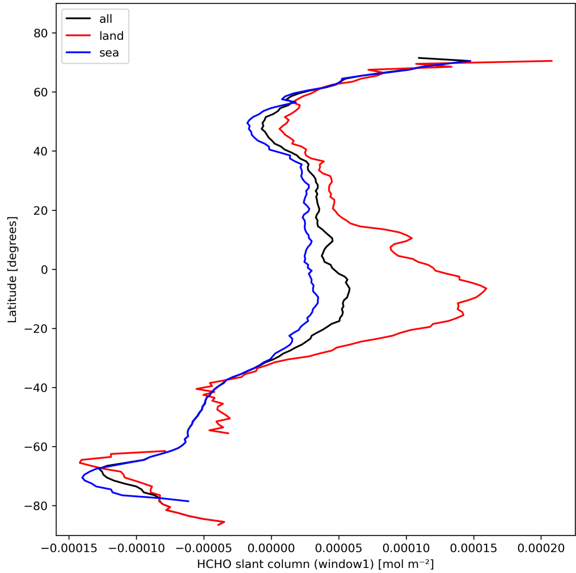
Figure 24: Zonal average of “HCHO slant column (window1)” for 2023-10-30 to 2023-11-01.
