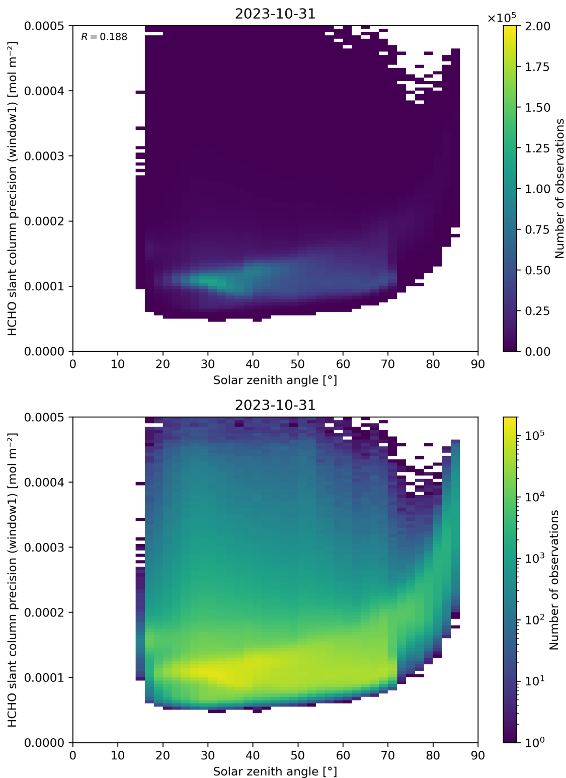
Figure 174: Scatter density plot of “Solar zenith angle” against “HCHO slant column precision (window1)” for 2023-10-30 to 2023-11-01.
