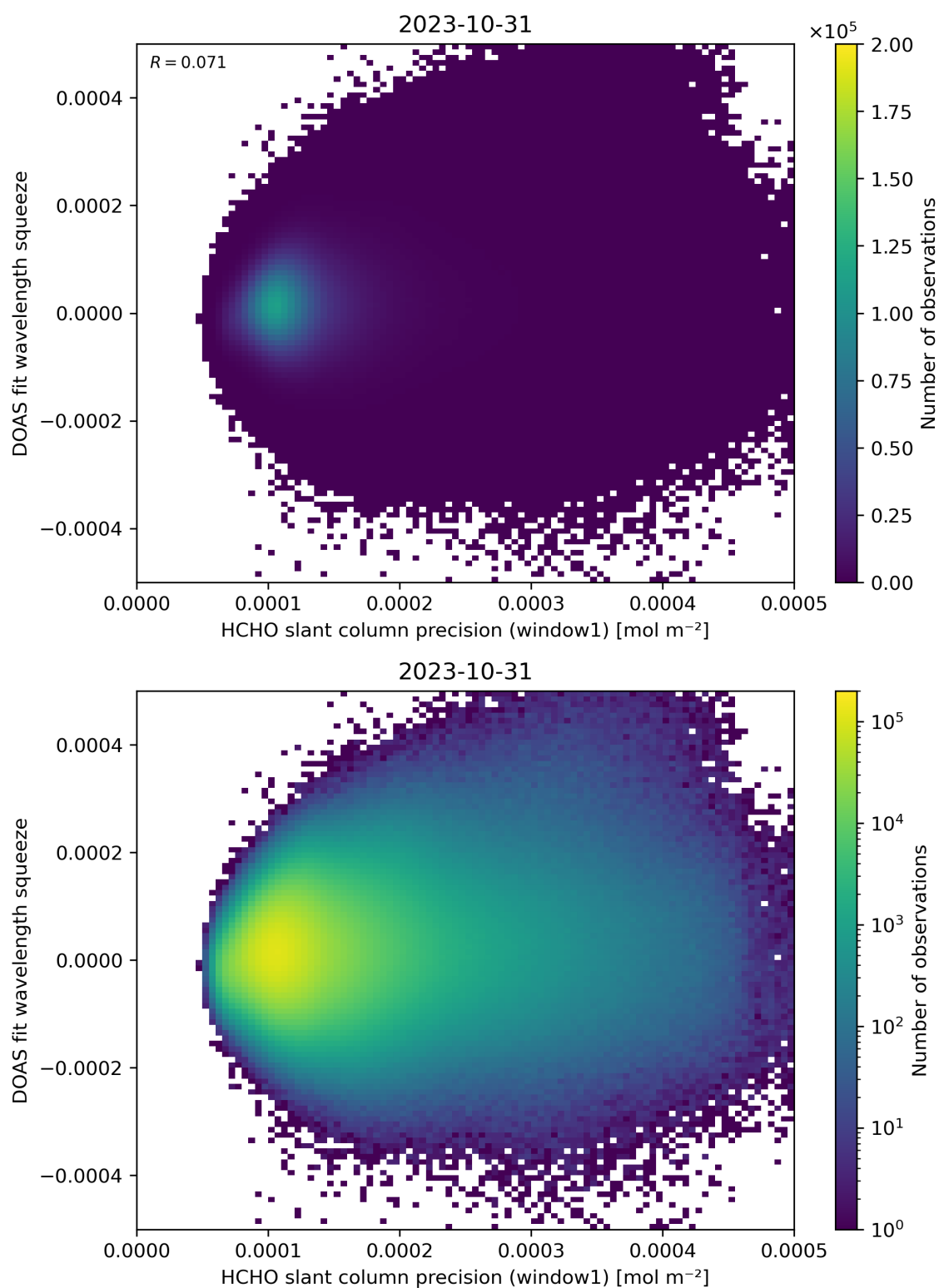
Figure 90: Scatter density plot of “HCHO slant column precision (window1)” against “DOAS fit wavelength squeeze” for 2023-10-30 to 2023-11-01.
