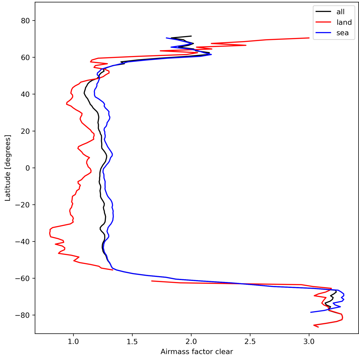
Figure 28: Zonal average of “Airmass factor clear” for 2023-10-30 to 2023-11-01.
