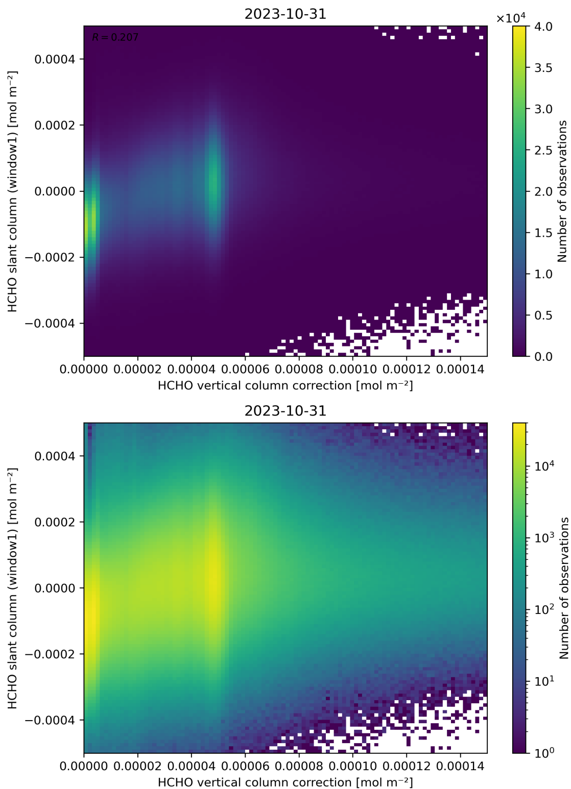
Figure 118: Scatter density plot of “HCHO vertical column correction” against “HCHO slant column (window1)” for 2023-10-30 to 2023-11-01.
