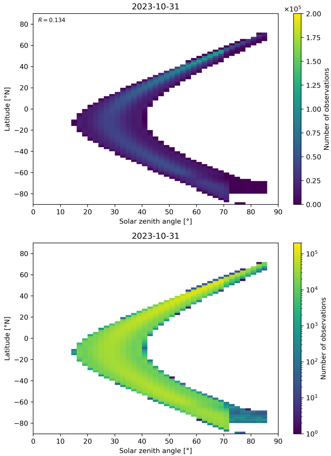
Figure 181: Scatter density plot of “Solar zenith angle” against “Latitude” for 2023-10-30 to 2023-11-01.
