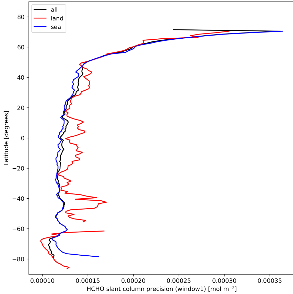
Figure 25: Zonal average of “HCHO slant column precision (window1)” for 2023-10-30 to 2023-11-01.
