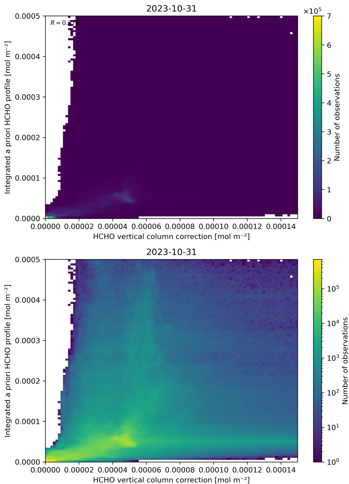
Figure 122: Scatter density plot of “HCHO vertical column correction” against “Integrated a priori HCHO profile” for 2023-10-30 to 2023-11-01.
