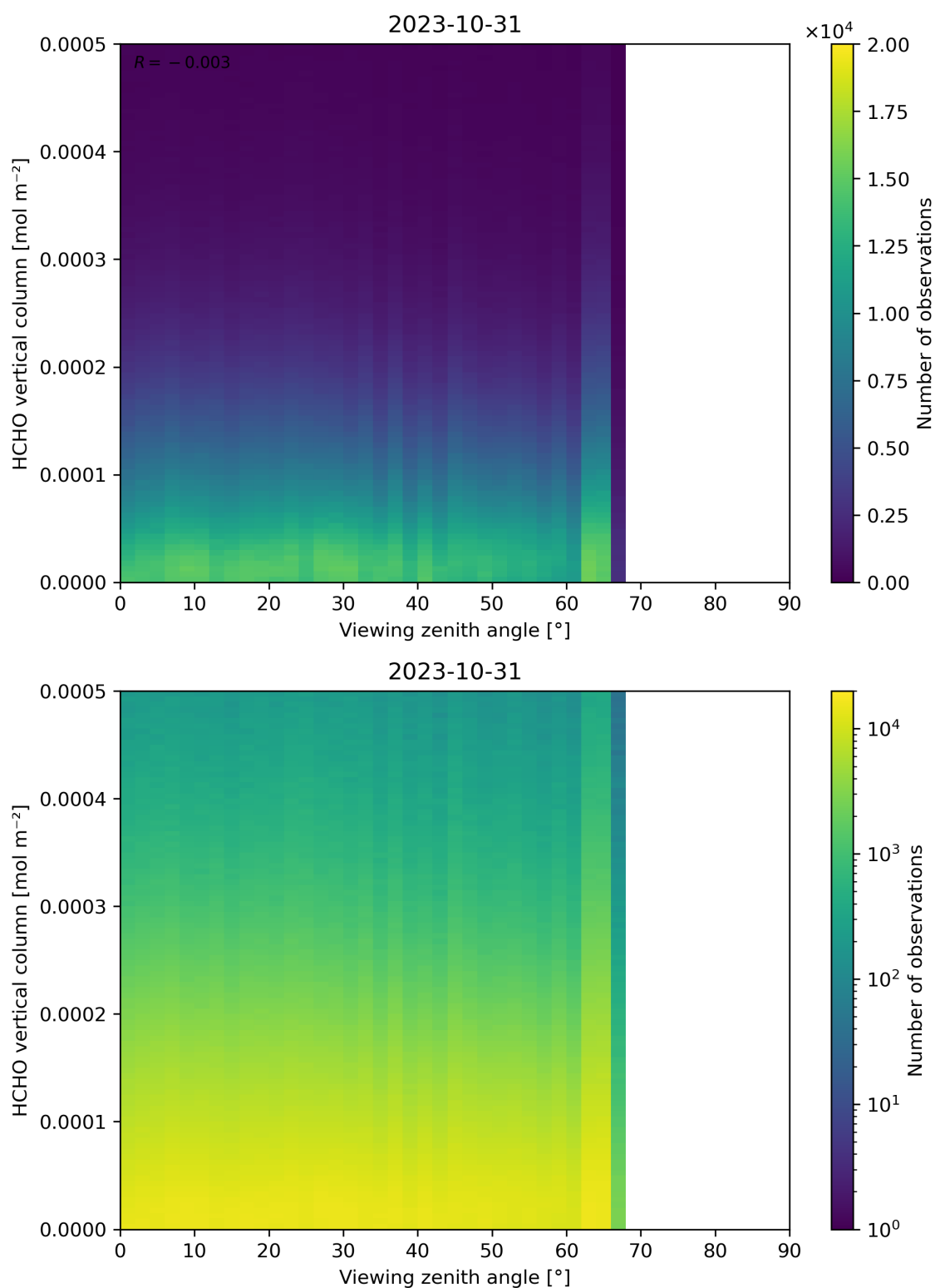
Figure 192: Scatter density plot of “Viewing zenith angle” against “HCHO vertical column” for 2023-10-30 to 2023-11-01.
