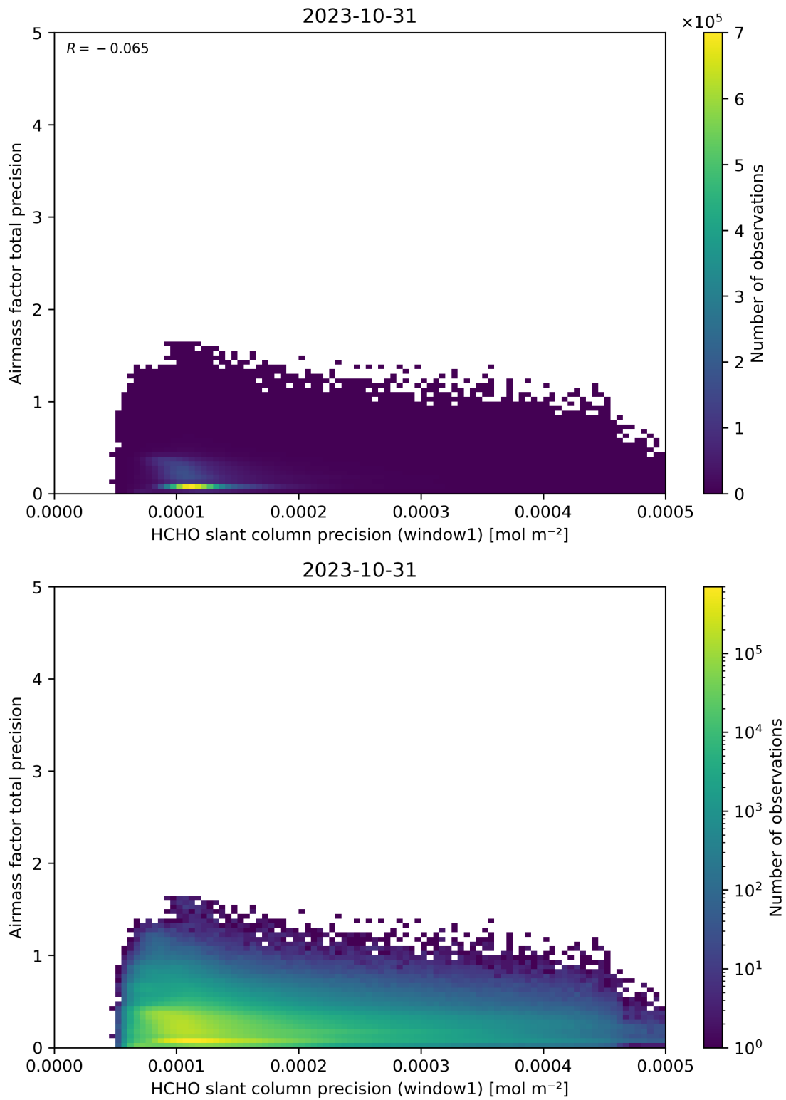
Figure 95: Scatter density plot of “HCHO slant column precision (window1)” against “Airmass factor total precision” for 2023-10-30 to 2023-11-01.
