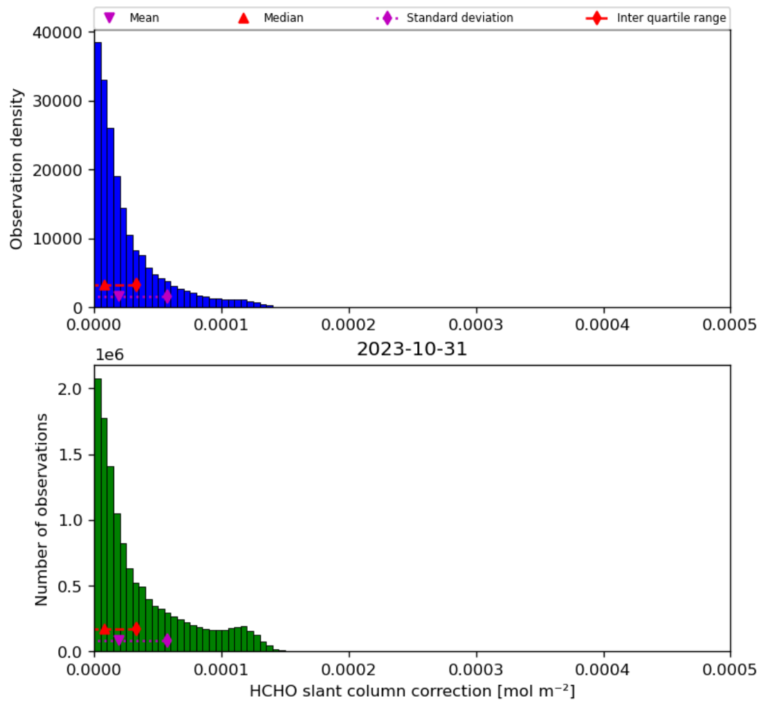
Figure 47: Histogram of “HCHO slant column correction” for 2023-10-30 to 2023-11-01
