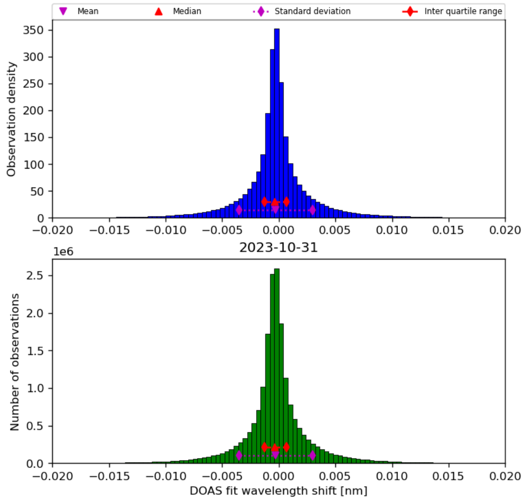
Figure 44: Histogram of “DOAS fit wavelength shift” for 2023-10-30 to 2023-11-01
