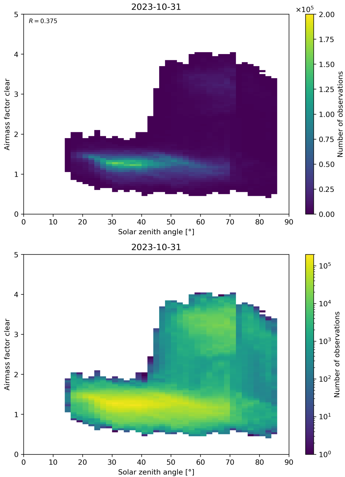
Figure 170: Scatter density plot of “Solar zenith angle” against “Airmass factor clear” for 2023-10-30 to 2023-11-01.
