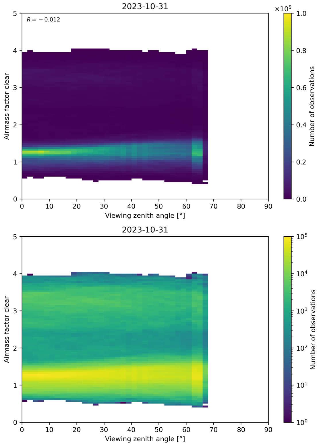
Figure 185: Scatter density plot of “Viewing zenith angle” against “Airmass factor clear” for 2023-10-30 to 2023-11-01.
