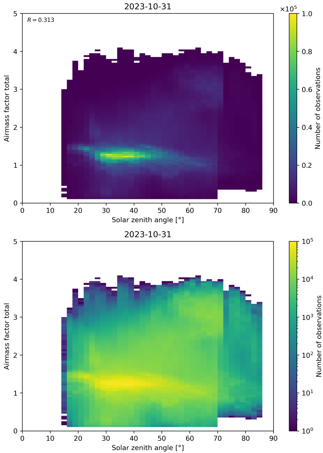
Figure 175: Scatter density plot of “Solar zenith angle” against “Airmass factor total” for 2023-10-30 to 2023-11-01.
