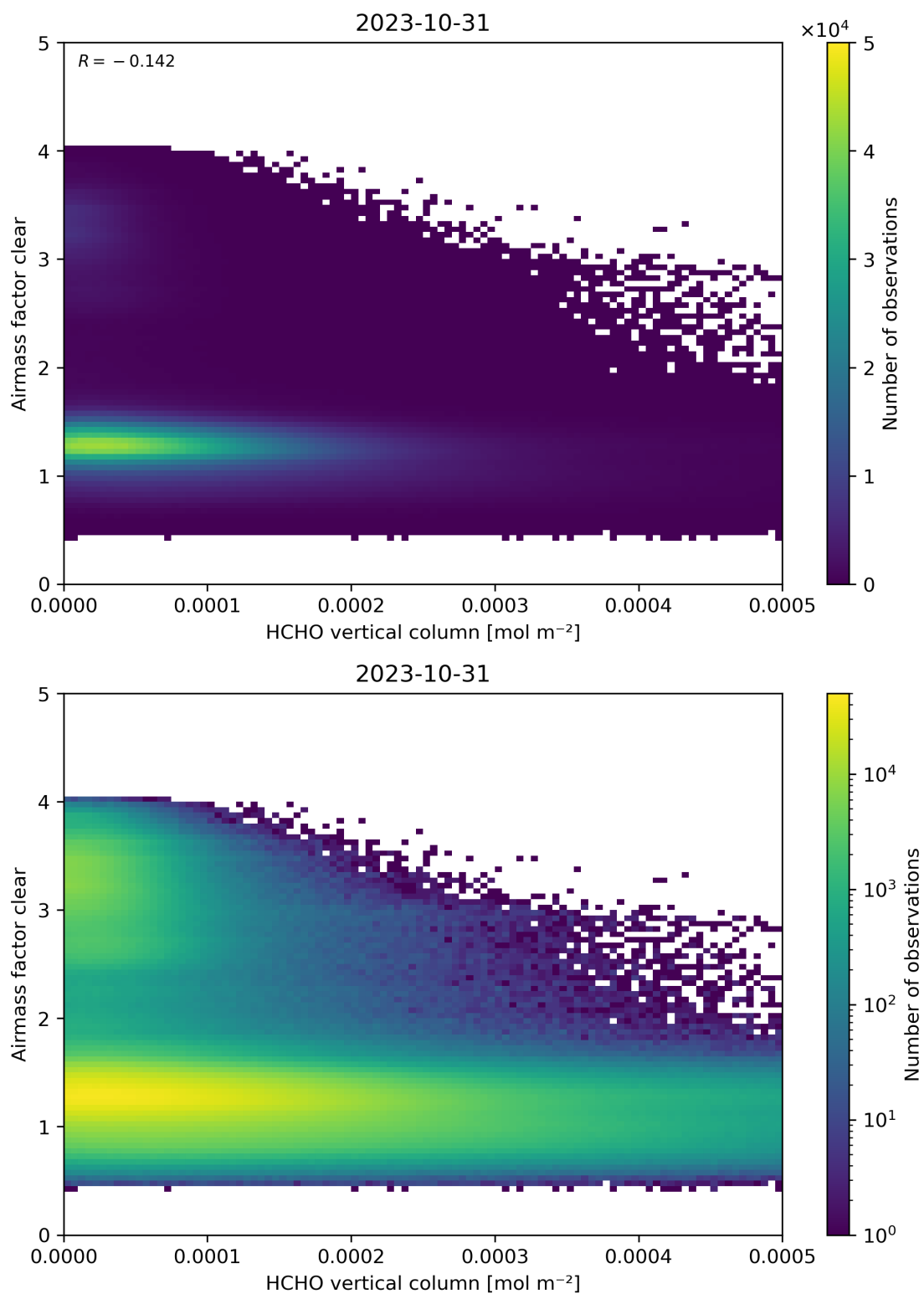
Figure 126: Scatter density plot of “HCHO vertical column” against “Airmass factor clear” for 2023-10-30 to 2023-11-01.
