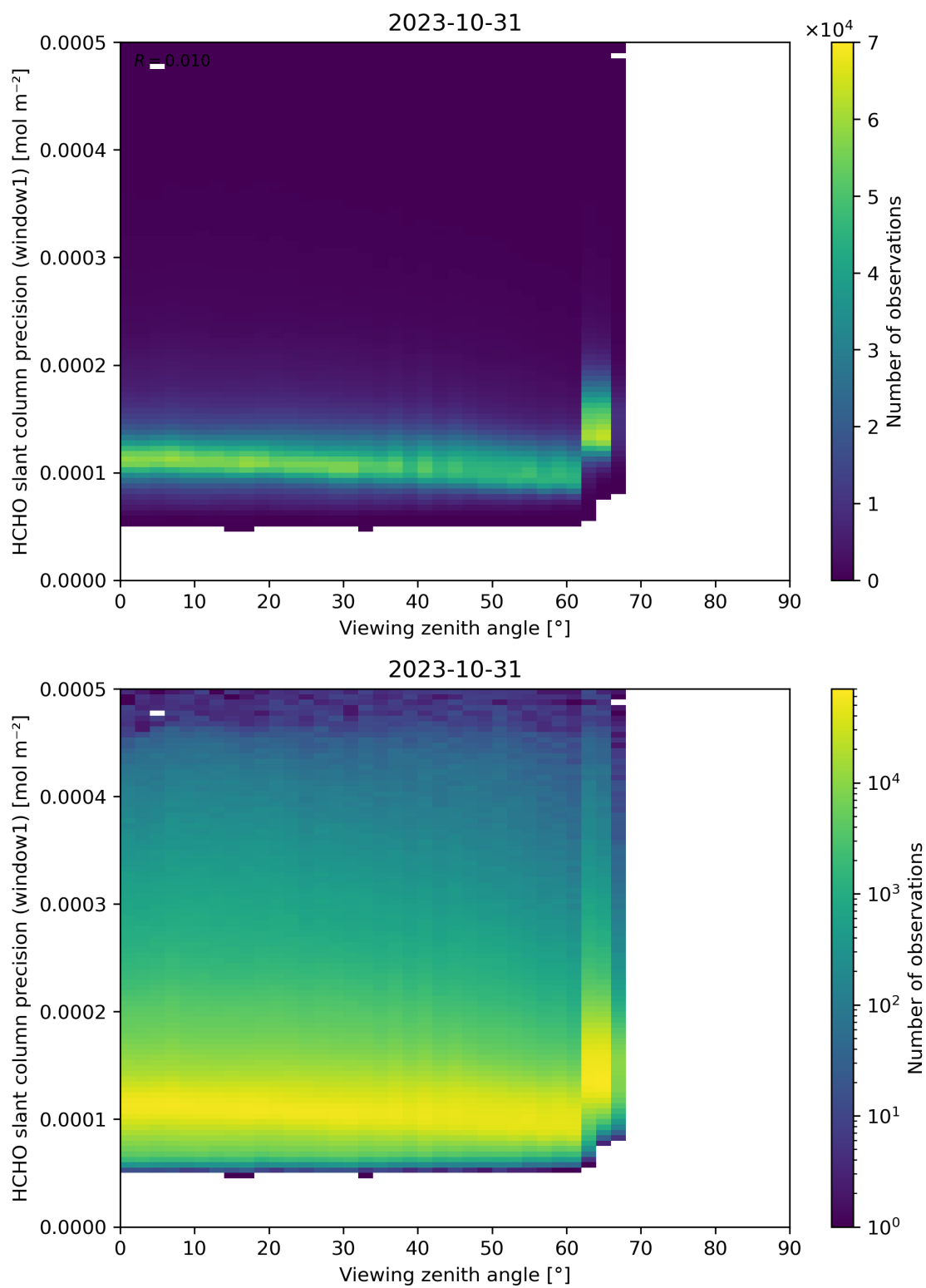
Figure 189: Scatter density plot of “Viewing zenith angle” against “HCHO slant column precision (window1)” for 2023-10-30 to 2023-11-01.
