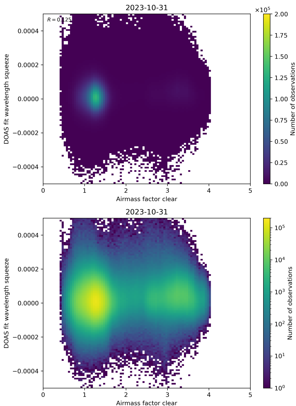
Figure 73: Scatter density plot of “Airmass factor clear” against “DOAS fit wavelength squeeze” for 2023-10-30 to 2023-11-01.
