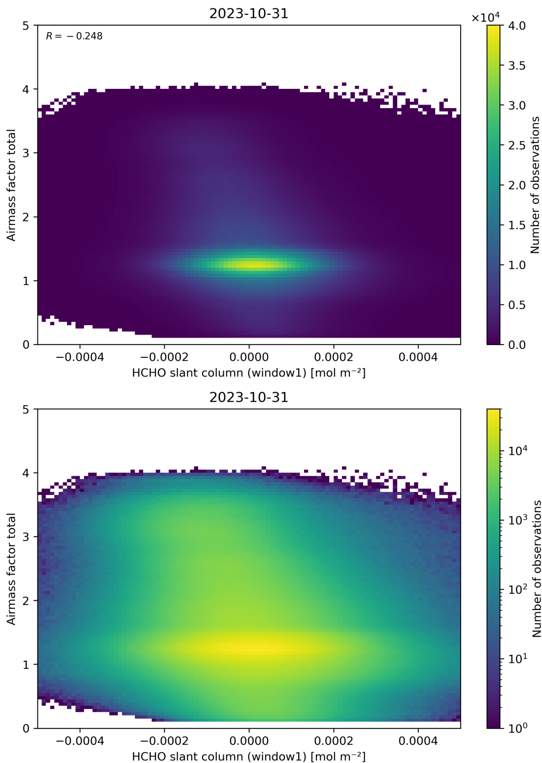
Figure 85: Scatter density plot of “HCHO slant column (window1)” against “Airmass factor total” for 2023-10-30 to 2023-11-01.
