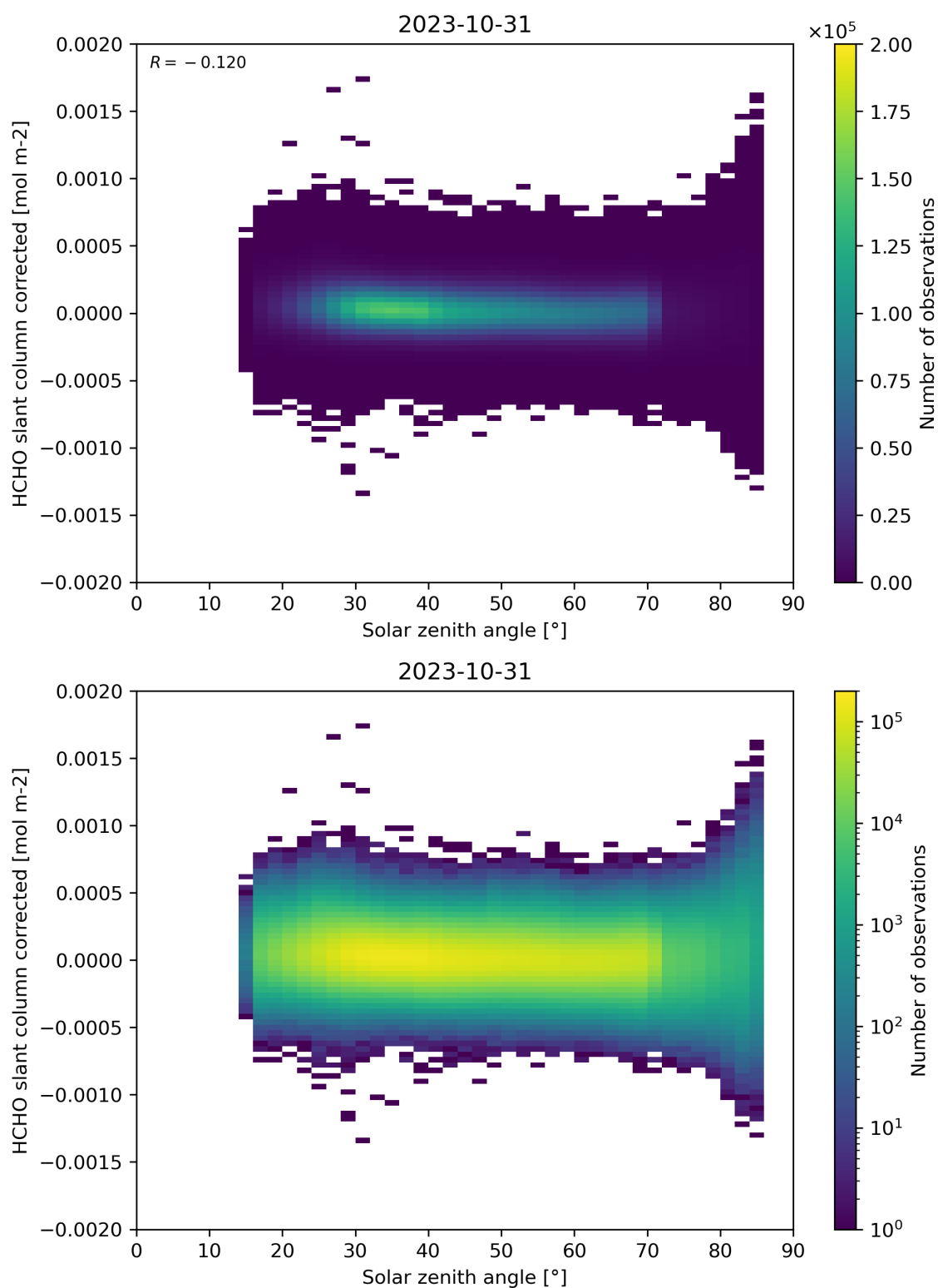
Figure 171: Scatter density plot of “Solar zenith angle” against “HCHO slant column corrected” for 2023-10-30 to 2023-11-01.
