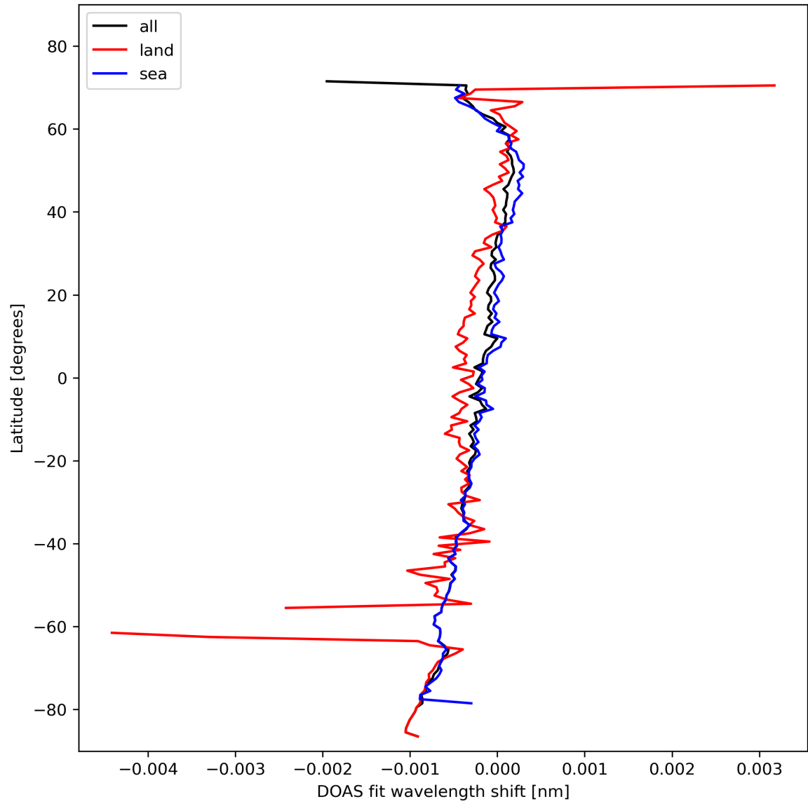
Figure 30: Zonal average of "DOAS fit wavelength shift" for 2023-10-30 to 2023-11-01.
