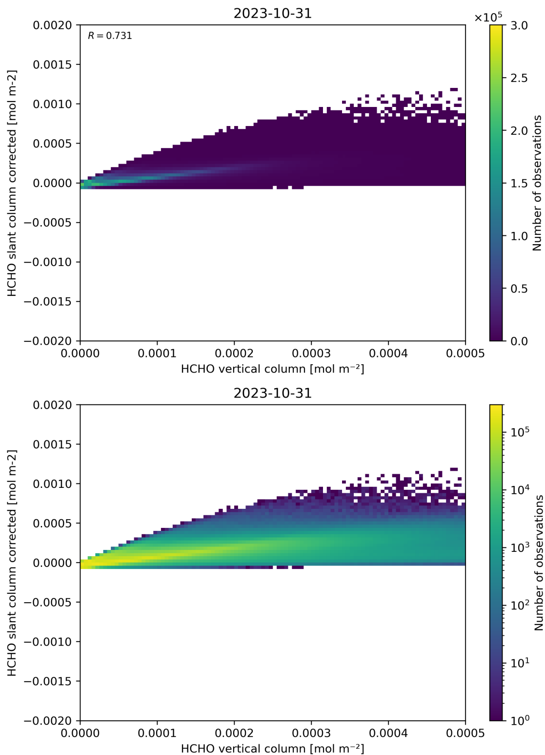
Figure 127: Scatter density plot of “HCHO vertical column” against “HCHO slant column corrected” for 2023-10-30 to 2023-11-01.
