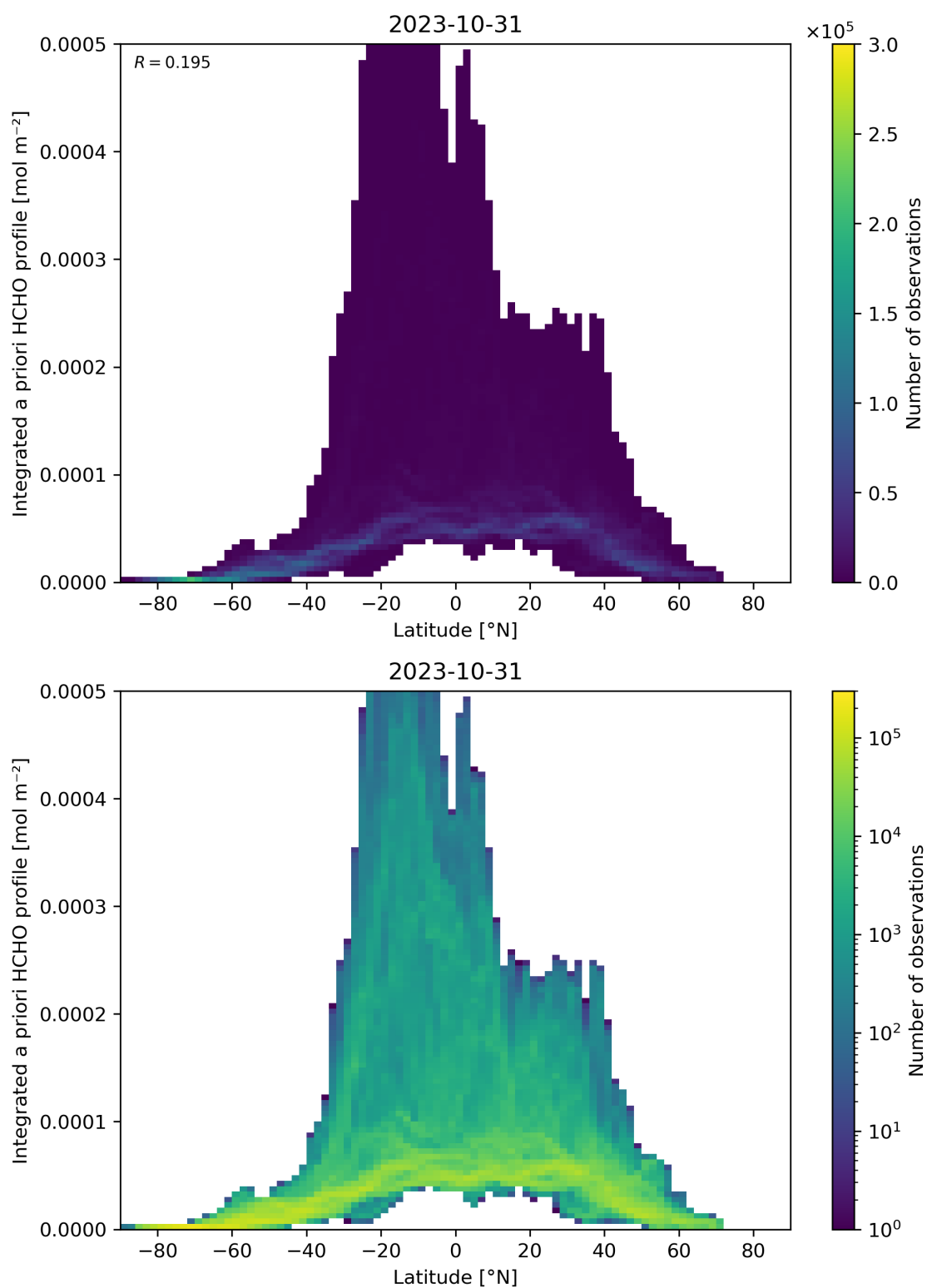
Figure 166: Scatter density plot of “Latitude” against “Integrated a priori HCHO profile” for 2023-10-30 to 2023-11-01.
