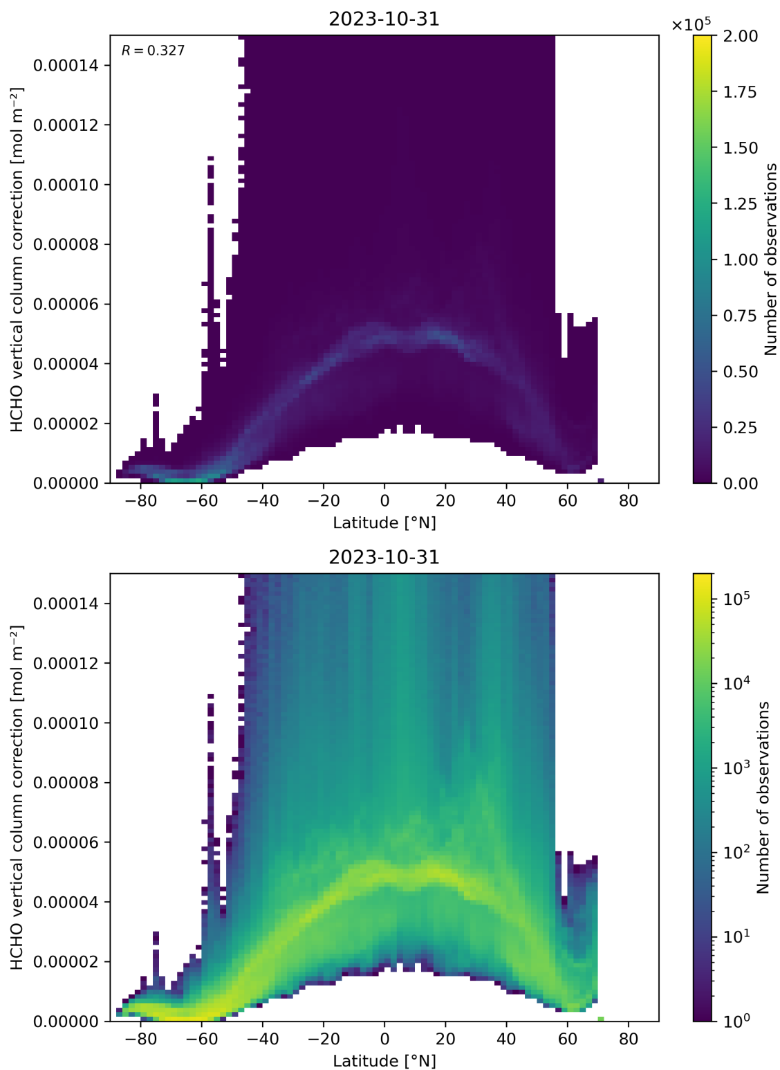
Figure 164: Scatter density plot of “Latitude” against “HCHO vertical column correction” for 2023-10-30 to 2023-11-01.
