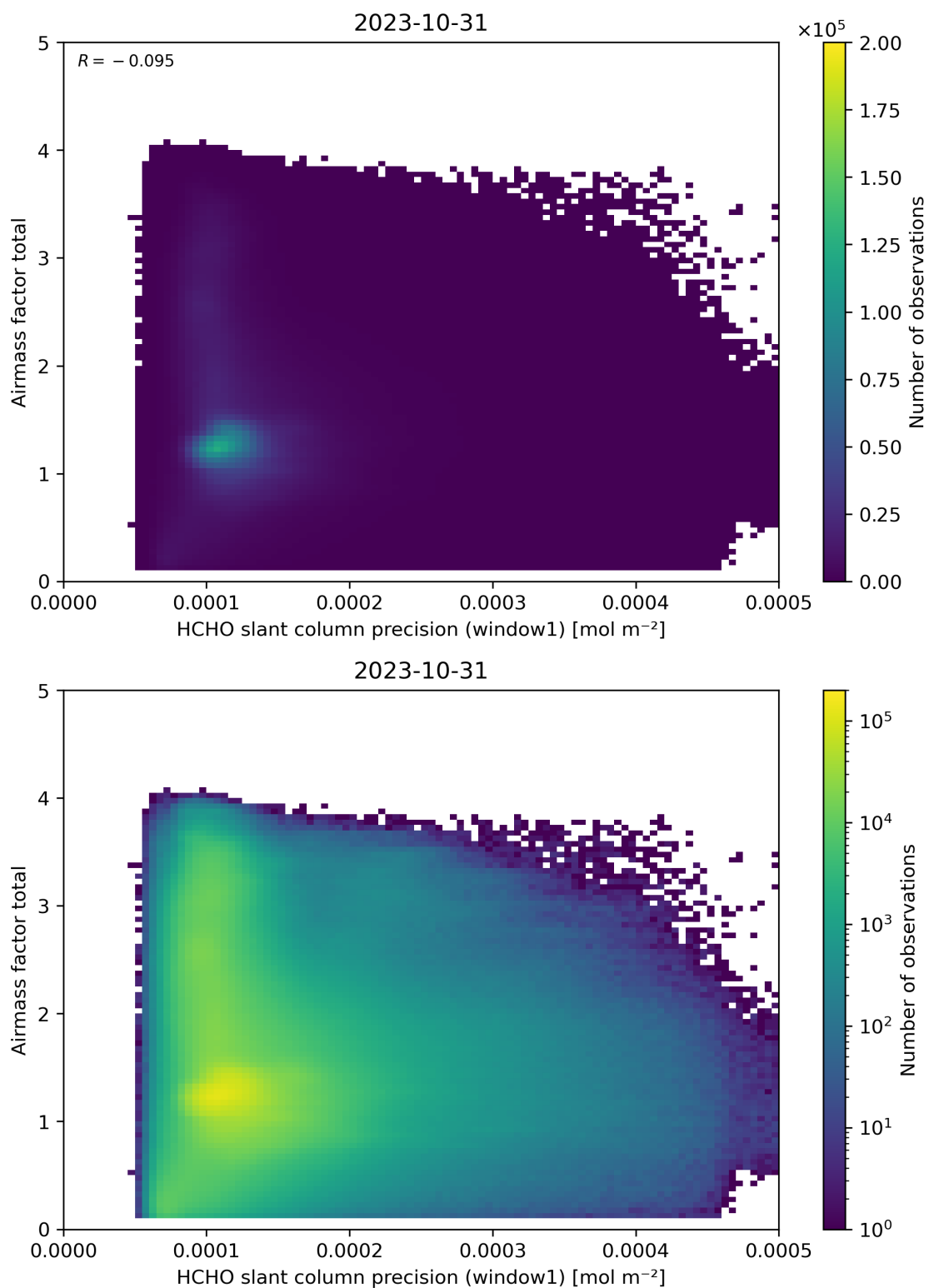
Figure 94: Scatter density plot of “HCHO slant column precision (window1)” against “Airmass factor total” for 2023-10-30 to 2023-11-01.
