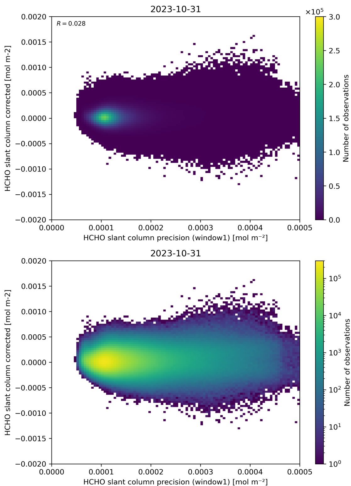
Figure 92: Scatter density plot of “HCHO slant column precision (window1)” against “HCHO slant column corrected” for 2023-10-30 to 2023-11-01.
