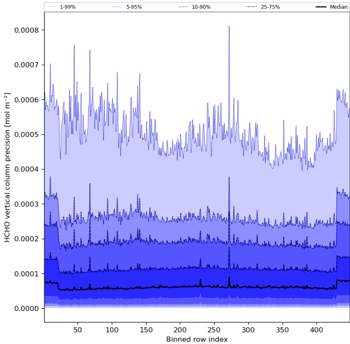
Figure 50: Along track statistics of “HCHO vertical column precision” for 2023-10-30 to 2023-11-01
