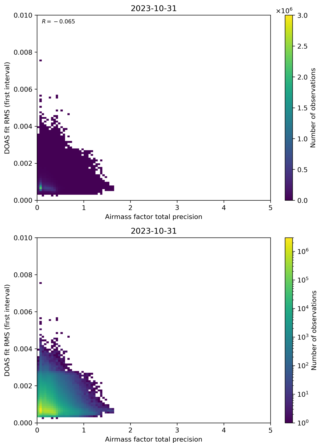
Figure 105: Scatter density plot of “Airmass factor total precision” against “DOAS fit RMS (first interval)” for 2023-10-30 to 2023-11-01.
