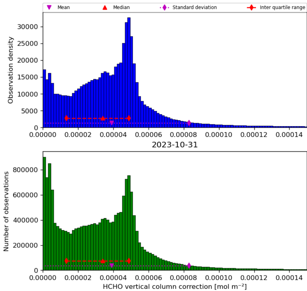
Figure 37: Histogram of “HCHO vertical column correction” for 2023-10-30 to 2023-11-01
