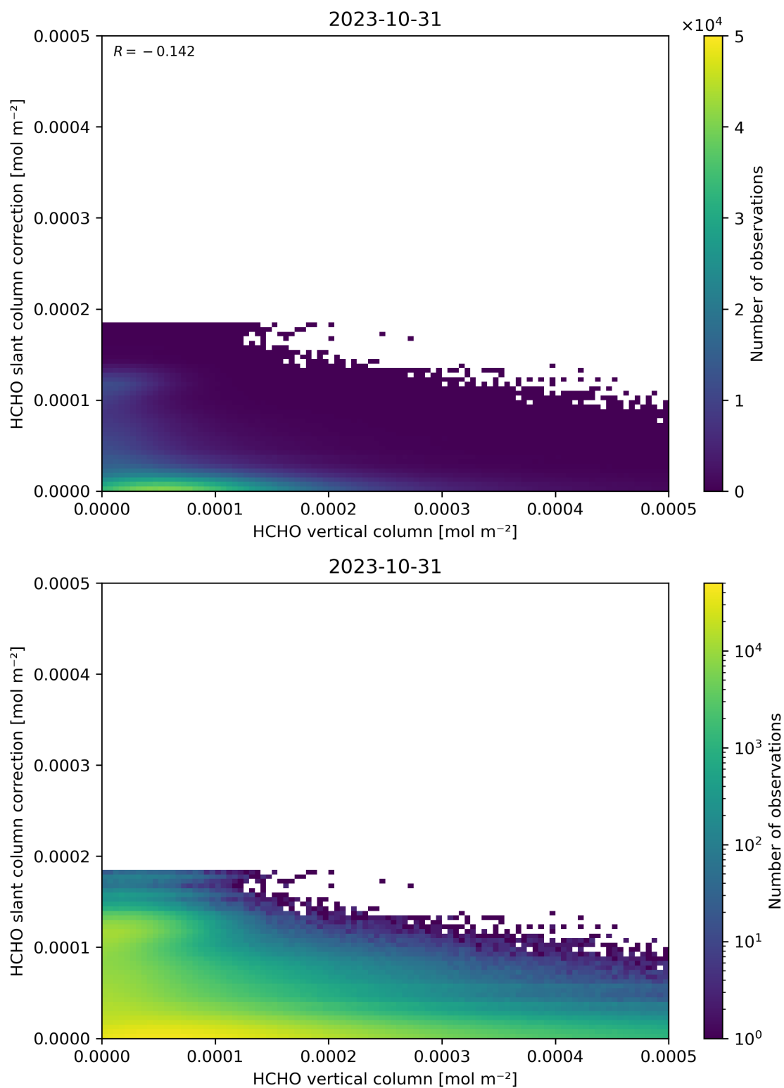
Figure 128: Scatter density plot of “HCHO vertical column” against “HCHO slant column correction” for 2023-10-30 to 2023-11-01.
