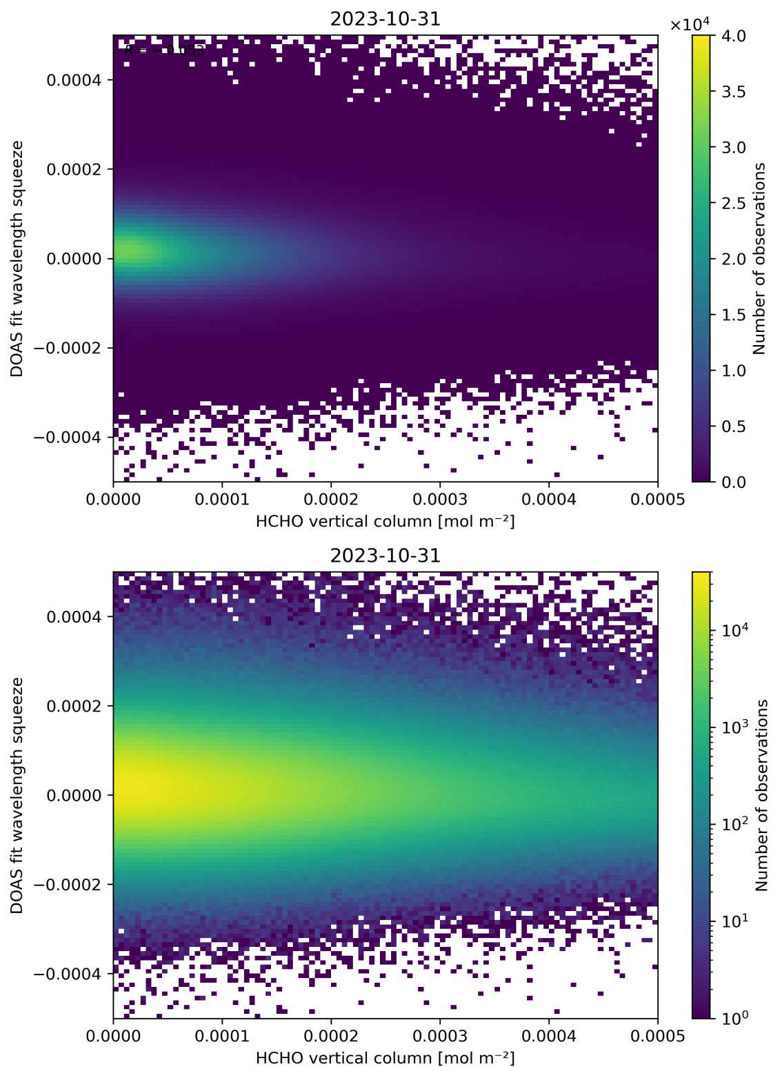
Figure 125: Scatter density plot of “HCHO vertical column” against “DOAS fit wavelength squeeze” for 2023-10-30 to 2023-11-01.
