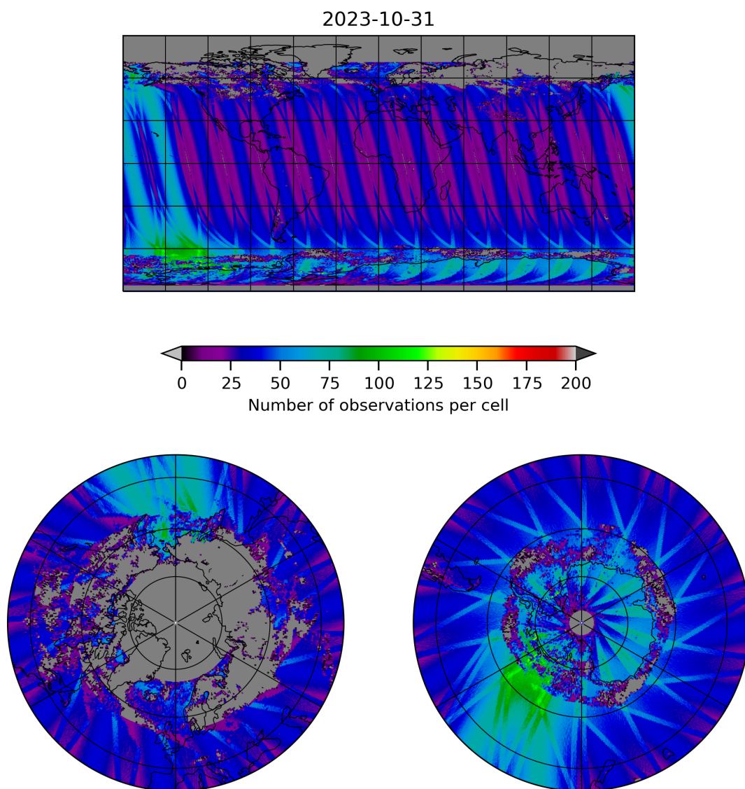
Figure 19: Map of the number of observations for 2023-10-30 to 2023-11-01
