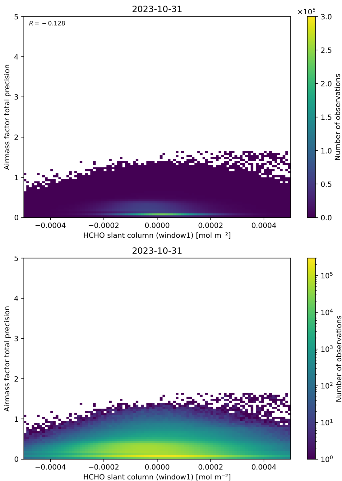
Figure 86: Scatter density plot of “HCHO slant column (window1)” against “Airmass factor total precision” for 2023-10-30 to 2023-11-01.
