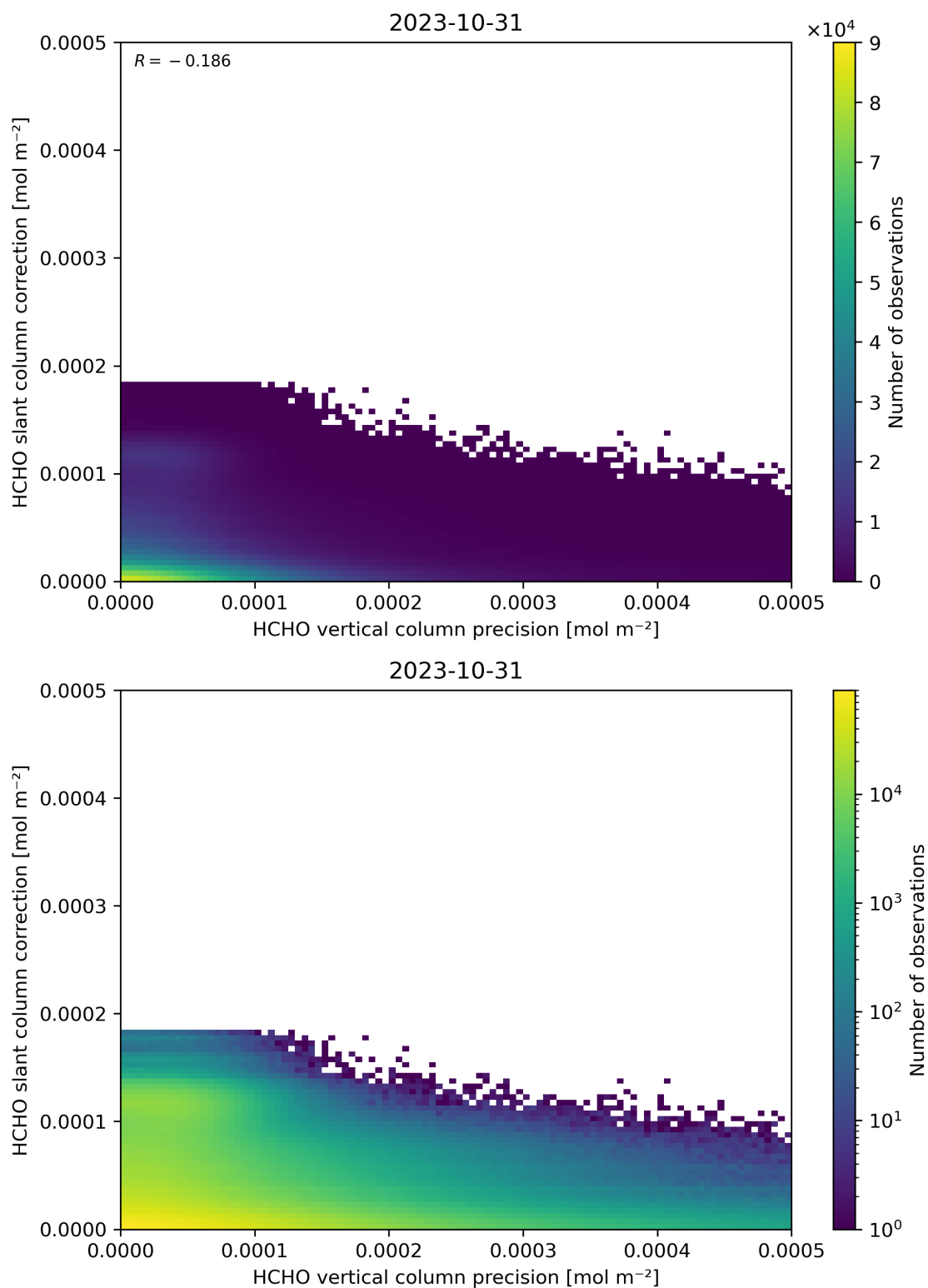
Figure 141: Scatter density plot of “HCHO vertical column precision” against “HCHO slant column correction” for 2023-10-30 to 2023-11-01.
