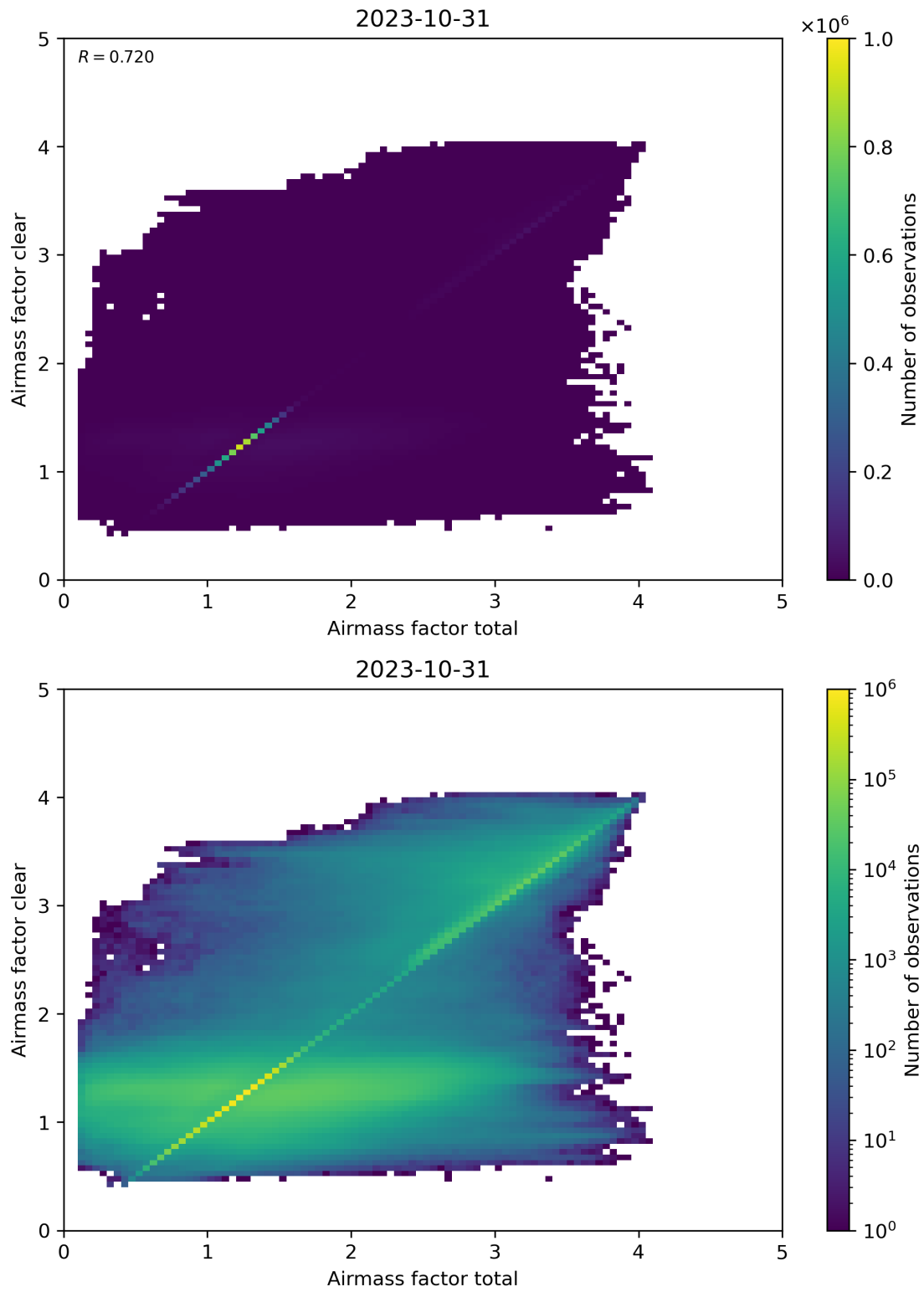
Figure 100: Scatter density plot of “Airmass factor total” against “Airmass factor clear” for 2023-10-30 to 2023-11-01.
