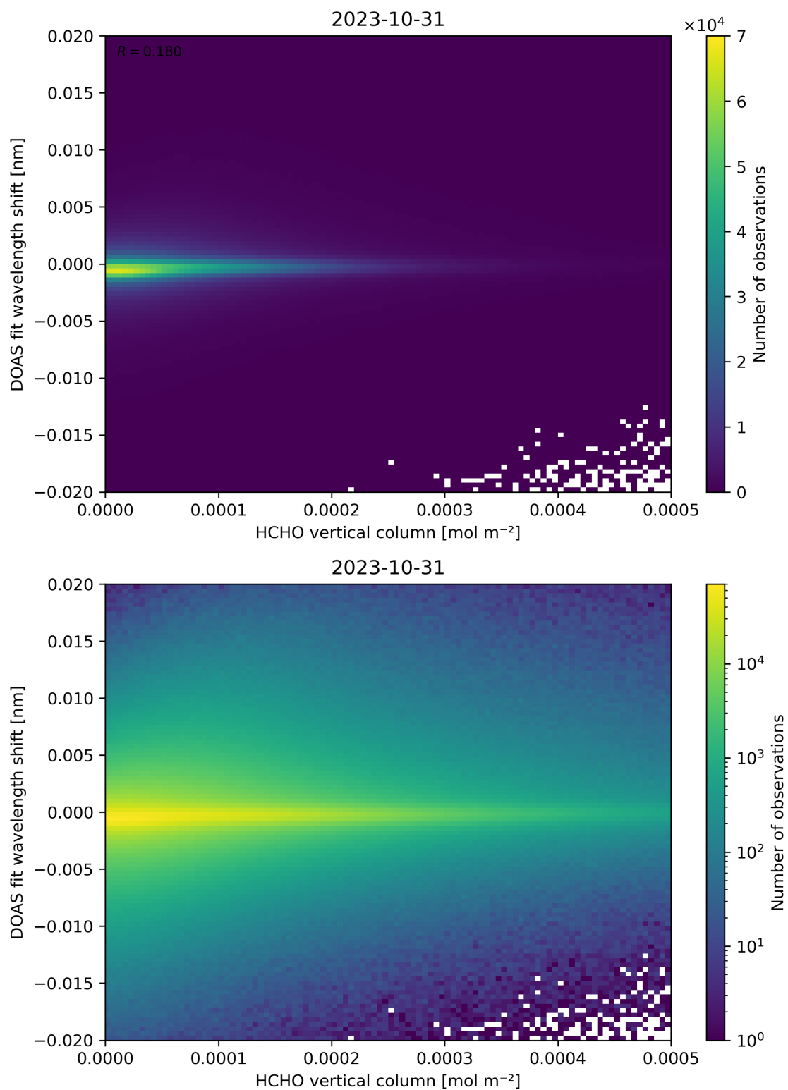
Figure 124: Scatter density plot of “HCHO vertical column” against “DOAS fit wavelength shift” for 2023-10-30 to 2023-11-01.
