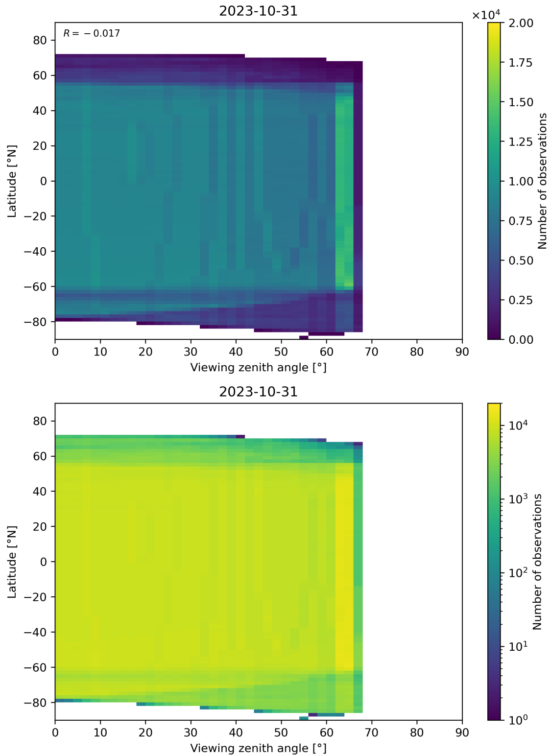
Figure 196: Scatter density plot of “Viewing zenith angle” against “Latitude” for 2023-10-30 to 2023-11-01.
