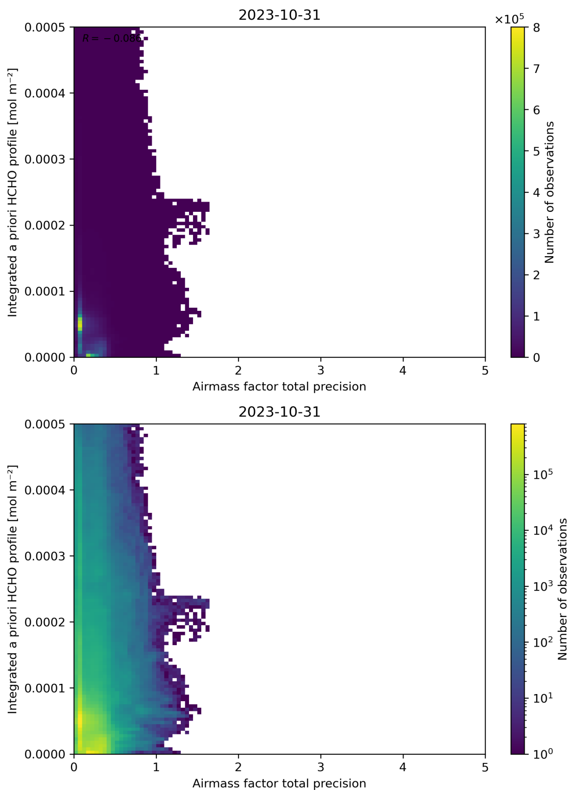
Figure 111: Scatter density plot of “Airmass factor total precision” against “Integrated a priori HCHO profile” for 2023-10-30 to 2023-11-01.
