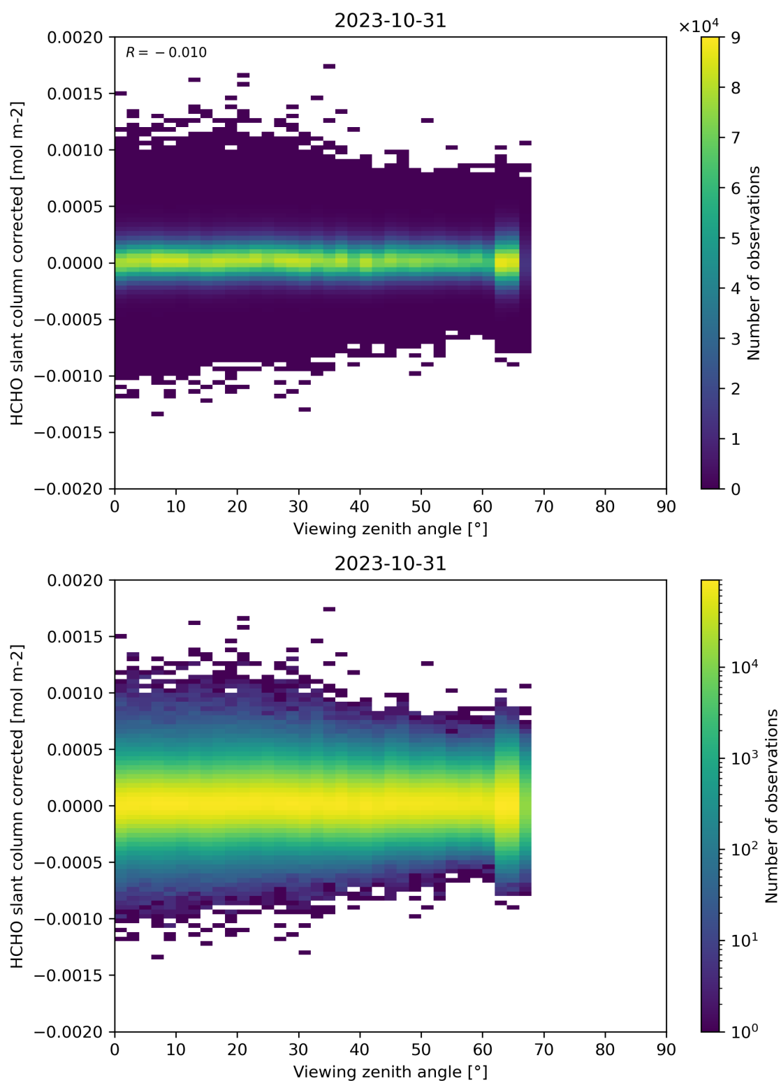
Figure 186: Scatter density plot of “Viewing zenith angle” against “HCHO slant column corrected” for 2023-10-30 to 2023-11-01.
