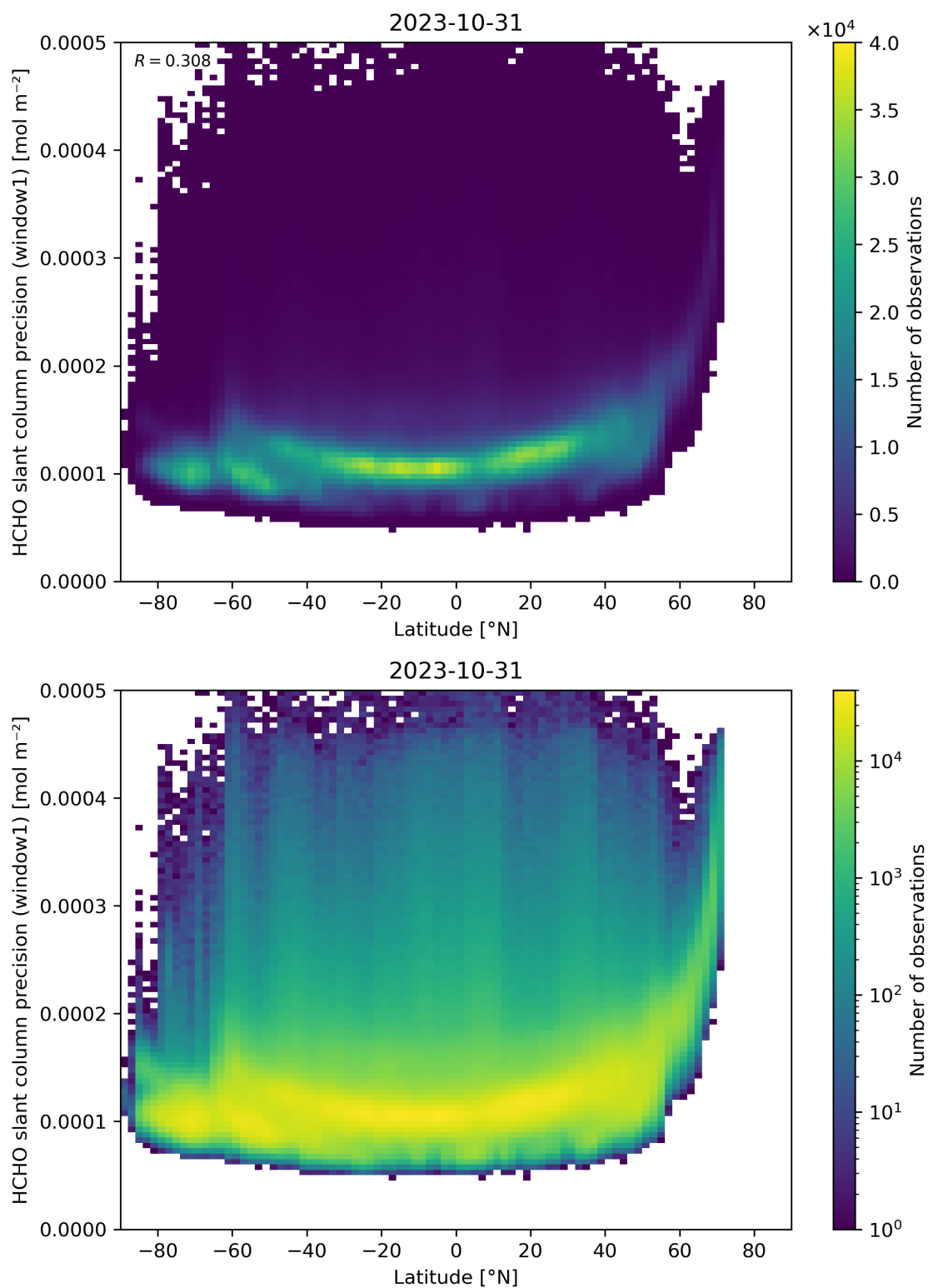
Figure 160: Scatter density plot of “Latitude” against “HCHO slant column precision (window1)” for 2023-10-30 to 2023-11-01.
