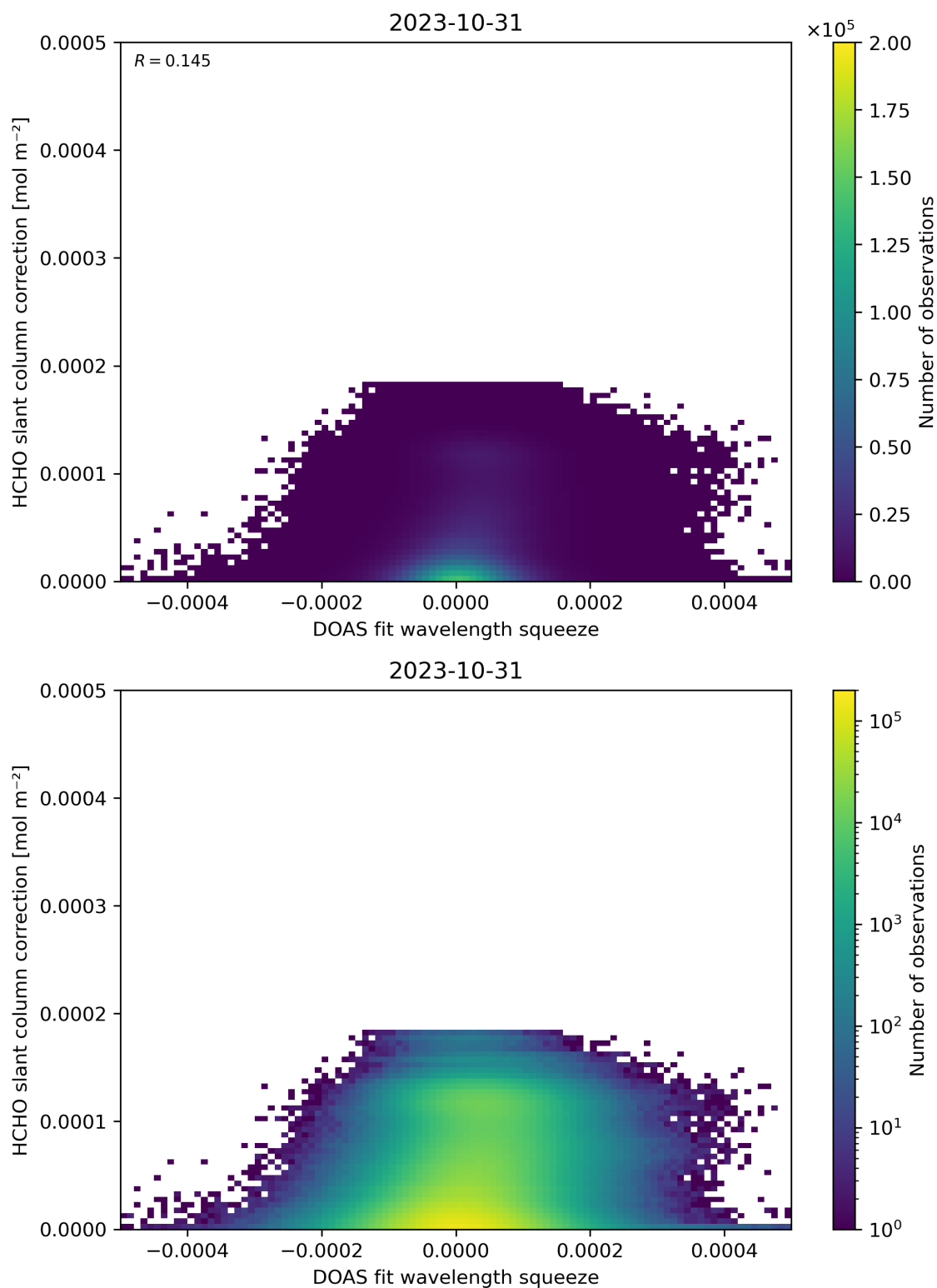
Figure 70: Scatter density plot of “DOAS fit wavelength squeeze” against “HCHO slant column correction” for 2023-10-30 to 2023-11-01.
