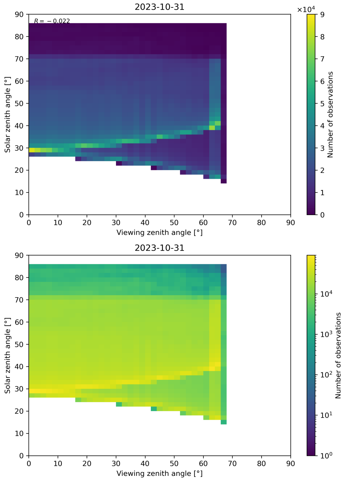
Figure 197: Scatter density plot of “Viewing zenith angle” against “Solar zenith angle” for 2023-10-30 to 2023-11-01.
