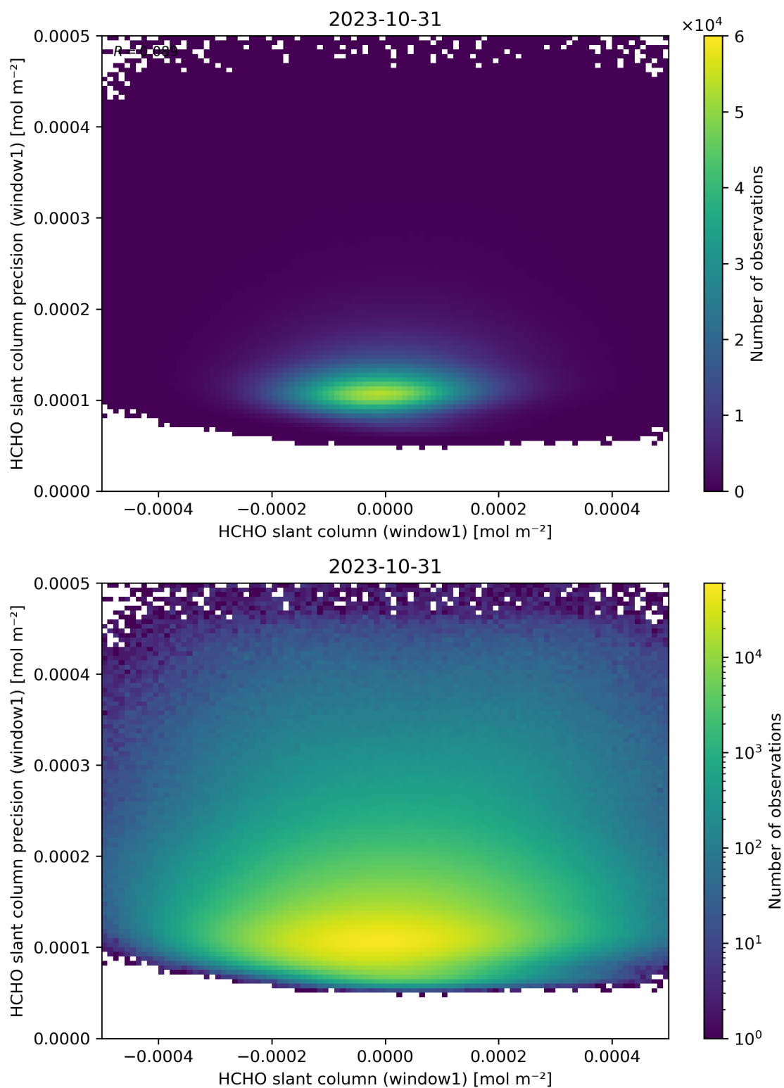
Figure 84: Scatter density plot of “HCHO slant column (window1)” against “HCHO slant column precision (window1)” for 2023-10-30 to 2023-11-01.
