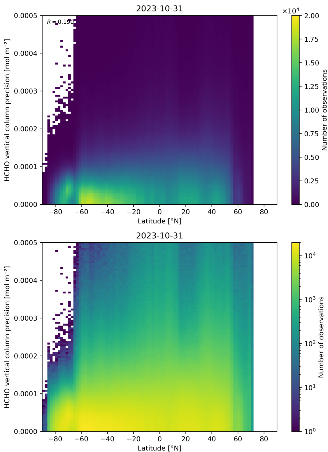
Figure 165: Scatter density plot of “Latitude” against “HCHO vertical column precision” for 2023-10-30 to 2023-11-01.
