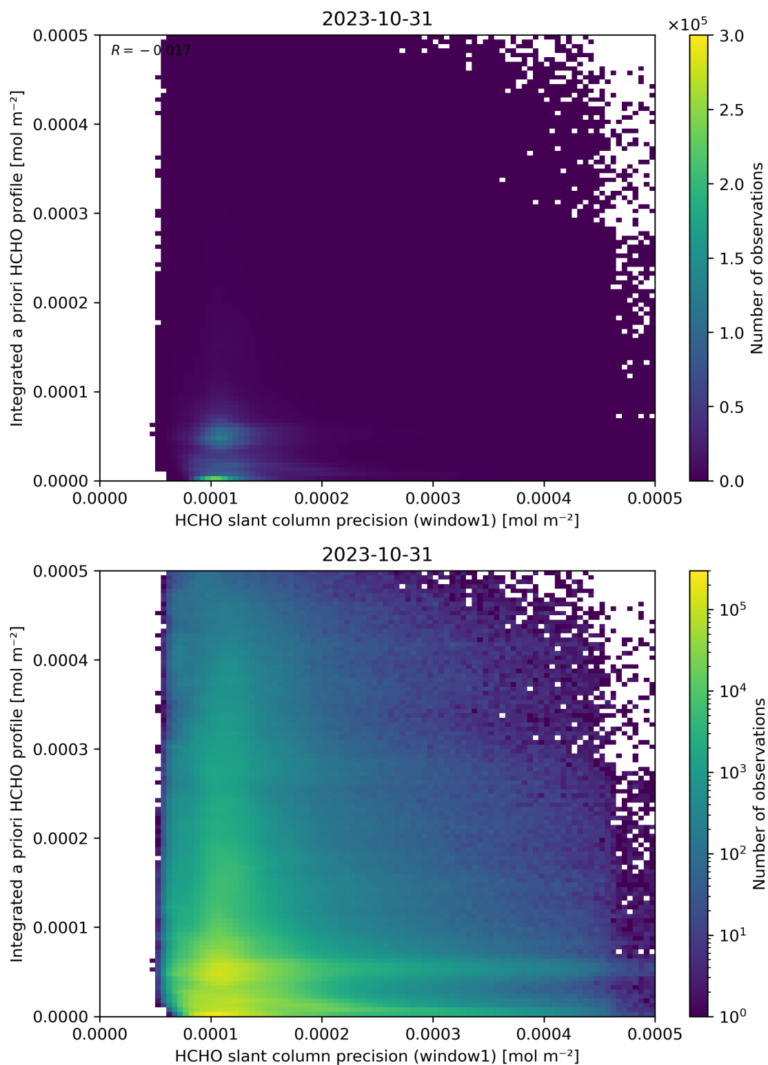
Figure 96: Scatter density plot of “HCHO slant column precision (window1)” against “Integrated a priori HCHO profile” for 2023-10-30 to 2023-11-01.
