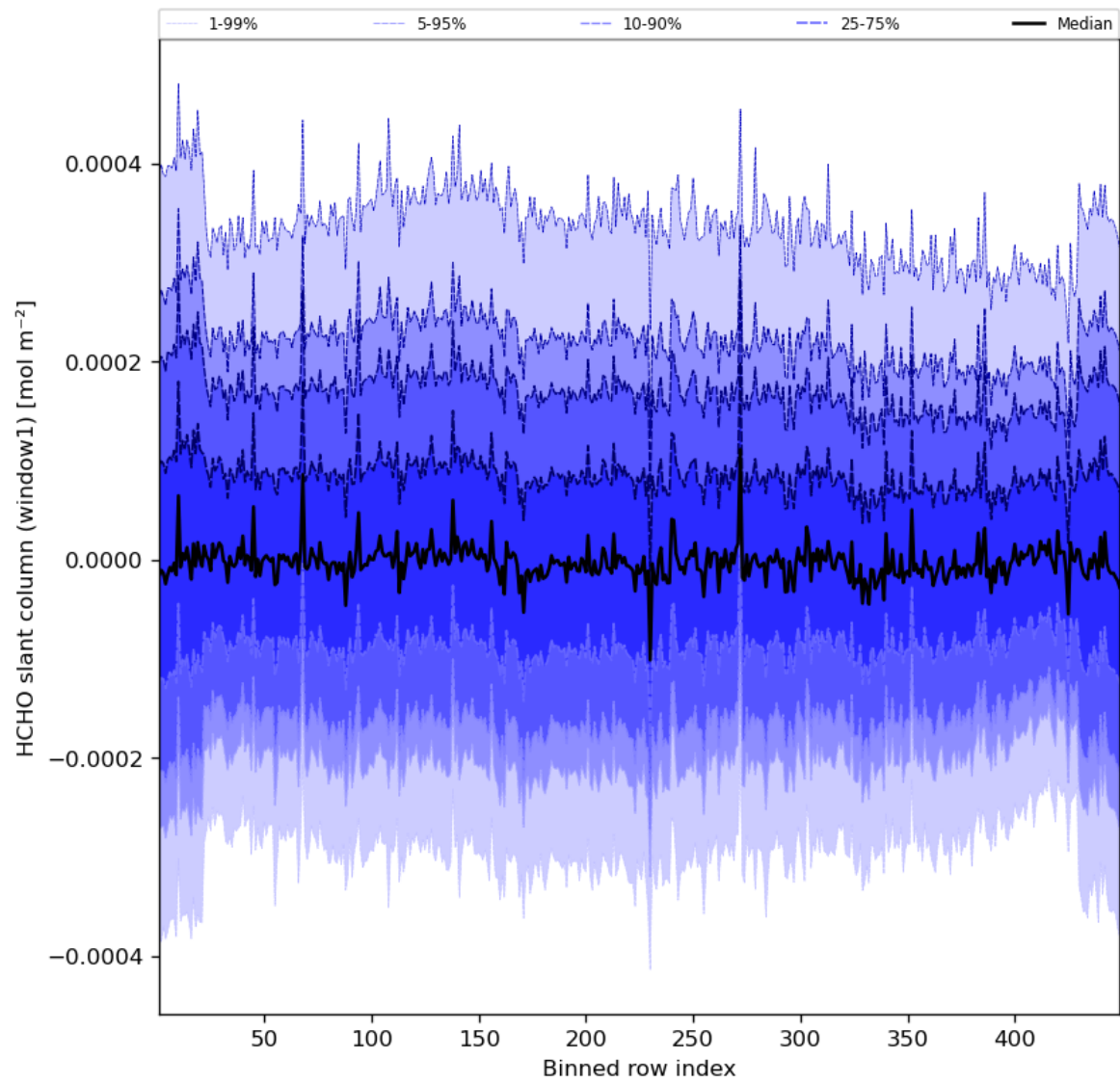
Figure 52: Along track statistics of “HCHO slant column (window1)” for 2023-10-30 to 2023-11-01
