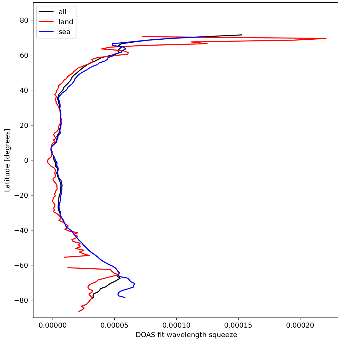
Figure 31: Zonal average of “DOAS fit wavelength squeeze” for 2023-10-30 to 2023-11-01.
