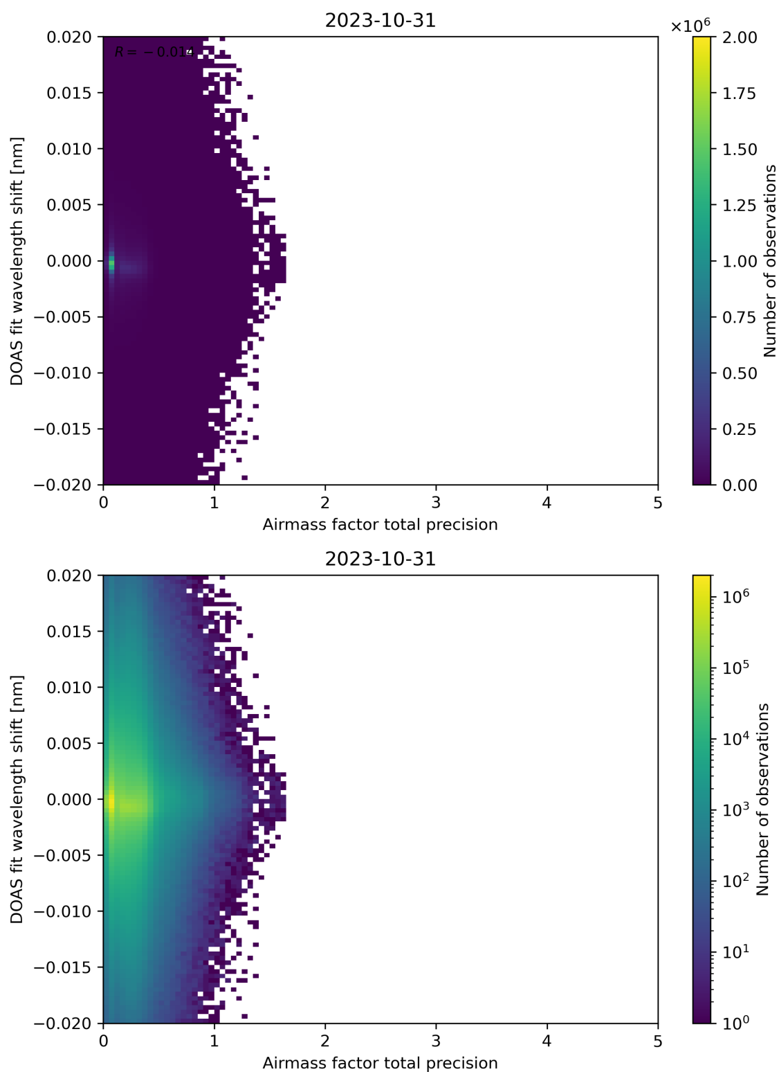
Figure 106: Scatter density plot of “Airmass factor total precision” against “DOAS fit wavelength shift” for 2023-10-30 to 2023-11-01.
