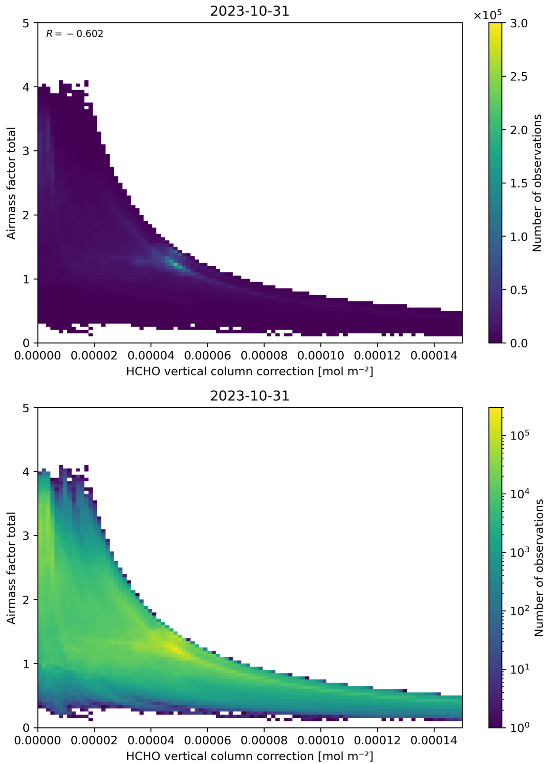
Figure 120: Scatter density plot of “HCHO vertical column correction” against “Airmass factor total” for 2023-10-30 to 2023-11-01.
