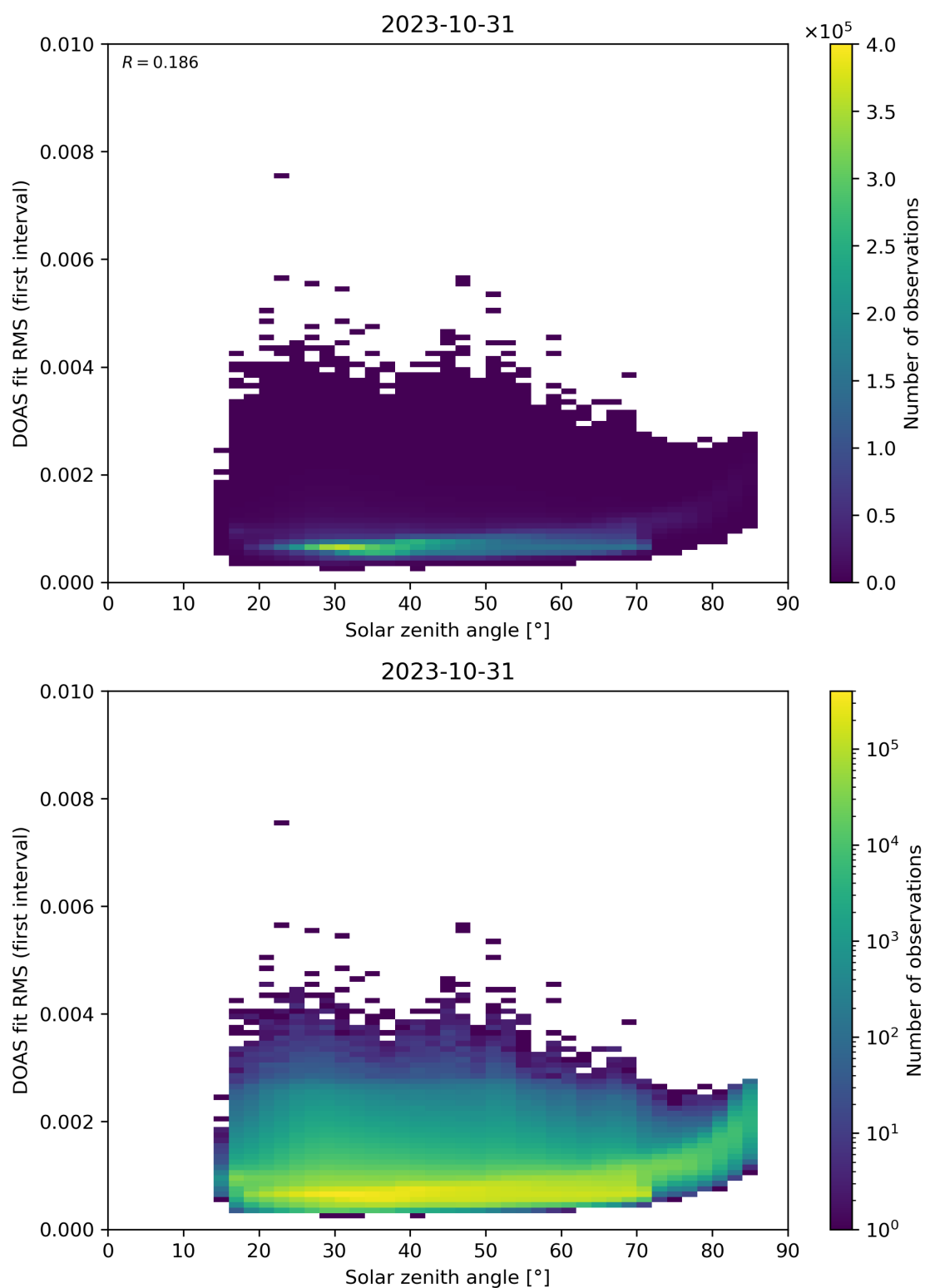
Figure 167: Scatter density plot of “Solar zenith angle” against “DOAS fit RMS (first interval)” for 2023-10-30 to 2023-11-01.
