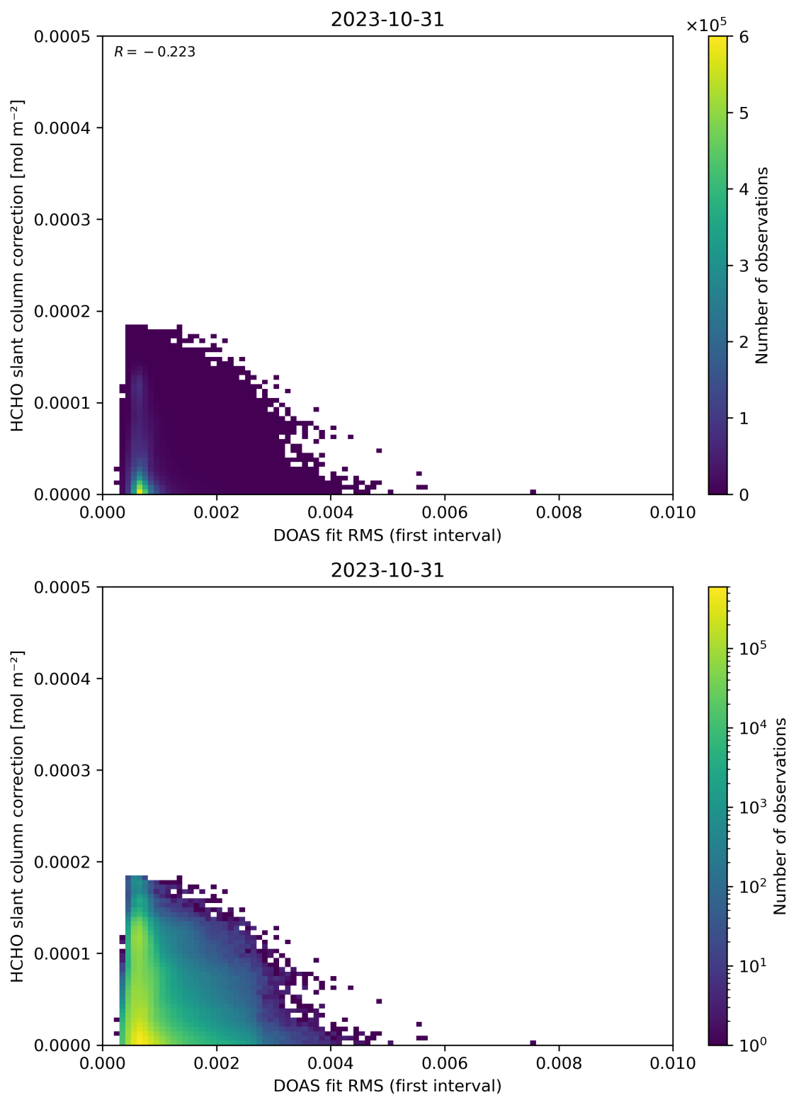
Figure 63: Scatter density plot of “DOAS fit RMS (first interval)” against “HCHO slant column correction” for 2023-10-30 to 2023-11-01.
