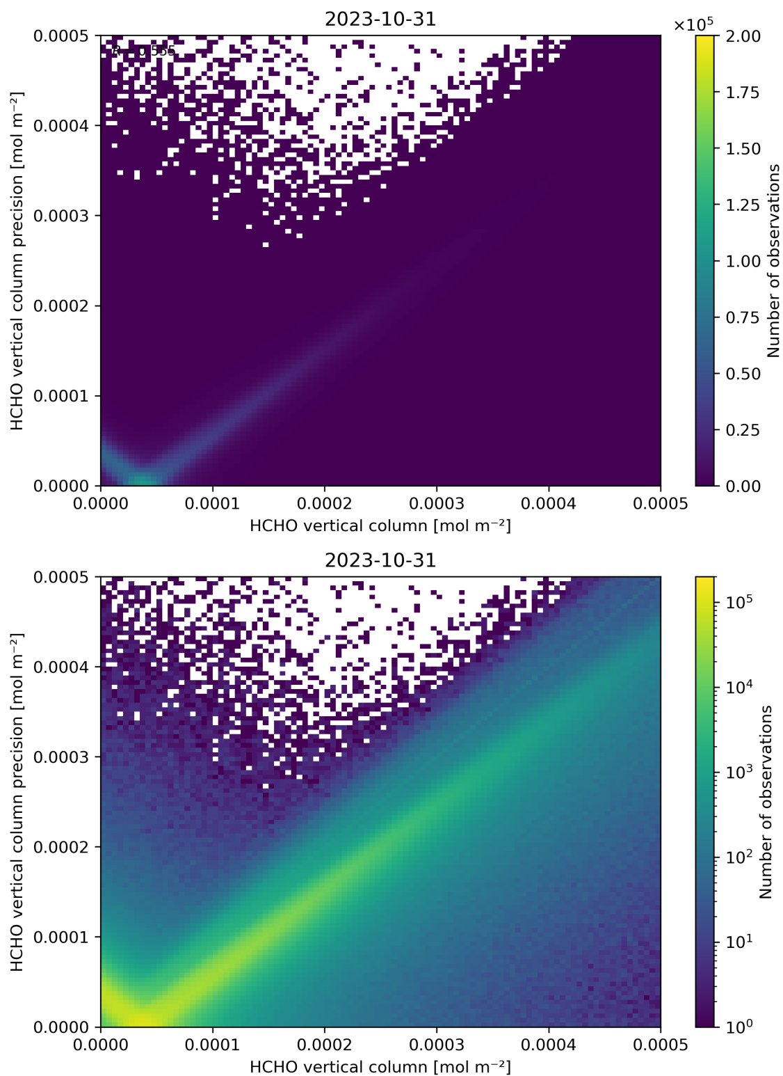
Figure 134: Scatter density plot of “HCHO vertical column” against “HCHO vertical column precision” for 2023-10-30 to 2023-11-01.
