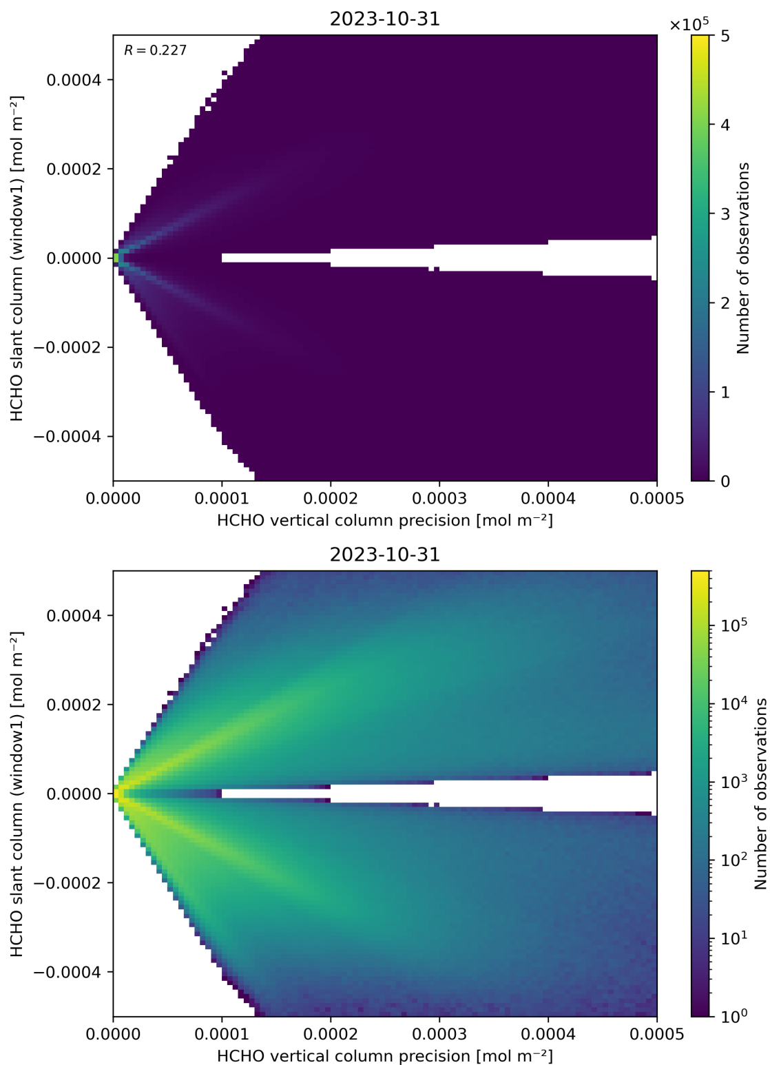
Figure 142: Scatter density plot of “HCHO vertical column precision” against “HCHO slant column (window1)” for 2023-10-30 to 2023-11-01.
