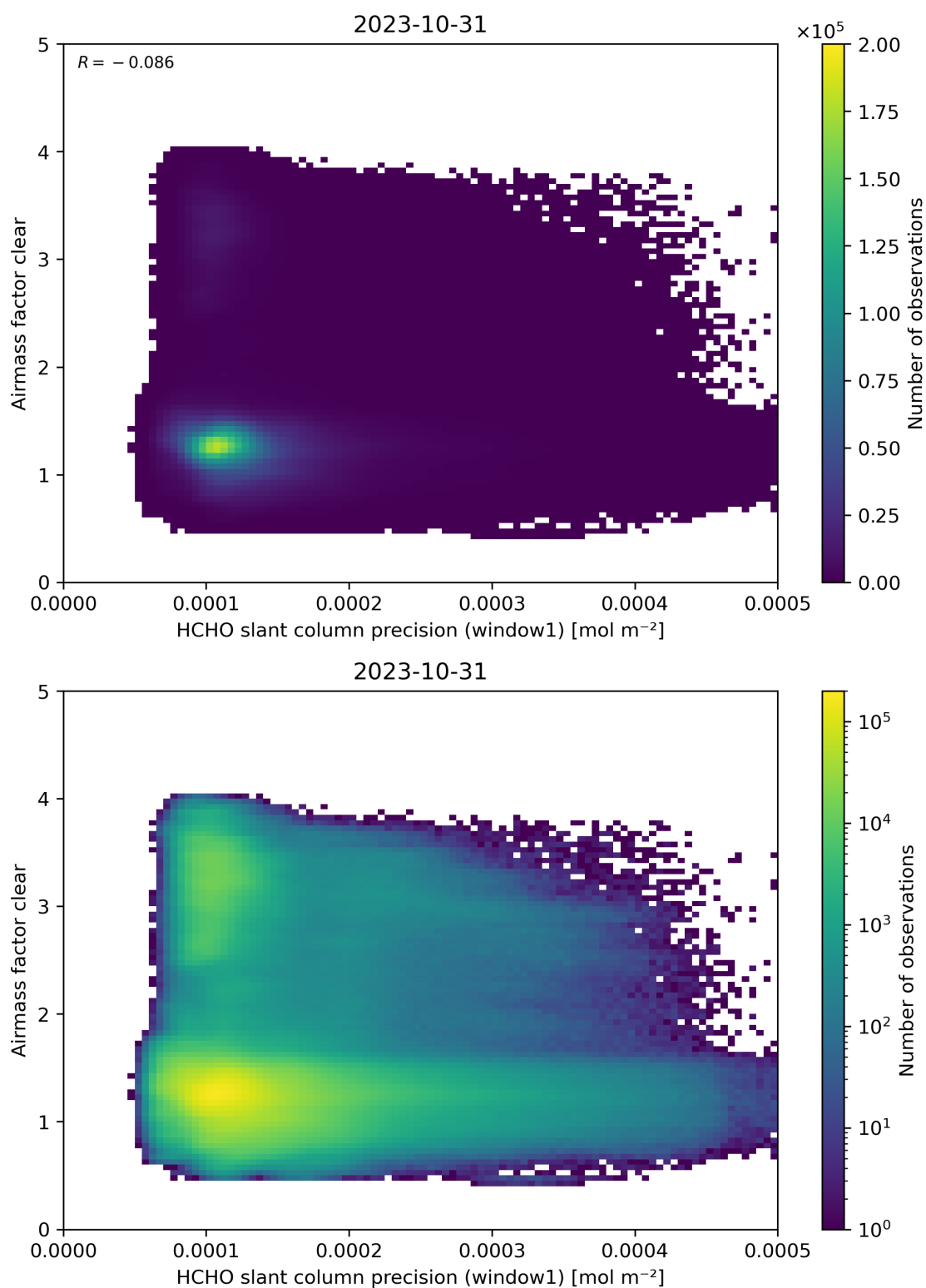
Figure 91: Scatter density plot of “HCHO slant column precision (window1)” against “Airmass factor clear” for 2023-10-30 to 2023-11-01.
