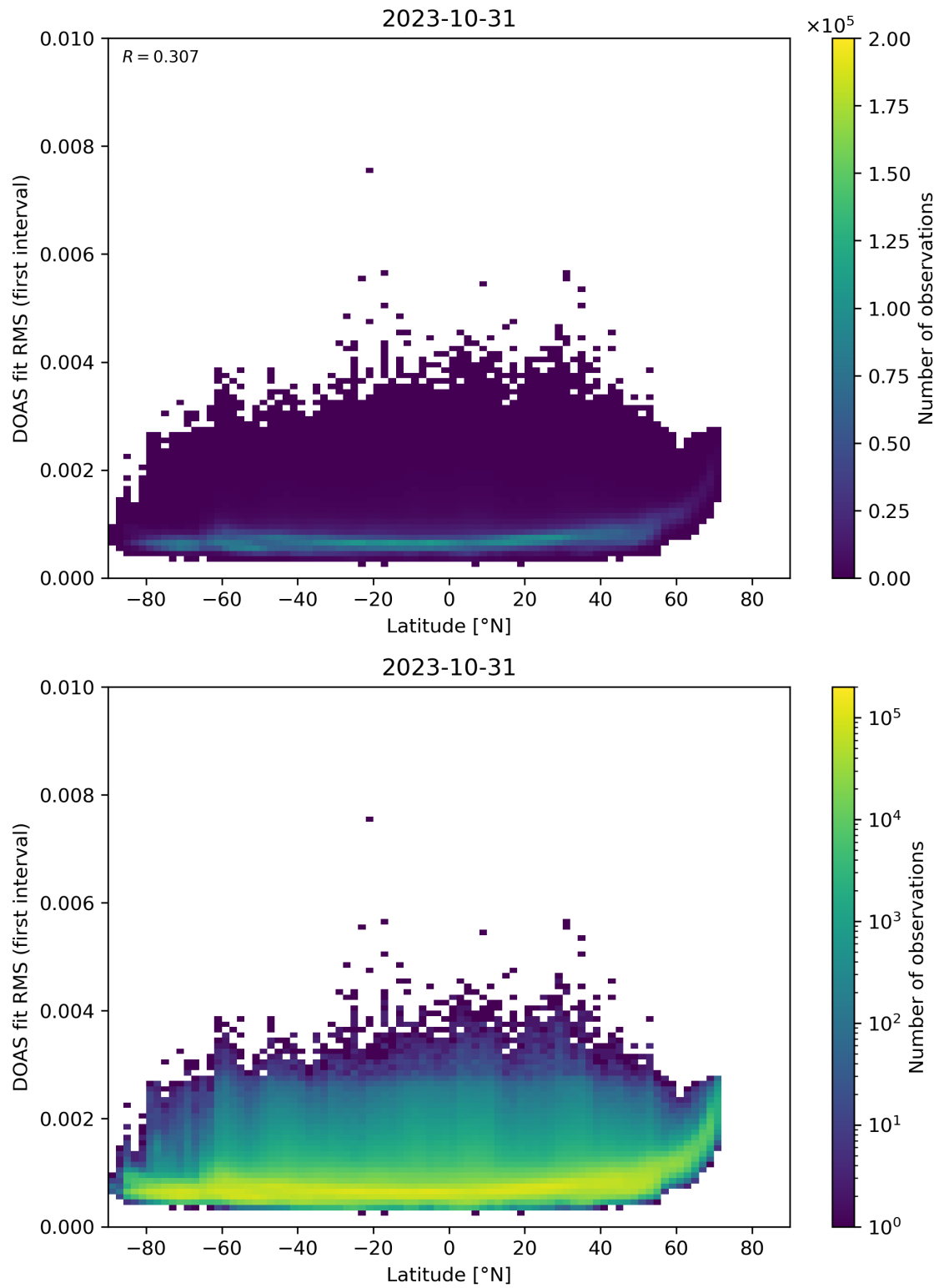
Figure 153: Scatter density plot of “Latitude” against “DOAS fit RMS (first interval)” for 2023-10-30 to 2023-11-01.
