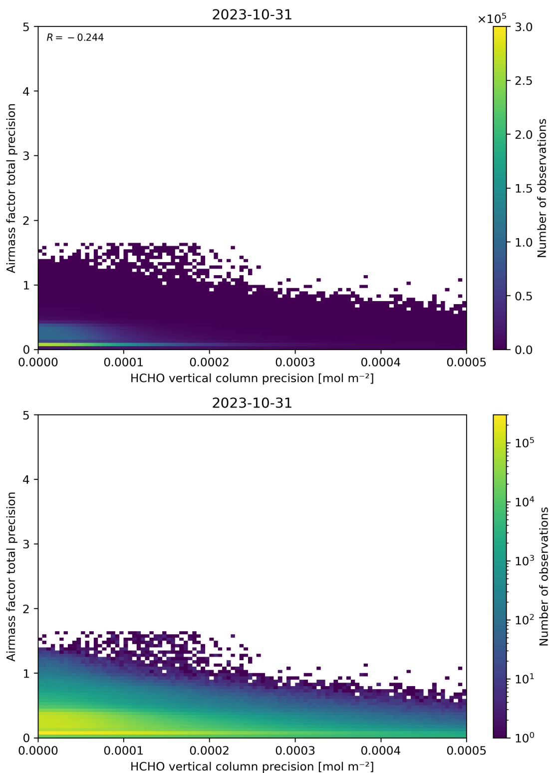
Figure 145: Scatter density plot of “HCHO vertical column precision” against “Airmass factor total precision” for 2023-10-30 to 2023-11-01.
