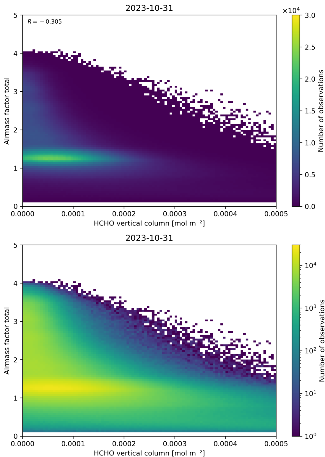
Figure 131: Scatter density plot of “HCHO vertical column” against “Airmass factor total” for 2023-10-30 to 2023-11-01.
