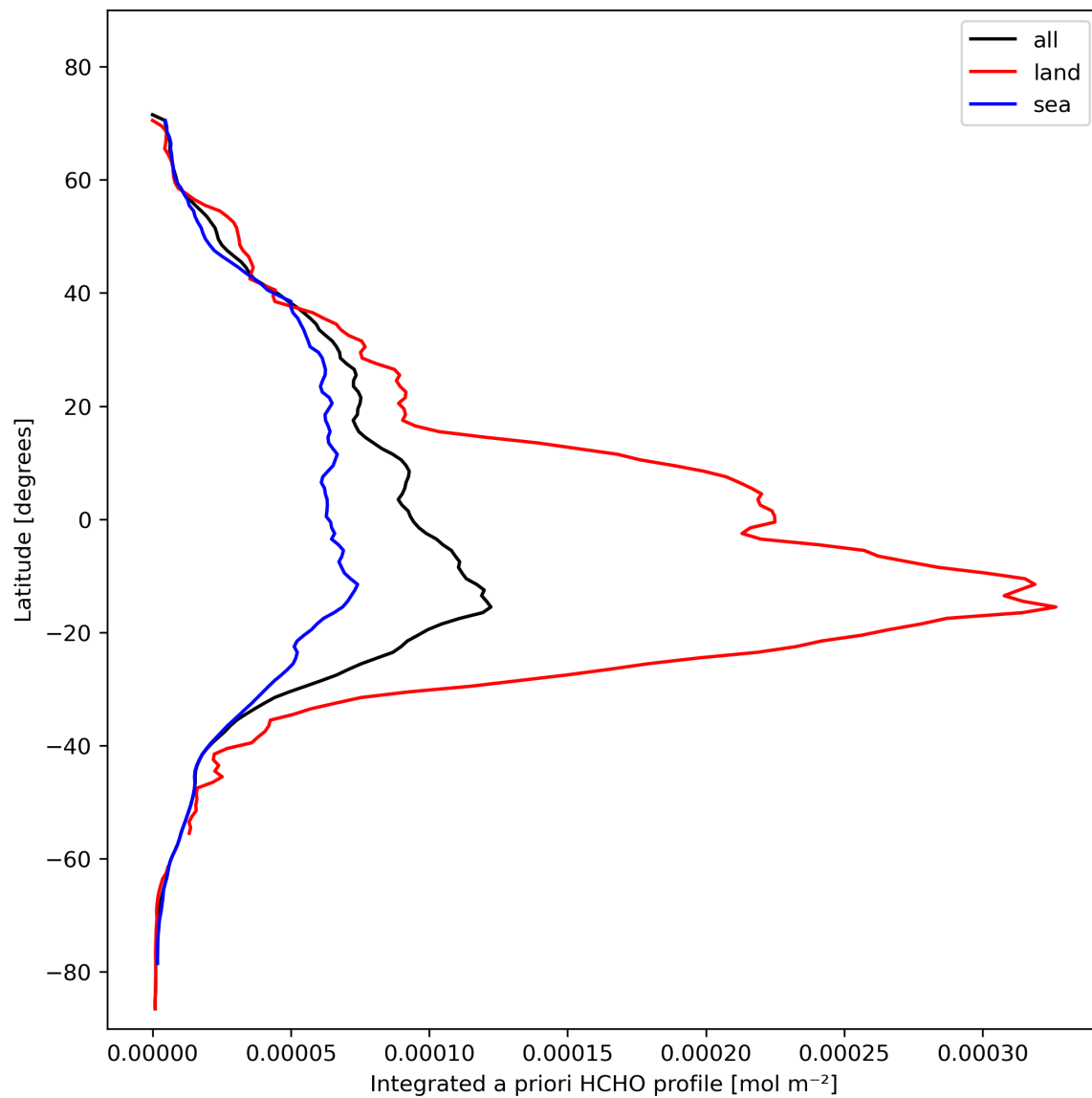
Figure 29: Zonal average of “Integrated a priori HCHO profile” for 2023-10-30 to 2023-11-01.
