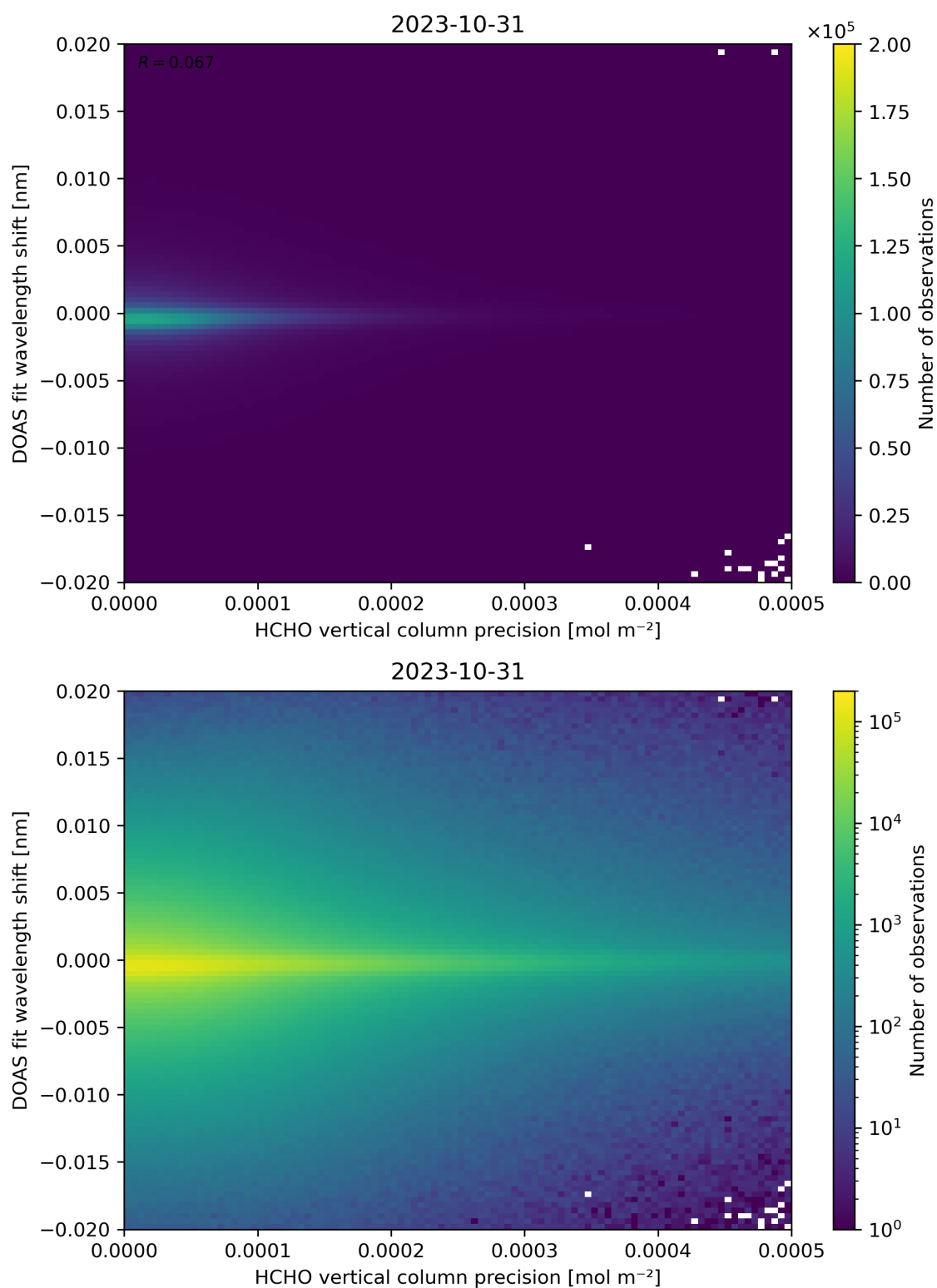
Figure 137: Scatter density plot of “HCHO vertical column precision” against “DOAS fit wavelength shift” for 2023-10-30 to 2023-11-01.
