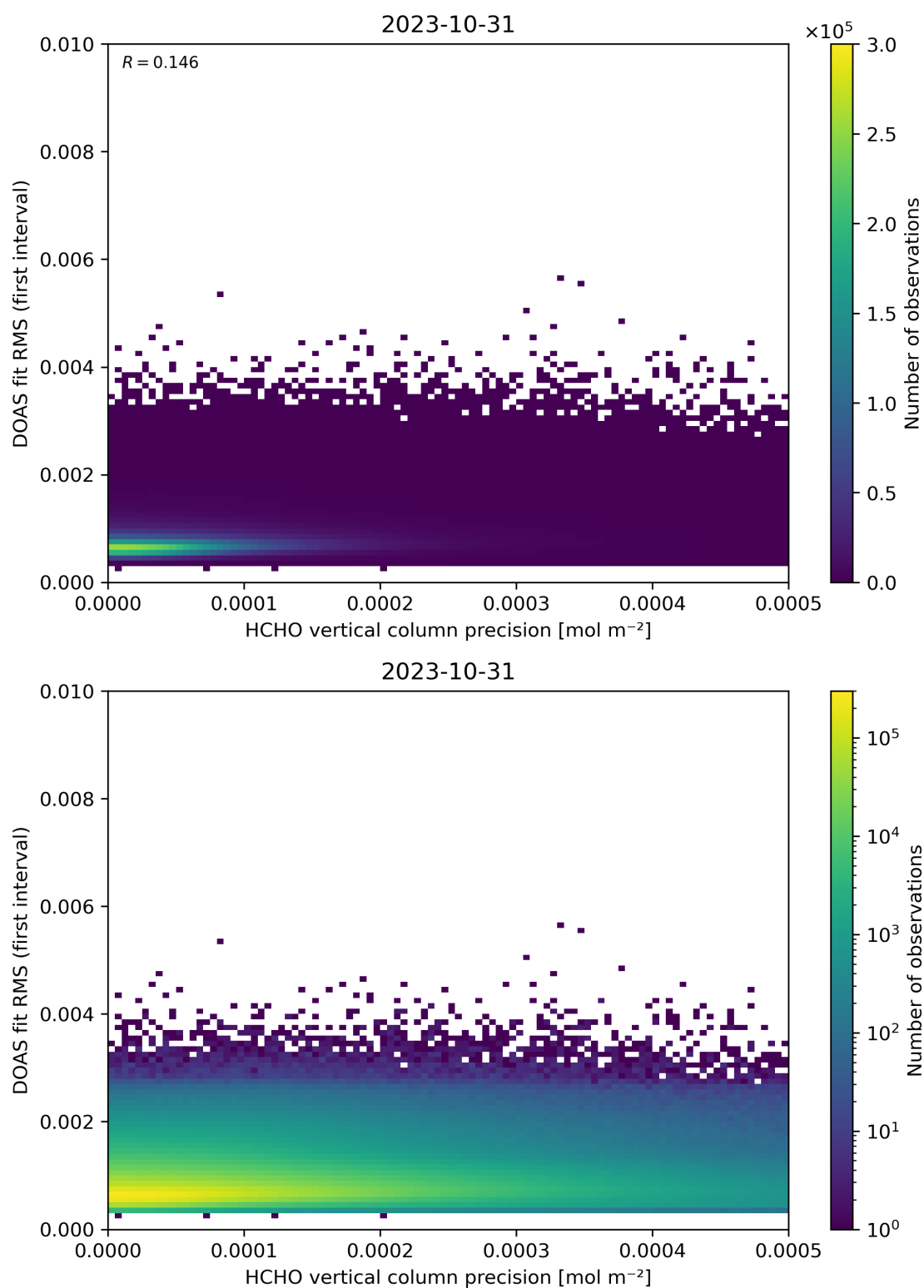
Figure 136: Scatter density plot of “HCHO vertical column precision” against “DOAS fit RMS (first interval)” for 2023-10-30 to 2023-11-01.
