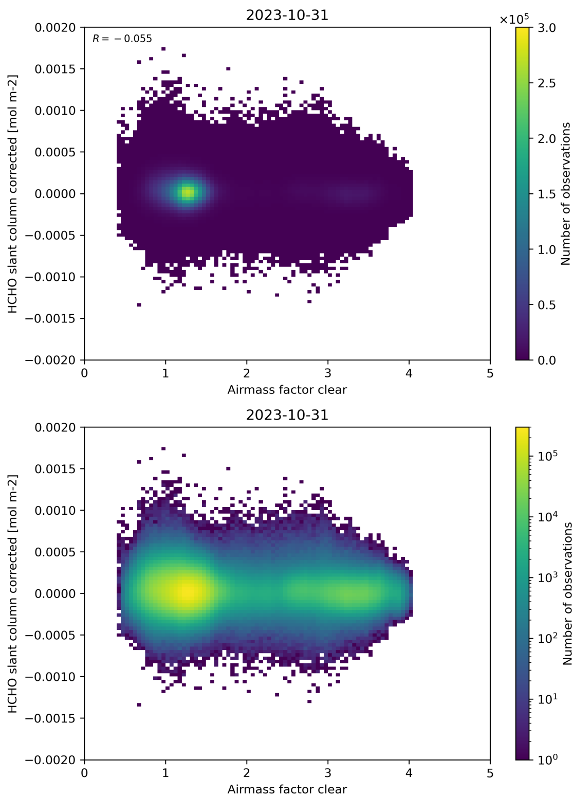
Figure 74: Scatter density plot of “Airmass factor clear” against “HCHO slant column corrected” for 2023-10-30 to 2023-11-01.
