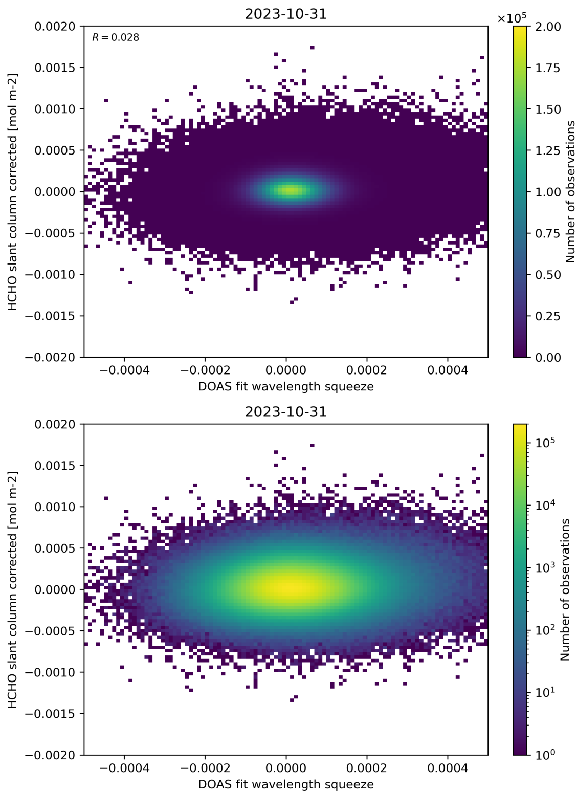
Figure 69: Scatter density plot of “DOAS fit wavelength squeeze” against “HCHO slant column corrected” for 2023-10-30 to 2023-11-01.
