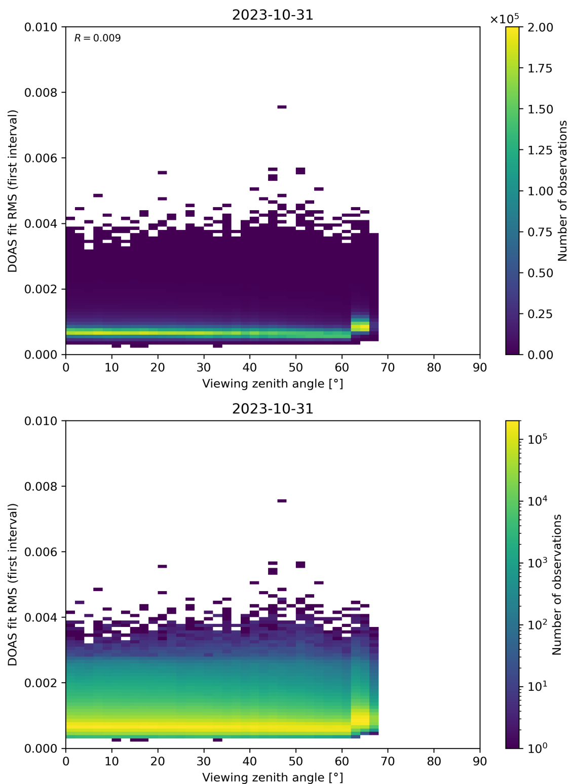
Figure 182: Scatter density plot of “Viewing zenith angle” against “DOAS fit RMS (first interval)” for 2023-10-30 to 2023-11-01.
