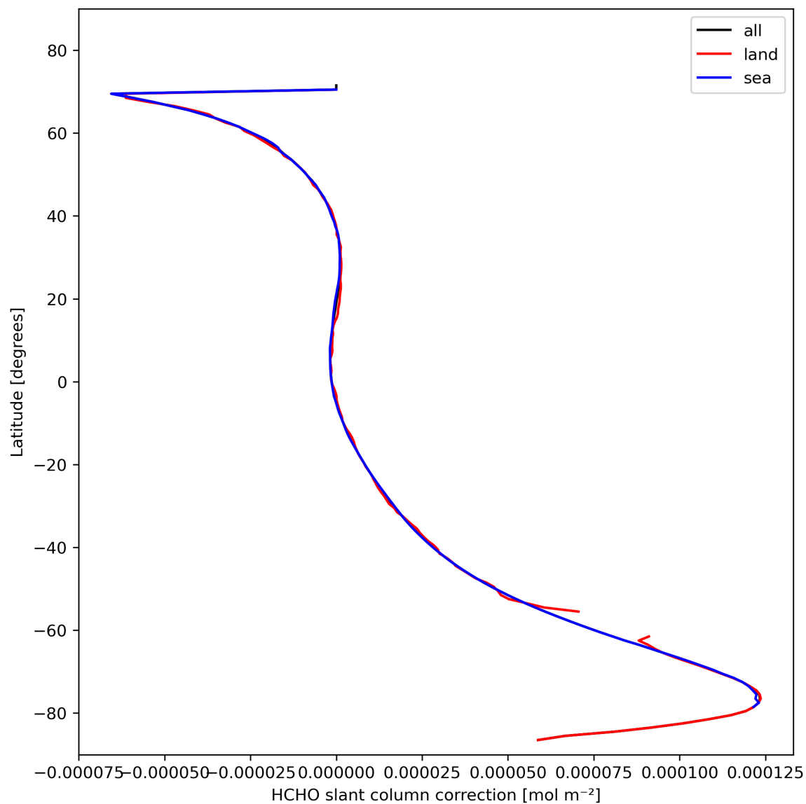
Figure 33: Zonal average of “HCHO slant column correction” for 2023-10-30 to 2023-11-01.
