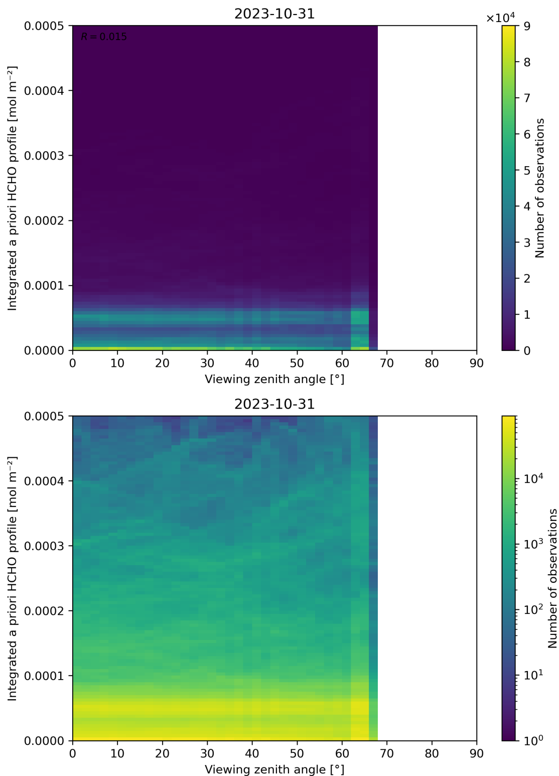
Figure 195: Scatter density plot of “Viewing zenith angle” against “Integrated a priori HCHO profile” for 2023-10-30 to 2023-11-01.
