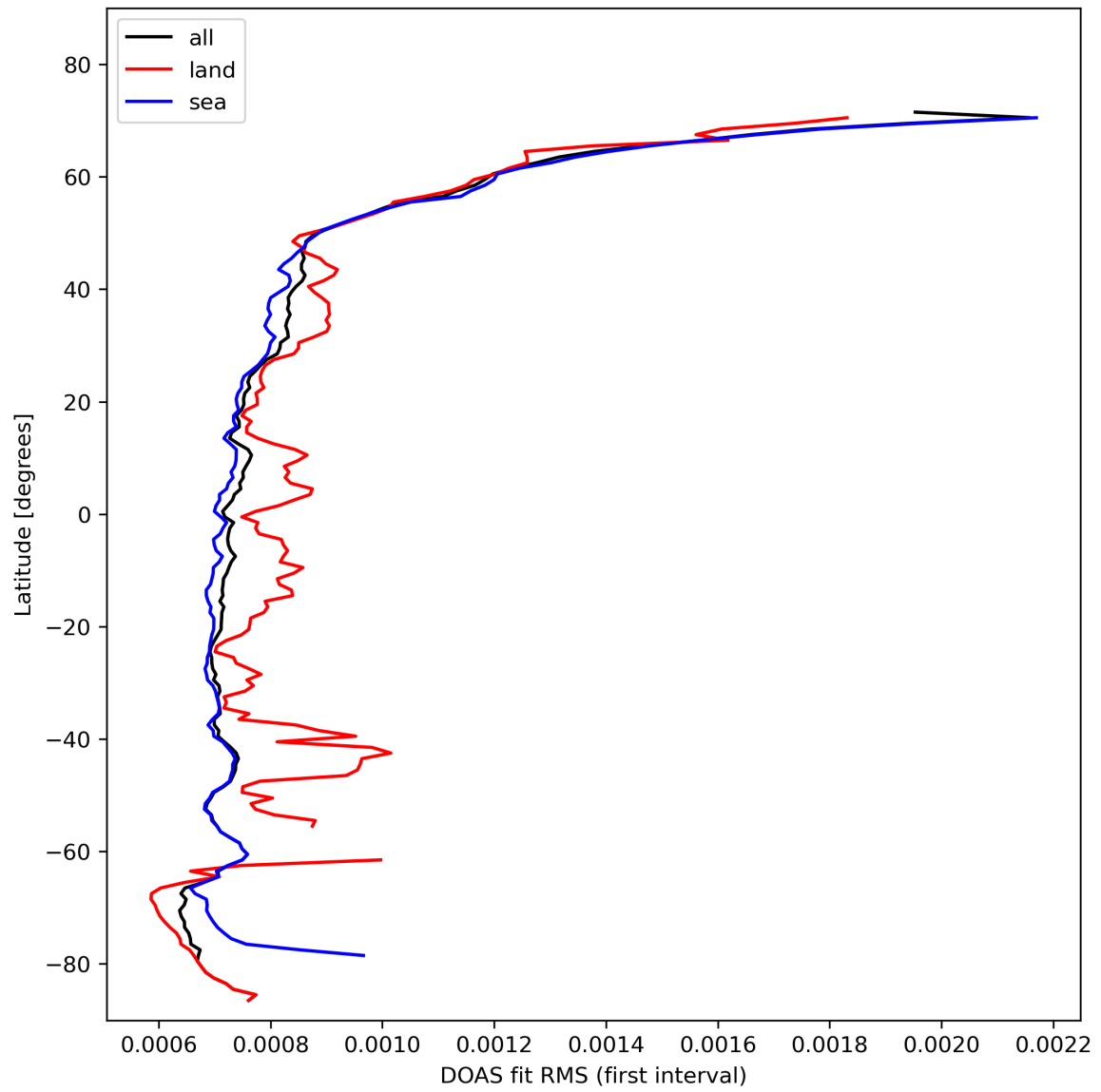
Figure 32: Zonal average of “DOAS fit RMS (first interval)” for 2023-10-30 to 2023-11-01.
