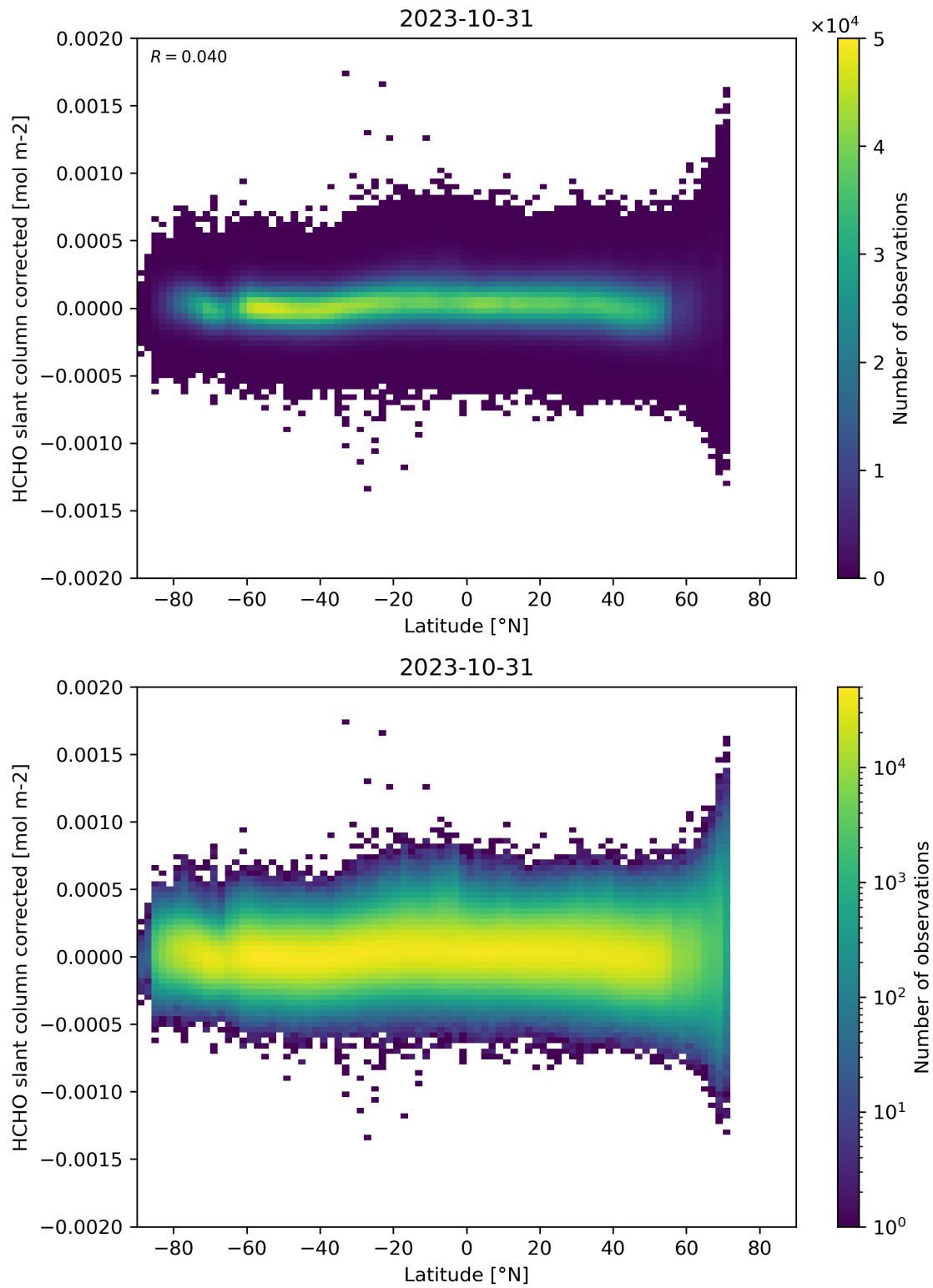
Figure 157: Scatter density plot of “Latitude” against “HCHO slant column corrected” for 2023-10-30 to 2023-11-01.
