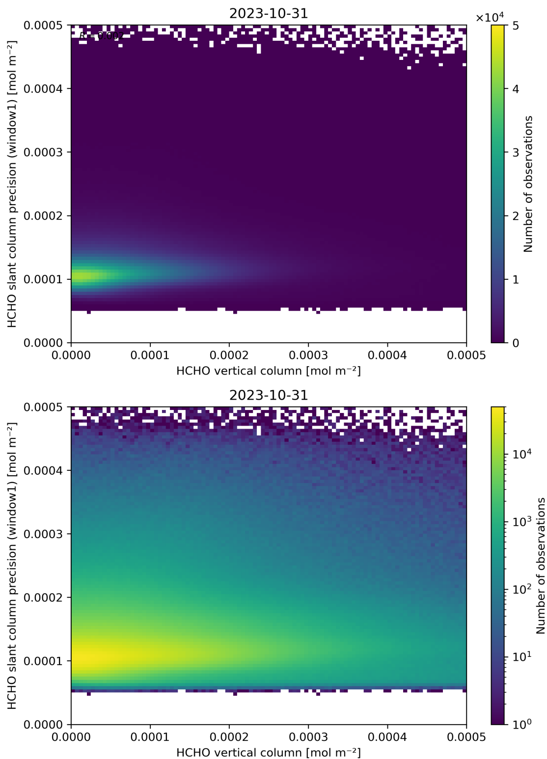
Figure 130: Scatter density plot of “HCHO vertical column” against “HCHO slant column precision (window1)” for 2023-10-30 to 2023-11-01.
