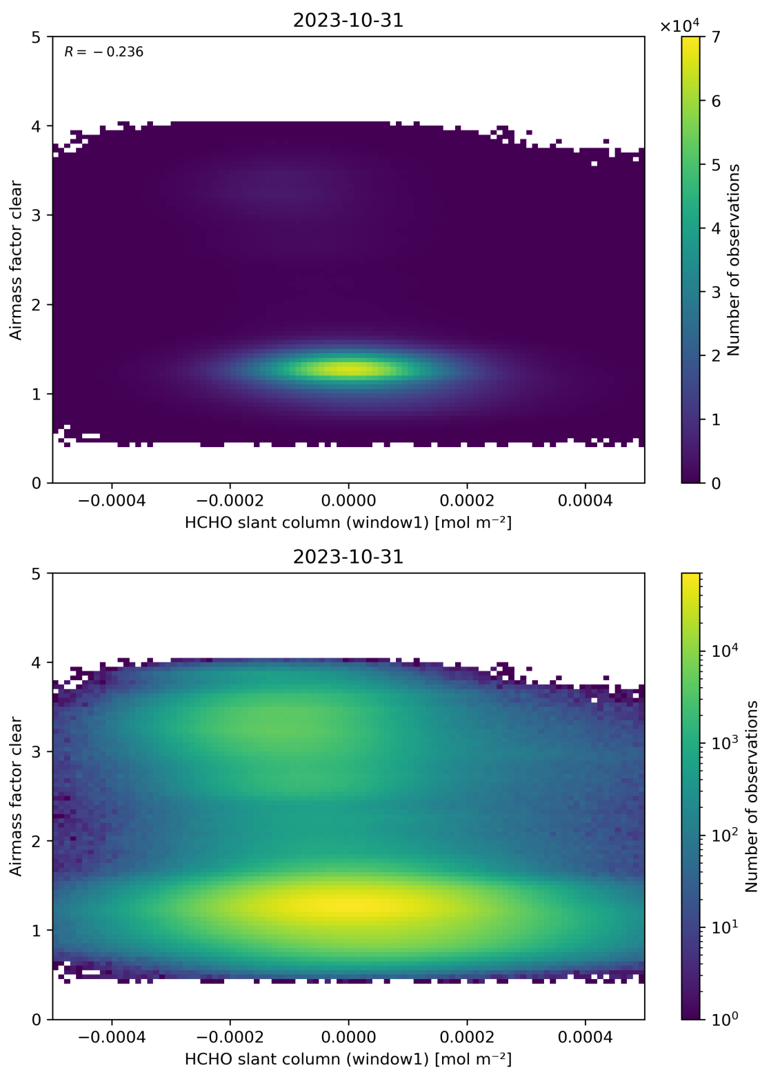
Figure 81: Scatter density plot of “HCHO slant column (window1)” against “Airmass factor clear” for 2023-10-30 to 2023-11-01.
