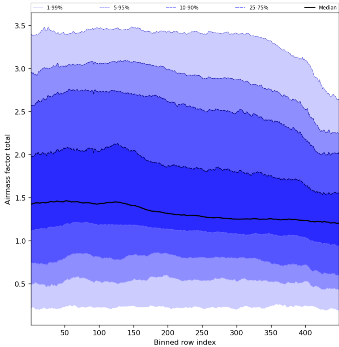
Figure 54: Along track statistics of “Airmass factor total” for 2023-11-03 to 2023-11-05
