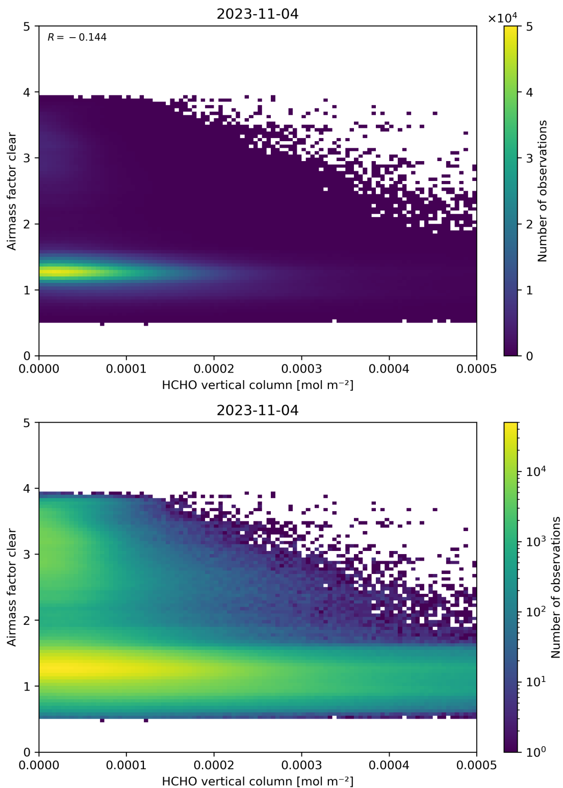
Figure 126: Scatter density plot of “HCHO vertical column” against “Airmass factor clear” for 2023-11-03 to 2023-11-05.
