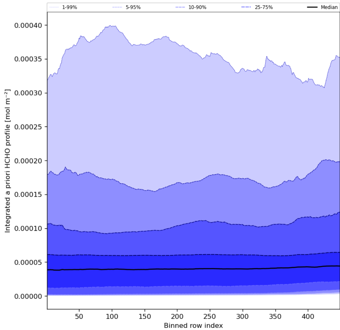
Figure 57: Along track statistics of “Integrated a priori HCHO profile” for 2023-11-03 to 2023-11-05
