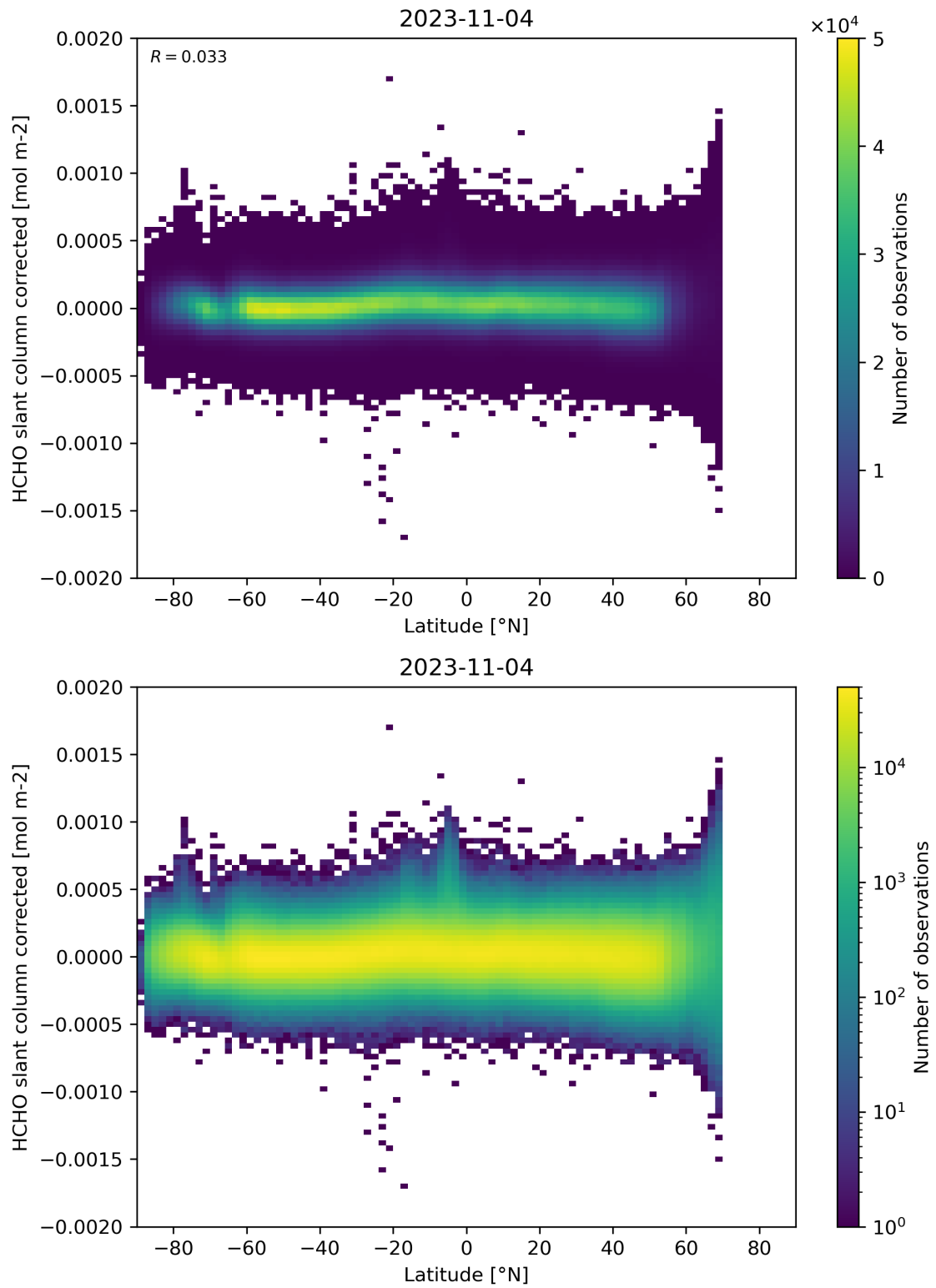
Figure 157: Scatter density plot of “Latitude” against “HCHO slant column corrected” for 2023-11-03 to 2023-11-05.
