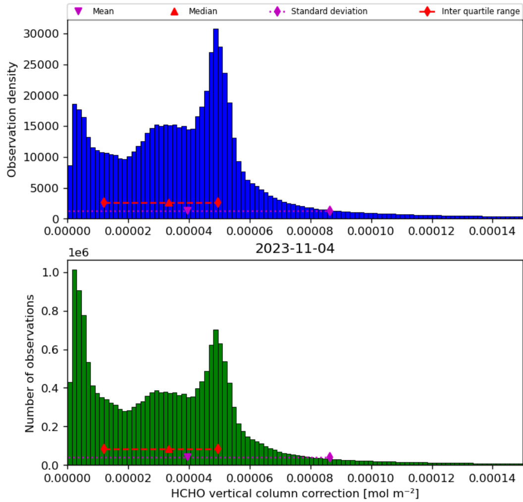
Figure 37: Histogram of “HCHO vertical column correction” for 2023-11-03 to 2023-11-05
