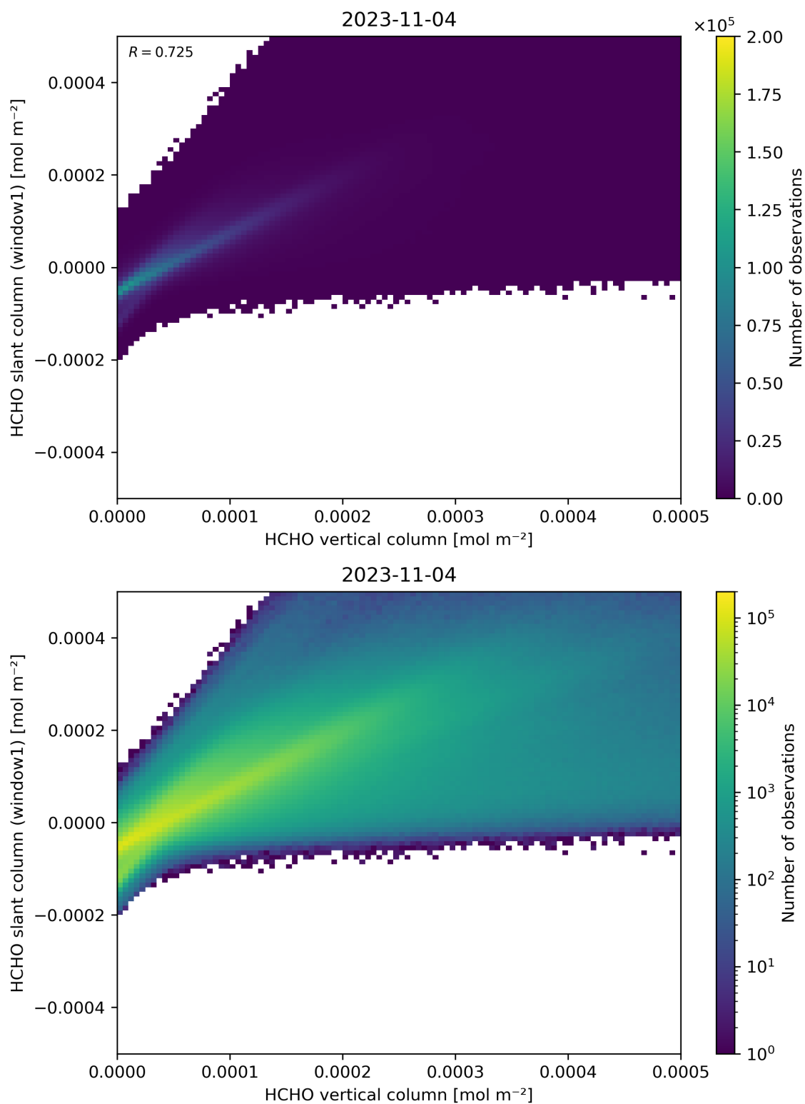
Figure 129: Scatter density plot of “HCHO vertical column” against “HCHO slant column (window1)” for 2023-11-03 to 2023-11-05.
