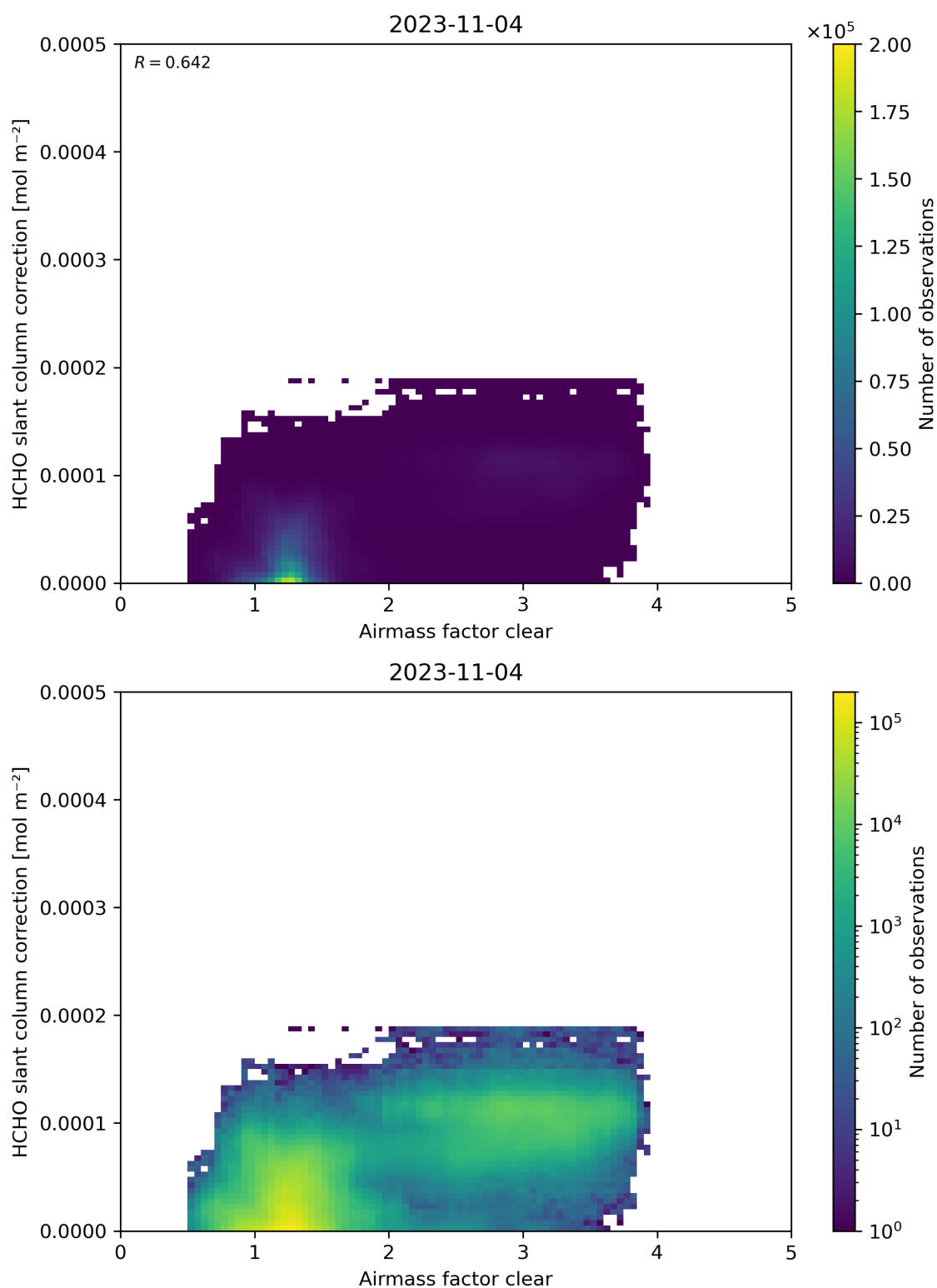
Figure 75: Scatter density plot of “Airmass factor clear” against “HCHO slant column correction” for 2023-11-03 to 2023-11-05.
