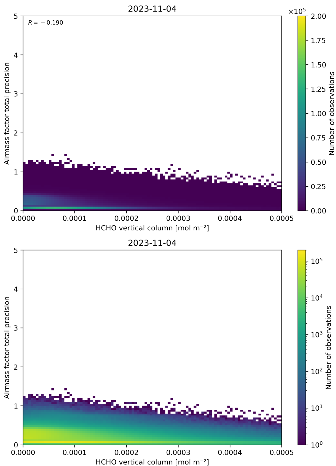
Figure 132: Scatter density plot of “HCHO vertical column” against “Airmass factor total precision” for 2023-11-03 to 2023-11-05.
