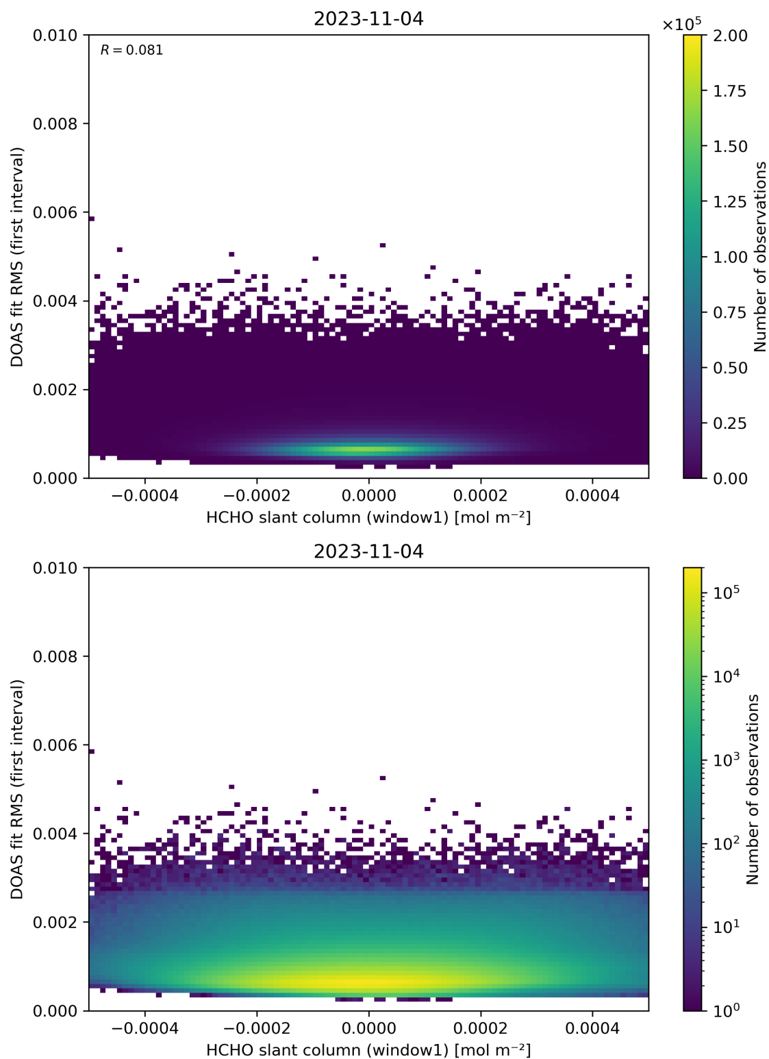
Figure 78: Scatter density plot of “HCHO slant column (window1)” against “DOAS fit RMS (first interval)” for 2023-11-03 to 2023-11-05.
