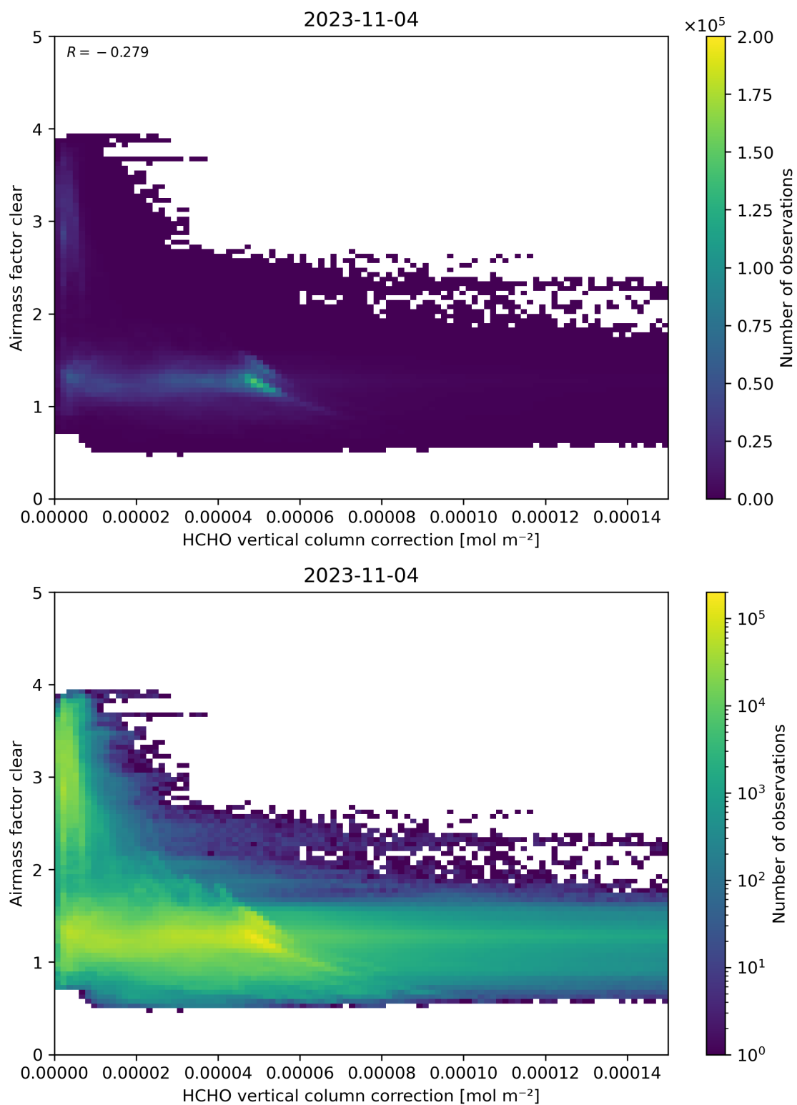
Figure 115: Scatter density plot of “HCHO vertical column correction” against “Airmass factor clear” for 2023-11-03 to 2023-11-05.
