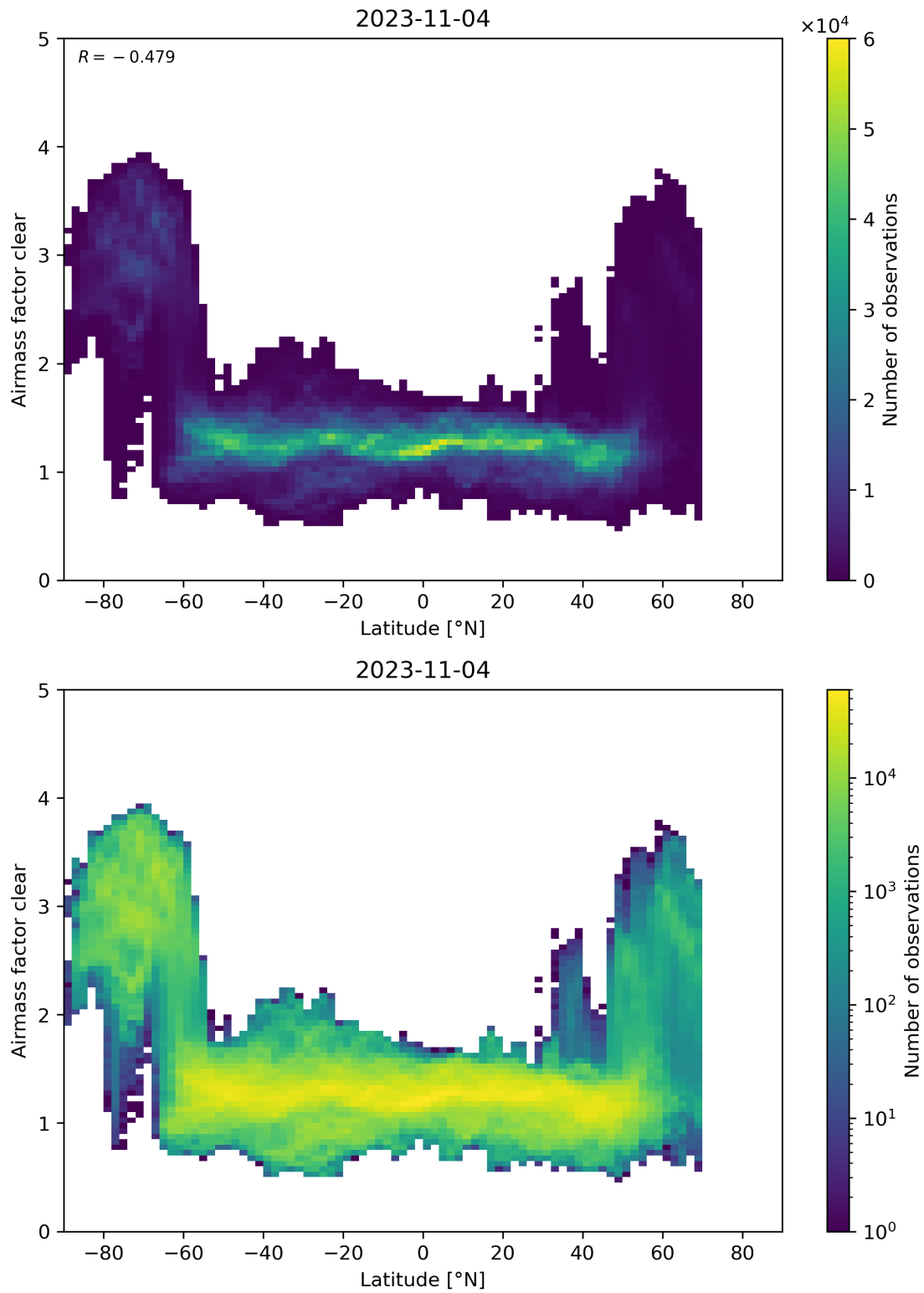
Figure 156: Scatter density plot of “Latitude” against “Airmass factor clear” for 2023-11-03 to 2023-11-05.
