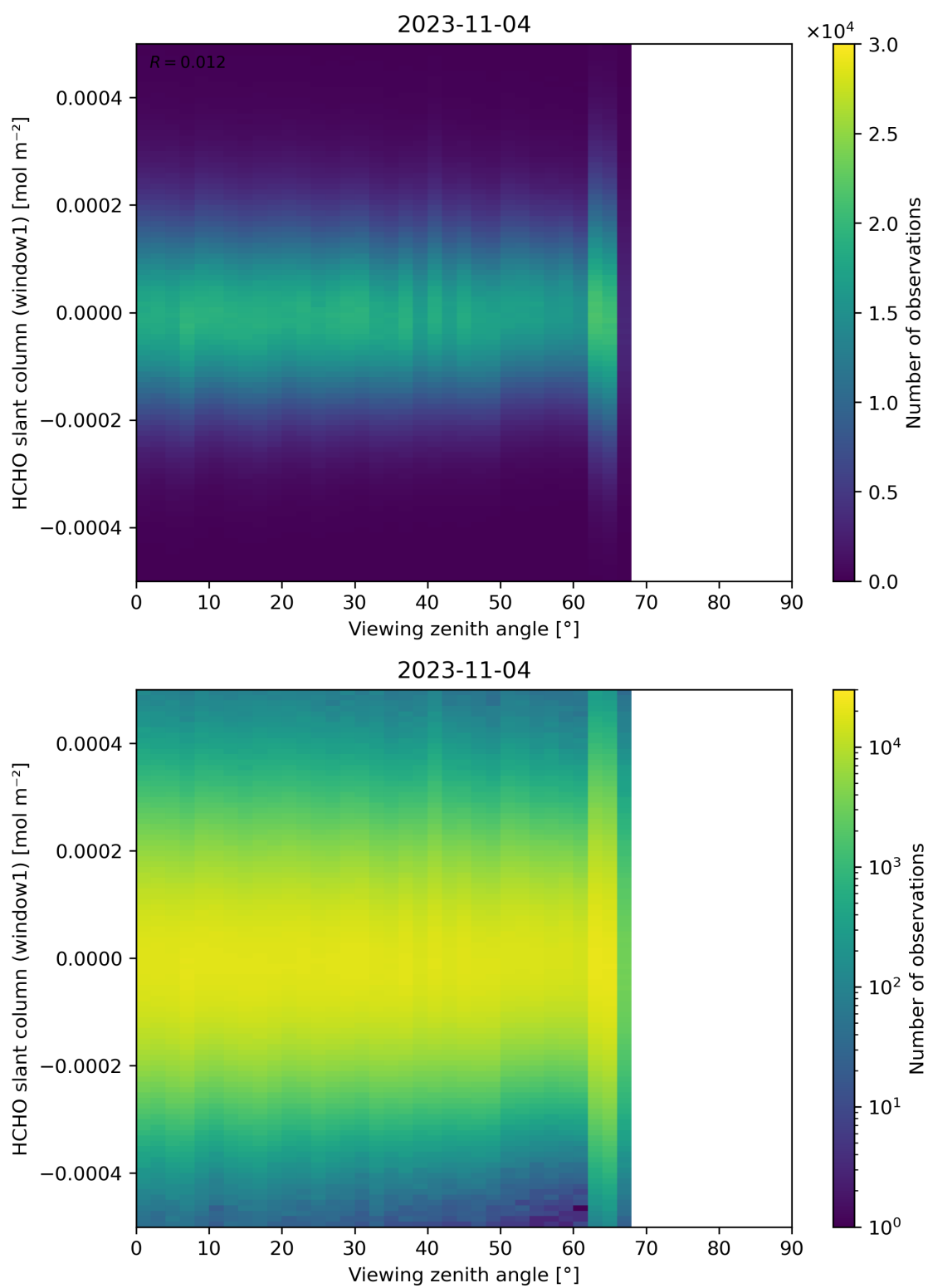
Figure 188: Scatter density plot of “Viewing zenith angle” against “HCHO slant column (window1)” for 2023-11-03 to 2023-11-05.
