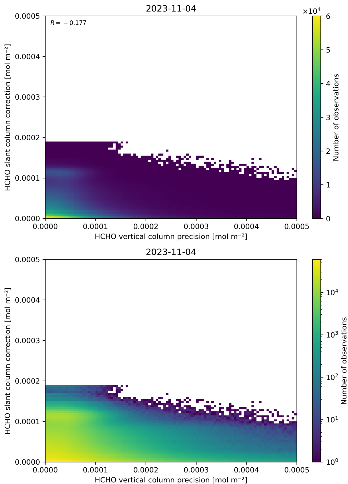
Figure 141: Scatter density plot of “HCHO vertical column precision” against “HCHO slant column correction” for 2023-11-03 to 2023-11-05.
