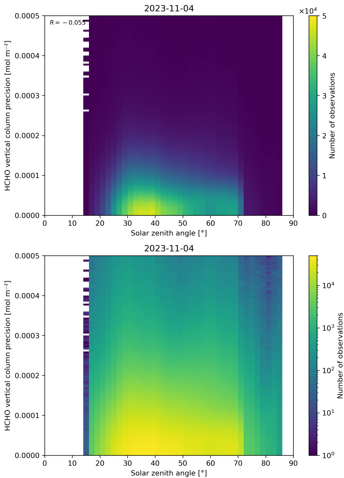
Figure 179: Scatter density plot of “Solar zenith angle” against “HCHO vertical column precision” for 2023-11-03 to 2023-11-05.
