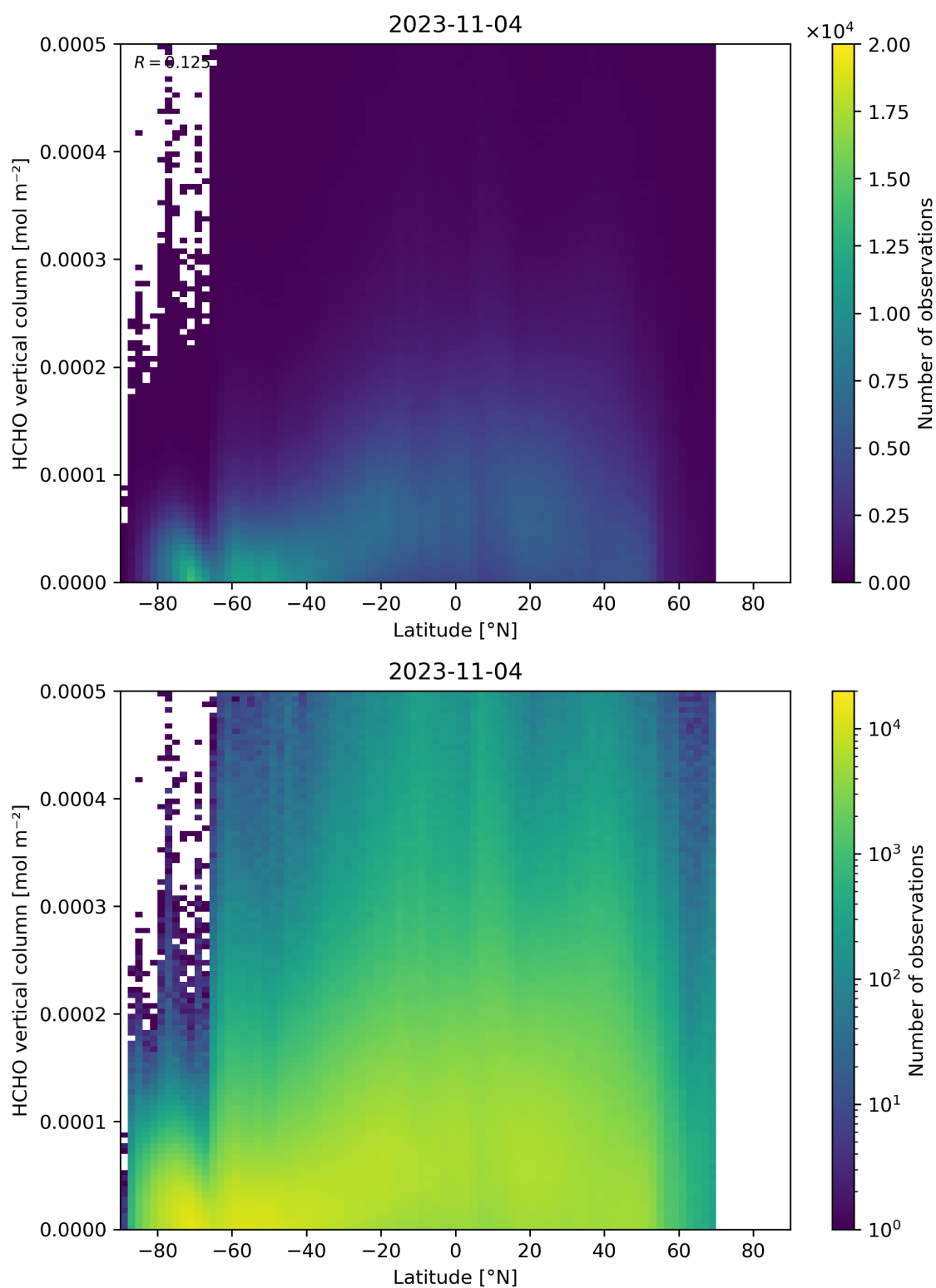
Figure 163: Scatter density plot of “Latitude” against “HCHO vertical column” for 2023-11-03 to 2023-11-05.
