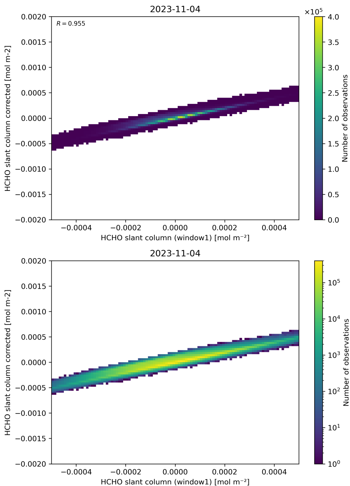
Figure 82: Scatter density plot of “HCHO slant column (window1)” against “HCHO slant column corrected” for 2023-11-03 to 2023-11-05.
