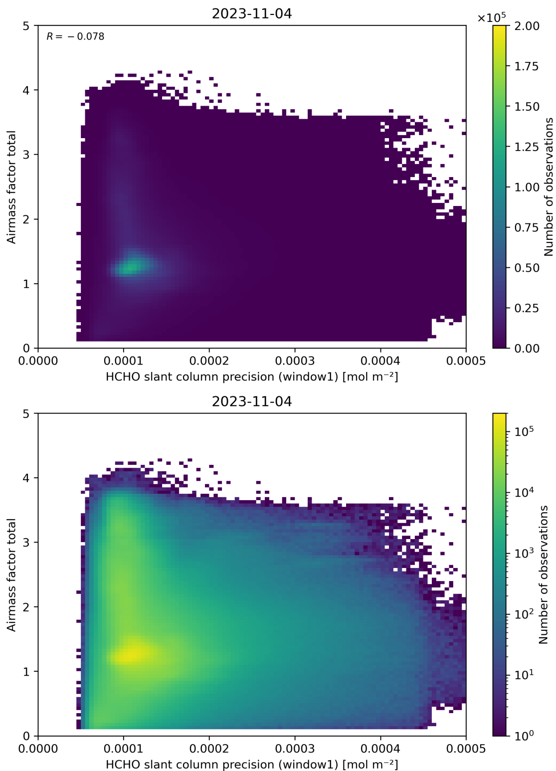
Figure 94: Scatter density plot of “HCHO slant column precision (window1)” against “Airmass factor total” for 2023-11-03 to 2023-11-05.
