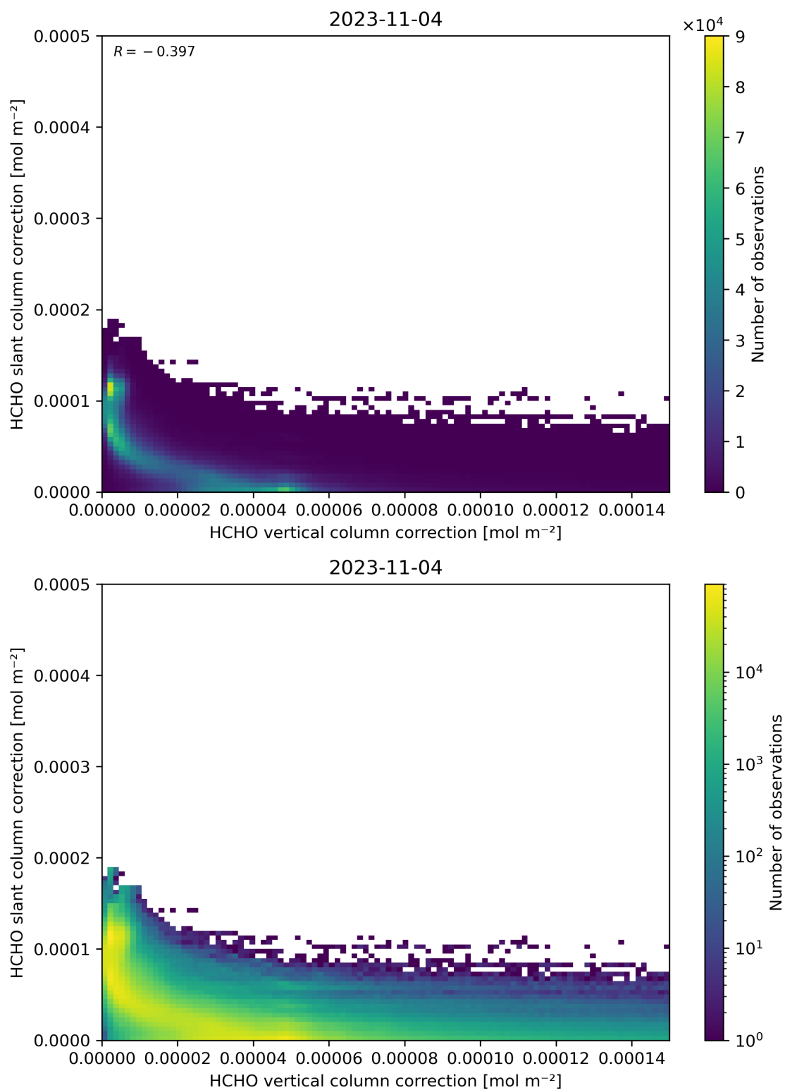
Figure 117: Scatter density plot of “HCHO vertical column correction” against “HCHO slant column correction” for 2023-11-03 to 2023-11-05.
