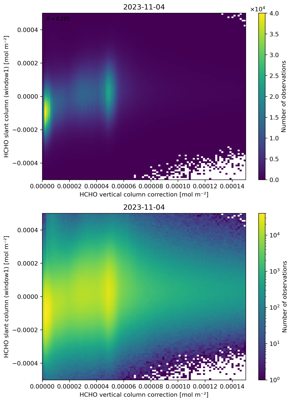
Figure 118: Scatter density plot of “HCHO vertical column correction” against “HCHO slant column (window1)” for 2023-11-03 to 2023-11-05.
