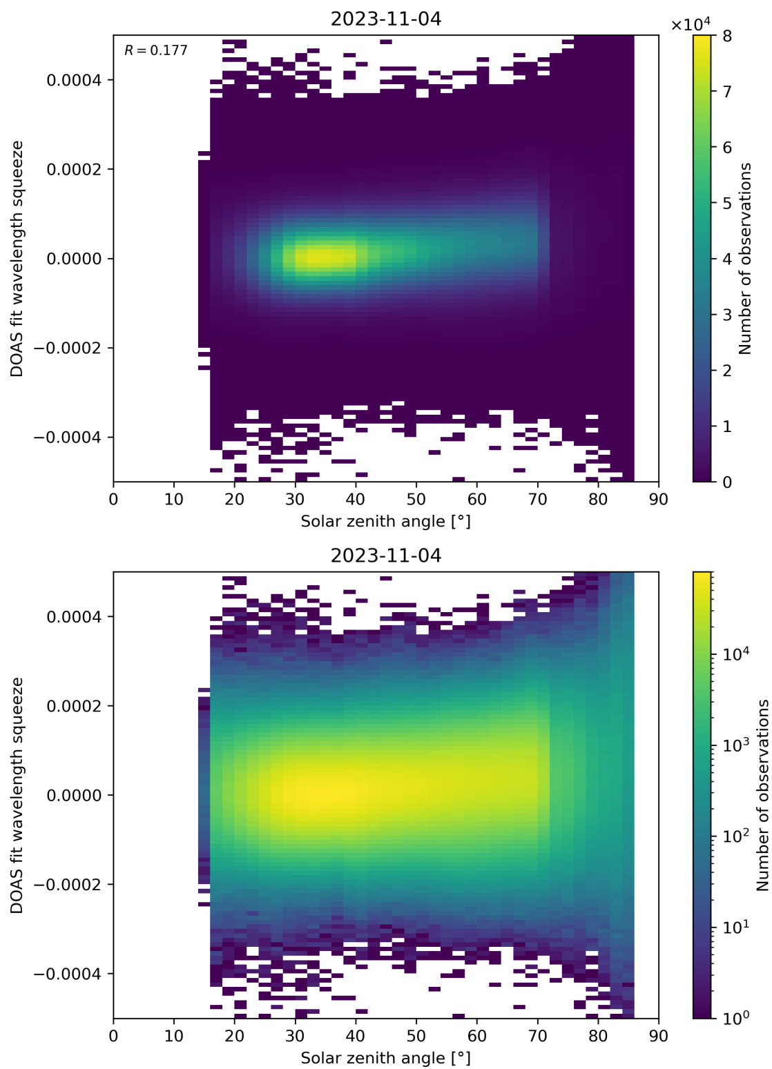
Figure 169: Scatter density plot of “Solar zenith angle” against “DOAS fit wavelength squeeze” for 2023-11-03 to 2023-11-05.
