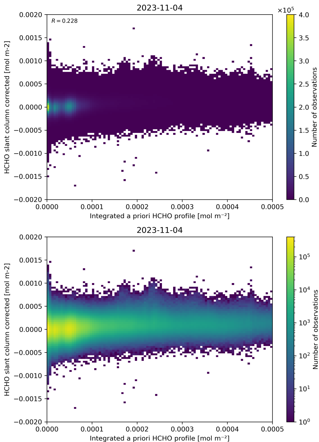
Figure 151: Scatter density plot of “Integrated a priori HCHO profile” against “HCHO slant column corrected” for 2023-11-03 to 2023-11-05.
