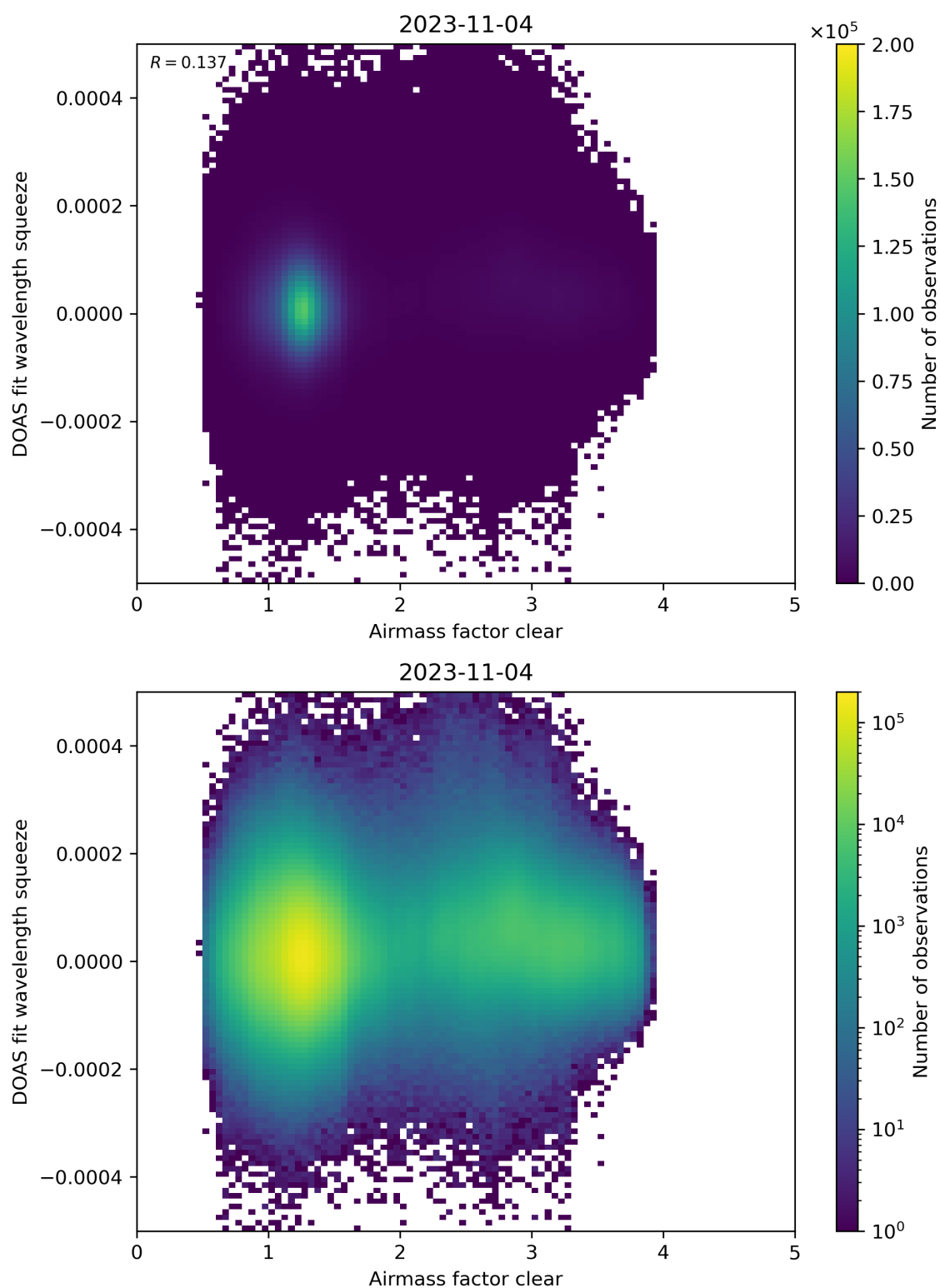
Figure 73: Scatter density plot of “Airmass factor clear” against “DOAS fit wavelength squeeze” for 2023-11-03 to 2023-11-05.
