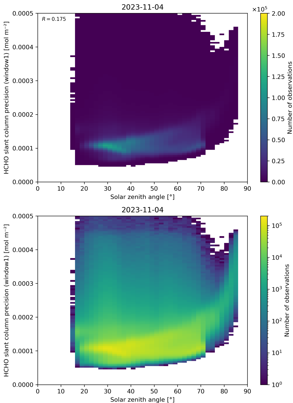
Figure 174: Scatter density plot of “Solar zenith angle” against “HCHO slant column precision (window1)” for 2023-11-03 to 2023-11-05.
