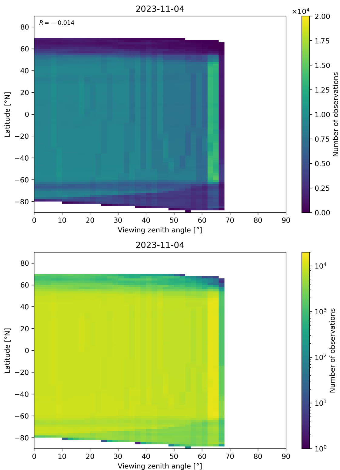
Figure 196: Scatter density plot of “Viewing zenith angle” against “Latitude” for 2023-11-03 to 2023-11-05.
