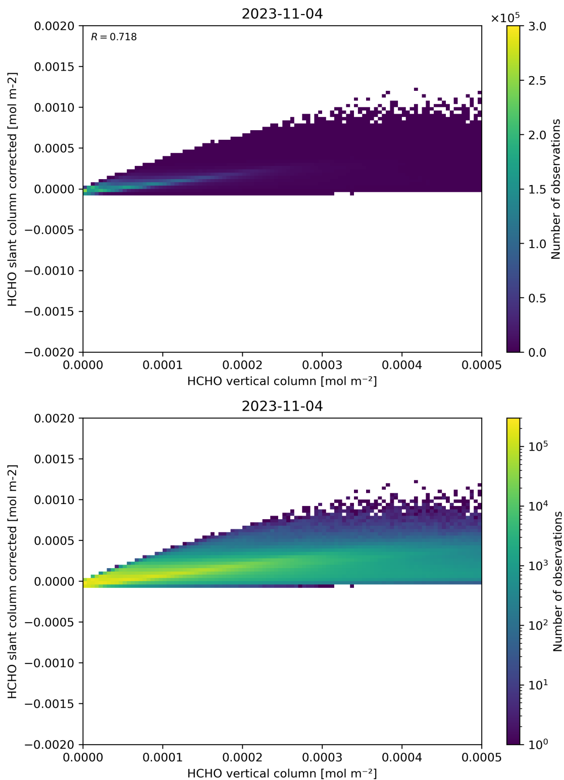
Figure 127: Scatter density plot of “HCHO vertical column” against “HCHO slant column corrected” for 2023-11-03 to 2023-11-05.
