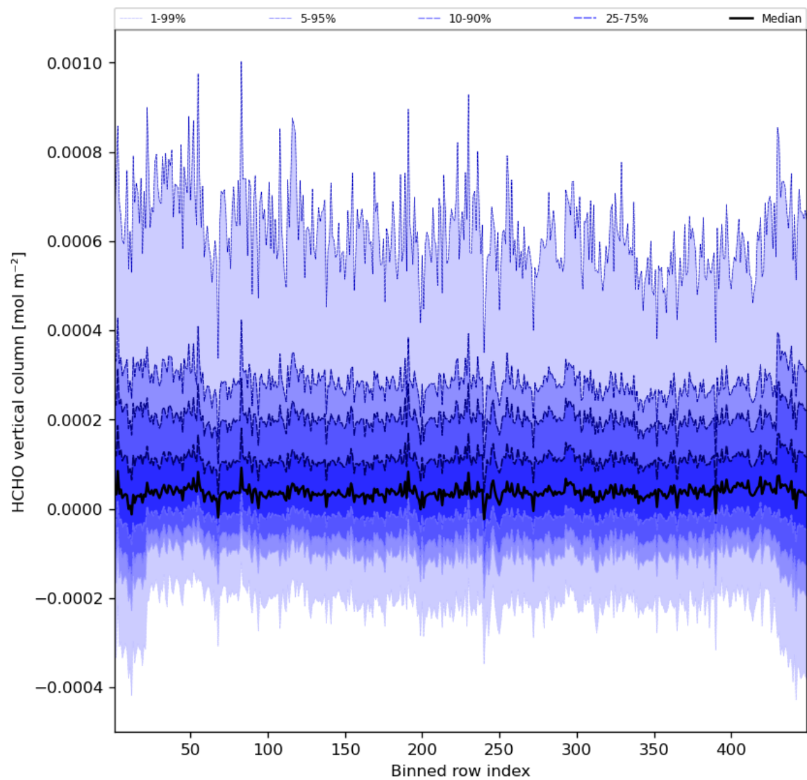
Figure 49: Along track statistics of “HCHO vertical column” for 2023-11-03 to 2023-11-05
