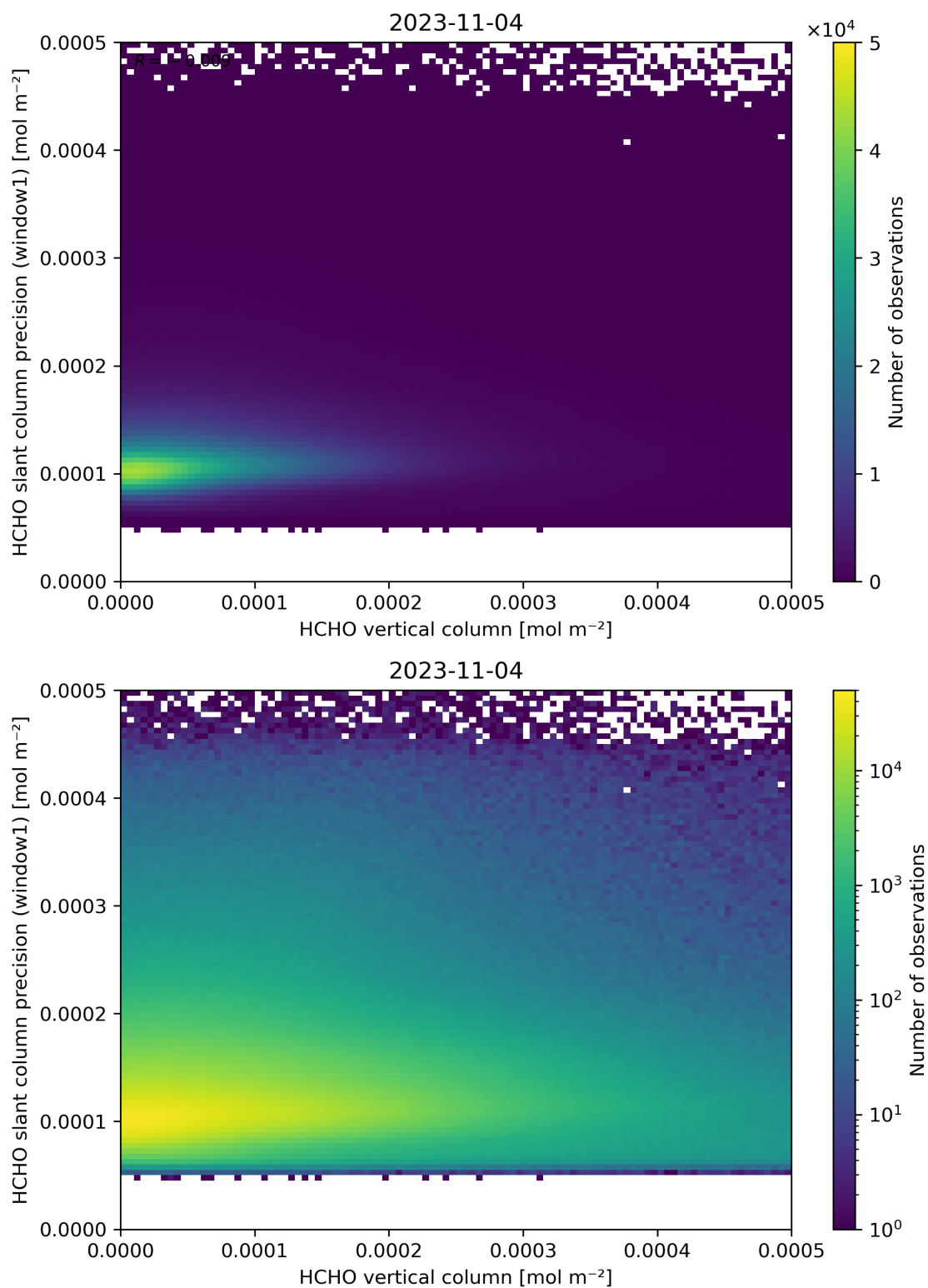
Figure 130: Scatter density plot of “HCHO vertical column” against “HCHO slant column precision (window1)” for 2023-11-03 to 2023-11-05.
