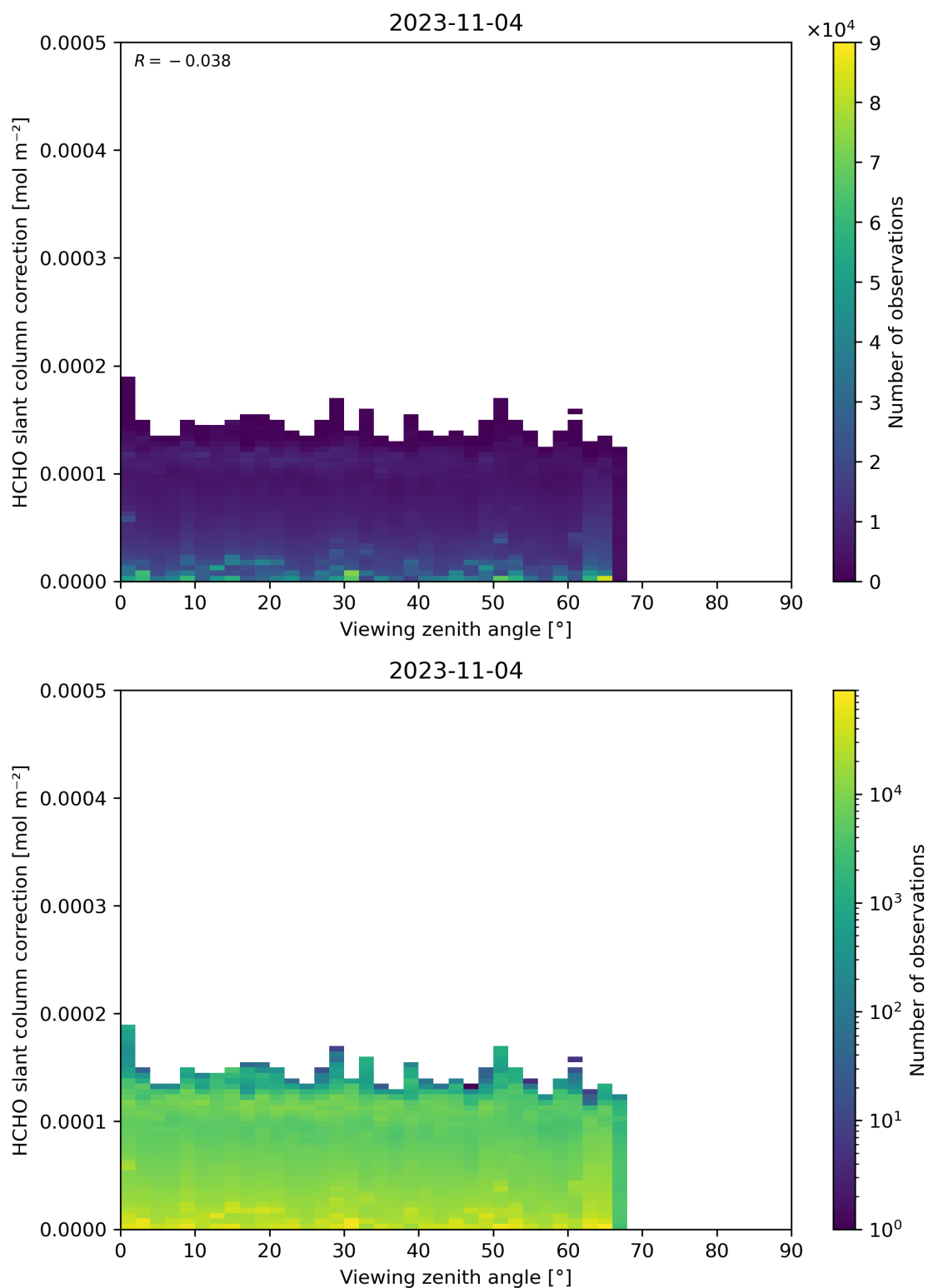
Figure 187: Scatter density plot of “Viewing zenith angle” against “HCHO slant column correction” for 2023-11-03 to 2023-11-05.
