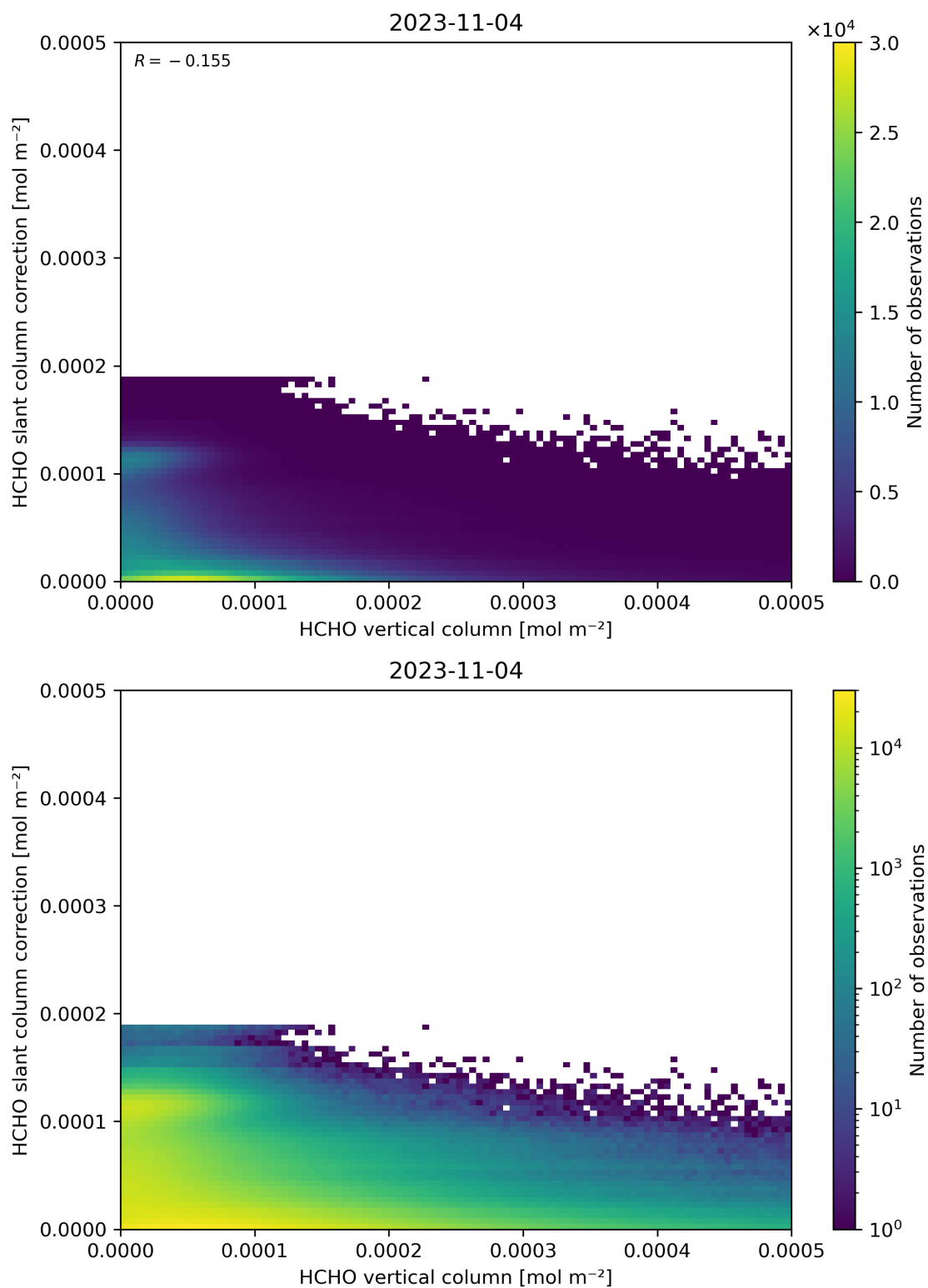
Figure 128: Scatter density plot of “HCHO vertical column” against “HCHO slant column correction” for 2023-11-03 to 2023-11-05.
