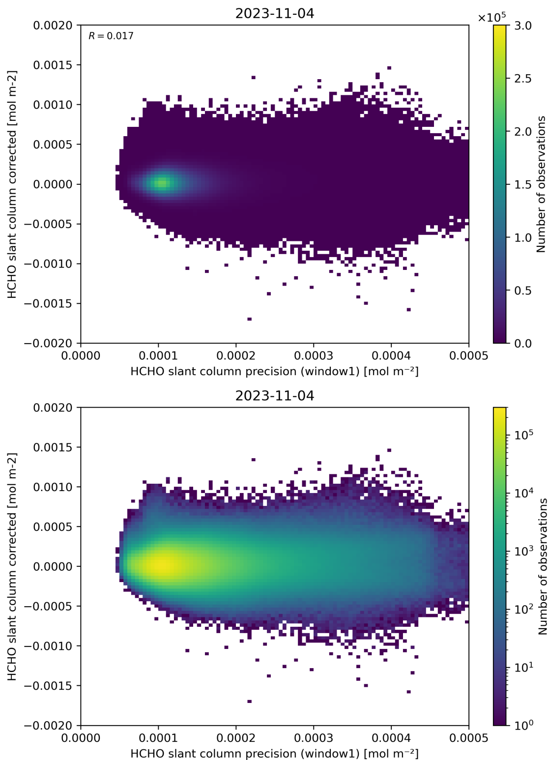
Figure 92: Scatter density plot of “HCHO slant column precision (window1)” against “HCHO slant column corrected” for 2023-11-03 to 2023-11-05.
