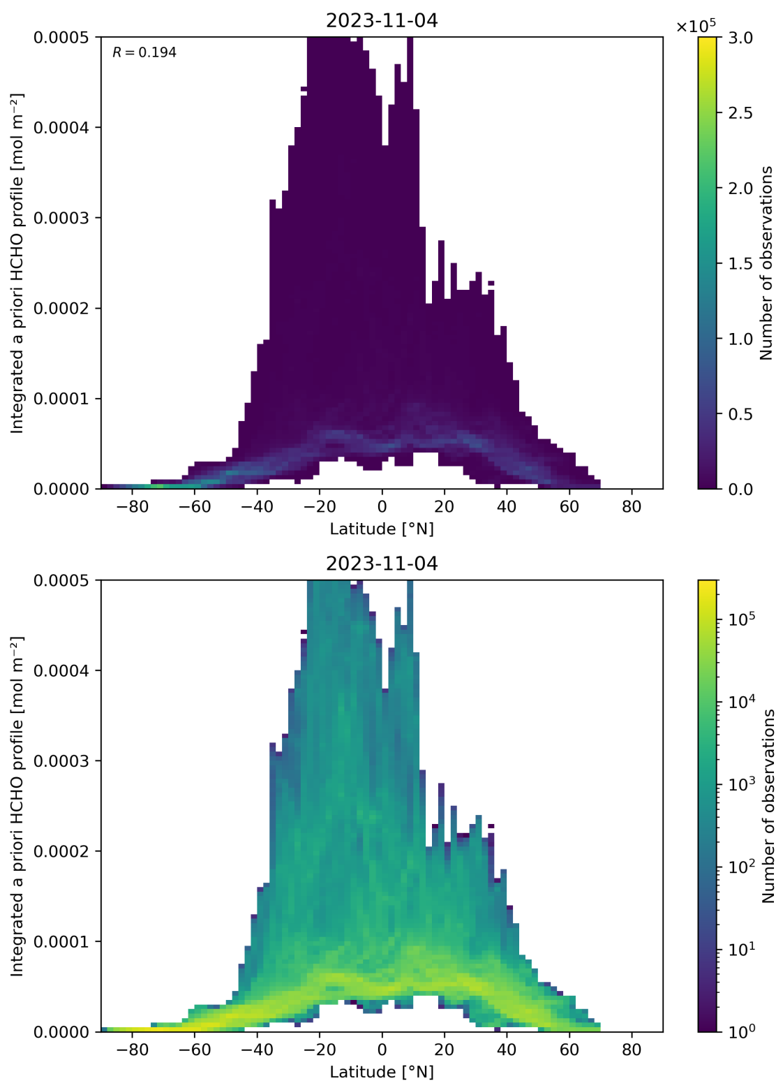
Figure 166: Scatter density plot of “Latitude” against “Integrated a priori HCHO profile” for 2023-11-03 to 2023-11-05.
