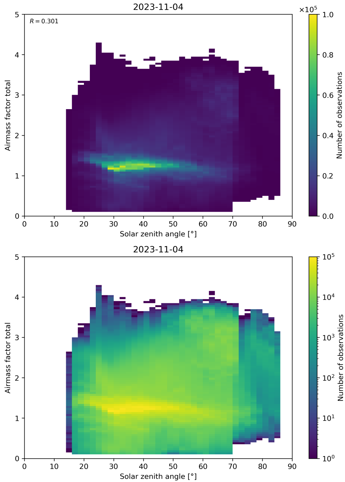
Figure 175: Scatter density plot of “Solar zenith angle” against “Airmass factor total” for 2023-11-03 to 2023-11-05.
