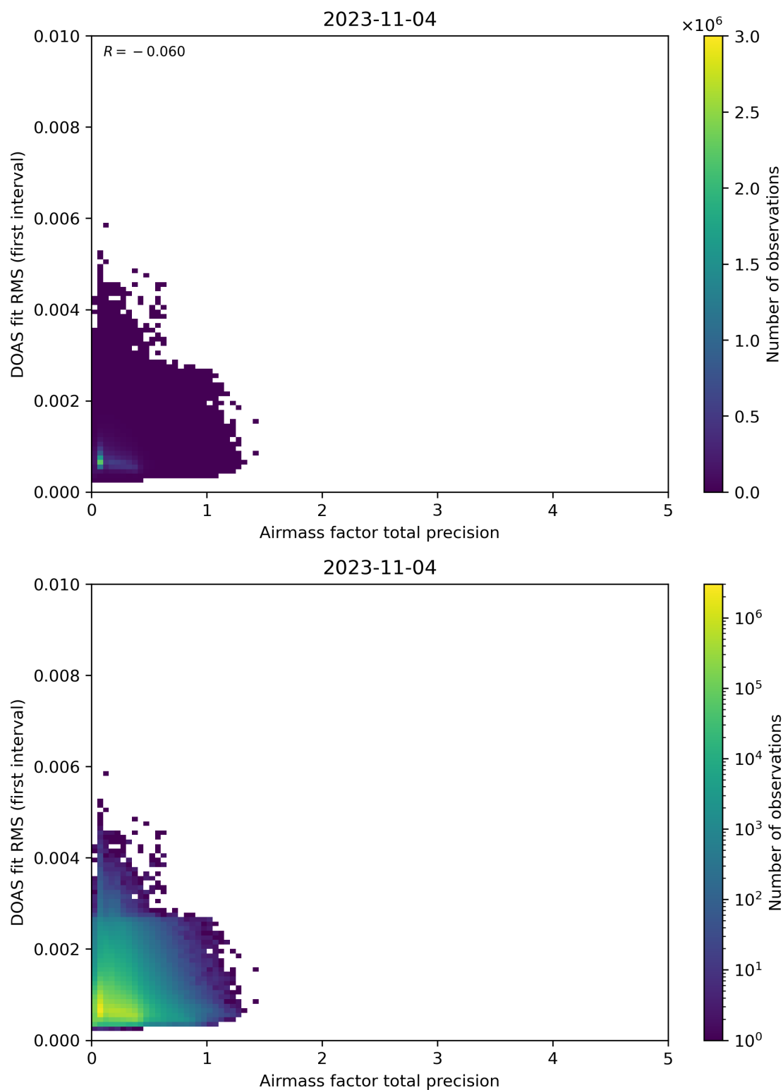
Figure 105: Scatter density plot of “Airmass factor total precision” against “DOAS fit RMS (first interval)” for 2023-11-03 to 2023-11-05.
