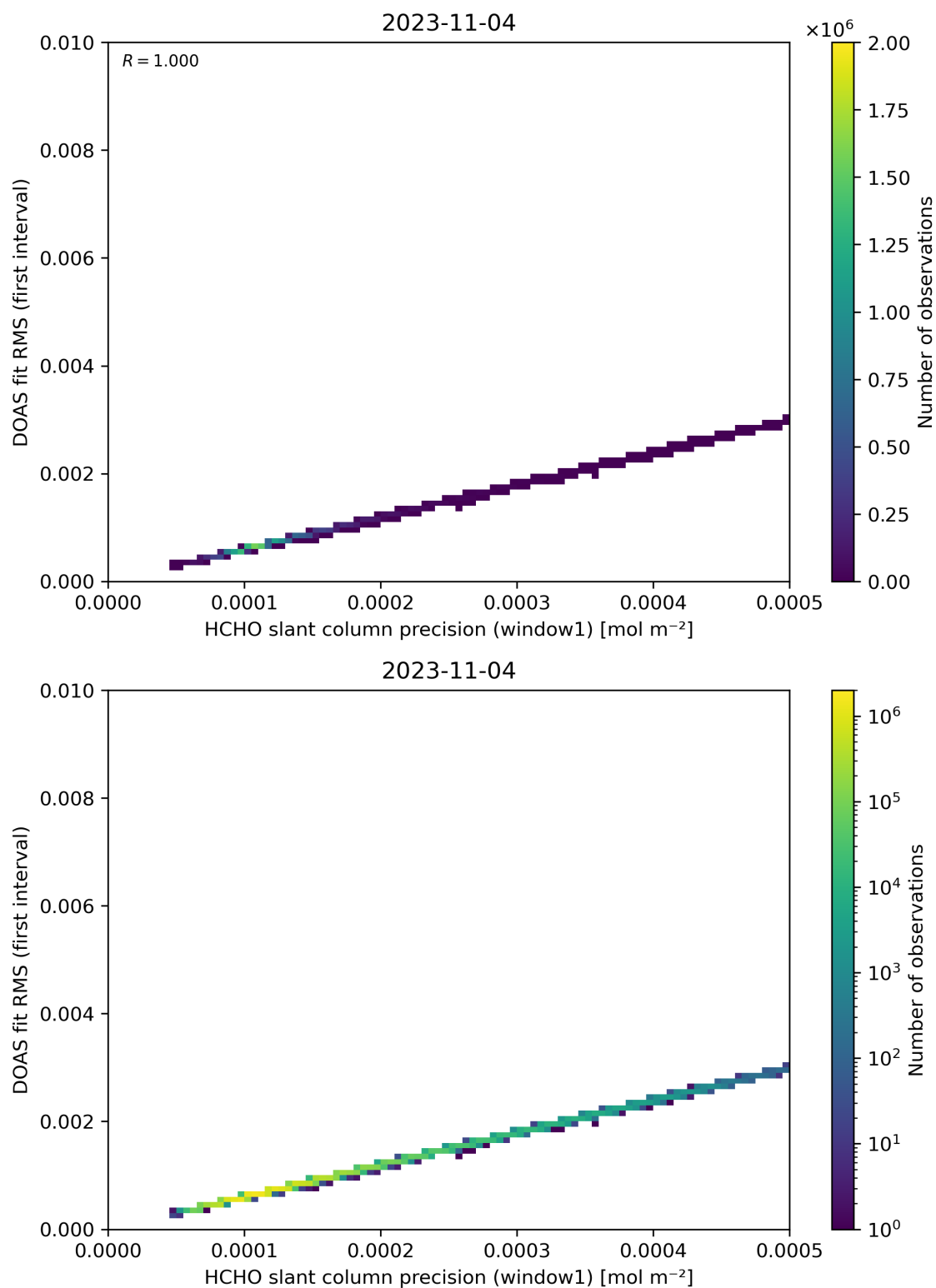
Figure 88: Scatter density plot of “HCHO slant column precision (window1)” against “DOAS fit RMS (first interval)” for 2023-11-03 to 2023-11-05.
