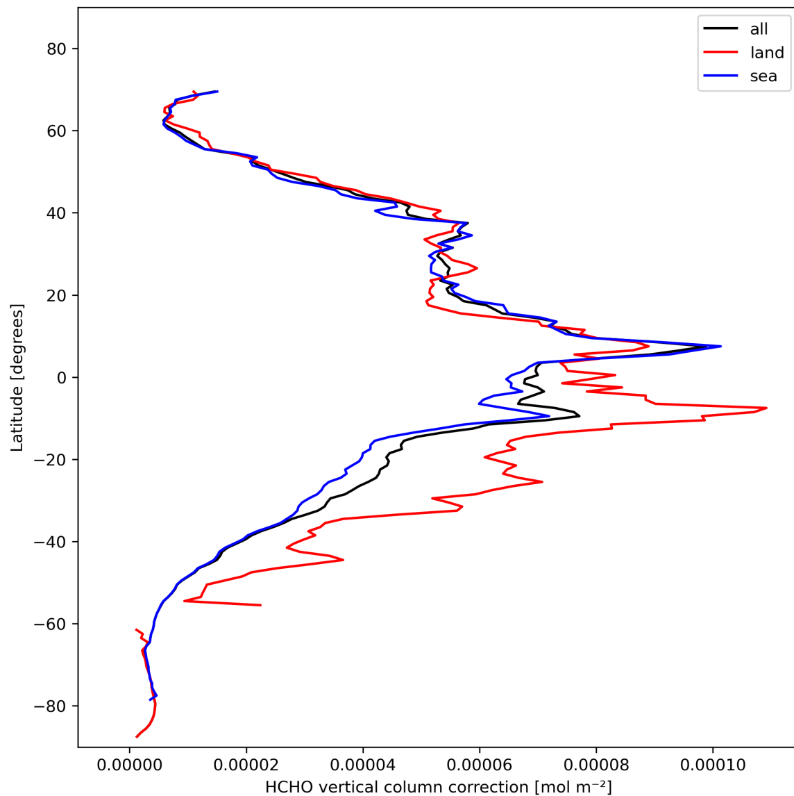
Figure 23: Zonal average of “HCHO vertical column correction” for 2023-11-03 to 2023-11-05.
