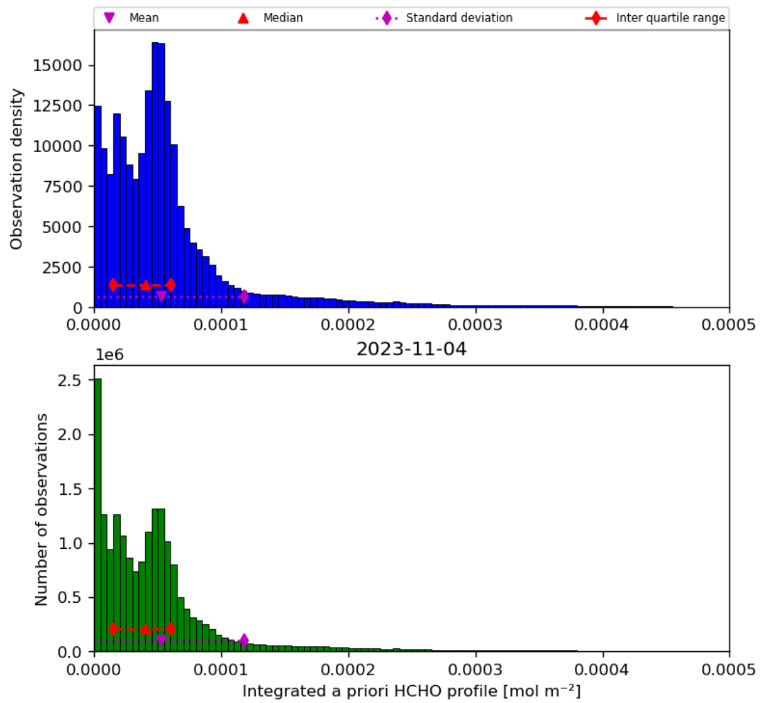
Figure 43: Histogram of “Integrated a priori HCHO profile” for 2023-11-03 to 2023-11-05
