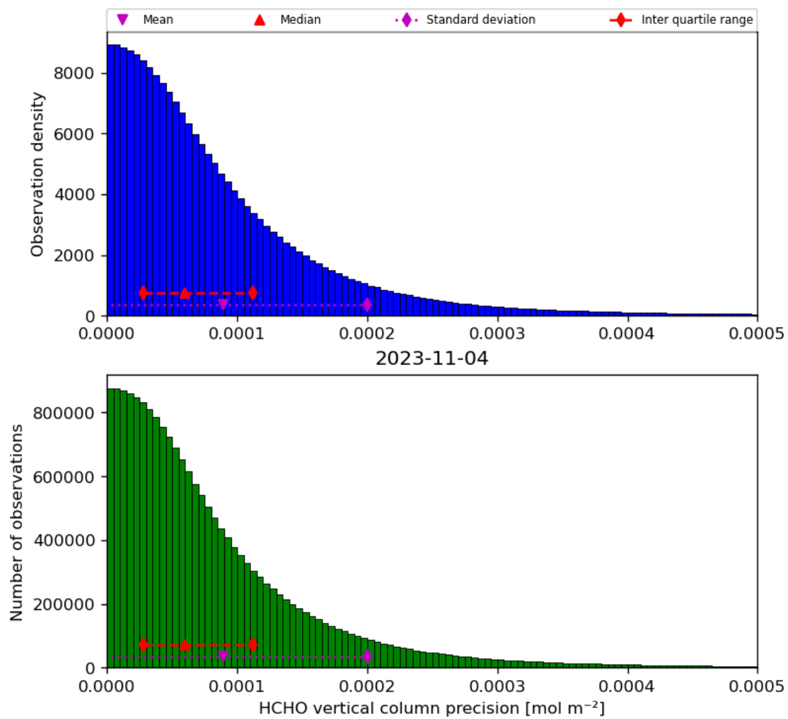
Figure 36: Histogram of “HCHO vertical column precision” for 2023-11-03 to 2023-11-05
