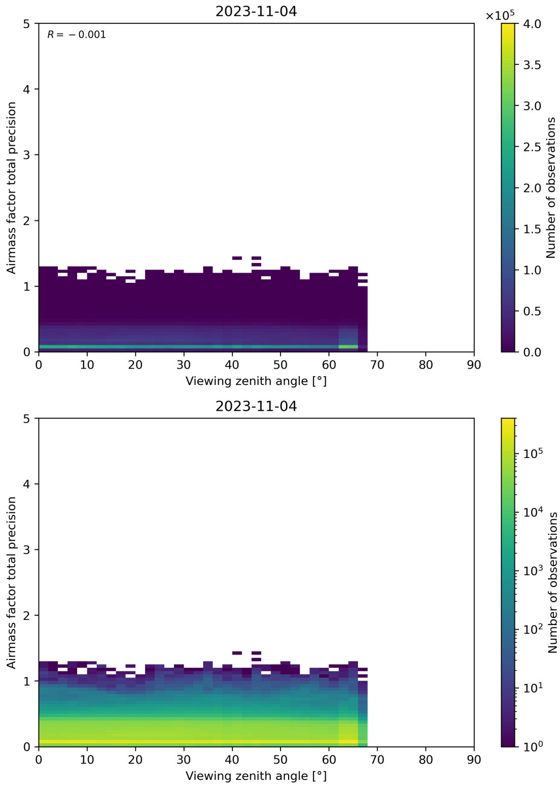
Figure 191: Scatter density plot of “Viewing zenith angle” against “Airmass factor total precision” for 2023-11-03 to 2023-11-05.
