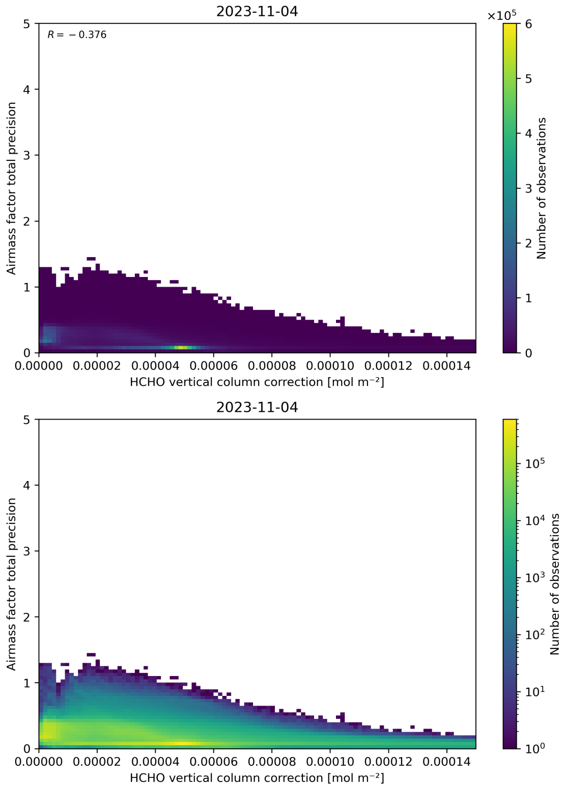
Figure 121: Scatter density plot of “HCHO vertical column correction” against “Airmass factor total precision” for 2023-11-03 to 2023-11-05.
