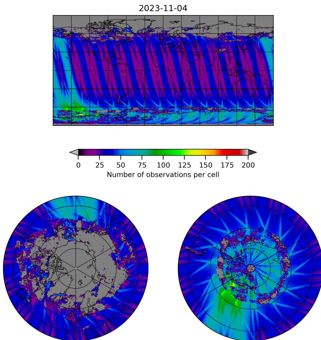
Figure 19: Map of the number of observations for 2023-11-03 to 2023-11-05
