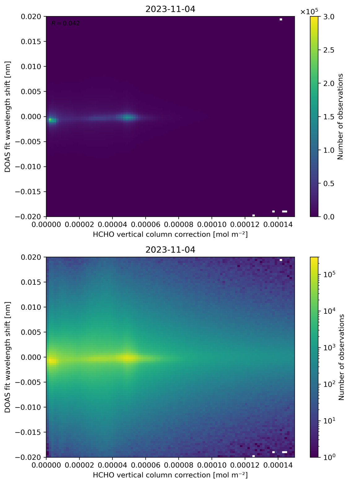
Figure 113: Scatter density plot of “HCHO vertical column correction” against “DOAS fit wavelength shift” for 2023-11-03 to 2023-11-05.
