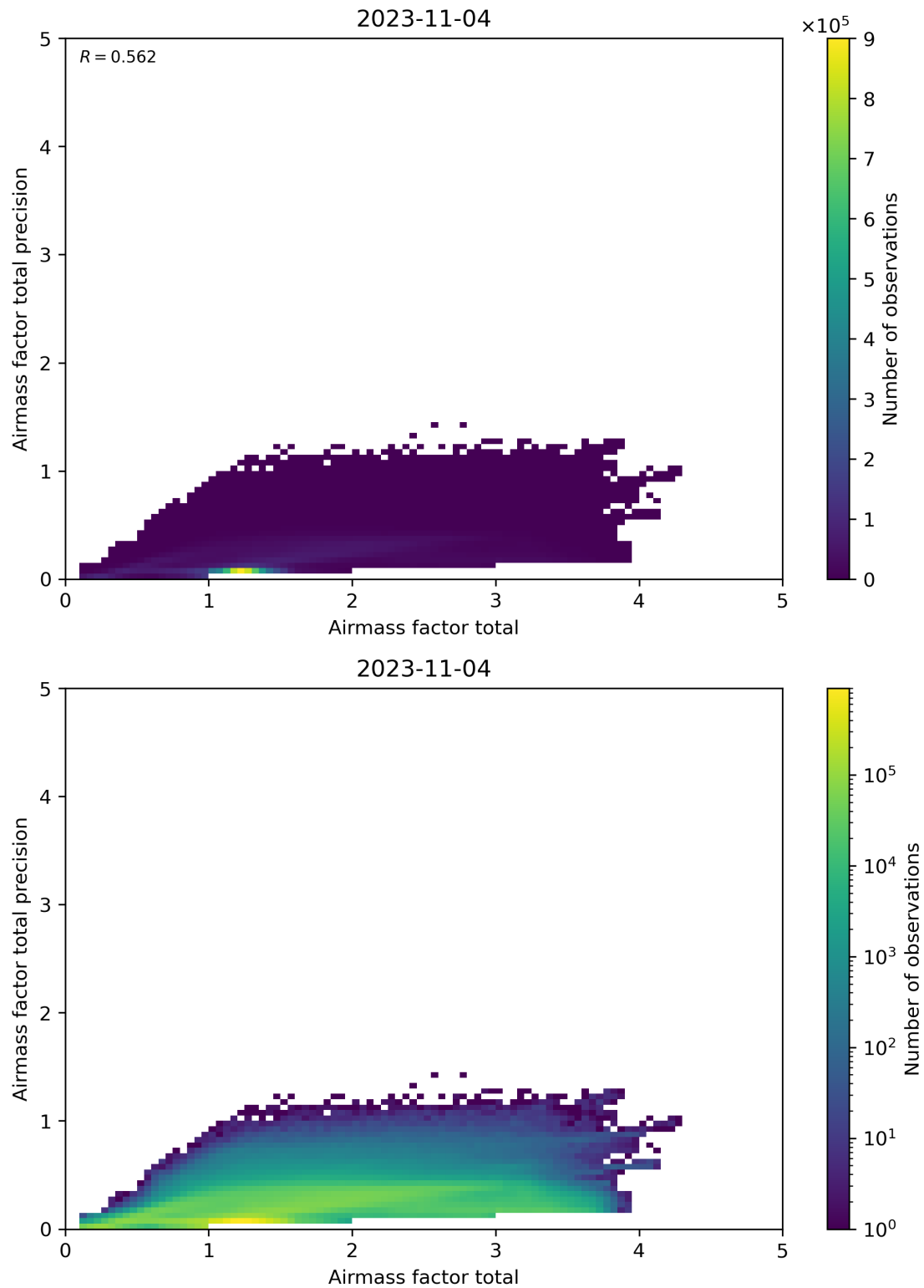
Figure 103: Scatter density plot of “Airmass factor total” against “Airmass factor total precision” for 2023-11-03 to 2023-11-05.
