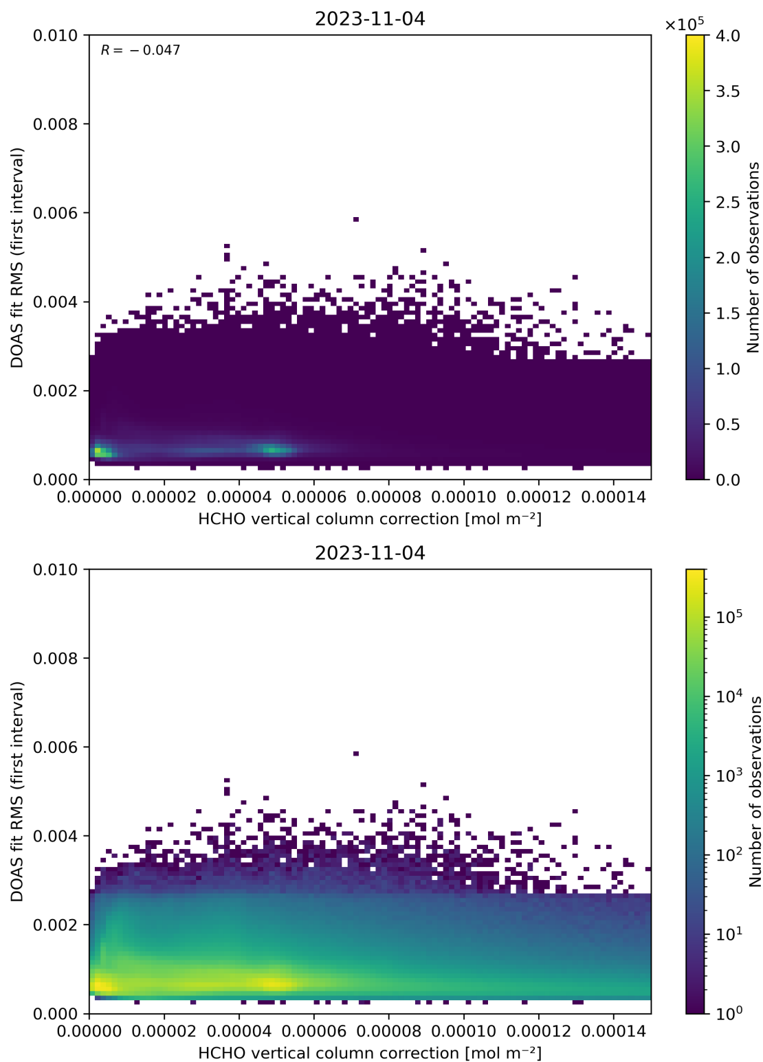
Figure 112: Scatter density plot of “HCHO vertical column correction” against “DOAS fit RMS (first interval)” for 2023-11-03 to 2023-11-05.
