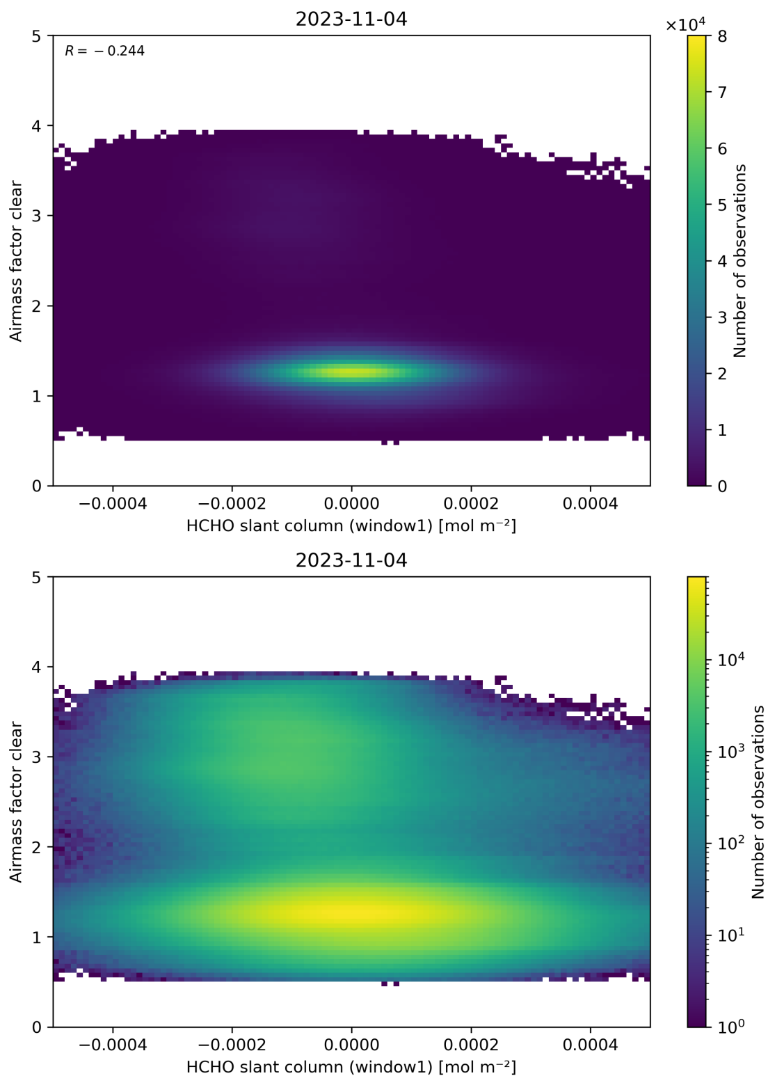
Figure 81: Scatter density plot of “HCHO slant column (window1)” against “Airmass factor clear” for 2023-11-03 to 2023-11-05.
