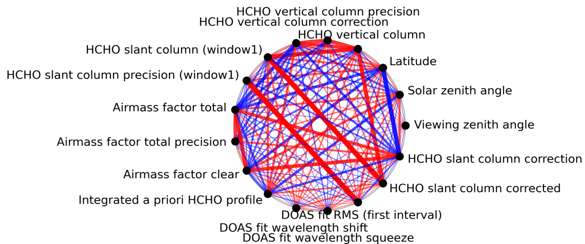
Figure 1: Map of correlation graph for 2023-11-03 to 2023-11-05.
