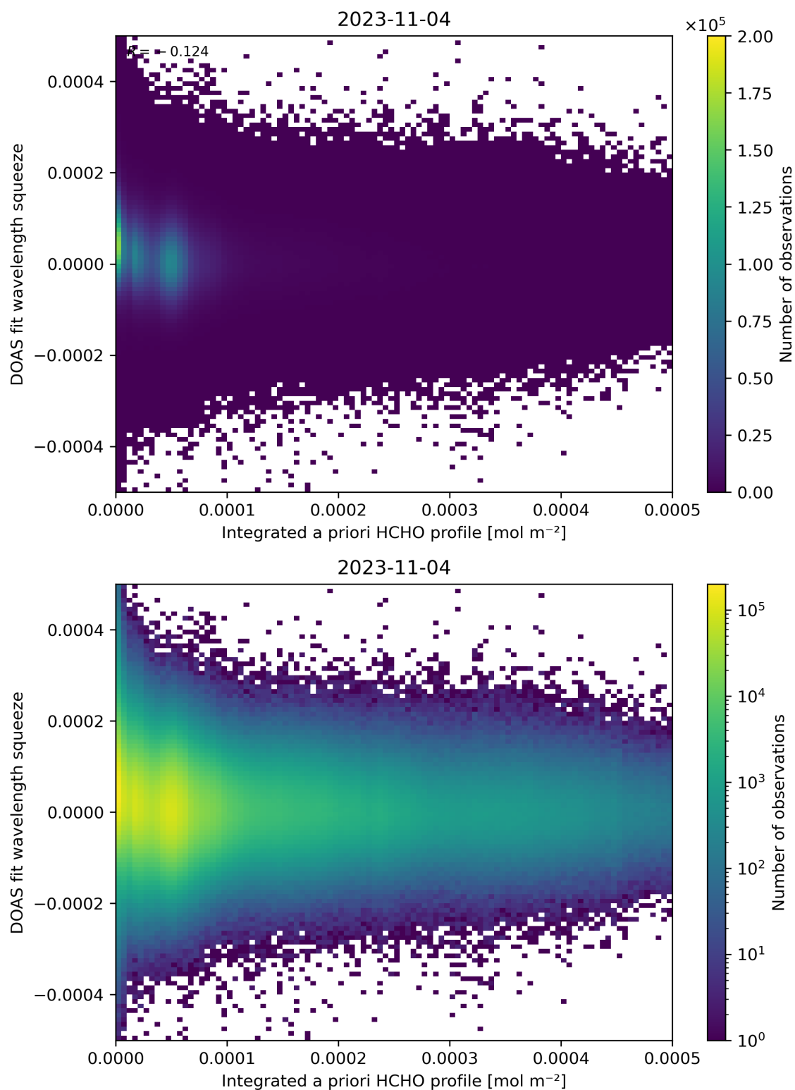
Figure 150: Scatter density plot of “Integrated a priori HCHO profile” against “DOAS fit wavelength squeeze” for 2023-11-03 to 2023-11-05.
