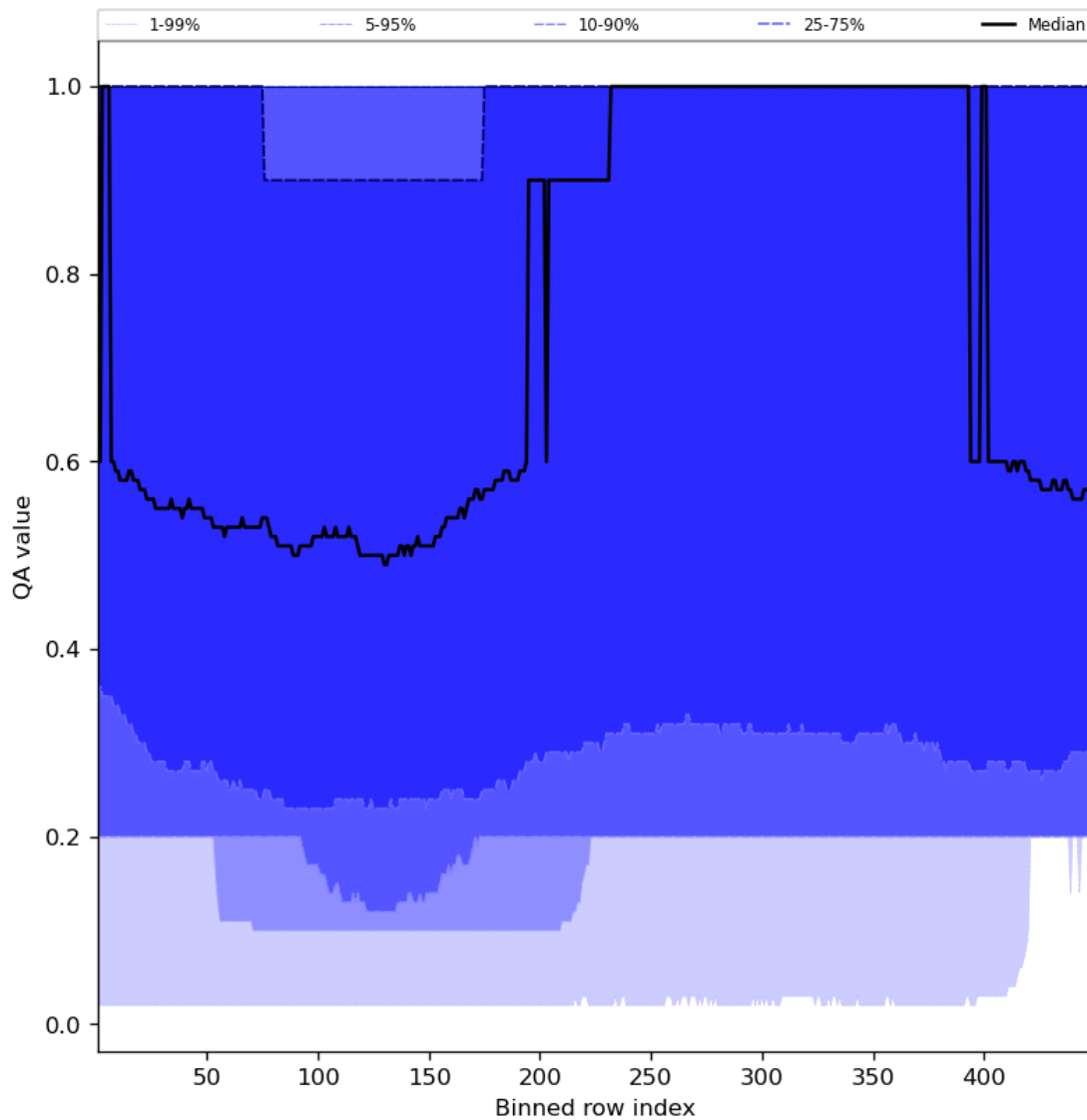
Figure 48: Along track statistics of “QA value” for 2023-11-03 to 2023-11-05
