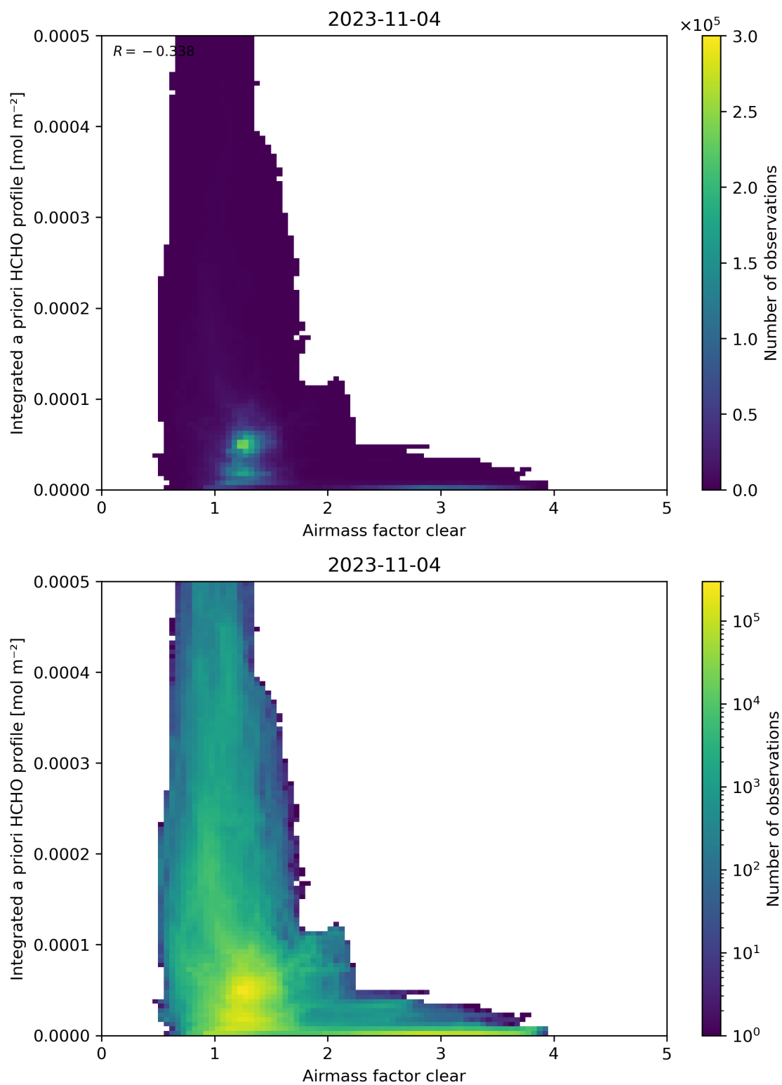
Figure 76: Scatter density plot of “Airmass factor clear” against “Integrated a priori HCHO profile” for 2023-11-03 to 2023-11-05.
