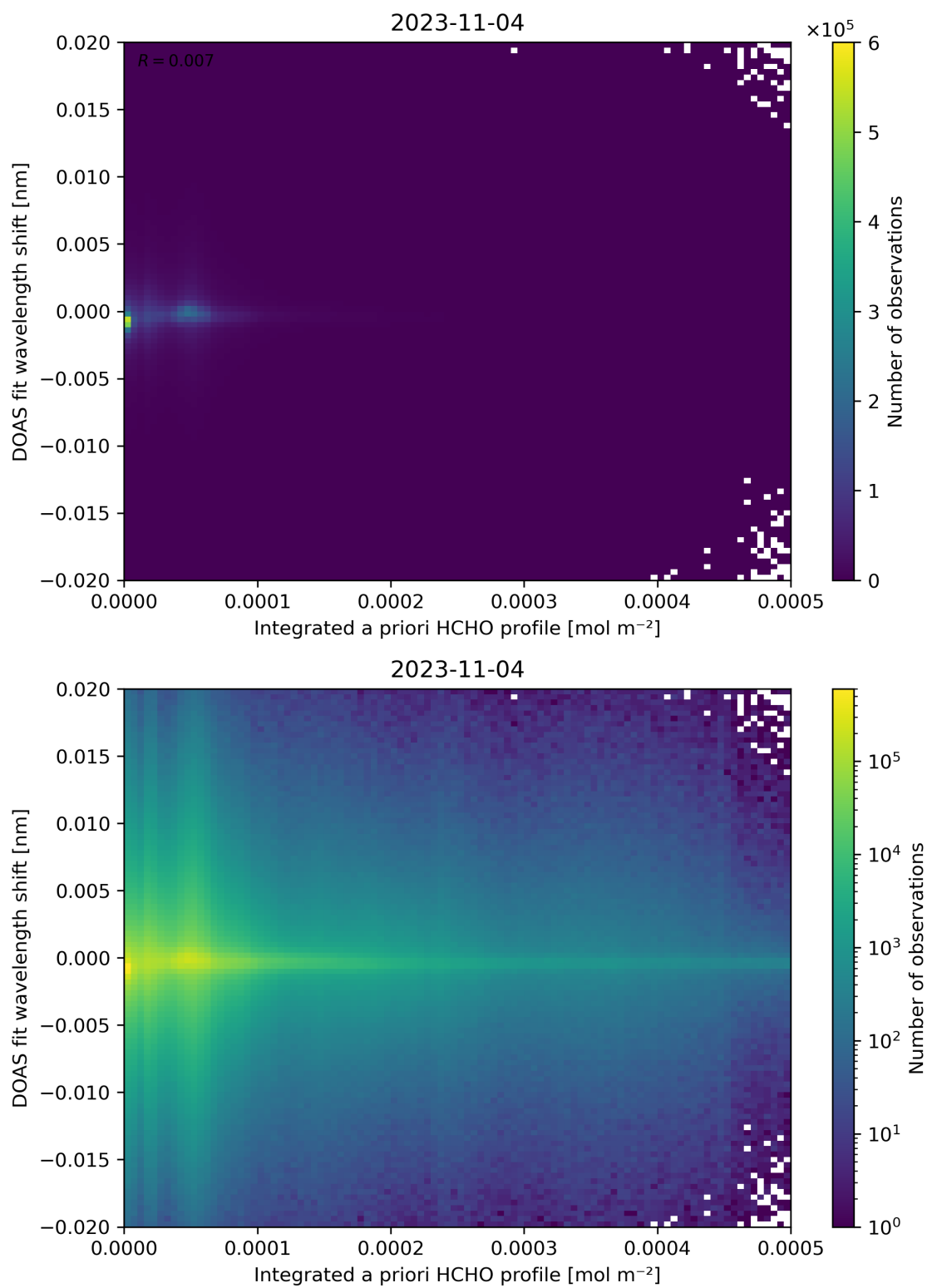
Figure 149: Scatter density plot of “Integrated a priori HCHO profile” against “DOAS fit wavelength shift” for 2023-11-03 to 2023-11-05.
