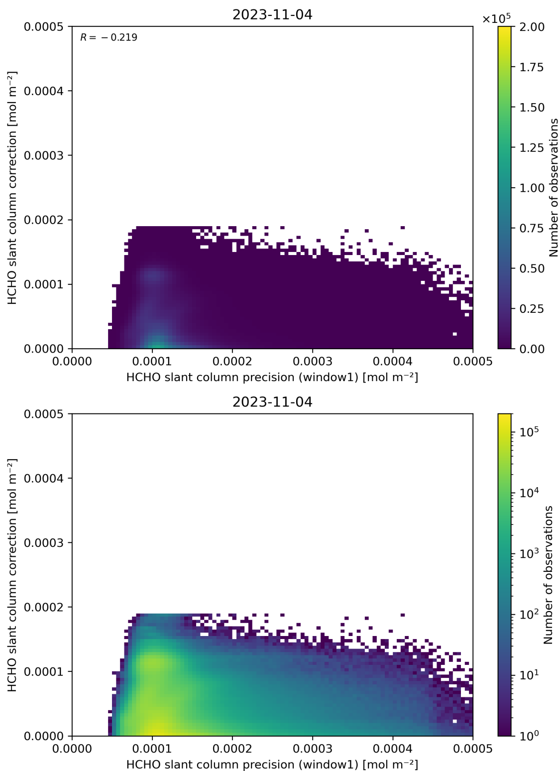
Figure 93: Scatter density plot of “HCHO slant column precision (window1)” against “HCHO slant column correction” for 2023-11-03 to 2023-11-05.
