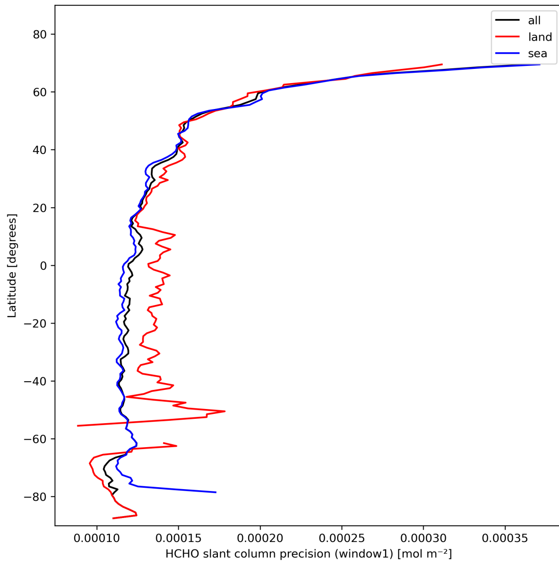
Figure 25: Zonal average of “HCHO slant column precision (window1)” for 2023-11-03 to 2023-11-05.
