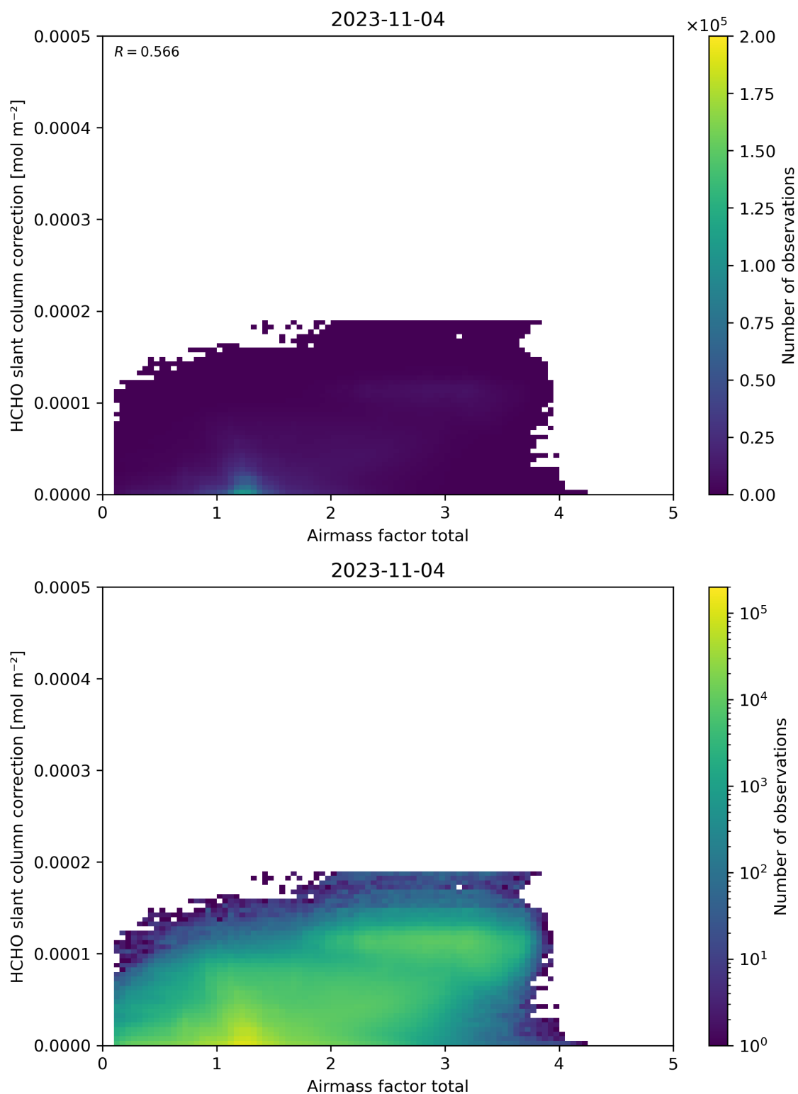
Figure 102: Scatter density plot of “Airmass factor total” against “HCHO slant column correction” for 2023-11-03 to 2023-11-05.
