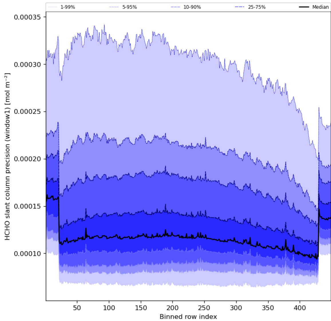
Figure 53: Along track statistics of “HCHO slant column precision (window1)” for 2023-11-03 to 2023-11-05
