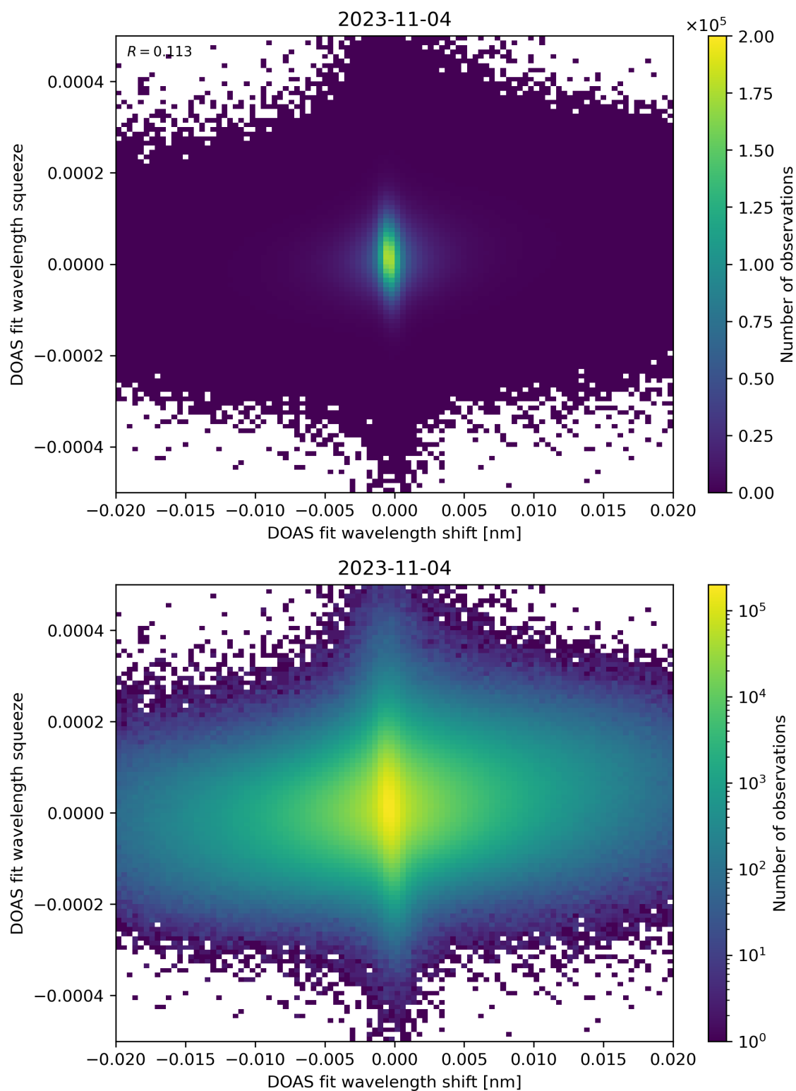
Figure 65: Scatter density plot of “DOAS fit wavelength shift” against “DOAS fit wavelength squeeze” for 2023-11-03 to 2023-11-05.
