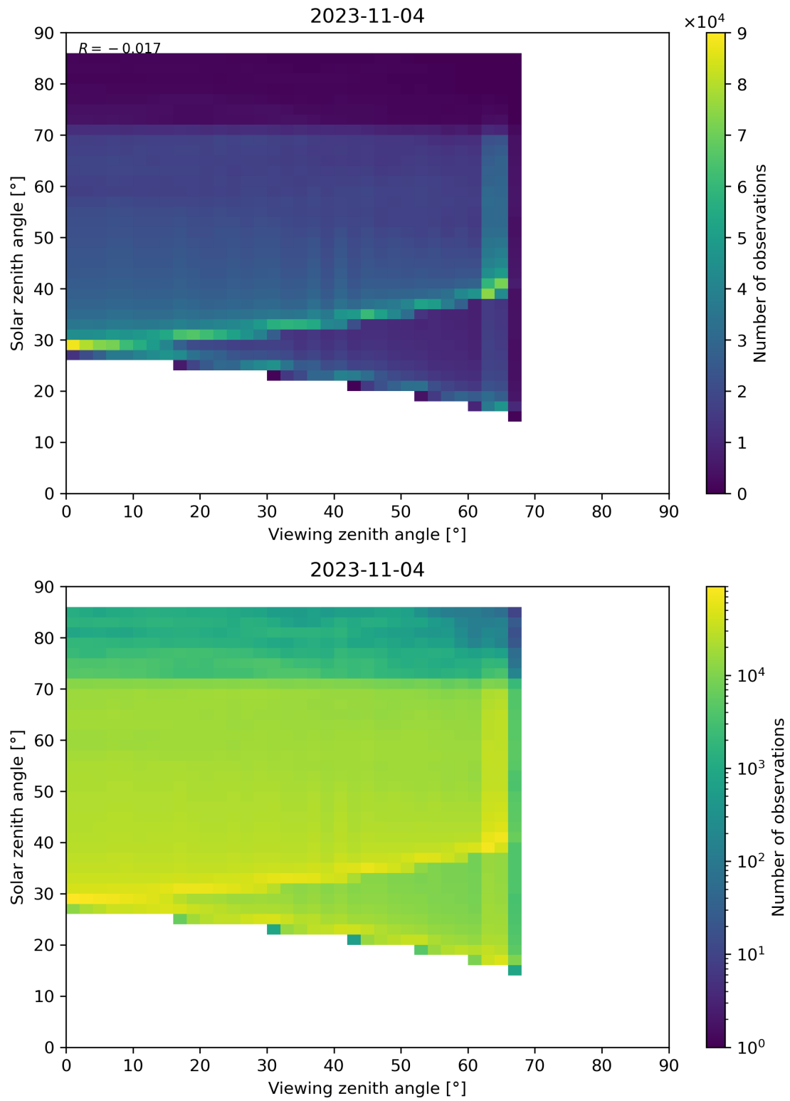
Figure 197: Scatter density plot of “Viewing zenith angle” against “Solar zenith angle” for 2023-11-03 to 2023-11-05.
