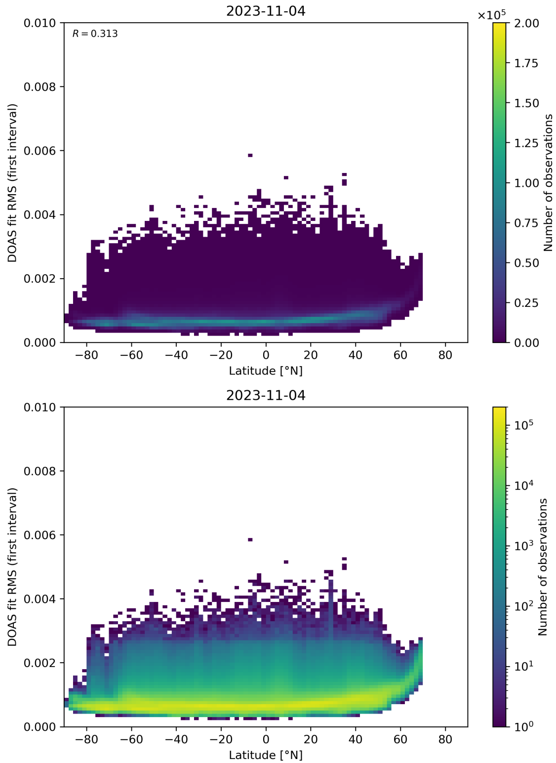
Figure 153: Scatter density plot of “Latitude” against “DOAS fit RMS (first interval)” for 2023-11-03 to 2023-11-05.
