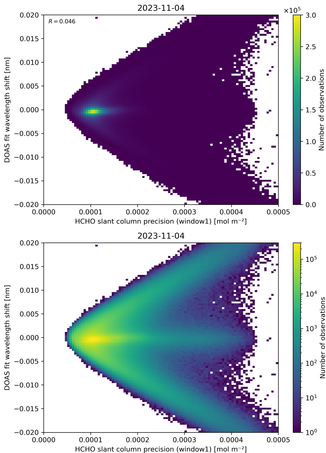
Figure 89: Scatter density plot of “HCHO slant column precision (window1)” against “DOAS fit wavelength shift” for 2023-11-03 to 2023-11-05.
