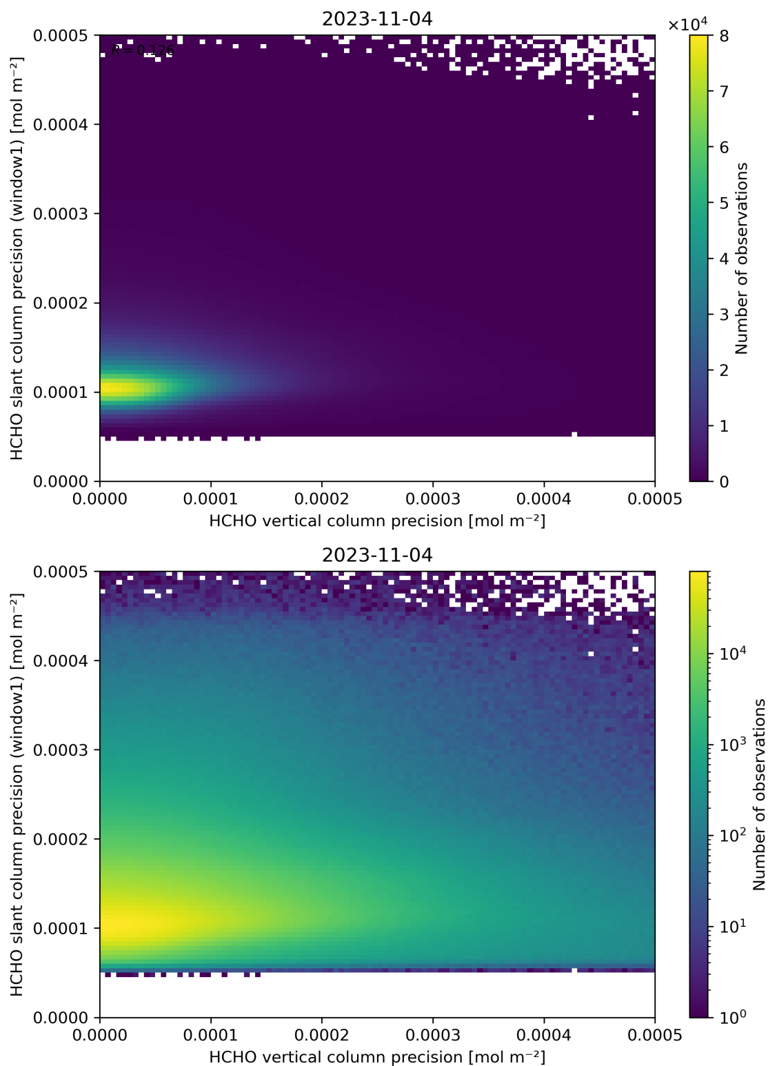
Figure 143: Scatter density plot of “HCHO vertical column precision” against “HCHO slant column precision (window1)” for 2023-11-03 to 2023-11-05.
