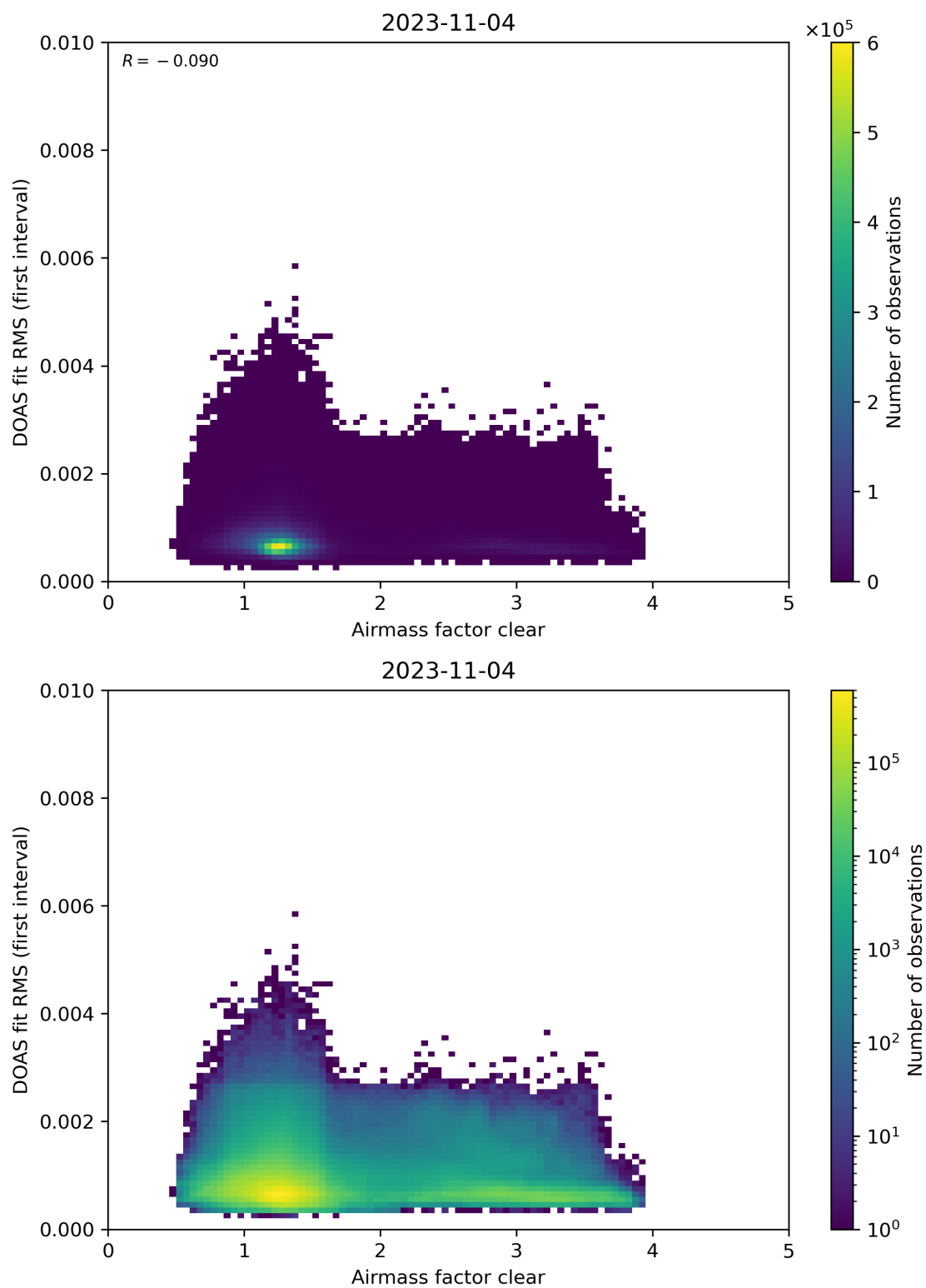
Figure 71: Scatter density plot of “Airmass factor clear” against “DOAS fit RMS (first interval)” for 2023-11-03 to 2023-11-05.
