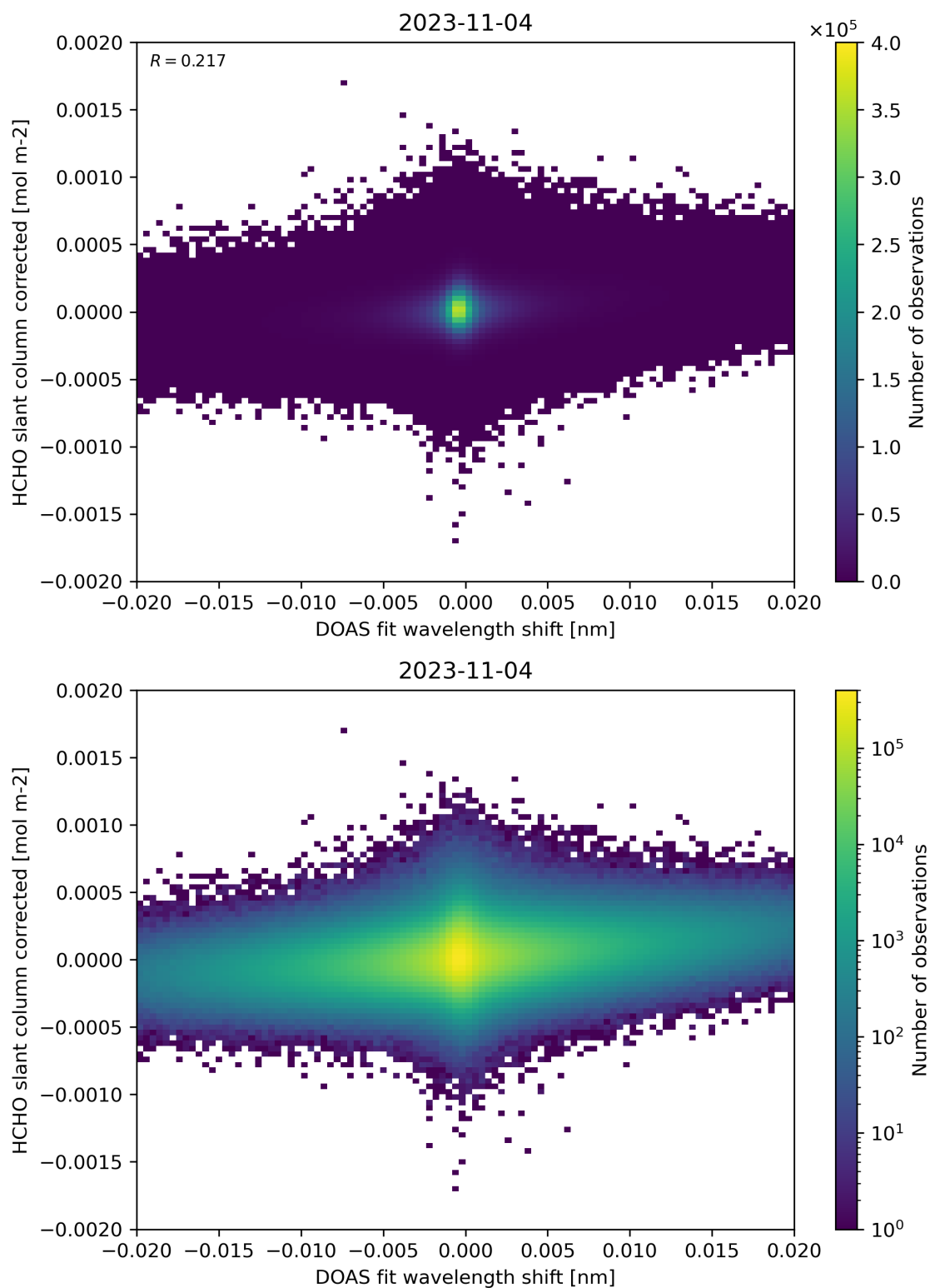
Figure 66: Scatter density plot of “DOAS fit wavelength shift” against “HCHO slant column corrected” for 2023-11-03 to 2023-11-05.
