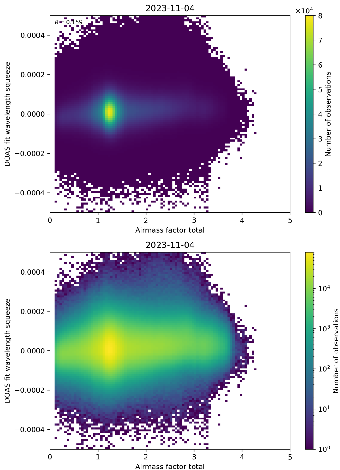
Figure 99: Scatter density plot of “Airmass factor total” against “DOAS fit wavelength squeeze” for 2023-11-03 to 2023-11-05.
