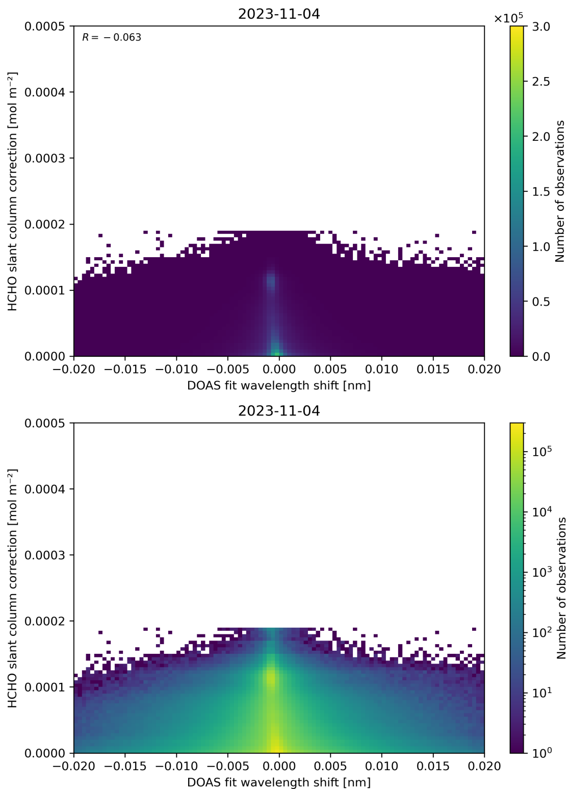
Figure 67: Scatter density plot of “DOAS fit wavelength shift” against “HCHO slant column correction” for 2023-11-03 to 2023-11-05.
