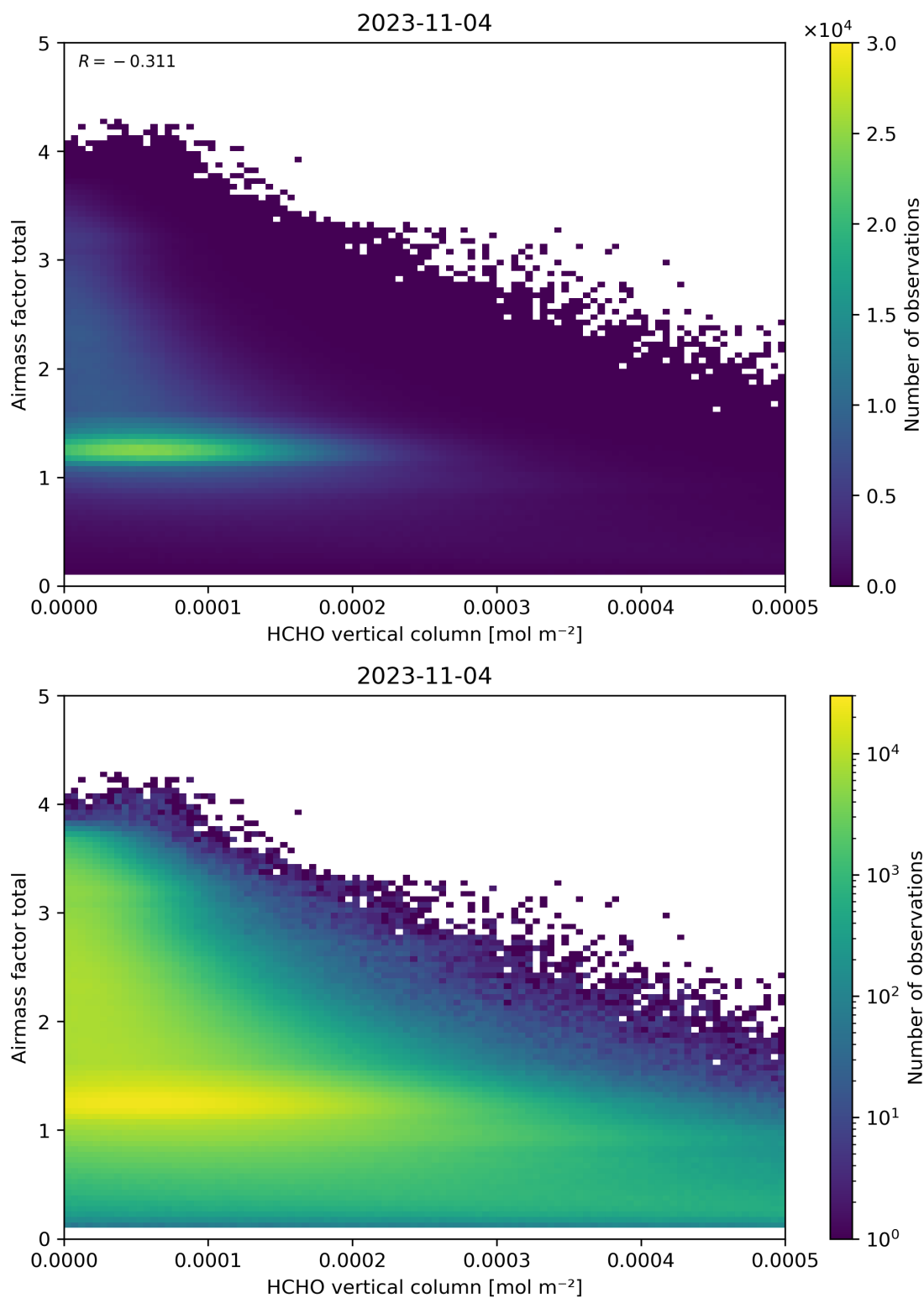
Figure 131: Scatter density plot of “HCHO vertical column” against “Airmass factor total” for 2023-11-03 to 2023-11-05.
