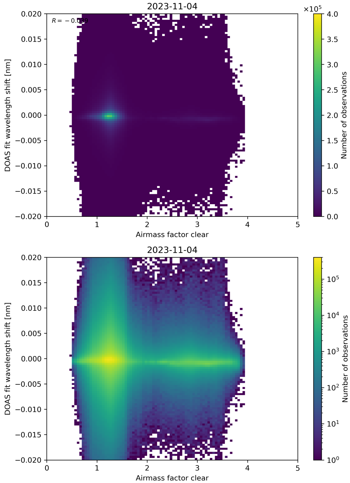
Figure 72: Scatter density plot of “Airmass factor clear” against “DOAS fit wavelength shift” for 2023-11-03 to 2023-11-05.
