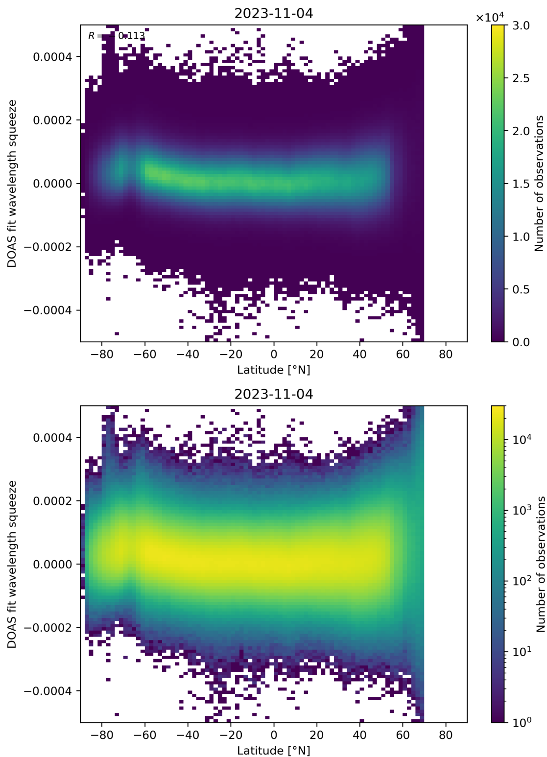
Figure 155: Scatter density plot of “Latitude” against “DOAS fit wavelength squeeze” for 2023-11-03 to 2023-11-05.
