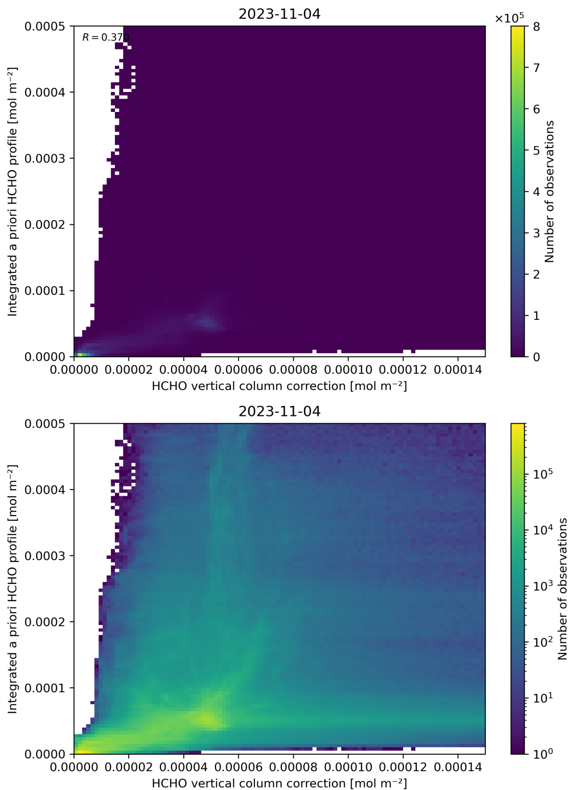
Figure 122: Scatter density plot of “HCHO vertical column correction” against “Integrated a priori HCHO profile” for 2023-11-03 to 2023-11-05.
