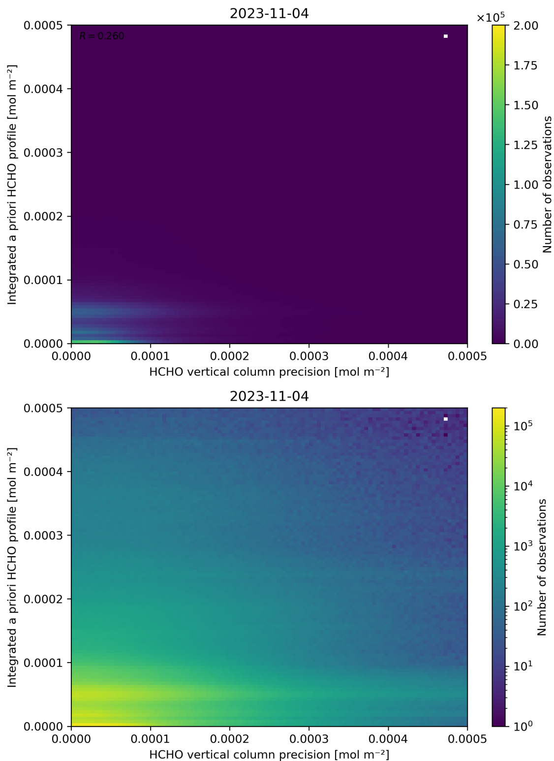
Figure 147: Scatter density plot of “HCHO vertical column precision” against “Integrated a priori HCHO profile” for 2023-11-03 to 2023-11-05.
