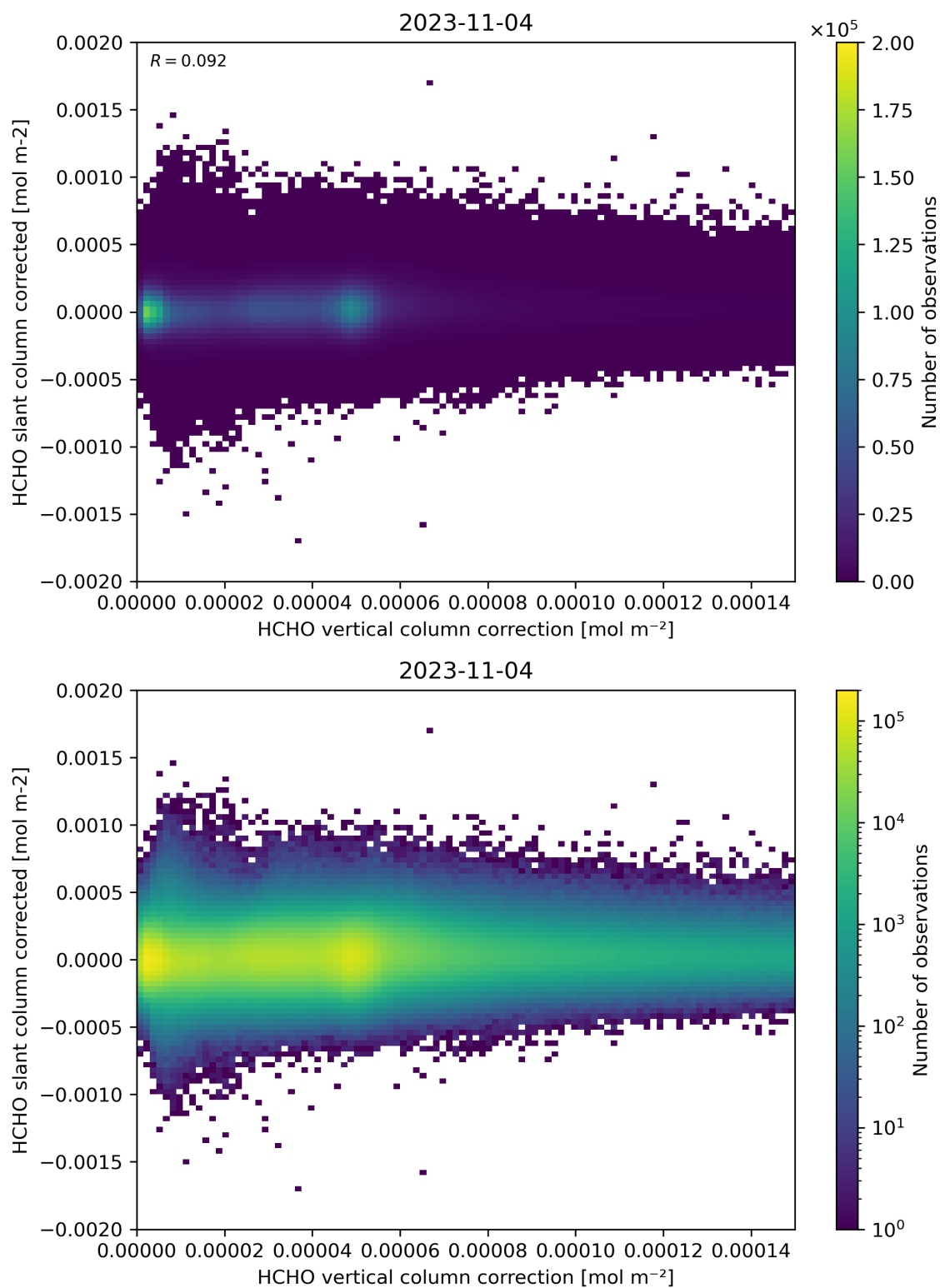
Figure 116: Scatter density plot of “HCHO vertical column correction” against “HCHO slant column corrected” for 2023-11-03 to 2023-11-05.
