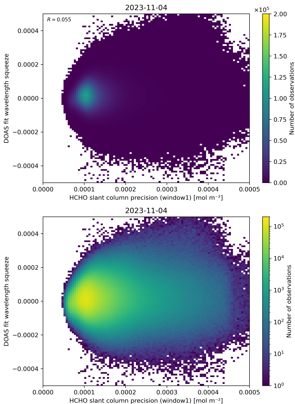
Figure 90: Scatter density plot of “HCHO slant column precision (window1)” against “DOAS fit wavelength squeeze” for 2023-11-03 to 2023-11-05.
