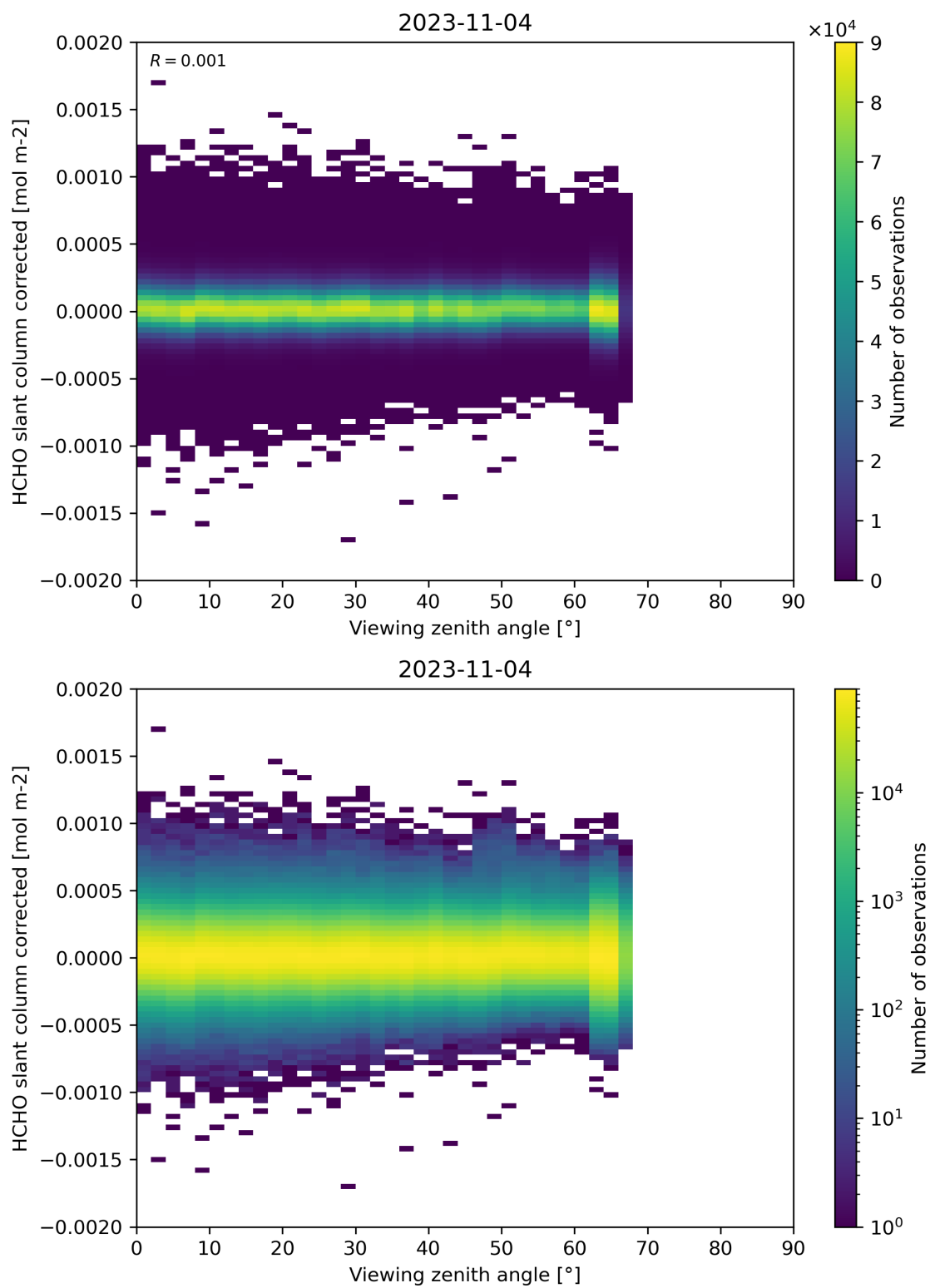
Figure 186: Scatter density plot of “Viewing zenith angle” against “HCHO slant column corrected” for 2023-11-03 to 2023-11-05.
