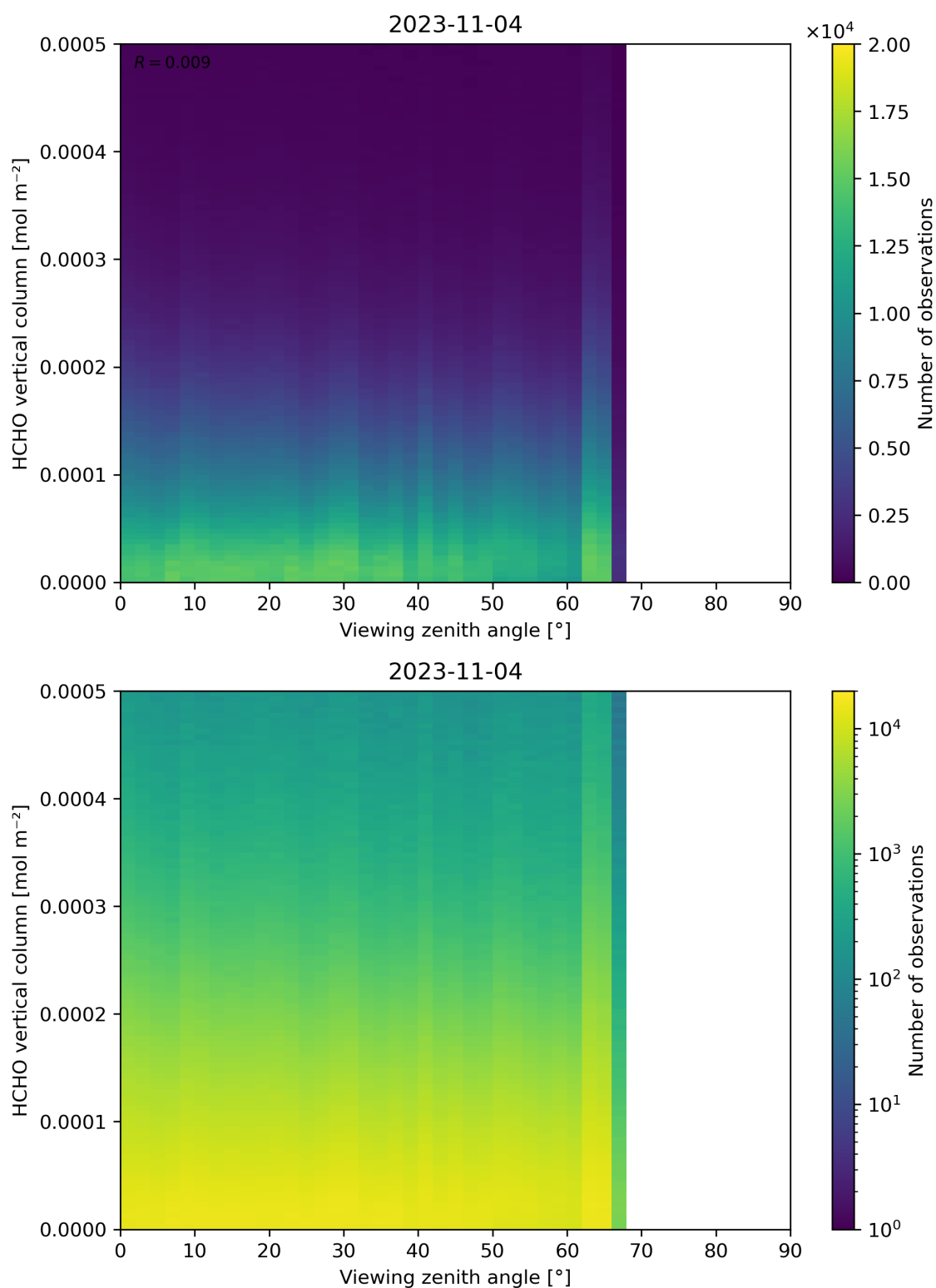
Figure 192: Scatter density plot of “Viewing zenith angle” against “HCHO vertical column” for 2023-11-03 to 2023-11-05.
