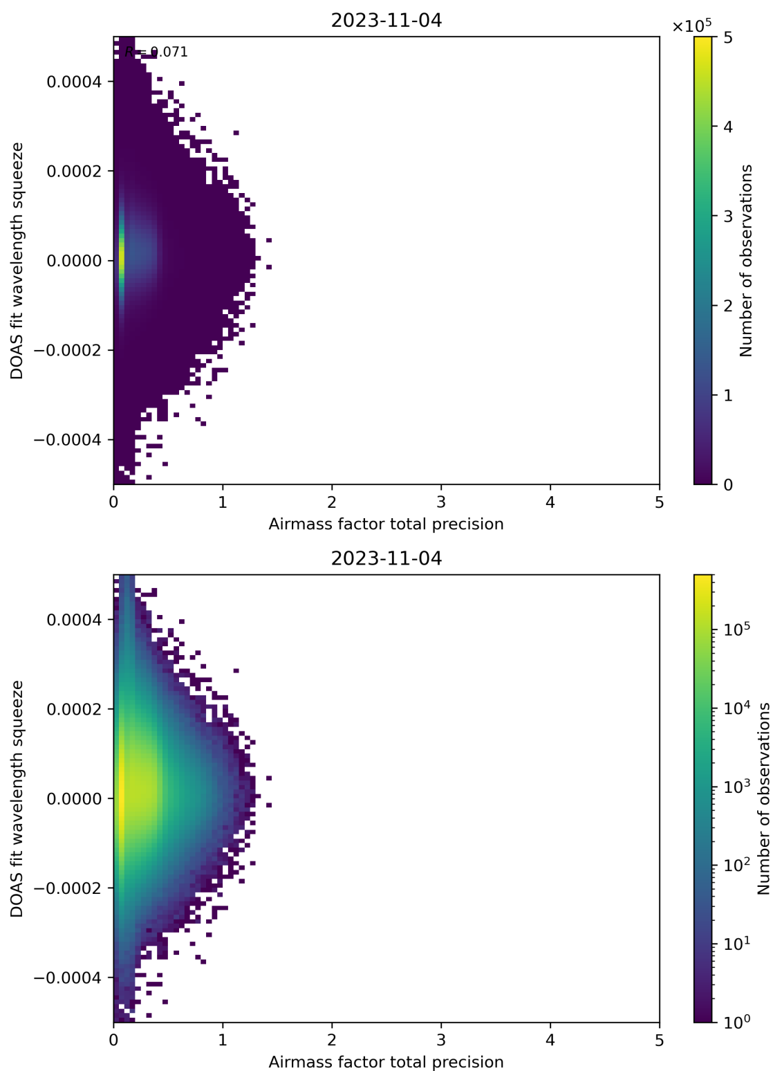
Figure 107: Scatter density plot of “Airmass factor total precision” against “DOAS fit wavelength squeeze” for 2023-11-03 to 2023-11-05.
