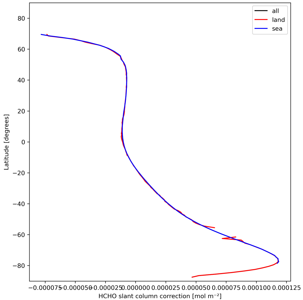
Figure 33: Zonal average of “HCHO slant column correction” for 2023-11-03 to 2023-11-05.
