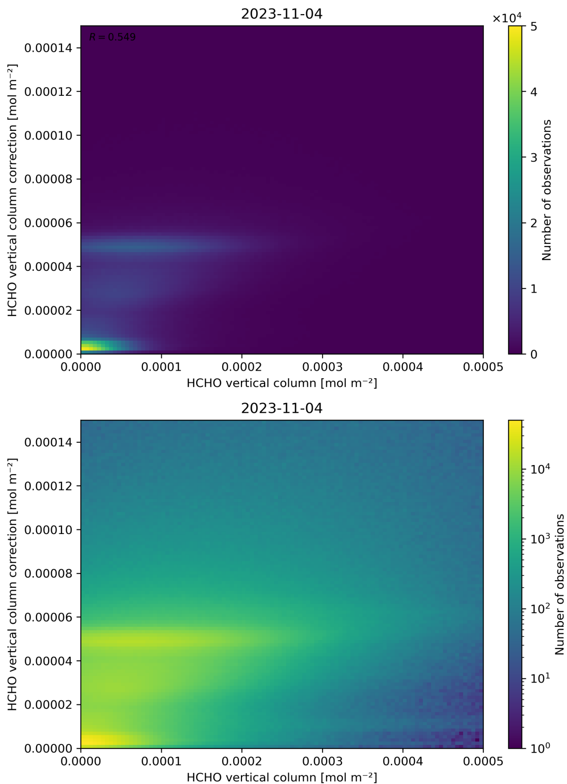
Figure 133: Scatter density plot of “HCHO vertical column” against “HCHO vertical column correction” for 2023-11-03 to 2023-11-05.
