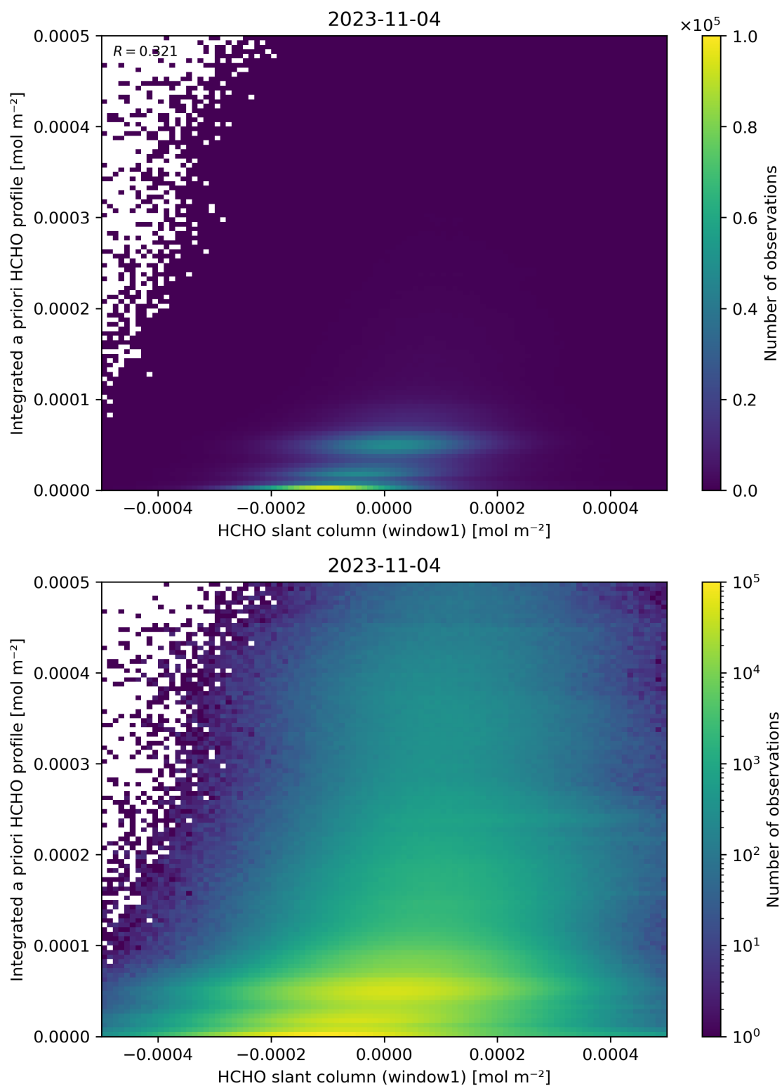
Figure 87: Scatter density plot of “HCHO slant column (window1)” against “Integrated a priori HCHO profile” for 2023-11-03 to 2023-11-05.
