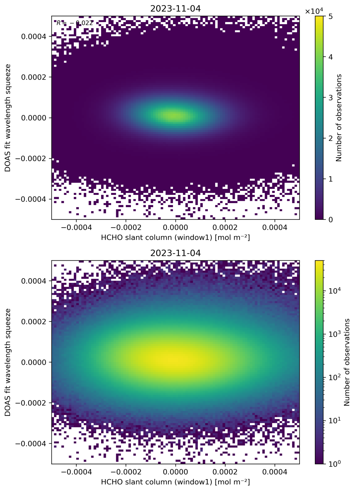
Figure 80: Scatter density plot of “HCHO slant column (window1)” against “DOAS fit wavelength squeeze” for 2023-11-03 to 2023-11-05.
