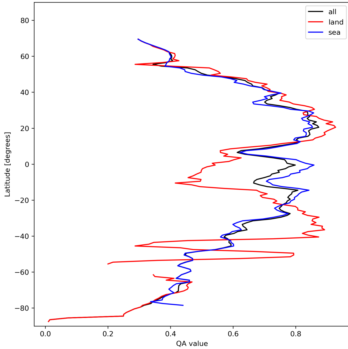
Figure 20: Zonal average of “QA value” for 2023-11-03 to 2023-11-05.
