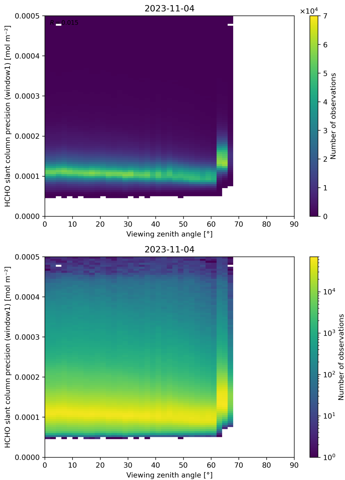
Figure 189: Scatter density plot of “Viewing zenith angle” against “HCHO slant column precision (window1)” for 2023-11-03 to 2023-11-05.
