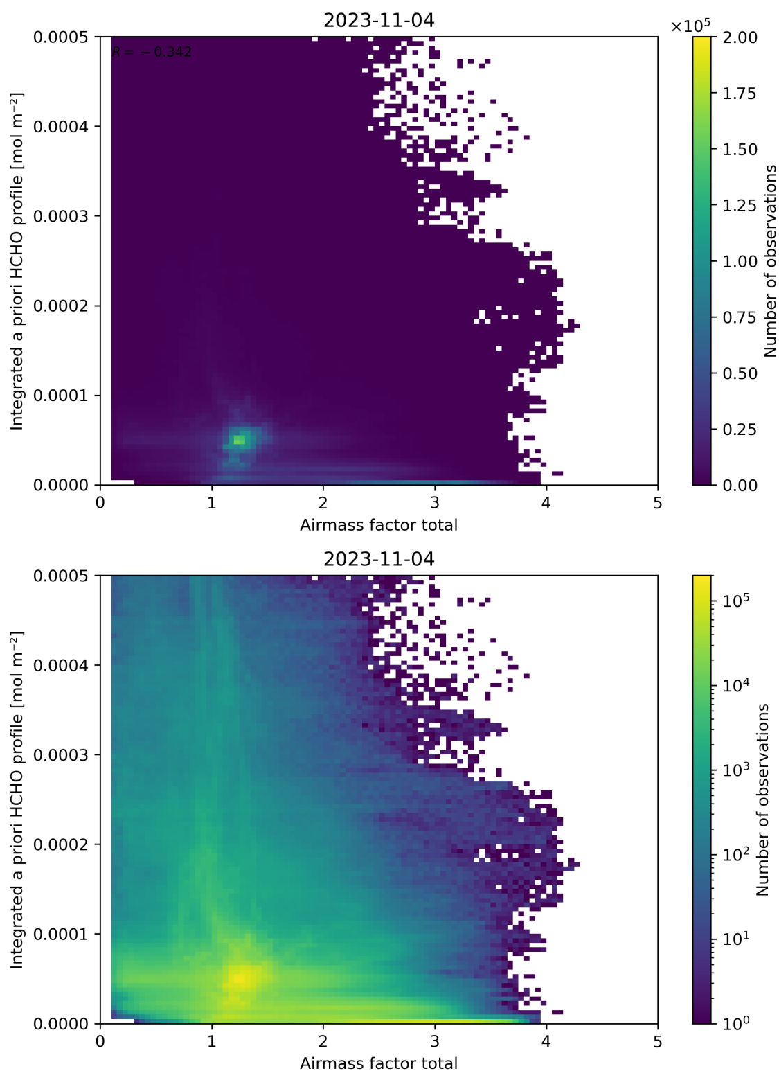
Figure 104: Scatter density plot of “Air mass factor total” against “Integrated a priori HCHO profile” for 2023-11-03 to 2023-11-05.
