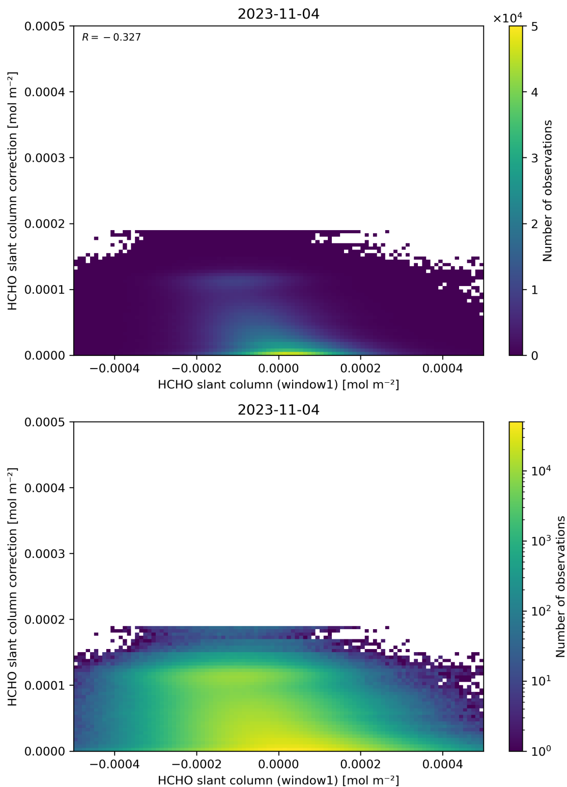
Figure 83: Scatter density plot of “HCHO slant column (window1)” against “HCHO slant column correction” for 2023-11-03 to 2023-11-05.
