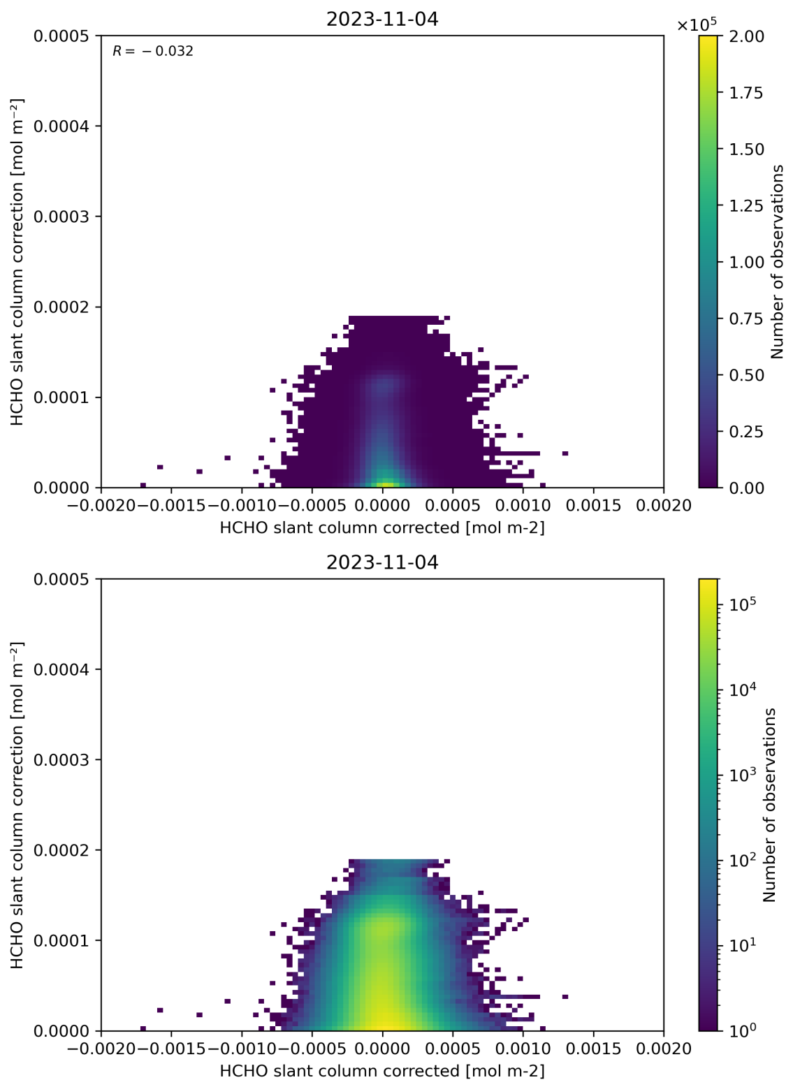
Figure 77: Scatter density plot of “HCHO slant column corrected” against “HCHO slant column correction” for 2023-11-03 to 2023-11-05.
