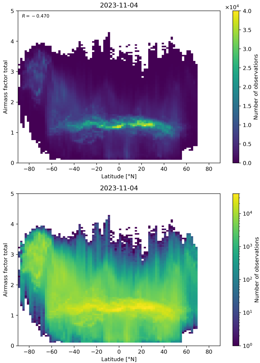
Figure 161: Scatter density plot of “Latitude” against “Airmass factor total” for 2023-11-03 to 2023-11-05.
