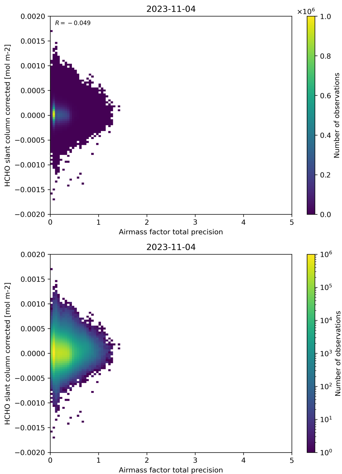
Figure 109: Scatter density plot of “Airmass factor total precision” against “HCHO slant column corrected” for 2023-11-03 to 2023-11-05.
