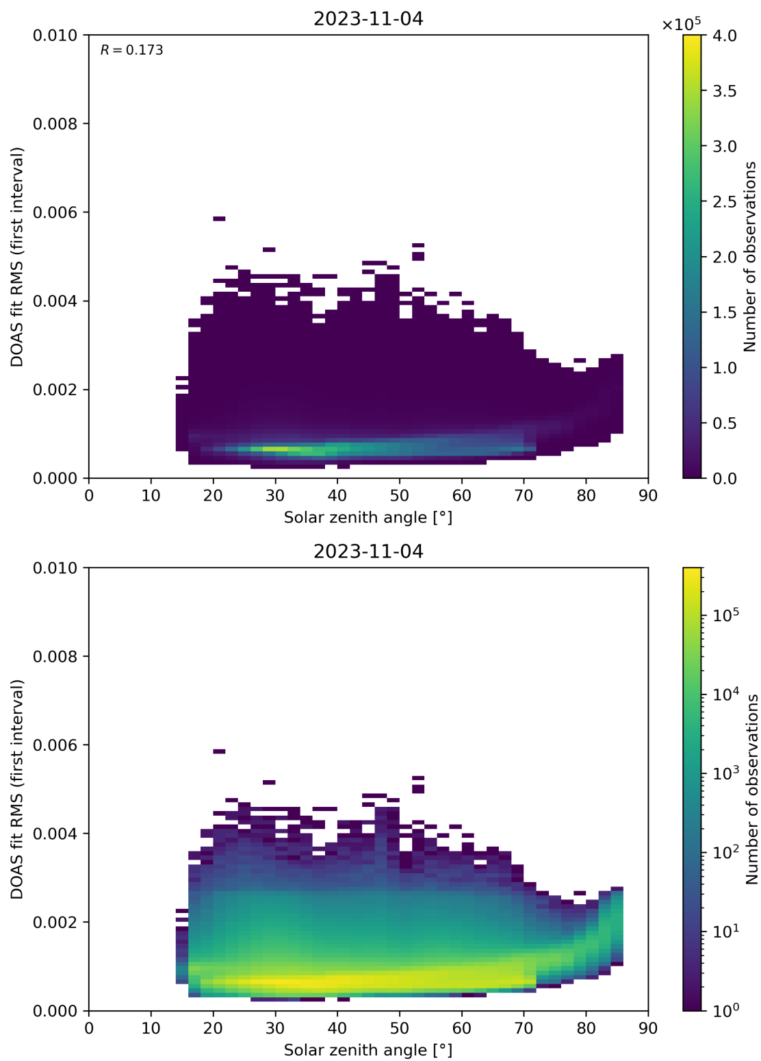
Figure 167: Scatter density plot of “Solar zenith angle” against “DOAS fit RMS (first interval)” for 2023-11-03 to 2023-11-05.
