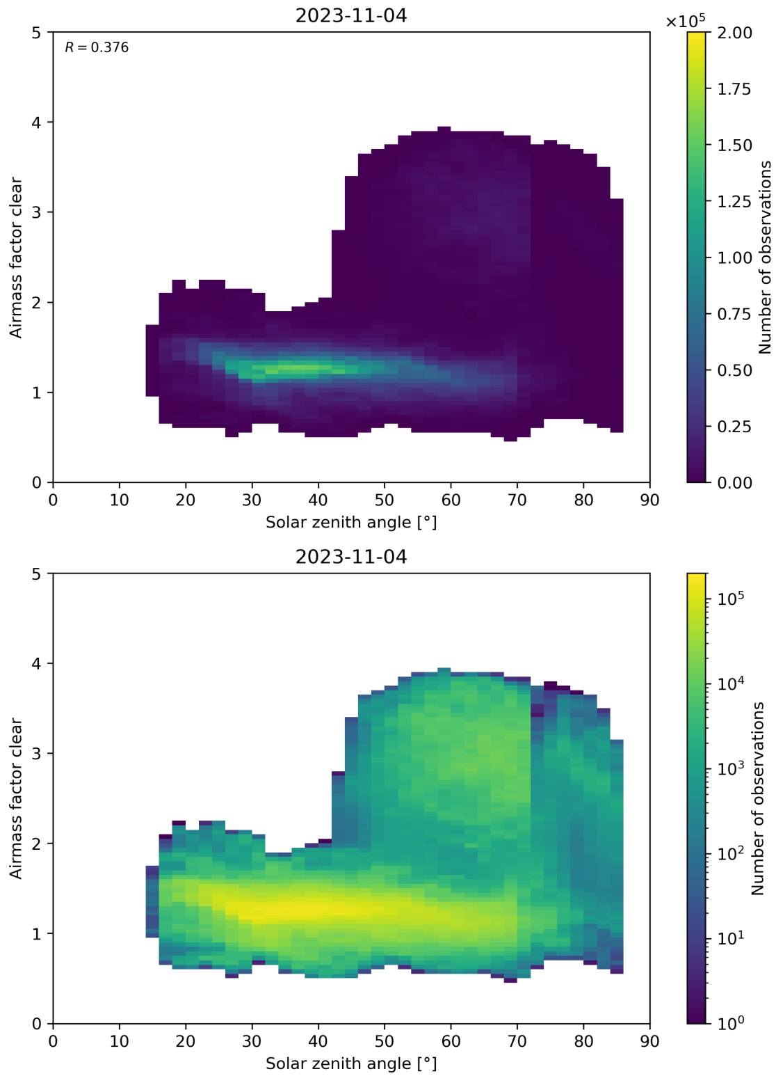
Figure 170: Scatter density plot of “Solar zenith angle” against “Airmass factor clear” for 2023-11-03 to 2023-11-05.
