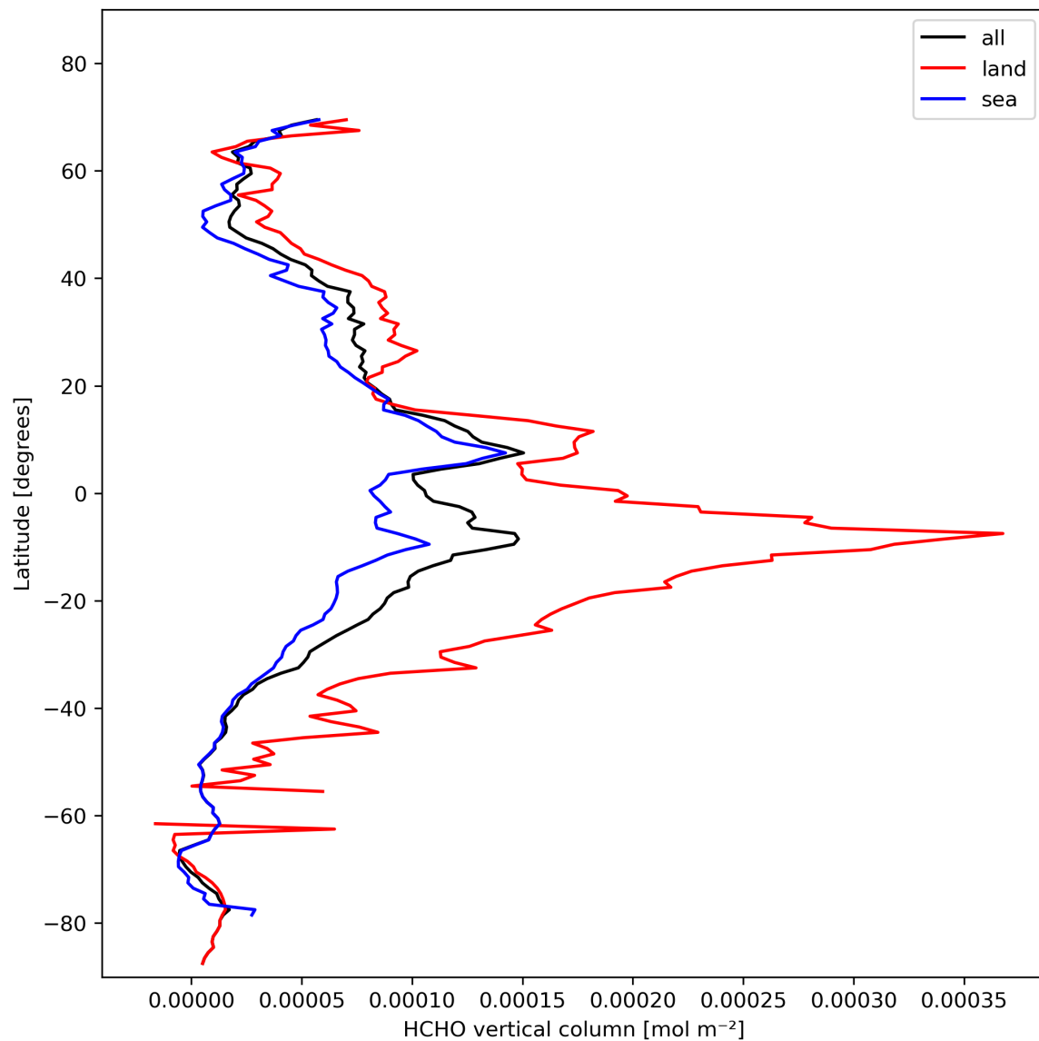
Figure 21: Zonal average of “HCHO vertical column” for 2023-11-03 to 2023-11-05.
