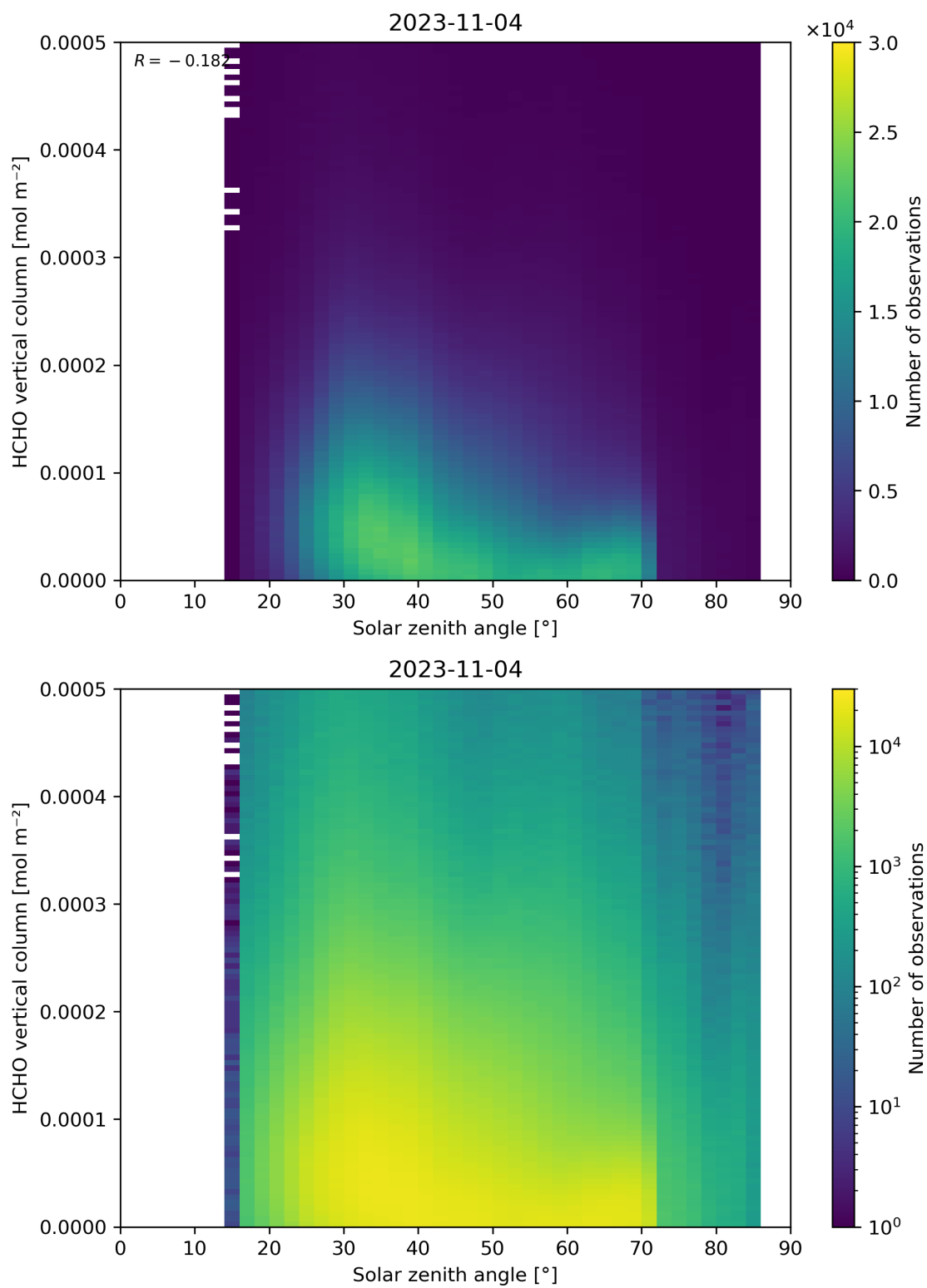
Figure 177: Scatter density plot of “Solar zenith angle” against “HCHO vertical column” for 2023-11-03 to 2023-11-05.
