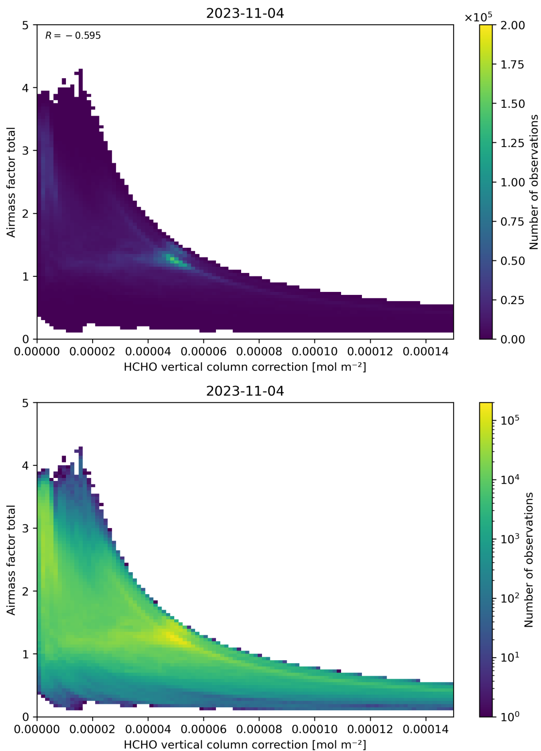
Figure 120: Scatter density plot of “HCHO vertical column correction” against “Airmass factor total” for 2023-11-03 to 2023-11-05.
