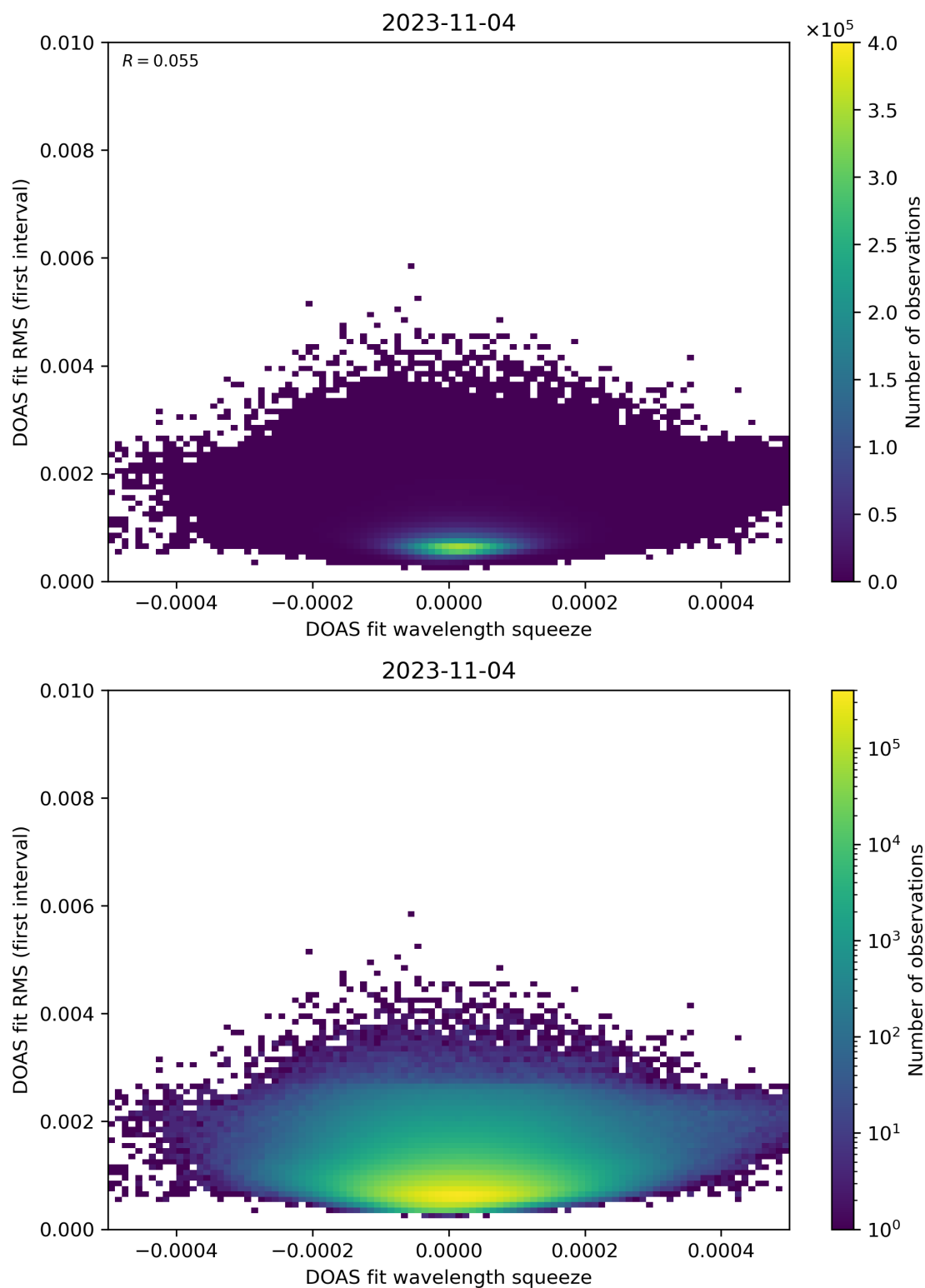
Figure 68: Scatter density plot of “DOAS fit wavelength squeeze” against “DOAS fit RMS (first interval)” for 2023-11-03 to 2023-11-05.
