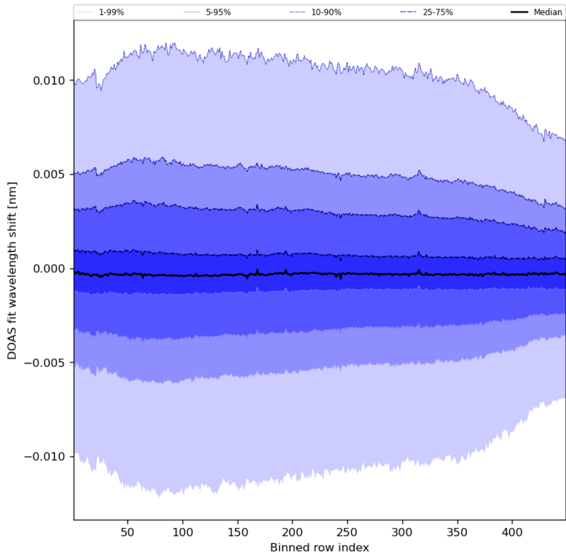
Figure 58: Along track statistics of “DOAS fit wavelength shift” for 2023-11-03 to 2023-11-05
