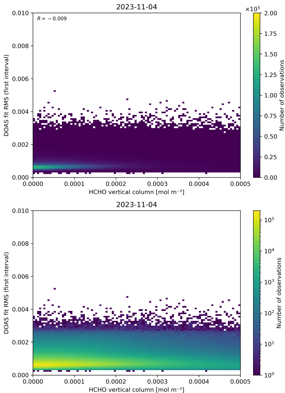
Figure 123: Scatter density plot of “HCHO vertical column” against “DOAS fit RMS (first interval)” for 2023-11-03 to 2023-11-05.
