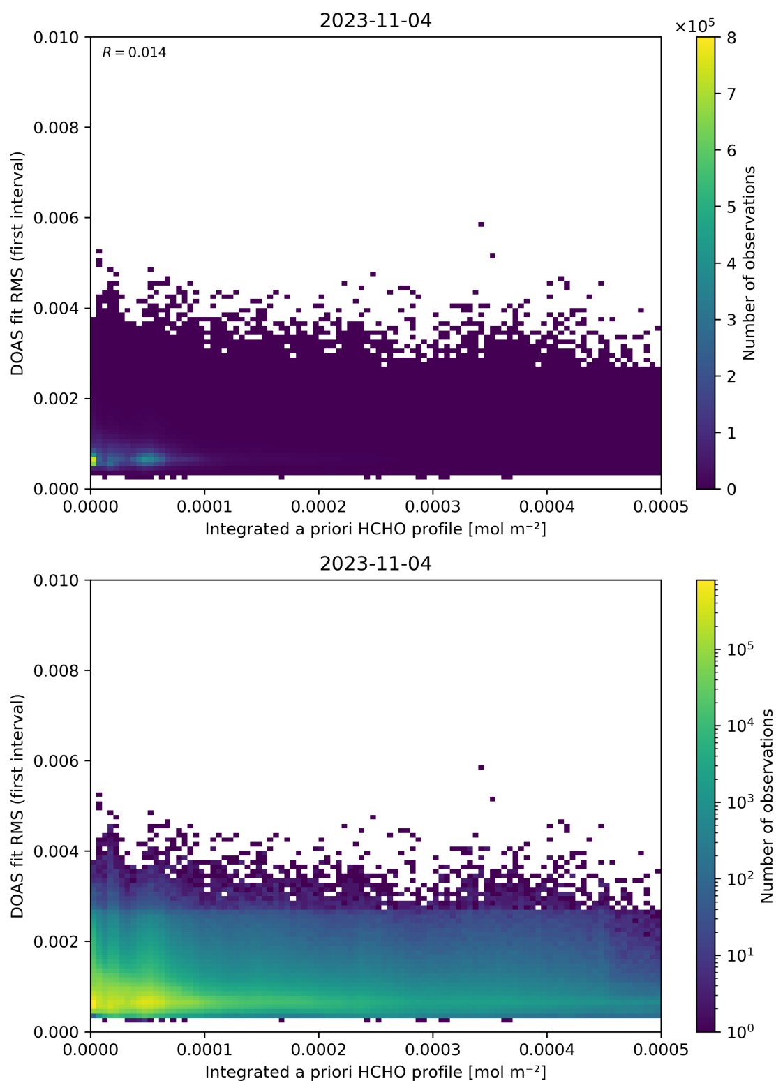
Figure 148: Scatter density plot of “Integrated a priori HCHO profile” against “DOAS fit RMS (first interval)” for 2023-11-03 to 2023-11-05.
