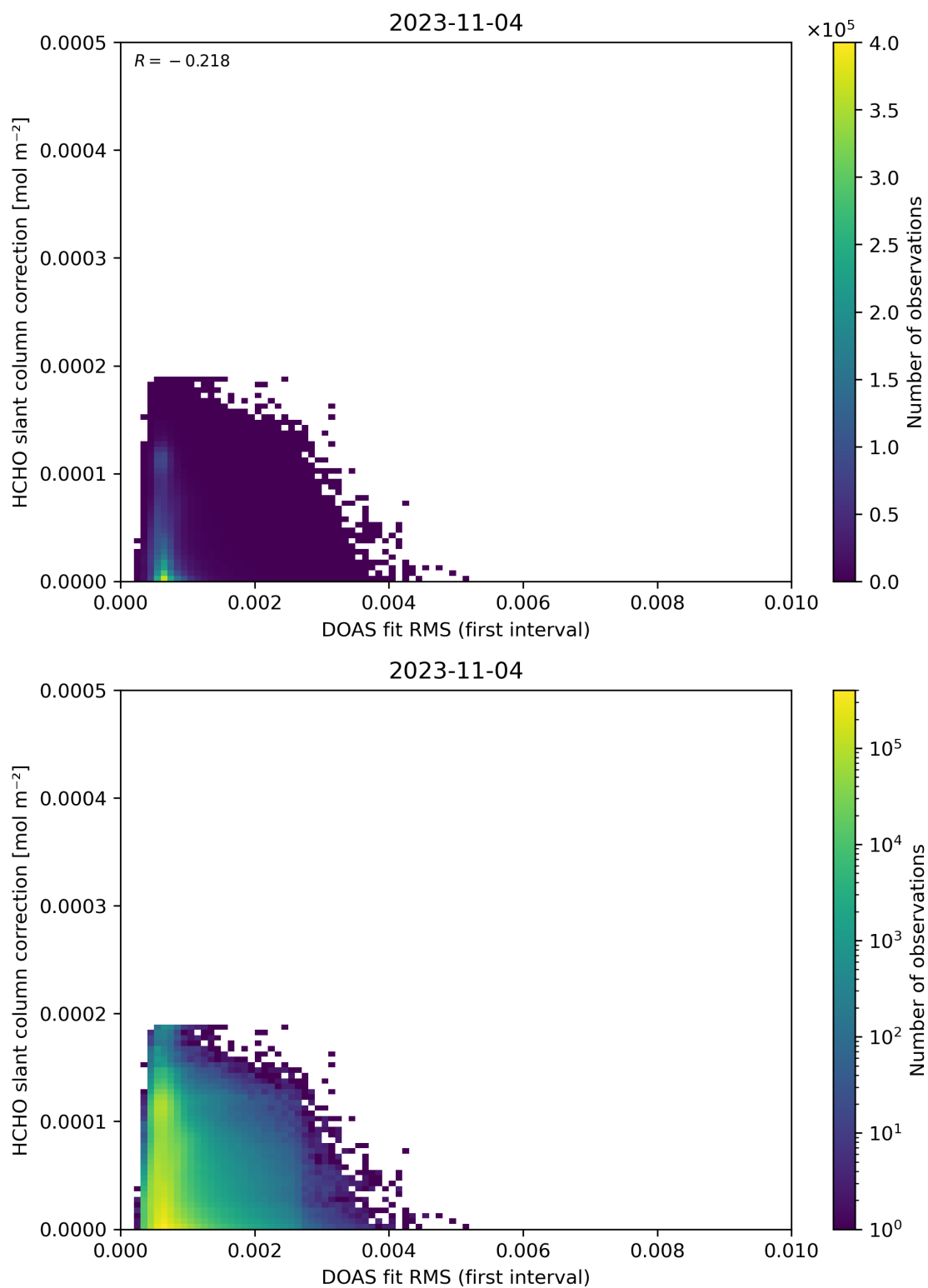
Figure 63: Scatter density plot of “DOAS fit RMS (first interval)” against “HCHO slant column correction” for 2023-11-03 to 2023-11-05.
