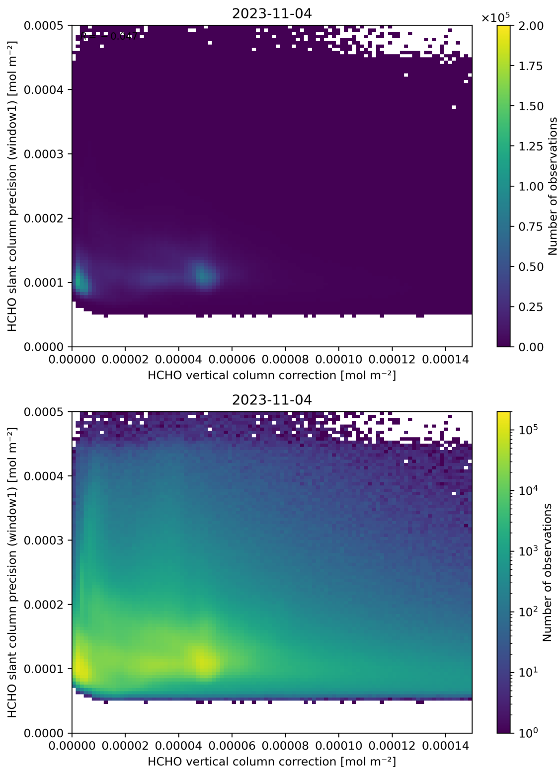
Figure 119: Scatter density plot of “HCHO vertical column correction” against “HCHO slant column precision (window1)” for 2023-11-03 to 2023-11-05.
