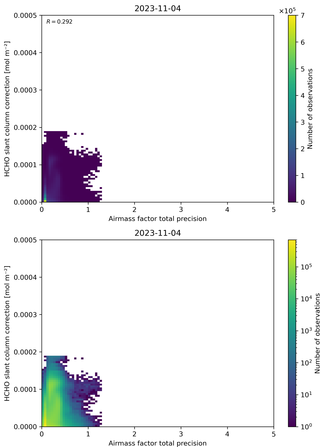
Figure 110: Scatter density plot of “Airmass factor total precision” against “HCHO slant column correction” for 2023-11-03 to 2023-11-05.
