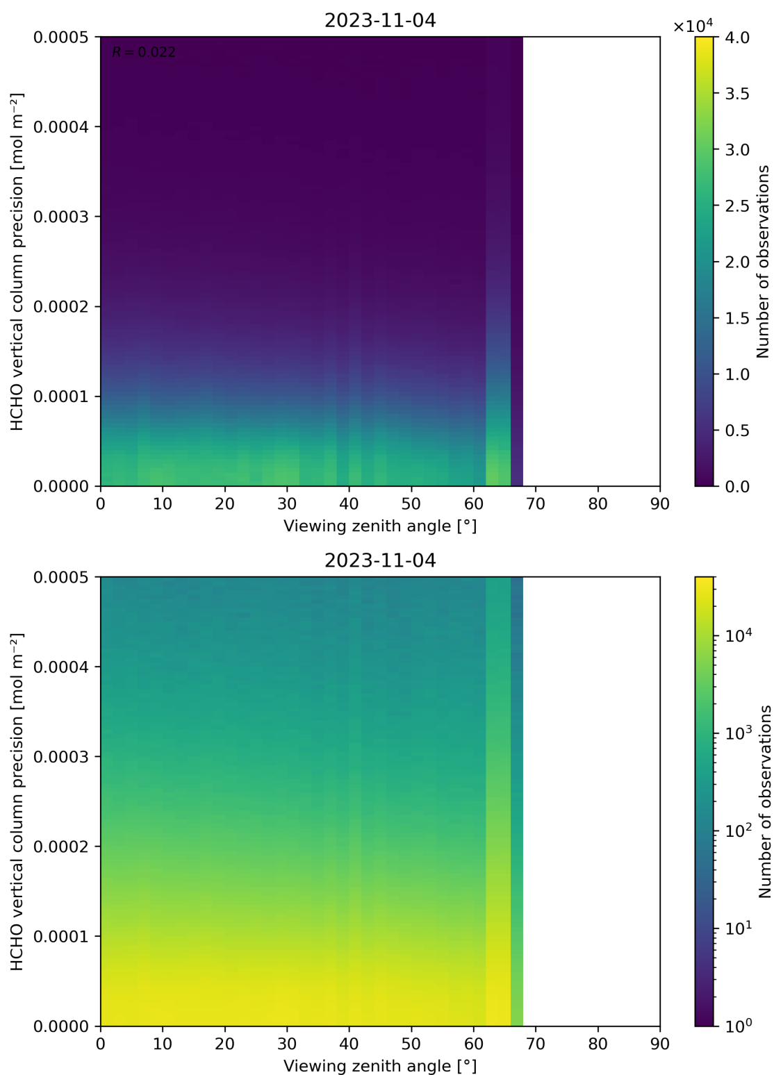
Figure 194: Scatter density plot of “Viewing zenith angle” against “HCHO vertical column precision” for 2023-11-03 to 2023-11-05.
