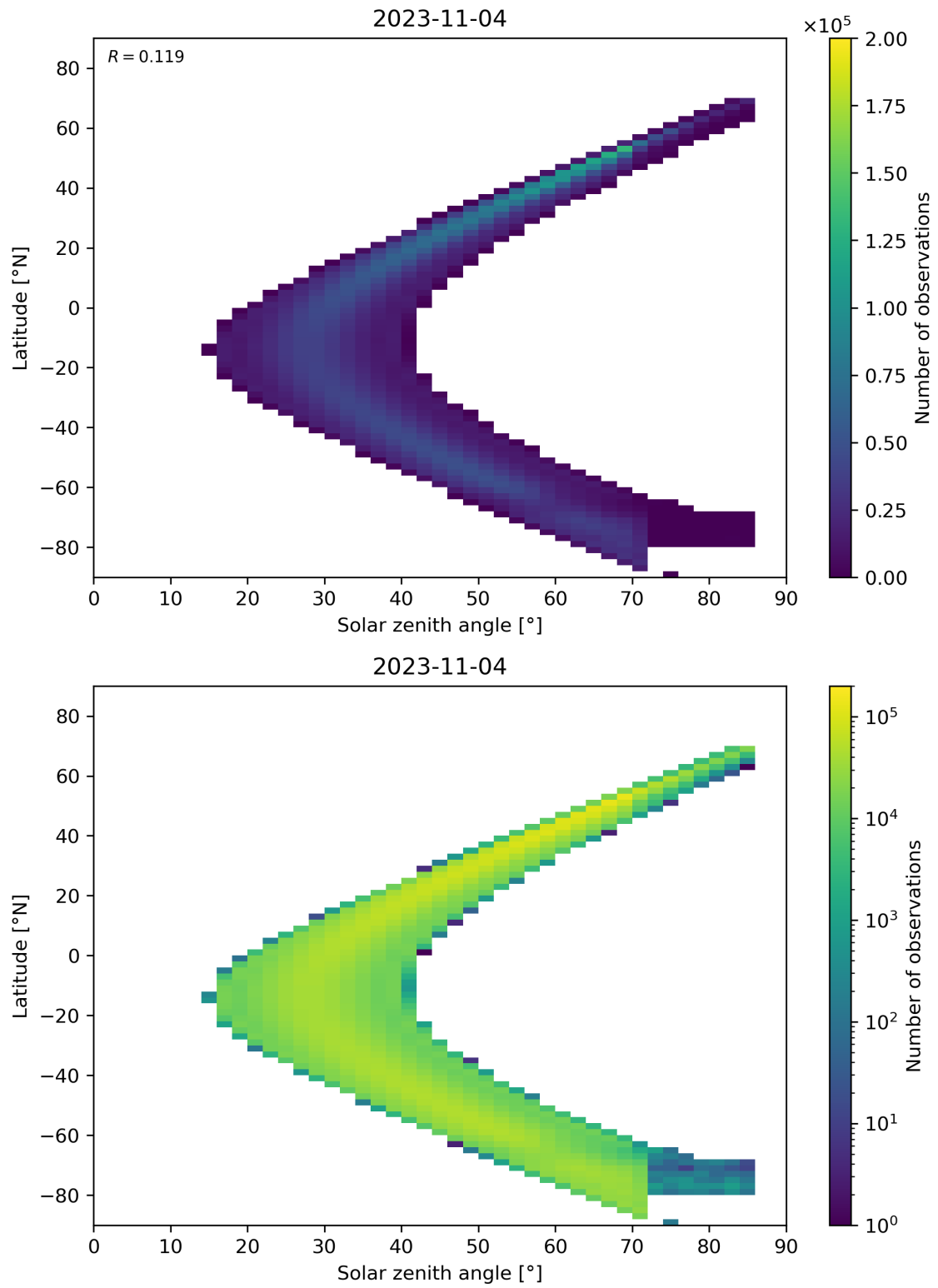
Figure 181: Scatter density plot of “Solar zenith angle” against “Latitude” for 2023-11-03 to 2023-11-05.
