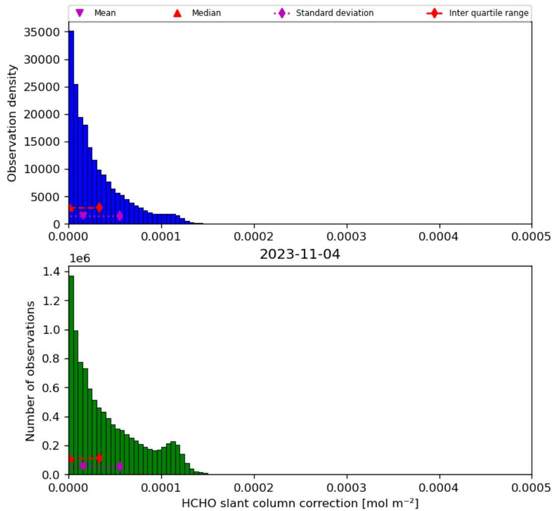
Figure 47: Histogram of “HCHO slant column correction” for 2023-11-03 to 2023-11-05
