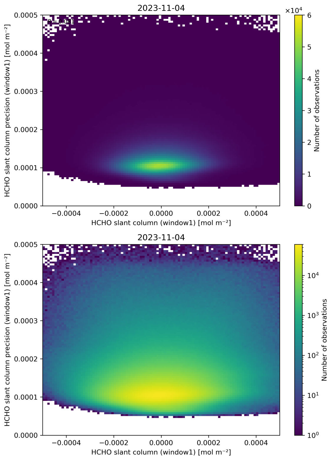
Figure 84: Scatter density plot of “HCHO slant column (window1)” against “HCHO slant column precision (window1)” for 2023-11-03 to 2023-11-05.
