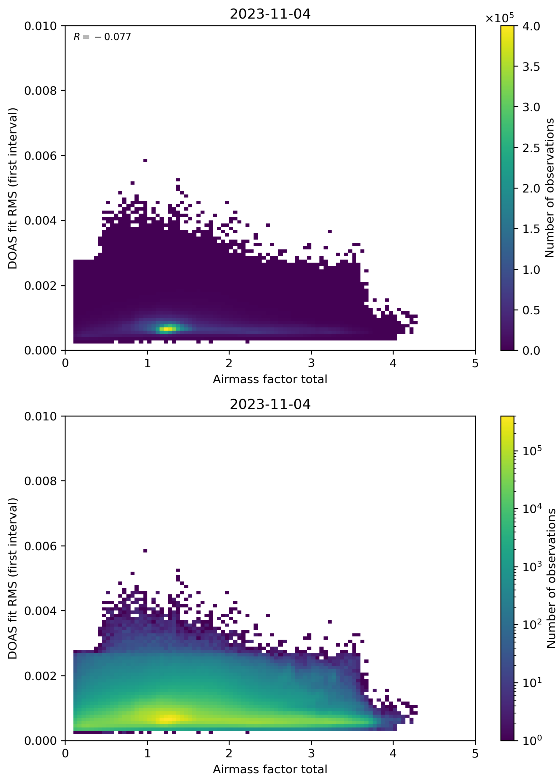
Figure 97: Scatter density plot of “Airmass factor total” against “DOAS fit RMS (first interval)” for 2023-11-03 to 2023-11-05.
