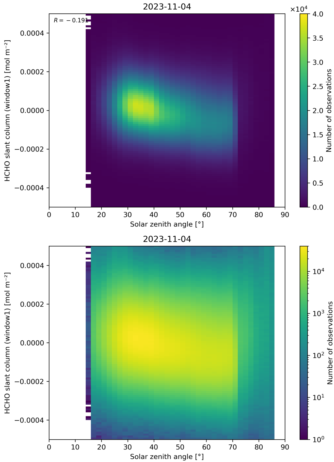
Figure 173: Scatter density plot of “Solar zenith angle” against “HCHO slant column (window1)” for 2023-11-03 to 2023-11-05.
