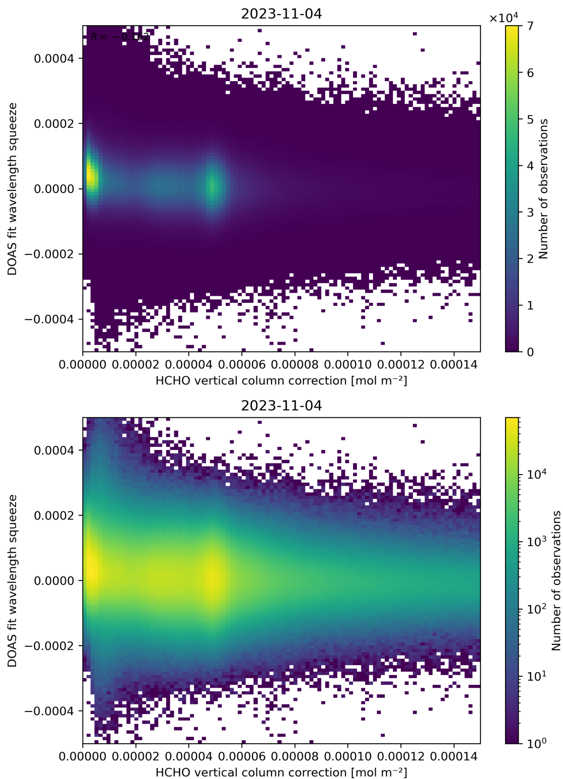
Figure 114: Scatter density plot of “HCHO vertical column correction” against “DOAS fit wavelength squeeze” for 2023-11-03 to 2023-11-05.
