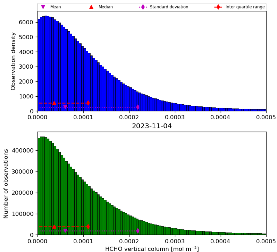
Figure 35: Histogram of “HCHO vertical column” for 2023-11-03 to 2023-11-05
