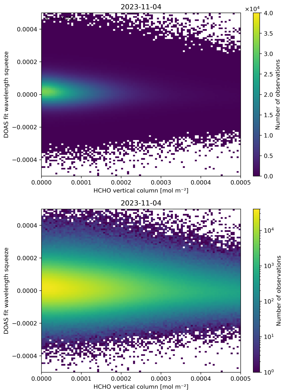
Figure 125: Scatter density plot of “HCHO vertical column” against “DOAS fit wavelength squeeze” for 2023-11-03 to 2023-11-05.
