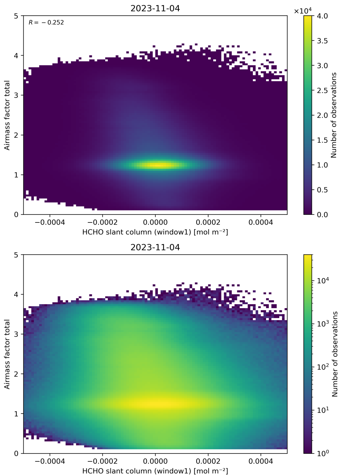
Figure 85: Scatter density plot of “HCHO slant column (window1)” against “Airmass factor total” for 2023-11-03 to 2023-11-05.
