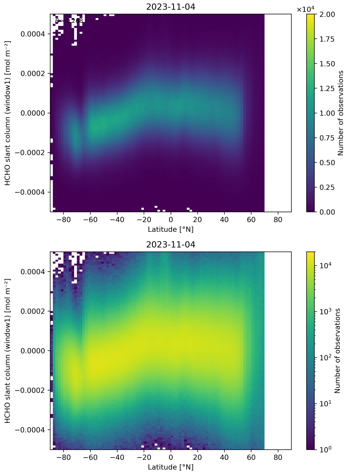
Figure 159: Scatter density plot of “Latitude” against “HCHO slant column (window1)” for 2023-11-03 to 2023-11-05.
