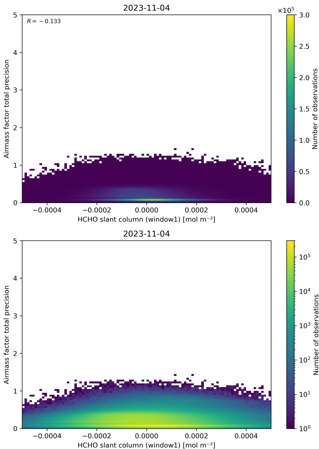
Figure 86: Scatter density plot of “HCHO slant column (window1)” against “Airmass factor total precision” for 2023-11-03 to 2023-11-05.
