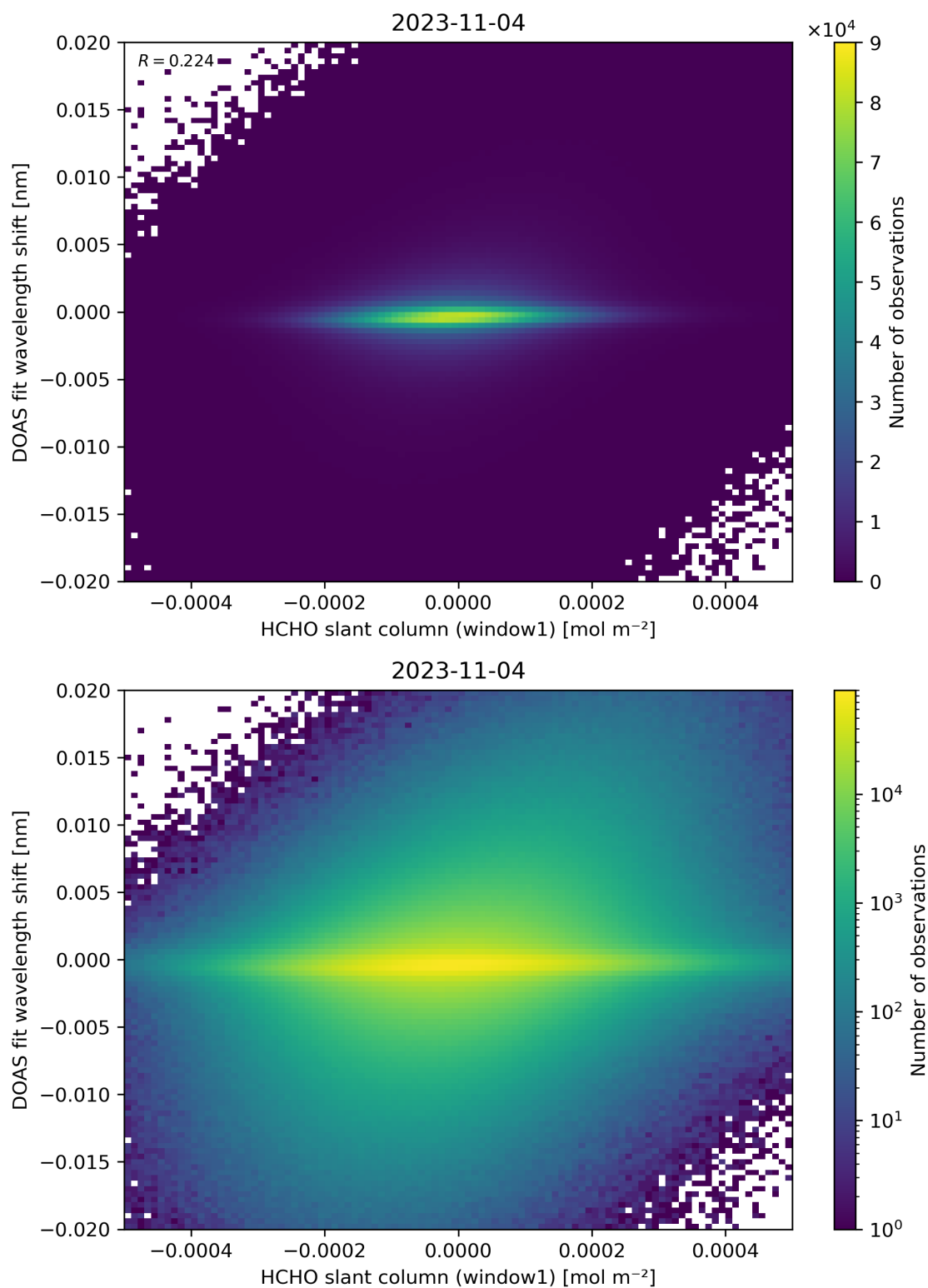
Figure 79: Scatter density plot of “HCHO slant column (window1)” against “DOAS fit wavelength shift” for 2023-11-03 to 2023-11-05.
