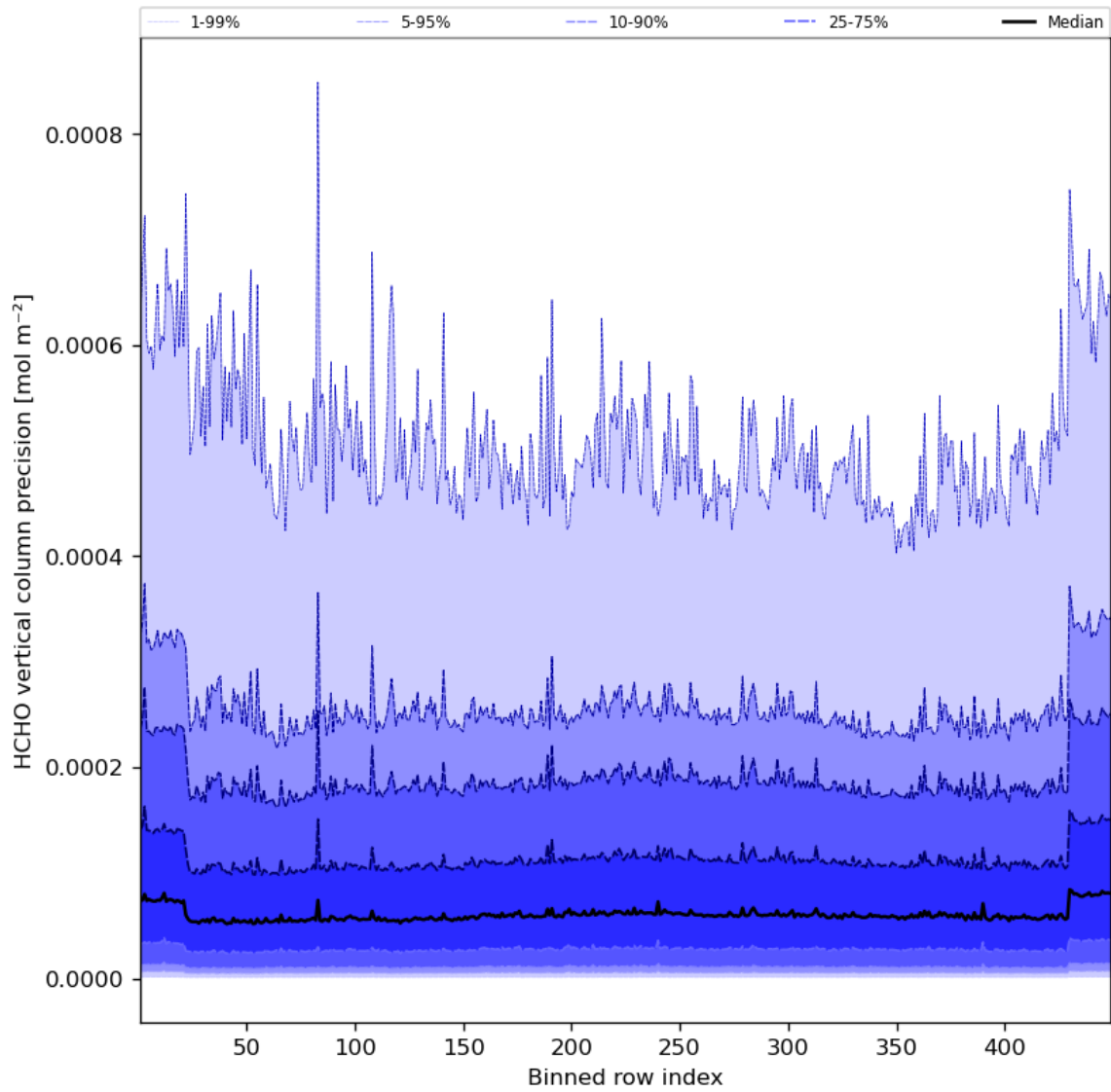
Figure 50: Along track statistics of “HCHO vertical column precision” for 2023-11-03 to 2023-11-05
