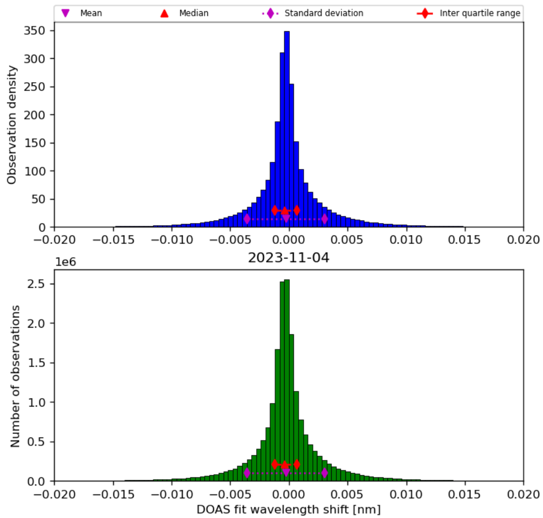
Figure 44: Histogram of “DOAS fit wavelength shift” for 2023-11-03 to 2023-11-05
