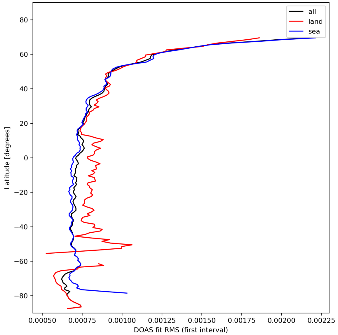
Figure 32: Zonal average of “DOAS fit RMS (first interval)” for 2023-11-03 to 2023-11-05.
