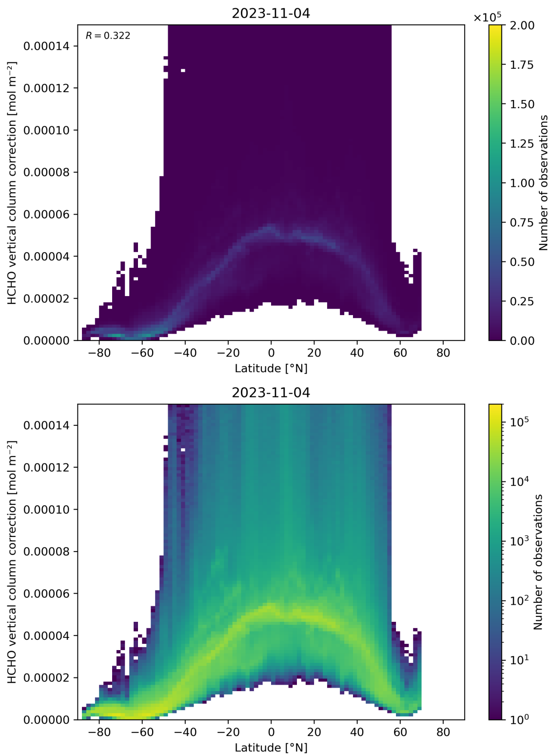
Figure 164: Scatter density plot of “Latitude” against “HCHO vertical column correction” for 2023-11-03 to 2023-11-05.
