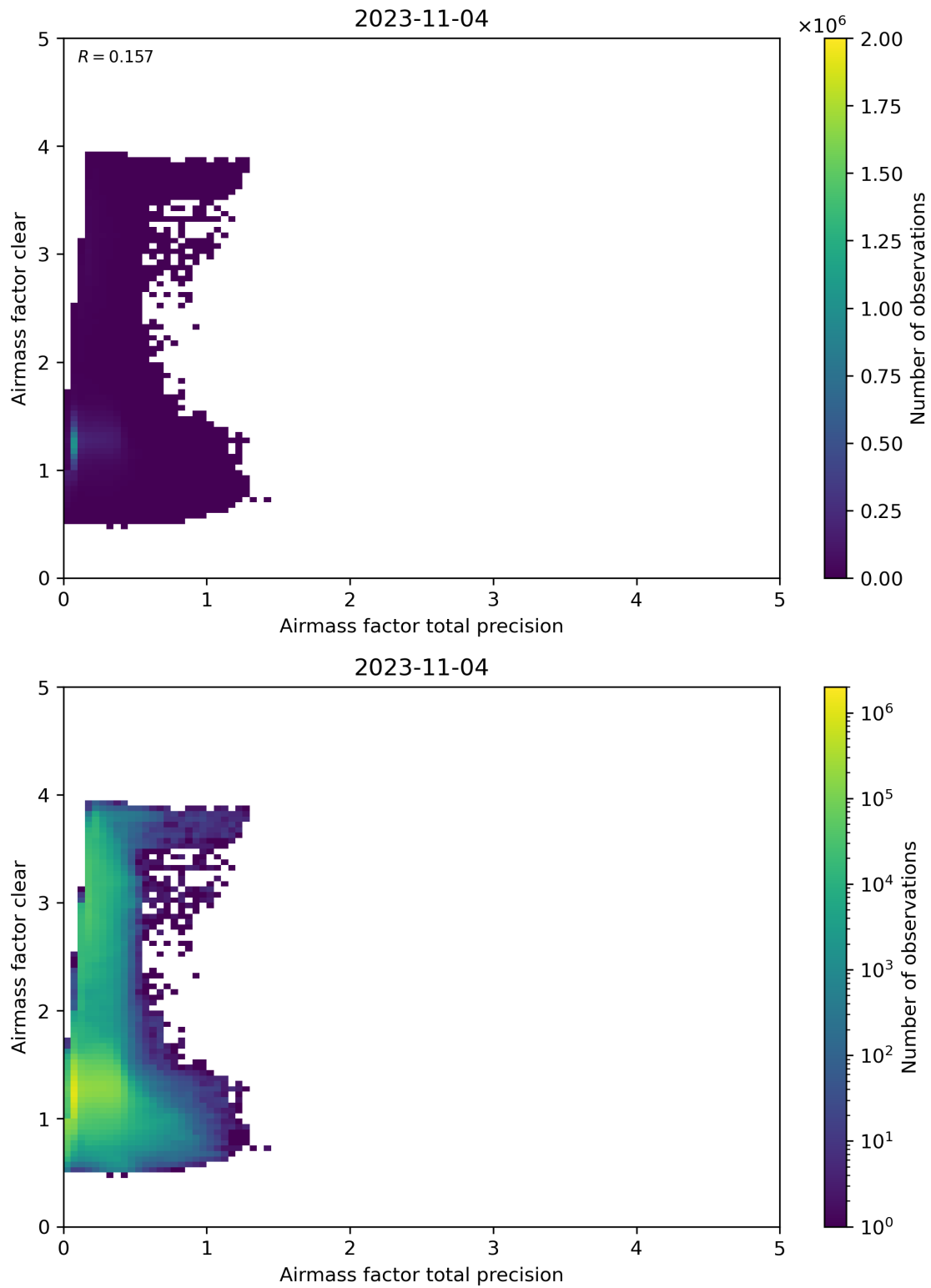
Figure 108: Scatter density plot of “Airmass factor total precision” against “Airmass factor clear” for 2023-11-03 to 2023-11-05.
