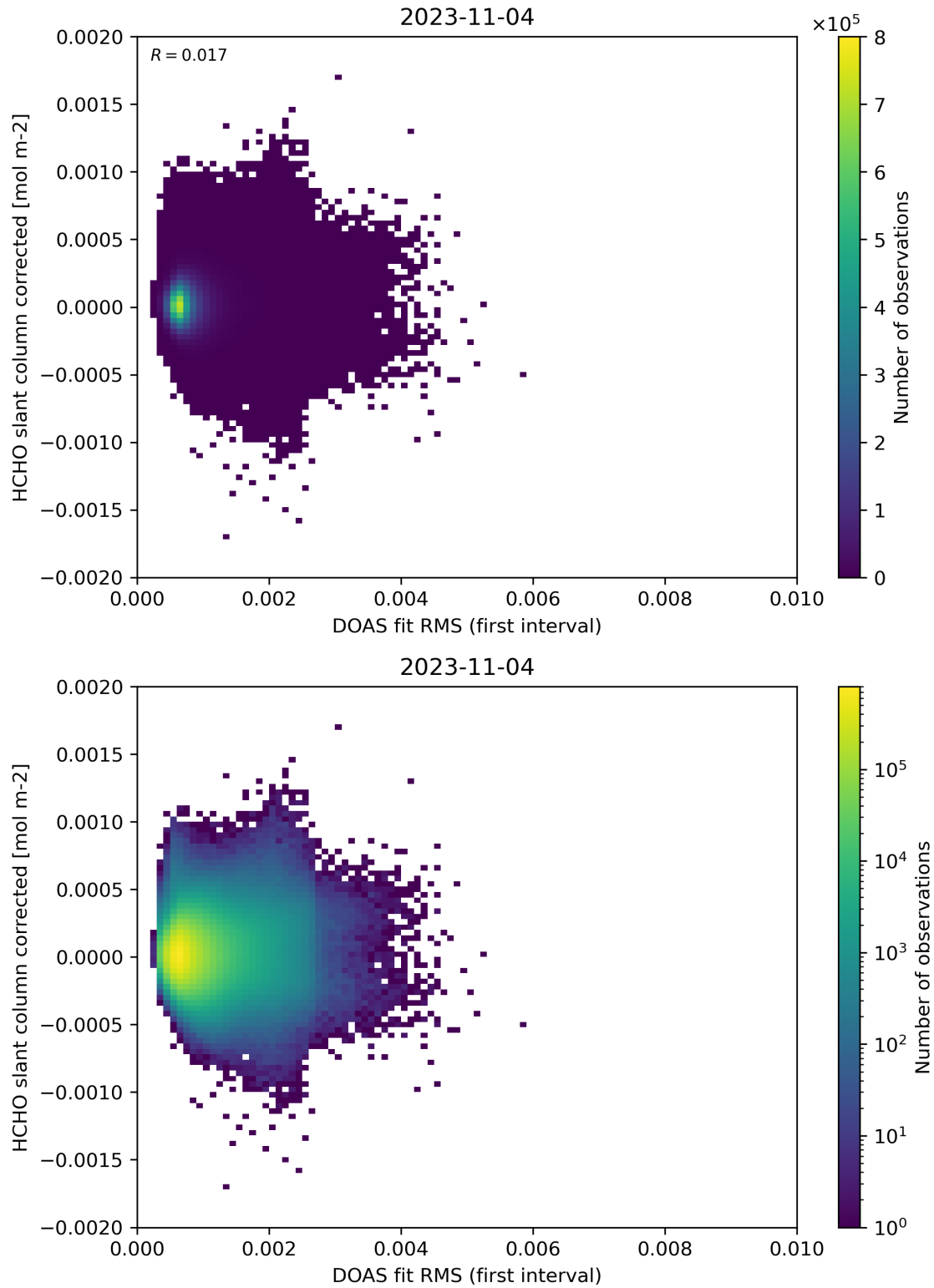
Figure 62: Scatter density plot of “DOAS fit RMS (first interval)” against “HCHO slant column corrected” for 2023-11-03 to 2023-11-05.
