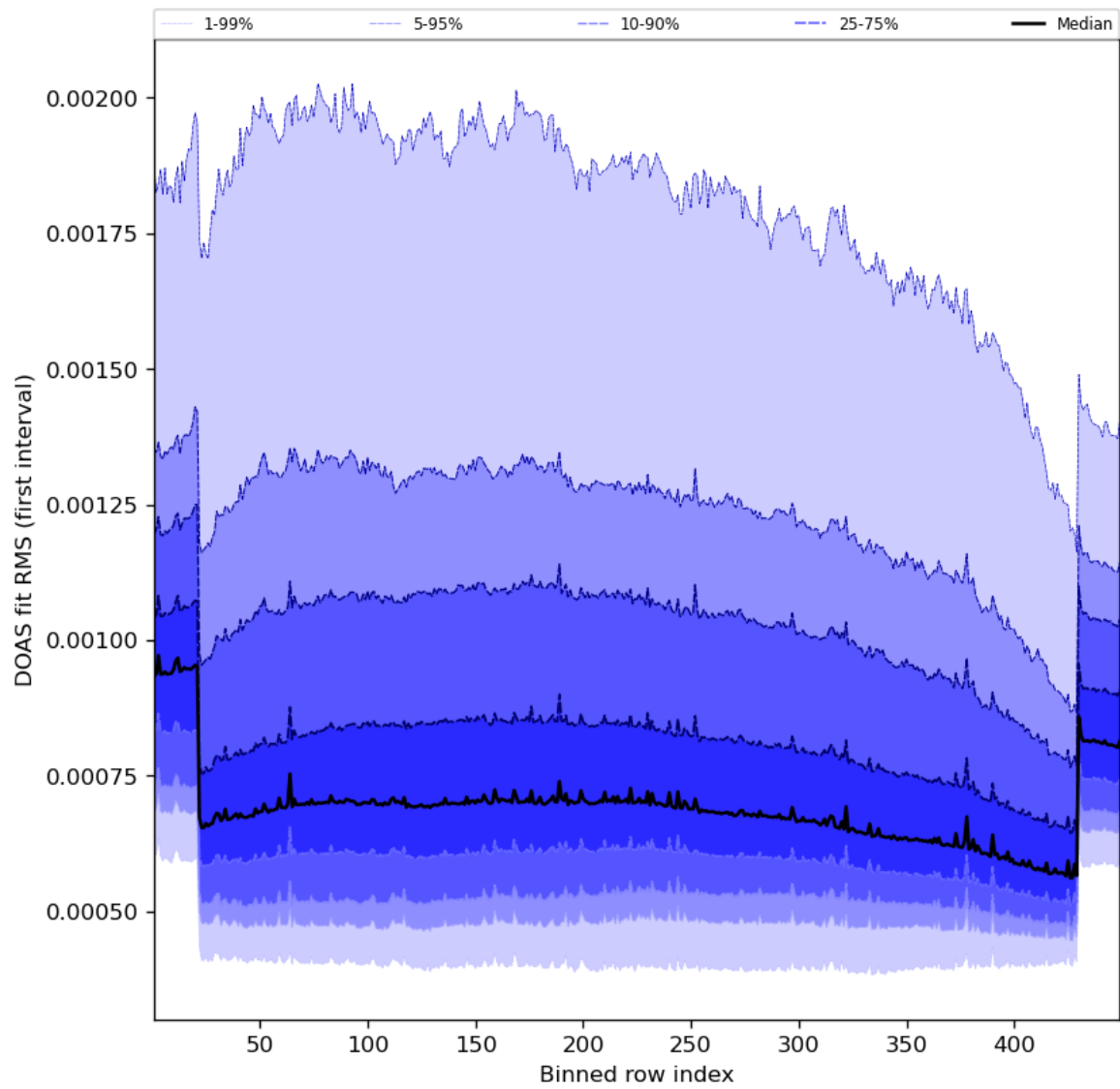
Figure 60: Along track statistics of “DOAS fit RMS (first interval)” for 2023-11-03 to 2023-11-05
