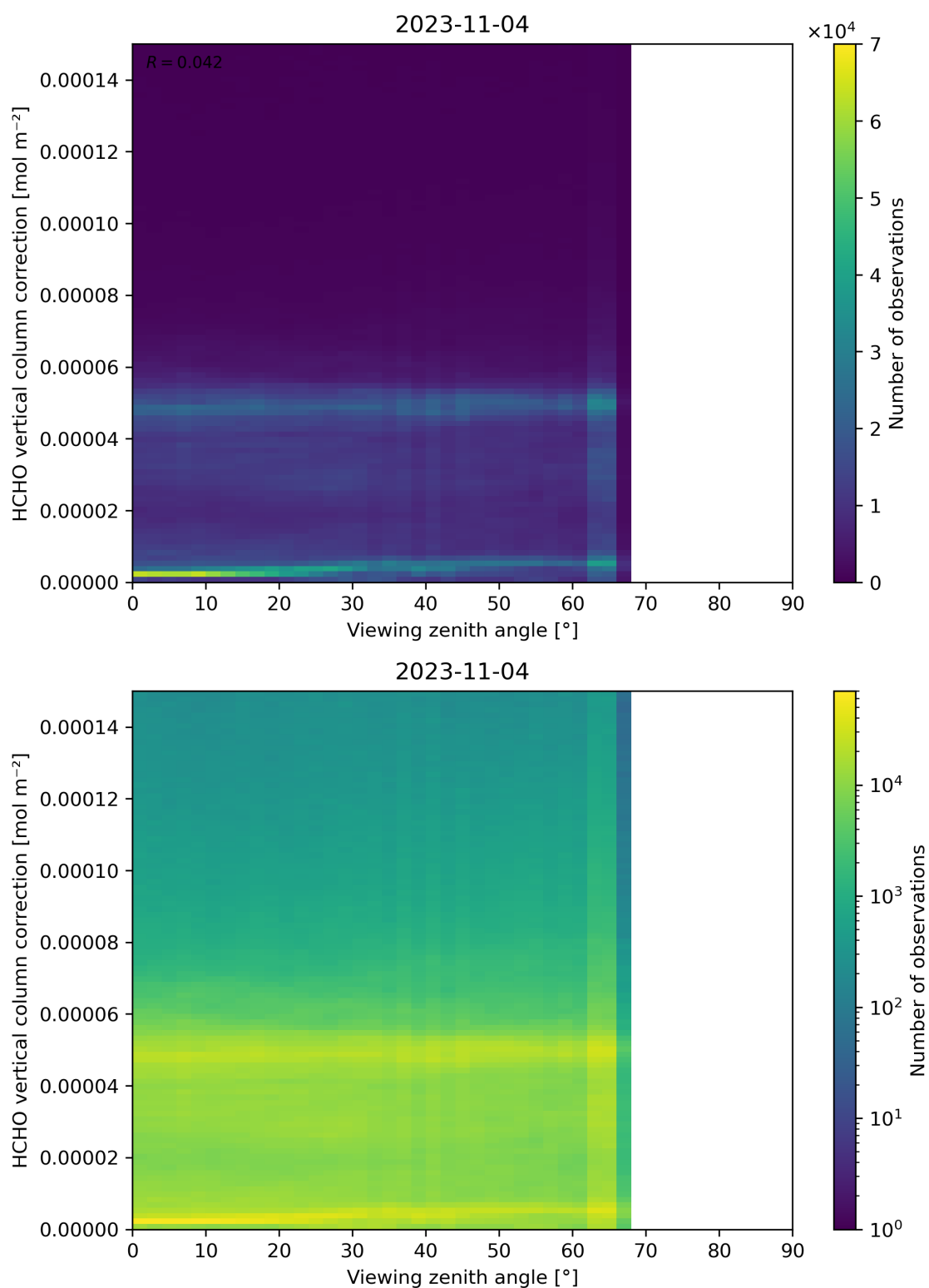
Figure 193: Scatter density plot of “Viewing zenith angle” against “HCHO vertical column correction” for 2023-11-03 to 2023-11-05.
