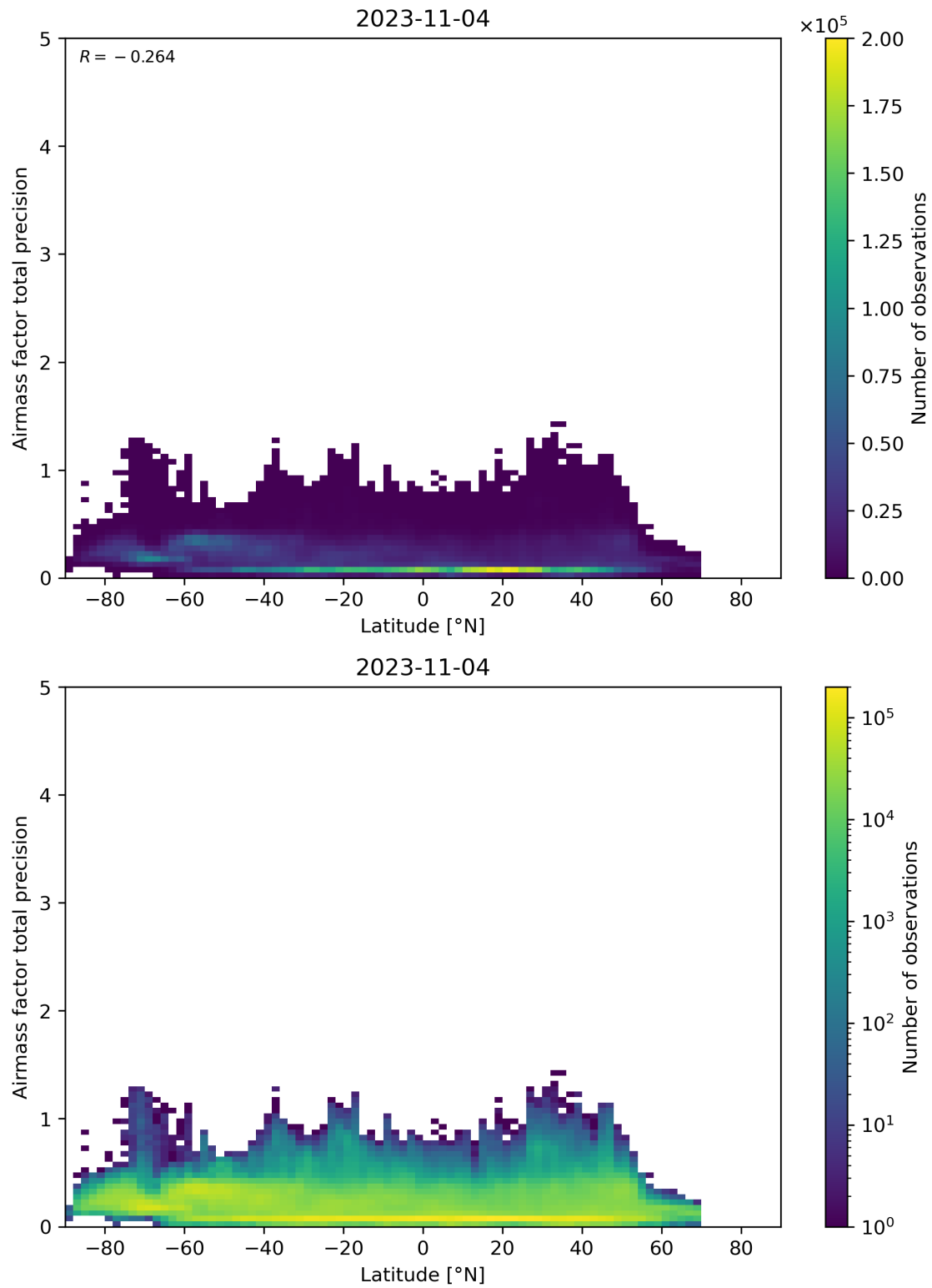
Figure 162: Scatter density plot of “Latitude” against “Airmass factor total precision” for 2023-11-03 to 2023-11-05.
