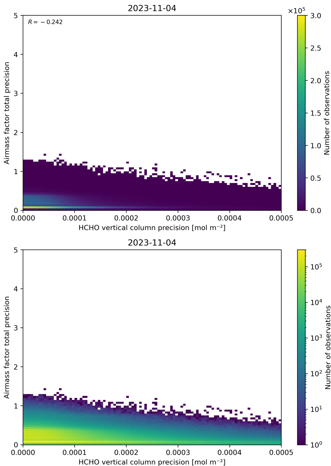
Figure 145: Scatter density plot of “HCHO vertical column precision” against “Airmass factor total precision” for 2023-11-03 to 2023-11-05.
