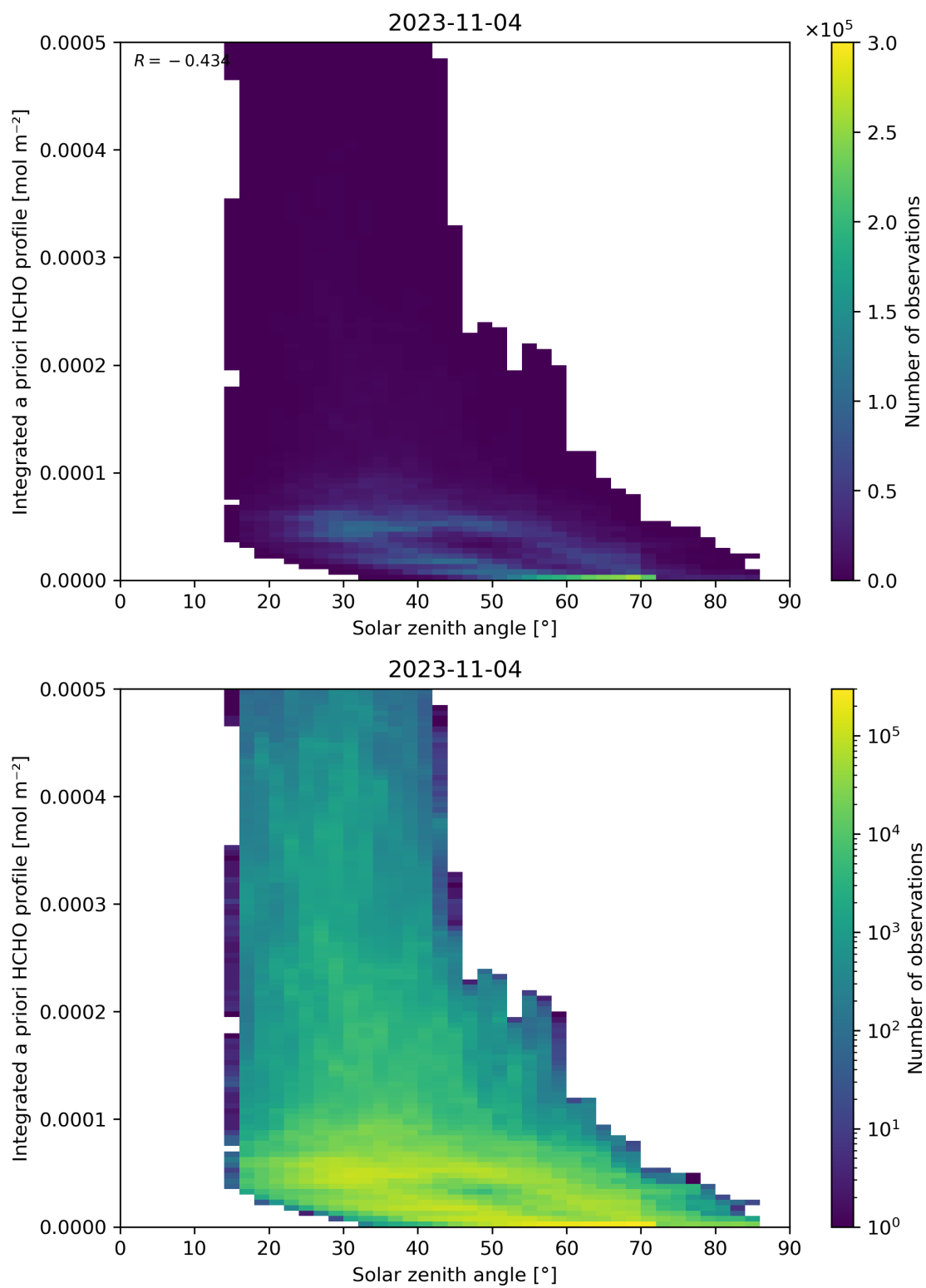
Figure 180: Scatter density plot of “Solar zenith angle” against “Integrated a priori HCHO profile” for 2023-11-03 to 2023-11-05.
