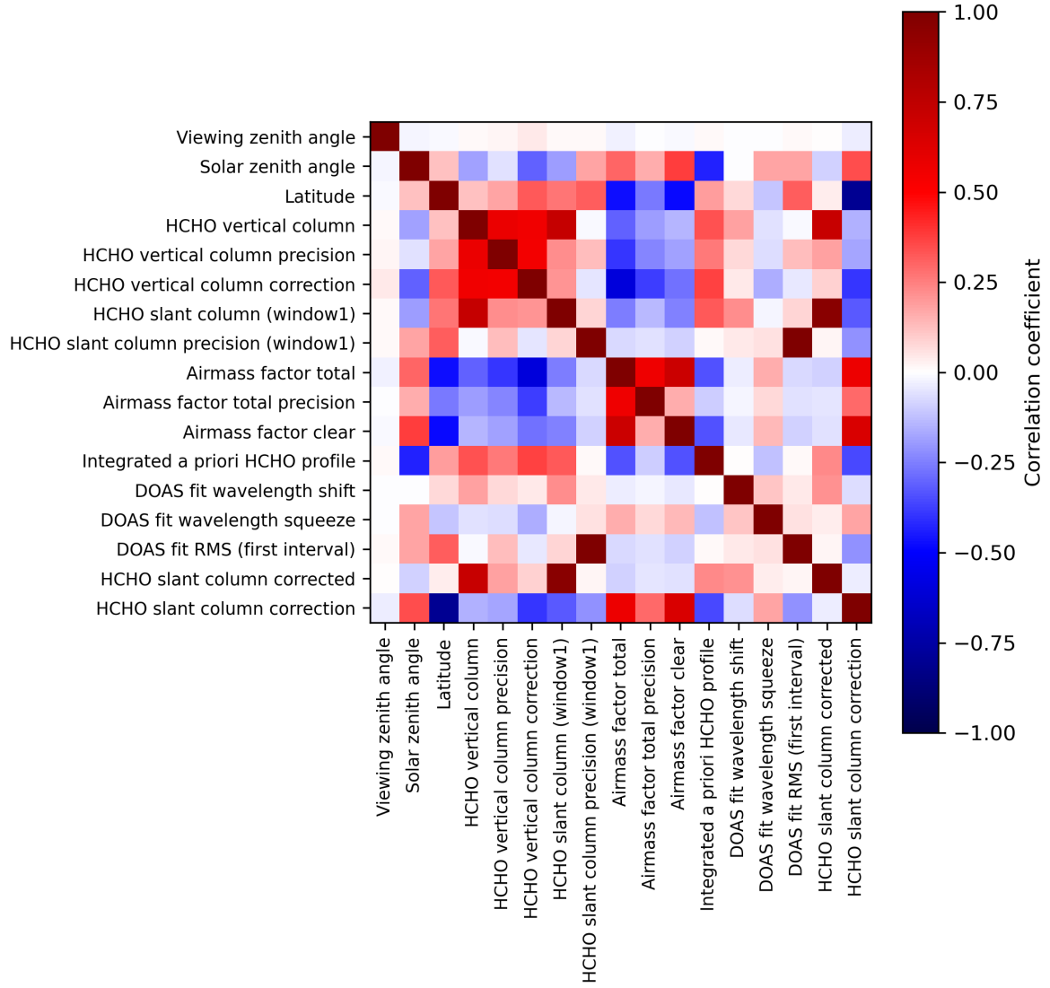
Figure 2: Map of correlation matrix for 2023-11-03 to 2023-11-05.
