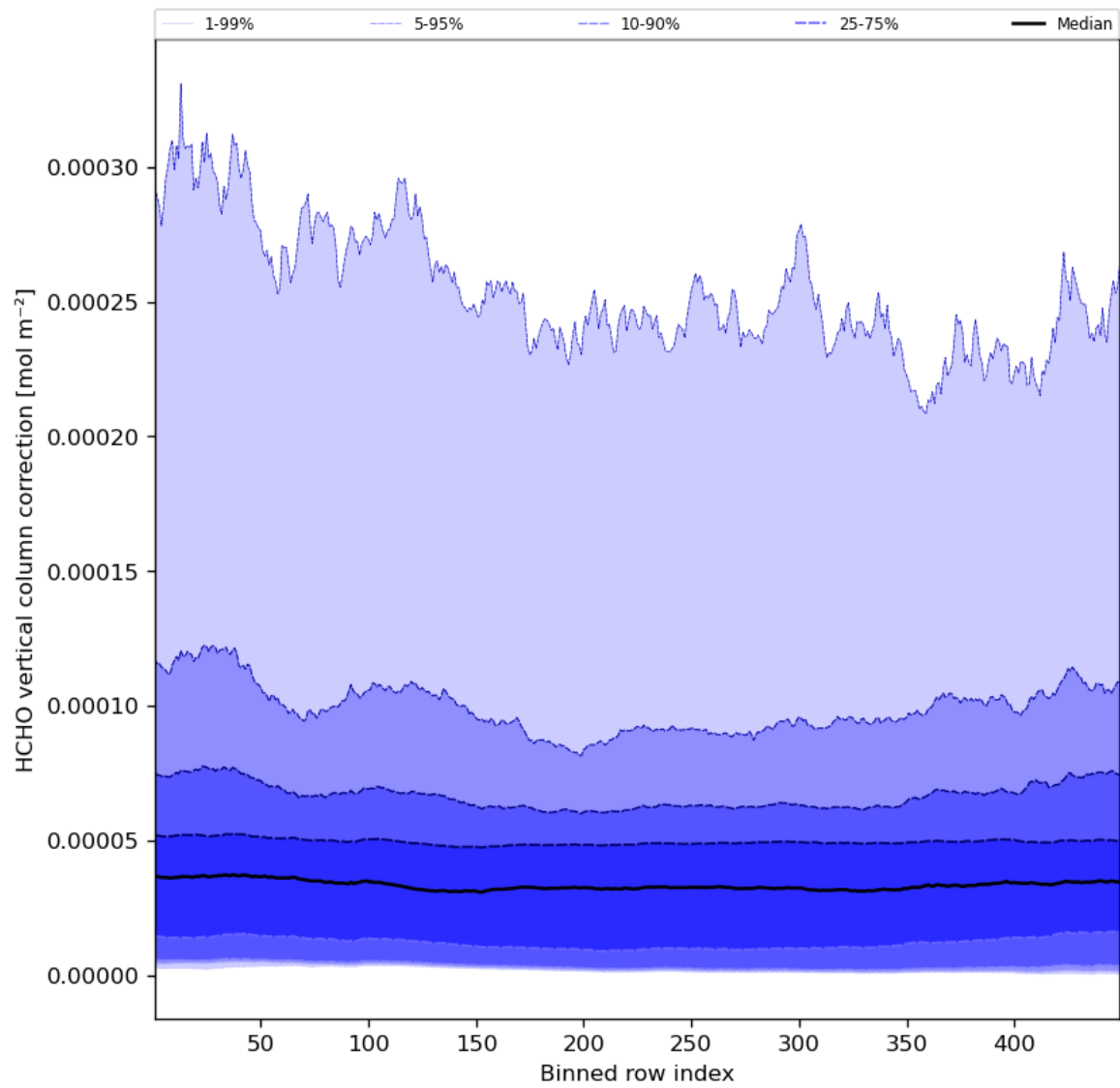
Figure 51: Along track statistics of “HCHO vertical column correction” for 2023-11-03 to 2023-11-05
