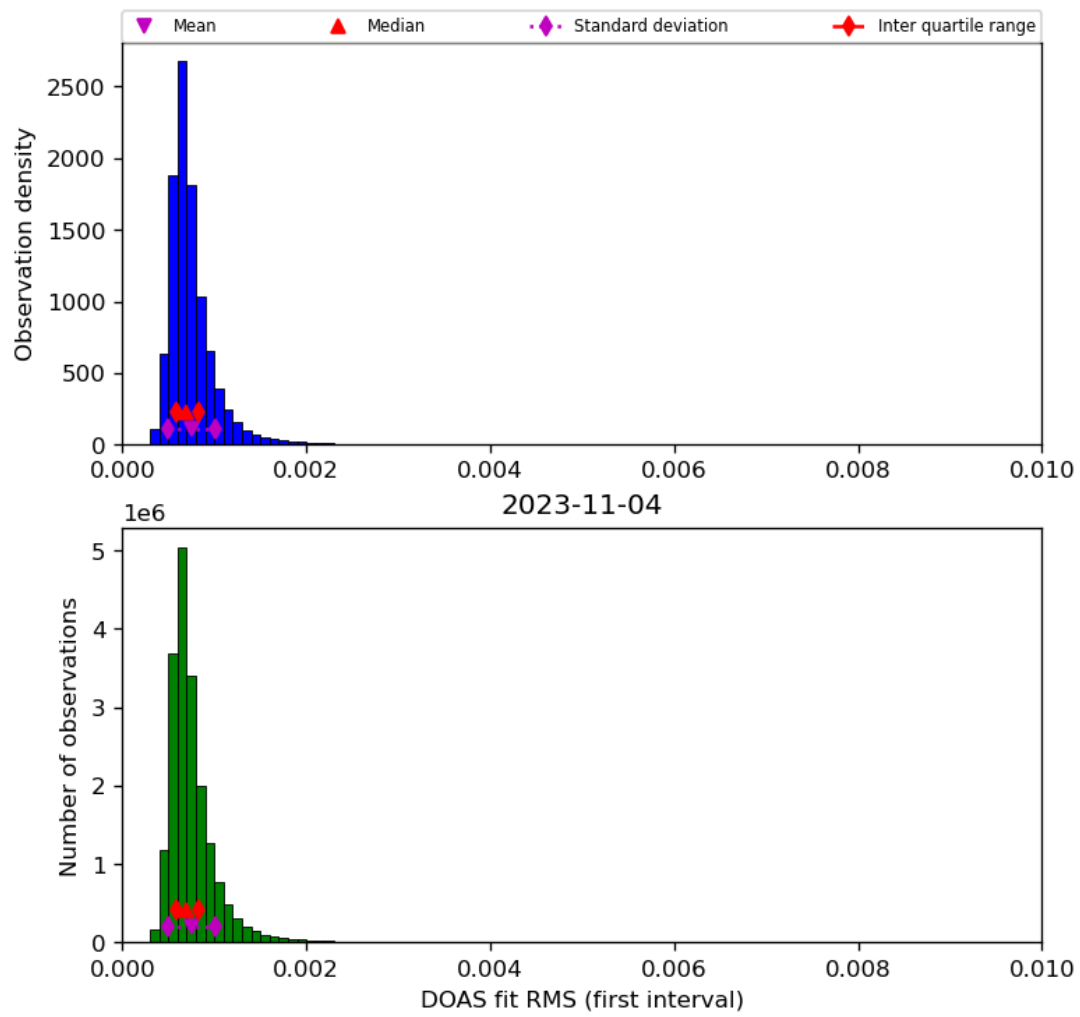
Figure 46: Histogram of “DOAS fit RMS (first interval)” for 2023-11-03 to 2023-11-05
