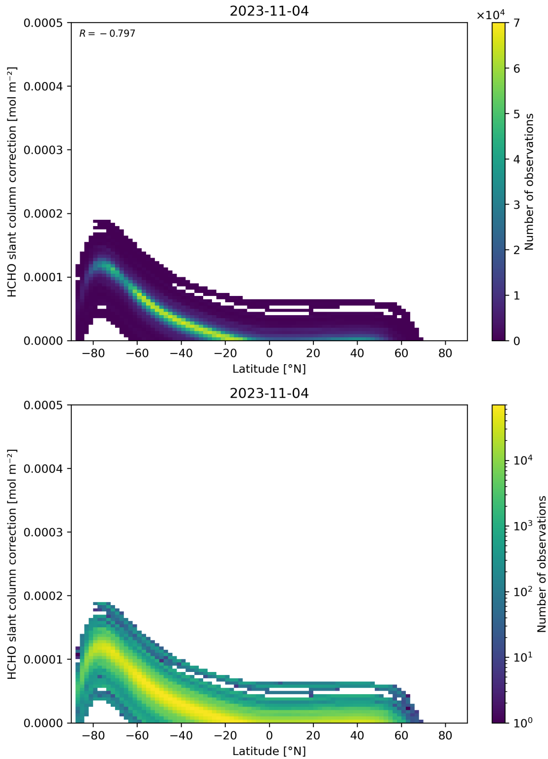
Figure 158: Scatter density plot of “Latitude” against “HCHO slant column correction” for 2023-11-03 to 2023-11-05.
