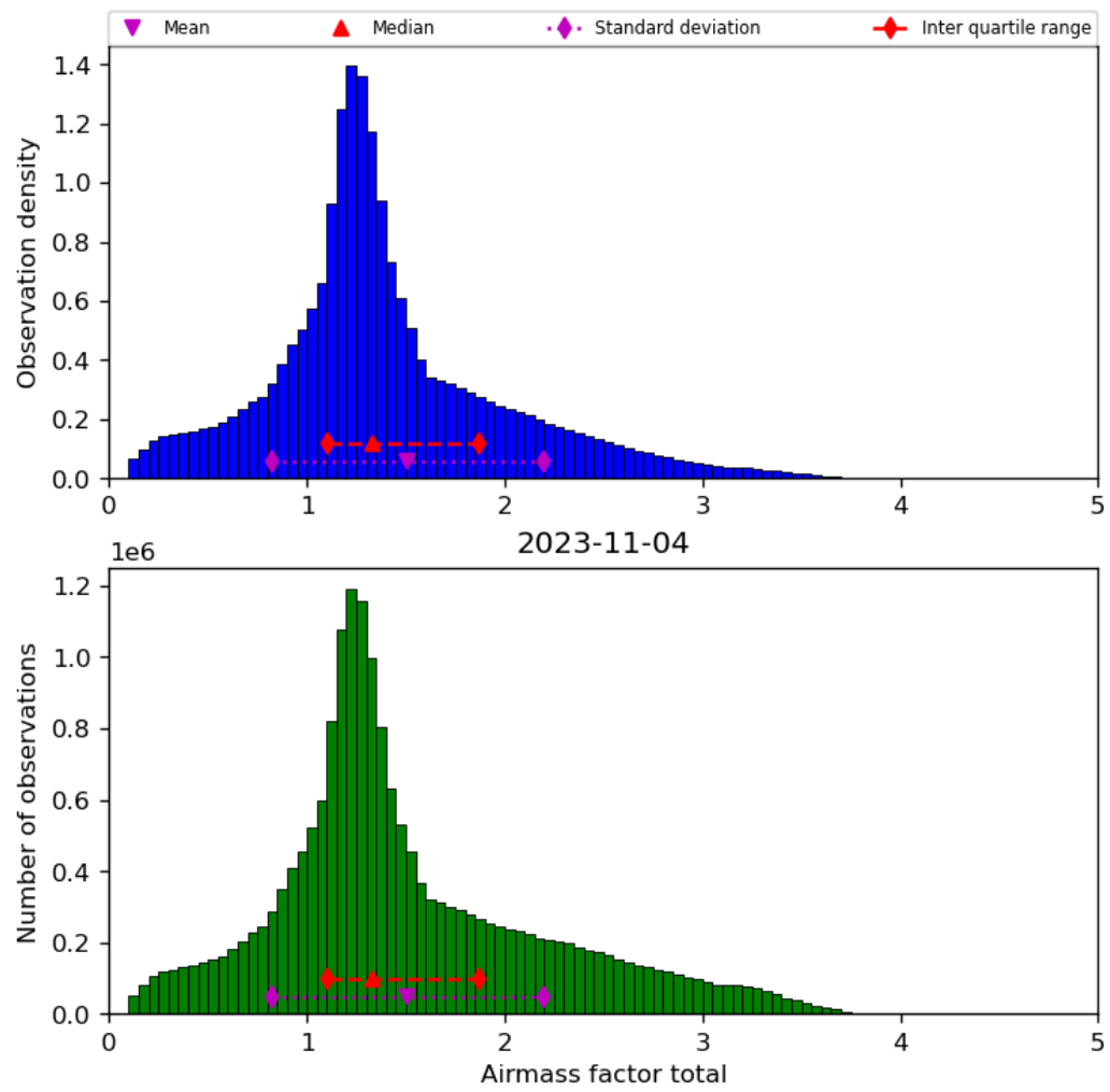
Figure 40: Histogram of “Airmass factor total” for 2023-11-03 to 2023-11-05
