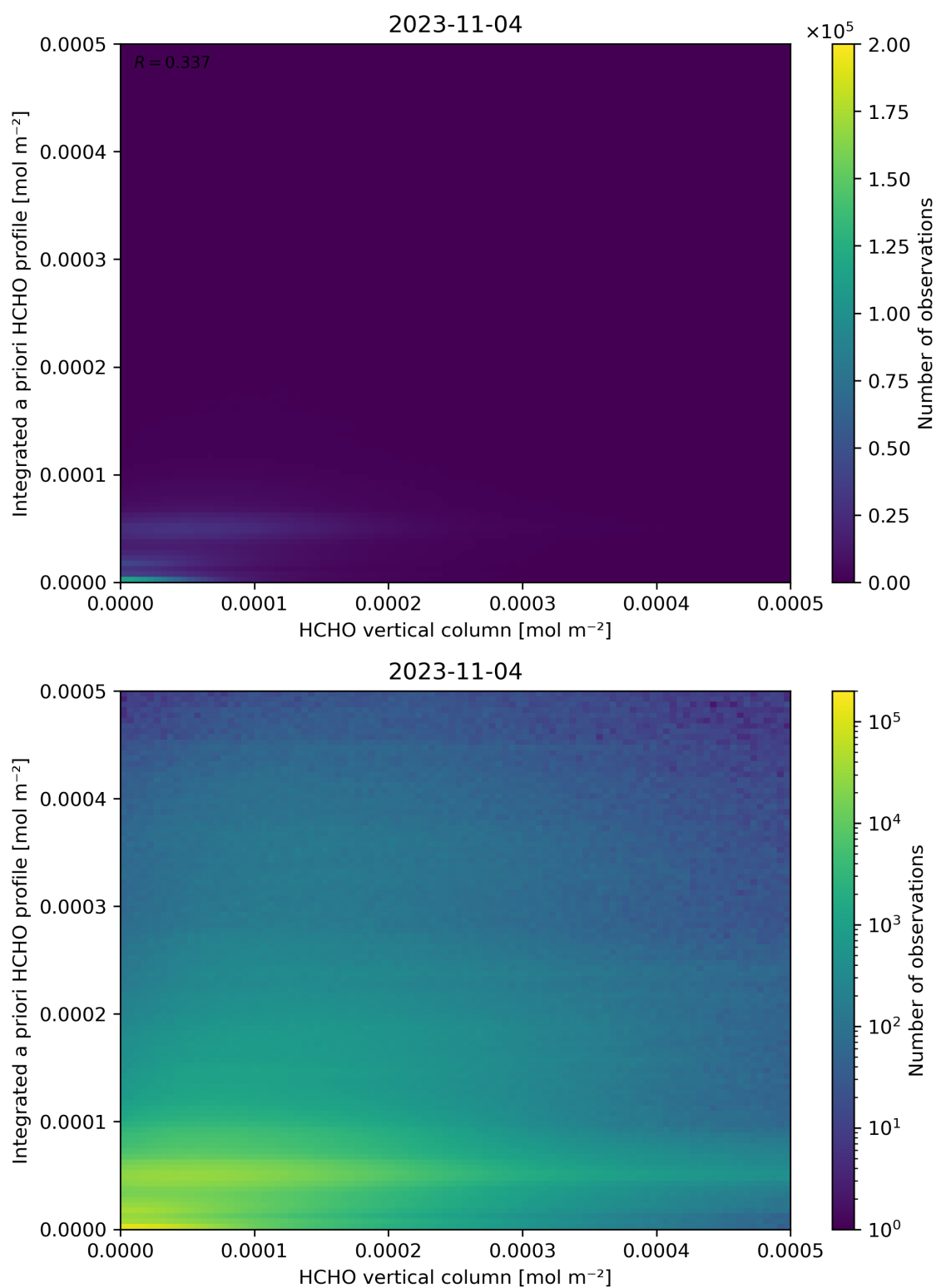
Figure 135: Scatter density plot of “HCHO vertical column” against “Integrated a priori HCHO profile” for 2023-11-03 to 2023-11-05.
