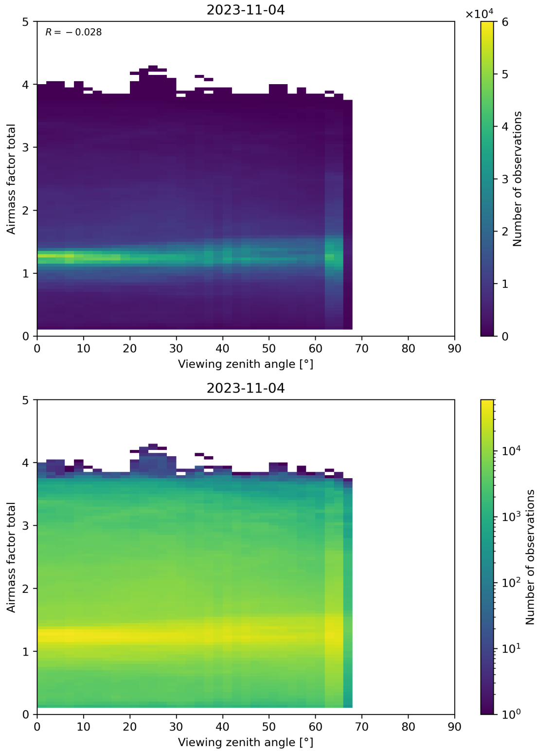
Figure 190: Scatter density plot of “Viewing zenith angle” against “Airmass factor total” for 2023-11-03 to 2023-11-05.
