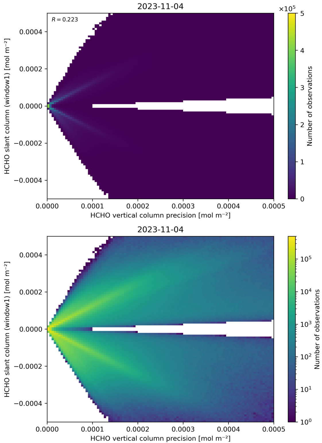
Figure 142: Scatter density plot of “HCHO vertical column precision” against “HCHO slant column (window1)” for 2023-11-03 to 2023-11-05.
