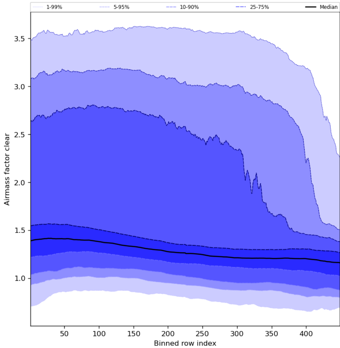
Figure 56: Along track statistics of “Airmass factor clear” for 2023-11-03 to 2023-11-05
