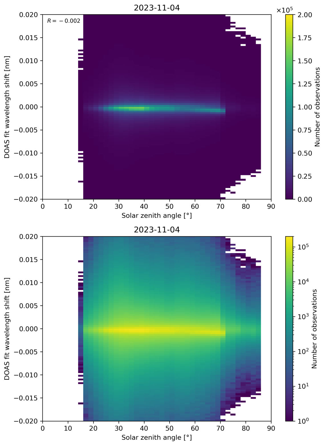
Figure 168: Scatter density plot of “Solar zenith angle” against “DOAS fit wavelength shift” for 2023-11-03 to 2023-11-05.
