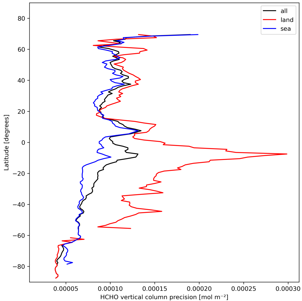
Figure 22: Zonal average of “HCHO vertical column precision” for 2023-11-03 to 2023-11-05.
