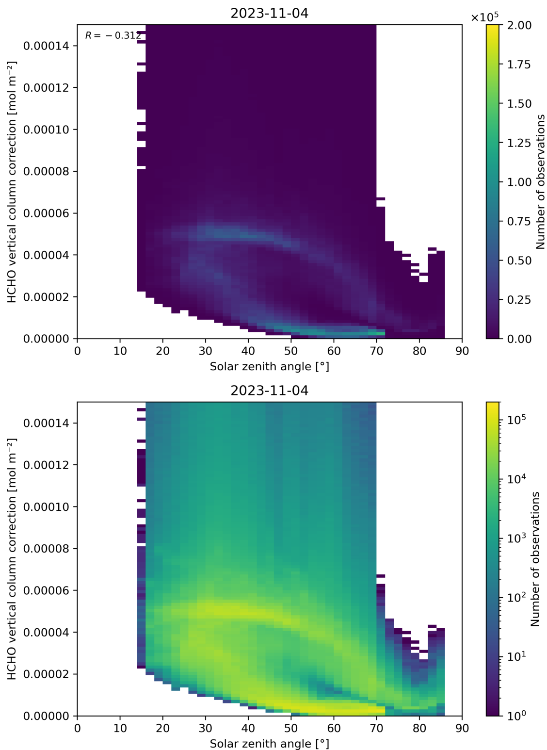
Figure 178: Scatter density plot of “Solar zenith angle” against “HCHO vertical column correction” for 2023-11-03 to 2023-11-05.
