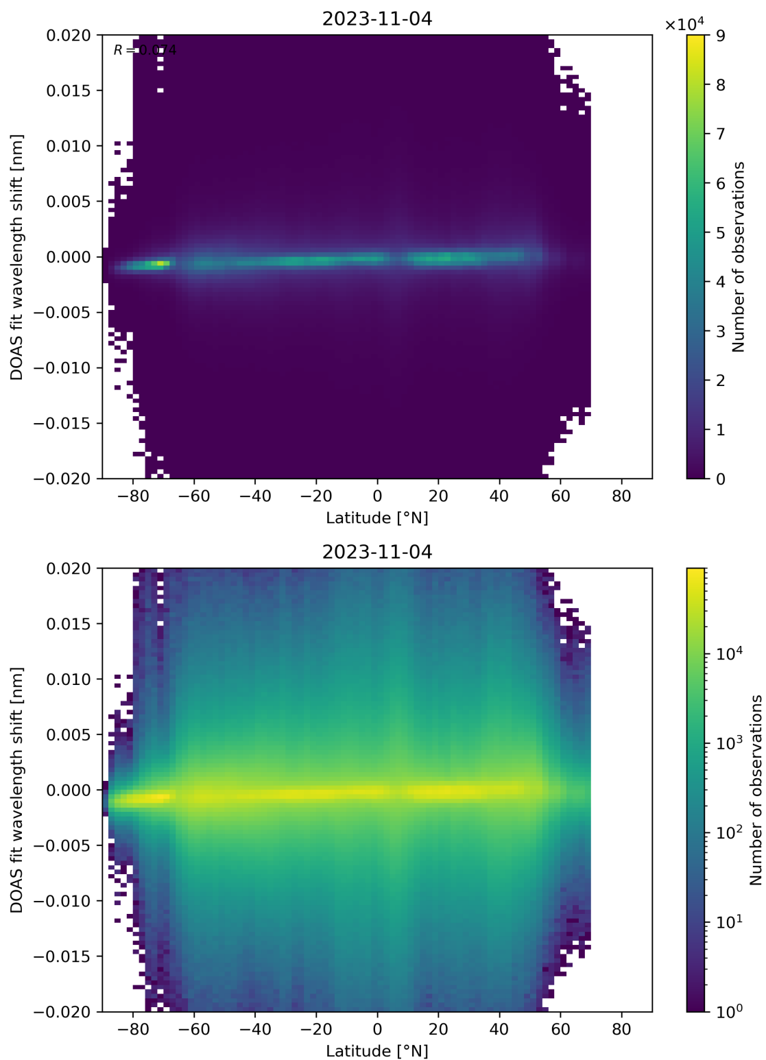
Figure 154: Scatter density plot of “Latitude” against “DOAS fit wavelength shift” for 2023-11-03 to 2023-11-05.
