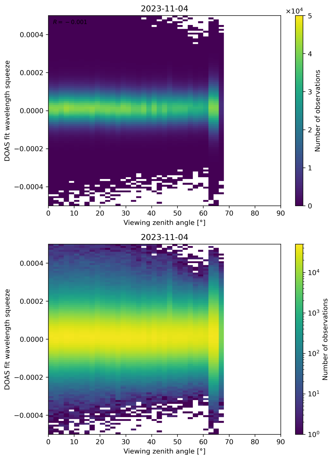
Figure 184: Scatter density plot of “Viewing zenith angle” against “DOAS fit wavelength squeeze” for 2023-11-03 to 2023-11-05.
