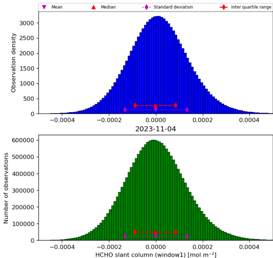
Figure 38: Histogram of “HCHO slant column (window1)” for 2023-11-03 to 2023-11-05
