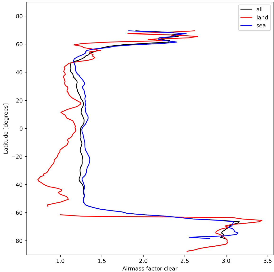
Figure 28: Zonal average of “Airmass factor clear” for 2023-11-03 to 2023-11-05.
