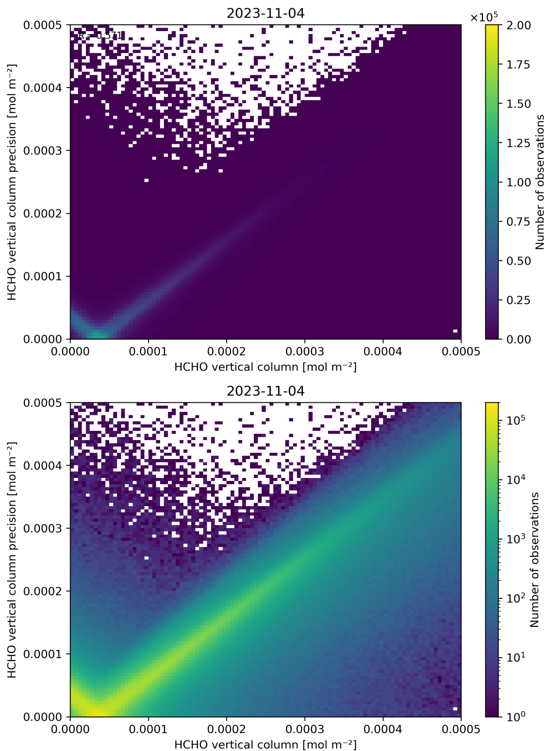
Figure 134: Scatter density plot of “HCHO vertical column” against “HCHO vertical column precision” for 2023-11-03 to 2023-11-05.
