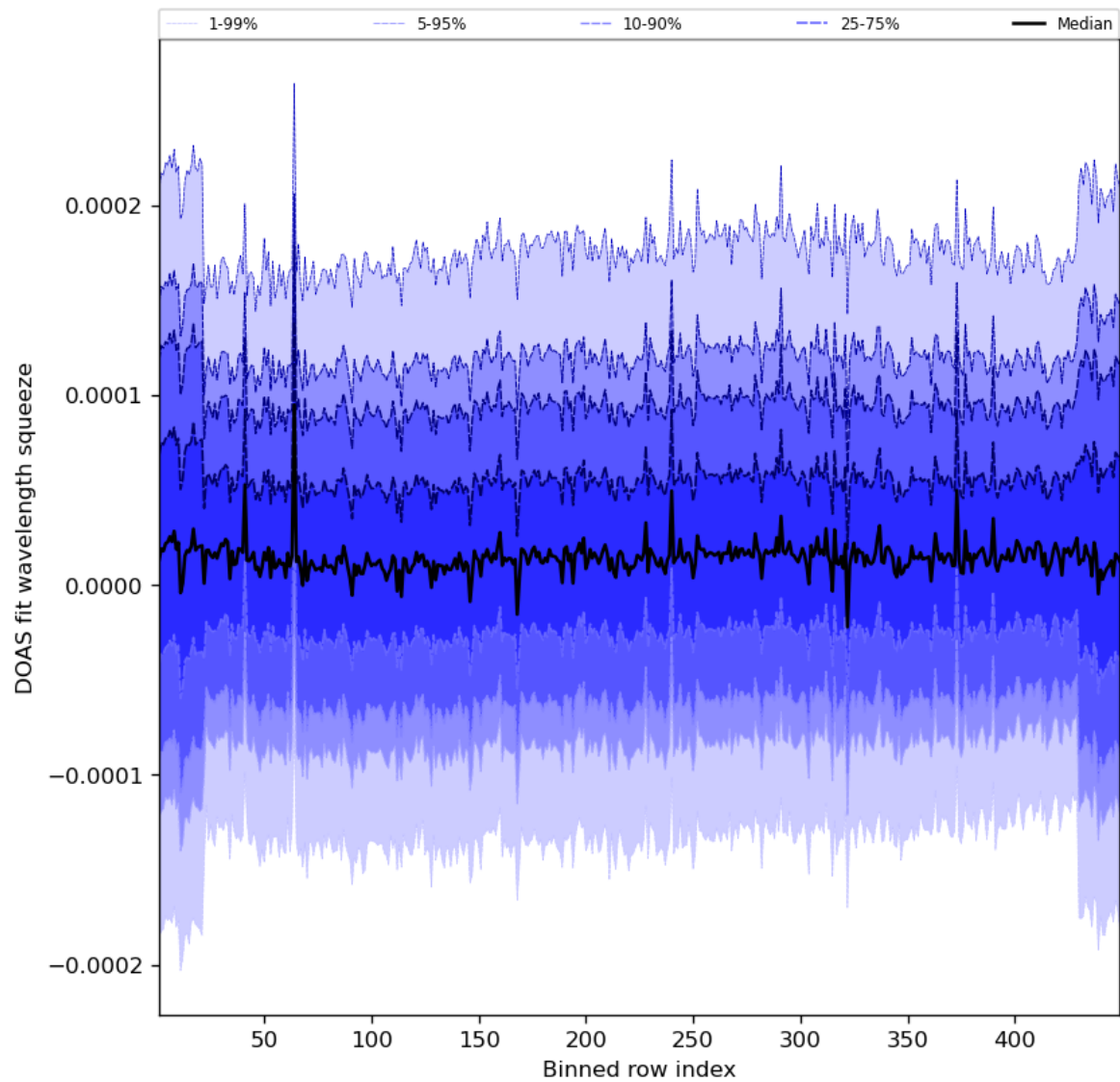
Figure 59: Along track statistics of “DOAS fit wavelength squeeze” for 2023-11-03 to 2023-11-05
