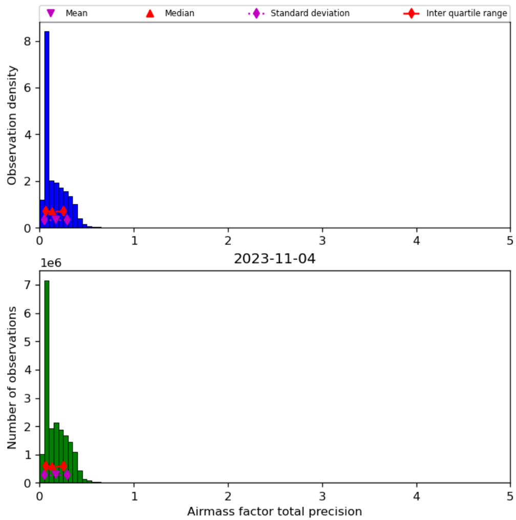
Figure 41: Histogram of “Airmass factor total precision” for 2023-11-03 to 2023-11-05
