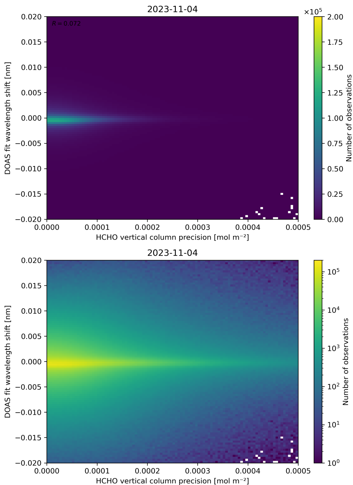
Figure 137: Scatter density plot of “HCHO vertical column precision” against “DOAS fit wavelength shift” for 2023-11-03 to 2023-11-05.
