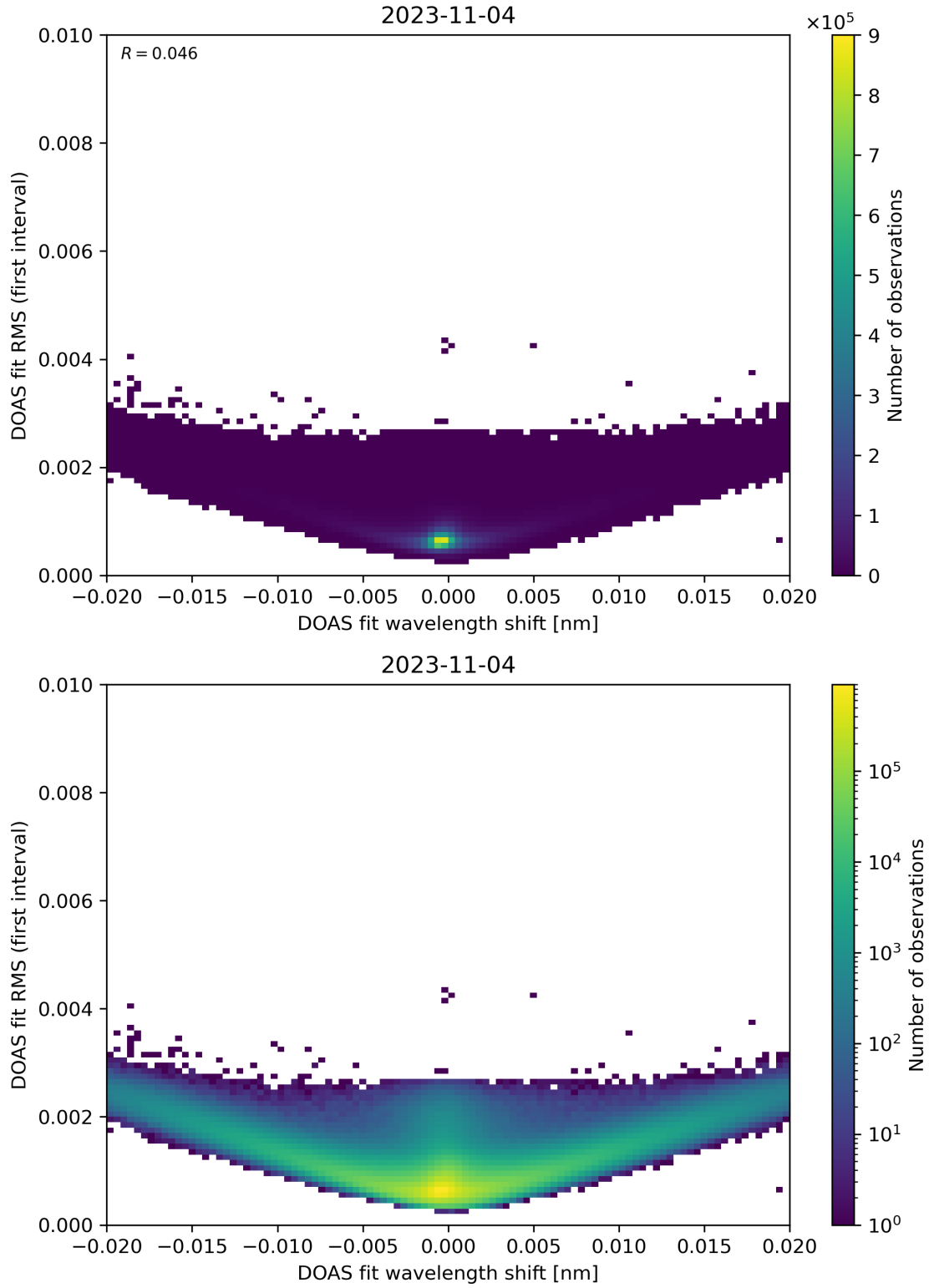
Figure 64: Scatter density plot of “DOAS fit wavelength shift” against “DOAS fit RMS (first interval)” for 2023-11-03 to 2023-11-05.
