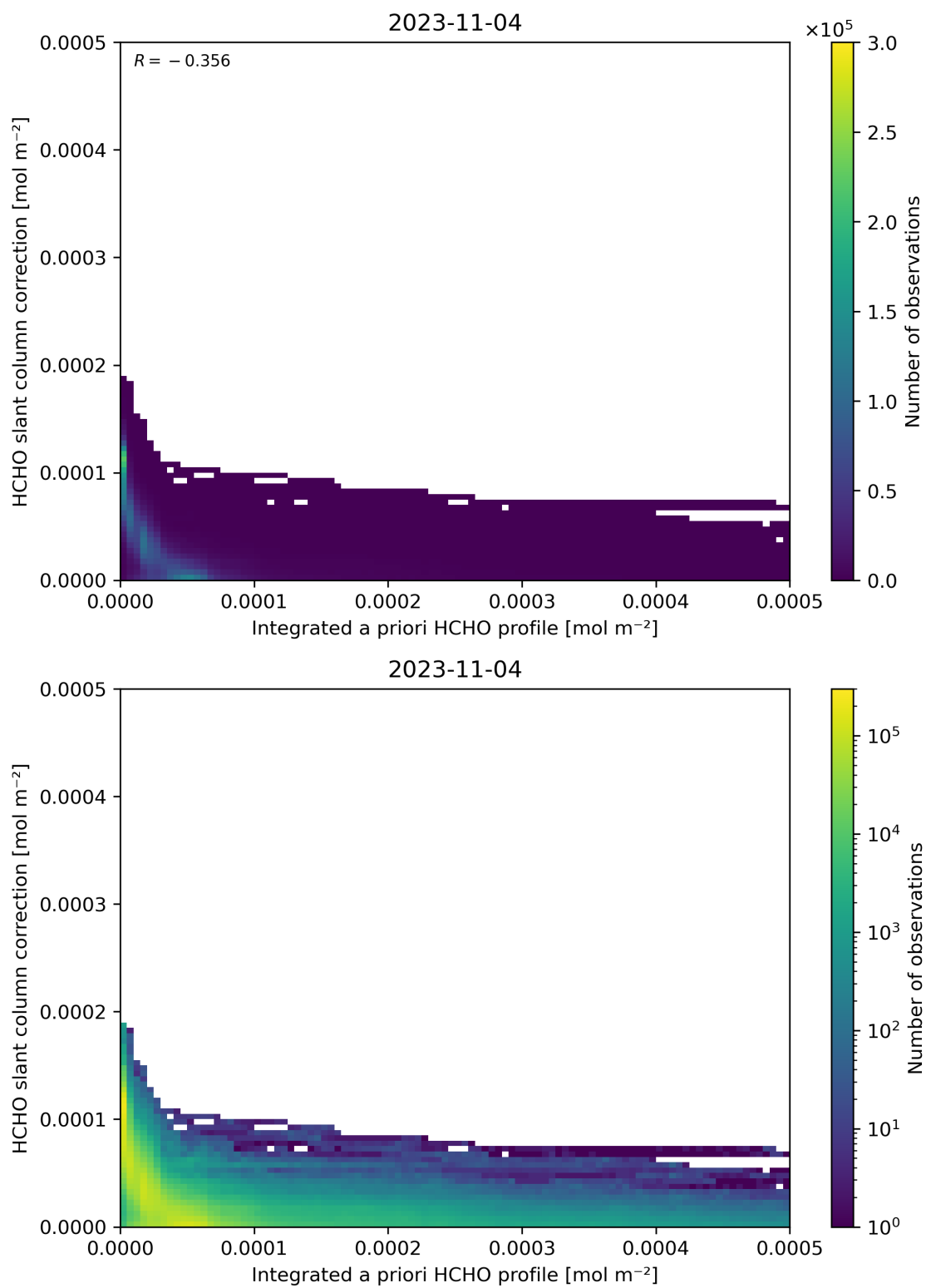
Figure 152: Scatter density plot of “Integrated a priori HCHO profile” against “HCHO slant column correction” for 2023-11-03 to 2023-11-05.
