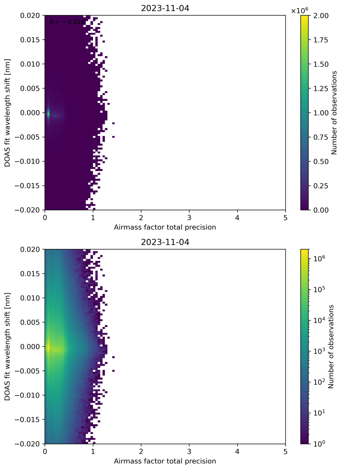
Figure 106: Scatter density plot of “Airmass factor total precision” against “DOAS fit wavelength shift” for 2023-11-03 to 2023-11-05.
