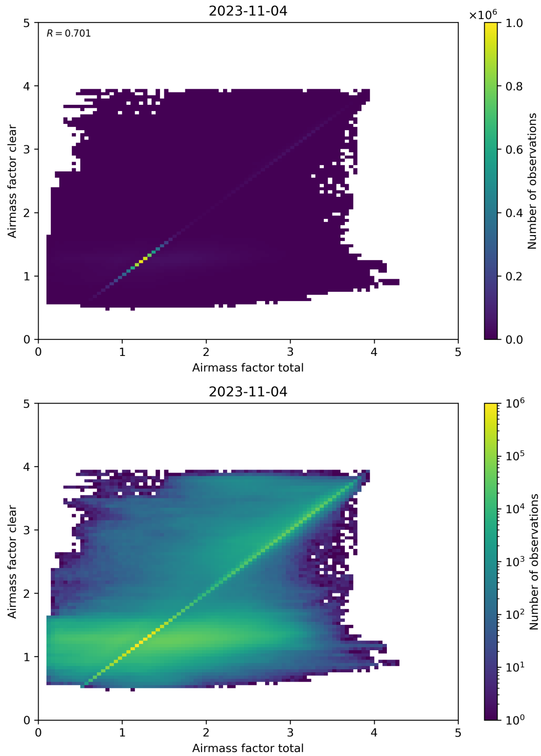
Figure 100: Scatter density plot of “Airmass factor total” against “Airmass factor clear” for 2023-11-03 to 2023-11-05.
