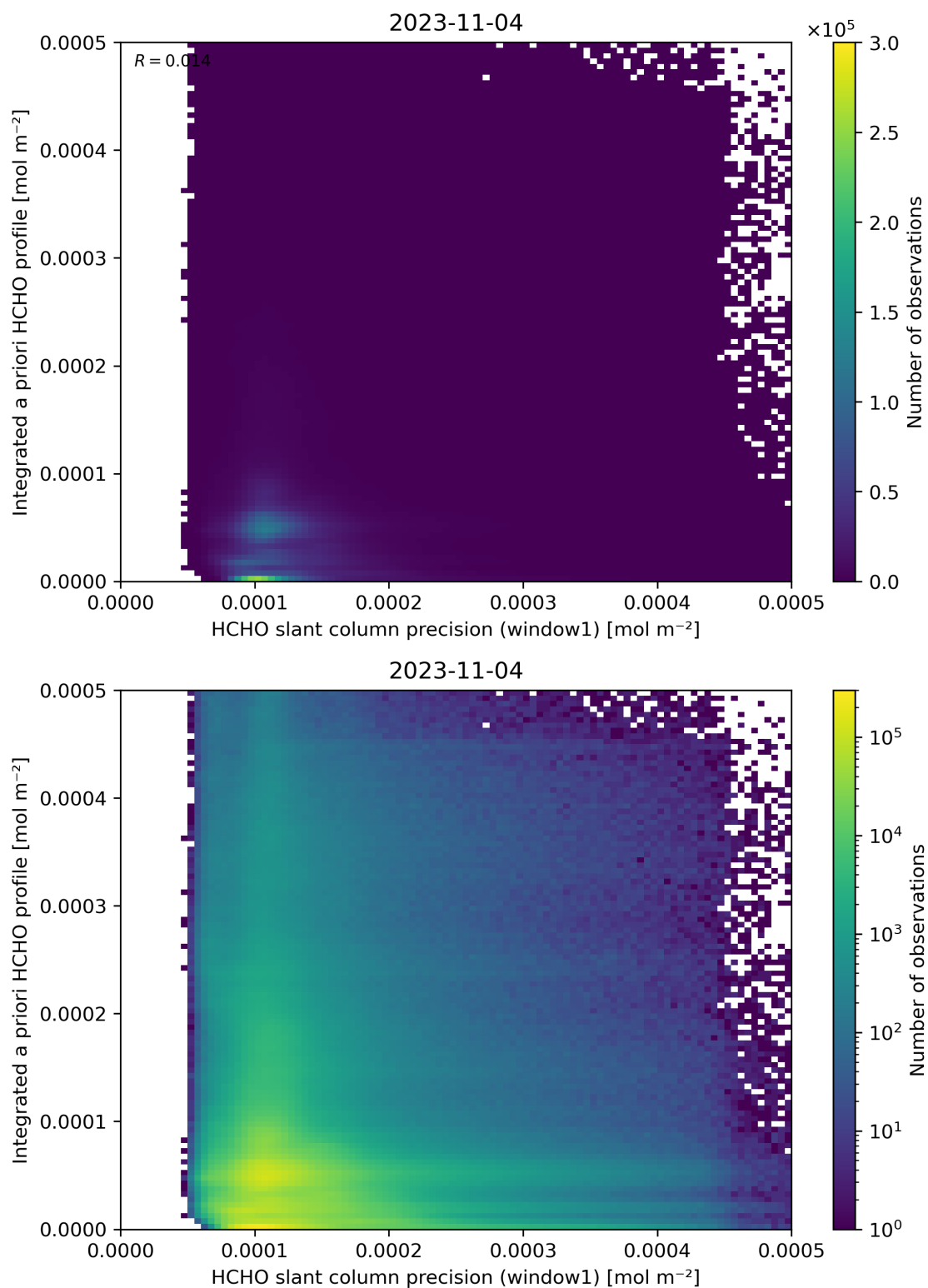
Figure 96: Scatter density plot of “HCHO slant column precision (window1)” against “Integrated a priori HCHO profile” for 2023-11-03 to 2023-11-05.
