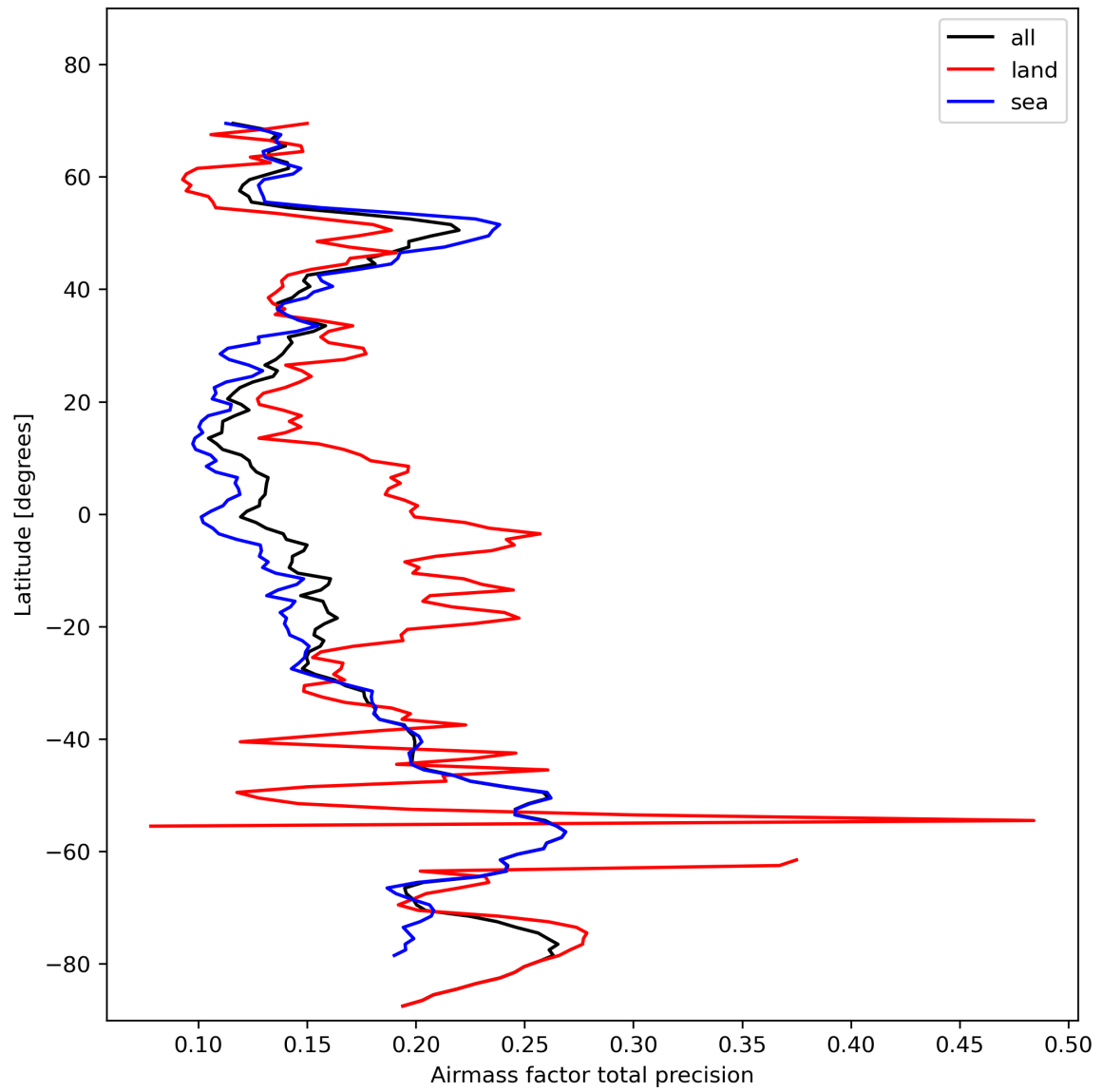
Figure 27: Zonal average of “Airmass factor total precision” for 2023-11-03 to 2023-11-05.
