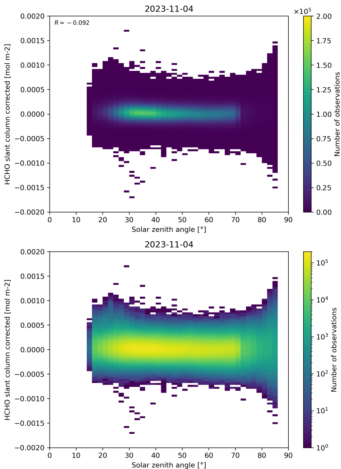
Figure 171: Scatter density plot of “Solar zenith angle” against “HCHO slant column corrected” for 2023-11-03 to 2023-11-05.
