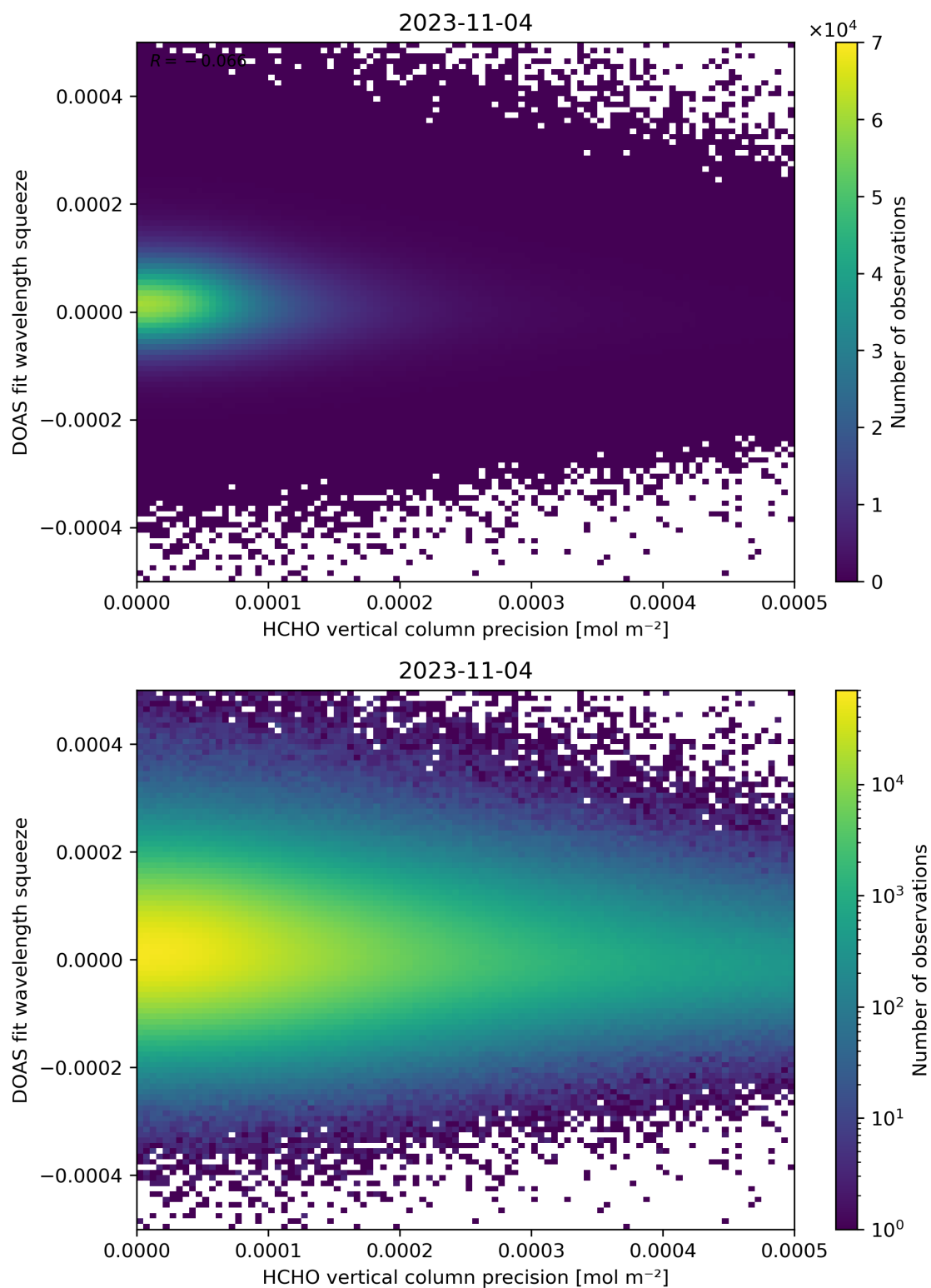
Figure 138: Scatter density plot of “HCHO vertical column precision” against “DOAS fit wavelength squeeze” for 2023-11-03 to 2023-11-05.
