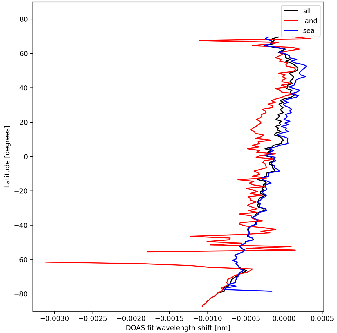
Figure 30: Zonal average of "DOAS fit wavelength shift" for 2023-11-03 to 2023-11-05.
