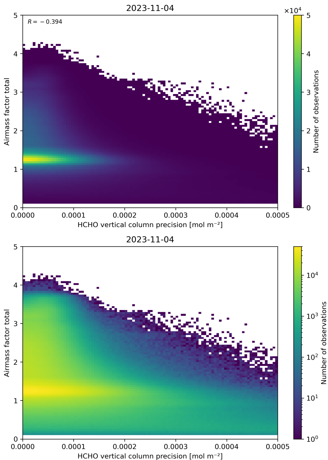
Figure 144: Scatter density plot of “HCHO vertical column precision” against “Airmass factor total” for 2023-11-03 to 2023-11-05.
