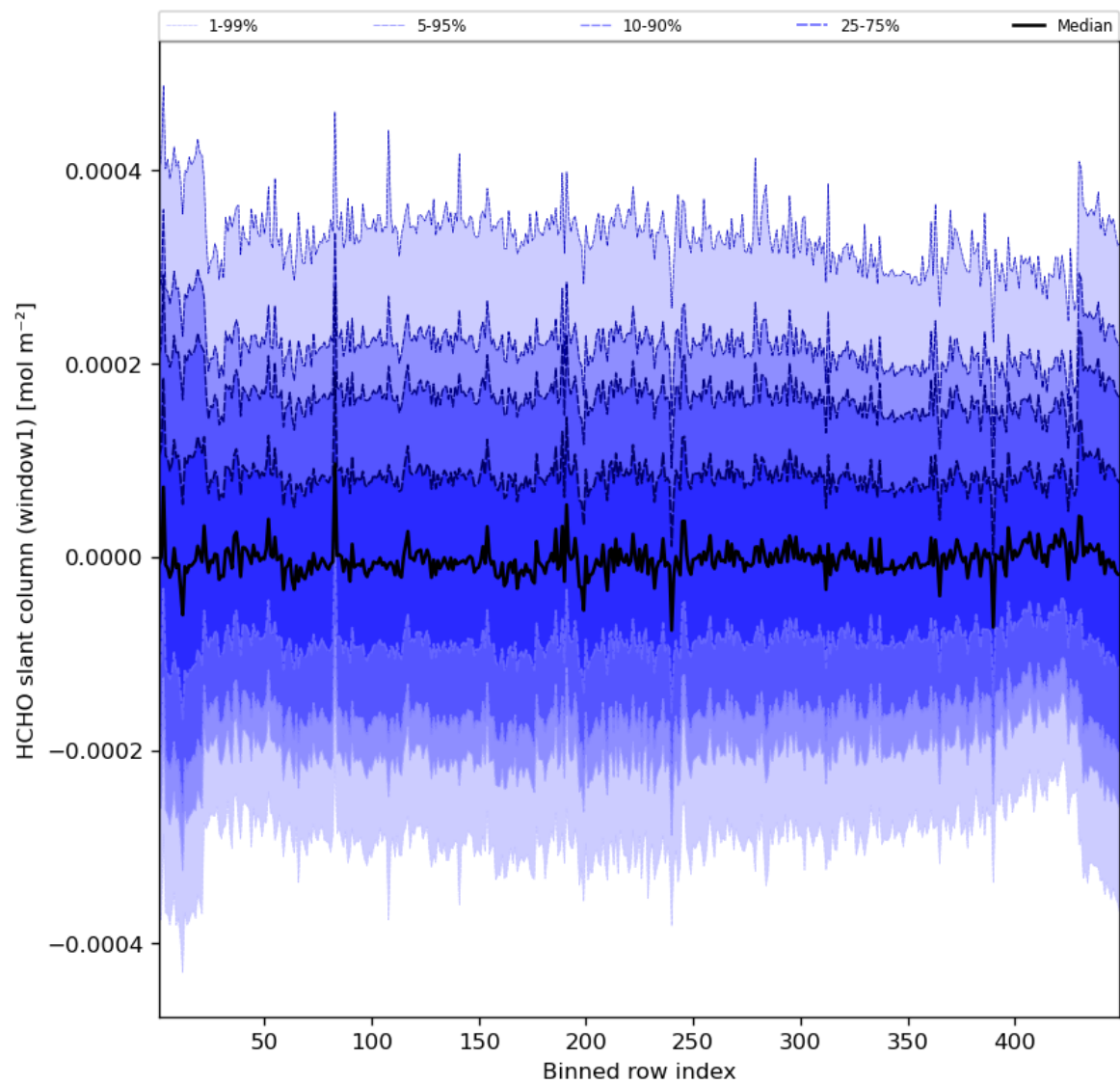
Figure 52: Along track statistics of “HCHO slant column (window1)” for 2023-11-03 to 2023-11-05
