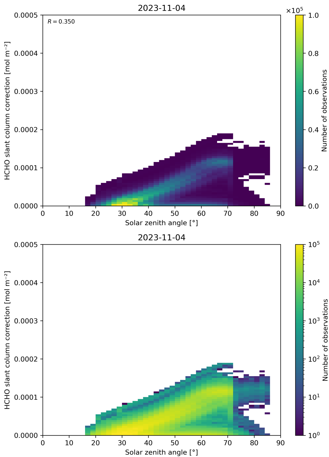
Figure 172: Scatter density plot of “Solar zenith angle” against “HCHO slant column correction” for 2023-11-03 to 2023-11-05.
