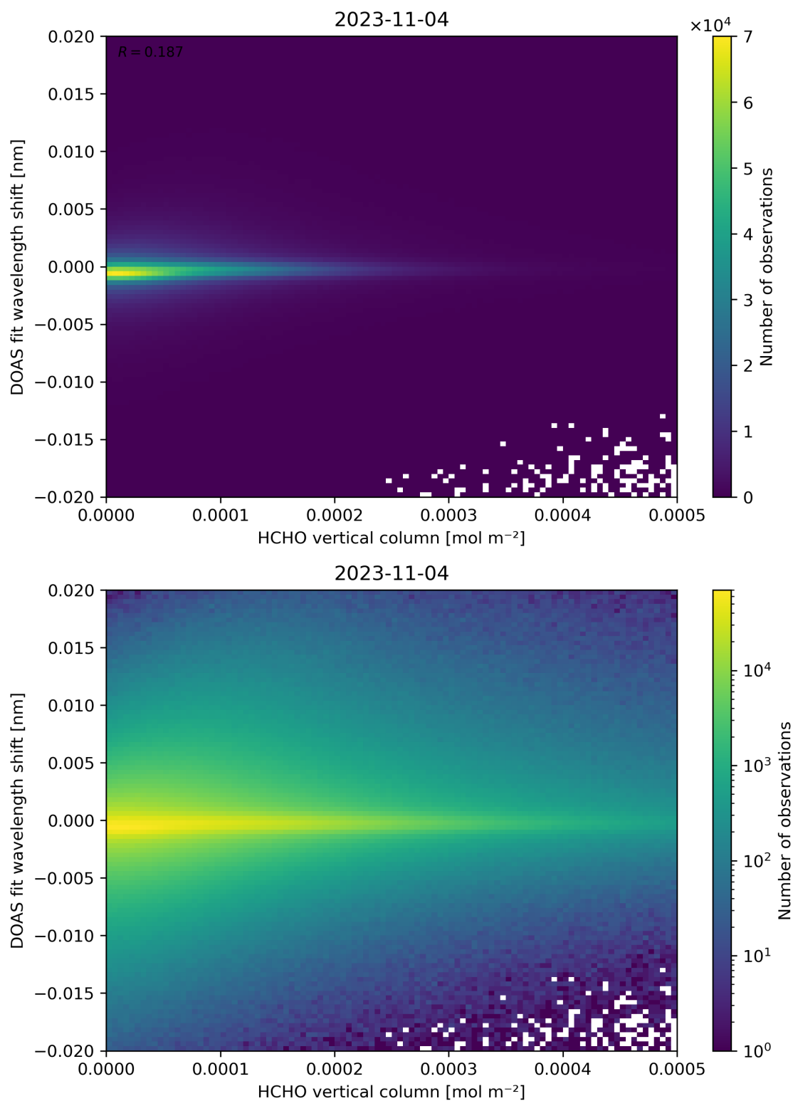
Figure 124: Scatter density plot of “HCHO vertical column” against “DOAS fit wavelength shift” for 2023-11-03 to 2023-11-05.
