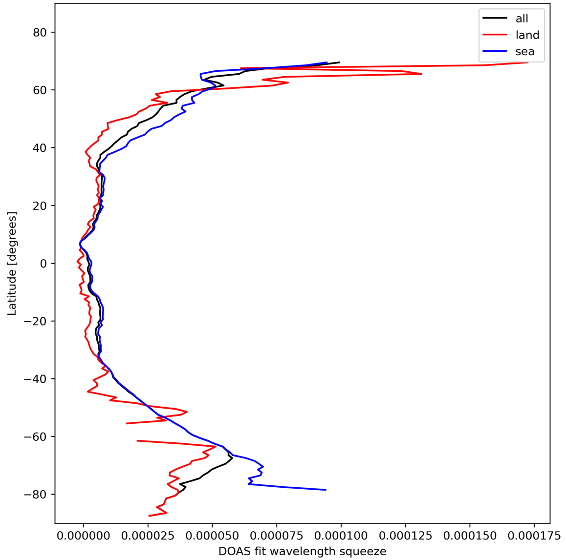
Figure 31: Zonal average of “DOAS fit wavelength squeeze” for 2023-11-03 to 2023-11-05.
