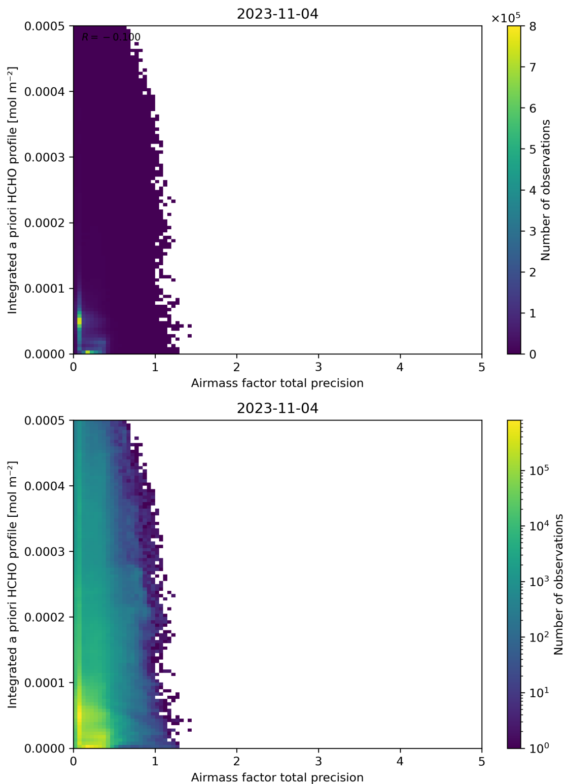
Figure 111: Scatter density plot of “Airmass factor total precision” against “Integrated a priori HCHO profile” for 2023-11-03 to 2023-11-05.
