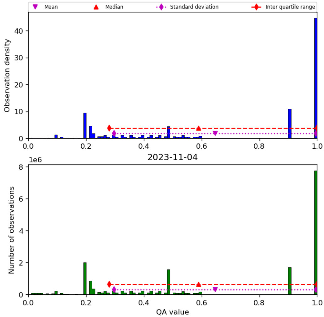
Figure 34: Histogram of “QA value” for 2023-11-03 to 2023-11-05
