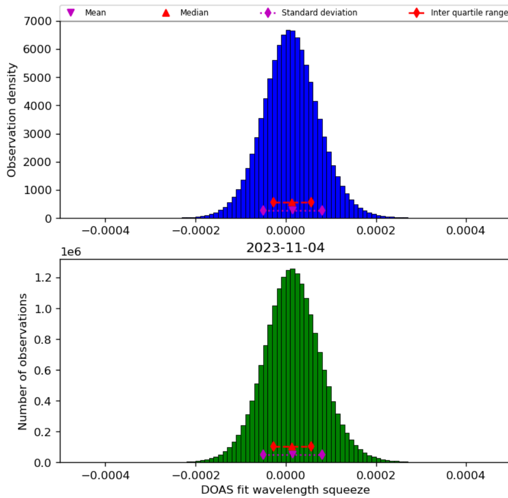
Figure 45: Histogram of “DOAS fit wavelength squeeze” for 2023-11-03 to 2023-11-05
