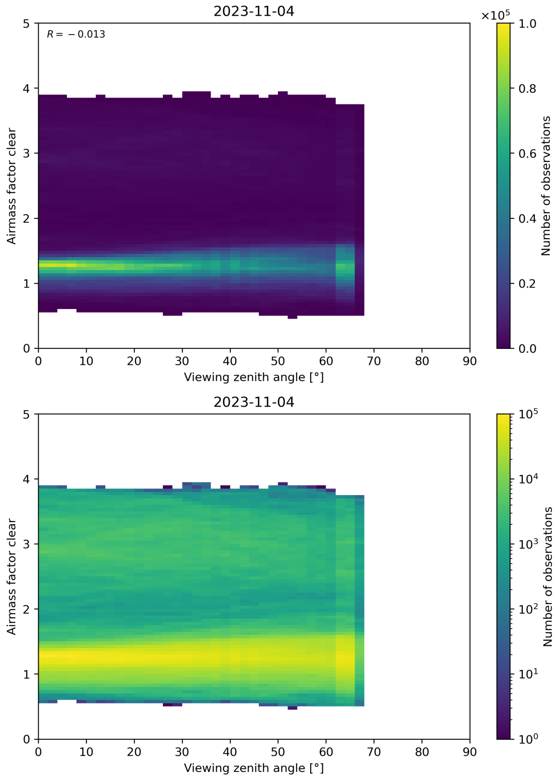
Figure 185: Scatter density plot of “Viewing zenith angle” against “Airmass factor clear” for 2023-11-03 to 2023-11-05.
