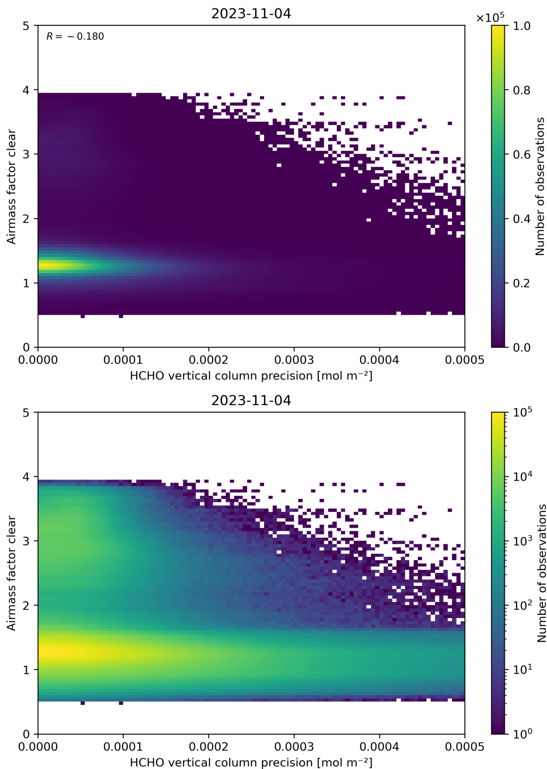
Figure 139: Scatter density plot of “HCHO vertical column precision” against “Airmass factor clear” for 2023-11-03 to 2023-11-05.
