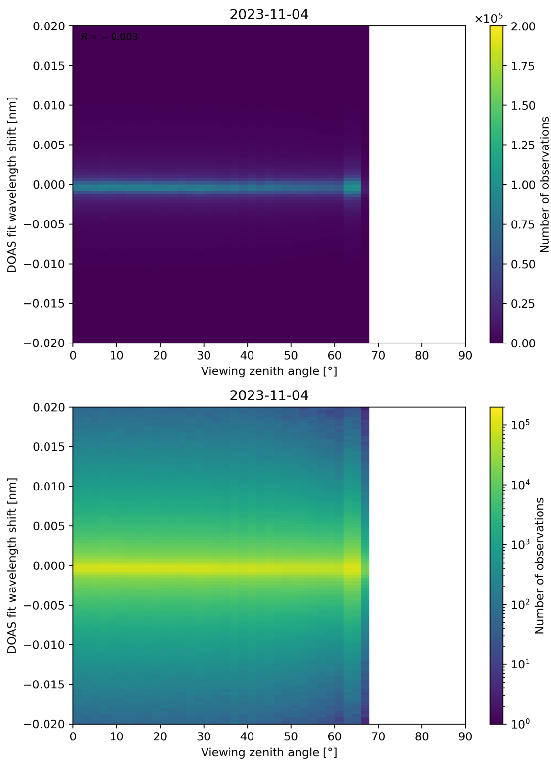
Figure 183: Scatter density plot of “Viewing zenith angle” against “DOAS fit wavelength shift” for 2023-11-03 to 2023-11-05.
