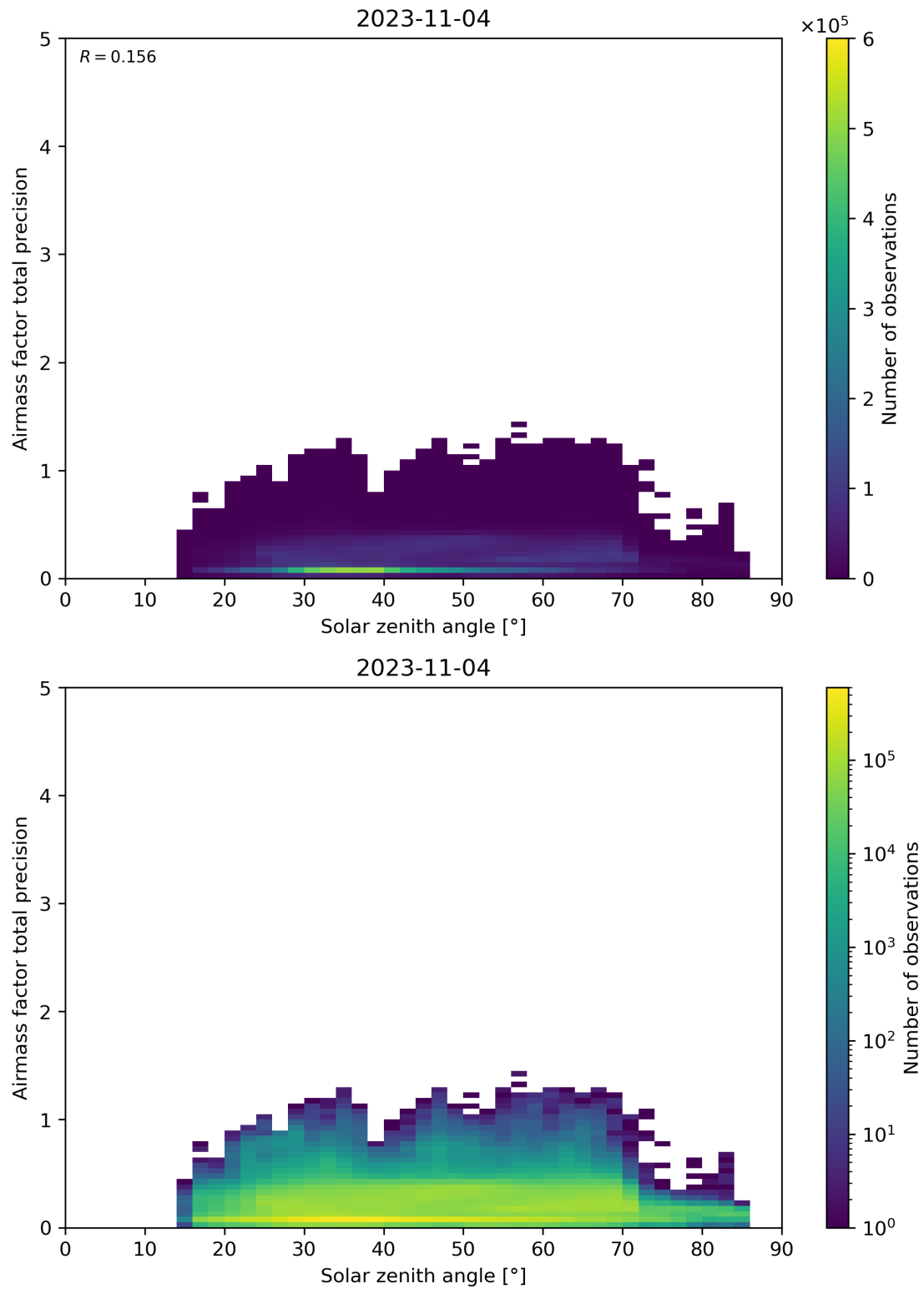
Figure 176: Scatter density plot of “Solar zenith angle” against “Airmass factor total precision” for 2023-11-03 to 2023-11-05.
