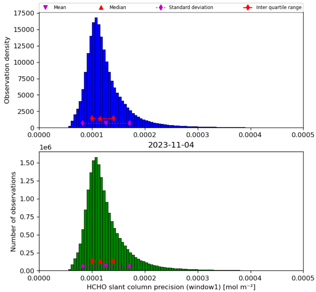
Figure 39: Histogram of “HCHO slant column precision (window1)” for 2023-11-03 to 2023-11-05
