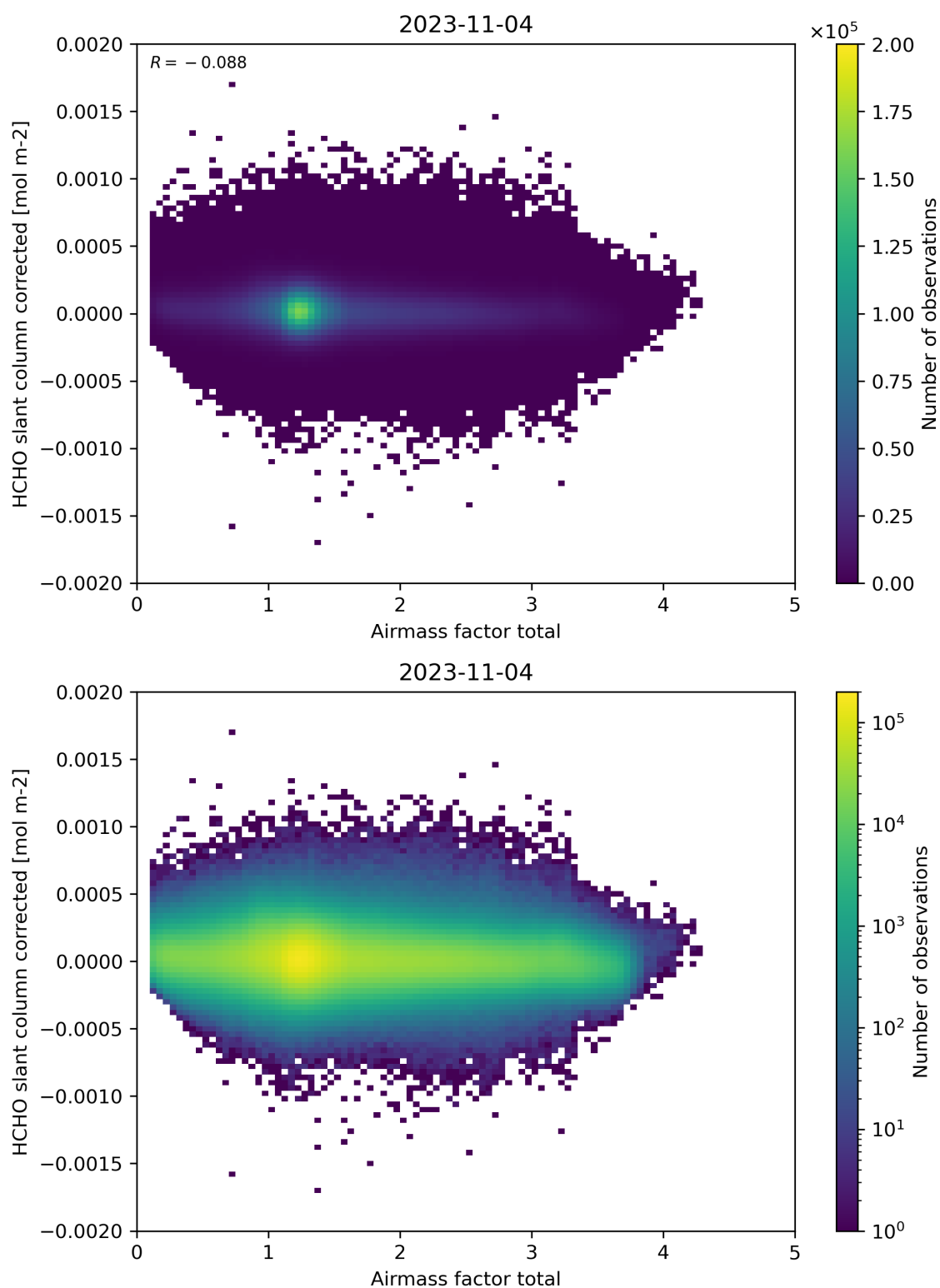
Figure 101: Scatter density plot of “Airmass factor total” against “HCHO slant column corrected” for 2023-11-03 to 2023-11-05.
