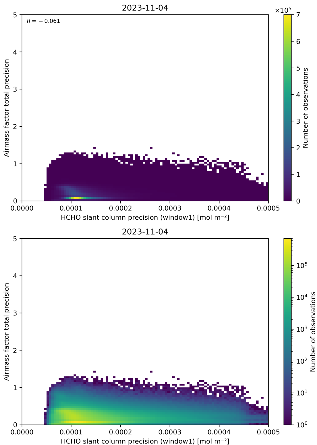
Figure 95: Scatter density plot of “HCHO slant column precision (window1)” against “Airmass factor total precision” for 2023-11-03 to 2023-11-05.
