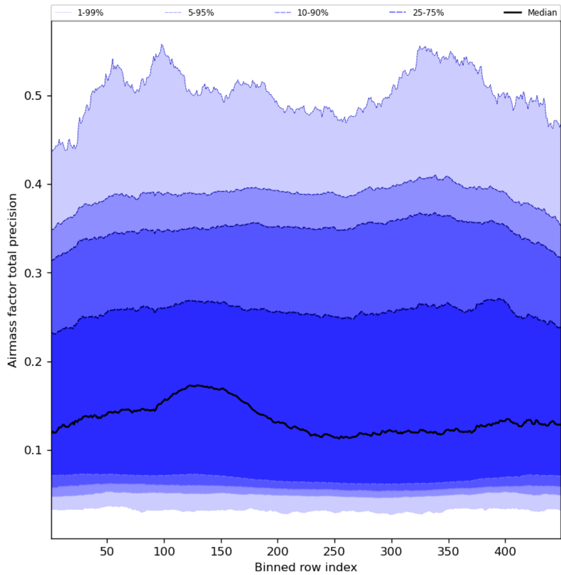
Figure 55: Along track statistics of “Airmass factor total precision” for 2023-11-03 to 2023-11-05
