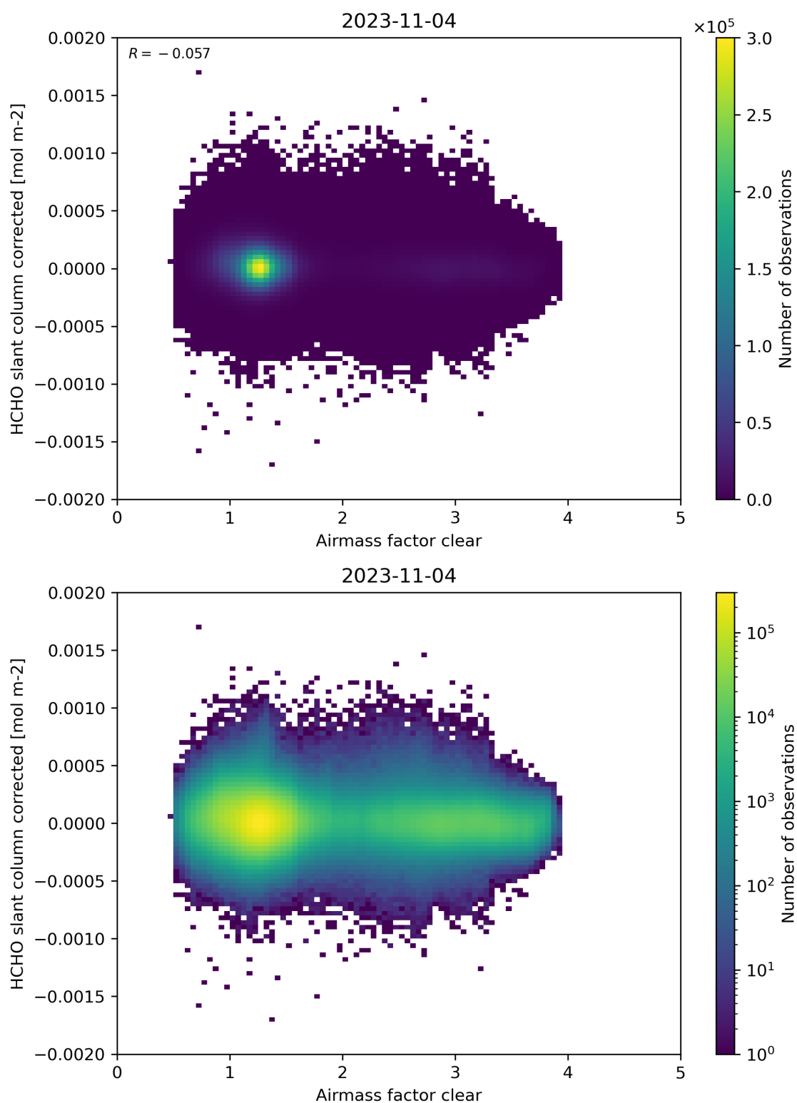
Figure 74: Scatter density plot of “Airmass factor clear” against “HCHO slant column corrected” for 2023-11-03 to 2023-11-05.
