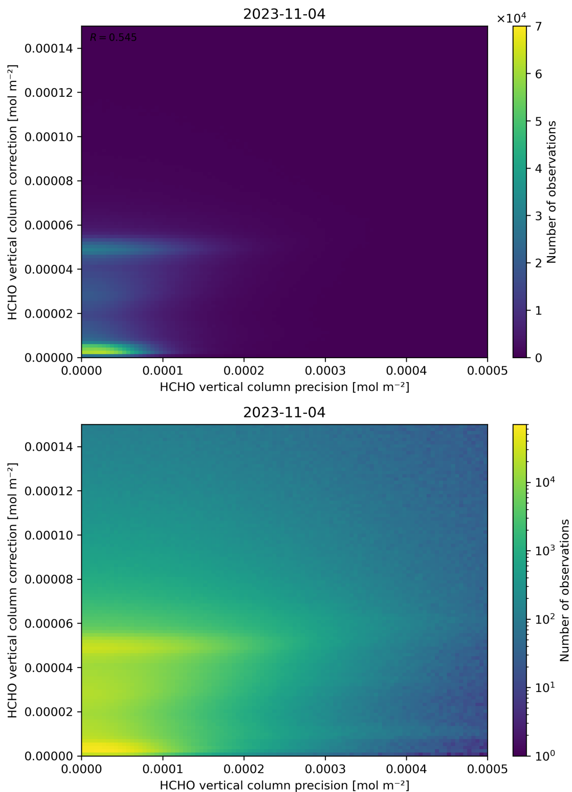
Figure 146: Scatter density plot of “HCHO vertical column precision” against “HCHO vertical column correction” for 2023-11-03 to 2023-11-05.
