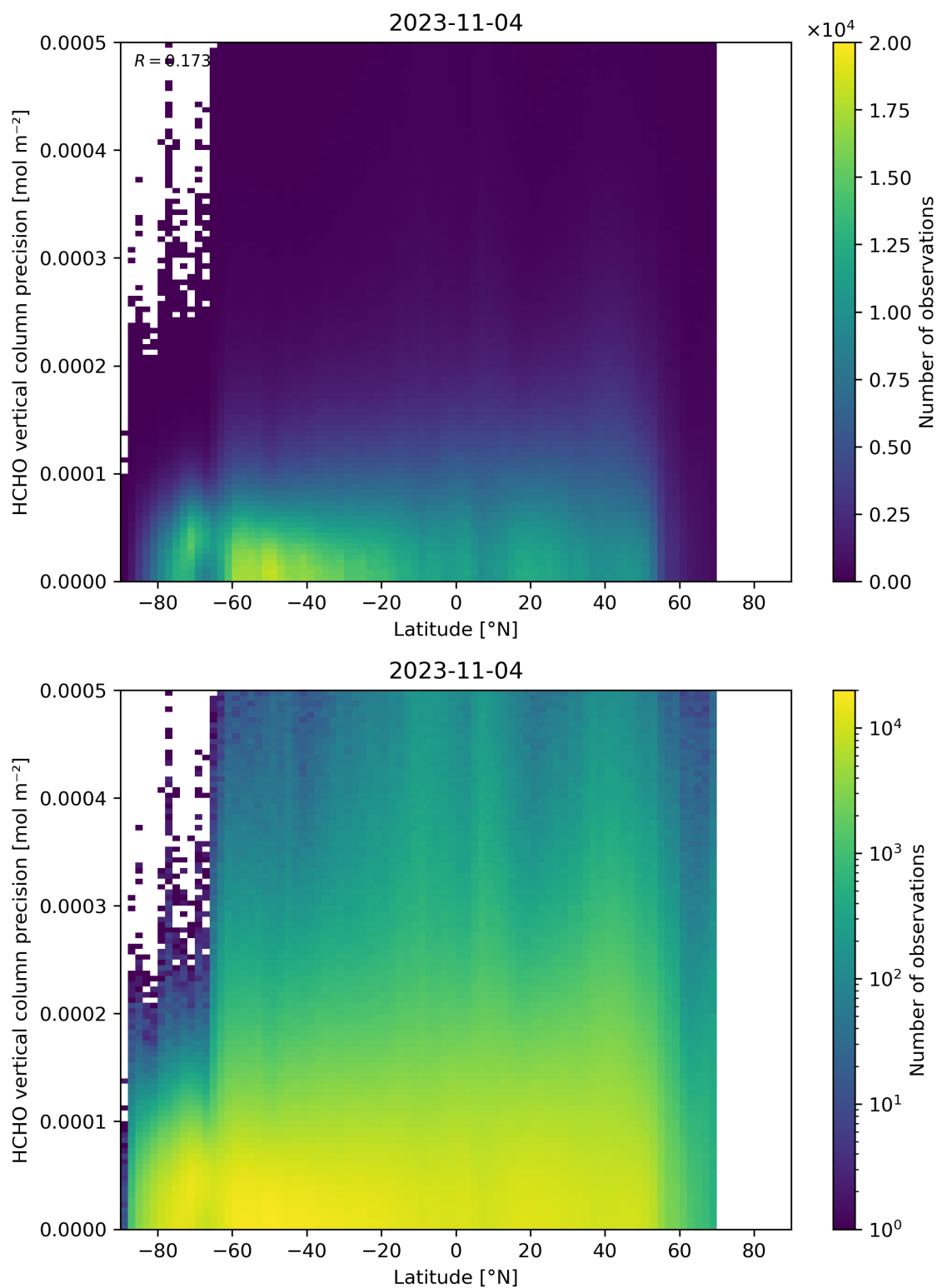
Figure 165: Scatter density plot of “Latitude” against “HCHO vertical column precision” for 2023-11-03 to 2023-11-05.
