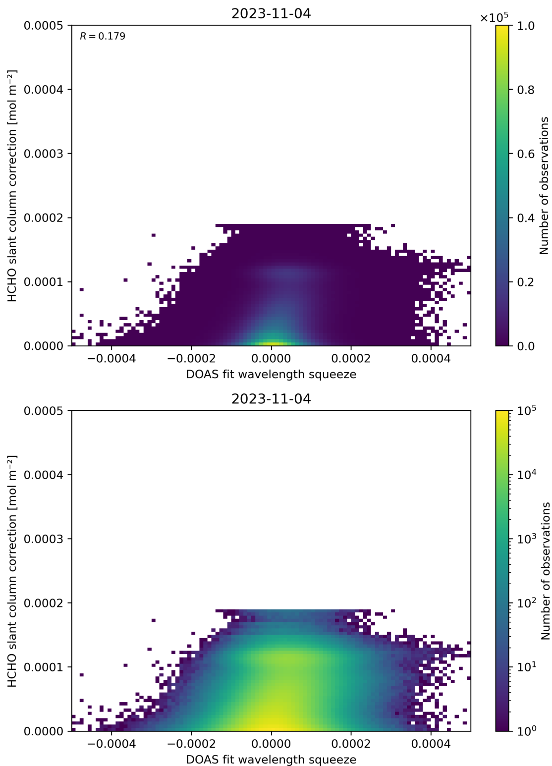
Figure 70: Scatter density plot of “DOAS fit wavelength squeeze” against “HCHO slant column correction” for 2023-11-03 to 2023-11-05.
