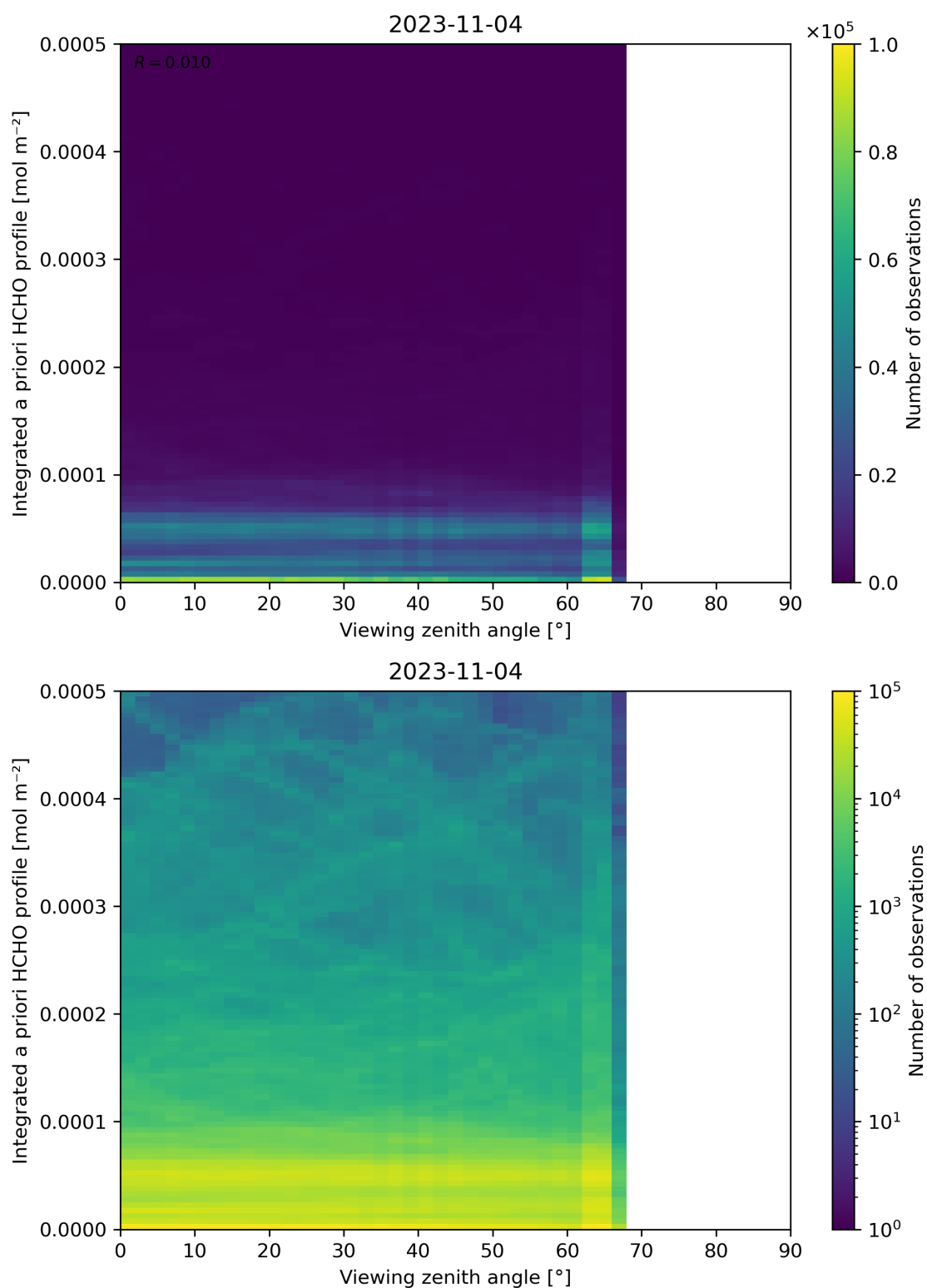
Figure 195: Scatter density plot of “Viewing zenith angle” against “Integrated a priori HCHO profile” for 2023-11-03 to 2023-11-05.
