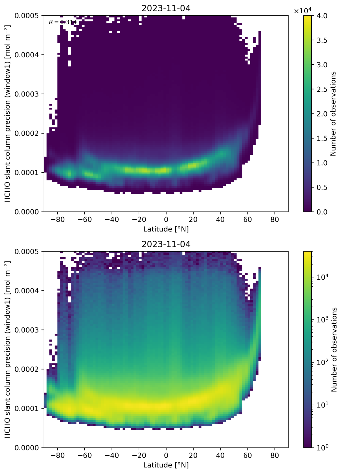
Figure 160: Scatter density plot of “Latitude” against “HCHO slant column precision (window1)” for 2023-11-03 to 2023-11-05.
