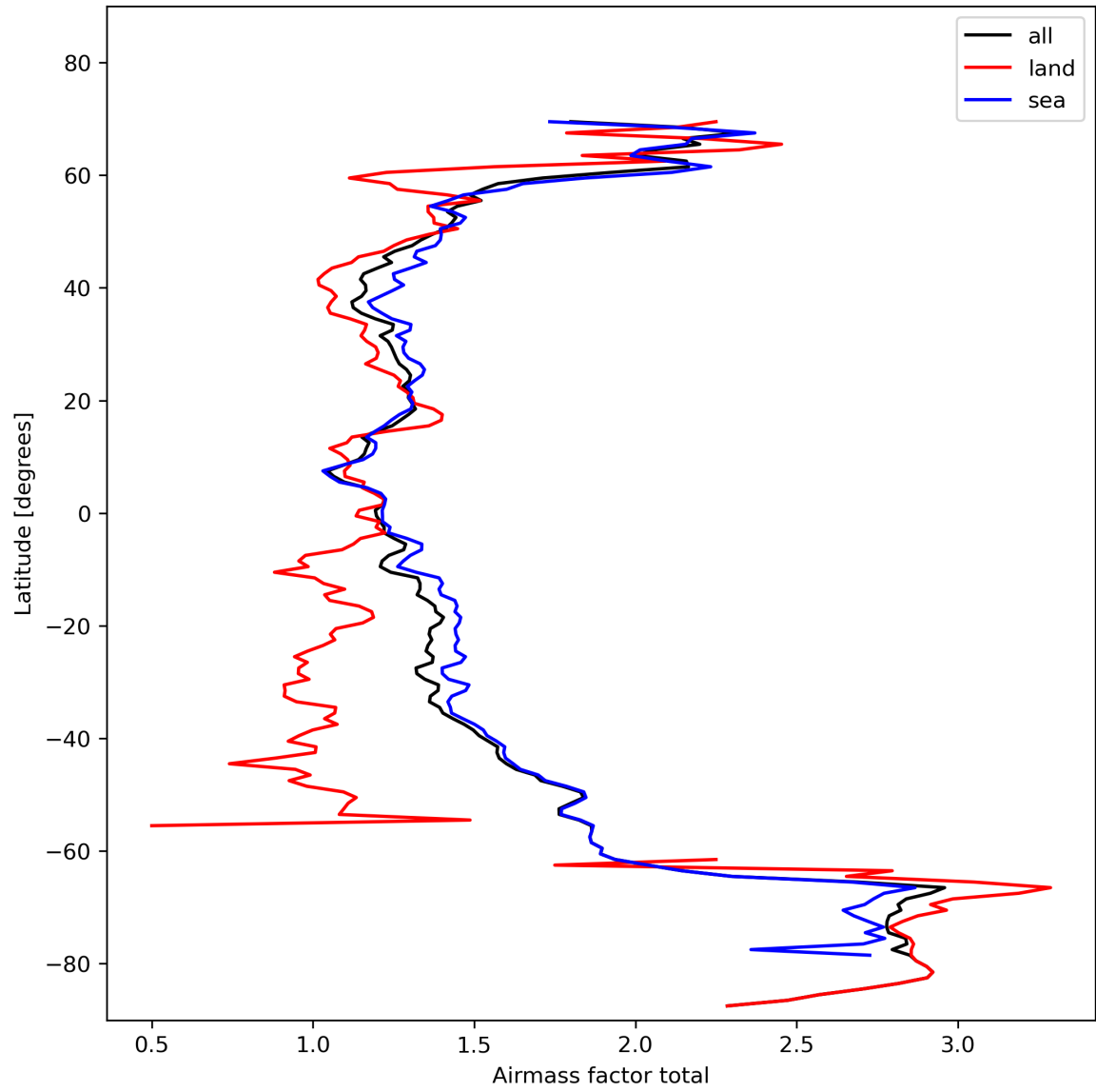
Figure 26: Zonal average of “Airmass factor total” for 2023-11-03 to 2023-11-05.
