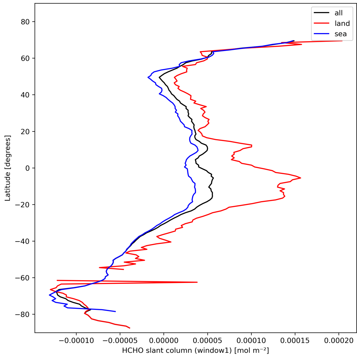
Figure 24: Zonal average of “HCHO slant column (window1)” for 2023-11-03 to 2023-11-05.
