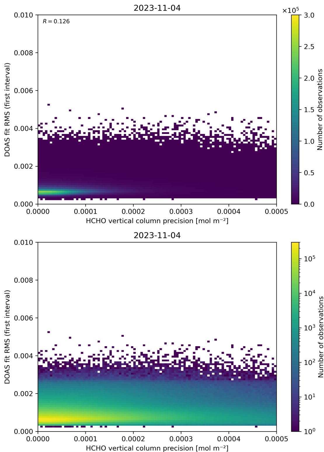
Figure 136: Scatter density plot of “HCHO vertical column precision” against “DOAS fit RMS (first interval)” for 2023-11-03 to 2023-11-05.
