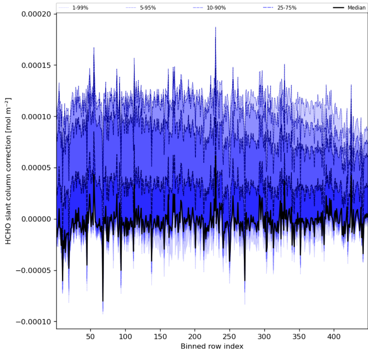
Figure 61: Along track statistics of “HCHO slant column correction” for 2023-11-03 to 2023-11-05
