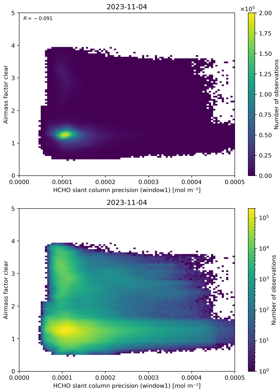
Figure 91: Scatter density plot of “HCHO slant column precision (window1)” against “Airmass factor clear” for 2023-11-03 to 2023-11-05.
