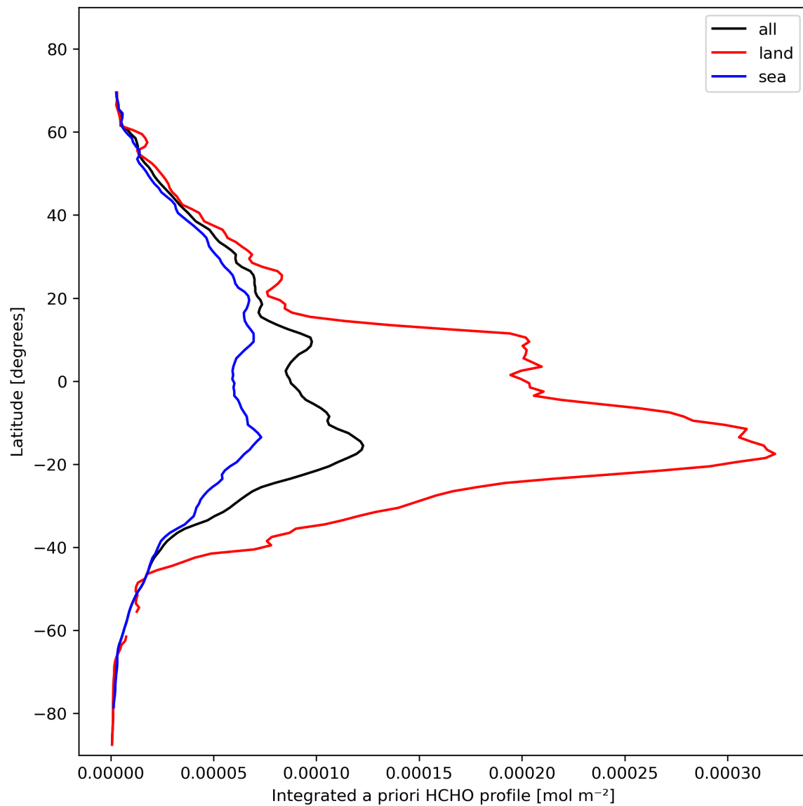
Figure 29: Zonal average of “Integrated a priori HCHO profile” for 2023-11-03 to 2023-11-05.
