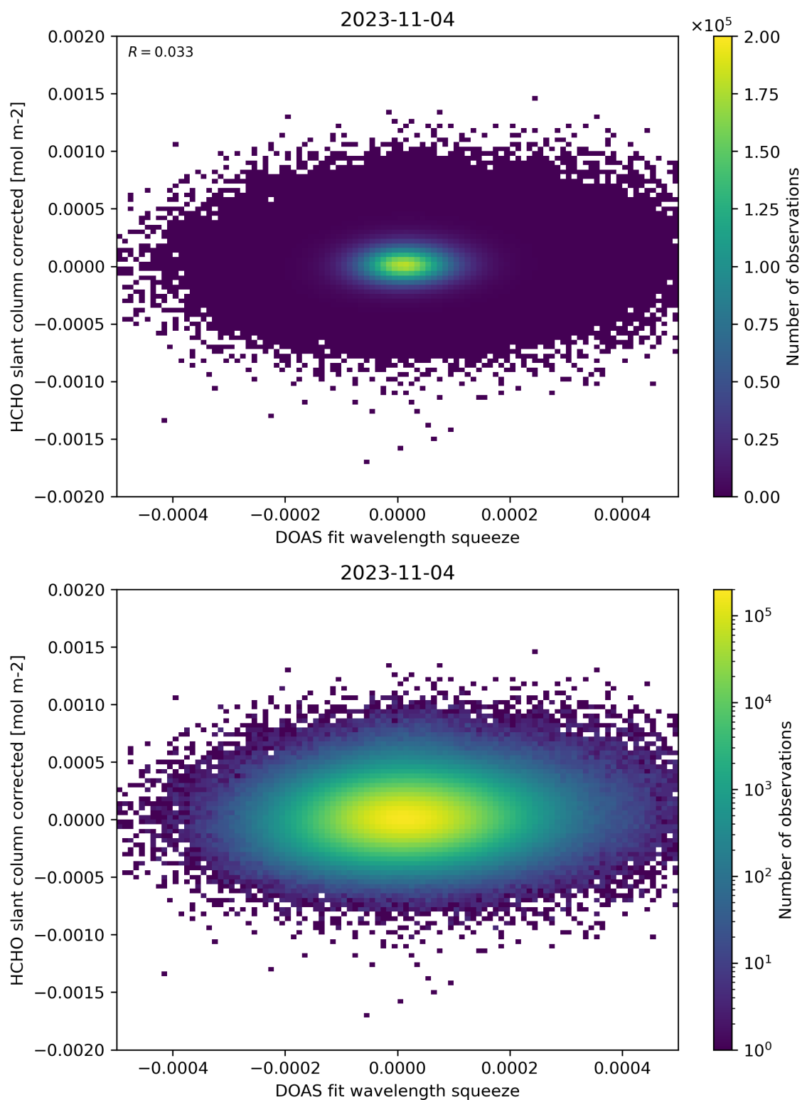
Figure 69: Scatter density plot of “DOAS fit wavelength squeeze” against “HCHO slant column corrected” for 2023-11-03 to 2023-11-05.
