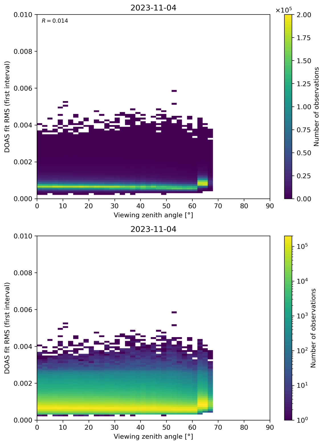
Figure 182: Scatter density plot of “Viewing zenith angle” against “DOAS fit RMS (first interval)” for 2023-11-03 to 2023-11-05.
