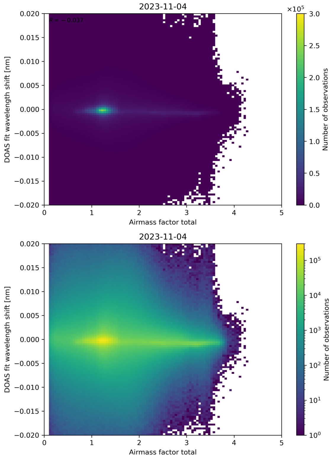
Figure 98: Scatter density plot of “Airmass factor total” against “DOAS fit wavelength shift” for 2023-11-03 to 2023-11-05.
