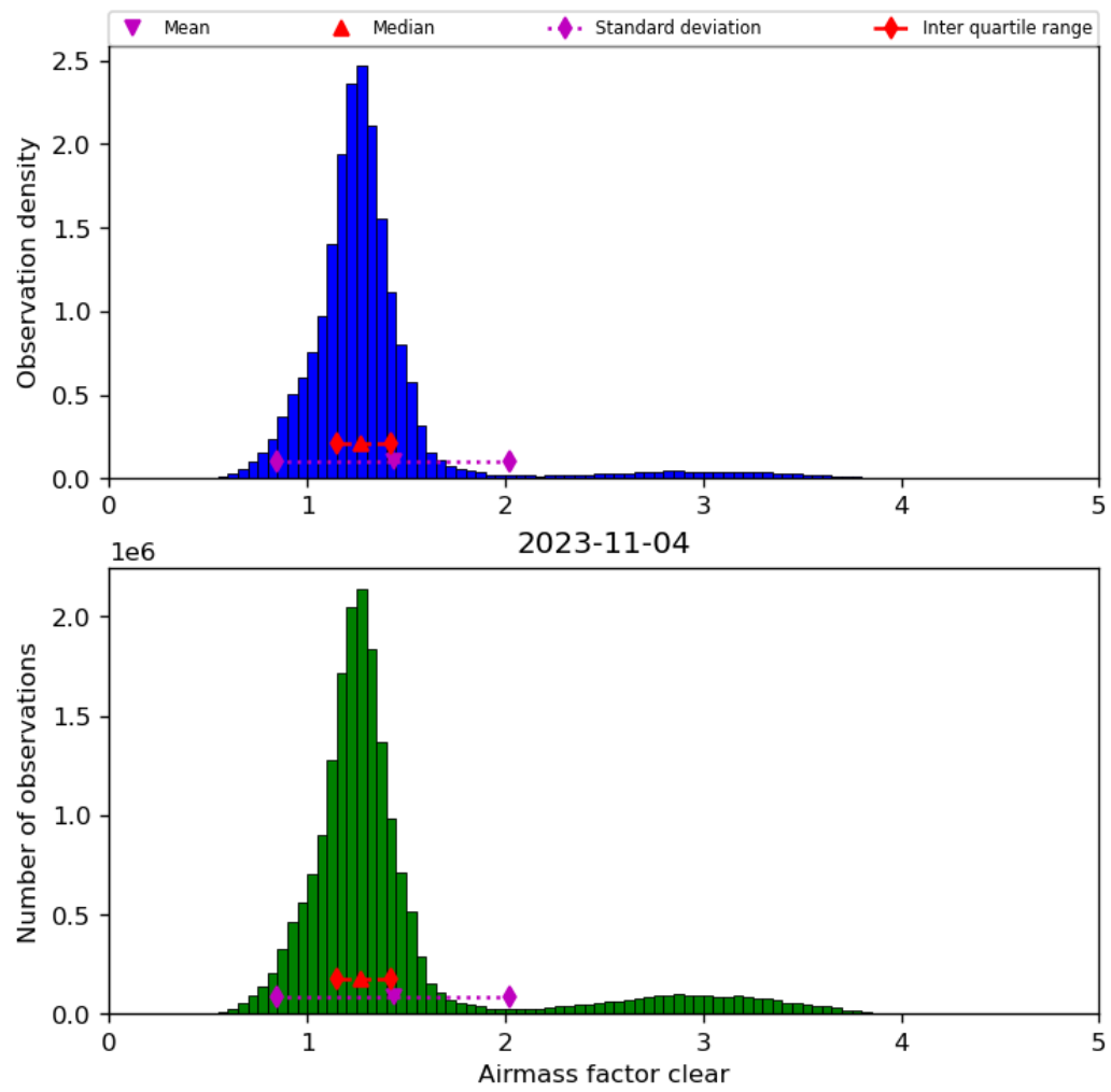
Figure 42: Histogram of “Airmass factor clear” for 2023-11-03 to 2023-11-05
