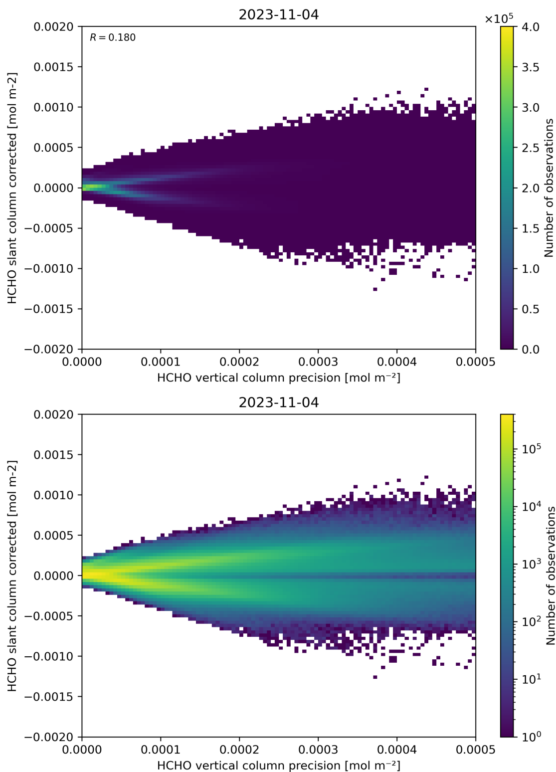
Figure 140: Scatter density plot of “HCHO vertical column precision” against “HCHO slant column corrected” for 2023-11-03 to 2023-11-05.
