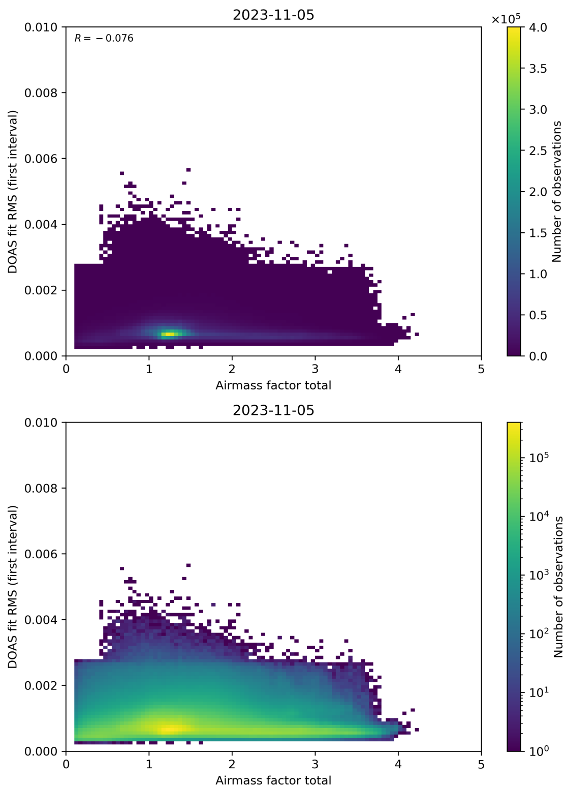
Figure 97: Scatter density plot of “Airmass factor total” against “DOAS fit RMS (first interval)” for 2023-11-04 to 2023-11-06.
