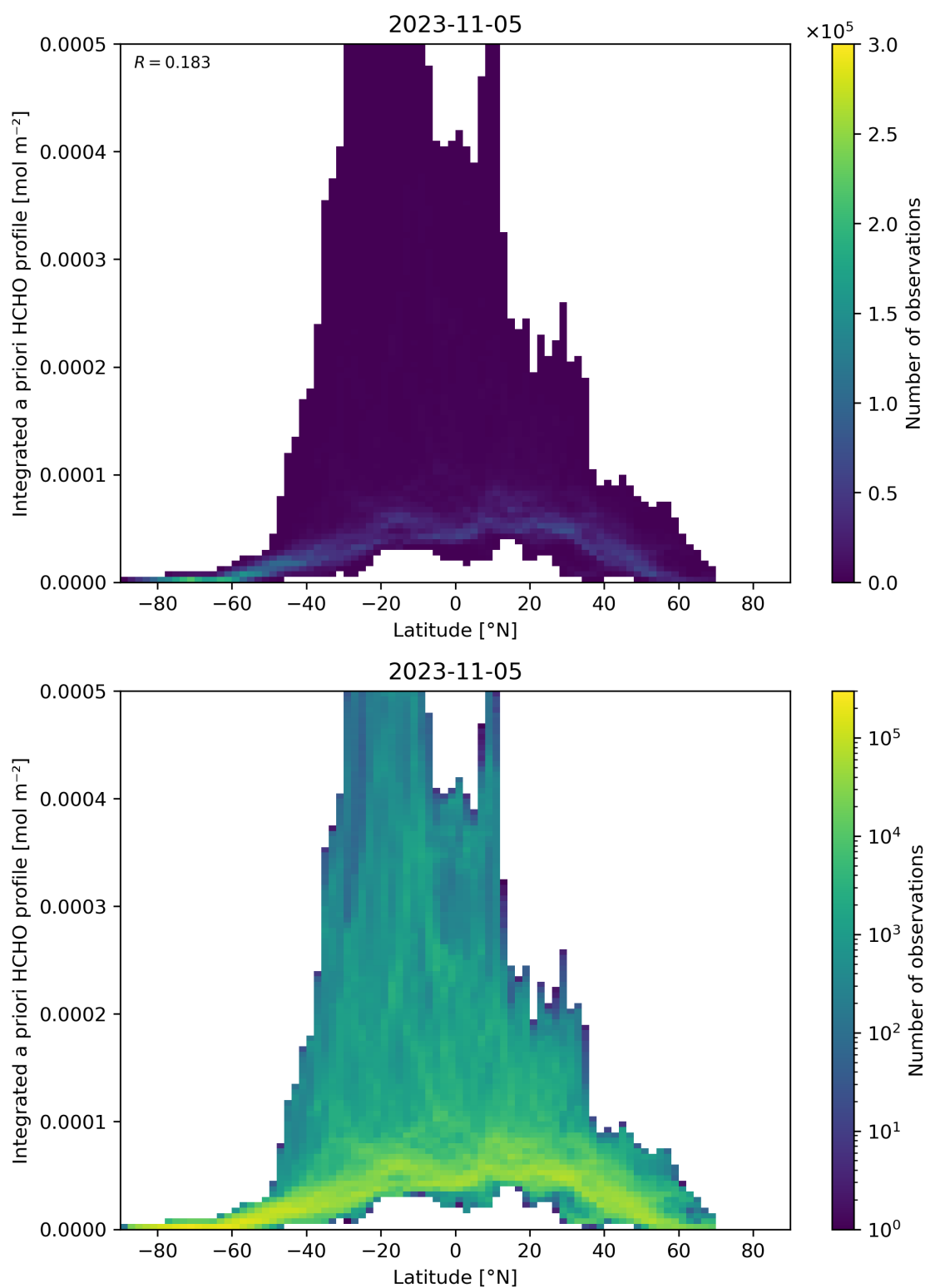
Figure 166: Scatter density plot of “Latitude” against “Integrated a priori HCHO profile” for 2023-11-04 to 2023-11-06.
