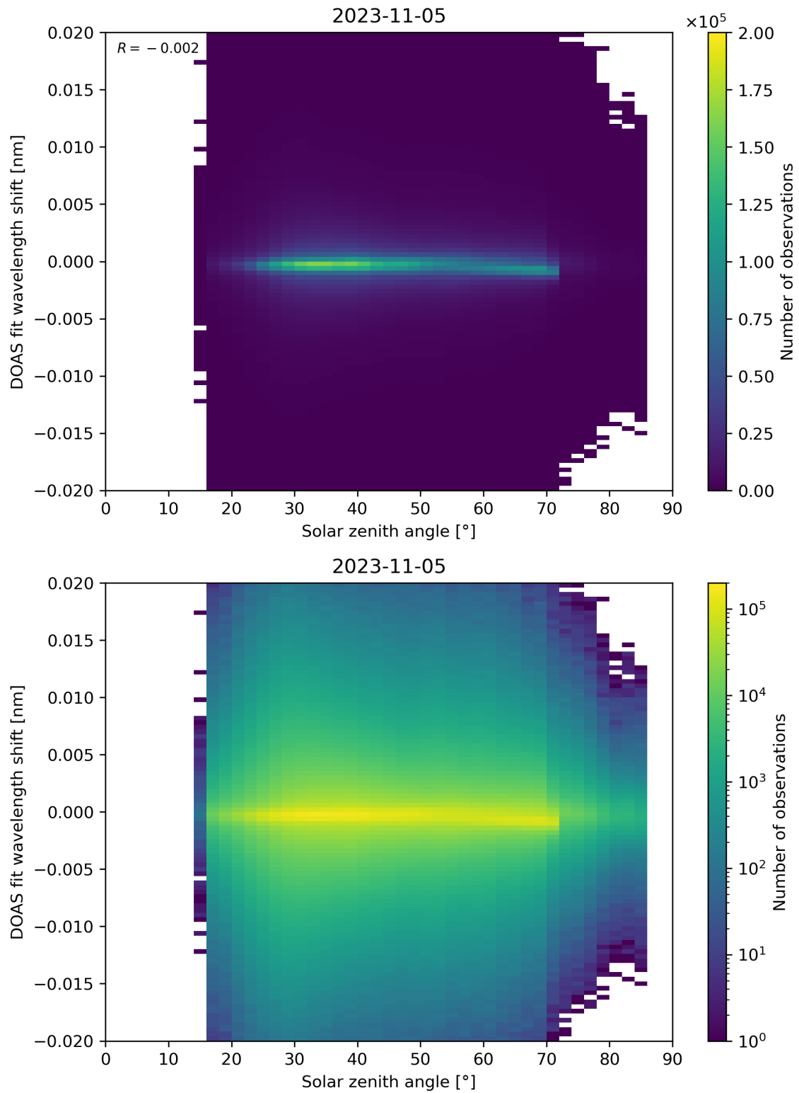
Figure 168: Scatter density plot of “Solar zenith angle” against “DOAS fit wavelength shift” for 2023-11-04 to 2023-11-06.
