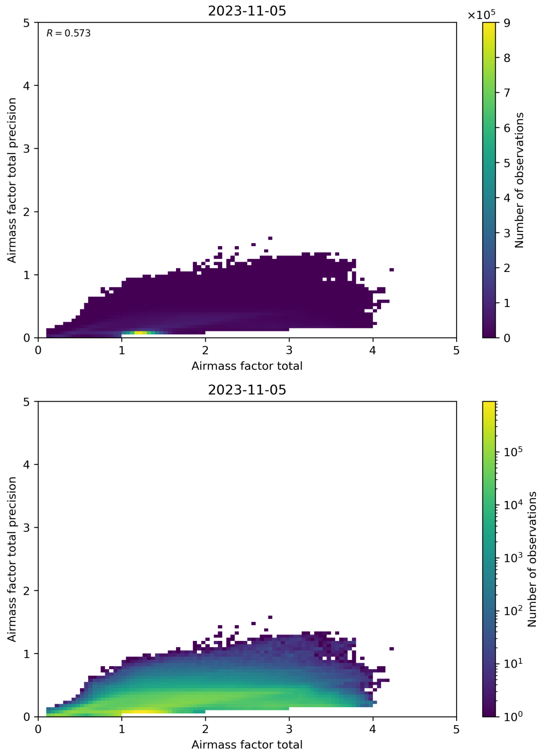
Figure 103: Scatter density plot of “Airmass factor total” against “Airmass factor total precision” for 2023-11-04 to 2023-11-06.
