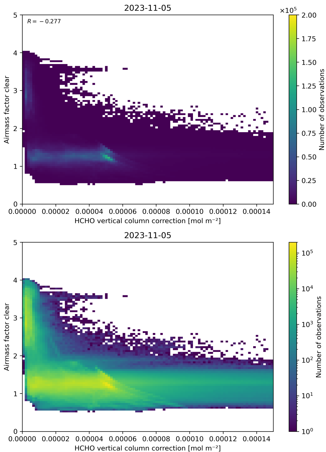
Figure 115: Scatter density plot of “HCHO vertical column correction” against “Airmass factor clear” for 2023-11-04 to 2023-11-06.
