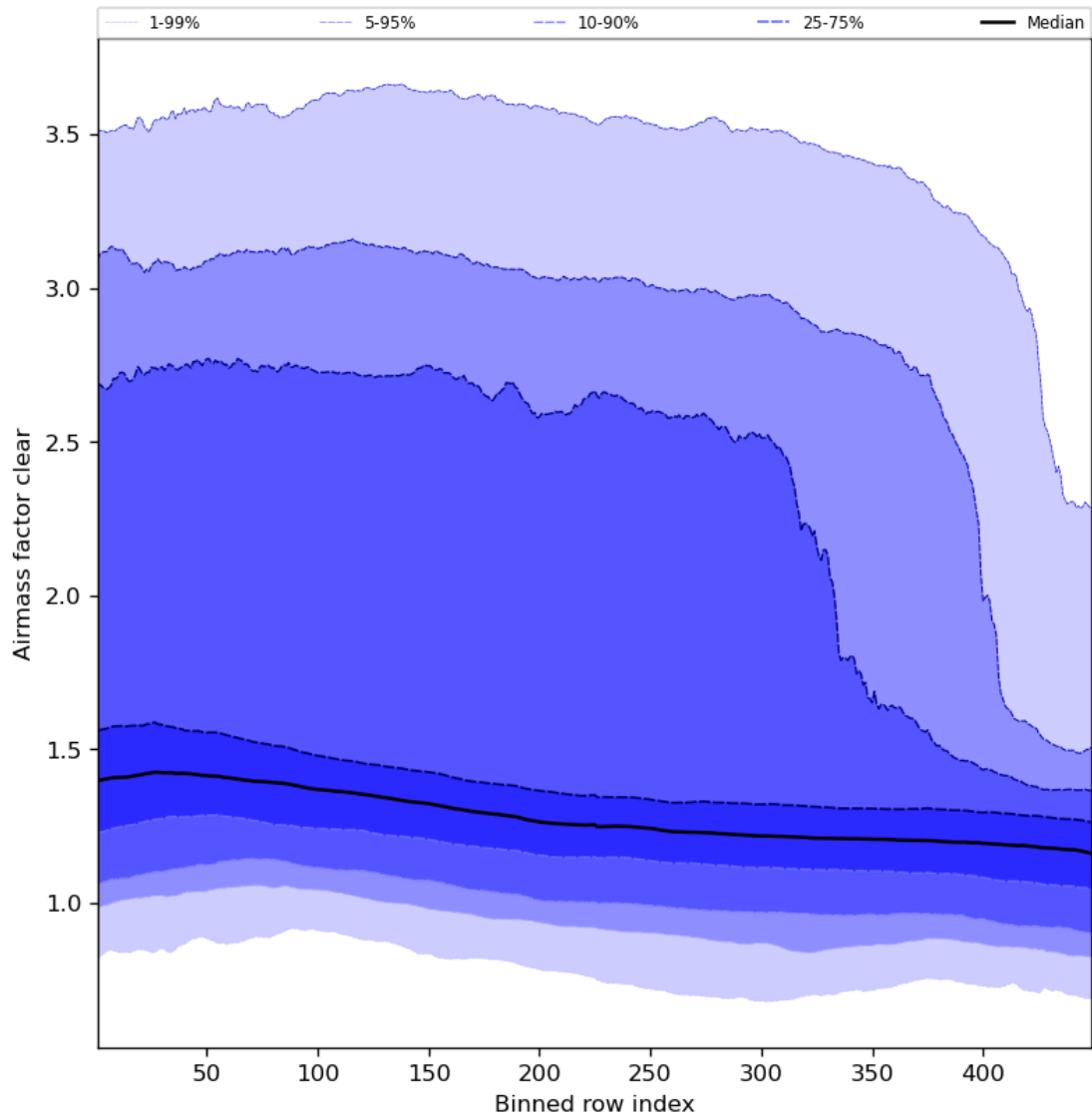
Figure 56: Along track statistics of “Airmass factor clear” for 2023-11-04 to 2023-11-06
