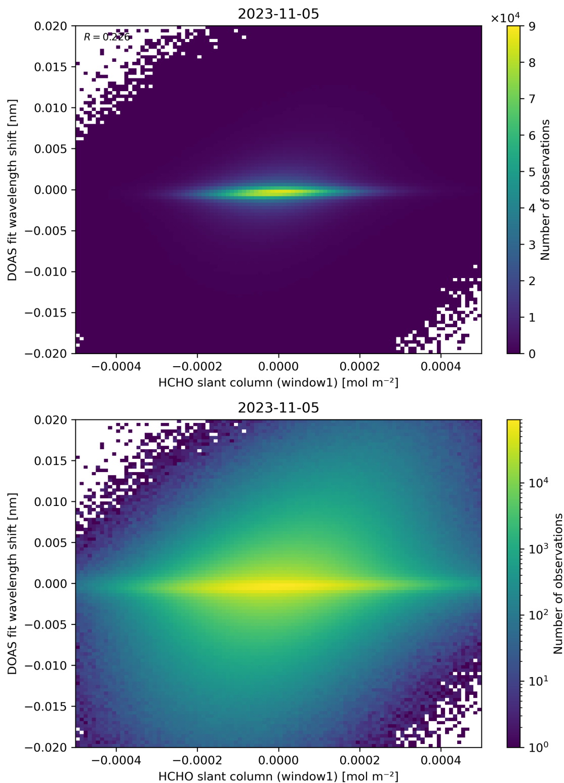
Figure 79: Scatter density plot of “HCHO slant column (window1)” against “DOAS fit wavelength shift” for 2023-11-04 to 2023-11-06.
