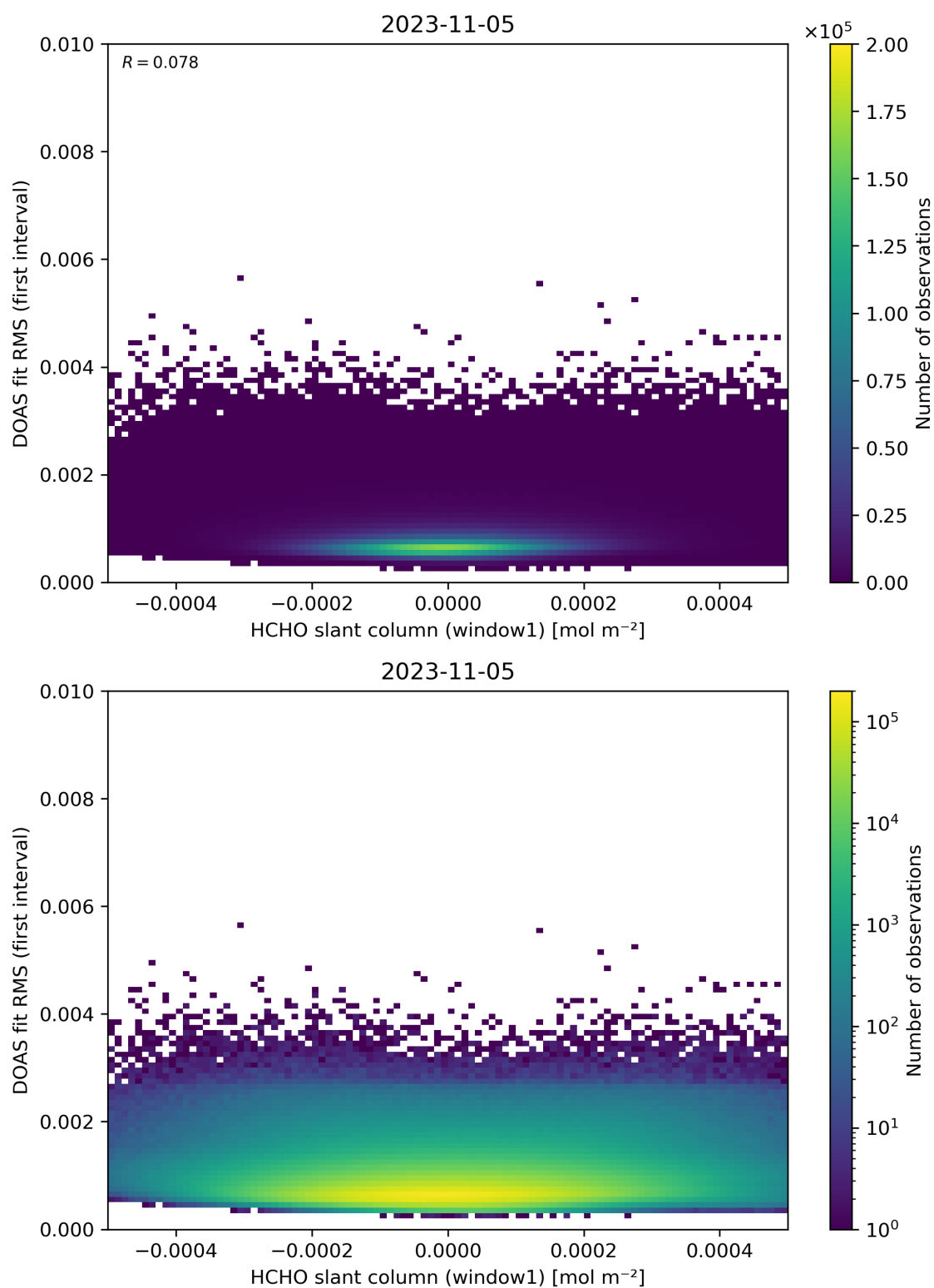
Figure 78: Scatter density plot of “HCHO slant column (window1)” against “DOAS fit RMS (first interval)” for 2023-11-04 to 2023-11-06.
