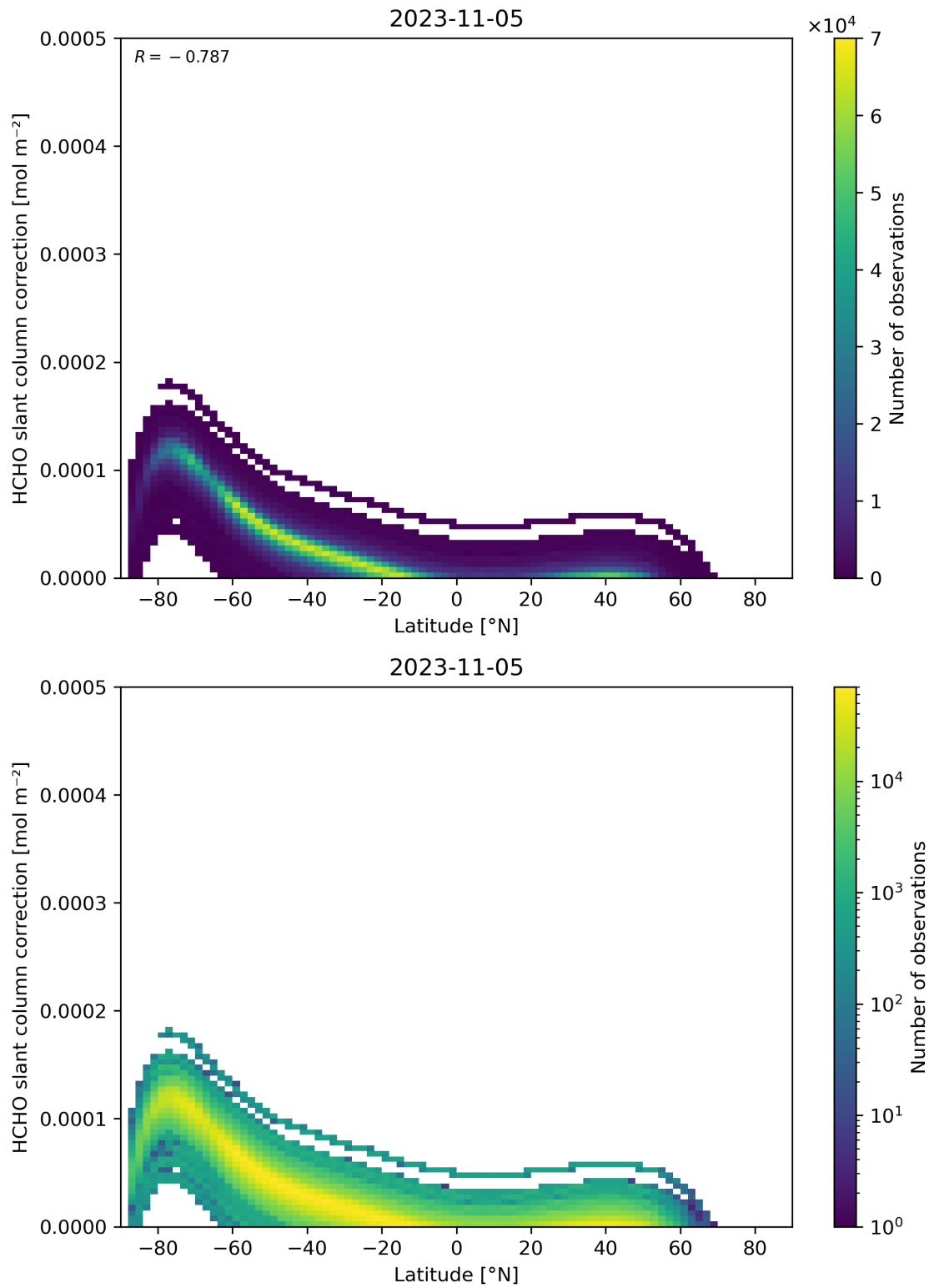
Figure 158: Scatter density plot of “Latitude” against “HCHO slant column correction” for 2023-11-04 to 2023-11-06.
