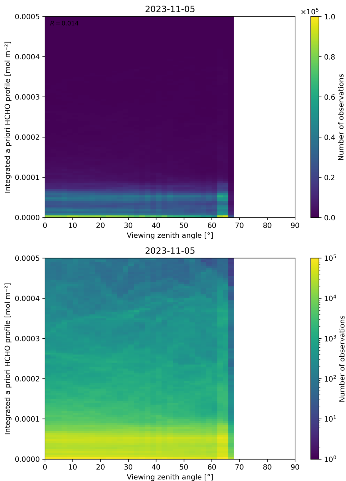
Figure 195: Scatter density plot of “Viewing zenith angle” against “Integrated a priori HCHO profile” for 2023-11-04 to 2023-11-06.
