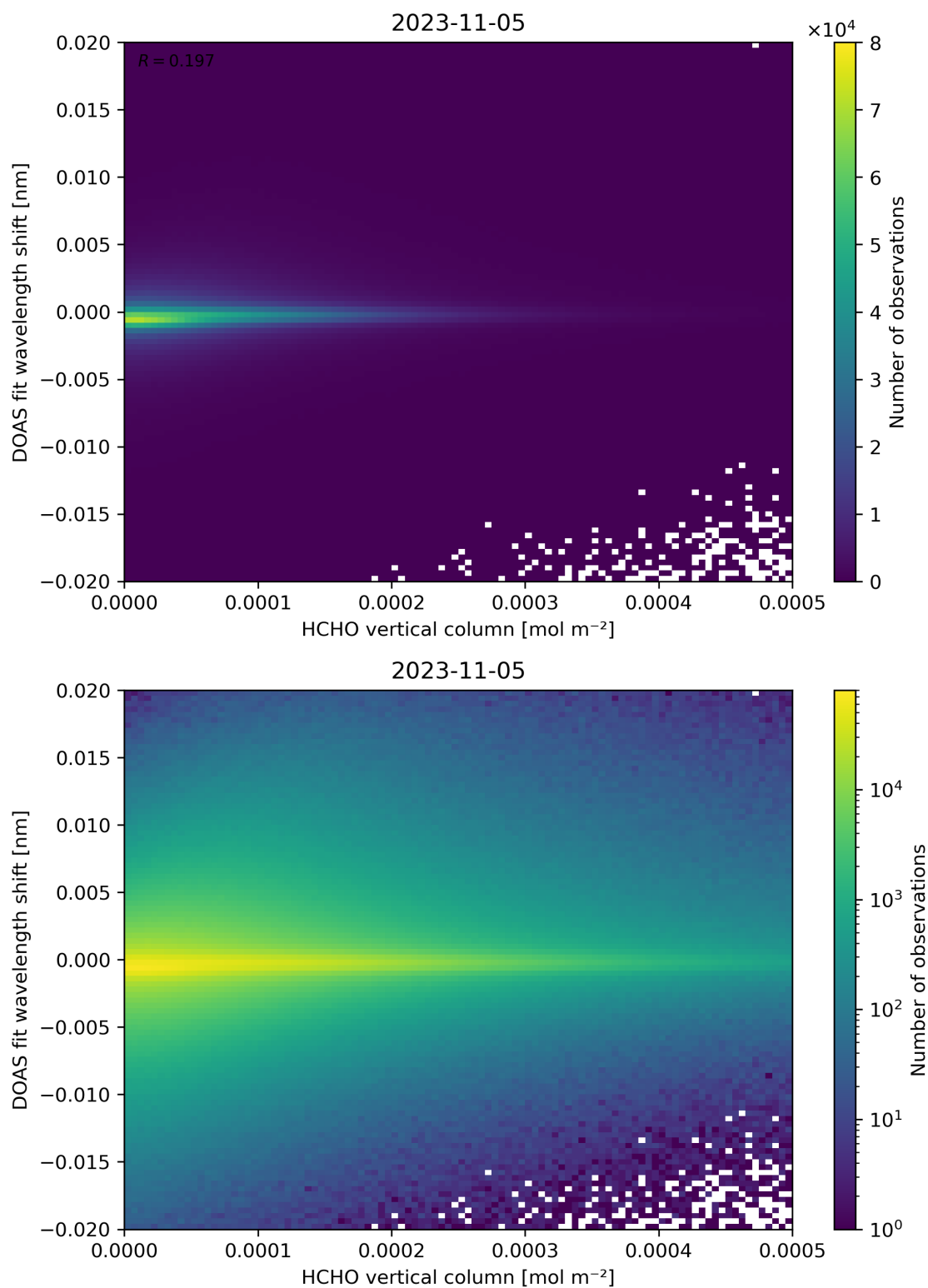
Figure 124: Scatter density plot of “HCHO vertical column” against “DOAS fit wavelength shift” for 2023-11-04 to 2023-11-06.
