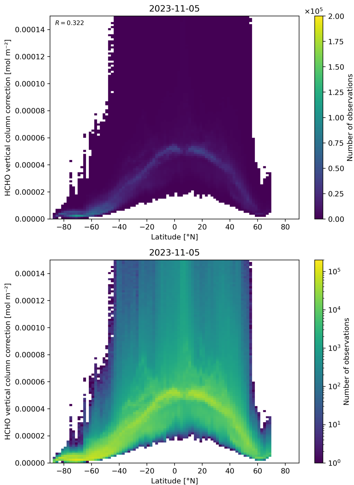
Figure 164: Scatter density plot of “Latitude” against “HCHO vertical column correction” for 2023-11-04 to 2023-11-06.
