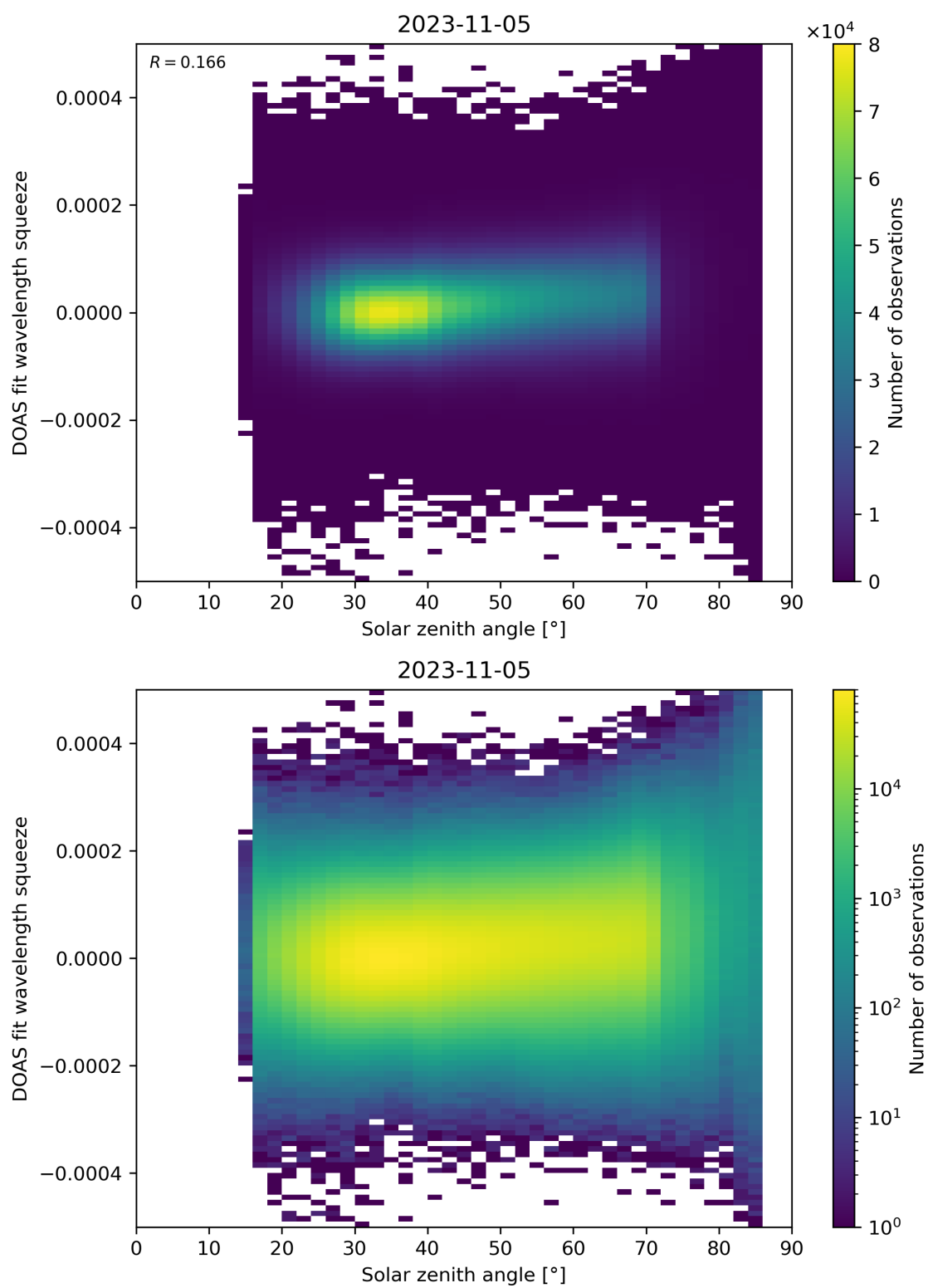
Figure 169: Scatter density plot of “Solar zenith angle” against “DOAS fit wavelength squeeze” for 2023-11-04 to 2023-11-06.
