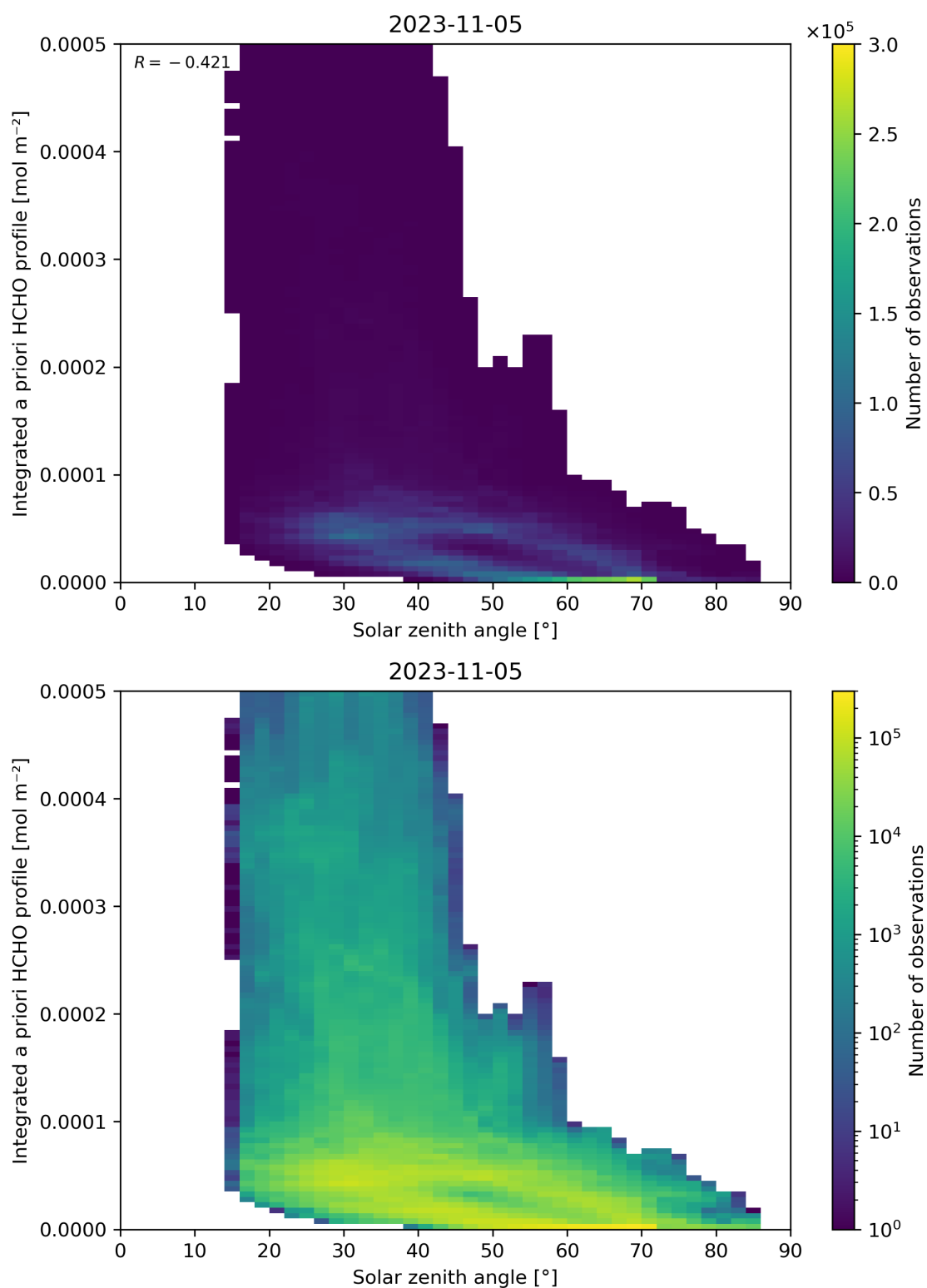
Figure 180: Scatter density plot of “Solar zenith angle” against “Integrated a priori HCHO profile” for 2023-11-04 to 2023-11-06.
