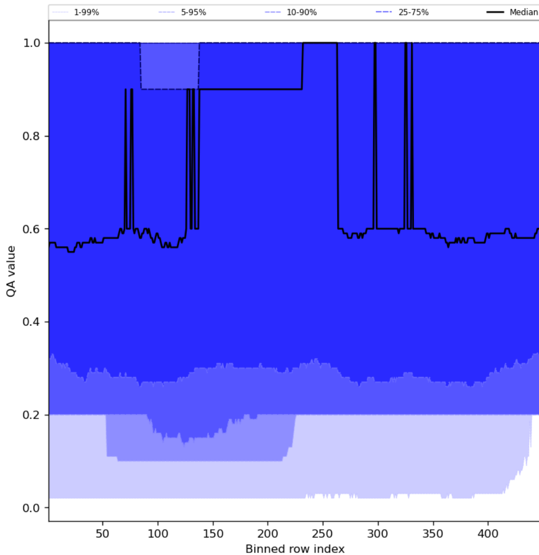
Figure 48: Along track statistics of “QA value” for 2023-11-04 to 2023-11-06
