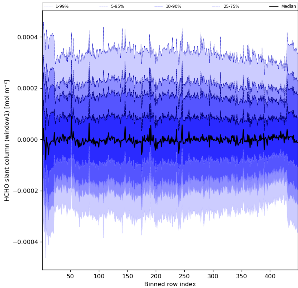
Figure 52: Along track statistics of “HCHO slant column (window1)” for 2023-11-04 to 2023-11-06
