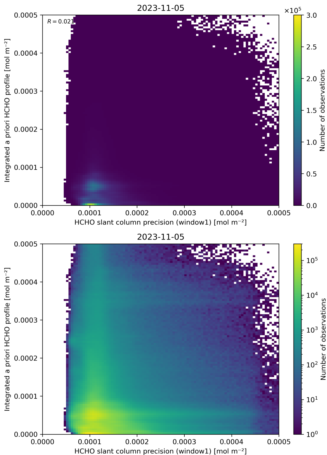
Figure 96: Scatter density plot of “HCHO slant column precision (window1)” against “Integrated a priori HCHO profile” for 2023-11-04 to 2023-11-06.
