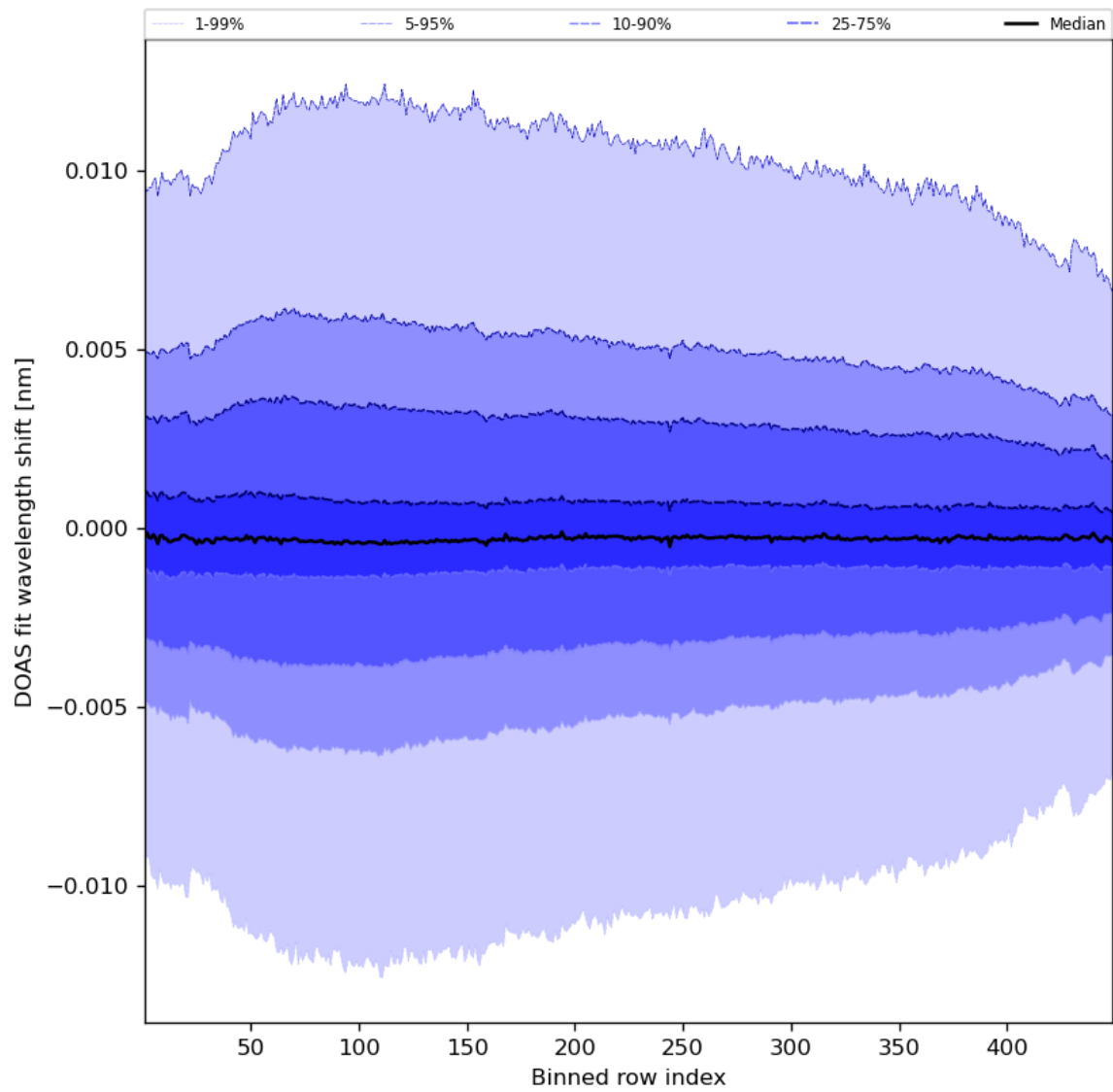
Figure 58: Along track statistics of “DOAS fit wavelength shift” for 2023-11-04 to 2023-11-06
