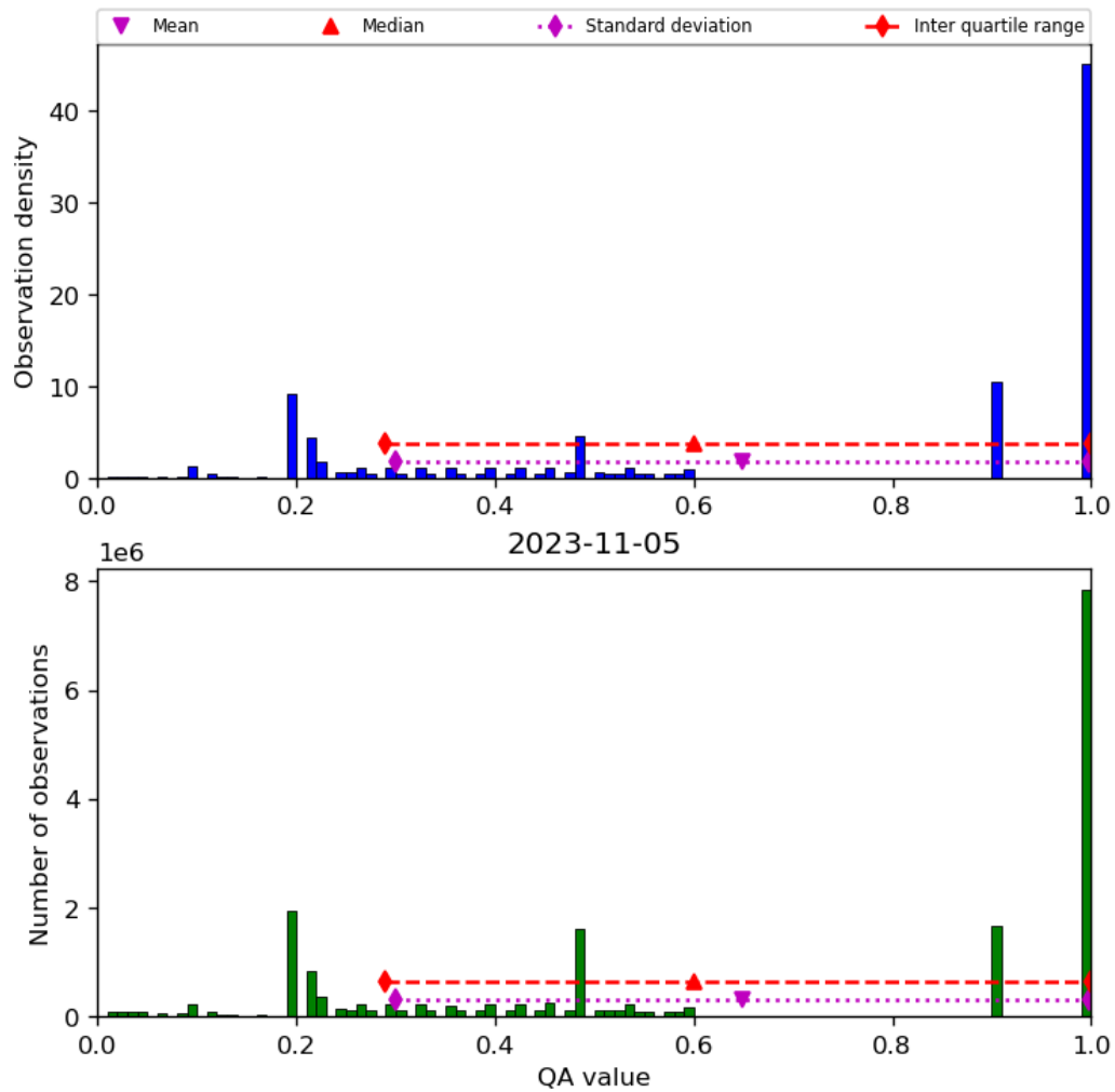
Figure 34: Histogram of “QA value” for 2023-11-04 to 2023-11-06
