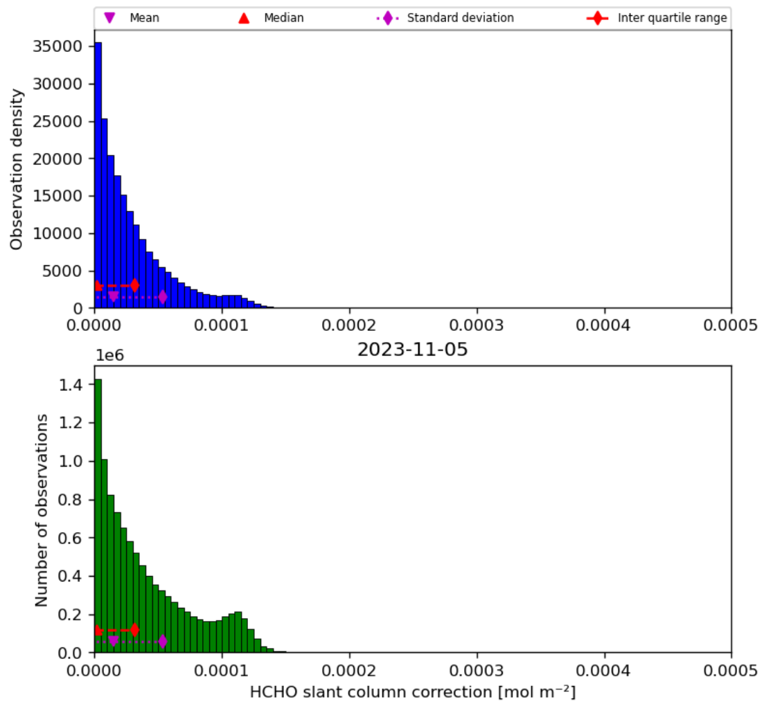
Figure 47: Histogram of “HCHO slant column correction” for 2023-11-04 to 2023-11-06
