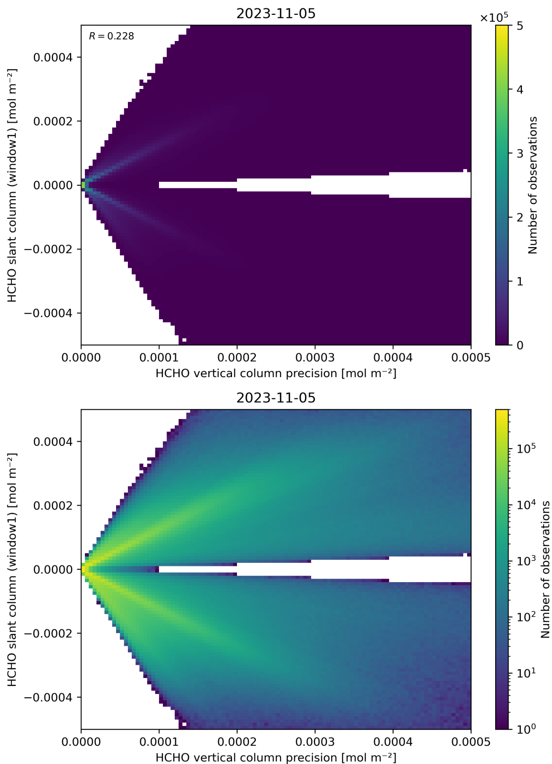
Figure 142: Scatter density plot of “HCHO vertical column precision” against “HCHO slant column (window1)” for 2023-11-04 to 2023-11-06.
