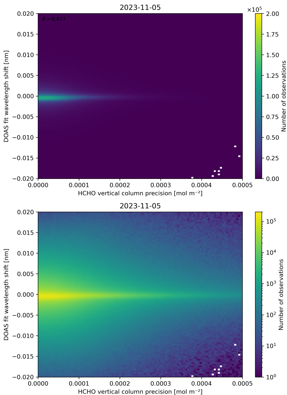
Figure 137: Scatter density plot of “HCHO vertical column precision” against “DOAS fit wavelength shift” for 2023-11-04 to 2023-11-06.
