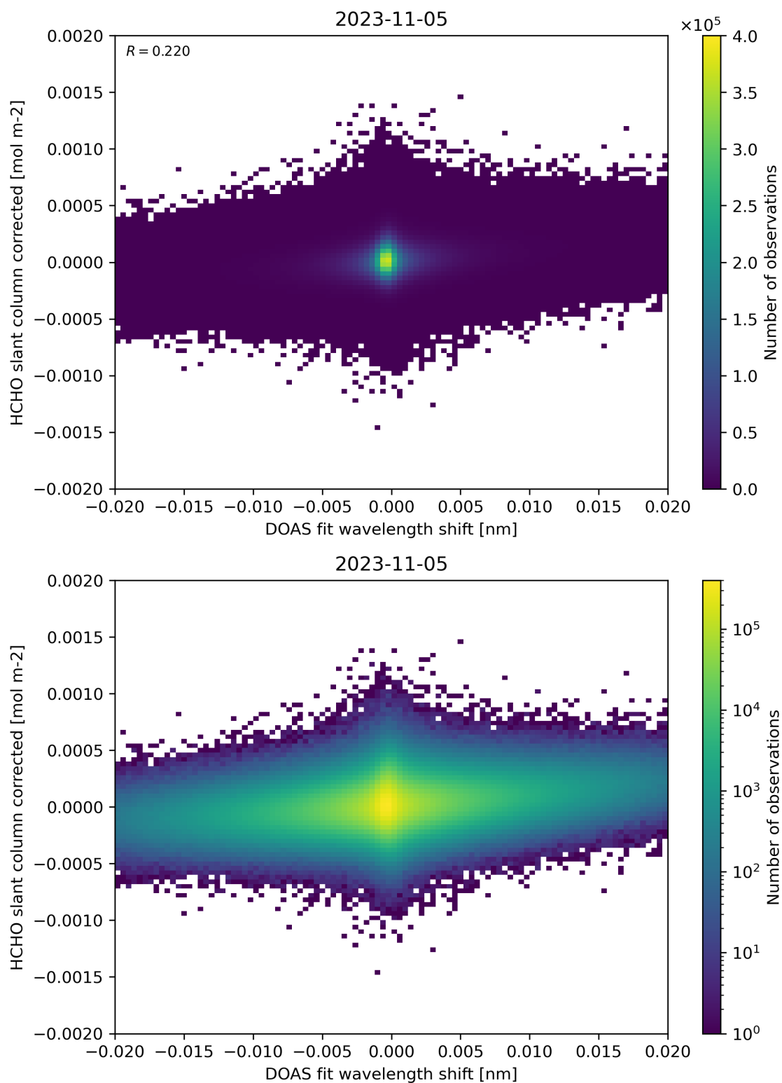
Figure 66: Scatter density plot of “DOAS fit wavelength shift” against “HCHO slant column corrected” for 2023-11-04 to 2023-11-06.
