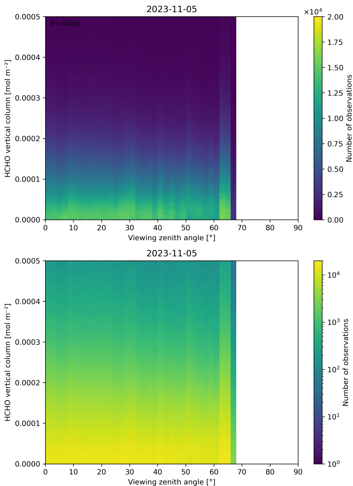
Figure 192: Scatter density plot of “Viewing zenith angle” against “HCHO vertical column” for 2023-11-04 to 2023-11-06.
