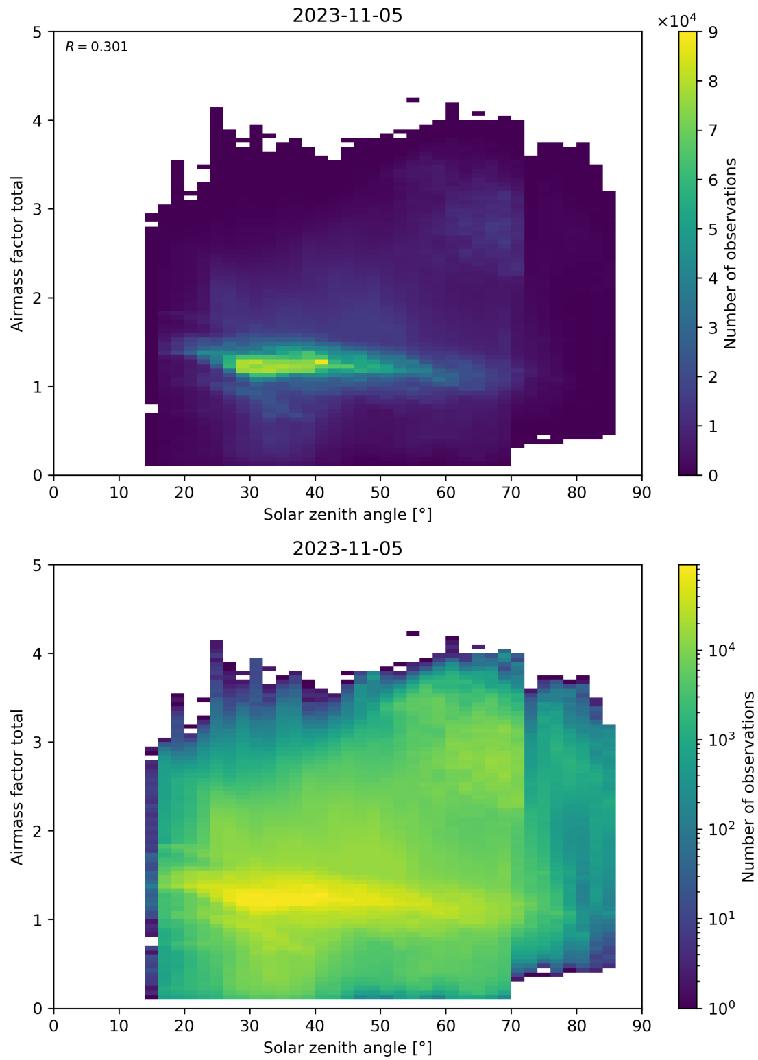
Figure 175: Scatter density plot of “Solar zenith angle” against “Airmass factor total” for 2023-11-04 to 2023-11-06.
