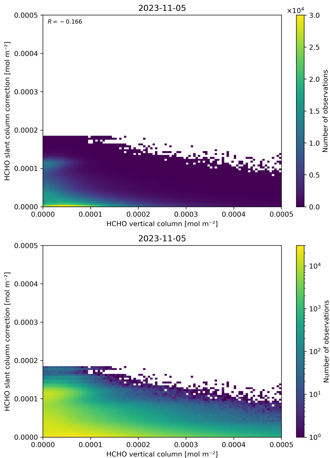
Figure 128: Scatter density plot of “HCHO vertical column” against “HCHO slant column correction” for 2023-11-04 to 2023-11-06.
