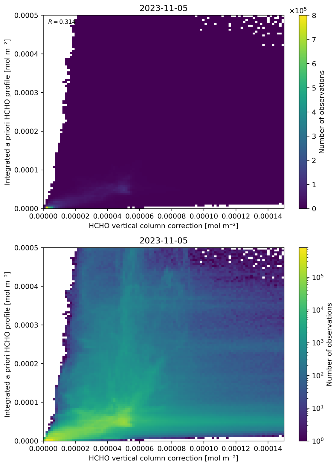
Figure 122: Scatter density plot of “HCHO vertical column correction” against “Integrated a priori HCHO profile” for 2023-11-04 to 2023-11-06.
