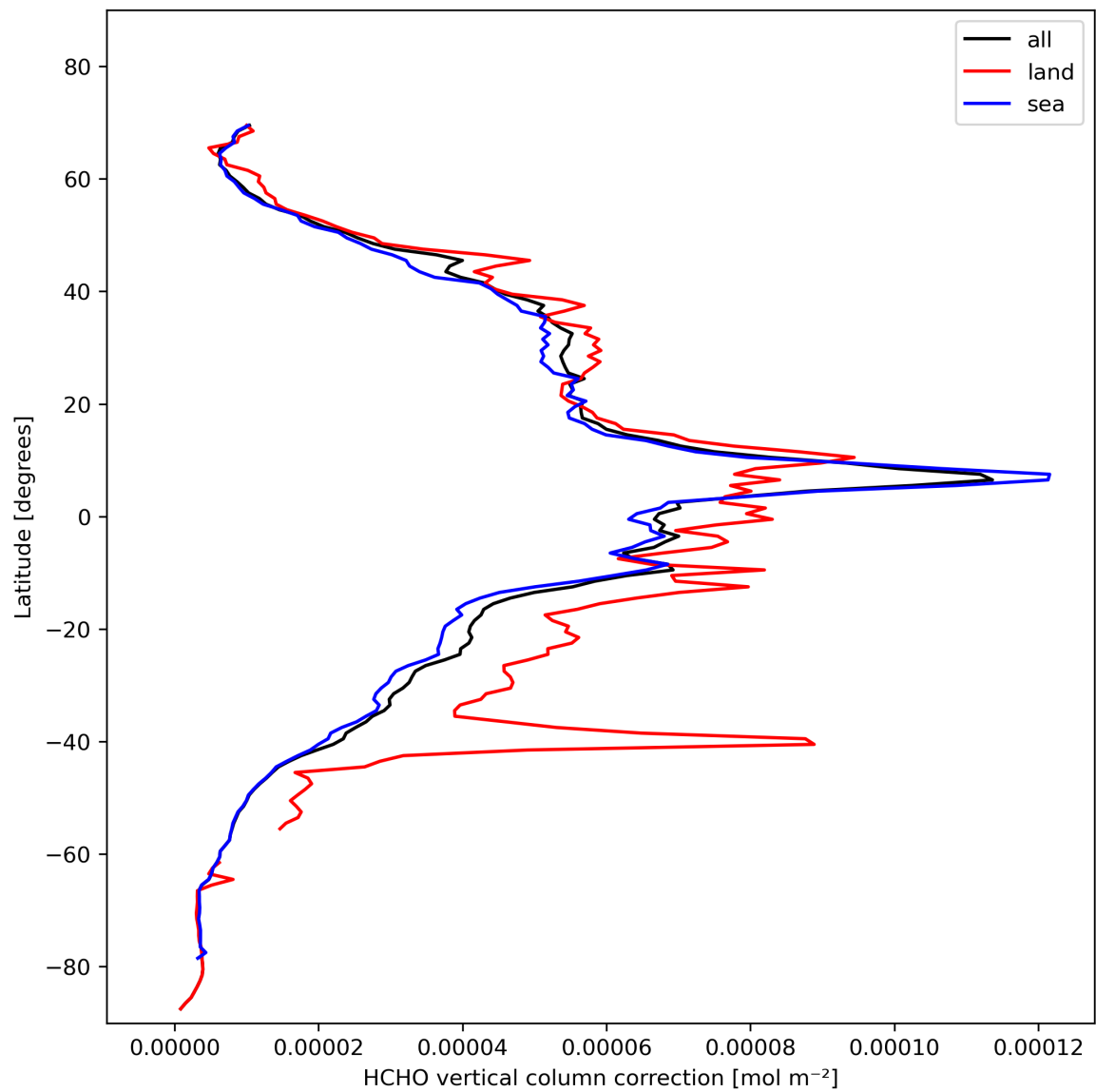
Figure 23: Zonal average of “HCHO vertical column correction” for 2023-11-04 to 2023-11-06.
