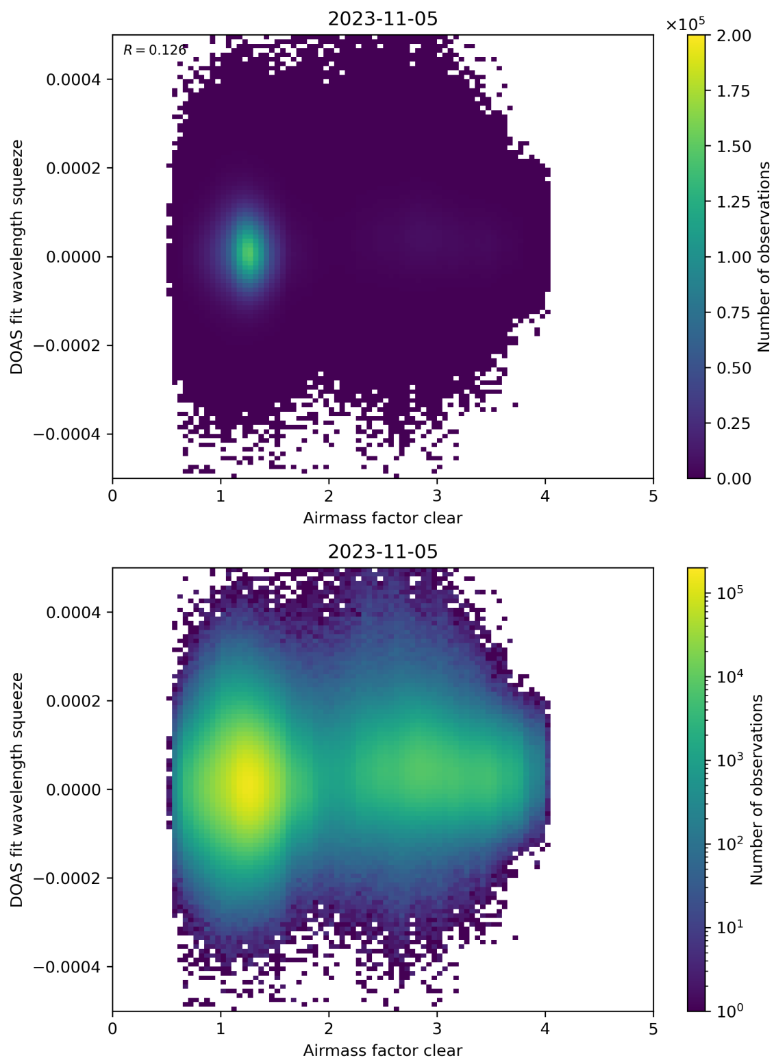
Figure 73: Scatter density plot of “Airmass factor clear” against “DOAS fit wavelength squeeze” for 2023-11-04 to 2023-11-06.
