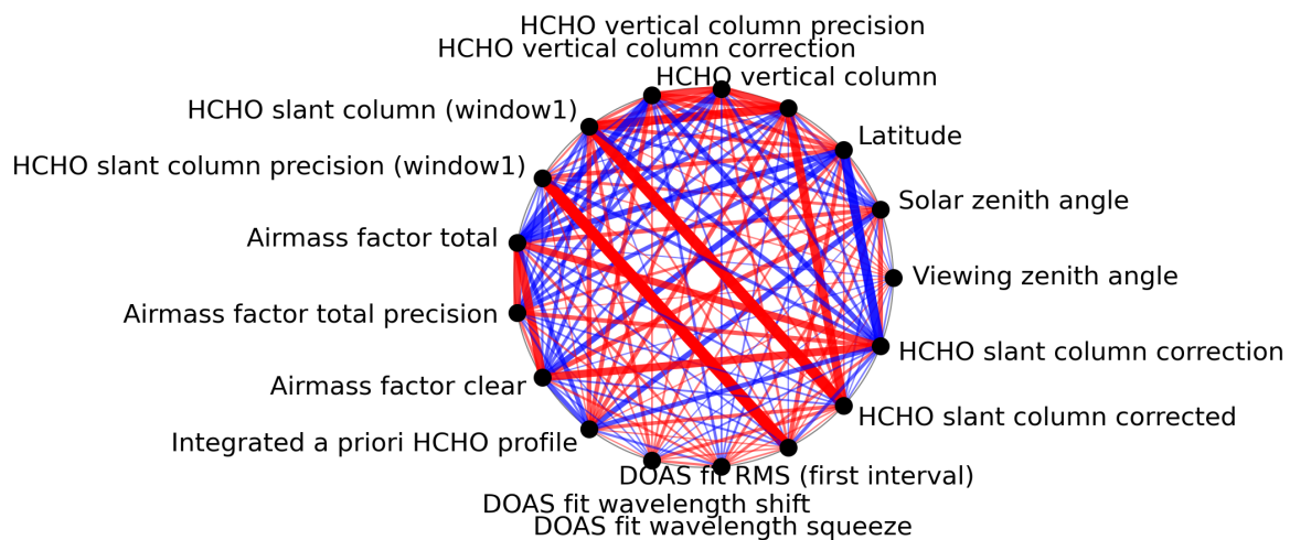
Figure 1: Map of correlation graph for 2023-11-04 to 2023-11-06.
