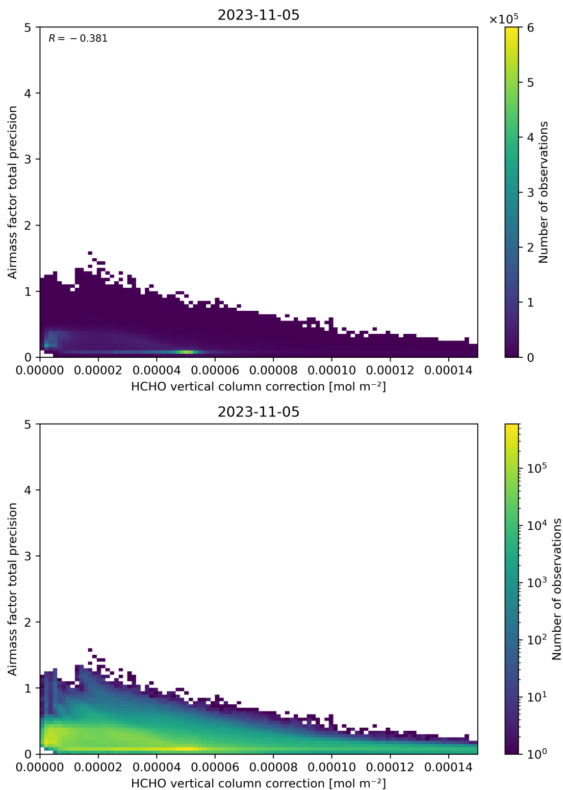
Figure 121: Scatter density plot of “HCHO vertical column correction” against “Airmass factor total precision” for 2023-11-04 to 2023-11-06.
