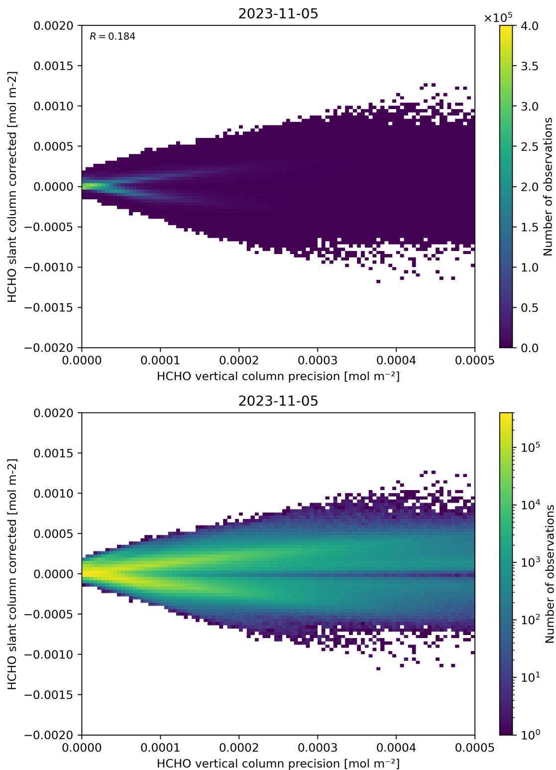
Figure 140: Scatter density plot of “HCHO vertical column precision” against “HCHO slant column corrected” for 2023-11-04 to 2023-11-06.
