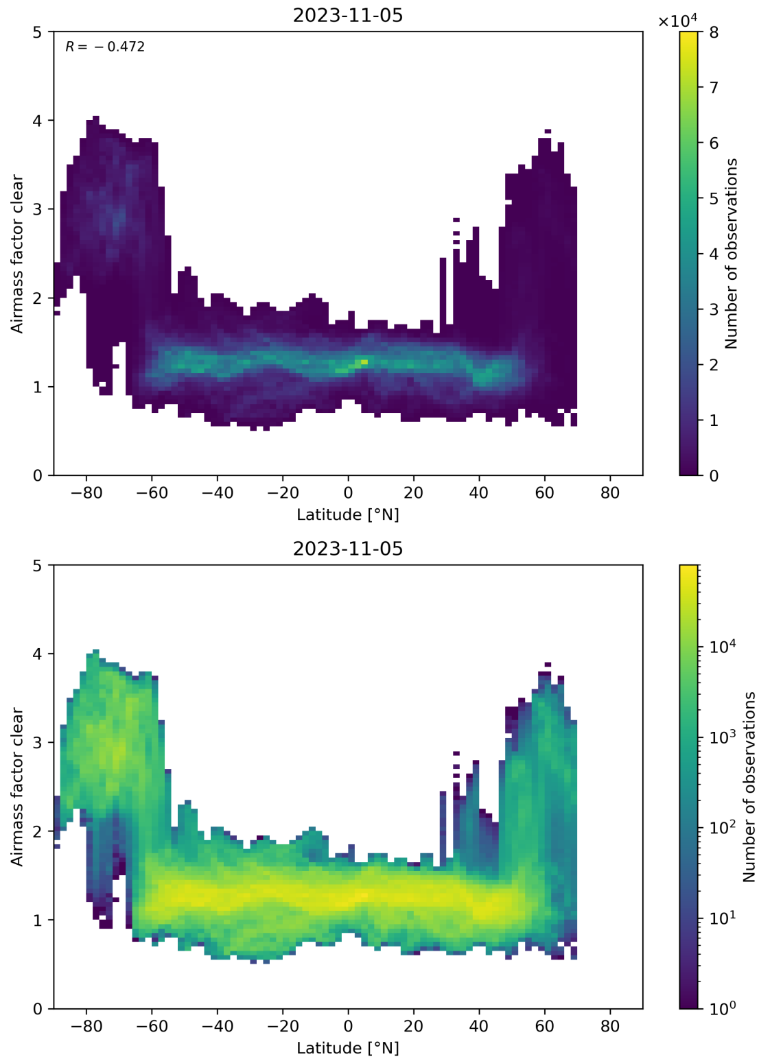
Figure 156: Scatter density plot of “Latitude” against “Airmass factor clear” for 2023-11-04 to 2023-11-06.
