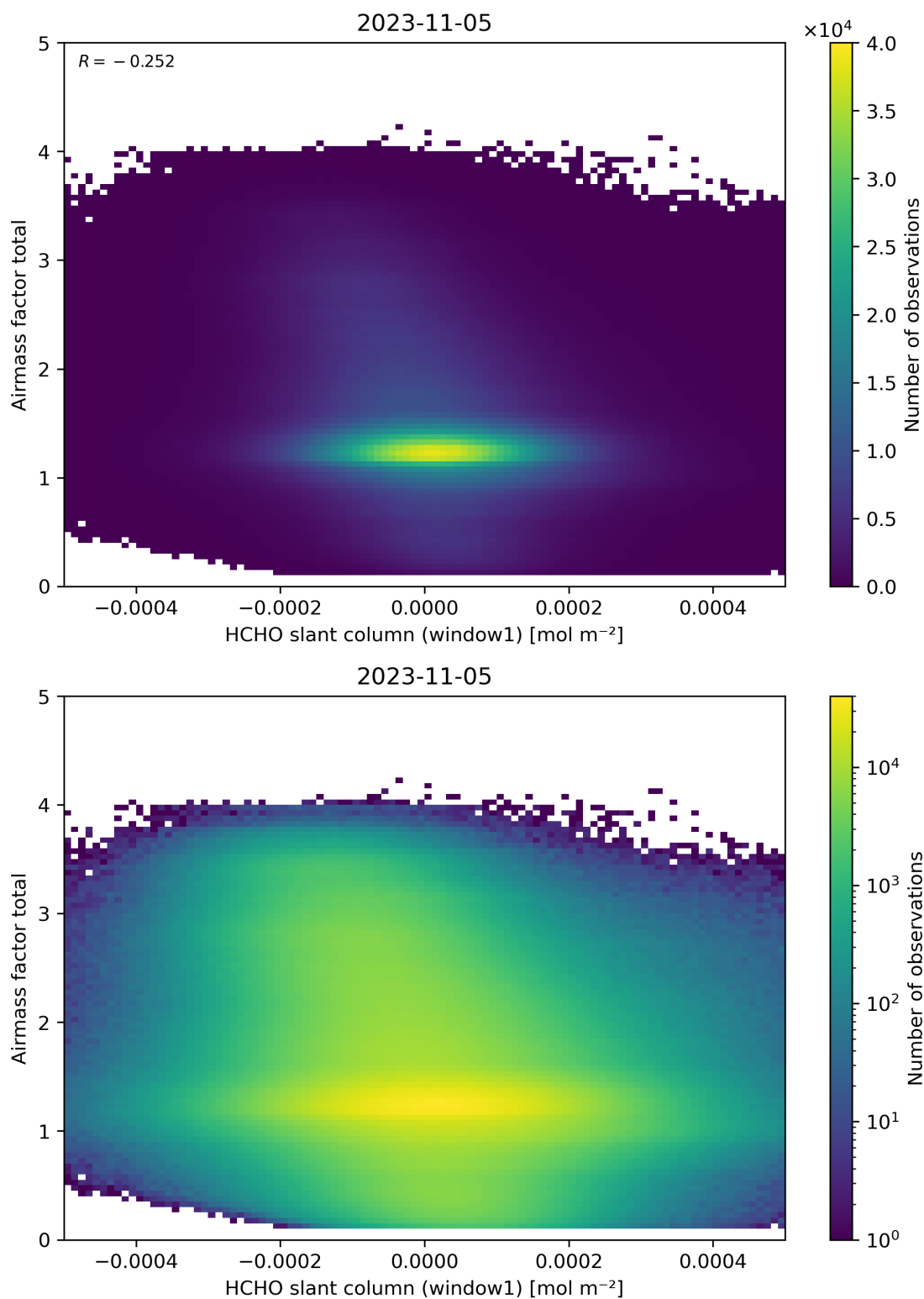
Figure 85: Scatter density plot of “HCHO slant column (window1)” against “Airmass factor total” for 2023-11-04 to 2023-11-06.
