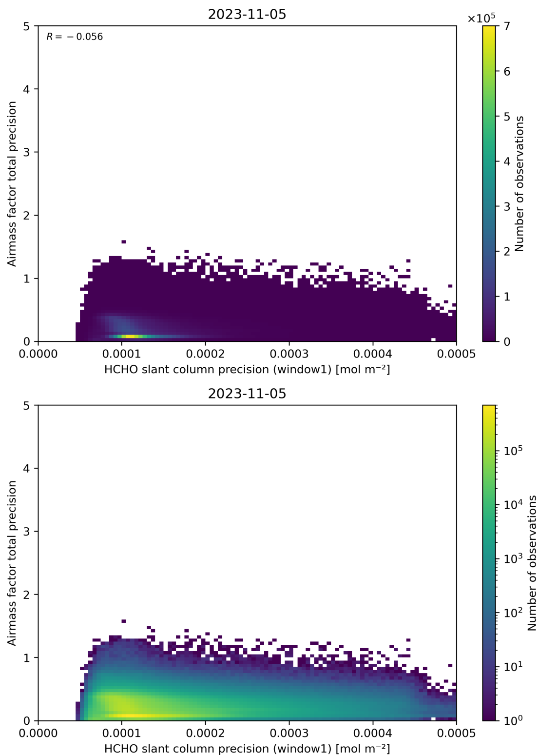
Figure 95: Scatter density plot of “HCHO slant column precision (window1)” against “Airmass factor total precision” for 2023-11-04 to 2023-11-06.
