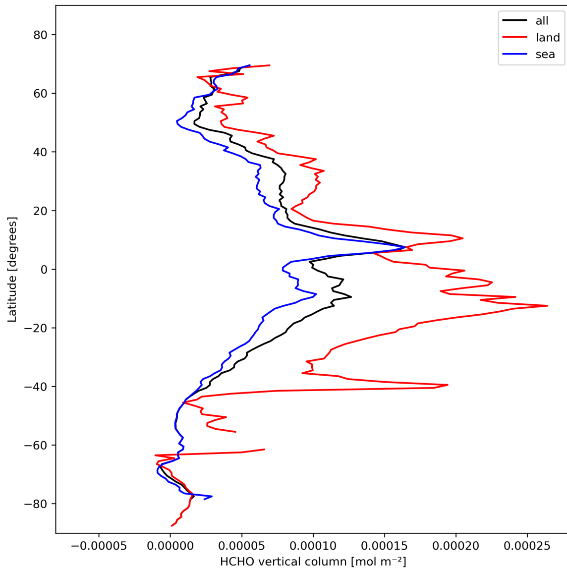
Figure 21: Zonal average of “HCHO vertical column” for 2023-11-04 to 2023-11-06.
