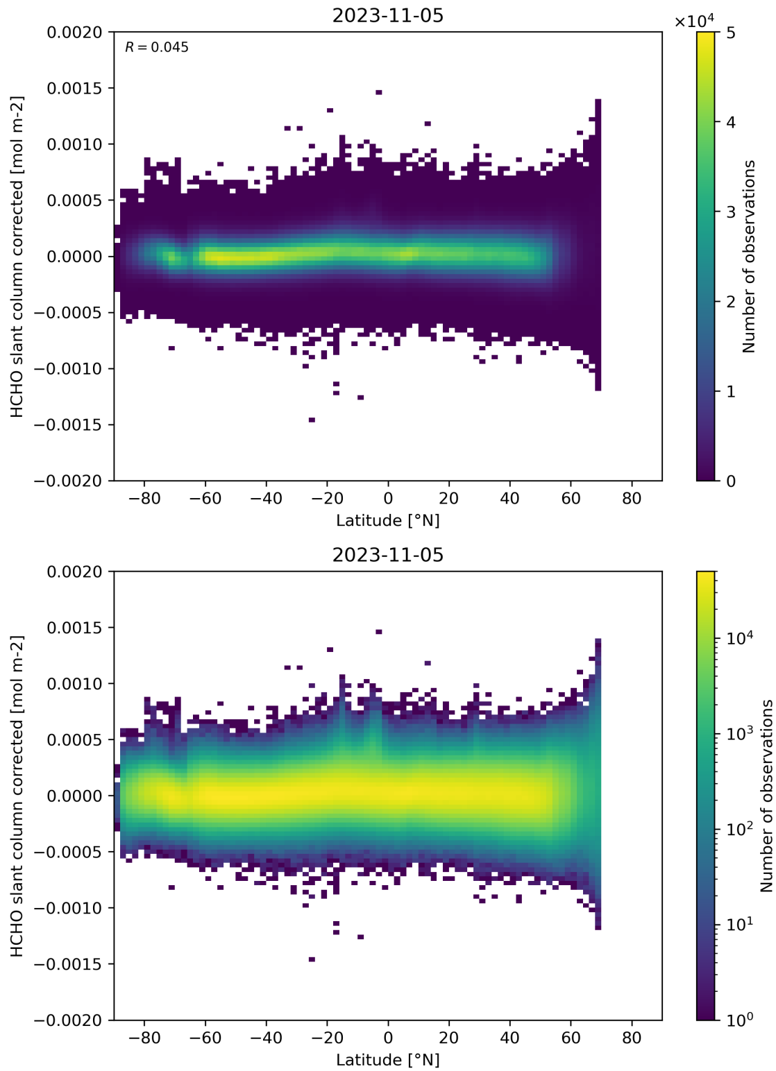
Figure 157: Scatter density plot of “Latitude” against “HCHO slant column corrected” for 2023-11-04 to 2023-11-06.
