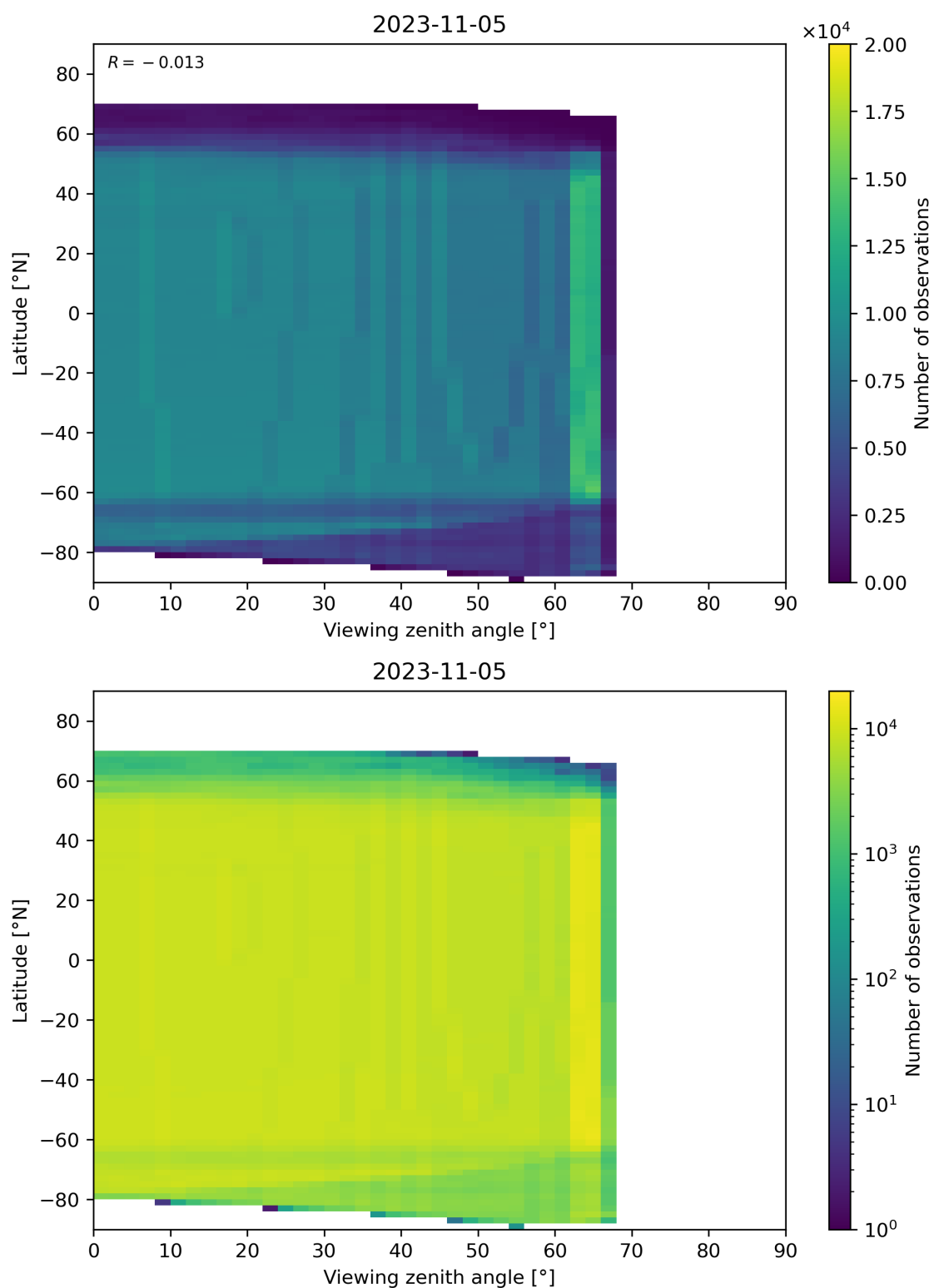
Figure 196: Scatter density plot of “Viewing zenith angle” against “Latitude” for 2023-11-04 to 2023-11-06.
