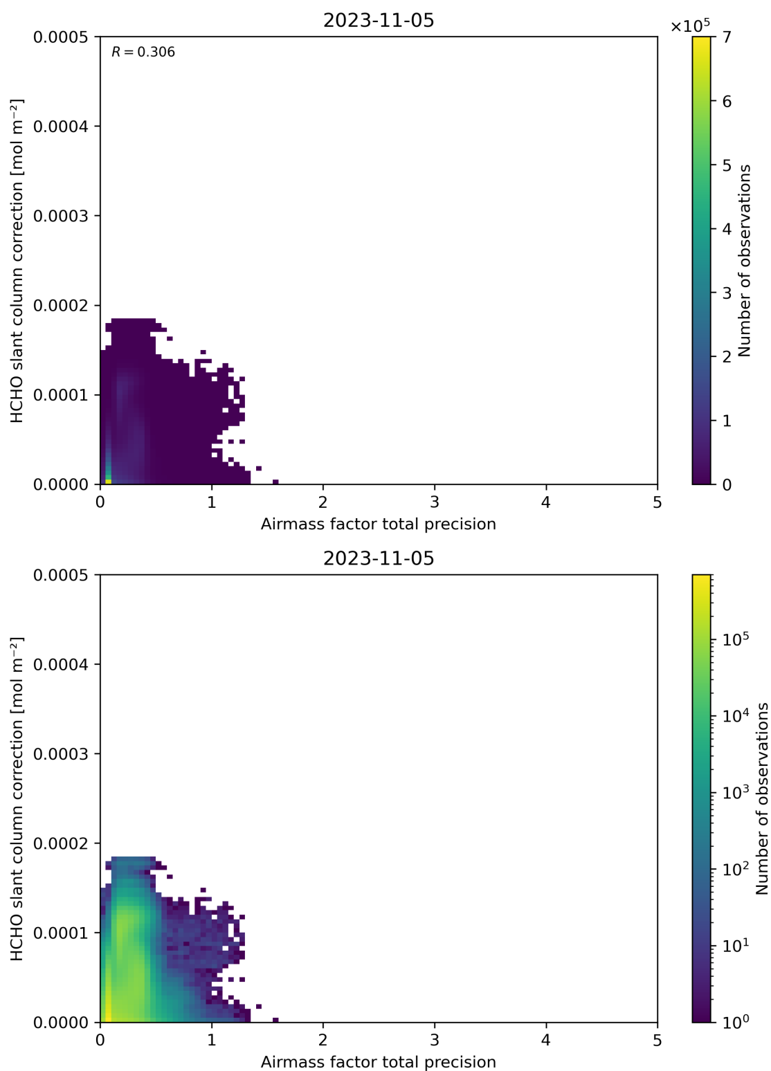
Figure 110: Scatter density plot of “Airmass factor total precision” against “HCHO slant column correction” for 2023-11-04 to 2023-11-06.
