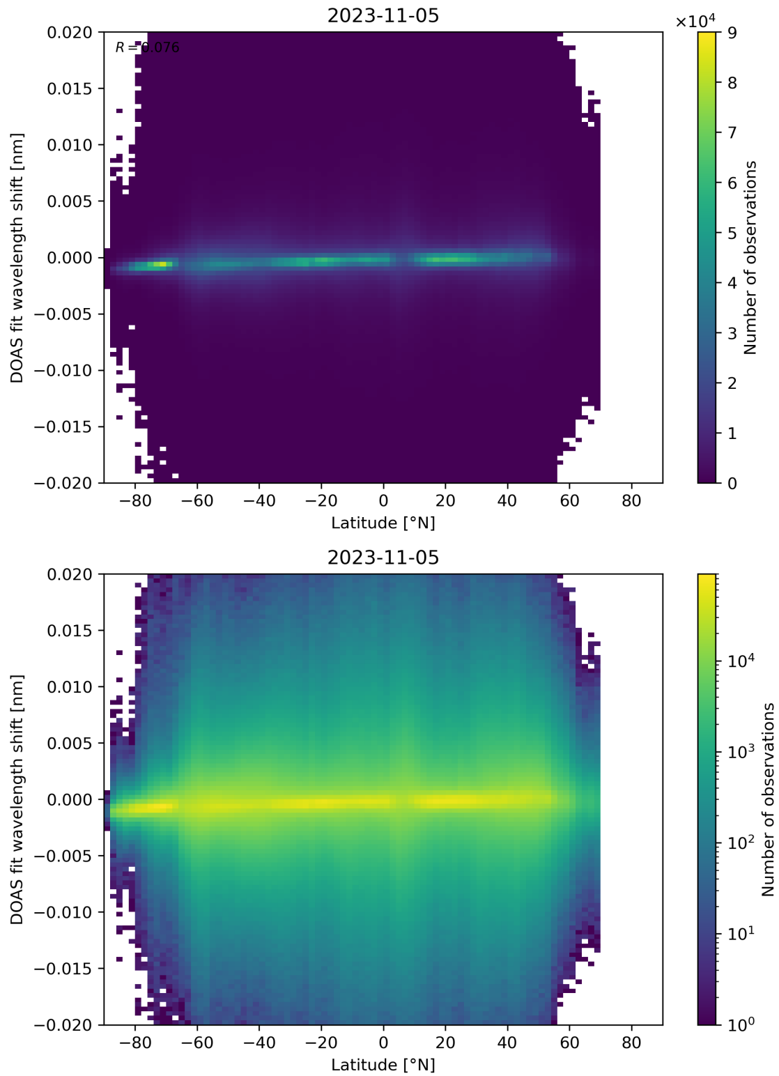
Figure 154: Scatter density plot of “Latitude” against “DOAS fit wavelength shift” for 2023-11-04 to 2023-11-06.
