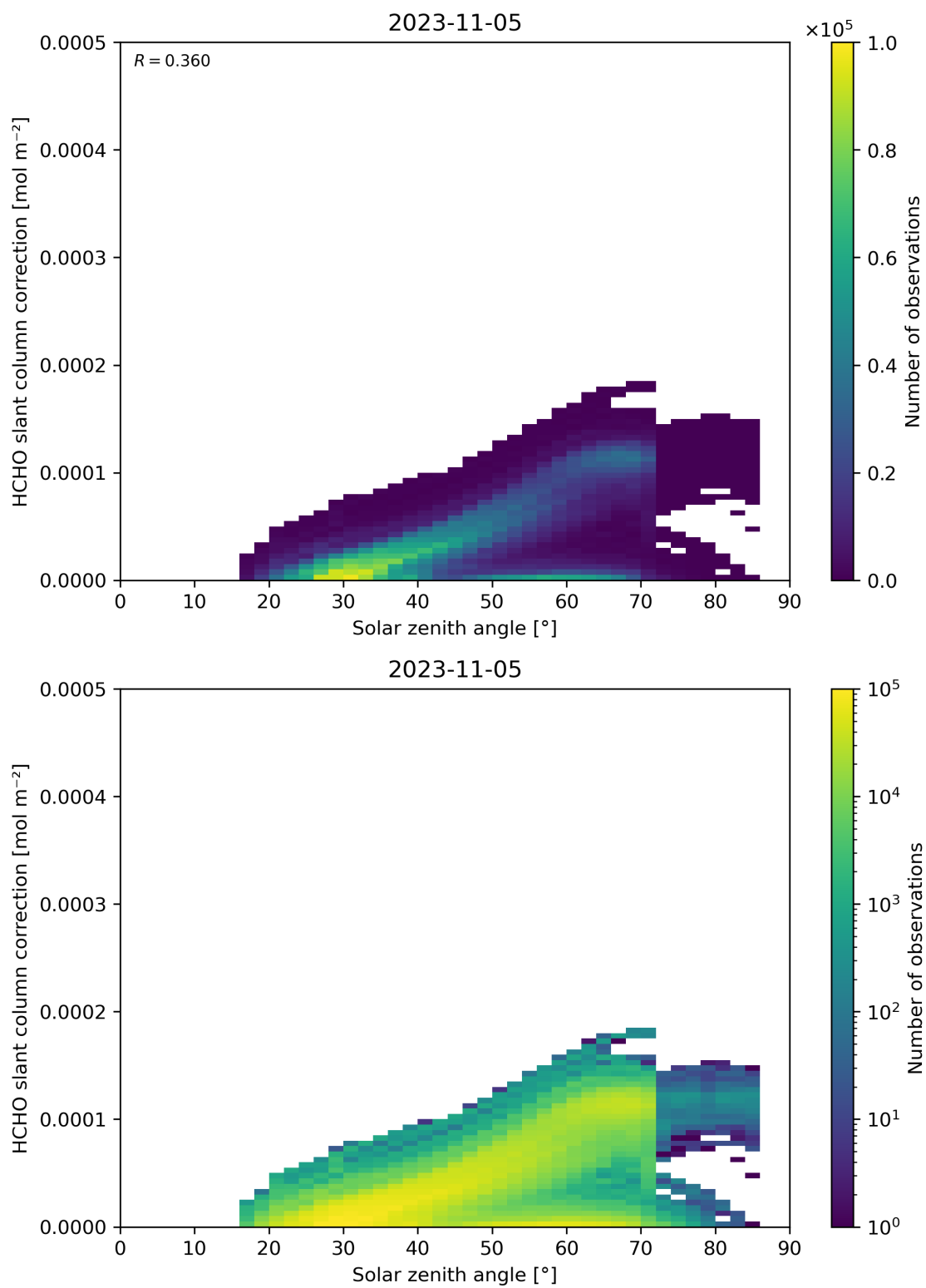
Figure 172: Scatter density plot of “Solar zenith angle” against “HCHO slant column correction” for 2023-11-04 to 2023-11-06.
