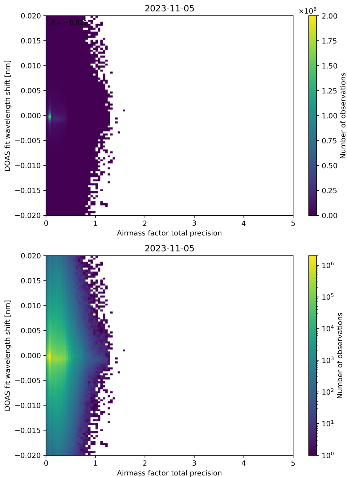
Figure 106: Scatter density plot of “Airmass factor total precision” against “DOAS fit wavelength shift” for 2023-11-04 to 2023-11-06.
