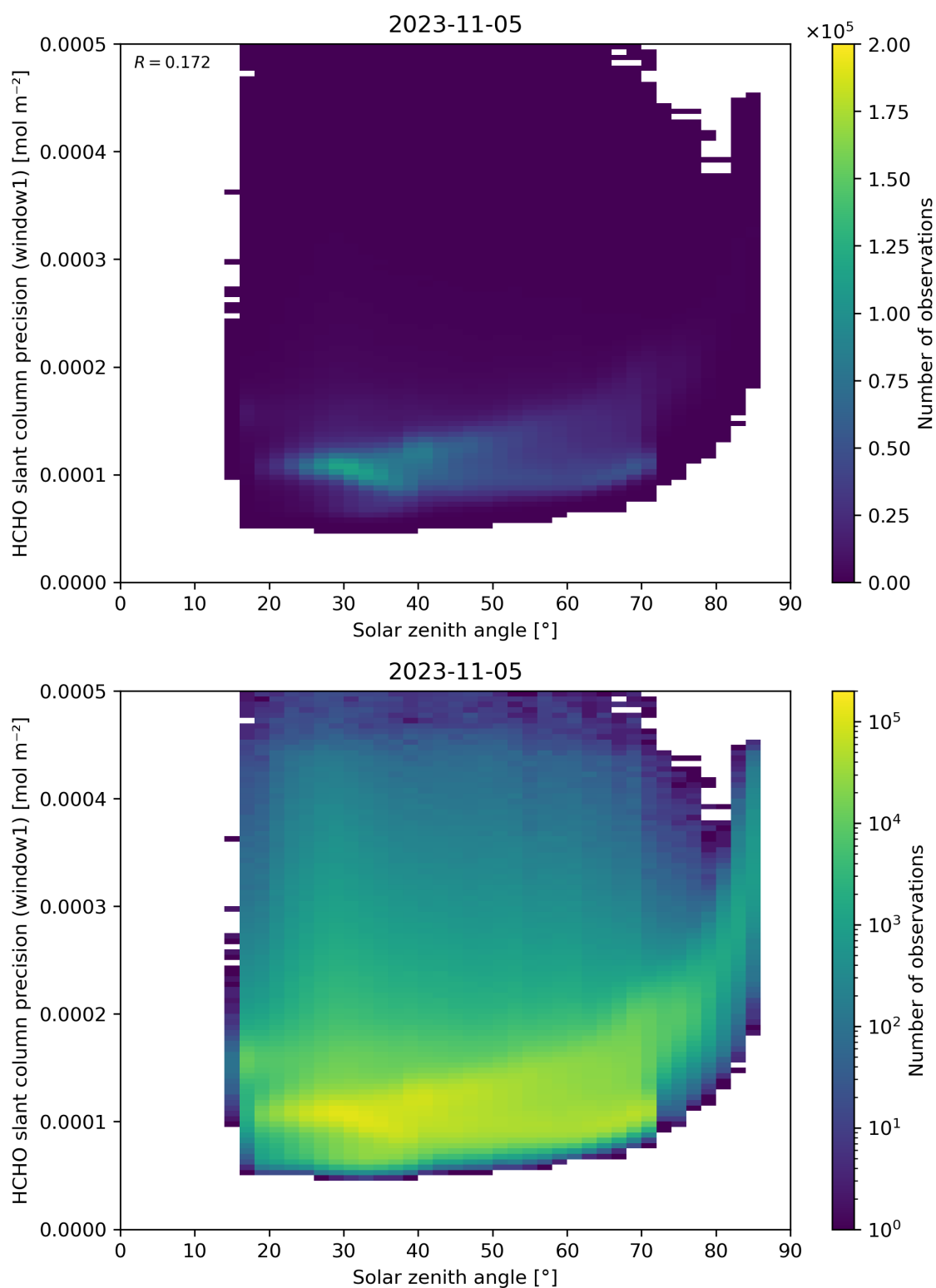
Figure 174: Scatter density plot of “Solar zenith angle” against “HCHO slant column precision (window1)” for 2023-11-04 to 2023-11-06.
