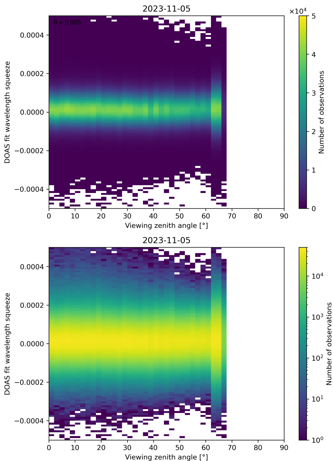
Figure 184: Scatter density plot of “Viewing zenith angle” against “DOAS fit wavelength squeeze” for 2023-11-04 to 2023-11-06.
