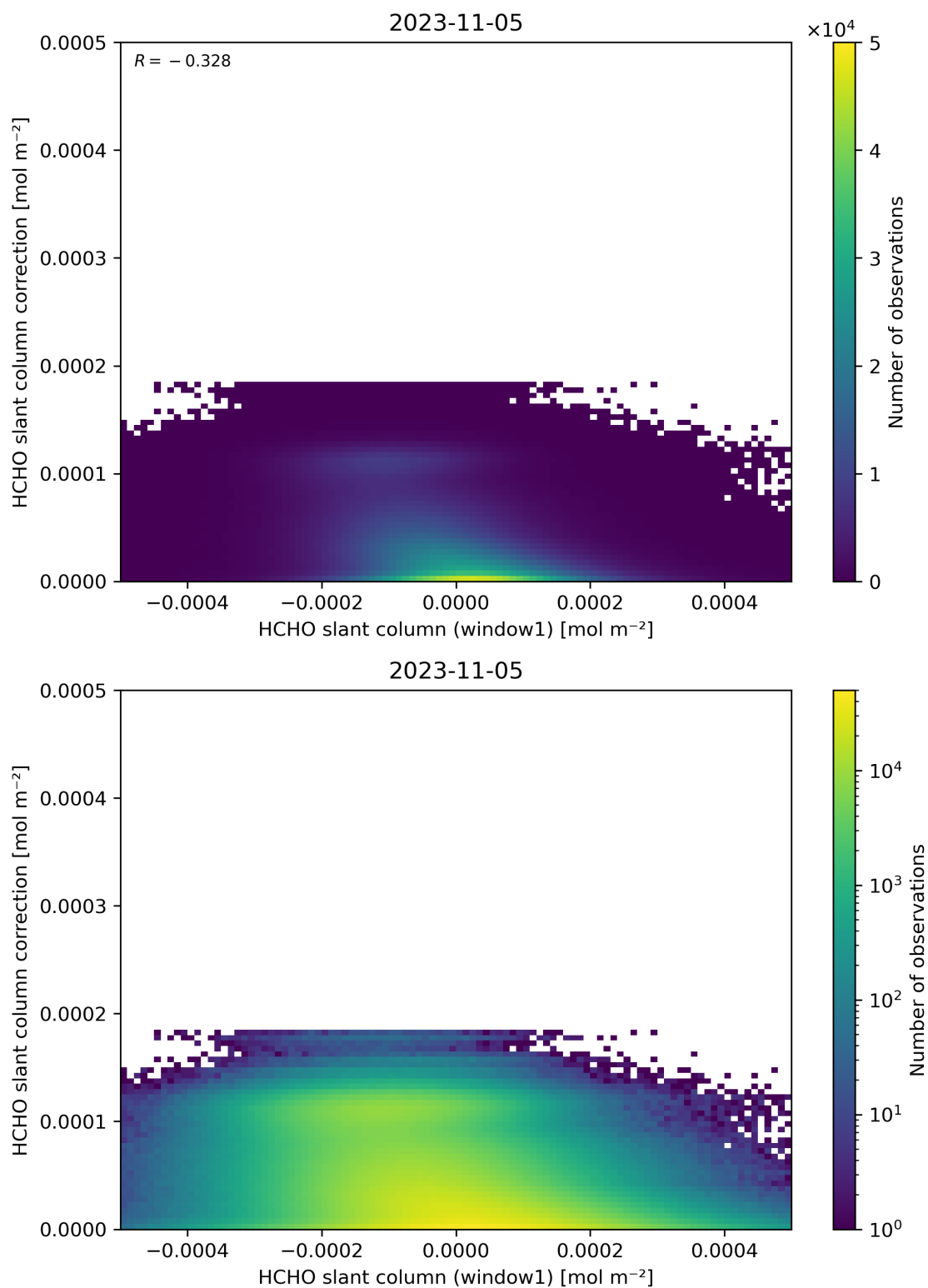
Figure 83: Scatter density plot of “HCHO slant column (window1)” against “HCHO slant column correction” for 2023-11-04 to 2023-11-06.
