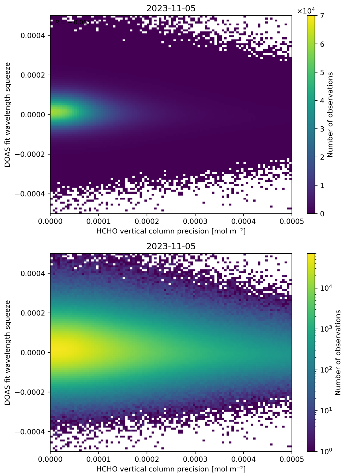
Figure 138: Scatter density plot of “HCHO vertical column precision” against “DOAS fit wavelength squeeze” for 2023-11-04 to 2023-11-06.
