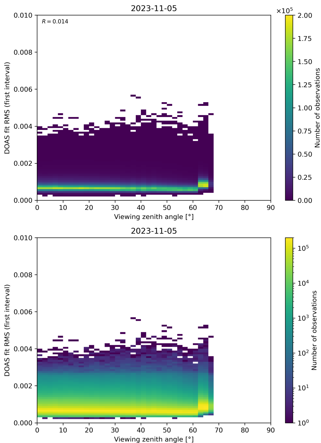
Figure 182: Scatter density plot of “Viewing zenith angle” against “DOAS fit RMS (first interval)” for 2023-11-04 to 2023-11-06.
