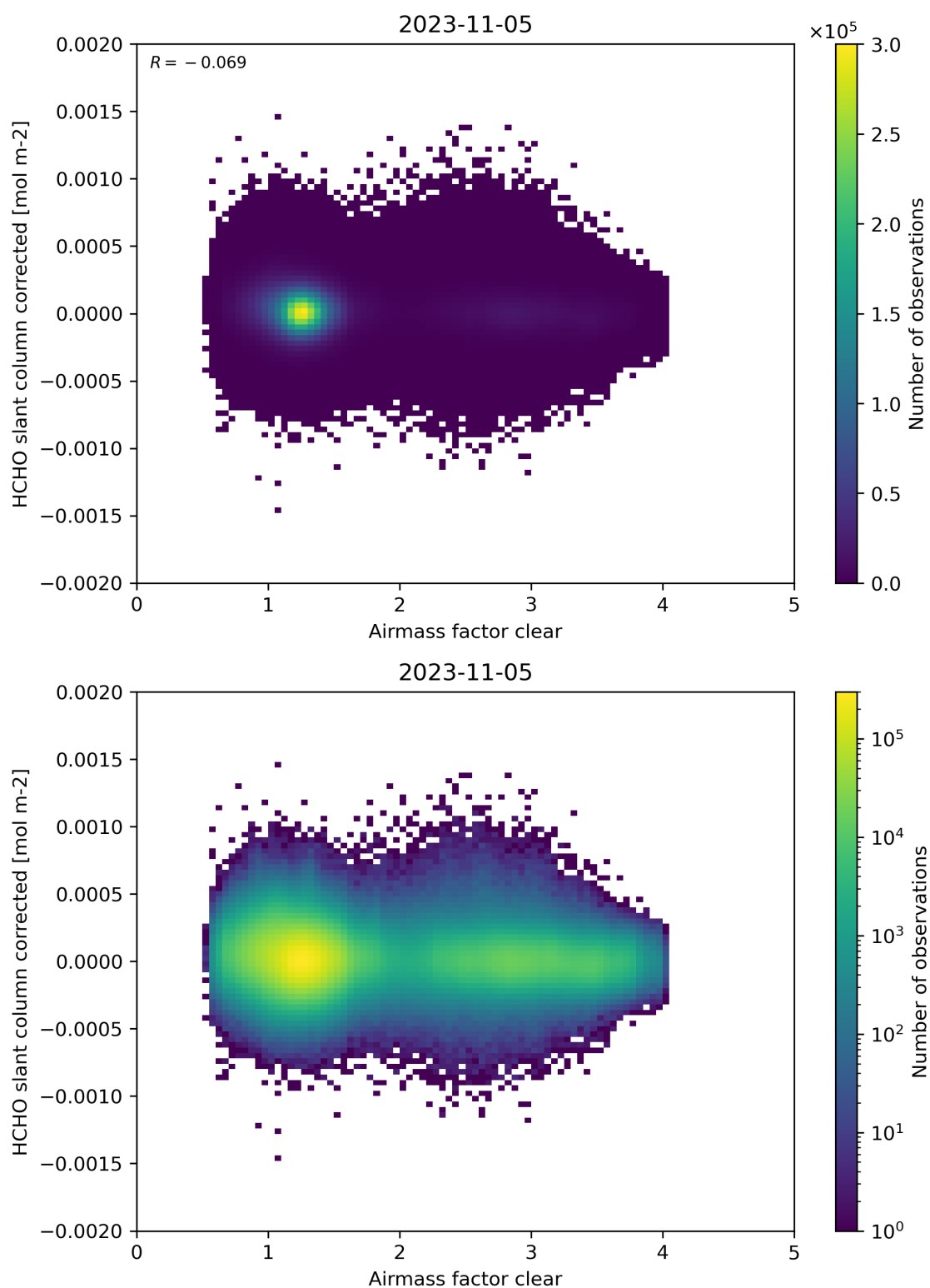
Figure 74: Scatter density plot of “Airmass factor clear” against “HCHO slant column corrected” for 2023-11-04 to 2023-11-06.
