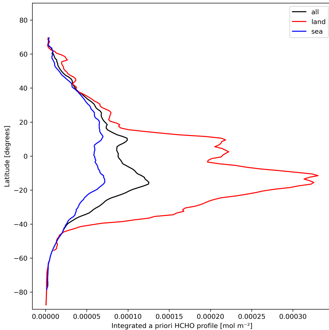
Figure 29: Zonal average of “Integrated a priori HCHO profile” for 2023-11-04 to 2023-11-06.
