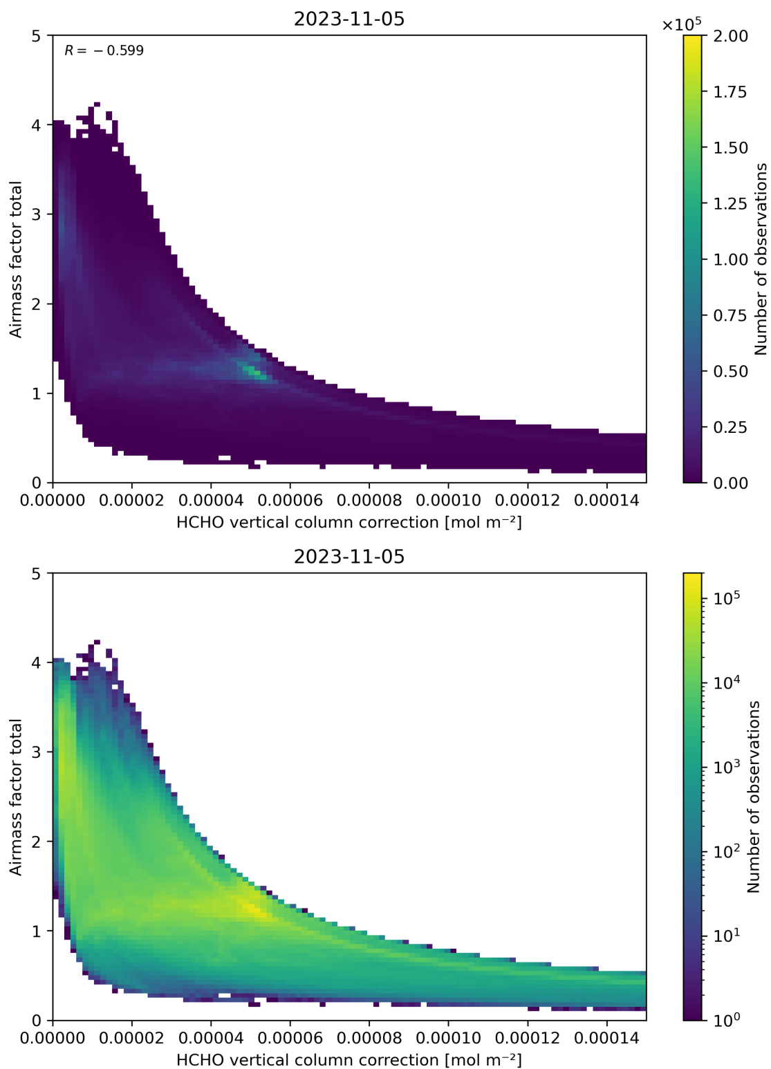
Figure 120: Scatter density plot of “HCHO vertical column correction” against “Airmass factor total” for 2023-11-04 to 2023-11-06.
