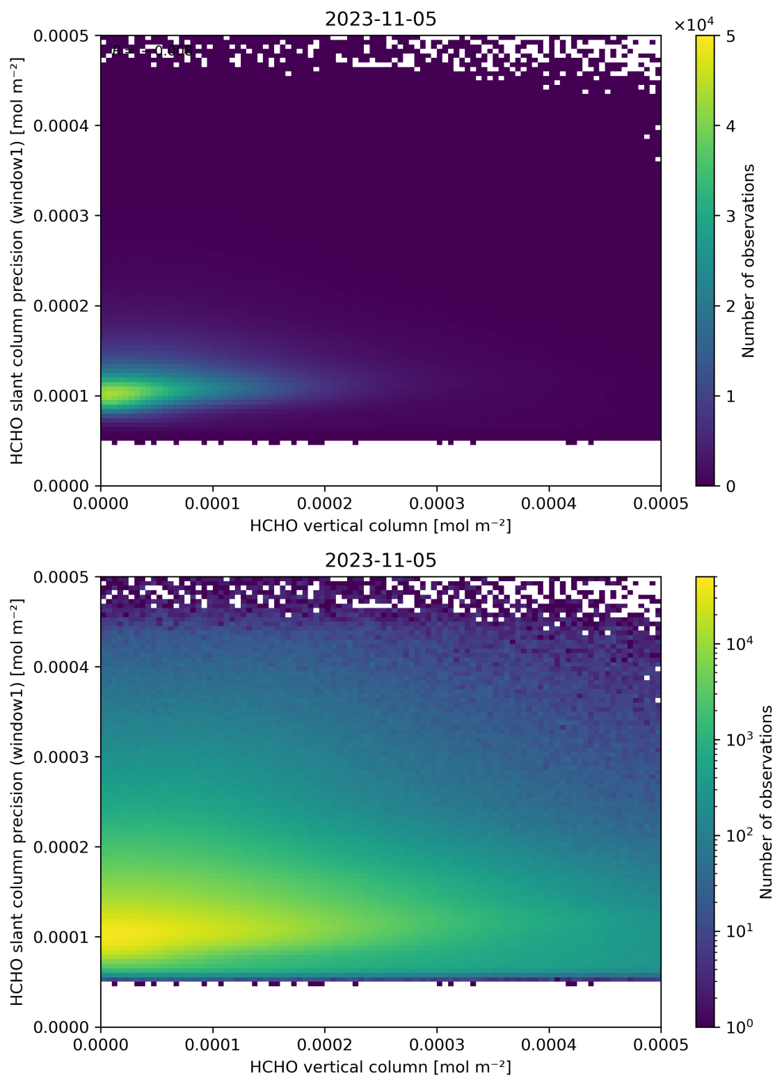
Figure 130: Scatter density plot of “HCHO vertical column” against “HCHO slant column precision (window1)” for 2023-11-04 to 2023-11-06.
