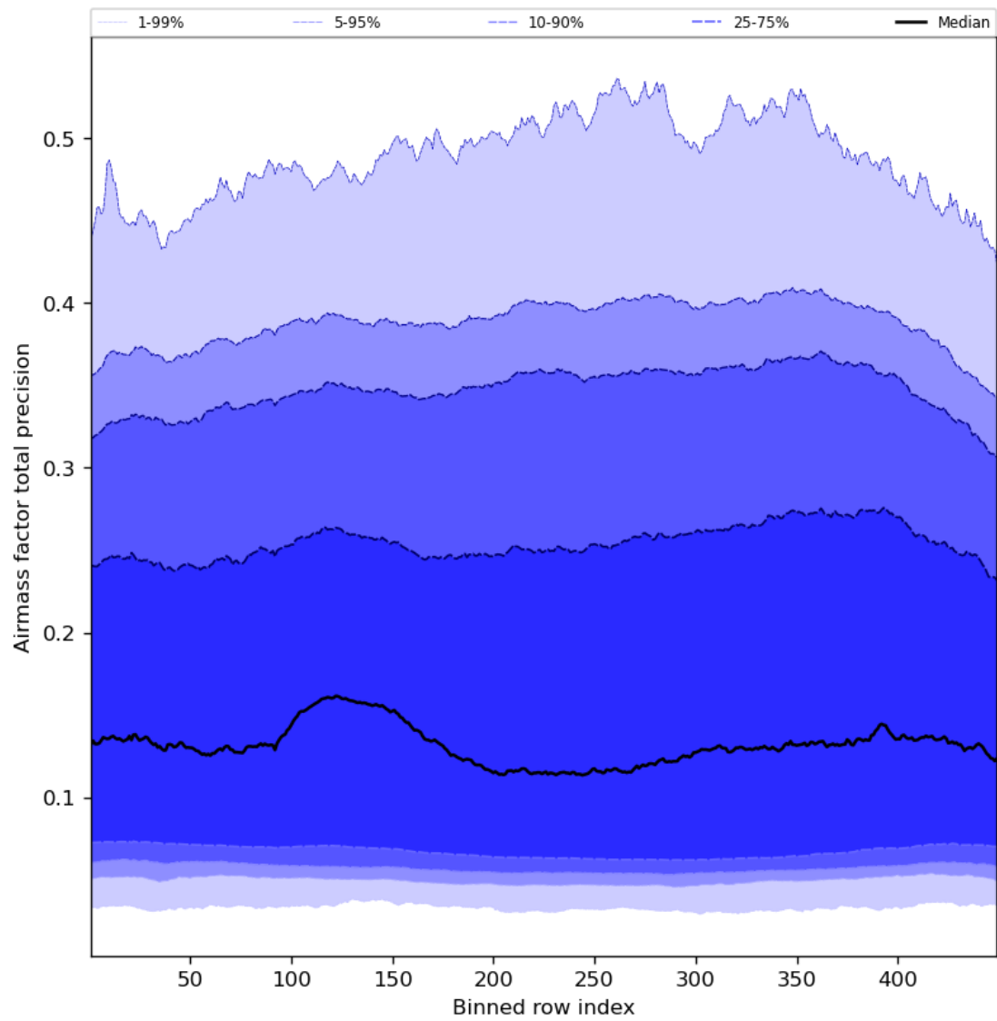
Figure 55: Along track statistics of “Airmass factor total precision” for 2023-11-04 to 2023-11-06
