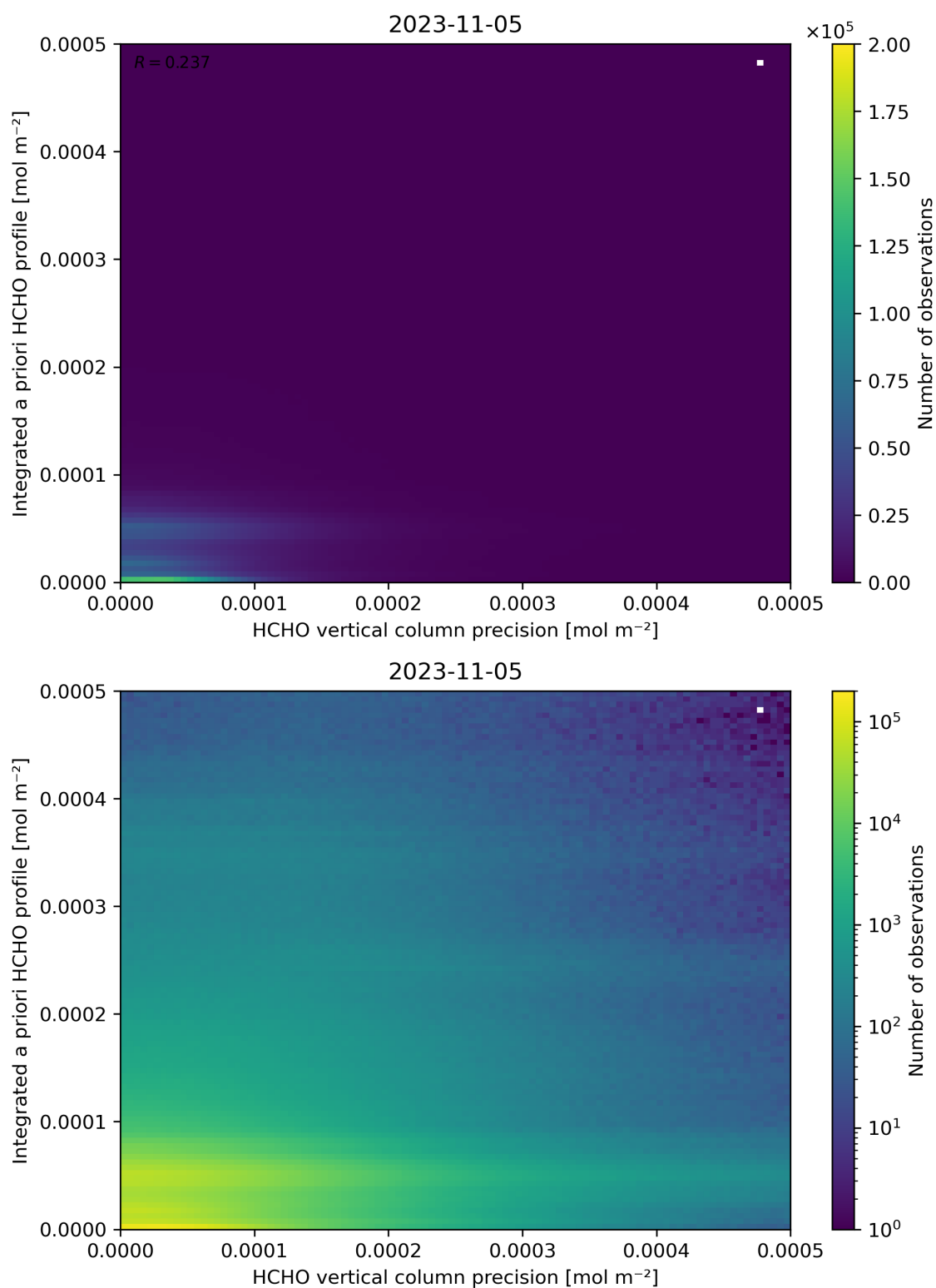
Figure 147: Scatter density plot of “HCHO vertical column precision” against “Integrated a priori HCHO profile” for 2023-11-04 to 2023-11-06.
