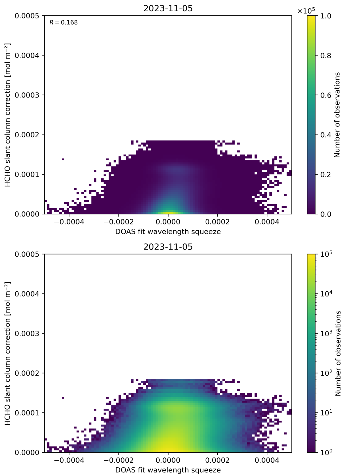
Figure 70: Scatter density plot of “DOAS fit wavelength squeeze” against “HCHO slant column correction” for 2023-11-04 to 2023-11-06.
