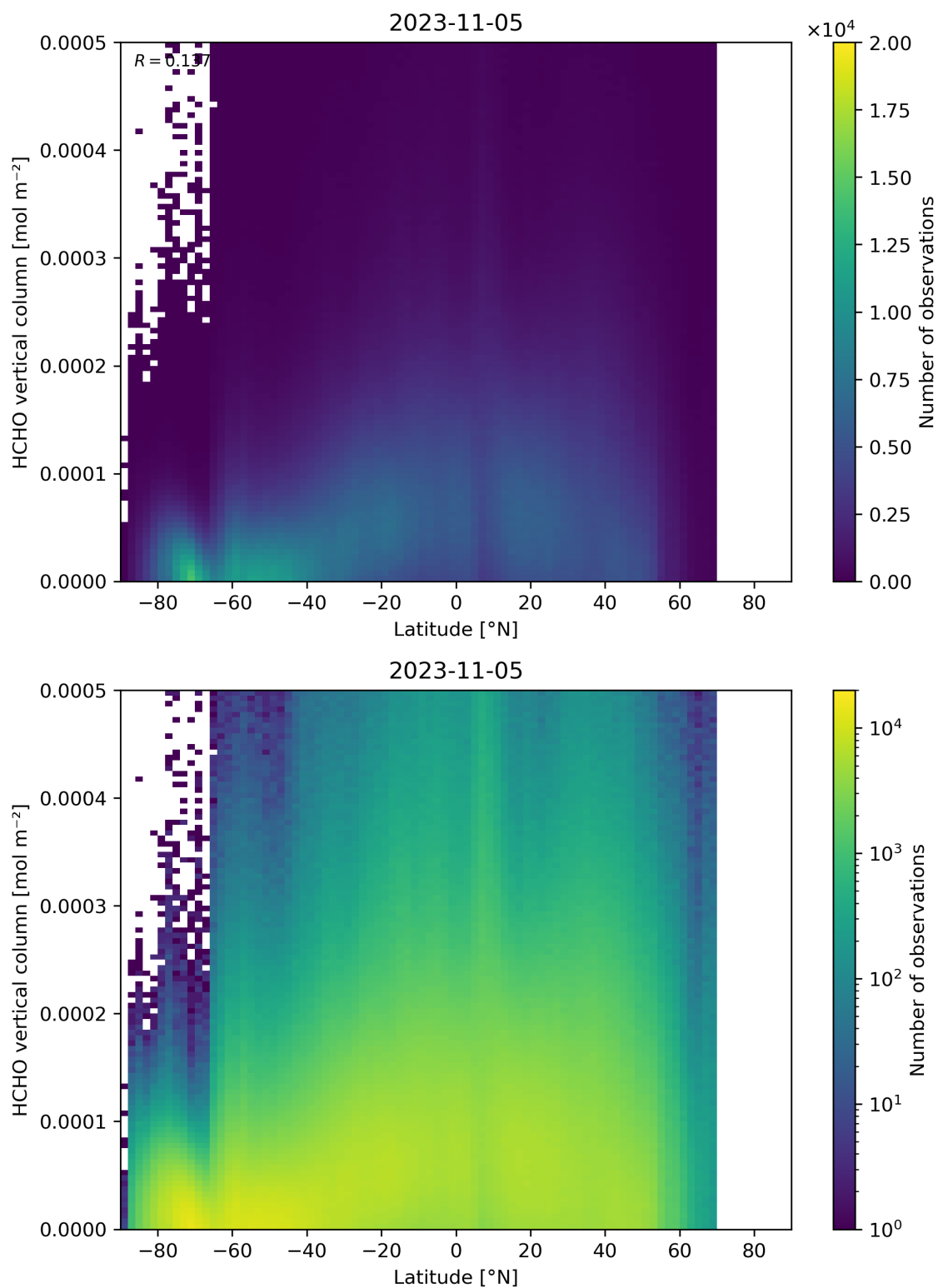
Figure 163: Scatter density plot of “Latitude” against “HCHO vertical column” for 2023-11-04 to 2023-11-06.
