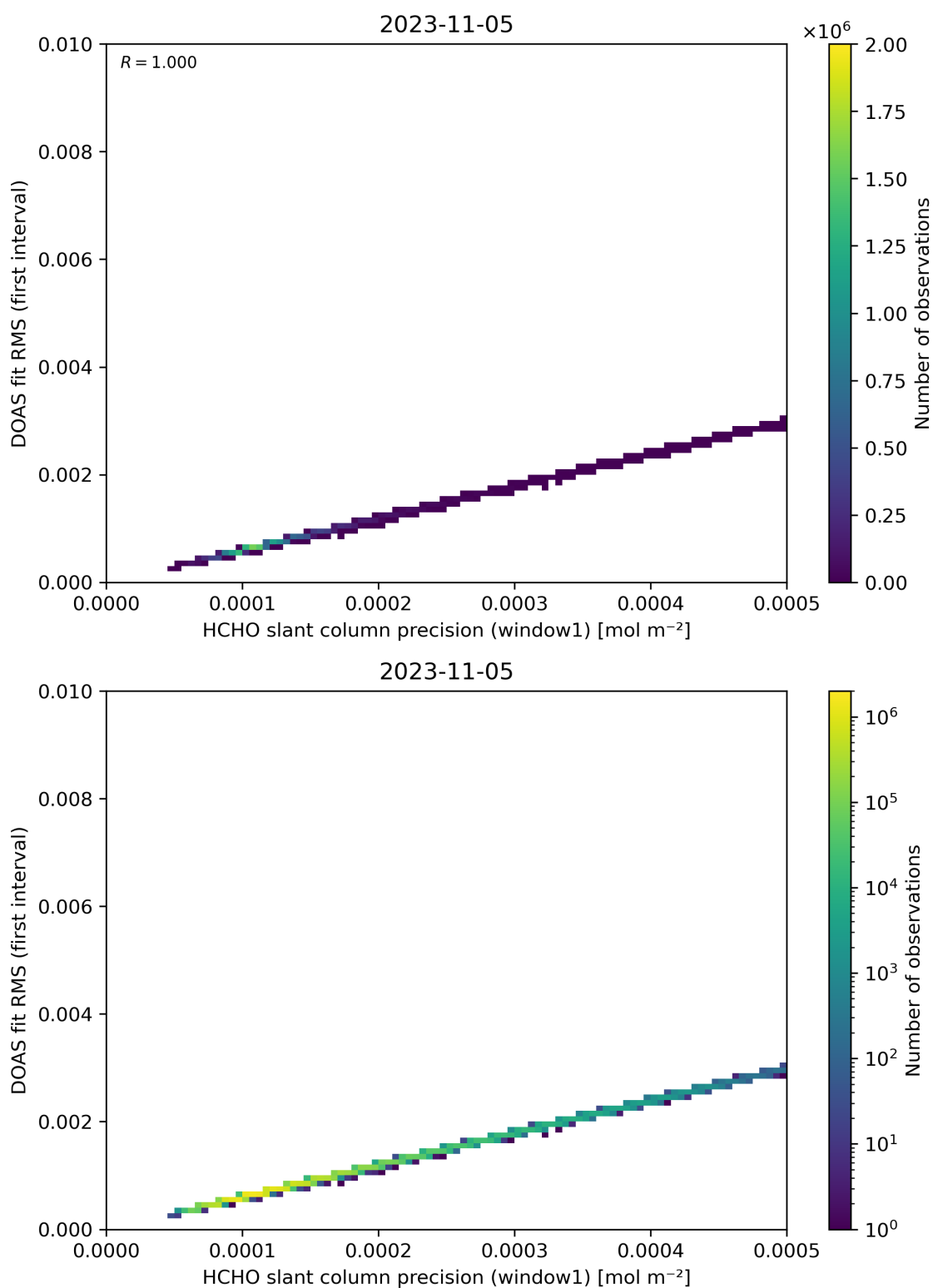
Figure 88: Scatter density plot of “HCHO slant column precision (window1)” against “DOAS fit RMS (first interval)” for 2023-11-04 to 2023-11-06.
