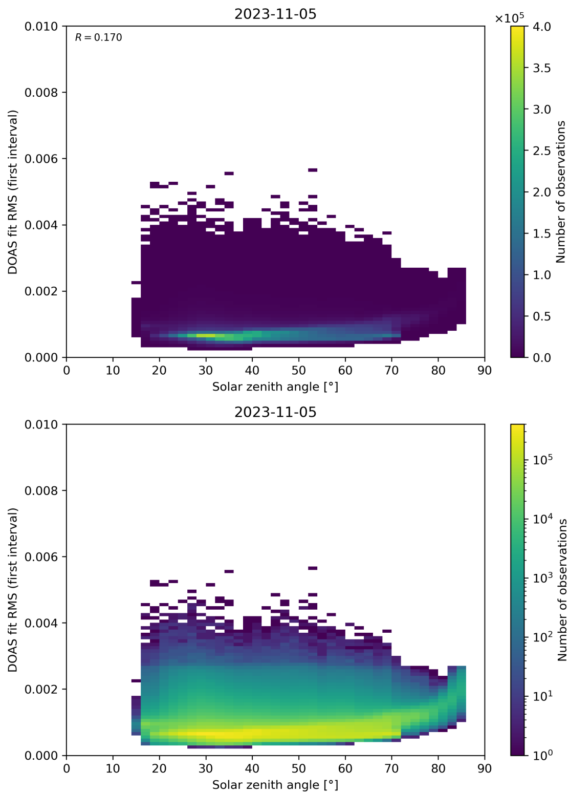
Figure 167: Scatter density plot of “Solar zenith angle” against “DOAS fit RMS (first interval)” for 2023-11-04 to 2023-11-06.
