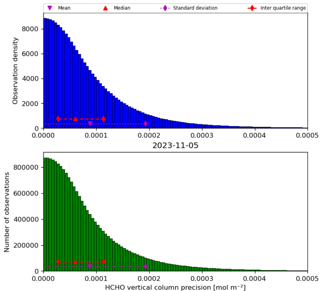
Figure 36: Histogram of “HCHO vertical column precision” for 2023-11-04 to 2023-11-06
