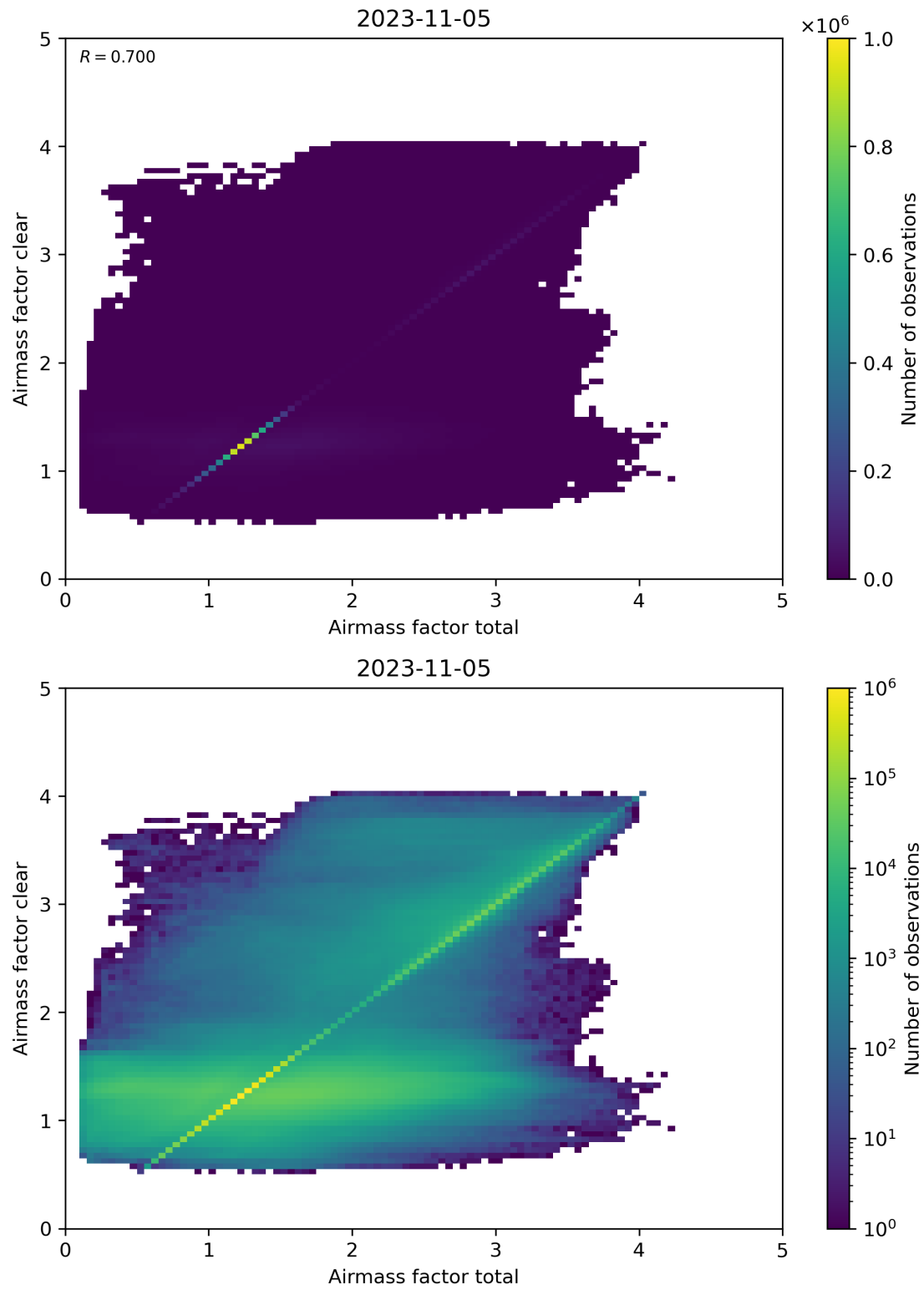
Figure 100: Scatter density plot of “Airmass factor total” against “Airmass factor clear” for 2023-11-04 to 2023-11-06.
