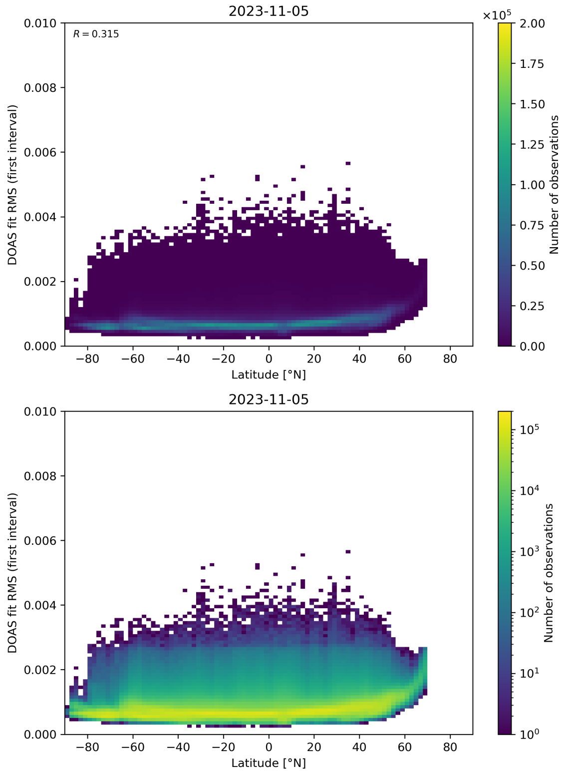
Figure 153: Scatter density plot of “Latitude” against “DOAS fit RMS (first interval)” for 2023-11-04 to 2023-11-06.
