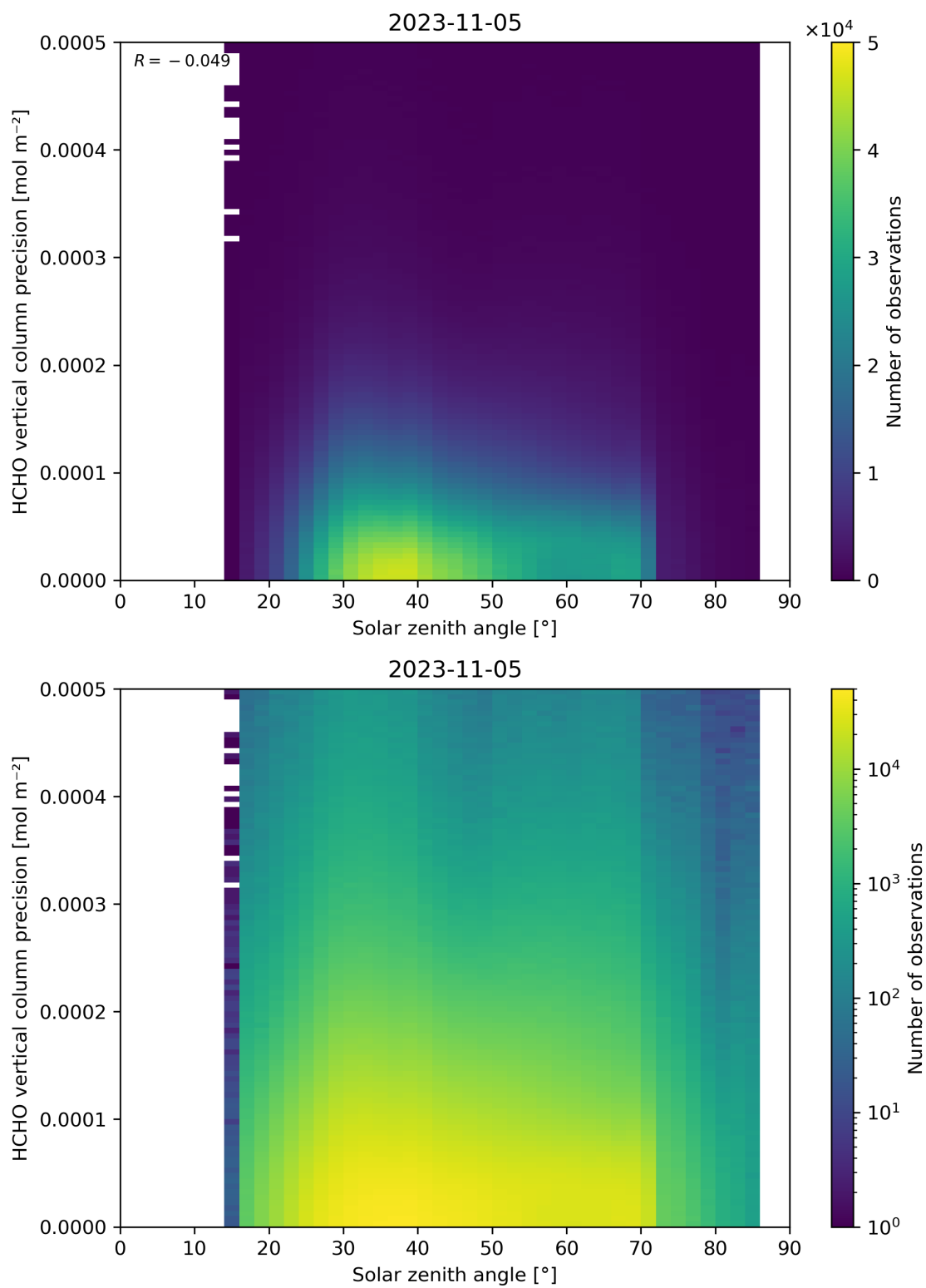
Figure 179: Scatter density plot of “Solar zenith angle” against “HCHO vertical column precision” for 2023-11-04 to 2023-11-06.
