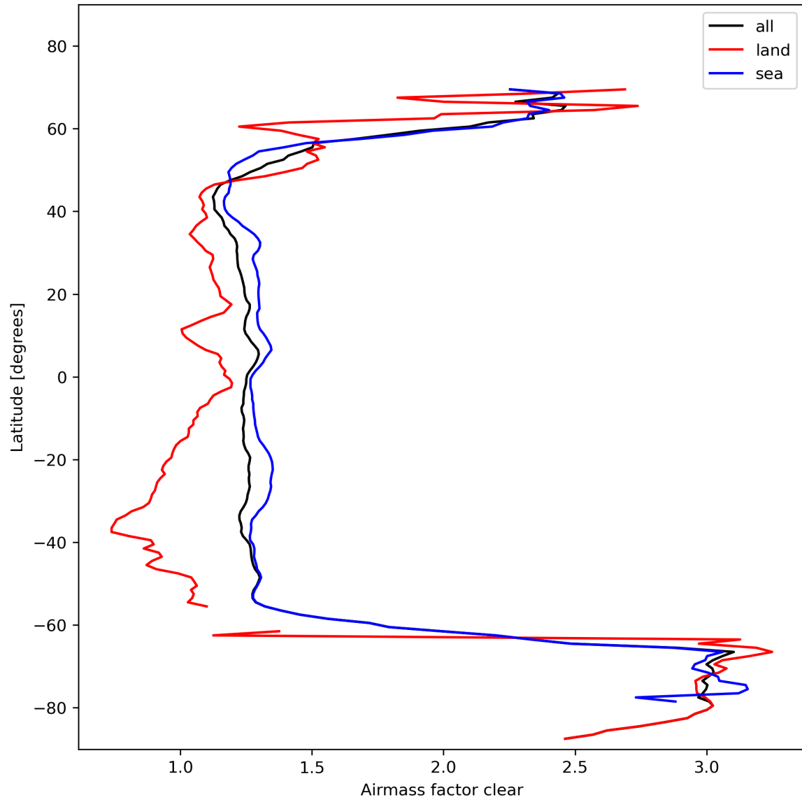
Figure 28: Zonal average of “Airmass factor clear” for 2023-11-04 to 2023-11-06.
