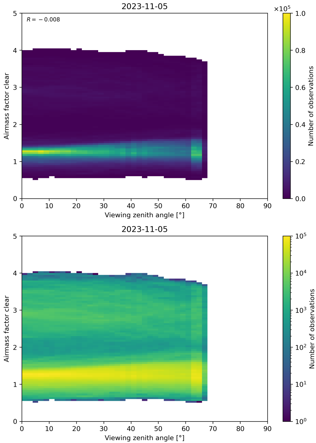
Figure 185: Scatter density plot of “Viewing zenith angle” against “Airmass factor clear” for 2023-11-04 to 2023-11-06.
