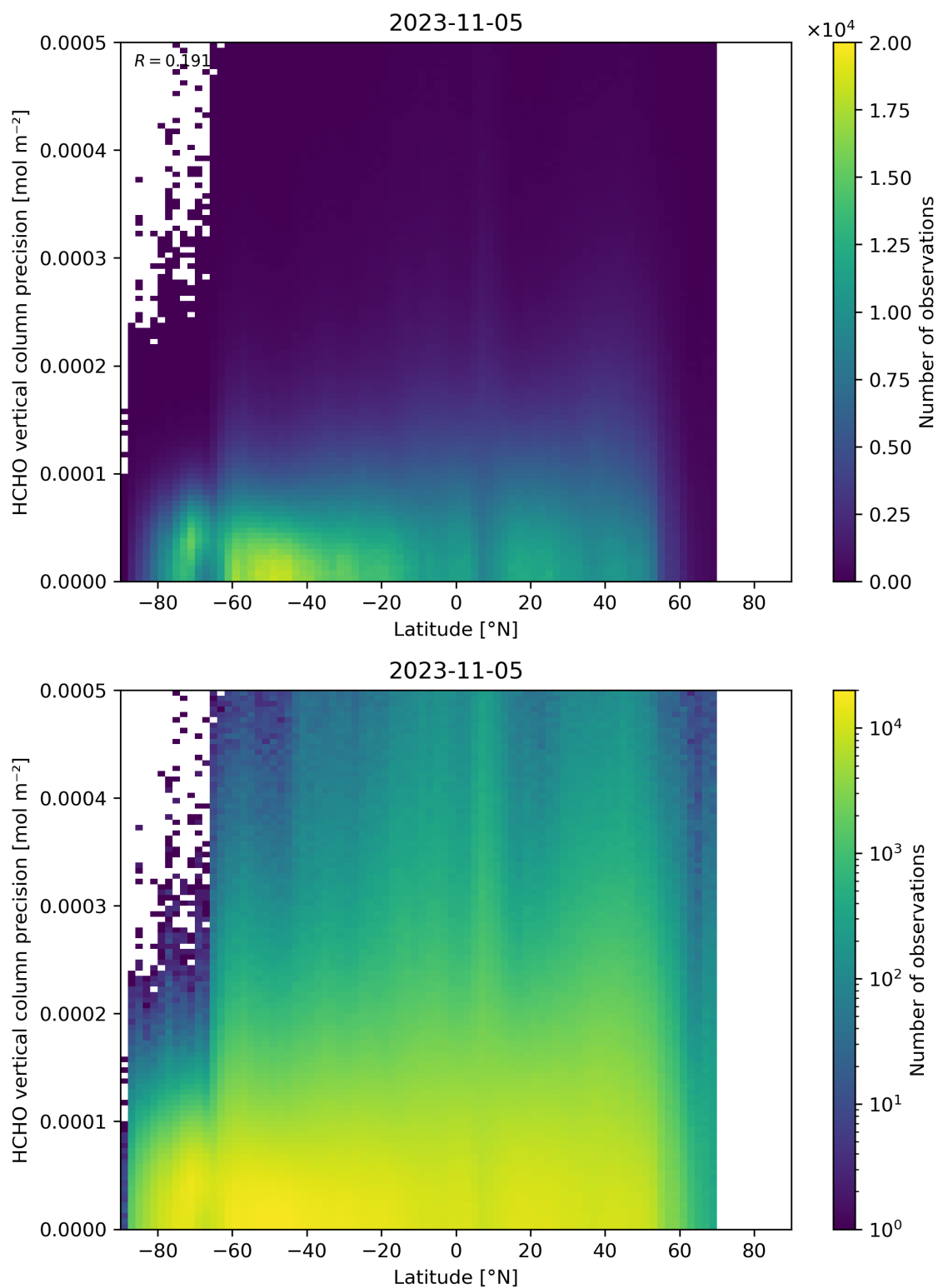
Figure 165: Scatter density plot of “Latitude” against “HCHO vertical column precision” for 2023-11-04 to 2023-11-06.
