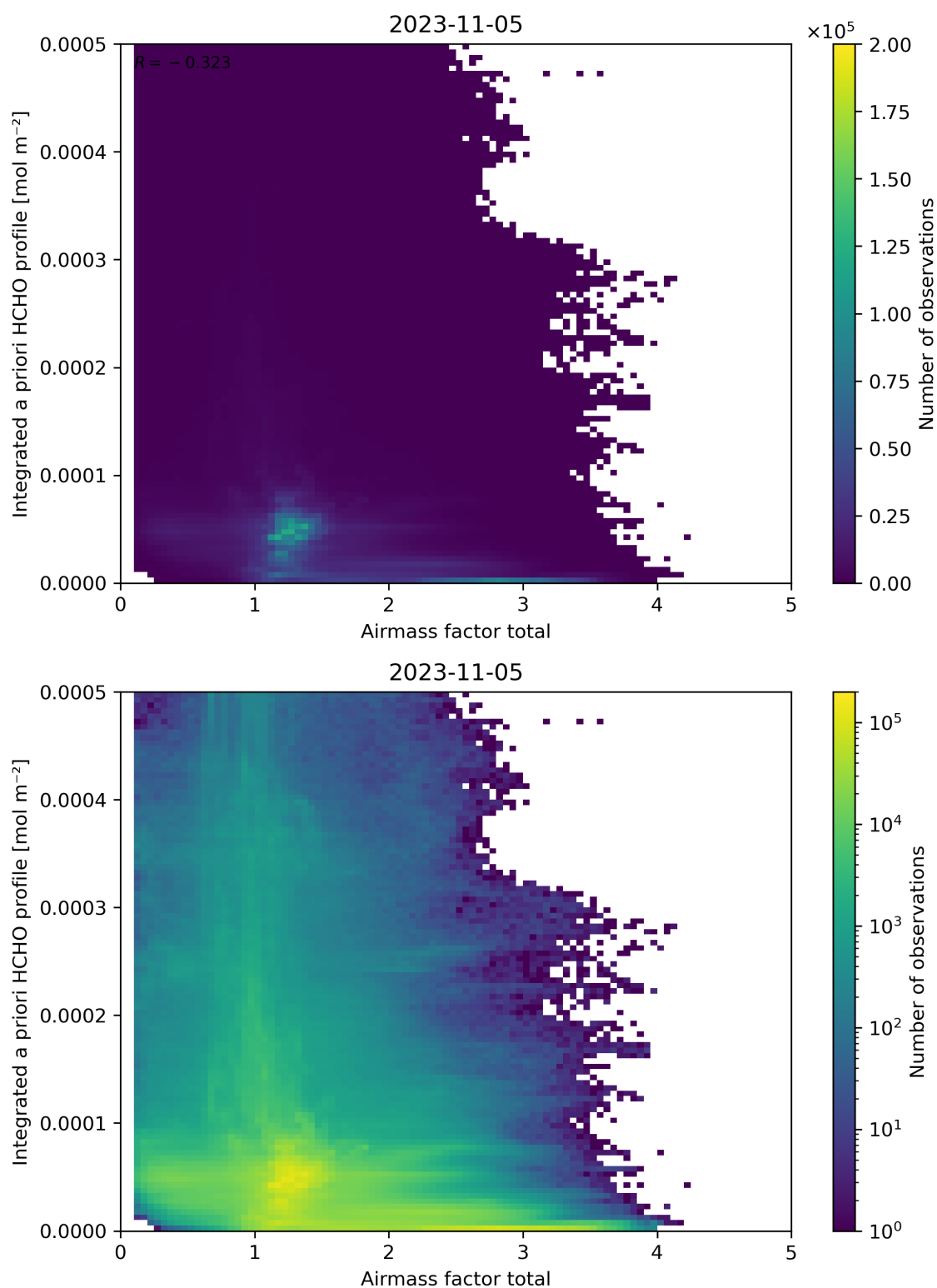
Figure 104: Scatter density plot of “Air mass factor total” against “Integrated a priori HCHO profile” for 2023-11-04 to 2023-11-06.
