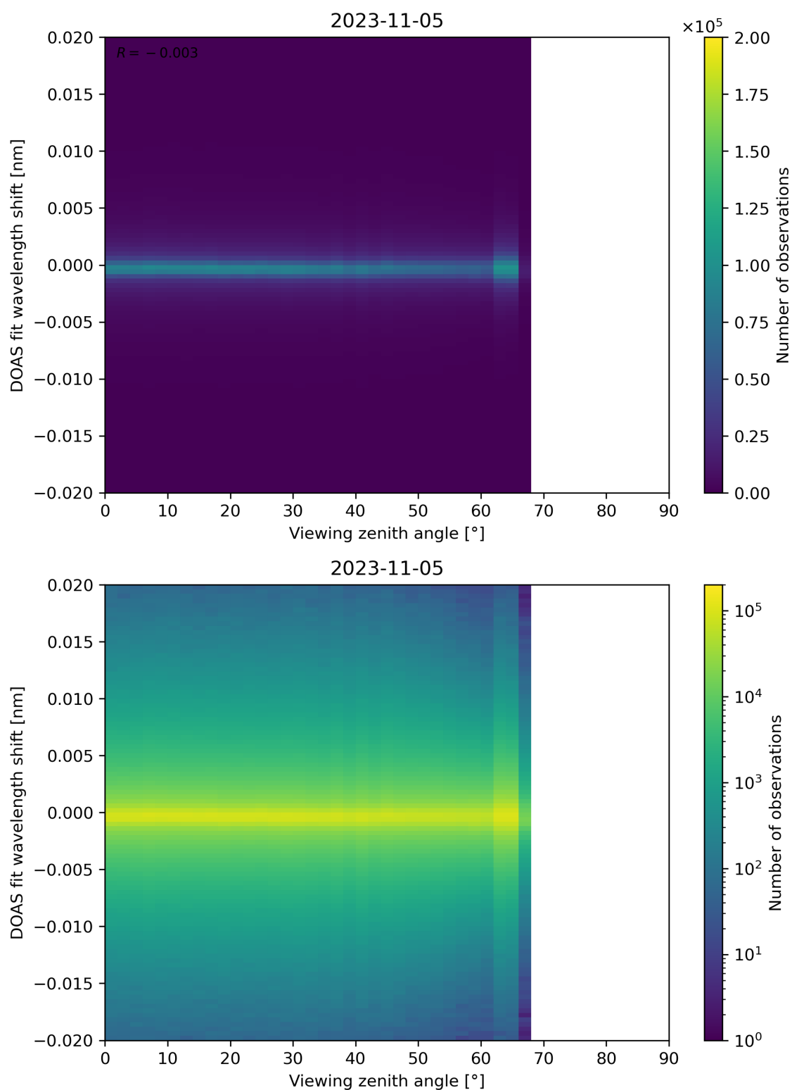
Figure 183: Scatter density plot of “Viewing zenith angle” against “DOAS fit wavelength shift” for 2023-11-04 to 2023-11-06.
