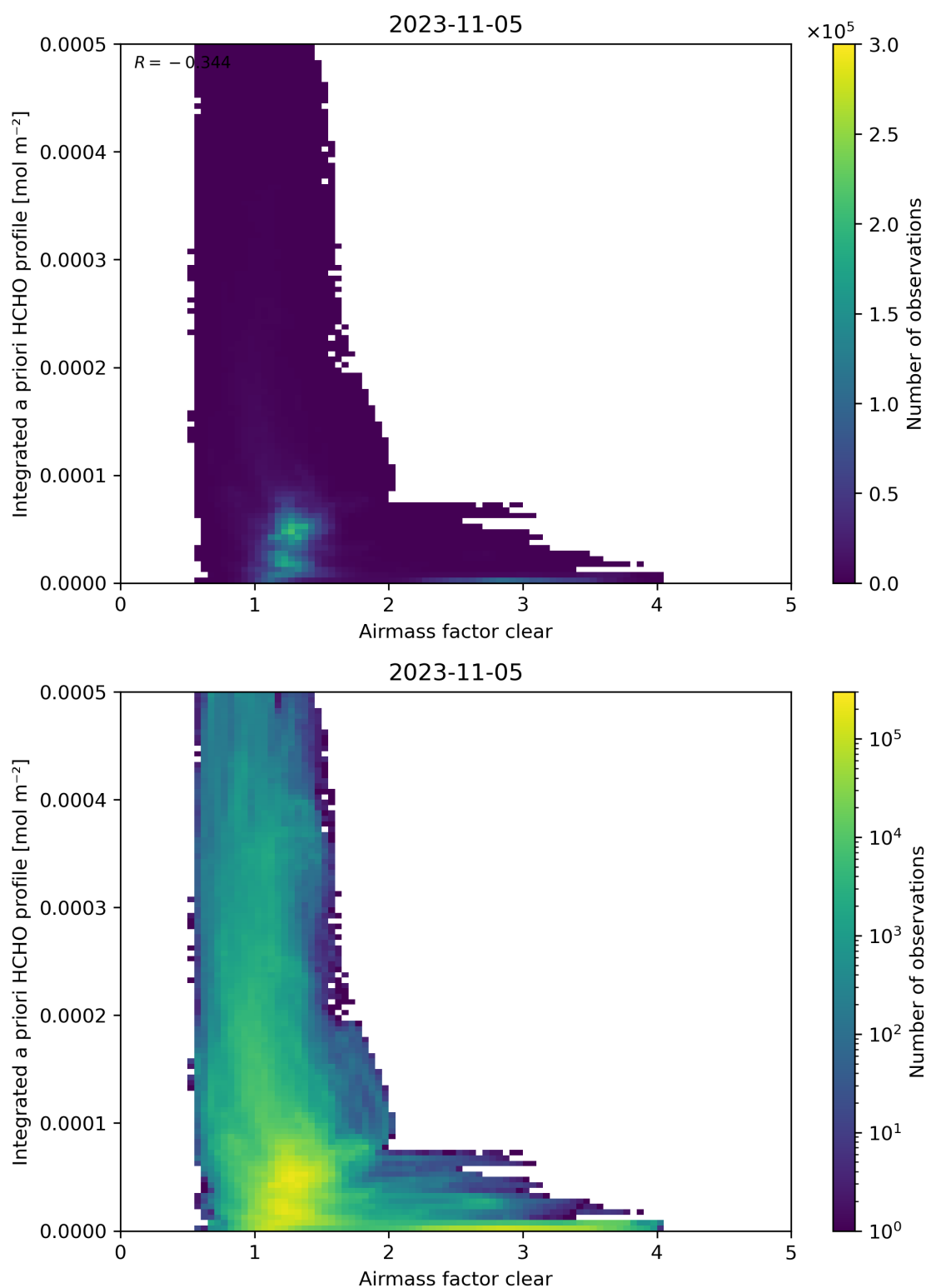
Figure 76: Scatter density plot of “Airmass factor clear” against “Integrated a priori HCHO profile” for 2023-11-04 to 2023-11-06.
