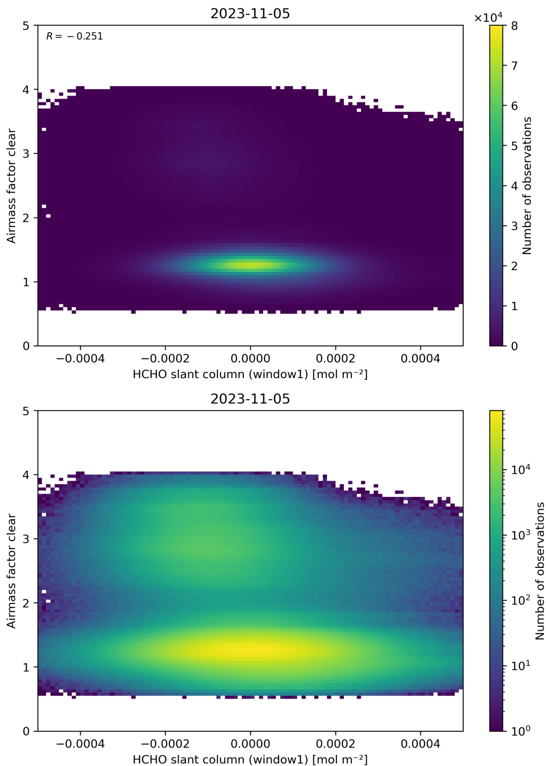
Figure 81: Scatter density plot of “HCHO slant column (window1)” against “Airmass factor clear” for 2023-11-04 to 2023-11-06.
