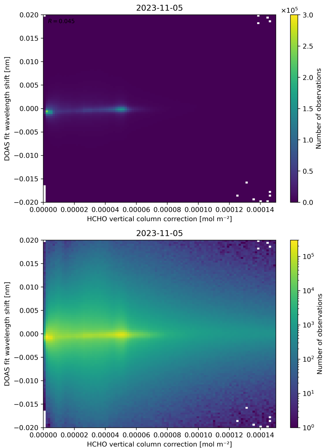
Figure 113: Scatter density plot of “HCHO vertical column correction” against “DOAS fit wavelength shift” for 2023-11-04 to 2023-11-06.
