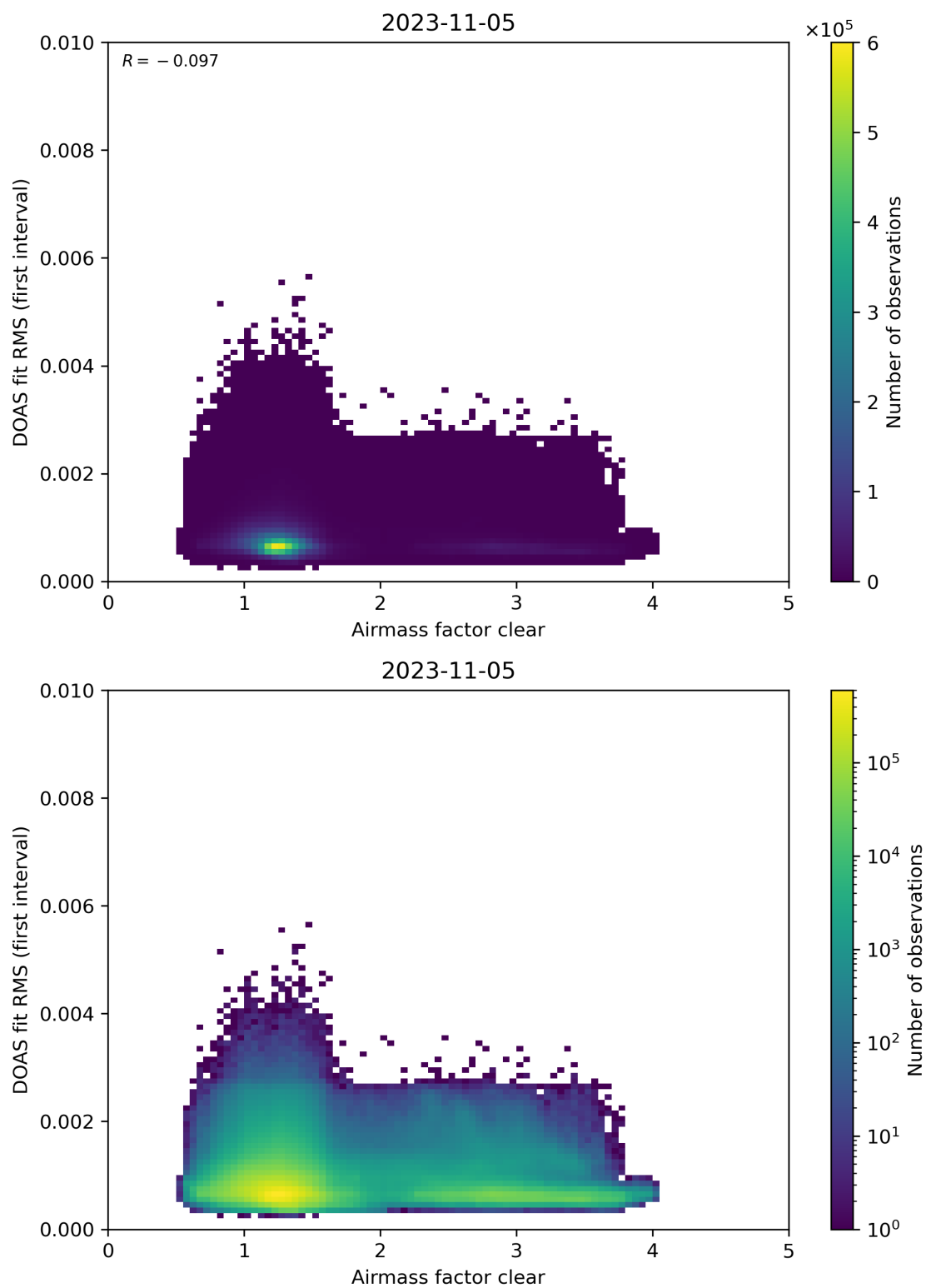
Figure 71: Scatter density plot of “Airmass factor clear” against “DOAS fit RMS (first interval)” for 2023-11-04 to 2023-11-06.
