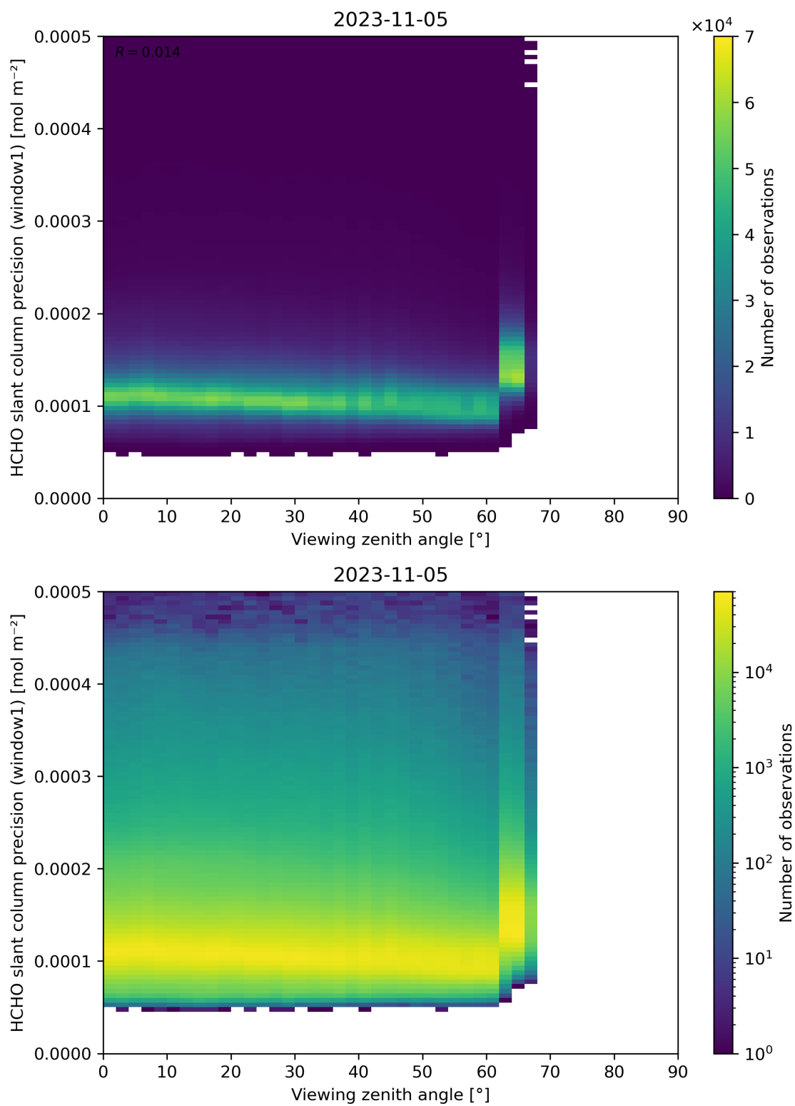
Figure 189: Scatter density plot of “Viewing zenith angle” against “HCHO slant column precision (window1)” for 2023-11-04 to 2023-11-06.
