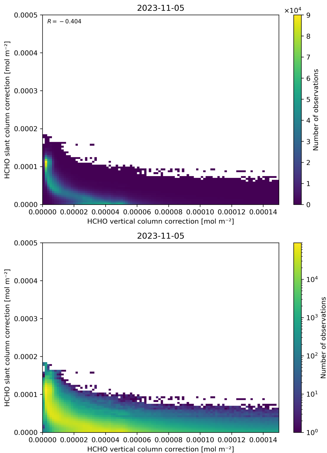
Figure 117: Scatter density plot of “HCHO vertical column correction” against “HCHO slant column correction” for 2023-11-04 to 2023-11-06.
