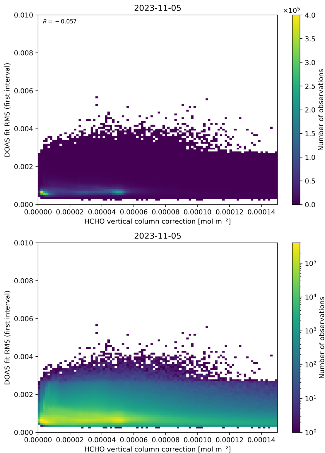
Figure 112: Scatter density plot of “HCHO vertical column correction” against “DOAS fit RMS (first interval)” for 2023-11-04 to 2023-11-06.
