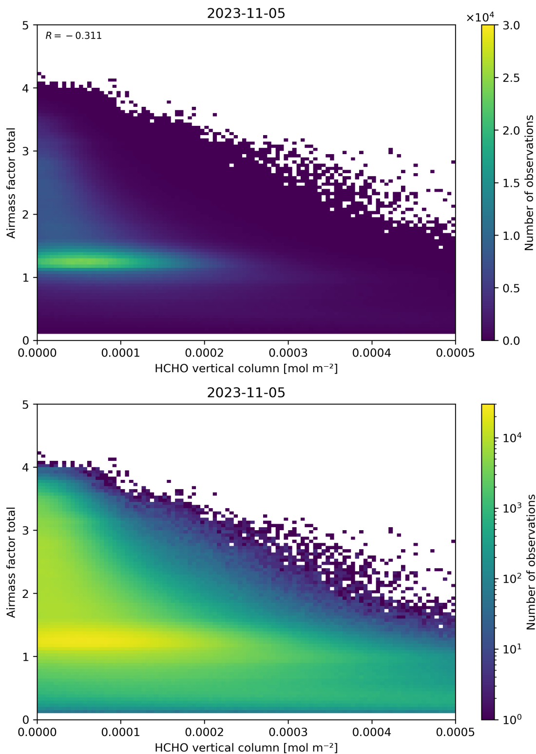
Figure 131: Scatter density plot of “HCHO vertical column” against “Airmass factor total” for 2023-11-04 to 2023-11-06.
