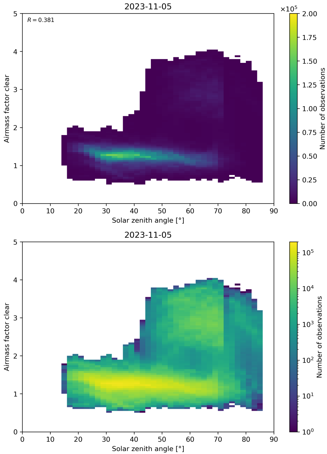
Figure 170: Scatter density plot of “Solar zenith angle” against “Airmass factor clear” for 2023-11-04 to 2023-11-06.
