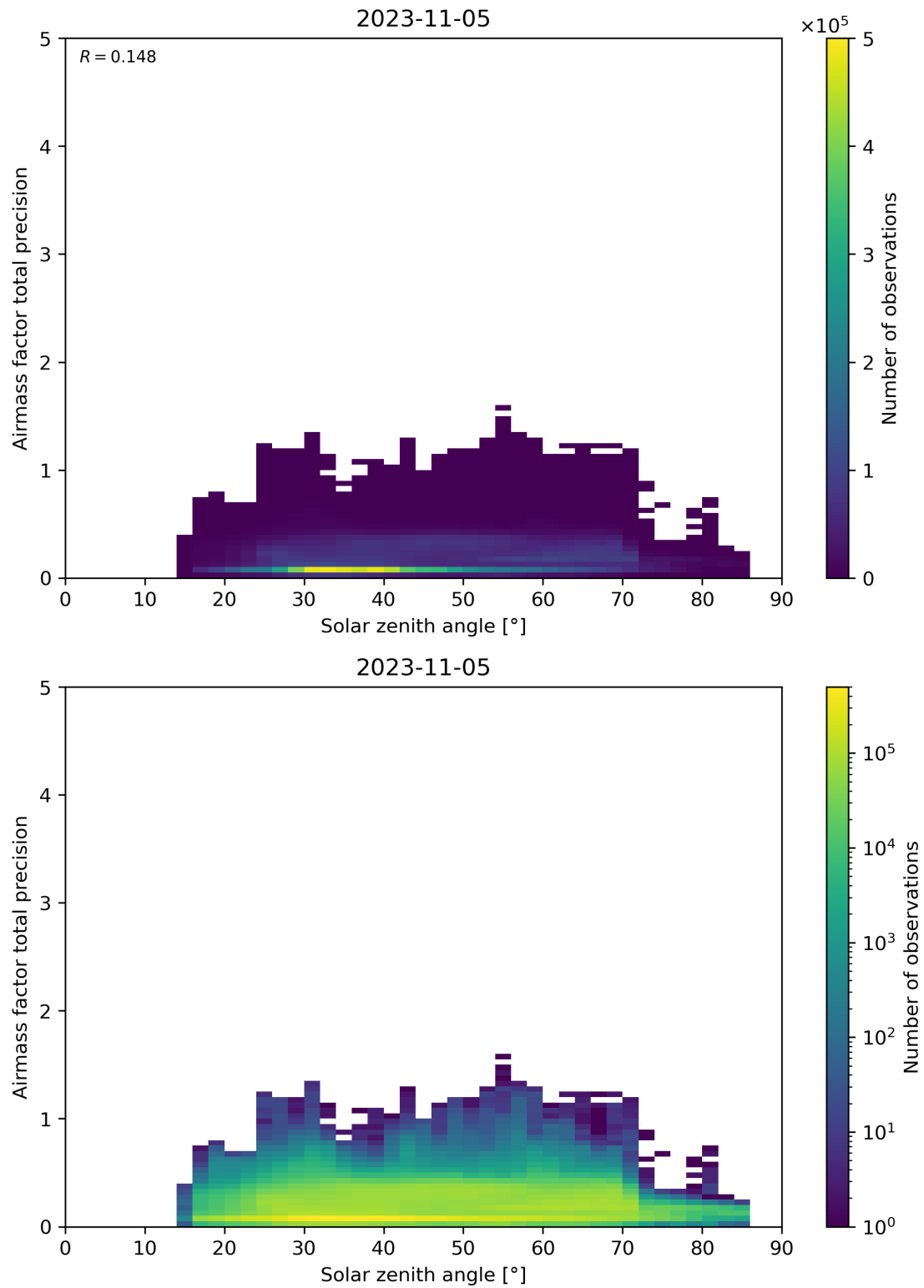
Figure 176: Scatter density plot of “Solar zenith angle” against “Airmass factor total precision” for 2023-11-04 to 2023-11-06.
