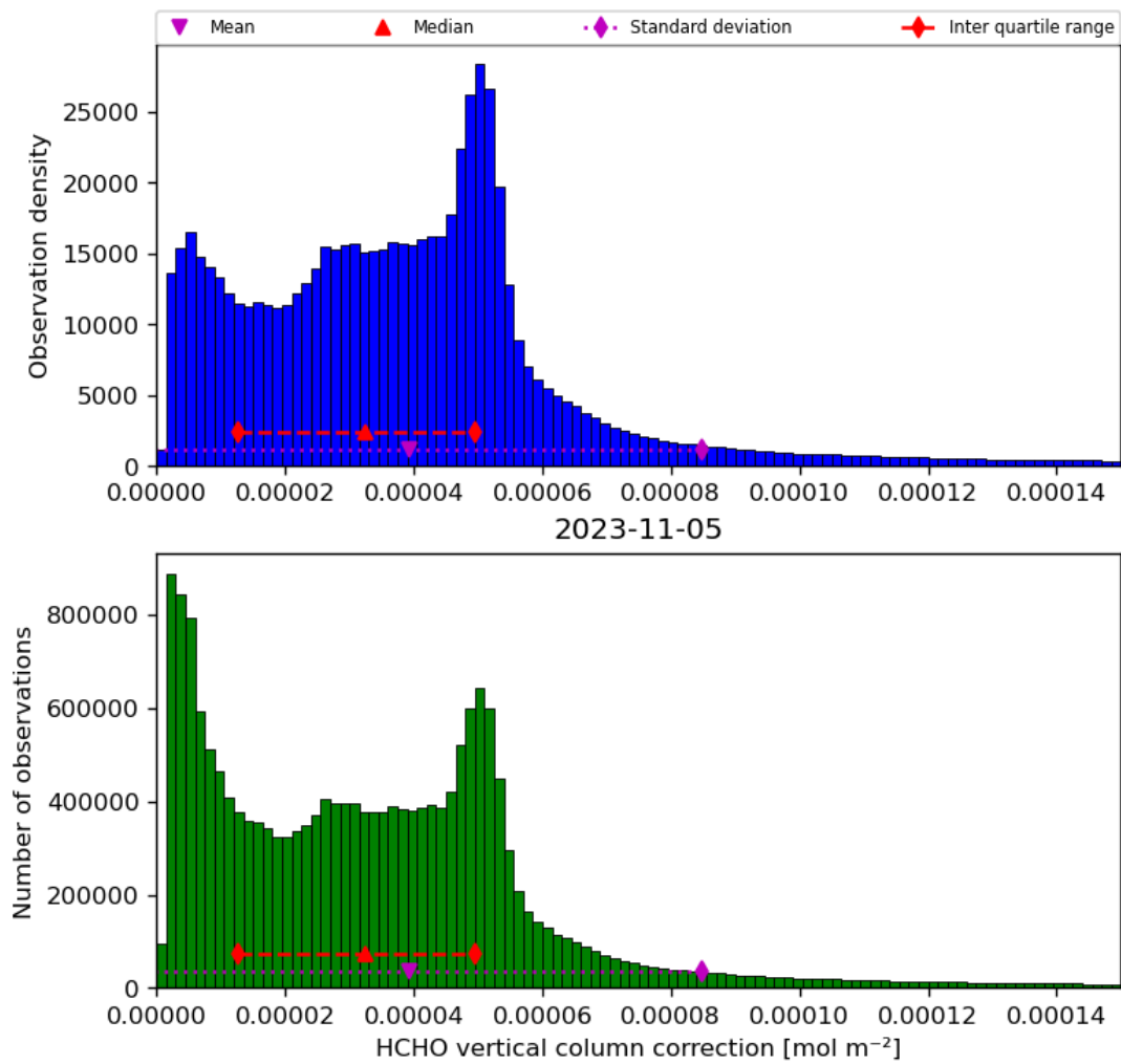
Figure 37: Histogram of “HCHO vertical column correction” for 2023-11-04 to 2023-11-06
