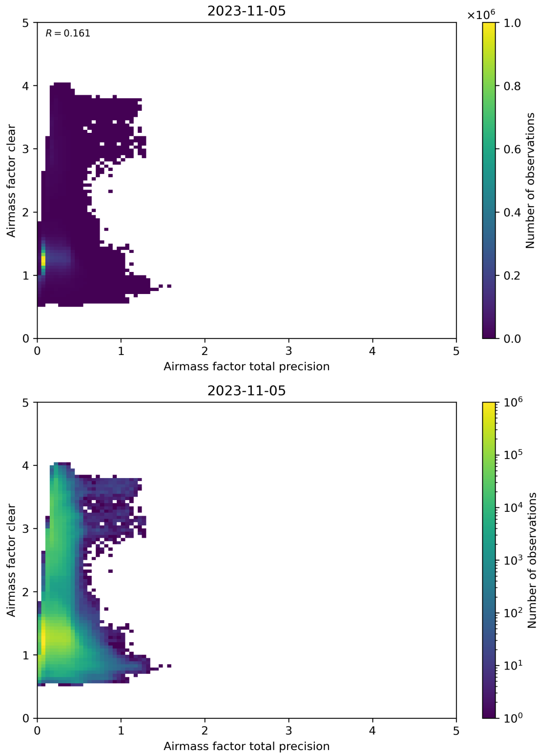
Figure 108: Scatter density plot of “Airmass factor total precision” against “Airmass factor clear” for 2023-11-04 to 2023-11-06.
