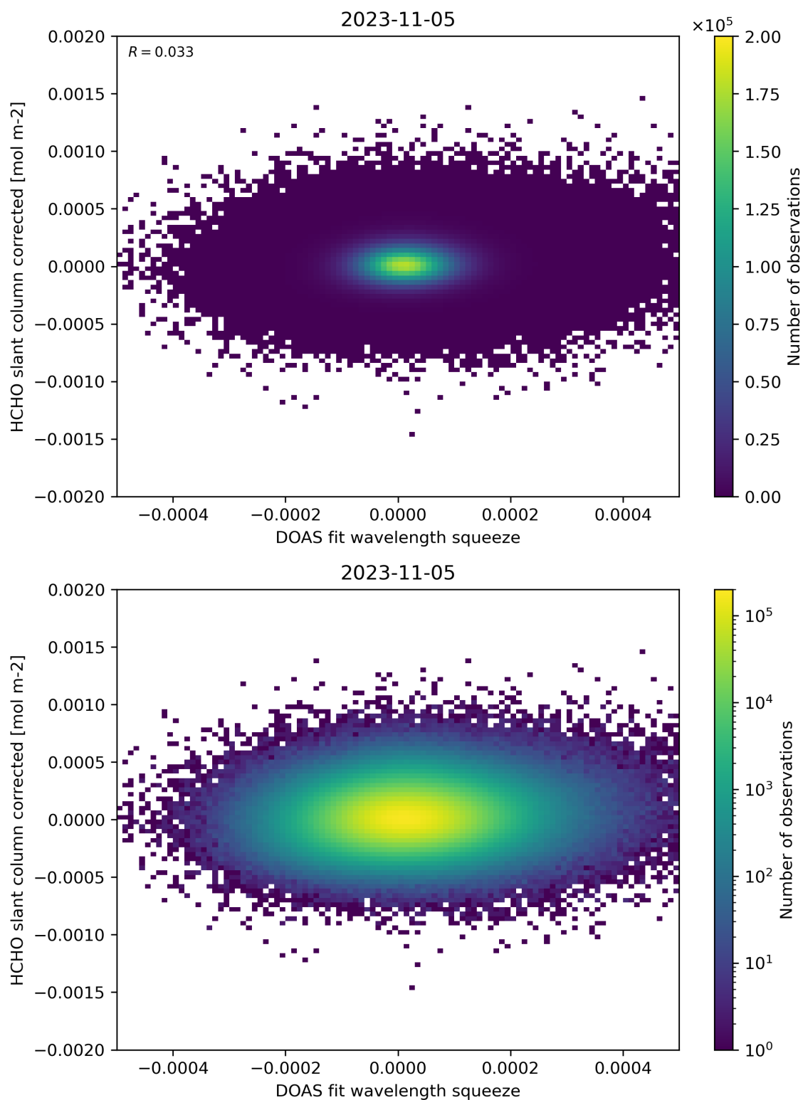
Figure 69: Scatter density plot of “DOAS fit wavelength squeeze” against “HCHO slant column corrected” for 2023-11-04 to 2023-11-06.
