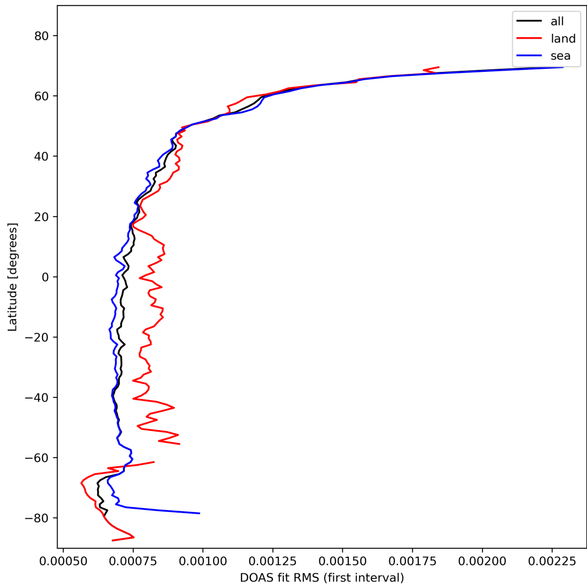
Figure 32: Zonal average of “DOAS fit RMS (first interval)” for 2023-11-04 to 2023-11-06.
