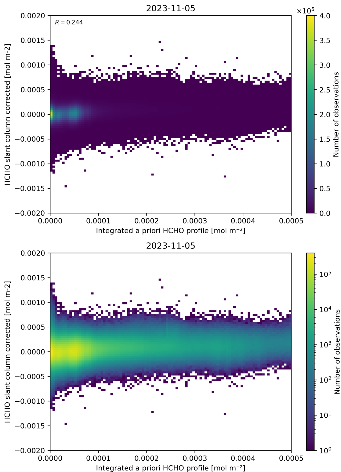
Figure 151: Scatter density plot of “Integrated a priori HCHO profile” against “HCHO slant column corrected” for 2023-11-04 to 2023-11-06.
