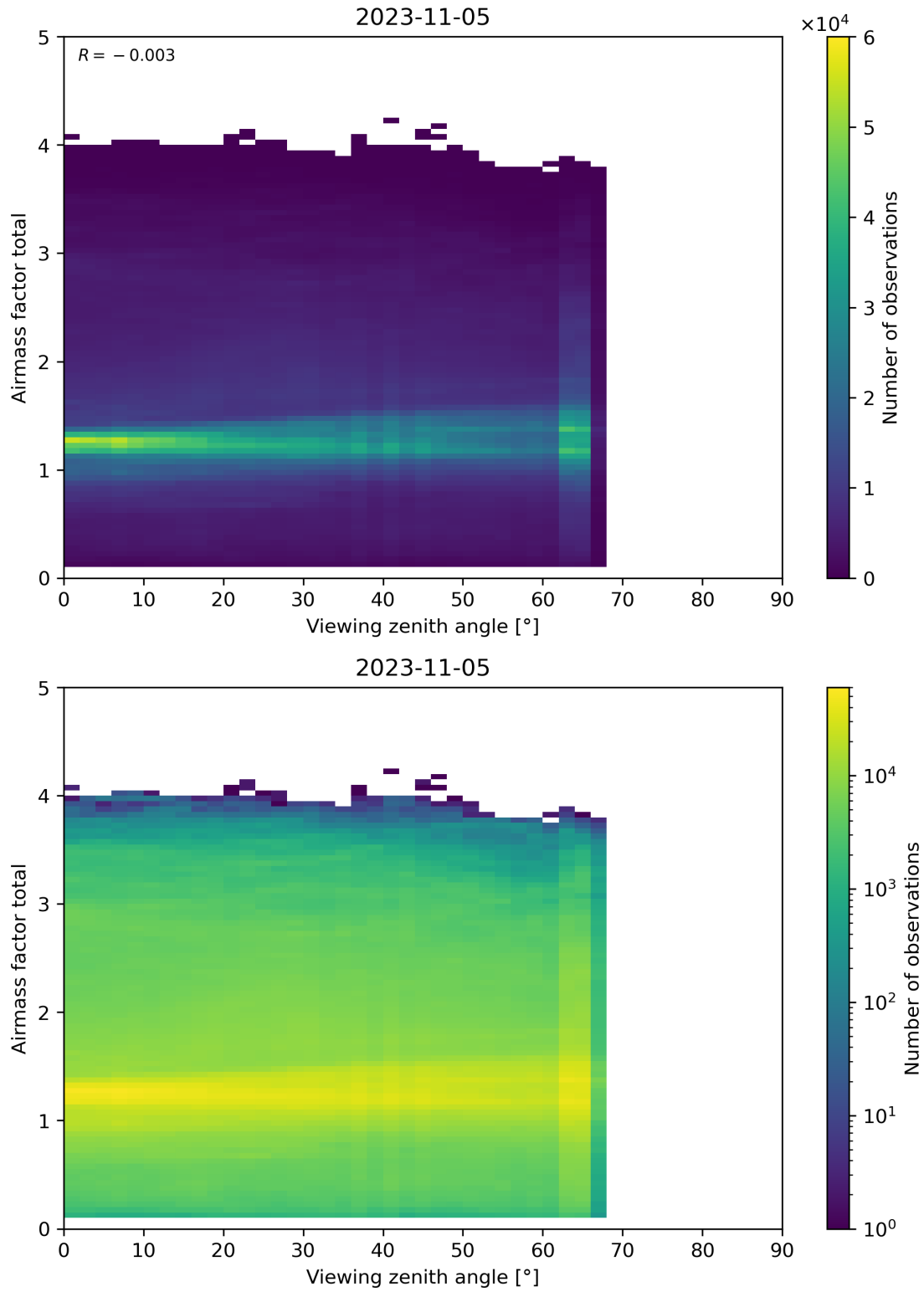
Figure 190: Scatter density plot of “Viewing zenith angle” against “Airmass factor total” for 2023-11-04 to 2023-11-06.
