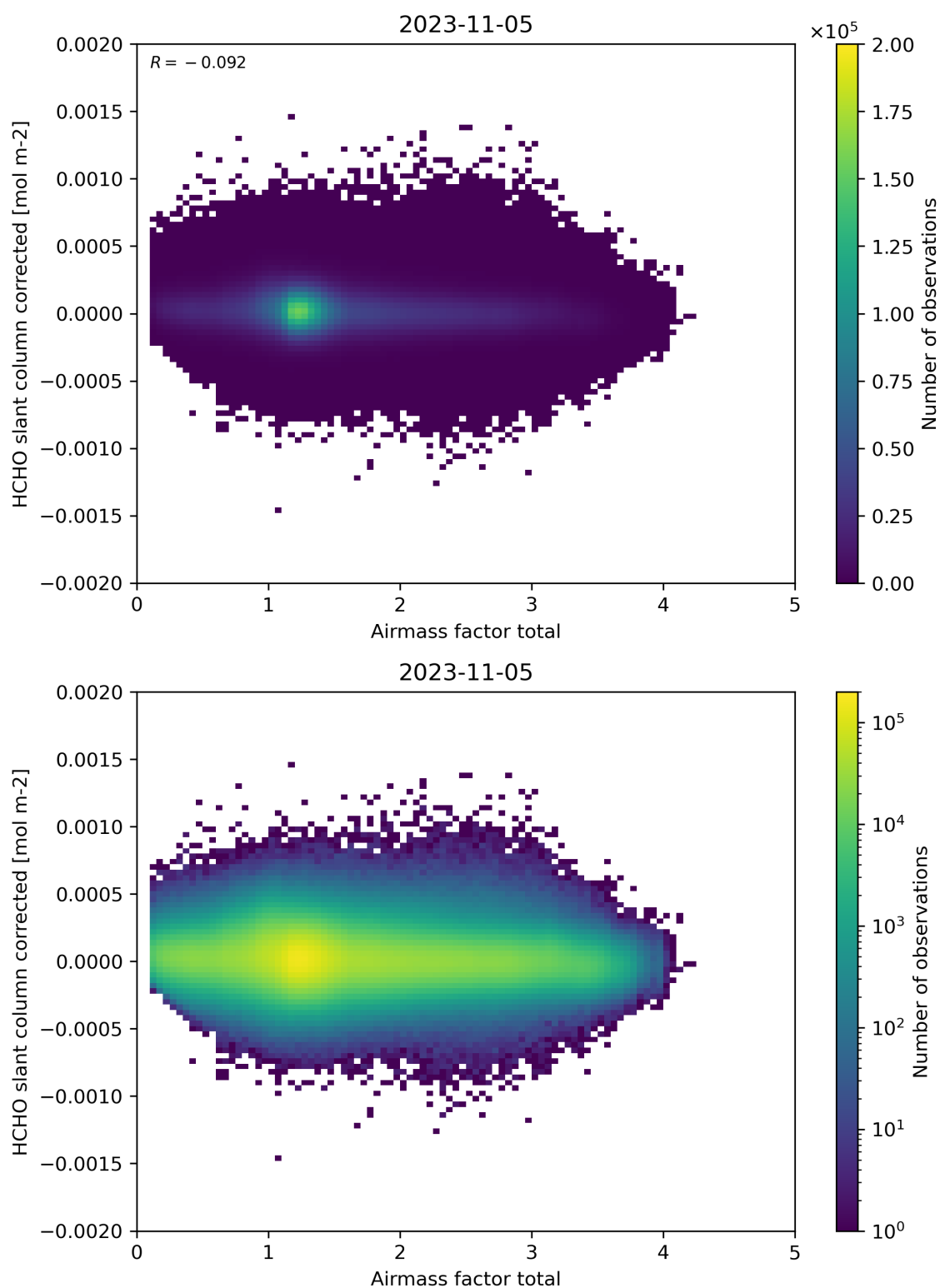
Figure 101: Scatter density plot of “Airmass factor total” against “HCHO slant column corrected” for 2023-11-04 to 2023-11-06.
