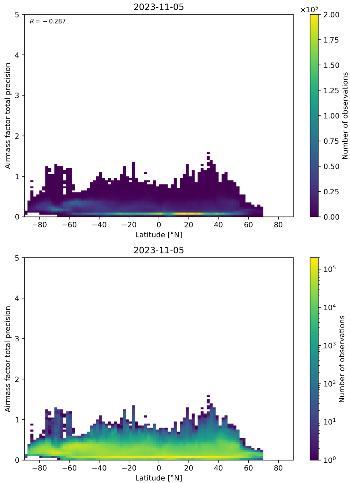
Figure 162: Scatter density plot of “Latitude” against “Airmass factor total precision” for 2023-11-04 to 2023-11-06.
