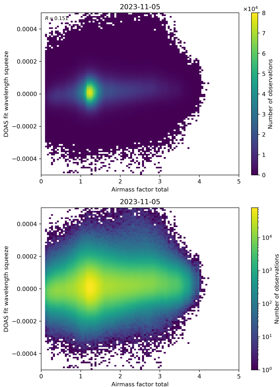
Figure 99: Scatter density plot of “Airmass factor total” against “DOAS fit wavelength squeeze” for 2023-11-04 to 2023-11-06.
