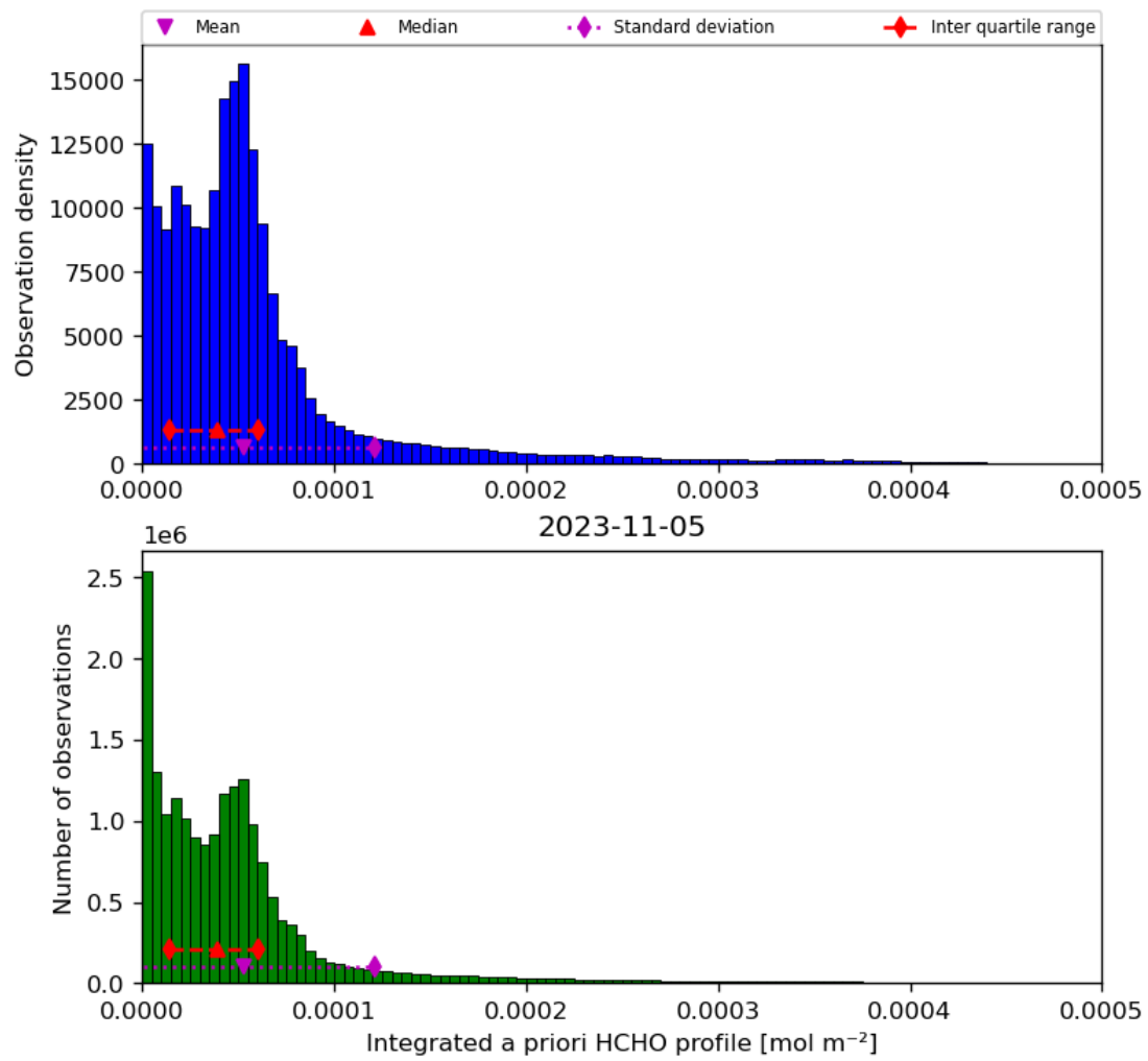
Figure 43: Histogram of “Integrated a priori HCHO profile” for 2023-11-04 to 2023-11-06
