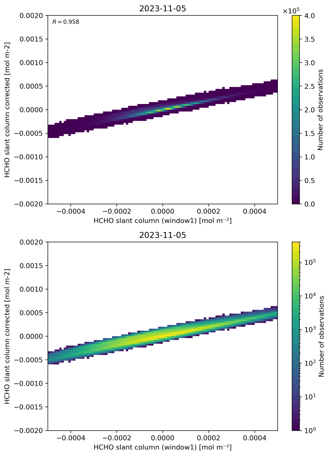
Figure 82: Scatter density plot of “HCHO slant column (window1)” against “HCHO slant column corrected” for 2023-11-04 to 2023-11-06.
