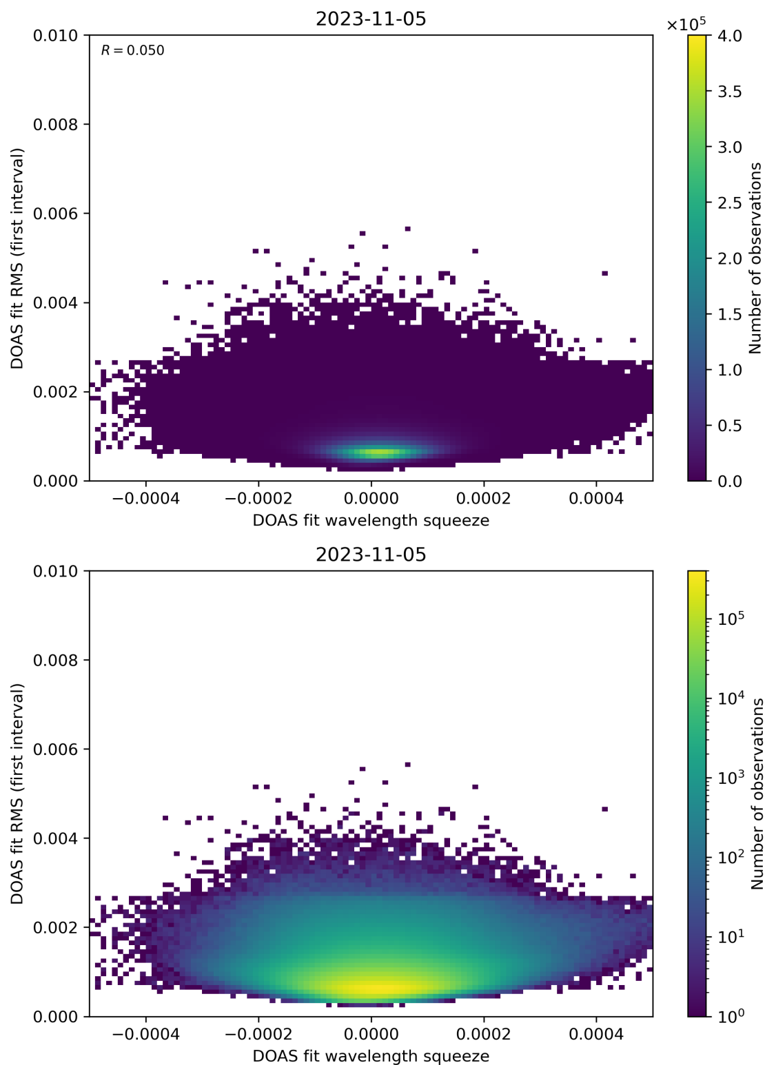
Figure 68: Scatter density plot of “DOAS fit wavelength squeeze” against “DOAS fit RMS (first interval)” for 2023-11-04 to 2023-11-06.
