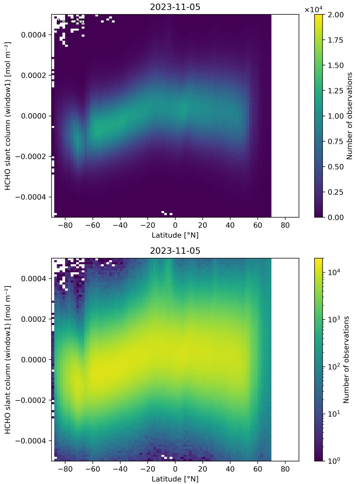
Figure 159: Scatter density plot of “Latitude” against “HCHO slant column (window1)” for 2023-11-04 to 2023-11-06.
