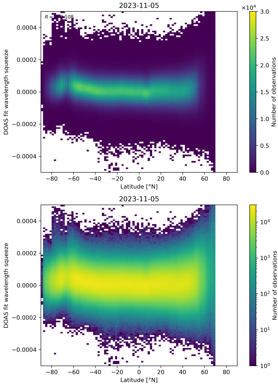
Figure 155: Scatter density plot of “Latitude” against “DOAS fit wavelength squeeze” for 2023-11-04 to 2023-11-06.
