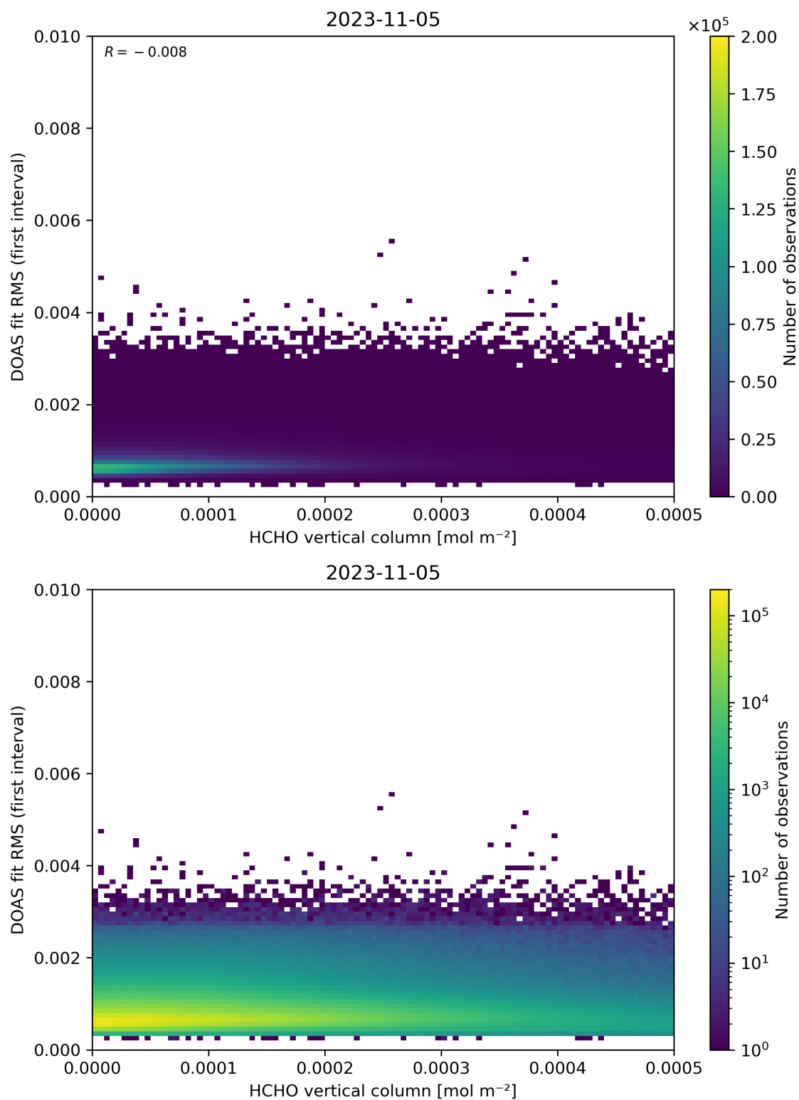
Figure 123: Scatter density plot of “HCHO vertical column” against “DOAS fit RMS (first interval)” for 2023-11-04 to 2023-11-06.
