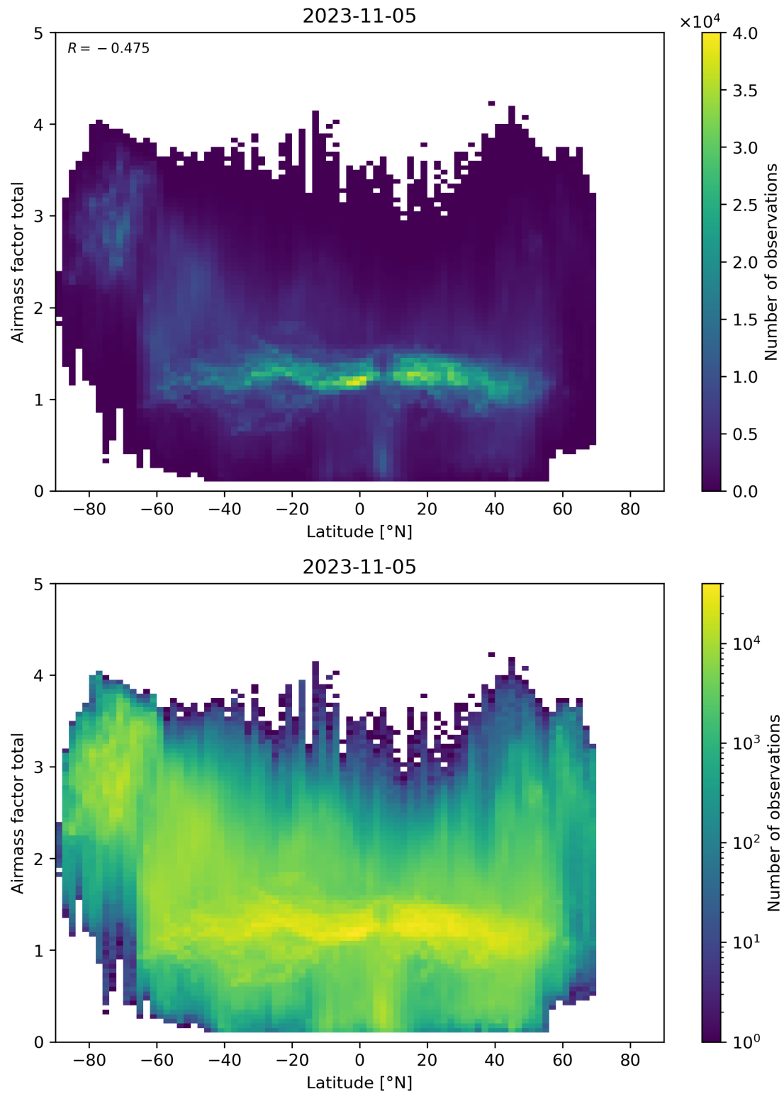
Figure 161: Scatter density plot of “Latitude” against “Airmass factor total” for 2023-11-04 to 2023-11-06.
