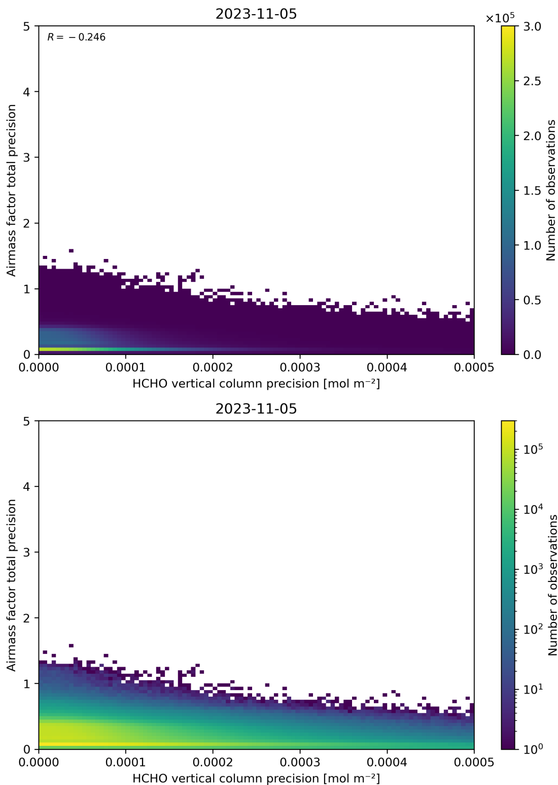
Figure 145: Scatter density plot of “HCHO vertical column precision” against “Airmass factor total precision” for 2023-11-04 to 2023-11-06.
