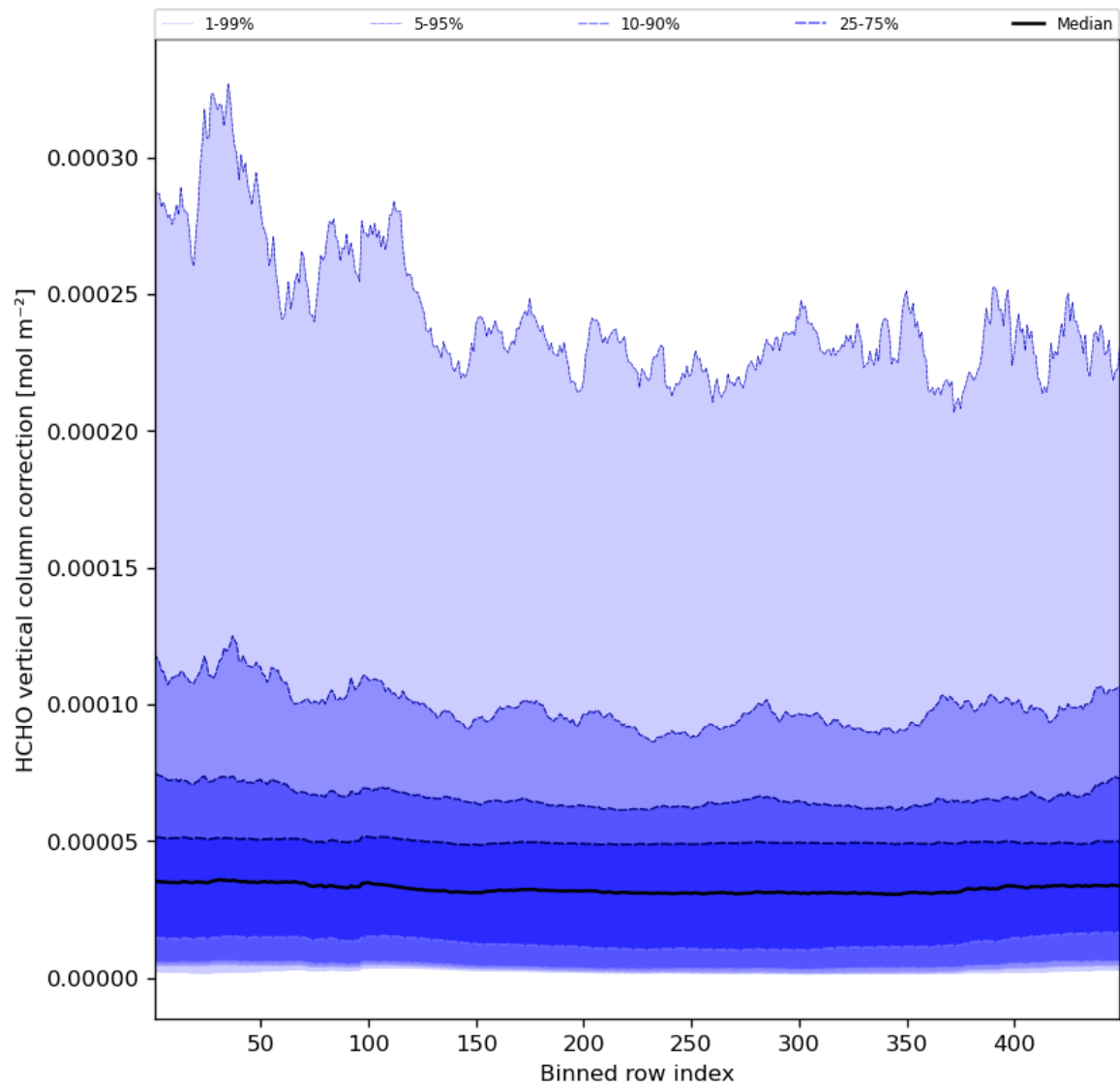
Figure 51: Along track statistics of “HCHO vertical column correction” for 2023-11-04 to 2023-11-06
