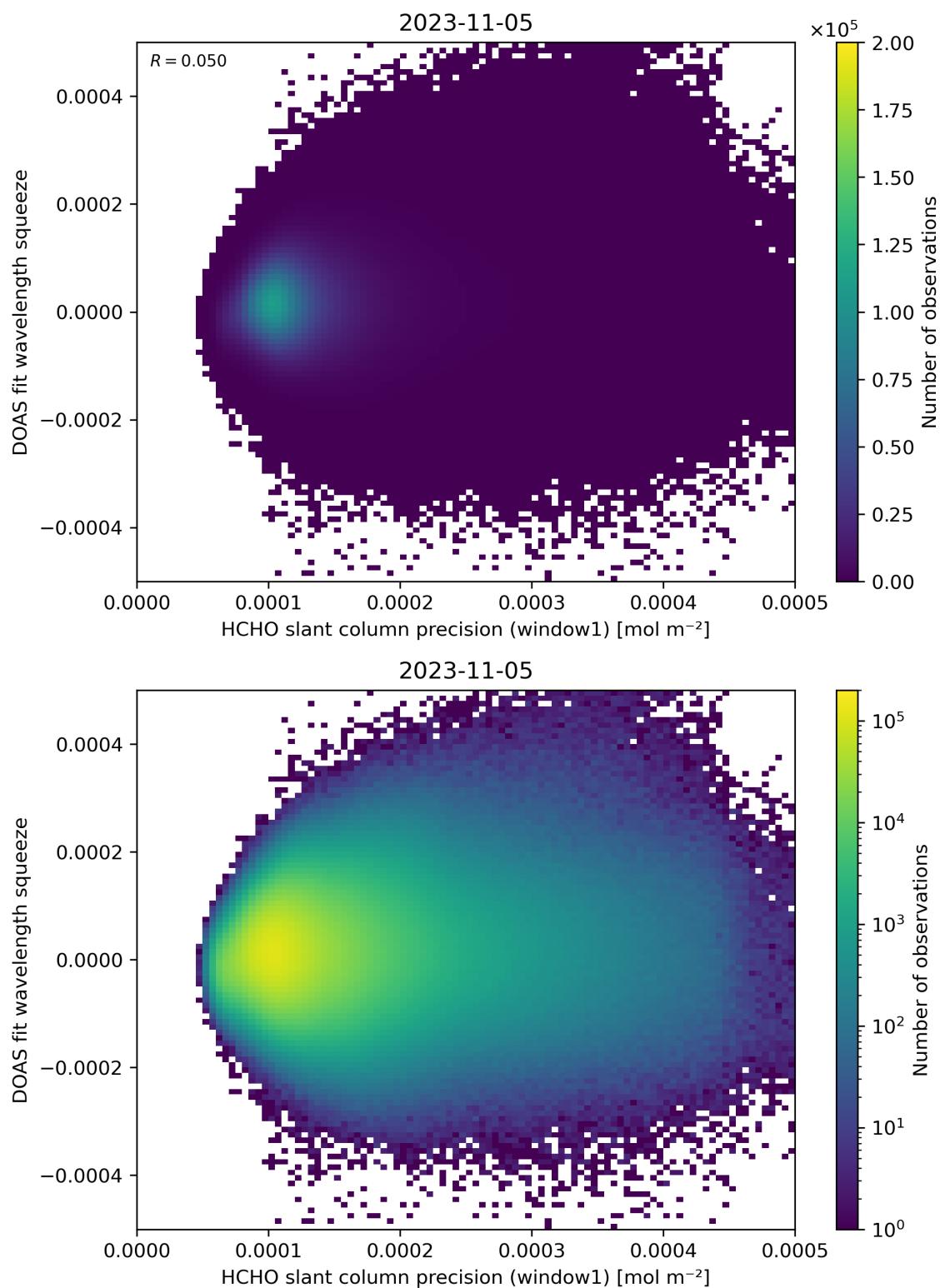
Figure 90: Scatter density plot of “HCHO slant column precision (window1)” against “DOAS fit wavelength squeeze” for 2023-11-04 to 2023-11-06.
