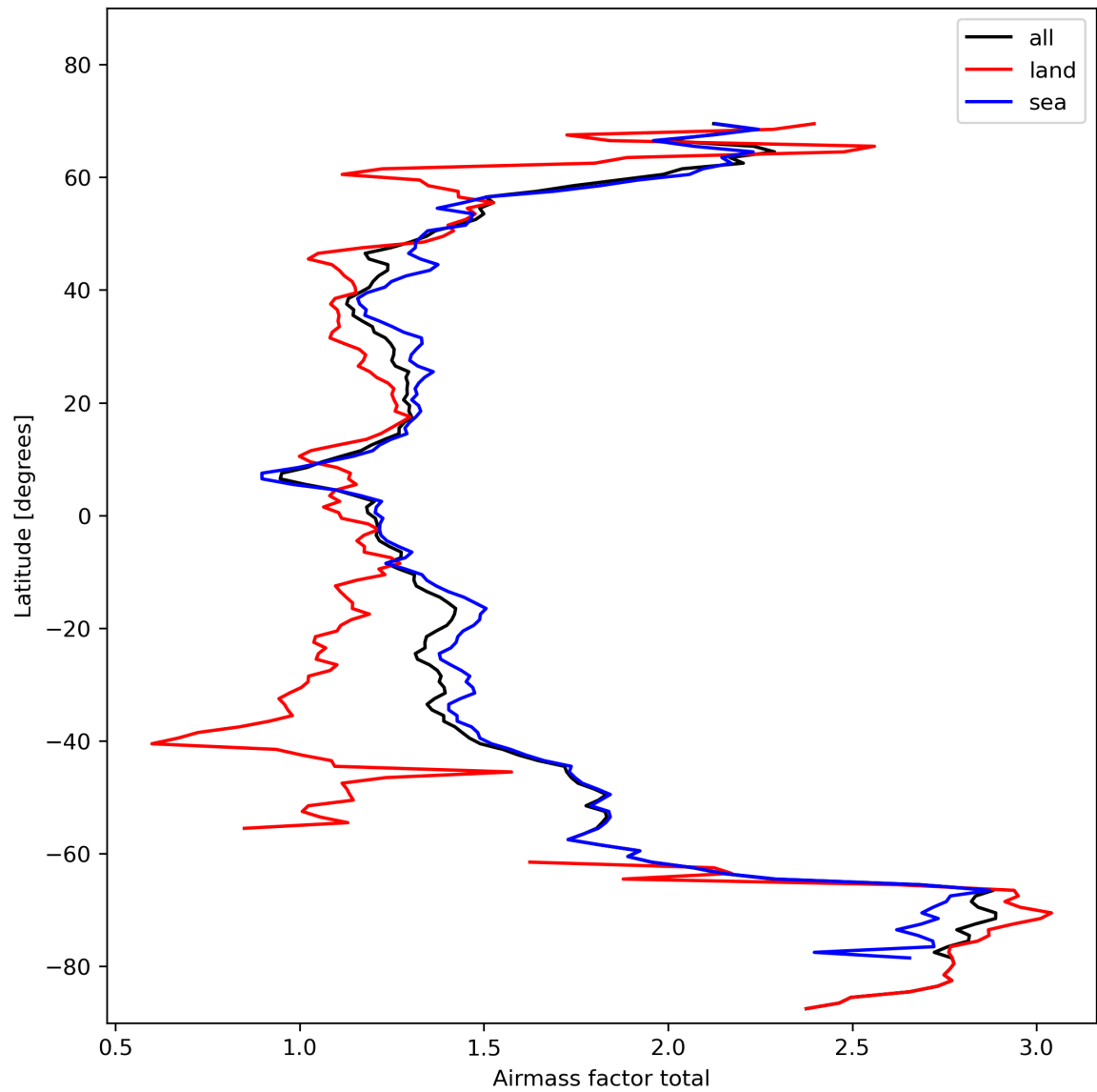
Figure 26: Zonal average of “Airmass factor total” for 2023-11-04 to 2023-11-06.
