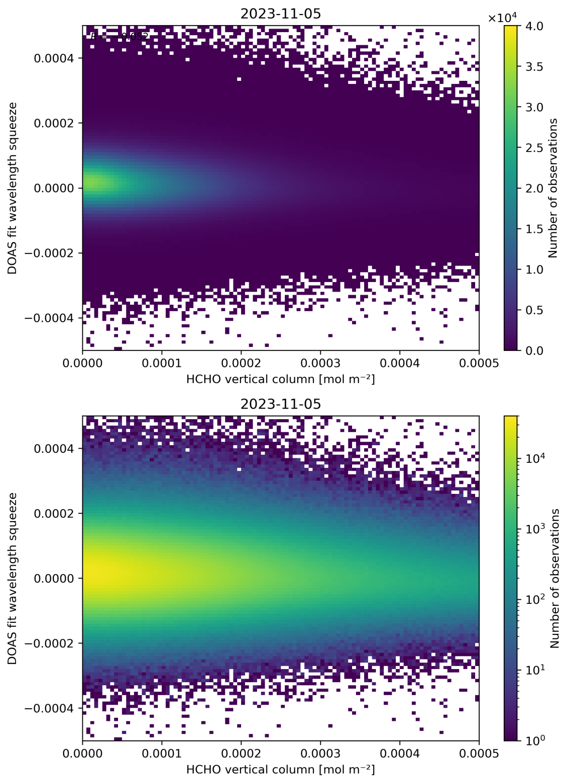
Figure 125: Scatter density plot of “HCHO vertical column” against “DOAS fit wavelength squeeze” for 2023-11-04 to 2023-11-06.
