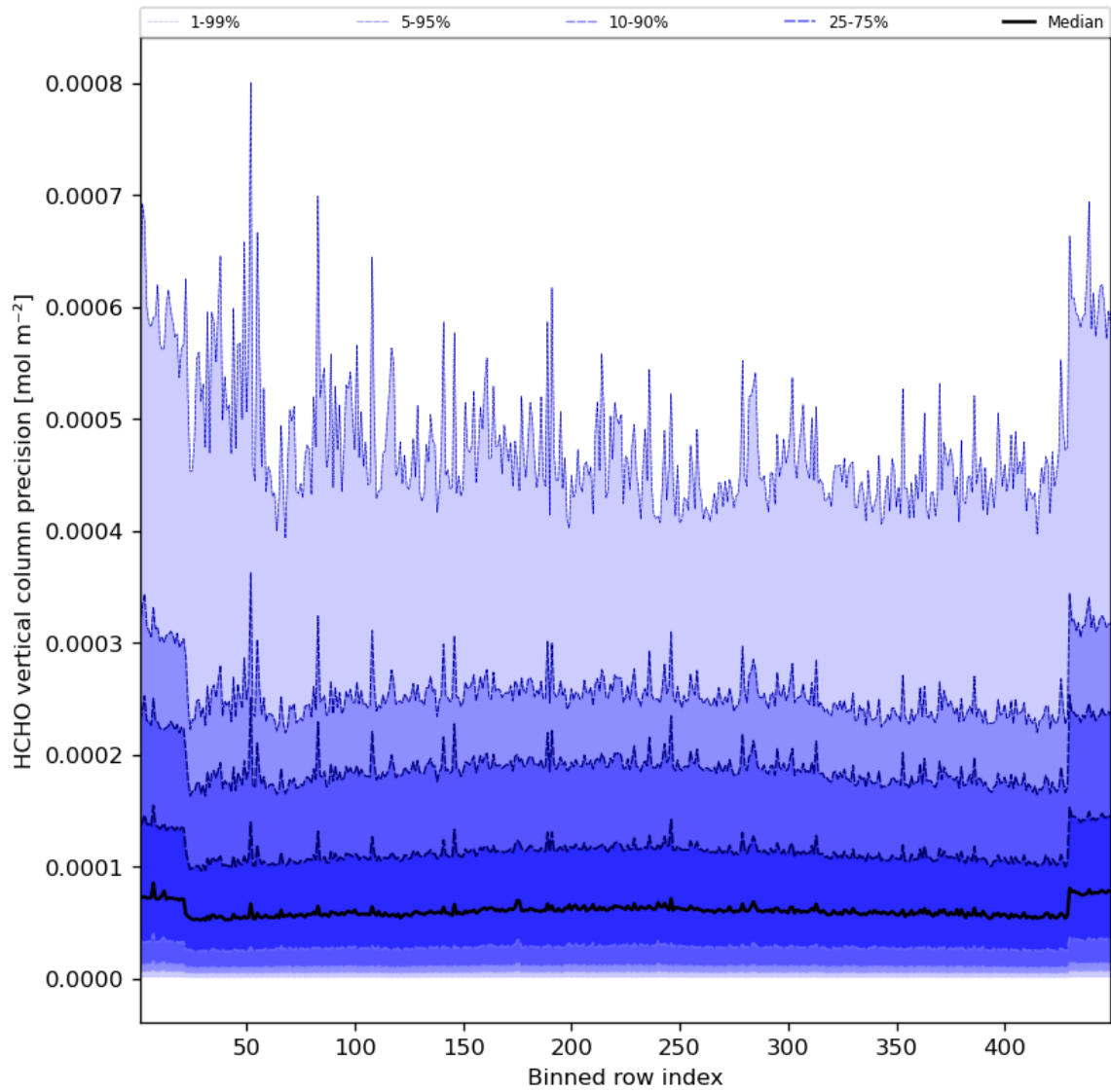
Figure 50: Along track statistics of "HCHO vertical column precision" for 2023-11-04 to 2023-11-06
