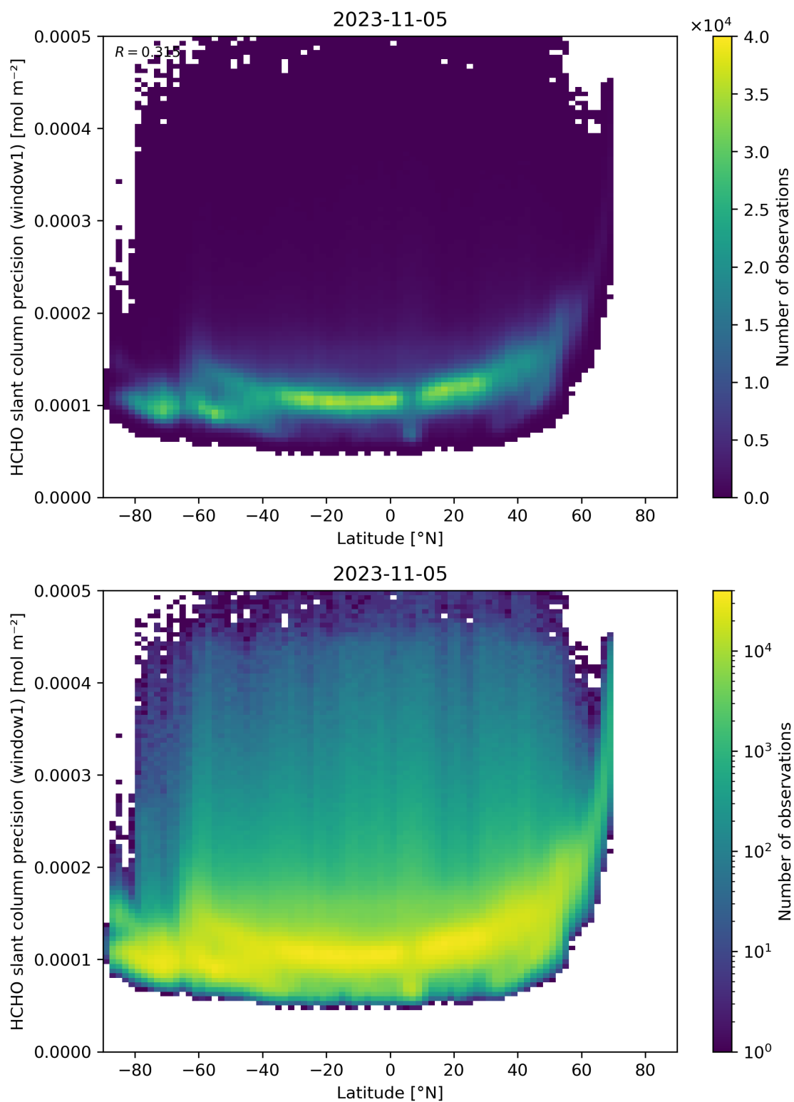
Figure 160: Scatter density plot of “Latitude” against “HCHO slant column precision (window1)” for 2023-11-04 to 2023-11-06.
