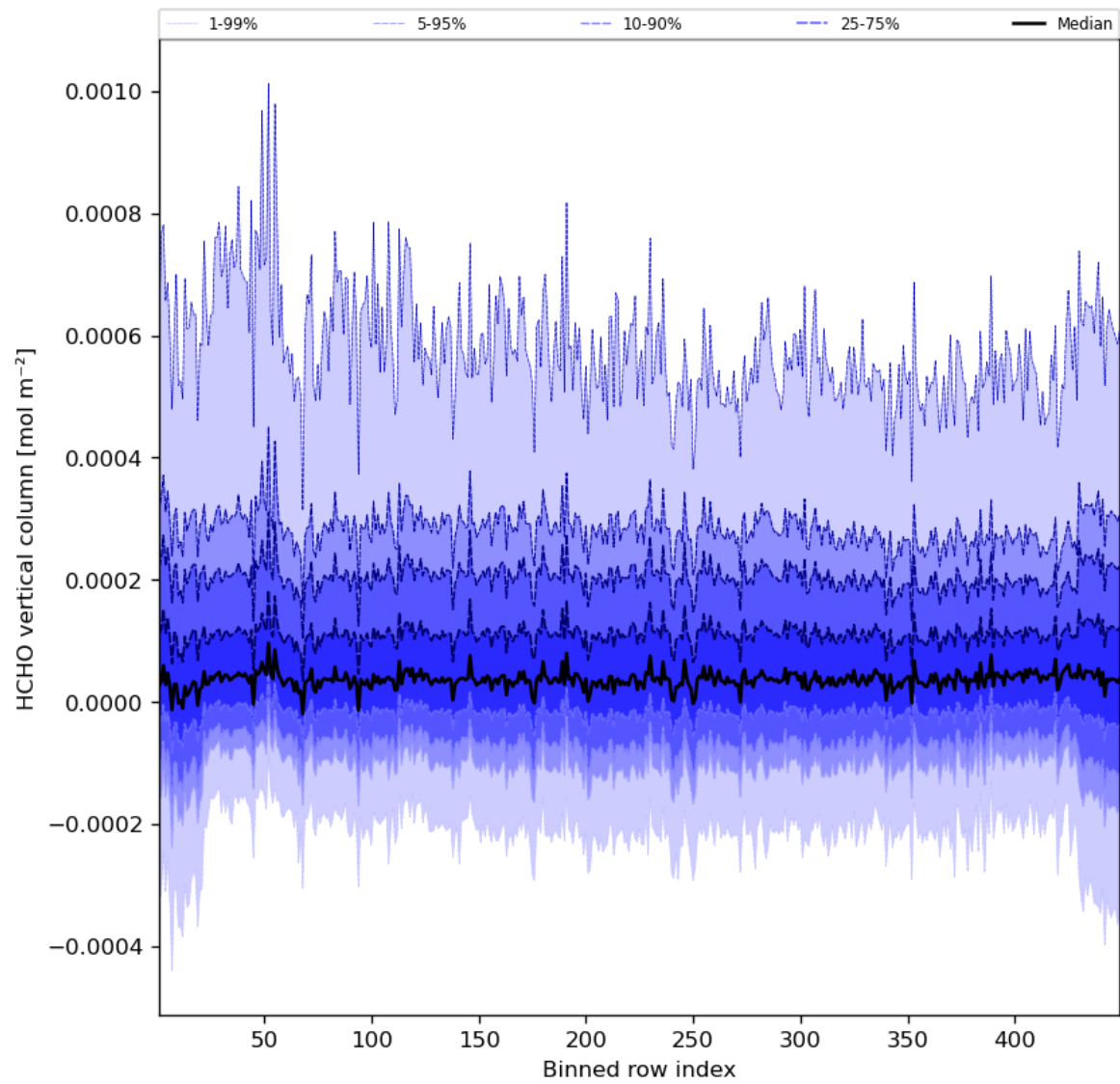
Figure 49: Along track statistics of “HCHO vertical column” for 2023-11-04 to 2023-11-06
