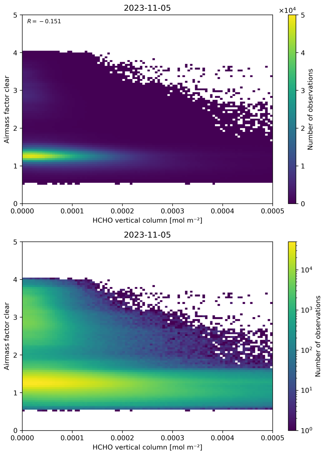
Figure 126: Scatter density plot of “HCHO vertical column” against “Airmass factor clear” for 2023-11-04 to 2023-11-06.
