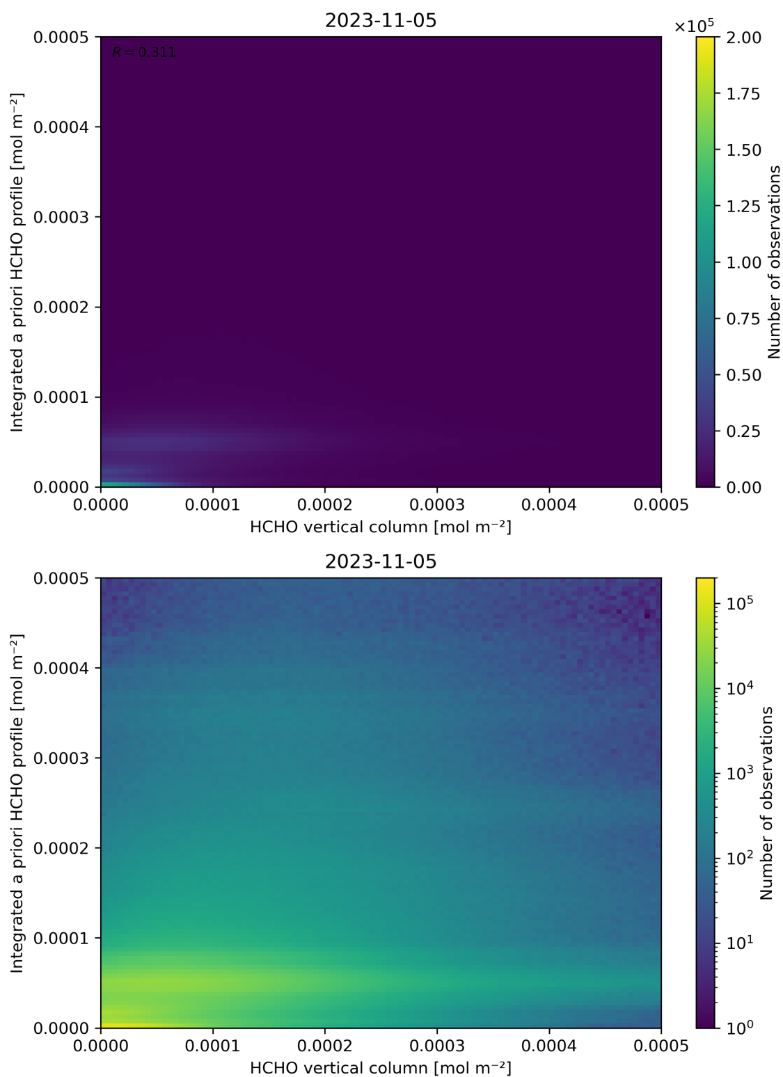
Figure 135: Scatter density plot of “HCHO vertical column” against “Integrated a priori HCHO profile” for 2023-11-04 to 2023-11-06.
