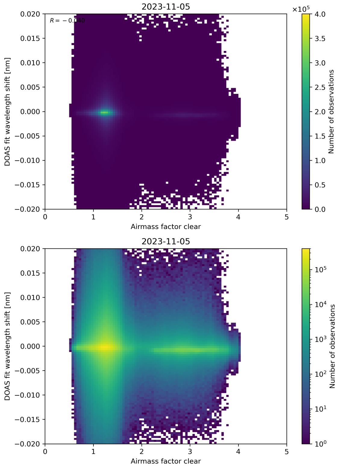
Figure 72: Scatter density plot of “Airmass factor clear” against “DOAS fit wavelength shift” for 2023-11-04 to 2023-11-06.
