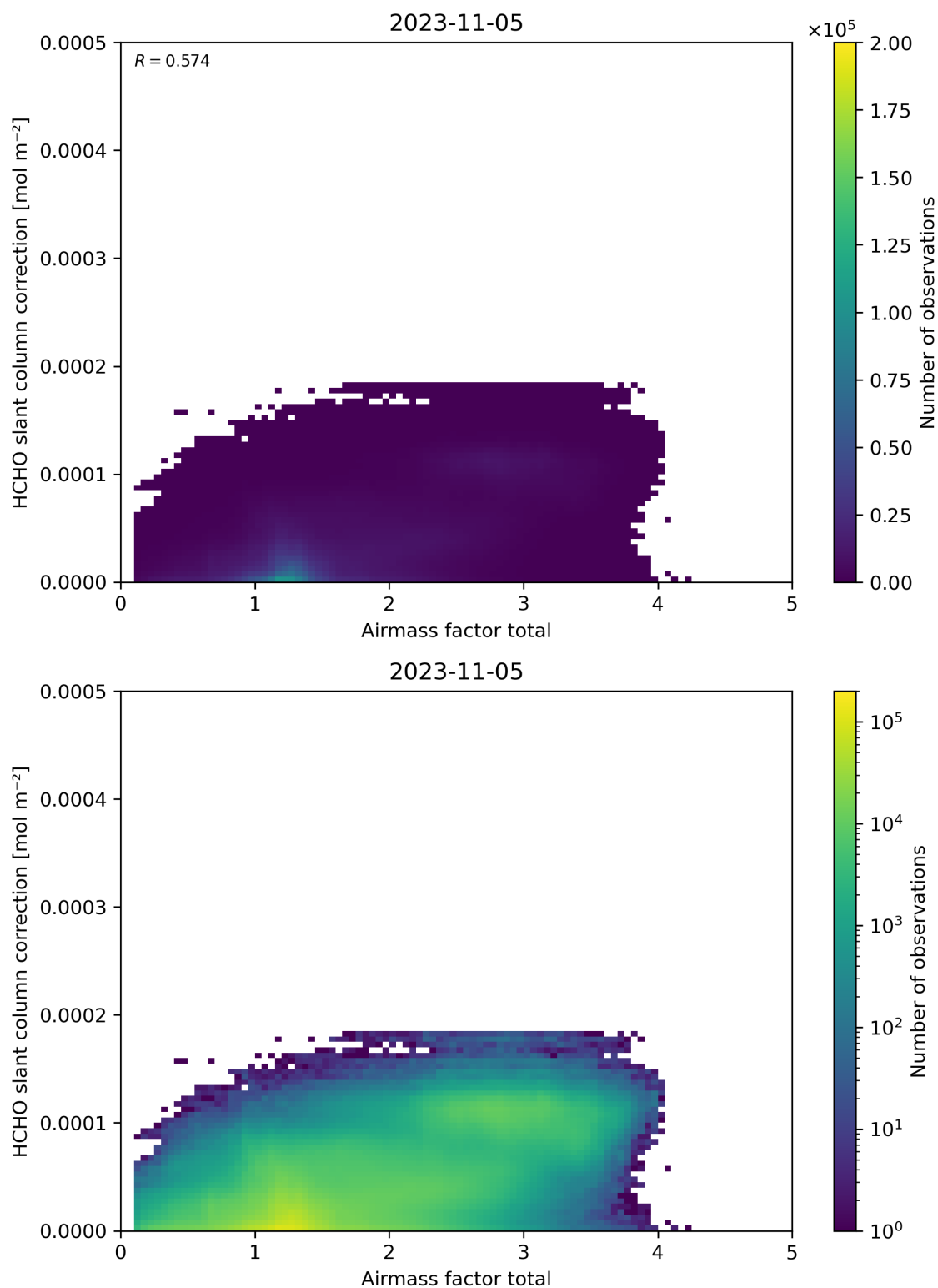
Figure 102: Scatter density plot of “Airmass factor total” against “HCHO slant column correction” for 2023-11-04 to 2023-11-06.
