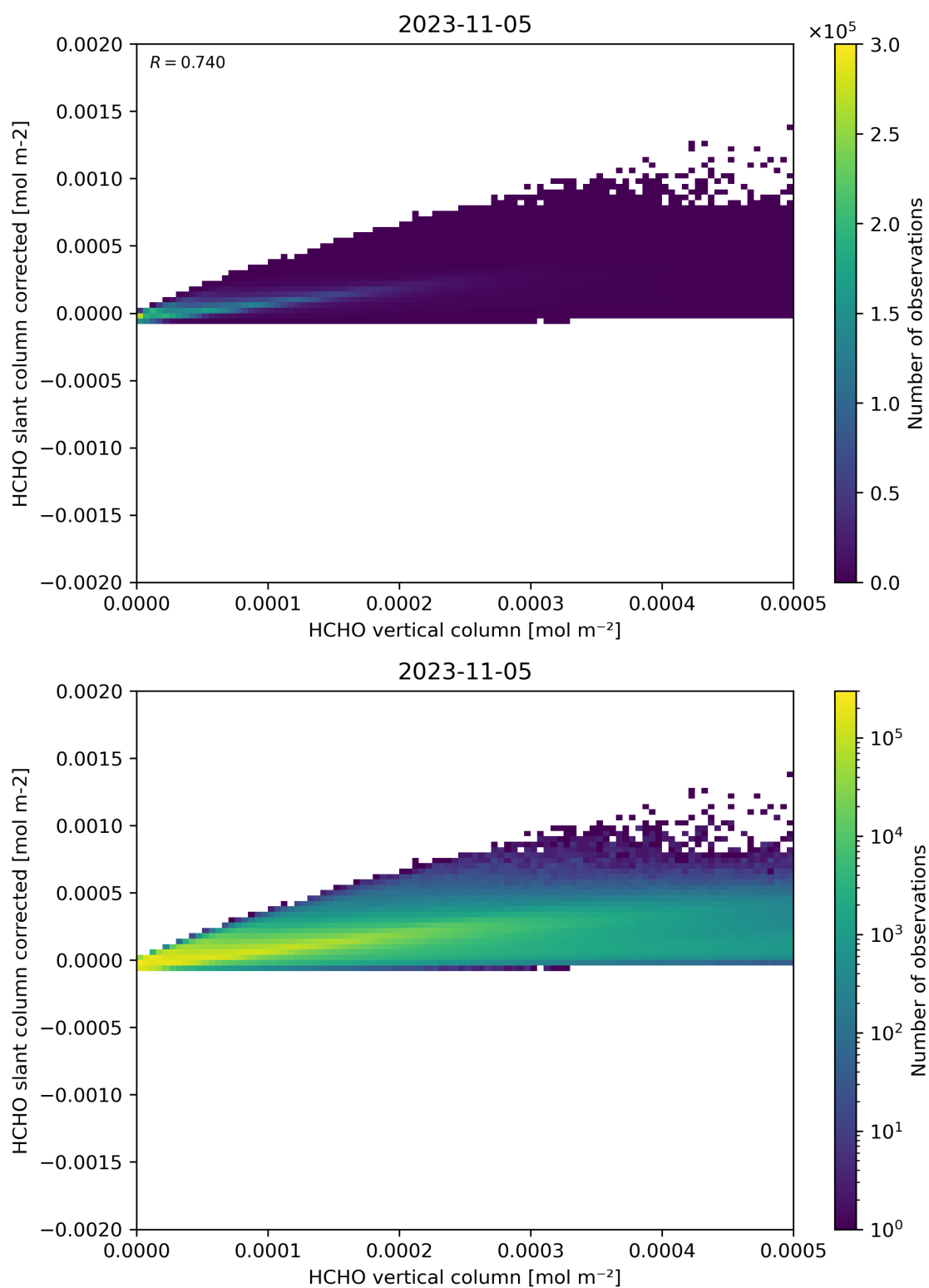
Figure 127: Scatter density plot of “HCHO vertical column” against “HCHO slant column corrected” for 2023-11-04 to 2023-11-06.
