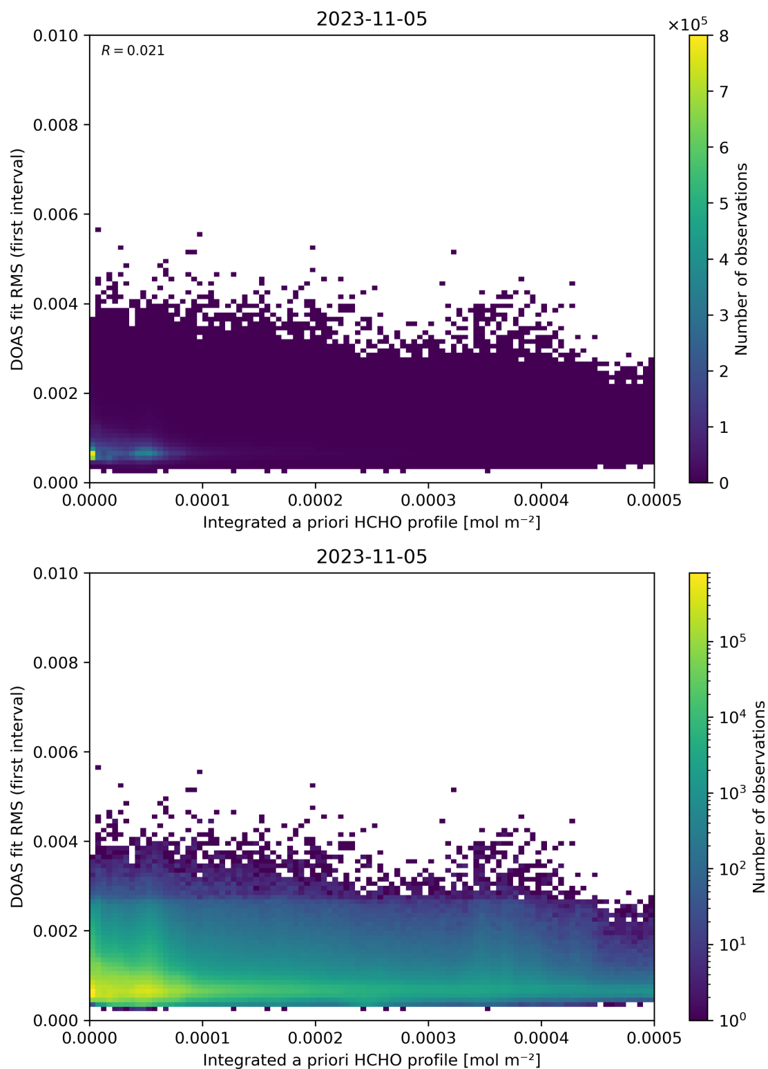
Figure 148: Scatter density plot of “Integrated a priori HCHO profile” against “DOAS fit RMS (first interval)” for 2023-11-04 to 2023-11-06.
