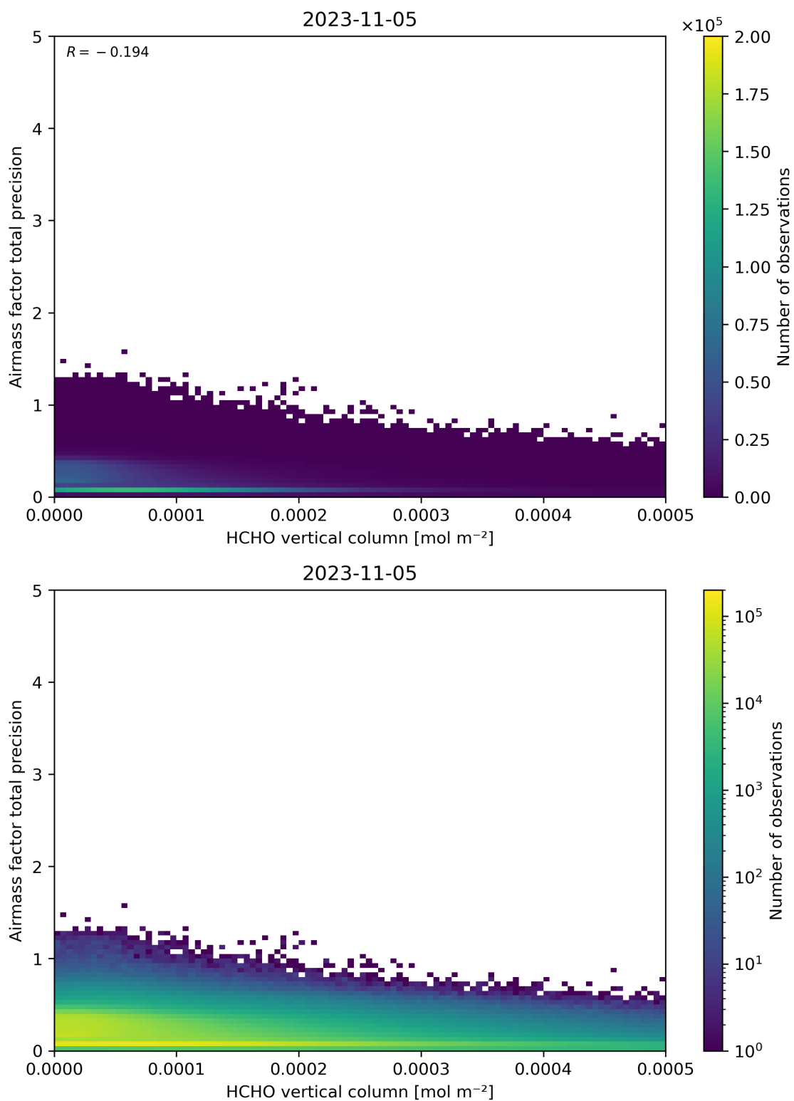
Figure 132: Scatter density plot of “HCHO vertical column” against “Airmass factor total precision” for 2023-11-04 to 2023-11-06.
