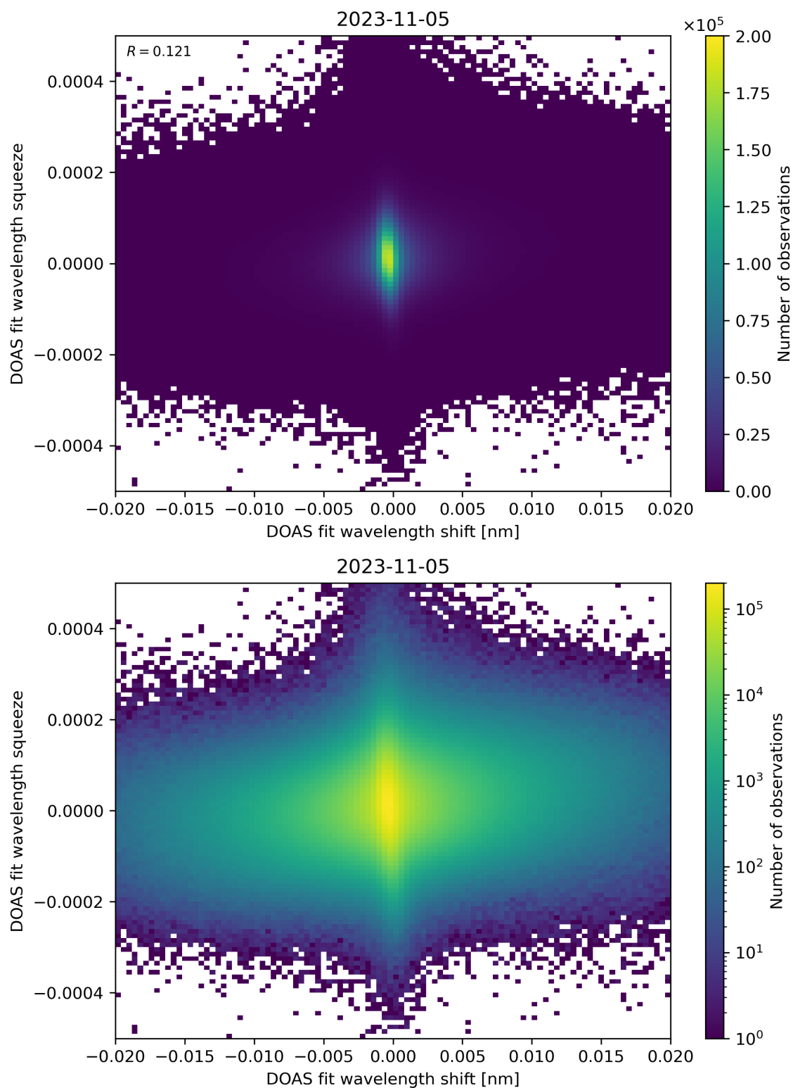
Figure 65: Scatter density plot of “DOAS fit wavelength shift” against “DOAS fit wavelength squeeze” for 2023-11-04 to 2023-11-06.
