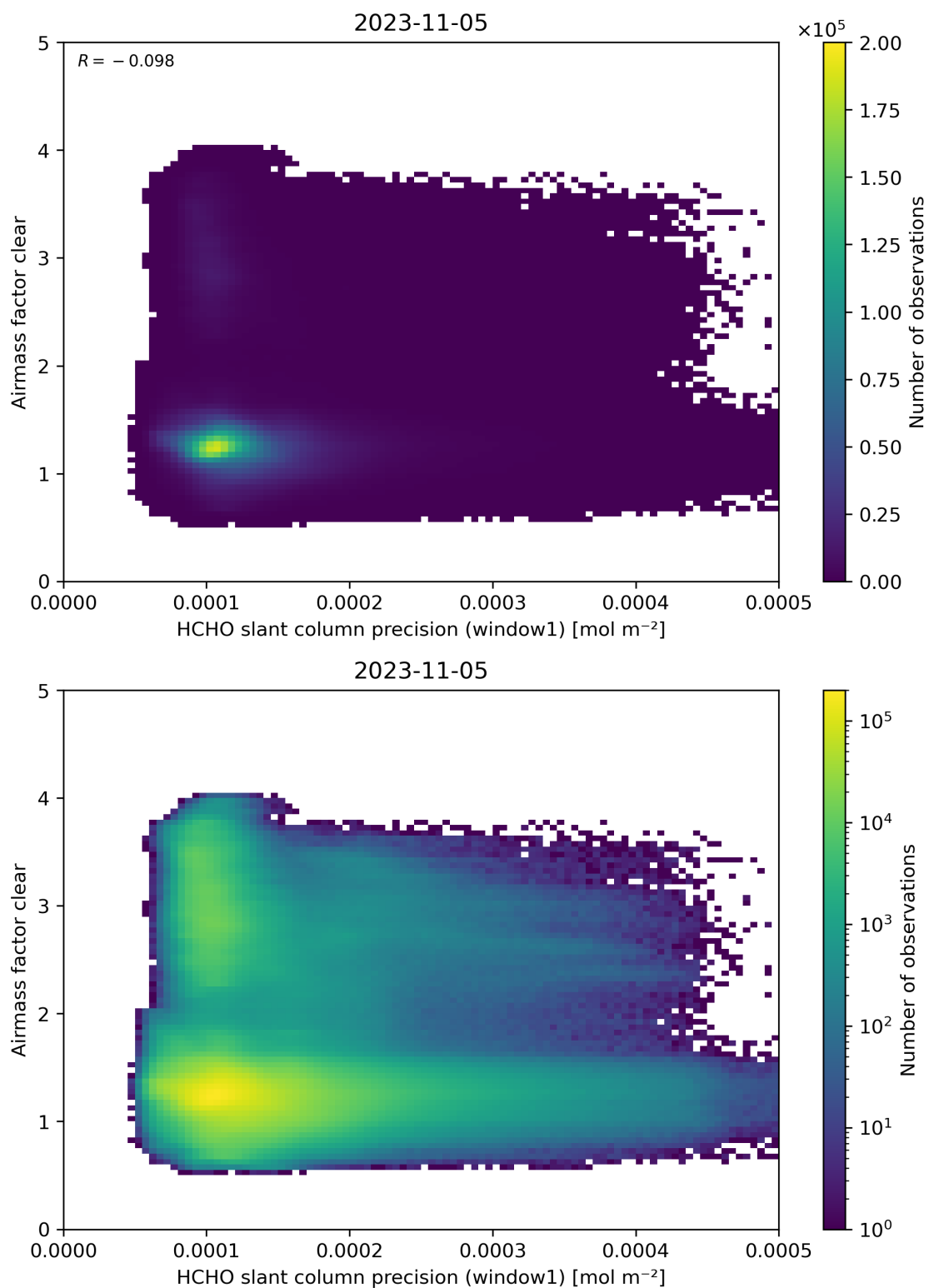
Figure 91: Scatter density plot of “HCHO slant column precision (window1)” against “Airmass factor clear” for 2023-11-04 to 2023-11-06.
