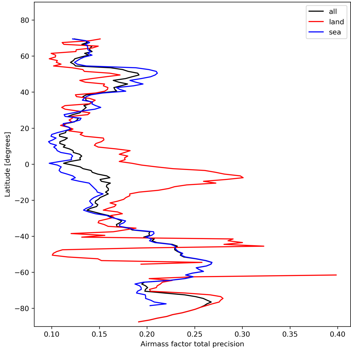
Figure 27: Zonal average of “Airmass factor total precision” for 2023-11-04 to 2023-11-06.
