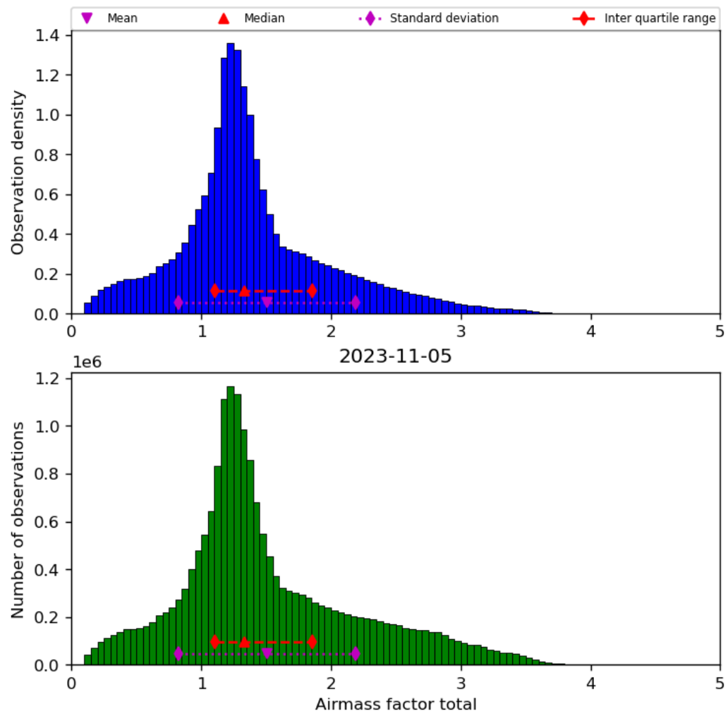
Figure 40: Histogram of “Airmass factor total” for 2023-11-04 to 2023-11-06
