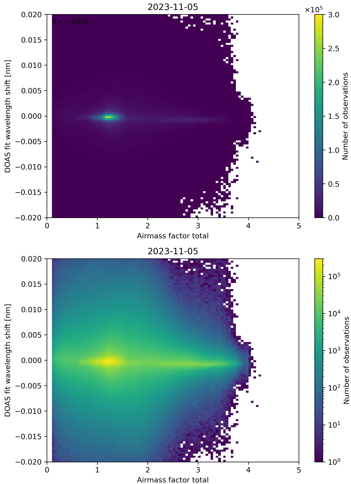
Figure 98: Scatter density plot of “Airmass factor total” against “DOAS fit wavelength shift” for 2023-11-04 to 2023-11-06.
