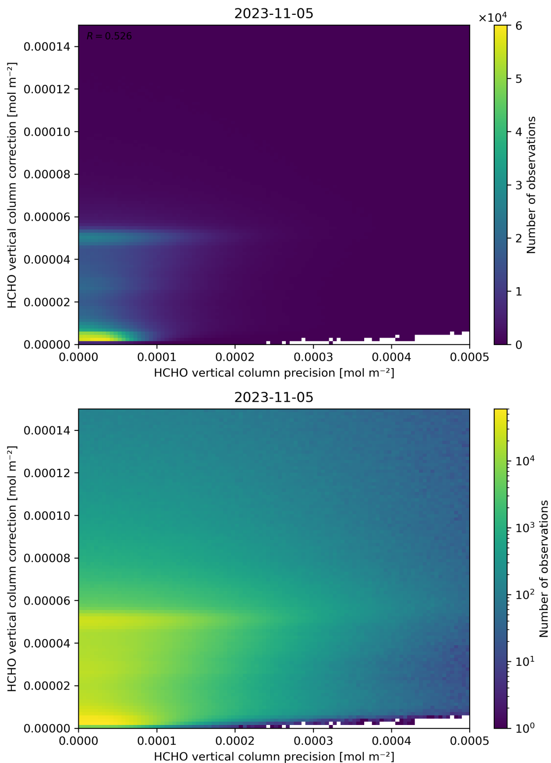
Figure 146: Scatter density plot of “HCHO vertical column precision” against “HCHO vertical column correction” for 2023-11-04 to 2023-11-06.
