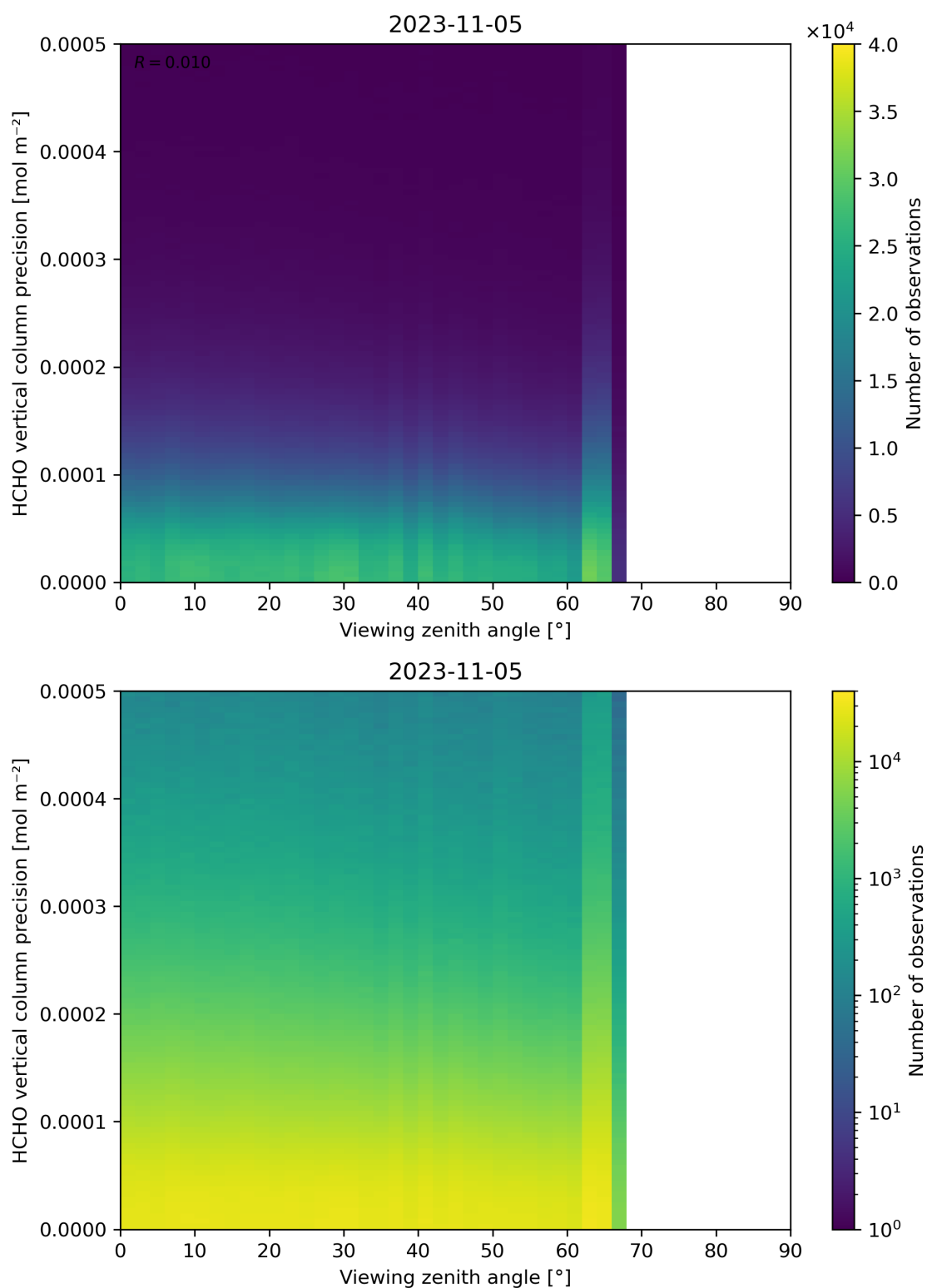
Figure 194: Scatter density plot of “Viewing zenith angle” against “HCHO vertical column precision” for 2023-11-04 to 2023-11-06.
