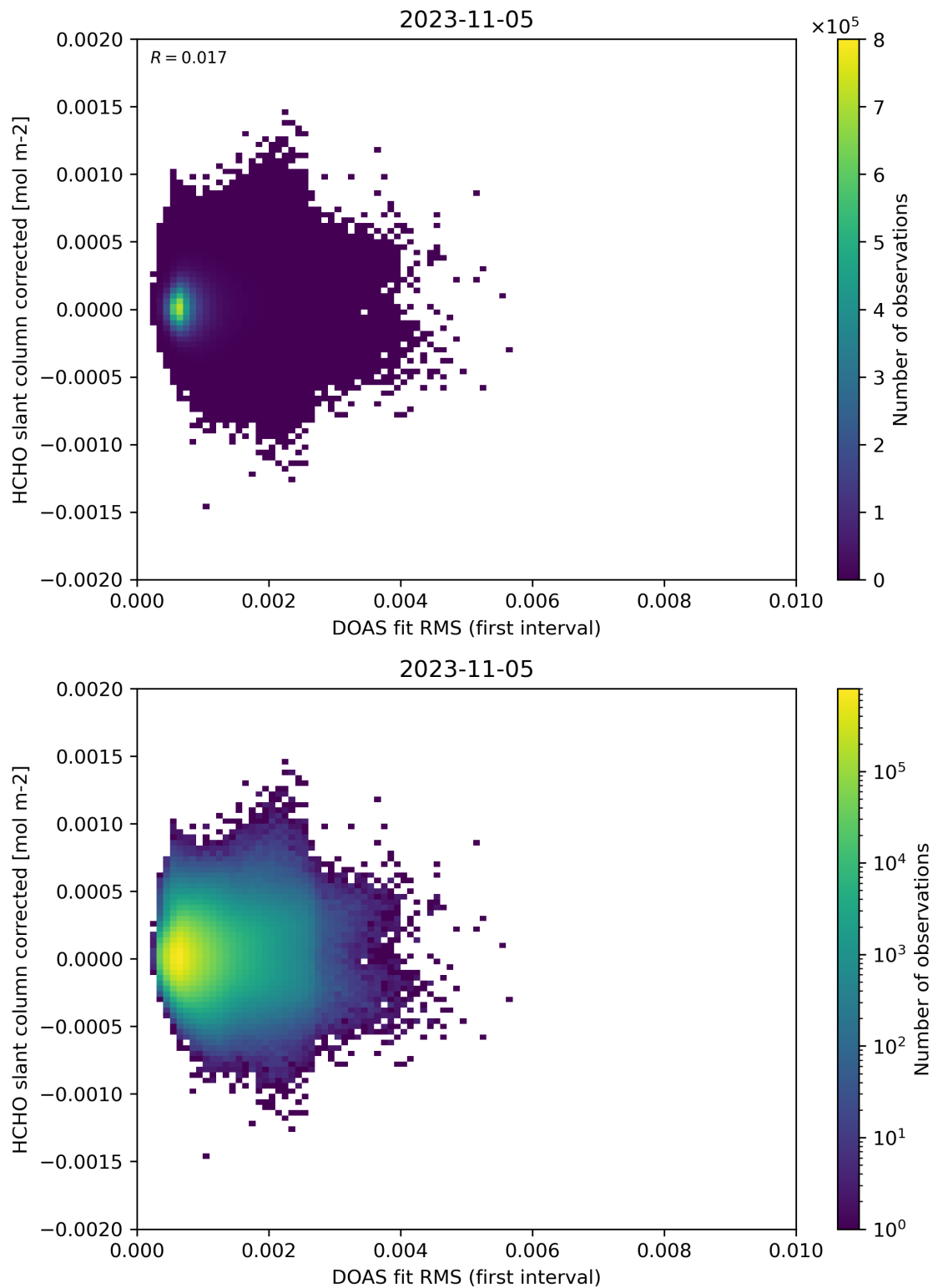
Figure 62: Scatter density plot of “DOAS fit RMS (first interval)” against “HCHO slant column corrected” for 2023-11-04 to 2023-11-06.
