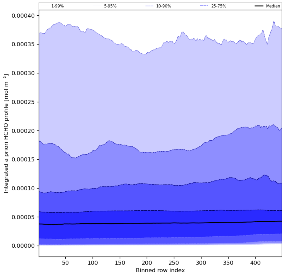
Figure 57: Along track statistics of “Integrated a priori HCHO profile” for 2023-11-04 to 2023-11-06
