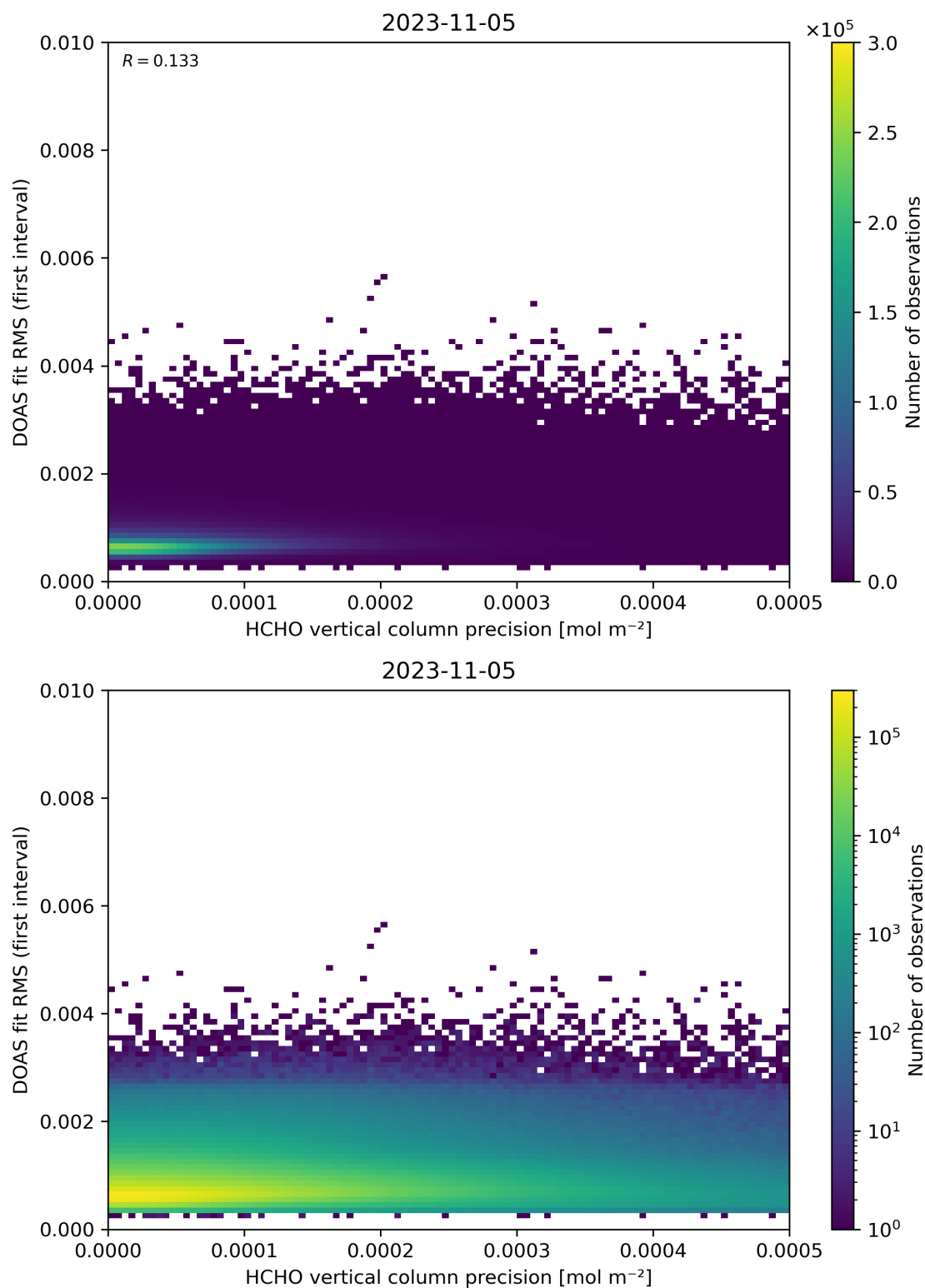
Figure 136: Scatter density plot of “HCHO vertical column precision” against “DOAS fit RMS (first interval)” for 2023-11-04 to 2023-11-06.
