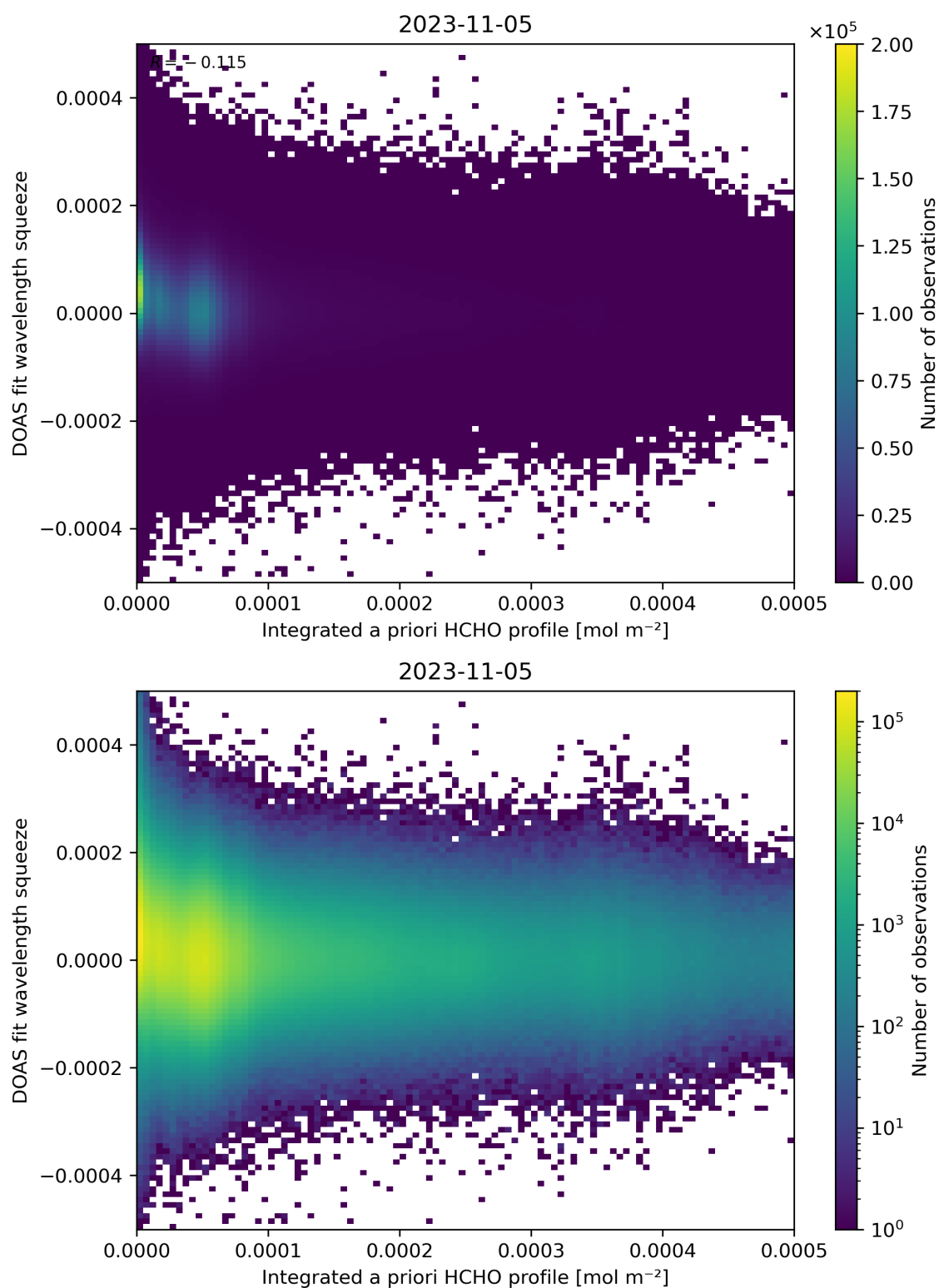
Figure 150: Scatter density plot of “Integrated a priori HCHO profile” against “DOAS fit wavelength squeeze” for 2023-11-04 to 2023-11-06.
