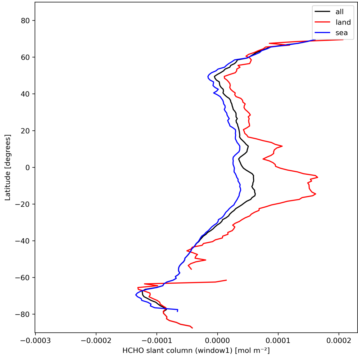
Figure 24: Zonal average of “HCHO slant column (window1)” for 2023-11-04 to 2023-11-06.
