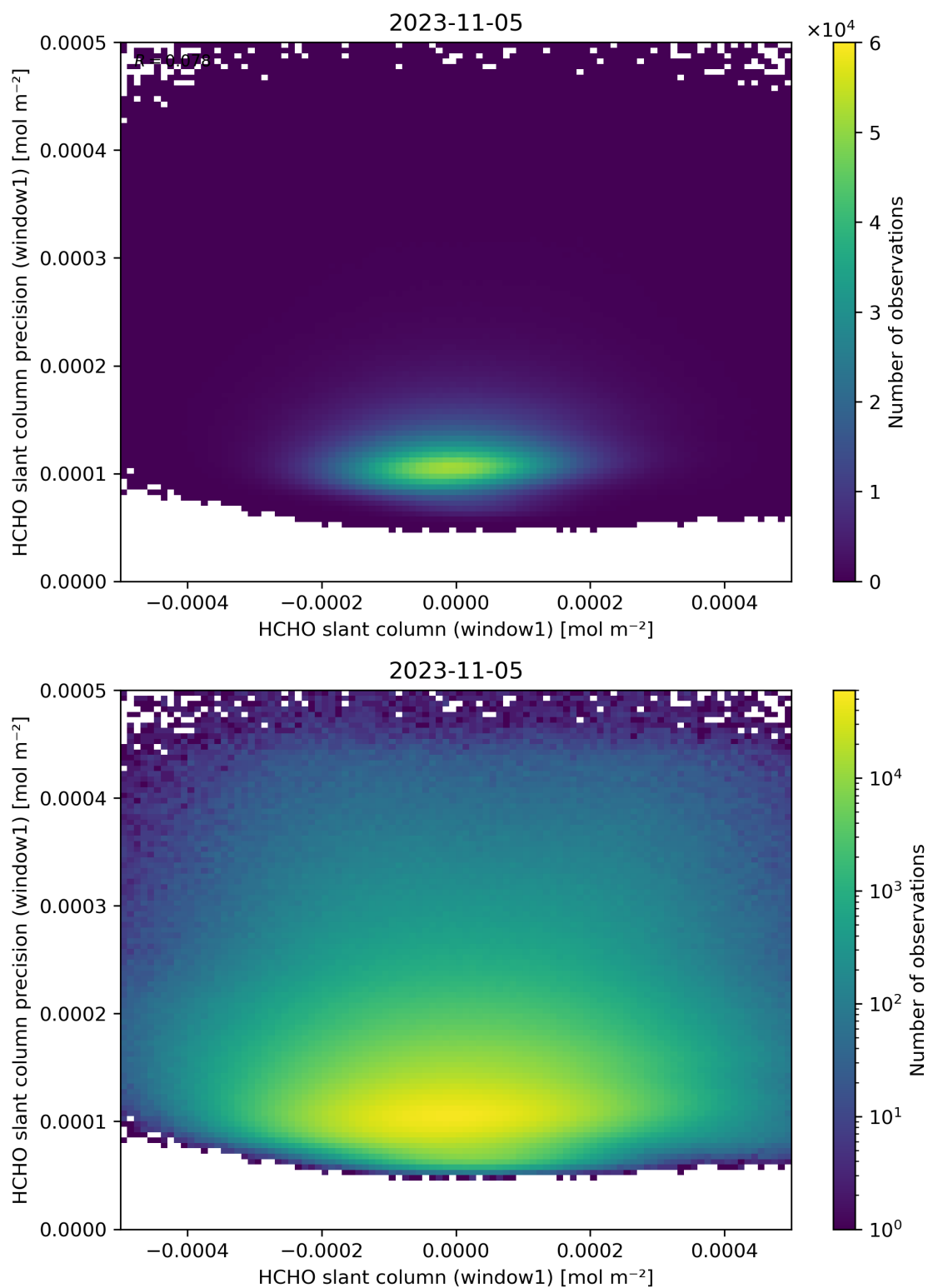
Figure 84: Scatter density plot of “HCHO slant column (window1)” against “HCHO slant column precision (window1)” for 2023-11-04 to 2023-11-06.
