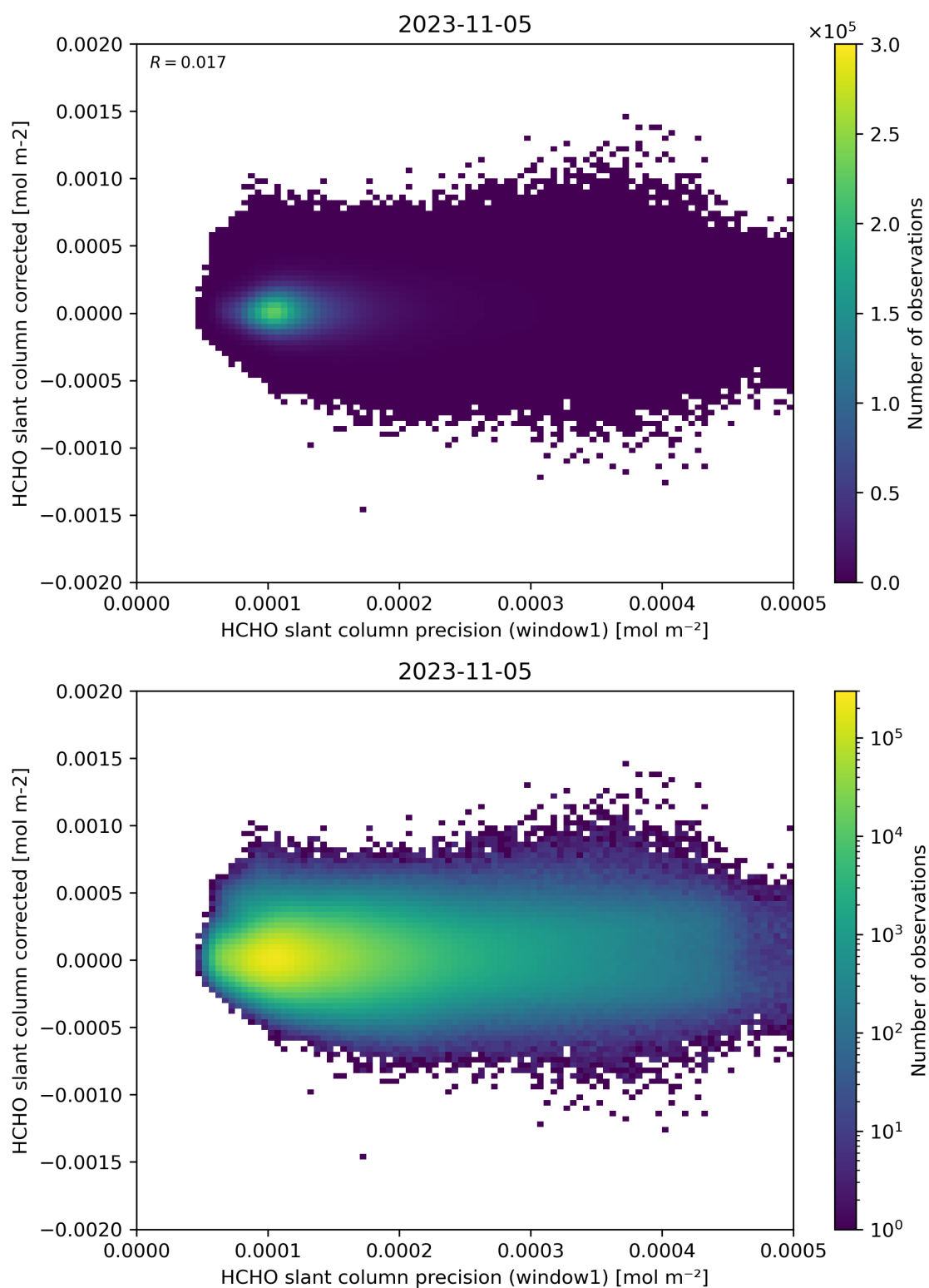
Figure 92: Scatter density plot of “HCHO slant column precision (window1)” against “HCHO slant column corrected” for 2023-11-04 to 2023-11-06.
