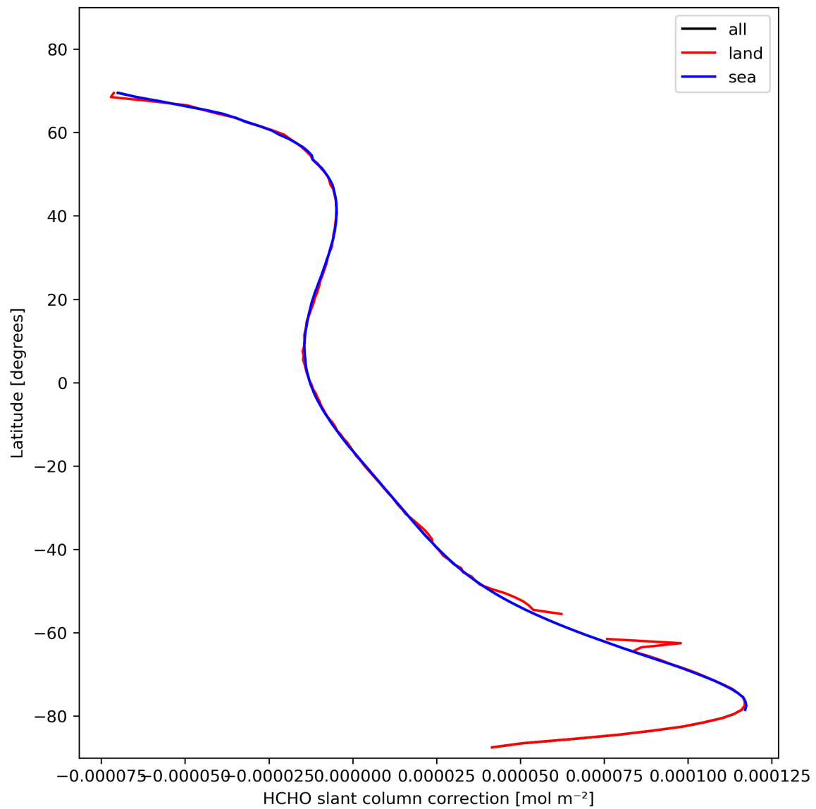
Figure 33: Zonal average of “HCHO slant column correction” for 2023-11-04 to 2023-11-06.
