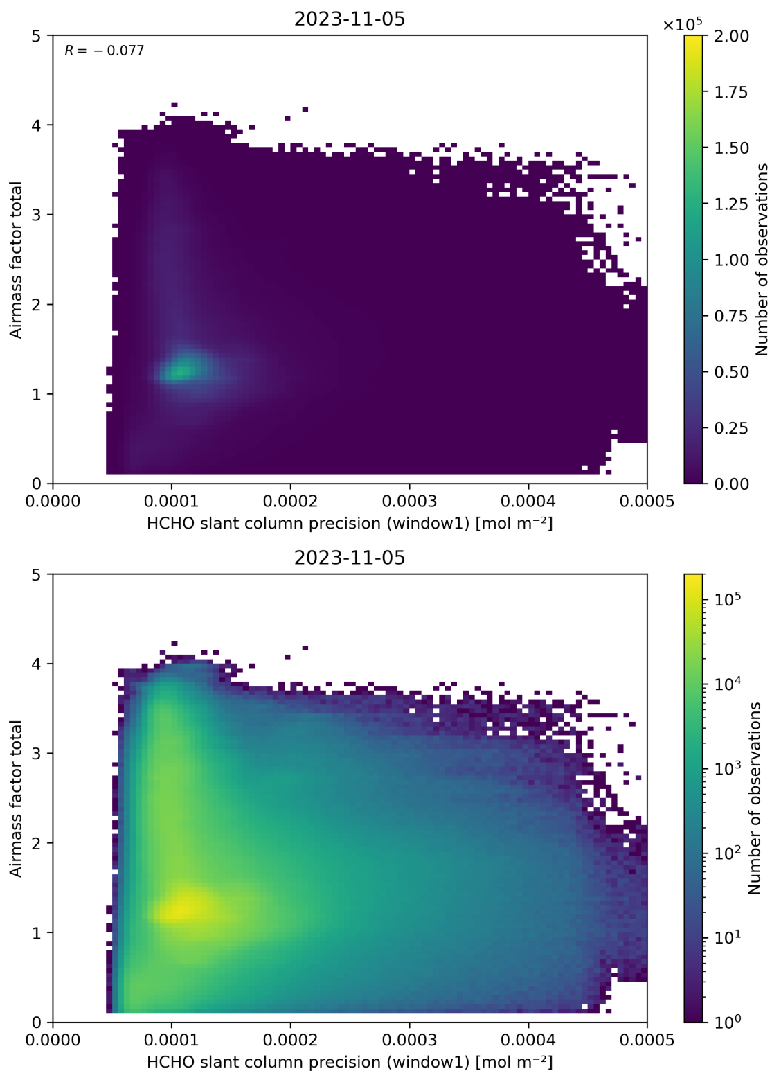
Figure 94: Scatter density plot of “HCHO slant column precision (window1)” against “Airmass factor total” for 2023-11-04 to 2023-11-06.
