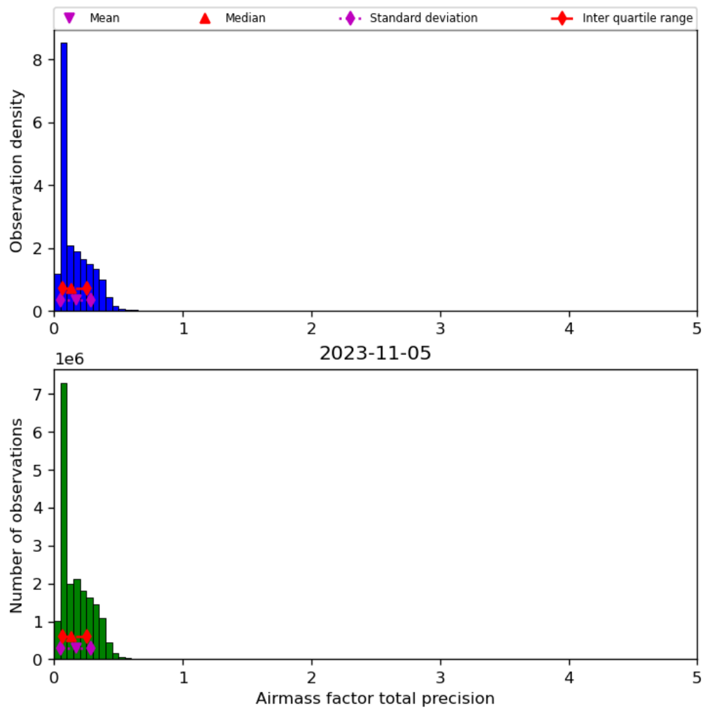
Figure 41: Histogram of “Airmass factor total precision” for 2023-11-04 to 2023-11-06
