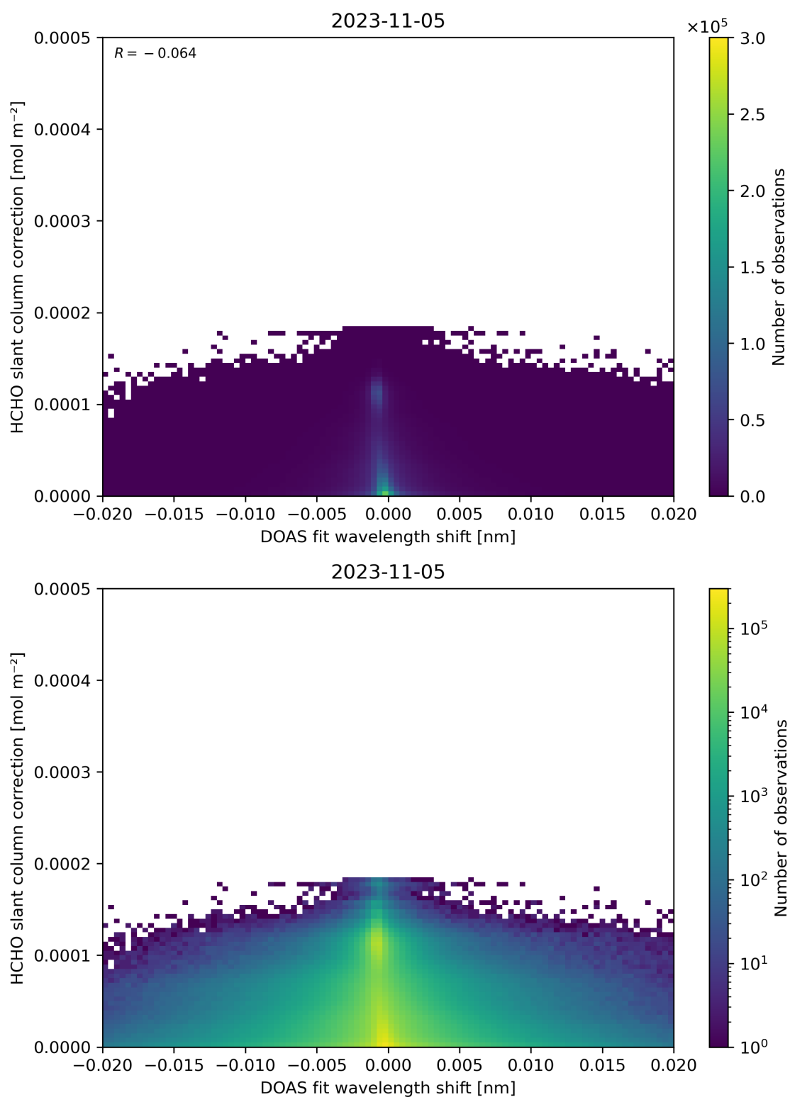
Figure 67: Scatter density plot of “DOAS fit wavelength shift” against “HCHO slant column correction” for 2023-11-04 to 2023-11-06.
