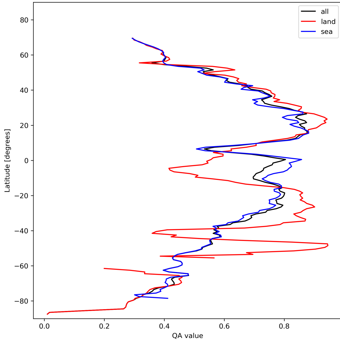
Figure 20: Zonal average of “QA value” for 2023-11-04 to 2023-11-06.
