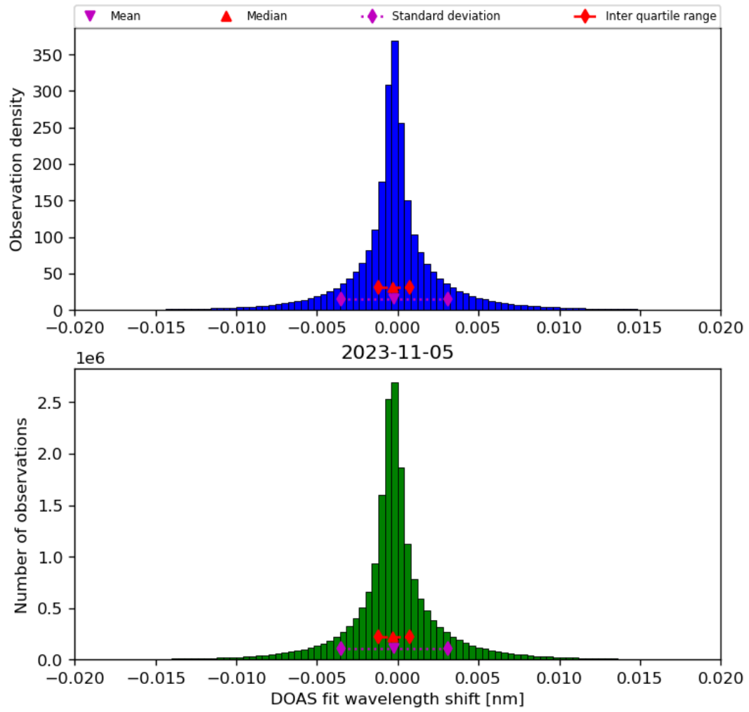
Figure 44: Histogram of “DOAS fit wavelength shift” for 2023-11-04 to 2023-11-06
