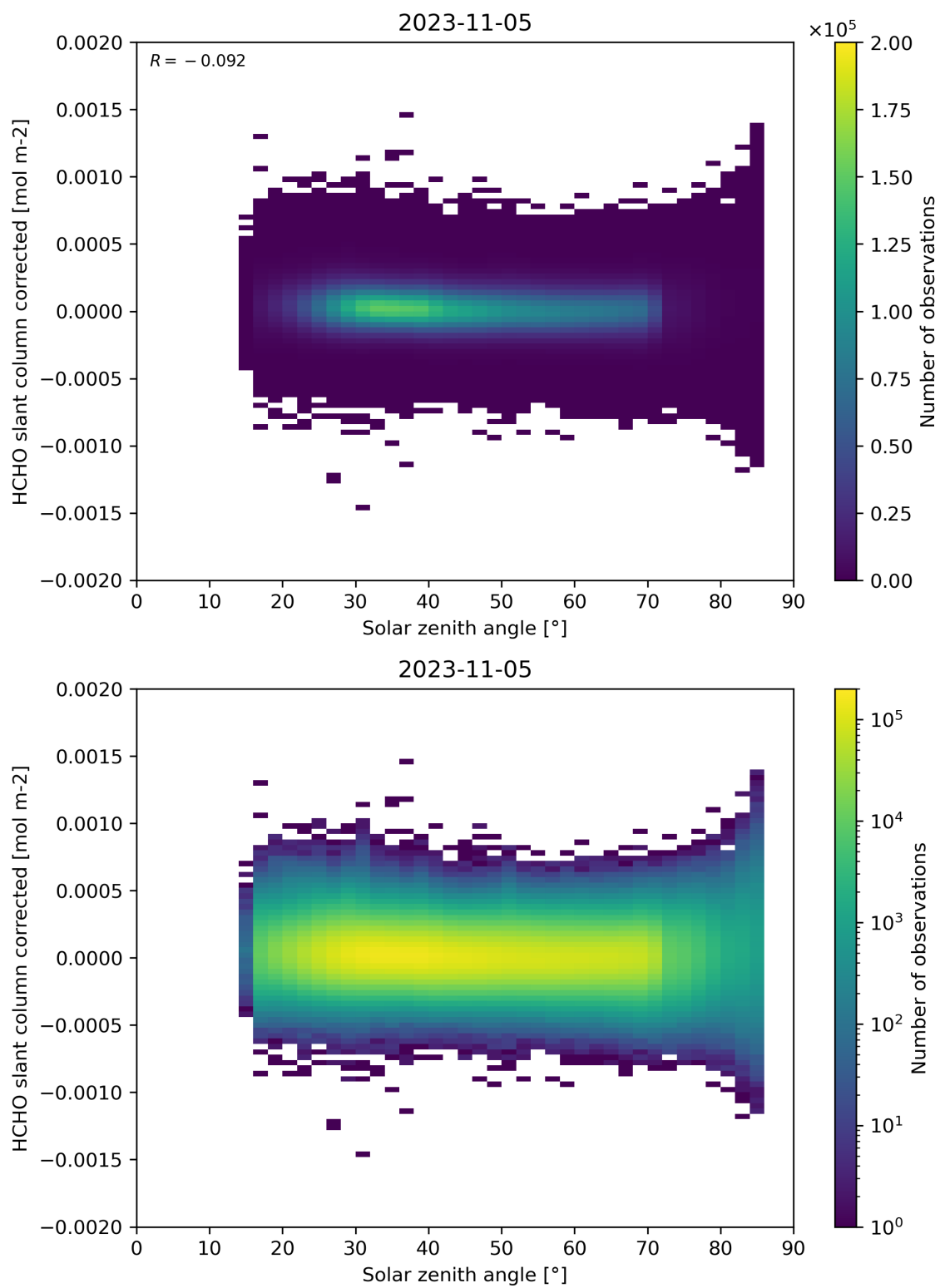
Figure 171: Scatter density plot of “Solar zenith angle” against “HCHO slant column corrected” for 2023-11-04 to 2023-11-06.
