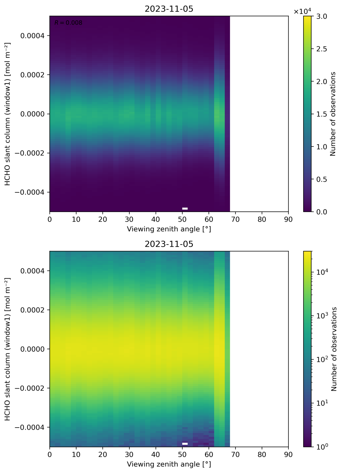
Figure 188: Scatter density plot of “Viewing zenith angle” against “HCHO slant column (window1)” for 2023-11-04 to 2023-11-06.
