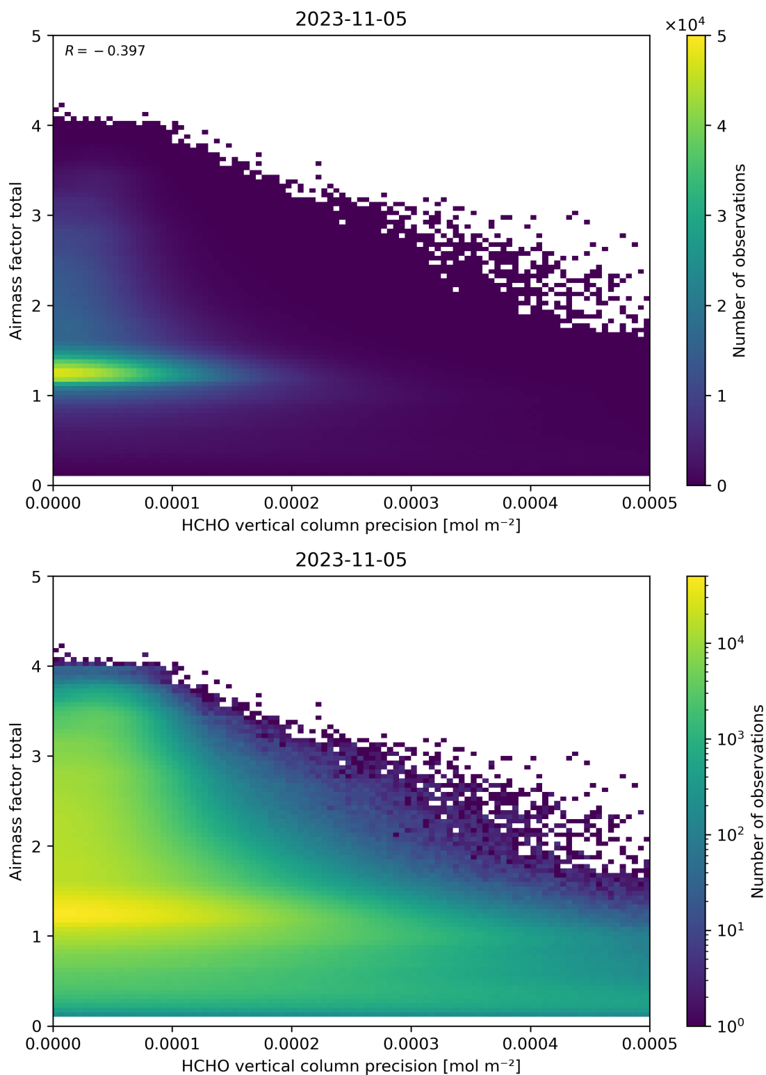
Figure 144: Scatter density plot of “HCHO vertical column precision” against “Airmass factor total” for 2023-11-04 to 2023-11-06.
