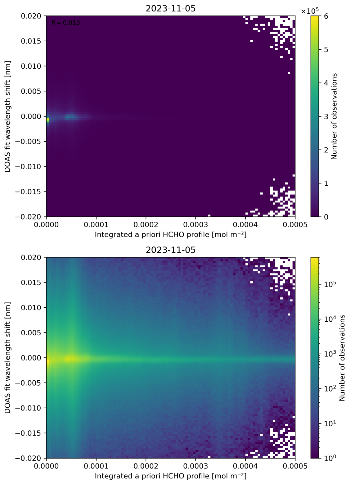
Figure 149: Scatter density plot of “Integrated a priori HCHO profile” against “DOAS fit wavelength shift” for 2023-11-04 to 2023-11-06.
