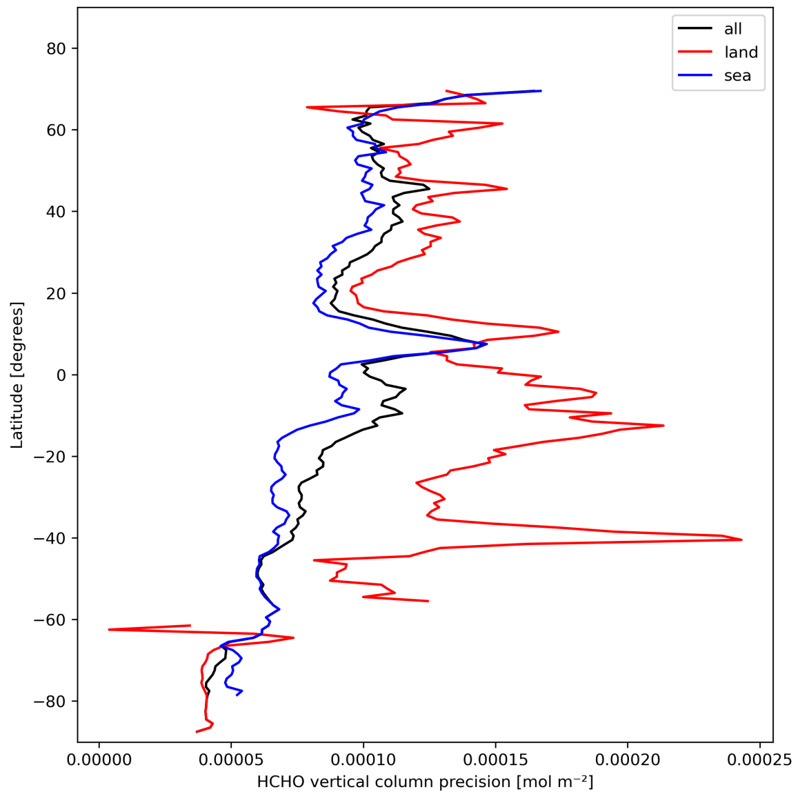
Figure 22: Zonal average of “HCHO vertical column precision” for 2023-11-04 to 2023-11-06.
