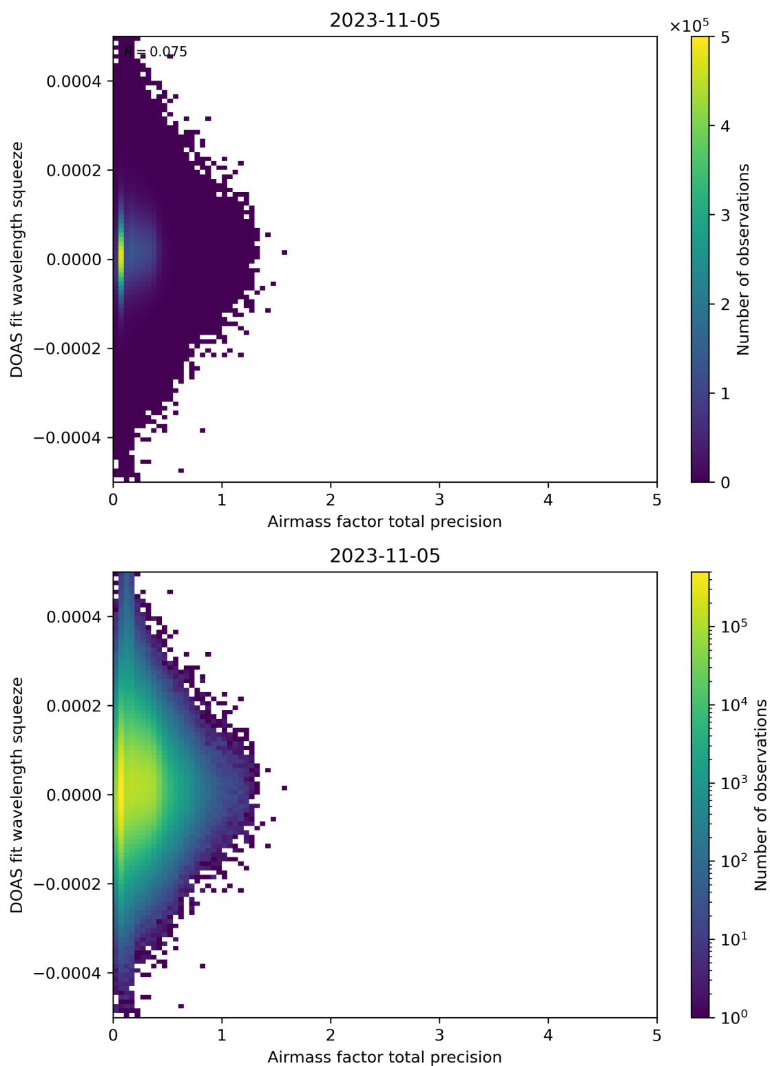
Figure 107: Scatter density plot of “Airmass factor total precision” against “DOAS fit wavelength squeeze” for 2023-11-04 to 2023-11-06.
