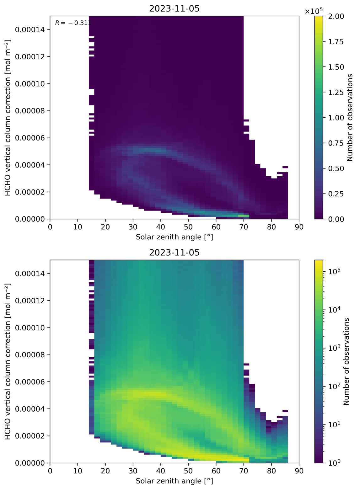
Figure 178: Scatter density plot of “Solar zenith angle” against “HCHO vertical column correction” for 2023-11-04 to 2023-11-06.
