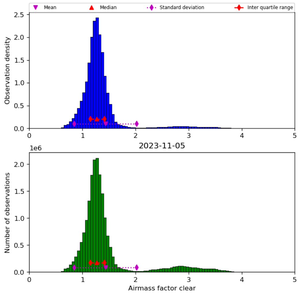
Figure 42: Histogram of “Airmass factor clear” for 2023-11-04 to 2023-11-06
