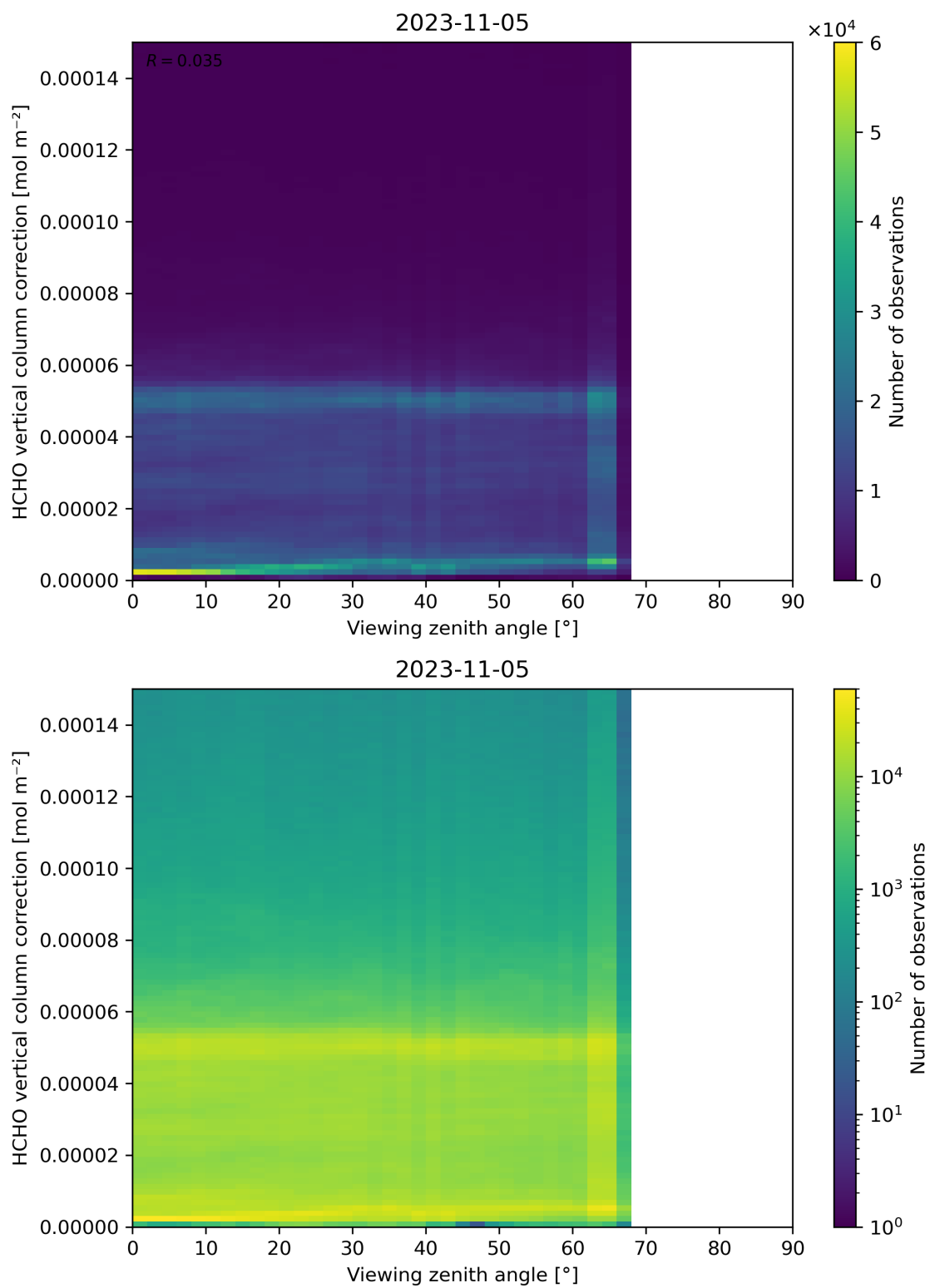
Figure 193: Scatter density plot of “Viewing zenith angle” against “HCHO vertical column correction” for 2023-11-04 to 2023-11-06.
