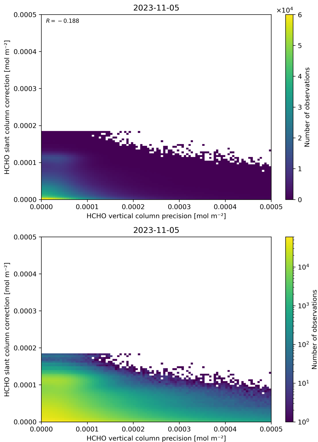
Figure 141: Scatter density plot of “HCHO vertical column precision” against “HCHO slant column correction” for 2023-11-04 to 2023-11-06.
