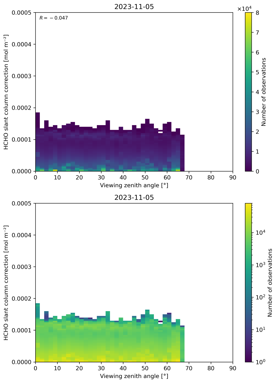
Figure 187: Scatter density plot of “Viewing zenith angle” against “HCHO slant column correction” for 2023-11-04 to 2023-11-06.
