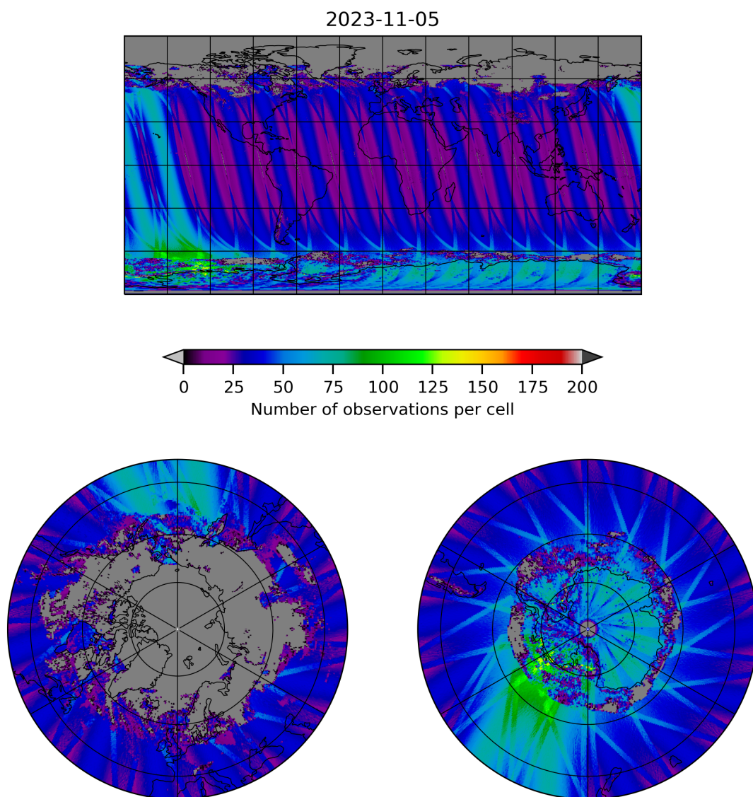
Figure 19: Map of the number of observations for 2023-11-04 to 2023-11-06
