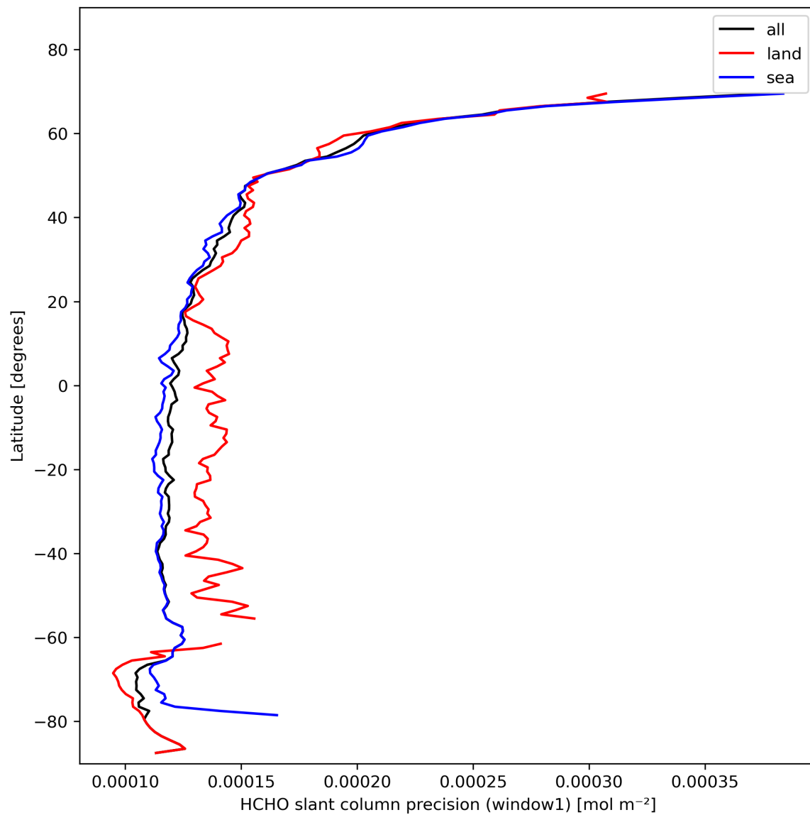
Figure 25: Zonal average of “HCHO slant column precision (window1)” for 2023-11-04 to 2023-11-06.
