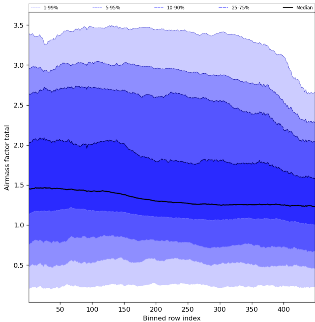
Figure 54: Along track statistics of “Airmass factor total” for 2023-11-04 to 2023-11-06
