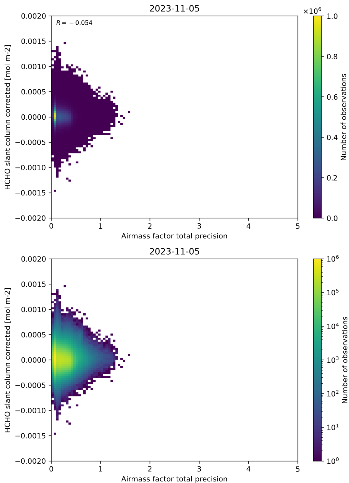
Figure 109: Scatter density plot of “Airmass factor total precision” against “HCHO slant column corrected” for 2023-11-04 to 2023-11-06.
