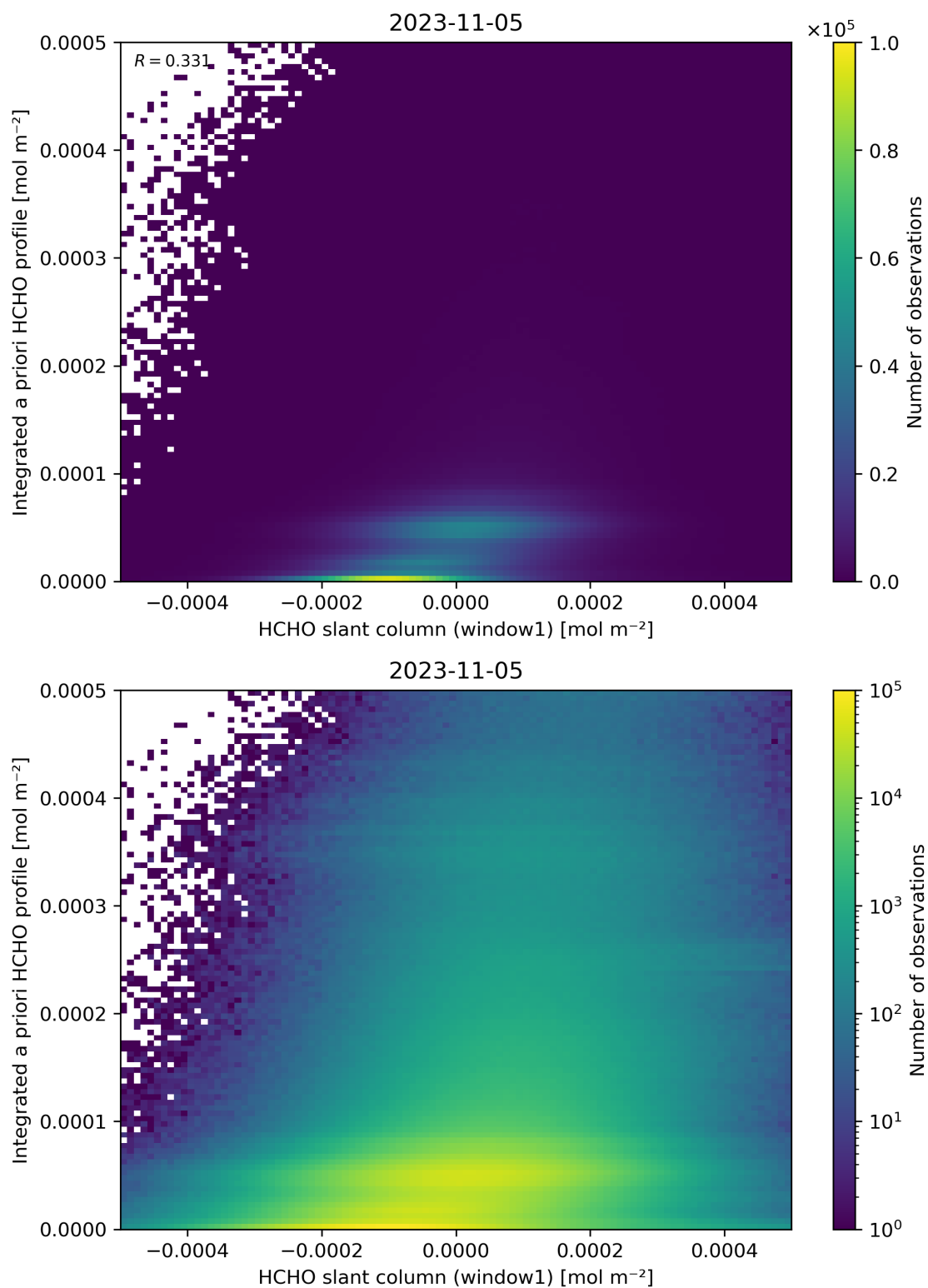
Figure 87: Scatter density plot of “HCHO slant column (window1)” against “Integrated a priori HCHO profile” for 2023-11-04 to 2023-11-06.
