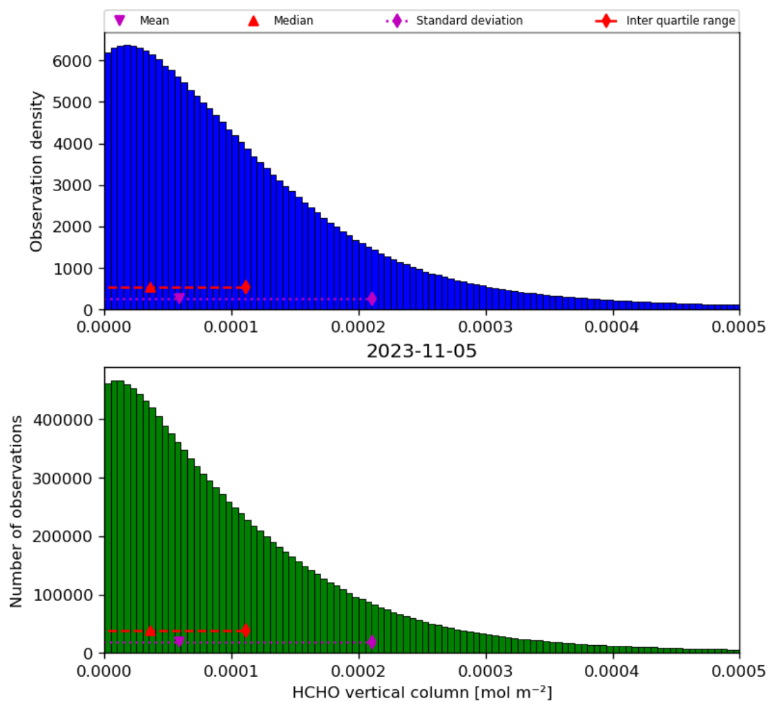
Figure 35: Histogram of “HCHO vertical column” for 2023-11-04 to 2023-11-06
