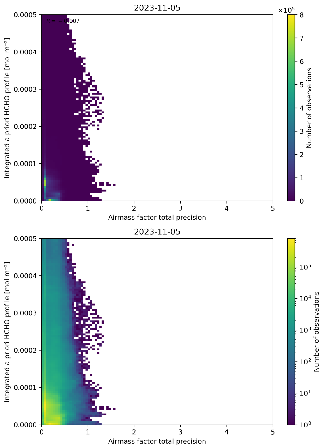
Figure 111: Scatter density plot of “Airmass factor total precision” against “Integrated a priori HCHO profile” for 2023-11-04 to 2023-11-06.
