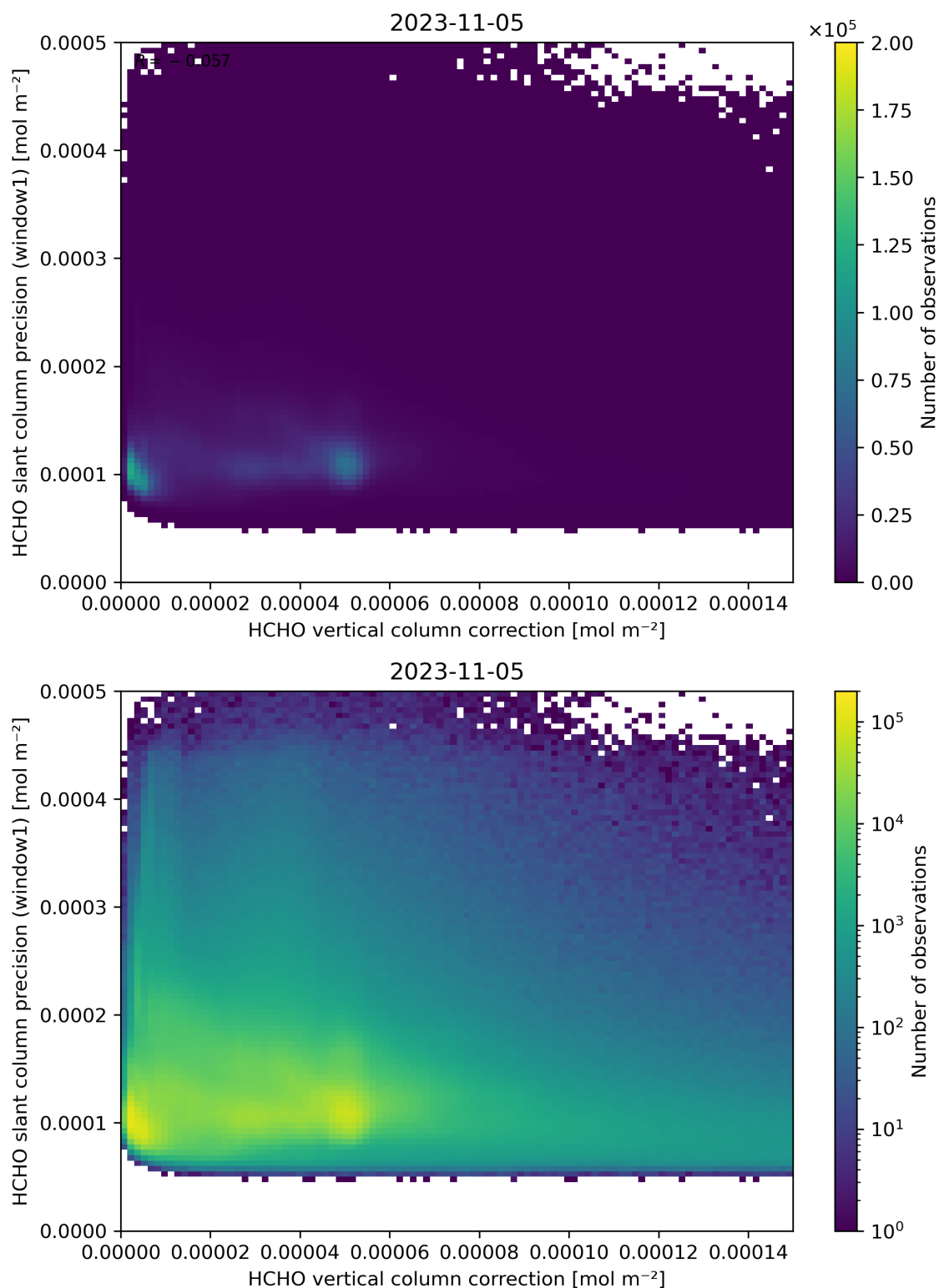
Figure 119: Scatter density plot of “HCHO vertical column correction” against “HCHO slant column precision (window1)” for 2023-11-04 to 2023-11-06.
