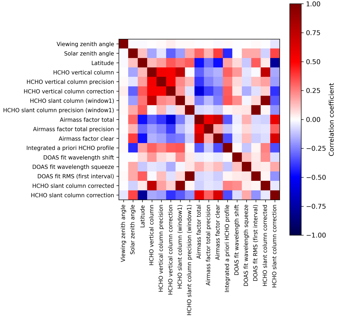
Figure 2: Map of correlation matrix for 2023-11-04 to 2023-11-06.
