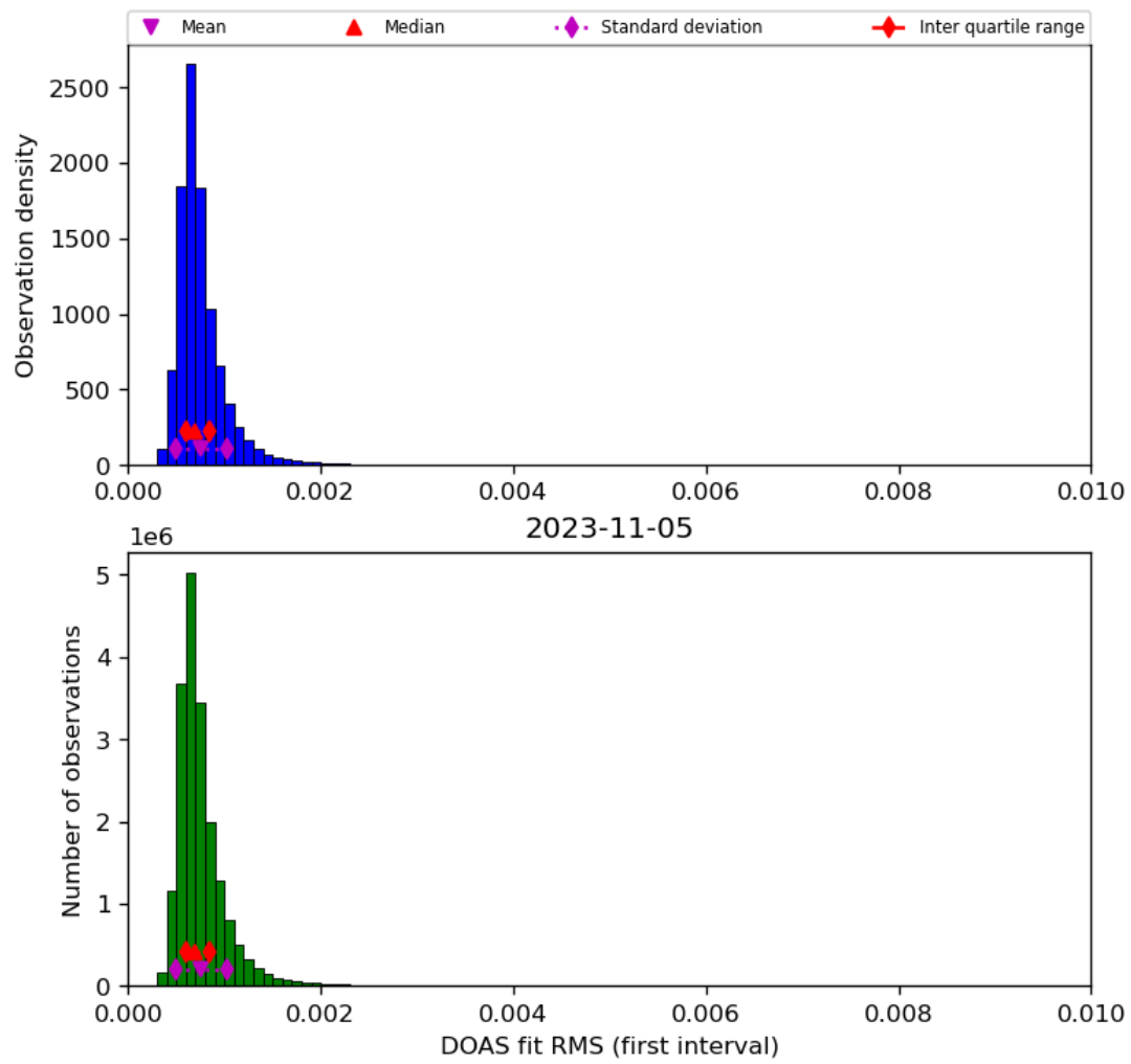
Figure 46: Histogram of “DOAS fit RMS (first interval)” for 2023-11-04 to 2023-11-06
