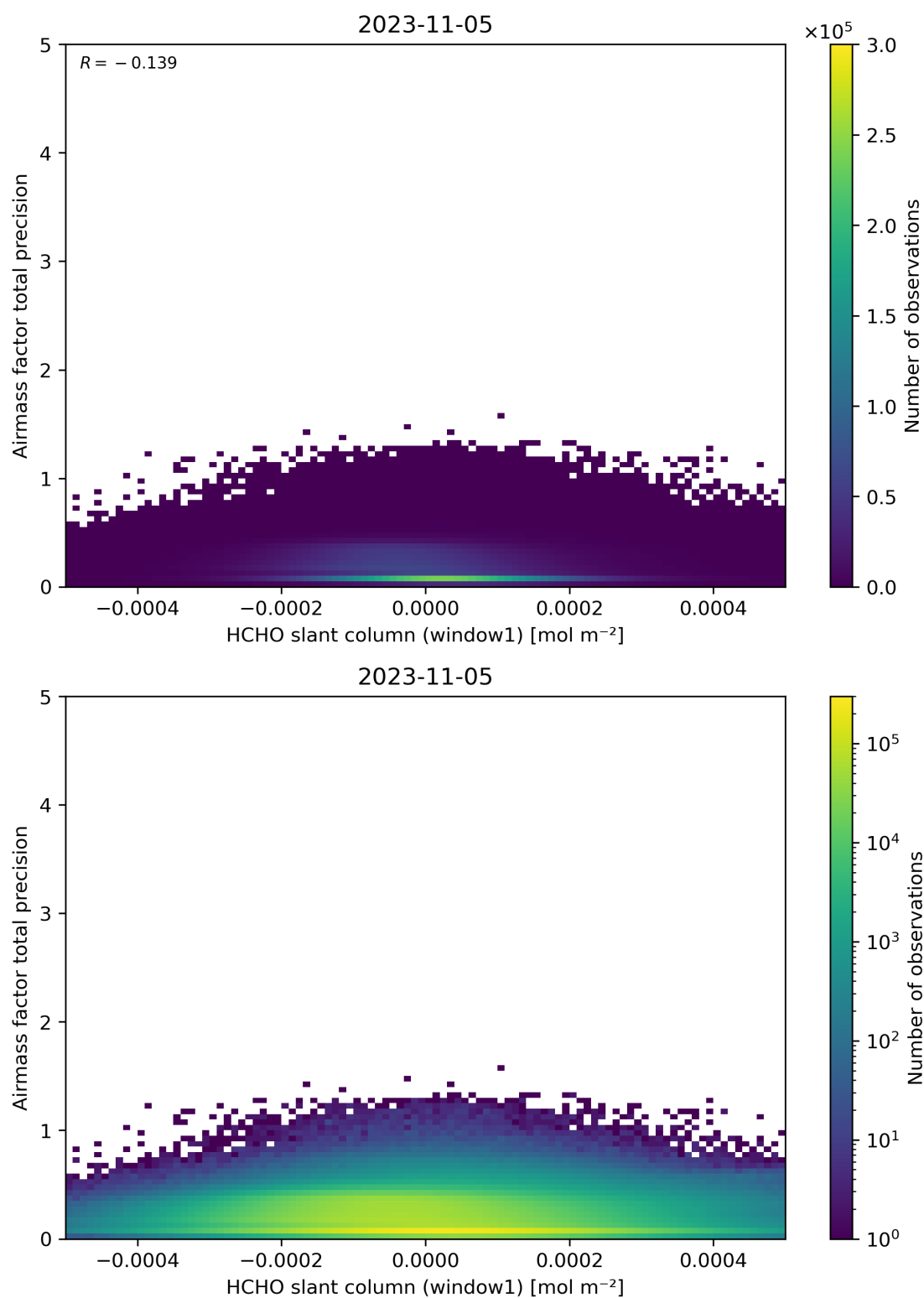
Figure 86: Scatter density plot of “HCHO slant column (window1)” against “Airmass factor total precision” for 2023-11-04 to 2023-11-06.
