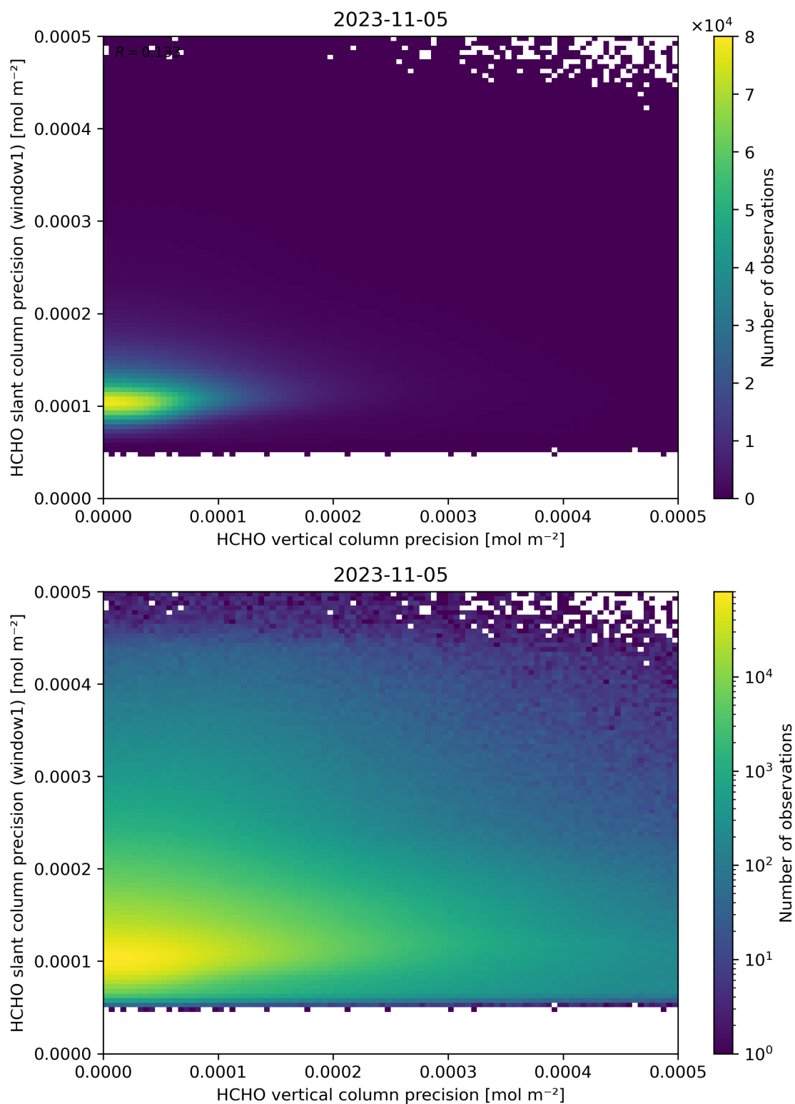
Figure 143: Scatter density plot of “HCHO vertical column precision” against “HCHO slant column precision (window1)” for 2023-11-04 to 2023-11-06.
