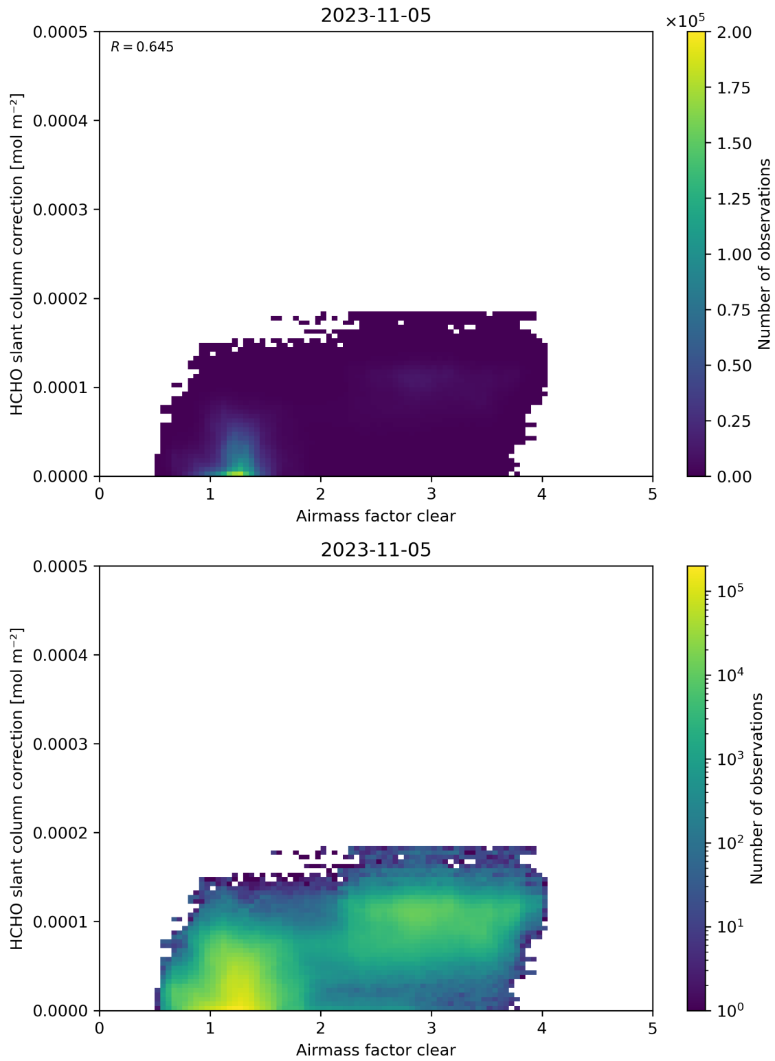
Figure 75: Scatter density plot of “Airmass factor clear” against “HCHO slant column correction” for 2023-11-04 to 2023-11-06.
