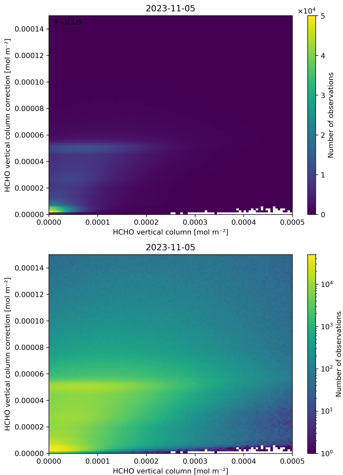
Figure 133: Scatter density plot of “HCHO vertical column” against “HCHO vertical column correction” for 2023-11-04 to 2023-11-06.
