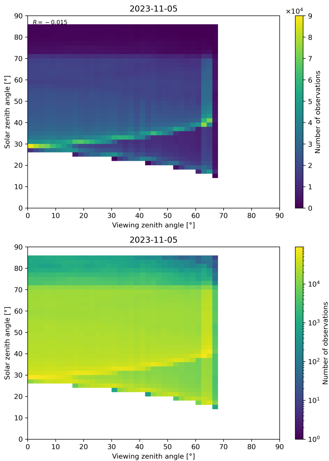
Figure 197: Scatter density plot of “Viewing zenith angle” against “Solar zenith angle” for 2023-11-04 to 2023-11-06.
