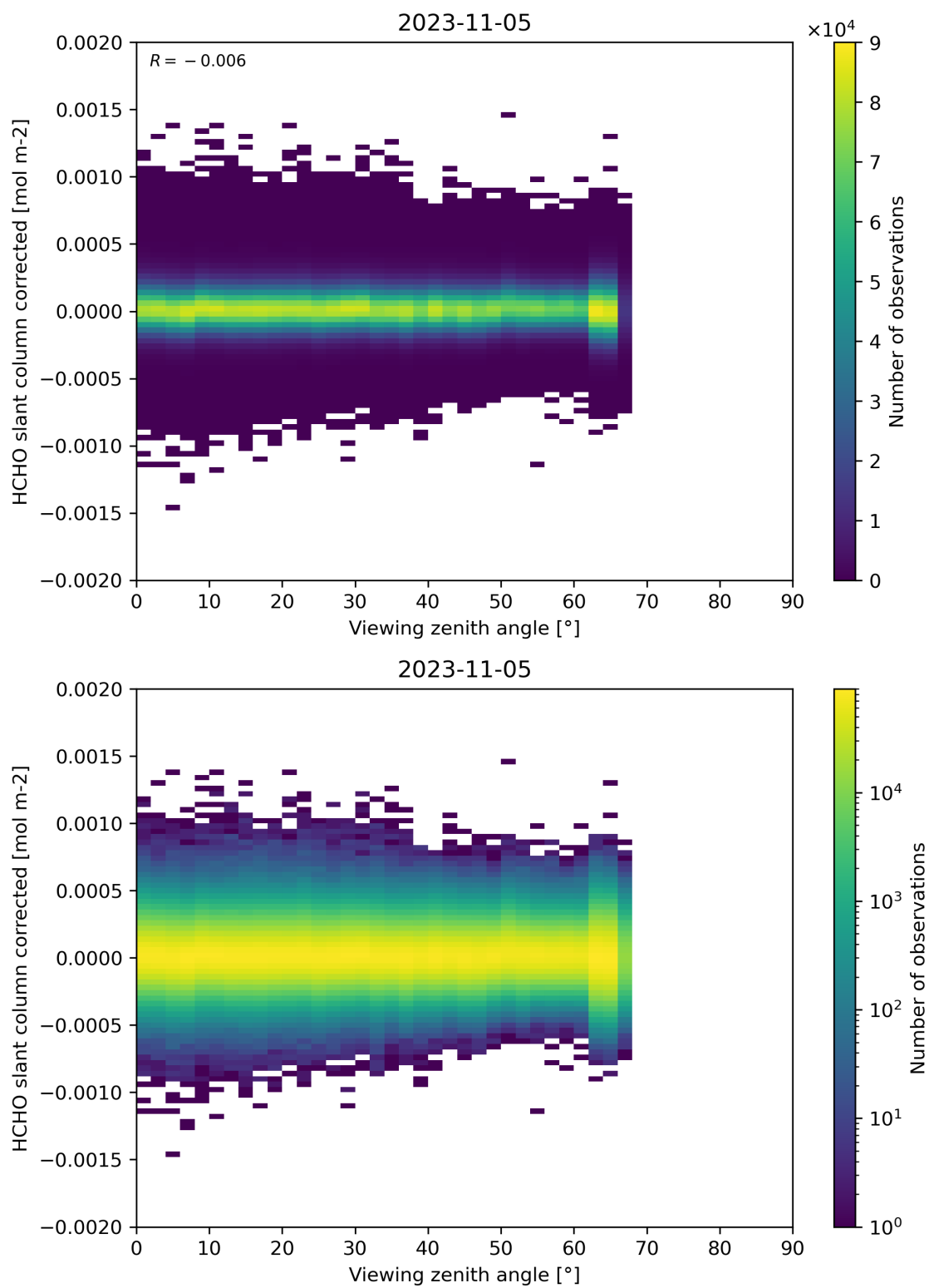
Figure 186: Scatter density plot of “Viewing zenith angle” against “HCHO slant column corrected” for 2023-11-04 to 2023-11-06.
