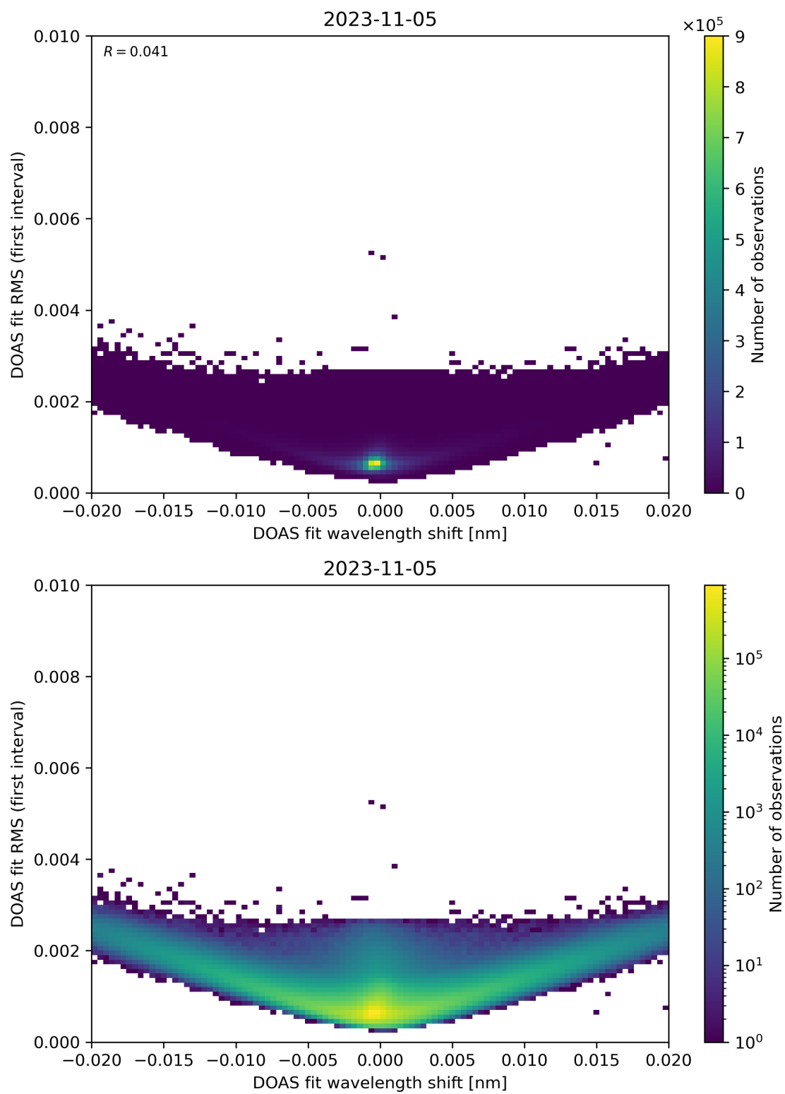
Figure 64: Scatter density plot of “DOAS fit wavelength shift” against “DOAS fit RMS (first interval)” for 2023-11-04 to 2023-11-06.
