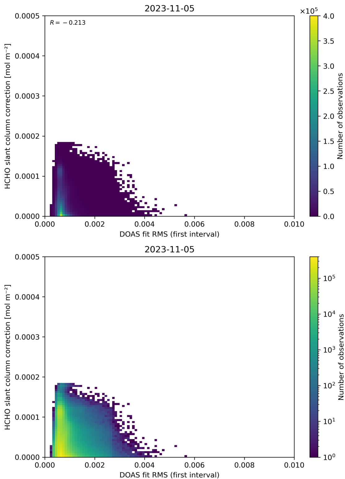
Figure 63: Scatter density plot of “DOAS fit RMS (first interval)” against “HCHO slant column correction” for 2023-11-04 to 2023-11-06.
