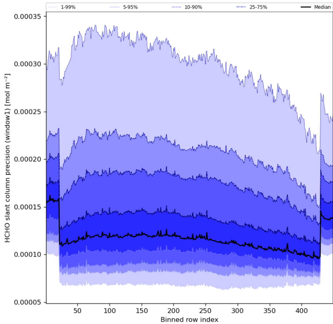
Figure 53: Along track statistics of “HCHO slant column precision (window1)” for 2023-11-04 to 2023-11-06
