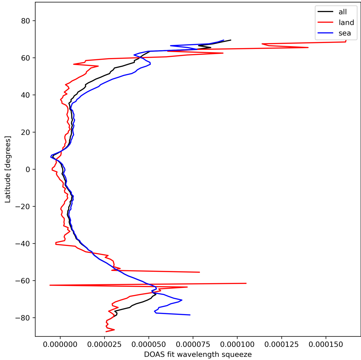
Figure 31: Zonal average of “DOAS fit wavelength squeeze” for 2023-11-04 to 2023-11-06.
