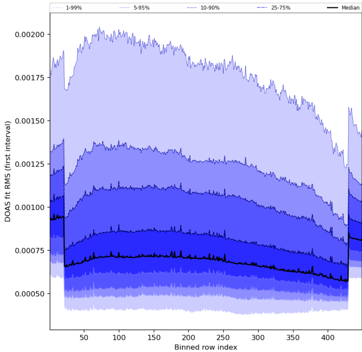
Figure 60: Along track statistics of “DOAS fit RMS (first interval)” for 2023-11-04 to 2023-11-06
