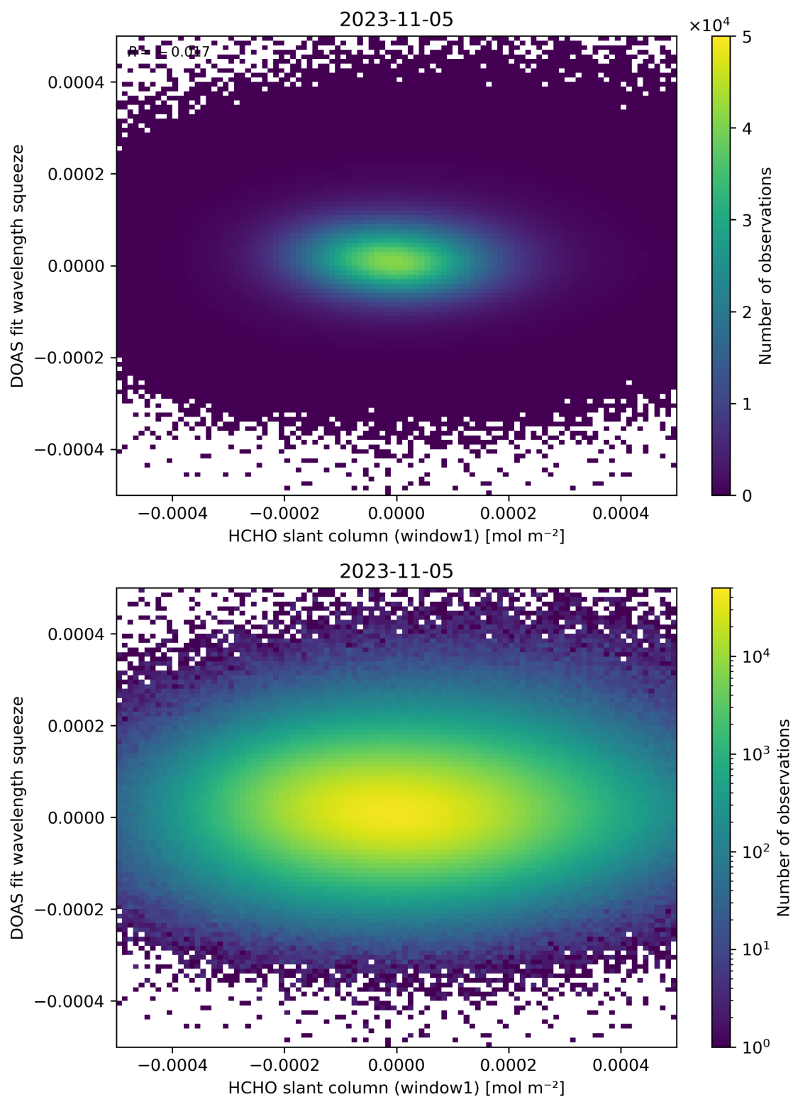
Figure 80: Scatter density plot of “HCHO slant column (window1)” against “DOAS fit wavelength squeeze” for 2023-11-04 to 2023-11-06.
