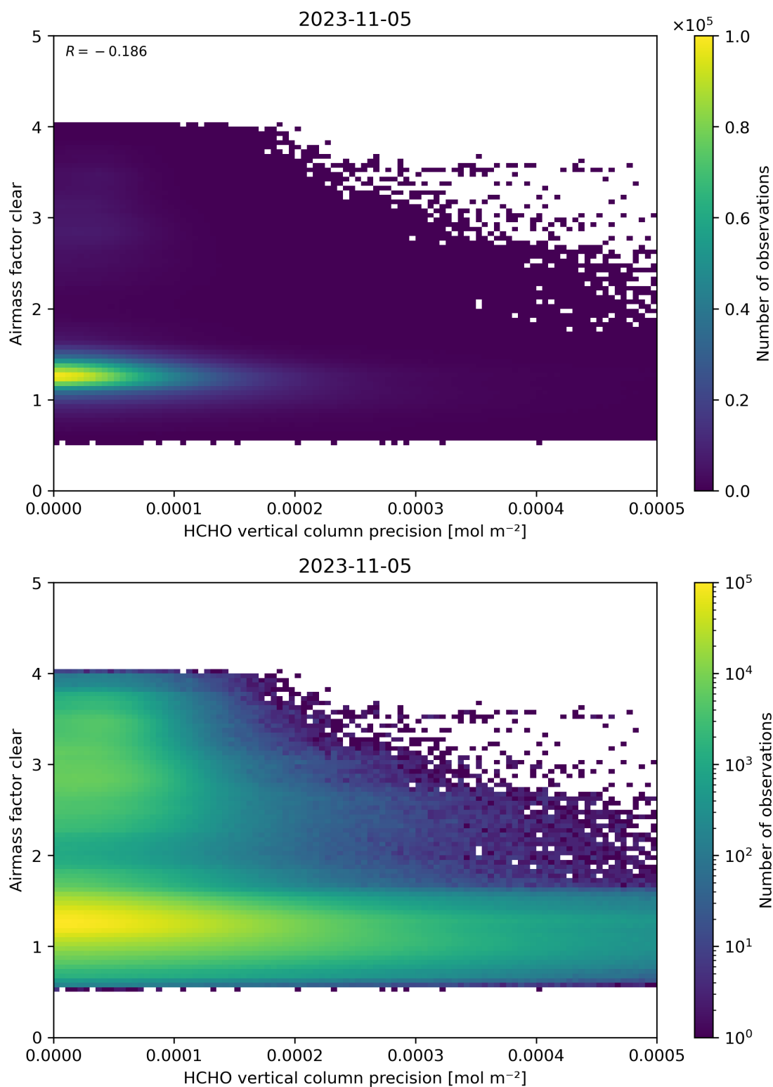
Figure 139: Scatter density plot of “HCHO vertical column precision” against “Airmass factor clear” for 2023-11-04 to 2023-11-06.
