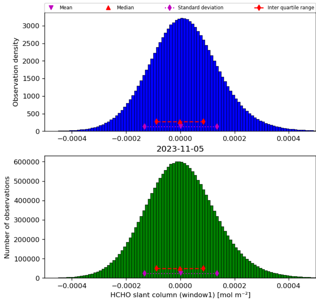
Figure 38: Histogram of “HCHO slant column (window1)” for 2023-11-04 to 2023-11-06
