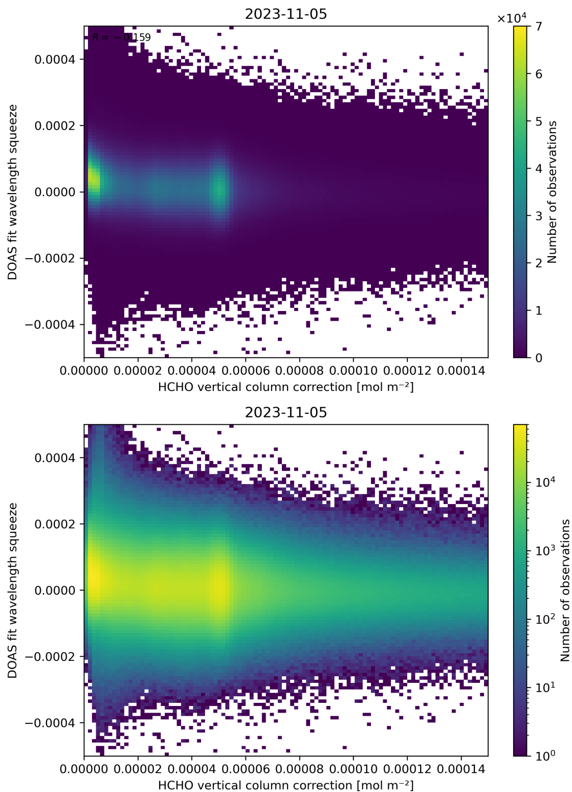
Figure 114: Scatter density plot of “HCHO vertical column correction” against “DOAS fit wavelength squeeze” for 2023-11-04 to 2023-11-06.
