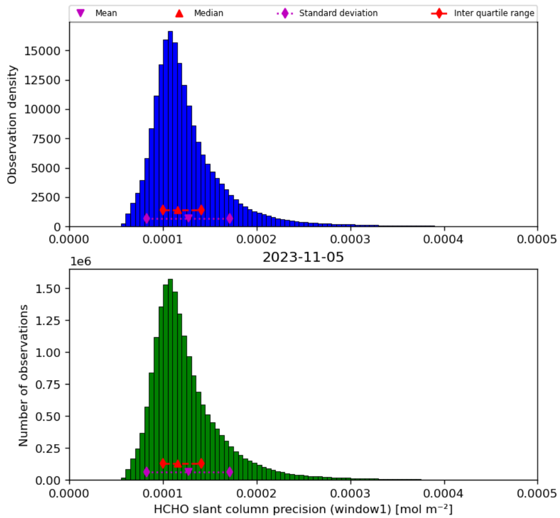
Figure 39: Histogram of “HCHO slant column precision (window1)” for 2023-11-04 to 2023-11-06
