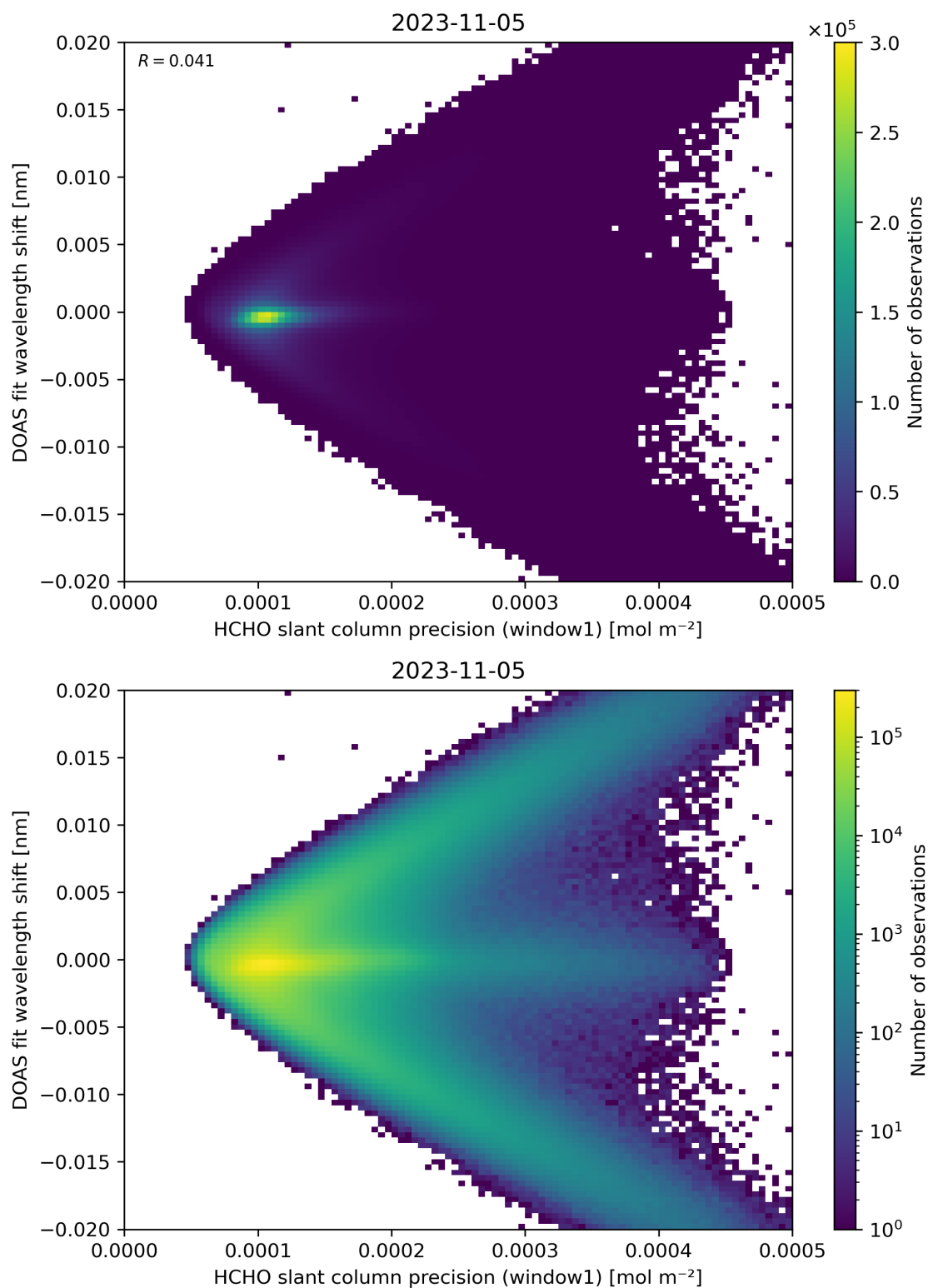
Figure 89: Scatter density plot of “HCHO slant column precision (window1)” against “DOAS fit wavelength shift” for 2023-11-04 to 2023-11-06.
