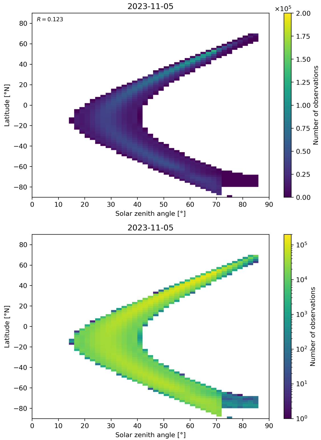
Figure 181: Scatter density plot of “Solar zenith angle” against “Latitude” for 2023-11-04 to 2023-11-06.
