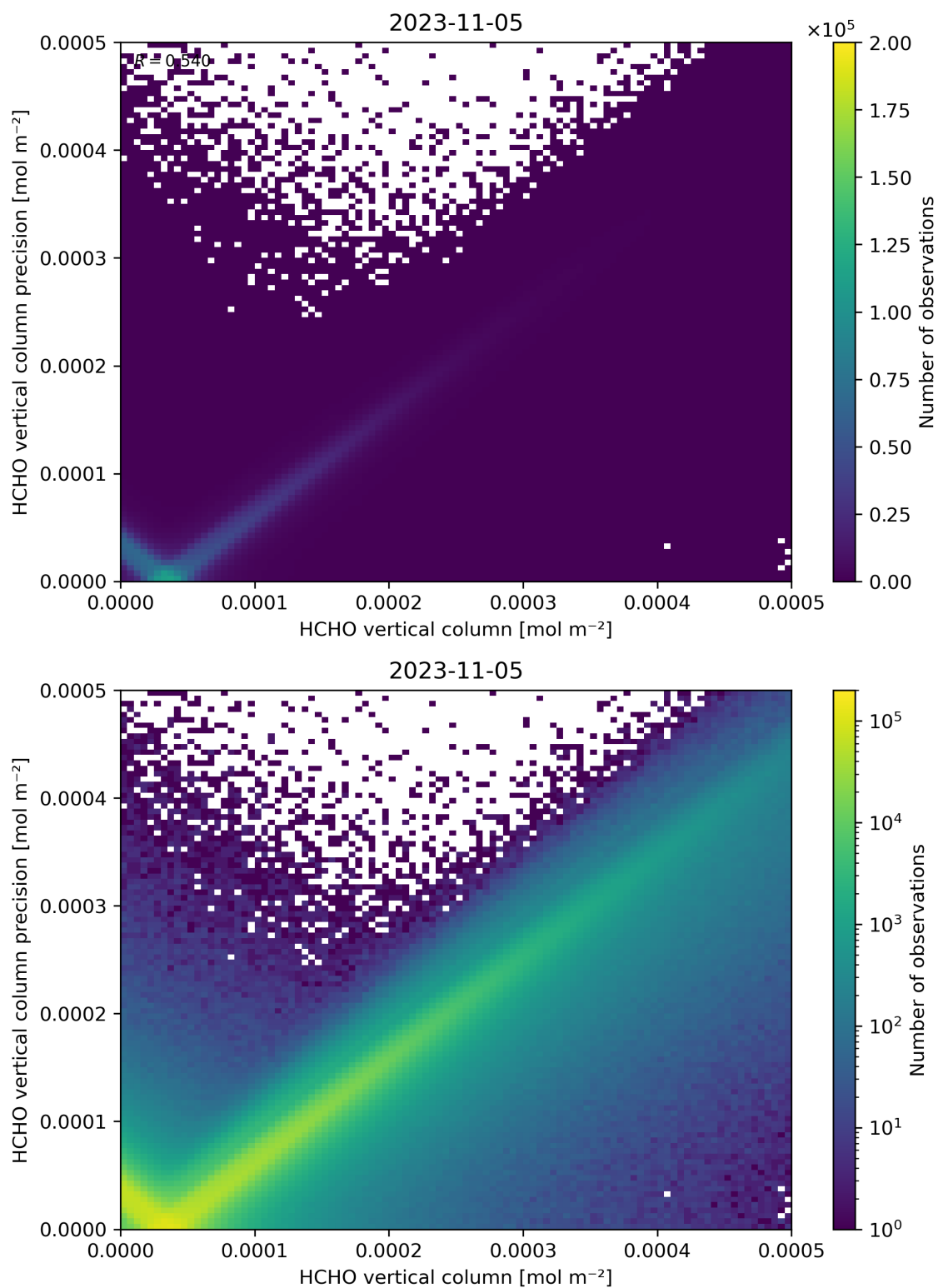
Figure 134: Scatter density plot of “HCHO vertical column” against “HCHO vertical column precision” for 2023-11-04 to 2023-11-06.
