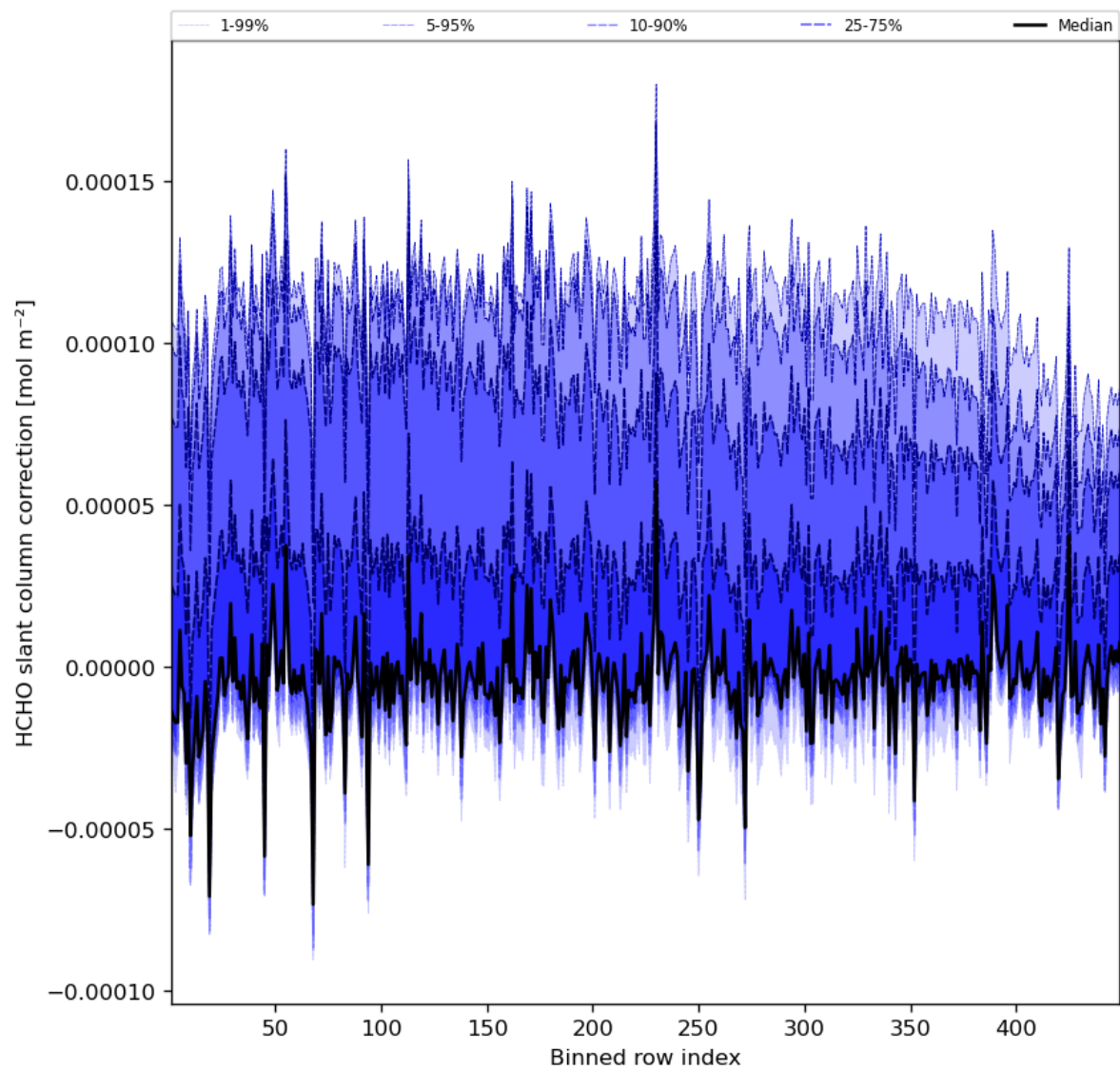
Figure 61: Along track statistics of “HCHO slant column correction” for 2023-11-04 to 2023-11-06
