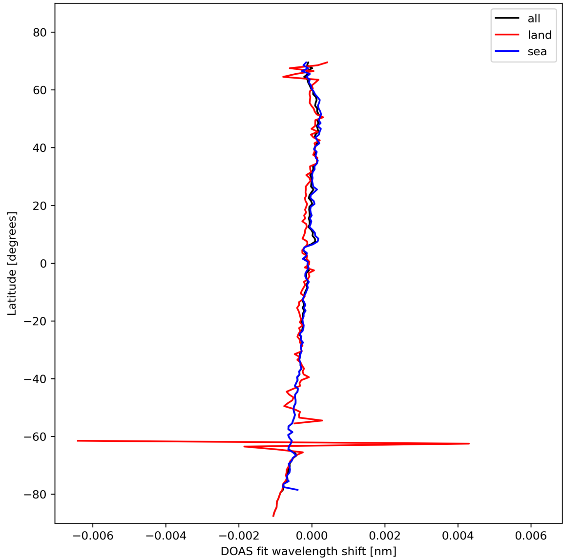
Figure 30: Zonal average of “DOAS fit wavelength shift” for 2023-11-04 to 2023-11-06.
