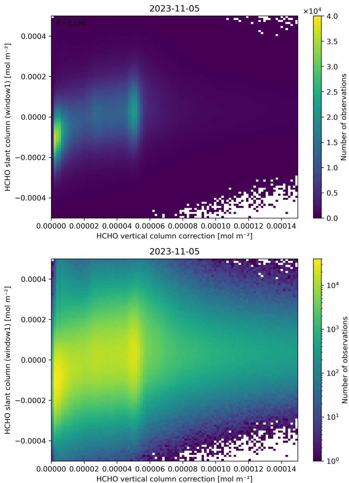
Figure 118: Scatter density plot of “HCHO vertical column correction” against “HCHO slant column (window1)” for 2023-11-04 to 2023-11-06.
