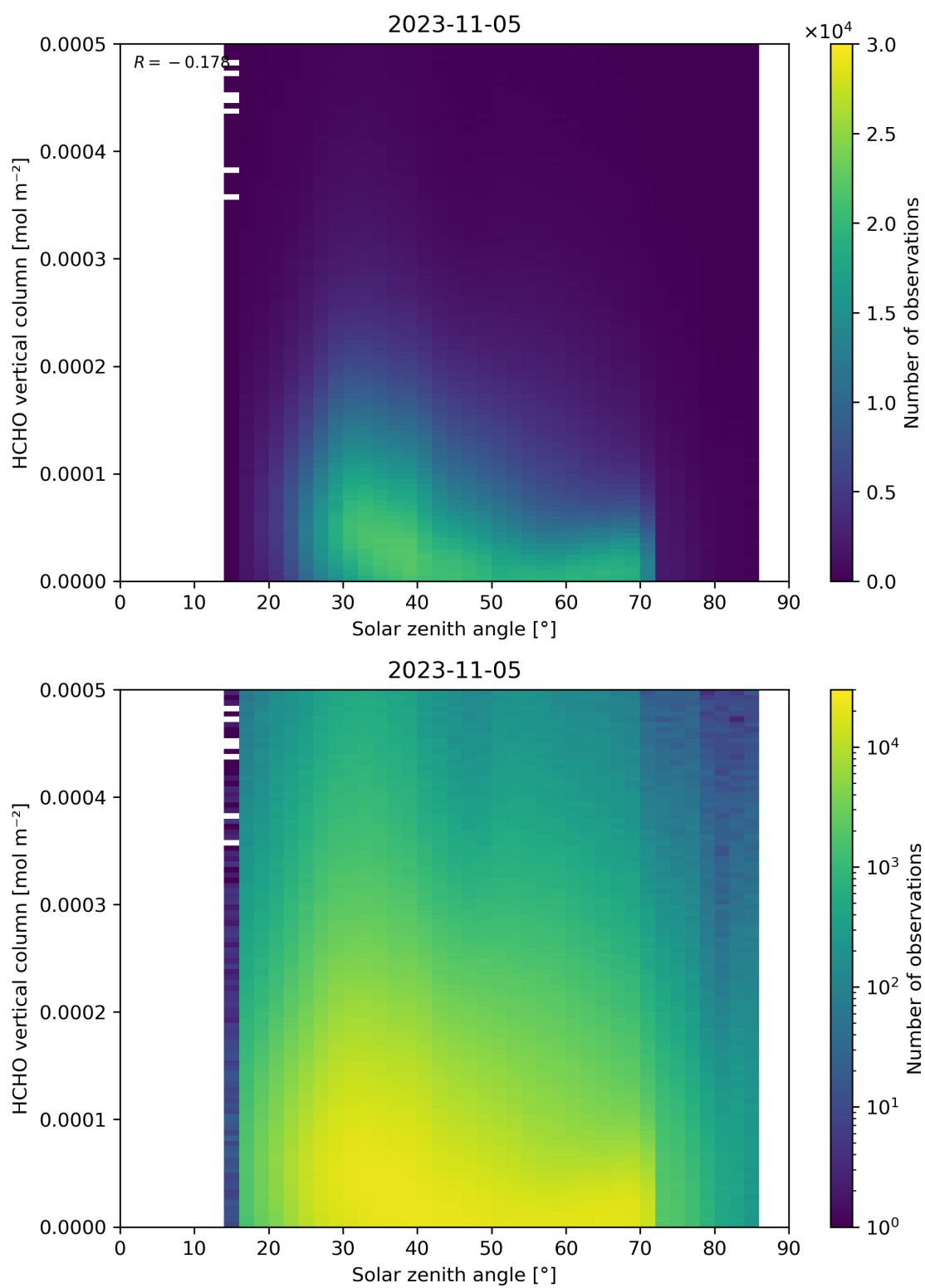
Figure 177: Scatter density plot of “Solar zenith angle” against “HCHO vertical column” for 2023-11-04 to 2023-11-06.
