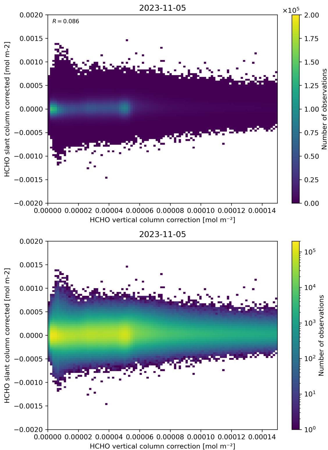
Figure 116: Scatter density plot of “HCHO vertical column correction” against “HCHO slant column corrected” for 2023-11-04 to 2023-11-06.
