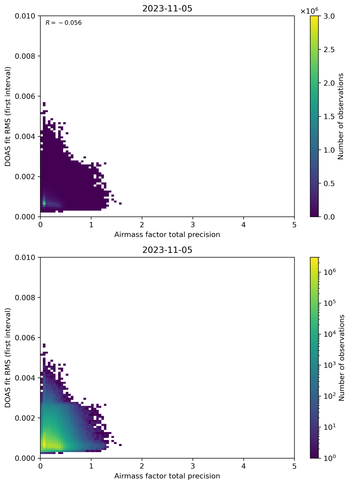
Figure 105: Scatter density plot of “Airmass factor total precision” against “DOAS fit RMS (first interval)” for 2023-11-04 to 2023-11-06.
