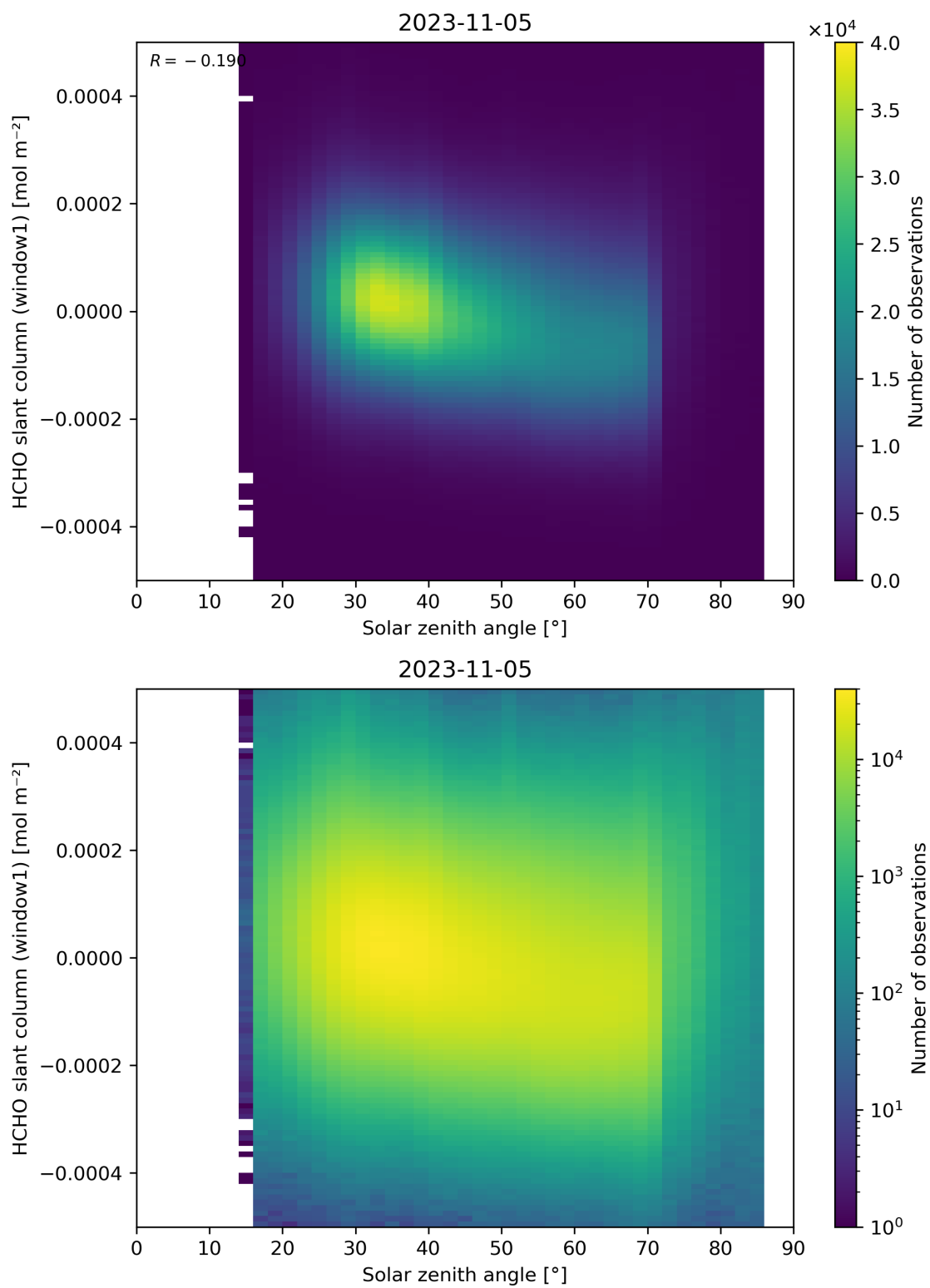
Figure 173: Scatter density plot of “Solar zenith angle” against “HCHO slant column (window1)” for 2023-11-04 to 2023-11-06.
