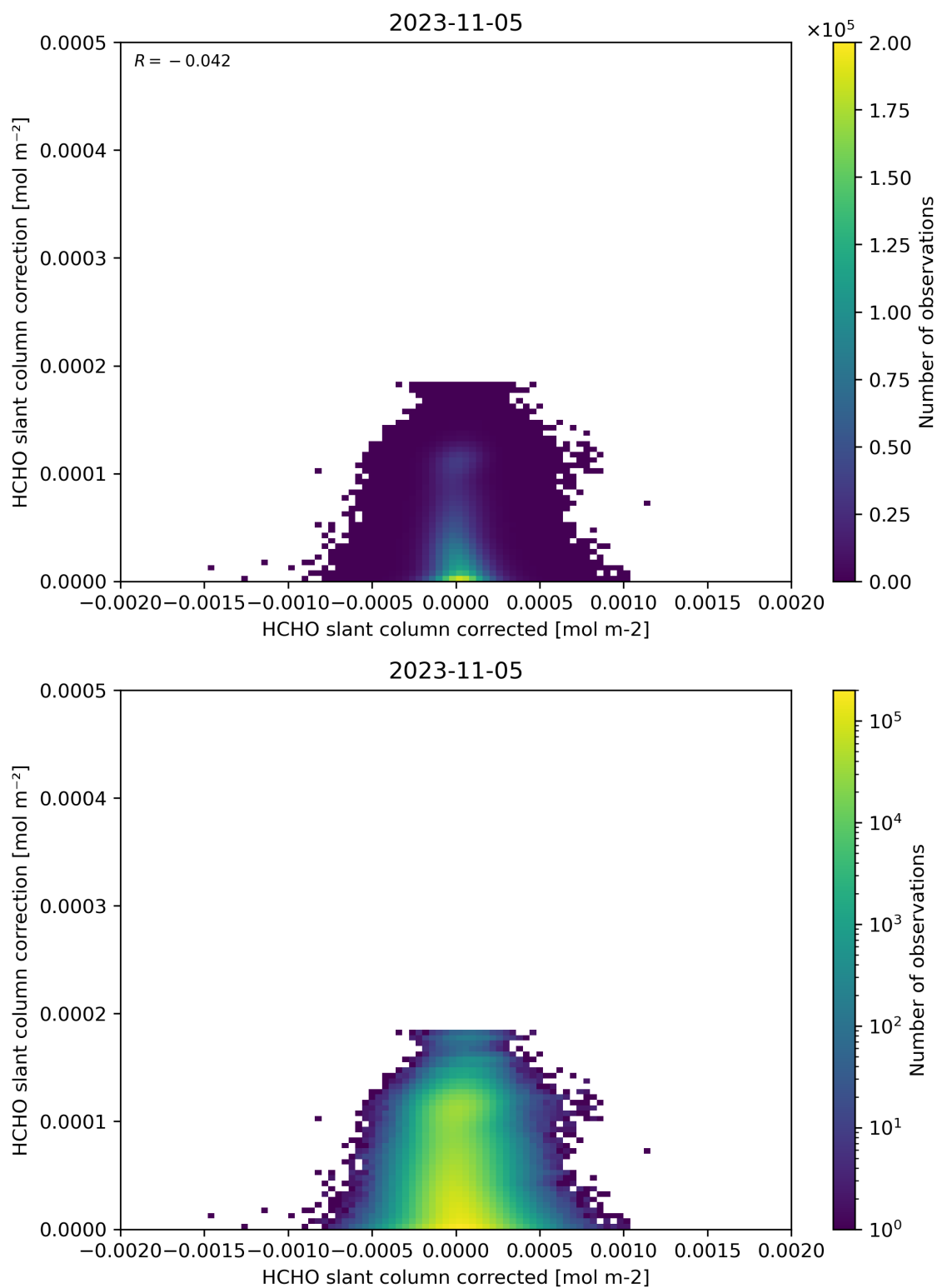
Figure 77: Scatter density plot of “HCHO slant column corrected” against “HCHO slant column correction” for 2023-11-04 to 2023-11-06.
