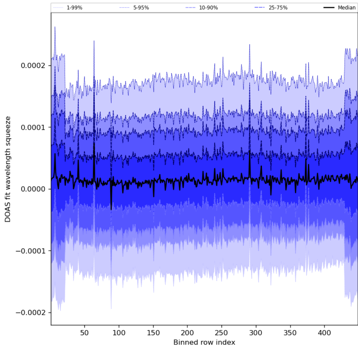
Figure 59: Along track statistics of “DOAS fit wavelength squeeze” for 2023-11-04 to 2023-11-06
