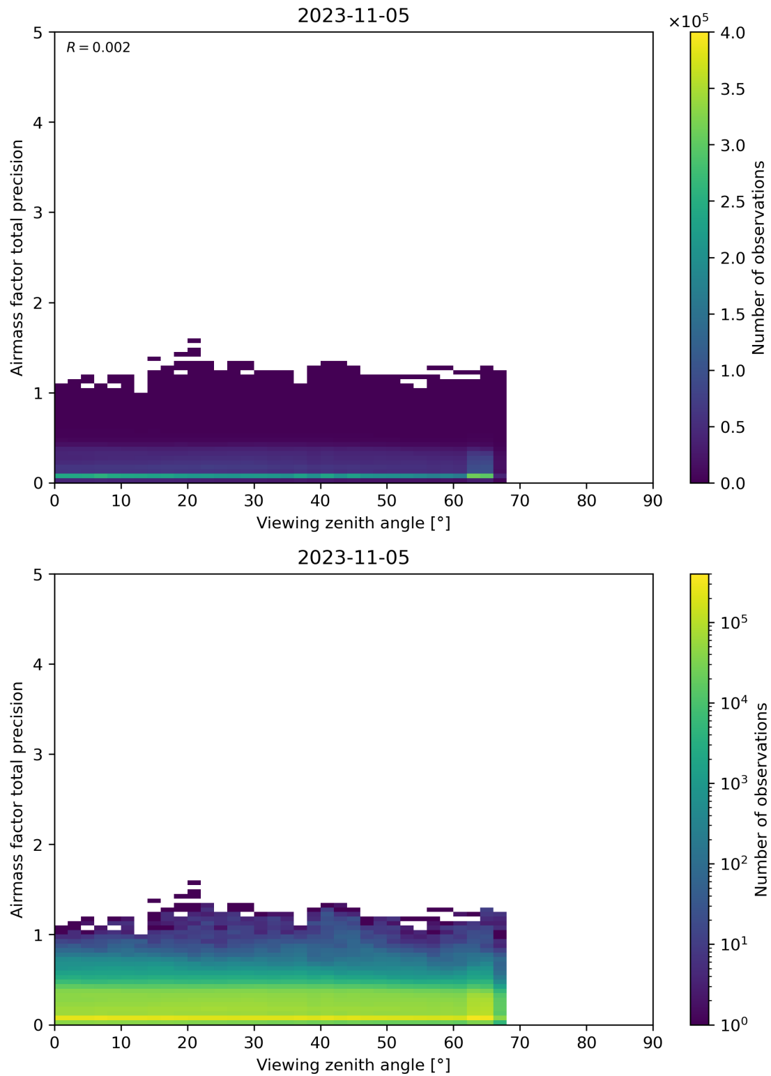
Figure 191: Scatter density plot of “Viewing zenith angle” against “Airmass factor total precision” for 2023-11-04 to 2023-11-06.
