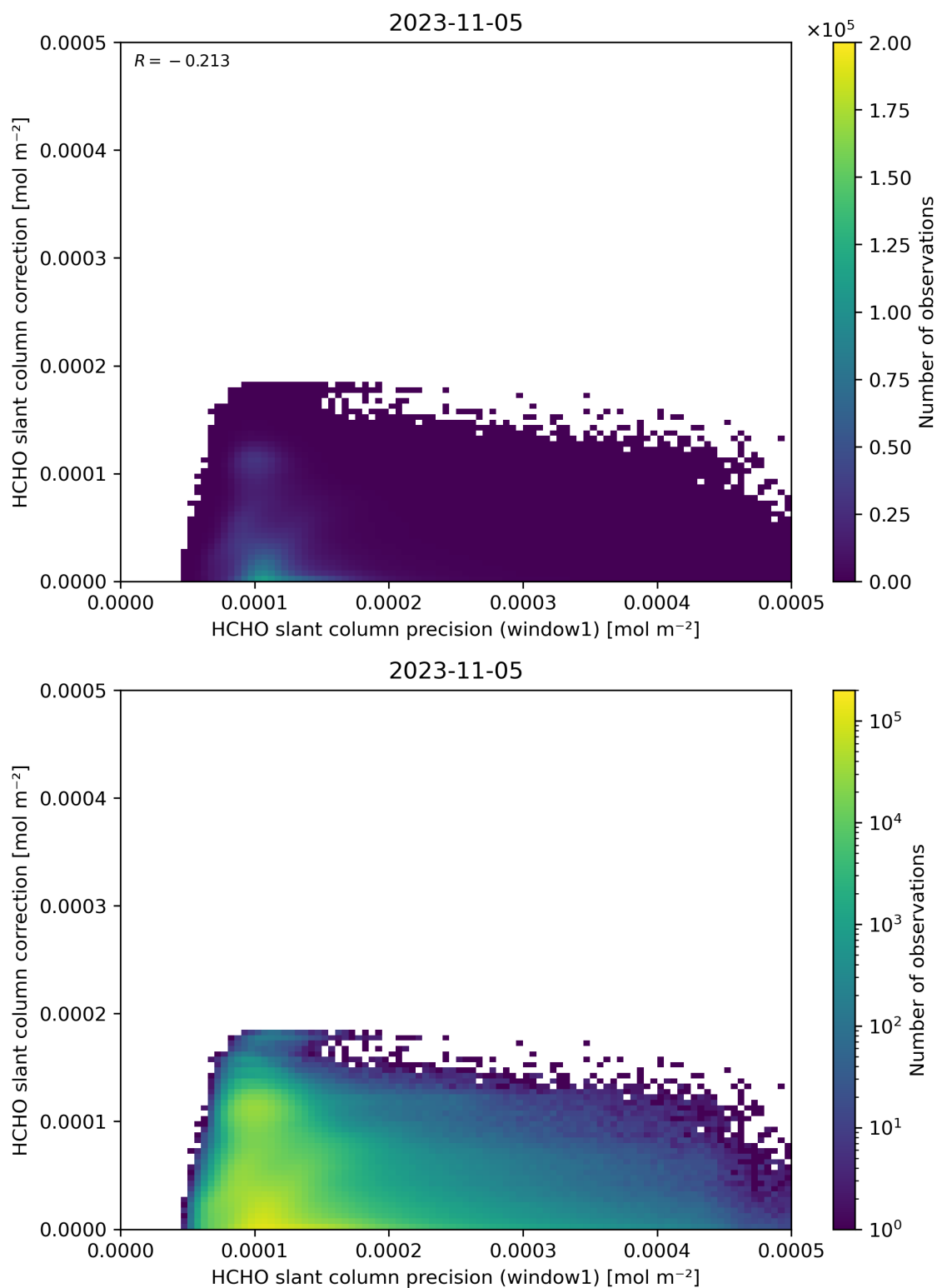
Figure 93: Scatter density plot of “HCHO slant column precision (window1)” against “HCHO slant column correction” for 2023-11-04 to 2023-11-06.
