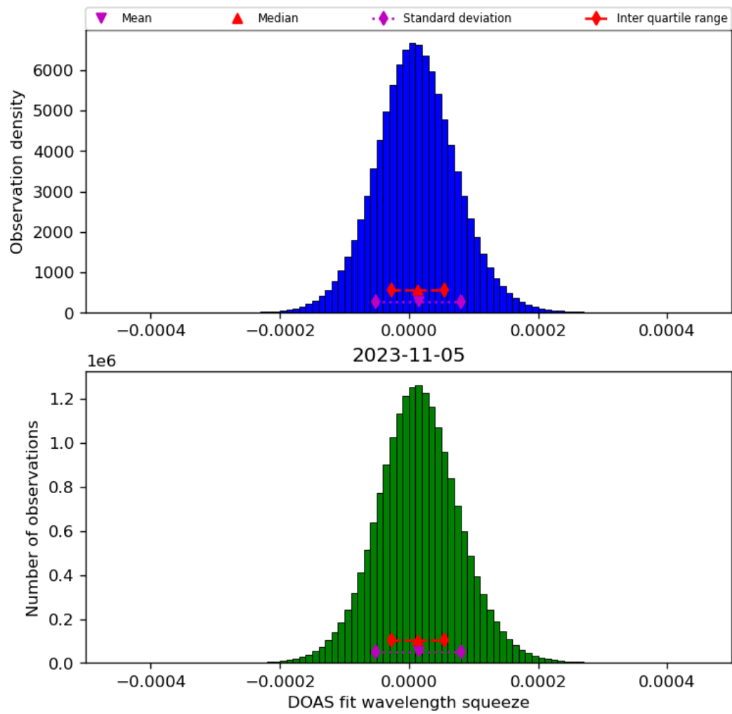
Figure 45: Histogram of “DOAS fit wavelength squeeze” for 2023-11-04 to 2023-11-06
