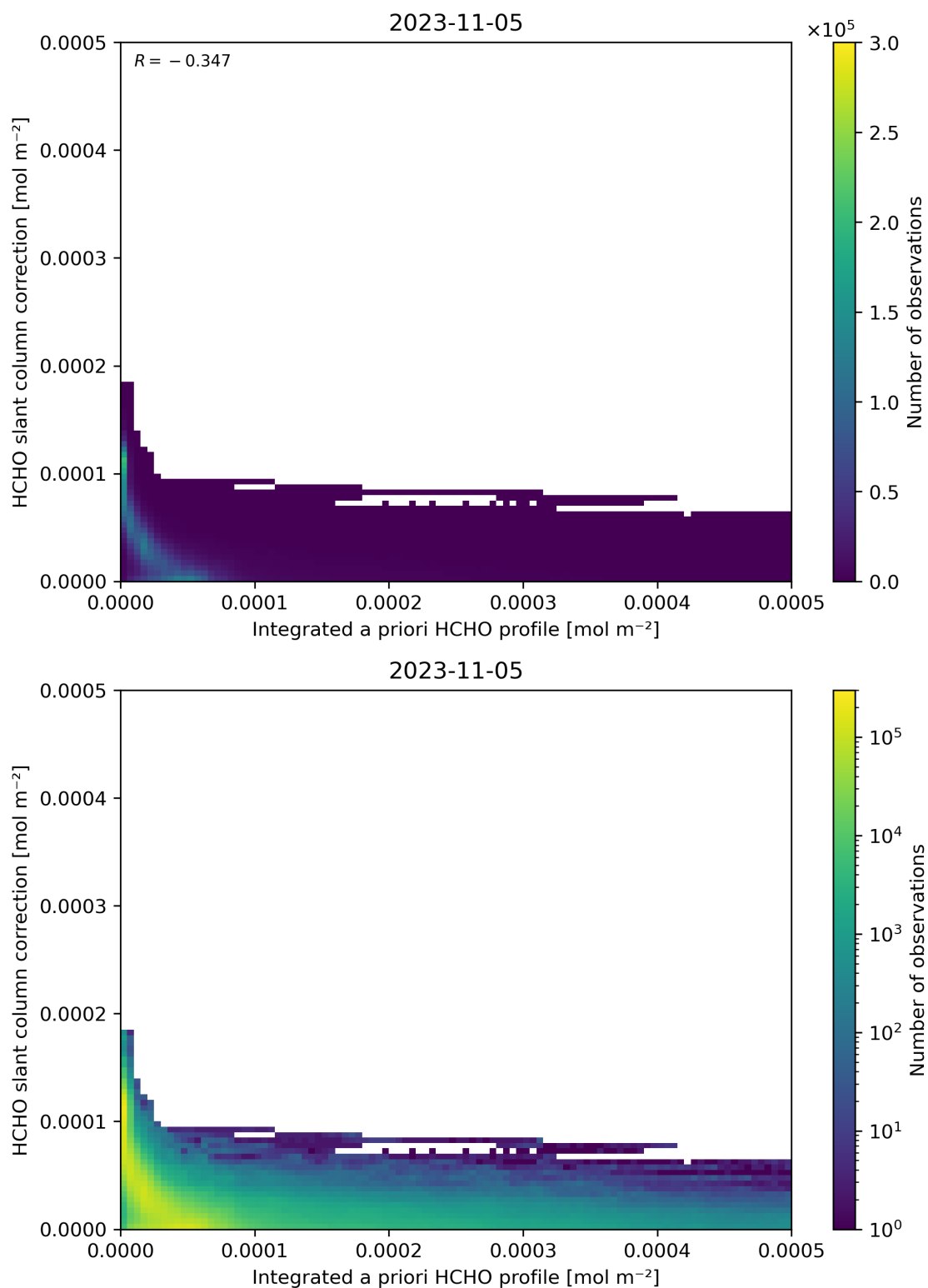
Figure 152: Scatter density plot of “Integrated a priori HCHO profile” against “HCHO slant column correction” for 2023-11-04 to 2023-11-06.
