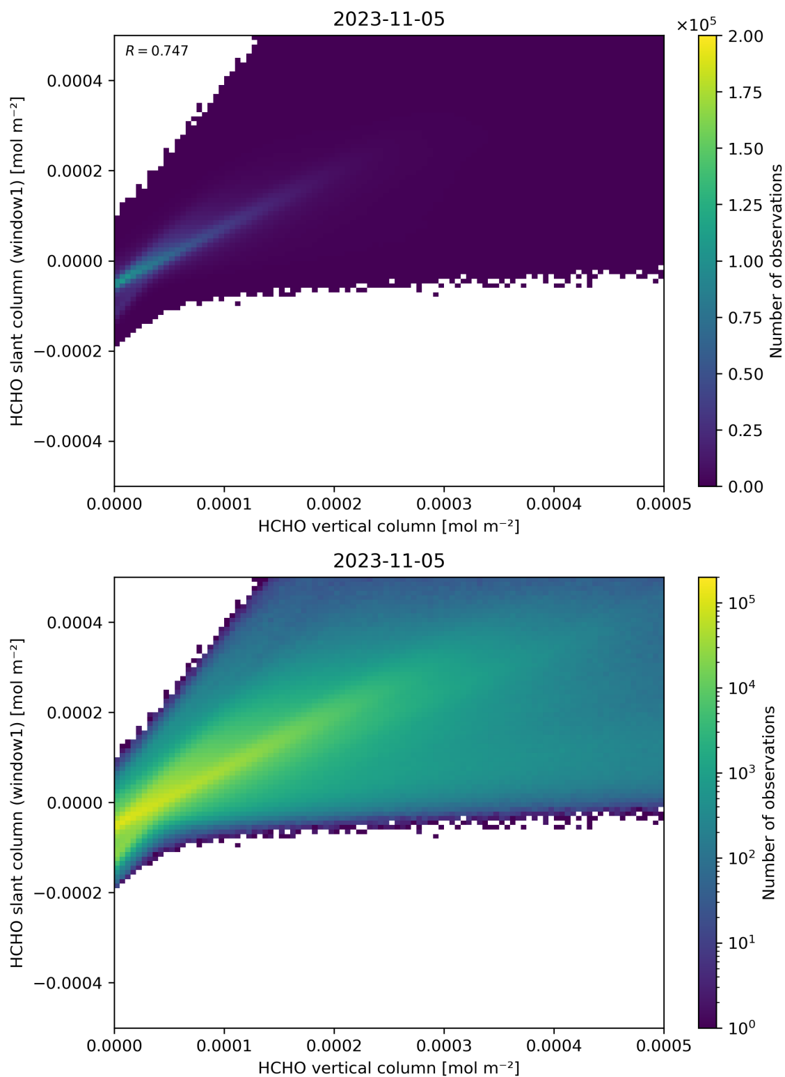
Figure 129: Scatter density plot of “HCHO vertical column” against “HCHO slant column (window1)” for 2023-11-04 to 2023-11-06.
