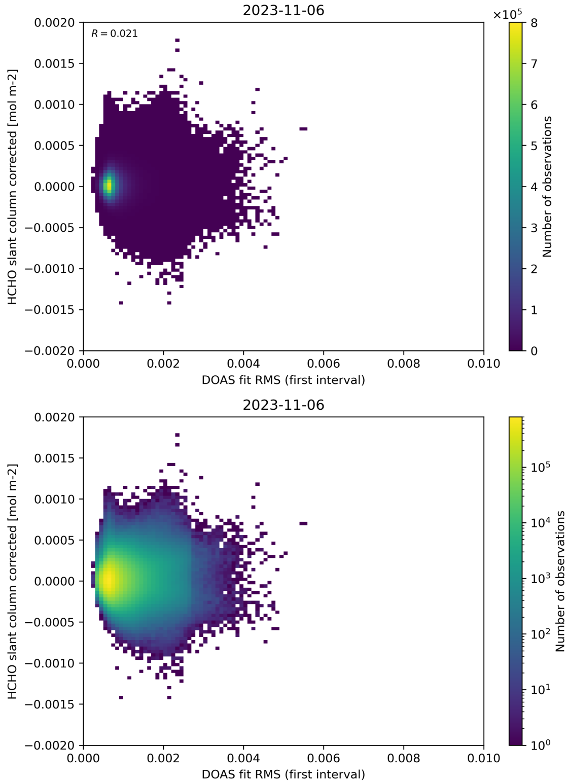
Figure 62: Scatter density plot of “DOAS fit RMS (first interval)” against “HCHO slant column corrected” for 2023-11-05 to 2023-11-07.
