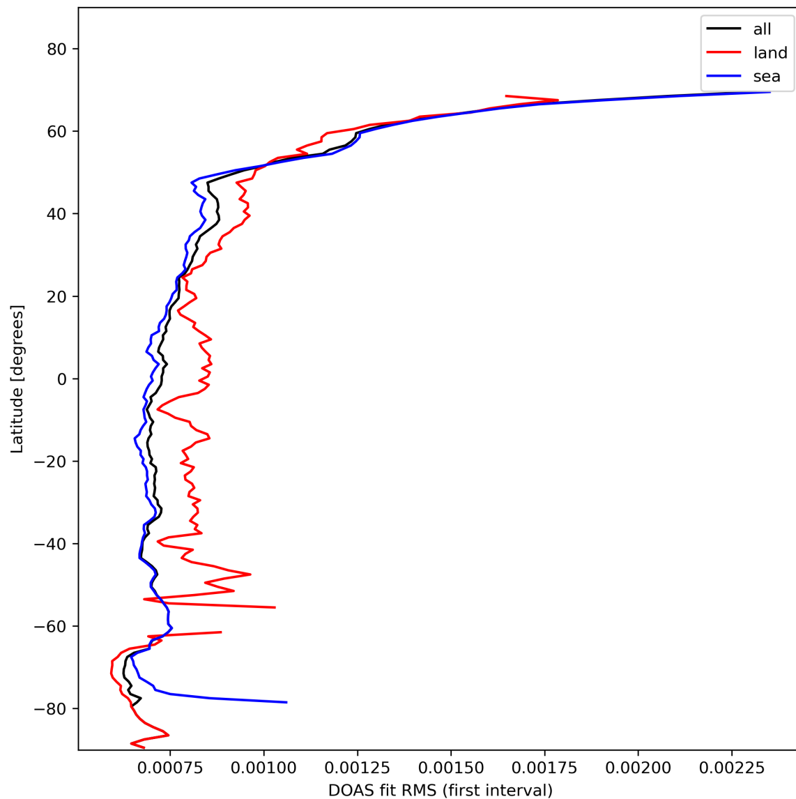
Figure 32: Zonal average of “DOAS fit RMS (first interval)” for 2023-11-05 to 2023-11-07.
