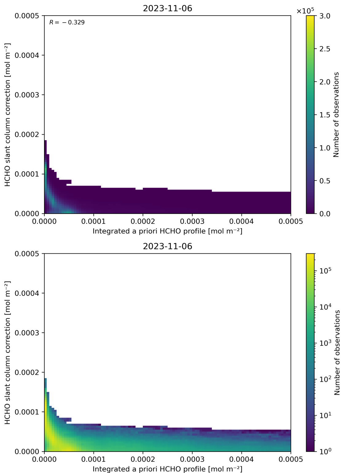
Figure 152: Scatter density plot of “Integrated a priori HCHO profile” against “HCHO slant column correction” for 2023-11-05 to 2023-11-07.
