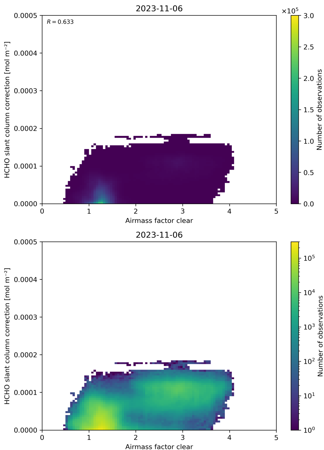
Figure 75: Scatter density plot of “Airmass factor clear” against “HCHO slant column correction” for 2023-11-05 to 2023-11-07.
