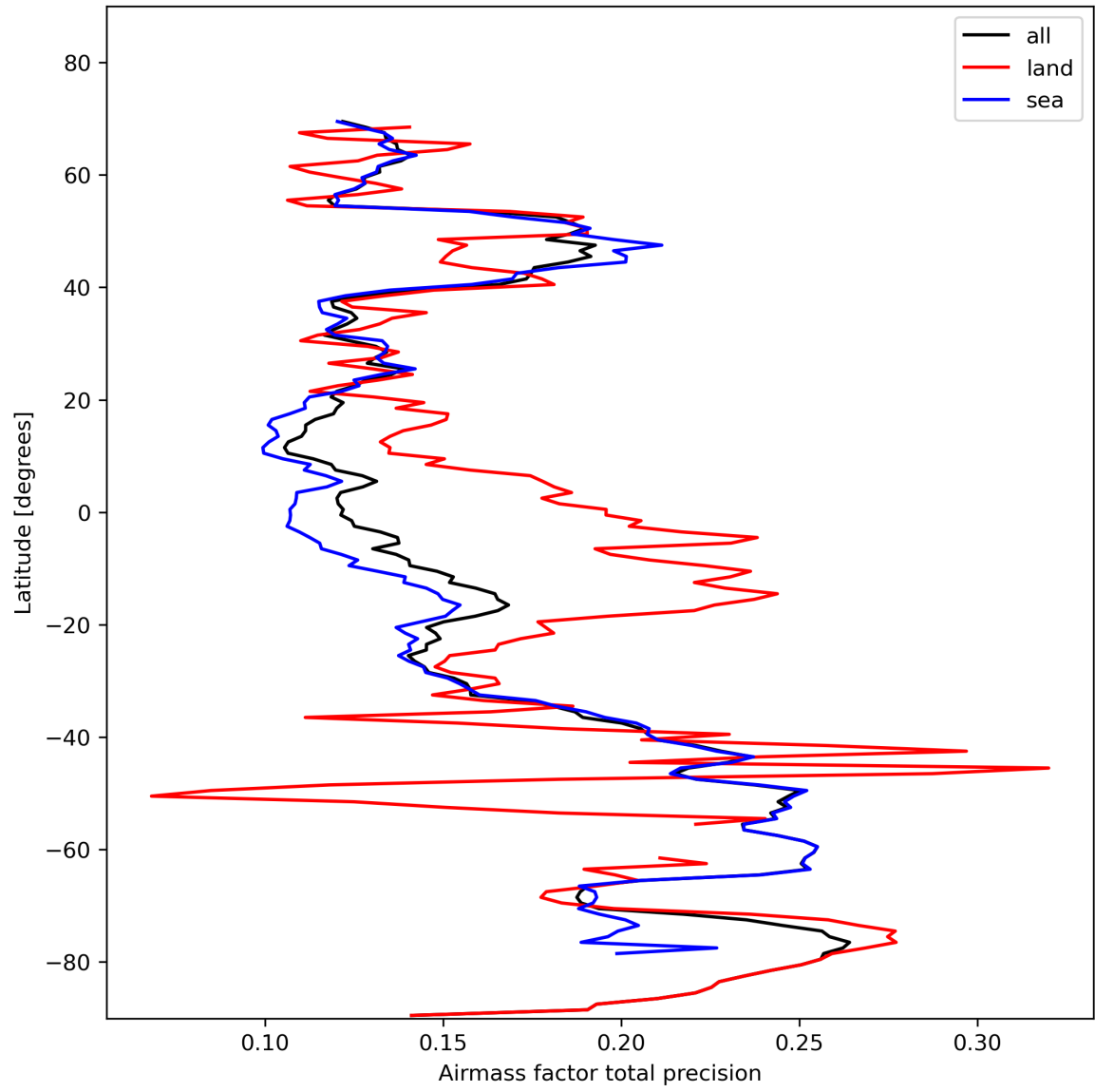
Figure 27: Zonal average of “Airmass factor total precision” for 2023-11-05 to 2023-11-07.
