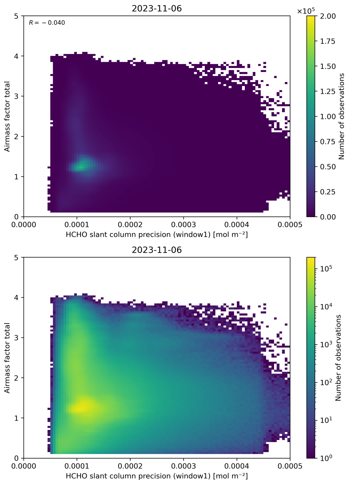
Figure 94: Scatter density plot of “HCHO slant column precision (window1)” against “Airmass factor total” for 2023-11-05 to 2023-11-07.
