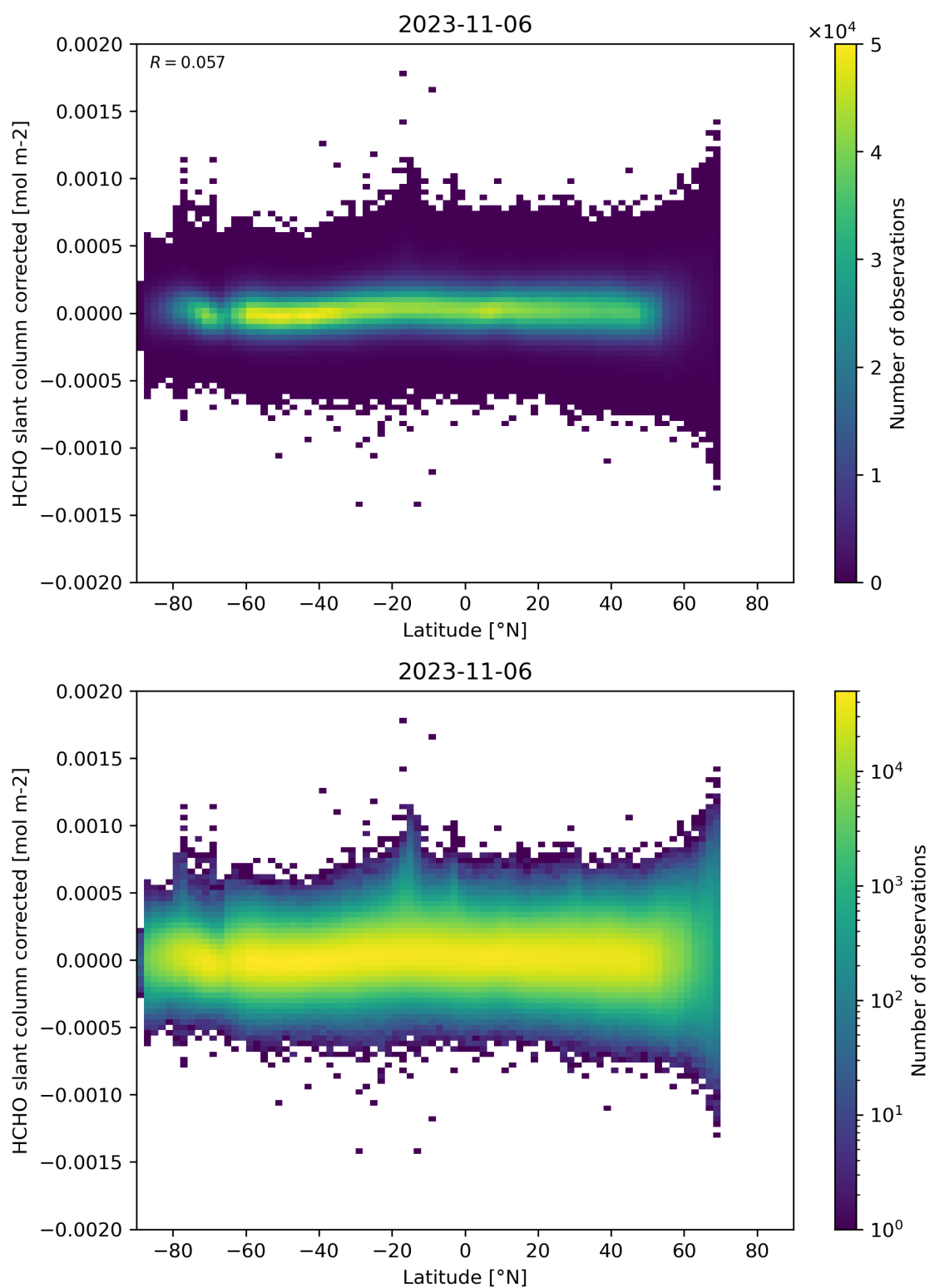
Figure 157: Scatter density plot of “Latitude” against “HCHO slant column corrected” for 2023-11-05 to 2023-11-07.
