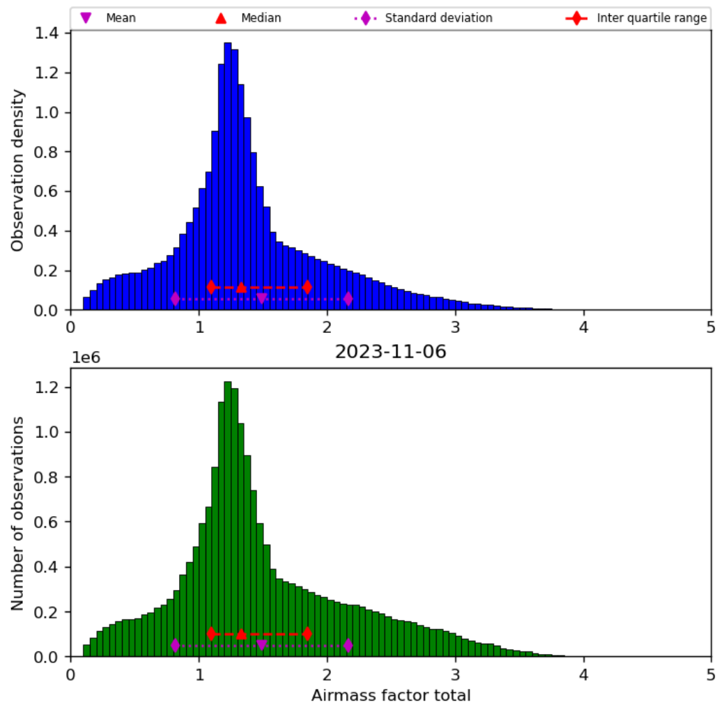
Figure 40: Histogram of “Airmass factor total” for 2023-11-05 to 2023-11-07
