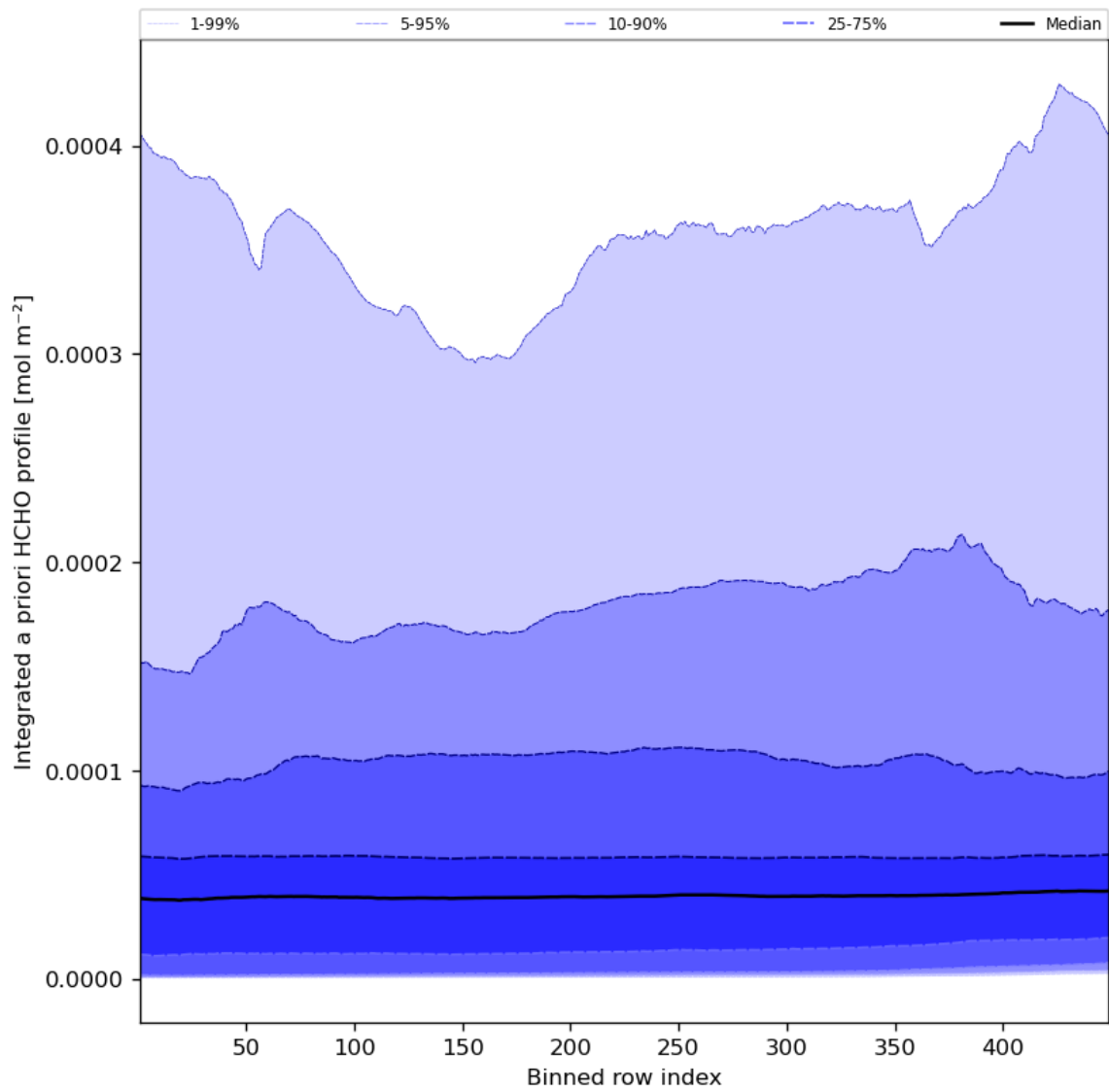
Figure 57: Along track statistics of “Integrated a priori HCHO profile” for 2023-11-05 to 2023-11-07
