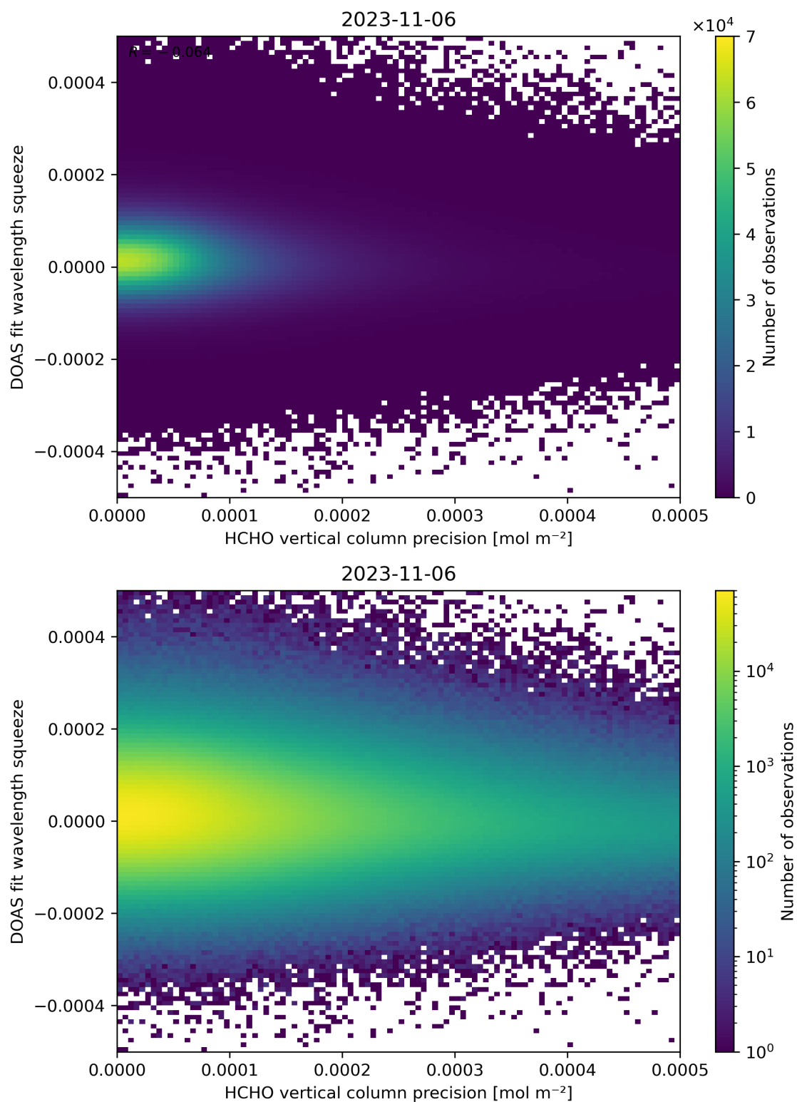
Figure 138: Scatter density plot of “HCHO vertical column precision” against “DOAS fit wavelength squeeze” for 2023-11-05 to 2023-11-07.
