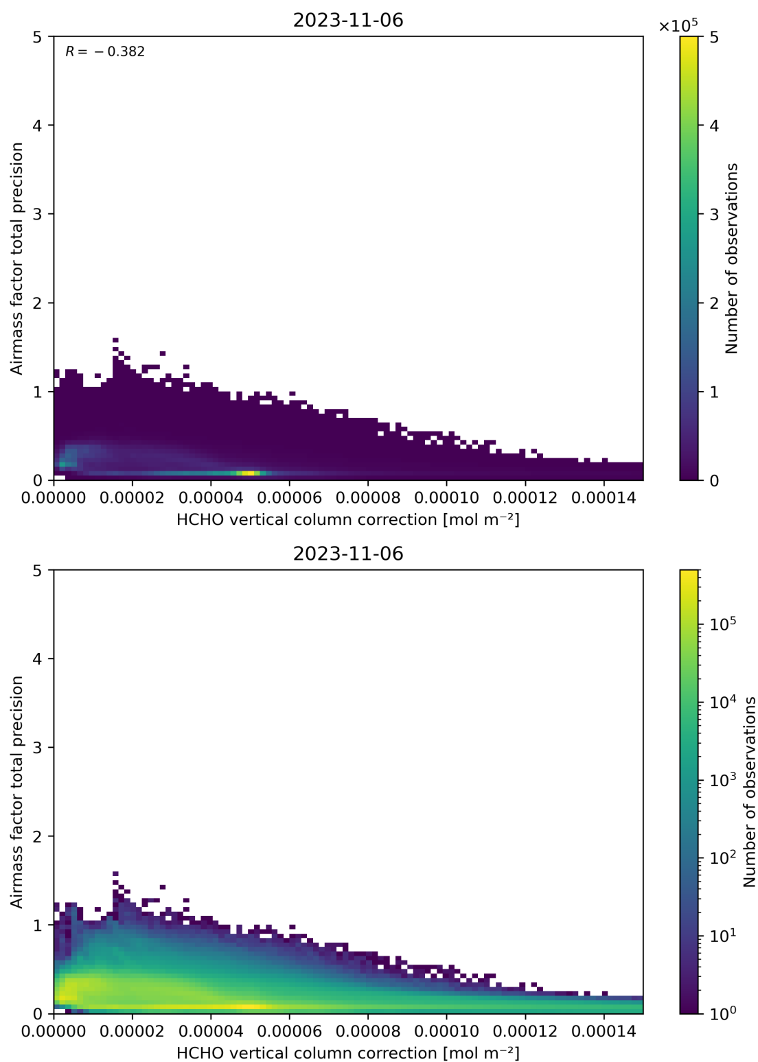
Figure 121: Scatter density plot of “HCHO vertical column correction” against “Airmass factor total precision” for 2023-11-05 to 2023-11-07.
