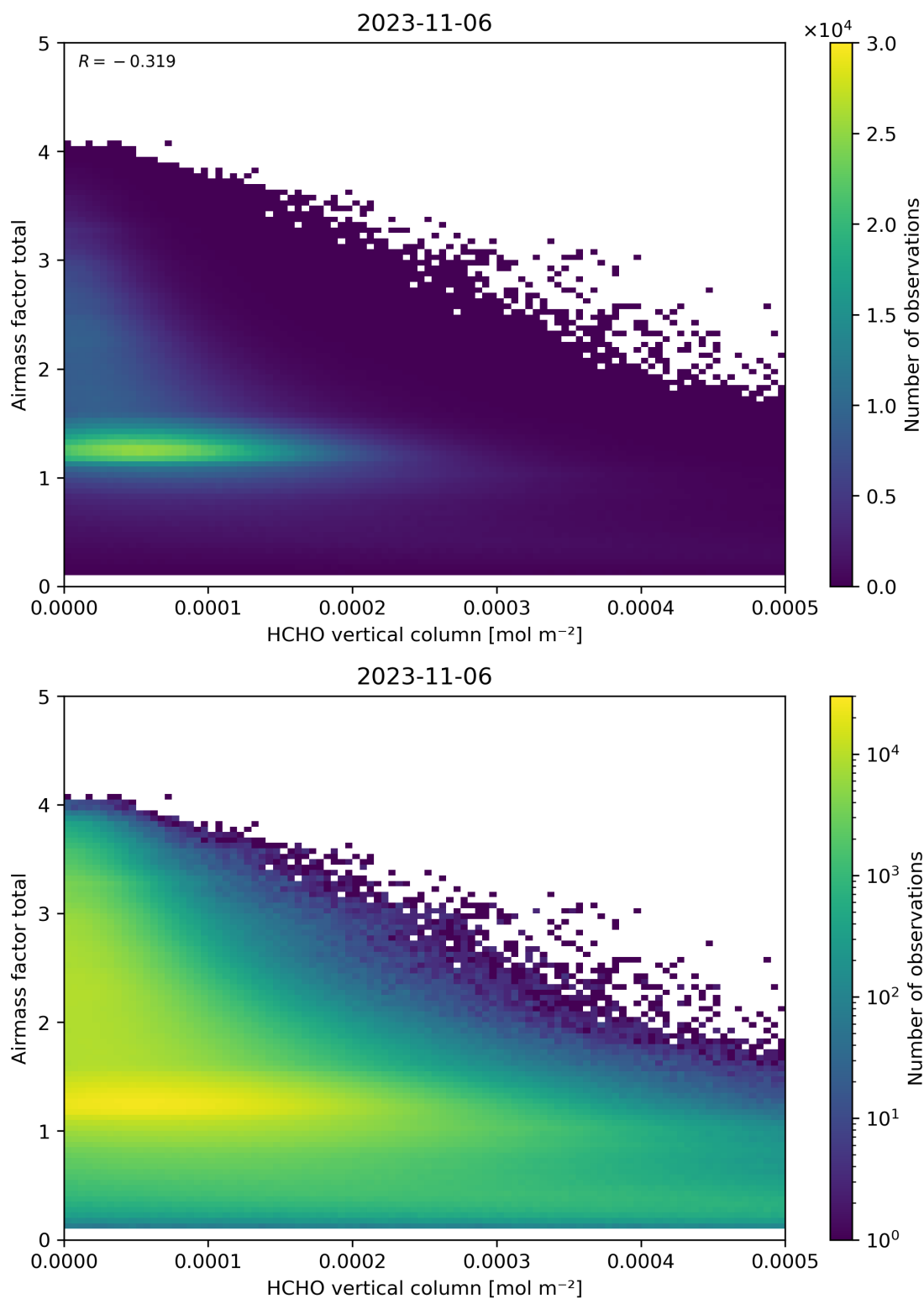
Figure 131: Scatter density plot of “HCHO vertical column” against “Airmass factor total” for 2023-11-05 to 2023-11-07.
