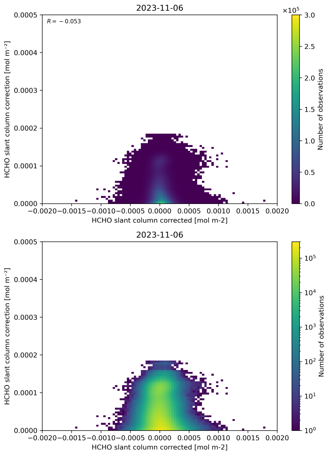
Figure 77: Scatter density plot of “HCHO slant column corrected” against “HCHO slant column correction” for 2023-11-05 to 2023-11-07.
