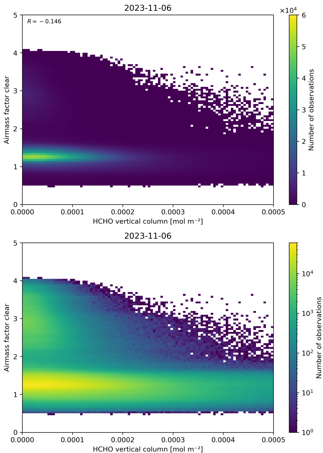
Figure 126: Scatter density plot of “HCHO vertical column” against “Airmass factor clear” for 2023-11-05 to 2023-11-07.
