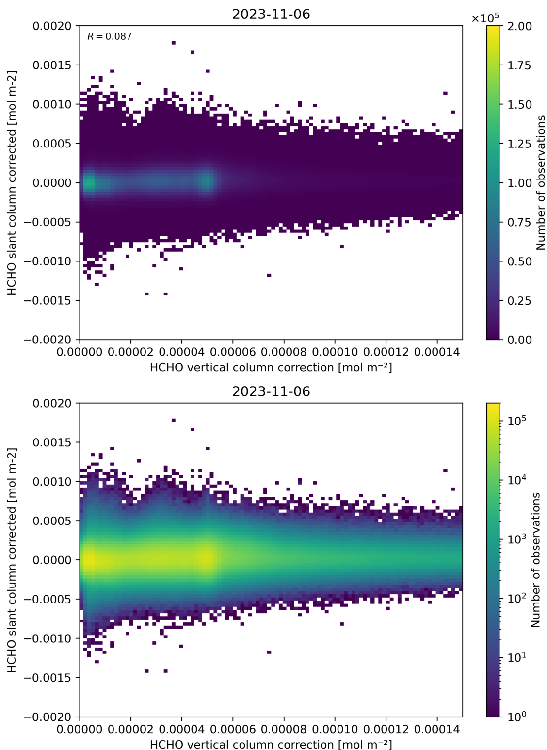
Figure 116: Scatter density plot of “HCHO vertical column correction” against “HCHO slant column corrected” for 2023-11-05 to 2023-11-07.
