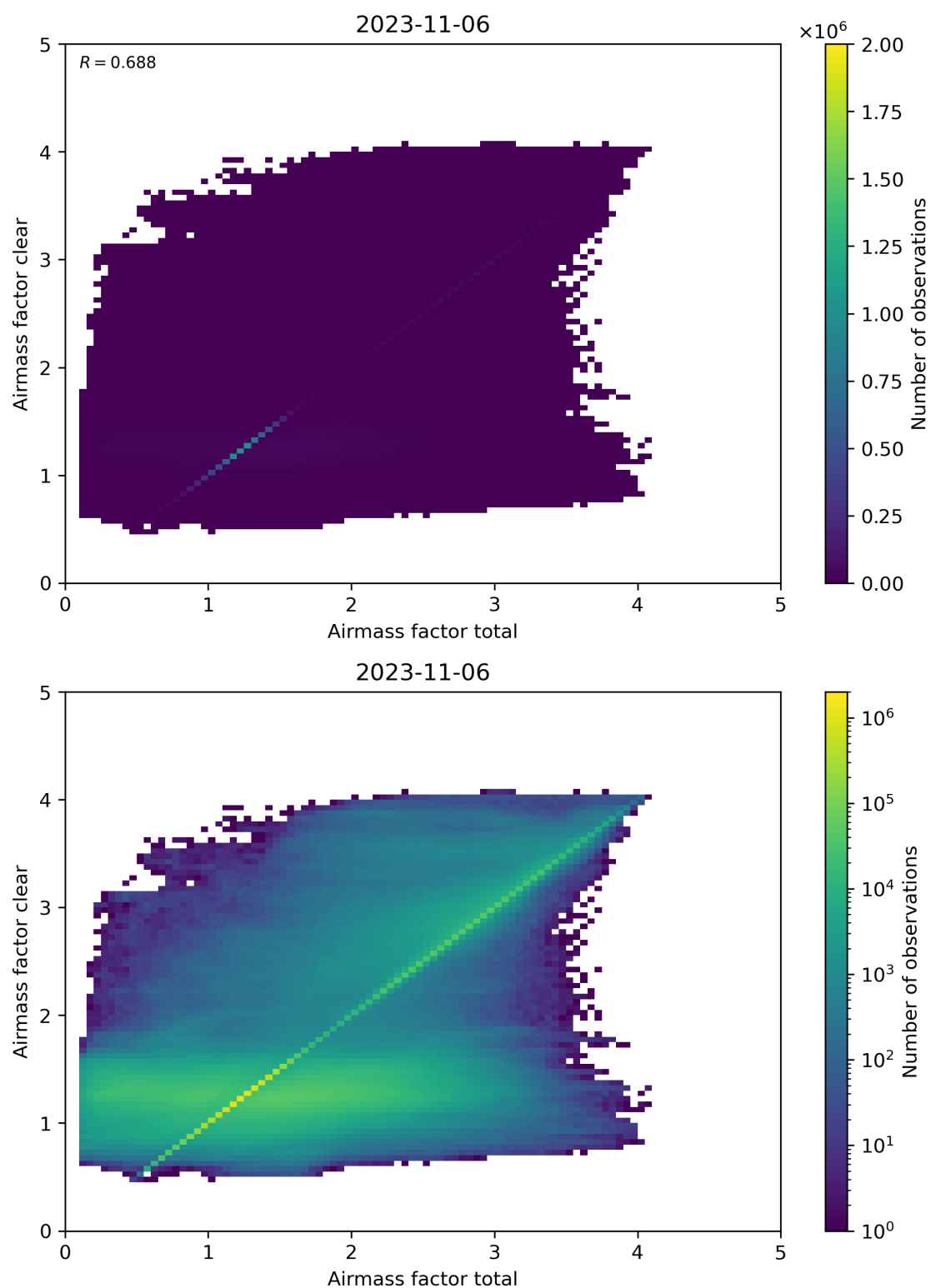
Figure 100: Scatter density plot of “Airmass factor total” against “Airmass factor clear” for 2023-11-05 to 2023-11-07.
