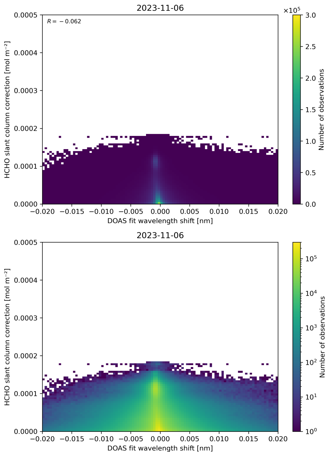
Figure 67: Scatter density plot of “DOAS fit wavelength shift” against “HCHO slant column correction” for 2023-11-05 to 2023-11-07.
