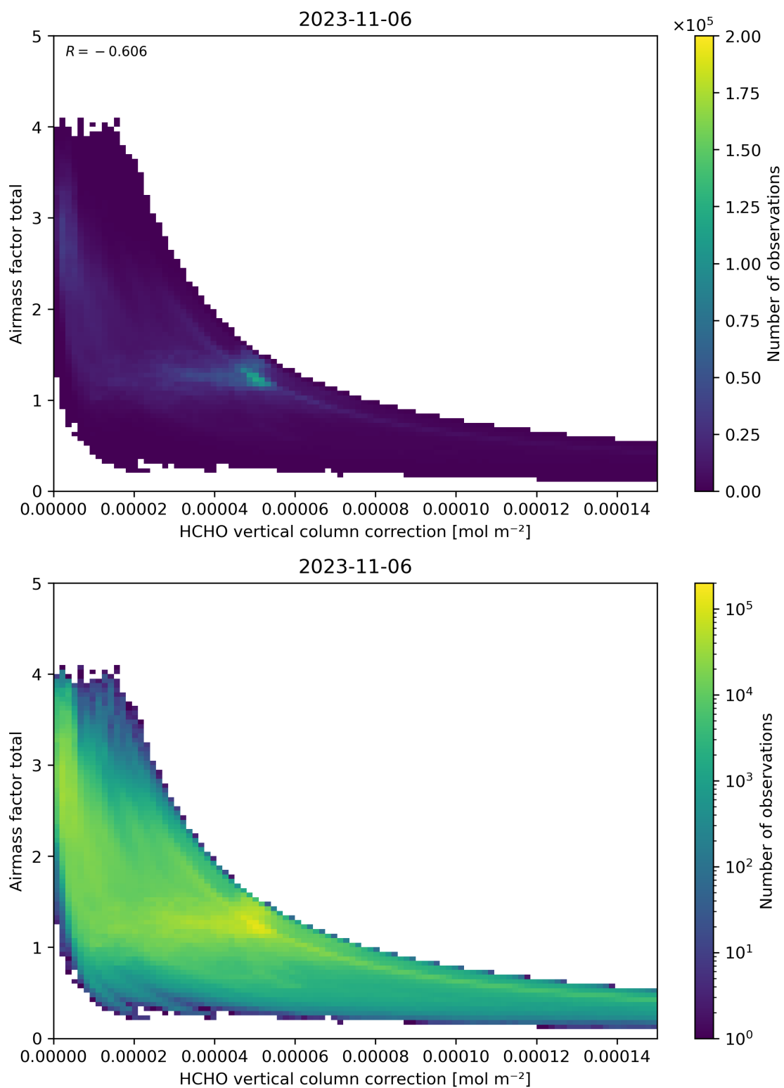
Figure 120: Scatter density plot of “HCHO vertical column correction” against “Airmass factor total” for 2023-11-05 to 2023-11-07.
