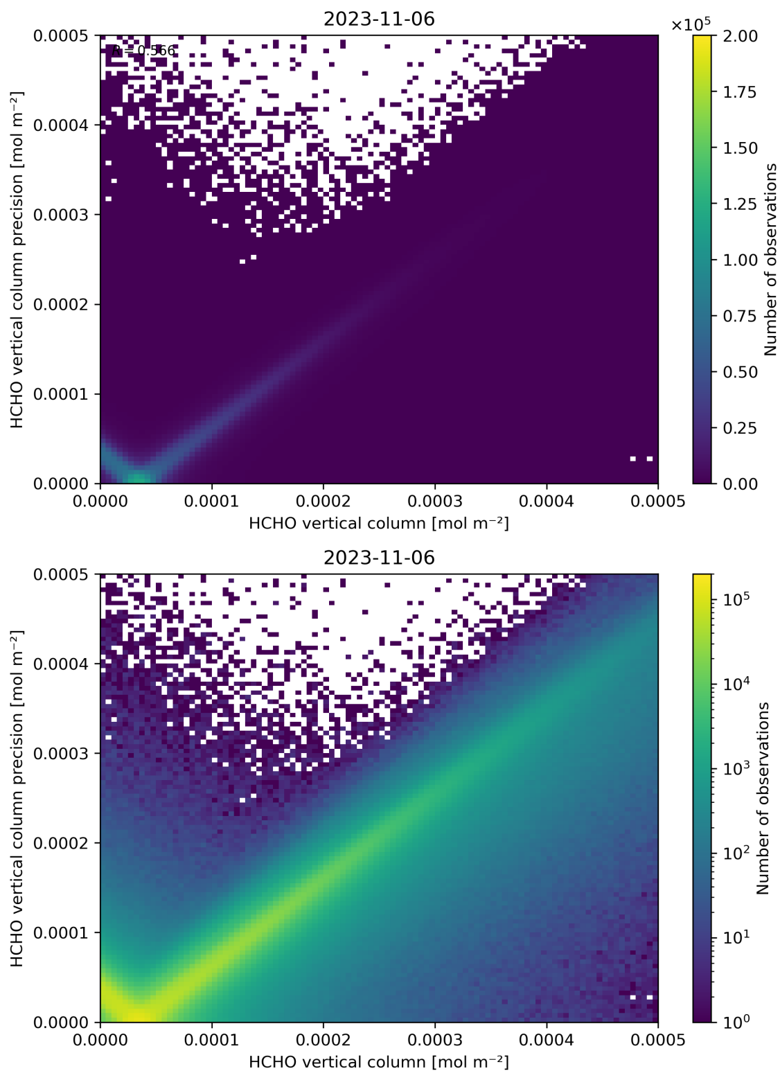
Figure 134: Scatter density plot of “HCHO vertical column” against “HCHO vertical column precision” for 2023-11-05 to 2023-11-07.
