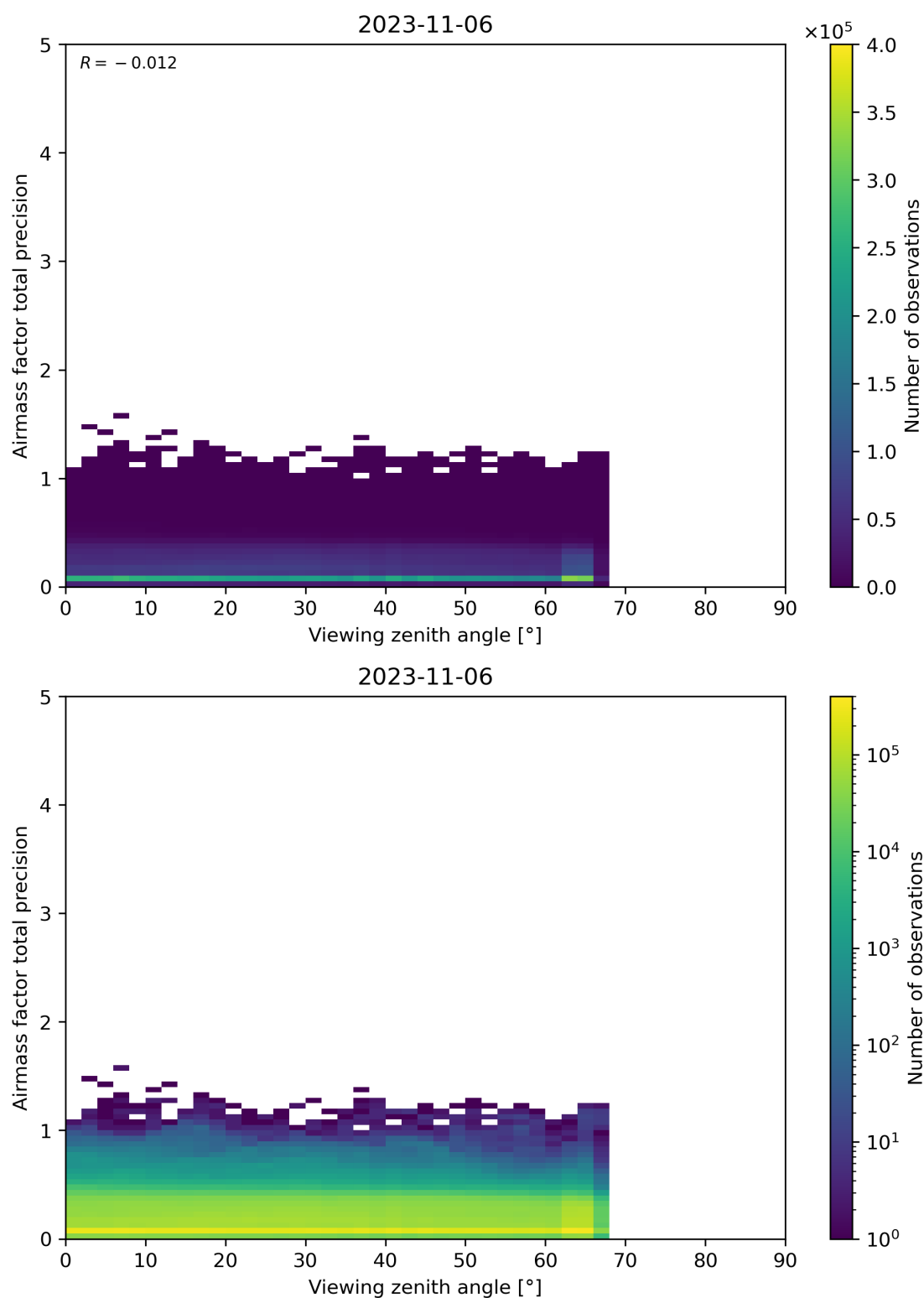
Figure 191: Scatter density plot of “Viewing zenith angle” against “Airmass factor total precision” for 2023-11-05 to 2023-11-07.
