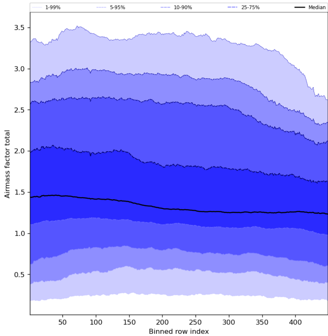
Figure 54: Along track statistics of “Airmass factor total” for 2023-11-05 to 2023-11-07
