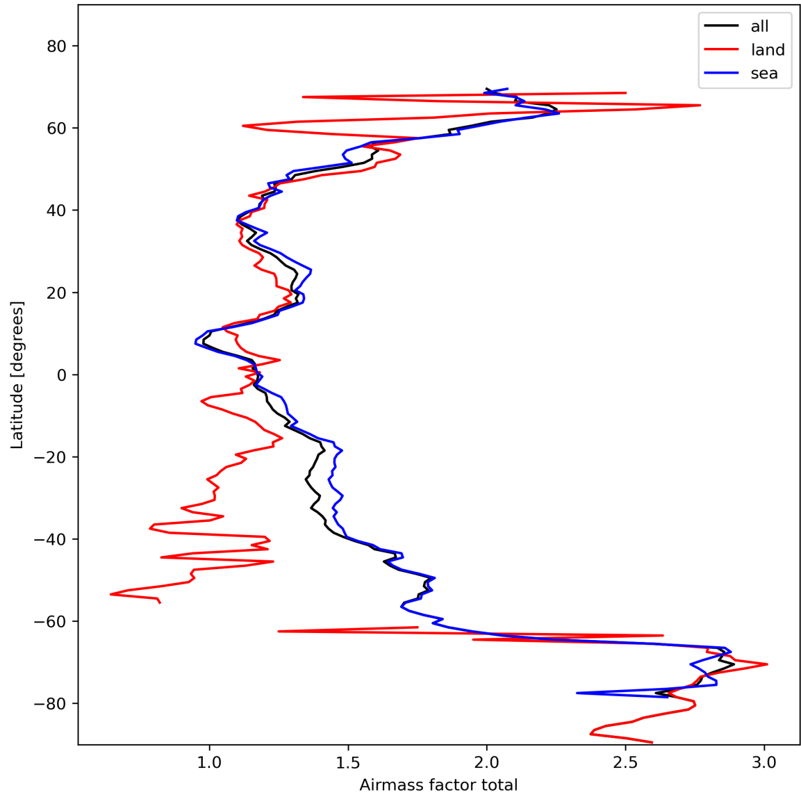
Figure 26: Zonal average of “Airmass factor total” for 2023-11-05 to 2023-11-07.
