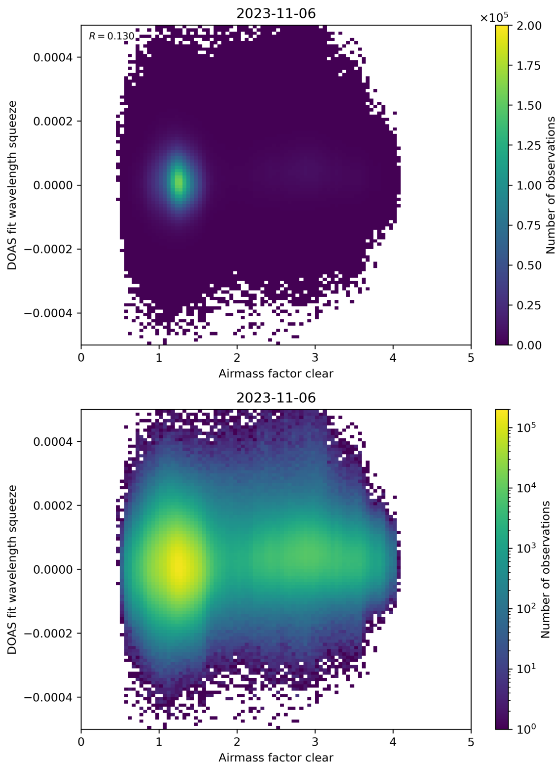
Figure 73: Scatter density plot of “Airmass factor clear” against “DOAS fit wavelength squeeze” for 2023-11-05 to 2023-11-07.
