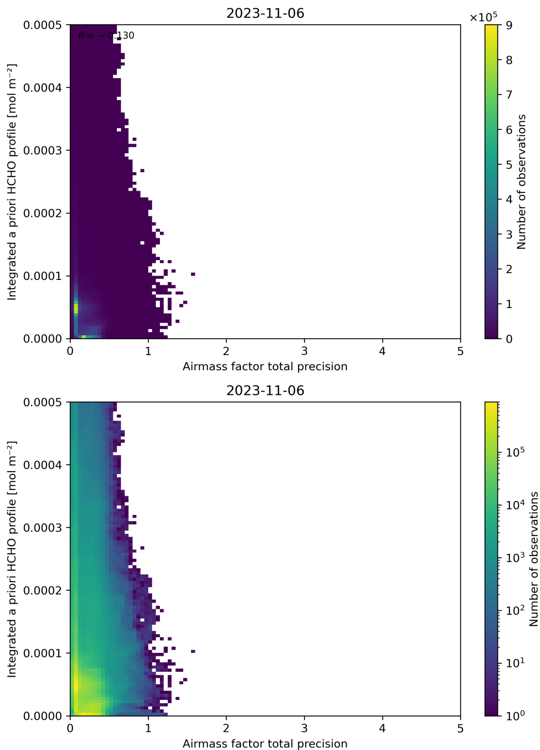
Figure 111: Scatter density plot of “Airmass factor total precision” against “Integrated a priori HCHO profile” for 2023-11-05 to 2023-11-07.
