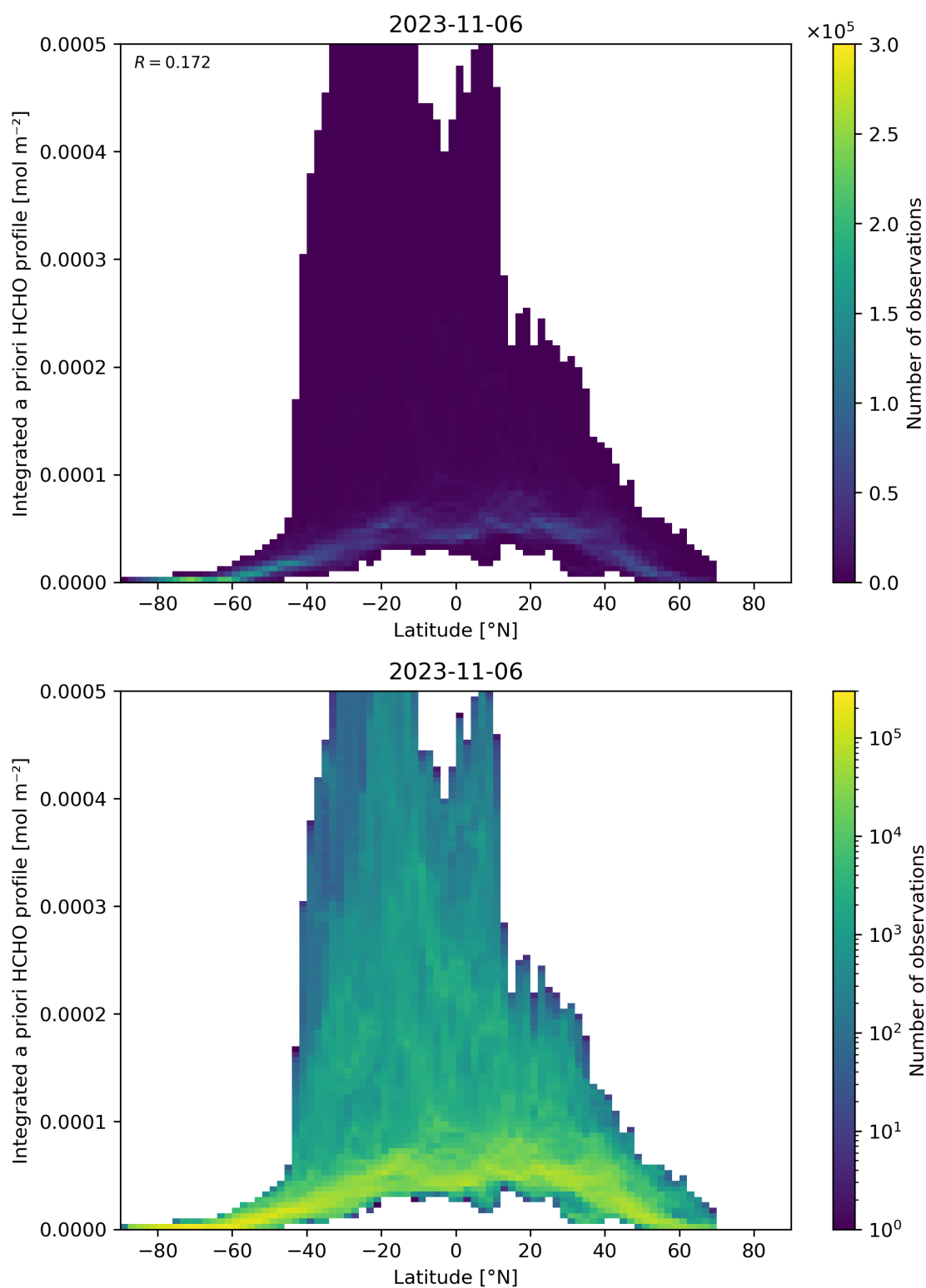
Figure 166: Scatter density plot of “Latitude” against “Integrated a priori HCHO profile” for 2023-11-05 to 2023-11-07.
