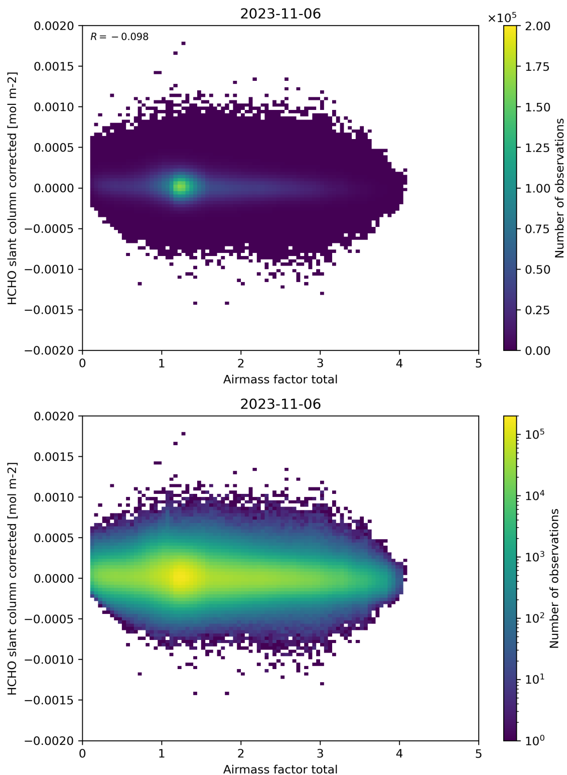
Figure 101: Scatter density plot of “Airmass factor total” against “HCHO slant column corrected” for 2023-11-05 to 2023-11-07.
