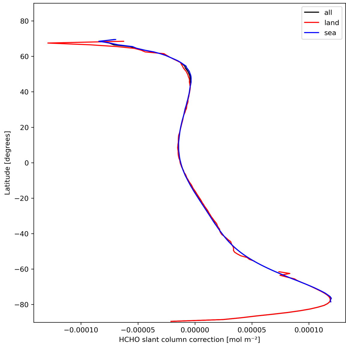
Figure 33: Zonal average of “HCHO slant column correction” for 2023-11-05 to 2023-11-07.
