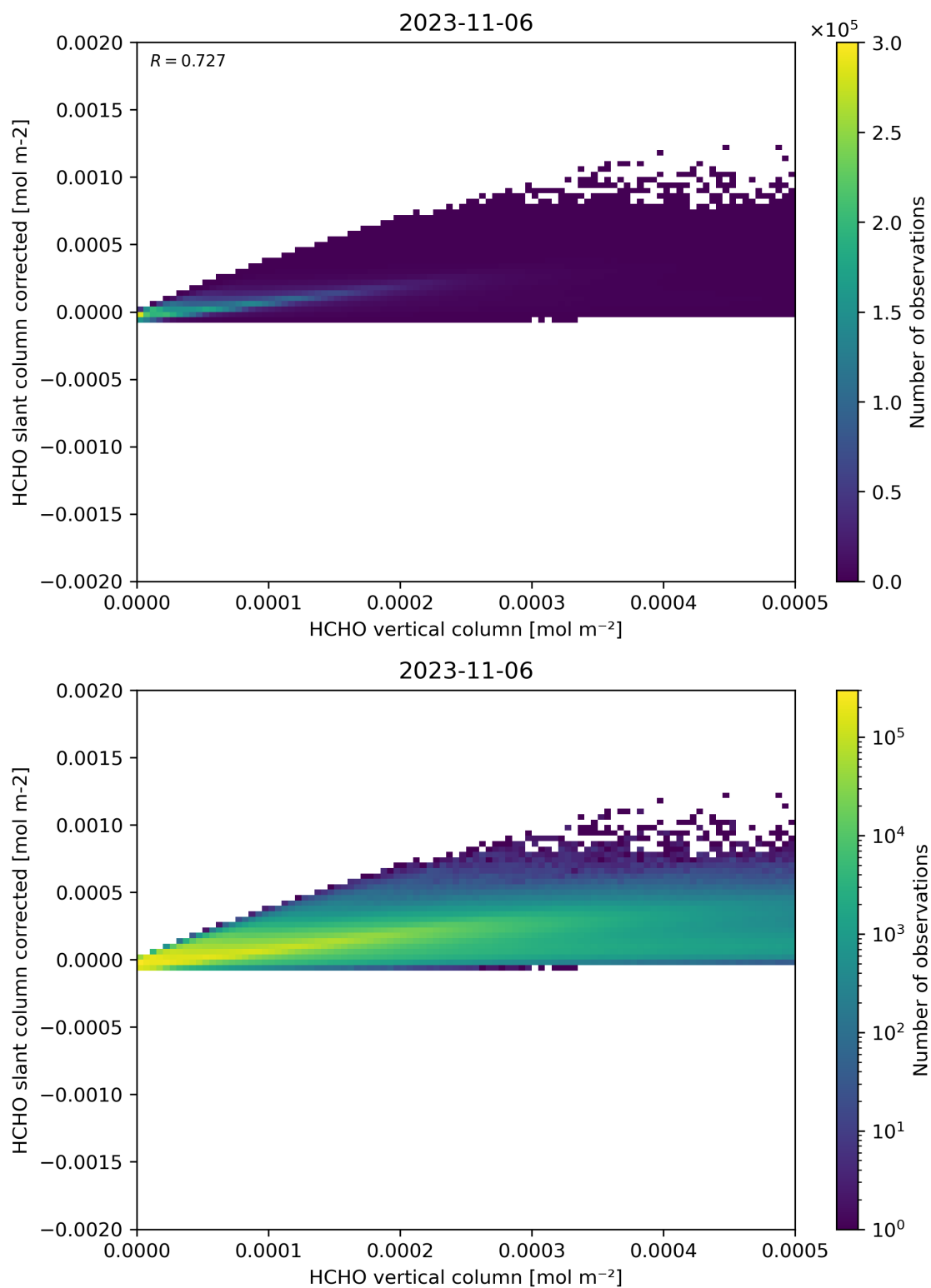
Figure 127: Scatter density plot of “HCHO vertical column” against “HCHO slant column corrected” for 2023-11-05 to 2023-11-07.
