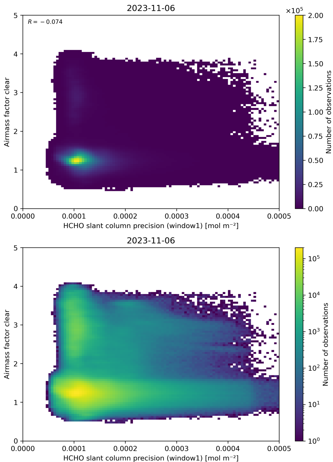
Figure 91: Scatter density plot of “HCHO slant column precision (window1)” against “Airmass factor clear” for 2023-11-05 to 2023-11-07.
