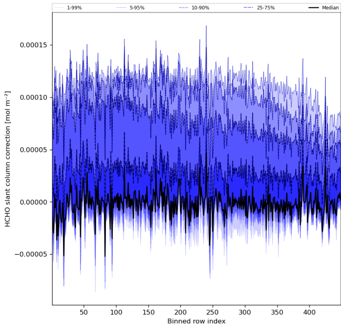
Figure 61: Along track statistics of “HCHO slant column correction” for 2023-11-05 to 2023-11-07
