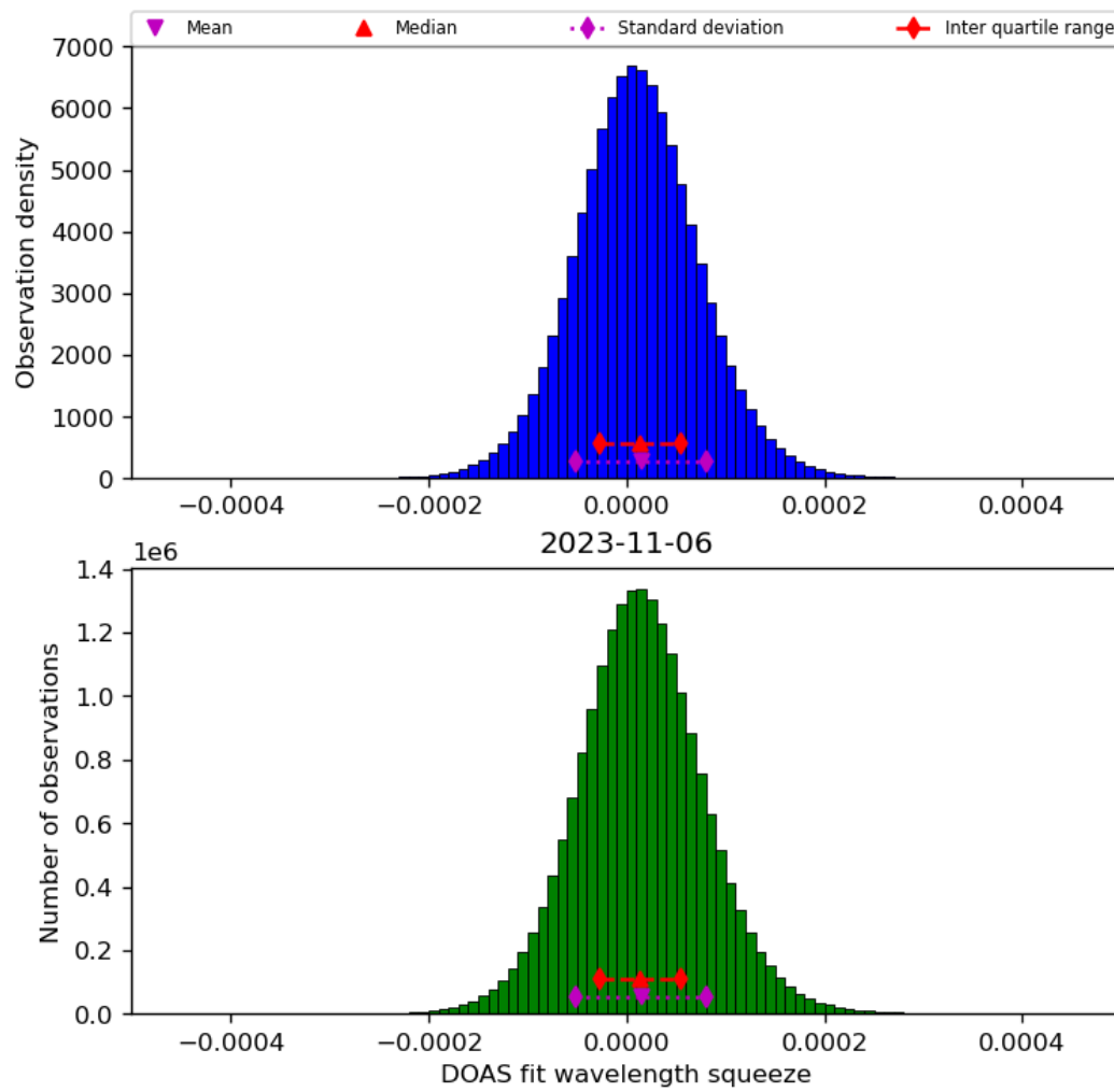
Figure 45: Histogram of “DOAS fit wavelength squeeze” for 2023-11-05 to 2023-11-07
