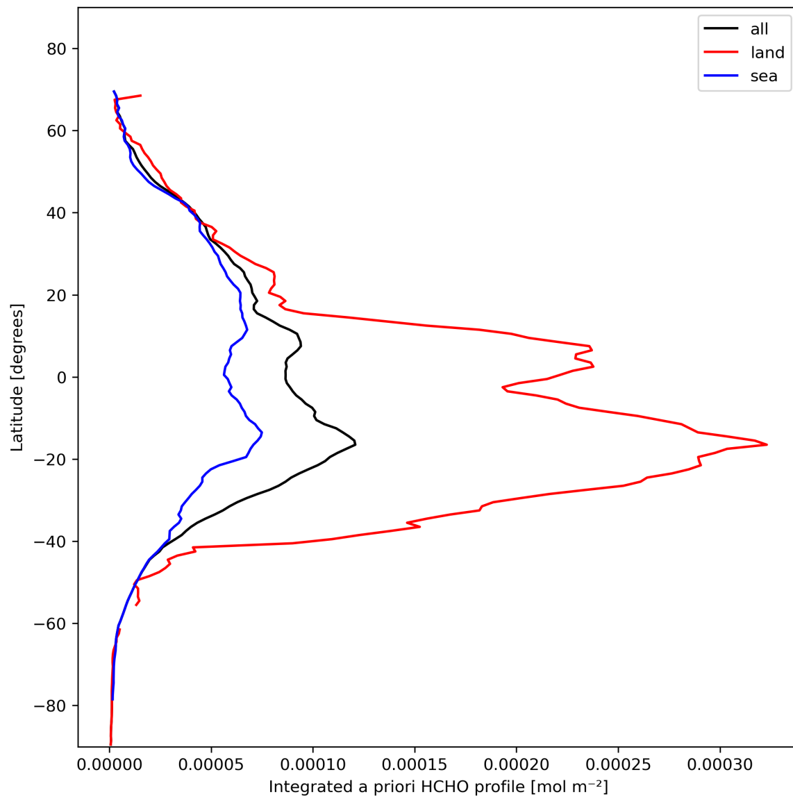
Figure 29: Zonal average of “Integrated a priori HCHO profile” for 2023-11-05 to 2023-11-07.
