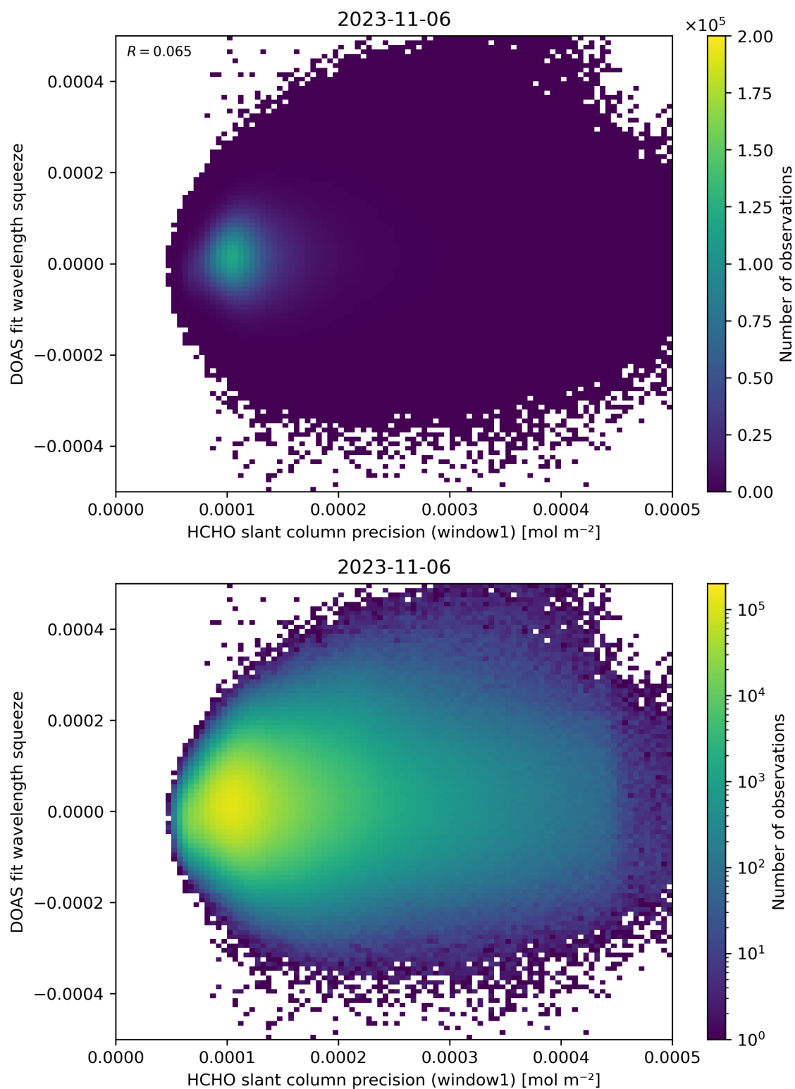
Figure 90: Scatter density plot of “HCHO slant column precision (window1)” against “DOAS fit wavelength squeeze” for 2023-11-05 to 2023-11-07.
