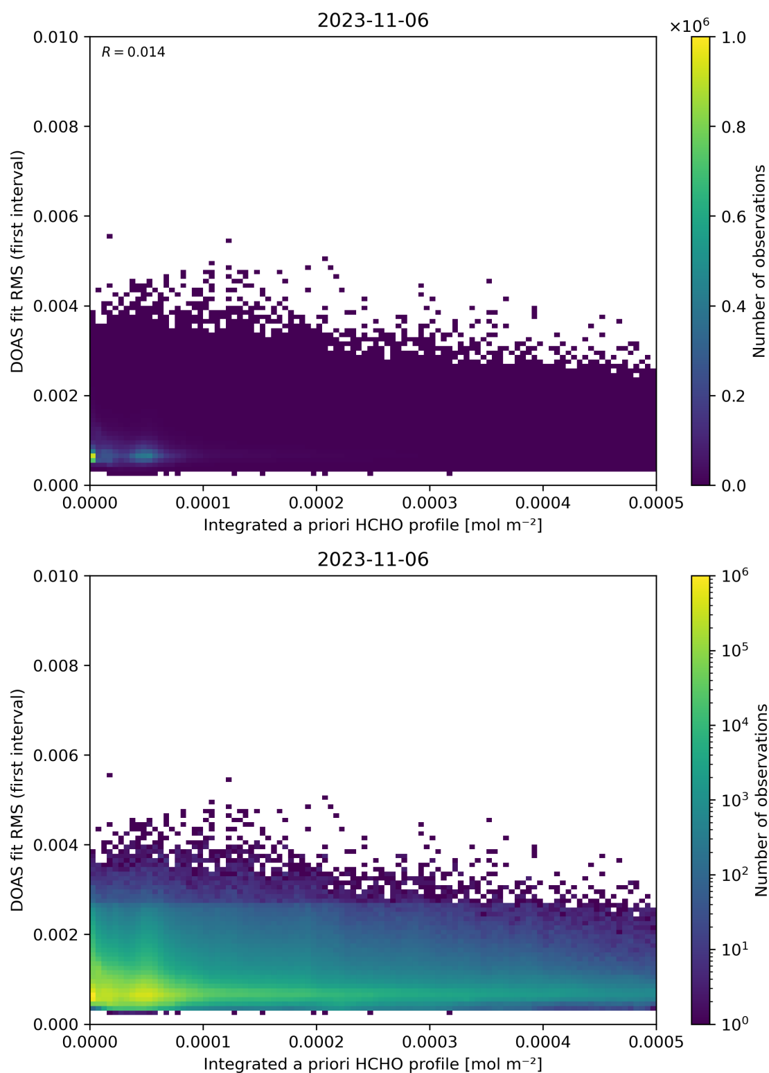
Figure 148: Scatter density plot of “Integrated a priori HCHO profile” against “DOAS fit RMS (first interval)” for 2023-11-05 to 2023-11-07.
