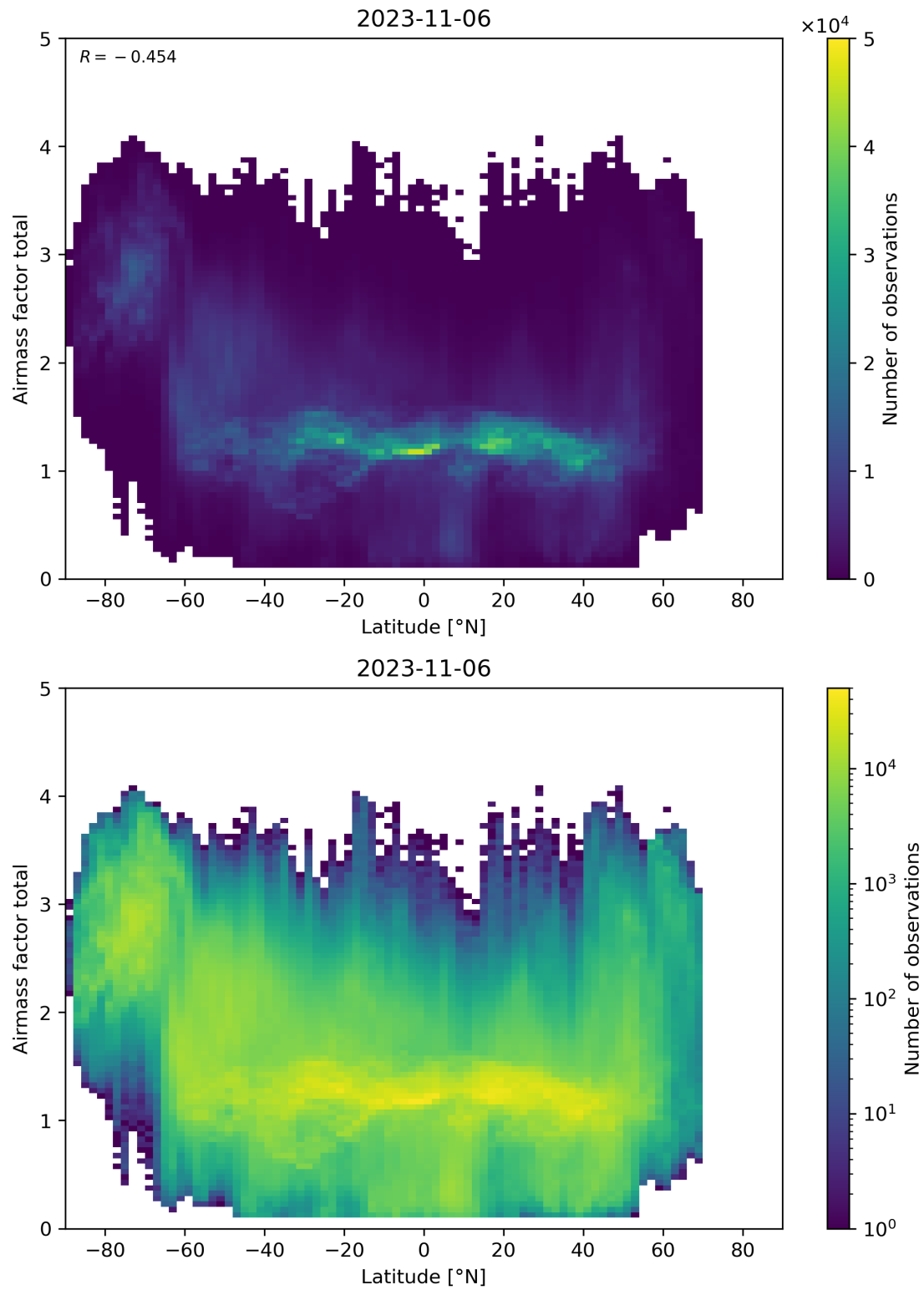
Figure 161: Scatter density plot of “Latitude” against “Airmass factor total” for 2023-11-05 to 2023-11-07.
