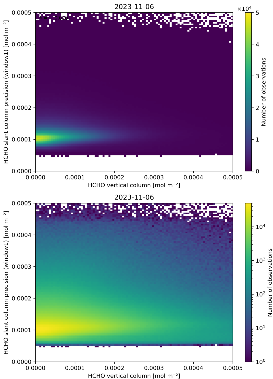
Figure 130: Scatter density plot of “HCHO vertical column” against “HCHO slant column precision (window1)” for 2023-11-05 to 2023-11-07.
