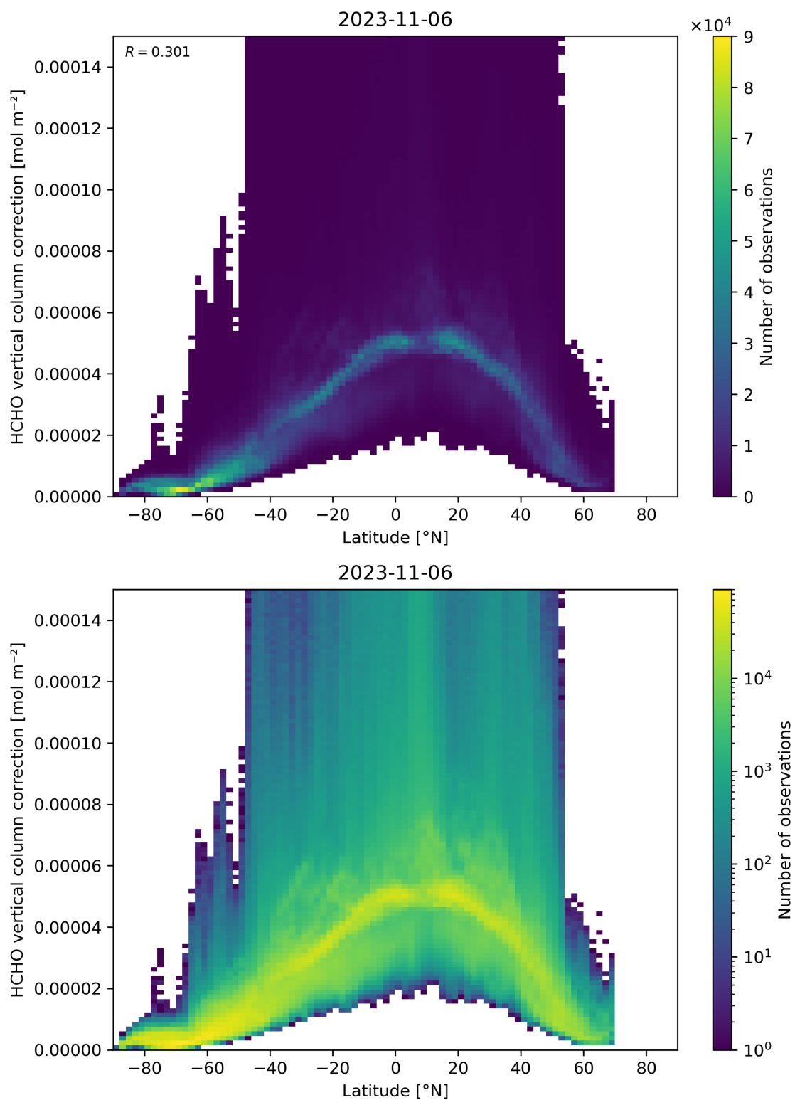
Figure 164: Scatter density plot of “Latitude” against “HCHO vertical column correction” for 2023-11-05 to 2023-11-07.
