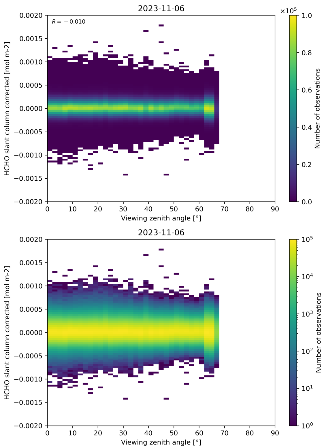
Figure 186: Scatter density plot of “Viewing zenith angle” against “HCHO slant column corrected” for 2023-11-05 to 2023-11-07.
