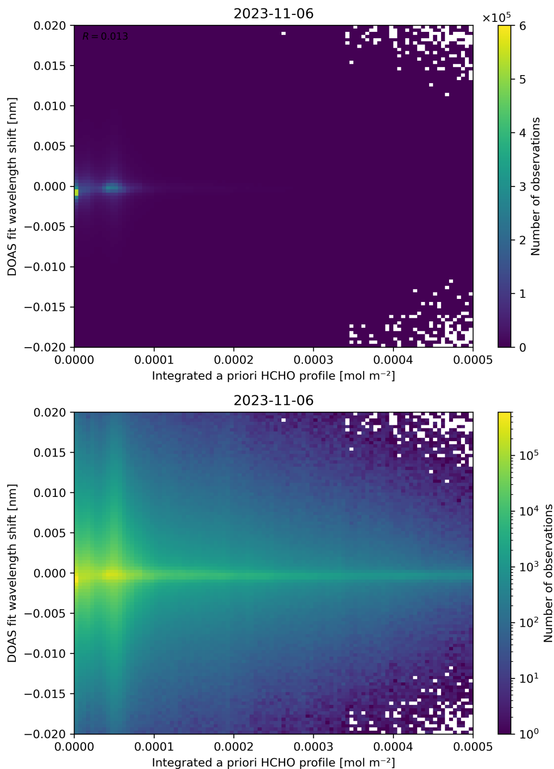
Figure 149: Scatter density plot of “Integrated a priori HCHO profile” against “DOAS fit wavelength shift” for 2023-11-05 to 2023-11-07.
