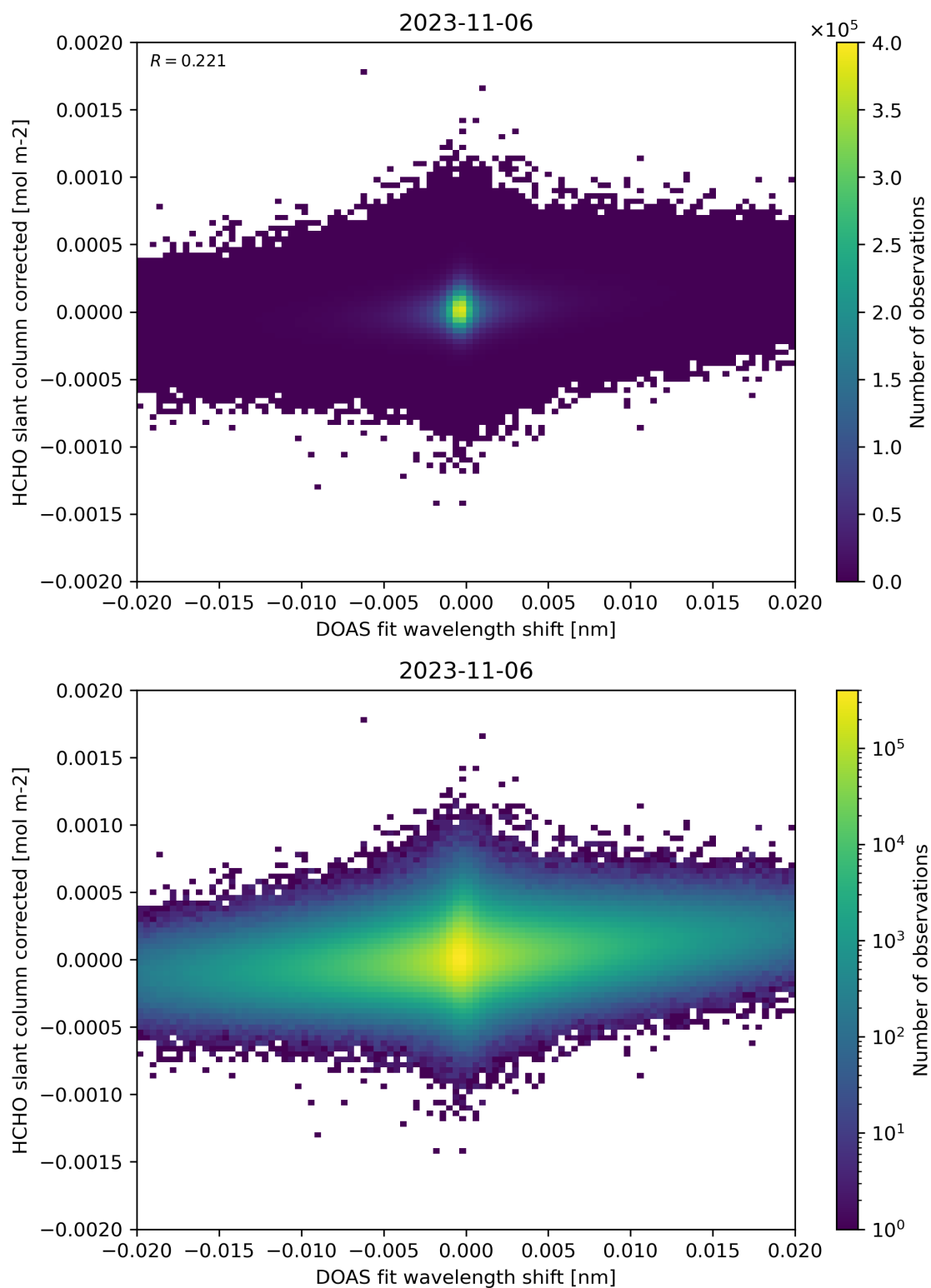
Figure 66: Scatter density plot of “DOAS fit wavelength shift” against “HCHO slant column corrected” for 2023-11-05 to 2023-11-07.
