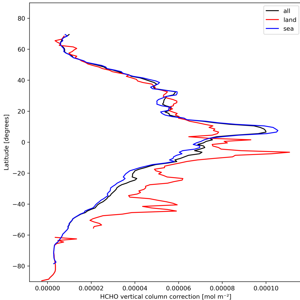
Figure 23: Zonal average of “HCHO vertical column correction” for 2023-11-05 to 2023-11-07.
