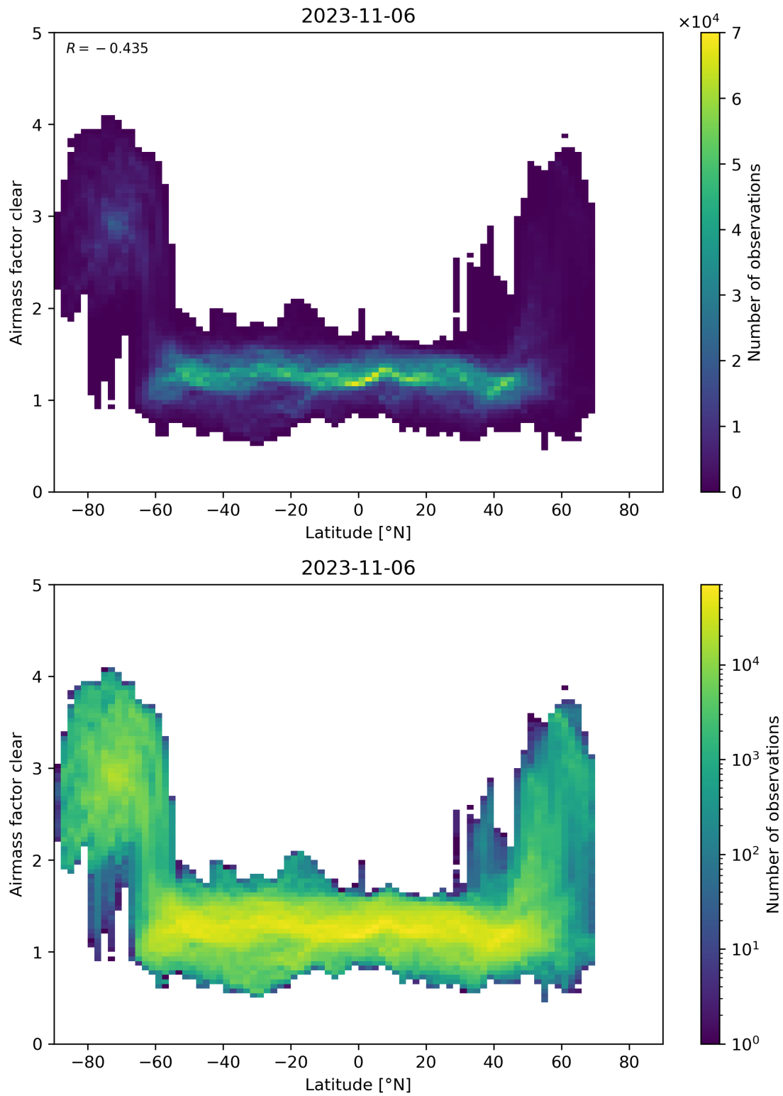
Figure 156: Scatter density plot of “Latitude” against “Airmass factor clear” for 2023-11-05 to 2023-11-07.
