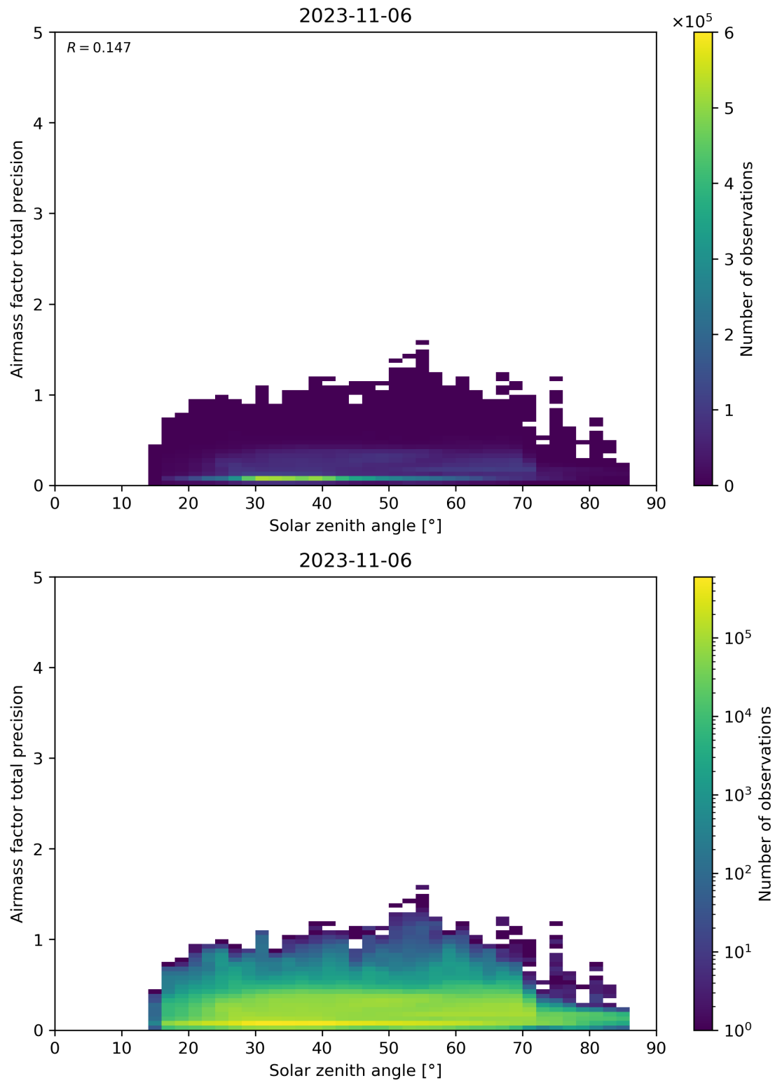
Figure 176: Scatter density plot of “Solar zenith angle” against “Airmass factor total precision” for 2023-11-05 to 2023-11-07.
