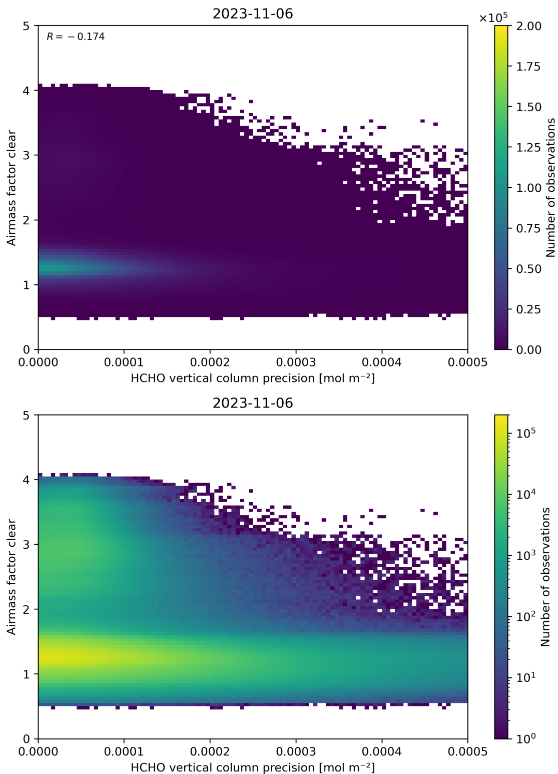
Figure 139: Scatter density plot of “HCHO vertical column precision” against “Airmass factor clear” for 2023-11-05 to 2023-11-07.
