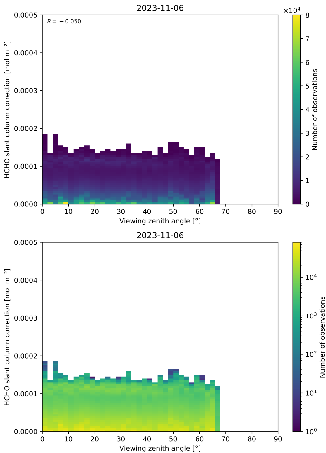
Figure 187: Scatter density plot of “Viewing zenith angle” against “HCHO slant column correction” for 2023-11-05 to 2023-11-07.
