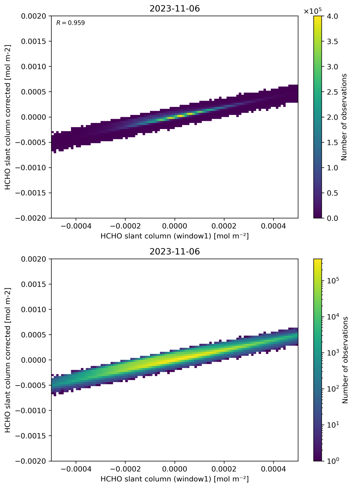
Figure 82: Scatter density plot of “HCHO slant column (window1)” against “HCHO slant column corrected” for 2023-11-05 to 2023-11-07.
