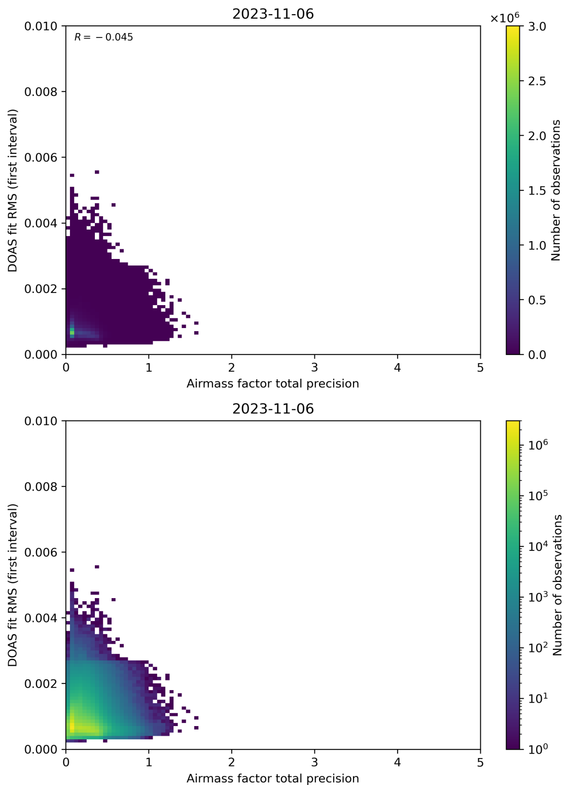
Figure 105: Scatter density plot of “Airmass factor total precision” against “DOAS fit RMS (first interval)” for 2023-11-05 to 2023-11-07.
