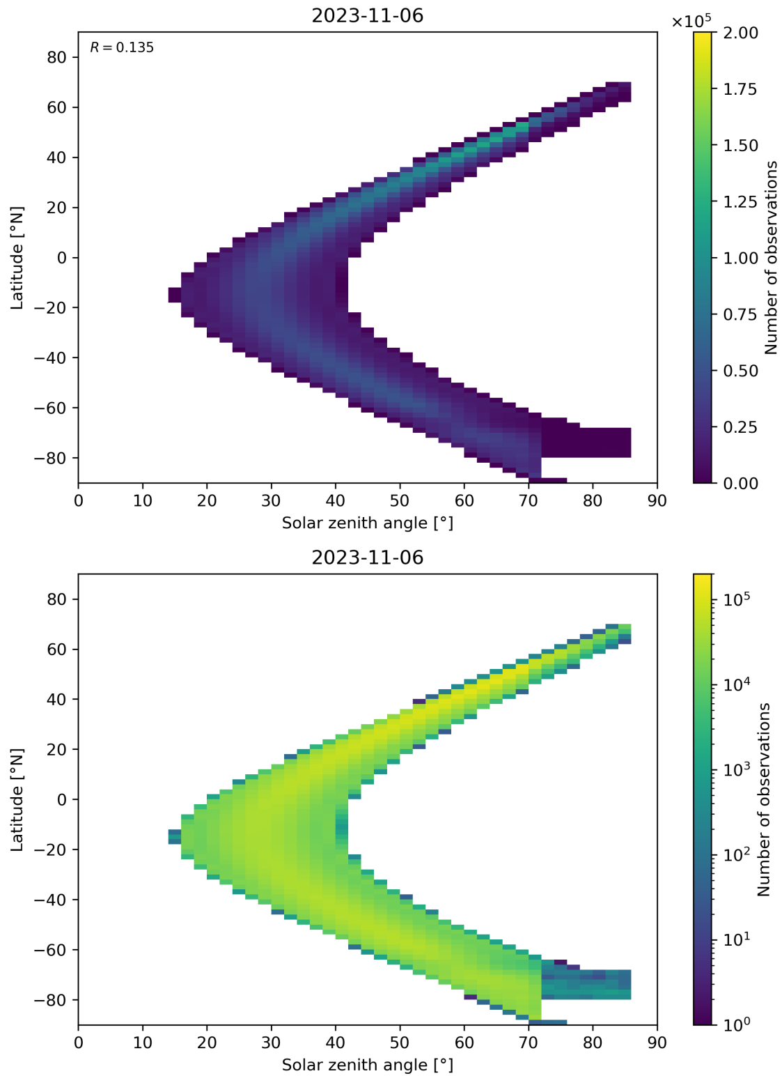
Figure 181: Scatter density plot of “Solar zenith angle” against “Latitude” for 2023-11-05 to 2023-11-07.
