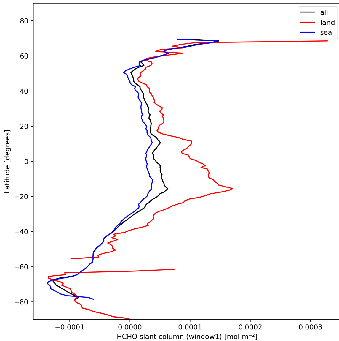
Figure 24: Zonal average of “HCHO slant column (window1)” for 2023-11-05 to 2023-11-07.
