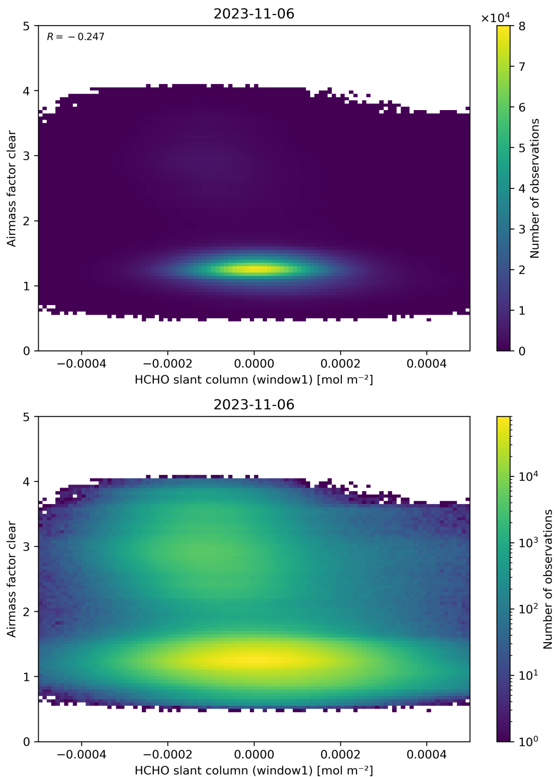
Figure 81: Scatter density plot of “HCHO slant column (window1)” against “Airmass factor clear” for 2023-11-05 to 2023-11-07.
