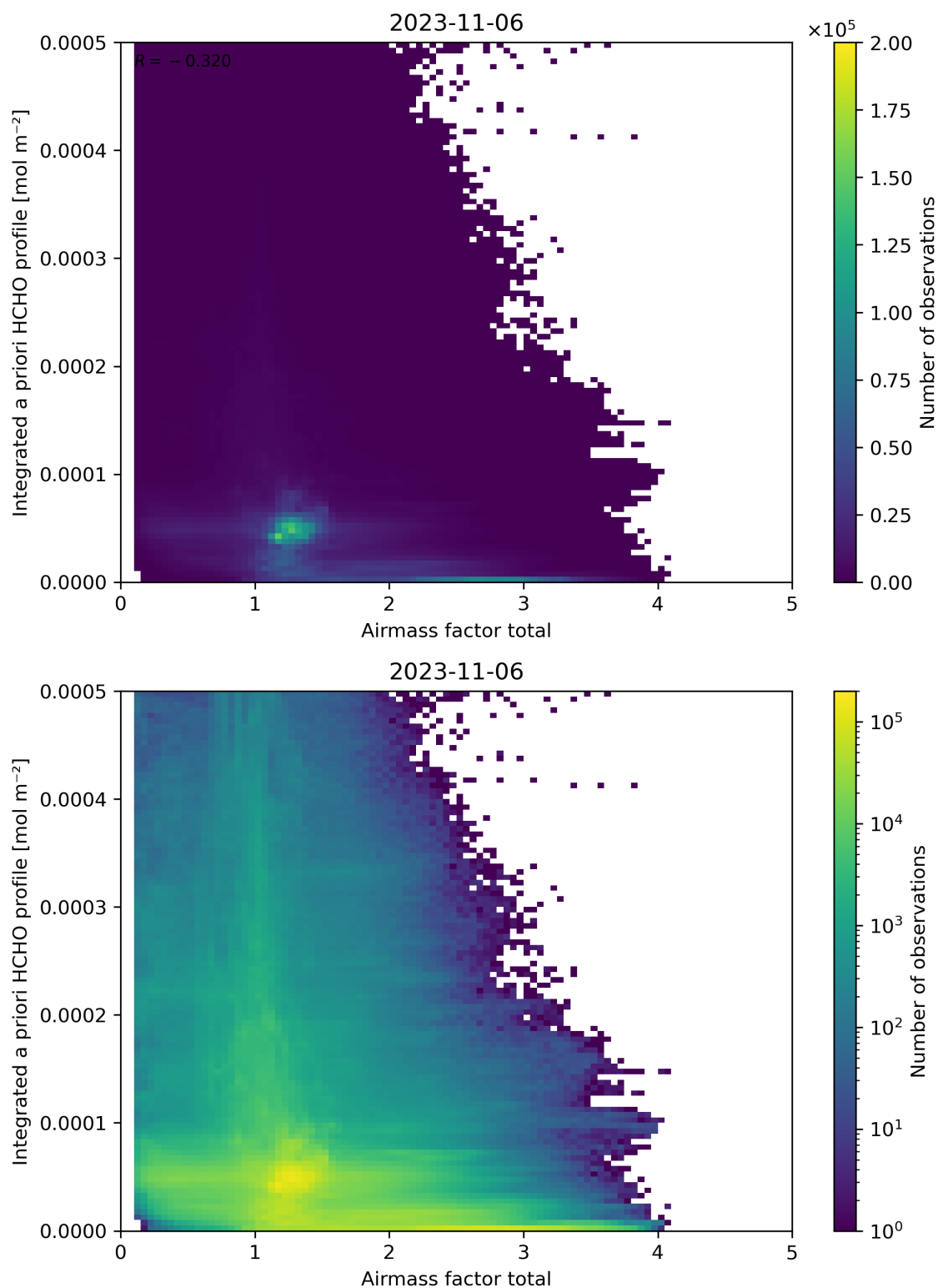
Figure 104: Scatter density plot of “Airmass factor total” against “Integrated a priori HCHO profile” for 2023-11-05 to 2023-11-07.
