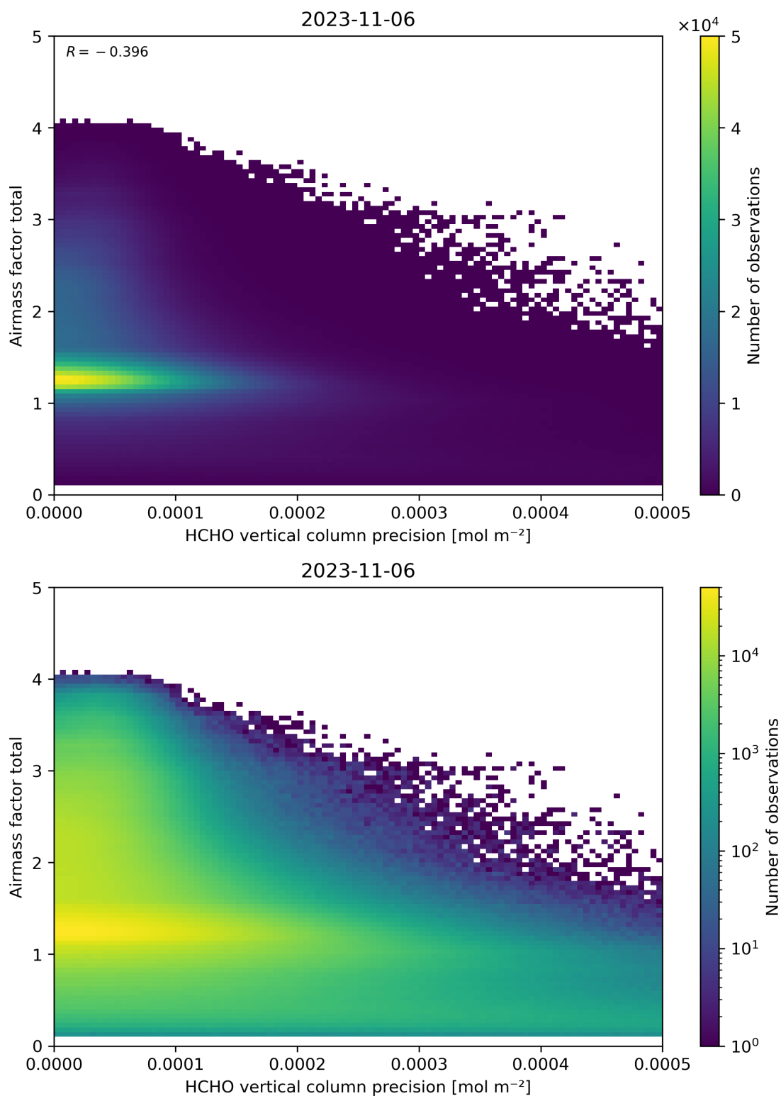
Figure 144: Scatter density plot of “HCHO vertical column precision” against “Airmass factor total” for 2023-11-05 to 2023-11-07.
