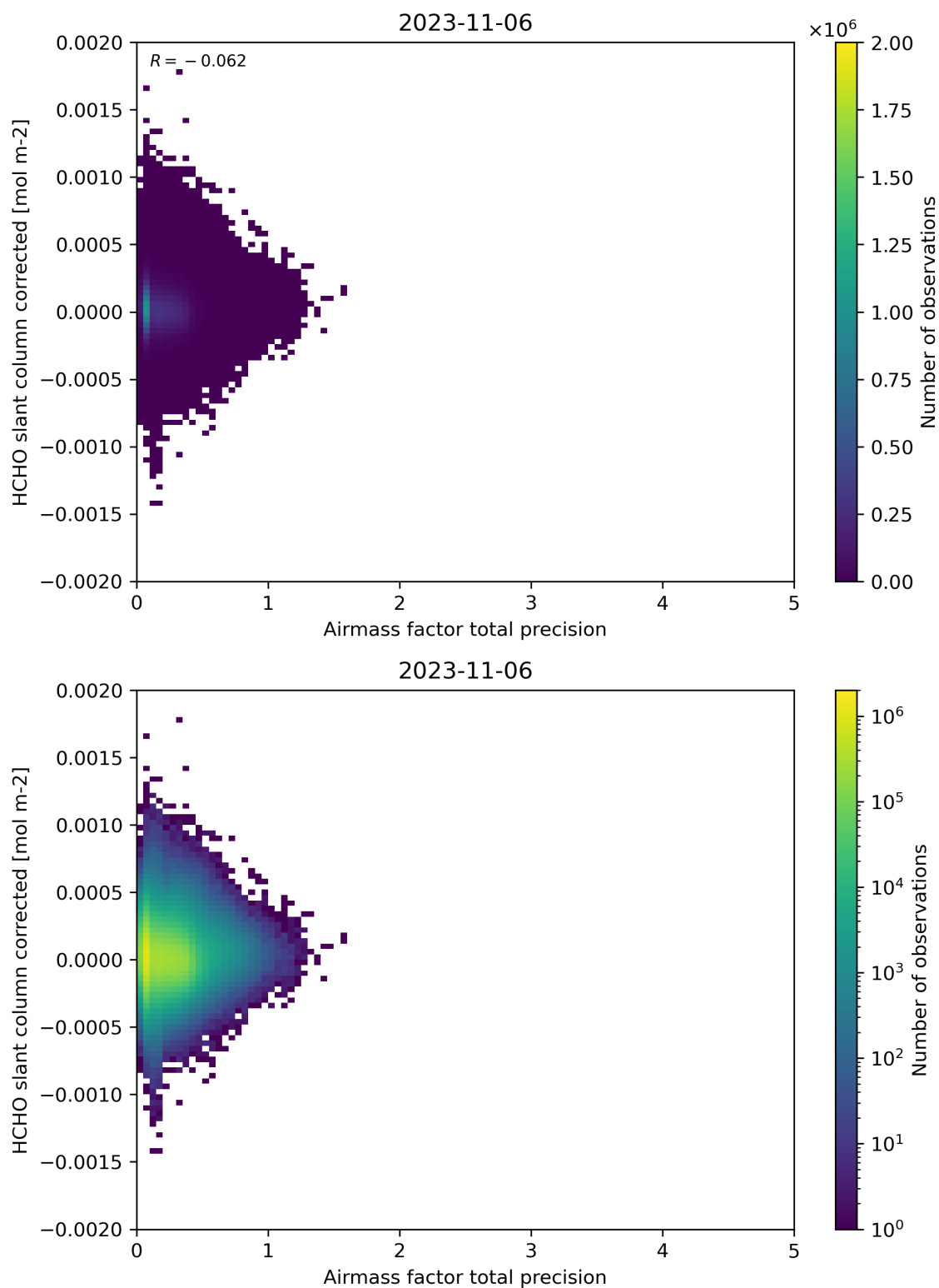
Figure 109: Scatter density plot of “Airmass factor total precision” against “HCHO slant column corrected” for 2023-11-05 to 2023-11-07.
