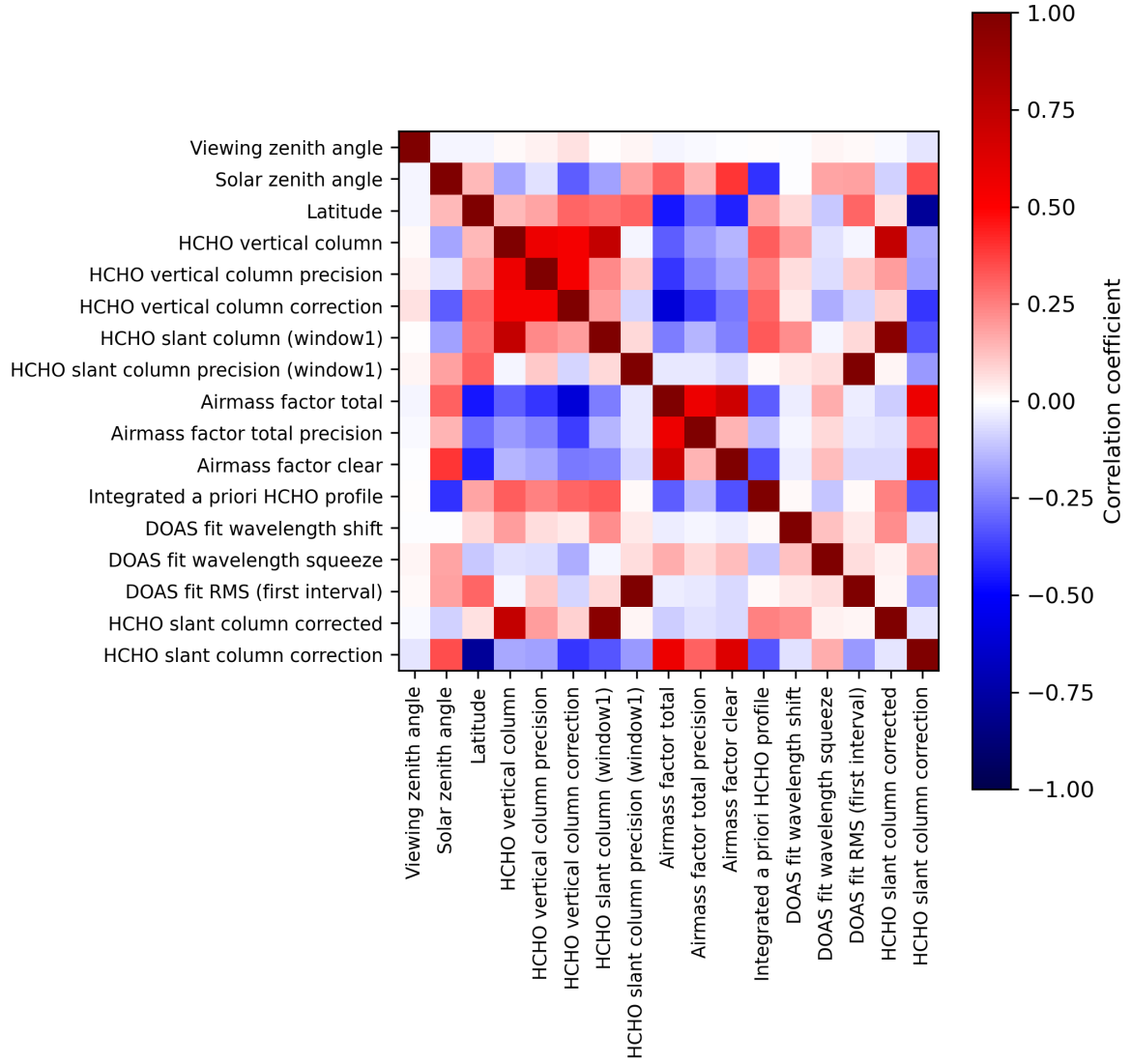
Figure 2: Map of correlation matrix for 2023-11-05 to 2023-11-07.
