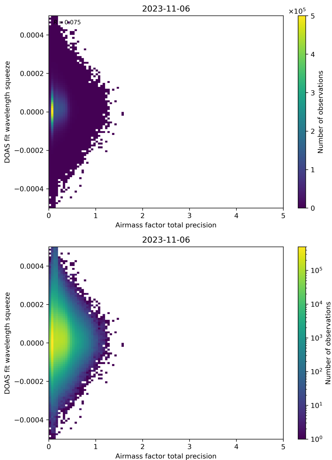
Figure 107: Scatter density plot of “Airmass factor total precision” against “DOAS fit wavelength squeeze” for 2023-11-05 to 2023-11-07.
