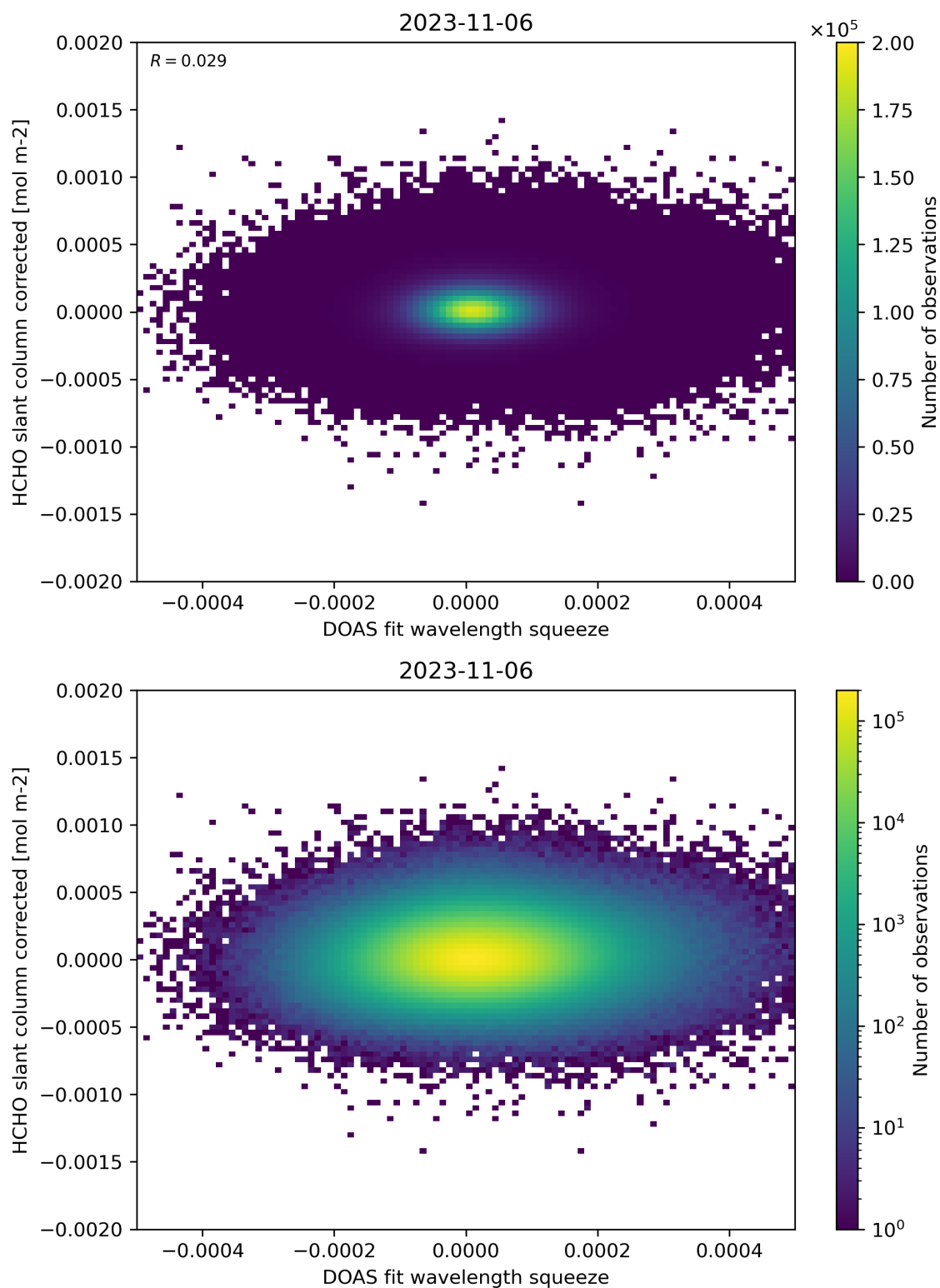
Figure 69: Scatter density plot of “DOAS fit wavelength squeeze” against “HCHO slant column corrected” for 2023-11-05 to 2023-11-07.
