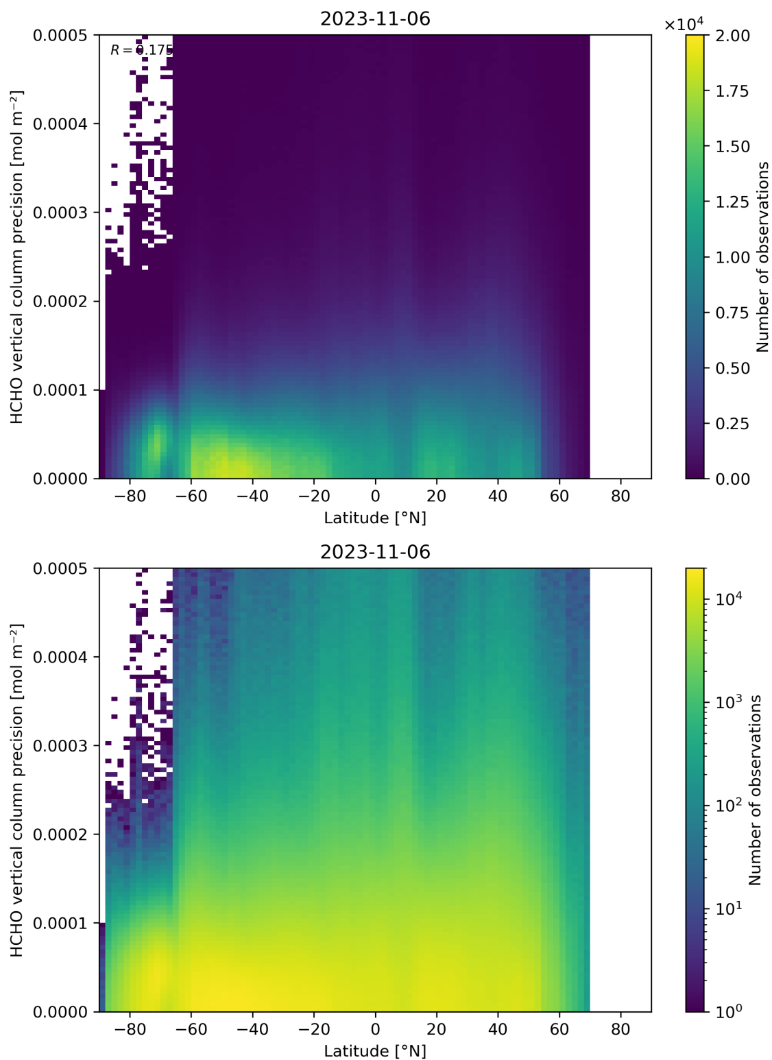
Figure 165: Scatter density plot of “Latitude” against “HCHO vertical column precision” for 2023-11-05 to 2023-11-07.
