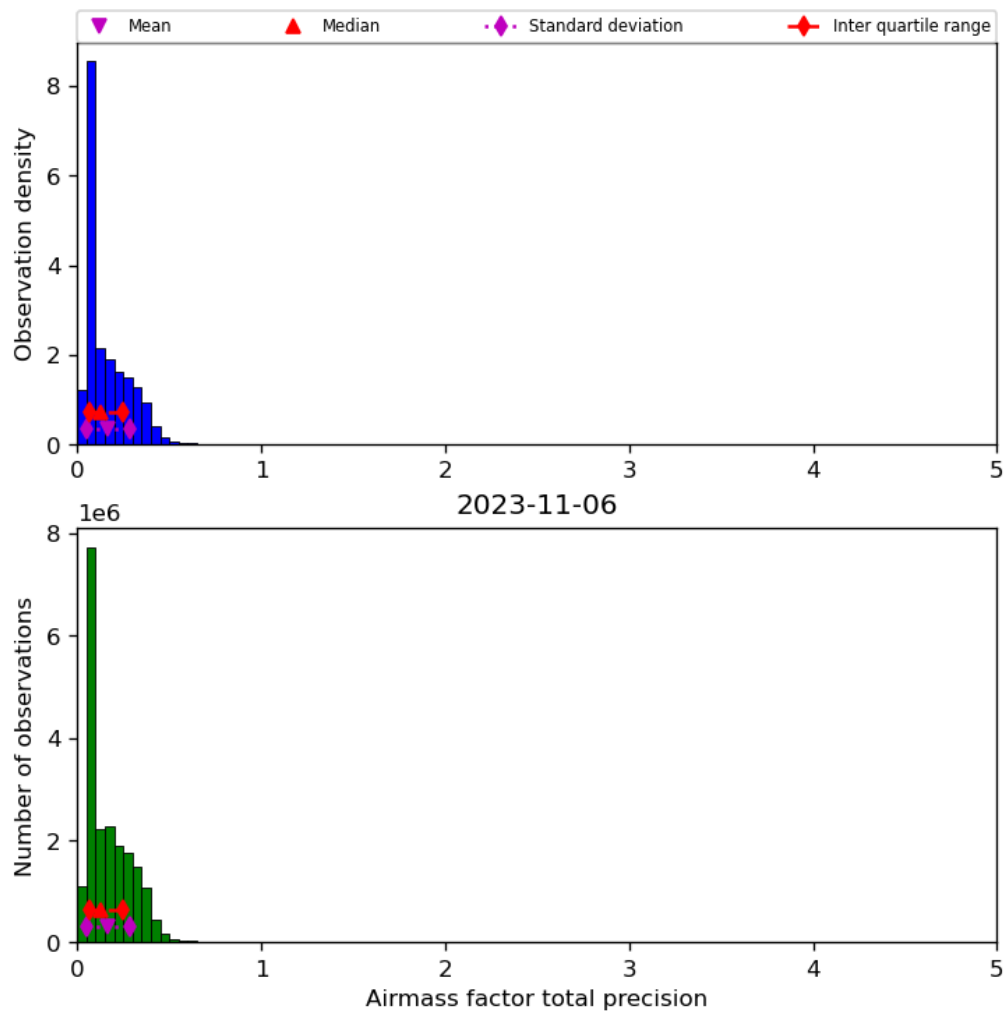
Figure 41: Histogram of “Airmass factor total precision” for 2023-11-05 to 2023-11-07
