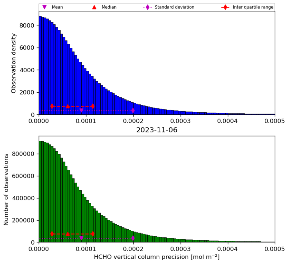
Figure 36: Histogram of “HCHO vertical column precision” for 2023-11-05 to 2023-11-07
