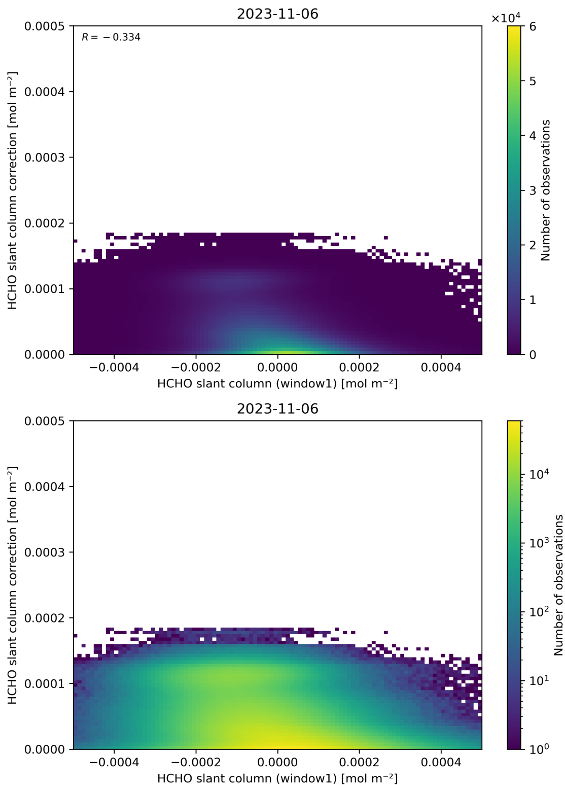
Figure 83: Scatter density plot of “HCHO slant column (window1)” against “HCHO slant column correction” for 2023-11-05 to 2023-11-07.
