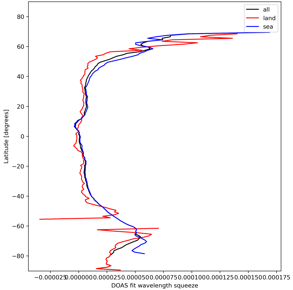
Figure 31: Zonal average of “DOAS fit wavelength squeeze” for 2023-11-05 to 2023-11-07.
