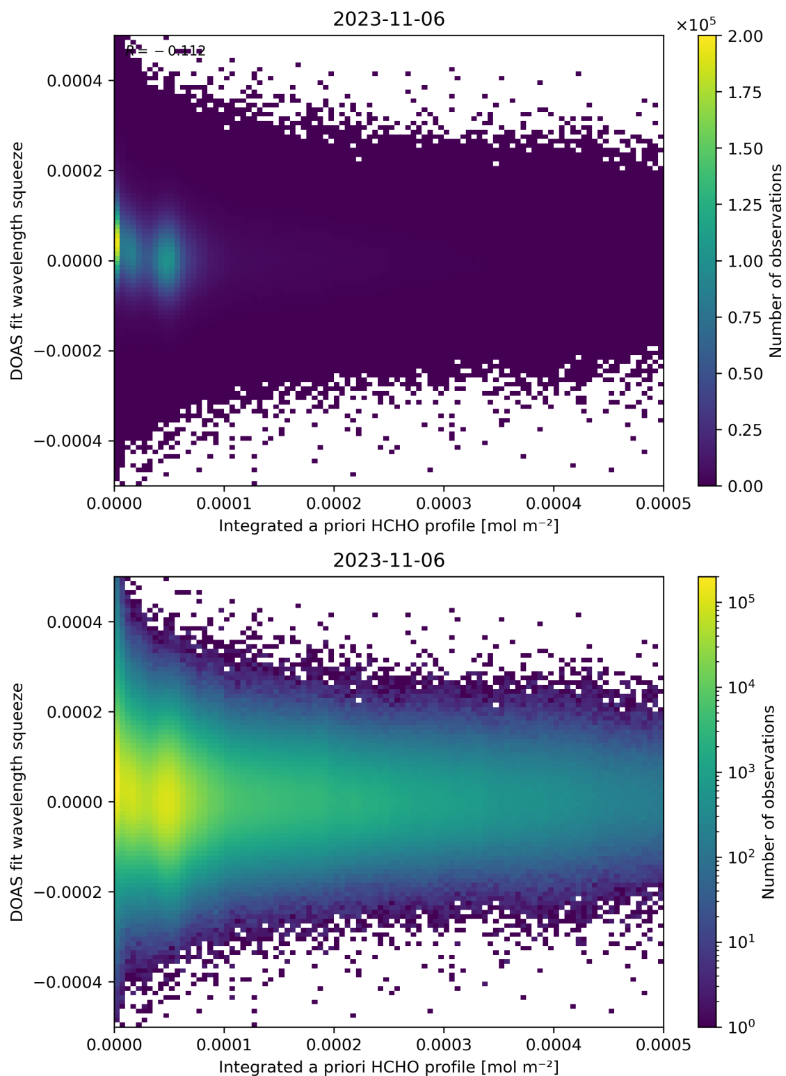
Figure 150: Scatter density plot of “Integrated a priori HCHO profile” against “DOAS fit wavelength squeeze” for 2023-11-05 to 2023-11-07.
