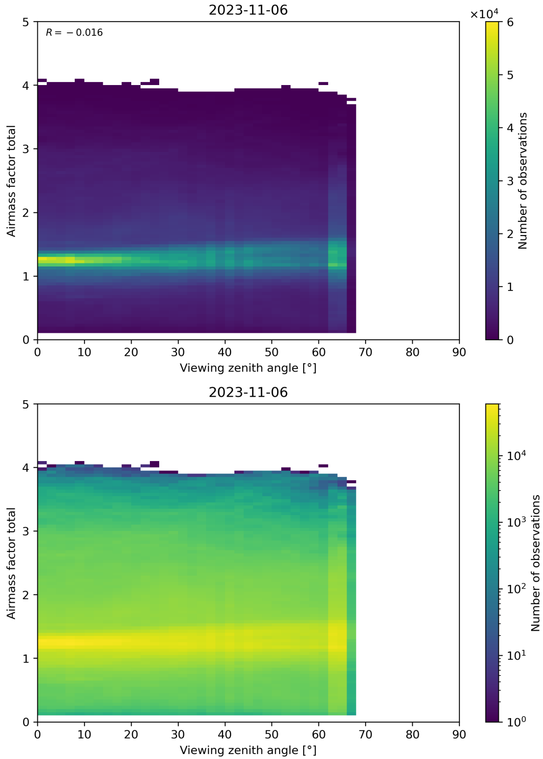
Figure 190: Scatter density plot of “Viewing zenith angle” against “Airmass factor total” for 2023-11-05 to 2023-11-07.
