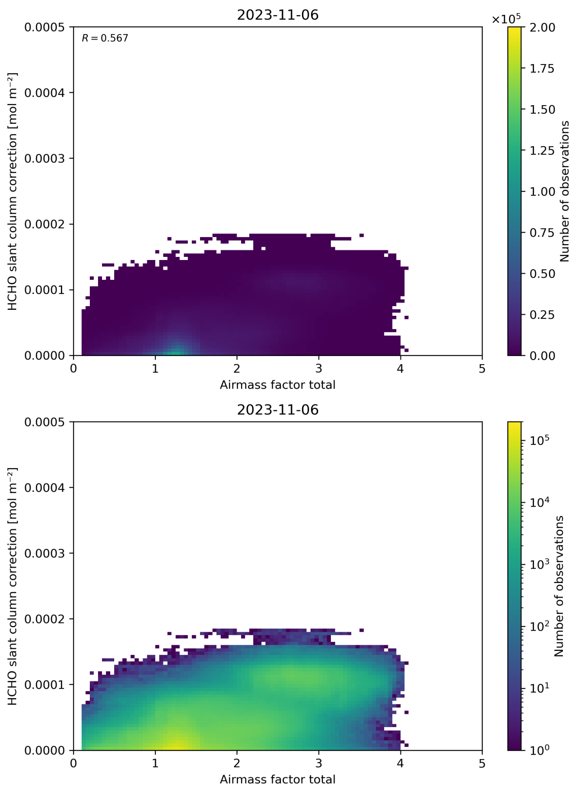
Figure 102: Scatter density plot of “Airmass factor total” against “HCHO slant column correction” for 2023-11-05 to 2023-11-07.
