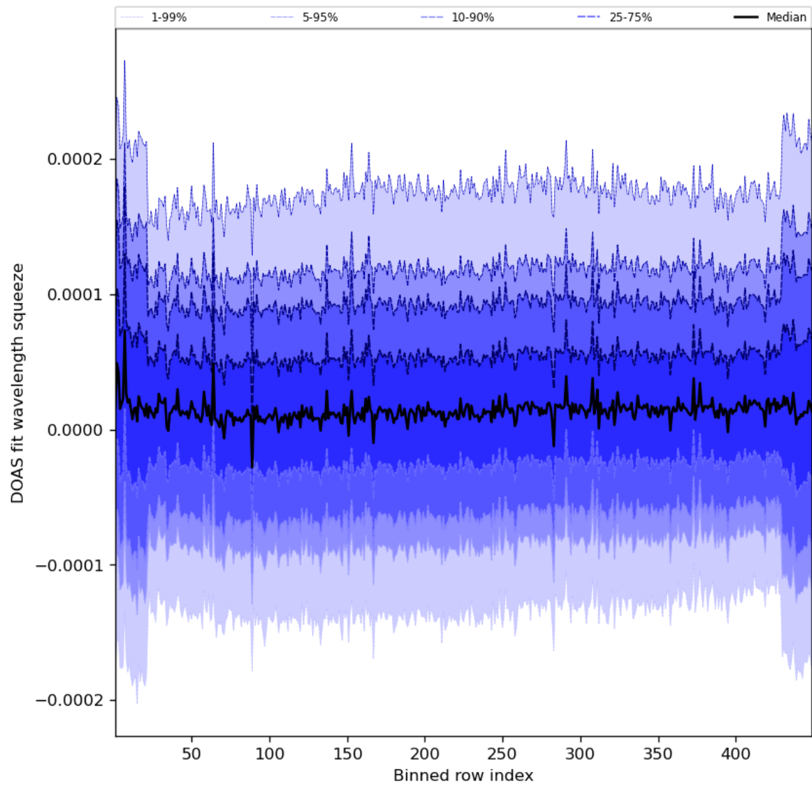
Figure 59: Along track statistics of “DOAS fit wavelength squeeze” for 2023-11-05 to 2023-11-07
