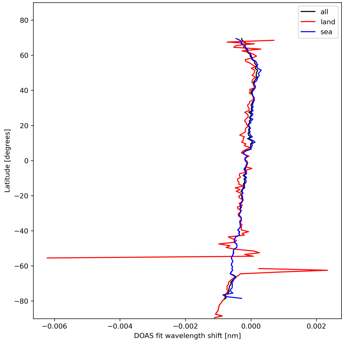
Figure 30: Zonal average of “DOAS fit wavelength shift” for 2023-11-05 to 2023-11-07.
