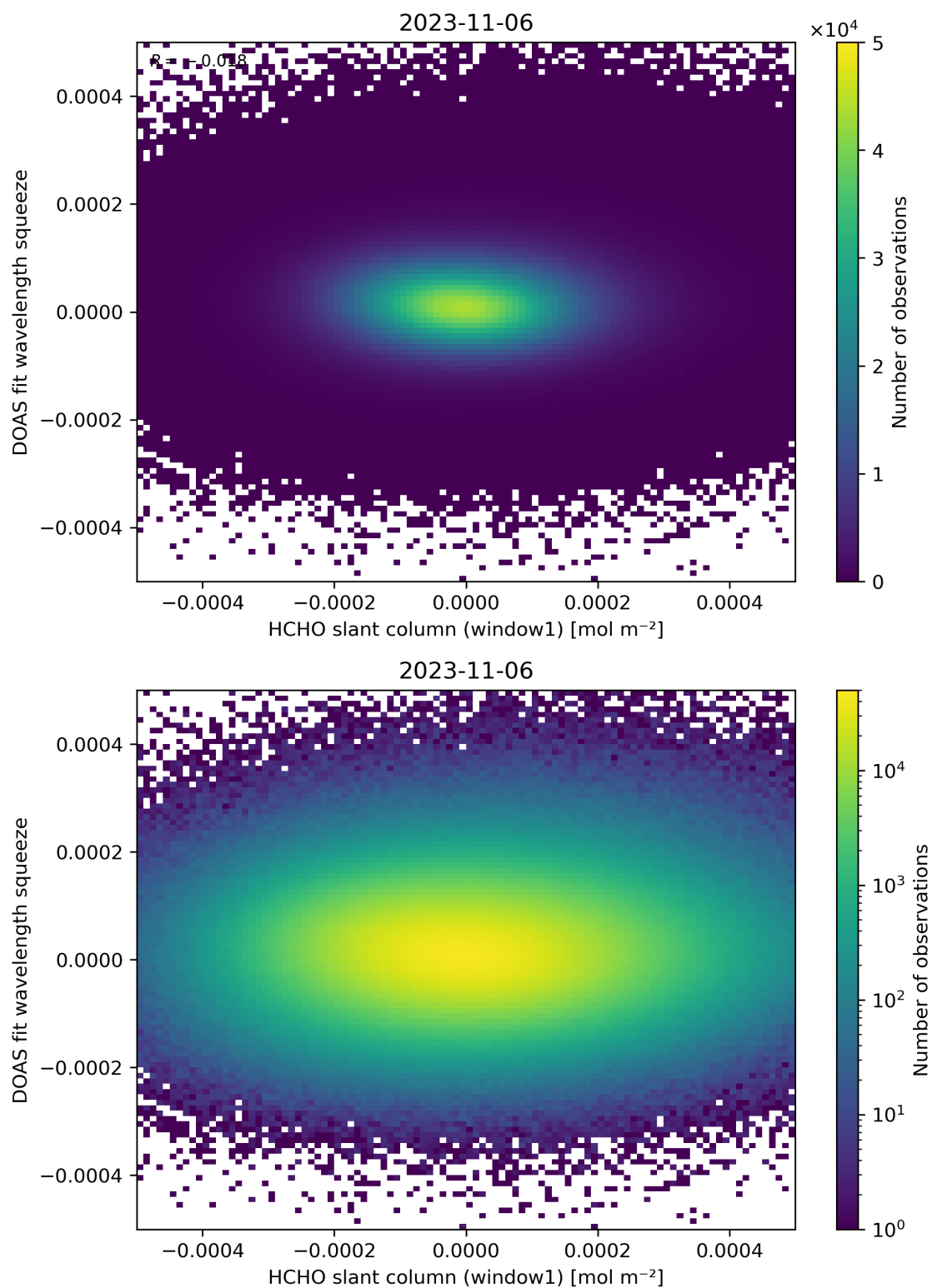
Figure 80: Scatter density plot of “HCHO slant column (window1)” against “DOAS fit wavelength squeeze” for 2023-11-05 to 2023-11-07.
