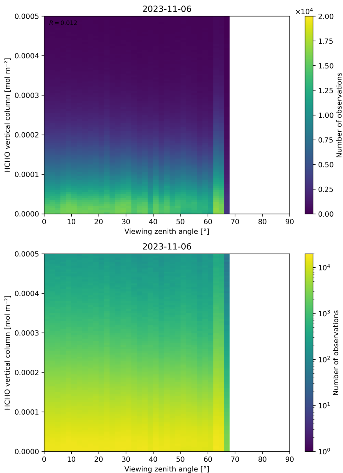
Figure 192: Scatter density plot of “Viewing zenith angle” against “HCHO vertical column” for 2023-11-05 to 2023-11-07.
