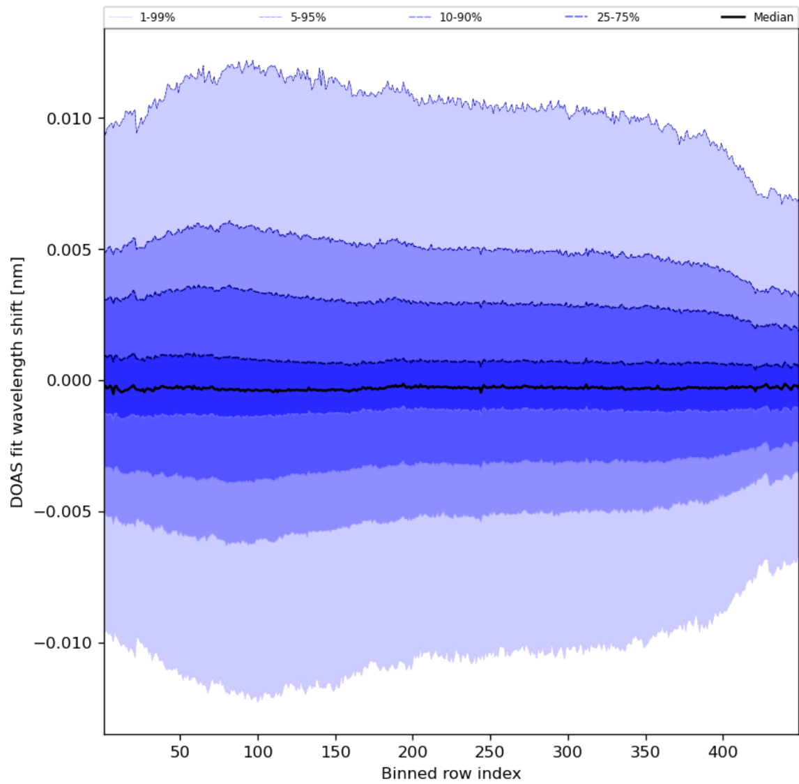
Figure 58: Along track statistics of “DOAS fit wavelength shift” for 2023-11-05 to 2023-11-07
