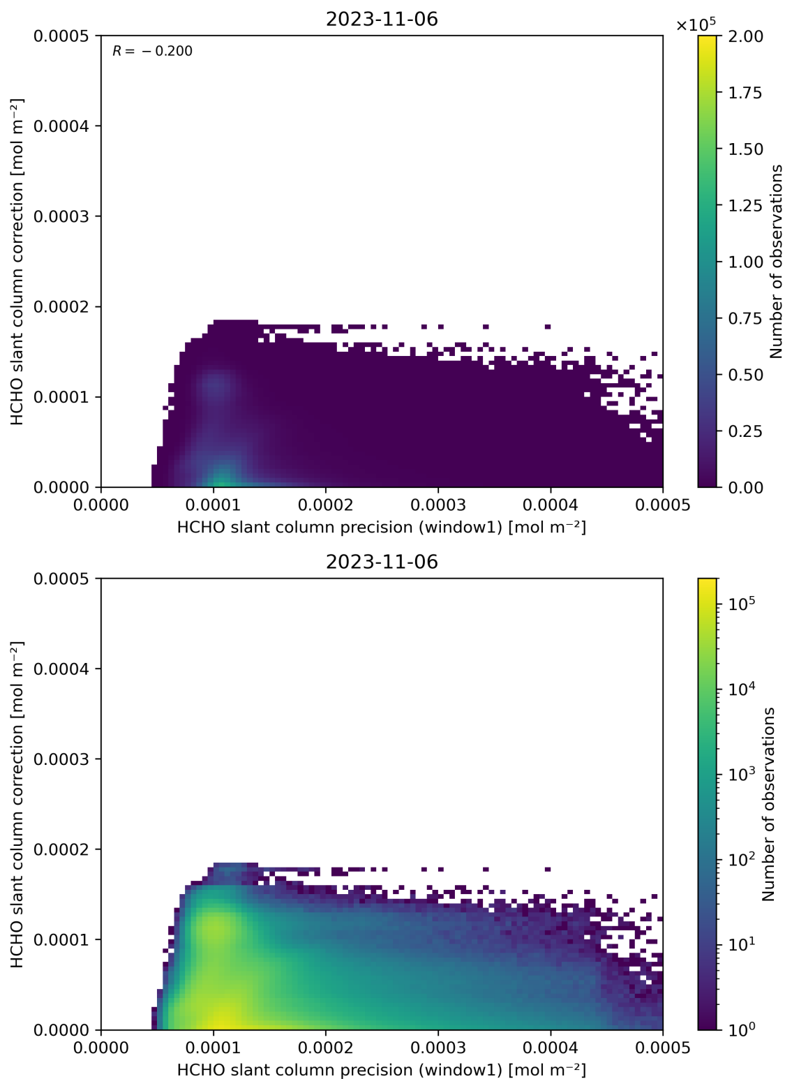
Figure 93: Scatter density plot of “HCHO slant column precision (window1)” against “HCHO slant column correction” for 2023-11-05 to 2023-11-07.
