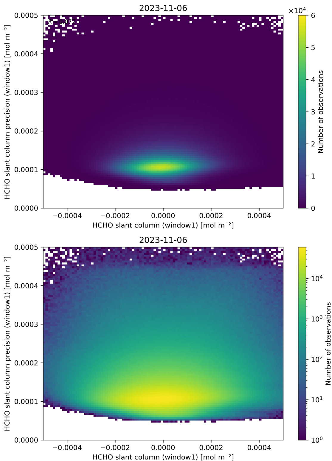
Figure 84: Scatter density plot of “HCHO slant column (window1)” against “HCHO slant column precision (window1)” for 2023-11-05 to 2023-11-07.
