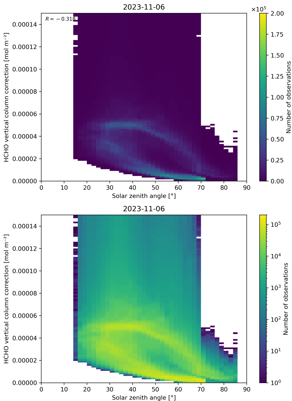
Figure 178: Scatter density plot of “Solar zenith angle” against “HCHO vertical column correction” for 2023-11-05 to 2023-11-07.
