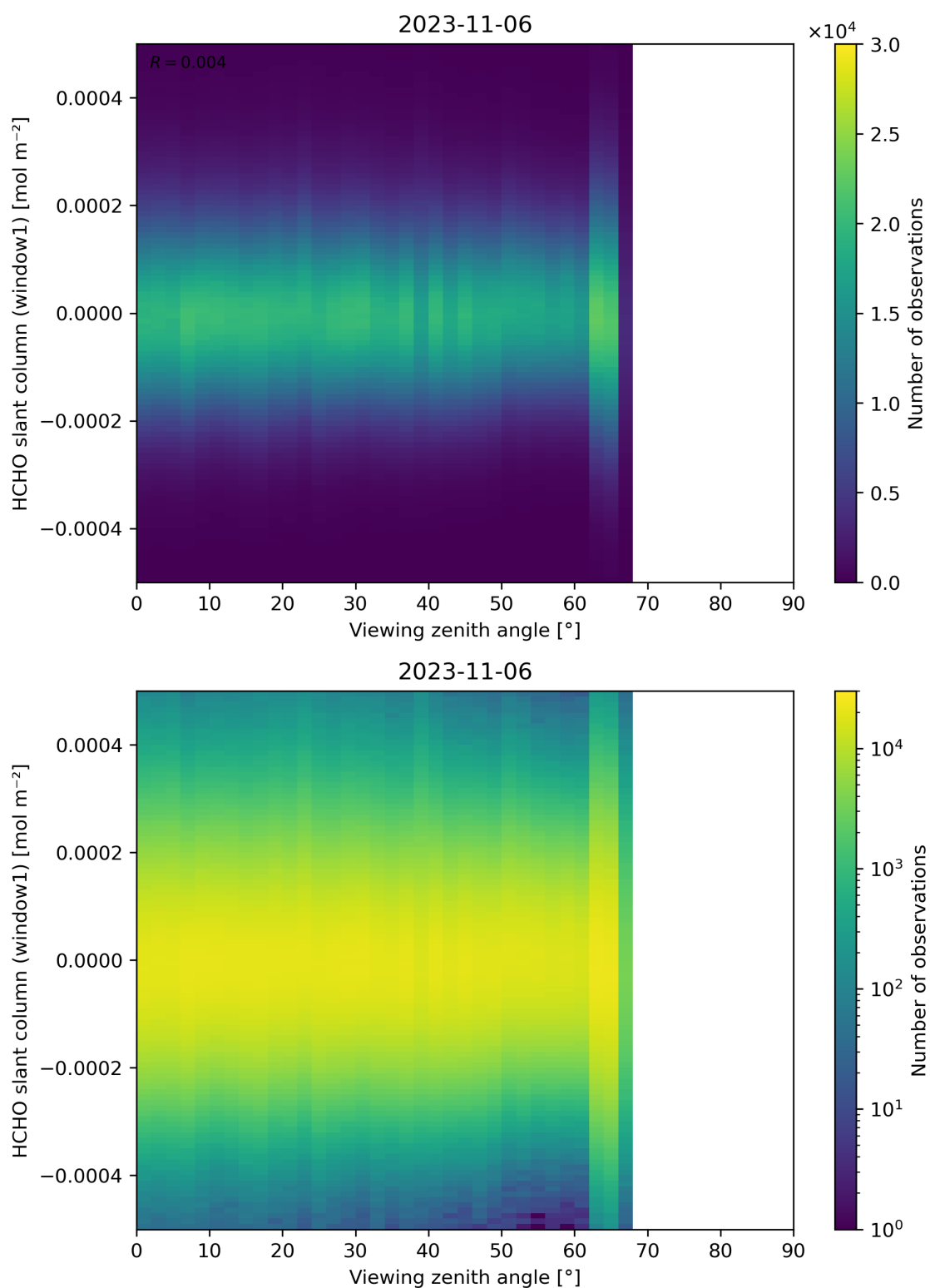
Figure 188: Scatter density plot of “Viewing zenith angle” against “HCHO slant column (window1)” for 2023-11-05 to 2023-11-07.
