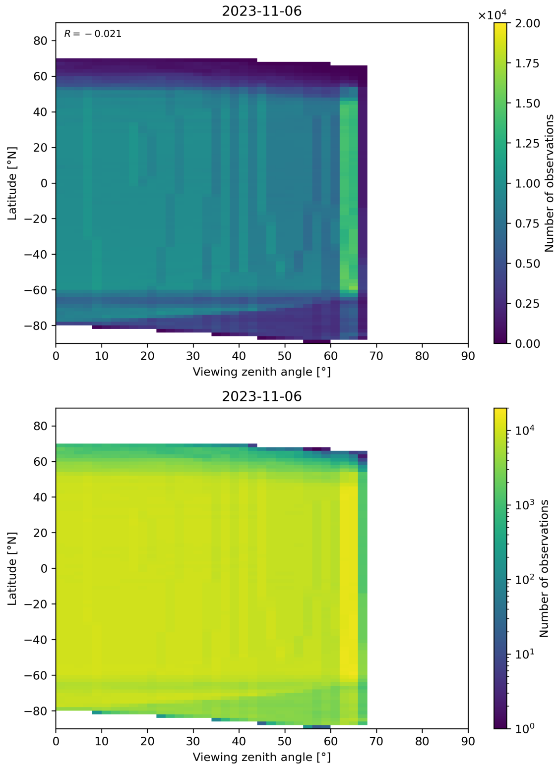
Figure 196: Scatter density plot of “Viewing zenith angle” against “Latitude” for 2023-11-05 to 2023-11-07.
