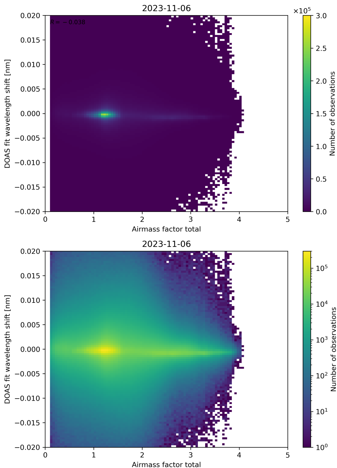
Figure 98: Scatter density plot of “Airmass factor total” against “DOAS fit wavelength shift” for 2023-11-05 to 2023-11-07.
