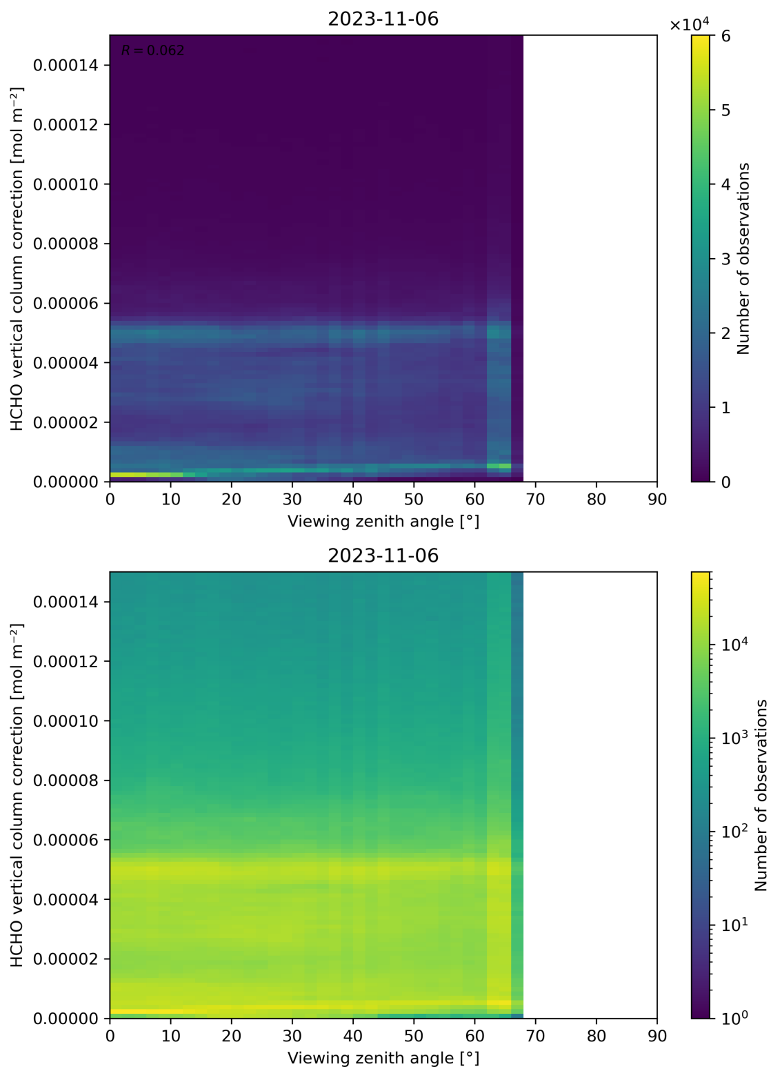
Figure 193: Scatter density plot of “Viewing zenith angle” against “HCHO vertical column correction” for 2023-11-05 to 2023-11-07.
