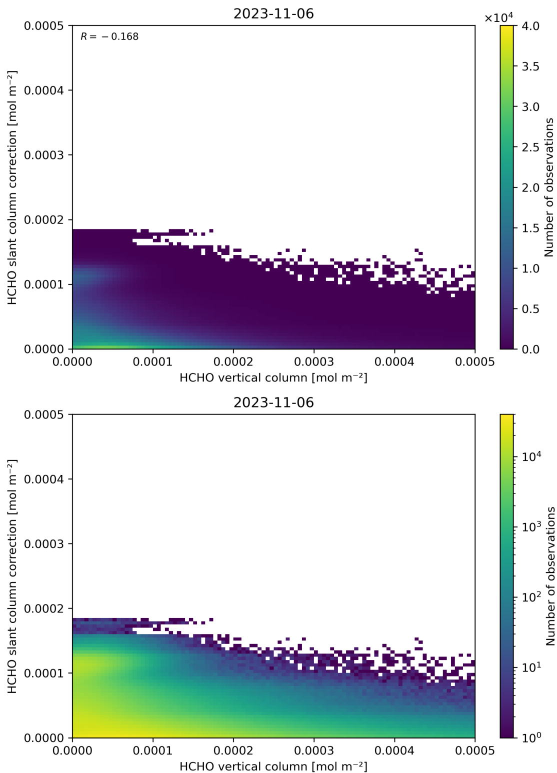
Figure 128: Scatter density plot of “HCHO vertical column” against “HCHO slant column correction” for 2023-11-05 to 2023-11-07.
