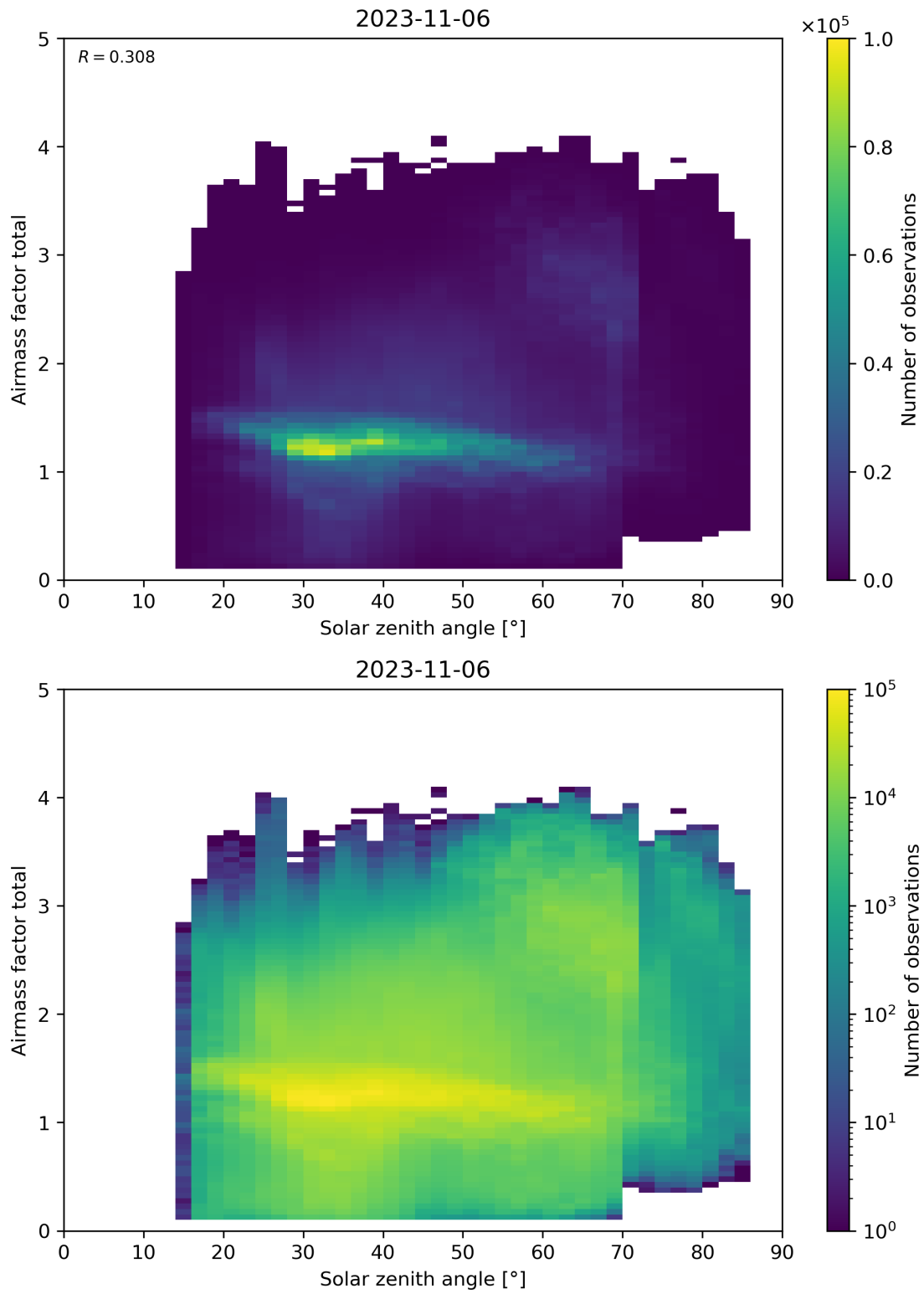
Figure 175: Scatter density plot of “Solar zenith angle” against “Airmass factor total” for 2023-11-05 to 2023-11-07.
