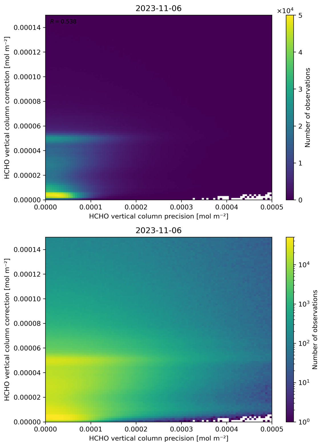
Figure 146: Scatter density plot of “HCHO vertical column precision” against “HCHO vertical column correction” for 2023-11-05 to 2023-11-07.
