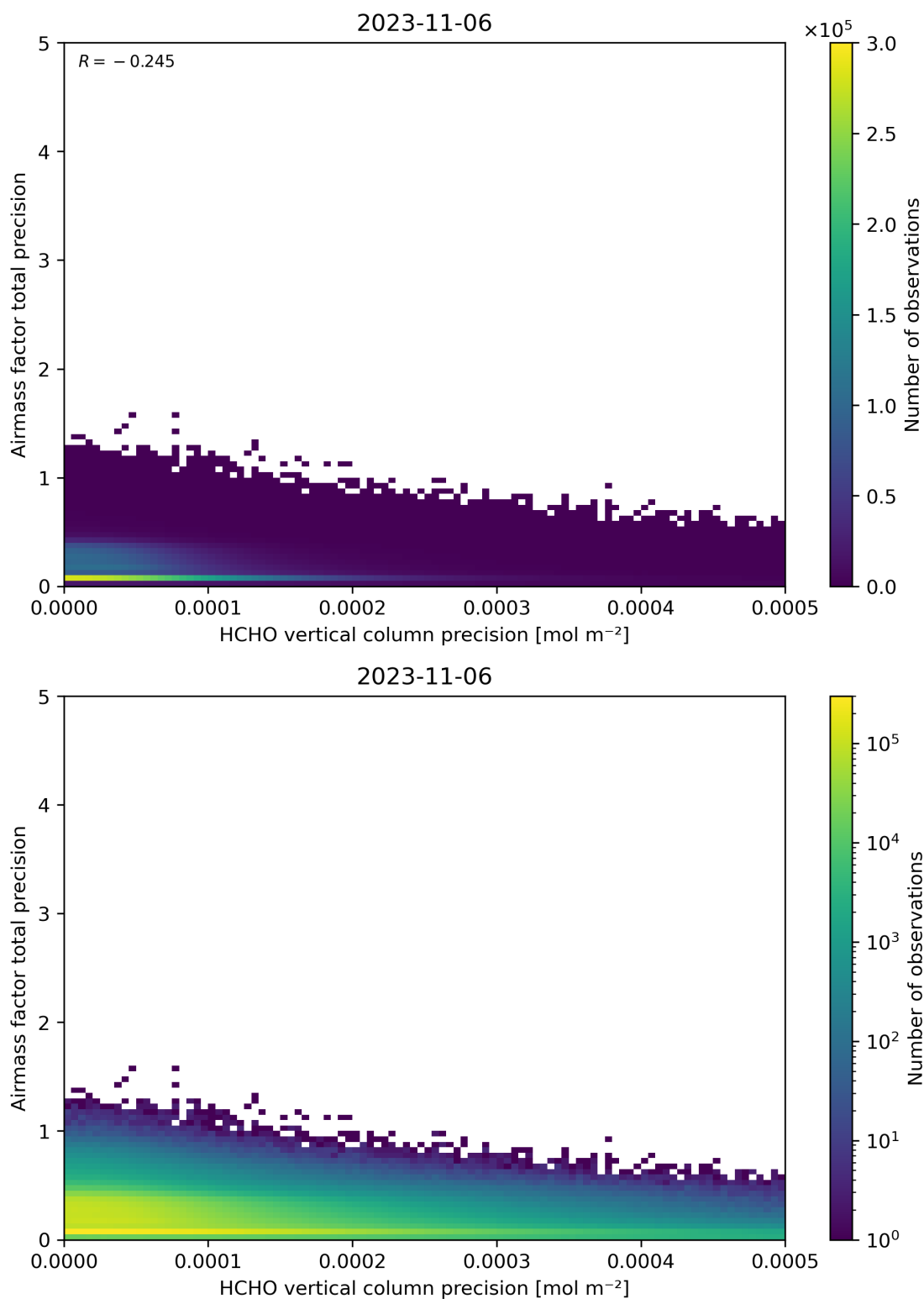
Figure 145: Scatter density plot of “HCHO vertical column precision” against “Airmass factor total precision” for 2023-11-05 to 2023-11-07.
