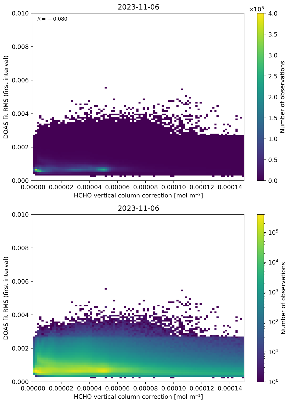
Figure 112: Scatter density plot of “HCHO vertical column correction” against “DOAS fit RMS (first interval)” for 2023-11-05 to 2023-11-07.
