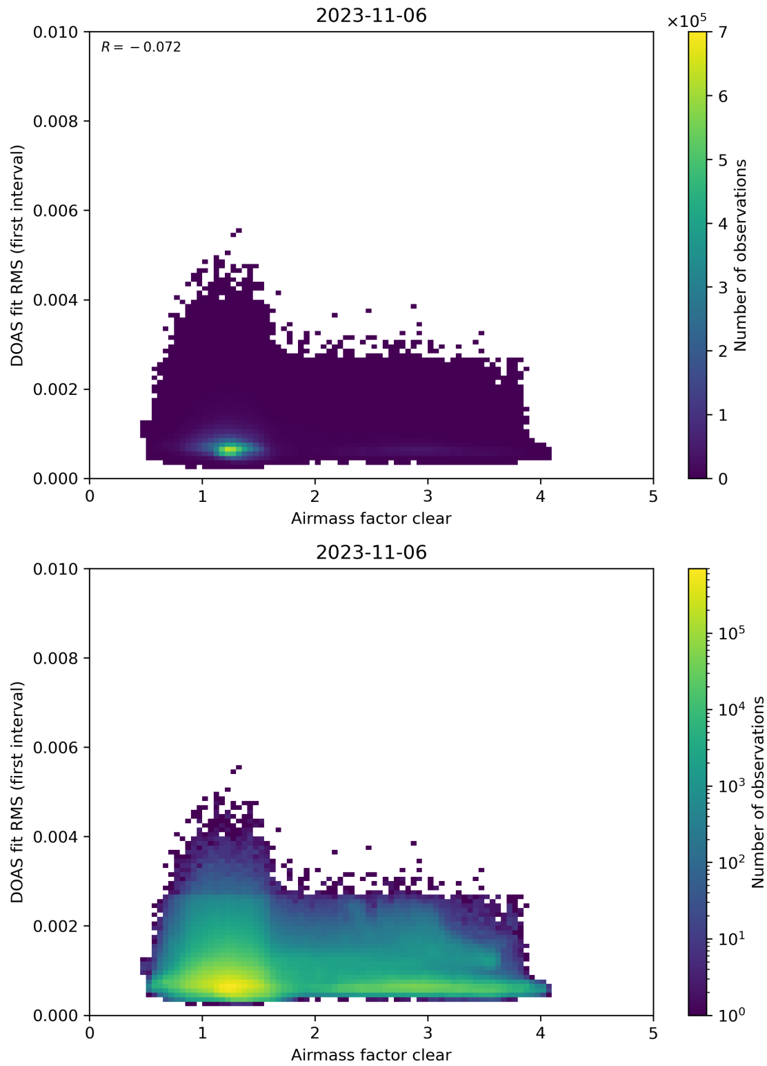
Figure 71: Scatter density plot of “Airmass factor clear” against “DOAS fit RMS (first interval)” for 2023-11-05 to 2023-11-07.
