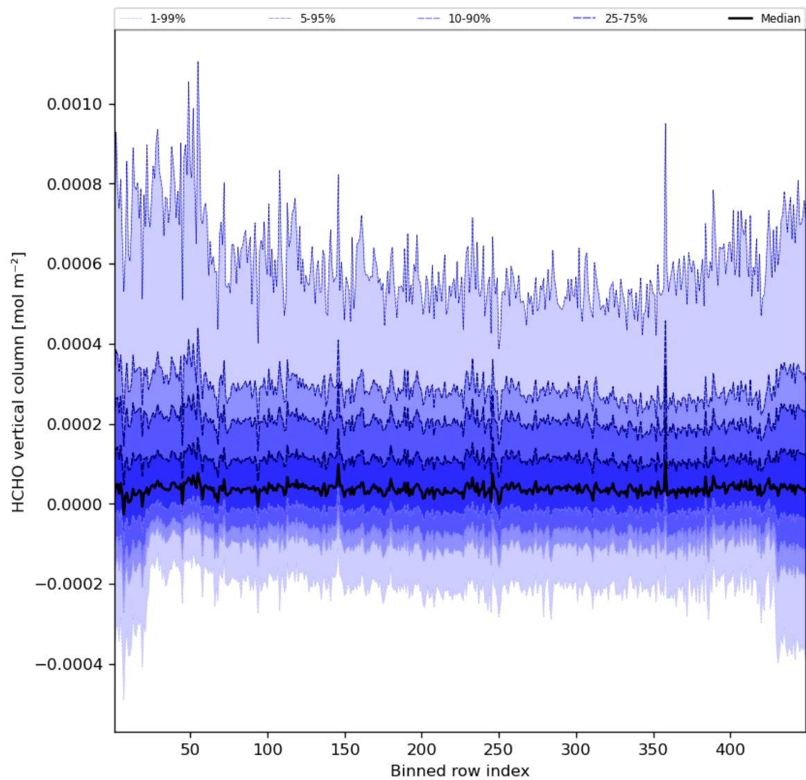
Figure 49: Along track statistics of “HCHO vertical column” for 2023-11-05 to 2023-11-07
