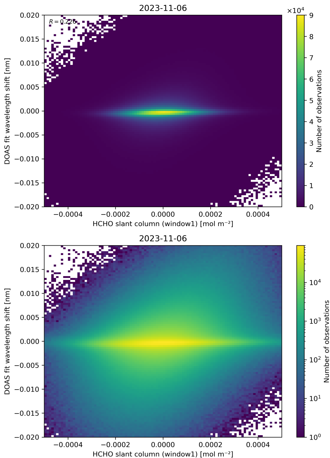
Figure 79: Scatter density plot of “HCHO slant column (window1)” against “DOAS fit wavelength shift” for 2023-11-05 to 2023-11-07.
