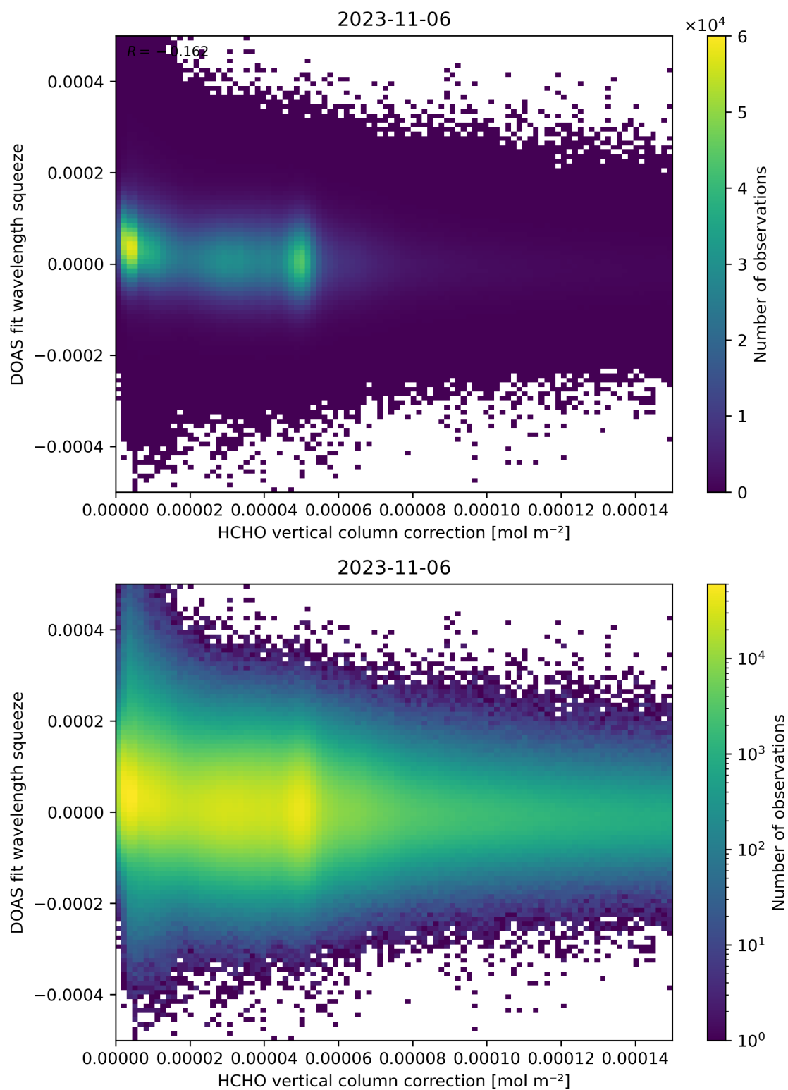
Figure 114: Scatter density plot of “HCHO vertical column correction” against “DOAS fit wavelength squeeze” for 2023-11-05 to 2023-11-07.
