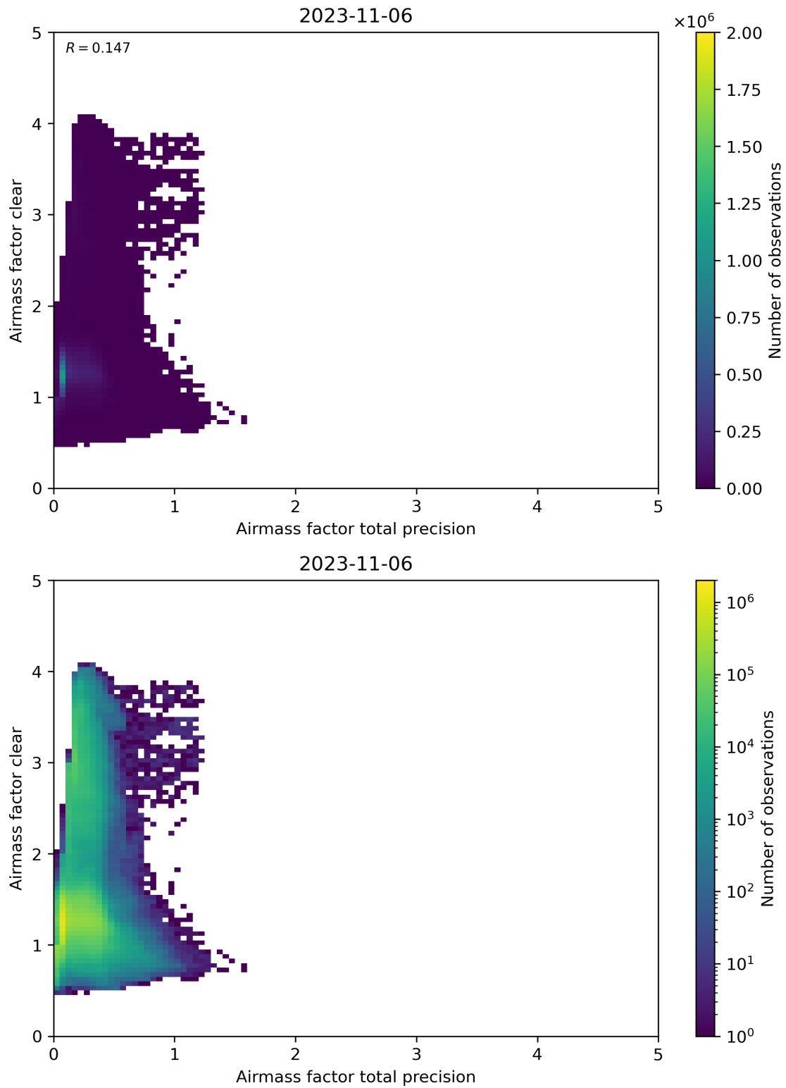
Figure 108: Scatter density plot of “Airmass factor total precision” against “Airmass factor clear” for 2023-11-05 to 2023-11-07.
