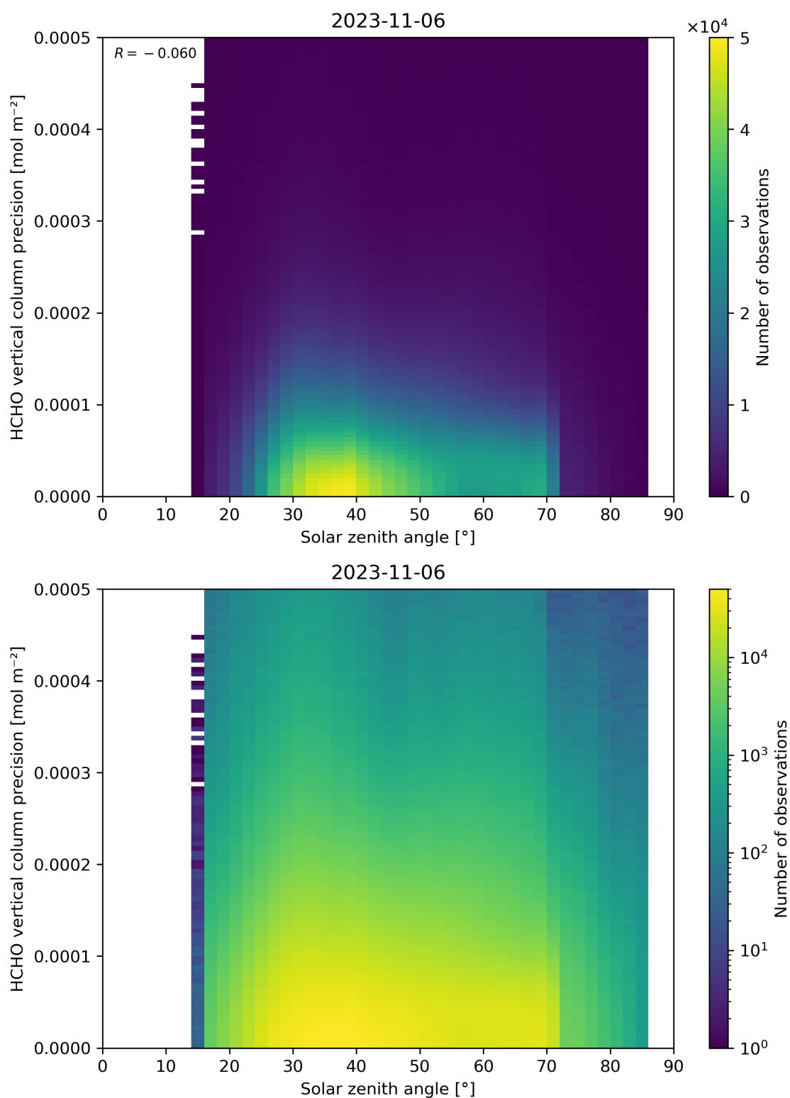
Figure 179: Scatter density plot of “Solar zenith angle” against “HCHO vertical column precision” for 2023-11-05 to 2023-11-07.
