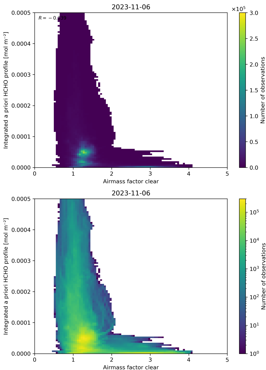
Figure 76: Scatter density plot of “Airmass factor clear” against “Integrated a priori HCHO profile” for 2023-11-05 to 2023-11-07.
