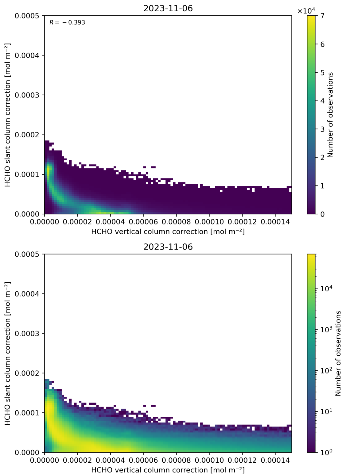
Figure 117: Scatter density plot of “HCHO vertical column correction” against “HCHO slant column correction” for 2023-11-05 to 2023-11-07.
