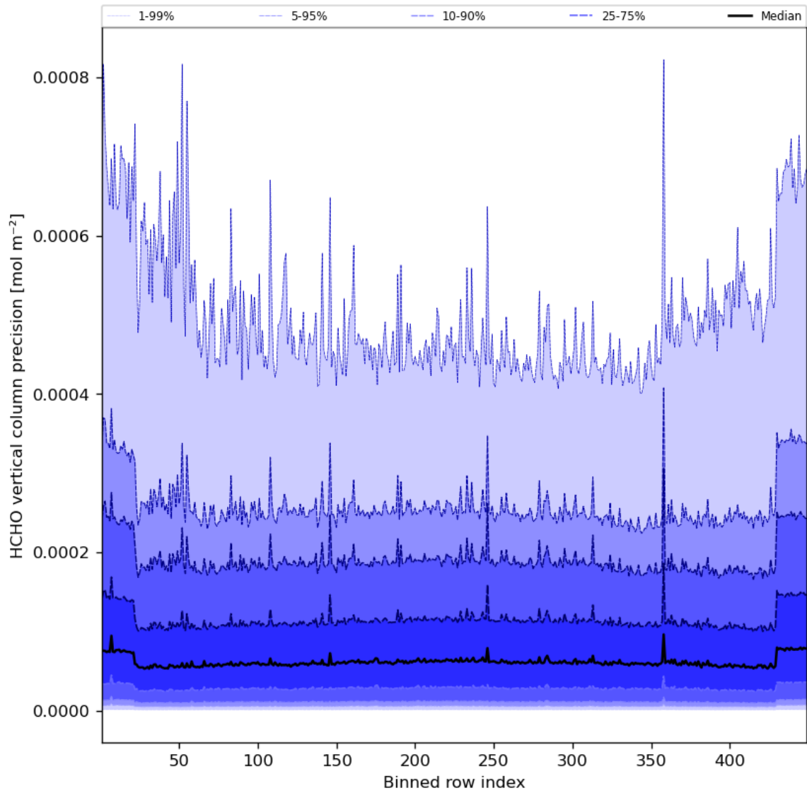
Figure 50: Along track statistics of “HCHO vertical column precision” for 2023-11-05 to 2023-11-07
