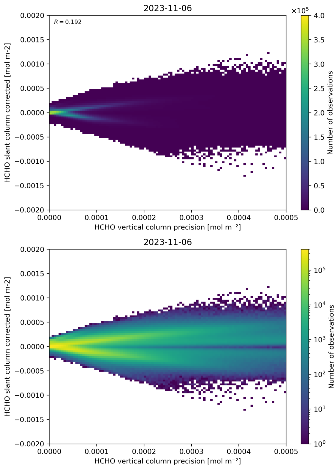
Figure 140: Scatter density plot of “HCHO vertical column precision” against “HCHO slant column corrected” for 2023-11-05 to 2023-11-07.
