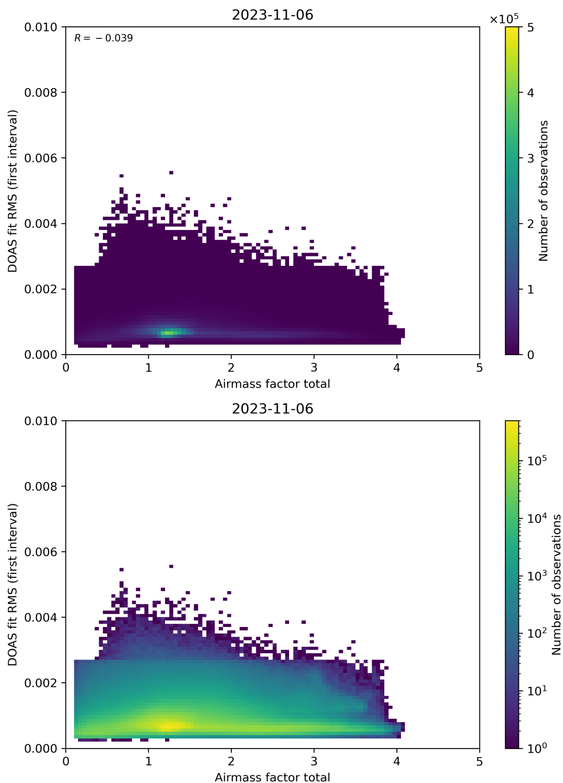
Figure 97: Scatter density plot of “Airmass factor total” against “DOAS fit RMS (first interval)” for 2023-11-05 to 2023-11-07.
