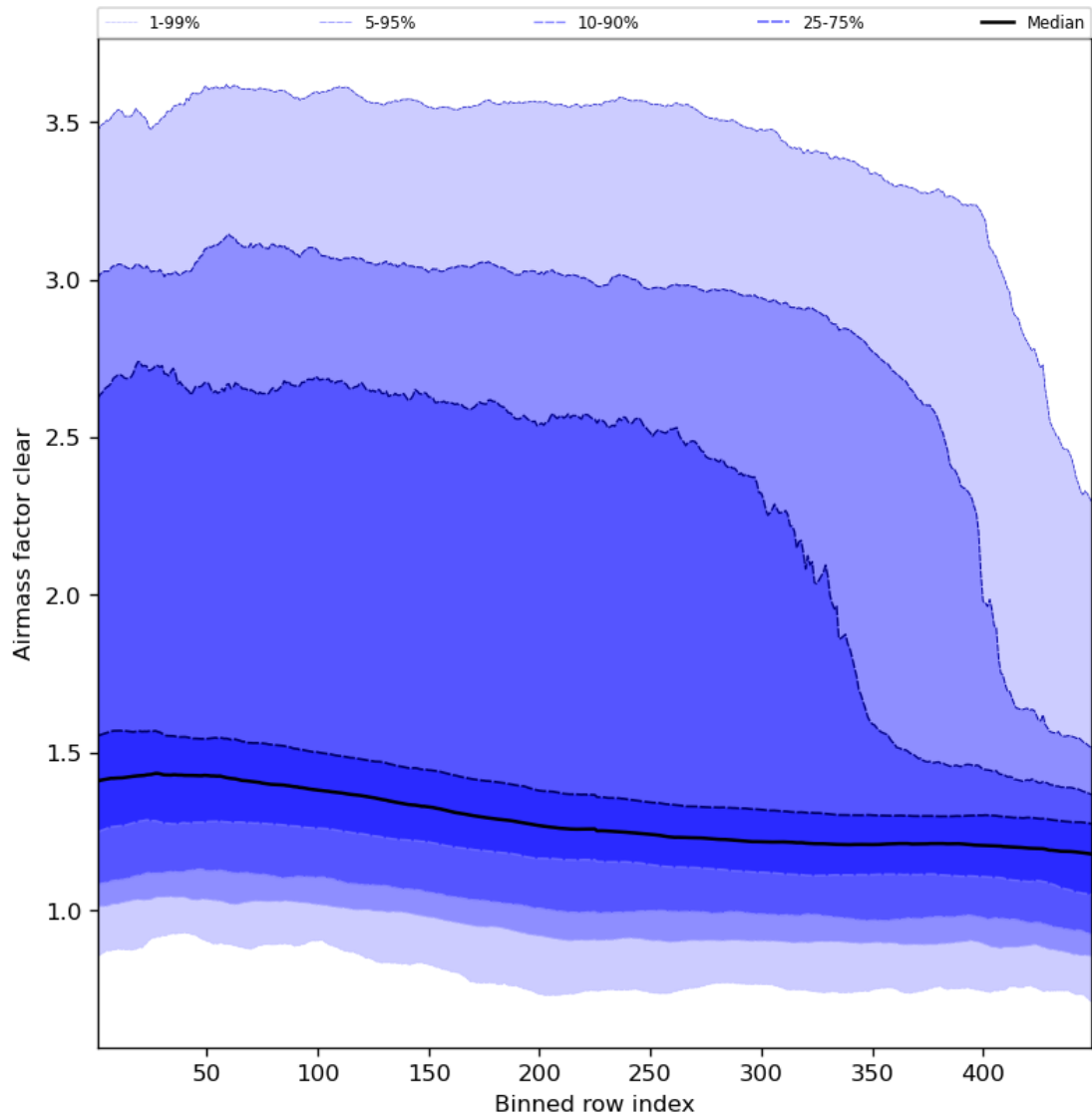
Figure 56: Along track statistics of “Airmass factor clear” for 2023-11-05 to 2023-11-07
