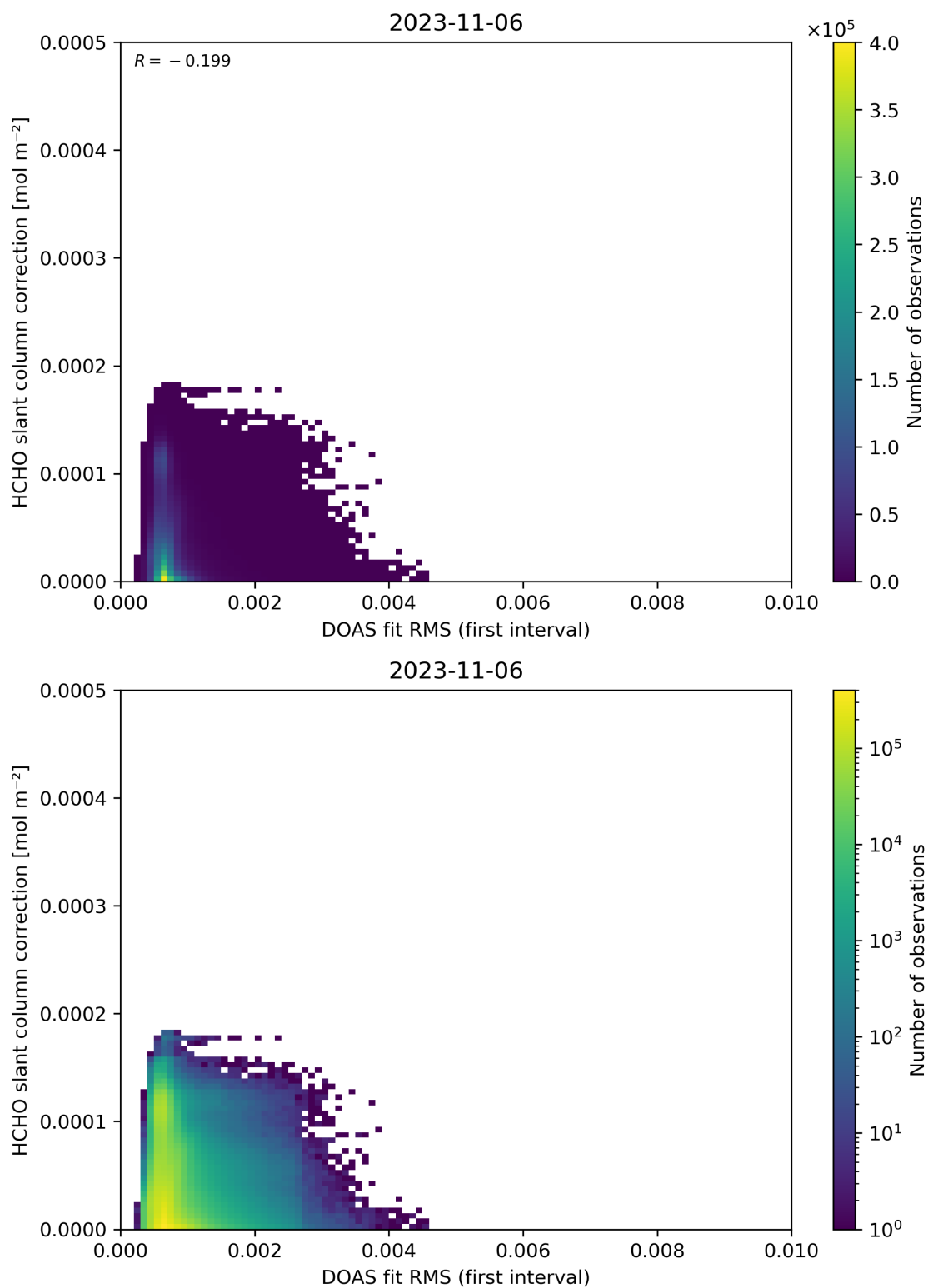
Figure 63: Scatter density plot of “DOAS fit RMS (first interval)” against “HCHO slant column correction” for 2023-11-05 to 2023-11-07.
