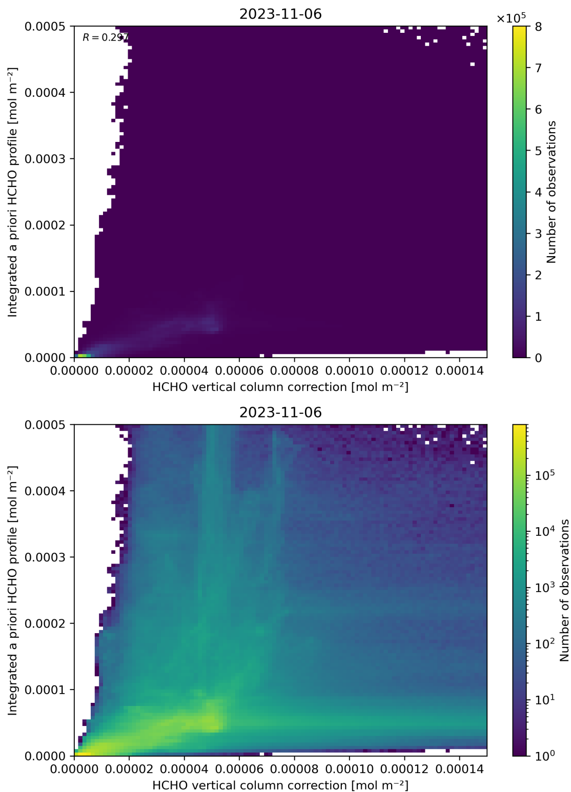
Figure 122: Scatter density plot of “HCHO vertical column correction” against “Integrated a priori HCHO profile” for 2023-11-05 to 2023-11-07.
