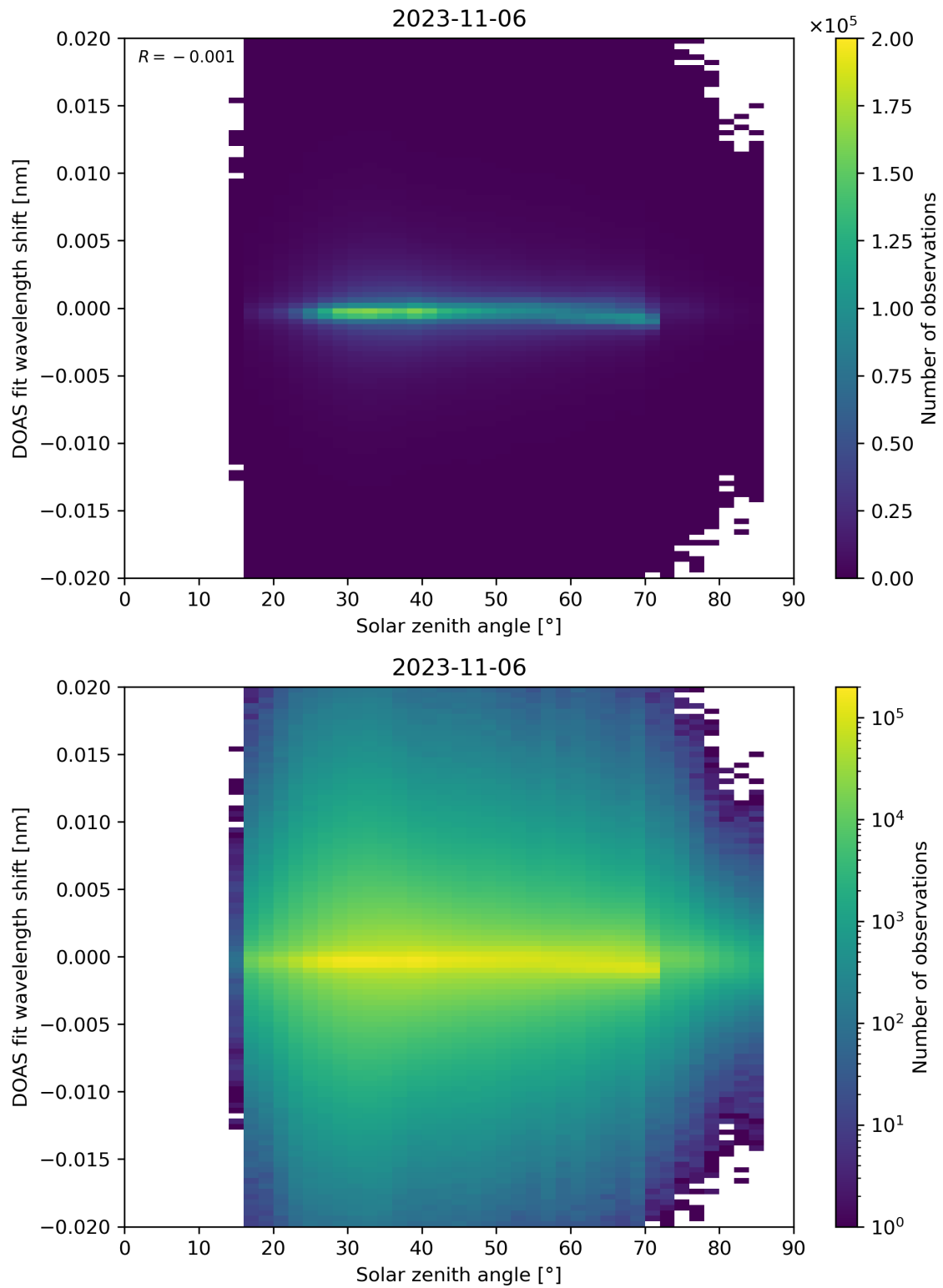
Figure 168: Scatter density plot of “Solar zenith angle” against “DOAS fit wavelength shift” for 2023-11-05 to 2023-11-07.
