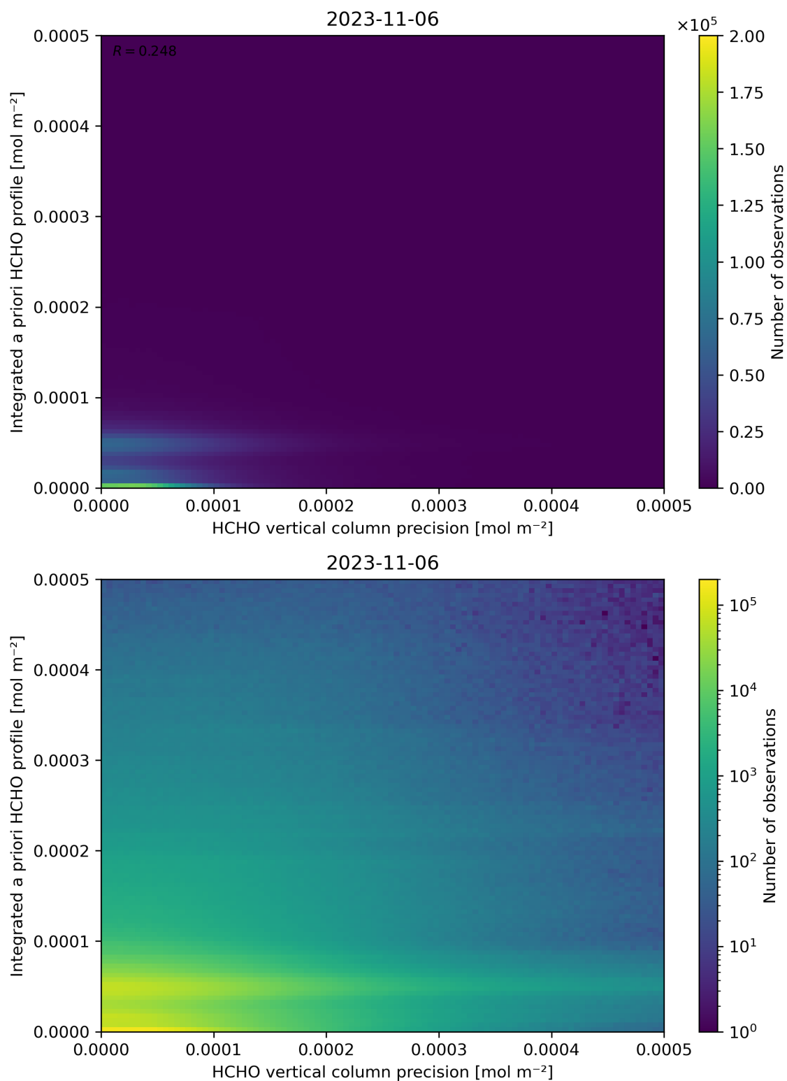
Figure 147: Scatter density plot of “HCHO vertical column precision” against “Integrated a priori HCHO profile” for 2023-11-05 to 2023-11-07.
