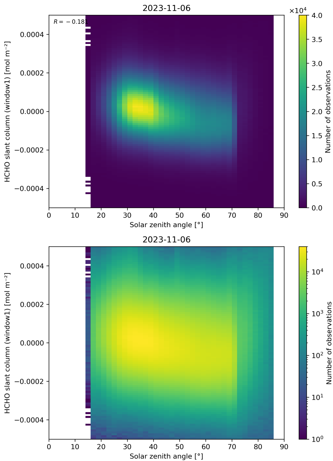
Figure 173: Scatter density plot of “Solar zenith angle” against “HCHO slant column (window1)” for 2023-11-05 to 2023-11-07.
