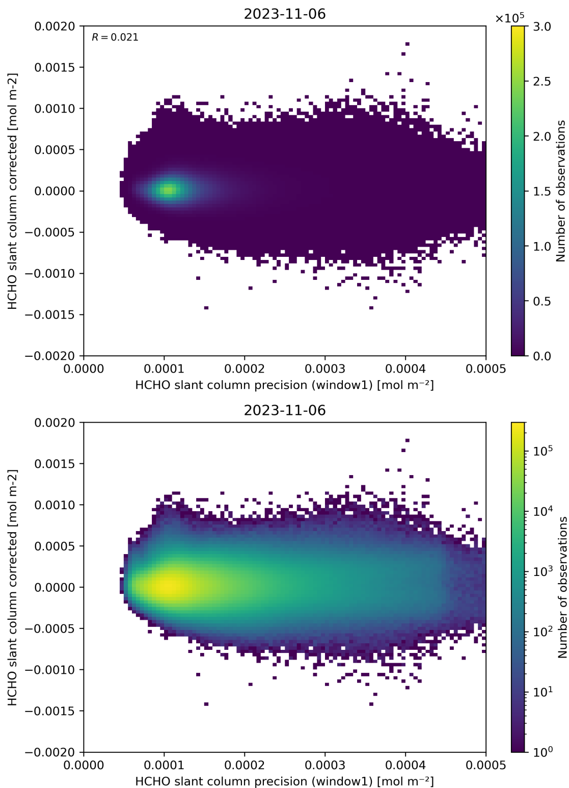
Figure 92: Scatter density plot of “HCHO slant column precision (window1)” against “HCHO slant column corrected” for 2023-11-05 to 2023-11-07.
