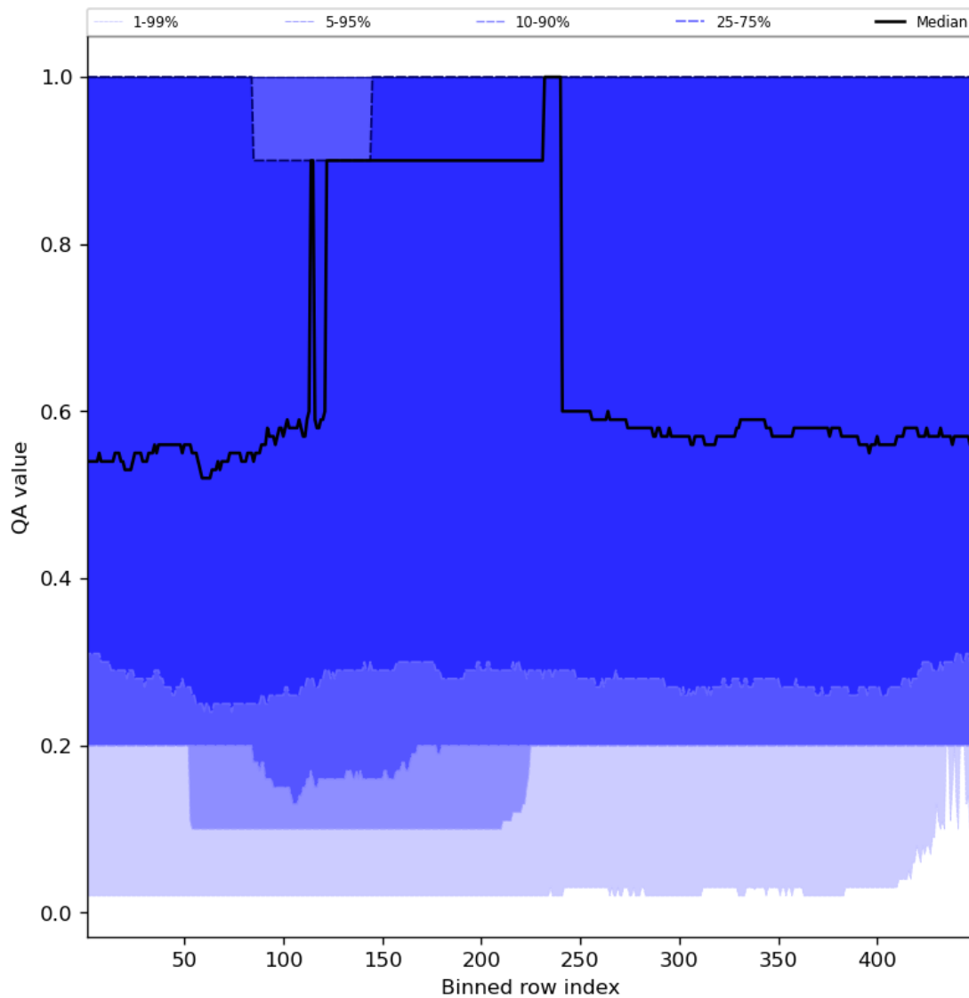
Figure 48: Along track statistics of “QA value” for 2023-11-05 to 2023-11-07
