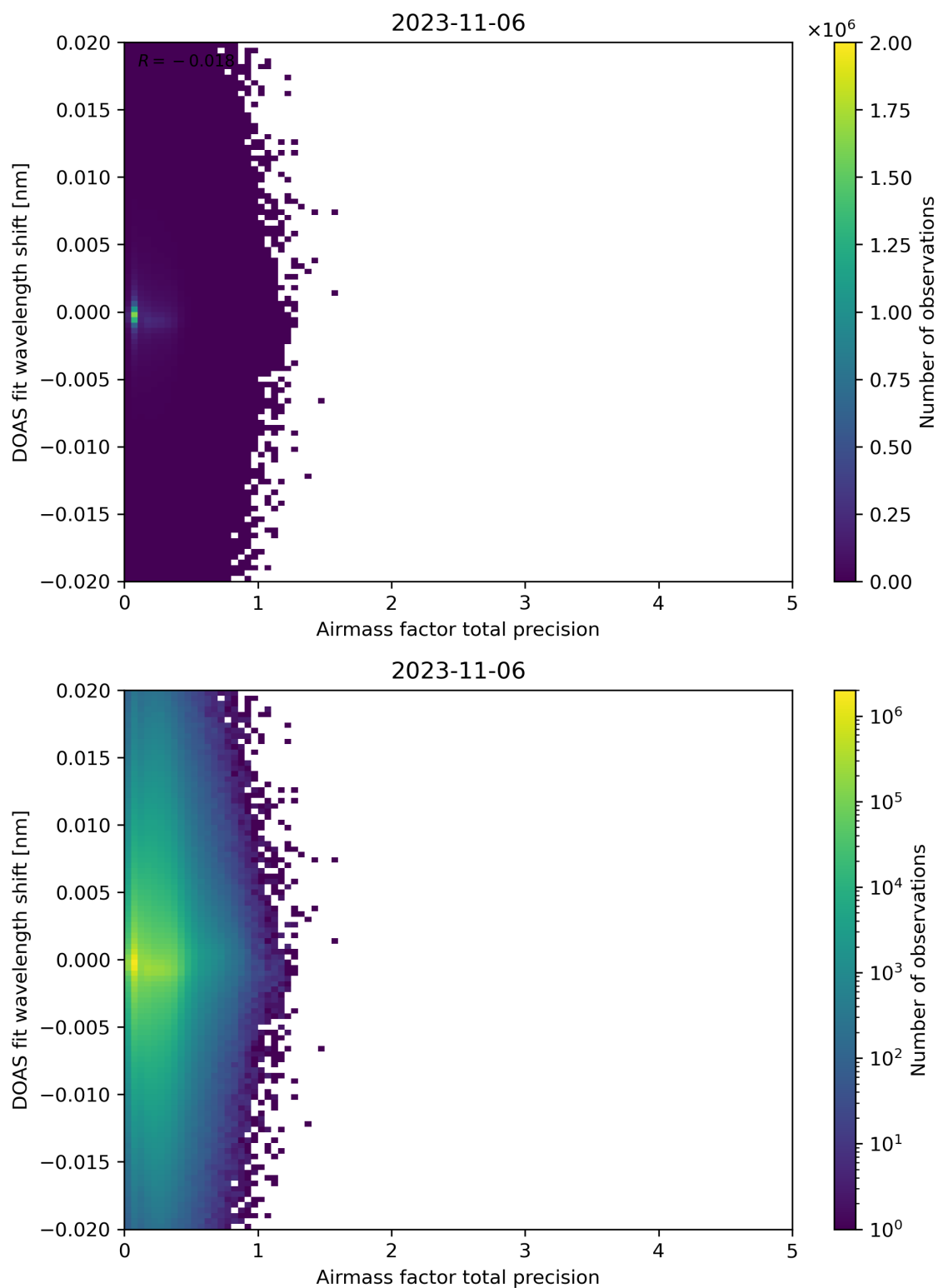
Figure 106: Scatter density plot of “Airmass factor total precision” against “DOAS fit wavelength shift” for 2023-11-05 to 2023-11-07.
