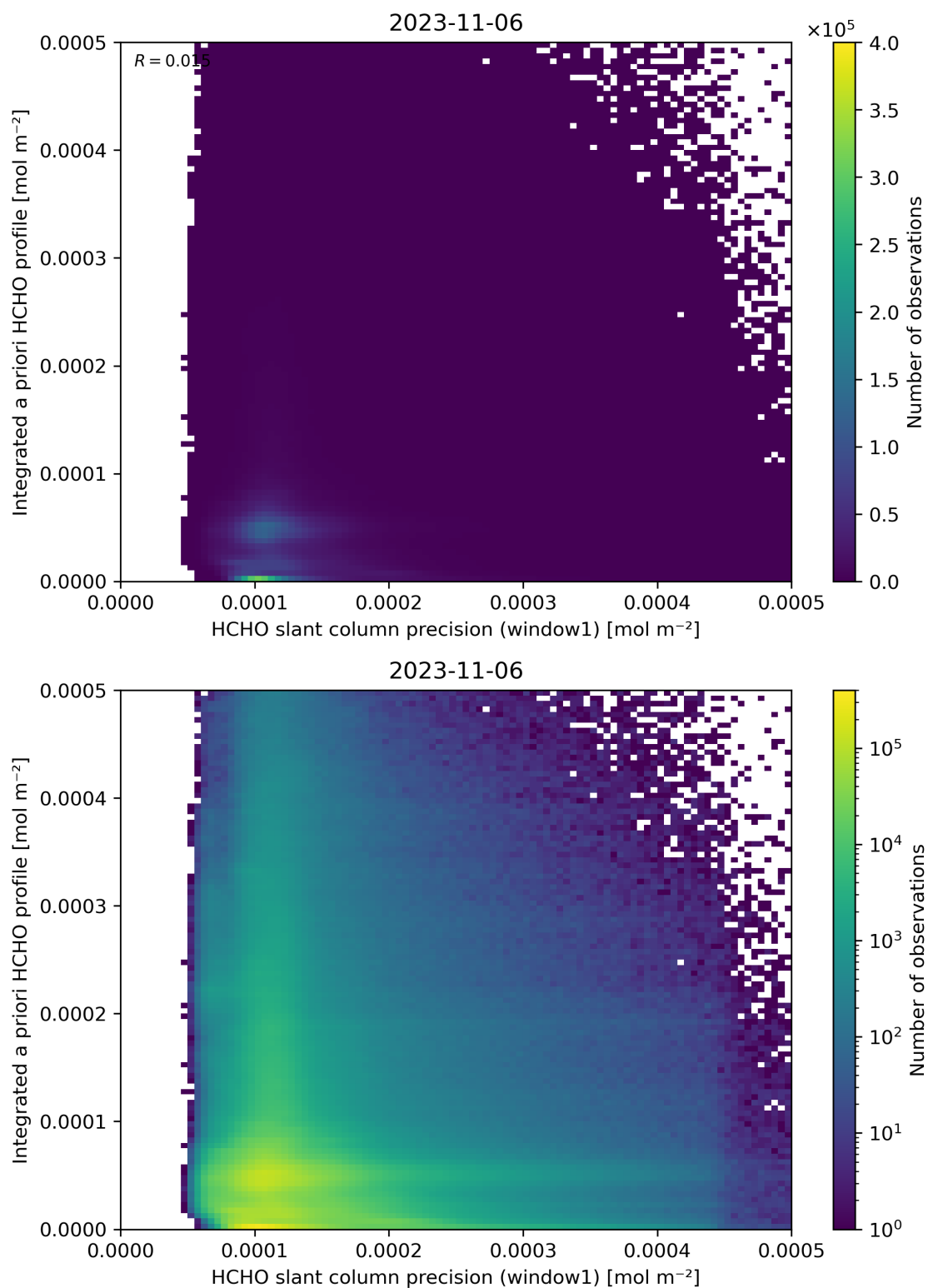
Figure 96: Scatter density plot of “HCHO slant column precision (window1)” against “Integrated a priori HCHO profile” for 2023-11-05 to 2023-11-07.
