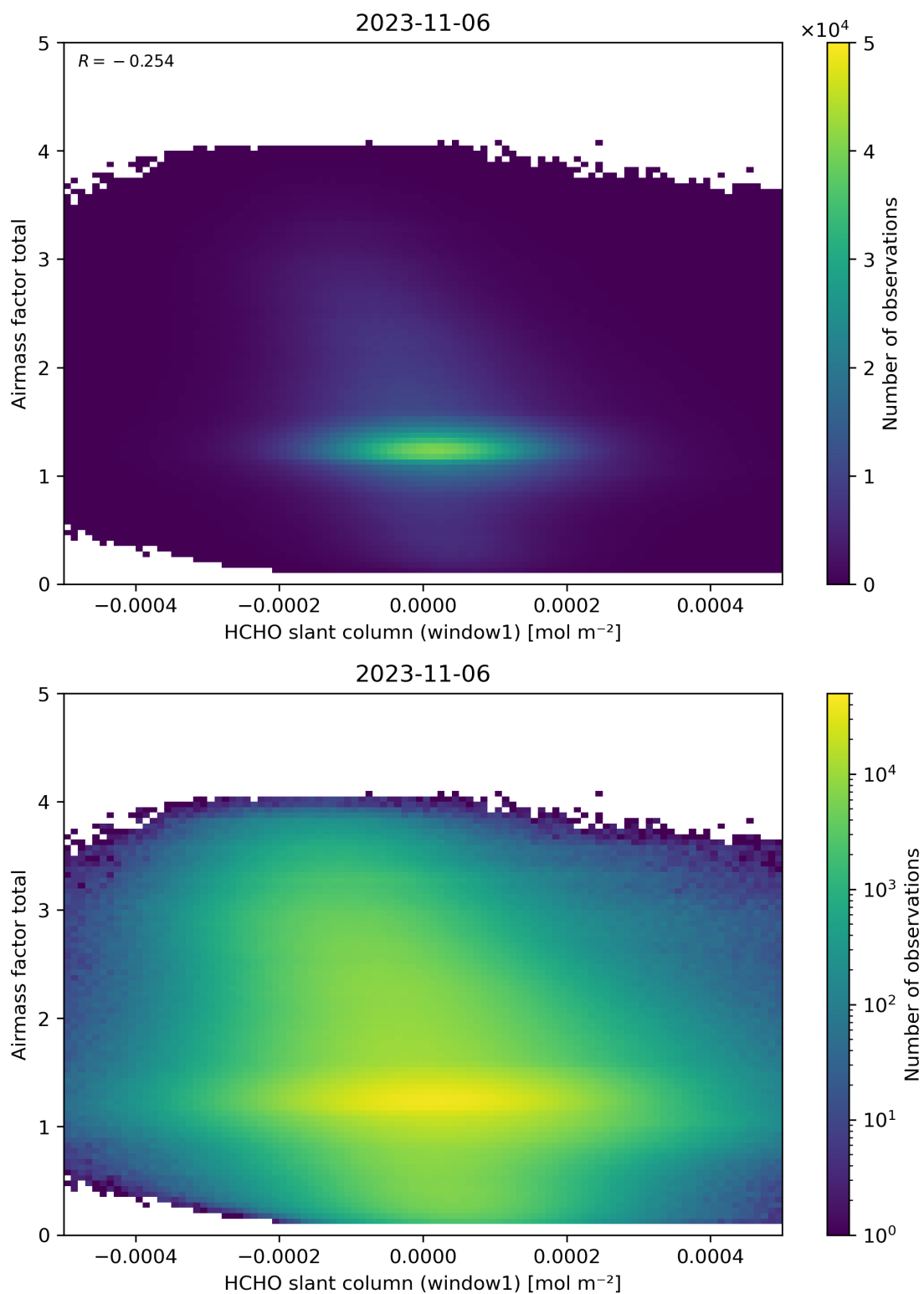
Figure 85: Scatter density plot of “HCHO slant column (window1)” against “Airmass factor total” for 2023-11-05 to 2023-11-07.
