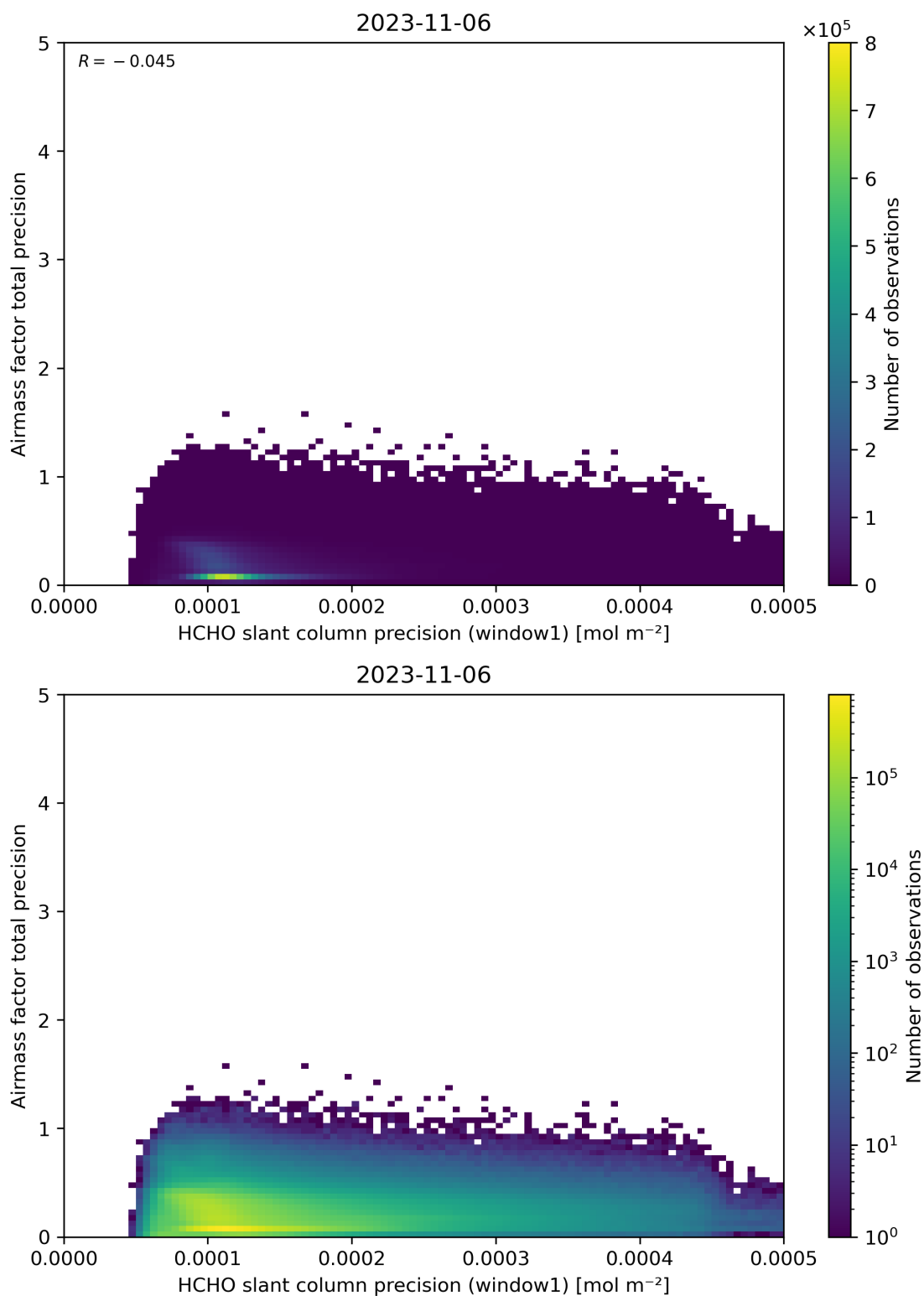
Figure 95: Scatter density plot of “HCHO slant column precision (window1)” against “Airmass factor total precision” for 2023-11-05 to 2023-11-07.
