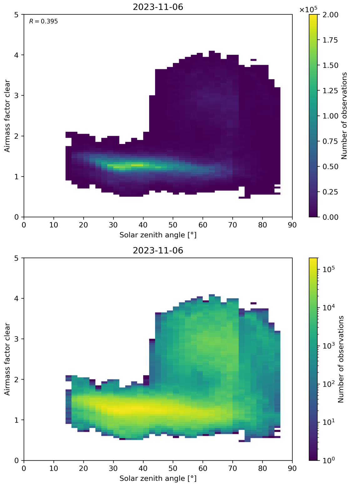
Figure 170: Scatter density plot of “Solar zenith angle” against “Airmass factor clear” for 2023-11-05 to 2023-11-07.
