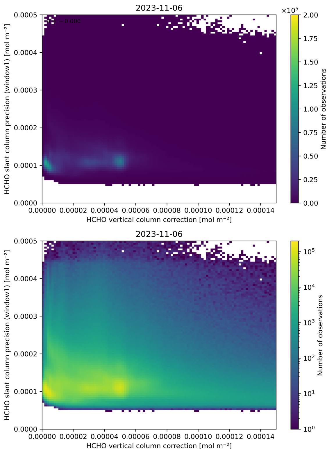
Figure 119: Scatter density plot of “HCHO vertical column correction” against “HCHO slant column precision (window1)” for 2023-11-05 to 2023-11-07.
