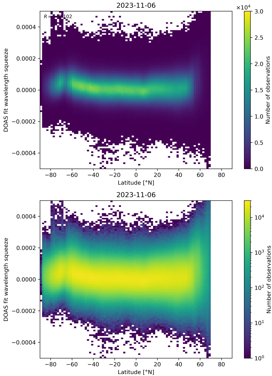
Figure 155: Scatter density plot of “Latitude” against “DOAS fit wavelength squeeze” for 2023-11-05 to 2023-11-07.
