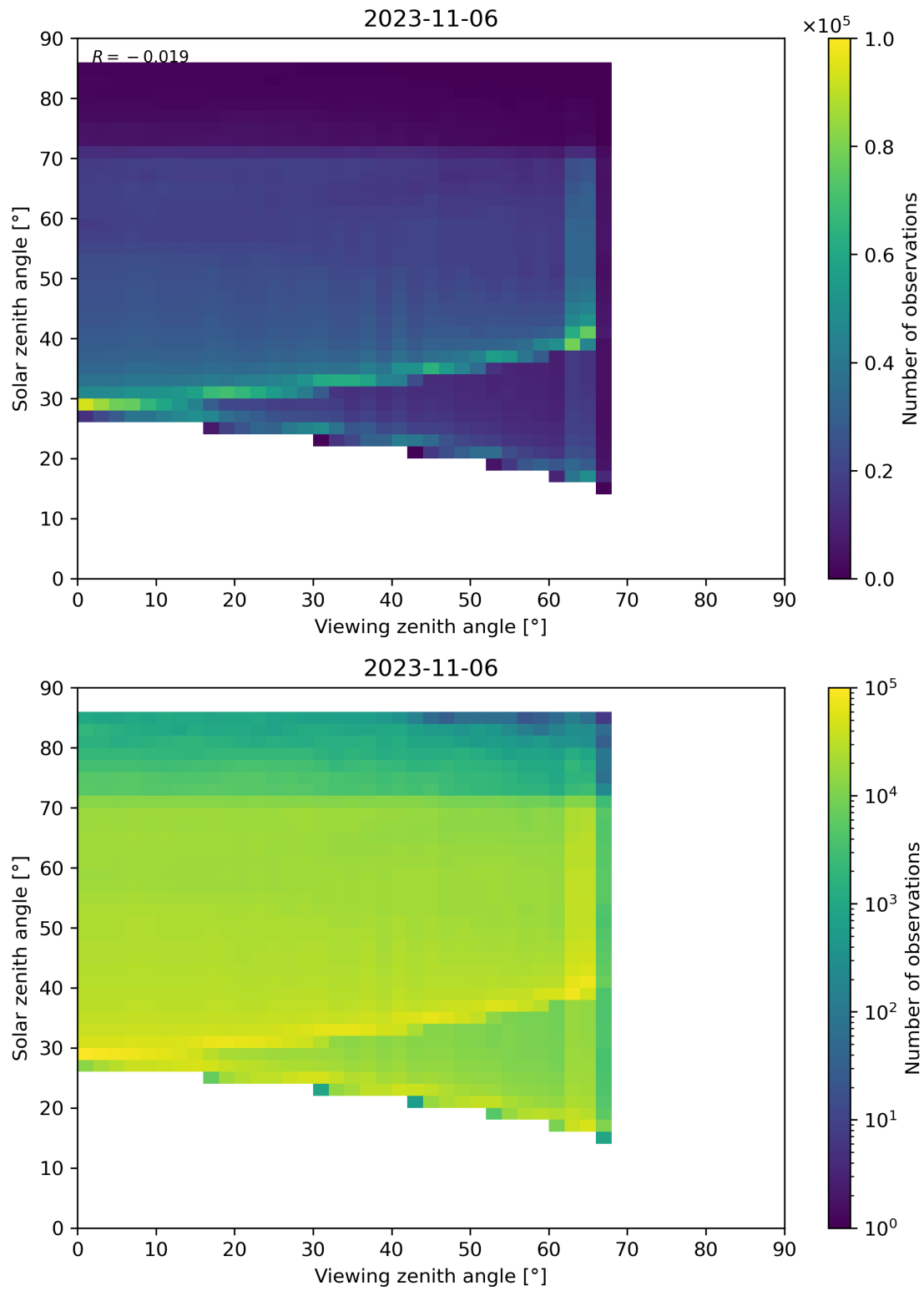
Figure 197: Scatter density plot of “Viewing zenith angle” against “Solar zenith angle” for 2023-11-05 to 2023-11-07.
