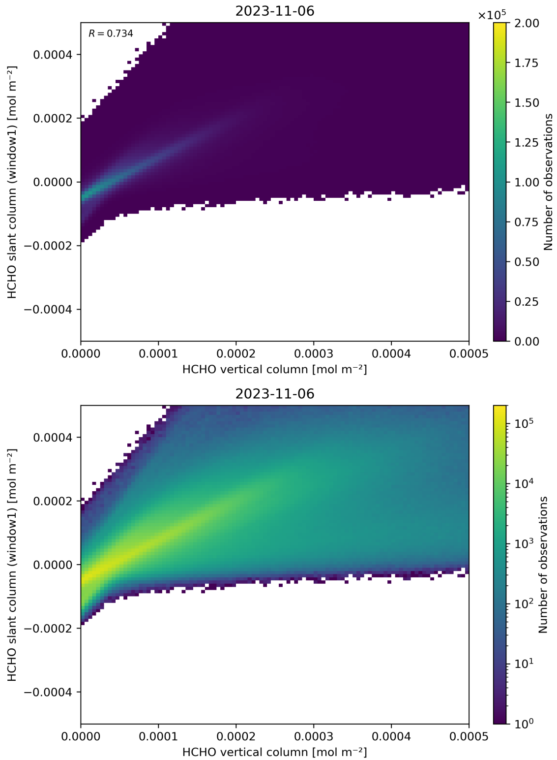
Figure 129: Scatter density plot of “HCHO vertical column” against “HCHO slant column (window1)” for 2023-11-05 to 2023-11-07.
