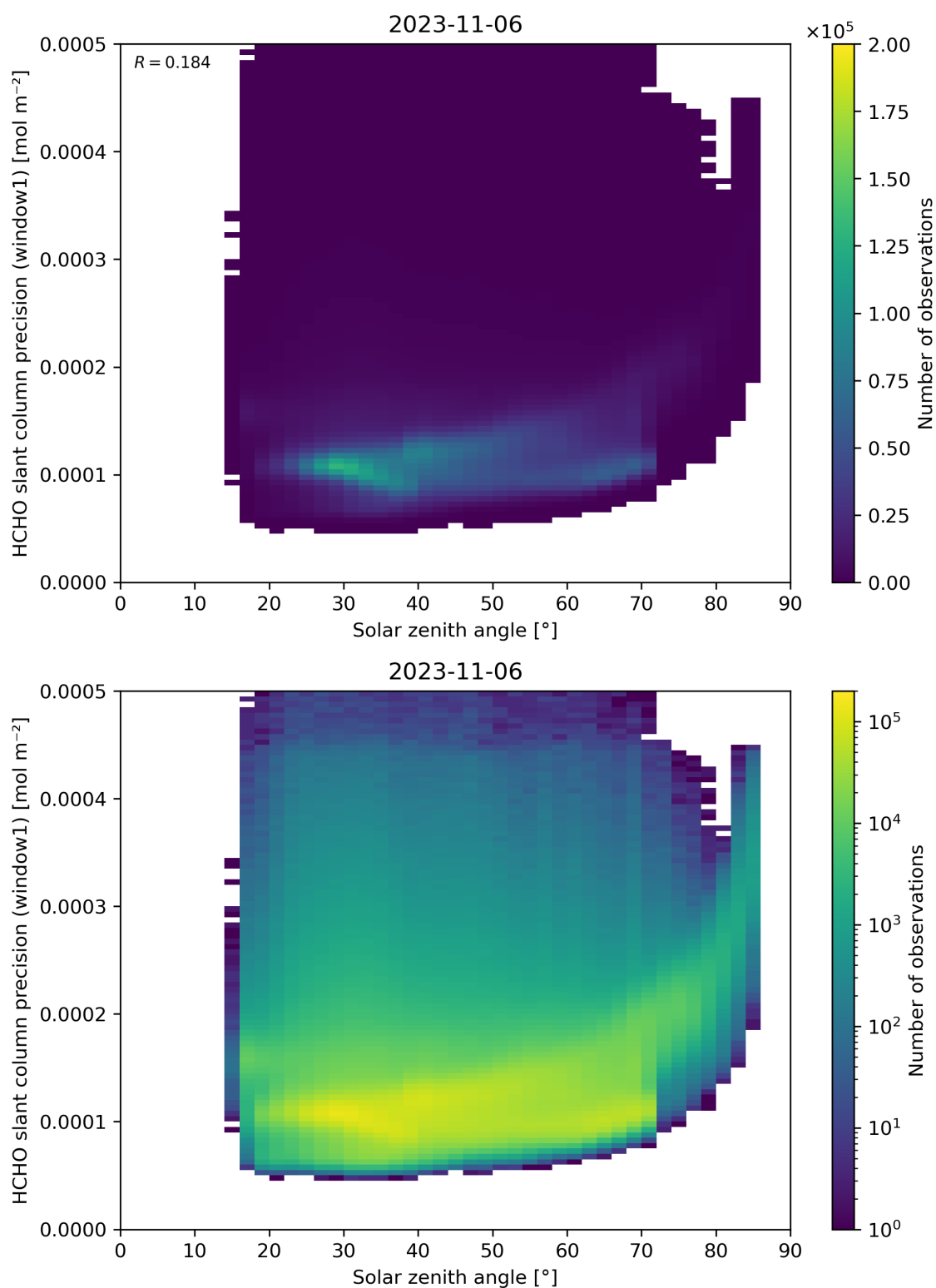
Figure 174: Scatter density plot of “Solar zenith angle” against “HCHO slant column precision (window1)” for 2023-11-05 to 2023-11-07.
