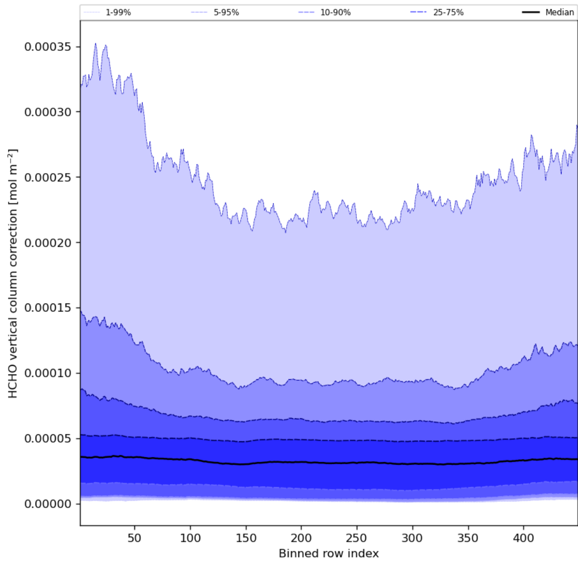
Figure 51: Along track statistics of “HCHO vertical column correction” for 2023-11-05 to 2023-11-07
