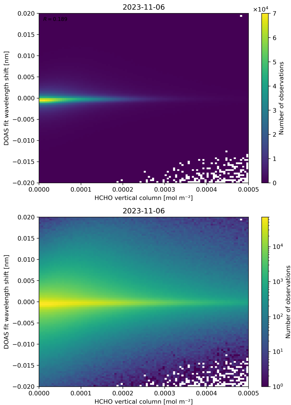
Figure 124: Scatter density plot of “HCHO vertical column” against “DOAS fit wavelength shift” for 2023-11-05 to 2023-11-07.
