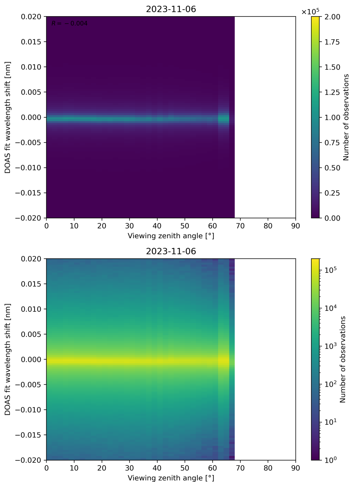
Figure 183: Scatter density plot of “Viewing zenith angle” against “DOAS fit wavelength shift” for 2023-11-05 to 2023-11-07.
