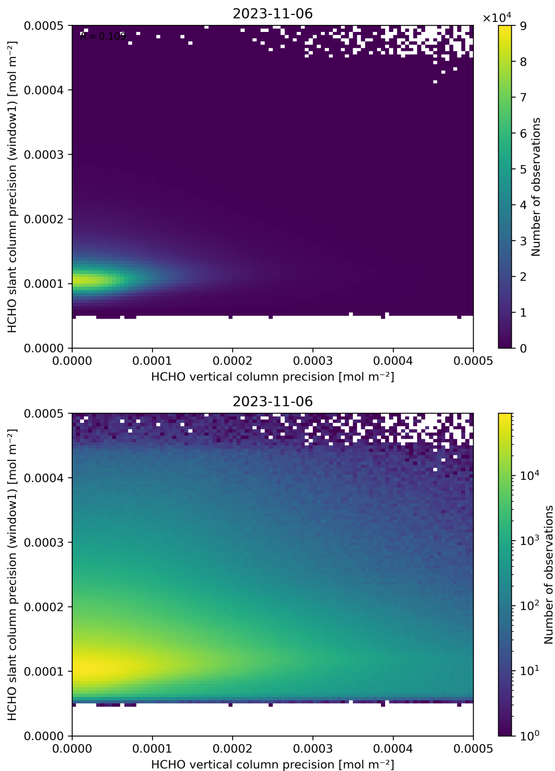
Figure 143: Scatter density plot of “HCHO vertical column precision” against “HCHO slant column precision (window1)” for 2023-11-05 to 2023-11-07.
