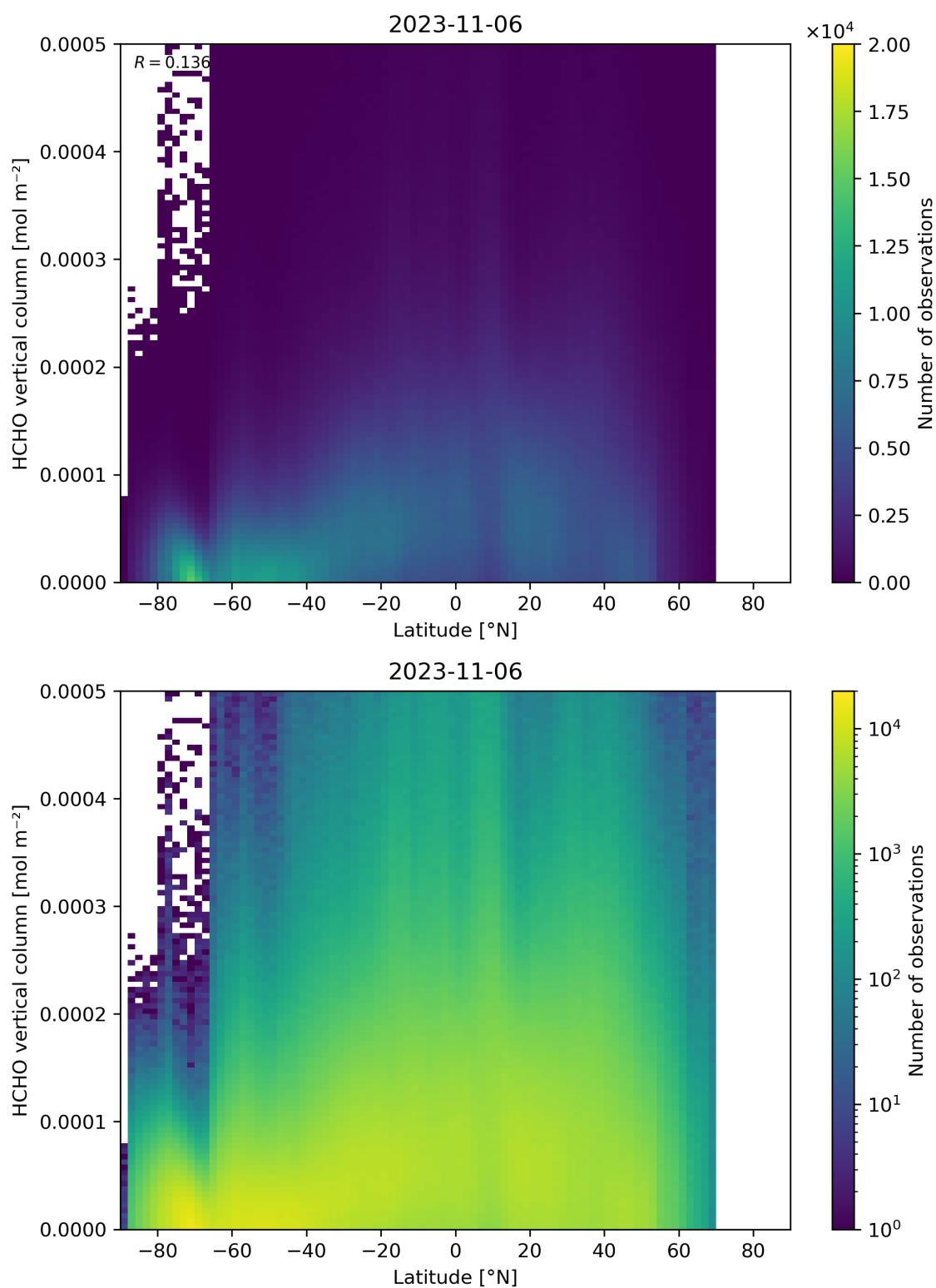
Figure 163: Scatter density plot of “Latitude” against “HCHO vertical column” for 2023-11-05 to 2023-11-07.
