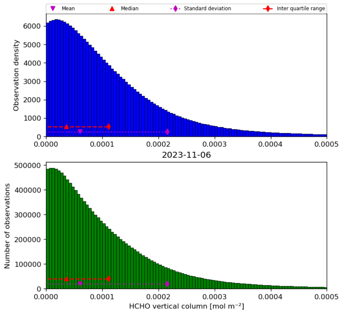
Figure 35: Histogram of “HCHO vertical column” for 2023-11-05 to 2023-11-07
