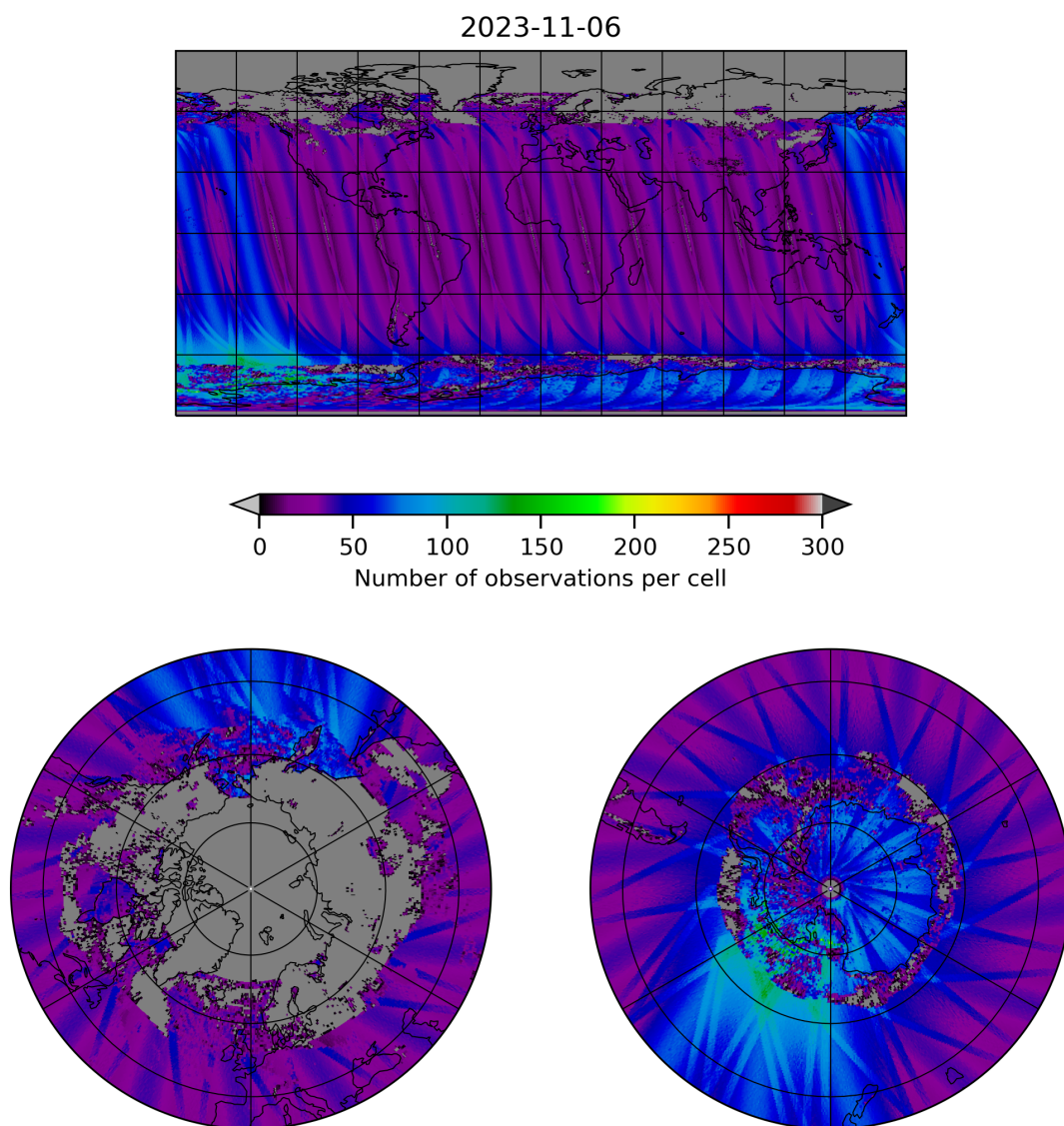
Figure 19: Map of the number of observations for 2023-11-05 to 2023-11-07
