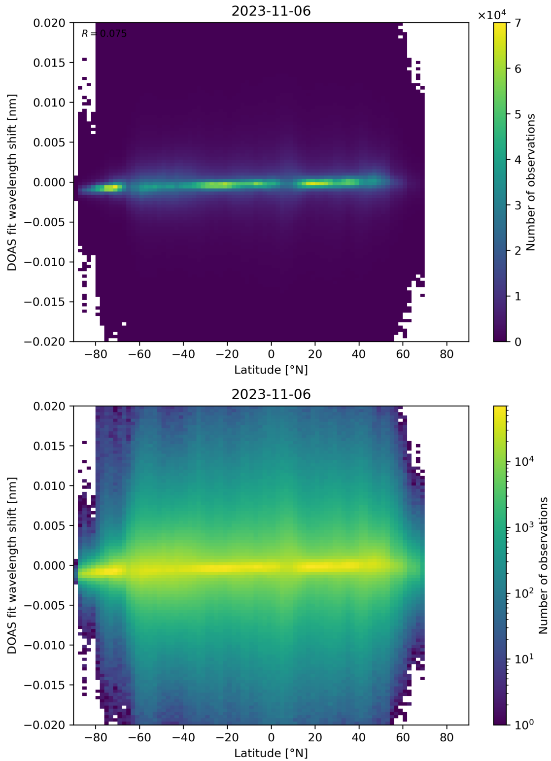
Figure 154: Scatter density plot of “Latitude” against “DOAS fit wavelength shift” for 2023-11-05 to 2023-11-07.
