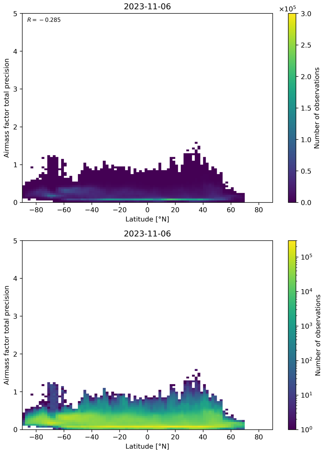
Figure 162: Scatter density plot of “Latitude” against “Airmass factor total precision” for 2023-11-05 to 2023-11-07.
