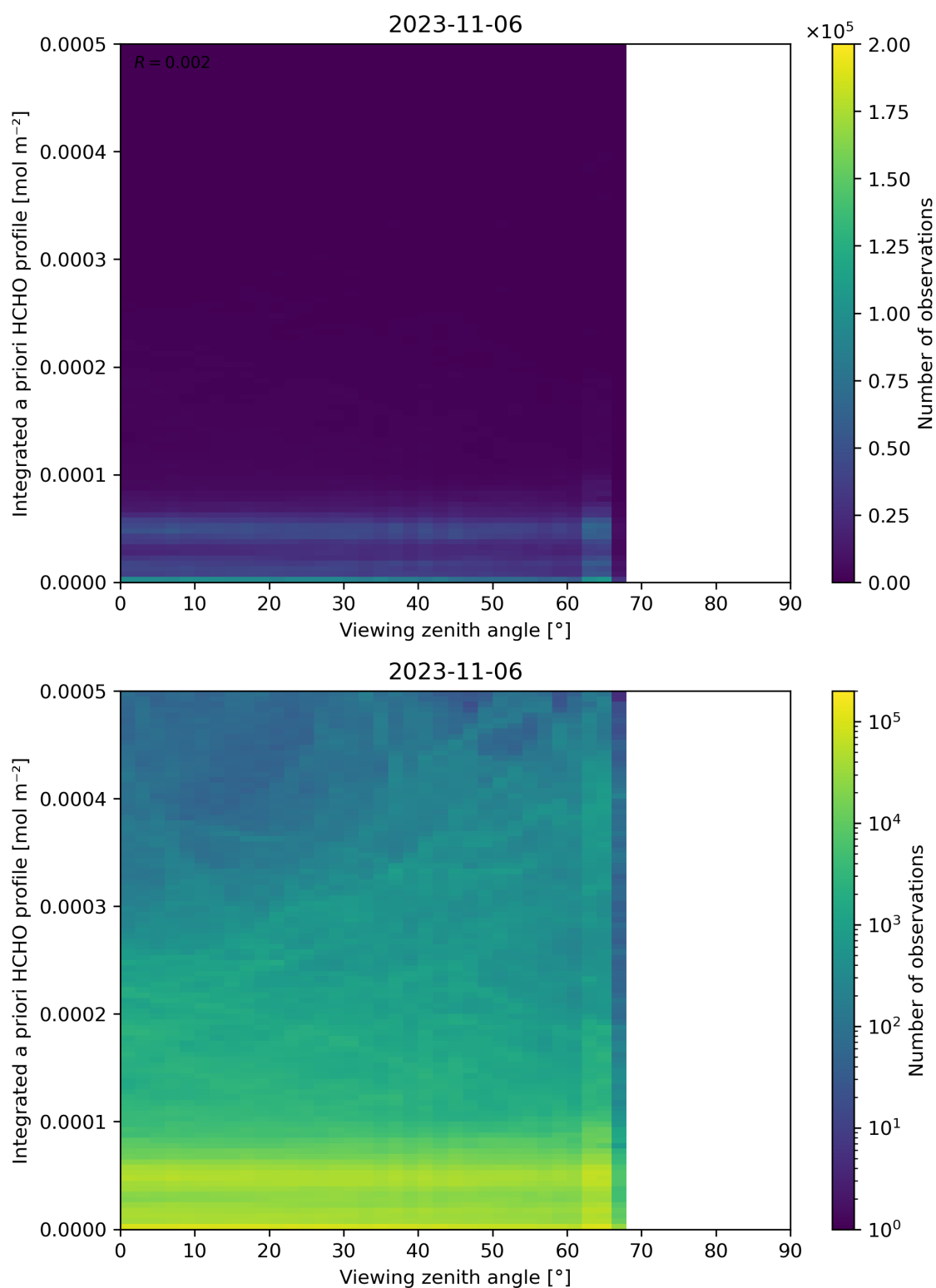
Figure 195: Scatter density plot of “Viewing zenith angle” against “Integrated a priori HCHO profile” for 2023-11-05 to 2023-11-07.
