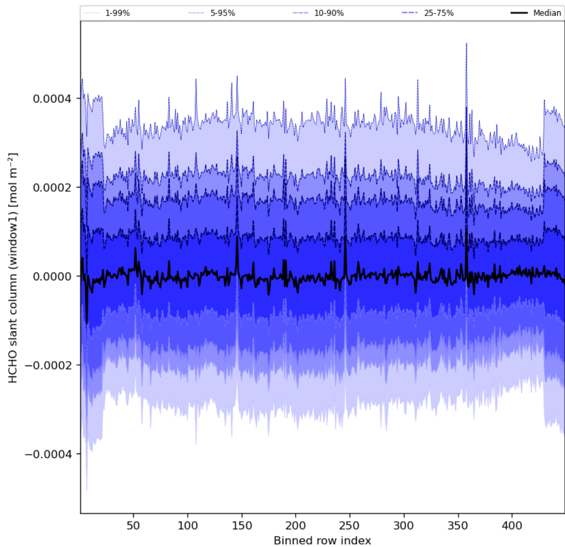
Figure 52: Along track statistics of “HCHO slant column (window1)” for 2023-11-05 to 2023-11-07
