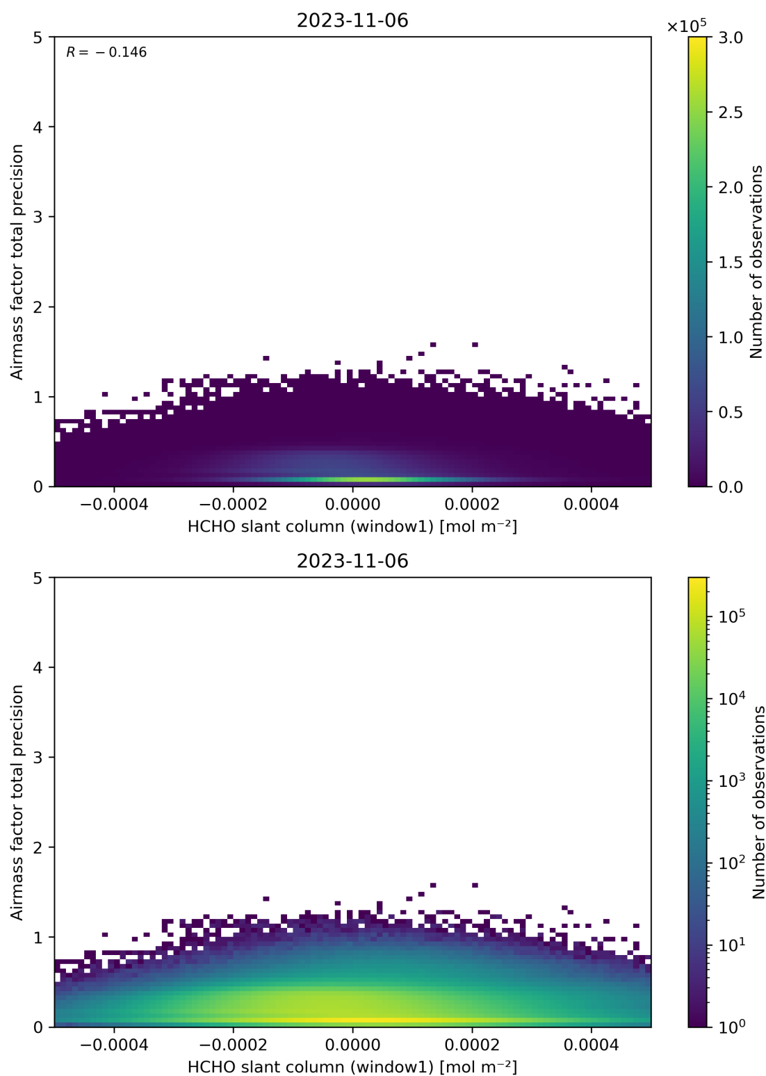
Figure 86: Scatter density plot of “HCHO slant column (window1)” against “Airmass factor total precision” for 2023-11-05 to 2023-11-07.
