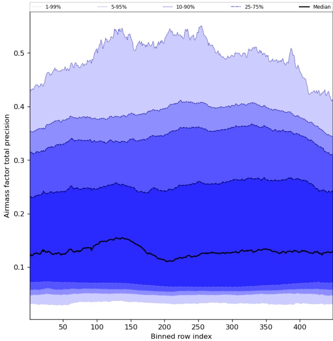
Figure 55: Along track statistics of “Airmass factor total precision” for 2023-11-05 to 2023-11-07
