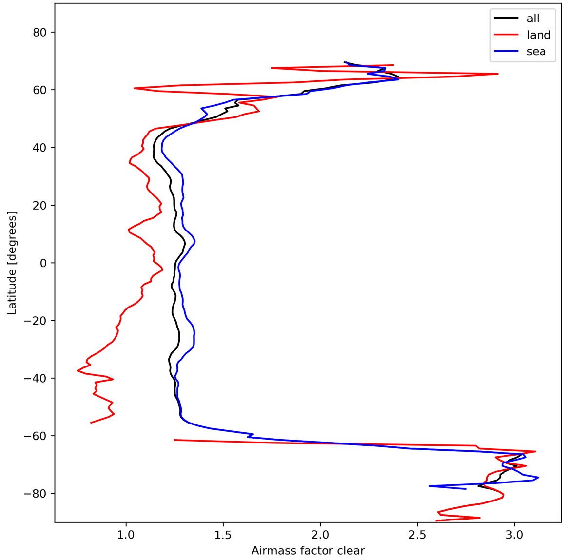
Figure 28: Zonal average of “Airmass factor clear” for 2023-11-05 to 2023-11-07.
