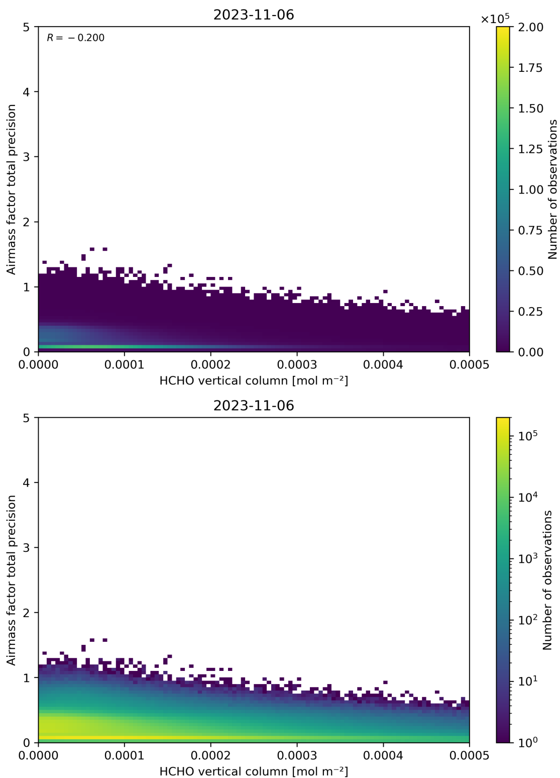
Figure 132: Scatter density plot of “HCHO vertical column” against “Airmass factor total precision” for 2023-11-05 to 2023-11-07.
