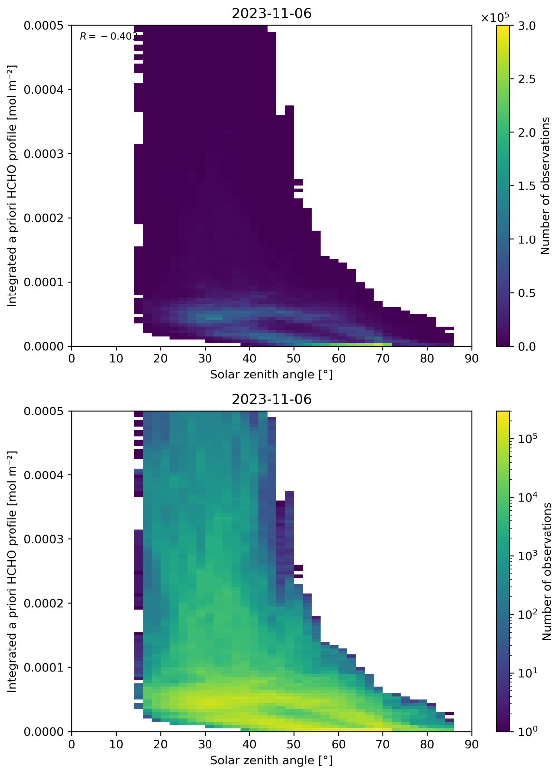
Figure 180: Scatter density plot of “Solar zenith angle” against “Integrated a priori HCHO profile” for 2023-11-05 to 2023-11-07.
