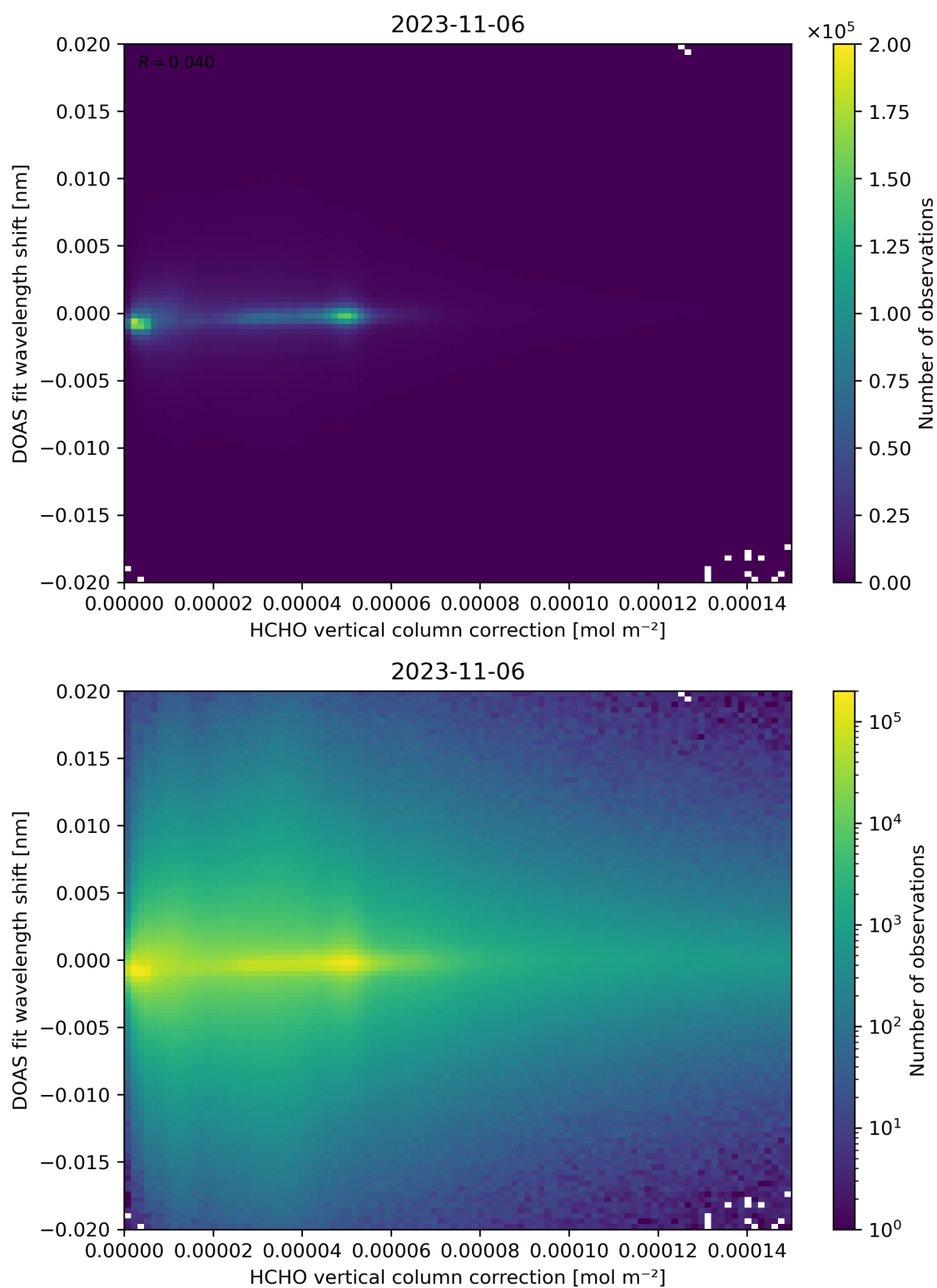
Figure 113: Scatter density plot of “HCHO vertical column correction” against “DOAS fit wavelength shift” for 2023-11-05 to 2023-11-07.
