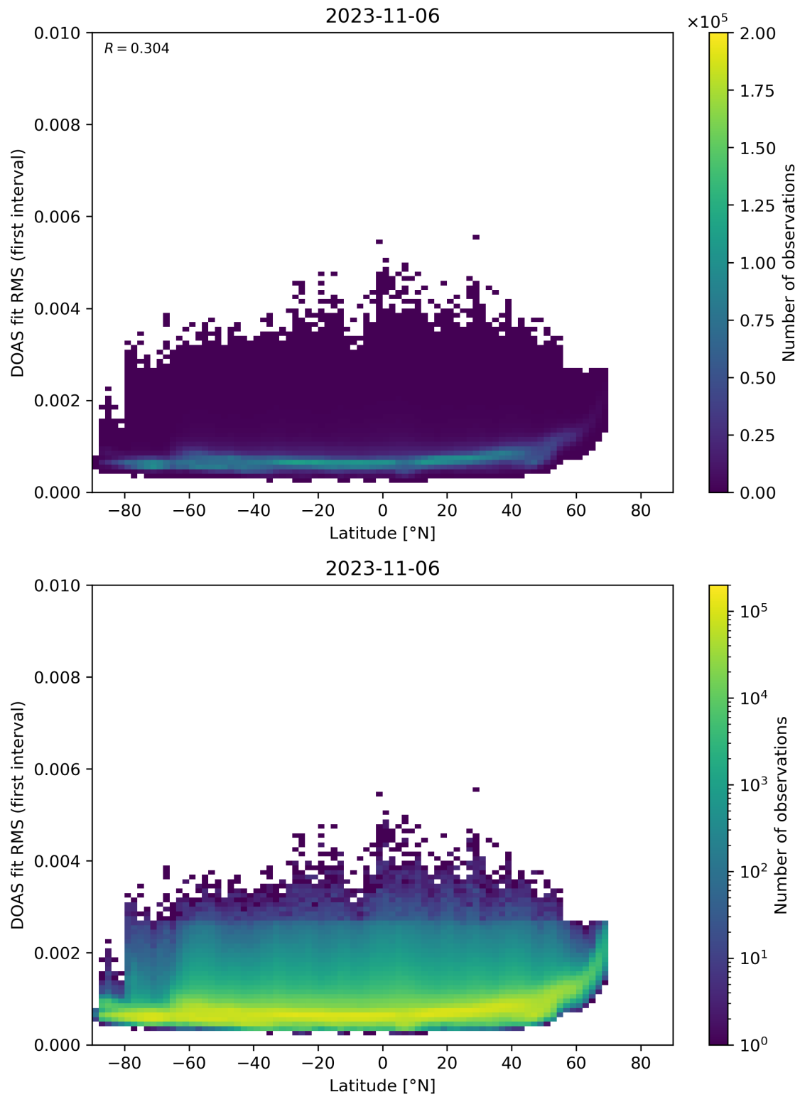
Figure 153: Scatter density plot of “Latitude” against “DOAS fit RMS (first interval)” for 2023-11-05 to 2023-11-07.
