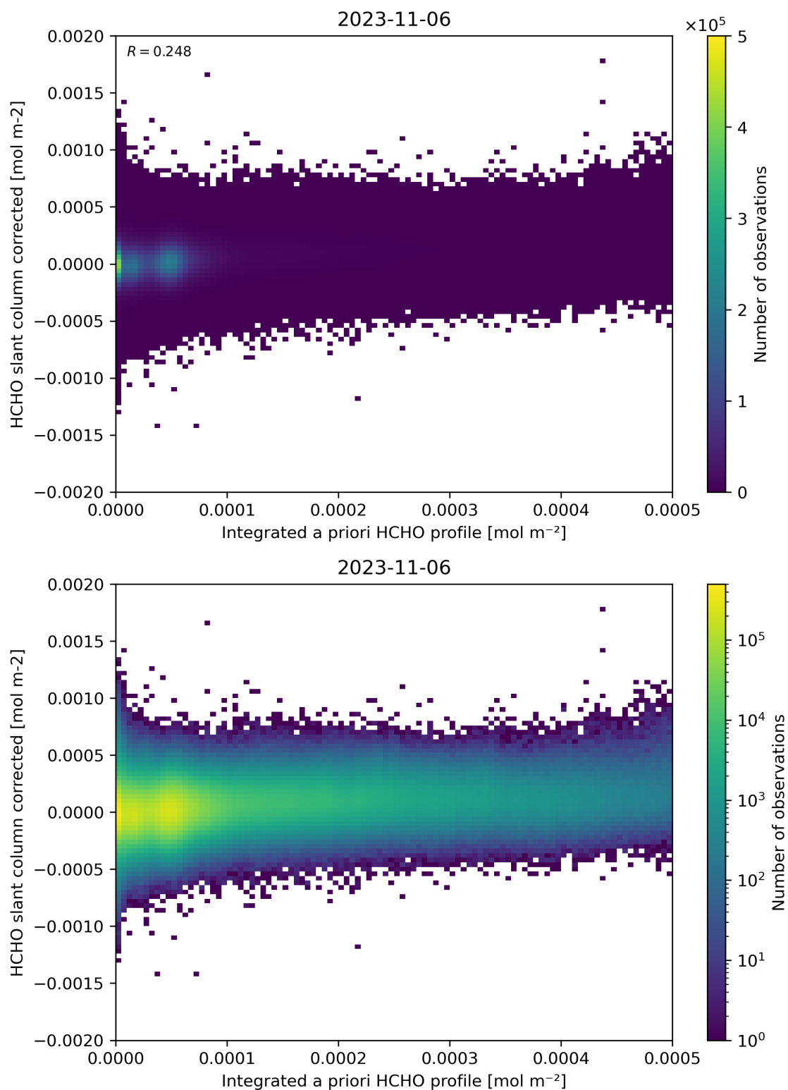
Figure 151: Scatter density plot of “Integrated a priori HCHO profile” against “HCHO slant column corrected” for 2023-11-05 to 2023-11-07.
