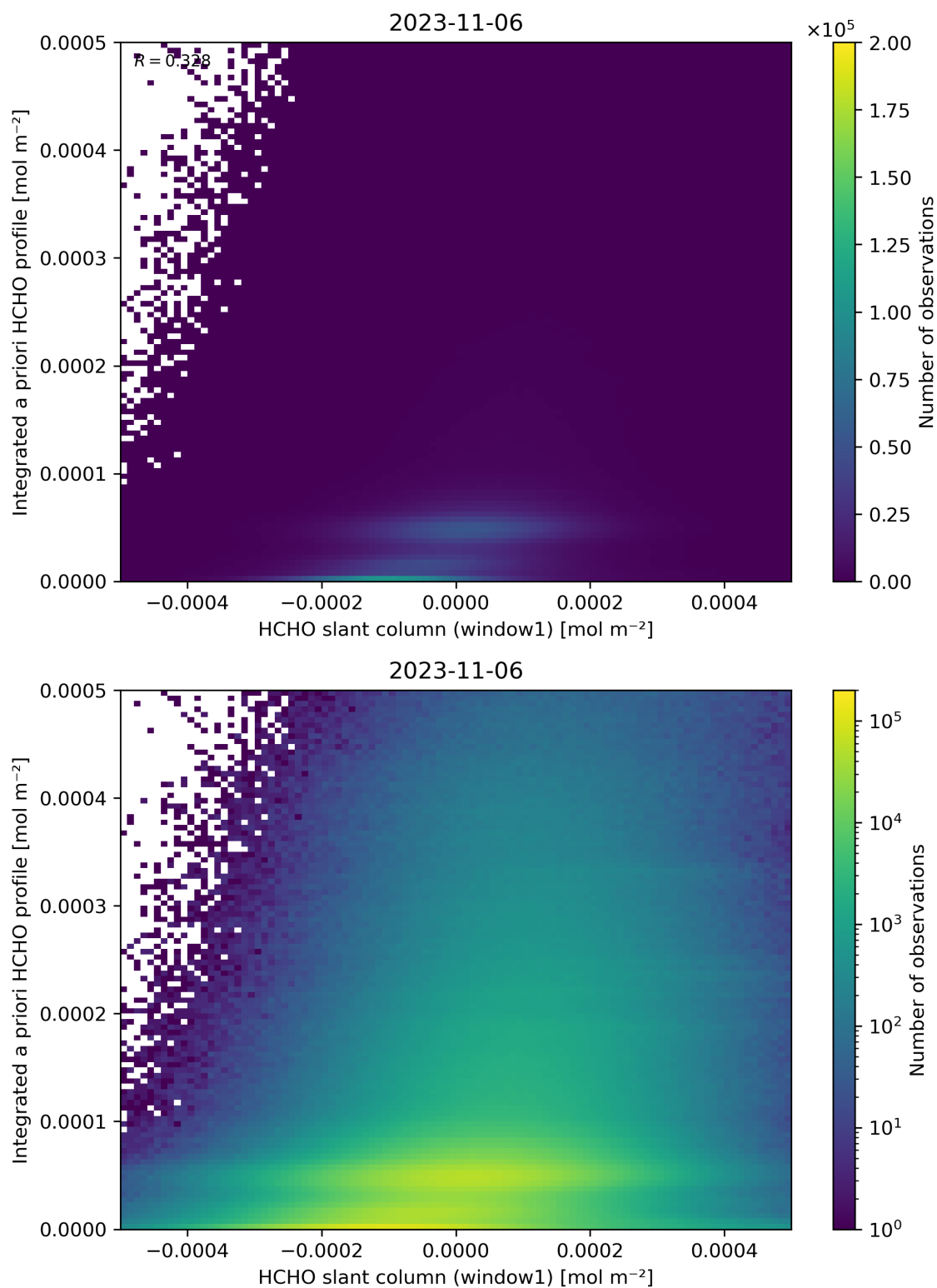
Figure 87: Scatter density plot of “HCHO slant column (window1)” against “Integrated a priori HCHO profile” for 2023-11-05 to 2023-11-07.
