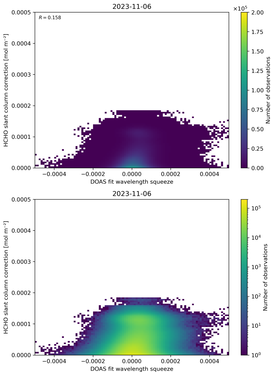
Figure 70: Scatter density plot of “DOAS fit wavelength squeeze” against “HCHO slant column correction” for 2023-11-05 to 2023-11-07.
