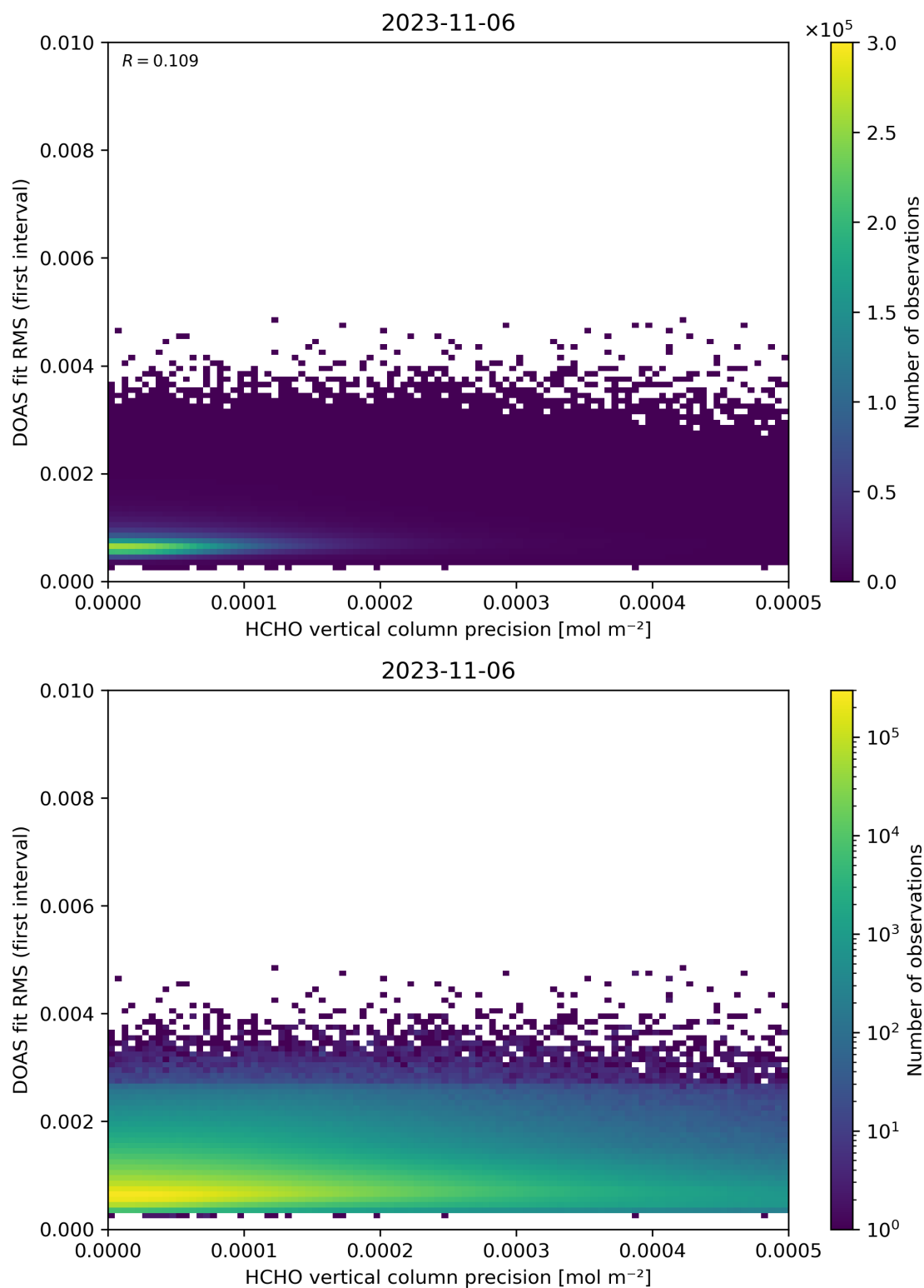
Figure 136: Scatter density plot of “HCHO vertical column precision” against “DOAS fit RMS (first interval)” for 2023-11-05 to 2023-11-07.
