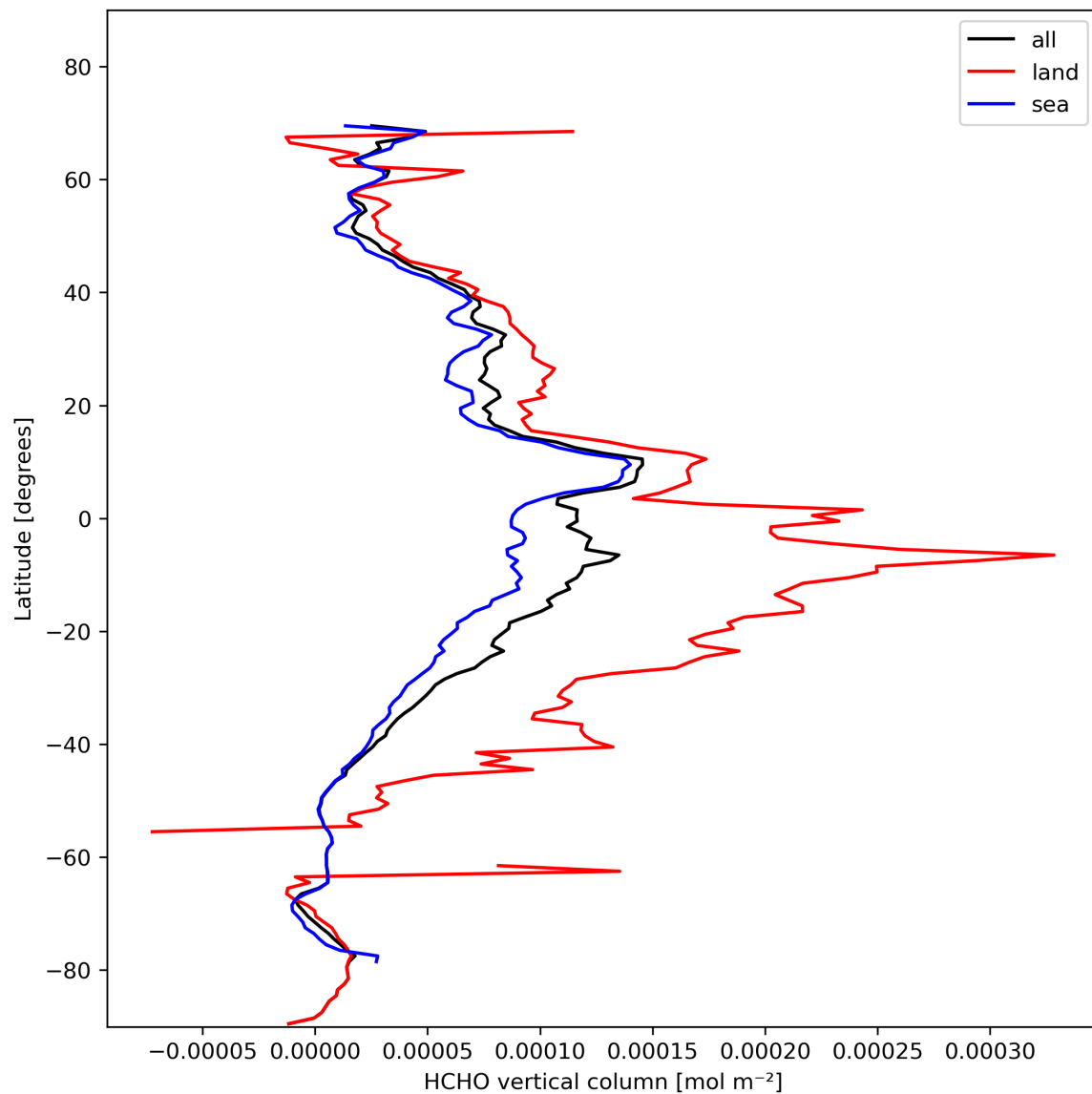
Figure 21: Zonal average of “HCHO vertical column” for 2023-11-05 to 2023-11-07.
