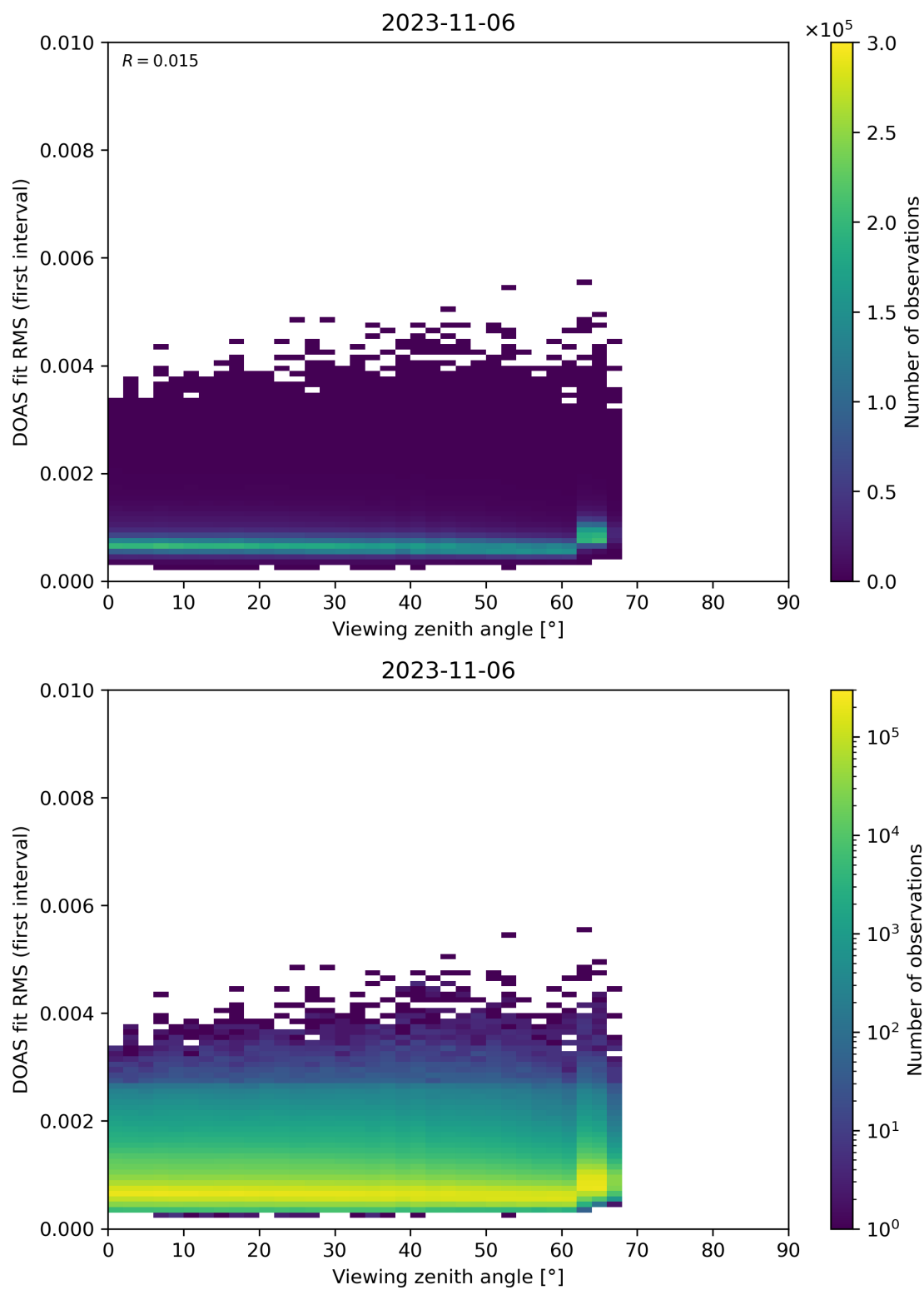
Figure 182: Scatter density plot of “Viewing zenith angle” against “DOAS fit RMS (first interval)” for 2023-11-05 to 2023-11-07.
