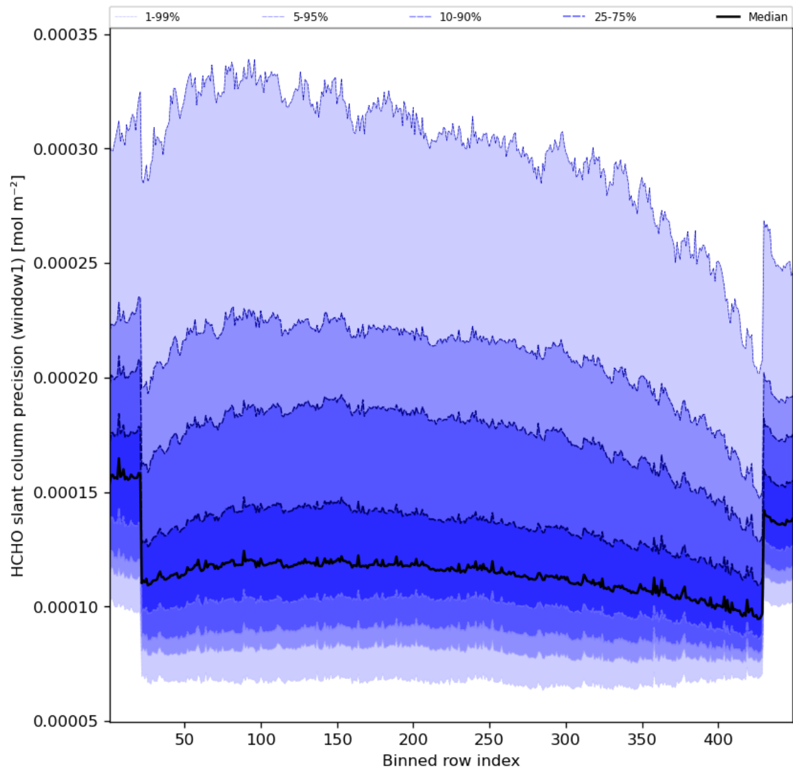
Figure 53: Along track statistics of “HCHO slant column precision (window1)” for 2023-11-05 to 2023-11-07
