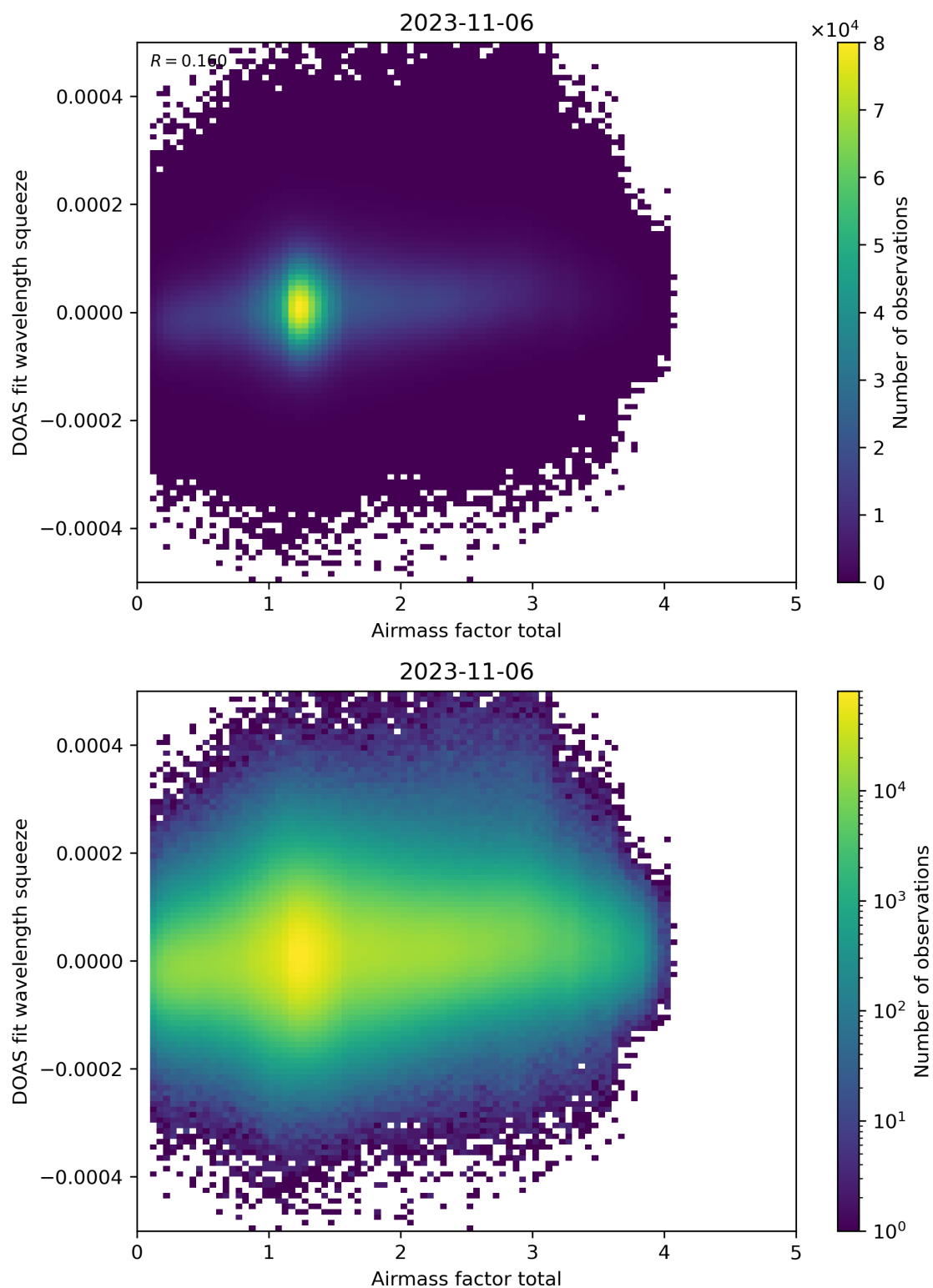
Figure 99: Scatter density plot of “Airmass factor total” against “DOAS fit wavelength squeeze” for 2023-11-05 to 2023-11-07.
