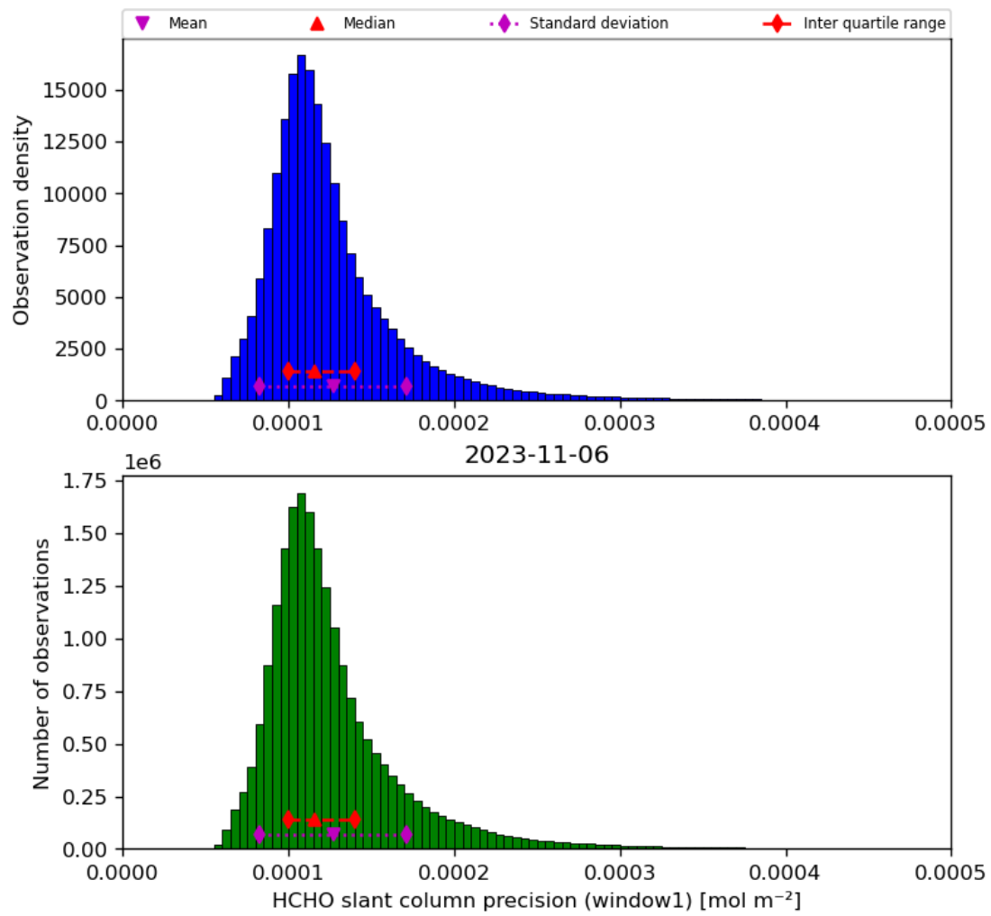
Figure 39: Histogram of “HCHO slant column precision (window1)” for 2023-11-05 to 2023-11-07
