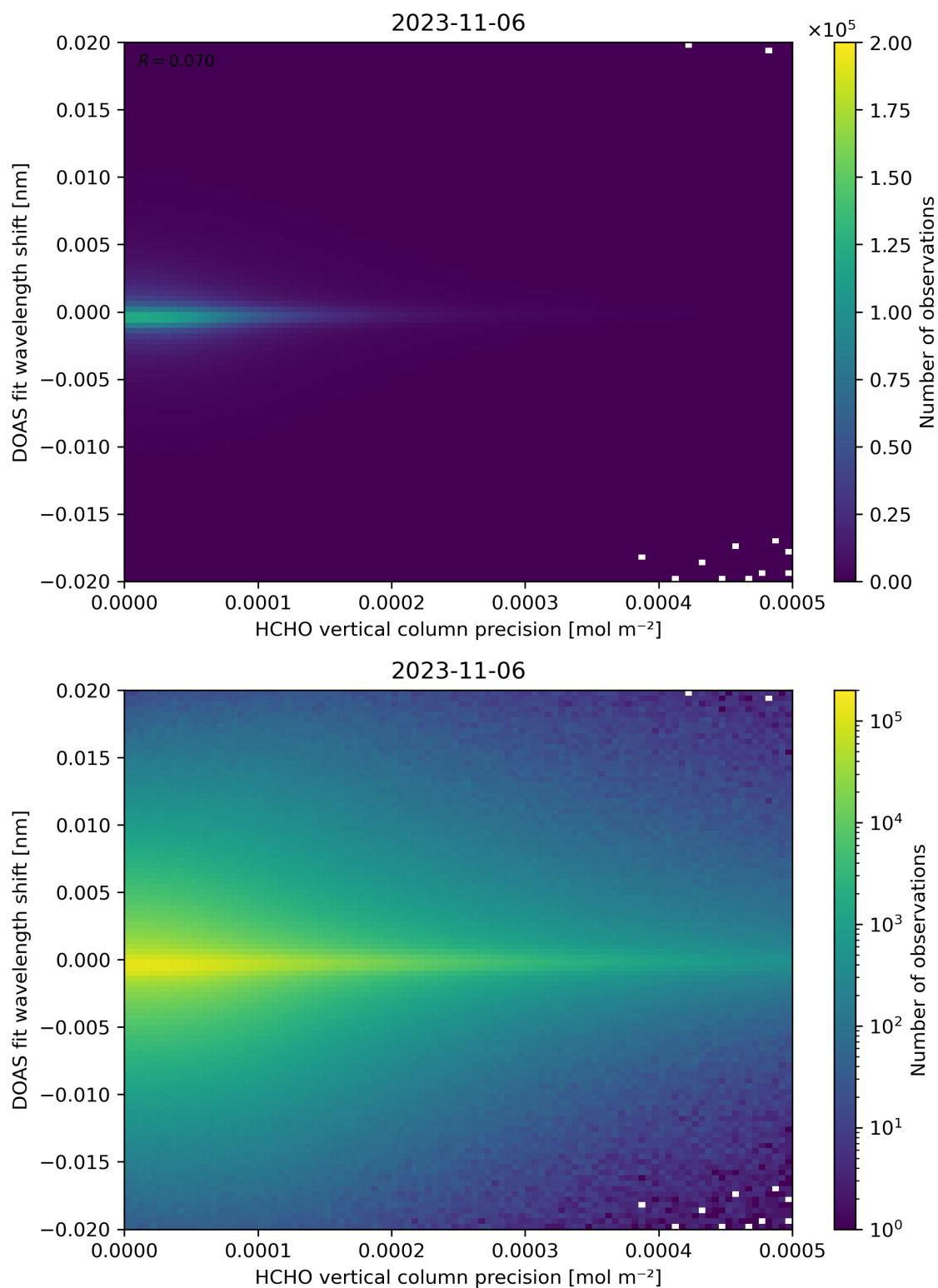
Figure 137: Scatter density plot of “HCHO vertical column precision” against “DOAS fit wavelength shift” for 2023-11-05 to 2023-11-07.
