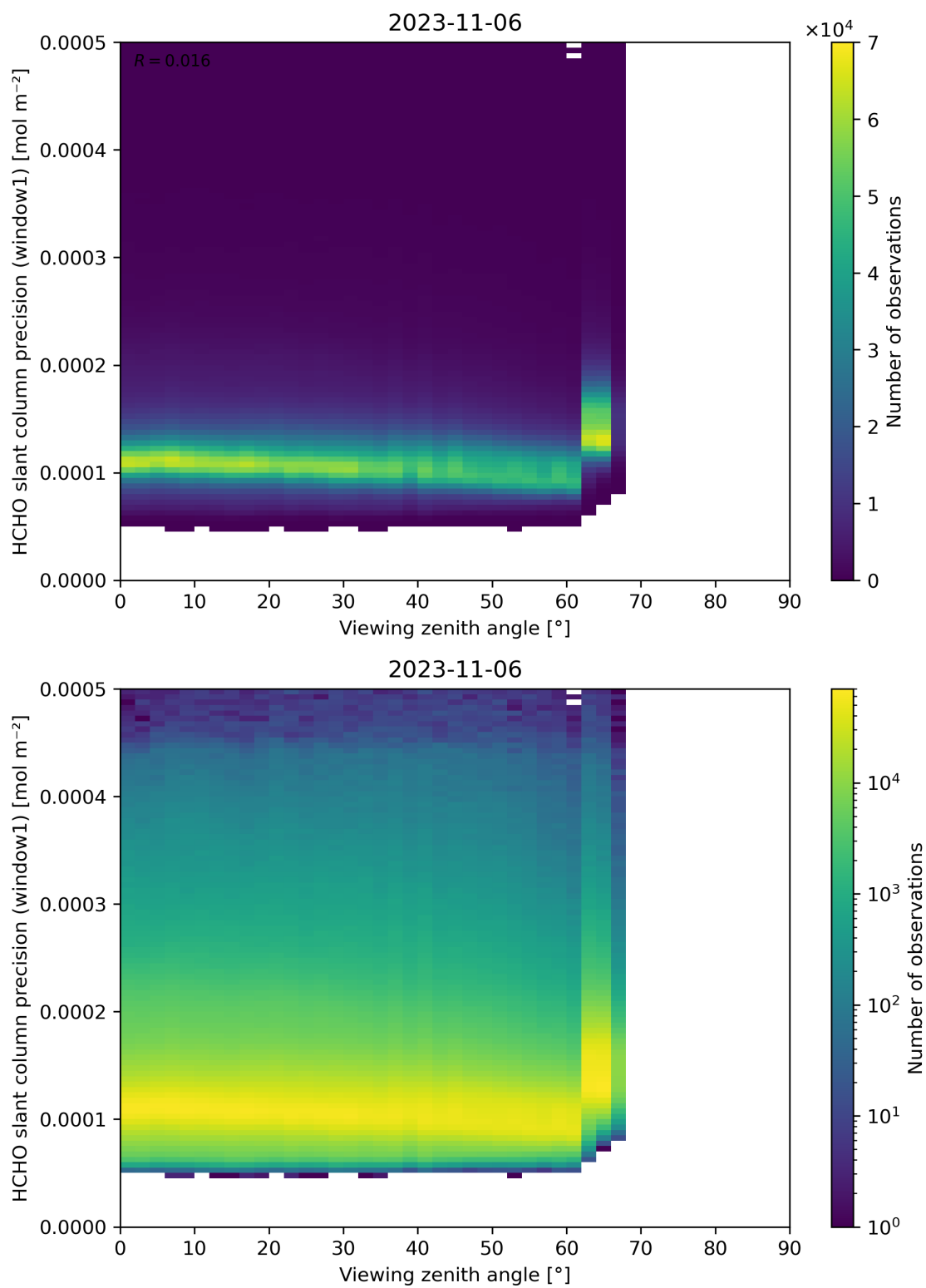
Figure 189: Scatter density plot of “Viewing zenith angle” against “HCHO slant column precision (window1)” for 2023-11-05 to 2023-11-07.
