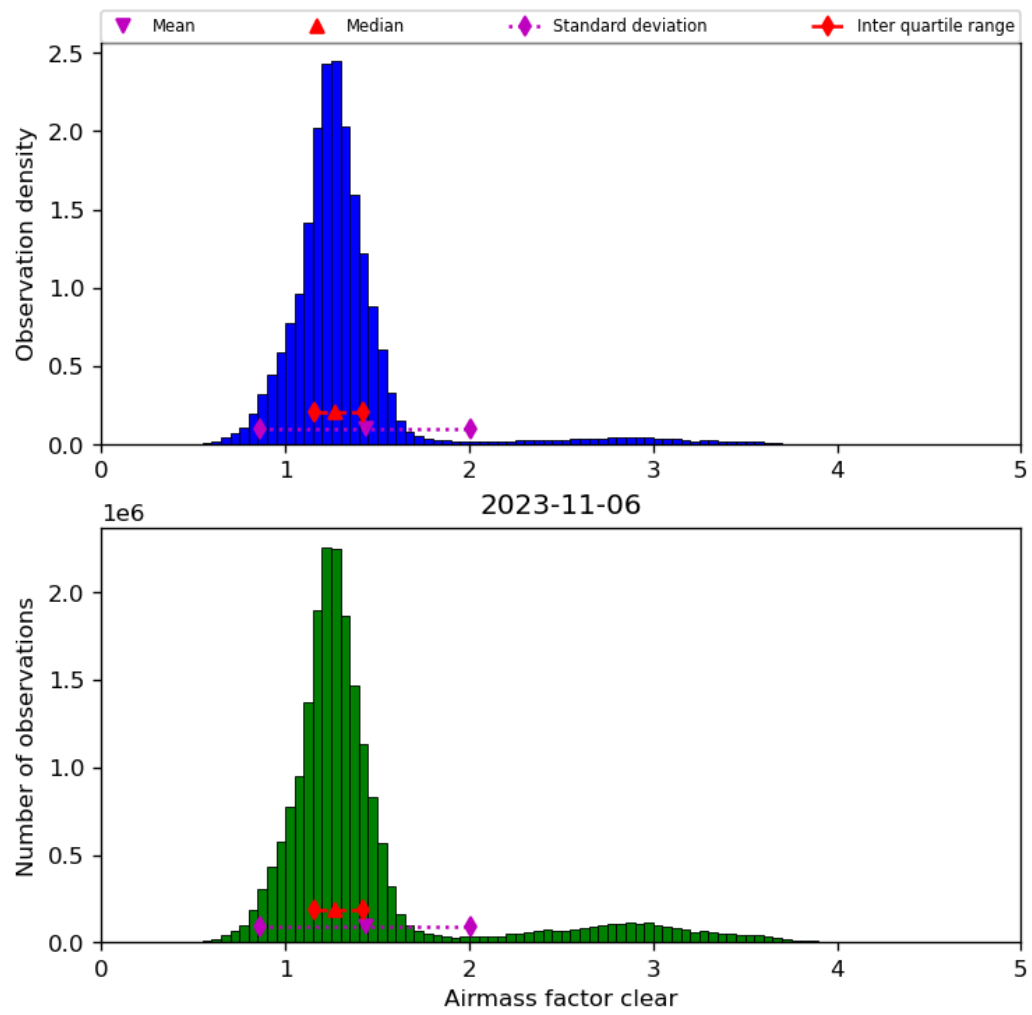
Figure 42: Histogram of “Airmass factor clear” for 2023-11-05 to 2023-11-07
