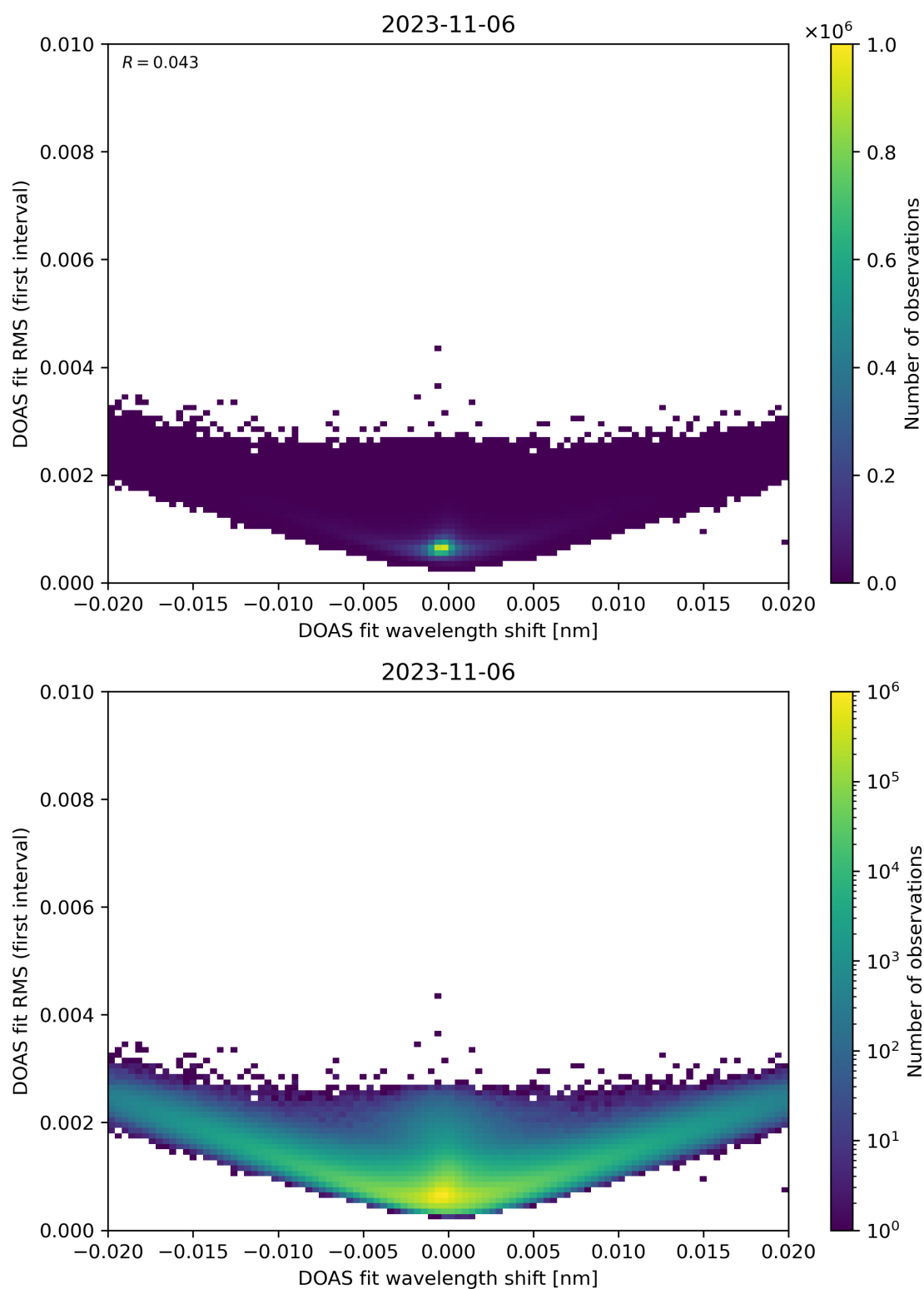
Figure 64: Scatter density plot of “DOAS fit wavelength shift” against “DOAS fit RMS (first interval)” for 2023-11-05 to 2023-11-07.
