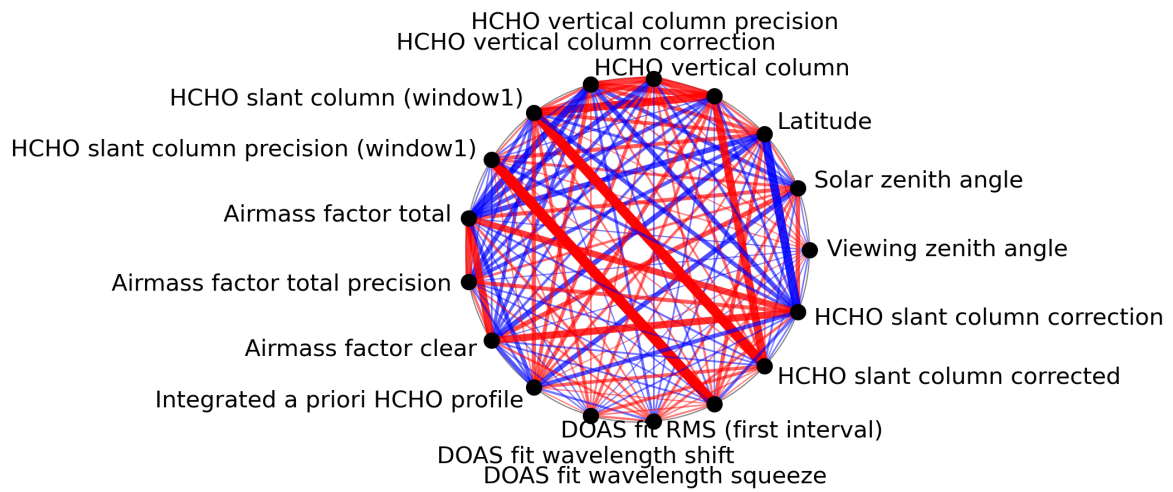
Figure 1: Map of correlation graph for 2023-11-05 to 2023-11-07.
