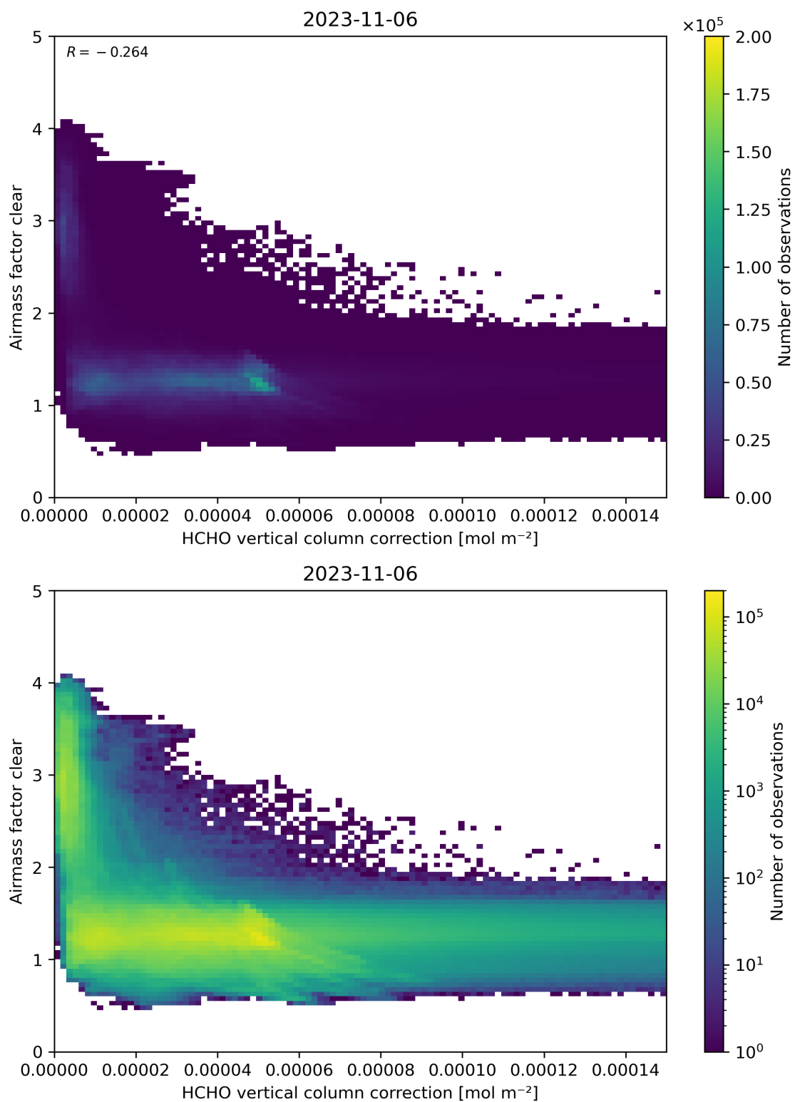
Figure 115: Scatter density plot of “HCHO vertical column correction” against “Airmass factor clear” for 2023-11-05 to 2023-11-07.
