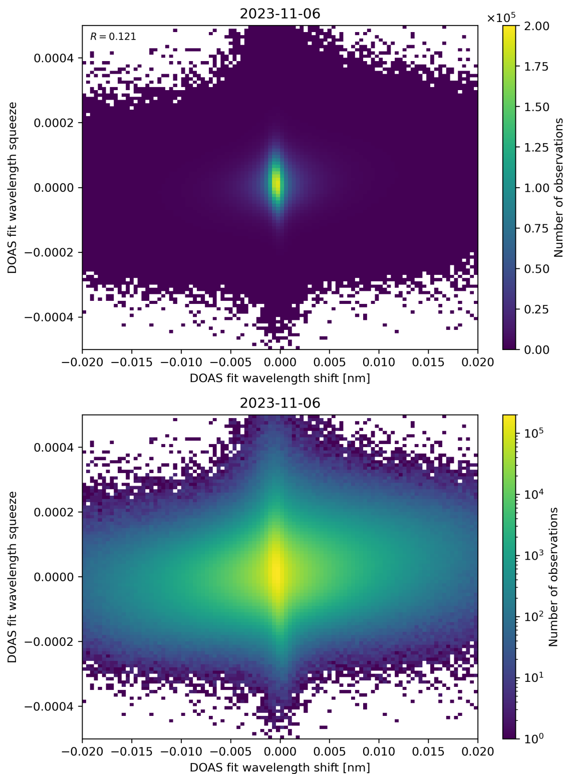
Figure 65: Scatter density plot of “DOAS fit wavelength shift” against “DOAS fit wavelength squeeze” for 2023-11-05 to 2023-11-07.
