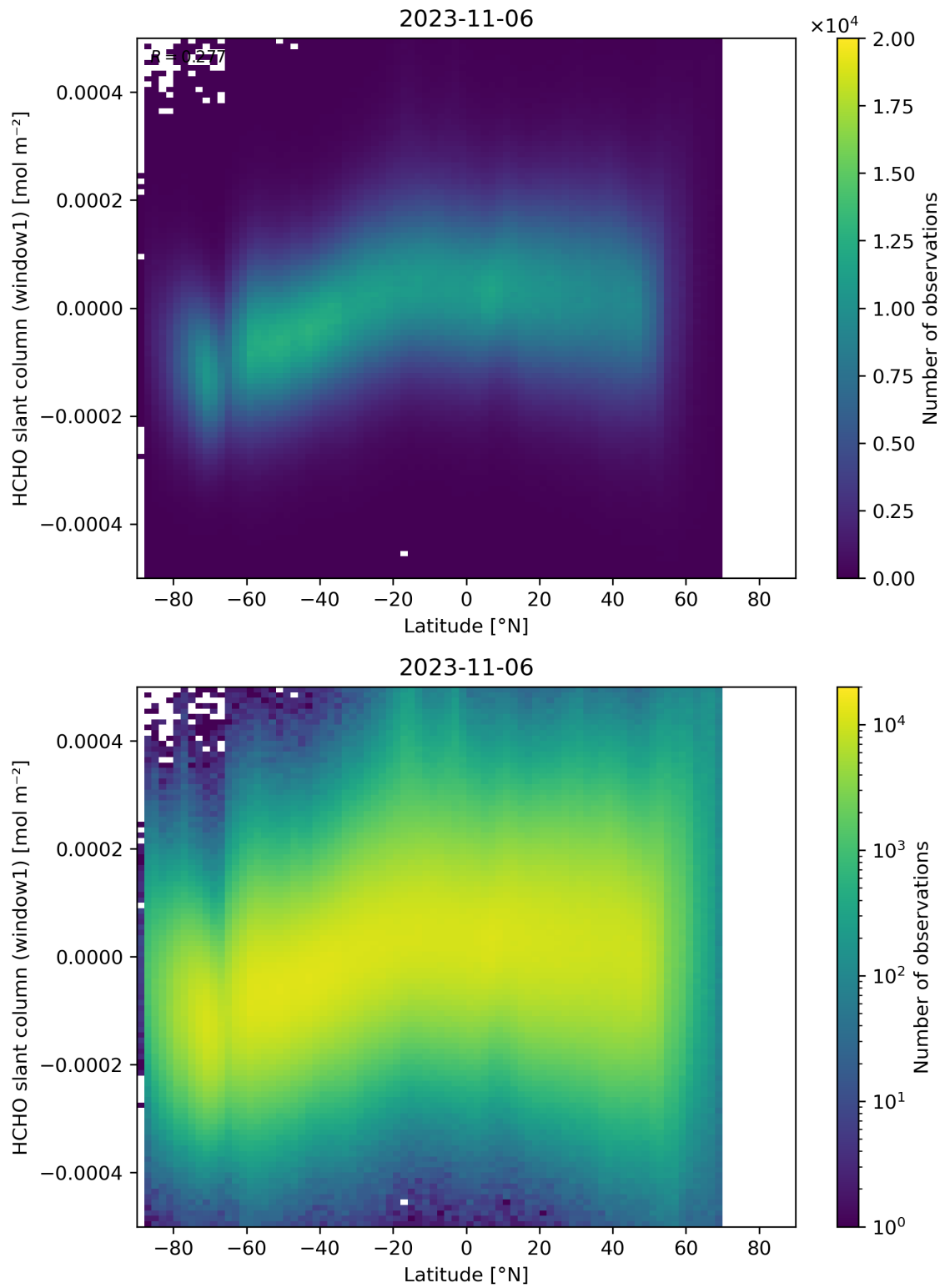
Figure 159: Scatter density plot of “Latitude” against “HCHO slant column (window1)” for 2023-11-05 to 2023-11-07.
