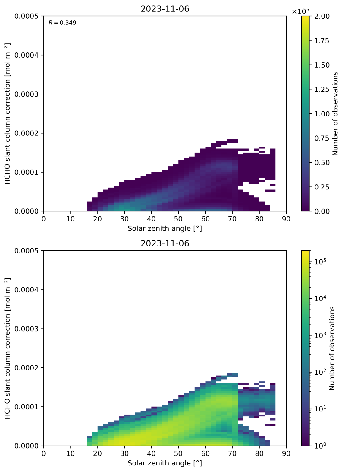
Figure 172: Scatter density plot of “Solar zenith angle” against “HCHO slant column correction” for 2023-11-05 to 2023-11-07.
