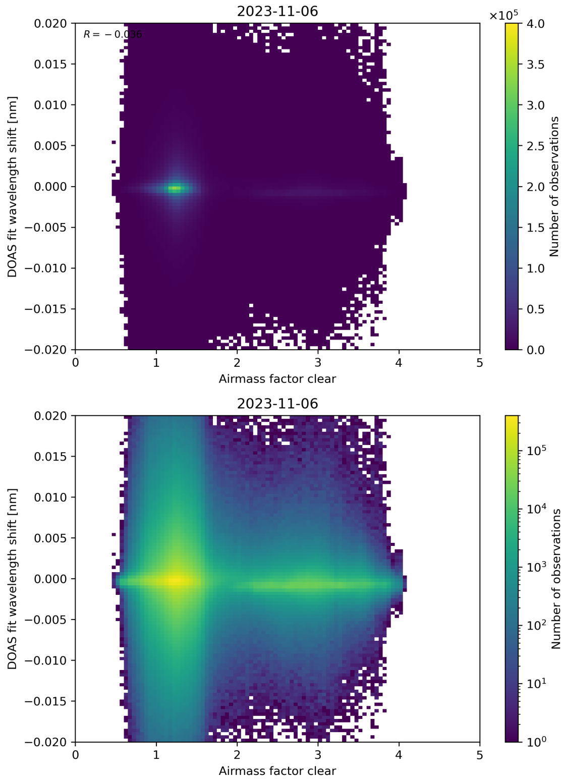
Figure 72: Scatter density plot of “Airmass factor clear” against “DOAS fit wavelength shift” for 2023-11-05 to 2023-11-07.
