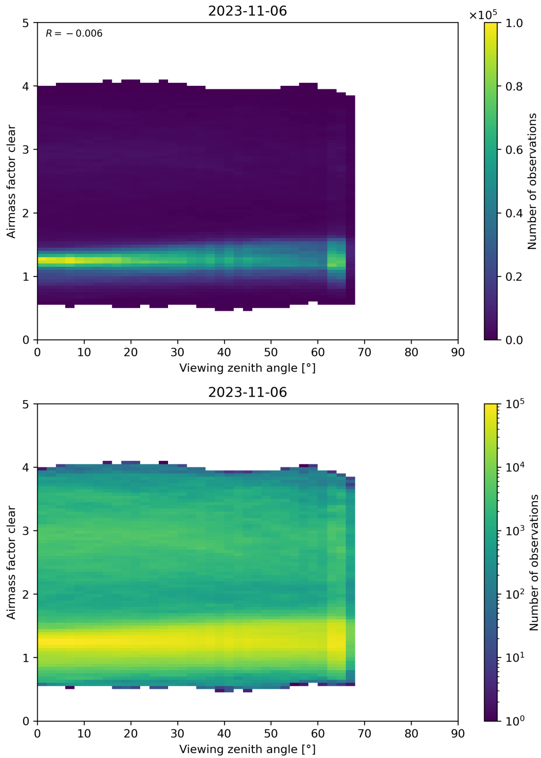
Figure 185: Scatter density plot of “Viewing zenith angle” against “Airmass factor clear” for 2023-11-05 to 2023-11-07.
