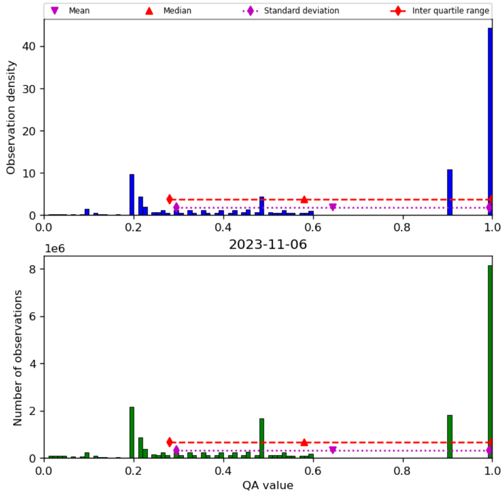
Figure 34: Histogram of “QA value” for 2023-11-05 to 2023-11-07
