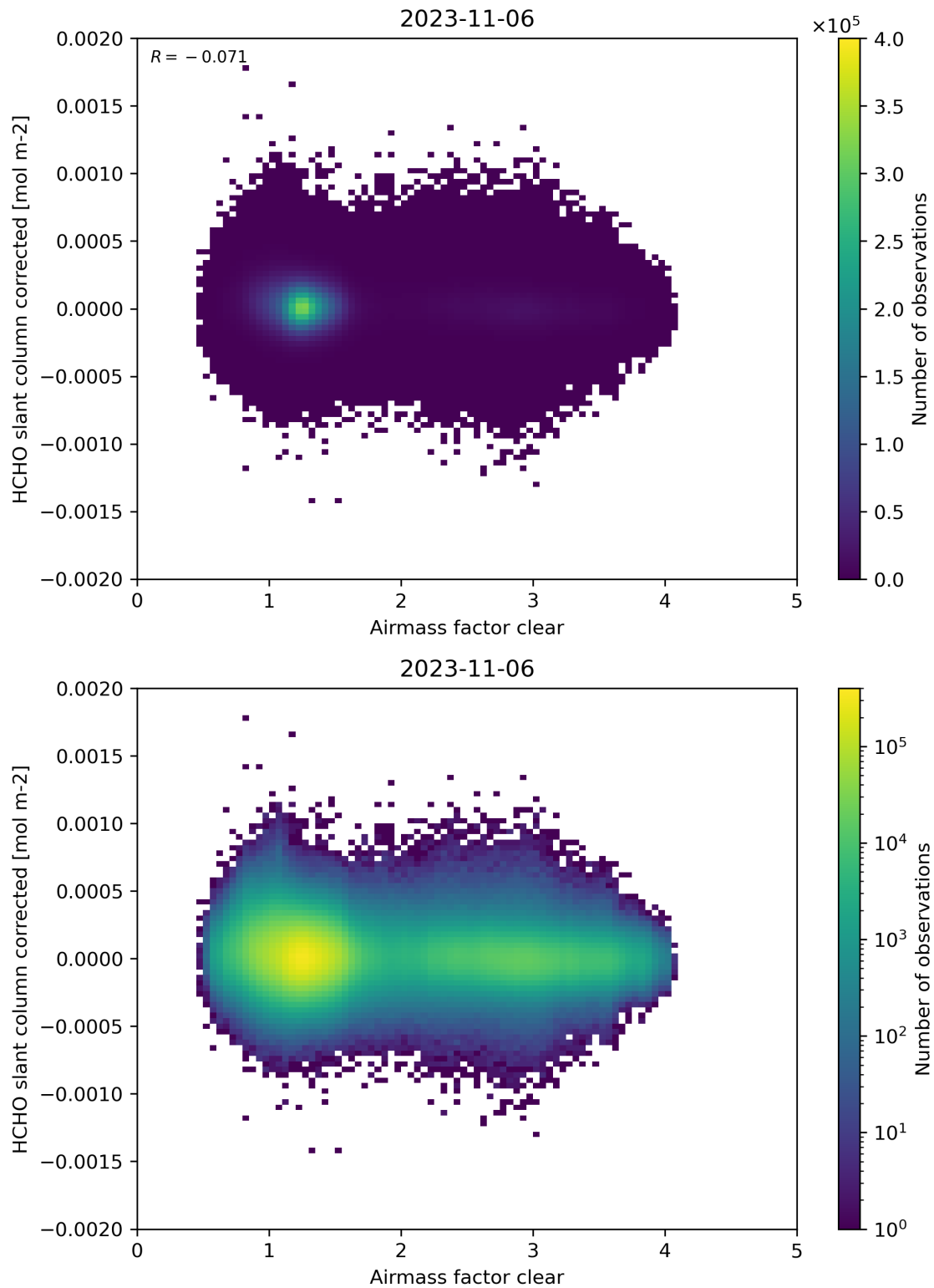
Figure 74: Scatter density plot of “Airmass factor clear” against “HCHO slant column corrected” for 2023-11-05 to 2023-11-07.
