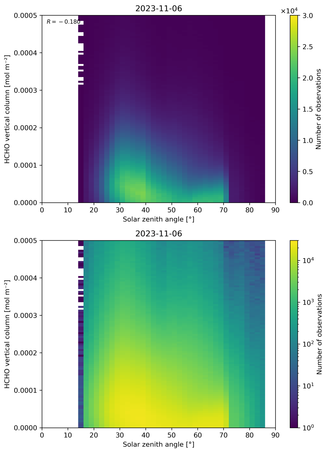
Figure 177: Scatter density plot of “Solar zenith angle” against “HCHO vertical column” for 2023-11-05 to 2023-11-07.
