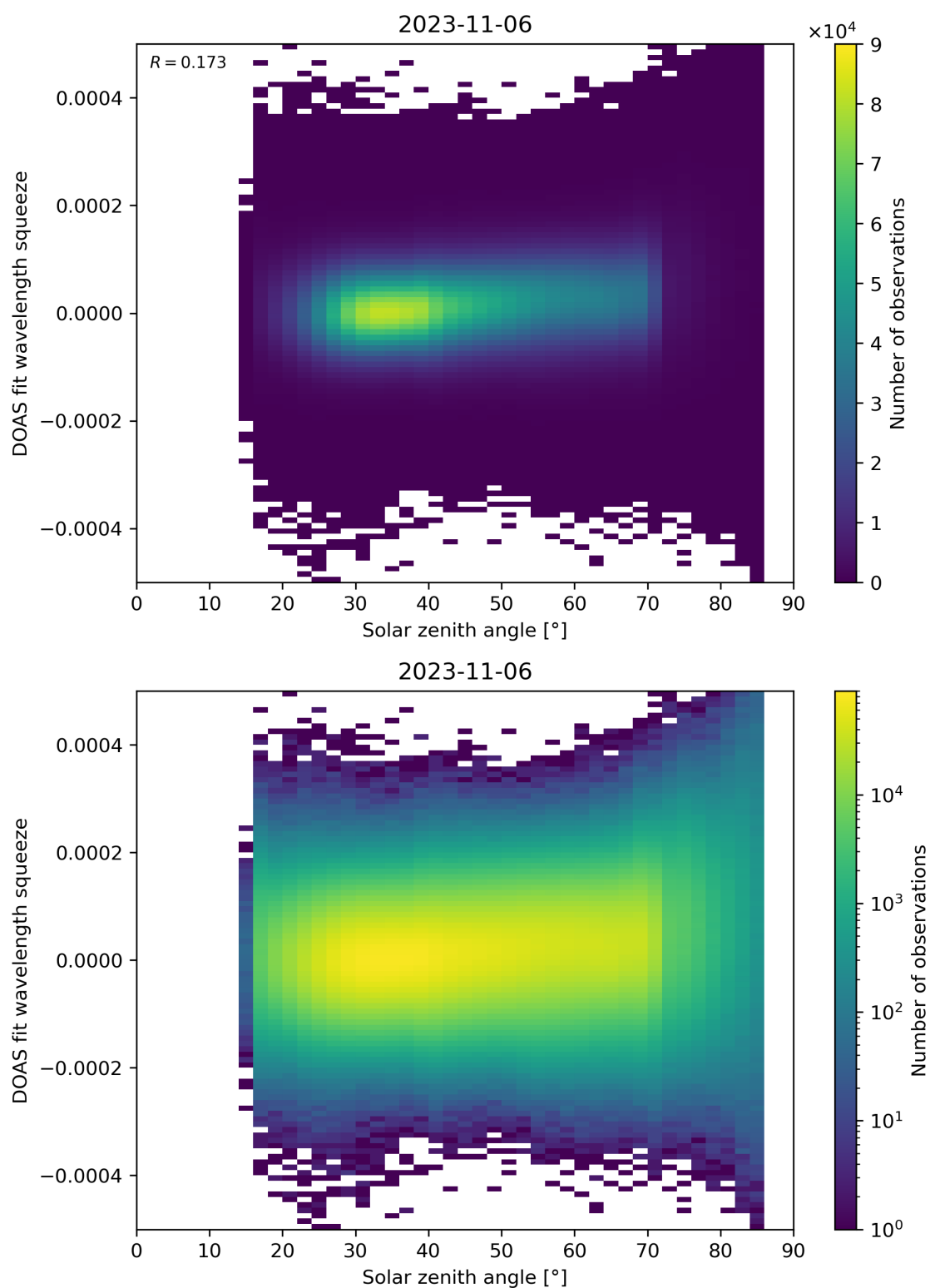
Figure 169: Scatter density plot of “Solar zenith angle” against “DOAS fit wavelength squeeze” for 2023-11-05 to 2023-11-07.
