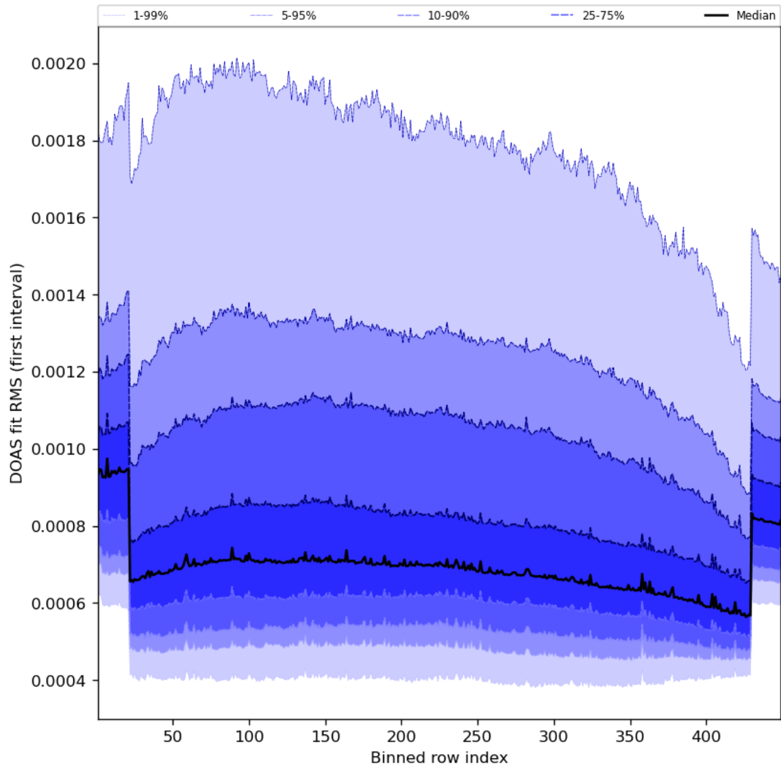
Figure 60: Along track statistics of “DOAS fit RMS (first interval)” for 2023-11-05 to 2023-11-07
