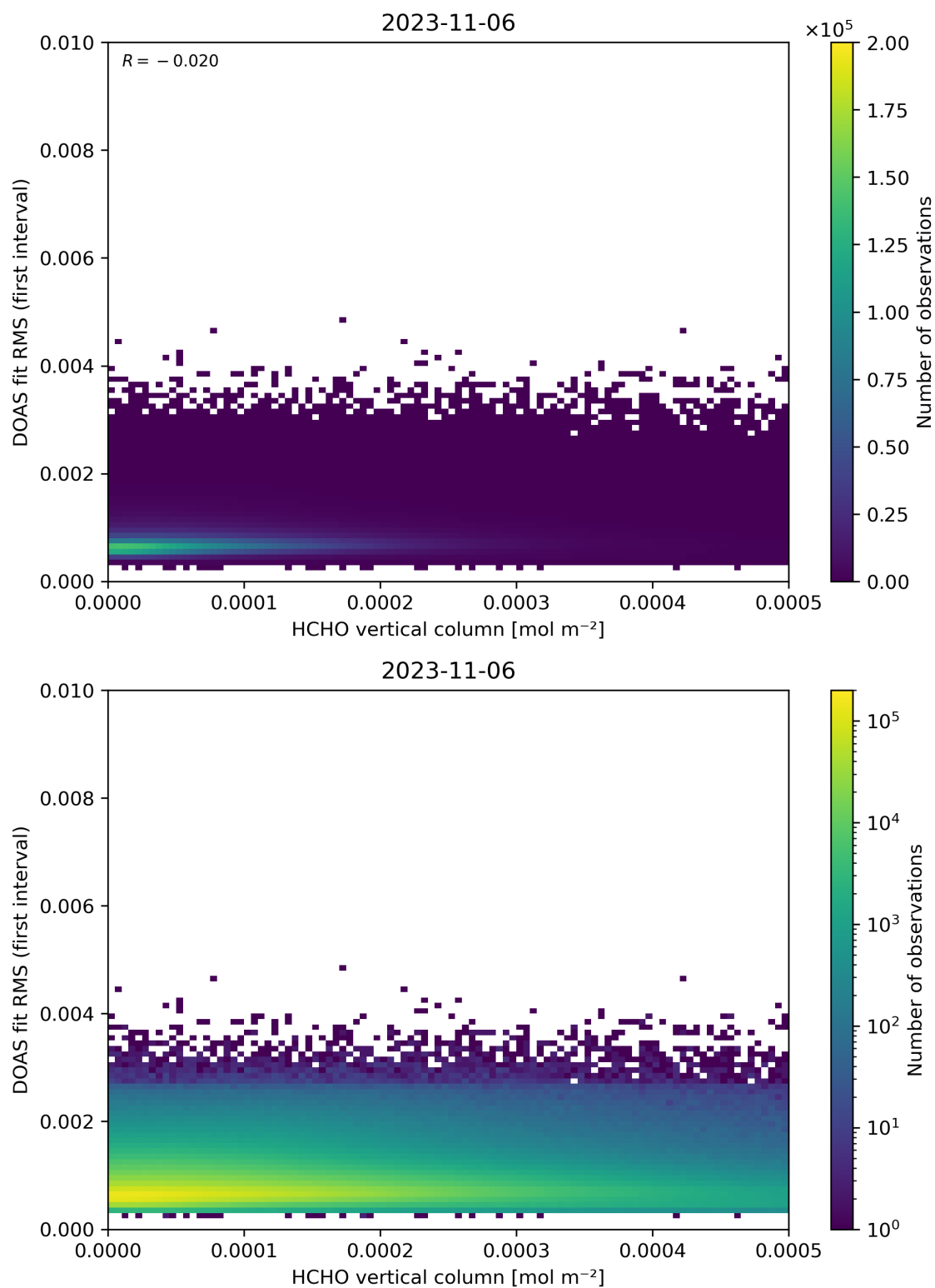
Figure 123: Scatter density plot of “HCHO vertical column” against “DOAS fit RMS (first interval)” for 2023-11-05 to 2023-11-07.
