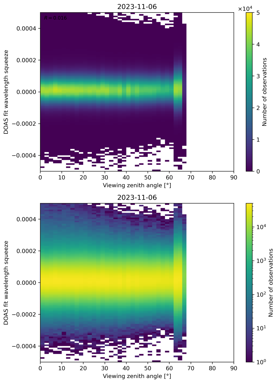
Figure 184: Scatter density plot of “Viewing zenith angle” against “DOAS fit wavelength squeeze” for 2023-11-05 to 2023-11-07.
