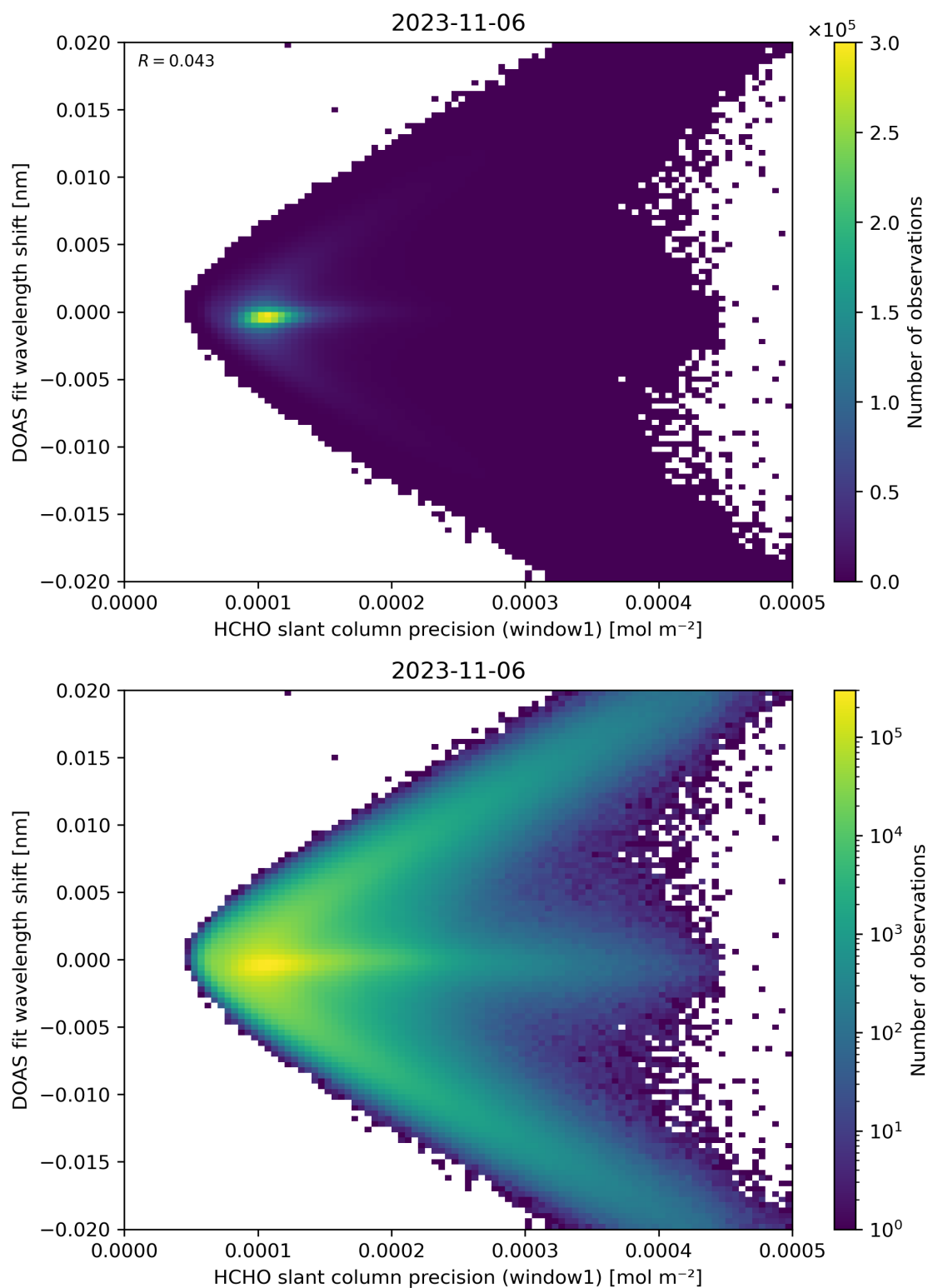
Figure 89: Scatter density plot of “HCHO slant column precision (window1)” against “DOAS fit wavelength shift” for 2023-11-05 to 2023-11-07.
