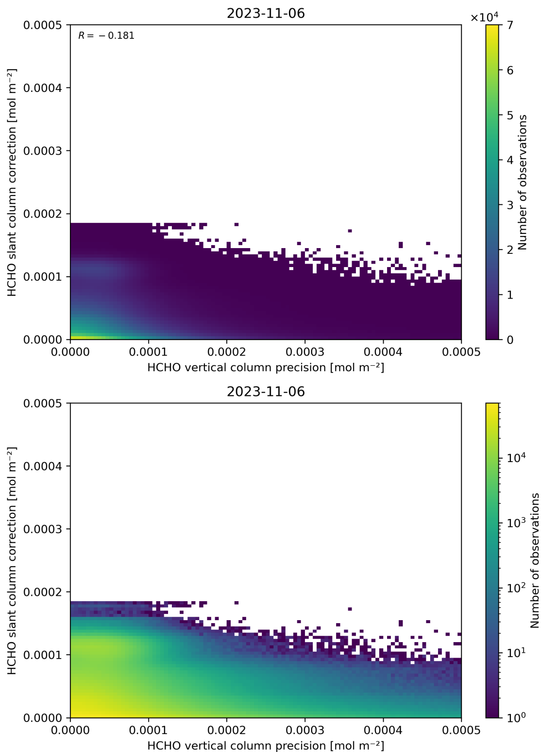
Figure 141: Scatter density plot of “HCHO vertical column precision” against “HCHO slant column correction” for 2023-11-05 to 2023-11-07.
