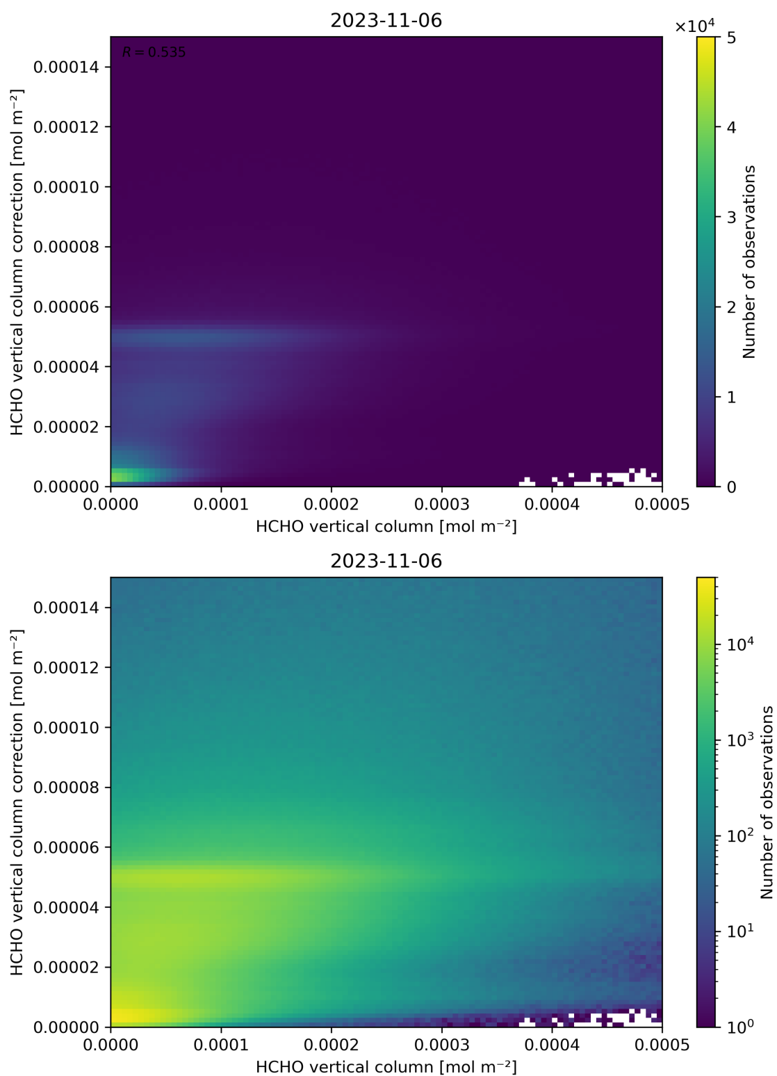
Figure 133: Scatter density plot of “HCHO vertical column” against “HCHO vertical column correction” for 2023-11-05 to 2023-11-07.
