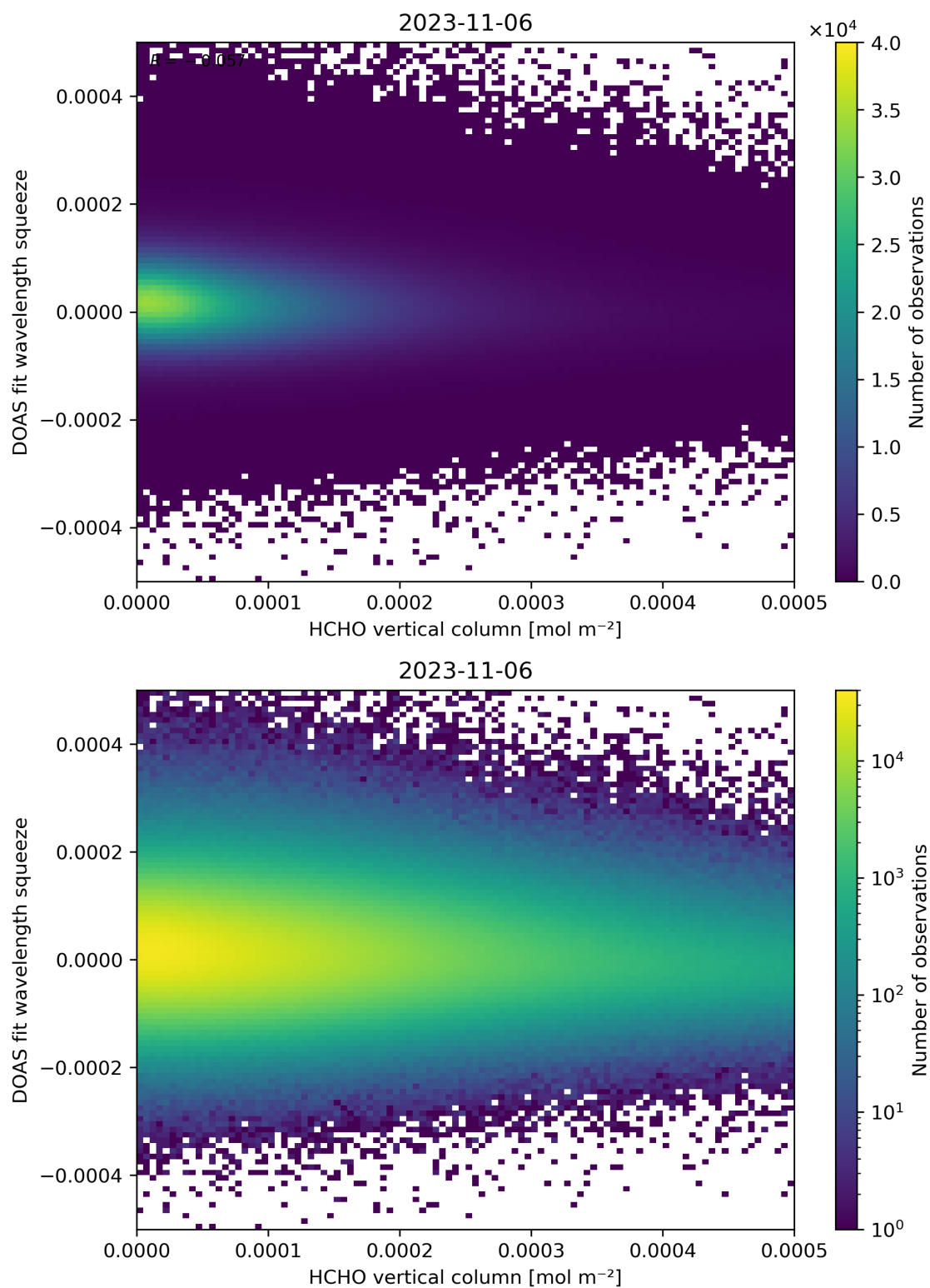
Figure 125: Scatter density plot of “HCHO vertical column” against “DOAS fit wavelength squeeze” for 2023-11-05 to 2023-11-07.
