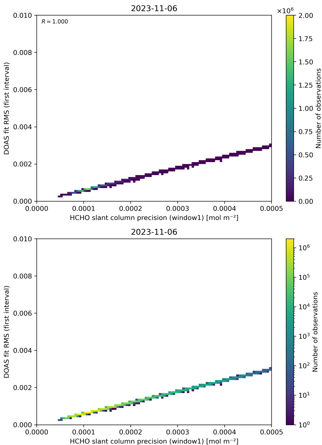
Figure 88: Scatter density plot of “HCHO slant column precision (window1)” against “DOAS fit RMS (first interval)” for 2023-11-05 to 2023-11-07.
