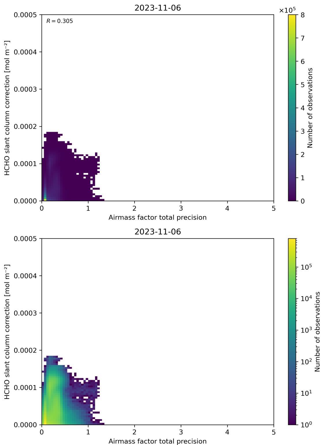
Figure 110: Scatter density plot of “Airmass factor total precision” against “HCHO slant column correction” for 2023-11-05 to 2023-11-07.
