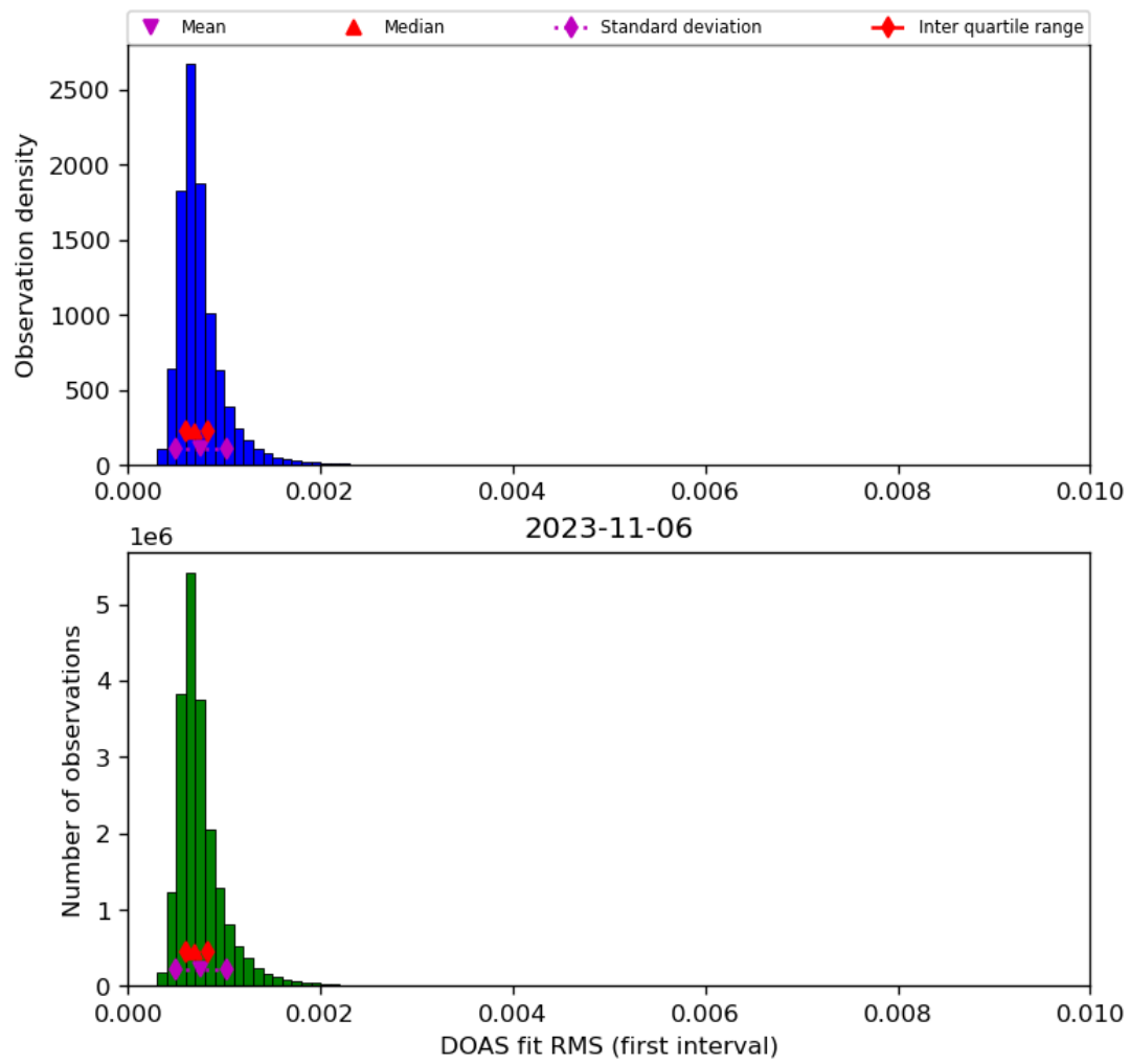
Figure 46: Histogram of “DOAS fit RMS (first interval)” for 2023-11-05 to 2023-11-07
