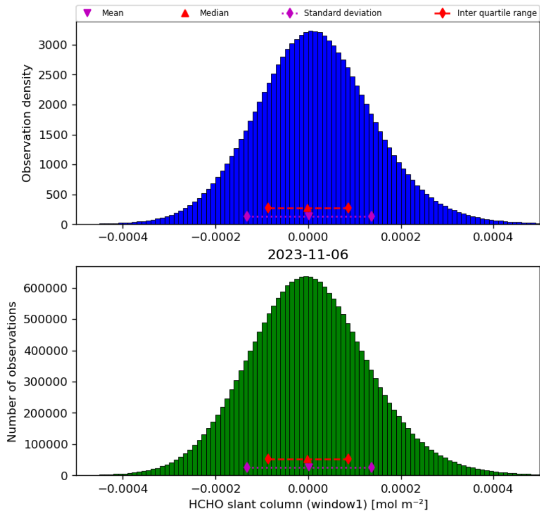
Figure 38: Histogram of “HCHO slant column (window1)” for 2023-11-05 to 2023-11-07
