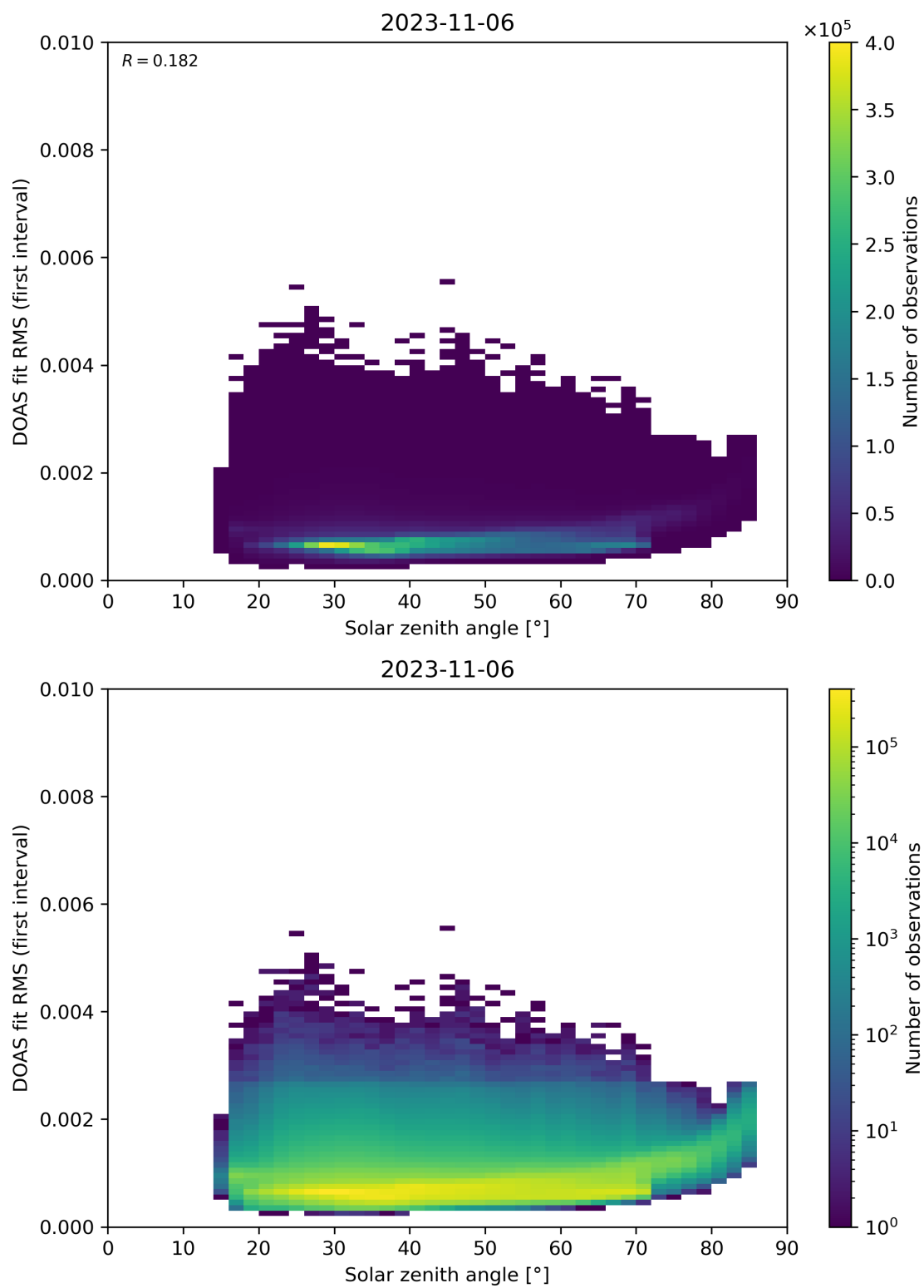
Figure 167: Scatter density plot of “Solar zenith angle” against “DOAS fit RMS (first interval)” for 2023-11-05 to 2023-11-07.
