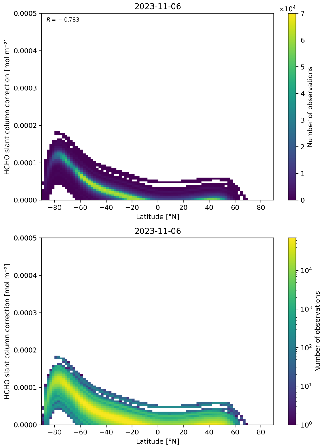
Figure 158: Scatter density plot of “Latitude” against “HCHO slant column correction” for 2023-11-05 to 2023-11-07.
