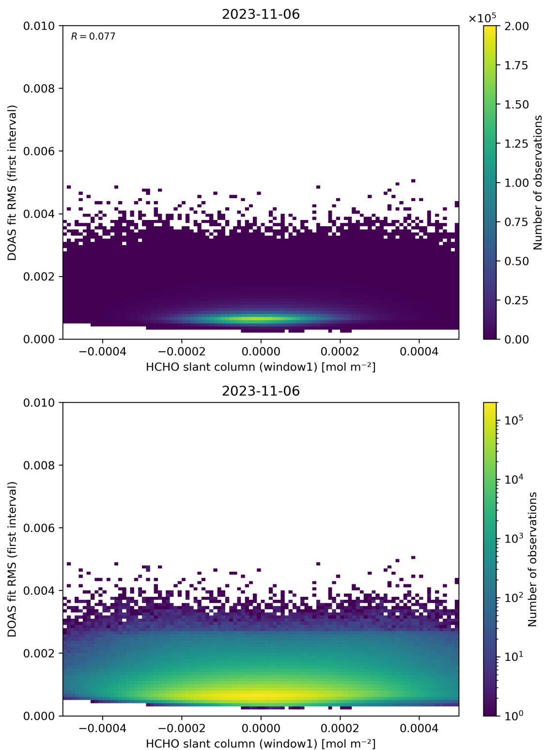
Figure 78: Scatter density plot of “HCHO slant column (window1)” against “DOAS fit RMS (first interval)” for 2023-11-05 to 2023-11-07.
