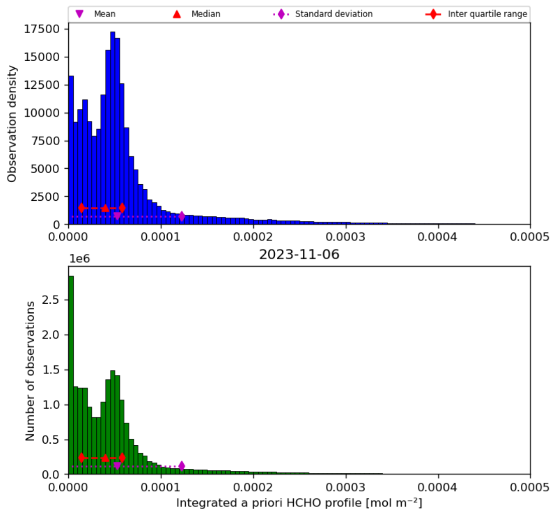
Figure 43: Histogram of “Integrated a priori HCHO profile” for 2023-11-05 to 2023-11-07
