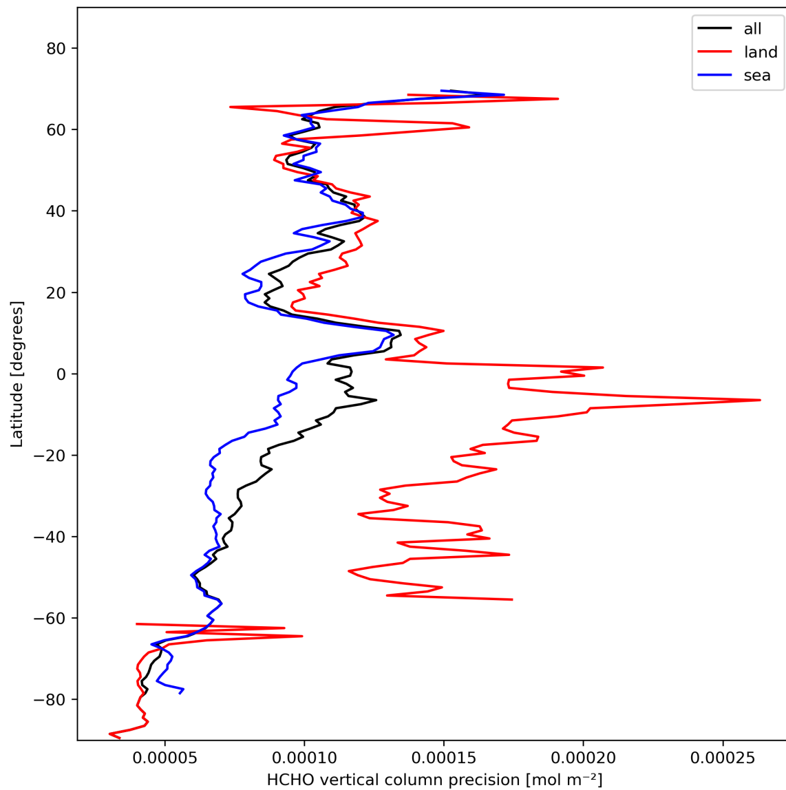
Figure 22: Zonal average of “HCHO vertical column precision” for 2023-11-05 to 2023-11-07.
