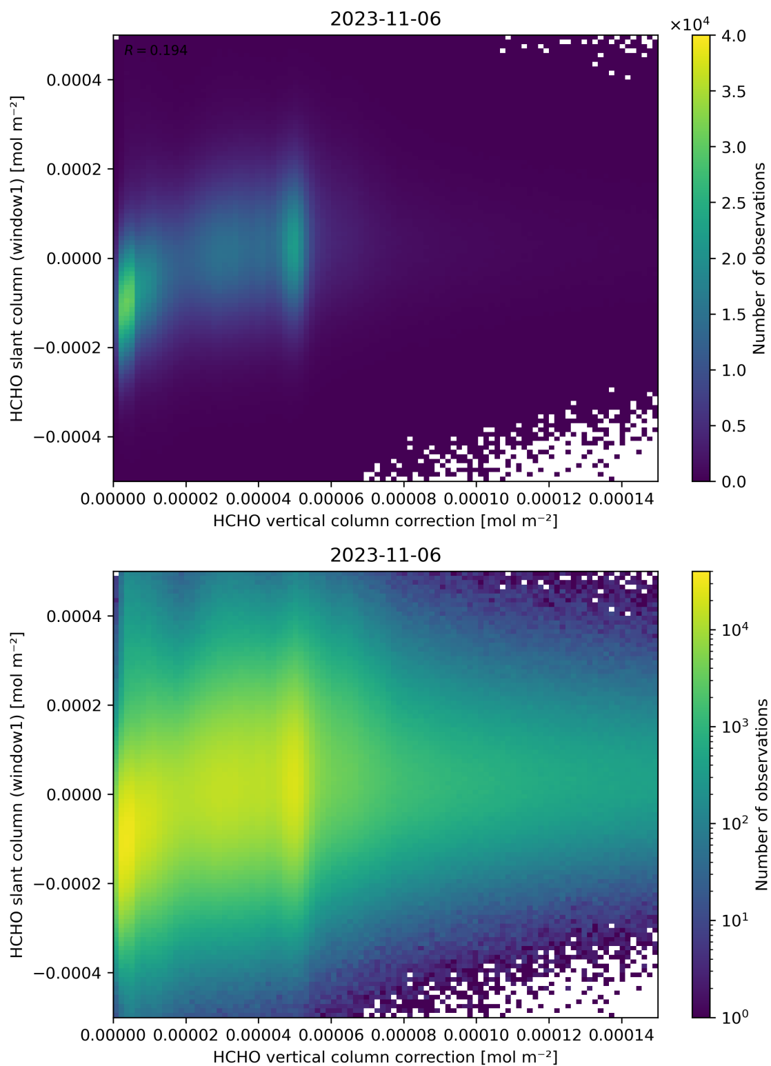
Figure 118: Scatter density plot of “HCHO vertical column correction” against “HCHO slant column (window1)” for 2023-11-05 to 2023-11-07.
