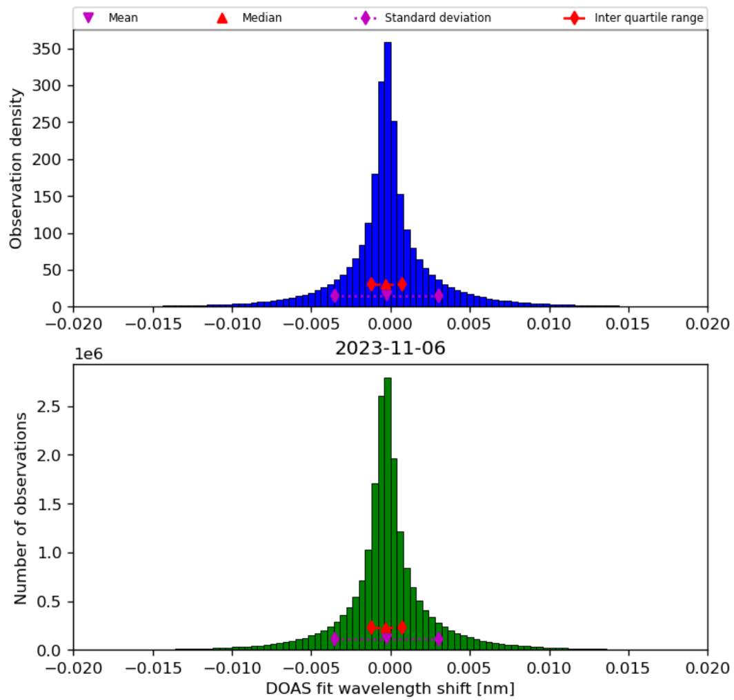
Figure 44: Histogram of “DOAS fit wavelength shift” for 2023-11-05 to 2023-11-07
