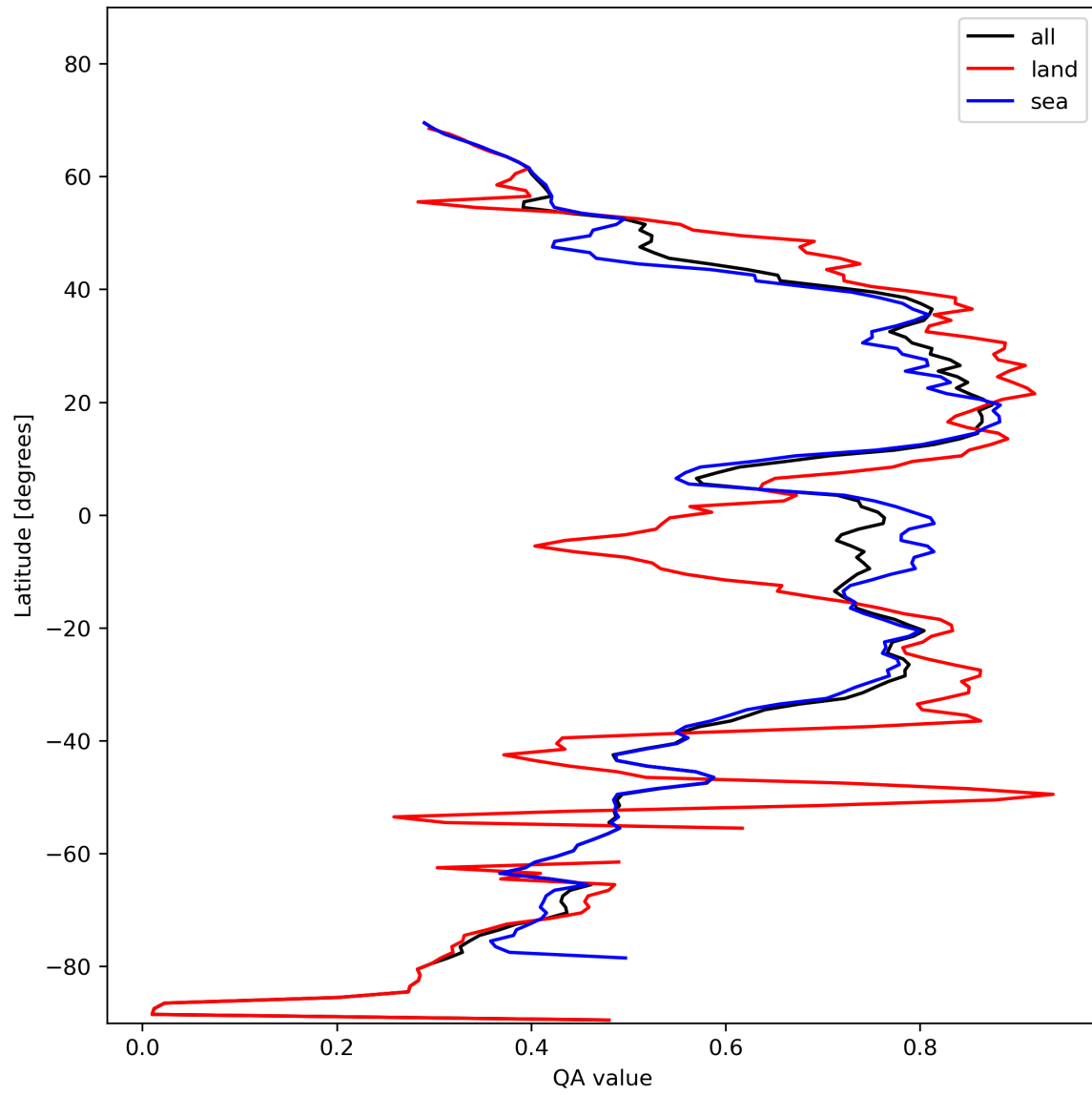
Figure 20: Zonal average of “QA value” for 2023-11-05 to 2023-11-07.
