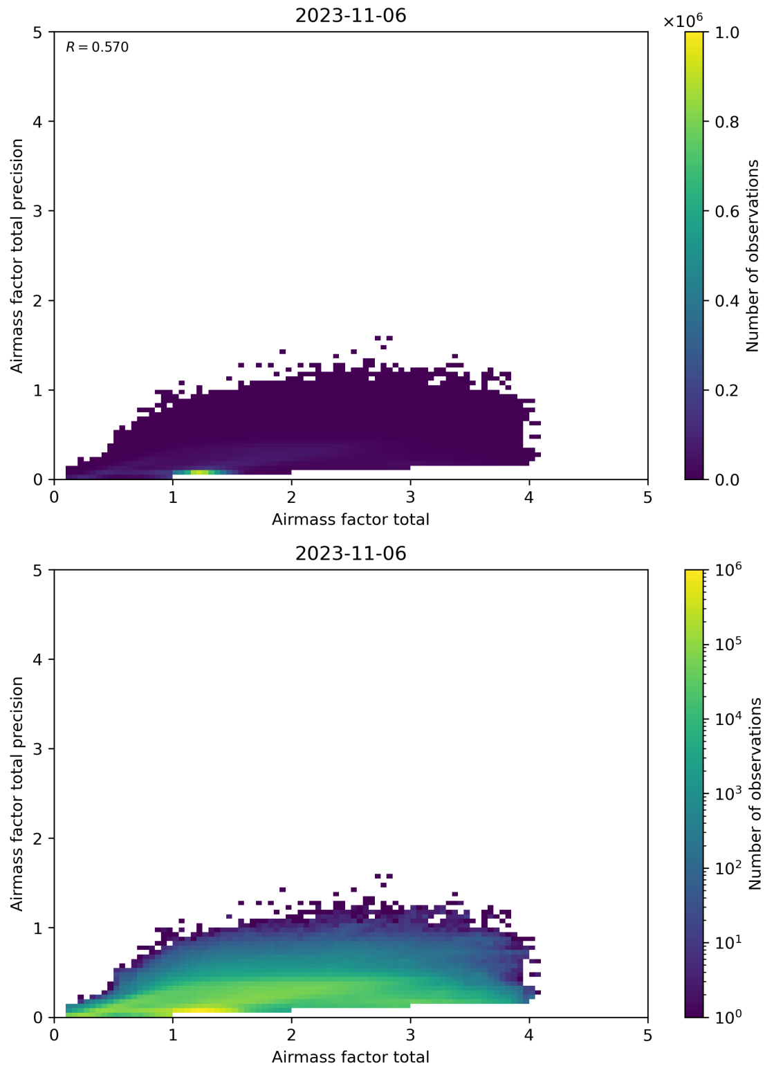
Figure 103: Scatter density plot of “Airmass factor total” against “Airmass factor total precision” for 2023-11-05 to 2023-11-07.
