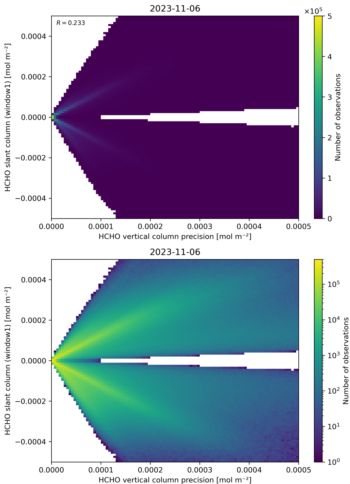
Figure 142: Scatter density plot of “HCHO vertical column precision” against “HCHO slant column (window1)” for 2023-11-05 to 2023-11-07.
