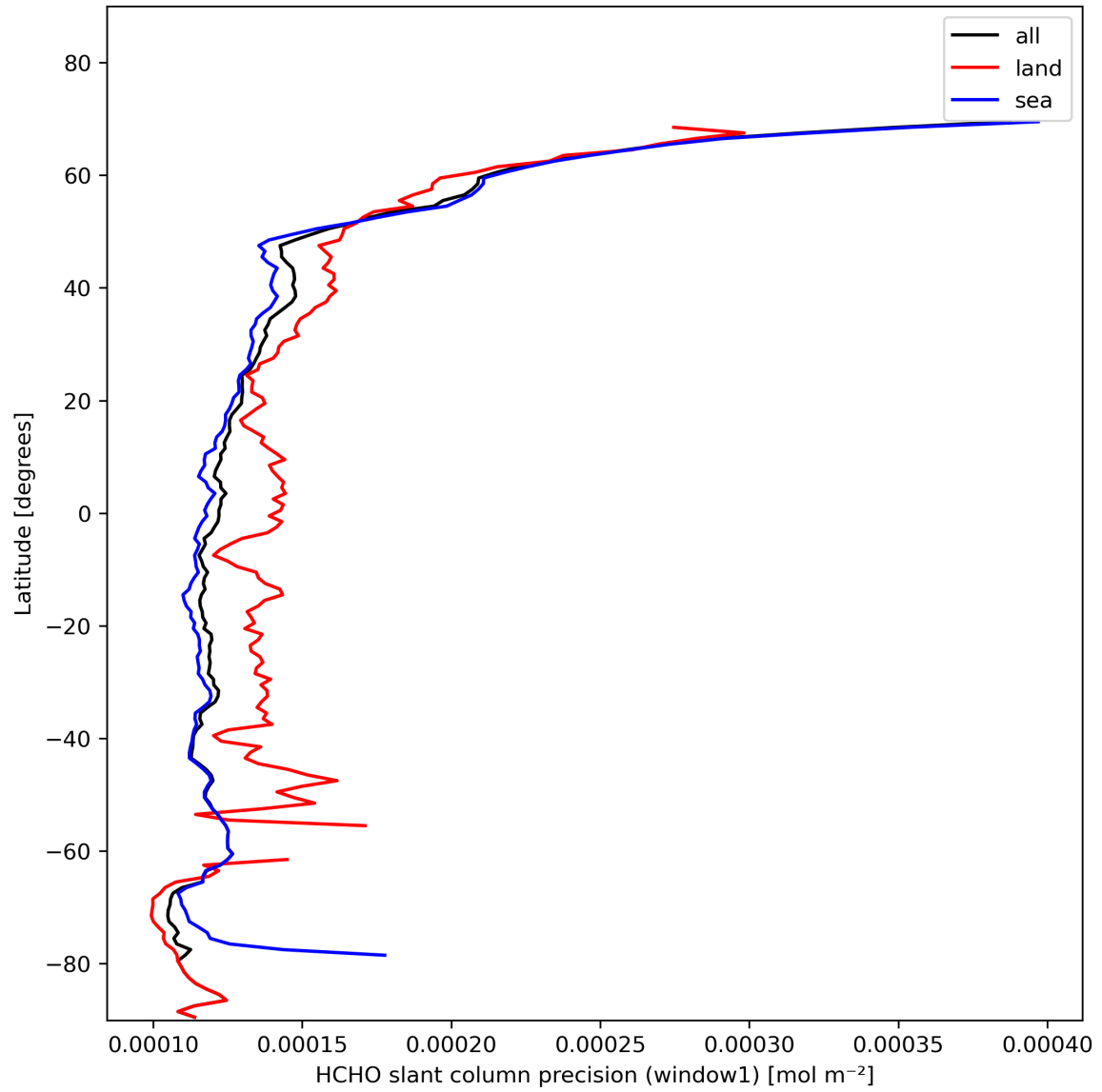
Figure 25: Zonal average of “HCHO slant column precision (window1)” for 2023-11-05 to 2023-11-07.
