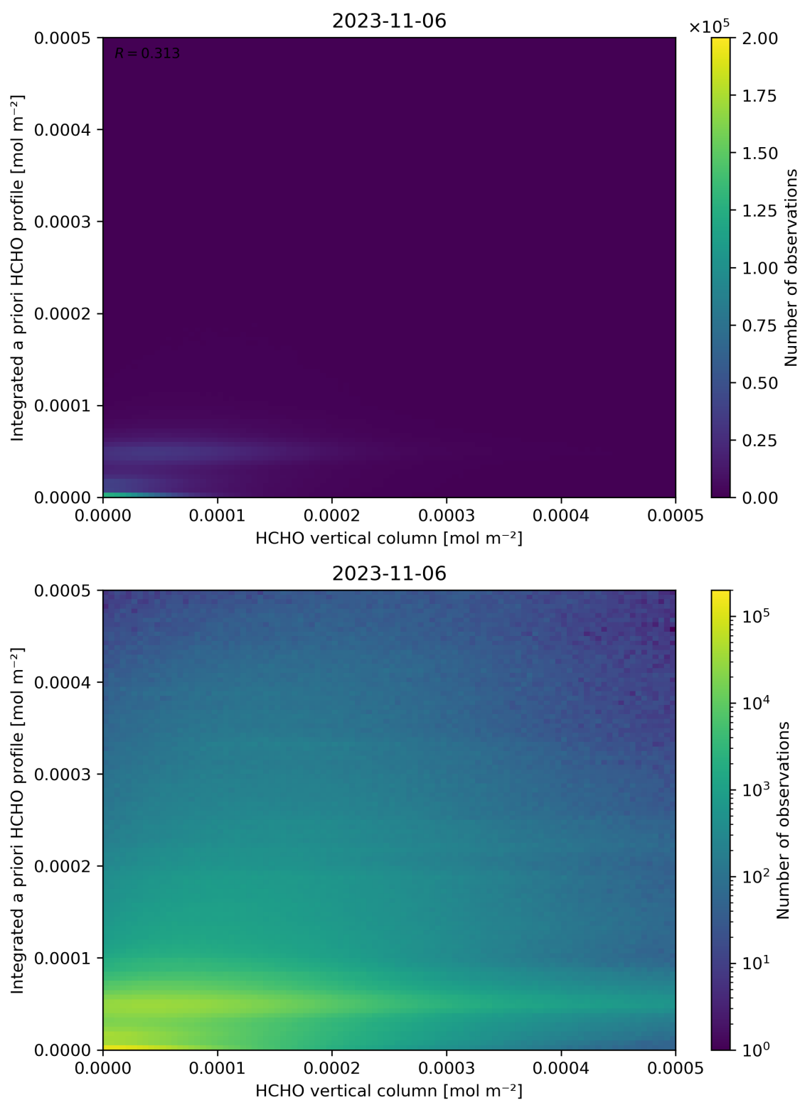
Figure 135: Scatter density plot of “HCHO vertical column” against “Integrated a priori HCHO profile” for 2023-11-05 to 2023-11-07.
