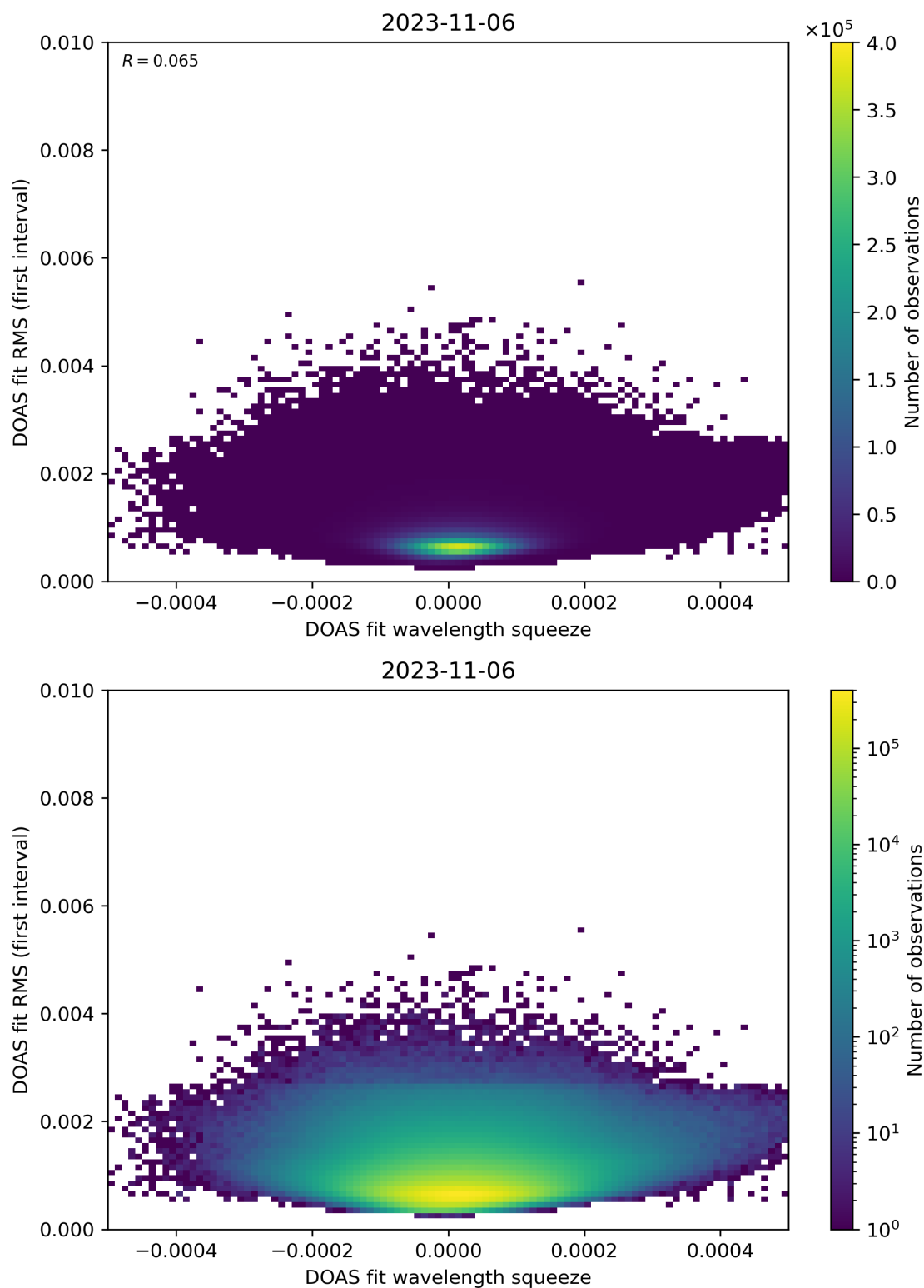
Figure 68: Scatter density plot of “DOAS fit wavelength squeeze” against “DOAS fit RMS (first interval)” for 2023-11-05 to 2023-11-07.
