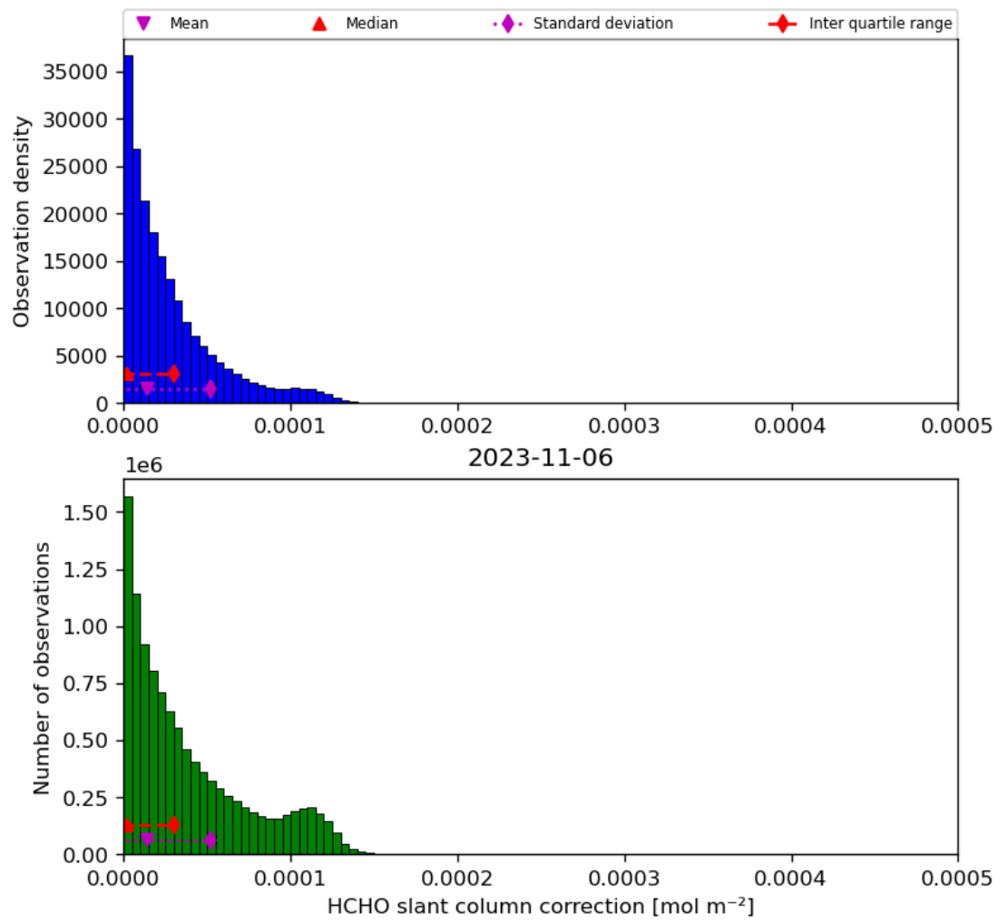
Figure 47: Histogram of “HCHO slant column correction” for 2023-11-05 to 2023-11-07
