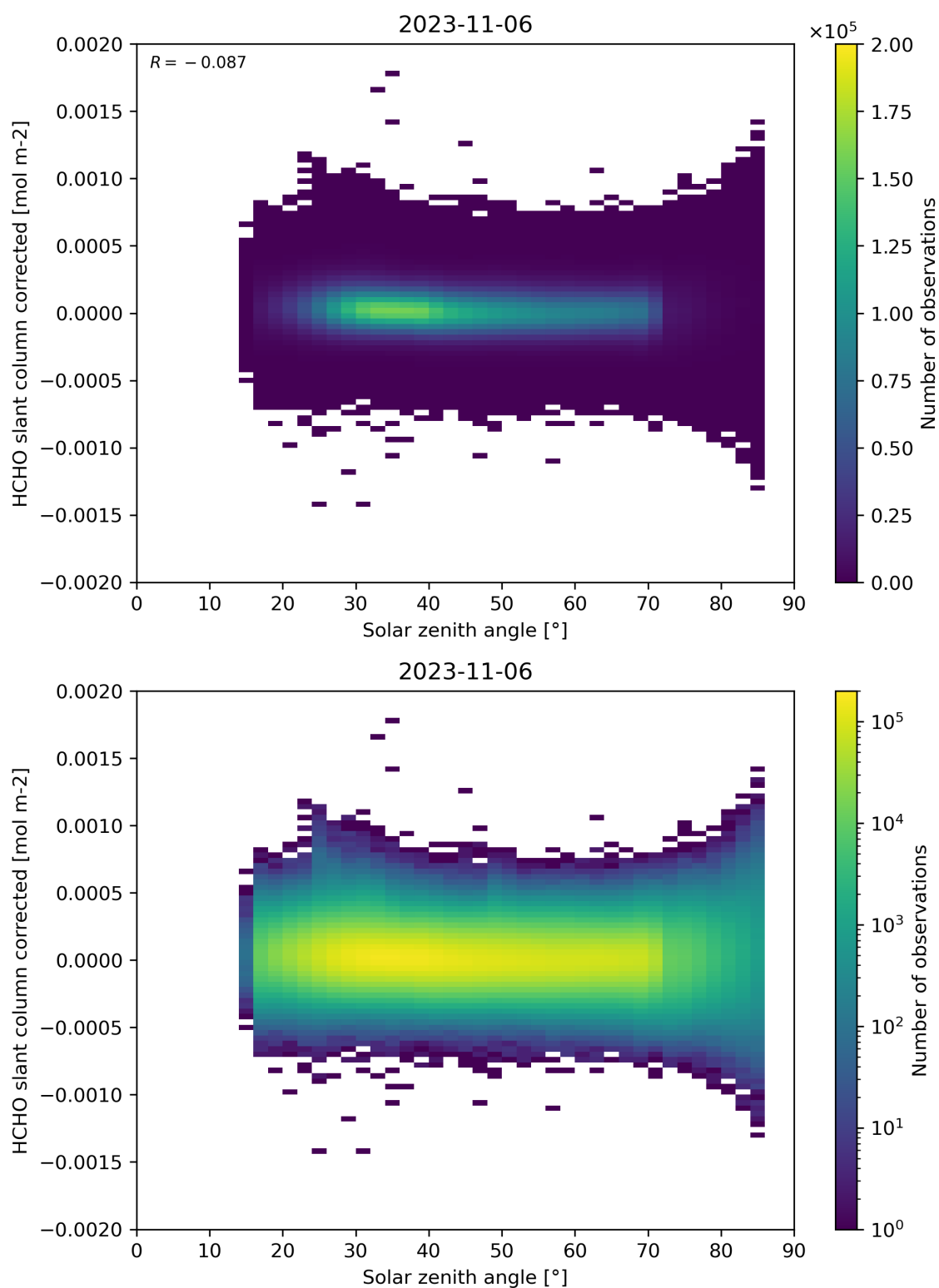
Figure 171: Scatter density plot of “Solar zenith angle” against “HCHO slant column corrected” for 2023-11-05 to 2023-11-07.
