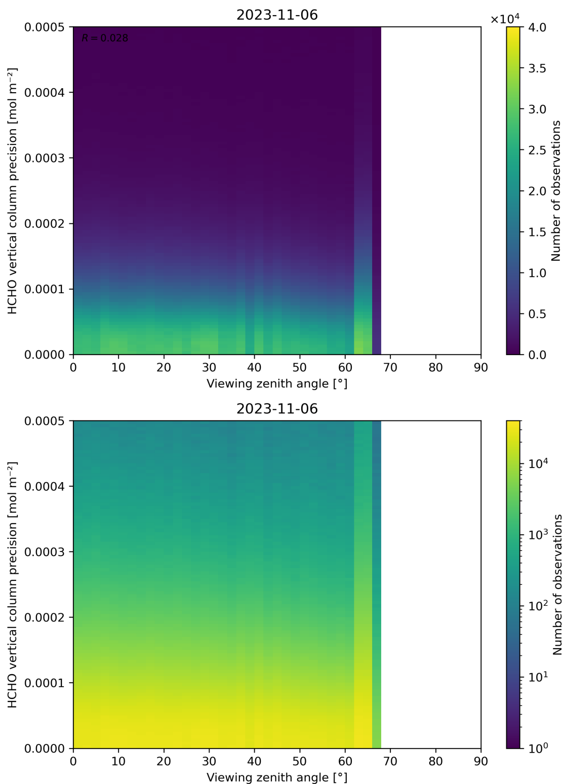
Figure 194: Scatter density plot of “Viewing zenith angle” against “HCHO vertical column precision” for 2023-11-05 to 2023-11-07.
