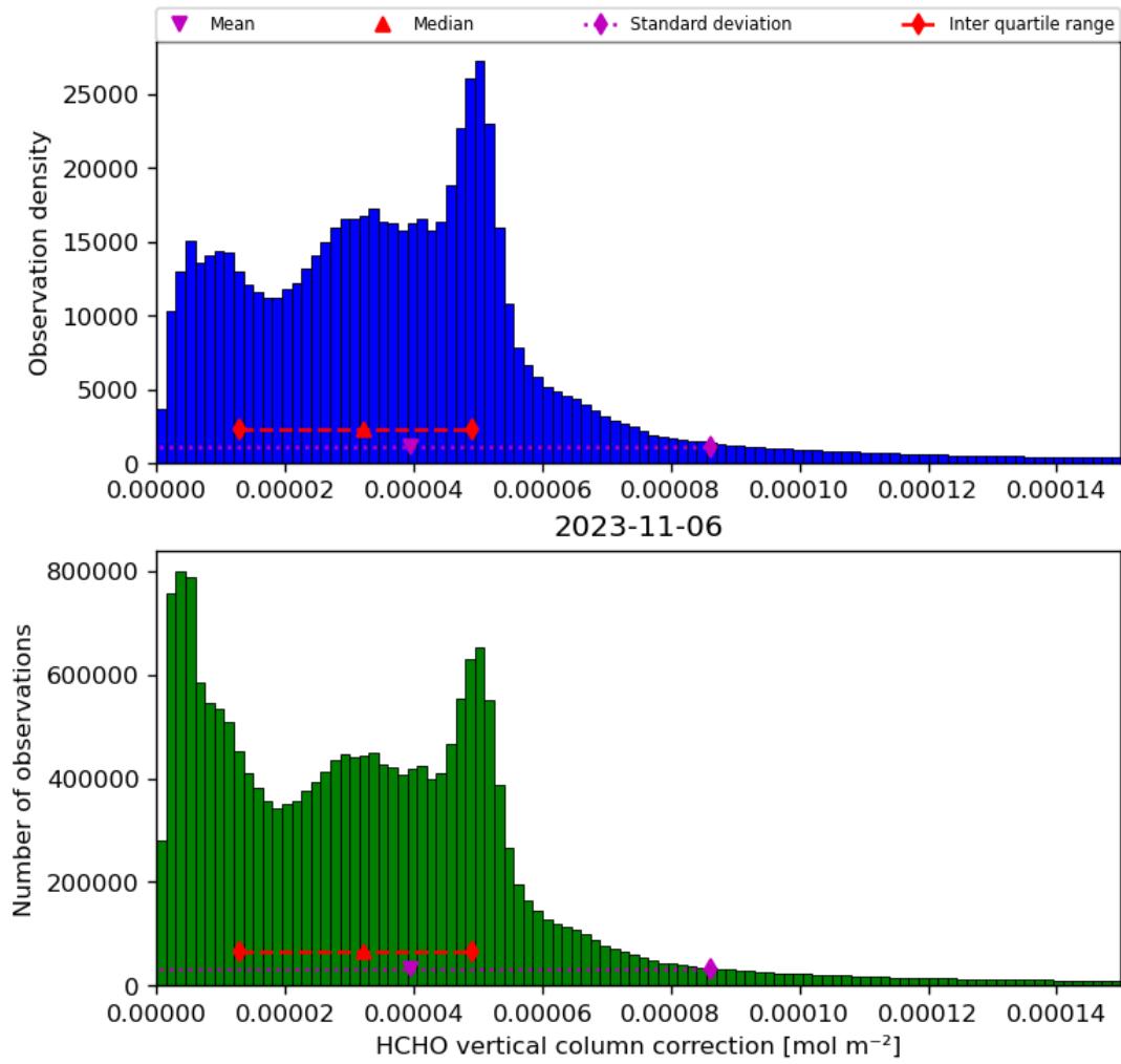
Figure 37: Histogram of “HCHO vertical column correction” for 2023-11-05 to 2023-11-07
