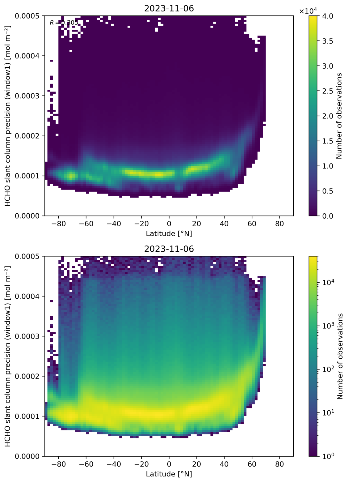
Figure 160: Scatter density plot of “Latitude” against “HCHO slant column precision (window1)” for 2023-11-05 to 2023-11-07.
