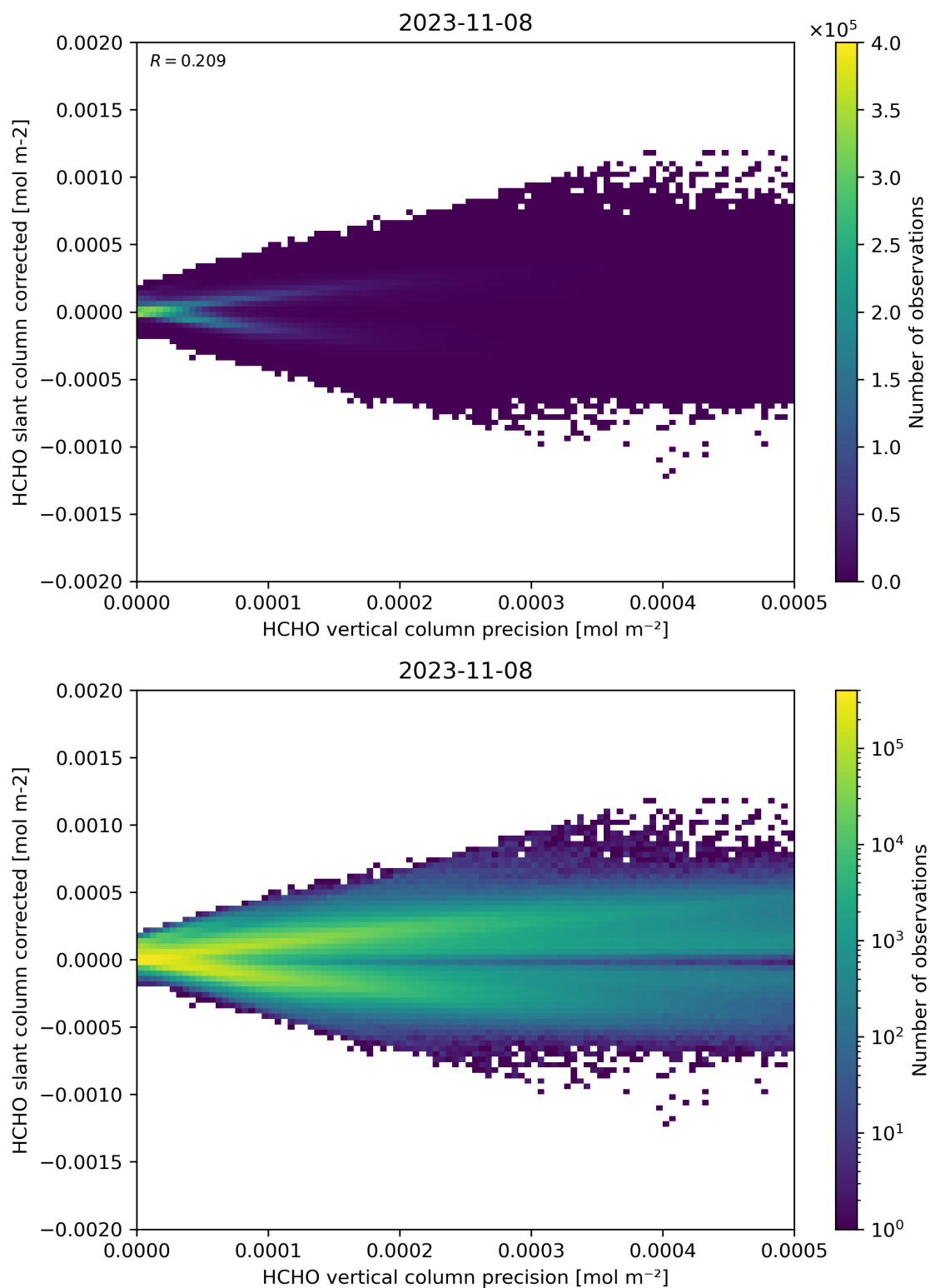
Figure 140: Scatter density plot of “HCHO vertical column precision” against “HCHO slant column corrected” for 2023-11-07 to 2023-11-09.
