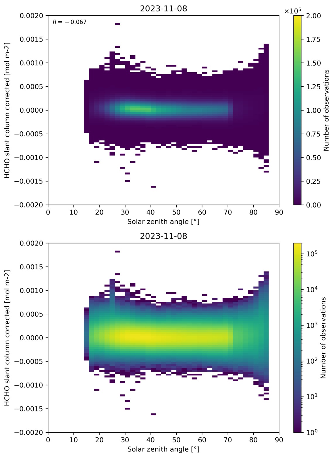
Figure 171: Scatter density plot of “Solar zenith angle” against “HCHO slant column corrected” for 2023-11-07 to 2023-11-09.
