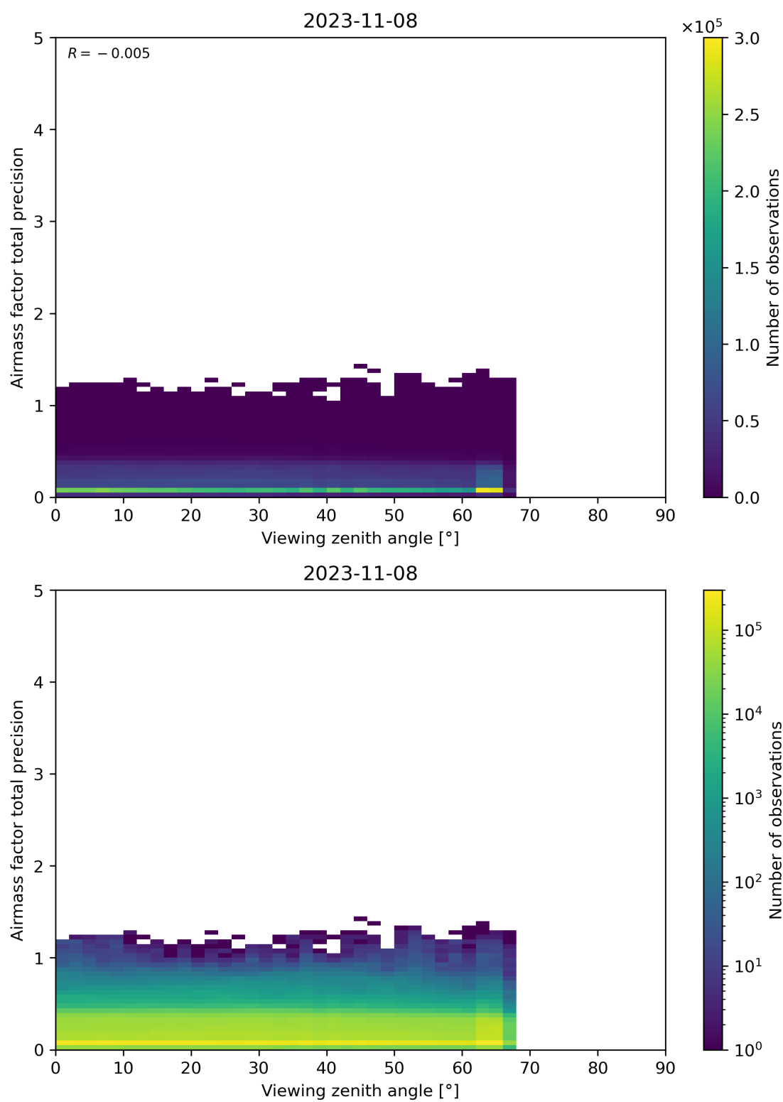
Figure 191: Scatter density plot of “Viewing zenith angle” against “Airmass factor total precision” for 2023-11-07 to 2023-11-09.
