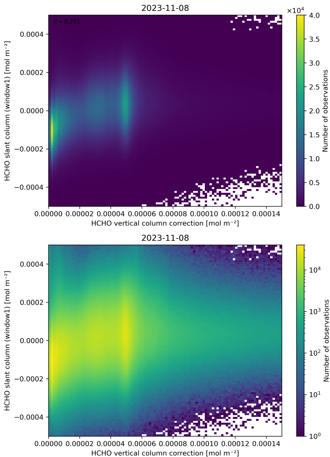
Figure 118: Scatter density plot of “HCHO vertical column correction” against “HCHO slant column (window1)” for 2023-11-07 to 2023-11-09.
