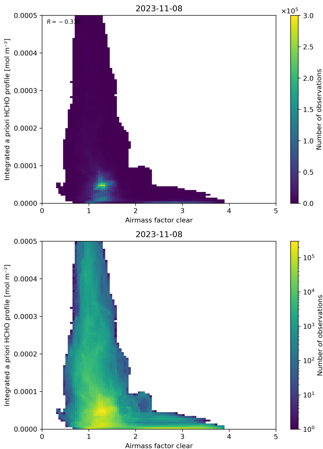
Figure 76: Scatter density plot of “Airmass factor clear” against “Integrated a priori HCHO profile” for 2023-11-07 to 2023-11-09.
