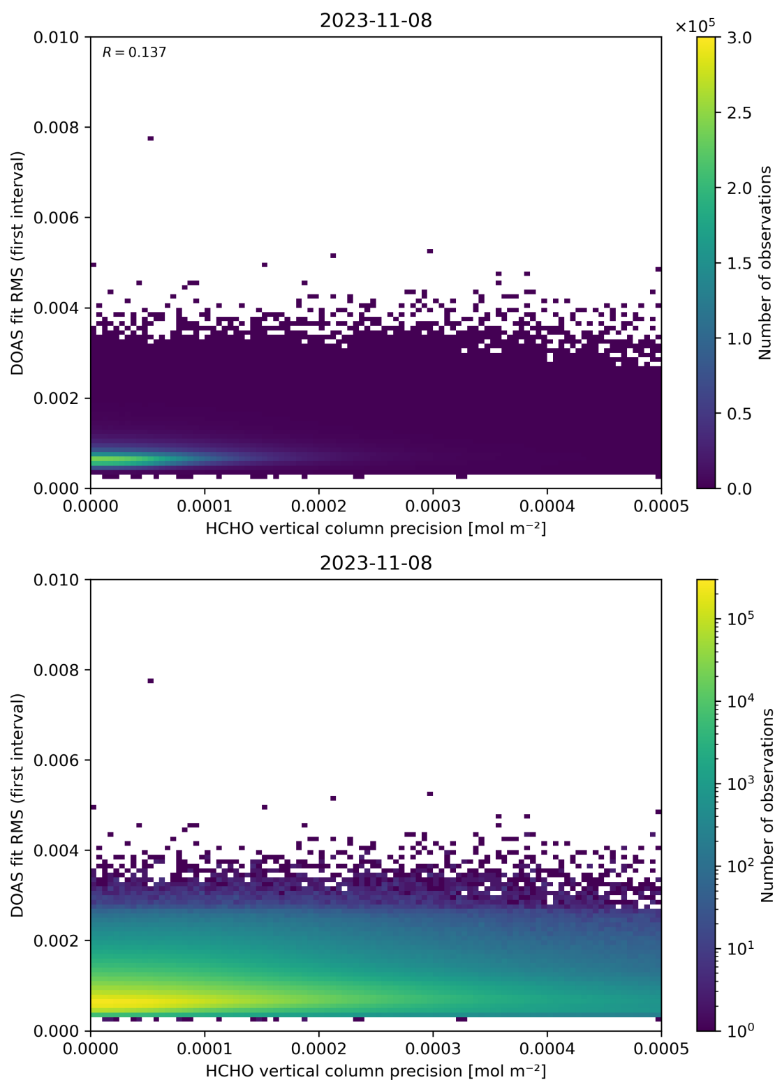
Figure 136: Scatter density plot of “HCHO vertical column precision” against “DOAS fit RMS (first interval)” for 2023-11-07 to 2023-11-09.
