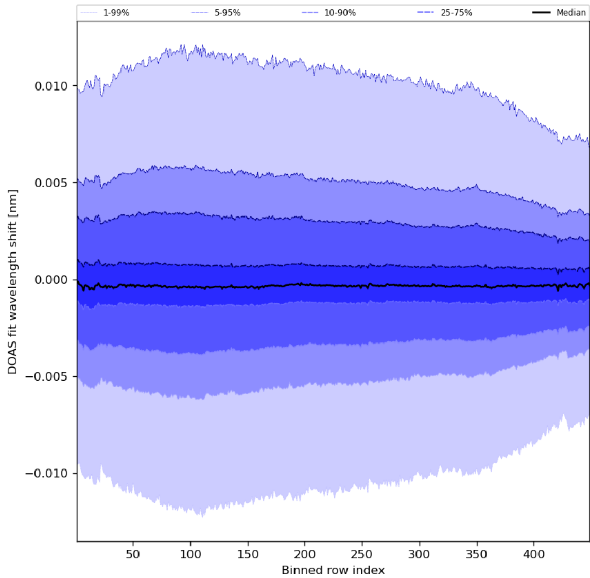
Figure 58: Along track statistics of “DOAS fit wavelength shift” for 2023-11-07 to 2023-11-09
