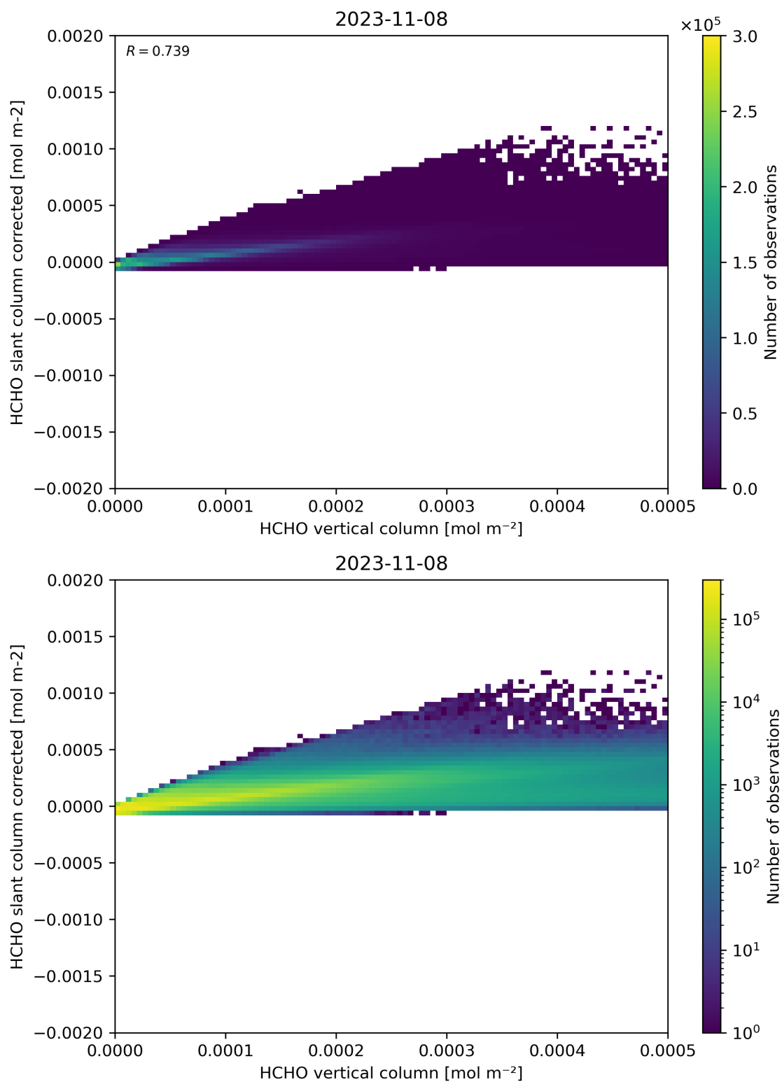
Figure 127: Scatter density plot of “HCHO vertical column” against “HCHO slant column corrected” for 2023-11-07 to 2023-11-09.
