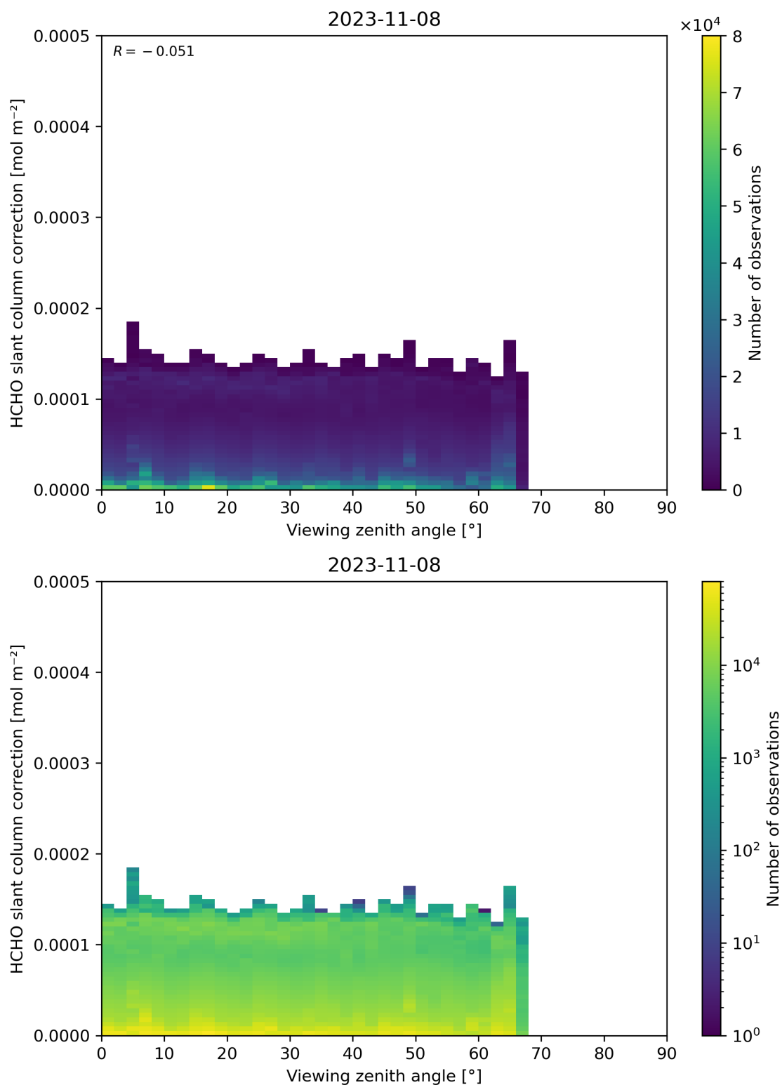
Figure 187: Scatter density plot of “Viewing zenith angle” against “HCHO slant column correction” for 2023-11-07 to 2023-11-09.
