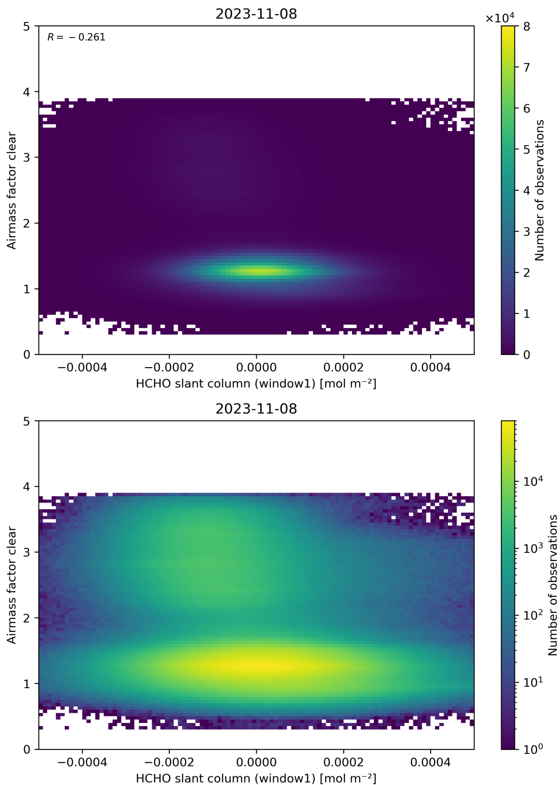
Figure 81: Scatter density plot of “HCHO slant column (window1)” against “Airmass factor clear” for 2023-11-07 to 2023-11-09.
