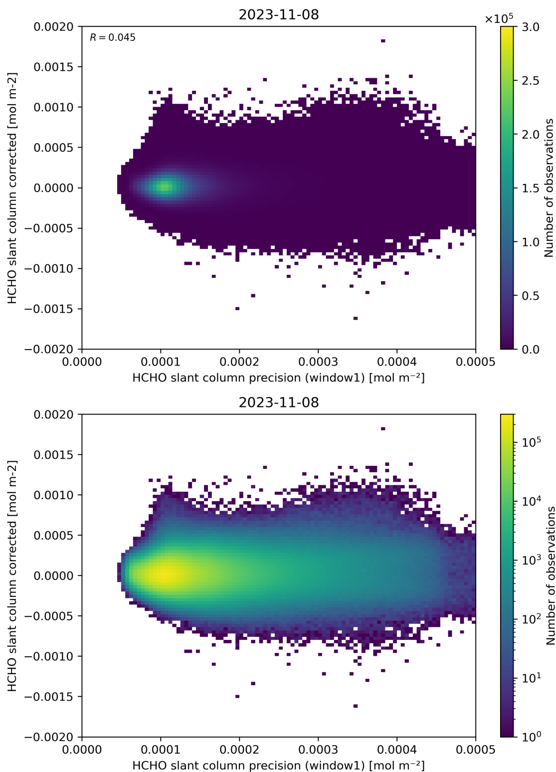
Figure 92: Scatter density plot of “HCHO slant column precision (window1)” against “HCHO slant column corrected” for 2023-11-07 to 2023-11-09.
