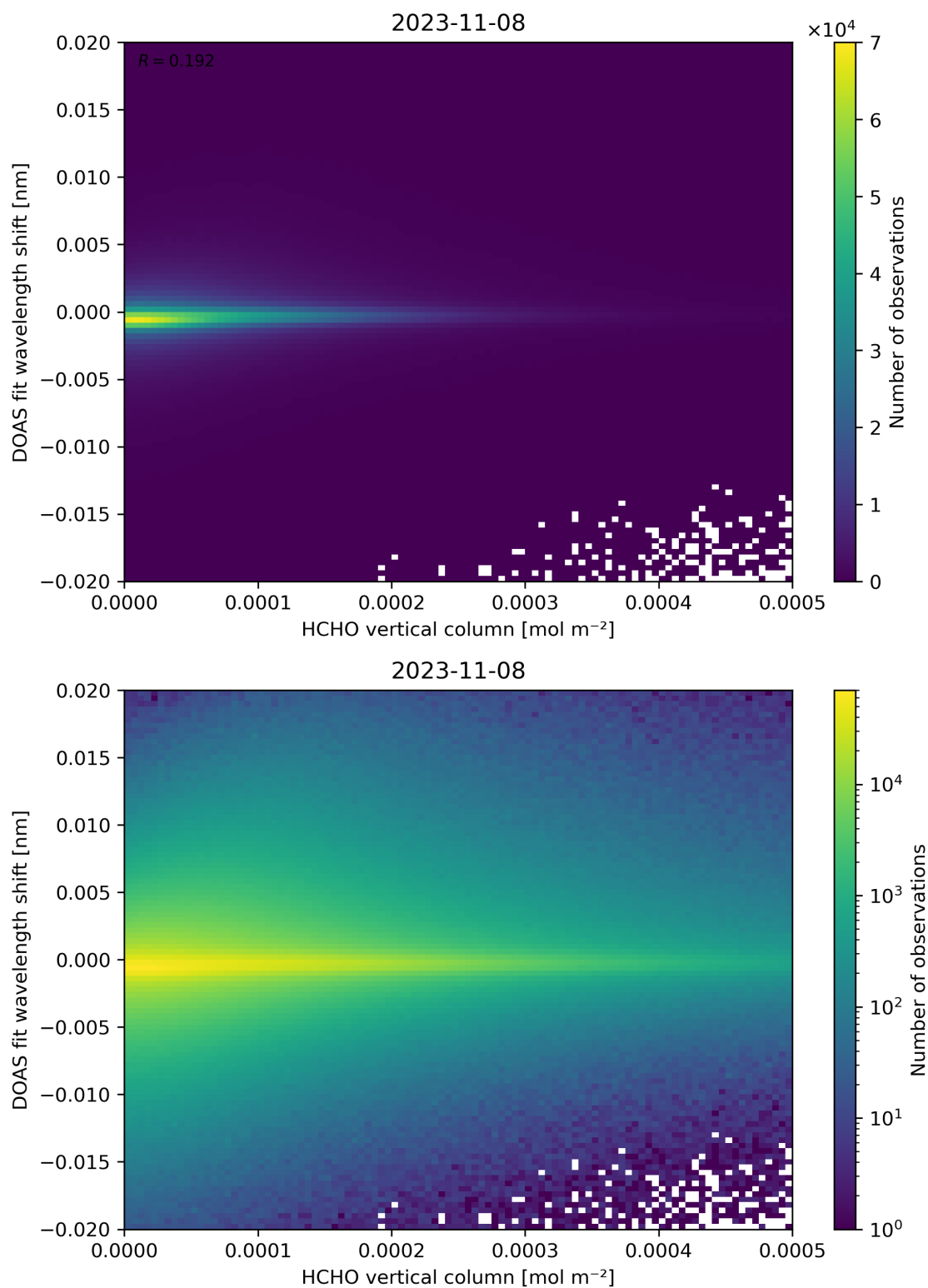
Figure 124: Scatter density plot of “HCHO vertical column” against “DOAS fit wavelength shift” for 2023-11-07 to 2023-11-09.
