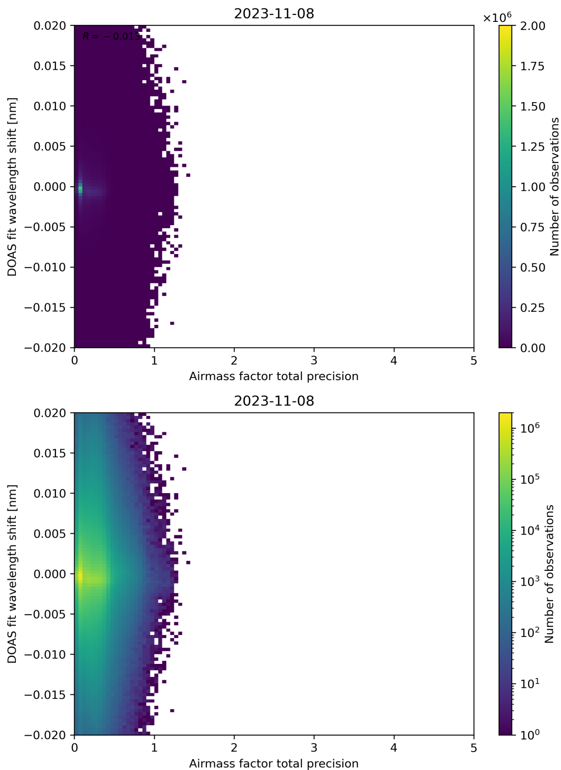
Figure 106: Scatter density plot of “Airmass factor total precision” against “DOAS fit wavelength shift” for 2023-11-07 to 2023-11-09.
