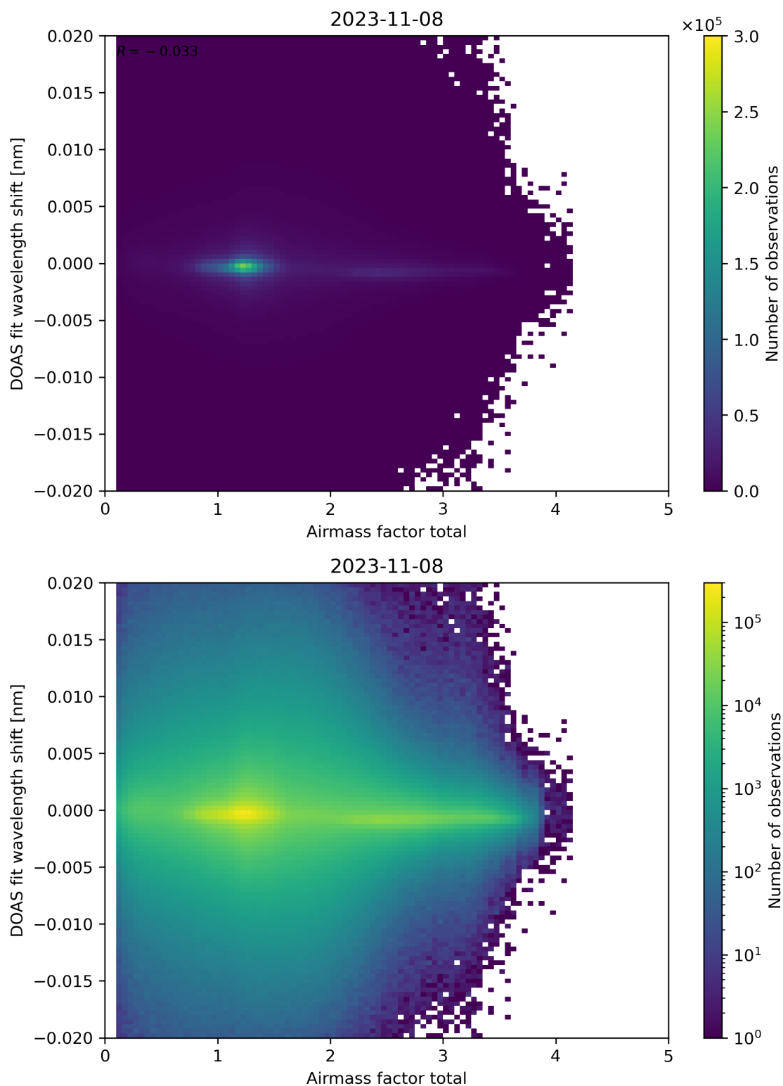
Figure 98: Scatter density plot of “Airmass factor total” against “DOAS fit wavelength shift” for 2023-11-07 to 2023-11-09.
