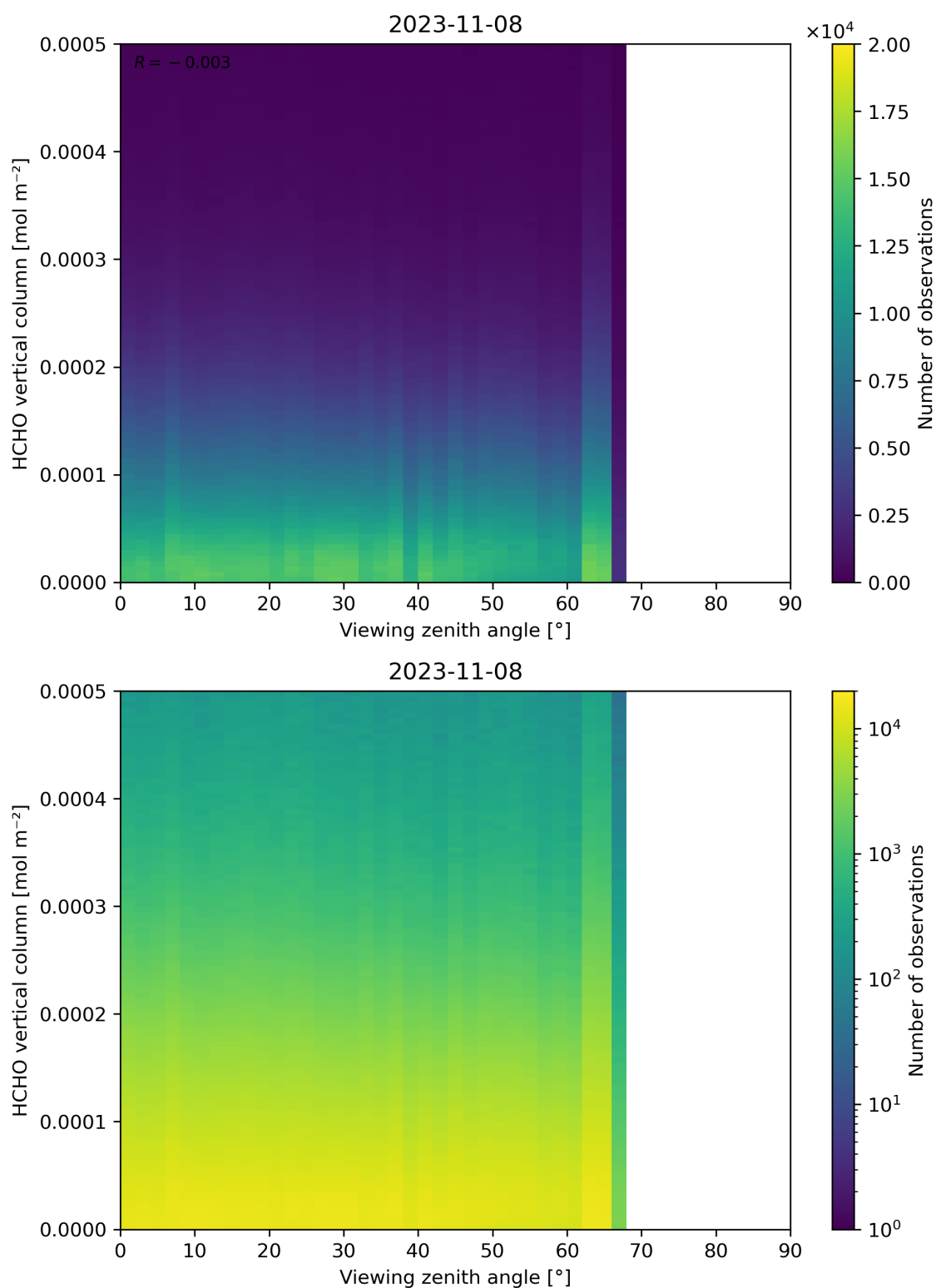
Figure 192: Scatter density plot of “Viewing zenith angle” against “HCHO vertical column” for 2023-11-07 to 2023-11-09.
