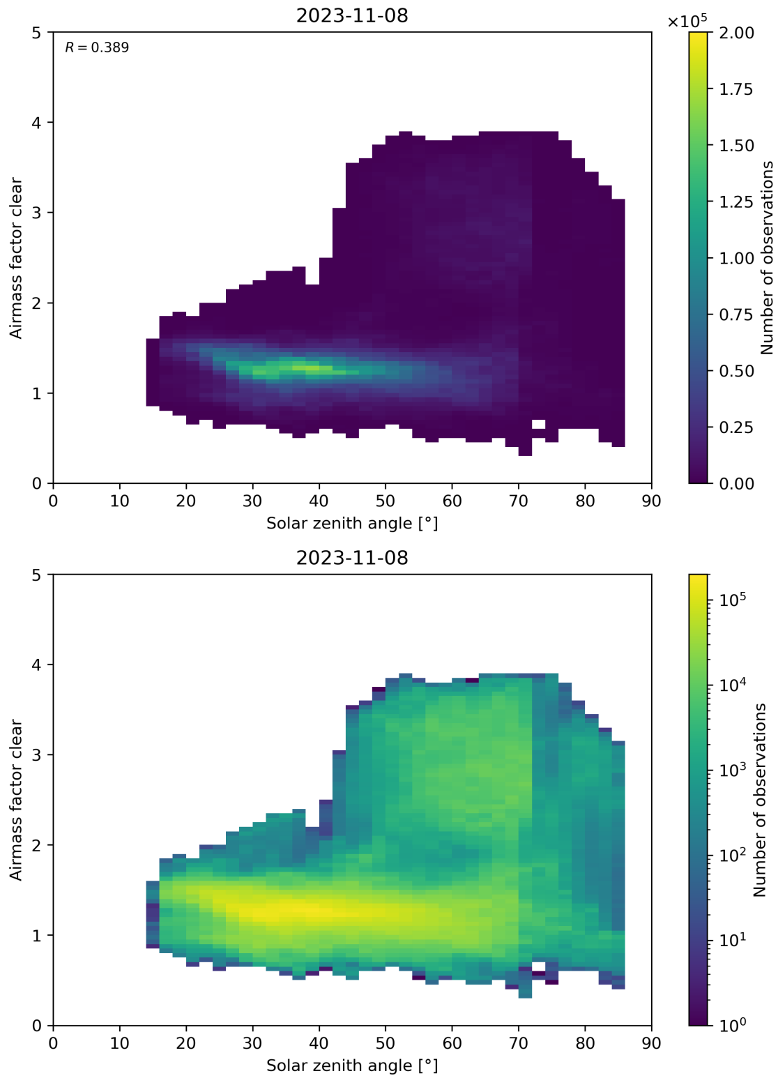
Figure 170: Scatter density plot of “Solar zenith angle” against “Airmass factor clear” for 2023-11-07 to 2023-11-09.
