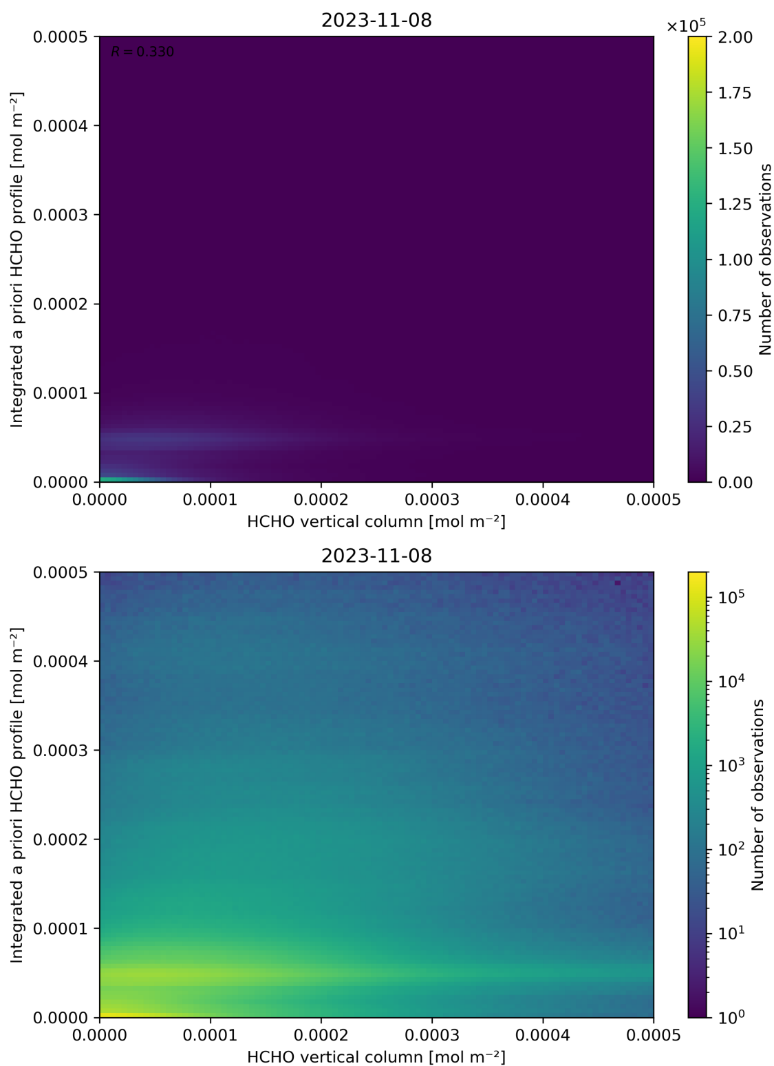
Figure 135: Scatter density plot of “HCHO vertical column” against “Integrated a priori HCHO profile” for 2023-11-07 to 2023-11-09.
