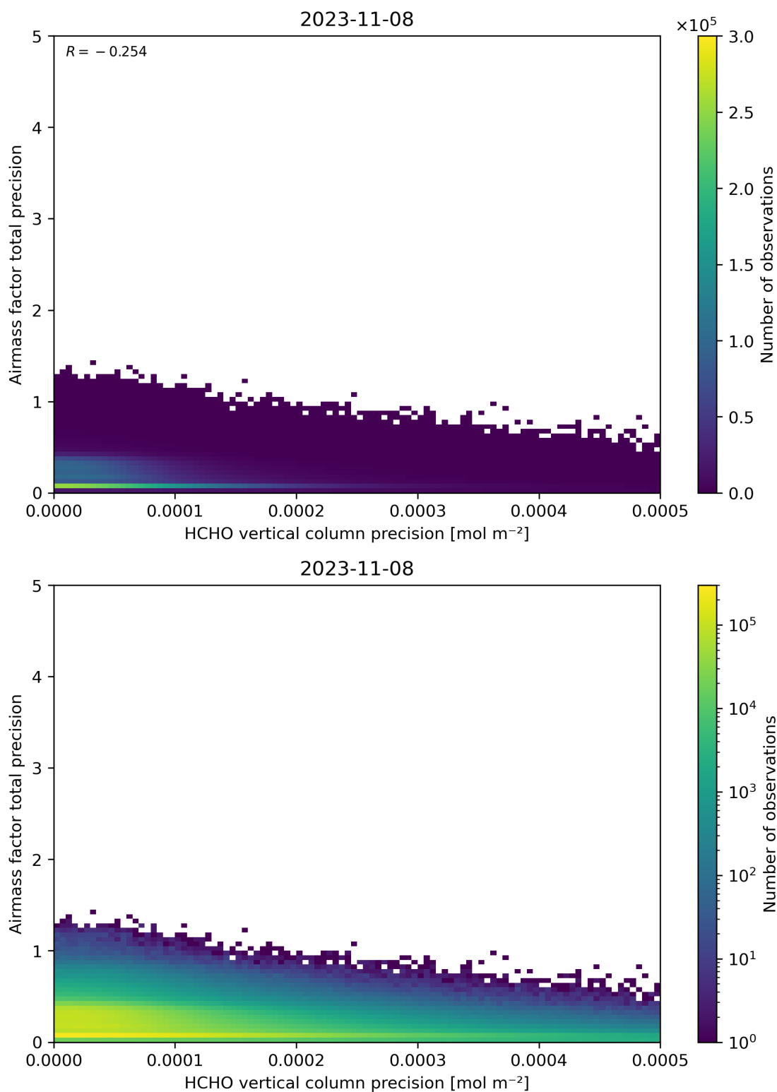
Figure 145: Scatter density plot of “HCHO vertical column precision” against “Airmass factor total precision” for 2023-11-07 to 2023-11-09.
