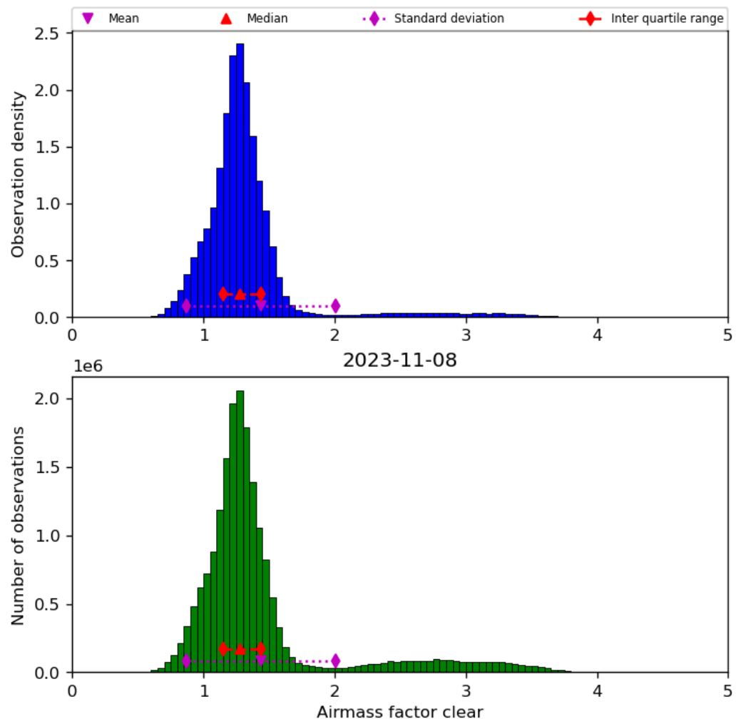
Figure 42: Histogram of “Airmass factor clear” for 2023-11-07 to 2023-11-09
