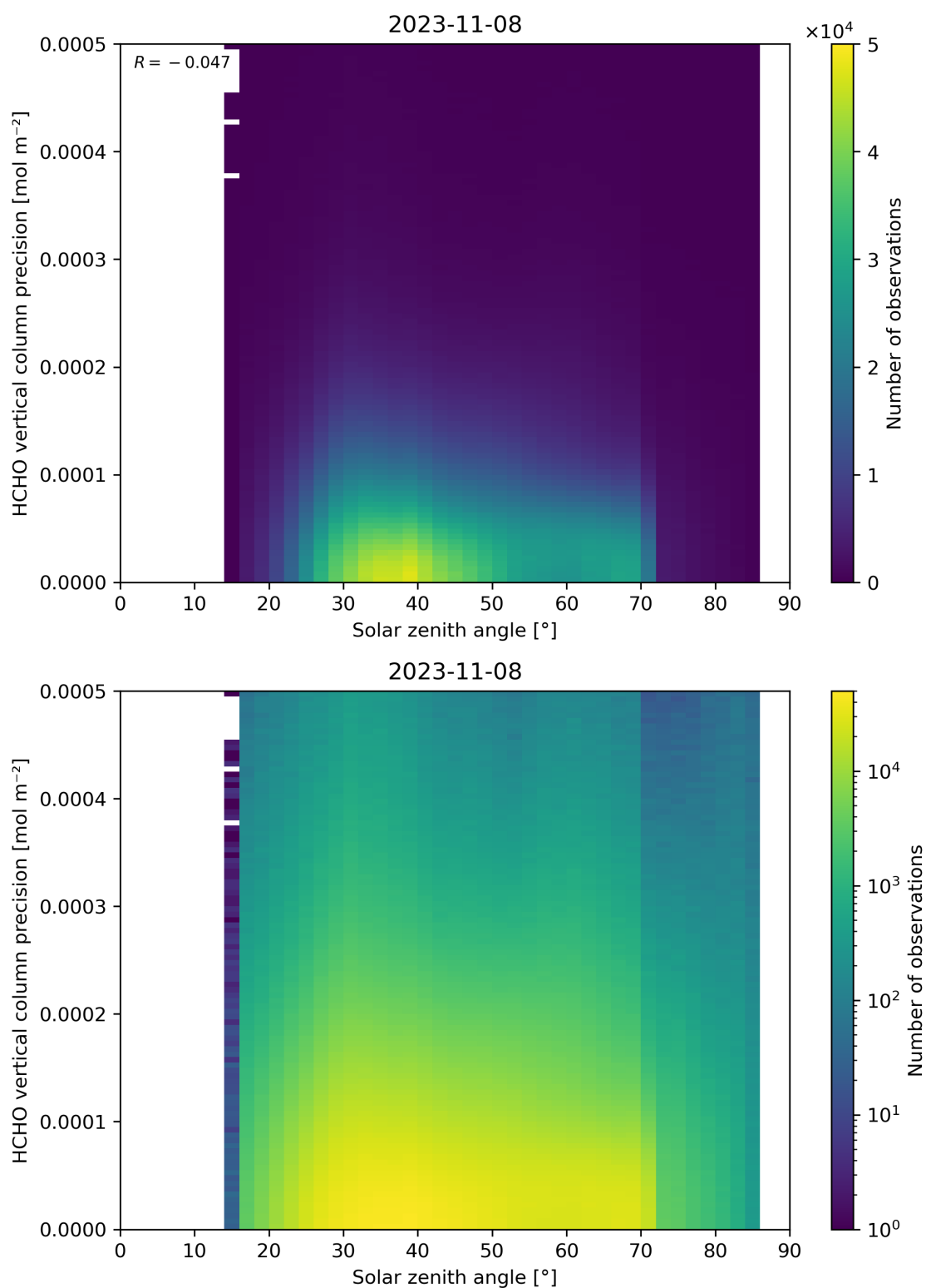
Figure 179: Scatter density plot of “Solar zenith angle” against “HCHO vertical column precision” for 2023-11-07 to 2023-11-09.
