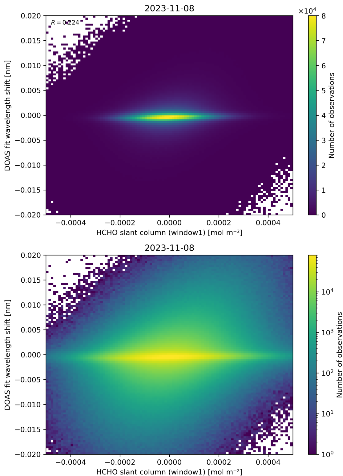
Figure 79: Scatter density plot of “HCHO slant column (window1)” against “DOAS fit wavelength shift” for 2023-11-07 to 2023-11-09.
