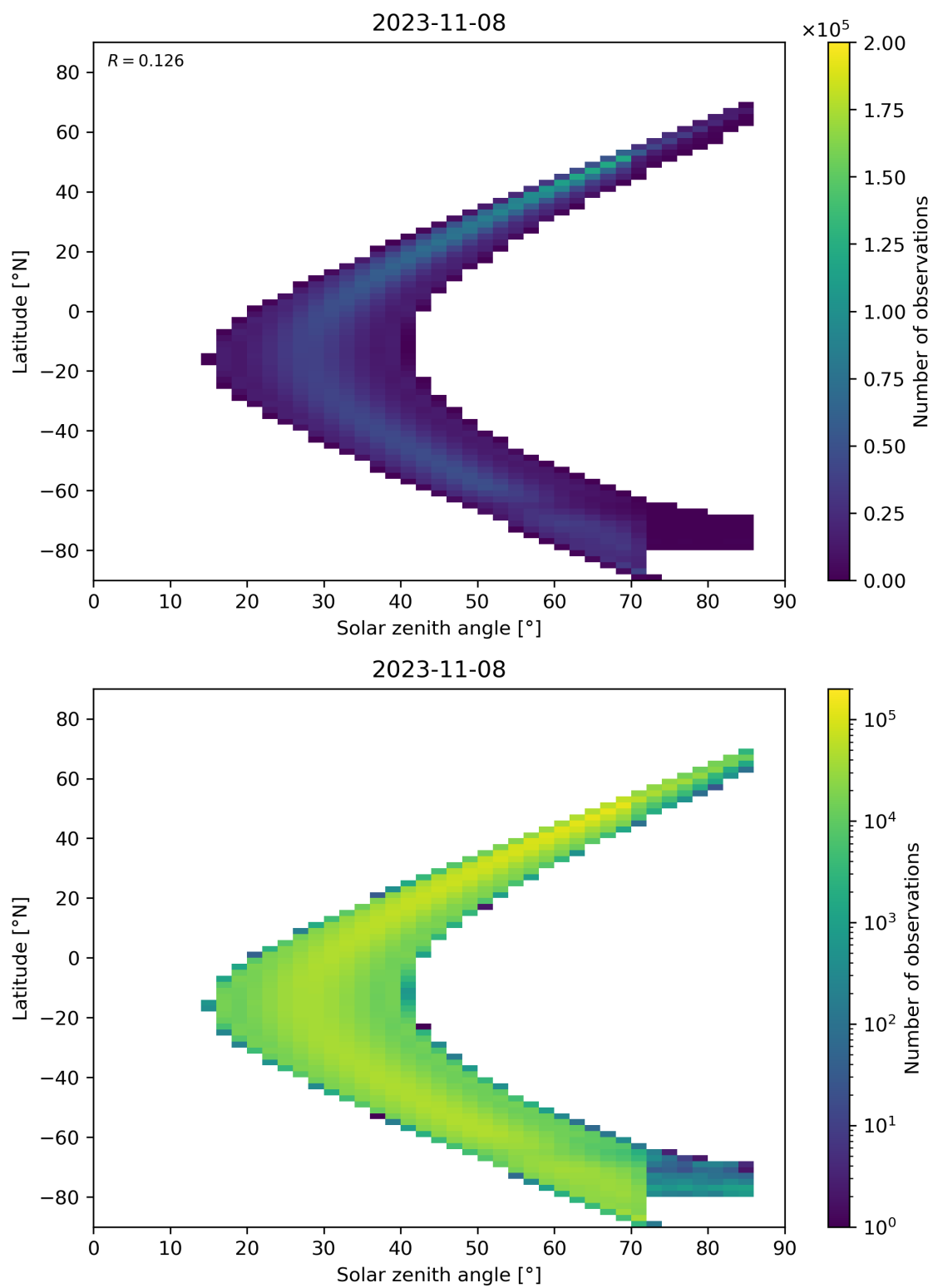
Figure 181: Scatter density plot of “Solar zenith angle” against “Latitude” for 2023-11-07 to 2023-11-09.
