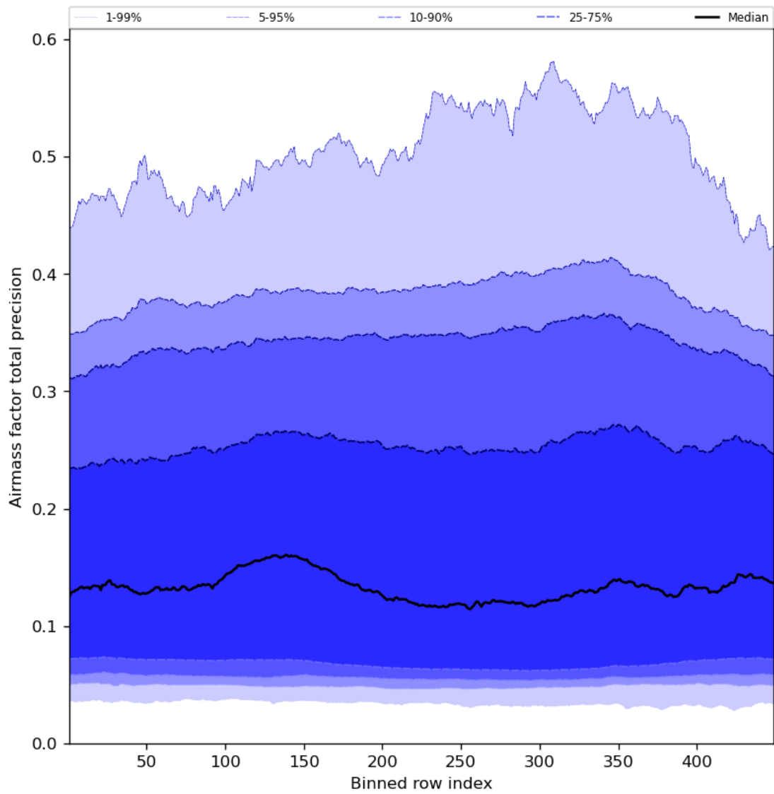
Figure 55: Along track statistics of “Airmass factor total precision” for 2023-11-07 to 2023-11-09
