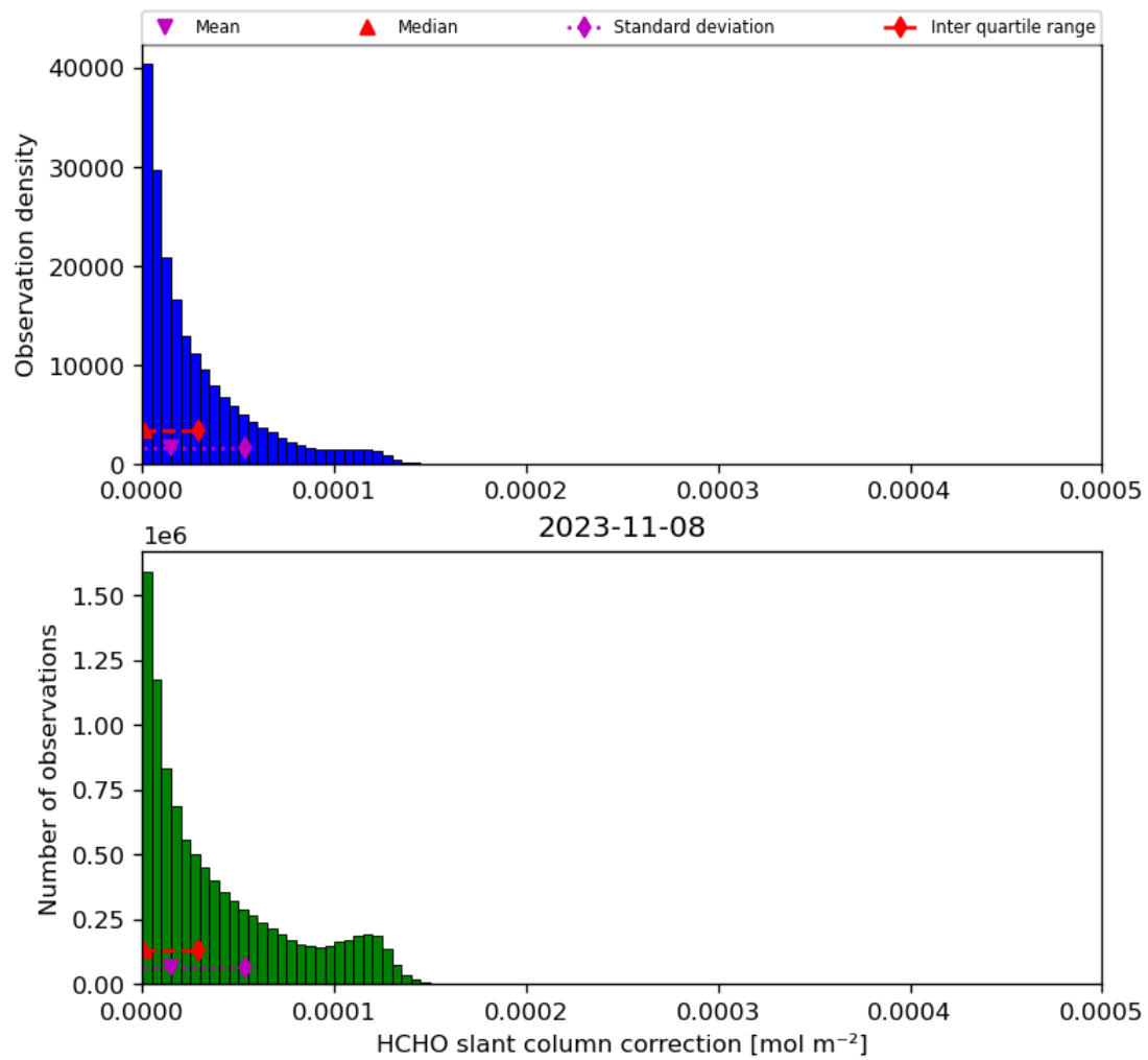
Figure 47: Histogram of “HCHO slant column correction” for 2023-11-07 to 2023-11-09
