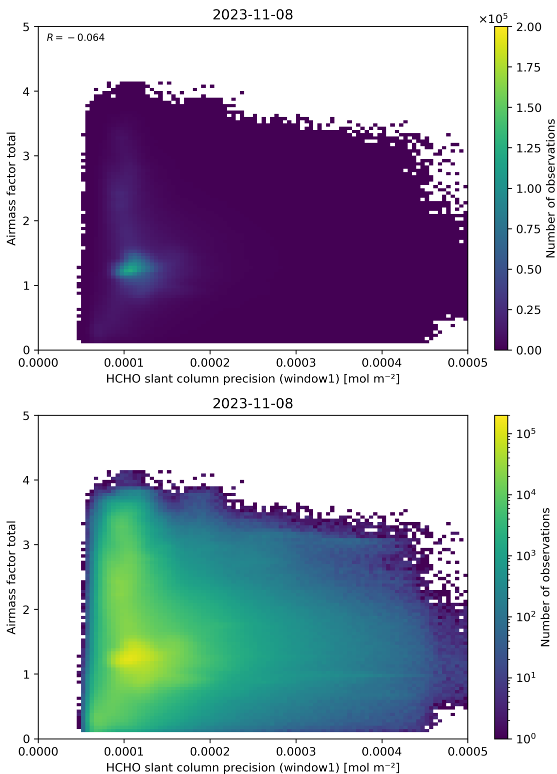
Figure 94: Scatter density plot of “HCHO slant column precision (window1)” against “Airmass factor total” for 2023-11-07 to 2023-11-09.
