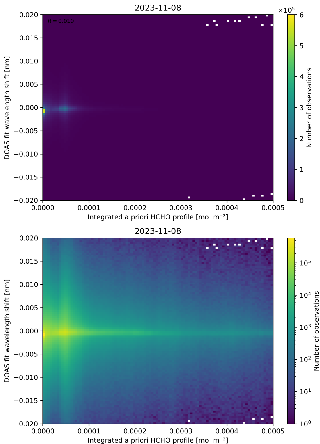
Figure 149: Scatter density plot of “Integrated a priori HCHO profile” against “DOAS fit wavelength shift” for 2023-11-07 to 2023-11-09.
