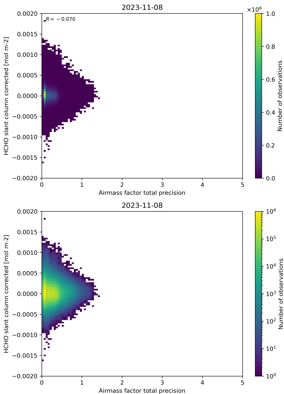
Figure 109: Scatter density plot of “Airmass factor total precision” against “HCHO slant column corrected” for 2023-11-07 to 2023-11-09.
