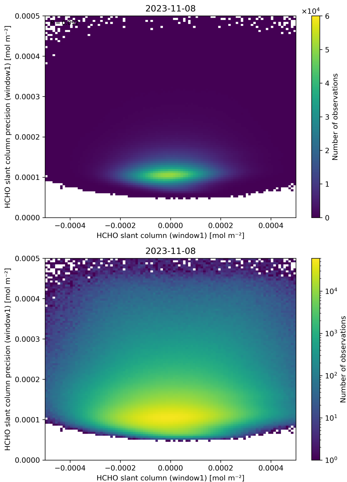
Figure 84: Scatter density plot of “HCHO slant column (window1)” against “HCHO slant column precision (window1)” for 2023-11-07 to 2023-11-09.
