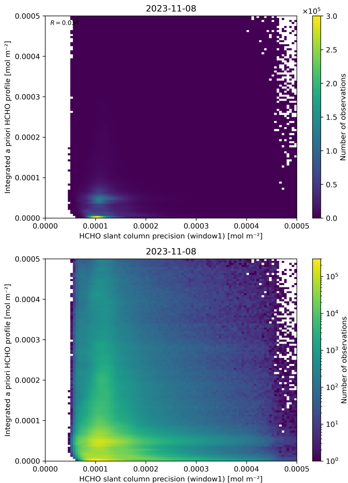
Figure 96: Scatter density plot of “HCHO slant column precision (window1)” against “Integrated a priori HCHO profile” for 2023-11-07 to 2023-11-09.
