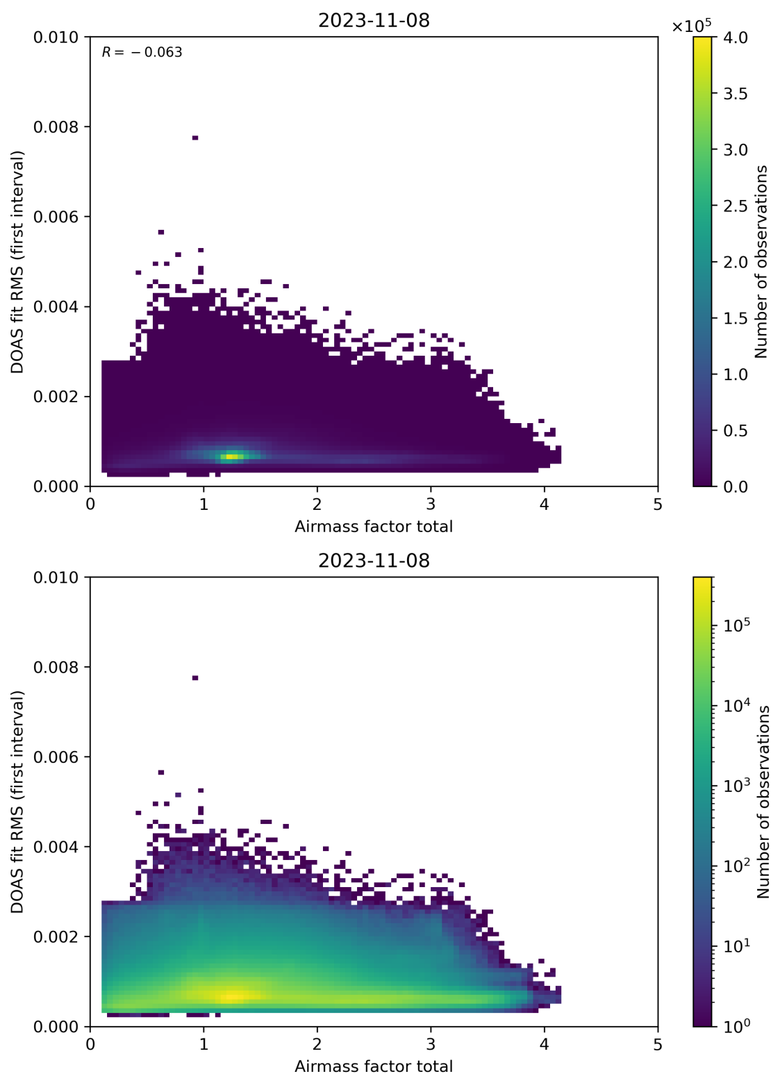
Figure 97: Scatter density plot of “Airmass factor total” against “DOAS fit RMS (first interval)” for 2023-11-07 to 2023-11-09.
