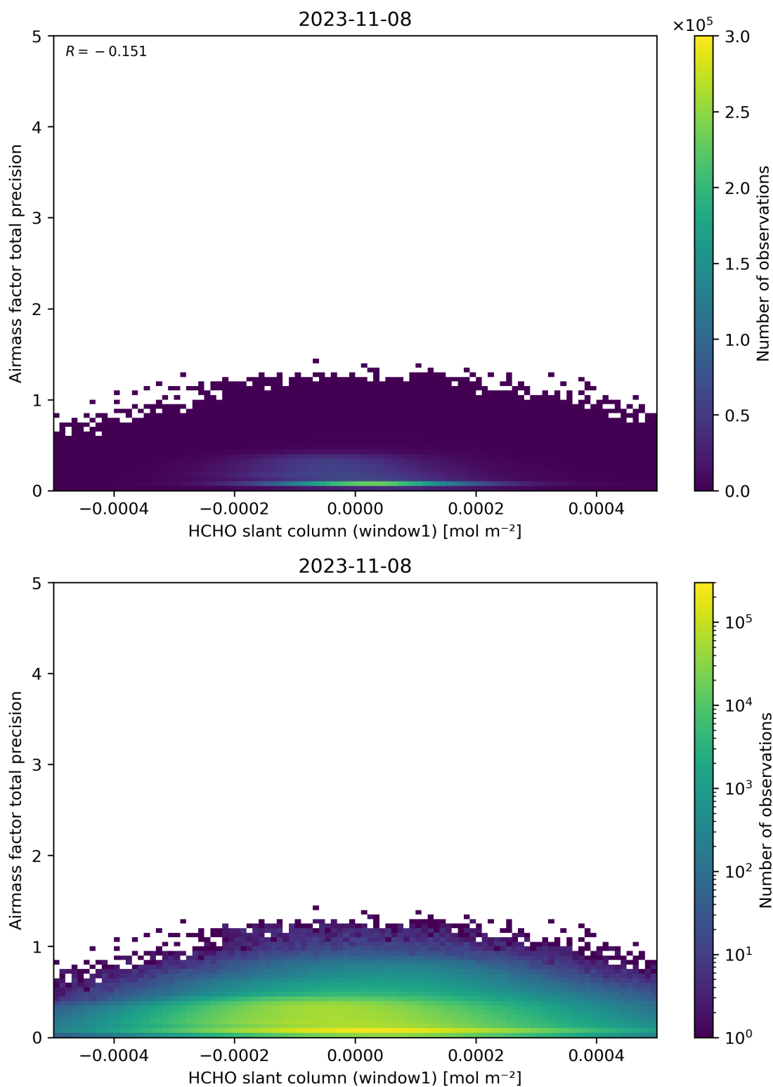
Figure 86: Scatter density plot of “HCHO slant column (window1)” against “Airmass factor total precision” for 2023-11-07 to 2023-11-09.
