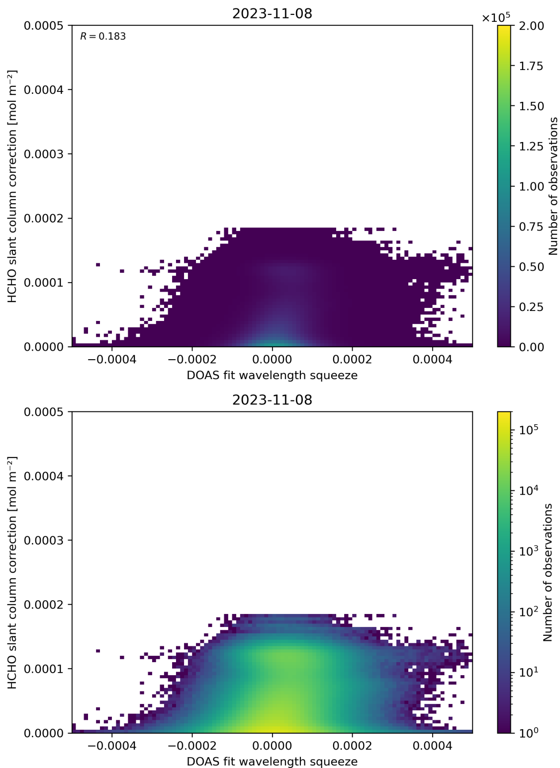
Figure 70: Scatter density plot of “DOAS fit wavelength squeeze” against “HCHO slant column correction” for 2023-11-07 to 2023-11-09.
