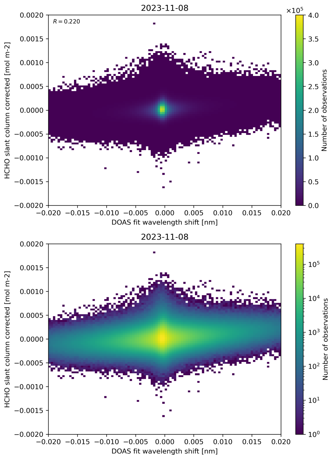
Figure 66: Scatter density plot of “DOAS fit wavelength shift” against “HCHO slant column corrected” for 2023-11-07 to 2023-11-09.
