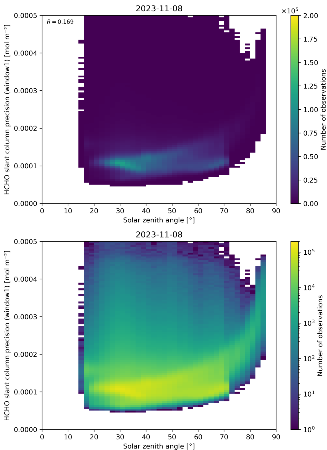
Figure 174: Scatter density plot of “Solar zenith angle” against “HCHO slant column precision (window1)” for 2023-11-07 to 2023-11-09.
