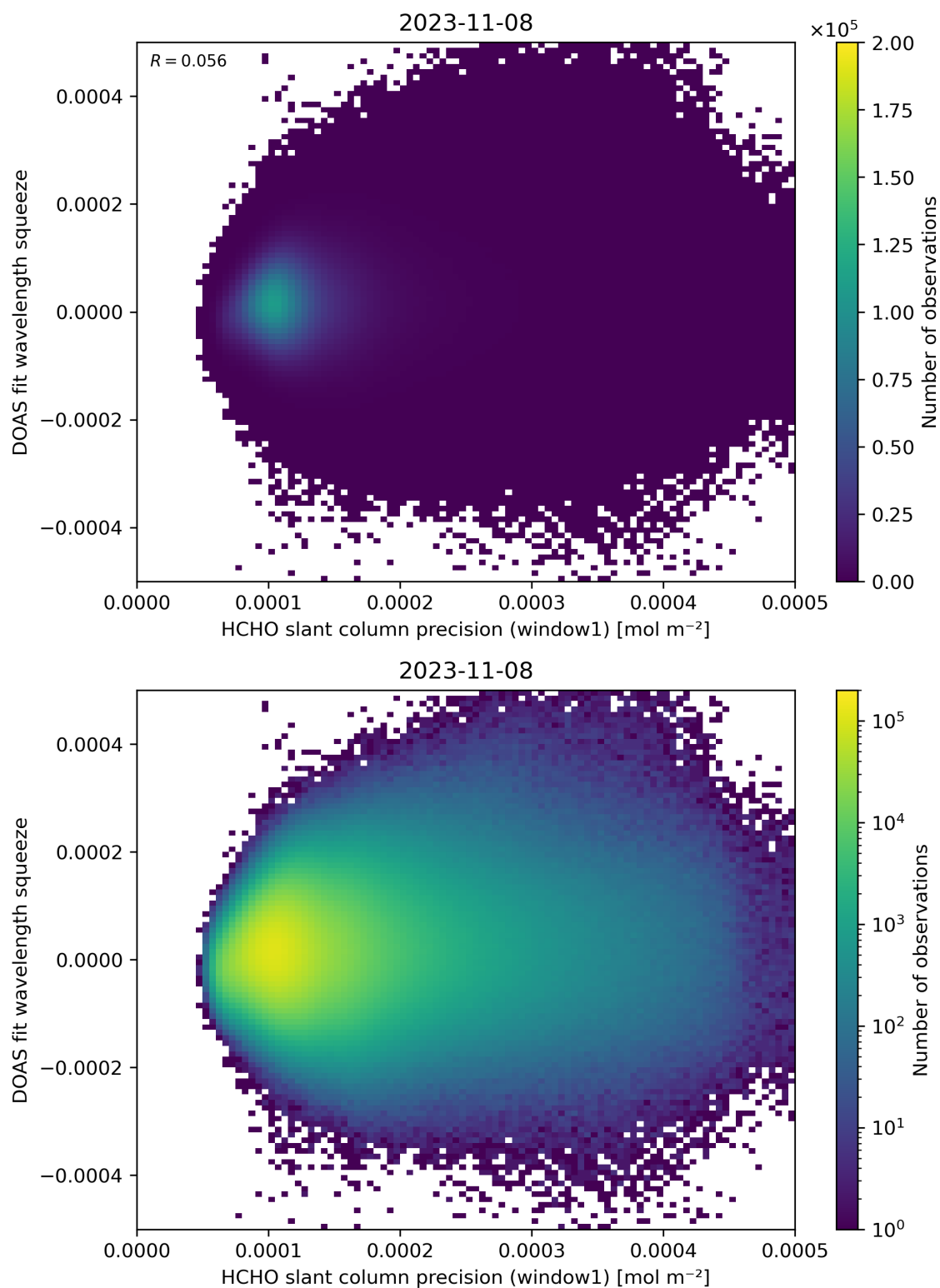
Figure 90: Scatter density plot of “HCHO slant column precision (window1)” against “DOAS fit wavelength squeeze” for 2023-11-07 to 2023-11-09.
