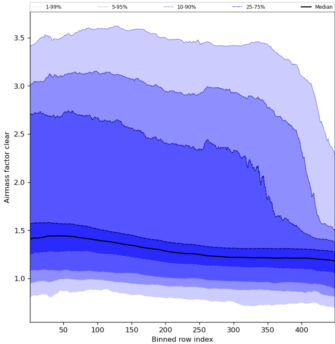
Figure 56: Along track statistics of “Airmass factor clear” for 2023-11-07 to 2023-11-09
