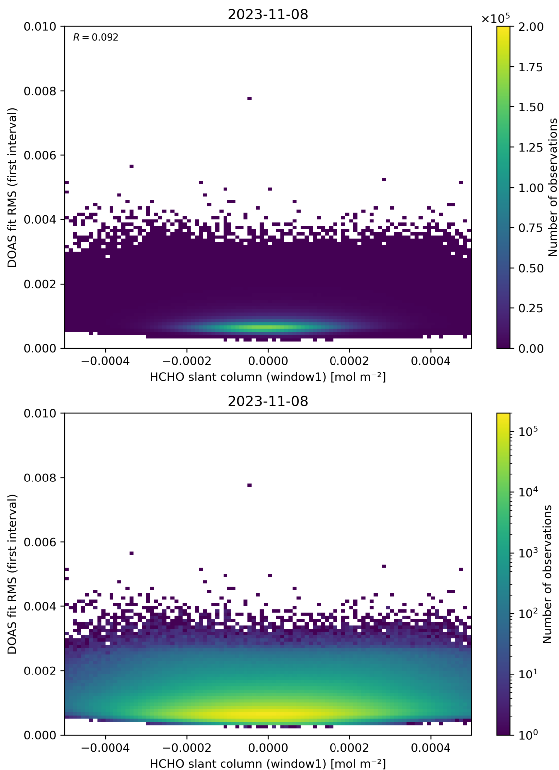
Figure 78: Scatter density plot of “HCHO slant column (window1)” against “DOAS fit RMS (first interval)” for 2023-11-07 to 2023-11-09.
