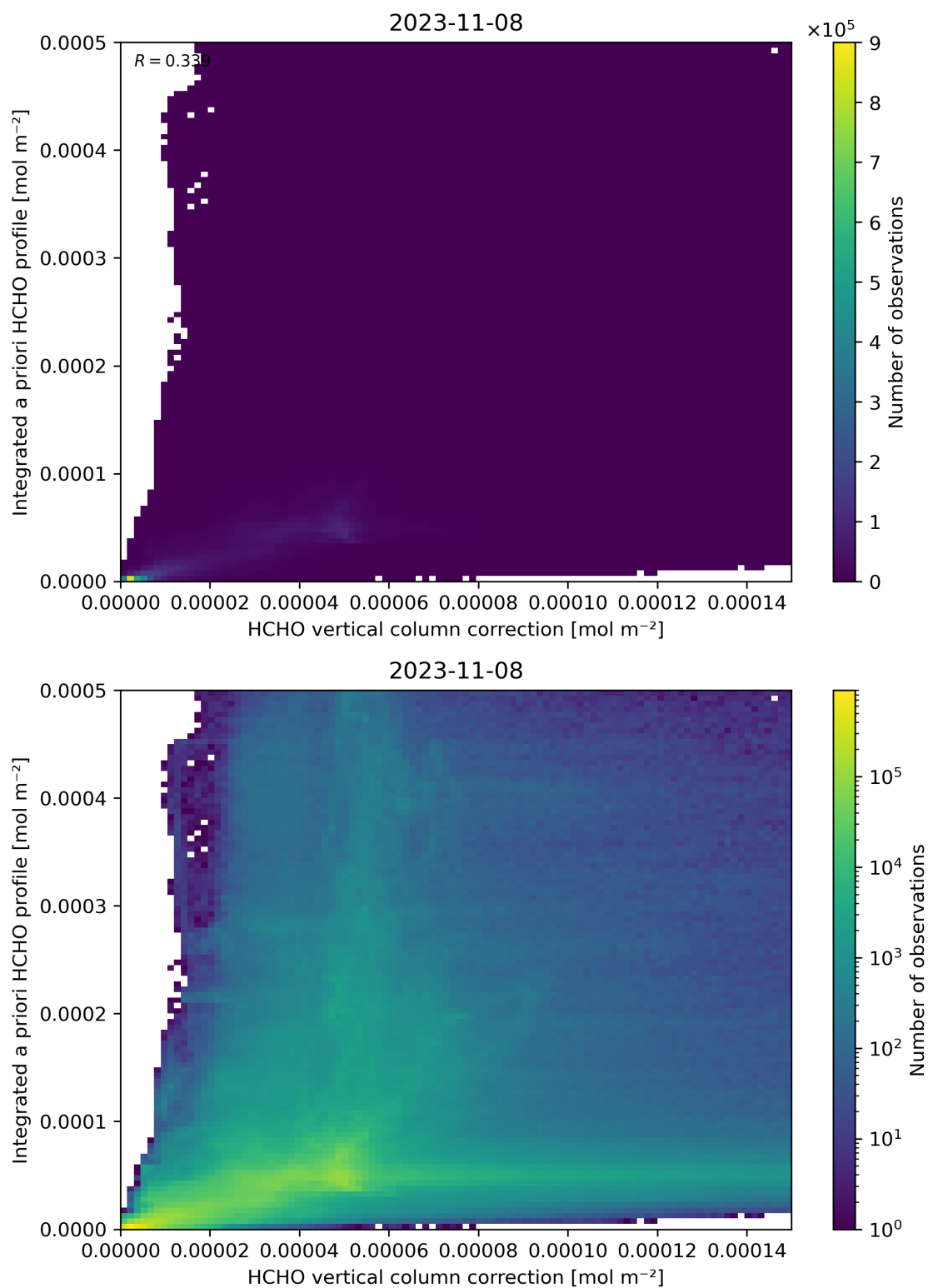
Figure 122: Scatter density plot of “HCHO vertical column correction” against “Integrated a priori HCHO profile” for 2023-11-07 to 2023-11-09.
