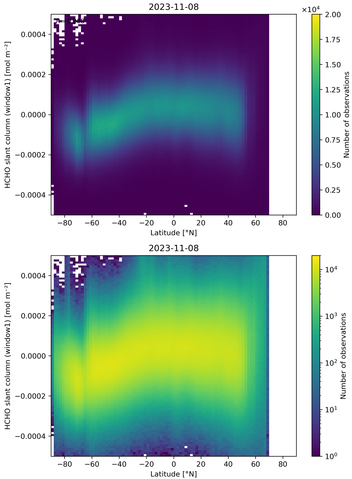
Figure 159: Scatter density plot of “Latitude” against “HCHO slant column (window1)” for 2023-11-07 to 2023-11-09.
