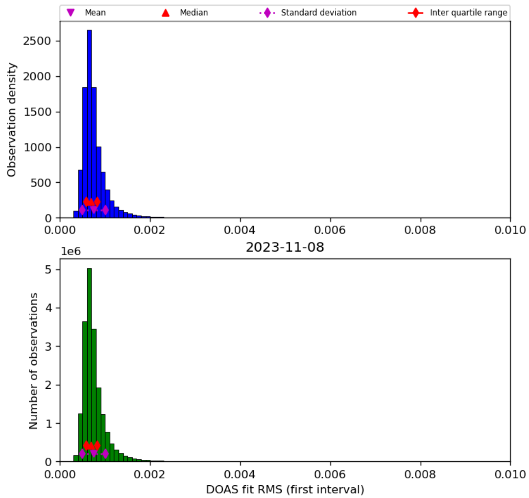
Figure 46: Histogram of “DOAS fit RMS (first interval)” for 2023-11-07 to 2023-11-09
