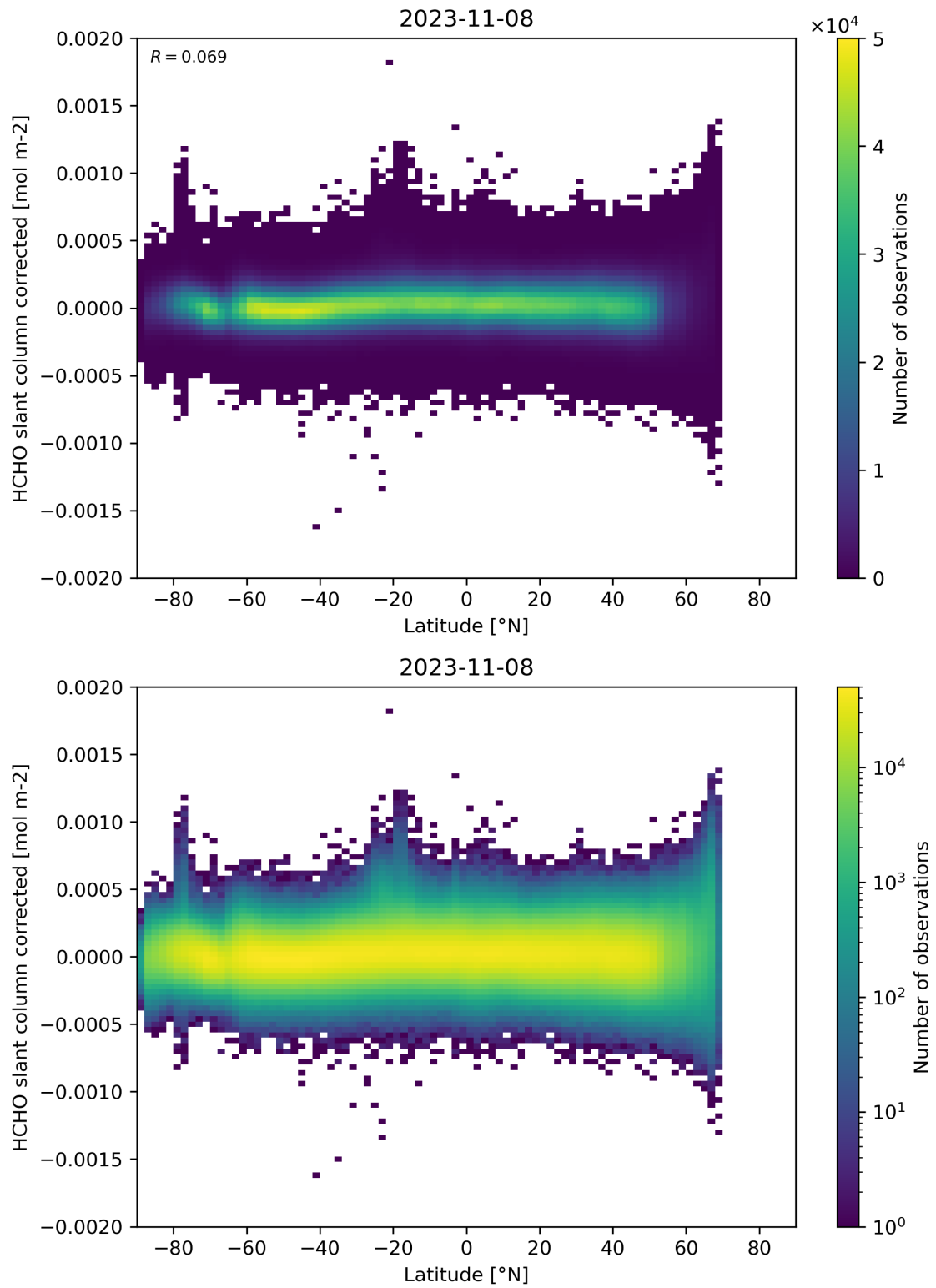
Figure 157: Scatter density plot of “Latitude” against “HCHO slant column corrected” for 2023-11-07 to 2023-11-09.
