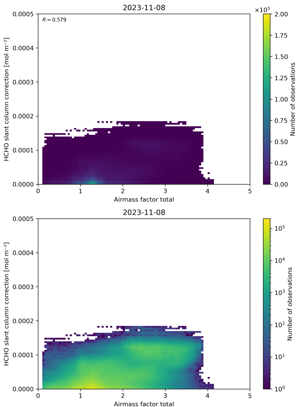
Figure 102: Scatter density plot of “Airmass factor total” against “HCHO slant column correction” for 2023-11-07 to 2023-11-09.
