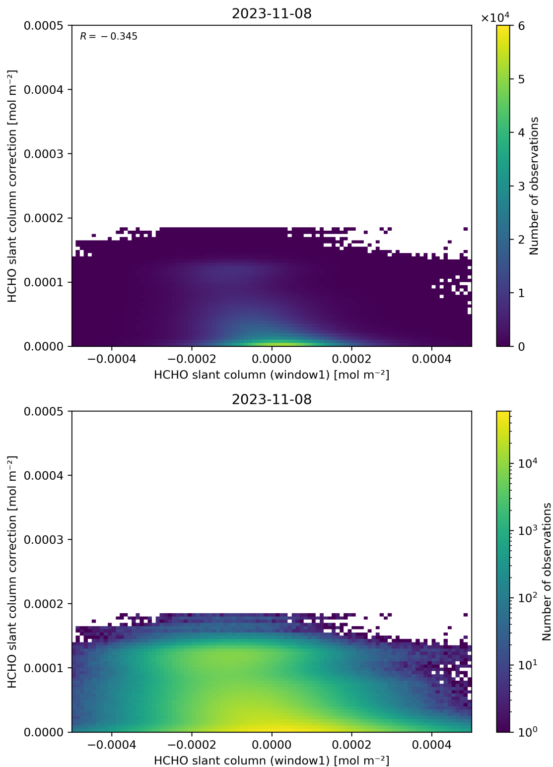
Figure 83: Scatter density plot of “HCHO slant column (window1)” against “HCHO slant column correction” for 2023-11-07 to 2023-11-09.
