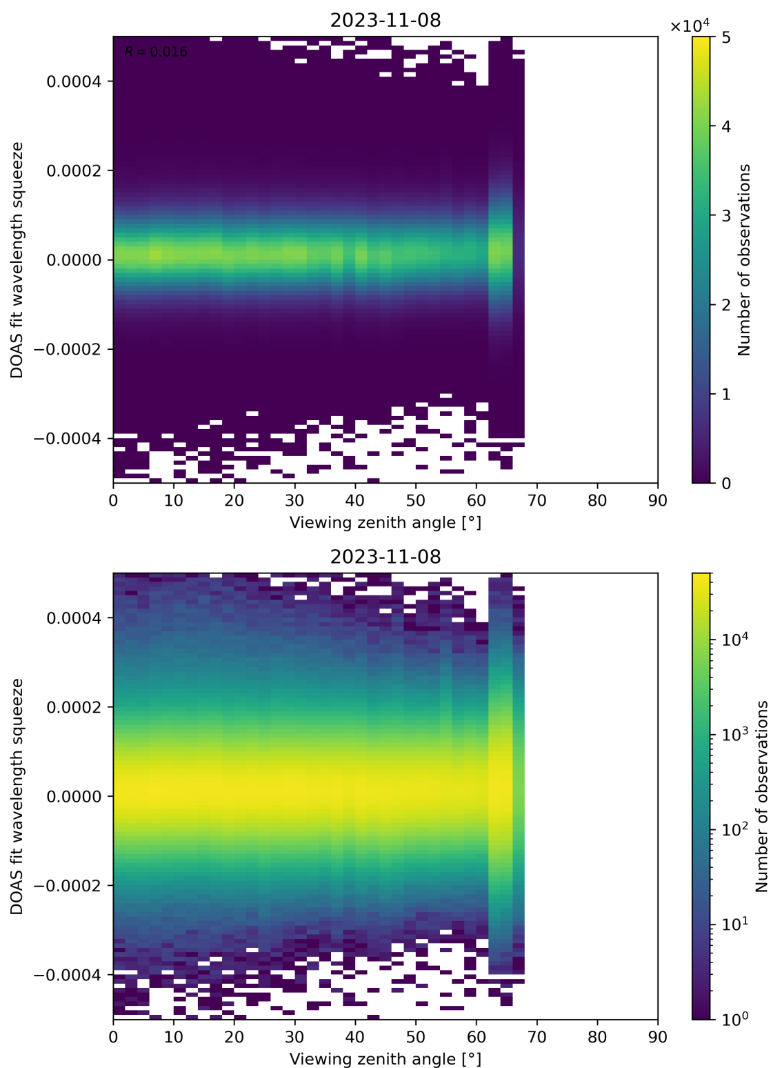
Figure 184: Scatter density plot of “Viewing zenith angle” against “DOAS fit wavelength squeeze” for 2023-11-07 to 2023-11-09.
