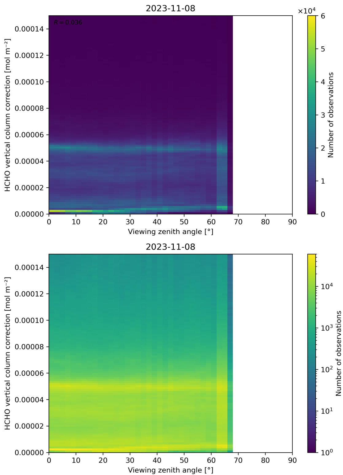
Figure 193: Scatter density plot of “Viewing zenith angle” against “HCHO vertical column correction” for 2023-11-07 to 2023-11-09.
