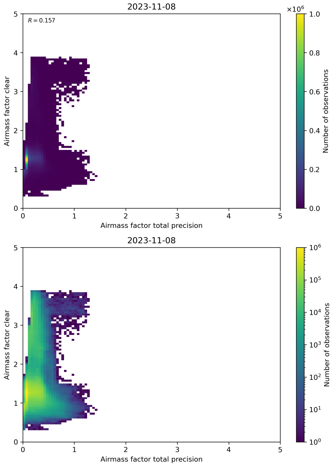
Figure 108: Scatter density plot of “Airmass factor total precision” against “Airmass factor clear” for 2023-11-07 to 2023-11-09.
