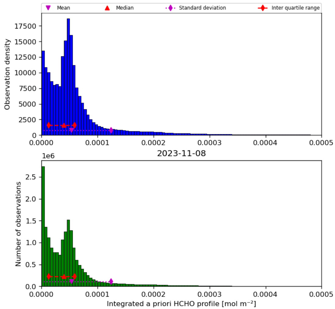
Figure 43: Histogram of “Integrated a priori HCHO profile” for 2023-11-07 to 2023-11-09
