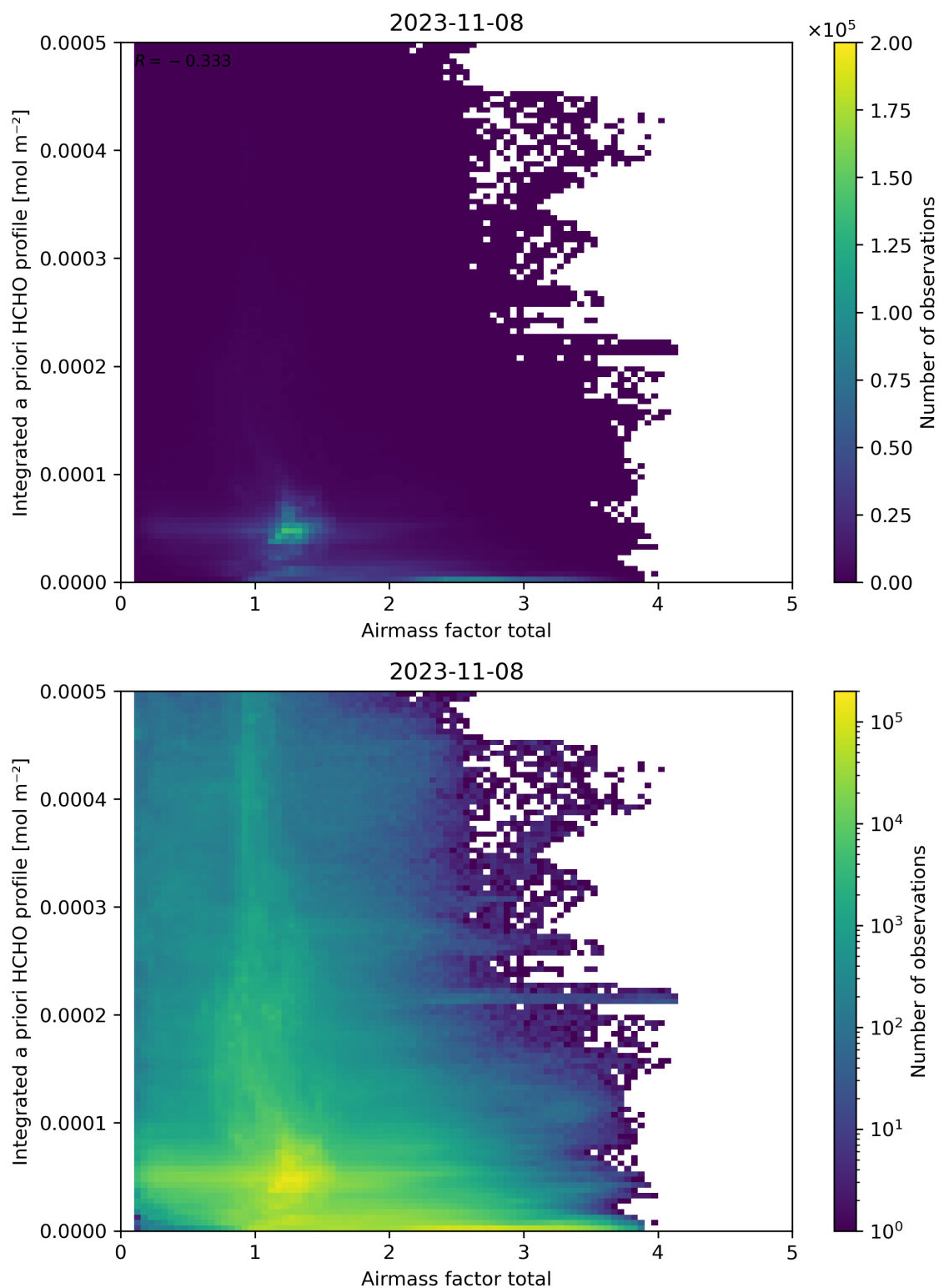
Figure 104: Scatter density plot of “Airmass factor total” against “Integrated a priori HCHO profile” for 2023-11-07 to 2023-11-09.
