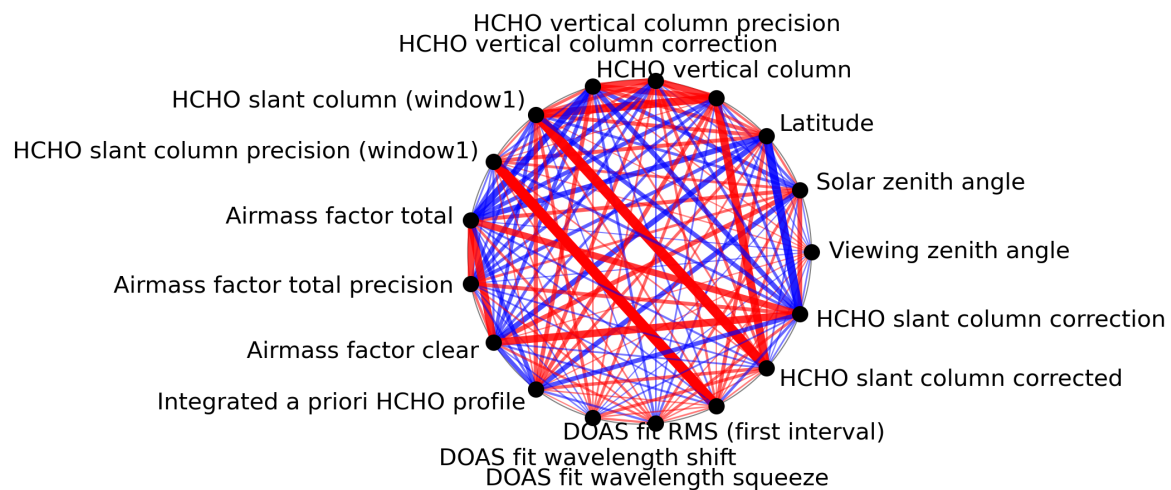
Figure 1: Map of correlation graph for 2023-11-07 to 2023-11-09.
