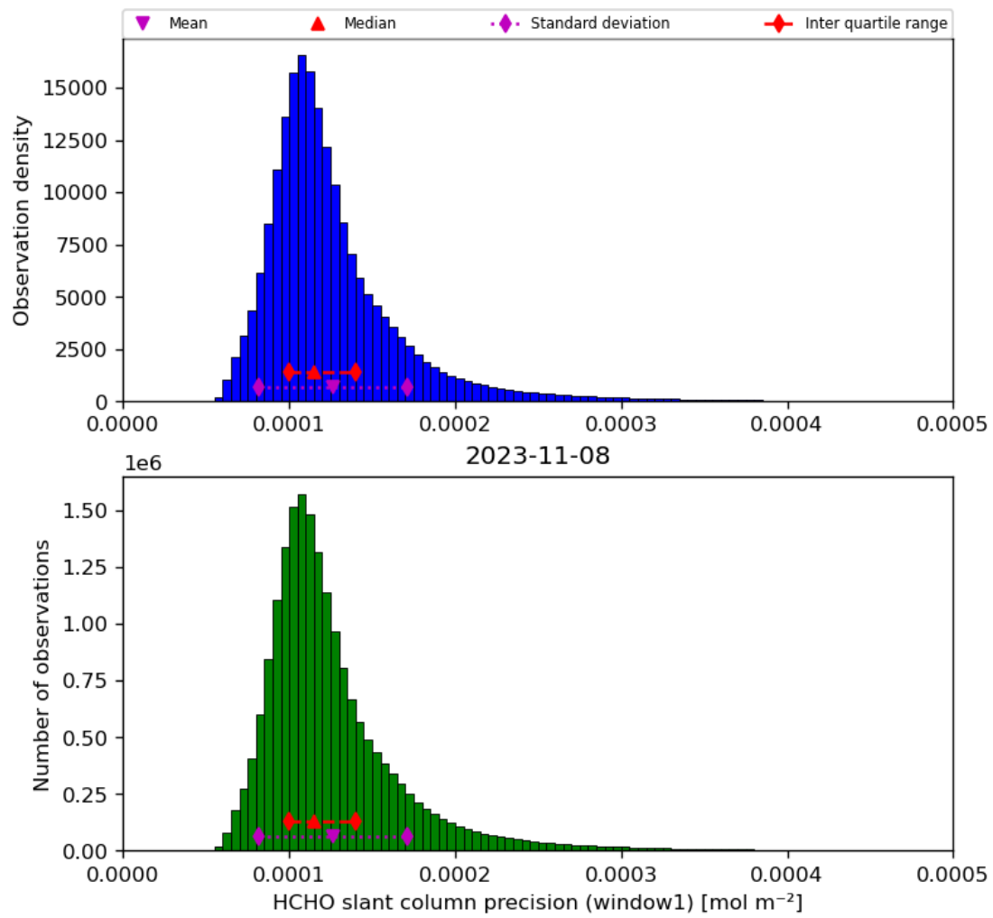
Figure 39: Histogram of “HCHO slant column precision (window1)” for 2023-11-07 to 2023-11-09
