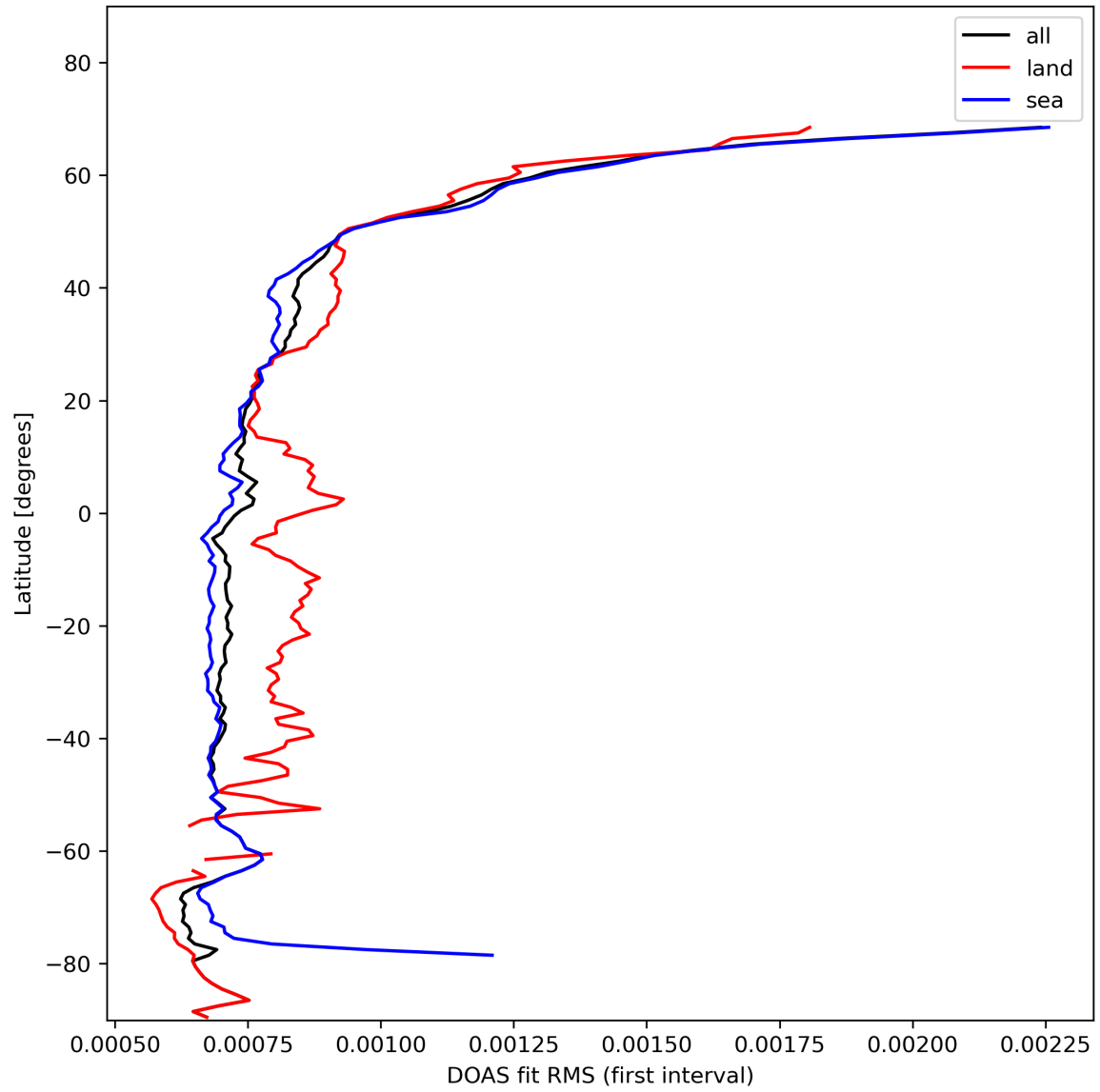
Figure 32: Zonal average of “DOAS fit RMS (first interval)” for 2023-11-07 to 2023-11-09.
