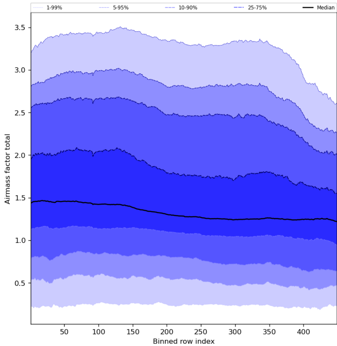
Figure 54: Along track statistics of “Airmass factor total” for 2023-11-07 to 2023-11-09
