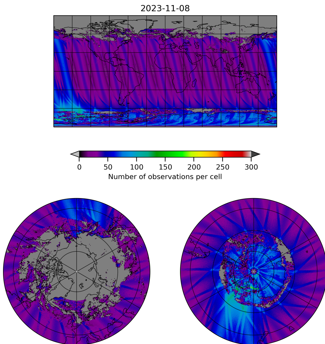
Figure 19: Map of the number of observations for 2023-11-07 to 2023-11-09
