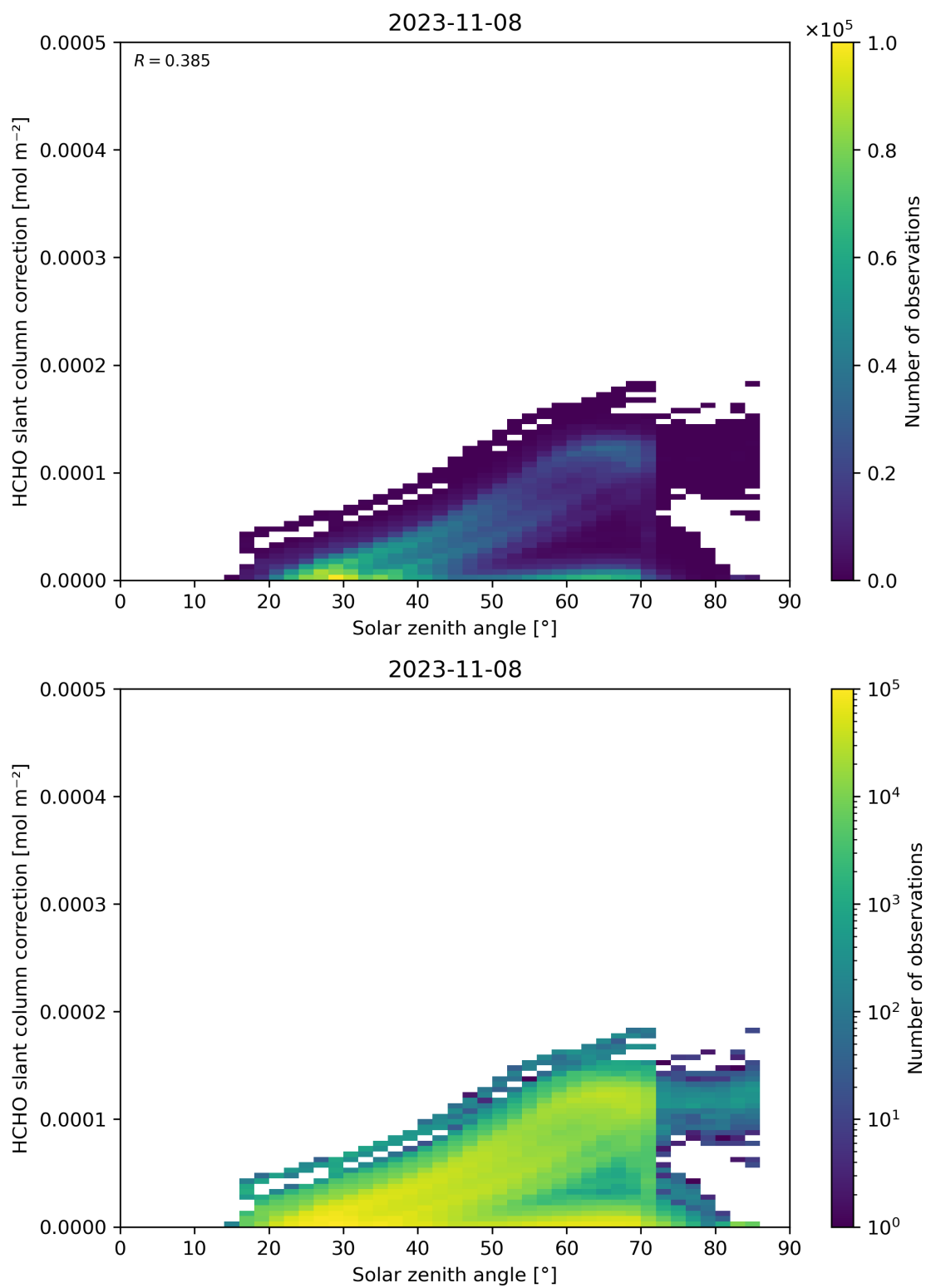
Figure 172: Scatter density plot of “Solar zenith angle” against “HCHO slant column correction” for 2023-11-07 to 2023-11-09.
