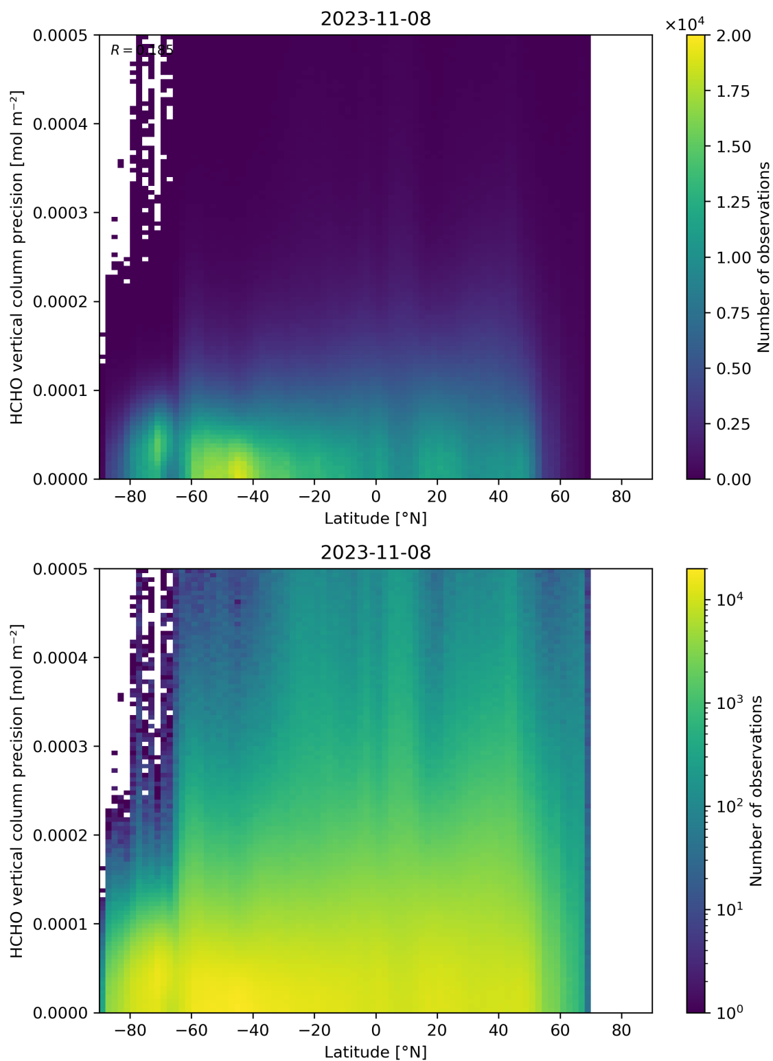
Figure 165: Scatter density plot of “Latitude” against “HCHO vertical column precision” for 2023-11-07 to 2023-11-09.
