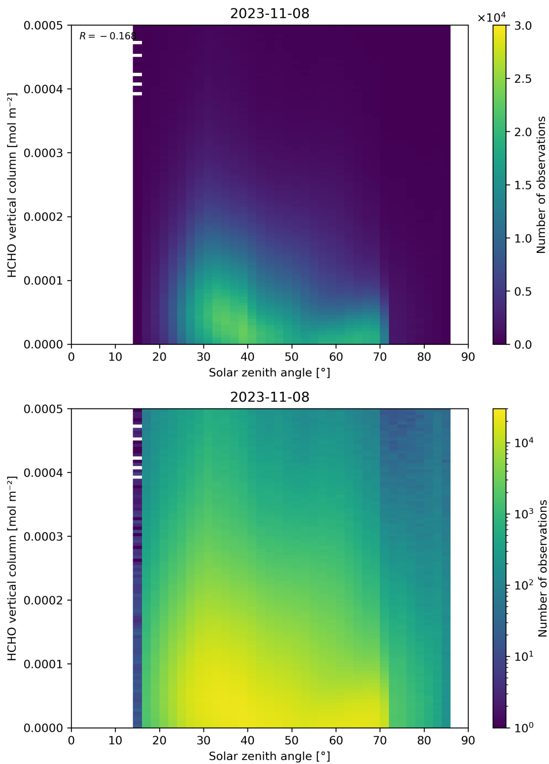
Figure 177: Scatter density plot of “Solar zenith angle” against “HCHO vertical column” for 2023-11-07 to 2023-11-09.
