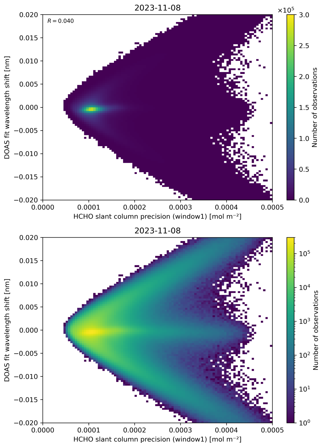
Figure 89: Scatter density plot of “HCHO slant column precision (window1)” against “DOAS fit wavelength shift” for 2023-11-07 to 2023-11-09.
