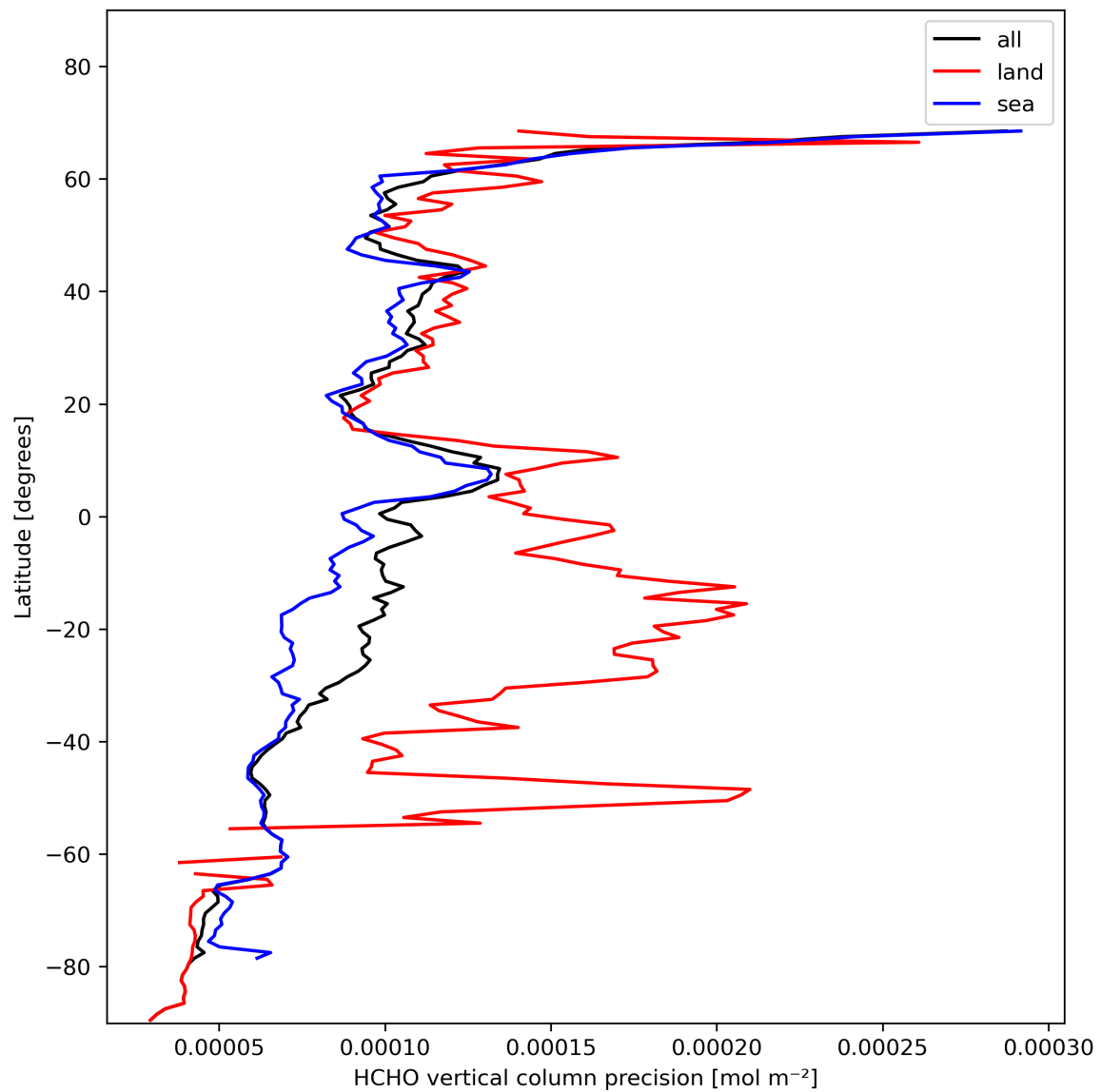
Figure 22: Zonal average of “HCHO vertical column precision” for 2023-11-07 to 2023-11-09.
