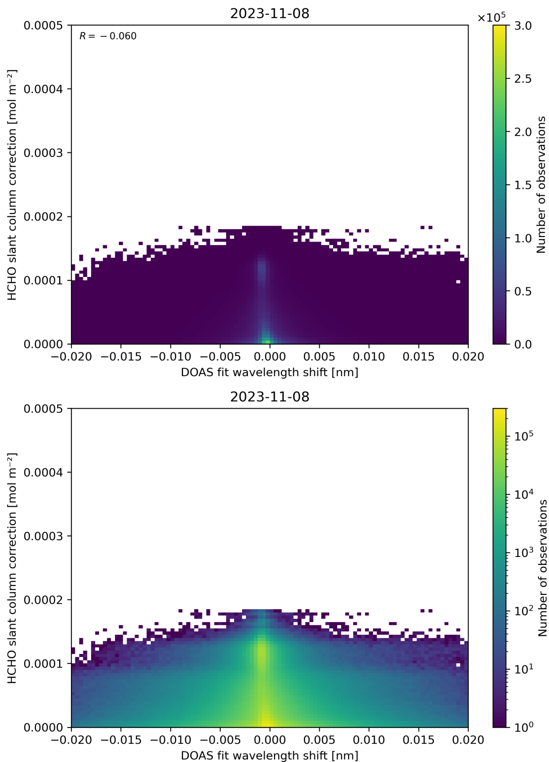
Figure 67: Scatter density plot of “DOAS fit wavelength shift” against “HCHO slant column correction” for 2023-11-07 to 2023-11-09.
