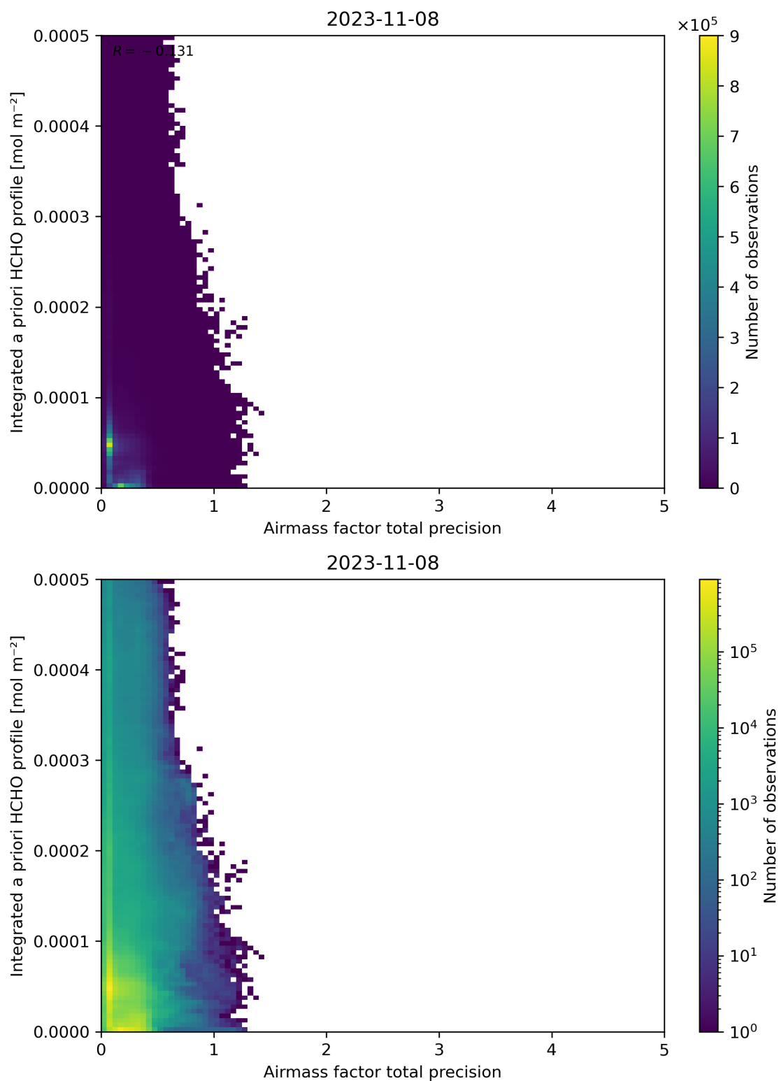
Figure 111: Scatter density plot of “Airmass factor total precision” against “Integrated a priori HCHO profile” for 2023-11-07 to 2023-11-09.
