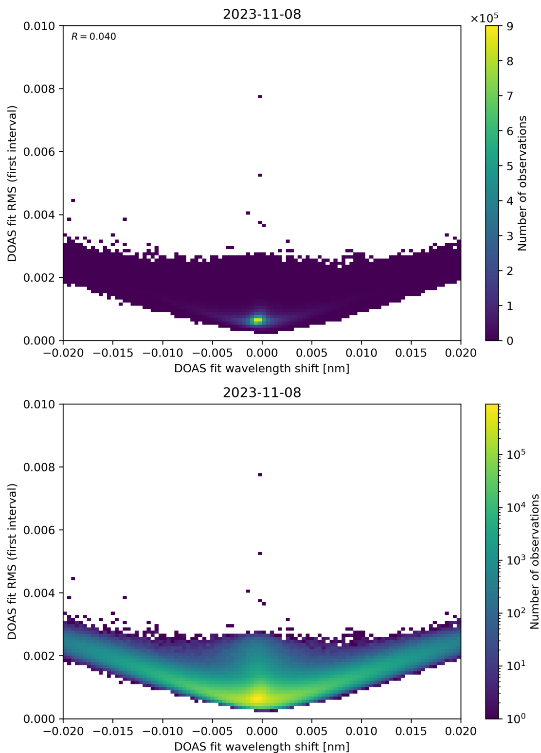
Figure 64: Scatter density plot of “DOAS fit wavelength shift” against “DOAS fit RMS (first interval)” for 2023-11-07 to 2023-11-09.
