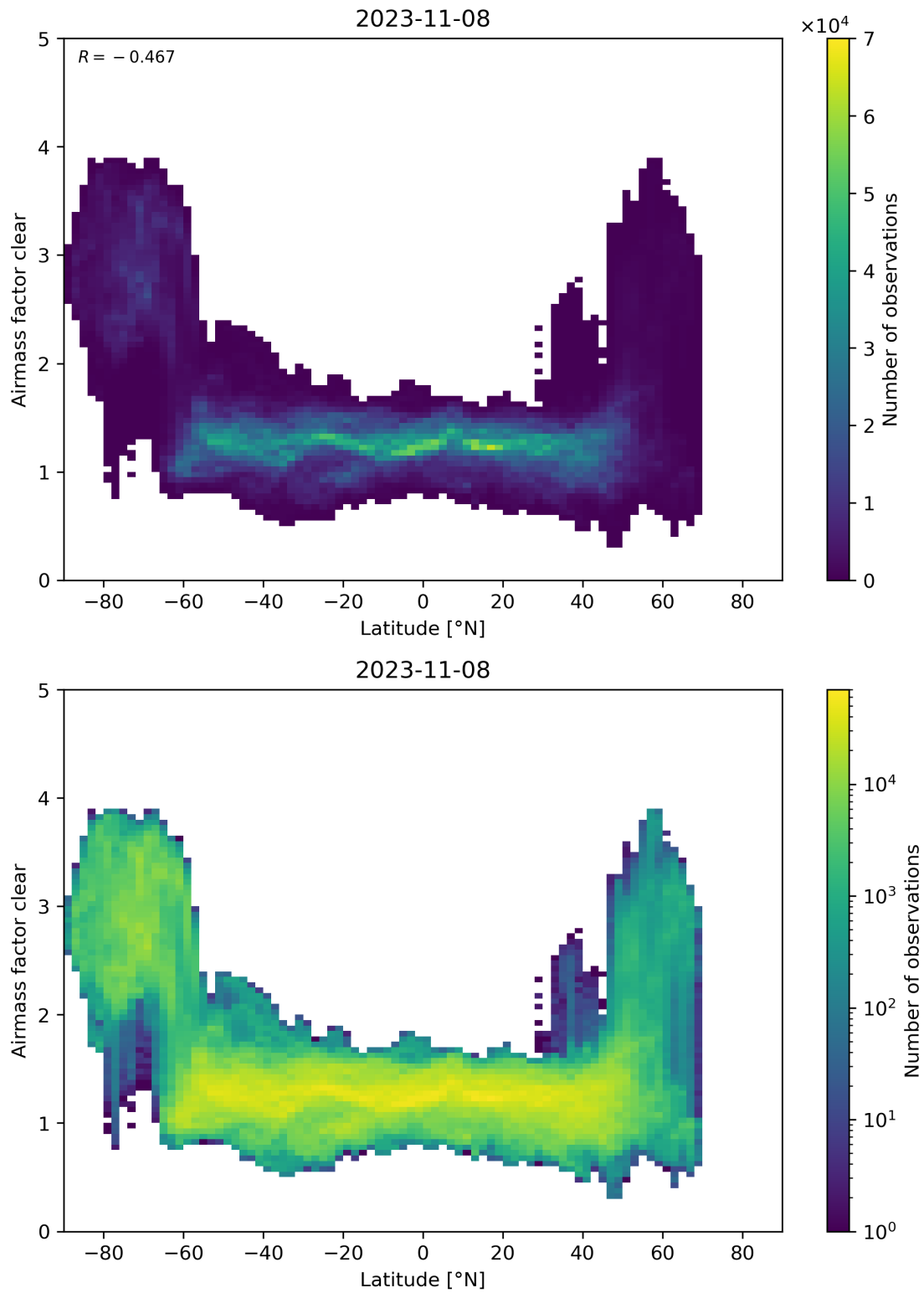
Figure 156: Scatter density plot of “Latitude” against “Airmass factor clear” for 2023-11-07 to 2023-11-09.
