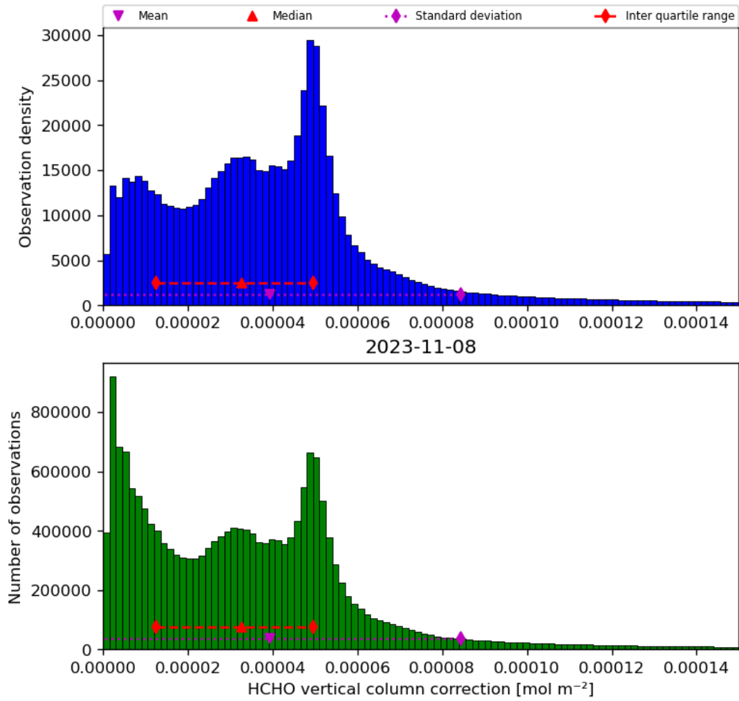
Figure 37: Histogram of “HCHO vertical column correction” for 2023-11-07 to 2023-11-09
