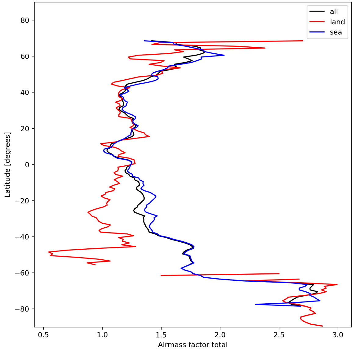
Figure 26: Zonal average of “Airmass factor total” for 2023-11-07 to 2023-11-09.
