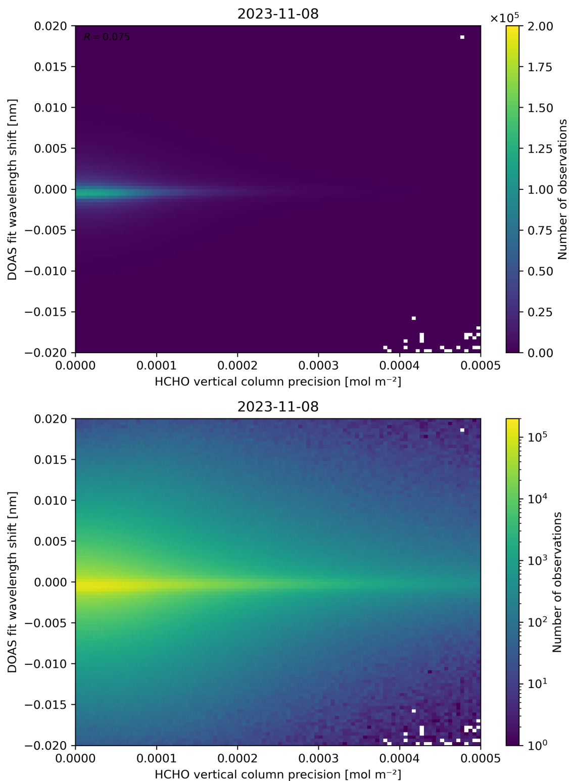
Figure 137: Scatter density plot of “HCHO vertical column precision” against “DOAS fit wavelength shift” for 2023-11-07 to 2023-11-09.
