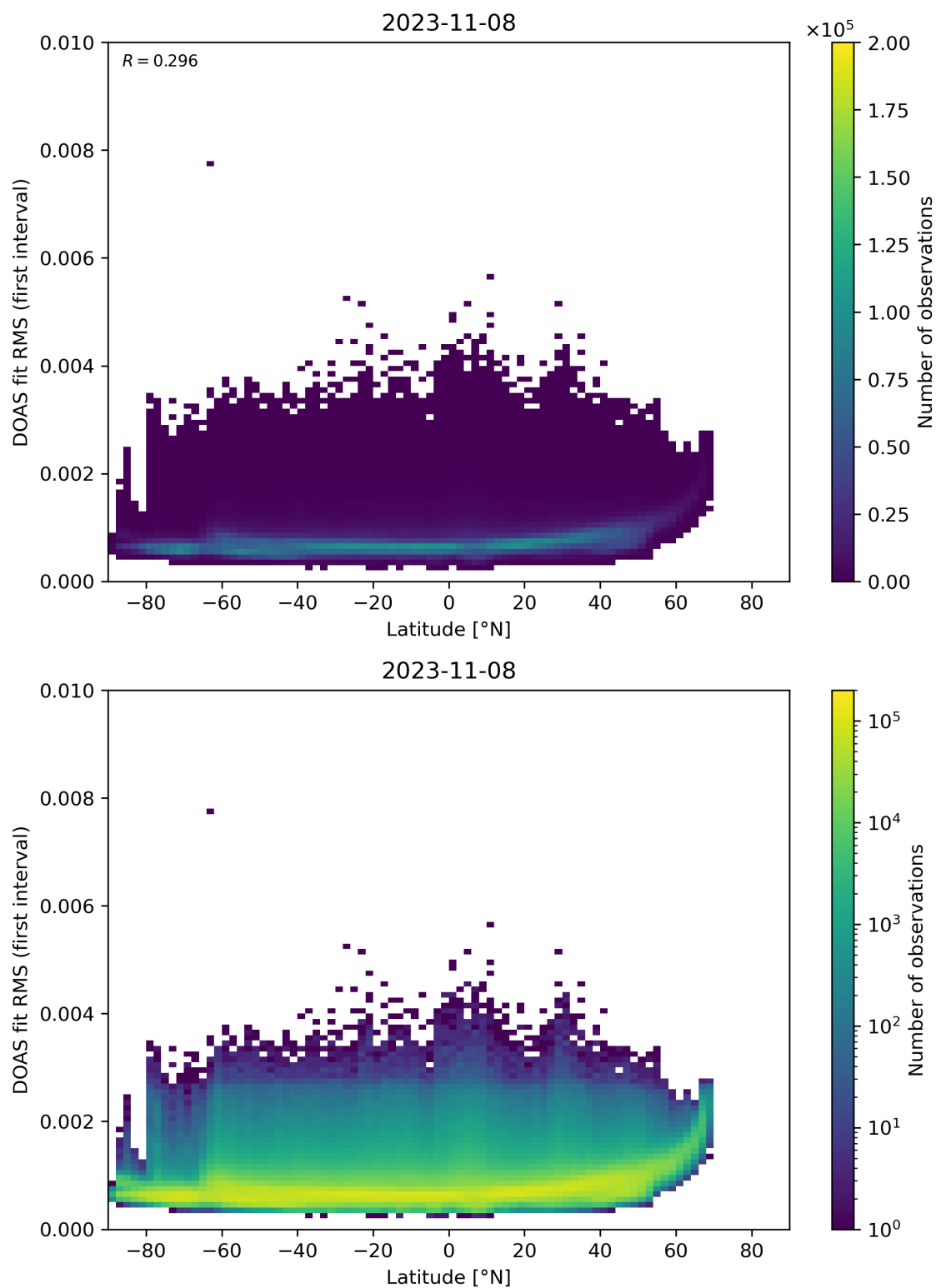
Figure 153: Scatter density plot of “Latitude” against “DOAS fit RMS (first interval)” for 2023-11-07 to 2023-11-09.
