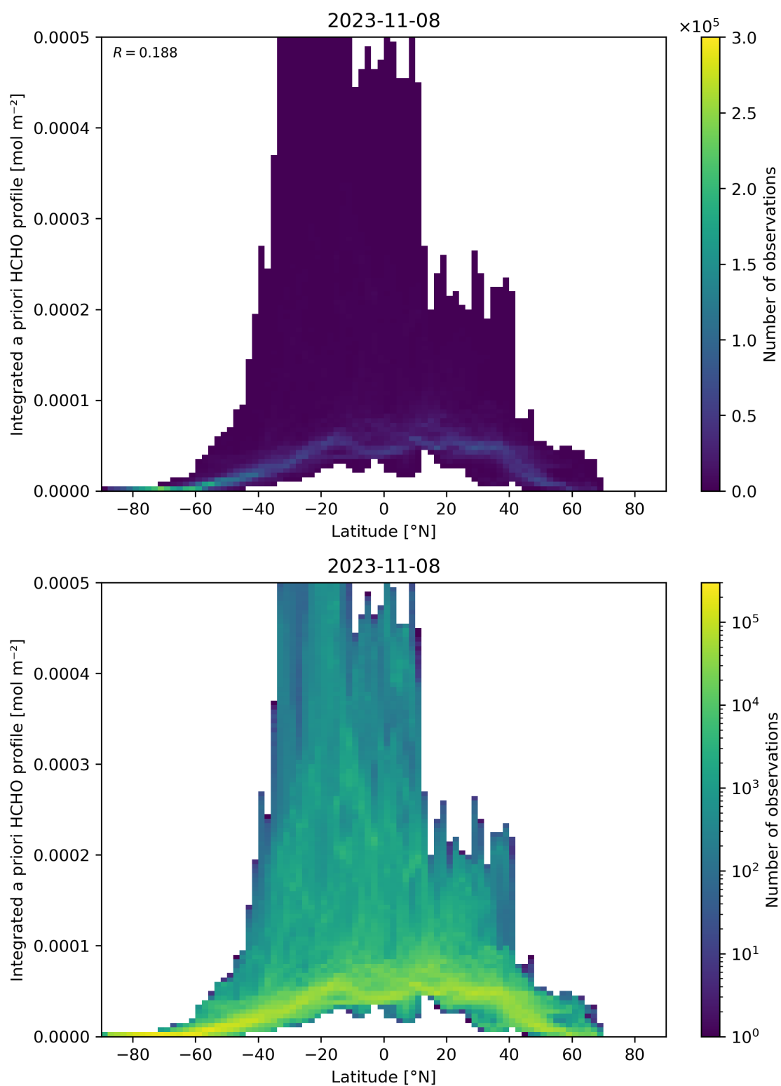
Figure 166: Scatter density plot of “Latitude” against “Integrated a priori HCHO profile” for 2023-11-07 to 2023-11-09.
