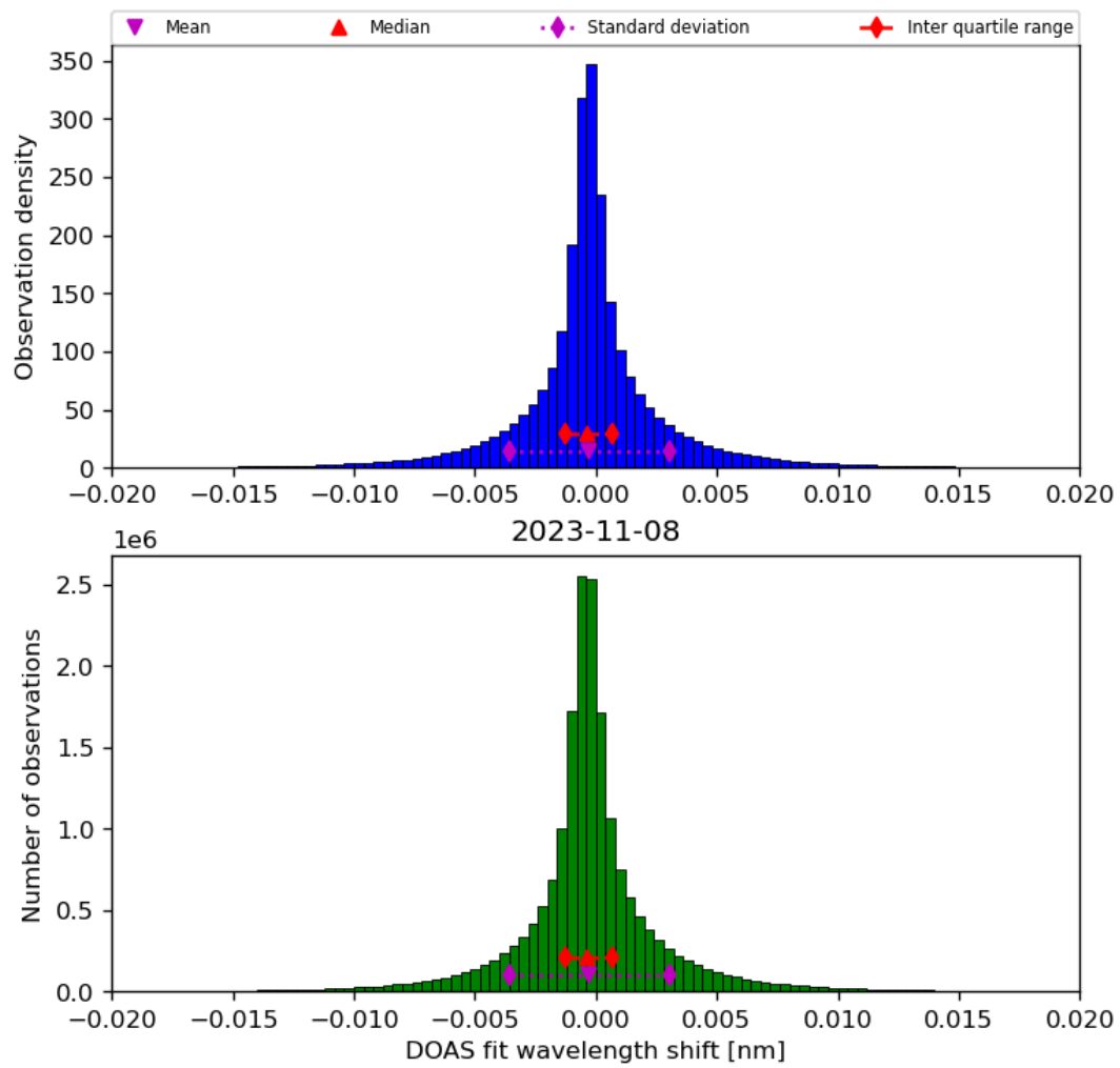
Figure 44: Histogram of “DOAS fit wavelength shift” for 2023-11-07 to 2023-11-09
