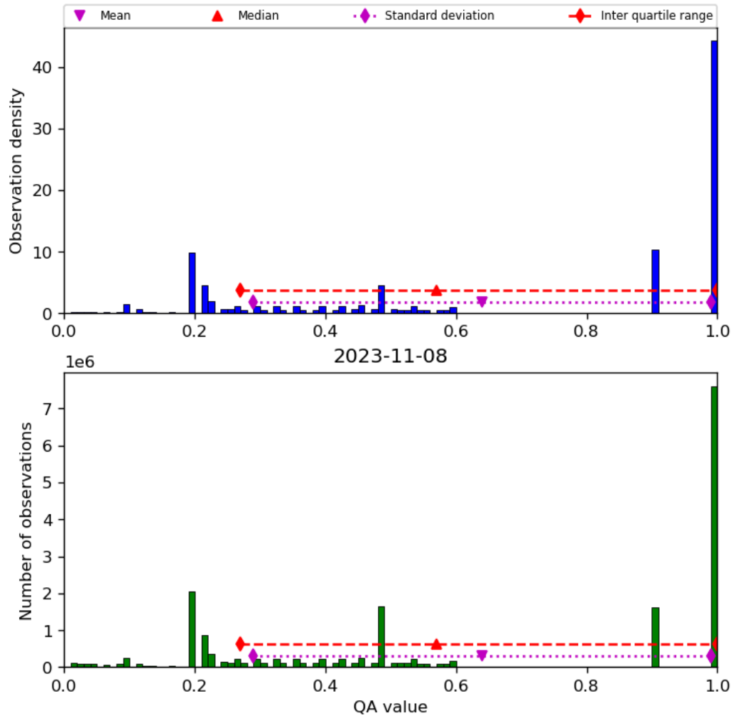
Figure 34: Histogram of “QA value” for 2023-11-07 to 2023-11-09
