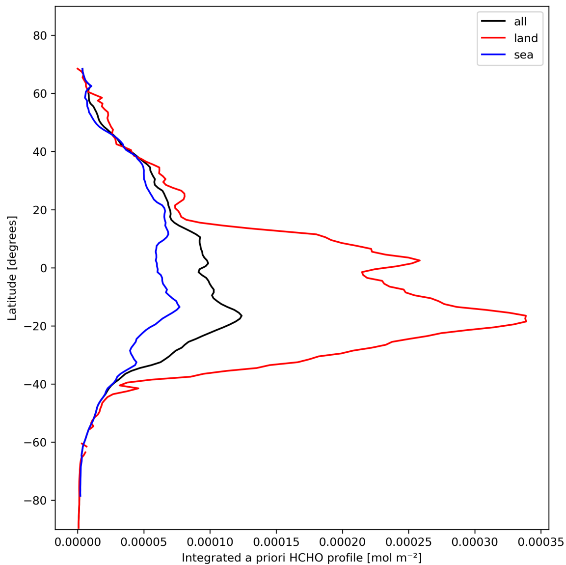
Figure 29: Zonal average of “Integrated a priori HCHO profile” for 2023-11-07 to 2023-11-09.
