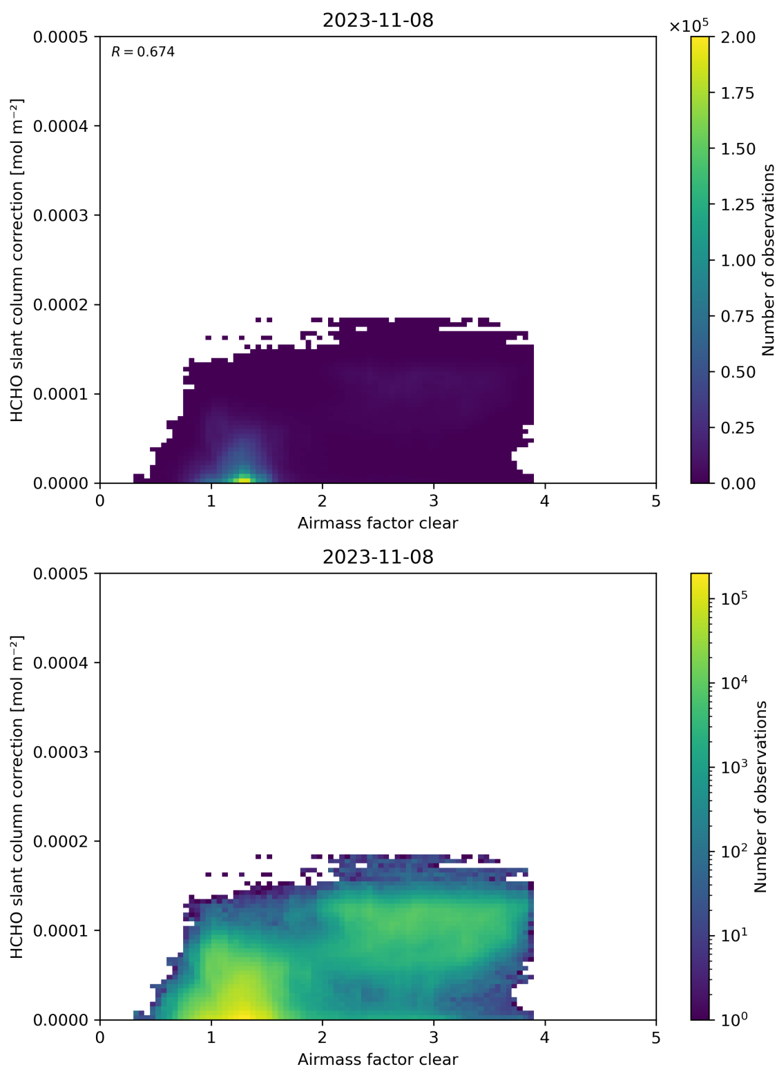
Figure 75: Scatter density plot of “Airmass factor clear” against “HCHO slant column correction” for 2023-11-07 to 2023-11-09.
