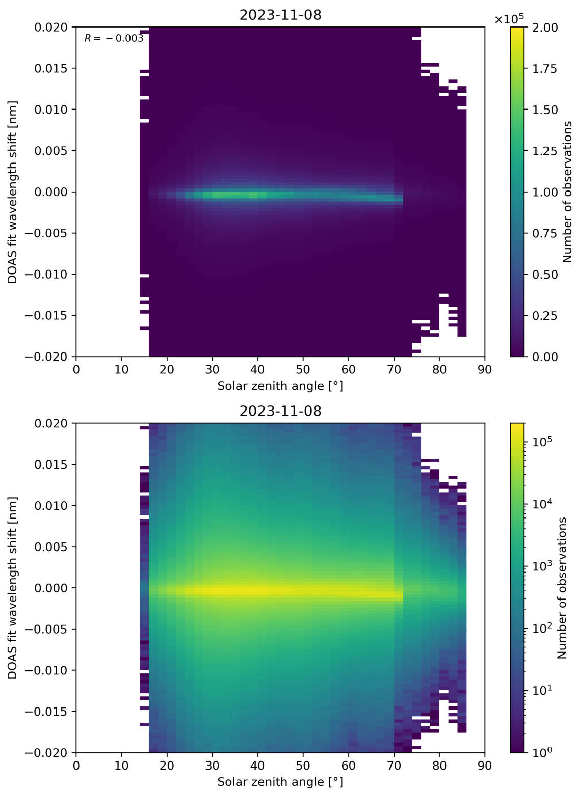
Figure 168: Scatter density plot of “Solar zenith angle” against “DOAS fit wavelength shift” for 2023-11-07 to 2023-11-09.
