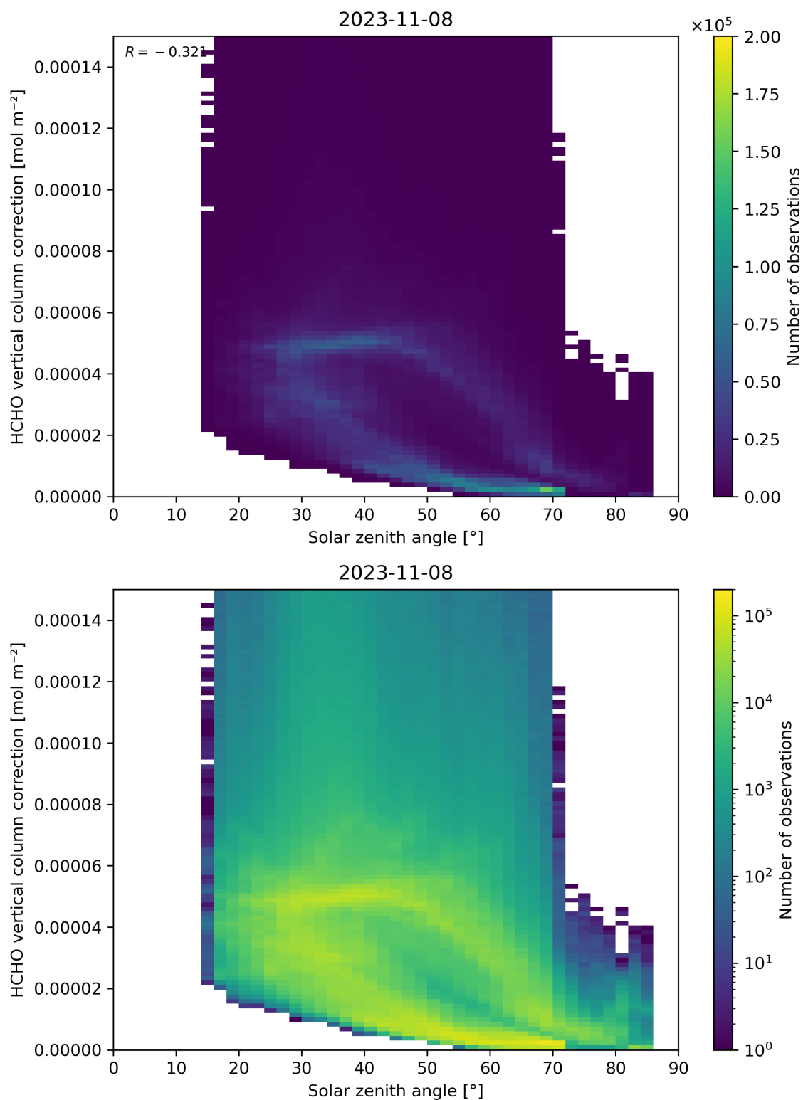
Figure 178: Scatter density plot of “Solar zenith angle” against “HCHO vertical column correction” for 2023-11-07 to 2023-11-09.
