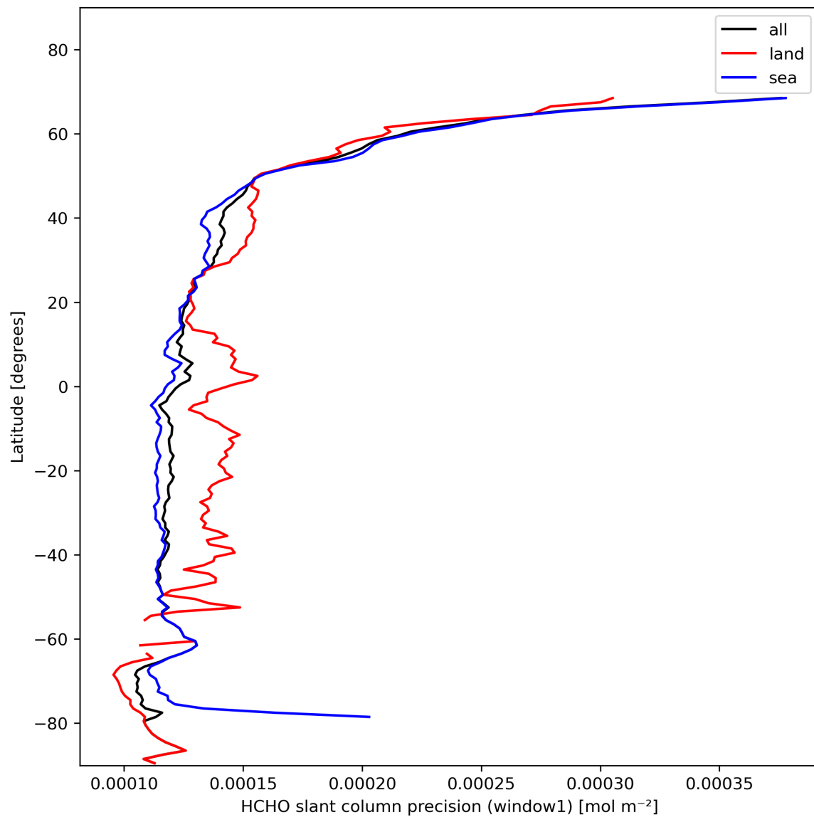
Figure 25: Zonal average of “HCHO slant column precision (window1)” for 2023-11-07 to 2023-11-09.
