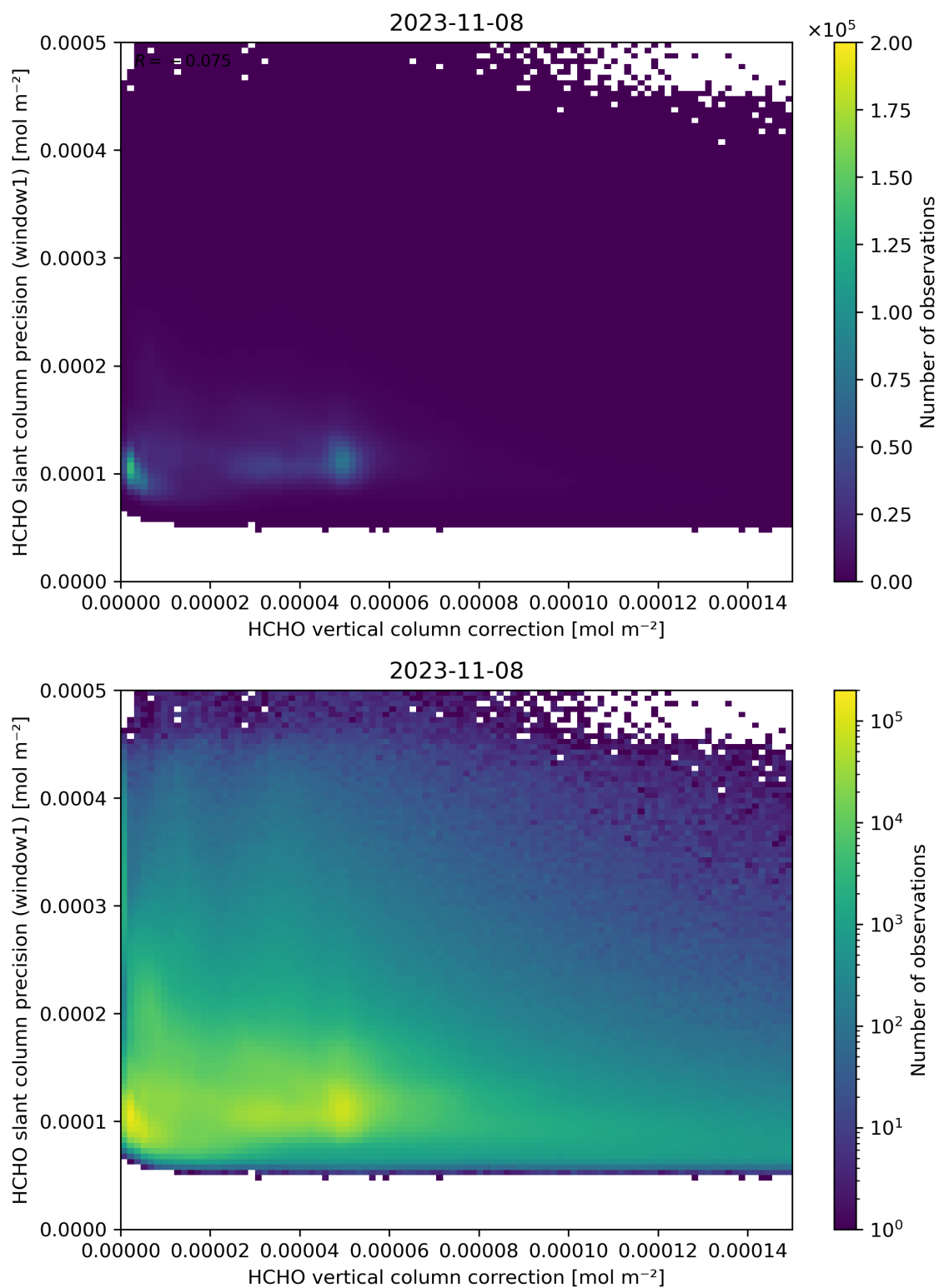
Figure 119: Scatter density plot of “HCHO vertical column correction” against “HCHO slant column precision (window1)” for 2023-11-07 to 2023-11-09.
