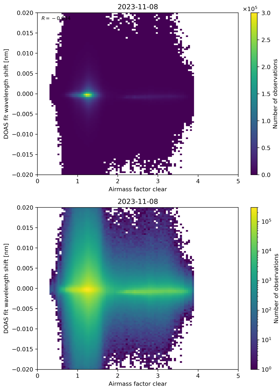
Figure 72: Scatter density plot of “Airmass factor clear” against “DOAS fit wavelength shift” for 2023-11-07 to 2023-11-09.
