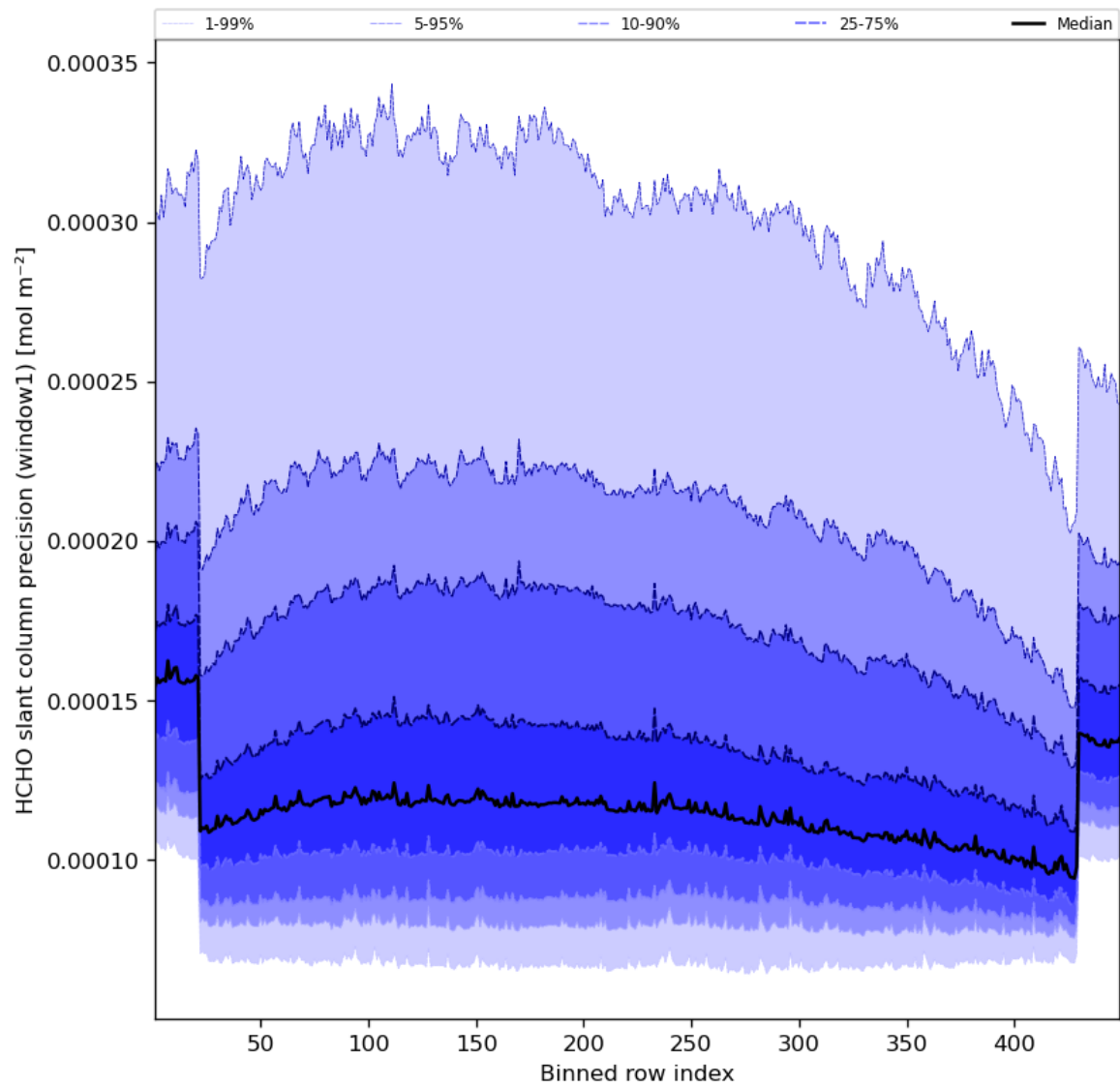
Figure 53: Along track statistics of “HCHO slant column precision (window1)” for 2023-11-07 to 2023-11-09
