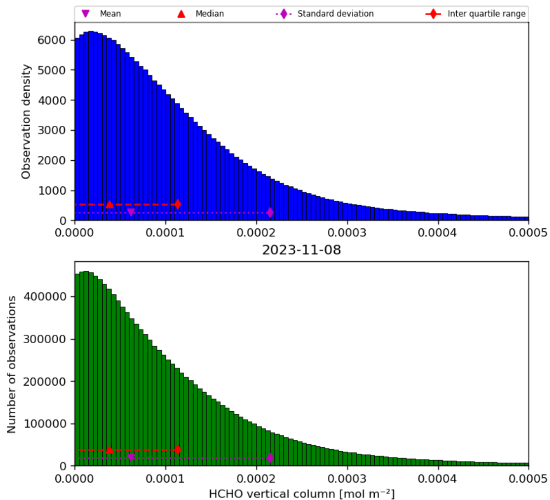
Figure 35: Histogram of “HCHO vertical column” for 2023-11-07 to 2023-11-09
