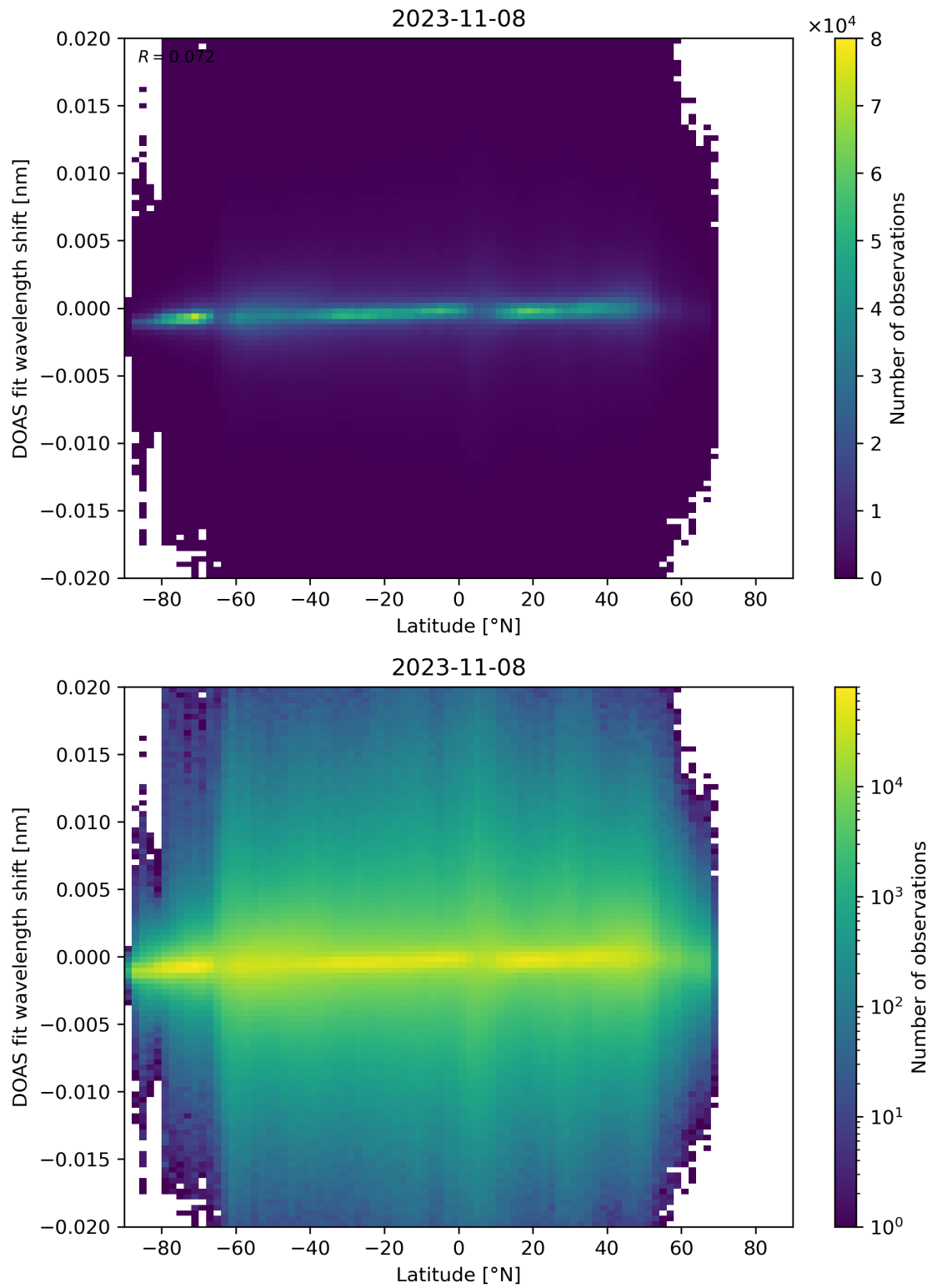
Figure 154: Scatter density plot of “Latitude” against “DOAS fit wavelength shift” for 2023-11-07 to 2023-11-09.
