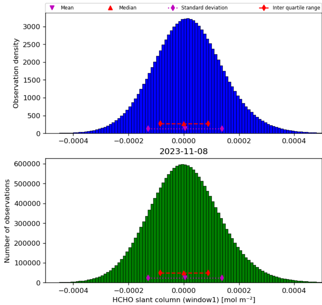
Figure 38: Histogram of “HCHO slant column (window1)” for 2023-11-07 to 2023-11-09
