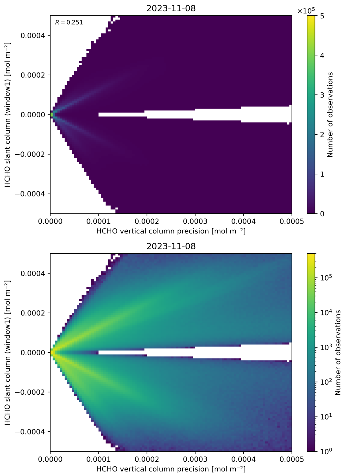
Figure 142: Scatter density plot of “HCHO vertical column precision” against “HCHO slant column (window1)” for 2023-11-07 to 2023-11-09.
