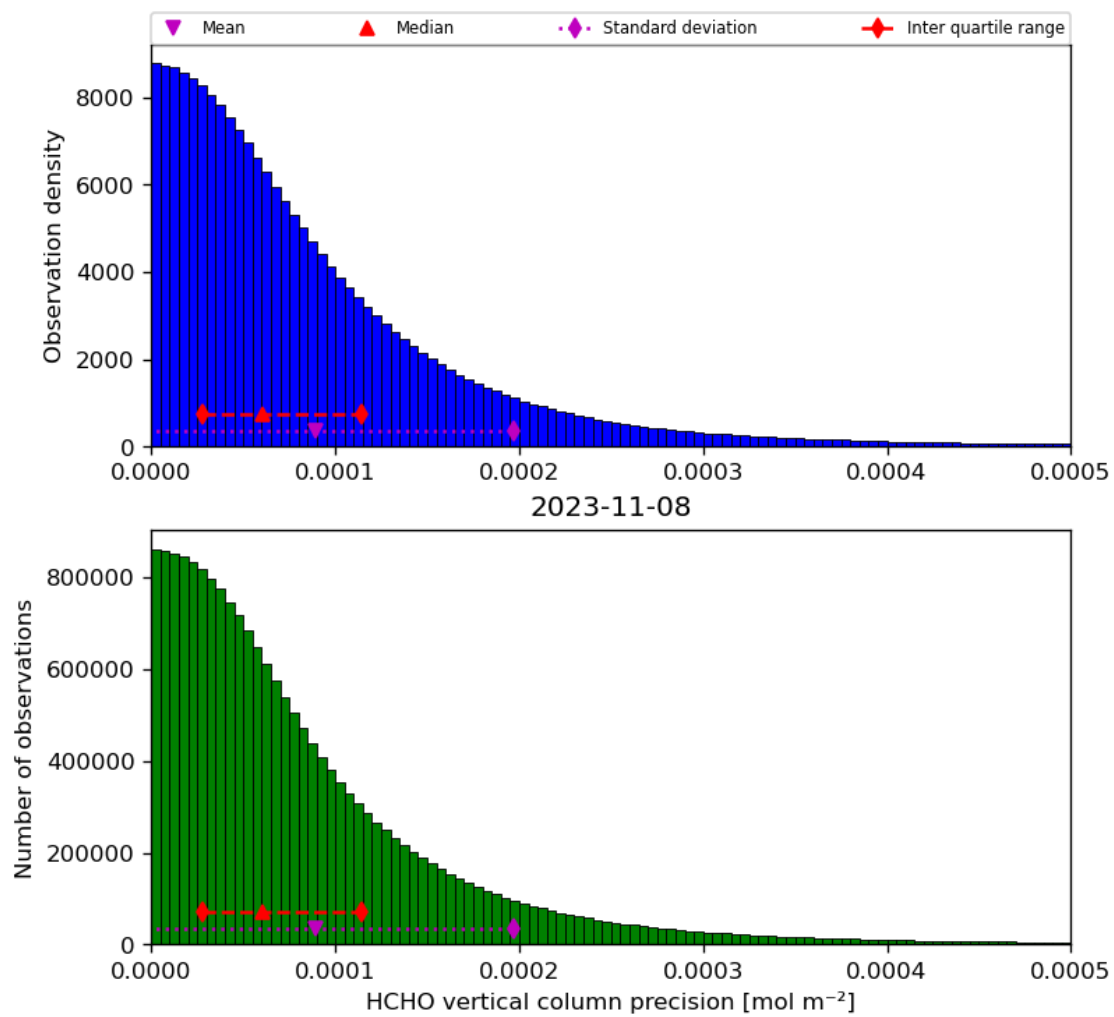
Figure 36: Histogram of “HCHO vertical column precision” for 2023-11-07 to 2023-11-09
