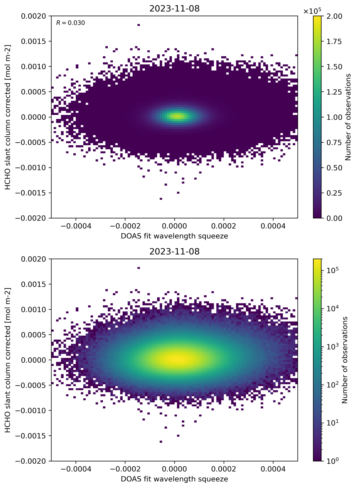
Figure 69: Scatter density plot of “DOAS fit wavelength squeeze” against “HCHO slant column corrected” for 2023-11-07 to 2023-11-09.
