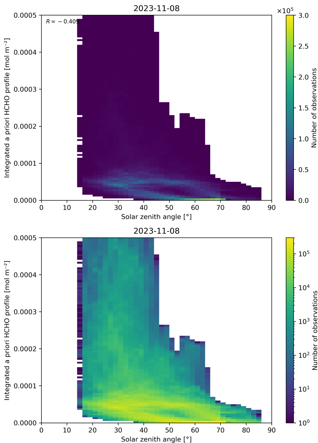
Figure 180: Scatter density plot of “Solar zenith angle” against “Integrated a priori HCHO profile” for 2023-11-07 to 2023-11-09.
