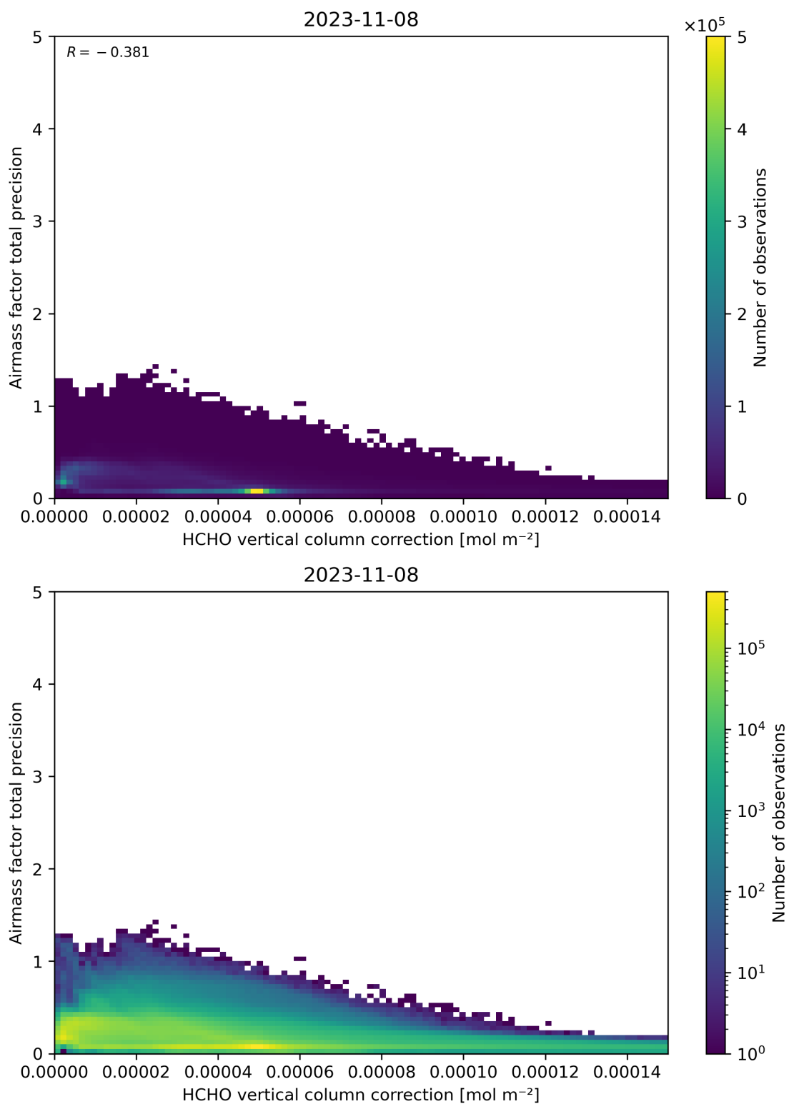
Figure 121: Scatter density plot of “HCHO vertical column correction” against “Airmass factor total precision” for 2023-11-07 to 2023-11-09.
