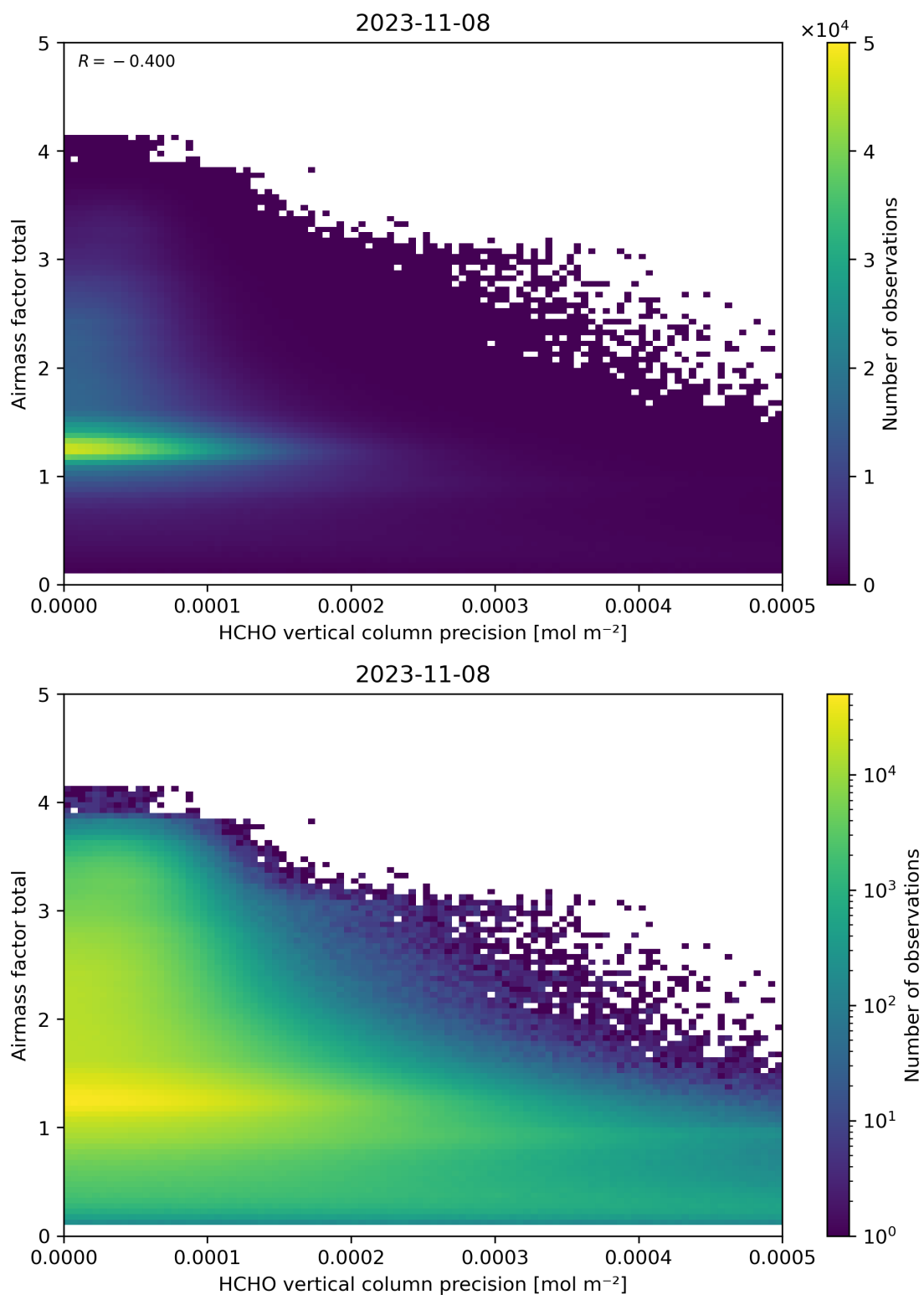
Figure 144: Scatter density plot of “HCHO vertical column precision” against “Airmass factor total” for 2023-11-07 to 2023-11-09.
