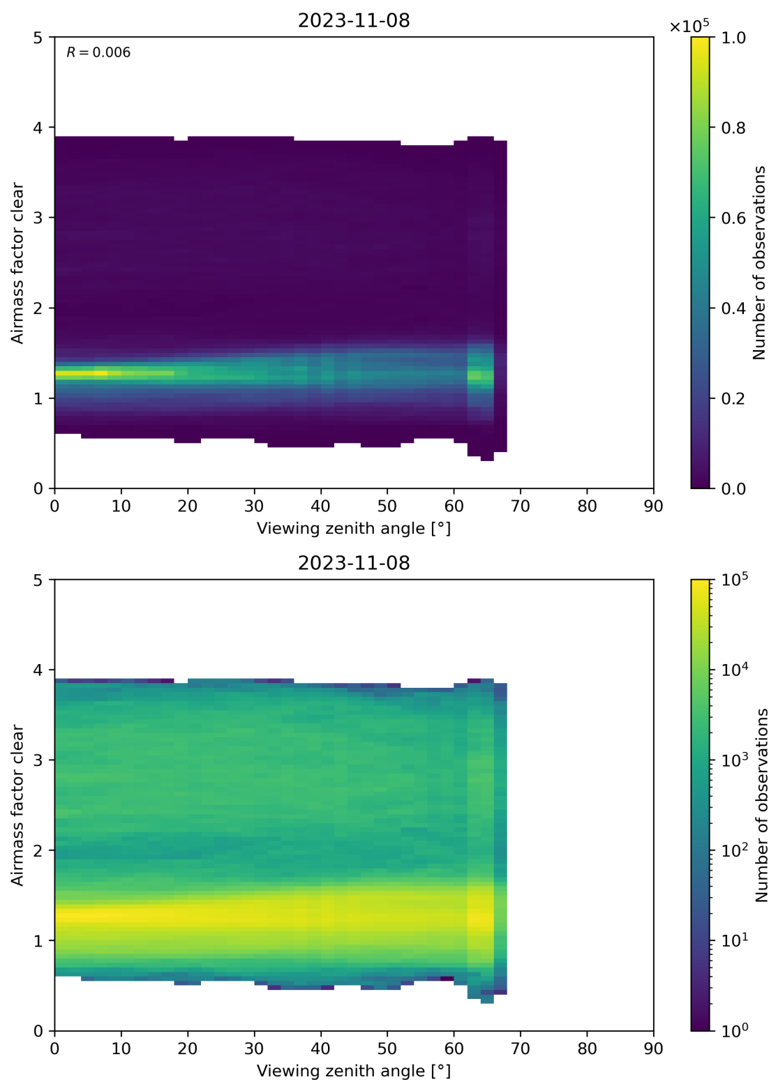
Figure 185: Scatter density plot of “Viewing zenith angle” against “Airmass factor clear” for 2023-11-07 to 2023-11-09.
