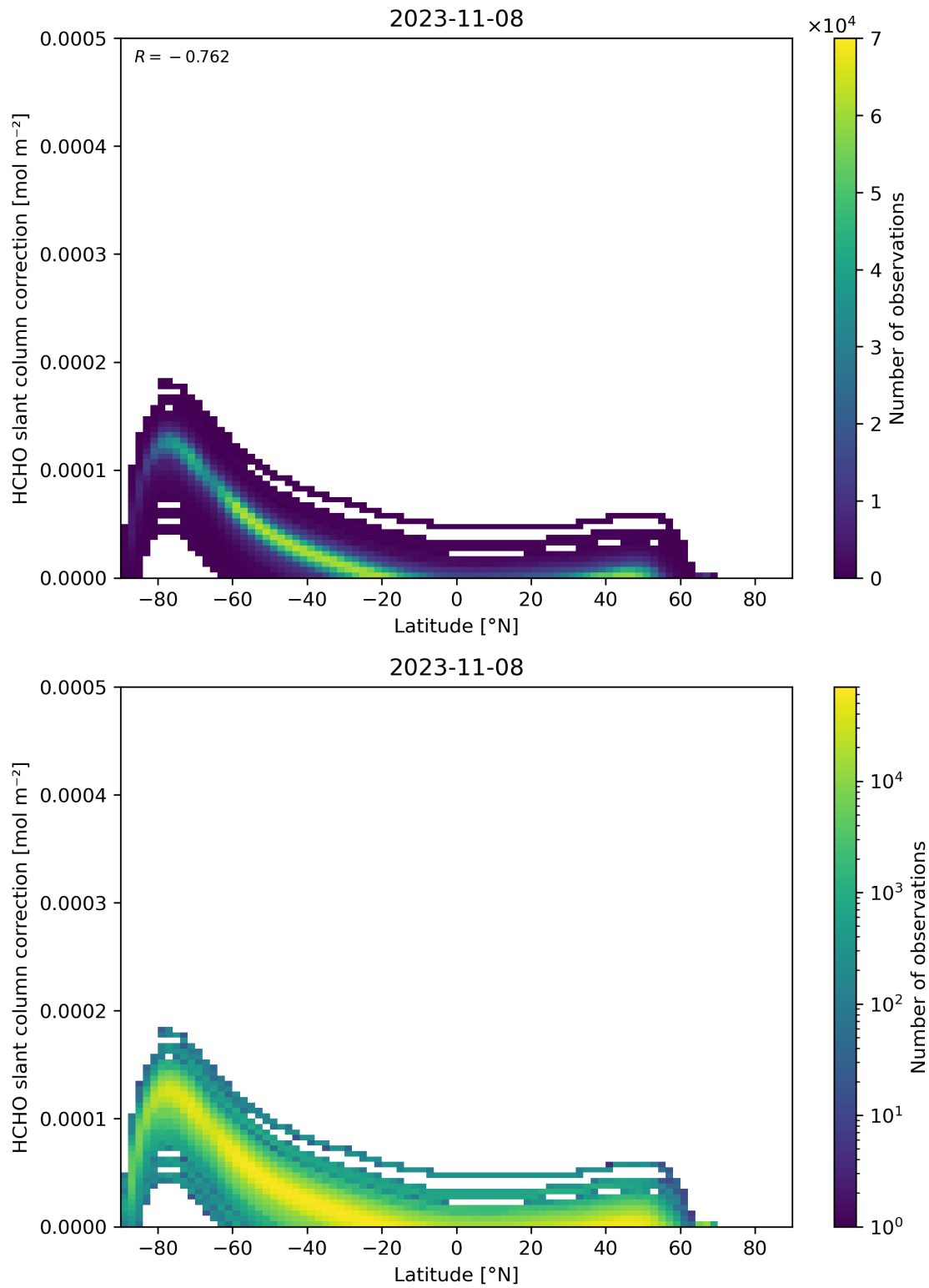
Figure 158: Scatter density plot of “Latitude” against “HCHO slant column correction” for 2023-11-07 to 2023-11-09.
