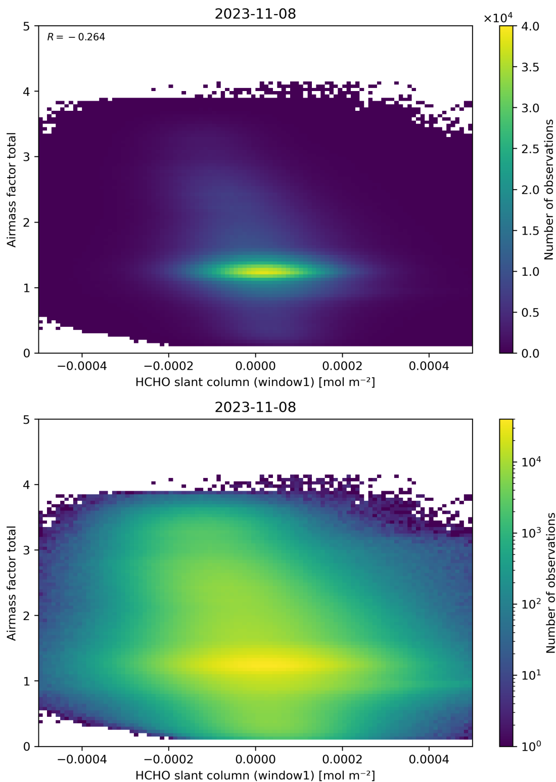
Figure 85: Scatter density plot of “HCHO slant column (window1)” against “Airmass factor total” for 2023-11-07 to 2023-11-09.
