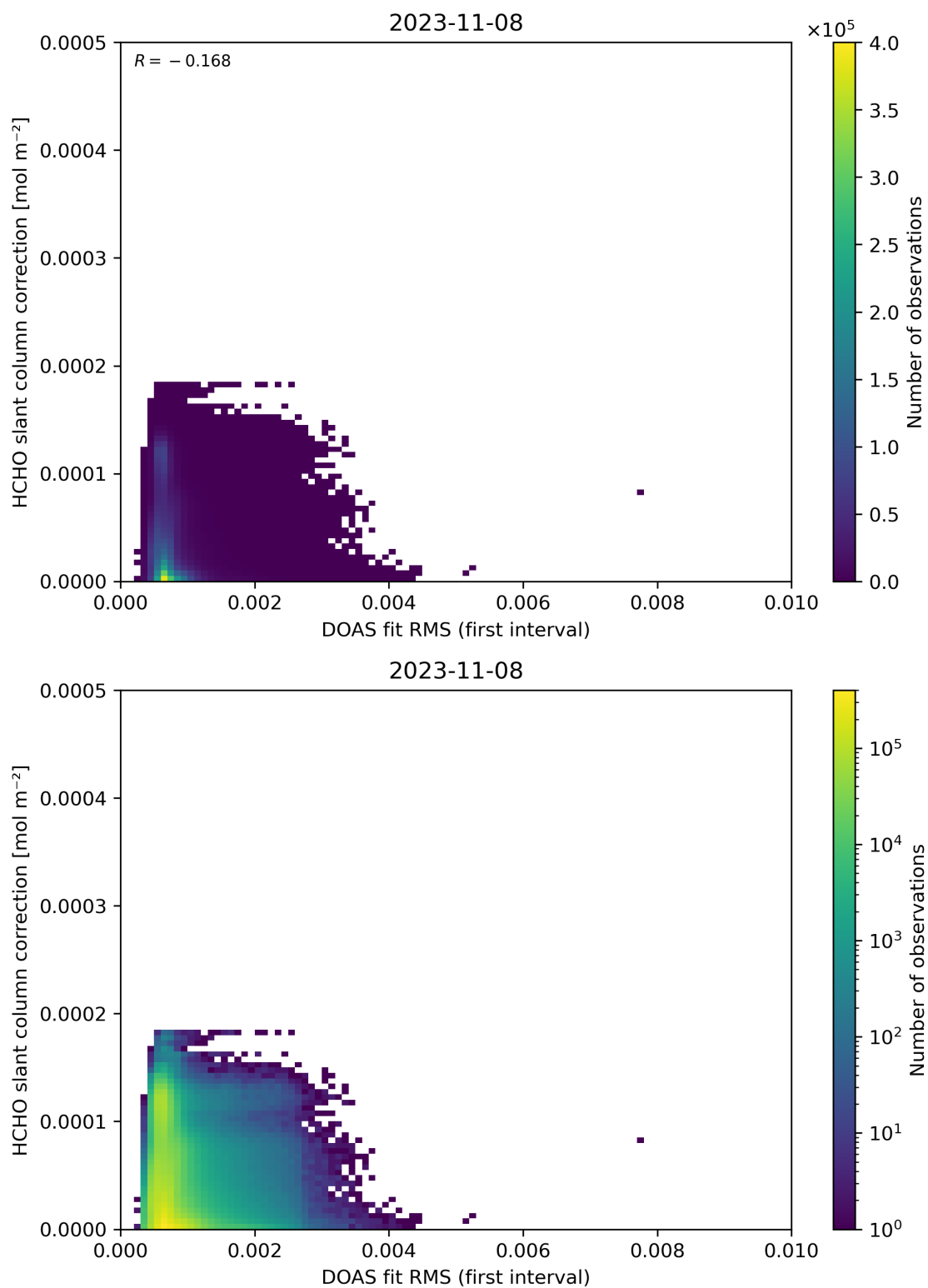
Figure 63: Scatter density plot of “DOAS fit RMS (first interval)” against “HCHO slant column correction” for 2023-11-07 to 2023-11-09.
