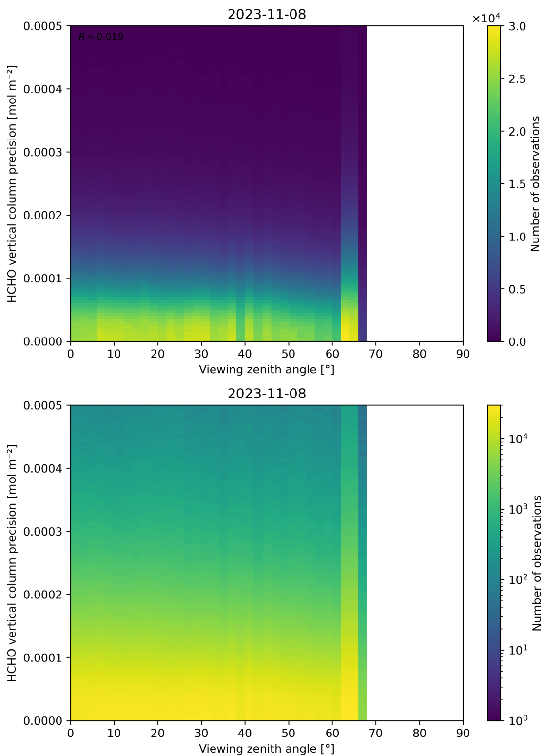
Figure 194: Scatter density plot of “Viewing zenith angle” against “HCHO vertical column precision” for 2023-11-07 to 2023-11-09.
