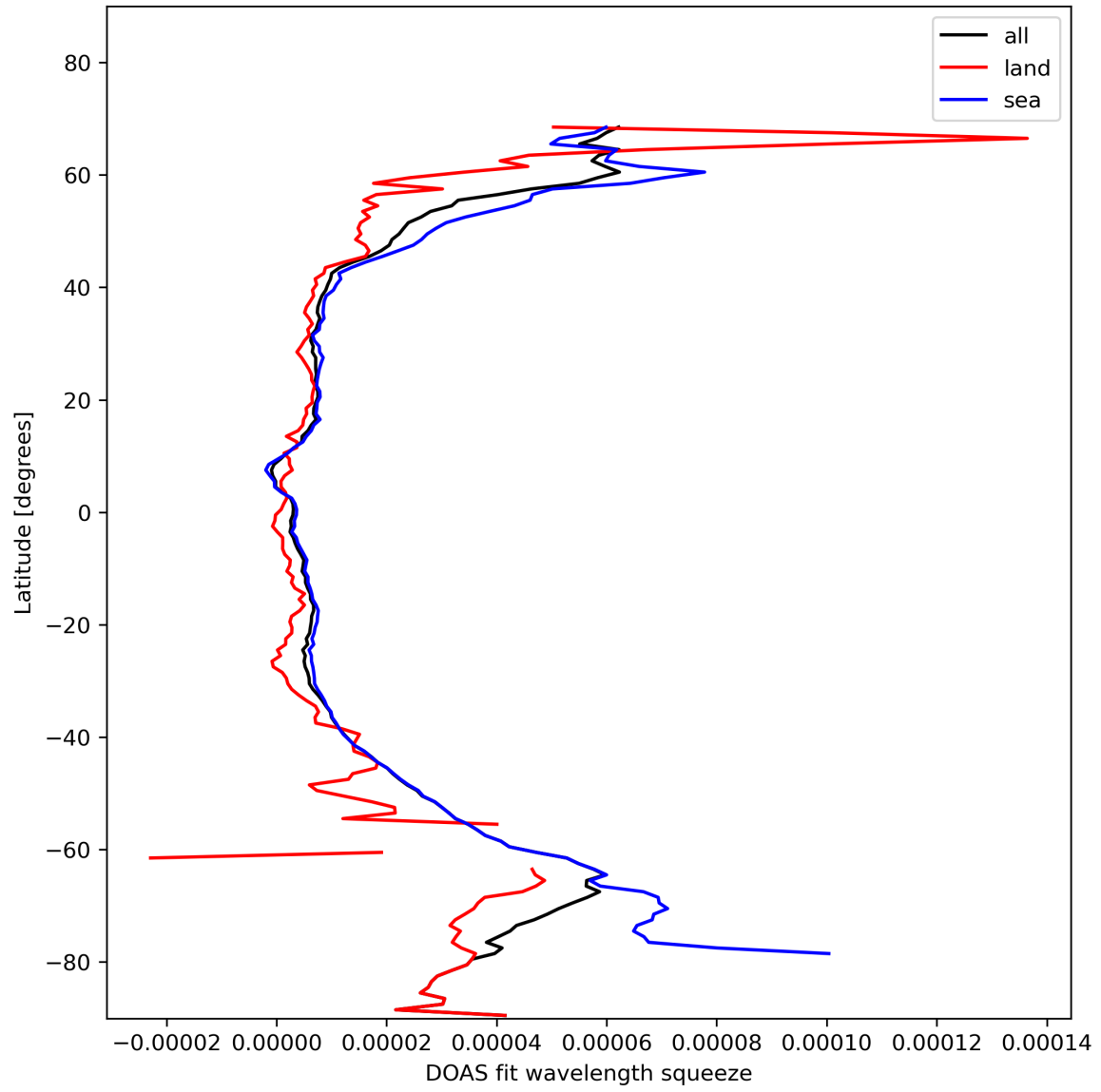
Figure 31: Zonal average of “DOAS fit wavelength squeeze” for 2023-11-07 to 2023-11-09.
