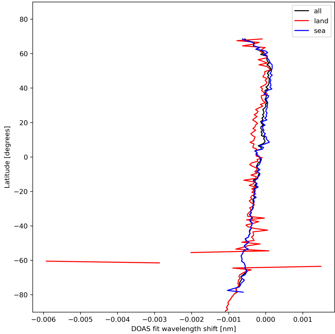
Figure 30: Zonal average of "DOAS fit wavelength shift" for 2023-11-07 to 2023-11-09.
