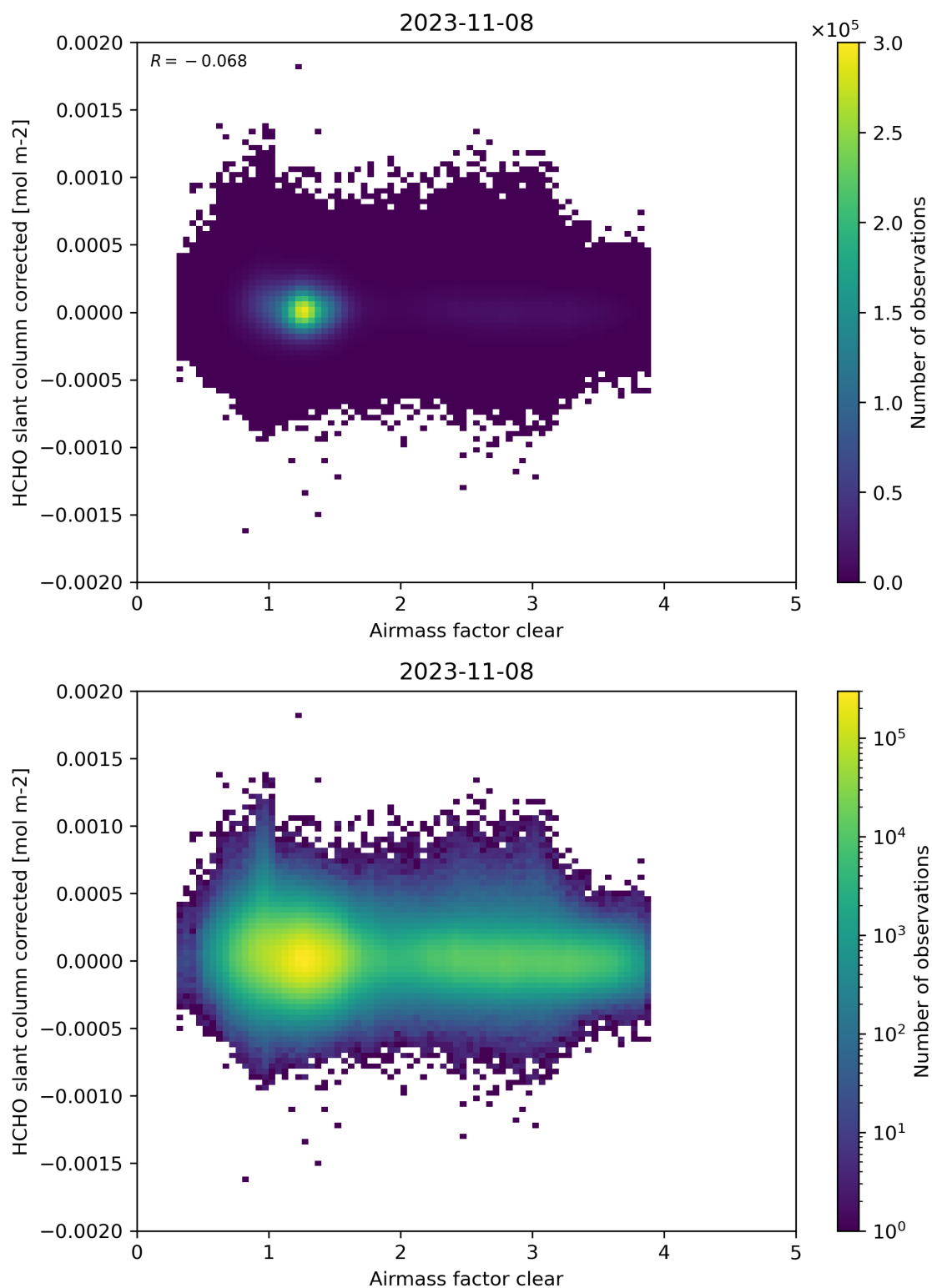
Figure 74: Scatter density plot of “Airmass factor clear” against “HCHO slant column corrected” for 2023-11-07 to 2023-11-09.
