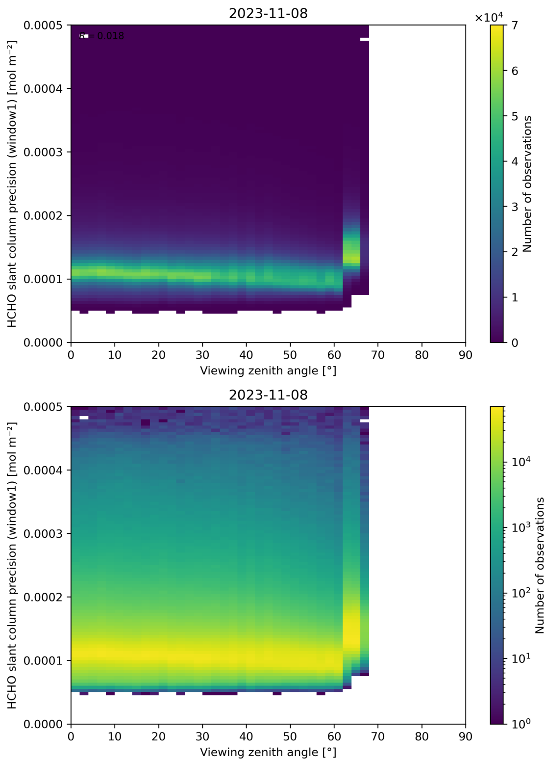
Figure 189: Scatter density plot of “Viewing zenith angle” against “HCHO slant column precision (window1)” for 2023-11-07 to 2023-11-09.
