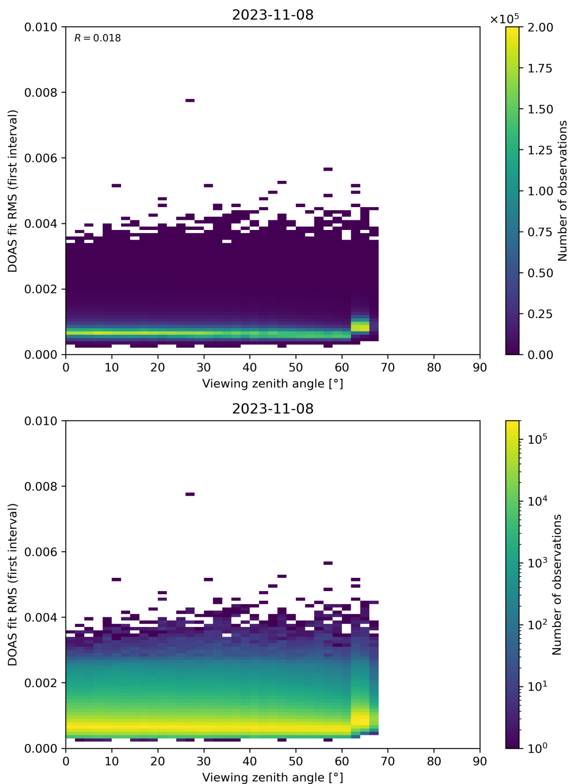
Figure 182: Scatter density plot of “Viewing zenith angle” against “DOAS fit RMS (first interval)” for 2023-11-07 to 2023-11-09.
