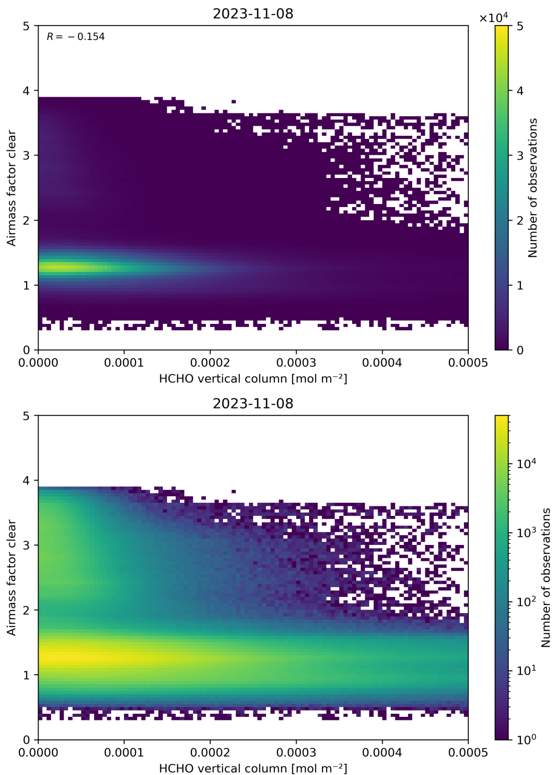
Figure 126: Scatter density plot of “HCHO vertical column” against “Airmass factor clear” for 2023-11-07 to 2023-11-09.
