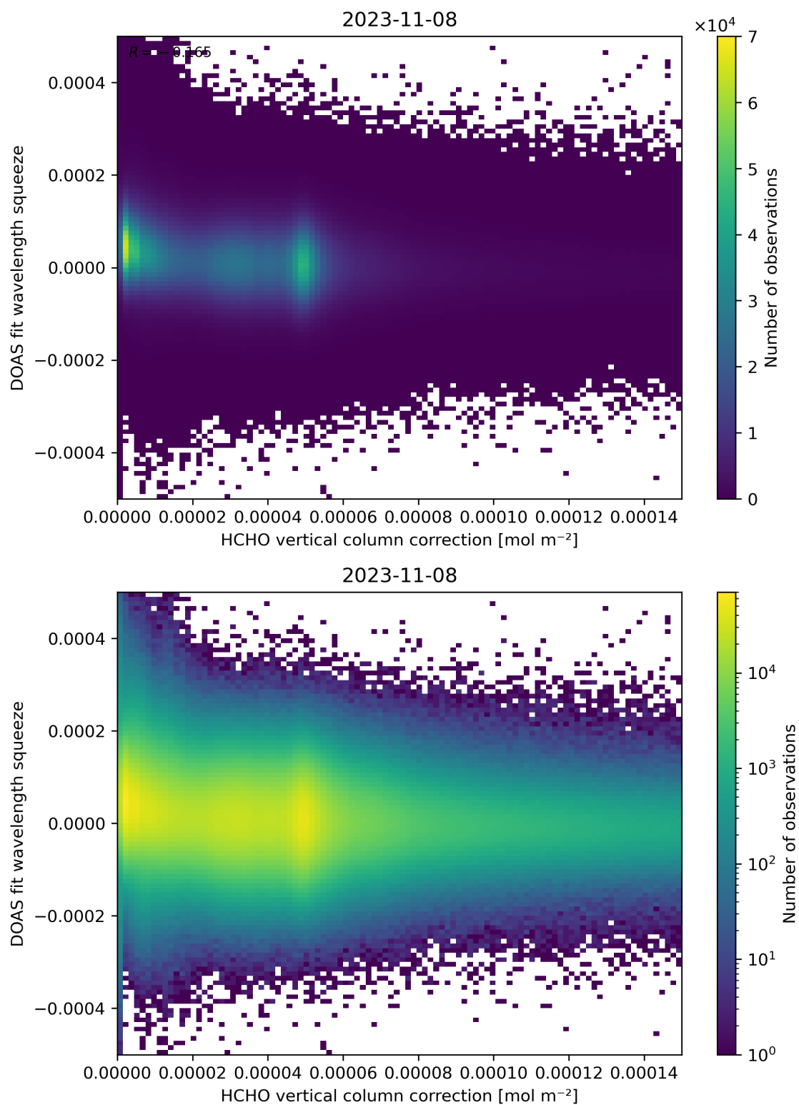
Figure 114: Scatter density plot of “HCHO vertical column correction” against “DOAS fit wavelength squeeze” for 2023-11-07 to 2023-11-09.
