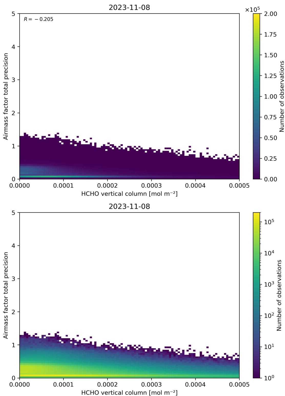
Figure 132: Scatter density plot of “HCHO vertical column” against “Airmass factor total precision” for 2023-11-07 to 2023-11-09.
