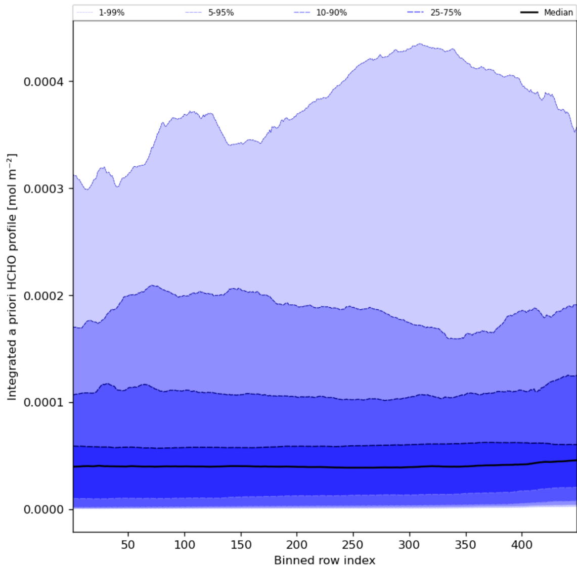
Figure 57: Along track statistics of “Integrated a priori HCHO profile” for 2023-11-07 to 2023-11-09
