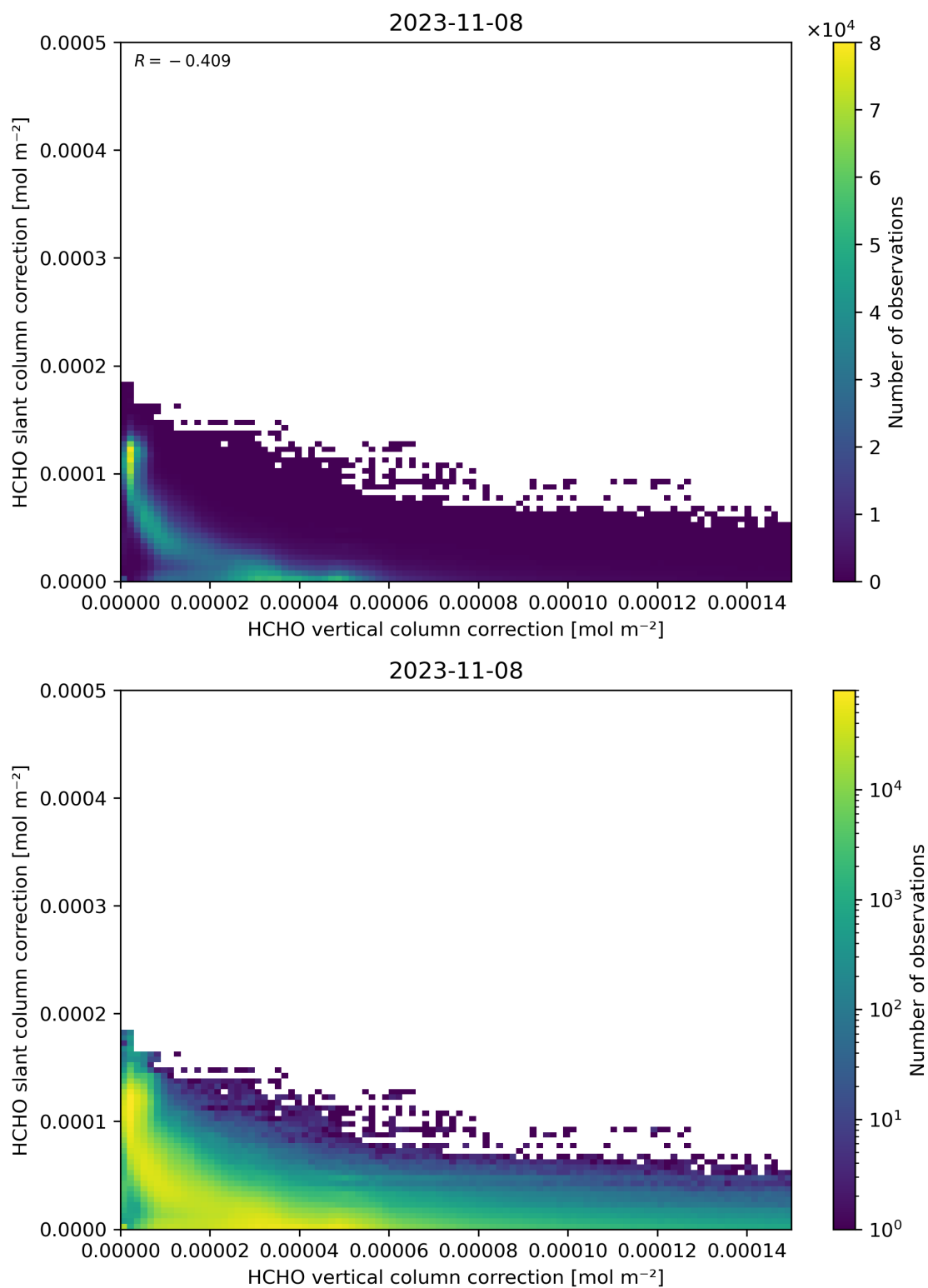
Figure 117: Scatter density plot of “HCHO vertical column correction” against “HCHO slant column correction” for 2023-11-07 to 2023-11-09.
