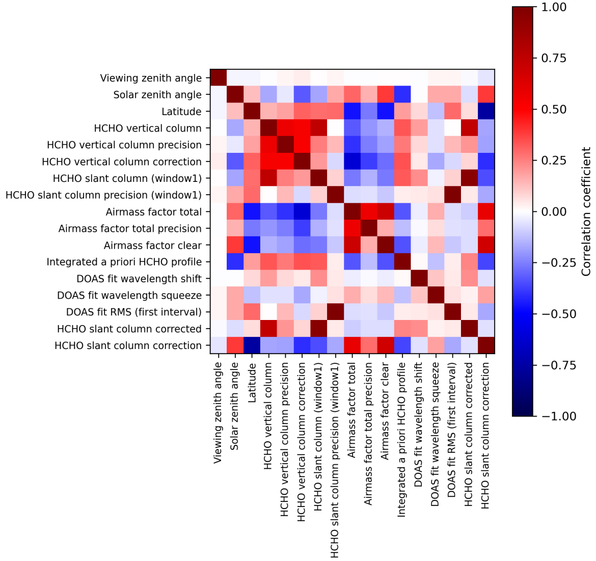
Figure 2: Map of correlation matrix for 2023-11-07 to 2023-11-09.
