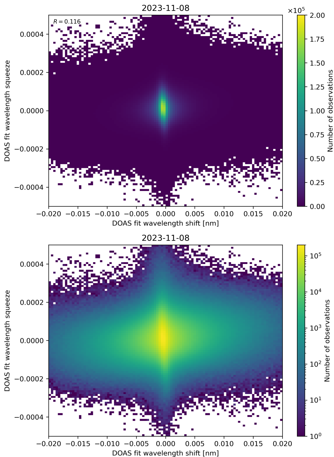
Figure 65: Scatter density plot of “DOAS fit wavelength shift” against “DOAS fit wavelength squeeze” for 2023-11-07 to 2023-11-09.
