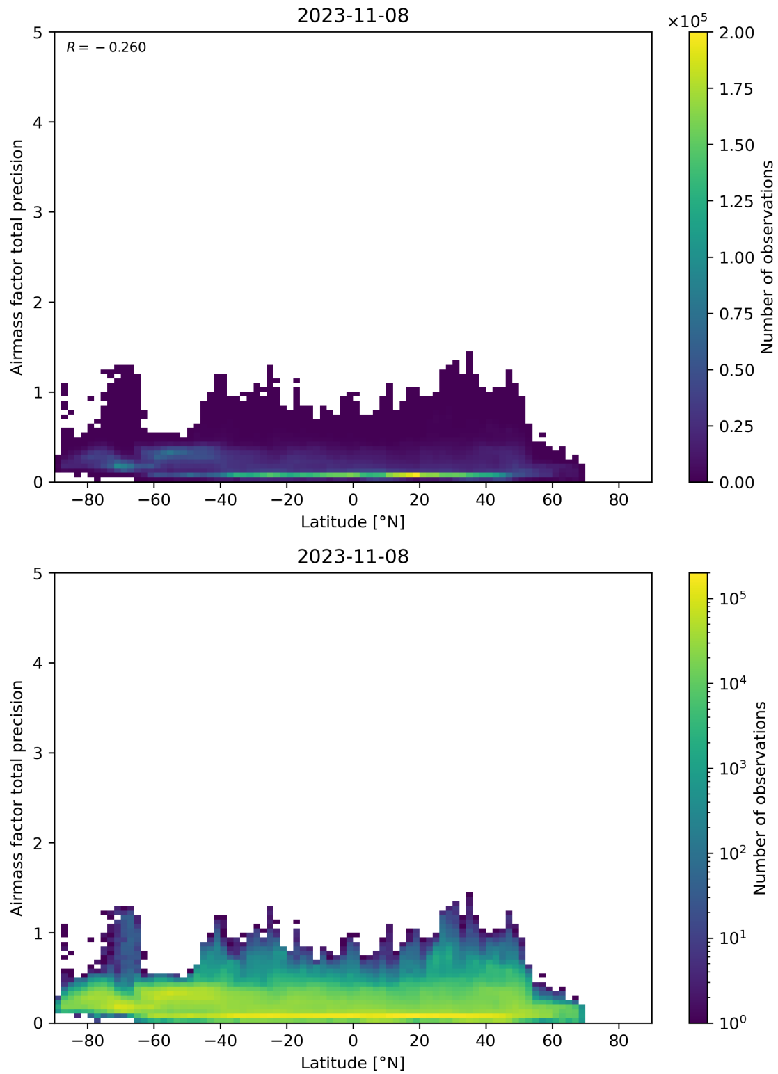
Figure 162: Scatter density plot of “Latitude” against “Airmass factor total precision” for 2023-11-07 to 2023-11-09.
