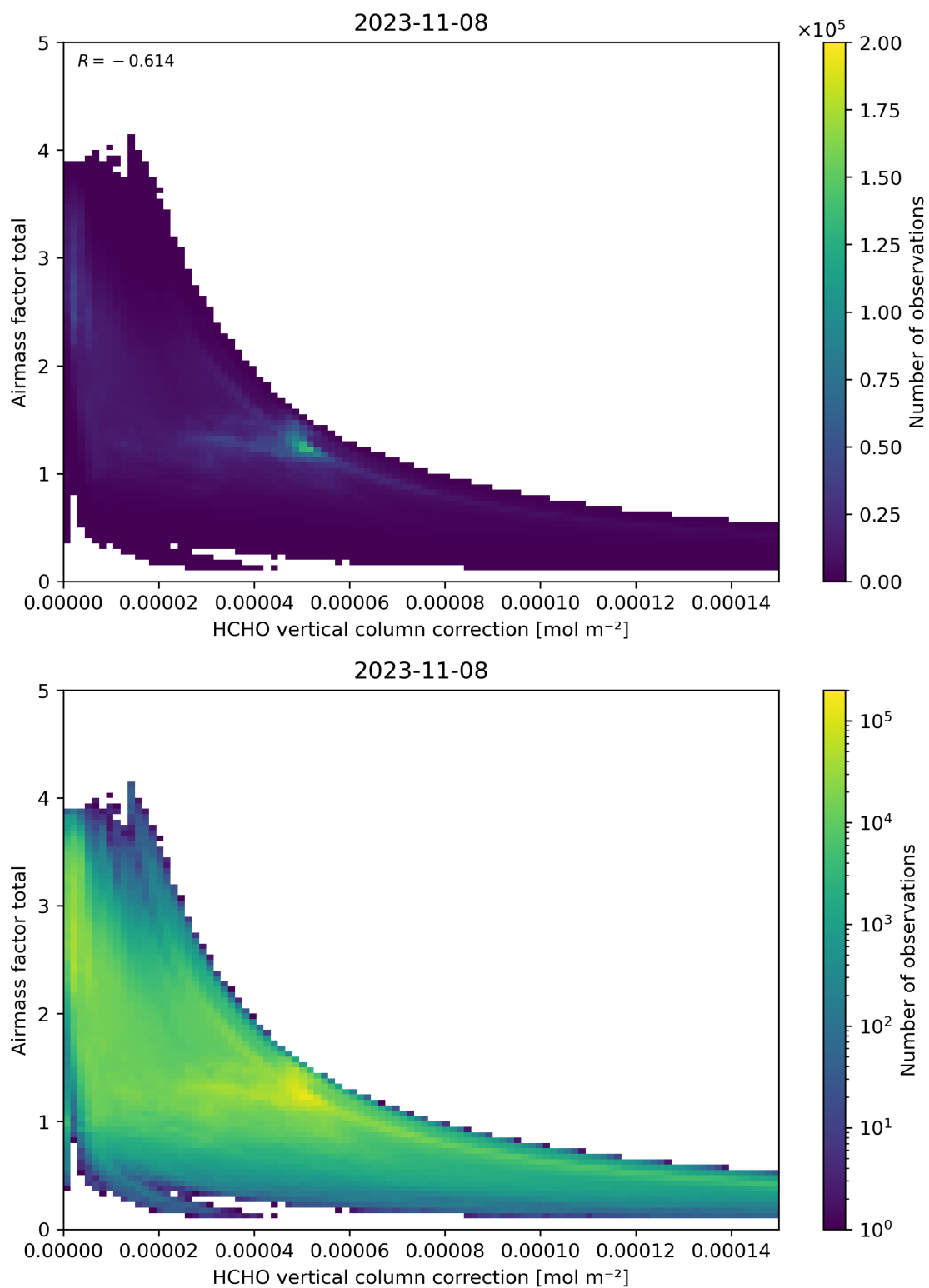
Figure 120: Scatter density plot of “HCHO vertical column correction” against “Airmass factor total” for 2023-11-07 to 2023-11-09.
