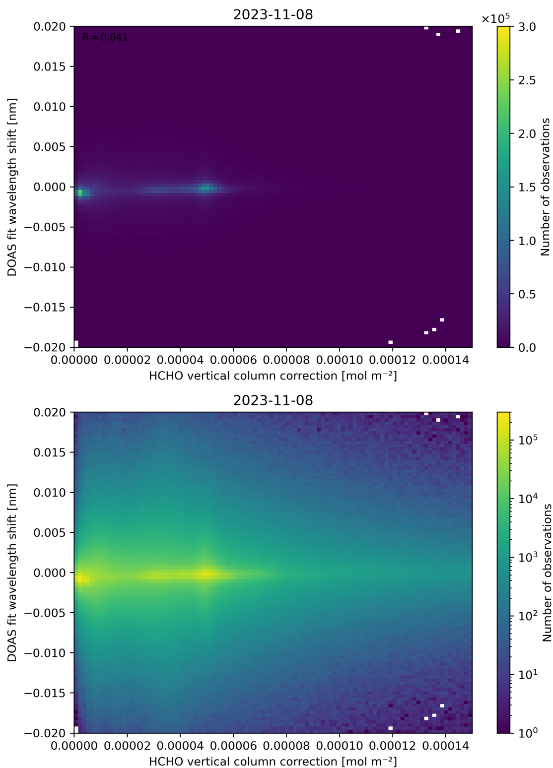
Figure 113: Scatter density plot of “HCHO vertical column correction” against “DOAS fit wavelength shift” for 2023-11-07 to 2023-11-09.
