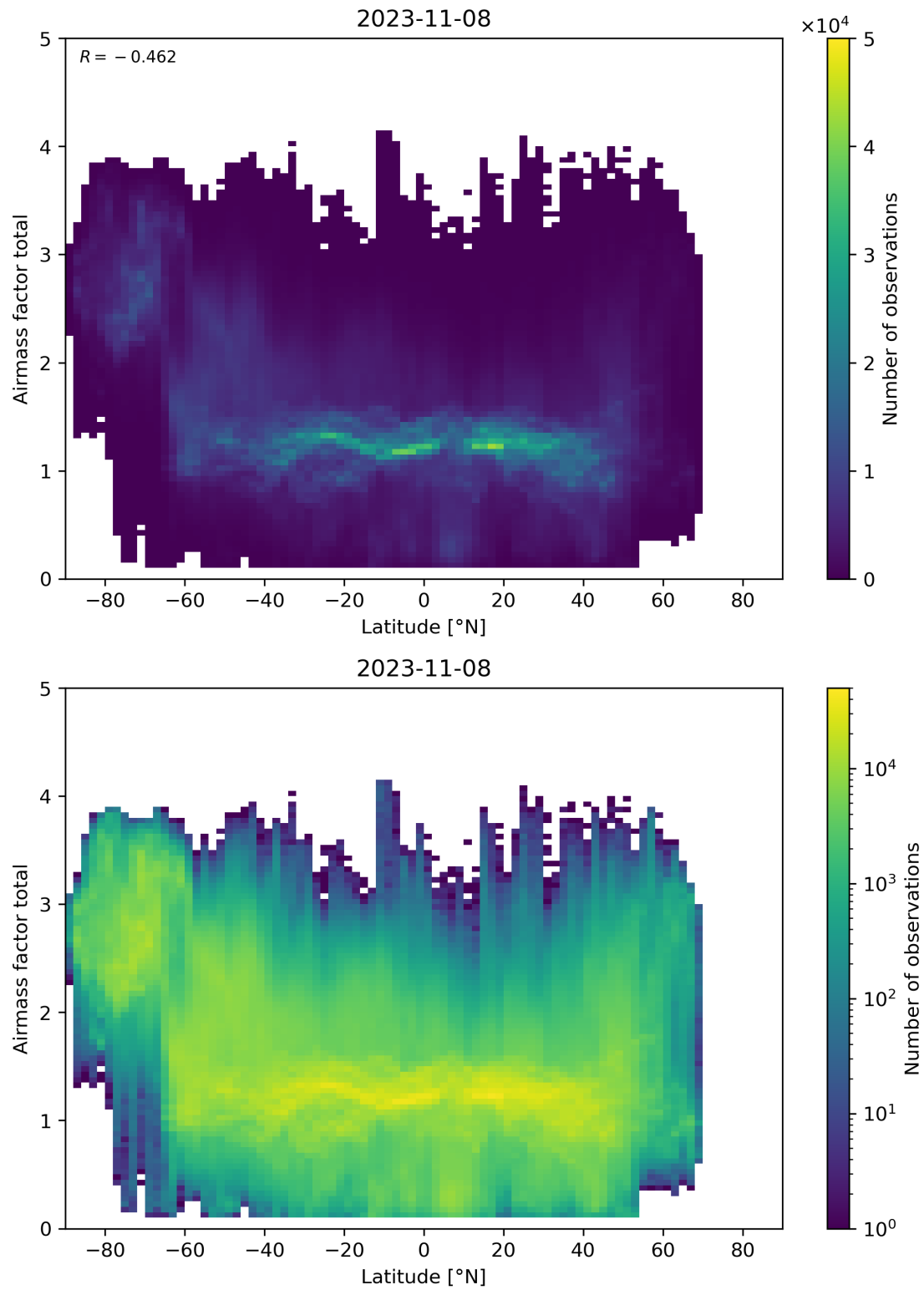
Figure 161: Scatter density plot of “Latitude” against “Airmass factor total” for 2023-11-07 to 2023-11-09.
