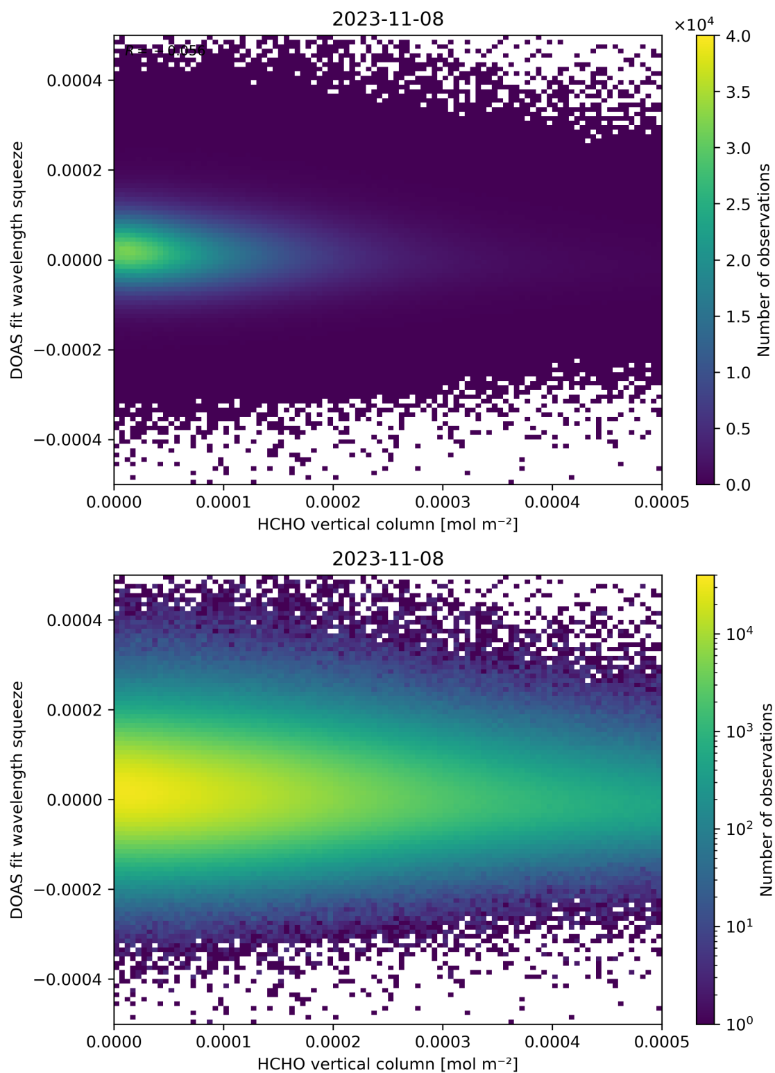
Figure 125: Scatter density plot of “HCHO vertical column” against “DOAS fit wavelength squeeze” for 2023-11-07 to 2023-11-09.
