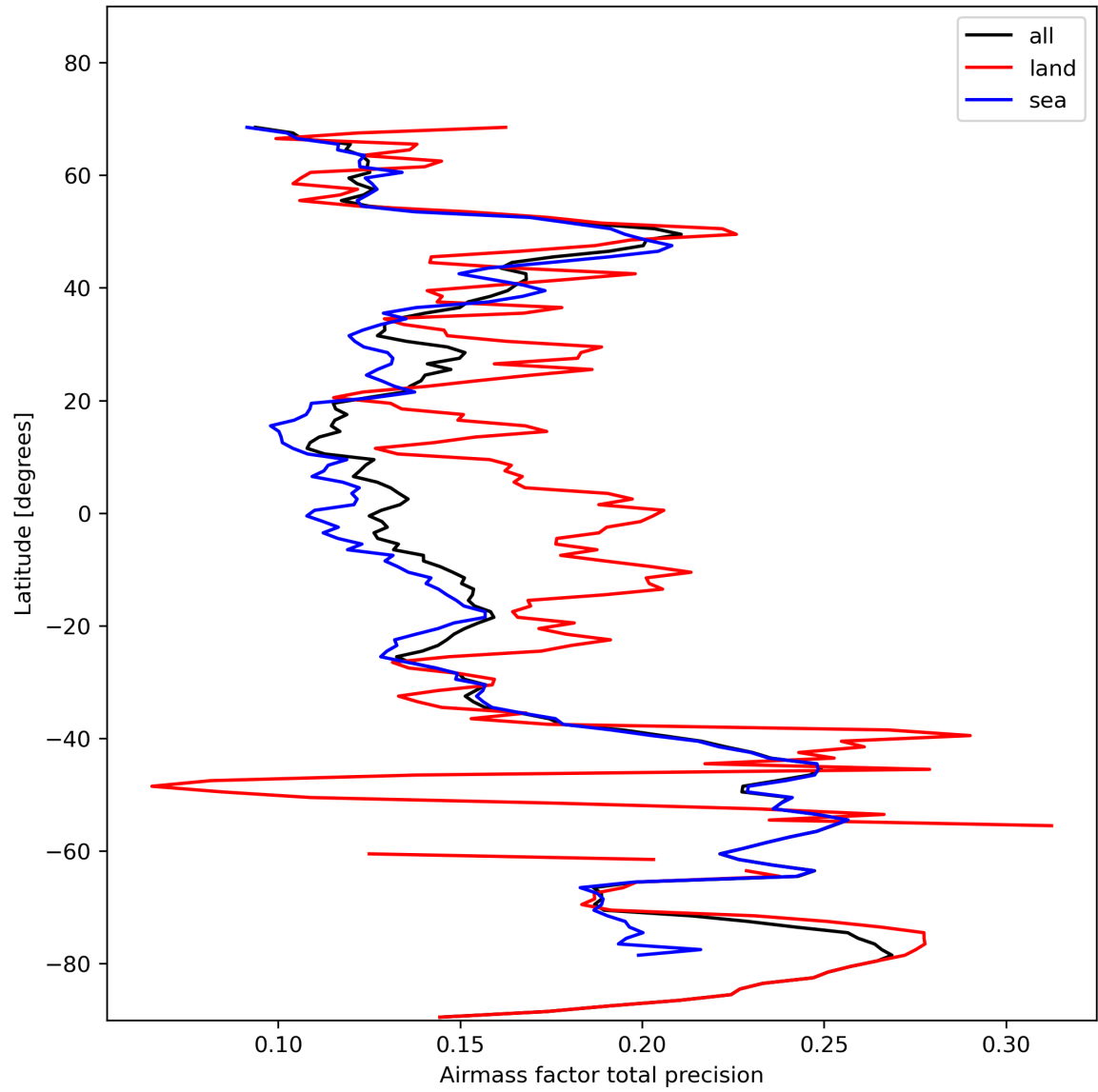
Figure 27: Zonal average of “Airmass factor total precision” for 2023-11-07 to 2023-11-09.
