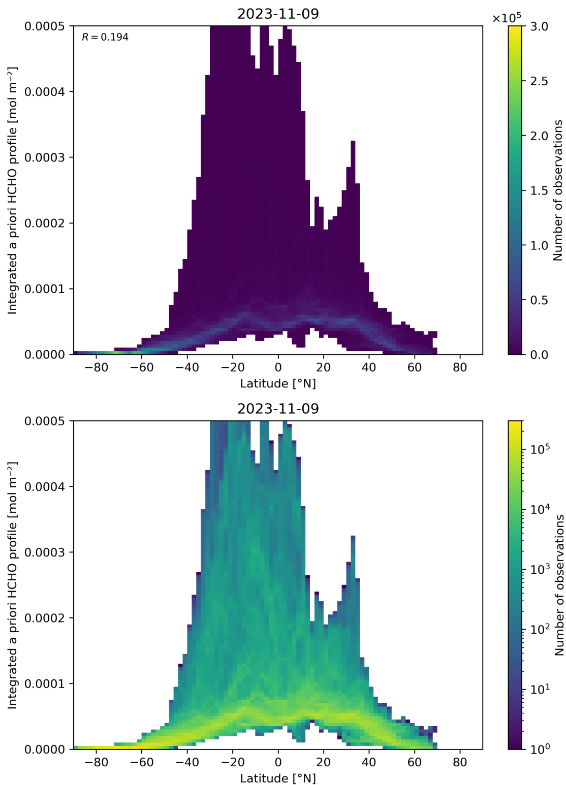
Figure 166: Scatter density plot of “Latitude” against “Integrated a priori HCHO profile” for 2023-11-08 to 2023-11-10.
