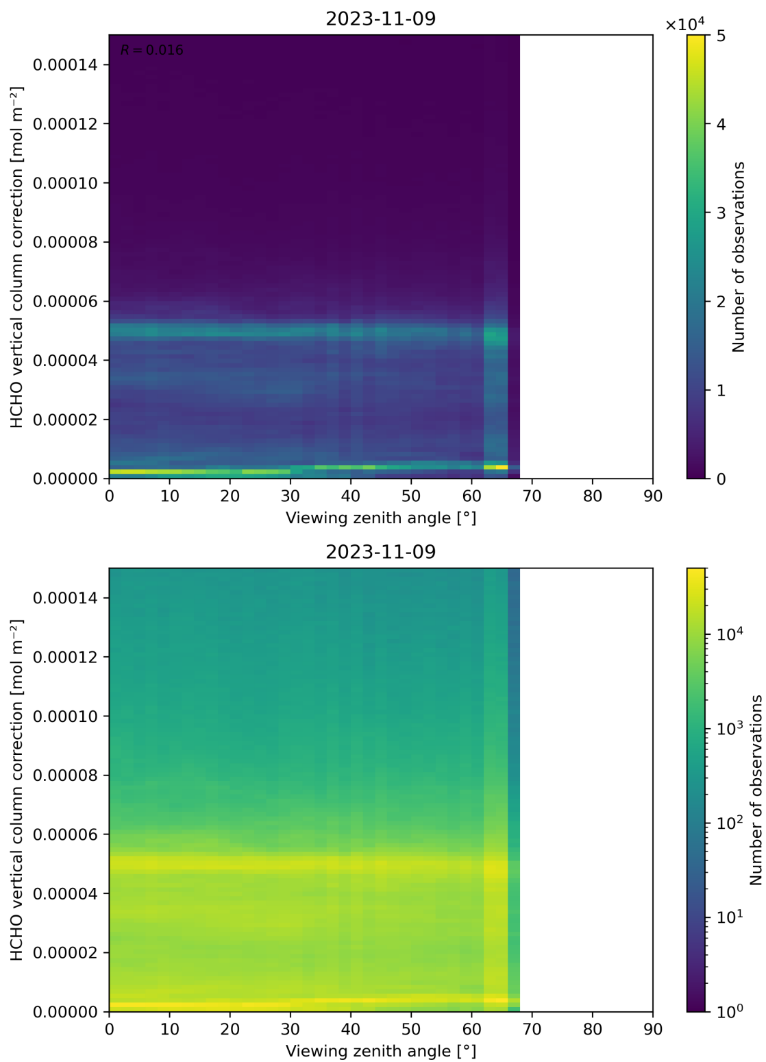
Figure 193: Scatter density plot of “Viewing zenith angle” against “HCHO vertical column correction” for 2023-11-08 to 2023-11-10.
