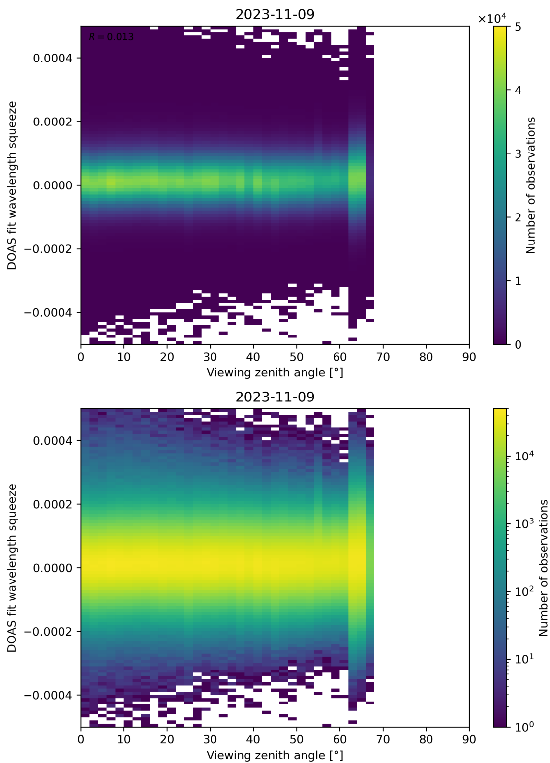
Figure 184: Scatter density plot of “Viewing zenith angle” against “DOAS fit wavelength squeeze” for 2023-11-08 to 2023-11-10.
