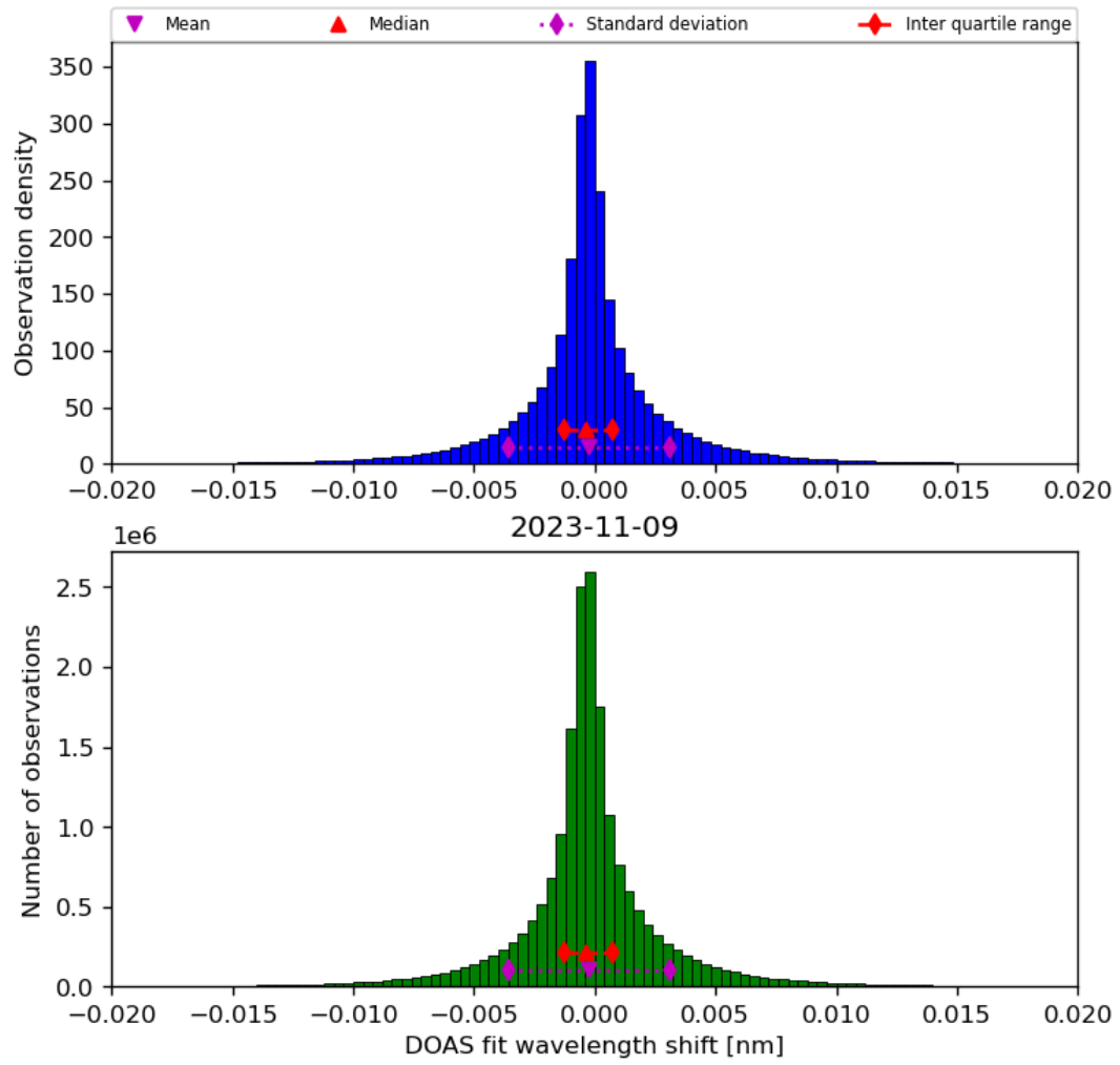
Figure 44: Histogram of “DOAS fit wavelength shift” for 2023-11-08 to 2023-11-10
