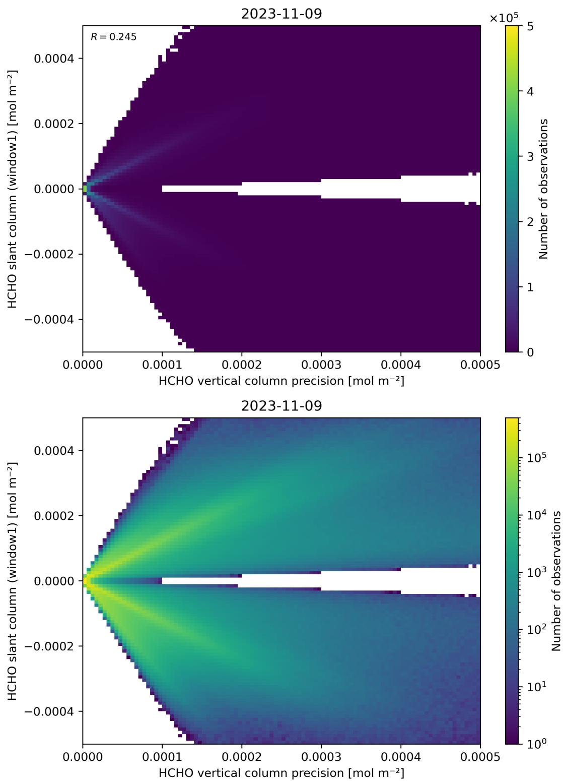
Figure 142: Scatter density plot of “HCHO vertical column precision” against “HCHO slant column (window1)” for 2023-11-08 to 2023-11-10.
