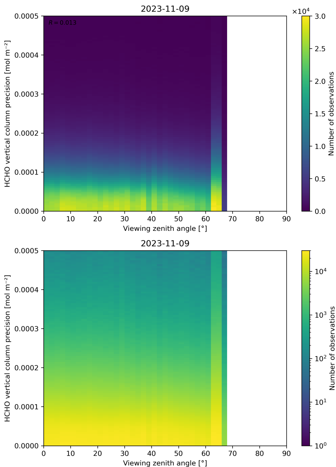
Figure 194: Scatter density plot of “Viewing zenith angle” against “HCHO vertical column precision” for 2023-11-08 to 2023-11-10.
