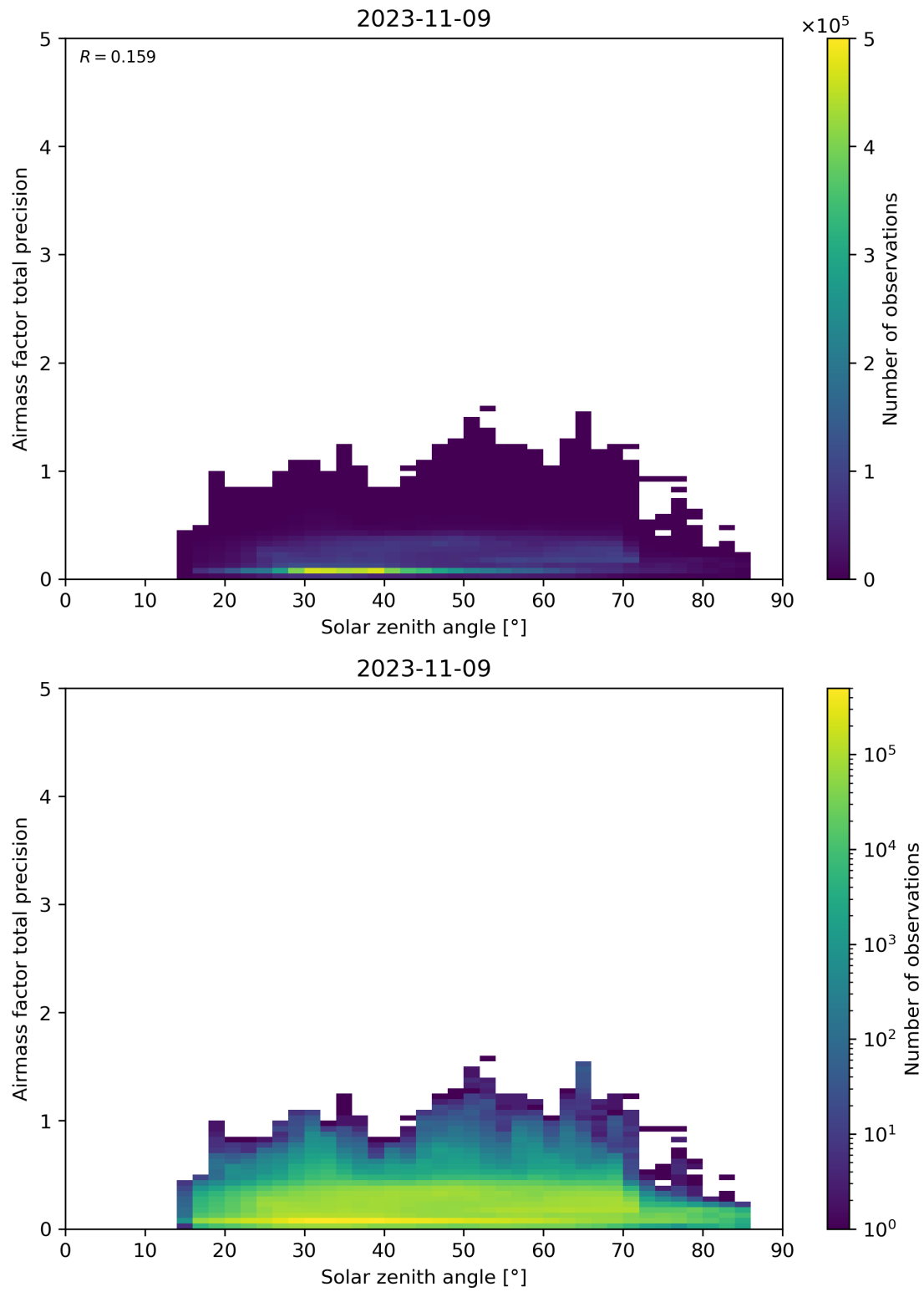
Figure 176: Scatter density plot of “Solar zenith angle” against “Airmass factor total precision” for 2023-11-08 to 2023-11-10.
