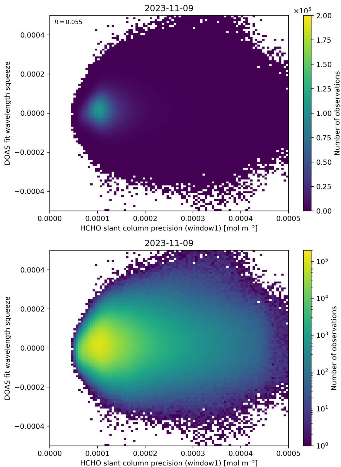
Figure 90: Scatter density plot of “HCHO slant column precision (window1)” against “DOAS fit wavelength squeeze” for 2023-11-08 to 2023-11-10.
