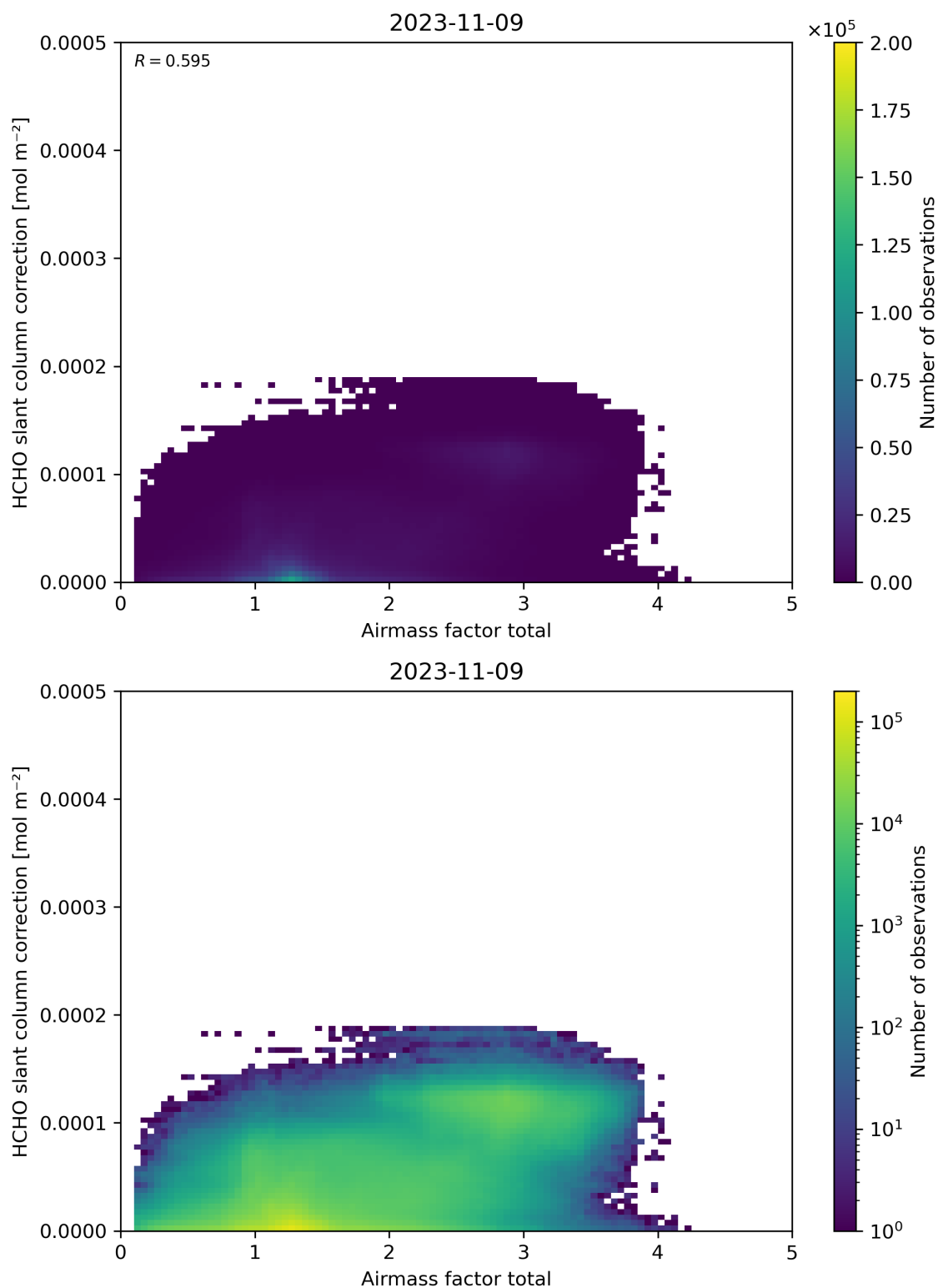
Figure 102: Scatter density plot of “Airmass factor total” against “HCHO slant column correction” for 2023-11-08 to 2023-11-10.
