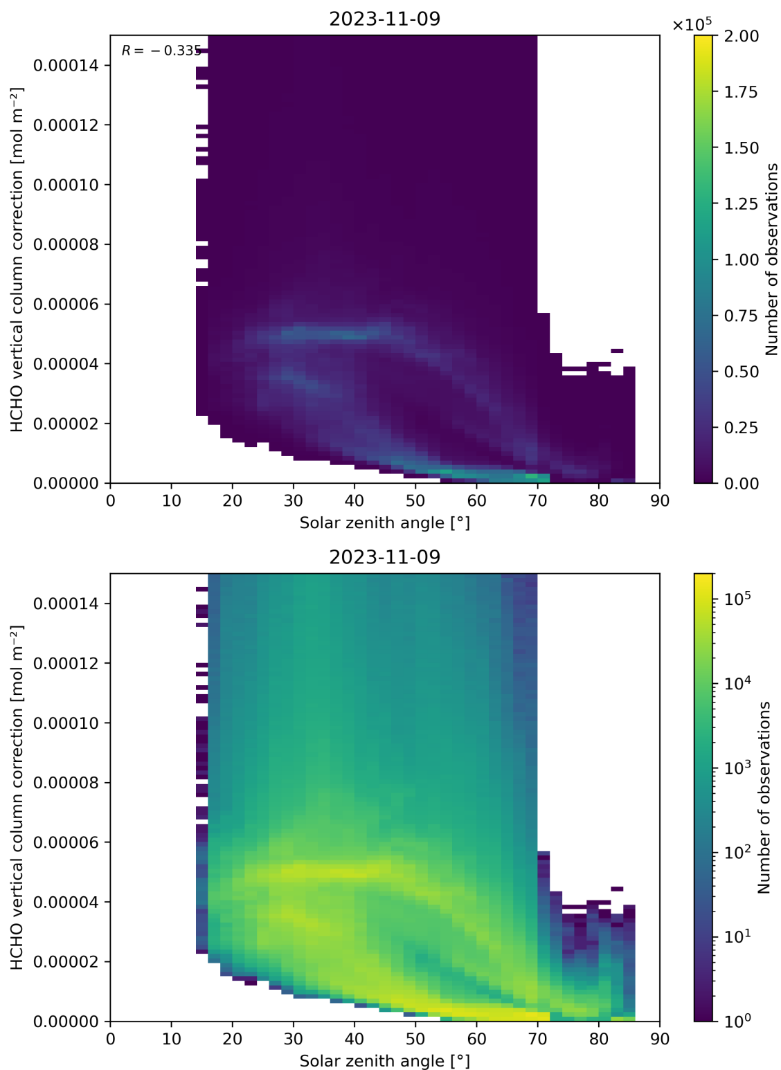
Figure 178: Scatter density plot of “Solar zenith angle” against “HCHO vertical column correction” for 2023-11-08 to 2023-11-10.
