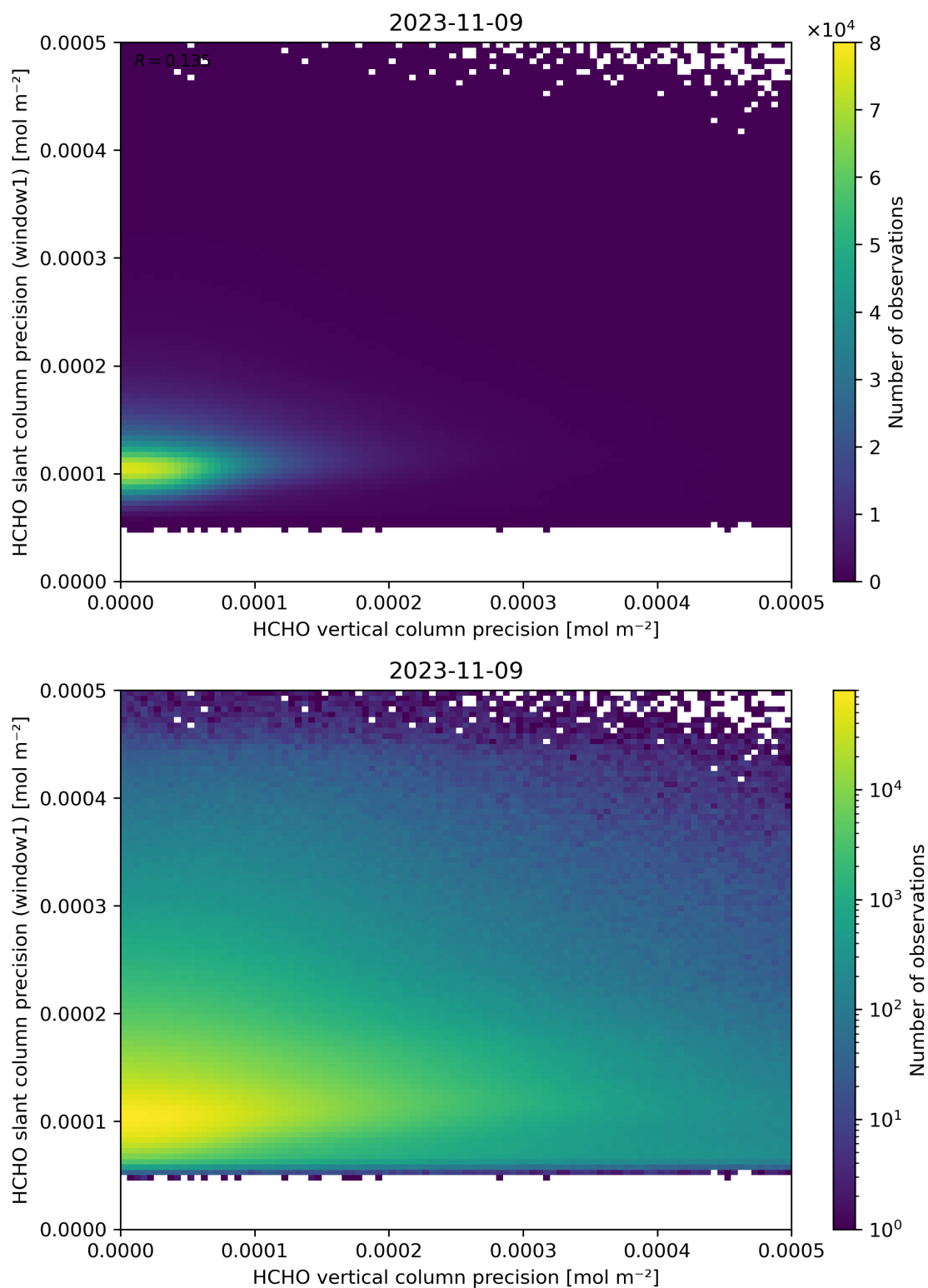
Figure 143: Scatter density plot of “HCHO vertical column precision” against “HCHO slant column precision (window1)” for 2023-11-08 to 2023-11-10.
