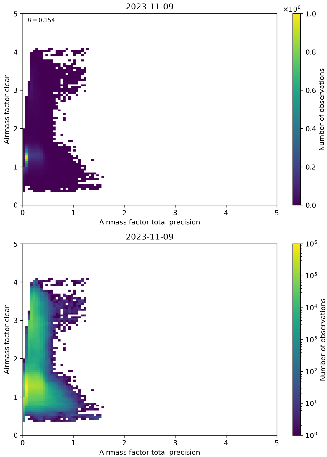
Figure 108: Scatter density plot of “Airmass factor total precision” against “Airmass factor clear” for 2023-11-08 to 2023-11-10.
