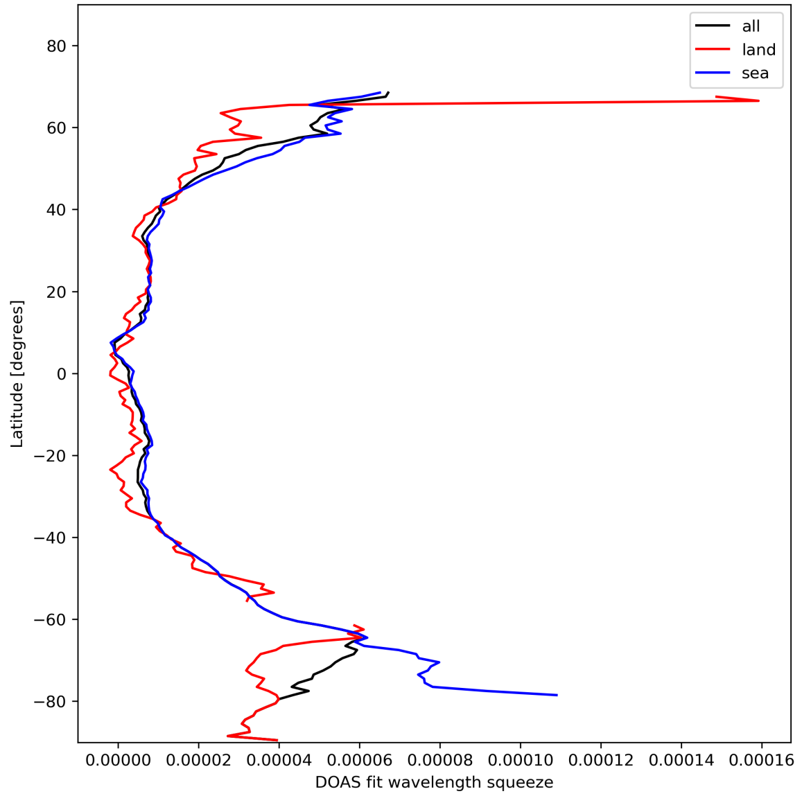
Figure 31: Zonal average of “DOAS fit wavelength squeeze” for 2023-11-08 to 2023-11-10.
