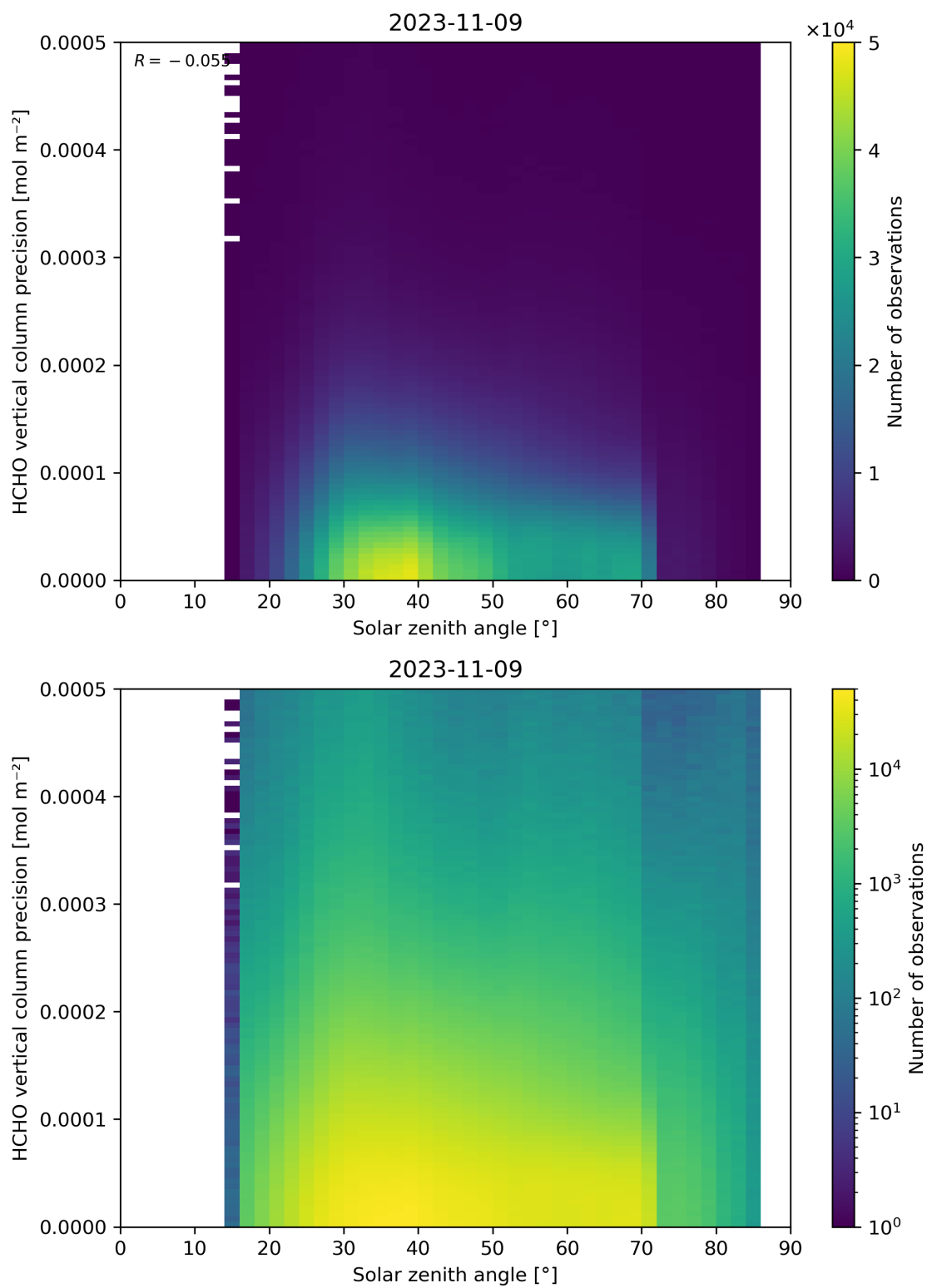
Figure 179: Scatter density plot of “Solar zenith angle” against “HCHO vertical column precision” for 2023-11-08 to 2023-11-10.
