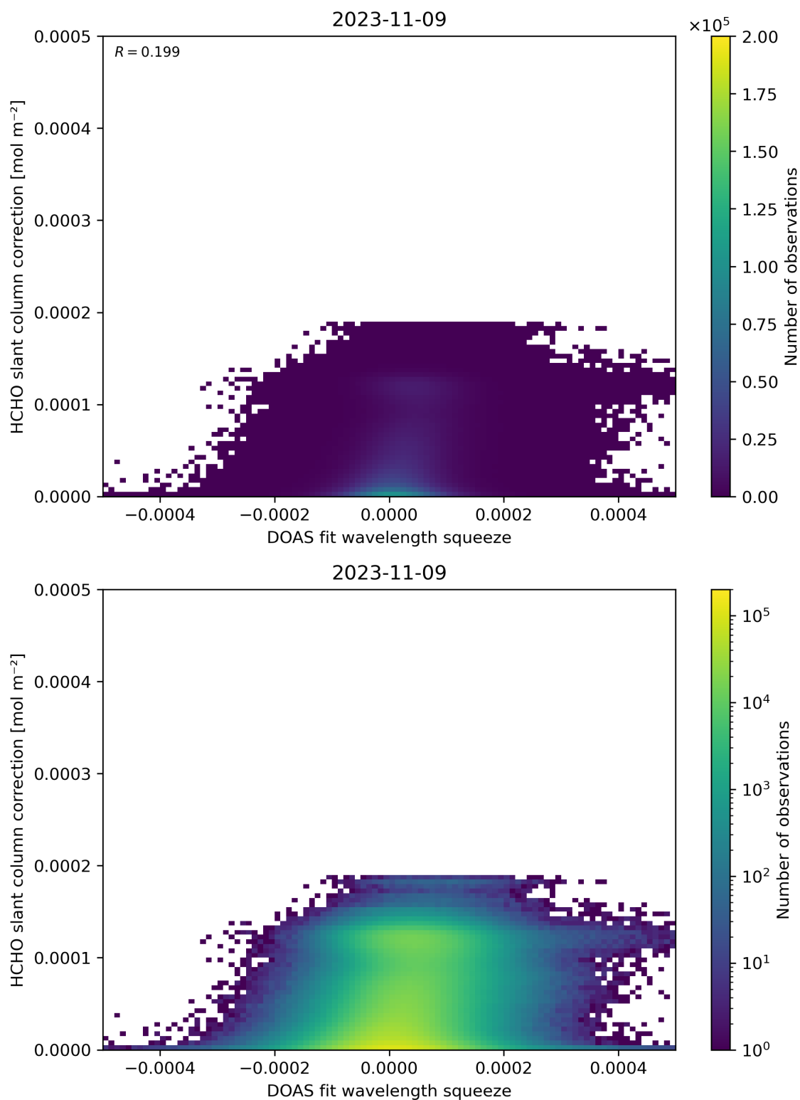
Figure 70: Scatter density plot of “DOAS fit wavelength squeeze” against “HCHO slant column correction” for 2023-11-08 to 2023-11-10.
