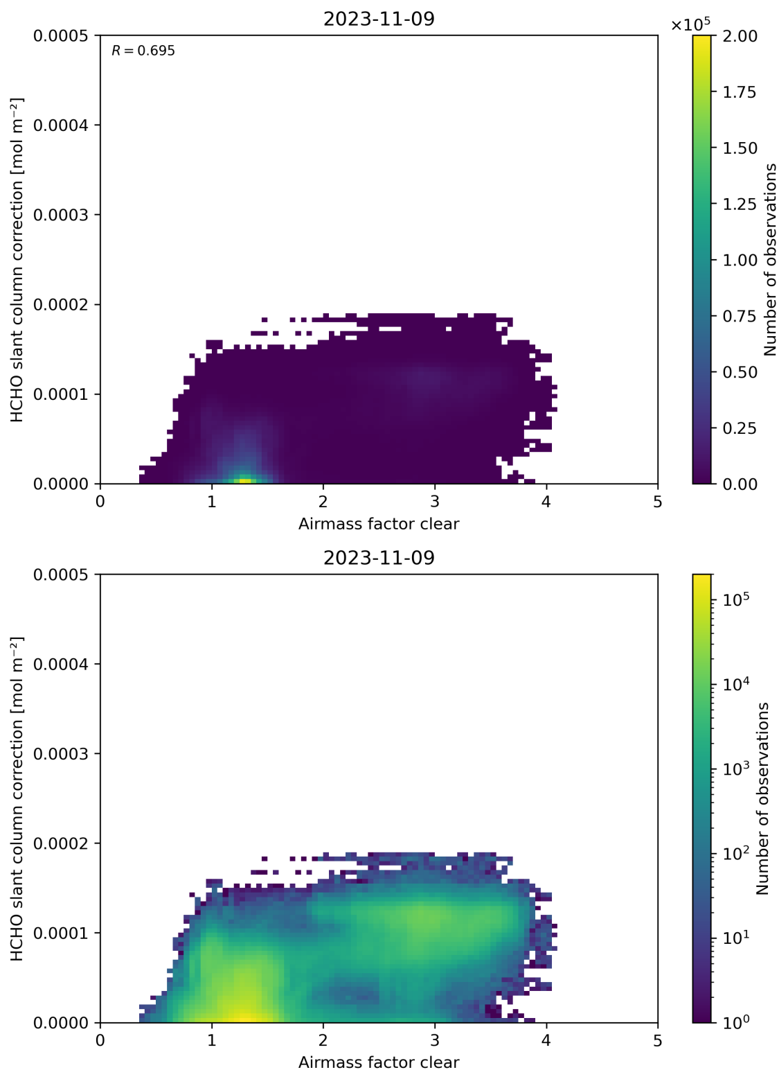
Figure 75: Scatter density plot of “Airmass factor clear” against “HCHO slant column correction” for 2023-11-08 to 2023-11-10.
