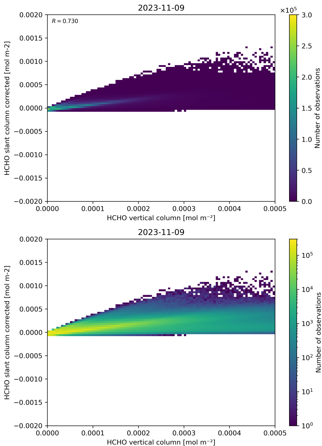
Figure 127: Scatter density plot of “HCHO vertical column” against “HCHO slant column corrected” for 2023-11-08 to 2023-11-10.
