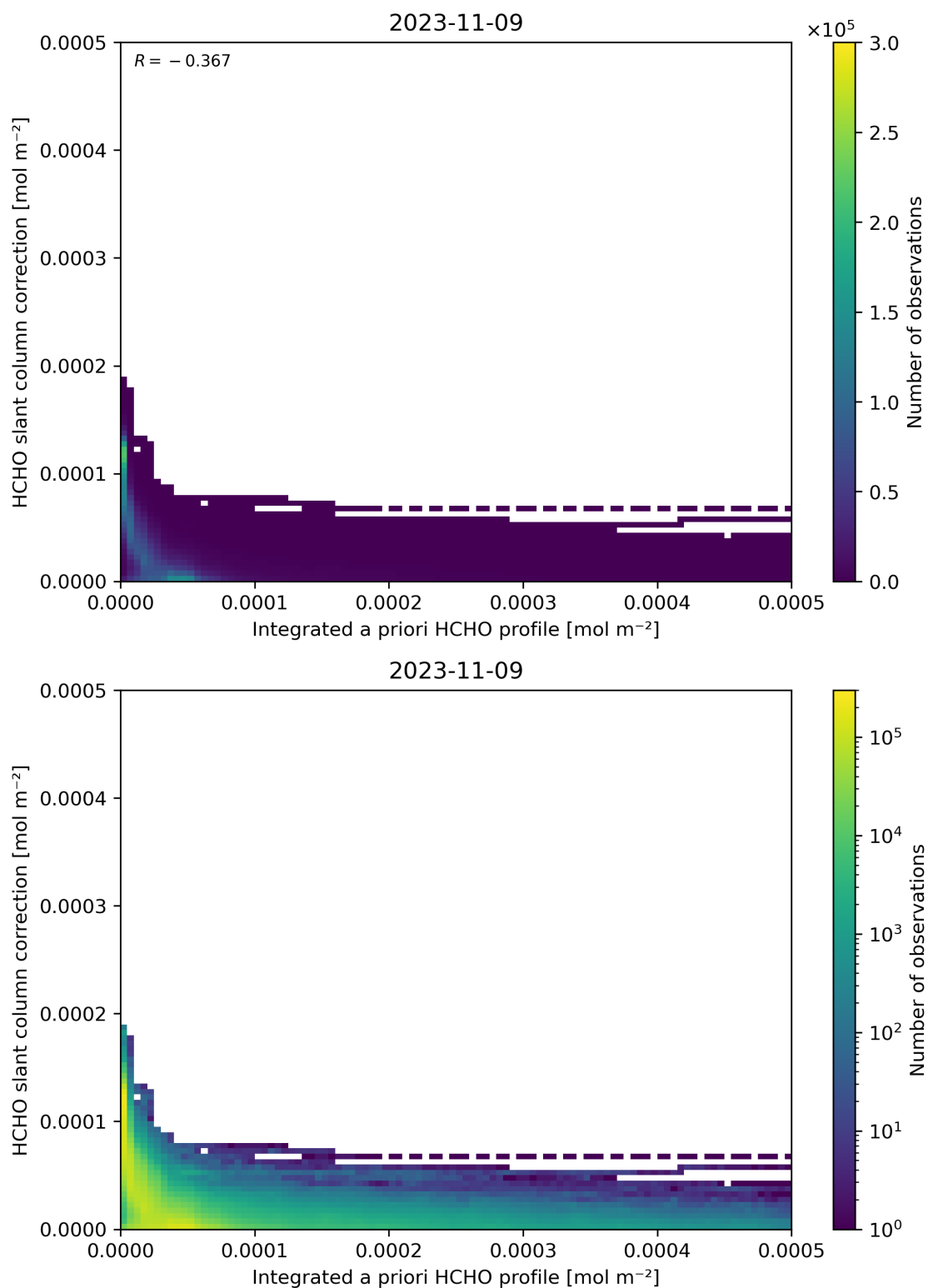
Figure 152: Scatter density plot of “Integrated a priori HCHO profile” against “HCHO slant column correction” for 2023-11-08 to 2023-11-10.
