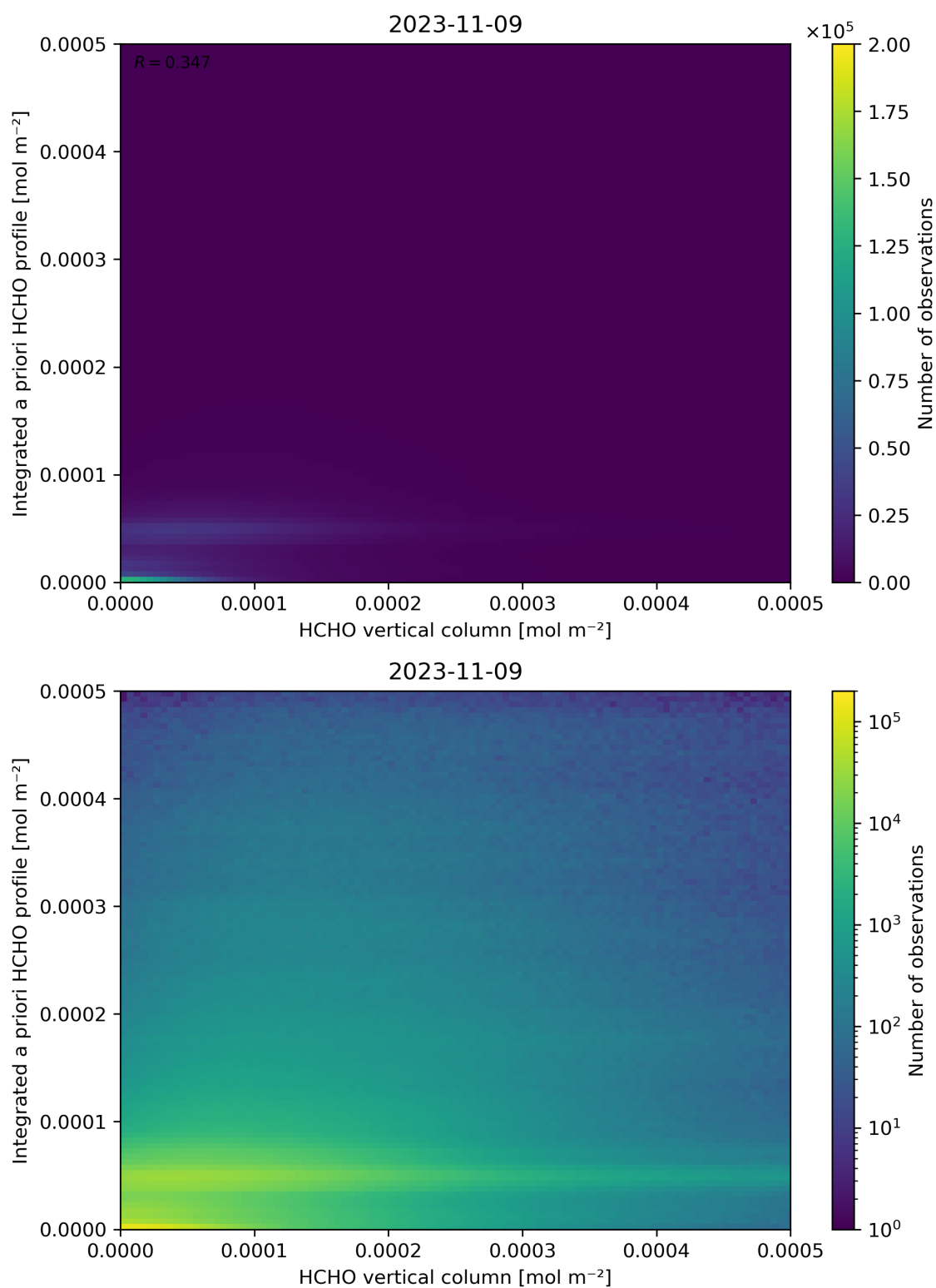
Figure 135: Scatter density plot of “HCHO vertical column” against “Integrated a priori HCHO profile” for 2023-11-08 to 2023-11-10.
