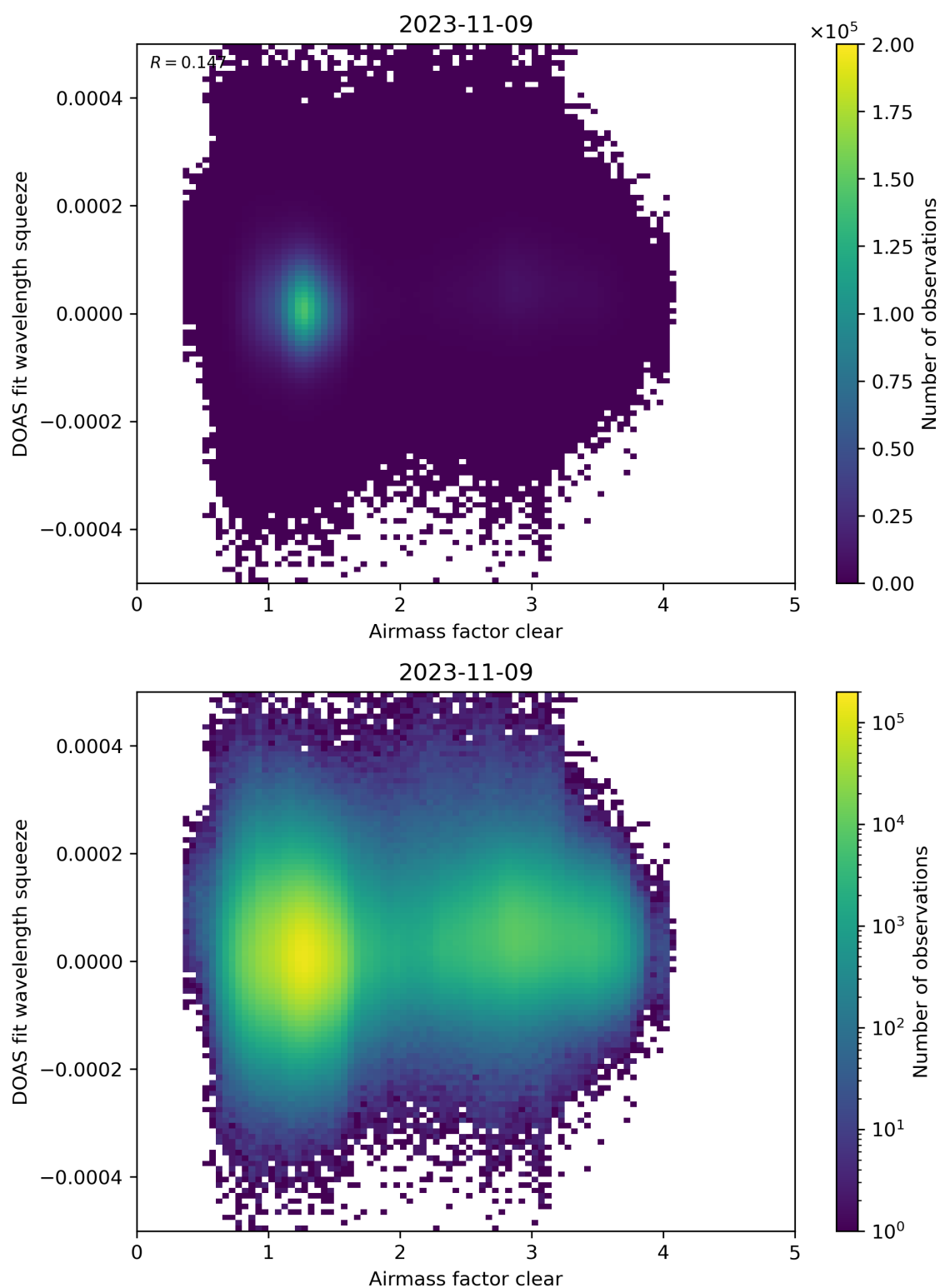
Figure 73: Scatter density plot of “Airmass factor clear” against “DOAS fit wavelength squeeze” for 2023-11-08 to 2023-11-10.
