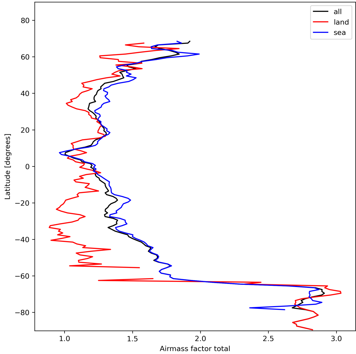
Figure 26: Zonal average of “Airmass factor total” for 2023-11-08 to 2023-11-10.
