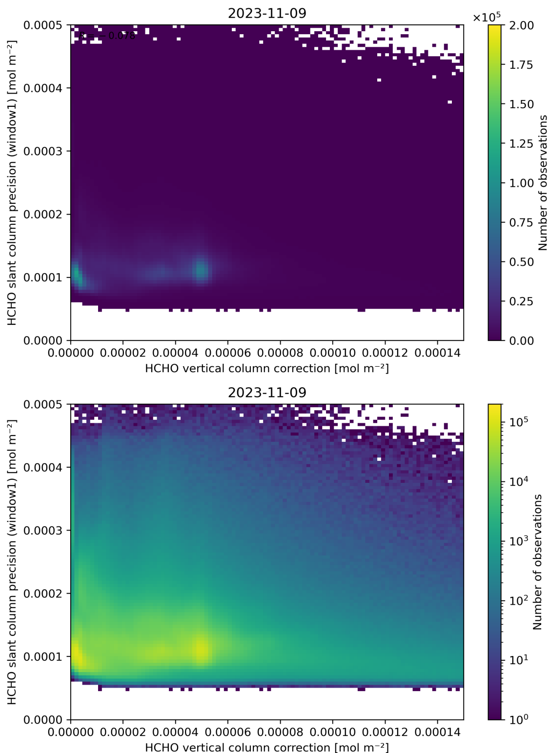
Figure 119: Scatter density plot of “HCHO vertical column correction” against “HCHO slant column precision (window1)” for 2023-11-08 to 2023-11-10.
