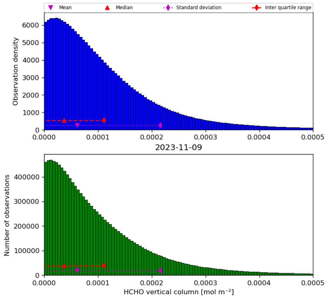
Figure 35: Histogram of “HCHO vertical column” for 2023-11-08 to 2023-11-10
