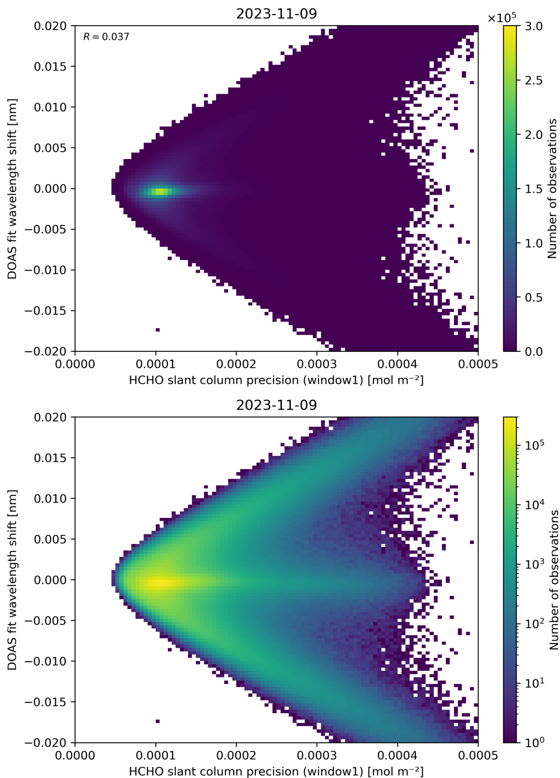
Figure 89: Scatter density plot of “HCHO slant column precision (window1)” against “DOAS fit wavelength shift” for 2023-11-08 to 2023-11-10.
