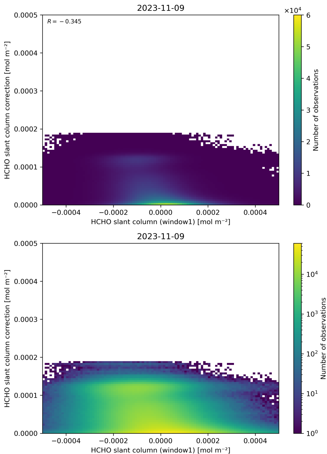
Figure 83: Scatter density plot of “HCHO slant column (window1)” against “HCHO slant column correction” for 2023-11-08 to 2023-11-10.
