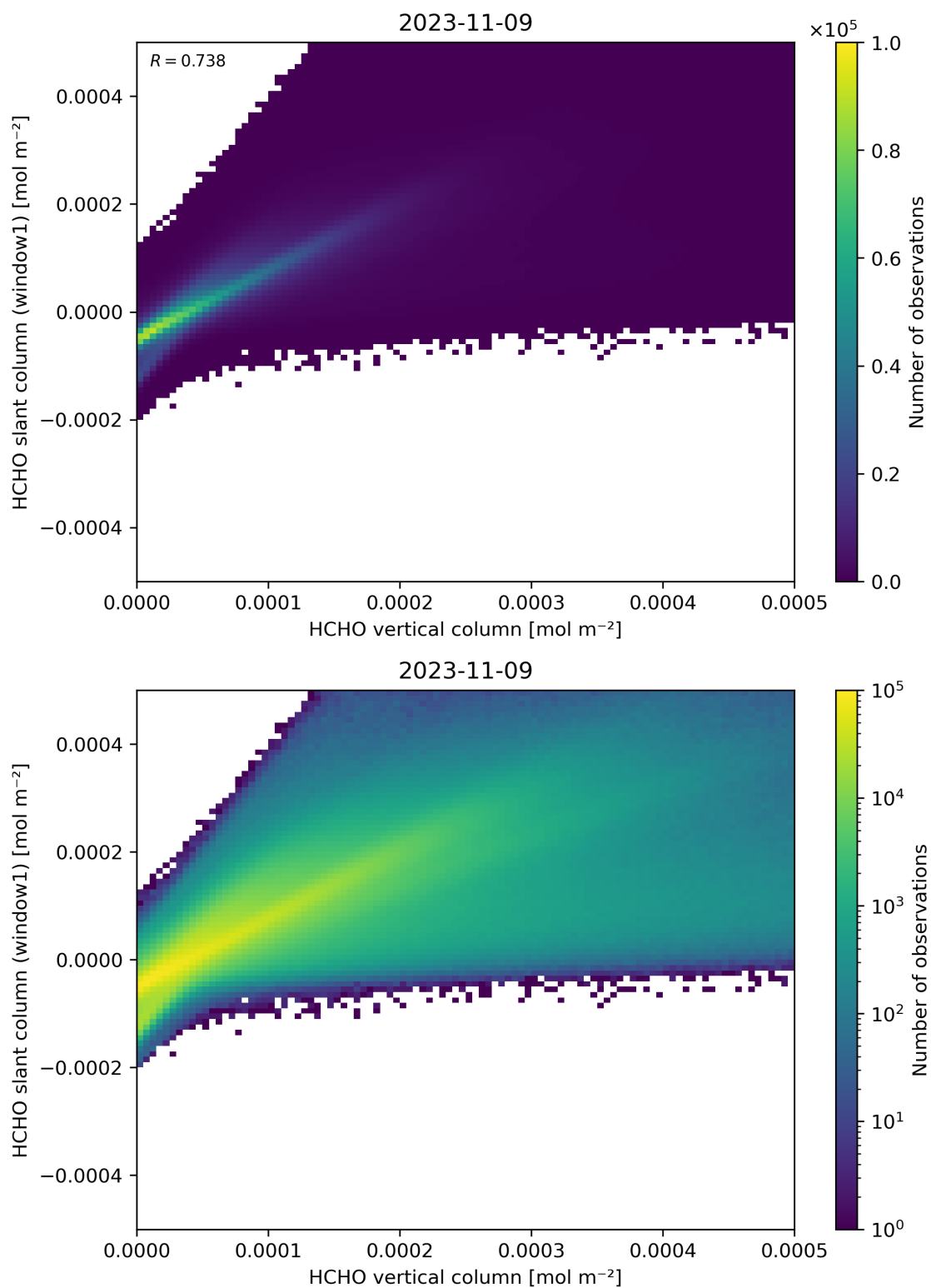
Figure 129: Scatter density plot of “HCHO vertical column” against “HCHO slant column (window1)” for 2023-11-08 to 2023-11-10.
