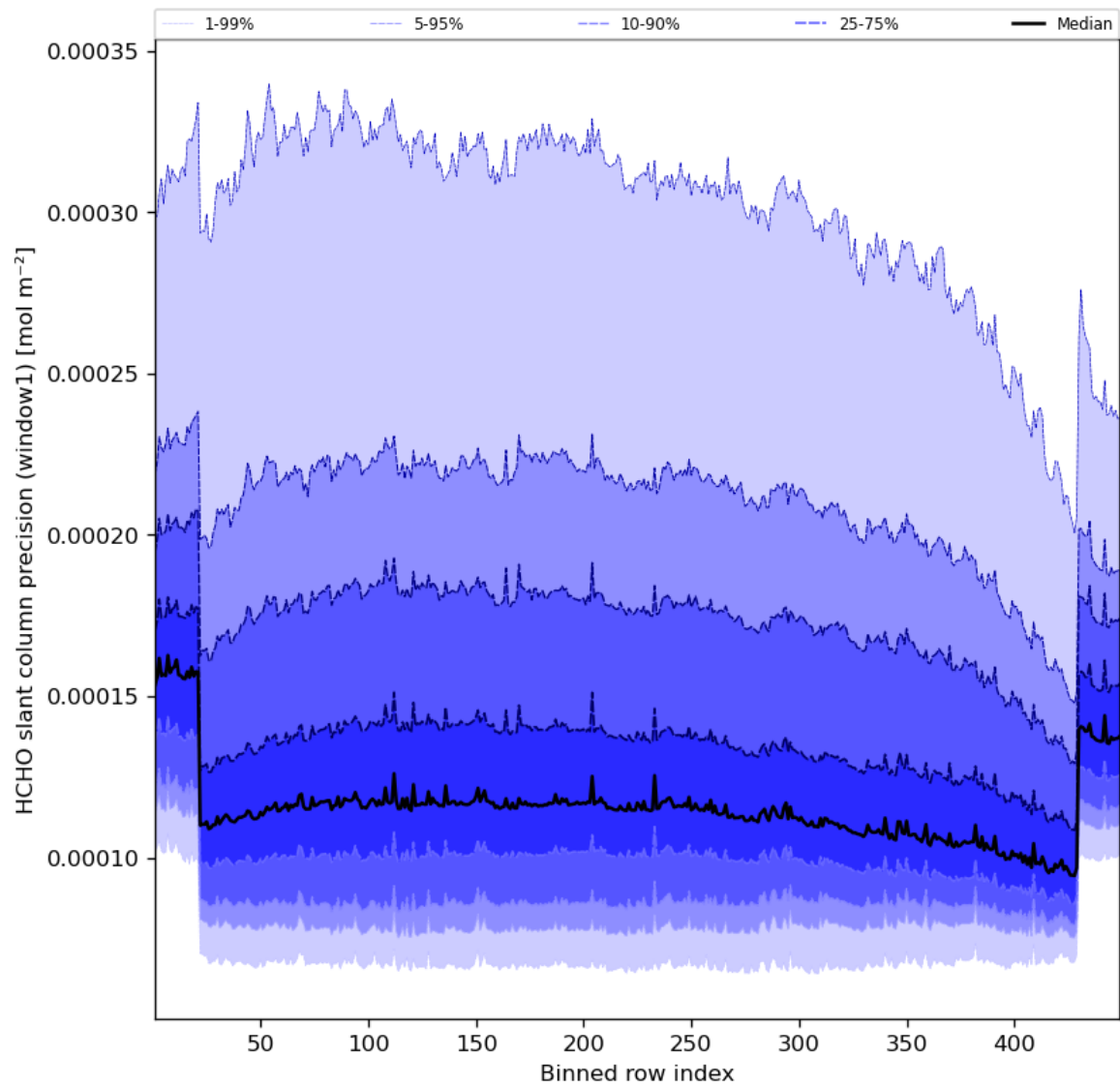
Figure 53: Along track statistics of “HCHO slant column precision (window1)” for 2023-11-08 to 2023-11-10
