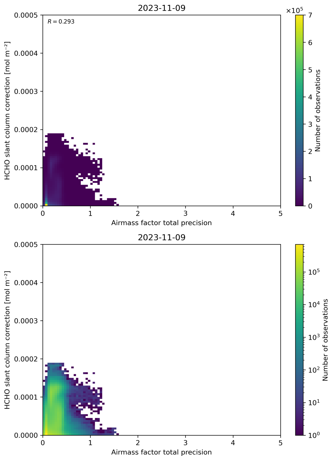
Figure 110: Scatter density plot of “Airmass factor total precision” against “HCHO slant column correction” for 2023-11-08 to 2023-11-10.
