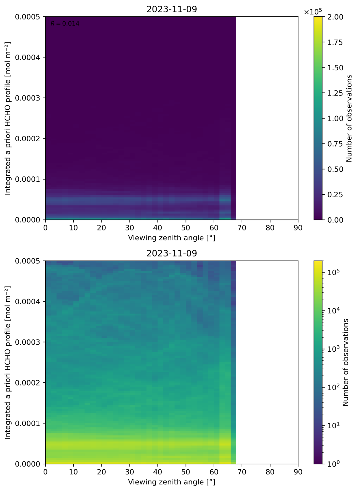
Figure 195: Scatter density plot of “Viewing zenith angle” against “Integrated a priori HCHO profile” for 2023-11-08 to 2023-11-10.
