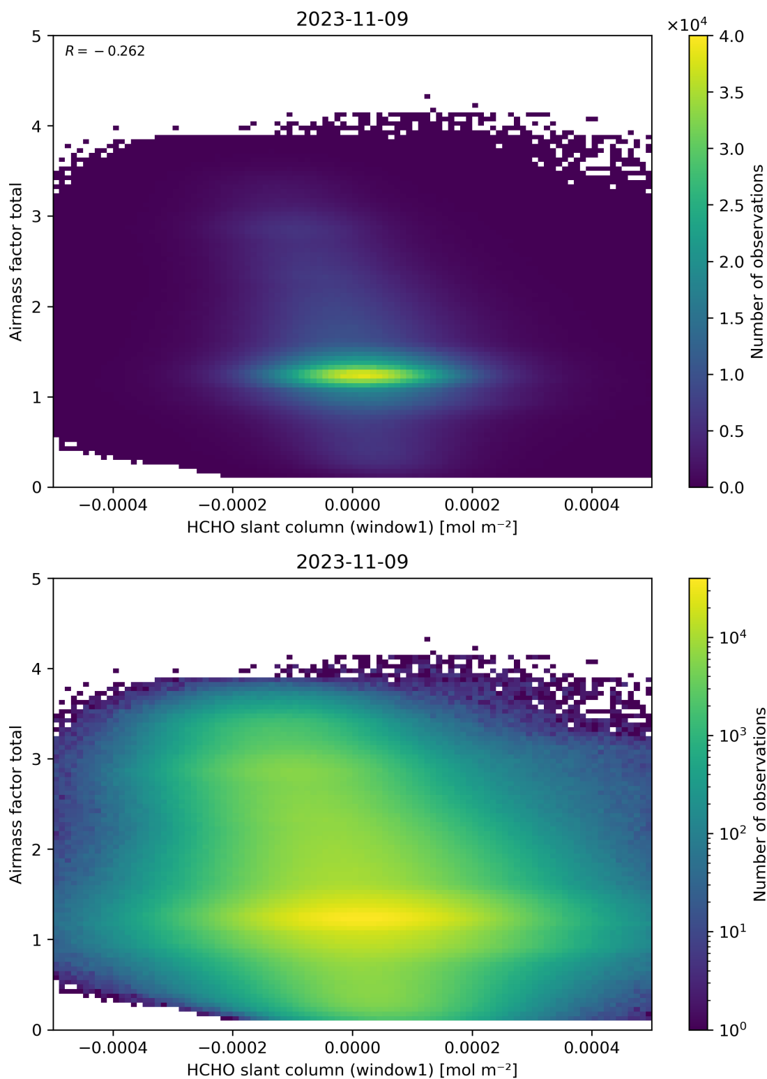
Figure 85: Scatter density plot of “HCHO slant column (window1)” against “Airmass factor total” for 2023-11-08 to 2023-11-10.
