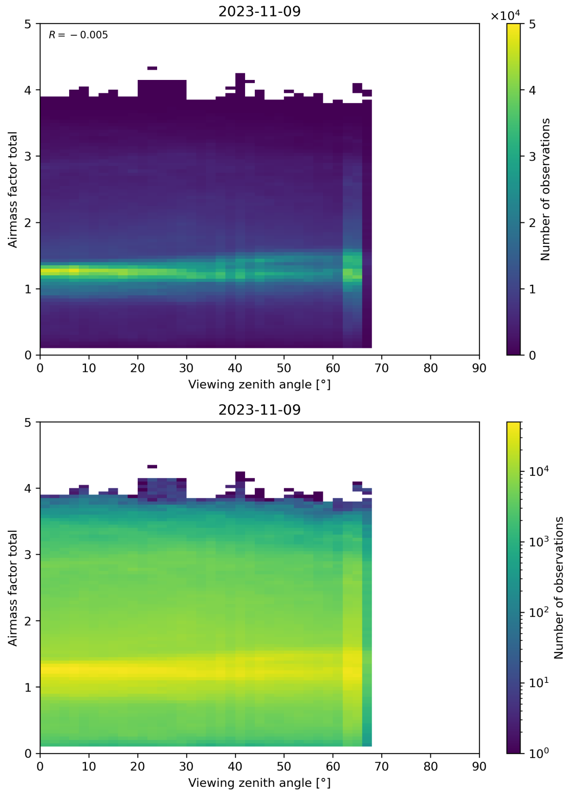
Figure 190: Scatter density plot of “Viewing zenith angle” against “Airmass factor total” for 2023-11-08 to 2023-11-10.
