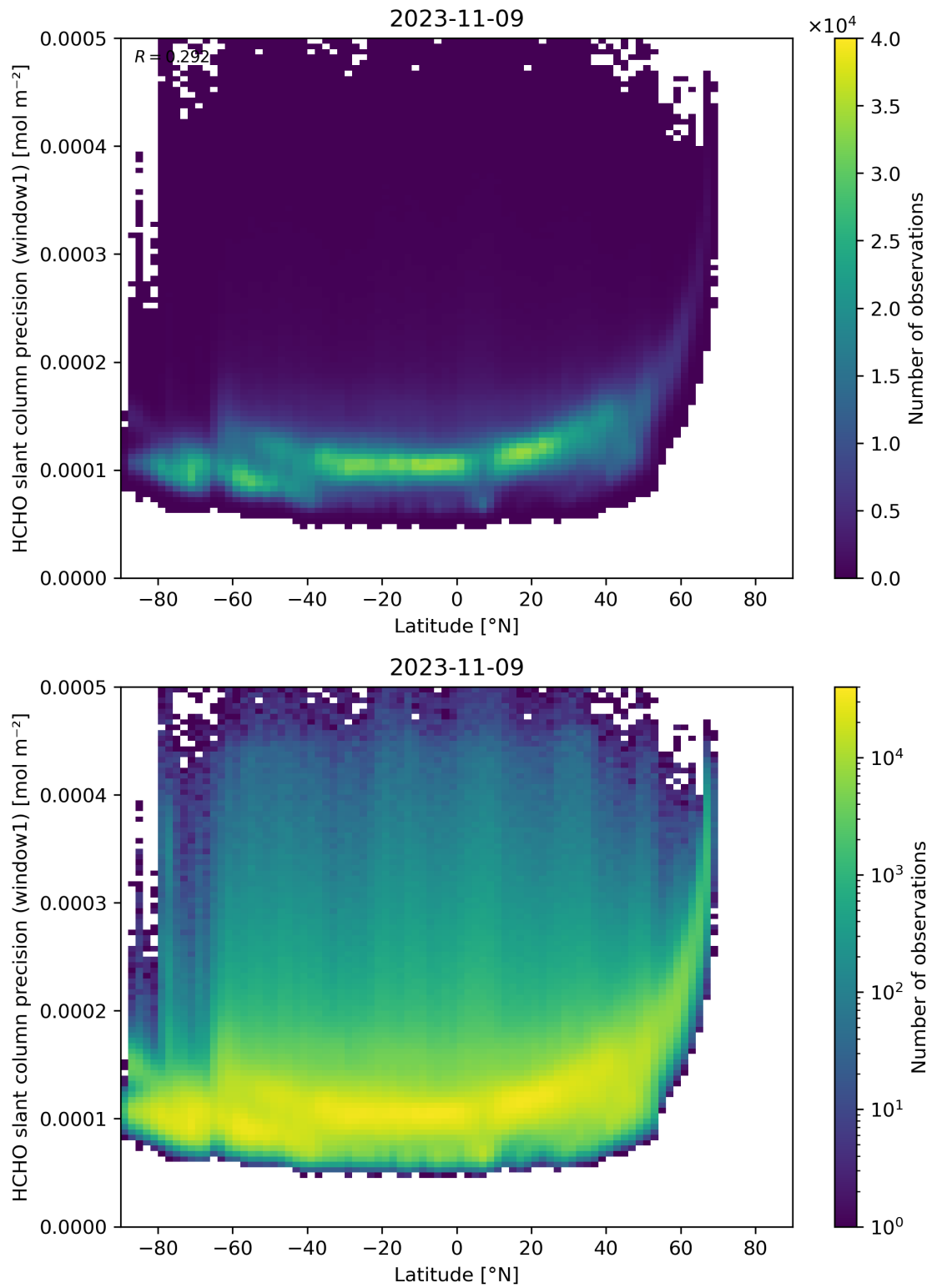
Figure 160: Scatter density plot of “Latitude” against “HCHO slant column precision (window1)” for 2023-11-08 to 2023-11-10.
