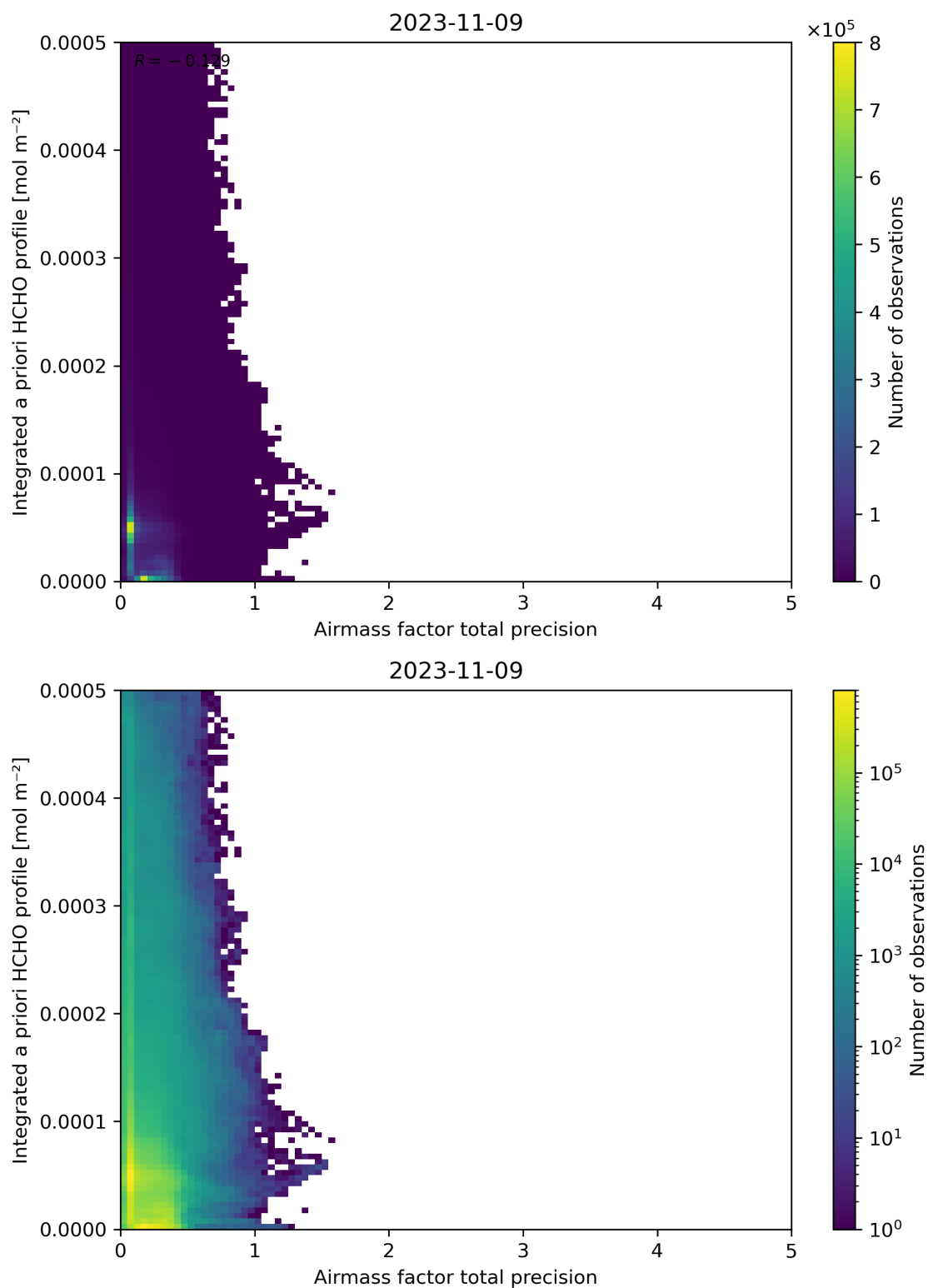
Figure 111: Scatter density plot of “Airmass factor total precision” against “Integrated a priori HCHO profile” for 2023-11-08 to 2023-11-10.
