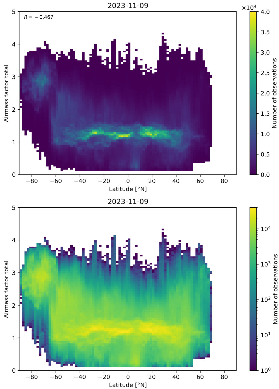
Figure 161: Scatter density plot of “Latitude” against “Airmass factor total” for 2023-11-08 to 2023-11-10.
