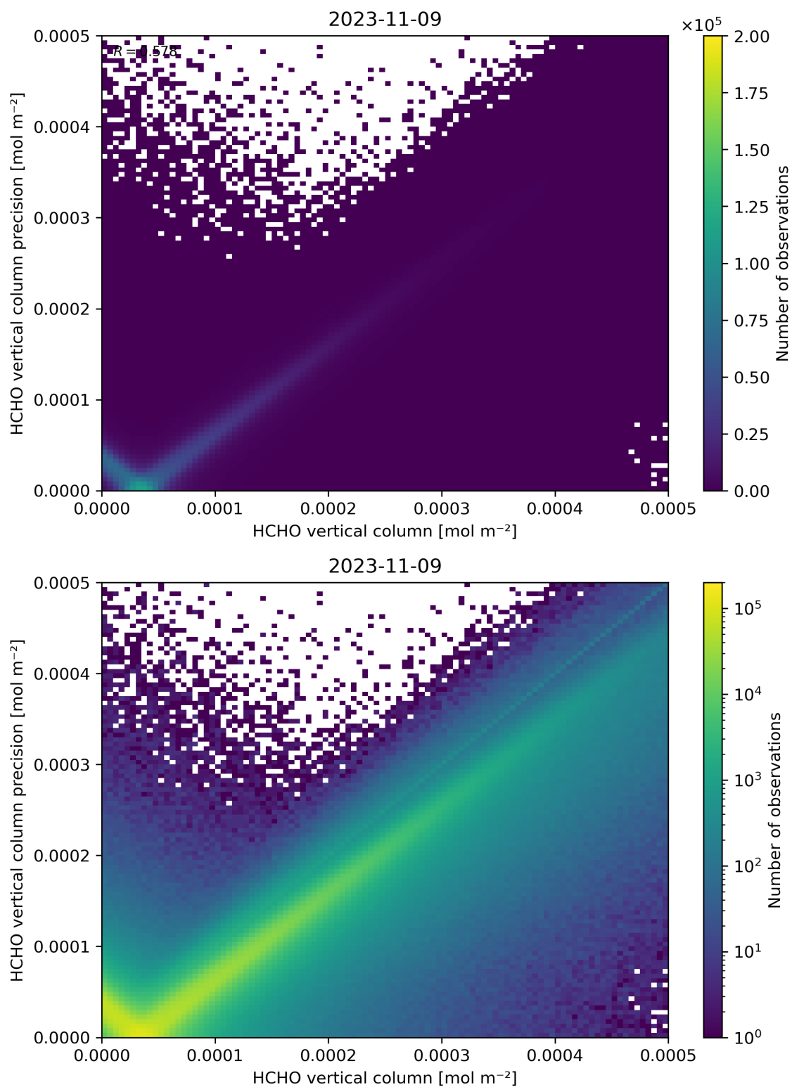
Figure 134: Scatter density plot of “HCHO vertical column” against “HCHO vertical column precision” for 2023-11-08 to 2023-11-10.
