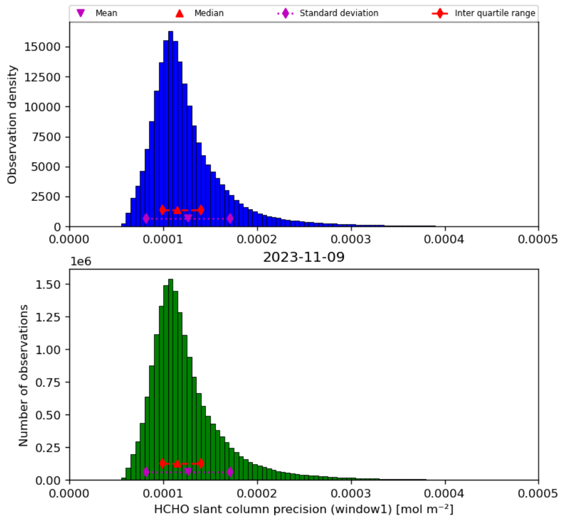
Figure 39: Histogram of “HCHO slant column precision (window1)” for 2023-11-08 to 2023-11-10
