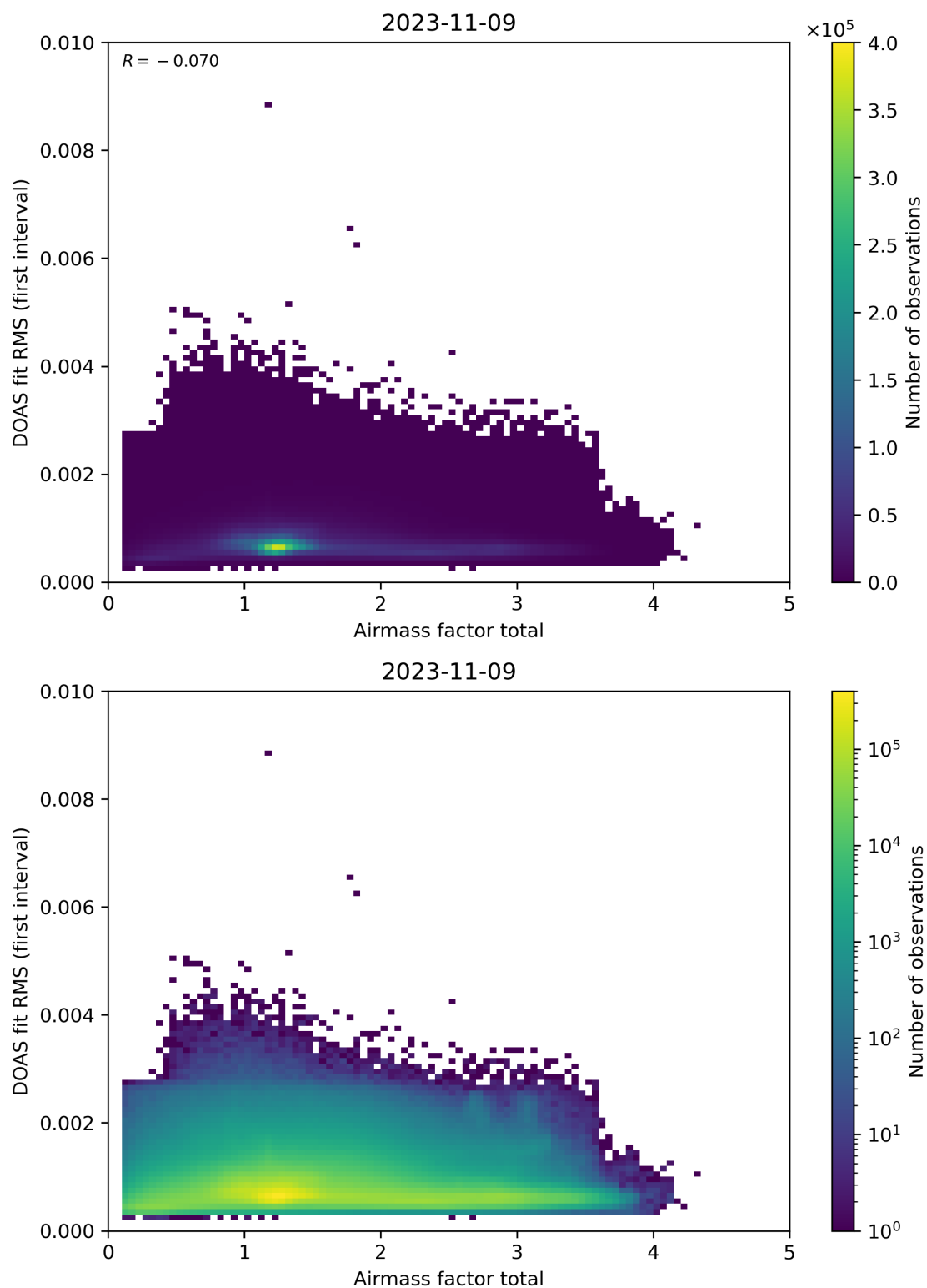
Figure 97: Scatter density plot of “Airmass factor total” against “DOAS fit RMS (first interval)” for 2023-11-08 to 2023-11-10.
