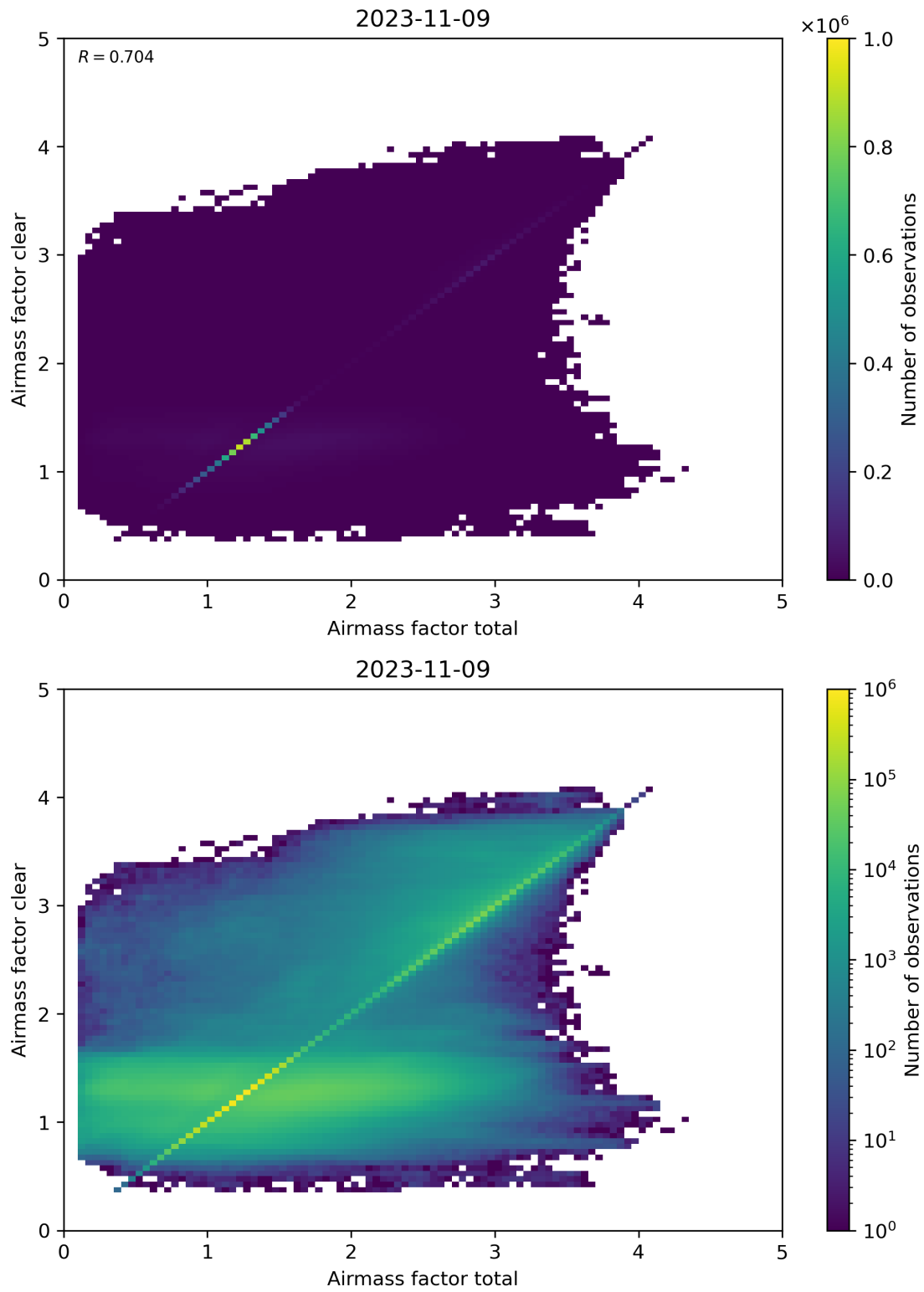
Figure 100: Scatter density plot of “Airmass factor total” against “Airmass factor clear” for 2023-11-08 to 2023-11-10.
