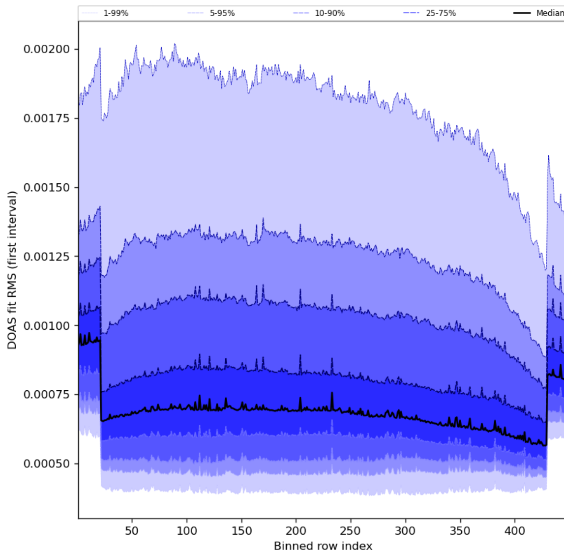
Figure 60: Along track statistics of “DOAS fit RMS (first interval)” for 2023-11-08 to 2023-11-10
