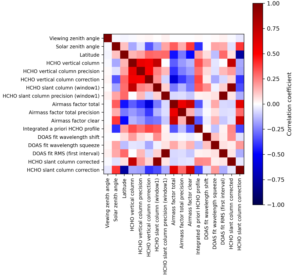
Figure 2: Map of correlation matrix for 2023-11-08 to 2023-11-10.
