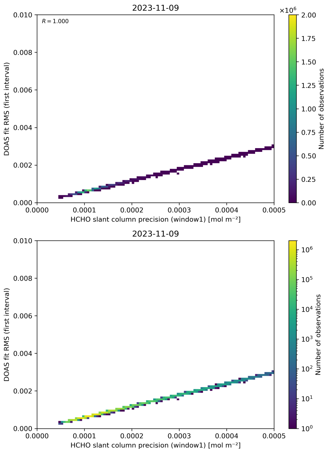
Figure 88: Scatter density plot of “HCHO slant column precision (window1)” against “DOAS fit RMS (first interval)” for 2023-11-08 to 2023-11-10.
