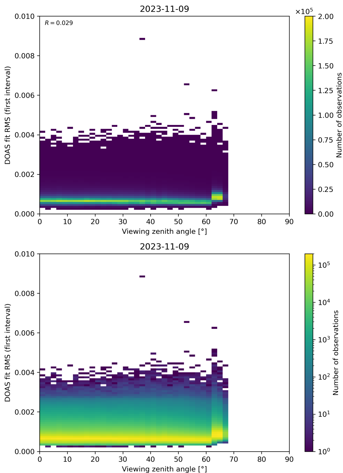
Figure 182: Scatter density plot of “Viewing zenith angle” against “DOAS fit RMS (first interval)” for 2023-11-08 to 2023-11-10.
