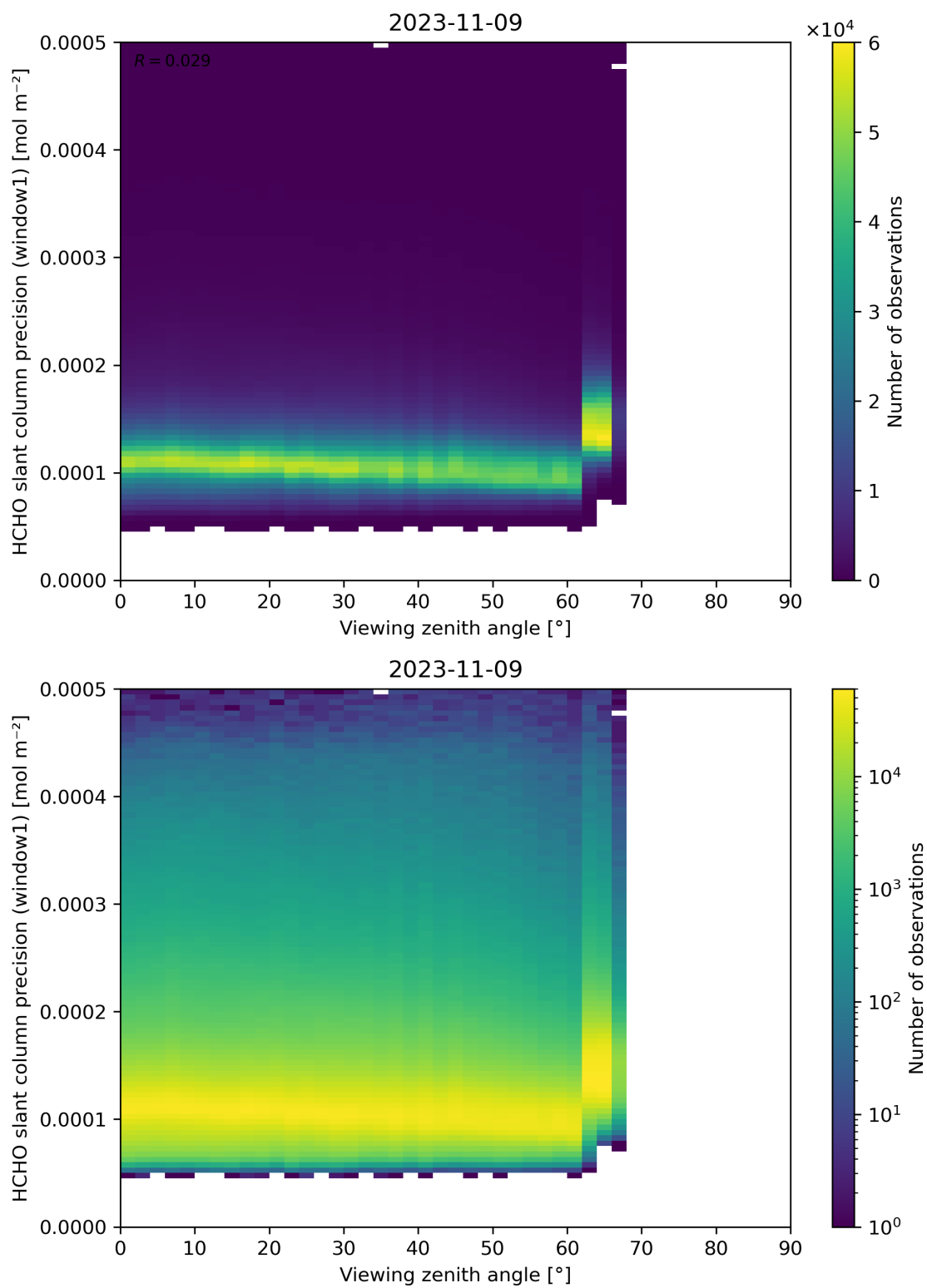
Figure 189: Scatter density plot of “Viewing zenith angle” against “HCHO slant column precision (window1)” for 2023-11-08 to 2023-11-10.
