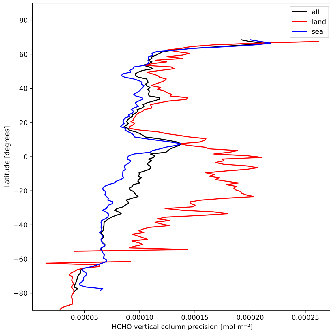
Figure 22: Zonal average of “HCHO vertical column precision” for 2023-11-08 to 2023-11-10.
