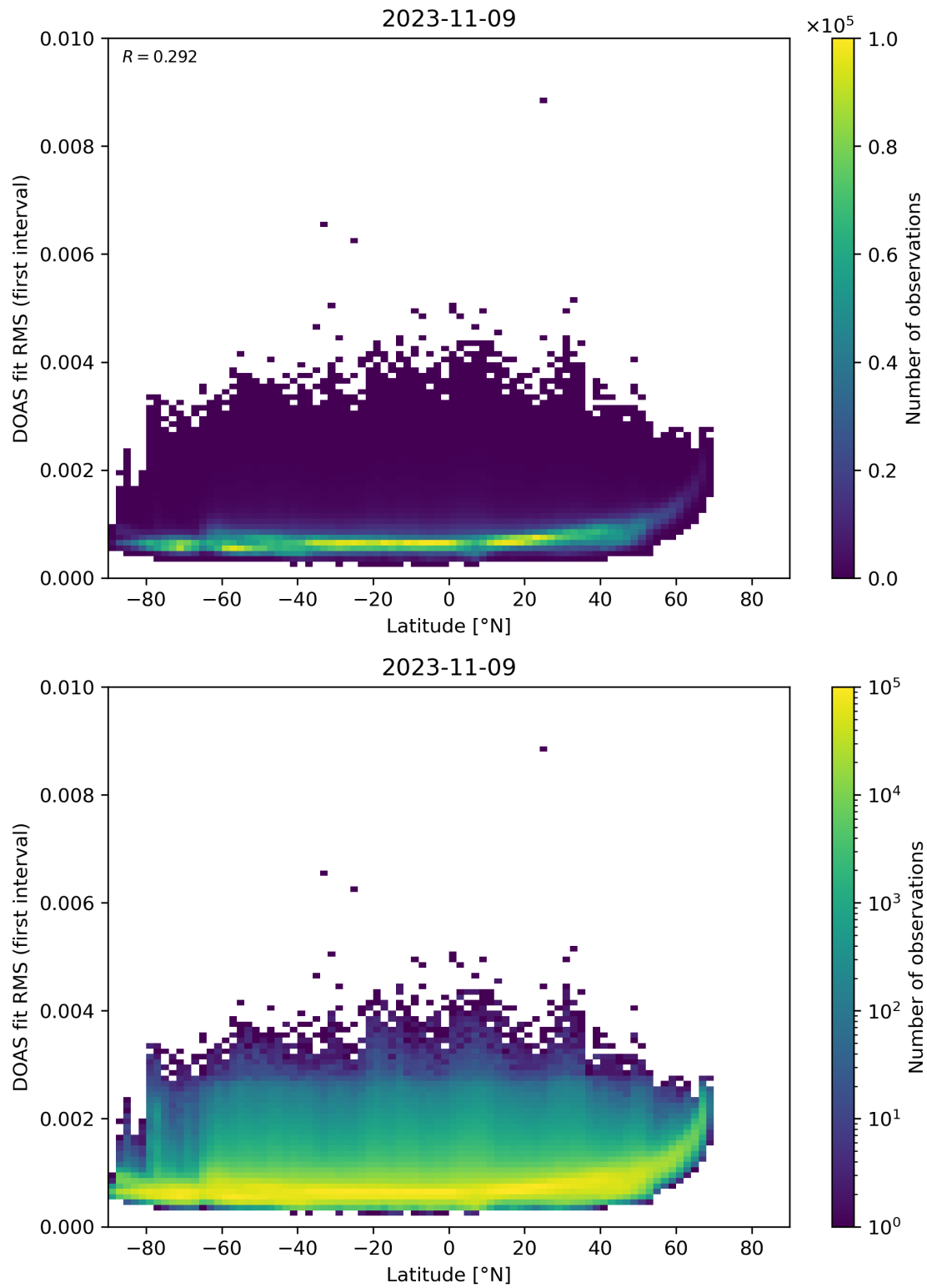
Figure 153: Scatter density plot of “Latitude” against “DOAS fit RMS (first interval)” for 2023-11-08 to 2023-11-10.
