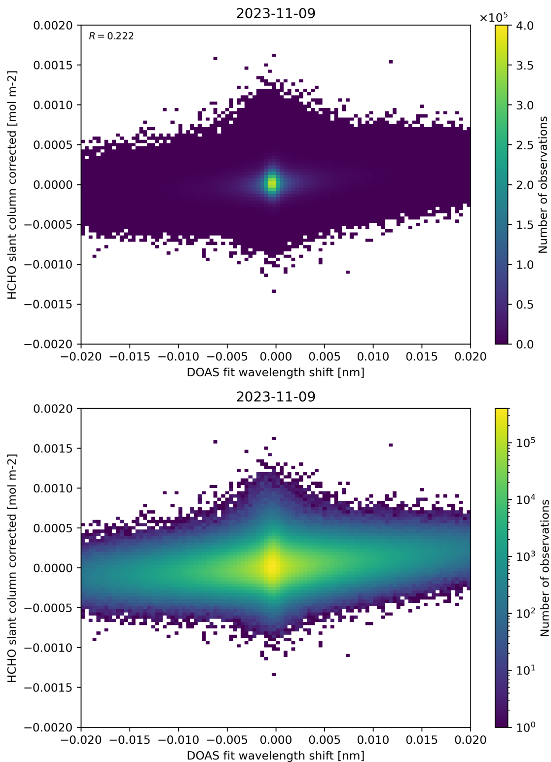
Figure 66: Scatter density plot of “DOAS fit wavelength shift” against “HCHO slant column corrected” for 2023-11-08 to 2023-11-10.
