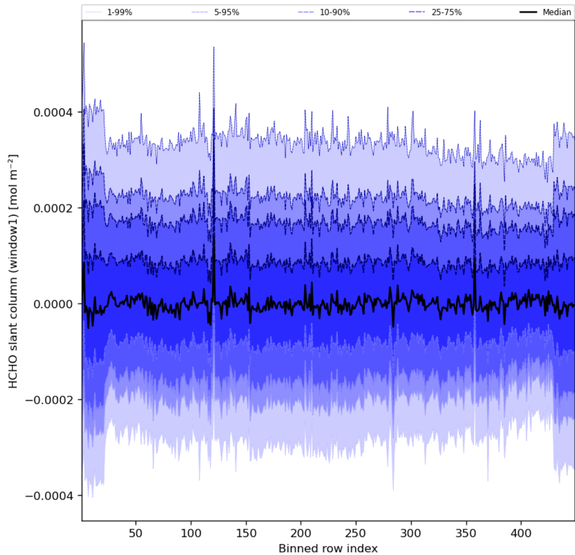
Figure 52: Along track statistics of “HCHO slant column (window1)” for 2023-11-08 to 2023-11-10
