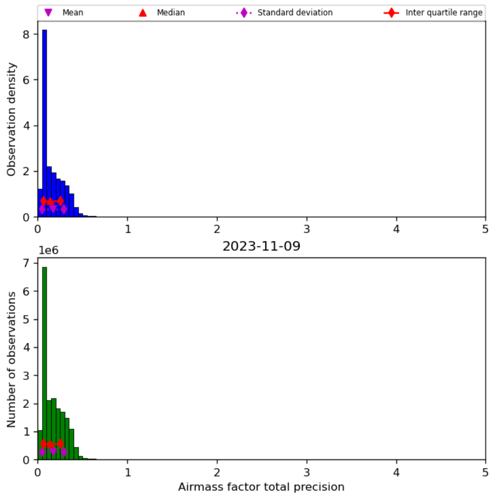
Figure 41: Histogram of “Airmass factor total precision” for 2023-11-08 to 2023-11-10
