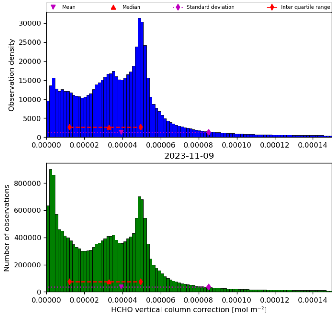
Figure 37: Histogram of “HCHO vertical column correction” for 2023-11-08 to 2023-11-10
