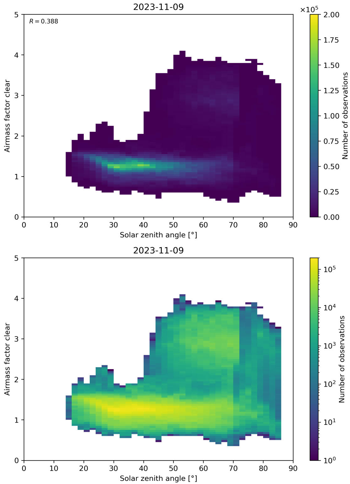
Figure 170: Scatter density plot of “Solar zenith angle” against “Airmass factor clear” for 2023-11-08 to 2023-11-10.
