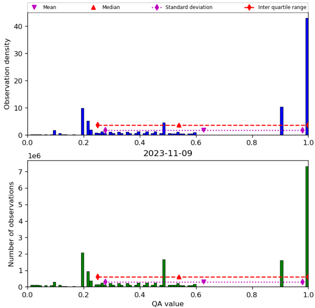
Figure 34: Histogram of “QA value” for 2023-11-08 to 2023-11-10
