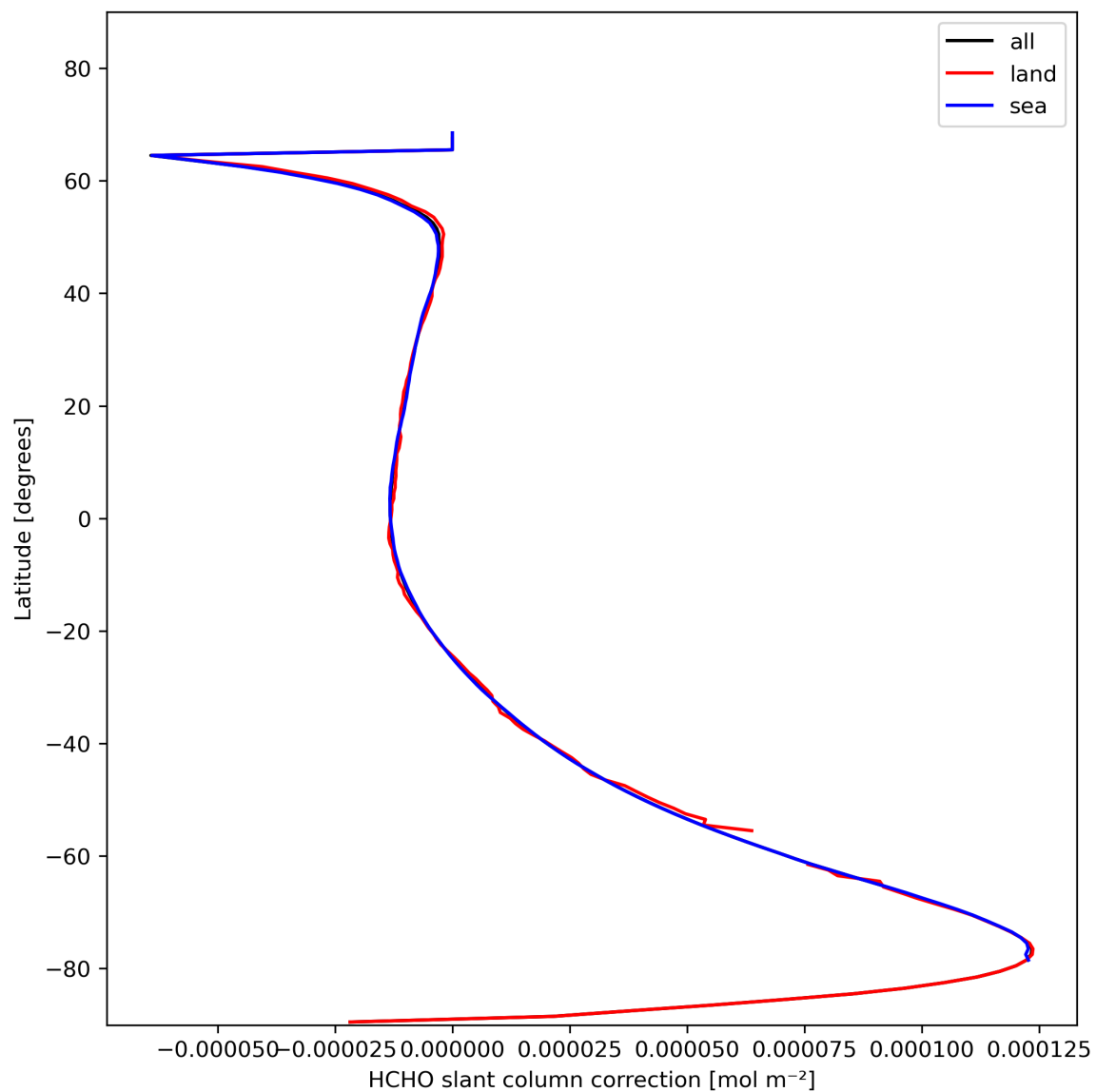
Figure 33: Zonal average of “HCHO slant column correction” for 2023-11-08 to 2023-11-10.
