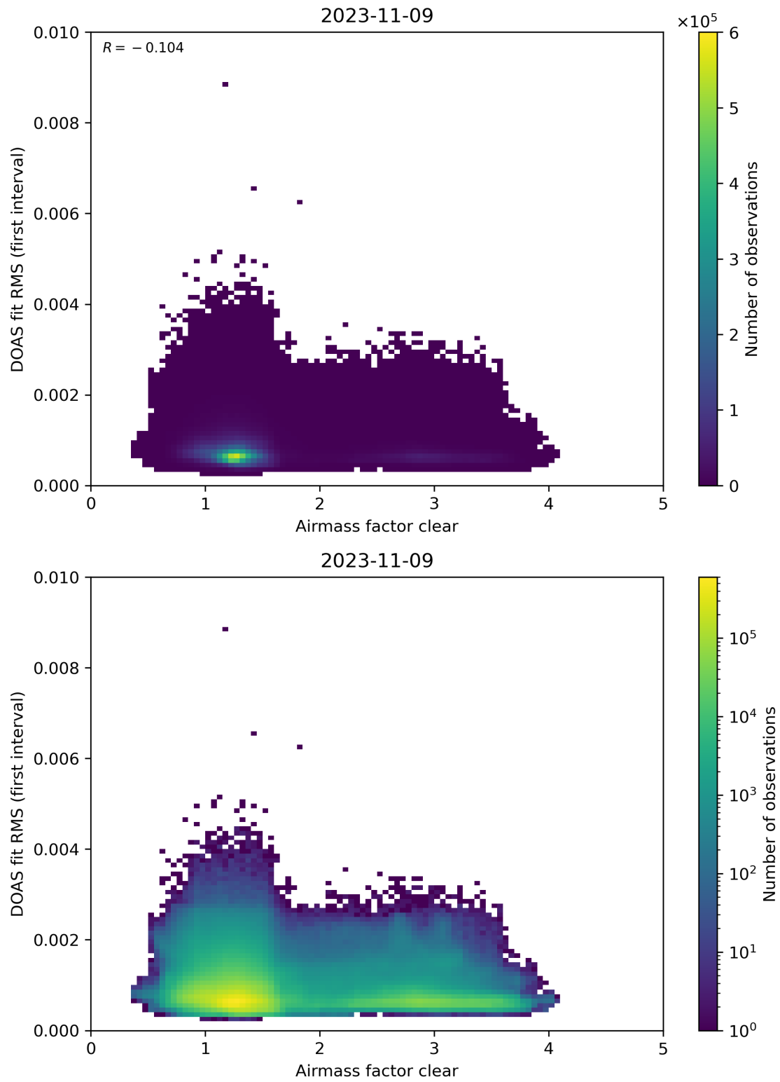
Figure 71: Scatter density plot of “Airmass factor clear” against “DOAS fit RMS (first interval)” for 2023-11-08 to 2023-11-10.
