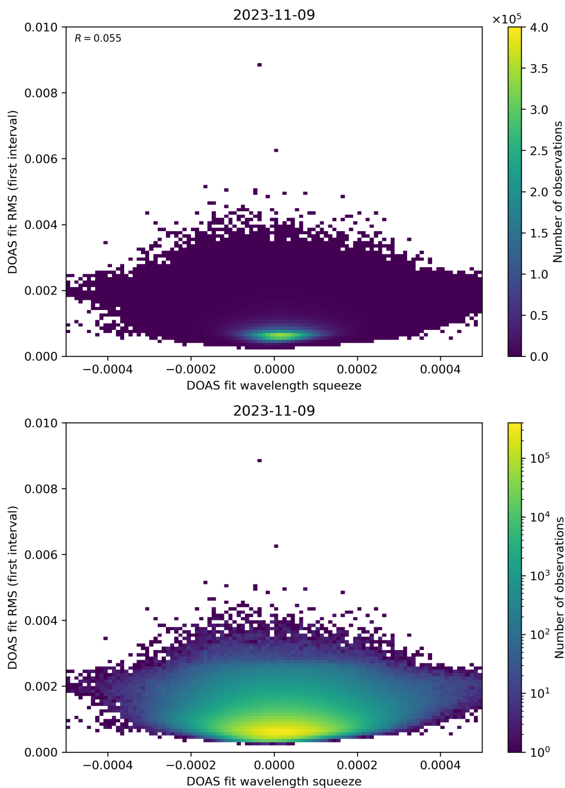
Figure 68: Scatter density plot of “DOAS fit wavelength squeeze” against “DOAS fit RMS (first interval)” for 2023-11-08 to 2023-11-10.
