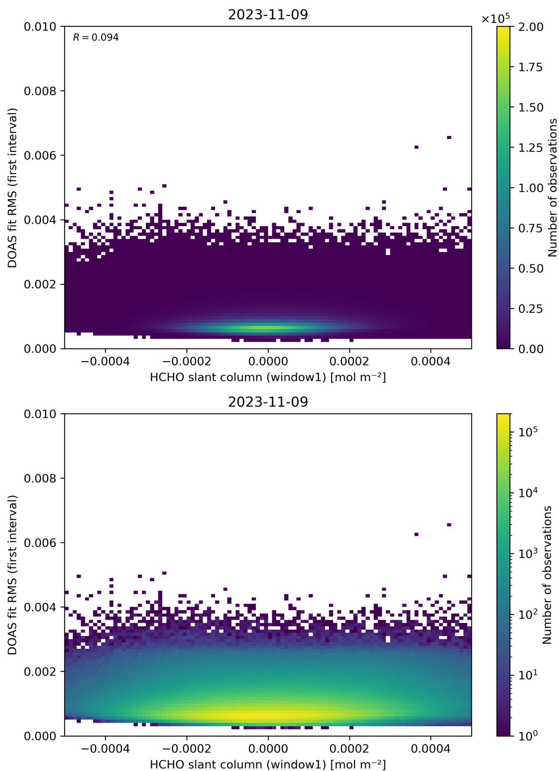
Figure 78: Scatter density plot of “HCHO slant column (window1)” against “DOAS fit RMS (first interval)” for 2023-11-08 to 2023-11-10.
