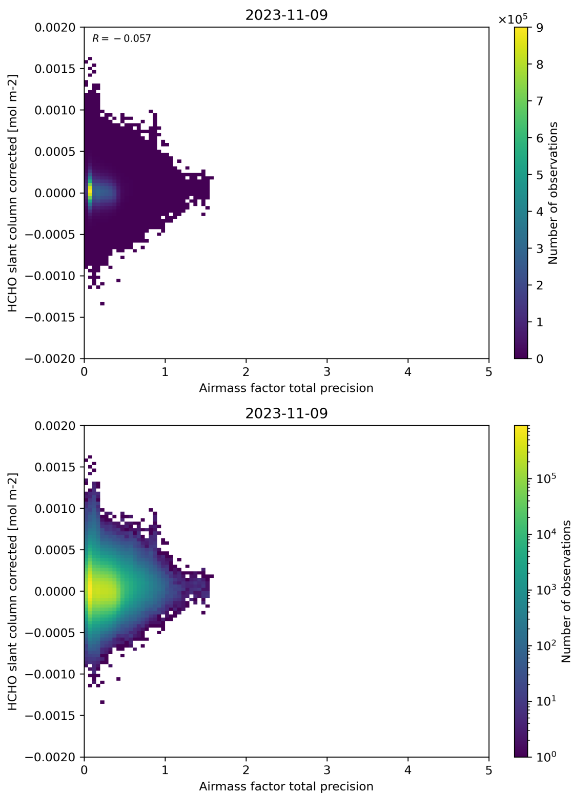
Figure 109: Scatter density plot of “Airmass factor total precision” against “HCHO slant column corrected” for 2023-11-08 to 2023-11-10.
