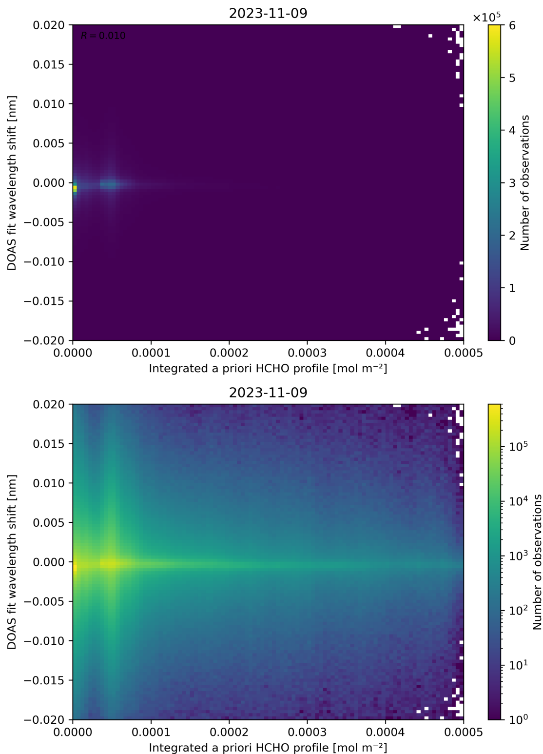
Figure 149: Scatter density plot of “Integrated a priori HCHO profile” against “DOAS fit wavelength shift” for 2023-11-08 to 2023-11-10.
