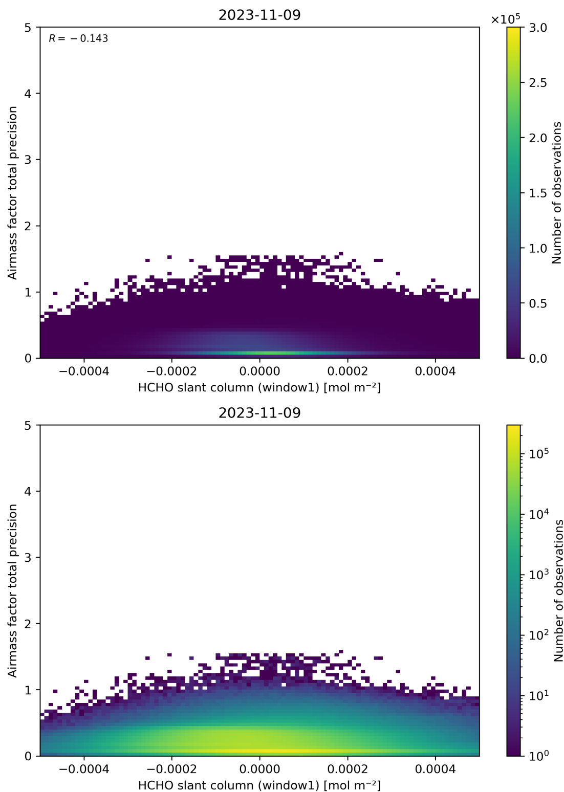
Figure 86: Scatter density plot of “HCHO slant column (window1)” against “Airmass factor total precision” for 2023-11-08 to 2023-11-10.
