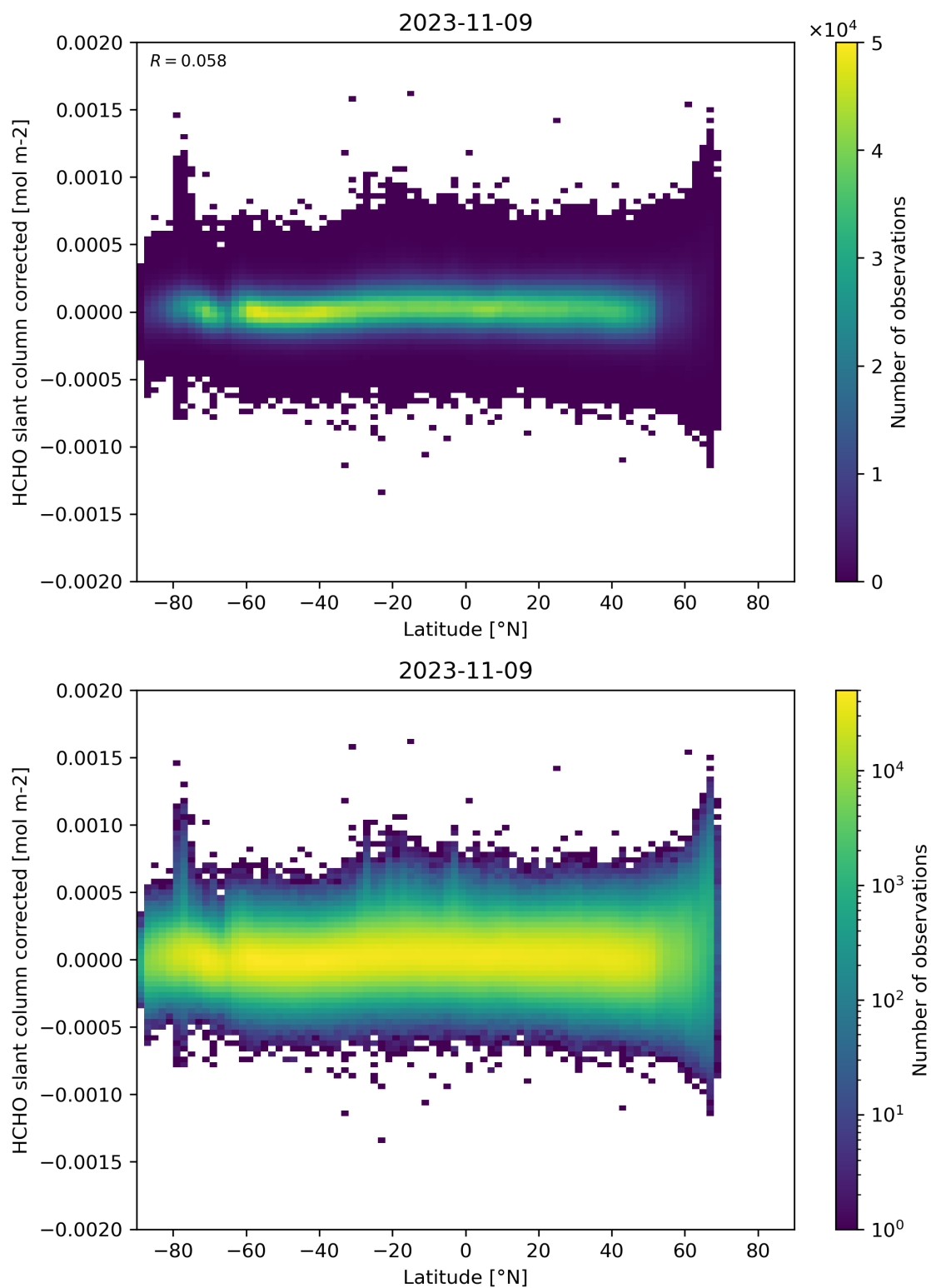
Figure 157: Scatter density plot of “Latitude” against “HCHO slant column corrected” for 2023-11-08 to 2023-11-10.
