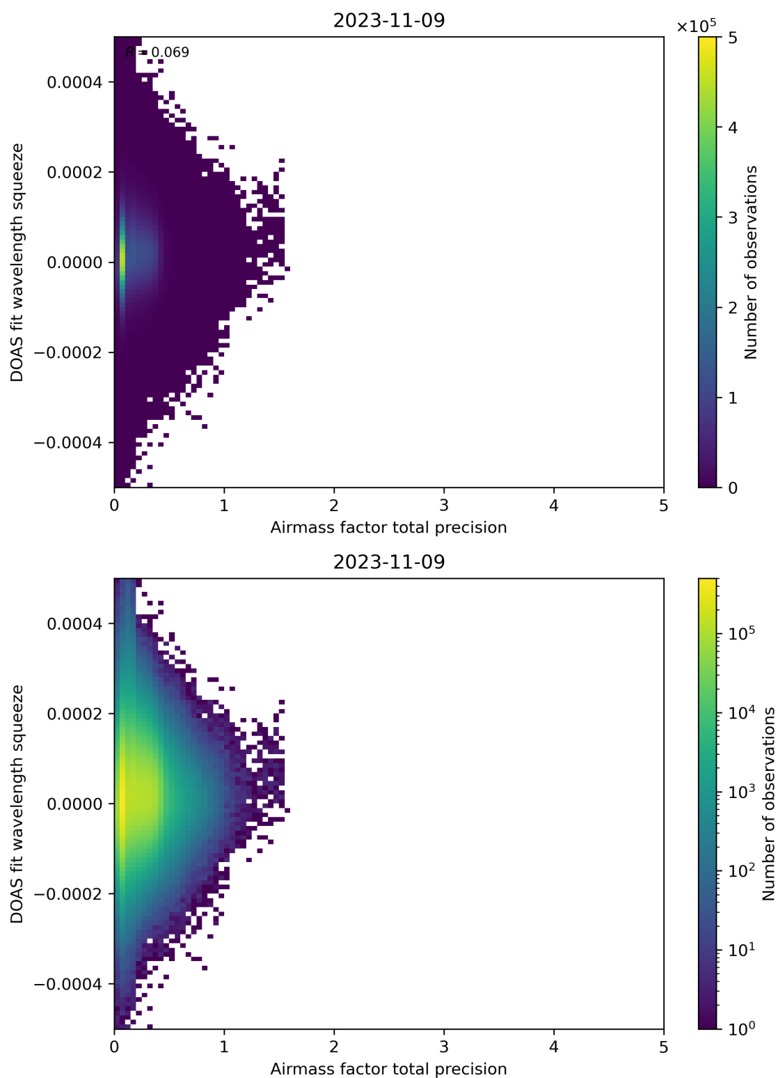
Figure 107: Scatter density plot of “Airmass factor total precision” against “DOAS fit wavelength squeeze” for 2023-11-08 to 2023-11-10.
