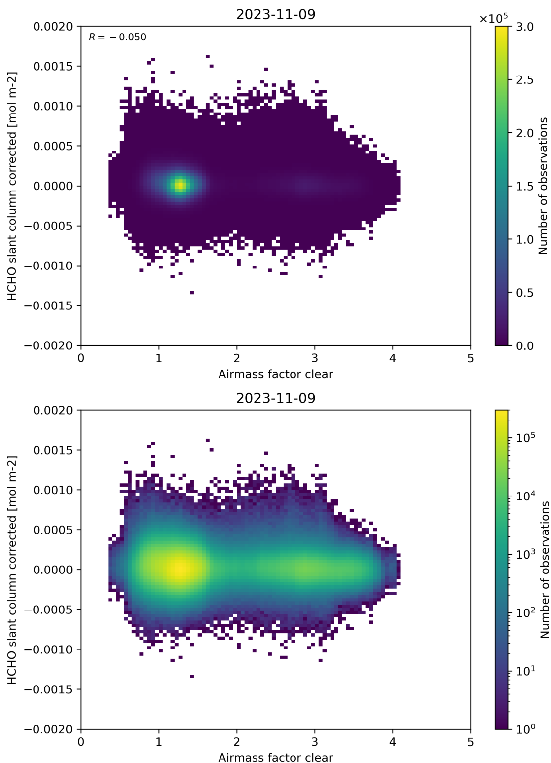
Figure 74: Scatter density plot of “Airmass factor clear” against “HCHO slant column corrected” for 2023-11-08 to 2023-11-10.
