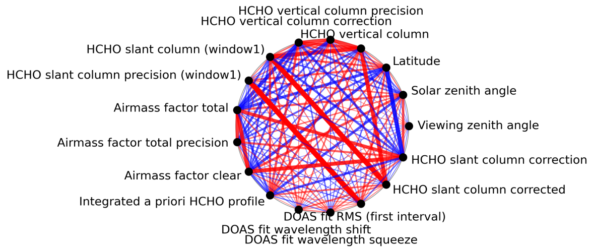
Figure 1: Map of correlation graph for 2023-11-08 to 2023-11-10.
