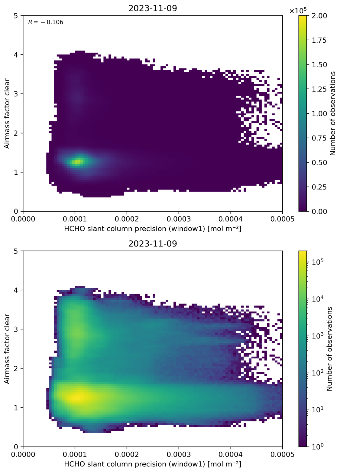
Figure 91: Scatter density plot of “HCHO slant column precision (window1)” against “Airmass factor clear” for 2023-11-08 to 2023-11-10.
