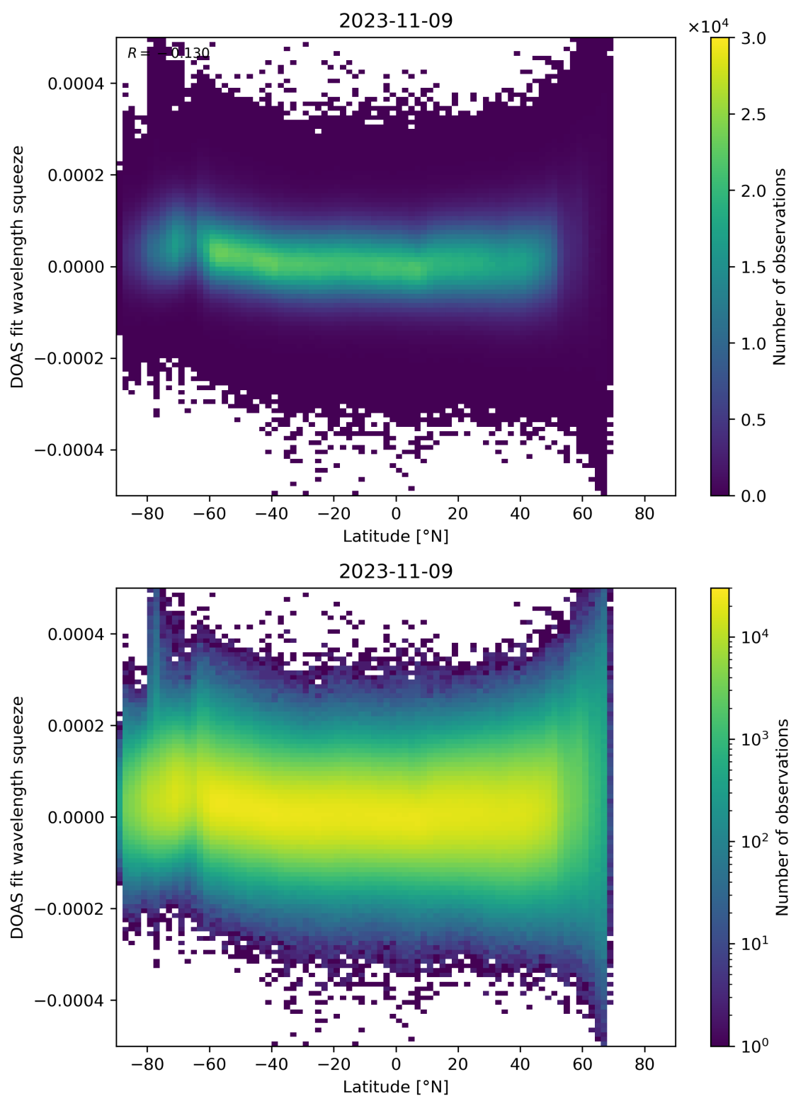
Figure 155: Scatter density plot of “Latitude” against “DOAS fit wavelength squeeze” for 2023-11-08 to 2023-11-10.
