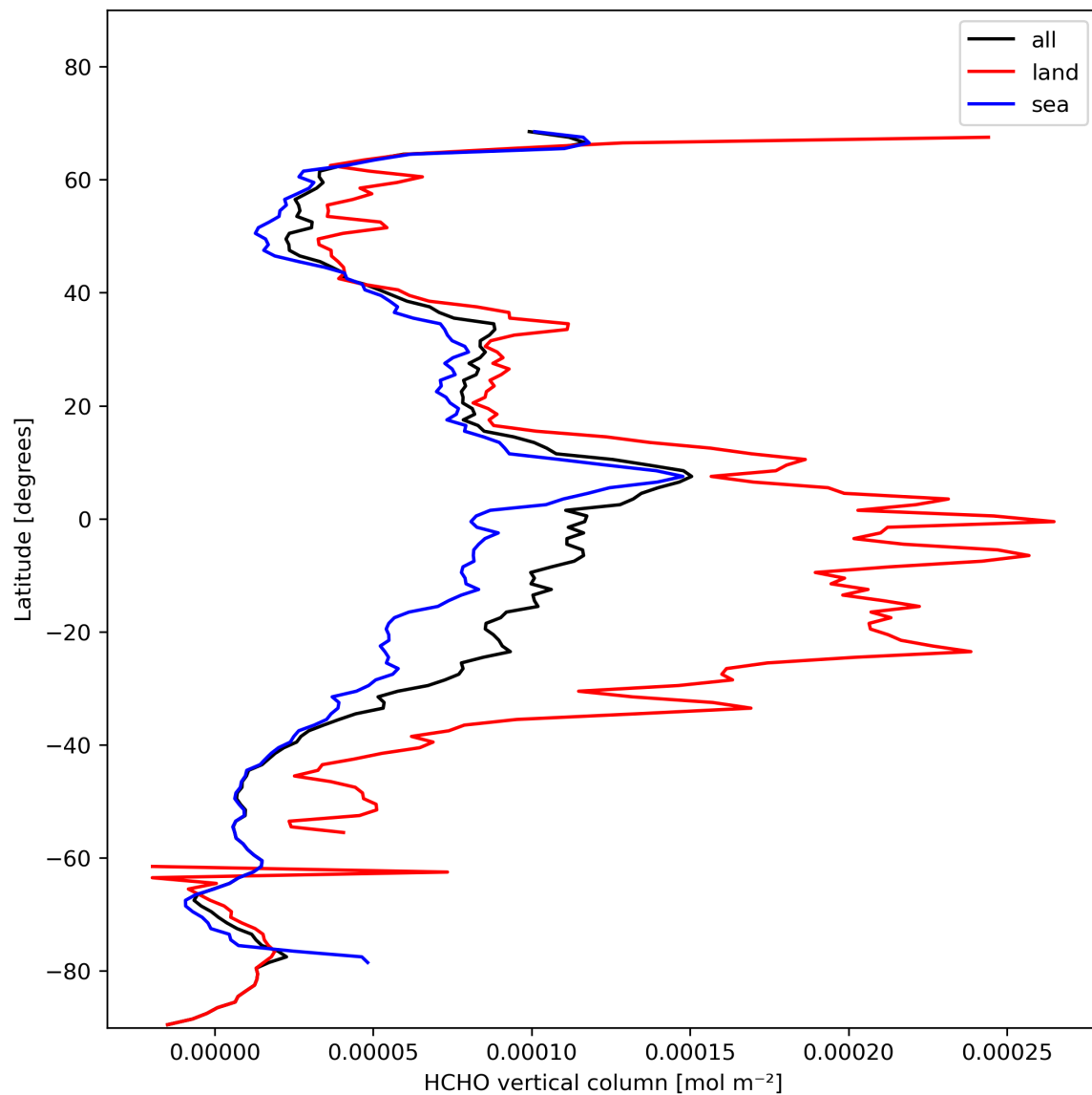
Figure 21: Zonal average of “HCHO vertical column” for 2023-11-08 to 2023-11-10.
