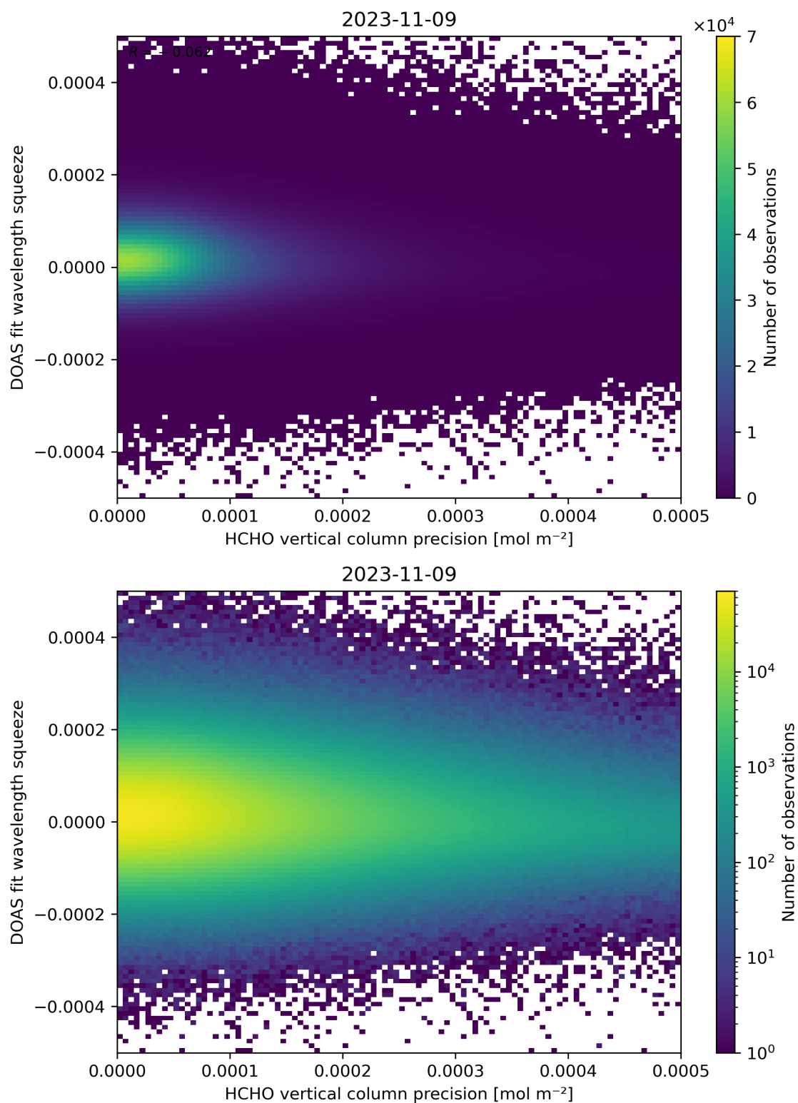
Figure 138: Scatter density plot of “HCHO vertical column precision” against “DOAS fit wavelength squeeze” for 2023-11-08 to 2023-11-10.
