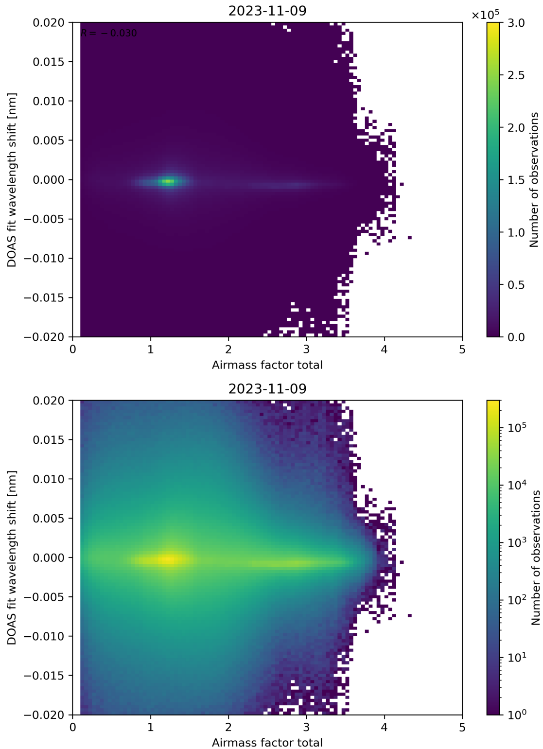
Figure 98: Scatter density plot of “Airmass factor total” against “DOAS fit wavelength shift” for 2023-11-08 to 2023-11-10.
