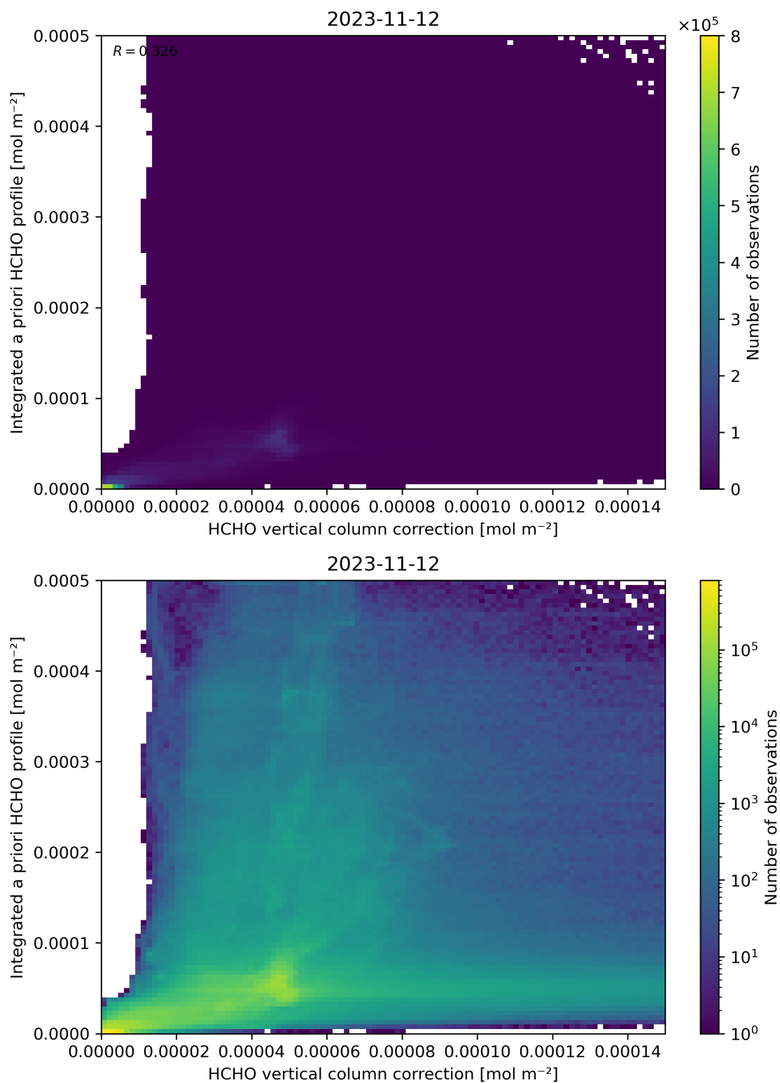
Figure 122: Scatter density plot of “HCHO vertical column correction” against “Integrated a priori HCHO profile” for 2023-11-12 to 2023-11-13.
