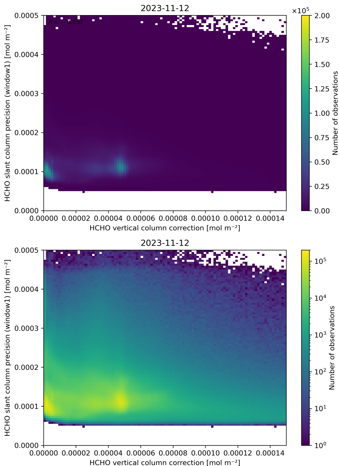
Figure 119: Scatter density plot of “HCHO vertical column correction” against “HCHO slant column precision (window1)” for 2023-11-12 to 2023-11-13.
