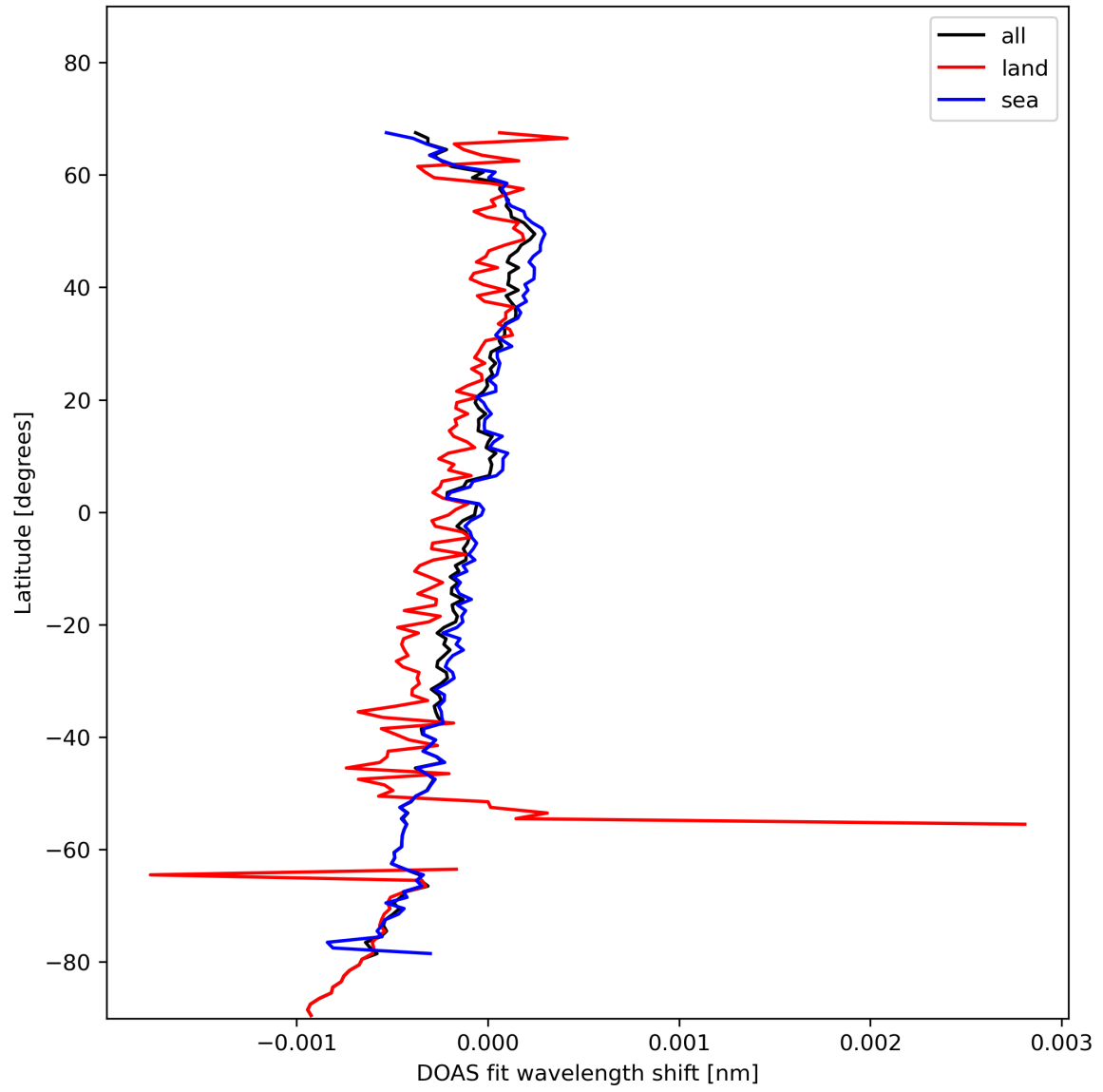
Figure 30: Zonal average of “DOAS fit wavelength shift” for 2023-11-12 to 2023-11-13.
