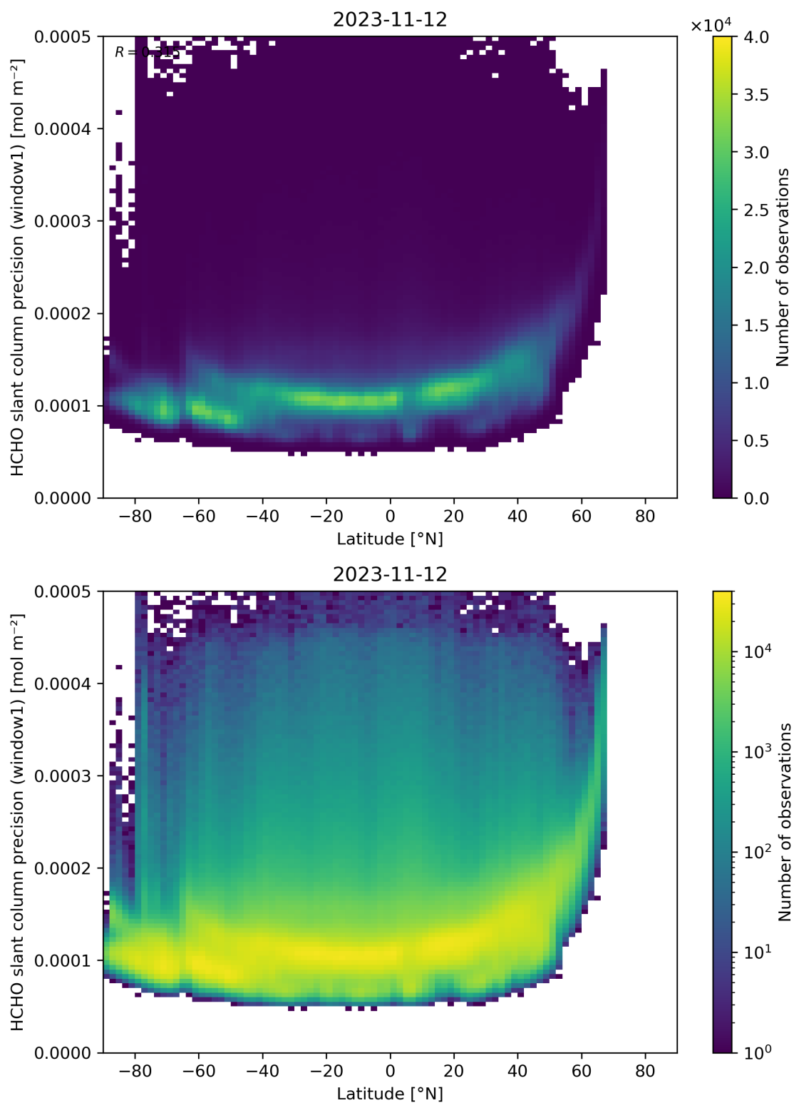
Figure 160: Scatter density plot of “Latitude” against “HCHO slant column precision (window1)” for 2023-11-12 to 2023-11-13.
