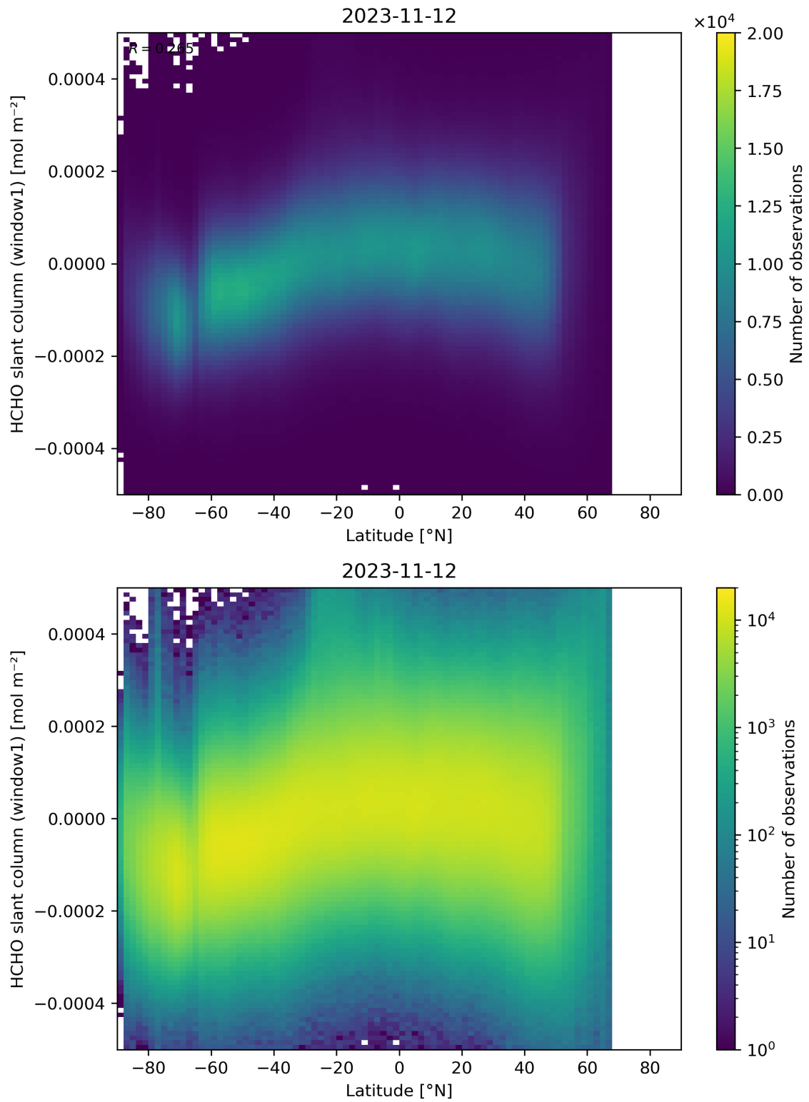
Figure 159: Scatter density plot of “Latitude” against “HCHO slant column (window1)” for 2023-11-12 to 2023-11-13.
