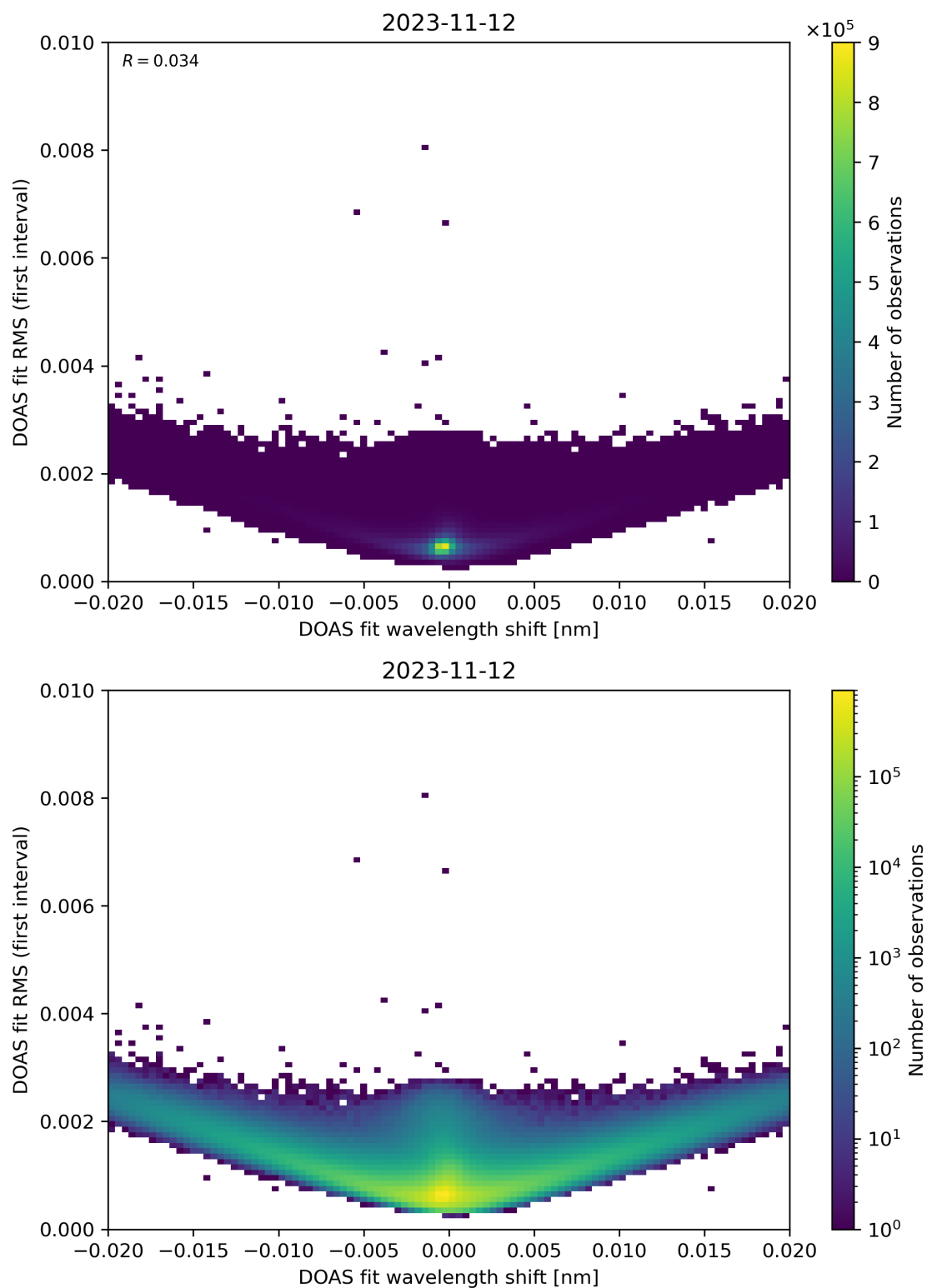
Figure 64: Scatter density plot of “DOAS fit wavelength shift” against “DOAS fit RMS (first interval)” for 2023-11-12 to 2023-11-13.
