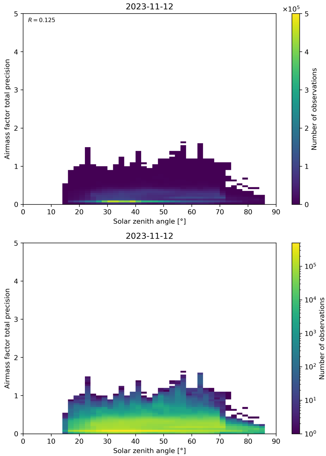
Figure 176: Scatter density plot of “Solar zenith angle” against “Airmass factor total precision” for 2023-11-12 to 2023-11-13.
