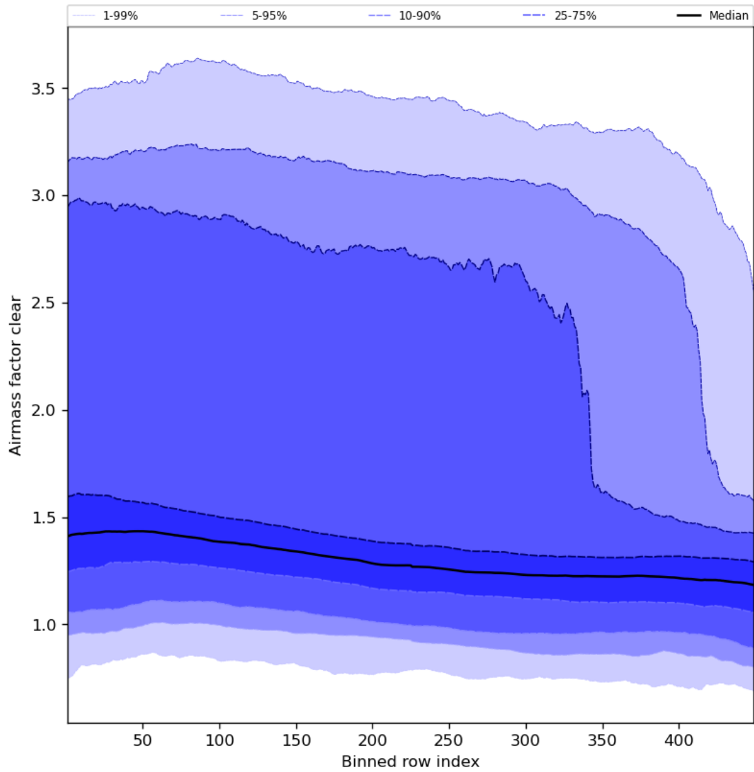
Figure 56: Along track statistics of “Airmass factor clear” for 2023-11-12 to 2023-11-13
