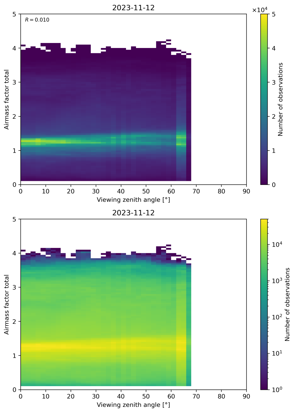
Figure 190: Scatter density plot of “Viewing zenith angle” against “Airmass factor total” for 2023-11-12 to 2023-11-13.
