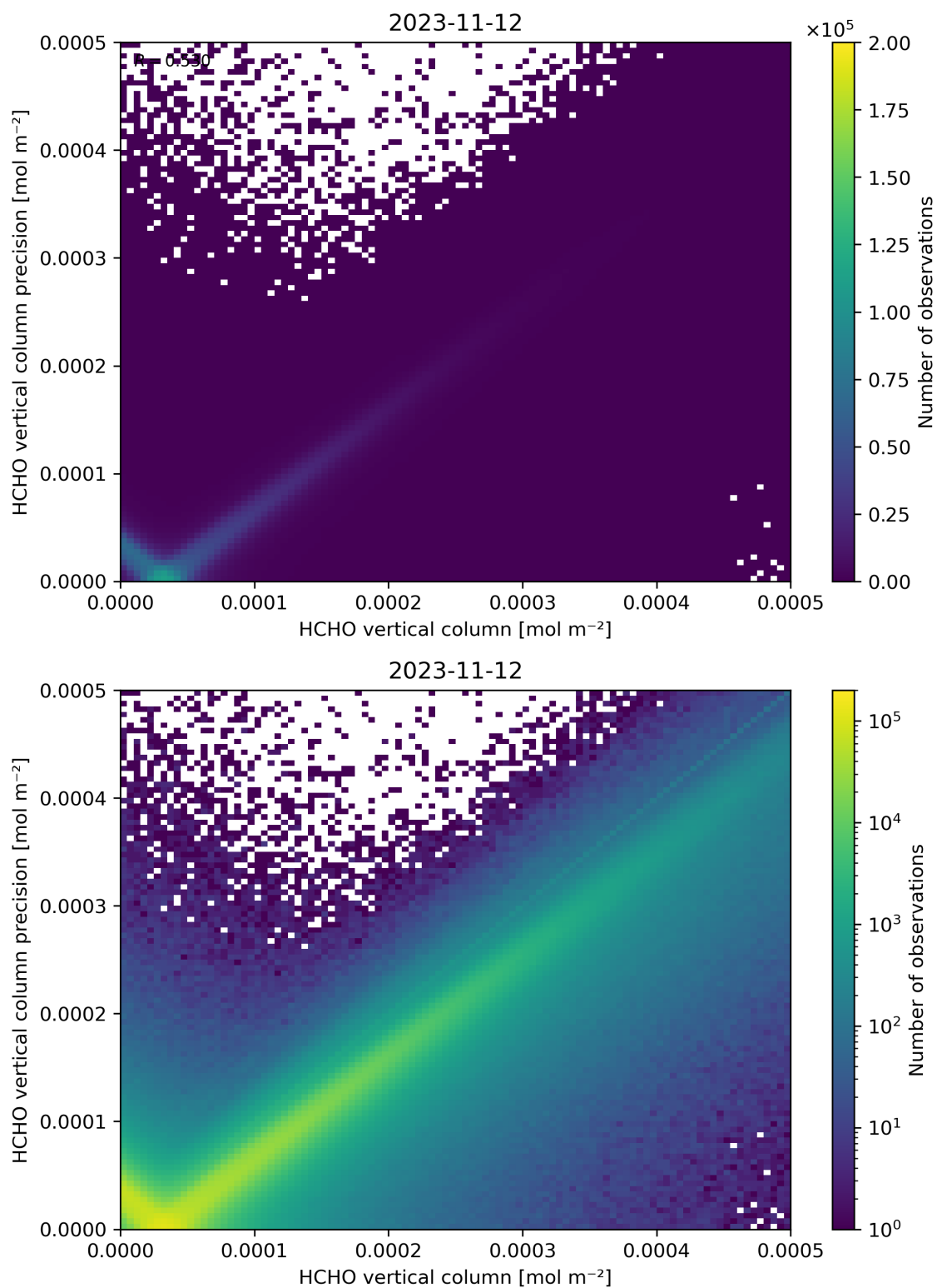
Figure 134: Scatter density plot of “HCHO vertical column” against “HCHO vertical column precision” for 2023-11-12 to 2023-11-13.
