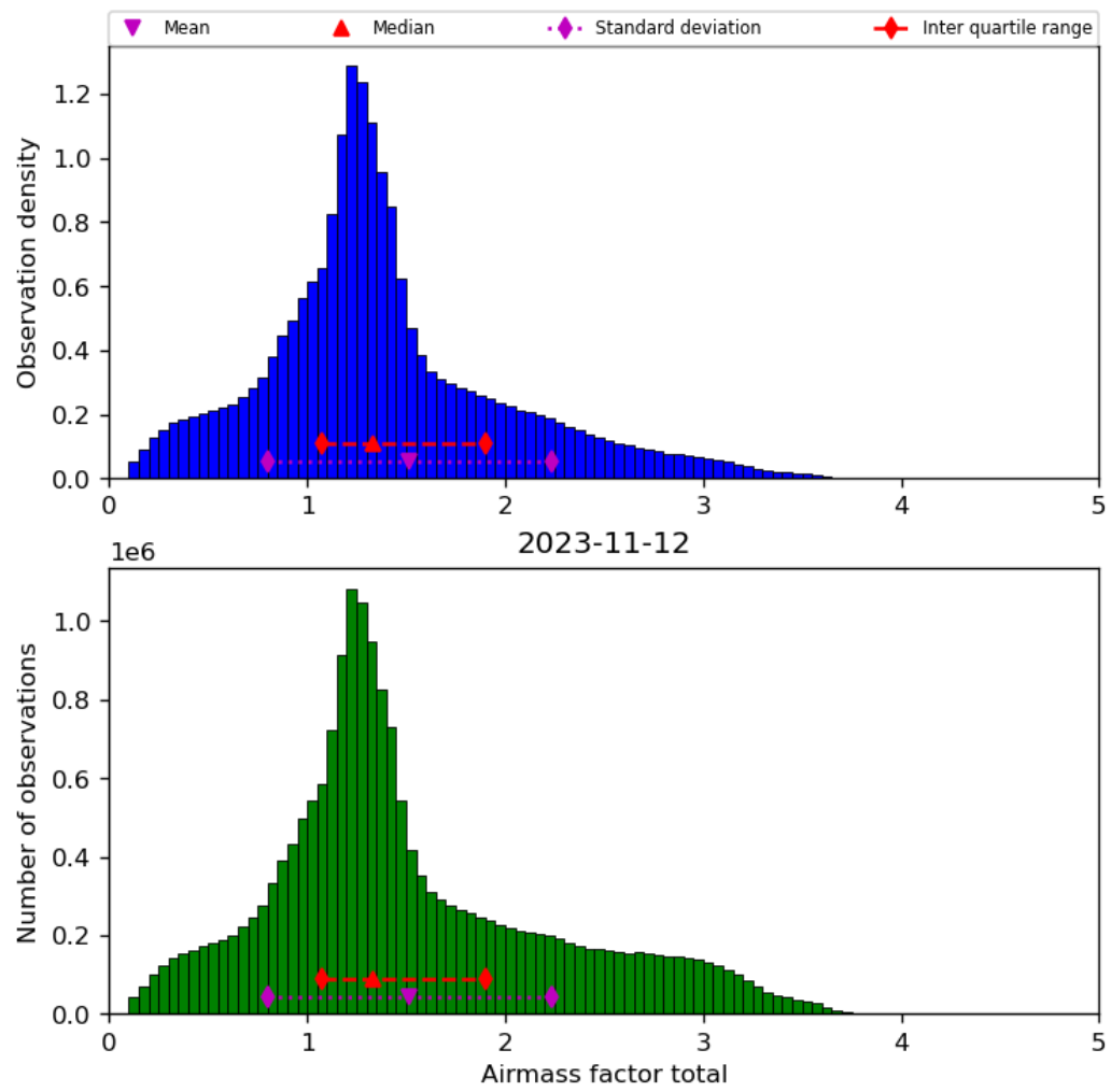
Figure 40: Histogram of “Airmass factor total” for 2023-11-12 to 2023-11-13
