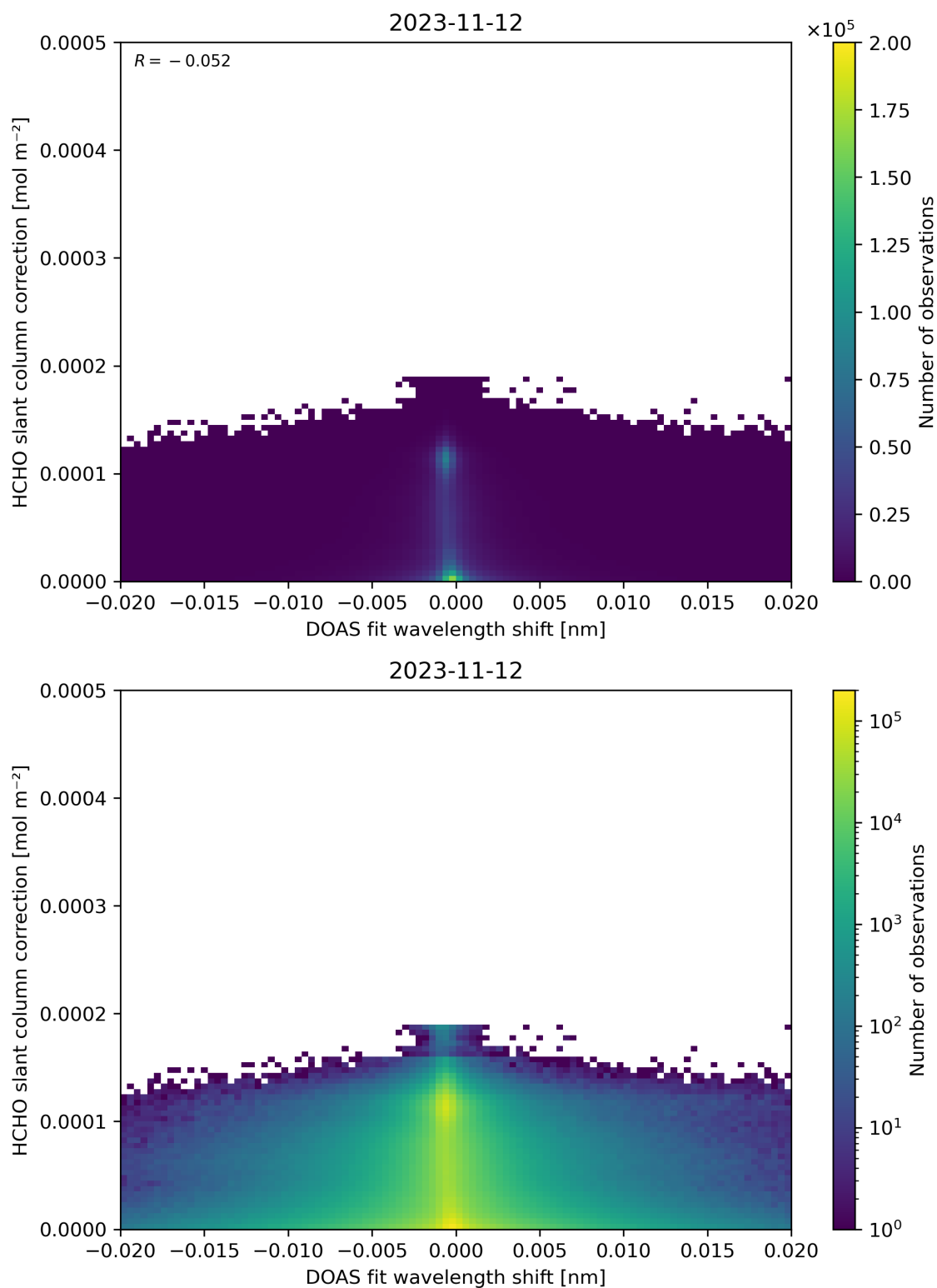
Figure 67: Scatter density plot of “DOAS fit wavelength shift” against “HCHO slant column correction” for 2023-11-12 to 2023-11-13.
