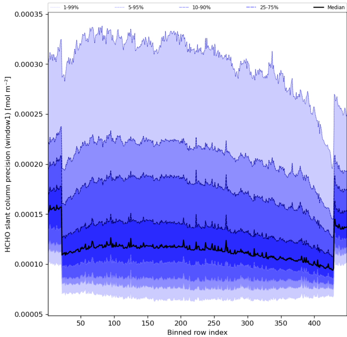
Figure 53: Along track statistics of “HCHO slant column precision (window1)” for 2023-11-12 to 2023-11-13
