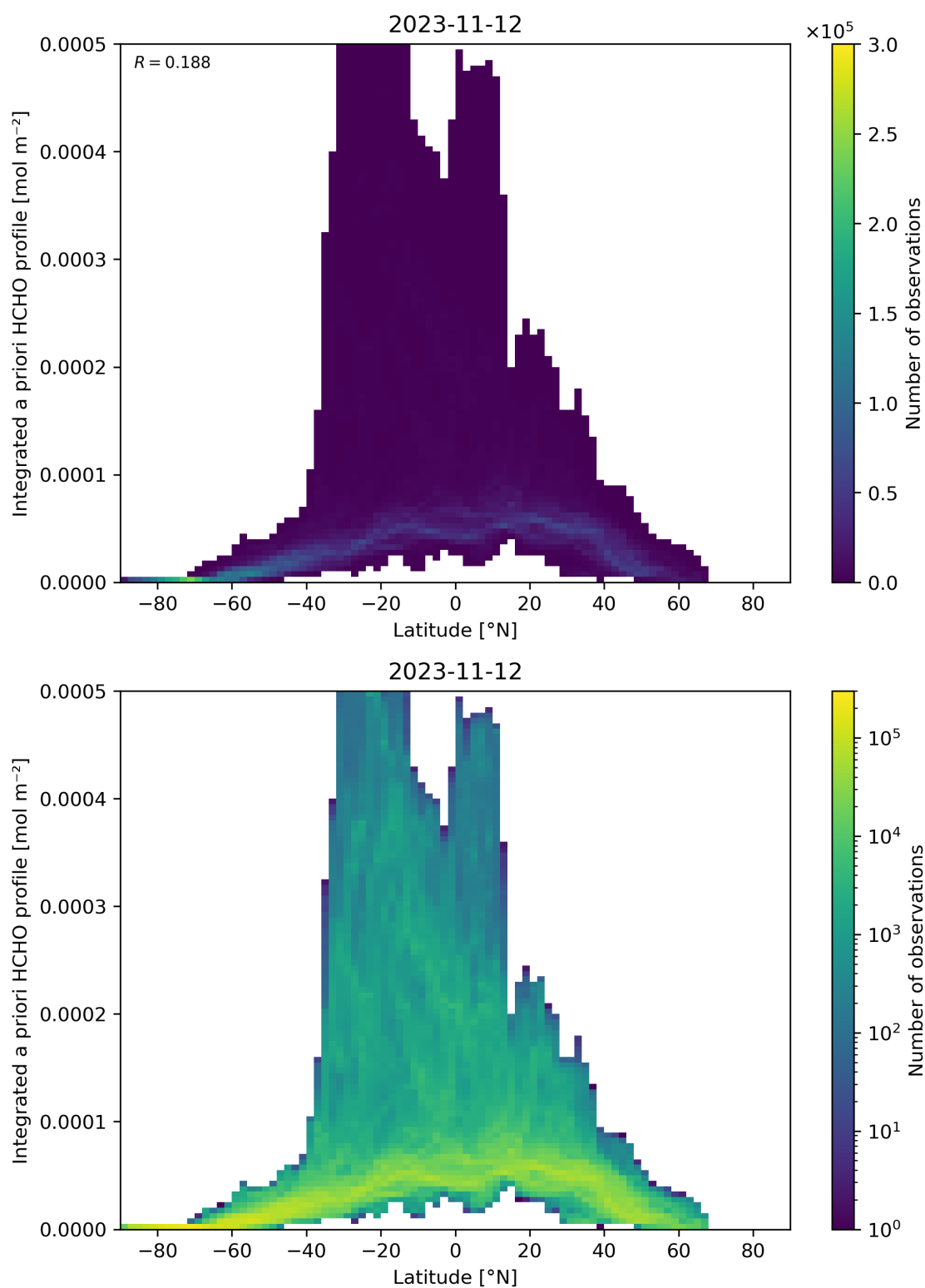
Figure 166: Scatter density plot of “Latitude” against “Integrated a priori HCHO profile” for 2023-11-12 to 2023-11-13.
