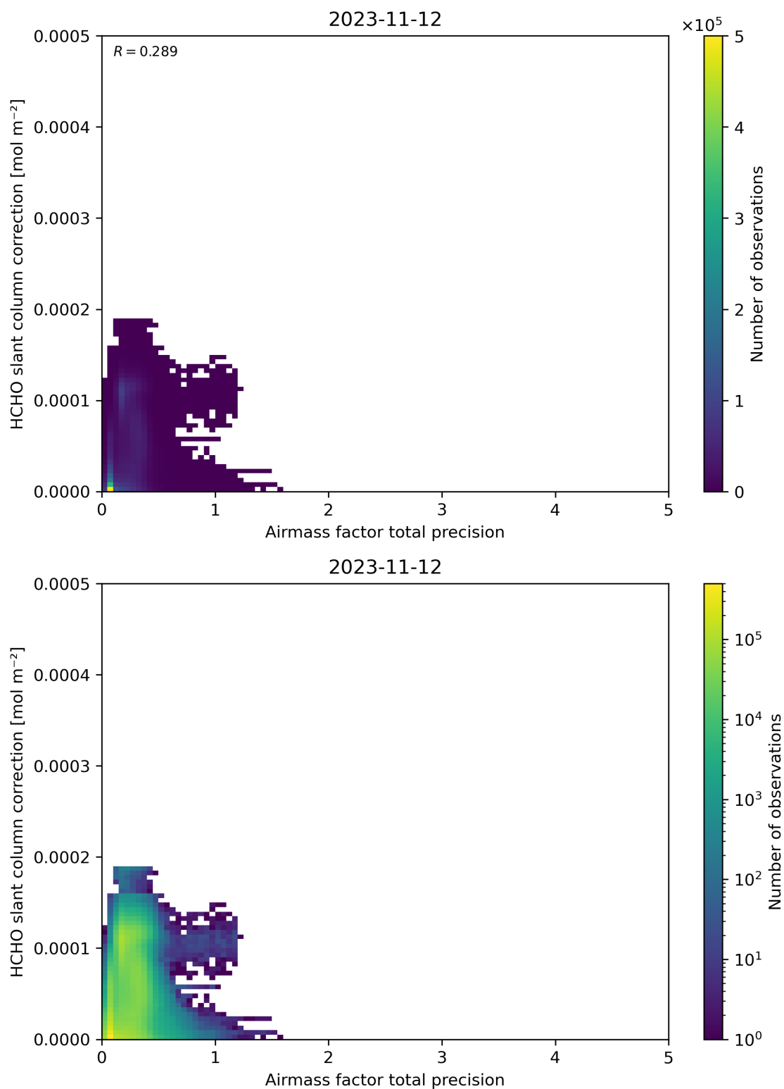
Figure 110: Scatter density plot of “Airmass factor total precision” against “HCHO slant column correction” for 2023-11-12 to 2023-11-13.
