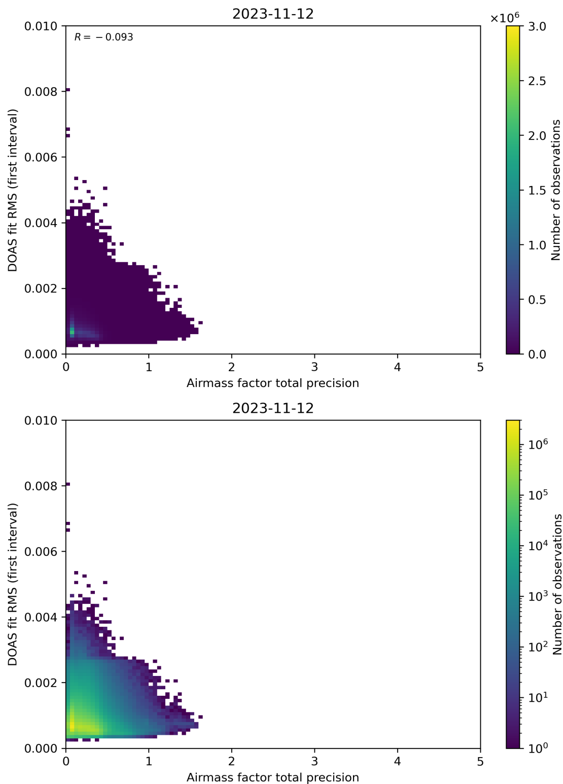
Figure 105: Scatter density plot of “Airmass factor total precision” against “DOAS fit RMS (first interval)” for 2023-11-12 to 2023-11-13.
