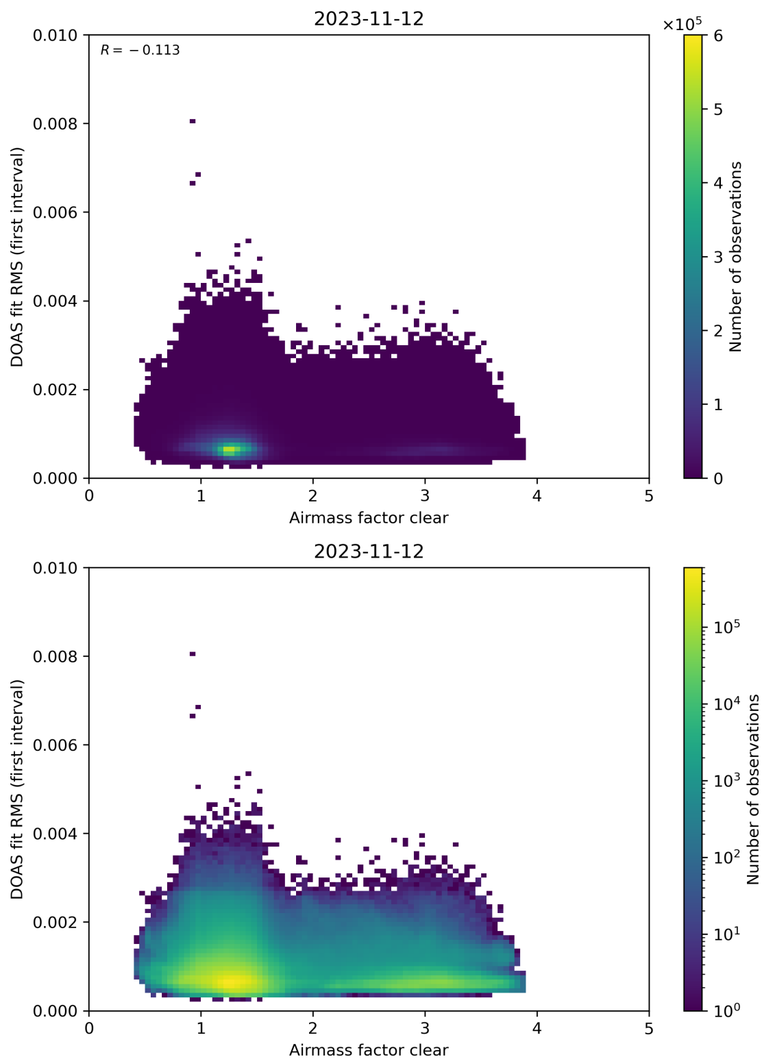
Figure 71: Scatter density plot of “Airmass factor clear” against “DOAS fit RMS (first interval)” for 2023-11-12 to 2023-11-13.
