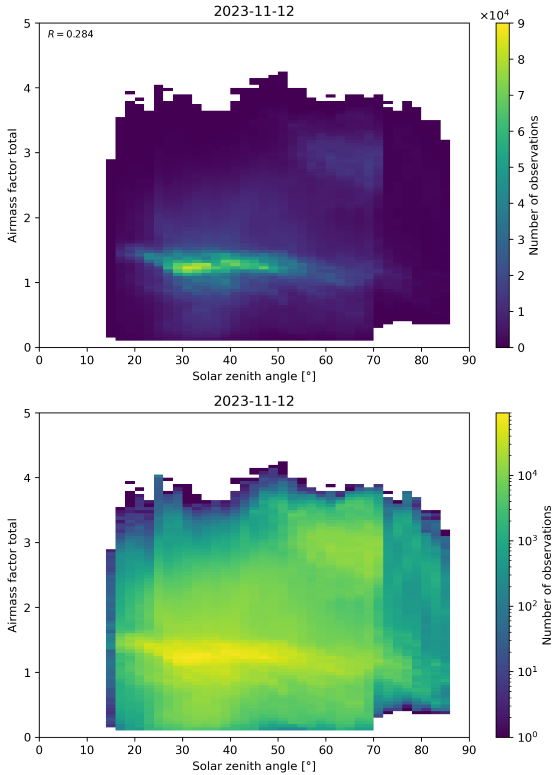
Figure 175: Scatter density plot of “Solar zenith angle” against “Airmass factor total” for 2023-11-12 to 2023-11-13.
