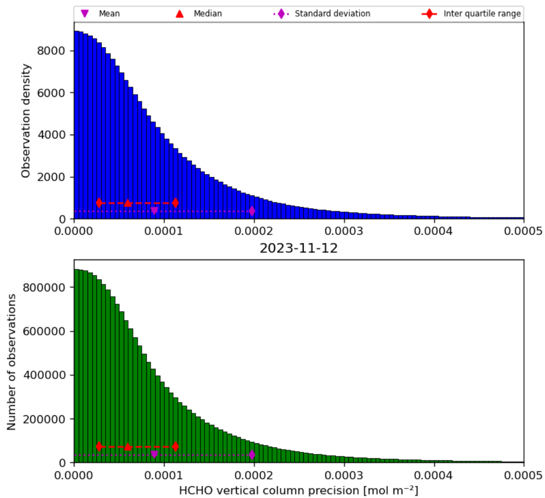
Figure 36: Histogram of “HCHO vertical column precision” for 2023-11-12 to 2023-11-13
