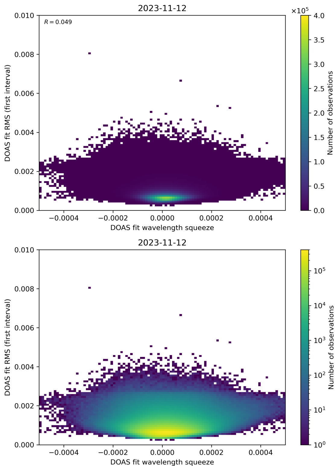
Figure 68: Scatter density plot of “DOAS fit wavelength squeeze” against “DOAS fit RMS (first interval)” for 2023-11-12 to 2023-11-13.
