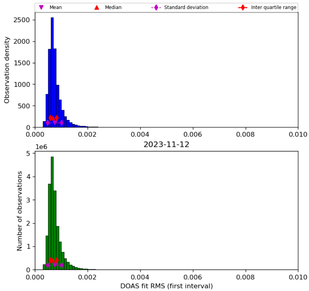
Figure 46: Histogram of “DOAS fit RMS (first interval)” for 2023-11-12 to 2023-11-13
