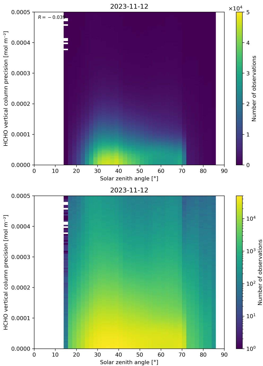
Figure 179: Scatter density plot of “Solar zenith angle” against “HCHO vertical column precision” for 2023-11-12 to 2023-11-13.
