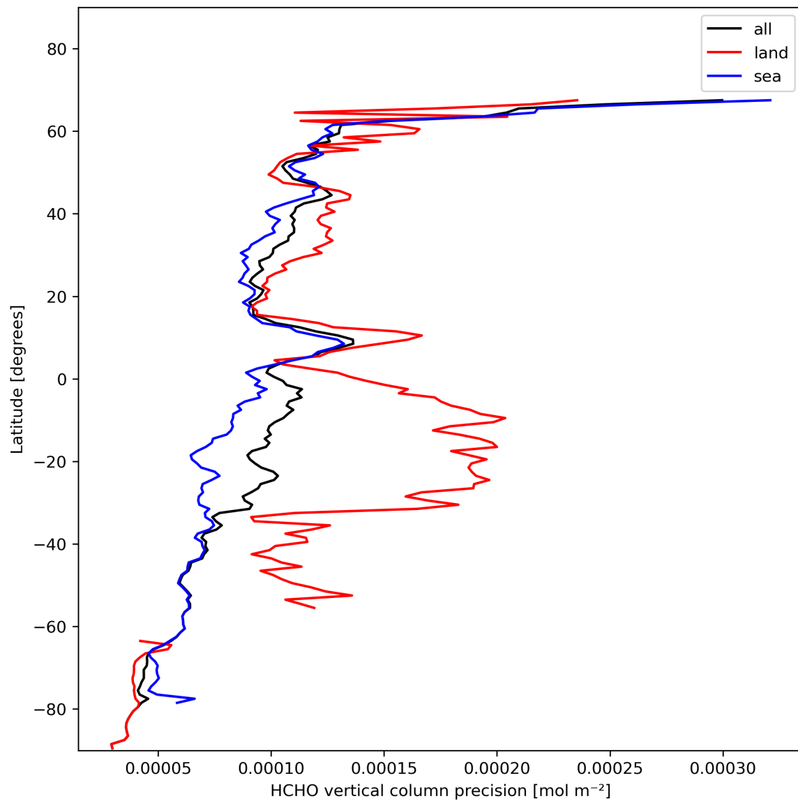
Figure 22: Zonal average of “HCHO vertical column precision” for 2023-11-12 to 2023-11-13.
