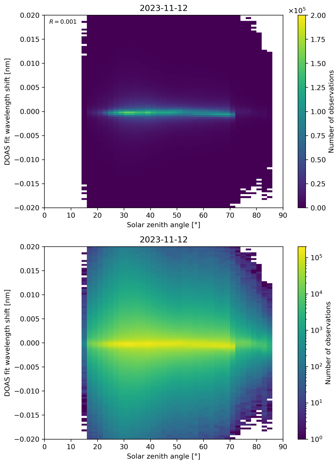
Figure 168: Scatter density plot of “Solar zenith angle” against “DOAS fit wavelength shift” for 2023-11-12 to 2023-11-13.
