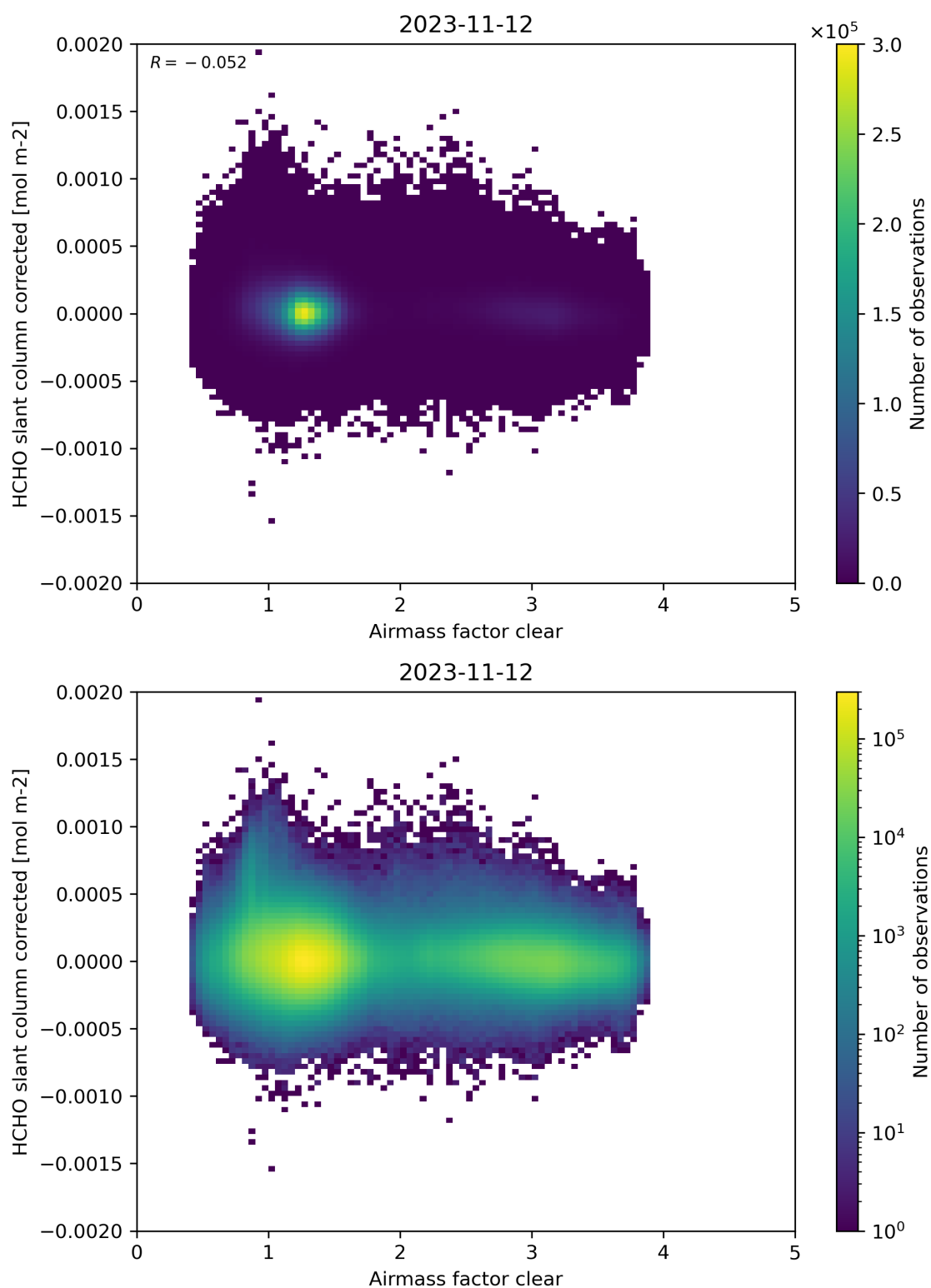
Figure 74: Scatter density plot of “Airmass factor clear” against “HCHO slant column corrected” for 2023-11-12 to 2023-11-13.
