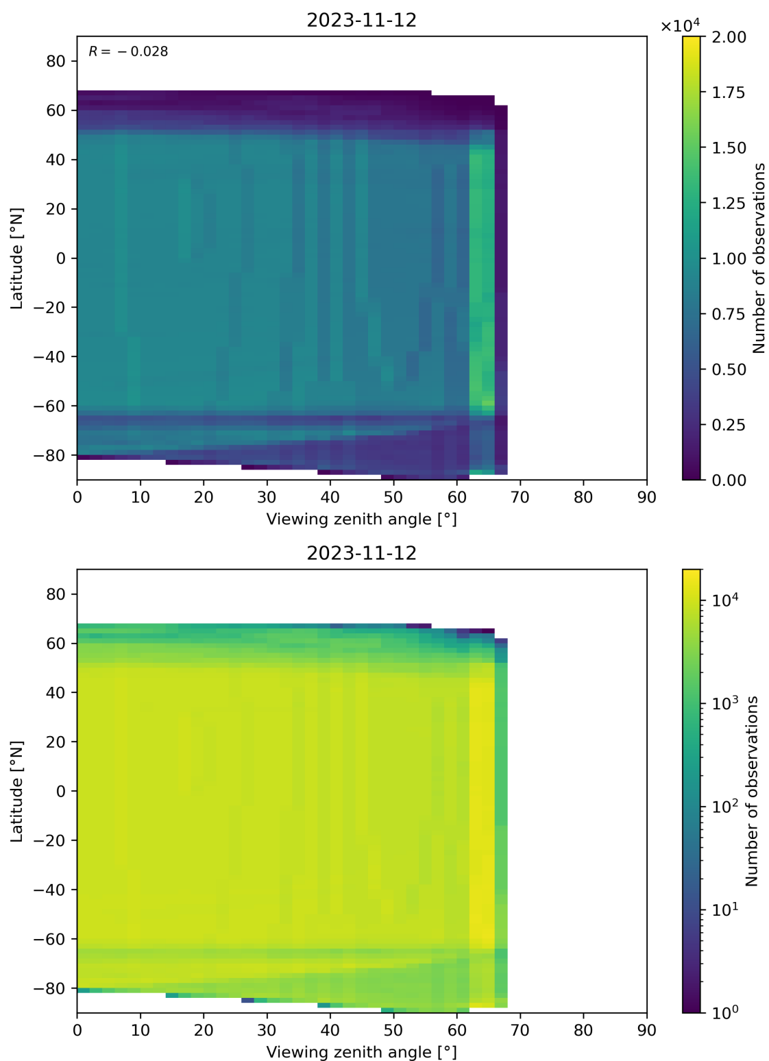
Figure 196: Scatter density plot of “Viewing zenith angle” against “Latitude” for 2023-11-12 to 2023-11-13.
