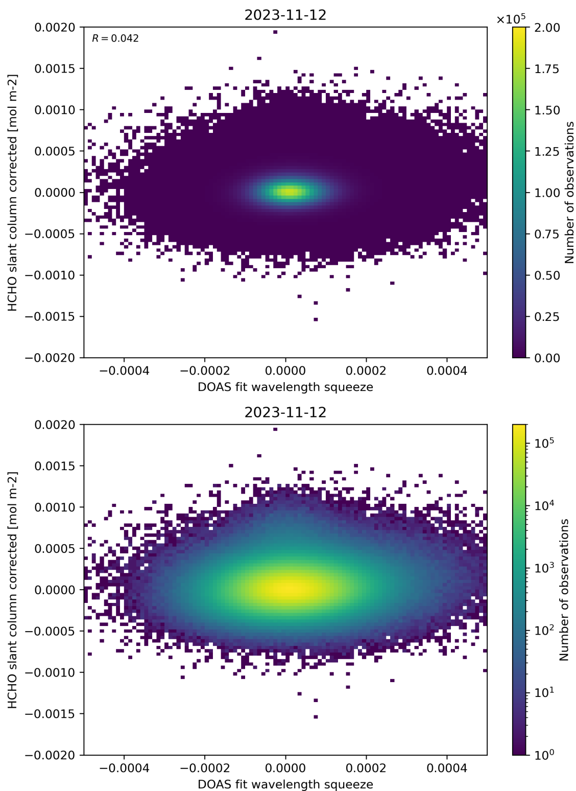
Figure 69: Scatter density plot of “DOAS fit wavelength squeeze” against “HCHO slant column corrected” for 2023-11-12 to 2023-11-13.
