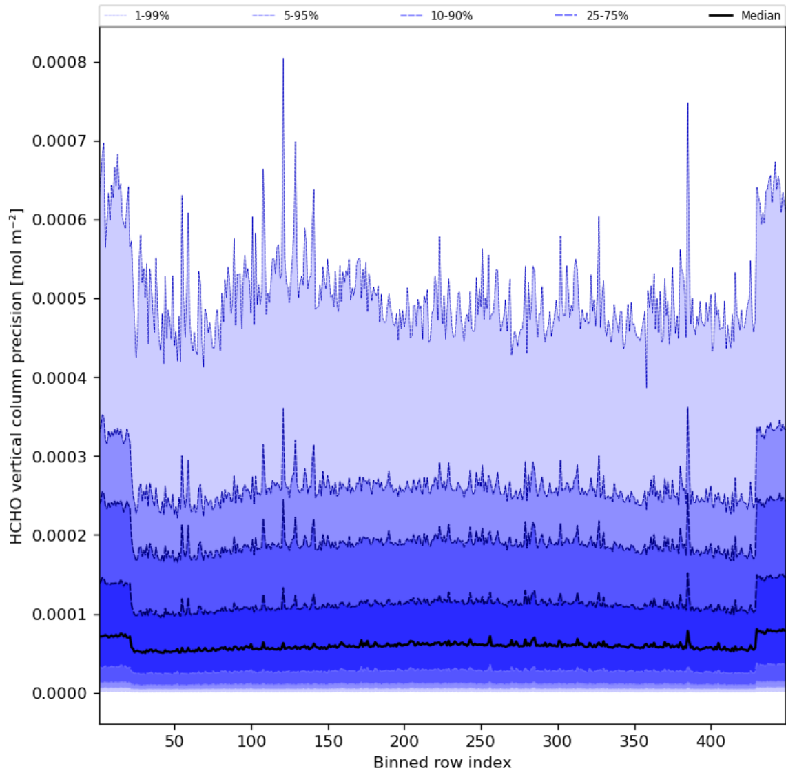
Figure 50: Along track statistics of “HCHO vertical column precision” for 2023-11-12 to 2023-11-13
