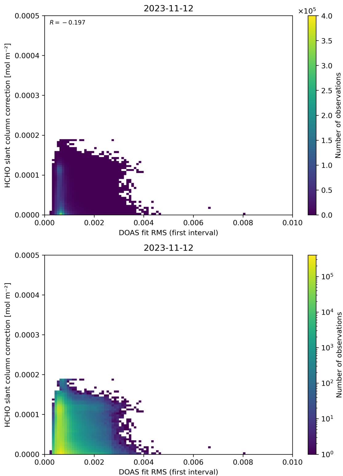
Figure 63: Scatter density plot of “DOAS fit RMS (first interval)” against “HCHO slant column correction” for 2023-11-12 to 2023-11-13.
