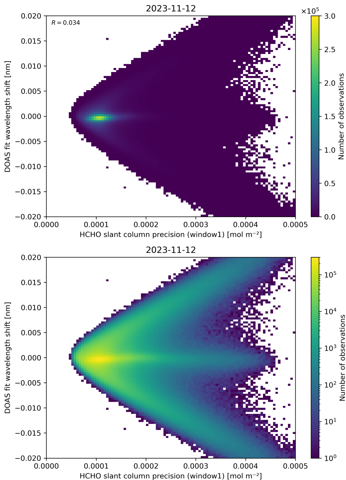
Figure 89: Scatter density plot of “HCHO slant column precision (window1)” against “DOAS fit wavelength shift” for 2023-11-12 to 2023-11-13.
