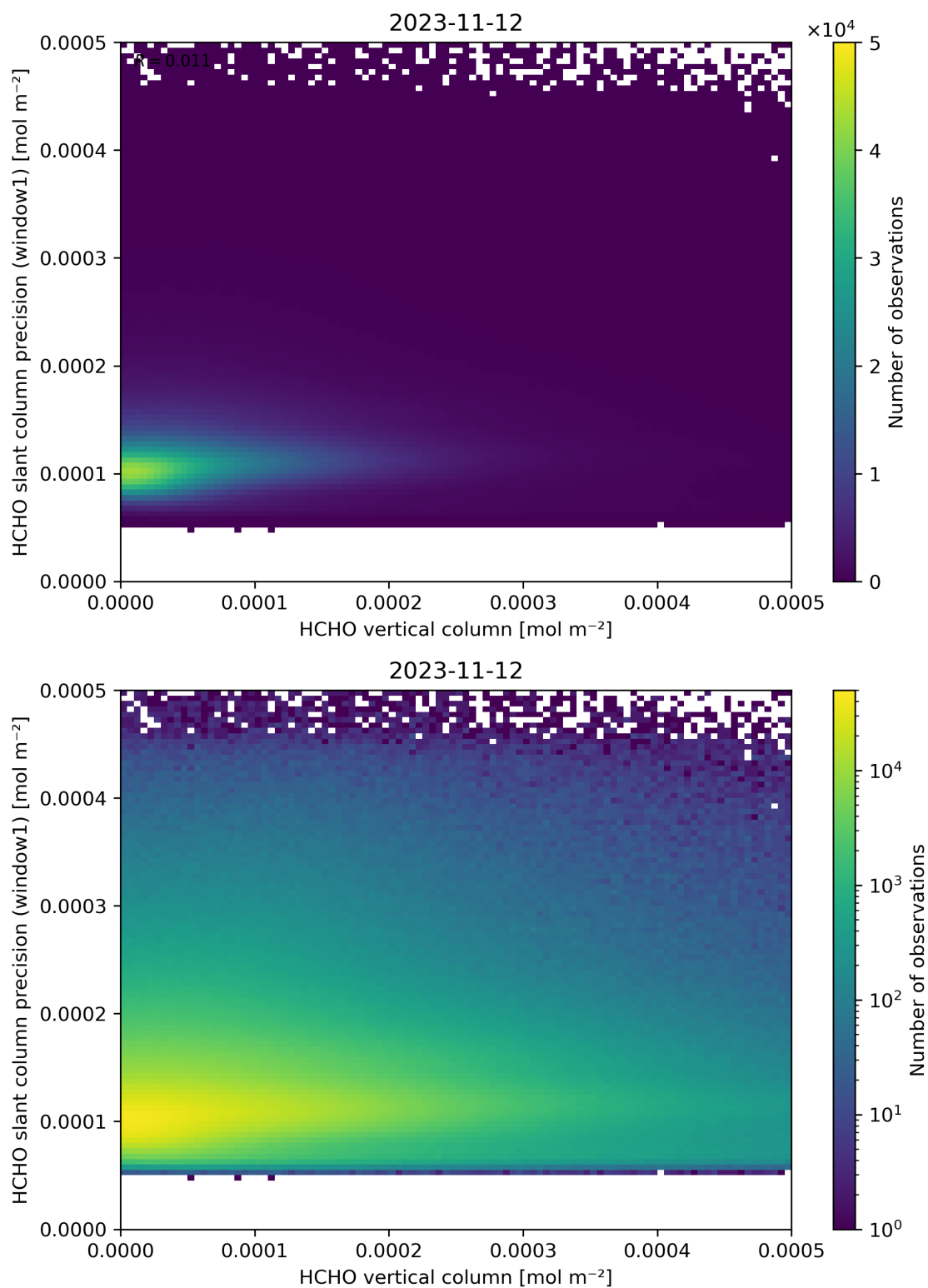
Figure 130: Scatter density plot of “HCHO vertical column” against “HCHO slant column precision (window1)” for 2023-11-12 to 2023-11-13.
