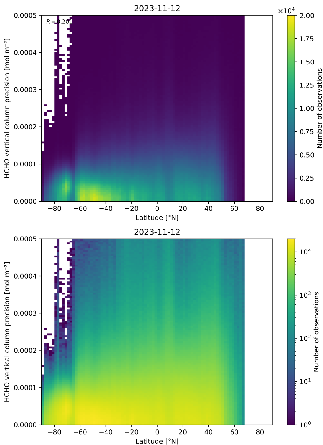
Figure 165: Scatter density plot of “Latitude” against “HCHO vertical column precision” for 2023-11-12 to 2023-11-13.
