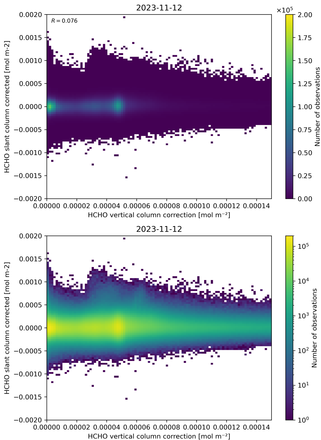
Figure 116: Scatter density plot of “HCHO vertical column correction” against “HCHO slant column corrected” for 2023-11-12 to 2023-11-13.
