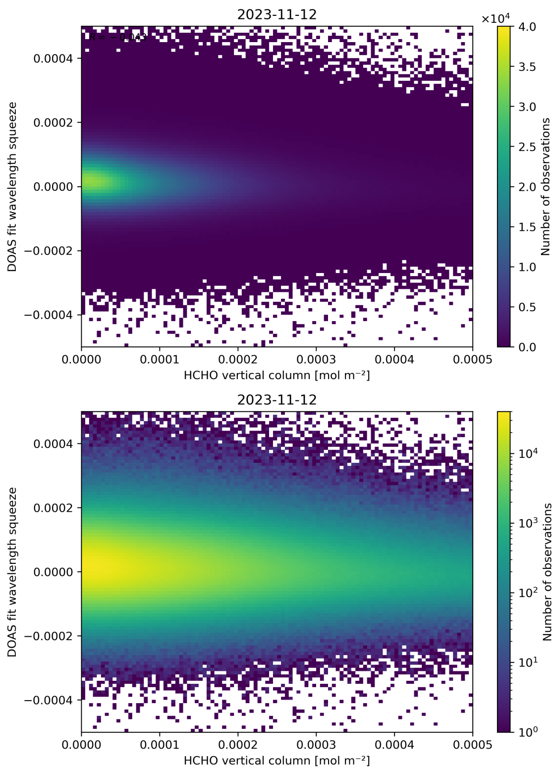
Figure 125: Scatter density plot of “HCHO vertical column” against “DOAS fit wavelength squeeze” for 2023-11-12 to 2023-11-13.
