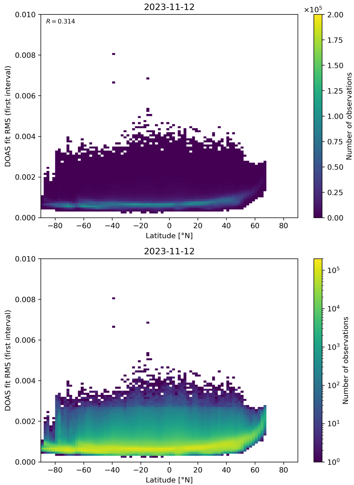
Figure 153: Scatter density plot of “Latitude” against “DOAS fit RMS (first interval)” for 2023-11-12 to 2023-11-13.
