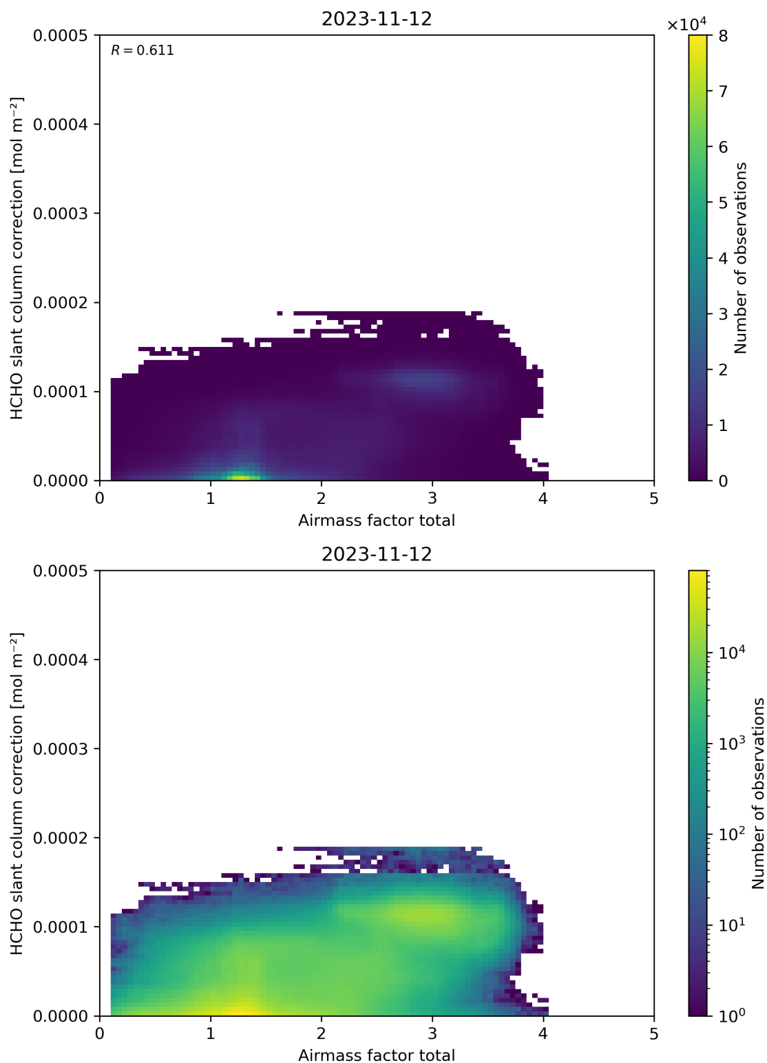
Figure 102: Scatter density plot of “Airmass factor total” against “HCHO slant column correction” for 2023-11-12 to 2023-11-13.
