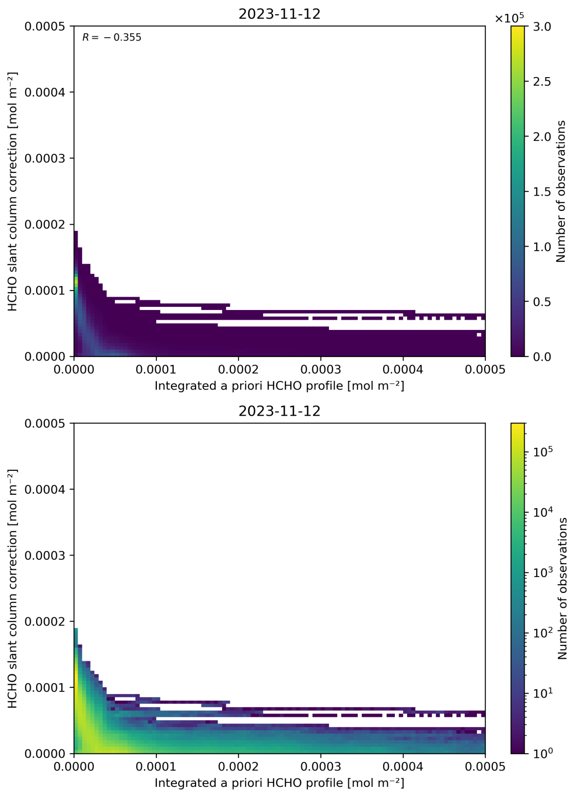
Figure 152: Scatter density plot of “Integrated a priori HCHO profile” against “HCHO slant column correction” for 2023-11-12 to 2023-11-13.
