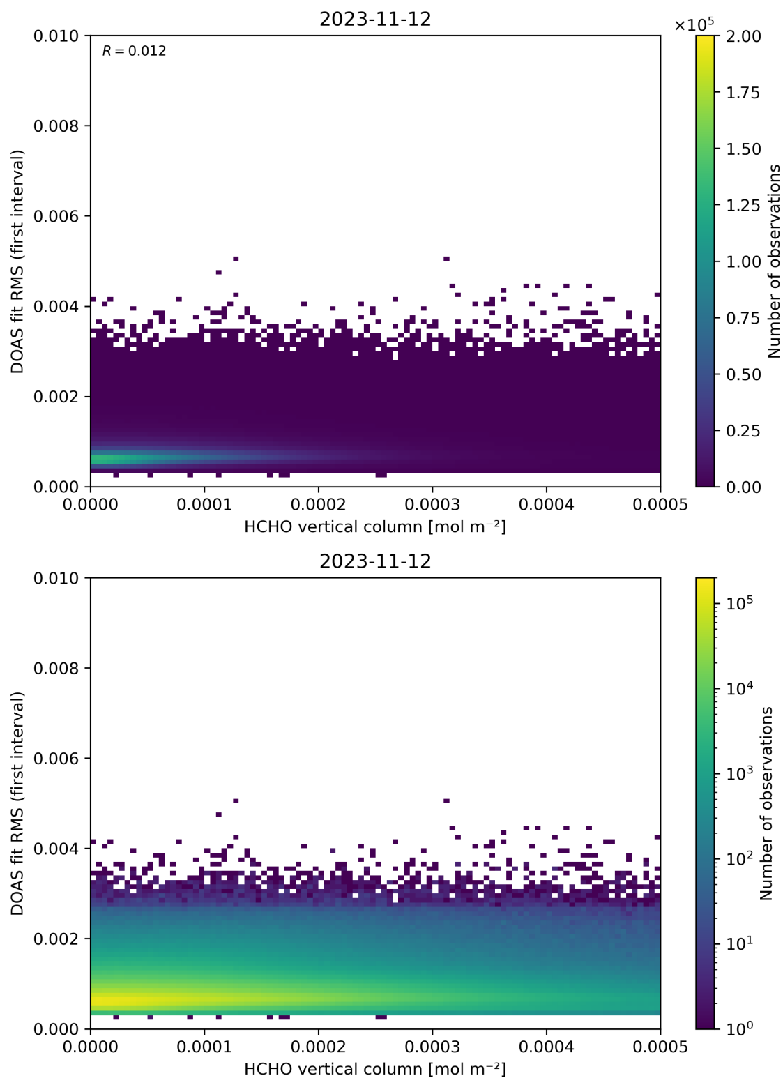
Figure 123: Scatter density plot of “HCHO vertical column” against “DOAS fit RMS (first interval)” for 2023-11-12 to 2023-11-13.
