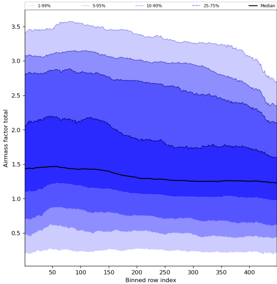
Figure 54: Along track statistics of “Airmass factor total” for 2023-11-12 to 2023-11-13
