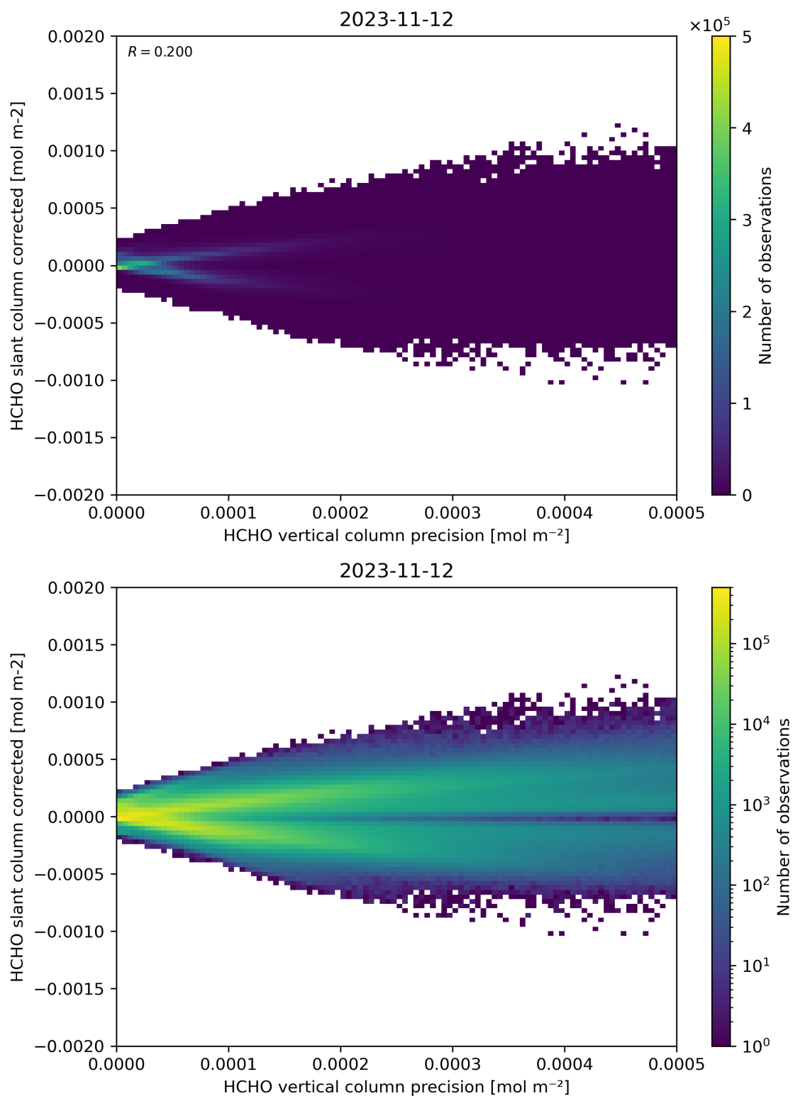
Figure 140: Scatter density plot of “HCHO vertical column precision” against “HCHO slant column corrected” for 2023-11-12 to 2023-11-13.
