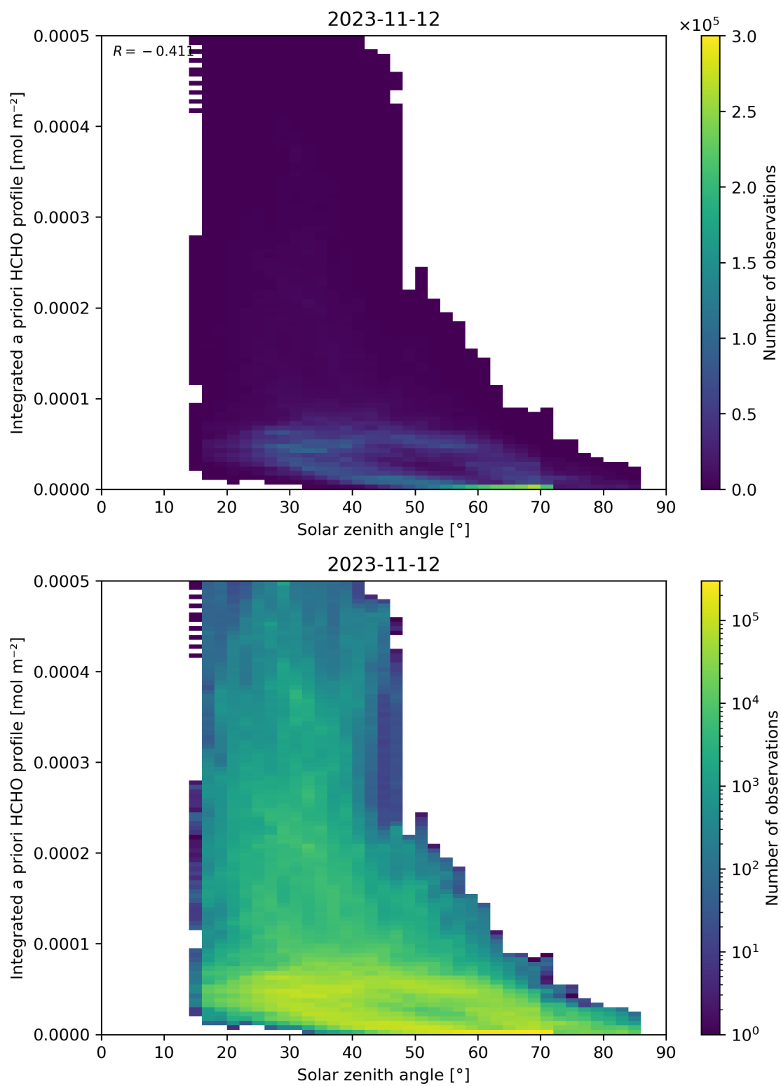
Figure 180: Scatter density plot of “Solar zenith angle” against “Integrated a priori HCHO profile” for 2023-11-12 to 2023-11-13.
