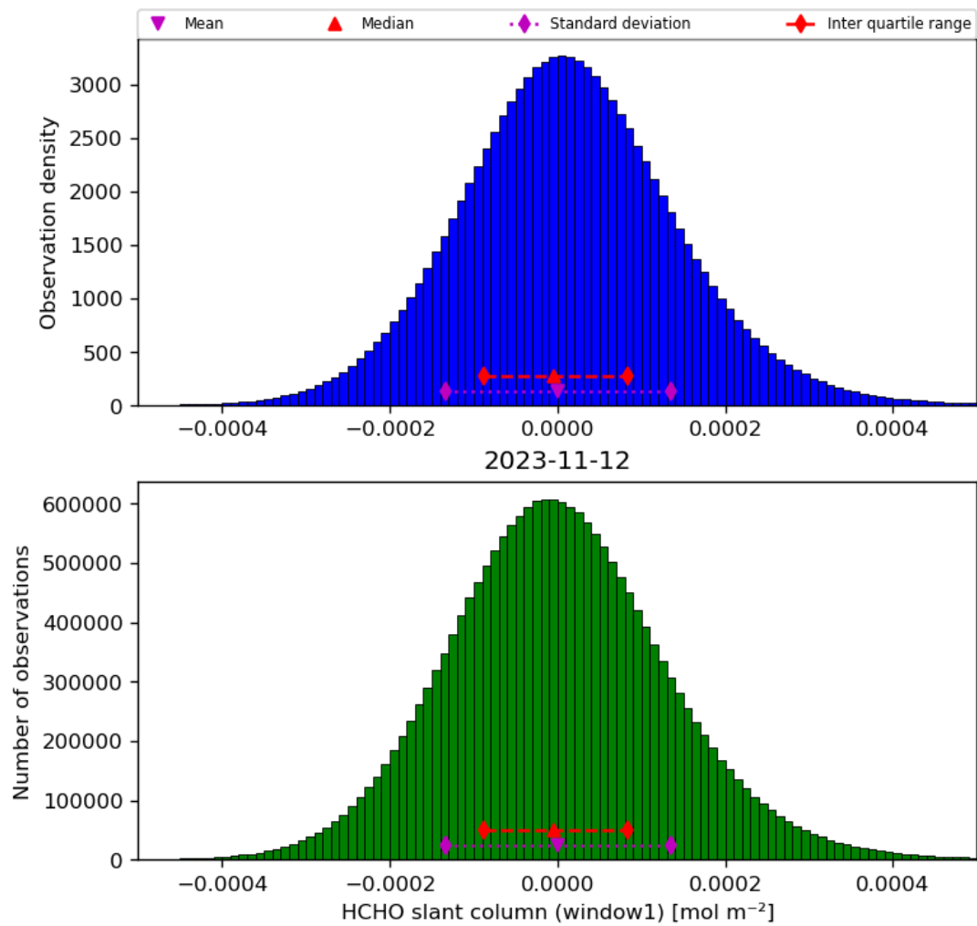
Figure 38: Histogram of “HCHO slant column (window1)” for 2023-11-12 to 2023-11-13
