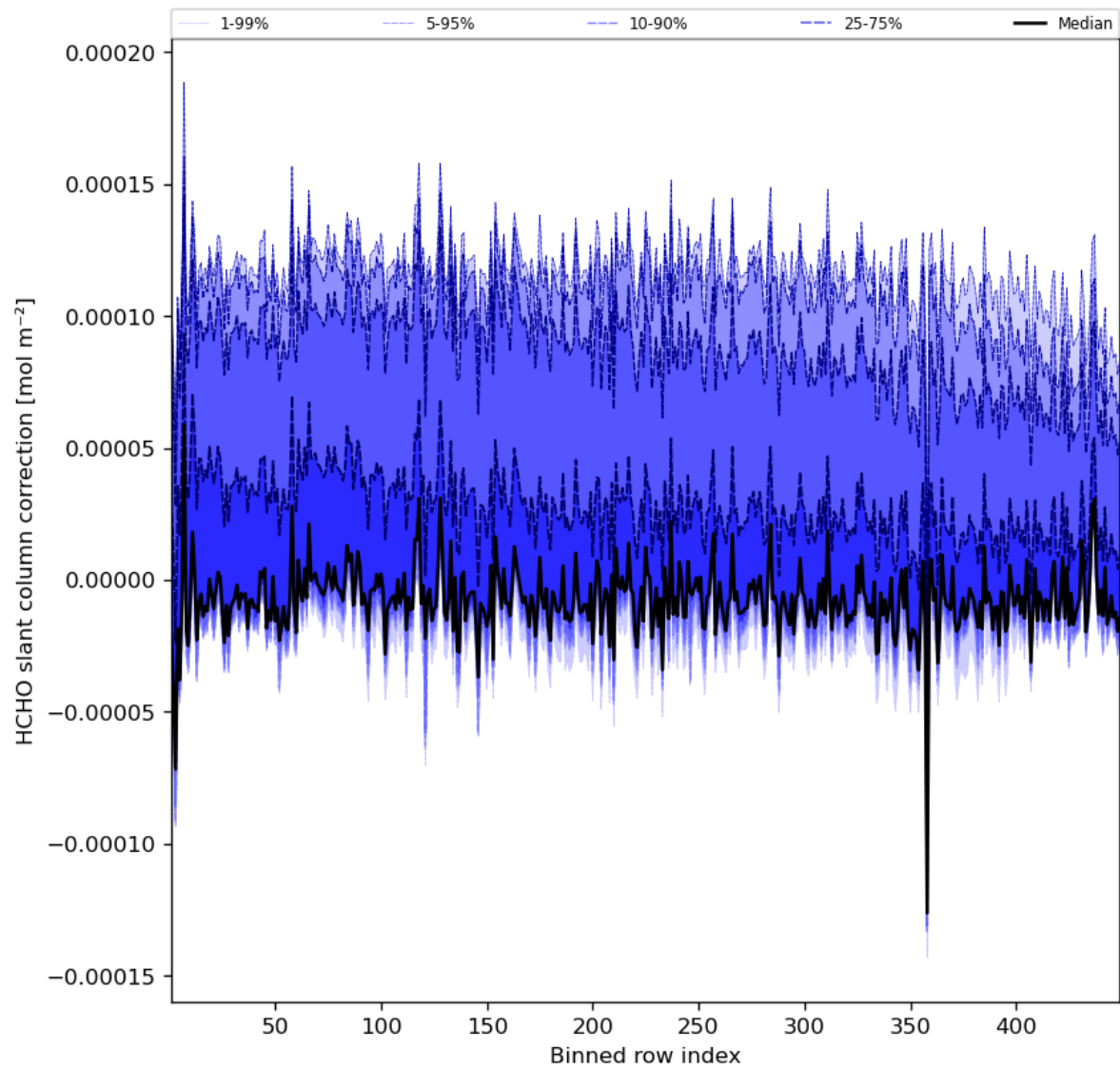
Figure 61: Along track statistics of “HCHO slant column correction” for 2023-11-12 to 2023-11-13
