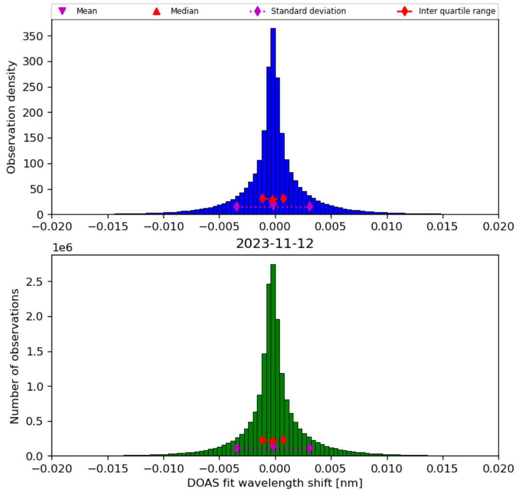
Figure 44: Histogram of “DOAS fit wavelength shift” for 2023-11-12 to 2023-11-13
