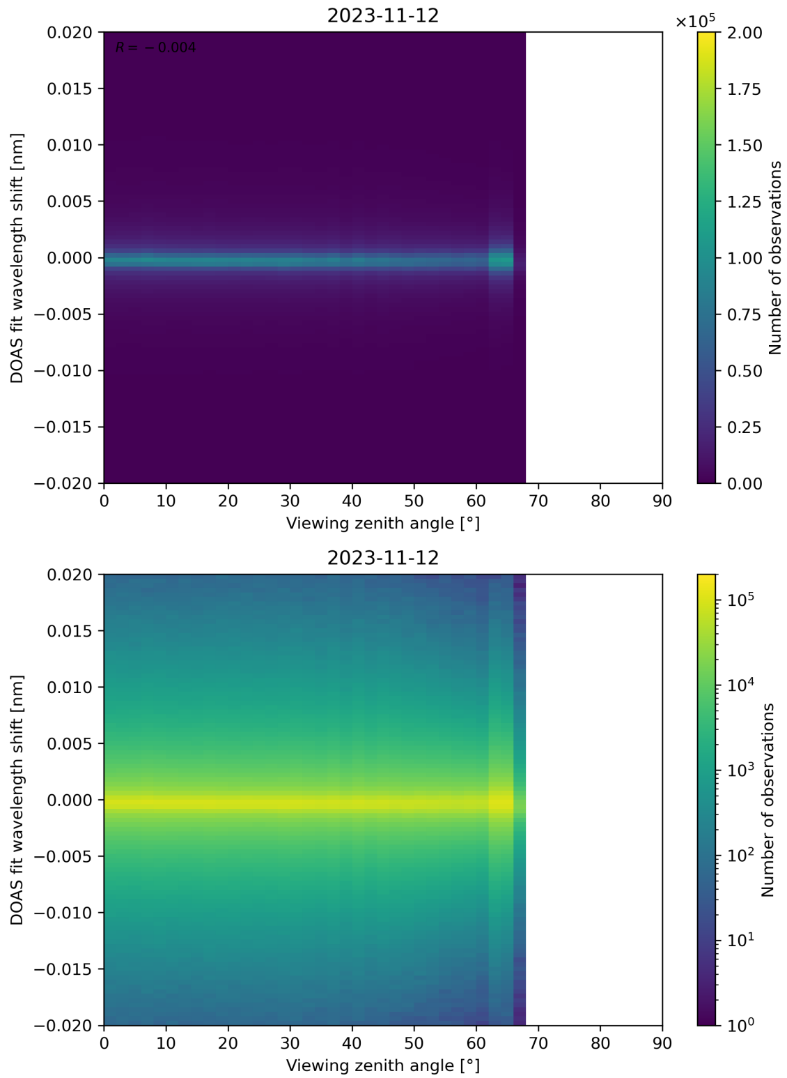
Figure 183: Scatter density plot of “Viewing zenith angle” against “DOAS fit wavelength shift” for 2023-11-12 to 2023-11-13.
