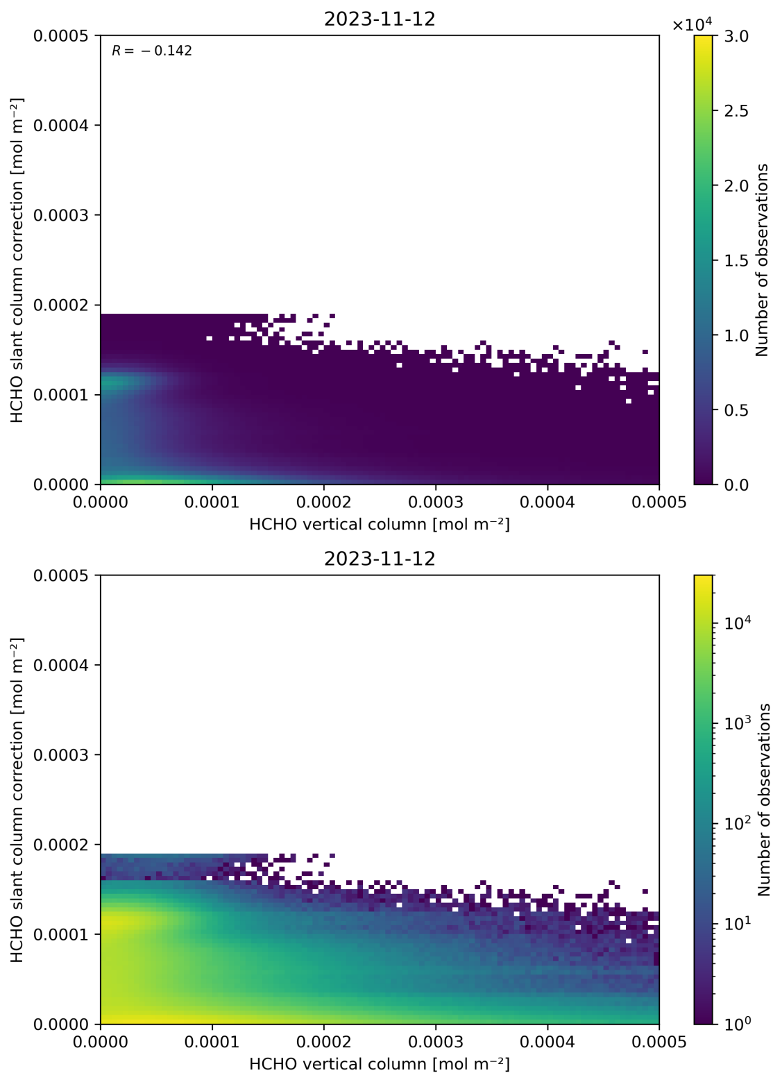
Figure 128: Scatter density plot of “HCHO vertical column” against “HCHO slant column correction” for 2023-11-12 to 2023-11-13.
