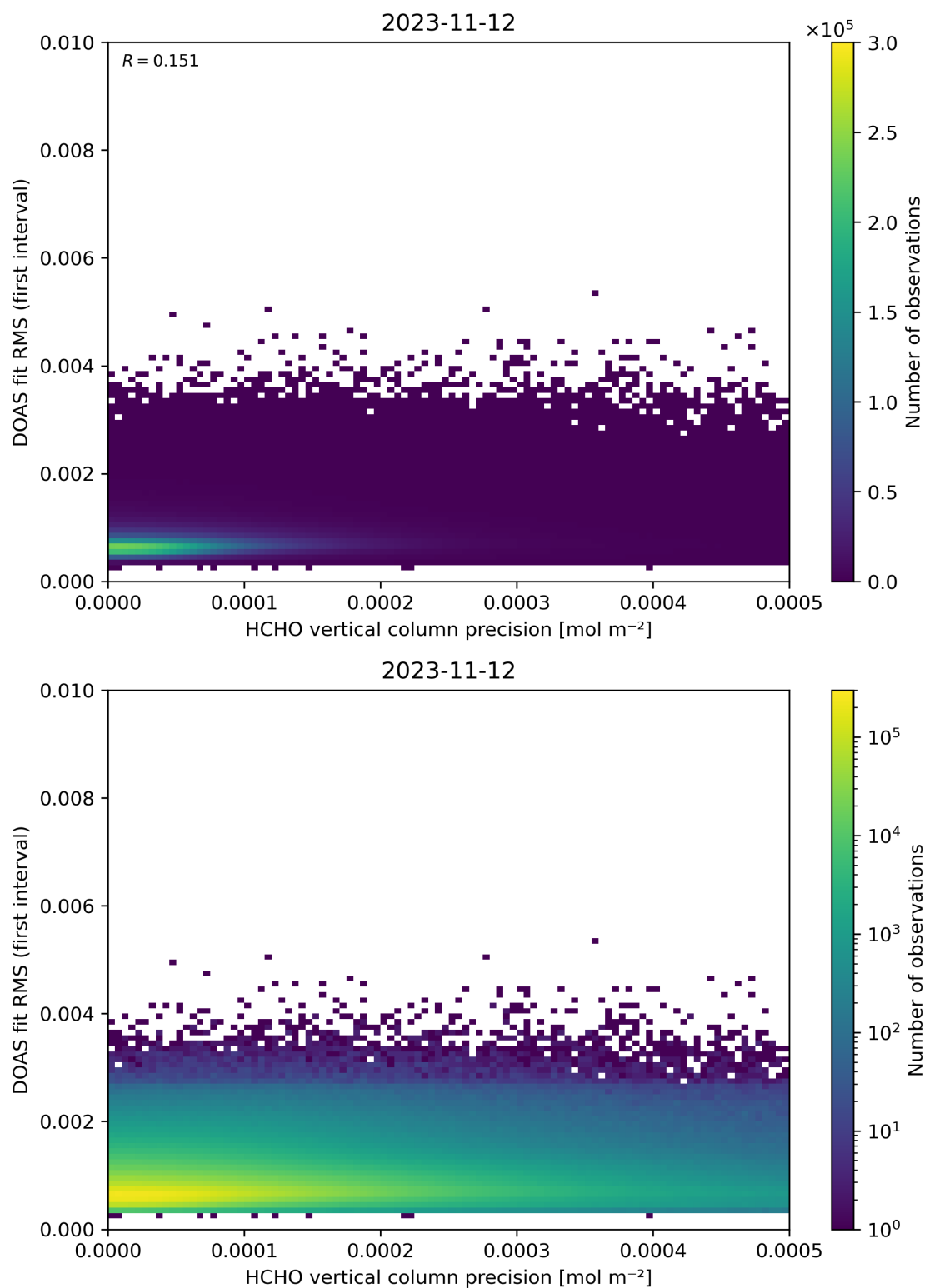
Figure 136: Scatter density plot of “HCHO vertical column precision” against “DOAS fit RMS (first interval)” for 2023-11-12 to 2023-11-13.
