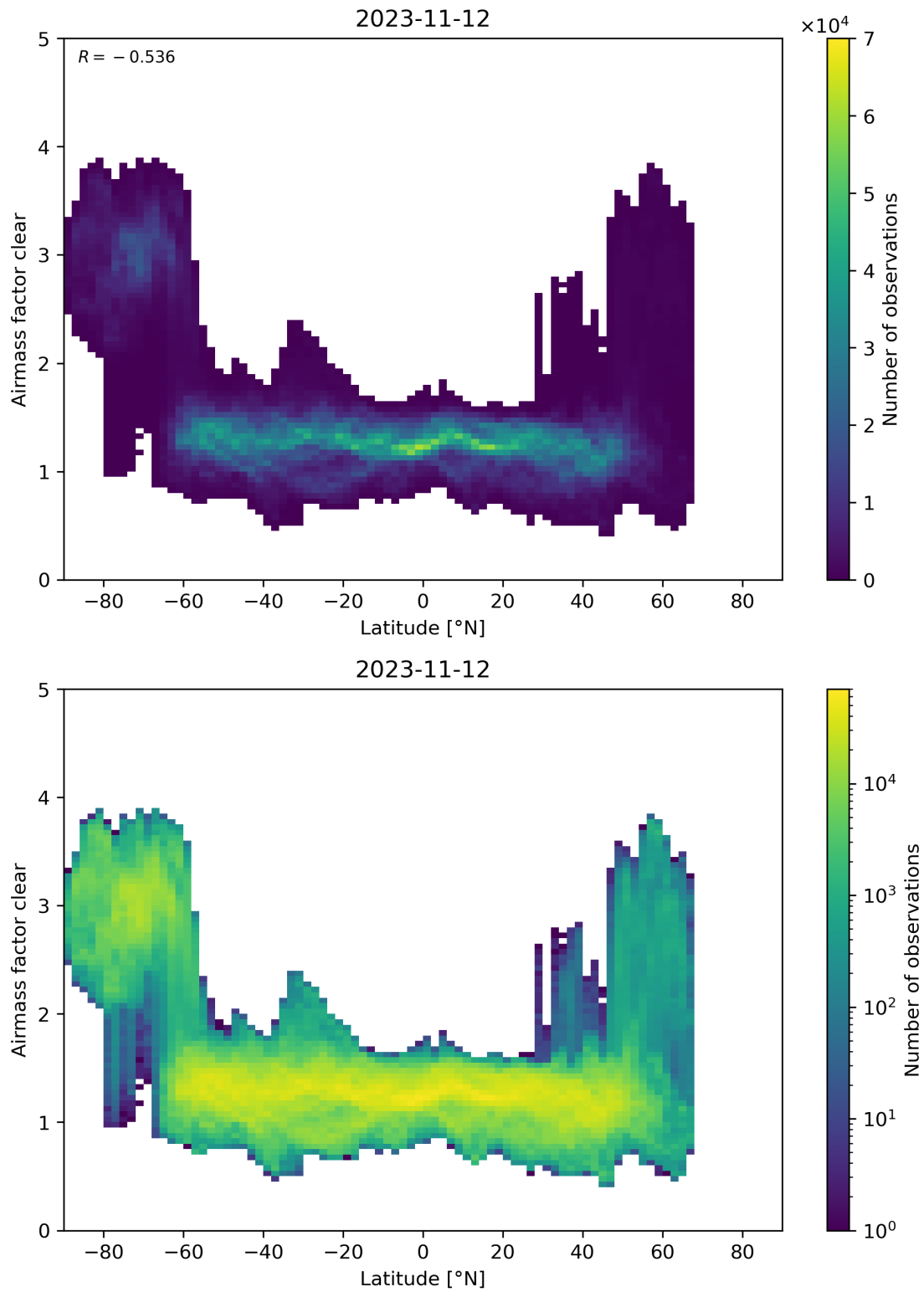
Figure 156: Scatter density plot of “Latitude” against “Airmass factor clear” for 2023-11-12 to 2023-11-13.
