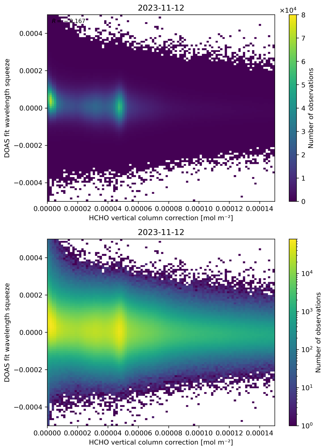
Figure 114: Scatter density plot of “HCHO vertical column correction” against “DOAS fit wavelength squeeze” for 2023-11-12 to 2023-11-13.
