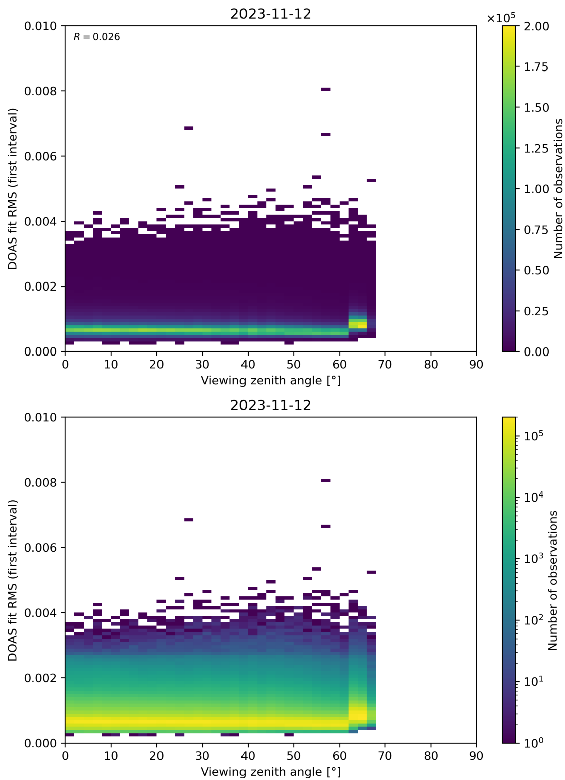
Figure 182: Scatter density plot of “Viewing zenith angle” against “DOAS fit RMS (first interval)” for 2023-11-12 to 2023-11-13.
