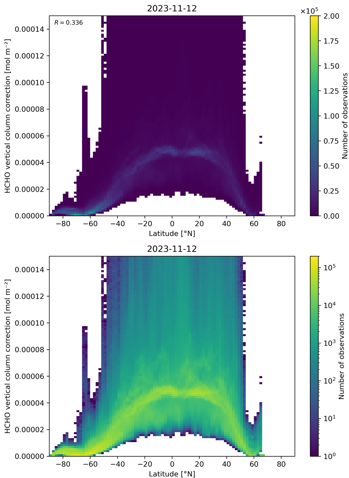
Figure 164: Scatter density plot of “Latitude” against “HCHO vertical column correction” for 2023-11-12 to 2023-11-13.
