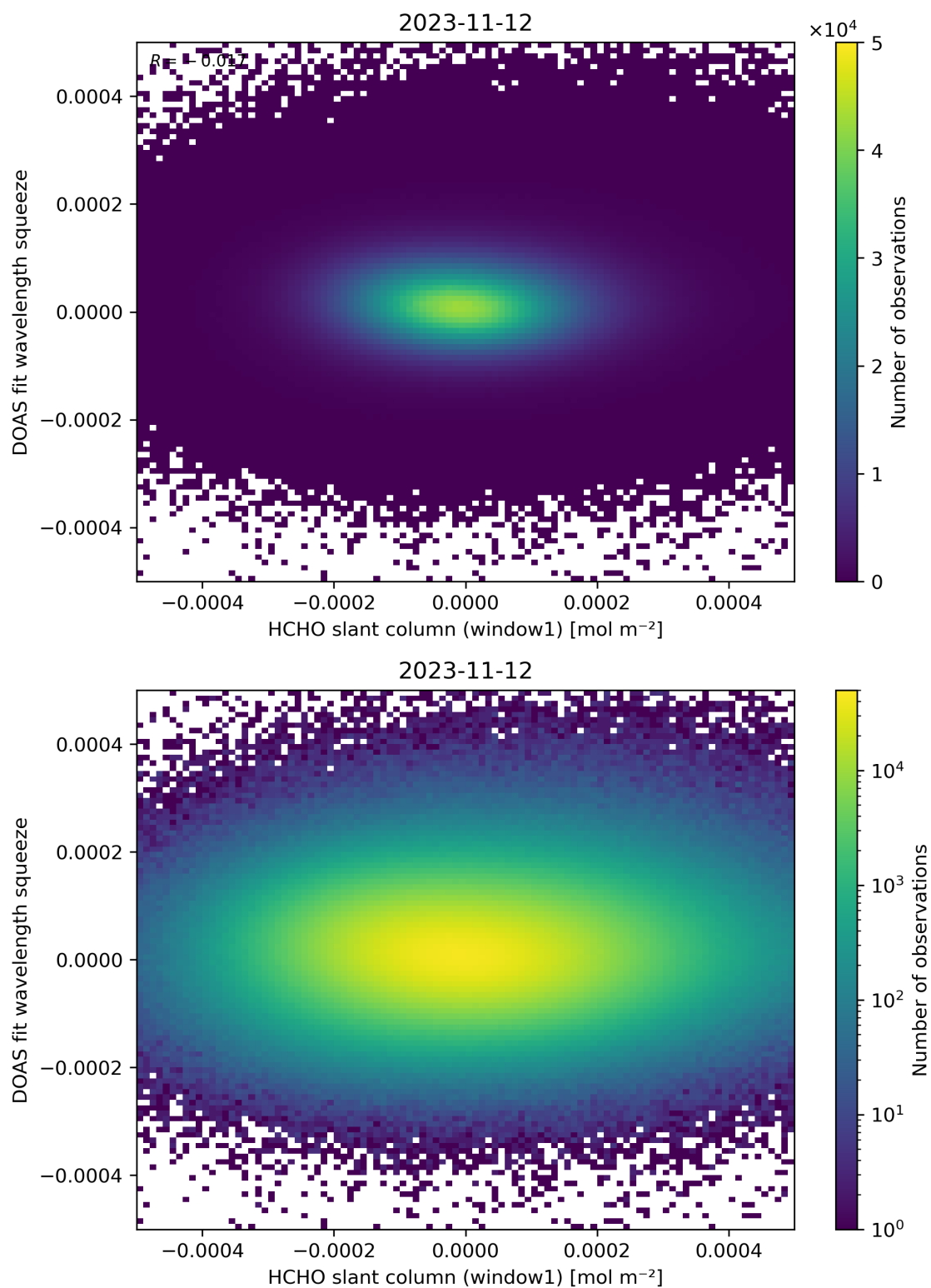
Figure 80: Scatter density plot of “HCHO slant column (window1)” against “DOAS fit wavelength squeeze” for 2023-11-12 to 2023-11-13.
