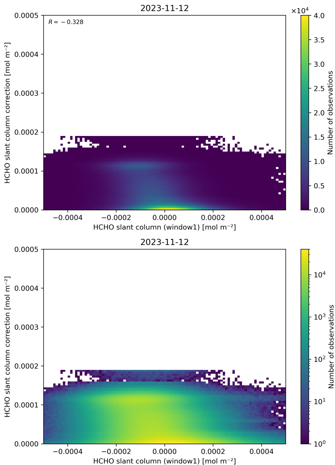
Figure 83: Scatter density plot of “HCHO slant column (window1)” against “HCHO slant column correction” for 2023-11-12 to 2023-11-13.
