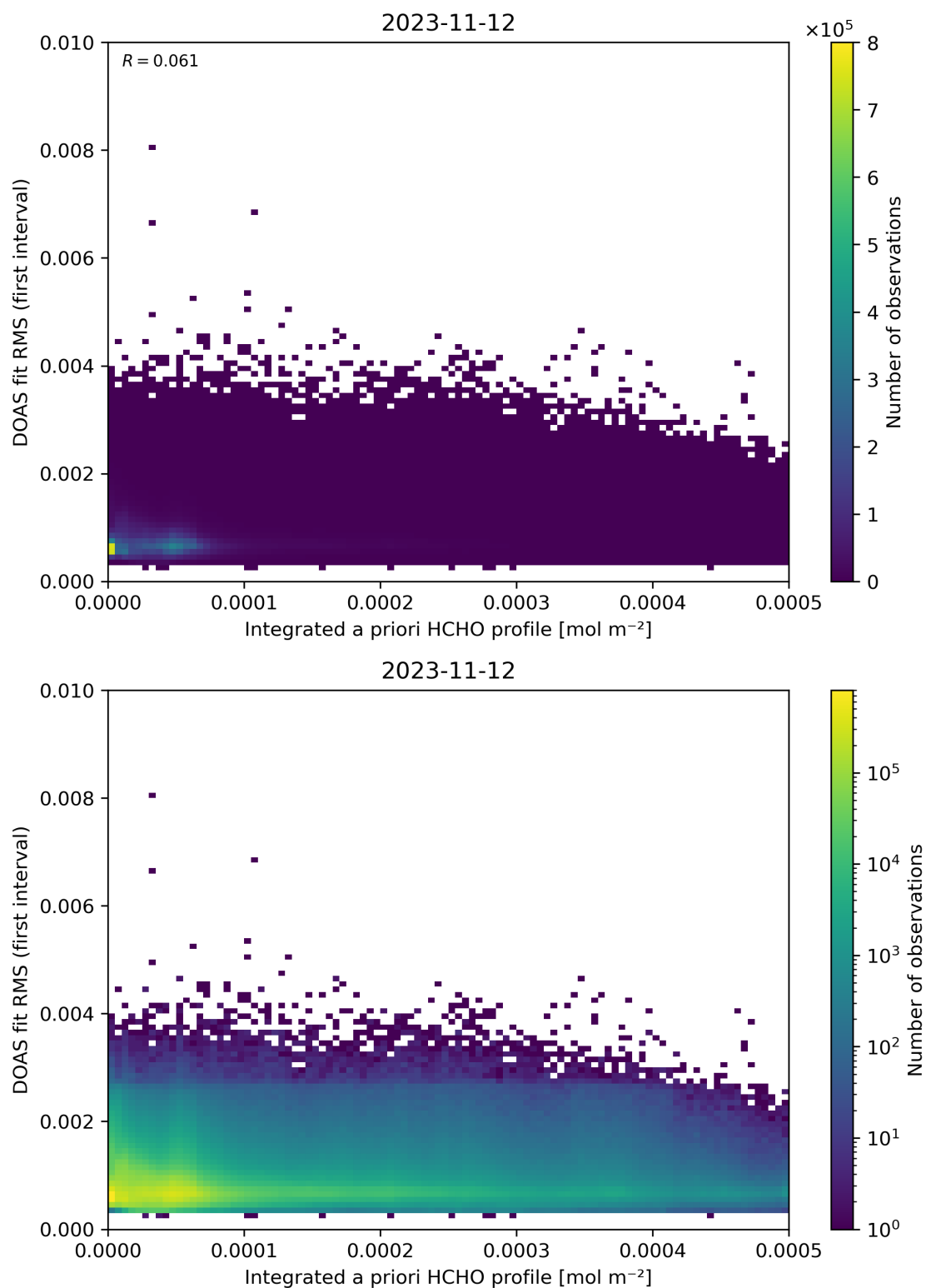
Figure 148: Scatter density plot of “Integrated a priori HCHO profile” against “DOAS fit RMS (first interval)” for 2023-11-12 to 2023-11-13.
