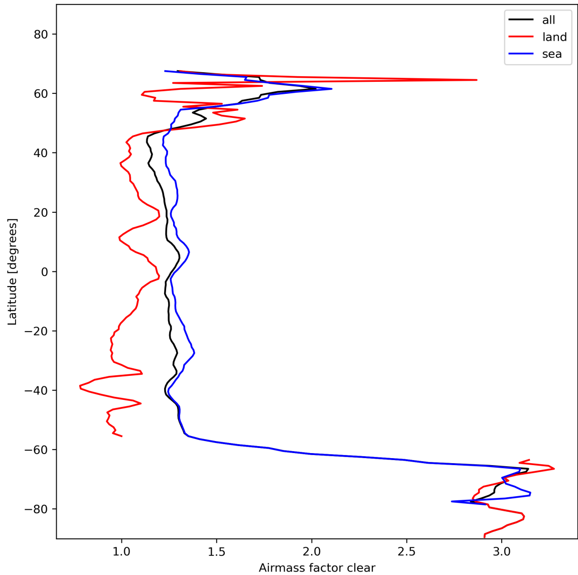
Figure 28: Zonal average of “Airmass factor clear” for 2023-11-12 to 2023-11-13.
