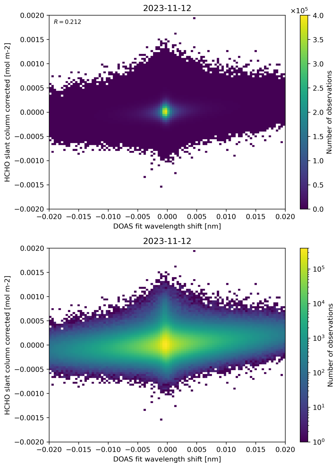
Figure 66: Scatter density plot of “DOAS fit wavelength shift” against “HCHO slant column corrected” for 2023-11-12 to 2023-11-13.
