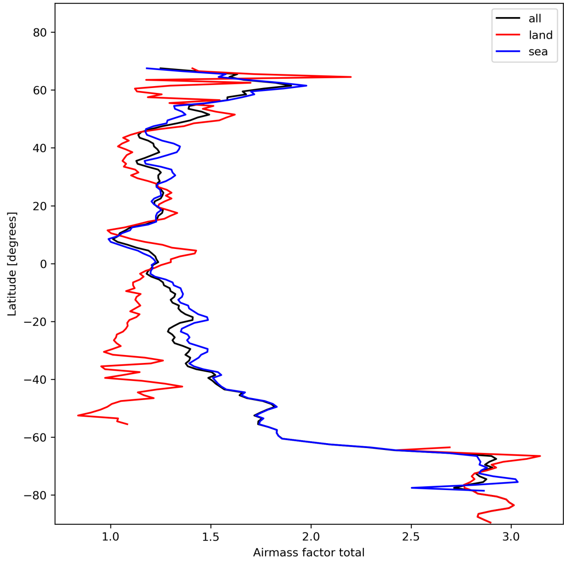
Figure 26: Zonal average of “Airmass factor total” for 2023-11-12 to 2023-11-13.
