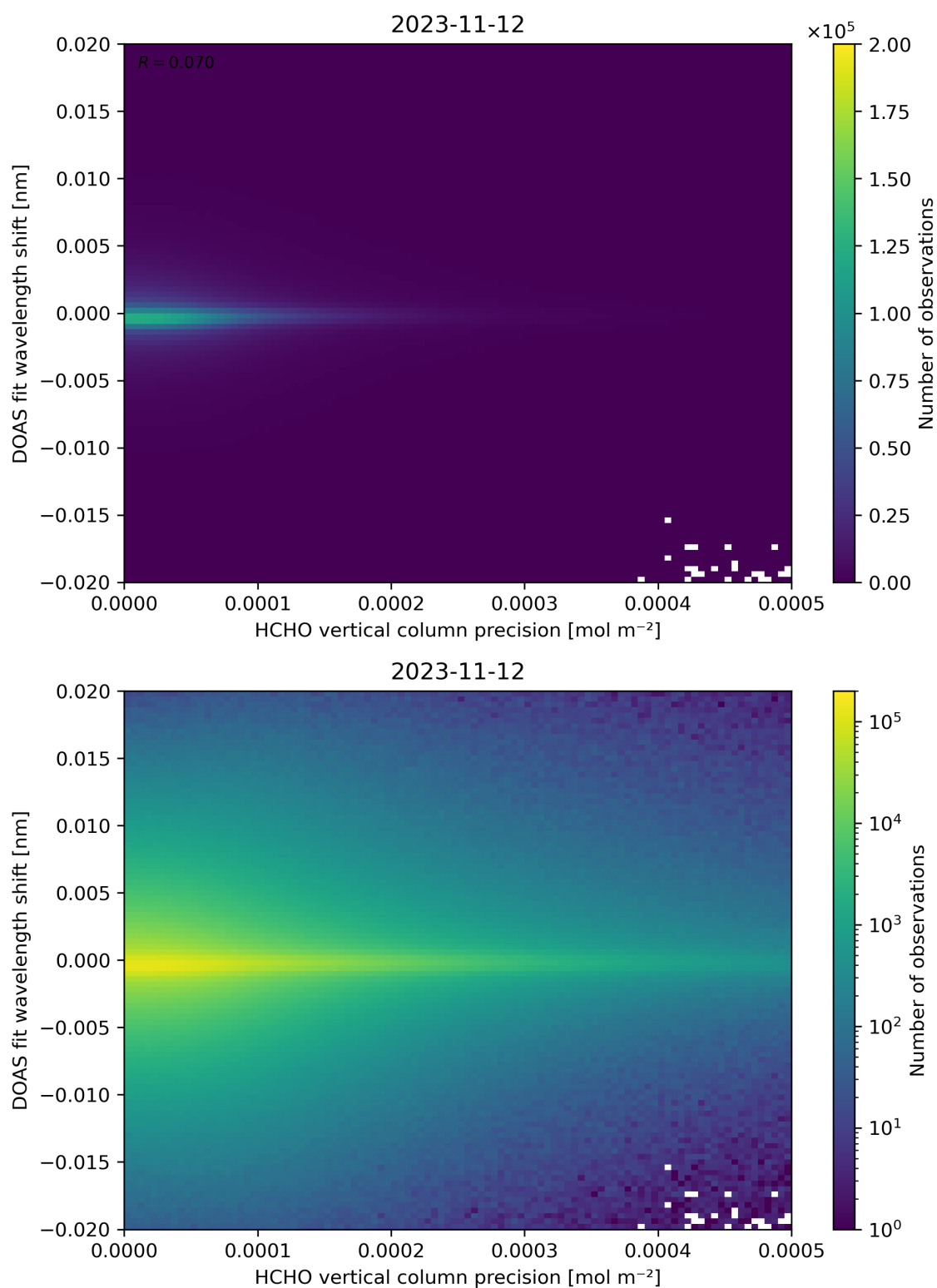
Figure 137: Scatter density plot of “HCHO vertical column precision” against “DOAS fit wavelength shift” for 2023-11-12 to 2023-11-13.
