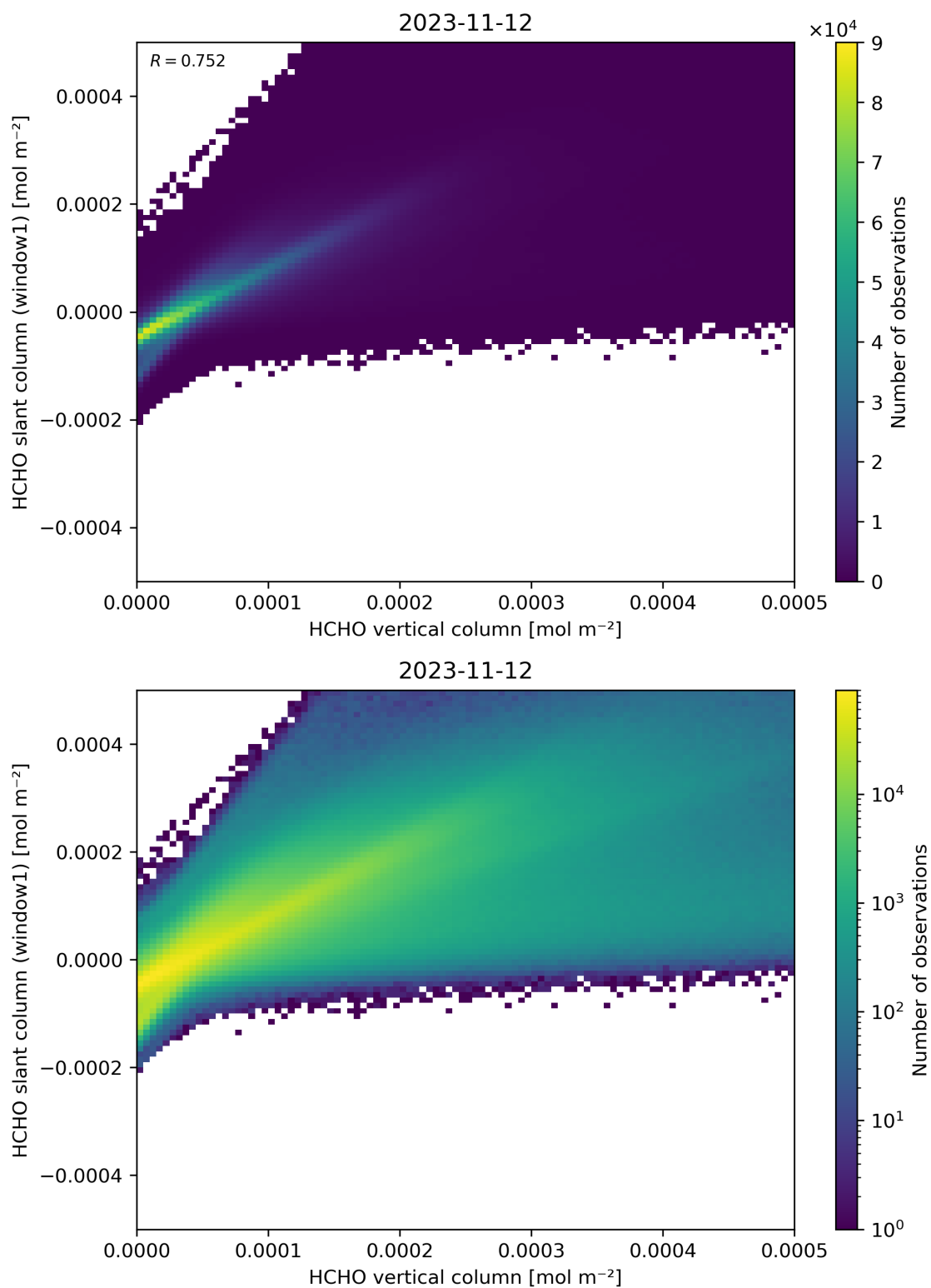
Figure 129: Scatter density plot of “HCHO vertical column” against “HCHO slant column (window1)” for 2023-11-12 to 2023-11-13.
