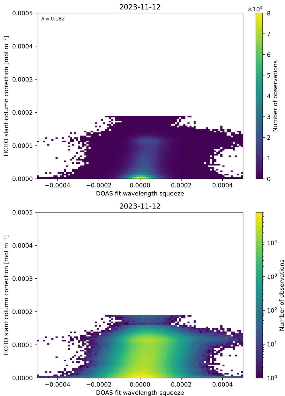
Figure 70: Scatter density plot of “DOAS fit wavelength squeeze” against “HCHO slant column correction” for 2023-11-12 to 2023-11-13.
