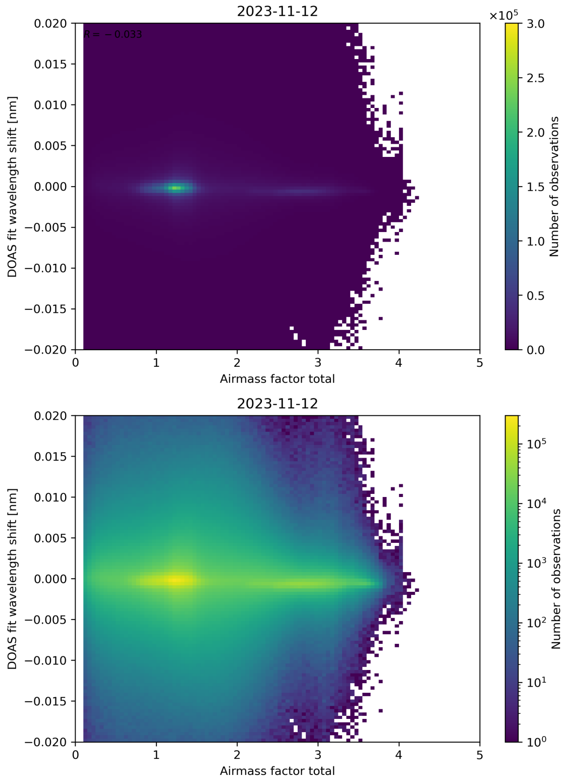
Figure 98: Scatter density plot of “Airmass factor total” against “DOAS fit wavelength shift” for 2023-11-12 to 2023-11-13.
