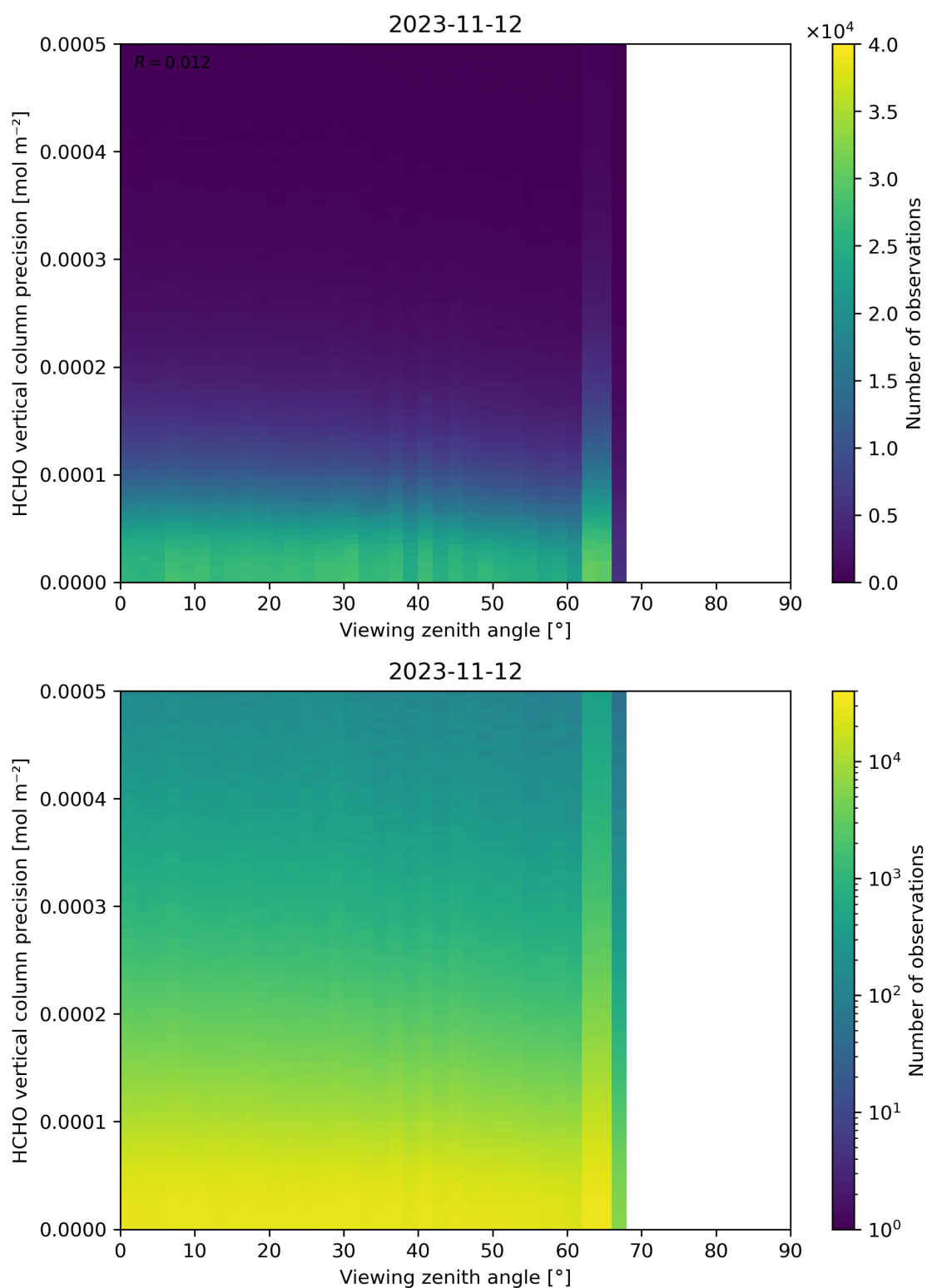
Figure 194: Scatter density plot of “Viewing zenith angle” against “HCHO vertical column precision” for 2023-11-12 to 2023-11-13.
