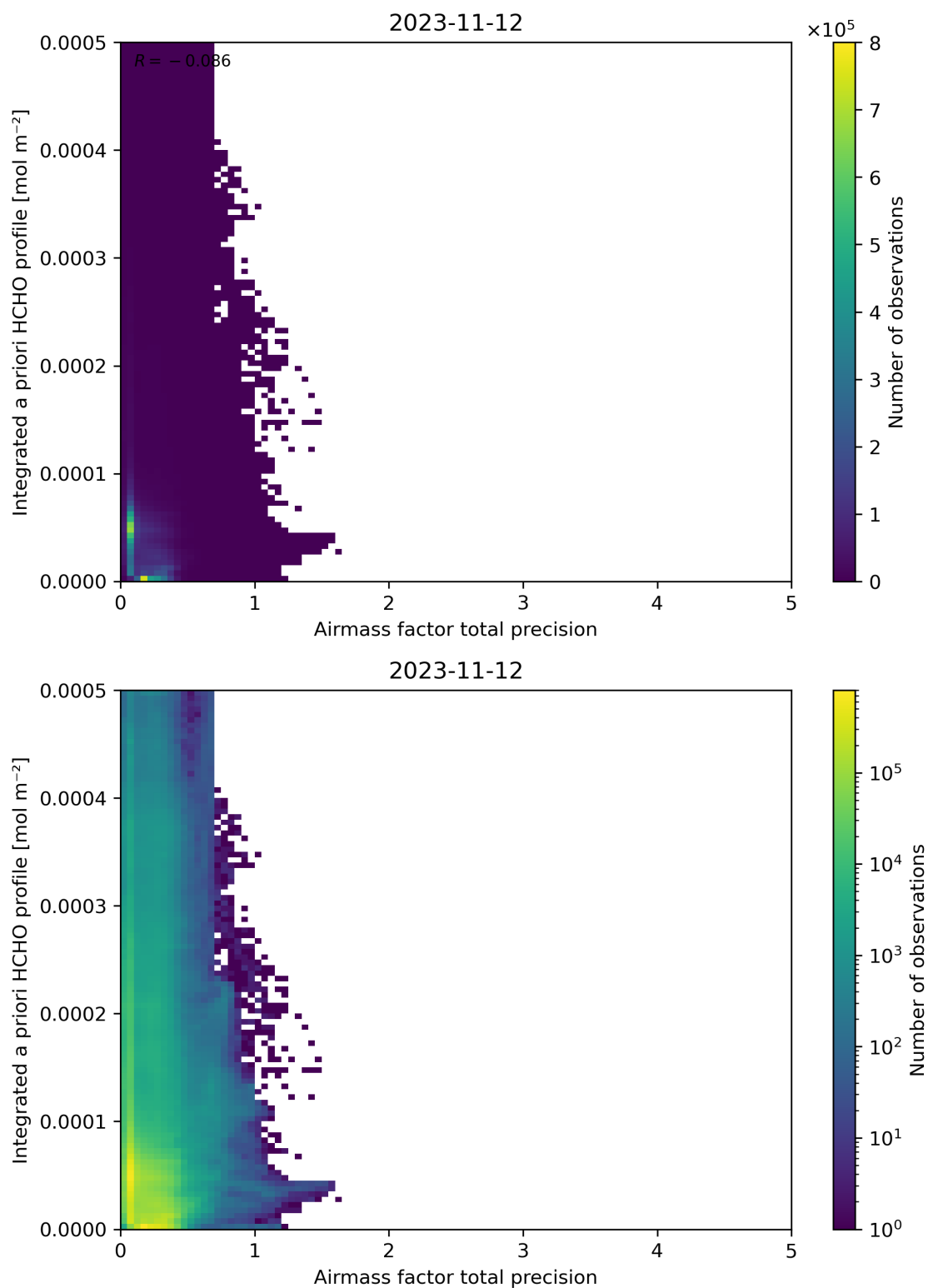
Figure 111: Scatter density plot of “Airmass factor total precision” against “Integrated a priori HCHO profile” for 2023-11-12 to 2023-11-13.
