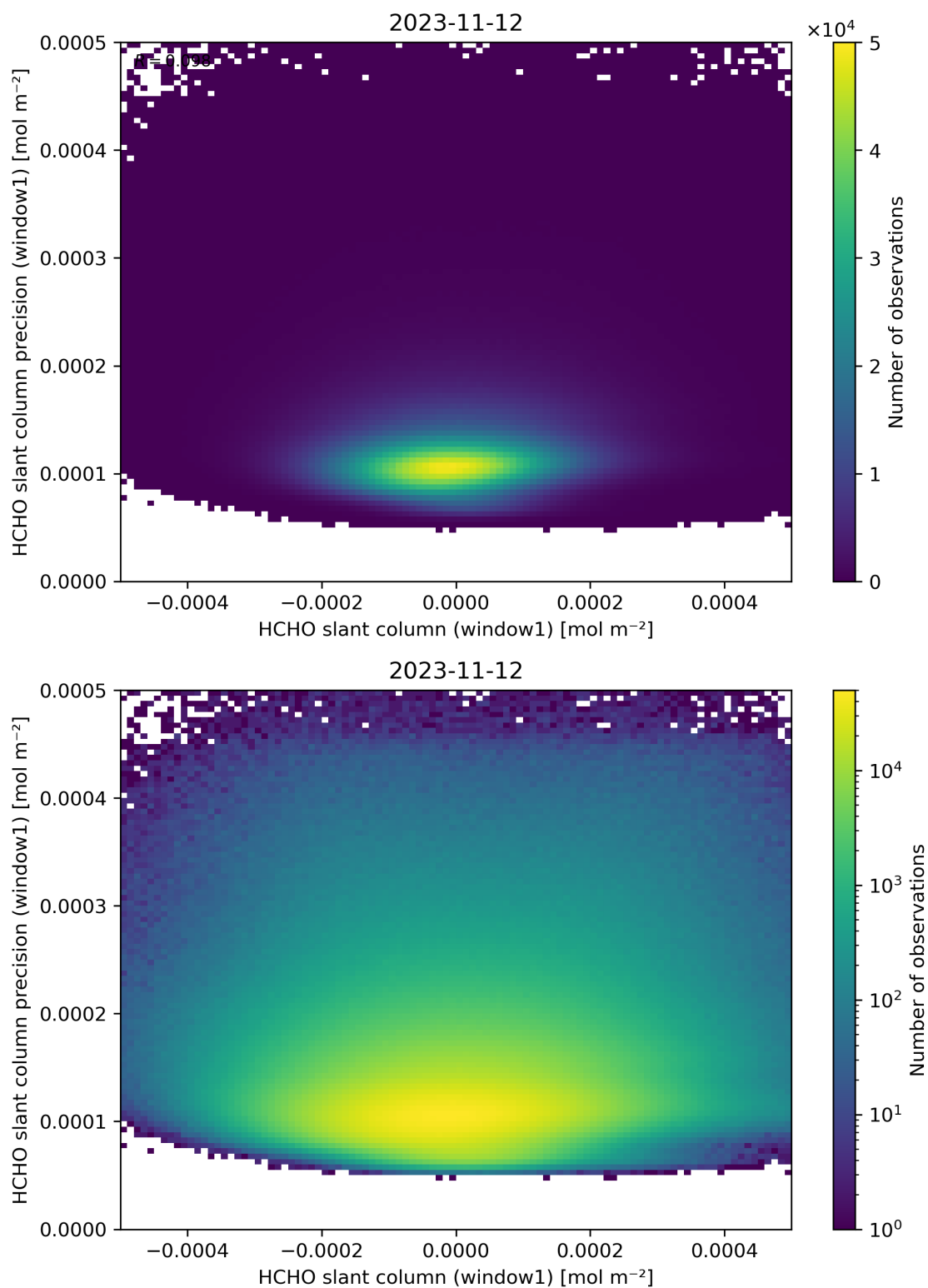
Figure 84: Scatter density plot of “HCHO slant column (window1)” against “HCHO slant column precision (window1)” for 2023-11-12 to 2023-11-13.
