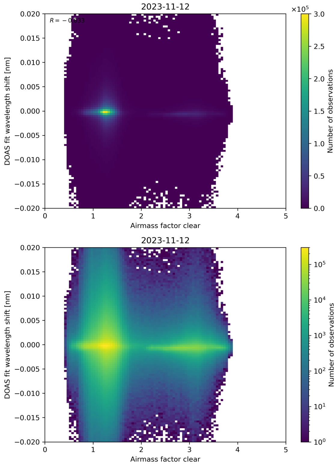
Figure 72: Scatter density plot of “Airmass factor clear” against “DOAS fit wavelength shift” for 2023-11-12 to 2023-11-13.
