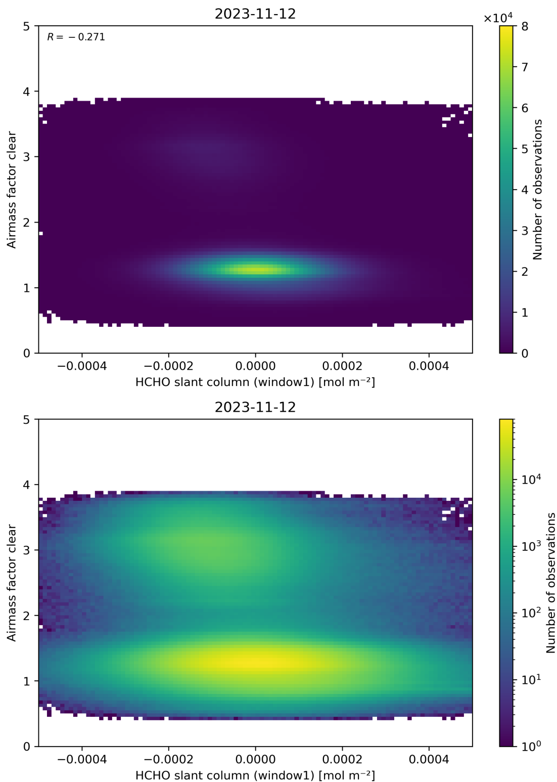
Figure 81: Scatter density plot of “HCHO slant column (window1)” against “Airmass factor clear” for 2023-11-12 to 2023-11-13.
