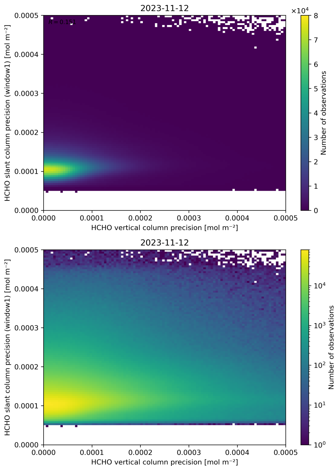
Figure 143: Scatter density plot of “HCHO vertical column precision” against “HCHO slant column precision (window1)” for 2023-11-12 to 2023-11-13.
