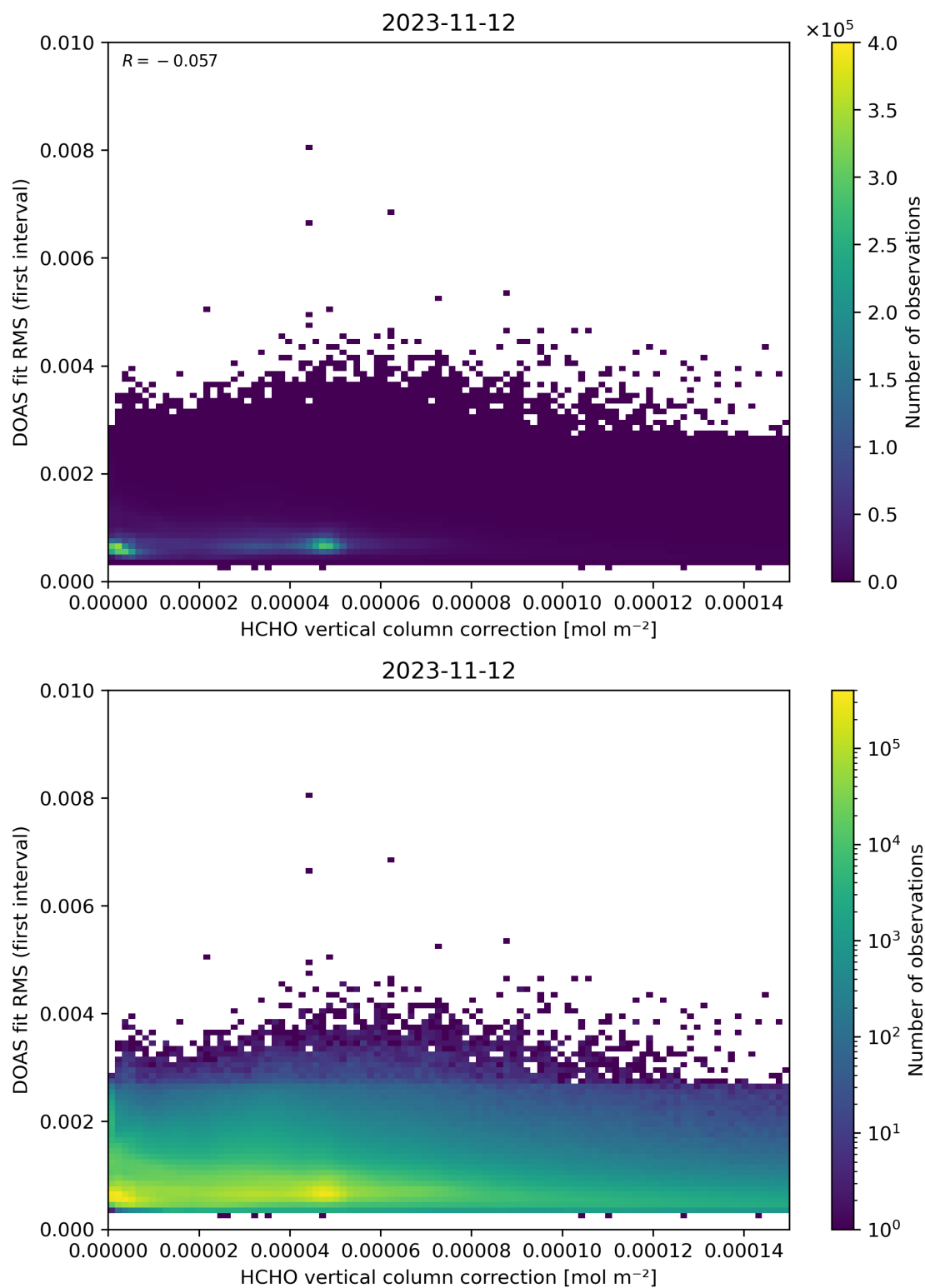
Figure 112: Scatter density plot of “HCHO vertical column correction” against “DOAS fit RMS (first interval)” for 2023-11-12 to 2023-11-13.
