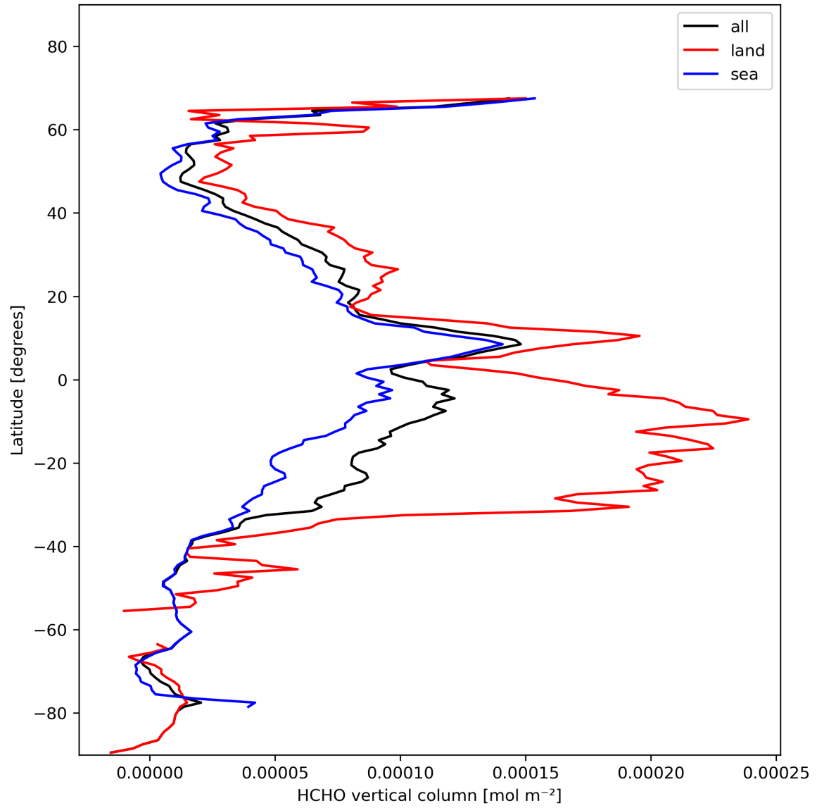
Figure 21: Zonal average of “HCHO vertical column” for 2023-11-12 to 2023-11-13.
