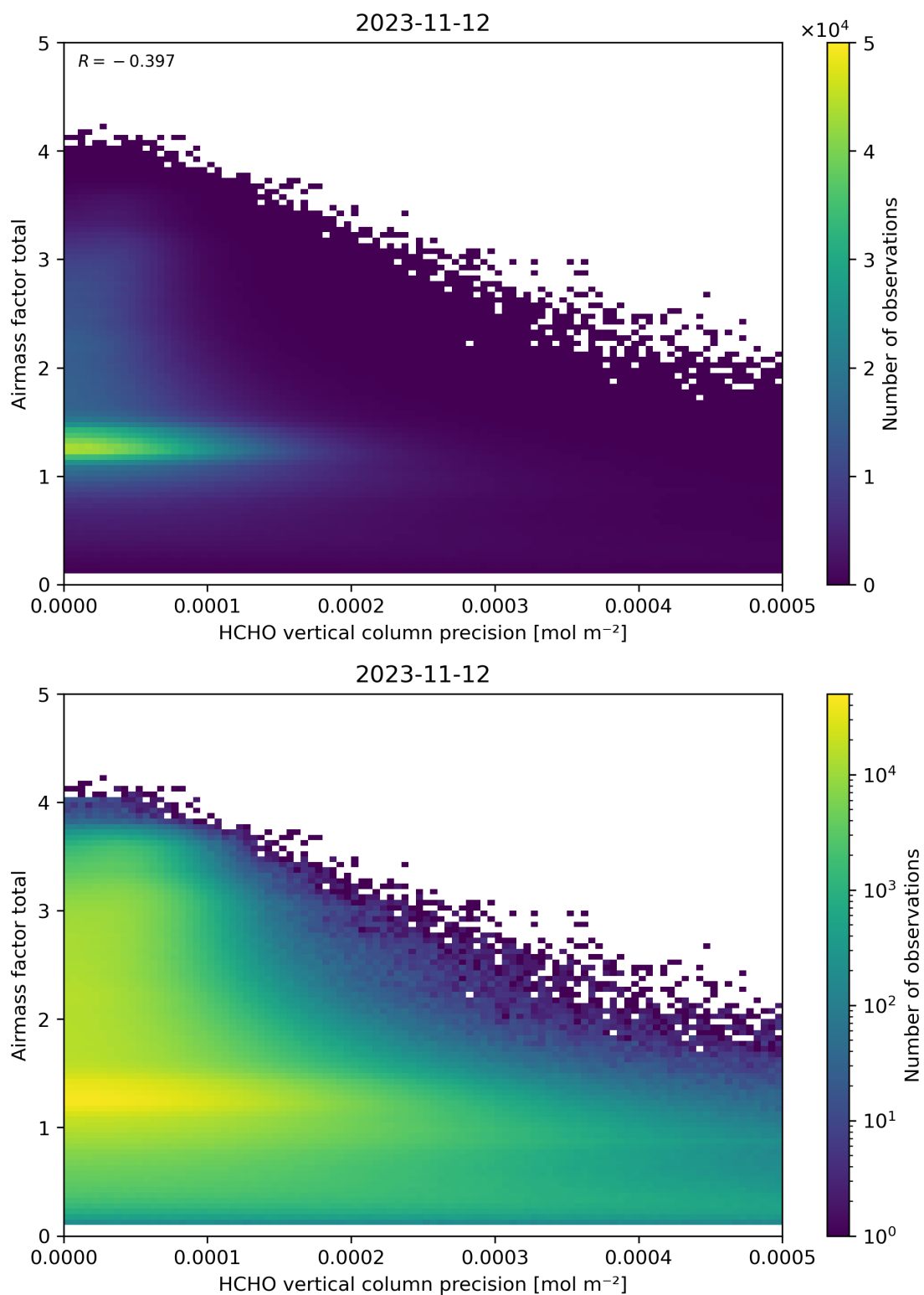
Figure 144: Scatter density plot of “HCHO vertical column precision” against “Airmass factor total” for 2023-11-12 to 2023-11-13.
