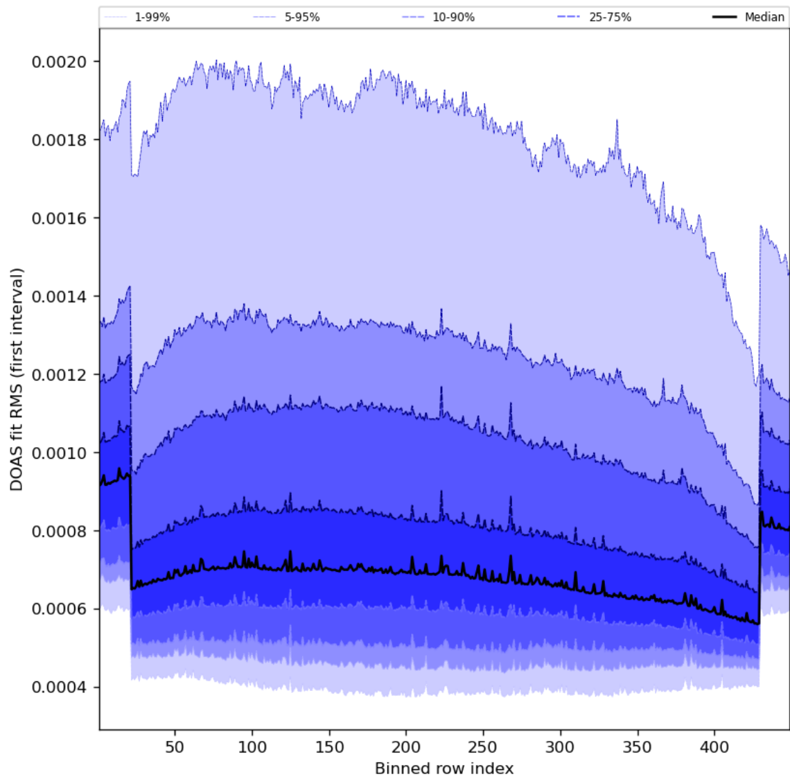
Figure 60: Along track statistics of “DOAS fit RMS (first interval)” for 2023-11-12 to 2023-11-13
