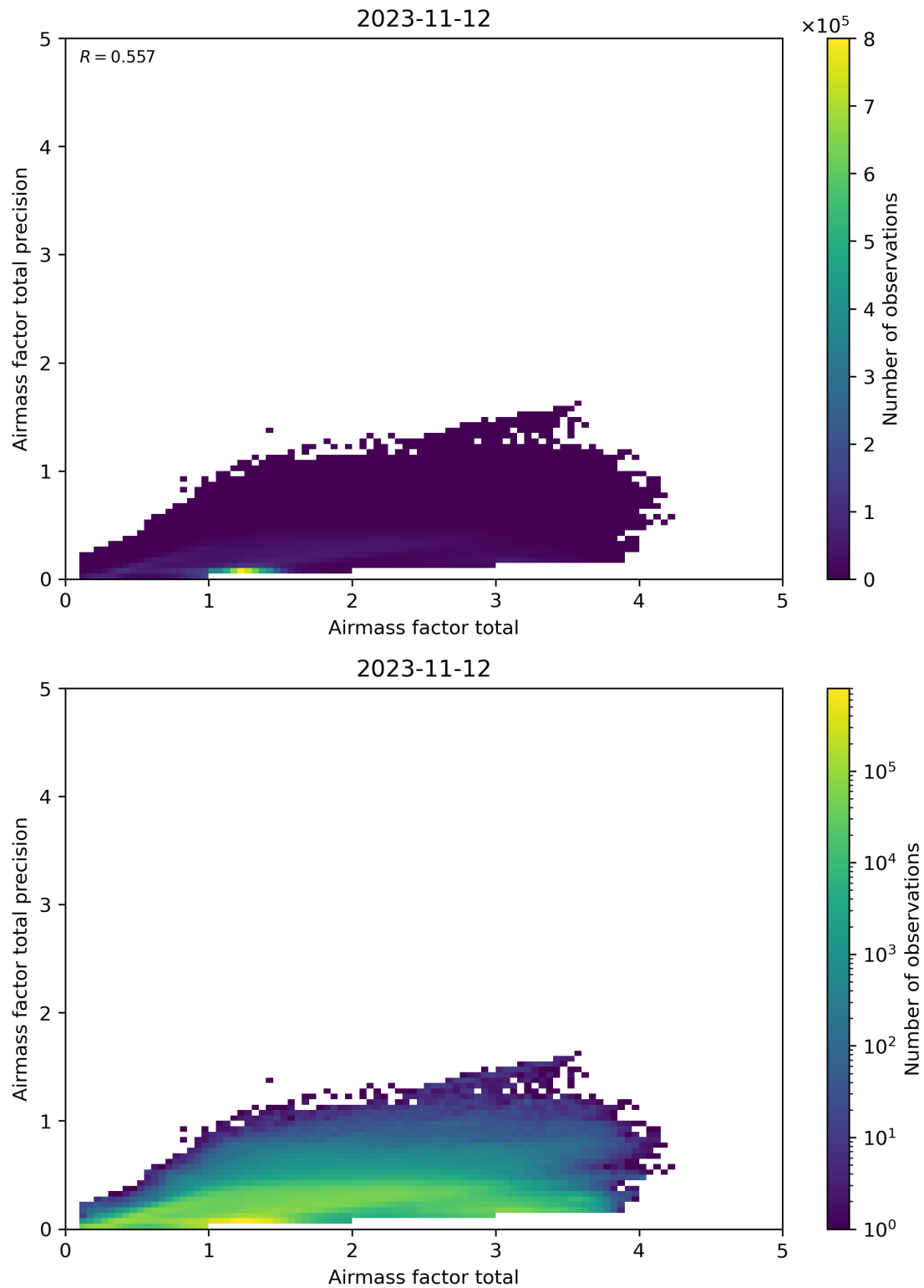
Figure 103: Scatter density plot of “Airmass factor total” against “Airmass factor total precision” for 2023-11-12 to 2023-11-13.
