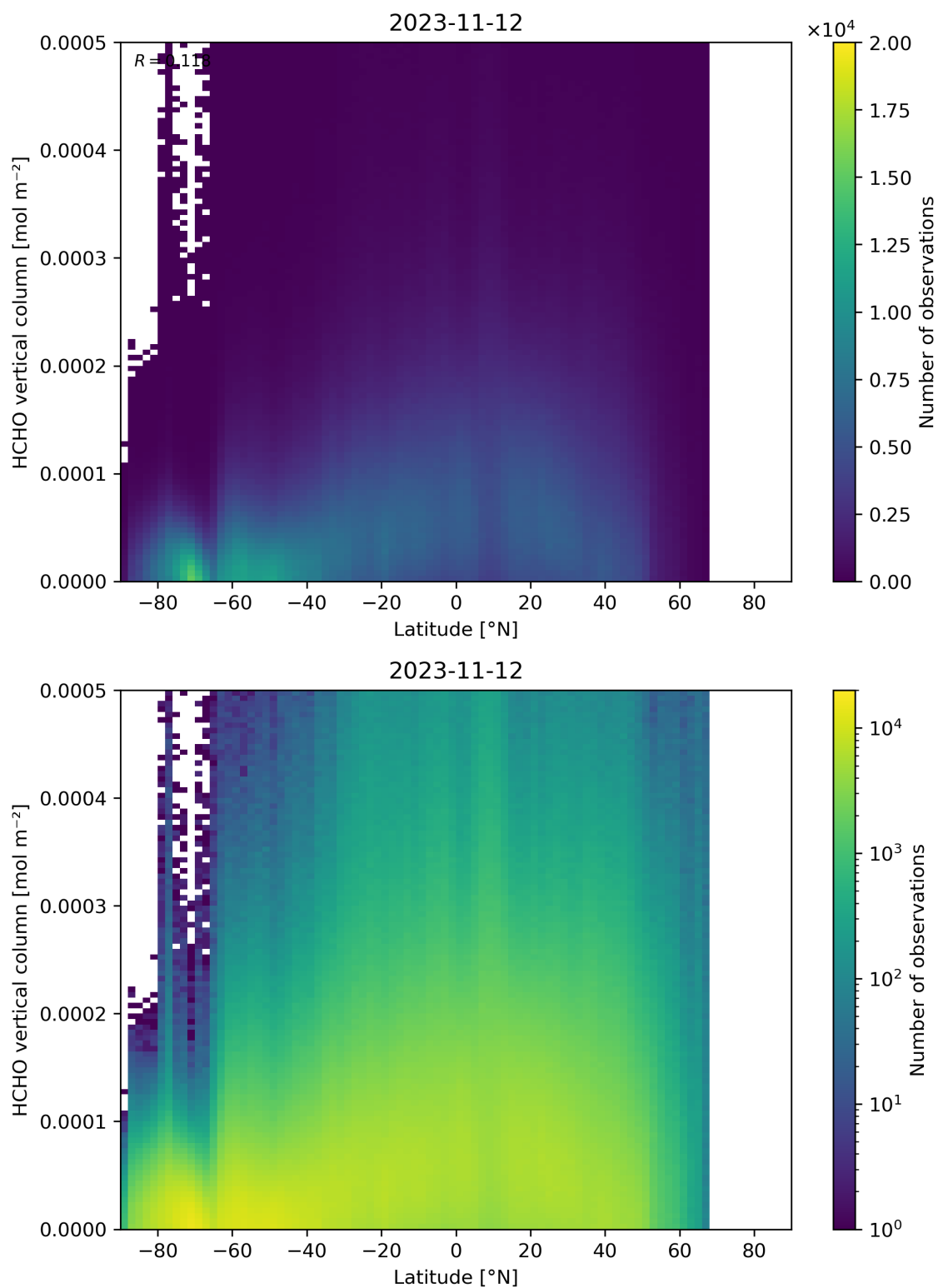
Figure 163: Scatter density plot of “Latitude” against “HCHO vertical column” for 2023-11-12 to 2023-11-13.
