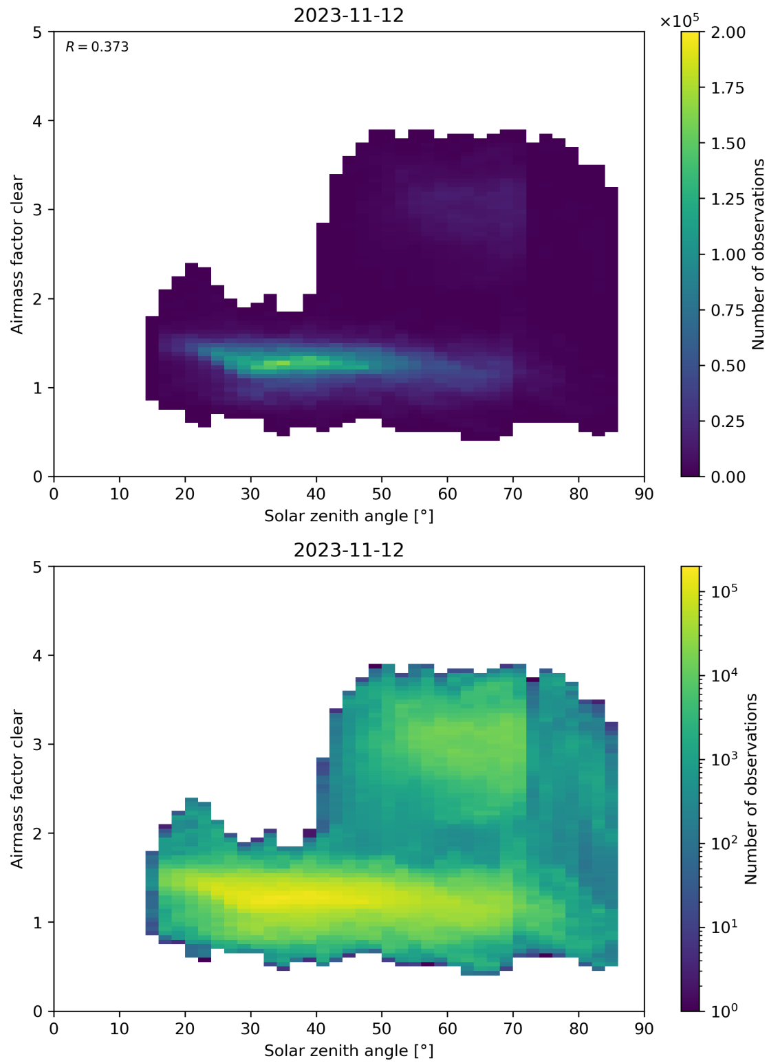
Figure 170: Scatter density plot of “Solar zenith angle” against “Airmass factor clear” for 2023-11-12 to 2023-11-13.
