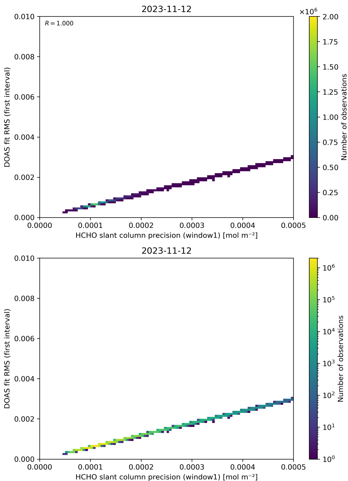
Figure 88: Scatter density plot of “HCHO slant column precision (window1)” against “DOAS fit RMS (first interval)” for 2023-11-12 to 2023-11-13.
