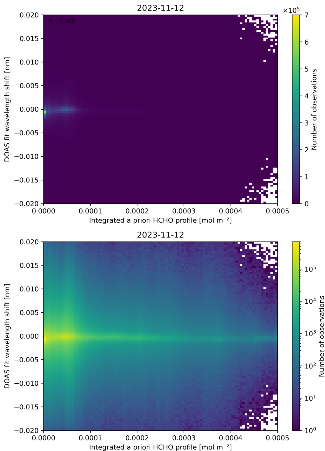
Figure 149: Scatter density plot of “Integrated a priori HCHO profile” against “DOAS fit wavelength shift” for 2023-11-12 to 2023-11-13.
