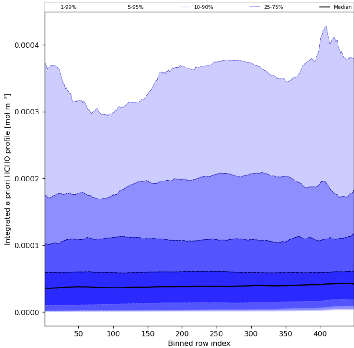
Figure 57: Along track statistics of "Integrated a priori HCHO profile" for 2023-11-12 to 2023-11-13
