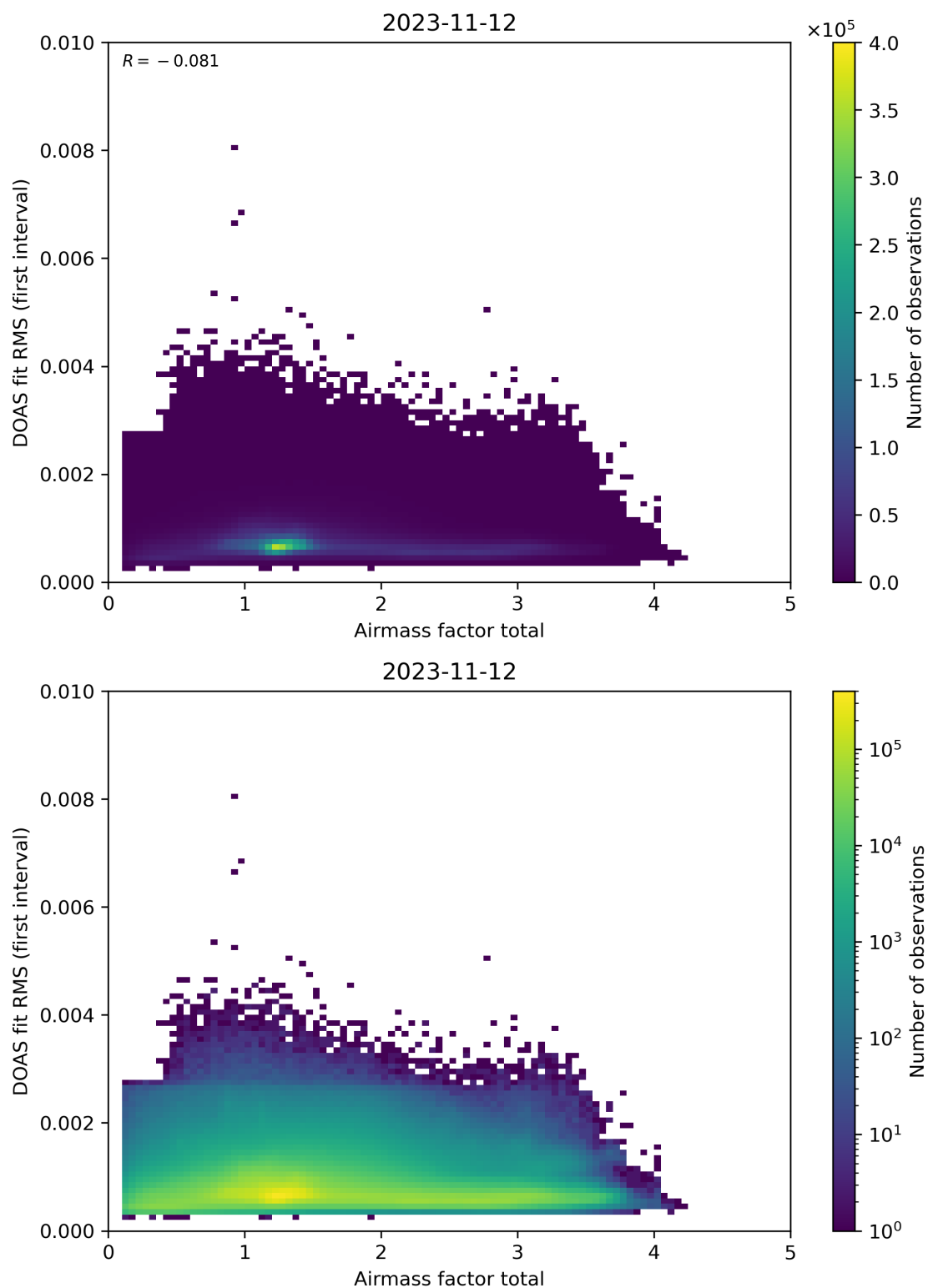
Figure 97: Scatter density plot of “Airmass factor total” against “DOAS fit RMS (first interval)” for 2023-11-12 to 2023-11-13.
