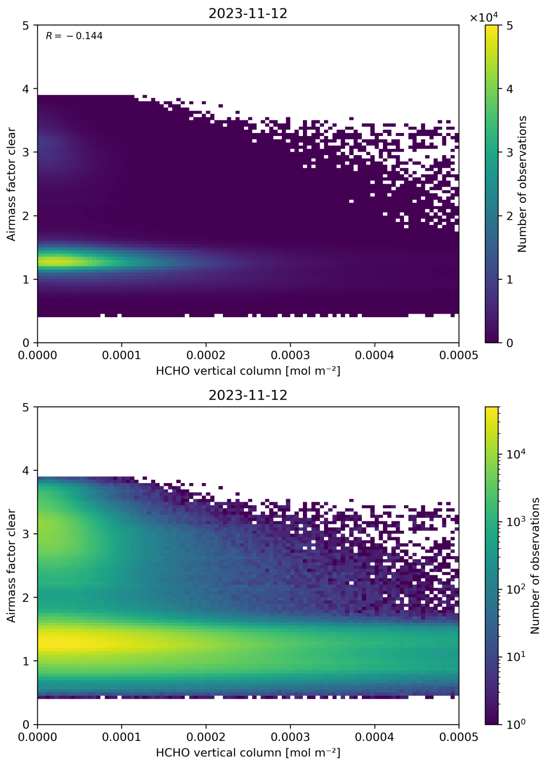
Figure 126: Scatter density plot of “HCHO vertical column” against “Airmass factor clear” for 2023-11-12 to 2023-11-13.
