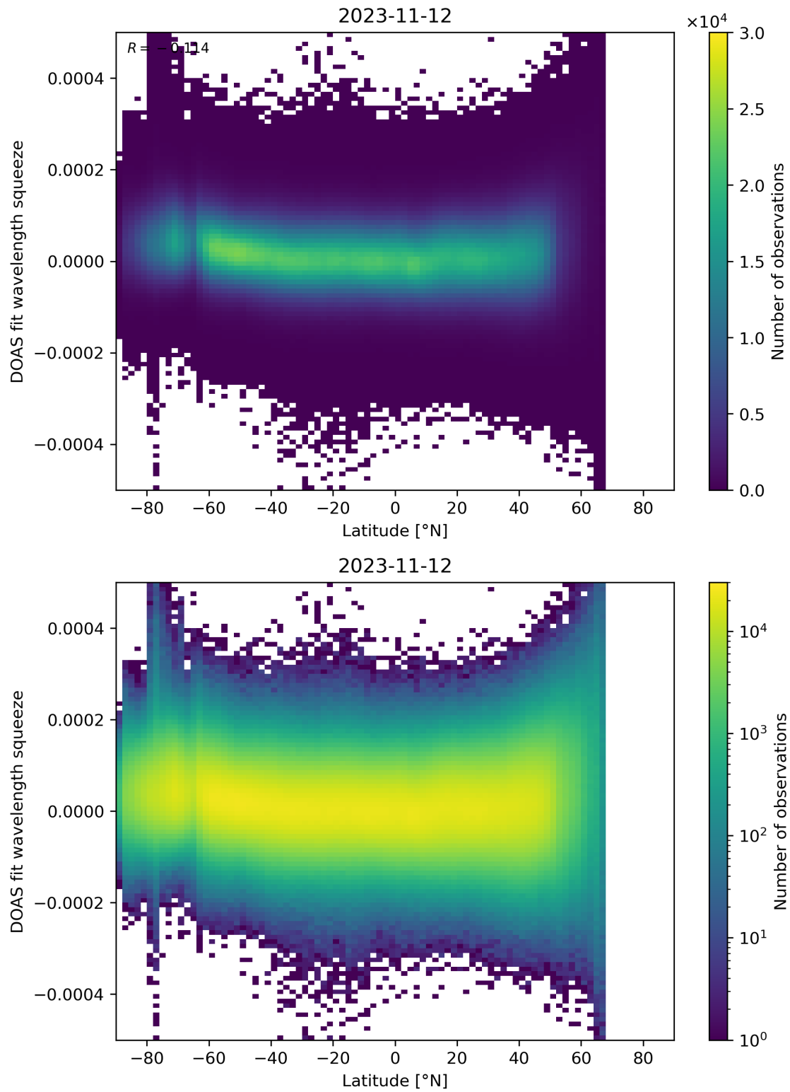
Figure 155: Scatter density plot of “Latitude” against “DOAS fit wavelength squeeze” for 2023-11-12 to 2023-11-13.
