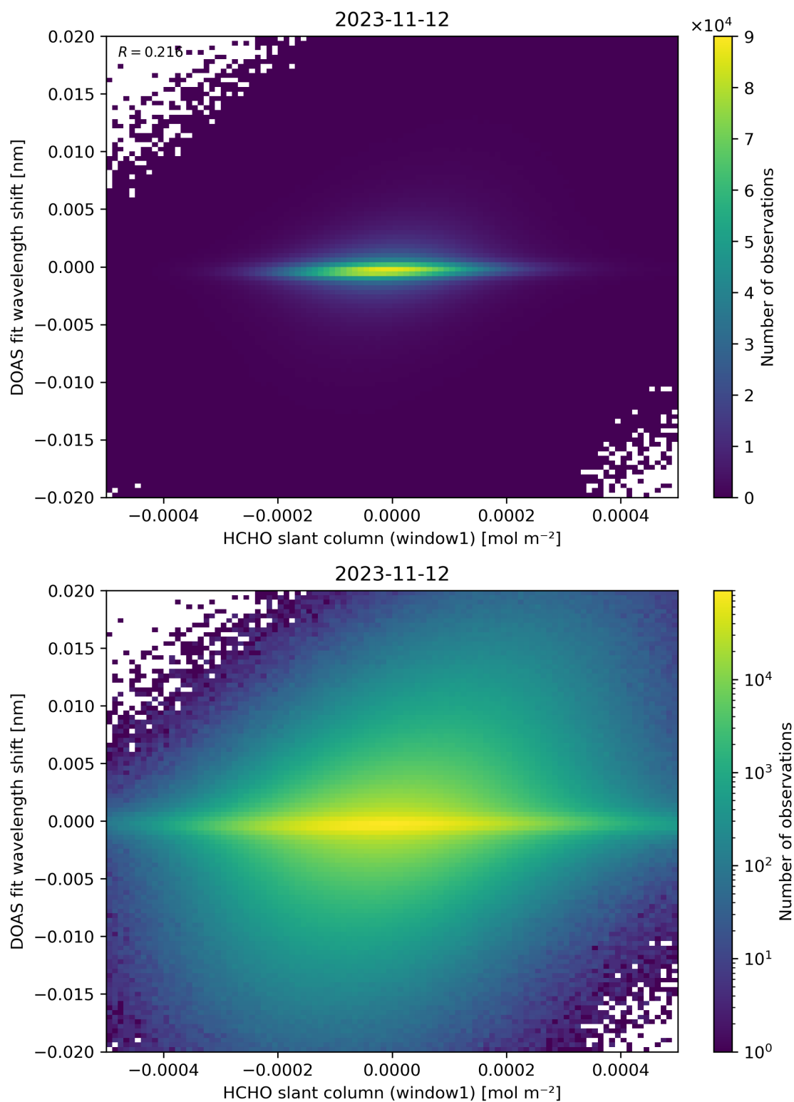
Figure 79: Scatter density plot of “HCHO slant column (window1)” against “DOAS fit wavelength shift” for 2023-11-12 to 2023-11-13.
