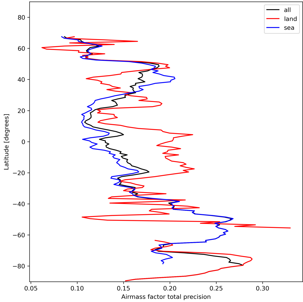
Figure 27: Zonal average of “Airmass factor total precision” for 2023-11-12 to 2023-11-13.
