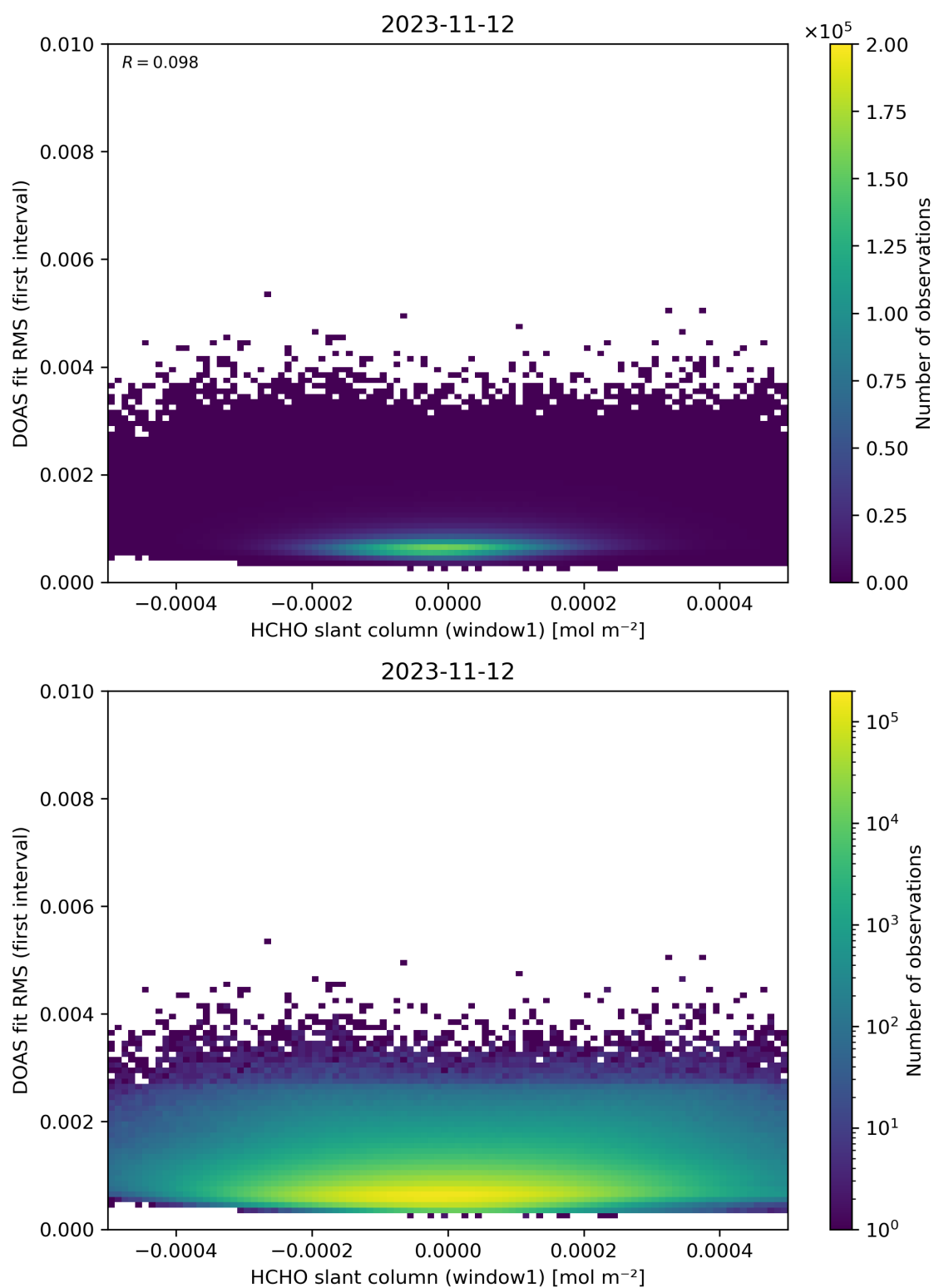
Figure 78: Scatter density plot of “HCHO slant column (window1)” against “DOAS fit RMS (first interval)” for 2023-11-12 to 2023-11-13.
