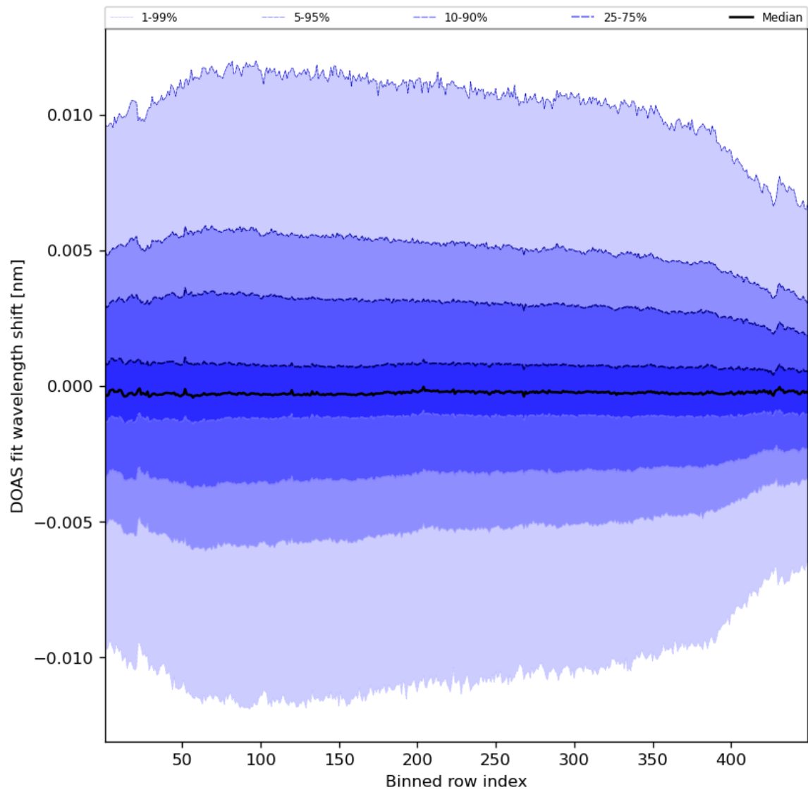
Figure 58: Along track statistics of “DOAS fit wavelength shift” for 2023-11-12 to 2023-11-13
