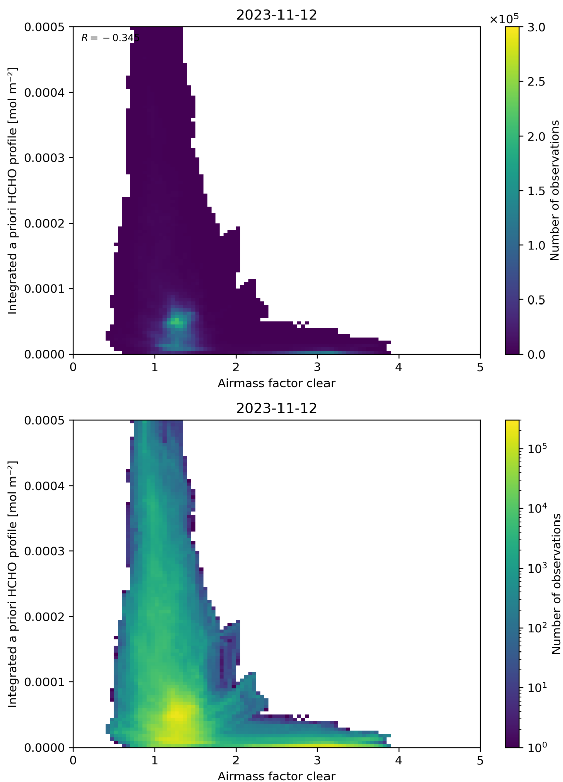
Figure 76: Scatter density plot of “Airmass factor clear” against “Integrated a priori HCHO profile” for 2023-11-12 to 2023-11-13.
