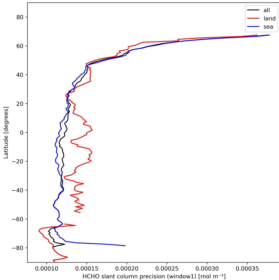
Figure 25: Zonal average of “HCHO slant column precision (window1)” for 2023-11-12 to 2023-11-13.
