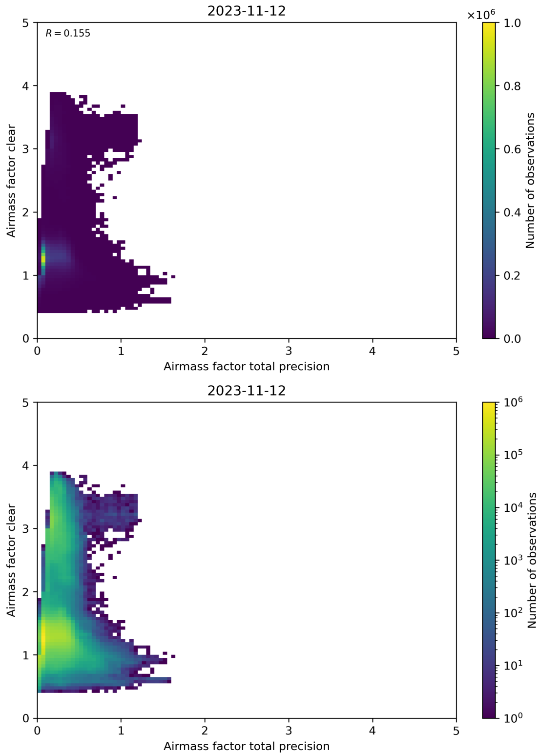
Figure 108: Scatter density plot of “Airmass factor total precision” against “Airmass factor clear” for 2023-11-12 to 2023-11-13.
