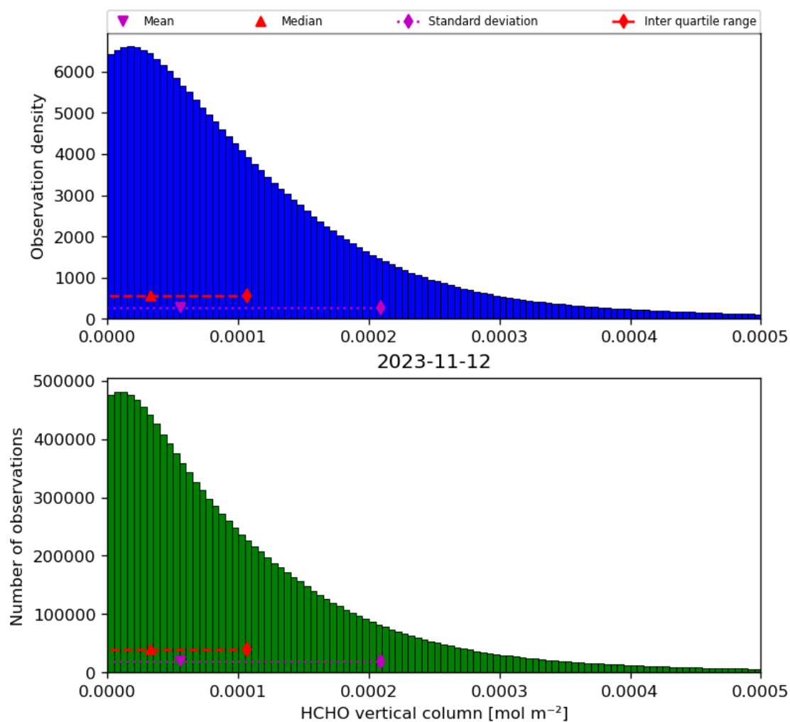
Figure 35: Histogram of “HCHO vertical column” for 2023-11-12 to 2023-11-13
