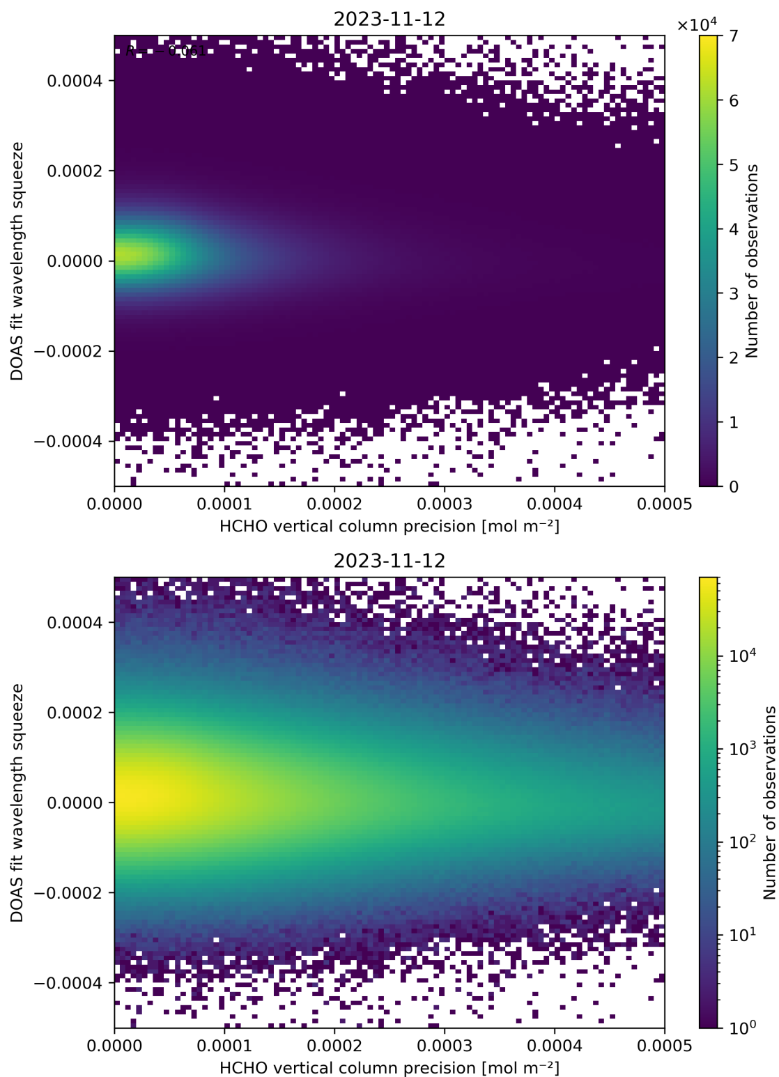
Figure 138: Scatter density plot of “HCHO vertical column precision” against “DOAS fit wavelength squeeze” for 2023-11-12 to 2023-11-13.
