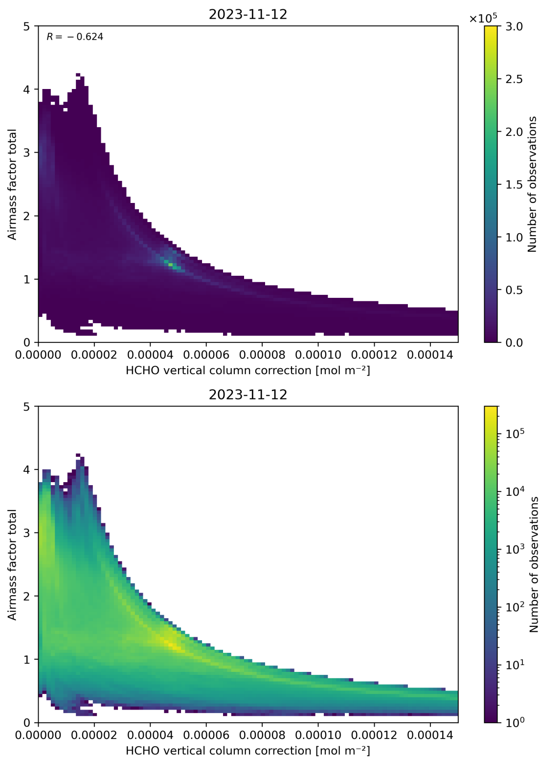
Figure 120: Scatter density plot of “HCHO vertical column correction” against “Airmass factor total” for 2023-11-12 to 2023-11-13.
