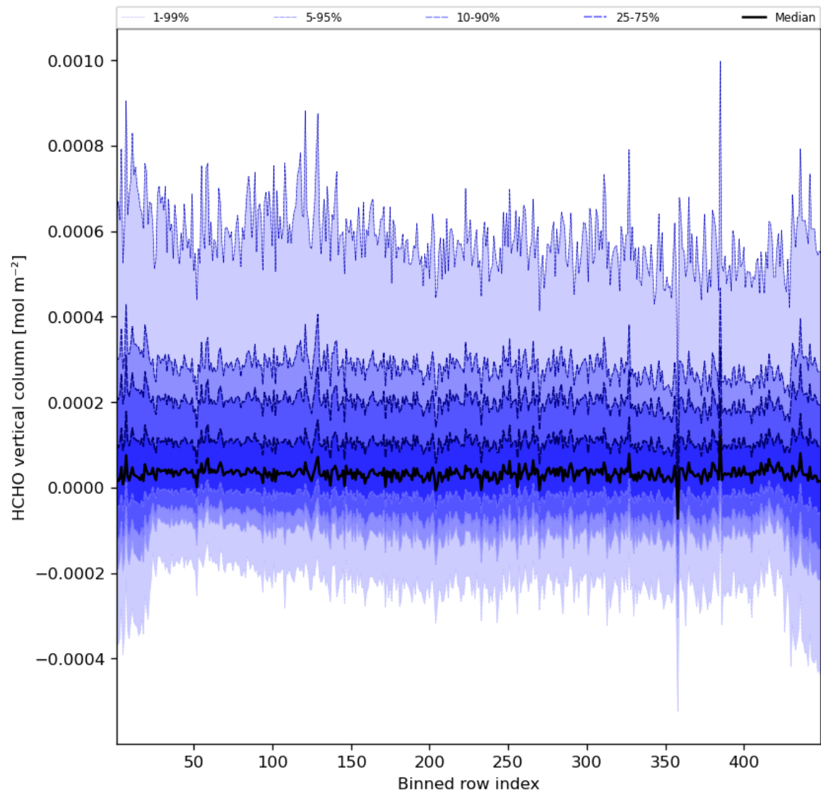
Figure 49: Along track statistics of “HCHO vertical column” for 2023-11-12 to 2023-11-13
