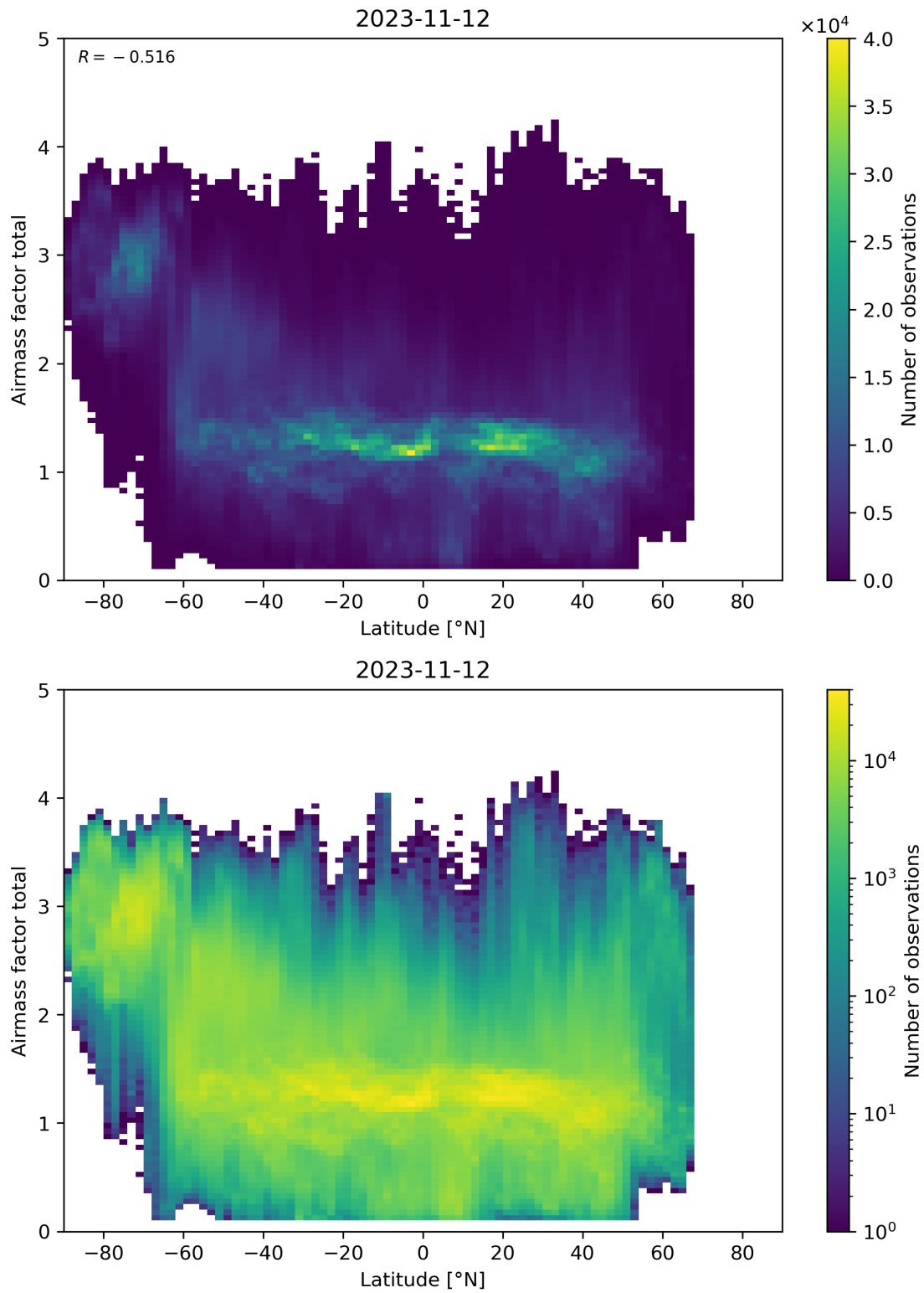
Figure 161: Scatter density plot of “Latitude” against “Airmass factor total” for 2023-11-12 to 2023-11-13.
