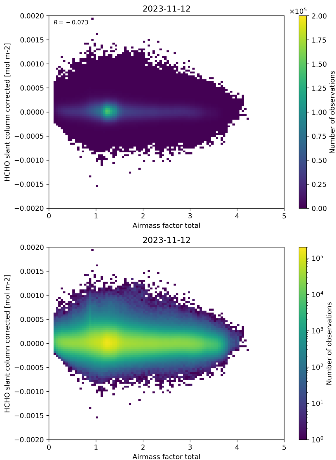
Figure 101: Scatter density plot of “Airmass factor total” against “HCHO slant column corrected” for 2023-11-12 to 2023-11-13.
