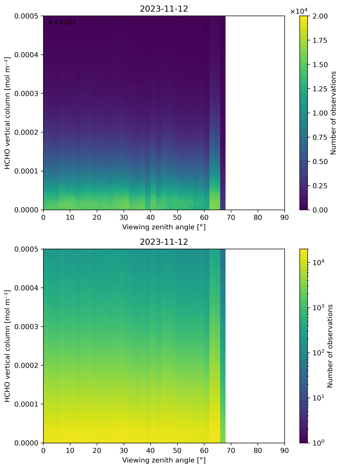
Figure 192: Scatter density plot of “Viewing zenith angle” against “HCHO vertical column” for 2023-11-12 to 2023-11-13.
