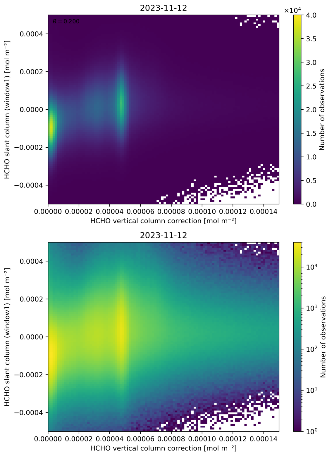
Figure 118: Scatter density plot of “HCHO vertical column correction” against “HCHO slant column (window1)” for 2023-11-12 to 2023-11-13.
