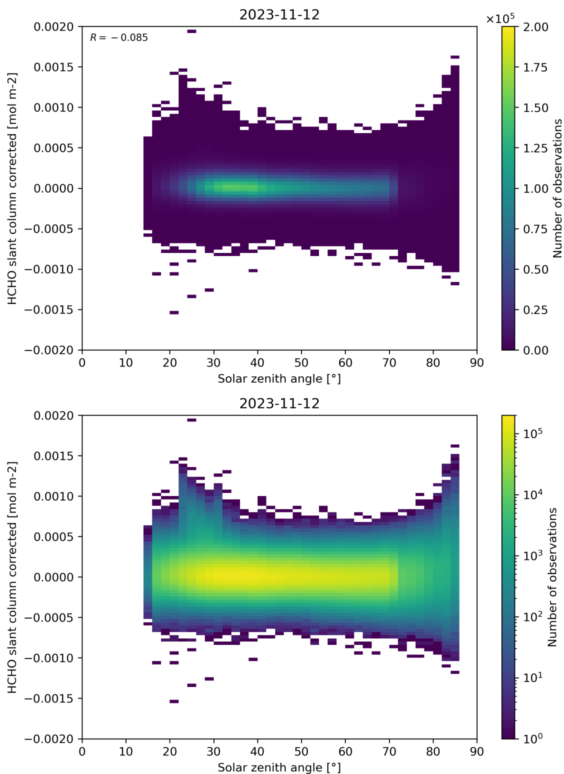
Figure 171: Scatter density plot of “Solar zenith angle” against “HCHO slant column corrected” for 2023-11-12 to 2023-11-13.
