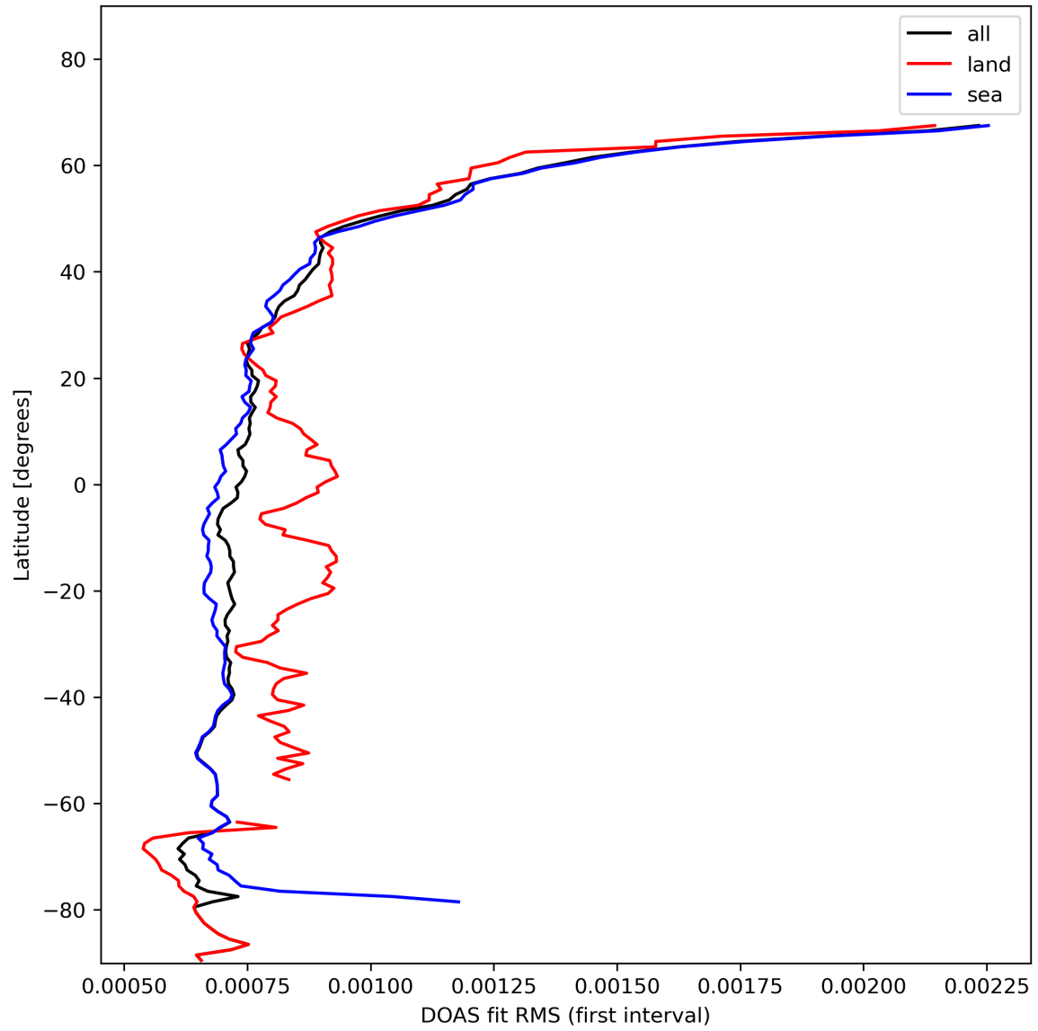
Figure 32: Zonal average of “DOAS fit RMS (first interval)” for 2023-11-12 to 2023-11-13.
