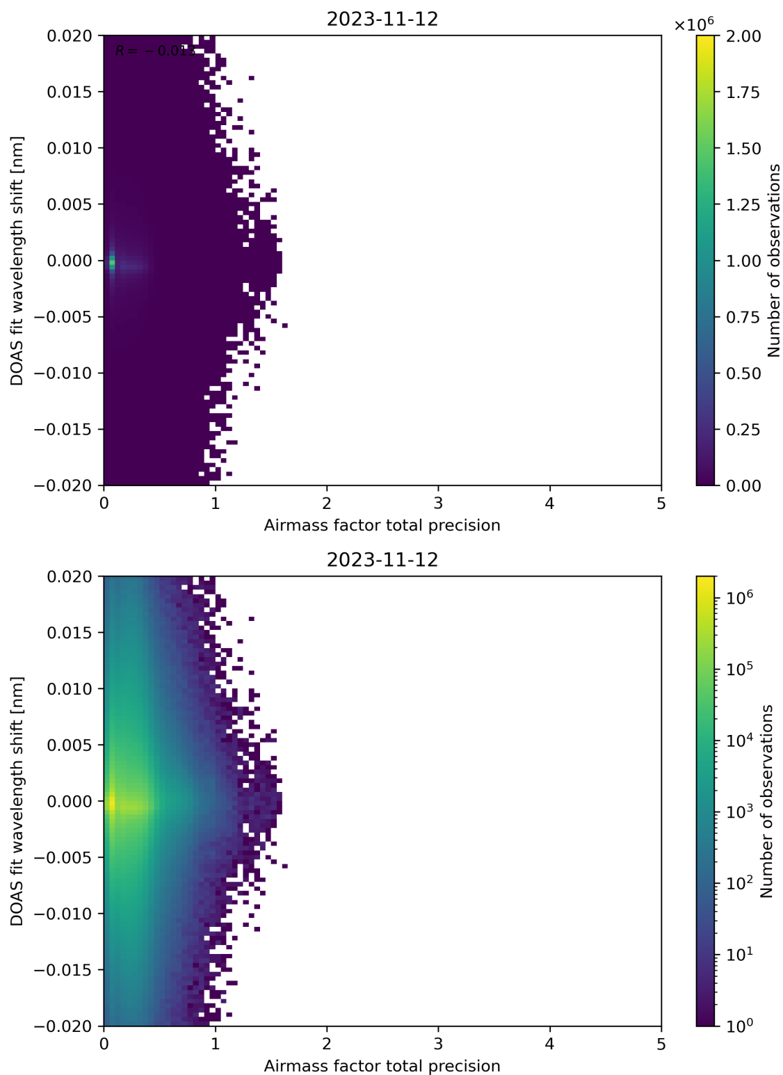
Figure 106: Scatter density plot of “Airmass factor total precision” against “DOAS fit wavelength shift” for 2023-11-12 to 2023-11-13.
