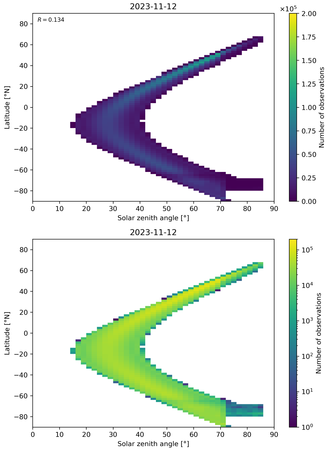
Figure 181: Scatter density plot of “Solar zenith angle” against “Latitude” for 2023-11-12 to 2023-11-13.
