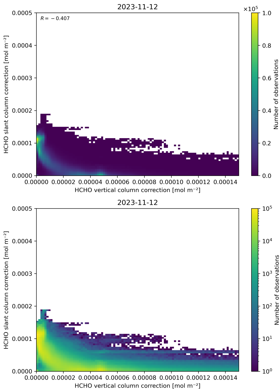
Figure 117: Scatter density plot of “HCHO vertical column correction” against “HCHO slant column correction” for 2023-11-12 to 2023-11-13.
