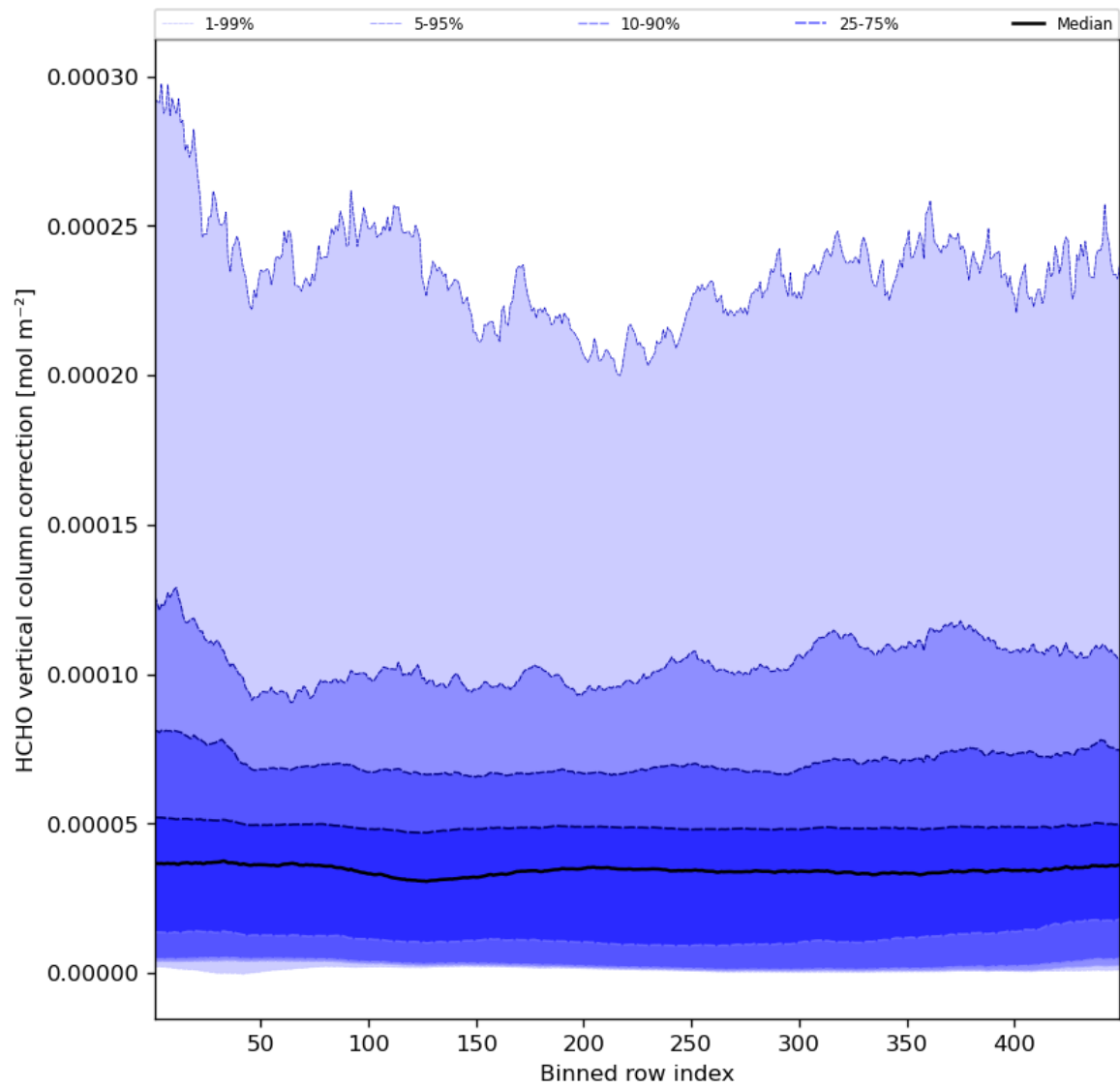
Figure 51: Along track statistics of “HCHO vertical column correction” for 2023-11-12 to 2023-11-13
