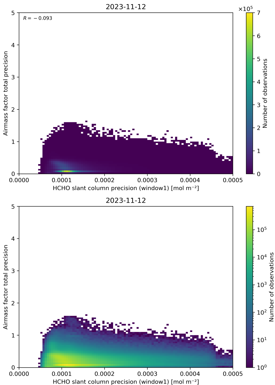
Figure 95: Scatter density plot of “HCHO slant column precision (window1)” against “Airmass factor total precision” for 2023-11-12 to 2023-11-13.
