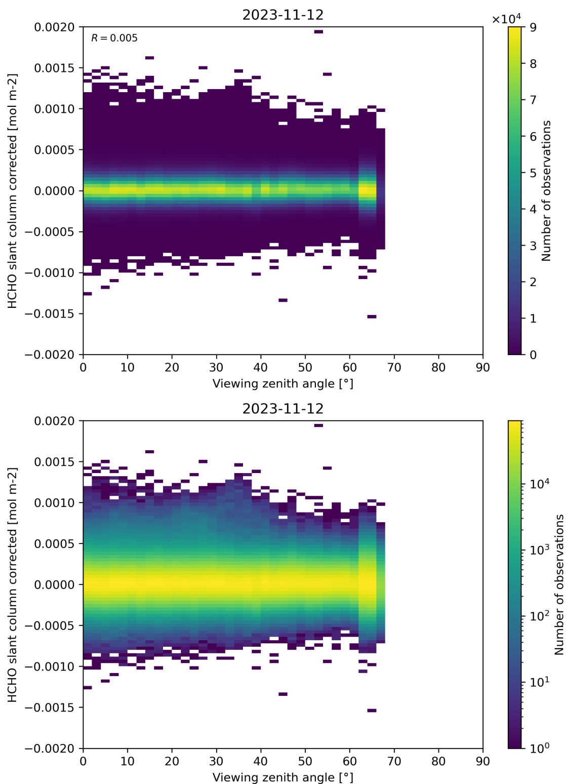
Figure 186: Scatter density plot of “Viewing zenith angle” against “HCHO slant column corrected” for 2023-11-12 to 2023-11-13.
