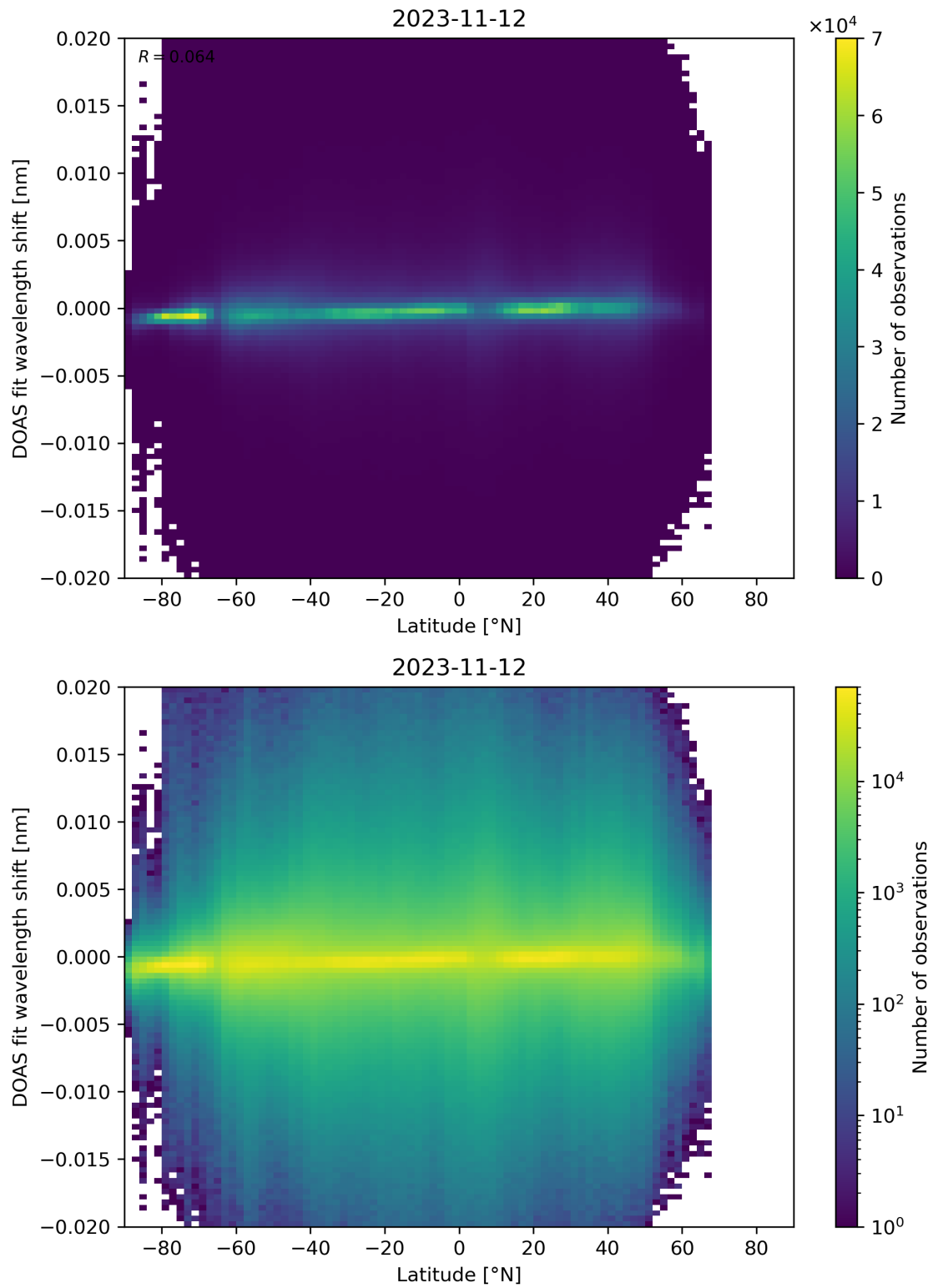
Figure 154: Scatter density plot of “Latitude” against “DOAS fit wavelength shift” for 2023-11-12 to 2023-11-13.
