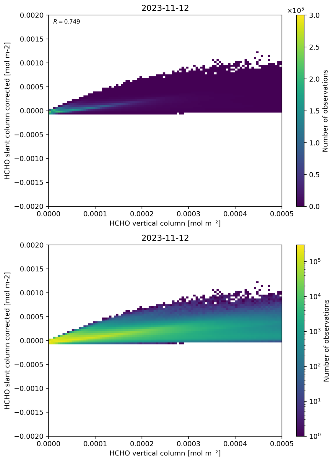
Figure 127: Scatter density plot of “HCHO vertical column” against “HCHO slant column corrected” for 2023-11-12 to 2023-11-13.
