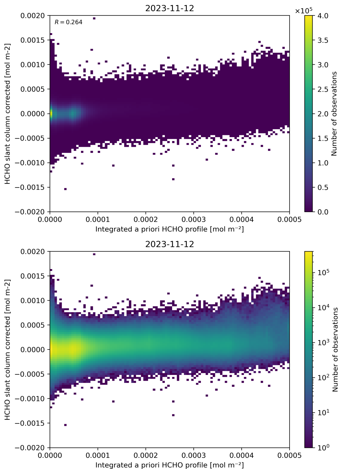
Figure 151: Scatter density plot of “Integrated a priori HCHO profile” against “HCHO slant column corrected” for 2023-11-12 to 2023-11-13.
