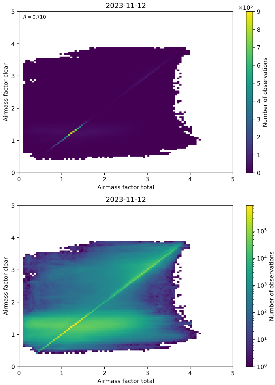
Figure 100: Scatter density plot of “Airmass factor total” against “Airmass factor clear” for 2023-11-12 to 2023-11-13.
