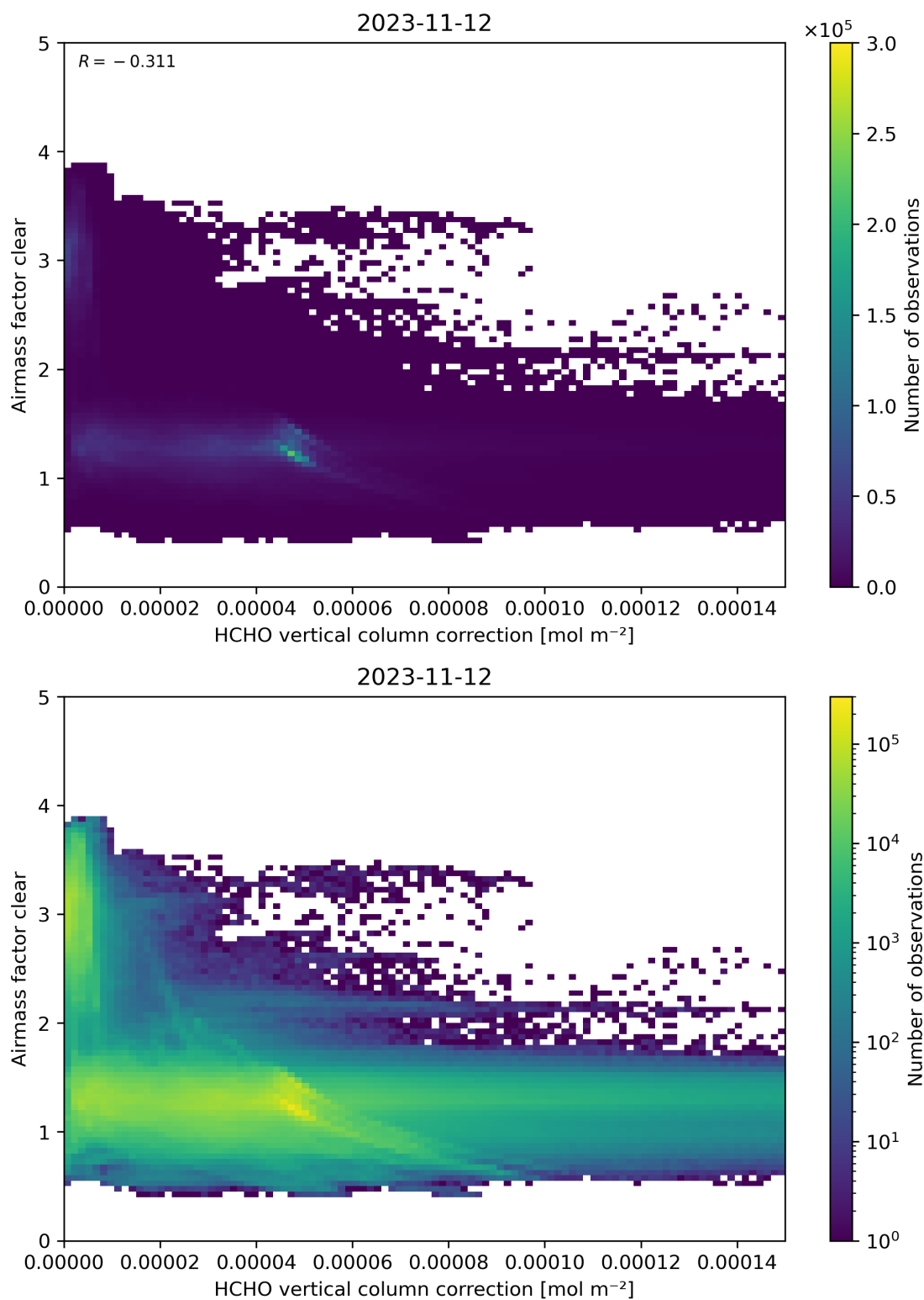
Figure 115: Scatter density plot of “HCHO vertical column correction” against “Airmass factor clear” for 2023-11-12 to 2023-11-13.
