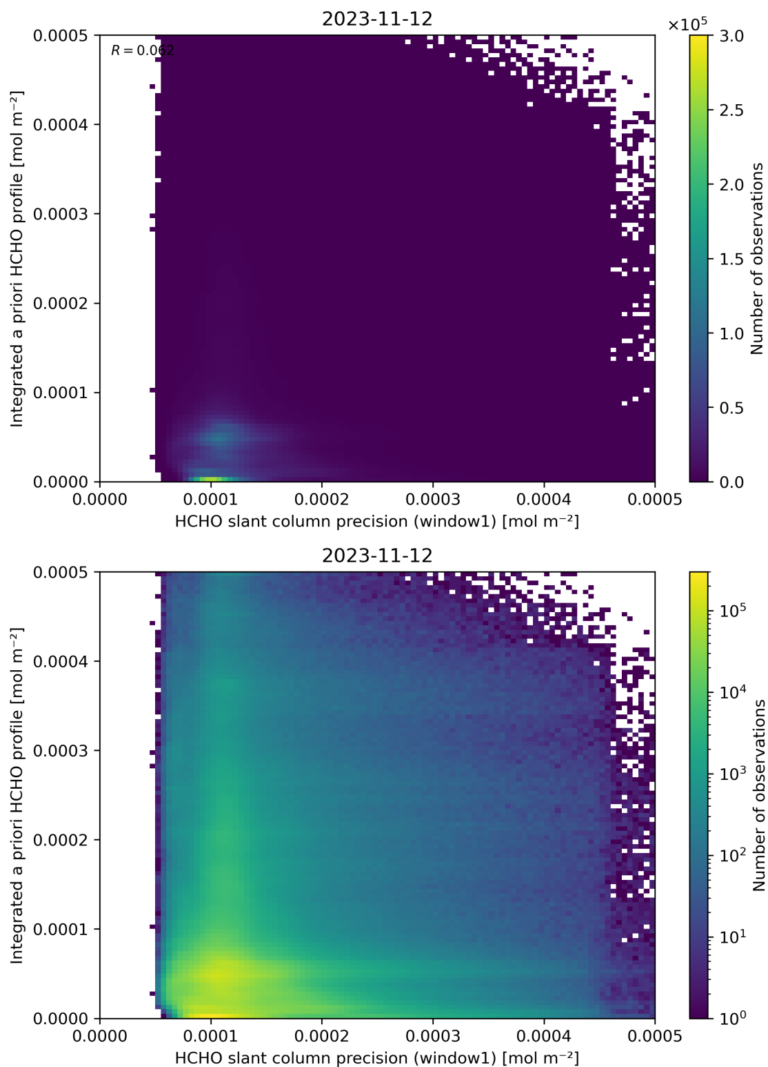
Figure 96: Scatter density plot of “HCHO slant column precision (window1)” against “Integrated a priori HCHO profile” for 2023-11-12 to 2023-11-13.
