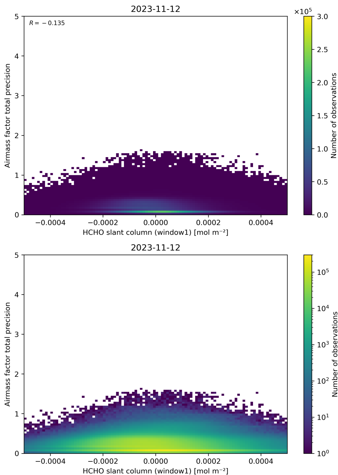
Figure 86: Scatter density plot of “HCHO slant column (window1)” against “Airmass factor total precision” for 2023-11-12 to 2023-11-13.
