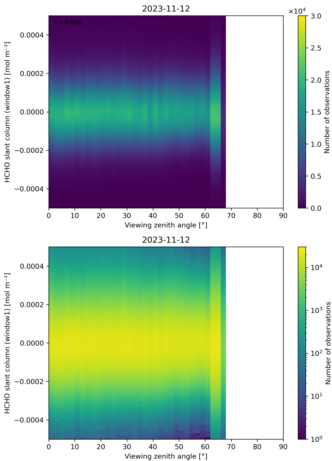
Figure 188: Scatter density plot of “Viewing zenith angle” against “HCHO slant column (window1)” for 2023-11-12 to 2023-11-13.
