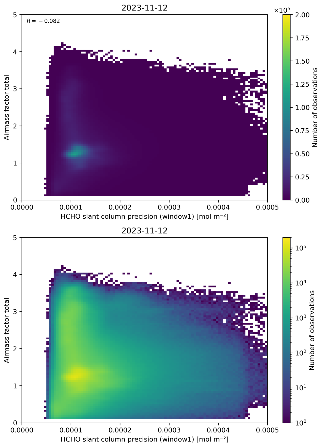
Figure 94: Scatter density plot of “HCHO slant column precision (window1)” against “Airmass factor total” for 2023-11-12 to 2023-11-13.
