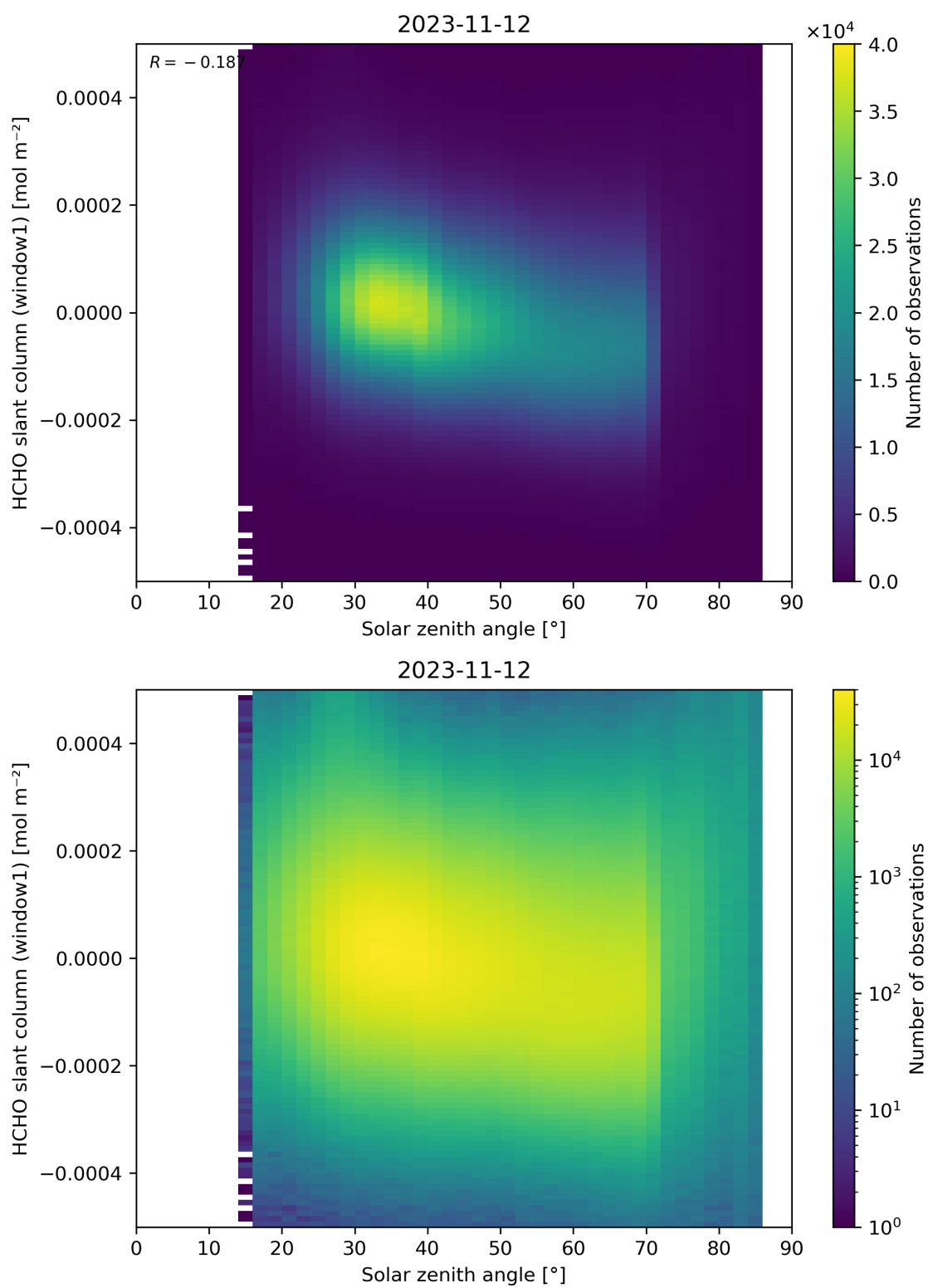
Figure 173: Scatter density plot of “Solar zenith angle” against “HCHO slant column (window1)” for 2023-11-12 to 2023-11-13.
