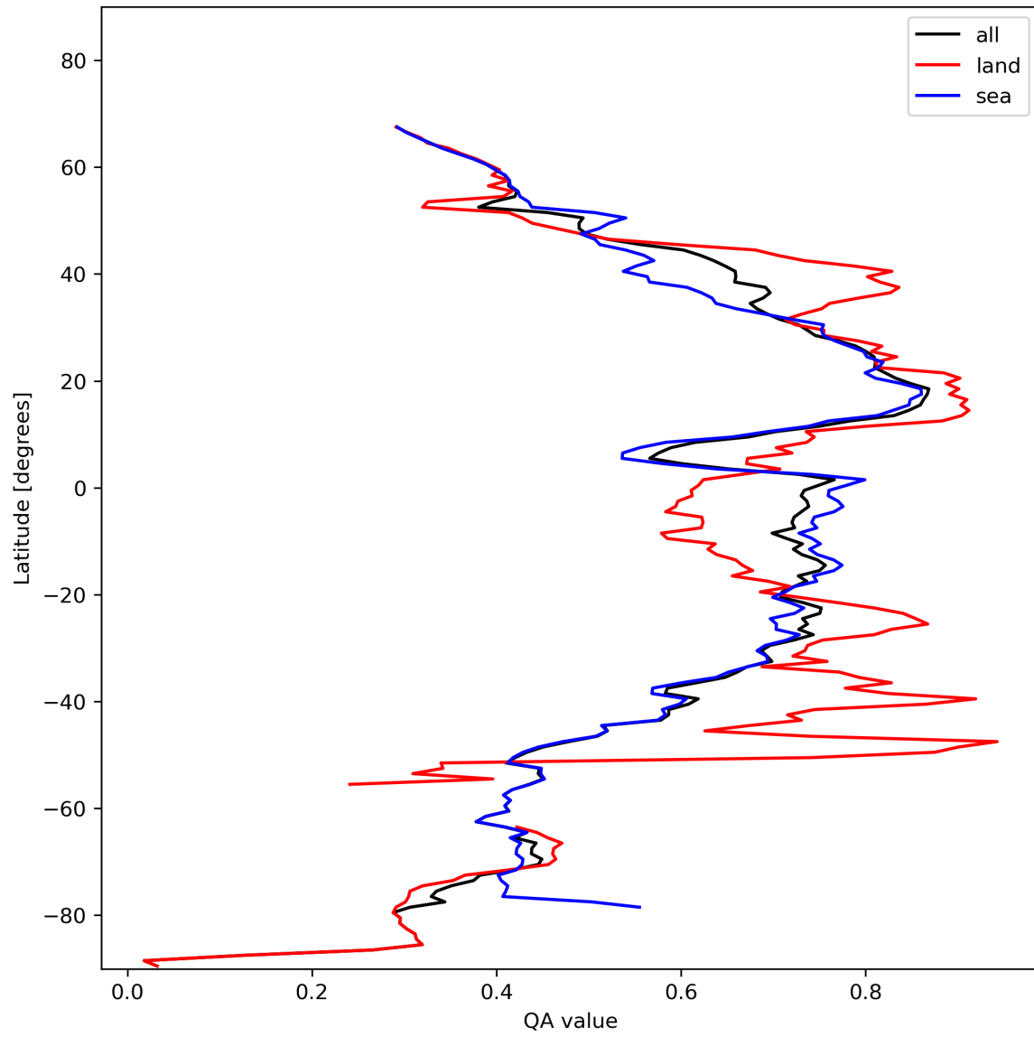
Figure 20: Zonal average of “QA value” for 2023-11-12 to 2023-11-13.
