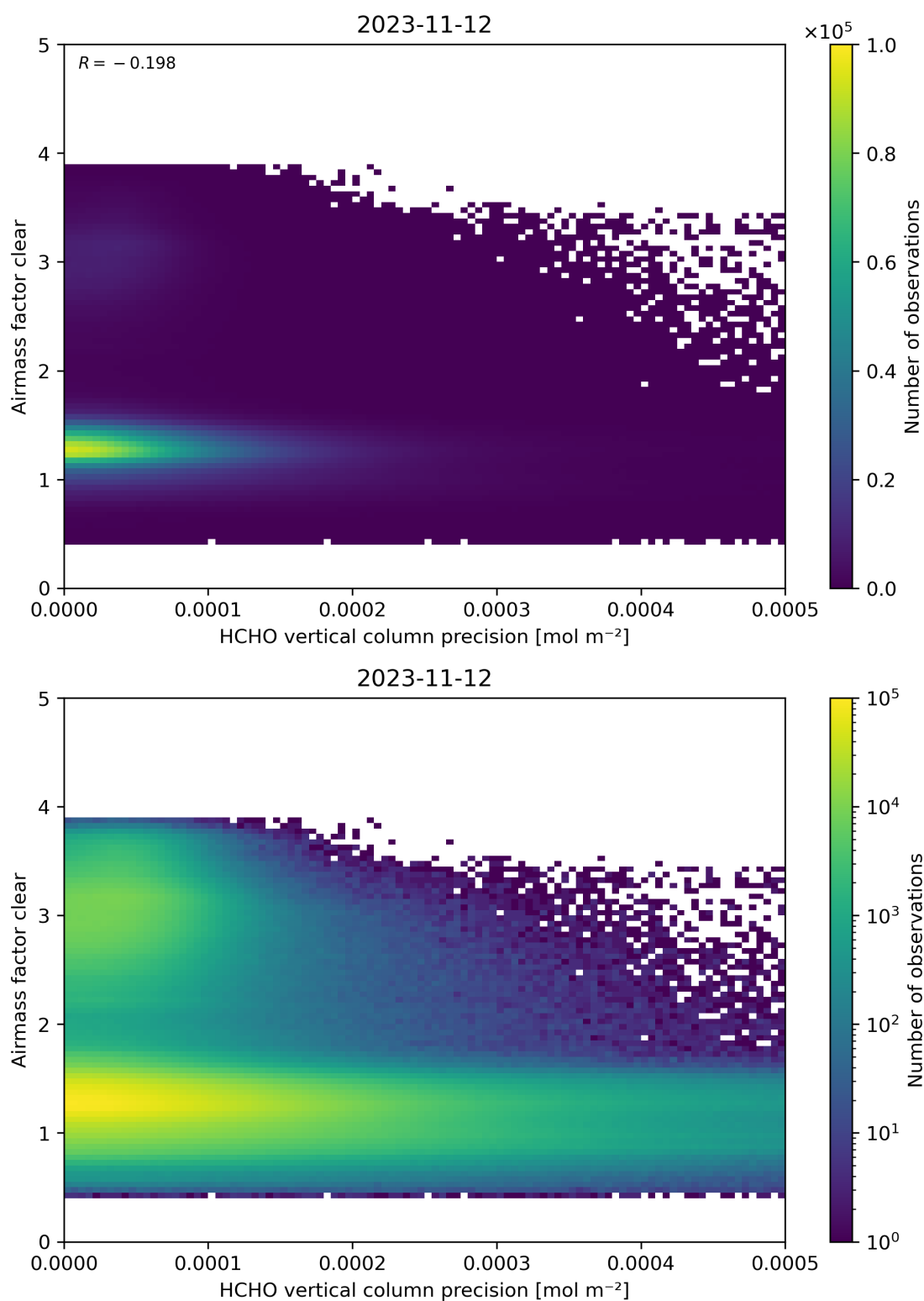
Figure 139: Scatter density plot of “HCHO vertical column precision” against “Airmass factor clear” for 2023-11-12 to 2023-11-13.
