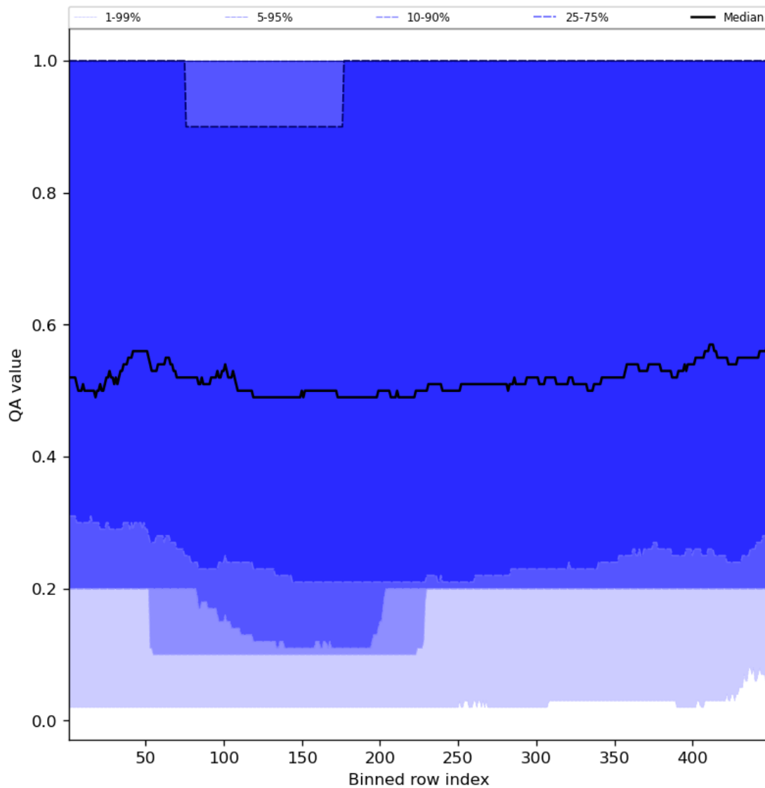
Figure 48: Along track statistics of “QA value” for 2023-11-12 to 2023-11-13
