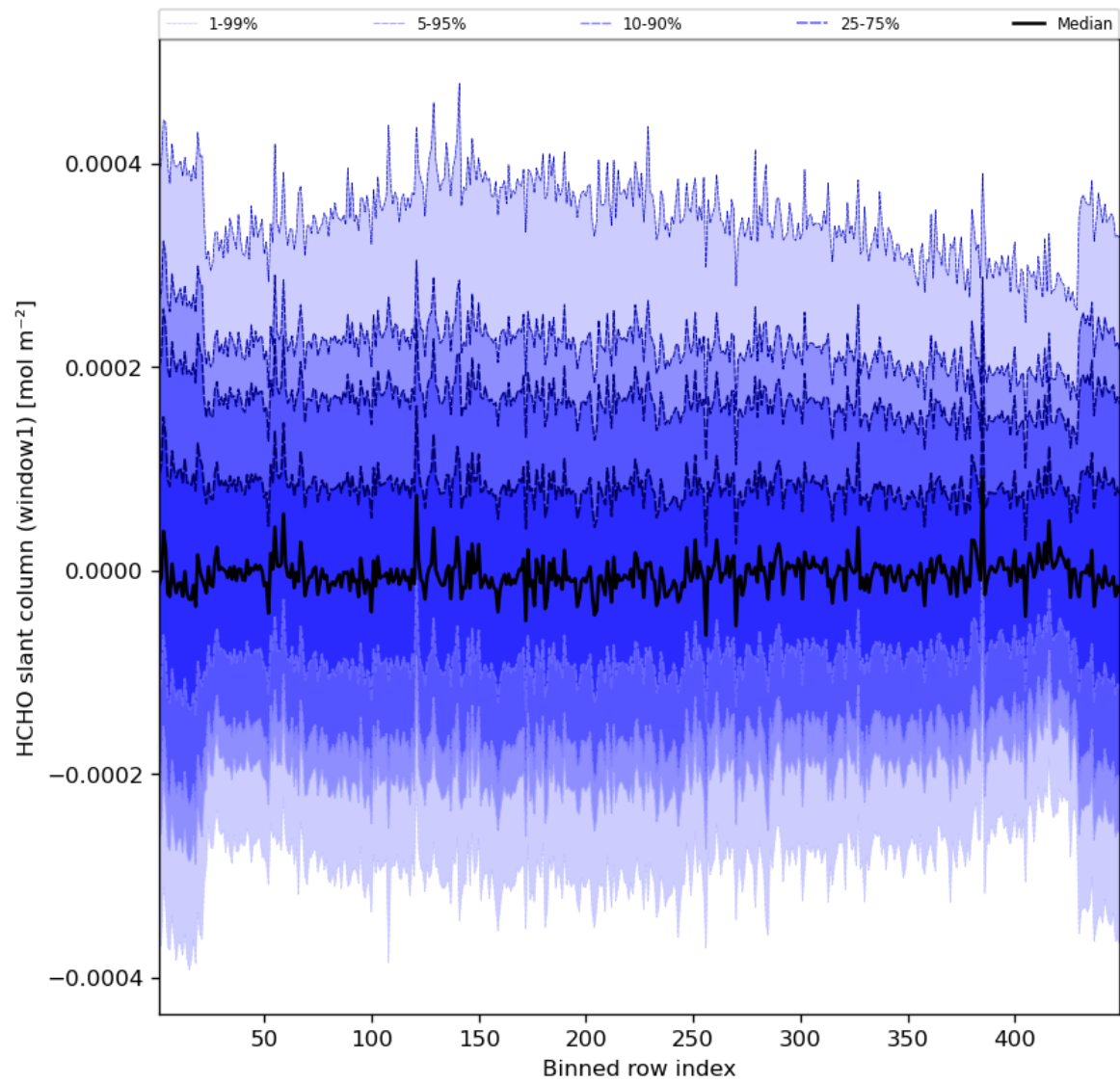
Figure 52: Along track statistics of “HCHO slant column (window1)” for 2023-11-12 to 2023-11-13
