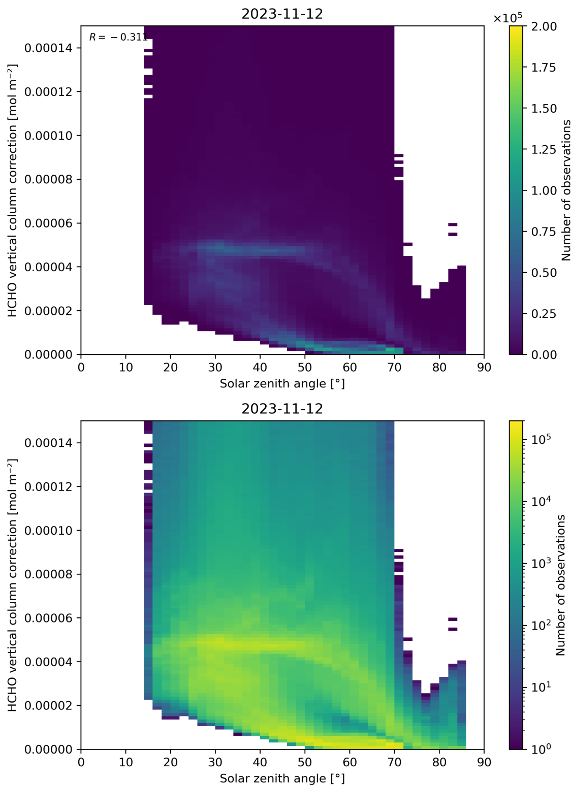
Figure 178: Scatter density plot of “Solar zenith angle” against “HCHO vertical column correction” for 2023-11-12 to 2023-11-13.
