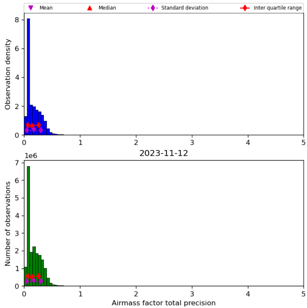
Figure 41: Histogram of “Airmass factor total precision” for 2023-11-12 to 2023-11-13
