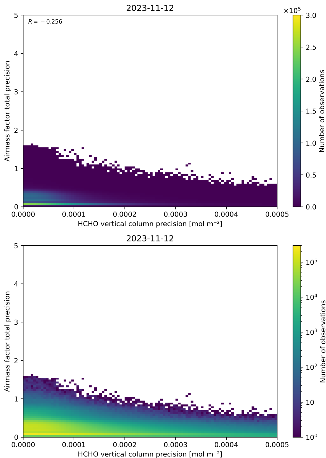
Figure 145: Scatter density plot of “HCHO vertical column precision” against “Airmass factor total precision” for 2023-11-12 to 2023-11-13.
