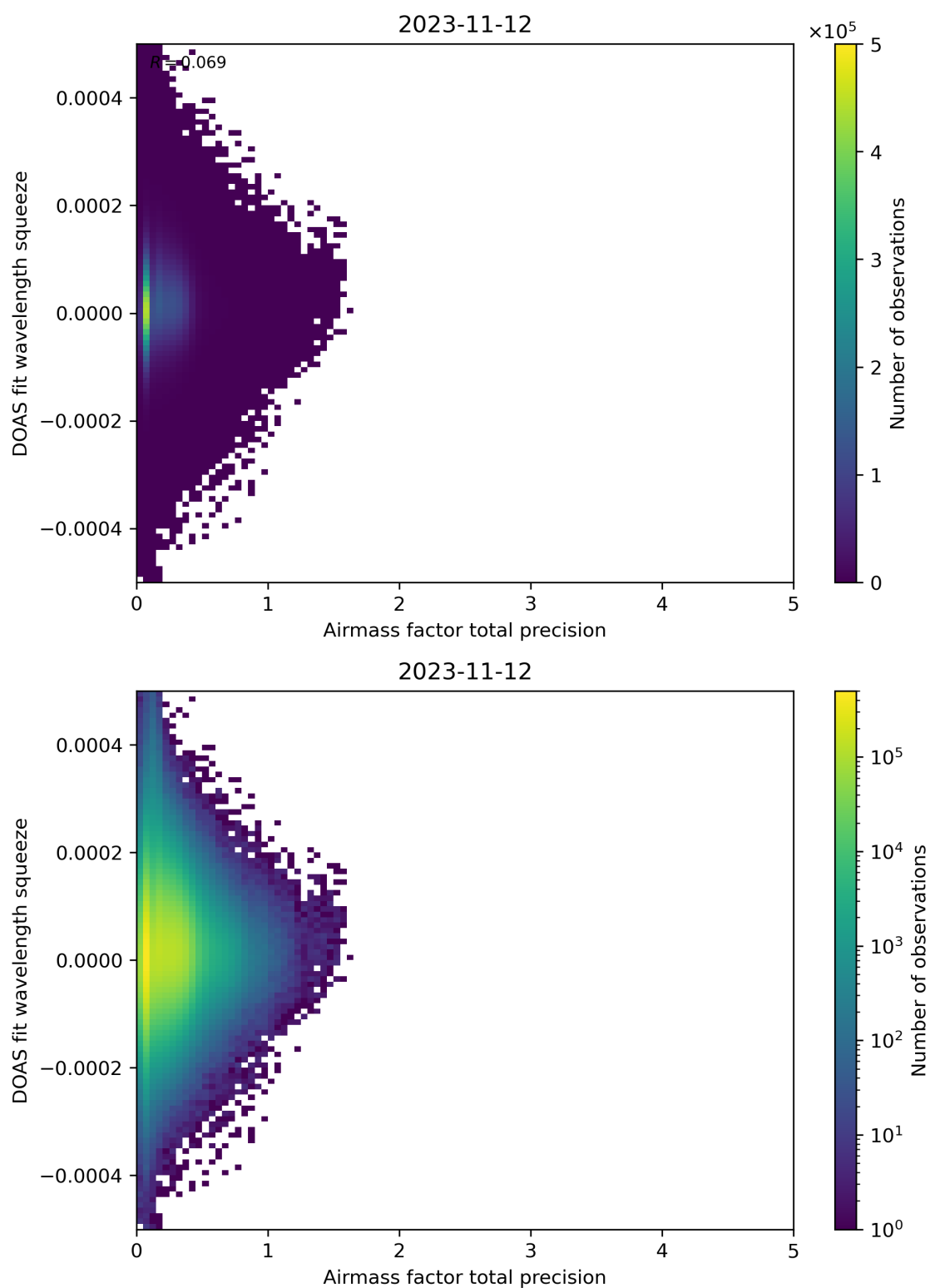
Figure 107: Scatter density plot of “Airmass factor total precision” against “DOAS fit wavelength squeeze” for 2023-11-12 to 2023-11-13.
