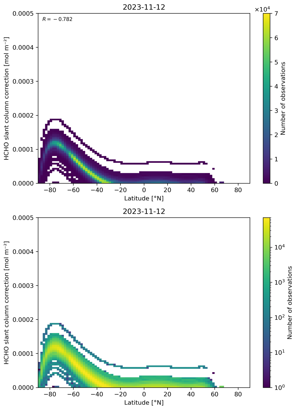
Figure 158: Scatter density plot of “Latitude” against “HCHO slant column correction” for 2023-11-12 to 2023-11-13.
