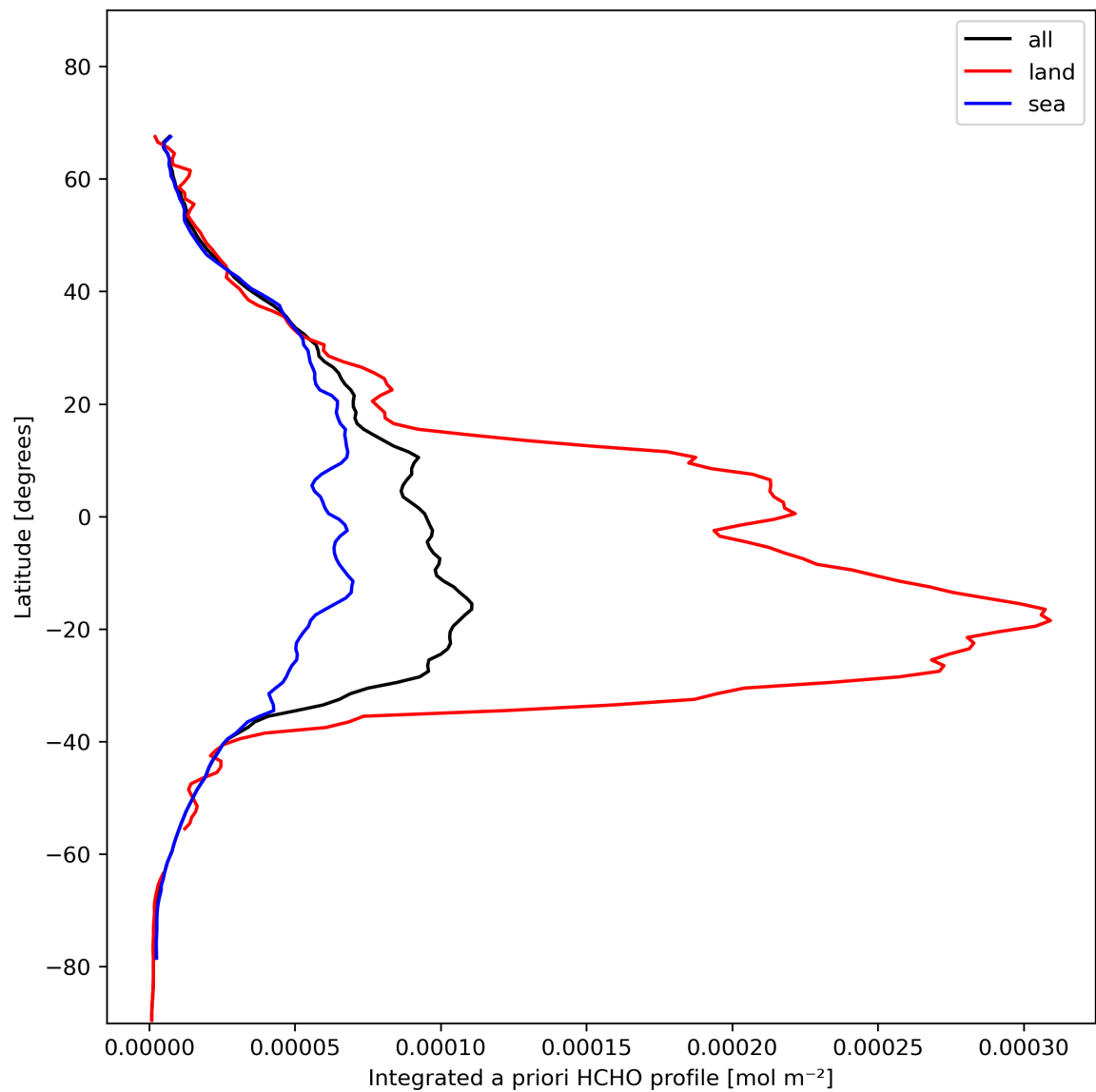
Figure 29: Zonal average of “Integrated a priori HCHO profile” for 2023-11-12 to 2023-11-13.
