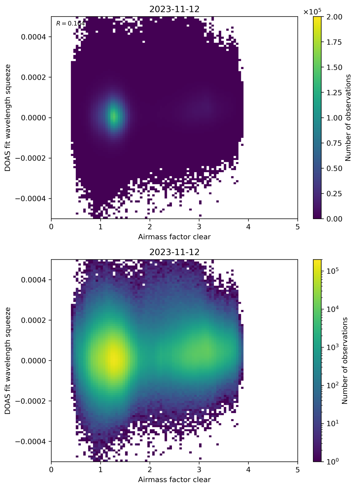
Figure 73: Scatter density plot of “Airmass factor clear” against “DOAS fit wavelength squeeze” for 2023-11-12 to 2023-11-13.
