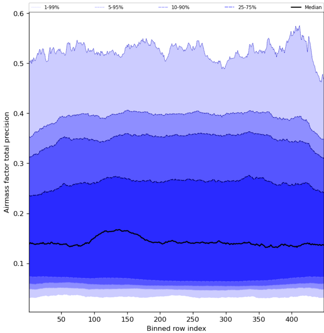
Figure 55: Along track statistics of “Airmass factor total precision” for 2023-11-12 to 2023-11-13
