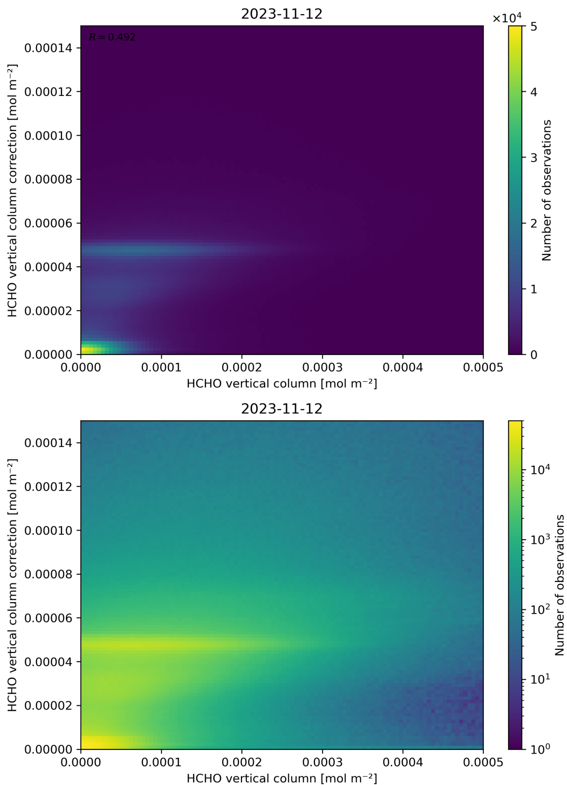
Figure 133: Scatter density plot of “HCHO vertical column” against “HCHO vertical column correction” for 2023-11-12 to 2023-11-13.
