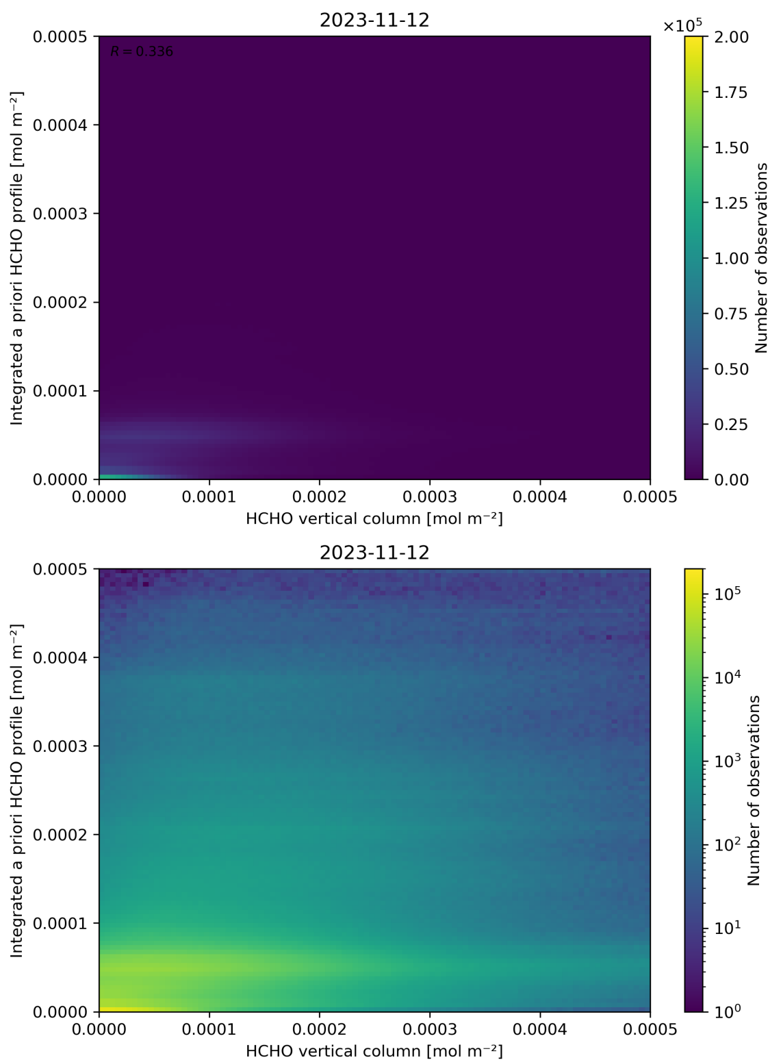
Figure 135: Scatter density plot of “HCHO vertical column” against “Integrated a priori HCHO profile” for 2023-11-12 to 2023-11-13.
