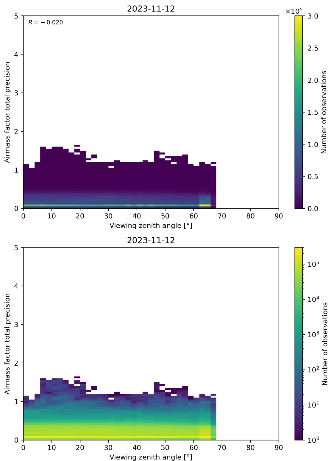
Figure 191: Scatter density plot of “Viewing zenith angle” against “Airmass factor total precision” for 2023-11-12 to 2023-11-13.
