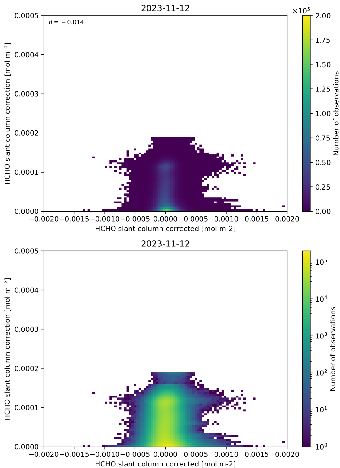
Figure 77: Scatter density plot of “HCHO slant column corrected” against “HCHO slant column correction” for 2023-11-12 to 2023-11-13.
