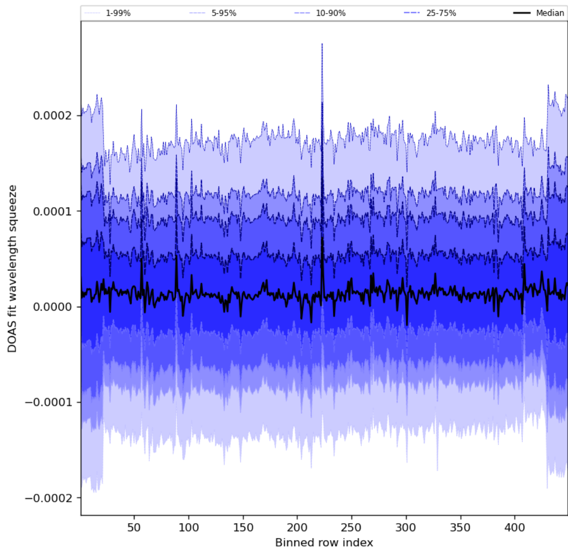
Figure 59: Along track statistics of “DOAS fit wavelength squeeze” for 2023-11-12 to 2023-11-13
