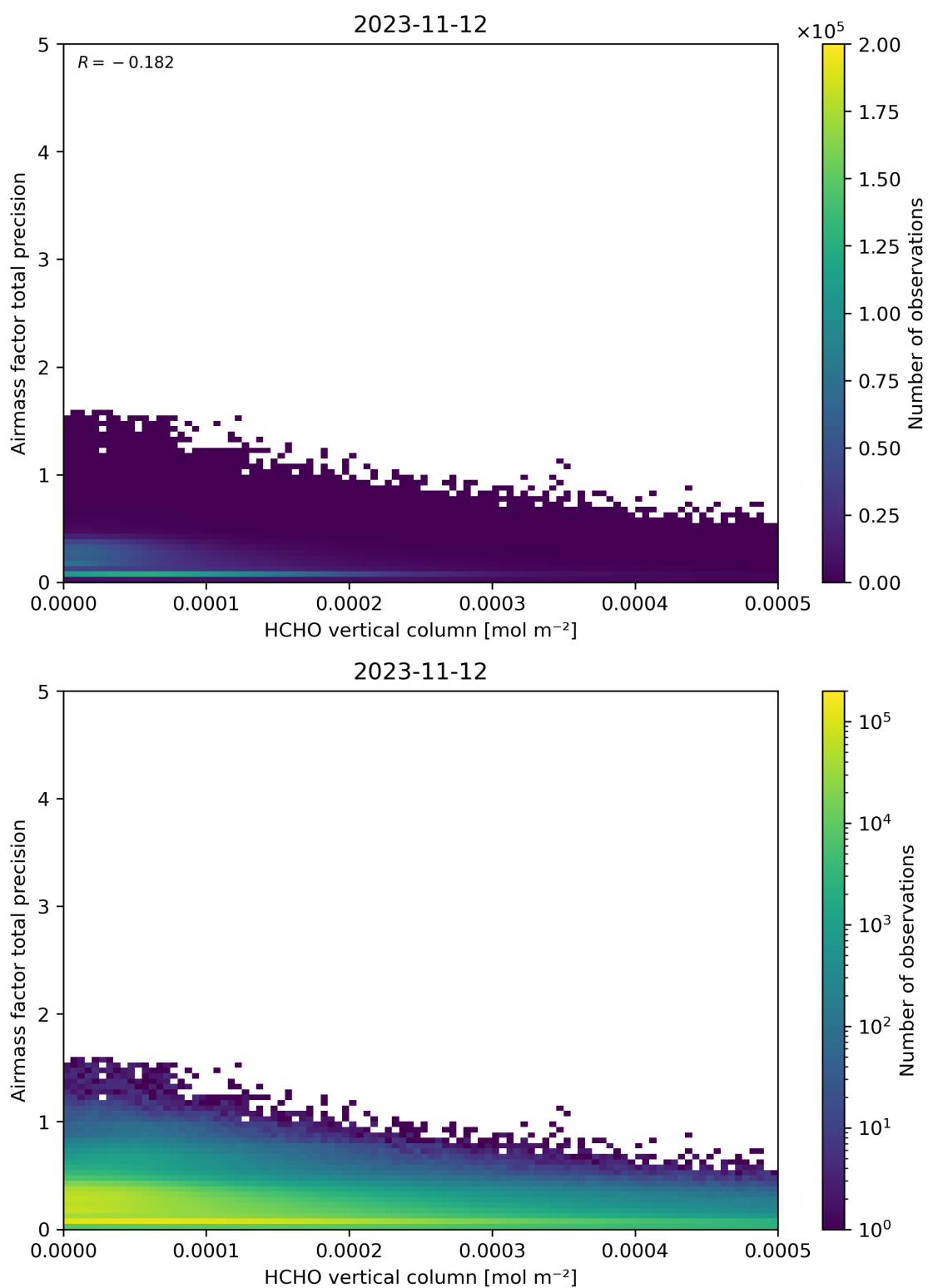
Figure 132: Scatter density plot of “HCHO vertical column” against “Airmass factor total precision” for 2023-11-12 to 2023-11-13.
