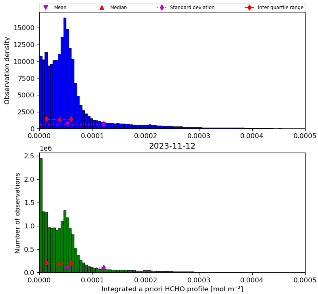
Figure 43: Histogram of “Integrated a priori HCHO profile” for 2023-11-12 to 2023-11-13
