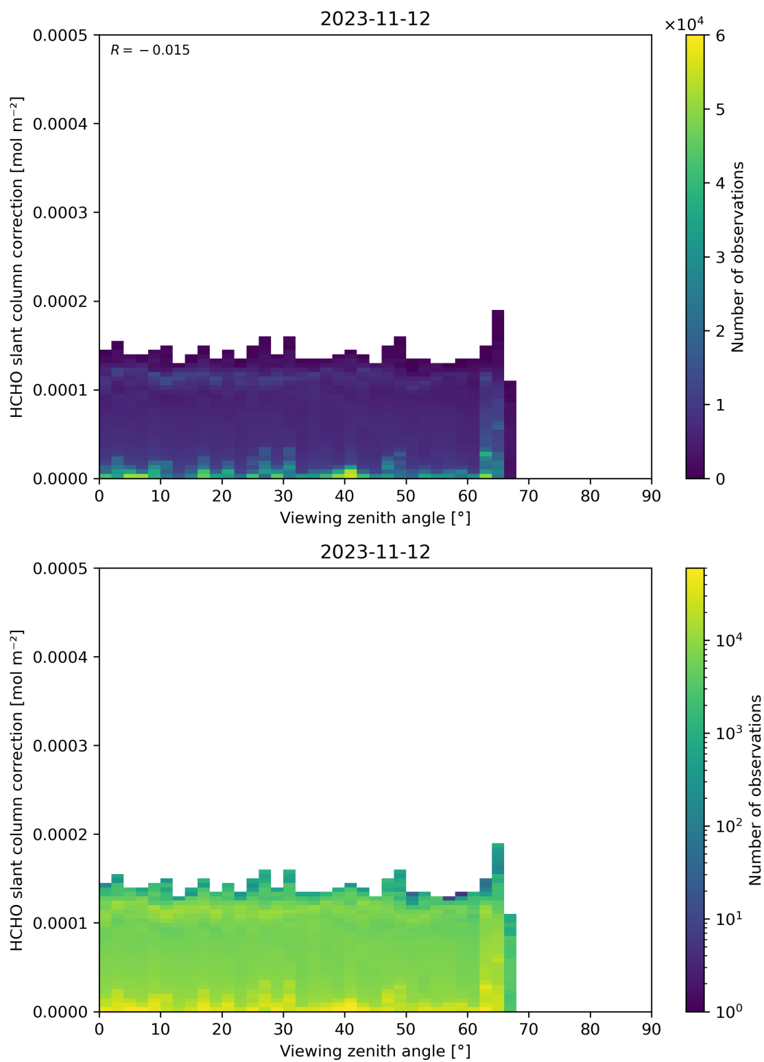
Figure 187: Scatter density plot of “Viewing zenith angle” against “HCHO slant column correction” for 2023-11-12 to 2023-11-13.
