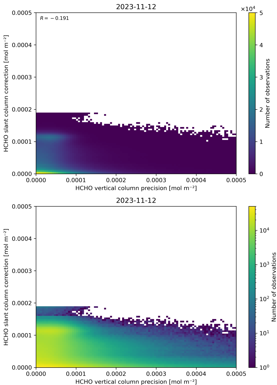
Figure 141: Scatter density plot of “HCHO vertical column precision” against “HCHO slant column correction” for 2023-11-12 to 2023-11-13.
