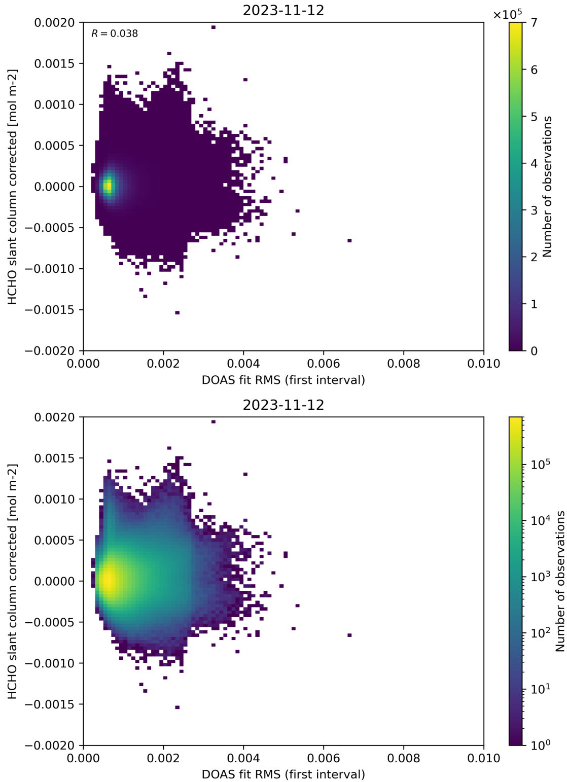
Figure 62: Scatter density plot of “DOAS fit RMS (first interval)” against “HCHO slant column corrected” for 2023-11-12 to 2023-11-13.
