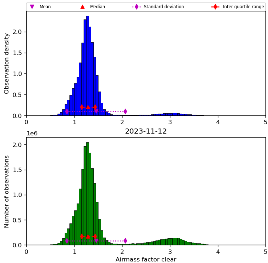
Figure 42: Histogram of “Airmass factor clear” for 2023-11-12 to 2023-11-13
