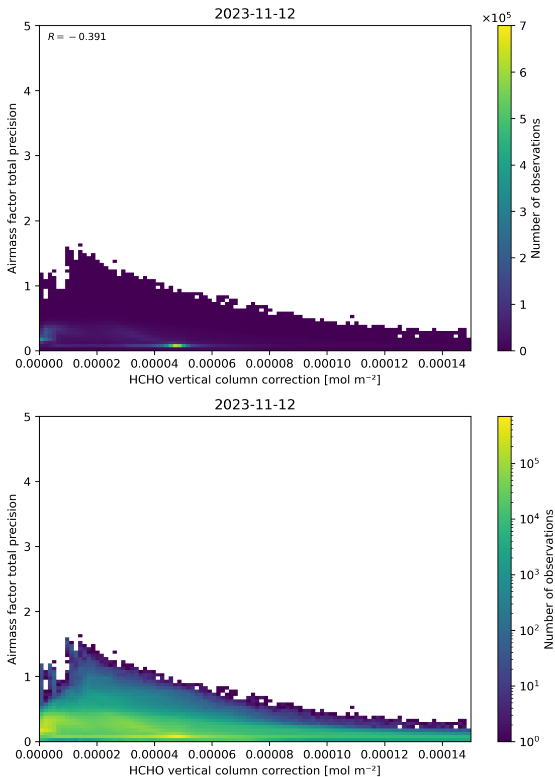
Figure 121: Scatter density plot of “HCHO vertical column correction” against “Airmass factor total precision” for 2023-11-12 to 2023-11-13.
