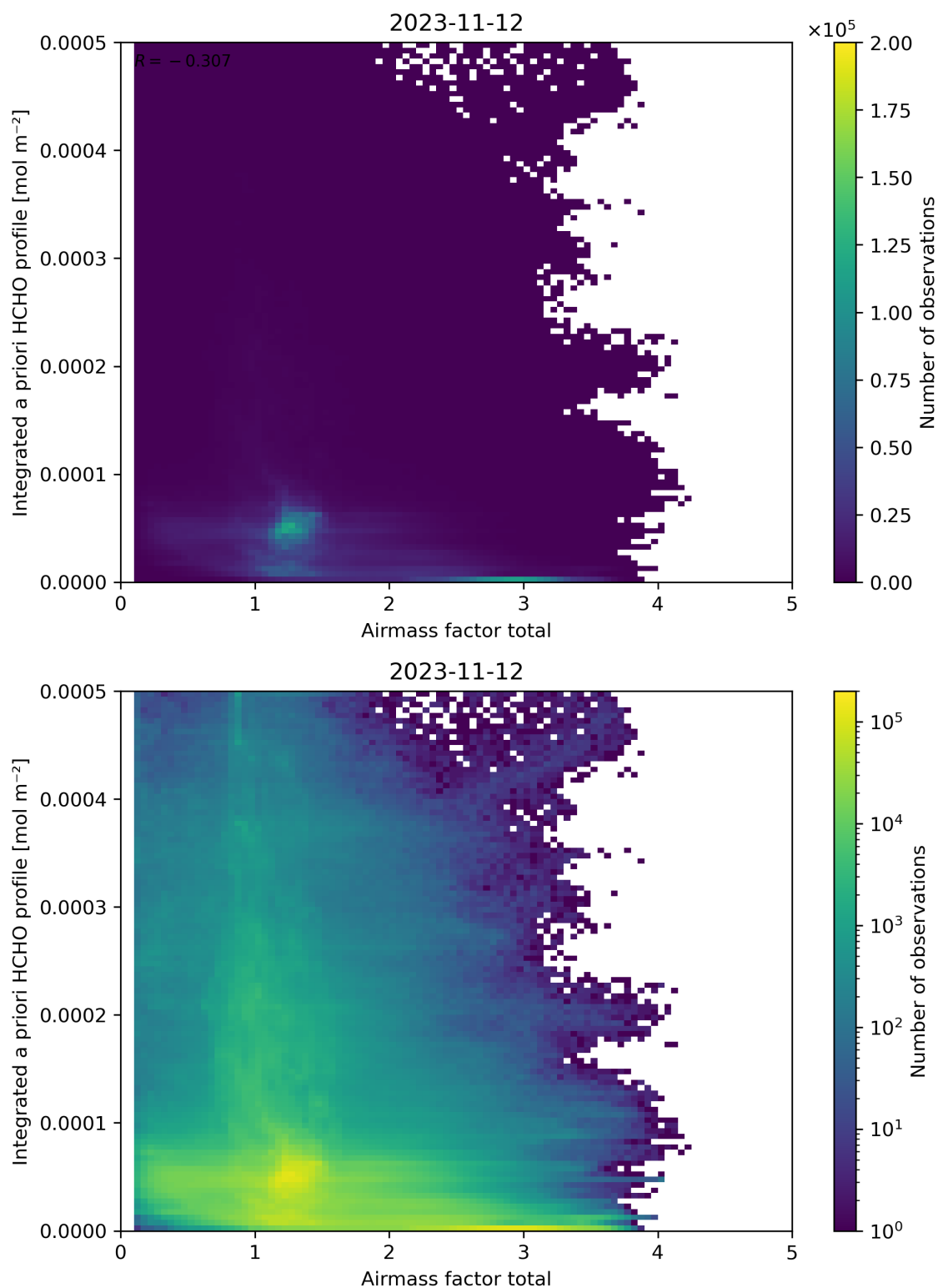
Figure 104: Scatter density plot of “Airmass factor total” against “Integrated a priori HCHO profile” for 2023-11-12 to 2023-11-13.
