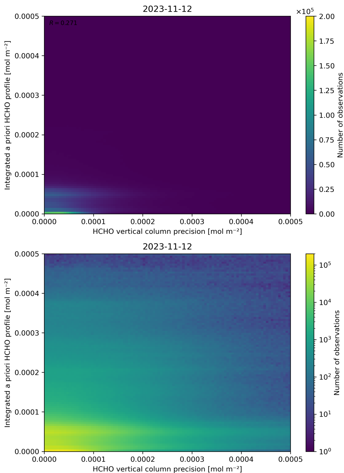
Figure 147: Scatter density plot of “HCHO vertical column precision” against “Integrated a priori HCHO profile” for 2023-11-12 to 2023-11-13.
