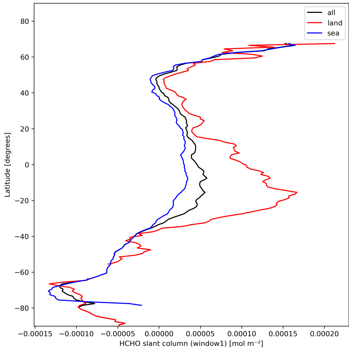
Figure 24: Zonal average of “HCHO slant column (window1)” for 2023-11-12 to 2023-11-13.
