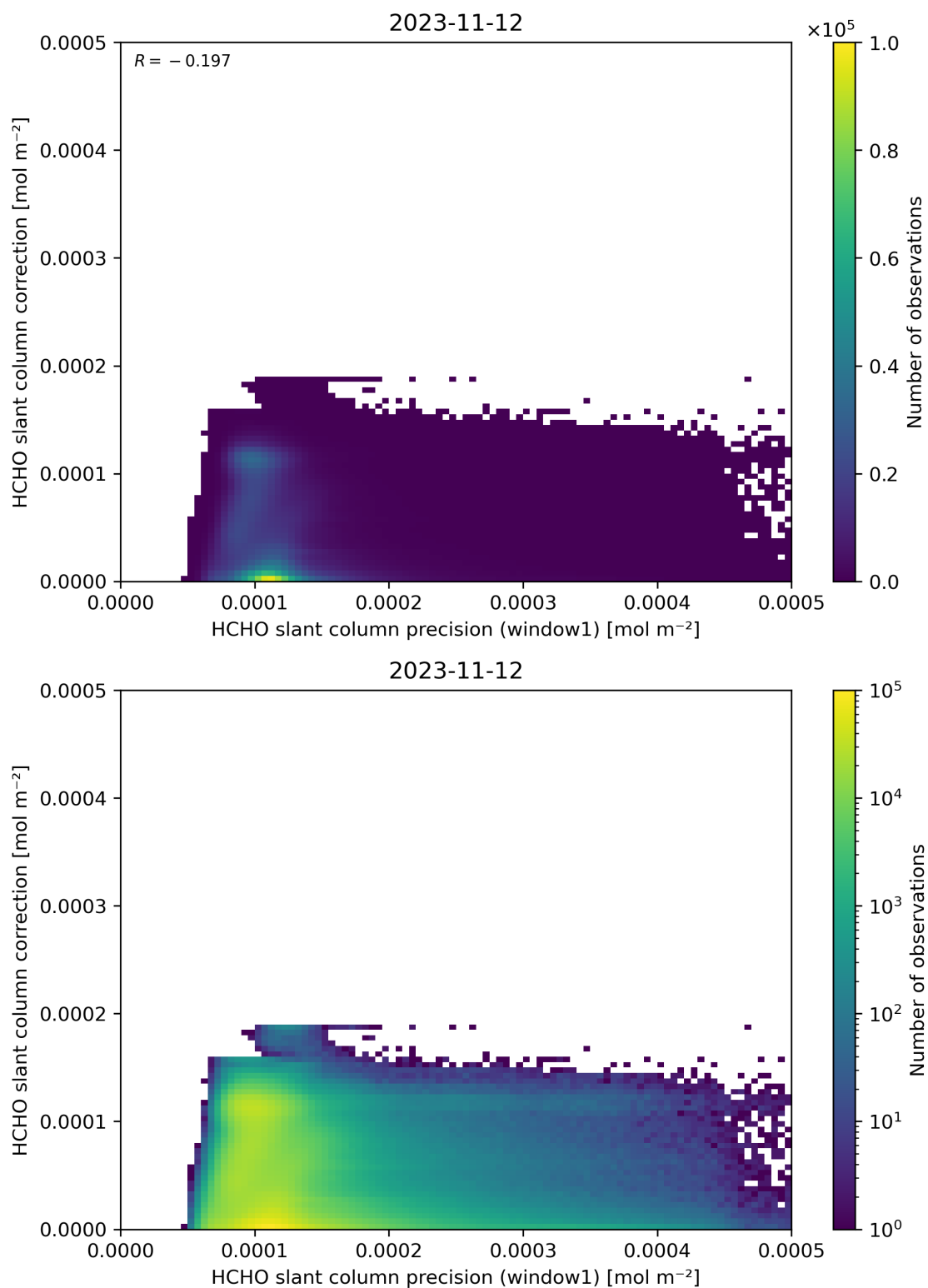
Figure 93: Scatter density plot of “HCHO slant column precision (window1)” against “HCHO slant column correction” for 2023-11-12 to 2023-11-13.
