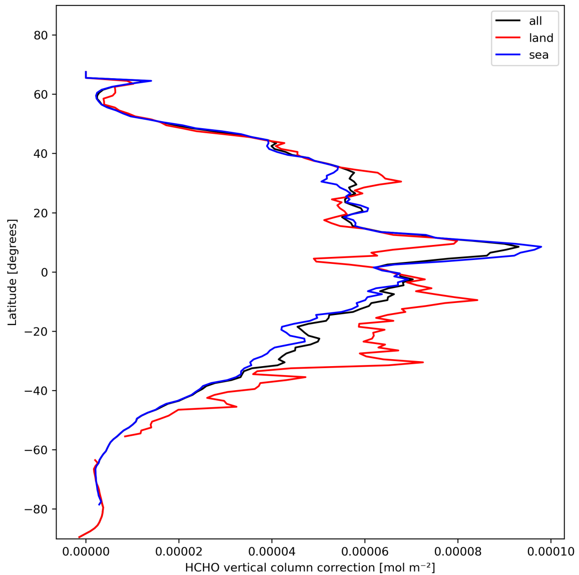
Figure 23: Zonal average of “HCHO vertical column correction” for 2023-11-12 to 2023-11-13.
