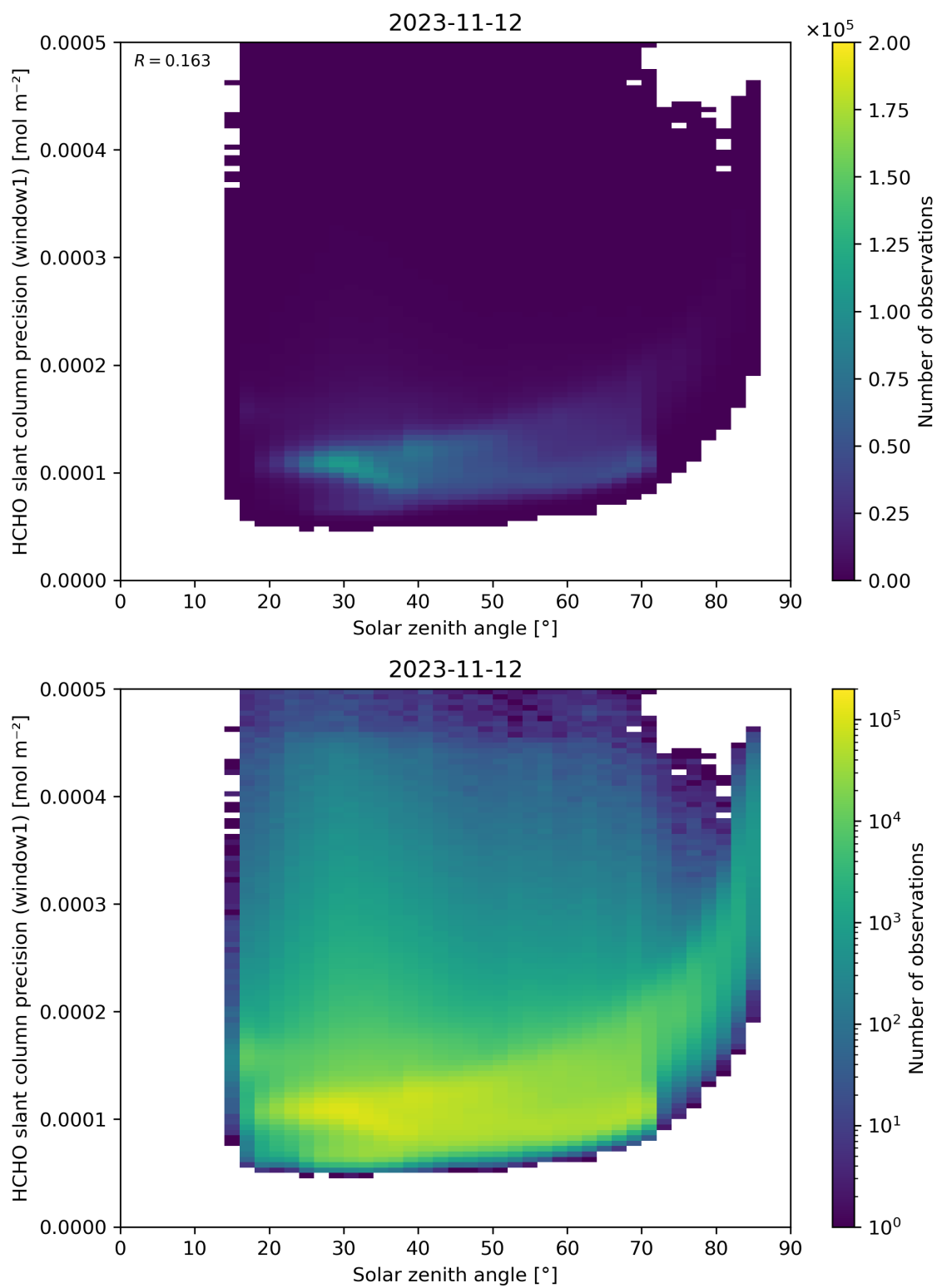
Figure 174: Scatter density plot of “Solar zenith angle” against “HCHO slant column precision (window1)” for 2023-11-12 to 2023-11-13.
