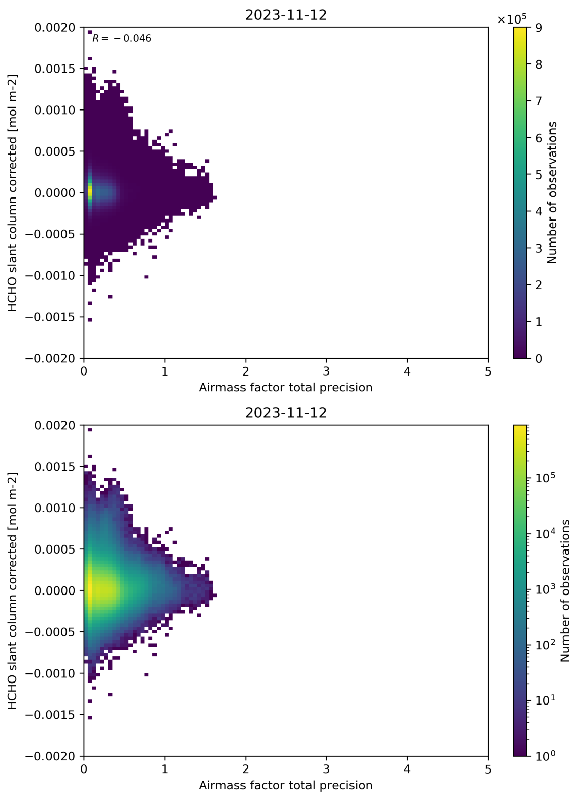
Figure 109: Scatter density plot of “Airmass factor total precision” against “HCHO slant column corrected” for 2023-11-12 to 2023-11-13.
