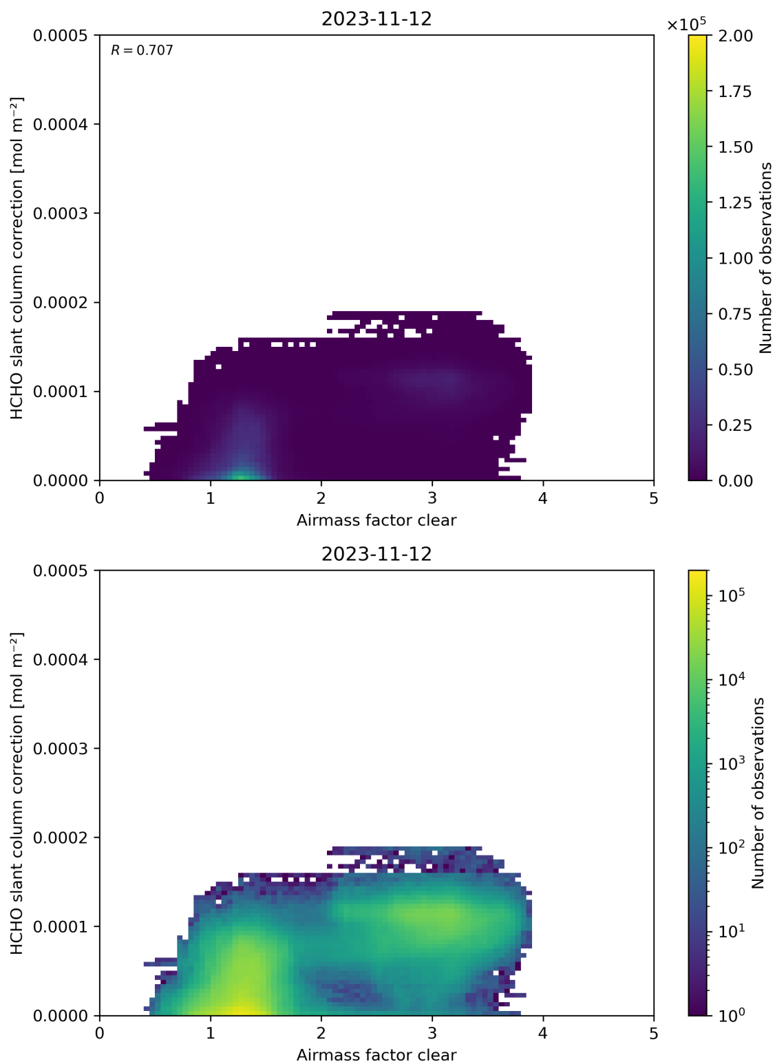
Figure 75: Scatter density plot of “Airmass factor clear” against “HCHO slant column correction” for 2023-11-12 to 2023-11-13.
