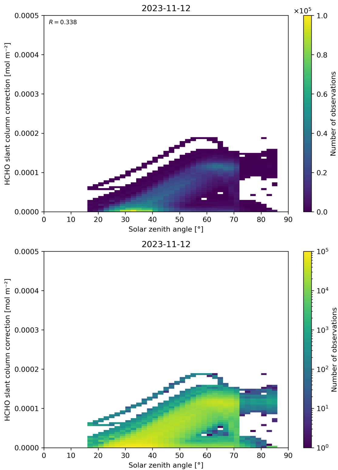
Figure 172: Scatter density plot of “Solar zenith angle” against “HCHO slant column correction” for 2023-11-12 to 2023-11-13.
