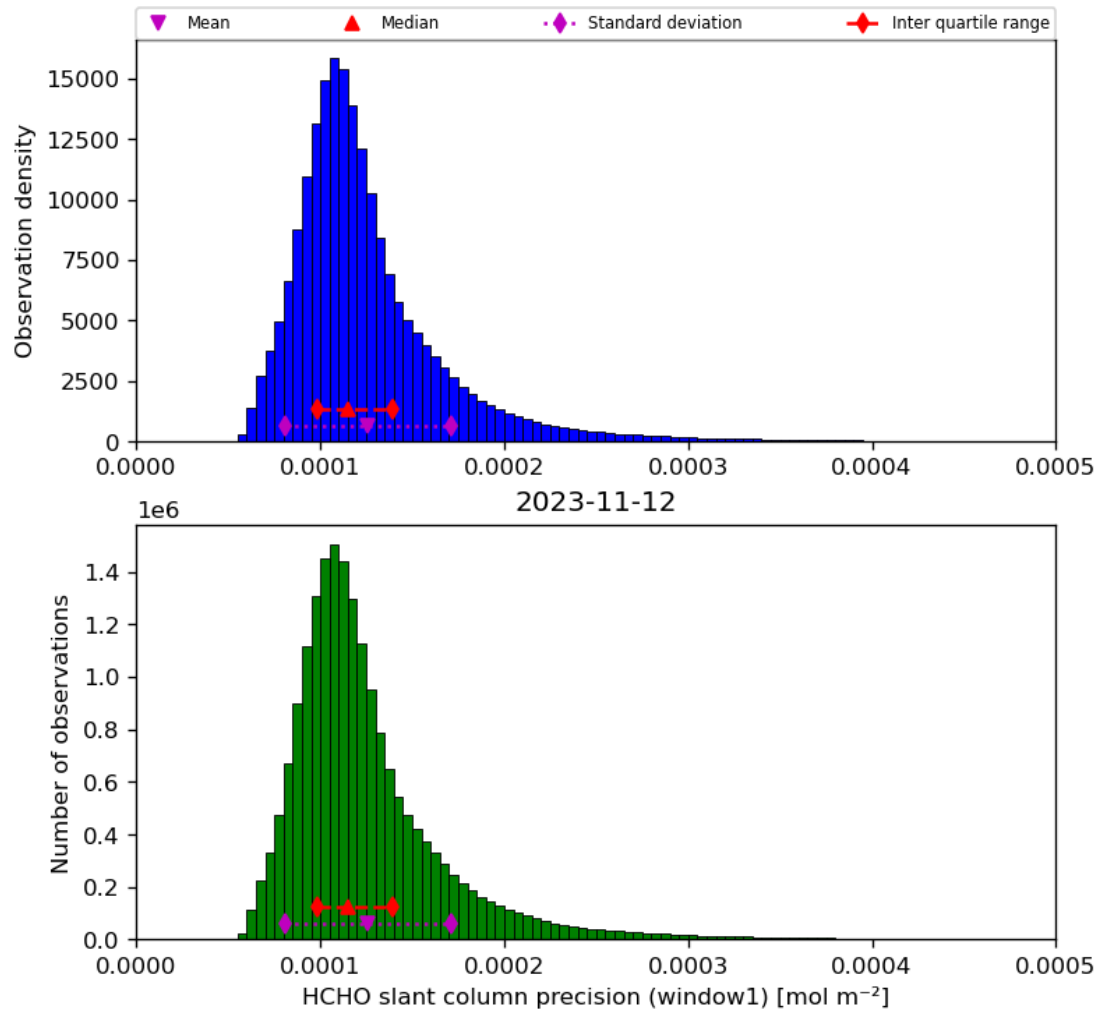
Figure 39: Histogram of “HCHO slant column precision (window1)” for 2023-11-12 to 2023-11-13
