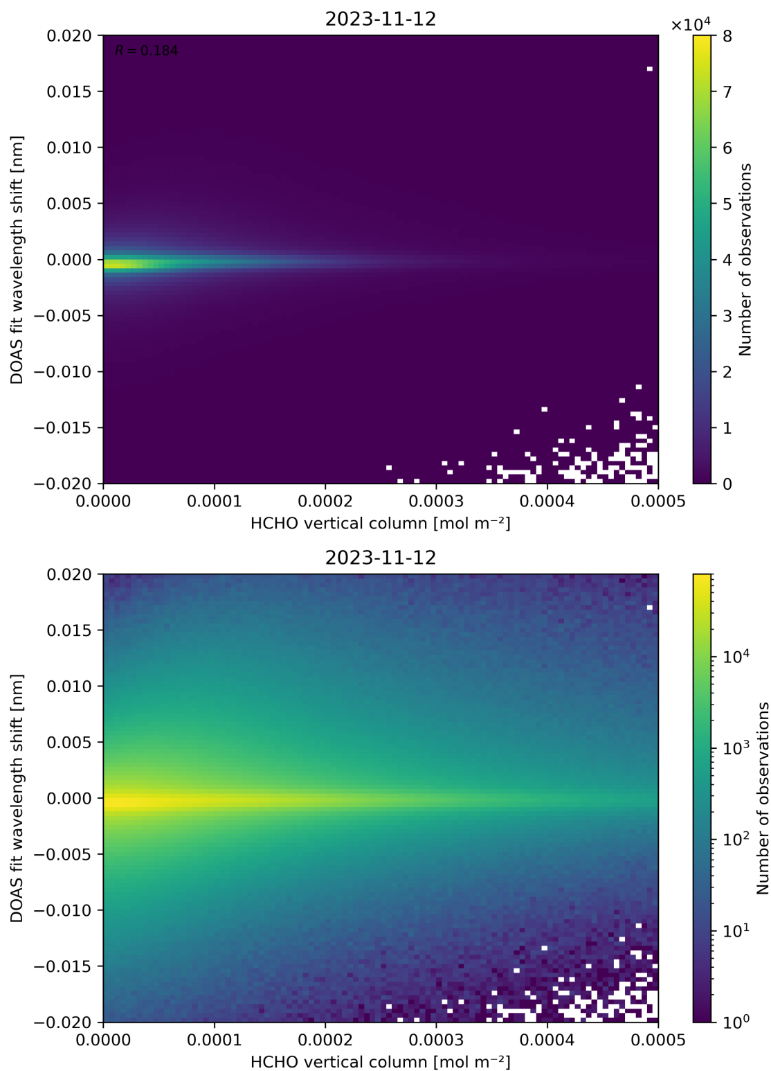
Figure 124: Scatter density plot of “HCHO vertical column” against “DOAS fit wavelength shift” for 2023-11-12 to 2023-11-13.
