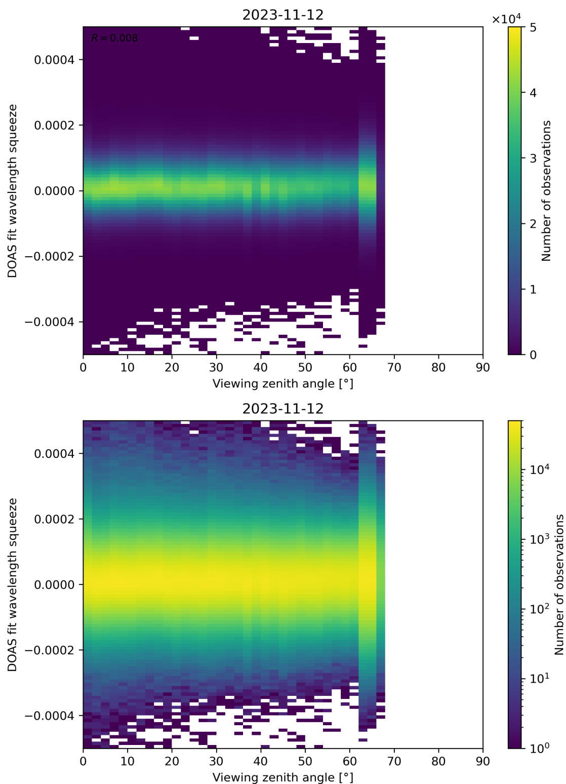
Figure 184: Scatter density plot of “Viewing zenith angle” against “DOAS fit wavelength squeeze” for 2023-11-12 to 2023-11-13.
