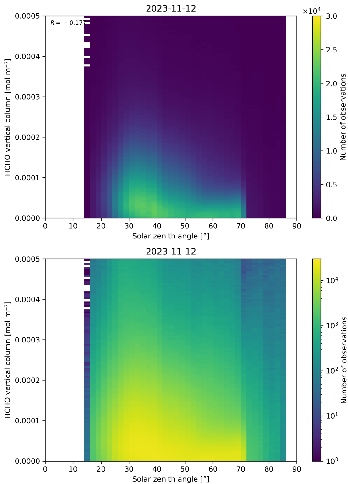
Figure 177: Scatter density plot of “Solar zenith angle” against “HCHO vertical column” for 2023-11-12 to 2023-11-13.
