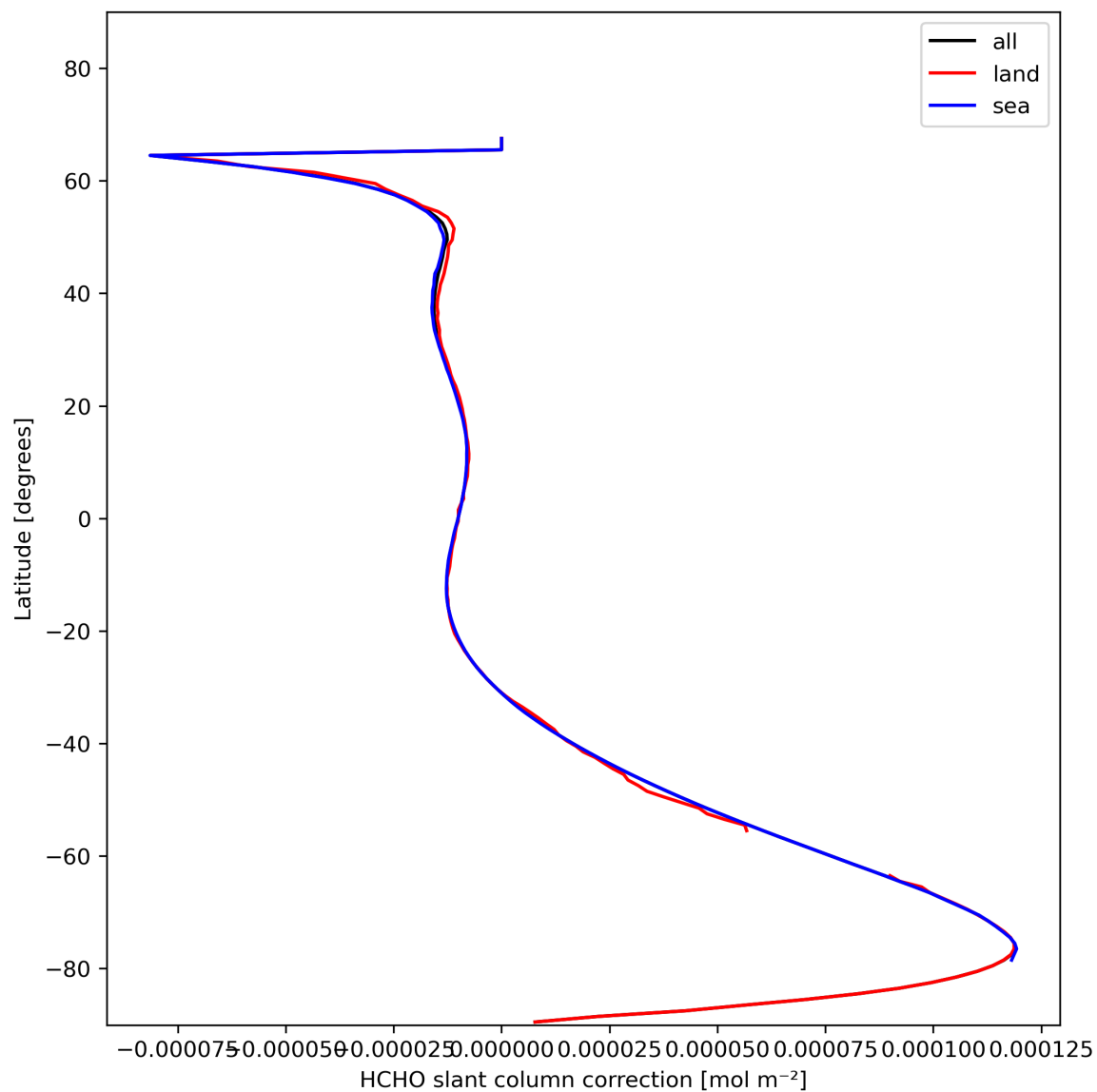
Figure 33: Zonal average of “HCHO slant column correction” for 2023-11-12 to 2023-11-13.
