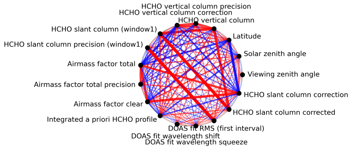
Figure 1: Map of correlation graph for 2023-11-12 to 2023-11-13.
