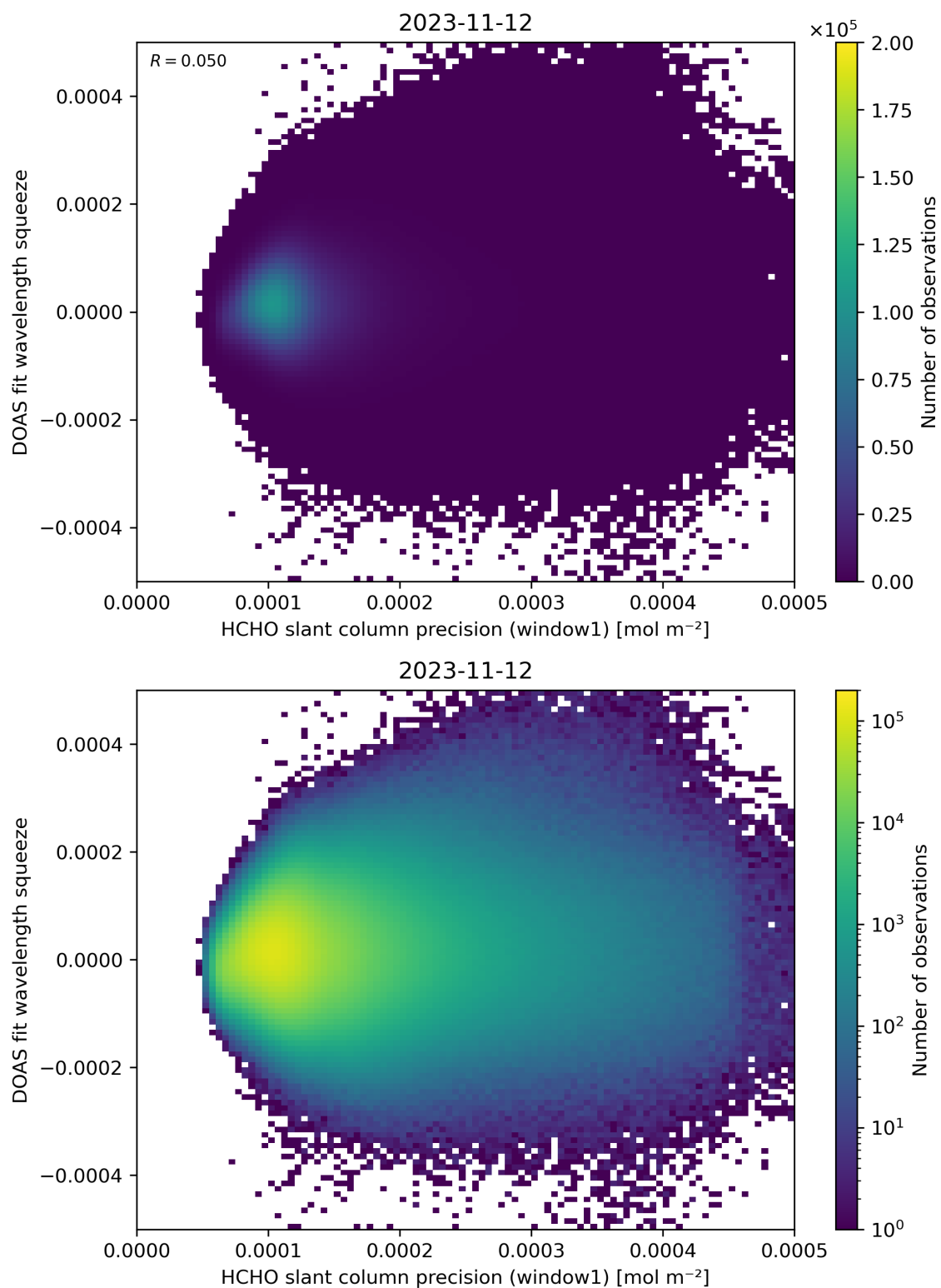
Figure 90: Scatter density plot of “HCHO slant column precision (window1)” against “DOAS fit wavelength squeeze” for 2023-11-12 to 2023-11-13.
