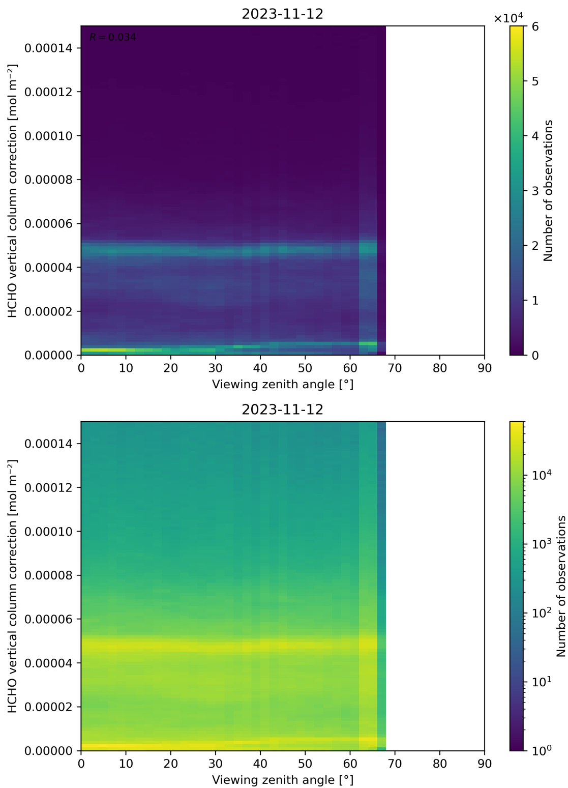
Figure 193: Scatter density plot of “Viewing zenith angle” against “HCHO vertical column correction” for 2023-11-12 to 2023-11-13.
