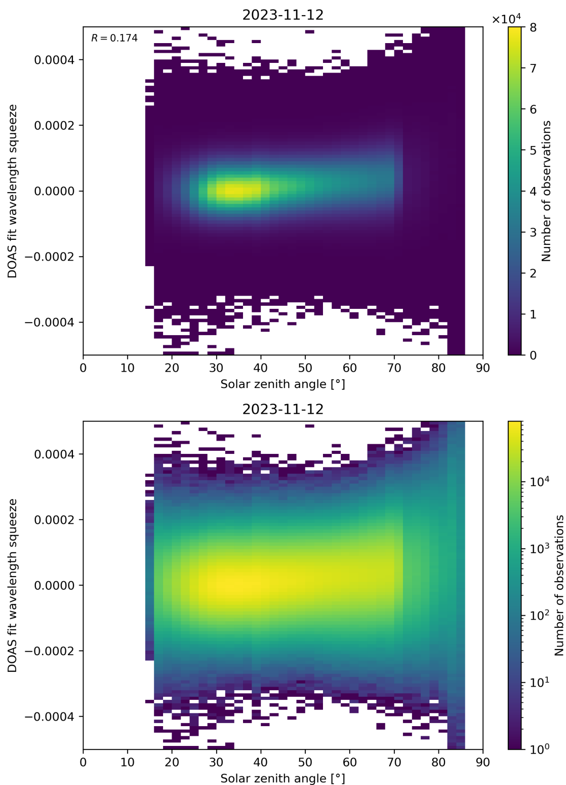
Figure 169: Scatter density plot of “Solar zenith angle” against “DOAS fit wavelength squeeze” for 2023-11-12 to 2023-11-13.
