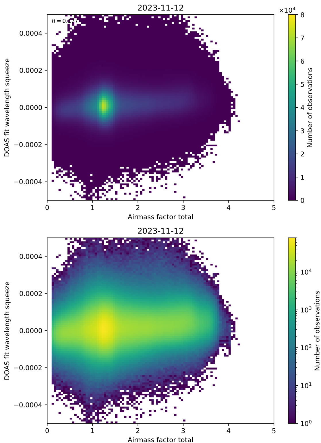
Figure 99: Scatter density plot of “Airmass factor total” against “DOAS fit wavelength squeeze” for 2023-11-12 to 2023-11-13.
