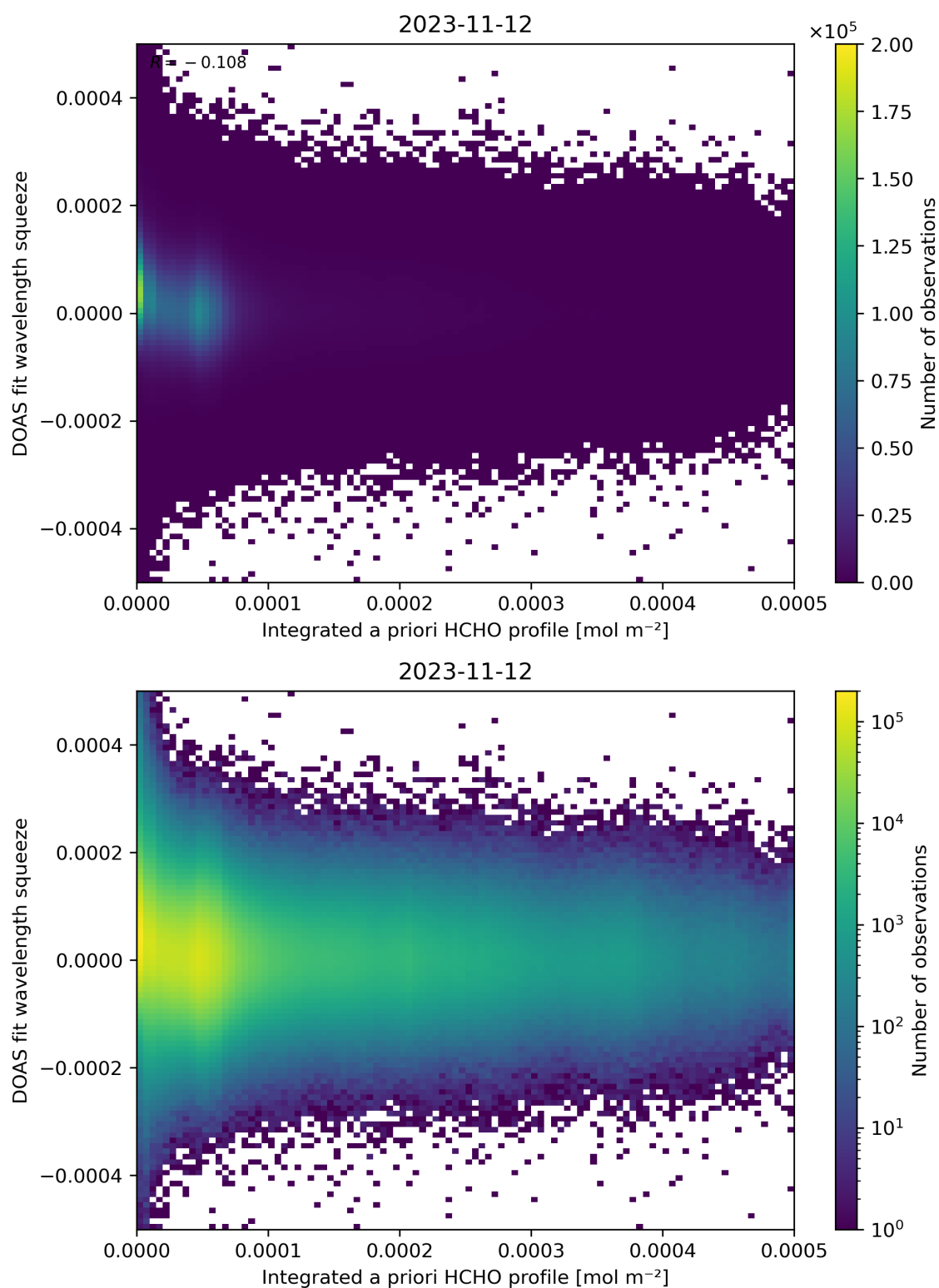
Figure 150: Scatter density plot of “Integrated a priori HCHO profile” against “DOAS fit wavelength squeeze” for 2023-11-12 to 2023-11-13.
