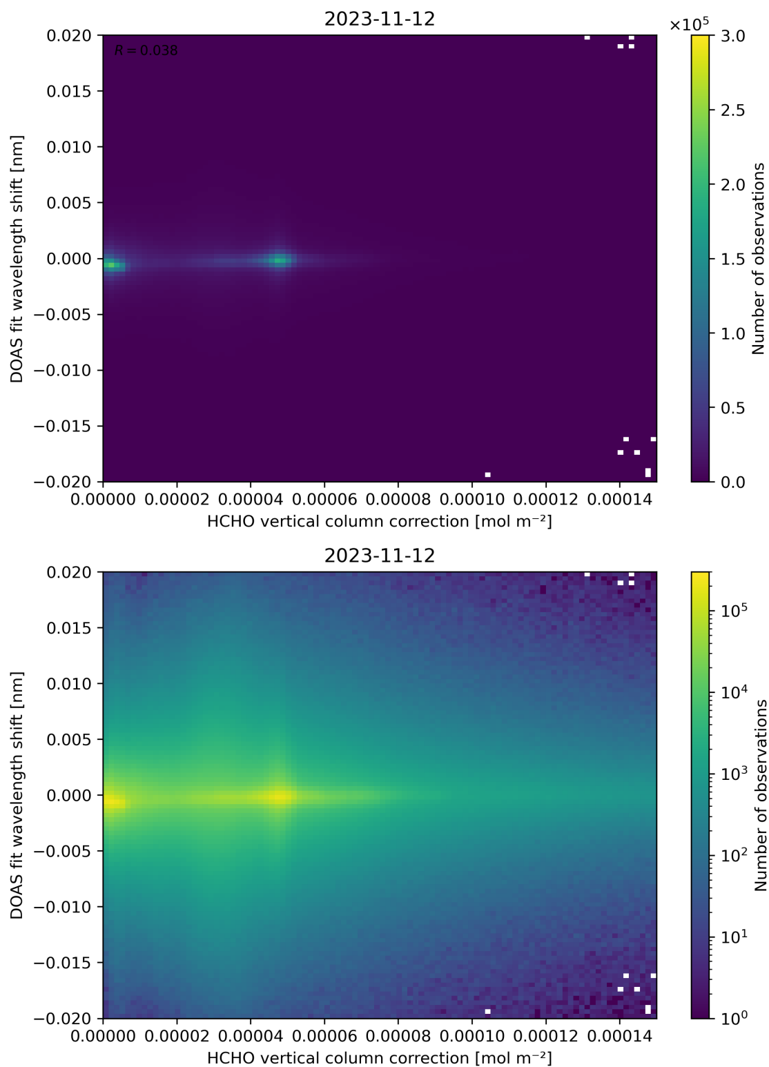
Figure 113: Scatter density plot of “HCHO vertical column correction” against “DOAS fit wavelength shift” for 2023-11-12 to 2023-11-13.
