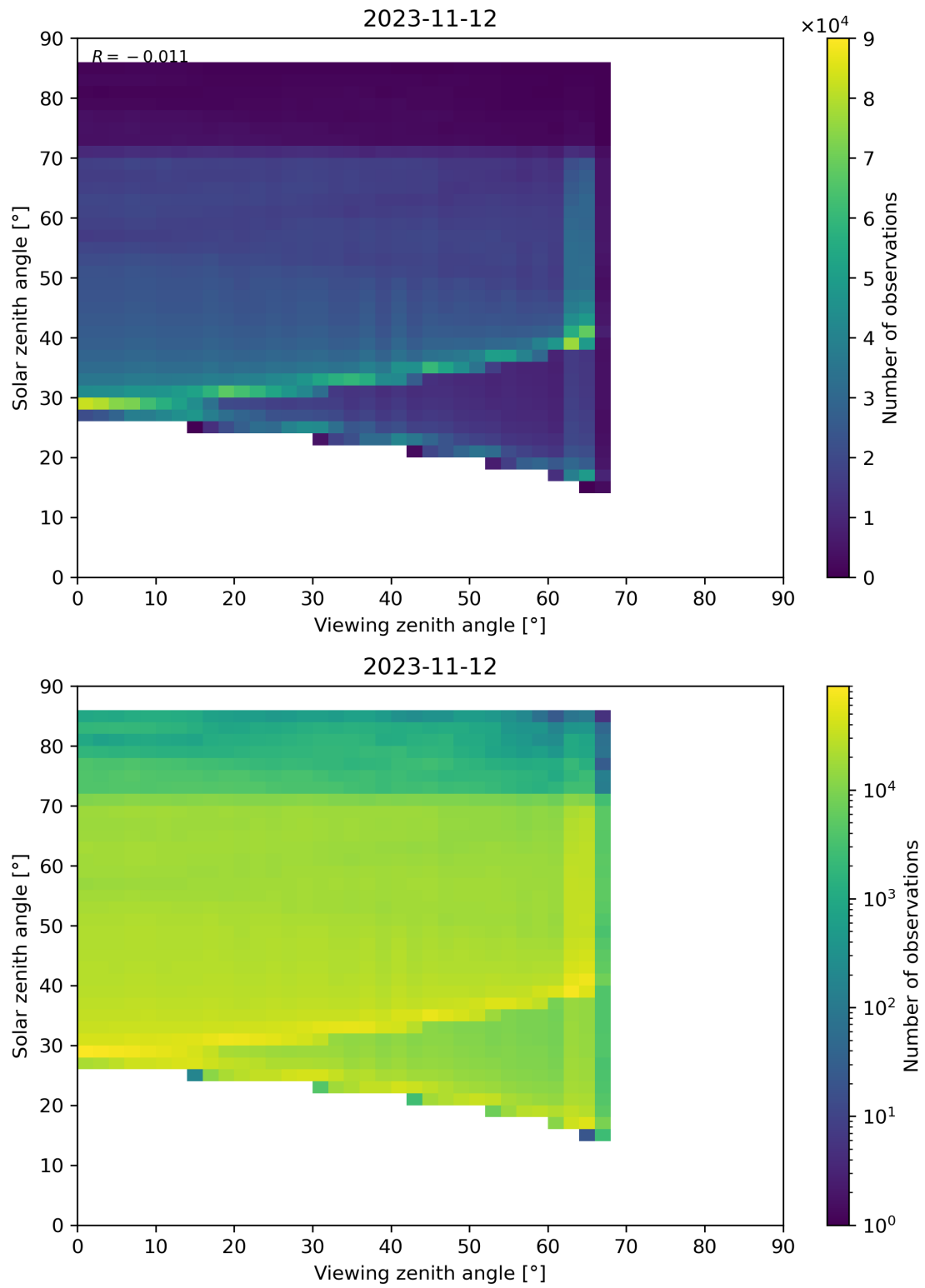
Figure 197: Scatter density plot of “Viewing zenith angle” against “Solar zenith angle” for 2023-11-12 to 2023-11-13.
