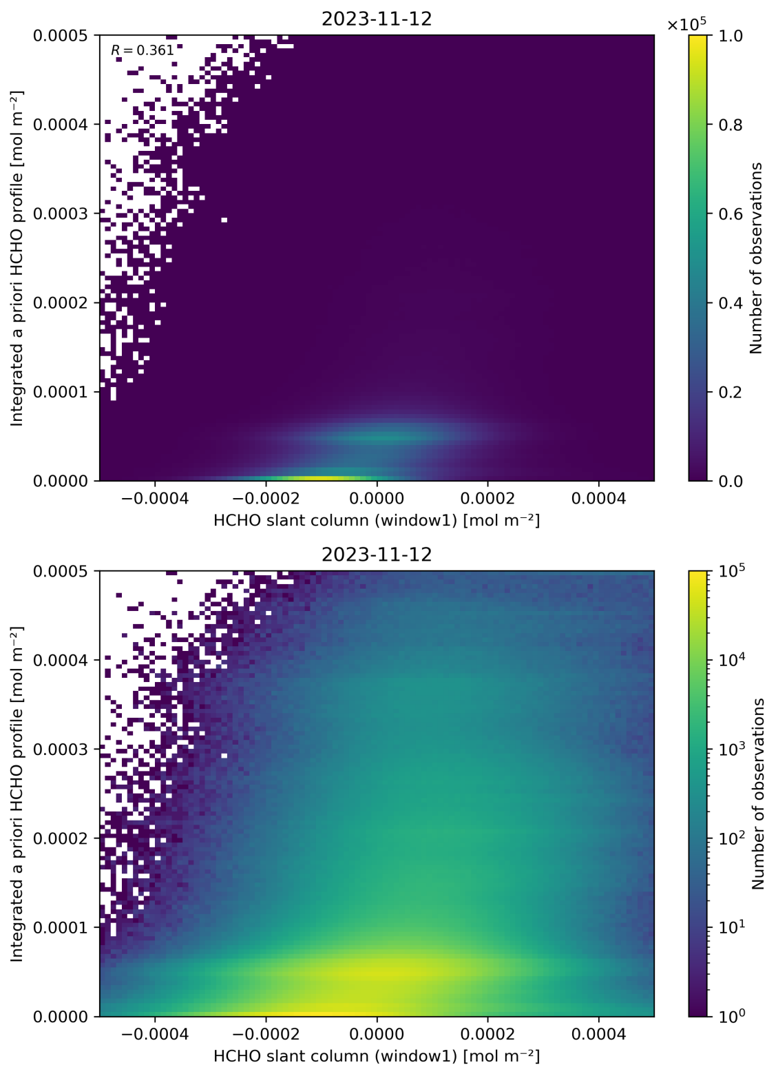
Figure 87: Scatter density plot of “HCHO slant column (window1)” against “Integrated a priori HCHO profile” for 2023-11-12 to 2023-11-13.
