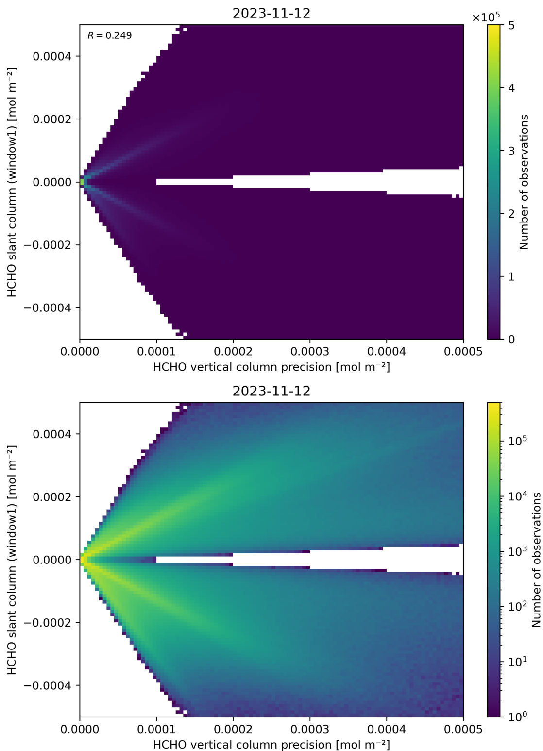
Figure 142: Scatter density plot of “HCHO vertical column precision” against “HCHO slant column (window1)” for 2023-11-12 to 2023-11-13.
