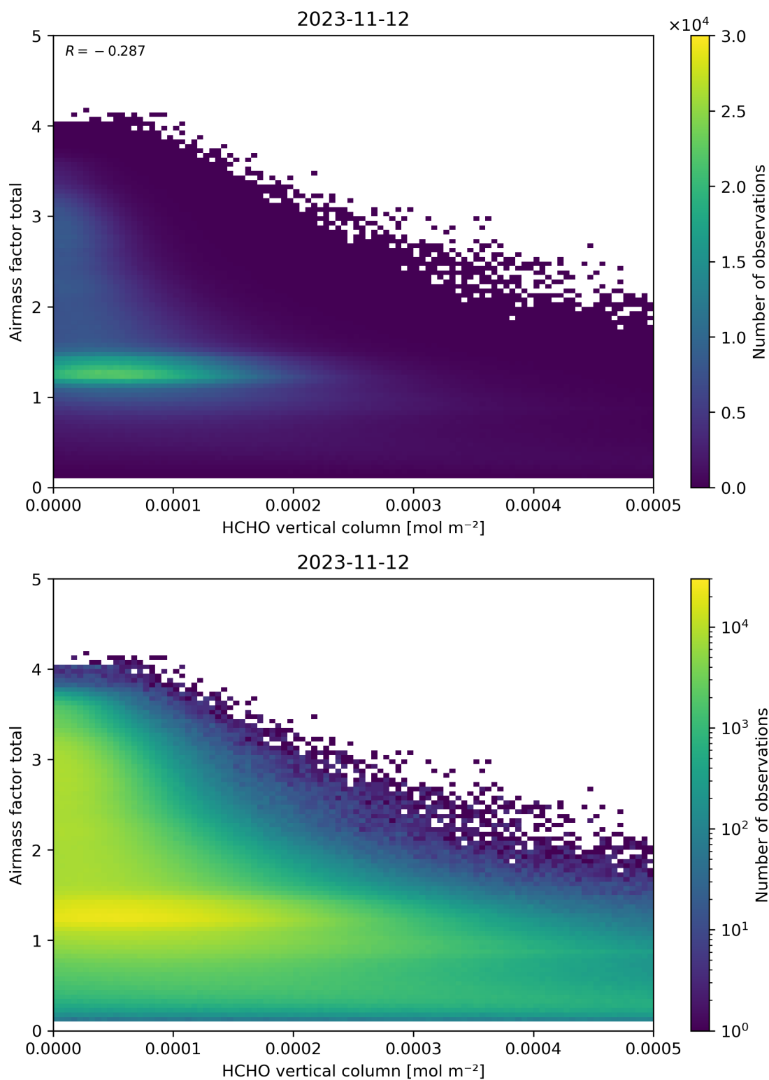
Figure 131: Scatter density plot of “HCHO vertical column” against “Airmass factor total” for 2023-11-12 to 2023-11-13.
