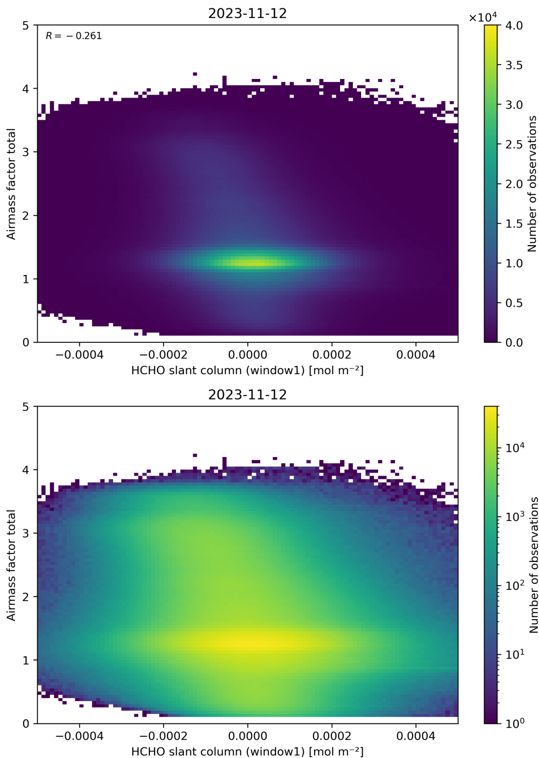
Figure 85: Scatter density plot of “HCHO slant column (window1)” against “Airmass factor total” for 2023-11-12 to 2023-11-13.
