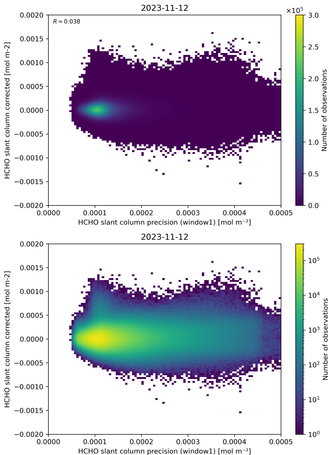
Figure 92: Scatter density plot of “HCHO slant column precision (window1)” against “HCHO slant column corrected” for 2023-11-12 to 2023-11-13.
