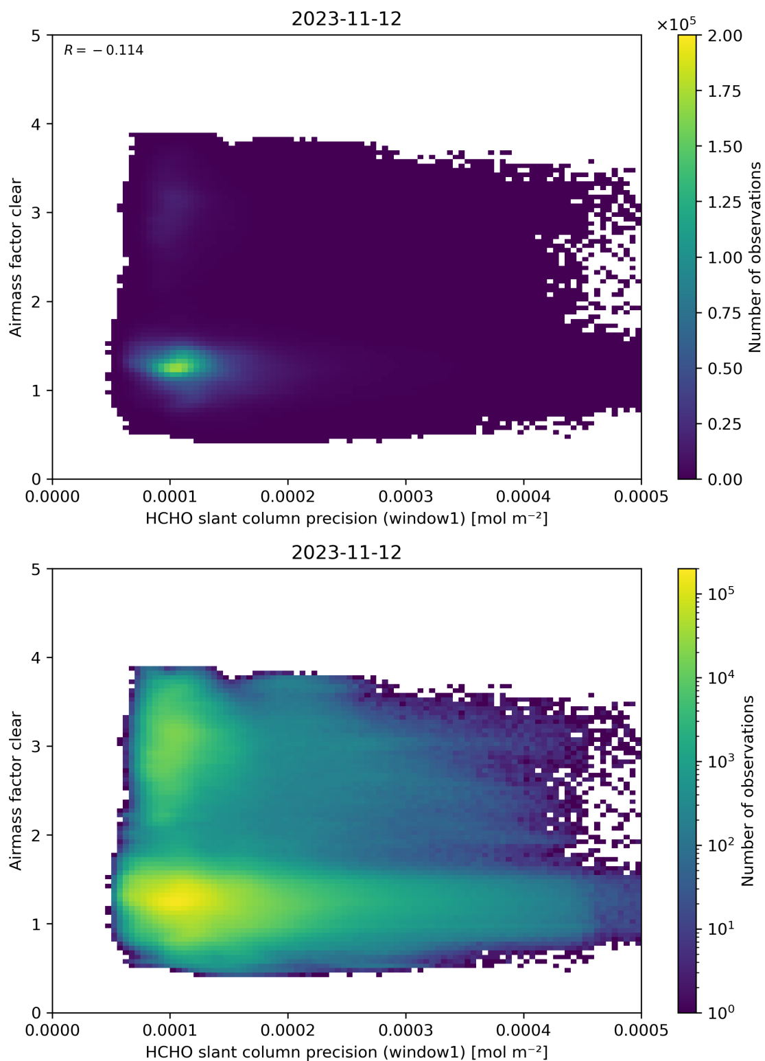
Figure 91: Scatter density plot of “HCHO slant column precision (window1)” against “Airmass factor clear” for 2023-11-12 to 2023-11-13.
