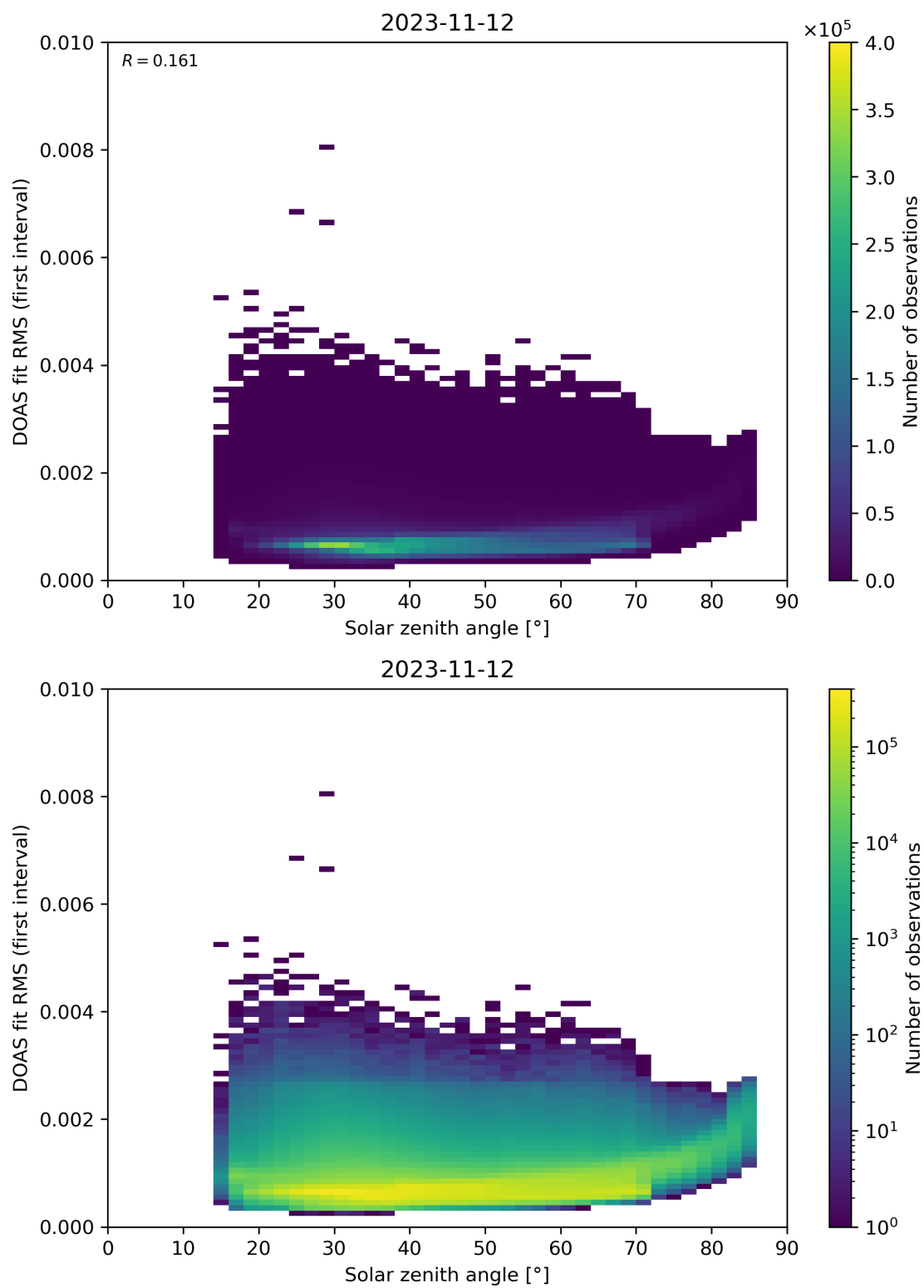
Figure 167: Scatter density plot of “Solar zenith angle” against “DOAS fit RMS (first interval)” for 2023-11-12 to 2023-11-13.
