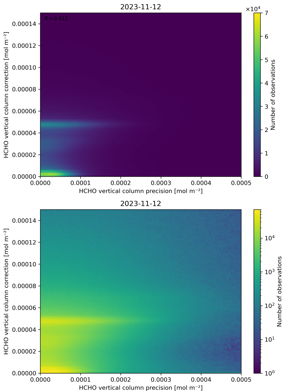
Figure 146: Scatter density plot of “HCHO vertical column precision” against “HCHO vertical column correction” for 2023-11-12 to 2023-11-13.
