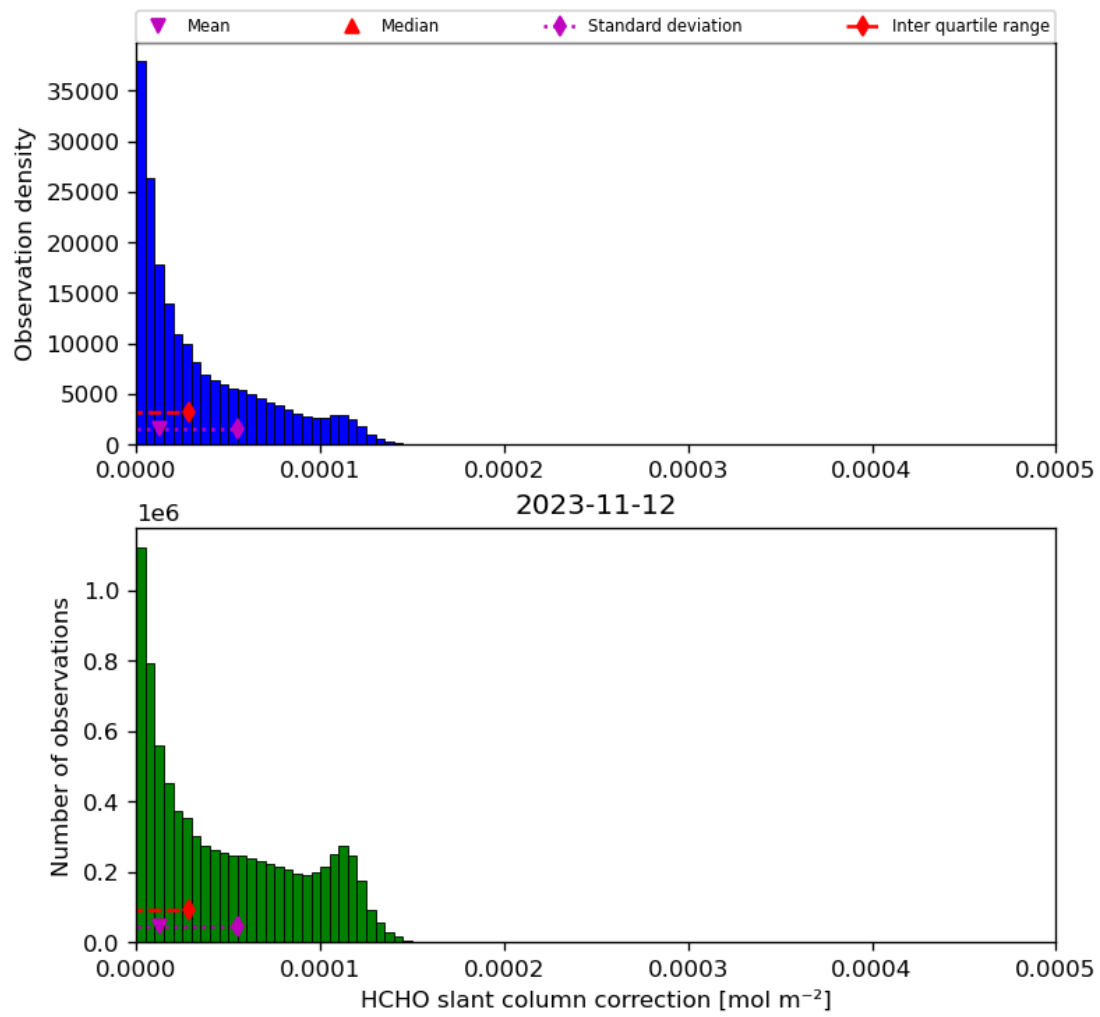
Figure 47: Histogram of “HCHO slant column correction” for 2023-11-12 to 2023-11-13
