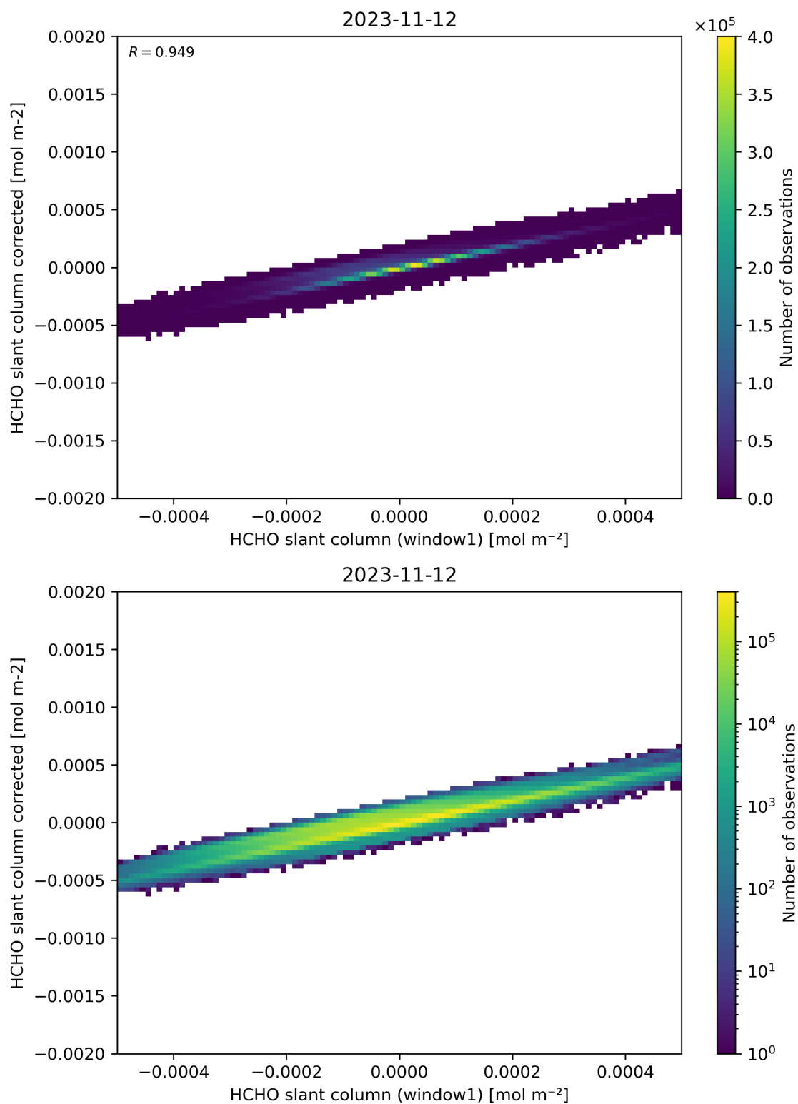
Figure 82: Scatter density plot of “HCHO slant column (window1)” against “HCHO slant column corrected” for 2023-11-12 to 2023-11-13.
