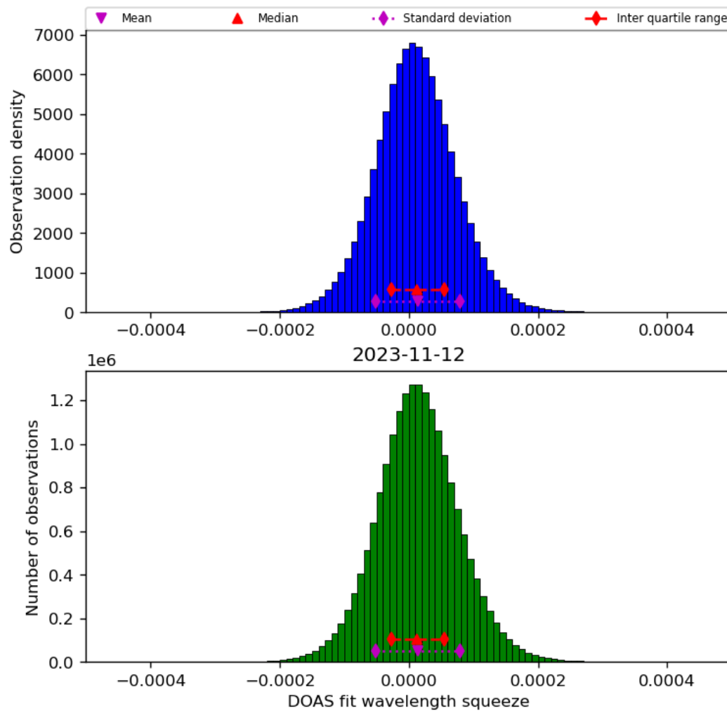
Figure 45: Histogram of “DOAS fit wavelength squeeze” for 2023-11-12 to 2023-11-13
