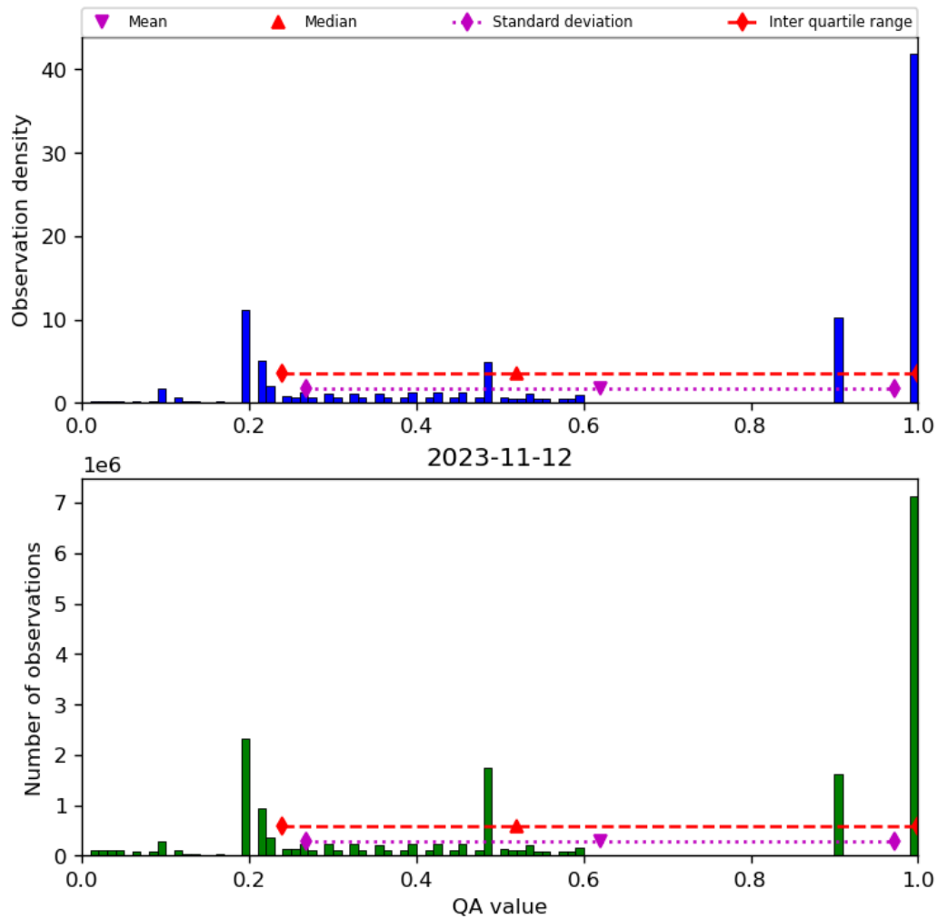
Figure 34: Histogram of “QA value” for 2023-11-12 to 2023-11-13
