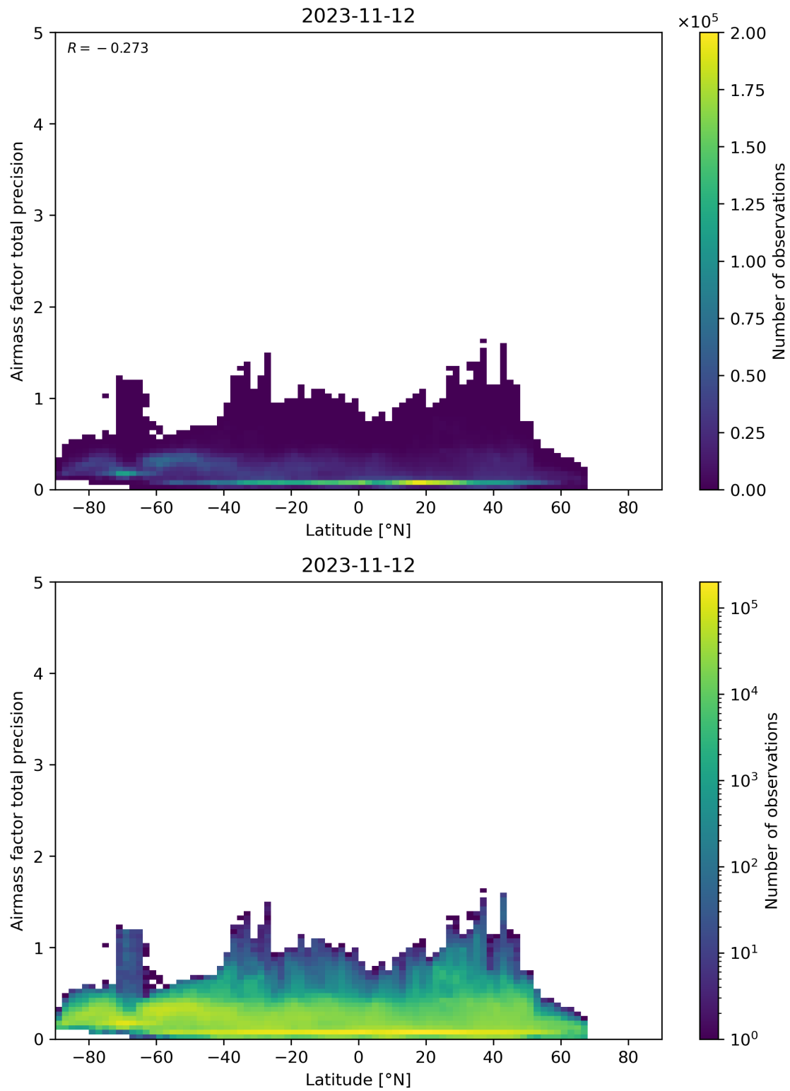
Figure 162: Scatter density plot of “Latitude” against “Airmass factor total precision” for 2023-11-12 to 2023-11-13.
