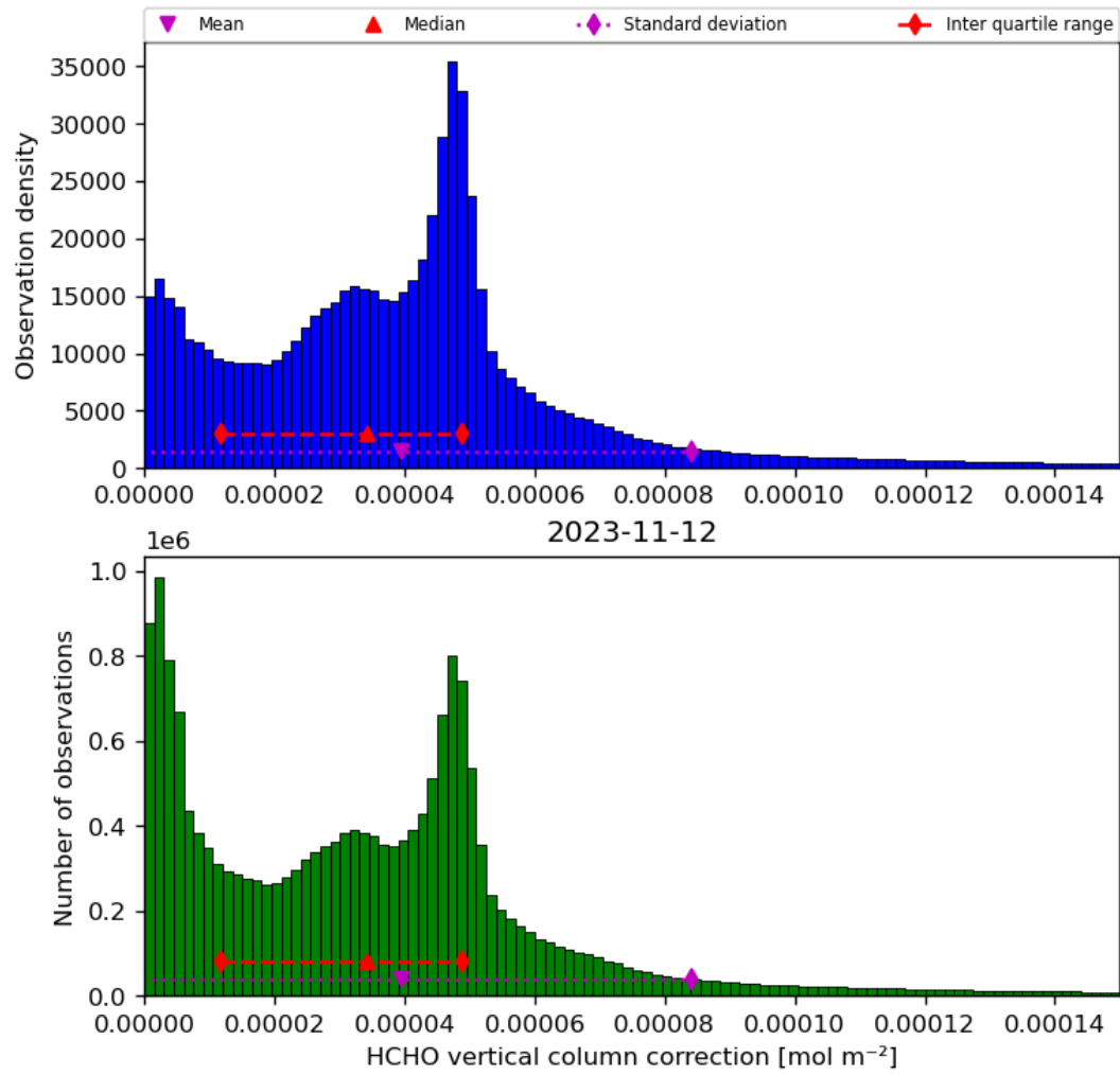
Figure 37: Histogram of “HCHO vertical column correction” for 2023-11-12 to 2023-11-13
