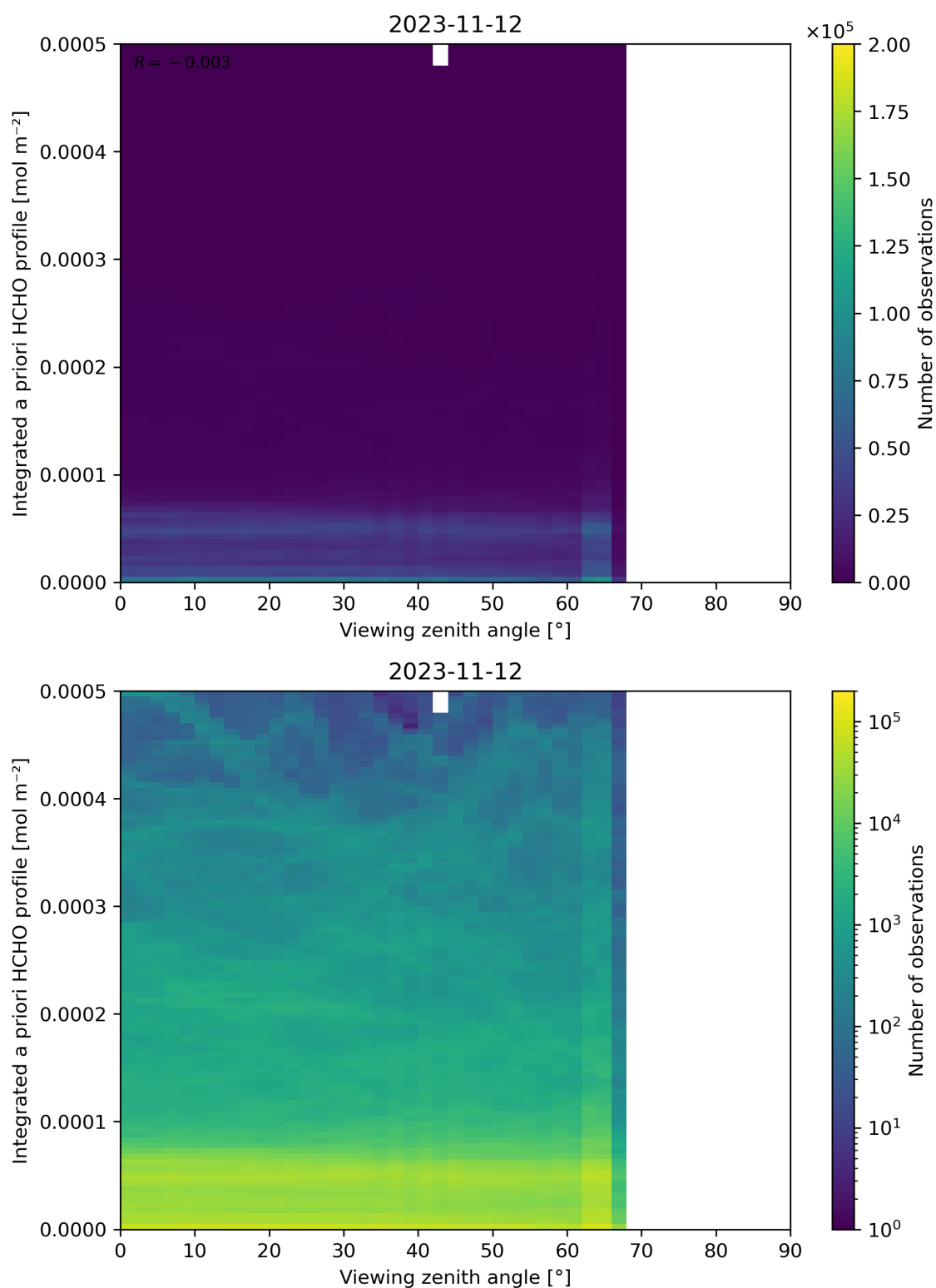
Figure 195: Scatter density plot of “Viewing zenith angle” against “Integrated a priori HCHO profile” for 2023-11-12 to 2023-11-13.
