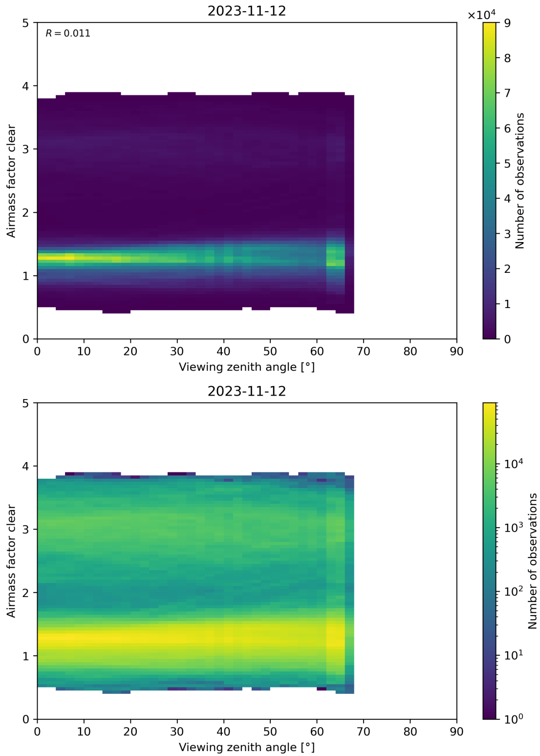
Figure 185: Scatter density plot of “Viewing zenith angle” against “Airmass factor clear” for 2023-11-12 to 2023-11-13.
