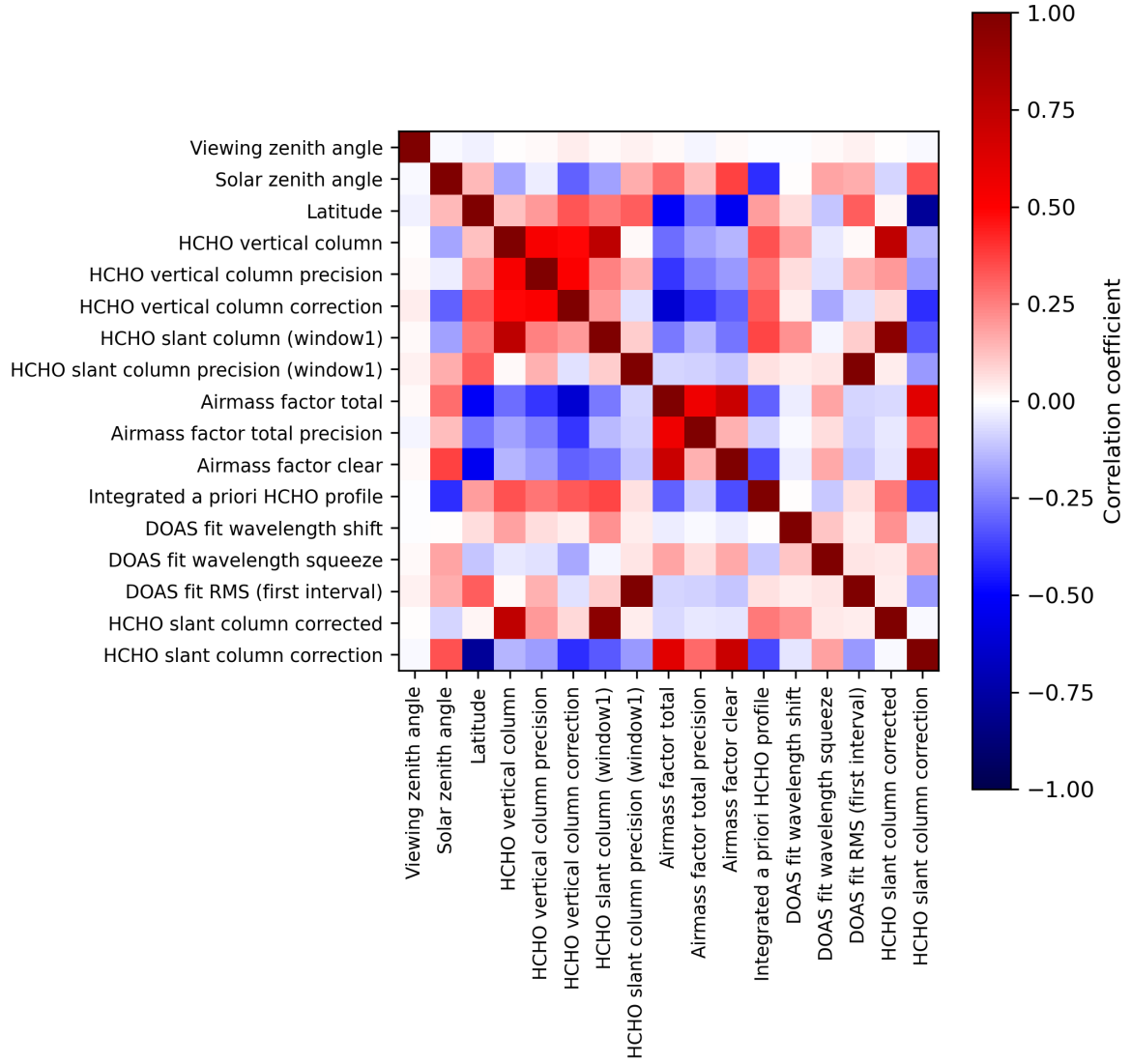
Figure 2: Map of correlation matrix for 2023-11-12 to 2023-11-13.
