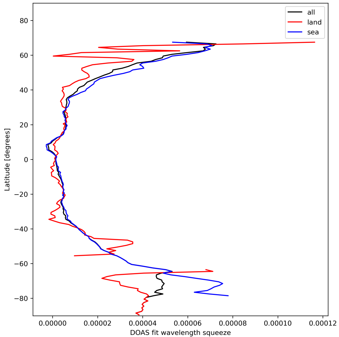
Figure 31: Zonal average of “DOAS fit wavelength squeeze” for 2023-11-12 to 2023-11-13.
