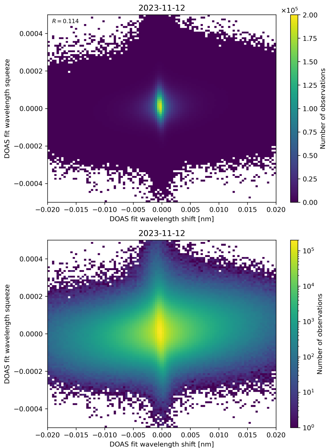
Figure 65: Scatter density plot of “DOAS fit wavelength shift” against “DOAS fit wavelength squeeze” for 2023-11-12 to 2023-11-13.
