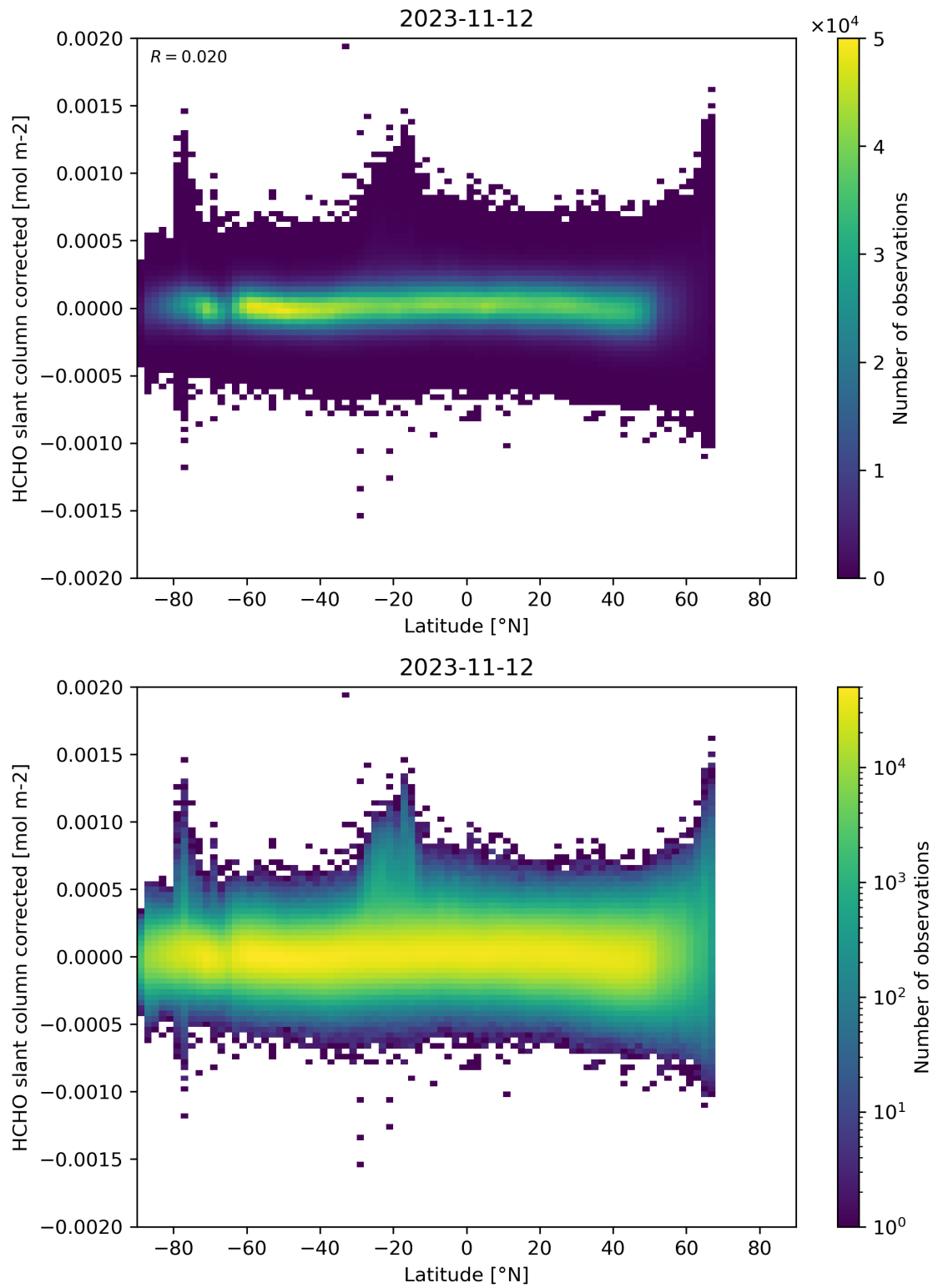
Figure 157: Scatter density plot of “Latitude” against “HCHO slant column corrected” for 2023-11-12 to 2023-11-13.
