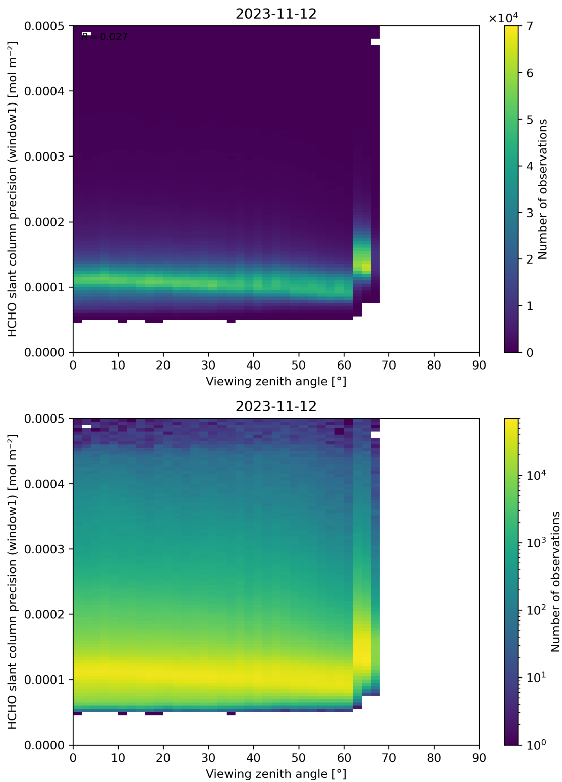
Figure 189: Scatter density plot of “Viewing zenith angle” against “HCHO slant column precision (window1)” for 2023-11-12 to 2023-11-13.
