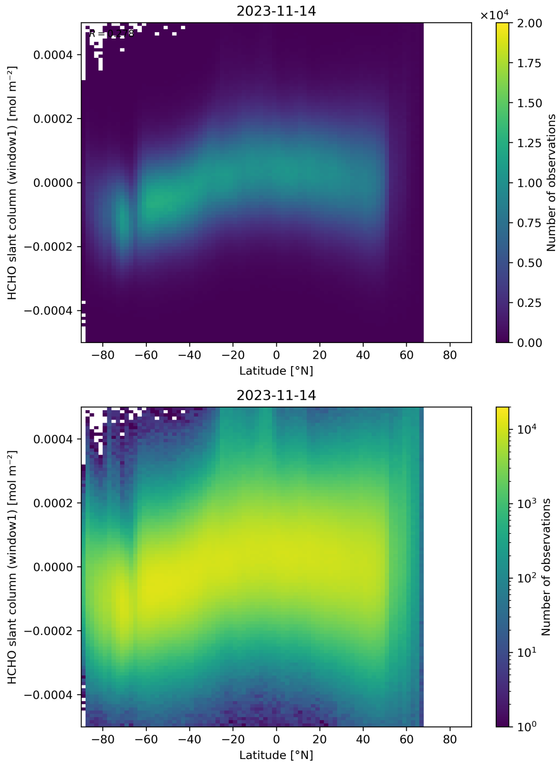
Figure 159: Scatter density plot of “Latitude” against “HCHO slant column (window1)” for 2023-11-13 to 2023-11-15.
