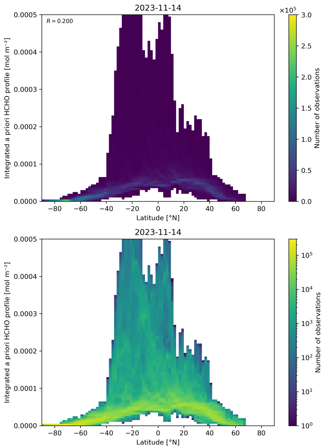
Figure 166: Scatter density plot of “Latitude” against “Integrated a priori HCHO profile” for 2023-11-13 to 2023-11-15.
