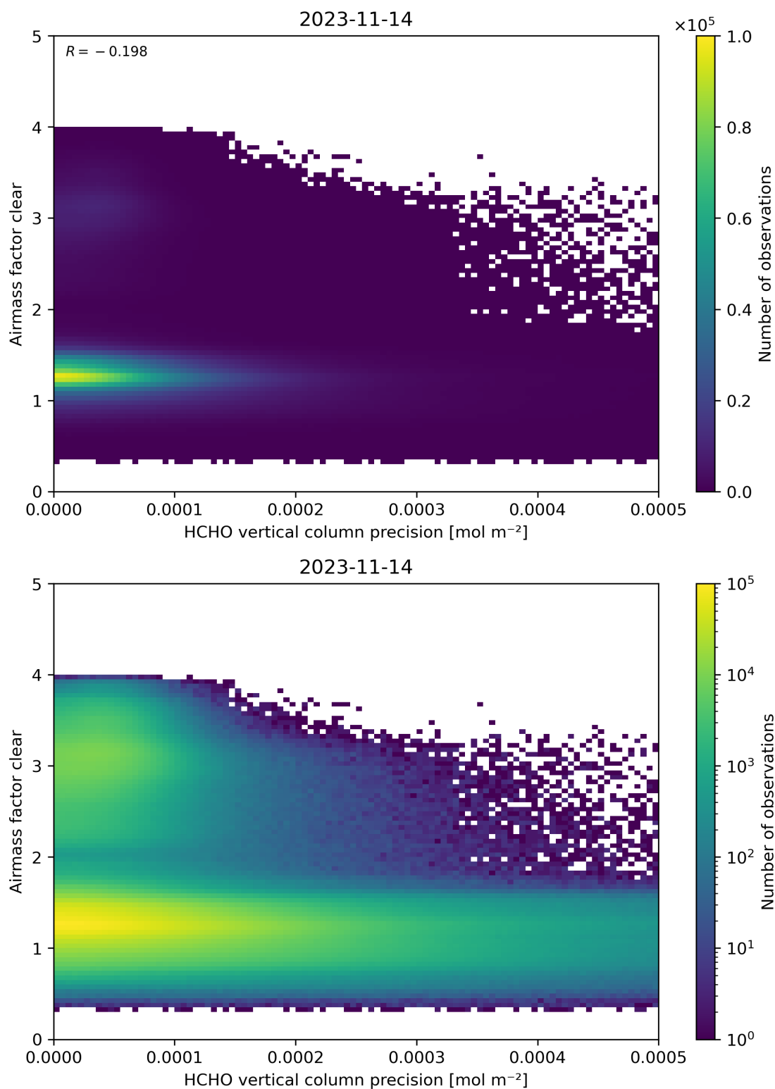
Figure 139: Scatter density plot of “HCHO vertical column precision” against “Airmass factor clear” for 2023-11-13 to 2023-11-15.
