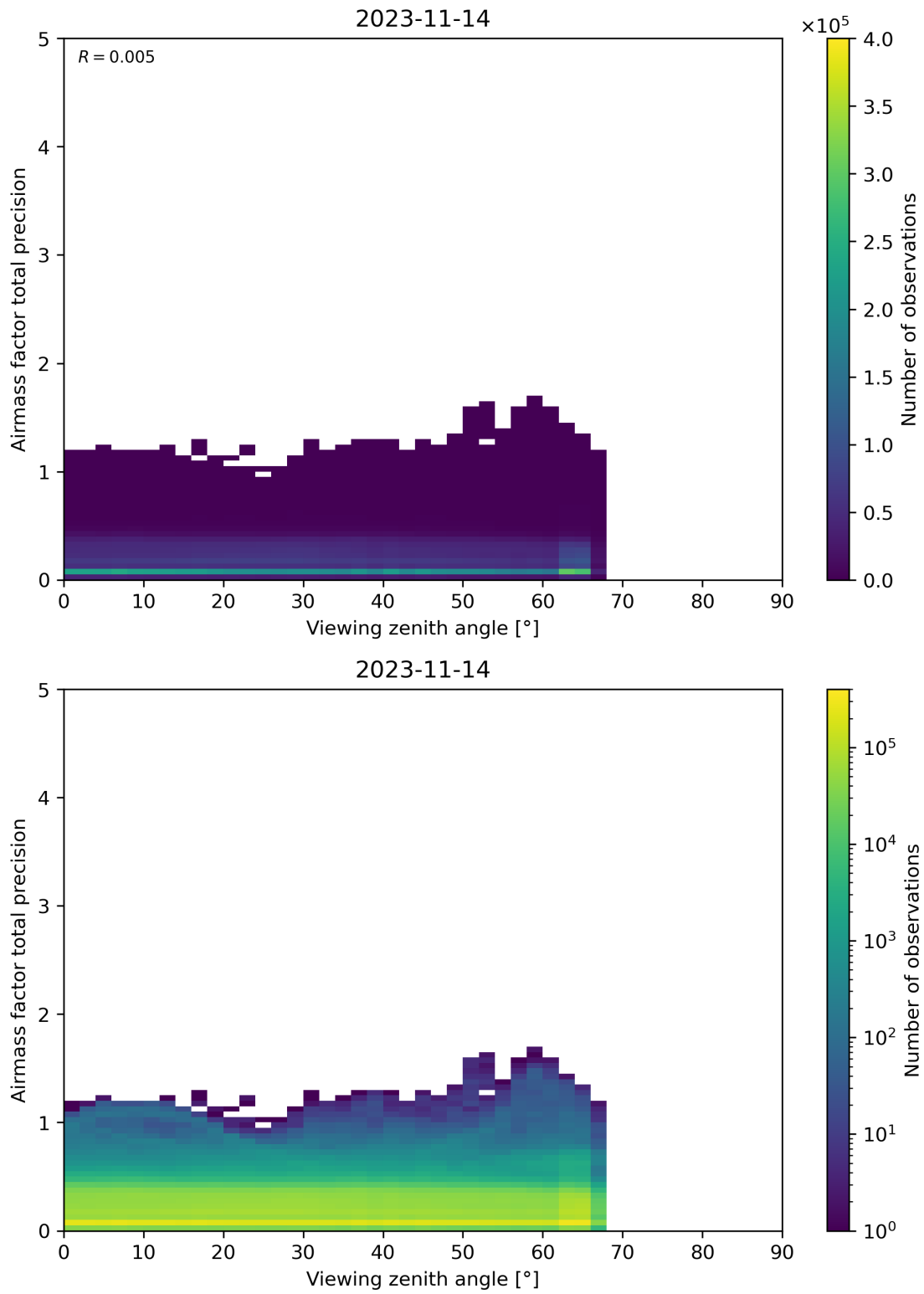
Figure 191: Scatter density plot of “Viewing zenith angle” against “Airmass factor total precision” for 2023-11-13 to 2023-11-15.
