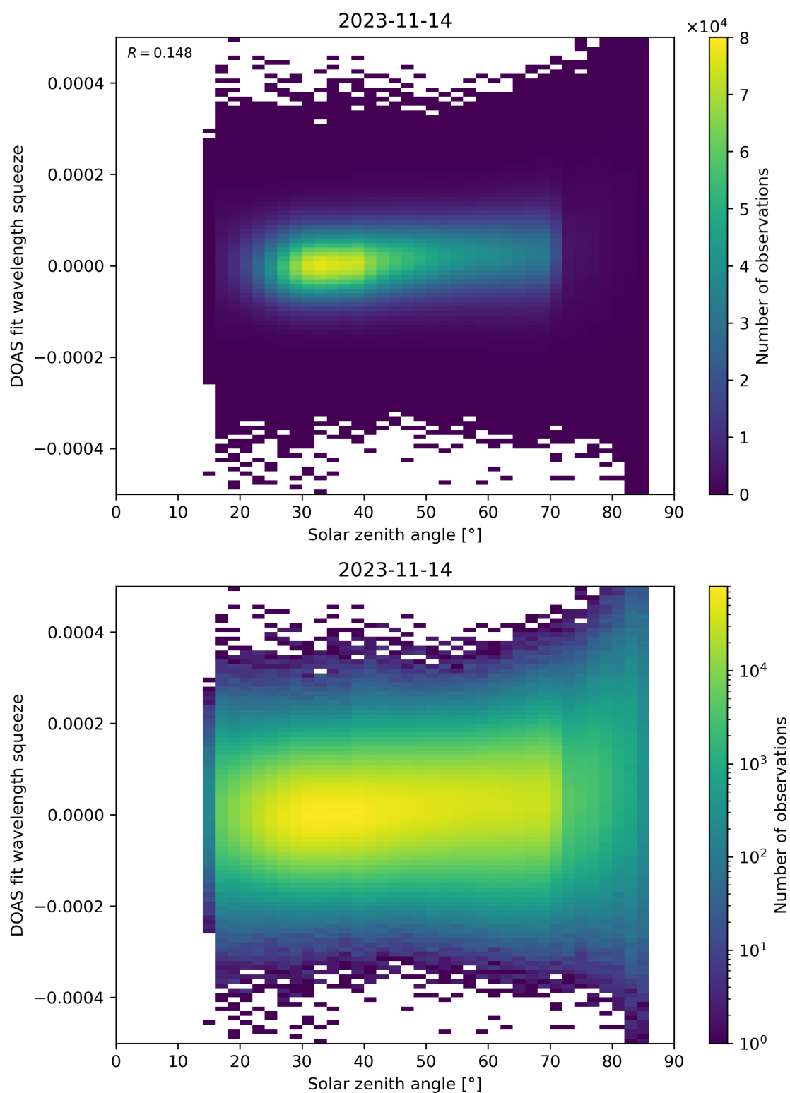
Figure 169: Scatter density plot of “Solar zenith angle” against “DOAS fit wavelength squeeze” for 2023-11-13 to 2023-11-15.
