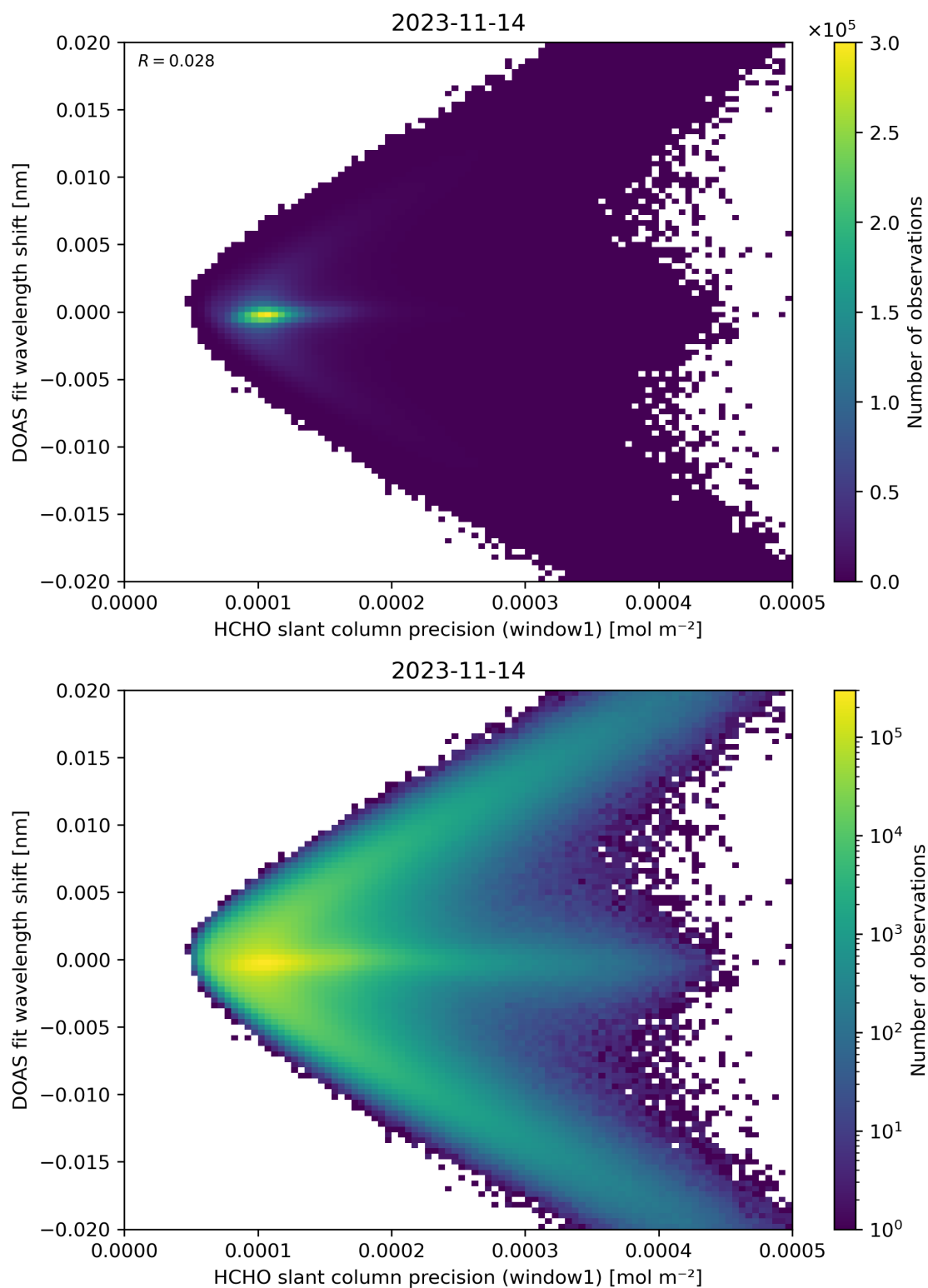
Figure 89: Scatter density plot of “HCHO slant column precision (window1)” against “DOAS fit wavelength shift” for 2023-11-13 to 2023-11-15.
