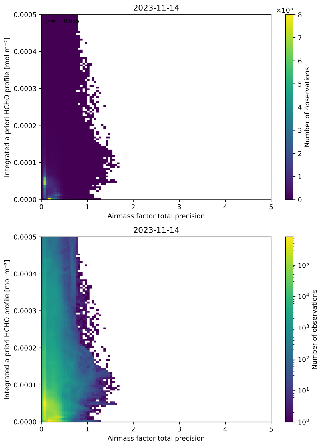
Figure 111: Scatter density plot of “Airmass factor total precision” against “Integrated a priori HCHO profile” for 2023-11-13 to 2023-11-15.
