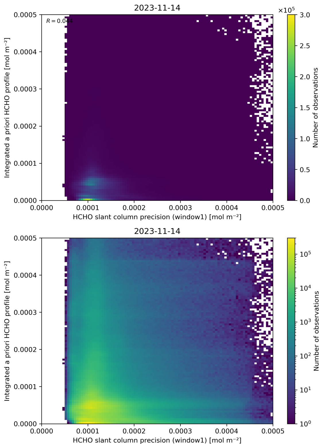
Figure 96: Scatter density plot of “HCHO slant column precision (window1)” against “Integrated a priori HCHO profile” for 2023-11-13 to 2023-11-15.
