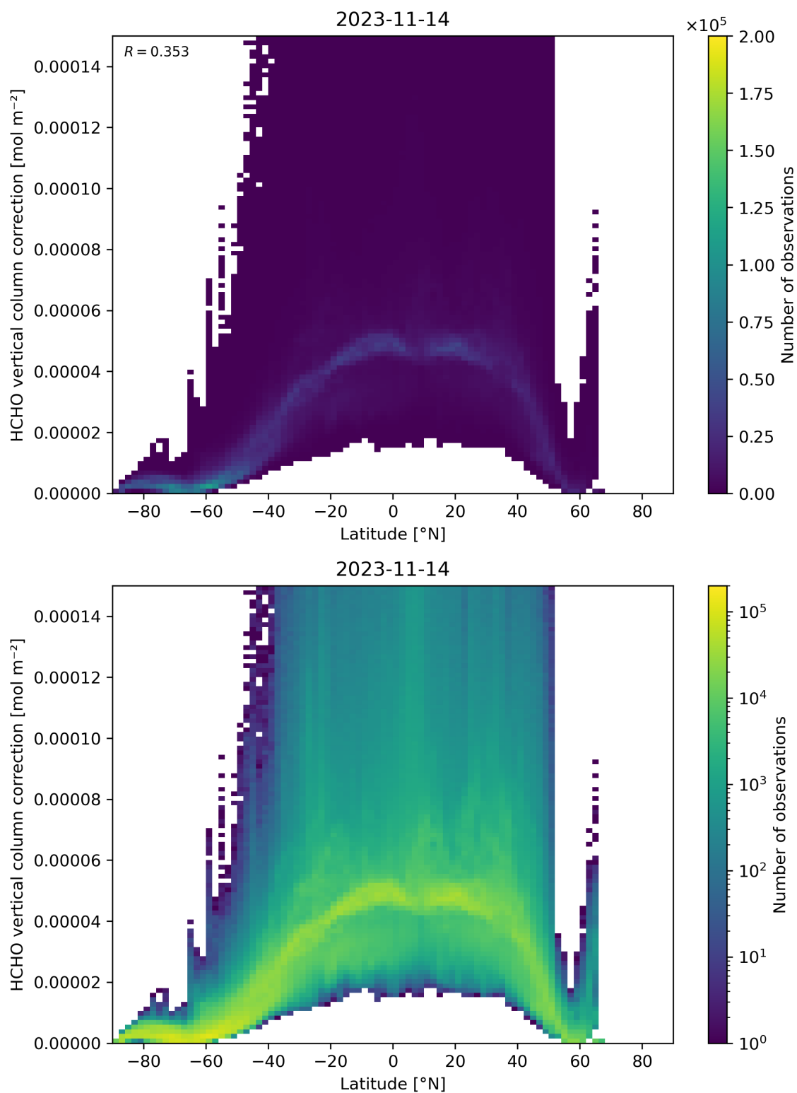
Figure 164: Scatter density plot of “Latitude” against “HCHO vertical column correction” for 2023-11-13 to 2023-11-15.
