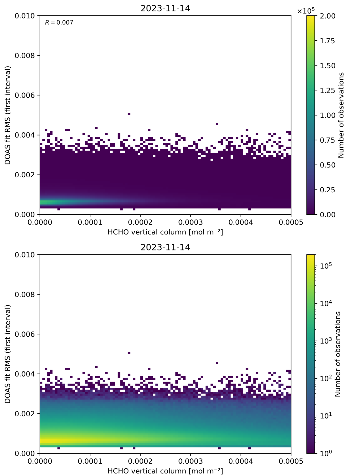
Figure 123: Scatter density plot of “HCHO vertical column” against “DOAS fit RMS (first interval)” for 2023-11-13 to 2023-11-15.
