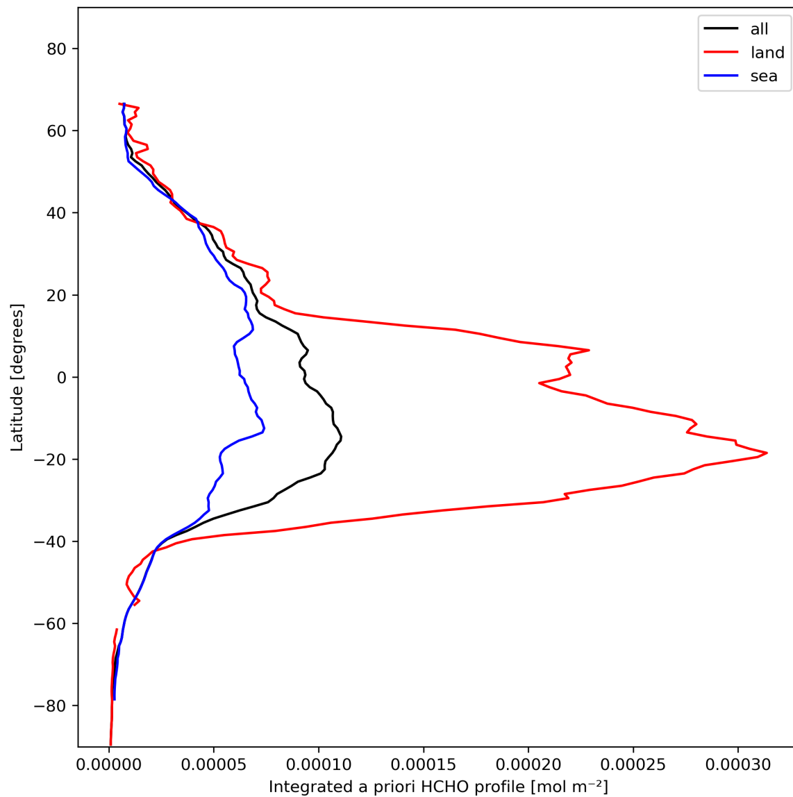
Figure 29: Zonal average of “Integrated a priori HCHO profile” for 2023-11-13 to 2023-11-15.
