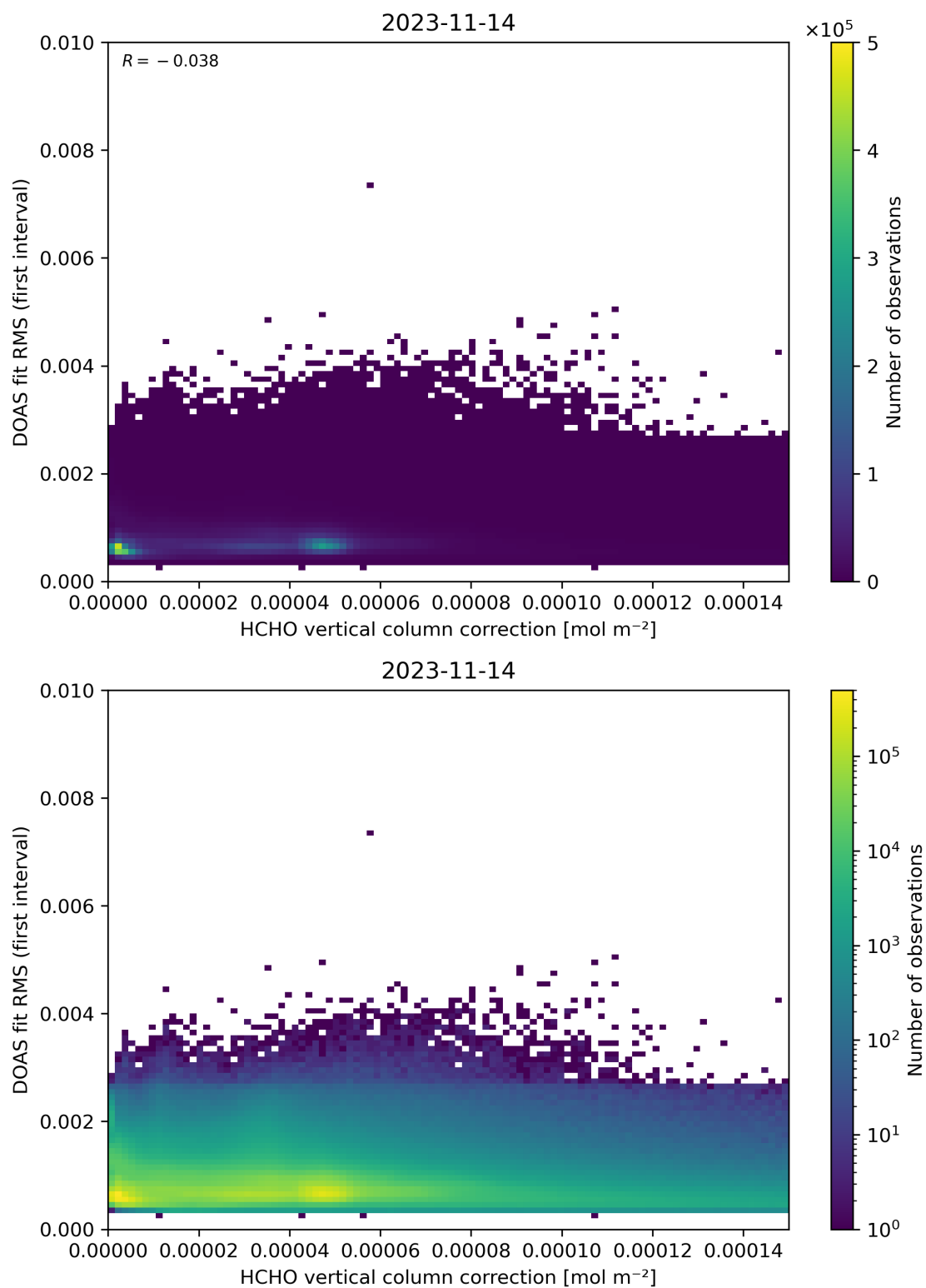
Figure 112: Scatter density plot of “HCHO vertical column correction” against “DOAS fit RMS (first interval)” for 2023-11-13 to 2023-11-15.
