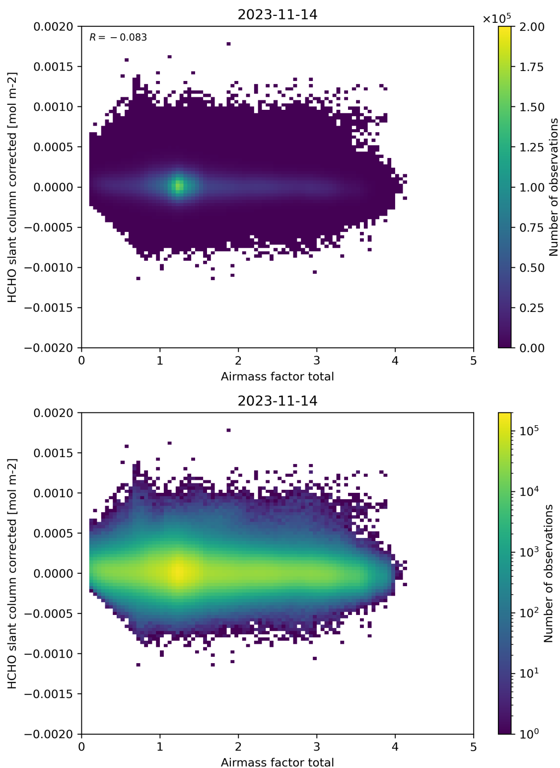
Figure 101: Scatter density plot of “Airmass factor total” against “HCHO slant column corrected” for 2023-11-13 to 2023-11-15.
