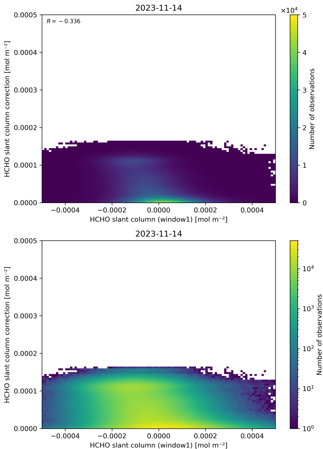
Figure 83: Scatter density plot of “HCHO slant column (window1)” against “HCHO slant column correction” for 2023-11-13 to 2023-11-15.
