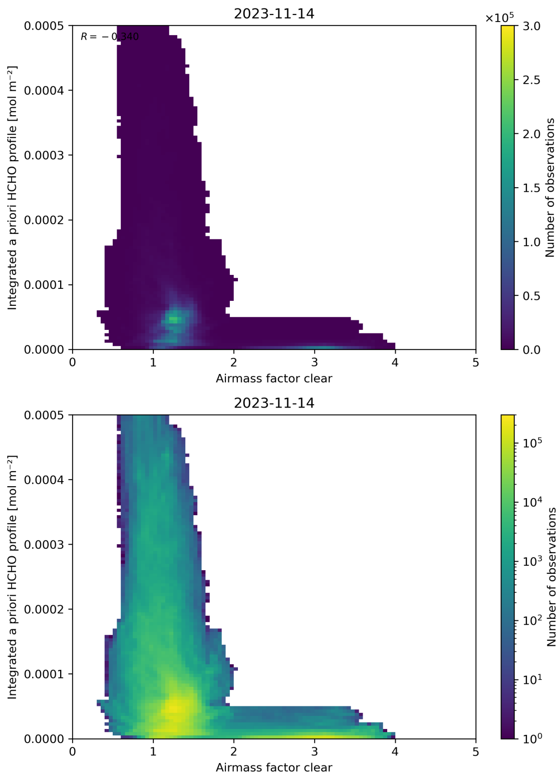
Figure 76: Scatter density plot of “Airmass factor clear” against “Integrated a priori HCHO profile” for 2023-11-13 to 2023-11-15.
