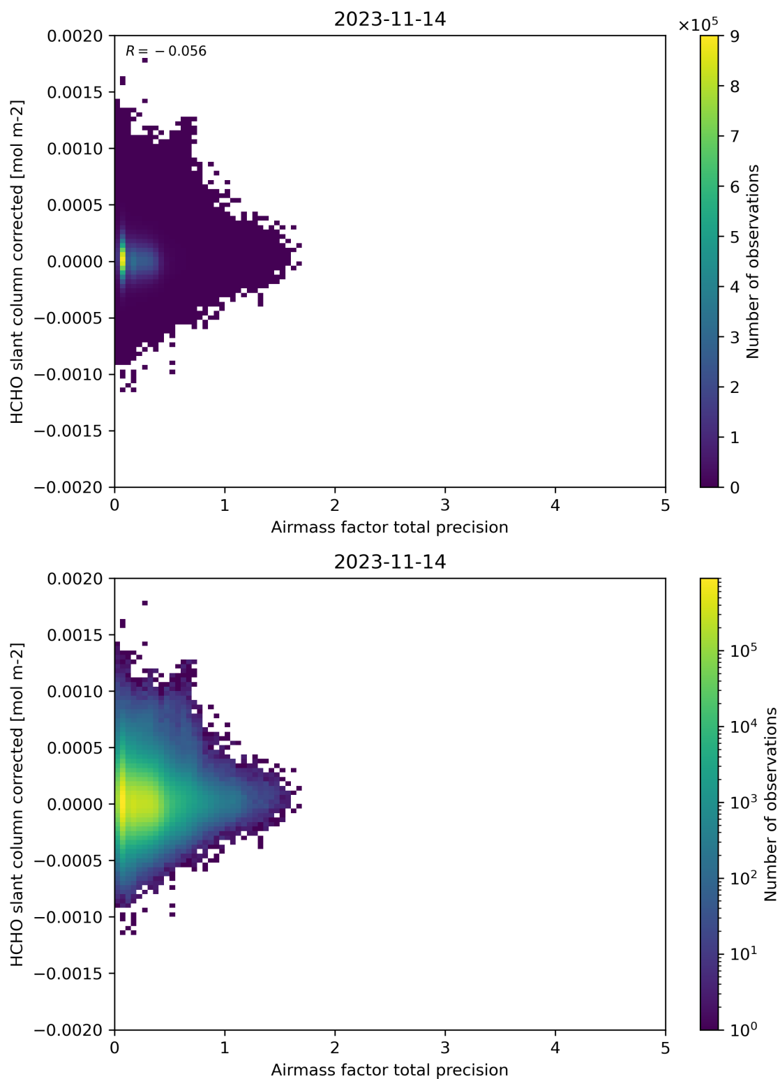
Figure 109: Scatter density plot of “Airmass factor total precision” against “HCHO slant column corrected” for 2023-11-13 to 2023-11-15.
