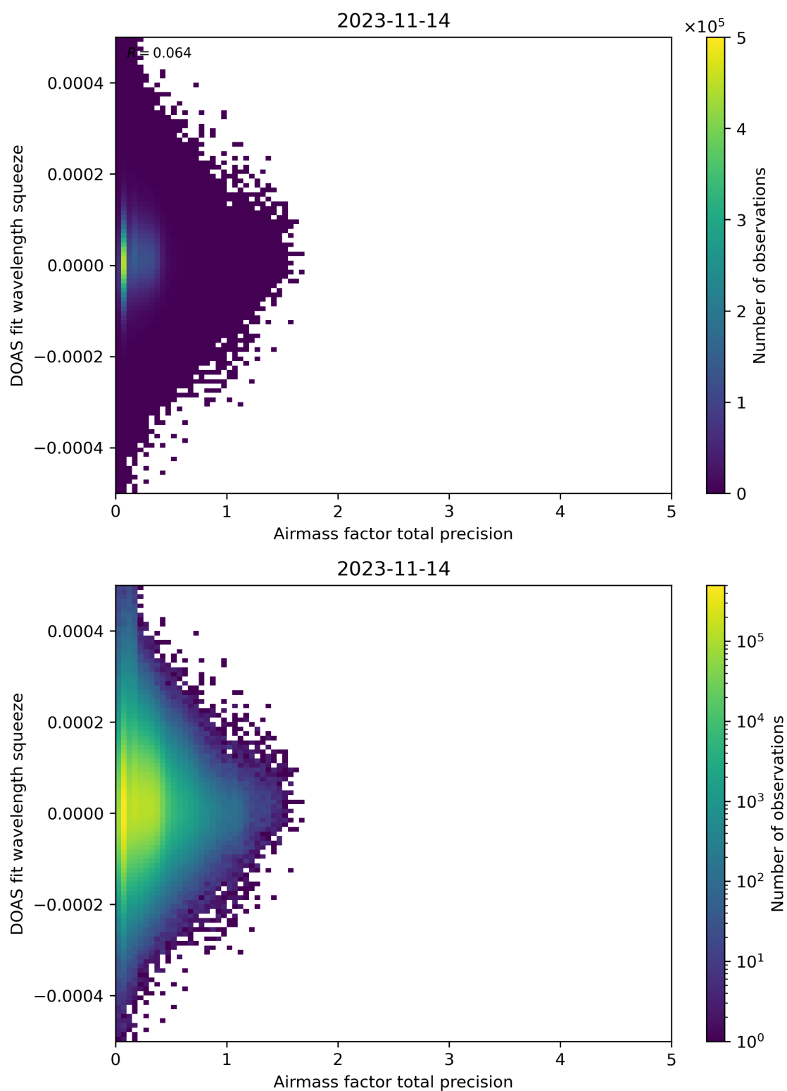
Figure 107: Scatter density plot of “Airmass factor total precision” against “DOAS fit wavelength squeeze” for 2023-11-13 to 2023-11-15.
