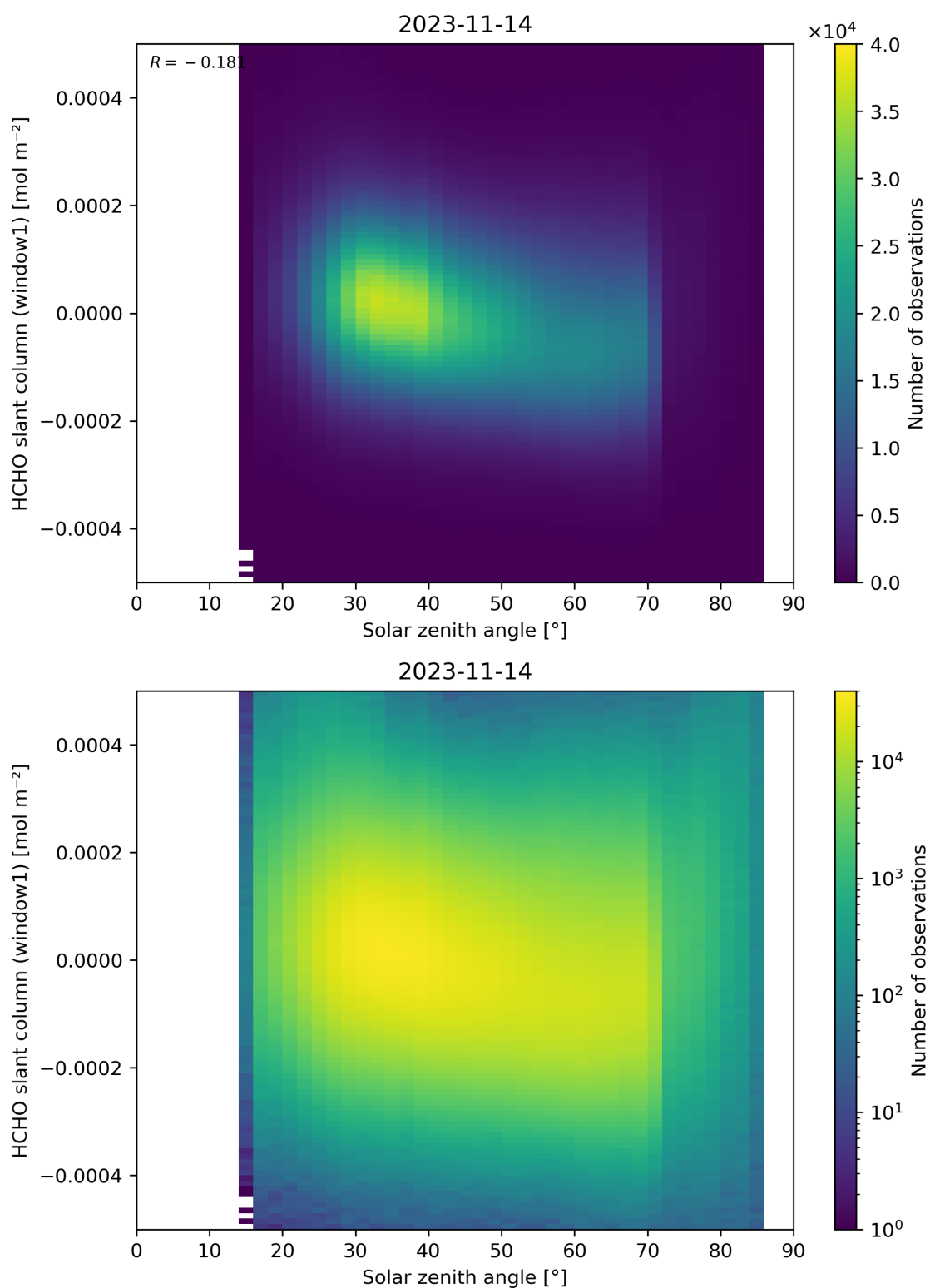
Figure 173: Scatter density plot of “Solar zenith angle” against “HCHO slant column (window1)” for 2023-11-13 to 2023-11-15.
