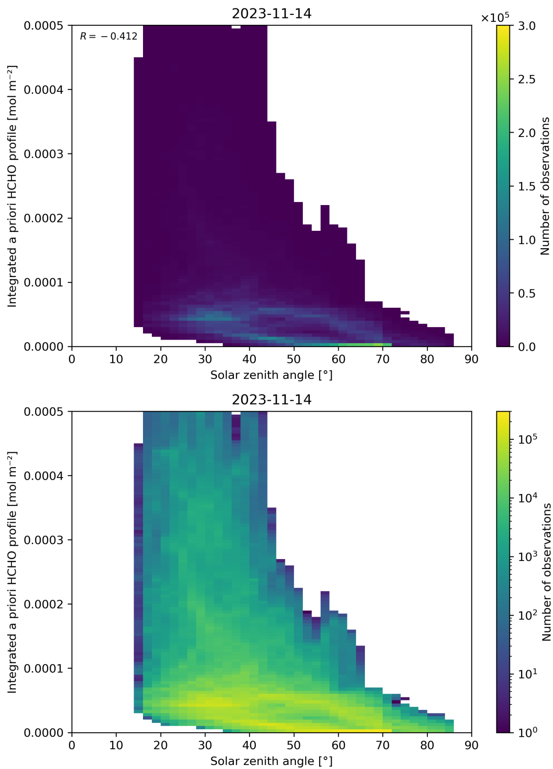
Figure 180: Scatter density plot of “Solar zenith angle” against “Integrated a priori HCHO profile” for 2023-11-13 to 2023-11-15.
