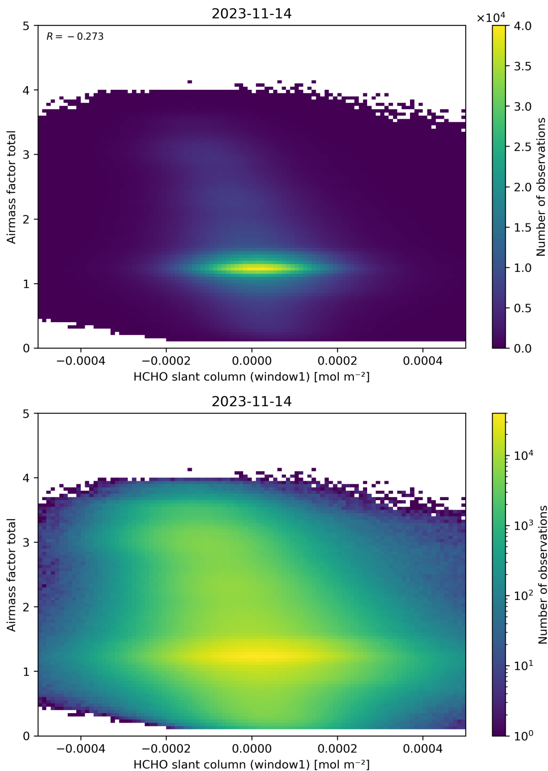
Figure 85: Scatter density plot of “HCHO slant column (window1)” against “Airmass factor total” for 2023-11-13 to 2023-11-15.
