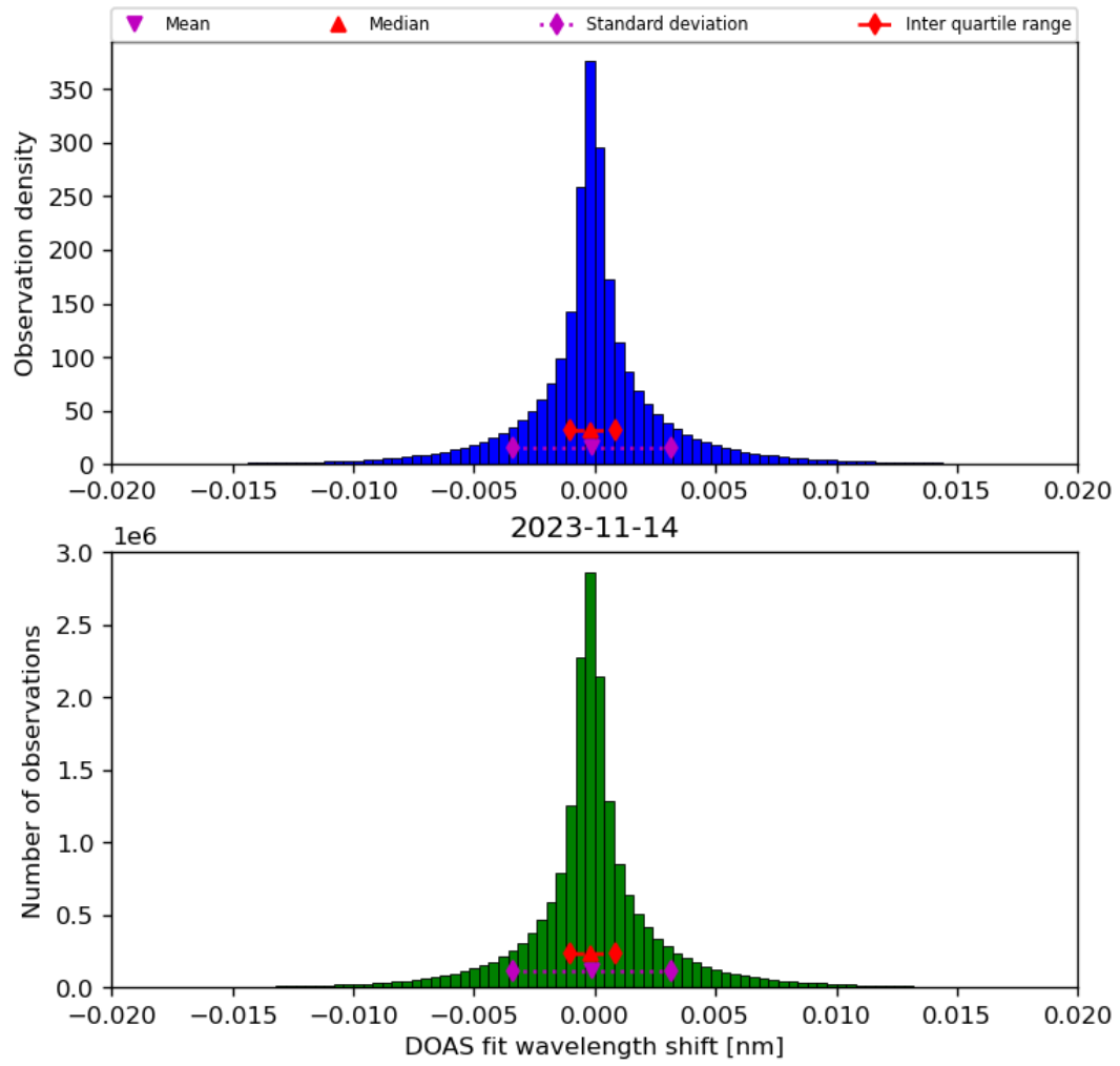
Figure 44: Histogram of “DOAS fit wavelength shift” for 2023-11-13 to 2023-11-15
