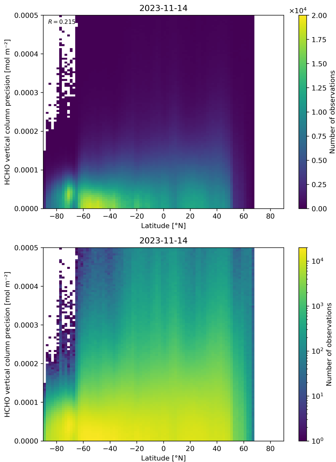
Figure 165: Scatter density plot of “Latitude” against “HCHO vertical column precision” for 2023-11-13 to 2023-11-15.
