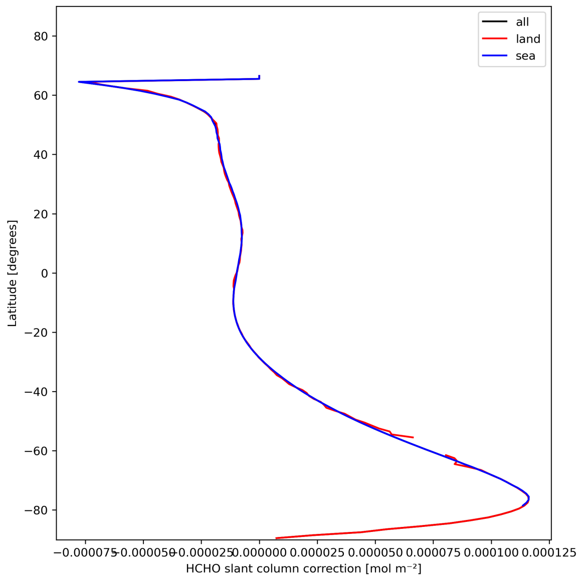
Figure 33: Zonal average of “HCHO slant column correction” for 2023-11-13 to 2023-11-15.
