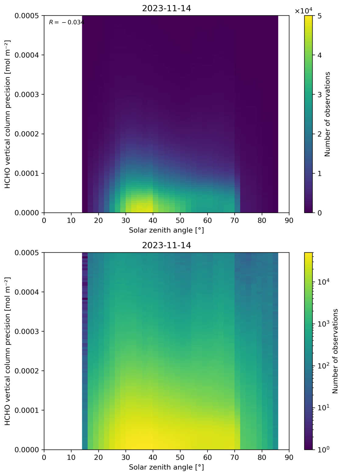
Figure 179: Scatter density plot of “Solar zenith angle” against “HCHO vertical column precision” for 2023-11-13 to 2023-11-15.
