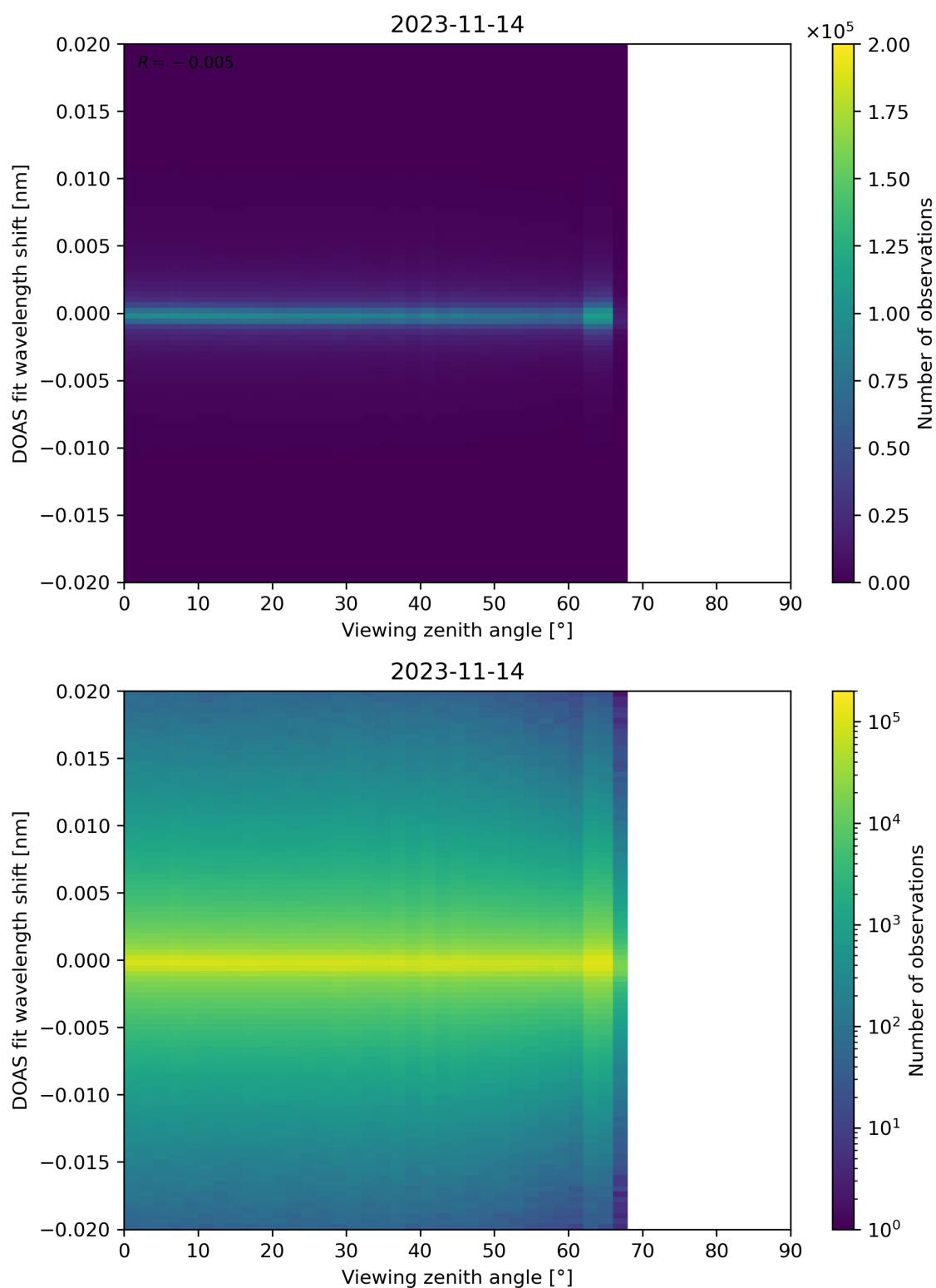
Figure 183: Scatter density plot of “Viewing zenith angle” against “DOAS fit wavelength shift” for 2023-11-13 to 2023-11-15.
