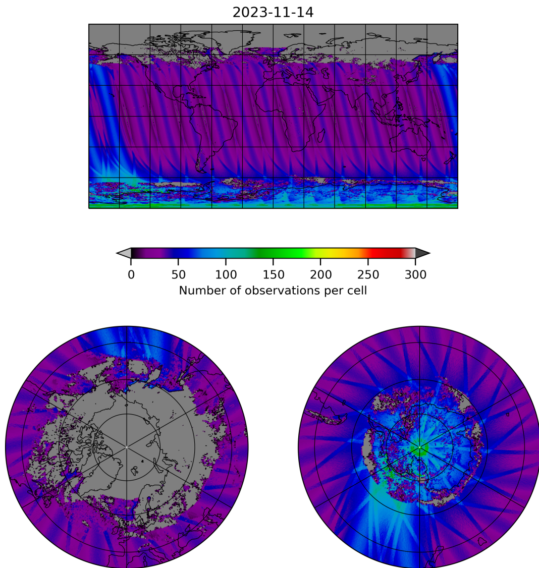
Figure 19: Map of the number of observations for 2023-11-13 to 2023-11-15
