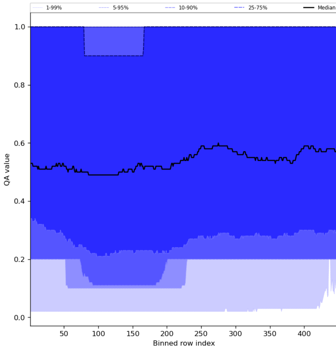
Figure 48: Along track statistics of "QA value" for 2023-11-13 to 2023-11-15
