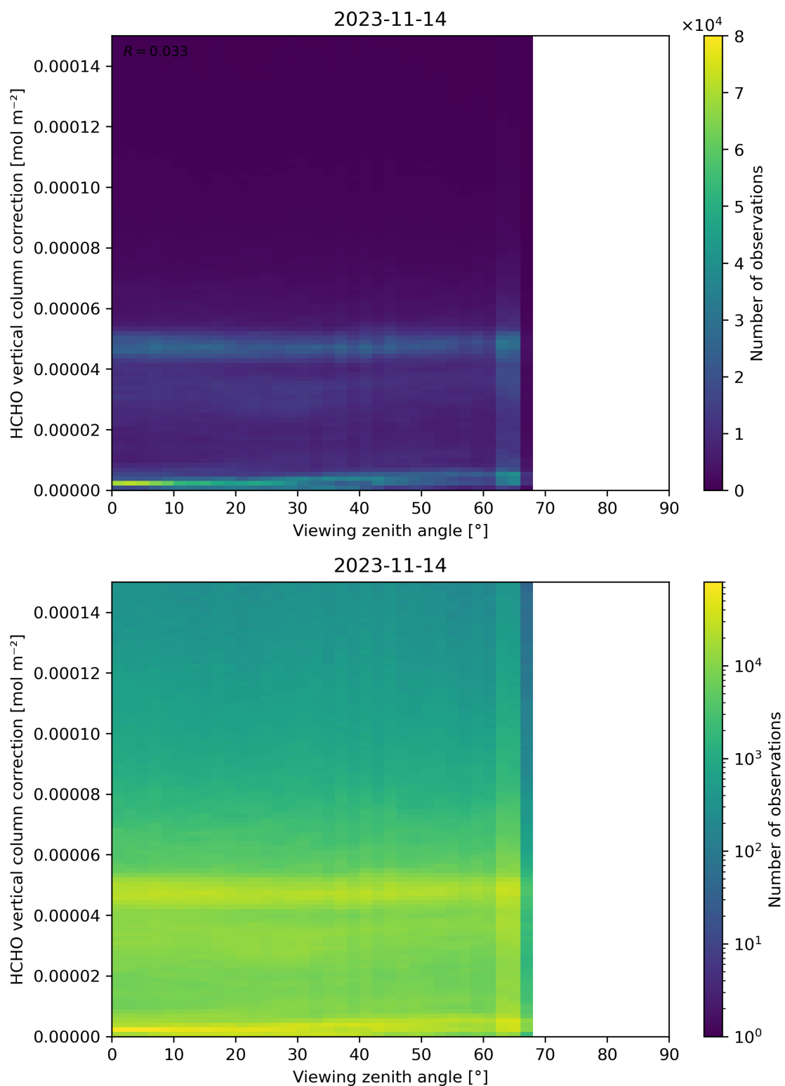
Figure 193: Scatter density plot of “Viewing zenith angle” against “HCHO vertical column correction” for 2023-11-13 to 2023-11-15.
