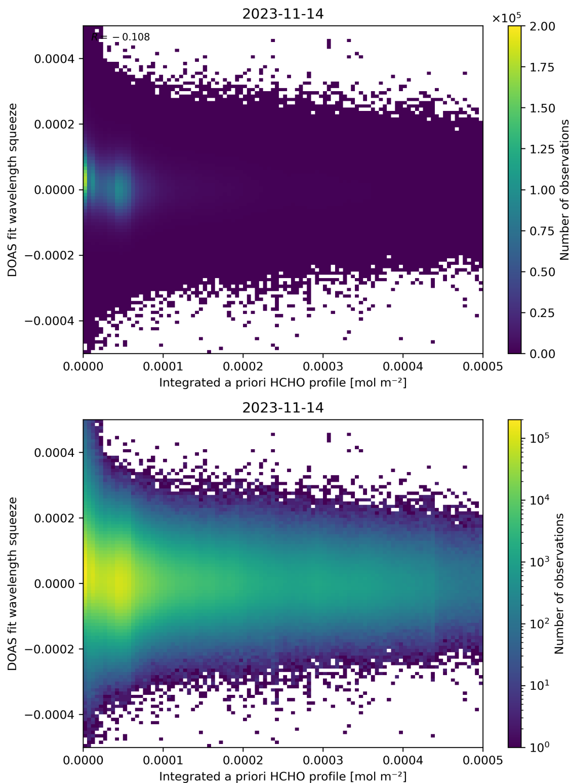
Figure 150: Scatter density plot of “Integrated a priori HCHO profile” against “DOAS fit wavelength squeeze” for 2023-11-13 to 2023-11-15.
