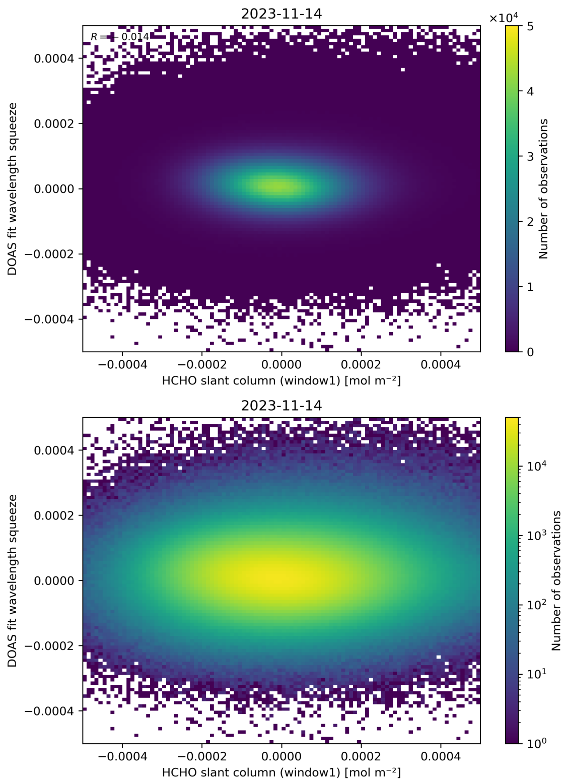
Figure 80: Scatter density plot of “HCHO slant column (window1)” against “DOAS fit wavelength squeeze” for 2023-11-13 to 2023-11-15.
