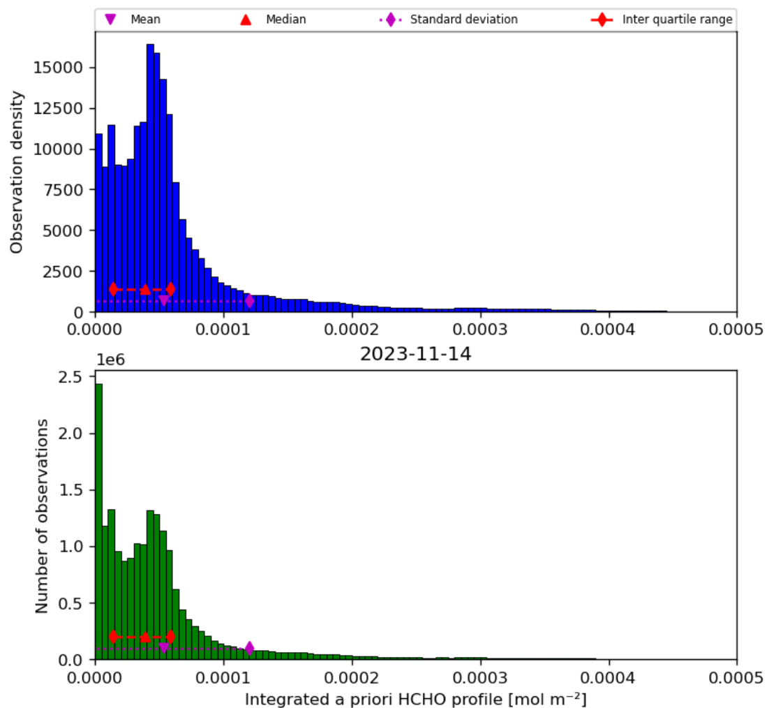
Figure 43: Histogram of “Integrated a priori HCHO profile” for 2023-11-13 to 2023-11-15
