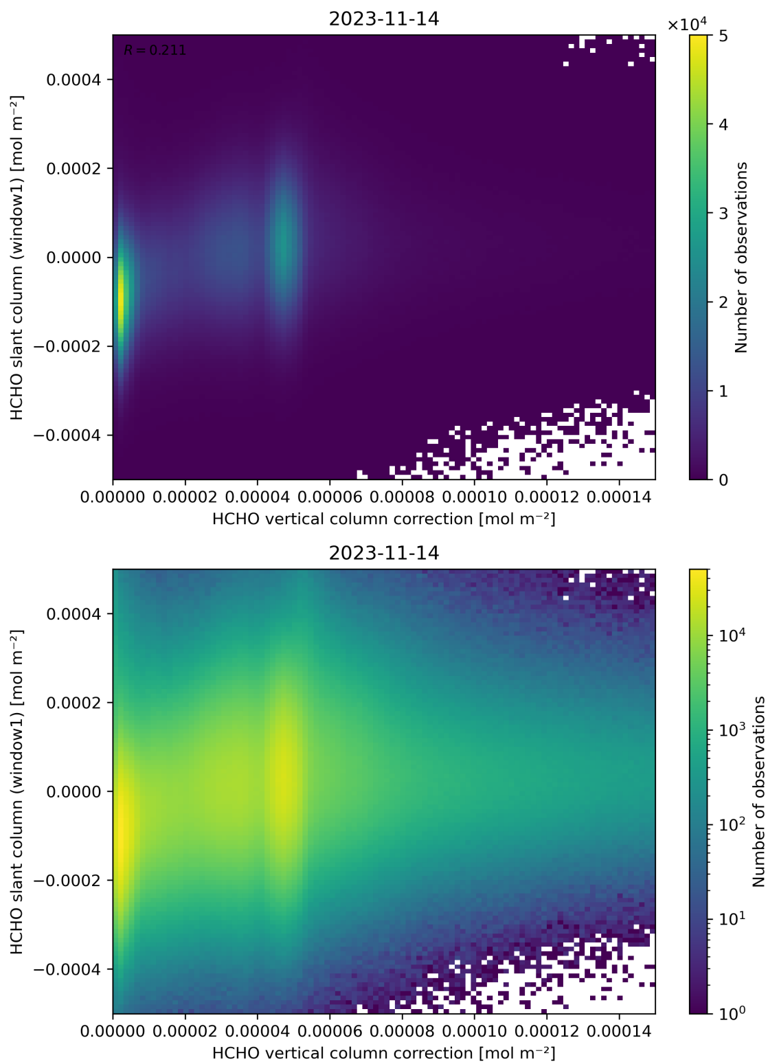
Figure 118: Scatter density plot of “HCHO vertical column correction” against “HCHO slant column (window1)” for 2023-11-13 to 2023-11-15.
