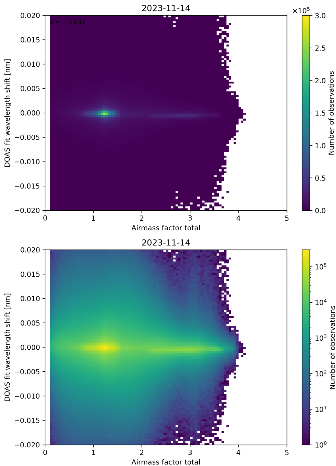
Figure 98: Scatter density plot of “Airmass factor total” against “DOAS fit wavelength shift” for 2023-11-13 to 2023-11-15.
