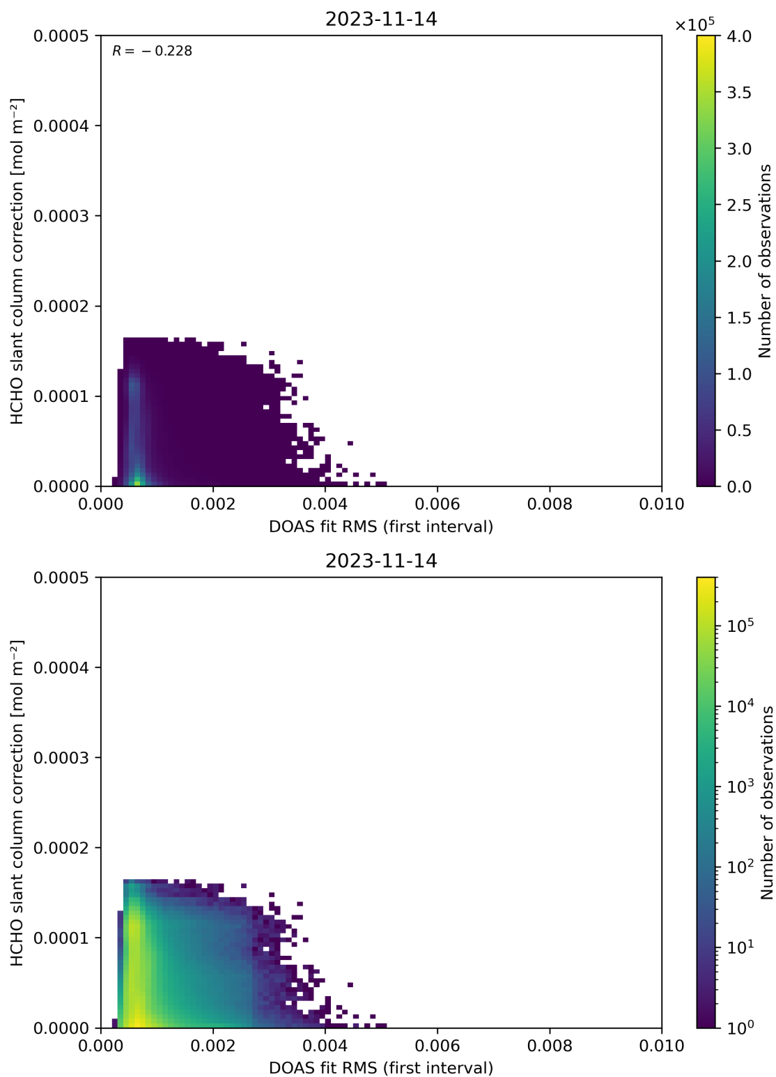
Figure 63: Scatter density plot of “DOAS fit RMS (first interval)” against “HCHO slant column correction” for 2023-11-13 to 2023-11-15.
