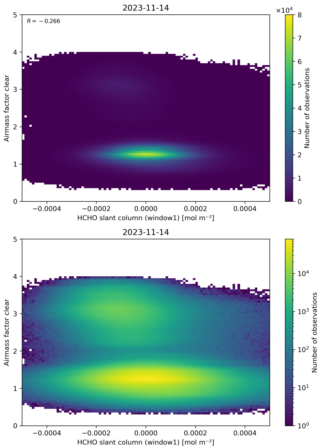
Figure 81: Scatter density plot of “HCHO slant column (window1)” against “Airmass factor clear” for 2023-11-13 to 2023-11-15.
