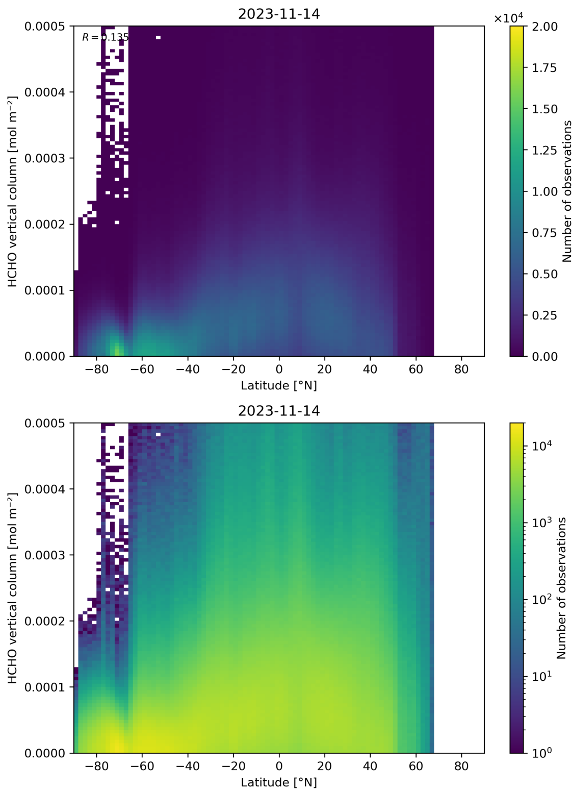
Figure 163: Scatter density plot of “Latitude” against “HCHO vertical column” for 2023-11-13 to 2023-11-15.
