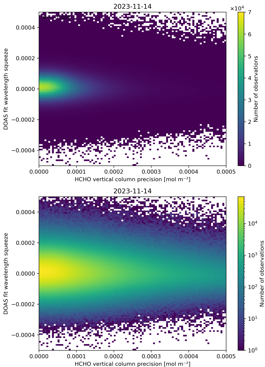
Figure 138: Scatter density plot of “HCHO vertical column precision” against “DOAS fit wavelength squeeze” for 2023-11-13 to 2023-11-15.
