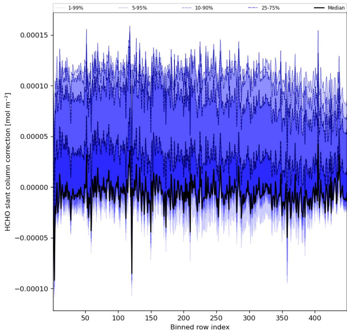
Figure 61: Along track statistics of “HCHO slant column correction” for 2023-11-13 to 2023-11-15
