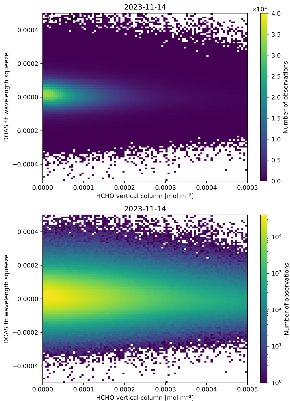
Figure 125: Scatter density plot of “HCHO vertical column” against “DOAS fit wavelength squeeze” for 2023-11-13 to 2023-11-15.
