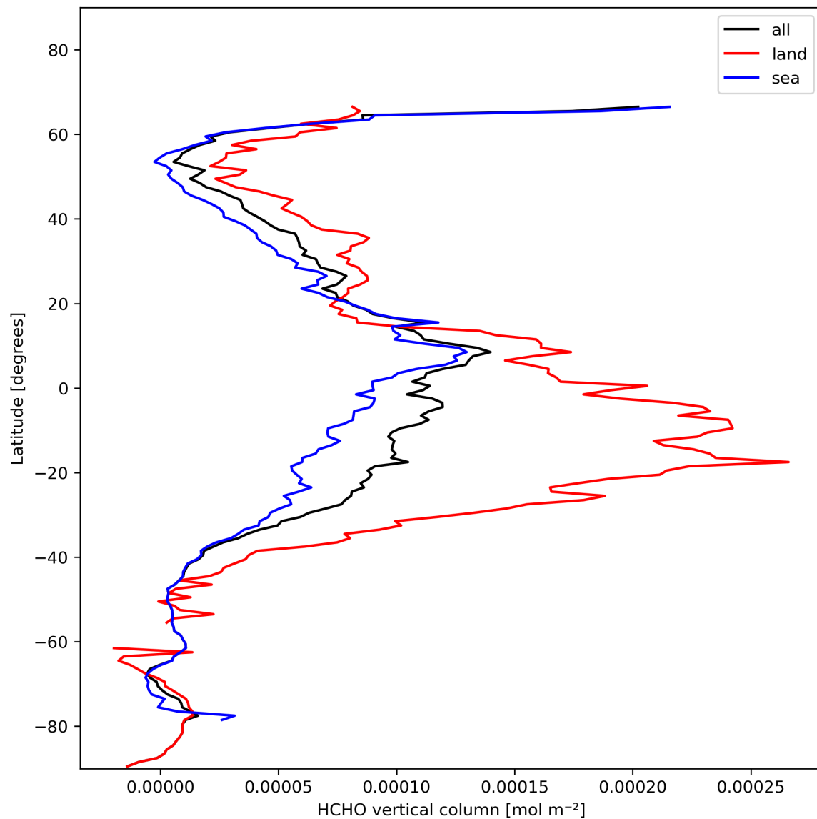
Figure 21: Zonal average of “HCHO vertical column” for 2023-11-13 to 2023-11-15.
