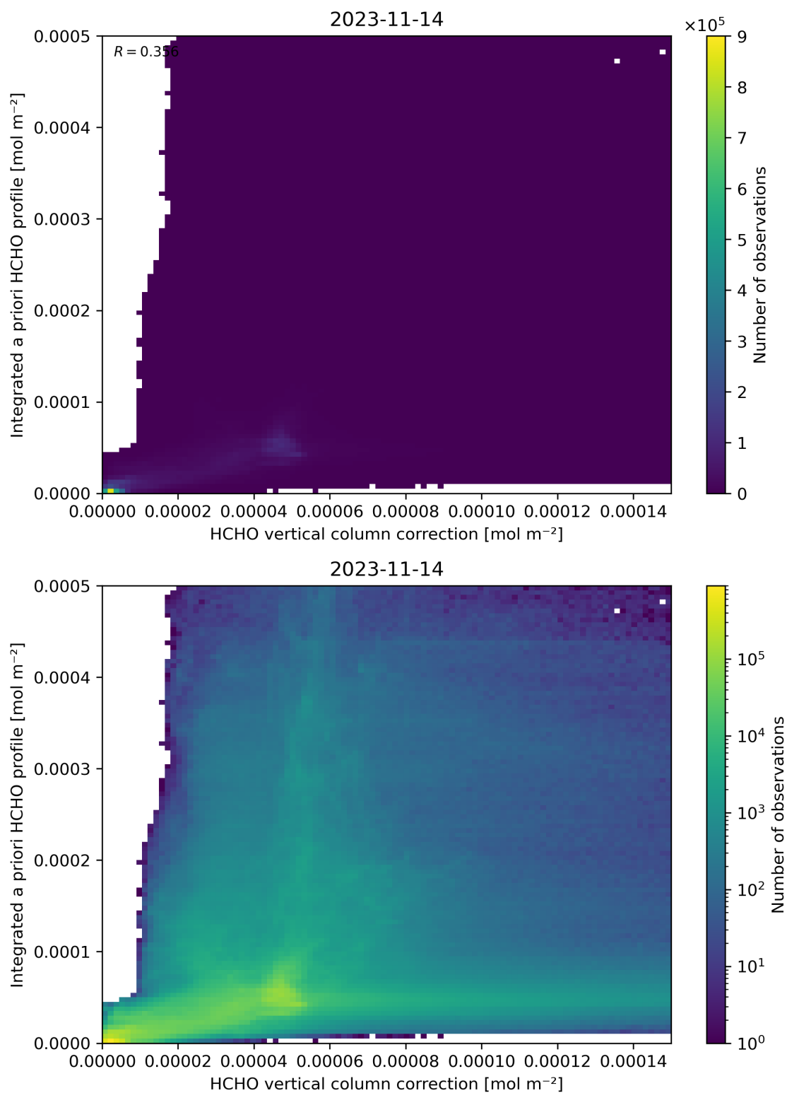
Figure 122: Scatter density plot of “HCHO vertical column correction” against “Integrated a priori HCHO profile” for 2023-11-13 to 2023-11-15.
