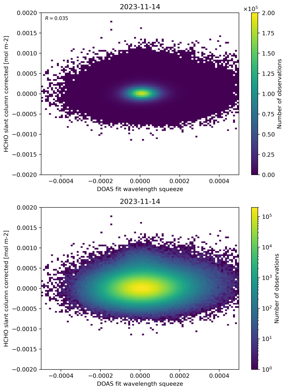
Figure 69: Scatter density plot of “DOAS fit wavelength squeeze” against “HCHO slant column corrected” for 2023-11-13 to 2023-11-15.
