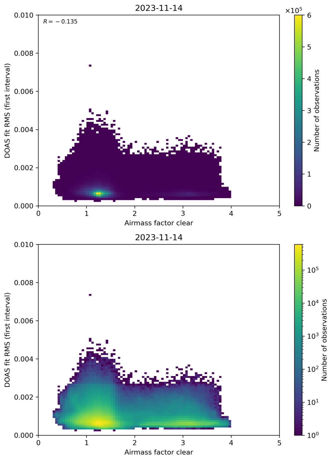
Figure 71: Scatter density plot of “Airmass factor clear” against “DOAS fit RMS (first interval)” for 2023-11-13 to 2023-11-15.
