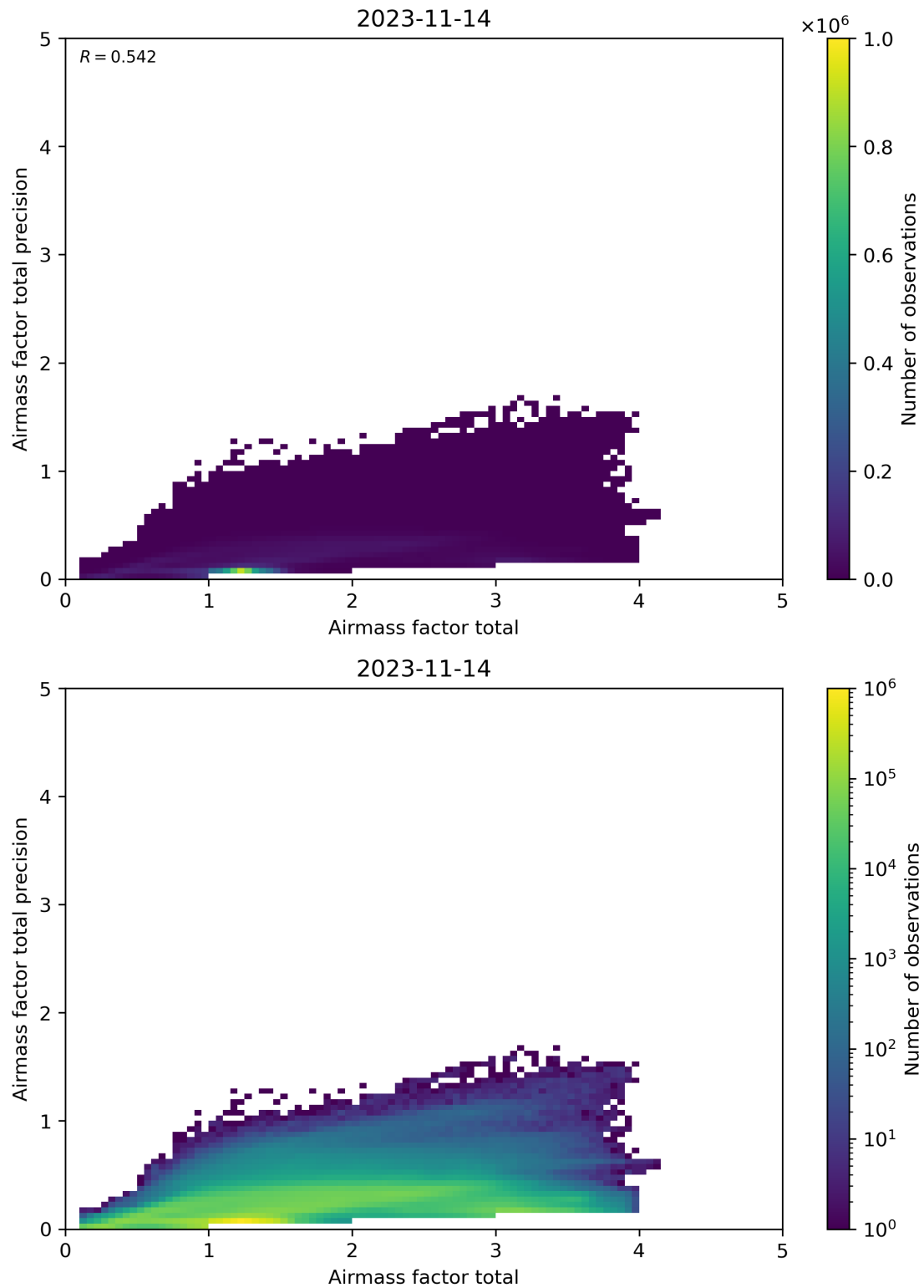
Figure 103: Scatter density plot of “Airmass factor total” against “Airmass factor total precision” for 2023-11-13 to 2023-11-15.
