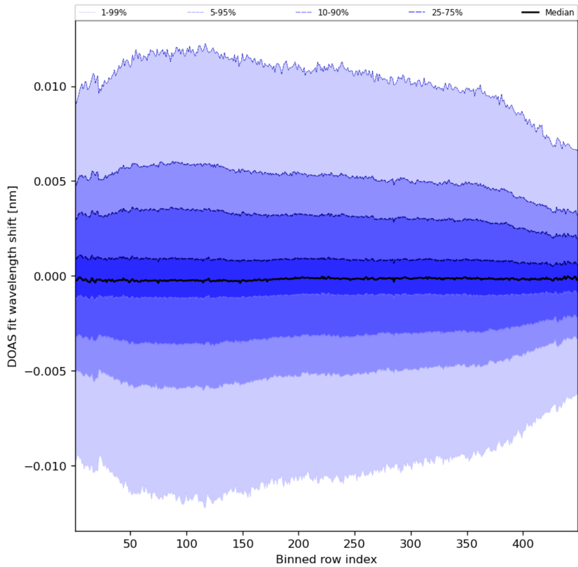
Figure 58: Along track statistics of “DOAS fit wavelength shift” for 2023-11-13 to 2023-11-15
