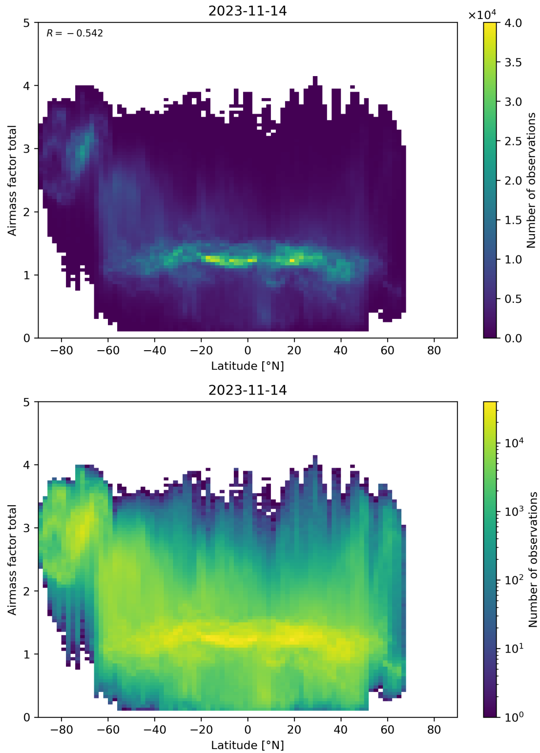
Figure 161: Scatter density plot of “Latitude” against “Airmass factor total” for 2023-11-13 to 2023-11-15.
