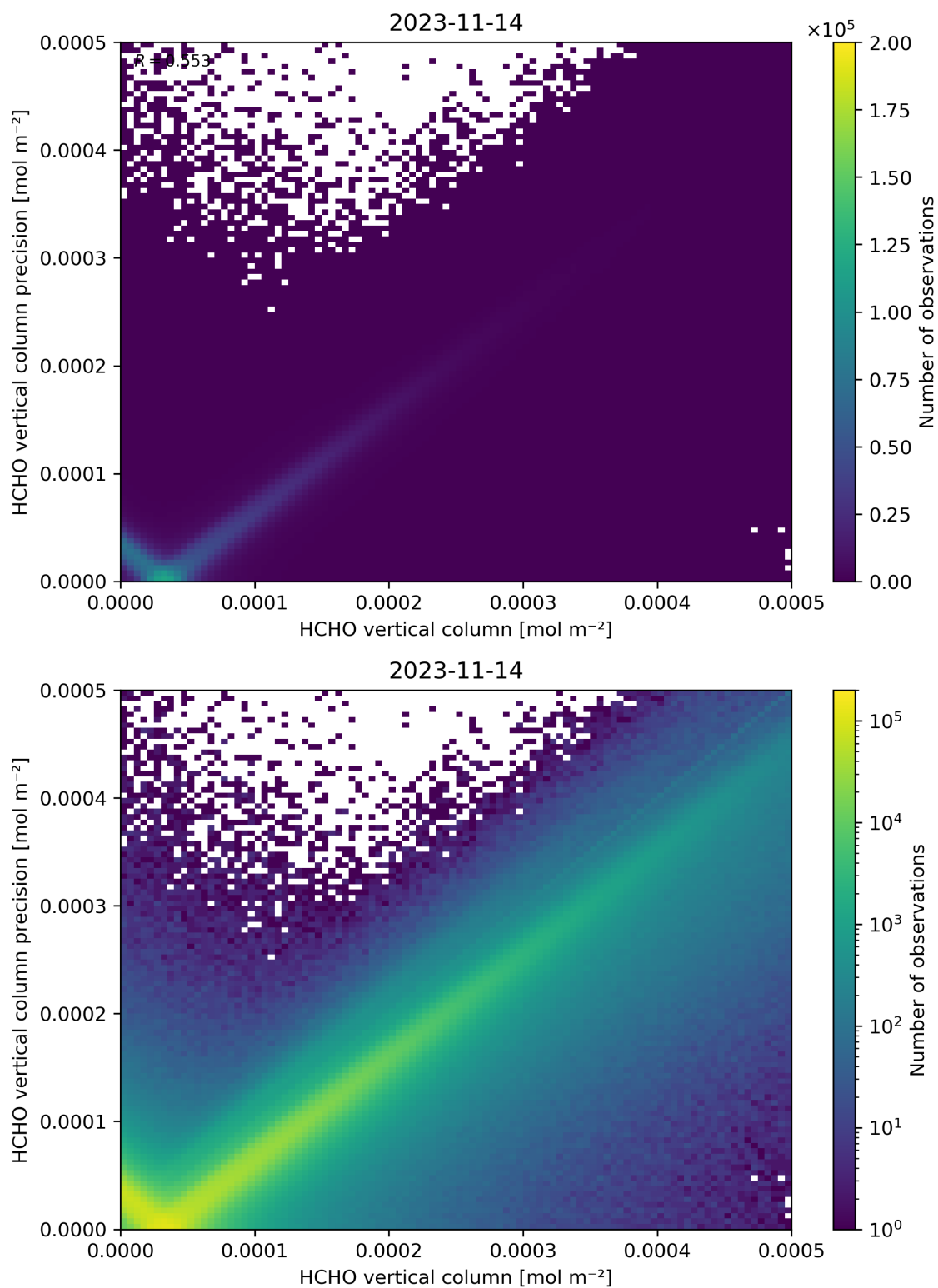
Figure 134: Scatter density plot of “HCHO vertical column” against “HCHO vertical column precision” for 2023-11-13 to 2023-11-15.
