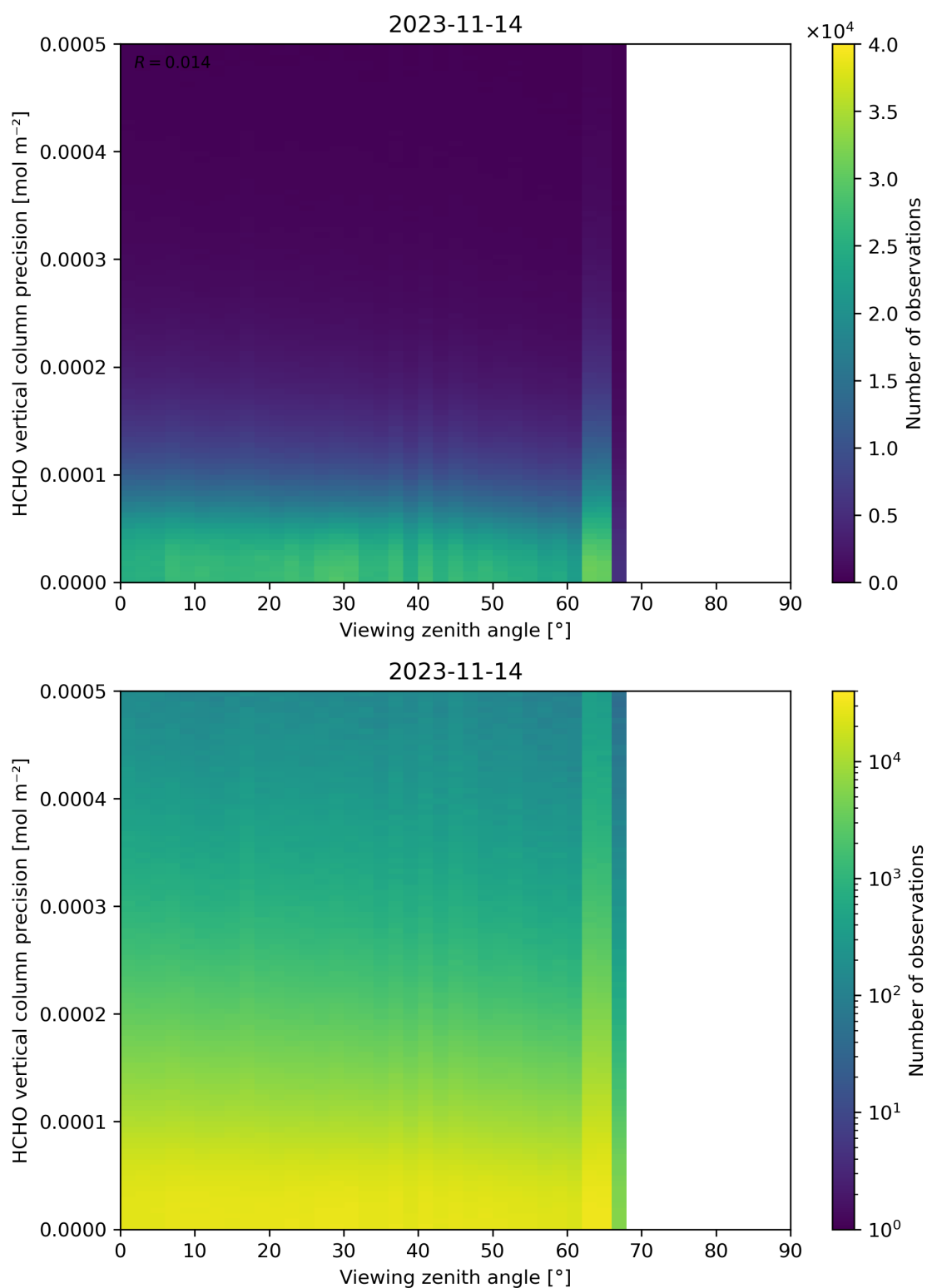
Figure 194: Scatter density plot of “Viewing zenith angle” against “HCHO vertical column precision” for 2023-11-13 to 2023-11-15.
