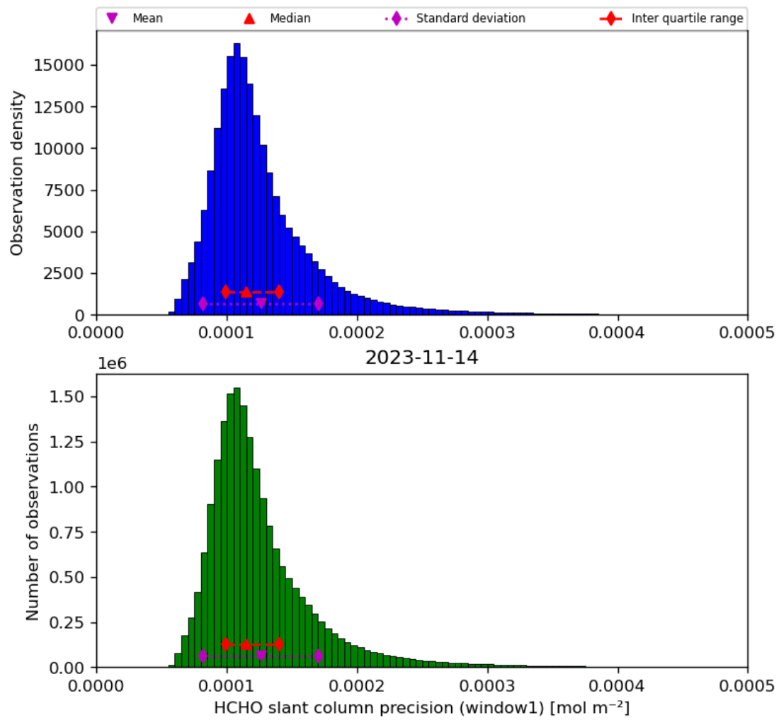
Figure 39: Histogram of “HCHO slant column precision (window1)” for 2023-11-13 to 2023-11-15
