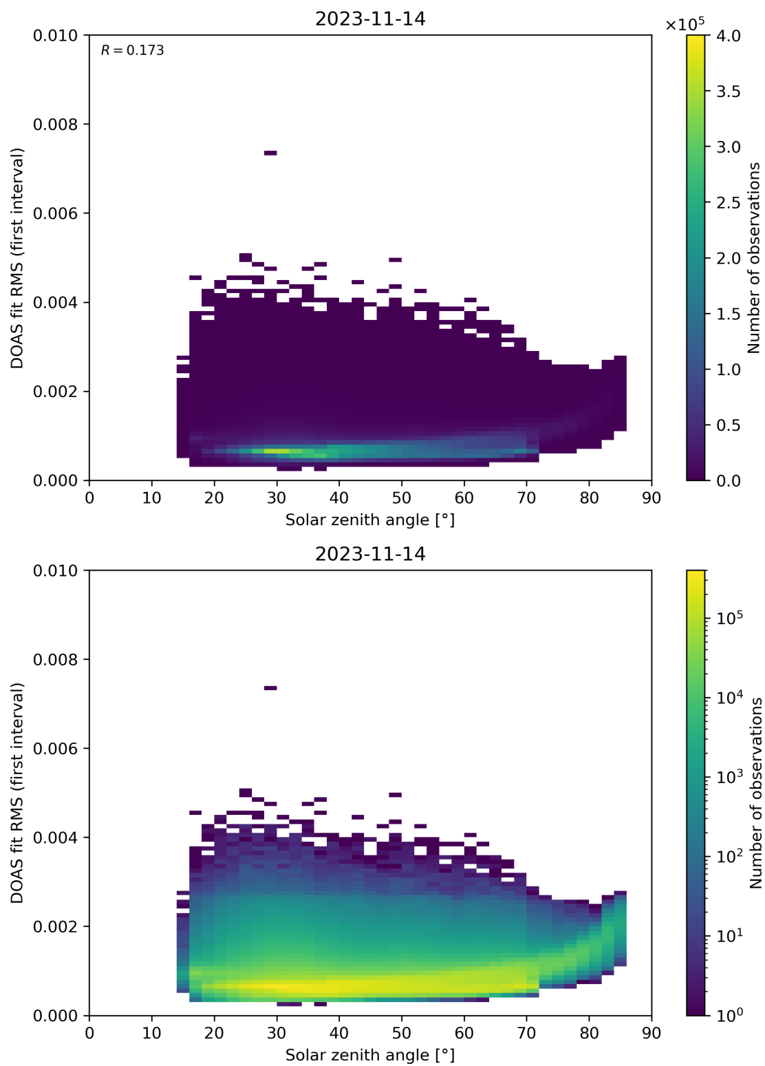
Figure 167: Scatter density plot of “Solar zenith angle” against “DOAS fit RMS (first interval)” for 2023-11-13 to 2023-11-15.
