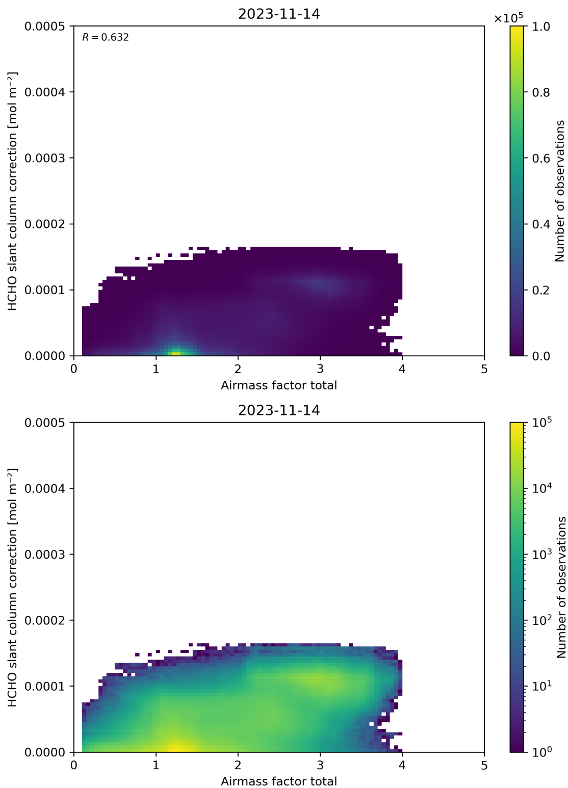
Figure 102: Scatter density plot of “Airmass factor total” against “HCHO slant column correction” for 2023-11-13 to 2023-11-15.
