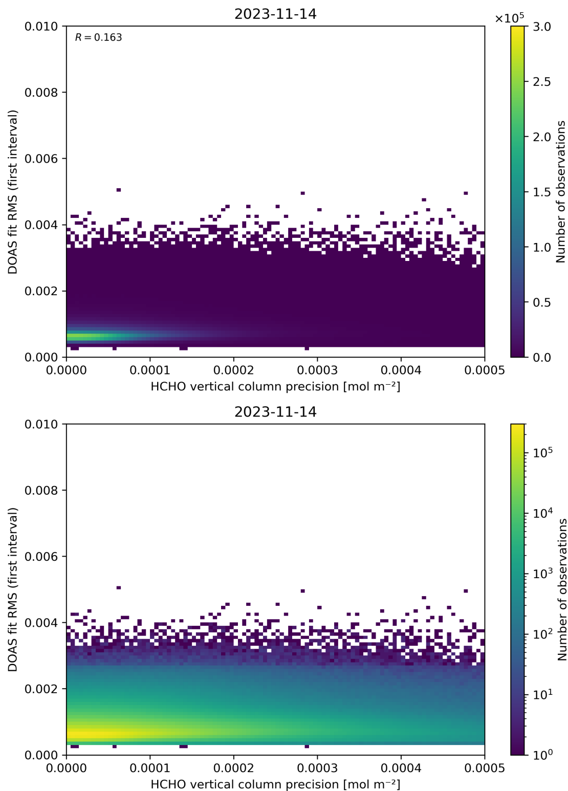
Figure 136: Scatter density plot of “HCHO vertical column precision” against “DOAS fit RMS (first interval)” for 2023-11-13 to 2023-11-15.
