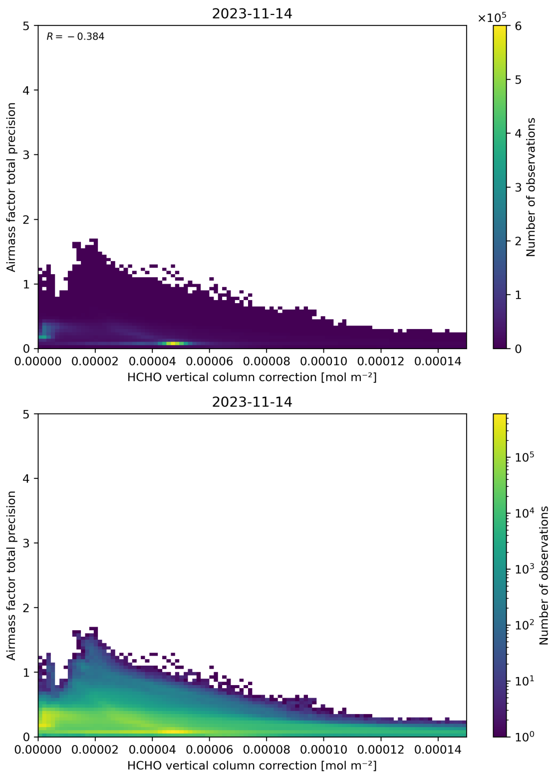
Figure 121: Scatter density plot of “HCHO vertical column correction” against “Airmass factor total precision” for 2023-11-13 to 2023-11-15.
