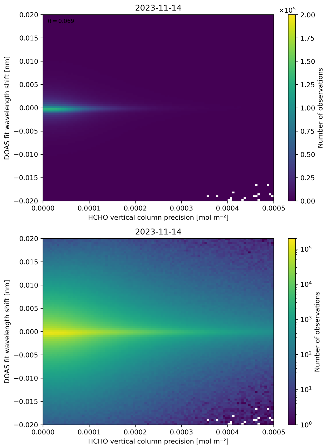
Figure 137: Scatter density plot of “HCHO vertical column precision” against “DOAS fit wavelength shift” for 2023-11-13 to 2023-11-15.
