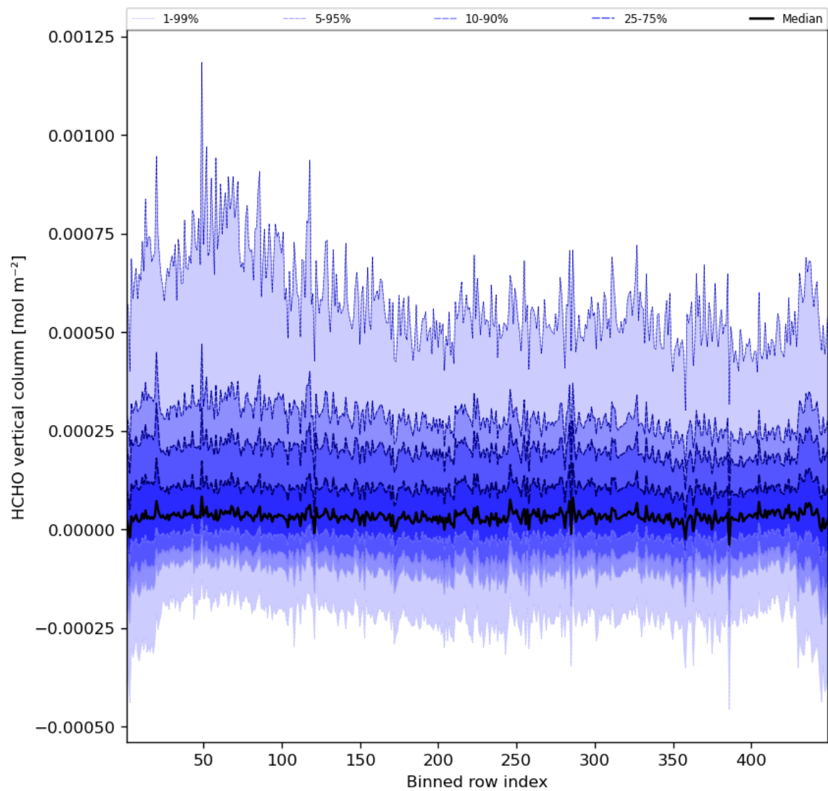
Figure 49: Along track statistics of “HCHO vertical column” for 2023-11-13 to 2023-11-15
