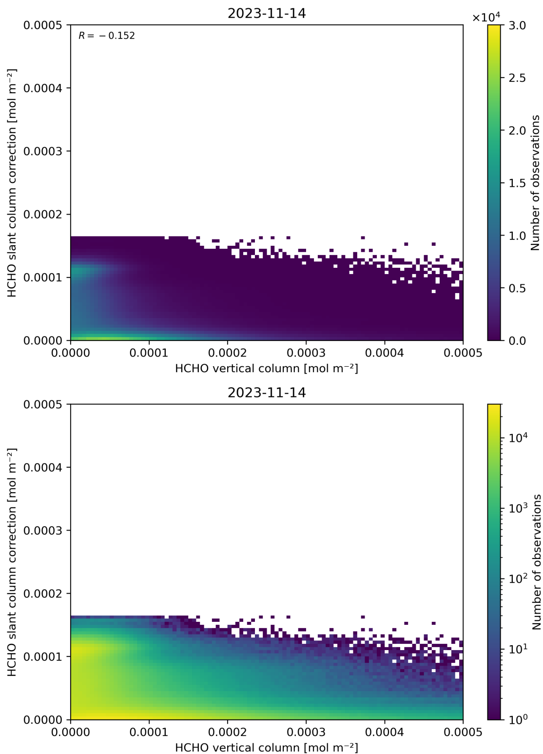
Figure 128: Scatter density plot of “HCHO vertical column” against “HCHO slant column correction” for 2023-11-13 to 2023-11-15.
