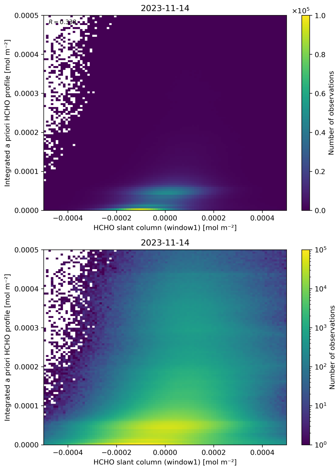
Figure 87: Scatter density plot of “HCHO slant column (window1)” against “Integrated a priori HCHO profile” for 2023-11-13 to 2023-11-15.
