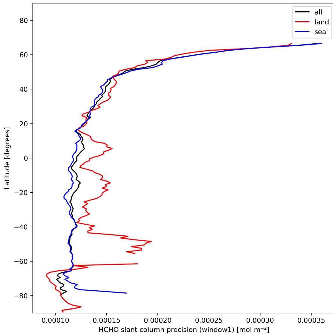
Figure 25: Zonal average of "HCHO slant column precision (window1)" for 2023-11-13 to 2023-11-15.
