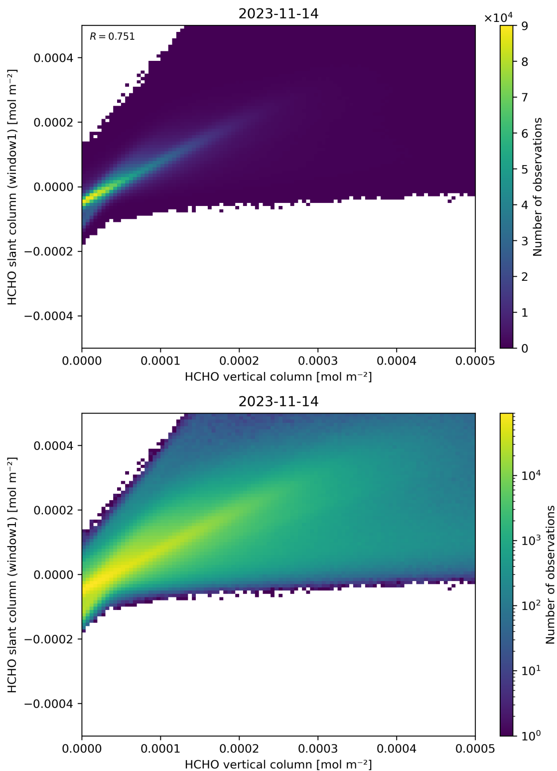
Figure 129: Scatter density plot of “HCHO vertical column” against “HCHO slant column (window1)” for 2023-11-13 to 2023-11-15.
