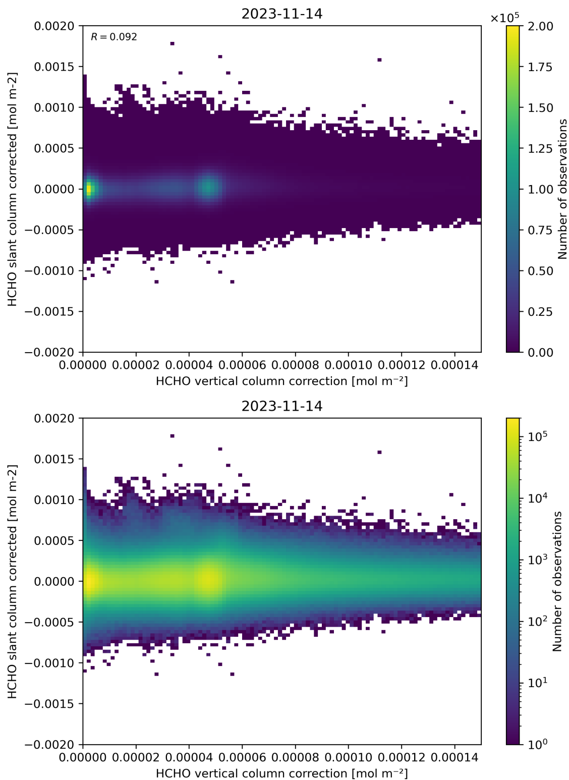
Figure 116: Scatter density plot of “HCHO vertical column correction” against “HCHO slant column corrected” for 2023-11-13 to 2023-11-15.
