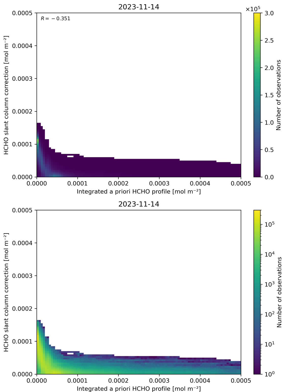
Figure 152: Scatter density plot of “Integrated a priori HCHO profile” against “HCHO slant column correction” for 2023-11-13 to 2023-11-15.
