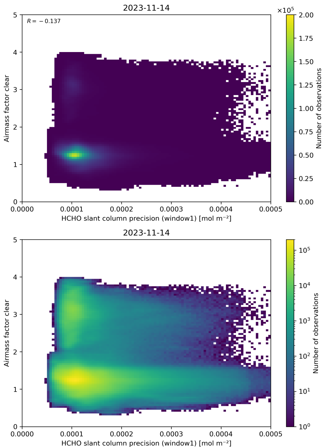
Figure 91: Scatter density plot of “HCHO slant column precision (window1)” against “Airmass factor clear” for 2023-11-13 to 2023-11-15.
