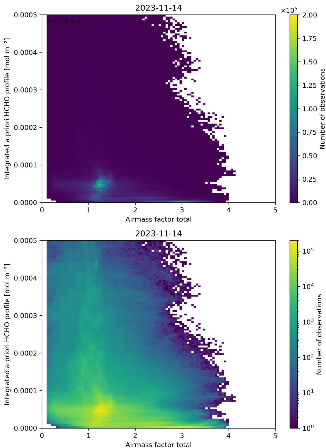
Figure 104: Scatter density plot of “Airmass factor total” against “Integrated a priori HCHO profile” for 2023-11-13 to 2023-11-15.
