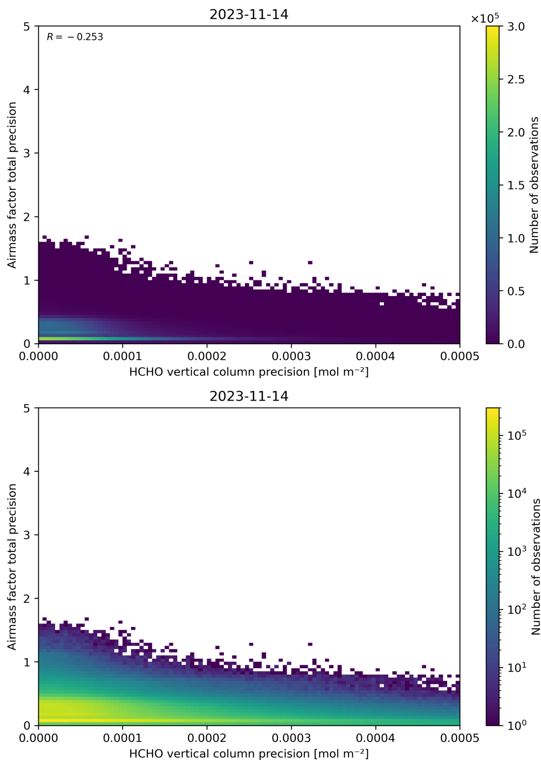
Figure 145: Scatter density plot of “HCHO vertical column precision” against “Airmass factor total precision” for 2023-11-13 to 2023-11-15.
