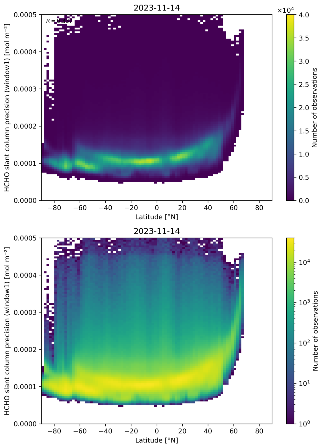
Figure 160: Scatter density plot of “Latitude” against “HCHO slant column precision (window1)” for 2023-11-13 to 2023-11-15.
