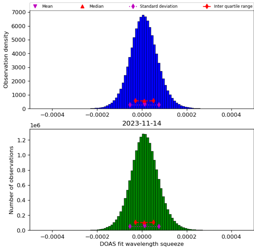
Figure 45: Histogram of “DOAS fit wavelength squeeze” for 2023-11-13 to 2023-11-15
