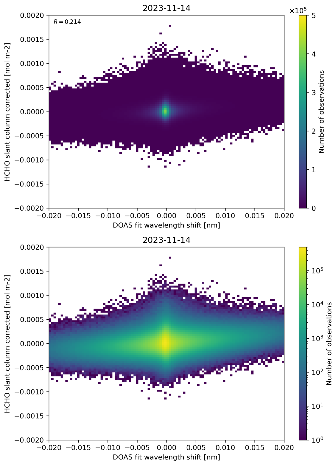
Figure 66: Scatter density plot of “DOAS fit wavelength shift” against “HCHO slant column corrected” for 2023-11-13 to 2023-11-15.
