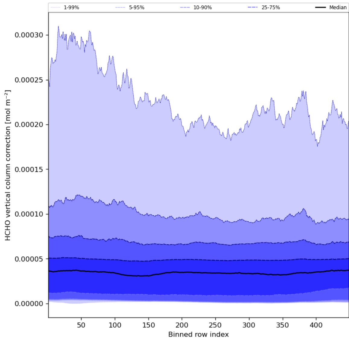
Figure 51: Along track statistics of “HCHO vertical column correction” for 2023-11-13 to 2023-11-15
