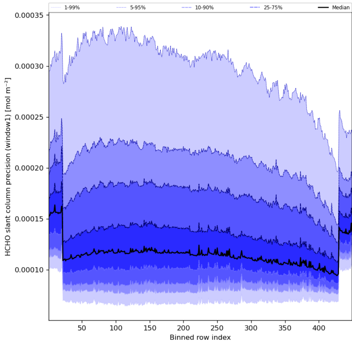
Figure 53: Along track statistics of “HCHO slant column precision (window1)” for 2023-11-13 to 2023-11-15
