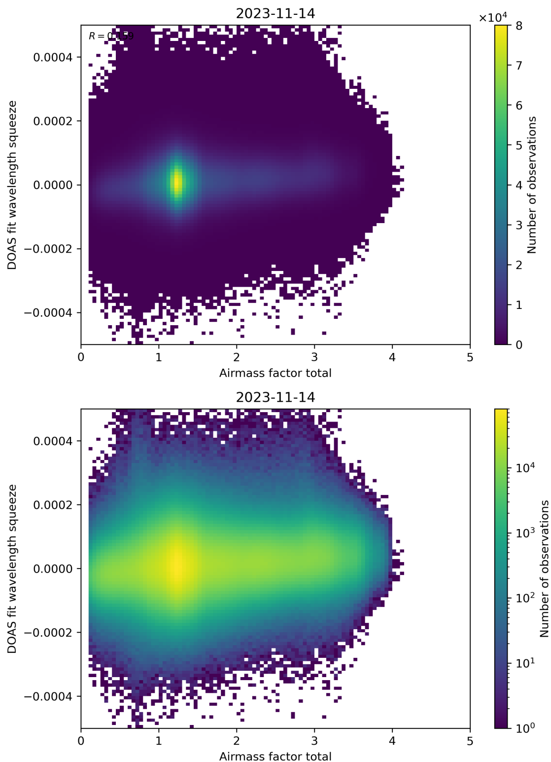
Figure 99: Scatter density plot of “Airmass factor total” against “DOAS fit wavelength squeeze” for 2023-11-13 to 2023-11-15.
