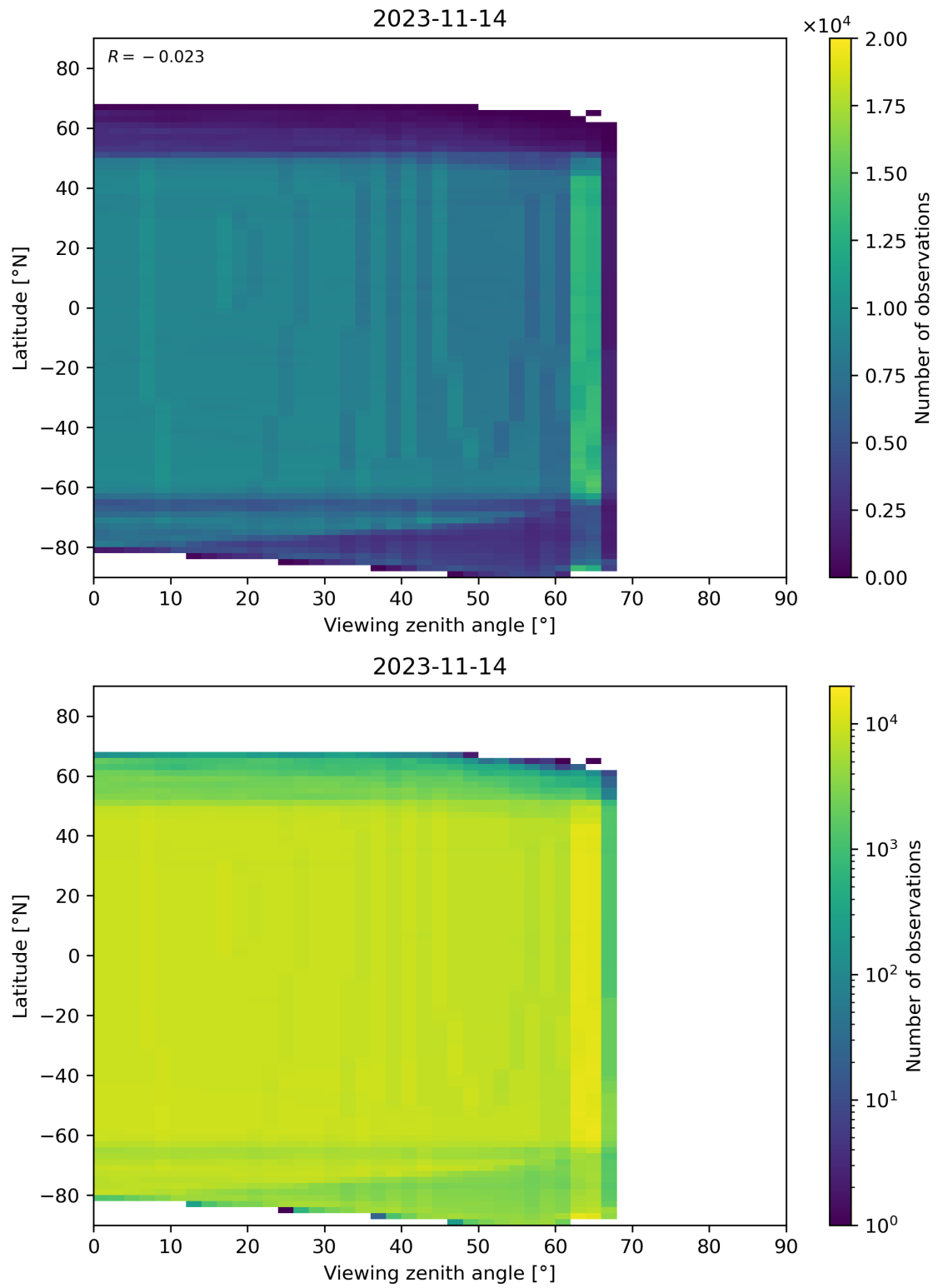
Figure 196: Scatter density plot of “Viewing zenith angle” against “Latitude” for 2023-11-13 to 2023-11-15.
