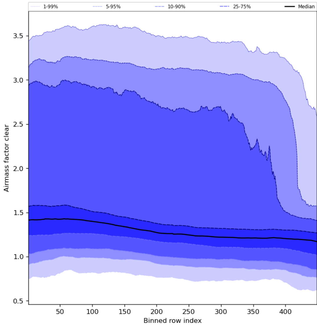
Figure 56: Along track statistics of “Airmass factor clear” for 2023-11-13 to 2023-11-15
