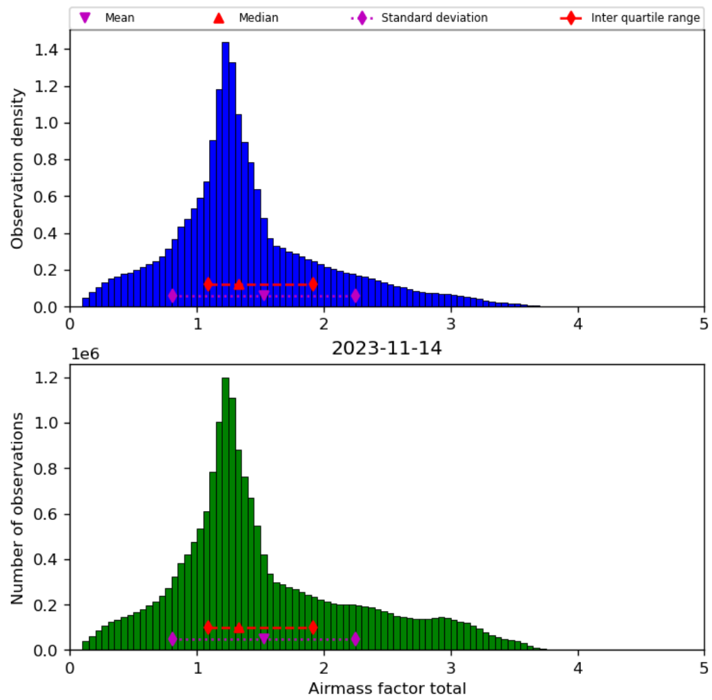
Figure 40: Histogram of “Airmass factor total” for 2023-11-13 to 2023-11-15
