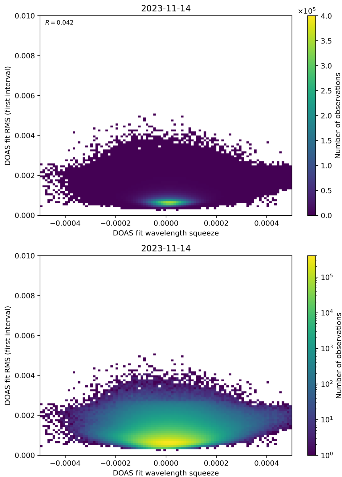
Figure 68: Scatter density plot of “DOAS fit wavelength squeeze” against “DOAS fit RMS (first interval)” for 2023-11-13 to 2023-11-15.
