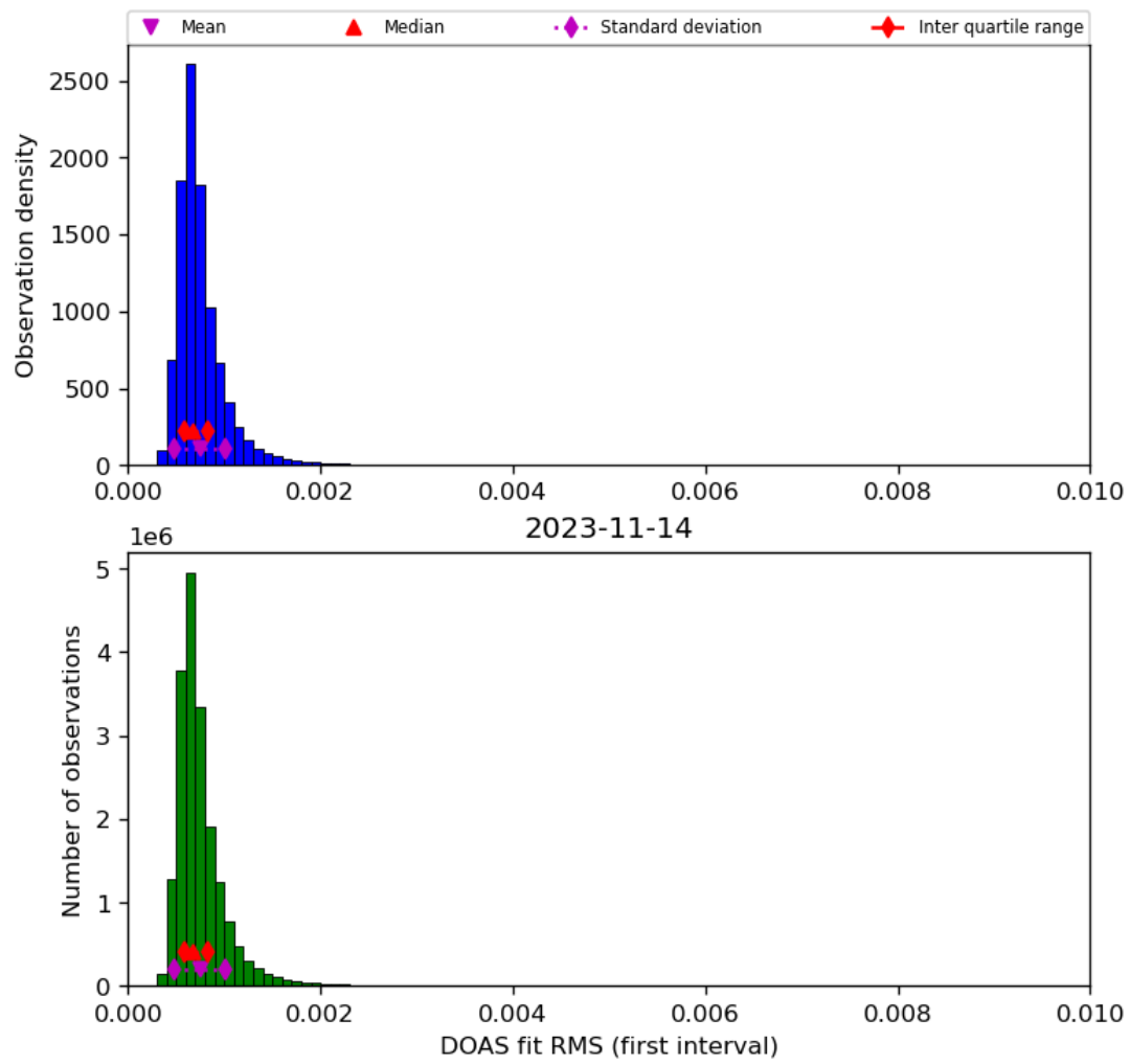
Figure 46: Histogram of “DOAS fit RMS (first interval)” for 2023-11-13 to 2023-11-15
