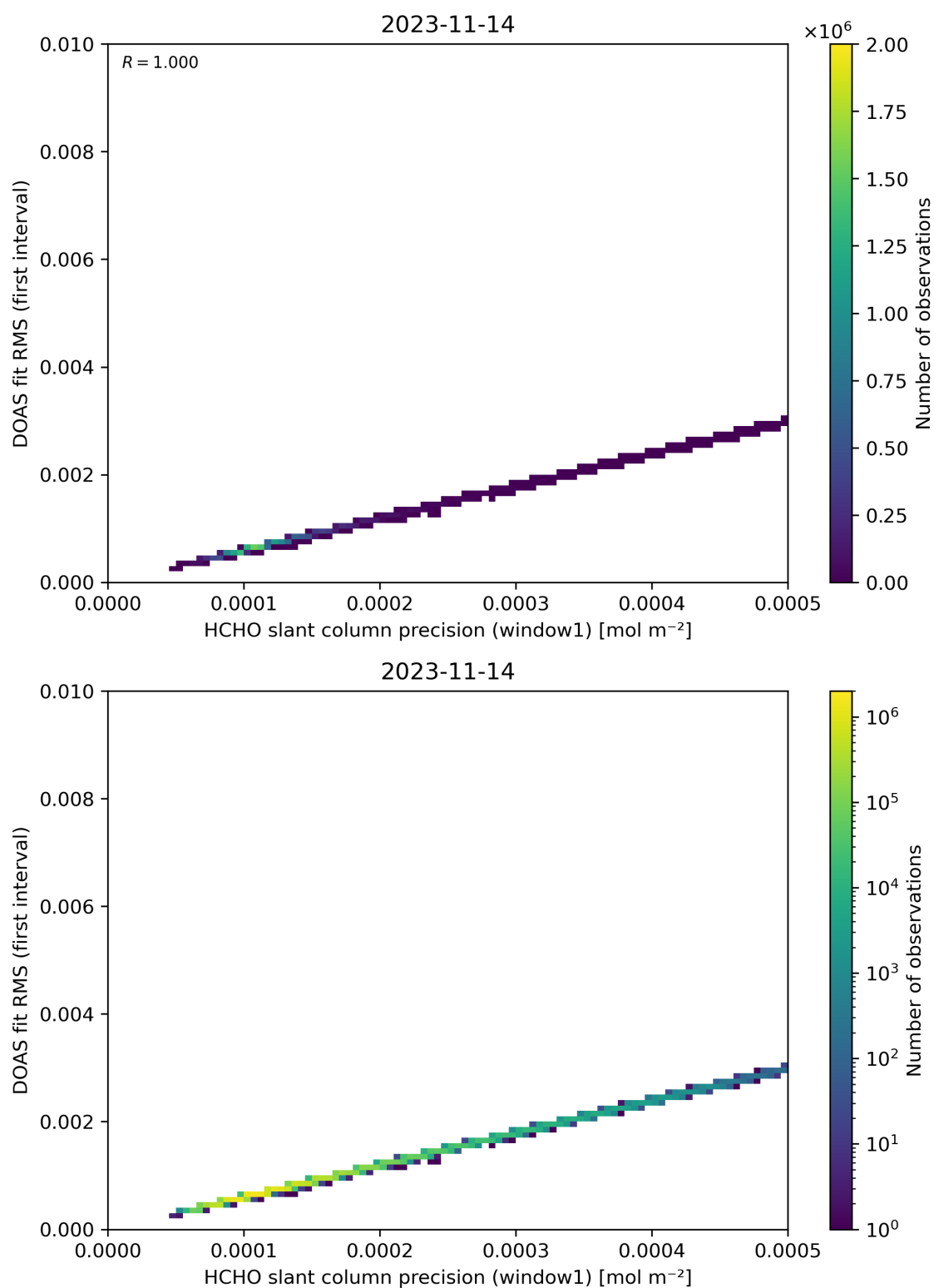
Figure 88: Scatter density plot of “HCHO slant column precision (window1)” against “DOAS fit RMS (first interval)” for 2023-11-13 to 2023-11-15.
