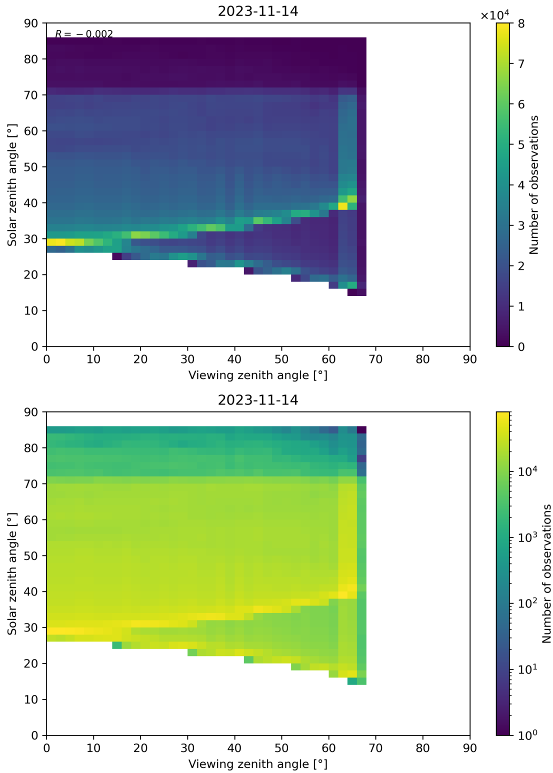
Figure 197: Scatter density plot of “Viewing zenith angle” against “Solar zenith angle” for 2023-11-13 to 2023-11-15.
