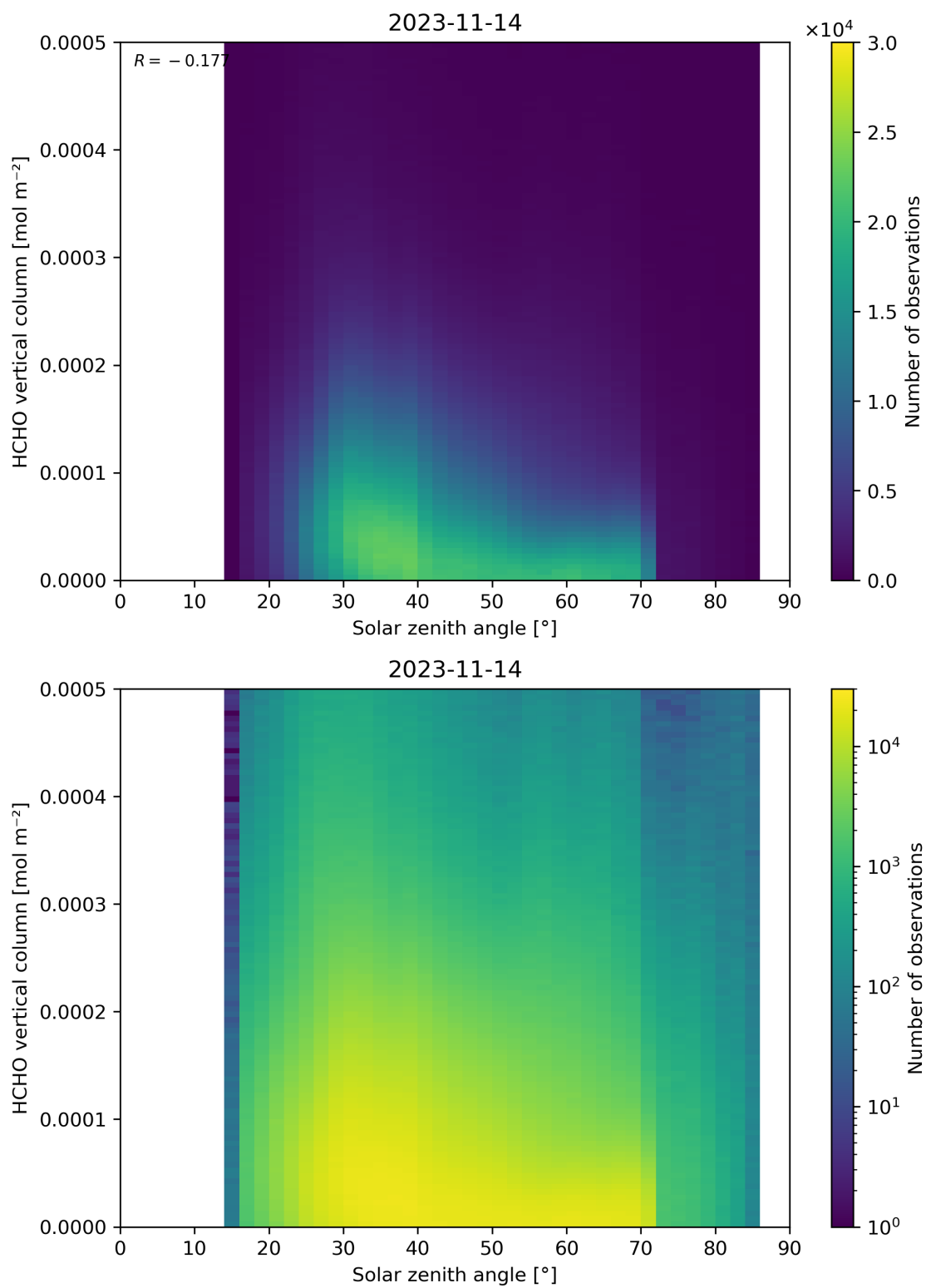
Figure 177: Scatter density plot of “Solar zenith angle” against “HCHO vertical column” for 2023-11-13 to 2023-11-15.
