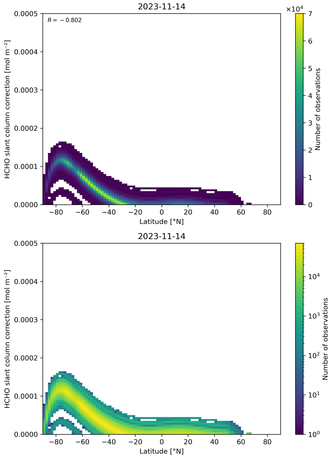
Figure 158: Scatter density plot of “Latitude” against “HCHO slant column correction” for 2023-11-13 to 2023-11-15.
