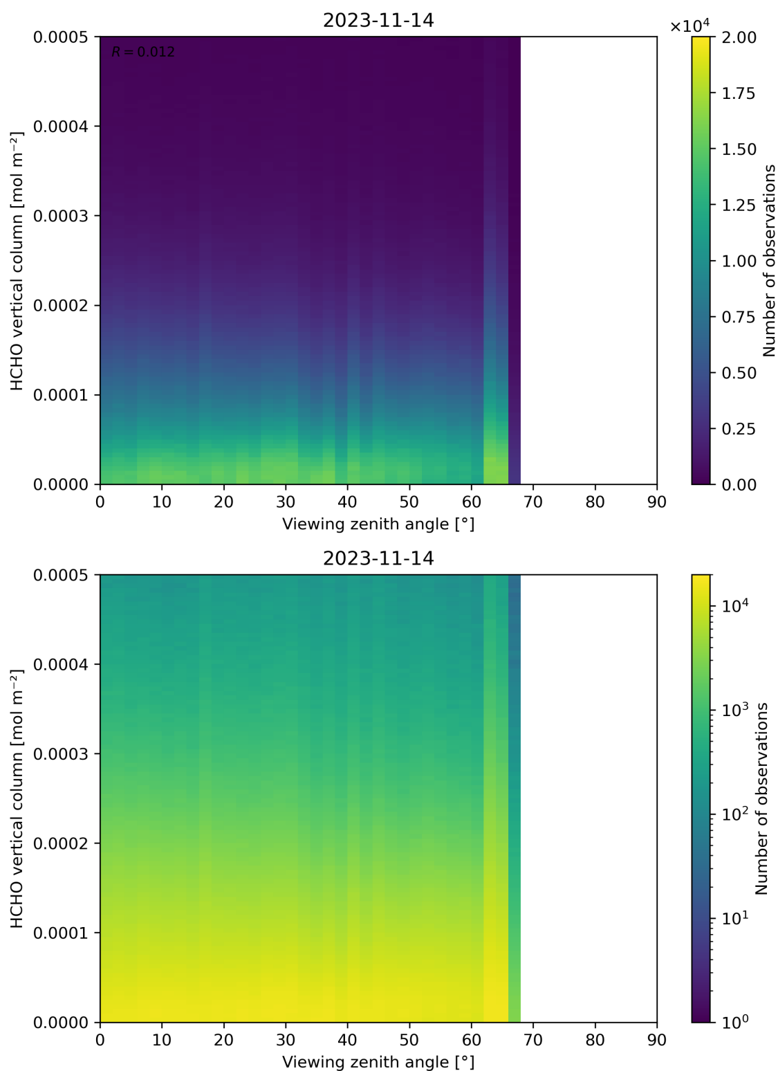
Figure 192: Scatter density plot of “Viewing zenith angle” against “HCHO vertical column” for 2023-11-13 to 2023-11-15.
