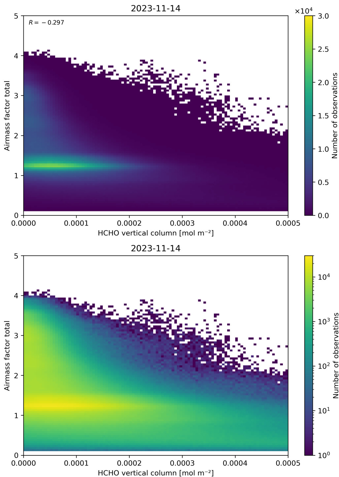
Figure 131: Scatter density plot of “HCHO vertical column” against “Airmass factor total” for 2023-11-13 to 2023-11-15.
