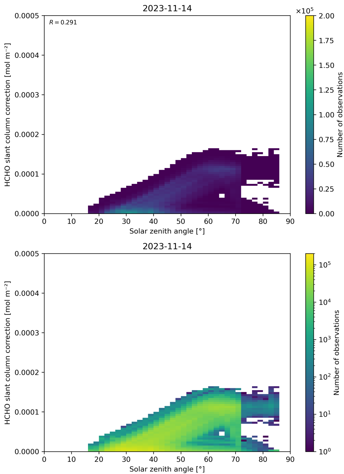
Figure 172: Scatter density plot of “Solar zenith angle” against “HCHO slant column correction” for 2023-11-13 to 2023-11-15.
