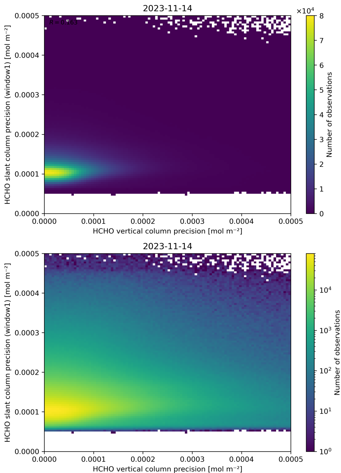
Figure 143: Scatter density plot of “HCHO vertical column precision” against “HCHO slant column precision (window1)” for 2023-11-13 to 2023-11-15.
