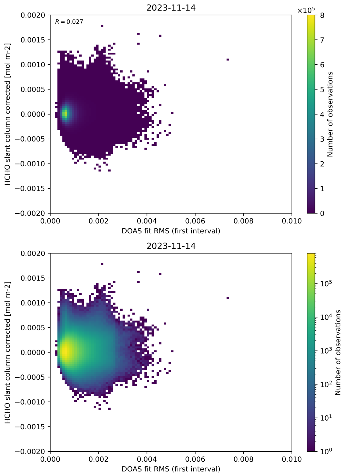
Figure 62: Scatter density plot of “DOAS fit RMS (first interval)” against “HCHO slant column corrected” for 2023-11-13 to 2023-11-15.
