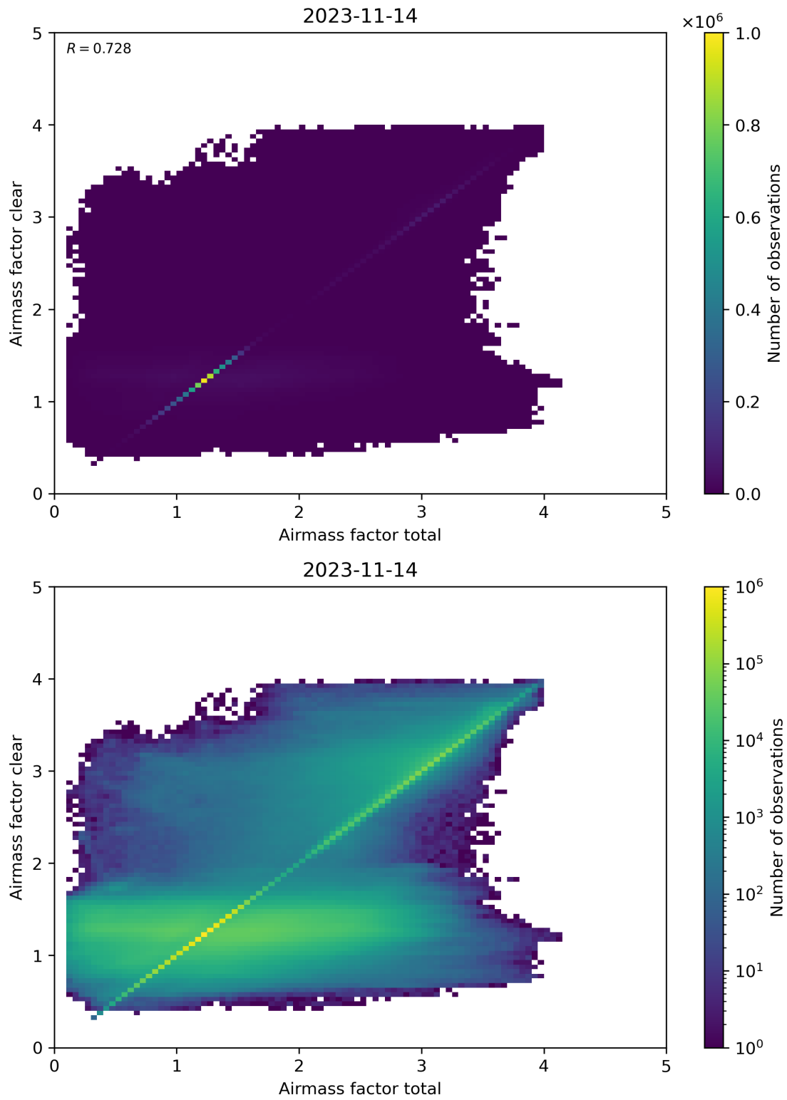
Figure 100: Scatter density plot of “Airmass factor total” against “Airmass factor clear” for 2023-11-13 to 2023-11-15.
