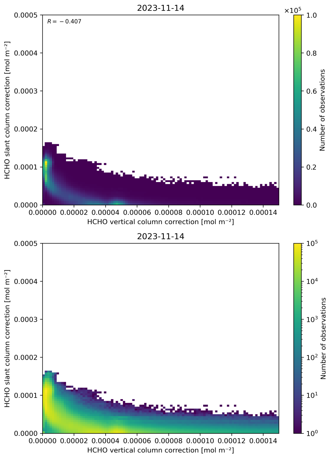
Figure 117: Scatter density plot of “HCHO vertical column correction” against “HCHO slant column correction” for 2023-11-13 to 2023-11-15.
