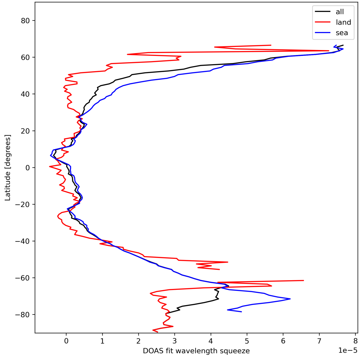
Figure 31: Zonal average of “DOAS fit wavelength squeeze” for 2023-11-13 to 2023-11-15.
