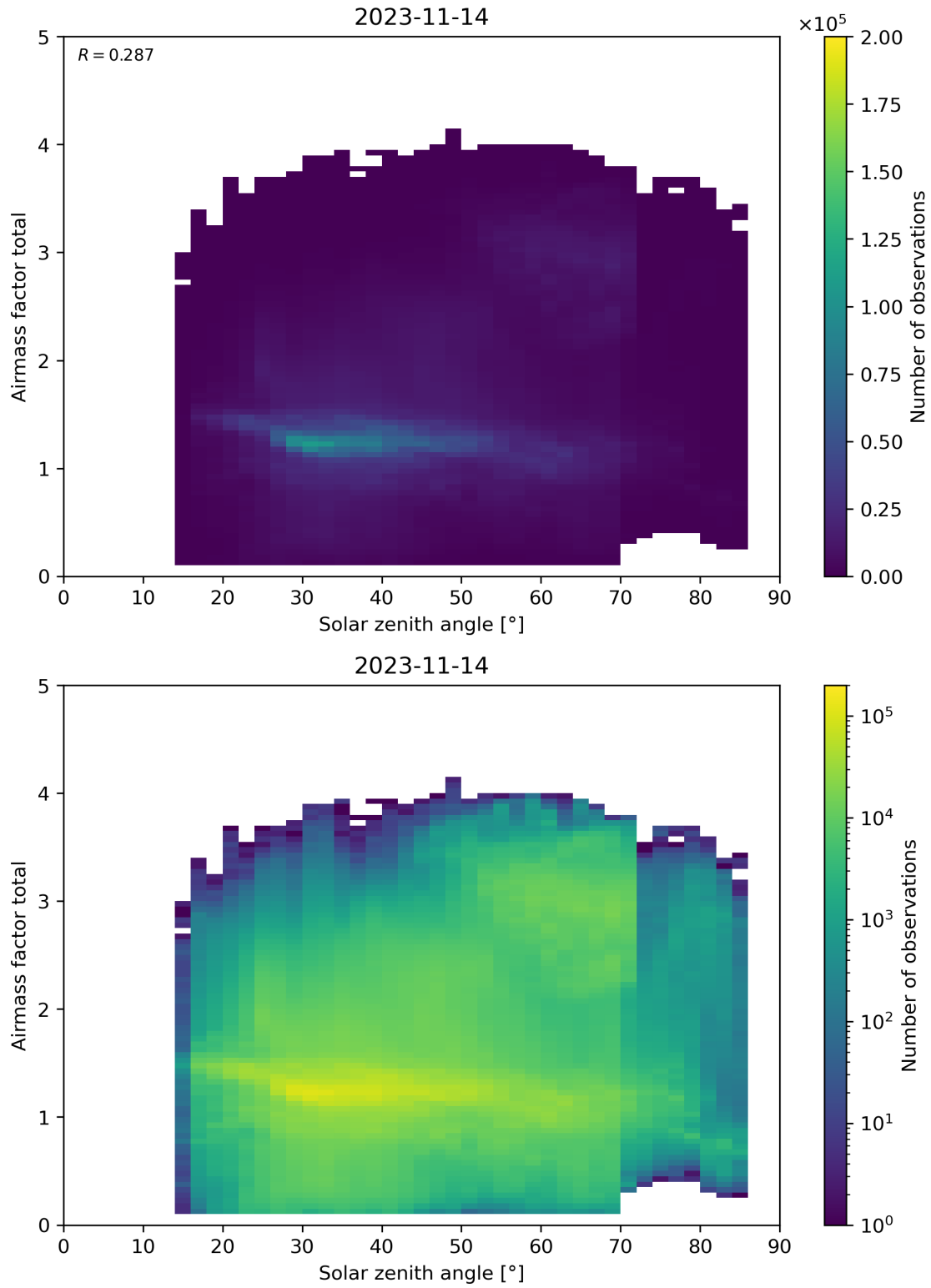
Figure 175: Scatter density plot of “Solar zenith angle” against “Airmass factor total” for 2023-11-13 to 2023-11-15.
