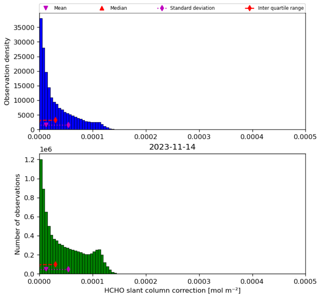
Figure 47: Histogram of “HCHO slant column correction” for 2023-11-13 to 2023-11-15
