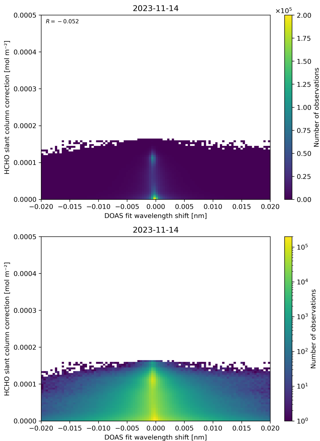
Figure 67: Scatter density plot of “DOAS fit wavelength shift” against “HCHO slant column correction” for 2023-11-13 to 2023-11-15.
