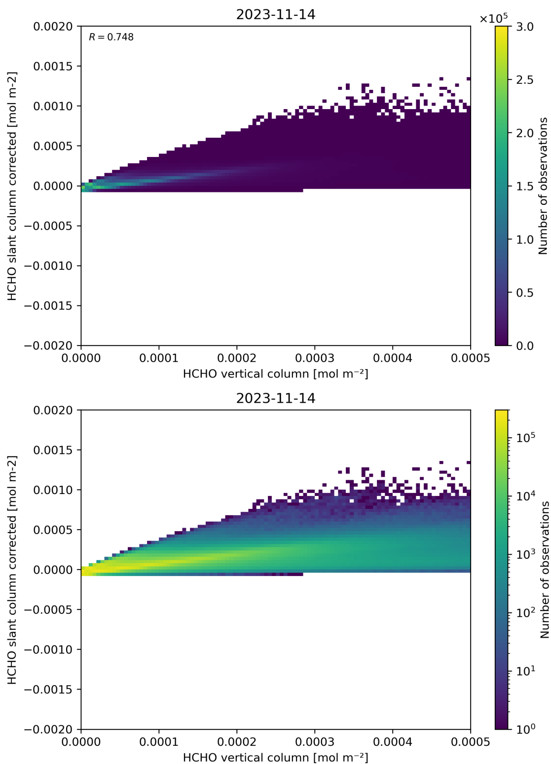
Figure 127: Scatter density plot of “HCHO vertical column” against “HCHO slant column corrected” for 2023-11-13 to 2023-11-15.
