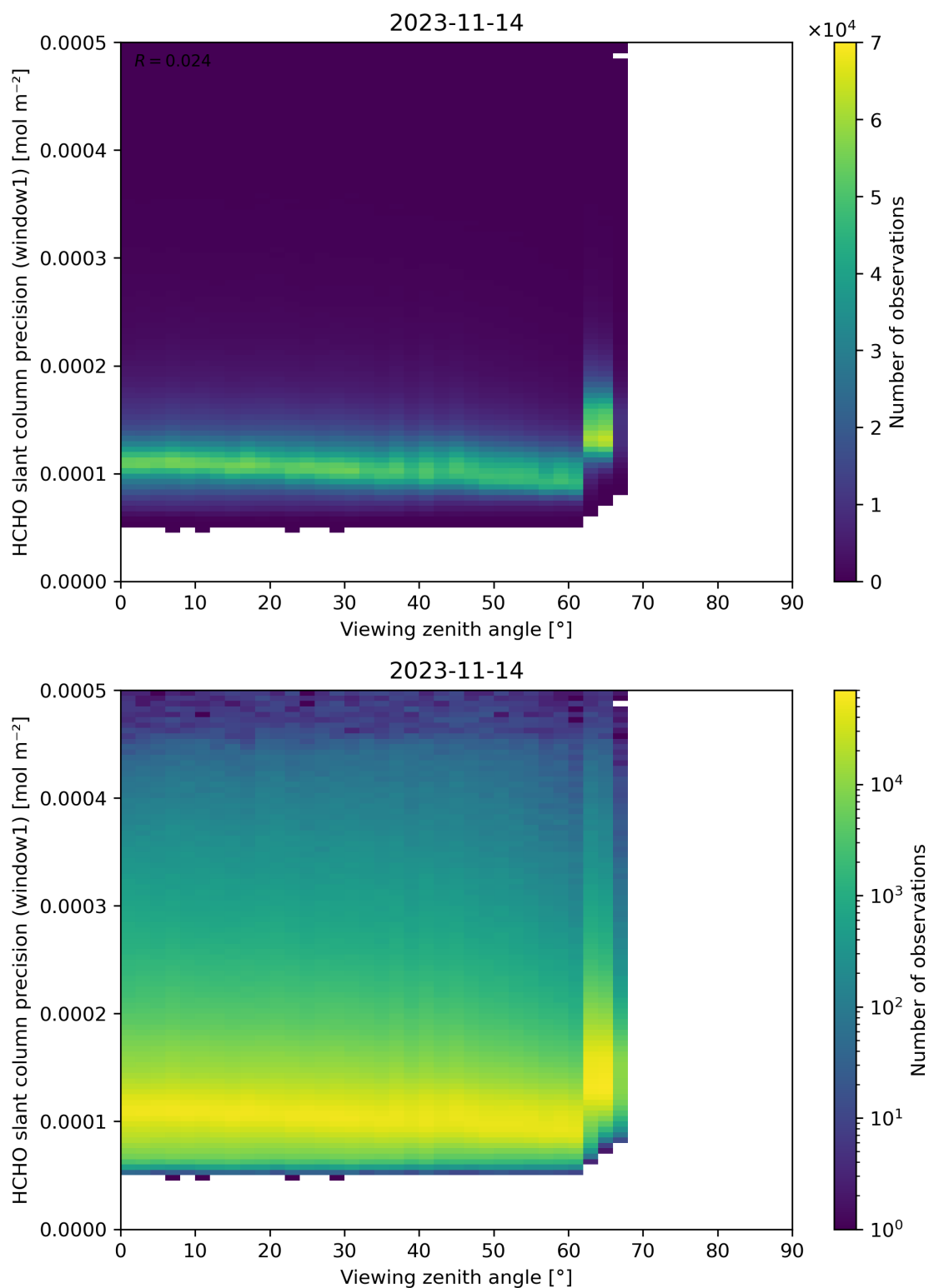
Figure 189: Scatter density plot of “Viewing zenith angle” against “HCHO slant column precision (window1)” for 2023-11-13 to 2023-11-15.
