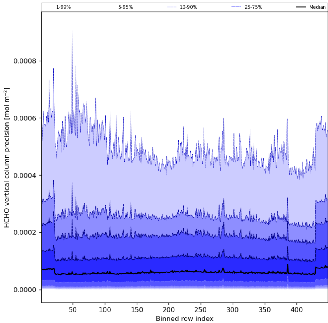
Figure 50: Along track statistics of “HCHO vertical column precision” for 2023-11-13 to 2023-11-15
