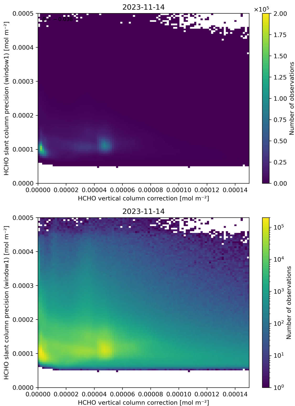
Figure 119: Scatter density plot of “HCHO vertical column correction” against “HCHO slant column precision (window1)” for 2023-11-13 to 2023-11-15.
