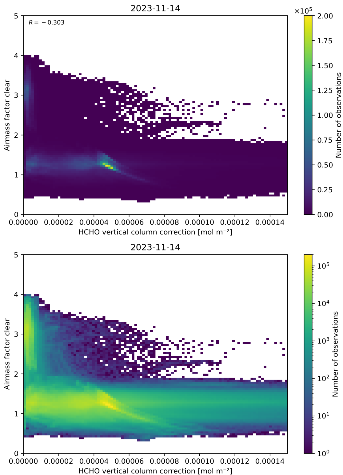
Figure 115: Scatter density plot of “HCHO vertical column correction” against “Airmass factor clear” for 2023-11-13 to 2023-11-15.
