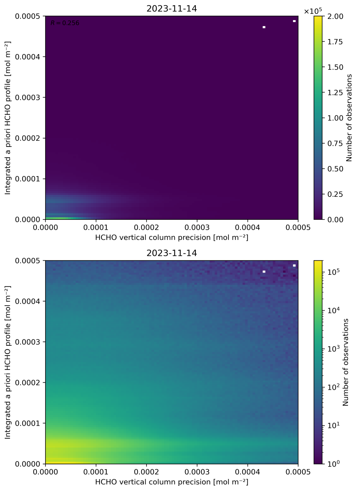
Figure 147: Scatter density plot of “HCHO vertical column precision” against “Integrated a priori HCHO profile” for 2023-11-13 to 2023-11-15.
