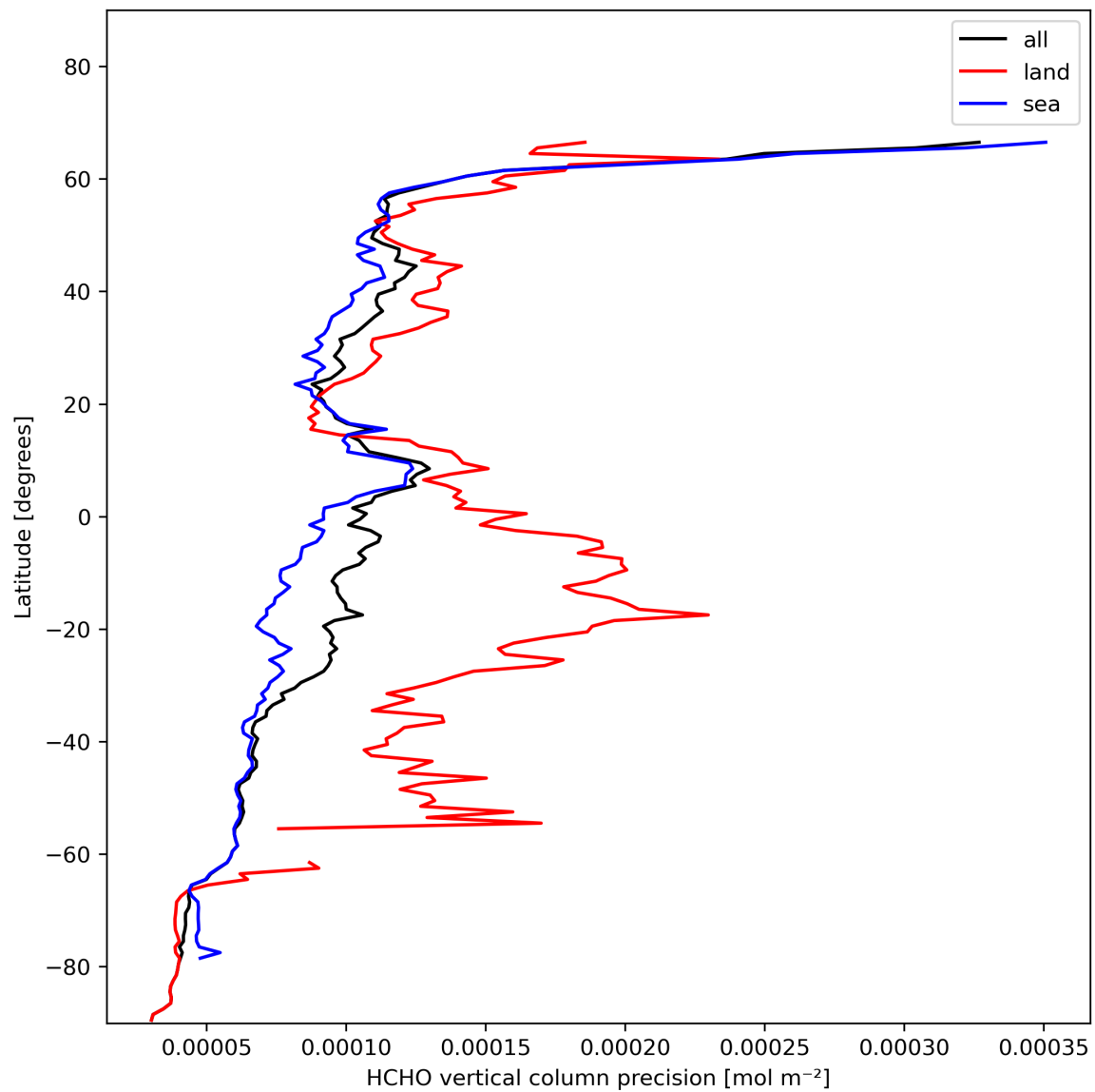
Figure 22: Zonal average of “HCHO vertical column precision” for 2023-11-13 to 2023-11-15.
