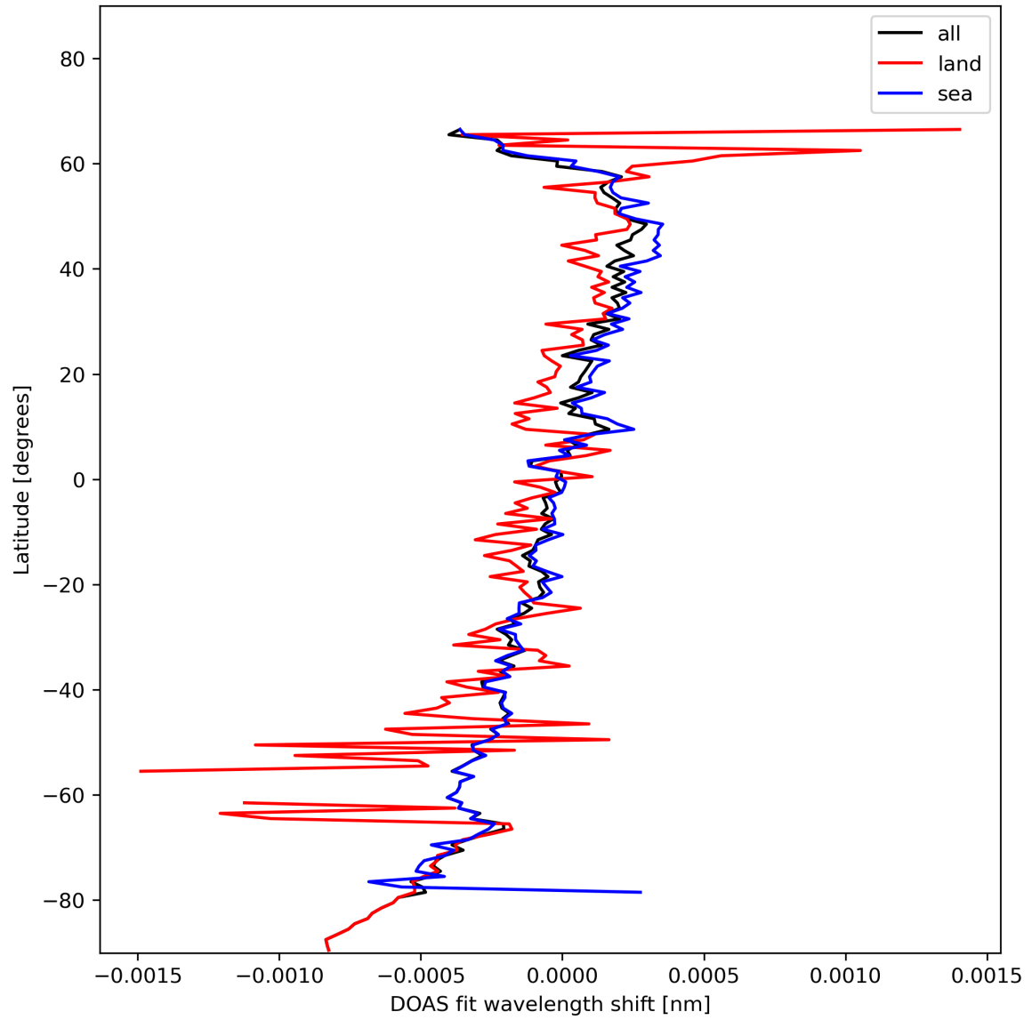
Figure 30: Zonal average of “DOAS fit wavelength shift” for 2023-11-13 to 2023-11-15.
