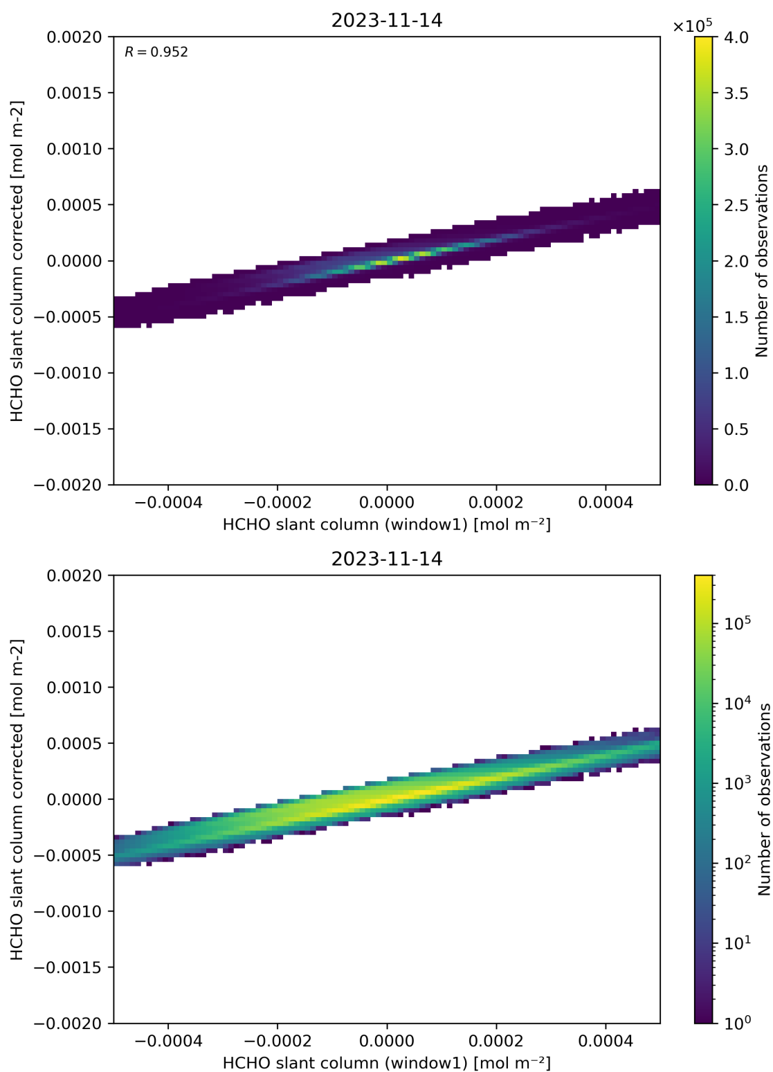
Figure 82: Scatter density plot of “HCHO slant column (window1)” against “HCHO slant column corrected” for 2023-11-13 to 2023-11-15.
