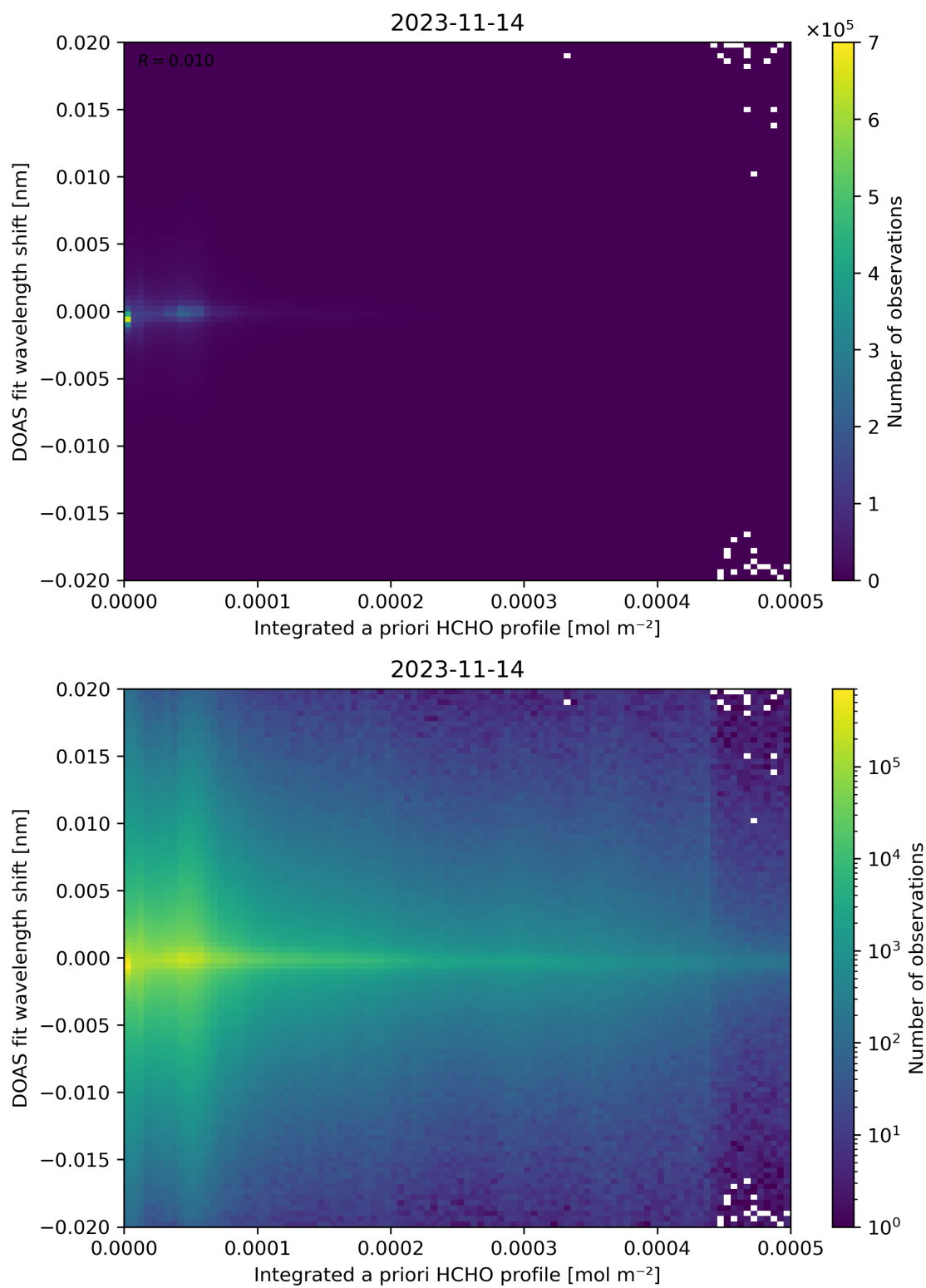
Figure 149: Scatter density plot of “Integrated a priori HCHO profile” against “DOAS fit wavelength shift” for 2023-11-13 to 2023-11-15.
