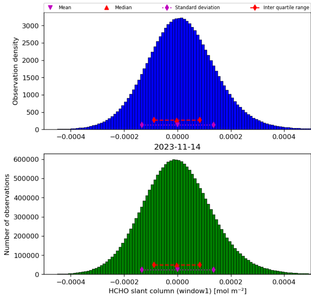
Figure 38: Histogram of “HCHO slant column (window1)” for 2023-11-13 to 2023-11-15
