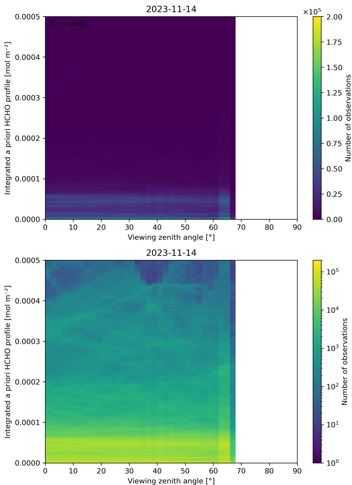
Figure 195: Scatter density plot of “Viewing zenith angle” against “Integrated a priori HCHO profile” for 2023-11-13 to 2023-11-15.
