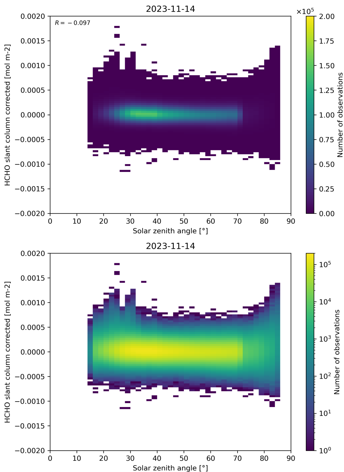
Figure 171: Scatter density plot of “Solar zenith angle” against “HCHO slant column corrected” for 2023-11-13 to 2023-11-15.
