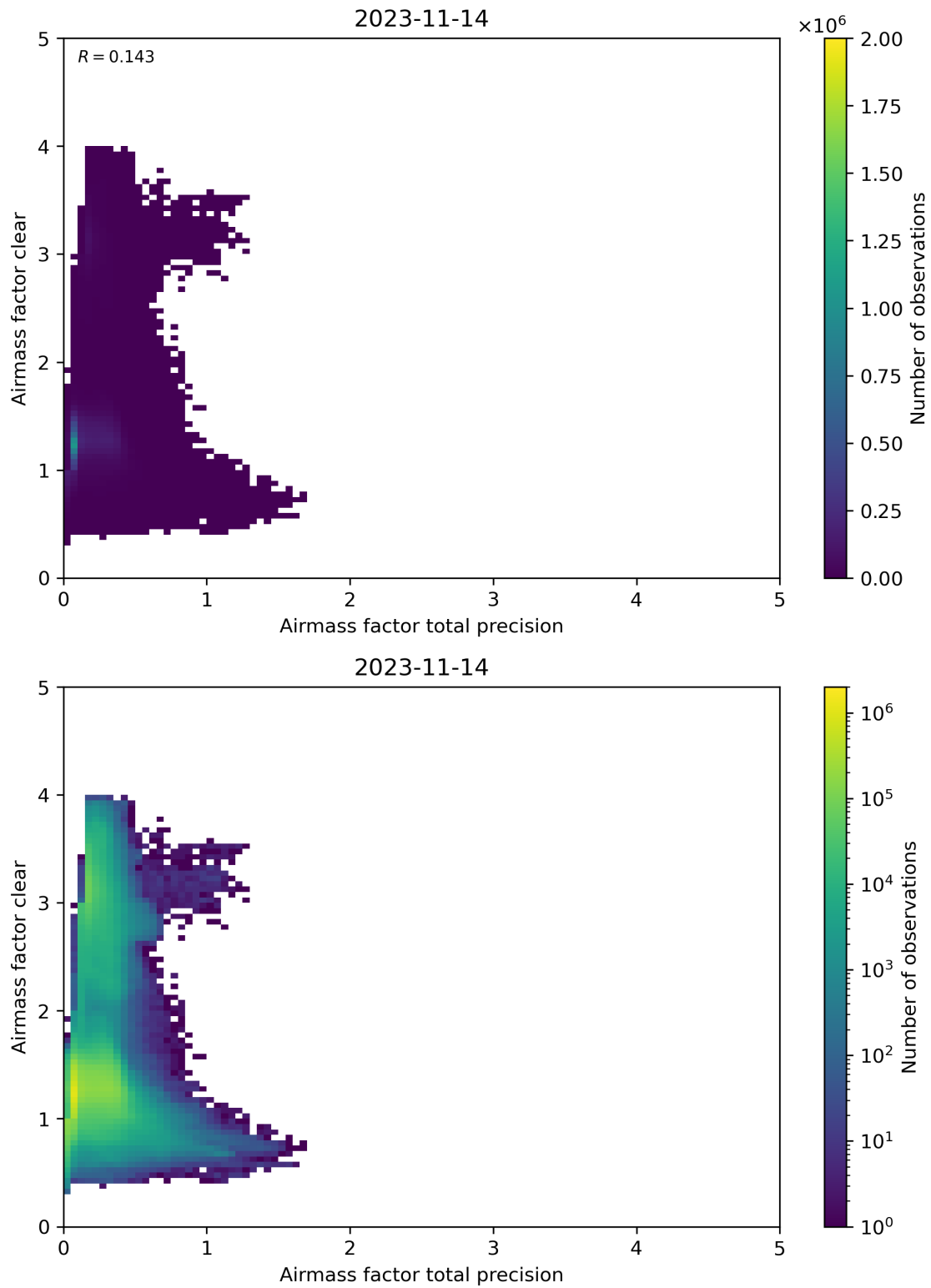
Figure 108: Scatter density plot of “Airmass factor total precision” against “Airmass factor clear” for 2023-11-13 to 2023-11-15.
