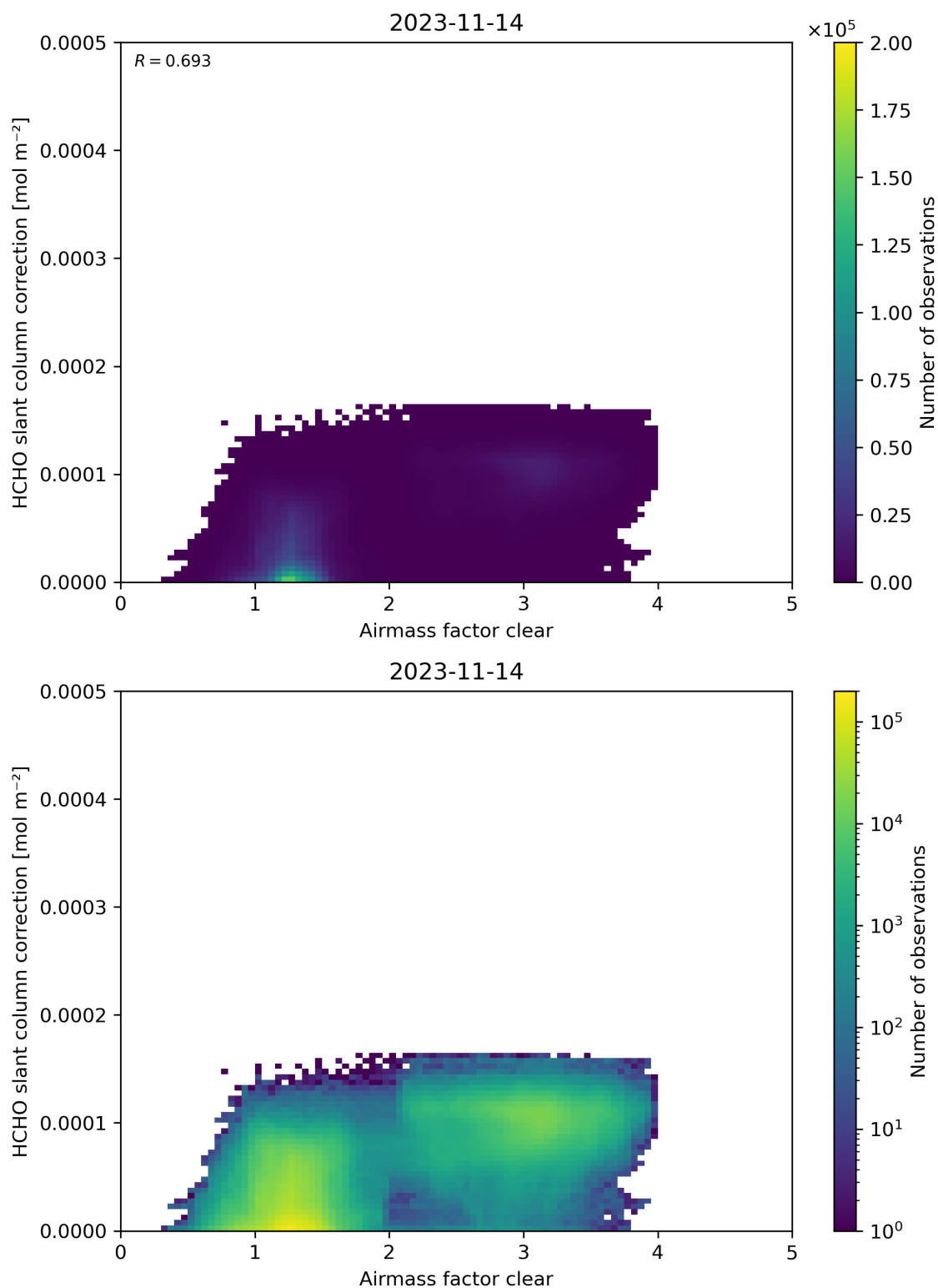
Figure 75: Scatter density plot of “Airmass factor clear” against “HCHO slant column correction” for 2023-11-13 to 2023-11-15.
