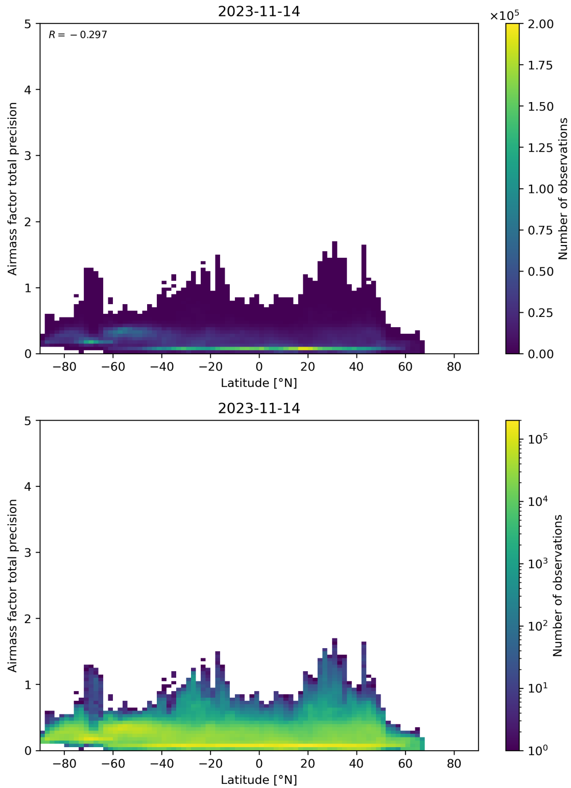
Figure 162: Scatter density plot of “Latitude” against “Airmass factor total precision” for 2023-11-13 to 2023-11-15.
