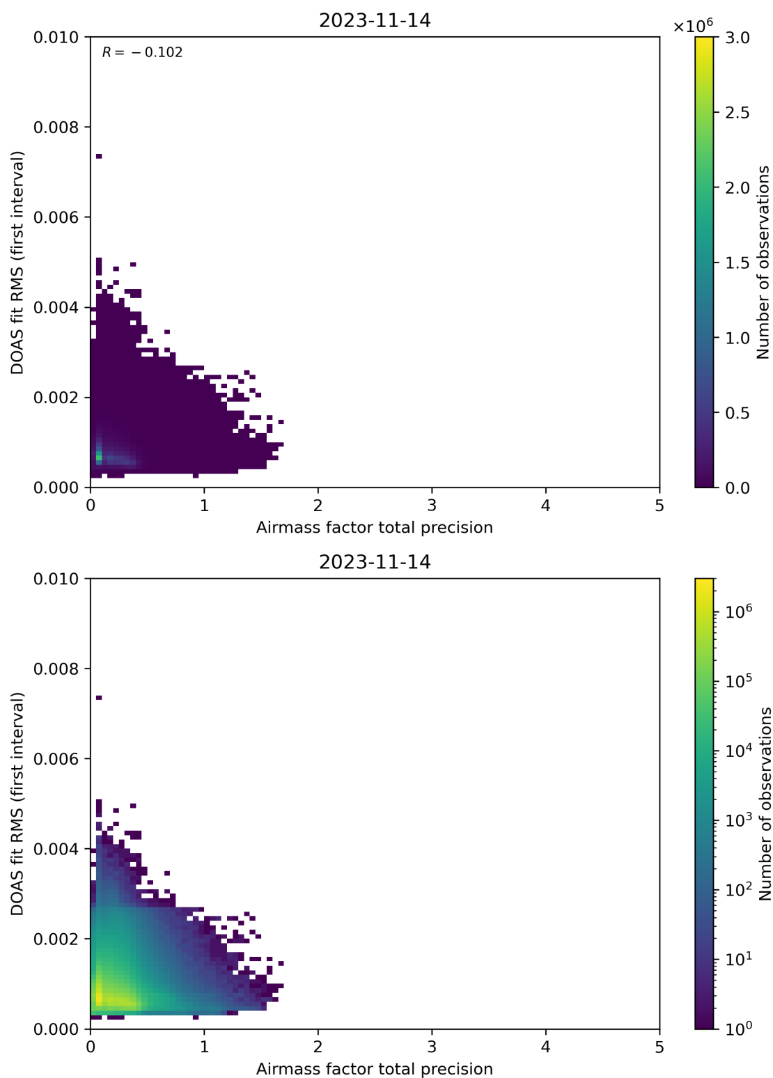
Figure 105: Scatter density plot of “Airmass factor total precision” against “DOAS fit RMS (first interval)” for 2023-11-13 to 2023-11-15.
