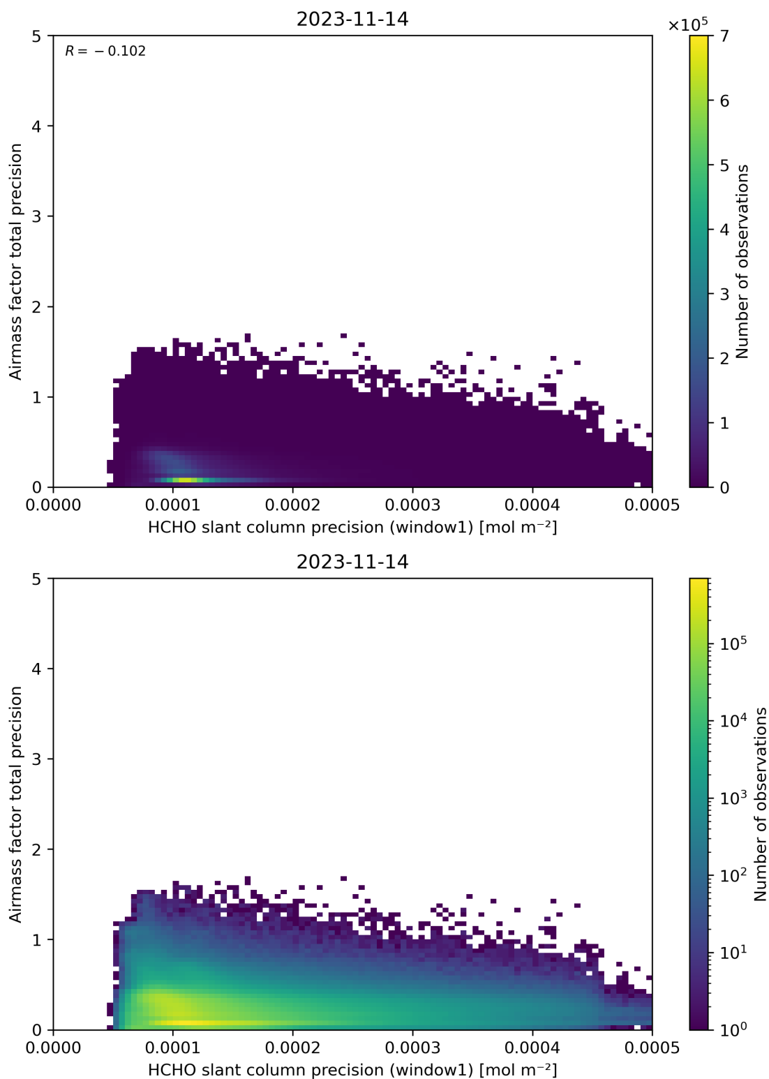
Figure 95: Scatter density plot of “HCHO slant column precision (window1)” against “Airmass factor total precision” for 2023-11-13 to 2023-11-15.
