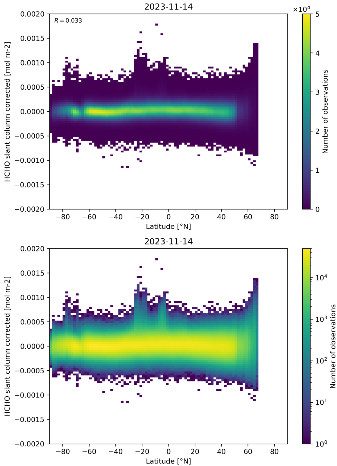
Figure 157: Scatter density plot of “Latitude” against “HCHO slant column corrected” for 2023-11-13 to 2023-11-15.
