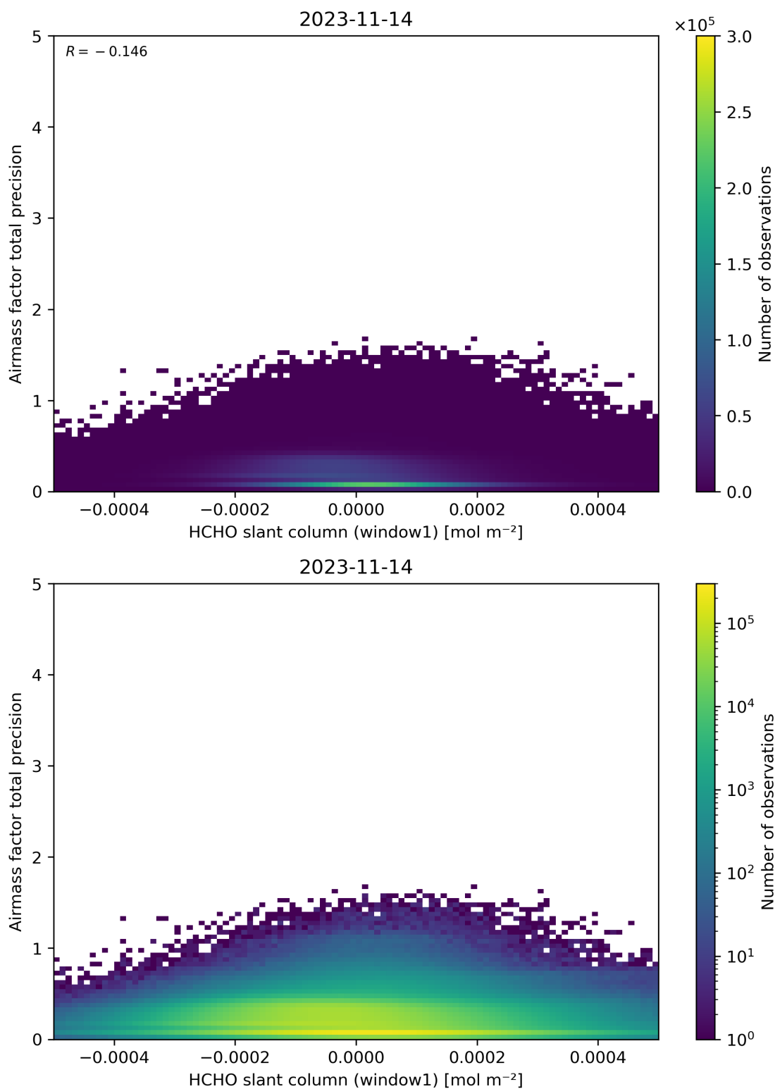
Figure 86: Scatter density plot of “HCHO slant column (window1)” against “Airmass factor total precision” for 2023-11-13 to 2023-11-15.
