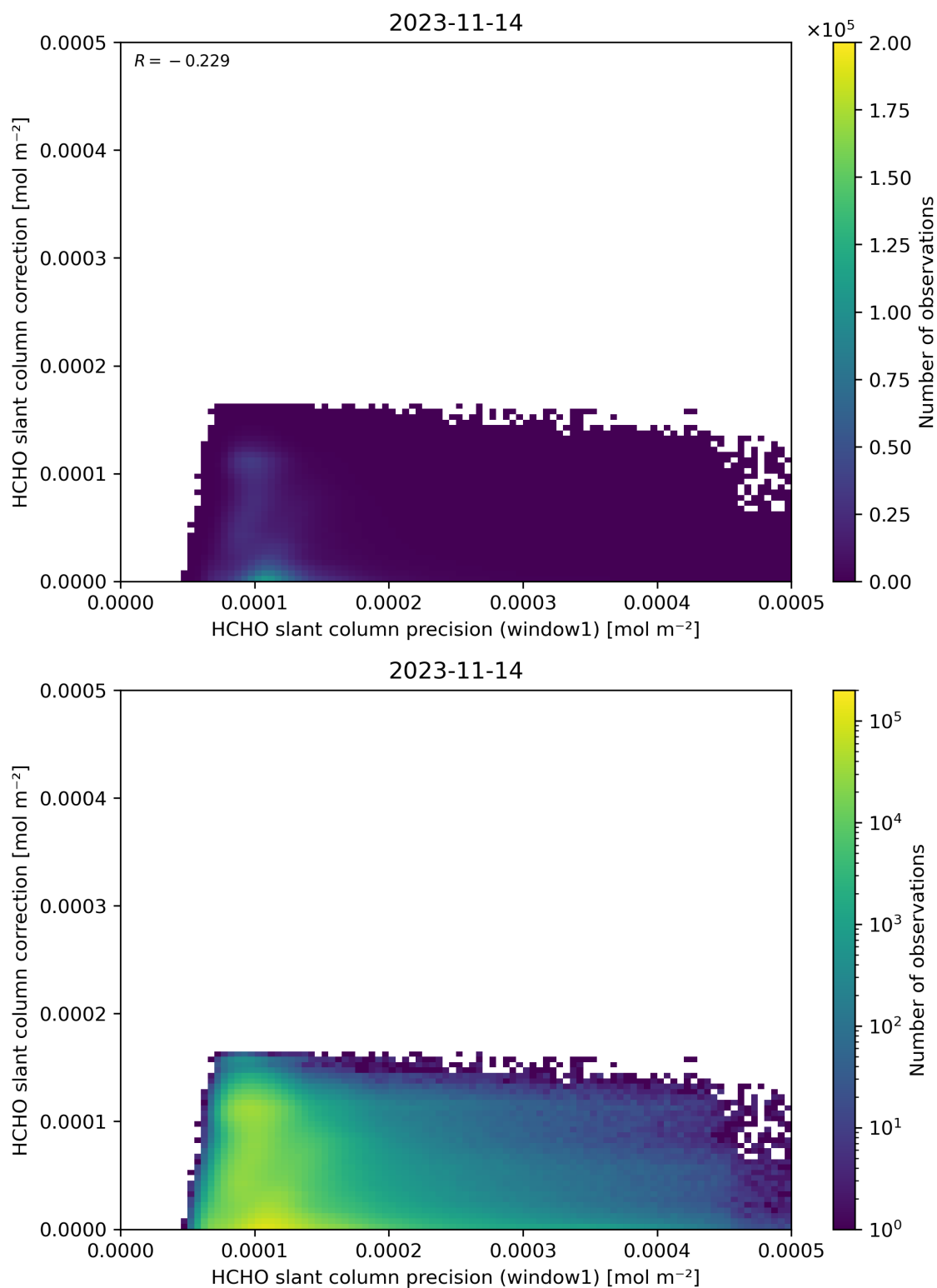
Figure 93: Scatter density plot of “HCHO slant column precision (window1)” against “HCHO slant column correction” for 2023-11-13 to 2023-11-15.
