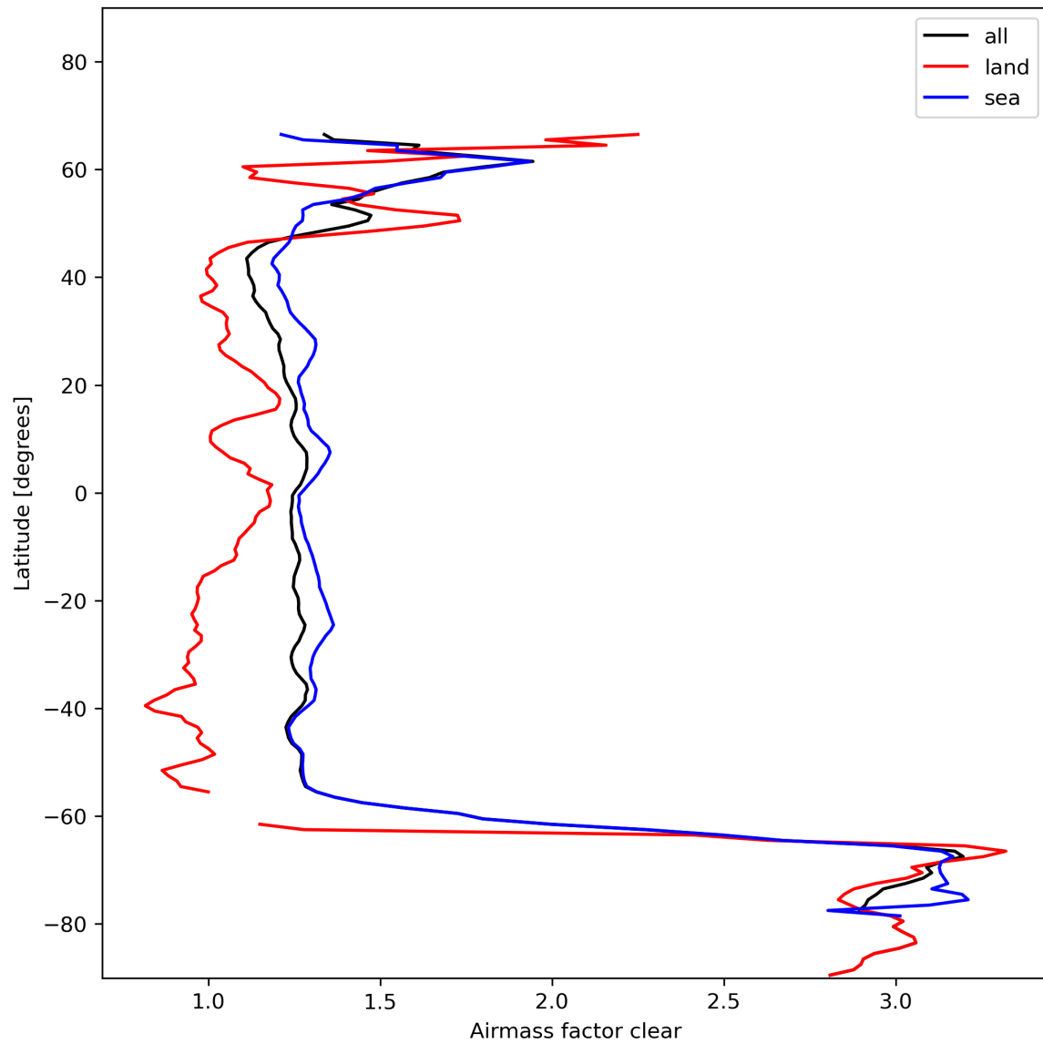
Figure 28: Zonal average of “Airmass factor clear” for 2023-11-13 to 2023-11-15.
