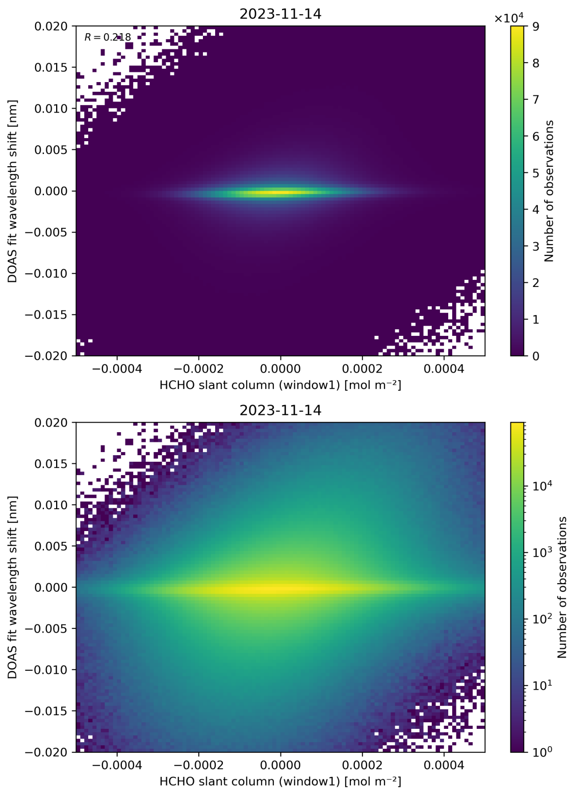
Figure 79: Scatter density plot of “HCHO slant column (window1)” against “DOAS fit wavelength shift” for 2023-11-13 to 2023-11-15.
