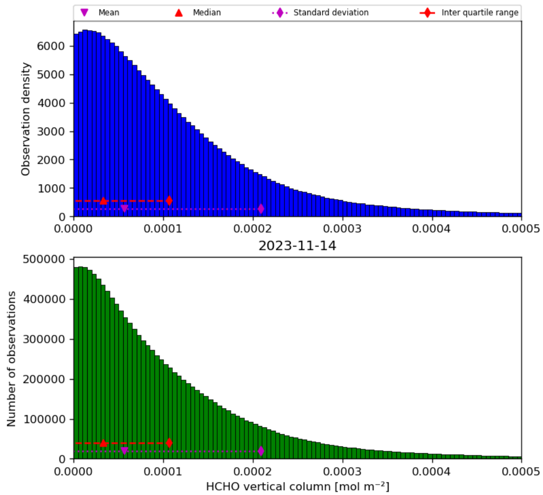
Figure 35: Histogram of “HCHO vertical column” for 2023-11-13 to 2023-11-15
