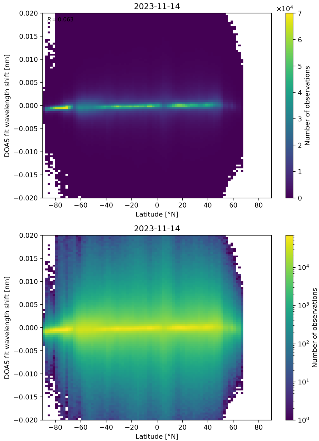
Figure 154: Scatter density plot of “Latitude” against “DOAS fit wavelength shift” for 2023-11-13 to 2023-11-15.
