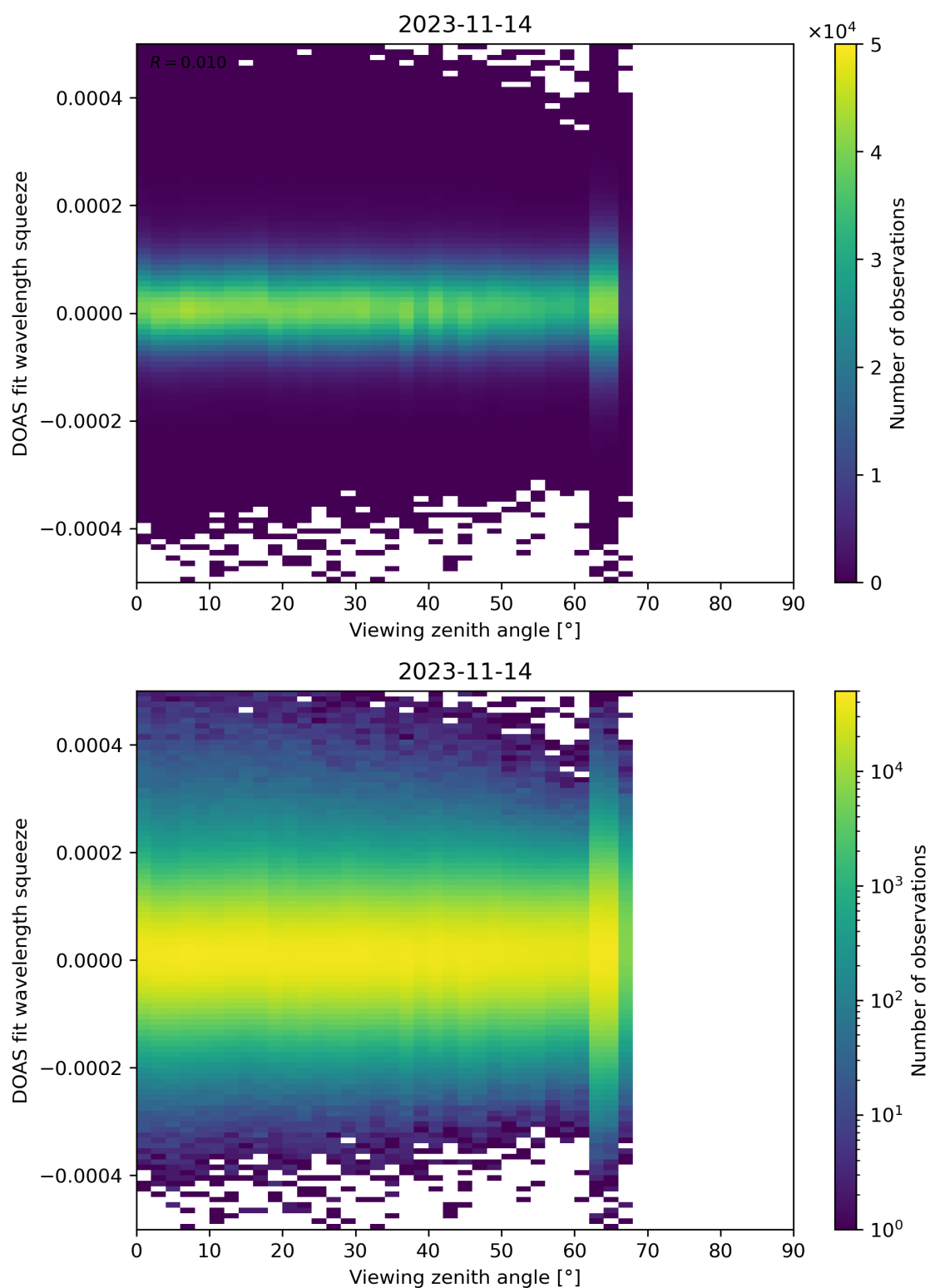
Figure 184: Scatter density plot of “Viewing zenith angle” against “DOAS fit wavelength squeeze” for 2023-11-13 to 2023-11-15.
