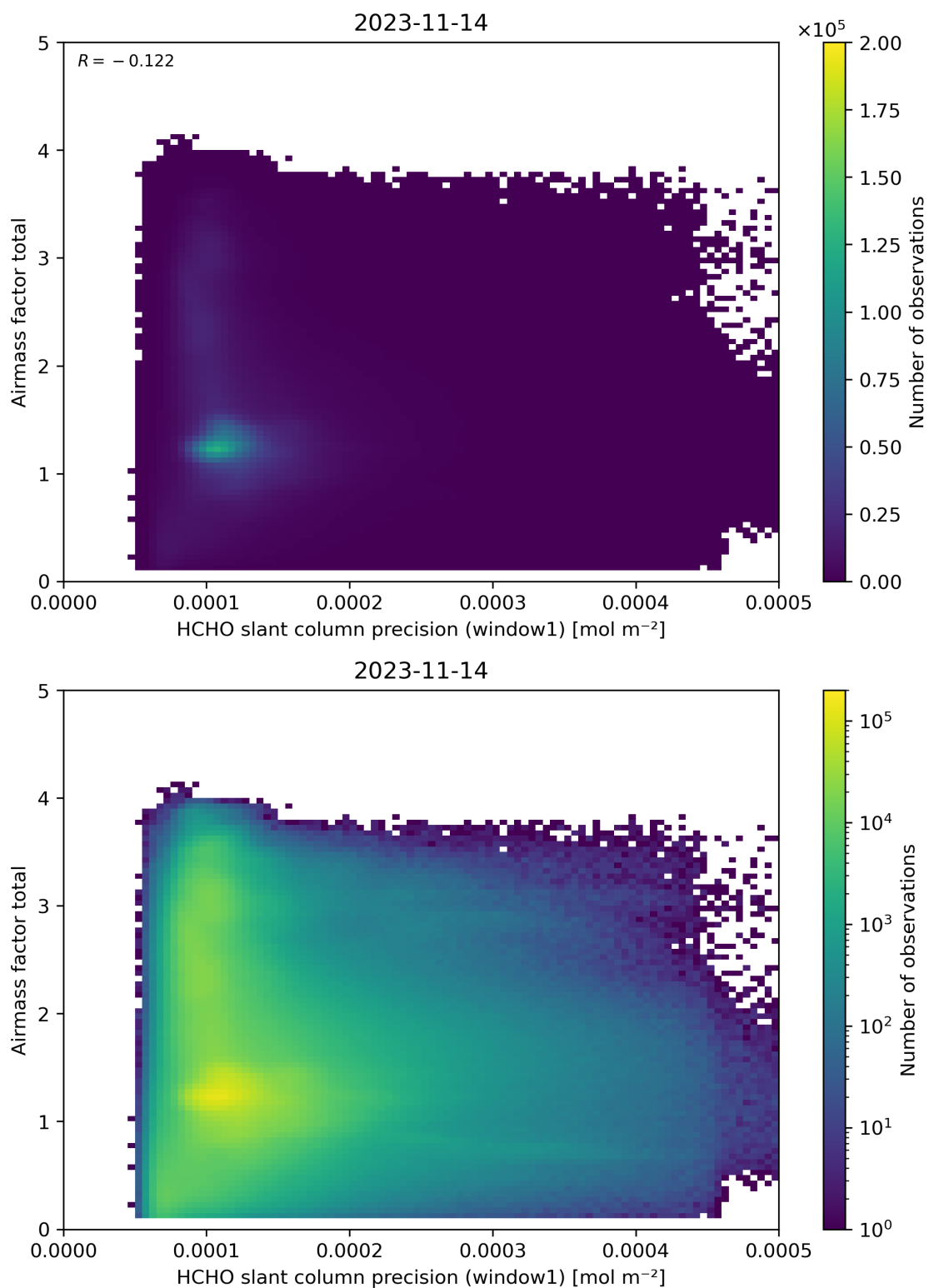
Figure 94: Scatter density plot of “HCHO slant column precision (window1)” against “Airmass factor total” for 2023-11-13 to 2023-11-15.
