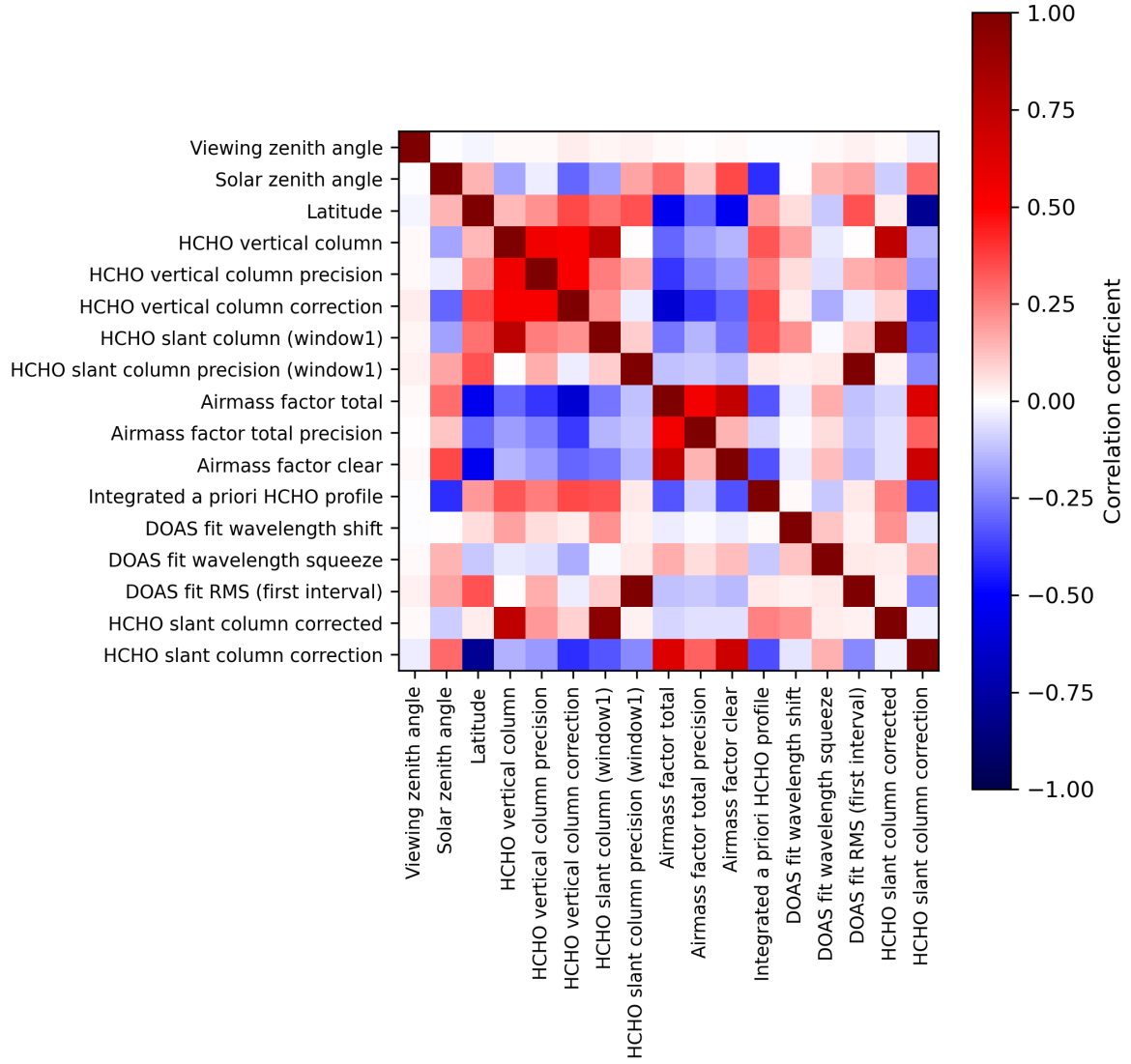
Figure 2: Map of correlation matrix for 2023-11-13 to 2023-11-15.
