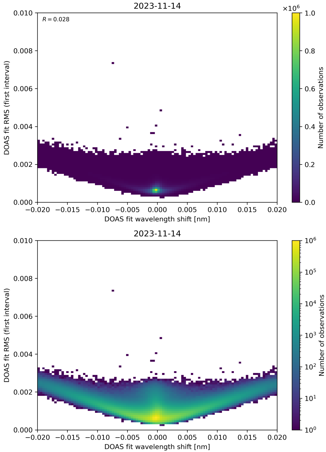
Figure 64: Scatter density plot of “DOAS fit wavelength shift” against “DOAS fit RMS (first interval)” for 2023-11-13 to 2023-11-15.
