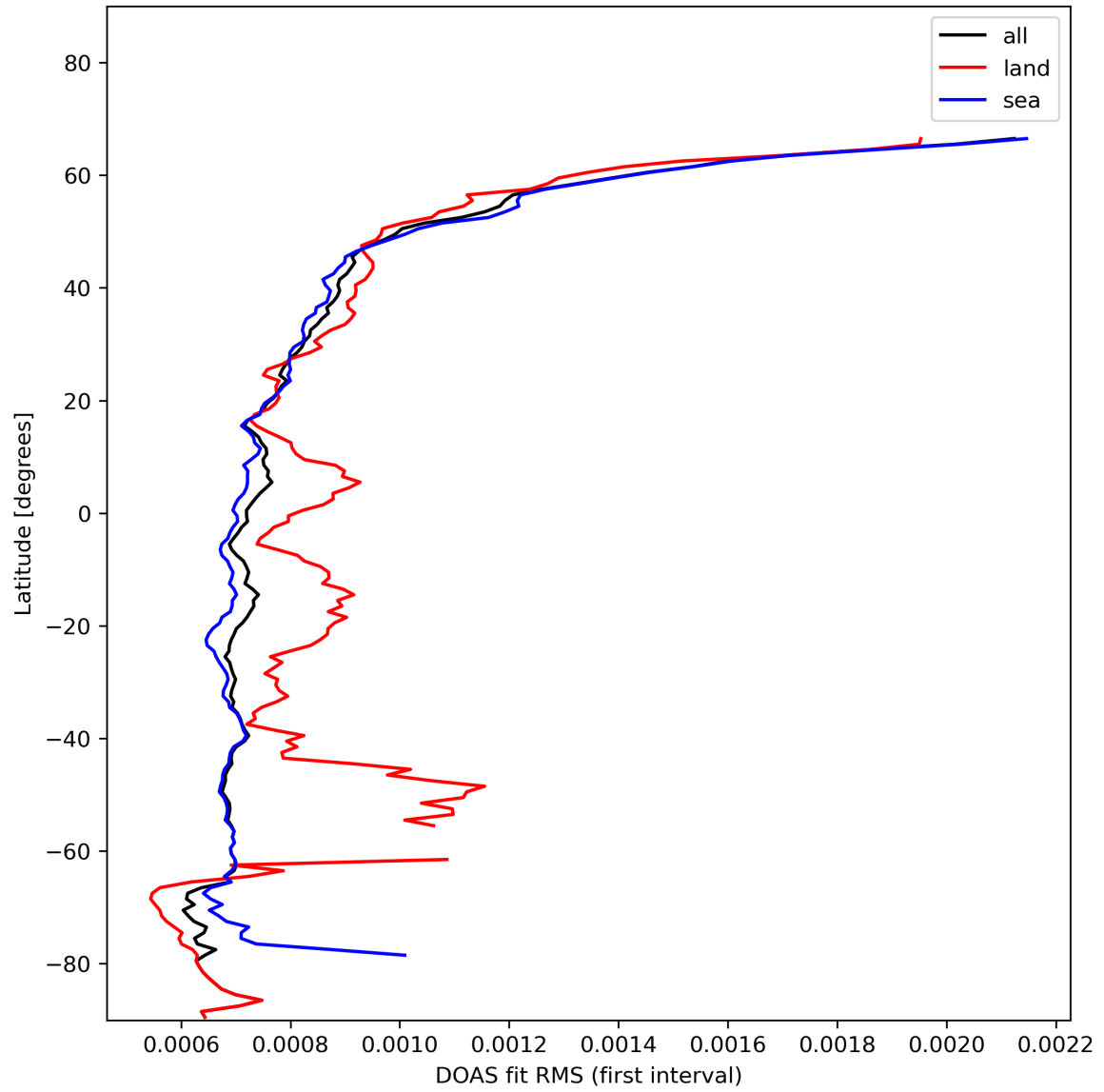
Figure 32: Zonal average of “DOAS fit RMS (first interval)” for 2023-11-13 to 2023-11-15.
