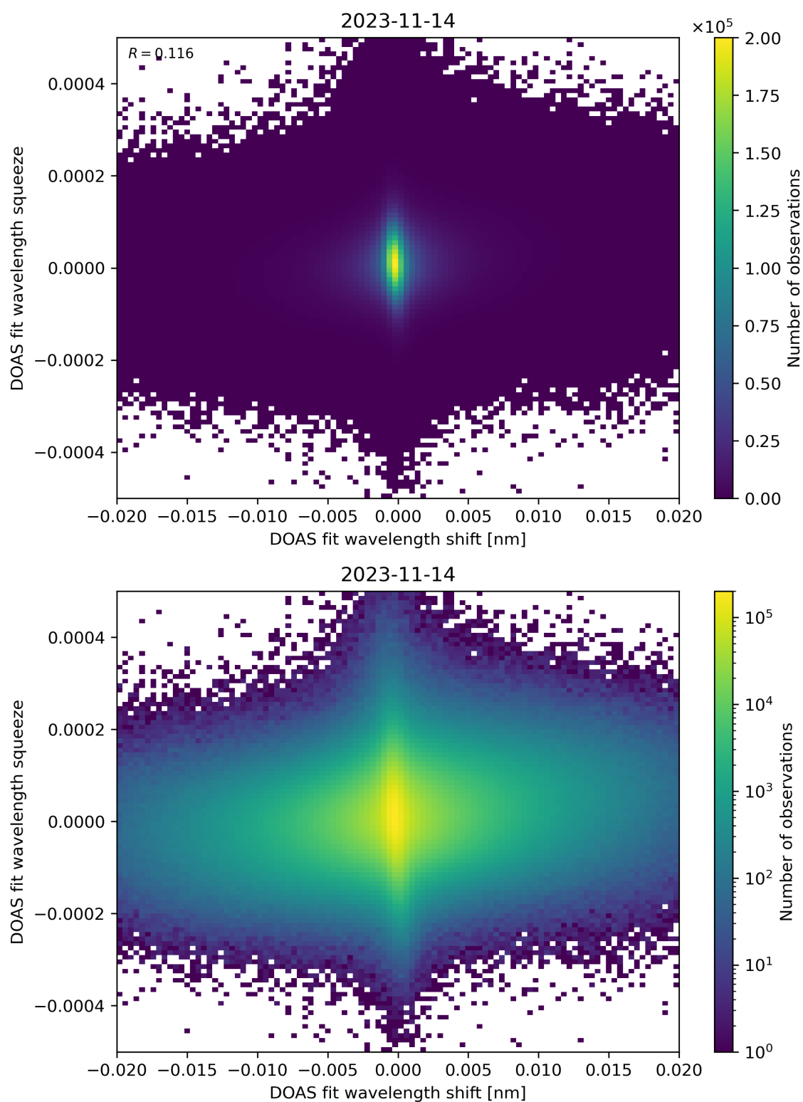
Figure 65: Scatter density plot of “DOAS fit wavelength shift” against “DOAS fit wavelength squeeze” for 2023-11-13 to 2023-11-15.
