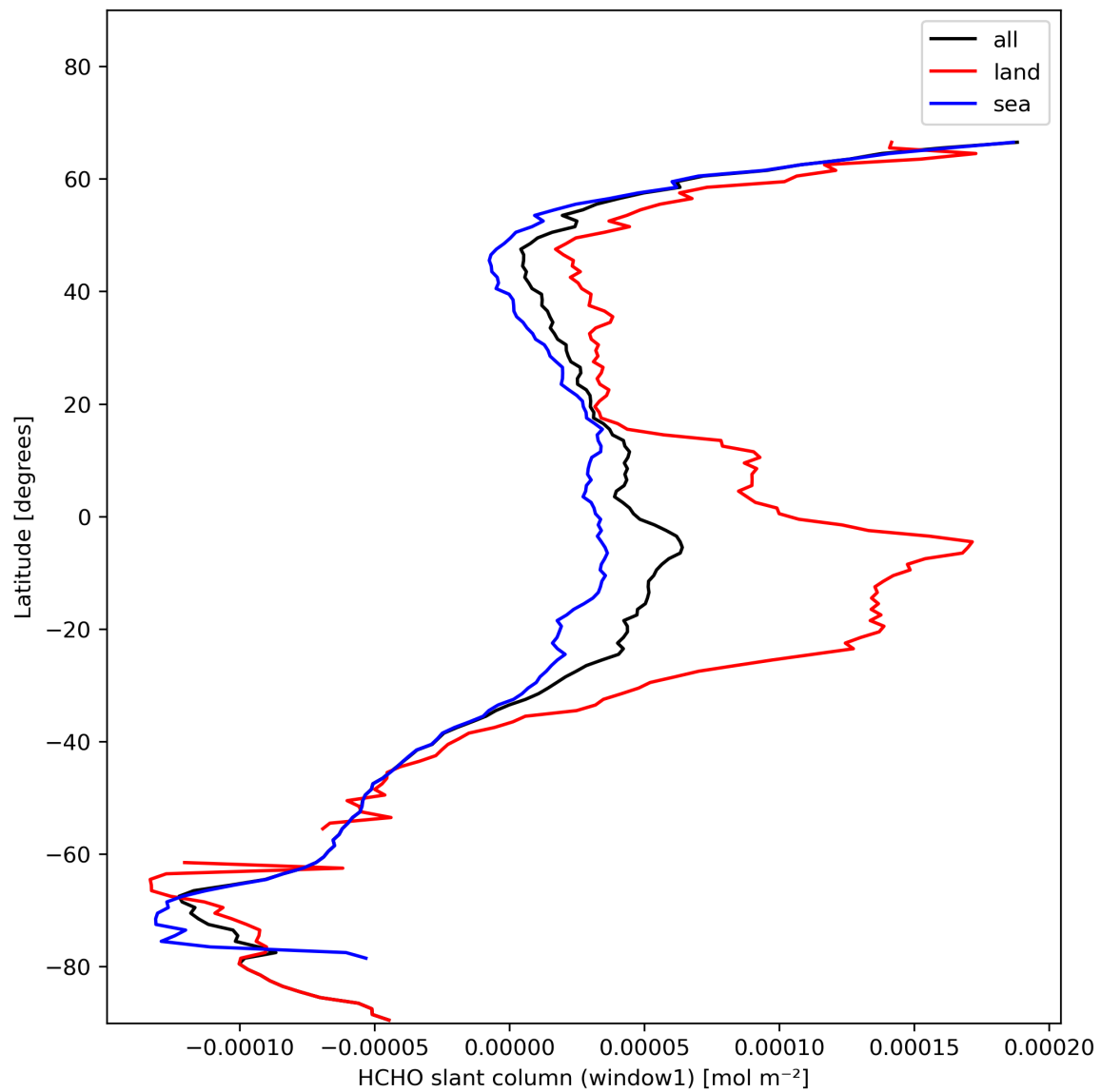
Figure 24: Zonal average of “HCHO slant column (window1)” for 2023-11-13 to 2023-11-15.
