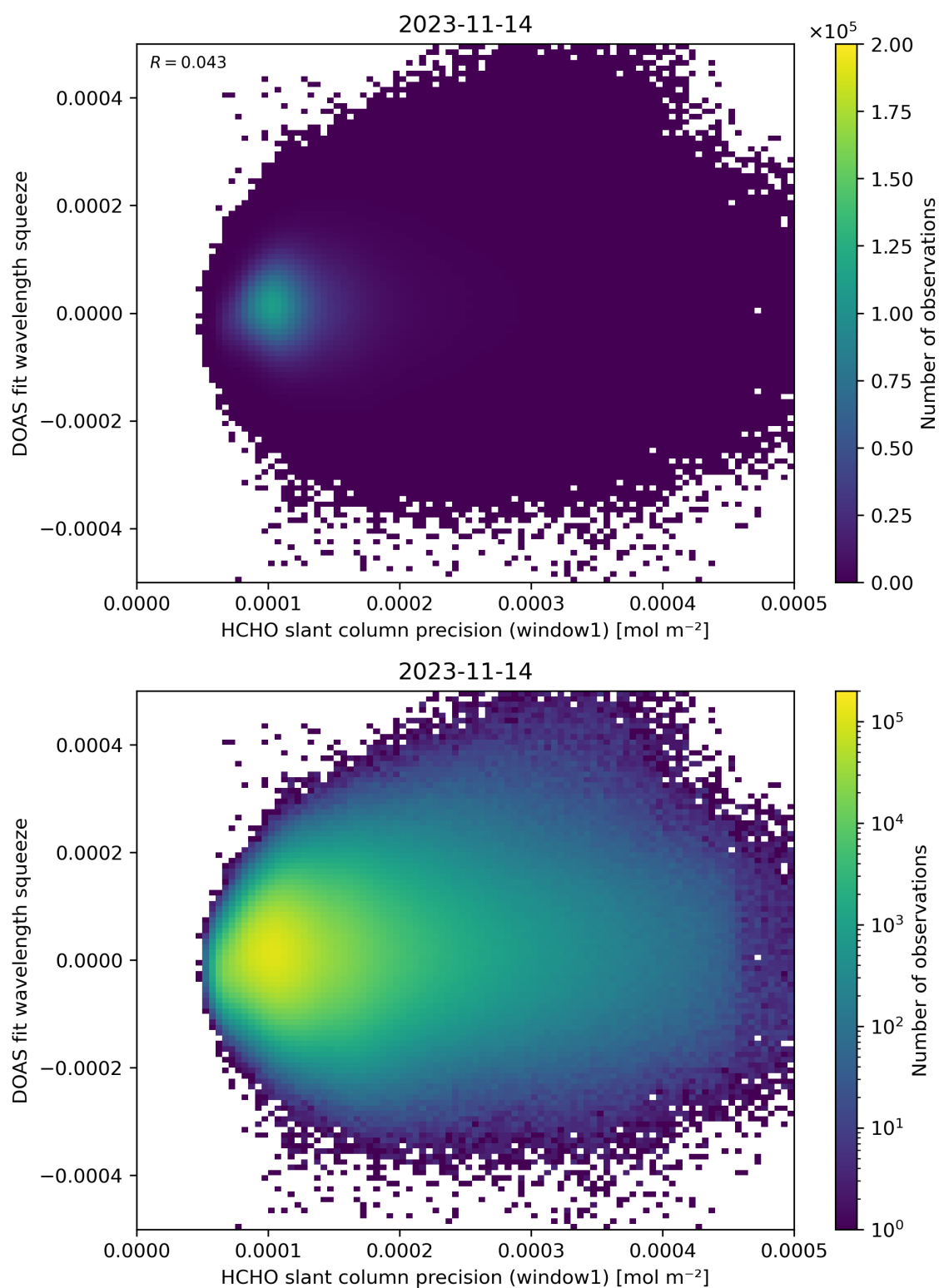
Figure 90: Scatter density plot of “HCHO slant column precision (window1)” against “DOAS fit wavelength squeeze” for 2023-11-13 to 2023-11-15.
