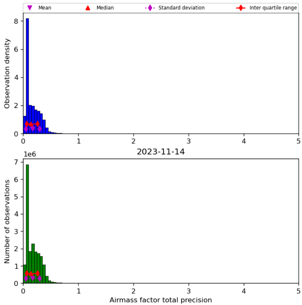
Figure 41: Histogram of “Airmass factor total precision” for 2023-11-13 to 2023-11-15
