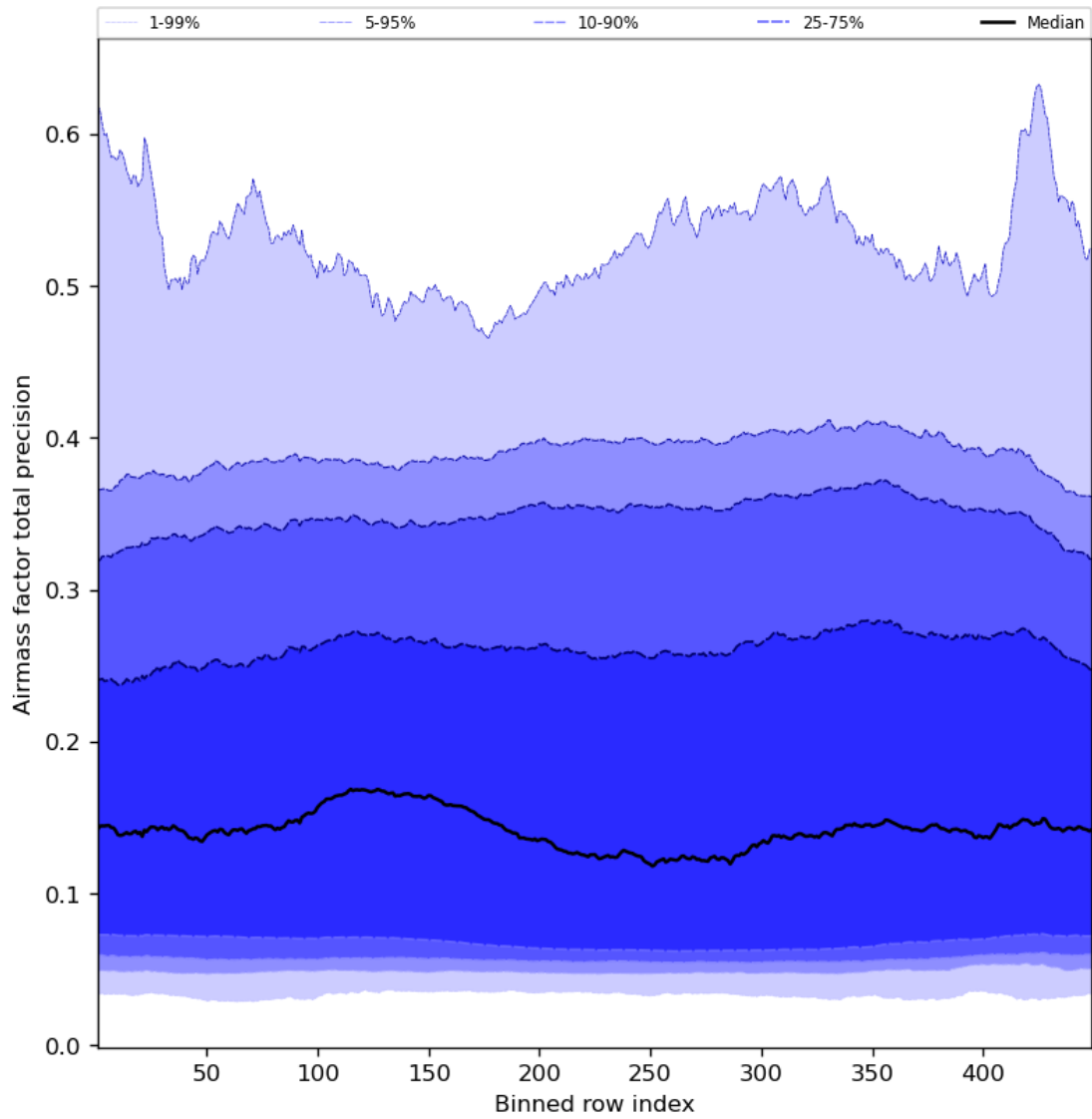
Figure 55: Along track statistics of “Airmass factor total precision” for 2023-11-13 to 2023-11-15
