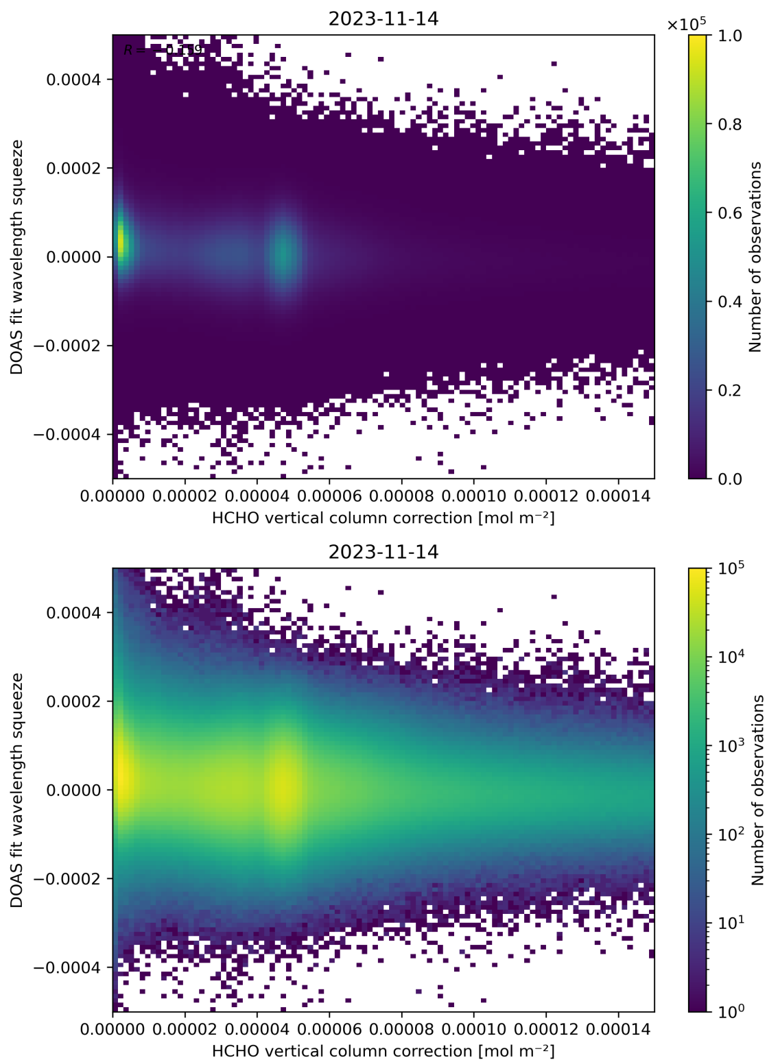
Figure 114: Scatter density plot of “HCHO vertical column correction” against “DOAS fit wavelength squeeze” for 2023-11-13 to 2023-11-15.
