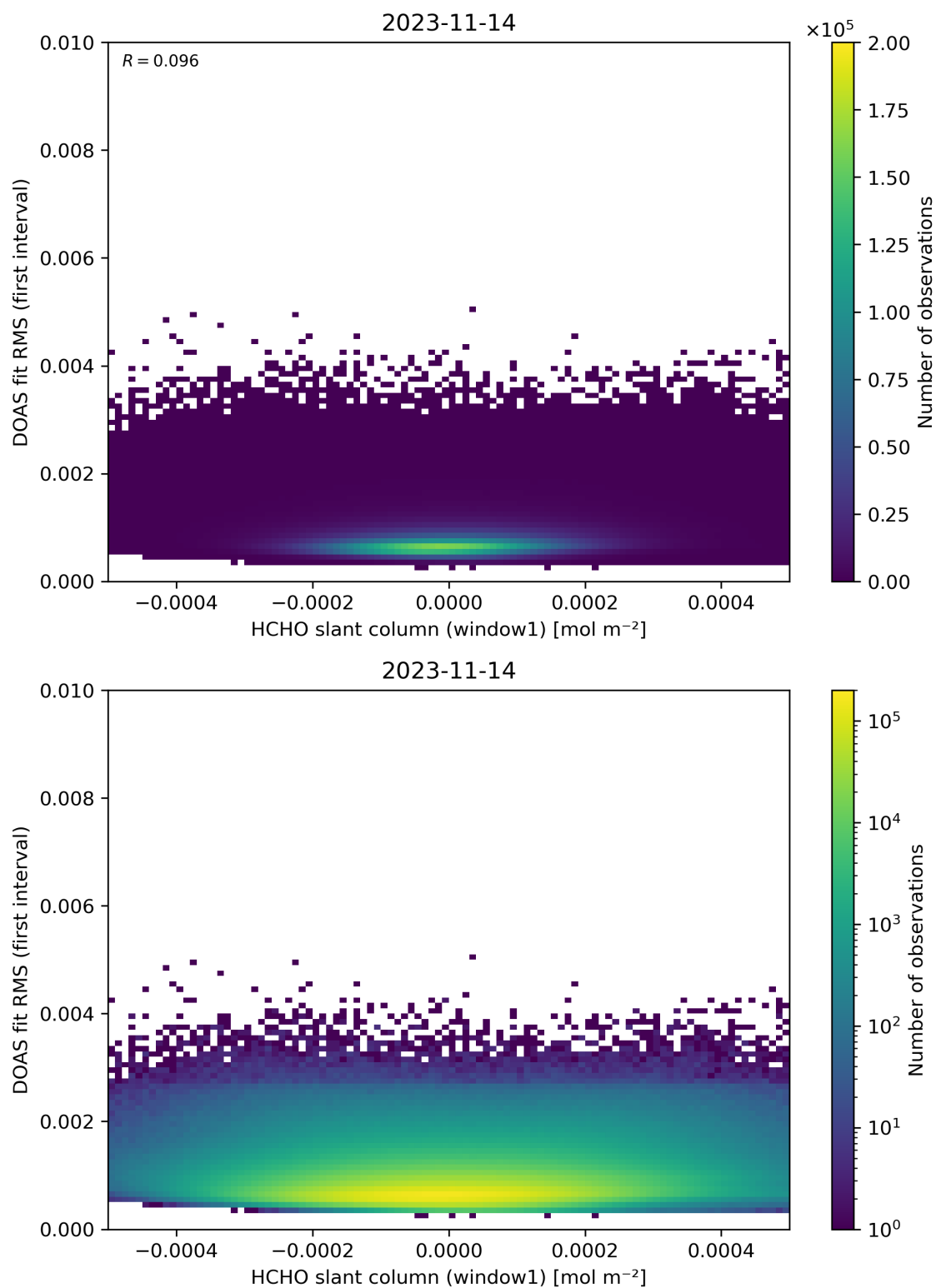
Figure 78: Scatter density plot of “HCHO slant column (window1)” against “DOAS fit RMS (first interval)” for 2023-11-13 to 2023-11-15.
