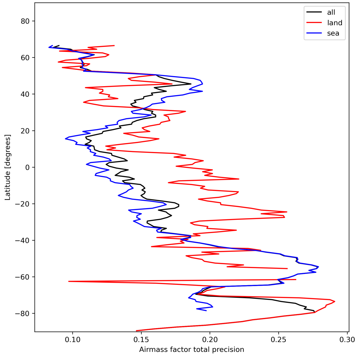
Figure 27: Zonal average of “Airmass factor total precision” for 2023-11-13 to 2023-11-15.
