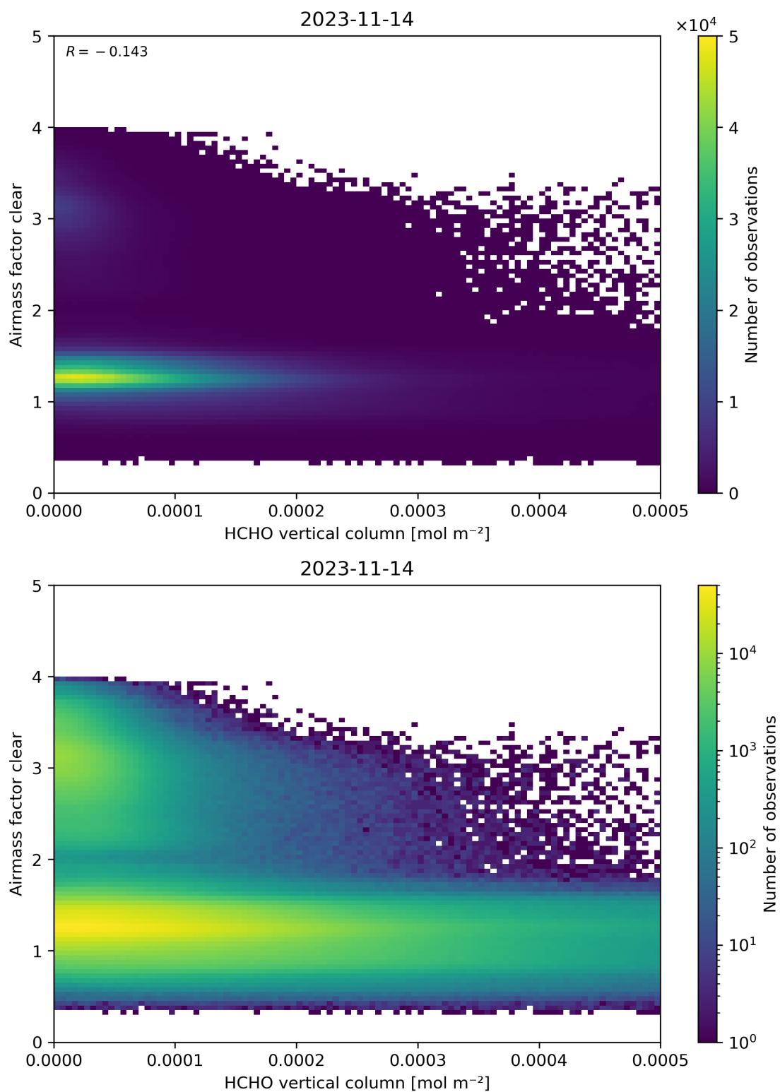
Figure 126: Scatter density plot of “HCHO vertical column” against “Airmass factor clear” for 2023-11-13 to 2023-11-15.
