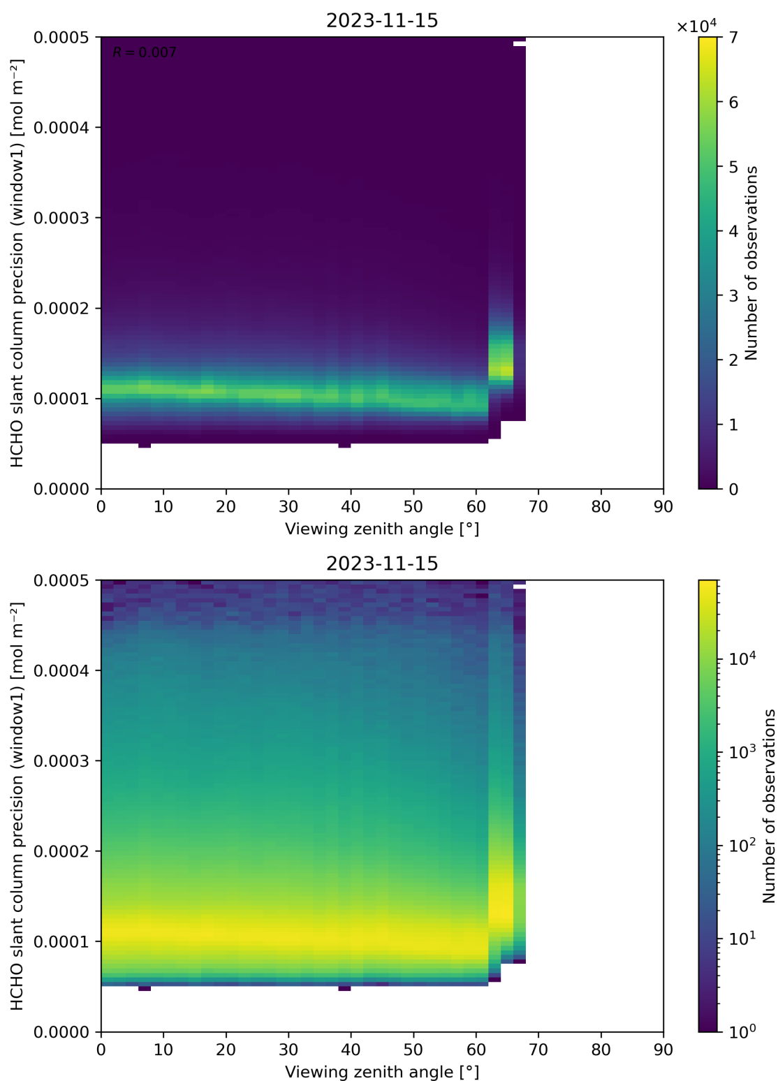
Figure 189: Scatter density plot of “Viewing zenith angle” against “HCHO slant column precision (window1)” for 2023-11-14 to 2023-11-16.
