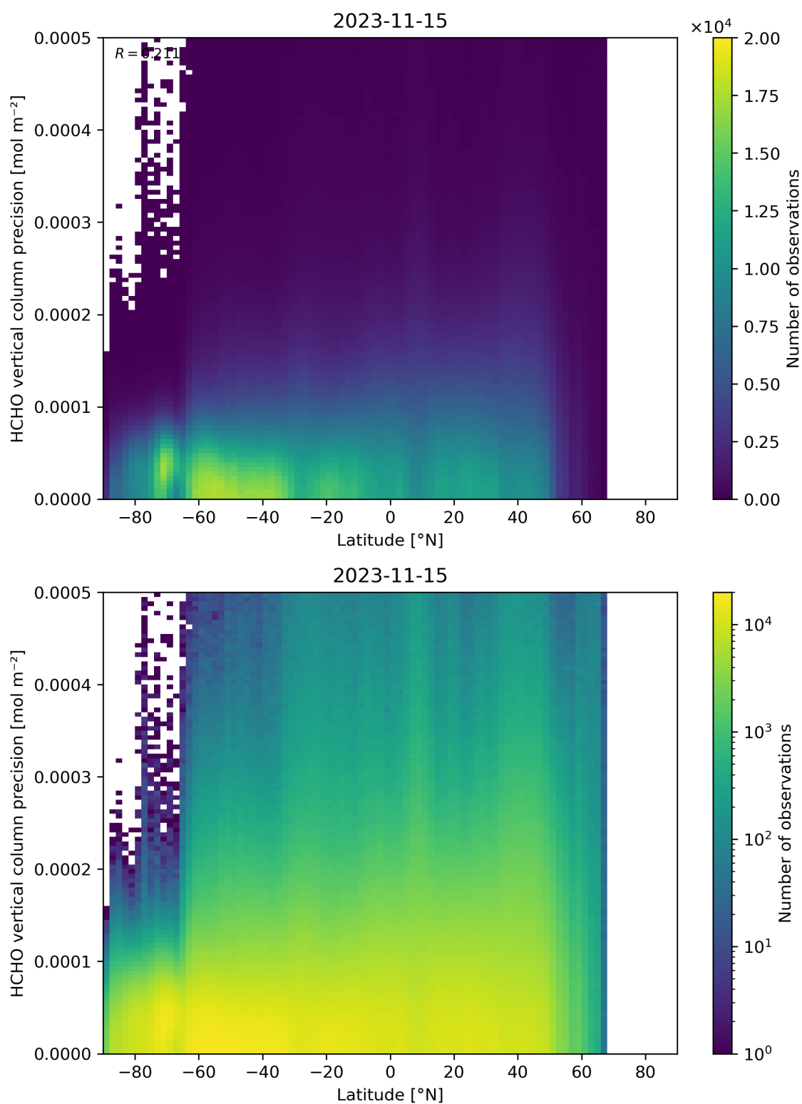
Figure 165: Scatter density plot of “Latitude” against “HCHO vertical column precision” for 2023-11-14 to 2023-11-16.
