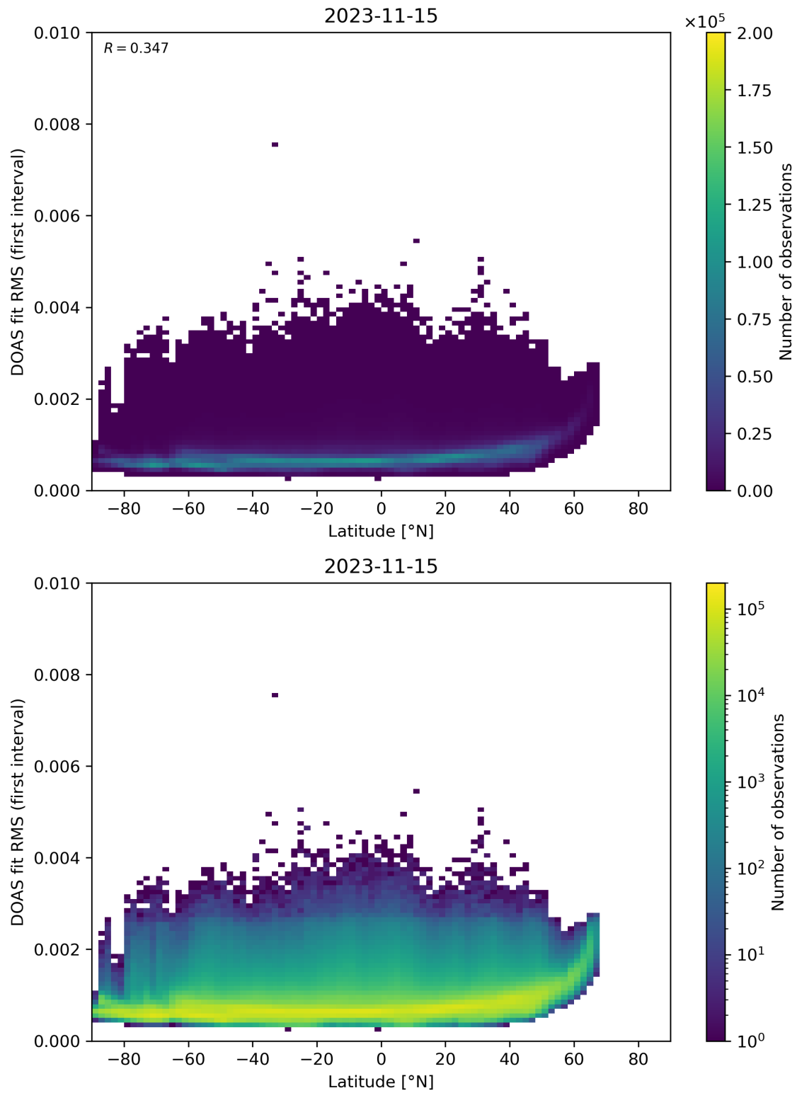
Figure 153: Scatter density plot of “Latitude” against “DOAS fit RMS (first interval)” for 2023-11-14 to 2023-11-16.
