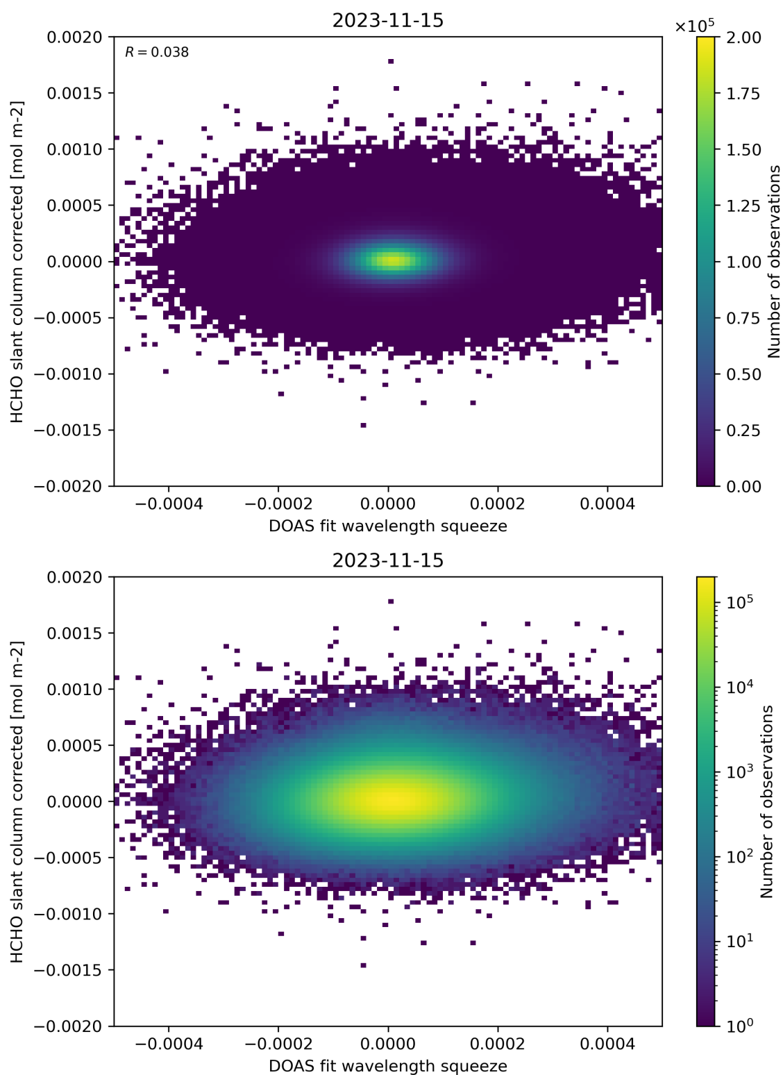
Figure 69: Scatter density plot of “DOAS fit wavelength squeeze” against “HCHO slant column corrected” for 2023-11-14 to 2023-11-16.
