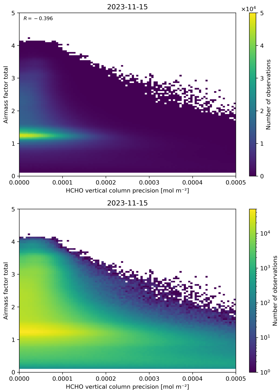
Figure 144: Scatter density plot of “HCHO vertical column precision” against “Airmass factor total” for 2023-11-14 to 2023-11-16.
