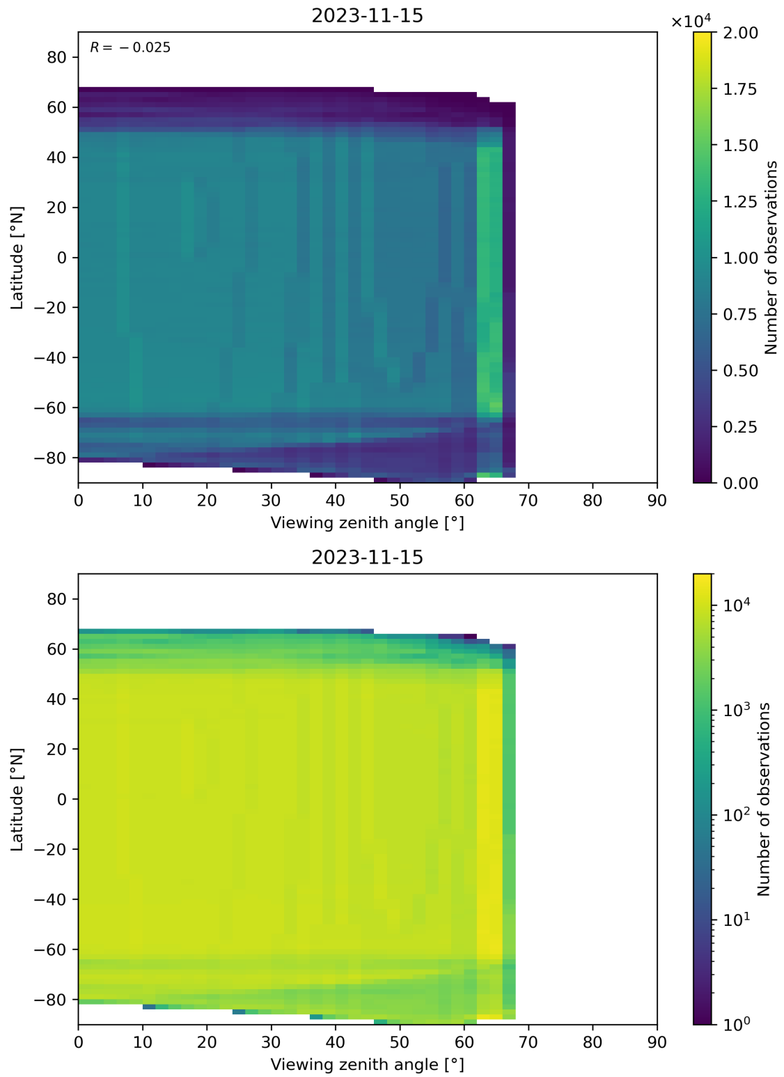
Figure 196: Scatter density plot of “Viewing zenith angle” against “Latitude” for 2023-11-14 to 2023-11-16.
