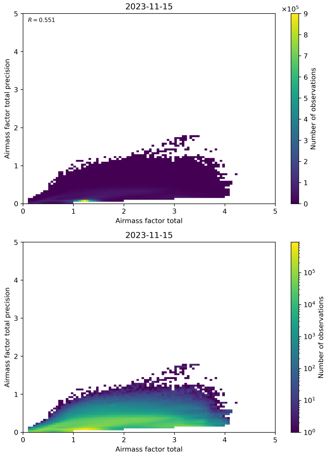
Figure 103: Scatter density plot of “Airmass factor total” against “Airmass factor total precision” for 2023-11-14 to 2023-11-16.
