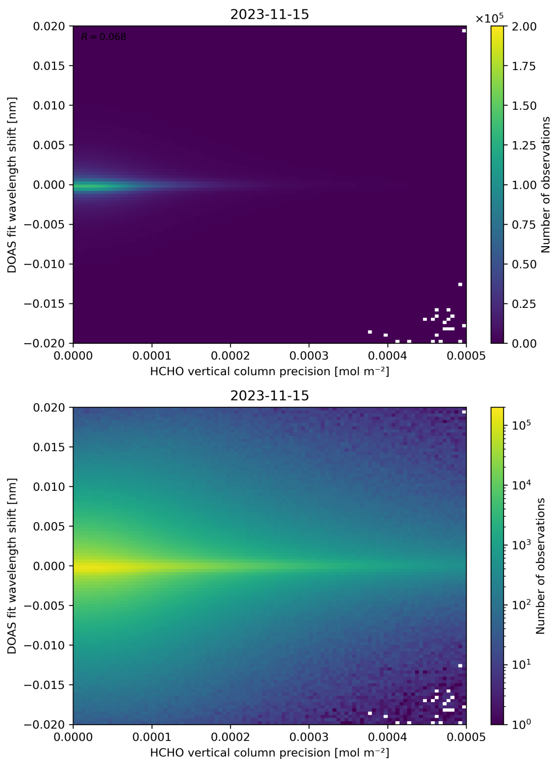
Figure 137: Scatter density plot of “HCHO vertical column precision” against “DOAS fit wavelength shift” for 2023-11-14 to 2023-11-16.
