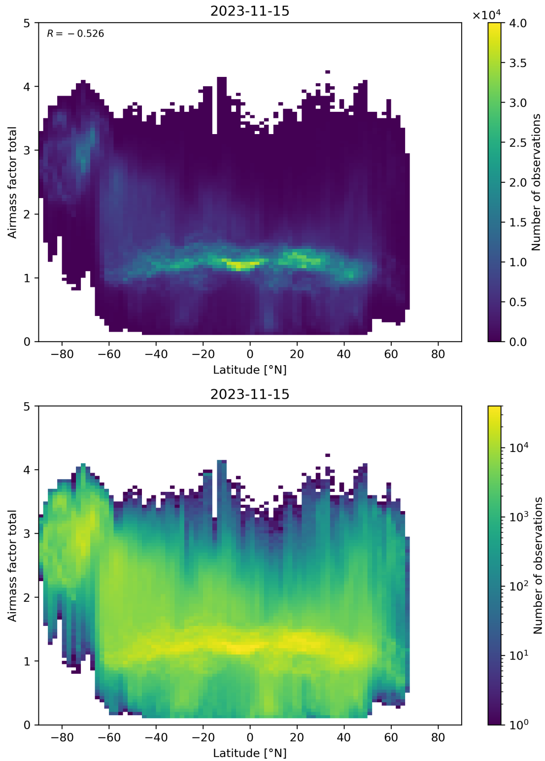
Figure 161: Scatter density plot of “Latitude” against “Airmass factor total” for 2023-11-14 to 2023-11-16.
