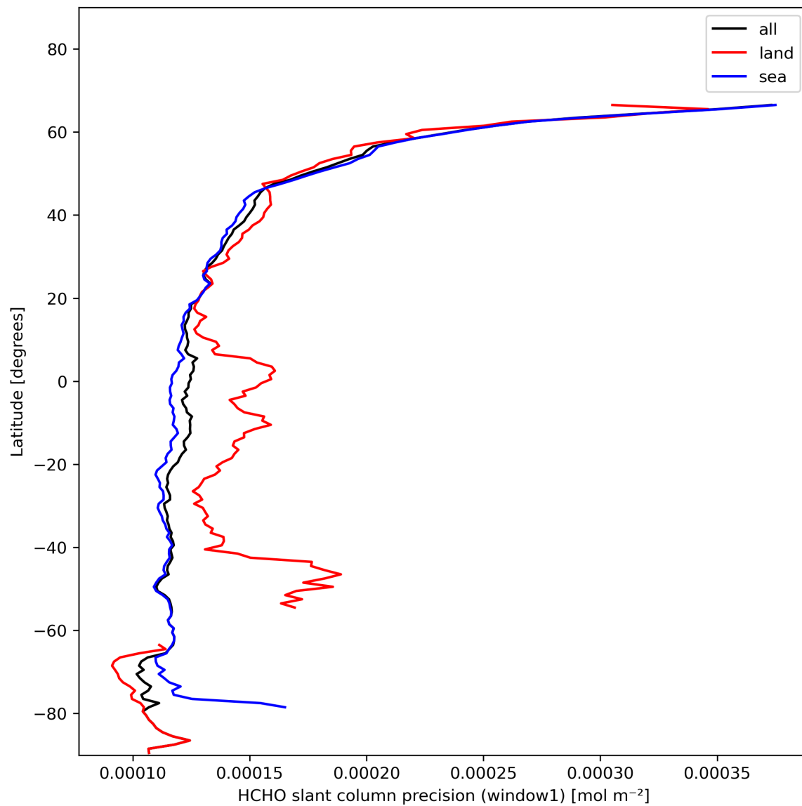
Figure 25: Zonal average of “HCHO slant column precision (window1)” for 2023-11-14 to 2023-11-16.
