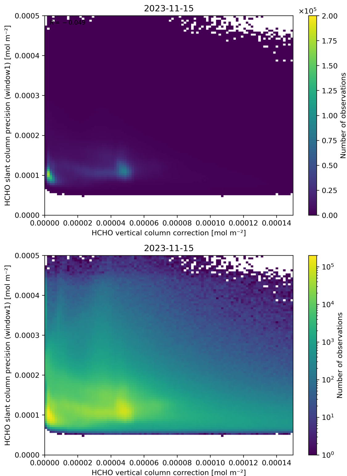
Figure 119: Scatter density plot of “HCHO vertical column correction” against “HCHO slant column precision (window1)” for 2023-11-14 to 2023-11-16.
