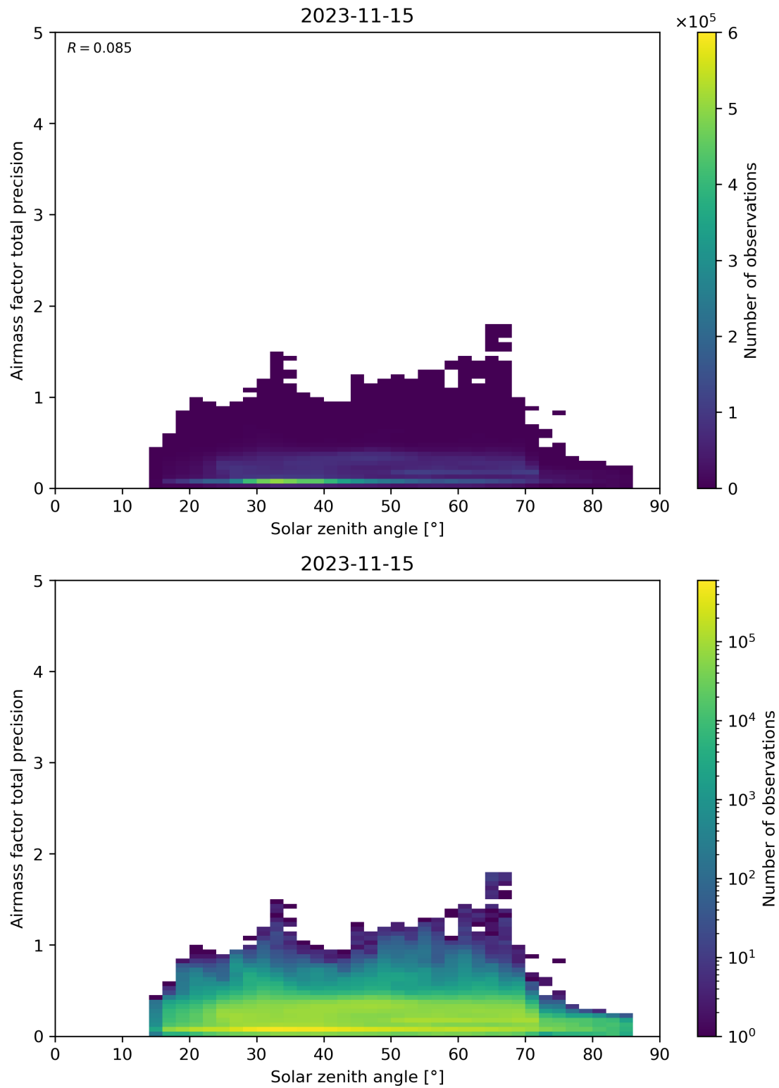
Figure 176: Scatter density plot of “Solar zenith angle” against “Airmass factor total precision” for 2023-11-14 to 2023-11-16.
