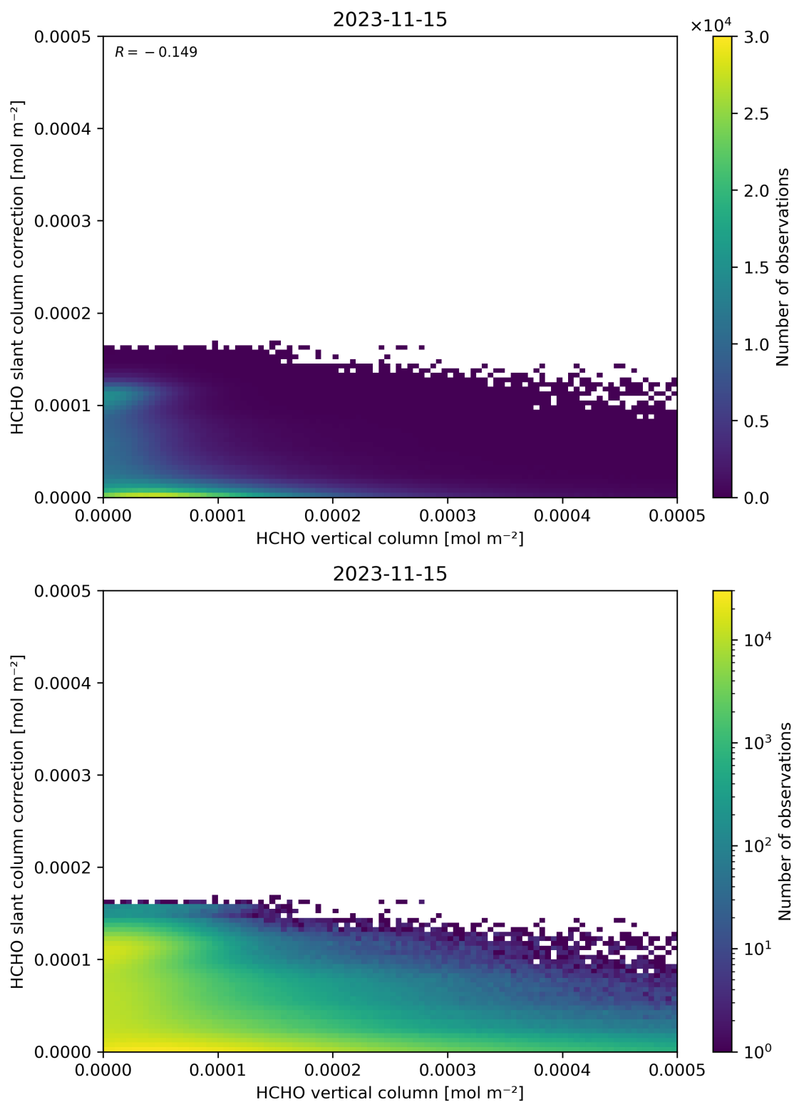
Figure 128: Scatter density plot of “HCHO vertical column” against “HCHO slant column correction” for 2023-11-14 to 2023-11-16.
