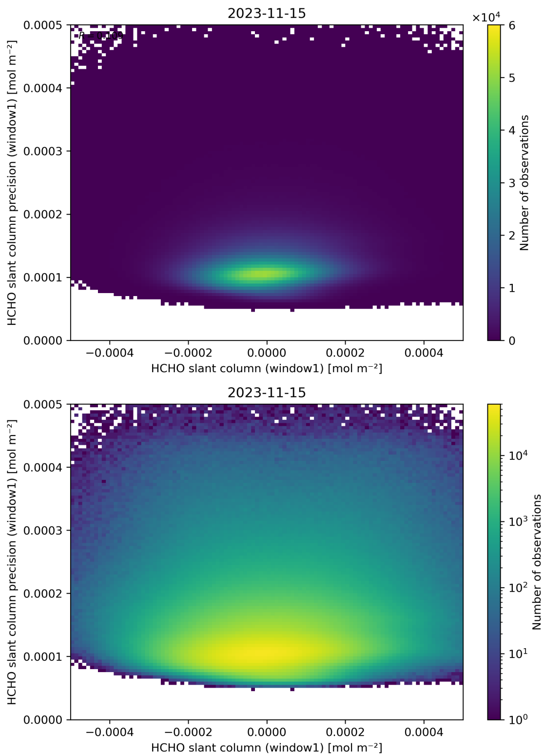
Figure 84: Scatter density plot of “HCHO slant column (window1)” against “HCHO slant column precision (window1)” for 2023-11-14 to 2023-11-16.
