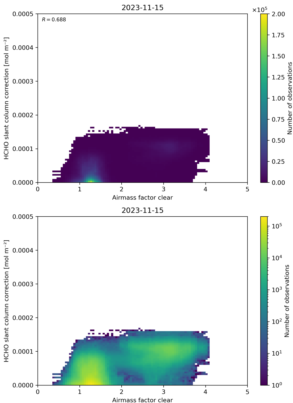
Figure 75: Scatter density plot of “Airmass factor clear” against “HCHO slant column correction” for 2023-11-14 to 2023-11-16.
