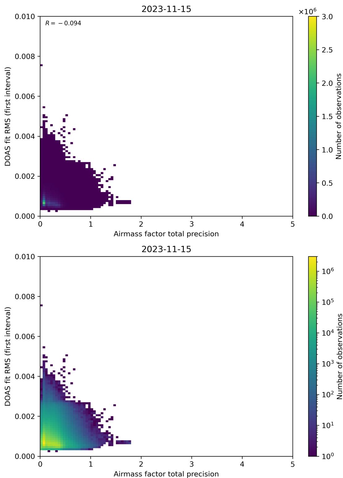
Figure 105: Scatter density plot of “Airmass factor total precision” against “DOAS fit RMS (first interval)” for 2023-11-14 to 2023-11-16.
