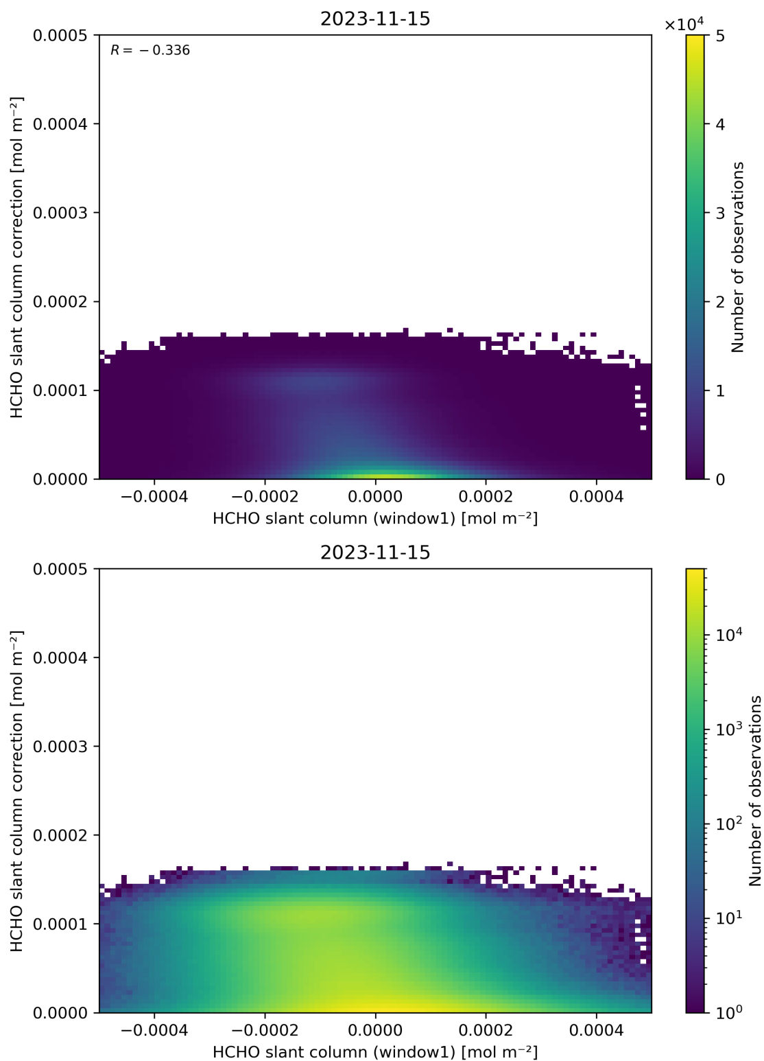
Figure 83: Scatter density plot of “HCHO slant column (window1)” against “HCHO slant column correction” for 2023-11-14 to 2023-11-16.
