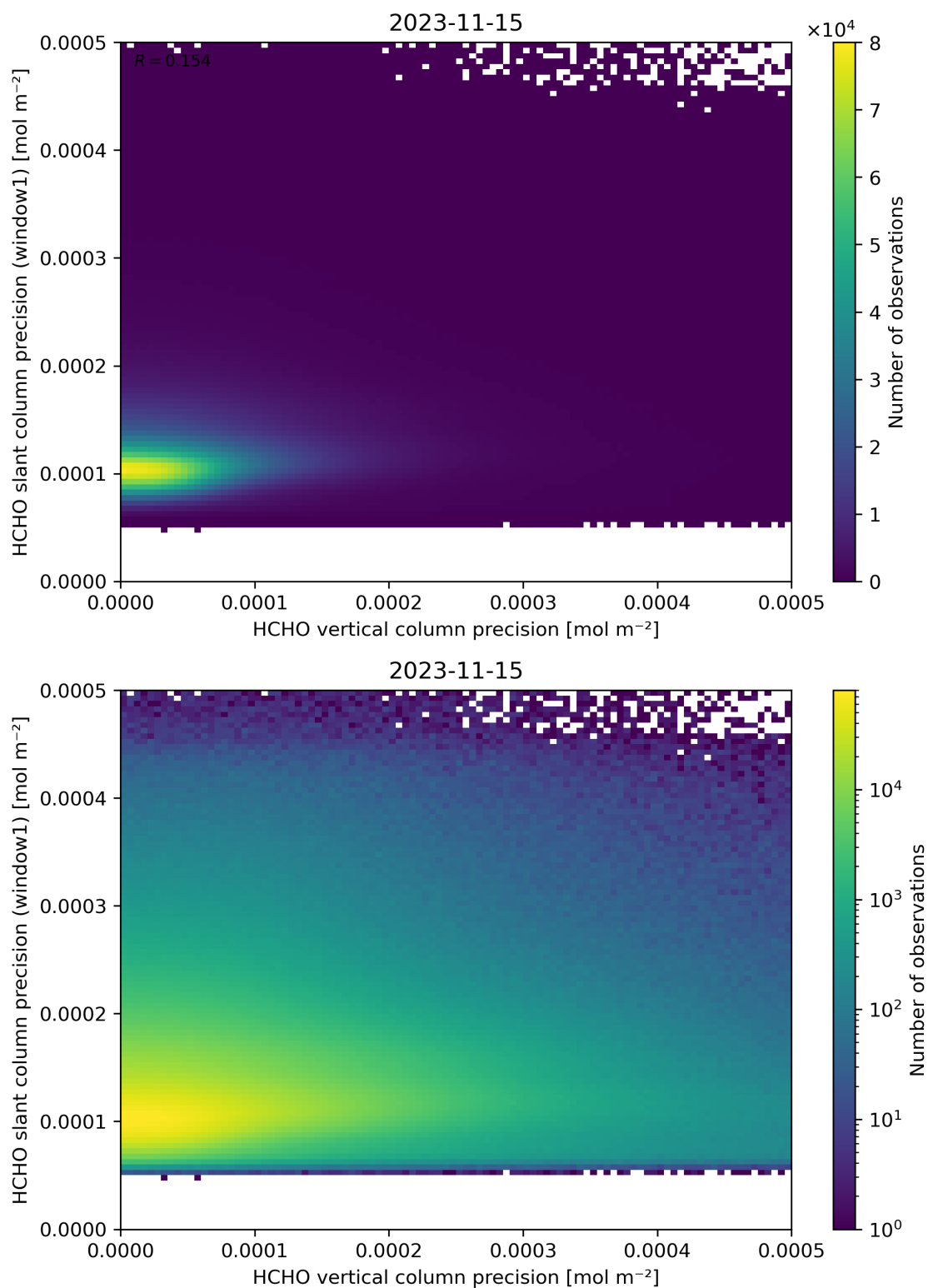
Figure 143: Scatter density plot of “HCHO vertical column precision” against “HCHO slant column precision (window1)” for 2023-11-14 to 2023-11-16.
