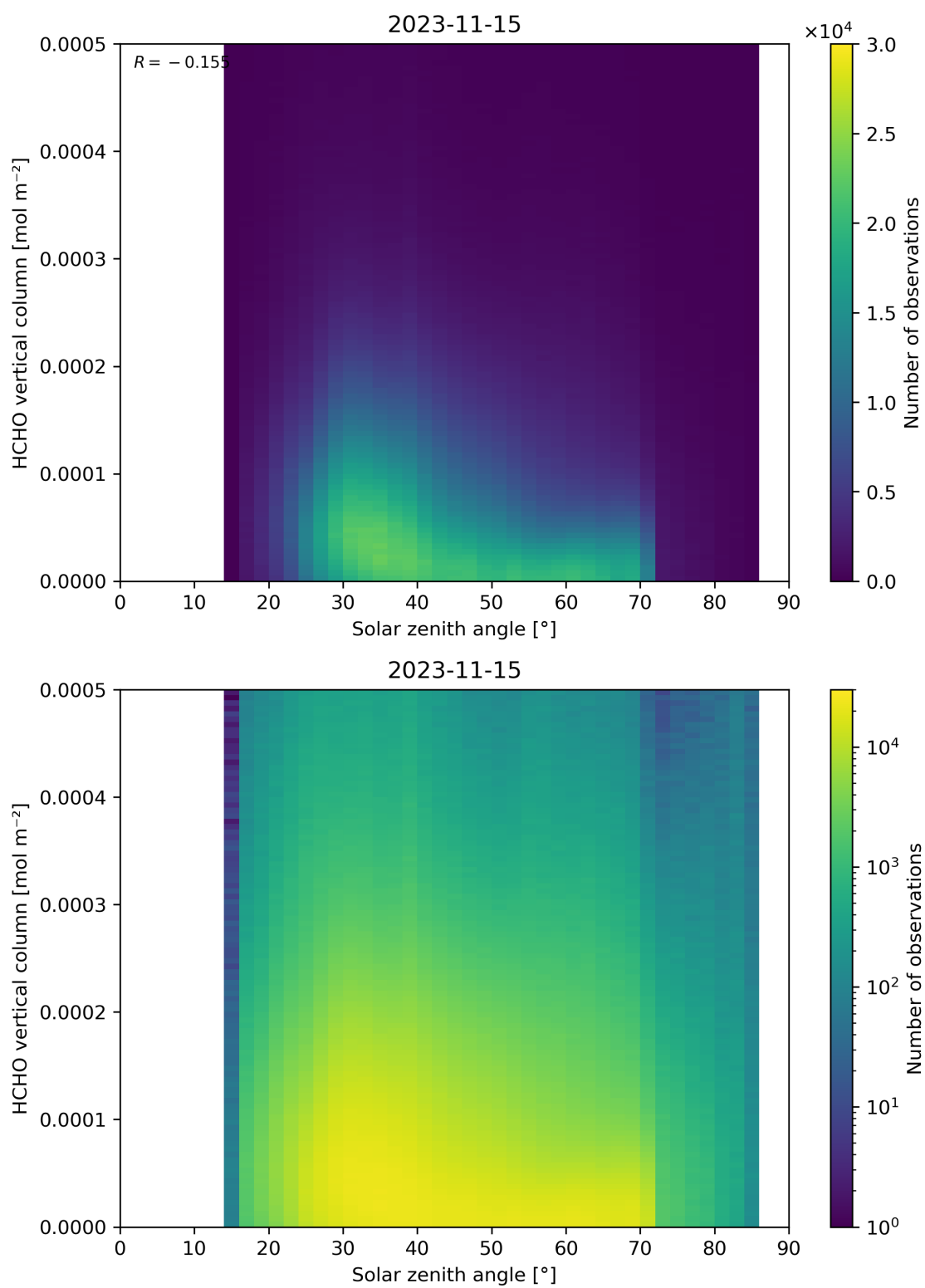
Figure 177: Scatter density plot of “Solar zenith angle” against “HCHO vertical column” for 2023-11-14 to 2023-11-16.
