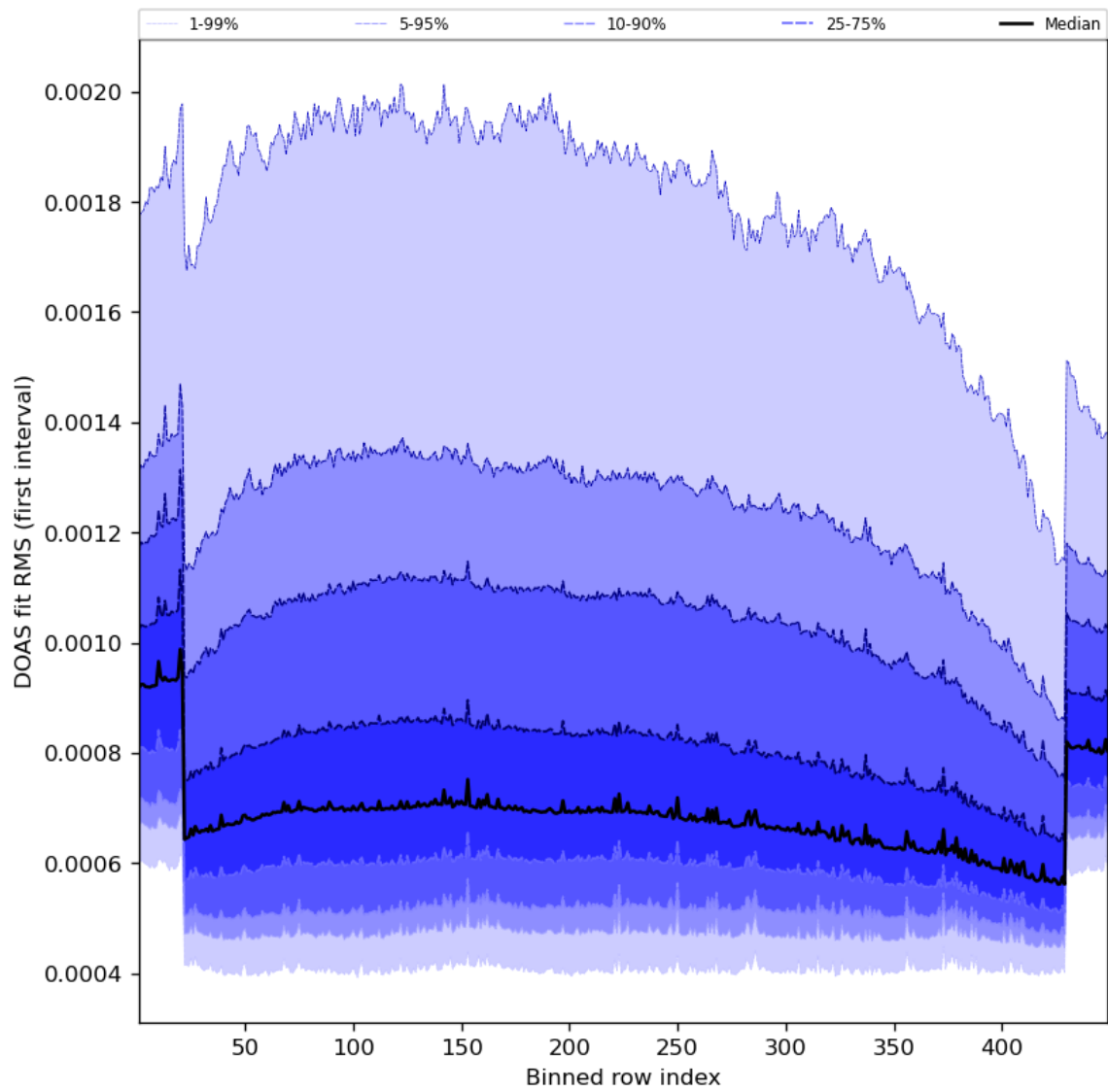
Figure 60: Along track statistics of “DOAS fit RMS (first interval)” for 2023-11-14 to 2023-11-16
