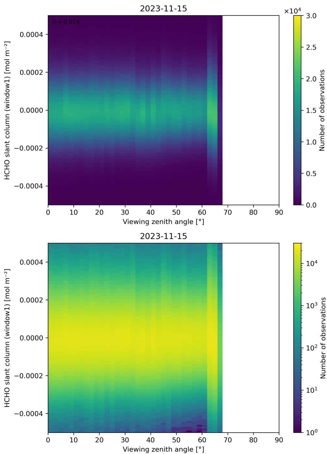
Figure 188: Scatter density plot of “Viewing zenith angle” against “HCHO slant column (window1)” for 2023-11-14 to 2023-11-16.
