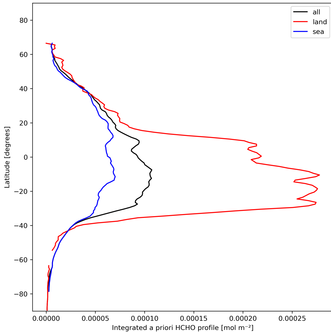
Figure 29: Zonal average of “Integrated a priori HCHO profile” for 2023-11-14 to 2023-11-16.
