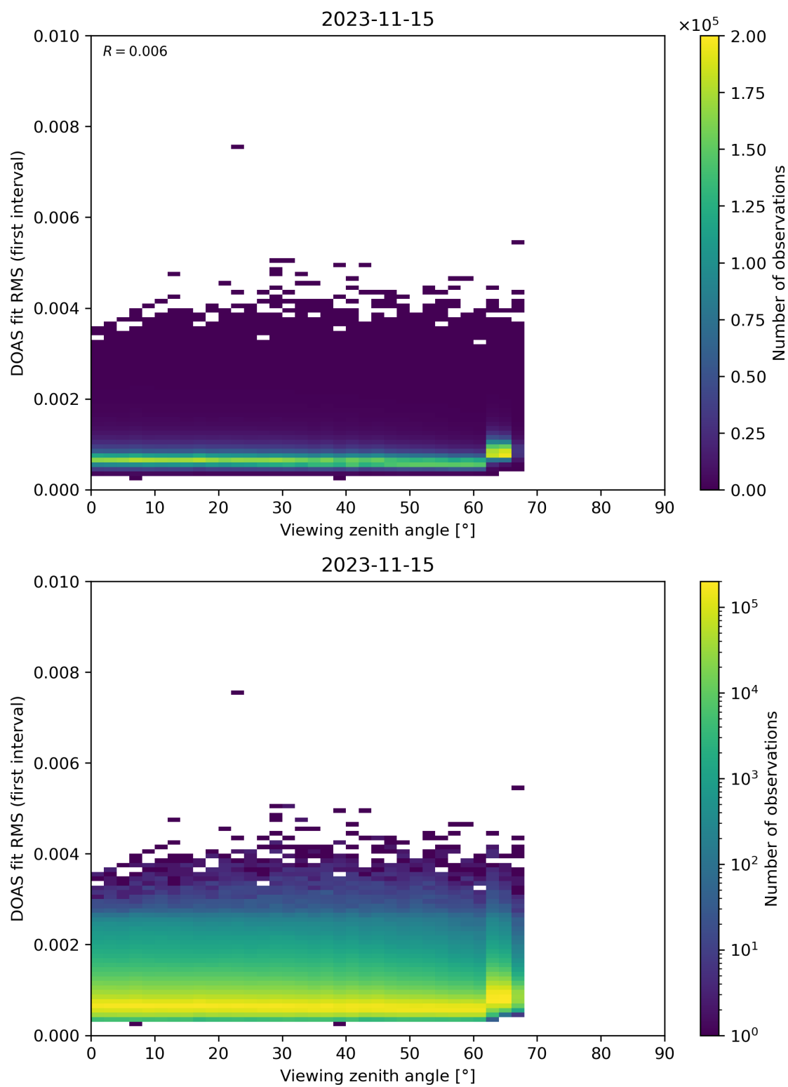
Figure 182: Scatter density plot of “Viewing zenith angle” against “DOAS fit RMS (first interval)” for 2023-11-14 to 2023-11-16.
