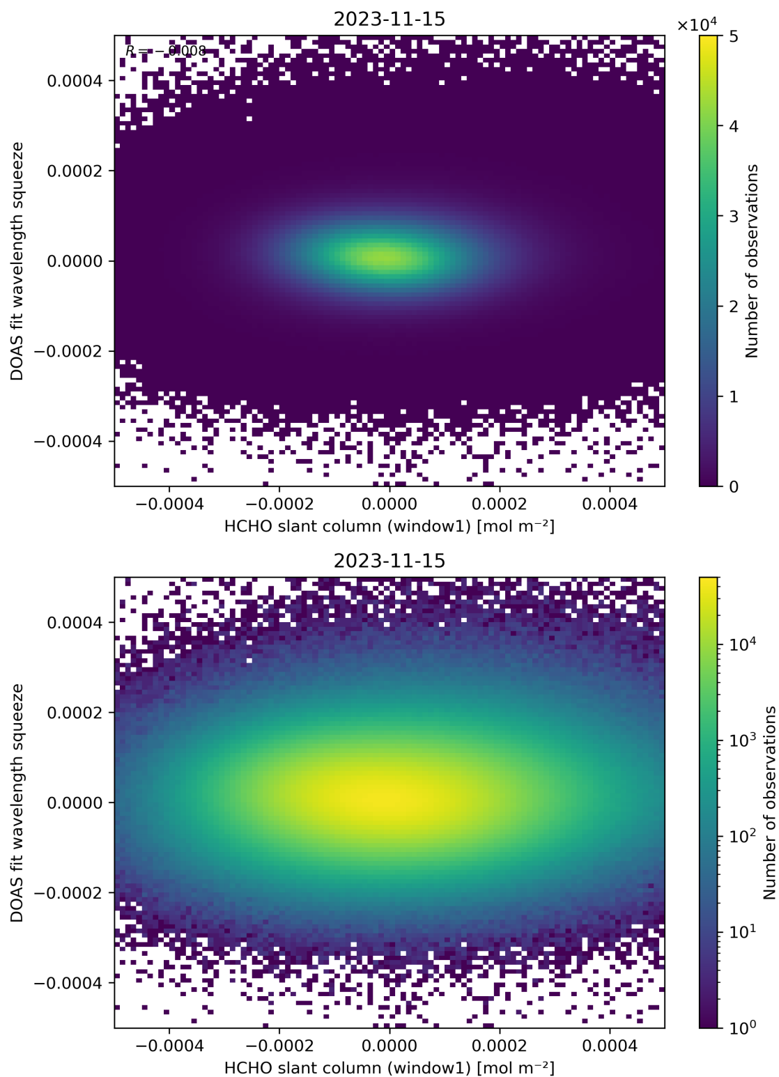
Figure 80: Scatter density plot of “HCHO slant column (window1)” against “DOAS fit wavelength squeeze” for 2023-11-14 to 2023-11-16.
