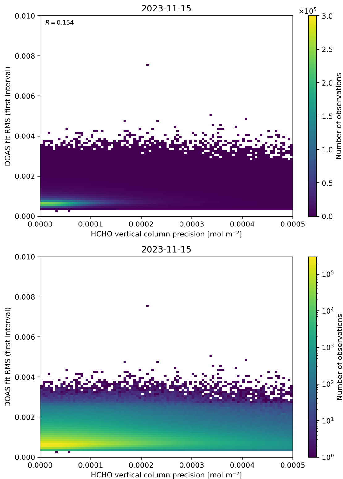
Figure 136: Scatter density plot of “HCHO vertical column precision” against “DOAS fit RMS (first interval)” for 2023-11-14 to 2023-11-16.
