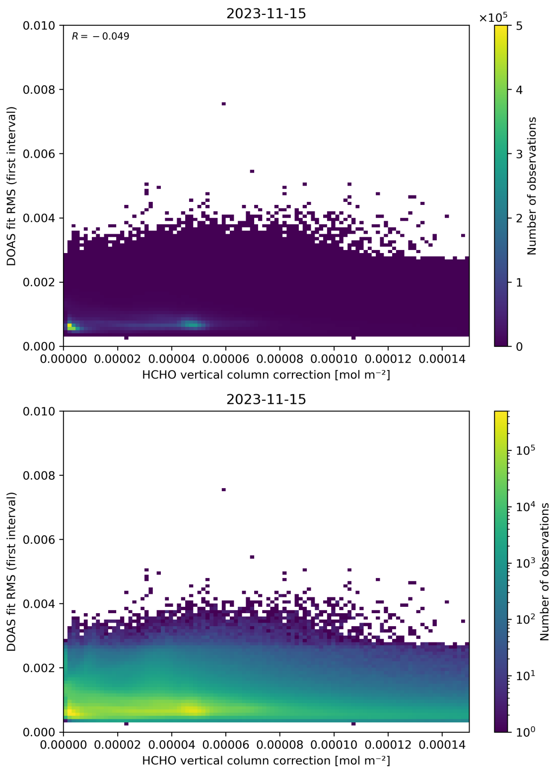
Figure 112: Scatter density plot of “HCHO vertical column correction” against “DOAS fit RMS (first interval)” for 2023-11-14 to 2023-11-16.
