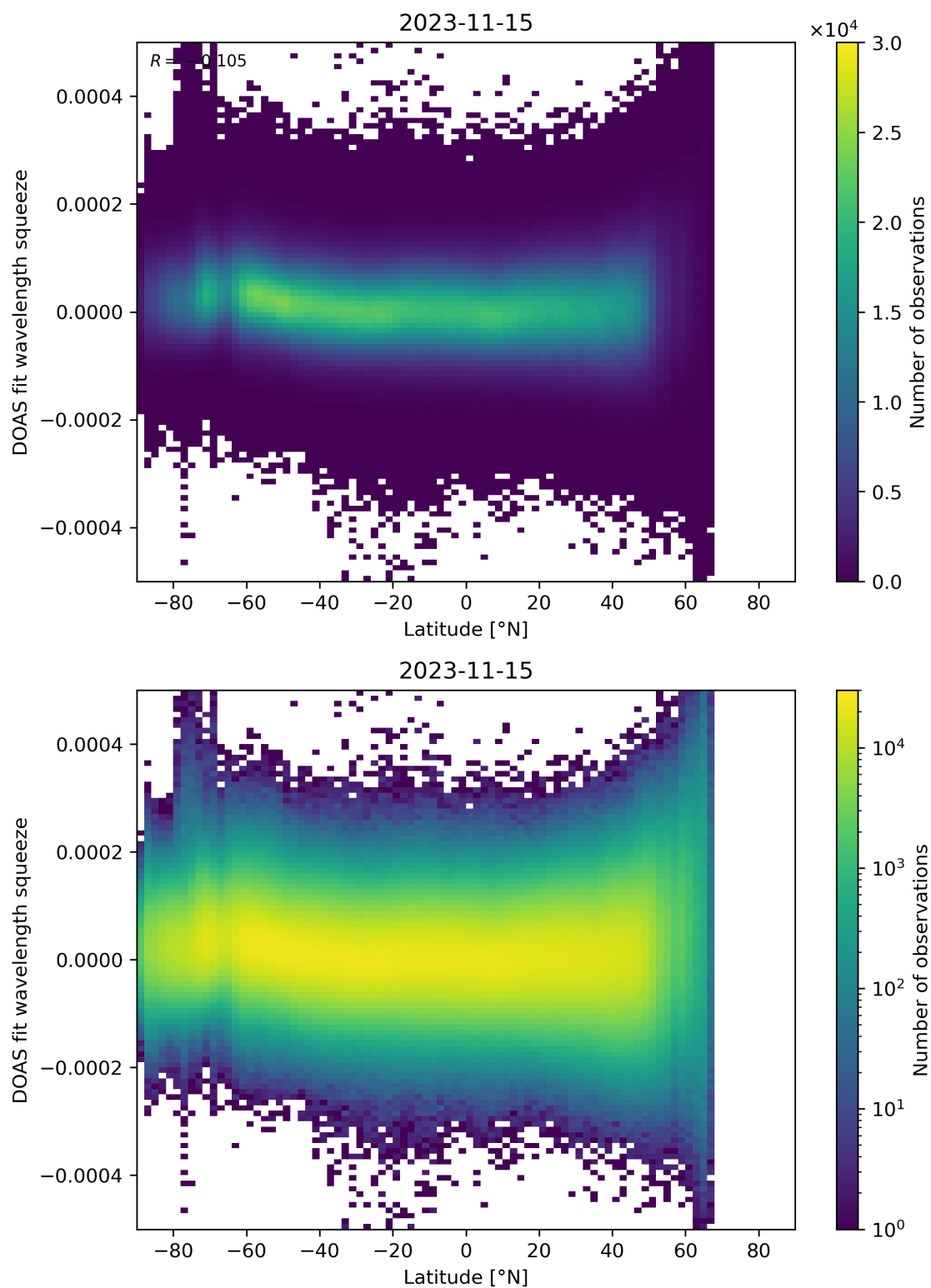
Figure 155: Scatter density plot of “Latitude” against “DOAS fit wavelength squeeze” for 2023-11-14 to 2023-11-16.
