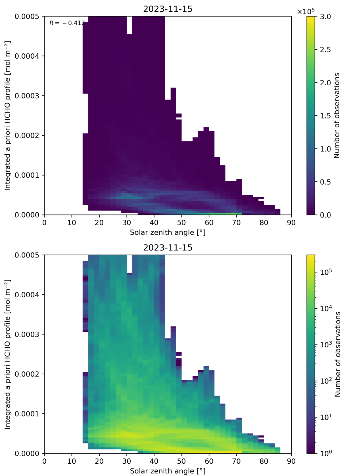
Figure 180: Scatter density plot of “Solar zenith angle” against “Integrated a priori HCHO profile” for 2023-11-14 to 2023-11-16.
