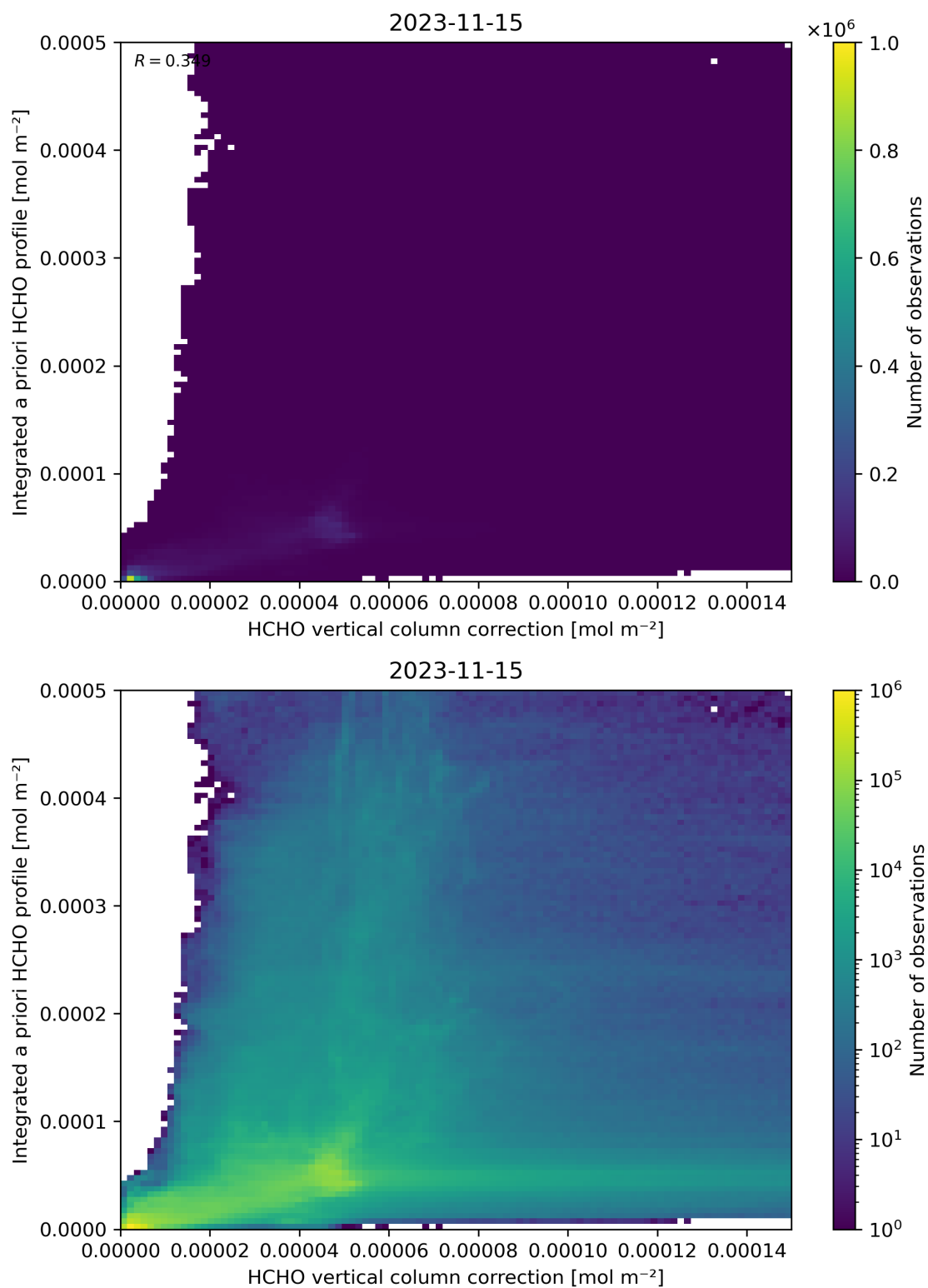
Figure 122: Scatter density plot of “HCHO vertical column correction” against “Integrated a priori HCHO profile” for 2023-11-14 to 2023-11-16.
