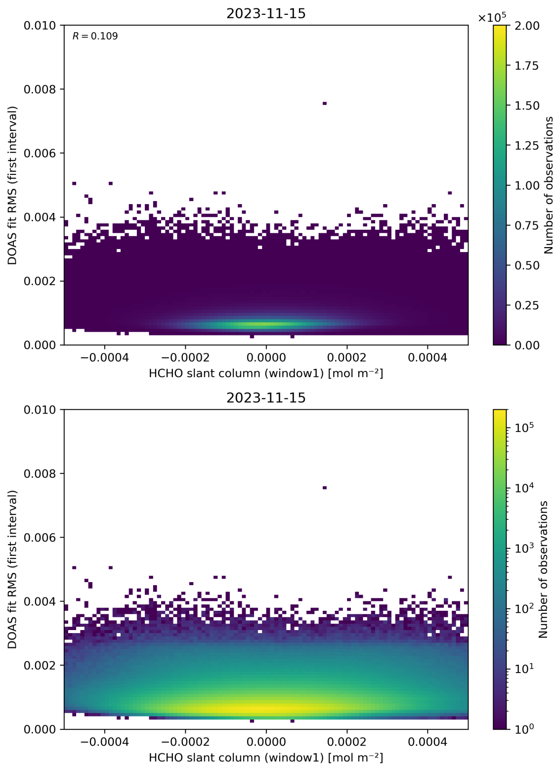
Figure 78: Scatter density plot of “HCHO slant column (window1)” against “DOAS fit RMS (first interval)” for 2023-11-14 to 2023-11-16.
