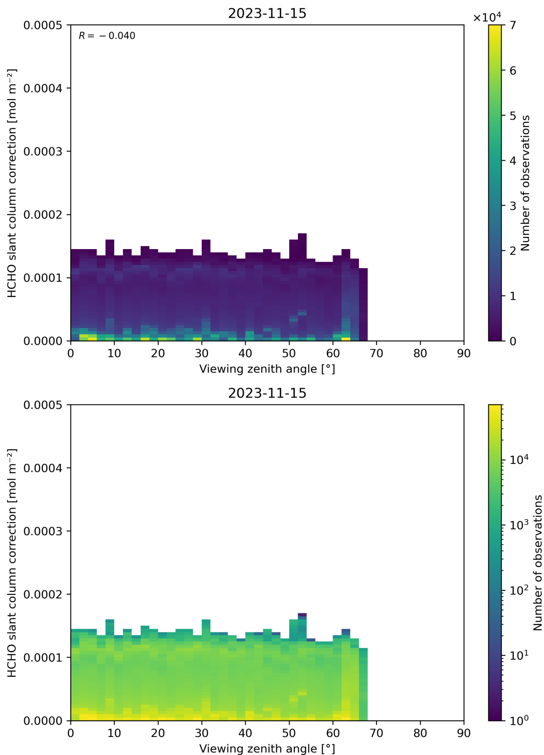
Figure 187: Scatter density plot of “Viewing zenith angle” against “HCHO slant column correction” for 2023-11-14 to 2023-11-16.
