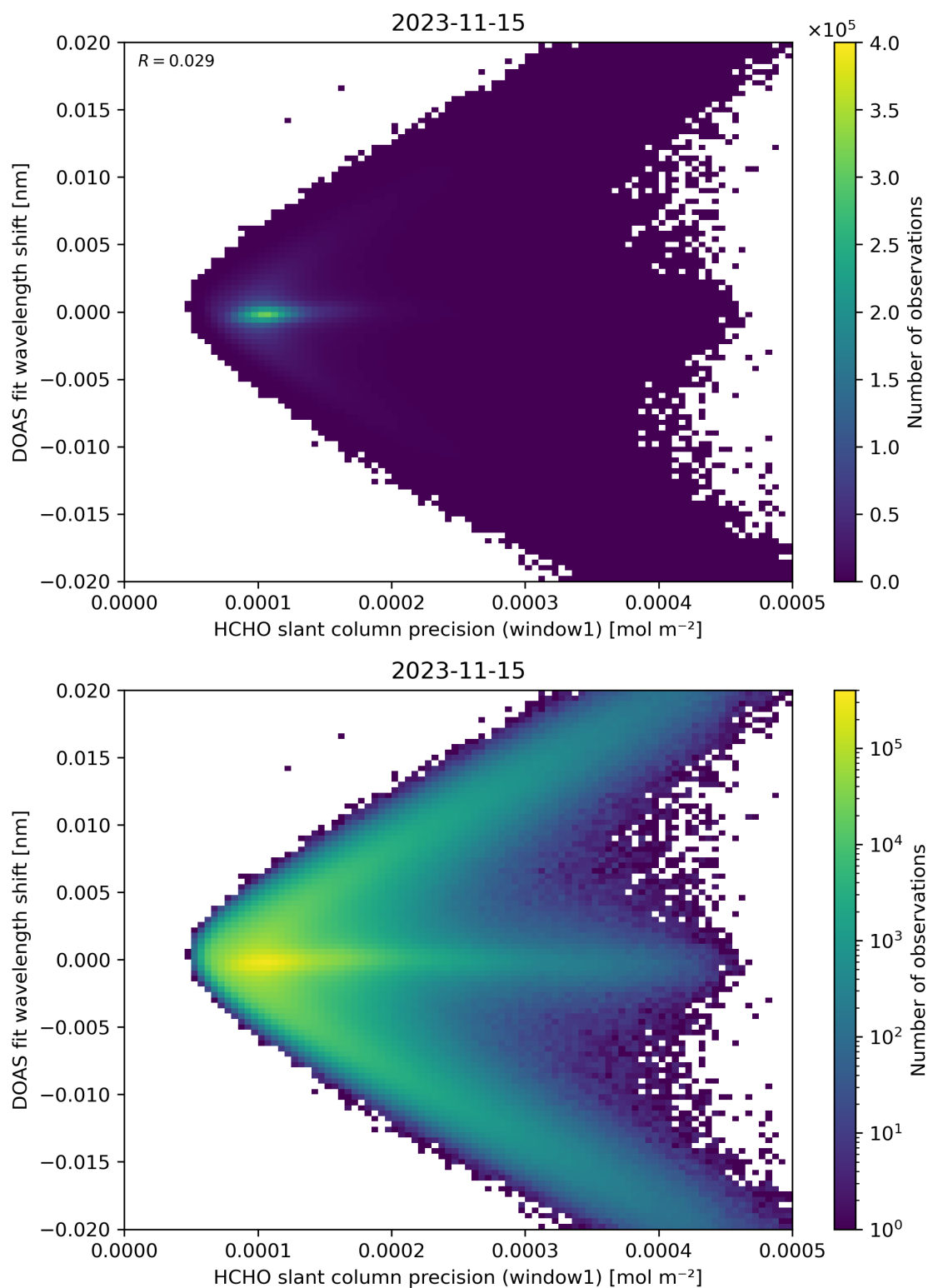
Figure 89: Scatter density plot of “HCHO slant column precision (window1)” against “DOAS fit wavelength shift” for 2023-11-14 to 2023-11-16.
