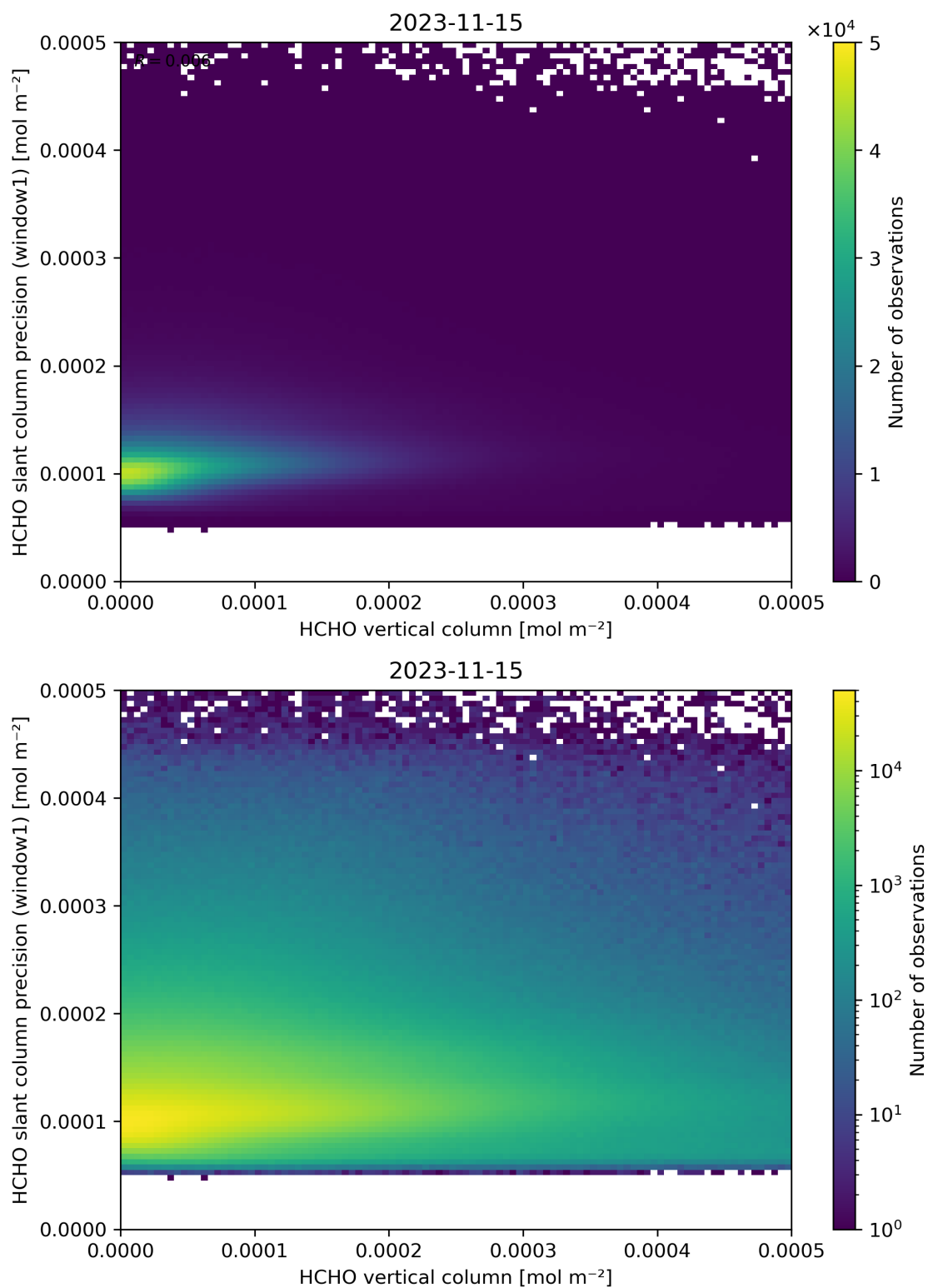
Figure 130: Scatter density plot of “HCHO vertical column” against “HCHO slant column precision (window1)” for 2023-11-14 to 2023-11-16.
