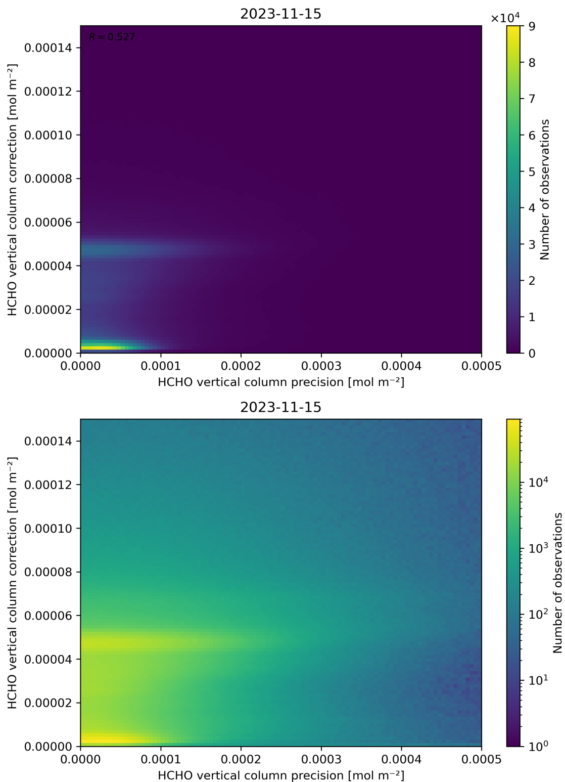
Figure 146: Scatter density plot of “HCHO vertical column precision” against “HCHO vertical column correction” for 2023-11-14 to 2023-11-16.
