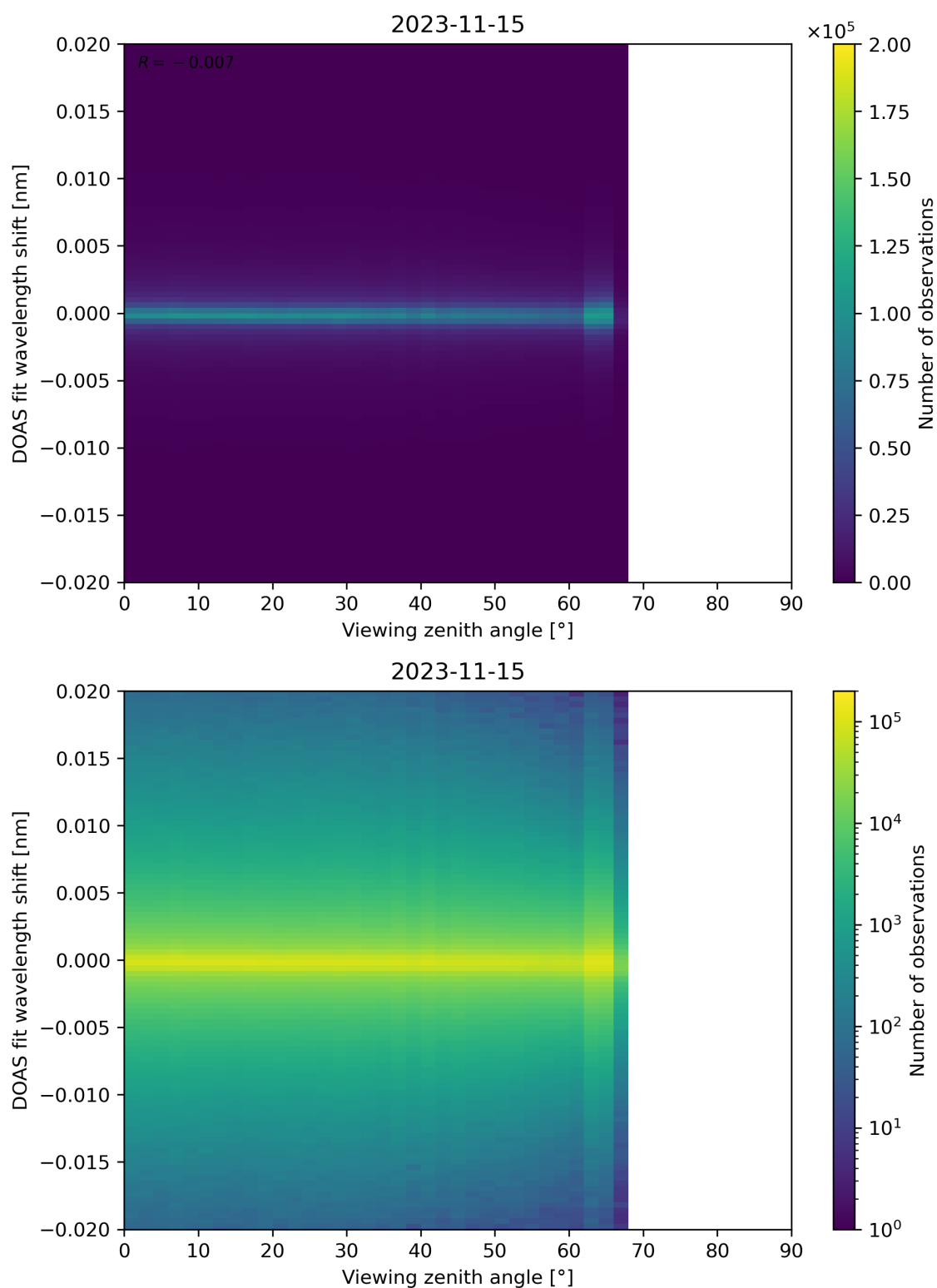
Figure 183: Scatter density plot of “Viewing zenith angle” against “DOAS fit wavelength shift” for 2023-11-14 to 2023-11-16.
