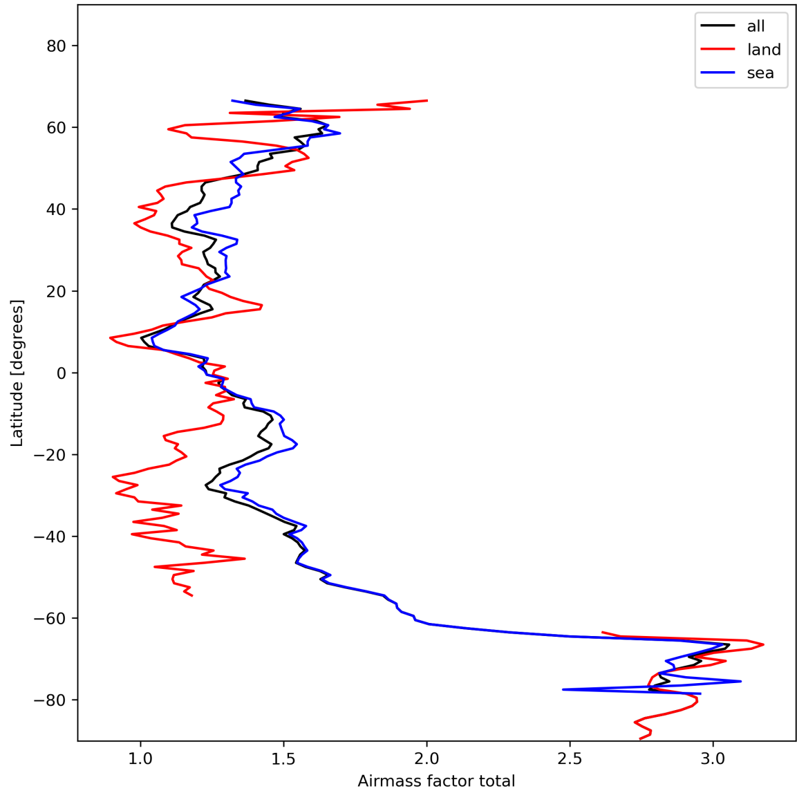
Figure 26: Zonal average of “Airmass factor total” for 2023-11-14 to 2023-11-16.
