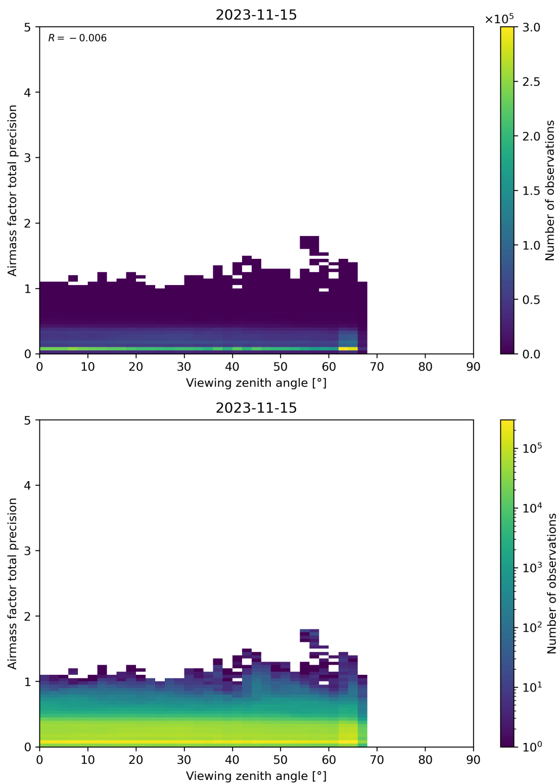
Figure 191: Scatter density plot of “Viewing zenith angle” against “Airmass factor total precision” for 2023-11-14 to 2023-11-16.
