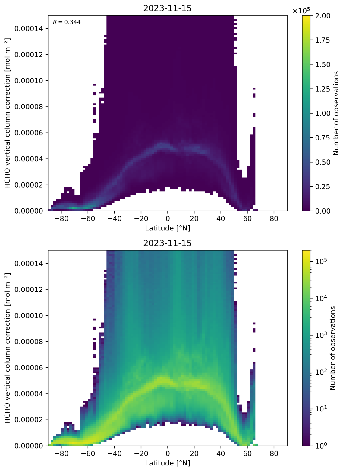
Figure 164: Scatter density plot of “Latitude” against “HCHO vertical column correction” for 2023-11-14 to 2023-11-16.
