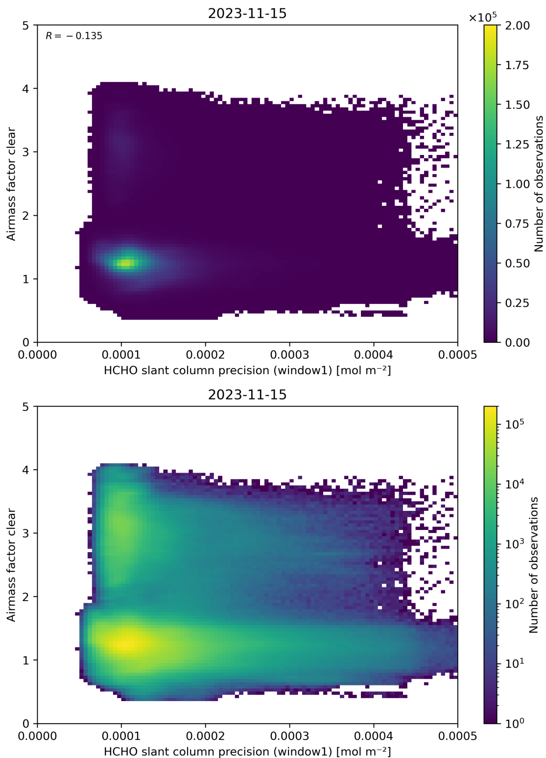
Figure 91: Scatter density plot of “HCHO slant column precision (window1)” against “Airmass factor clear” for 2023-11-14 to 2023-11-16.
