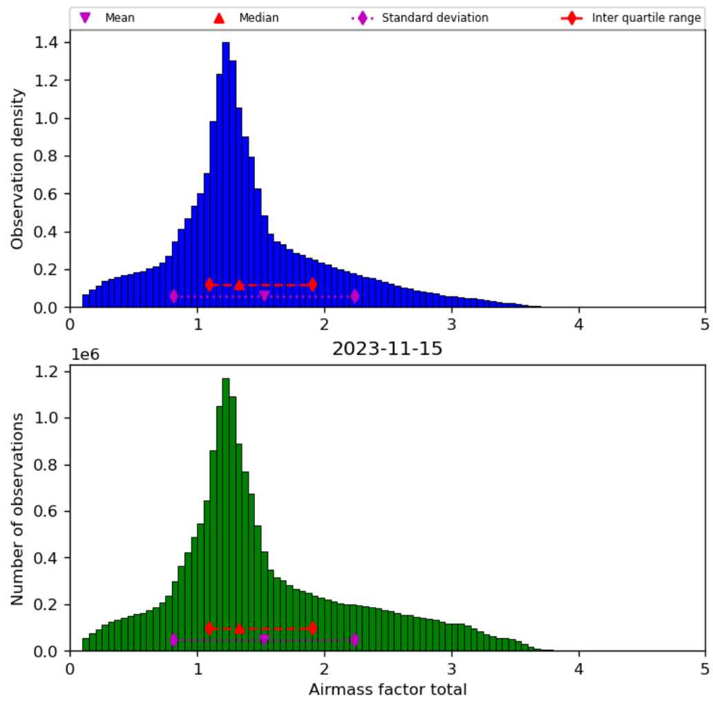
Figure 40: Histogram of “Airmass factor total” for 2023-11-14 to 2023-11-16
