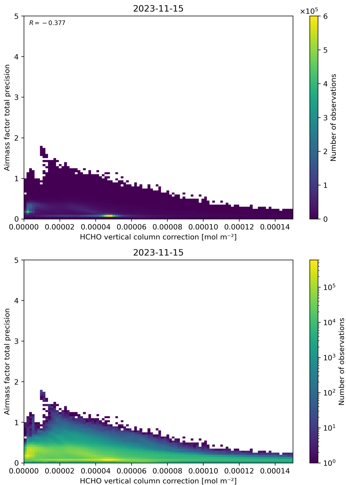
Figure 121: Scatter density plot of “HCHO vertical column correction” against “Airmass factor total precision” for 2023-11-14 to 2023-11-16.
