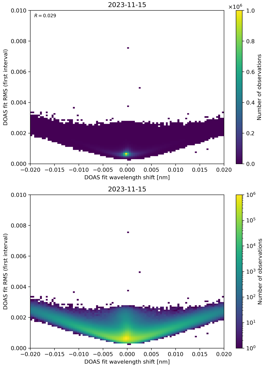
Figure 64: Scatter density plot of “DOAS fit wavelength shift” against “DOAS fit RMS (first interval)” for 2023-11-14 to 2023-11-16.
