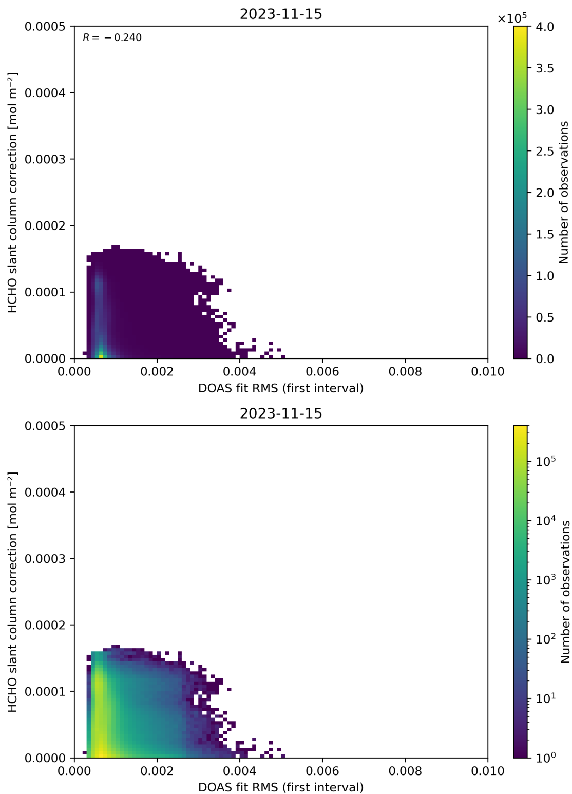
Figure 63: Scatter density plot of “DOAS fit RMS (first interval)” against “HCHO slant column correction” for 2023-11-14 to 2023-11-16.
