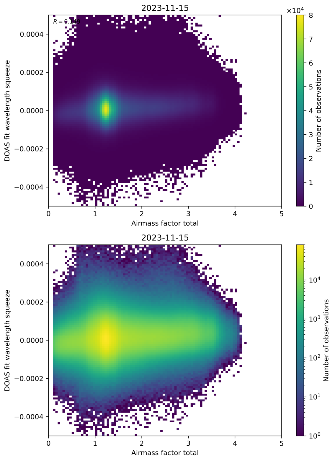
Figure 99: Scatter density plot of “Airmass factor total” against “DOAS fit wavelength squeeze” for 2023-11-14 to 2023-11-16.
