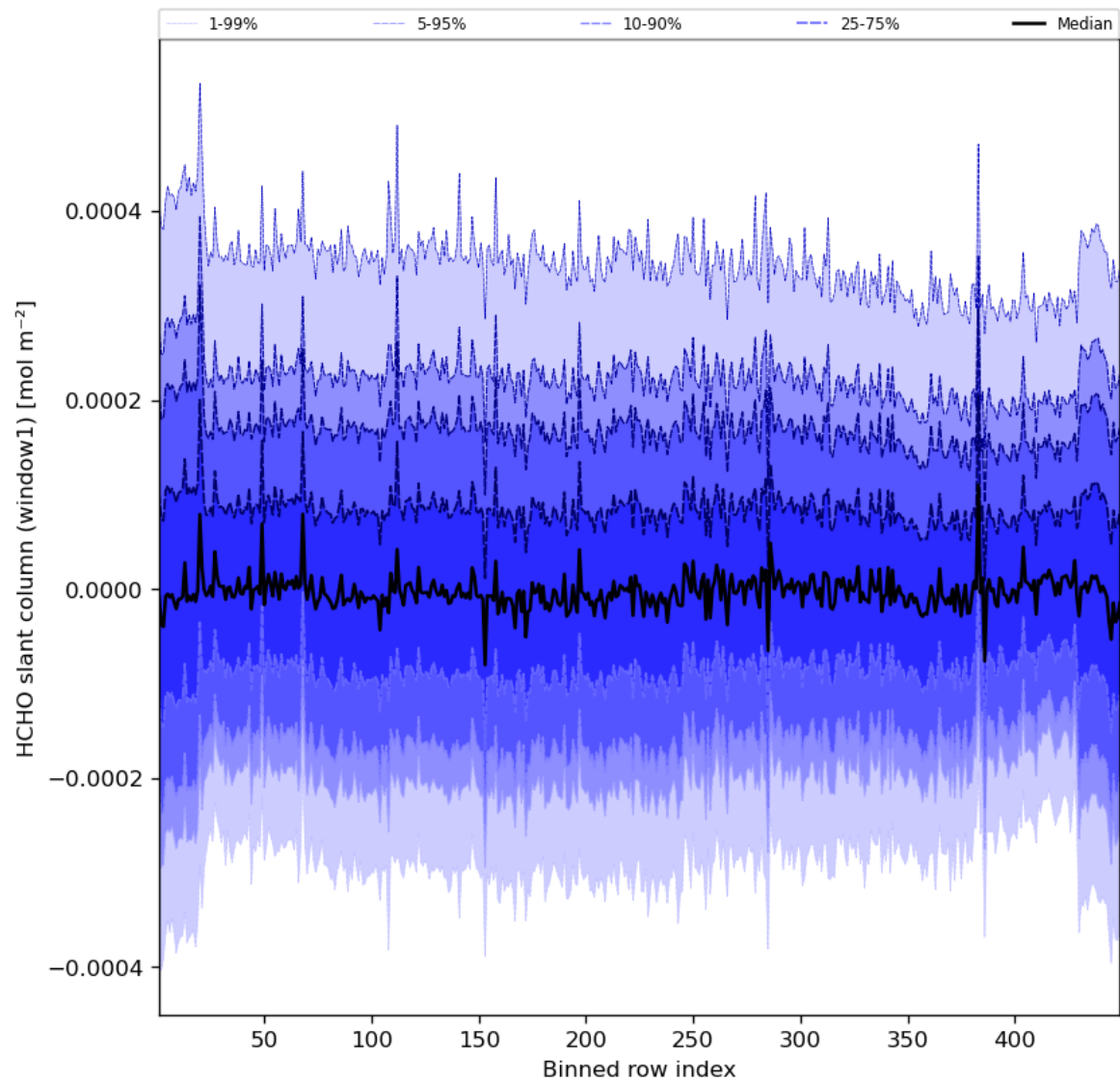
Figure 52: Along track statistics of “HCHO slant column (window1)” for 2023-11-14 to 2023-11-16
