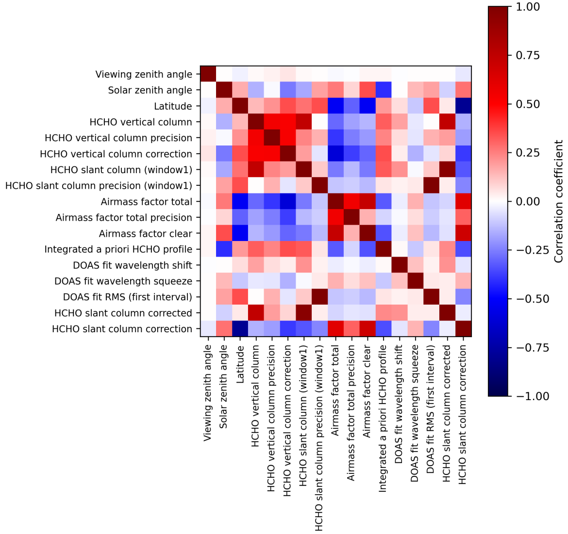
Figure 2: Map of correlation matrix for 2023-11-14 to 2023-11-16.
