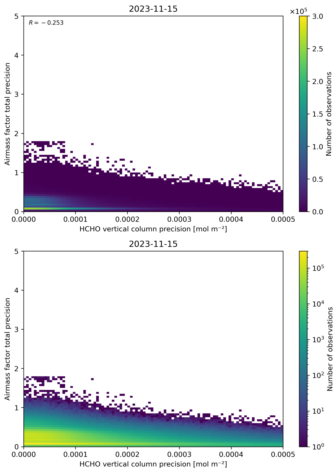
Figure 145: Scatter density plot of “HCHO vertical column precision” against “Airmass factor total precision” for 2023-11-14 to 2023-11-16.
