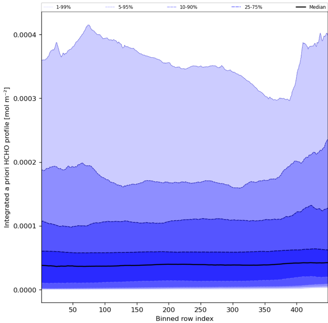
Figure 57: Along track statistics of "Integrated a priori HCHO profile" for 2023-11-14 to 2023-11-16
