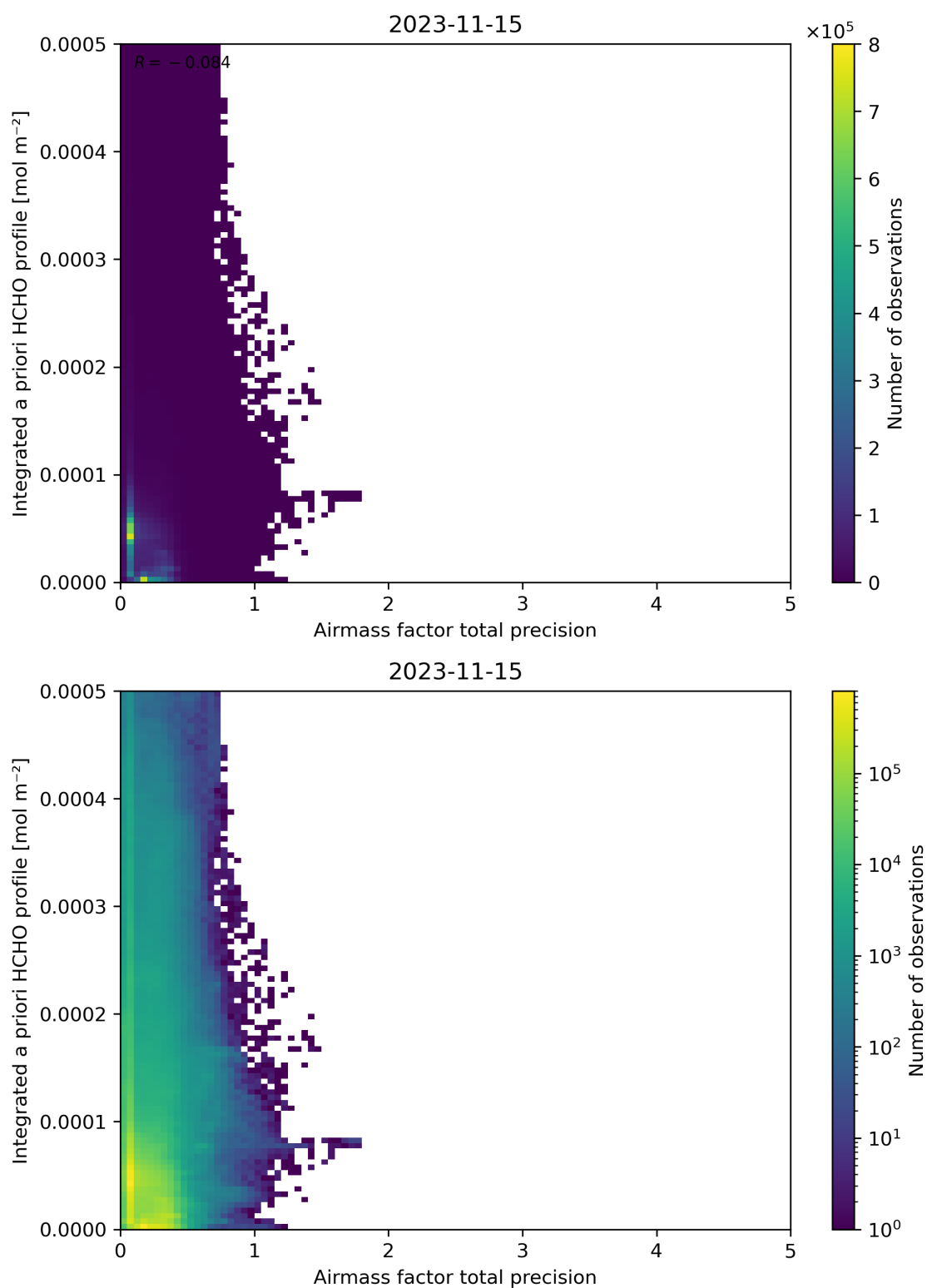
Figure 111: Scatter density plot of “Airmass factor total precision” against “Integrated a priori HCHO profile” for 2023-11-14 to 2023-11-16.
