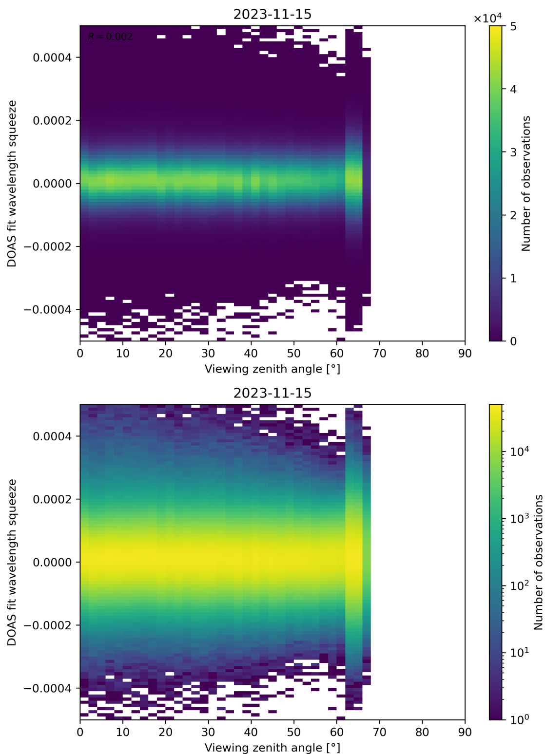
Figure 184: Scatter density plot of “Viewing zenith angle” against “DOAS fit wavelength squeeze” for 2023-11-14 to 2023-11-16.
