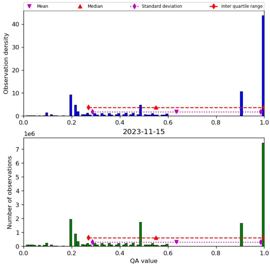
Figure 34: Histogram of “QA value” for 2023-11-14 to 2023-11-16
