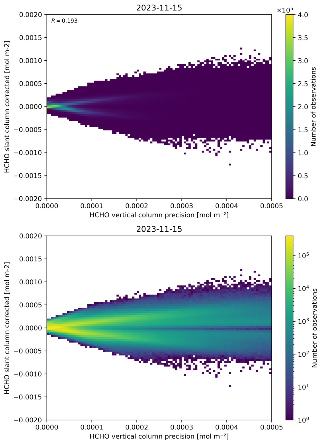
Figure 140: Scatter density plot of “HCHO vertical column precision” against “HCHO slant column corrected” for 2023-11-14 to 2023-11-16.
