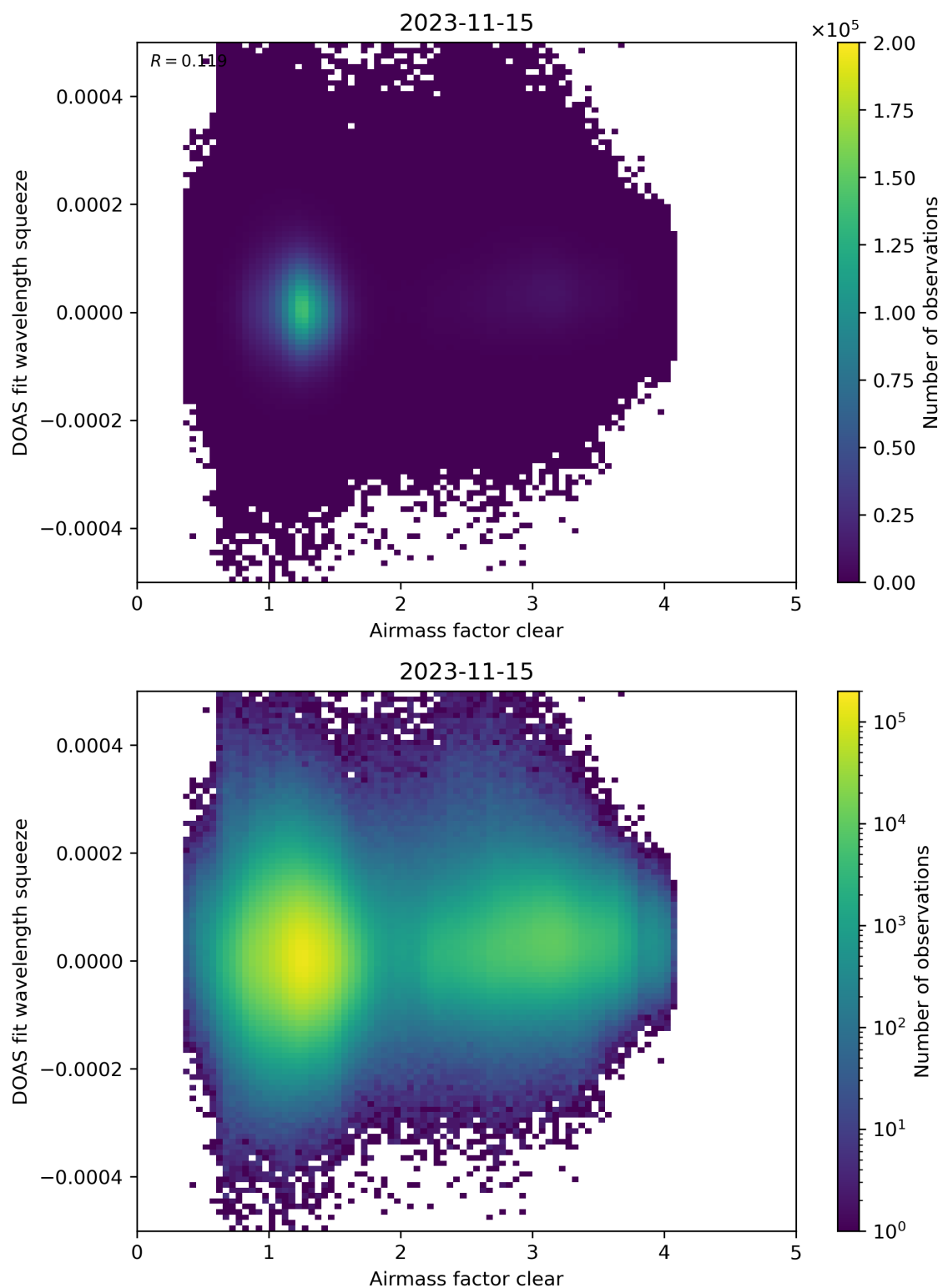
Figure 73: Scatter density plot of “Airmass factor clear” against “DOAS fit wavelength squeeze” for 2023-11-14 to 2023-11-16.
