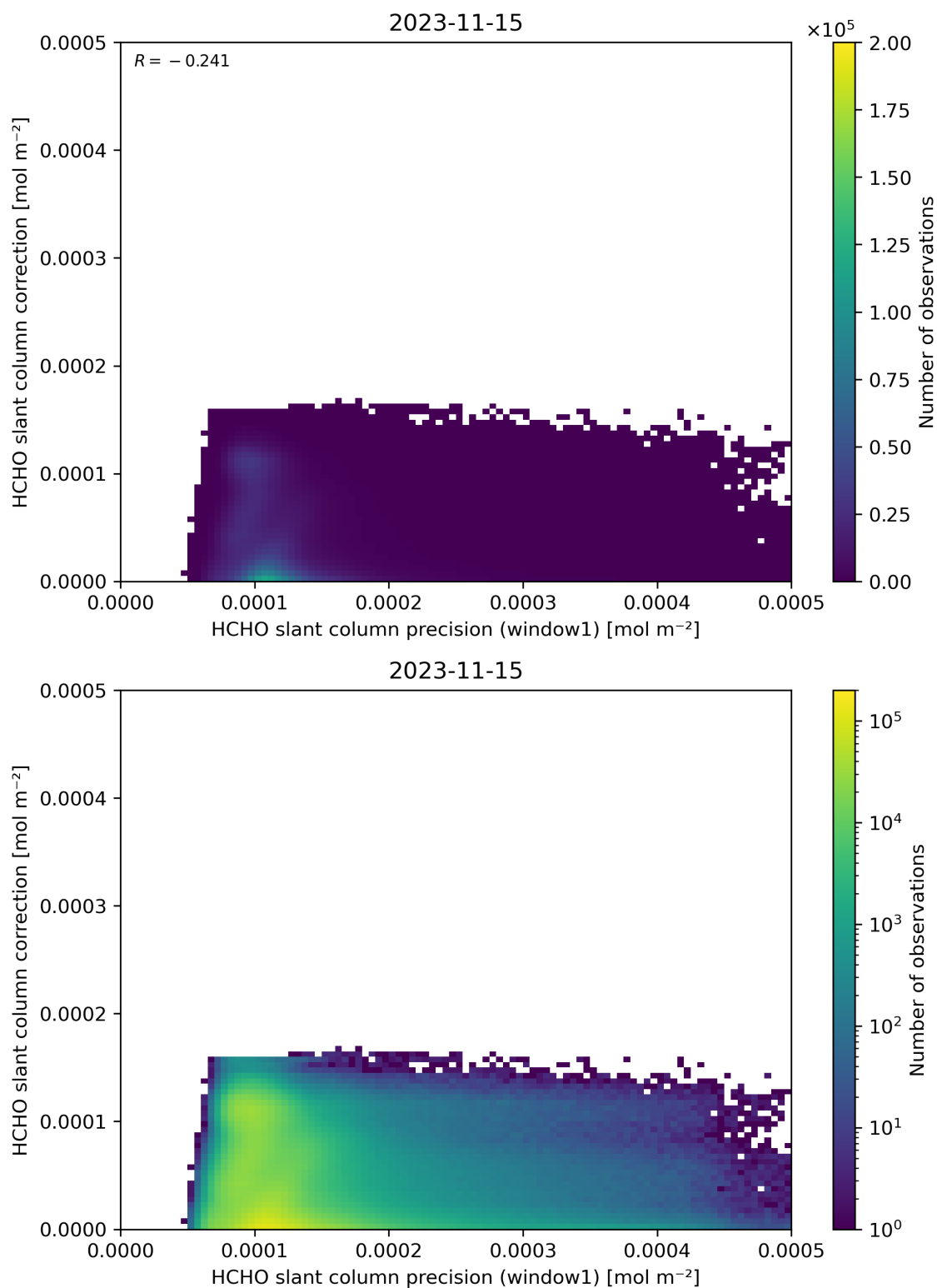
Figure 93: Scatter density plot of “HCHO slant column precision (window1)” against “HCHO slant column correction” for 2023-11-14 to 2023-11-16.
