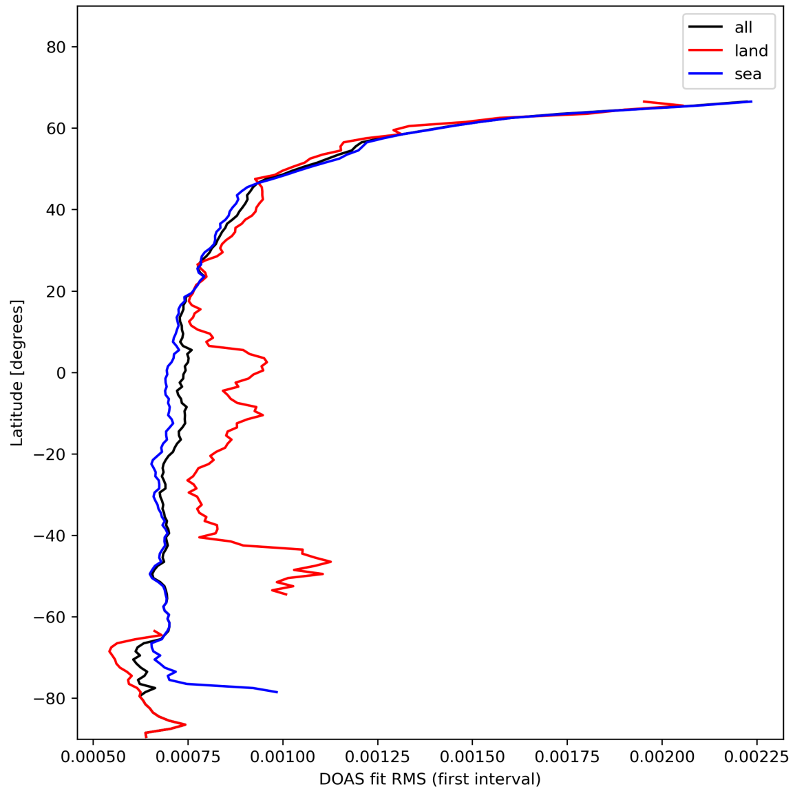
Figure 32: Zonal average of “DOAS fit RMS (first interval)” for 2023-11-14 to 2023-11-16.
