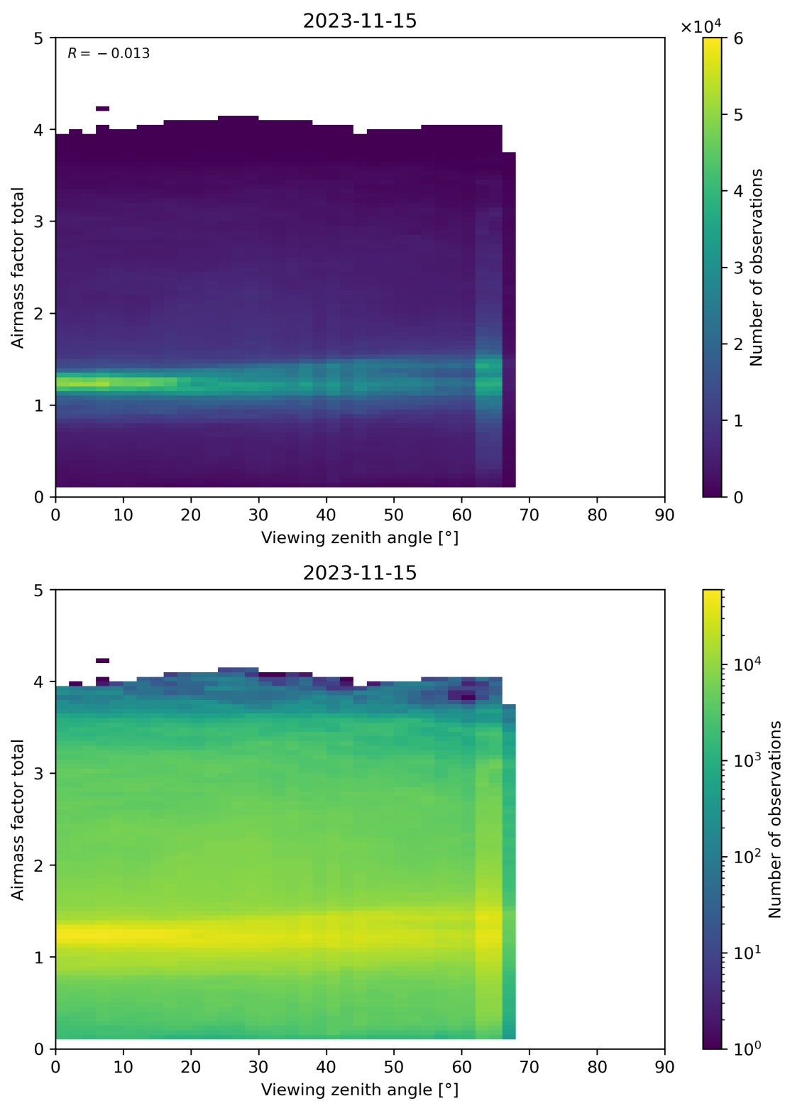
Figure 190: Scatter density plot of “Viewing zenith angle” against “Airmass factor total” for 2023-11-14 to 2023-11-16.
