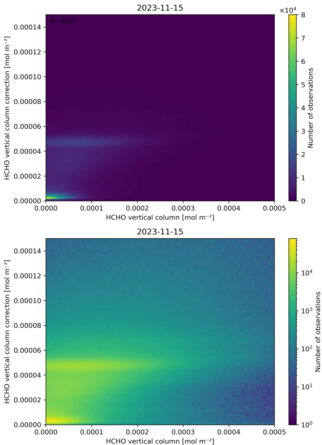
Figure 133: Scatter density plot of “HCHO vertical column” against “HCHO vertical column correction” for 2023-11-14 to 2023-11-16.
