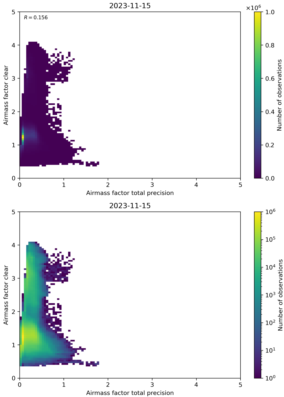
Figure 108: Scatter density plot of “Airmass factor total precision” against “Airmass factor clear” for 2023-11-14 to 2023-11-16.
