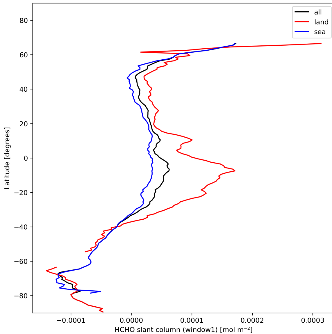
Figure 24: Zonal average of “HCHO slant column (window1)” for 2023-11-14 to 2023-11-16.
