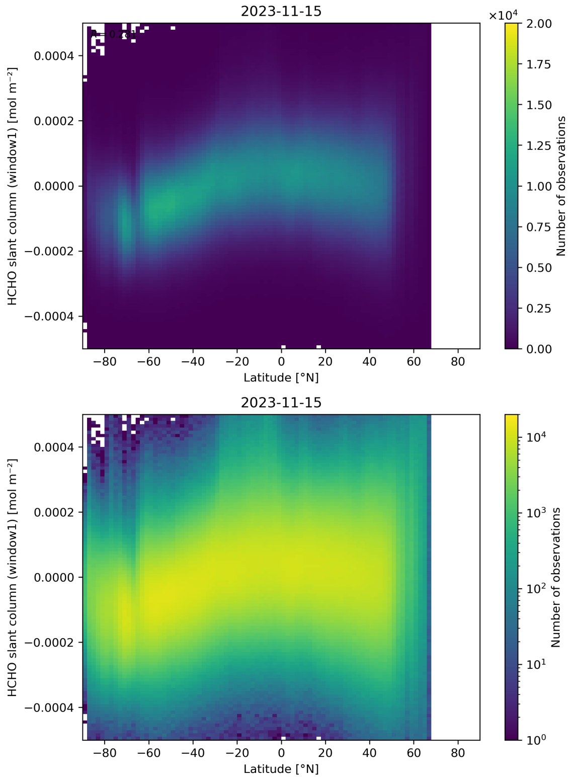
Figure 159: Scatter density plot of “Latitude” against “HCHO slant column (window1)” for 2023-11-14 to 2023-11-16.
