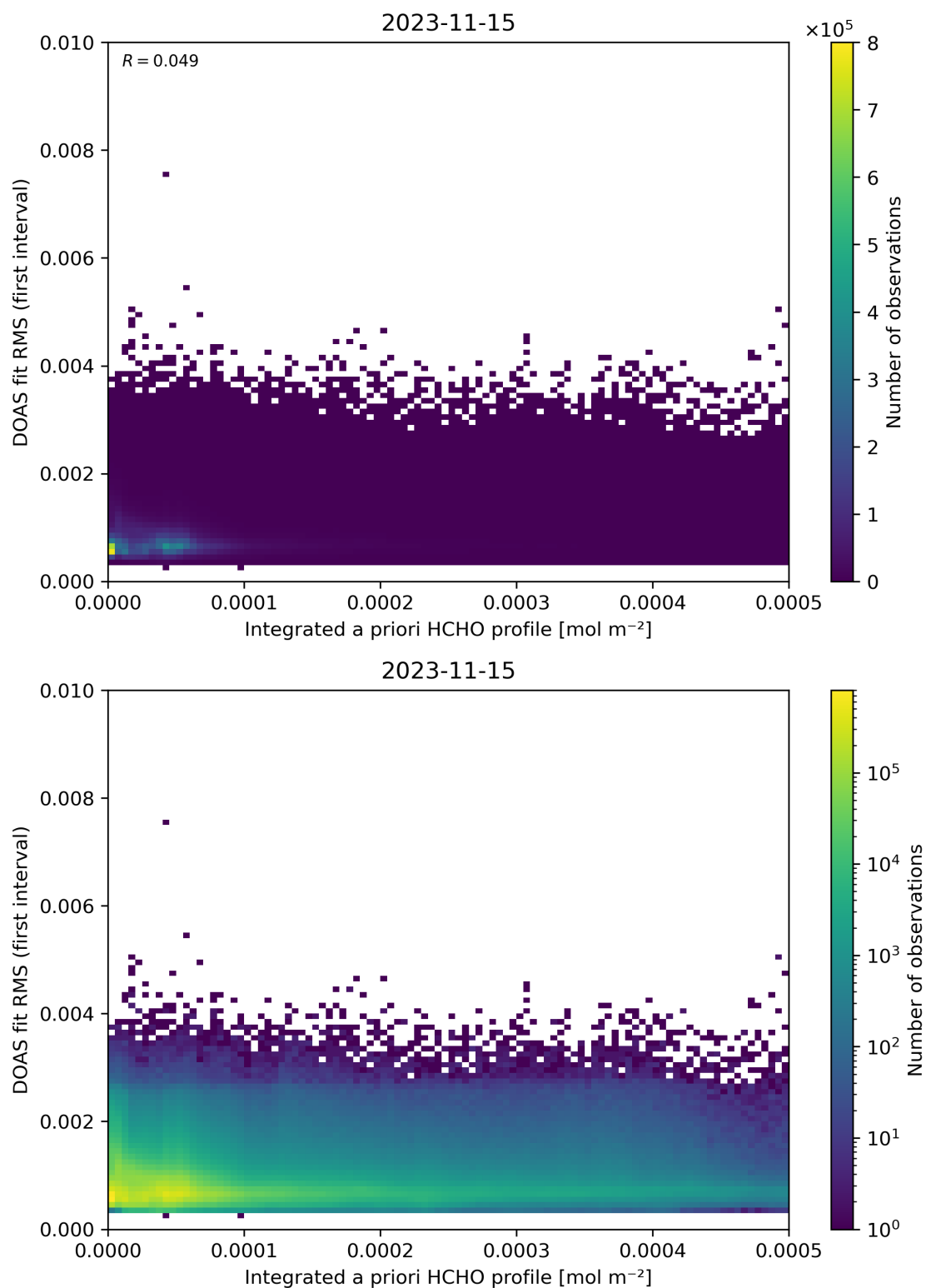
Figure 148: Scatter density plot of “Integrated a priori HCHO profile” against “DOAS fit RMS (first interval)” for 2023-11-14 to 2023-11-16.
