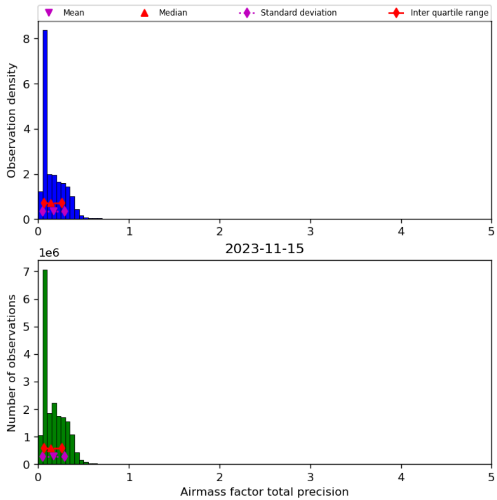
Figure 41: Histogram of “Airmass factor total precision” for 2023-11-14 to 2023-11-16
