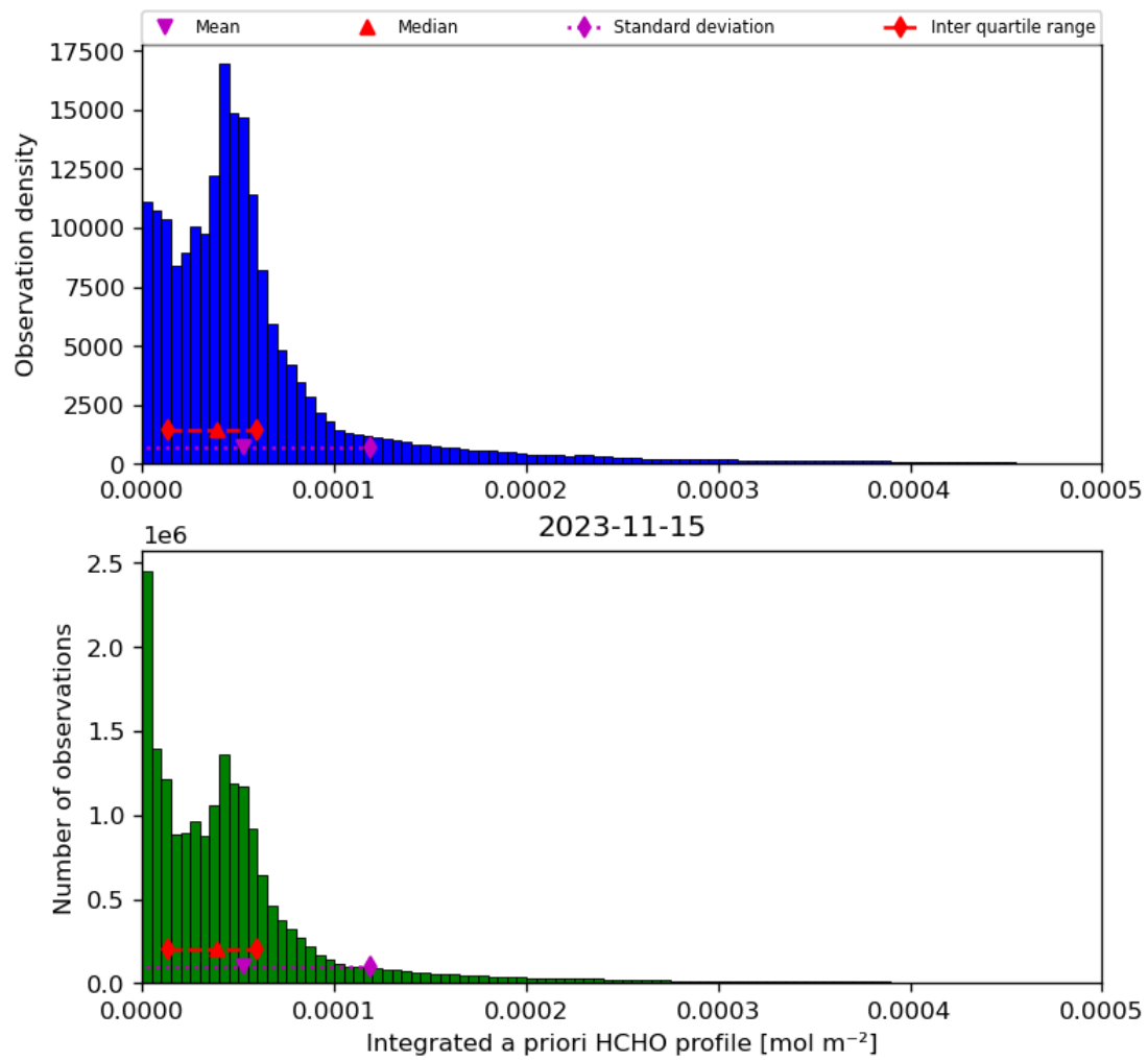
Figure 43: Histogram of “Integrated a priori HCHO profile” for 2023-11-14 to 2023-11-16
