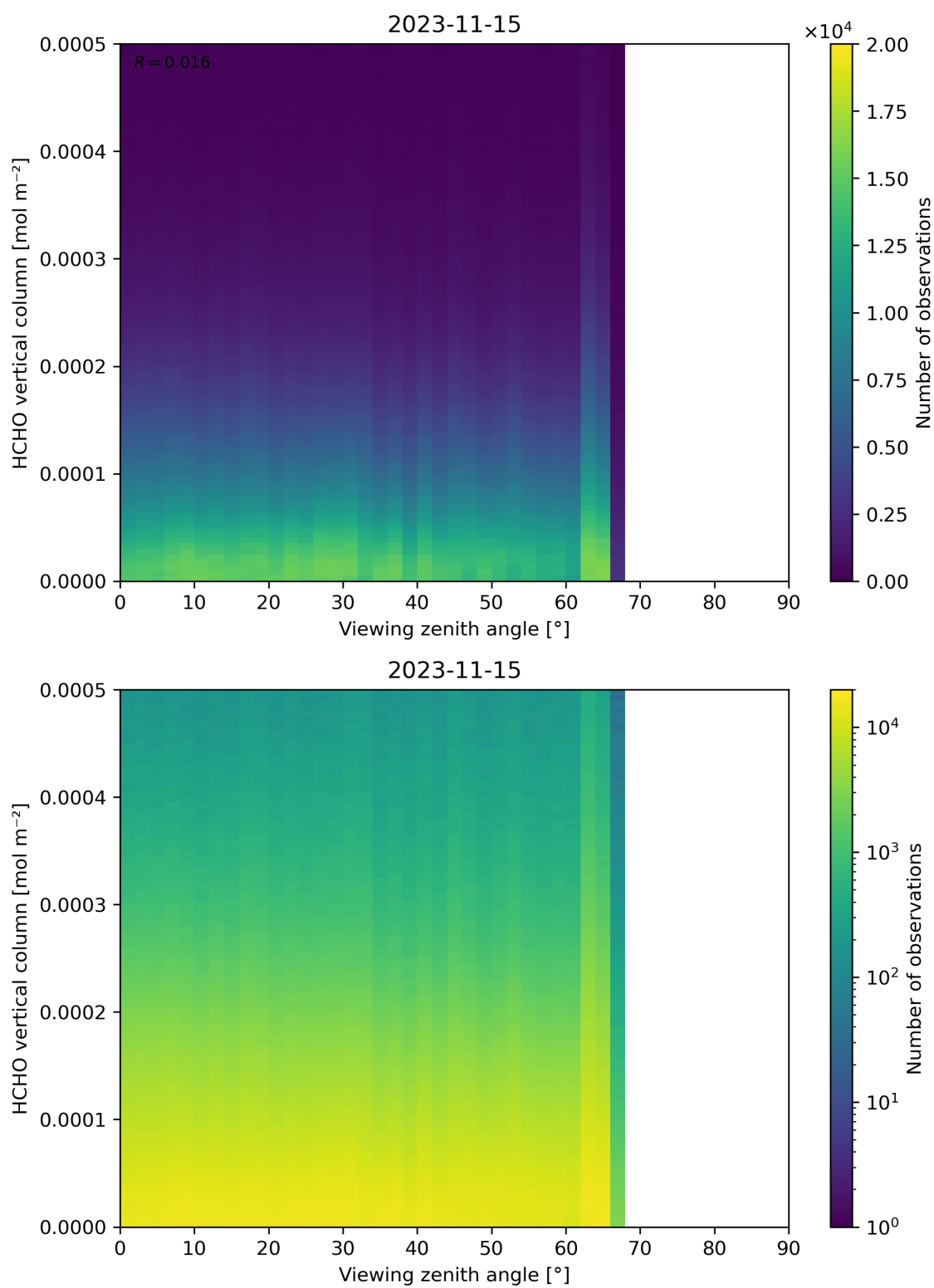
Figure 192: Scatter density plot of “Viewing zenith angle” against “HCHO vertical column” for 2023-11-14 to 2023-11-16.
