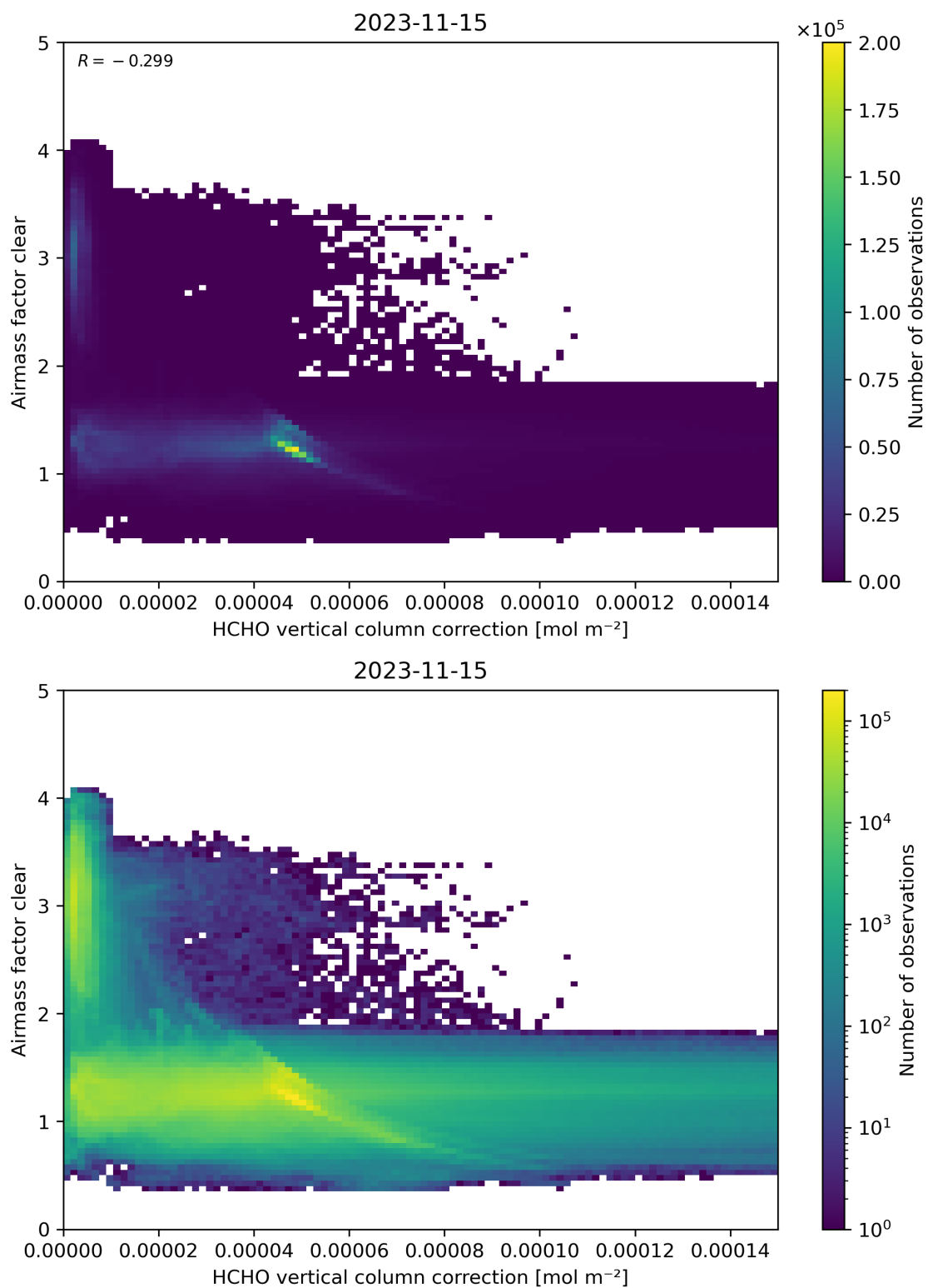
Figure 115: Scatter density plot of “HCHO vertical column correction” against “Airmass factor clear” for 2023-11-14 to 2023-11-16.
