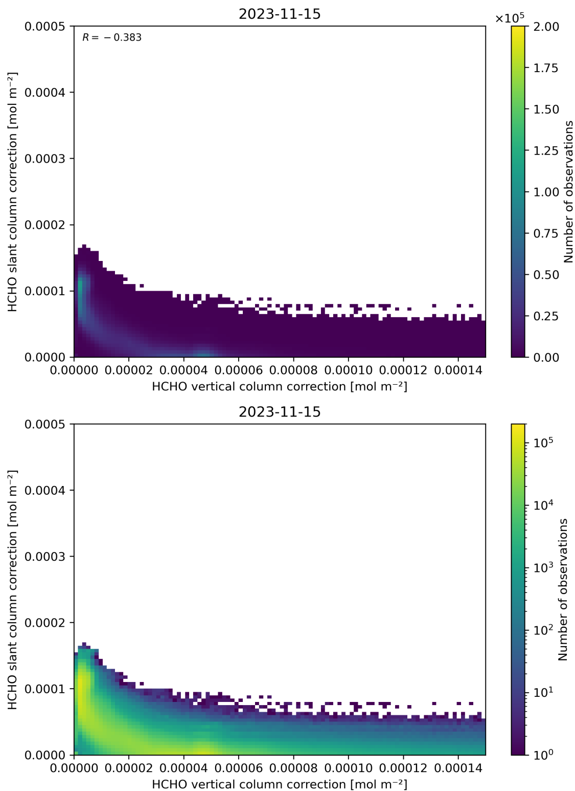
Figure 117: Scatter density plot of “HCHO vertical column correction” against “HCHO slant column correction” for 2023-11-14 to 2023-11-16.
