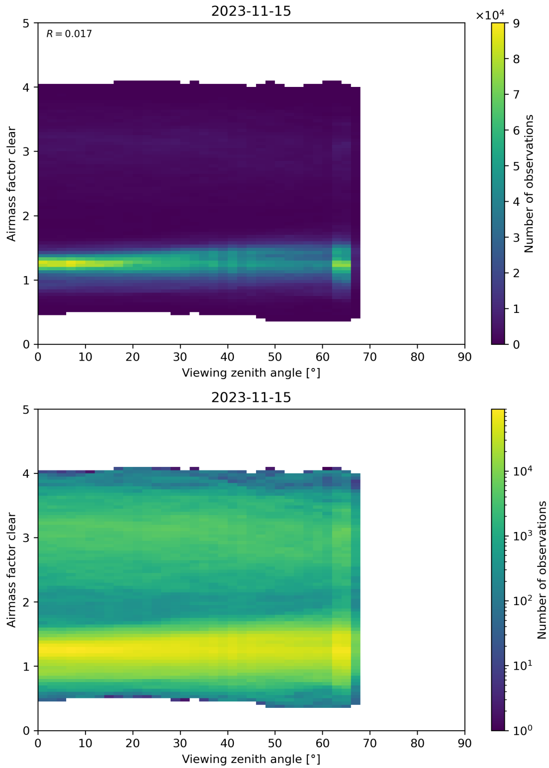
Figure 185: Scatter density plot of “Viewing zenith angle” against “Airmass factor clear” for 2023-11-14 to 2023-11-16.
