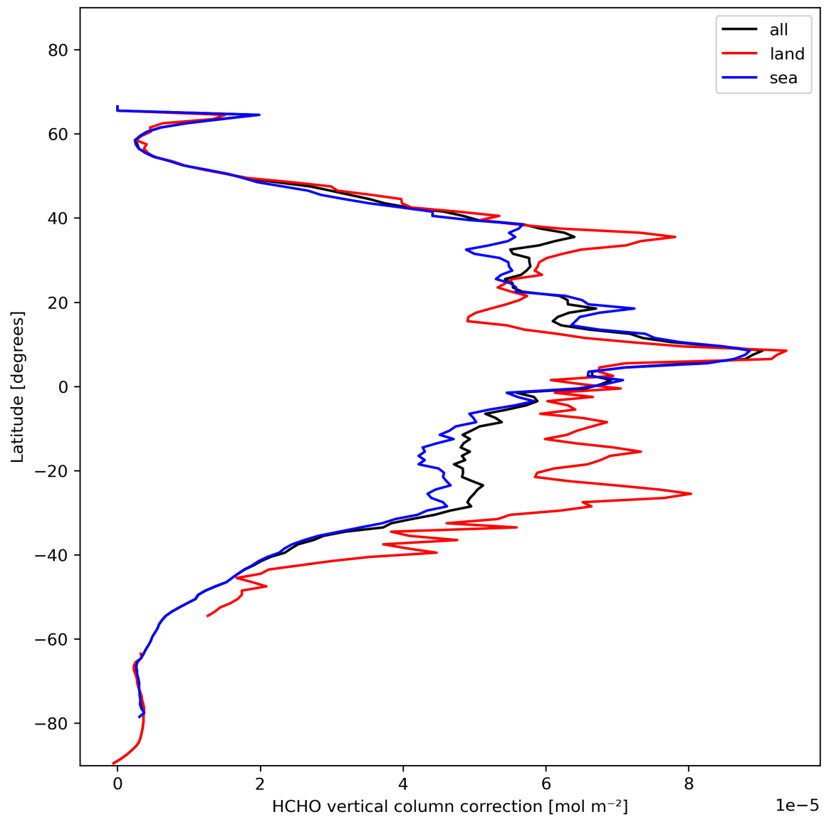
Figure 23: Zonal average of “HCHO vertical column correction” for 2023-11-14 to 2023-11-16.
