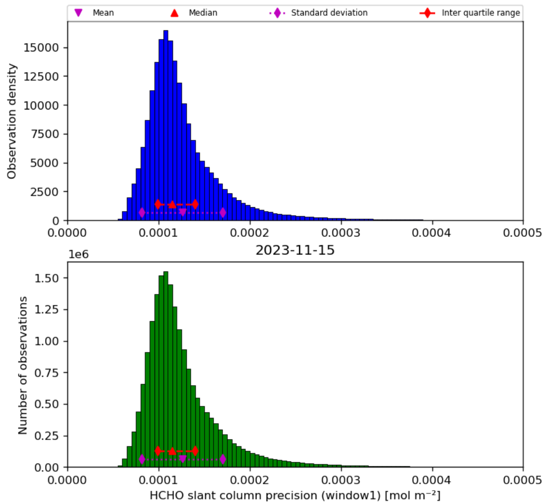
Figure 39: Histogram of “HCHO slant column precision (window1)” for 2023-11-14 to 2023-11-16
