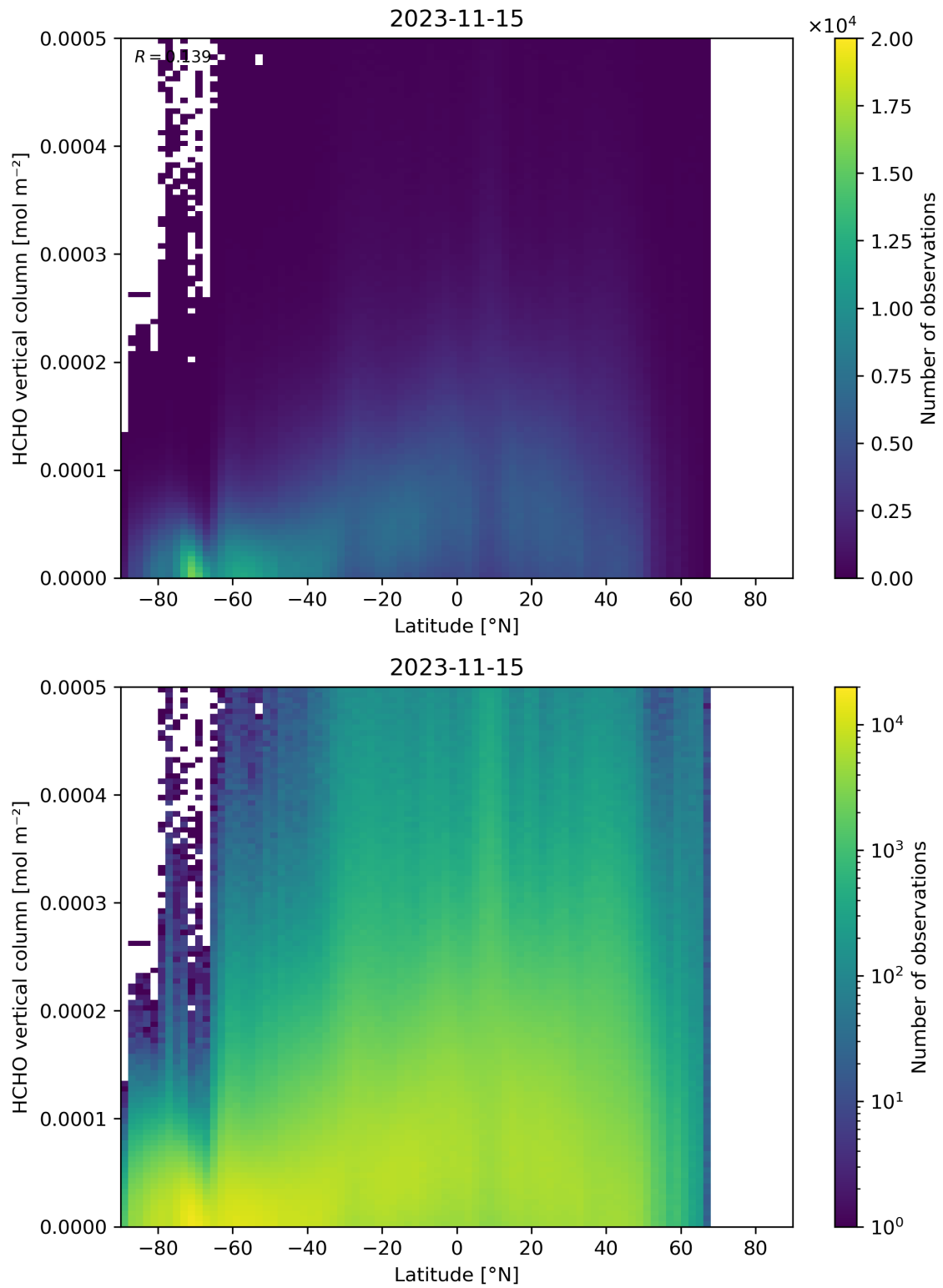
Figure 163: Scatter density plot of “Latitude” against “HCHO vertical column” for 2023-11-14 to 2023-11-16.
