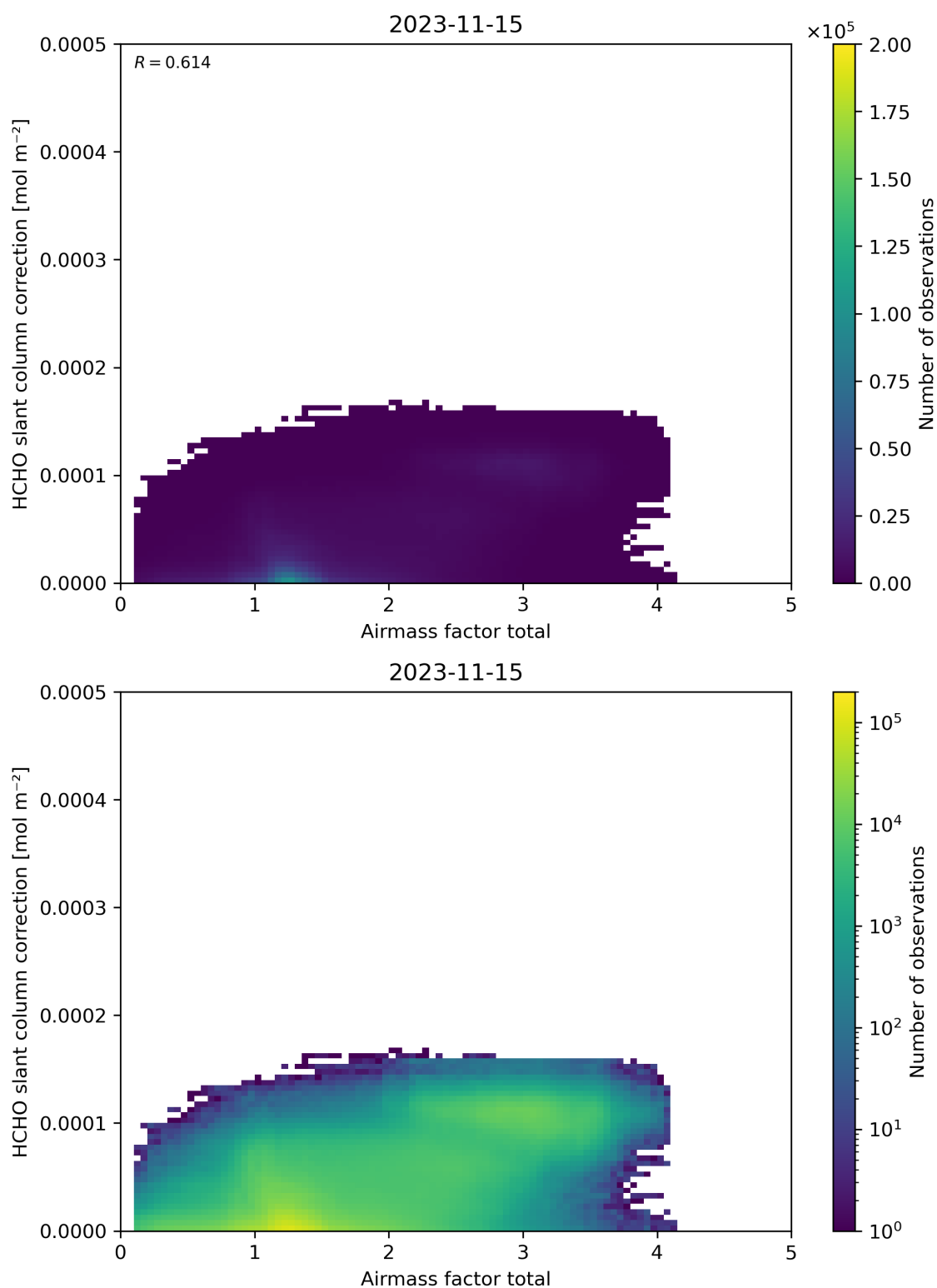
Figure 102: Scatter density plot of “Airmass factor total” against “HCHO slant column correction” for 2023-11-14 to 2023-11-16.
