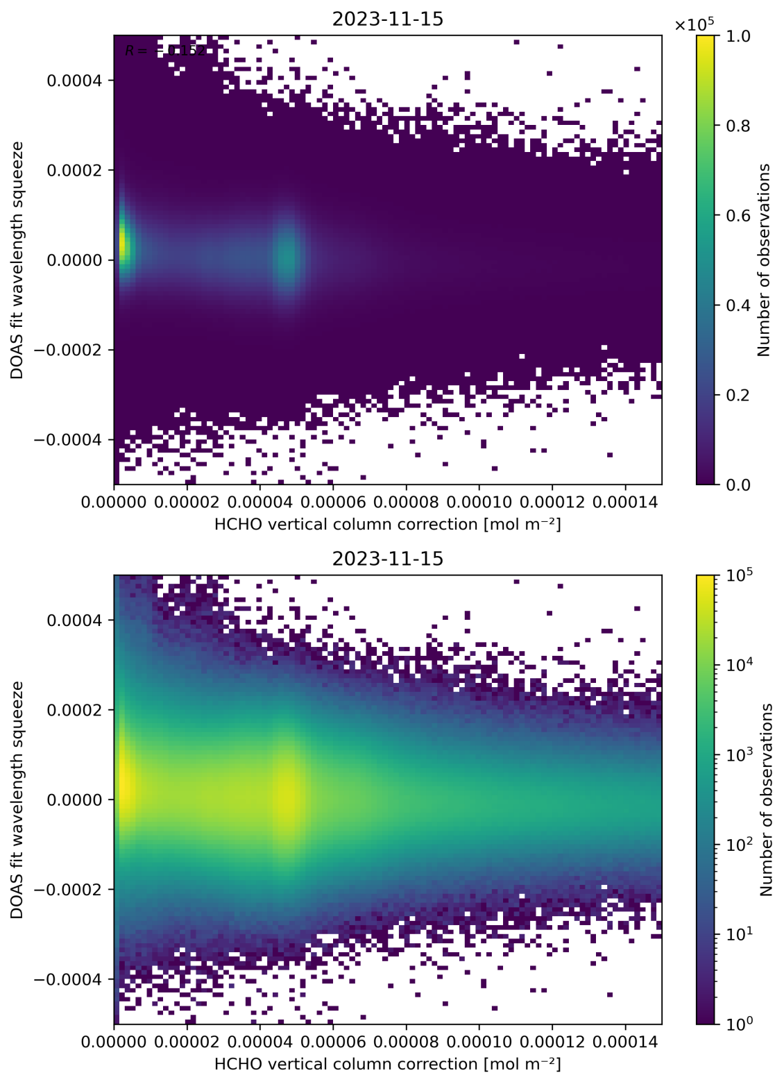
Figure 114: Scatter density plot of “HCHO vertical column correction” against “DOAS fit wavelength squeeze” for 2023-11-14 to 2023-11-16.
