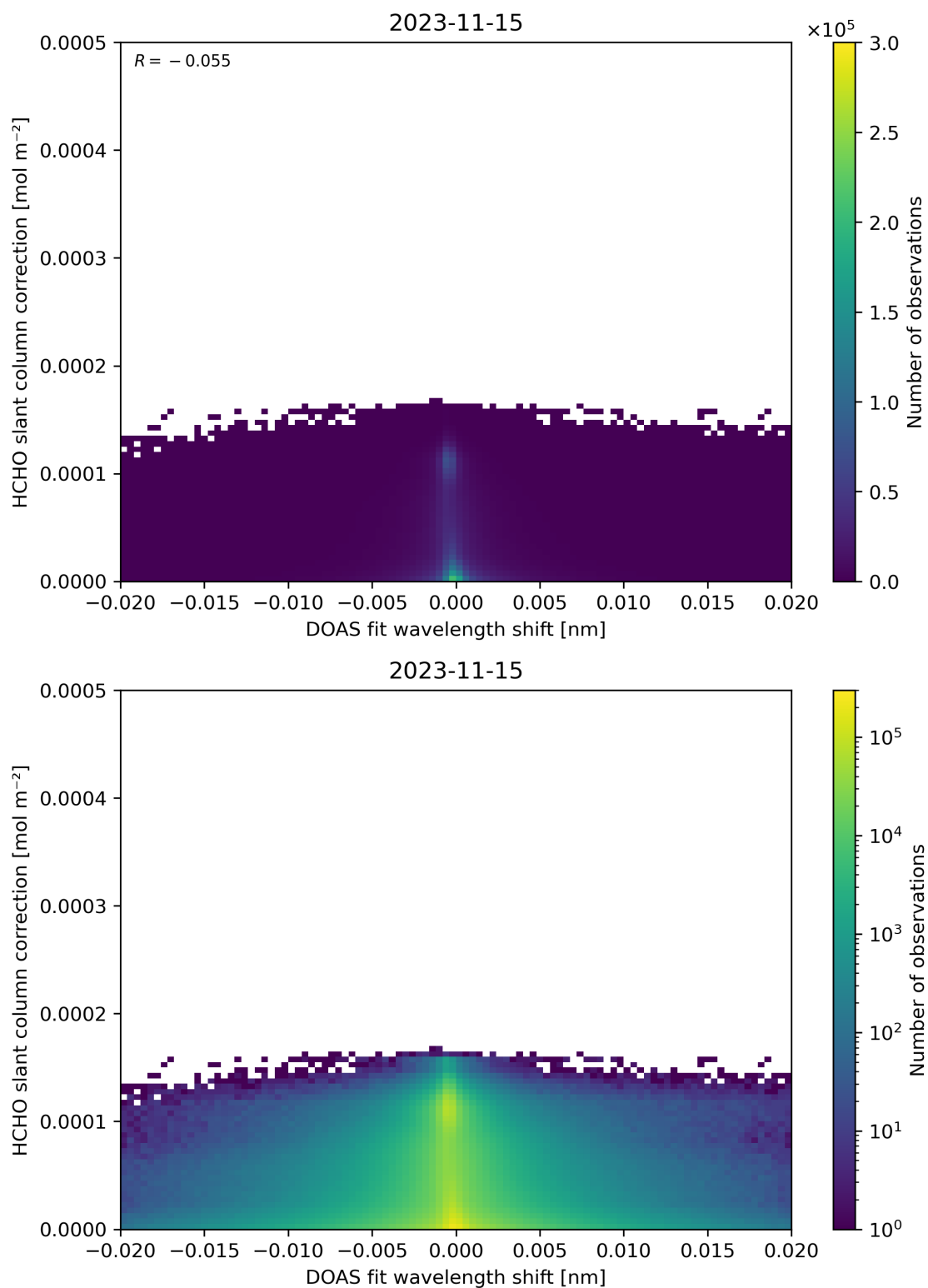
Figure 67: Scatter density plot of “DOAS fit wavelength shift” against “HCHO slant column correction” for 2023-11-14 to 2023-11-16.
