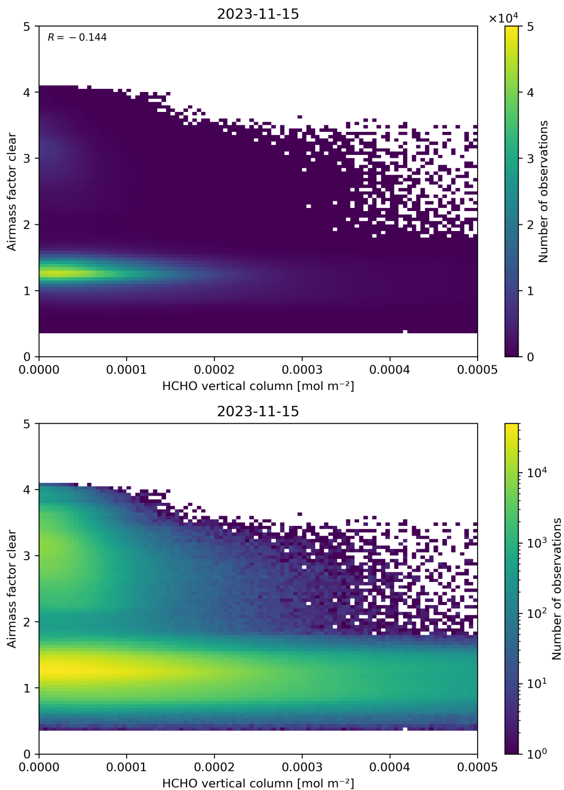
Figure 126: Scatter density plot of “HCHO vertical column” against “Airmass factor clear” for 2023-11-14 to 2023-11-16.
