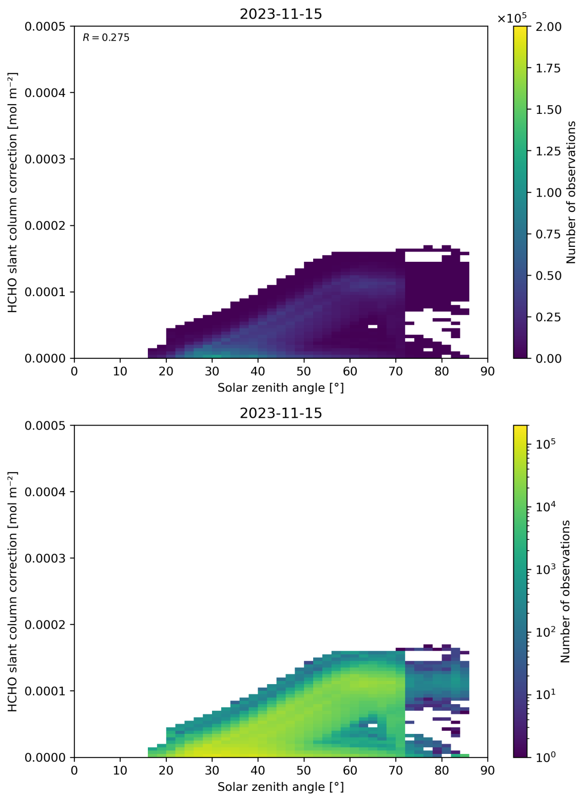
Figure 172: Scatter density plot of “Solar zenith angle” against “HCHO slant column correction” for 2023-11-14 to 2023-11-16.
