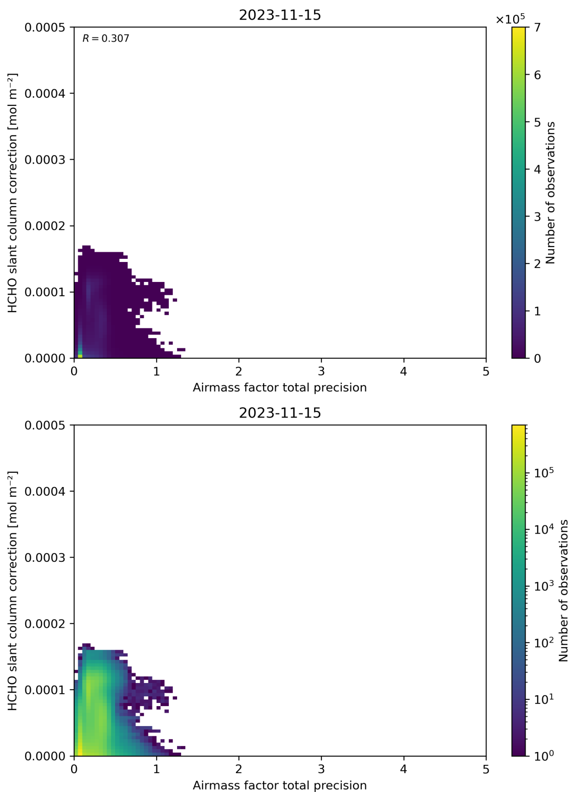
Figure 110: Scatter density plot of “Airmass factor total precision” against “HCHO slant column correction” for 2023-11-14 to 2023-11-16.
