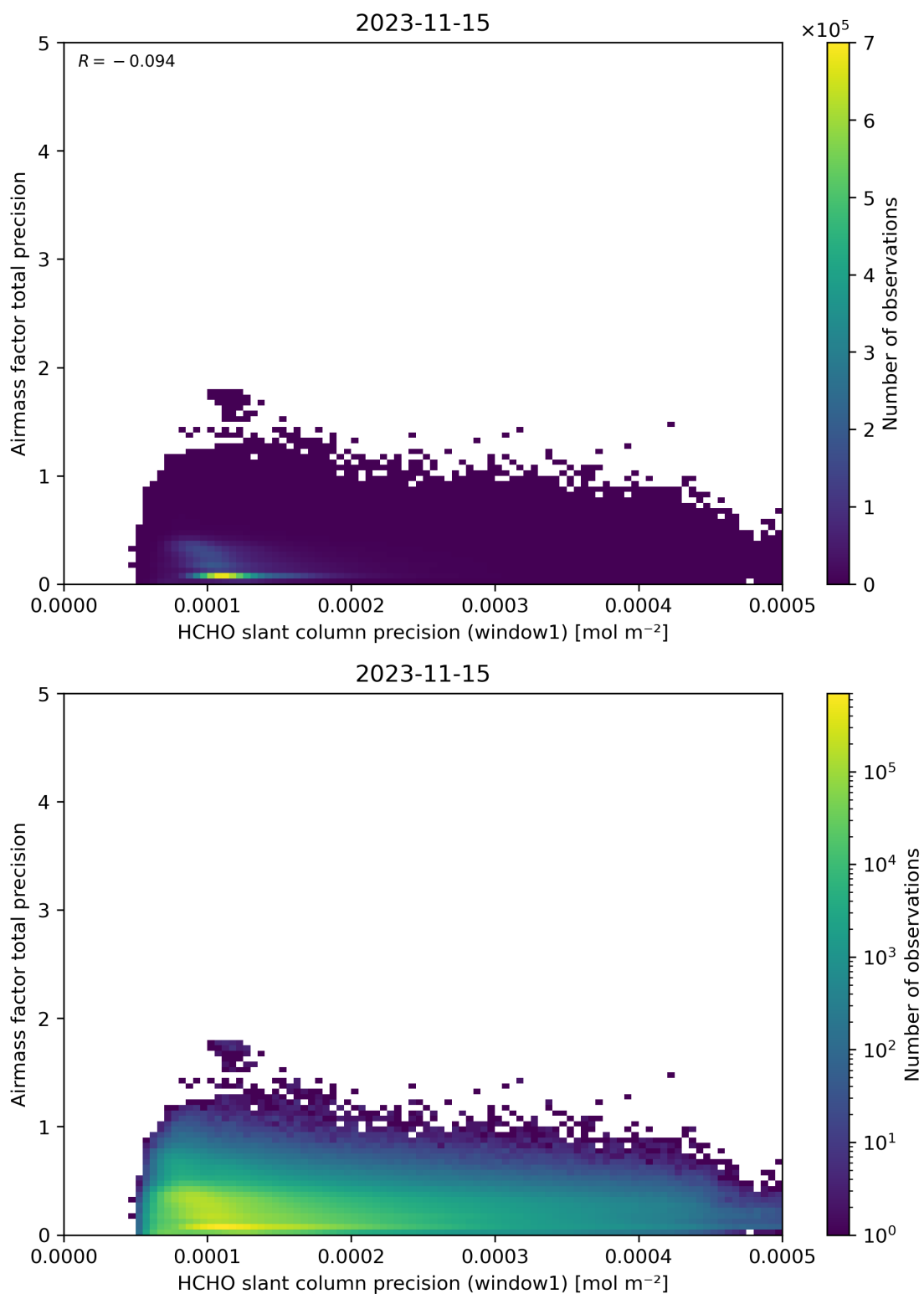
Figure 95: Scatter density plot of “HCHO slant column precision (window1)” against “Airmass factor total precision” for 2023-11-14 to 2023-11-16.
