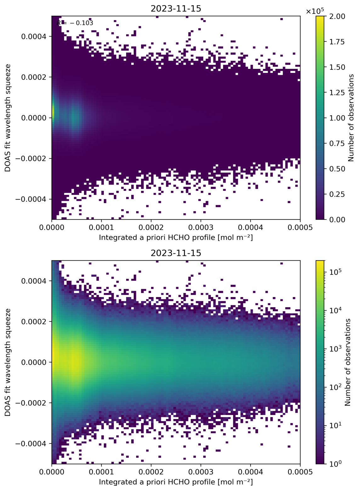
Figure 150: Scatter density plot of “Integrated a priori HCHO profile” against “DOAS fit wavelength squeeze” for 2023-11-14 to 2023-11-16.
