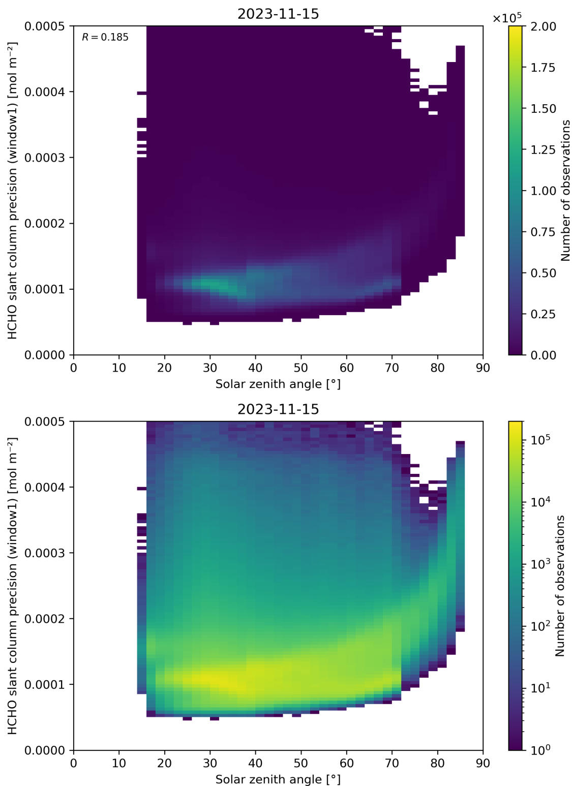
Figure 174: Scatter density plot of “Solar zenith angle” against “HCHO slant column precision (window1)” for 2023-11-14 to 2023-11-16.
