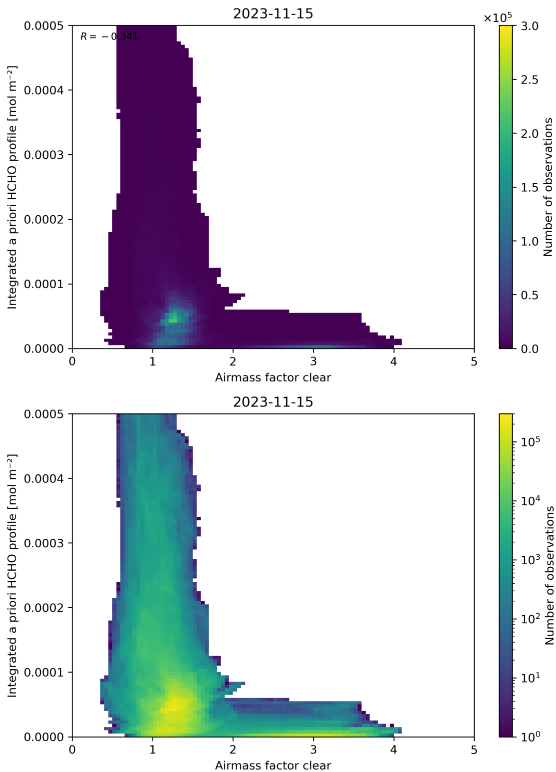
Figure 76: Scatter density plot of “Airmass factor clear” against “Integrated a priori HCHO profile” for 2023-11-14 to 2023-11-16.
