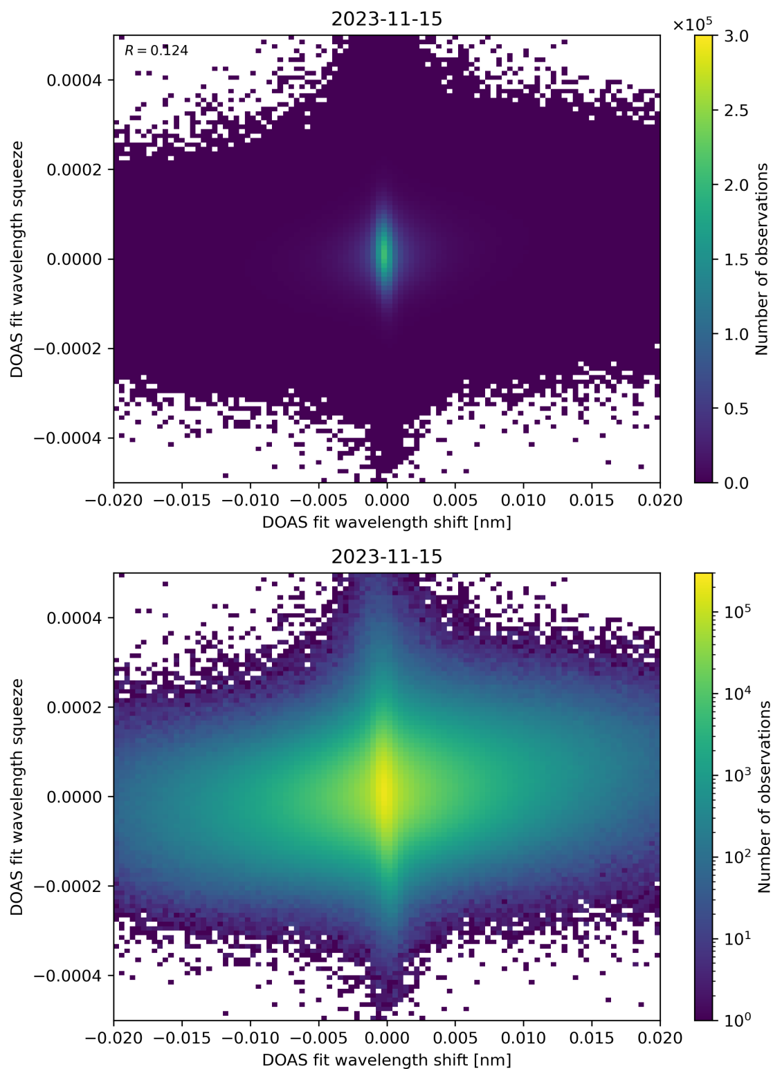
Figure 65: Scatter density plot of “DOAS fit wavelength shift” against “DOAS fit wavelength squeeze” for 2023-11-14 to 2023-11-16.
