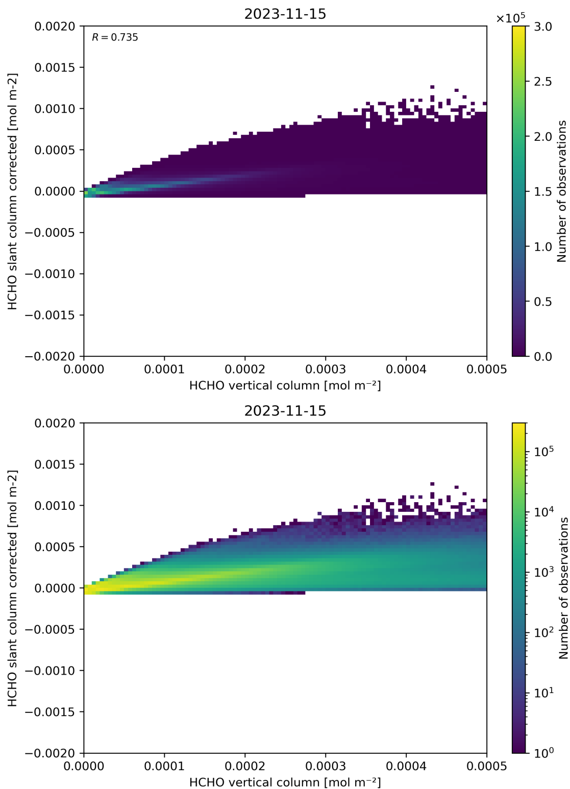
Figure 127: Scatter density plot of “HCHO vertical column” against “HCHO slant column corrected” for 2023-11-14 to 2023-11-16.
