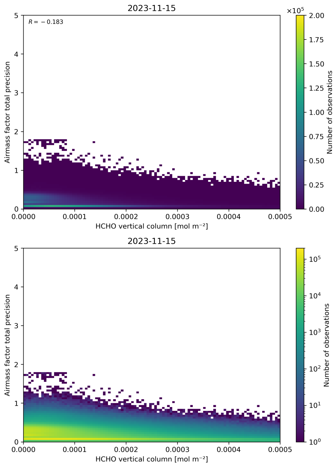
Figure 132: Scatter density plot of “HCHO vertical column” against “Airmass factor total precision” for 2023-11-14 to 2023-11-16.
