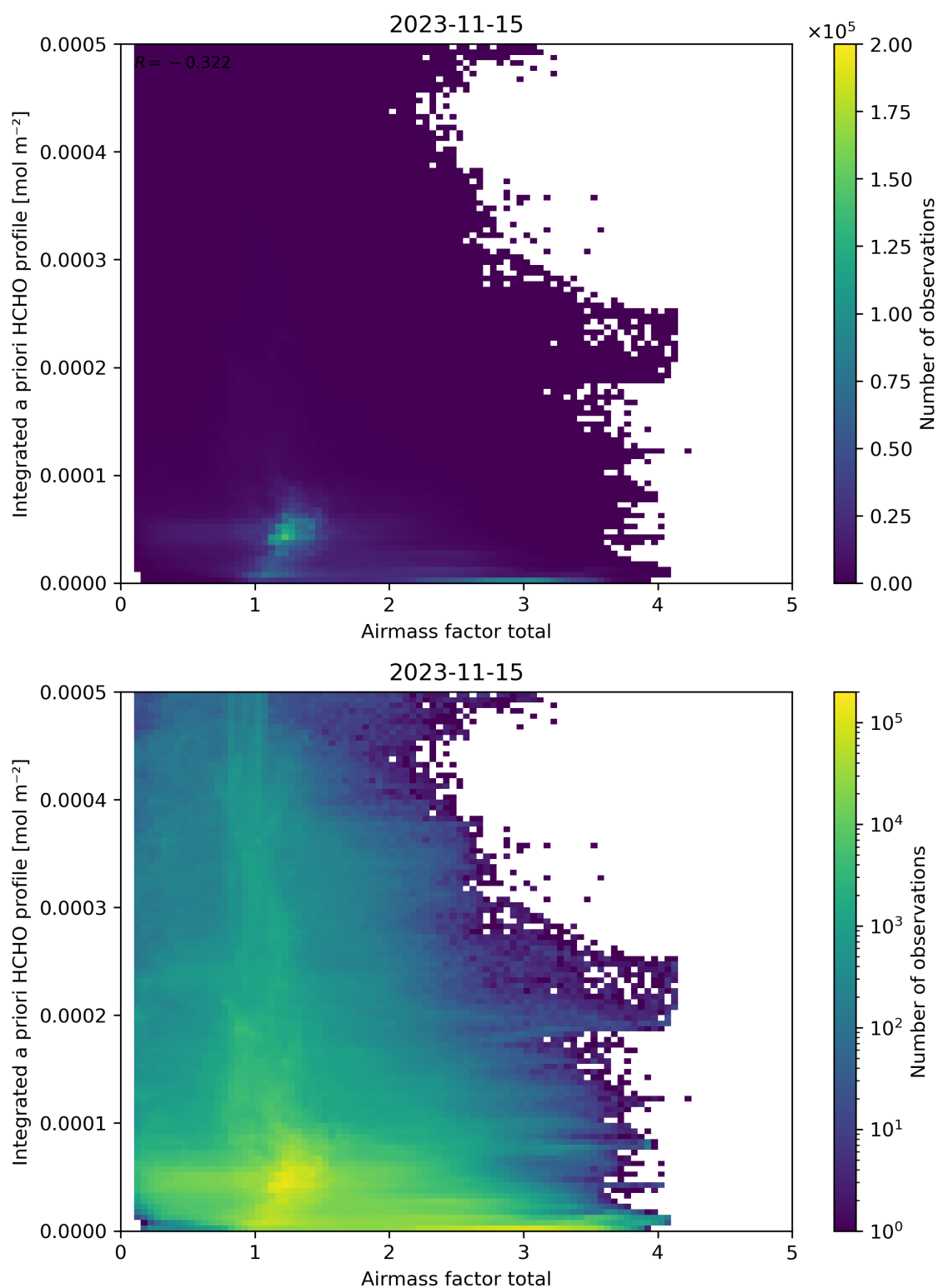
Figure 104: Scatter density plot of “Airmass factor total” against “Integrated a priori HCHO profile” for 2023-11-14 to 2023-11-16.
