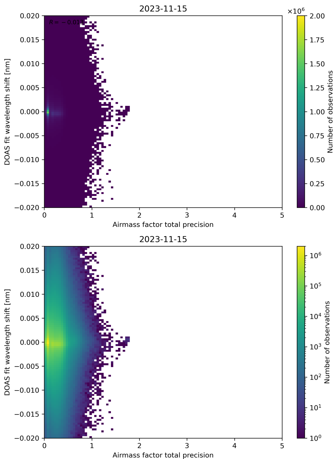
Figure 106: Scatter density plot of “Airmass factor total precision” against “DOAS fit wavelength shift” for 2023-11-14 to 2023-11-16.
