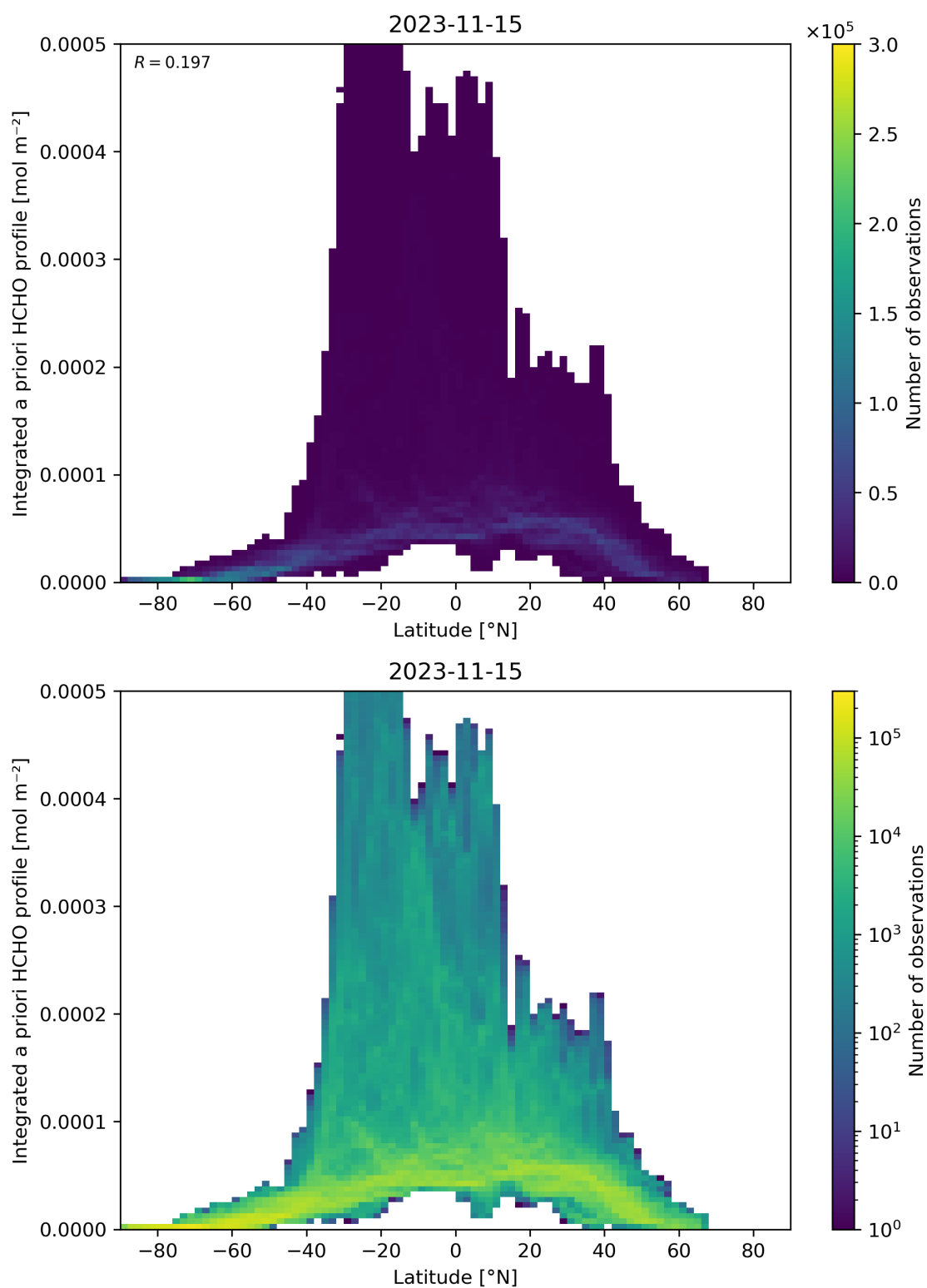
Figure 166: Scatter density plot of “Latitude” against “Integrated a priori HCHO profile” for 2023-11-14 to 2023-11-16.
