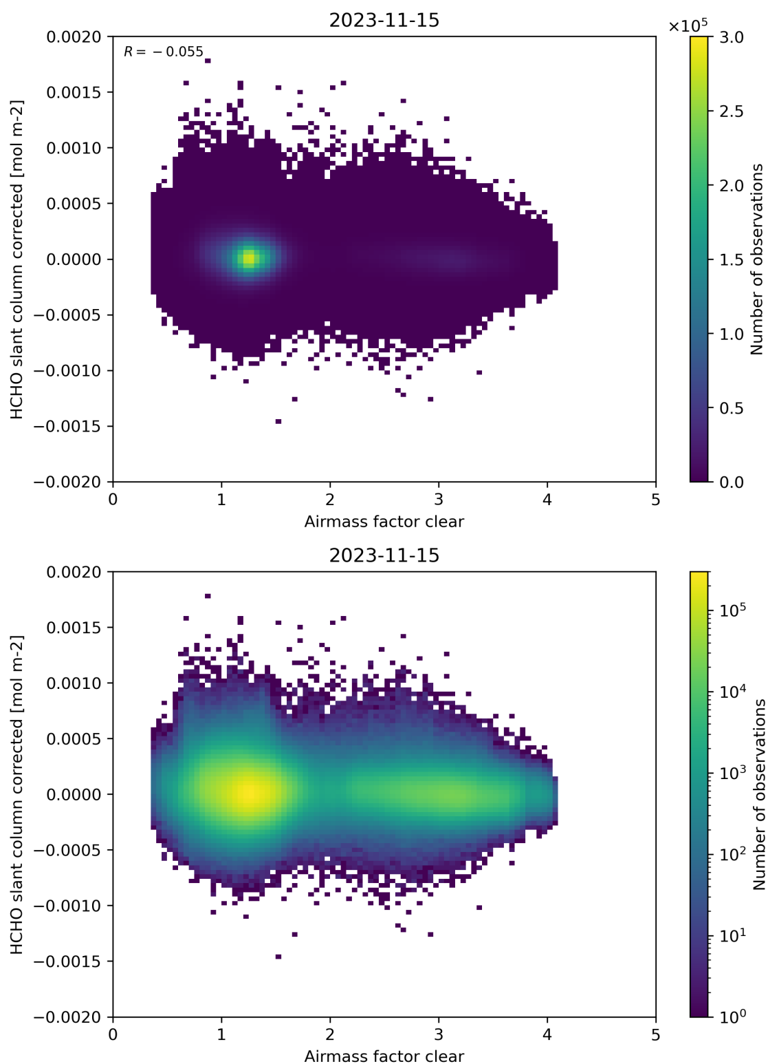
Figure 74: Scatter density plot of “Airmass factor clear” against “HCHO slant column corrected” for 2023-11-14 to 2023-11-16.
