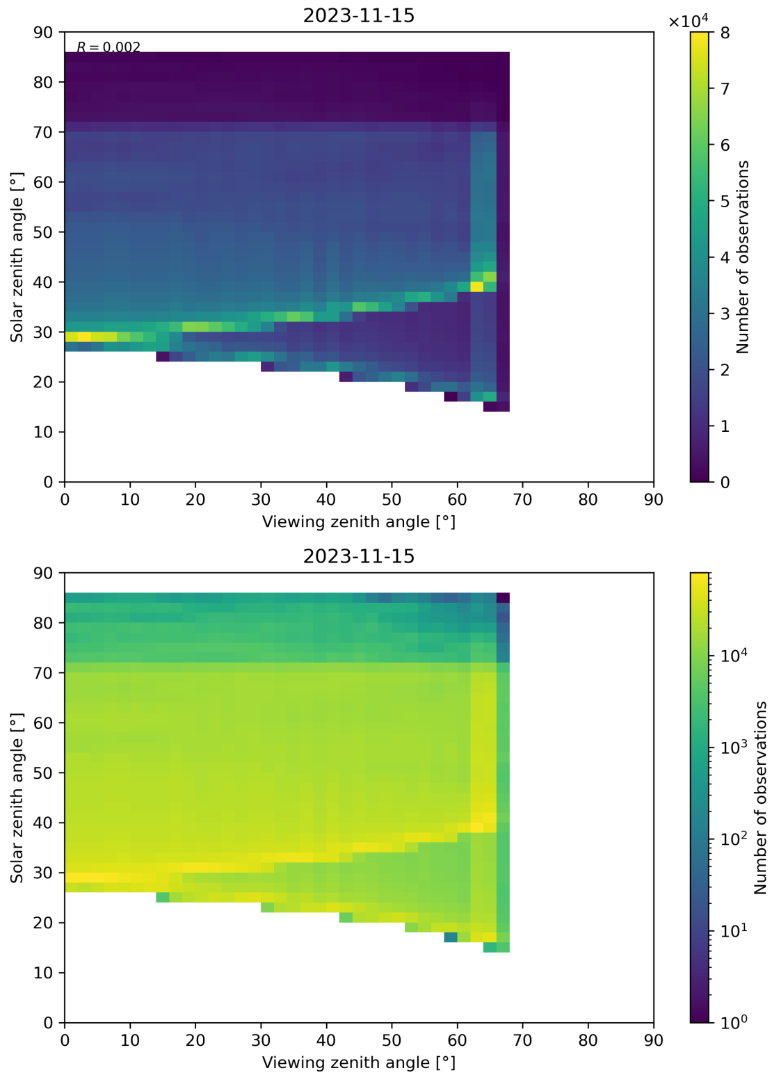
Figure 197: Scatter density plot of “Viewing zenith angle” against “Solar zenith angle” for 2023-11-14 to 2023-11-16.
