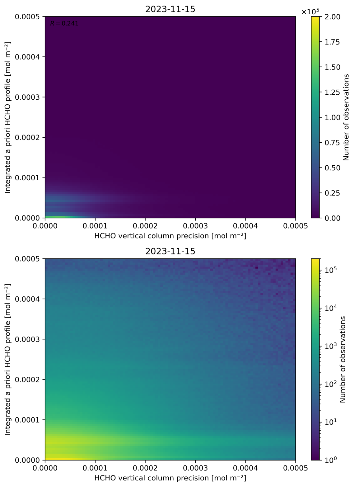
Figure 147: Scatter density plot of “HCHO vertical column precision” against “Integrated a priori HCHO profile” for 2023-11-14 to 2023-11-16.
