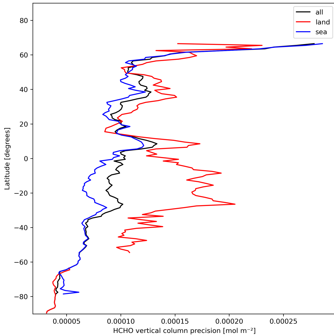
Figure 22: Zonal average of “HCHO vertical column precision” for 2023-11-14 to 2023-11-16.
