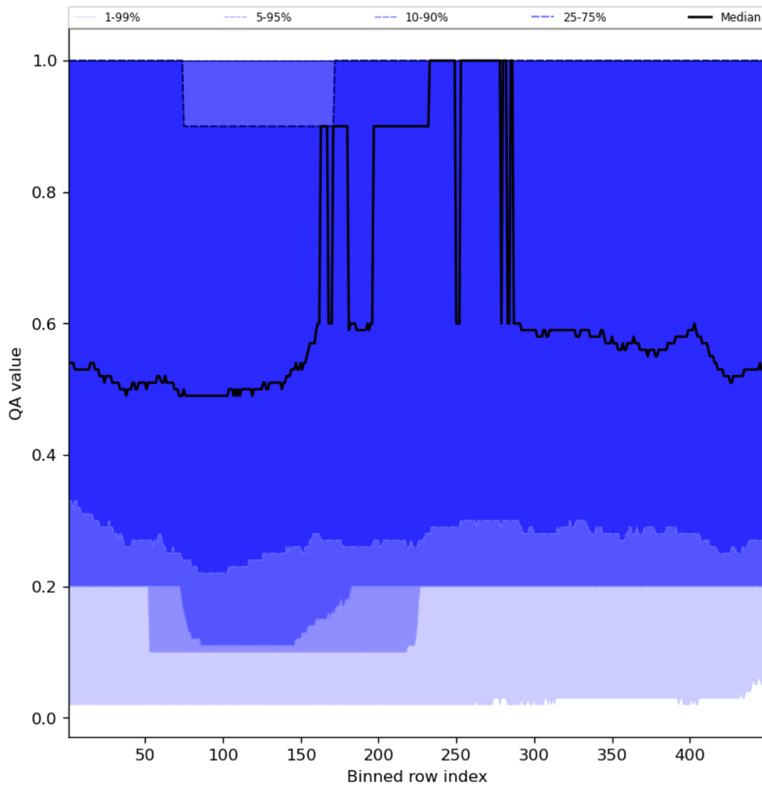
Figure 48: Along track statistics of “QA value” for 2023-11-14 to 2023-11-16
