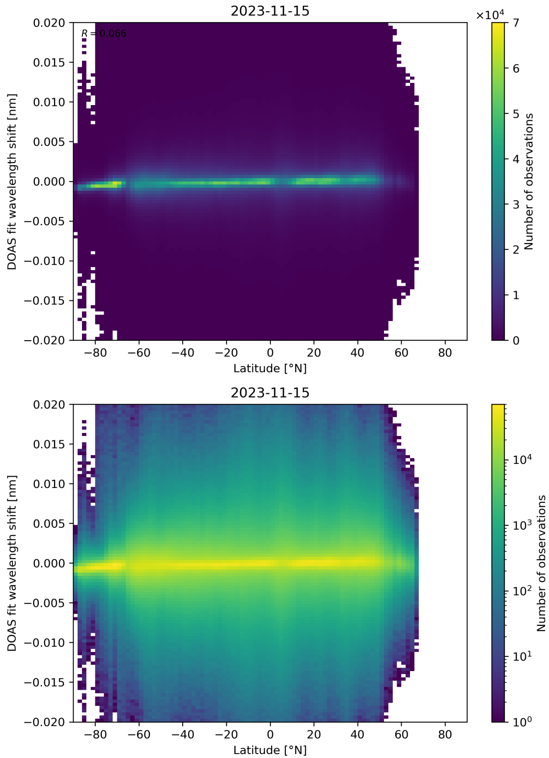
Figure 154: Scatter density plot of “Latitude” against “DOAS fit wavelength shift” for 2023-11-14 to 2023-11-16.
