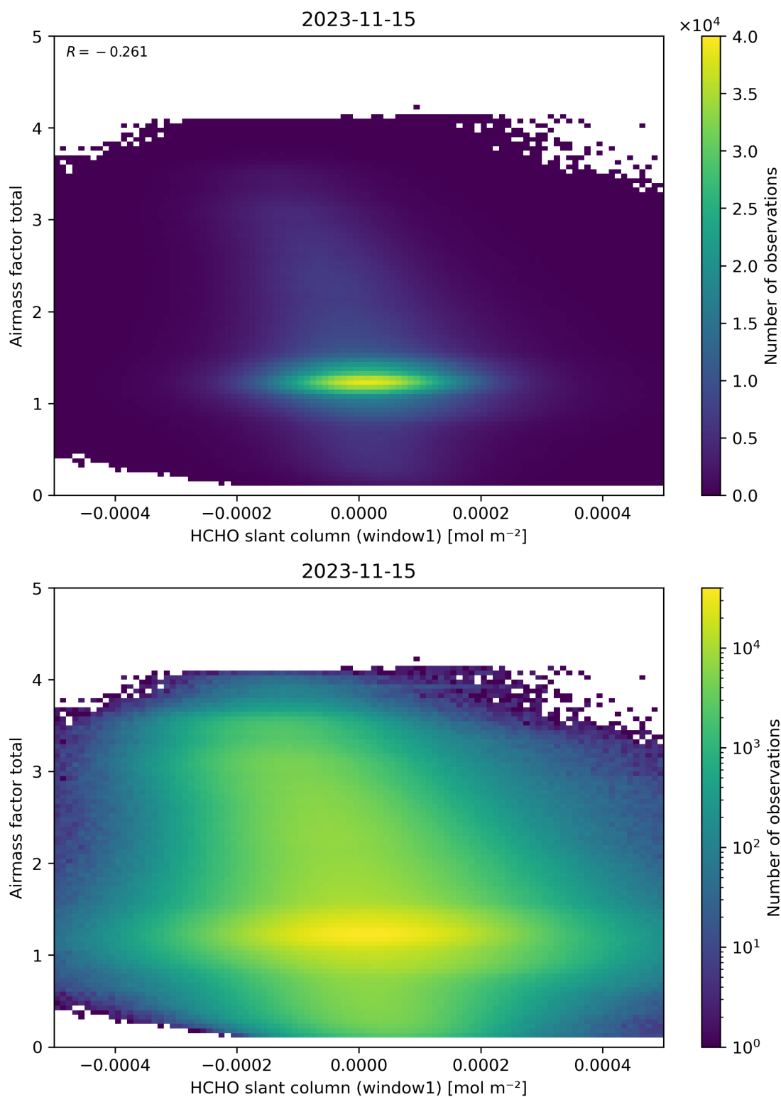
Figure 85: Scatter density plot of “HCHO slant column (window1)” against “Airmass factor total” for 2023-11-14 to 2023-11-16.
