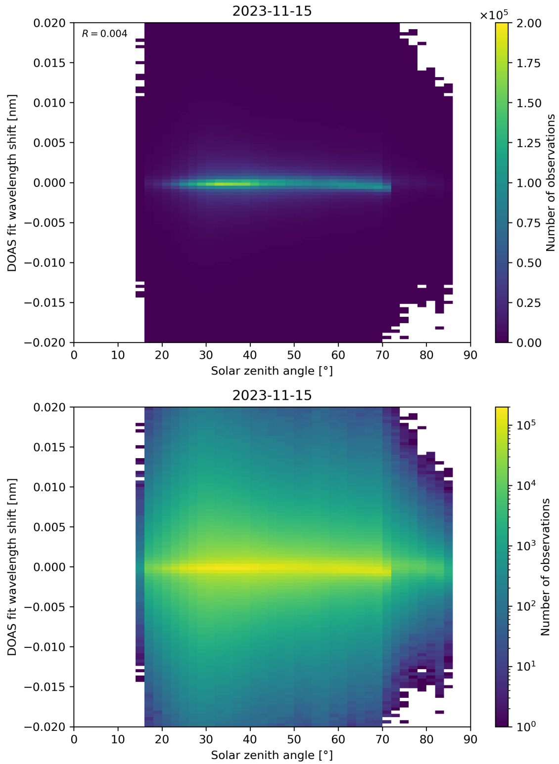
Figure 168: Scatter density plot of “Solar zenith angle” against “DOAS fit wavelength shift” for 2023-11-14 to 2023-11-16.
