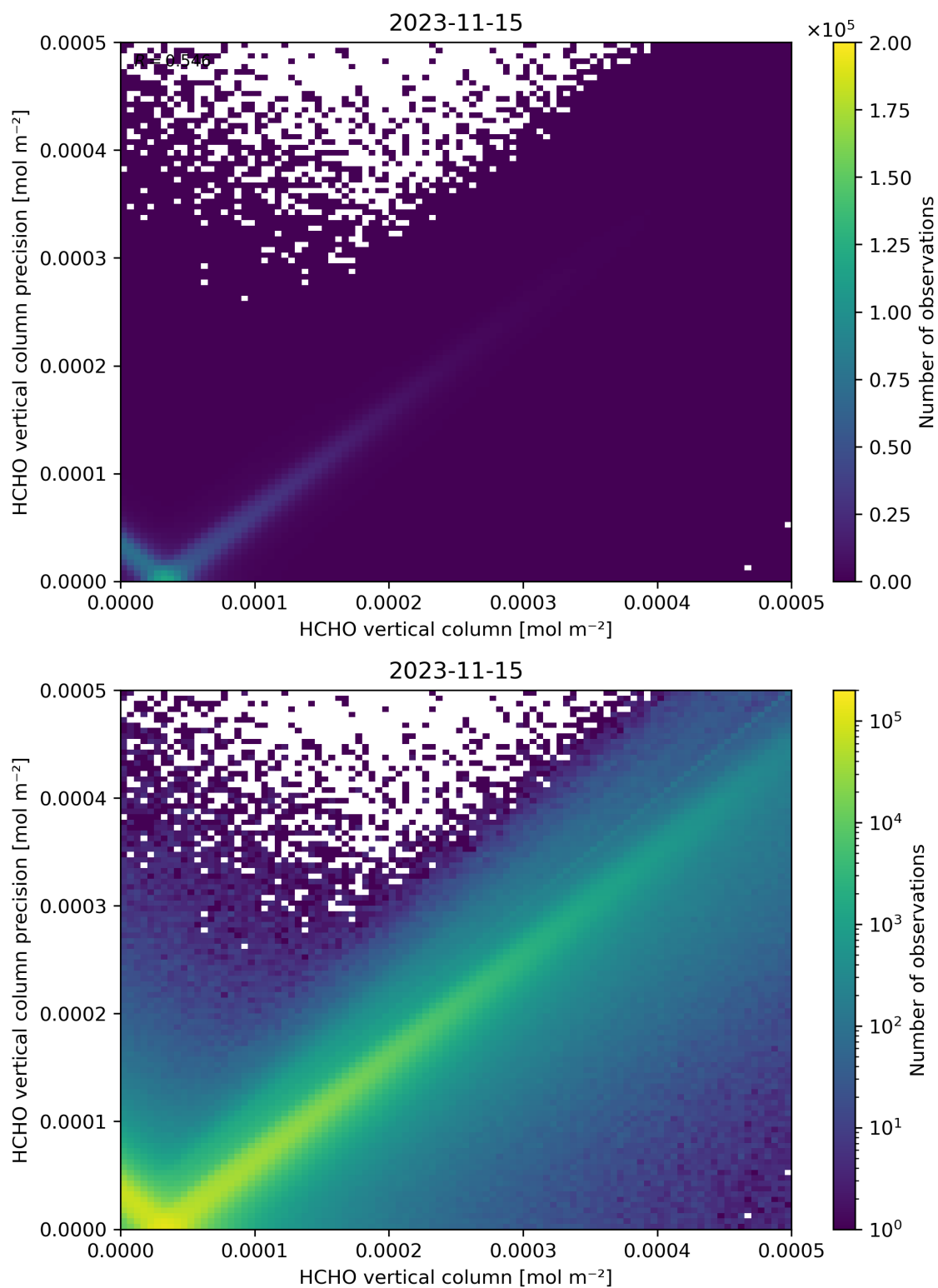
Figure 134: Scatter density plot of “HCHO vertical column” against “HCHO vertical column precision” for 2023-11-14 to 2023-11-16.
