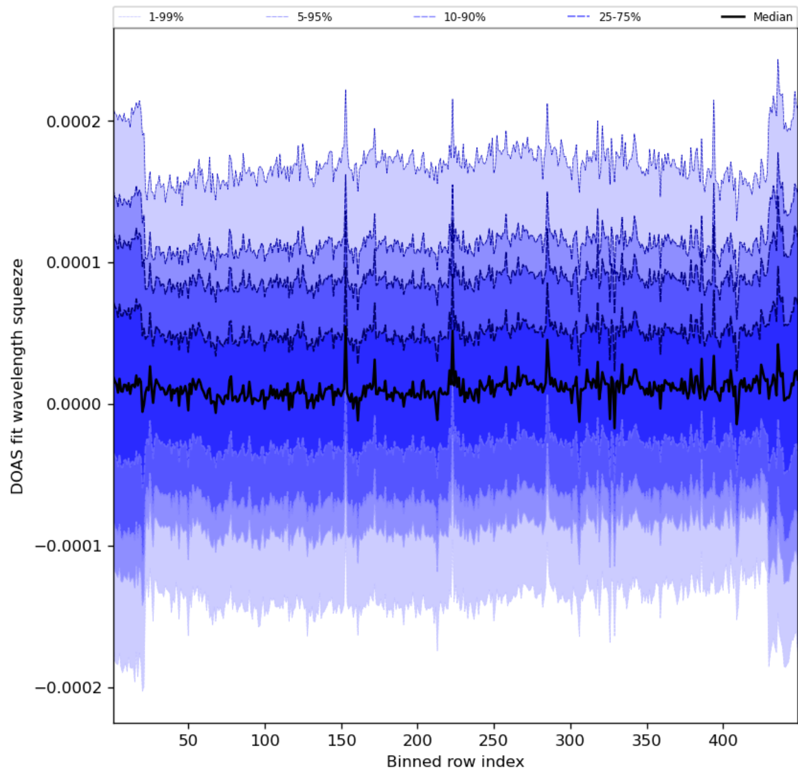
Figure 59: Along track statistics of “DOAS fit wavelength squeeze” for 2023-11-14 to 2023-11-16
