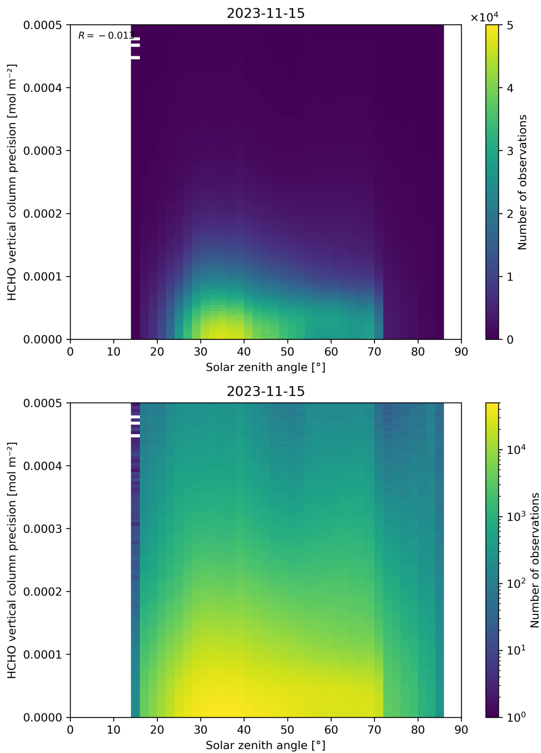
Figure 179: Scatter density plot of “Solar zenith angle” against “HCHO vertical column precision” for 2023-11-14 to 2023-11-16.
