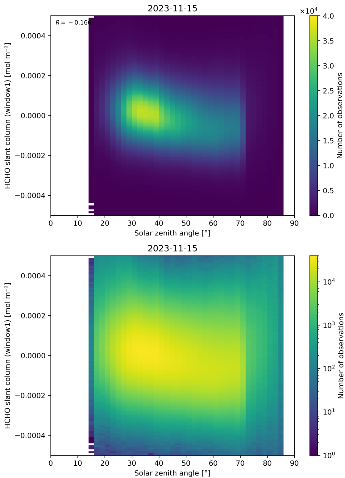
Figure 173: Scatter density plot of “Solar zenith angle” against “HCHO slant column (window1)” for 2023-11-14 to 2023-11-16.
