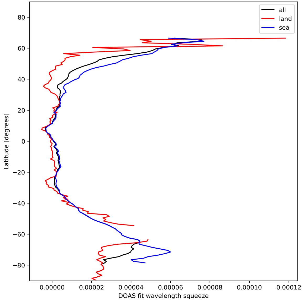
Figure 31: Zonal average of “DOAS fit wavelength squeeze” for 2023-11-14 to 2023-11-16.
