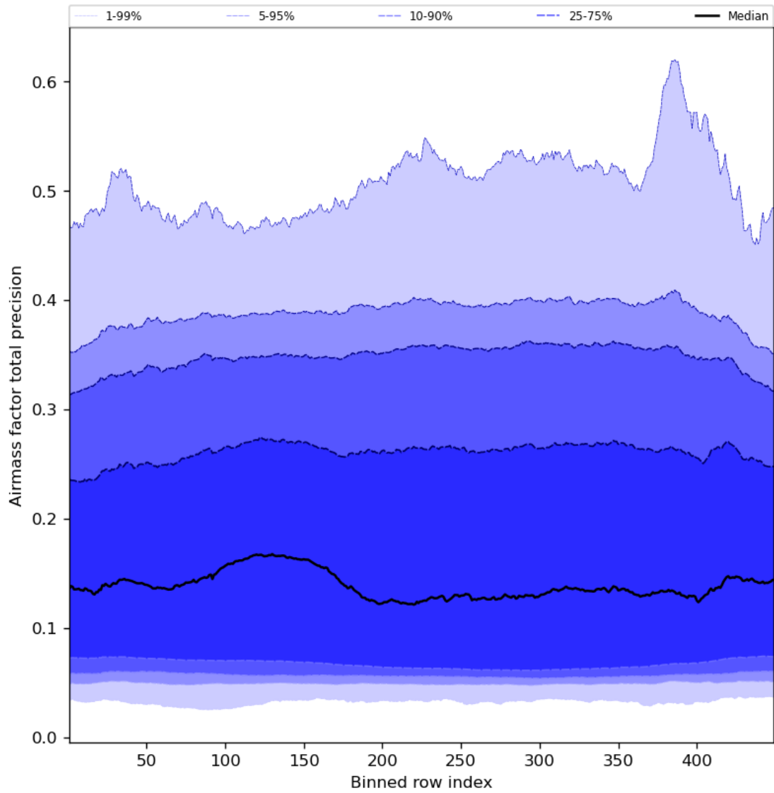
Figure 55: Along track statistics of “Airmass factor total precision” for 2023-11-14 to 2023-11-16
