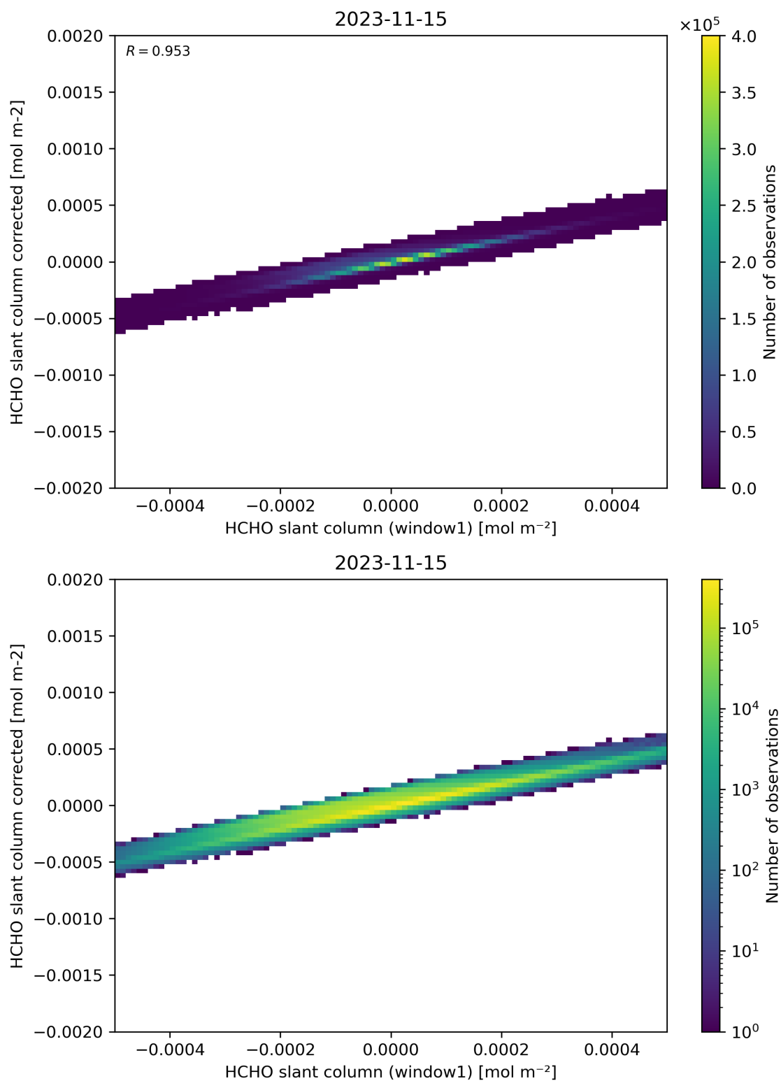
Figure 82: Scatter density plot of “HCHO slant column (window1)” against “HCHO slant column corrected” for 2023-11-14 to 2023-11-16.
