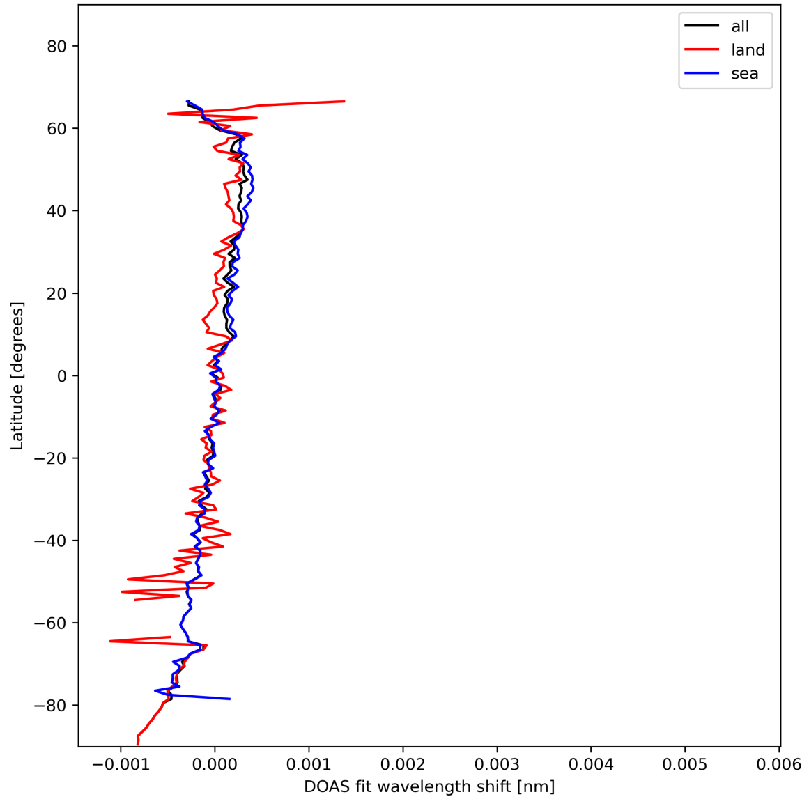
Figure 30: Zonal average of “DOAS fit wavelength shift” for 2023-11-14 to 2023-11-16.
