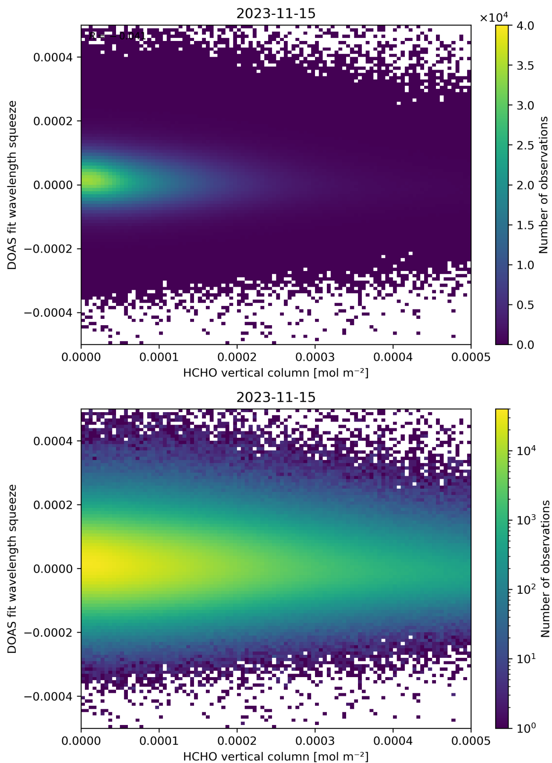
Figure 125: Scatter density plot of “HCHO vertical column” against “DOAS fit wavelength squeeze” for 2023-11-14 to 2023-11-16.
