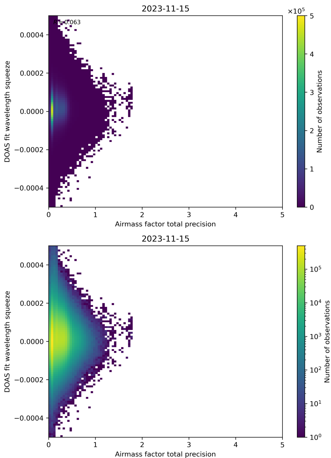
Figure 107: Scatter density plot of “Airmass factor total precision” against “DOAS fit wavelength squeeze” for 2023-11-14 to 2023-11-16.
