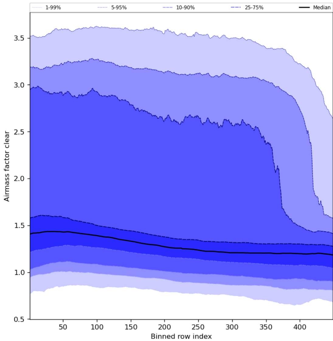
Figure 56: Along track statistics of “Airmass factor clear” for 2023-11-14 to 2023-11-16
