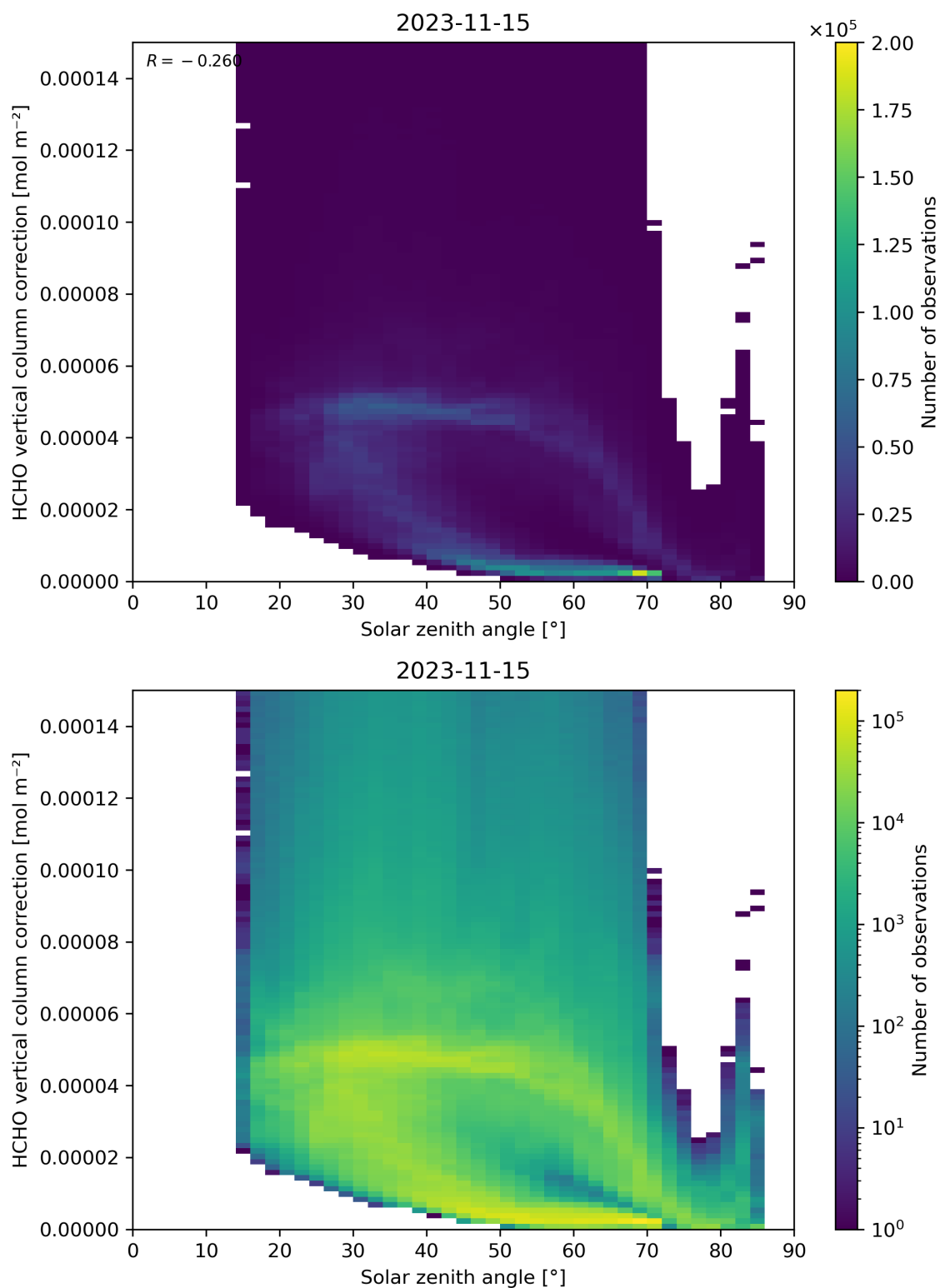
Figure 178: Scatter density plot of “Solar zenith angle” against “HCHO vertical column correction” for 2023-11-14 to 2023-11-16.
