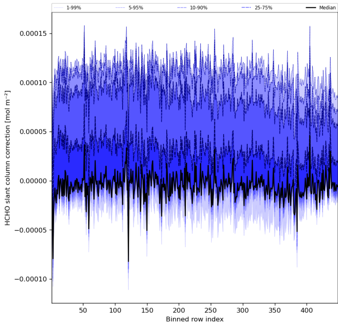
Figure 61: Along track statistics of “HCHO slant column correction” for 2023-11-14 to 2023-11-16
