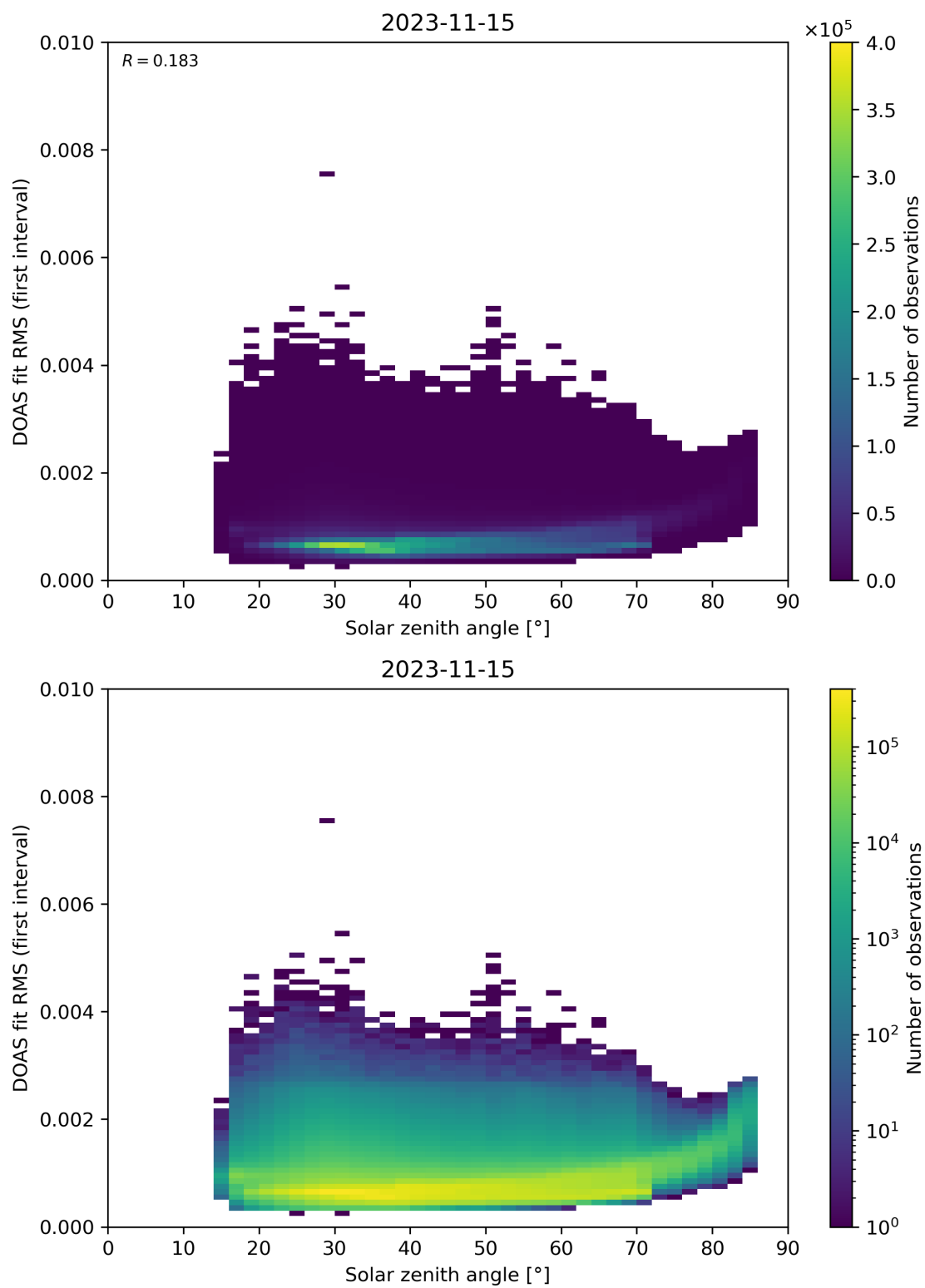
Figure 167: Scatter density plot of “Solar zenith angle” against “DOAS fit RMS (first interval)” for 2023-11-14 to 2023-11-16.
