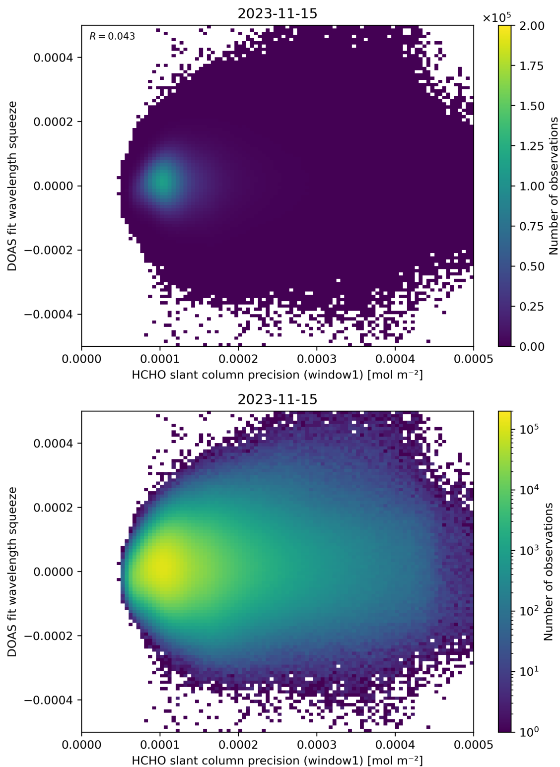
Figure 90: Scatter density plot of “HCHO slant column precision (window1)” against “DOAS fit wavelength squeeze” for 2023-11-14 to 2023-11-16.
