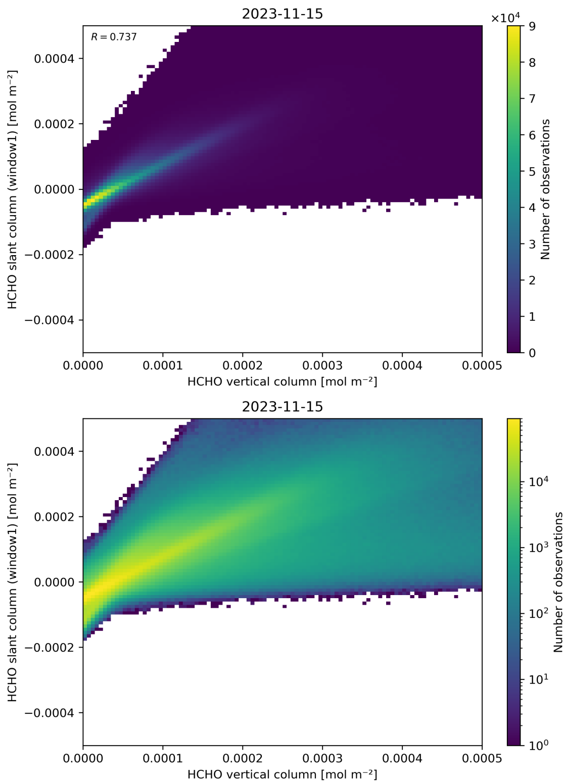
Figure 129: Scatter density plot of “HCHO vertical column” against “HCHO slant column (window1)” for 2023-11-14 to 2023-11-16.
