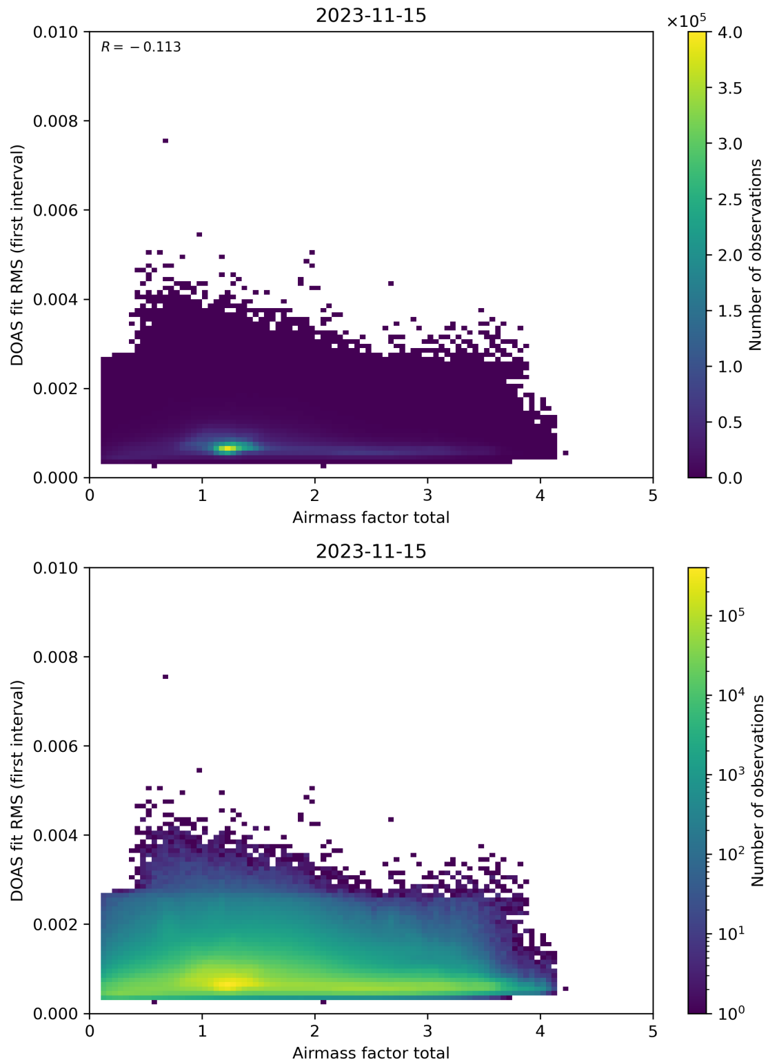
Figure 97: Scatter density plot of “Airmass factor total” against “DOAS fit RMS (first interval)” for 2023-11-14 to 2023-11-16.
