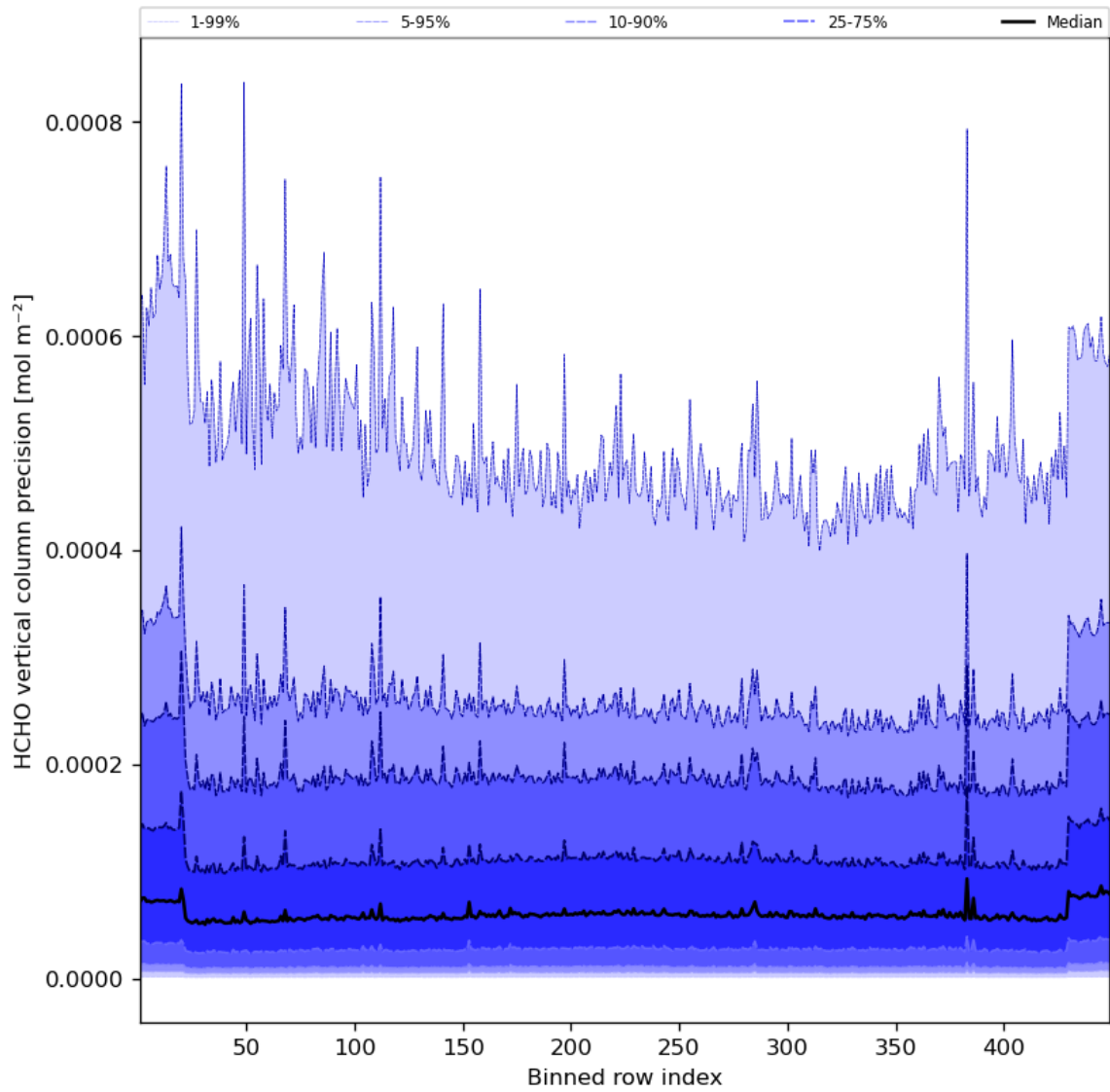
Figure 50: Along track statistics of “HCHO vertical column precision” for 2023-11-14 to 2023-11-16
