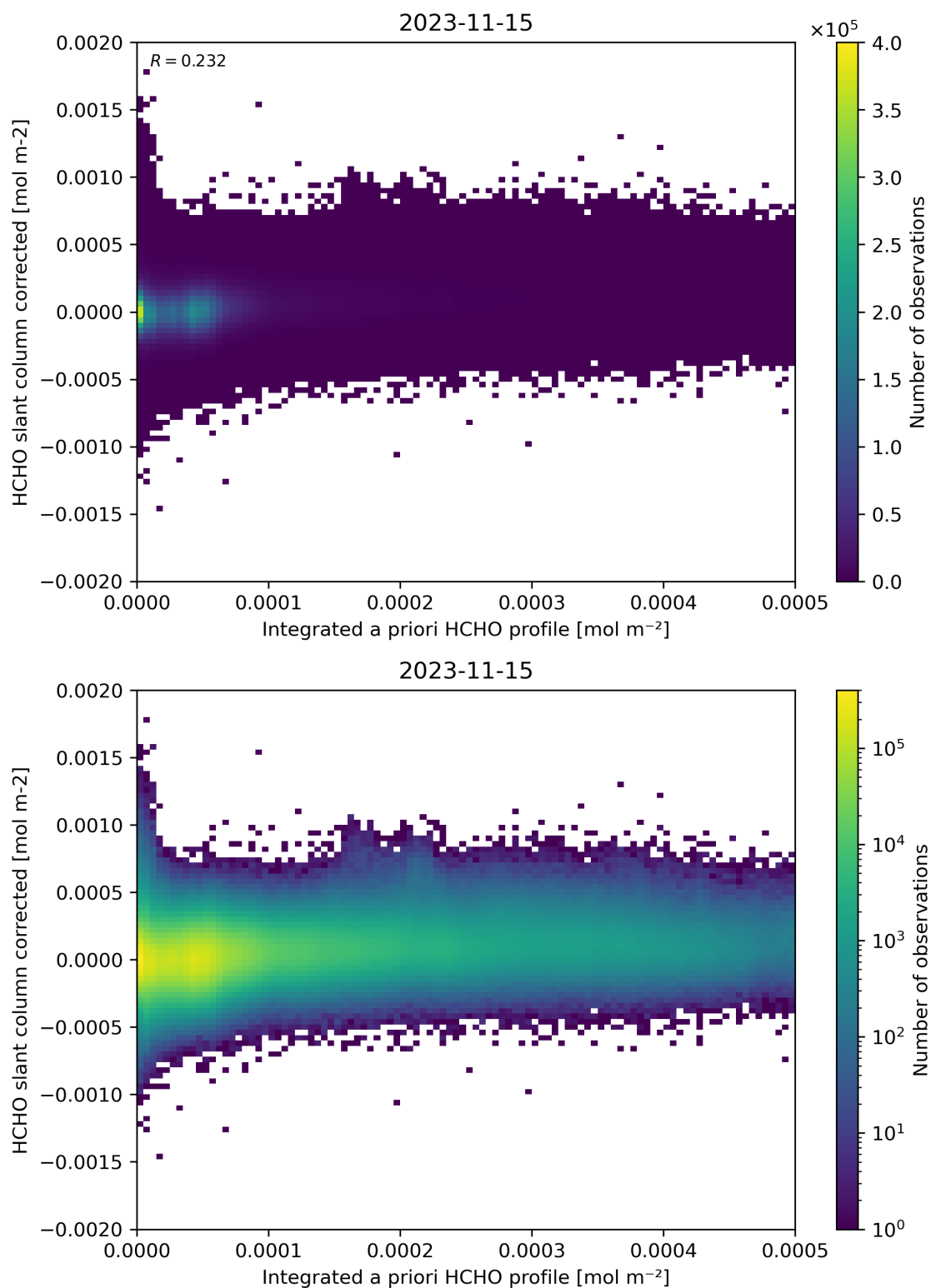
Figure 151: Scatter density plot of “Integrated a priori HCHO profile” against “HCHO slant column corrected” for 2023-11-14 to 2023-11-16.
