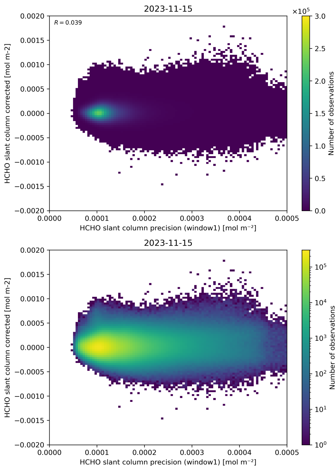
Figure 92: Scatter density plot of “HCHO slant column precision (window1)” against “HCHO slant column corrected” for 2023-11-14 to 2023-11-16.
