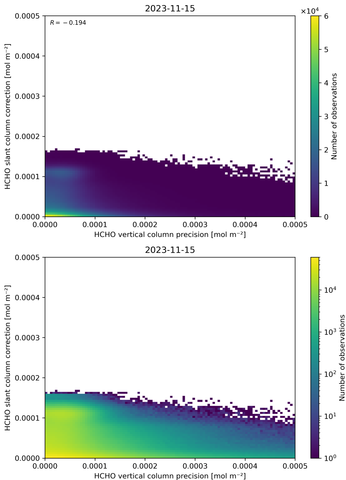
Figure 141: Scatter density plot of “HCHO vertical column precision” against “HCHO slant column correction” for 2023-11-14 to 2023-11-16.
