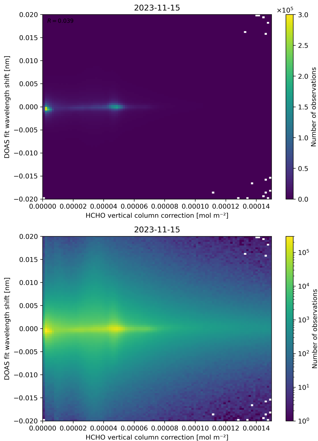
Figure 113: Scatter density plot of “HCHO vertical column correction” against “DOAS fit wavelength shift” for 2023-11-14 to 2023-11-16.
