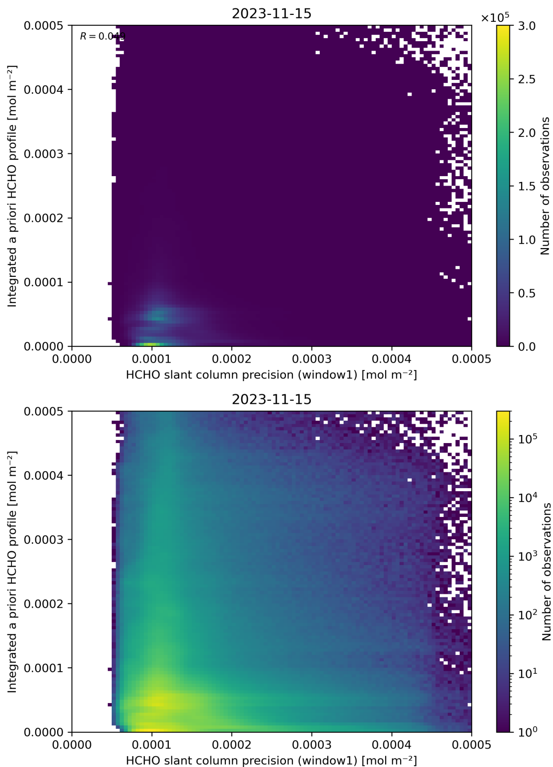
Figure 96: Scatter density plot of “HCHO slant column precision (window1)” against “Integrated a priori HCHO profile” for 2023-11-14 to 2023-11-16.
