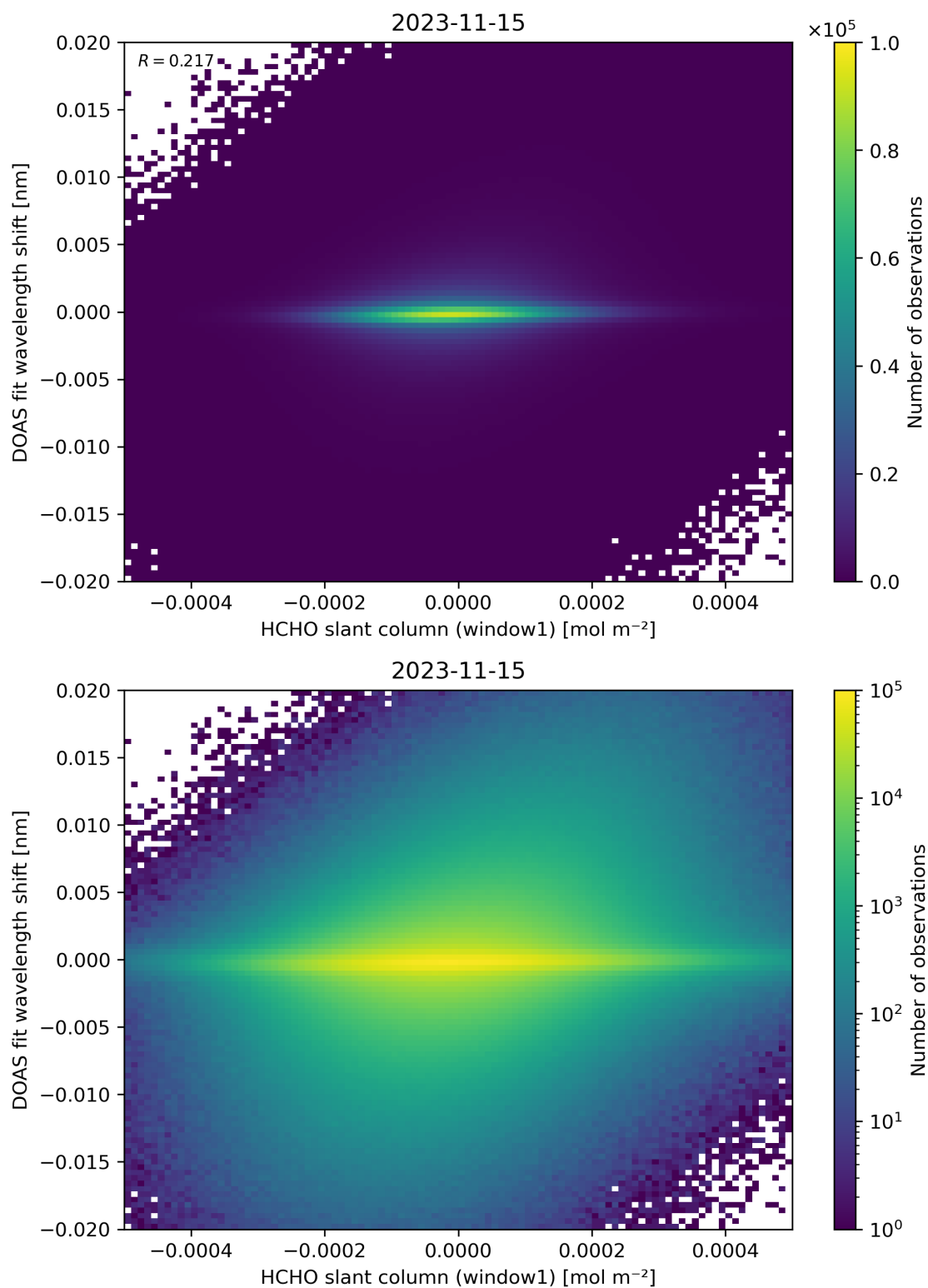
Figure 79: Scatter density plot of “HCHO slant column (window1)” against “DOAS fit wavelength shift” for 2023-11-14 to 2023-11-16.
