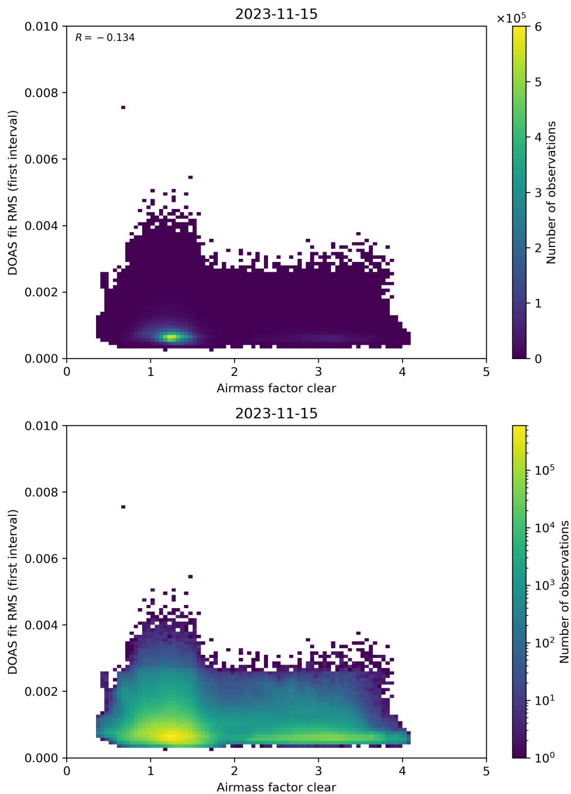
Figure 71: Scatter density plot of “Airmass factor clear” against “DOAS fit RMS (first interval)” for 2023-11-14 to 2023-11-16.
