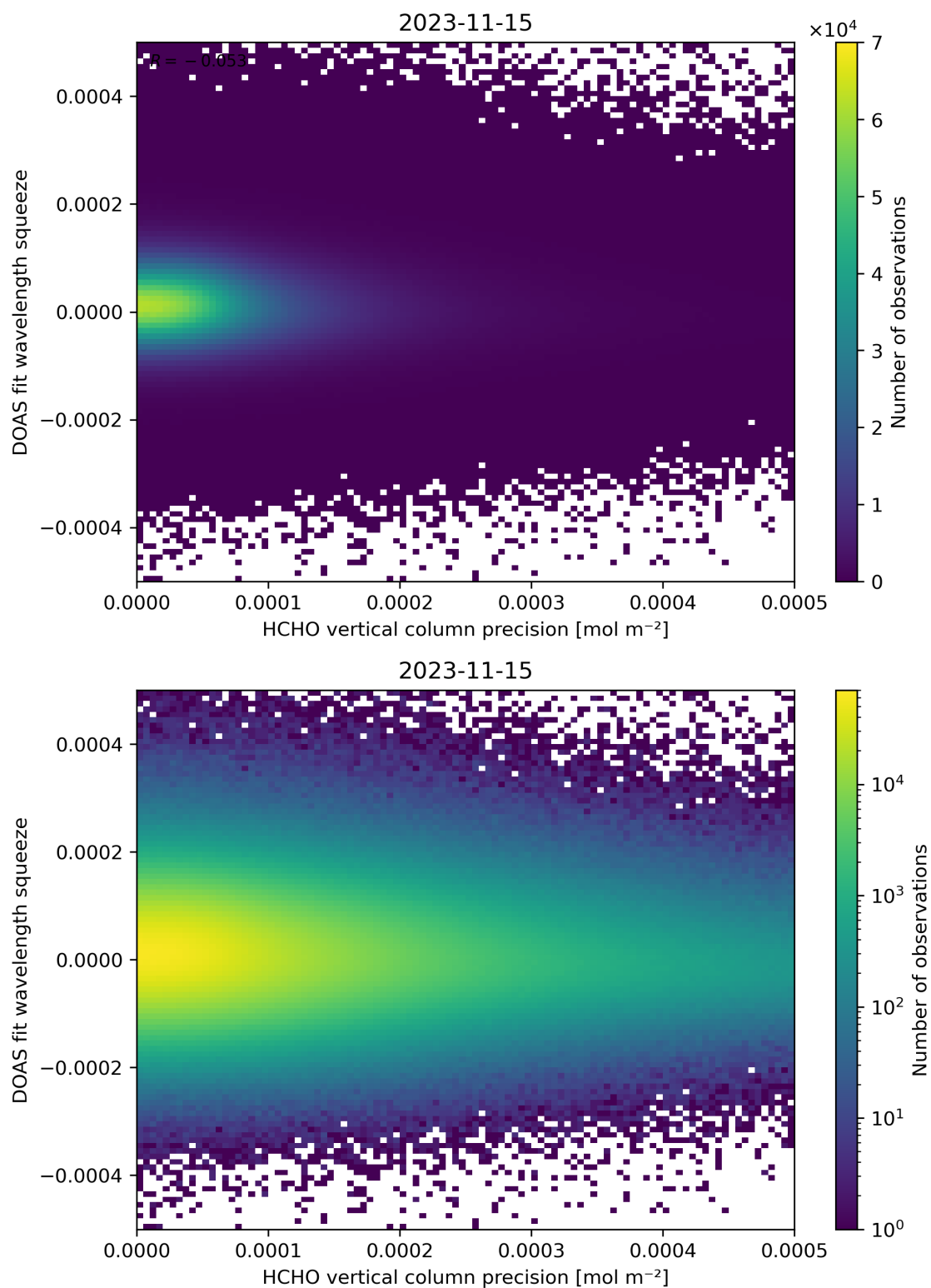
Figure 138: Scatter density plot of “HCHO vertical column precision” against “DOAS fit wavelength squeeze” for 2023-11-14 to 2023-11-16.
