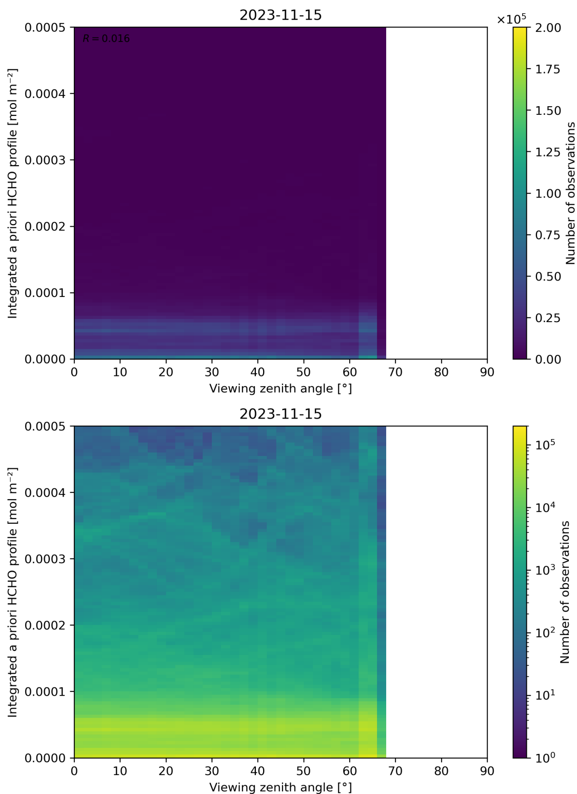
Figure 195: Scatter density plot of “Viewing zenith angle” against “Integrated a priori HCHO profile” for 2023-11-14 to 2023-11-16.
