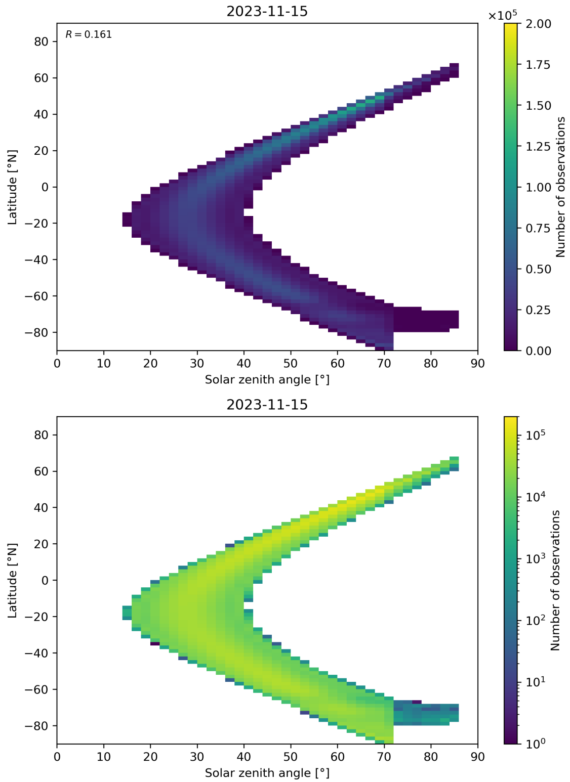
Figure 181: Scatter density plot of “Solar zenith angle” against “Latitude” for 2023-11-14 to 2023-11-16.
