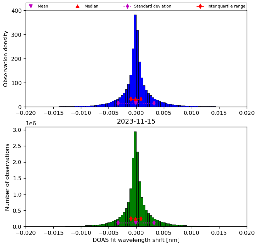
Figure 44: Histogram of “DOAS fit wavelength shift” for 2023-11-14 to 2023-11-16
