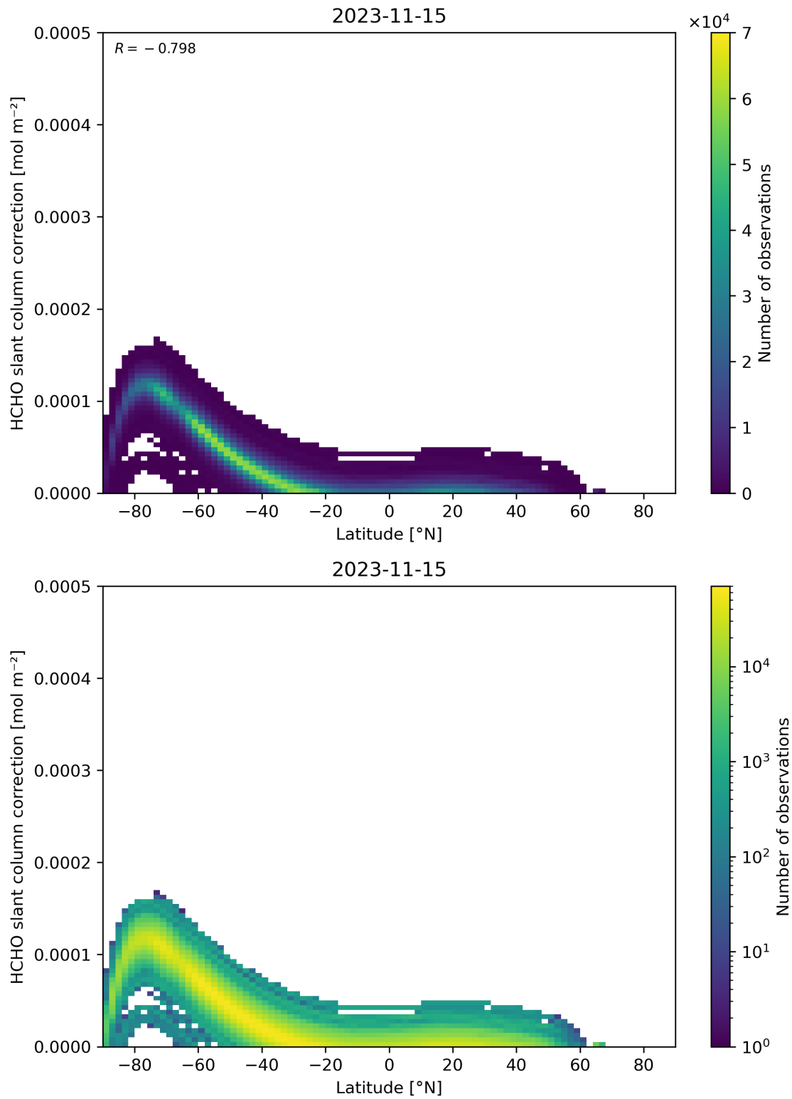
Figure 158: Scatter density plot of “Latitude” against “HCHO slant column correction” for 2023-11-14 to 2023-11-16.
