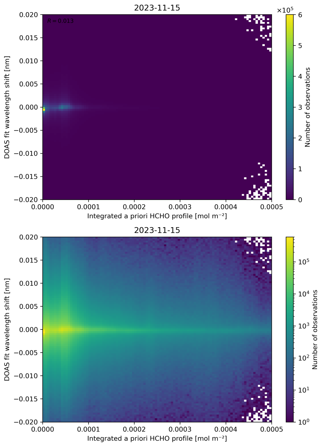
Figure 149: Scatter density plot of “Integrated a priori HCHO profile” against “DOAS fit wavelength shift” for 2023-11-14 to 2023-11-16.
