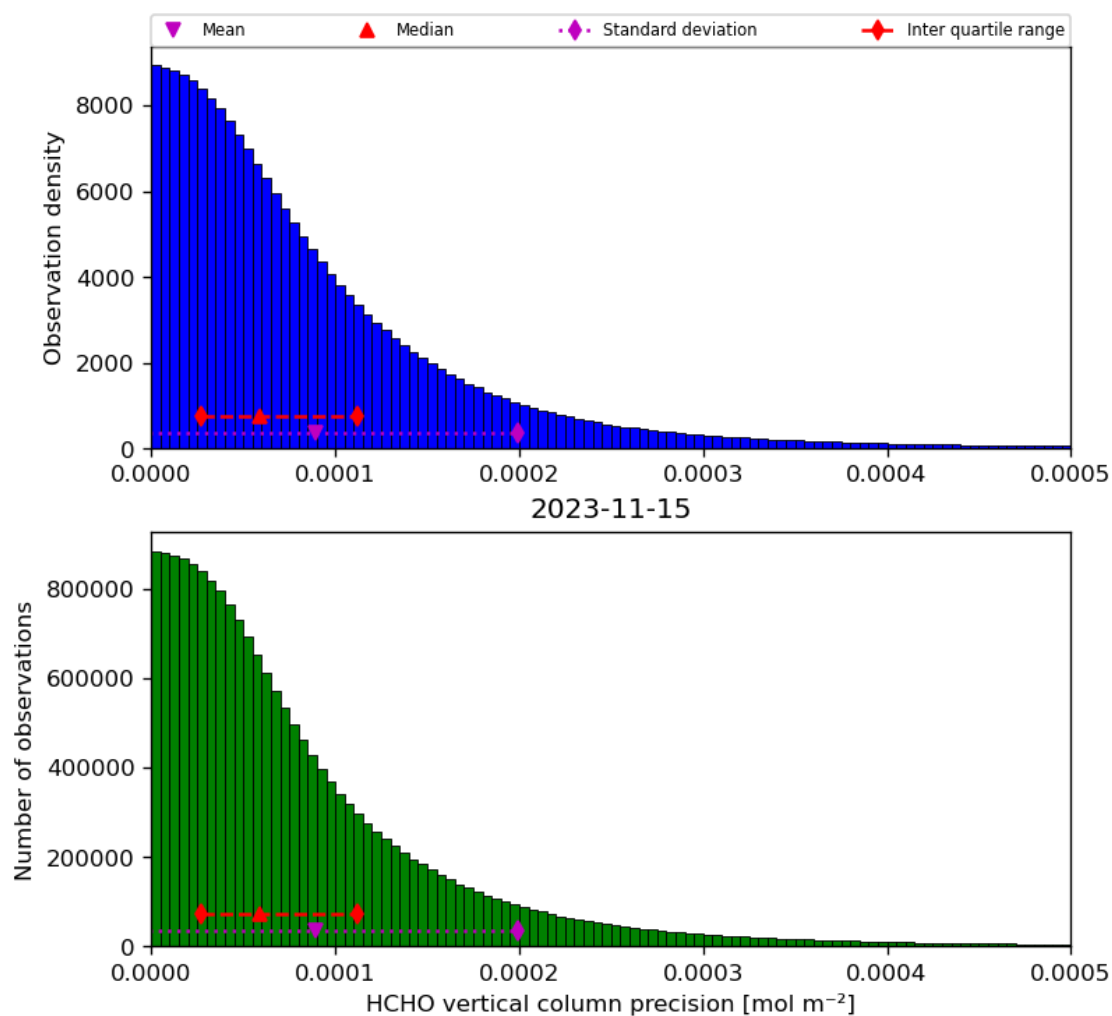
Figure 36: Histogram of “HCHO vertical column precision” for 2023-11-14 to 2023-11-16
