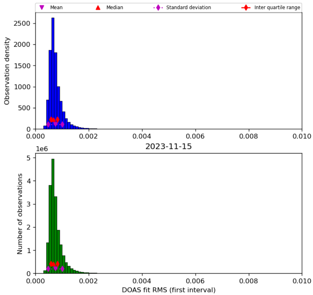
Figure 46: Histogram of “DOAS fit RMS (first interval)” for 2023-11-14 to 2023-11-16
