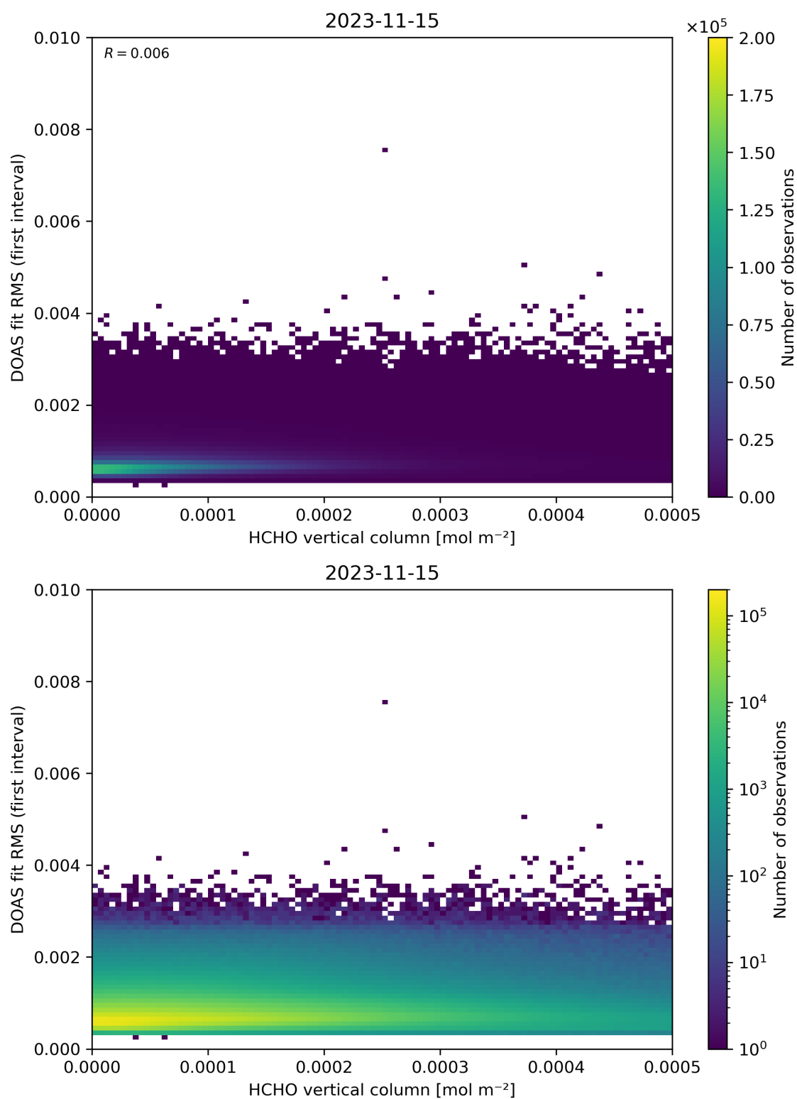
Figure 123: Scatter density plot of “HCHO vertical column” against “DOAS fit RMS (first interval)” for 2023-11-14 to 2023-11-16.
