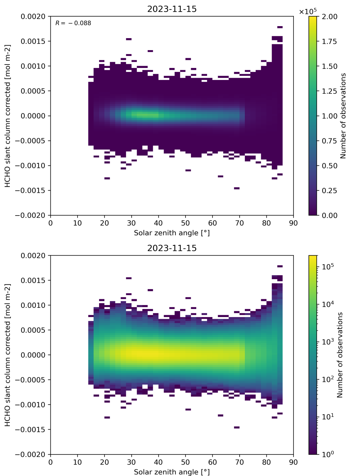
Figure 171: Scatter density plot of “Solar zenith angle” against “HCHO slant column corrected” for 2023-11-14 to 2023-11-16.
