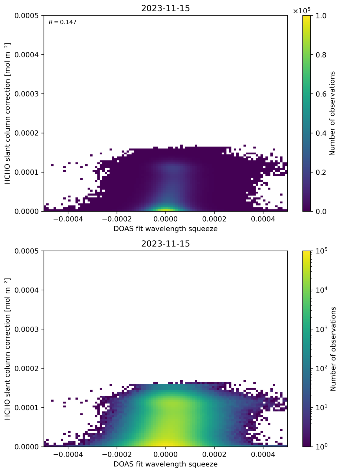
Figure 70: Scatter density plot of “DOAS fit wavelength squeeze” against “HCHO slant column correction” for 2023-11-14 to 2023-11-16.
