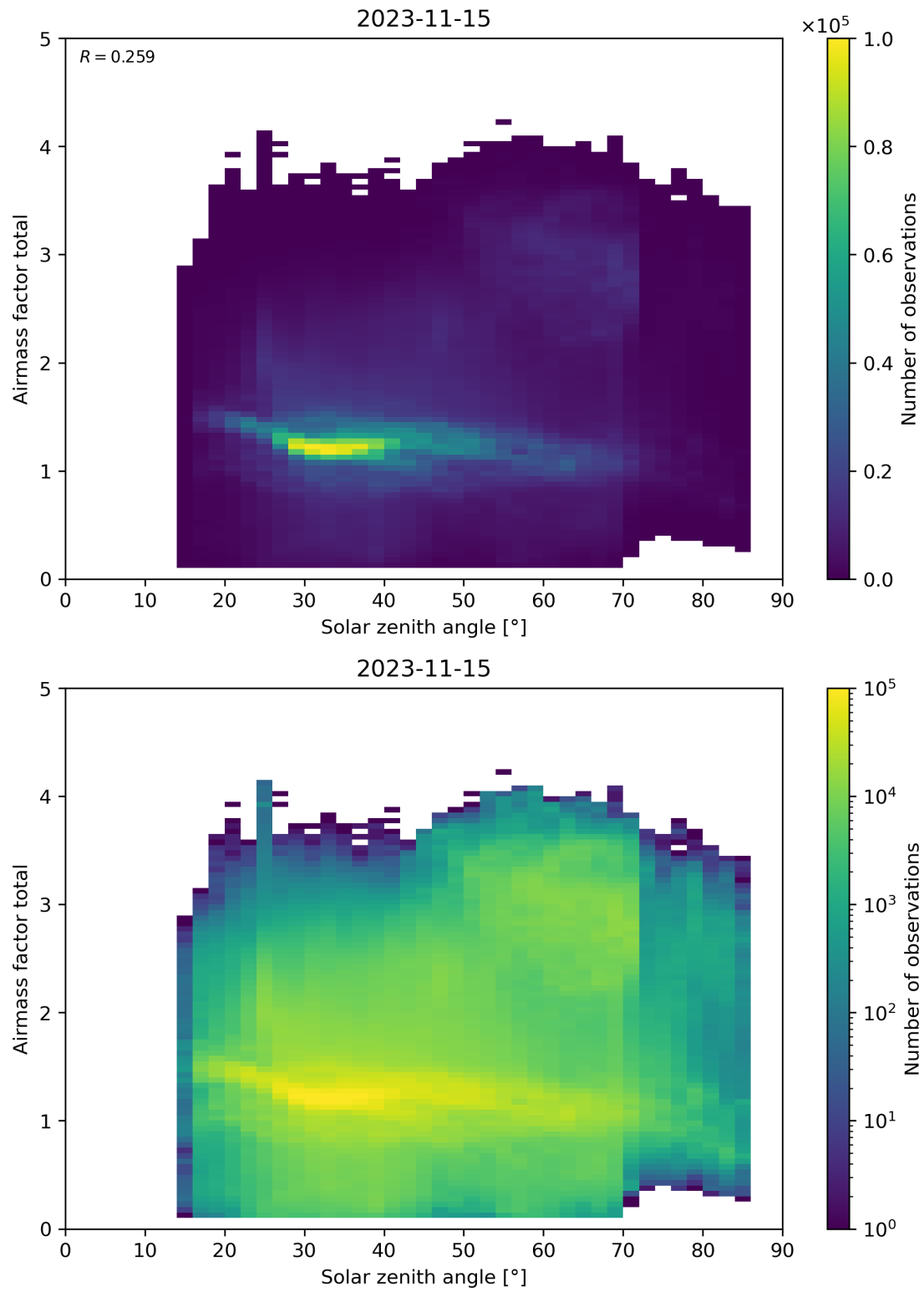
Figure 175: Scatter density plot of “Solar zenith angle” against “Airmass factor total” for 2023-11-14 to 2023-11-16.
