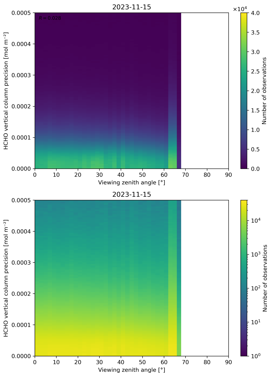
Figure 194: Scatter density plot of “Viewing zenith angle” against “HCHO vertical column precision” for 2023-11-14 to 2023-11-16.
