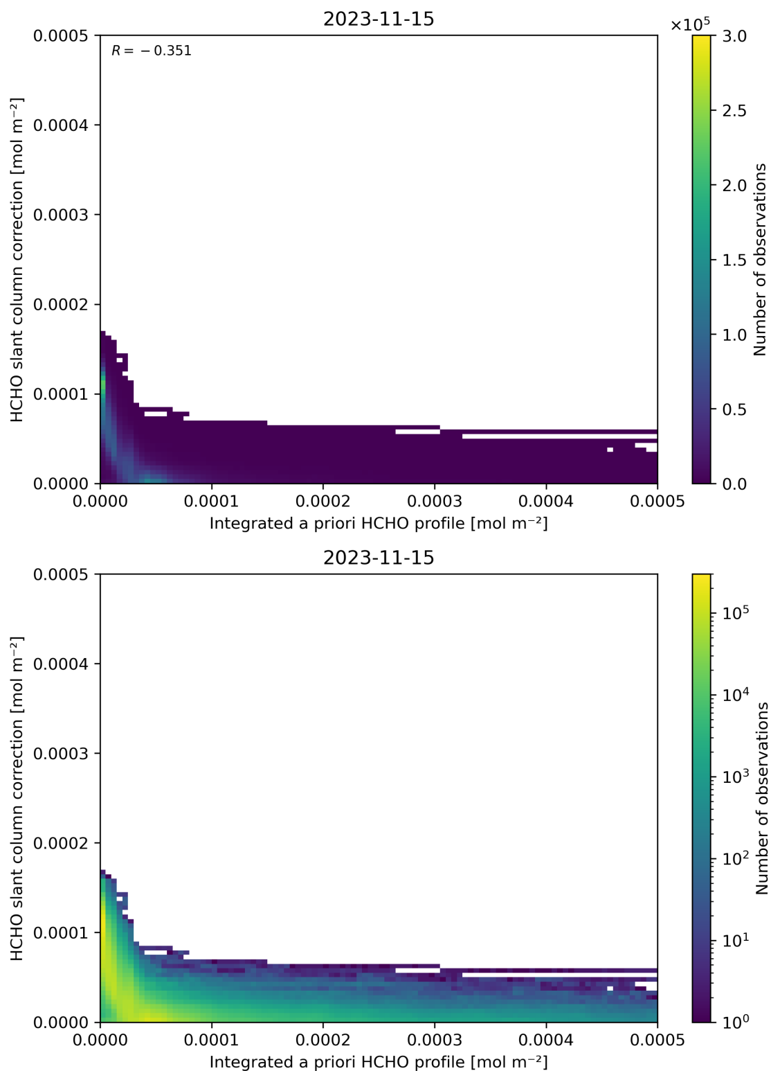
Figure 152: Scatter density plot of “Integrated a priori HCHO profile” against “HCHO slant column correction” for 2023-11-14 to 2023-11-16.
