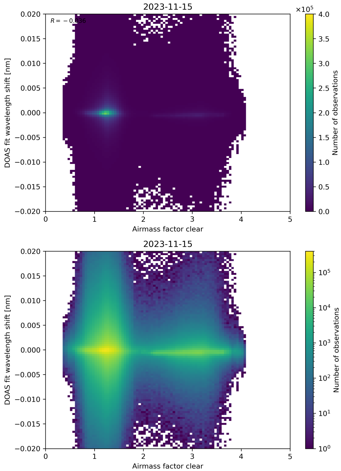
Figure 72: Scatter density plot of “Airmass factor clear” against “DOAS fit wavelength shift” for 2023-11-14 to 2023-11-16.
