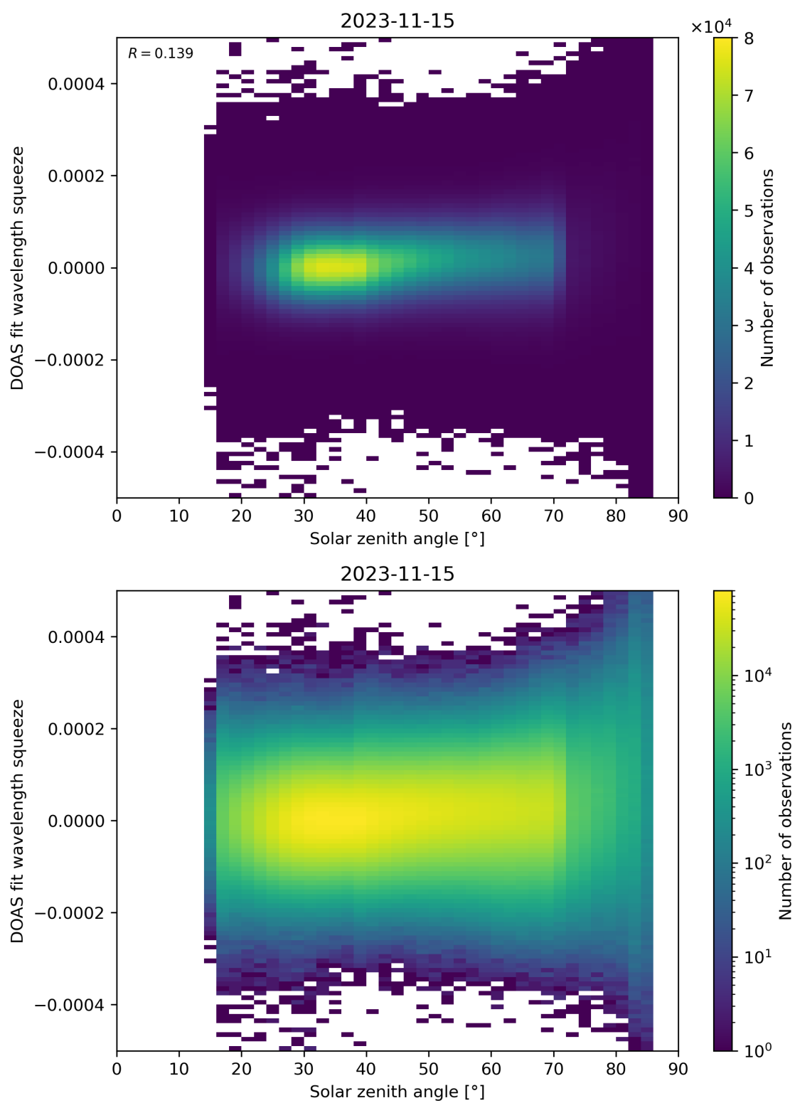
Figure 169: Scatter density plot of “Solar zenith angle” against “DOAS fit wavelength squeeze” for 2023-11-14 to 2023-11-16.
