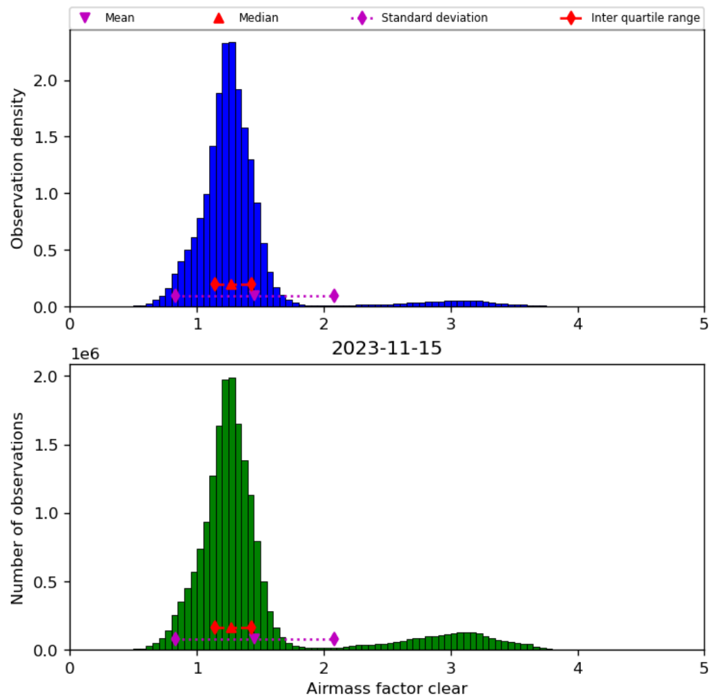
Figure 42: Histogram of “Airmass factor clear” for 2023-11-14 to 2023-11-16
