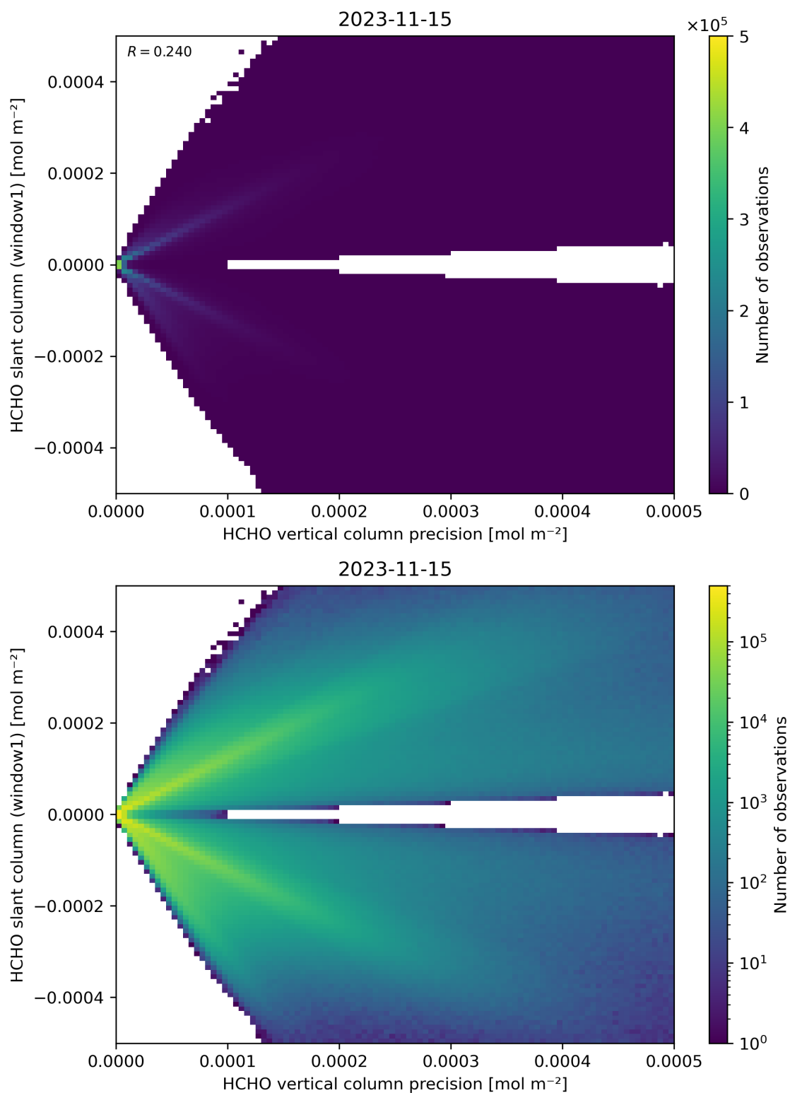
Figure 142: Scatter density plot of “HCHO vertical column precision” against “HCHO slant column (window1)” for 2023-11-14 to 2023-11-16.
