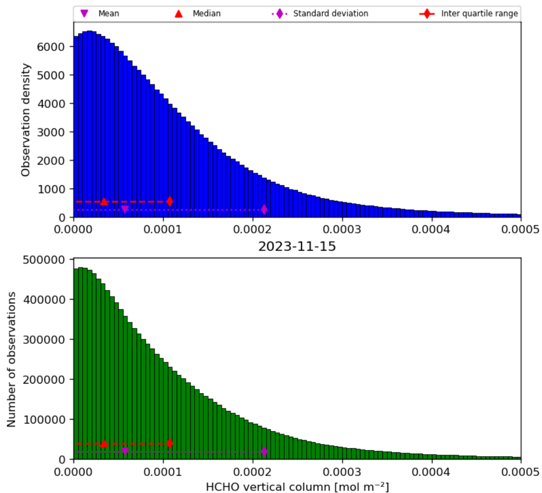
Figure 35: Histogram of “HCHO vertical column” for 2023-11-14 to 2023-11-16
