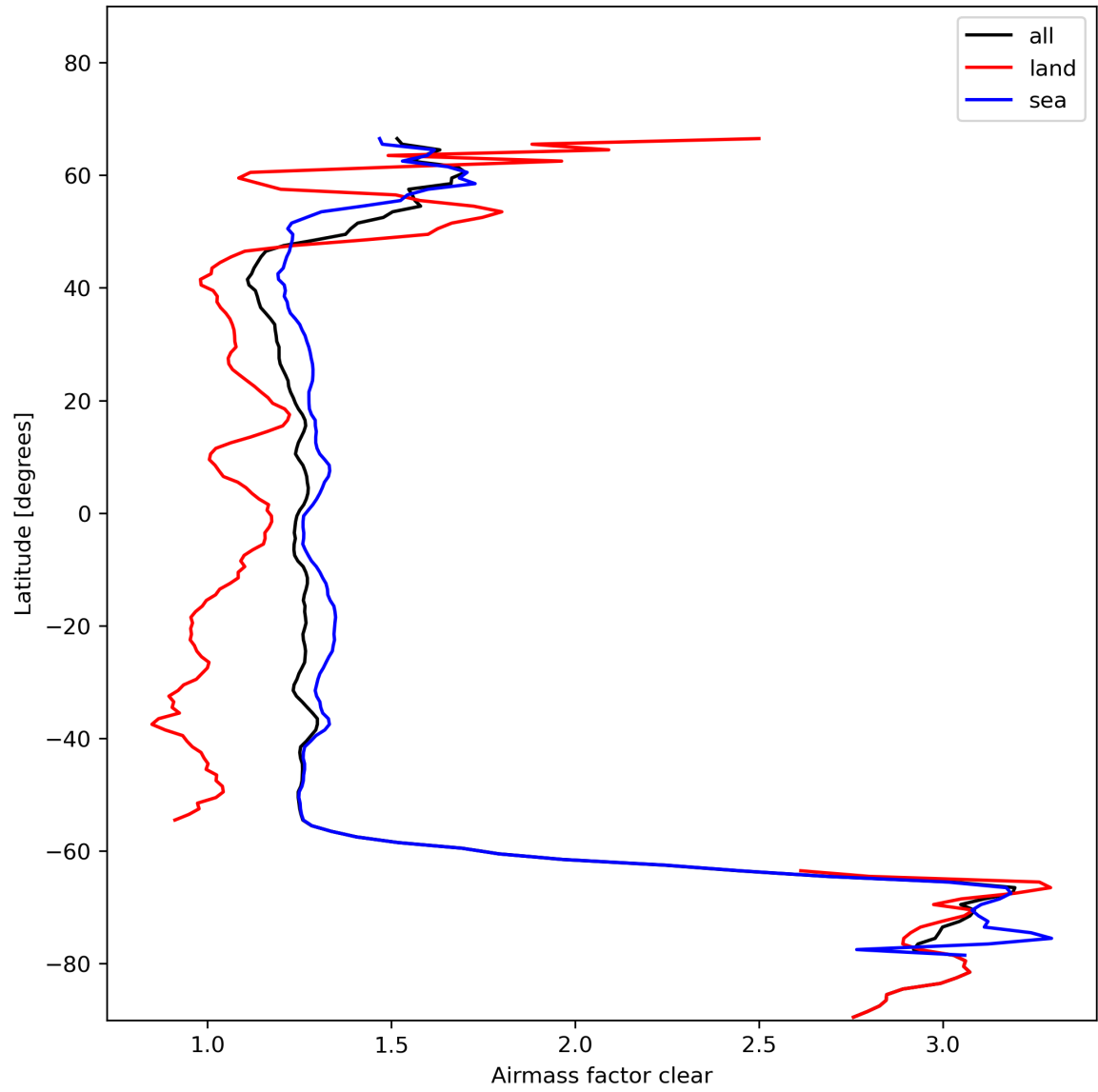
Figure 28: Zonal average of “Airmass factor clear” for 2023-11-14 to 2023-11-16.
