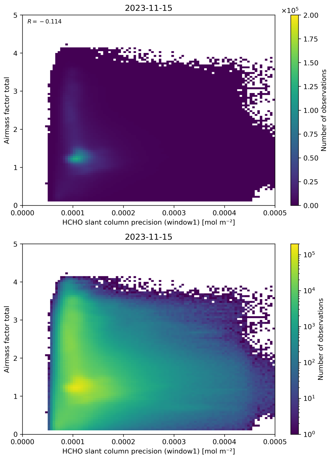
Figure 94: Scatter density plot of “HCHO slant column precision (window1)” against “Airmass factor total” for 2023-11-14 to 2023-11-16.
