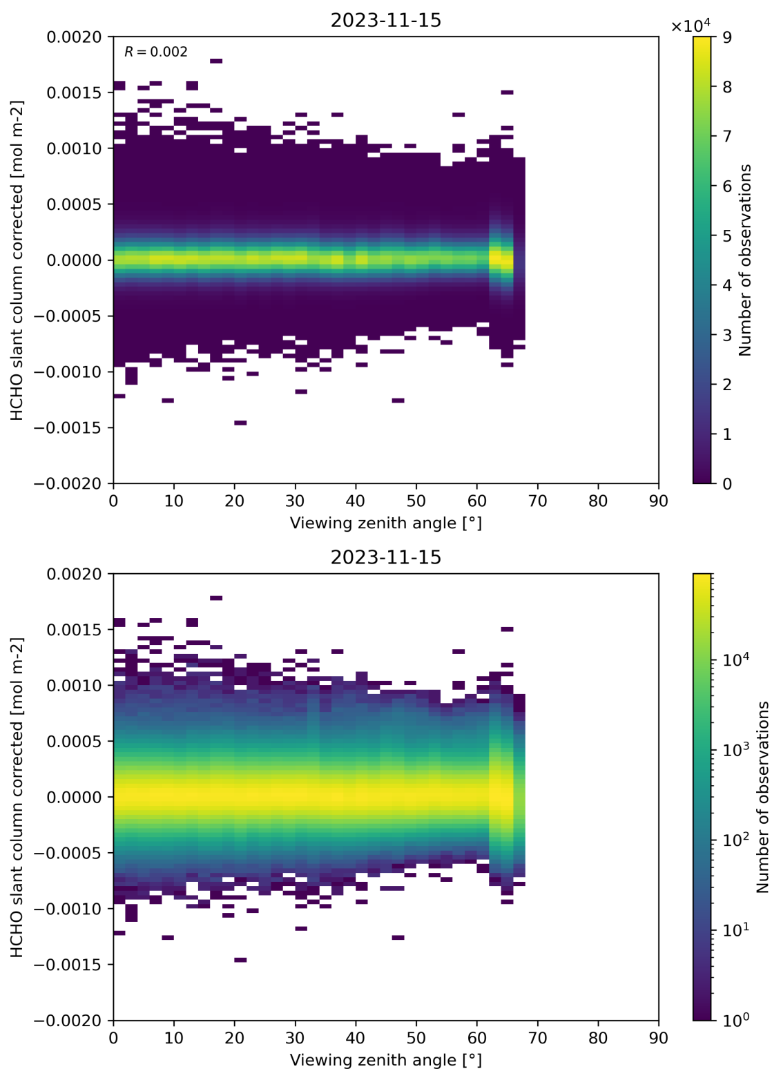
Figure 186: Scatter density plot of “Viewing zenith angle” against “HCHO slant column corrected” for 2023-11-14 to 2023-11-16.
