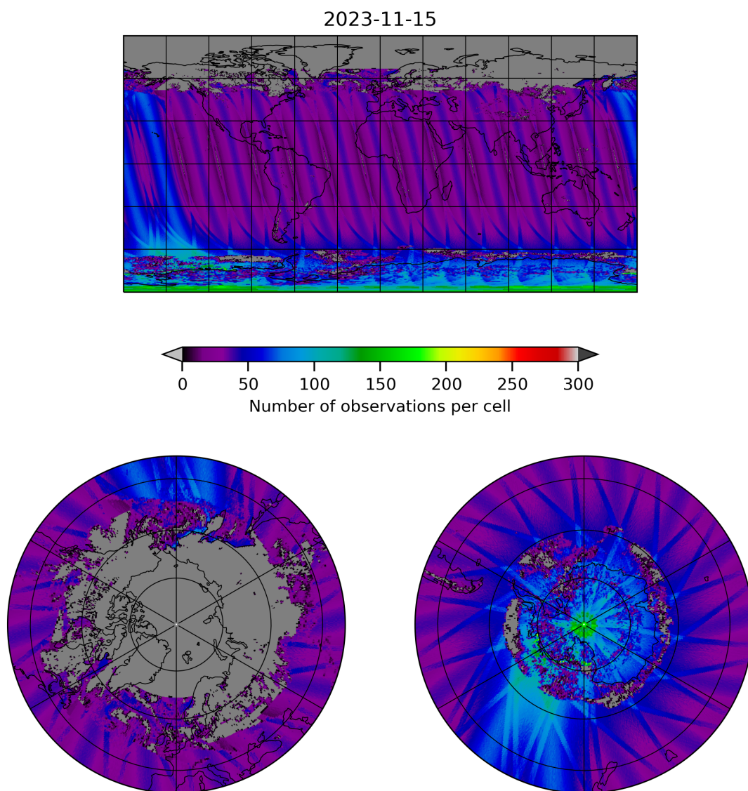
Figure 19: Map of the number of observations for 2023-11-14 to 2023-11-16
