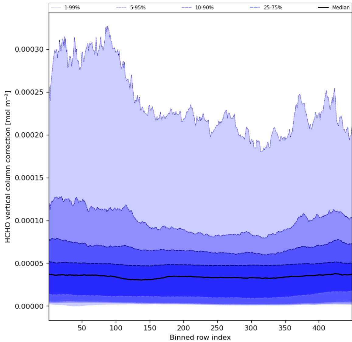
Figure 51: Along track statistics of “HCHO vertical column correction” for 2023-11-14 to 2023-11-16
