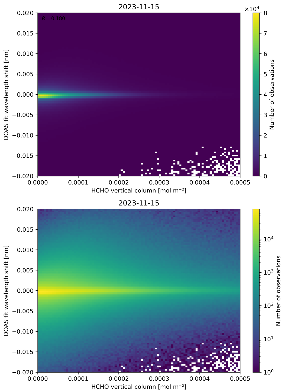
Figure 124: Scatter density plot of “HCHO vertical column” against “DOAS fit wavelength shift” for 2023-11-14 to 2023-11-16.
