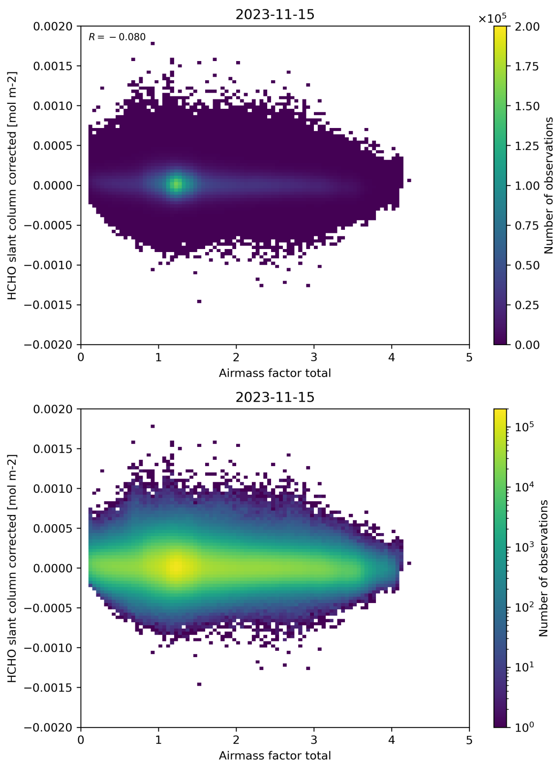
Figure 101: Scatter density plot of “Airmass factor total” against “HCHO slant column corrected” for 2023-11-14 to 2023-11-16.
