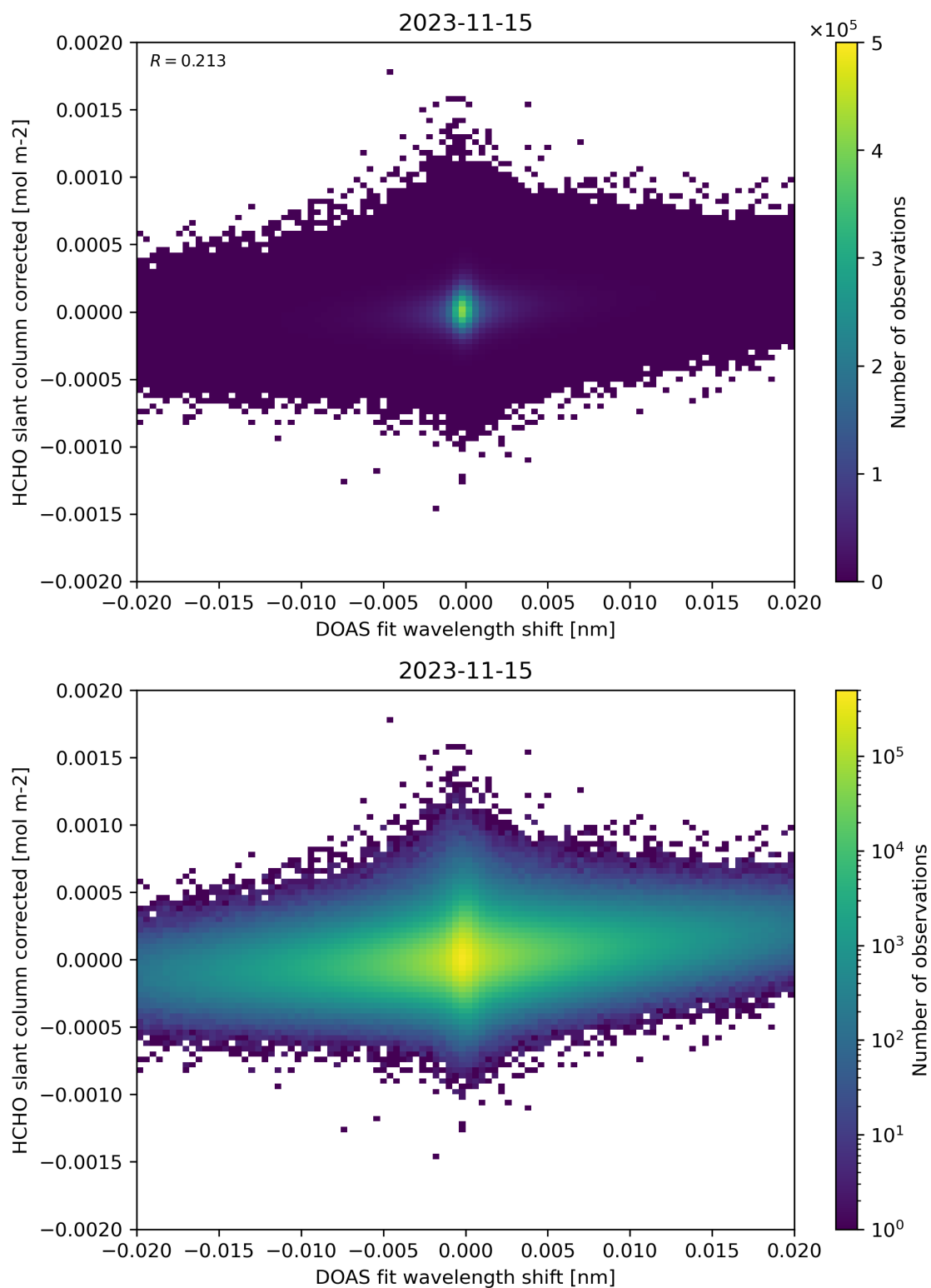
Figure 66: Scatter density plot of “DOAS fit wavelength shift” against “HCHO slant column corrected” for 2023-11-14 to 2023-11-16.
