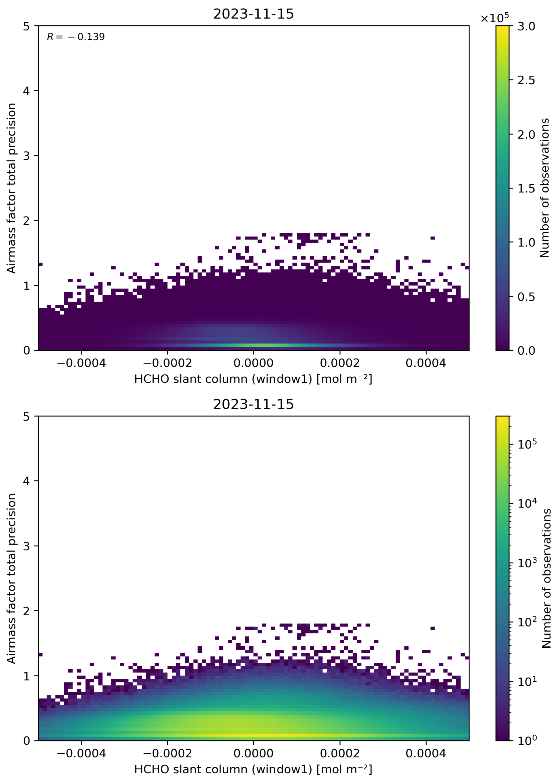
Figure 86: Scatter density plot of “HCHO slant column (window1)” against “Airmass factor total precision” for 2023-11-14 to 2023-11-16.
