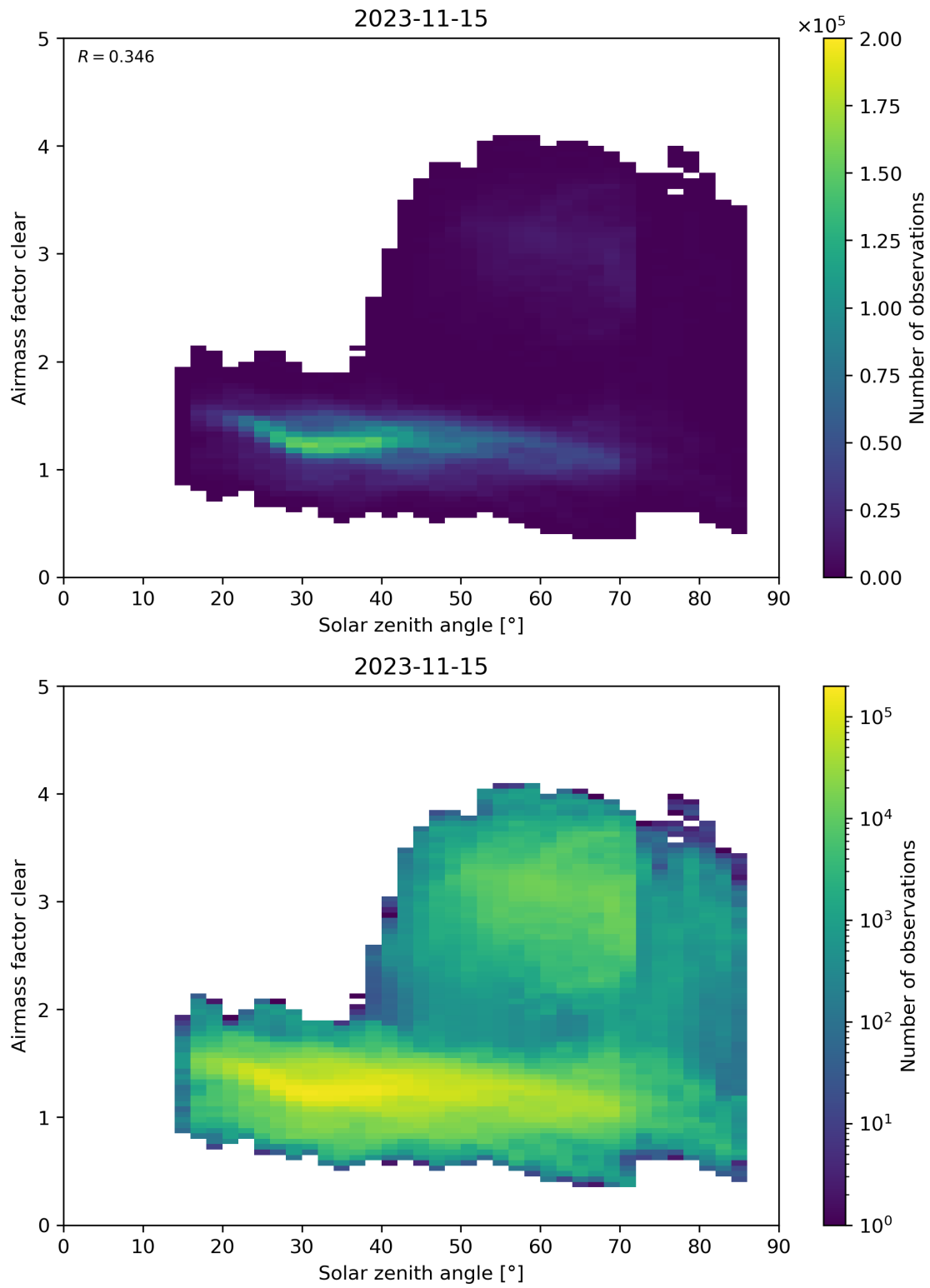
Figure 170: Scatter density plot of “Solar zenith angle” against “Airmass factor clear” for 2023-11-14 to 2023-11-16.
