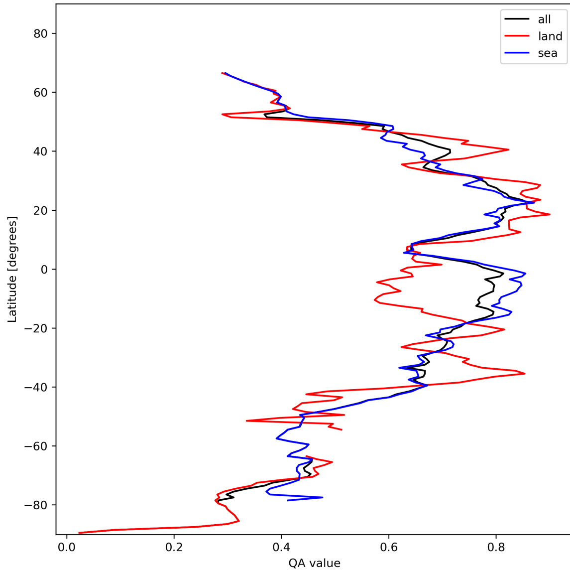
Figure 20: Zonal average of “QA value” for 2023-11-14 to 2023-11-16.
