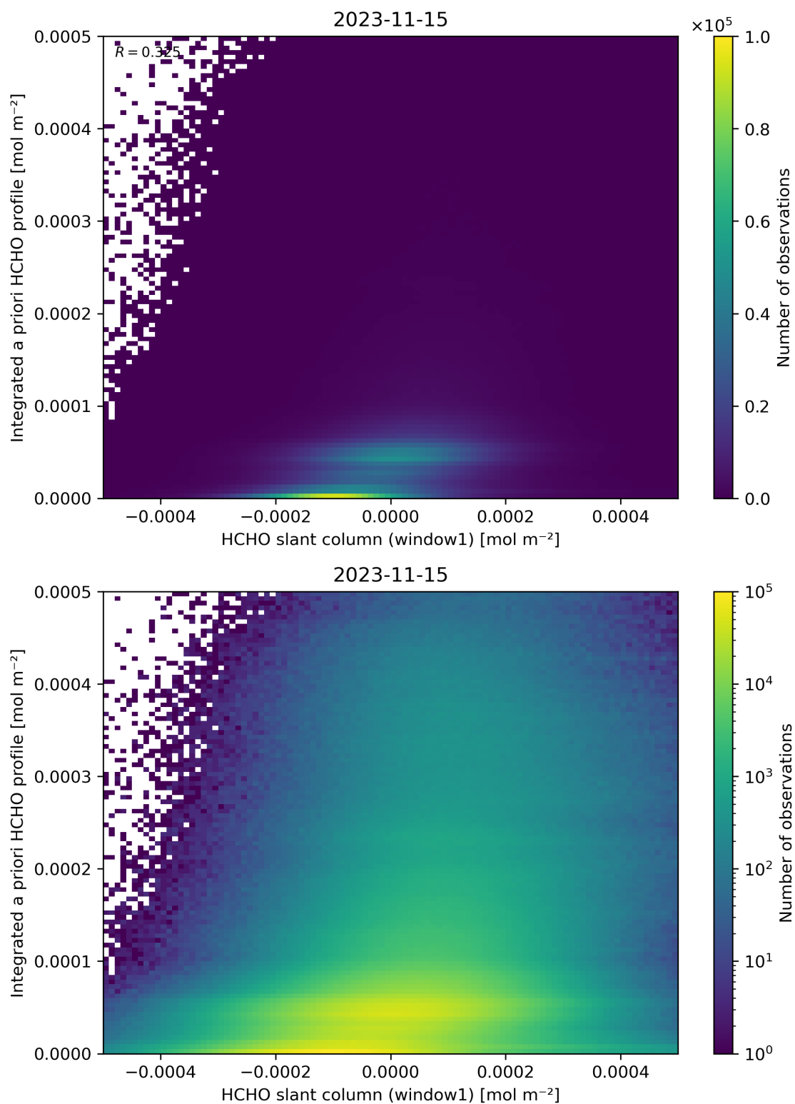
Figure 87: Scatter density plot of “HCHO slant column (window1)” against “Integrated a priori HCHO profile” for 2023-11-14 to 2023-11-16.
