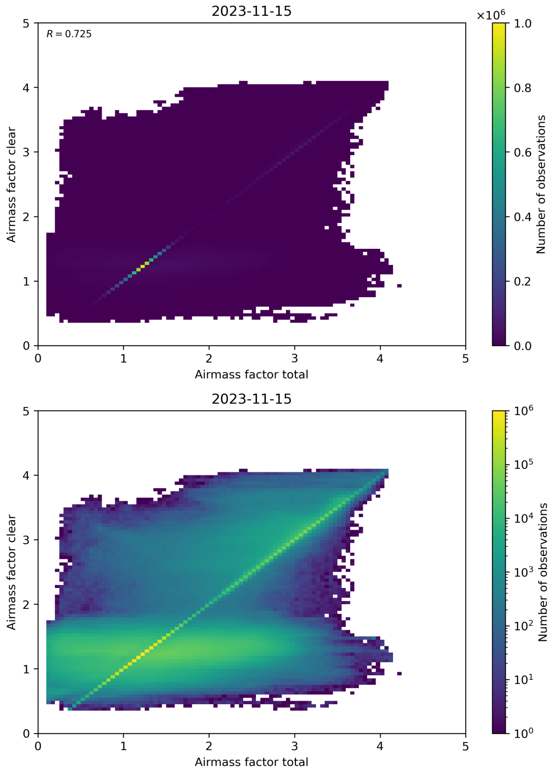
Figure 100: Scatter density plot of “Airmass factor total” against “Airmass factor clear” for 2023-11-14 to 2023-11-16.
