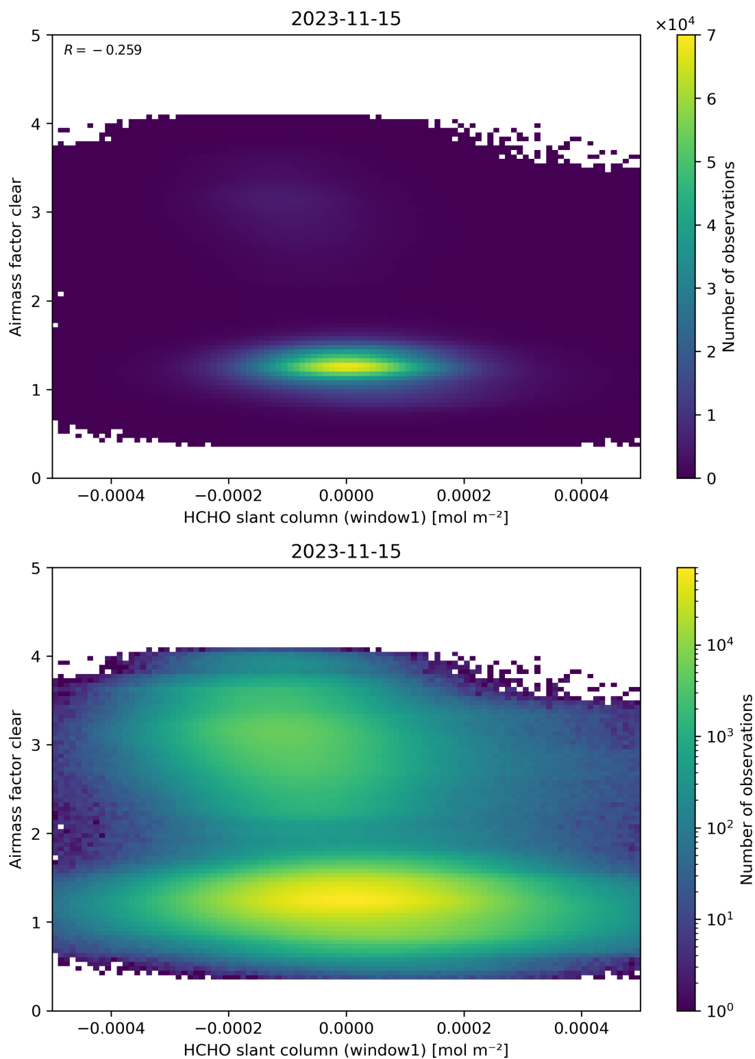
Figure 81: Scatter density plot of “HCHO slant column (window1)” against “Airmass factor clear” for 2023-11-14 to 2023-11-16.
