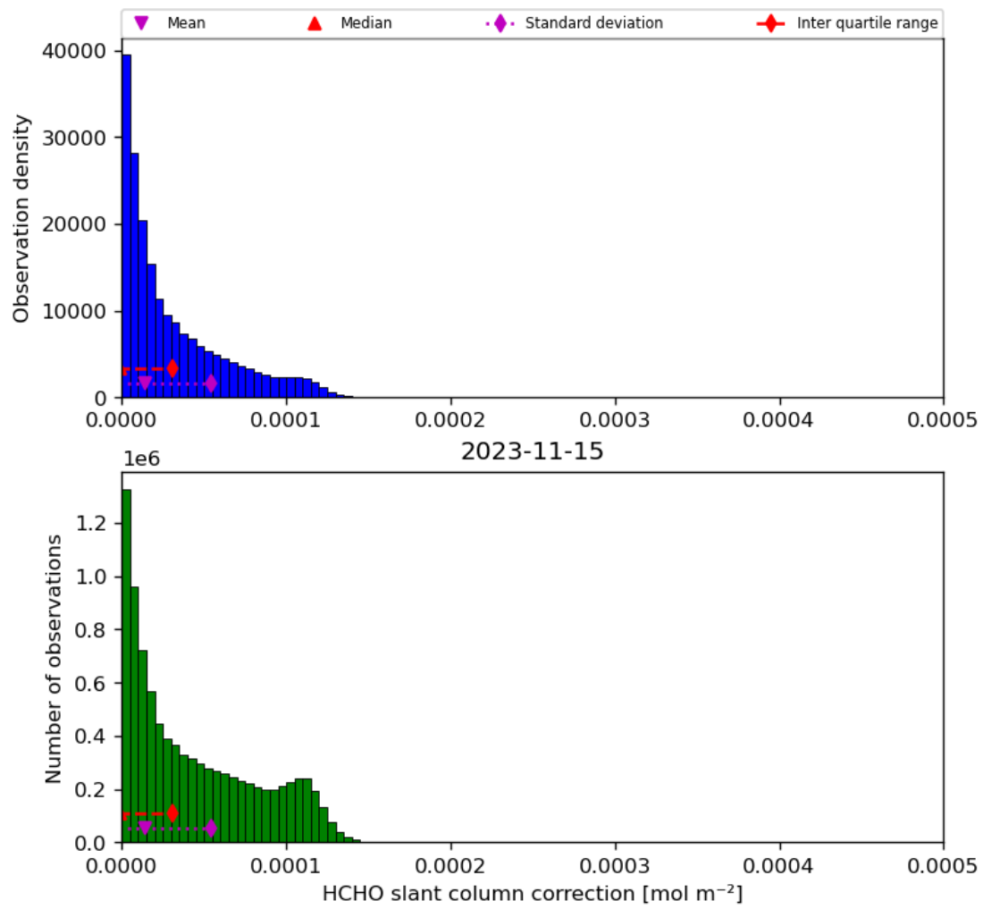
Figure 47: Histogram of “HCHO slant column correction” for 2023-11-14 to 2023-11-16
