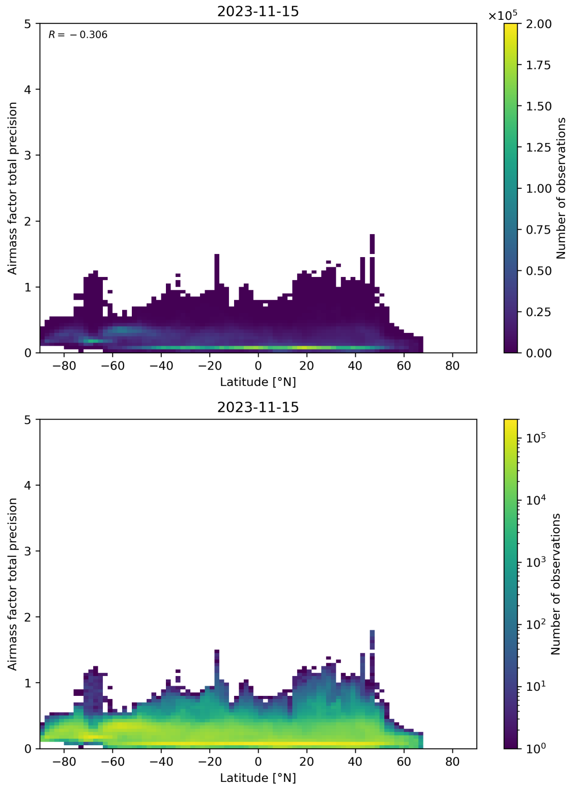
Figure 162: Scatter density plot of “Latitude” against “Airmass factor total precision” for 2023-11-14 to 2023-11-16.
