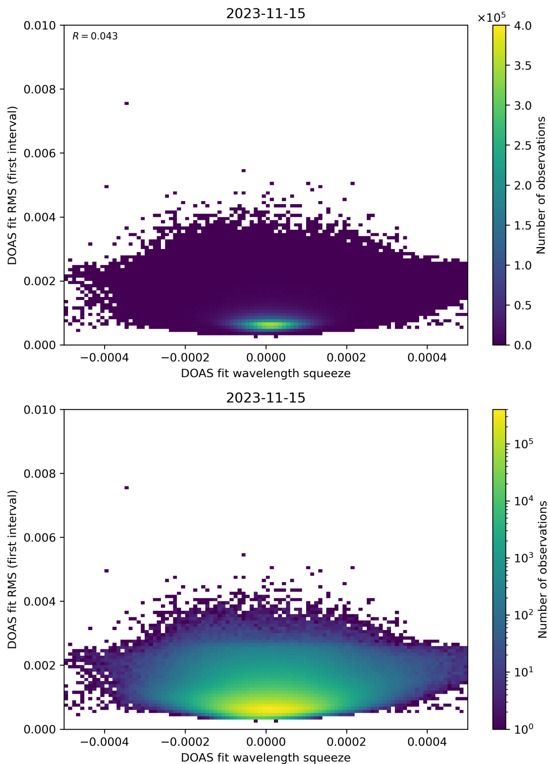
Figure 68: Scatter density plot of “DOAS fit wavelength squeeze” against “DOAS fit RMS (first interval)” for 2023-11-14 to 2023-11-16.
