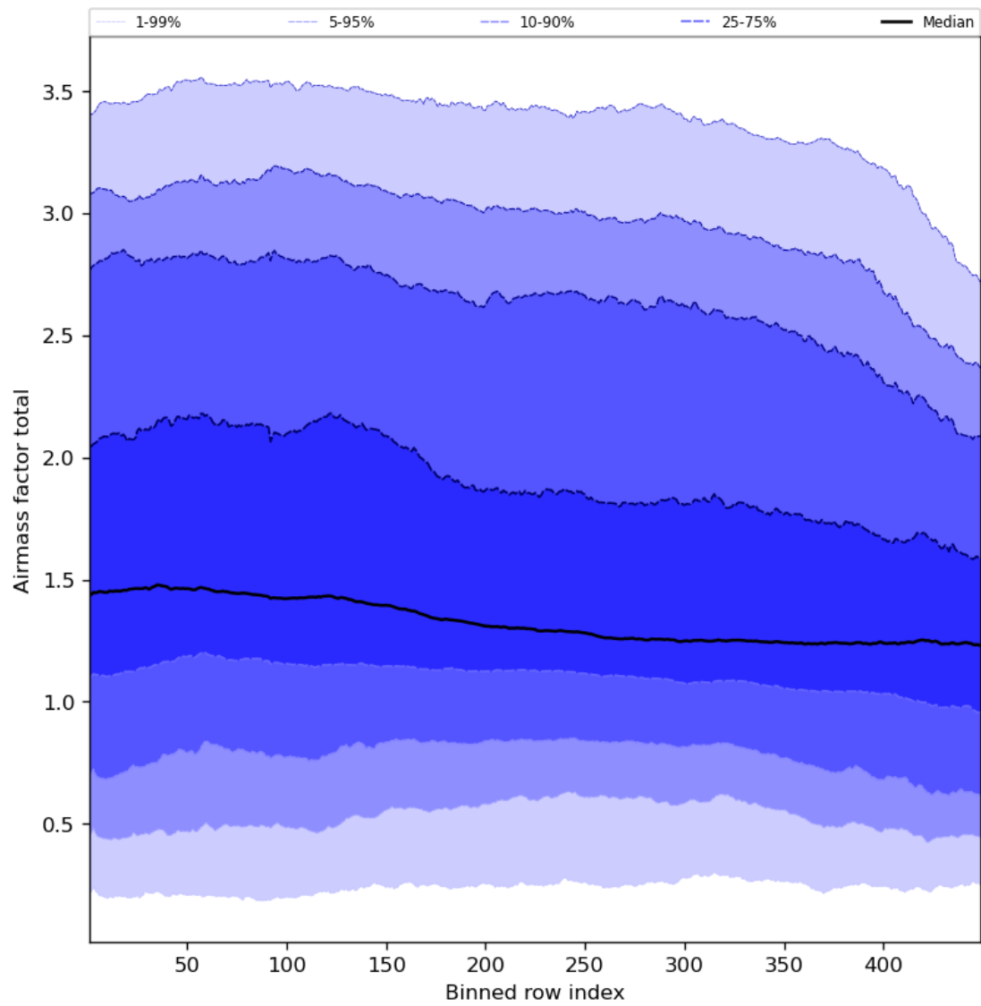
Figure 54: Along track statistics of “Airmass factor total” for 2023-11-14 to 2023-11-16
