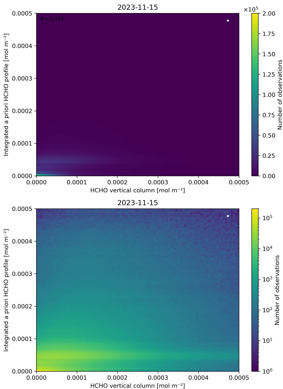
Figure 135: Scatter density plot of “HCHO vertical column” against “Integrated a priori HCHO profile” for 2023-11-14 to 2023-11-16.
