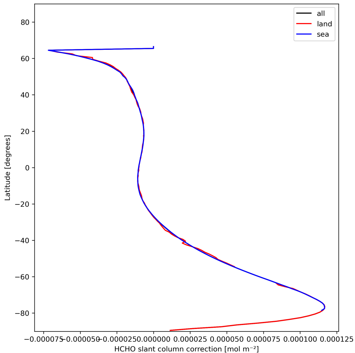
Figure 33: Zonal average of “HCHO slant column correction” for 2023-11-14 to 2023-11-16.
