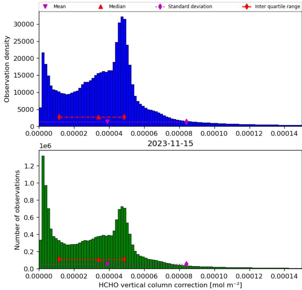
Figure 37: Histogram of “HCHO vertical column correction” for 2023-11-14 to 2023-11-16
