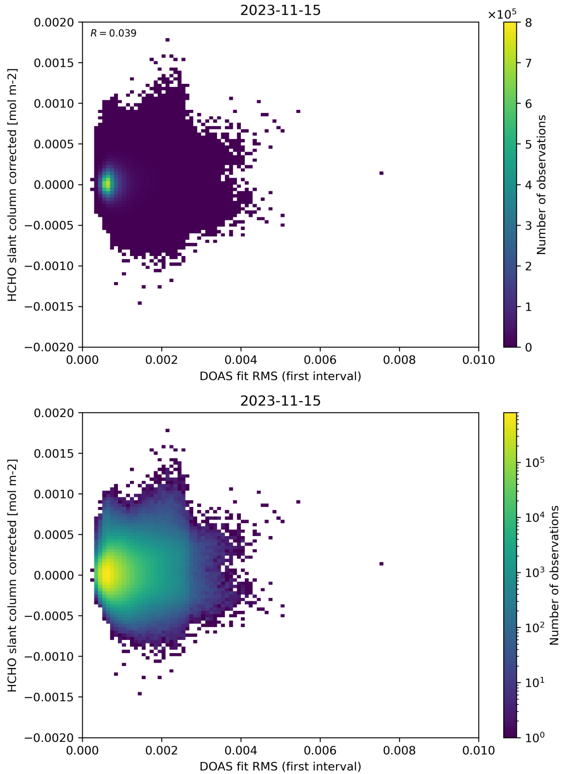
Figure 62: Scatter density plot of “DOAS fit RMS (first interval)” against “HCHO slant column corrected” for 2023-11-14 to 2023-11-16.
