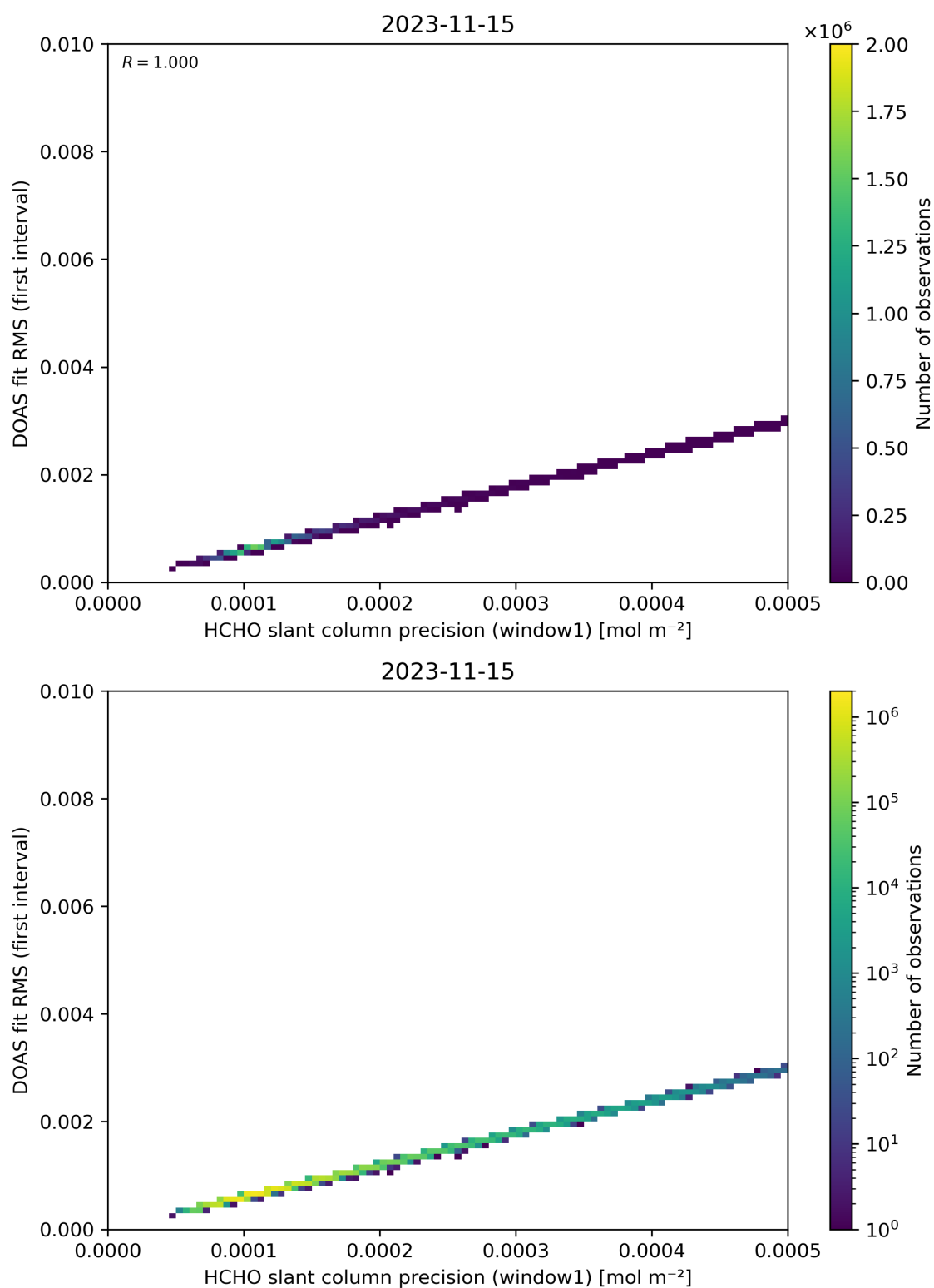
Figure 88: Scatter density plot of “HCHO slant column precision (window1)” against “DOAS fit RMS (first interval)” for 2023-11-14 to 2023-11-16.
