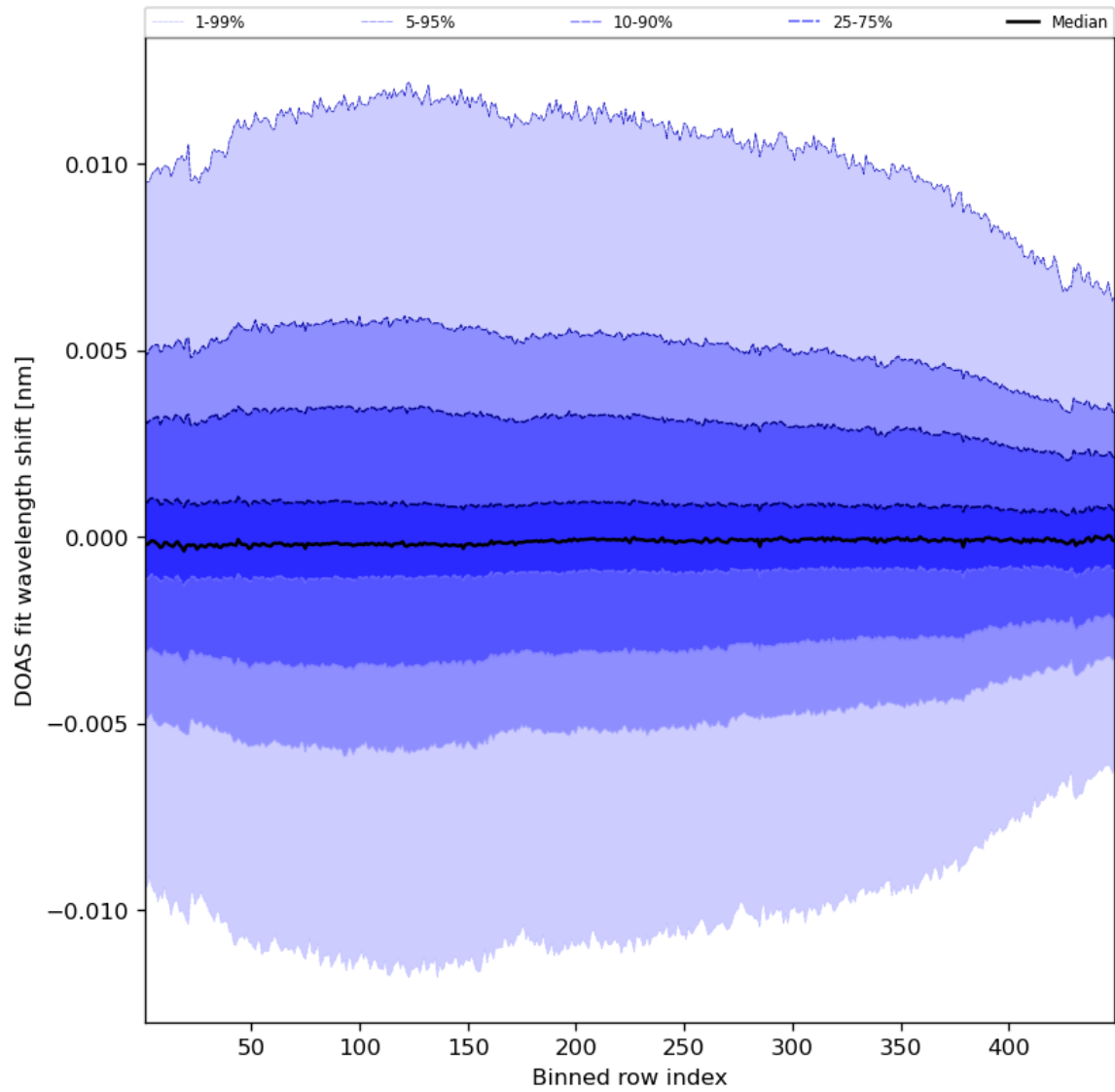
Figure 58: Along track statistics of “DOAS fit wavelength shift” for 2023-11-14 to 2023-11-16
