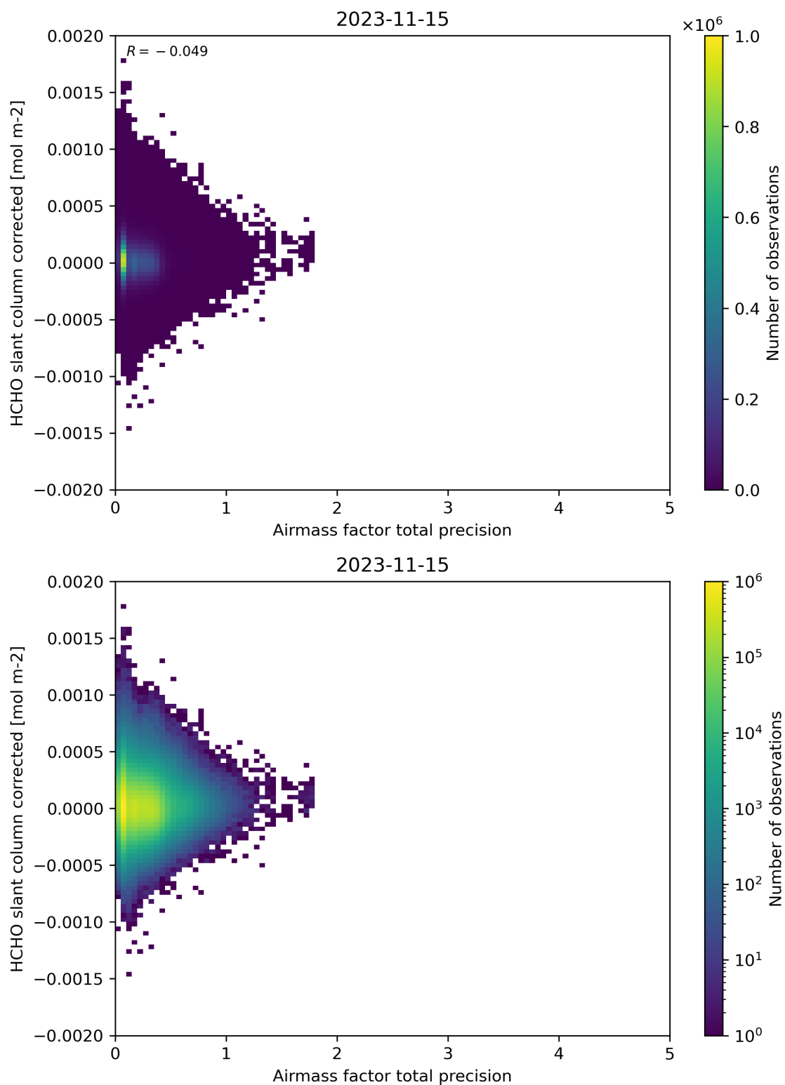
Figure 109: Scatter density plot of “Airmass factor total precision” against “HCHO slant column corrected” for 2023-11-14 to 2023-11-16.
