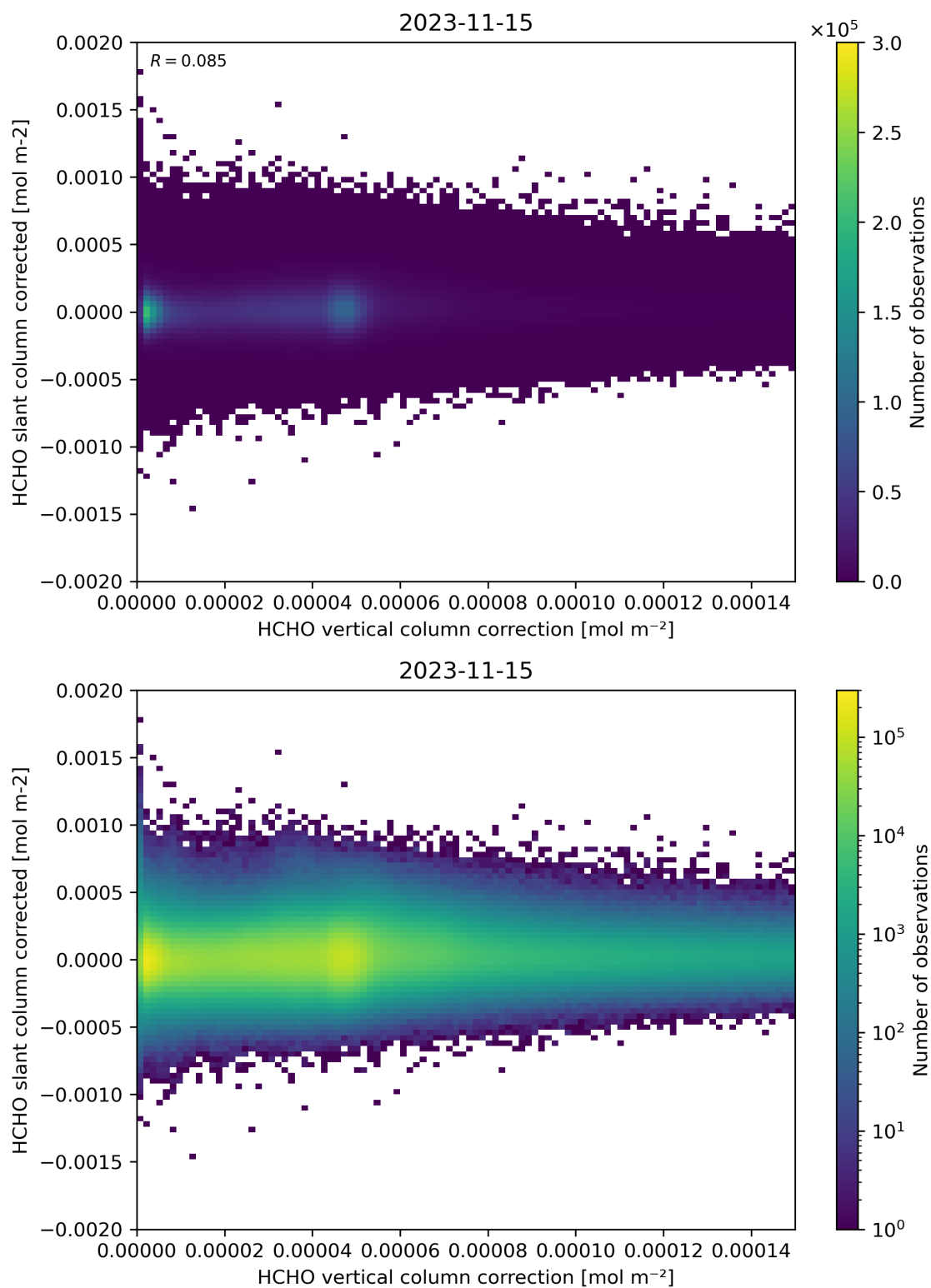
Figure 116: Scatter density plot of “HCHO vertical column correction” against “HCHO slant column corrected” for 2023-11-14 to 2023-11-16.
