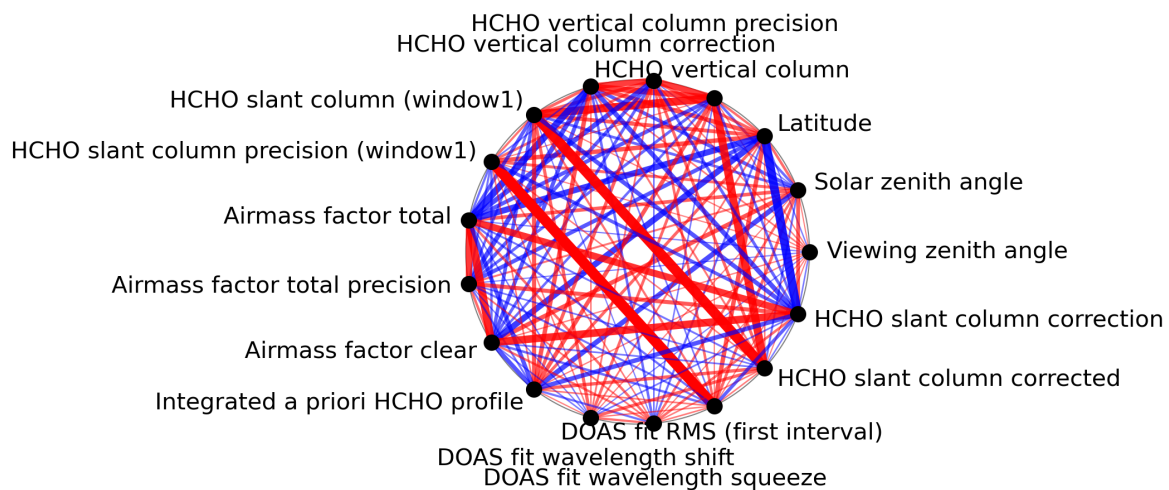
Figure 1: Map of correlation graph for 2023-11-14 to 2023-11-16.
