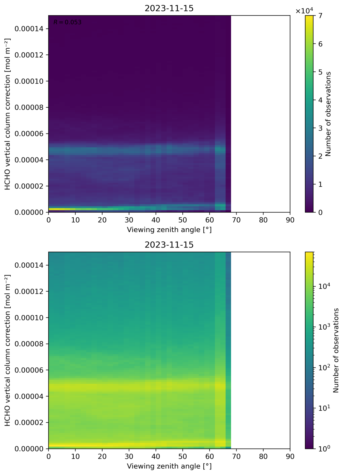
Figure 193: Scatter density plot of “Viewing zenith angle” against “HCHO vertical column correction” for 2023-11-14 to 2023-11-16.
