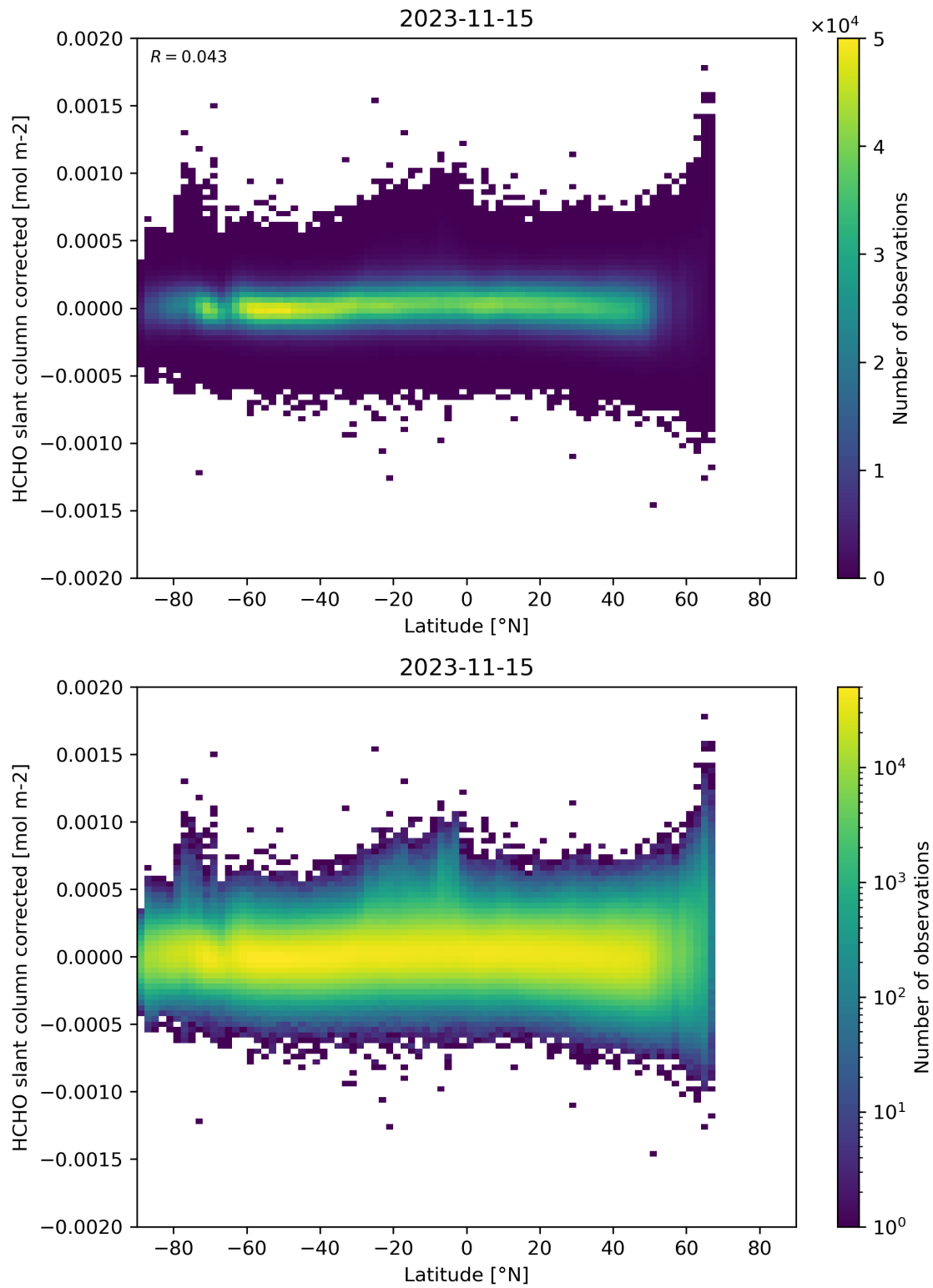
Figure 157: Scatter density plot of “Latitude” against “HCHO slant column corrected” for 2023-11-14 to 2023-11-16.
