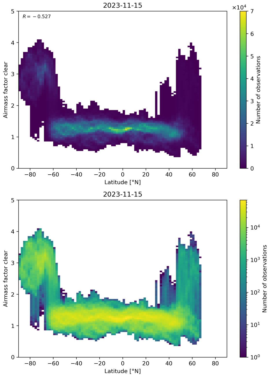
Figure 156: Scatter density plot of “Latitude” against “Airmass factor clear” for 2023-11-14 to 2023-11-16.
