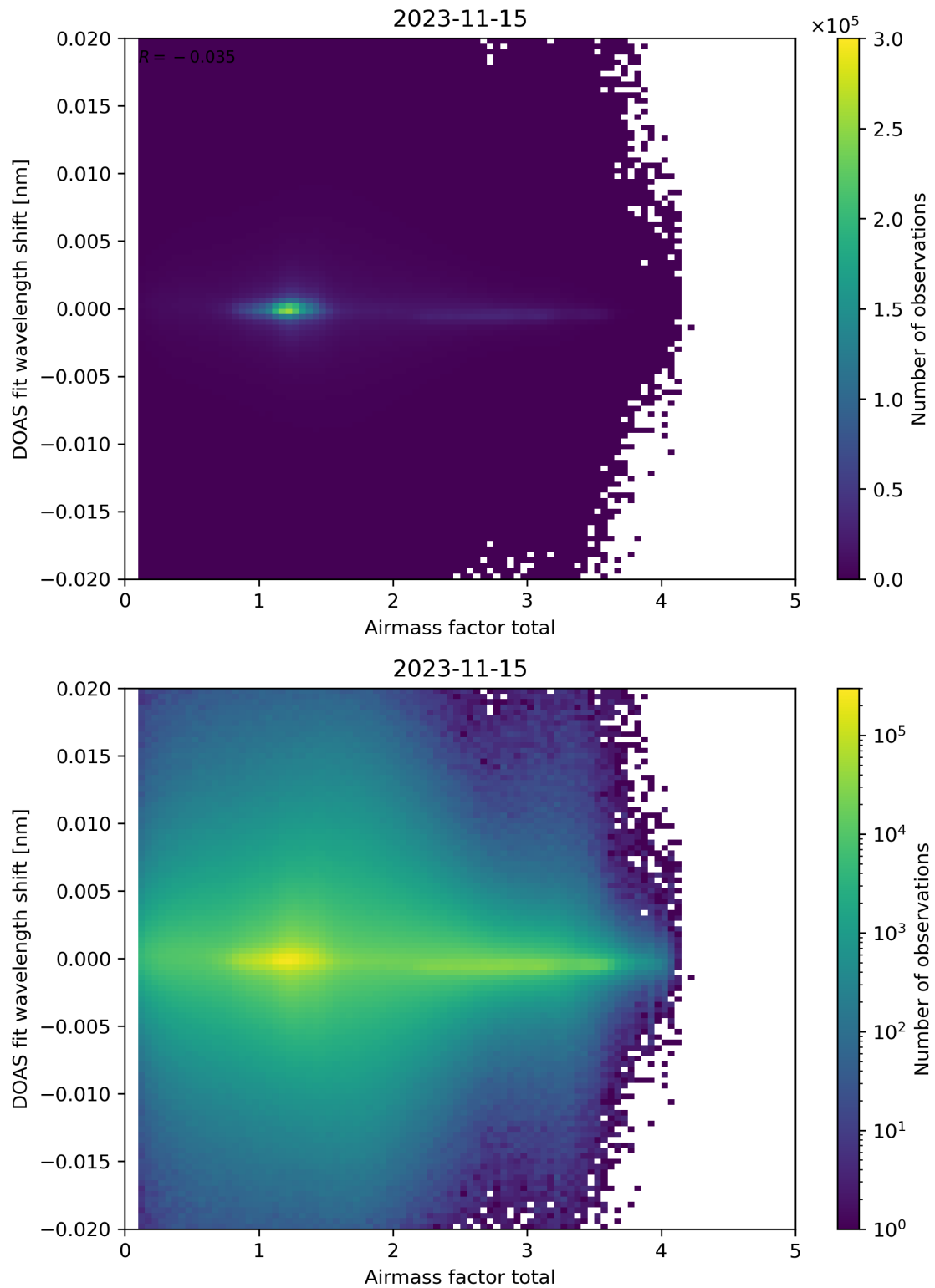
Figure 98: Scatter density plot of “Airmass factor total” against “DOAS fit wavelength shift” for 2023-11-14 to 2023-11-16.
