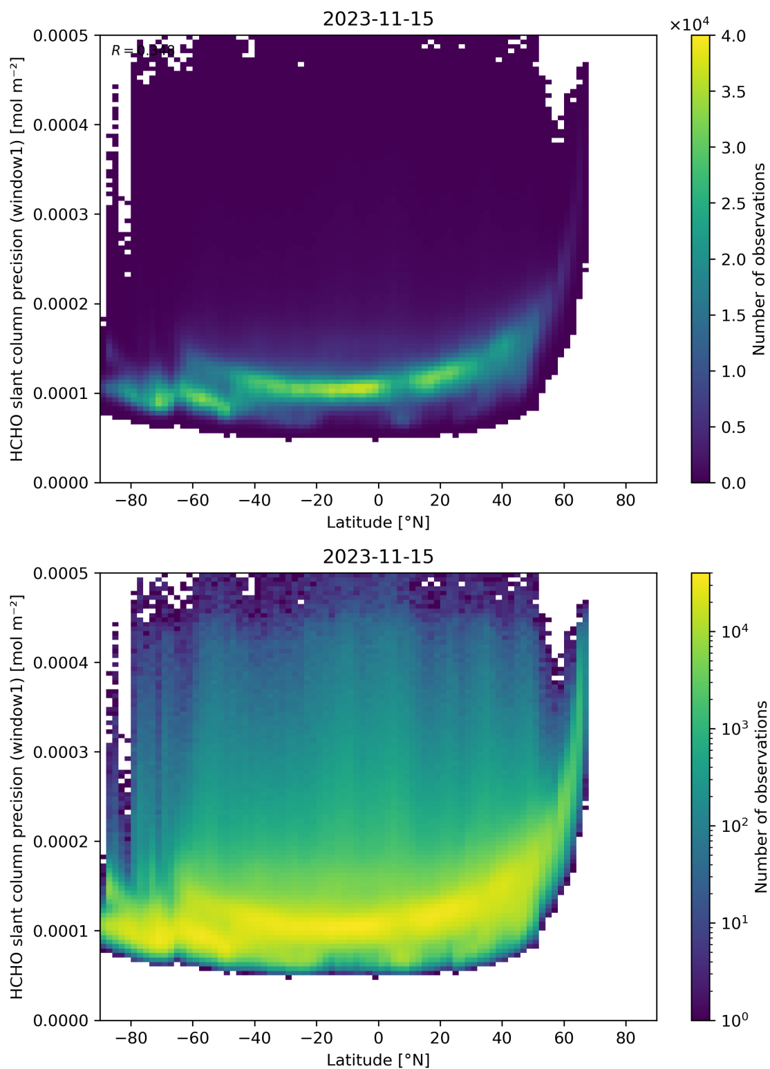
Figure 160: Scatter density plot of “Latitude” against “HCHO slant column precision (window1)” for 2023-11-14 to 2023-11-16.
