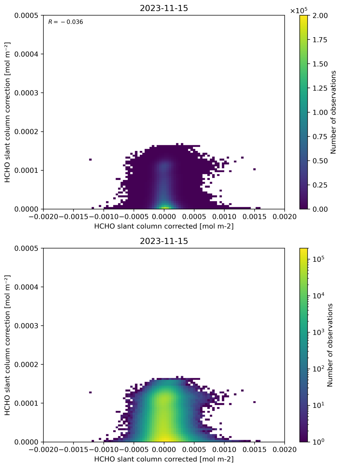
Figure 77: Scatter density plot of “HCHO slant column corrected” against “HCHO slant column correction” for 2023-11-14 to 2023-11-16.
