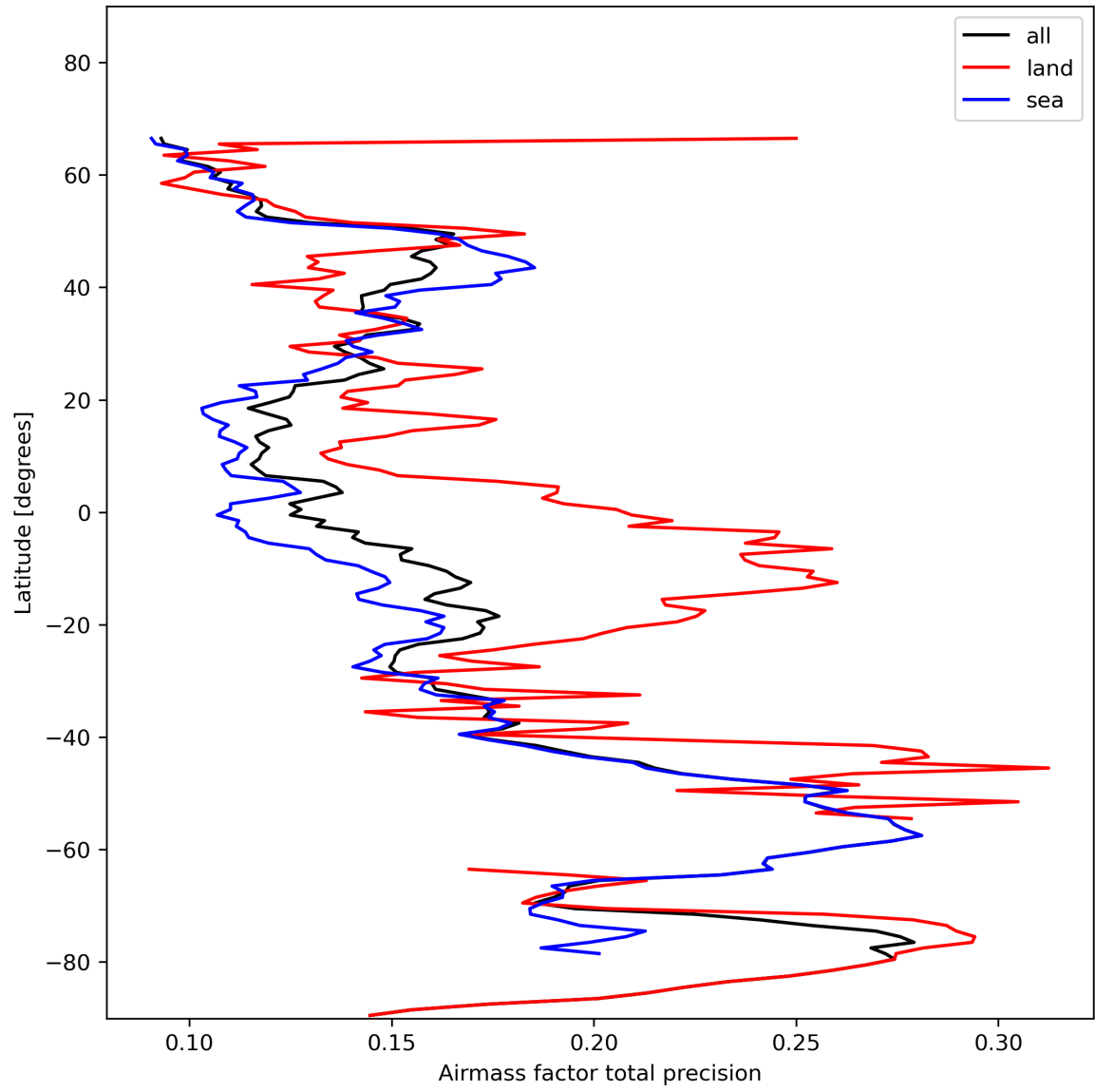
Figure 27: Zonal average of “Airmass factor total precision” for 2023-11-14 to 2023-11-16.
