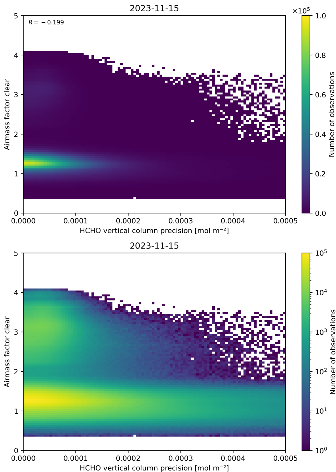
Figure 139: Scatter density plot of “HCHO vertical column precision” against “Airmass factor clear” for 2023-11-14 to 2023-11-16.
