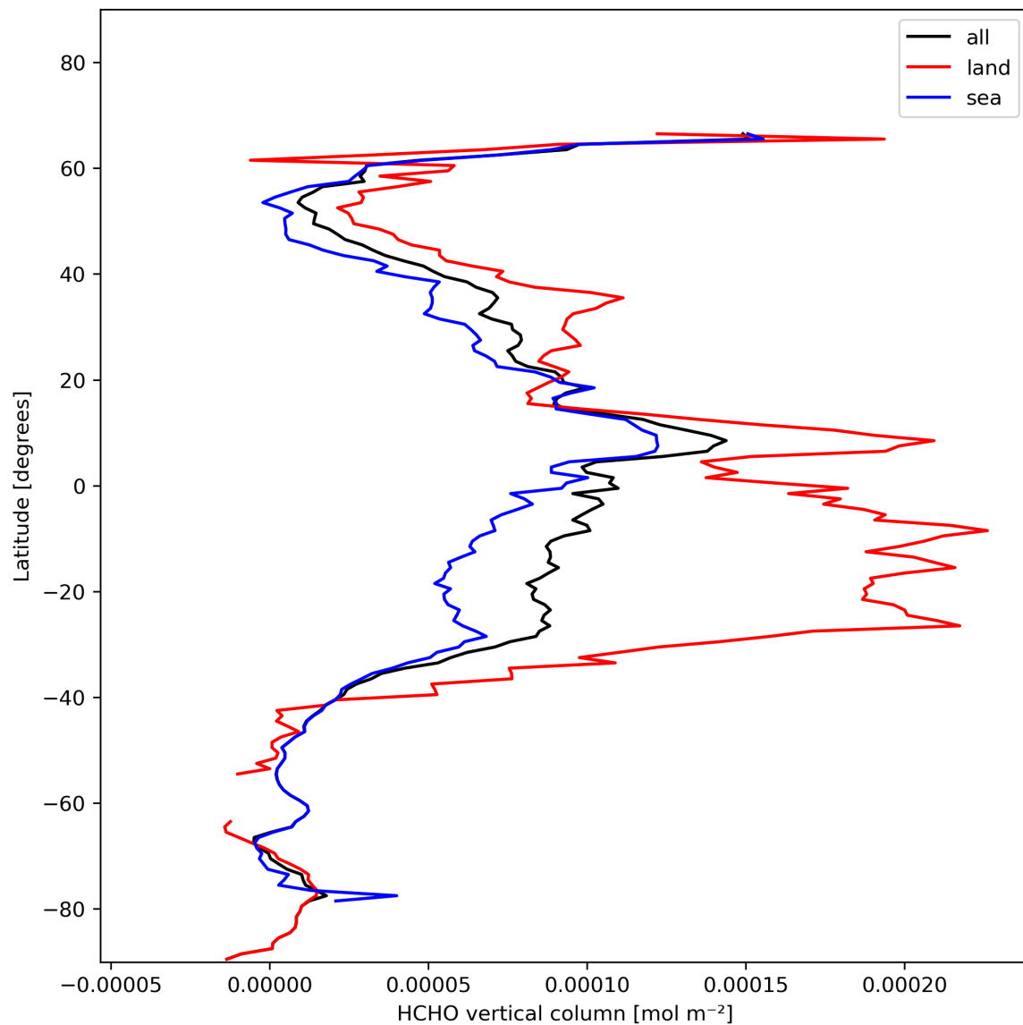
Figure 21: Zonal average of “HCHO vertical column” for 2023-11-14 to 2023-11-16.
