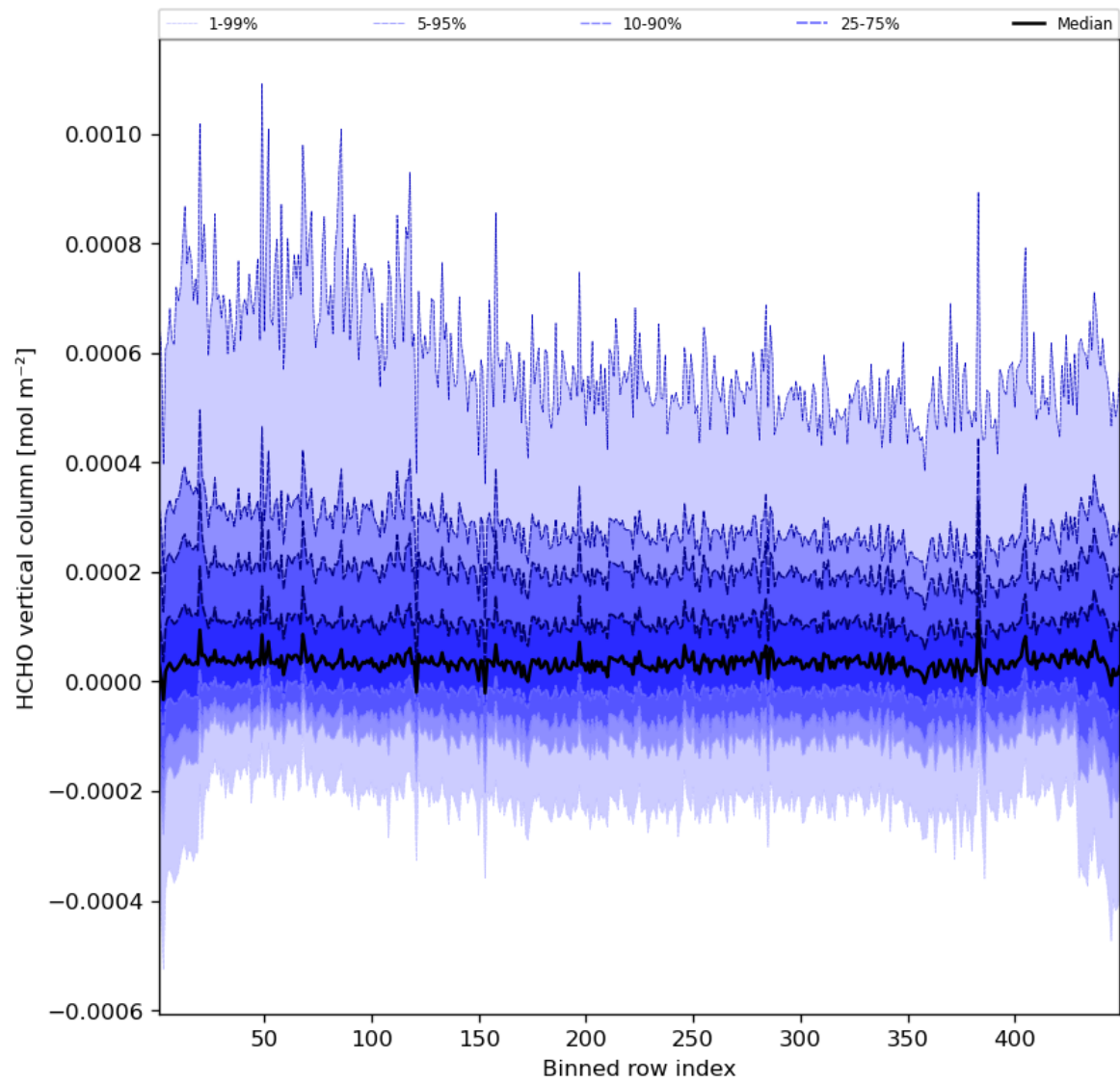
Figure 49: Along track statistics of “HCHO vertical column” for 2023-11-14 to 2023-11-16
