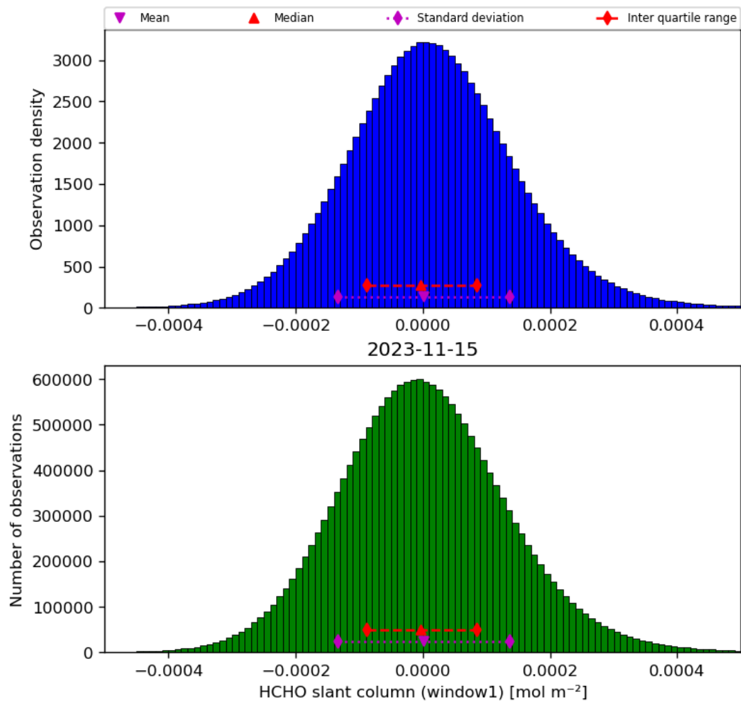
Figure 38: Histogram of “HCHO slant column (window1)” for 2023-11-14 to 2023-11-16
