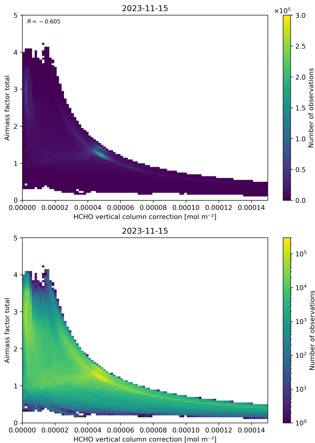
Figure 120: Scatter density plot of “HCHO vertical column correction” against “Airmass factor total” for 2023-11-14 to 2023-11-16.
