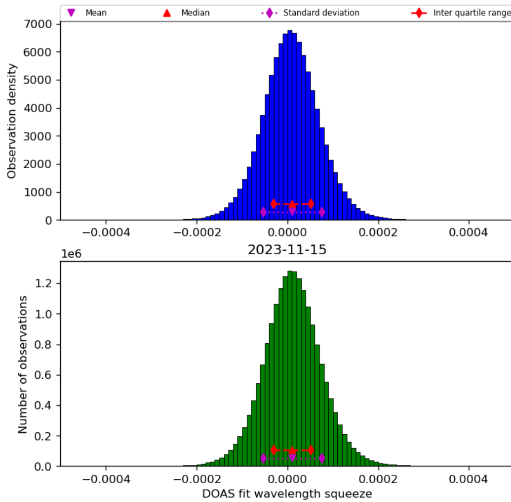
Figure 45: Histogram of “DOAS fit wavelength squeeze” for 2023-11-14 to 2023-11-16
