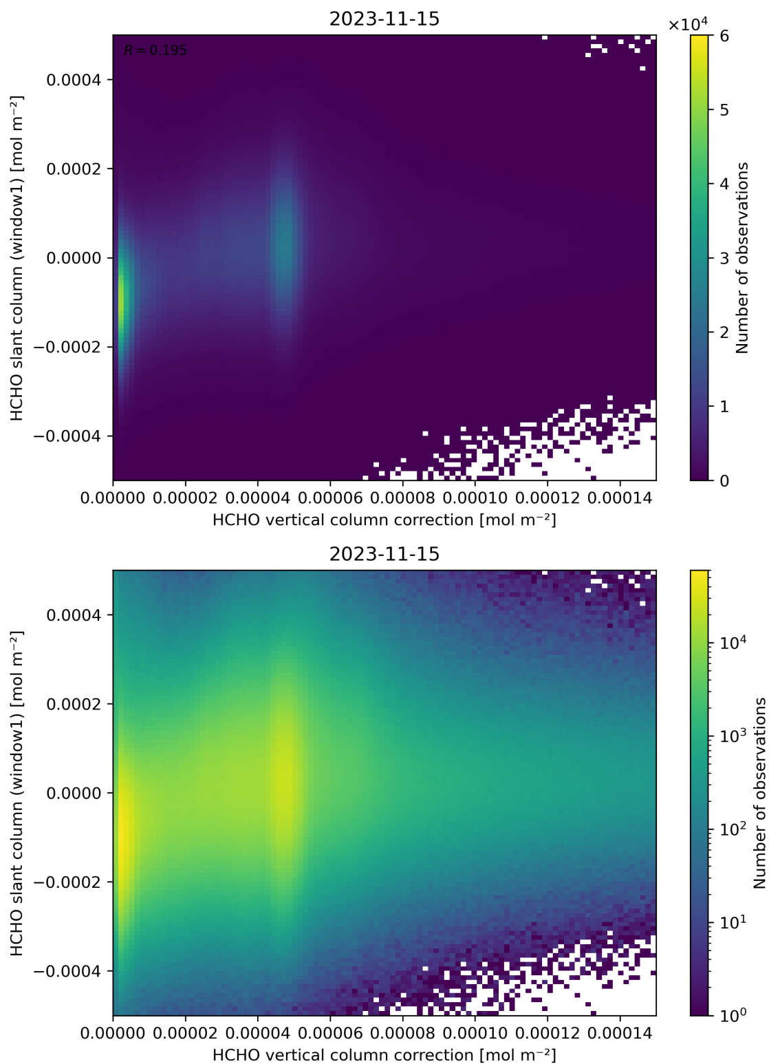
Figure 118: Scatter density plot of “HCHO vertical column correction” against “HCHO slant column (window1)” for 2023-11-14 to 2023-11-16.
