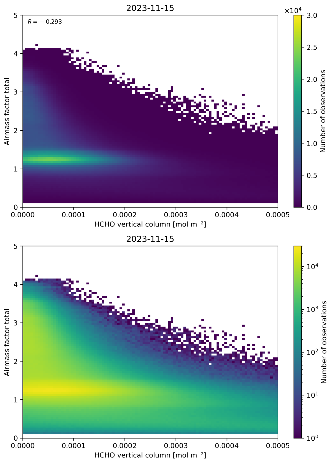
Figure 131: Scatter density plot of “HCHO vertical column” against “Airmass factor total” for 2023-11-14 to 2023-11-16.
