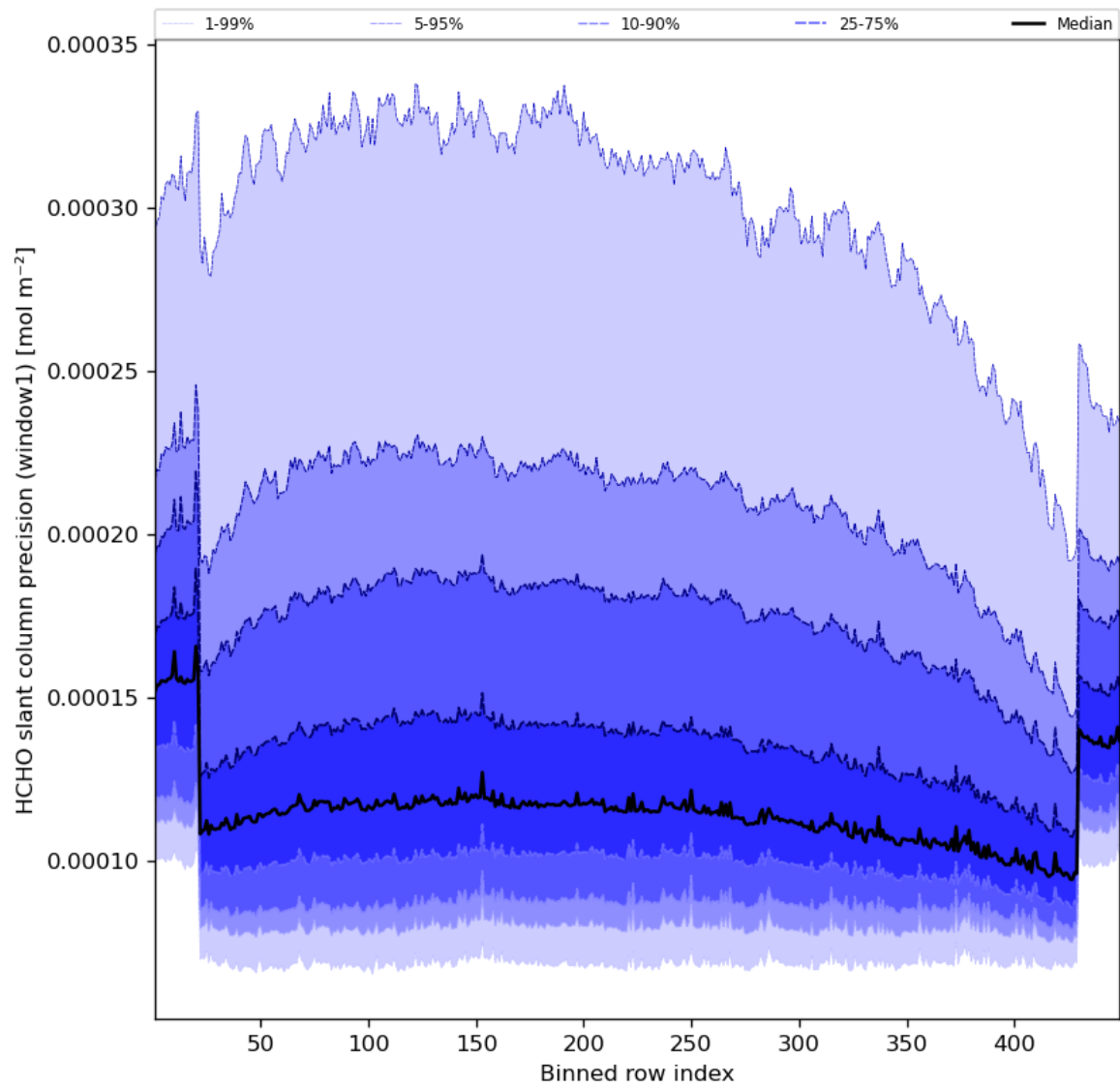
Figure 53: Along track statistics of “HCHO slant column precision (window1)” for 2023-11-14 to 2023-11-16
