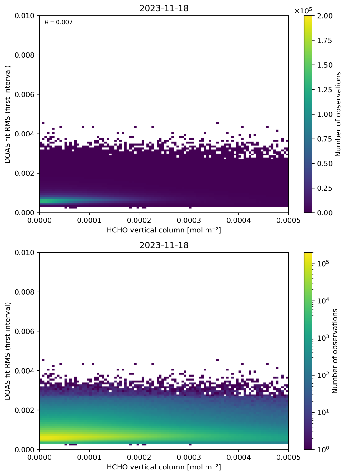
Figure 123: Scatter density plot of “HCHO vertical column” against “DOAS fit RMS (first interval)” for 2023-11-18 to 2023-11-19.
