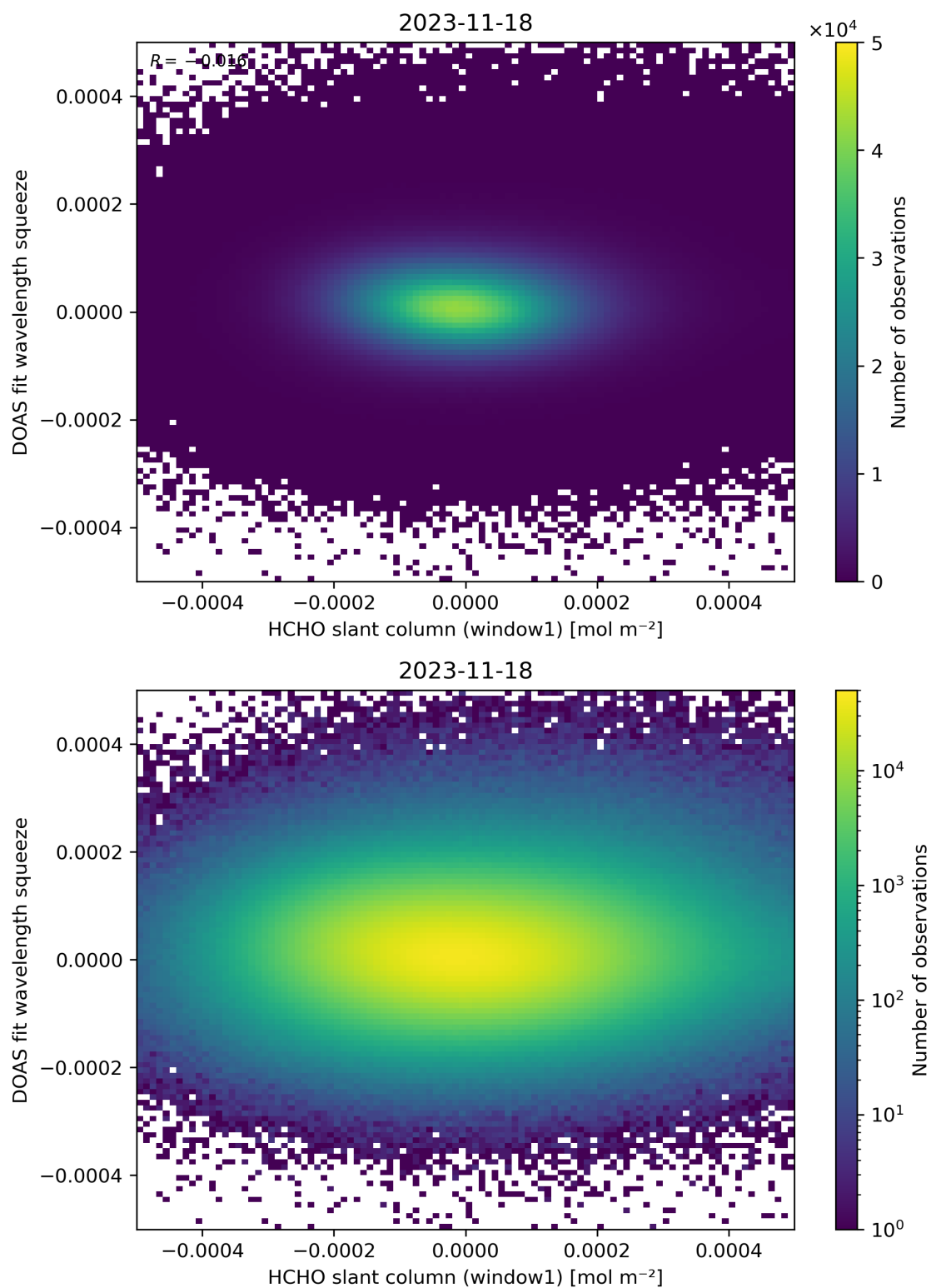
Figure 80: Scatter density plot of “HCHO slant column (window1)” against “DOAS fit wavelength squeeze” for 2023-11-18 to 2023-11-19.
