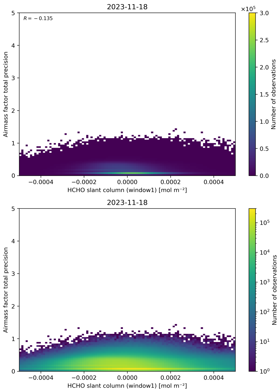
Figure 86: Scatter density plot of “HCHO slant column (window1)” against “Airmass factor total precision” for 2023-11-18 to 2023-11-19.
