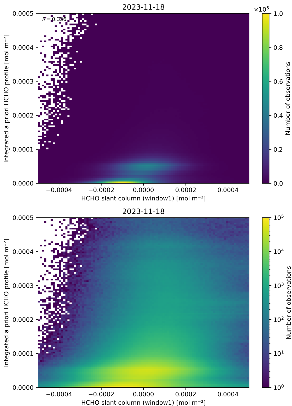
Figure 87: Scatter density plot of “HCHO slant column (window1)” against “Integrated a priori HCHO profile” for 2023-11-18 to 2023-11-19.
