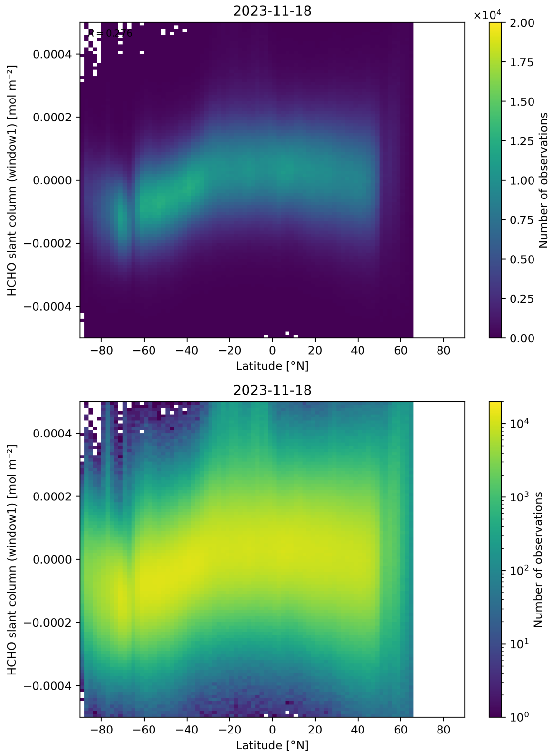
Figure 159: Scatter density plot of “Latitude” against “HCHO slant column (window1)” for 2023-11-18 to 2023-11-19.
