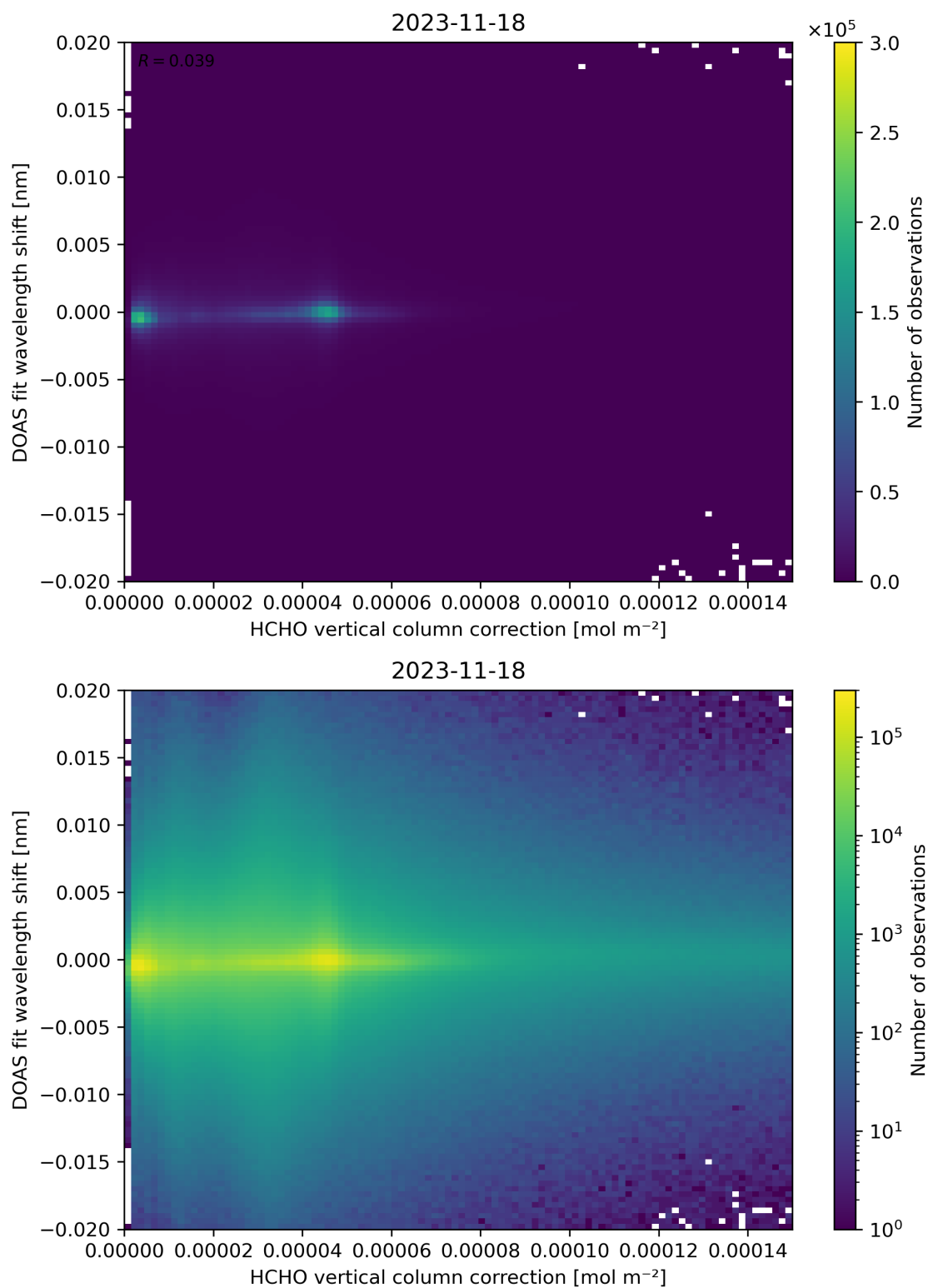
Figure 113: Scatter density plot of “HCHO vertical column correction” against “DOAS fit wavelength shift” for 2023-11-18 to 2023-11-19.
