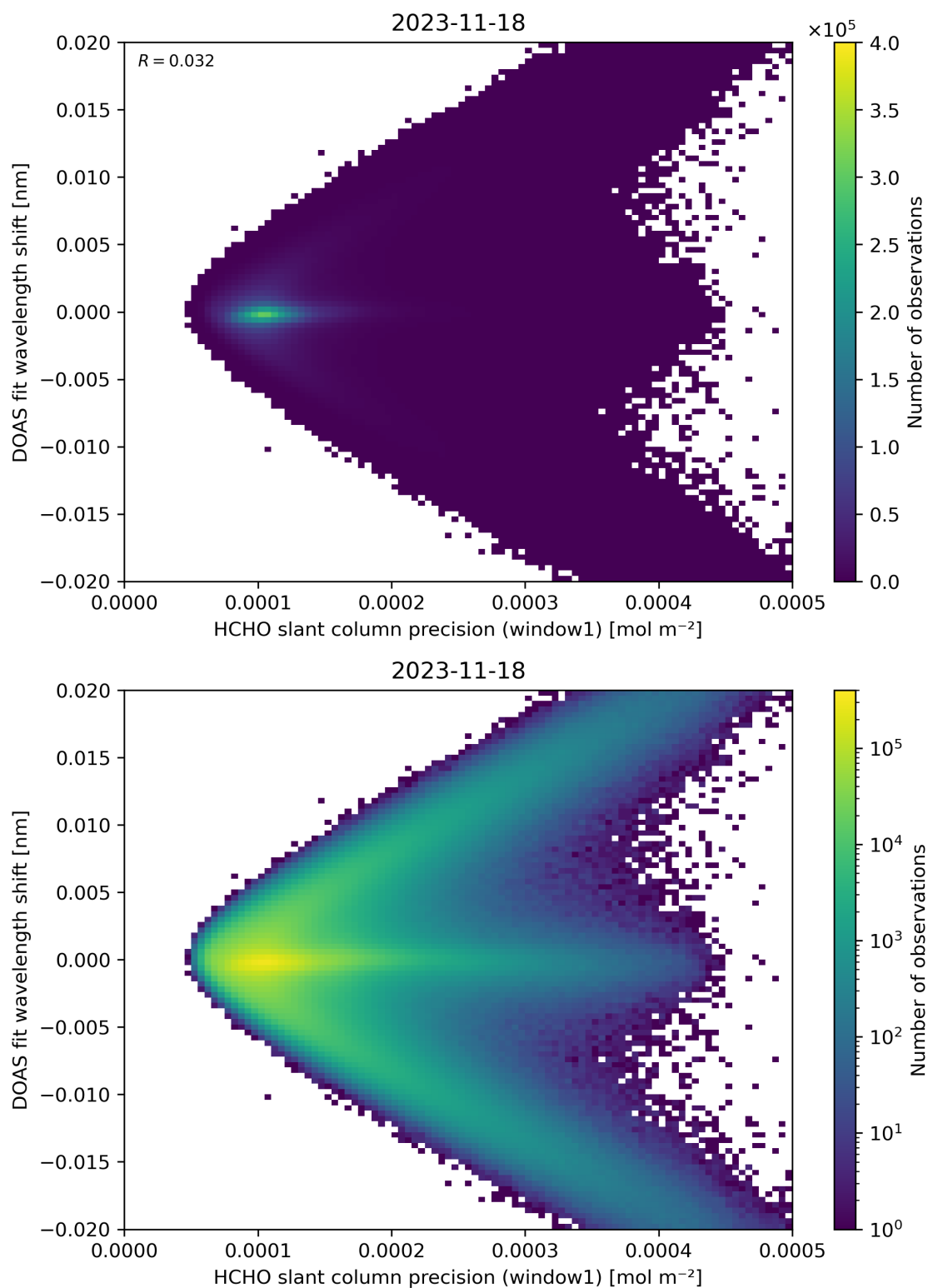
Figure 89: Scatter density plot of “HCHO slant column precision (window1)” against “DOAS fit wavelength shift” for 2023-11-18 to 2023-11-19.
