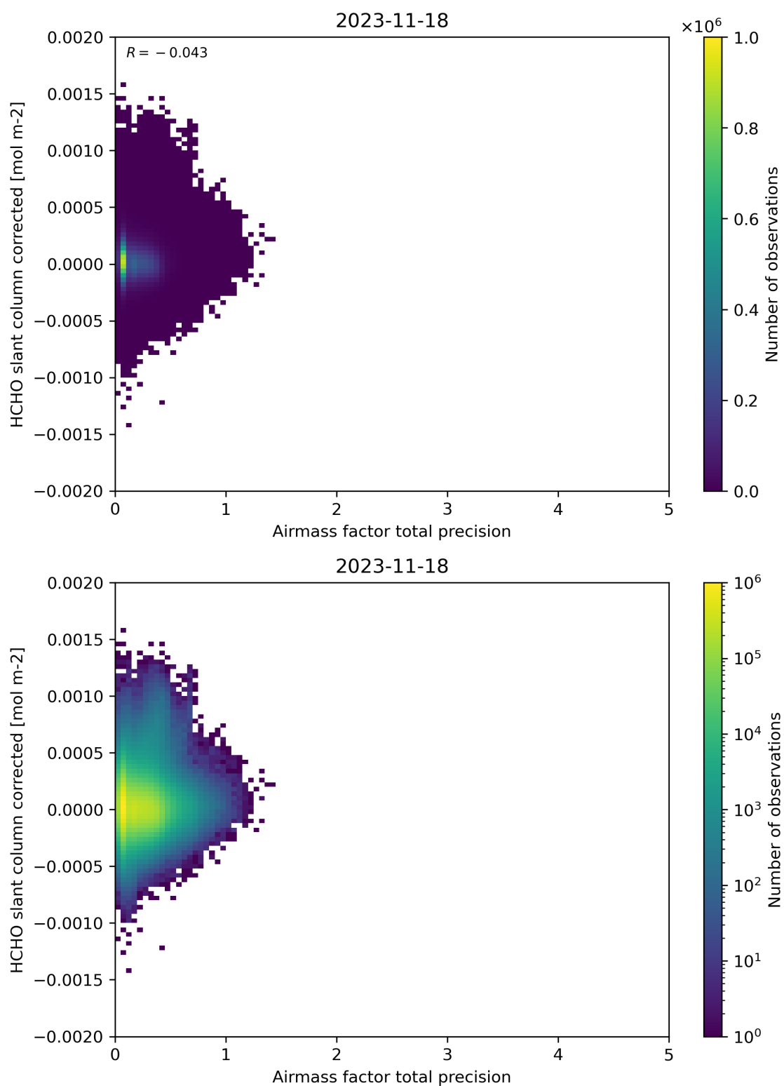
Figure 109: Scatter density plot of “Airmass factor total precision” against “HCHO slant column corrected” for 2023-11-18 to 2023-11-19.
