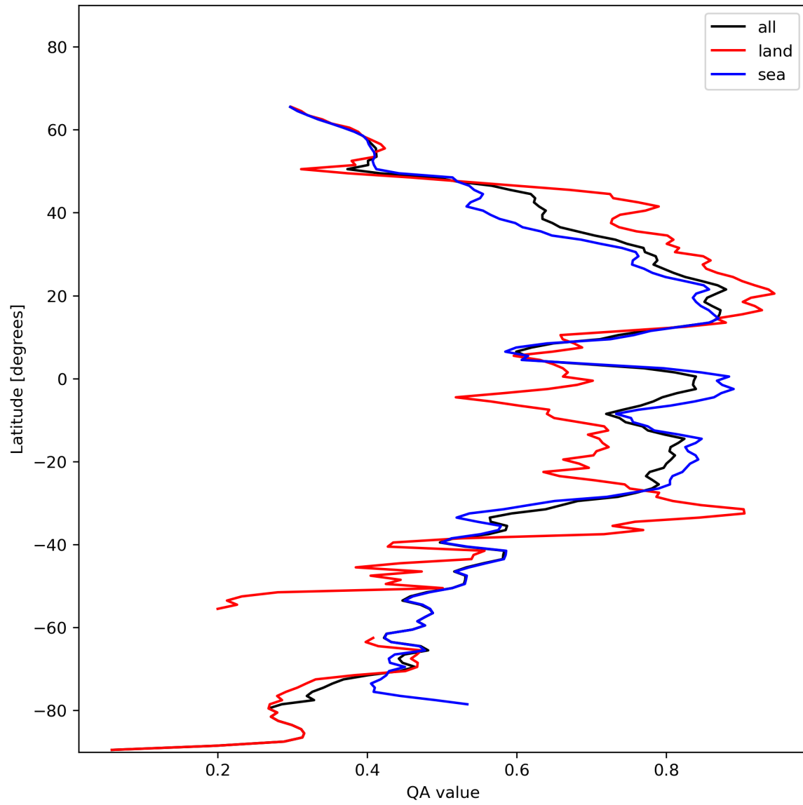
Figure 20: Zonal average of “QA value” for 2023-11-18 to 2023-11-19.
