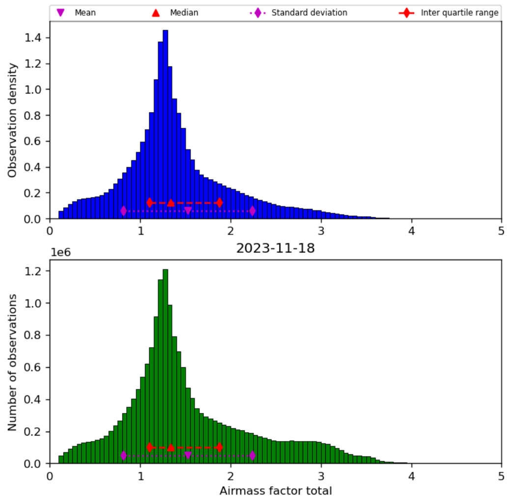
Figure 40: Histogram of “Airmass factor total” for 2023-11-18 to 2023-11-19
