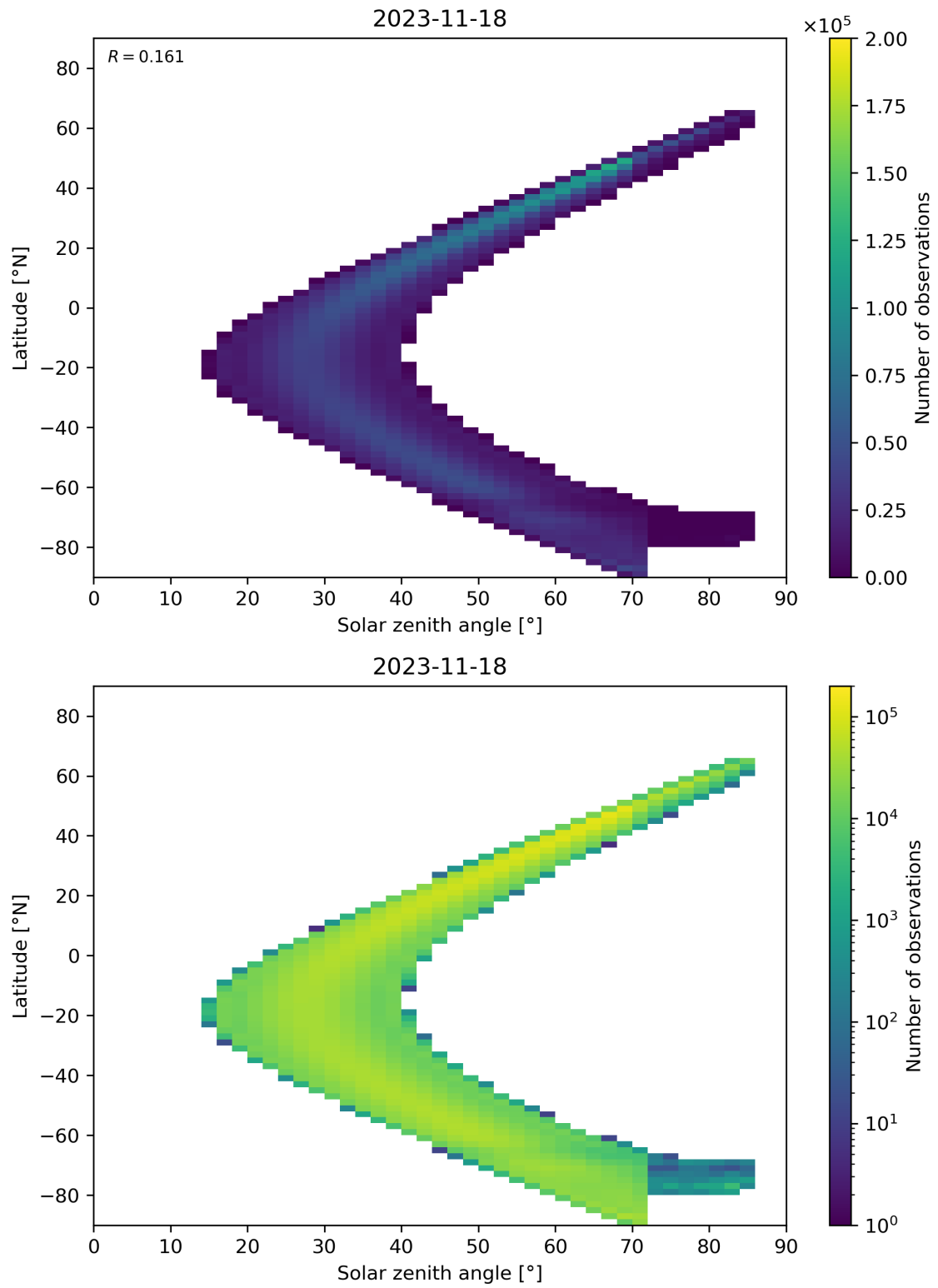
Figure 181: Scatter density plot of “Solar zenith angle” against “Latitude” for 2023-11-18 to 2023-11-19.
