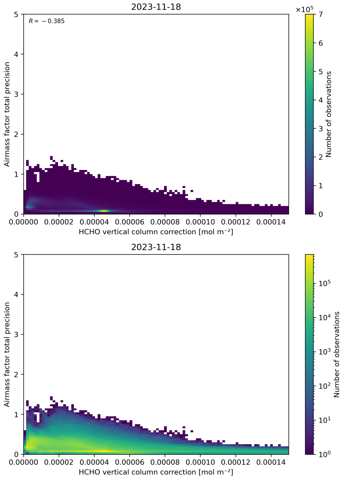
Figure 121: Scatter density plot of “HCHO vertical column correction” against “Airmass factor total precision” for 2023-11-18 to 2023-11-19.
