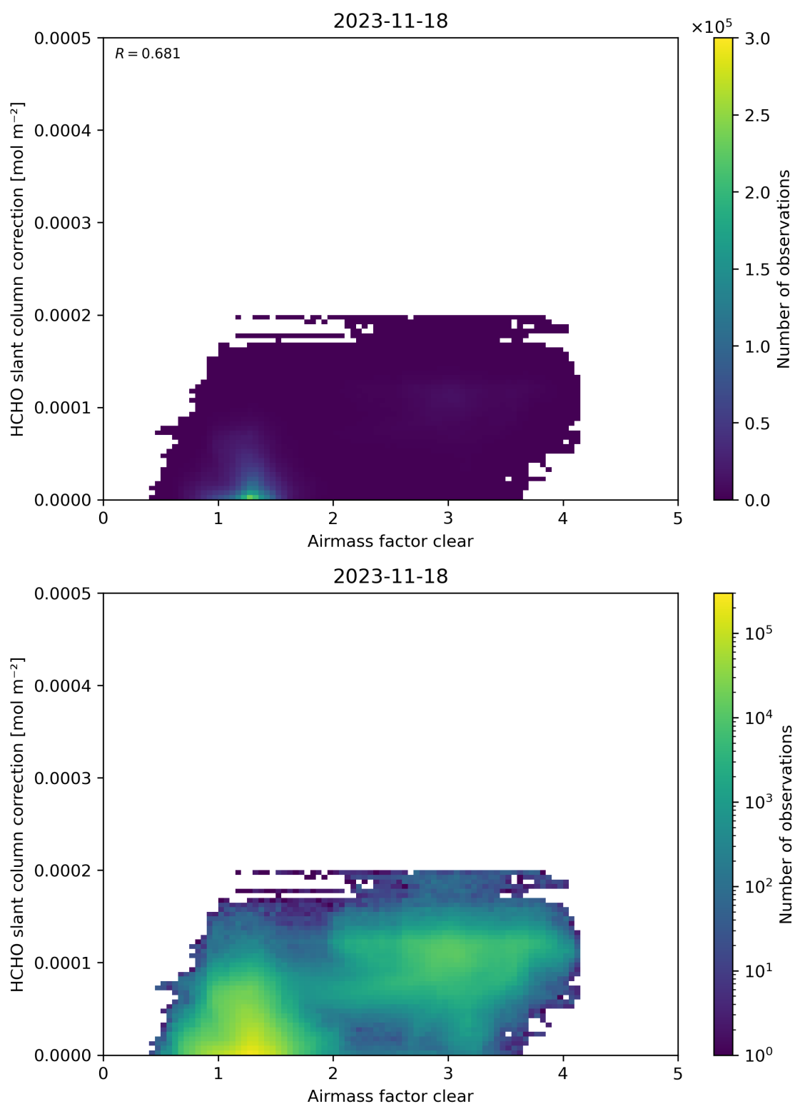
Figure 75: Scatter density plot of “Airmass factor clear” against “HCHO slant column correction” for 2023-11-18 to 2023-11-19.
