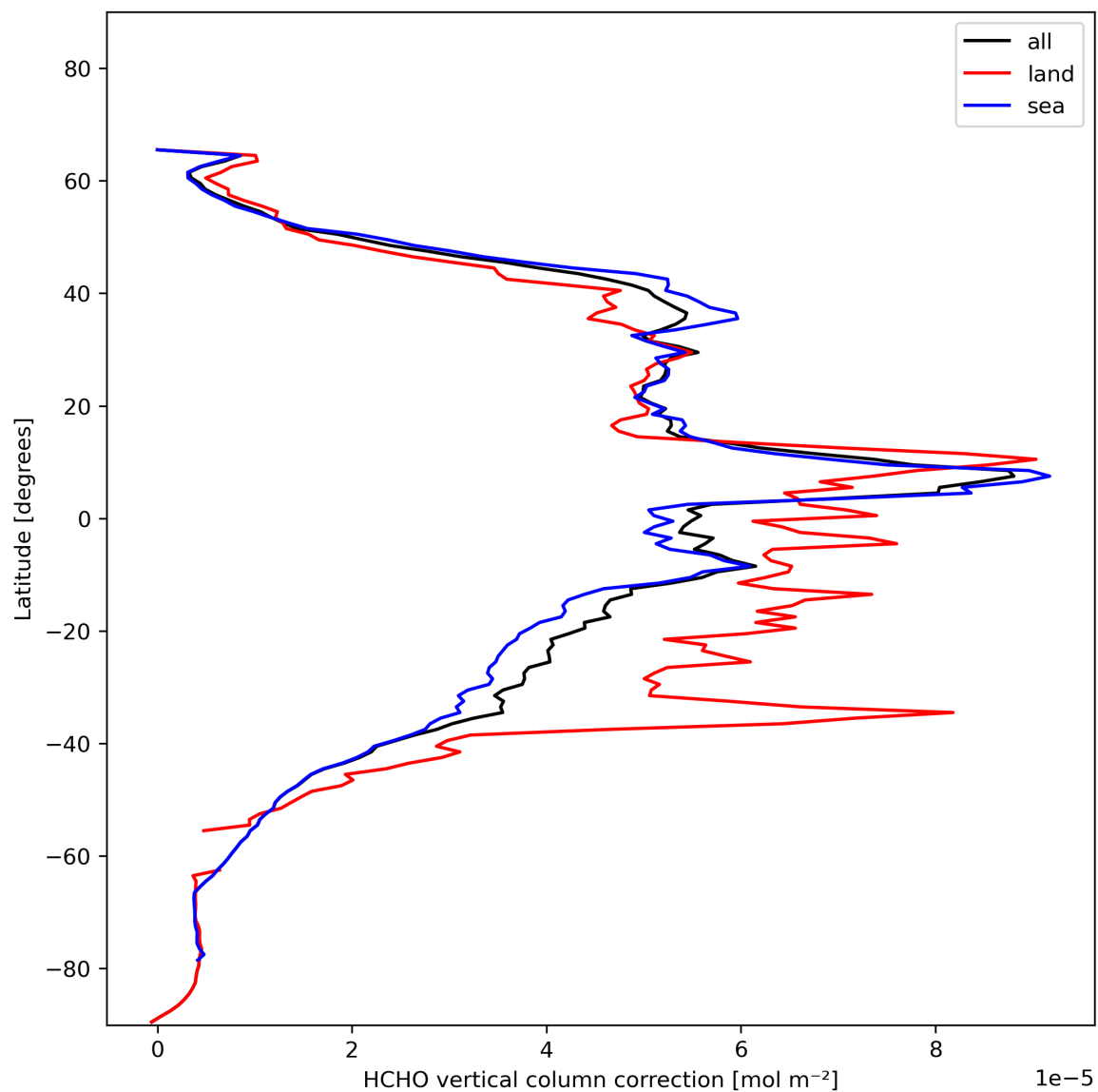
Figure 23: Zonal average of “HCHO vertical column correction” for 2023-11-18 to 2023-11-19.
