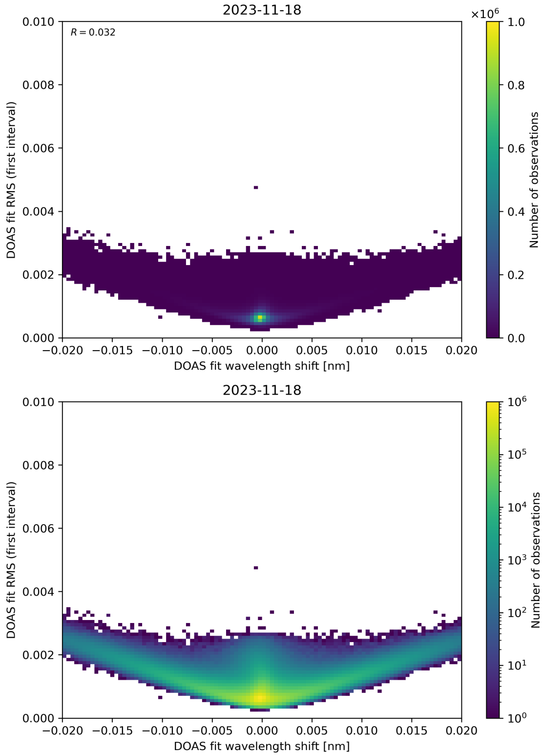
Figure 64: Scatter density plot of “DOAS fit wavelength shift” against “DOAS fit RMS (first interval)” for 2023-11-18 to 2023-11-19.
