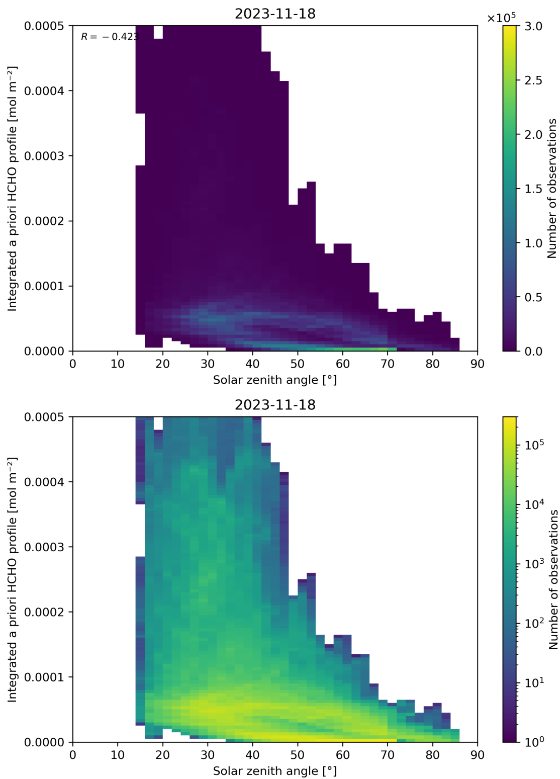
Figure 180: Scatter density plot of “Solar zenith angle” against “Integrated a priori HCHO profile” for 2023-11-18 to 2023-11-19.
