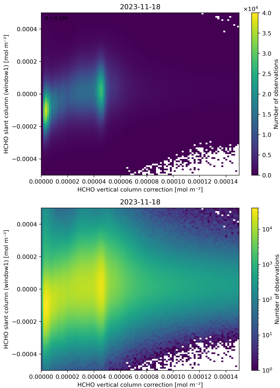
Figure 118: Scatter density plot of “HCHO vertical column correction” against “HCHO slant column (window1)” for 2023-11-18 to 2023-11-19.
