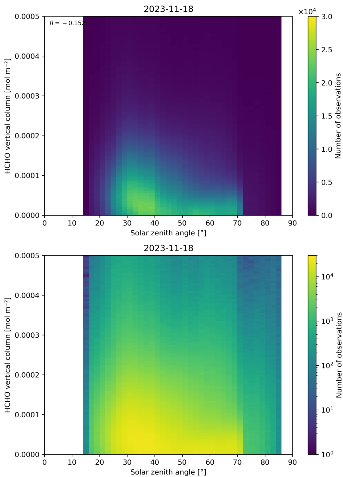
Figure 177: Scatter density plot of “Solar zenith angle” against “HCHO vertical column” for 2023-11-18 to 2023-11-19.
