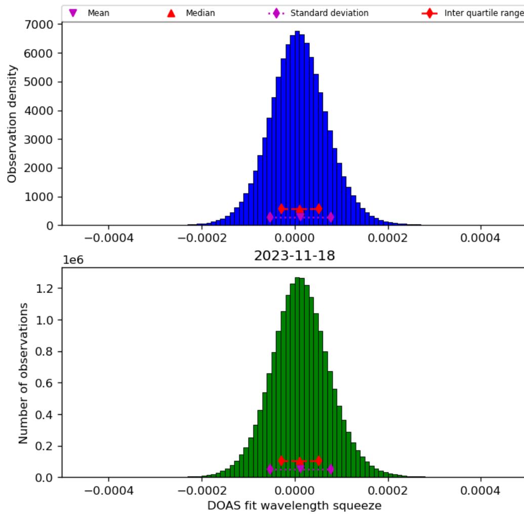
Figure 45: Histogram of “DOAS fit wavelength squeeze” for 2023-11-18 to 2023-11-19
