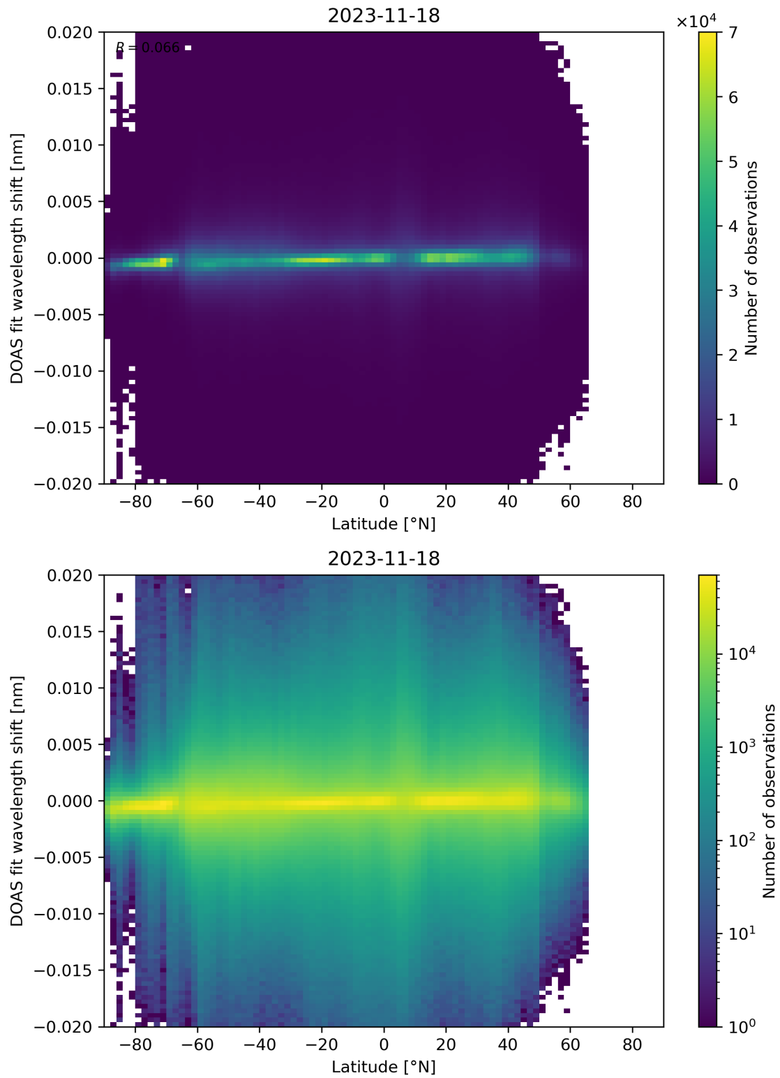
Figure 154: Scatter density plot of “Latitude” against “DOAS fit wavelength shift” for 2023-11-18 to 2023-11-19.
