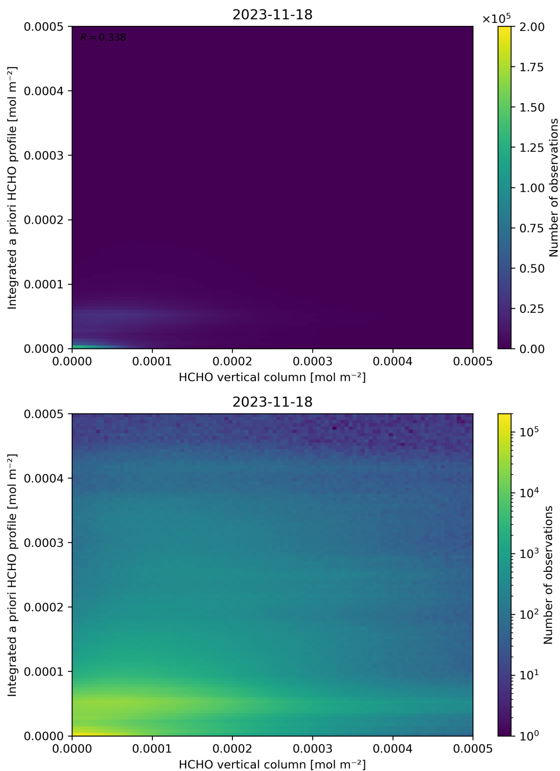
Figure 135: Scatter density plot of “HCHO vertical column” against “Integrated a priori HCHO profile” for 2023-11-18 to 2023-11-19.
