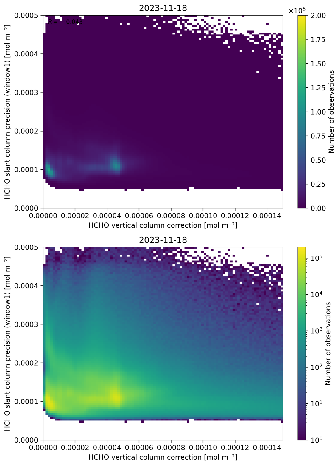
Figure 119: Scatter density plot of “HCHO vertical column correction” against “HCHO slant column precision (window1)” for 2023-11-18 to 2023-11-19.
