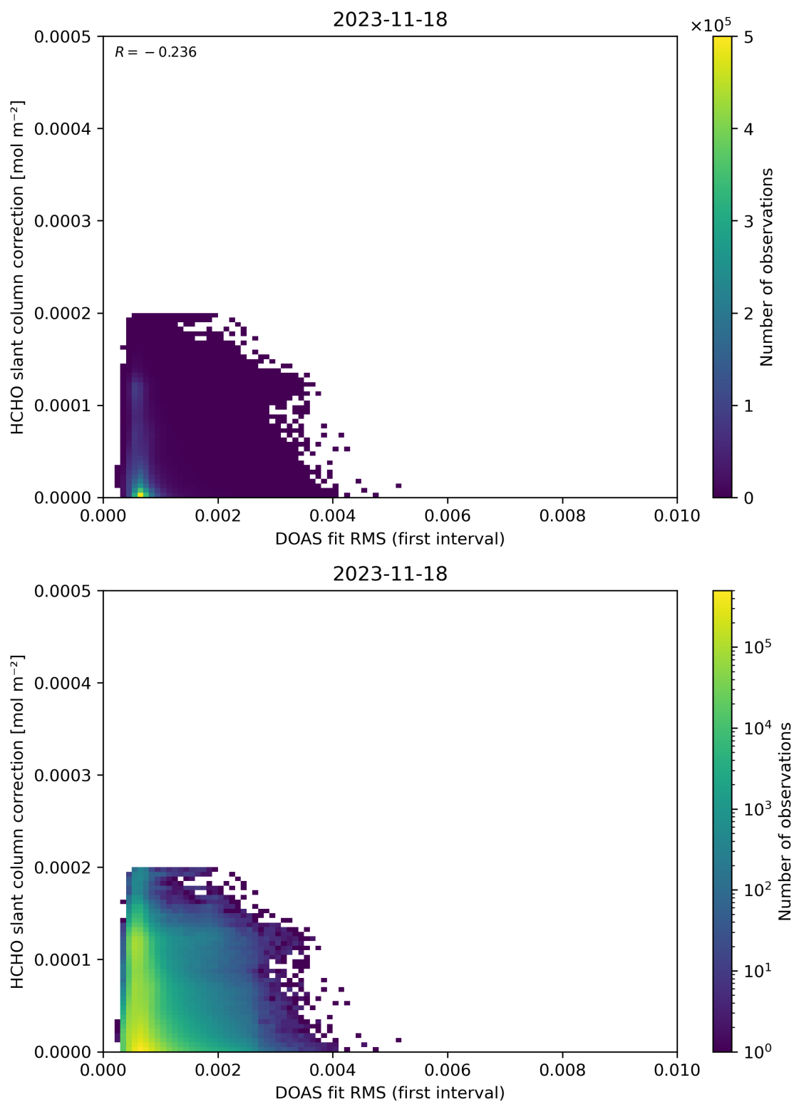
Figure 63: Scatter density plot of “DOAS fit RMS (first interval)” against “HCHO slant column correction” for 2023-11-18 to 2023-11-19.
