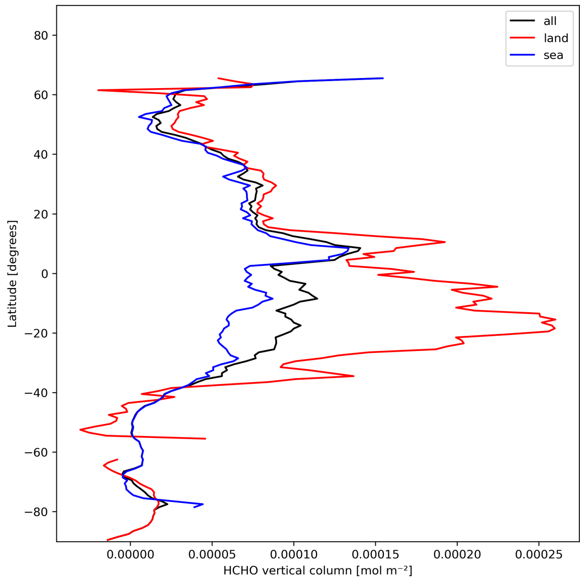
Figure 21: Zonal average of “HCHO vertical column” for 2023-11-18 to 2023-11-19.
