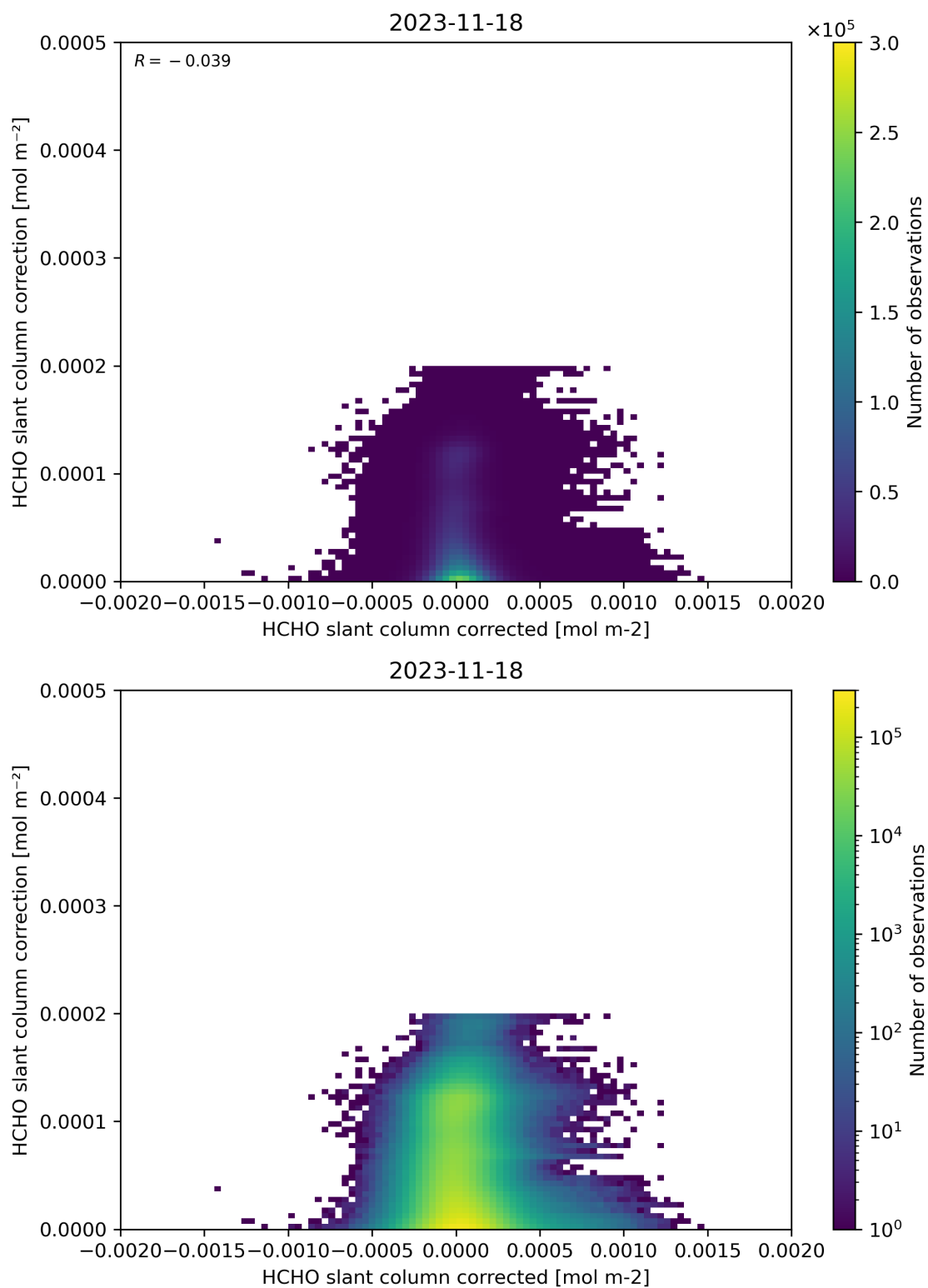
Figure 77: Scatter density plot of “HCHO slant column corrected” against “HCHO slant column correction” for 2023-11-18 to 2023-11-19.
