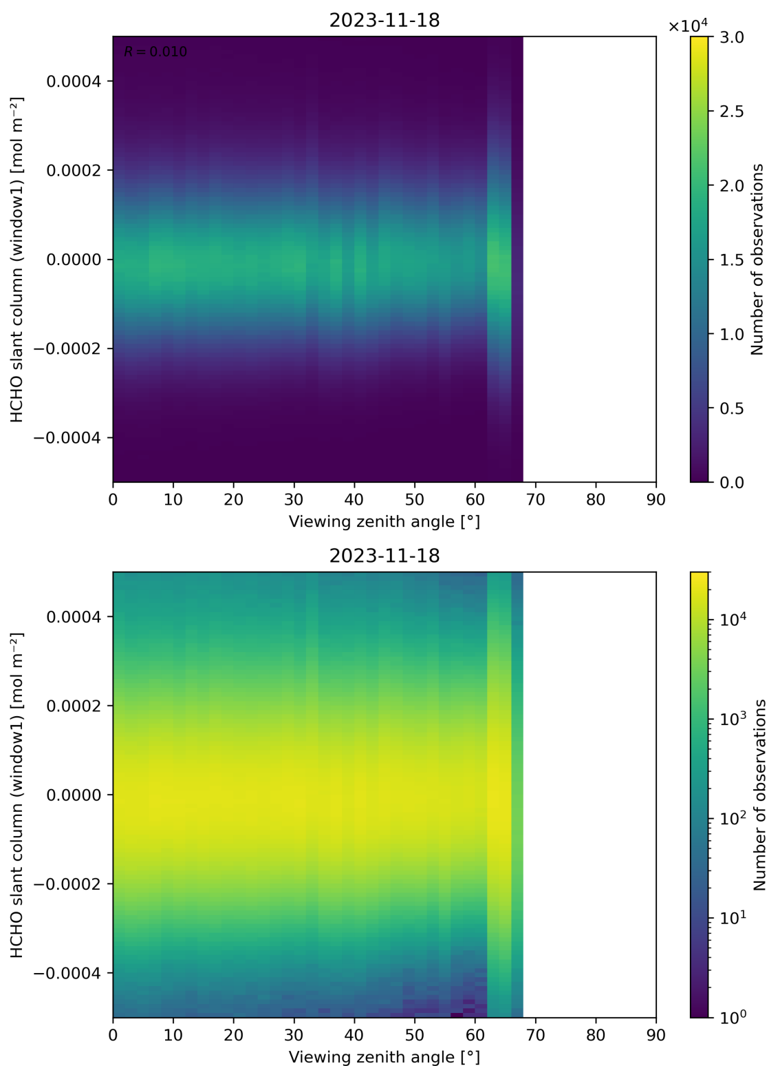
Figure 188: Scatter density plot of “Viewing zenith angle” against “HCHO slant column (window1)” for 2023-11-18 to 2023-11-19.
