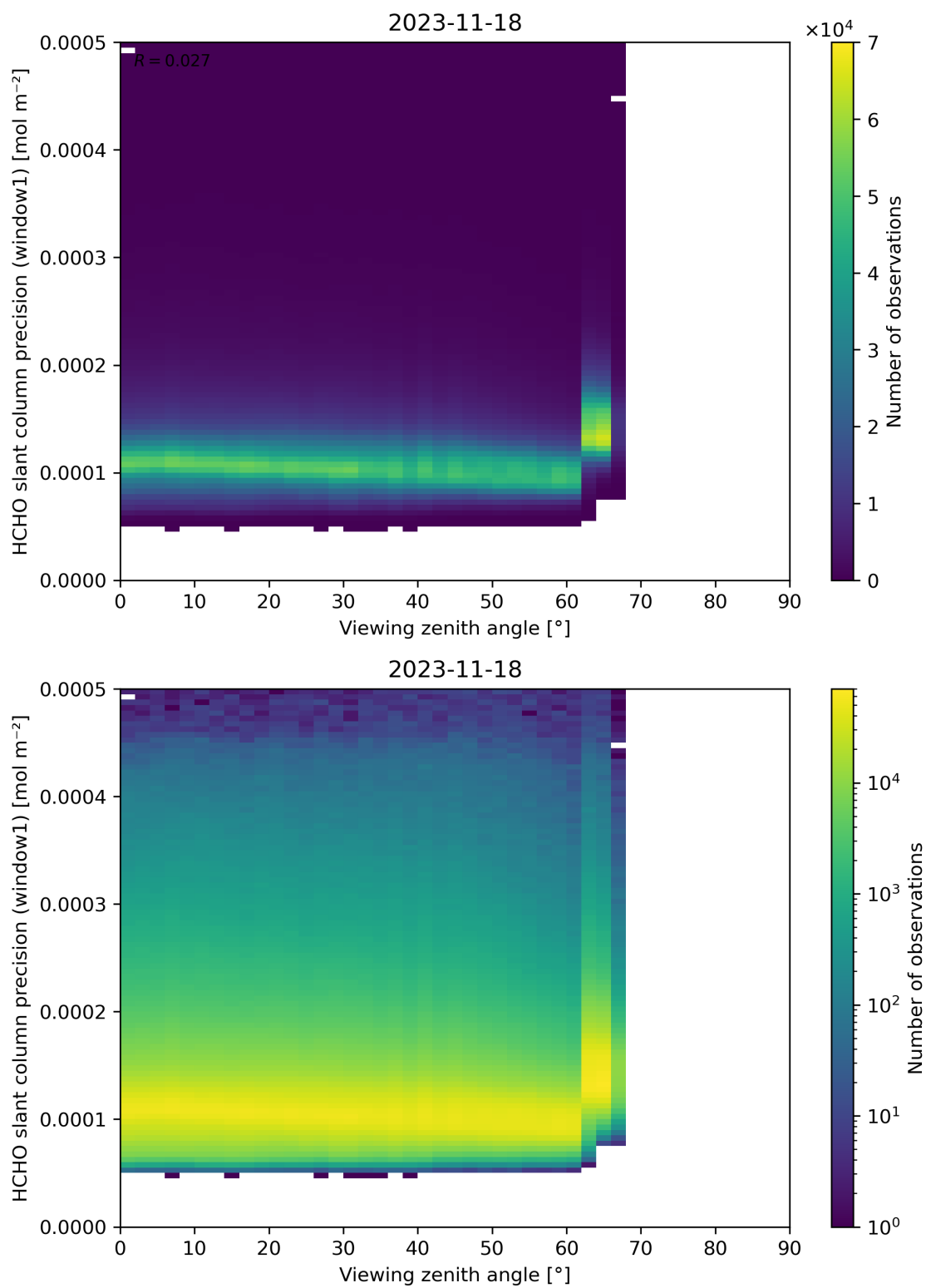
Figure 189: Scatter density plot of “Viewing zenith angle” against “HCHO slant column precision (window1)” for 2023-11-18 to 2023-11-19.
