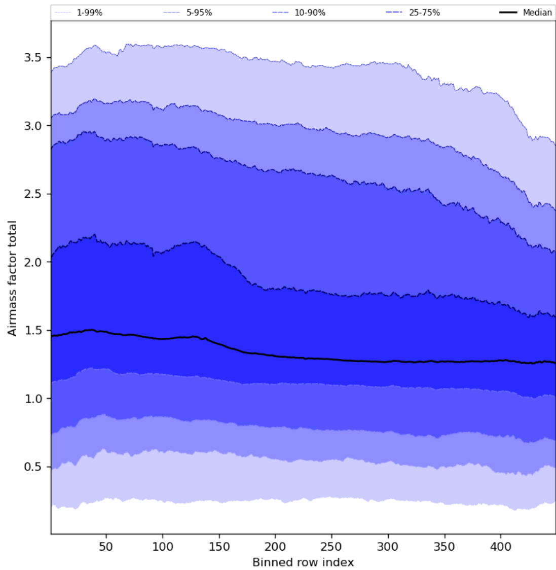
Figure 54: Along track statistics of “Airmass factor total” for 2023-11-18 to 2023-11-19
