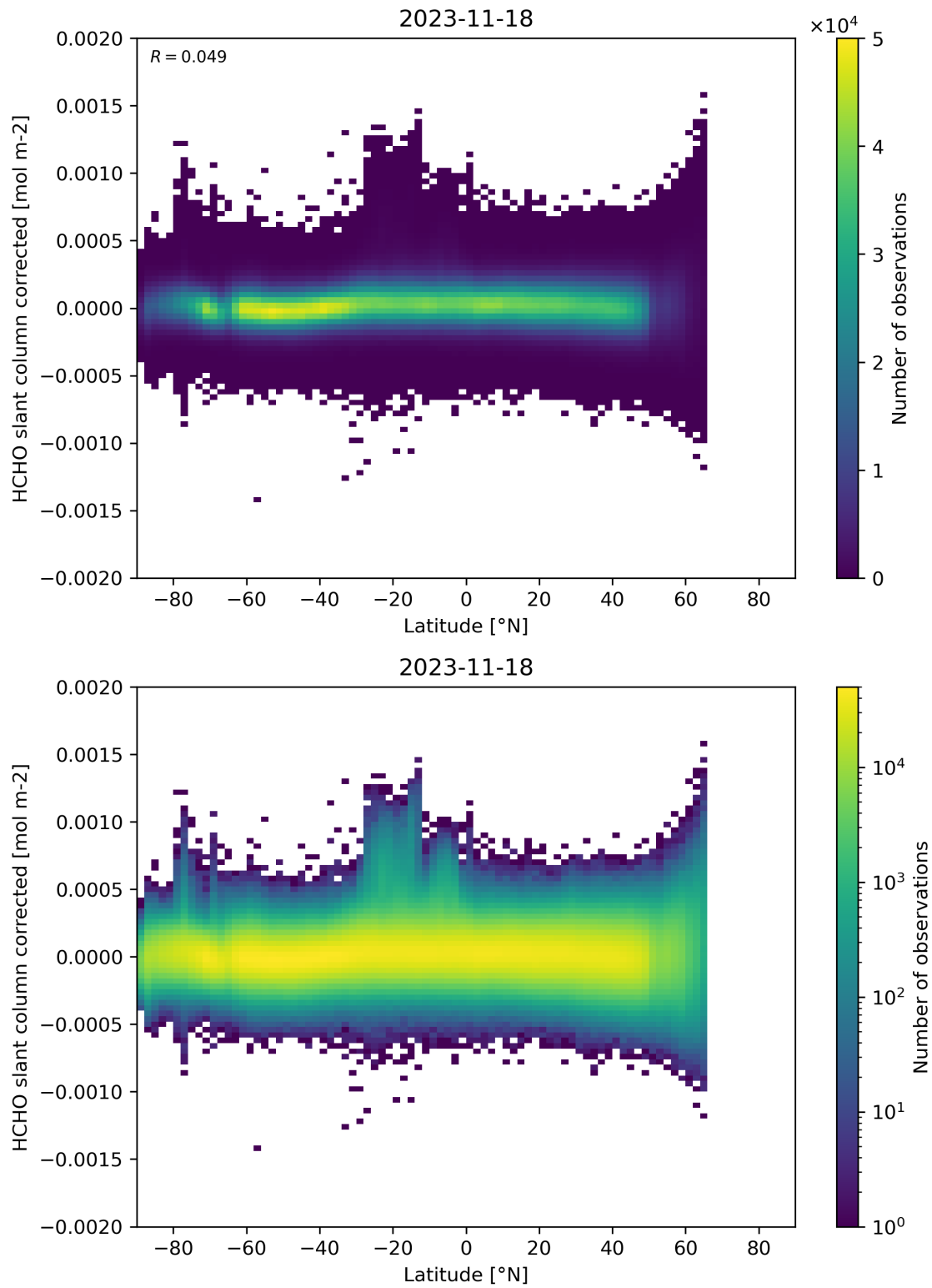
Figure 157: Scatter density plot of “Latitude” against “HCHO slant column corrected” for 2023-11-18 to 2023-11-19.
