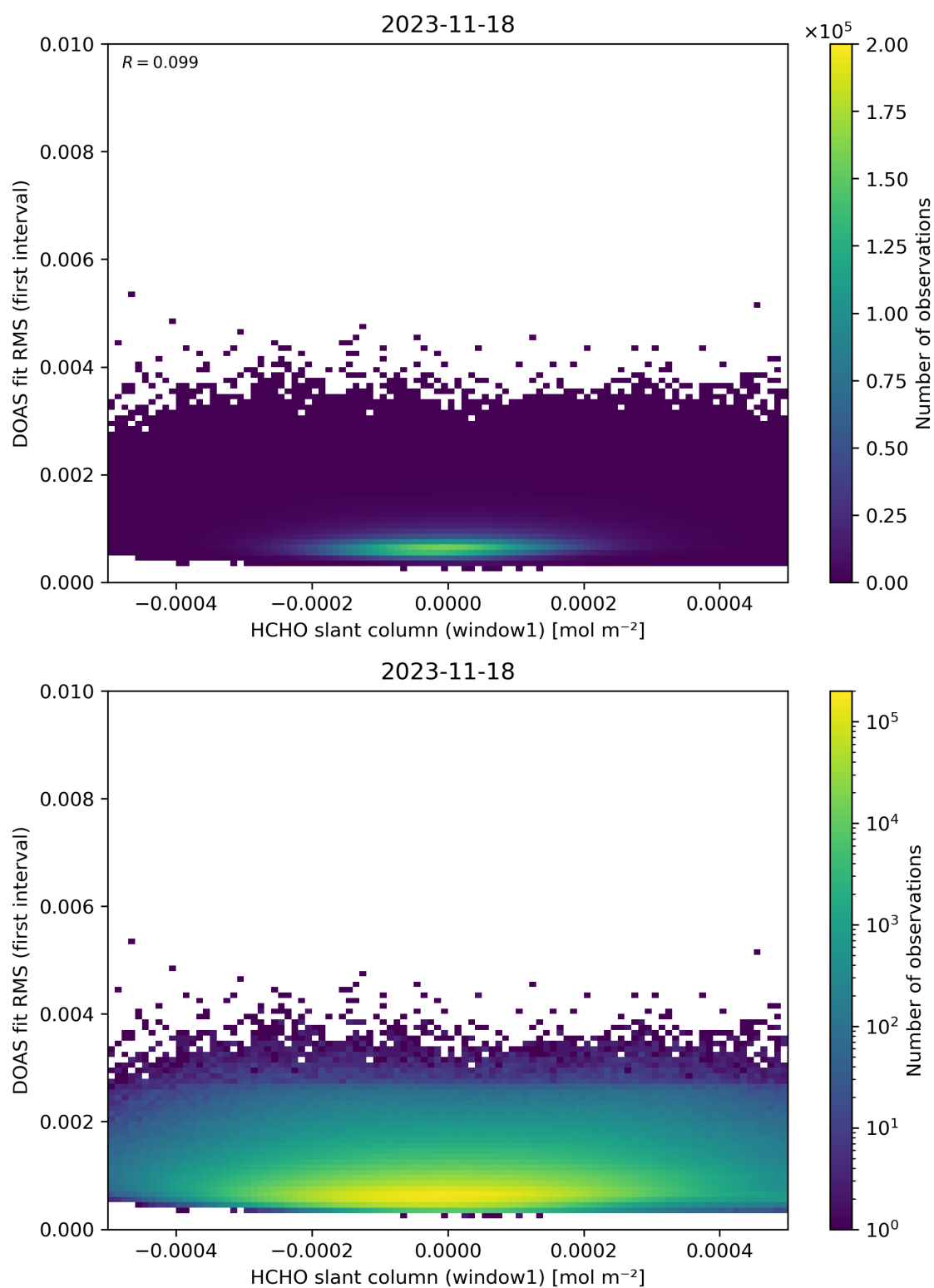
Figure 78: Scatter density plot of “HCHO slant column (window1)” against “DOAS fit RMS (first interval)” for 2023-11-18 to 2023-11-19.
