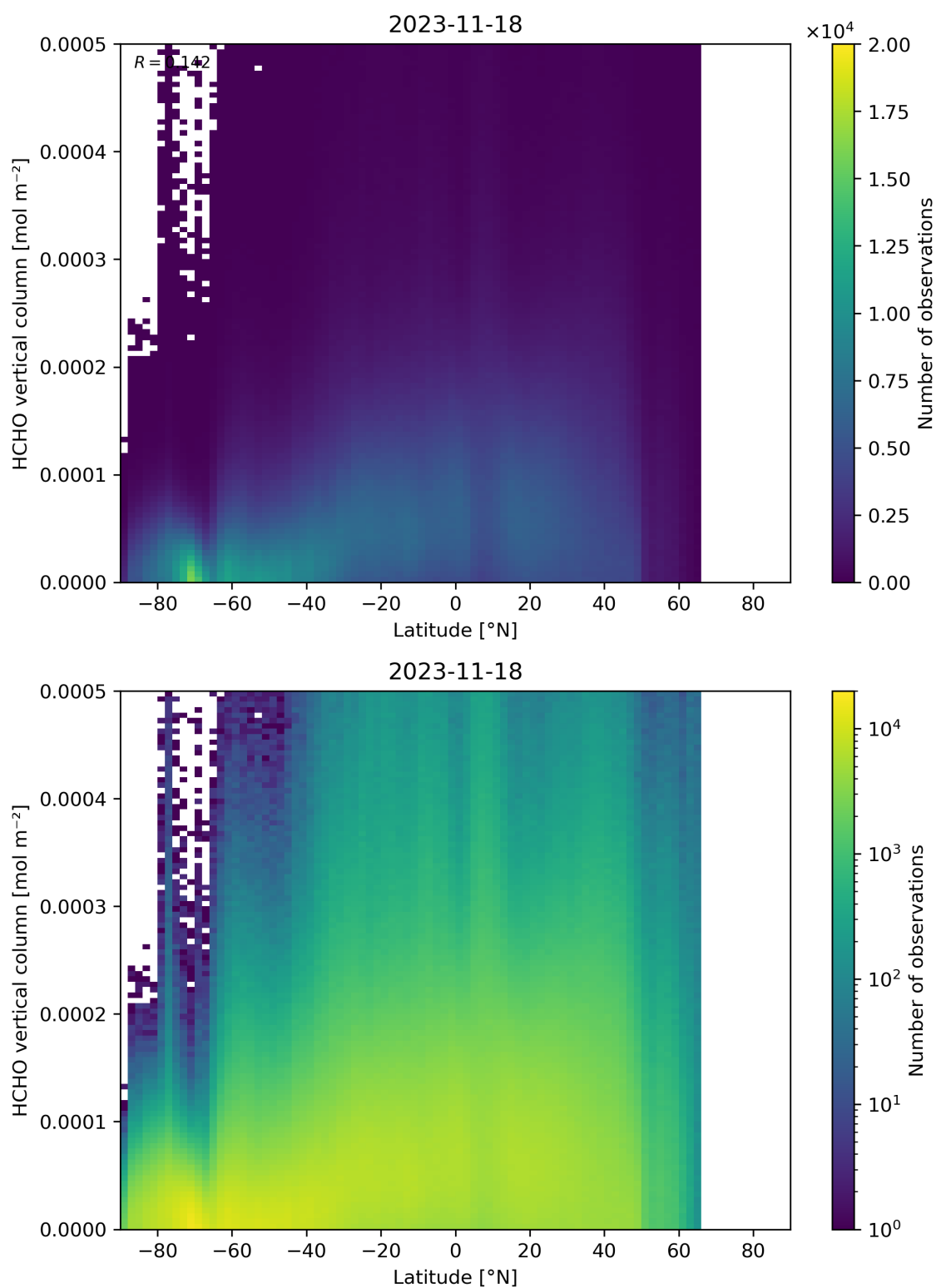
Figure 163: Scatter density plot of “Latitude” against “HCHO vertical column” for 2023-11-18 to 2023-11-19.
