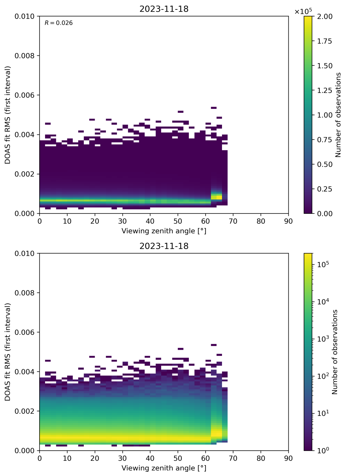
Figure 182: Scatter density plot of “Viewing zenith angle” against “DOAS fit RMS (first interval)” for 2023-11-18 to 2023-11-19.
