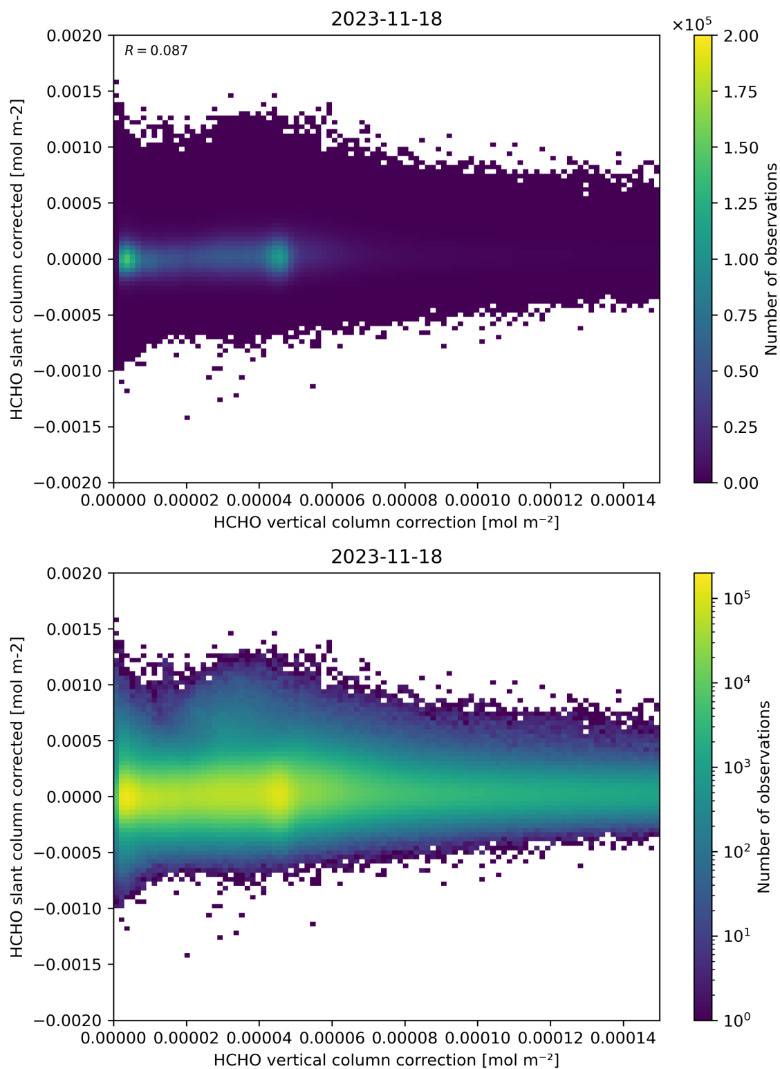
Figure 116: Scatter density plot of “HCHO vertical column correction” against “HCHO slant column corrected” for 2023-11-18 to 2023-11-19.
