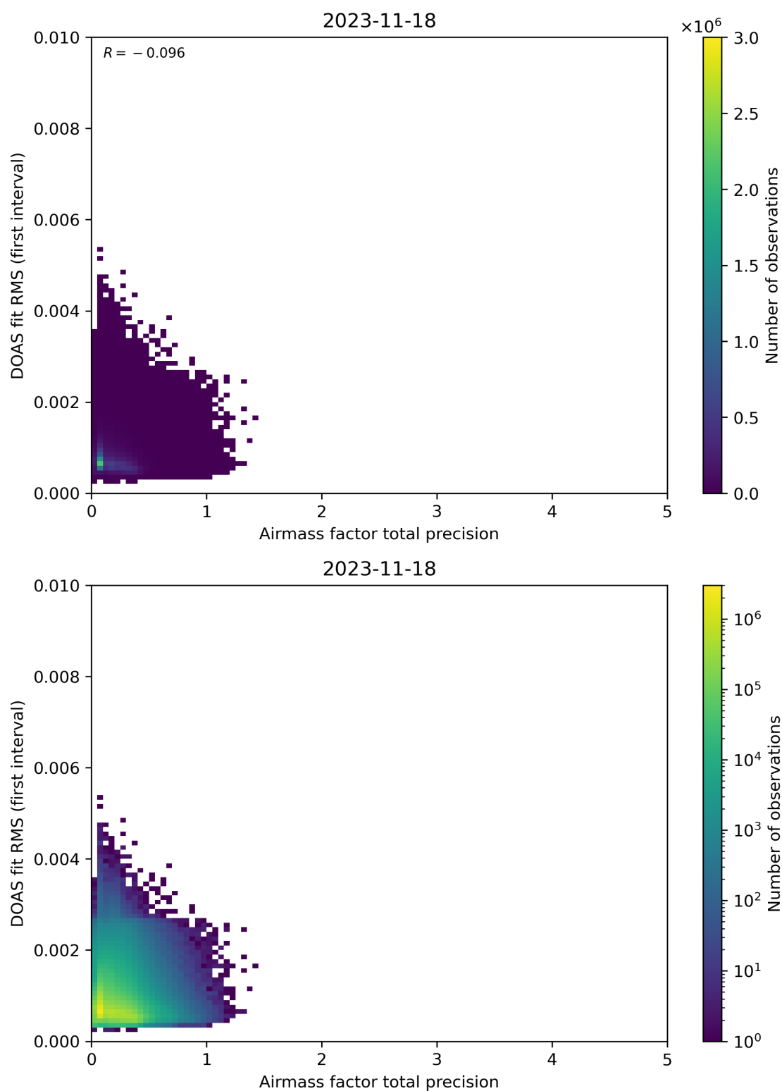
Figure 105: Scatter density plot of “Airmass factor total precision” against “DOAS fit RMS (first interval)” for 2023-11-18 to 2023-11-19.
