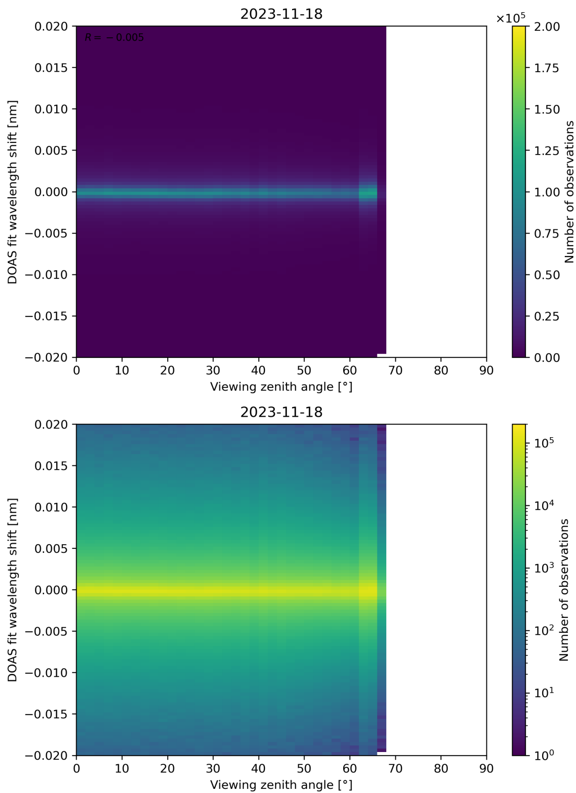
Figure 183: Scatter density plot of “Viewing zenith angle” against “DOAS fit wavelength shift” for 2023-11-18 to 2023-11-19.
