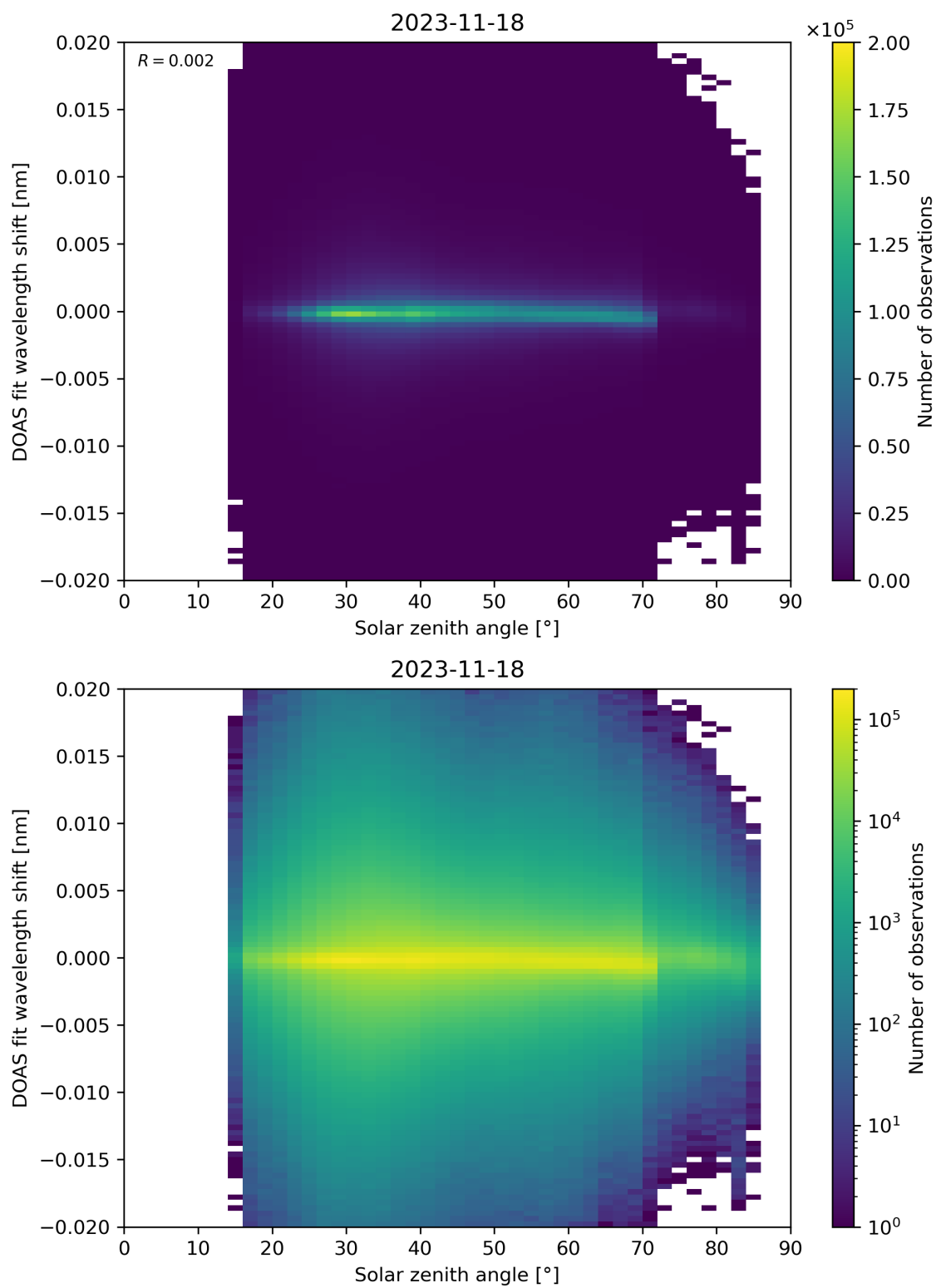
Figure 168: Scatter density plot of “Solar zenith angle” against “DOAS fit wavelength shift” for 2023-11-18 to 2023-11-19.
