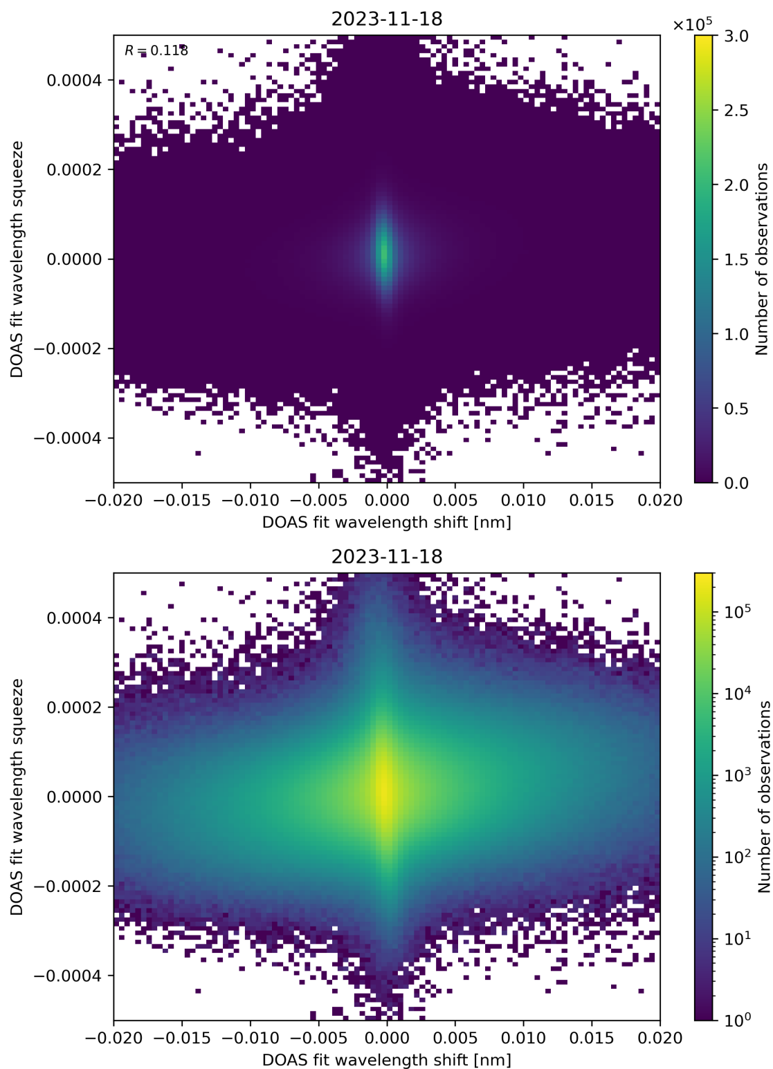
Figure 65: Scatter density plot of “DOAS fit wavelength shift” against “DOAS fit wavelength squeeze” for 2023-11-18 to 2023-11-19.
