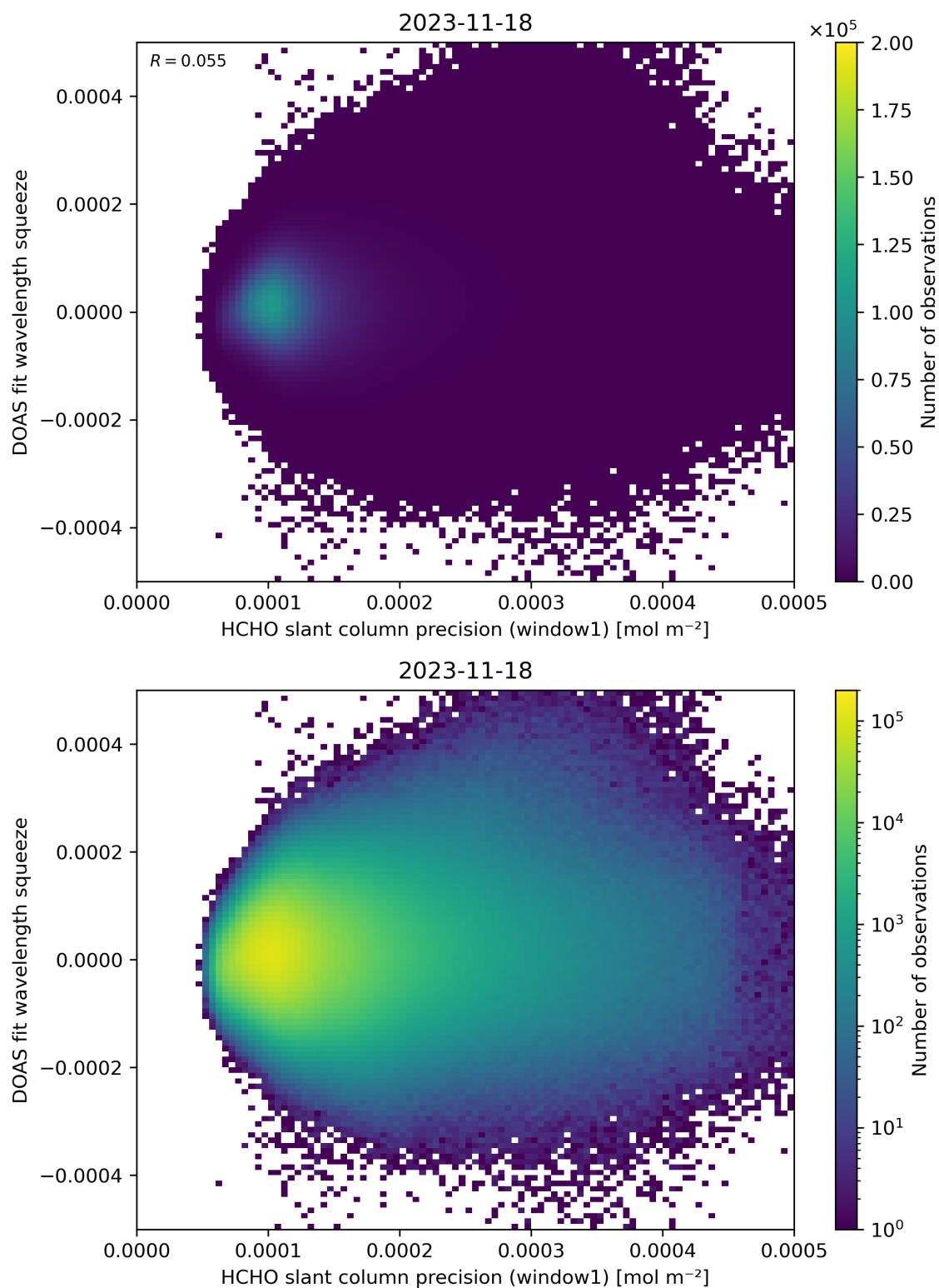
Figure 90: Scatter density plot of “HCHO slant column precision (window1)” against “DOAS fit wavelength squeeze” for 2023-11-18 to 2023-11-19.
