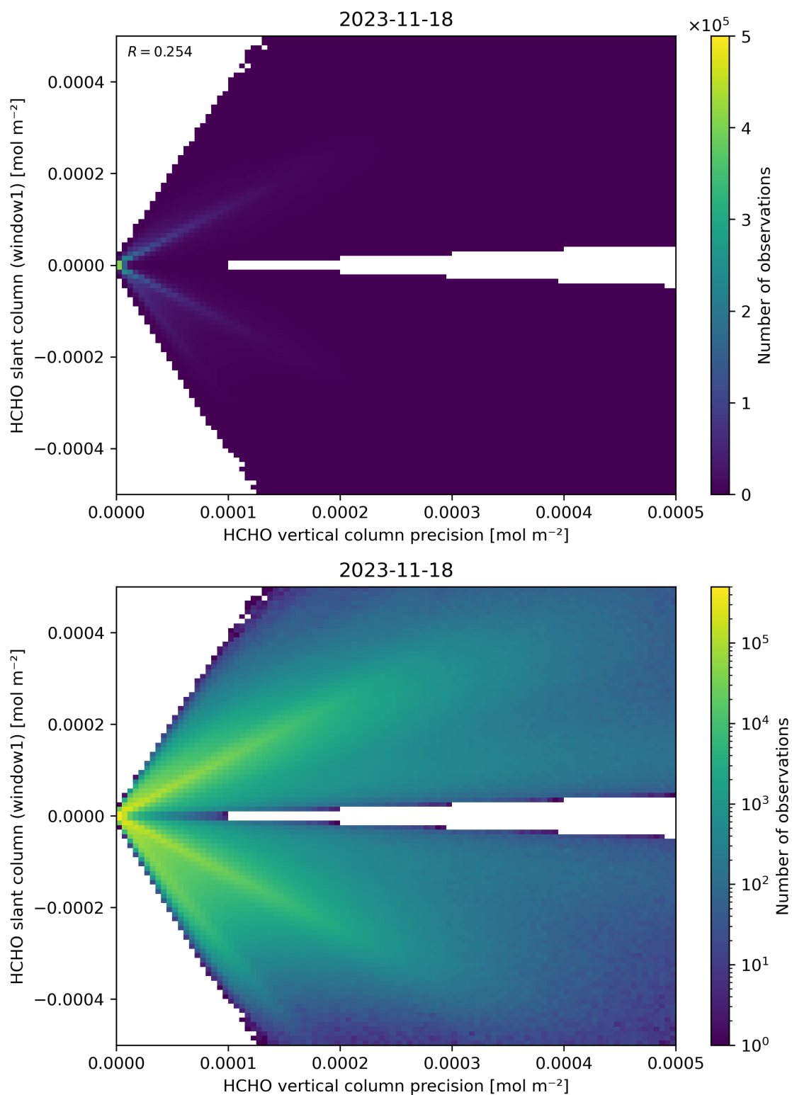
Figure 142: Scatter density plot of “HCHO vertical column precision” against “HCHO slant column (window1)” for 2023-11-18 to 2023-11-19.
