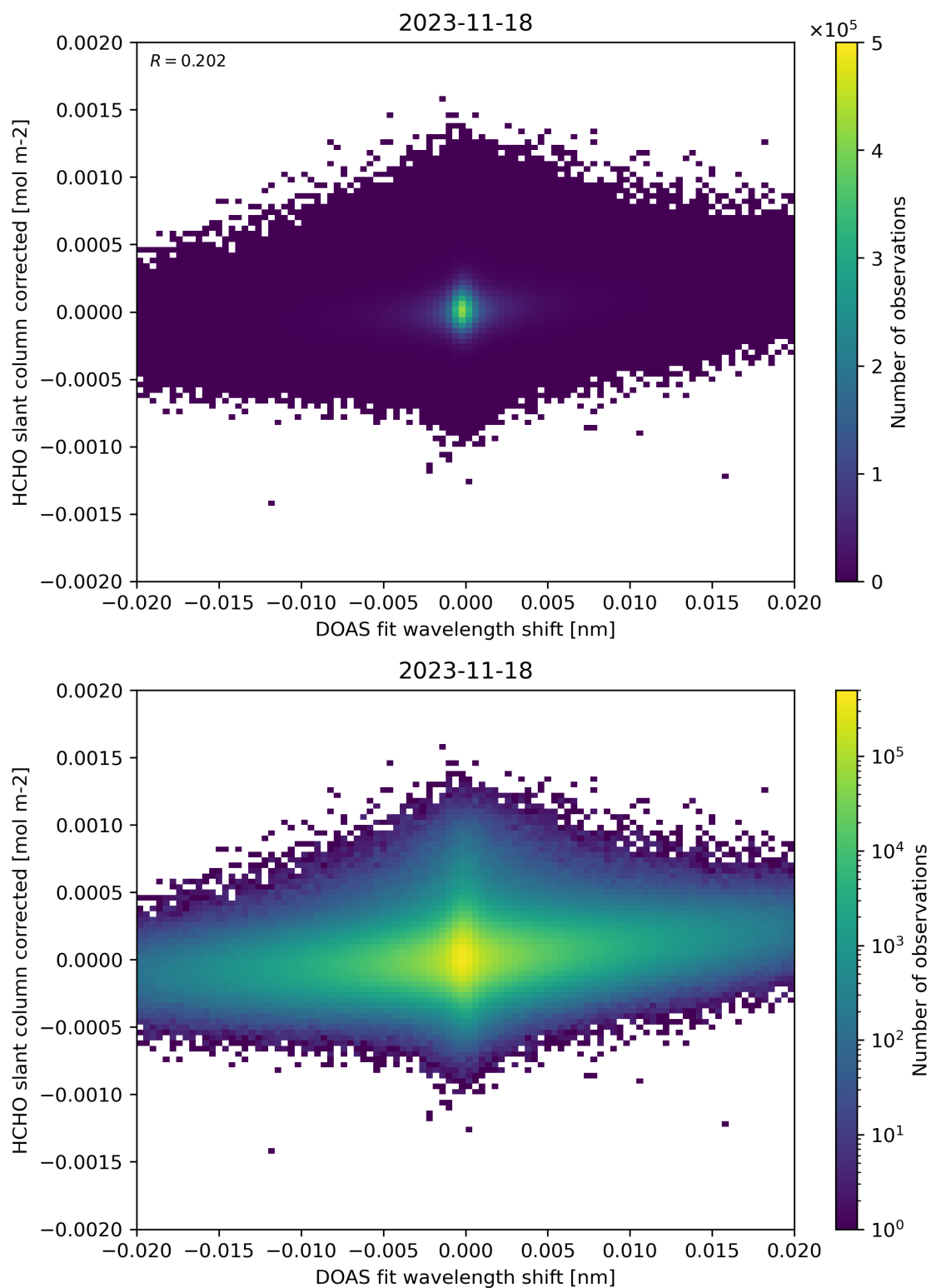
Figure 66: Scatter density plot of “DOAS fit wavelength shift” against “HCHO slant column corrected” for 2023-11-18 to 2023-11-19.
