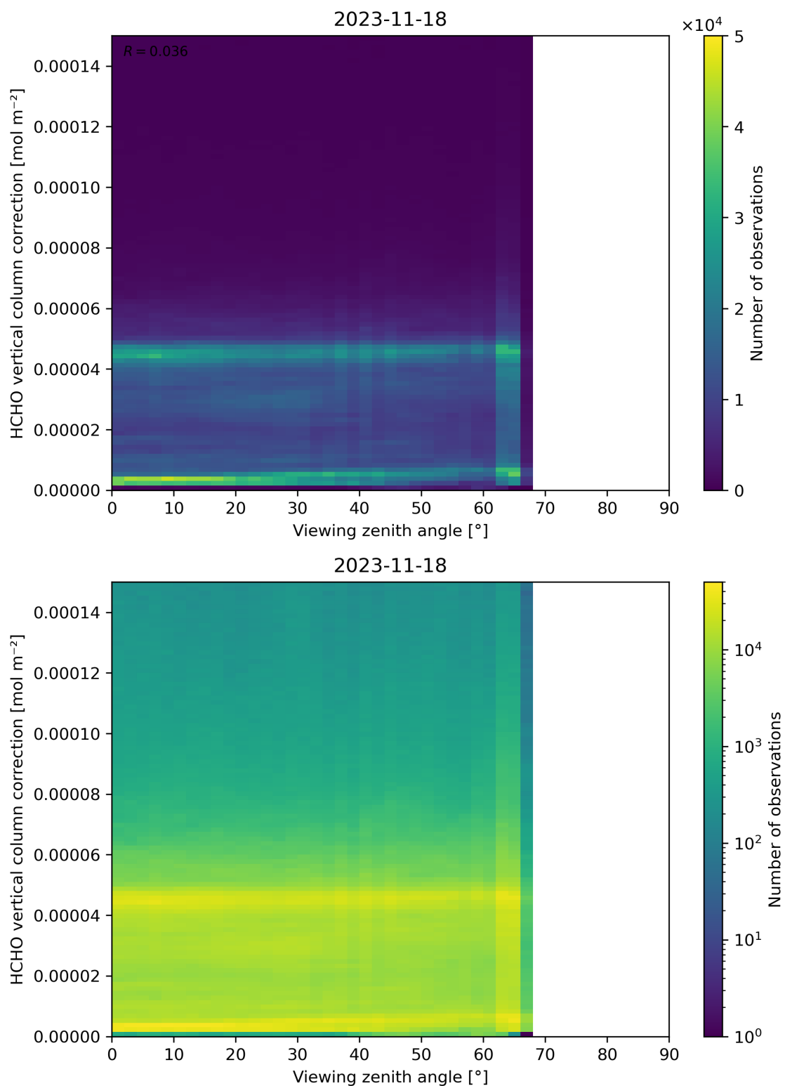
Figure 193: Scatter density plot of “Viewing zenith angle” against “HCHO vertical column correction” for 2023-11-18 to 2023-11-19.
