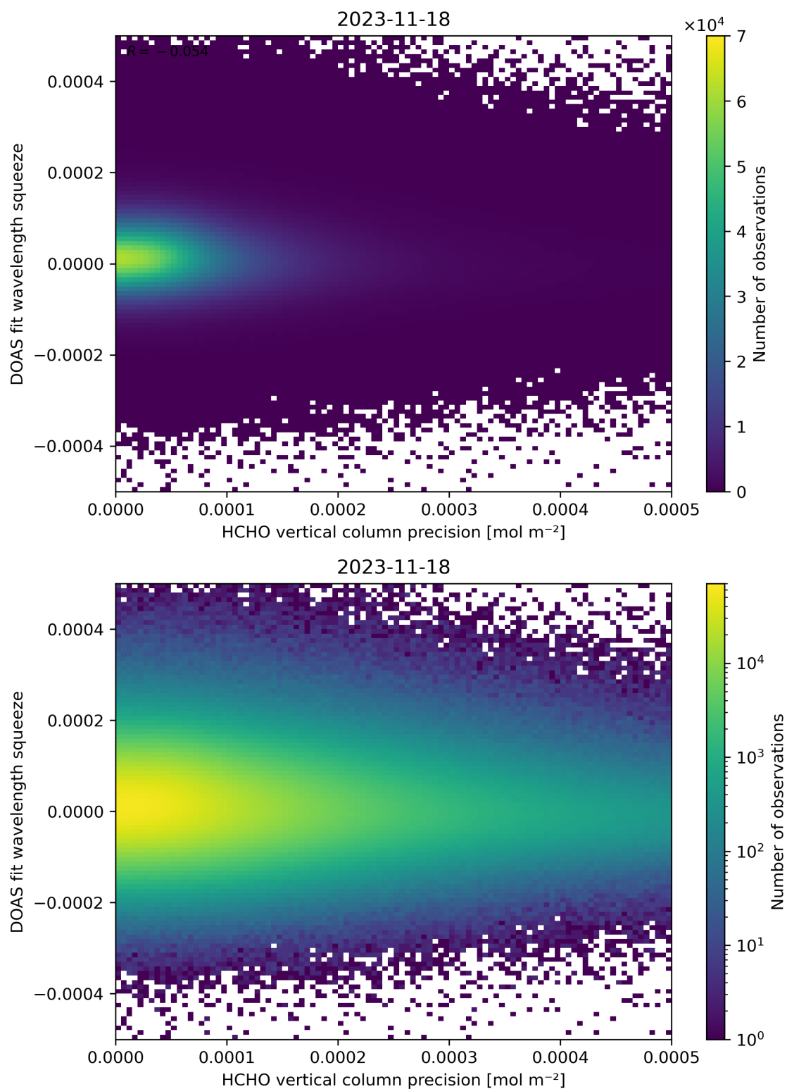
Figure 138: Scatter density plot of “HCHO vertical column precision” against “DOAS fit wavelength squeeze” for 2023-11-18 to 2023-11-19.
