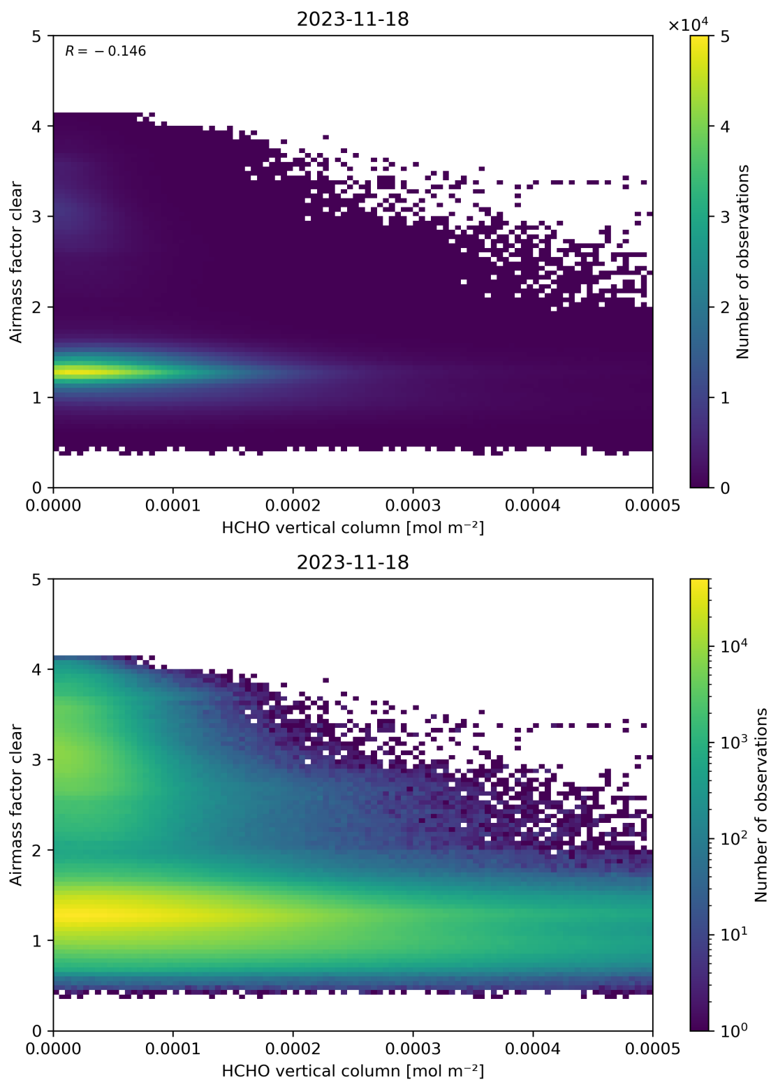
Figure 126: Scatter density plot of “HCHO vertical column” against “Airmass factor clear” for 2023-11-18 to 2023-11-19.
