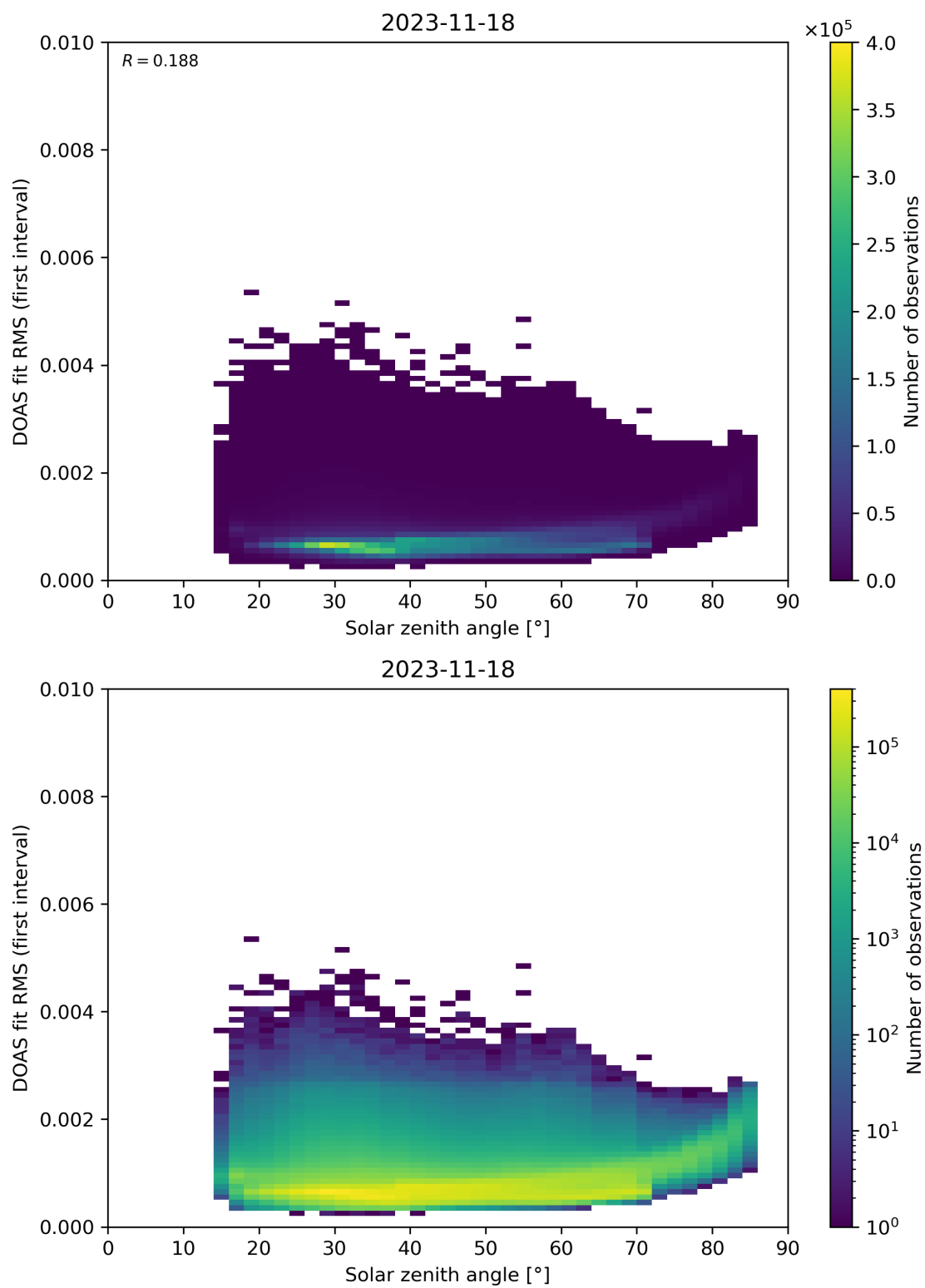
Figure 167: Scatter density plot of “Solar zenith angle” against “DOAS fit RMS (first interval)” for 2023-11-18 to 2023-11-19.
