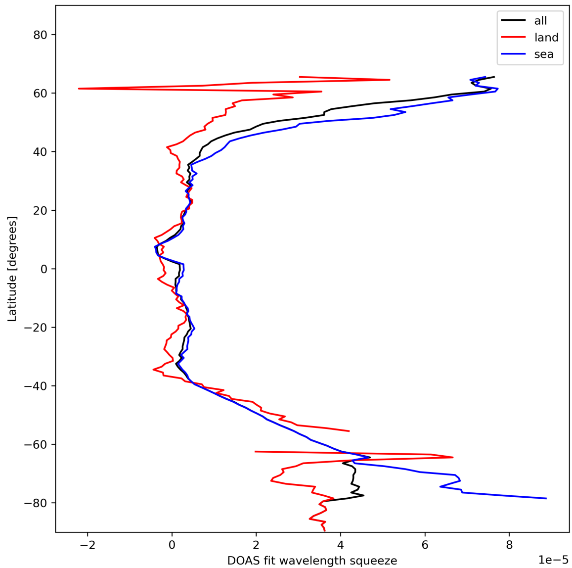
Figure 31: Zonal average of “DOAS fit wavelength squeeze” for 2023-11-18 to 2023-11-19.
