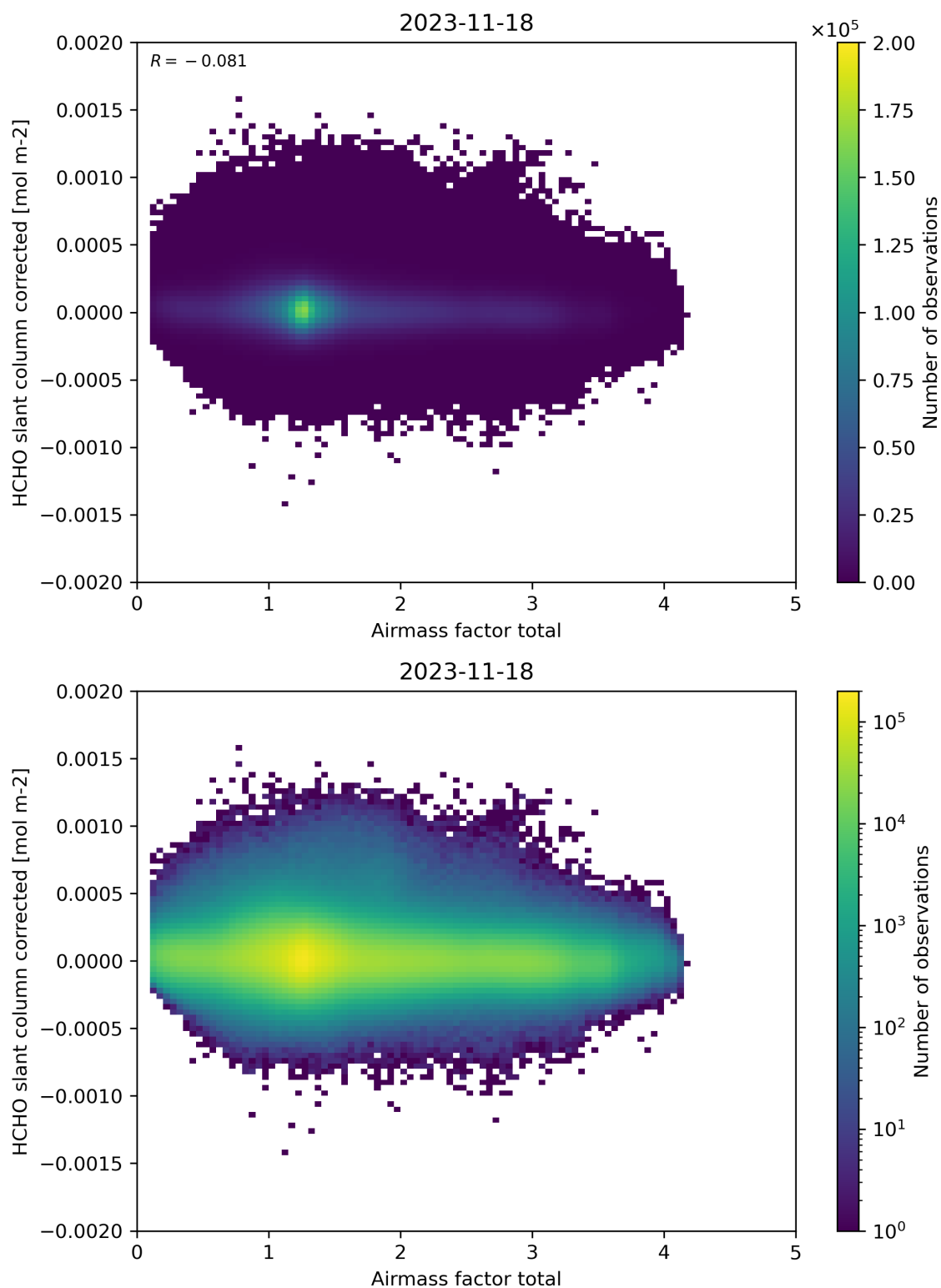
Figure 101: Scatter density plot of “Airmass factor total” against “HCHO slant column corrected” for 2023-11-18 to 2023-11-19.
