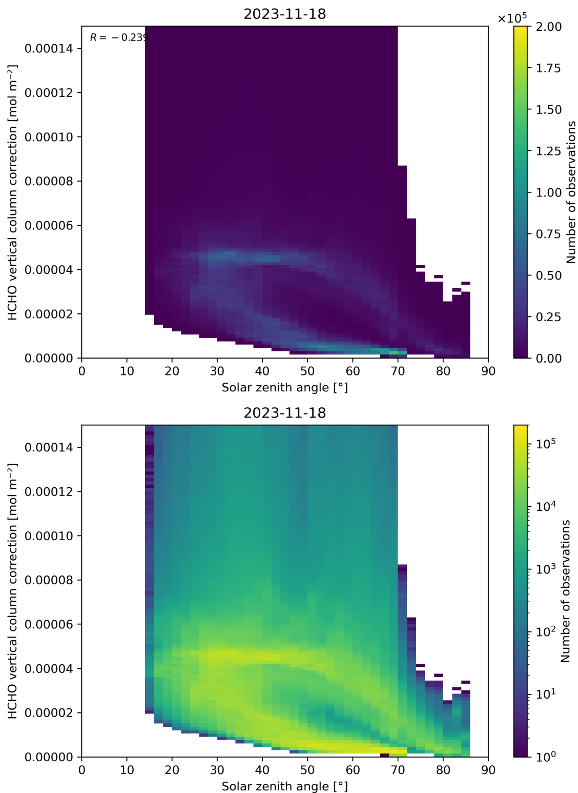
Figure 178: Scatter density plot of “Solar zenith angle” against “HCHO vertical column correction” for 2023-11-18 to 2023-11-19.
