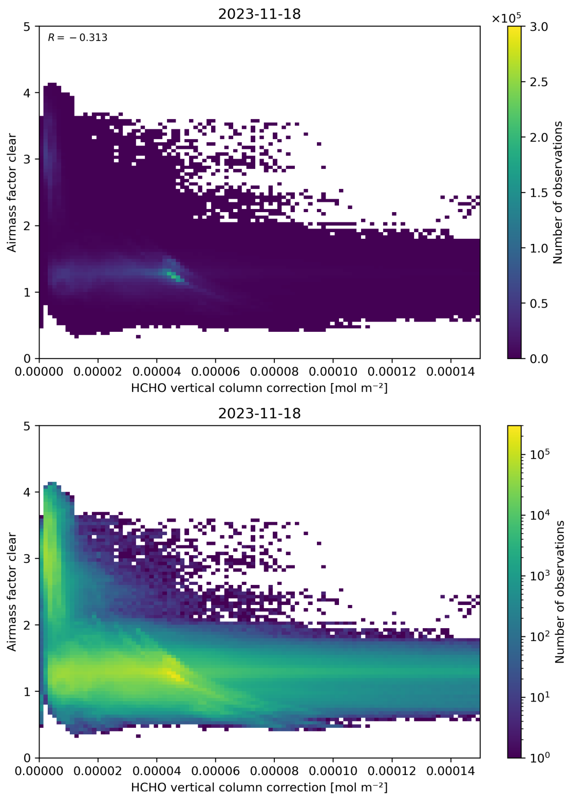
Figure 115: Scatter density plot of “HCHO vertical column correction” against “Airmass factor clear” for 2023-11-18 to 2023-11-19.
