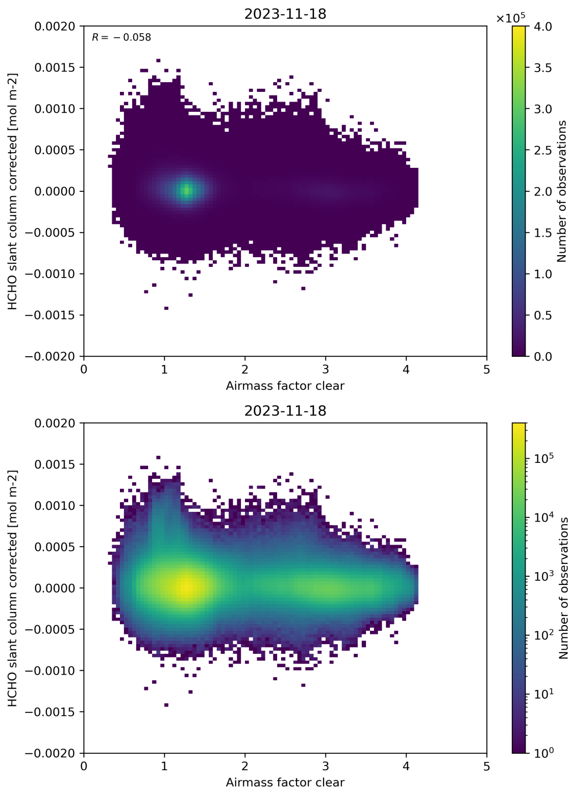
Figure 74: Scatter density plot of “Airmass factor clear” against “HCHO slant column corrected” for 2023-11-18 to 2023-11-19.
