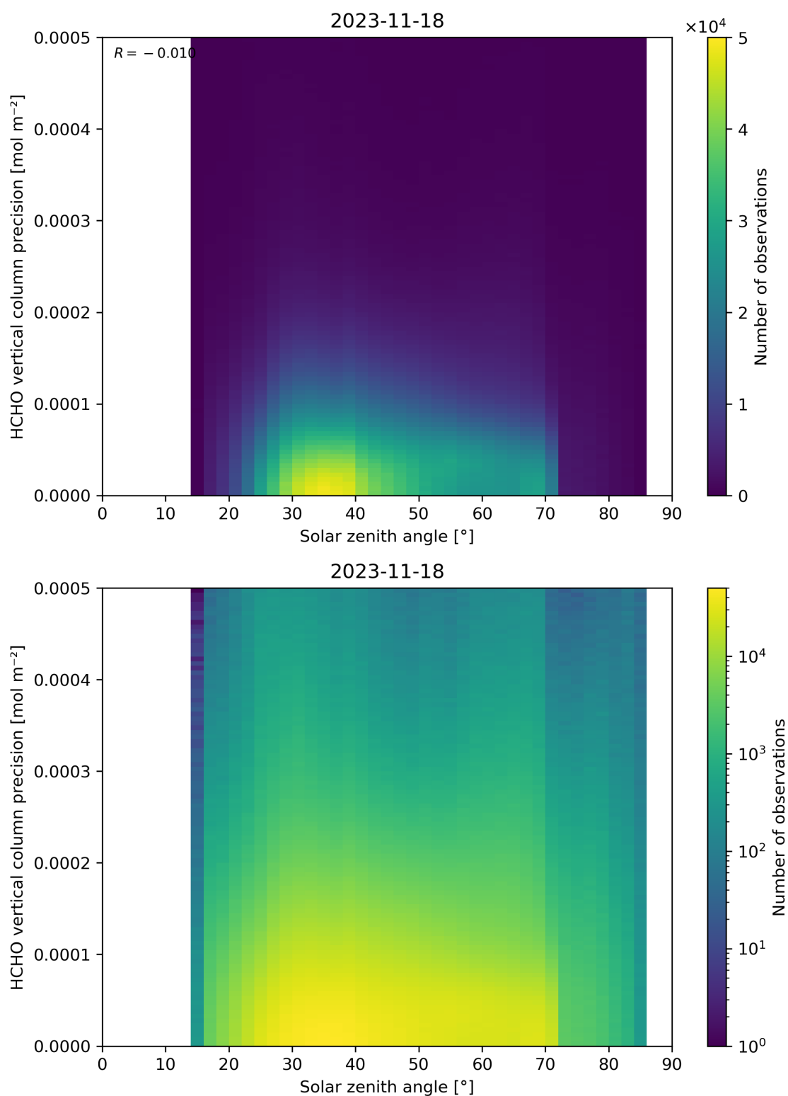
Figure 179: Scatter density plot of “Solar zenith angle” against “HCHO vertical column precision” for 2023-11-18 to 2023-11-19.
