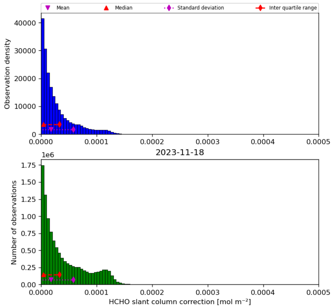
Figure 47: Histogram of “HCHO slant column correction” for 2023-11-18 to 2023-11-19
