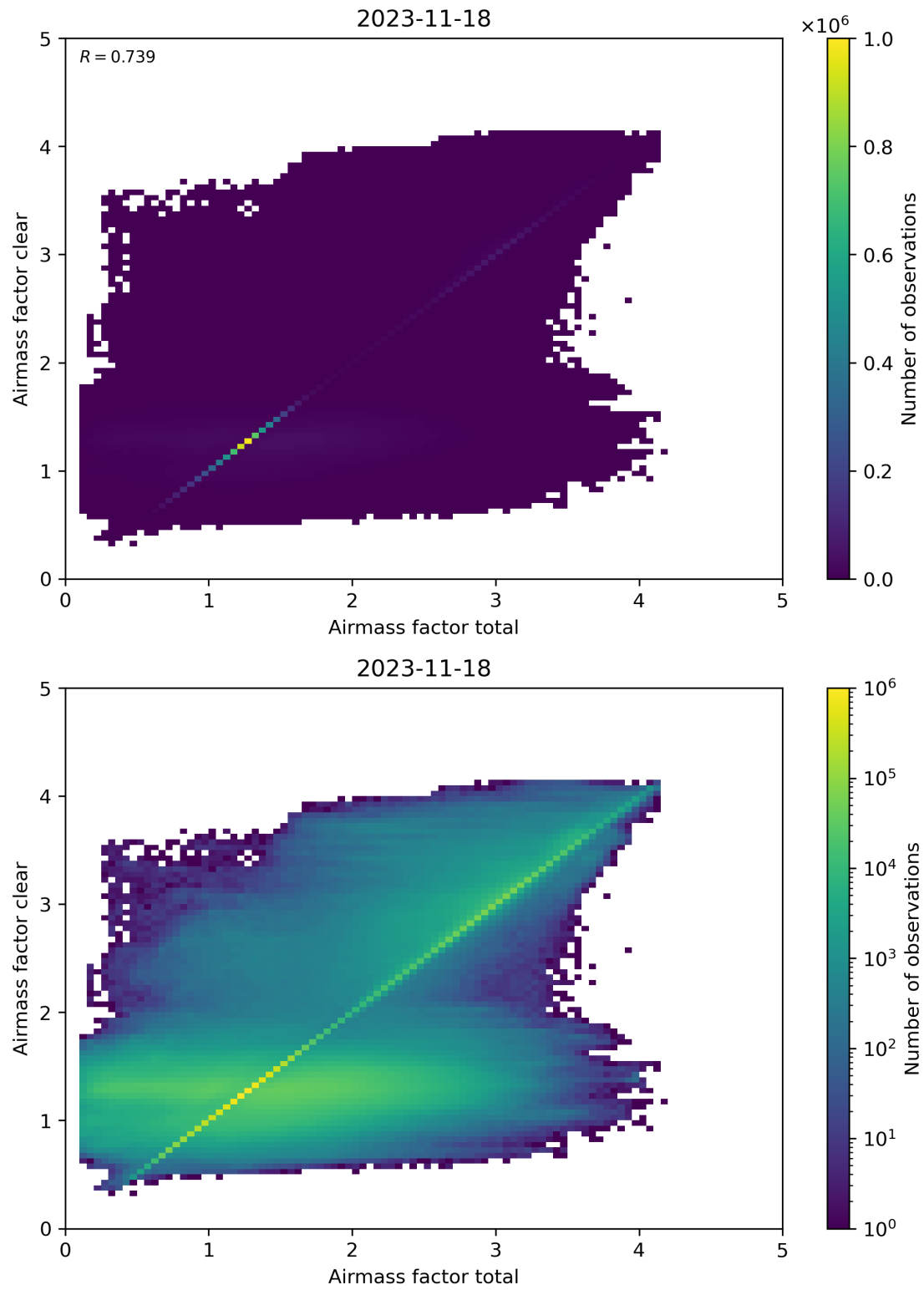
Figure 100: Scatter density plot of “Airmass factor total” against “Airmass factor clear” for 2023-11-18 to 2023-11-19.
