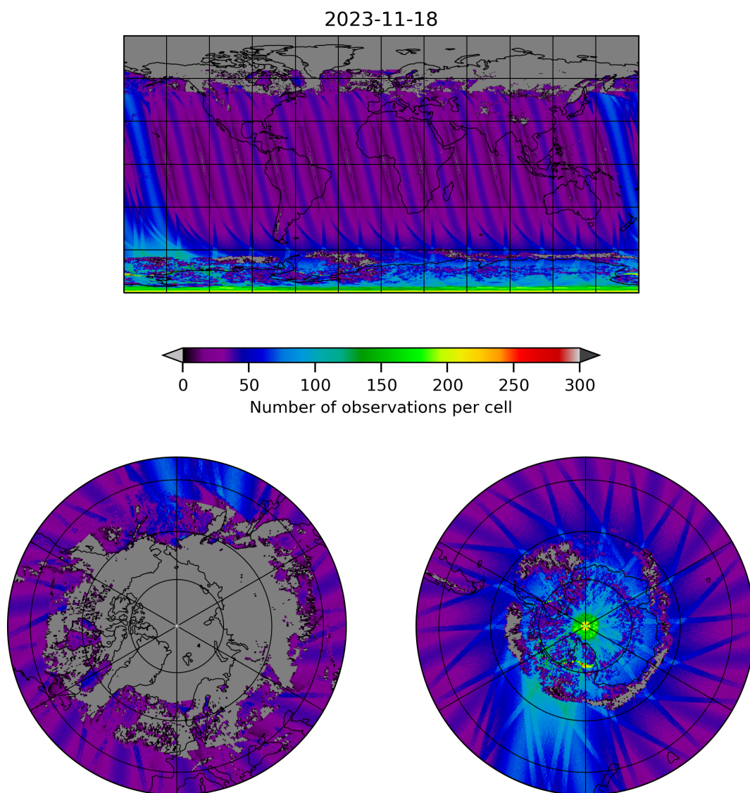
Figure 19: Map of the number of observations for 2023-11-18 to 2023-11-19
