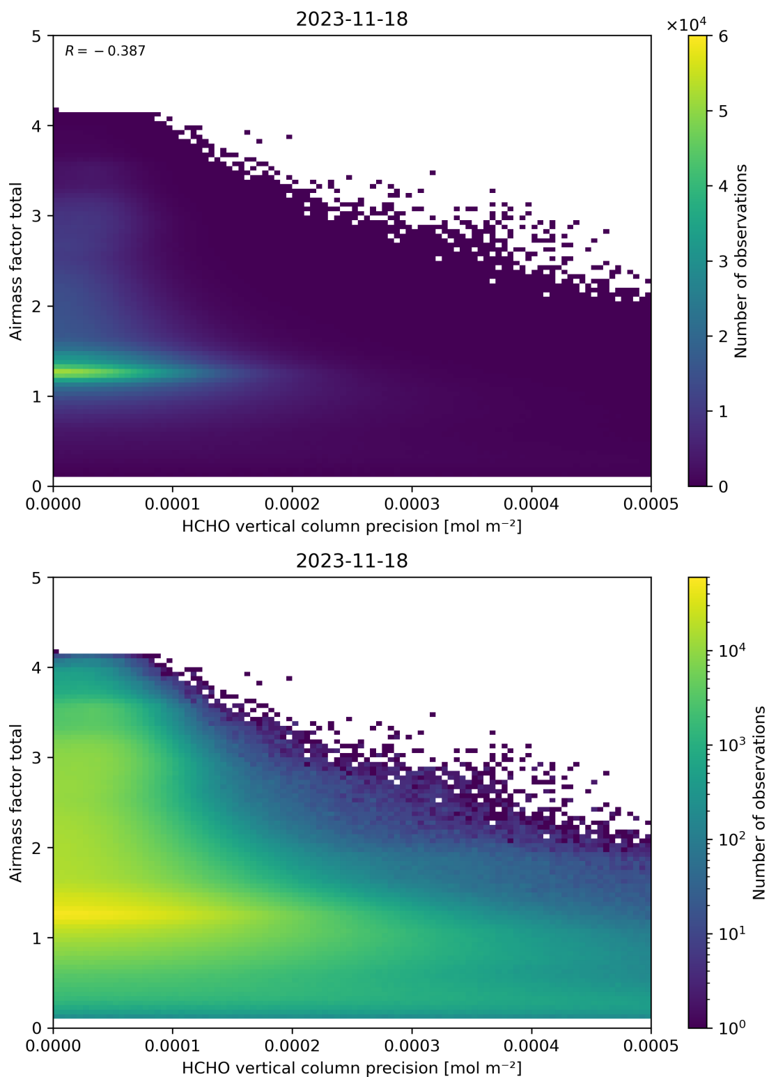
Figure 144: Scatter density plot of “HCHO vertical column precision” against “Airmass factor total” for 2023-11-18 to 2023-11-19.
