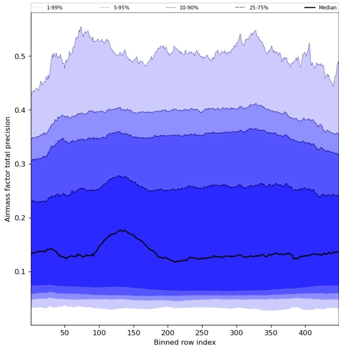
Figure 55: Along track statistics of “Airmass factor total precision” for 2023-11-18 to 2023-11-19
