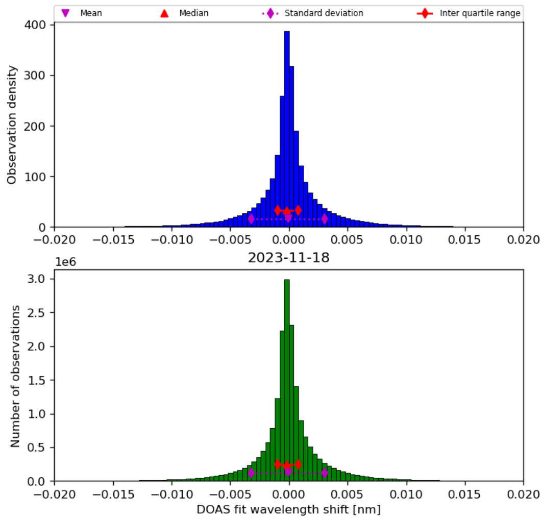
Figure 44: Histogram of “DOAS fit wavelength shift” for 2023-11-18 to 2023-11-19
