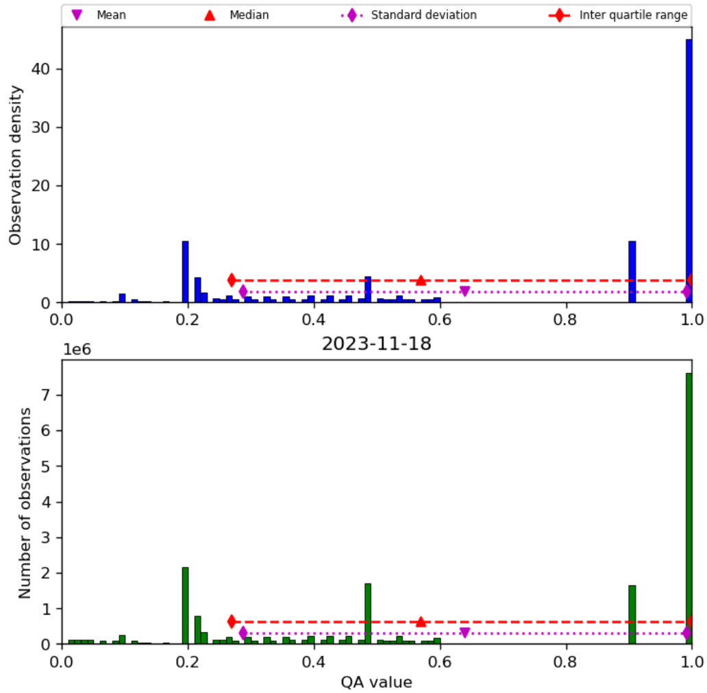
Figure 34: Histogram of “QA value” for 2023-11-18 to 2023-11-19
