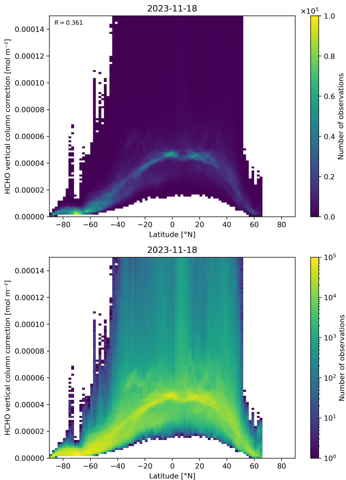
Figure 164: Scatter density plot of “Latitude” against “HCHO vertical column correction” for 2023-11-18 to 2023-11-19.
