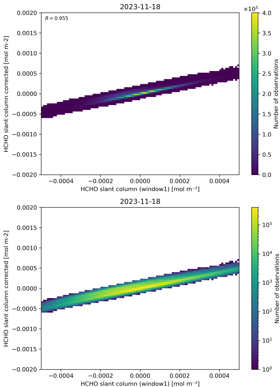
Figure 82: Scatter density plot of “HCHO slant column (window1)” against “HCHO slant column corrected” for 2023-11-18 to 2023-11-19.
