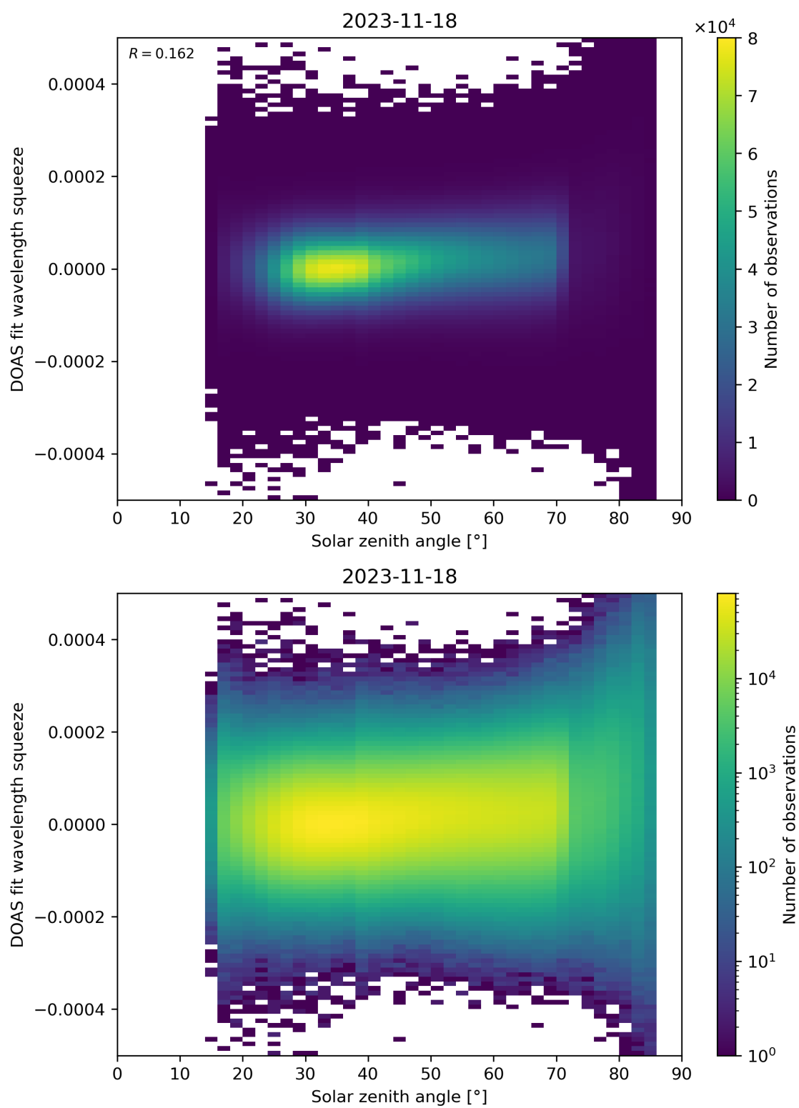
Figure 169: Scatter density plot of “Solar zenith angle” against “DOAS fit wavelength squeeze” for 2023-11-18 to 2023-11-19.
