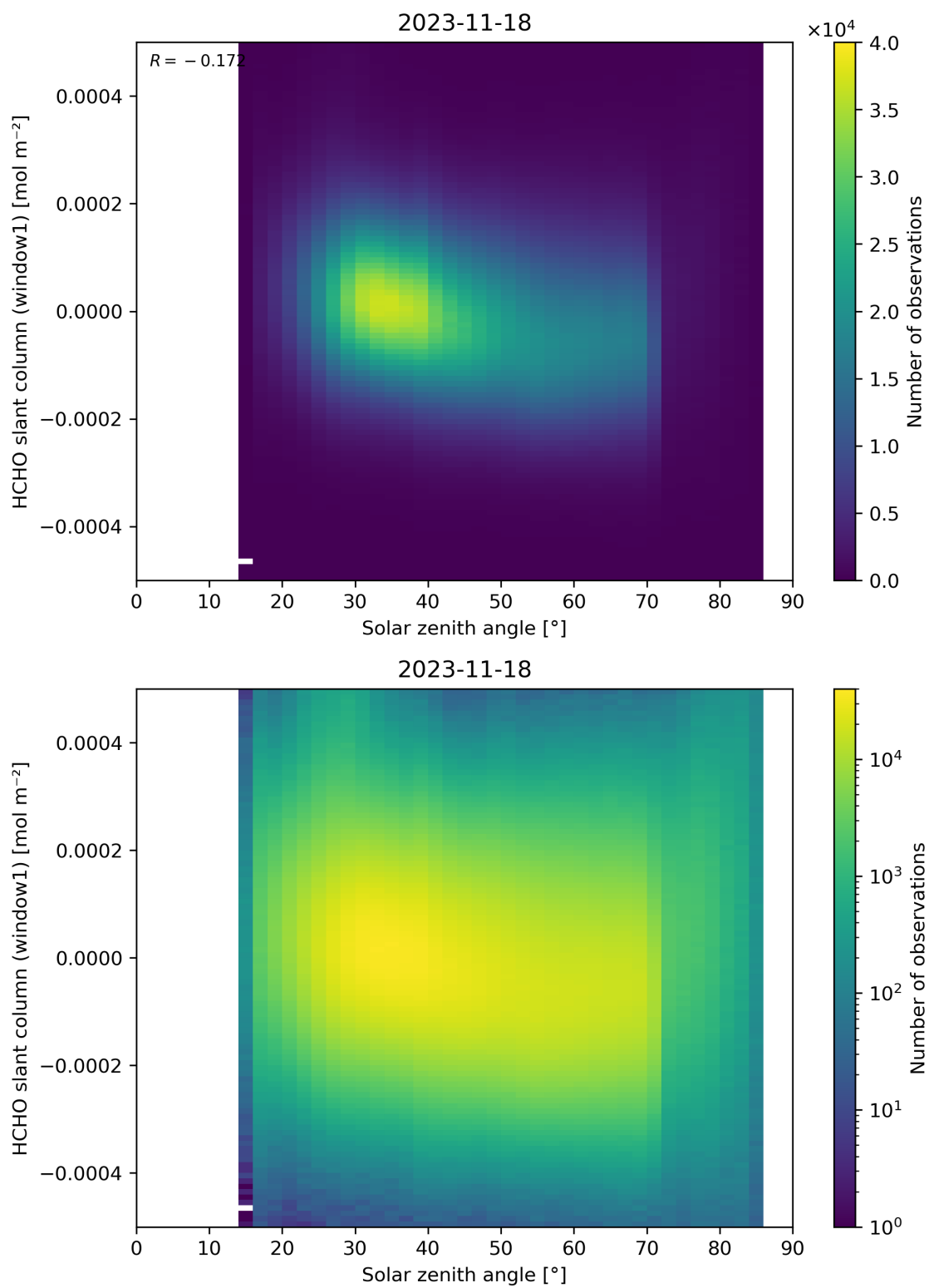
Figure 173: Scatter density plot of “Solar zenith angle” against “HCHO slant column (window1)” for 2023-11-18 to 2023-11-19.
