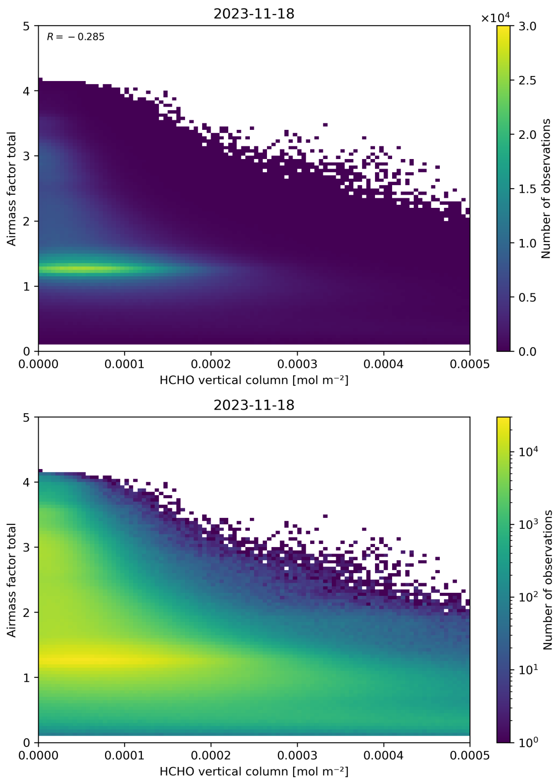
Figure 131: Scatter density plot of “HCHO vertical column” against “Airmass factor total” for 2023-11-18 to 2023-11-19.
