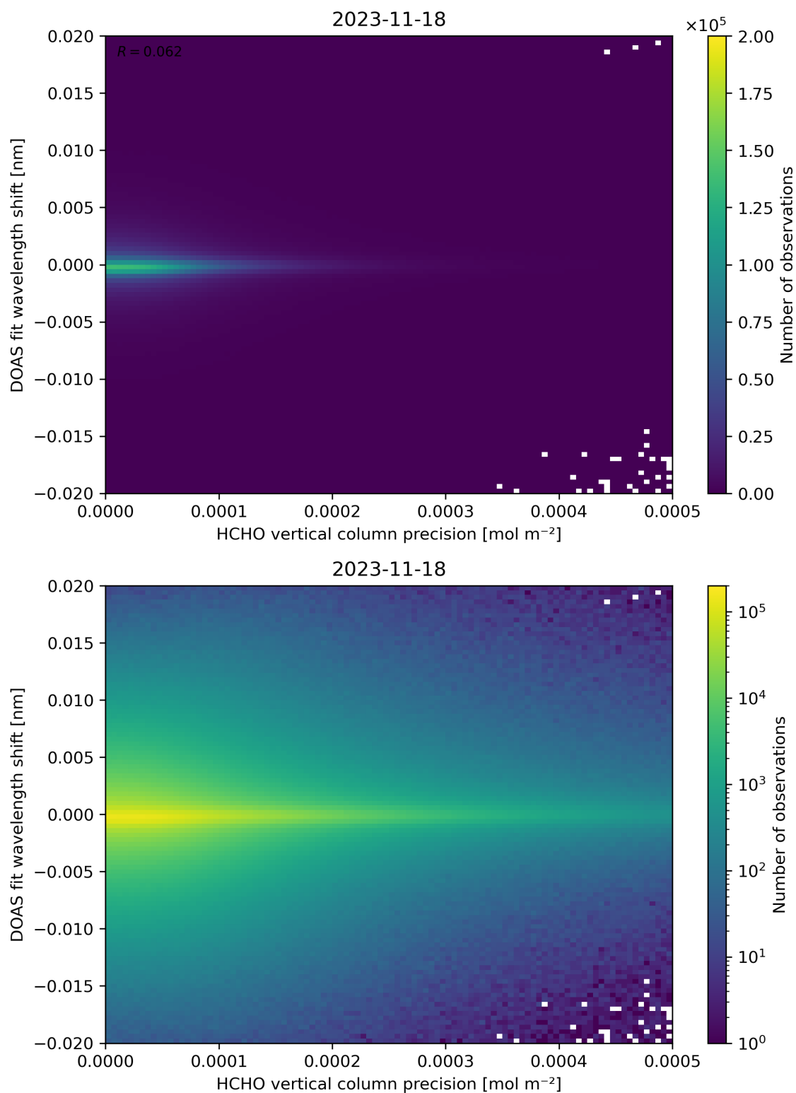
Figure 137: Scatter density plot of “HCHO vertical column precision” against “DOAS fit wavelength shift” for 2023-11-18 to 2023-11-19.
