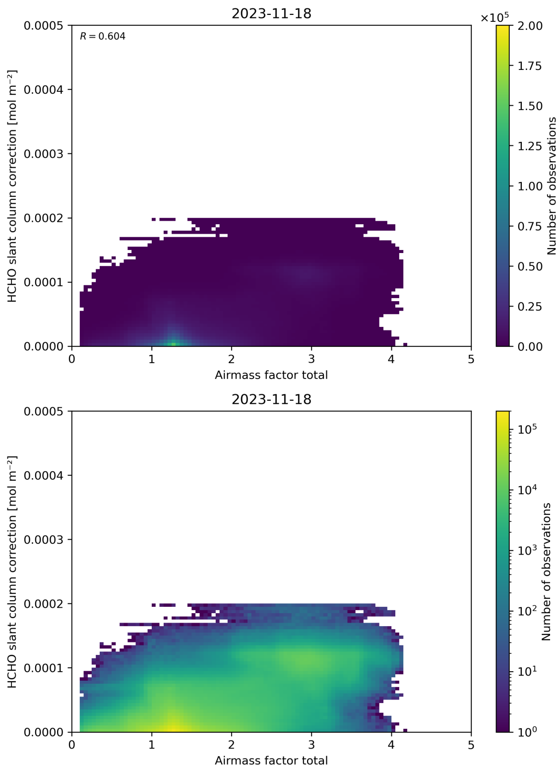
Figure 102: Scatter density plot of “Airmass factor total” against “HCHO slant column correction” for 2023-11-18 to 2023-11-19.
