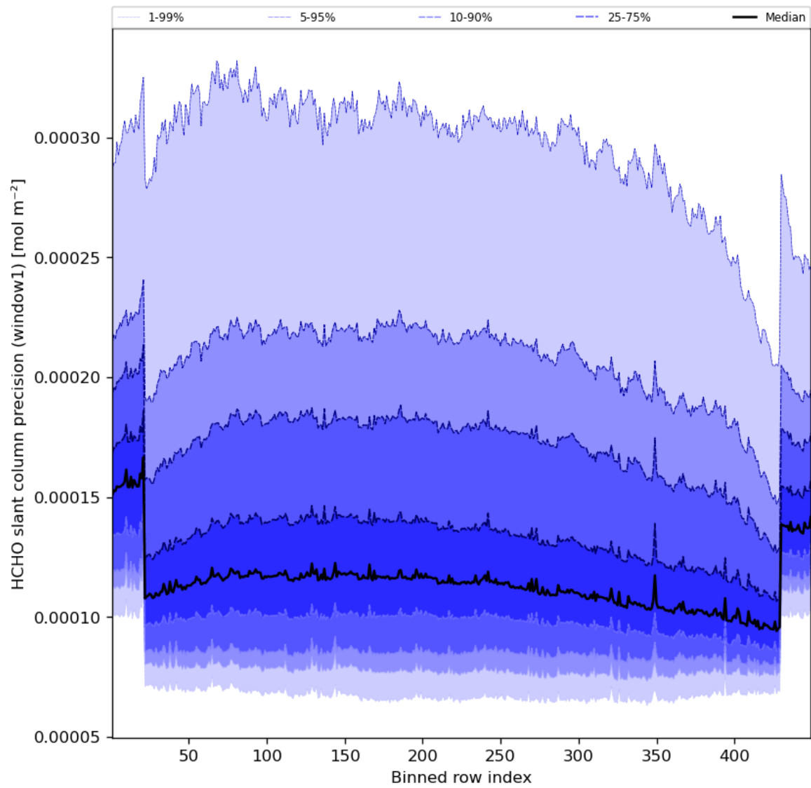
Figure 53: Along track statistics of “HCHO slant column precision (window1)” for 2023-11-18 to 2023-11-19
