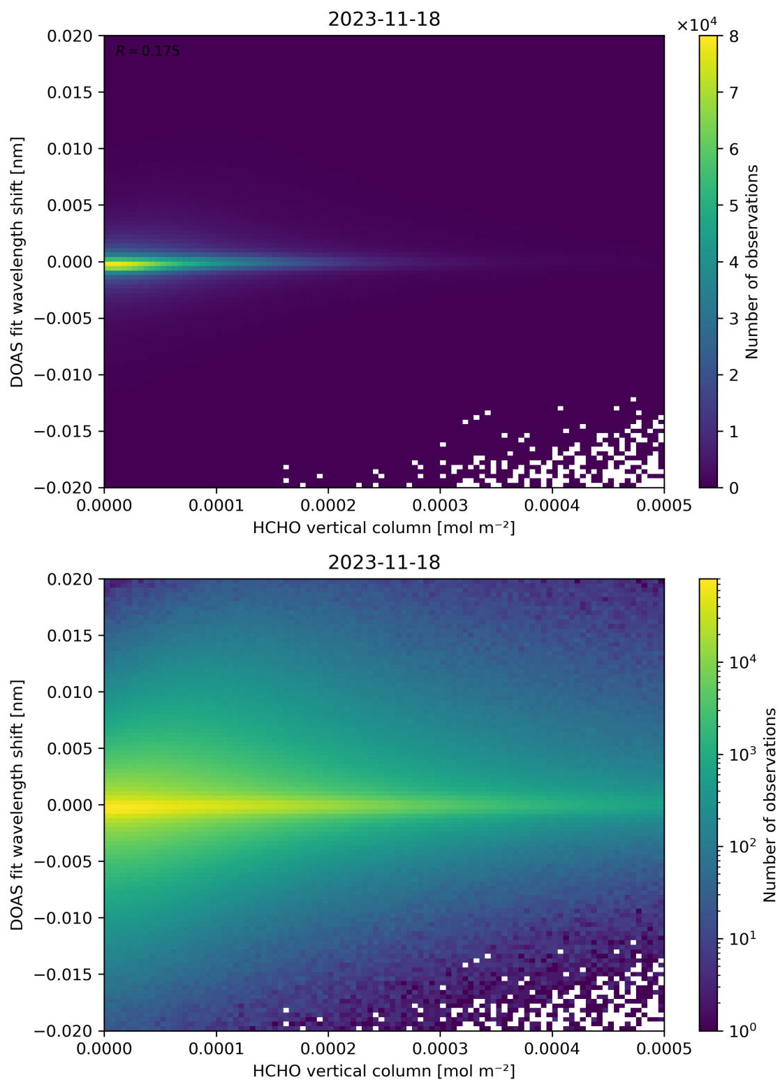
Figure 124: Scatter density plot of “HCHO vertical column” against “DOAS fit wavelength shift” for 2023-11-18 to 2023-11-19.
