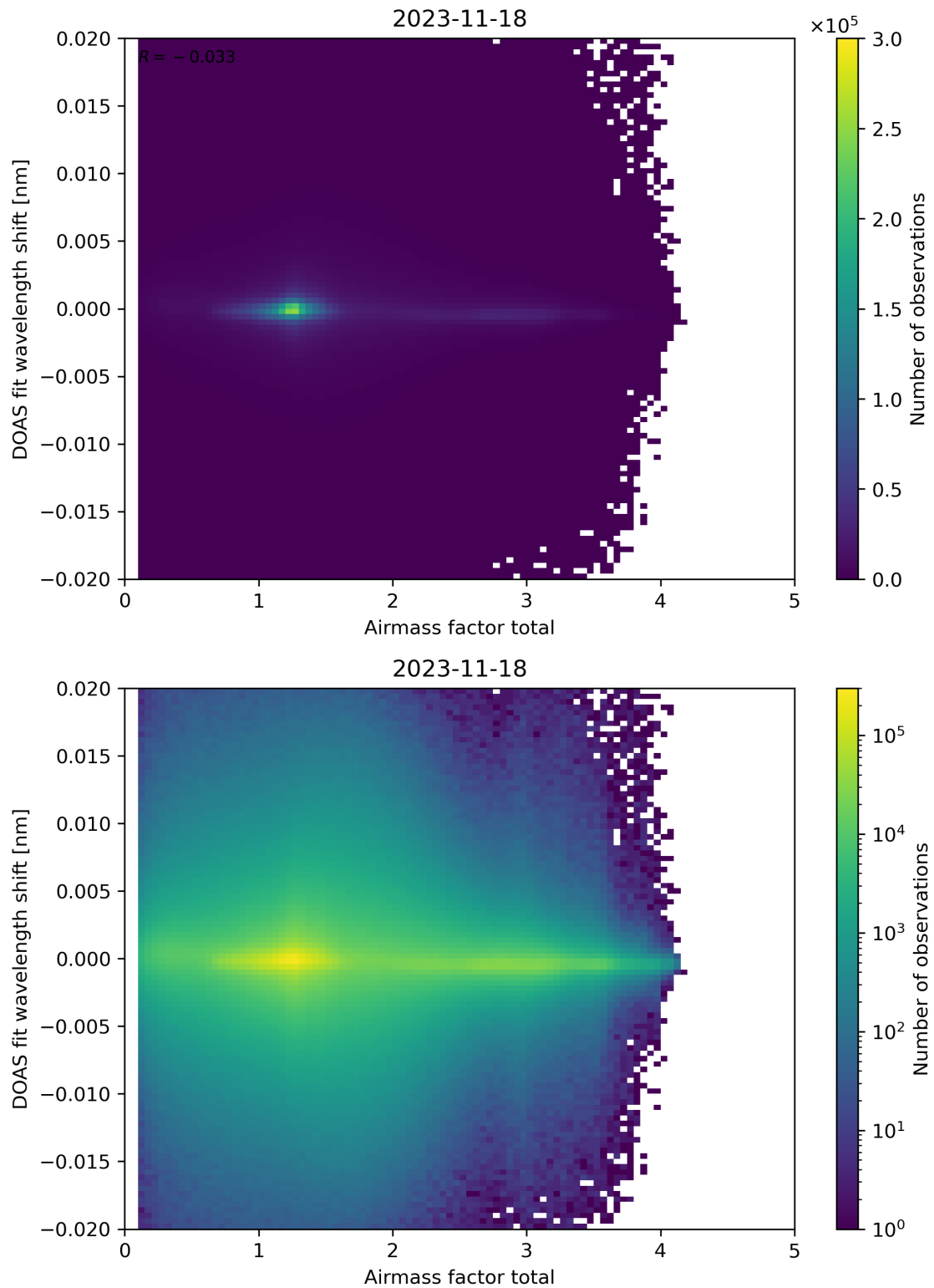
Figure 98: Scatter density plot of “Airmass factor total” against “DOAS fit wavelength shift” for 2023-11-18 to 2023-11-19.
