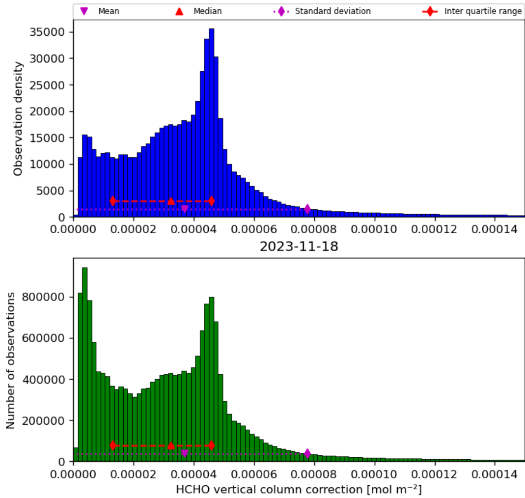
Figure 37: Histogram of “HCHO vertical column correction” for 2023-11-18 to 2023-11-19
