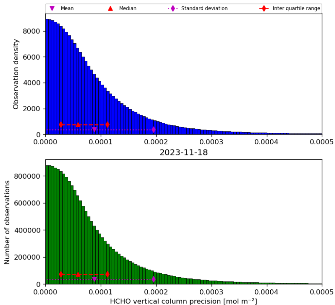
Figure 36: Histogram of “HCHO vertical column precision” for 2023-11-18 to 2023-11-19
