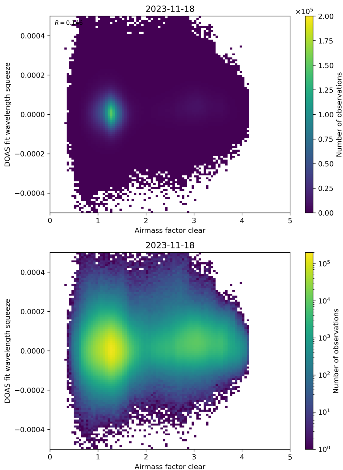
Figure 73: Scatter density plot of “Airmass factor clear” against “DOAS fit wavelength squeeze” for 2023-11-18 to 2023-11-19.
