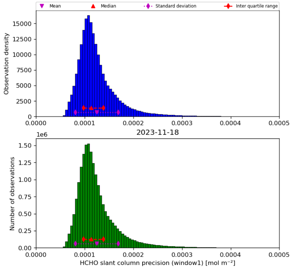
Figure 39: Histogram of “HCHO slant column precision (window1)” for 2023-11-18 to 2023-11-19
