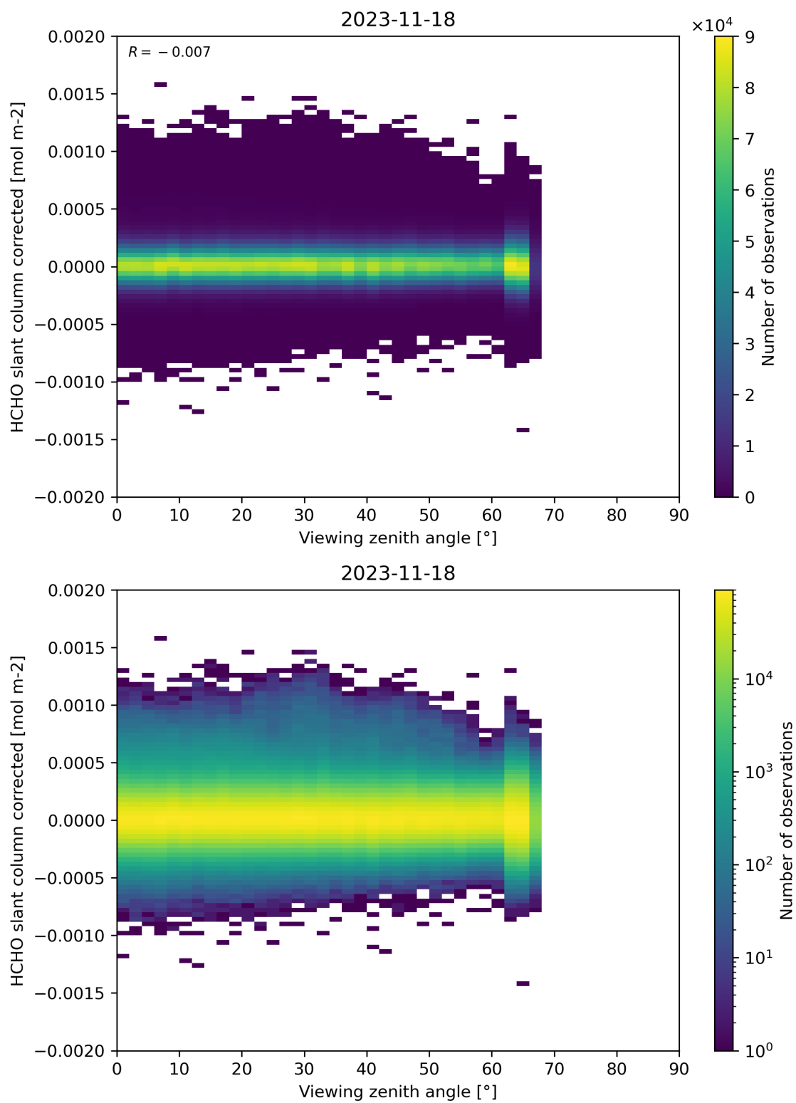
Figure 186: Scatter density plot of “Viewing zenith angle” against “HCHO slant column corrected” for 2023-11-18 to 2023-11-19.
