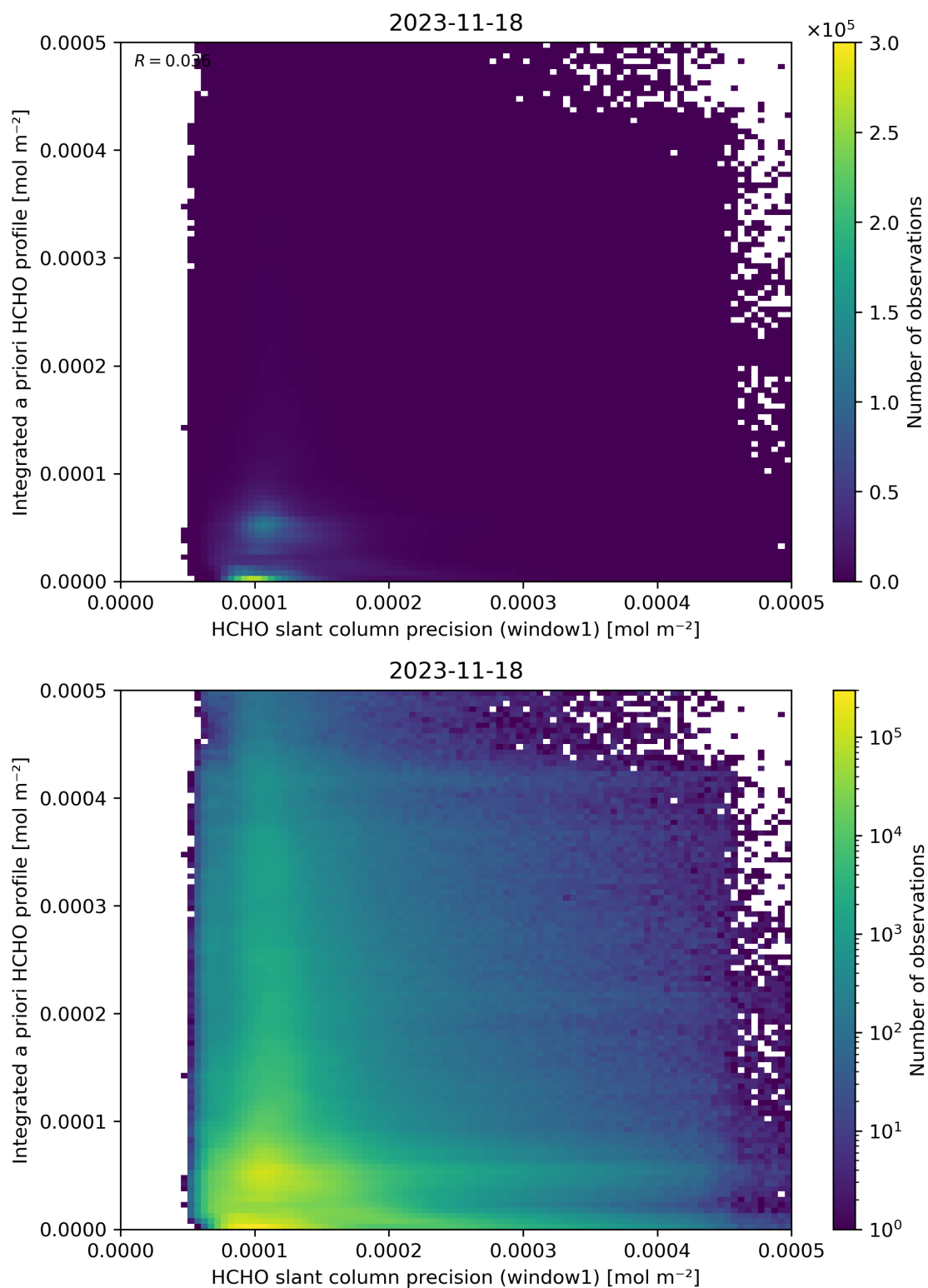
Figure 96: Scatter density plot of “HCHO slant column precision (window1)” against “Integrated a priori HCHO profile” for 2023-11-18 to 2023-11-19.
