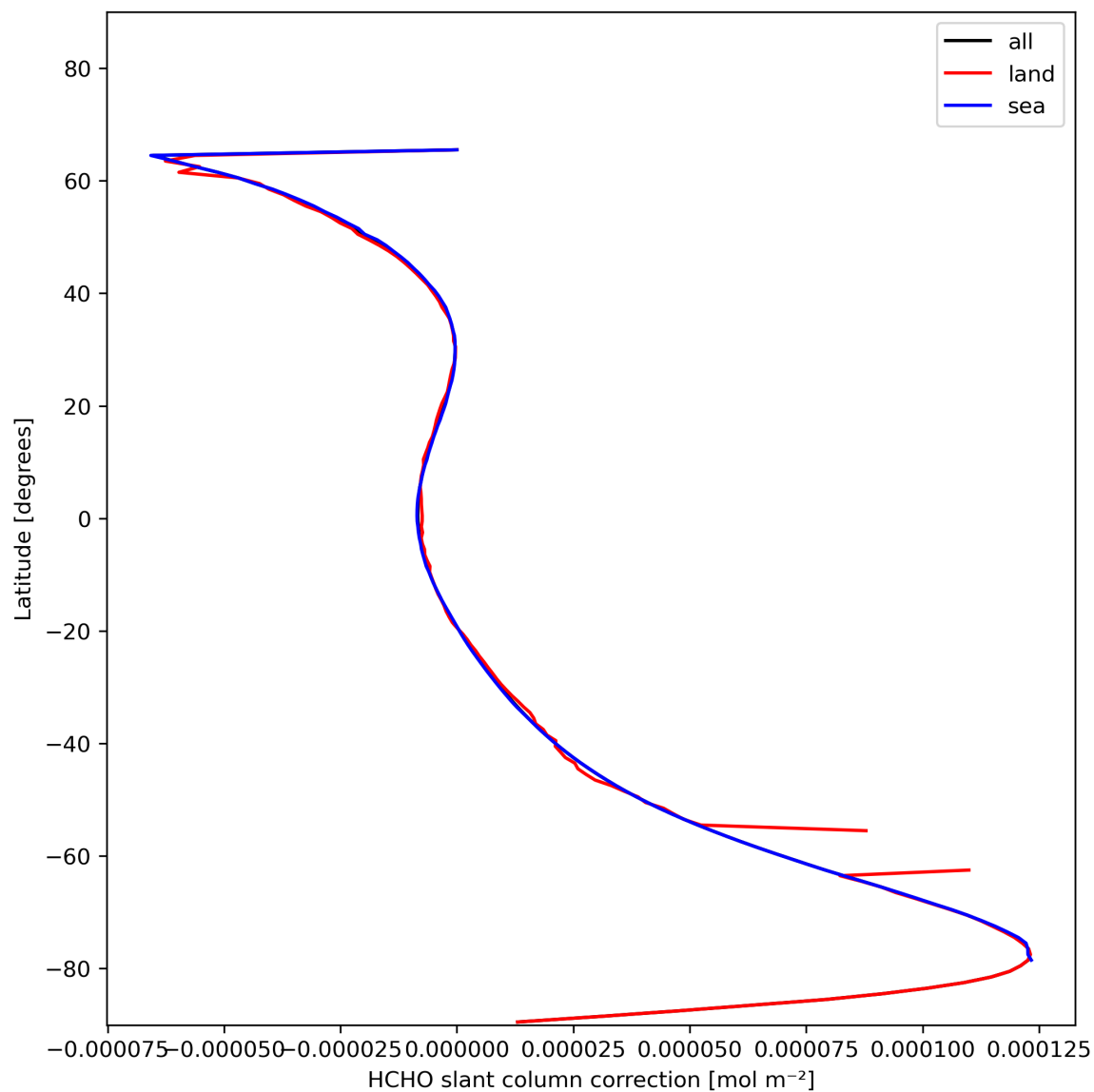
Figure 33: Zonal average of “HCHO slant column correction” for 2023-11-18 to 2023-11-19.
