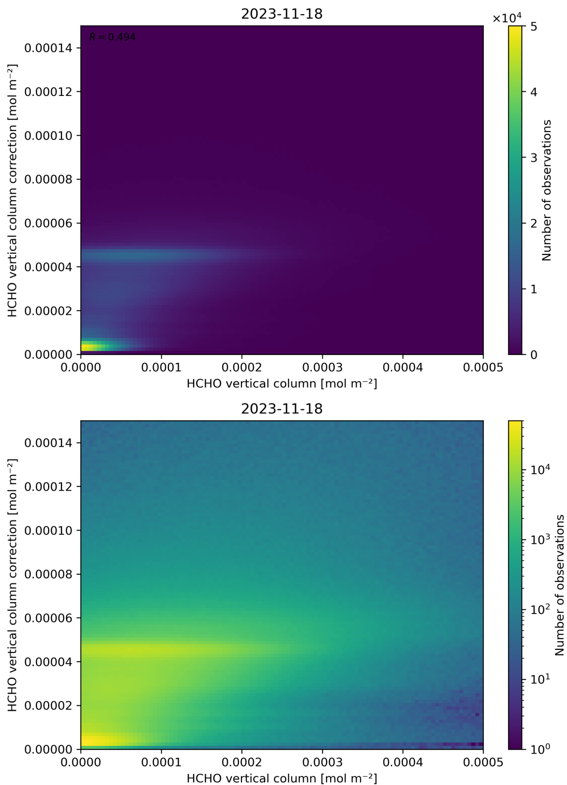
Figure 133: Scatter density plot of “HCHO vertical column” against “HCHO vertical column correction” for 2023-11-18 to 2023-11-19.
