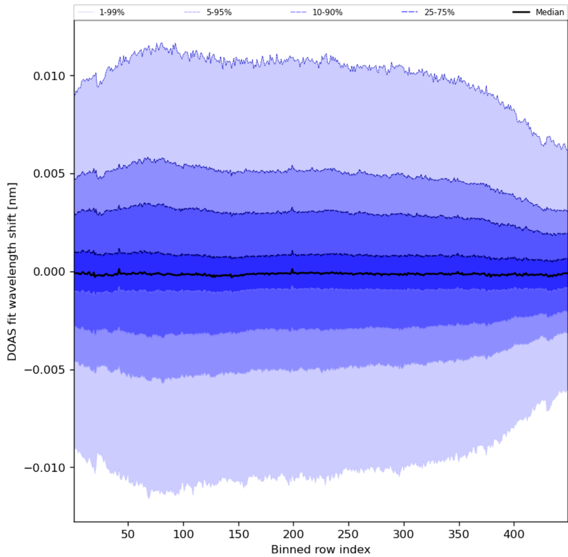
Figure 58: Along track statistics of “DOAS fit wavelength shift” for 2023-11-18 to 2023-11-19
