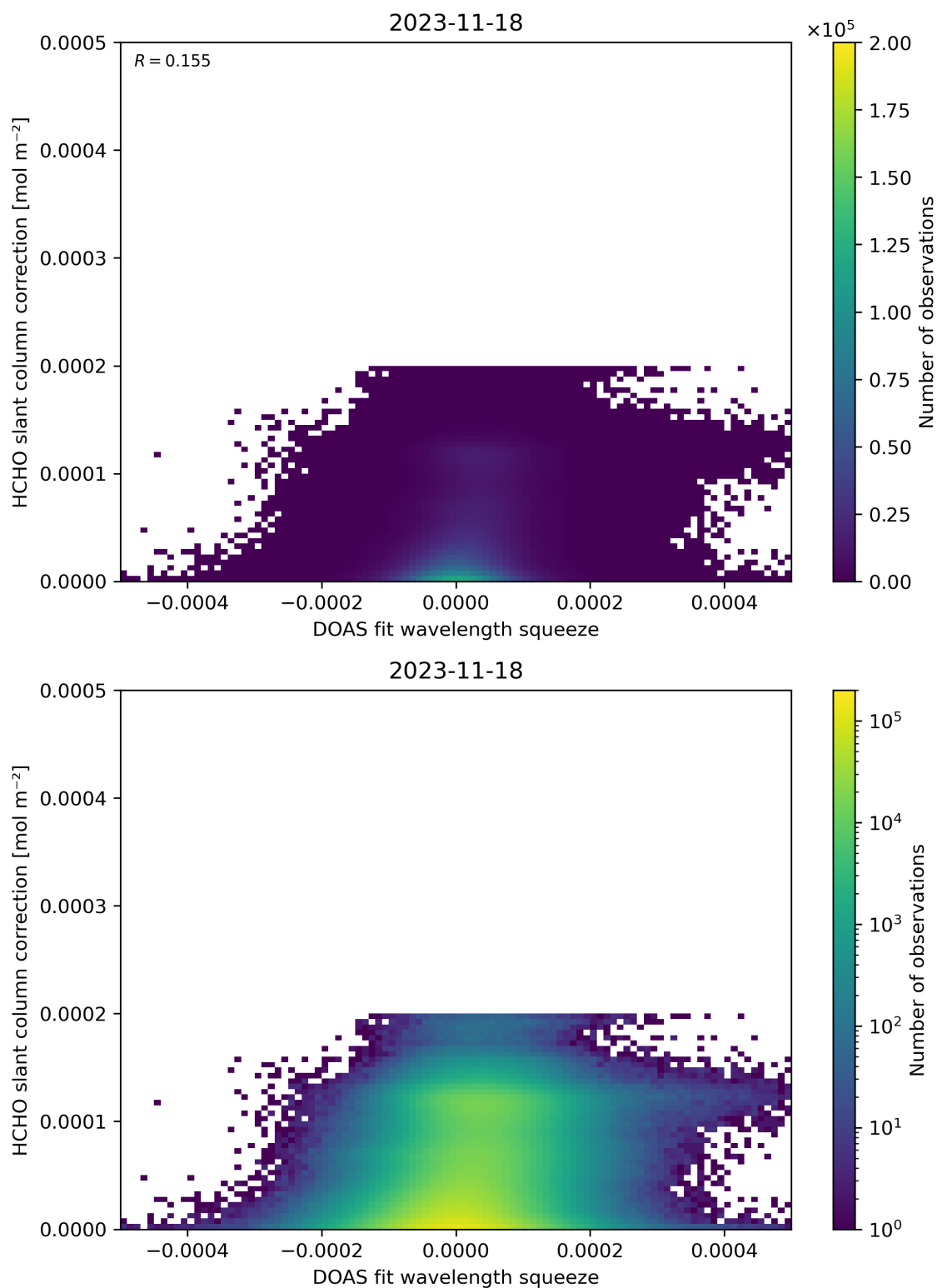
Figure 70: Scatter density plot of “DOAS fit wavelength squeeze” against “HCHO slant column correction” for 2023-11-18 to 2023-11-19.
