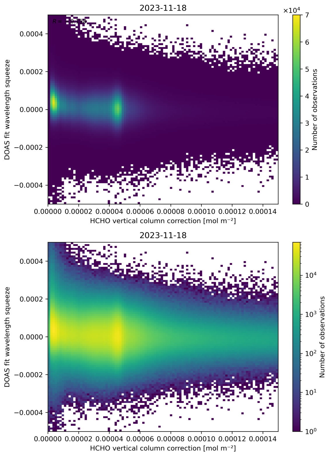
Figure 114: Scatter density plot of “HCHO vertical column correction” against “DOAS fit wavelength squeeze” for 2023-11-18 to 2023-11-19.
