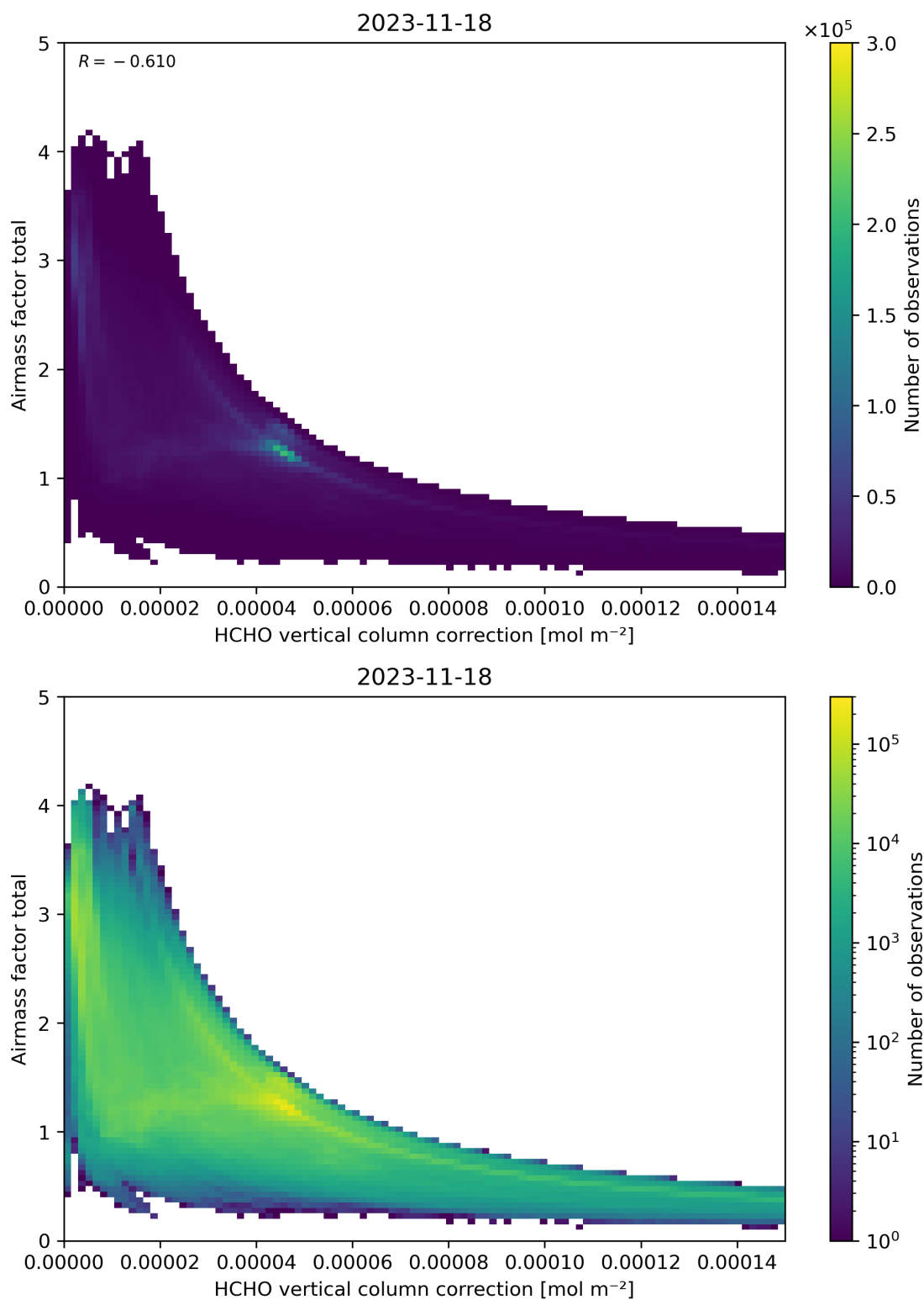
Figure 120: Scatter density plot of “HCHO vertical column correction” against “Airmass factor total” for 2023-11-18 to 2023-11-19.
