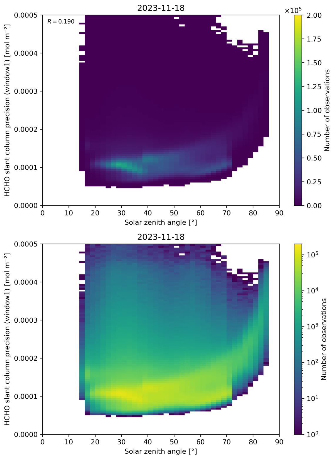
Figure 174: Scatter density plot of “Solar zenith angle” against “HCHO slant column precision (window1)” for 2023-11-18 to 2023-11-19.
