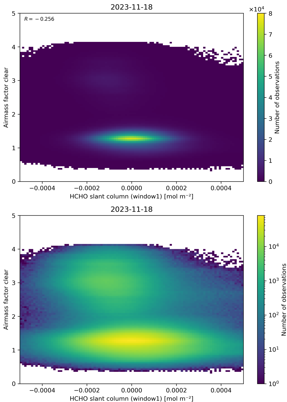
Figure 81: Scatter density plot of “HCHO slant column (window1)” against “Airmass factor clear” for 2023-11-18 to 2023-11-19.
