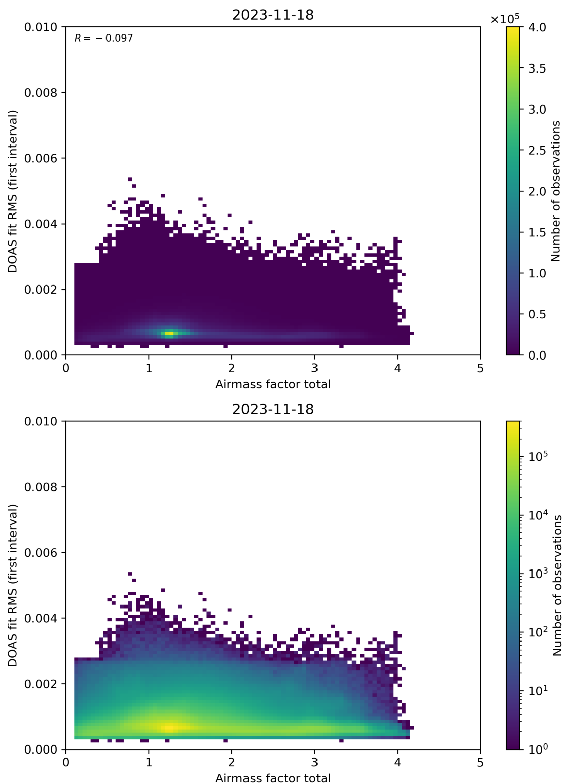
Figure 97: Scatter density plot of “Airmass factor total” against “DOAS fit RMS (first interval)” for 2023-11-18 to 2023-11-19.
