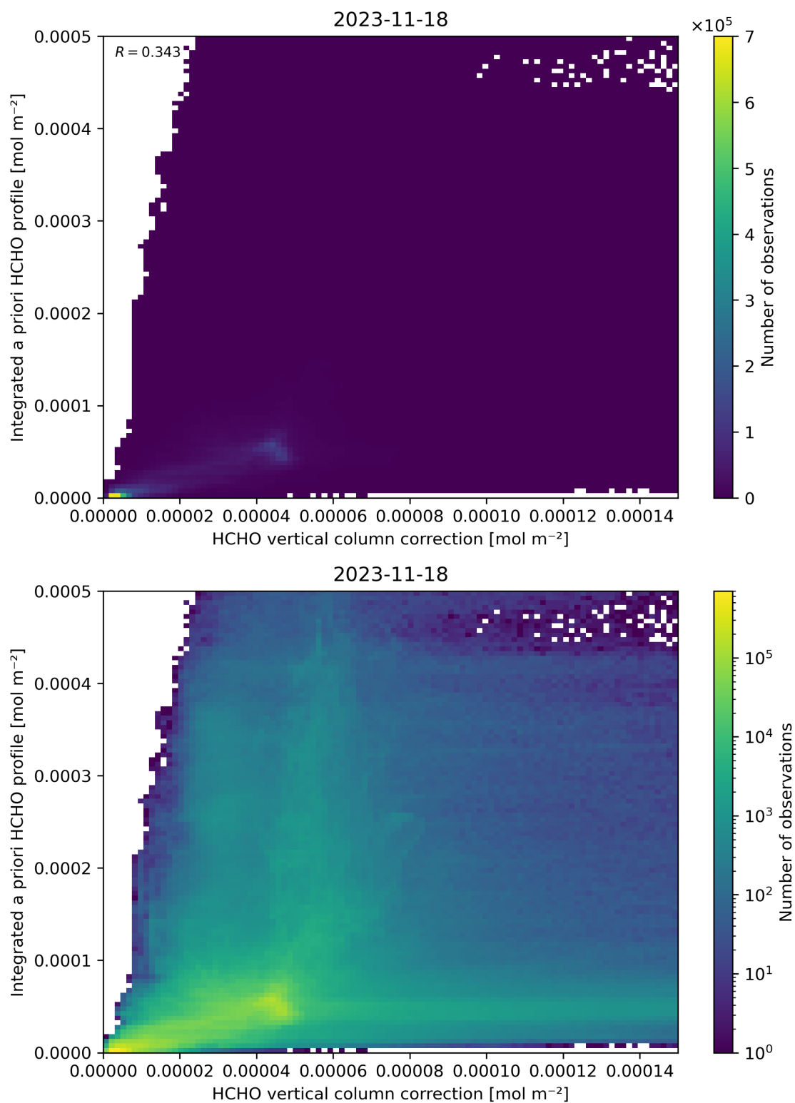
Figure 122: Scatter density plot of “HCHO vertical column correction” against “Integrated a priori HCHO profile” for 2023-11-18 to 2023-11-19.
