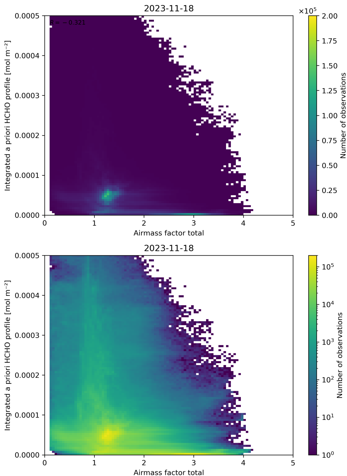
Figure 104: Scatter density plot of “Airmass factor total” against “Integrated a priori HCHO profile” for 2023-11-18 to 2023-11-19.
