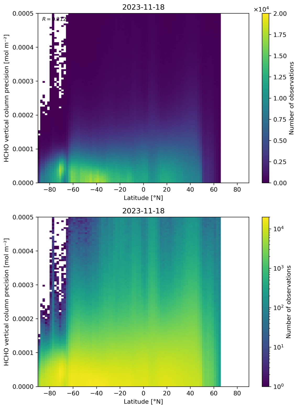
Figure 165: Scatter density plot of “Latitude” against “HCHO vertical column precision” for 2023-11-18 to 2023-11-19.
