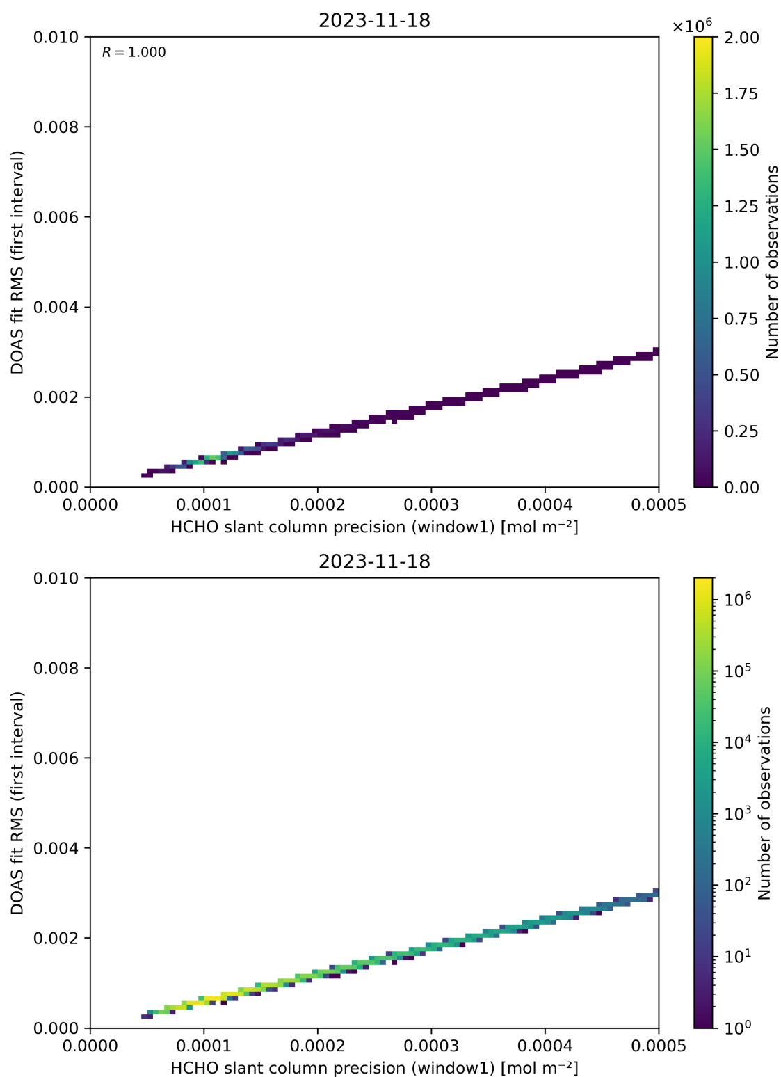
Figure 88: Scatter density plot of “HCHO slant column precision (window1)” against “DOAS fit RMS (first interval)” for 2023-11-18 to 2023-11-19.
