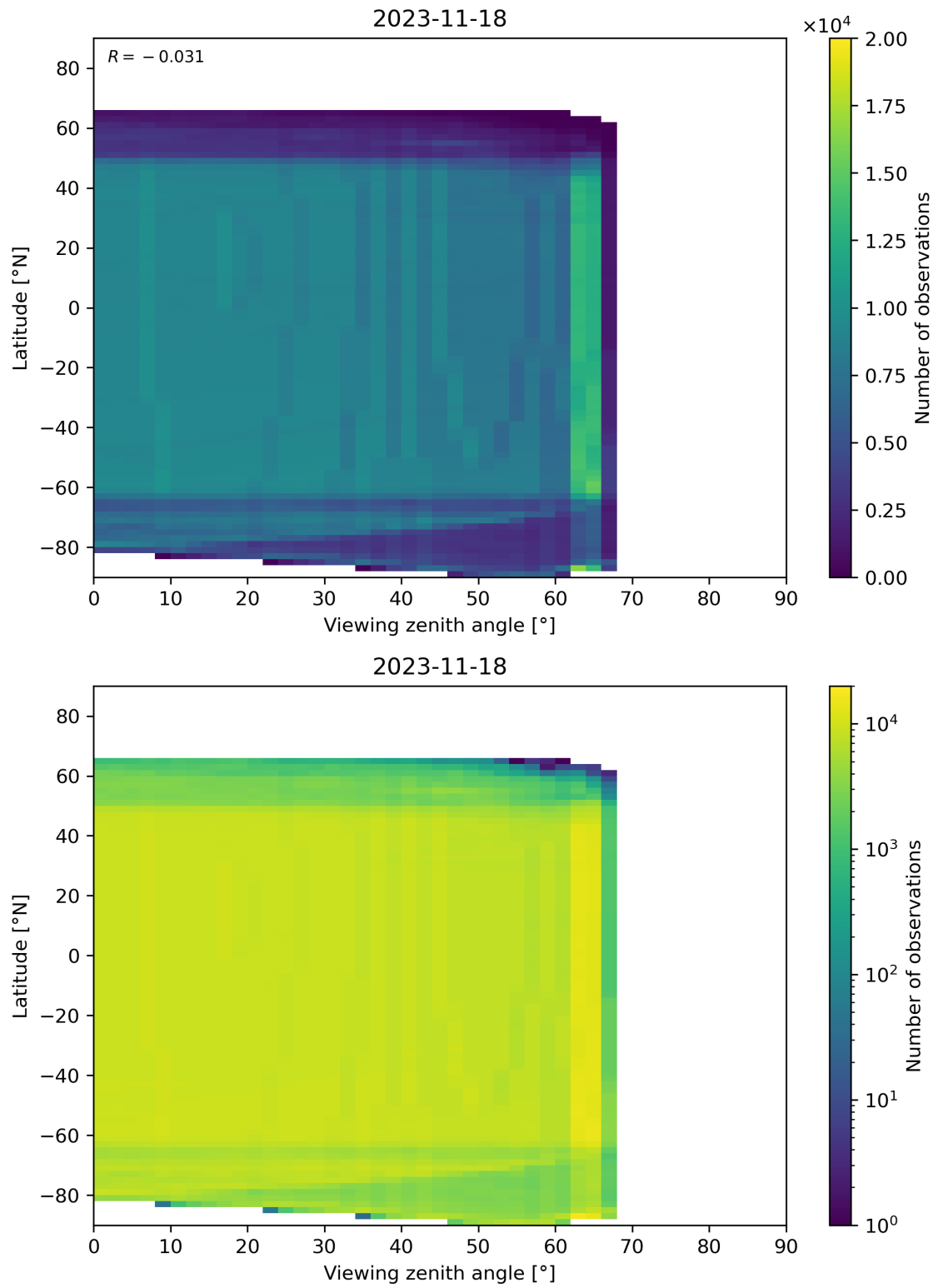
Figure 196: Scatter density plot of “Viewing zenith angle” against “Latitude” for 2023-11-18 to 2023-11-19.
