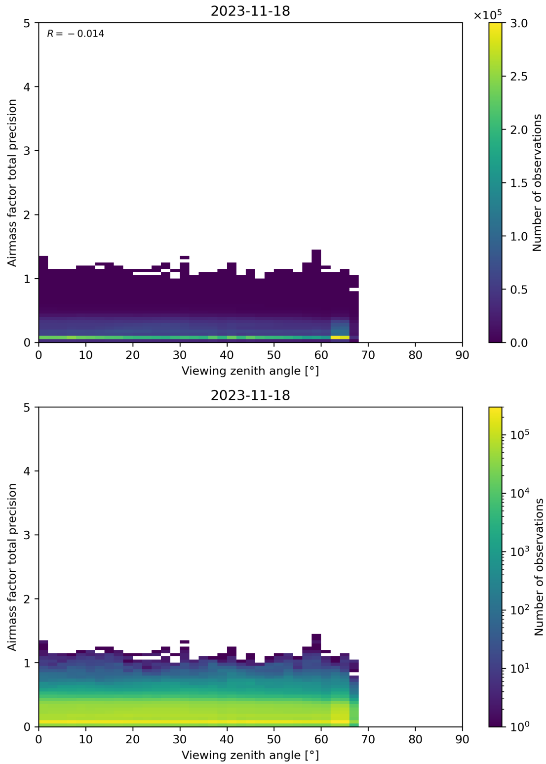
Figure 191: Scatter density plot of “Viewing zenith angle” against “Airmass factor total precision” for 2023-11-18 to 2023-11-19.
