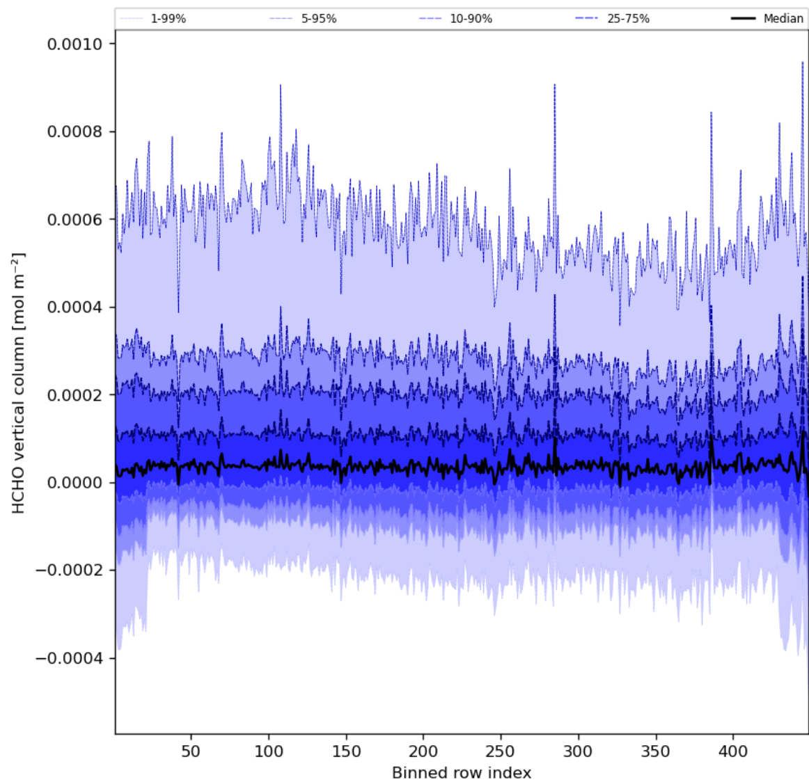
Figure 49: Along track statistics of “HCHO vertical column” for 2023-11-18 to 2023-11-19
