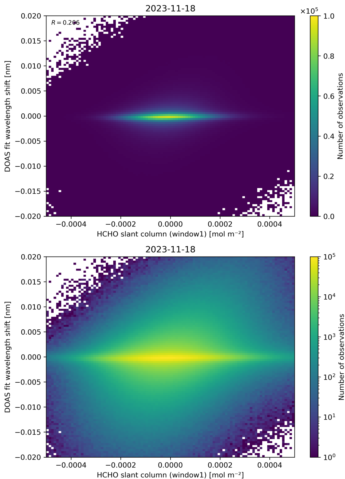
Figure 79: Scatter density plot of “HCHO slant column (window1)” against “DOAS fit wavelength shift” for 2023-11-18 to 2023-11-19.
