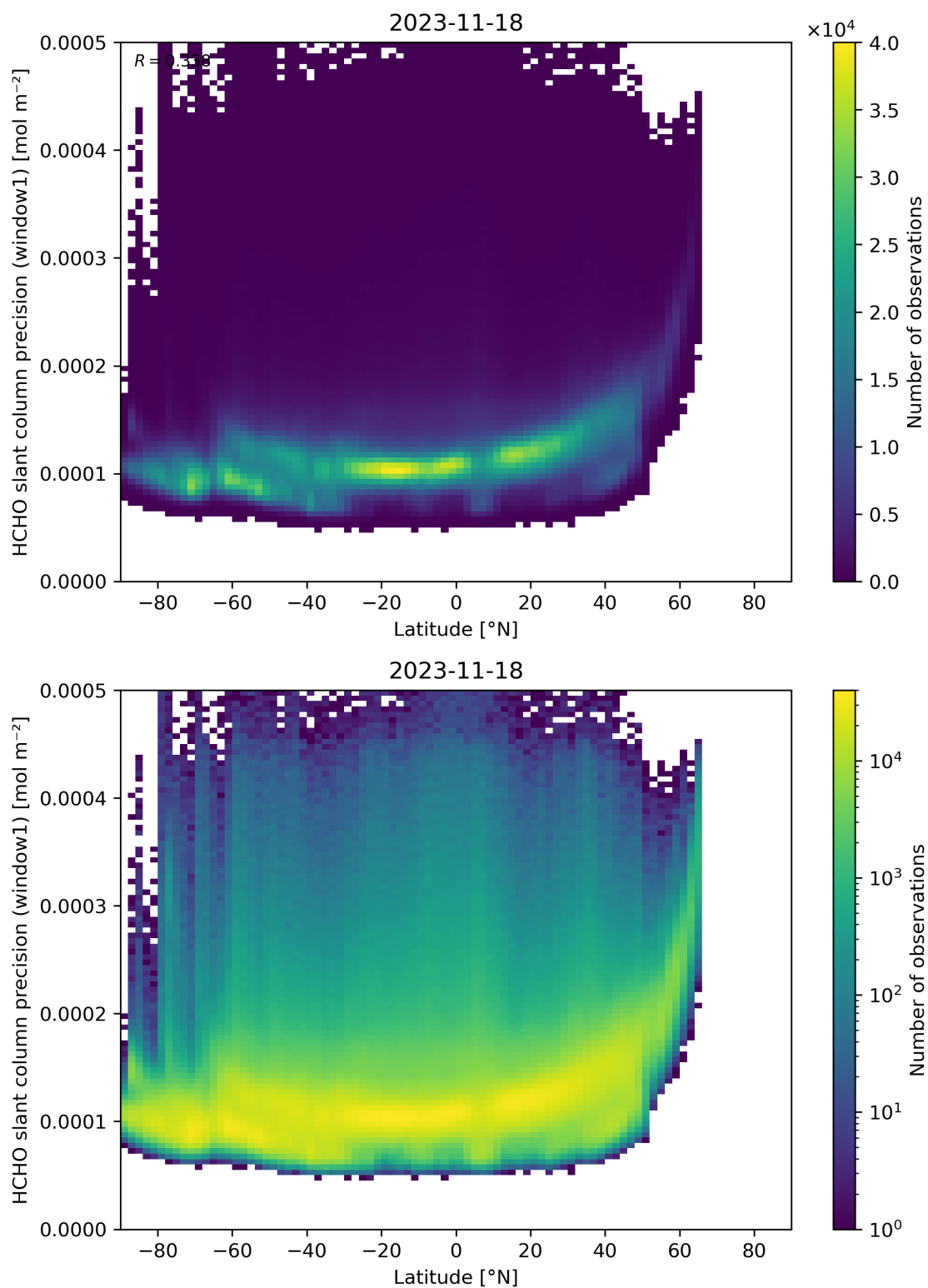
Figure 160: Scatter density plot of “Latitude” against “HCHO slant column precision (window1)” for 2023-11-18 to 2023-11-19.
