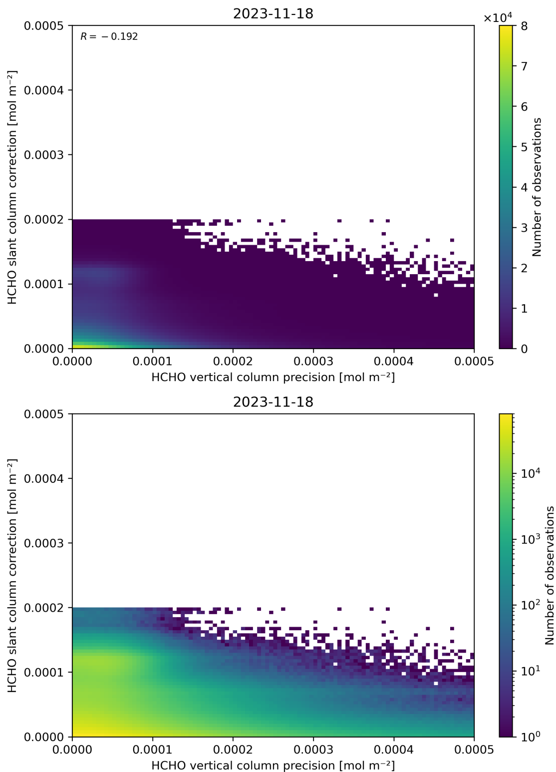
Figure 141: Scatter density plot of “HCHO vertical column precision” against “HCHO slant column correction” for 2023-11-18 to 2023-11-19.
