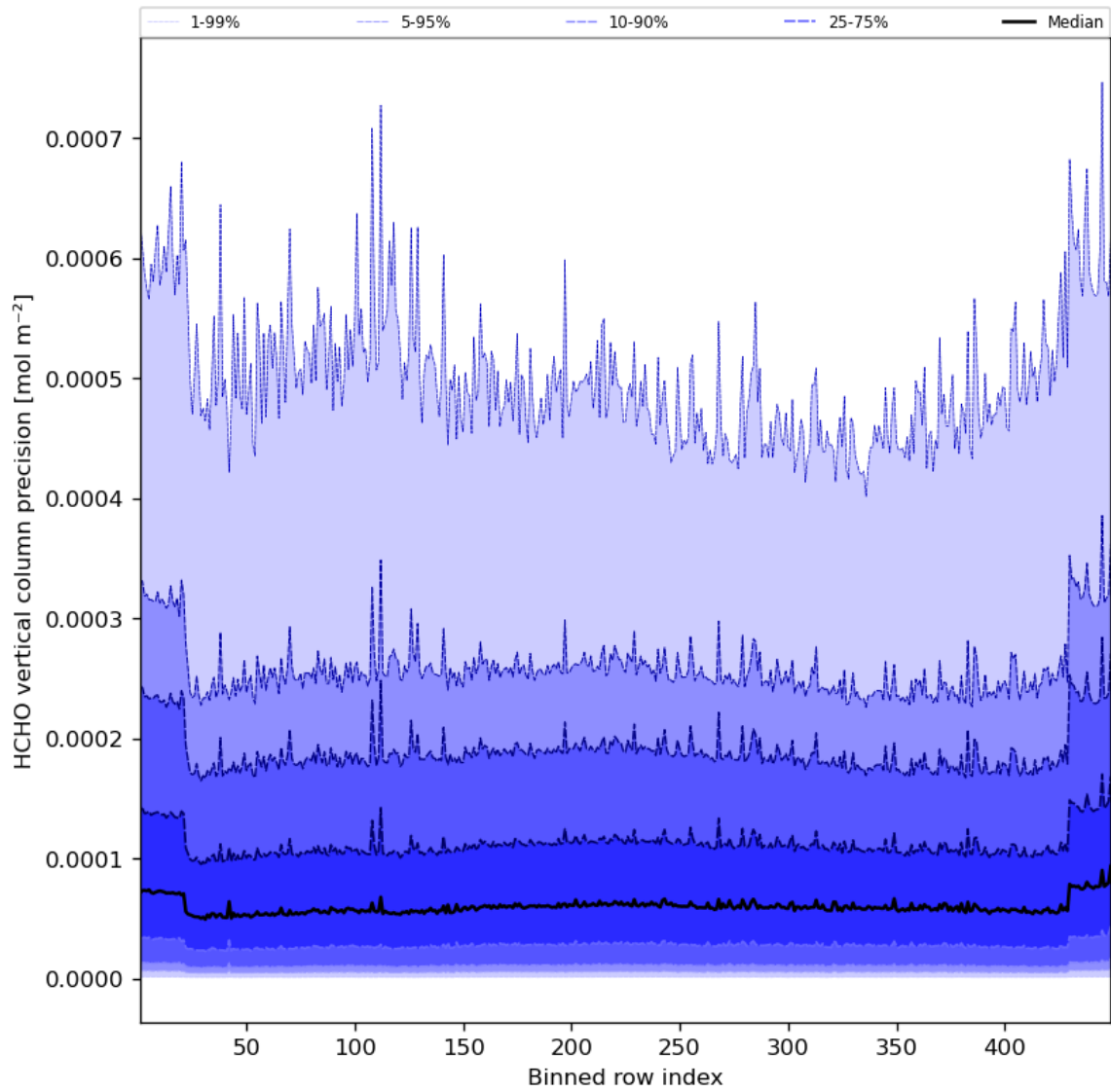
Figure 50: Along track statistics of “HCHO vertical column precision” for 2023-11-18 to 2023-11-19
