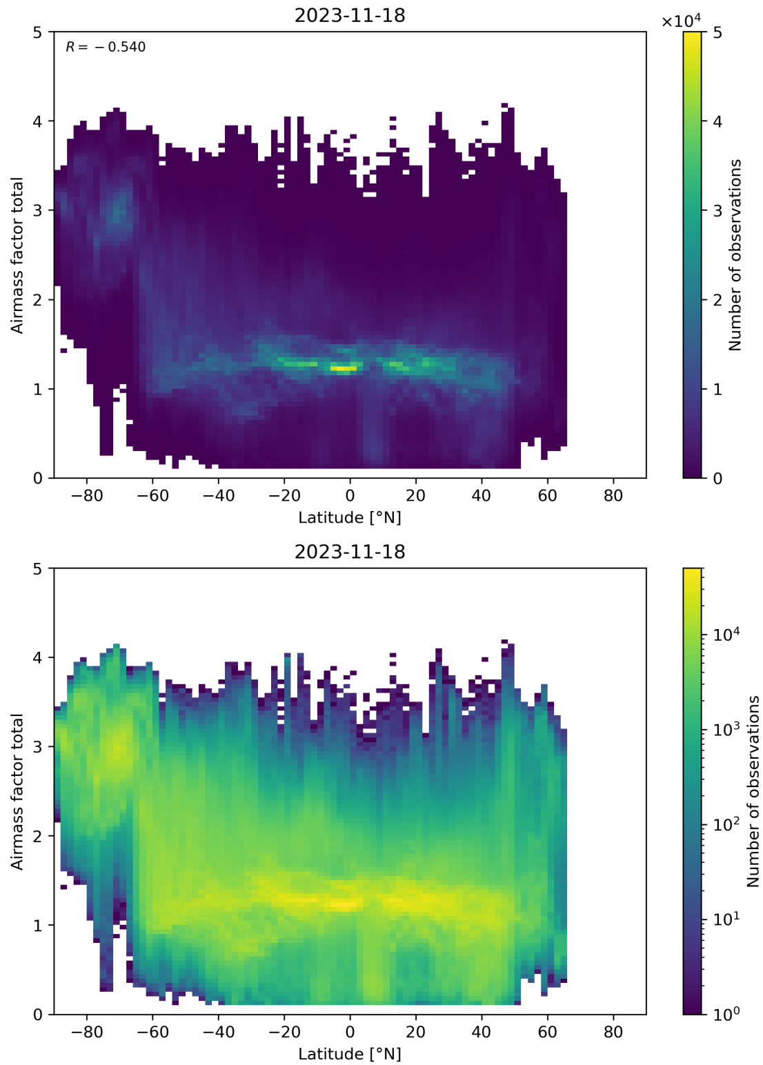
Figure 161: Scatter density plot of “Latitude” against “Airmass factor total” for 2023-11-18 to 2023-11-19.
