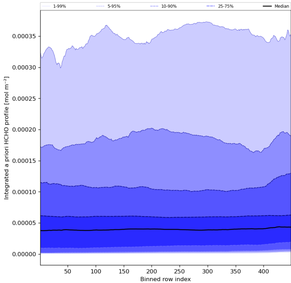
Figure 57: Along track statistics of “Integrated a priori HCHO profile” for 2023-11-18 to 2023-11-19
