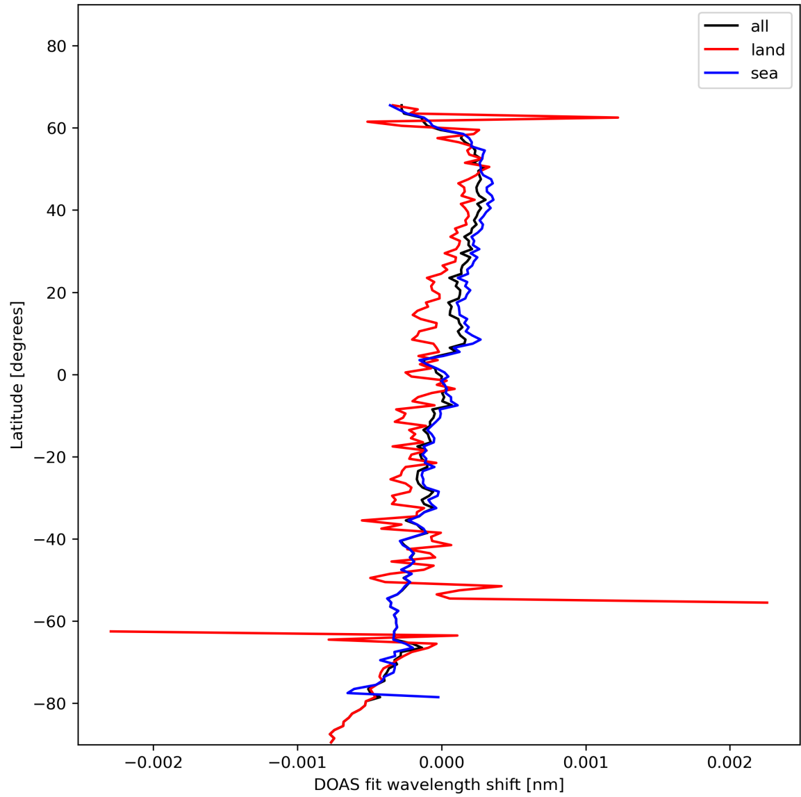
Figure 30: Zonal average of “DOAS fit wavelength shift” for 2023-11-18 to 2023-11-19.
