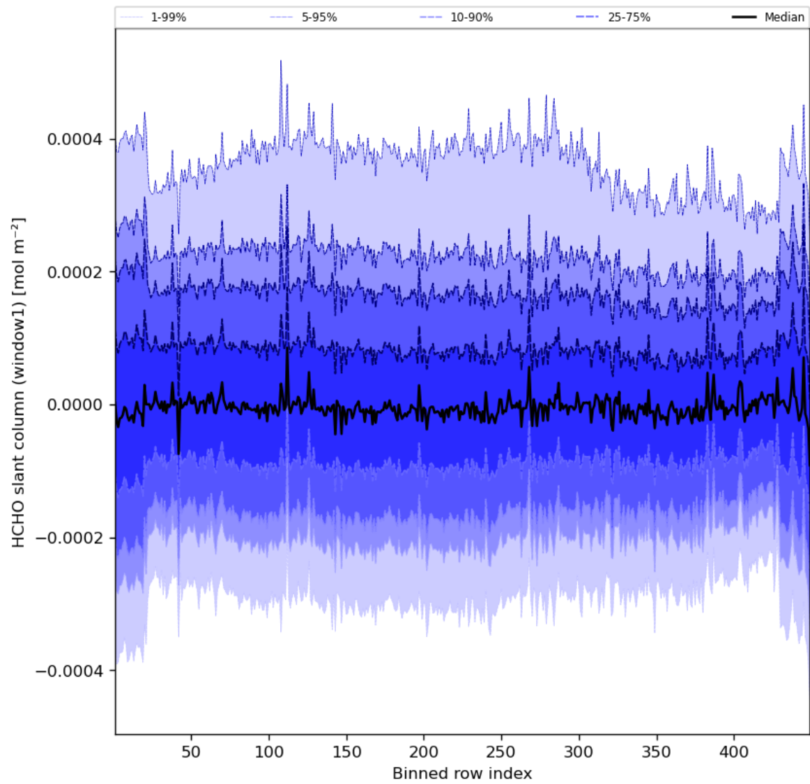
Figure 52: Along track statistics of “HCHO slant column (window1)” for 2023-11-18 to 2023-11-19
