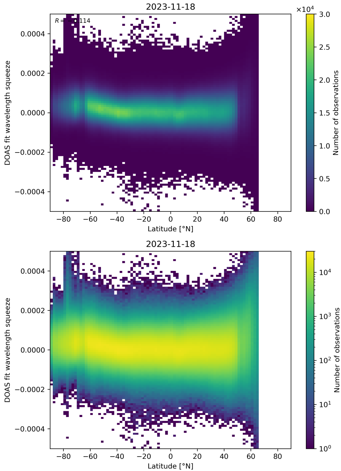
Figure 155: Scatter density plot of “Latitude” against “DOAS fit wavelength squeeze” for 2023-11-18 to 2023-11-19.
