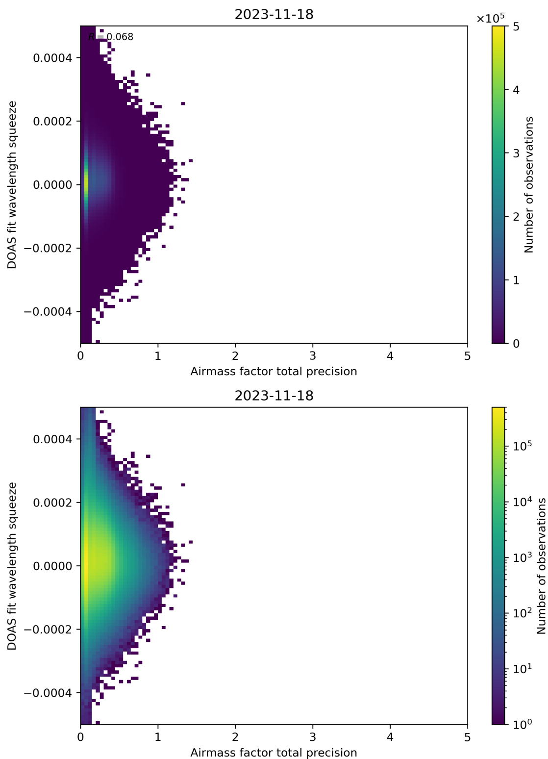
Figure 107: Scatter density plot of “Airmass factor total precision” against “DOAS fit wavelength squeeze” for 2023-11-18 to 2023-11-19.
