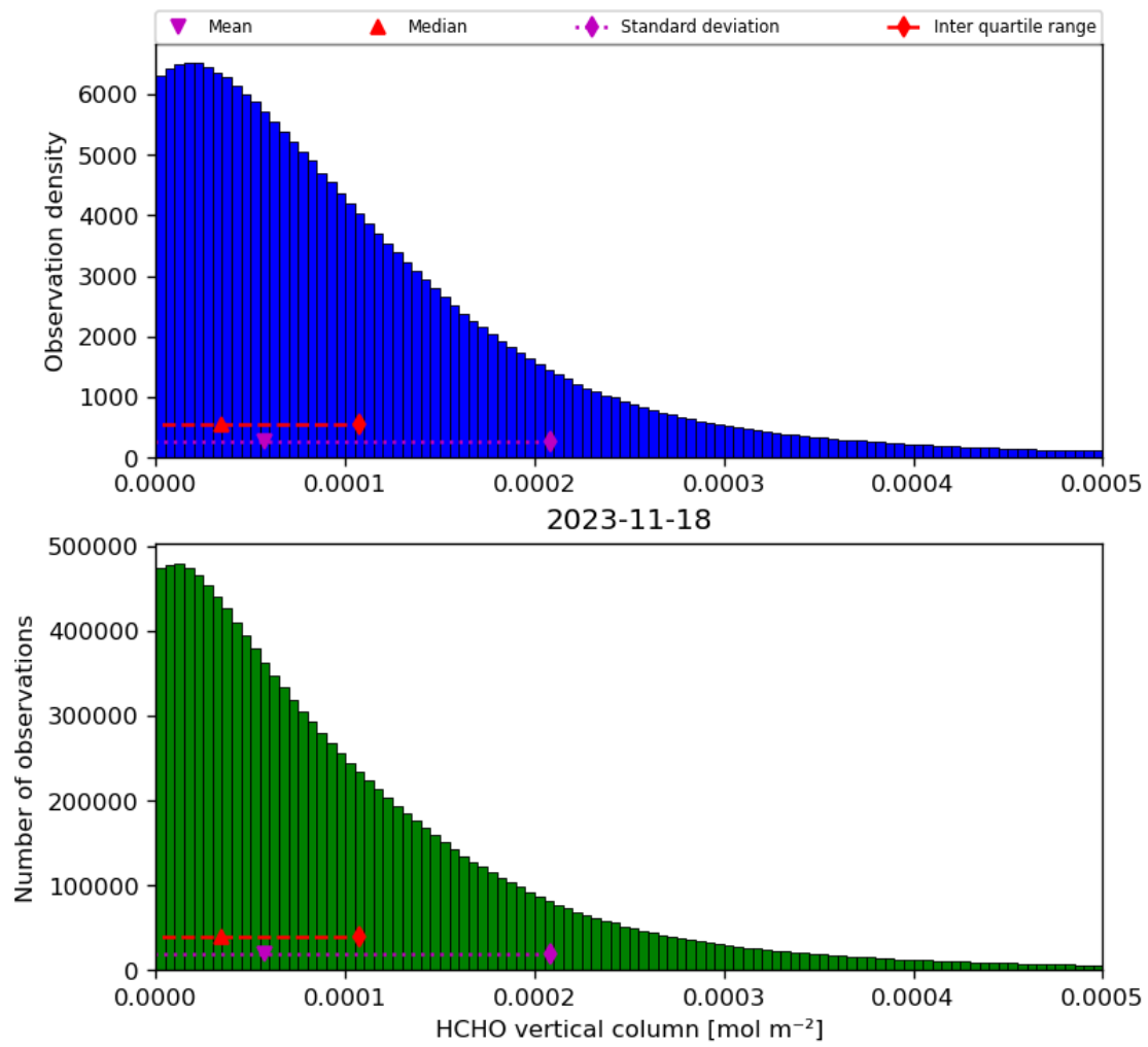
Figure 35: Histogram of “HCHO vertical column” for 2023-11-18 to 2023-11-19
