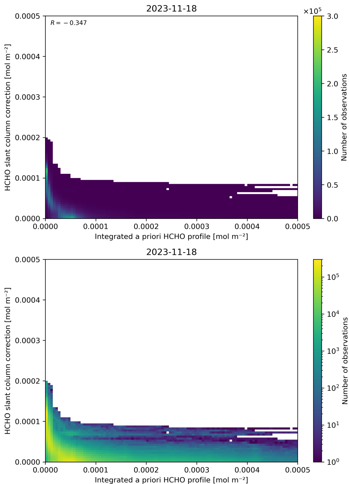
Figure 152: Scatter density plot of “Integrated a priori HCHO profile” against “HCHO slant column correction” for 2023-11-18 to 2023-11-19.
