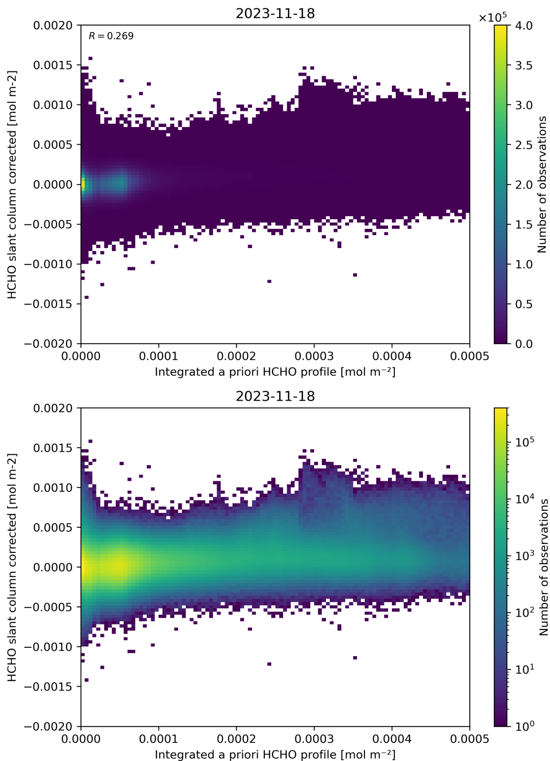
Figure 151: Scatter density plot of “Integrated a priori HCHO profile” against “HCHO slant column corrected” for 2023-11-18 to 2023-11-19.
