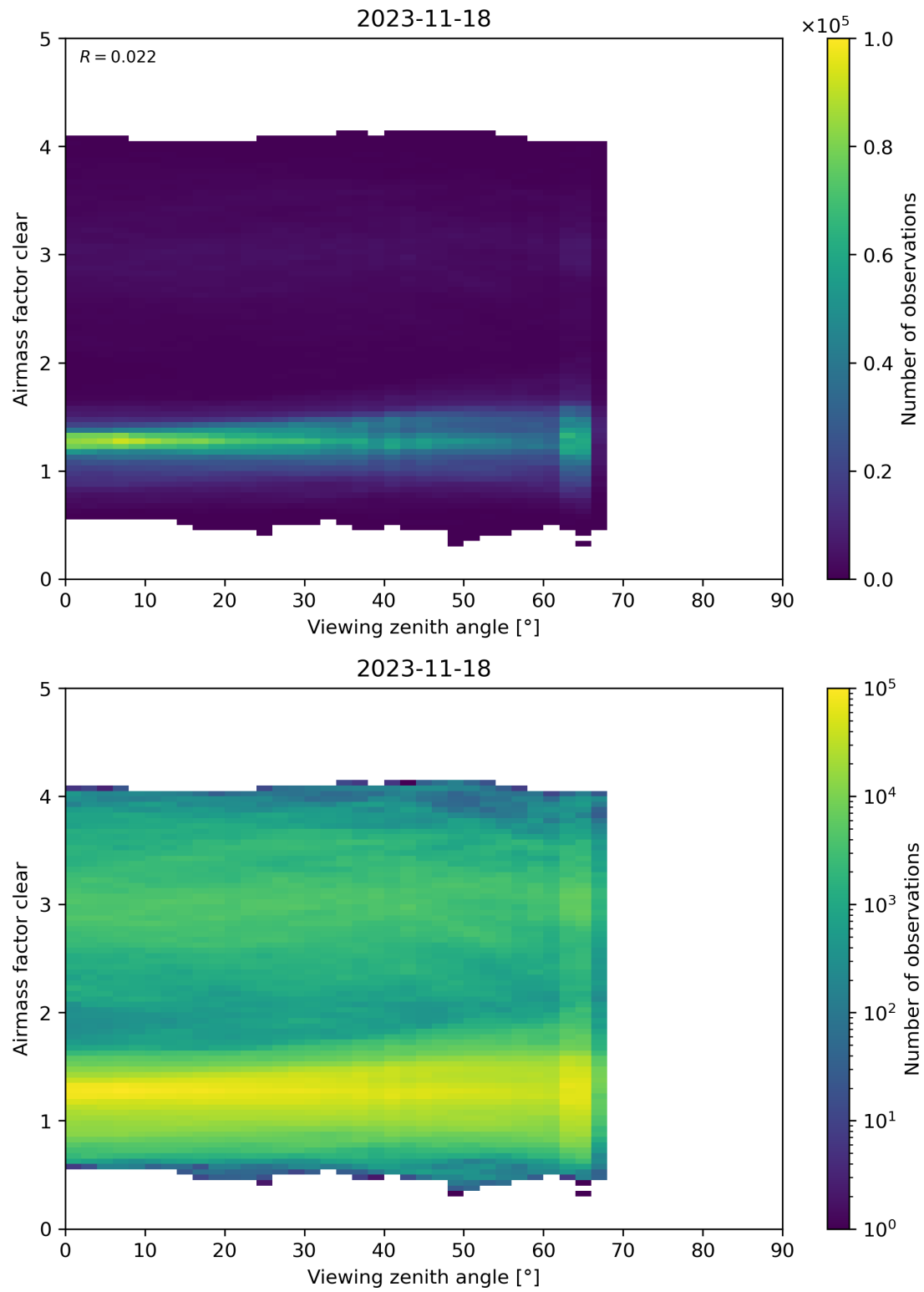
Figure 185: Scatter density plot of “Viewing zenith angle” against “Airmass factor clear” for 2023-11-18 to 2023-11-19.
