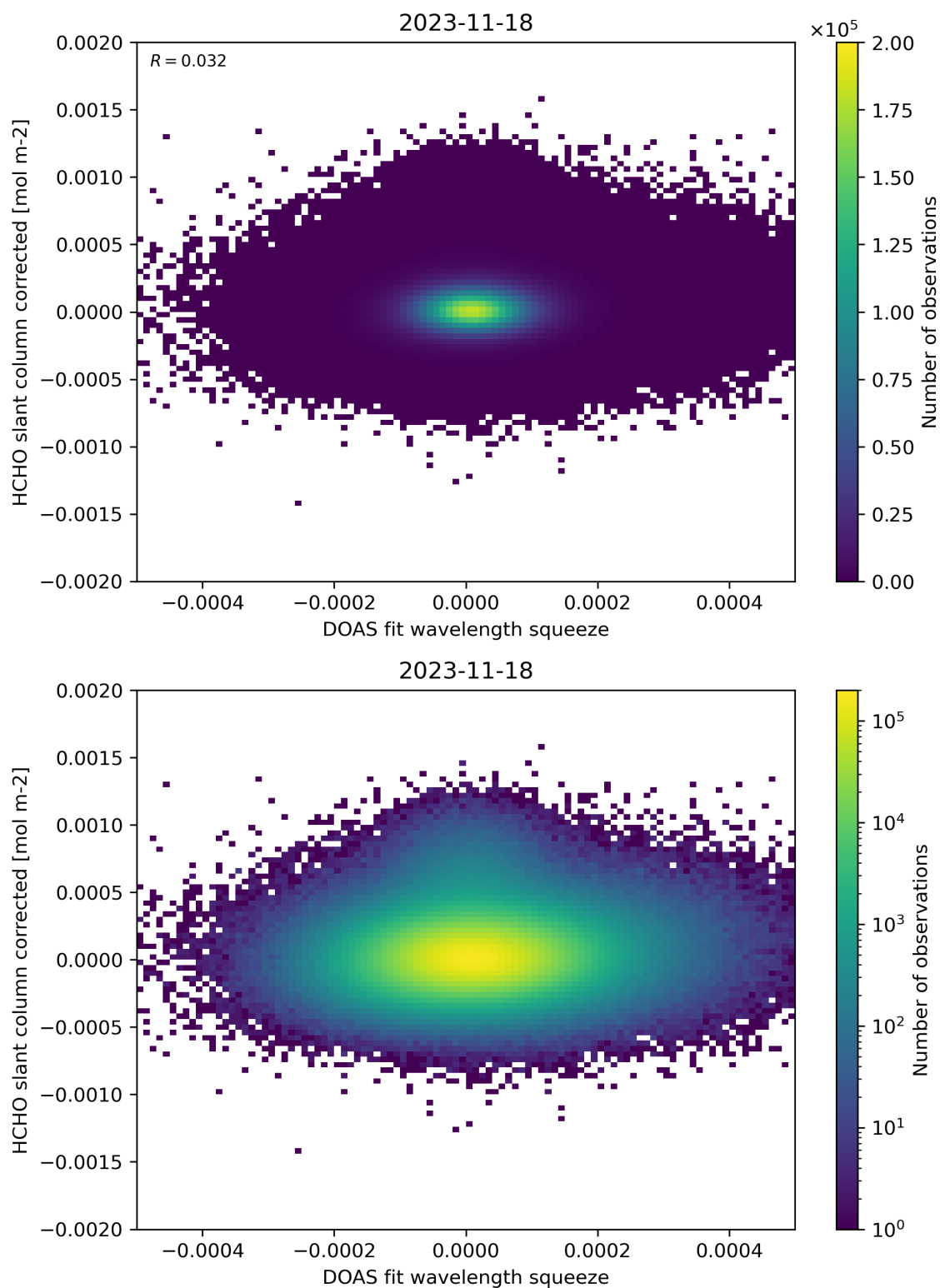
Figure 69: Scatter density plot of “DOAS fit wavelength squeeze” against “HCHO slant column corrected” for 2023-11-18 to 2023-11-19.
