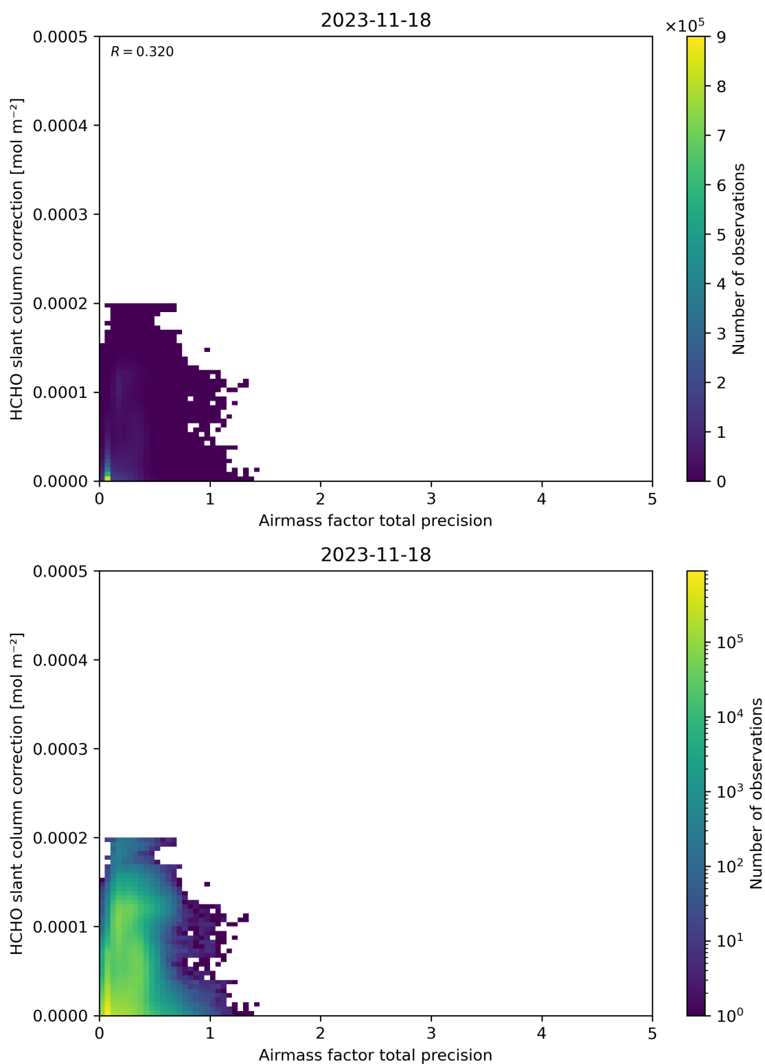
Figure 110: Scatter density plot of “Airmass factor total precision” against “HCHO slant column correction” for 2023-11-18 to 2023-11-19.
