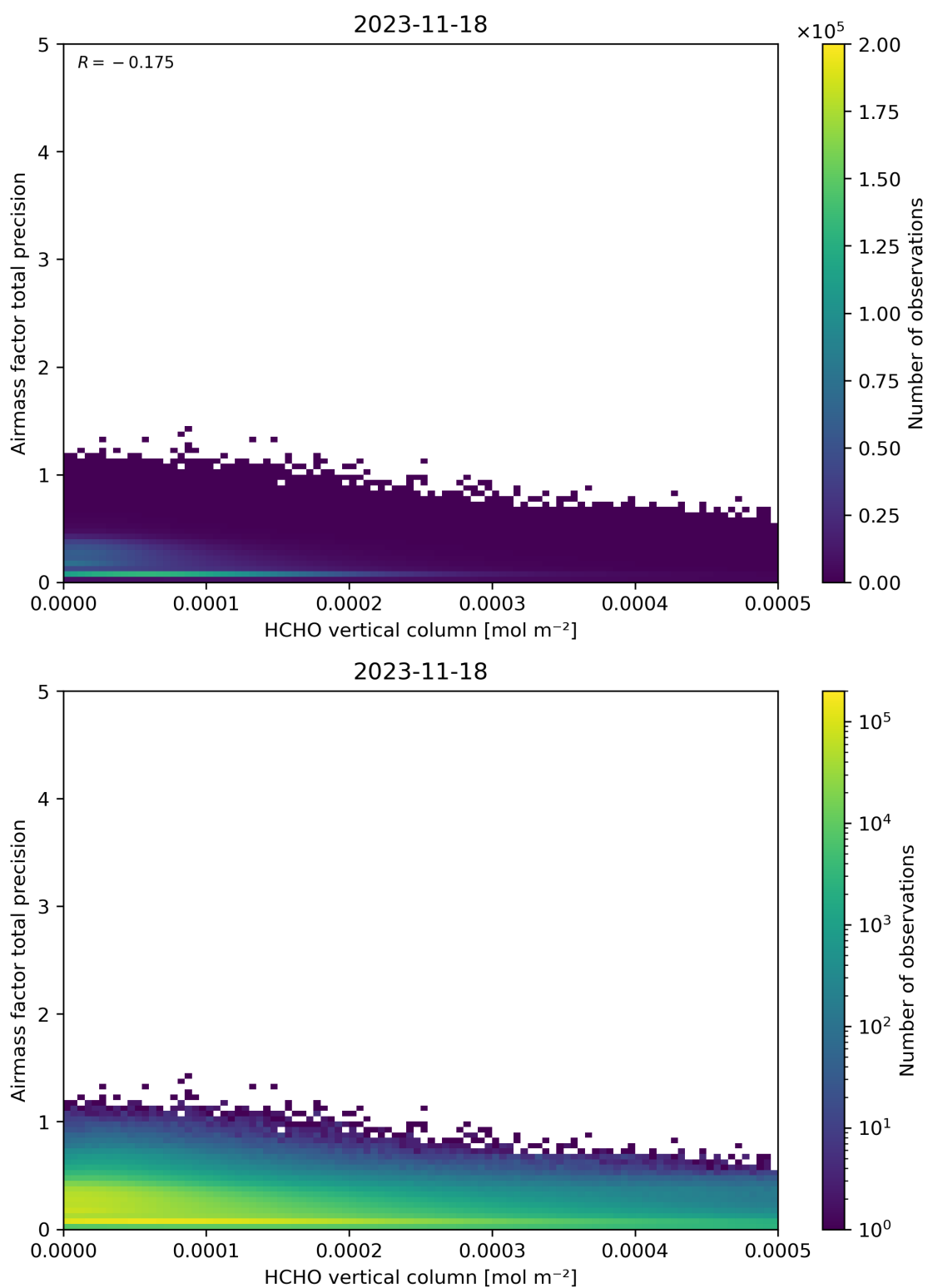
Figure 132: Scatter density plot of “HCHO vertical column” against “Airmass factor total precision” for 2023-11-18 to 2023-11-19.
