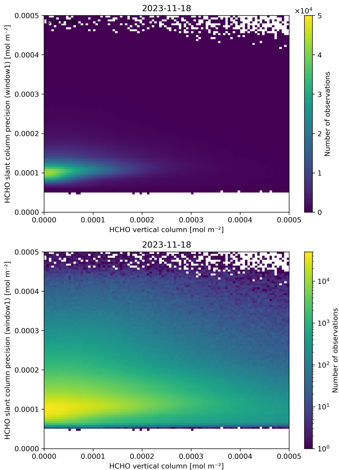
Figure 130: Scatter density plot of “HCHO vertical column” against “HCHO slant column precision (window1)” for 2023-11-18 to 2023-11-19.
