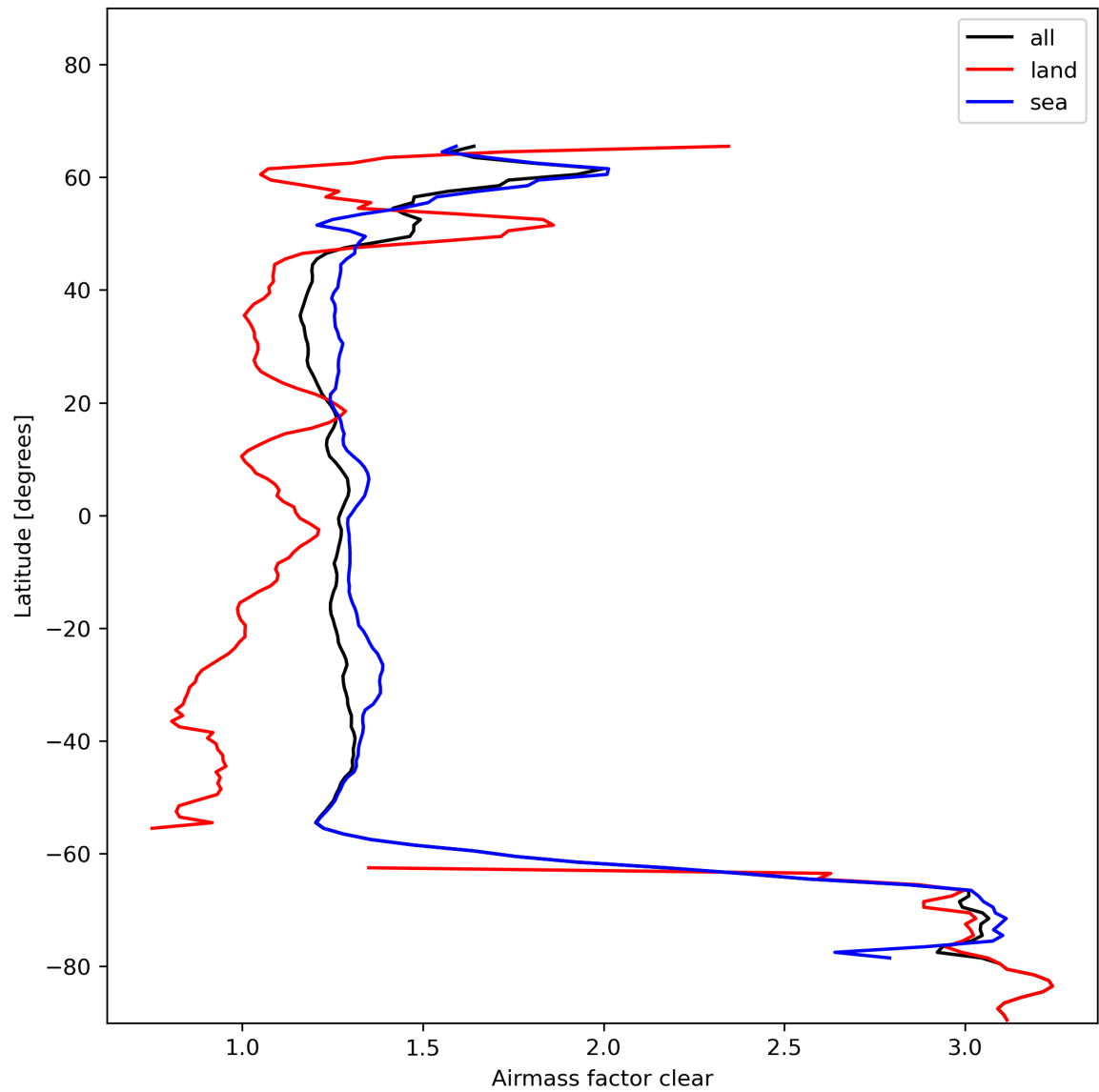
Figure 28: Zonal average of “Airmass factor clear” for 2023-11-18 to 2023-11-19.
