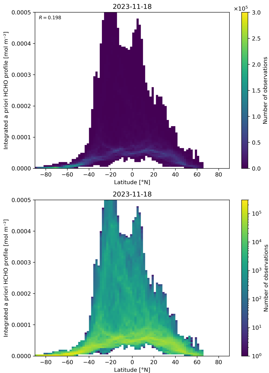
Figure 166: Scatter density plot of “Latitude” against “Integrated a priori HCHO profile” for 2023-11-18 to 2023-11-19.
