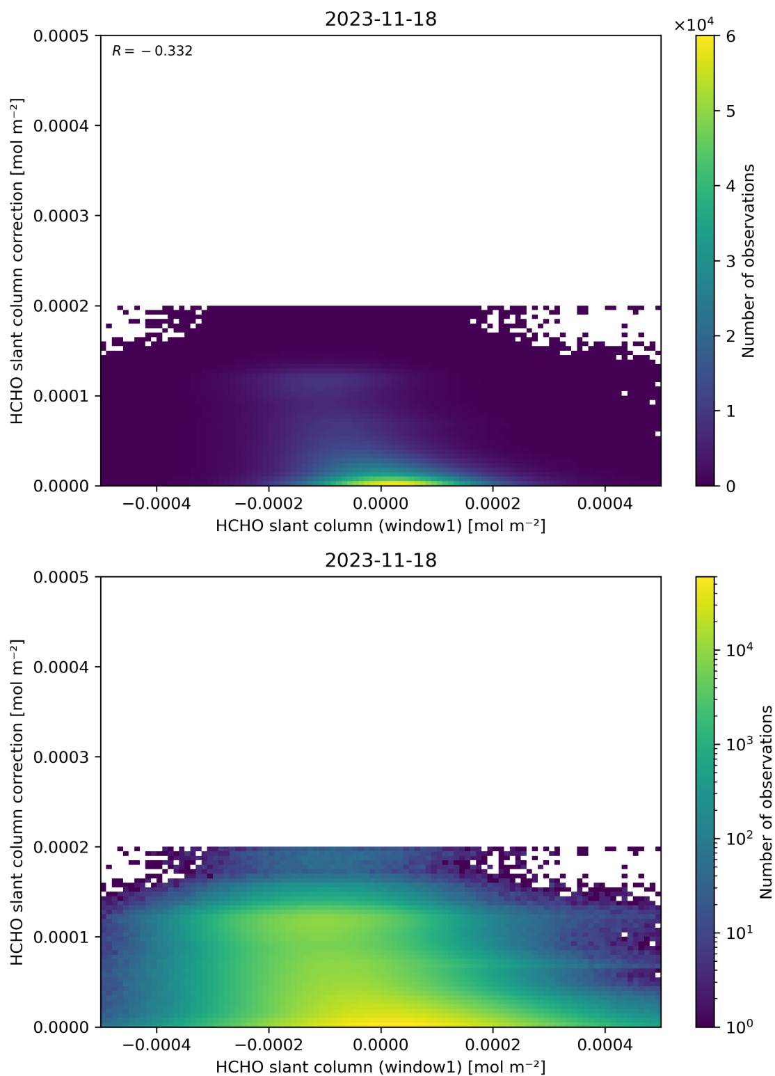
Figure 83: Scatter density plot of “HCHO slant column (window1)” against “HCHO slant column correction” for 2023-11-18 to 2023-11-19.
