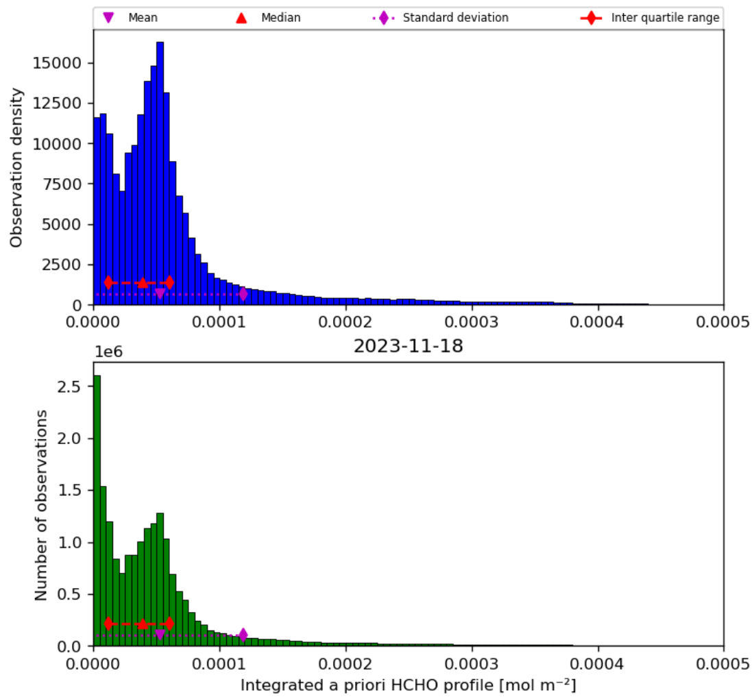
Figure 43: Histogram of “Integrated a priori HCHO profile” for 2023-11-18 to 2023-11-19
