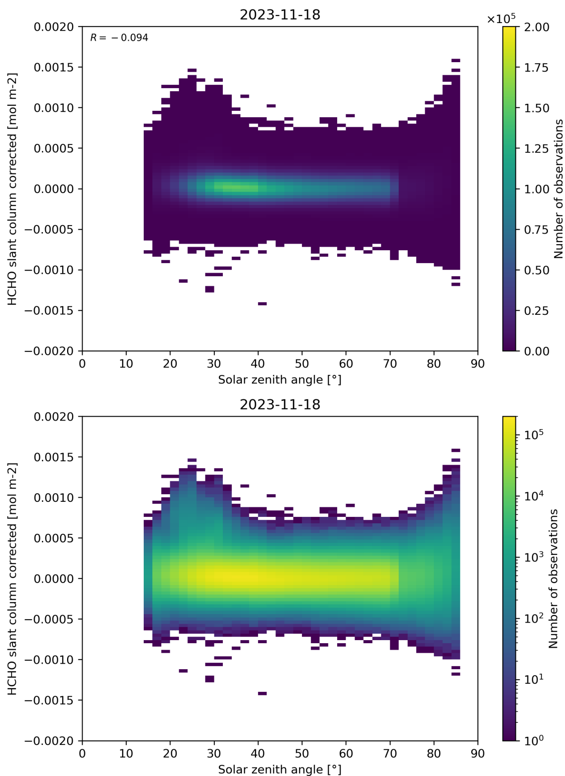
Figure 171: Scatter density plot of “Solar zenith angle” against “HCHO slant column corrected” for 2023-11-18 to 2023-11-19.
