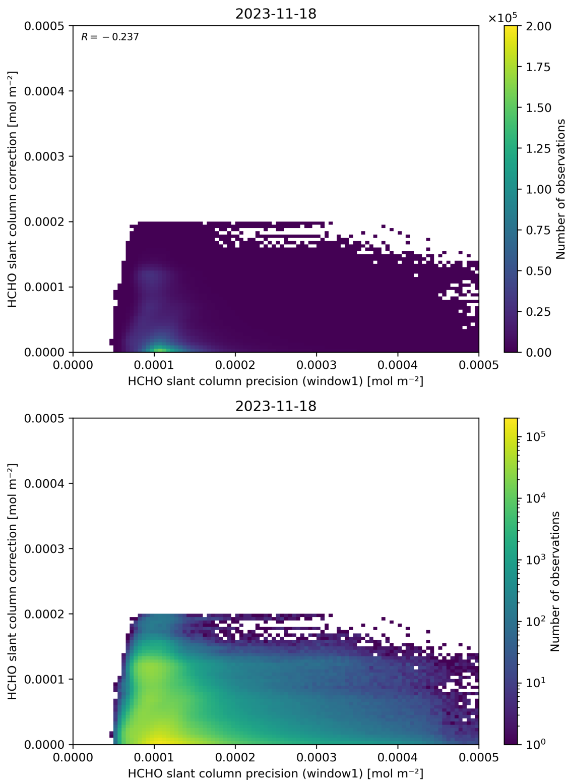
Figure 93: Scatter density plot of “HCHO slant column precision (window1)” against “HCHO slant column correction” for 2023-11-18 to 2023-11-19.
