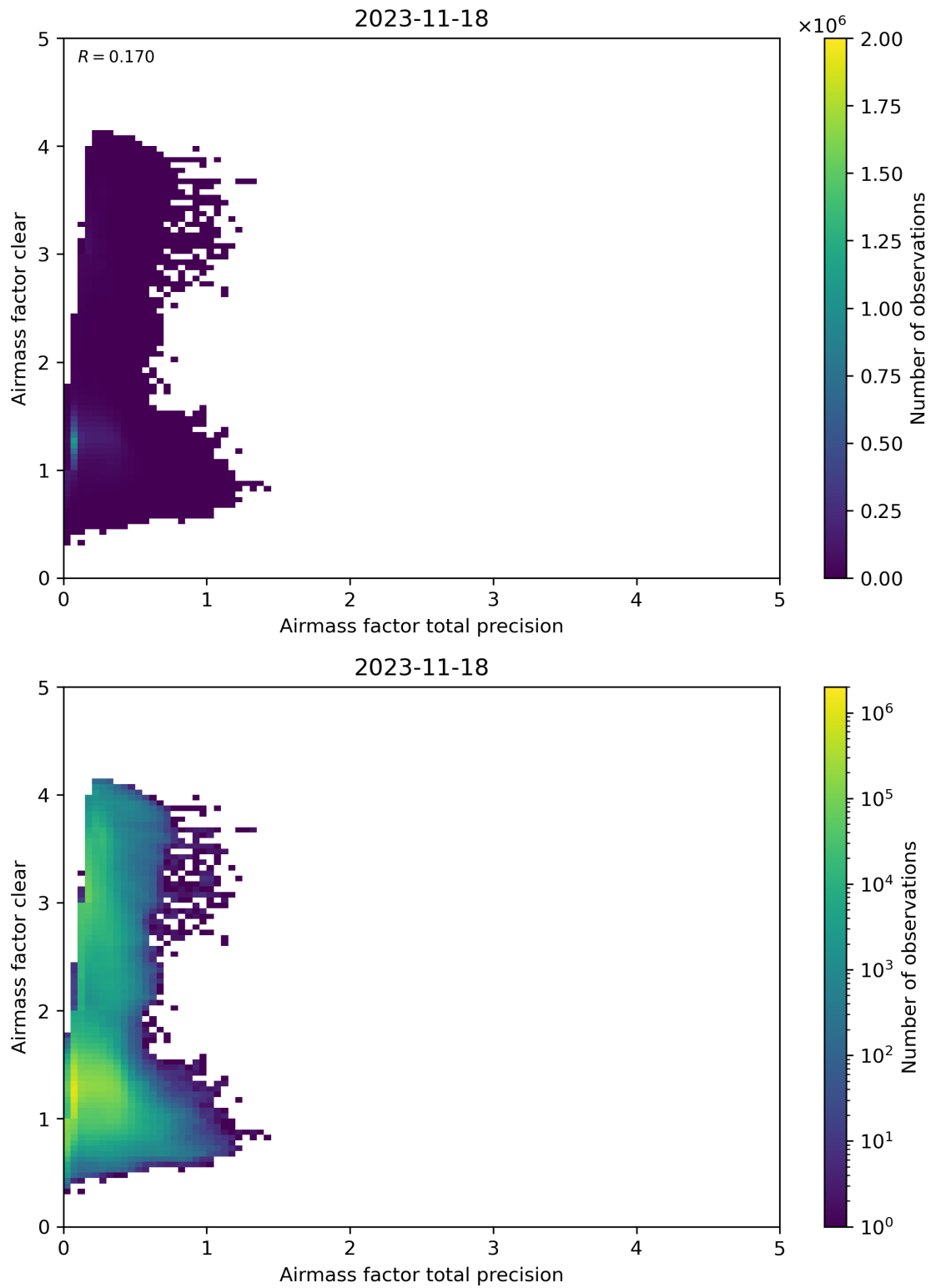
Figure 108: Scatter density plot of “Airmass factor total precision” against “Airmass factor clear” for 2023-11-18 to 2023-11-19.
