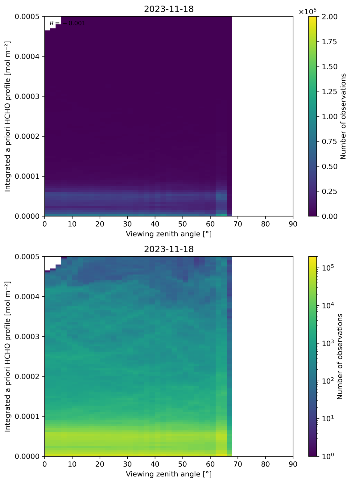
Figure 195: Scatter density plot of “Viewing zenith angle” against “Integrated a priori HCHO profile” for 2023-11-18 to 2023-11-19.
