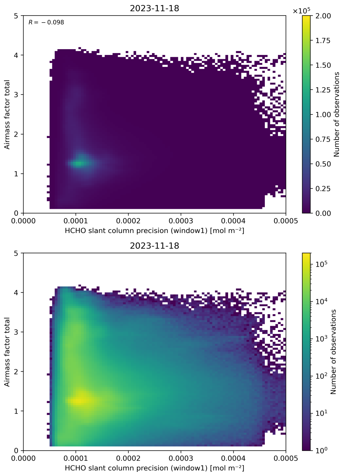
Figure 94: Scatter density plot of “HCHO slant column precision (window1)” against “Airmass factor total” for 2023-11-18 to 2023-11-19.
