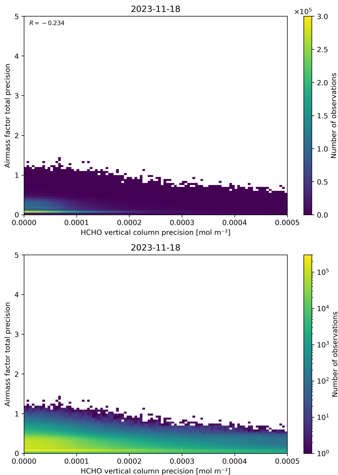
Figure 145: Scatter density plot of “HCHO vertical column precision” against “Airmass factor total precision” for 2023-11-18 to 2023-11-19.
