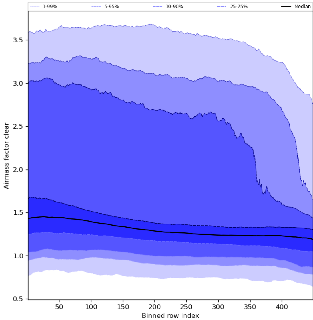
Figure 56: Along track statistics of “Airmass factor clear” for 2023-11-18 to 2023-11-19
