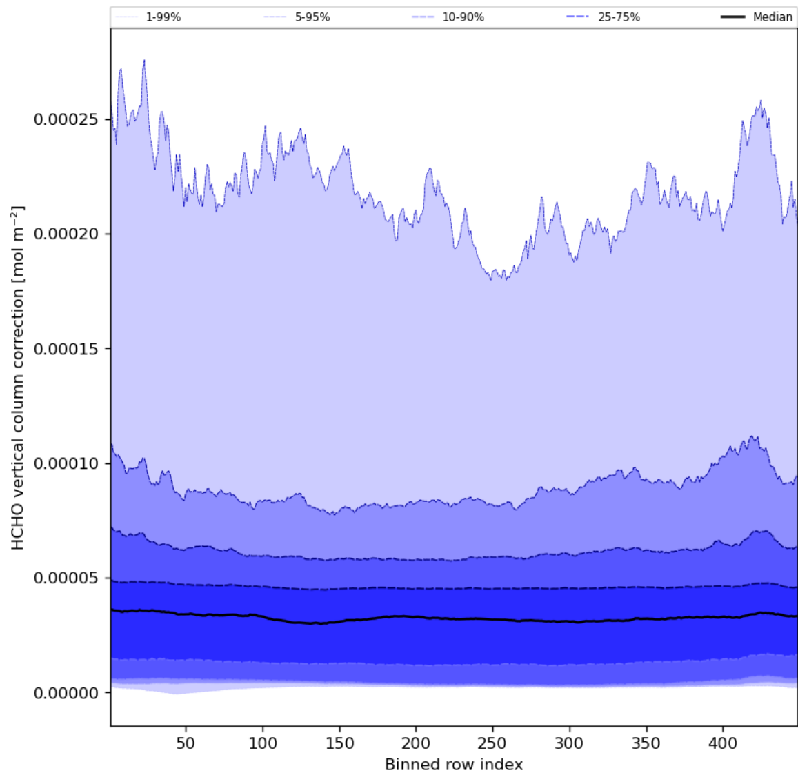
Figure 51: Along track statistics of “HCHO vertical column correction” for 2023-11-18 to 2023-11-19
