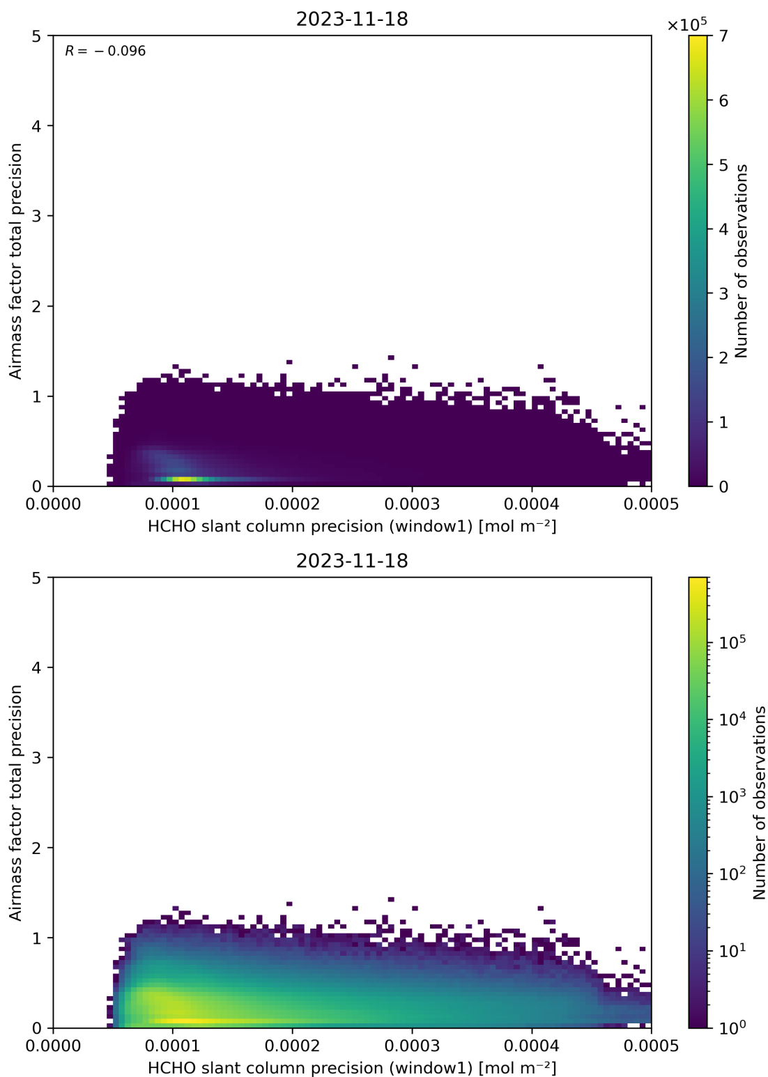
Figure 95: Scatter density plot of “HCHO slant column precision (window1)” against “Airmass factor total precision” for 2023-11-18 to 2023-11-19.
