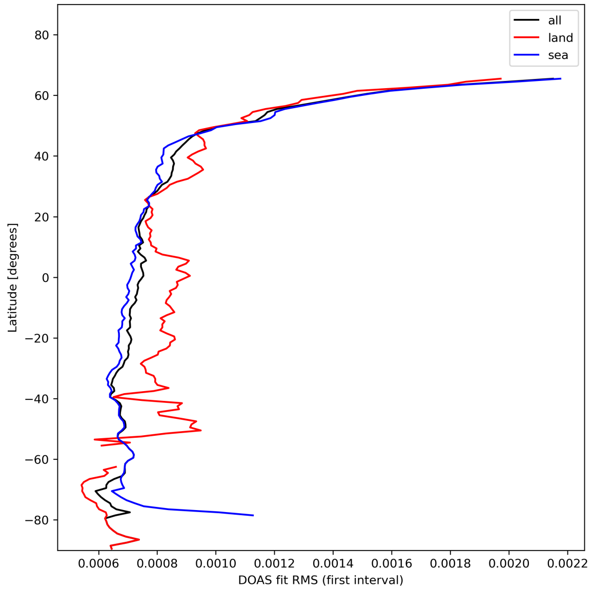
Figure 32: Zonal average of “DOAS fit RMS (first interval)” for 2023-11-18 to 2023-11-19.
