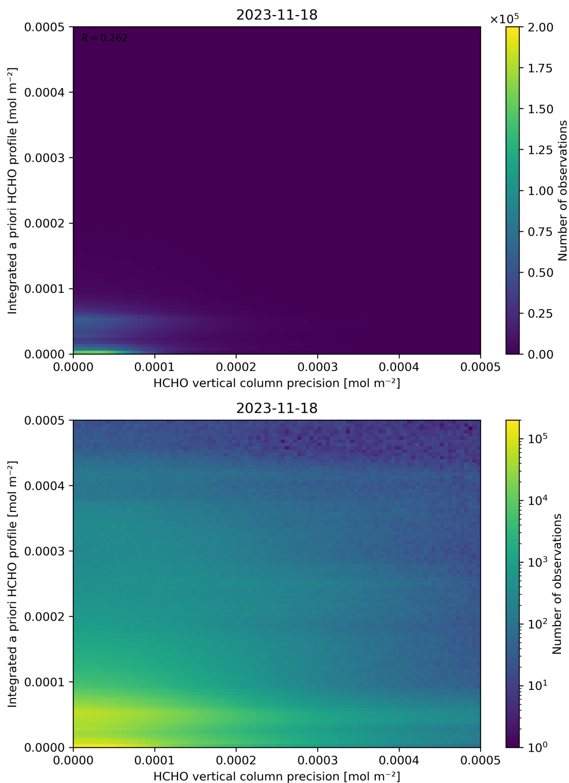
Figure 147: Scatter density plot of “HCHO vertical column precision” against “Integrated a priori HCHO profile” for 2023-11-18 to 2023-11-19.
