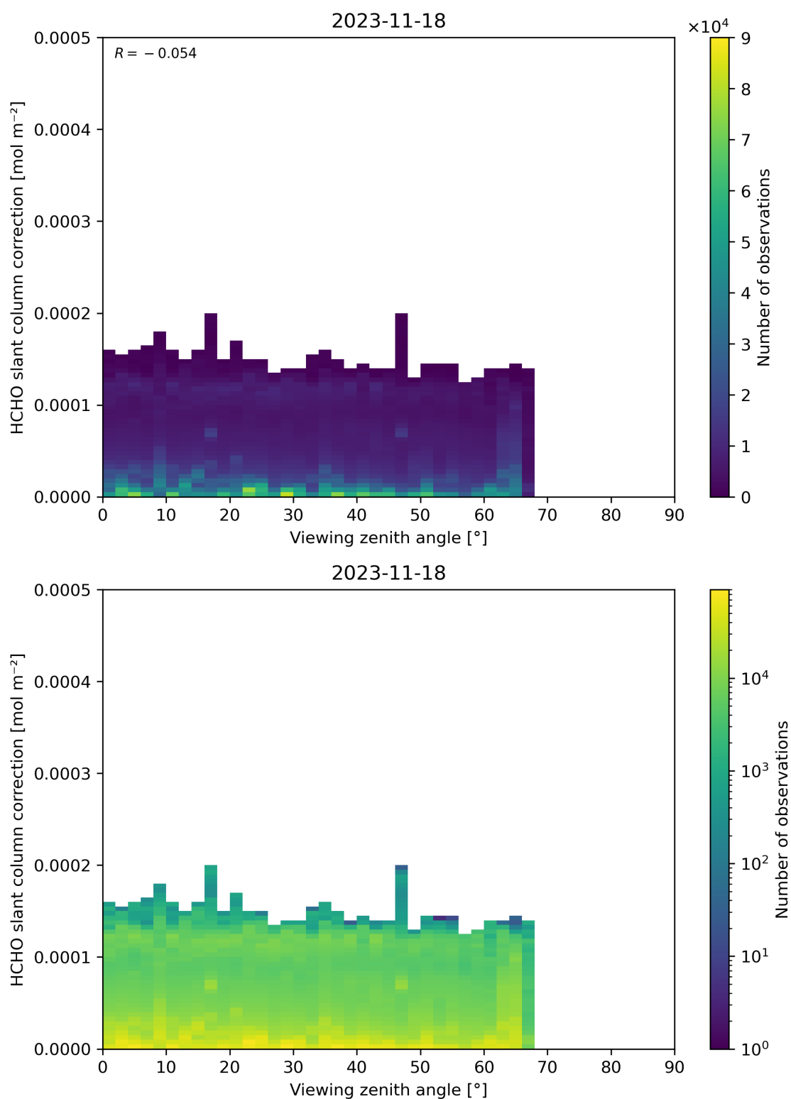
Figure 187: Scatter density plot of “Viewing zenith angle” against “HCHO slant column correction” for 2023-11-18 to 2023-11-19.
