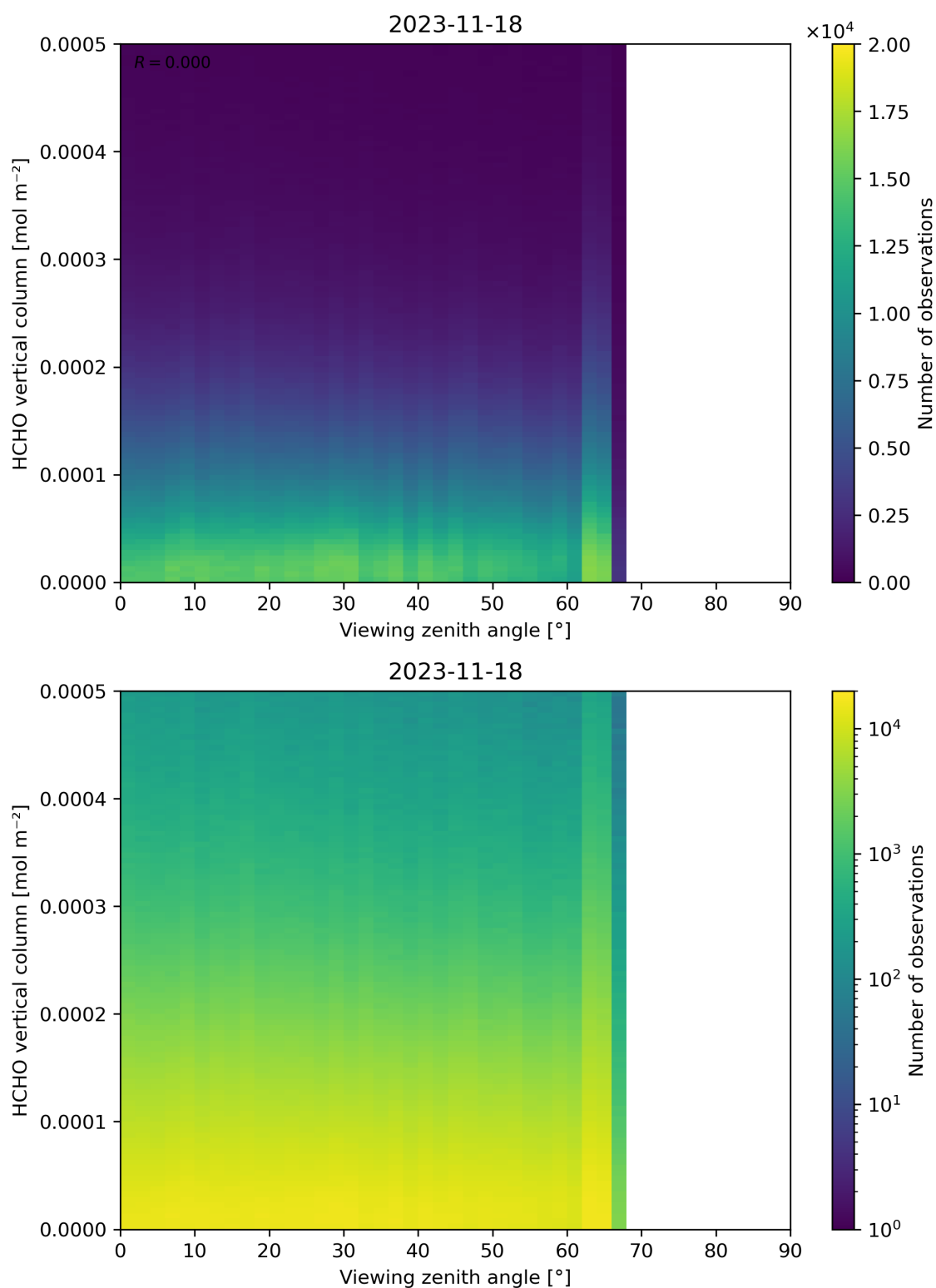
Figure 192: Scatter density plot of “Viewing zenith angle” against “HCHO vertical column” for 2023-11-18 to 2023-11-19.
