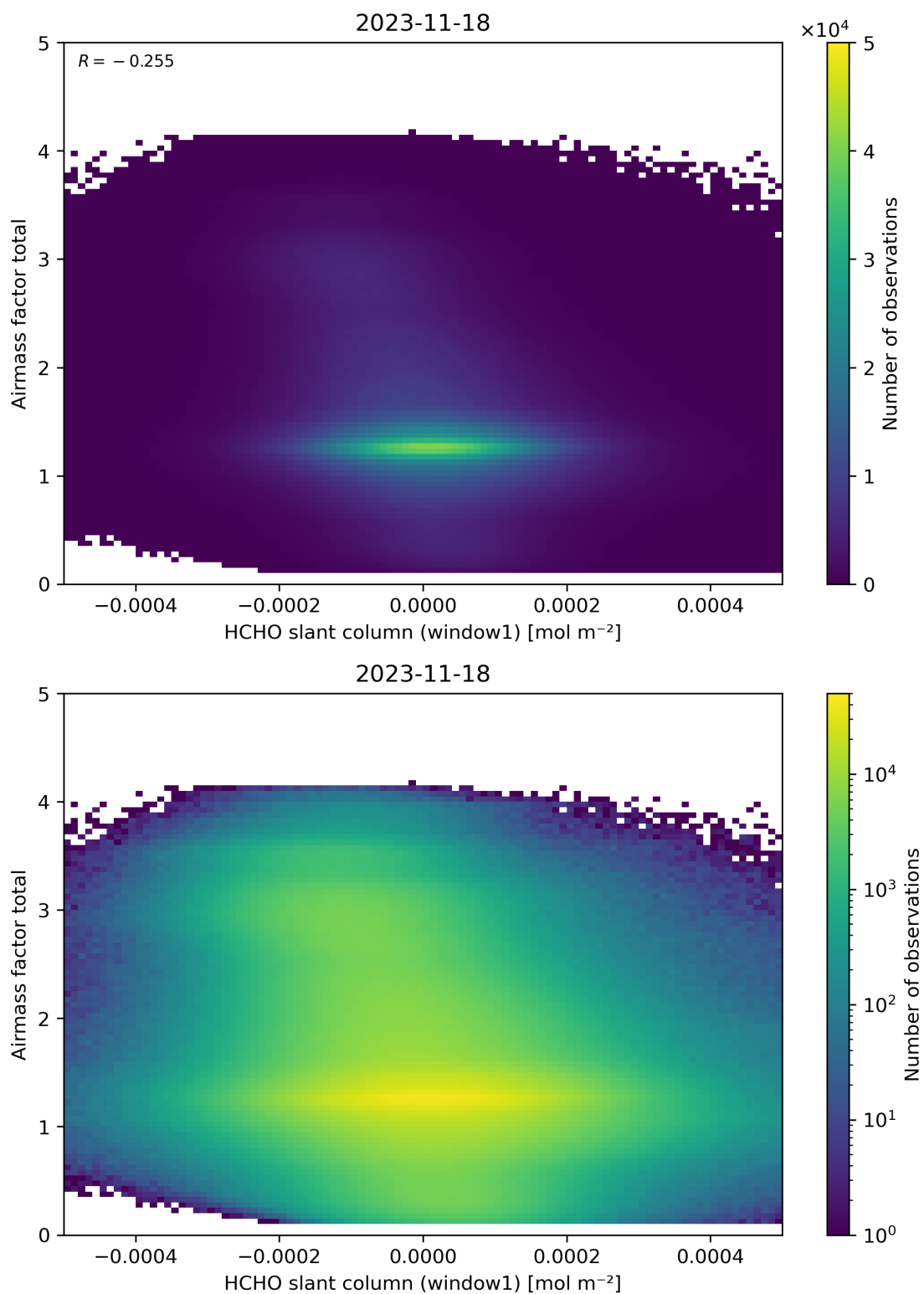
Figure 85: Scatter density plot of “HCHO slant column (window1)” against “Airmass factor total” for 2023-11-18 to 2023-11-19.
