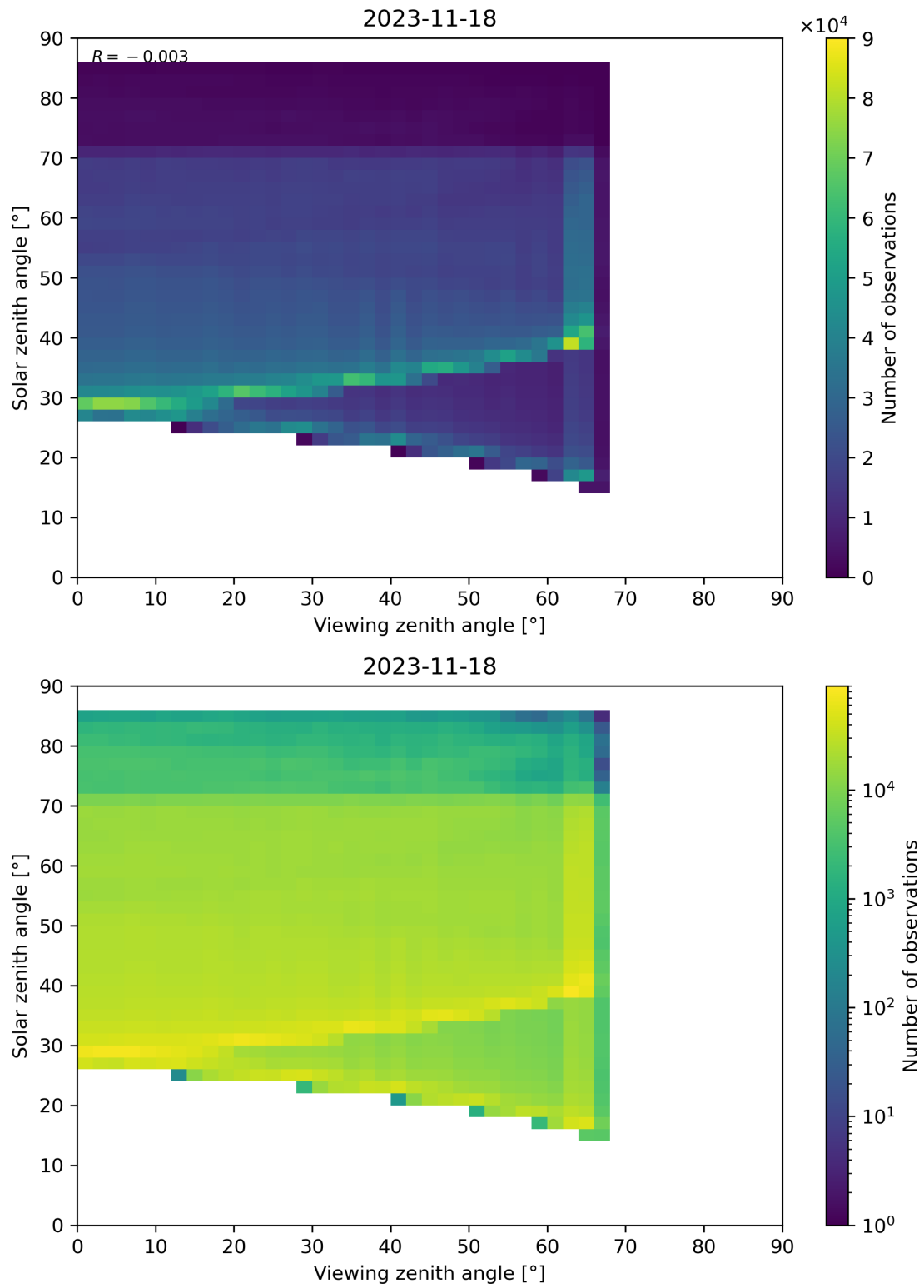
Figure 197: Scatter density plot of “Viewing zenith angle” against “Solar zenith angle” for 2023-11-18 to 2023-11-19.
