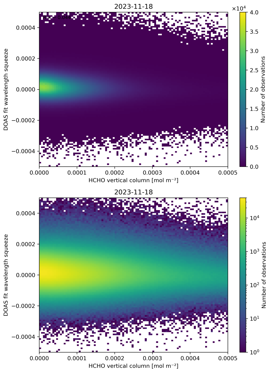
Figure 125: Scatter density plot of “HCHO vertical column” against “DOAS fit wavelength squeeze” for 2023-11-18 to 2023-11-19.
