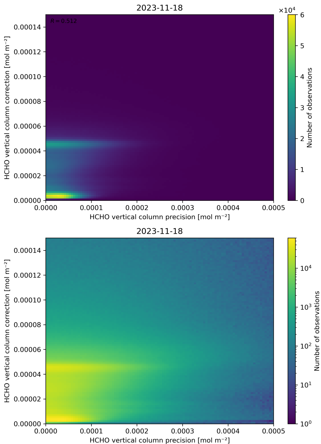
Figure 146: Scatter density plot of “HCHO vertical column precision” against “HCHO vertical column correction” for 2023-11-18 to 2023-11-19.
