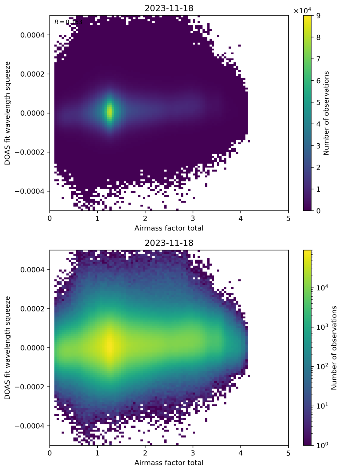
Figure 99: Scatter density plot of “Airmass factor total” against “DOAS fit wavelength squeeze” for 2023-11-18 to 2023-11-19.
