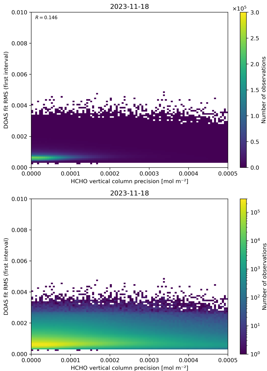
Figure 136: Scatter density plot of “HCHO vertical column precision” against “DOAS fit RMS (first interval)” for 2023-11-18 to 2023-11-19.
