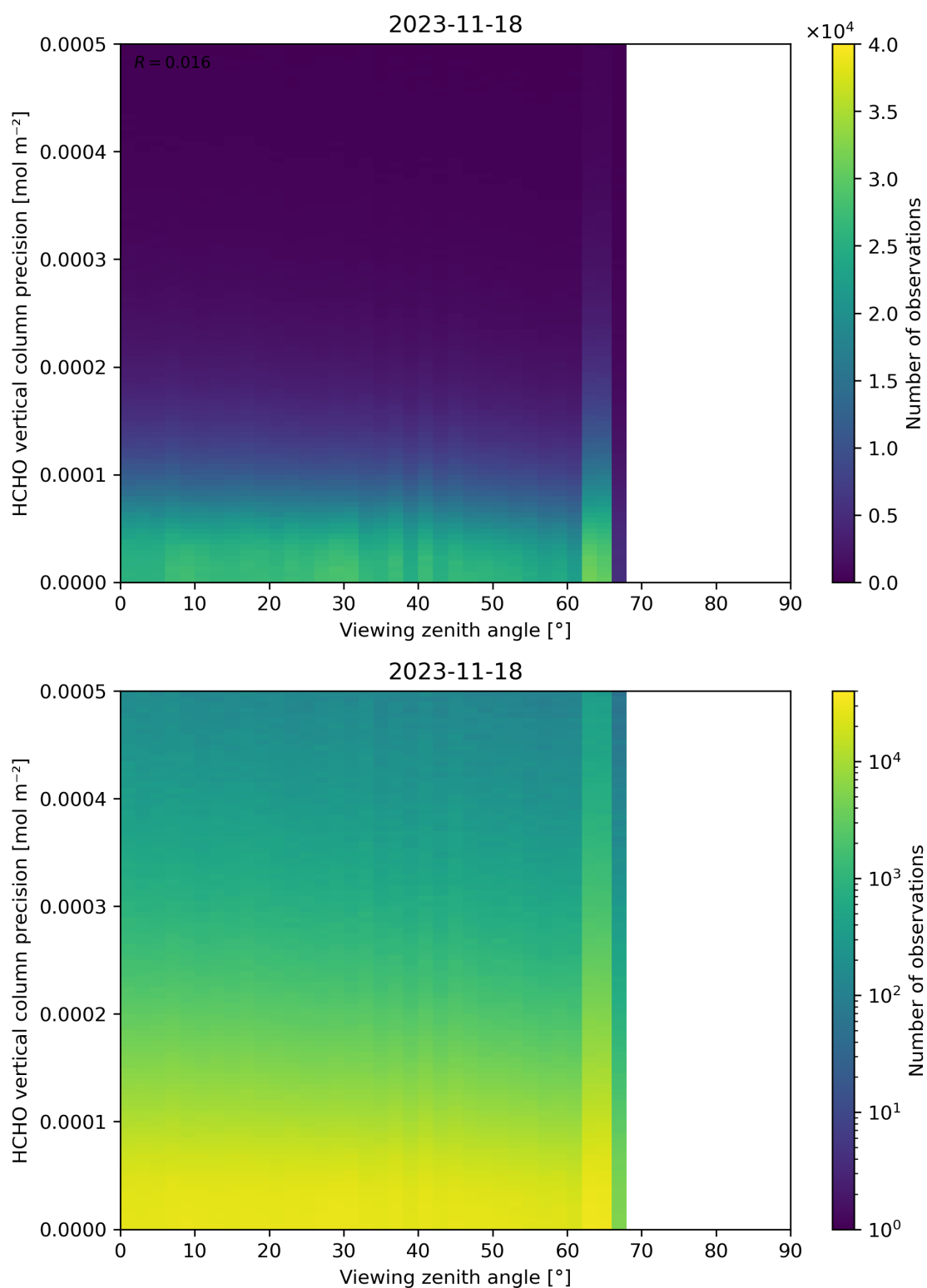
Figure 194: Scatter density plot of “Viewing zenith angle” against “HCHO vertical column precision” for 2023-11-18 to 2023-11-19.
