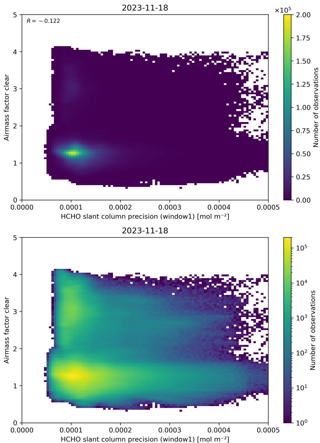
Figure 91: Scatter density plot of “HCHO slant column precision (window1)” against “Airmass factor clear” for 2023-11-18 to 2023-11-19.
