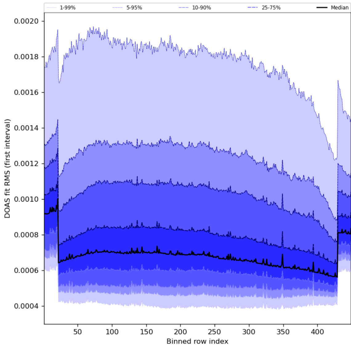
Figure 60: Along track statistics of “DOAS fit RMS (first interval)” for 2023-11-18 to 2023-11-19
