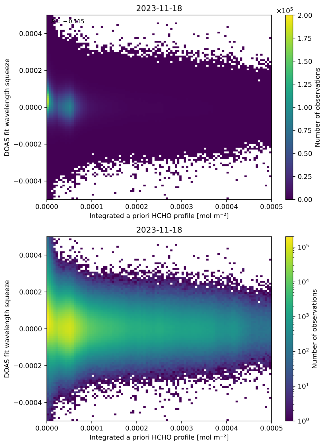
Figure 150: Scatter density plot of “Integrated a priori HCHO profile” against “DOAS fit wavelength squeeze” for 2023-11-18 to 2023-11-19.
