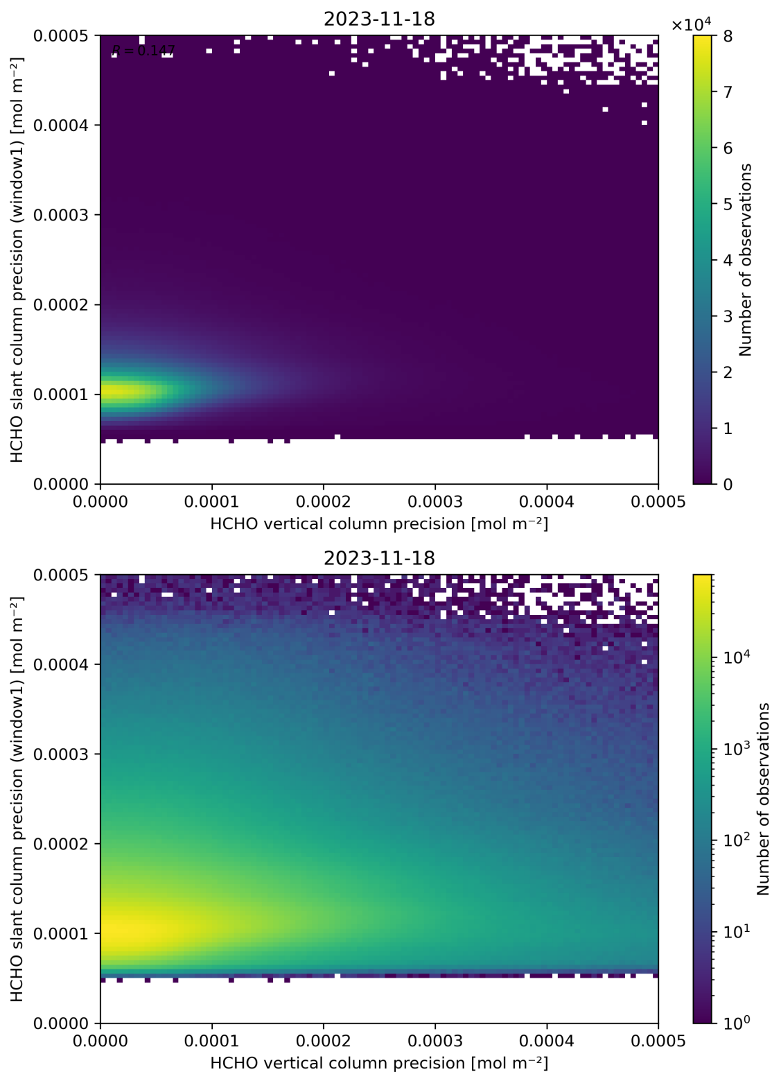
Figure 143: Scatter density plot of “HCHO vertical column precision” against “HCHO slant column precision (window1)” for 2023-11-18 to 2023-11-19.
