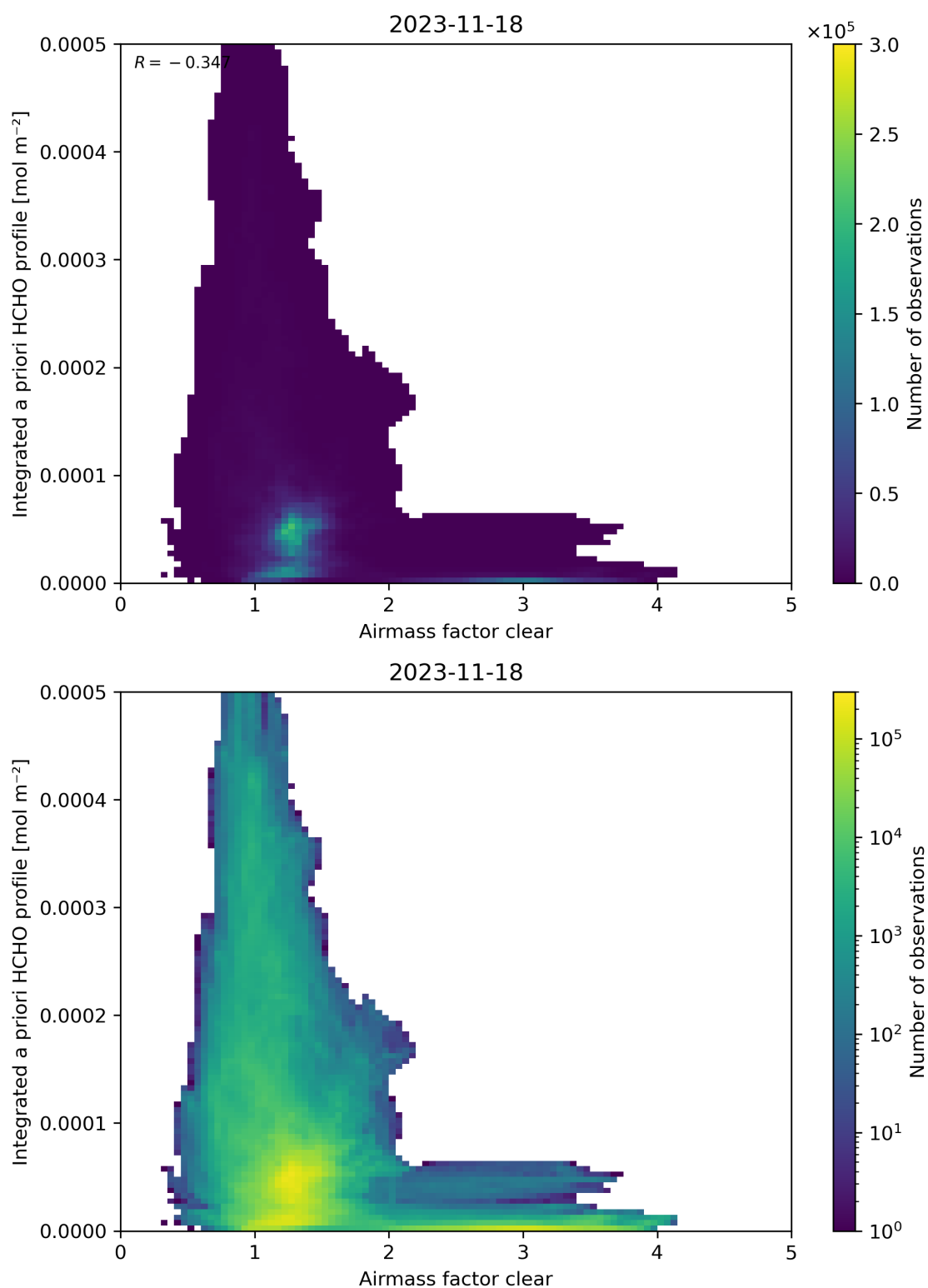
Figure 76: Scatter density plot of “Airmass factor clear” against “Integrated a priori HCHO profile” for 2023-11-18 to 2023-11-19.
