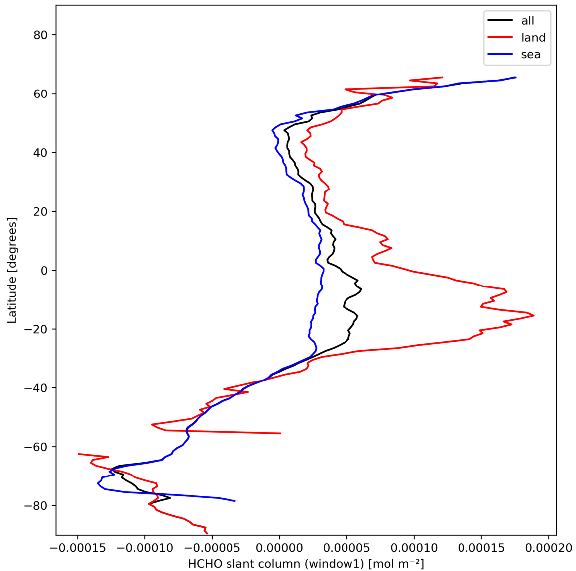
Figure 24: Zonal average of “HCHO slant column (window1)” for 2023-11-18 to 2023-11-19.
