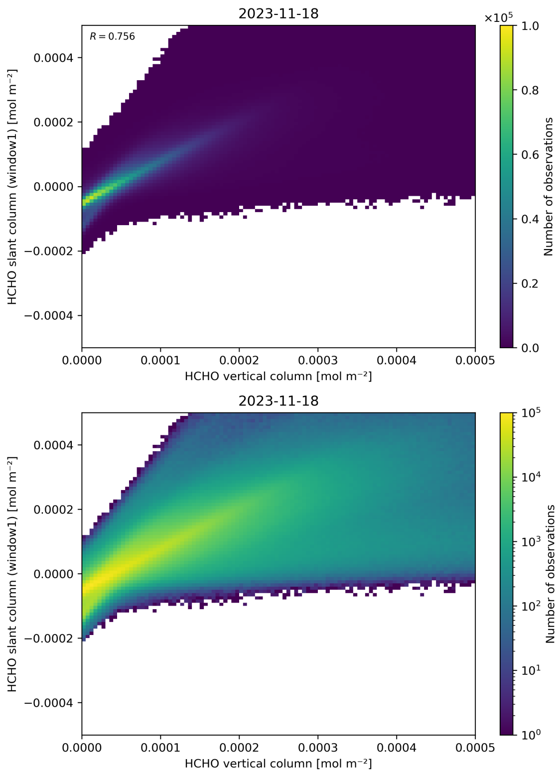
Figure 129: Scatter density plot of “HCHO vertical column” against “HCHO slant column (window1)” for 2023-11-18 to 2023-11-19.
