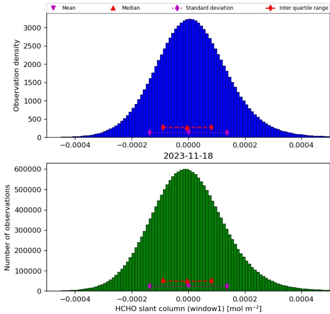
Figure 38: Histogram of “HCHO slant column (window1)” for 2023-11-18 to 2023-11-19
