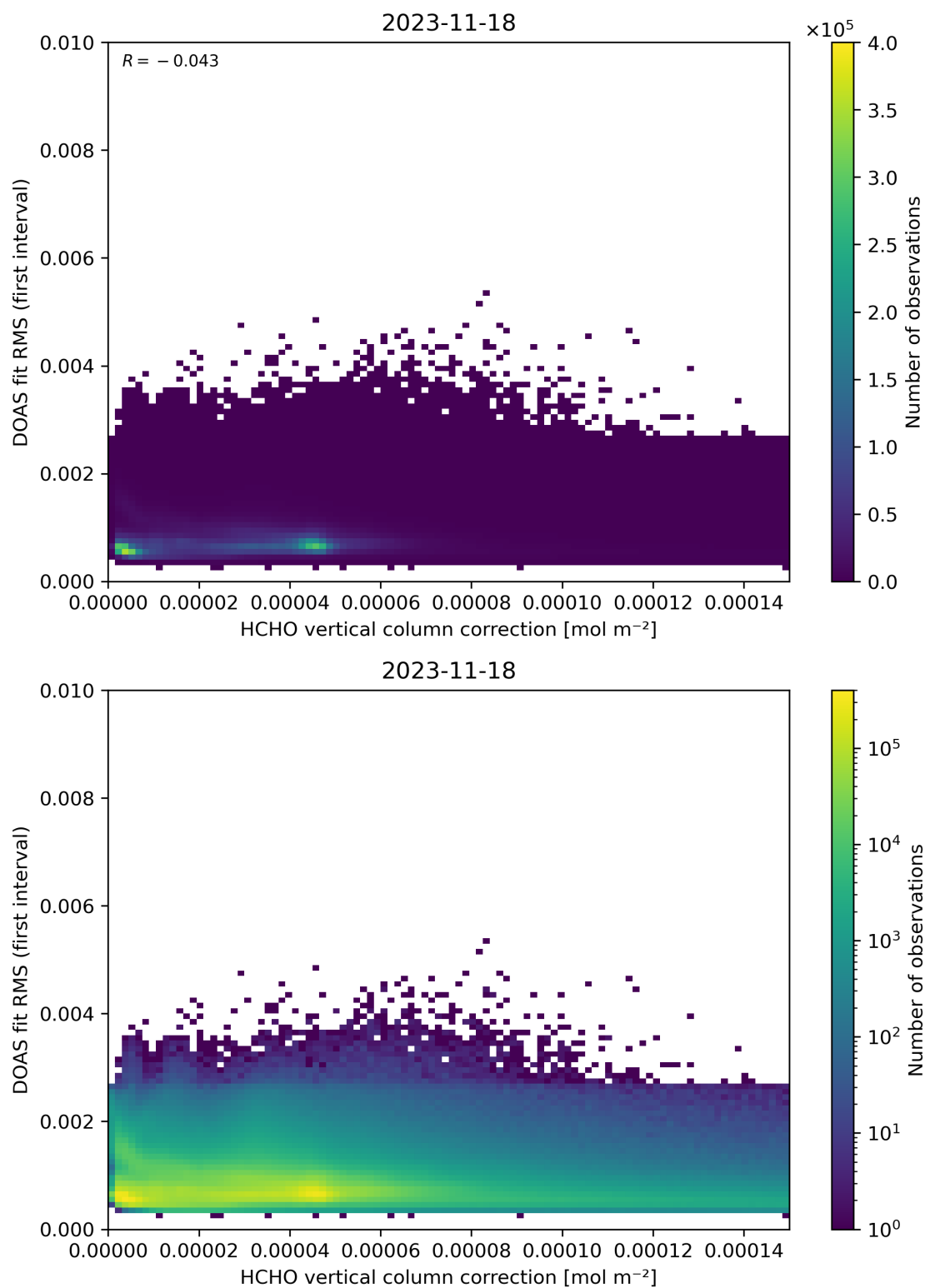
Figure 112: Scatter density plot of “HCHO vertical column correction” against “DOAS fit RMS (first interval)” for 2023-11-18 to 2023-11-19.
