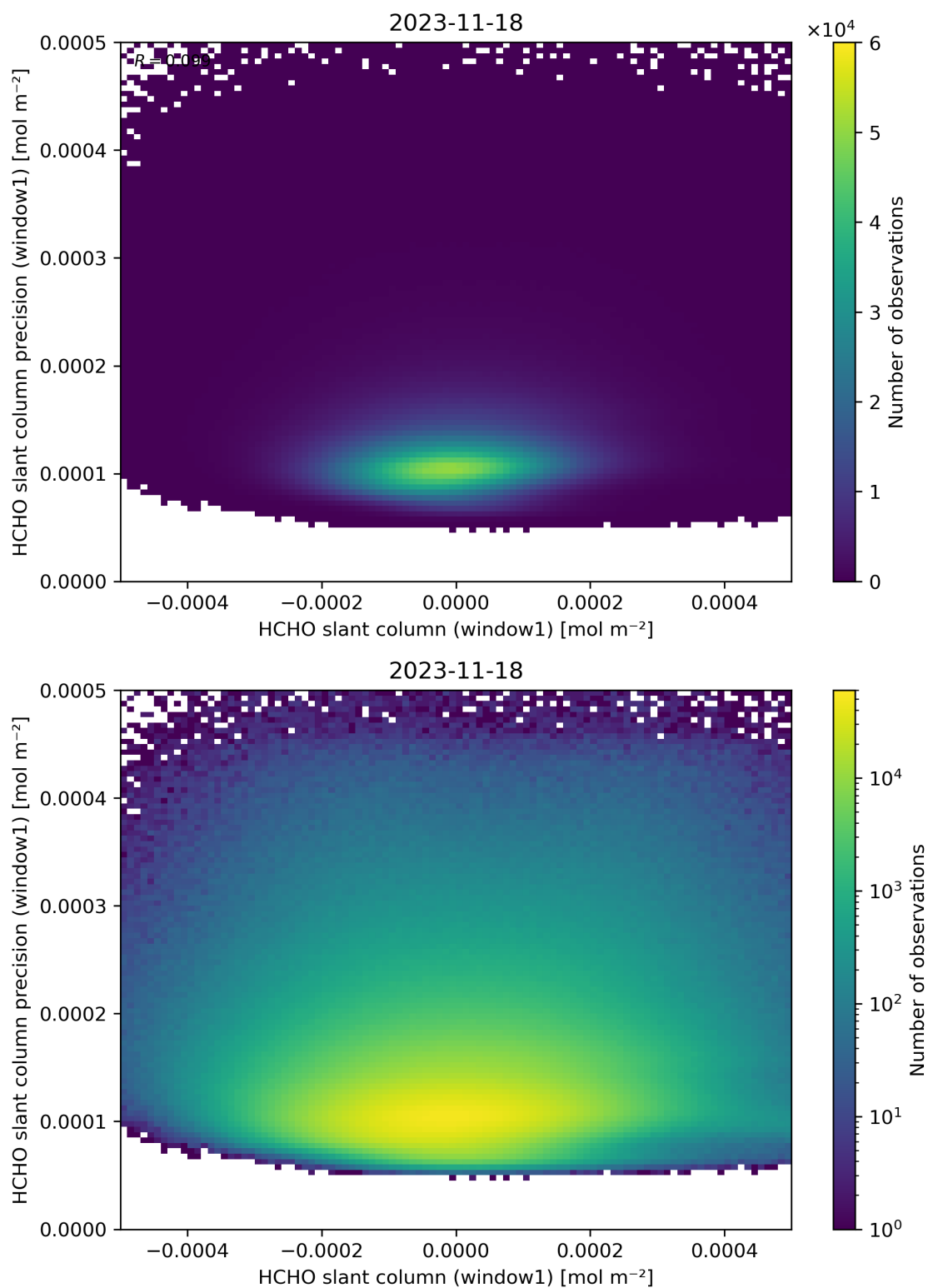
Figure 84: Scatter density plot of “HCHO slant column (window1)” against “HCHO slant column precision (window1)” for 2023-11-18 to 2023-11-19.
