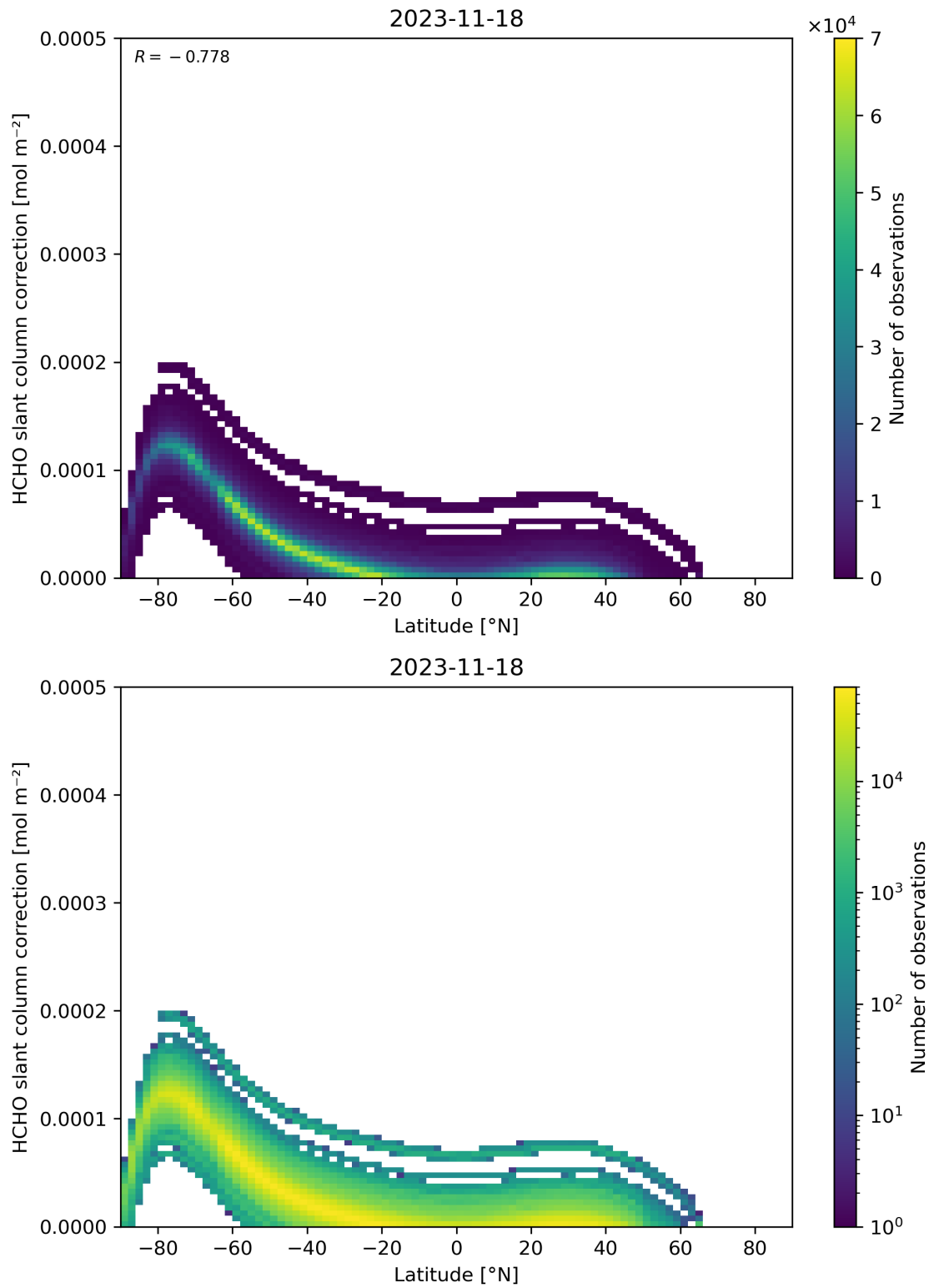
Figure 158: Scatter density plot of “Latitude” against “HCHO slant column correction” for 2023-11-18 to 2023-11-19.
