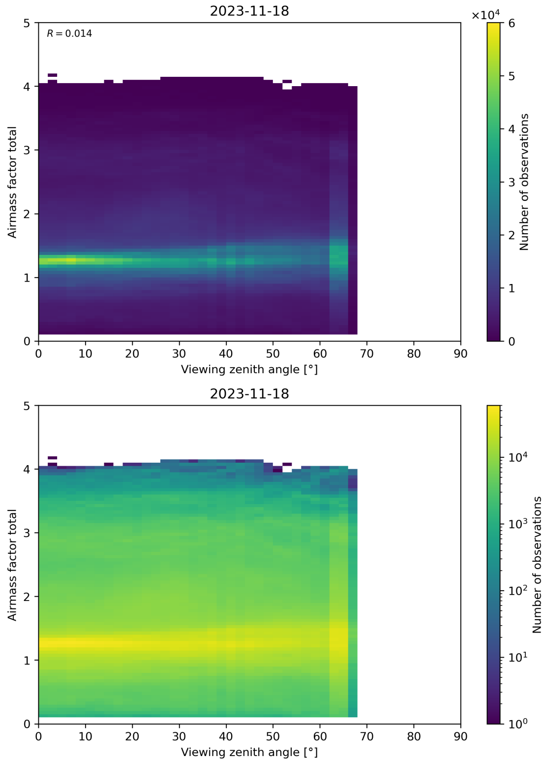
Figure 190: Scatter density plot of “Viewing zenith angle” against “Airmass factor total” for 2023-11-18 to 2023-11-19.
