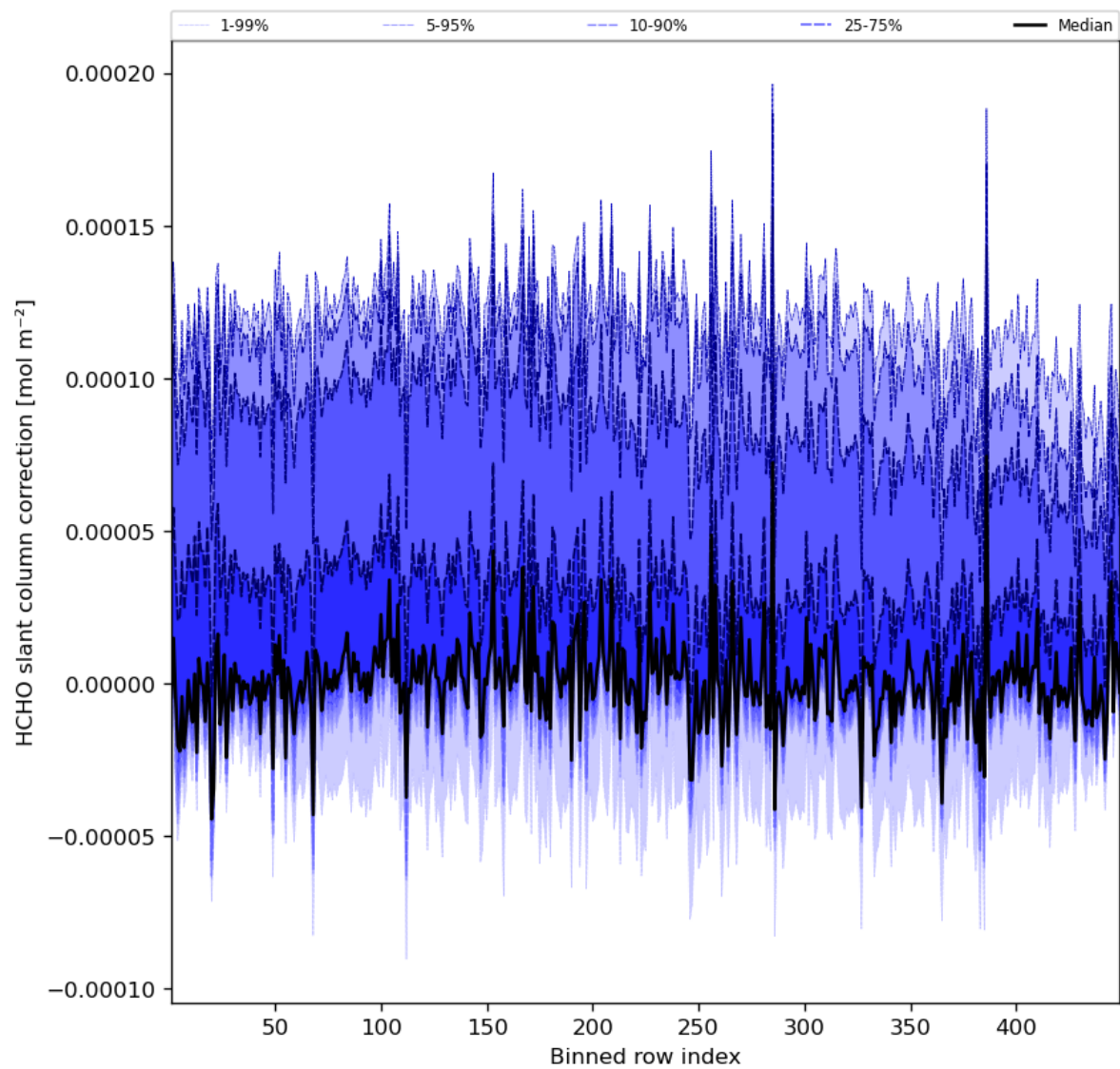
Figure 61: Along track statistics of “HCHO slant column correction” for 2023-11-18 to 2023-11-19
