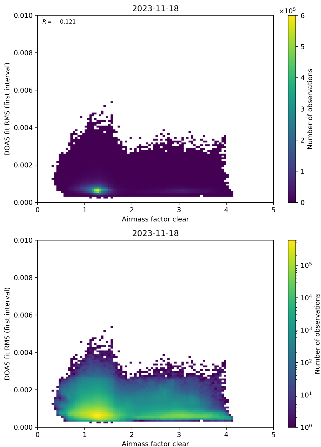
Figure 71: Scatter density plot of “Airmass factor clear” against “DOAS fit RMS (first interval)” for 2023-11-18 to 2023-11-19.
