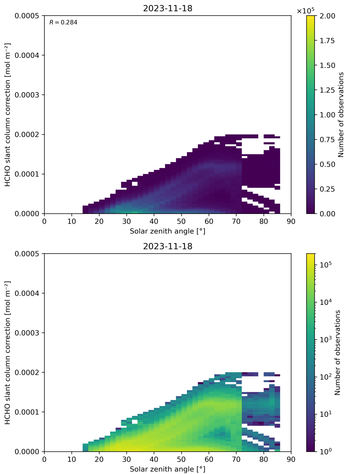
Figure 172: Scatter density plot of “Solar zenith angle” against “HCHO slant column correction” for 2023-11-18 to 2023-11-19.
