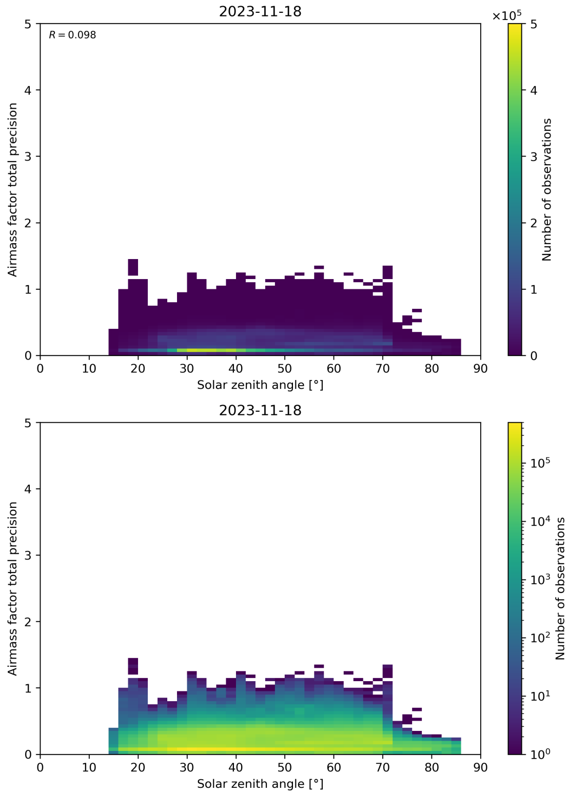
Figure 176: Scatter density plot of “Solar zenith angle” against “Airmass factor total precision” for 2023-11-18 to 2023-11-19.
