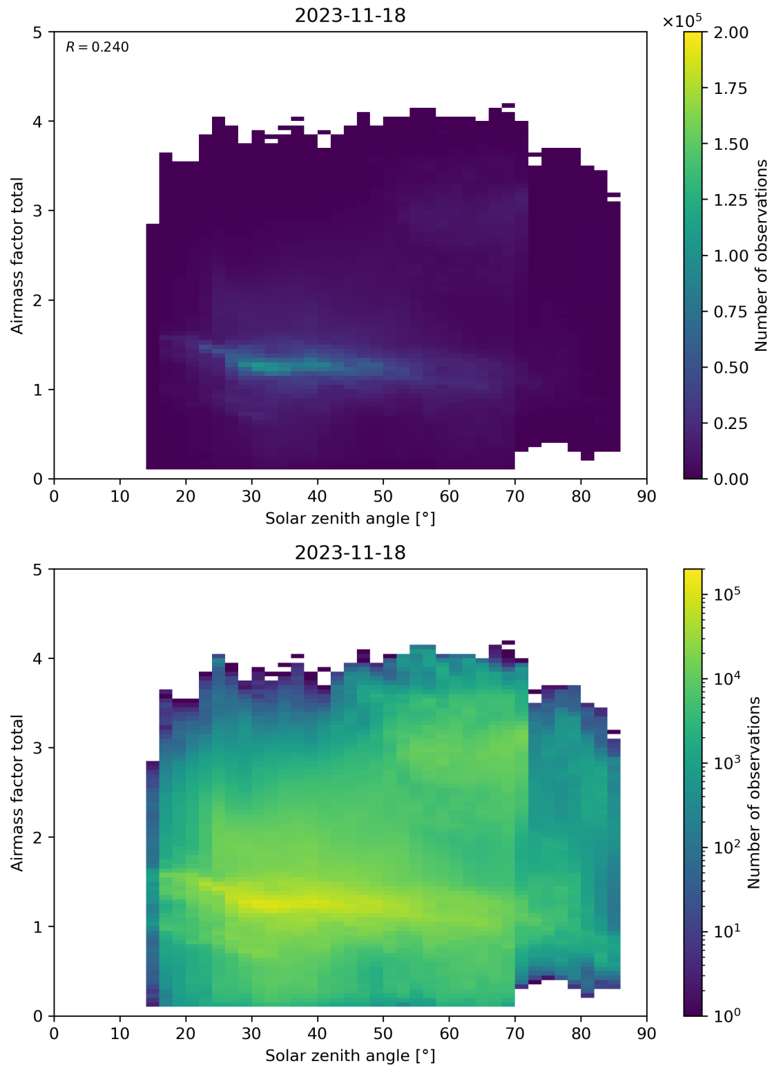
Figure 175: Scatter density plot of “Solar zenith angle” against “Airmass factor total” for 2023-11-18 to 2023-11-19.
