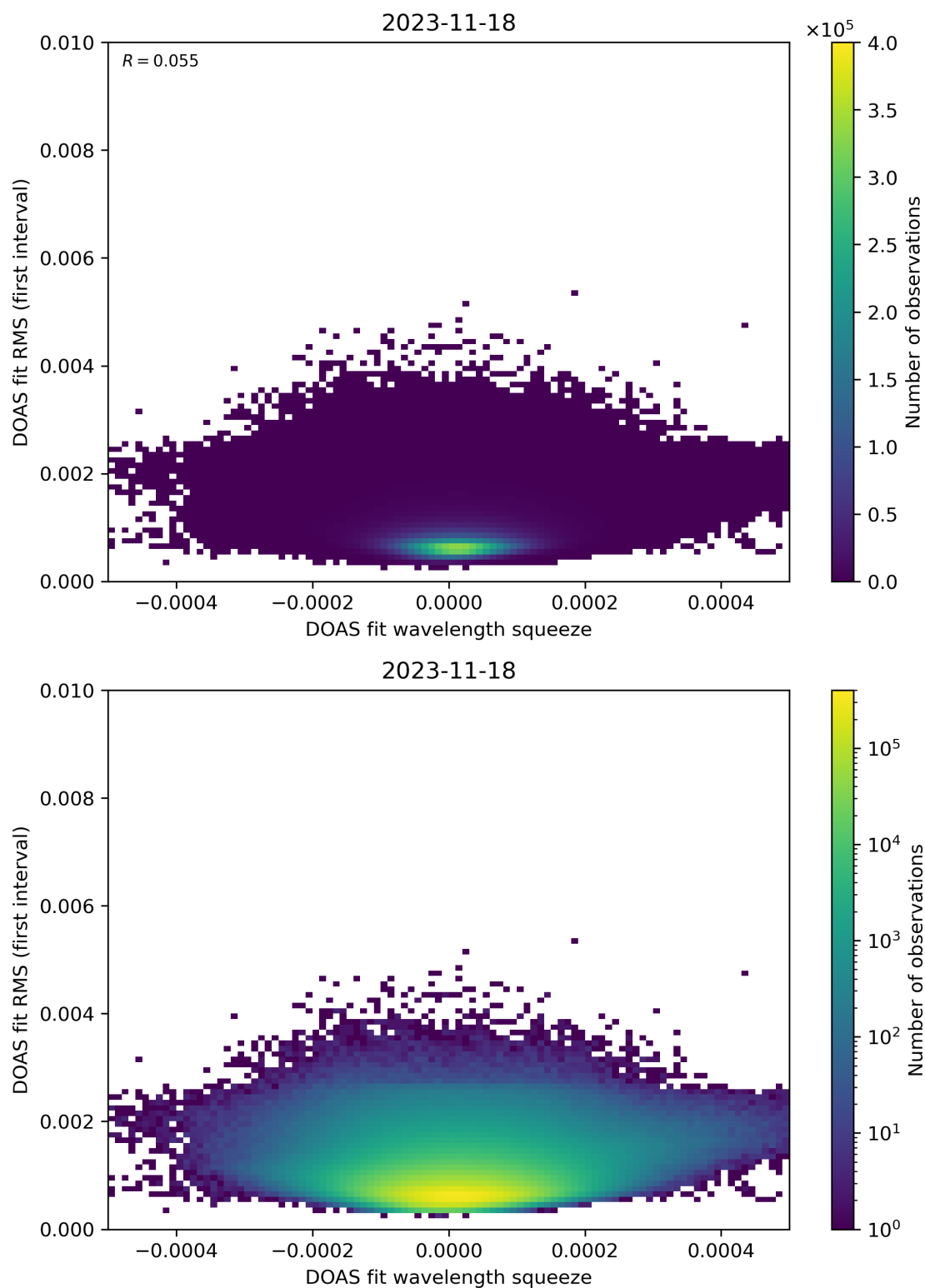
Figure 68: Scatter density plot of “DOAS fit wavelength squeeze” against “DOAS fit RMS (first interval)” for 2023-11-18 to 2023-11-19.
