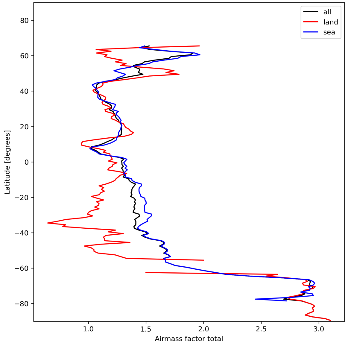
Figure 26: Zonal average of “Airmass factor total” for 2023-11-18 to 2023-11-19.
