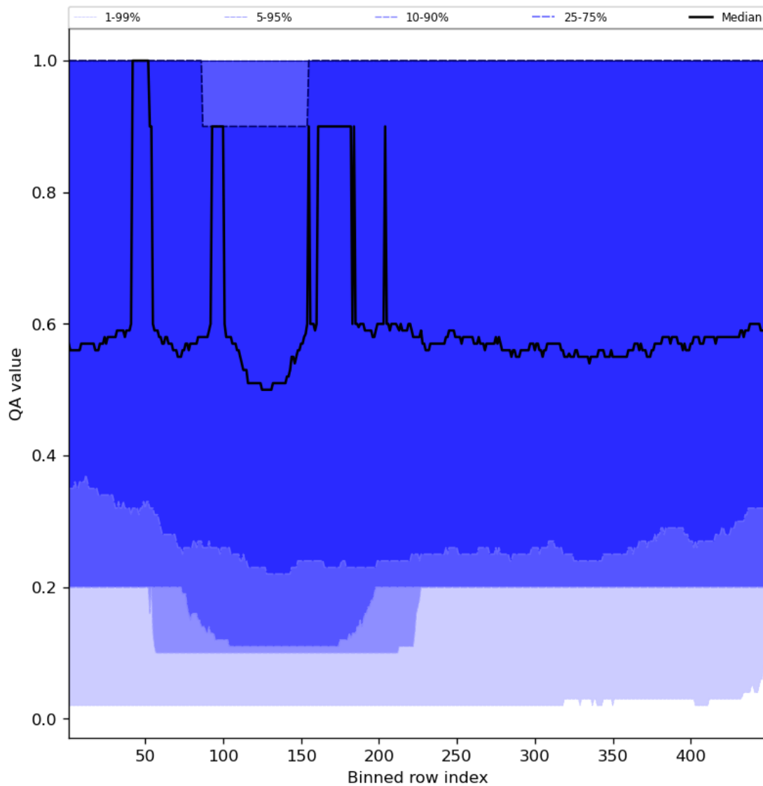
Figure 48: Along track statistics of “QA value” for 2023-11-18 to 2023-11-19
