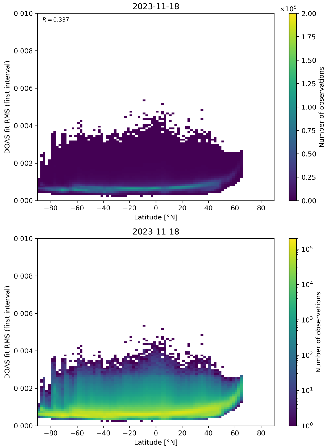
Figure 153: Scatter density plot of “Latitude” against “DOAS fit RMS (first interval)” for 2023-11-18 to 2023-11-19.
