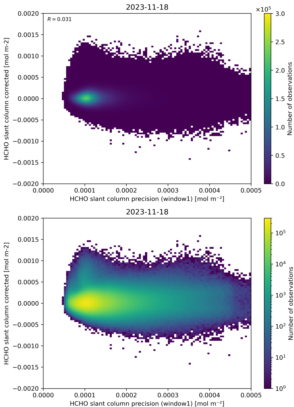
Figure 92: Scatter density plot of “HCHO slant column precision (window1)” against “HCHO slant column corrected” for 2023-11-18 to 2023-11-19.
