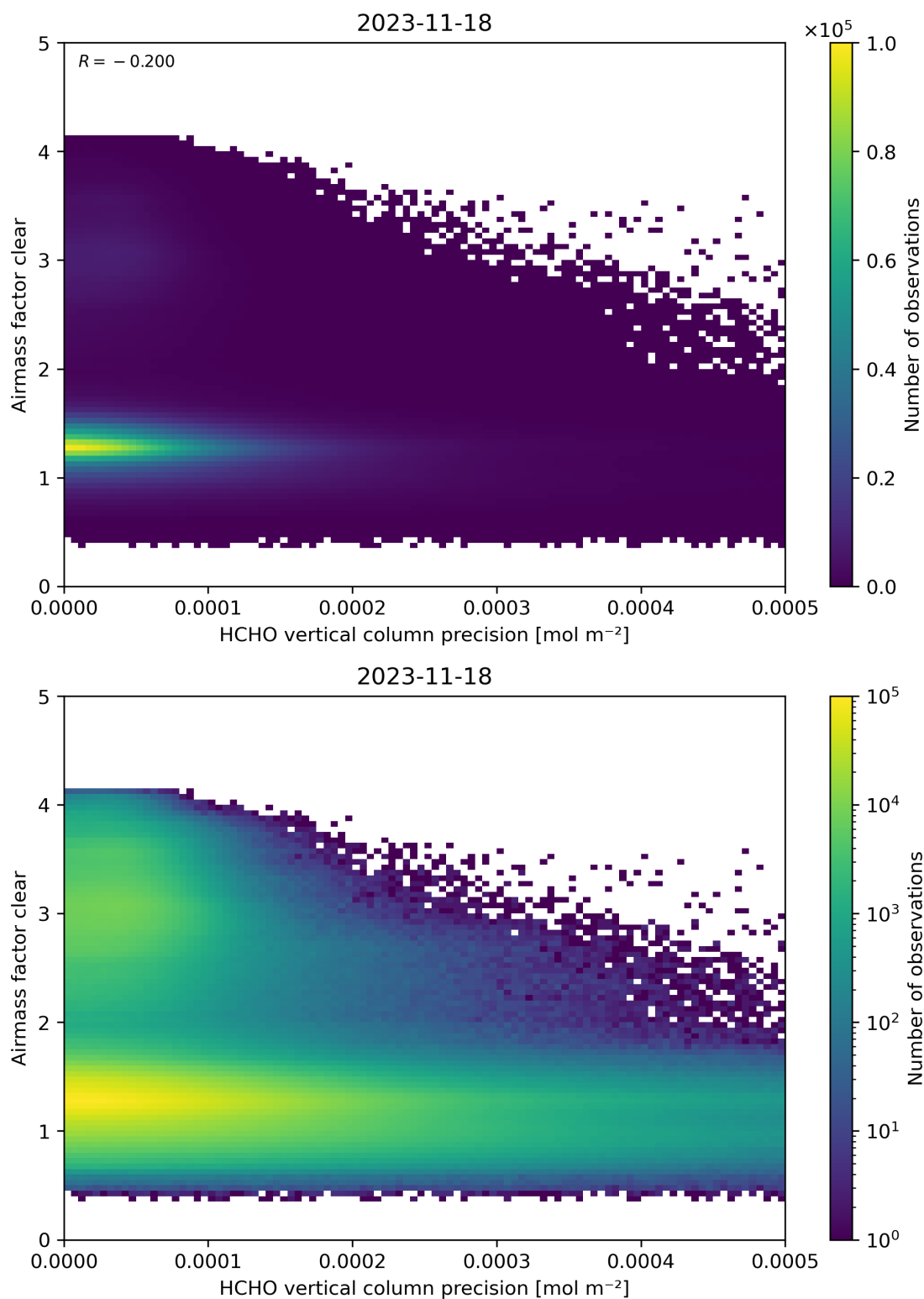
Figure 139: Scatter density plot of “HCHO vertical column precision” against “Airmass factor clear” for 2023-11-18 to 2023-11-19.
