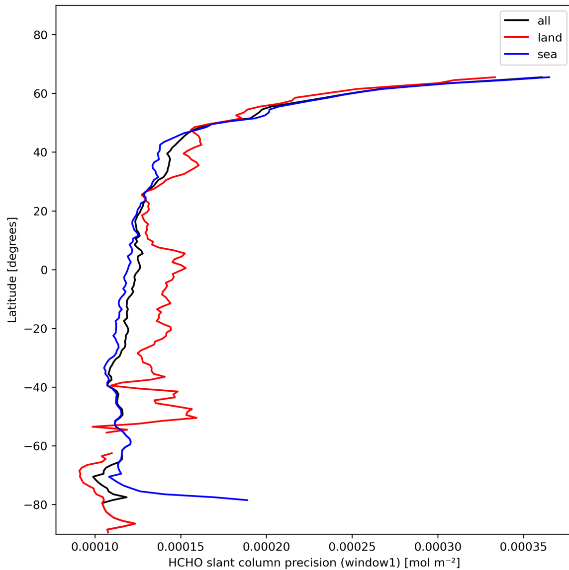
Figure 25: Zonal average of “HCHO slant column precision (window1)” for 2023-11-18 to 2023-11-19.
