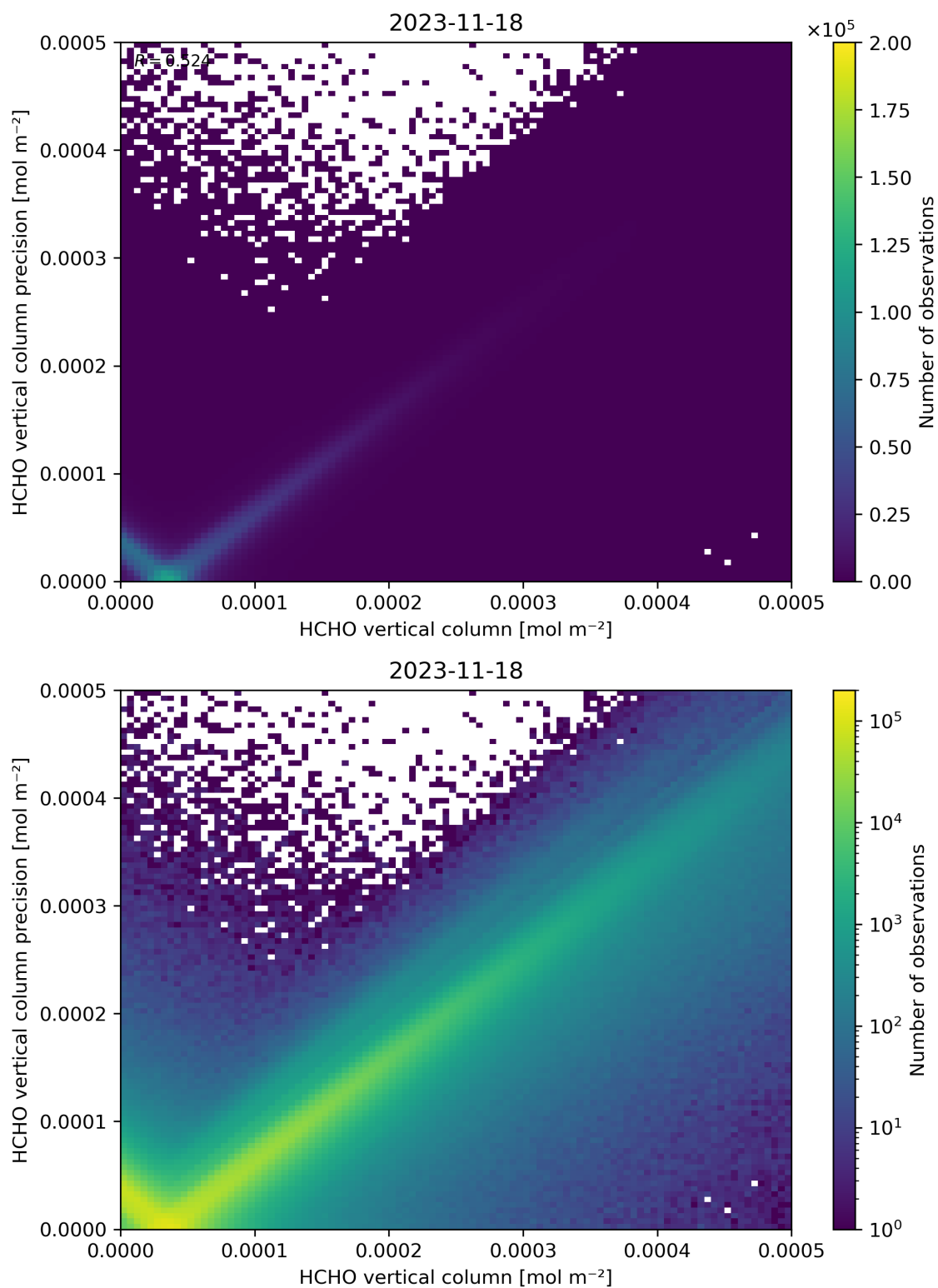
Figure 134: Scatter density plot of “HCHO vertical column” against “HCHO vertical column precision” for 2023-11-18 to 2023-11-19.
