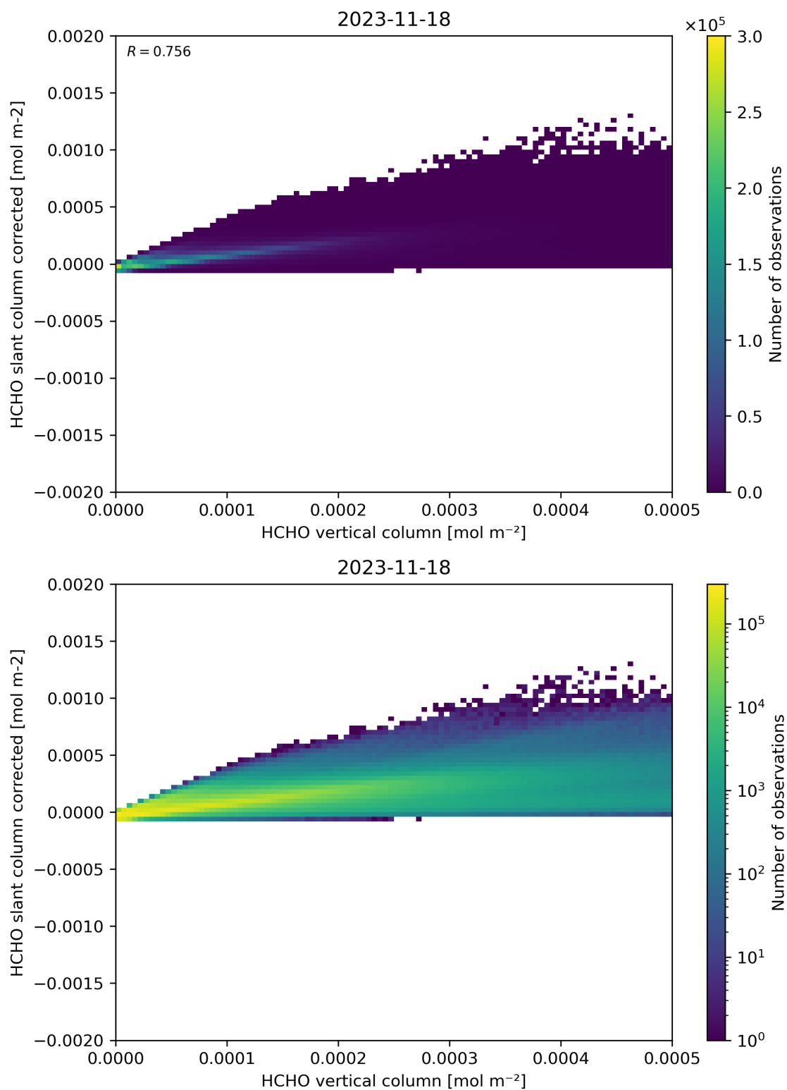
Figure 127: Scatter density plot of “HCHO vertical column” against “HCHO slant column corrected” for 2023-11-18 to 2023-11-19.
