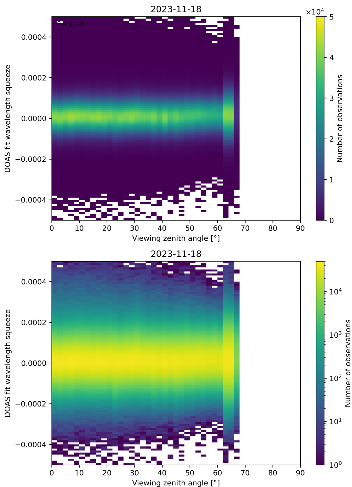
Figure 184: Scatter density plot of “Viewing zenith angle” against “DOAS fit wavelength squeeze” for 2023-11-18 to 2023-11-19.
