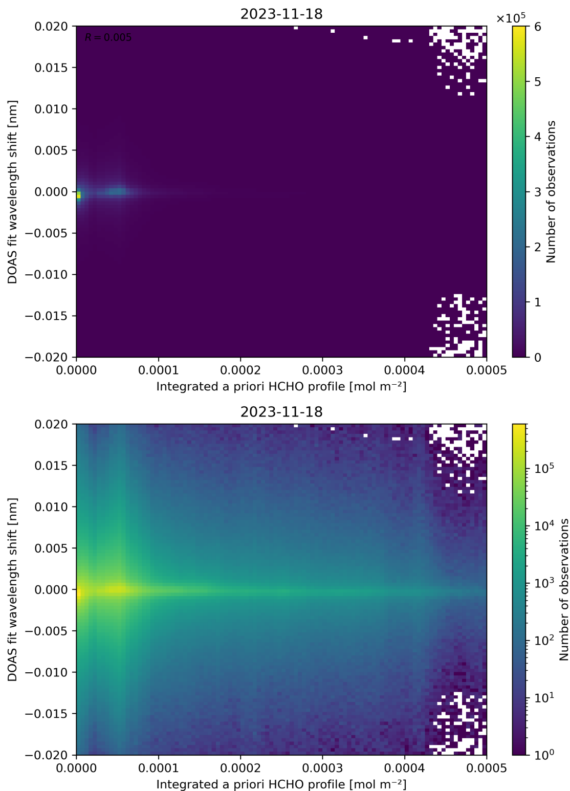
Figure 149: Scatter density plot of “Integrated a priori HCHO profile” against “DOAS fit wavelength shift” for 2023-11-18 to 2023-11-19.
