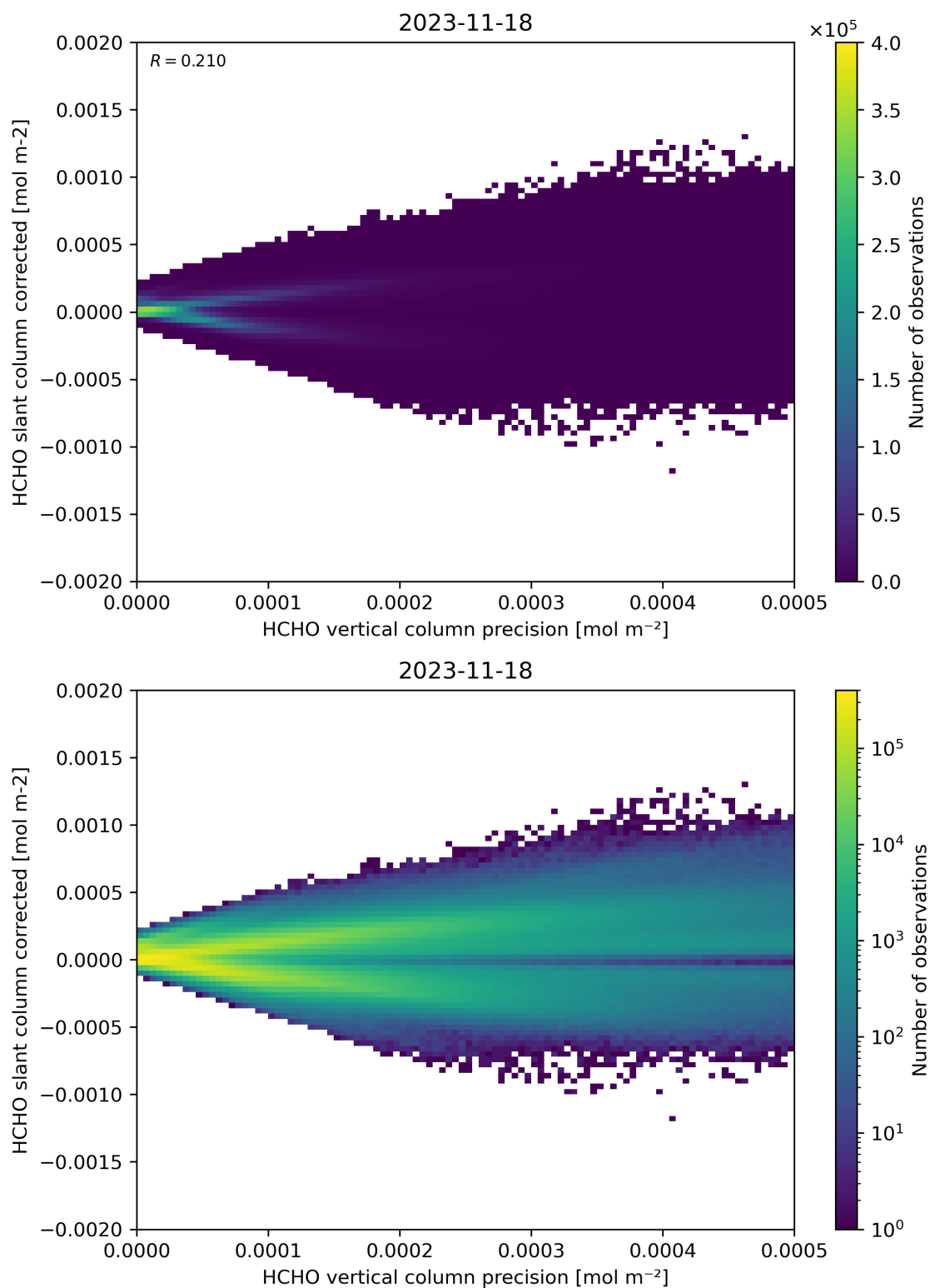
Figure 140: Scatter density plot of “HCHO vertical column precision” against “HCHO slant column corrected” for 2023-11-18 to 2023-11-19.
