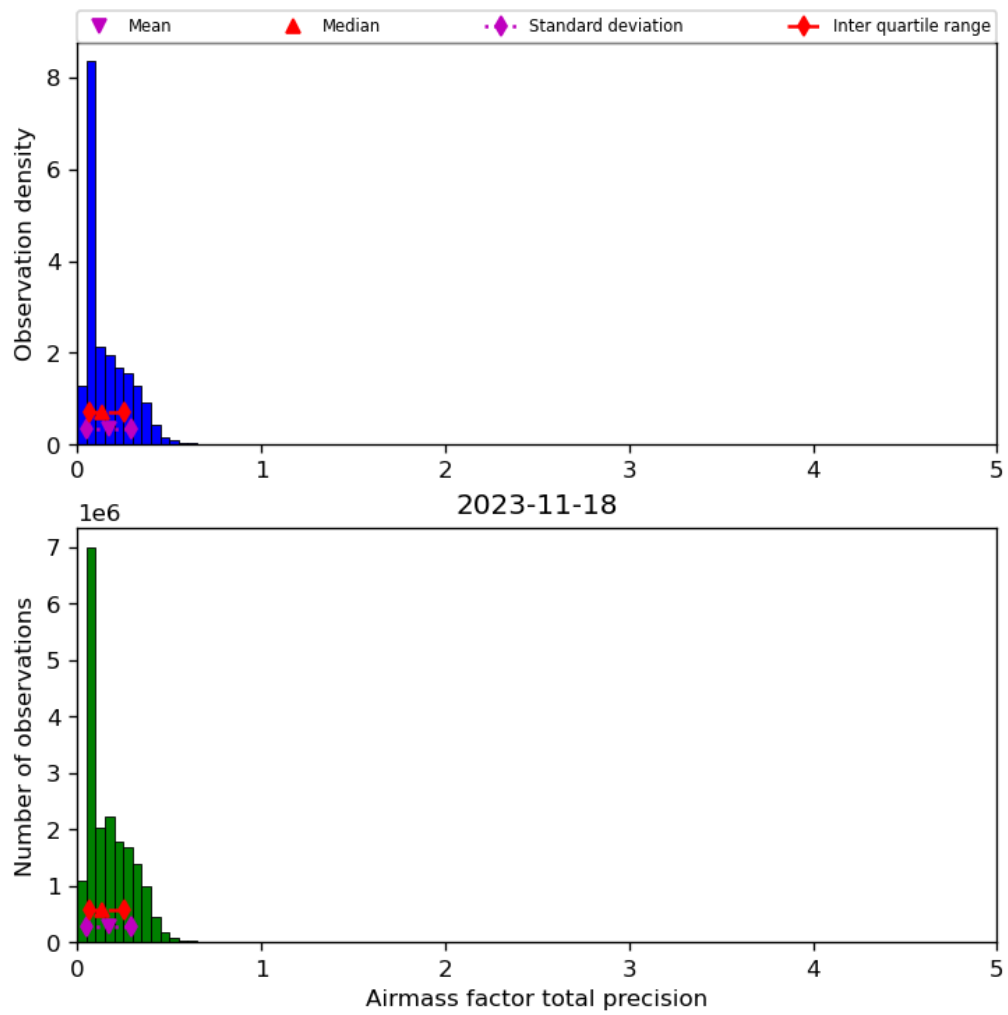
Figure 41: Histogram of “Airmass factor total precision” for 2023-11-18 to 2023-11-19
