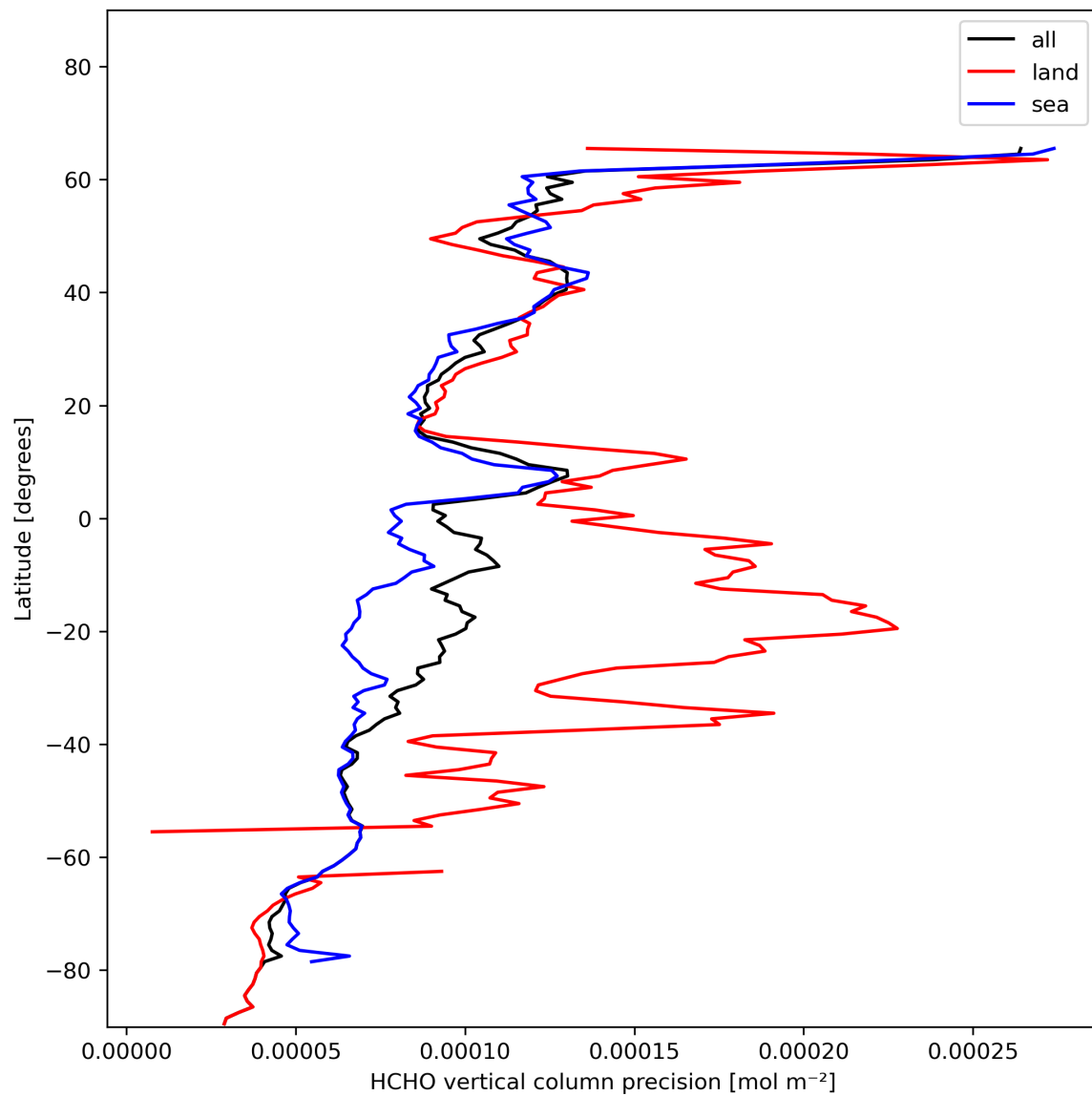
Figure 22: Zonal average of “HCHO vertical column precision” for 2023-11-18 to 2023-11-19.
