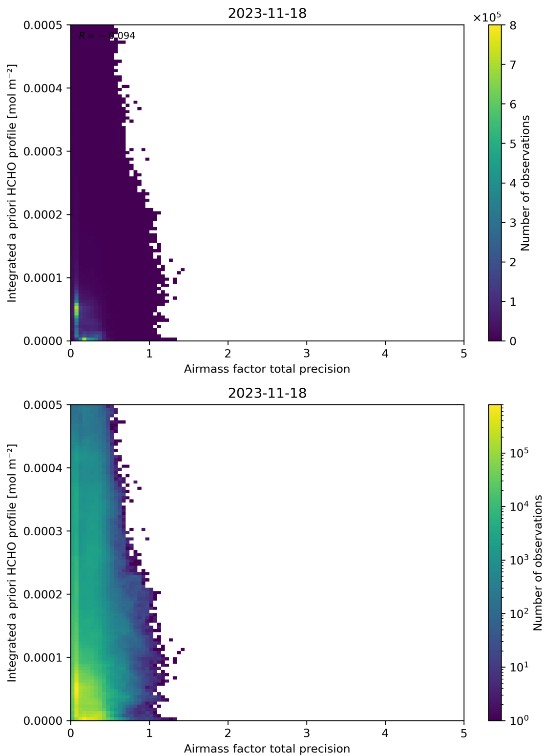
Figure 111: Scatter density plot of “Airmass factor total precision” against “Integrated a priori HCHO profile” for 2023-11-18 to 2023-11-19.
