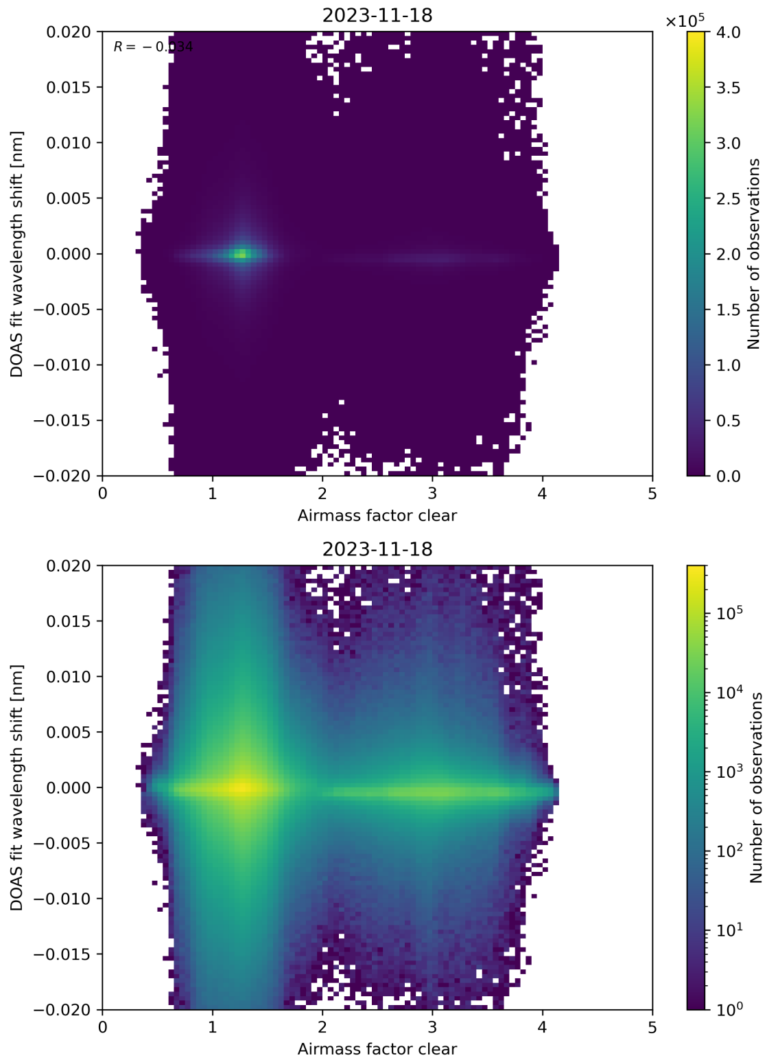
Figure 72: Scatter density plot of “Airmass factor clear” against “DOAS fit wavelength shift” for 2023-11-18 to 2023-11-19.
