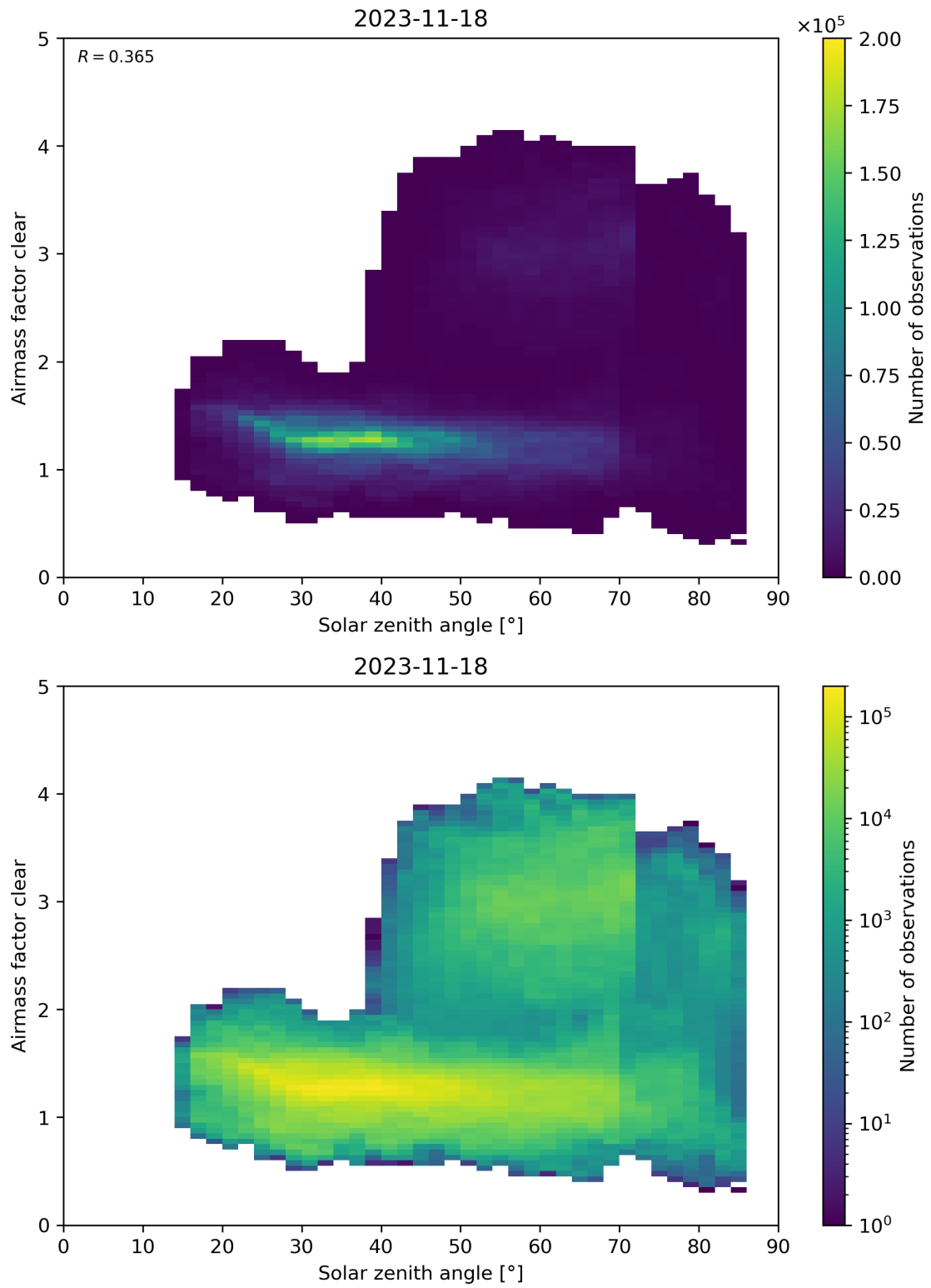
Figure 170: Scatter density plot of “Solar zenith angle” against “Airmass factor clear” for 2023-11-18 to 2023-11-19.
