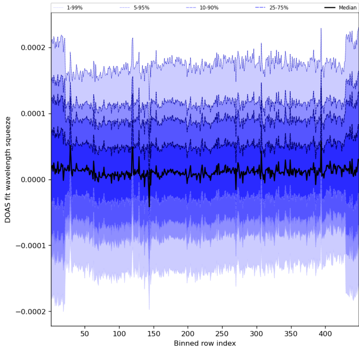
Figure 59: Along track statistics of “DOAS fit wavelength squeeze” for 2023-11-18 to 2023-11-19
