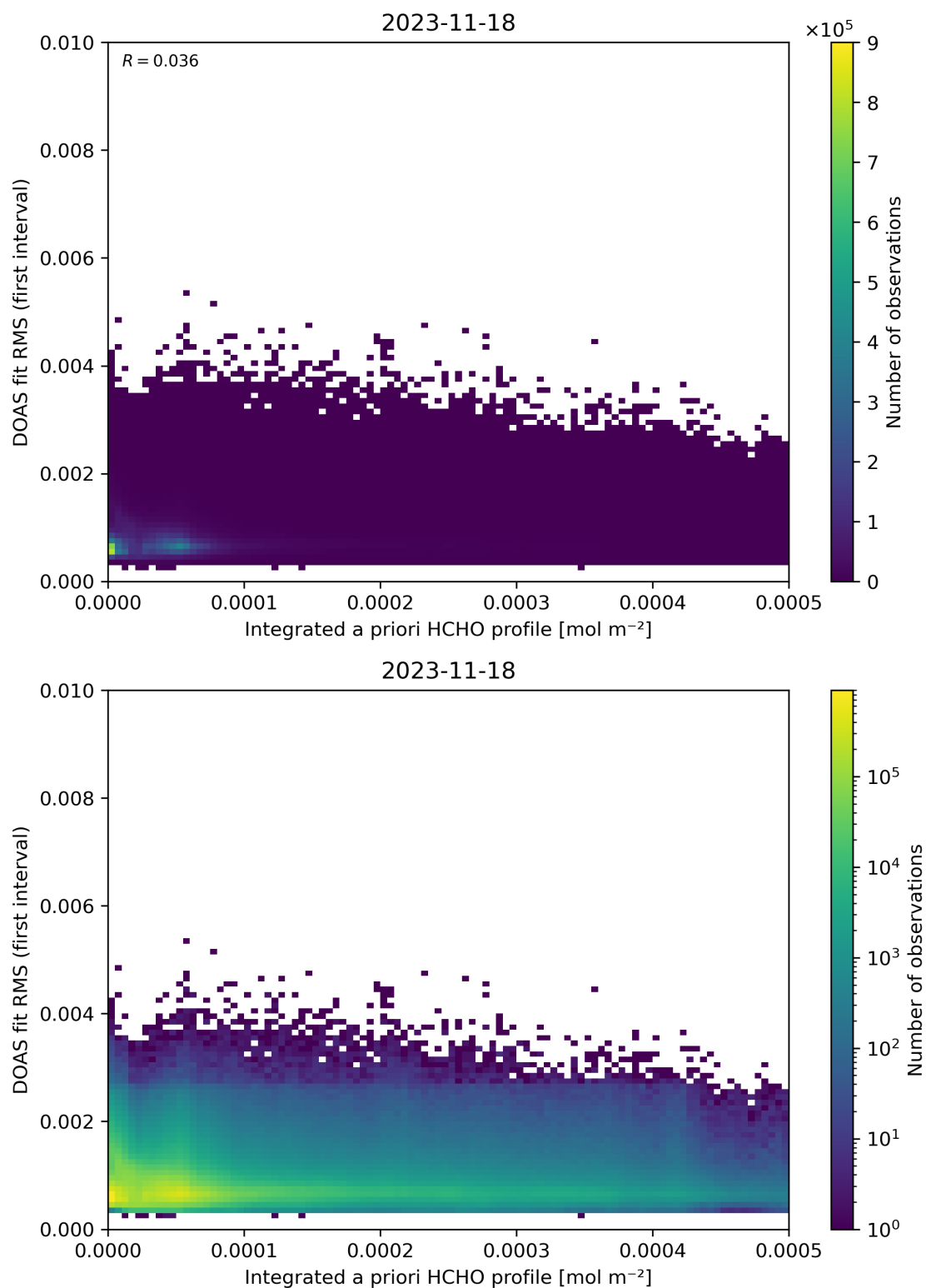
Figure 148: Scatter density plot of “Integrated a priori HCHO profile” against “DOAS fit RMS (first interval)” for 2023-11-18 to 2023-11-19.
