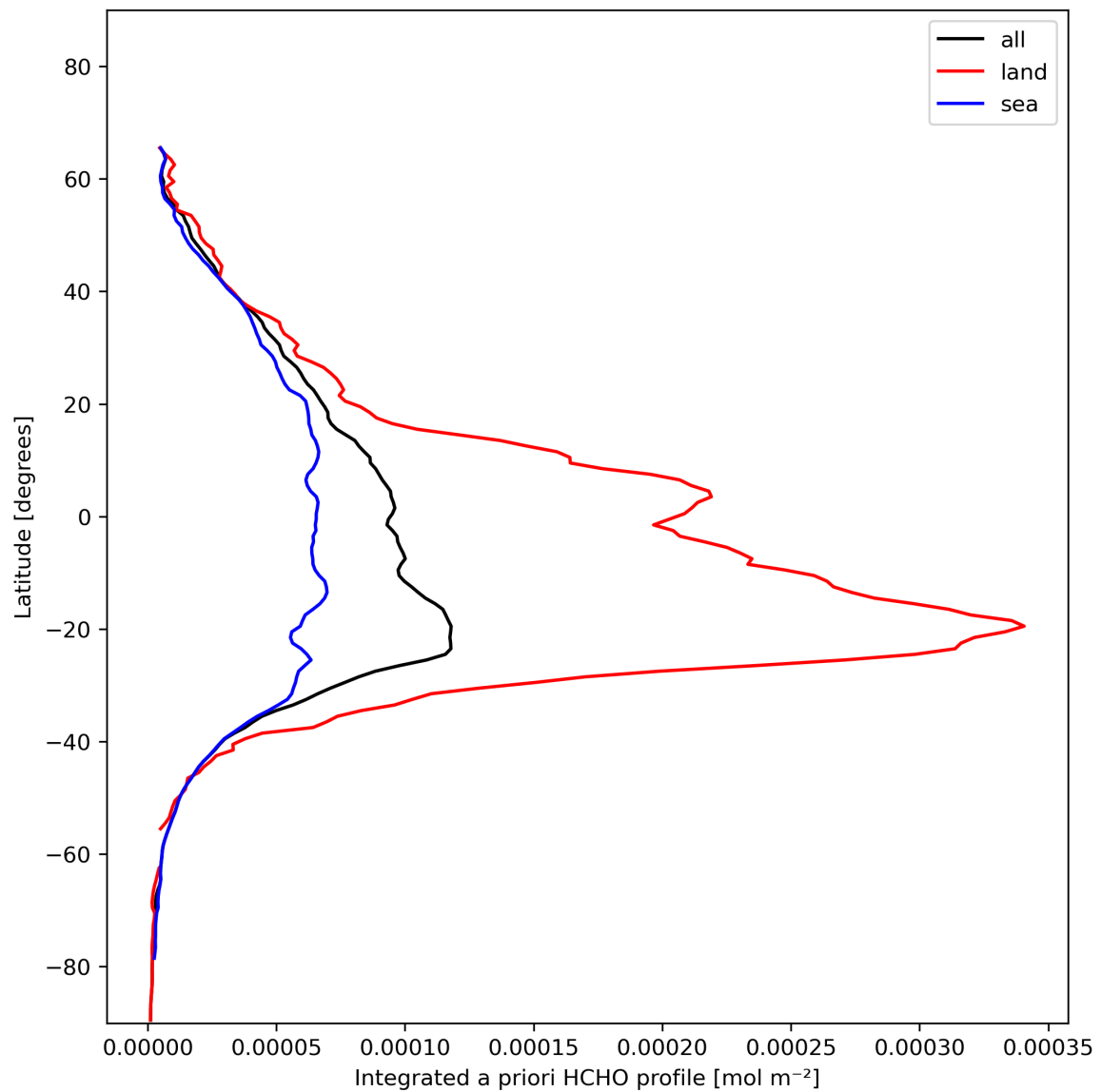
Figure 29: Zonal average of “Integrated a priori HCHO profile” for 2023-11-18 to 2023-11-19.
