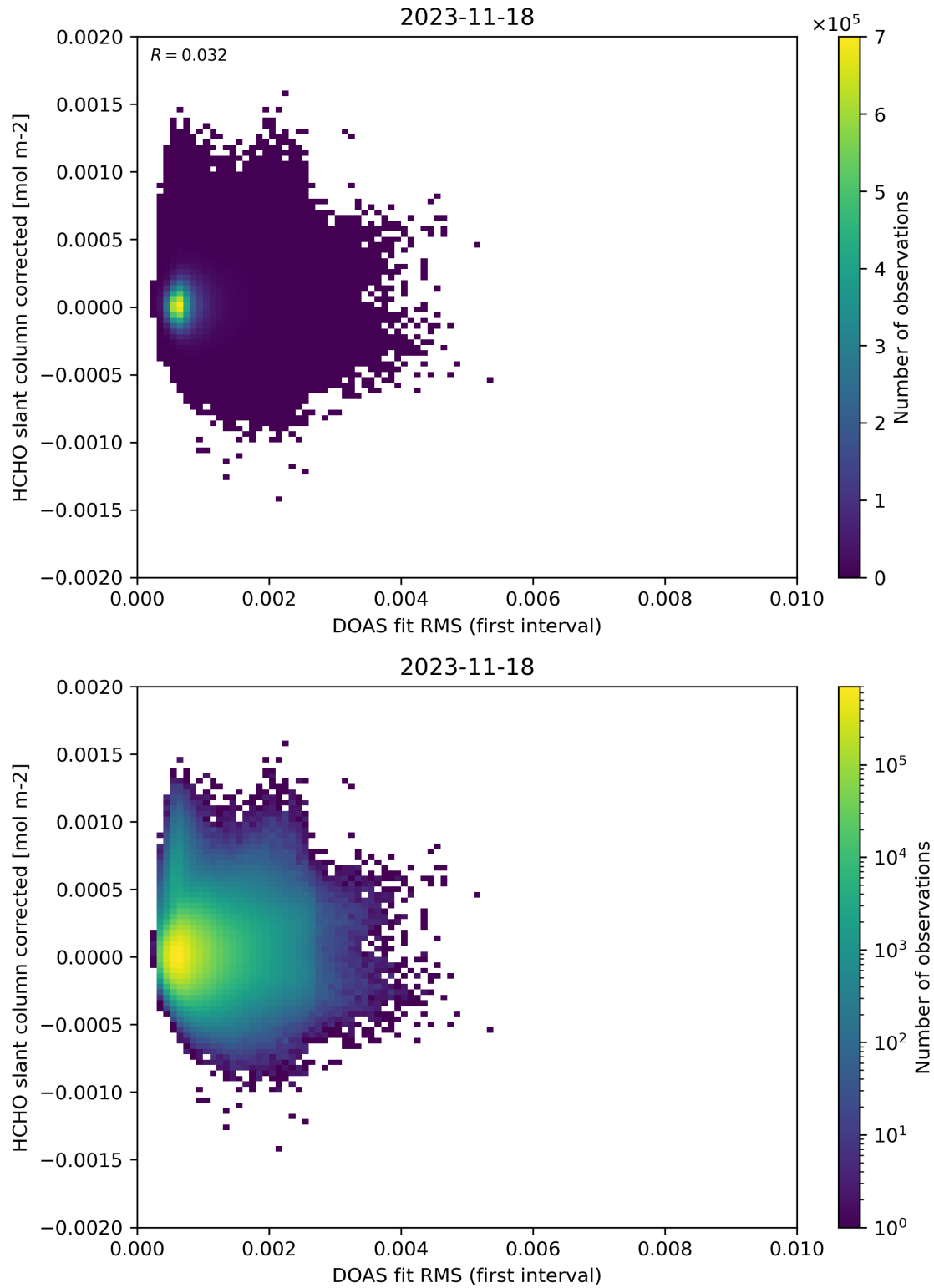
Figure 62: Scatter density plot of “DOAS fit RMS (first interval)” against “HCHO slant column corrected” for 2023-11-18 to 2023-11-19.
