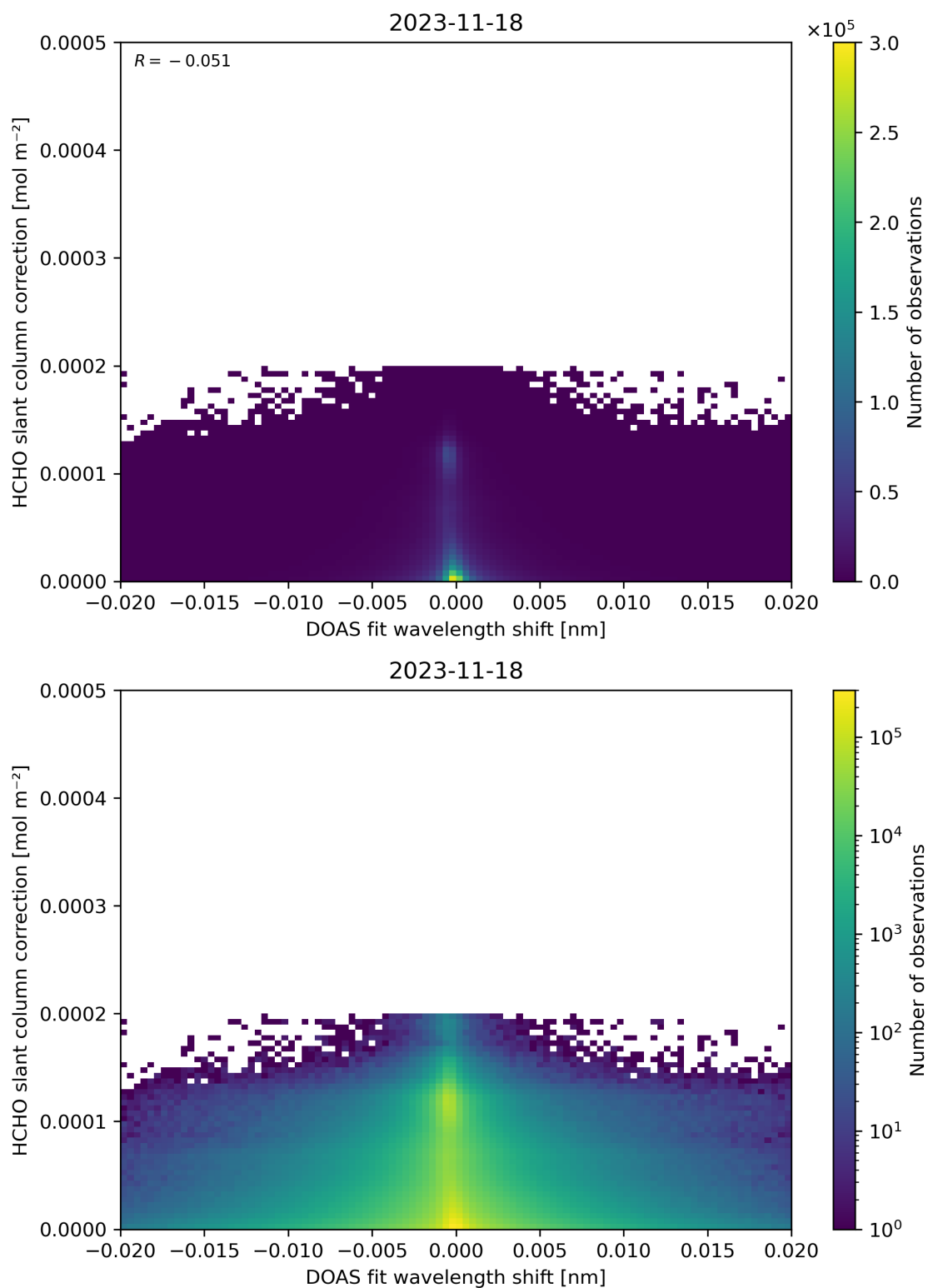
Figure 67: Scatter density plot of “DOAS fit wavelength shift” against “HCHO slant column correction” for 2023-11-18 to 2023-11-19.
