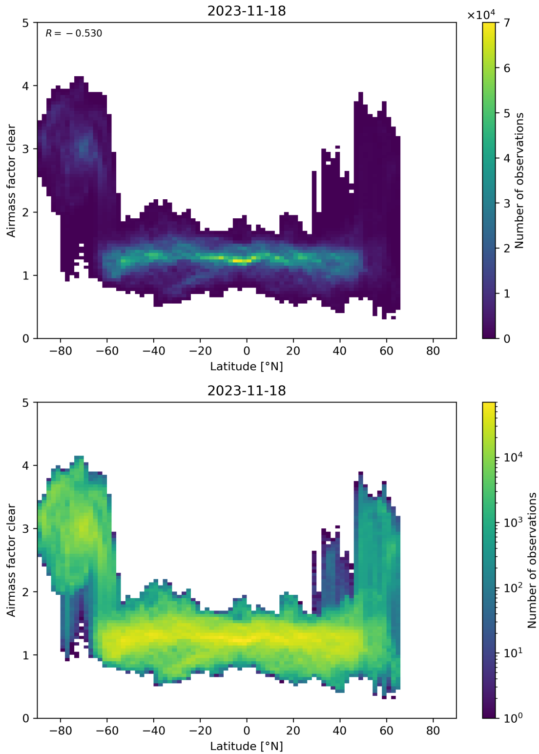
Figure 156: Scatter density plot of “Latitude” against “Airmass factor clear” for 2023-11-18 to 2023-11-19.
