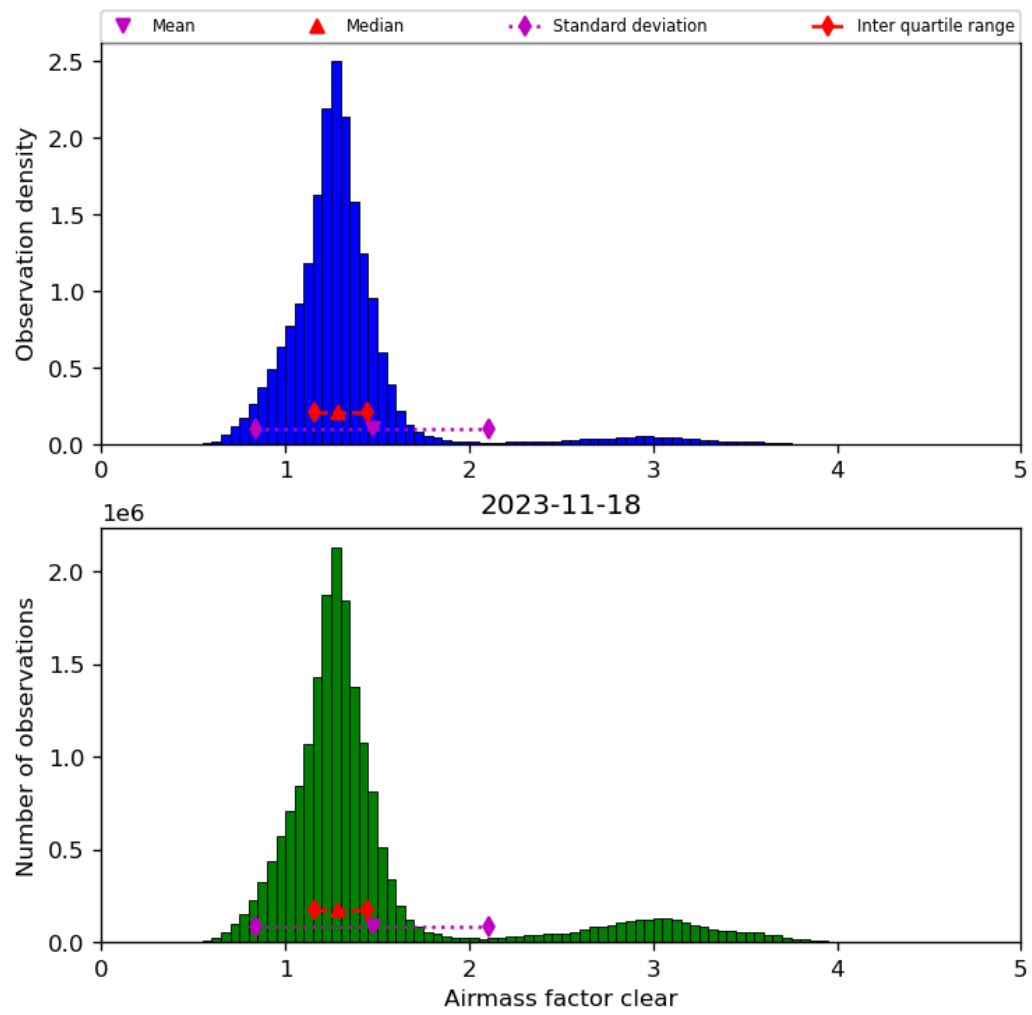
Figure 42: Histogram of “Airmass factor clear” for 2023-11-18 to 2023-11-19
