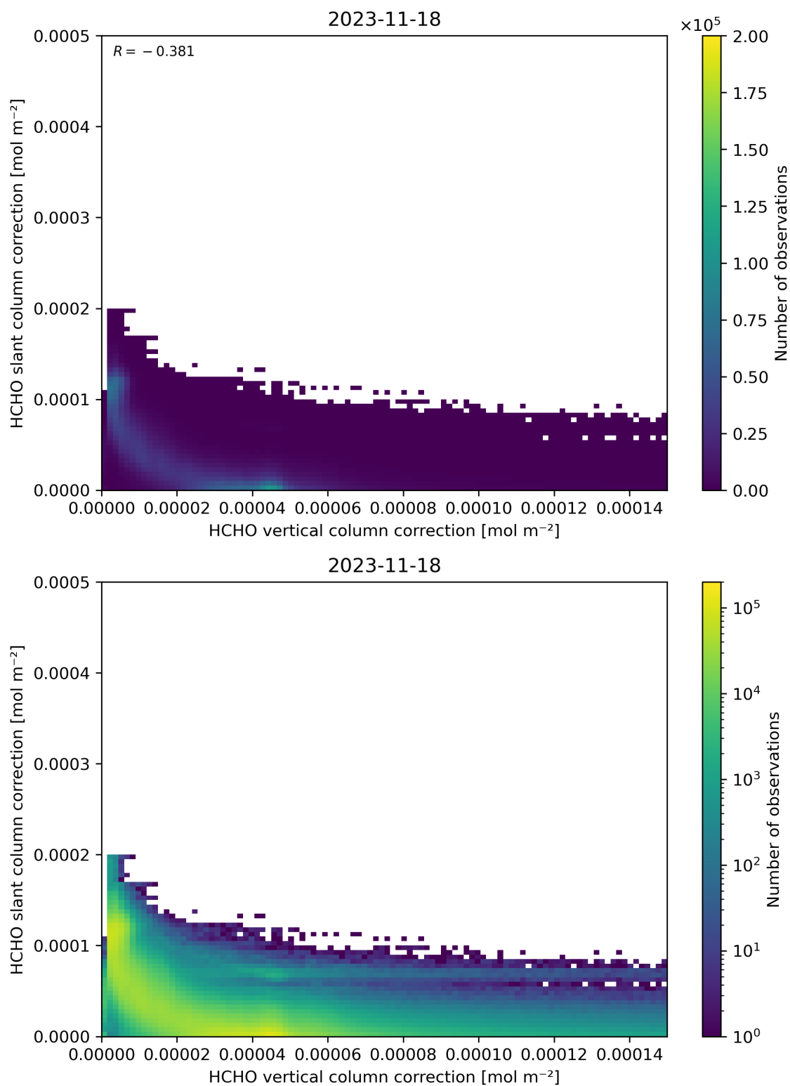
Figure 117: Scatter density plot of “HCHO vertical column correction” against “HCHO slant column correction” for 2023-11-18 to 2023-11-19.
