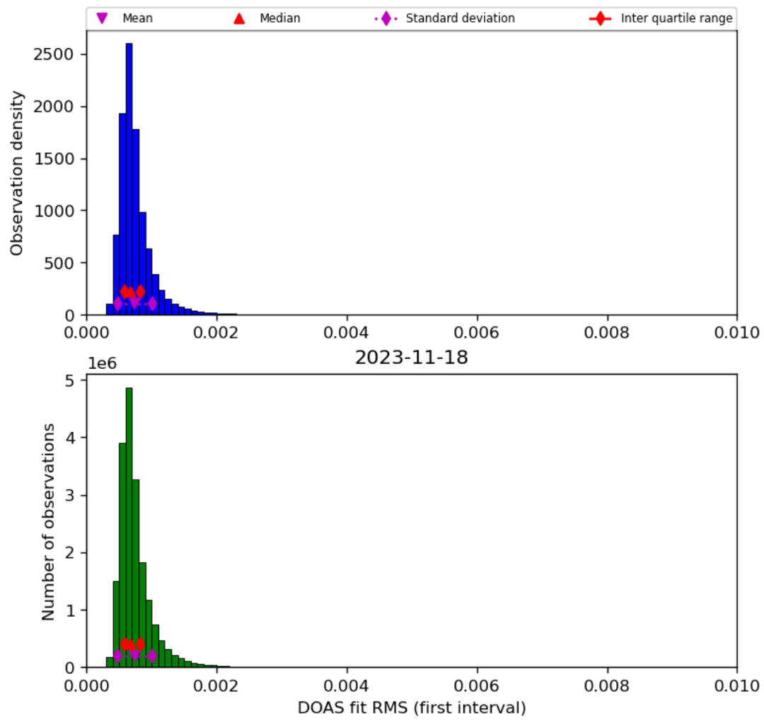
Figure 46: Histogram of “DOAS fit RMS (first interval)” for 2023-11-18 to 2023-11-19
