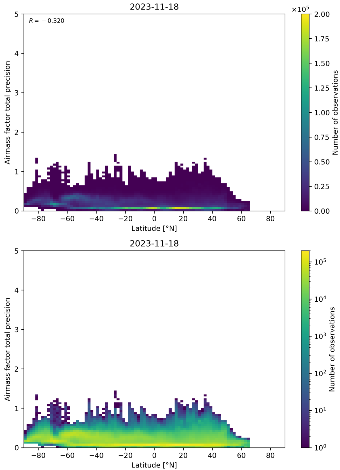
Figure 162: Scatter density plot of “Latitude” against “Airmass factor total precision” for 2023-11-18 to 2023-11-19.
