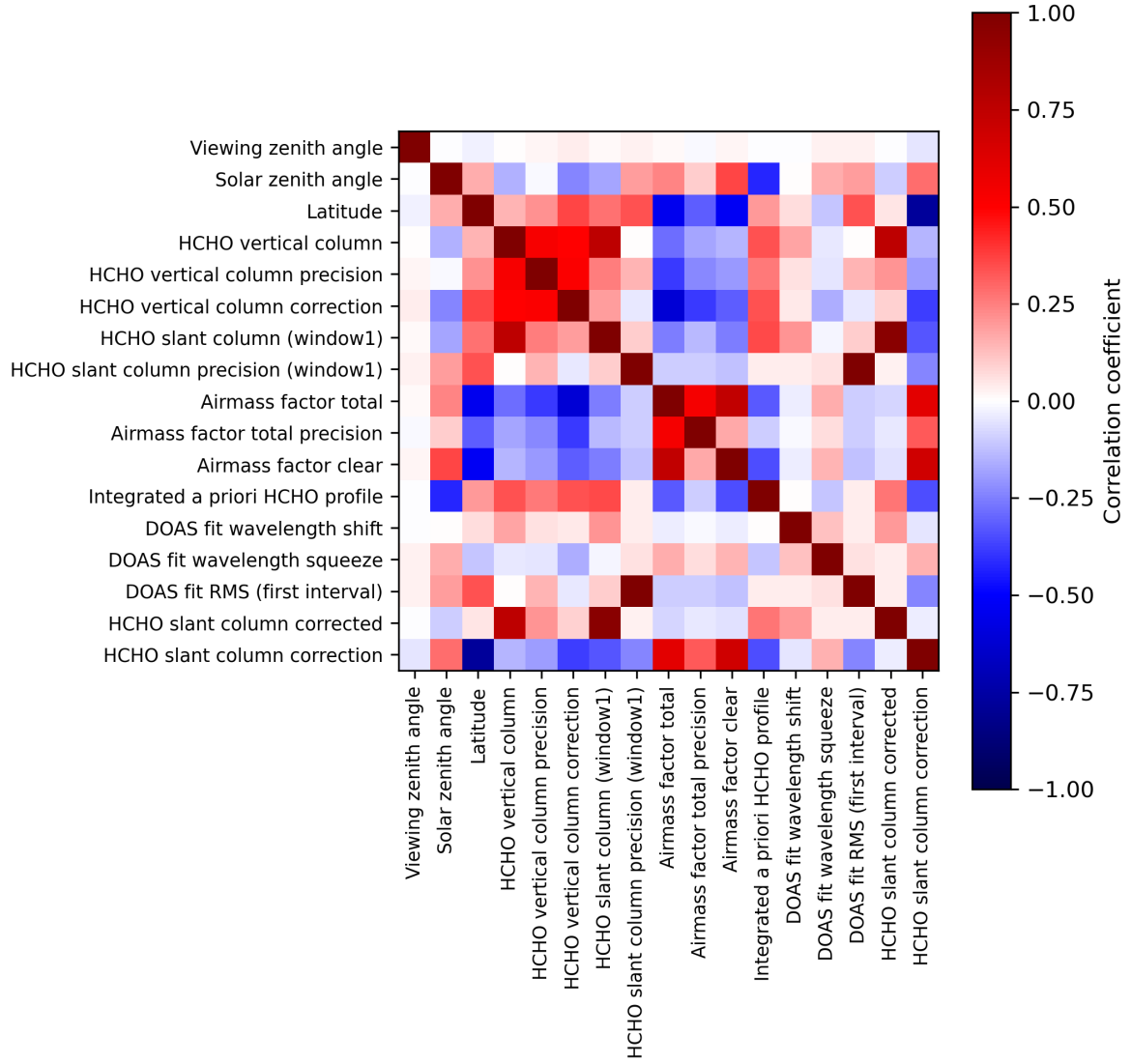
Figure 2: Map of correlation matrix for 2023-11-18 to 2023-11-19.
