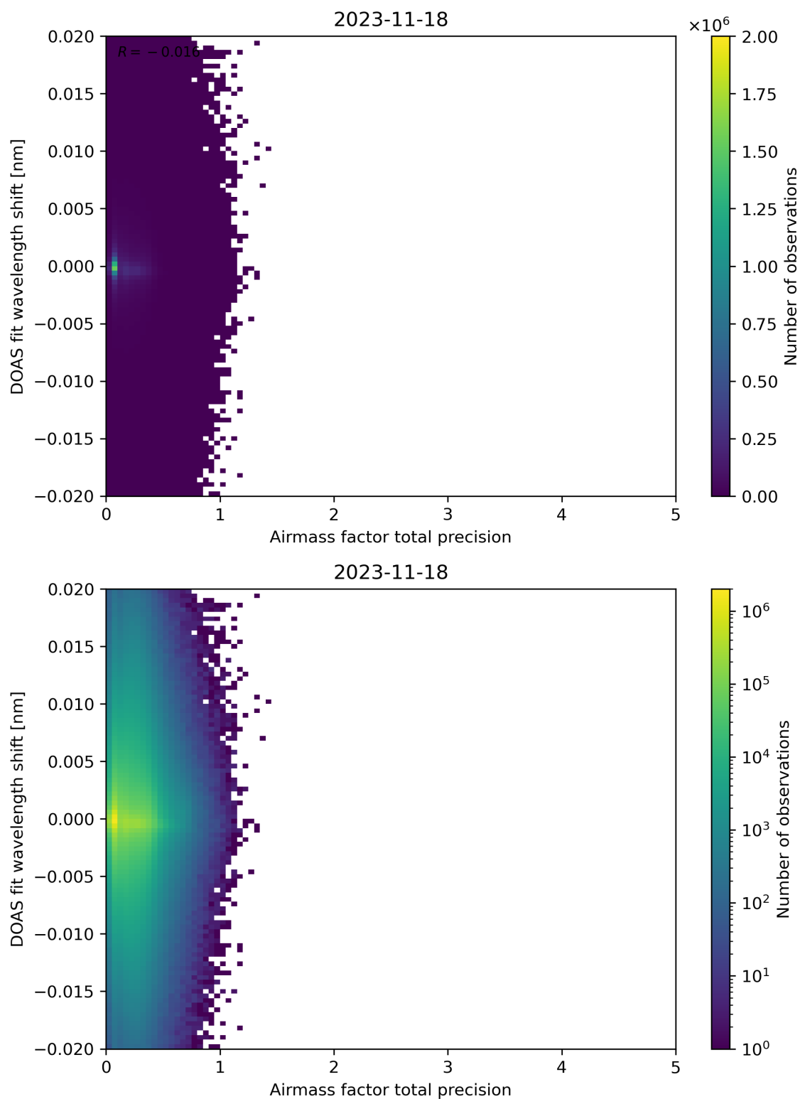
Figure 106: Scatter density plot of “Airmass factor total precision” against “DOAS fit wavelength shift” for 2023-11-18 to 2023-11-19.
