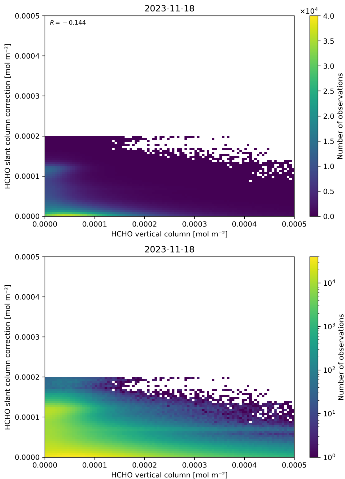
Figure 128: Scatter density plot of “HCHO vertical column” against “HCHO slant column correction” for 2023-11-18 to 2023-11-19.
