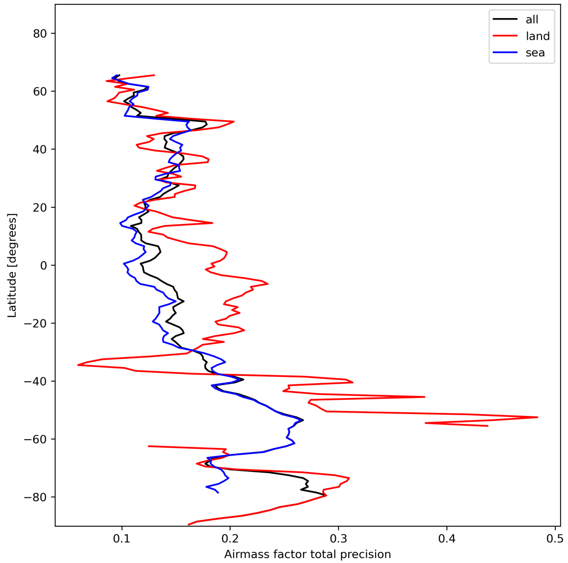
Figure 27: Zonal average of “Airmass factor total precision” for 2023-11-18 to 2023-11-19.
