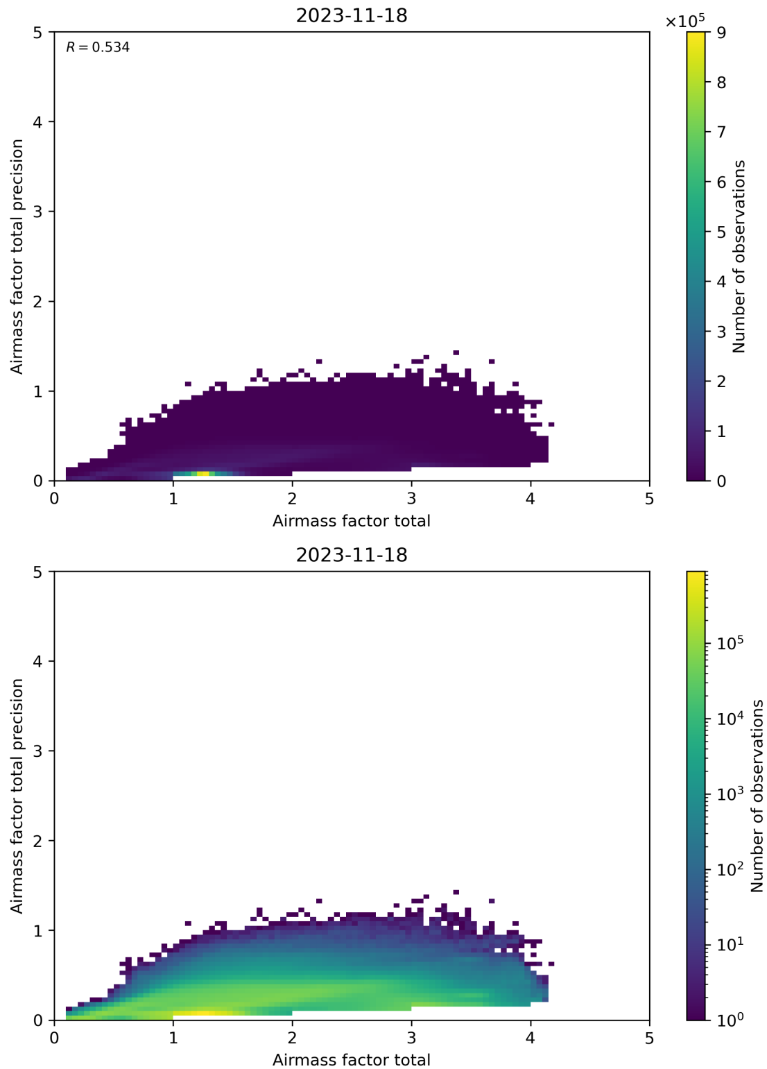
Figure 103: Scatter density plot of “Airmass factor total” against “Airmass factor total precision” for 2023-11-18 to 2023-11-19.
