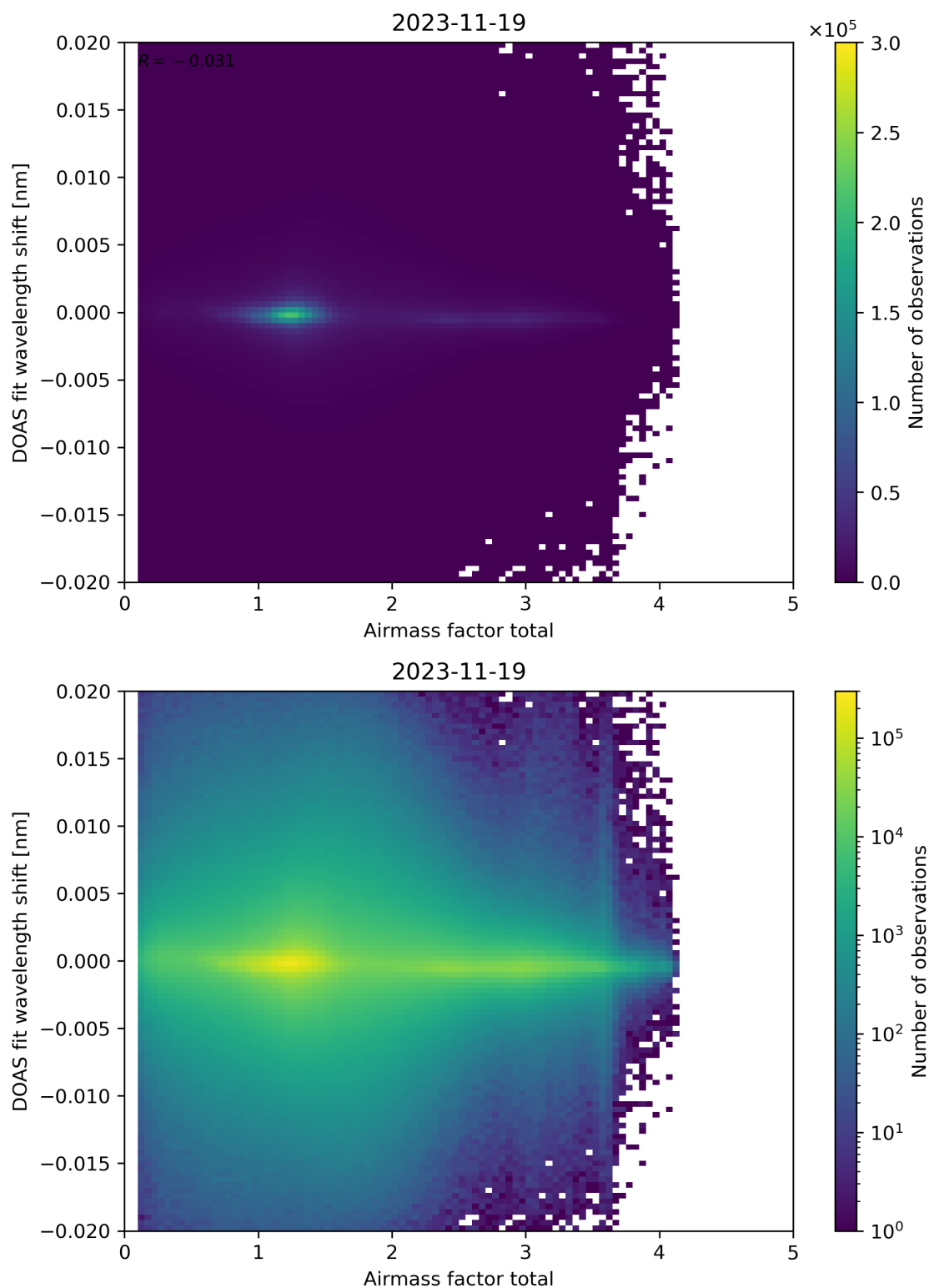
Figure 98: Scatter density plot of “Airmass factor total” against “DOAS fit wavelength shift” for 2023-11-18 to 2023-11-20.
