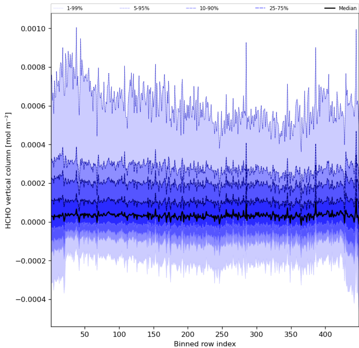
Figure 49: Along track statistics of “HCHO vertical column” for 2023-11-18 to 2023-11-20
