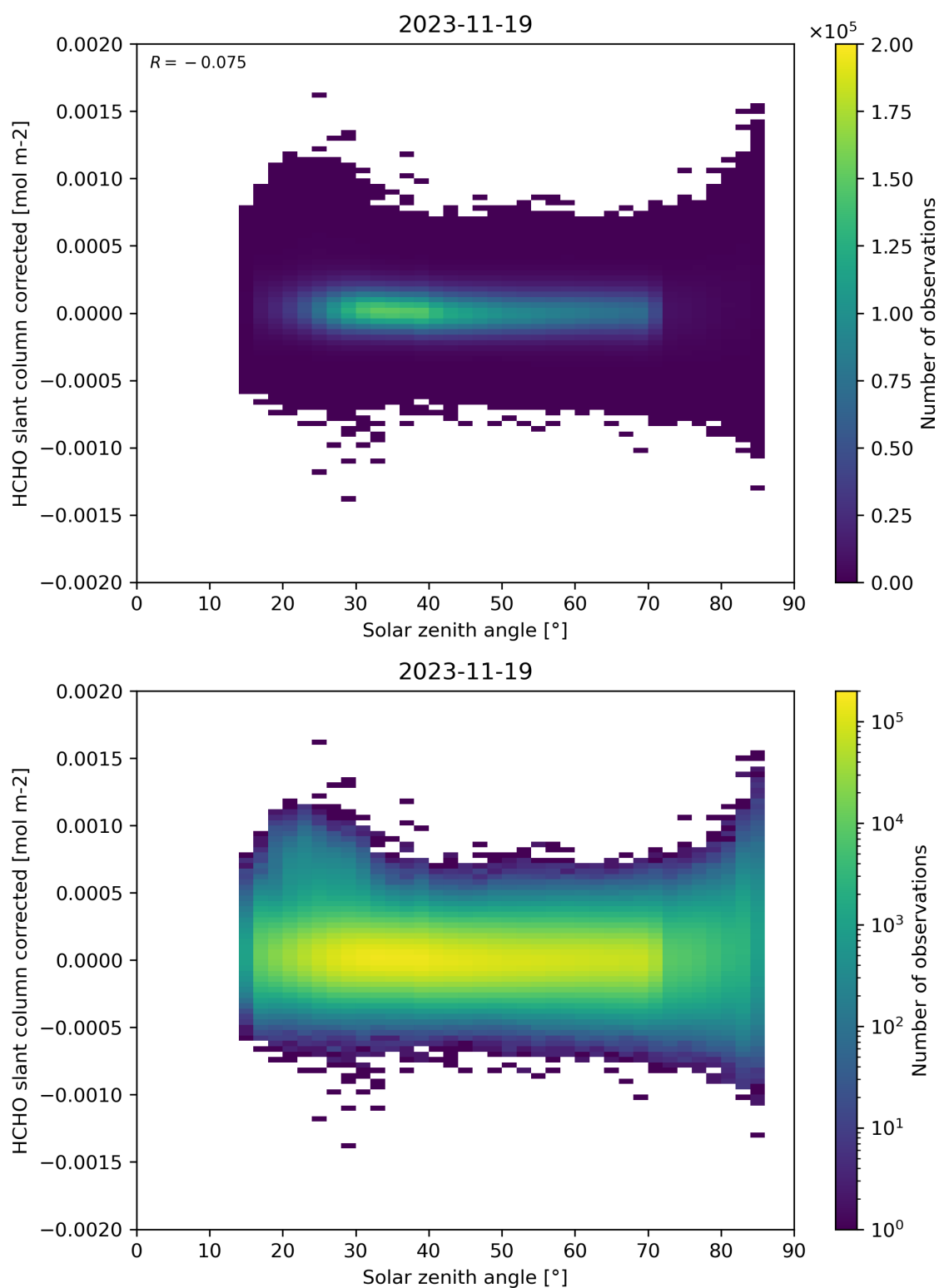
Figure 171: Scatter density plot of “Solar zenith angle” against “HCHO slant column corrected” for 2023-11-18 to 2023-11-20.
