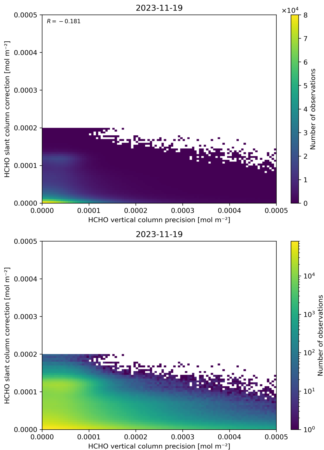
Figure 141: Scatter density plot of “HCHO vertical column precision” against “HCHO slant column correction” for 2023-11-18 to 2023-11-20.
