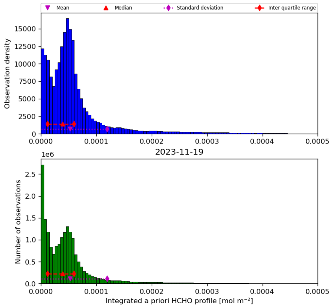
Figure 43: Histogram of “Integrated a priori HCHO profile” for 2023-11-18 to 2023-11-20
