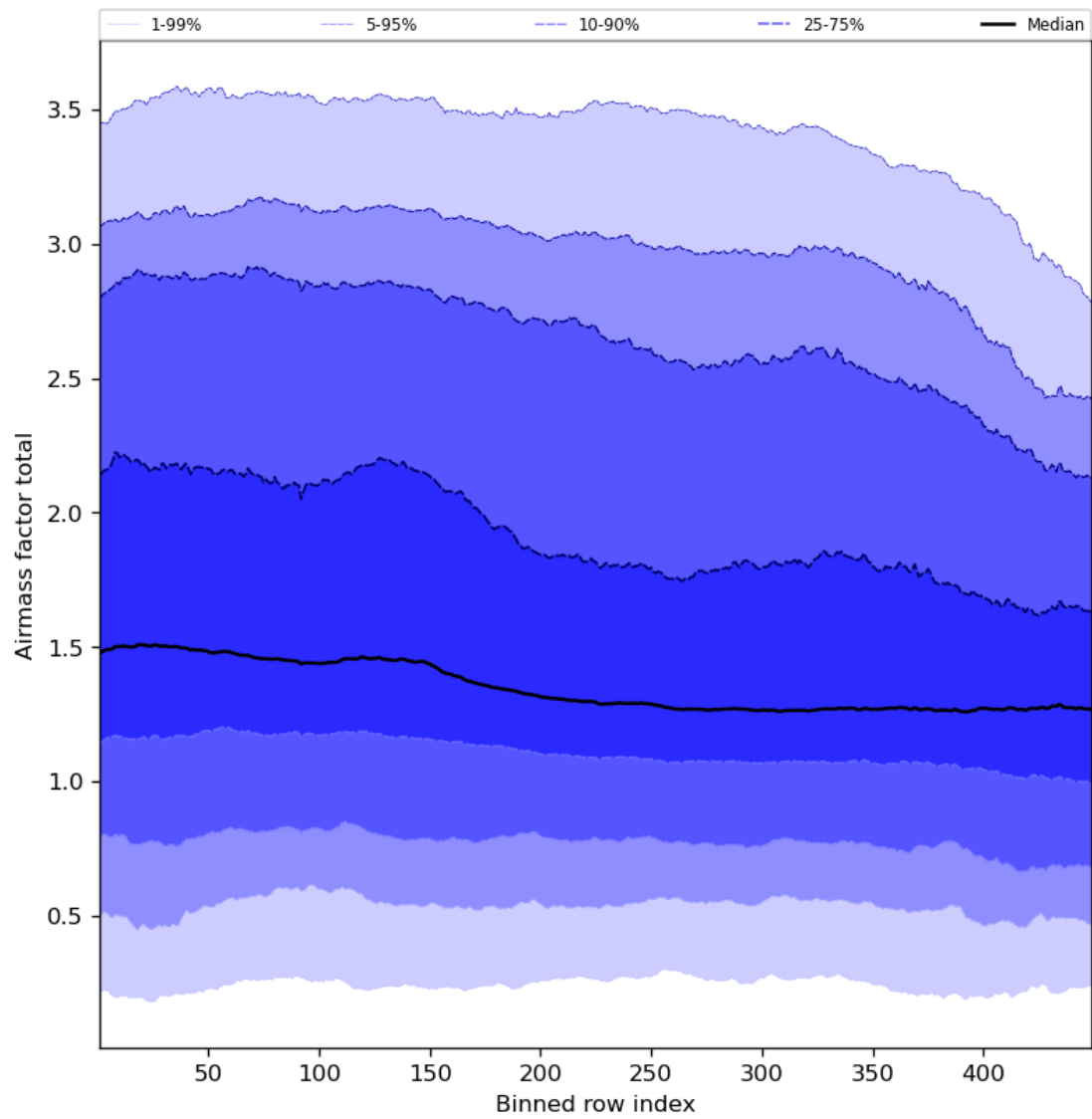
Figure 54: Along track statistics of “Airmass factor total” for 2023-11-18 to 2023-11-20
