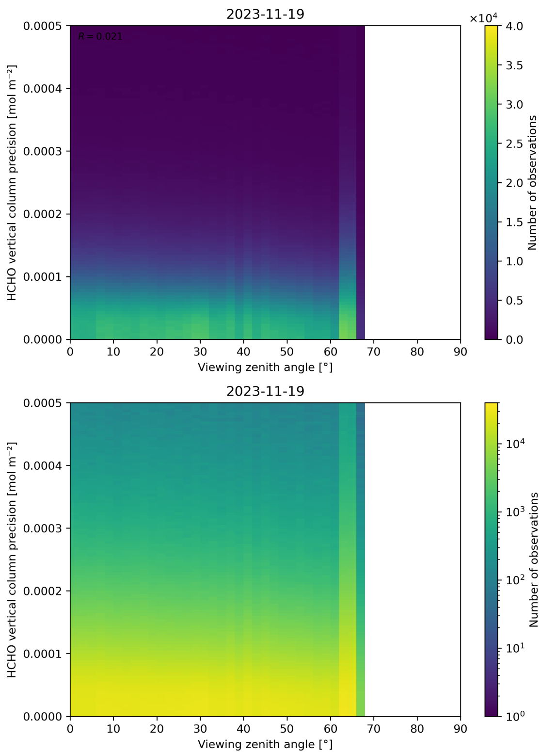
Figure 194: Scatter density plot of “Viewing zenith angle” against “HCHO vertical column precision” for 2023-11-18 to 2023-11-20.
