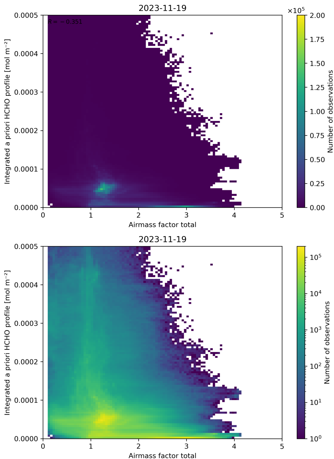
Figure 104: Scatter density plot of “Airmass factor total” against “Integrated a priori HCHO profile” for 2023-11-18 to 2023-11-20.
