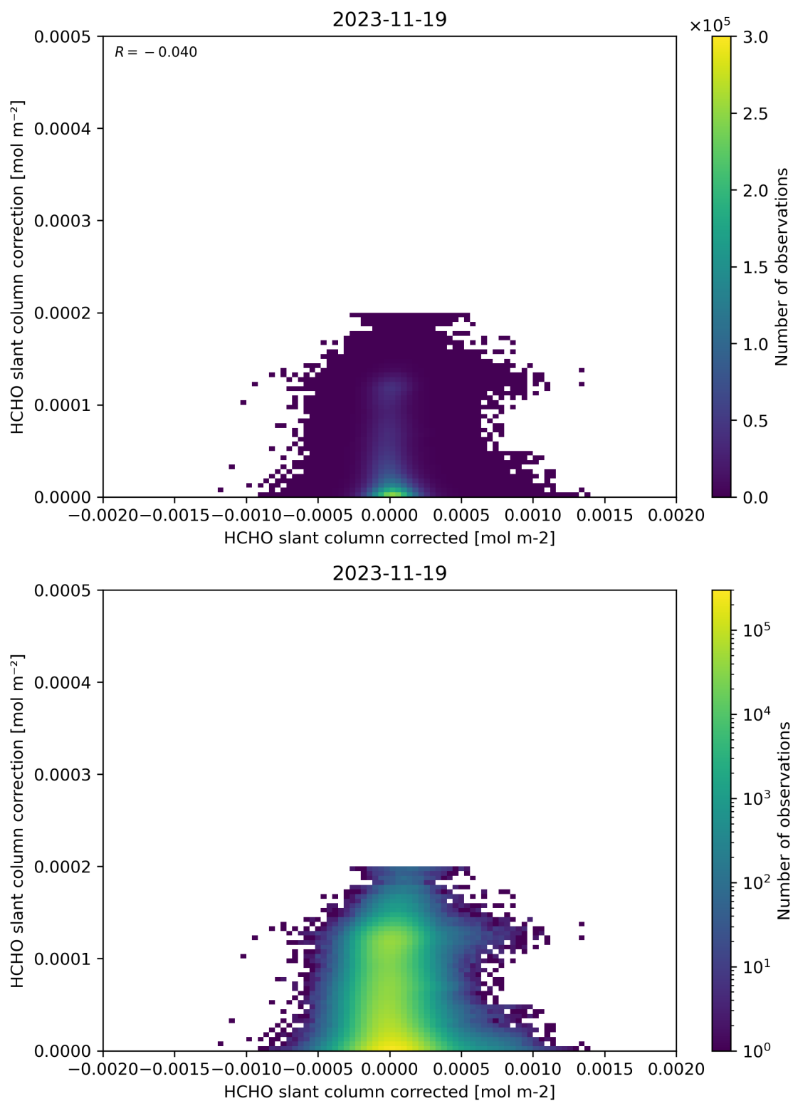
Figure 77: Scatter density plot of “HCHO slant column corrected” against “HCHO slant column correction” for 2023-11-18 to 2023-11-20.
