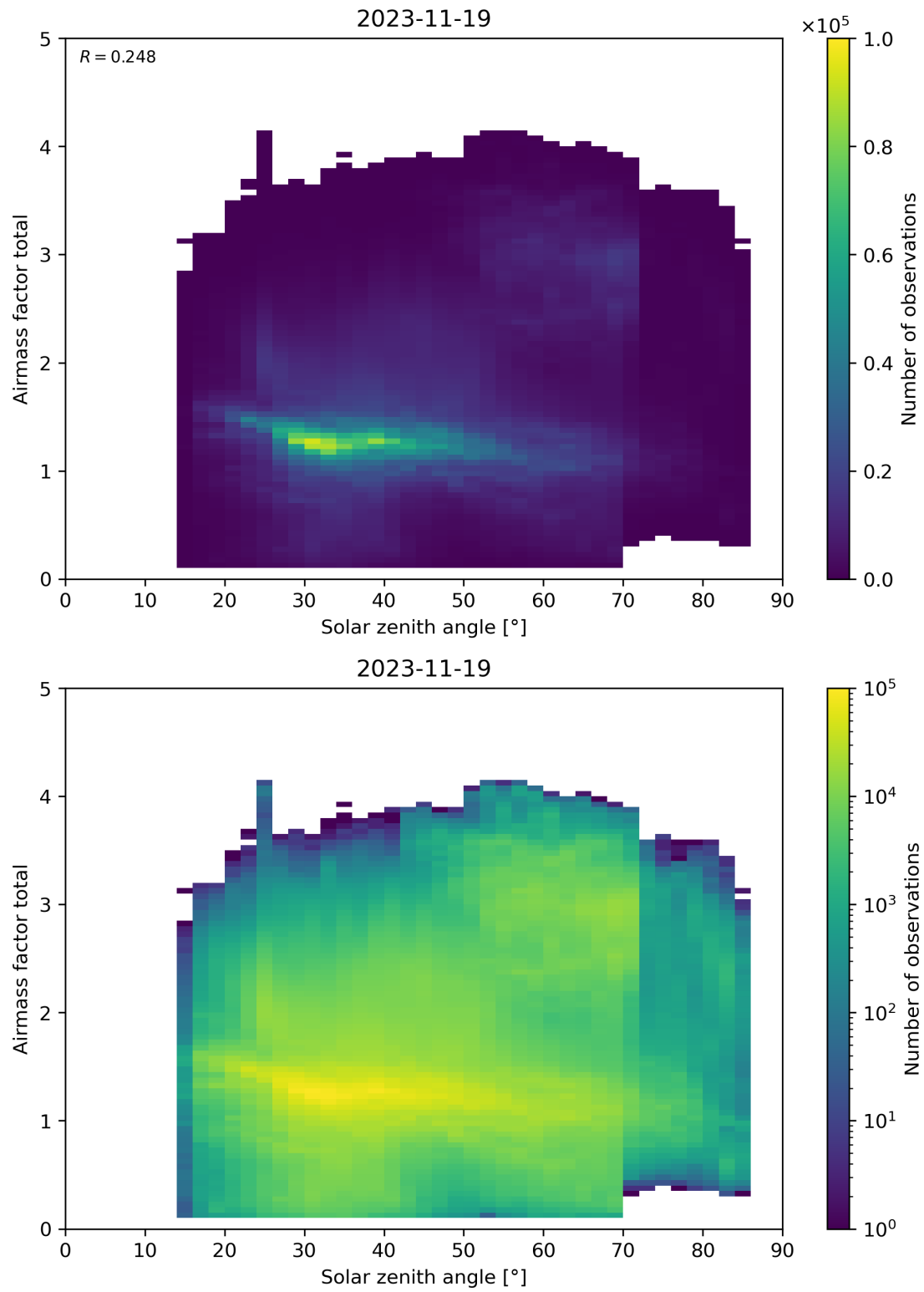
Figure 175: Scatter density plot of “Solar zenith angle” against “Airmass factor total” for 2023-11-18 to 2023-11-20.
