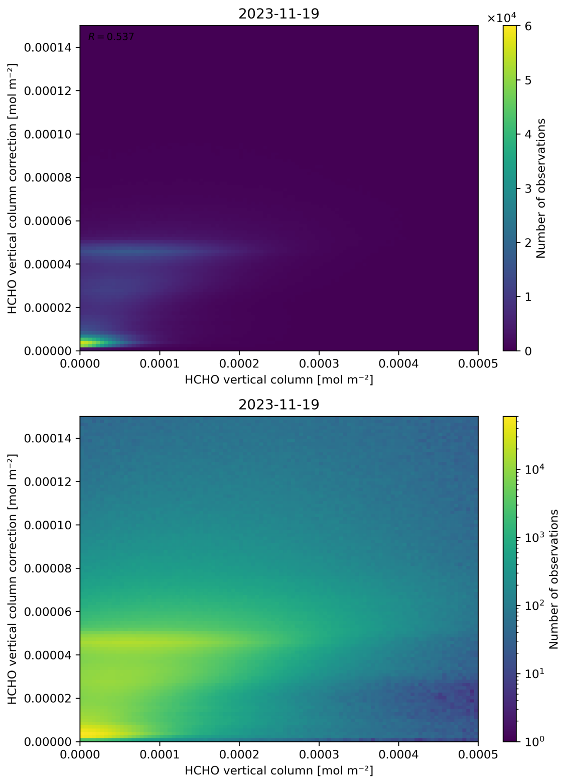
Figure 133: Scatter density plot of “HCHO vertical column” against “HCHO vertical column correction” for 2023-11-18 to 2023-11-20.
