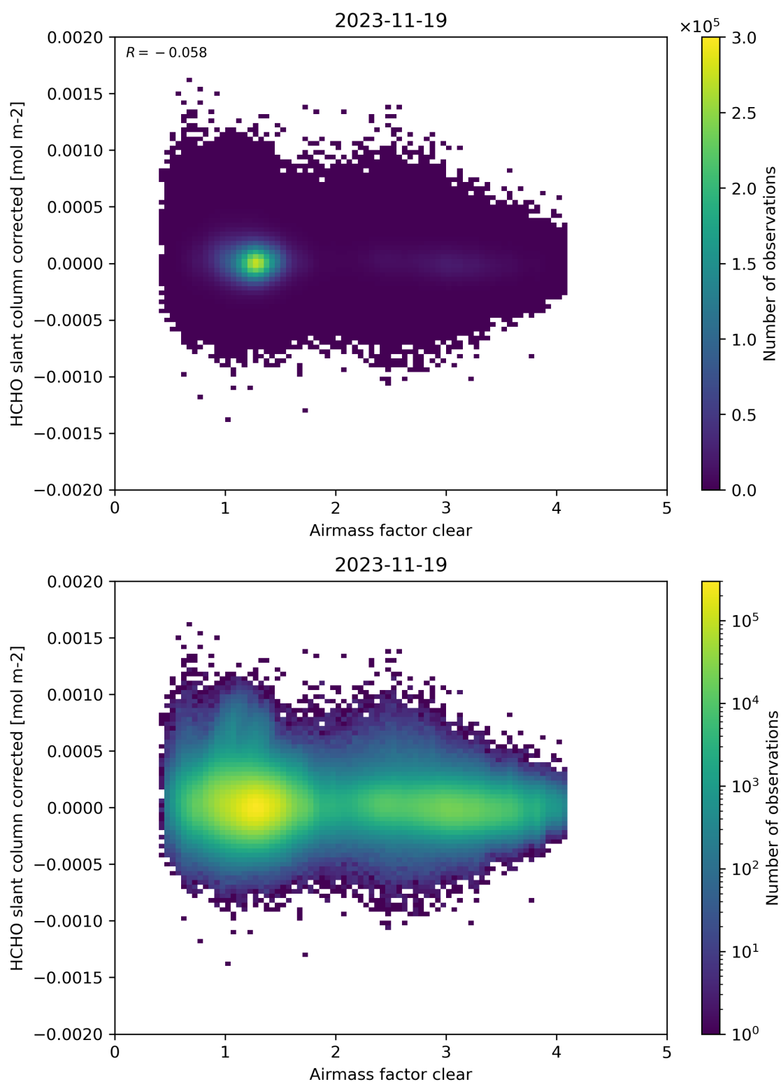
Figure 74: Scatter density plot of “Airmass factor clear” against “HCHO slant column corrected” for 2023-11-18 to 2023-11-20.
