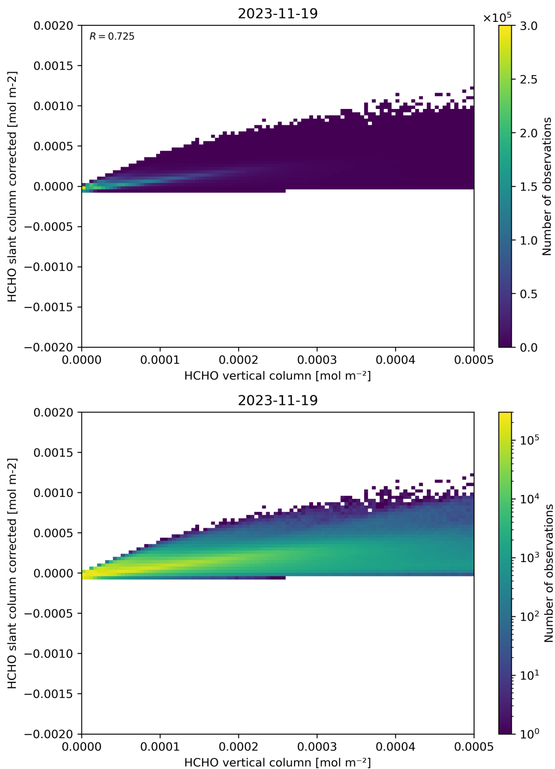
Figure 127: Scatter density plot of “HCHO vertical column” against “HCHO slant column corrected” for 2023-11-18 to 2023-11-20.
