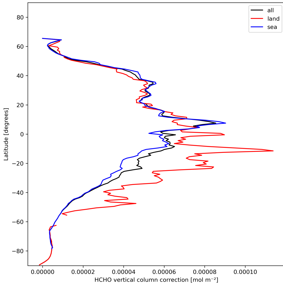
Figure 23: Zonal average of “HCHO vertical column correction” for 2023-11-18 to 2023-11-20.
