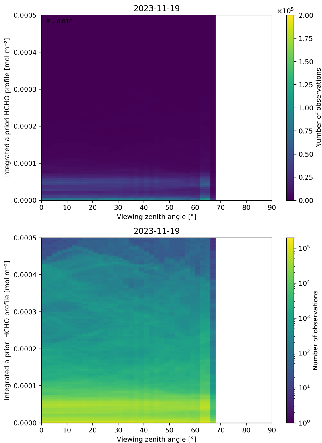
Figure 195: Scatter density plot of “Viewing zenith angle” against “Integrated a priori HCHO profile” for 2023-11-18 to 2023-11-20.
