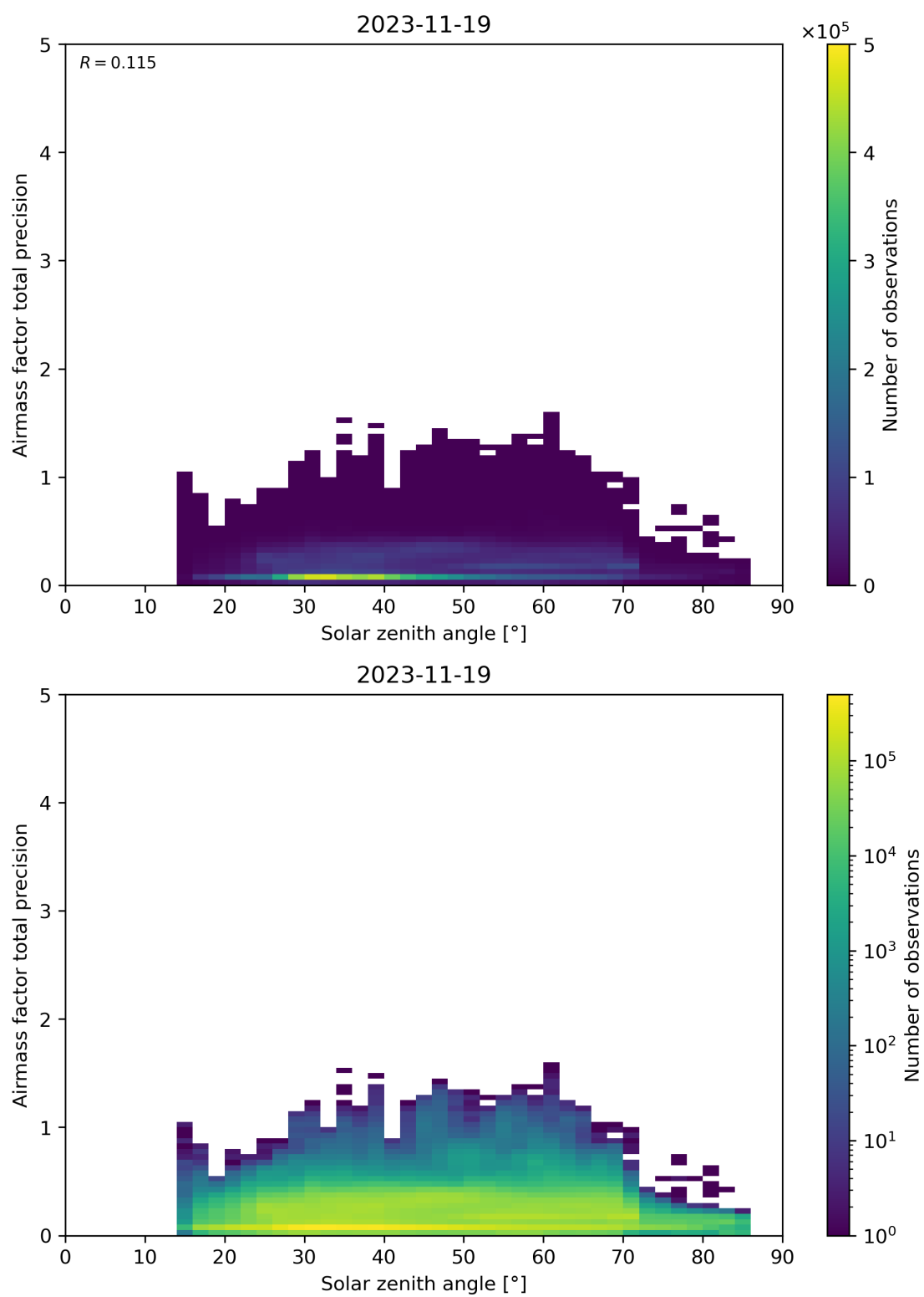
Figure 176: Scatter density plot of “Solar zenith angle” against “Airmass factor total precision” for 2023-11-18 to 2023-11-20.
