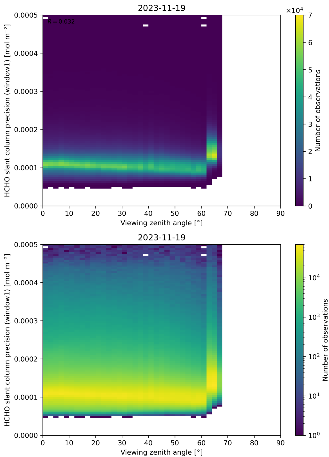
Figure 189: Scatter density plot of “Viewing zenith angle” against “HCHO slant column precision (window1)” for 2023-11-18 to 2023-11-20.
