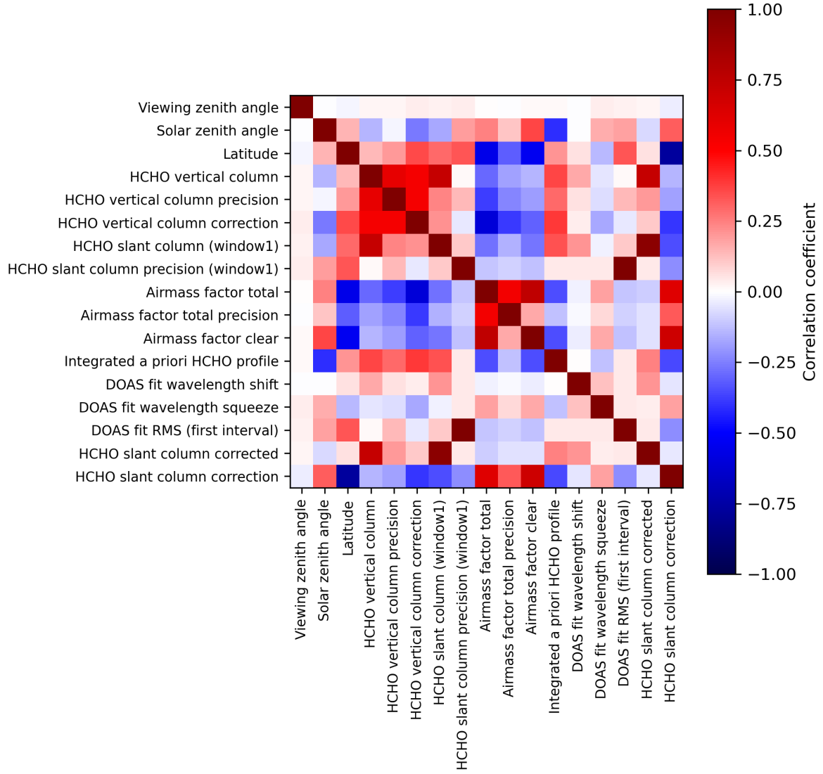
Figure 2: Map of correlation matrix for 2023-11-18 to 2023-11-20.
