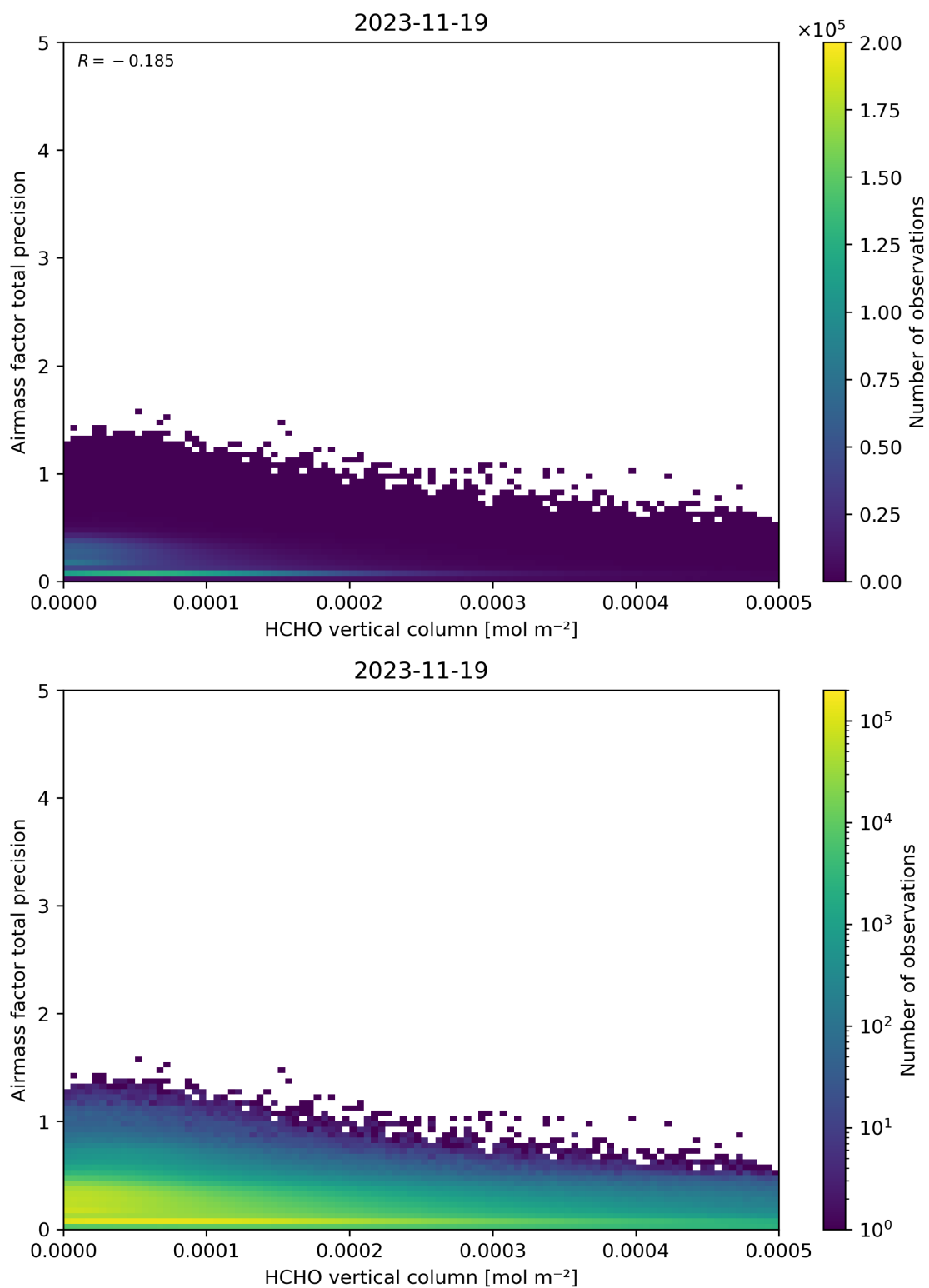
Figure 132: Scatter density plot of “HCHO vertical column” against “Airmass factor total precision” for 2023-11-18 to 2023-11-20.
