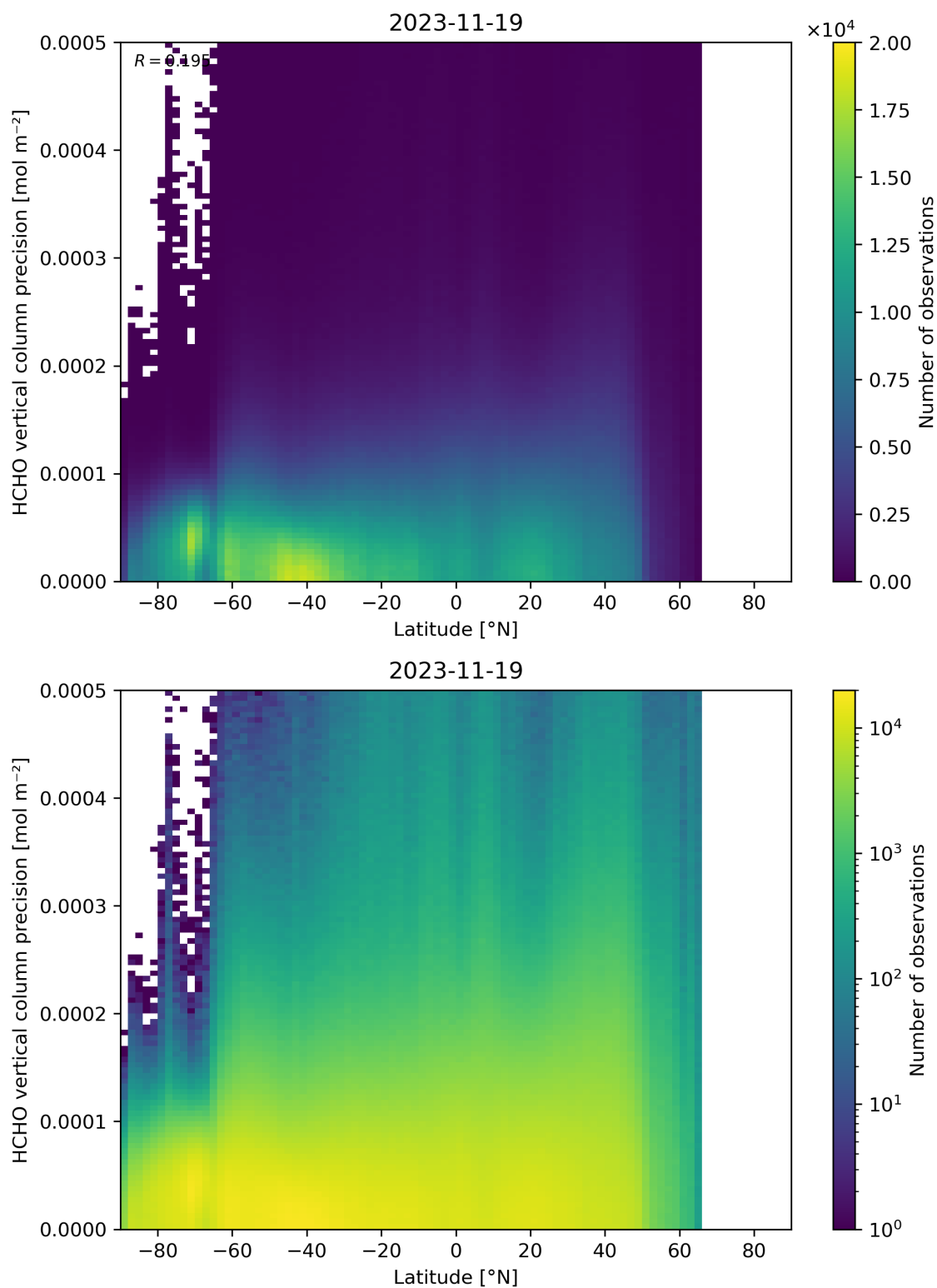
Figure 165: Scatter density plot of “Latitude” against “HCHO vertical column precision” for 2023-11-18 to 2023-11-20.
