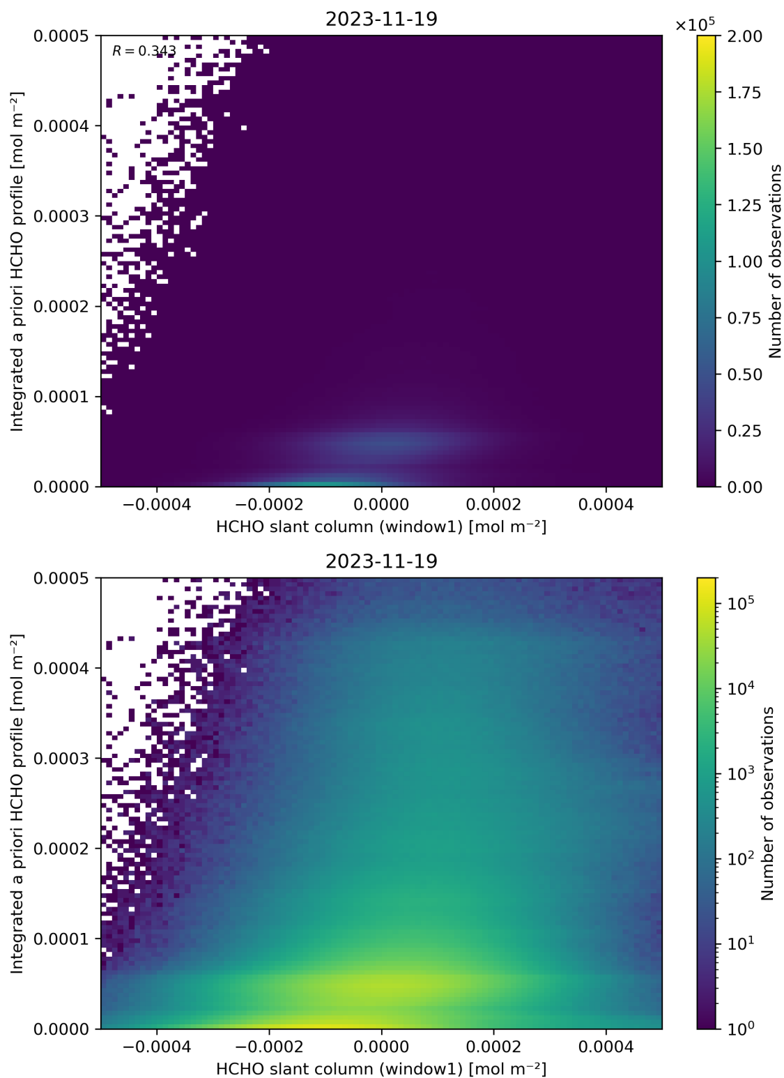
Figure 87: Scatter density plot of “HCHO slant column (window1)” against “Integrated a priori HCHO profile” for 2023-11-18 to 2023-11-20.
