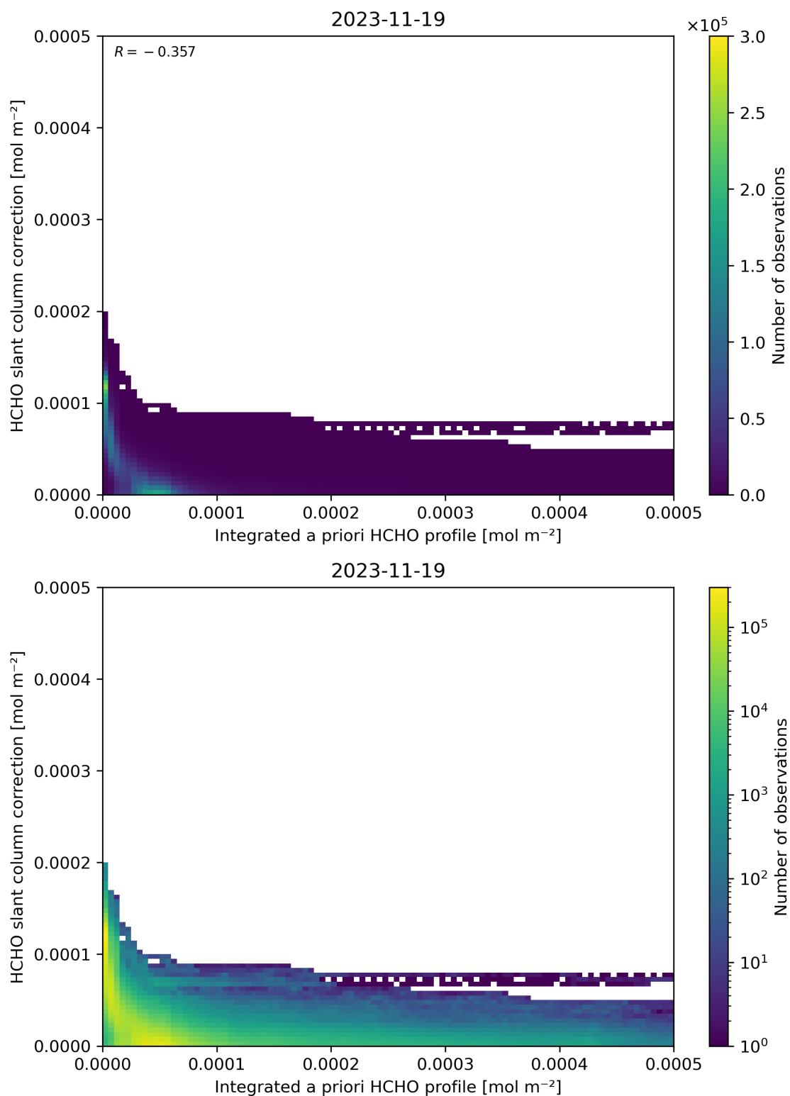
Figure 152: Scatter density plot of “Integrated a priori HCHO profile” against “HCHO slant column correction” for 2023-11-18 to 2023-11-20.
