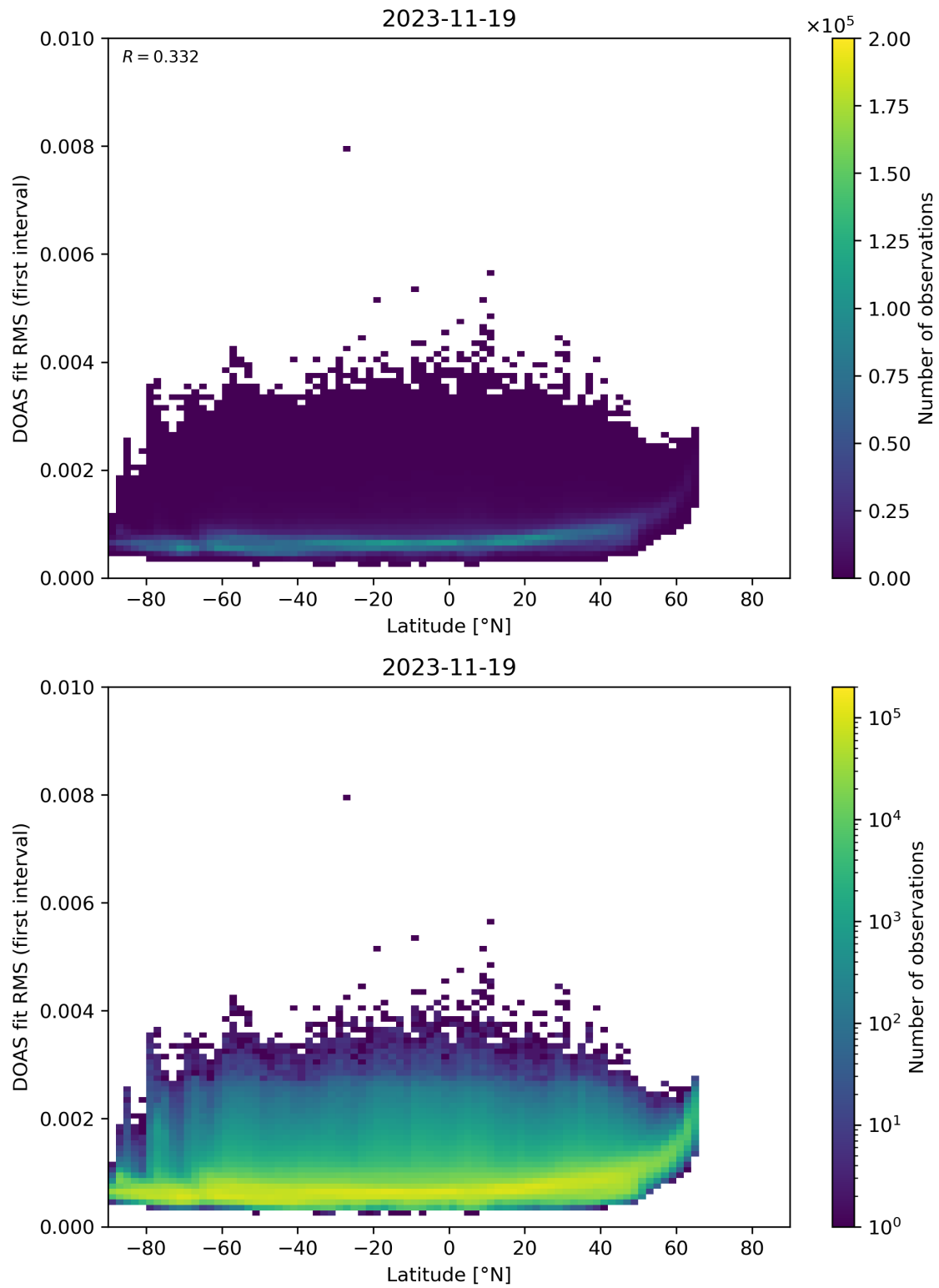
Figure 153: Scatter density plot of “Latitude” against “DOAS fit RMS (first interval)” for 2023-11-18 to 2023-11-20.
