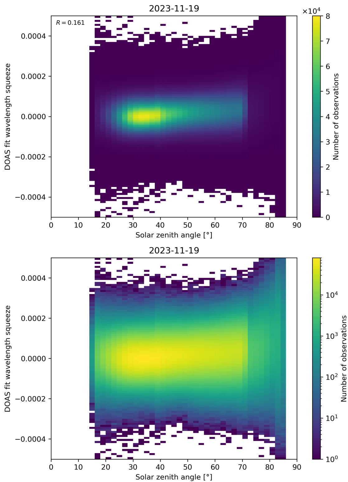
Figure 169: Scatter density plot of “Solar zenith angle” against “DOAS fit wavelength squeeze” for 2023-11-18 to 2023-11-20.
