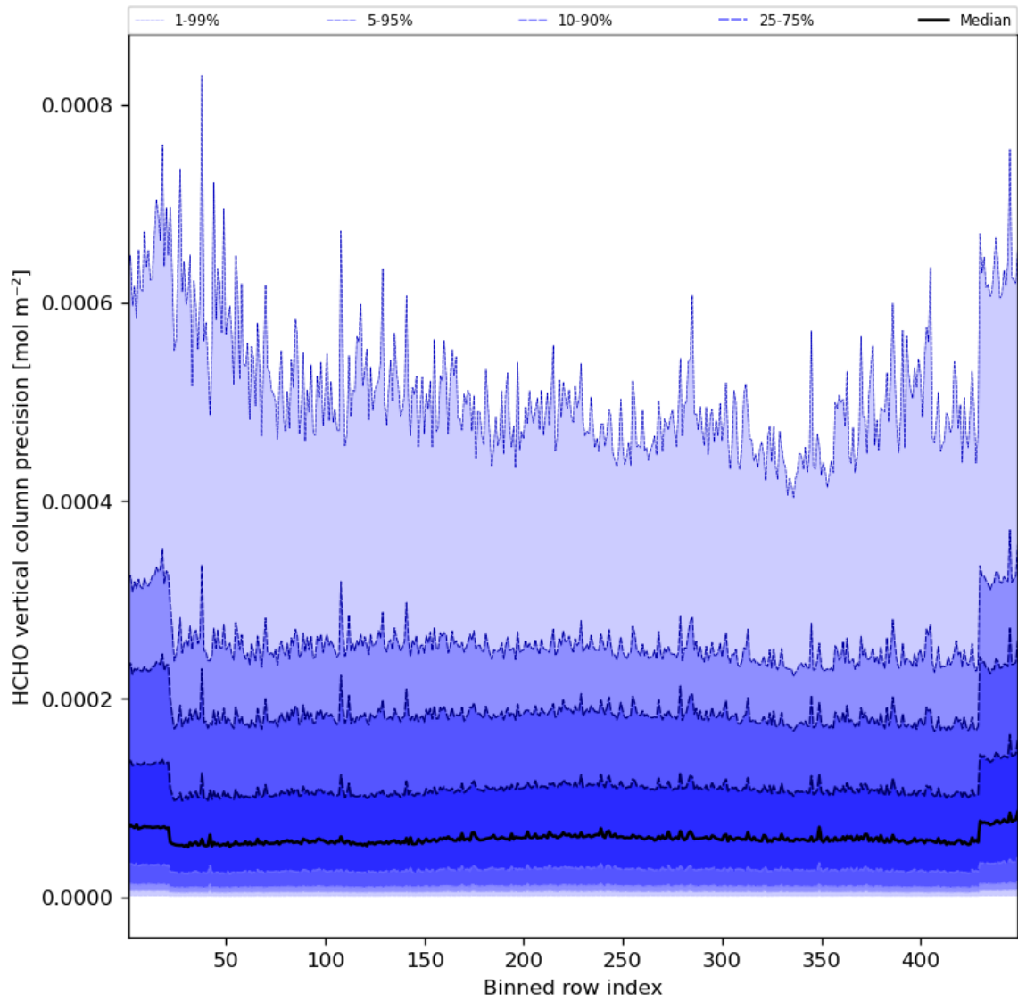
Figure 50: Along track statistics of “HCHO vertical column precision” for 2023-11-18 to 2023-11-20
