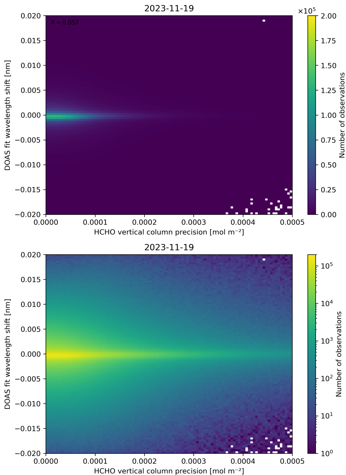
Figure 137: Scatter density plot of “HCHO vertical column precision” against “DOAS fit wavelength shift” for 2023-11-18 to 2023-11-20.
