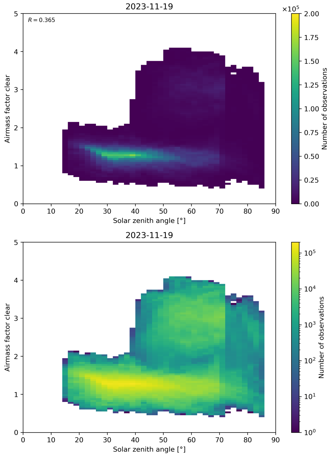
Figure 170: Scatter density plot of “Solar zenith angle” against “Airmass factor clear” for 2023-11-18 to 2023-11-20.
