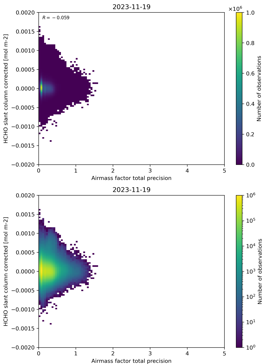
Figure 109: Scatter density plot of “Airmass factor total precision” against “HCHO slant column corrected” for 2023-11-18 to 2023-11-20.
