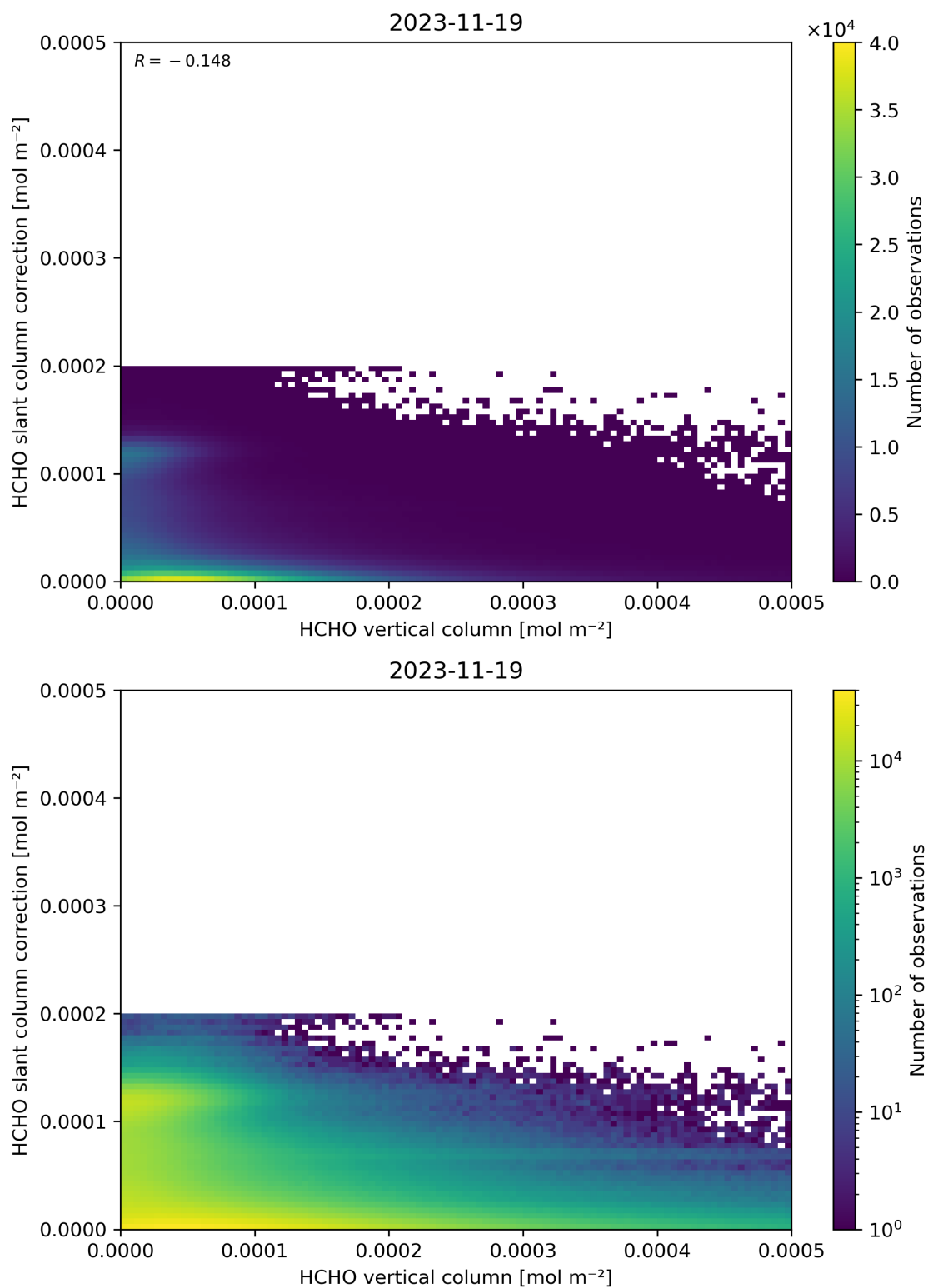
Figure 128: Scatter density plot of “HCHO vertical column” against “HCHO slant column correction” for 2023-11-18 to 2023-11-20.
