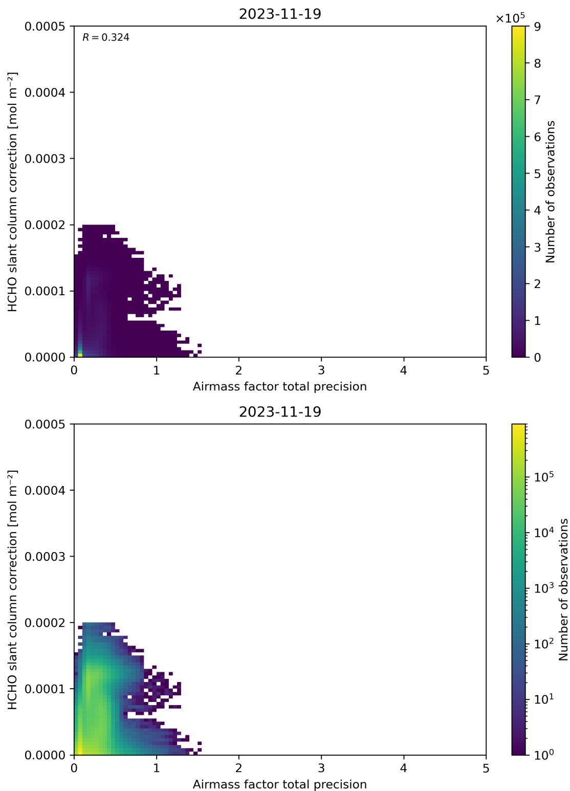
Figure 110: Scatter density plot of “Airmass factor total precision” against “HCHO slant column correction” for 2023-11-18 to 2023-11-20.
