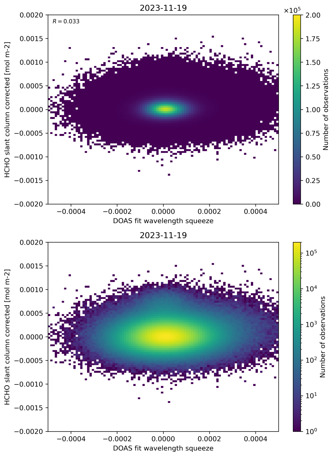
Figure 69: Scatter density plot of “DOAS fit wavelength squeeze” against “HCHO slant column corrected” for 2023-11-18 to 2023-11-20.
