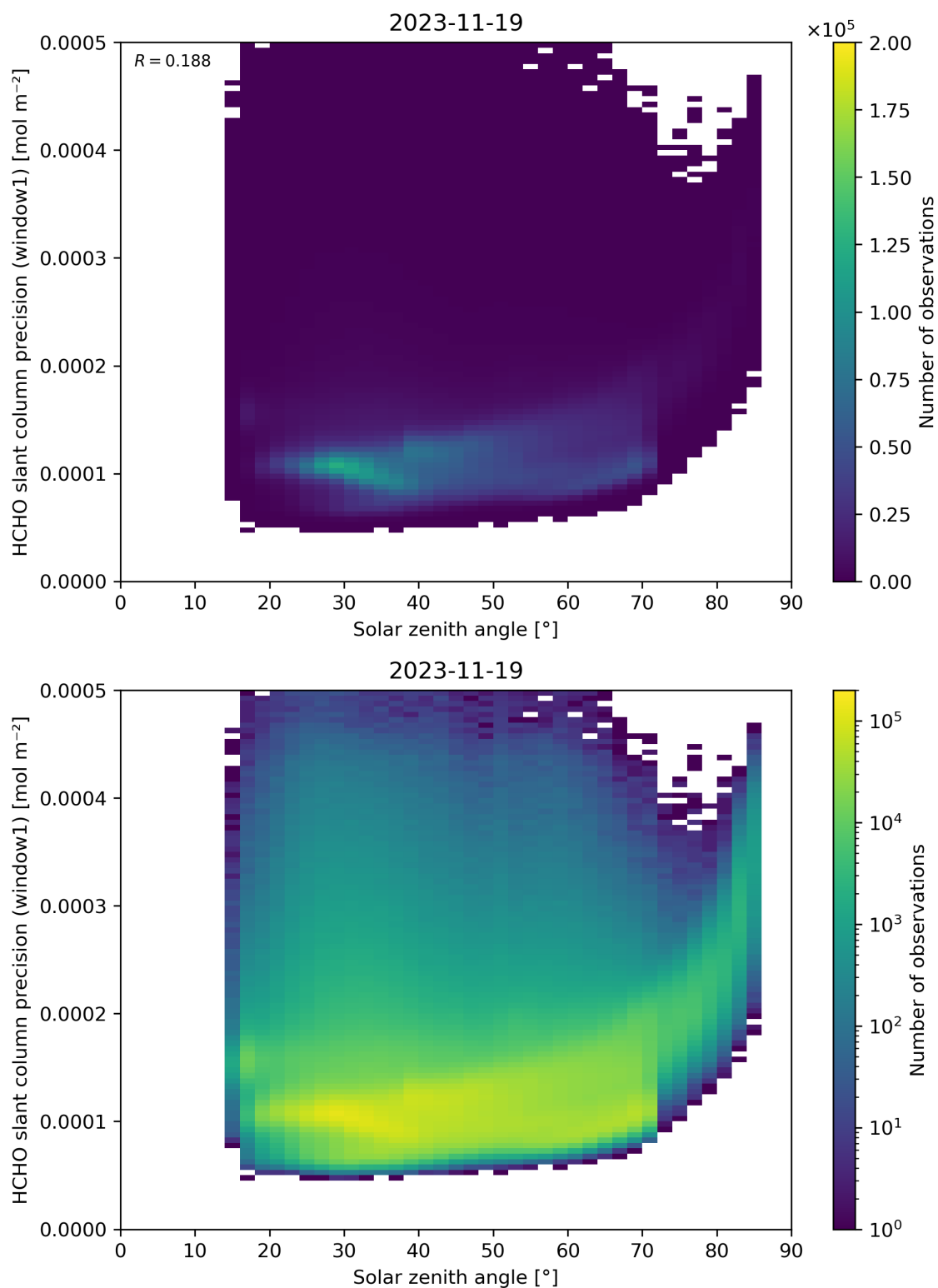
Figure 174: Scatter density plot of “Solar zenith angle” against “HCHO slant column precision (window1)” for 2023-11-18 to 2023-11-20.
