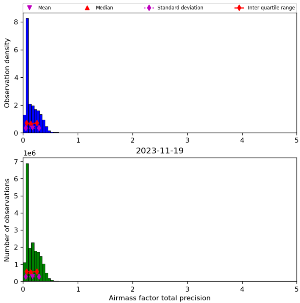
Figure 41: Histogram of “Airmass factor total precision” for 2023-11-18 to 2023-11-20
