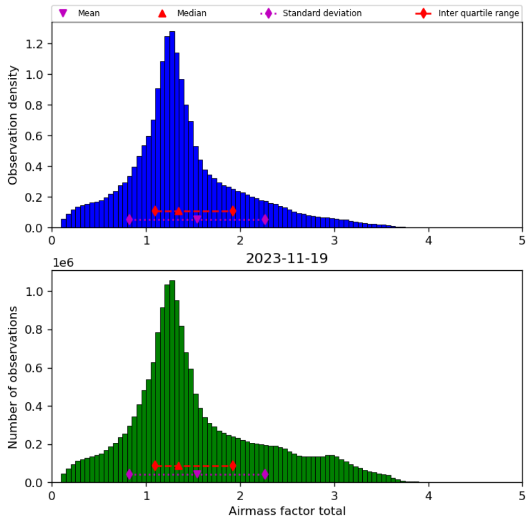
Figure 40: Histogram of “Airmass factor total” for 2023-11-18 to 2023-11-20
