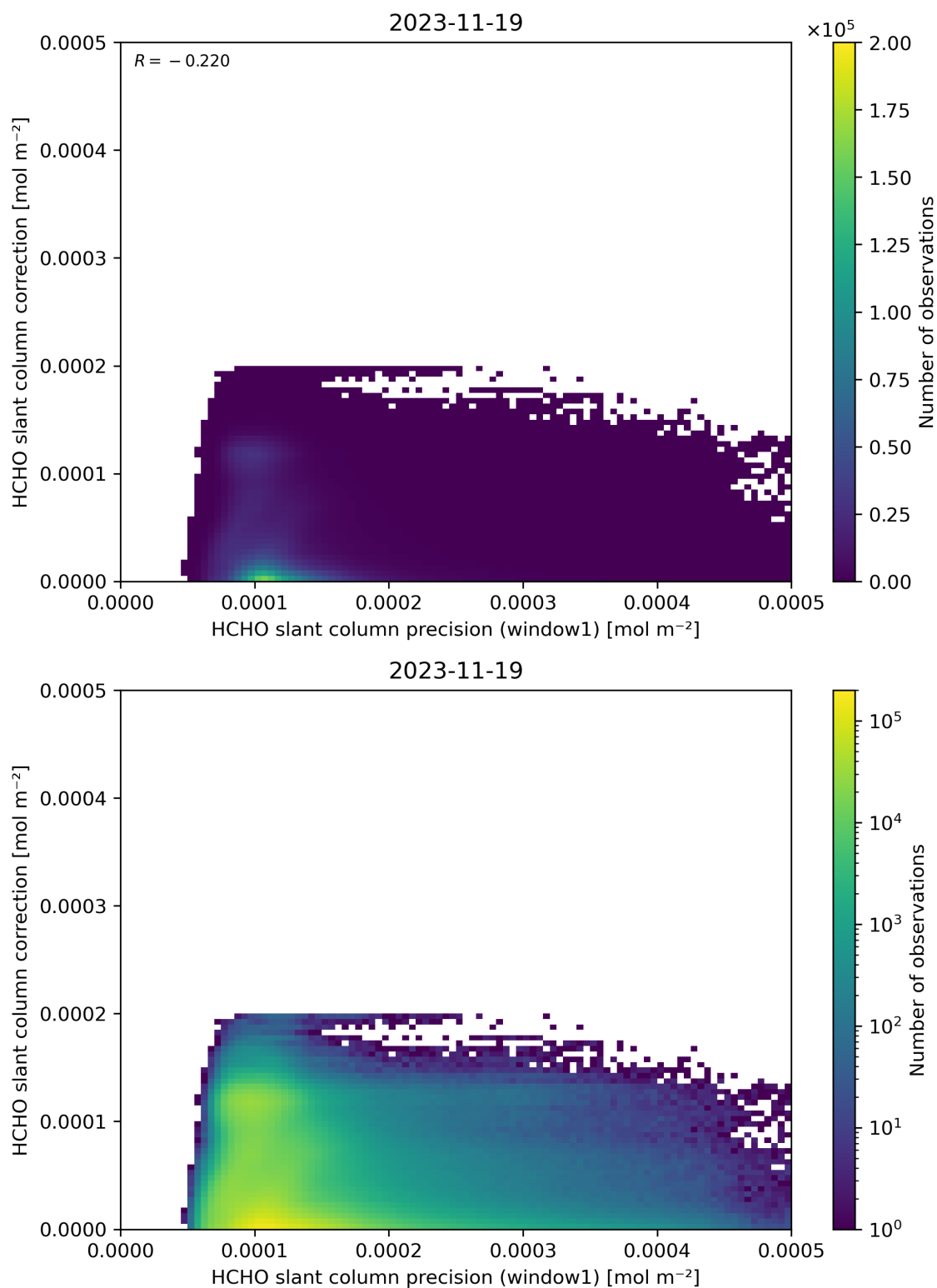
Figure 93: Scatter density plot of “HCHO slant column precision (window1)” against “HCHO slant column correction” for 2023-11-18 to 2023-11-20.
