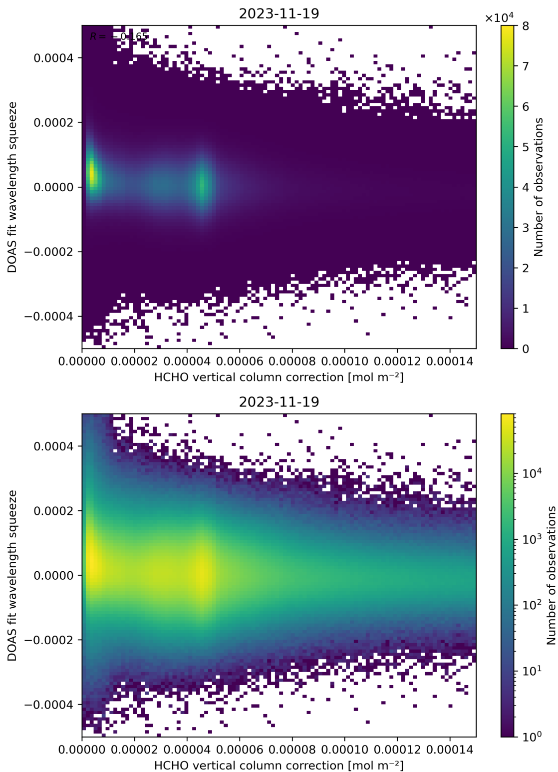
Figure 114: Scatter density plot of “HCHO vertical column correction” against “DOAS fit wavelength squeeze” for 2023-11-18 to 2023-11-20.
