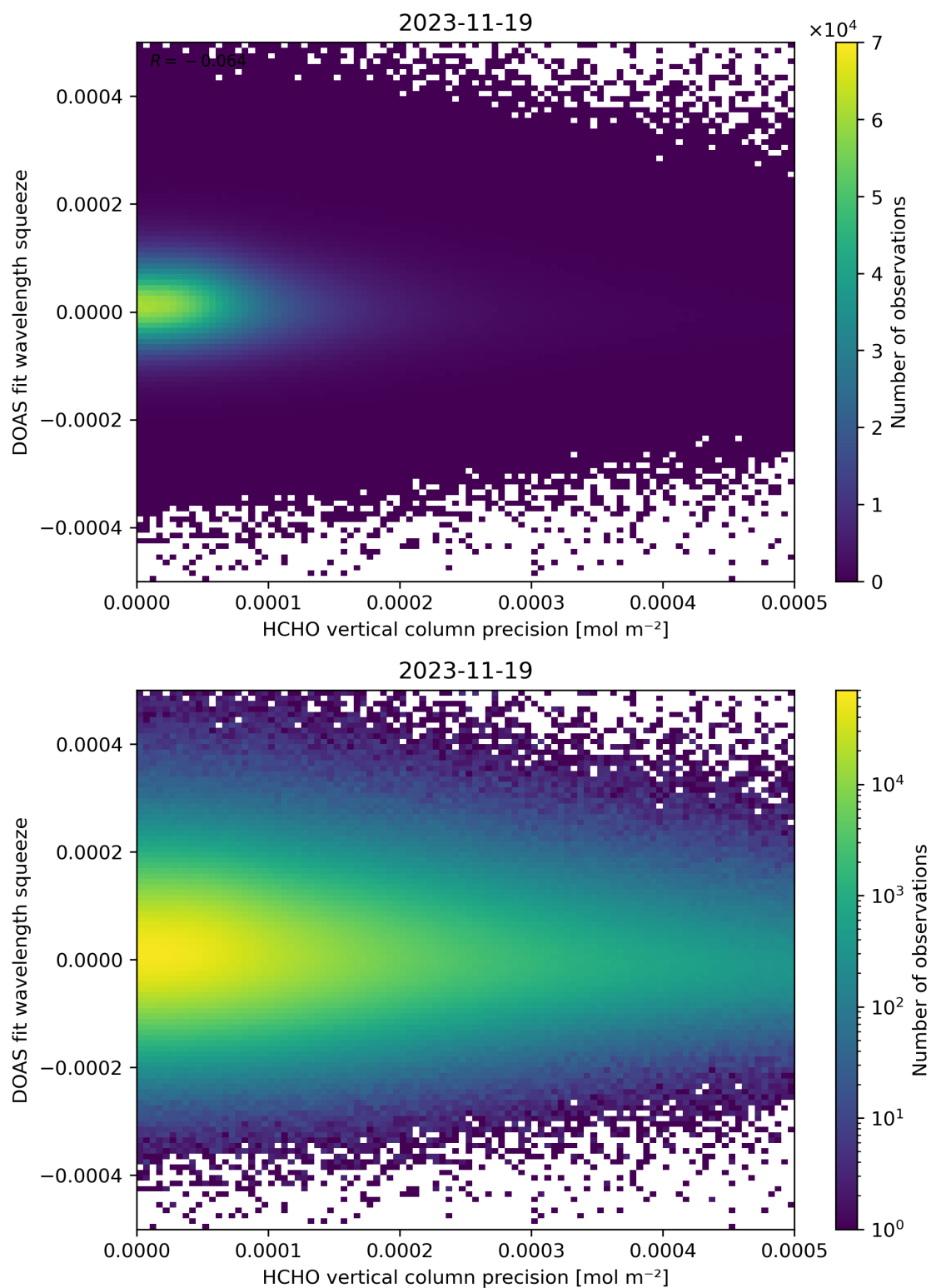
Figure 138: Scatter density plot of “HCHO vertical column precision” against “DOAS fit wavelength squeeze” for 2023-11-18 to 2023-11-20.
