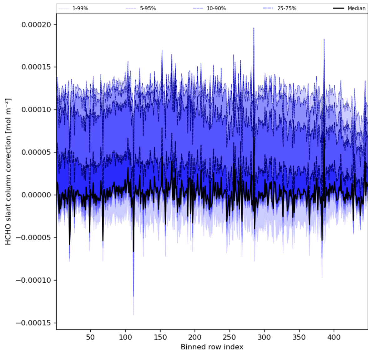
Figure 61: Along track statistics of “HCHO slant column correction” for 2023-11-18 to 2023-11-20
