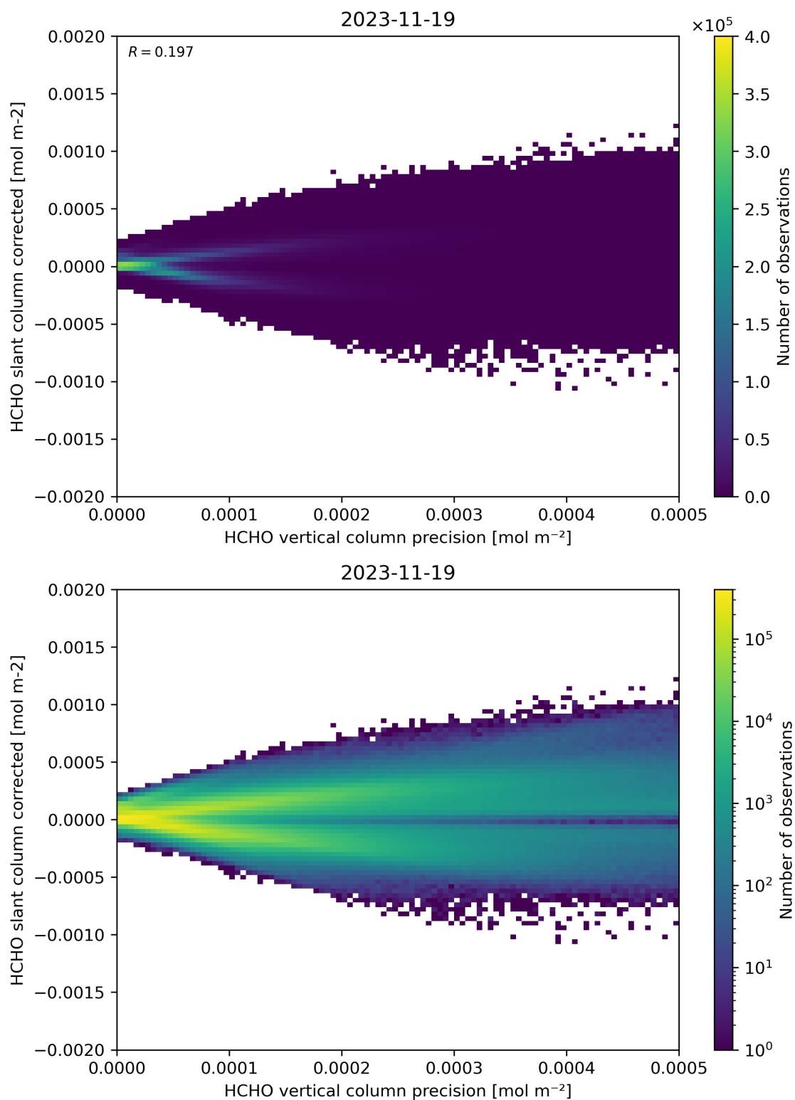
Figure 140: Scatter density plot of “HCHO vertical column precision” against “HCHO slant column corrected” for 2023-11-18 to 2023-11-20.
