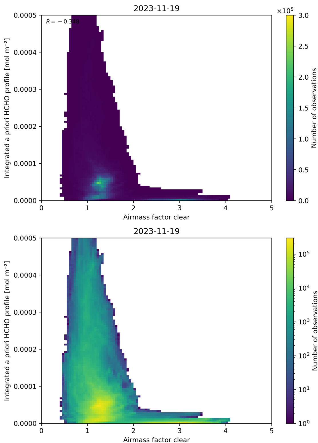
Figure 76: Scatter density plot of “Airmass factor clear” against “Integrated a priori HCHO profile” for 2023-11-18 to 2023-11-20.
