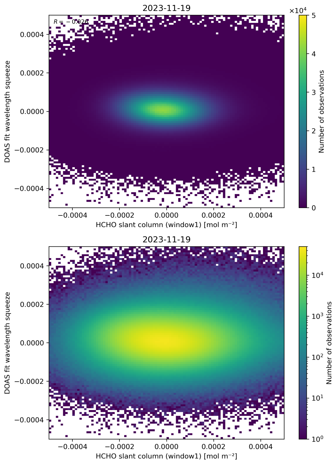
Figure 80: Scatter density plot of “HCHO slant column (window1)” against “DOAS fit wavelength squeeze” for 2023-11-18 to 2023-11-20.
