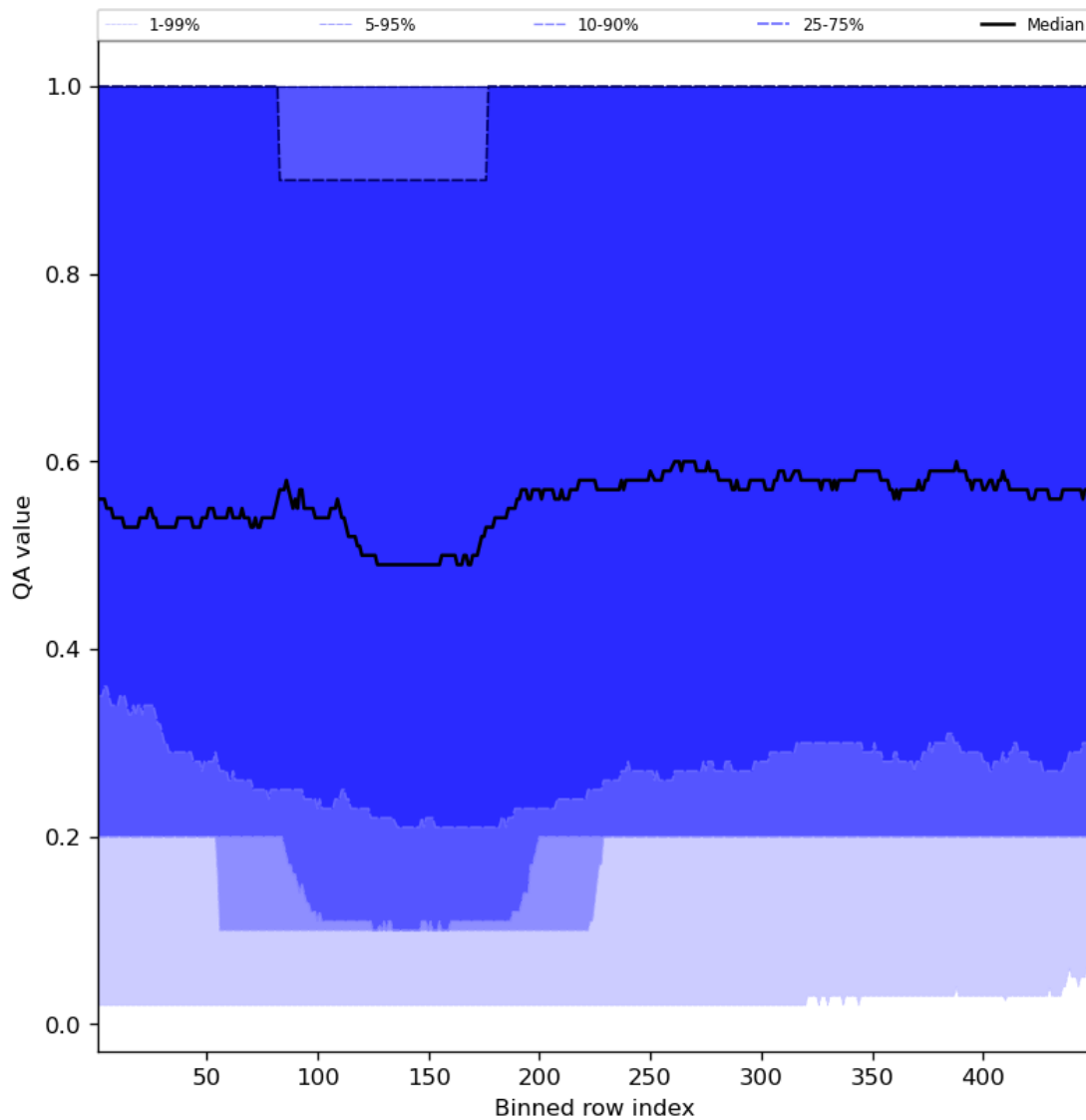
Figure 48: Along track statistics of “QA value” for 2023-11-18 to 2023-11-20
