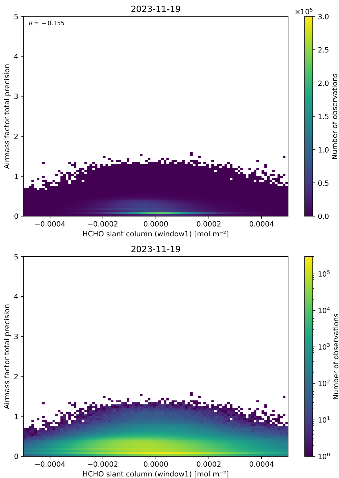
Figure 86: Scatter density plot of “HCHO slant column (window1)” against “Airmass factor total precision” for 2023-11-18 to 2023-11-20.
