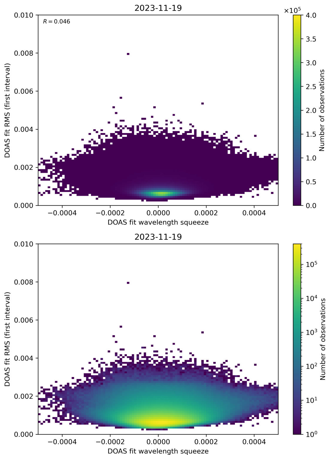
Figure 68: Scatter density plot of “DOAS fit wavelength squeeze” against “DOAS fit RMS (first interval)” for 2023-11-18 to 2023-11-20.
