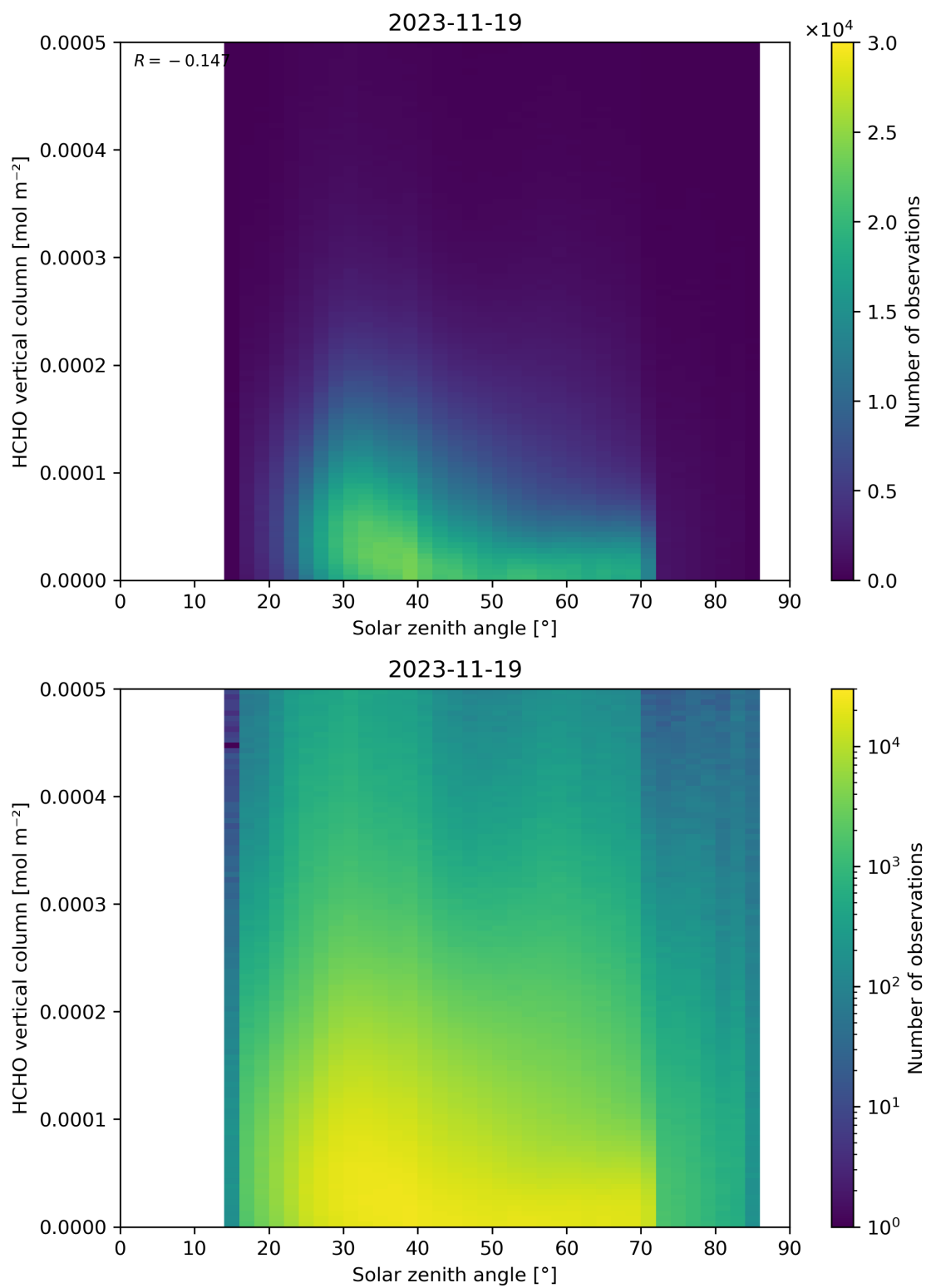
Figure 177: Scatter density plot of “Solar zenith angle” against “HCHO vertical column” for 2023-11-18 to 2023-11-20.
