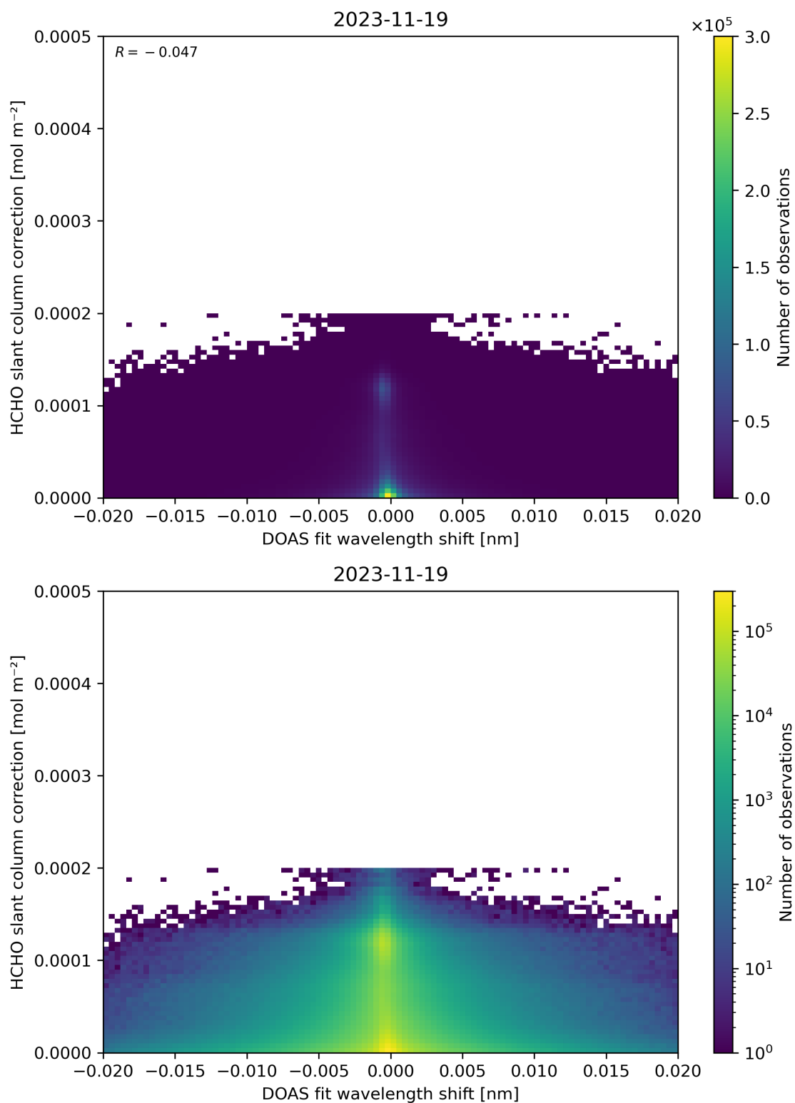
Figure 67: Scatter density plot of “DOAS fit wavelength shift” against “HCHO slant column correction” for 2023-11-18 to 2023-11-20.
