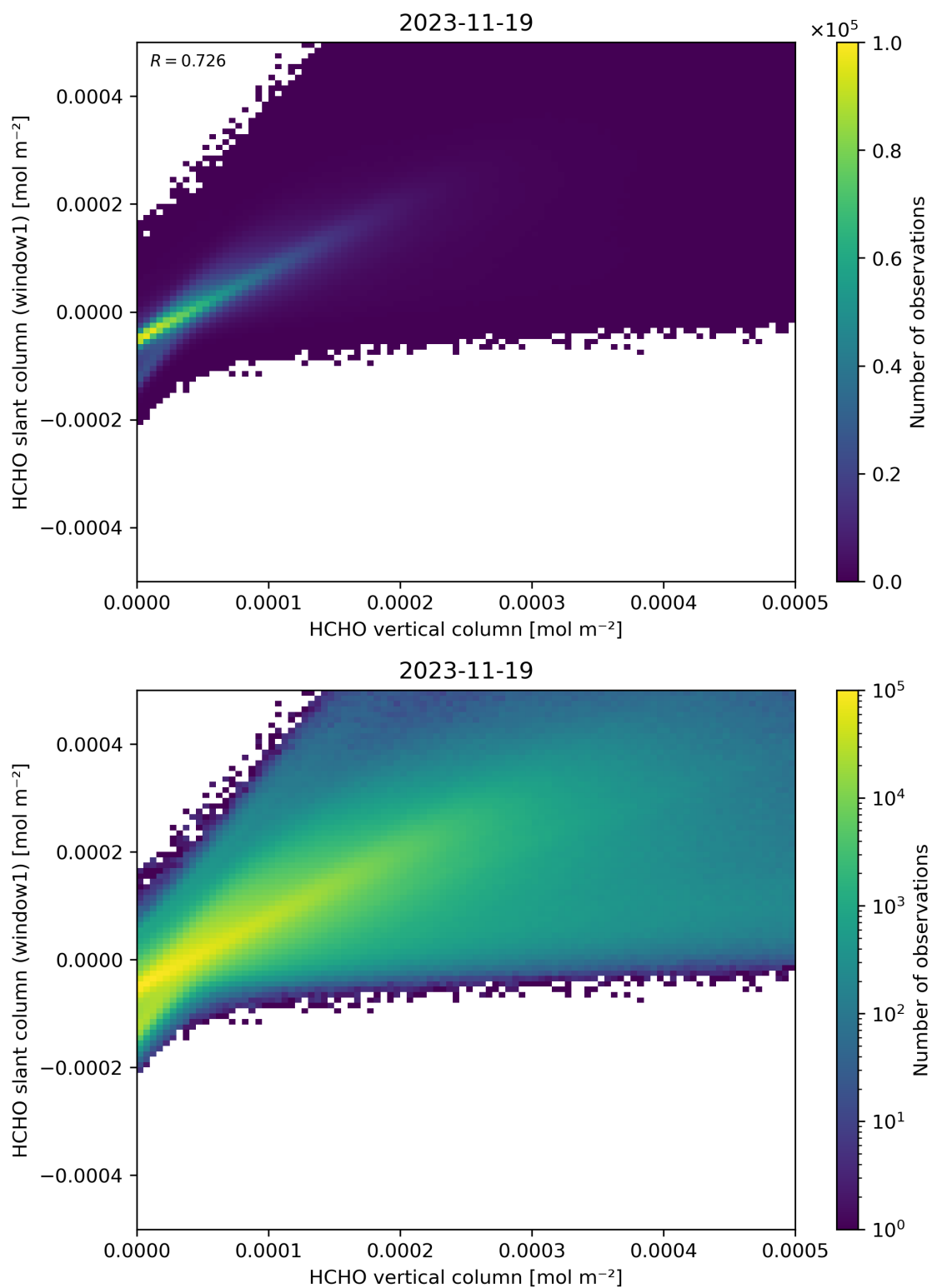
Figure 129: Scatter density plot of “HCHO vertical column” against “HCHO slant column (window1)” for 2023-11-18 to 2023-11-20.
