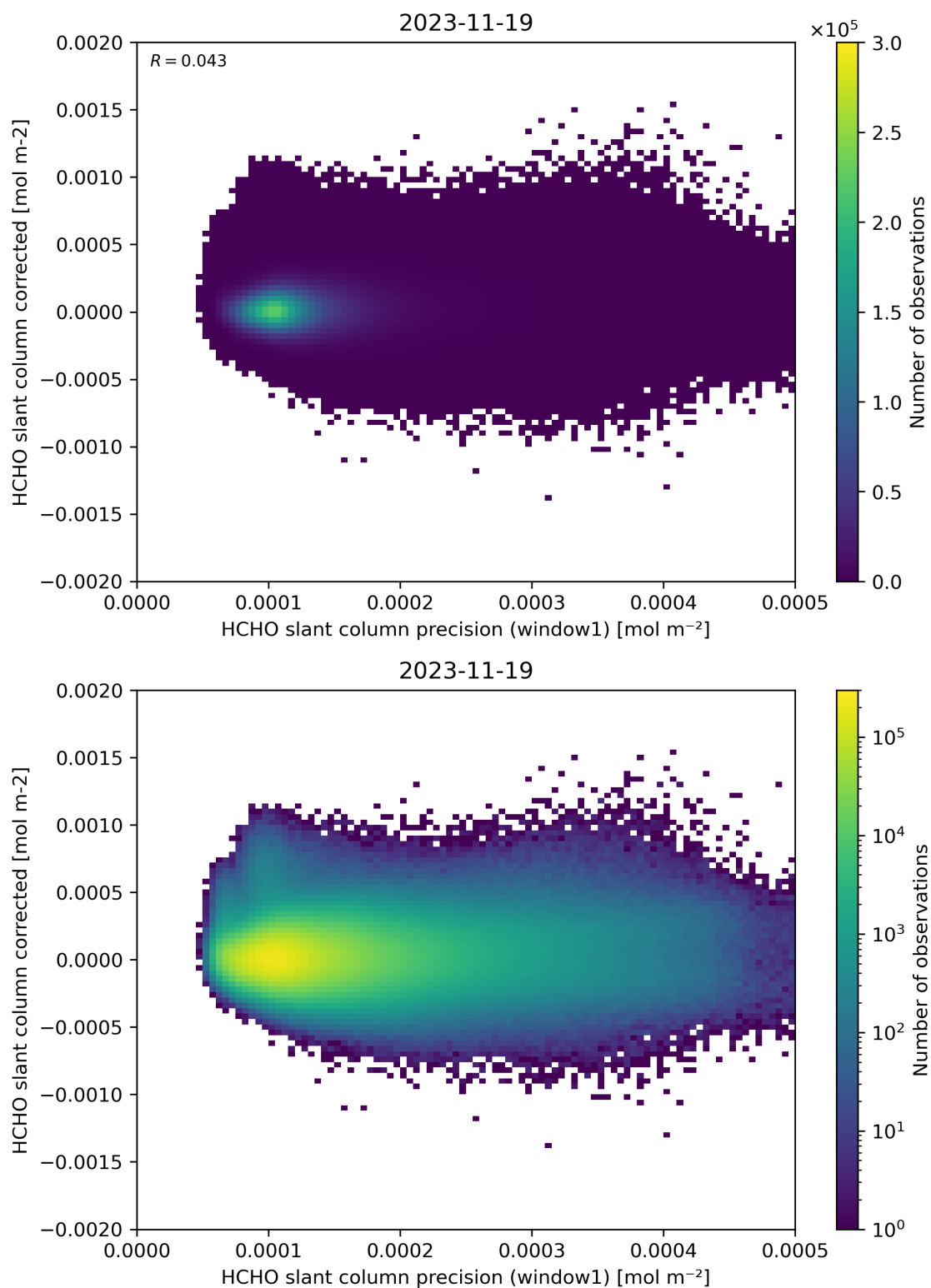
Figure 92: Scatter density plot of “HCHO slant column precision (window1)” against “HCHO slant column corrected” for 2023-11-18 to 2023-11-20.
