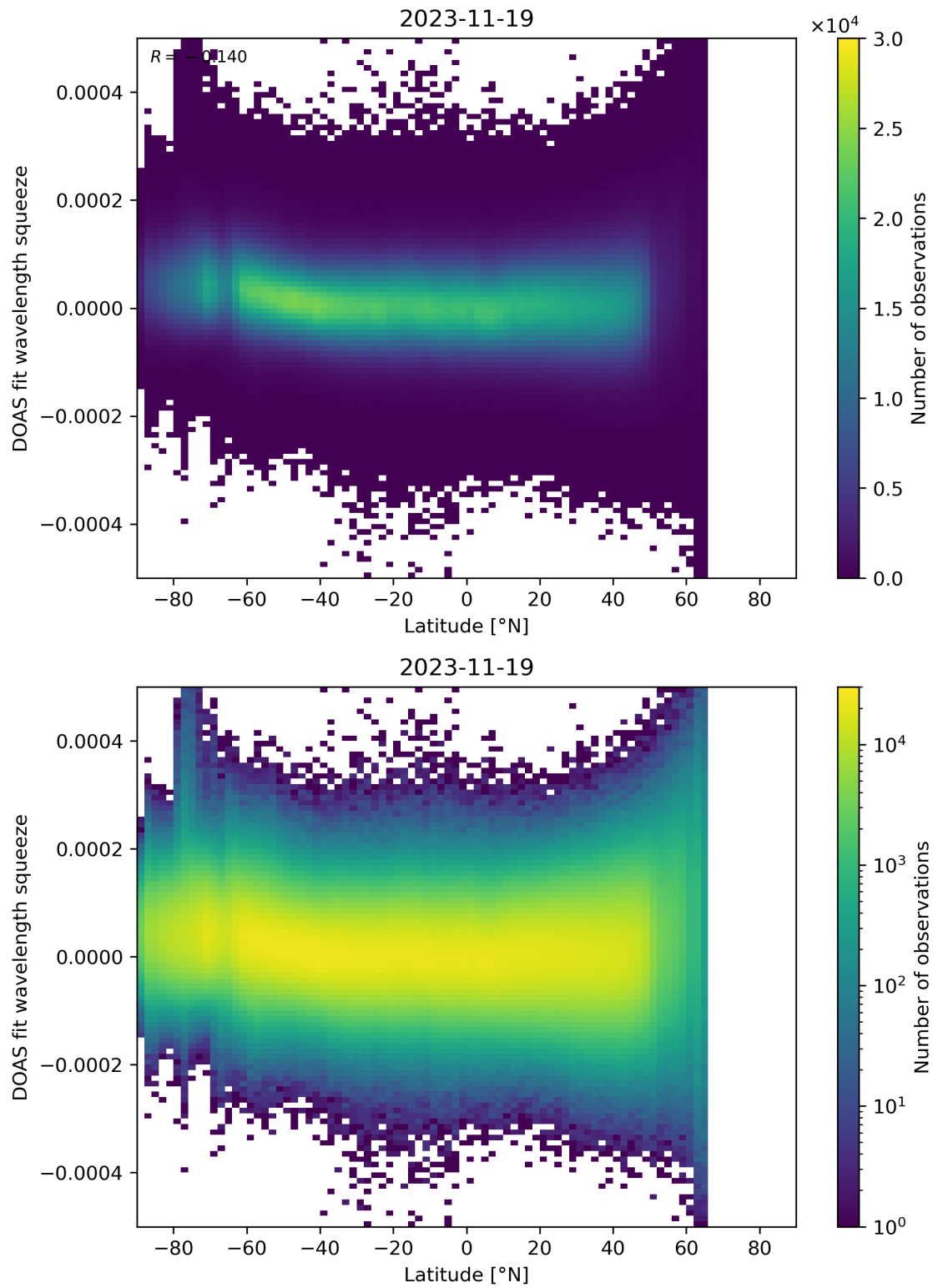
Figure 155: Scatter density plot of “Latitude” against “DOAS fit wavelength squeeze” for 2023-11-18 to 2023-11-20.
