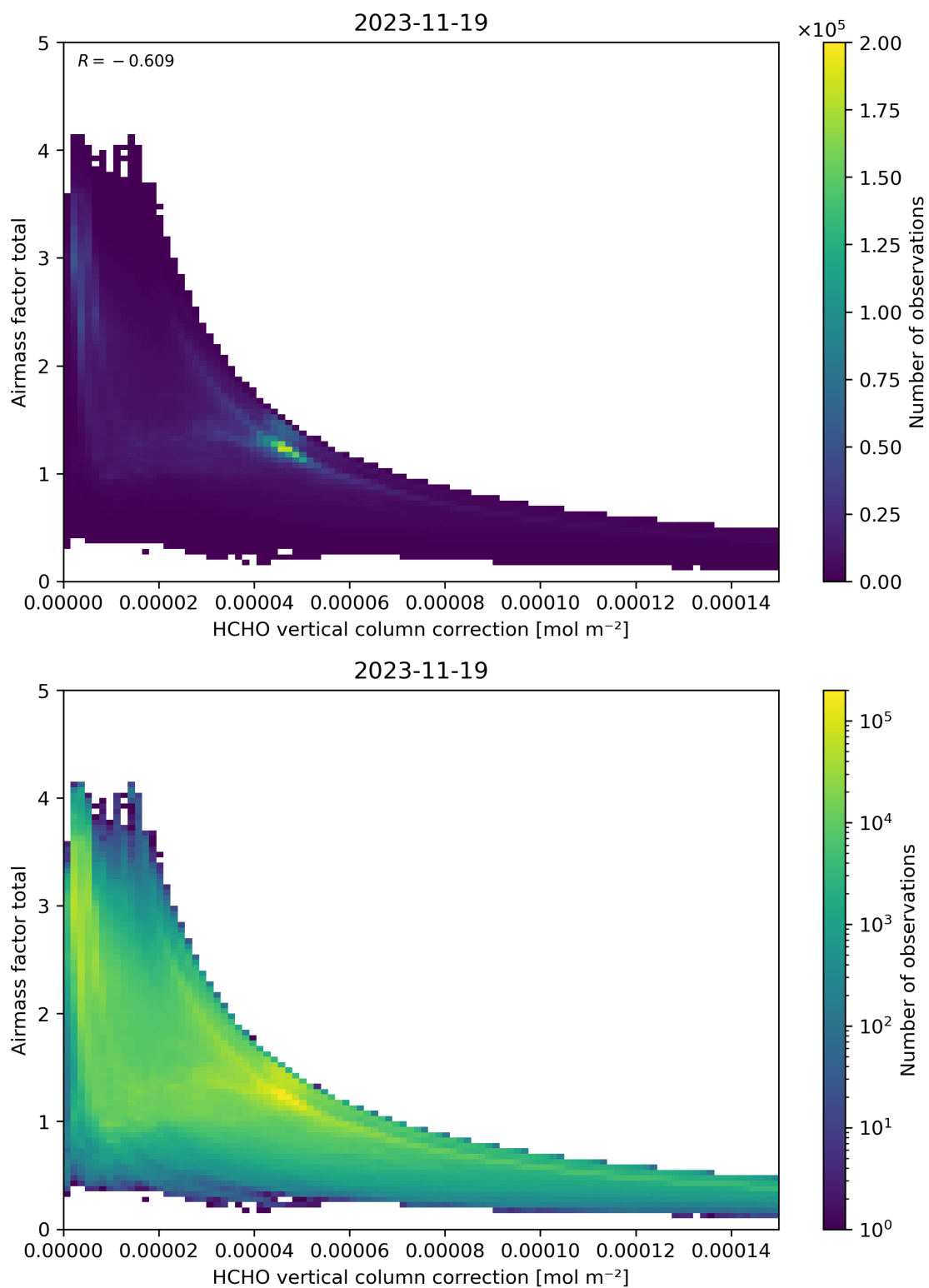
Figure 120: Scatter density plot of “HCHO vertical column correction” against “Airmass factor total” for 2023-11-18 to 2023-11-20.
