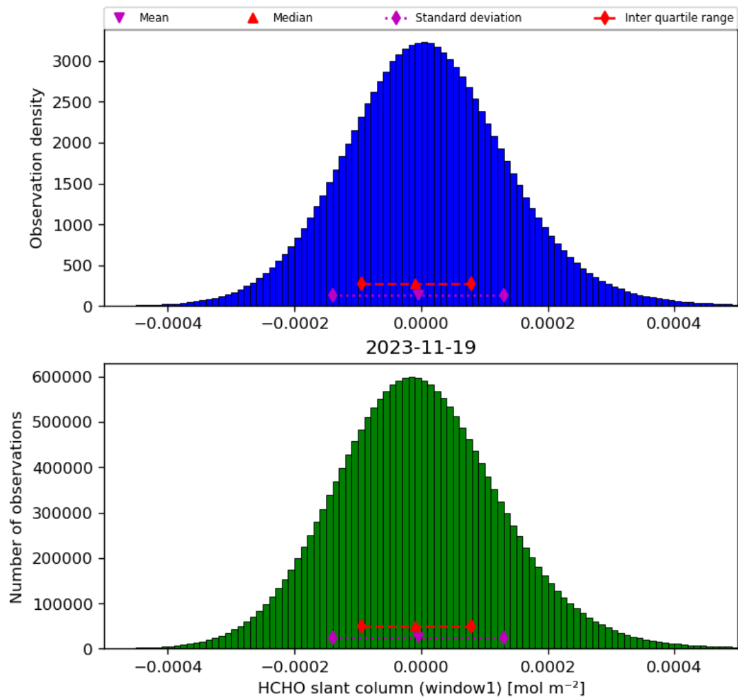
Figure 38: Histogram of “HCHO slant column (window1)” for 2023-11-18 to 2023-11-20
