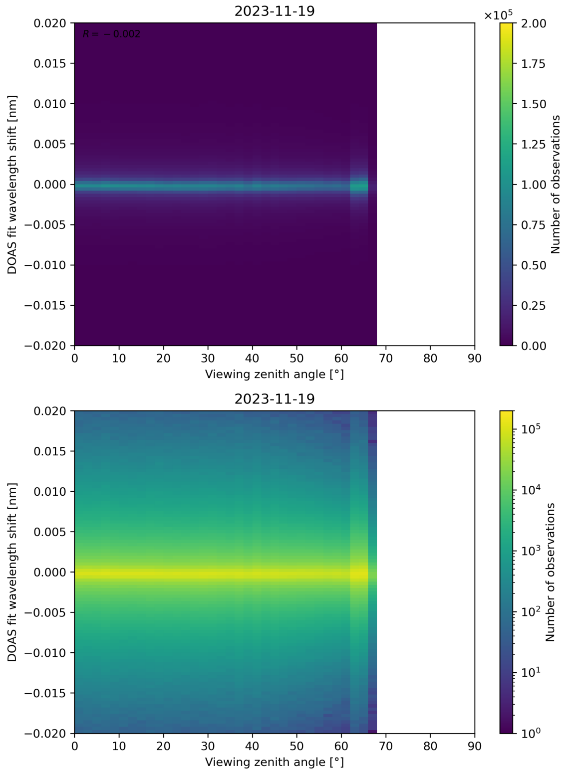
Figure 183: Scatter density plot of “Viewing zenith angle” against “DOAS fit wavelength shift” for 2023-11-18 to 2023-11-20.
