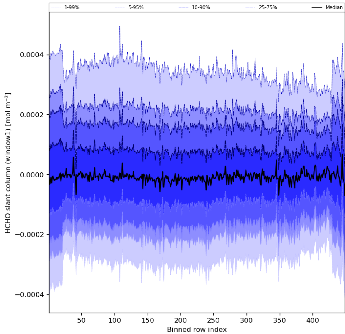
Figure 52: Along track statistics of “HCHO slant column (window1)” for 2023-11-18 to 2023-11-20
