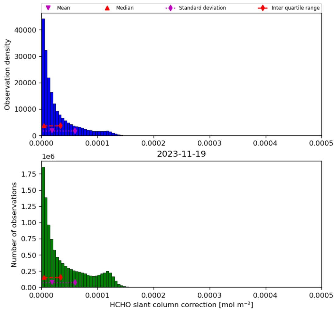
Figure 47: Histogram of “HCHO slant column correction” for 2023-11-18 to 2023-11-20
