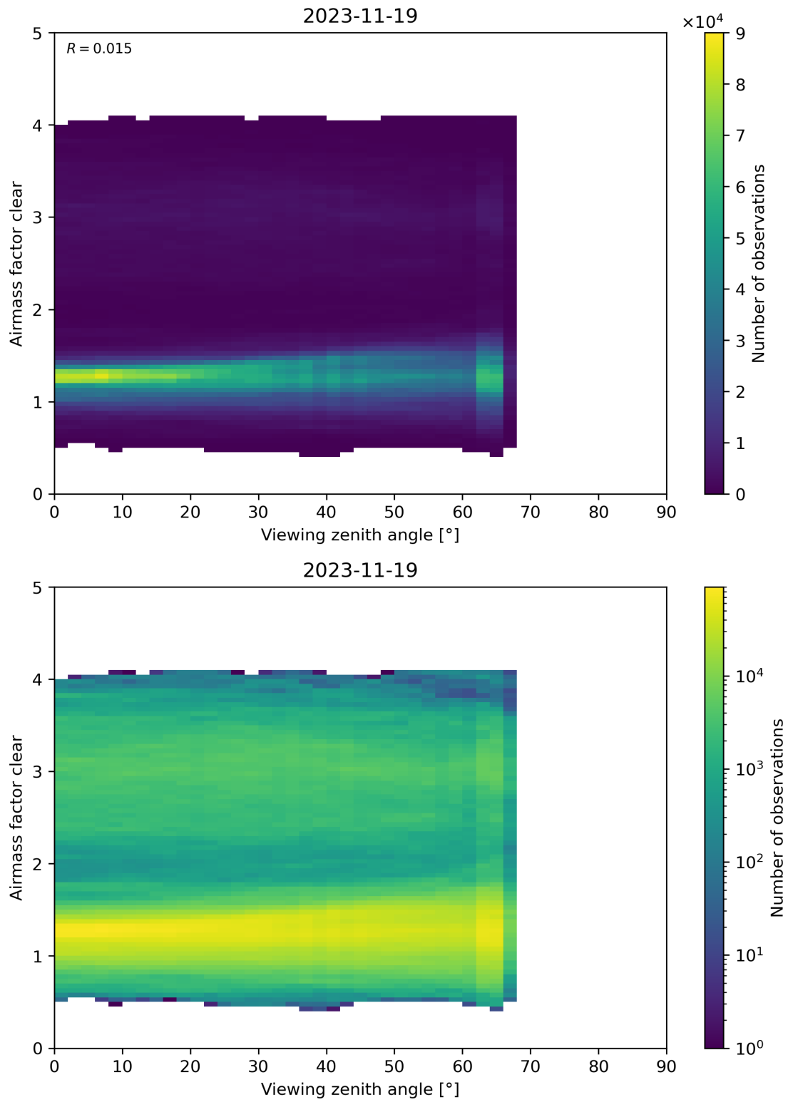
Figure 185: Scatter density plot of “Viewing zenith angle” against “Airmass factor clear” for 2023-11-18 to 2023-11-20.
