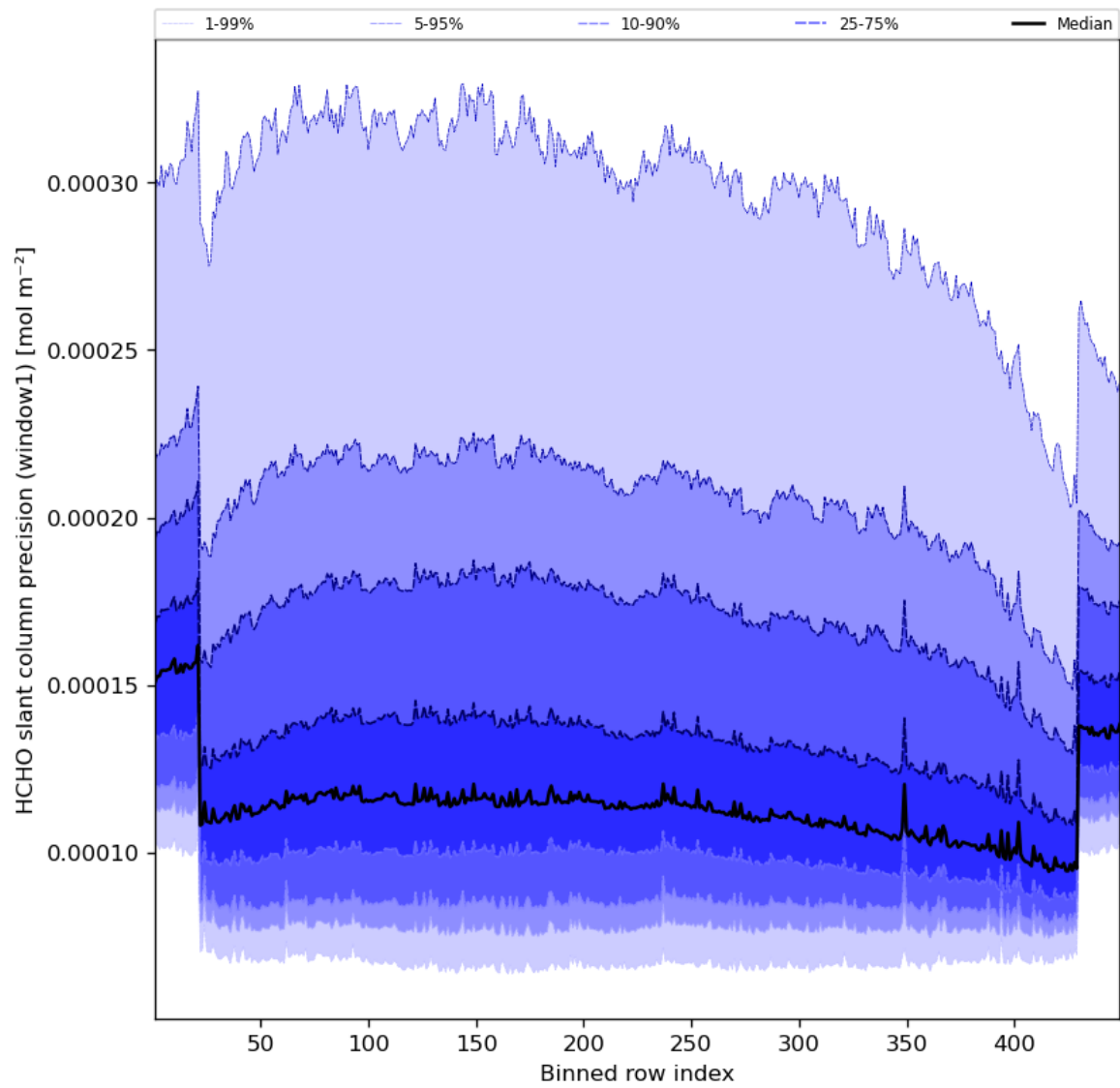
Figure 53: Along track statistics of “HCHO slant column precision (window1)” for 2023-11-18 to 2023-11-20
