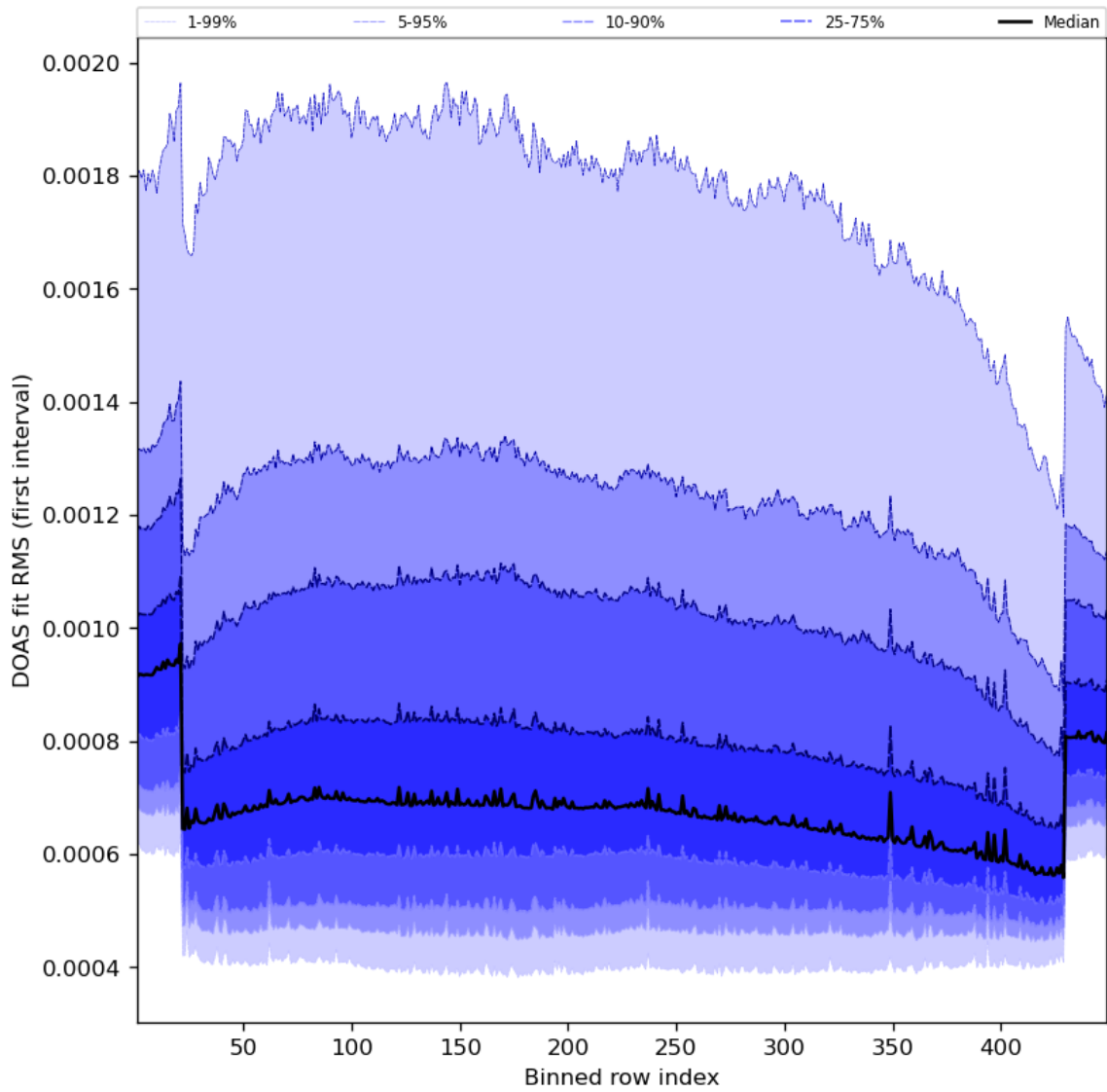
Figure 60: Along track statistics of “DOAS fit RMS (first interval)” for 2023-11-18 to 2023-11-20
