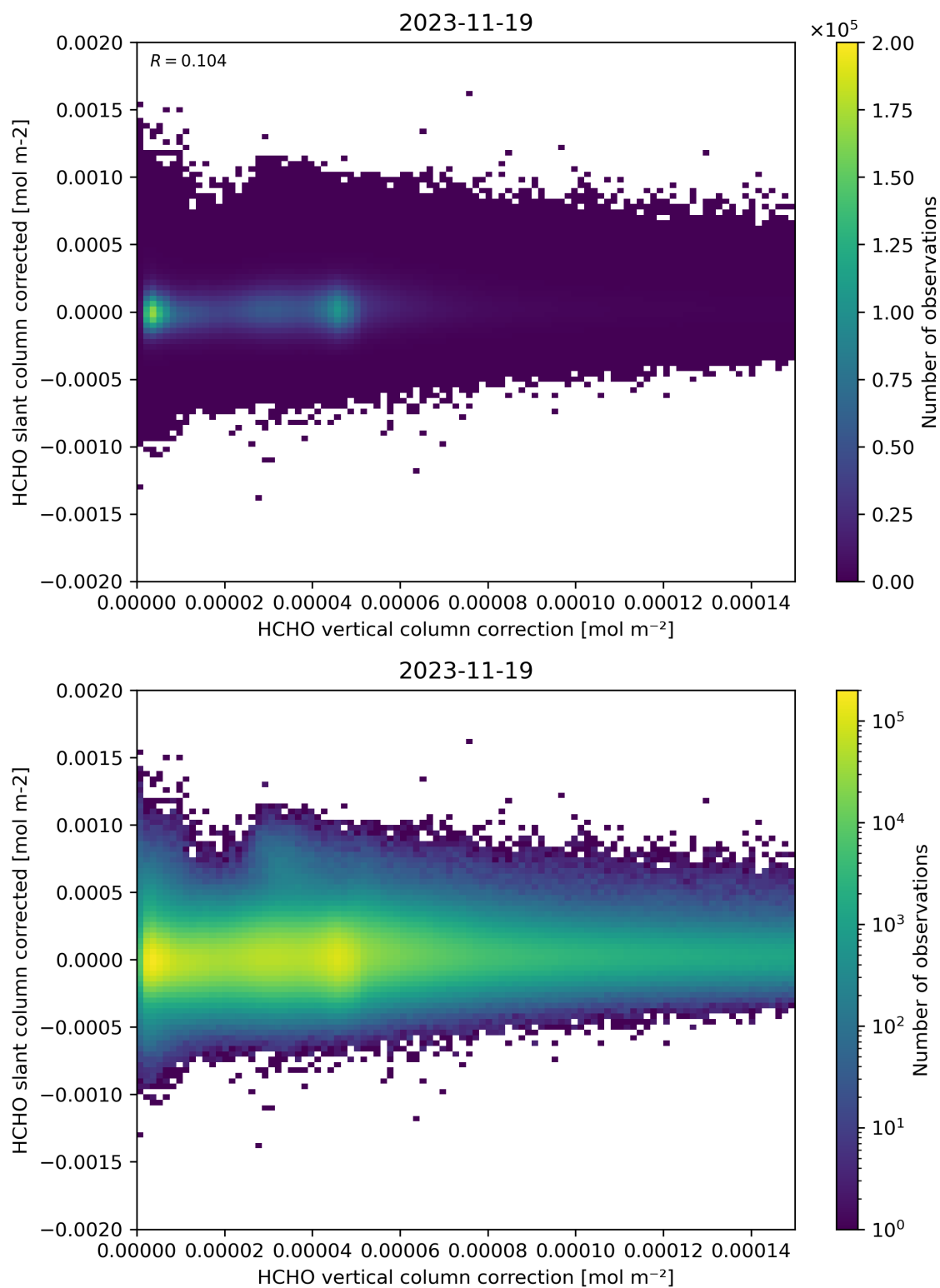
Figure 116: Scatter density plot of “HCHO vertical column correction” against “HCHO slant column corrected” for 2023-11-18 to 2023-11-20.
