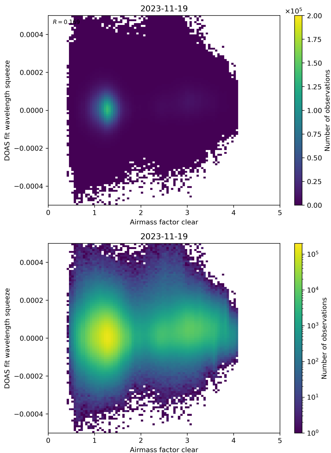
Figure 73: Scatter density plot of “Airmass factor clear” against “DOAS fit wavelength squeeze” for 2023-11-18 to 2023-11-20.
