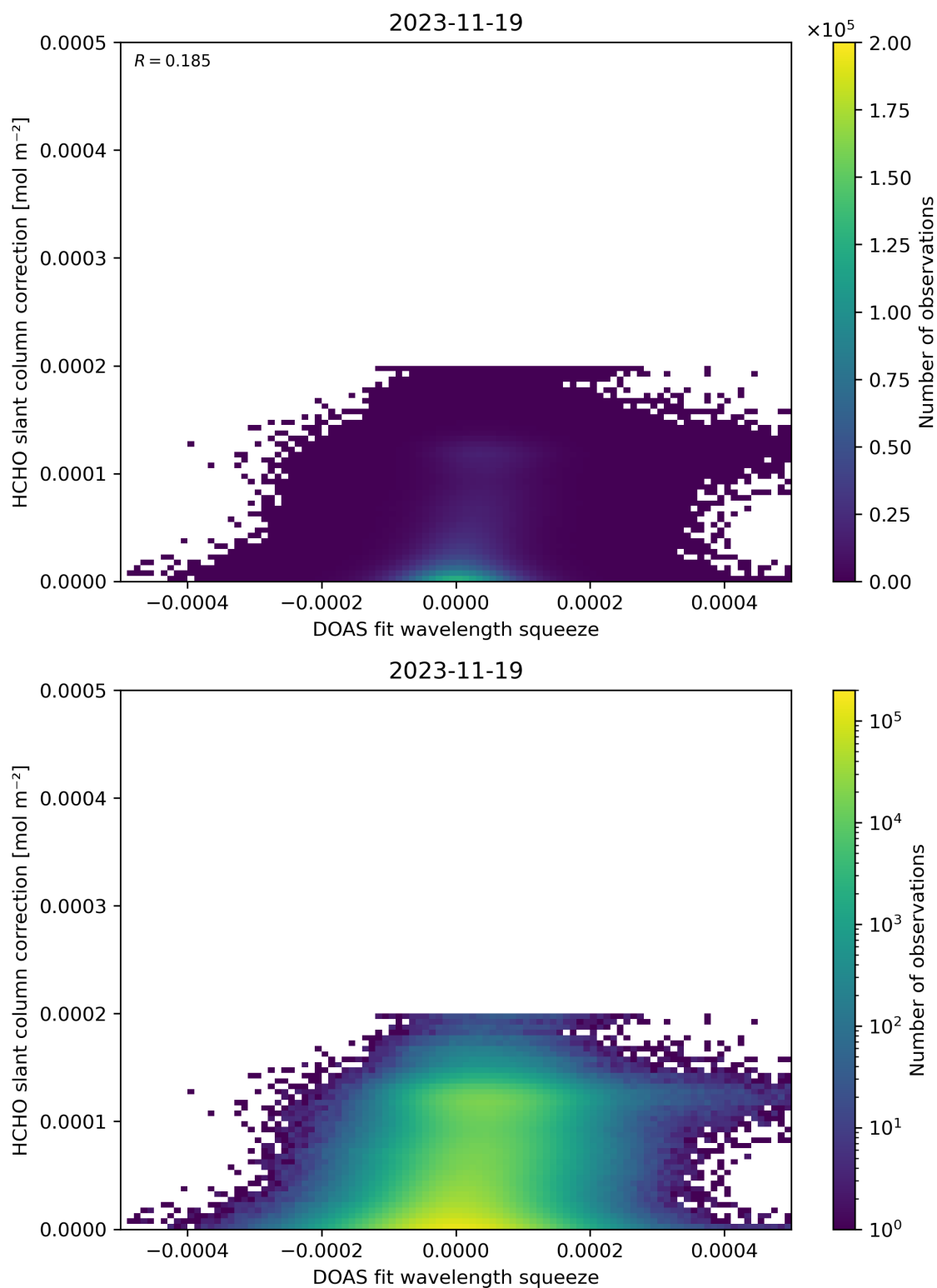
Figure 70: Scatter density plot of “DOAS fit wavelength squeeze” against “HCHO slant column correction” for 2023-11-18 to 2023-11-20.
