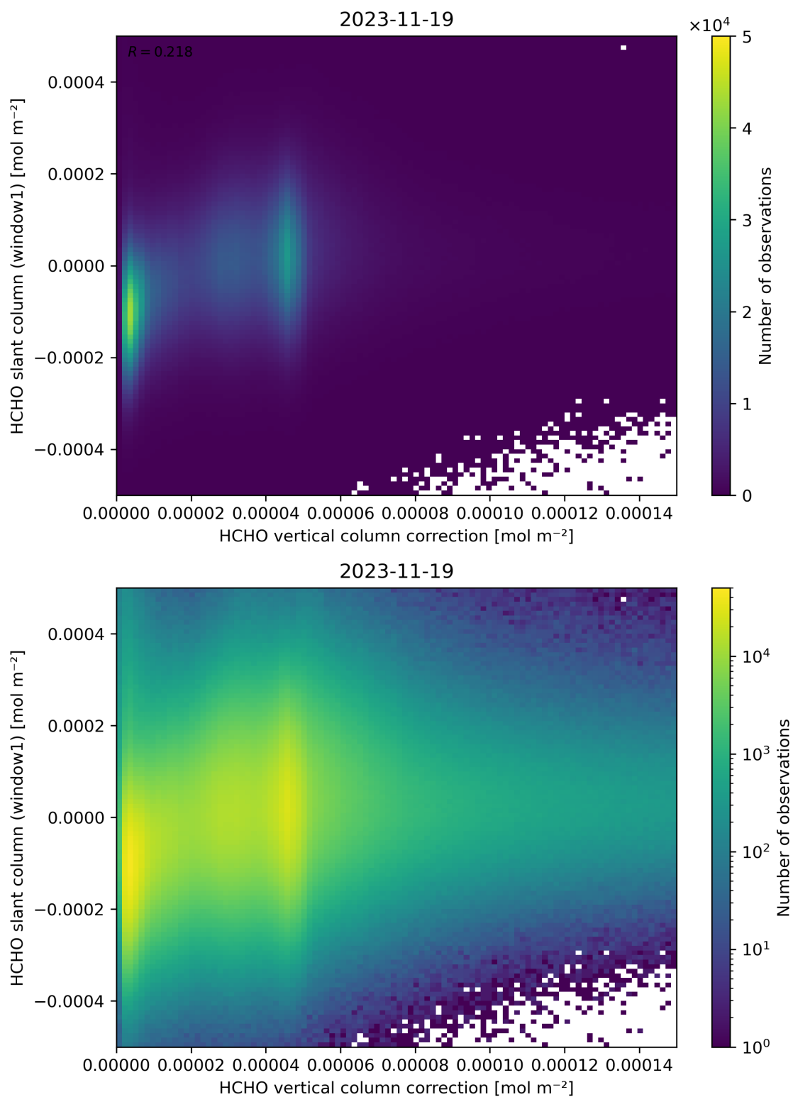
Figure 118: Scatter density plot of “HCHO vertical column correction” against “HCHO slant column (window1)” for 2023-11-18 to 2023-11-20.
