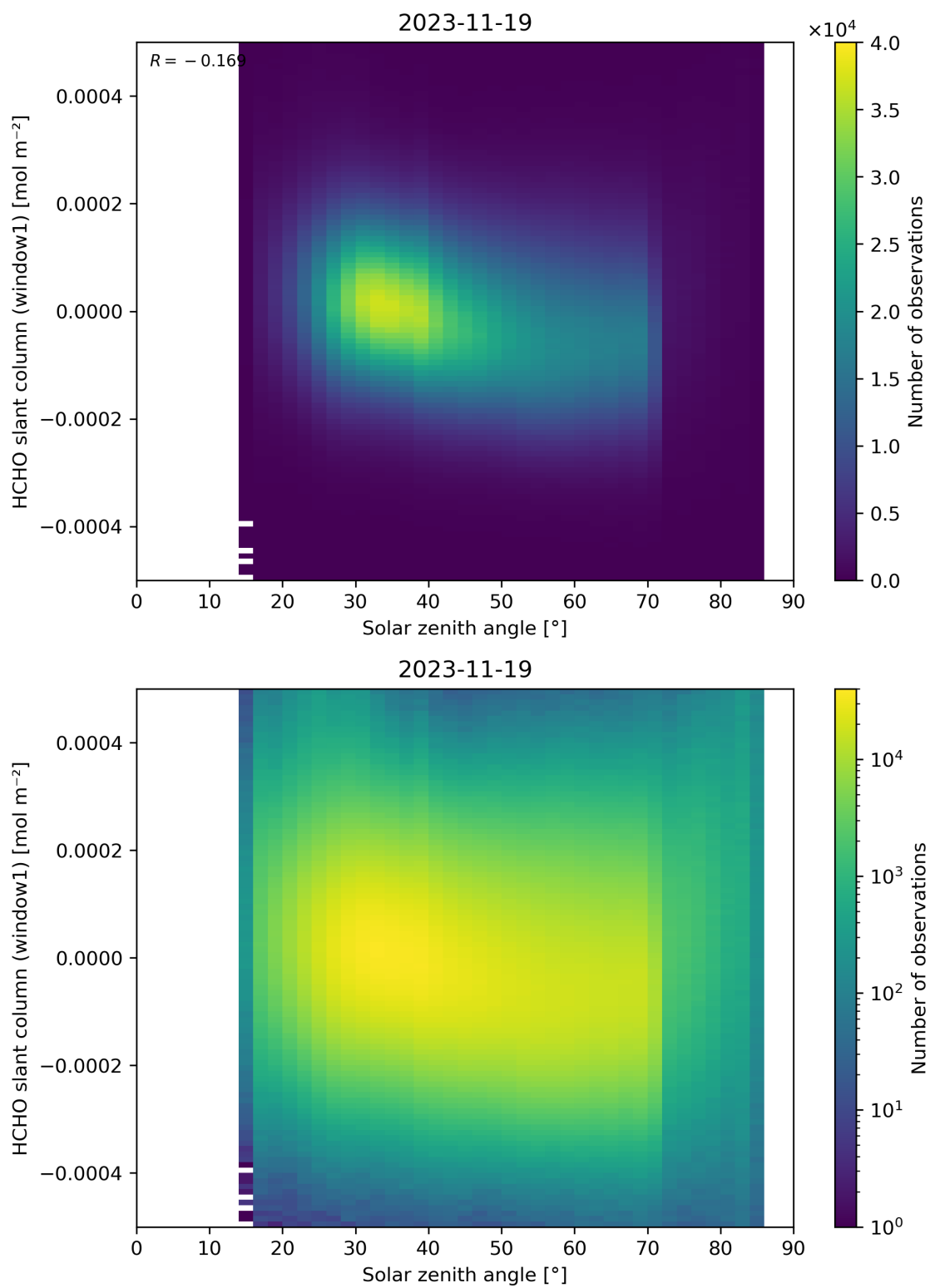
Figure 173: Scatter density plot of “Solar zenith angle” against “HCHO slant column (window1)” for 2023-11-18 to 2023-11-20.
