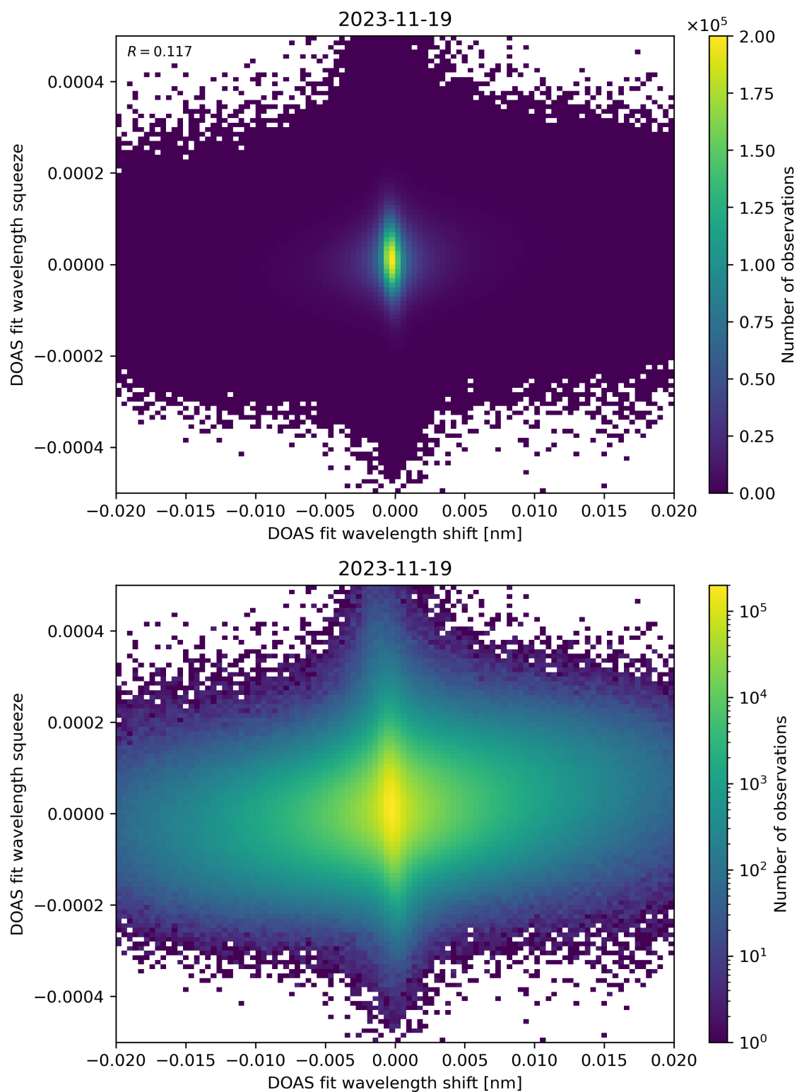
Figure 65: Scatter density plot of “DOAS fit wavelength shift” against “DOAS fit wavelength squeeze” for 2023-11-18 to 2023-11-20.
