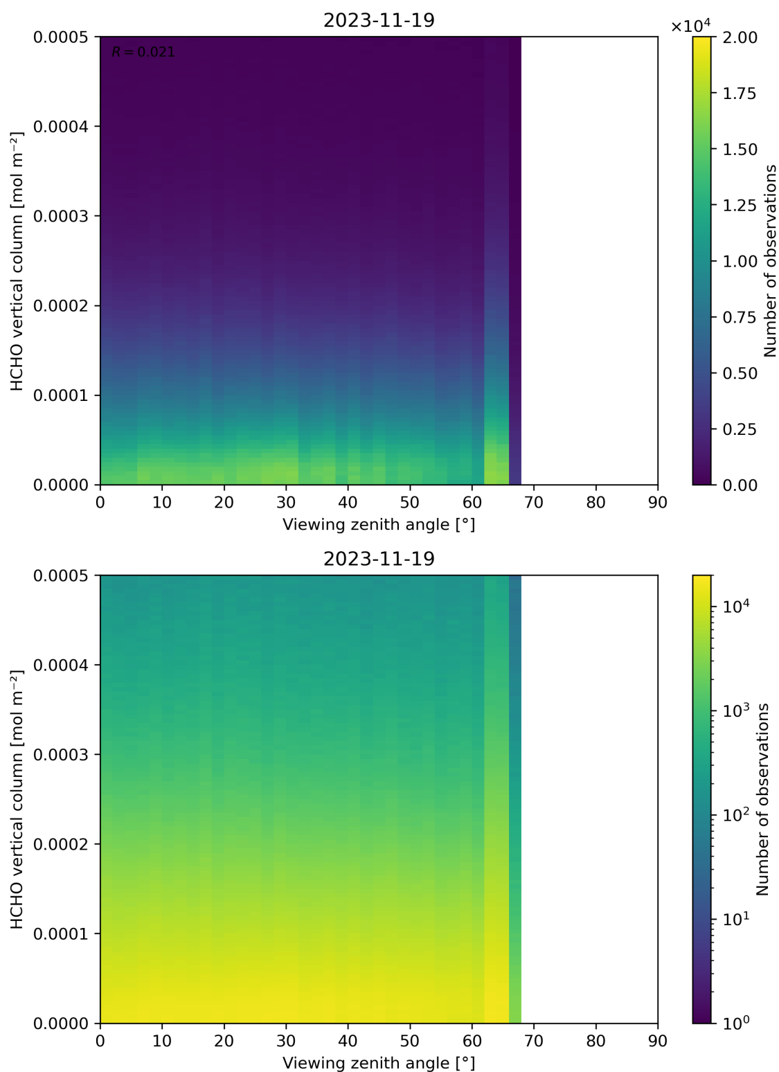
Figure 192: Scatter density plot of “Viewing zenith angle” against “HCHO vertical column” for 2023-11-18 to 2023-11-20.
