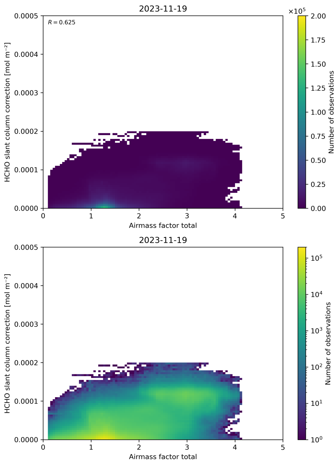
Figure 102: Scatter density plot of “Airmass factor total” against “HCHO slant column correction” for 2023-11-18 to 2023-11-20.
