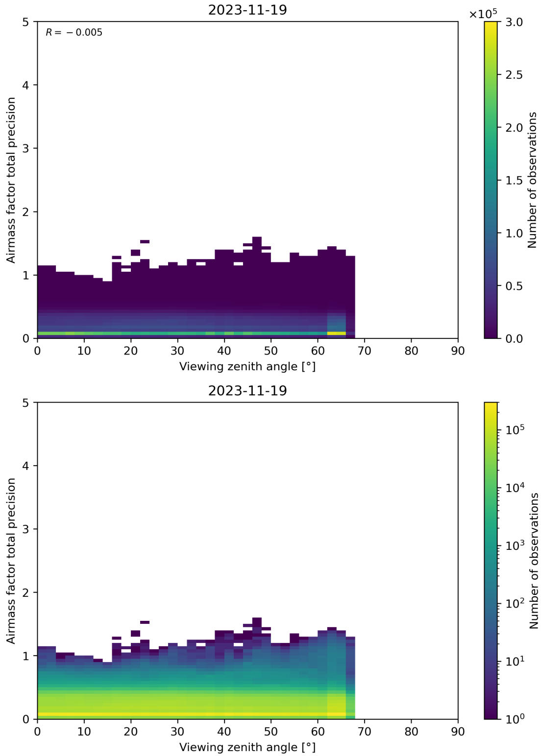
Figure 191: Scatter density plot of “Viewing zenith angle” against “Airmass factor total precision” for 2023-11-18 to 2023-11-20.
