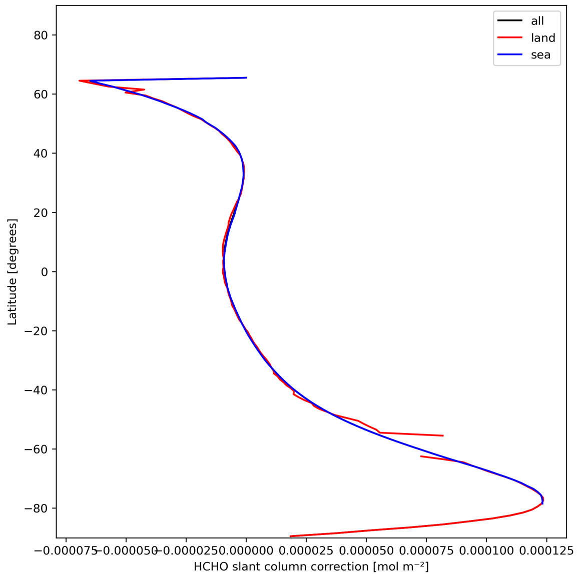
Figure 33: Zonal average of “HCHO slant column correction” for 2023-11-18 to 2023-11-20.
