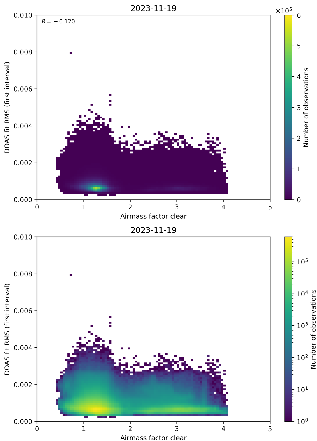
Figure 71: Scatter density plot of “Airmass factor clear” against “DOAS fit RMS (first interval)” for 2023-11-18 to 2023-11-20.
