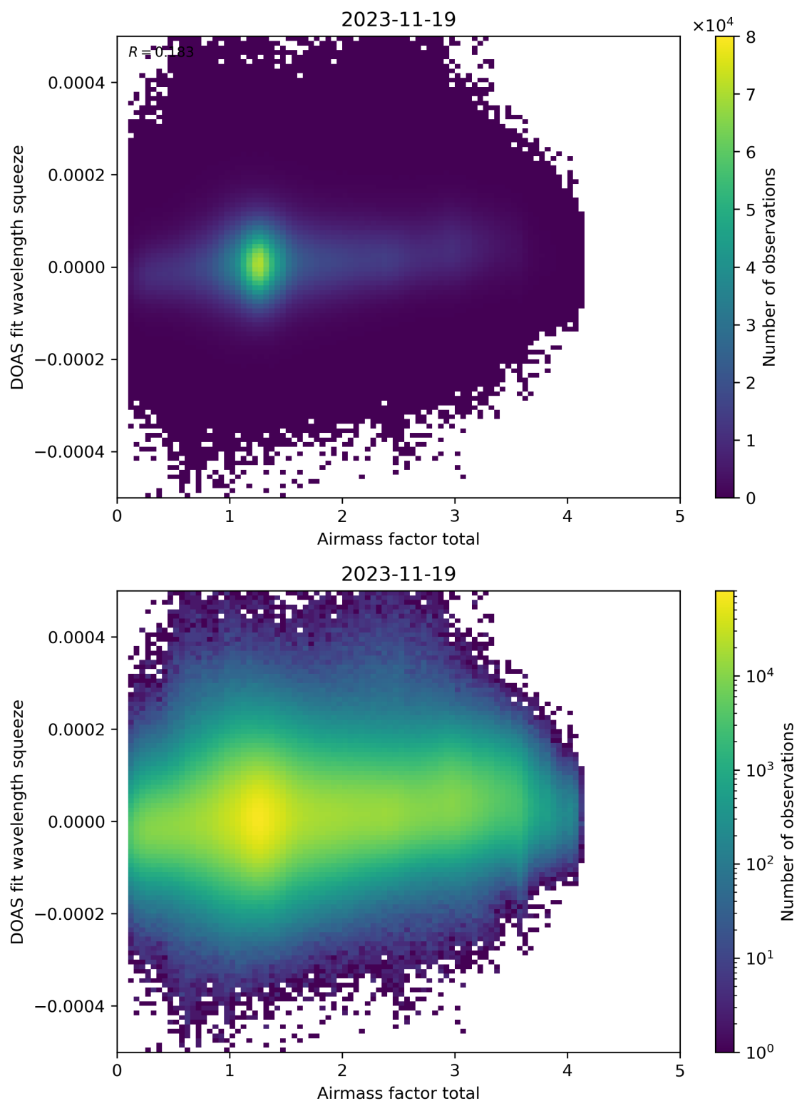
Figure 99: Scatter density plot of “Airmass factor total” against “DOAS fit wavelength squeeze” for 2023-11-18 to 2023-11-20.
