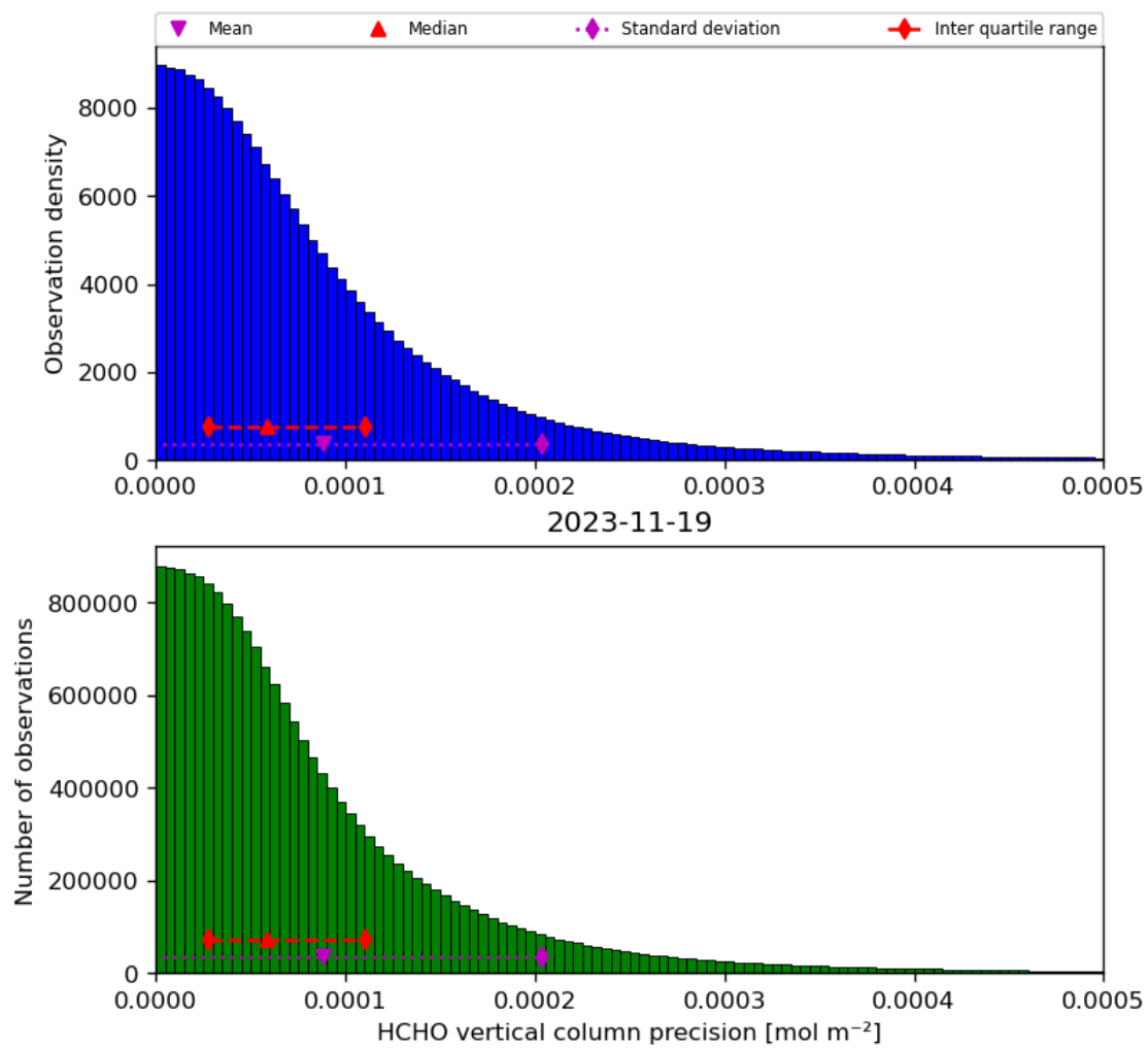
Figure 36: Histogram of “HCHO vertical column precision” for 2023-11-18 to 2023-11-20
