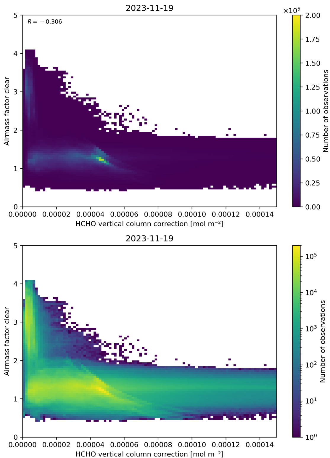
Figure 115: Scatter density plot of “HCHO vertical column correction” against “Airmass factor clear” for 2023-11-18 to 2023-11-20.
