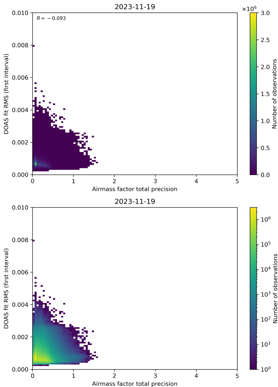
Figure 105: Scatter density plot of “Airmass factor total precision” against “DOAS fit RMS (first interval)” for 2023-11-18 to 2023-11-20.
