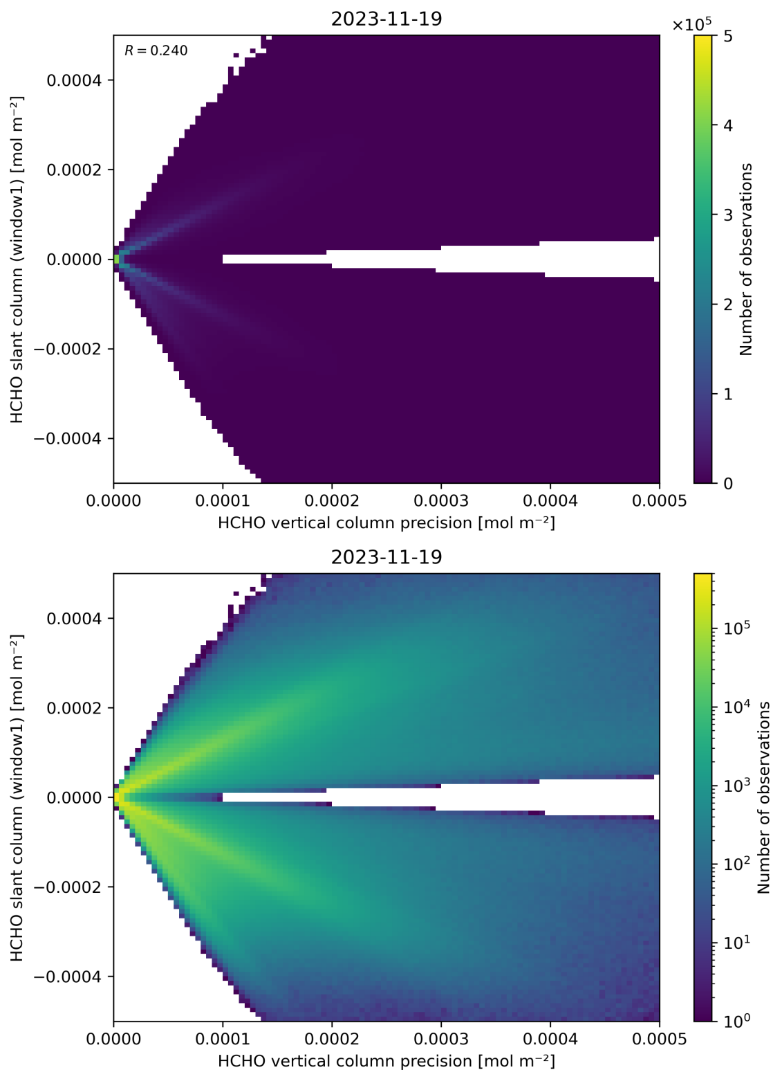
Figure 142: Scatter density plot of “HCHO vertical column precision” against “HCHO slant column (window1)” for 2023-11-18 to 2023-11-20.
