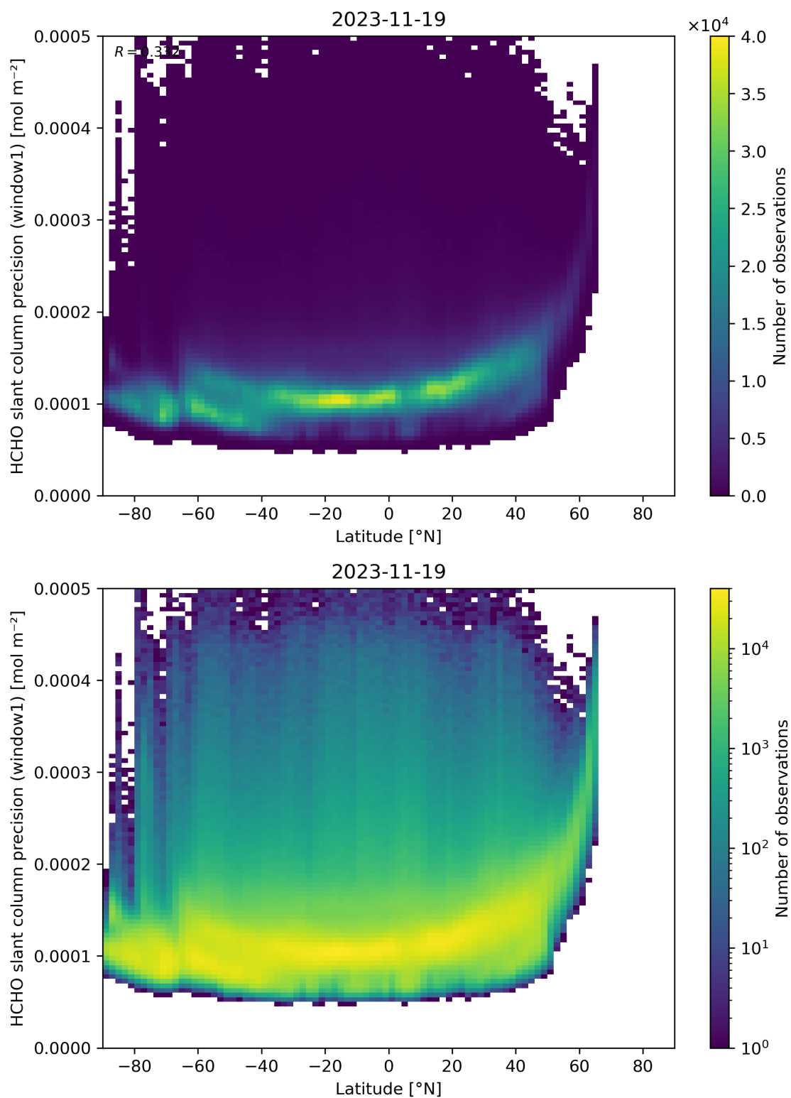
Figure 160: Scatter density plot of “Latitude” against “HCHO slant column precision (window1)” for 2023-11-18 to 2023-11-20.
