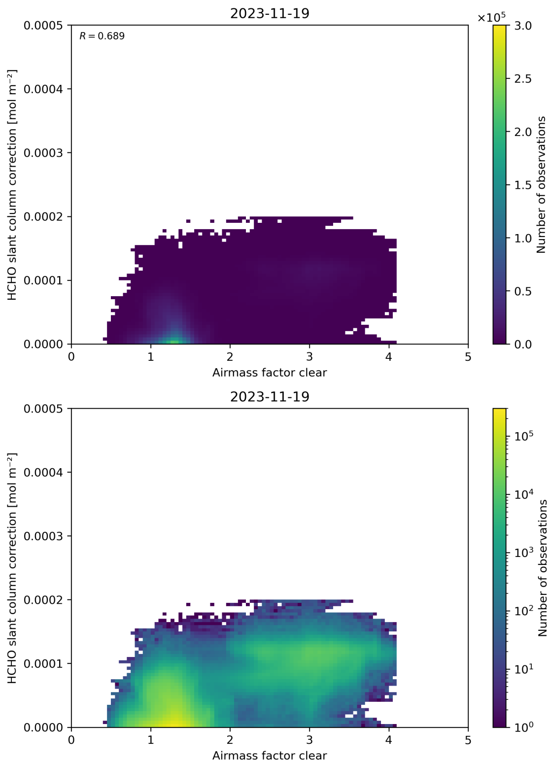
Figure 75: Scatter density plot of “Airmass factor clear” against “HCHO slant column correction” for 2023-11-18 to 2023-11-20.
