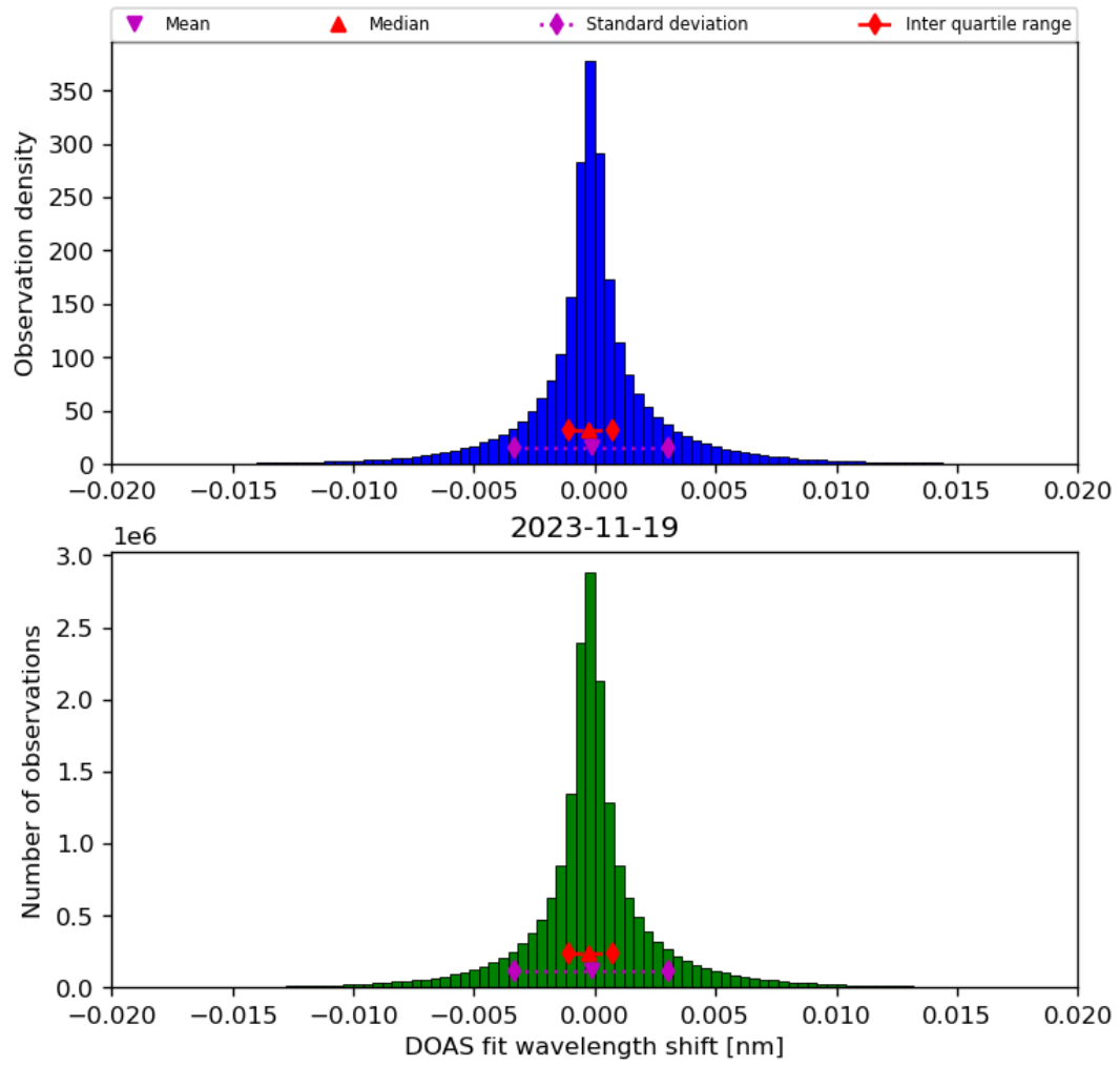
Figure 44: Histogram of “DOAS fit wavelength shift” for 2023-11-18 to 2023-11-20
