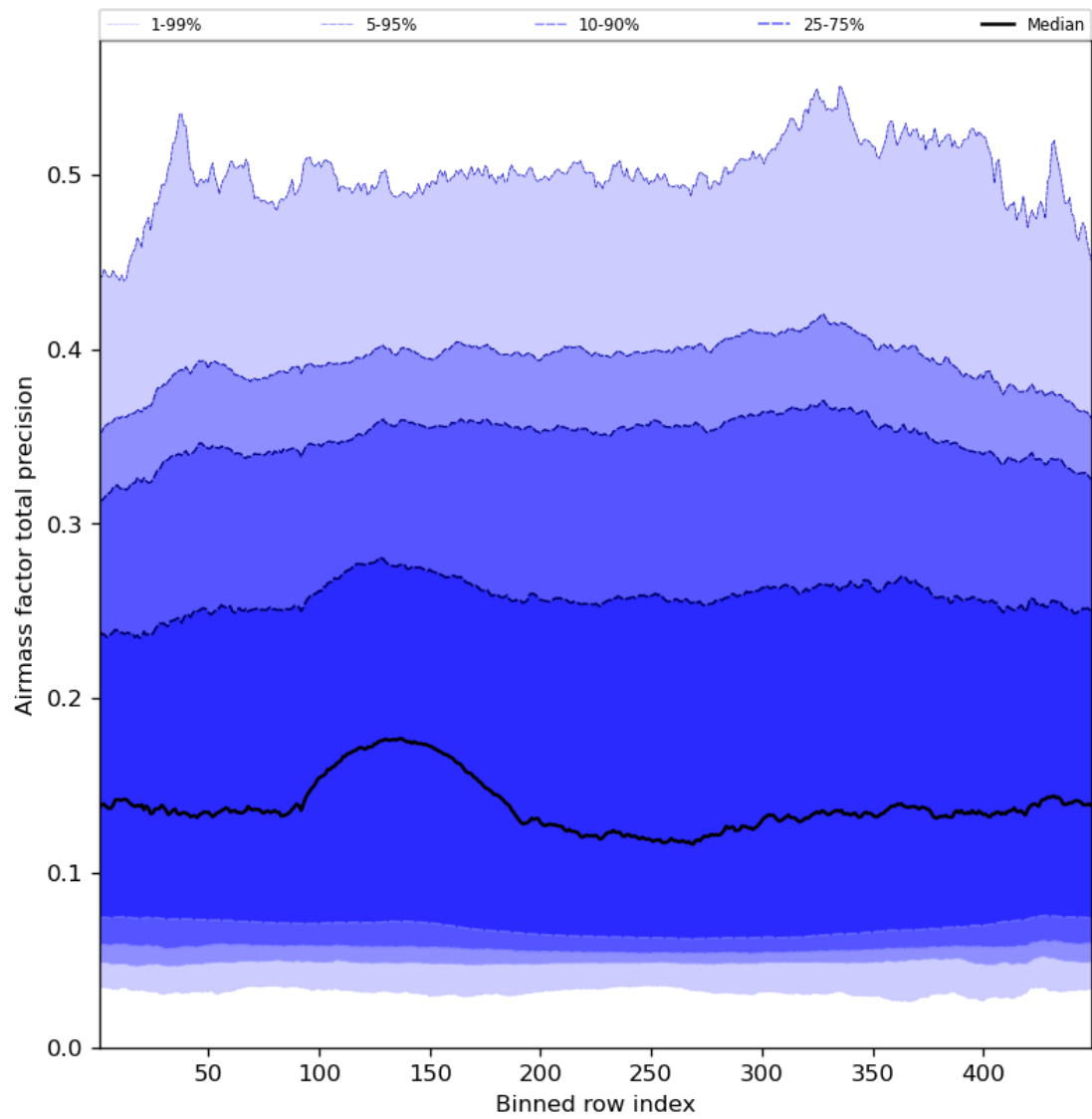
Figure 55: Along track statistics of “Airmass factor total precision” for 2023-11-18 to 2023-11-20
