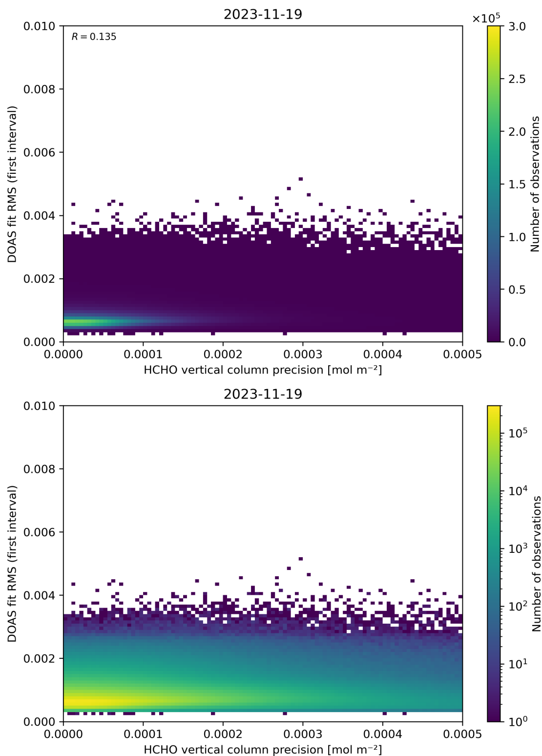
Figure 136: Scatter density plot of “HCHO vertical column precision” against “DOAS fit RMS (first interval)” for 2023-11-18 to 2023-11-20.
