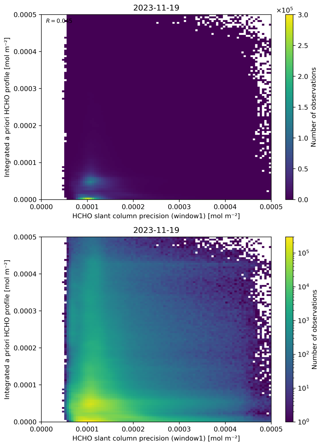
Figure 96: Scatter density plot of “HCHO slant column precision (window1)” against “Integrated a priori HCHO profile” for 2023-11-18 to 2023-11-20.
