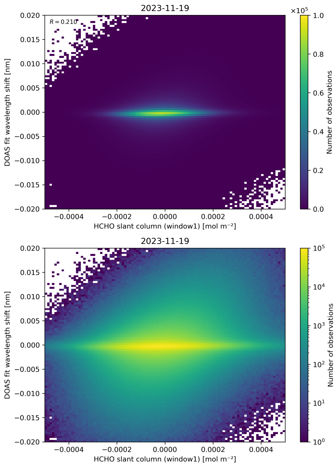
Figure 79: Scatter density plot of “HCHO slant column (window1)” against “DOAS fit wavelength shift” for 2023-11-18 to 2023-11-20.
