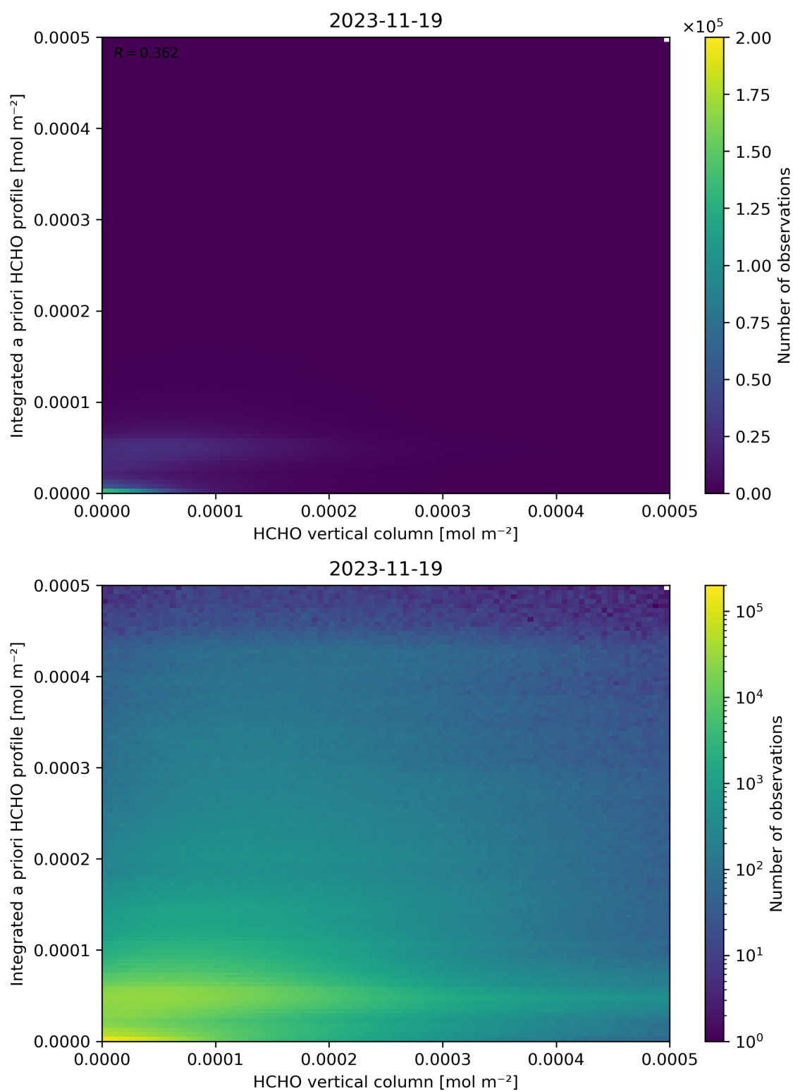
Figure 135: Scatter density plot of “HCHO vertical column” against “Integrated a priori HCHO profile” for 2023-11-18 to 2023-11-20.
