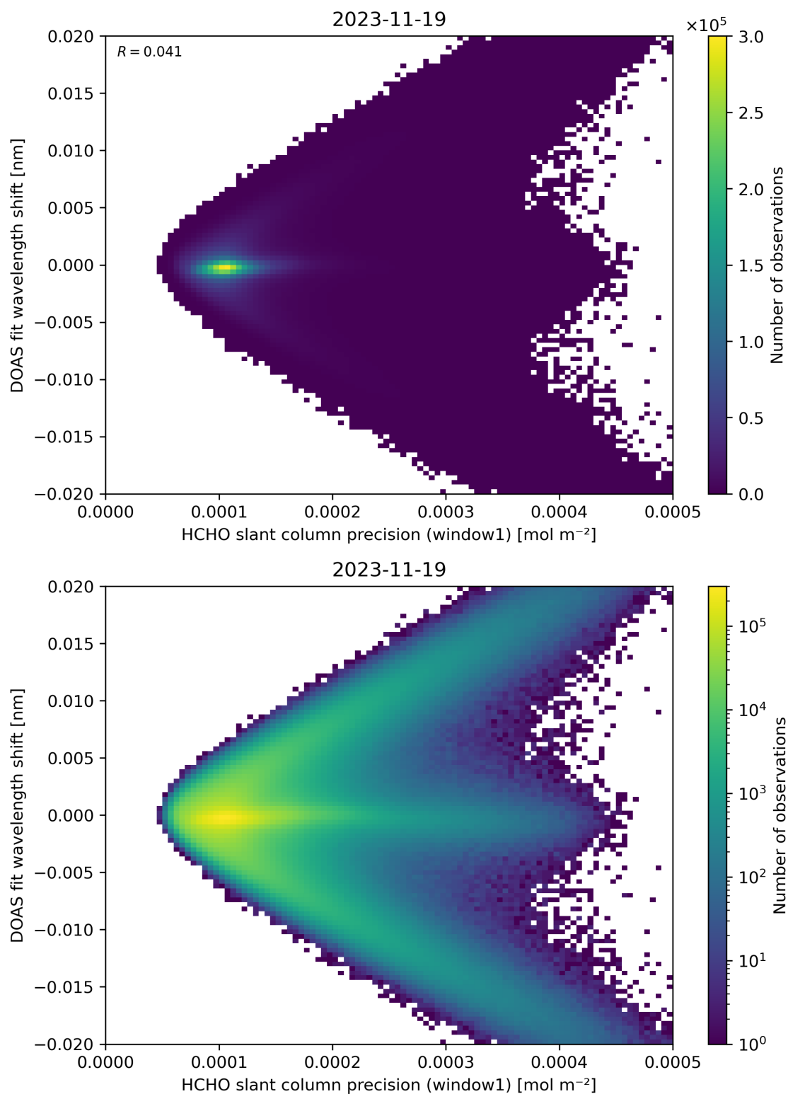
Figure 89: Scatter density plot of “HCHO slant column precision (window1)” against “DOAS fit wavelength shift” for 2023-11-18 to 2023-11-20.
