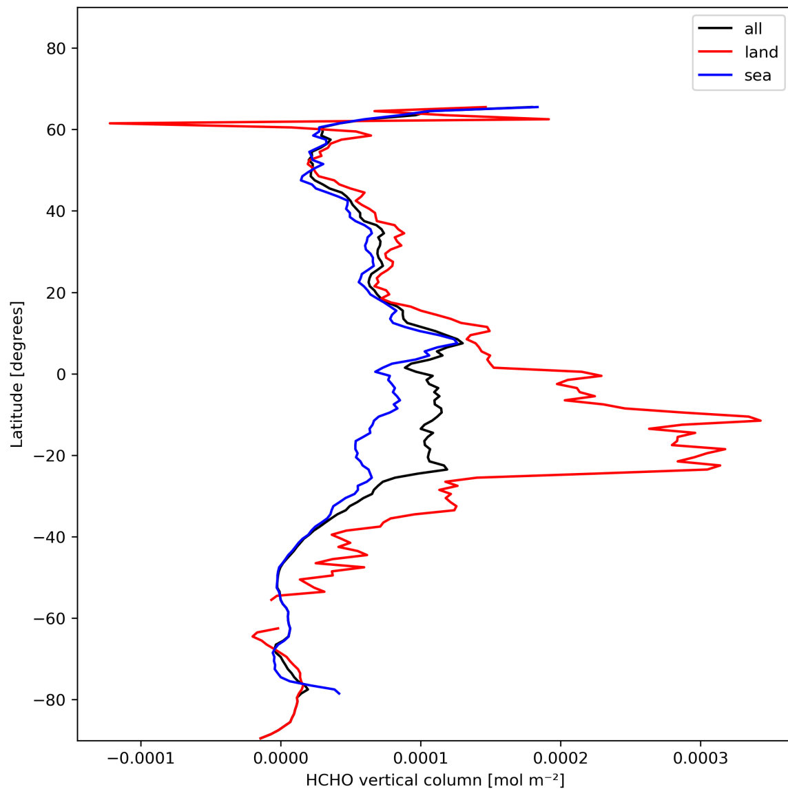
Figure 21: Zonal average of “HCHO vertical column” for 2023-11-18 to 2023-11-20.
