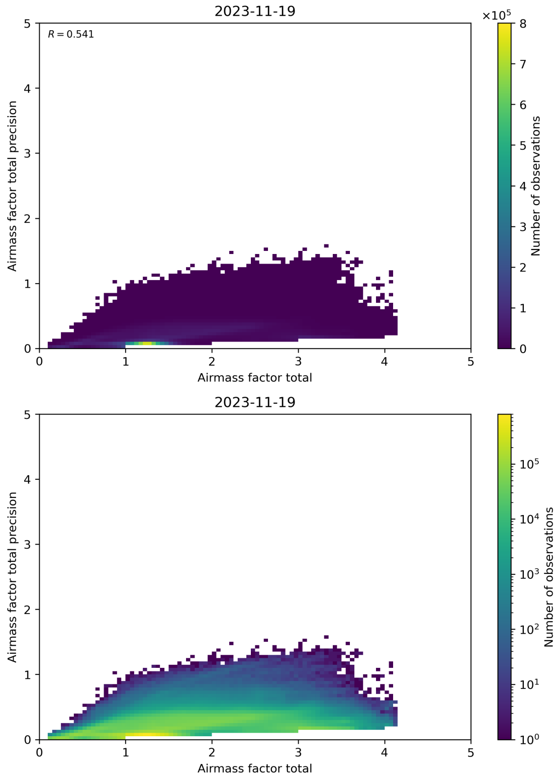
Figure 103: Scatter density plot of “Airmass factor total” against “Airmass factor total precision” for 2023-11-18 to 2023-11-20.
