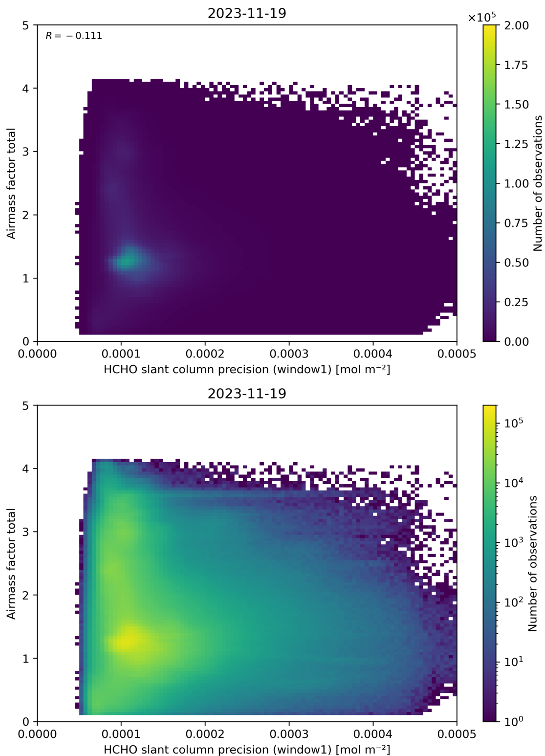
Figure 94: Scatter density plot of “HCHO slant column precision (window1)” against “Airmass factor total” for 2023-11-18 to 2023-11-20.
