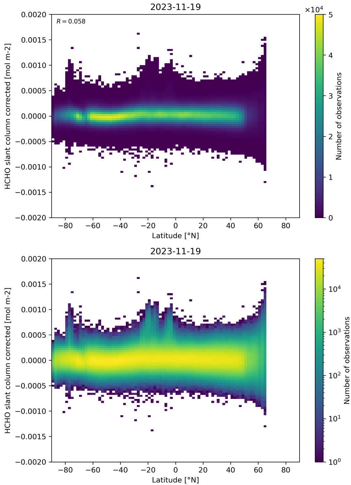
Figure 157: Scatter density plot of “Latitude” against “HCHO slant column corrected” for 2023-11-18 to 2023-11-20.
