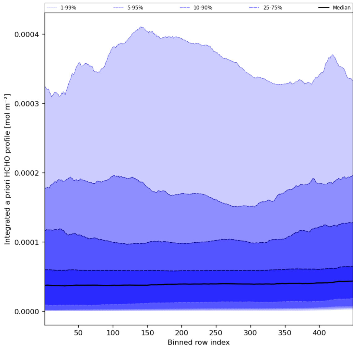
Figure 57: Along track statistics of “Integrated a priori HCHO profile” for 2023-11-18 to 2023-11-20
