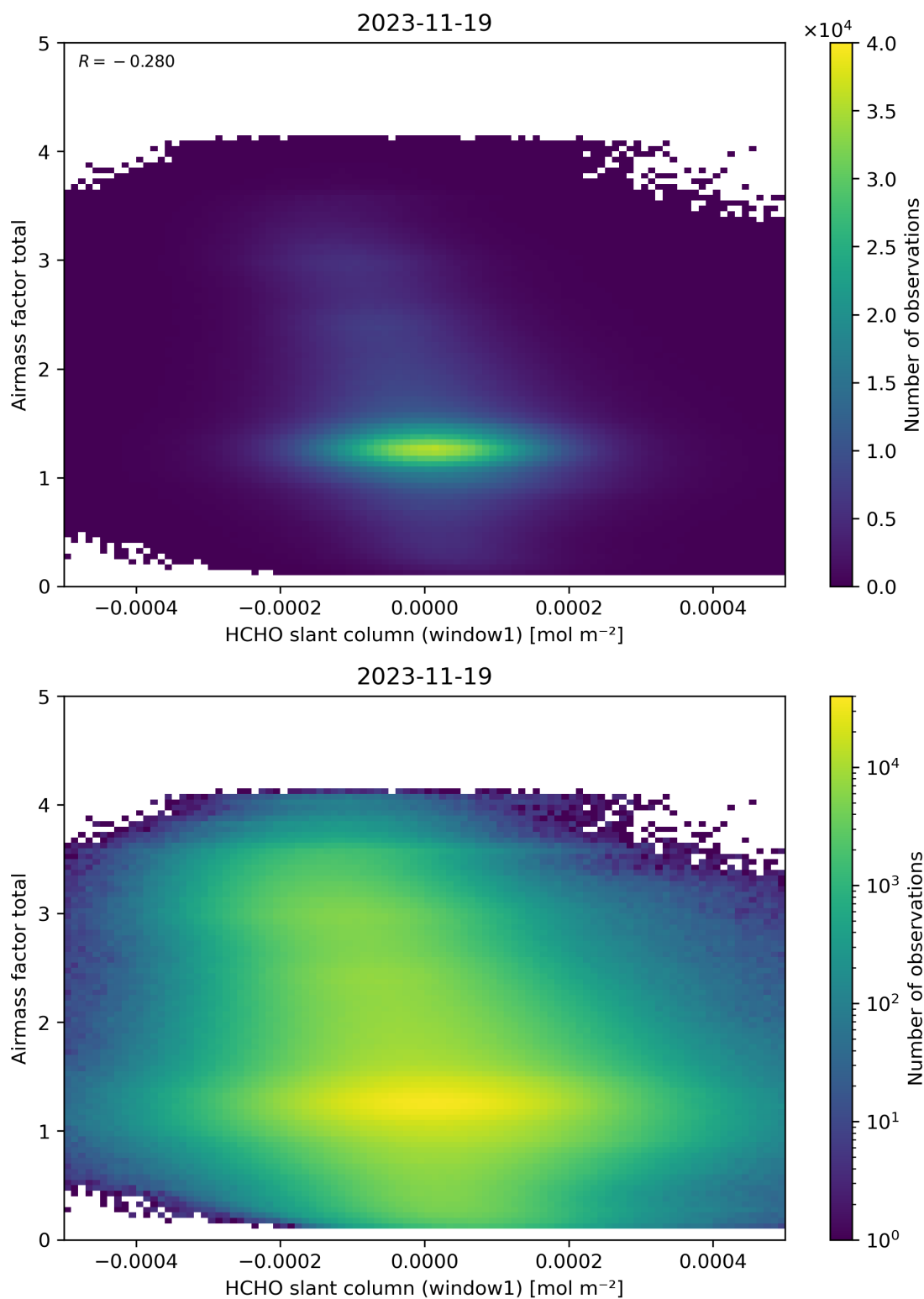
Figure 85: Scatter density plot of “HCHO slant column (window1)” against “Airmass factor total” for 2023-11-18 to 2023-11-20.
