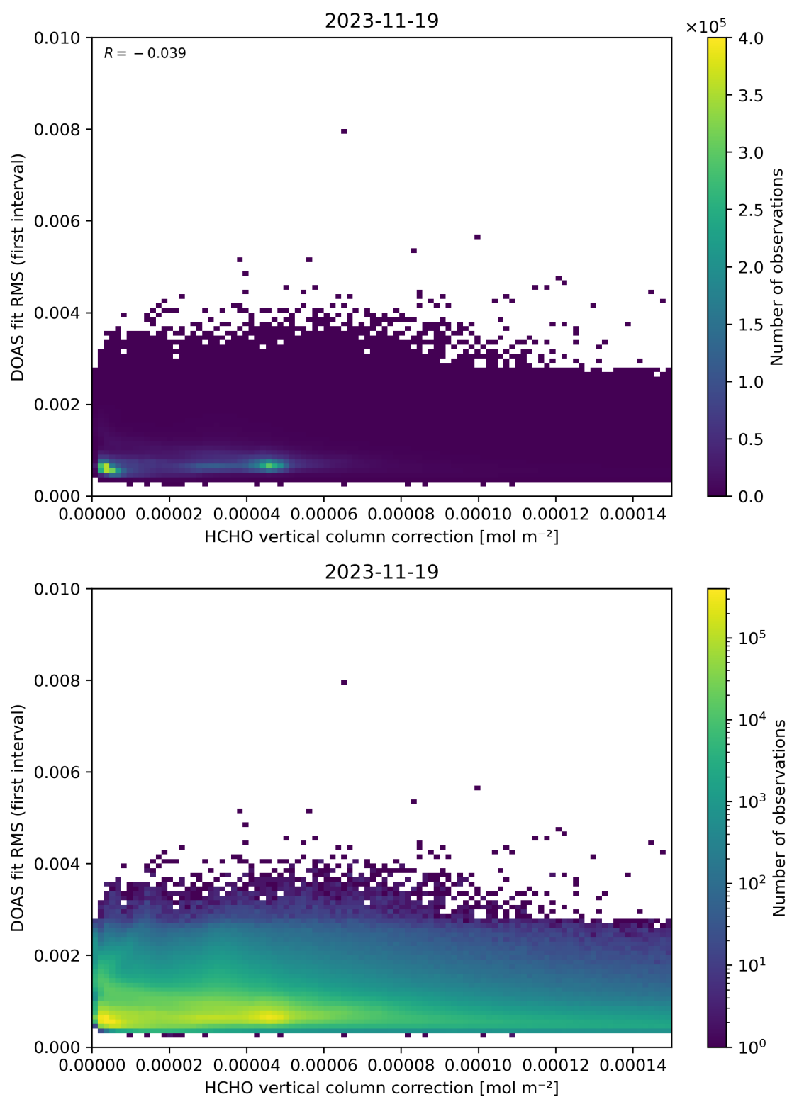
Figure 112: Scatter density plot of “HCHO vertical column correction” against “DOAS fit RMS (first interval)” for 2023-11-18 to 2023-11-20.
