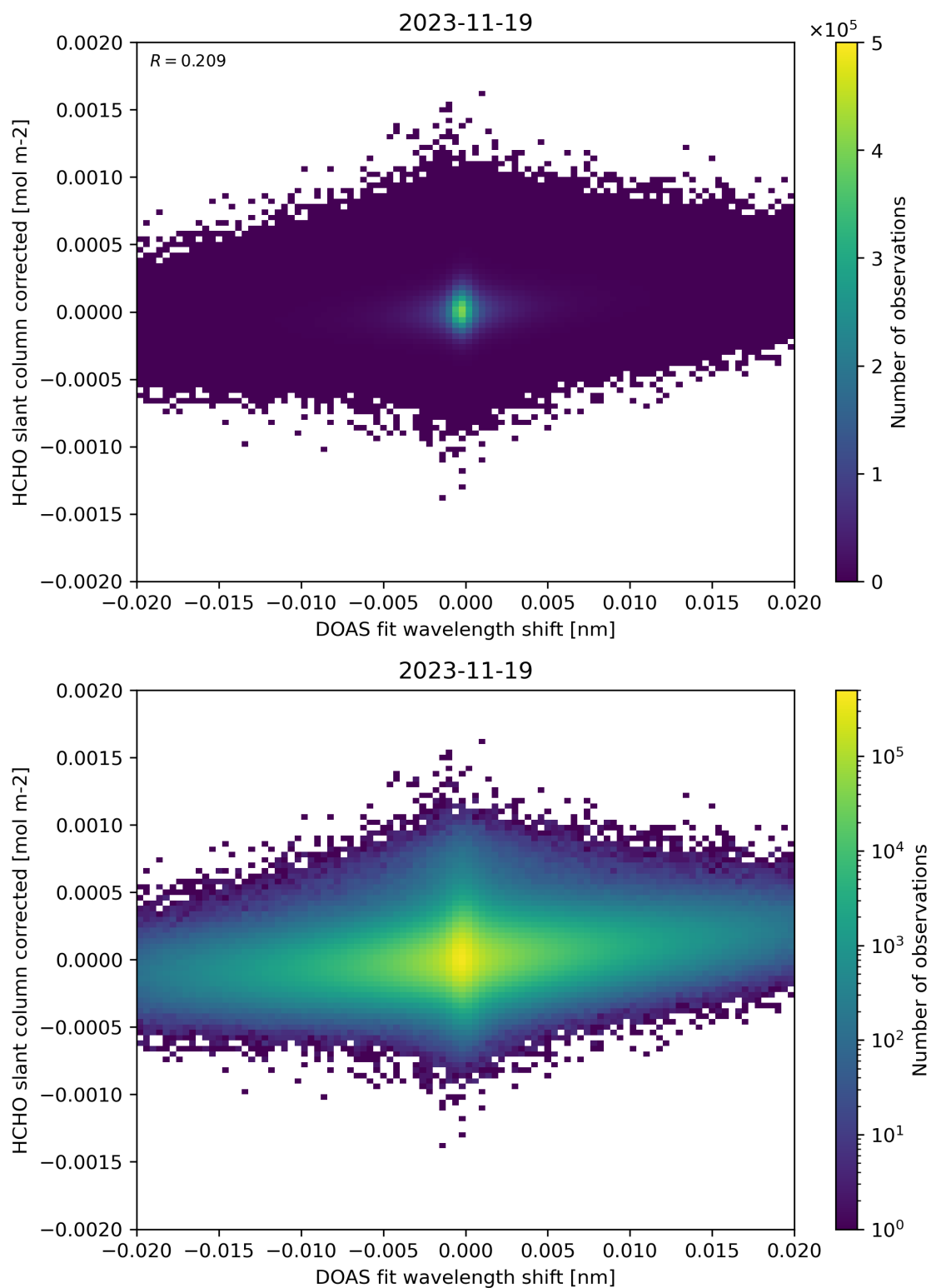
Figure 66: Scatter density plot of “DOAS fit wavelength shift” against “HCHO slant column corrected” for 2023-11-18 to 2023-11-20.
