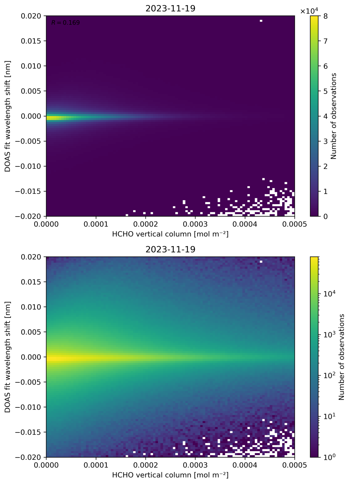
Figure 124: Scatter density plot of “HCHO vertical column” against “DOAS fit wavelength shift” for 2023-11-18 to 2023-11-20.
