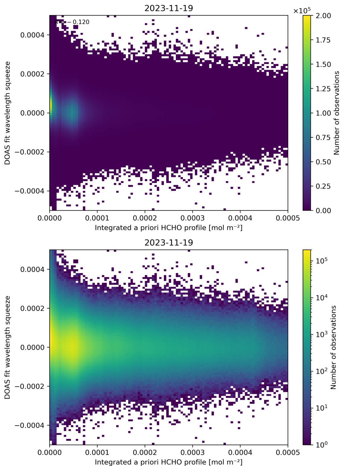
Figure 150: Scatter density plot of “Integrated a priori HCHO profile” against “DOAS fit wavelength squeeze” for 2023-11-18 to 2023-11-20.
