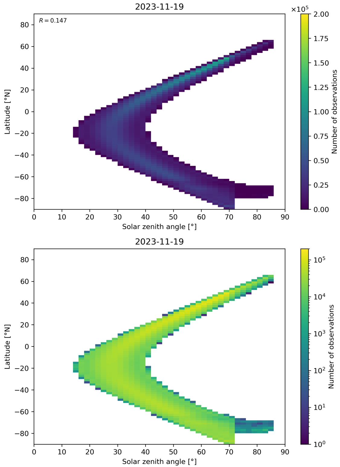
Figure 181: Scatter density plot of “Solar zenith angle” against “Latitude” for 2023-11-18 to 2023-11-20.
