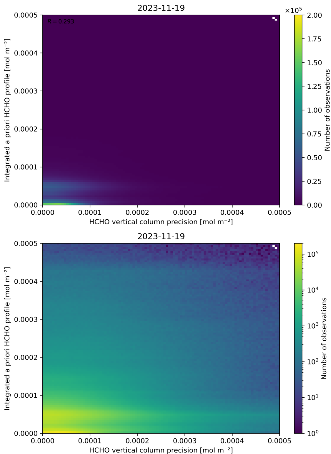
Figure 147: Scatter density plot of “HCHO vertical column precision” against “Integrated a priori HCHO profile” for 2023-11-18 to 2023-11-20.
