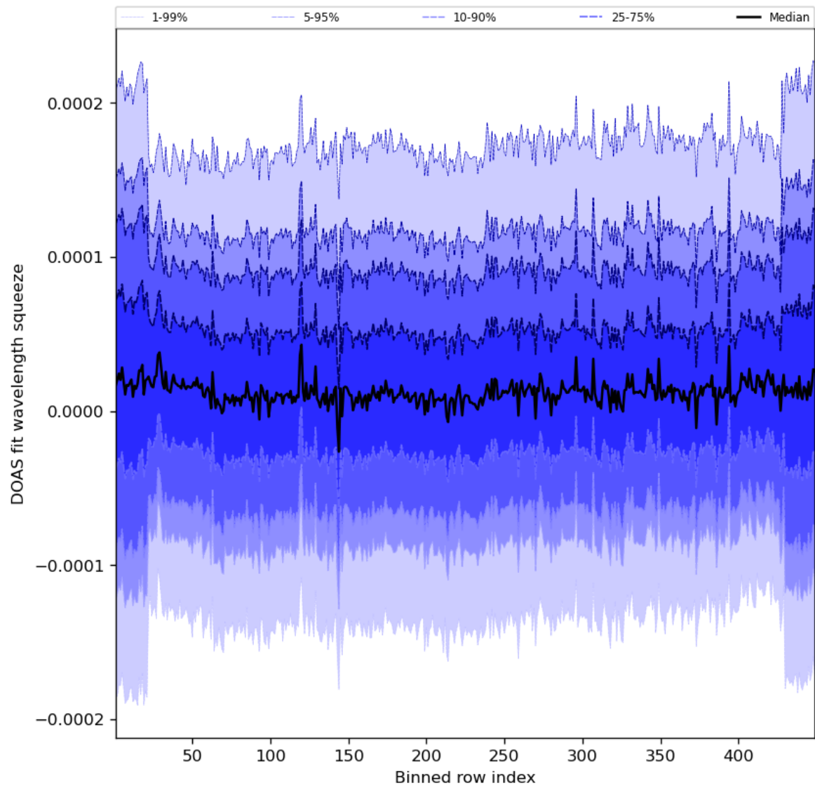
Figure 59: Along track statistics of “DOAS fit wavelength squeeze” for 2023-11-18 to 2023-11-20
