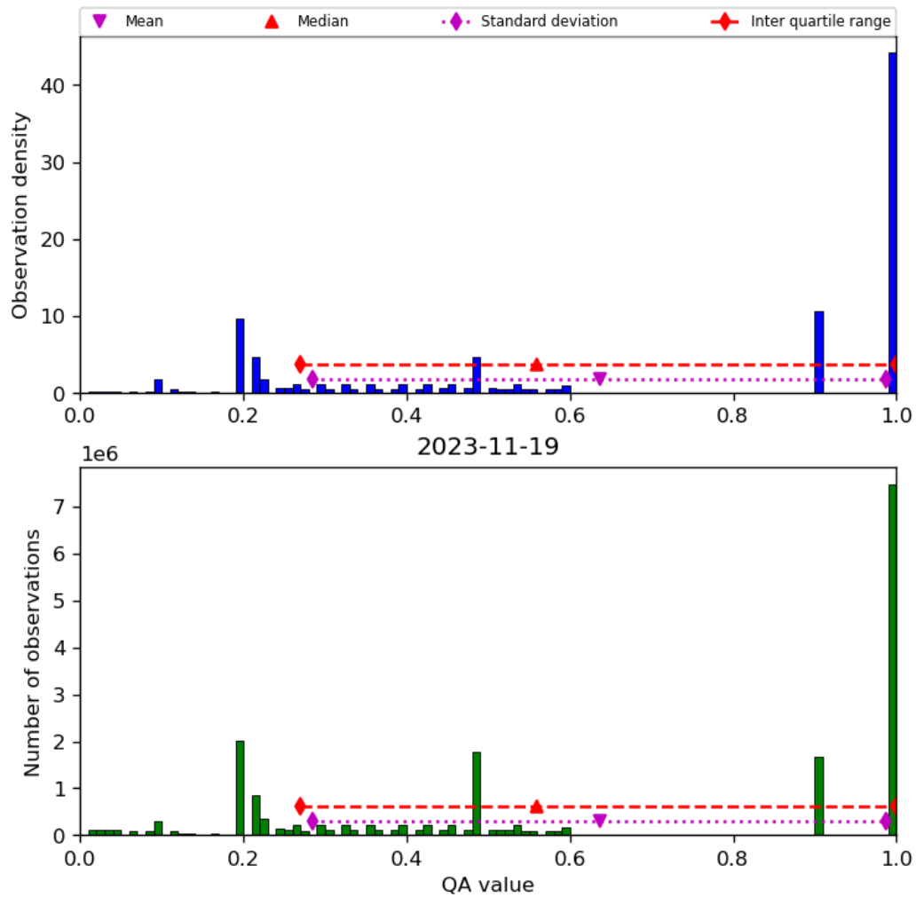
Figure 34: Histogram of “QA value” for 2023-11-18 to 2023-11-20
