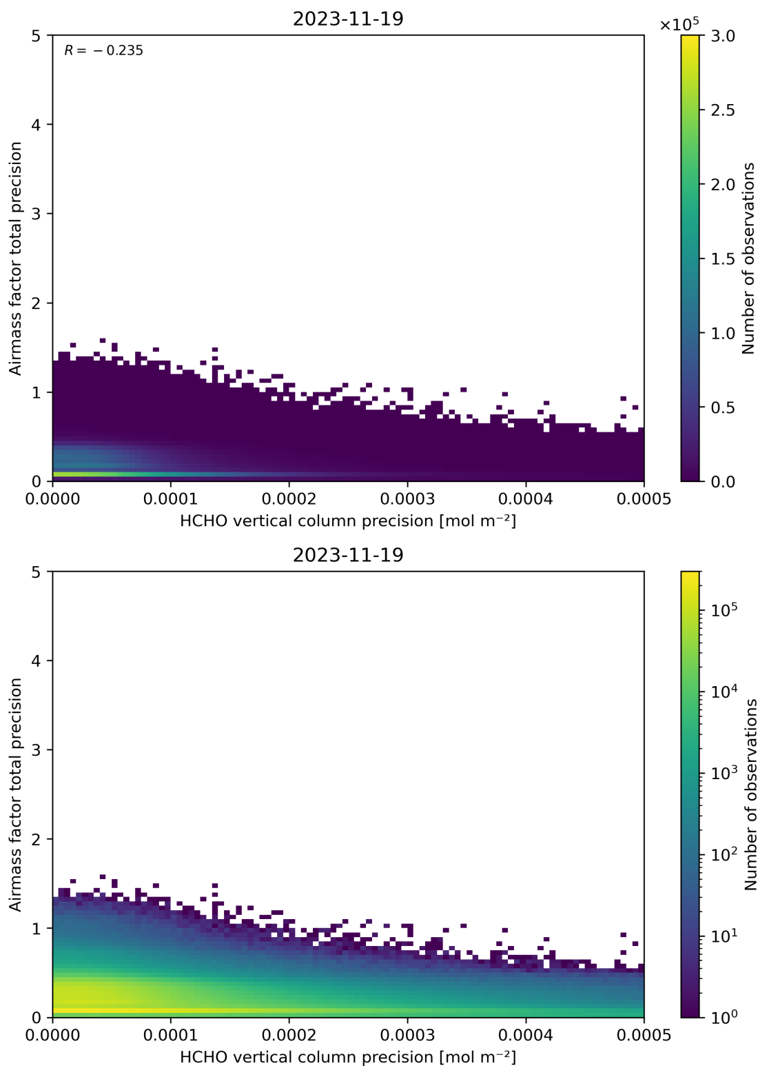
Figure 145: Scatter density plot of “HCHO vertical column precision” against “Airmass factor total precision” for 2023-11-18 to 2023-11-20.
