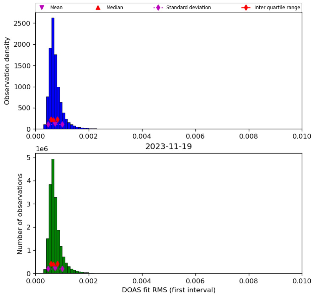
Figure 46: Histogram of “DOAS fit RMS (first interval)” for 2023-11-18 to 2023-11-20
