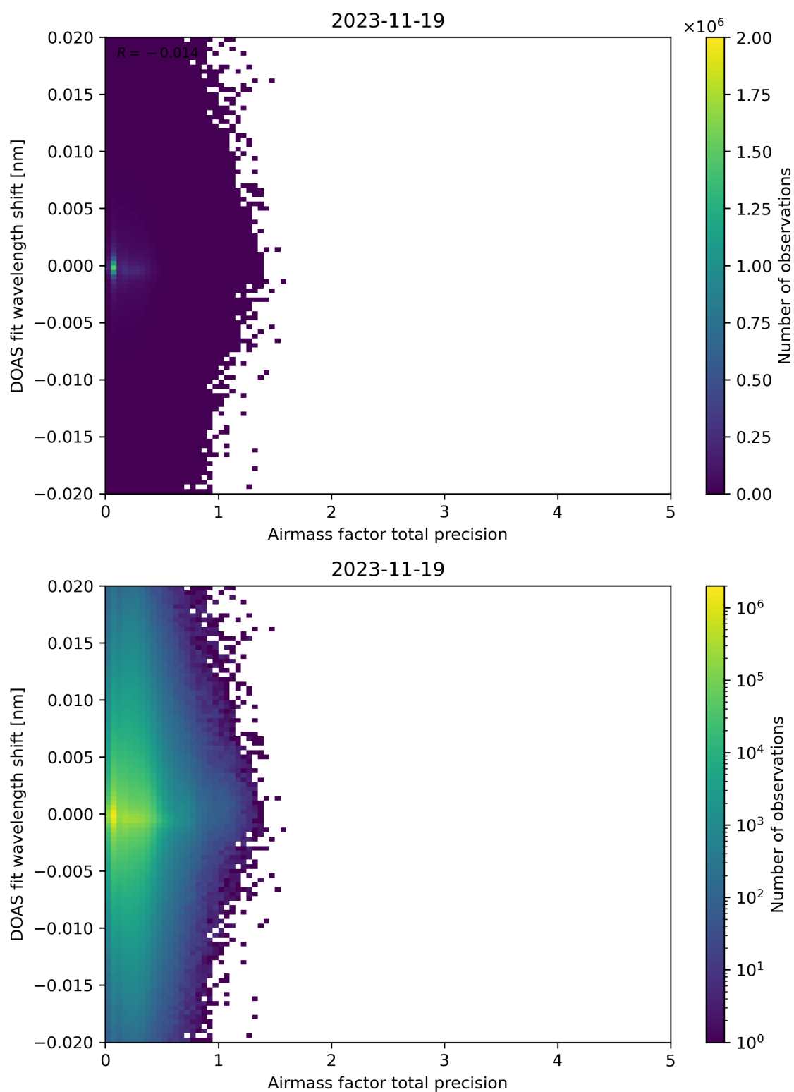
Figure 106: Scatter density plot of “Airmass factor total precision” against “DOAS fit wavelength shift” for 2023-11-18 to 2023-11-20.
