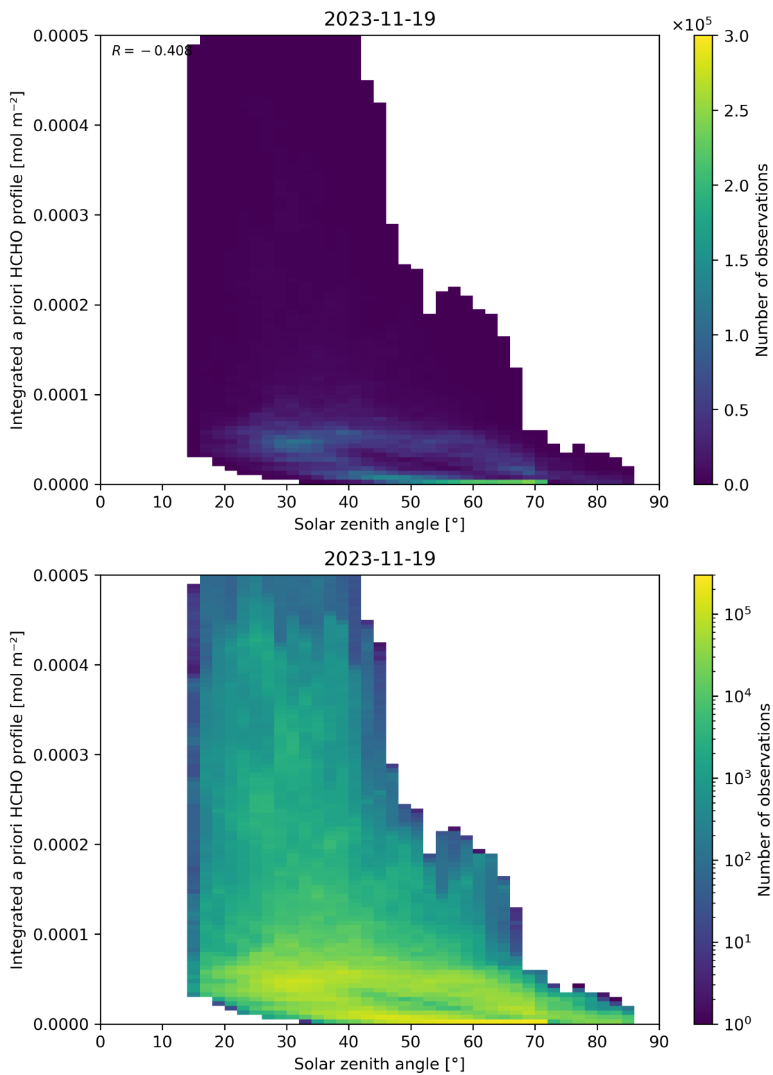
Figure 180: Scatter density plot of “Solar zenith angle” against “Integrated a priori HCHO profile” for 2023-11-18 to 2023-11-20.
