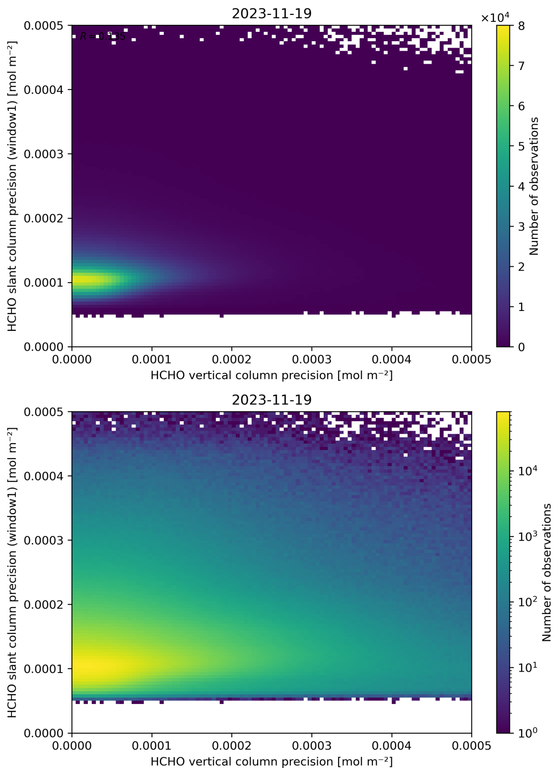
Figure 143: Scatter density plot of “HCHO vertical column precision” against “HCHO slant column precision (window1)” for 2023-11-18 to 2023-11-20.
