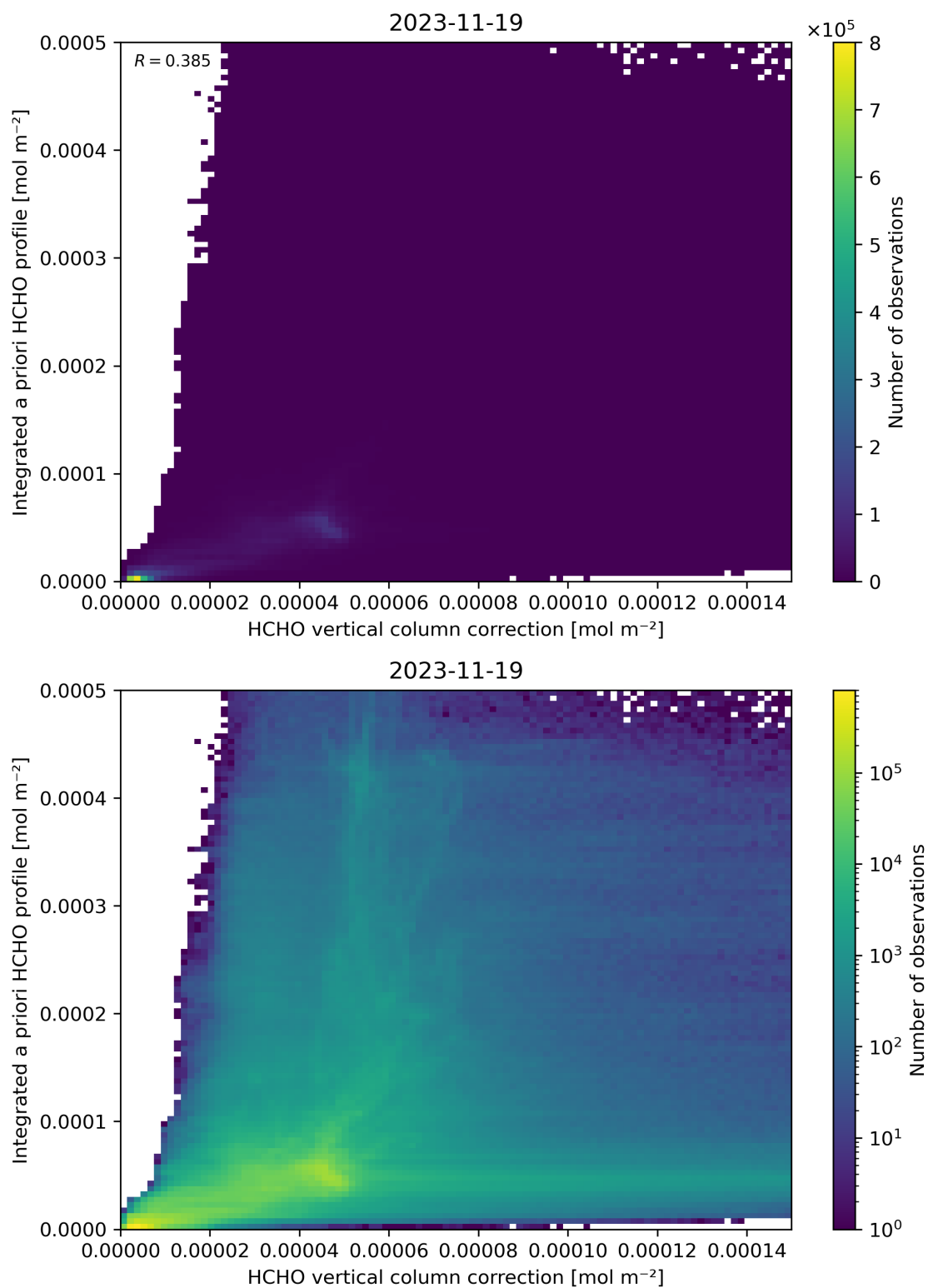
Figure 122: Scatter density plot of “HCHO vertical column correction” against “Integrated a priori HCHO profile” for 2023-11-18 to 2023-11-20.
