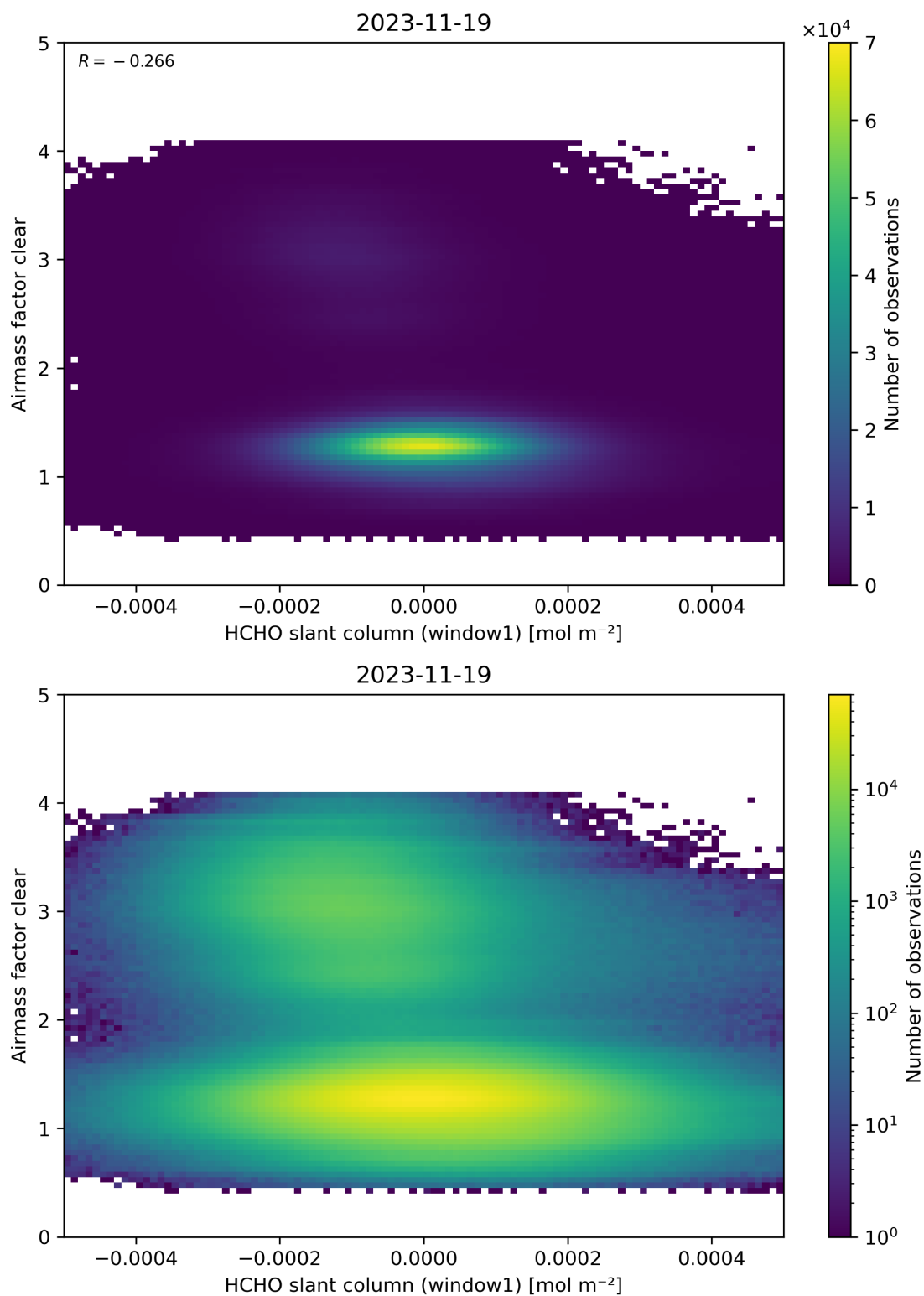
Figure 81: Scatter density plot of “HCHO slant column (window1)” against “Airmass factor clear” for 2023-11-18 to 2023-11-20.
