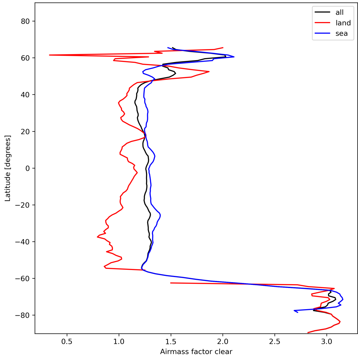
Figure 28: Zonal average of “Airmass factor clear” for 2023-11-18 to 2023-11-20.
