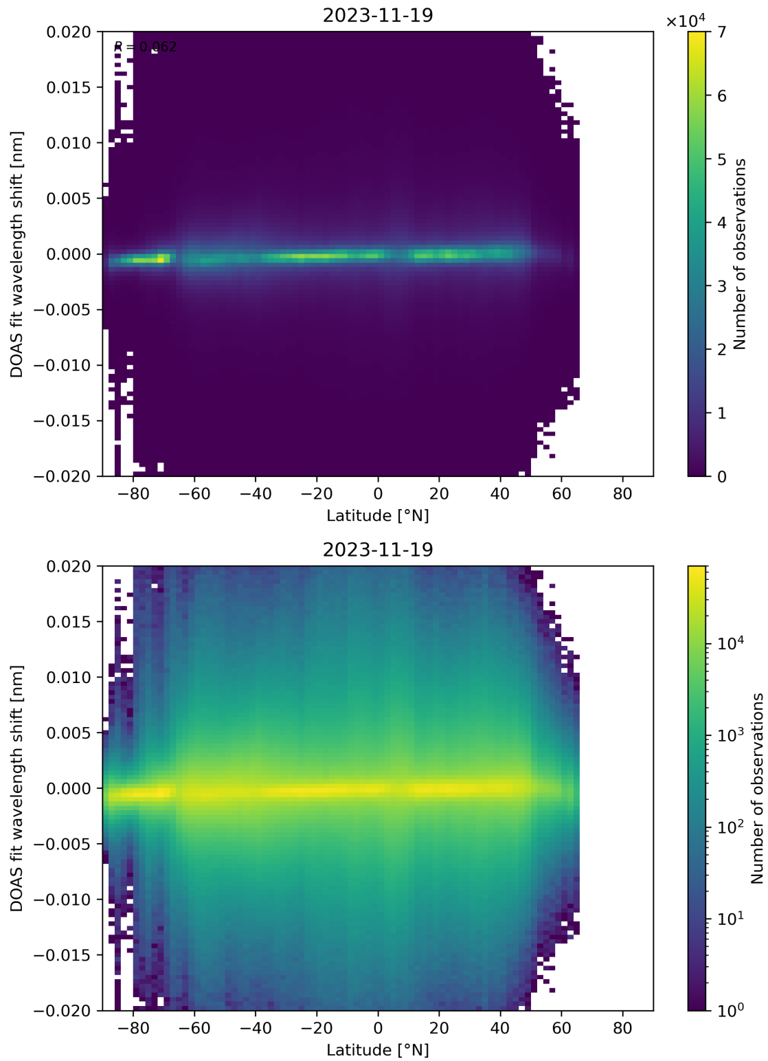
Figure 154: Scatter density plot of “Latitude” against “DOAS fit wavelength shift” for 2023-11-18 to 2023-11-20.
