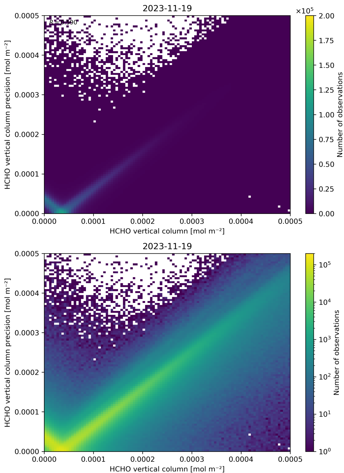
Figure 134: Scatter density plot of “HCHO vertical column” against “HCHO vertical column precision” for 2023-11-18 to 2023-11-20.
