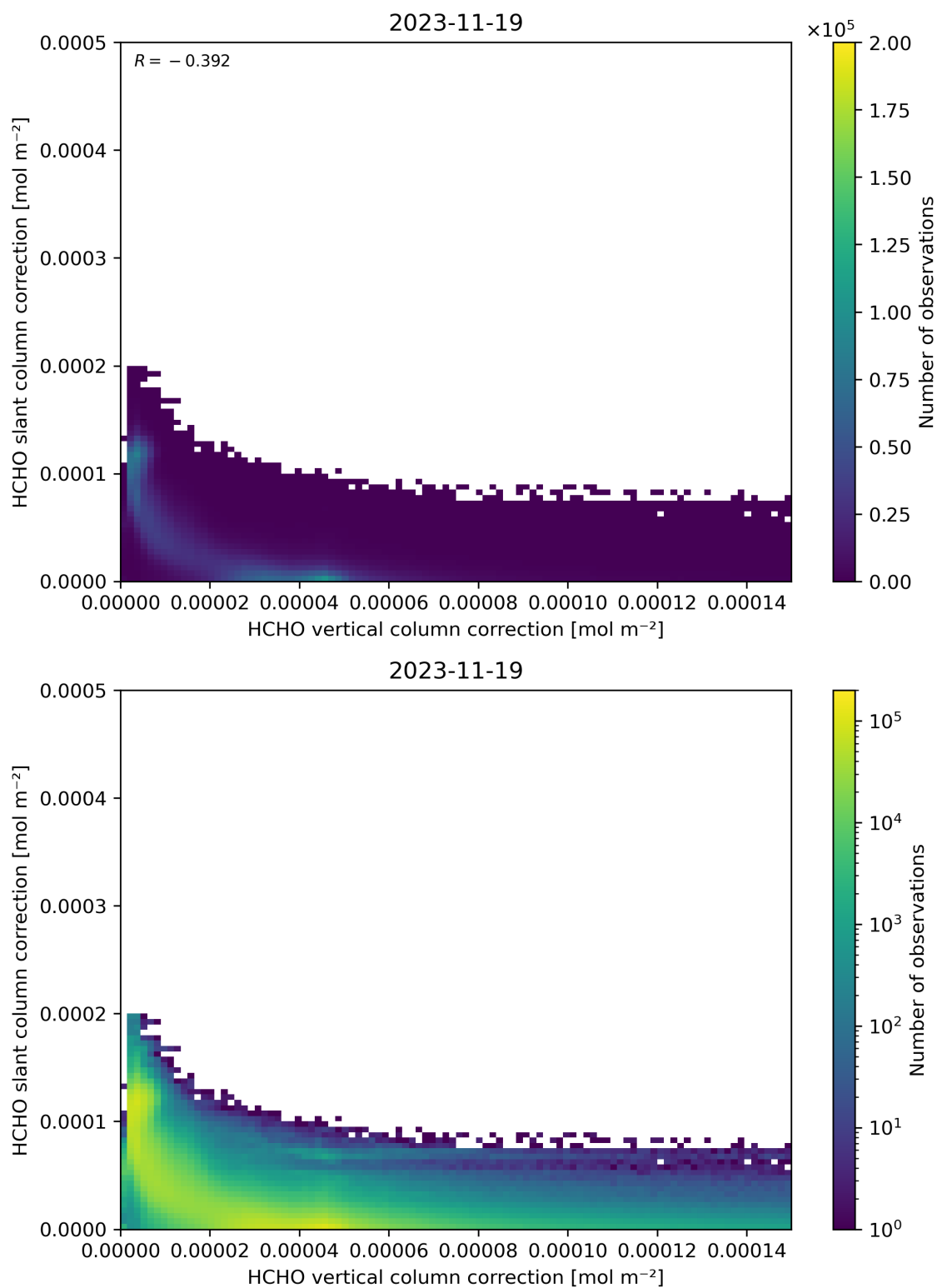
Figure 117: Scatter density plot of “HCHO vertical column correction” against “HCHO slant column correction” for 2023-11-18 to 2023-11-20.
