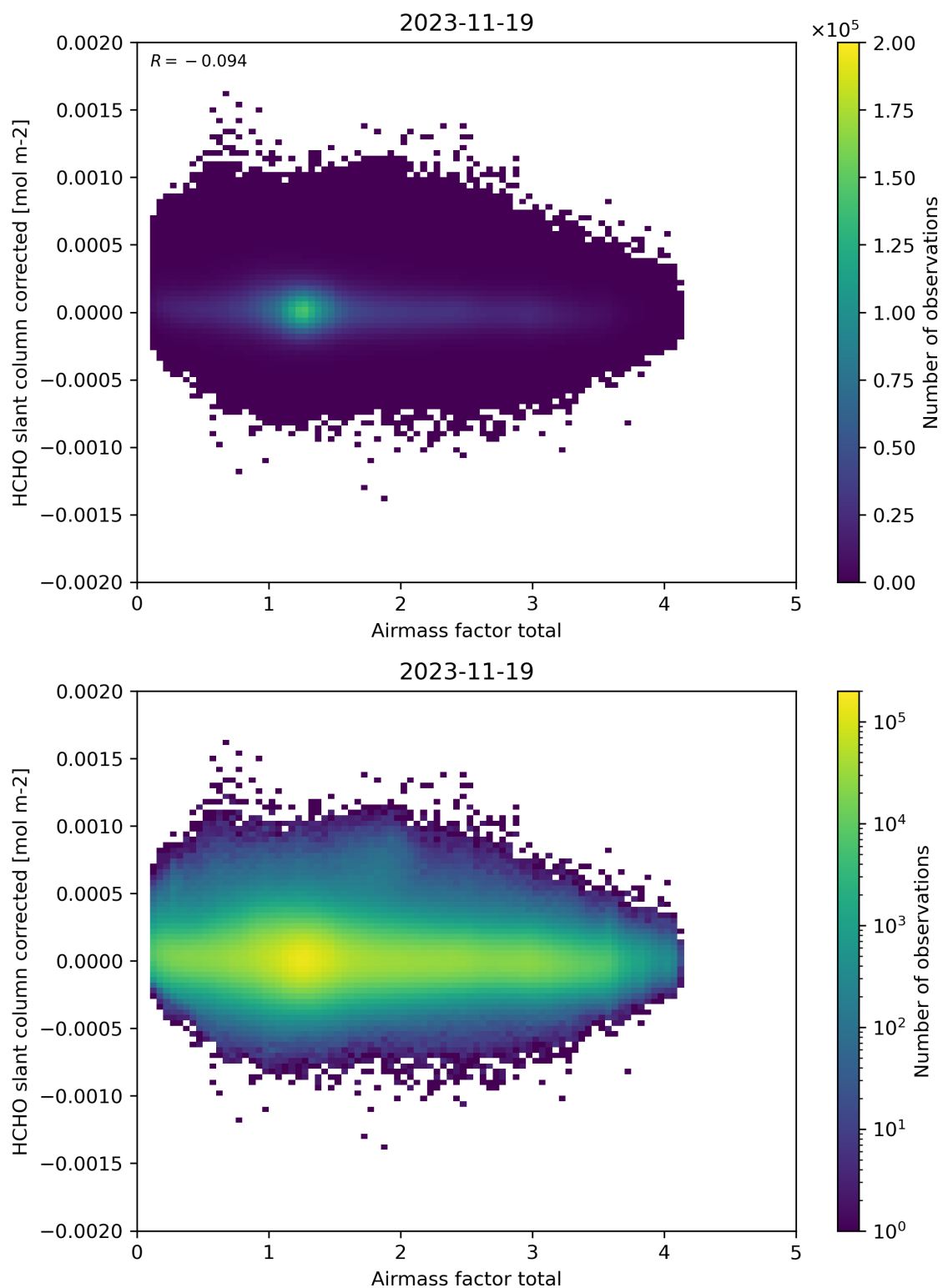
Figure 101: Scatter density plot of “Airmass factor total” against “HCHO slant column corrected” for 2023-11-18 to 2023-11-20.
