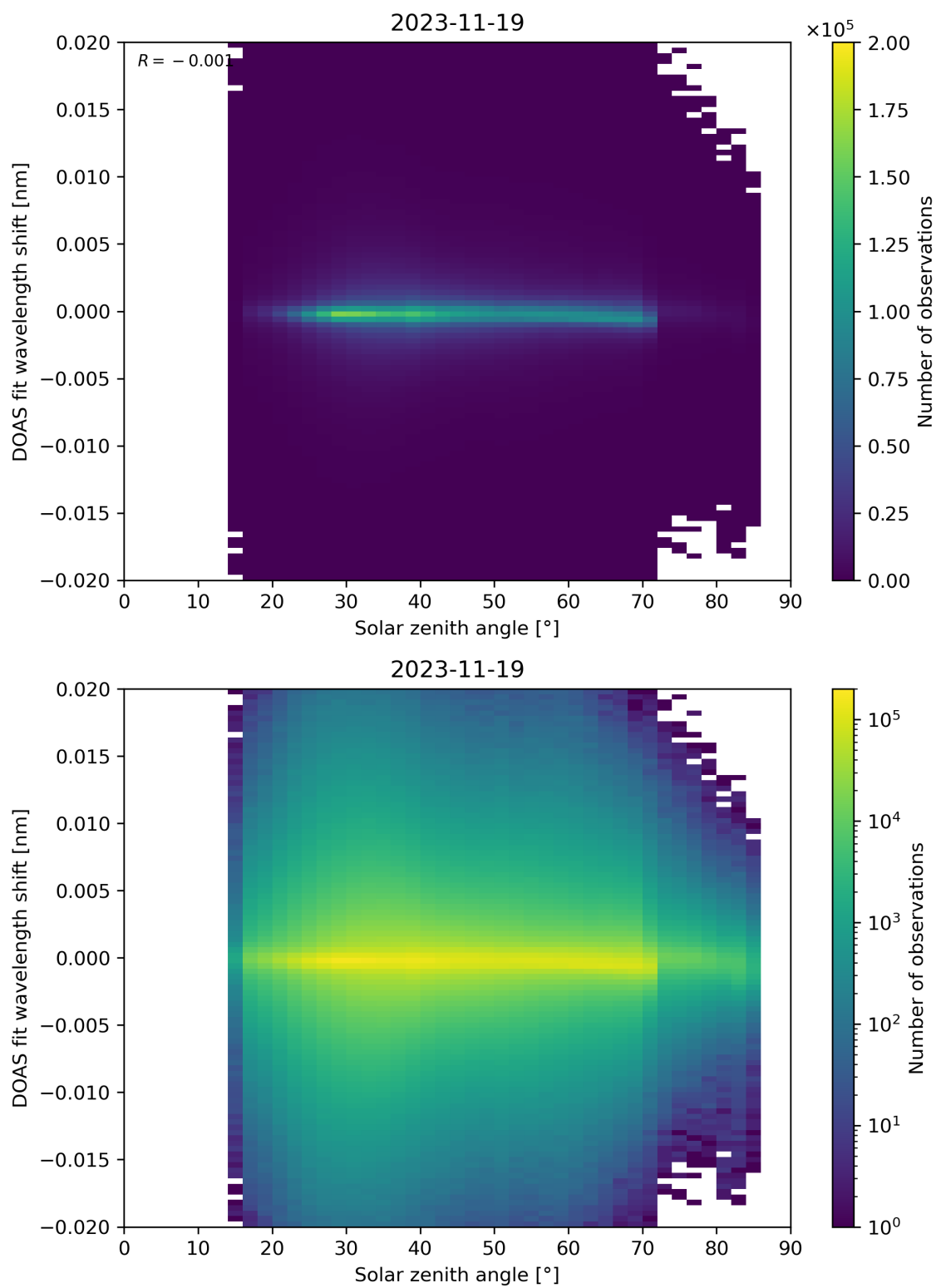
Figure 168: Scatter density plot of “Solar zenith angle” against “DOAS fit wavelength shift” for 2023-11-18 to 2023-11-20.
