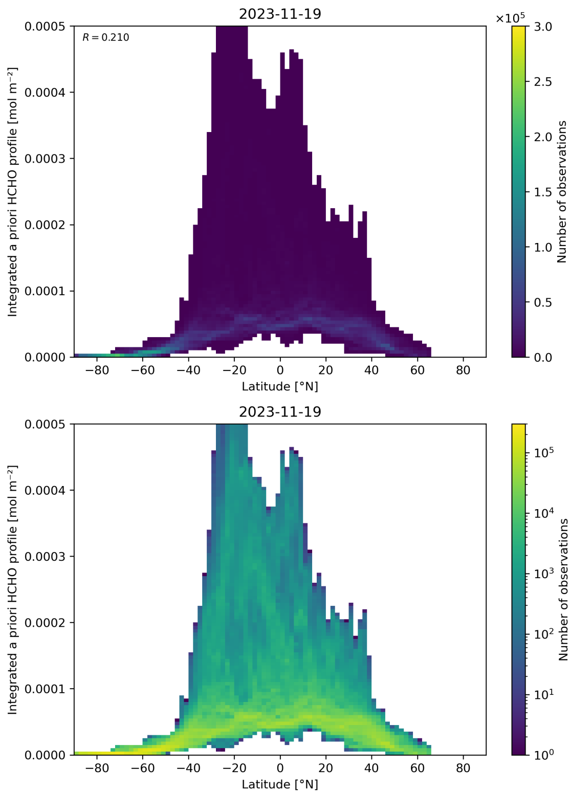
Figure 166: Scatter density plot of “Latitude” against “Integrated a priori HCHO profile” for 2023-11-18 to 2023-11-20.
