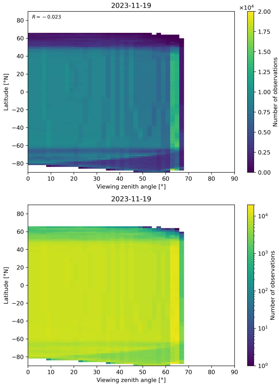
Figure 196: Scatter density plot of “Viewing zenith angle” against “Latitude” for 2023-11-18 to 2023-11-20.
