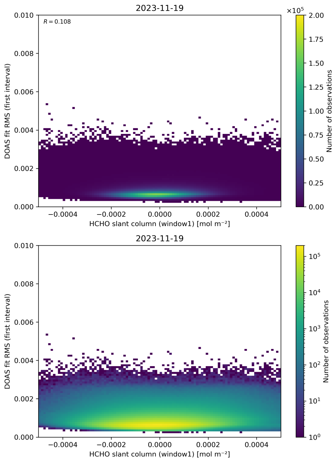
Figure 78: Scatter density plot of “HCHO slant column (window1)” against “DOAS fit RMS (first interval)” for 2023-11-18 to 2023-11-20.
