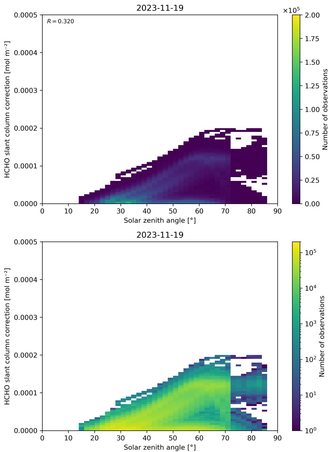
Figure 172: Scatter density plot of “Solar zenith angle” against “HCHO slant column correction” for 2023-11-18 to 2023-11-20.
