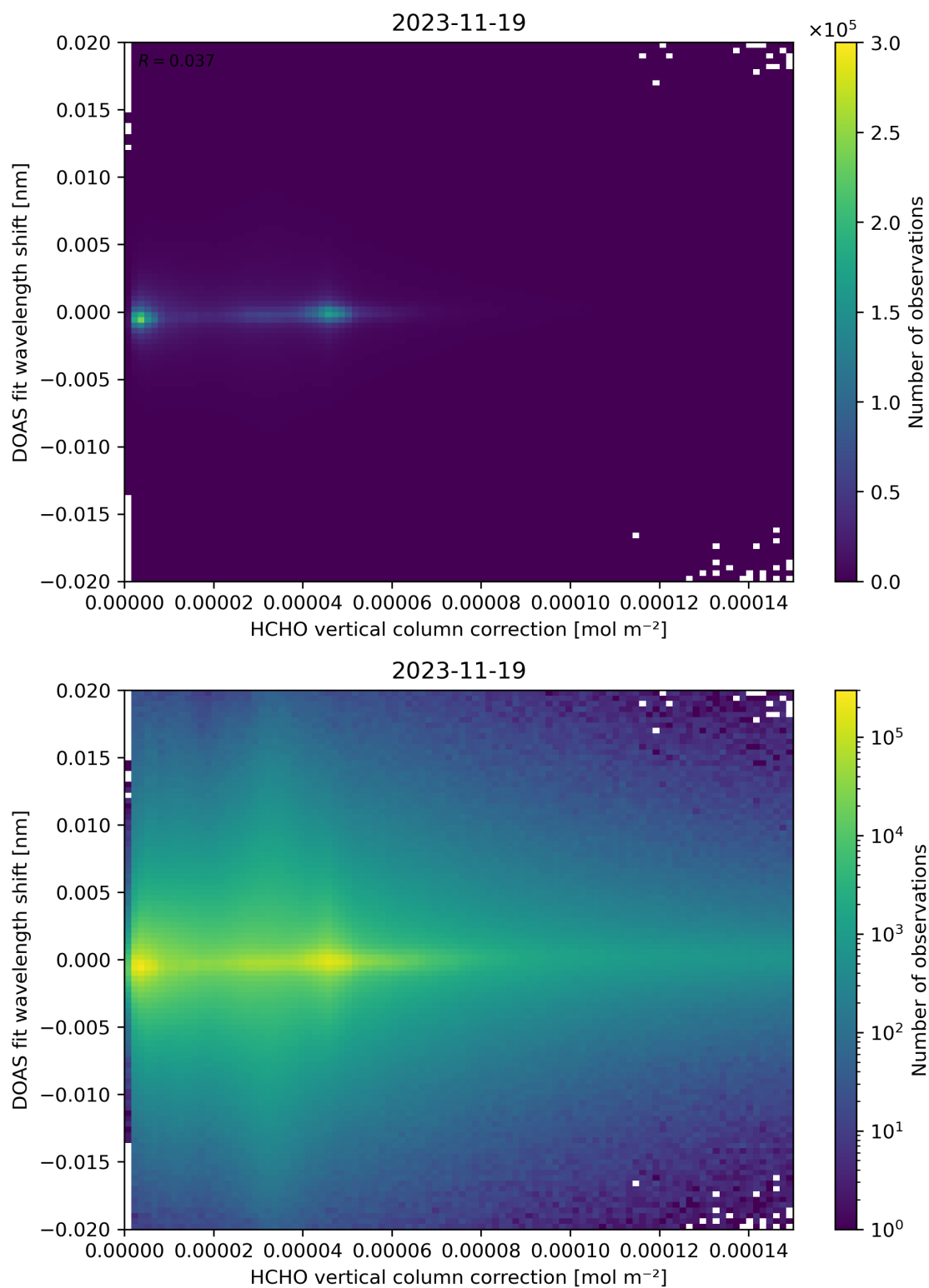
Figure 113: Scatter density plot of “HCHO vertical column correction” against “DOAS fit wavelength shift” for 2023-11-18 to 2023-11-20.
