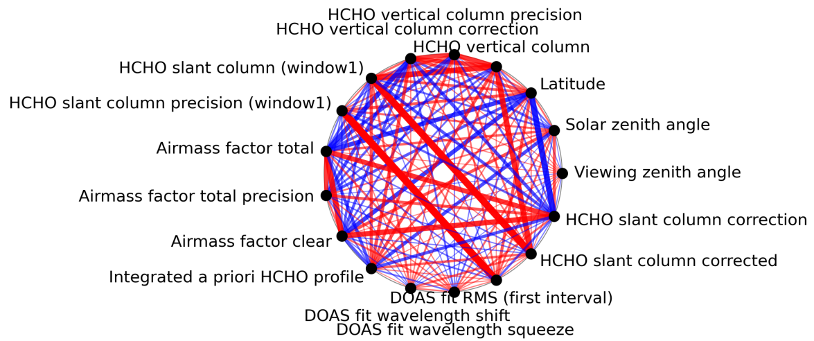
Figure 1: Map of correlation graph for 2023-11-18 to 2023-11-20.
