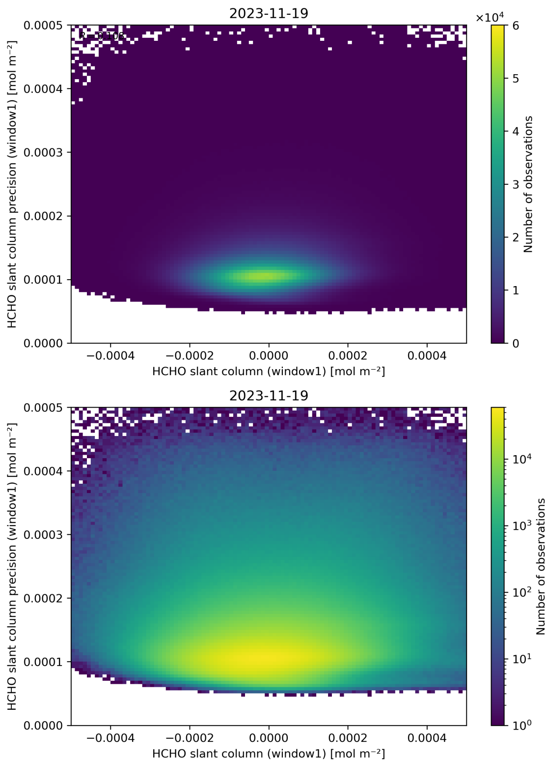
Figure 84: Scatter density plot of “HCHO slant column (window1)” against “HCHO slant column precision (window1)” for 2023-11-18 to 2023-11-20.
