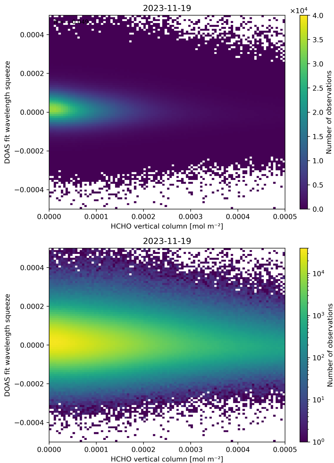
Figure 125: Scatter density plot of “HCHO vertical column” against “DOAS fit wavelength squeeze” for 2023-11-18 to 2023-11-20.
