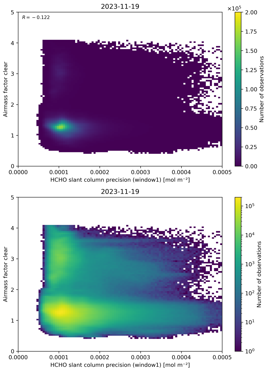
Figure 91: Scatter density plot of “HCHO slant column precision (window1)” against “Airmass factor clear” for 2023-11-18 to 2023-11-20.
