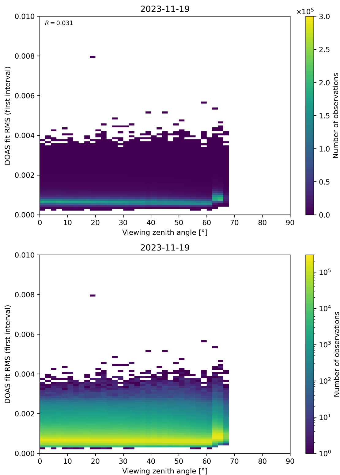
Figure 182: Scatter density plot of “Viewing zenith angle” against “DOAS fit RMS (first interval)” for 2023-11-18 to 2023-11-20.
