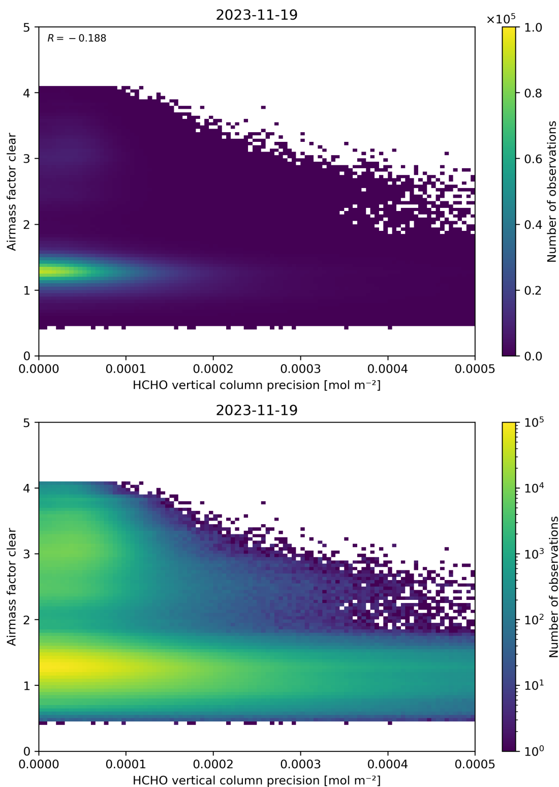
Figure 139: Scatter density plot of “HCHO vertical column precision” against “Airmass factor clear” for 2023-11-18 to 2023-11-20.
