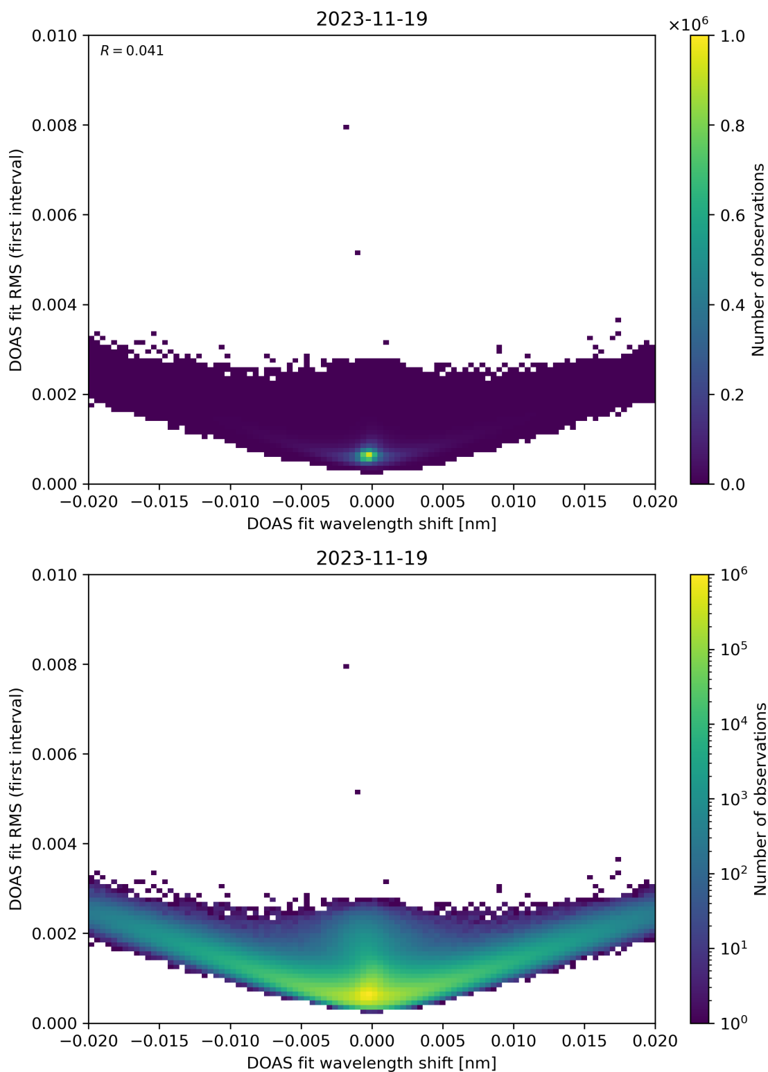
Figure 64: Scatter density plot of “DOAS fit wavelength shift” against “DOAS fit RMS (first interval)” for 2023-11-18 to 2023-11-20.
