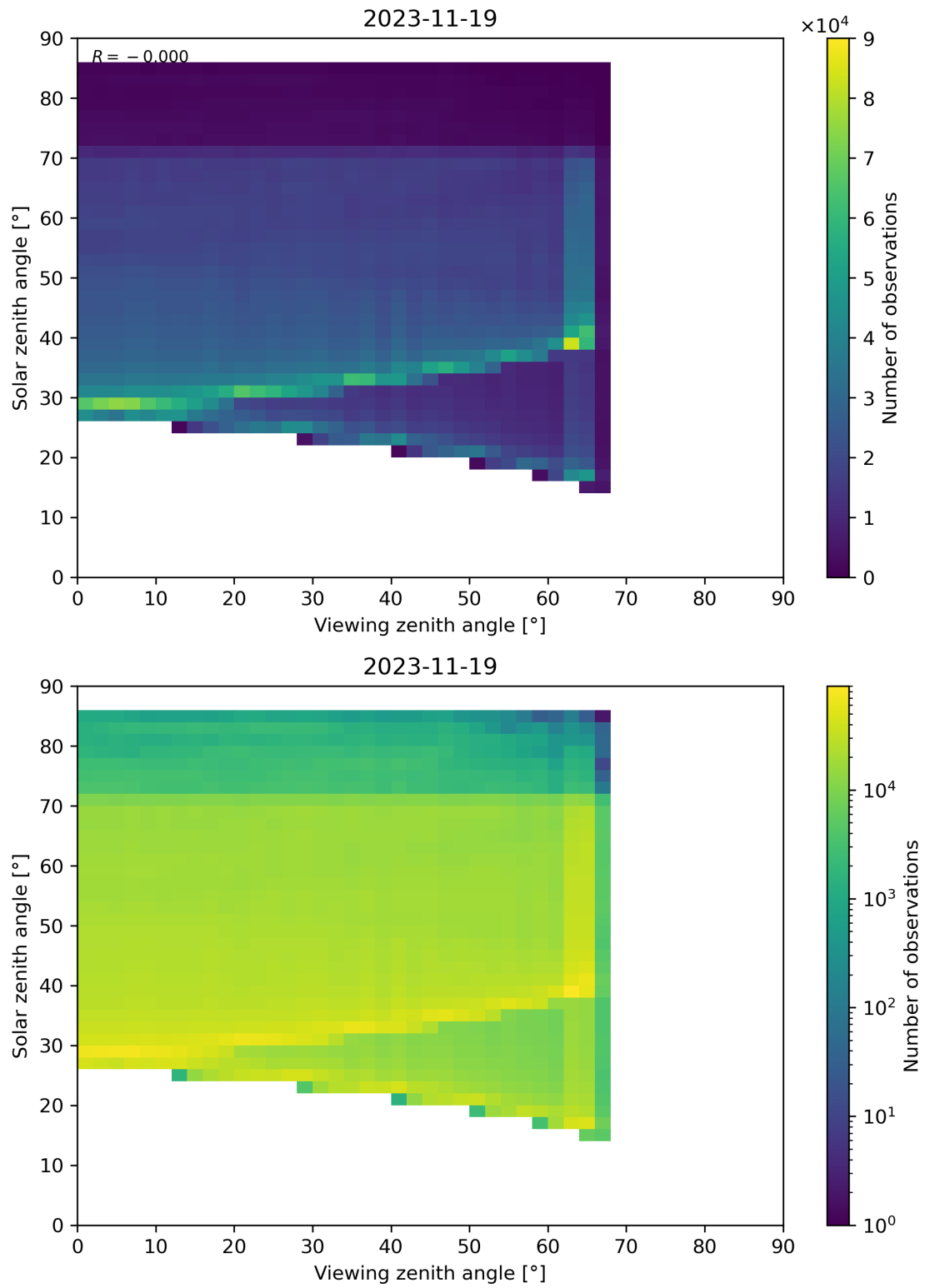
Figure 197: Scatter density plot of “Viewing zenith angle” against “Solar zenith angle” for 2023-11-18 to 2023-11-20.
