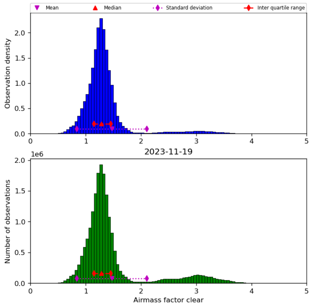
Figure 42: Histogram of “Airmass factor clear” for 2023-11-18 to 2023-11-20
