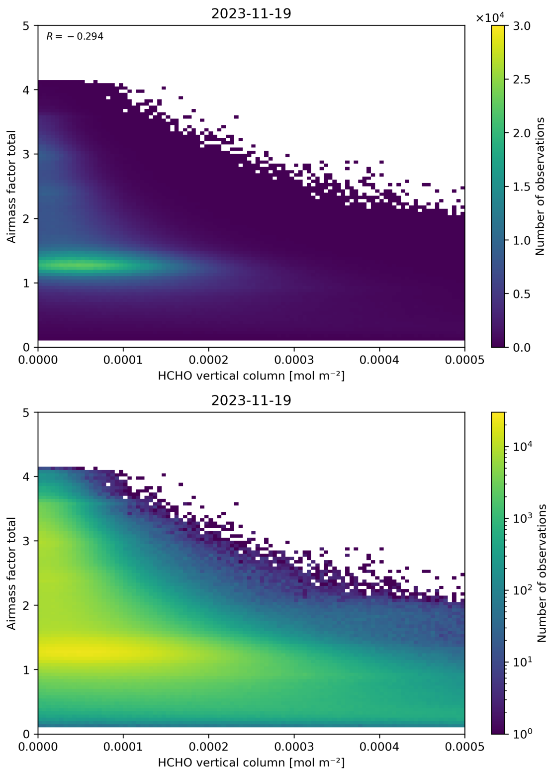
Figure 131: Scatter density plot of “HCHO vertical column” against “Airmass factor total” for 2023-11-18 to 2023-11-20.
