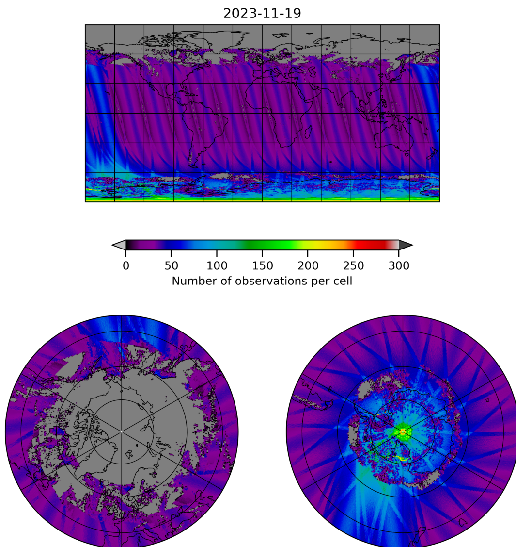
Figure 19: Map of the number of observations for 2023-11-18 to 2023-11-20
