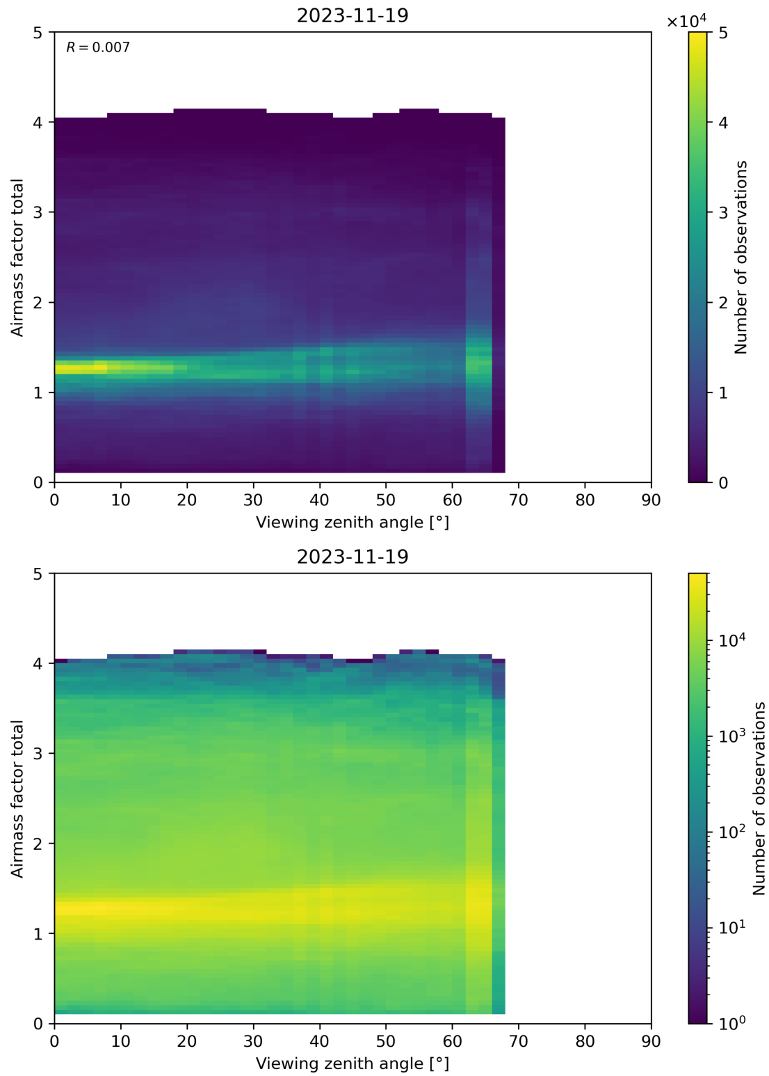
Figure 190: Scatter density plot of “Viewing zenith angle” against “Airmass factor total” for 2023-11-18 to 2023-11-20.
