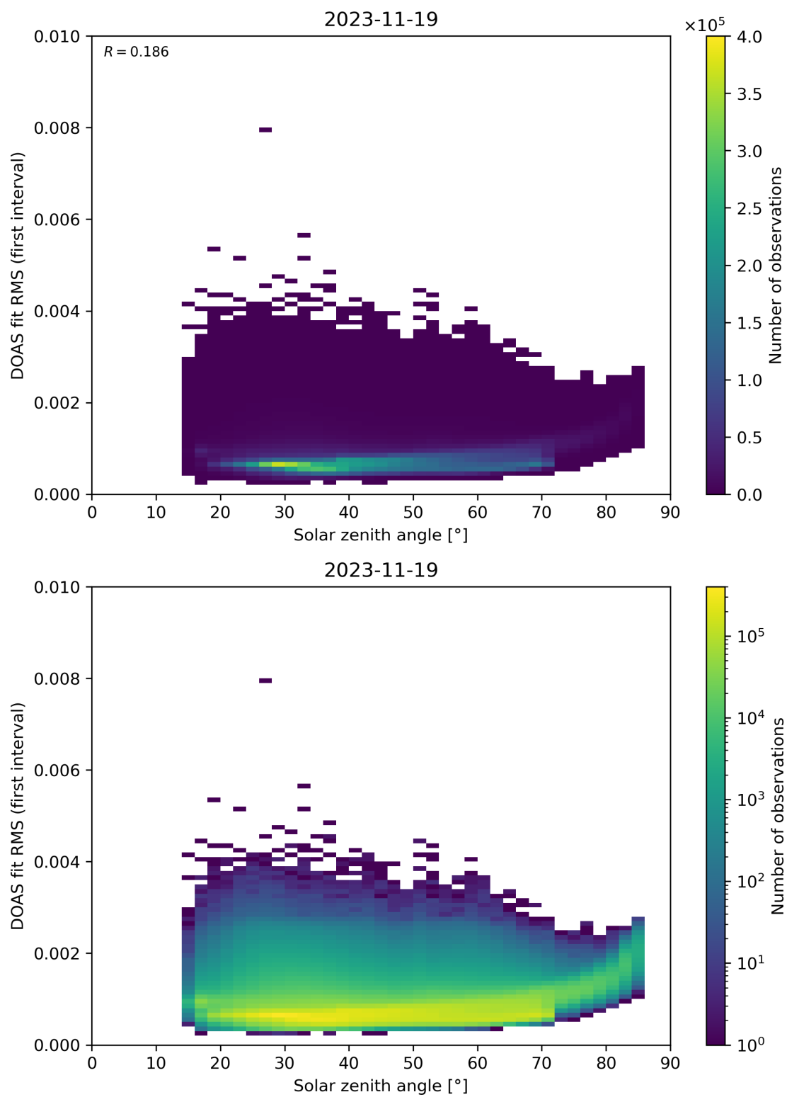
Figure 167: Scatter density plot of “Solar zenith angle” against “DOAS fit RMS (first interval)” for 2023-11-18 to 2023-11-20.
