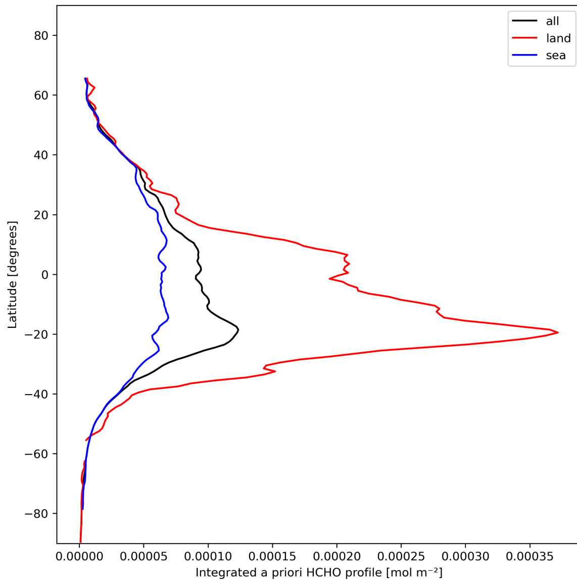
Figure 29: Zonal average of “Integrated a priori HCHO profile” for 2023-11-18 to 2023-11-20.
