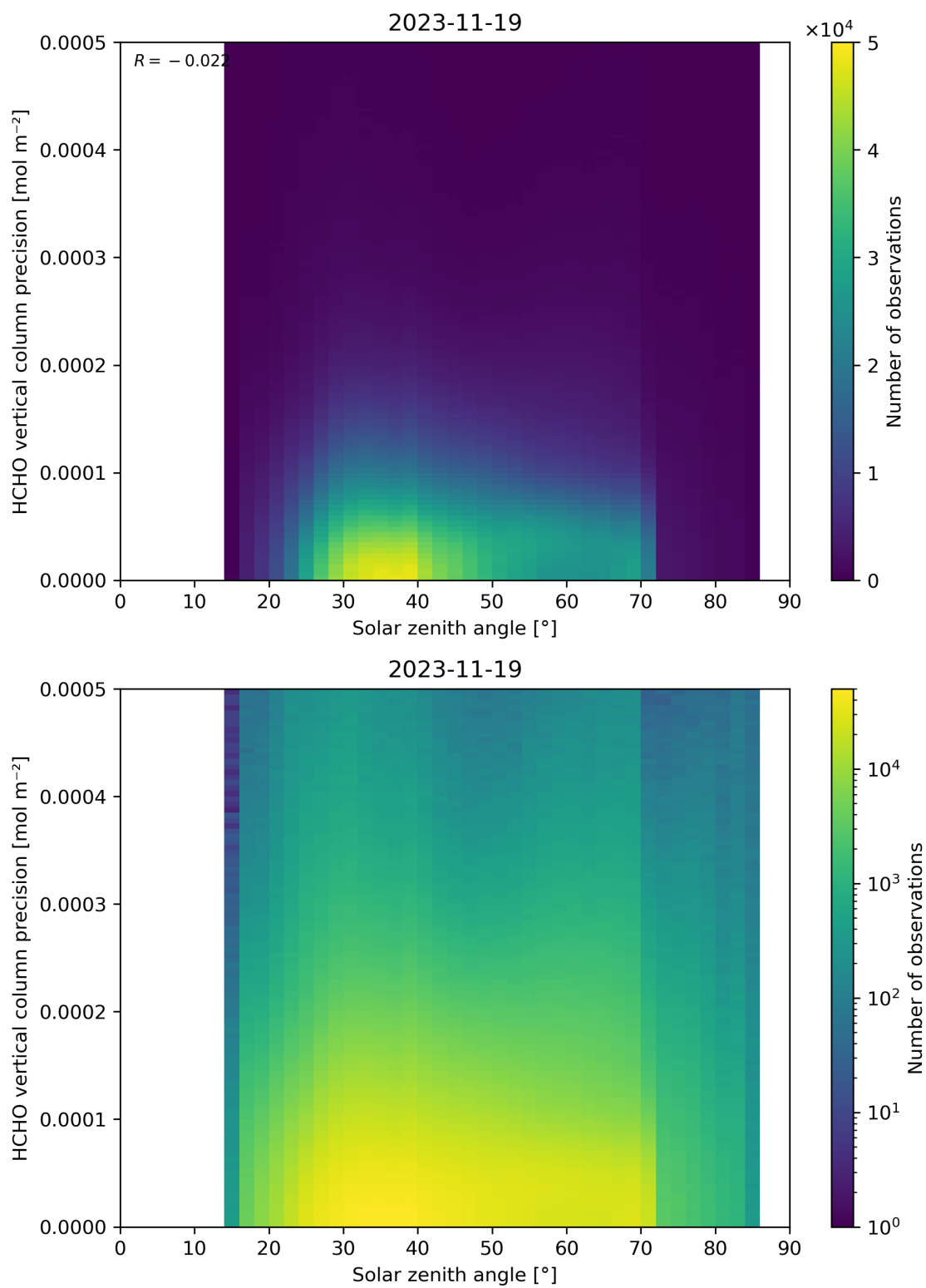
Figure 179: Scatter density plot of “Solar zenith angle” against “HCHO vertical column precision” for 2023-11-18 to 2023-11-20.
