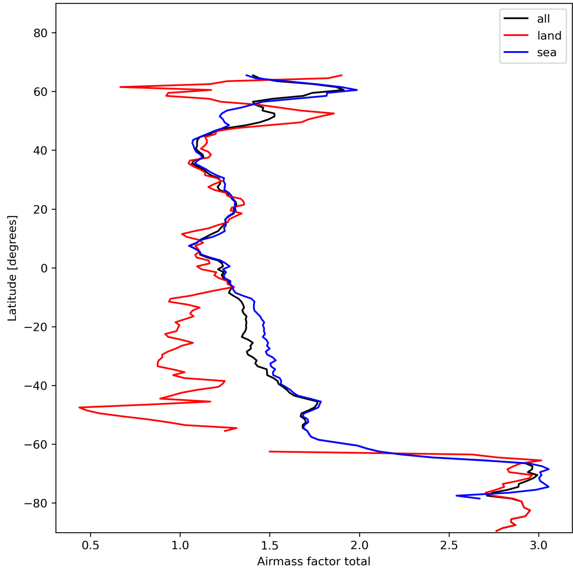
Figure 26: Zonal average of “Airmass factor total” for 2023-11-18 to 2023-11-20.
