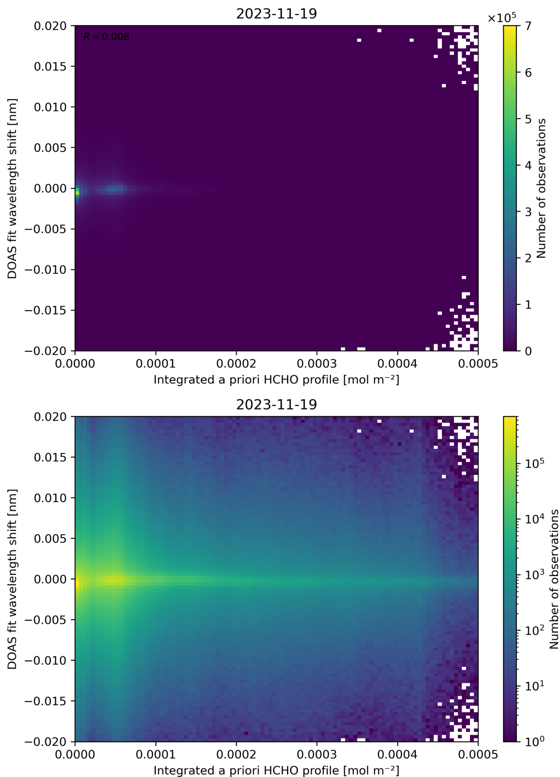
Figure 149: Scatter density plot of “Integrated a priori HCHO profile” against “DOAS fit wavelength shift” for 2023-11-18 to 2023-11-20.
