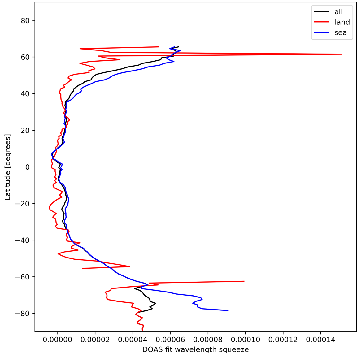
Figure 31: Zonal average of “DOAS fit wavelength squeeze” for 2023-11-18 to 2023-11-20.
