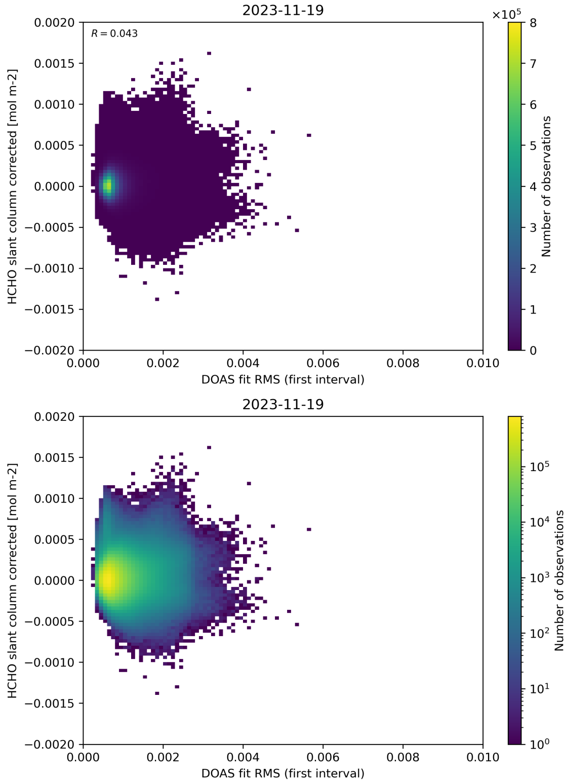
Figure 62: Scatter density plot of “DOAS fit RMS (first interval)” against “HCHO slant column corrected” for 2023-11-18 to 2023-11-20.
