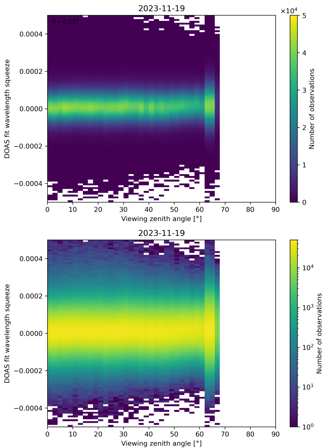
Figure 184: Scatter density plot of “Viewing zenith angle” against “DOAS fit wavelength squeeze” for 2023-11-18 to 2023-11-20.
