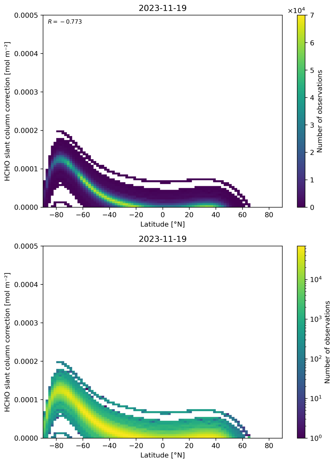
Figure 158: Scatter density plot of “Latitude” against “HCHO slant column correction” for 2023-11-18 to 2023-11-20.
