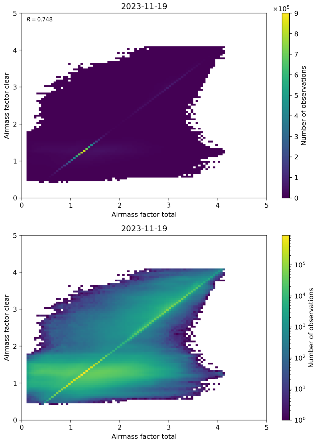
Figure 100: Scatter density plot of “Airmass factor total” against “Airmass factor clear” for 2023-11-18 to 2023-11-20.
