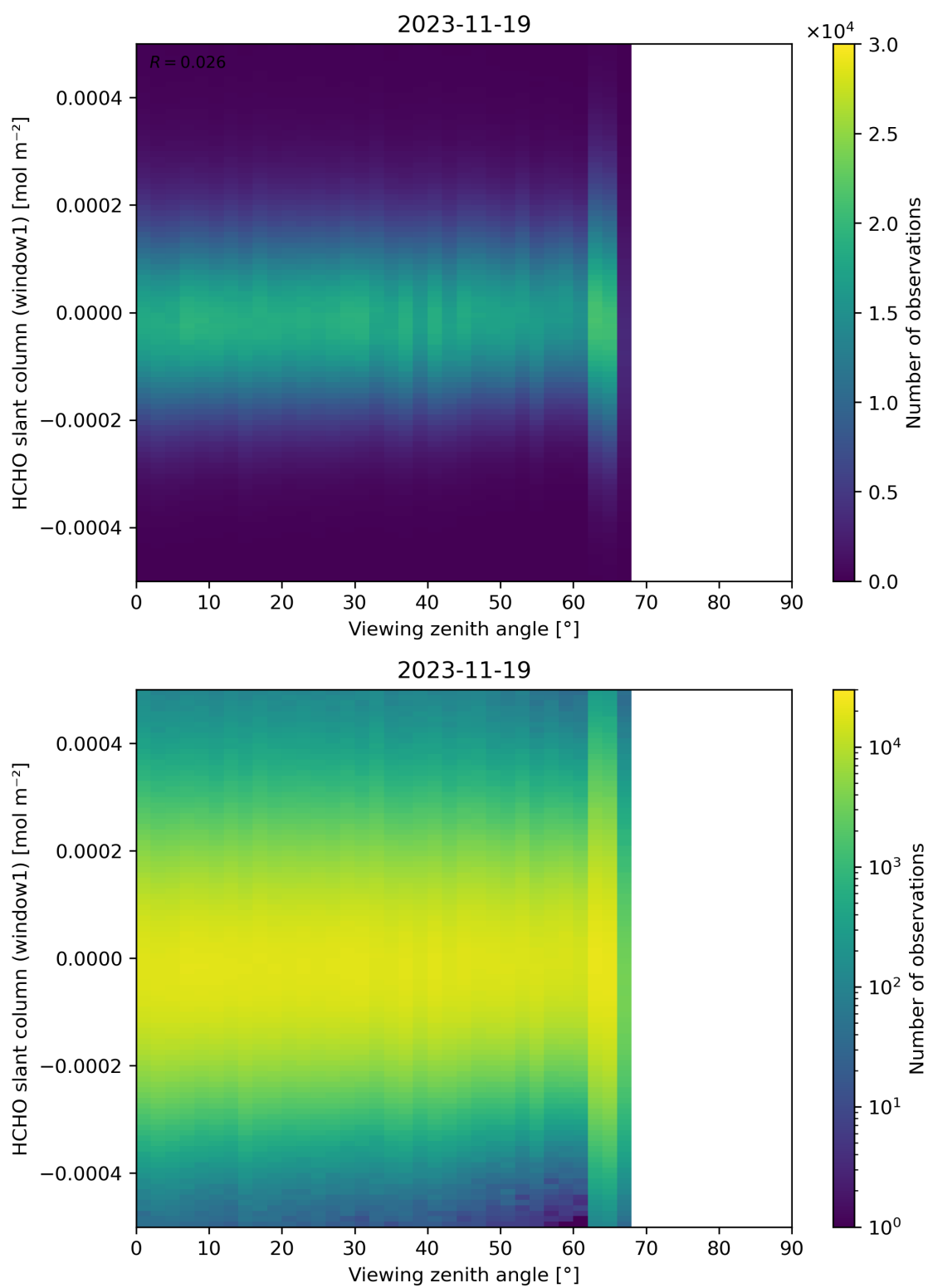
Figure 188: Scatter density plot of “Viewing zenith angle” against “HCHO slant column (window1)” for 2023-11-18 to 2023-11-20.
