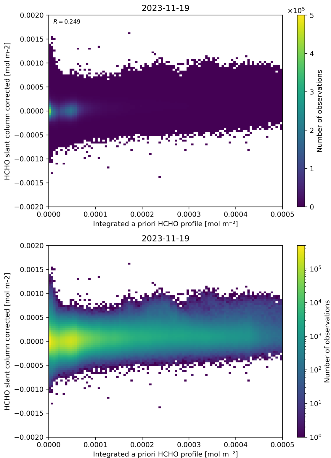
Figure 151: Scatter density plot of “Integrated a priori HCHO profile” against “HCHO slant column corrected” for 2023-11-18 to 2023-11-20.
