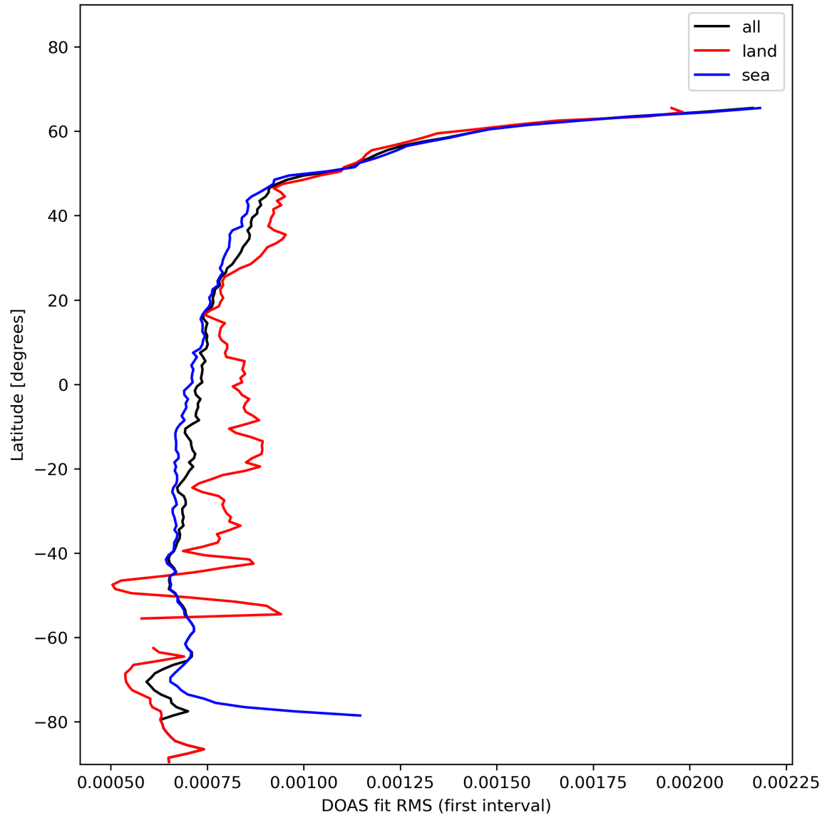
Figure 32: Zonal average of “DOAS fit RMS (first interval)” for 2023-11-18 to 2023-11-20.
