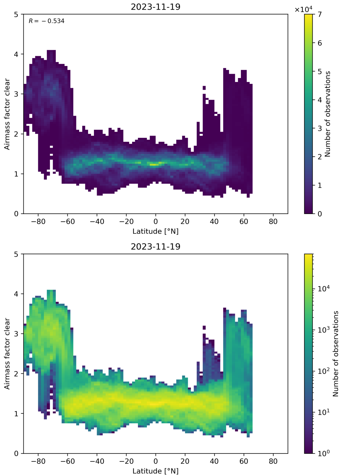
Figure 156: Scatter density plot of “Latitude” against “Airmass factor clear” for 2023-11-18 to 2023-11-20.
