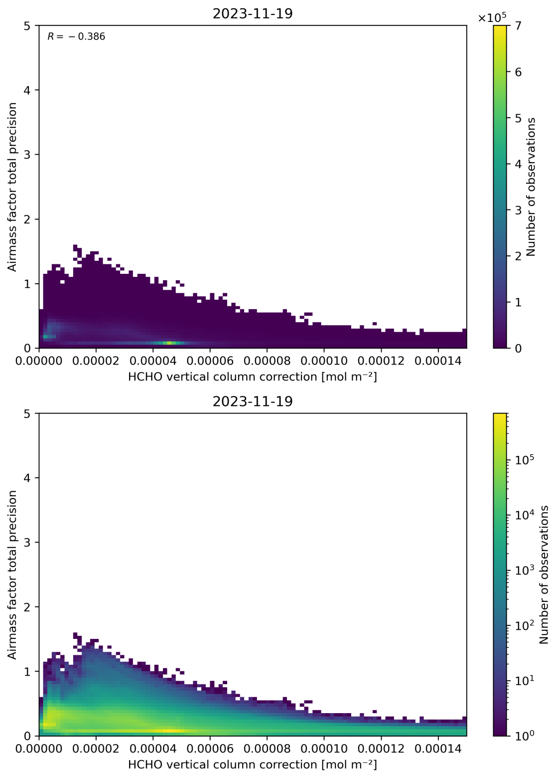
Figure 121: Scatter density plot of “HCHO vertical column correction” against “Airmass factor total precision” for 2023-11-18 to 2023-11-20.
