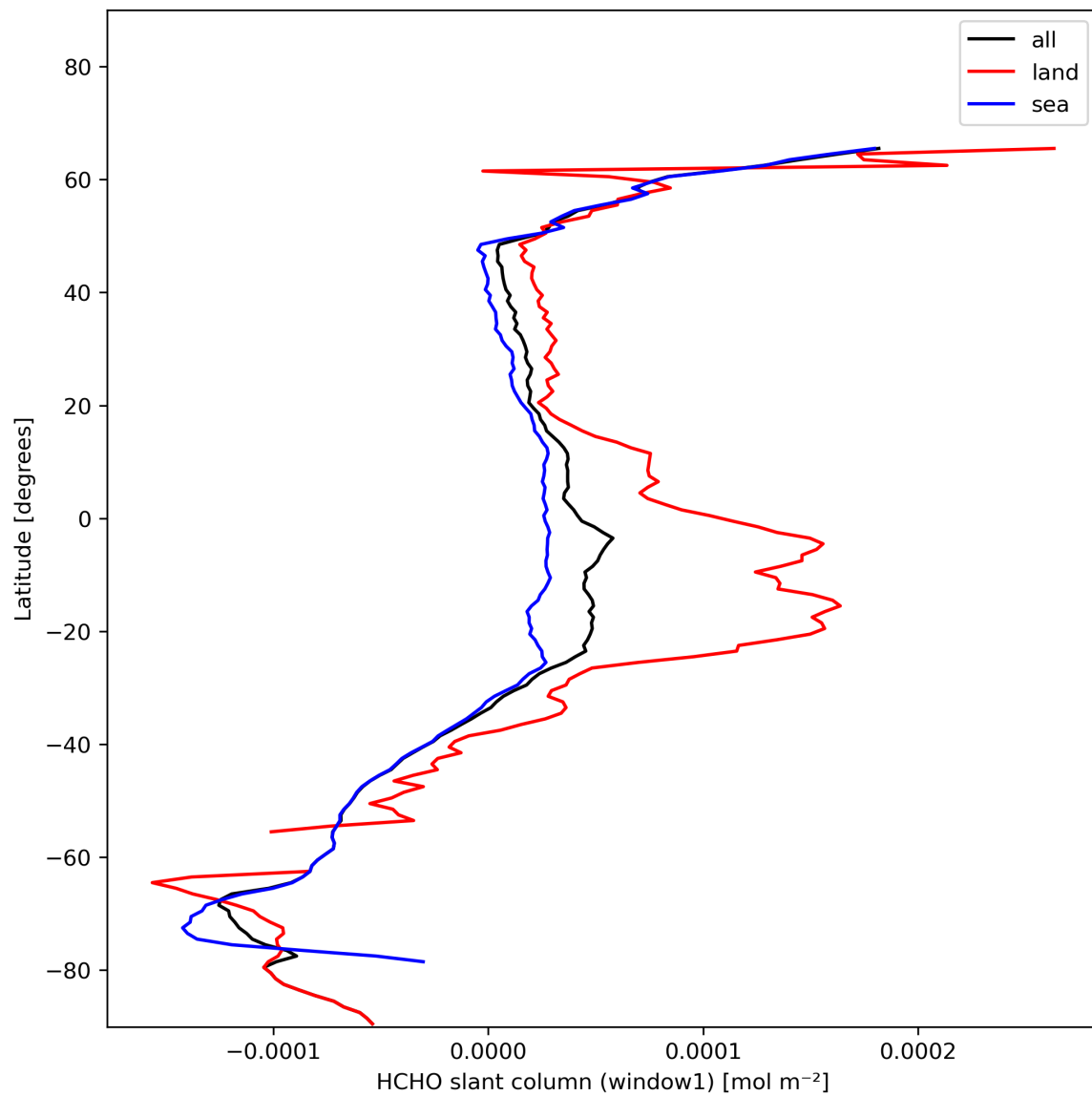
Figure 24: Zonal average of “HCHO slant column (window1)” for 2023-11-18 to 2023-11-20.
