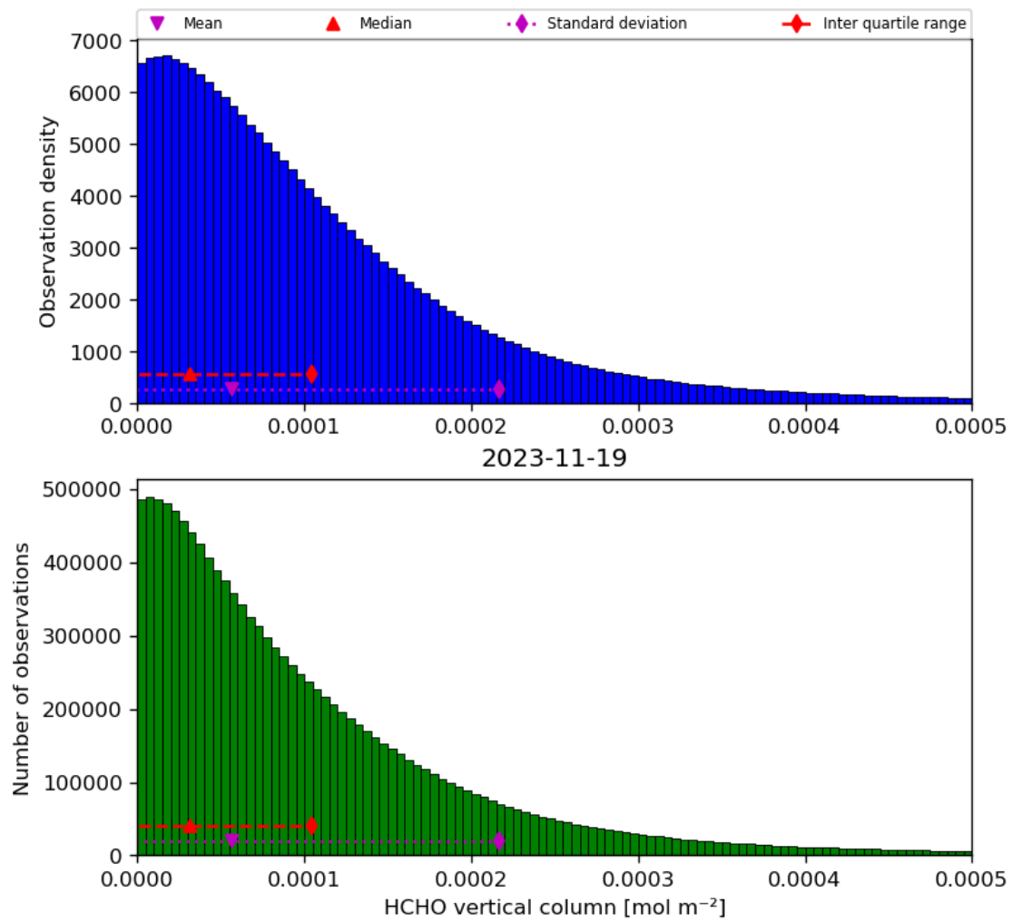
Figure 35: Histogram of “HCHO vertical column” for 2023-11-18 to 2023-11-20
