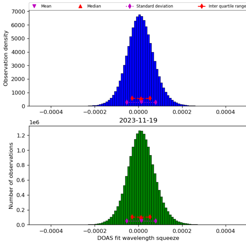
Figure 45: Histogram of “DOAS fit wavelength squeeze” for 2023-11-18 to 2023-11-20
