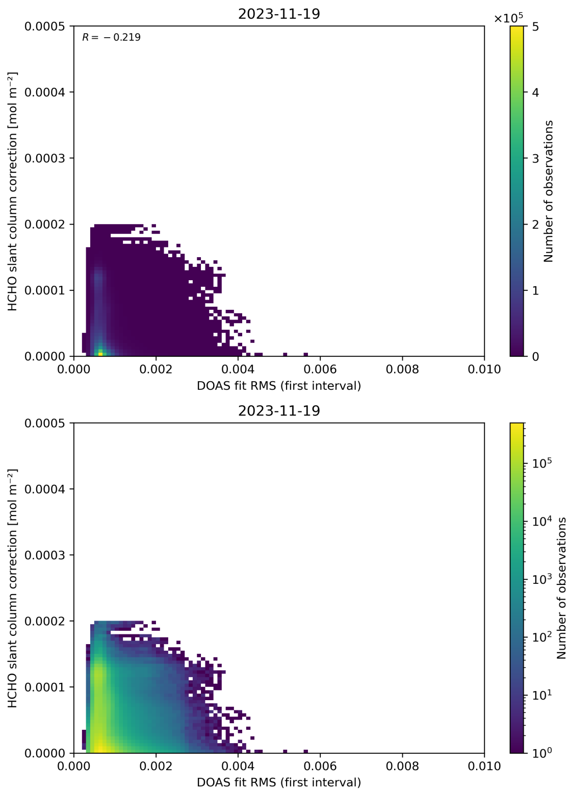
Figure 63: Scatter density plot of “DOAS fit RMS (first interval)” against “HCHO slant column correction” for 2023-11-18 to 2023-11-20.
