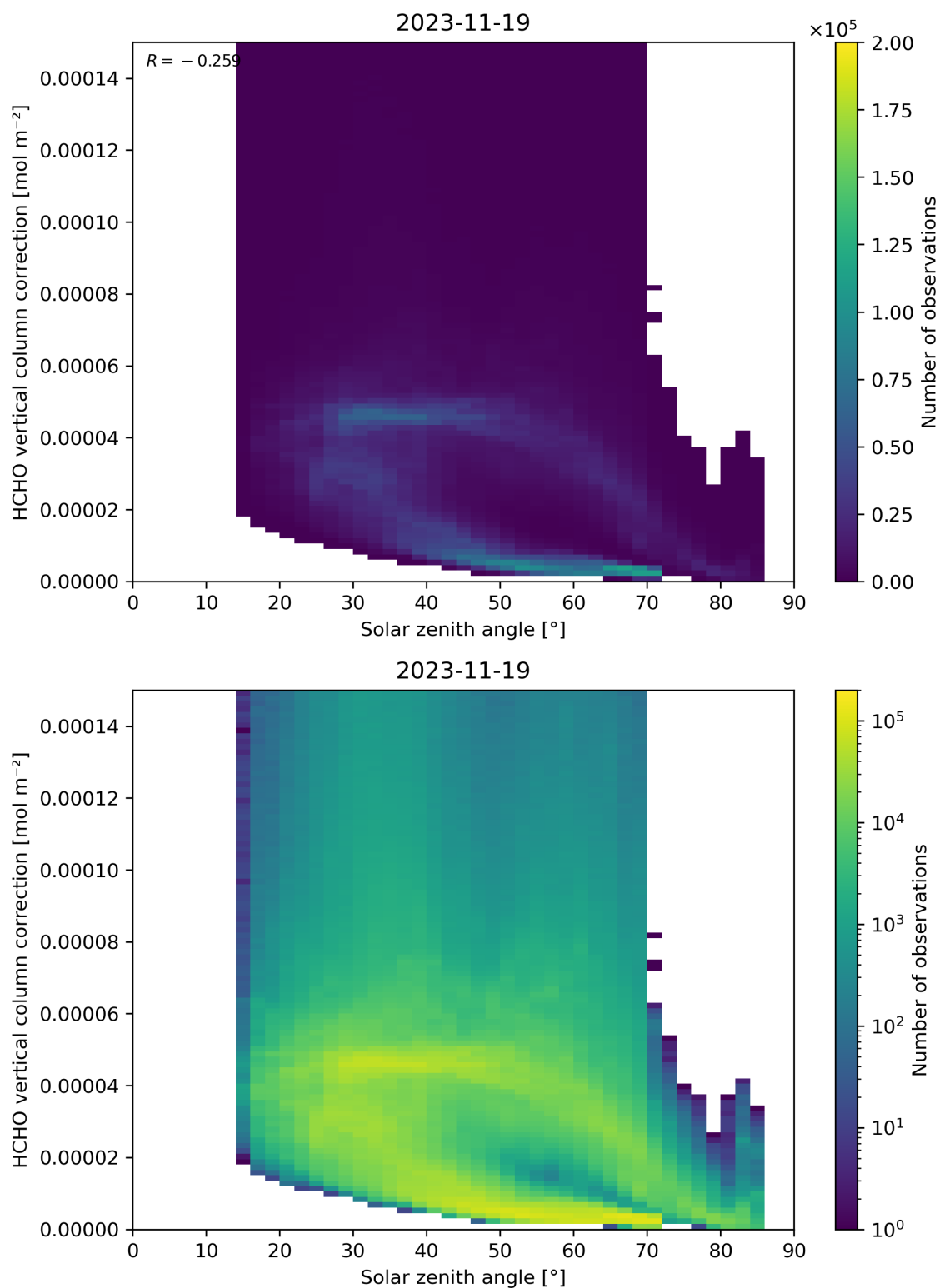
Figure 178: Scatter density plot of “Solar zenith angle” against “HCHO vertical column correction” for 2023-11-18 to 2023-11-20.
