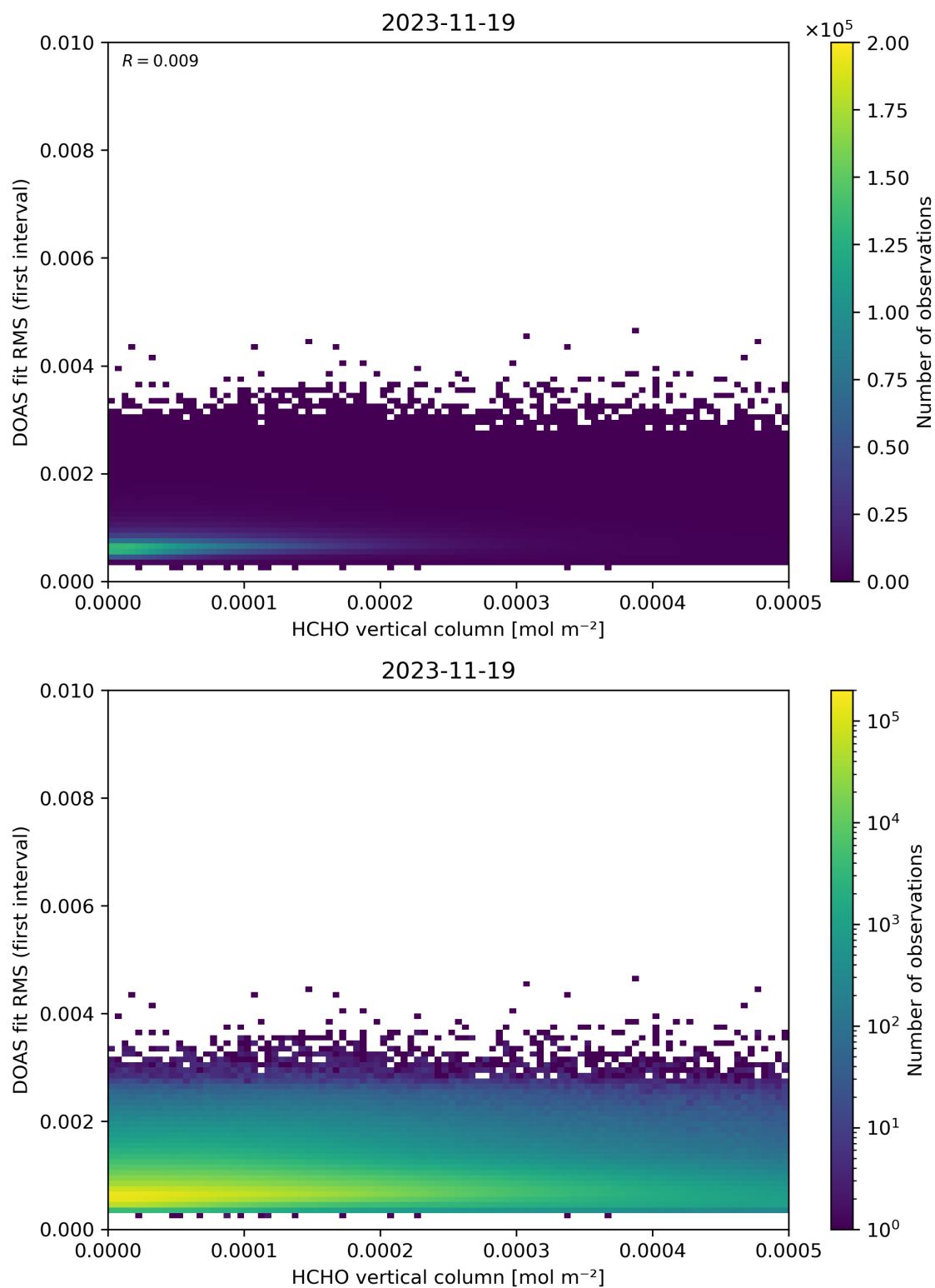
Figure 123: Scatter density plot of “HCHO vertical column” against “DOAS fit RMS (first interval)” for 2023-11-18 to 2023-11-20.
