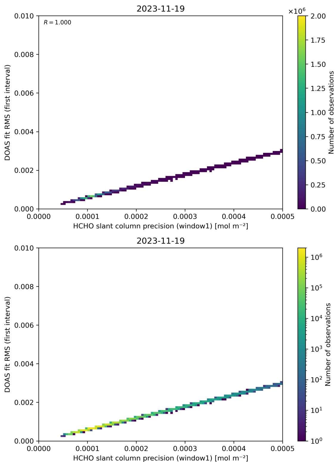
Figure 88: Scatter density plot of “HCHO slant column precision (window1)” against “DOAS fit RMS (first interval)” for 2023-11-18 to 2023-11-20.
