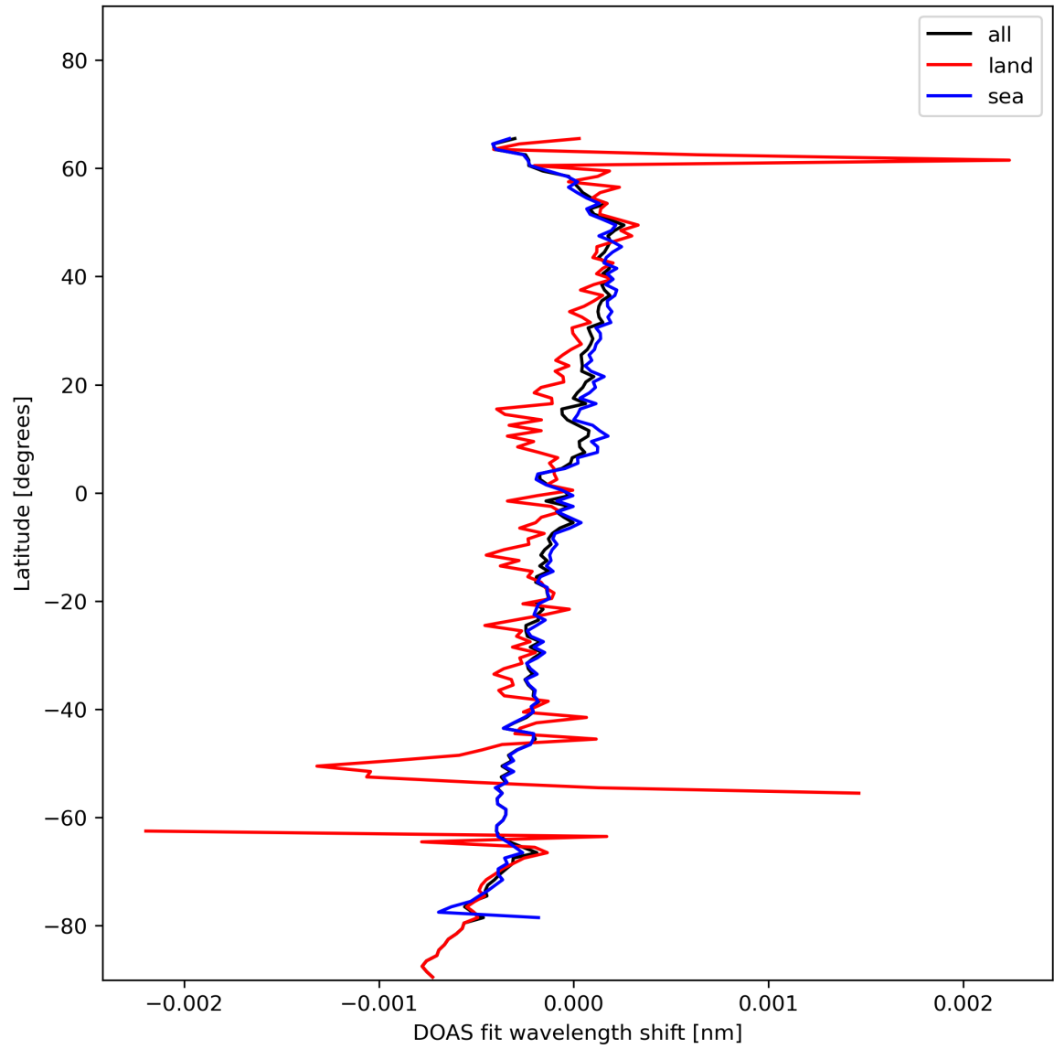
Figure 30: Zonal average of “DOAS fit wavelength shift” for 2023-11-18 to 2023-11-20.
