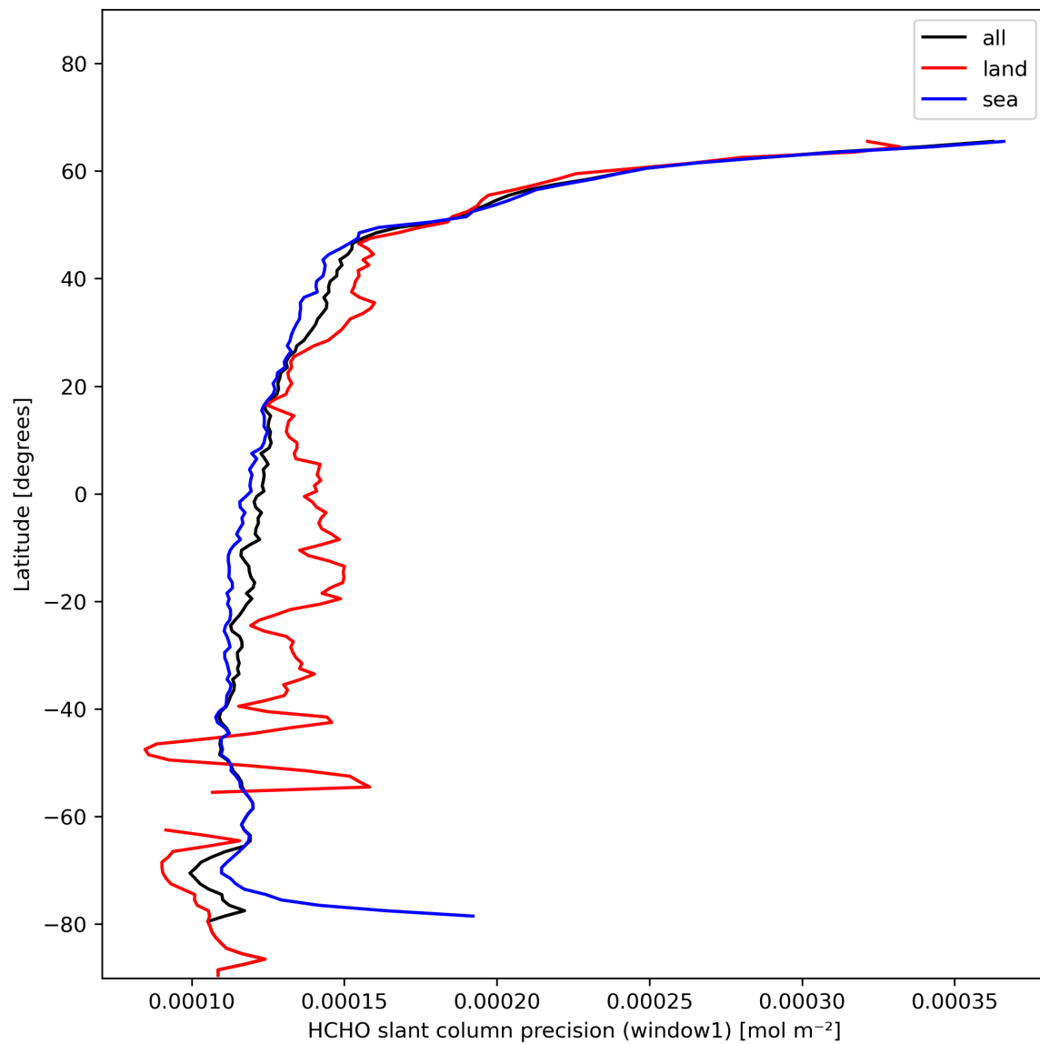
Figure 25: Zonal average of “HCHO slant column precision (window1)” for 2023-11-18 to 2023-11-20.
