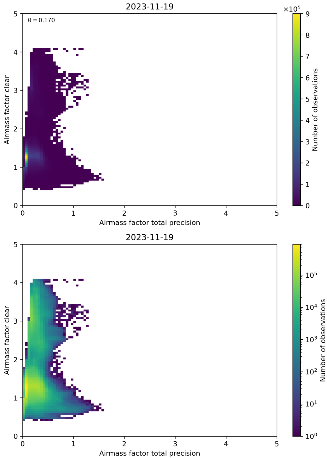
Figure 108: Scatter density plot of “Airmass factor total precision” against “Airmass factor clear” for 2023-11-18 to 2023-11-20.
