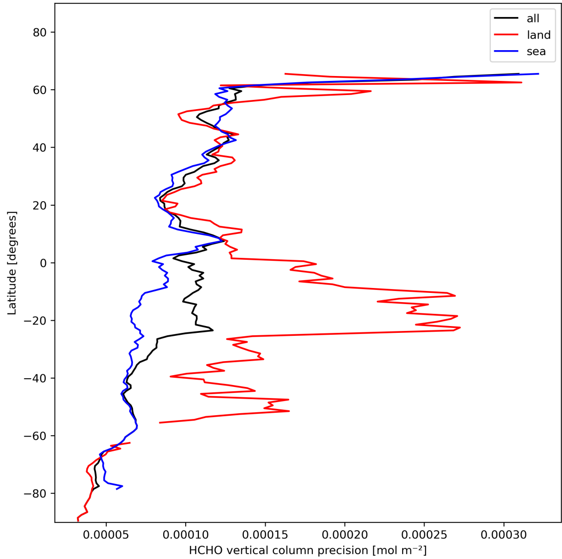
Figure 22: Zonal average of “HCHO vertical column precision” for 2023-11-18 to 2023-11-20.
