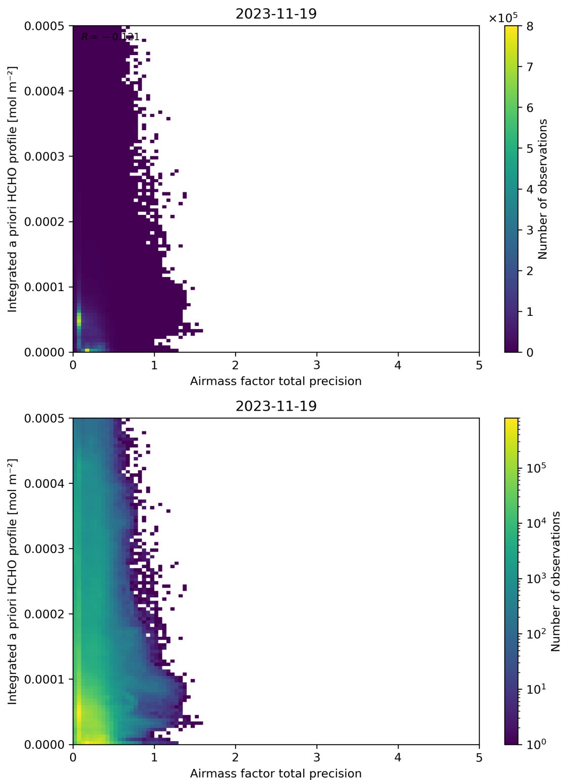
Figure 111: Scatter density plot of “Airmass factor total precision” against “Integrated a priori HCHO profile” for 2023-11-18 to 2023-11-20.
