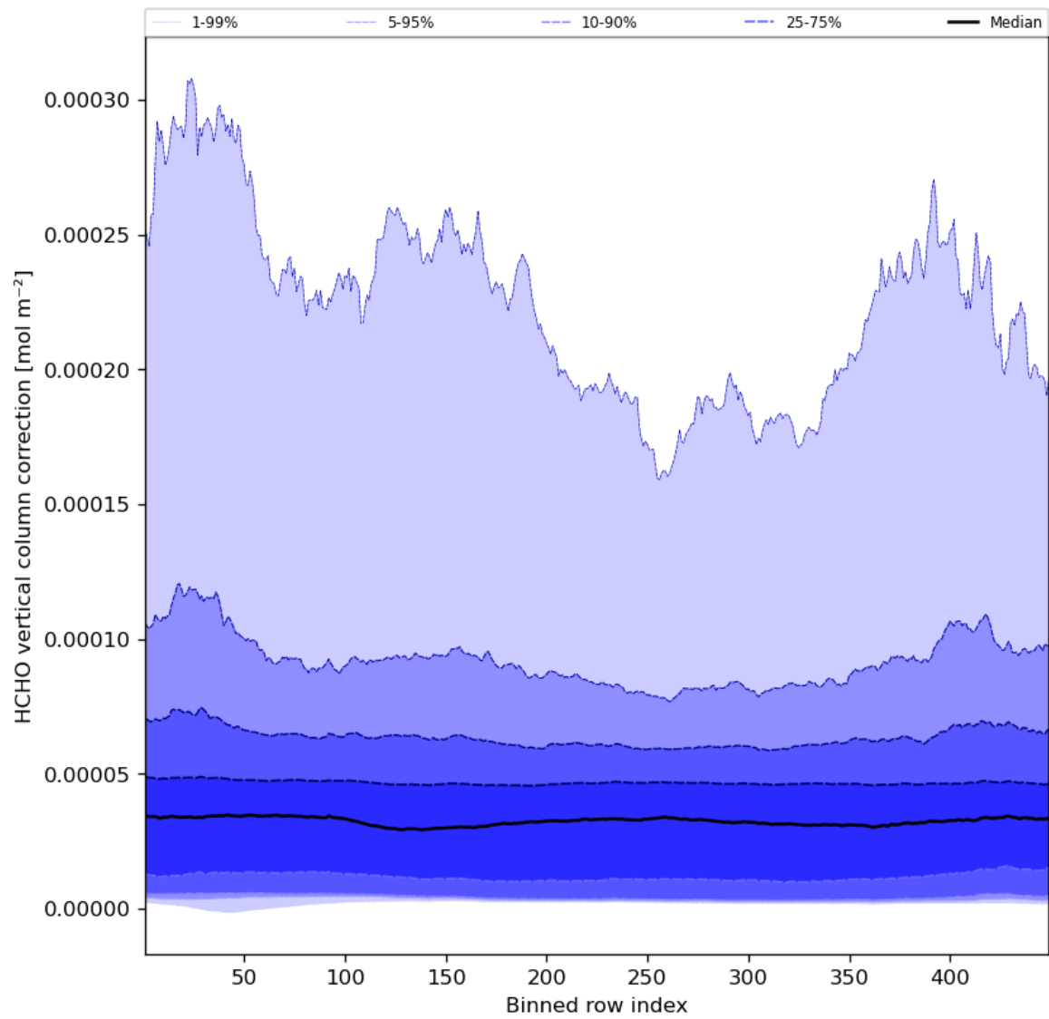
Figure 51: Along track statistics of "HCHO vertical column correction" for 2023-11-18 to 2023-11-20
