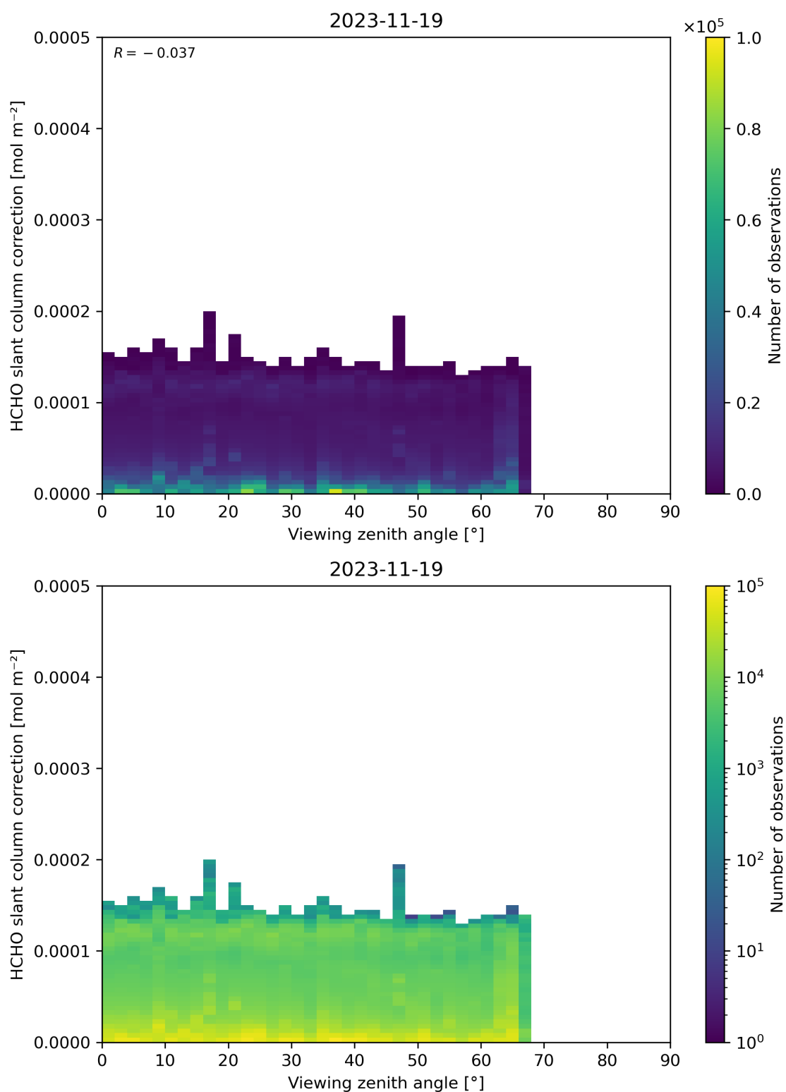
Figure 187: Scatter density plot of “Viewing zenith angle” against “HCHO slant column correction” for 2023-11-18 to 2023-11-20.
