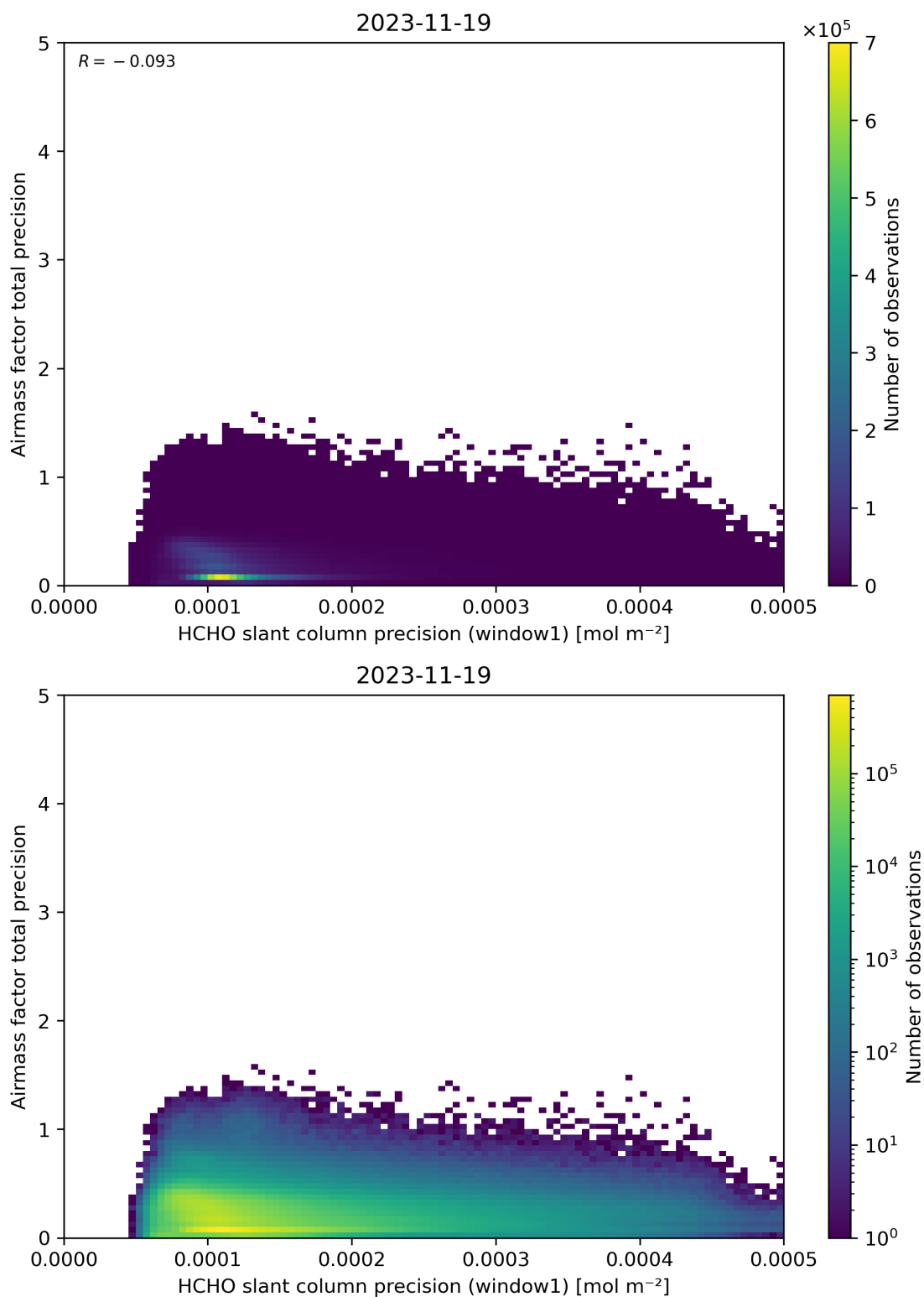
Figure 95: Scatter density plot of “HCHO slant column precision (window1)” against “Airmass factor total precision” for 2023-11-18 to 2023-11-20.
