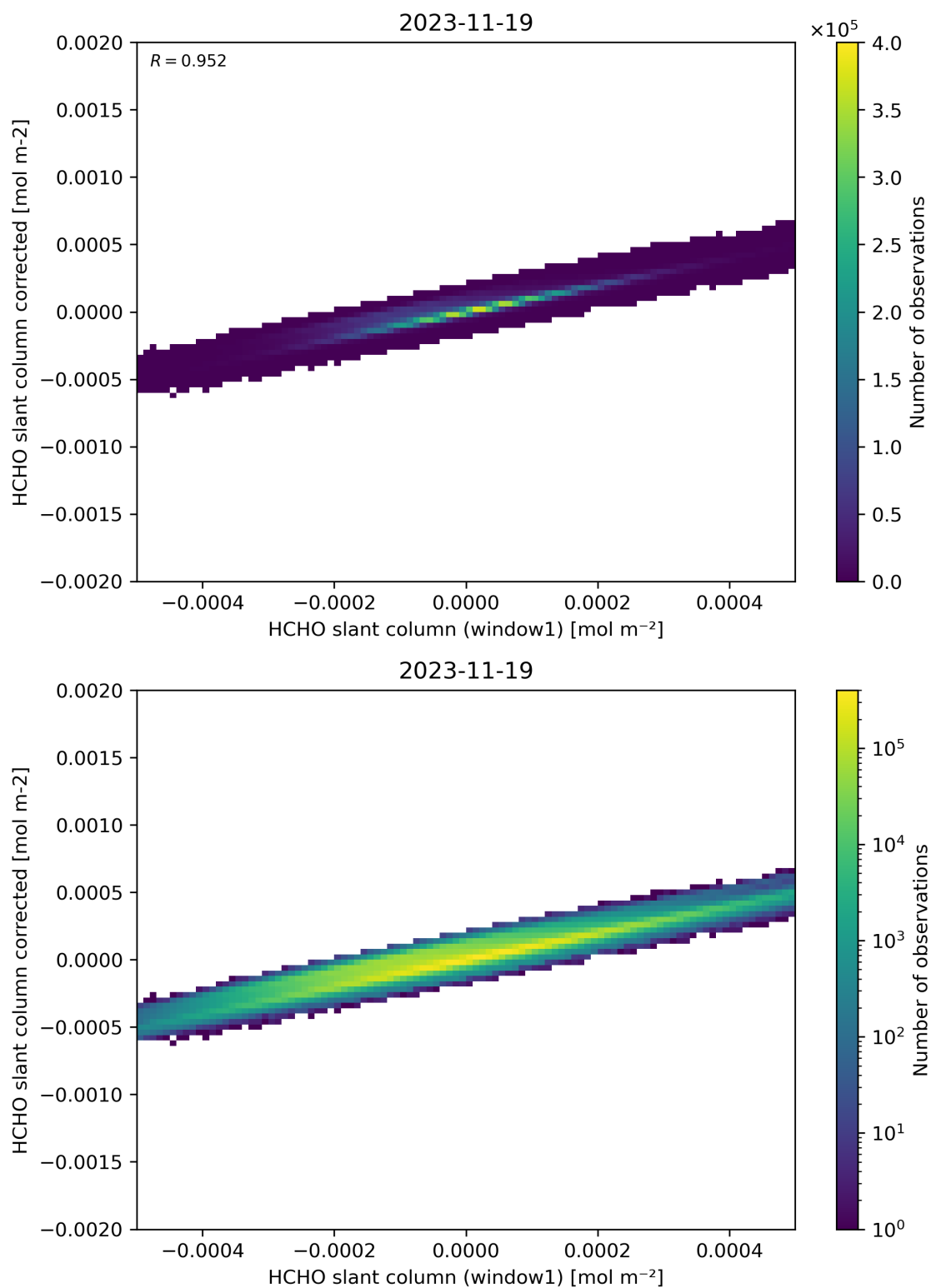
Figure 82: Scatter density plot of “HCHO slant column (window1)” against “HCHO slant column corrected” for 2023-11-18 to 2023-11-20.
