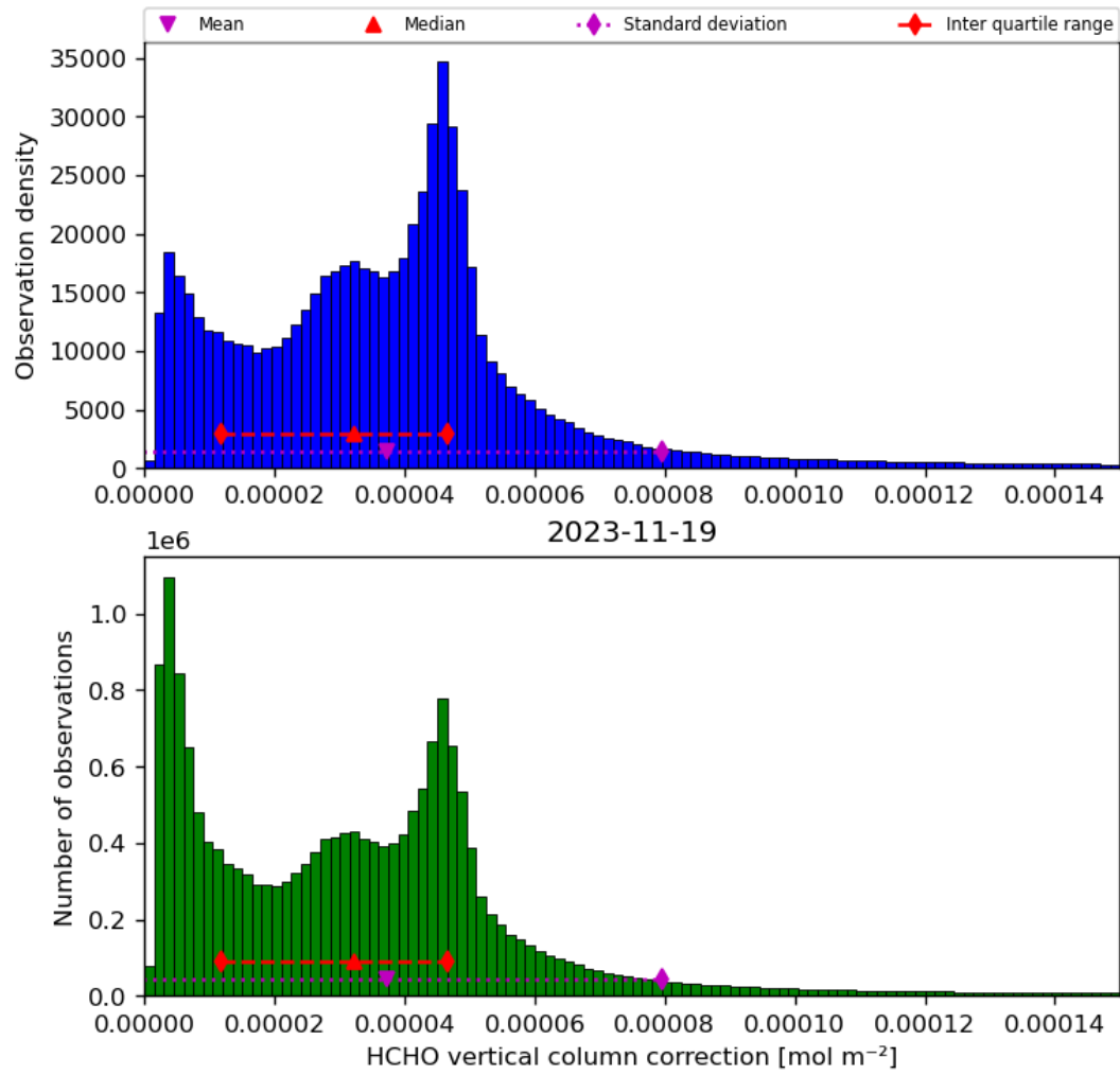
Figure 37: Histogram of “HCHO vertical column correction” for 2023-11-18 to 2023-11-20
