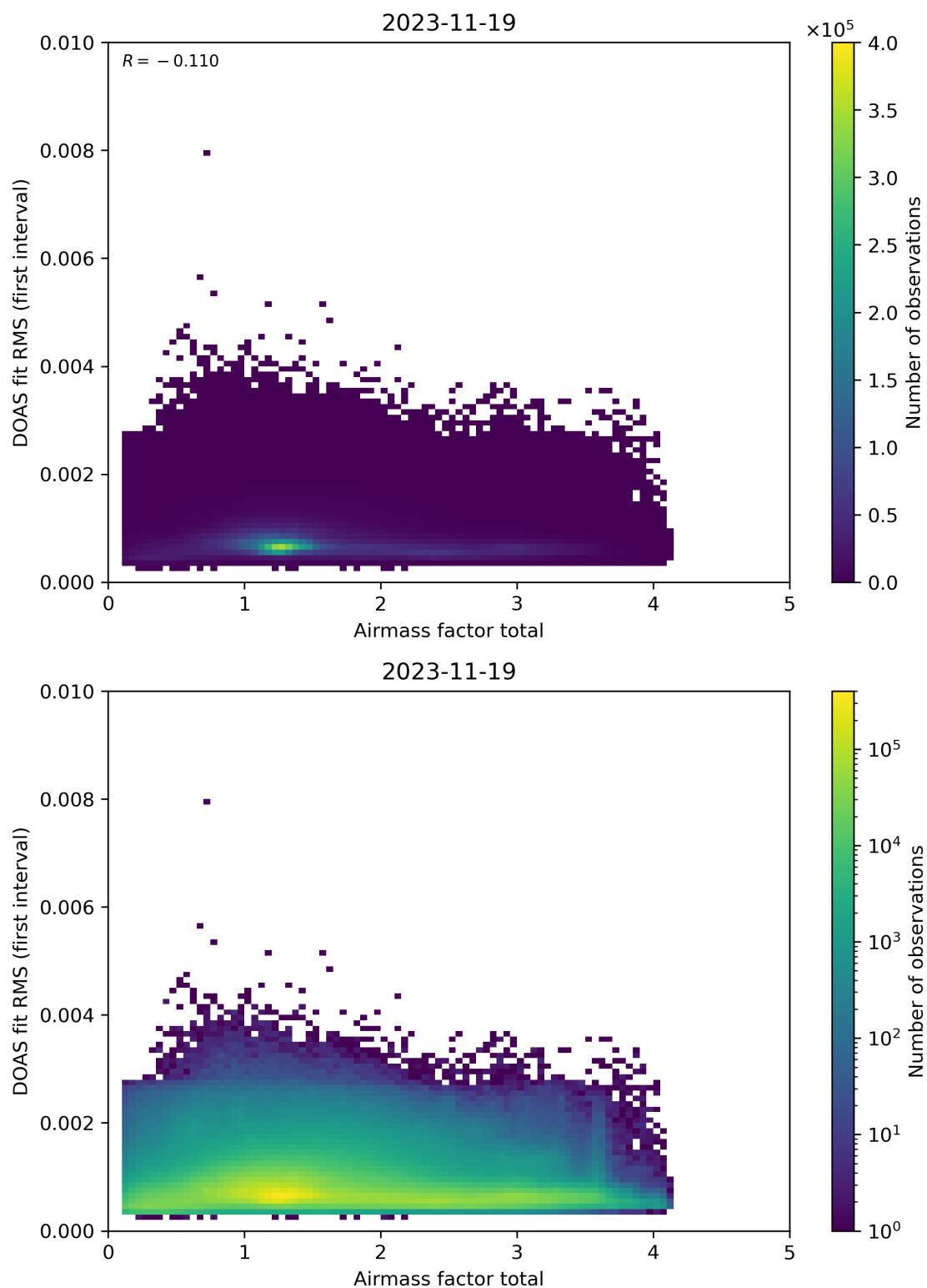
Figure 97: Scatter density plot of “Airmass factor total” against “DOAS fit RMS (first interval)” for 2023-11-18 to 2023-11-20.
