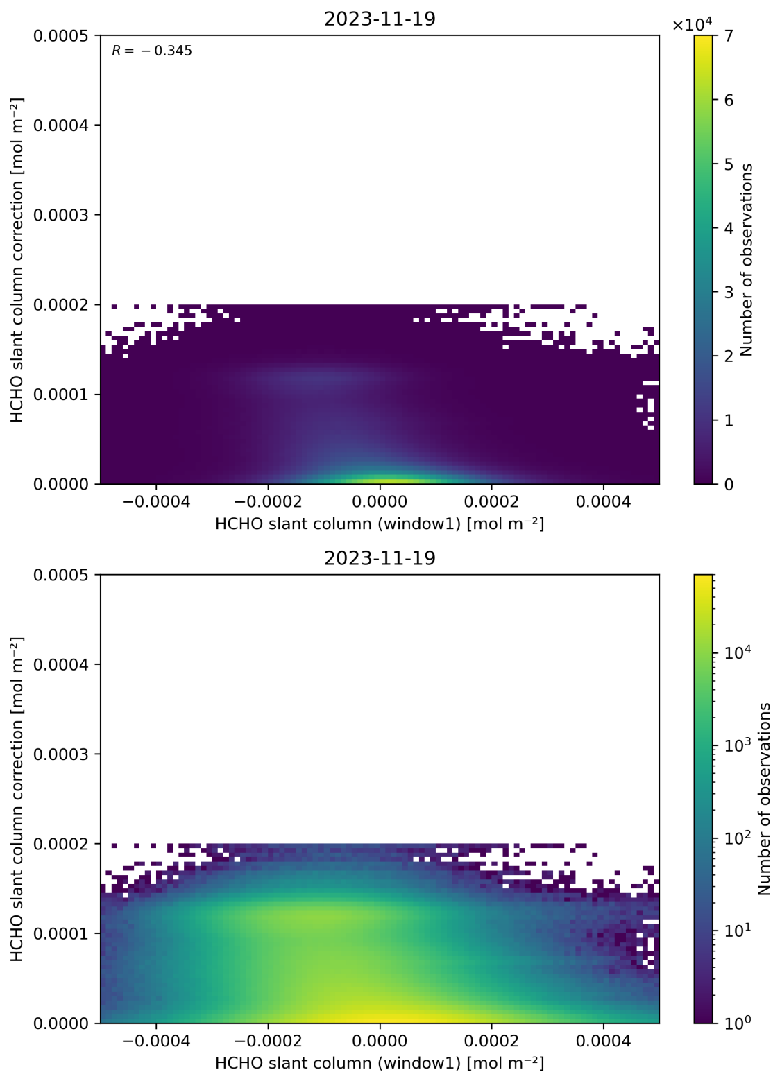
Figure 83: Scatter density plot of “HCHO slant column (window1)” against “HCHO slant column correction” for 2023-11-18 to 2023-11-20.
