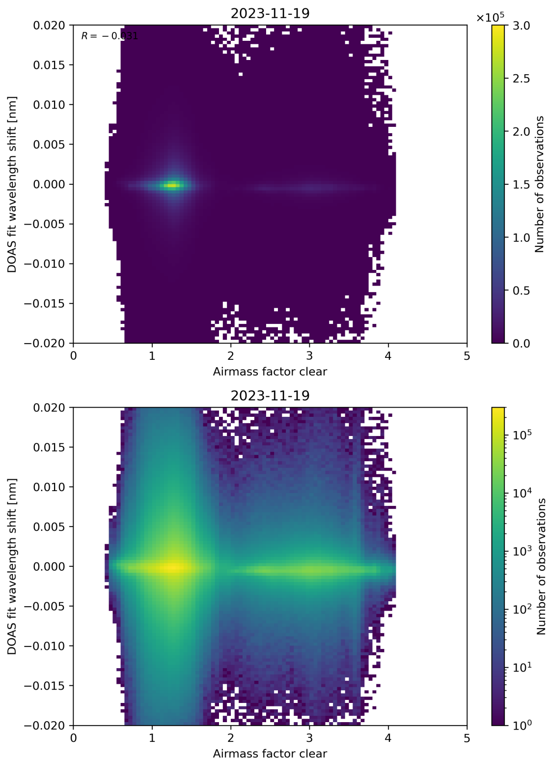
Figure 72: Scatter density plot of “Airmass factor clear” against “DOAS fit wavelength shift” for 2023-11-18 to 2023-11-20.
