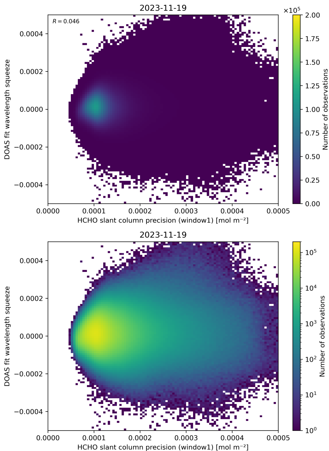
Figure 90: Scatter density plot of “HCHO slant column precision (window1)” against “DOAS fit wavelength squeeze” for 2023-11-18 to 2023-11-20.
