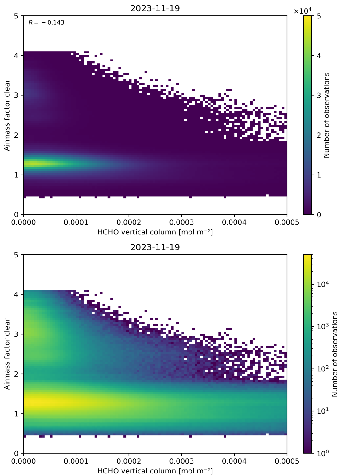
Figure 126: Scatter density plot of “HCHO vertical column” against “Airmass factor clear” for 2023-11-18 to 2023-11-20.
