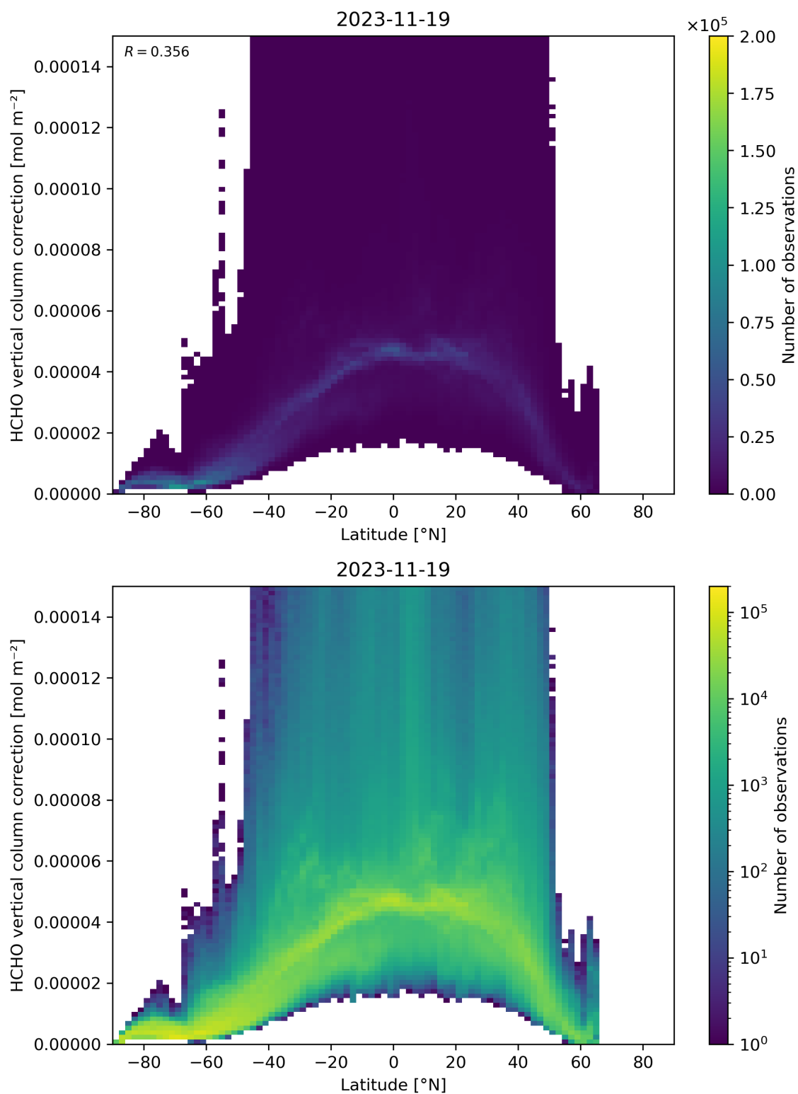
Figure 164: Scatter density plot of “Latitude” against “HCHO vertical column correction” for 2023-11-18 to 2023-11-20.
