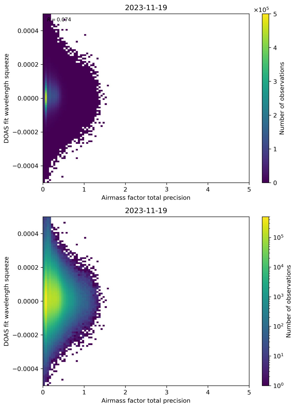
Figure 107: Scatter density plot of “Airmass factor total precision” against “DOAS fit wavelength squeeze” for 2023-11-18 to 2023-11-20.
