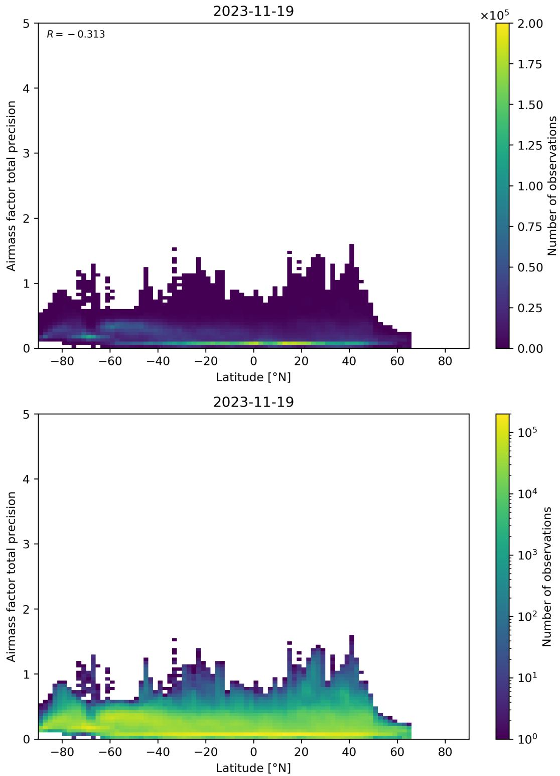
Figure 162: Scatter density plot of “Latitude” against “Airmass factor total precision” for 2023-11-18 to 2023-11-20.
