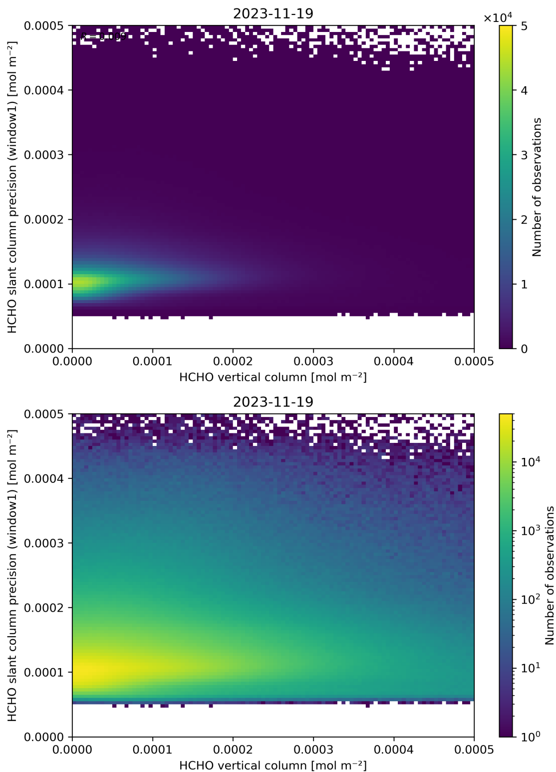
Figure 130: Scatter density plot of “HCHO vertical column” against “HCHO slant column precision (window1)” for 2023-11-18 to 2023-11-20.
