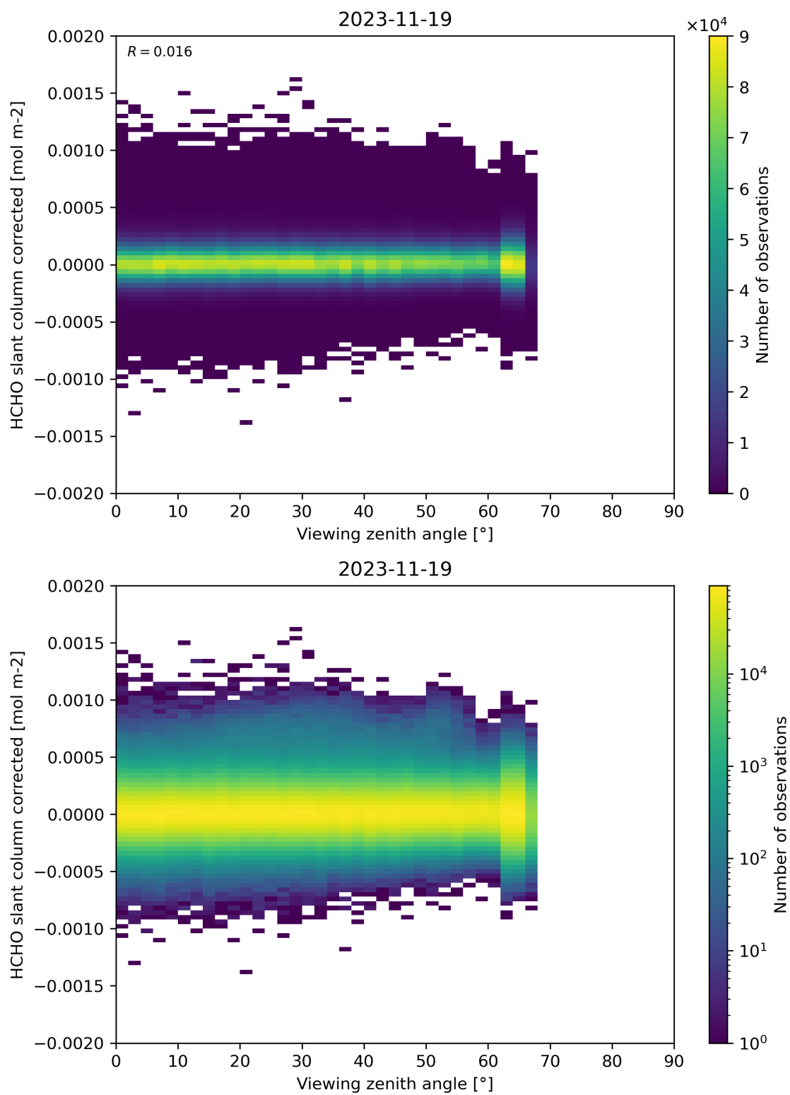
Figure 186: Scatter density plot of “Viewing zenith angle” against “HCHO slant column corrected” for 2023-11-18 to 2023-11-20.
