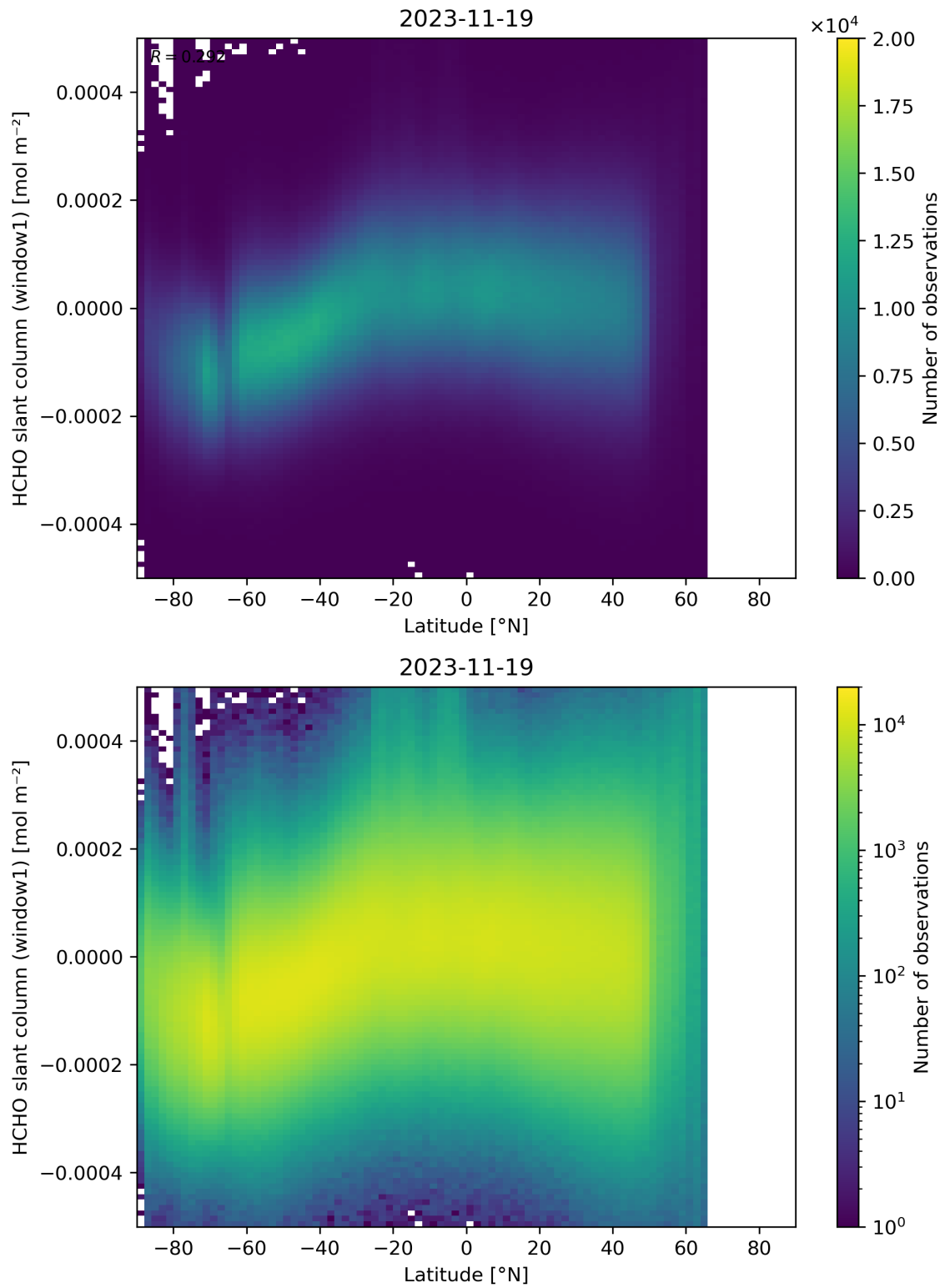
Figure 159: Scatter density plot of “Latitude” against “HCHO slant column (window1)” for 2023-11-18 to 2023-11-20.
