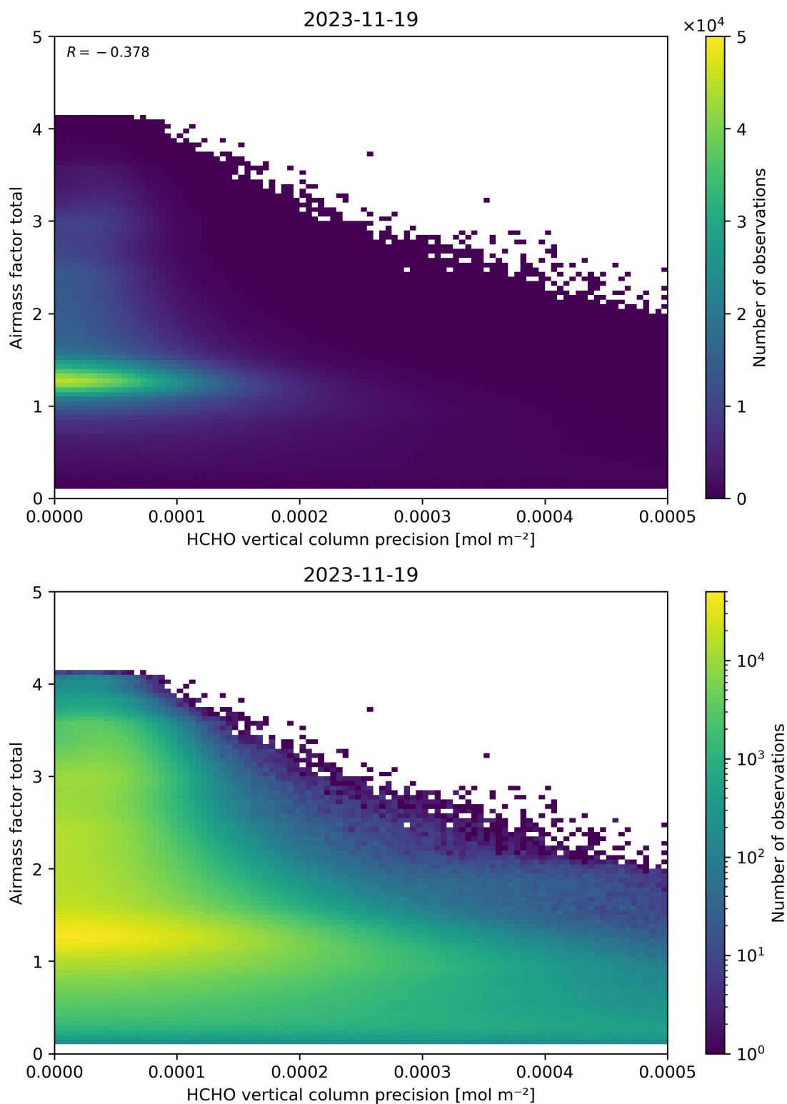
Figure 144: Scatter density plot of “HCHO vertical column precision” against “Airmass factor total” for 2023-11-18 to 2023-11-20.
