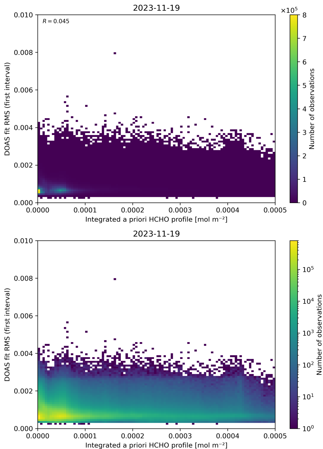
Figure 148: Scatter density plot of “Integrated a priori HCHO profile” against “DOAS fit RMS (first interval)” for 2023-11-18 to 2023-11-20.
