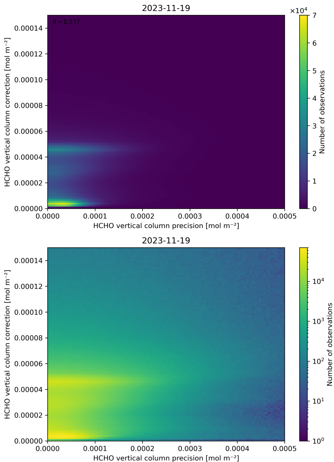
Figure 146: Scatter density plot of “HCHO vertical column precision” against “HCHO vertical column correction” for 2023-11-18 to 2023-11-20.
