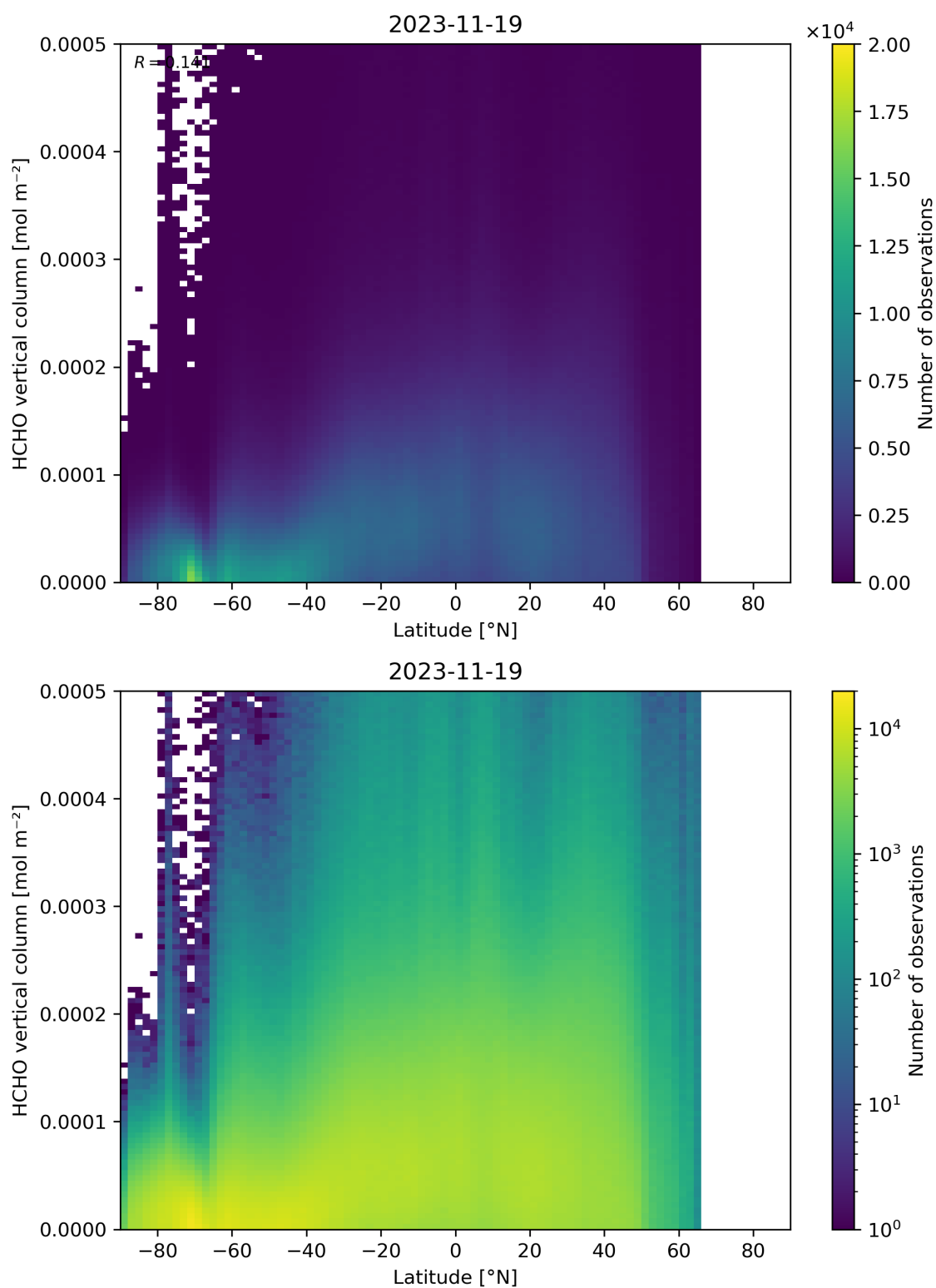
Figure 163: Scatter density plot of “Latitude” against “HCHO vertical column” for 2023-11-18 to 2023-11-20.
