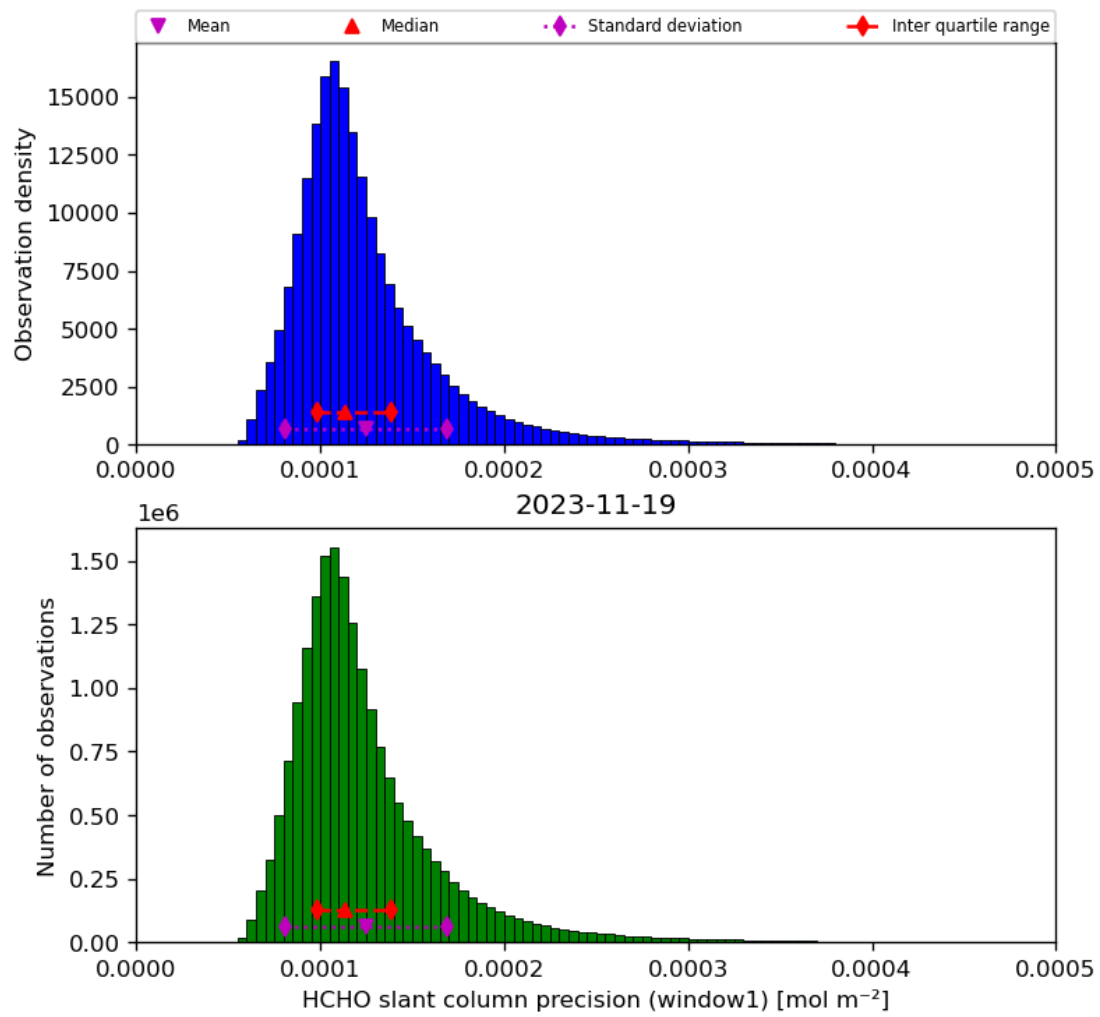
Figure 39: Histogram of “HCHO slant column precision (window1)” for 2023-11-18 to 2023-11-20
