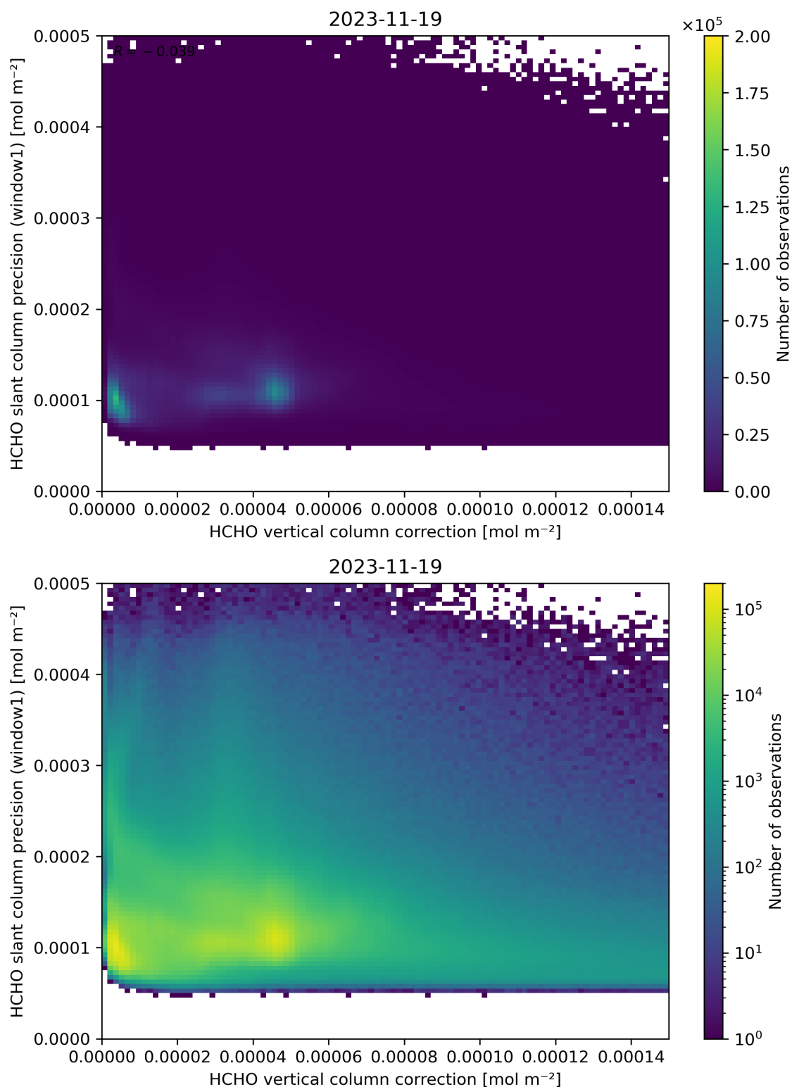
Figure 119: Scatter density plot of “HCHO vertical column correction” against “HCHO slant column precision (window1)” for 2023-11-18 to 2023-11-20.
