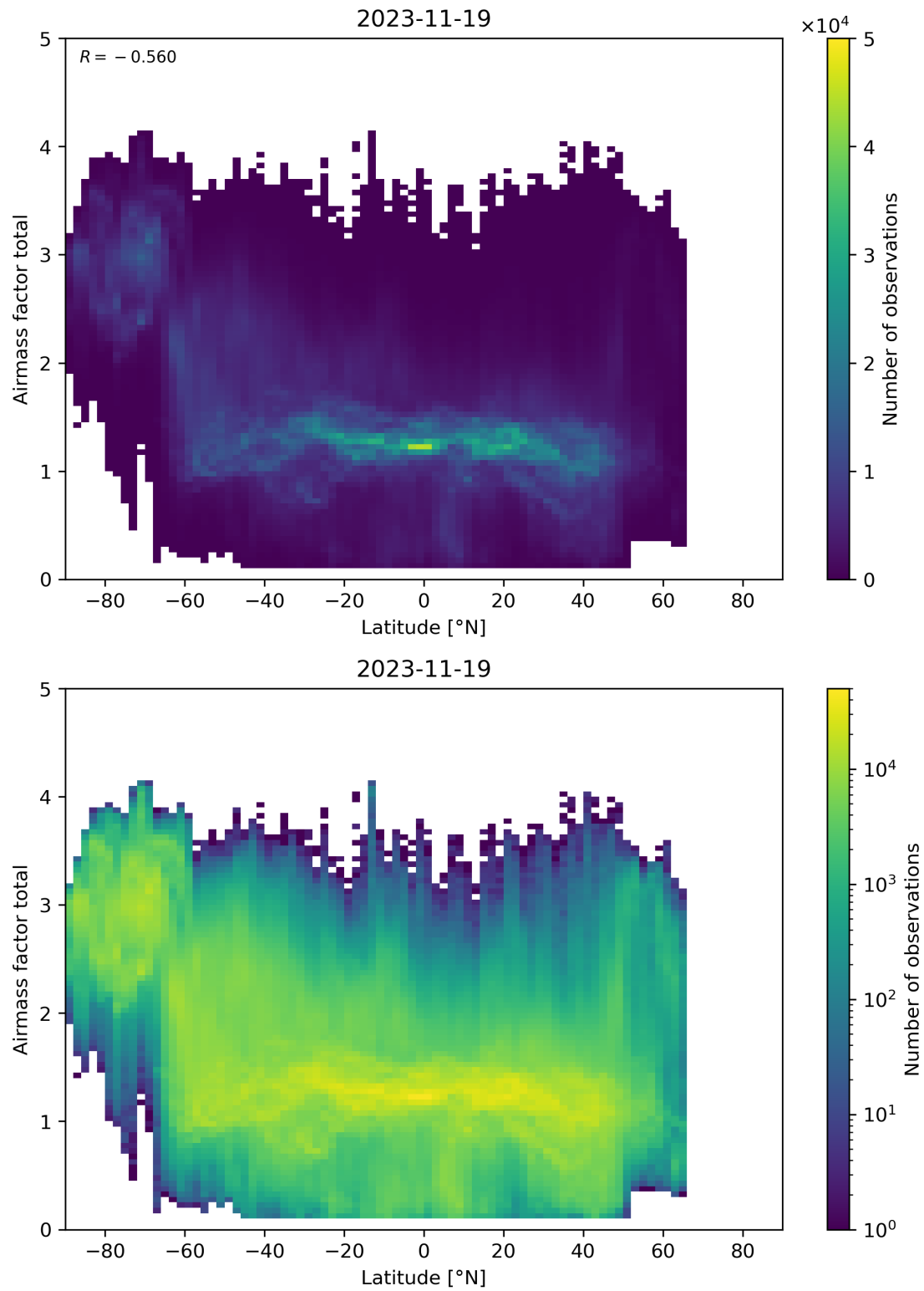
Figure 161: Scatter density plot of “Latitude” against “Airmass factor total” for 2023-11-18 to 2023-11-20.
