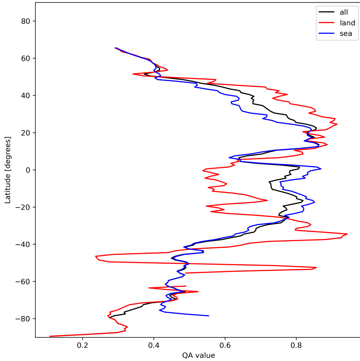
Figure 20: Zonal average of “QA value” for 2023-11-18 to 2023-11-20.
