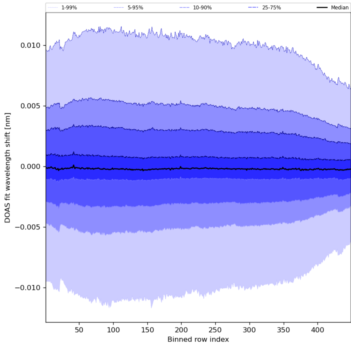
Figure 58: Along track statistics of “DOAS fit wavelength shift” for 2023-11-18 to 2023-11-20
