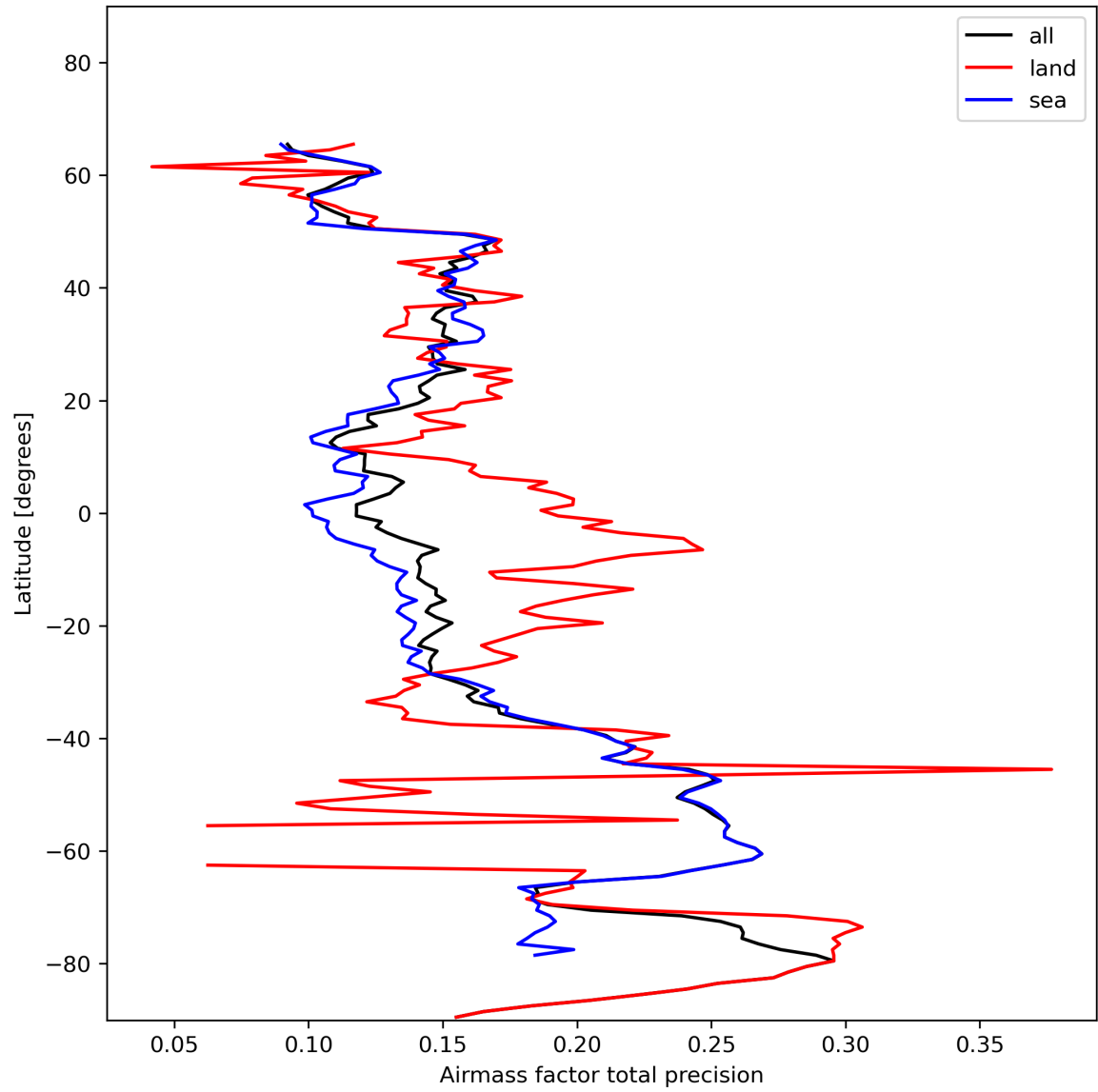
Figure 27: Zonal average of “Airmass factor total precision” for 2023-11-18 to 2023-11-20.
