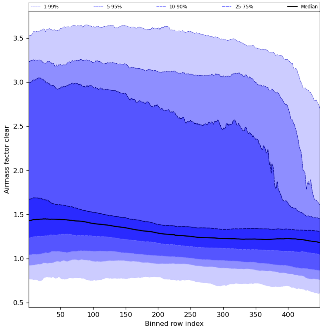
Figure 56: Along track statistics of “Airmass factor clear” for 2023-11-18 to 2023-11-20
