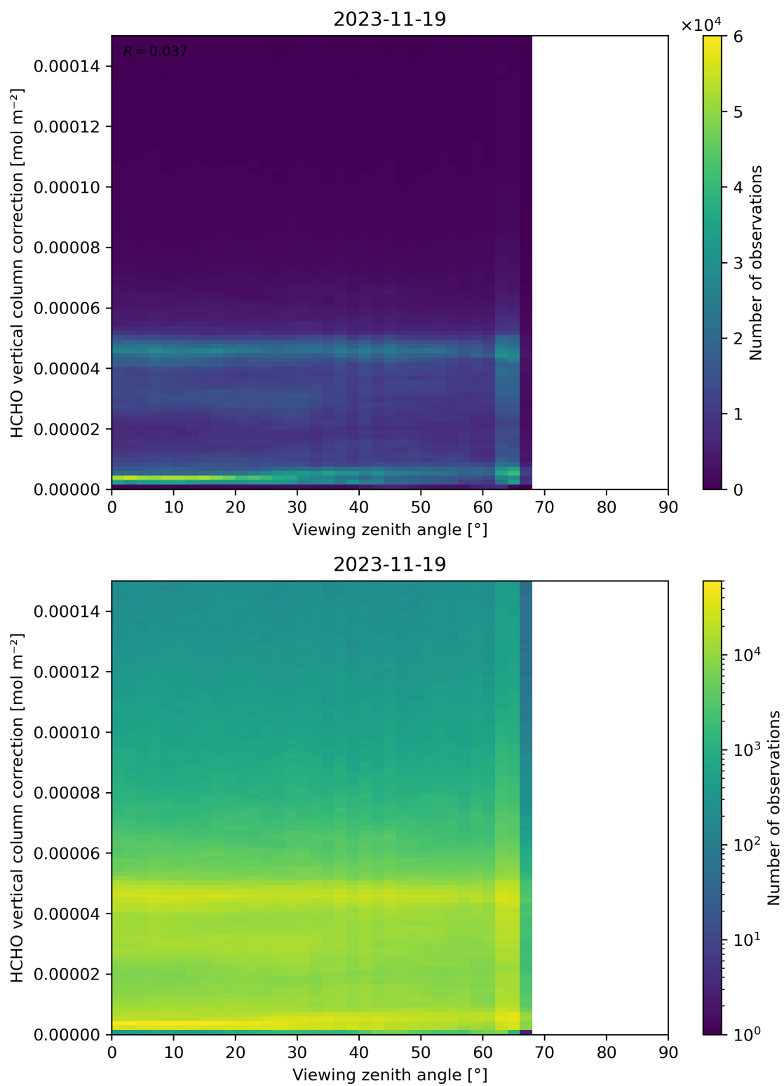
Figure 193: Scatter density plot of “Viewing zenith angle” against “HCHO vertical column correction” for 2023-11-18 to 2023-11-20.
