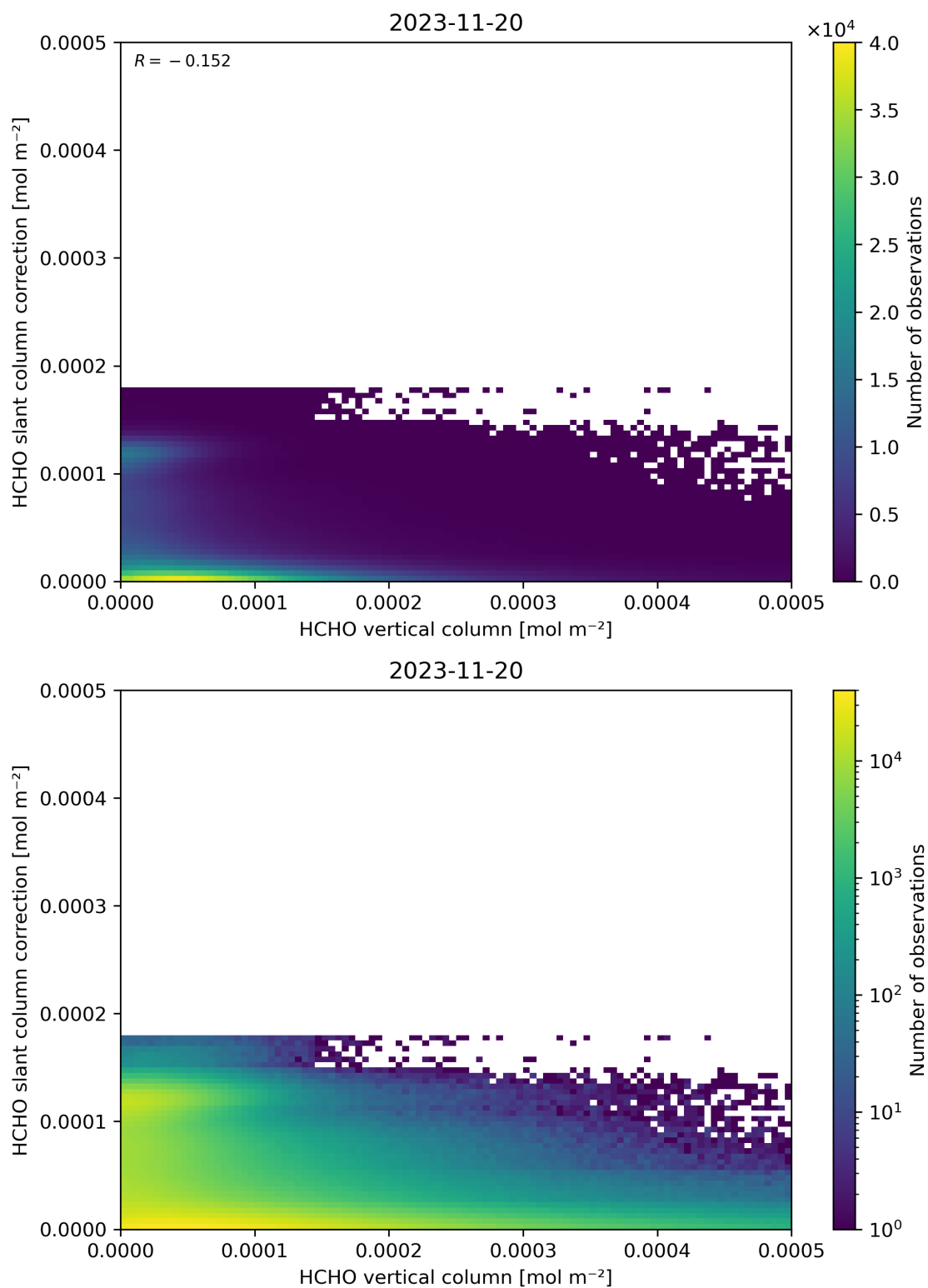
Figure 128: Scatter density plot of “HCHO vertical column” against “HCHO slant column correction” for 2023-11-19 to 2023-11-21.
