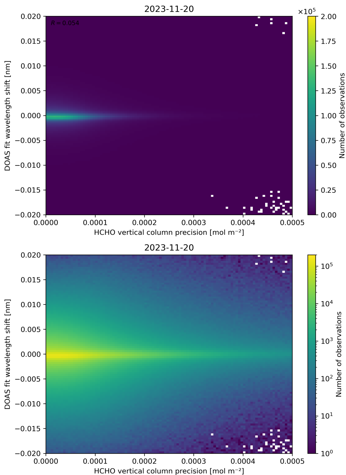
Figure 137: Scatter density plot of “HCHO vertical column precision” against “DOAS fit wavelength shift” for 2023-11-19 to 2023-11-21.
