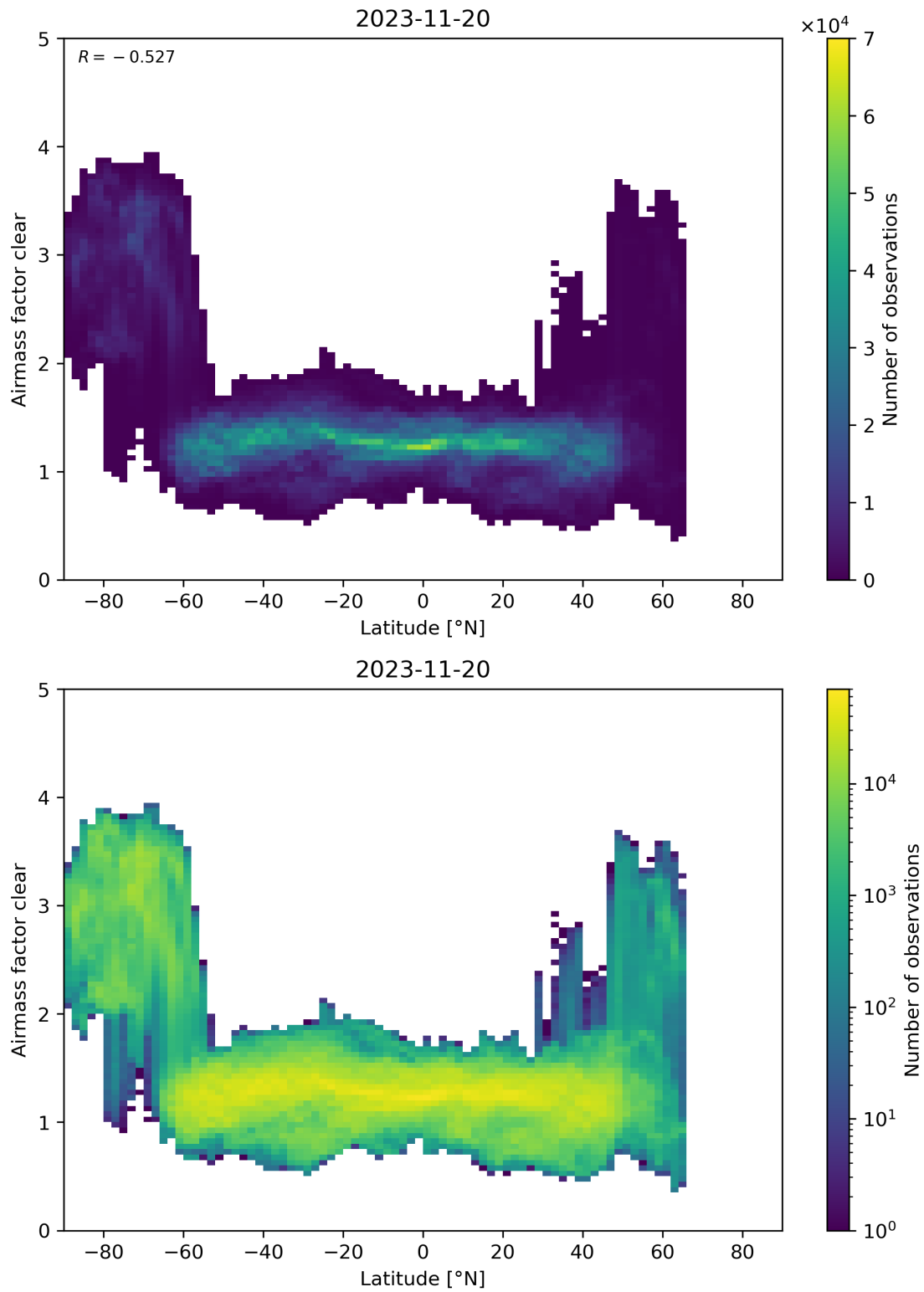
Figure 156: Scatter density plot of “Latitude” against “Airmass factor clear” for 2023-11-19 to 2023-11-21.
