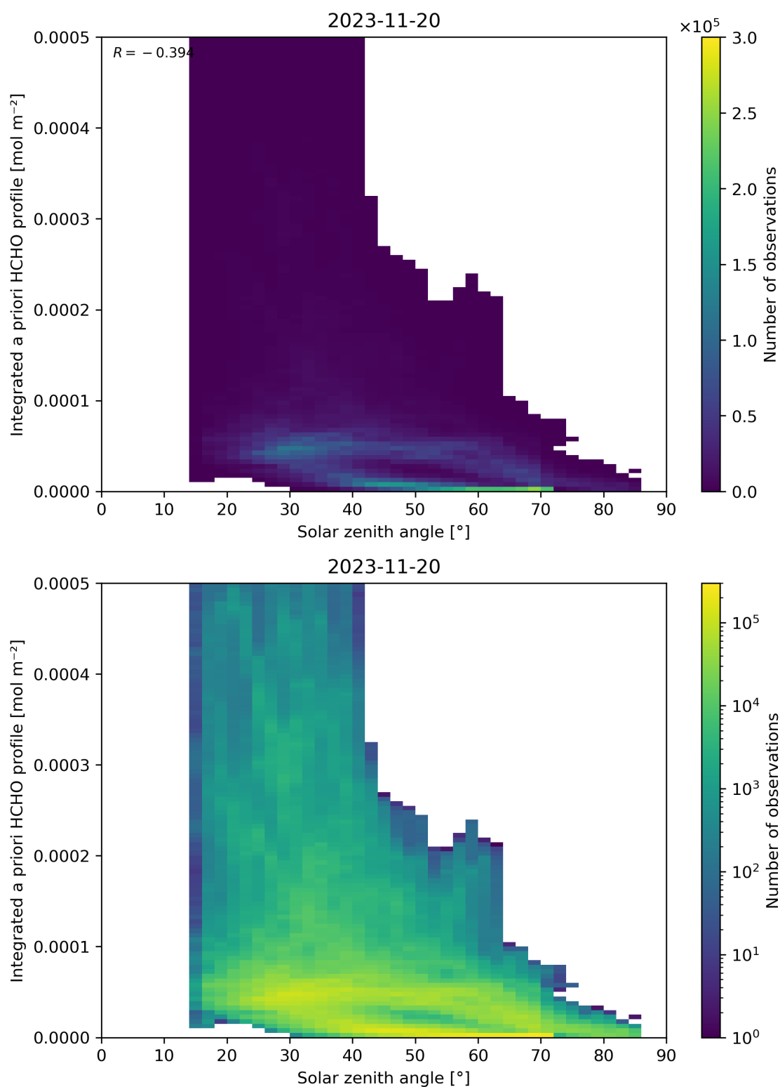
Figure 180: Scatter density plot of “Solar zenith angle” against “Integrated a priori HCHO profile” for 2023-11-19 to 2023-11-21.
