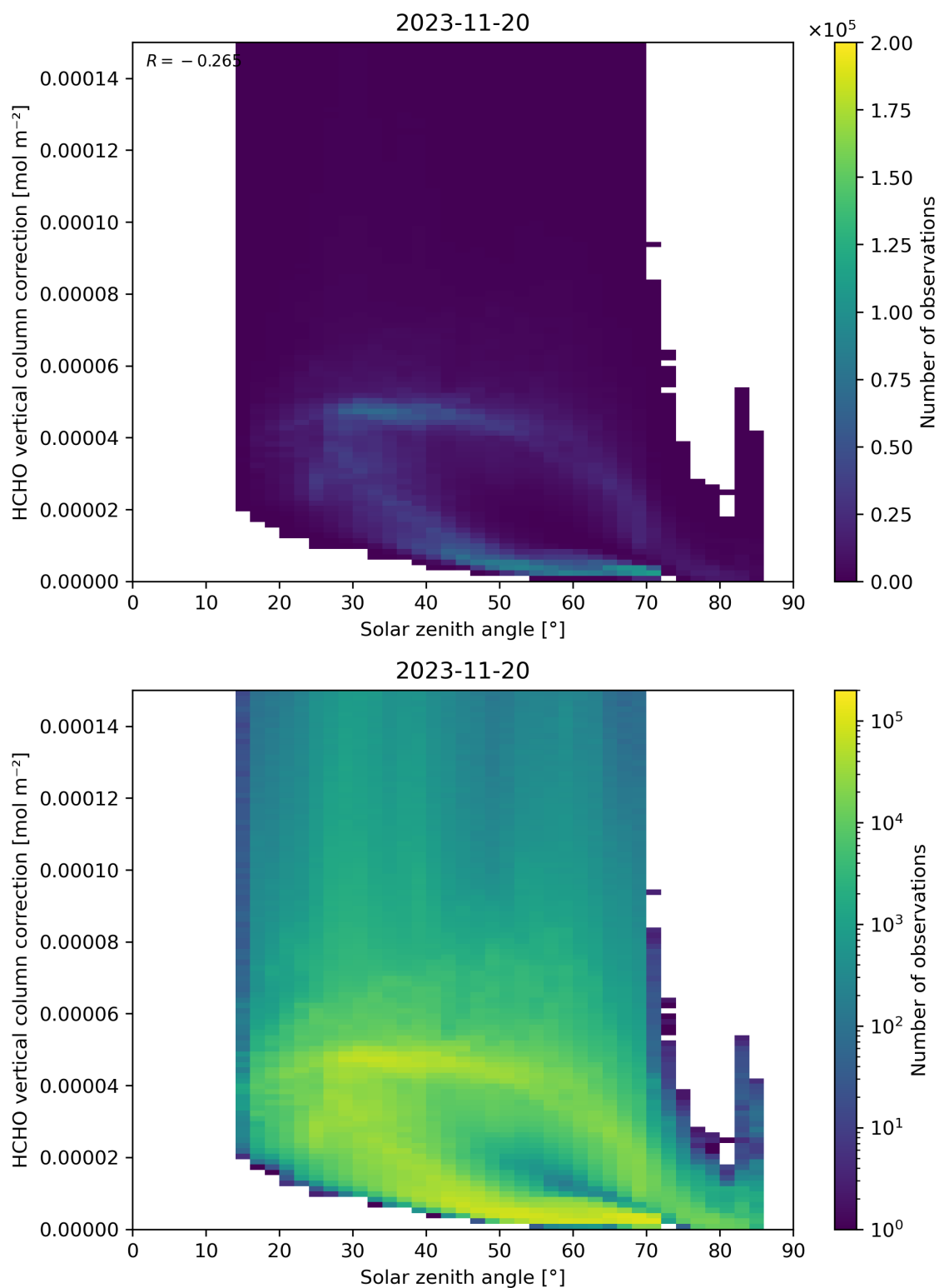
Figure 178: Scatter density plot of “Solar zenith angle” against “HCHO vertical column correction” for 2023-11-19 to 2023-11-21.
