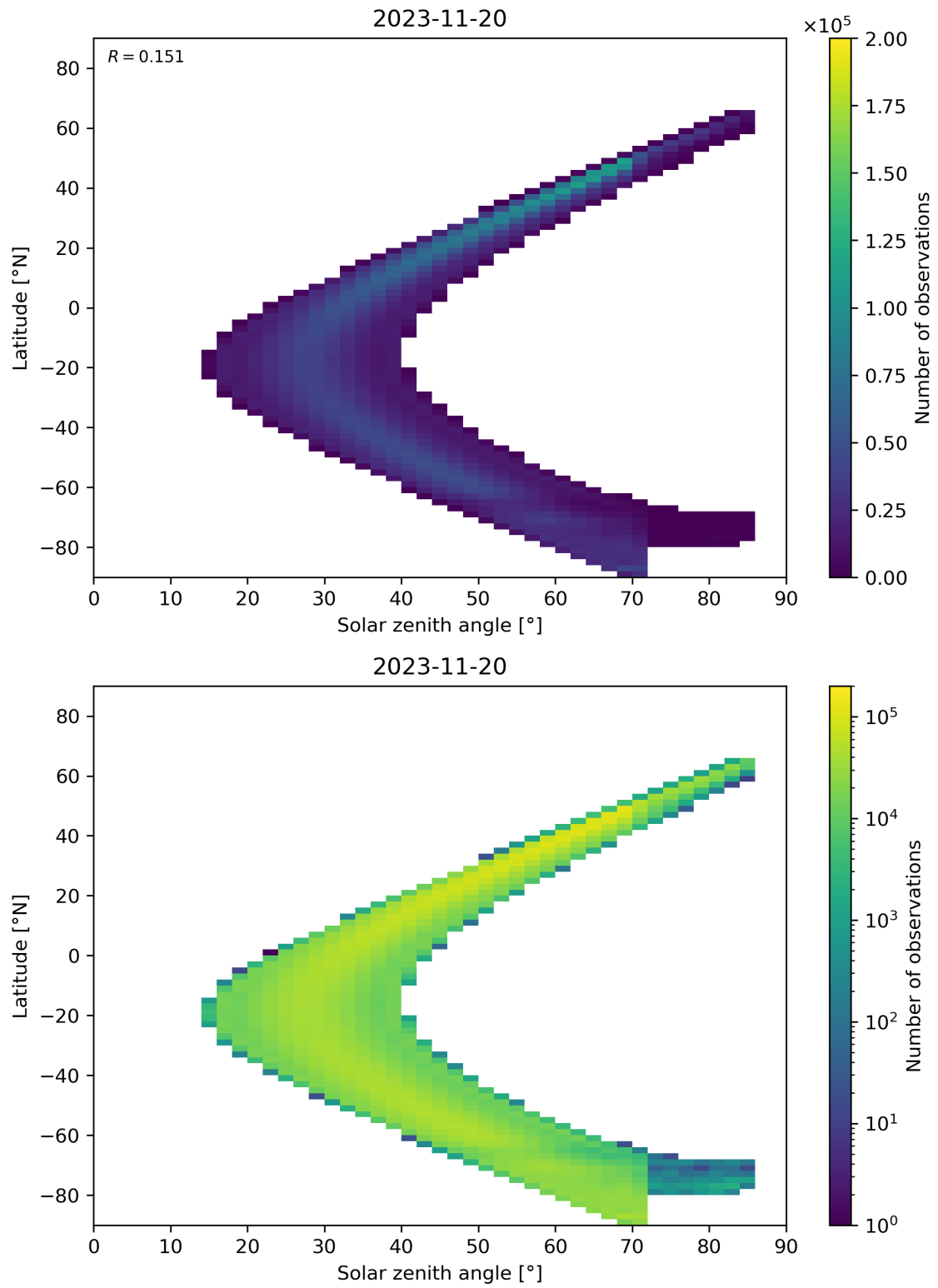
Figure 181: Scatter density plot of “Solar zenith angle” against “Latitude” for 2023-11-19 to 2023-11-21.
