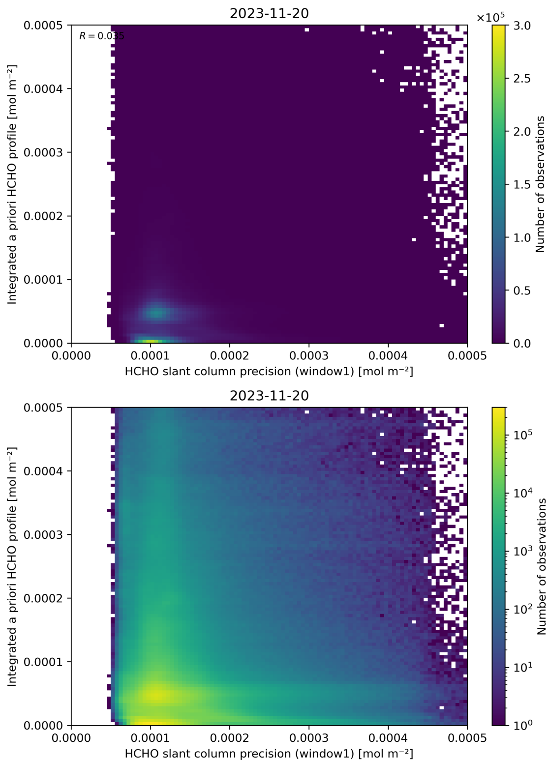
Figure 96: Scatter density plot of “HCHO slant column precision (window1)” against “Integrated a priori HCHO profile” for 2023-11-19 to 2023-11-21.
