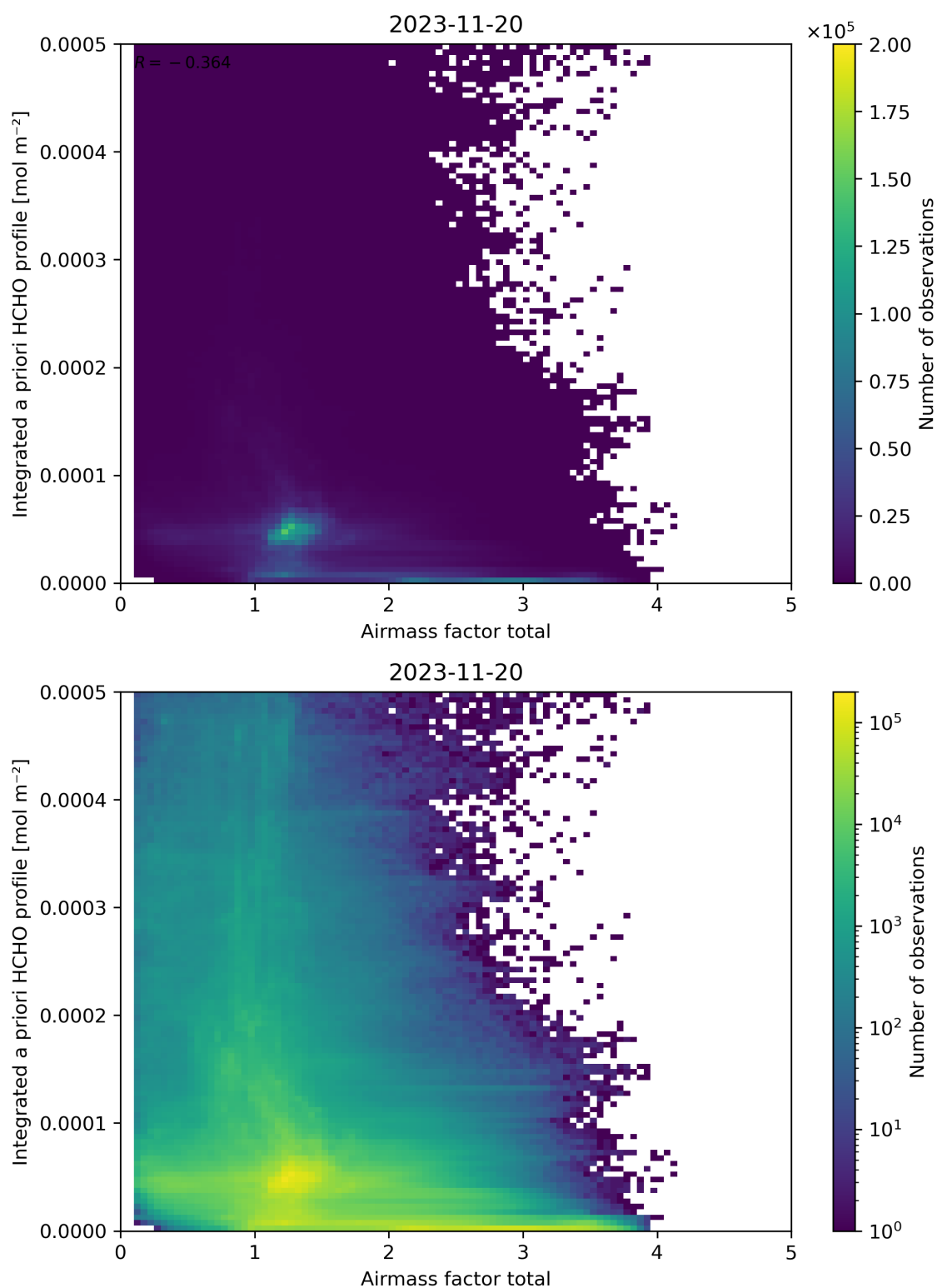
Figure 104: Scatter density plot of “Airmass factor total” against “Integrated a priori HCHO profile” for 2023-11-19 to 2023-11-21.
