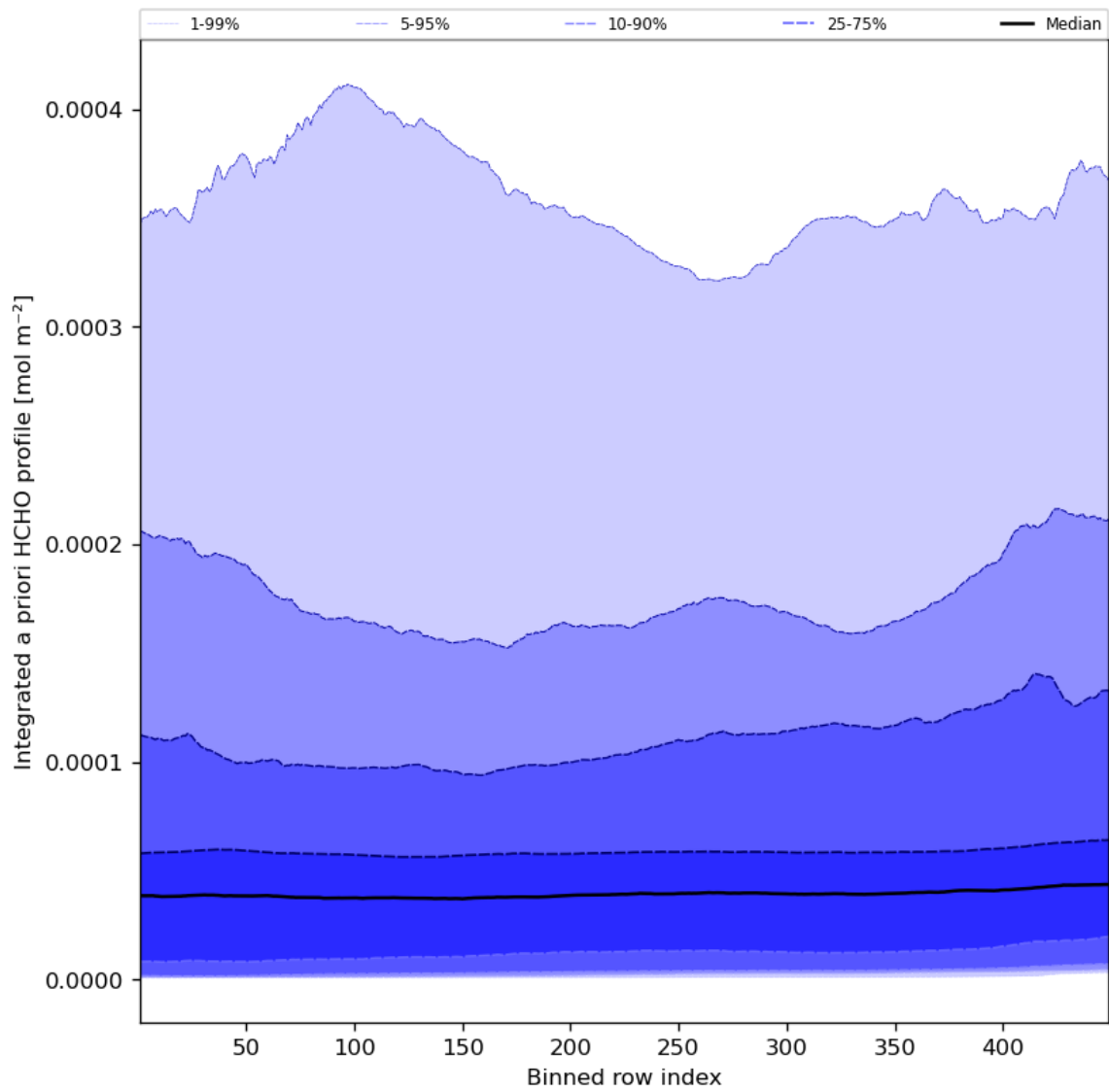
Figure 57: Along track statistics of "Integrated a priori HCHO profile" for 2023-11-19 to 2023-11-21
