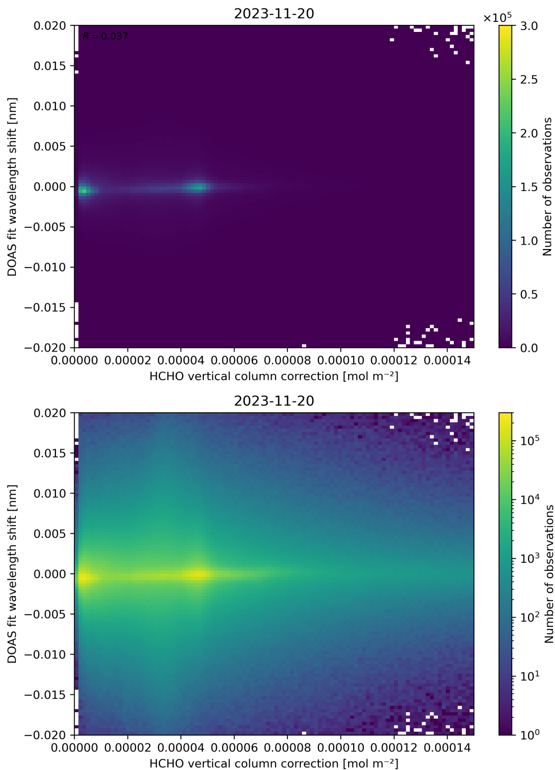
Figure 113: Scatter density plot of “HCHO vertical column correction” against “DOAS fit wavelength shift” for 2023-11-19 to 2023-11-21.
