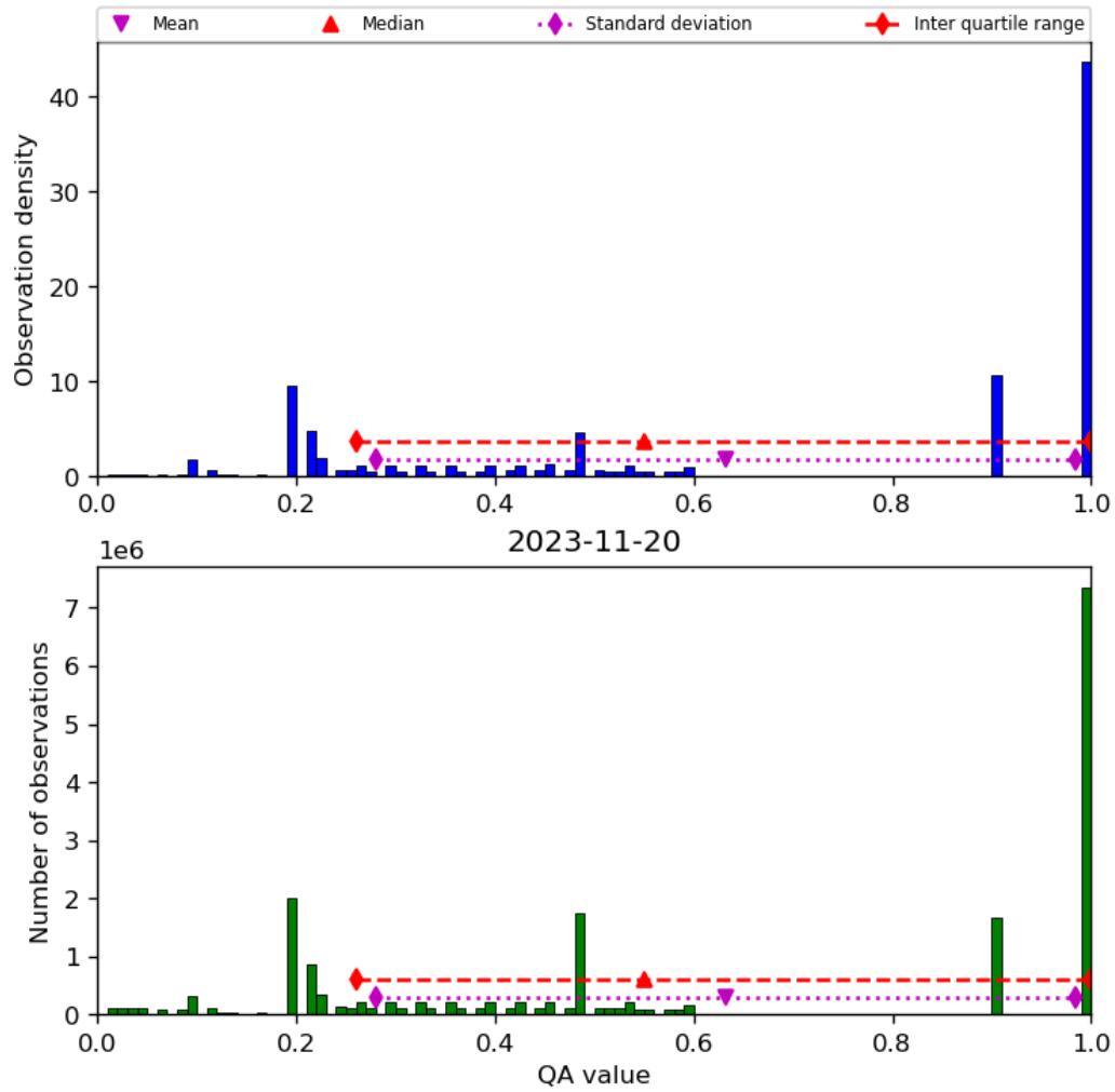
Figure 34: Histogram of “QA value” for 2023-11-19 to 2023-11-21
