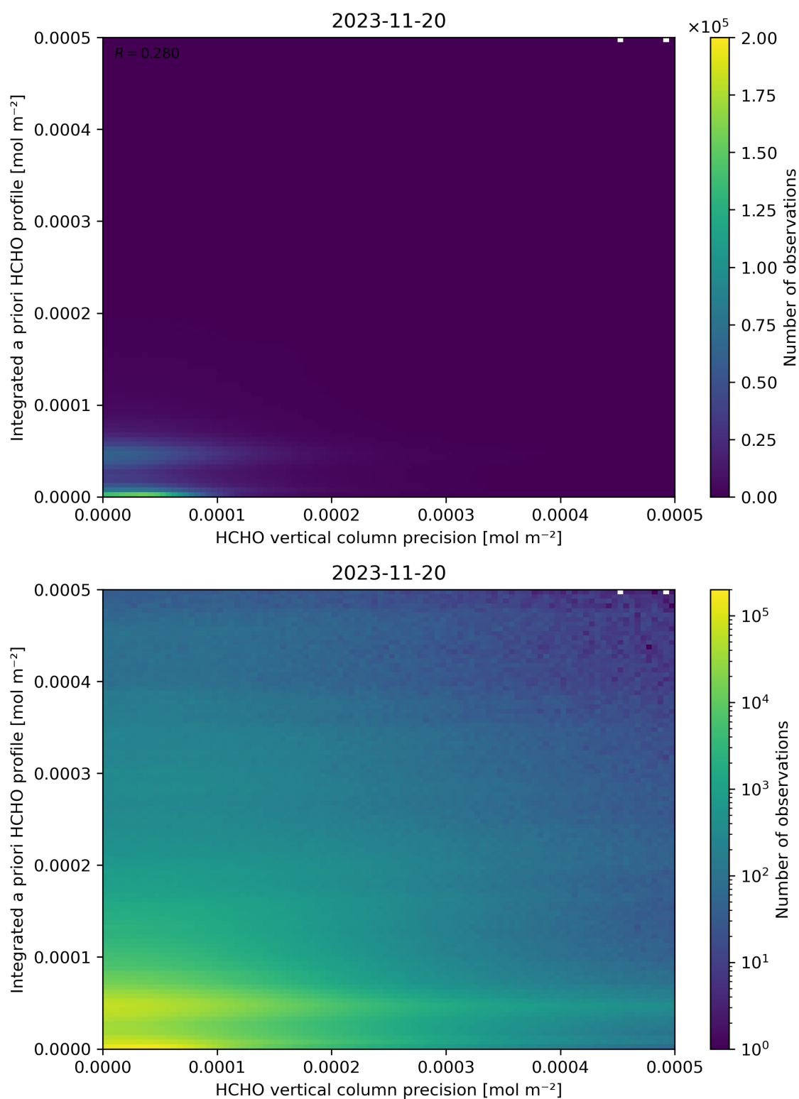
Figure 147: Scatter density plot of “HCHO vertical column precision” against “Integrated a priori HCHO profile” for 2023-11-19 to 2023-11-21.
