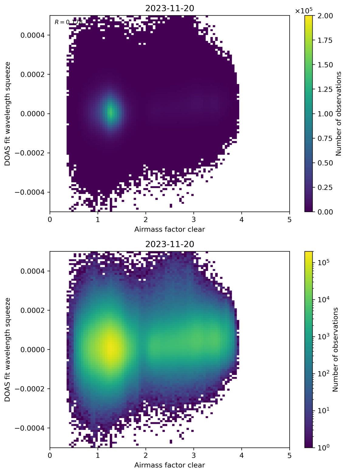
Figure 73: Scatter density plot of “Airmass factor clear” against “DOAS fit wavelength squeeze” for 2023-11-19 to 2023-11-21.
