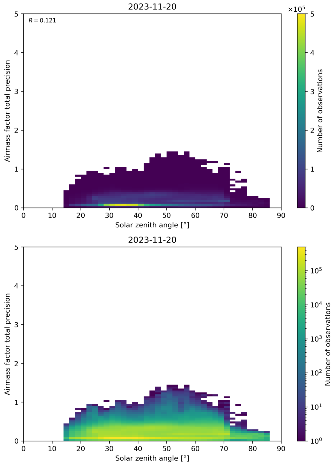
Figure 176: Scatter density plot of “Solar zenith angle” against “Airmass factor total precision” for 2023-11-19 to 2023-11-21.
