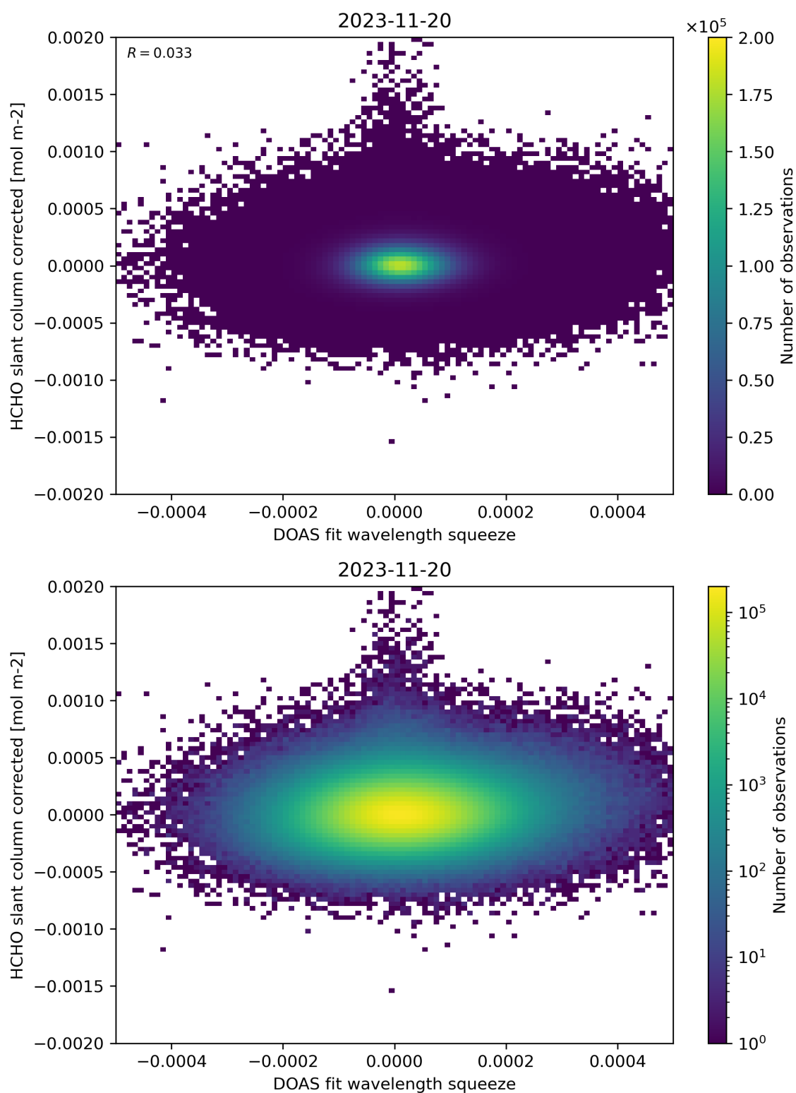
Figure 69: Scatter density plot of “DOAS fit wavelength squeeze” against “HCHO slant column corrected” for 2023-11-19 to 2023-11-21.
