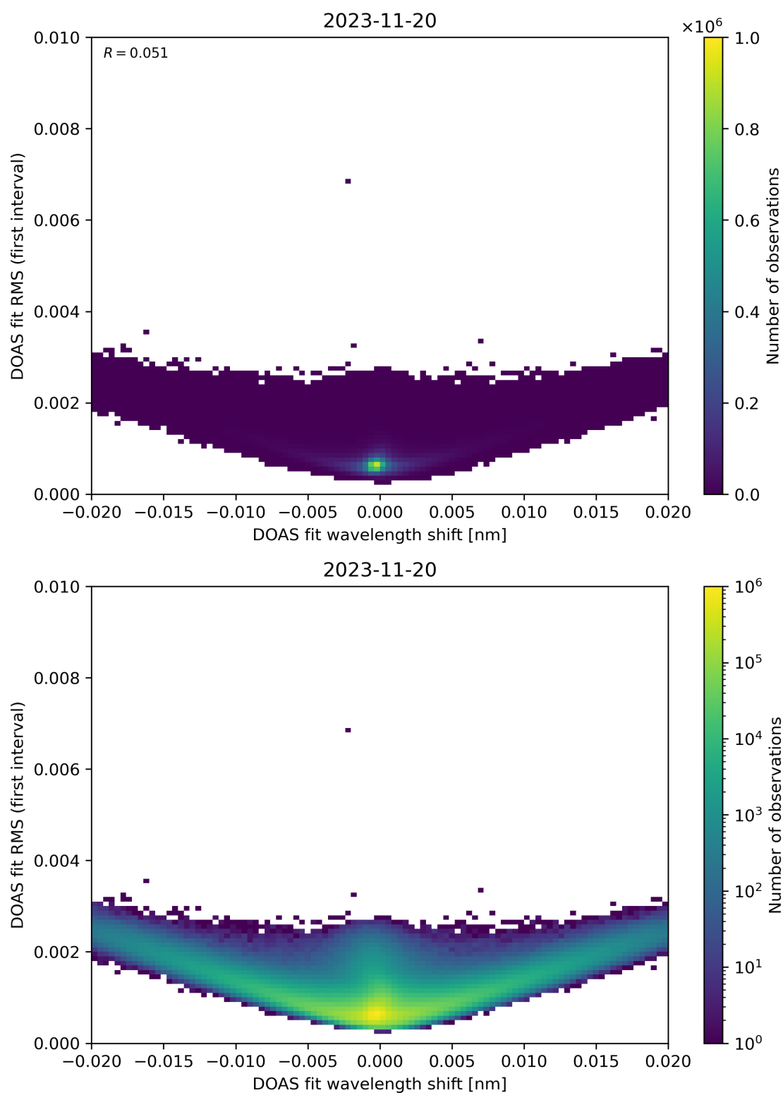
Figure 64: Scatter density plot of “DOAS fit wavelength shift” against “DOAS fit RMS (first interval)” for 2023-11-19 to 2023-11-21.
