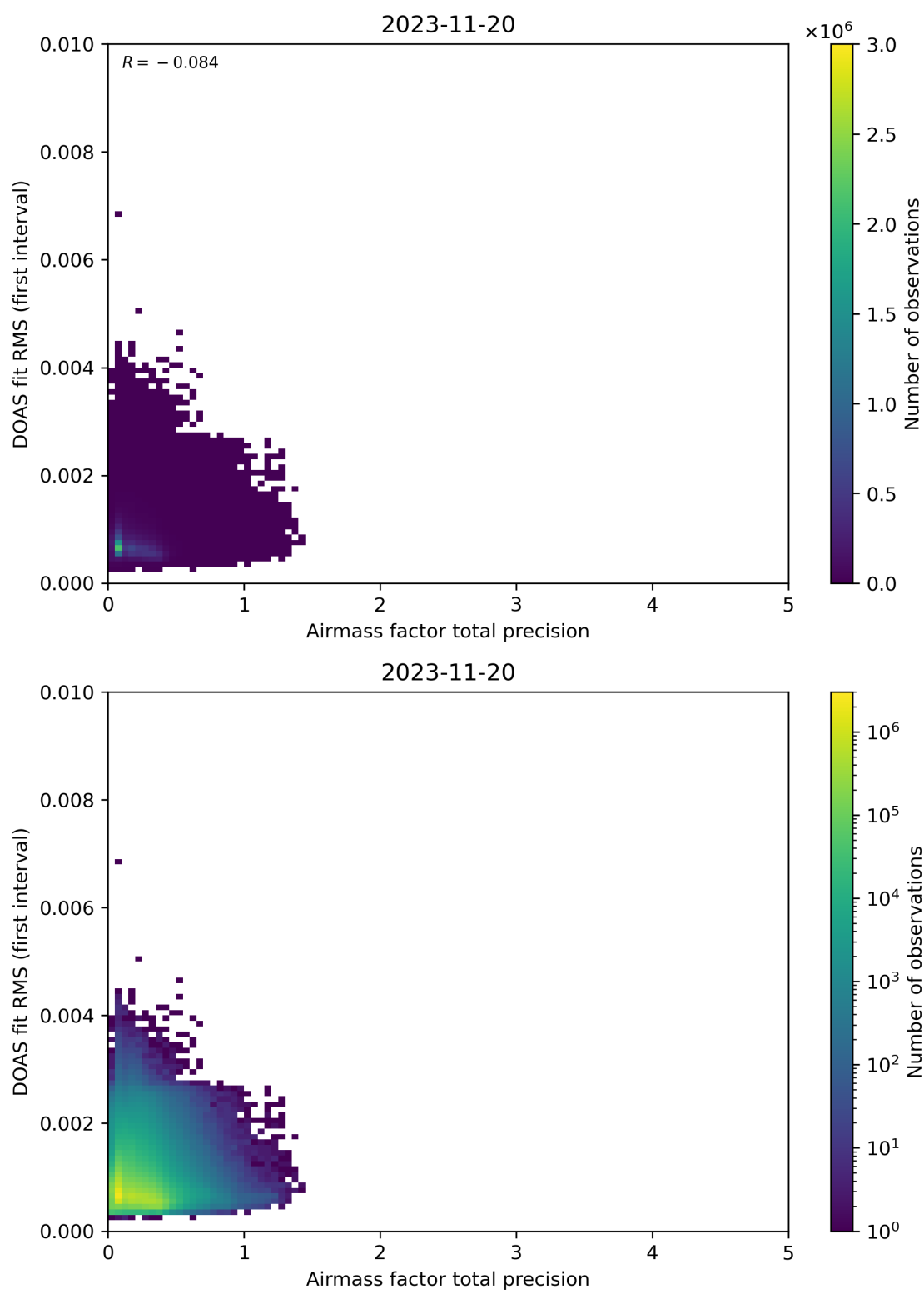
Figure 105: Scatter density plot of “Airmass factor total precision” against “DOAS fit RMS (first interval)” for 2023-11-19 to 2023-11-21.
