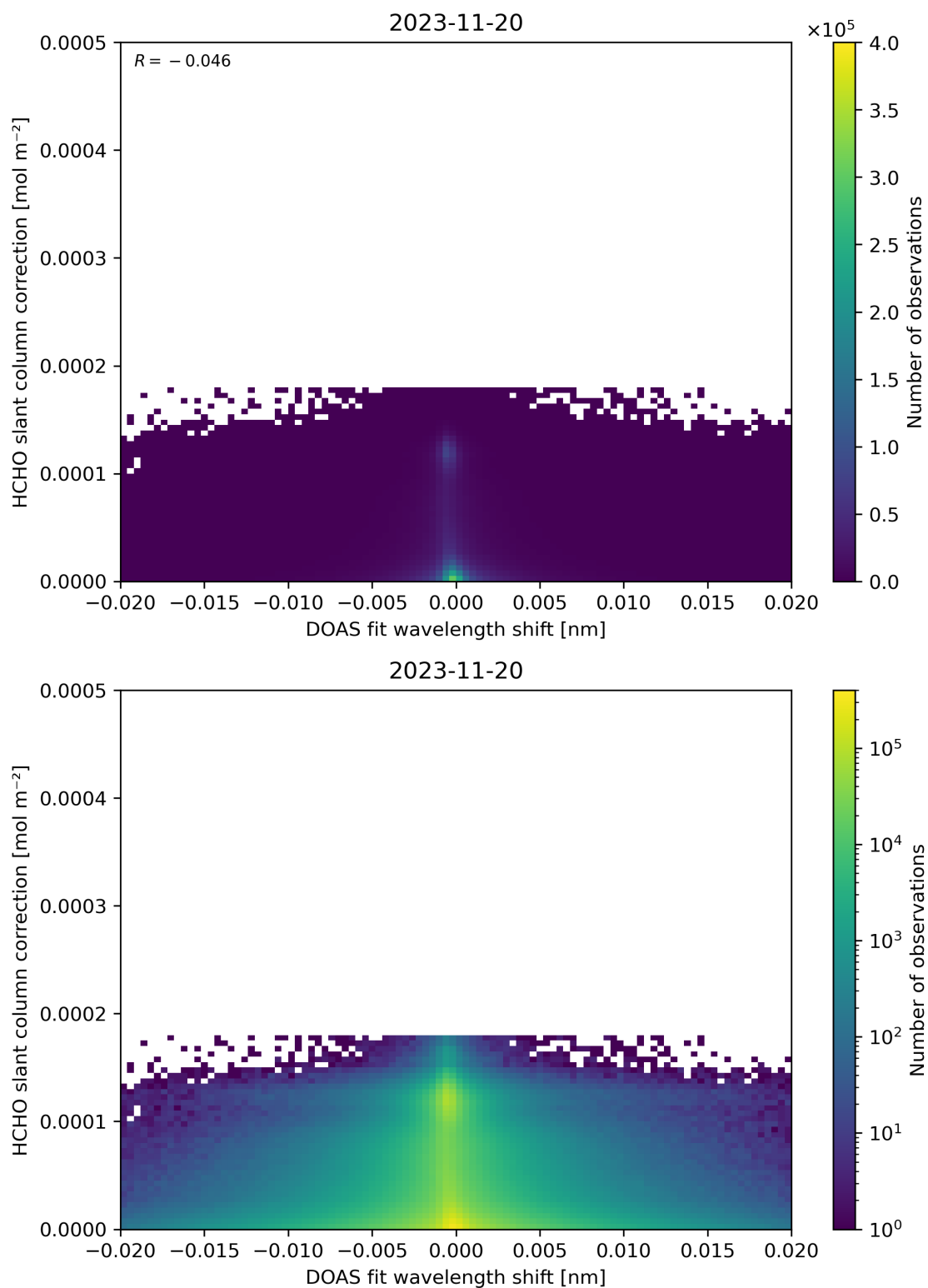
Figure 67: Scatter density plot of “DOAS fit wavelength shift” against “HCHO slant column correction” for 2023-11-19 to 2023-11-21.
