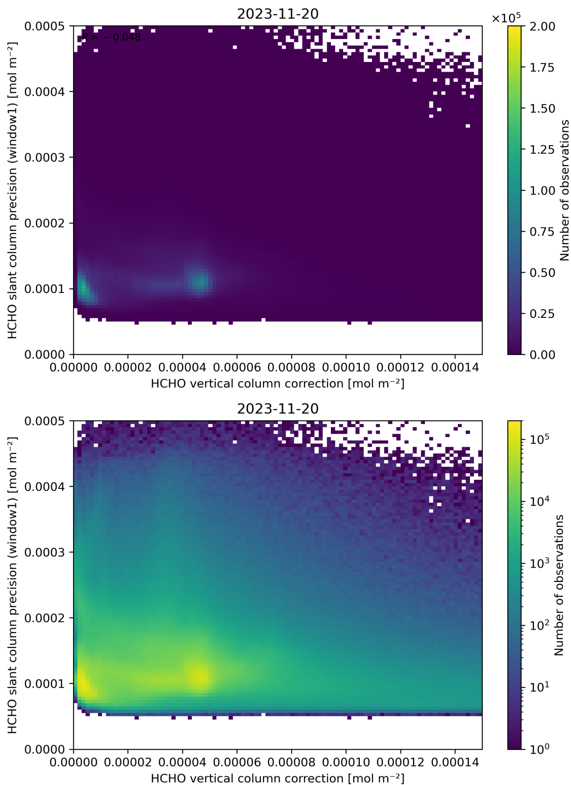
Figure 119: Scatter density plot of “HCHO vertical column correction” against “HCHO slant column precision (window1)” for 2023-11-19 to 2023-11-21.
