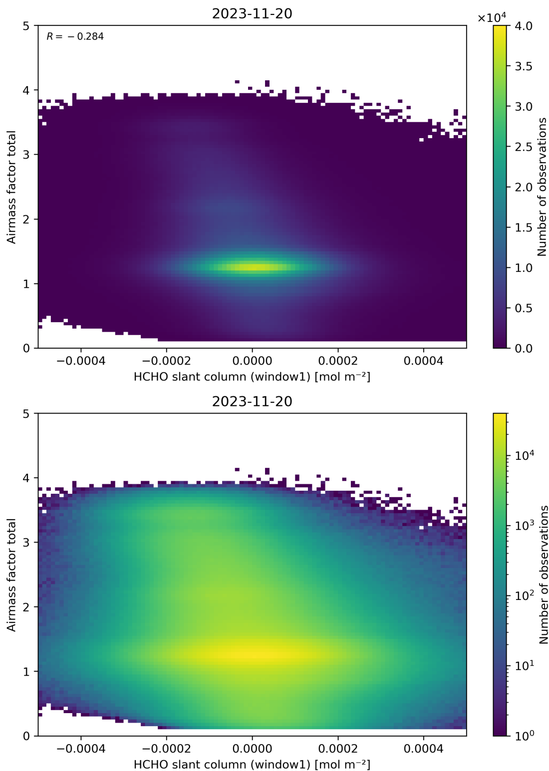
Figure 85: Scatter density plot of “HCHO slant column (window1)” against “Airmass factor total” for 2023-11-19 to 2023-11-21.
