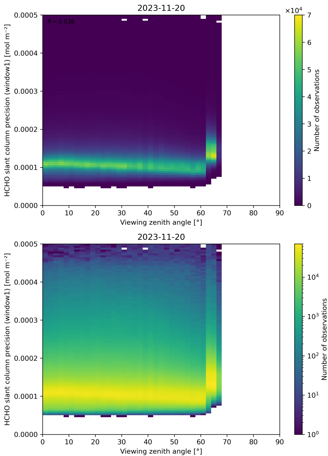
Figure 189: Scatter density plot of “Viewing zenith angle” against “HCHO slant column precision (window1)” for 2023-11-19 to 2023-11-21.
