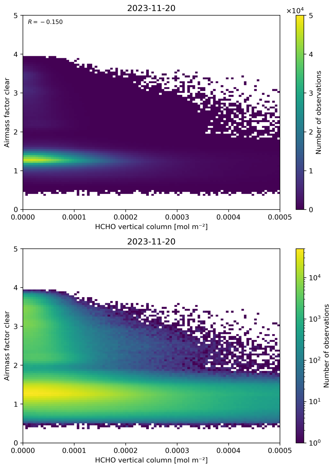
Figure 126: Scatter density plot of “HCHO vertical column” against “Airmass factor clear” for 2023-11-19 to 2023-11-21.
