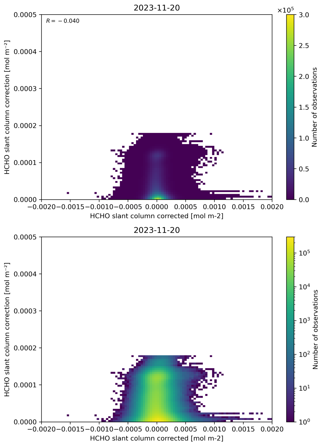
Figure 77: Scatter density plot of “HCHO slant column corrected” against “HCHO slant column correction” for 2023-11-19 to 2023-11-21.
