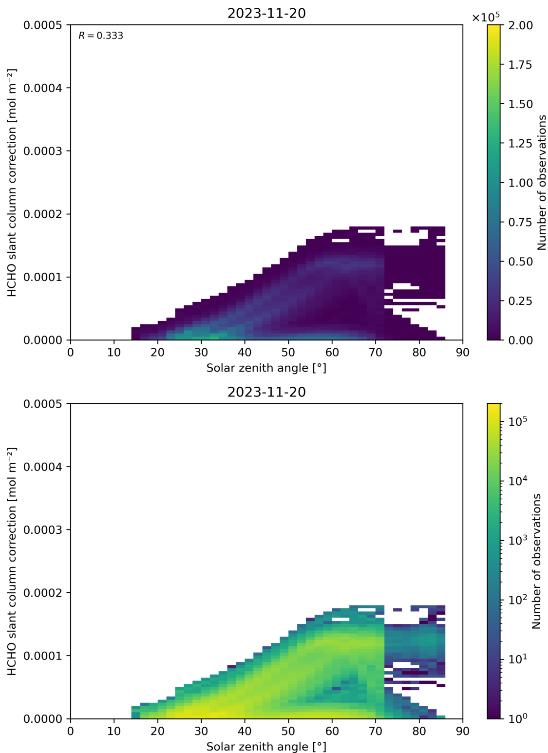
Figure 172: Scatter density plot of “Solar zenith angle” against “HCHO slant column correction” for 2023-11-19 to 2023-11-21.
