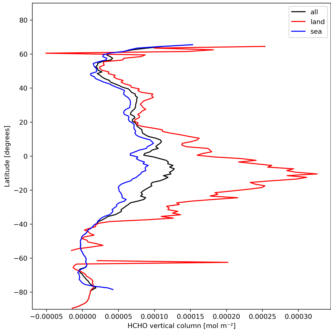
Figure 21: Zonal average of “HCHO vertical column” for 2023-11-19 to 2023-11-21.
