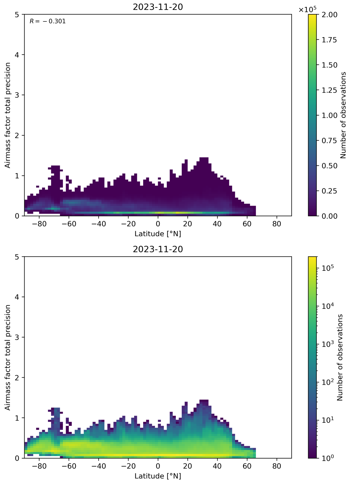
Figure 162: Scatter density plot of “Latitude” against “Airmass factor total precision” for 2023-11-19 to 2023-11-21.
