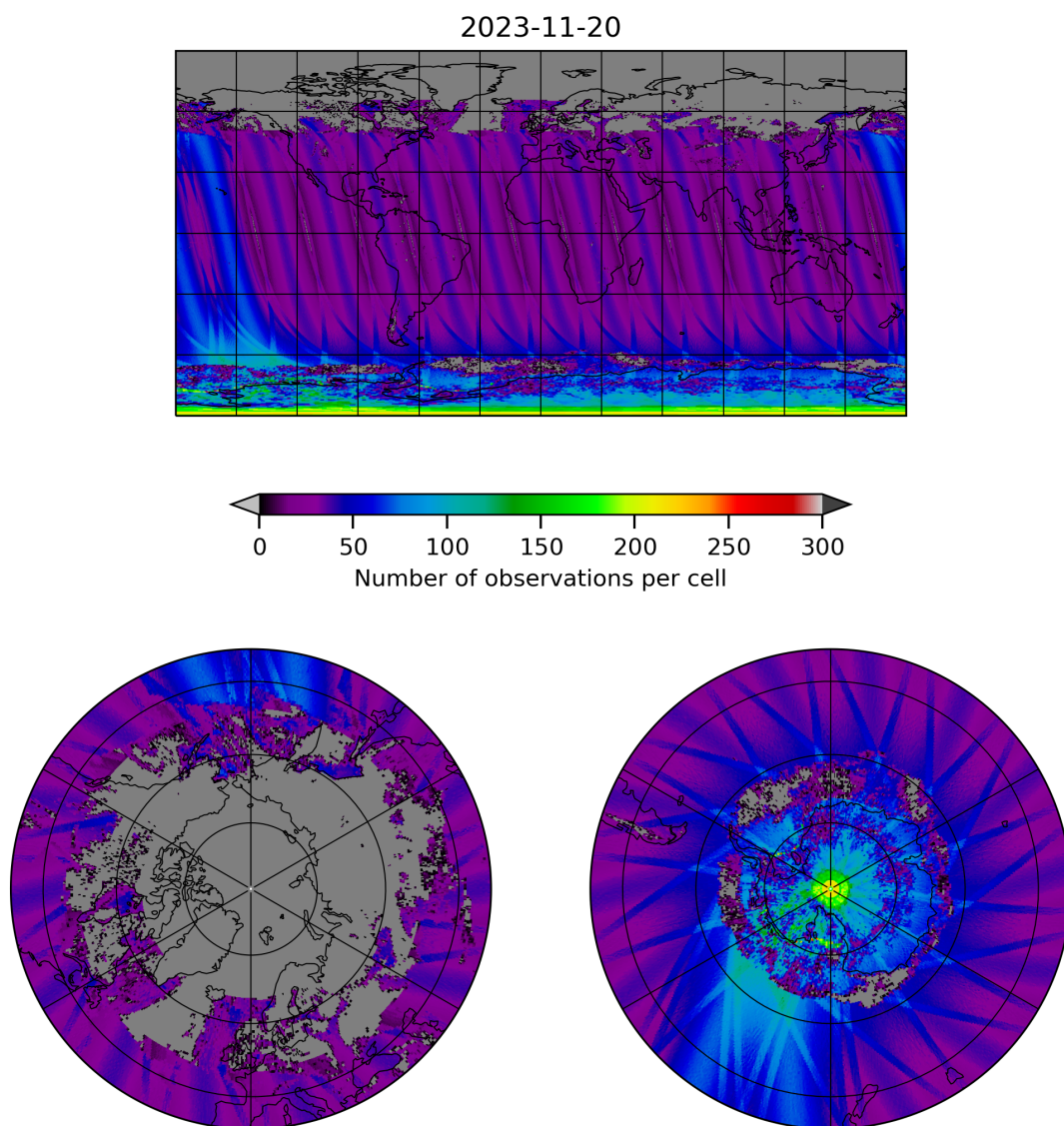
Figure 19: Map of the number of observations for 2023-11-19 to 2023-11-21
