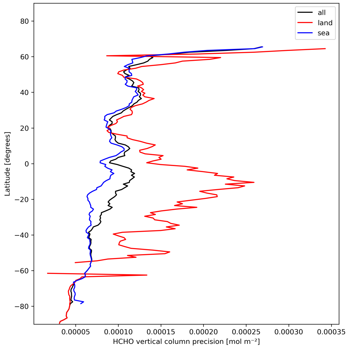
Figure 22: Zonal average of “HCHO vertical column precision” for 2023-11-19 to 2023-11-21.
