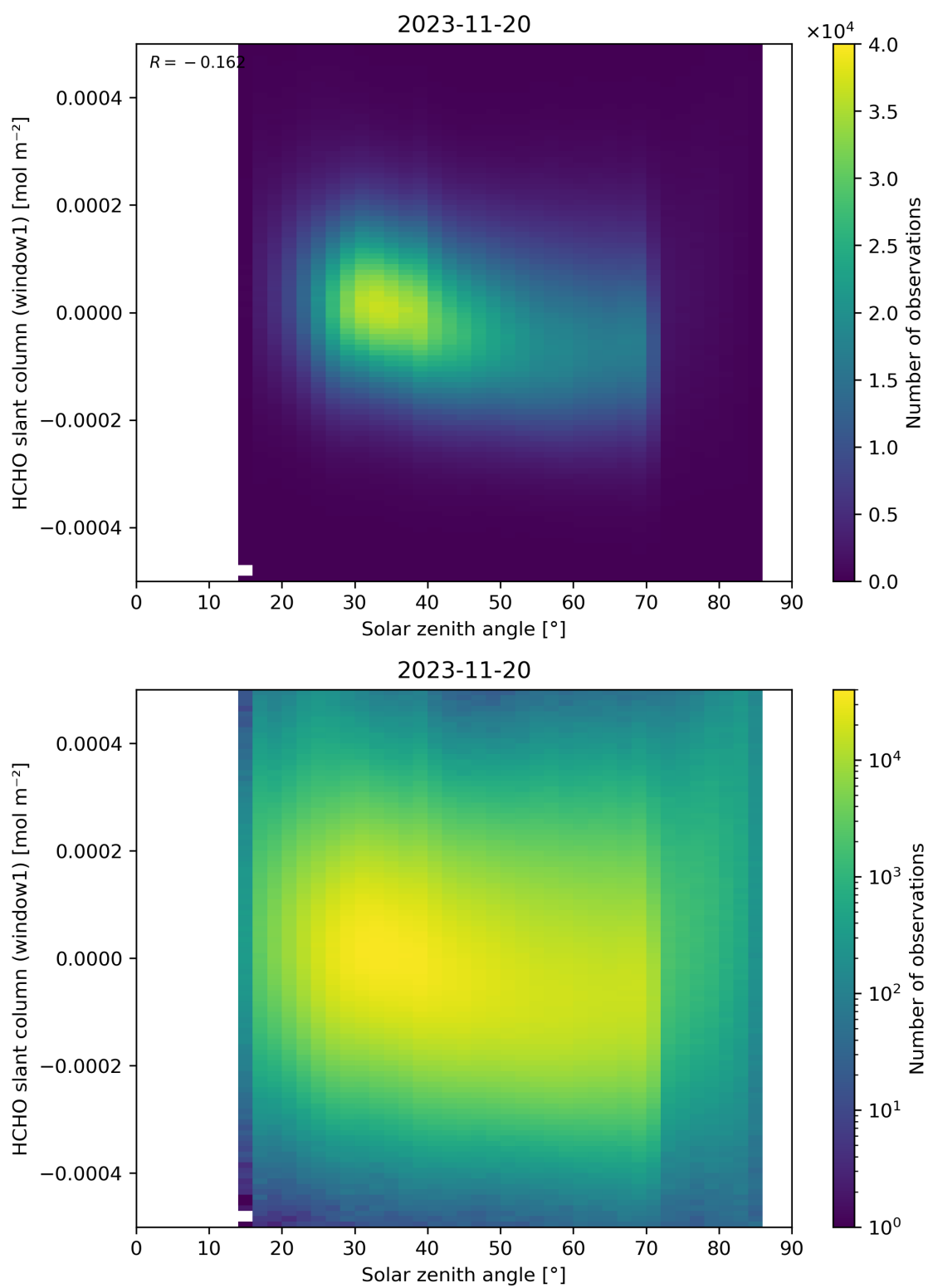
Figure 173: Scatter density plot of “Solar zenith angle” against “HCHO slant column (window1)” for 2023-11-19 to 2023-11-21.
