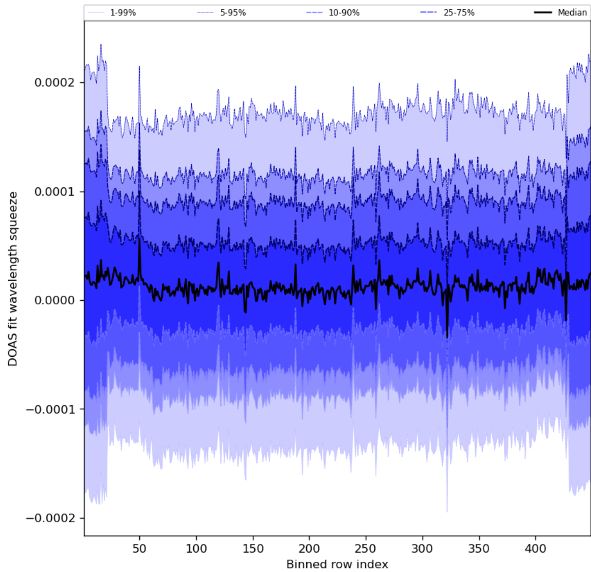
Figure 59: Along track statistics of “DOAS fit wavelength squeeze” for 2023-11-19 to 2023-11-21
