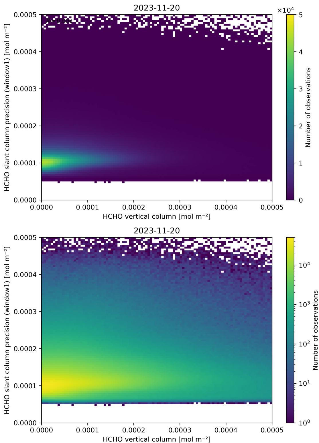
Figure 130: Scatter density plot of “HCHO vertical column” against “HCHO slant column precision (window1)” for 2023-11-19 to 2023-11-21.
