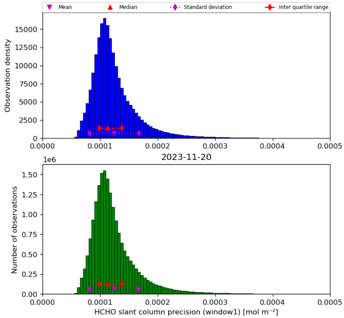
Figure 39: Histogram of “HCHO slant column precision (window1)” for 2023-11-19 to 2023-11-21
