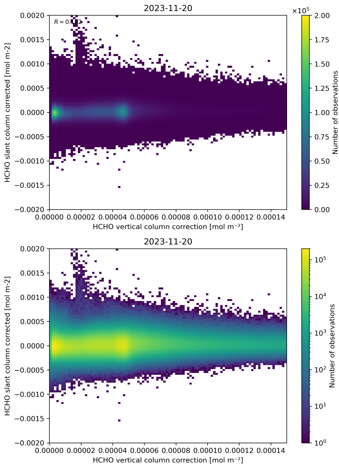
Figure 116: Scatter density plot of “HCHO vertical column correction” against “HCHO slant column corrected” for 2023-11-19 to 2023-11-21.
