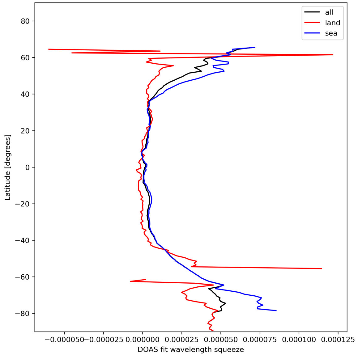
Figure 31: Zonal average of “DOAS fit wavelength squeeze” for 2023-11-19 to 2023-11-21.
