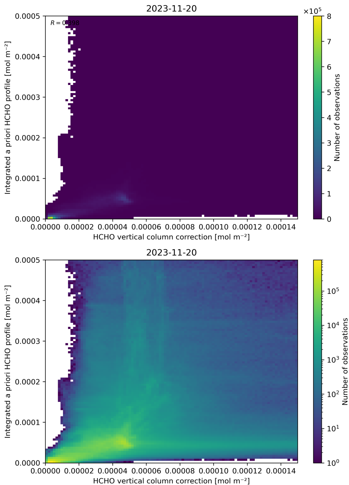
Figure 122: Scatter density plot of “HCHO vertical column correction” against “Integrated a priori HCHO profile” for 2023-11-19 to 2023-11-21.
