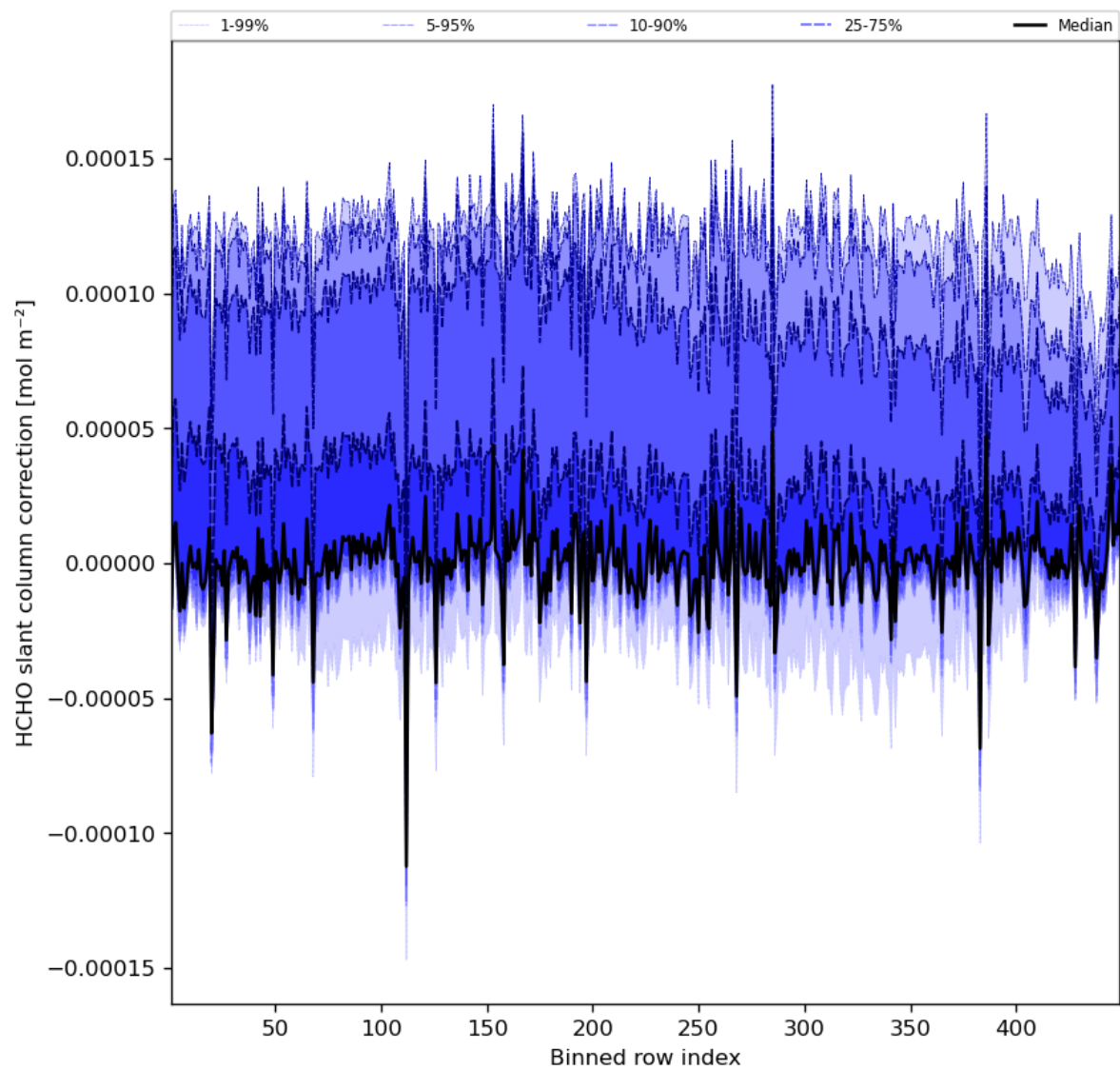
Figure 61: Along track statistics of “HCHO slant column correction” for 2023-11-19 to 2023-11-21
