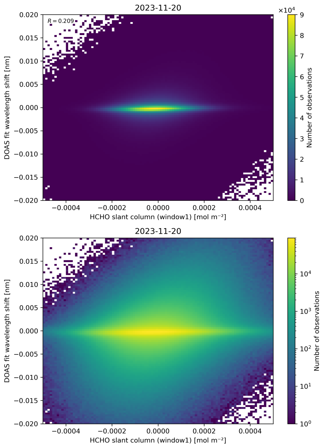
Figure 79: Scatter density plot of “HCHO slant column (window1)” against “DOAS fit wavelength shift” for 2023-11-19 to 2023-11-21.
