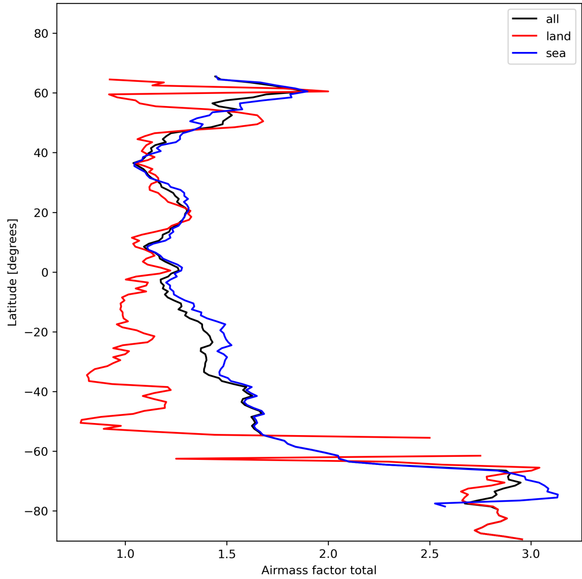
Figure 26: Zonal average of “Airmass factor total” for 2023-11-19 to 2023-11-21.
