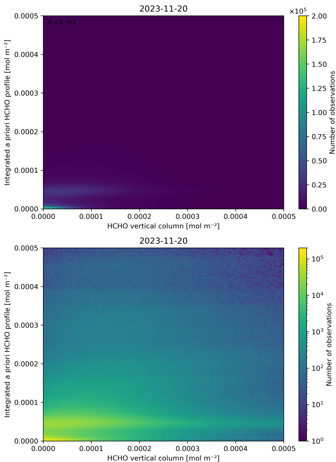
Figure 135: Scatter density plot of “HCHO vertical column” against “Integrated a priori HCHO profile” for 2023-11-19 to 2023-11-21.
