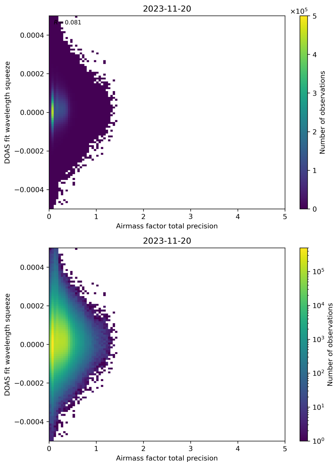
Figure 107: Scatter density plot of “Airmass factor total precision” against “DOAS fit wavelength squeeze” for 2023-11-19 to 2023-11-21.
