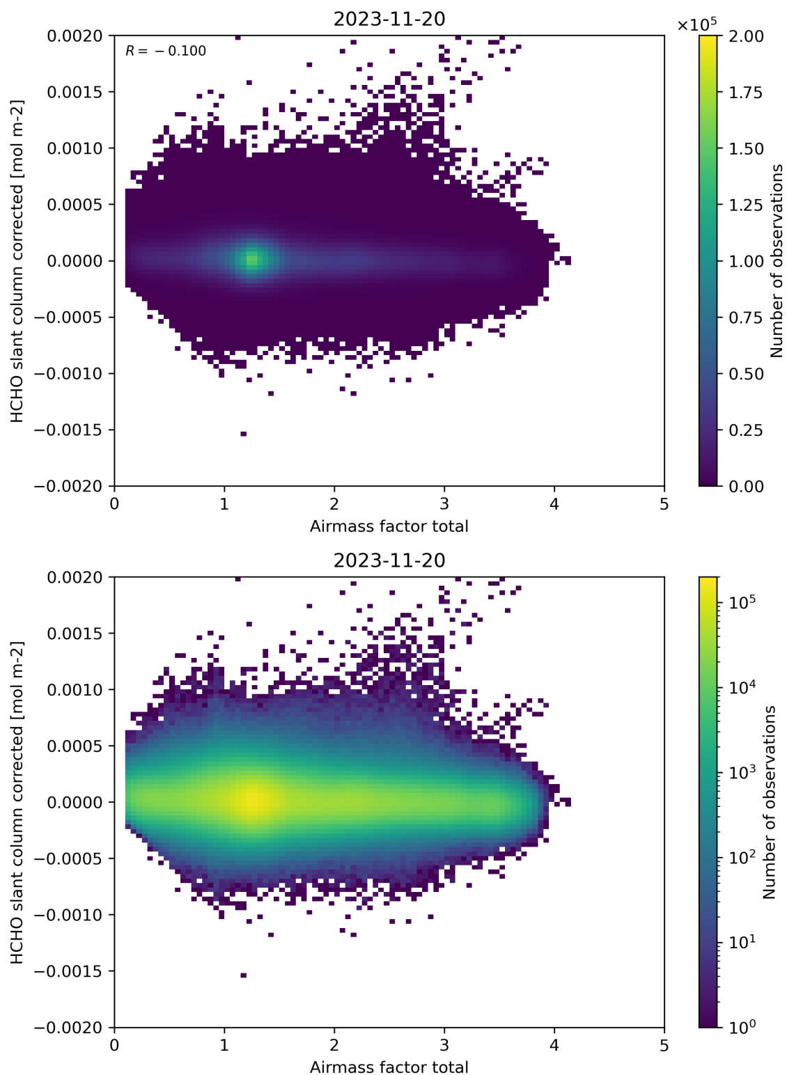
Figure 101: Scatter density plot of “Airmass factor total” against “HCHO slant column corrected” for 2023-11-19 to 2023-11-21.
