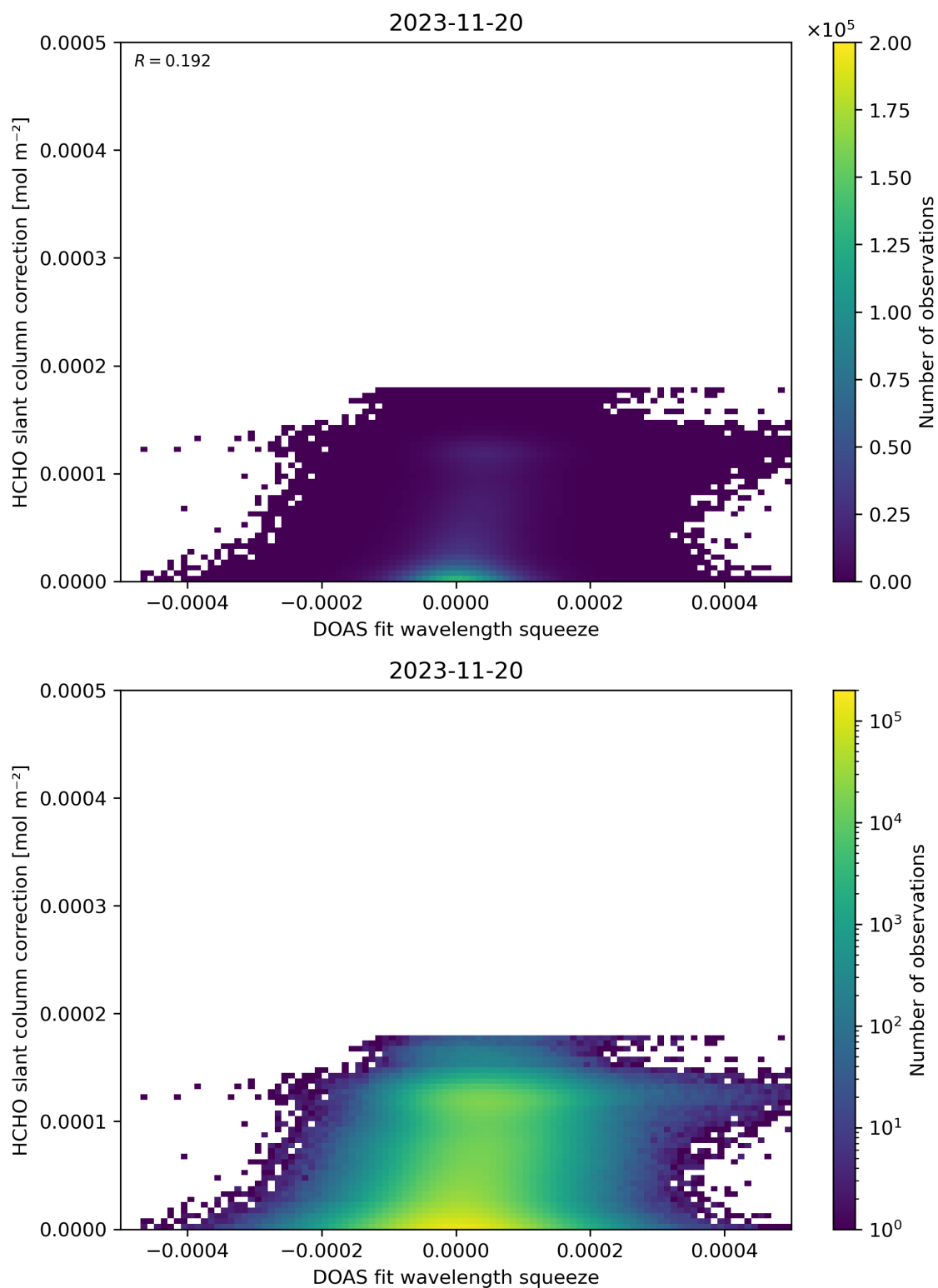
Figure 70: Scatter density plot of “DOAS fit wavelength squeeze” against “HCHO slant column correction” for 2023-11-19 to 2023-11-21.
