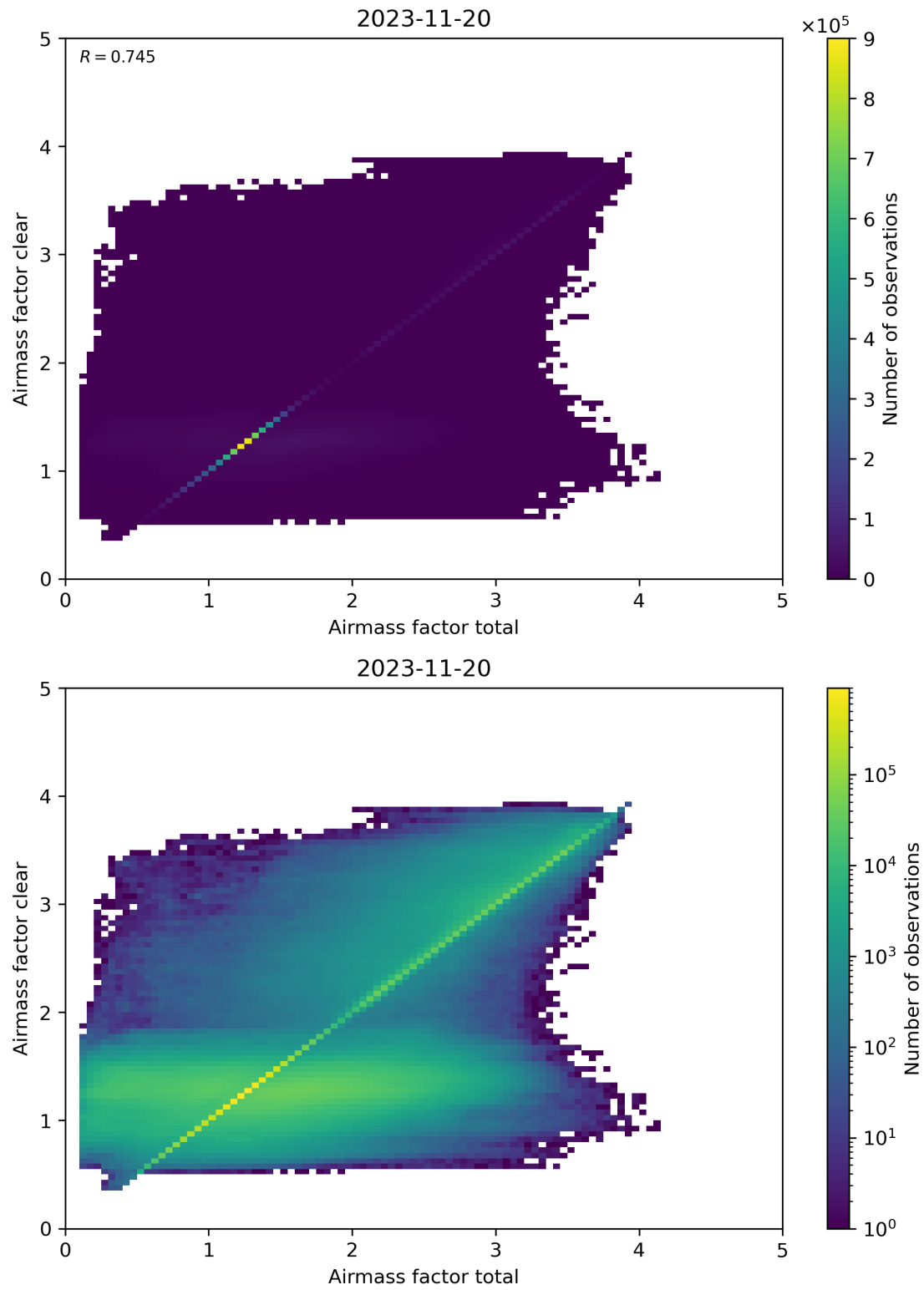
Figure 100: Scatter density plot of “Airmass factor total” against “Airmass factor clear” for 2023-11-19 to 2023-11-21.
