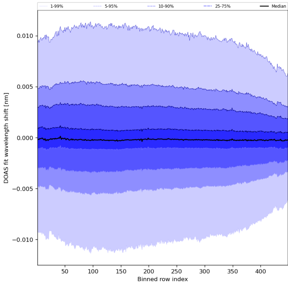
Figure 58: Along track statistics of “DOAS fit wavelength shift” for 2023-11-19 to 2023-11-21
