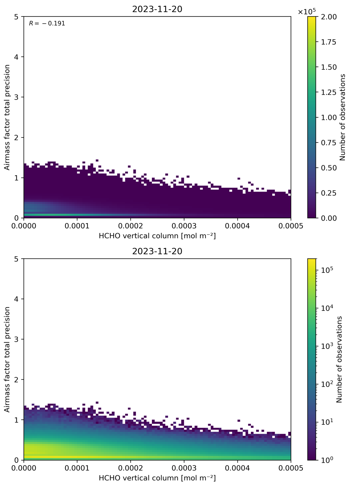
Figure 132: Scatter density plot of “HCHO vertical column” against “Airmass factor total precision” for 2023-11-19 to 2023-11-21.
