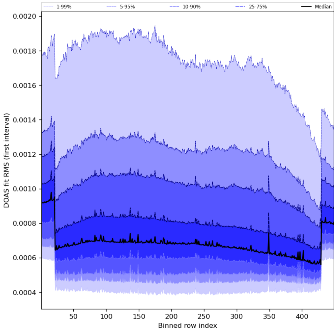
Figure 60: Along track statistics of “DOAS fit RMS (first interval)” for 2023-11-19 to 2023-11-21
