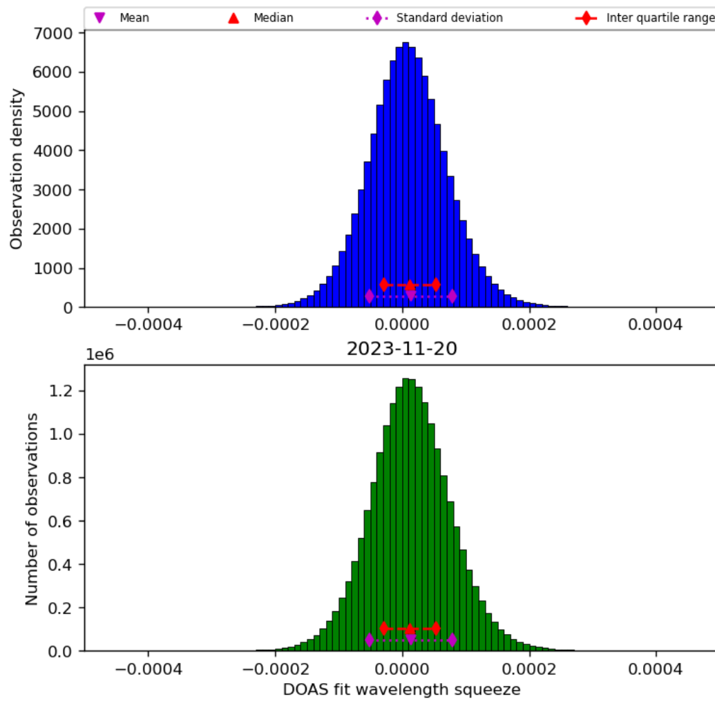
Figure 45: Histogram of “DOAS fit wavelength squeeze” for 2023-11-19 to 2023-11-21
