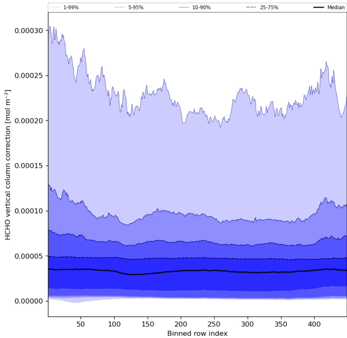
Figure 51: Along track statistics of “HCHO vertical column correction” for 2023-11-19 to 2023-11-21
