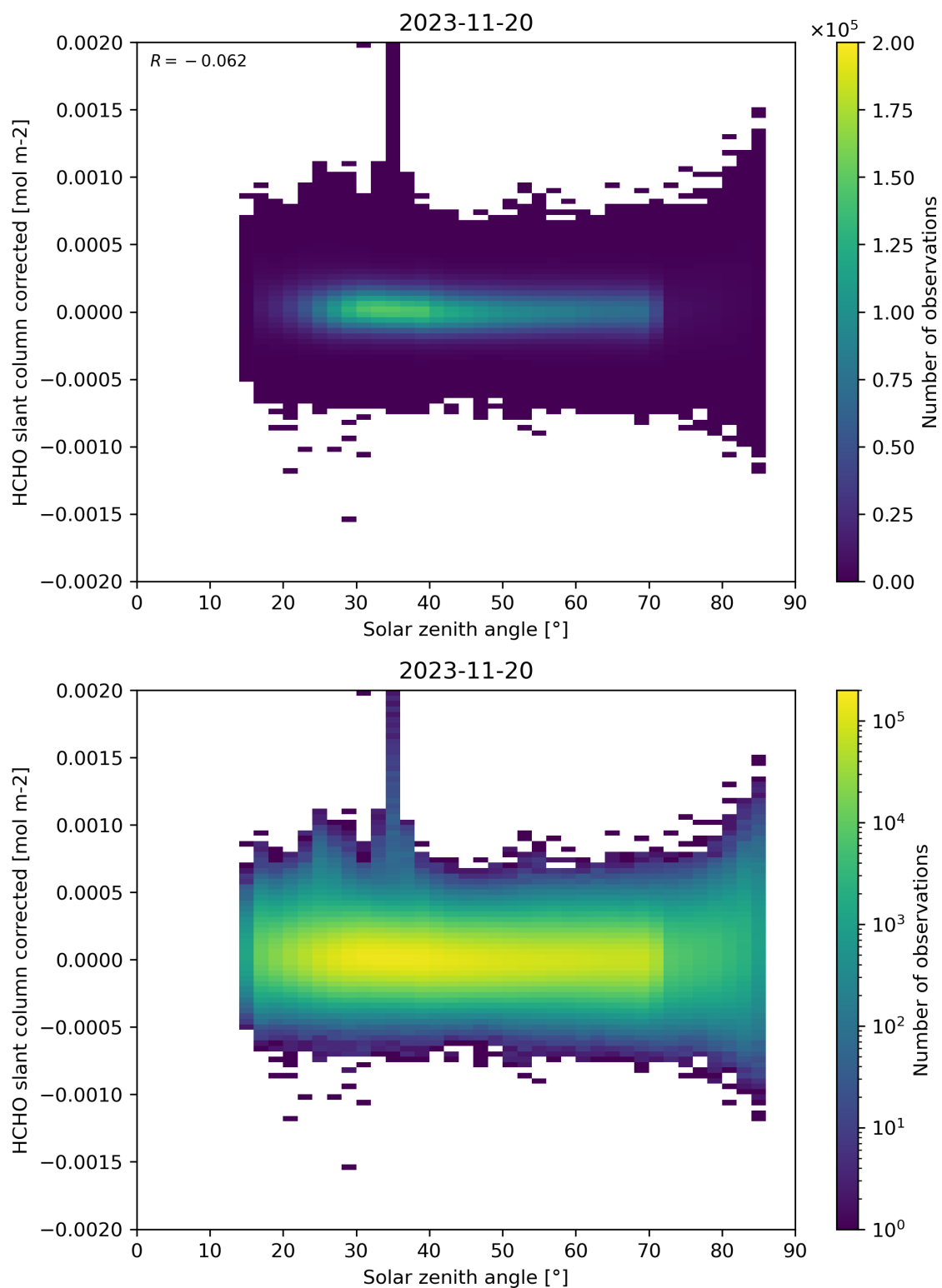
Figure 171: Scatter density plot of “Solar zenith angle” against “HCHO slant column corrected” for 2023-11-19 to 2023-11-21.
