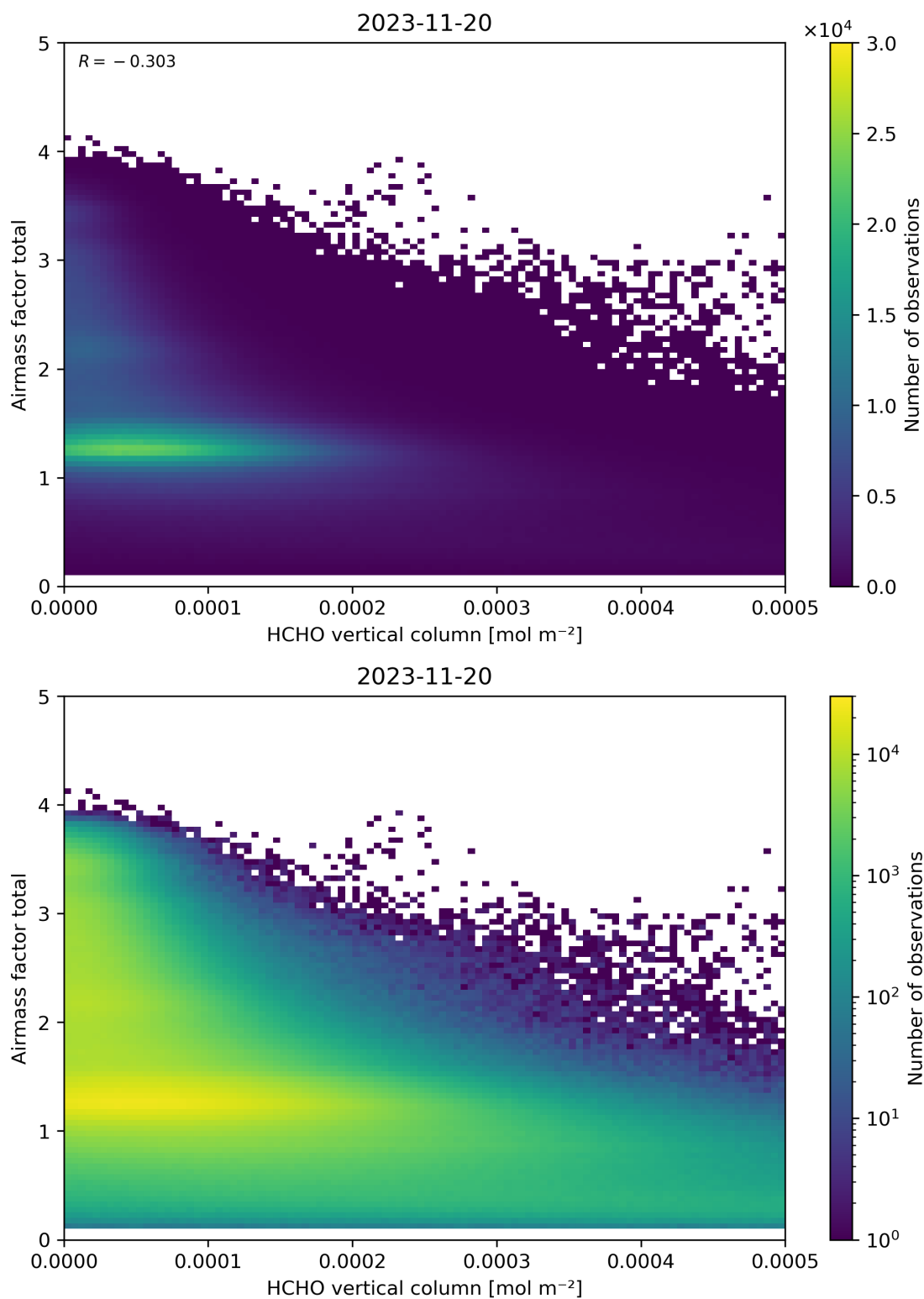
Figure 131: Scatter density plot of “HCHO vertical column” against “Airmass factor total” for 2023-11-19 to 2023-11-21.
