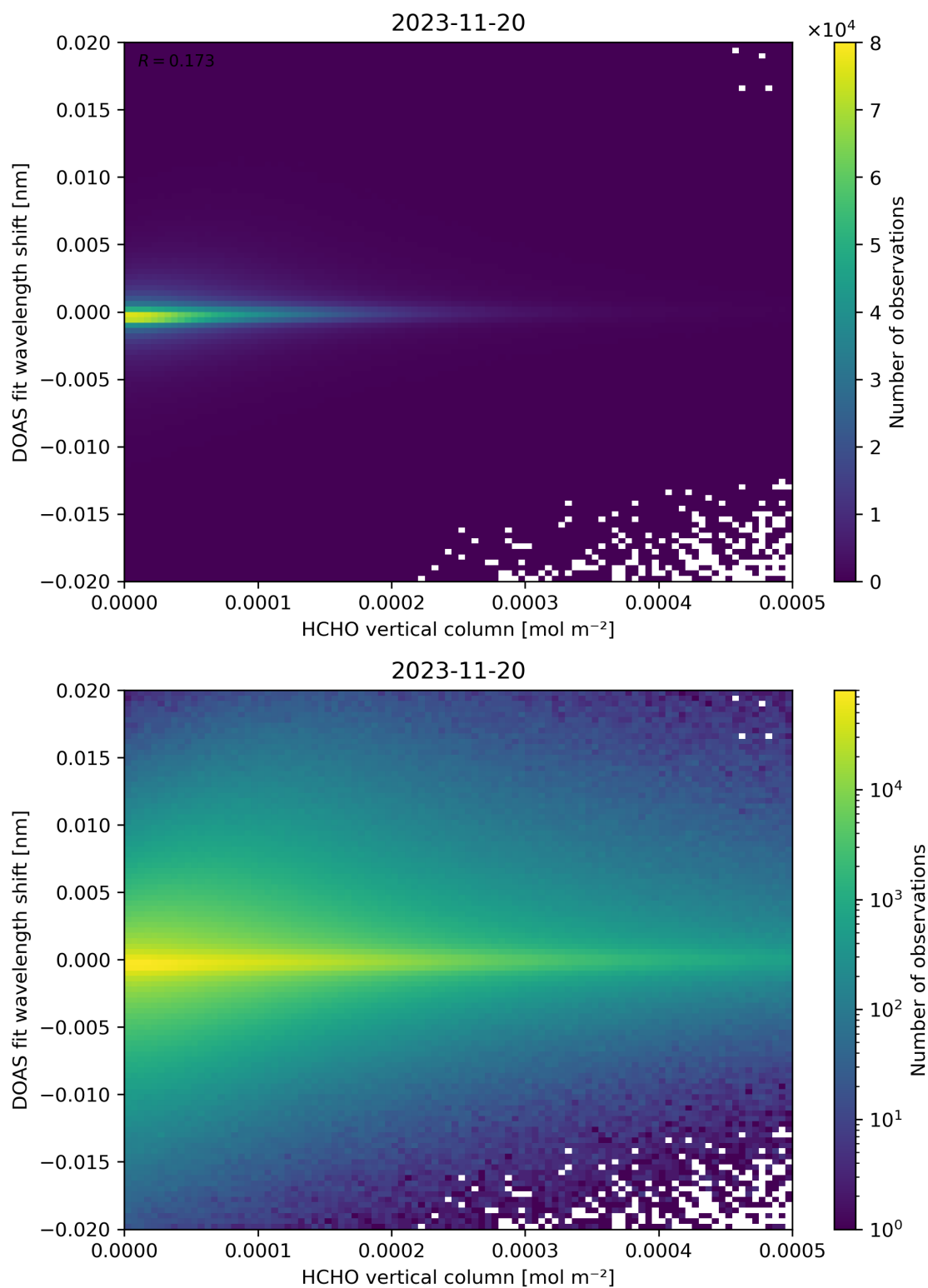
Figure 124: Scatter density plot of “HCHO vertical column” against “DOAS fit wavelength shift” for 2023-11-19 to 2023-11-21.
