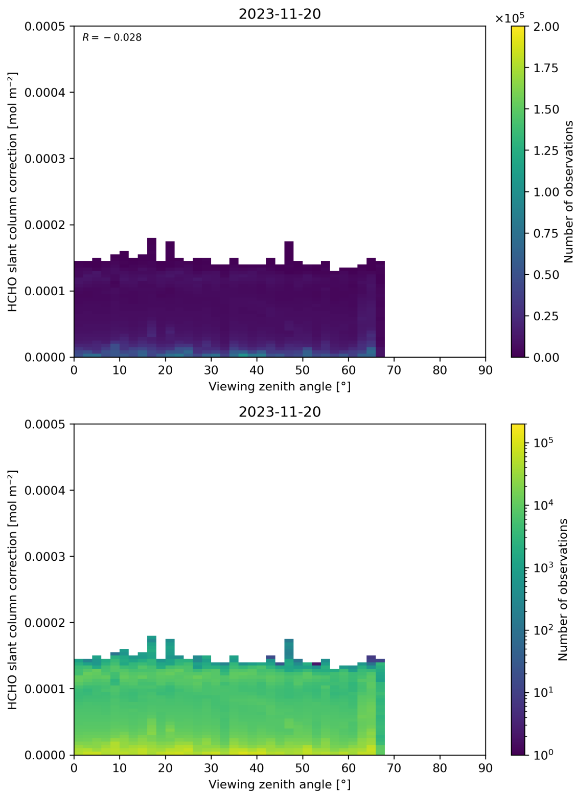
Figure 187: Scatter density plot of “Viewing zenith angle” against “HCHO slant column correction” for 2023-11-19 to 2023-11-21.
