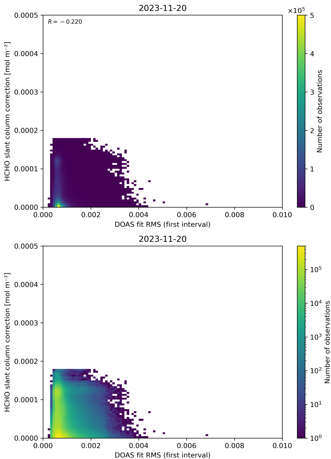
Figure 63: Scatter density plot of “DOAS fit RMS (first interval)” against “HCHO slant column correction” for 2023-11-19 to 2023-11-21.
