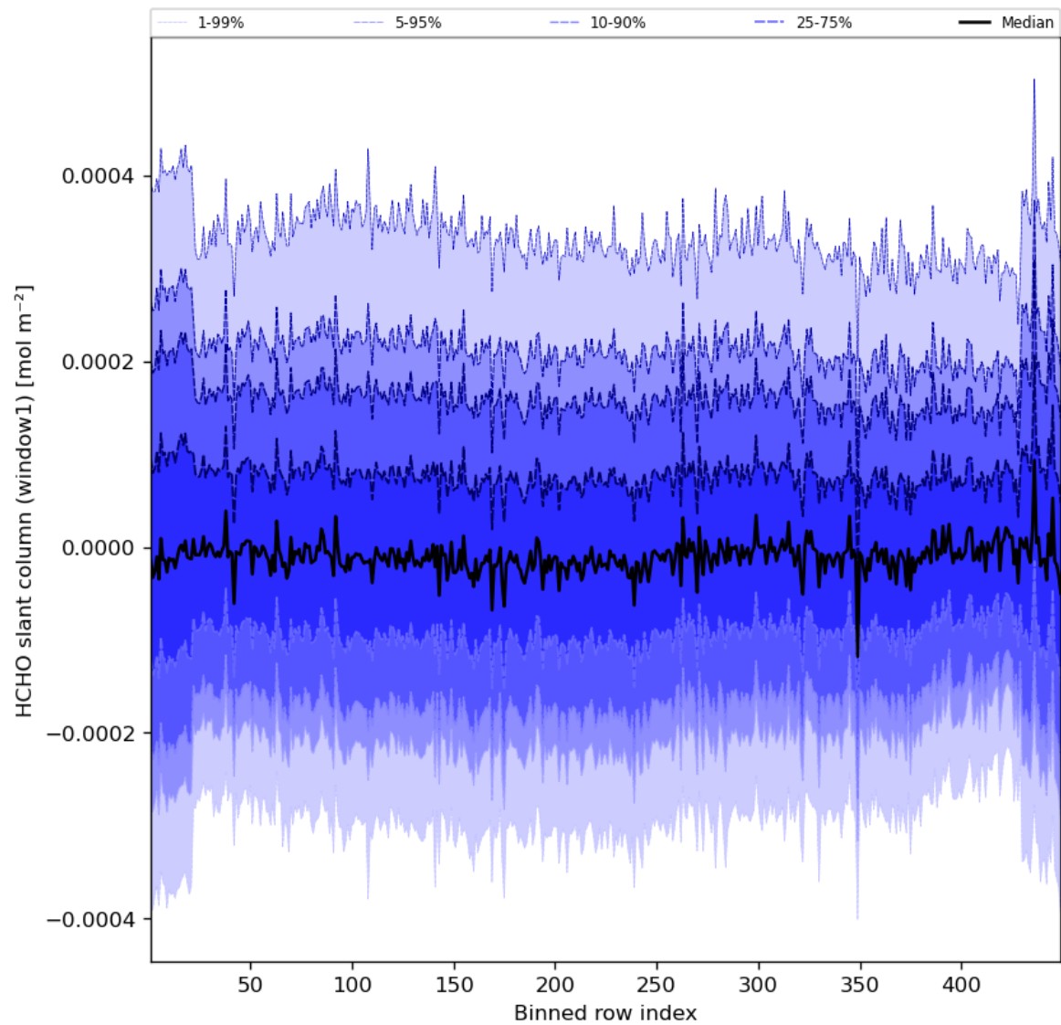
Figure 52: Along track statistics of “HCHO slant column (window1)” for 2023-11-19 to 2023-11-21
