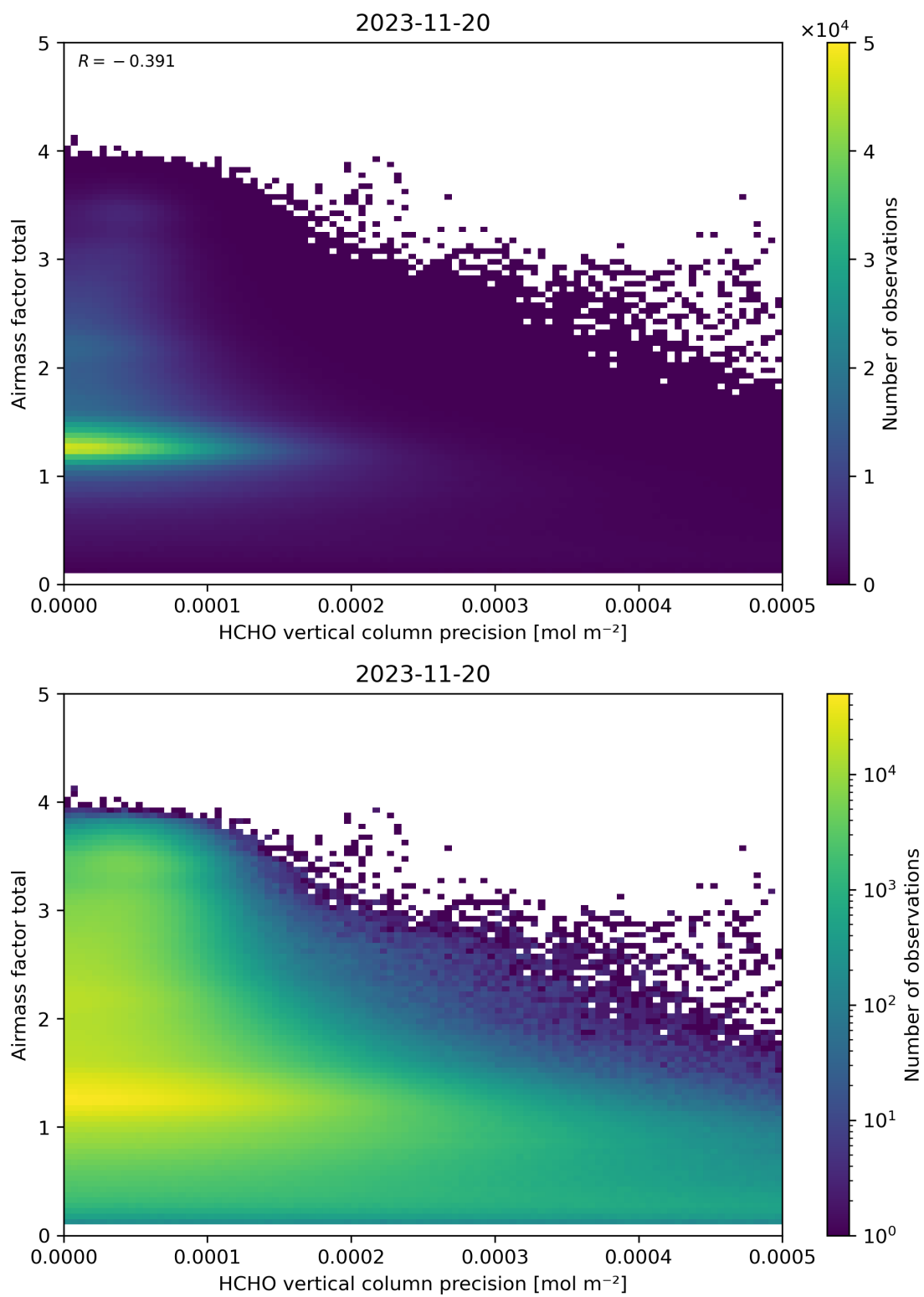
Figure 144: Scatter density plot of “HCHO vertical column precision” against “Airmass factor total” for 2023-11-19 to 2023-11-21.
