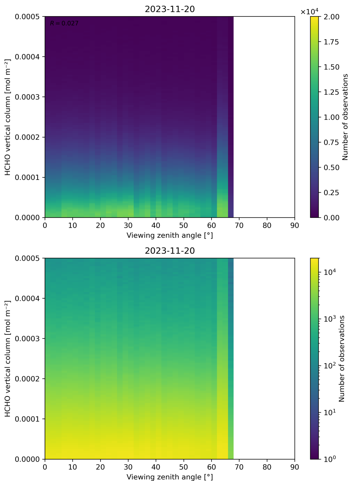
Figure 192: Scatter density plot of “Viewing zenith angle” against “HCHO vertical column” for 2023-11-19 to 2023-11-21.
