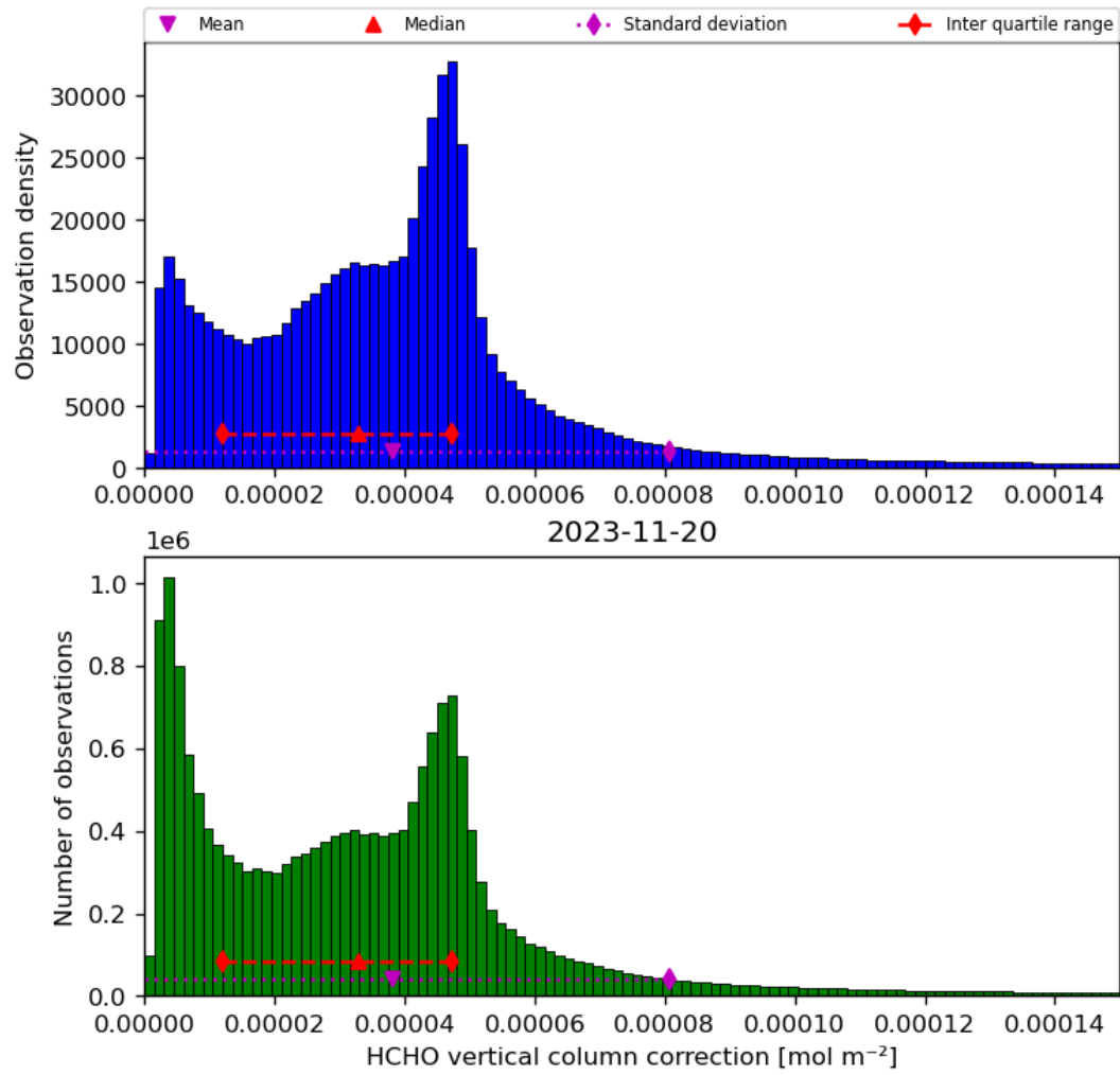
Figure 37: Histogram of “HCHO vertical column correction” for 2023-11-19 to 2023-11-21
