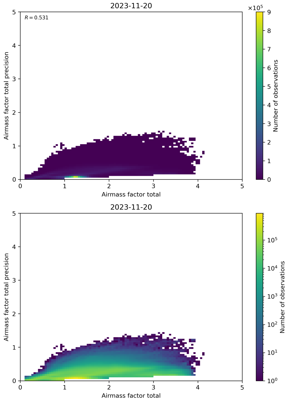
Figure 103: Scatter density plot of “Airmass factor total” against “Airmass factor total precision” for 2023-11-19 to 2023-11-21.
