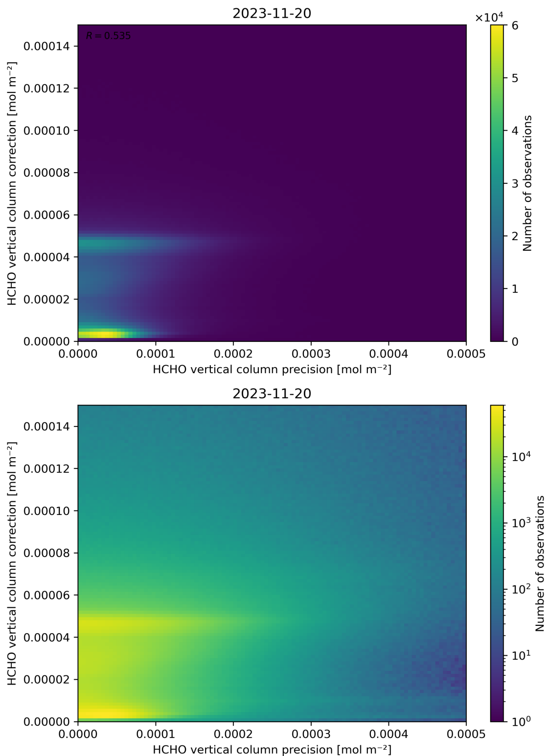
Figure 146: Scatter density plot of “HCHO vertical column precision” against “HCHO vertical column correction” for 2023-11-19 to 2023-11-21.
