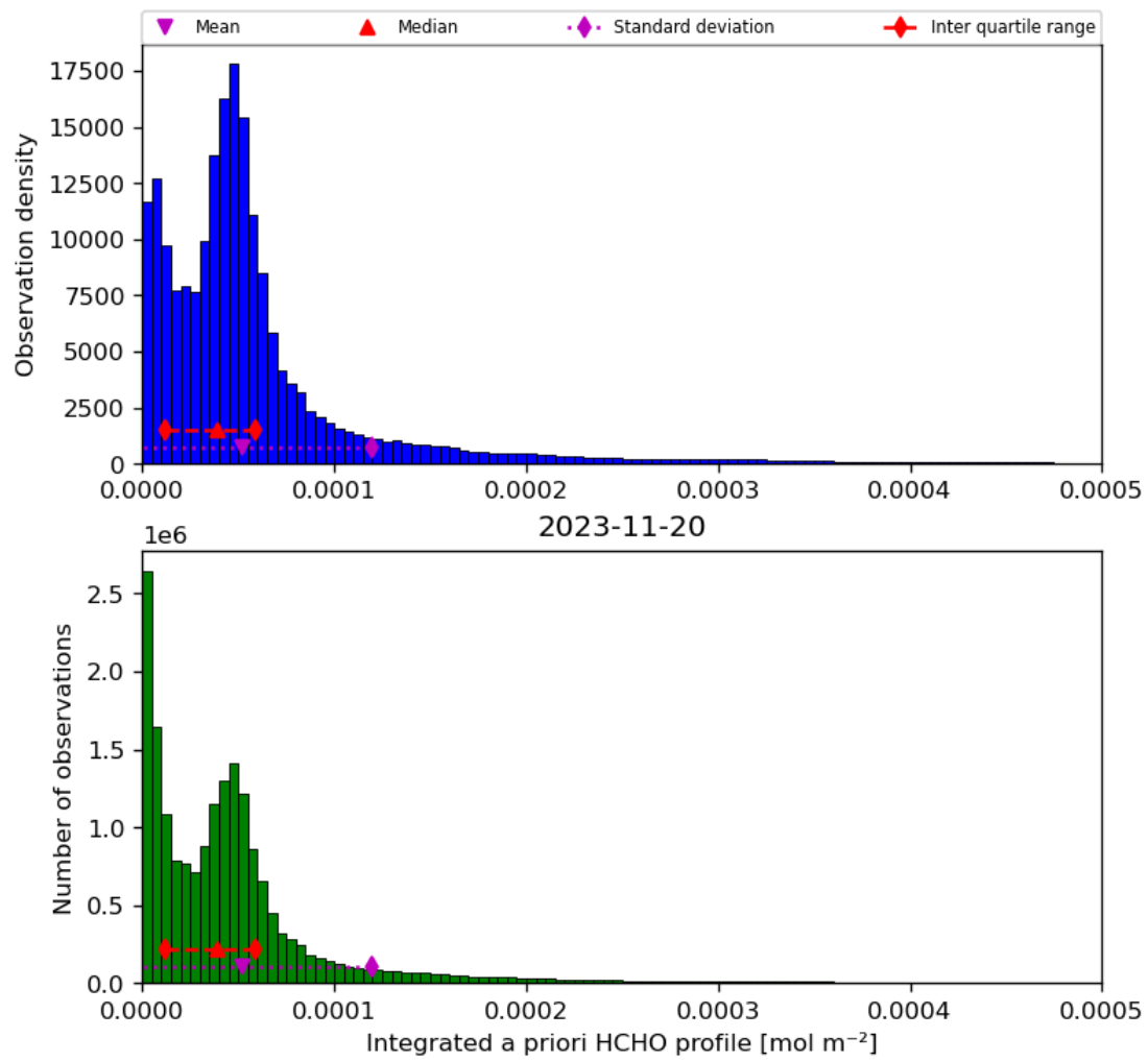
Figure 43: Histogram of “Integrated a priori HCHO profile” for 2023-11-19 to 2023-11-21
