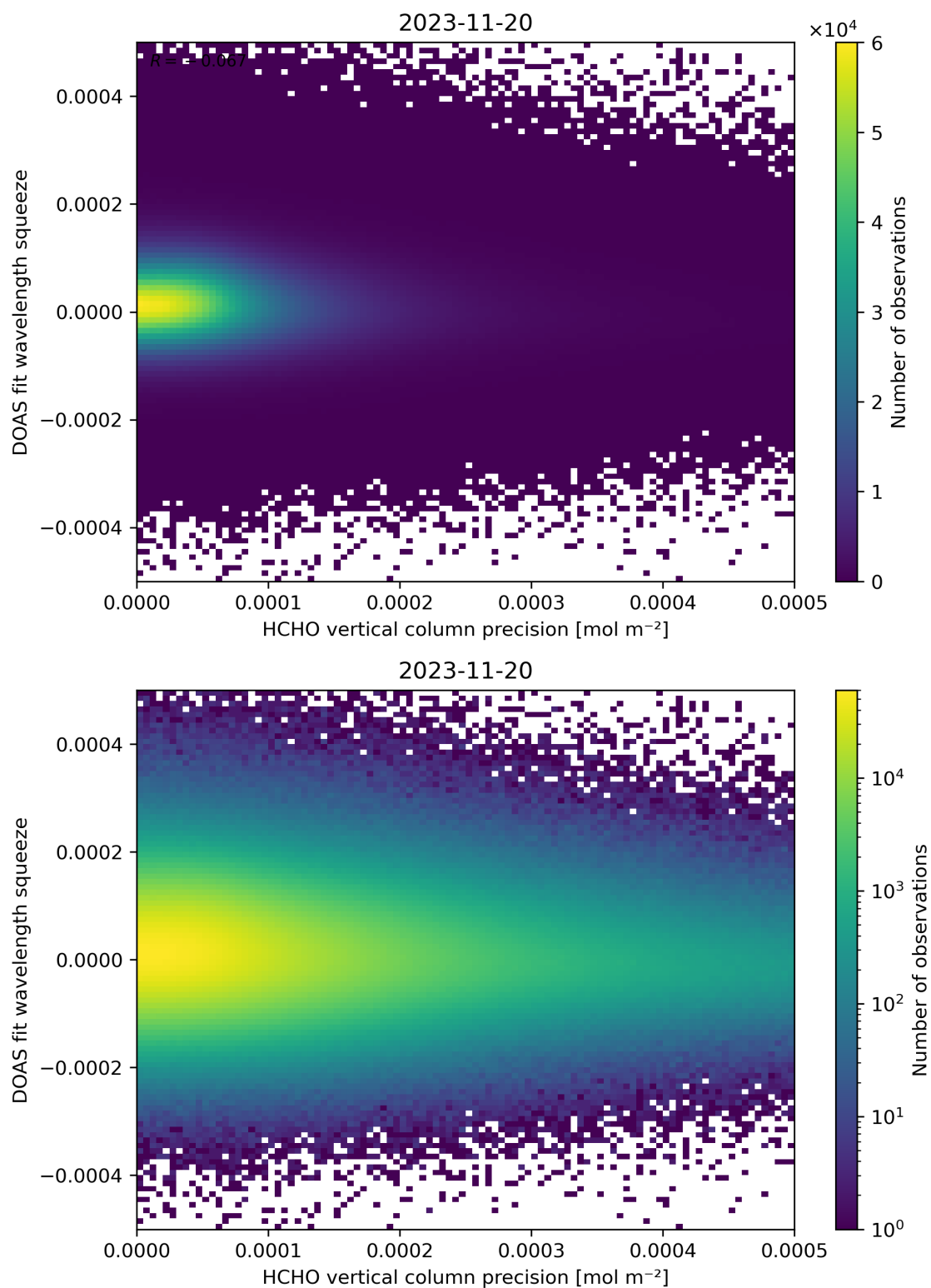
Figure 138: Scatter density plot of “HCHO vertical column precision” against “DOAS fit wavelength squeeze” for 2023-11-19 to 2023-11-21.
