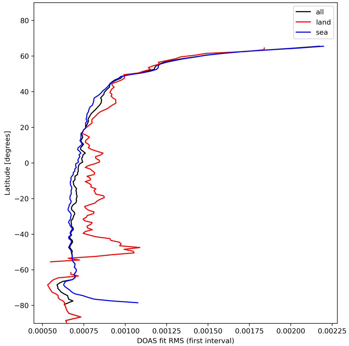
Figure 32: Zonal average of “DOAS fit RMS (first interval)” for 2023-11-19 to 2023-11-21.
