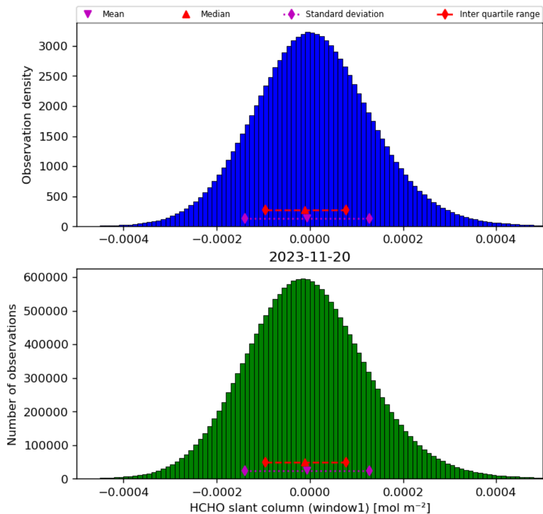
Figure 38: Histogram of “HCHO slant column (window1)” for 2023-11-19 to 2023-11-21
