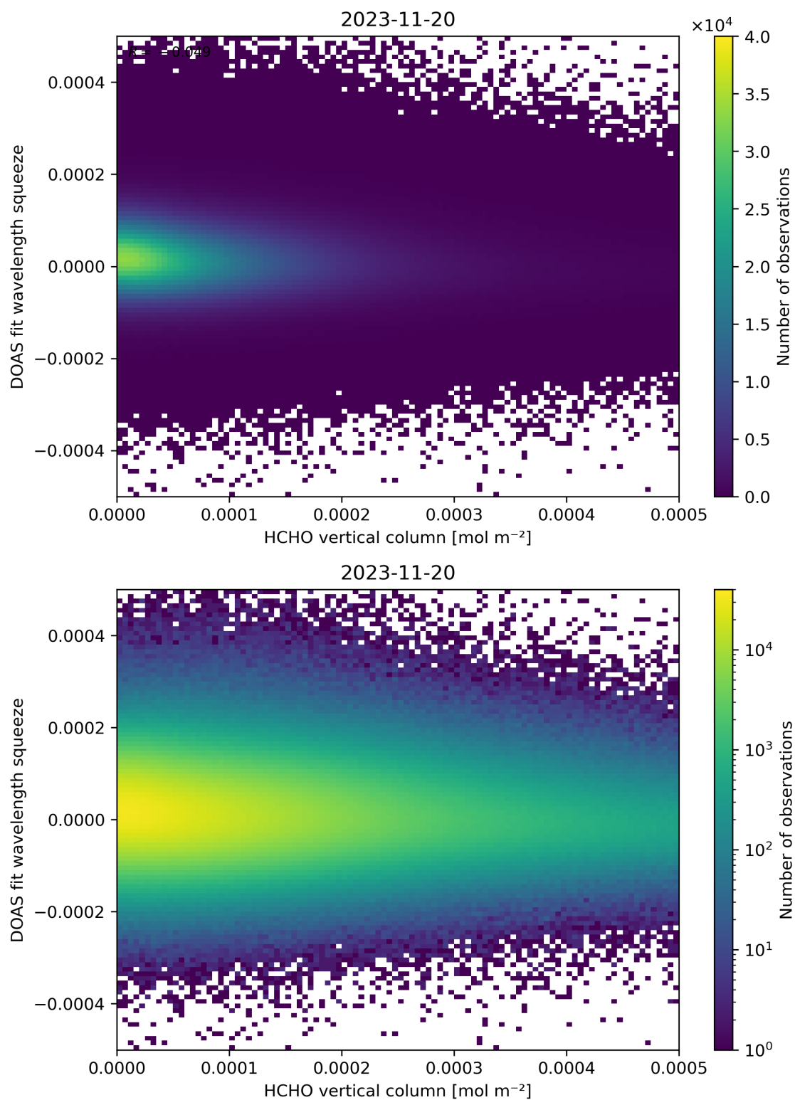
Figure 125: Scatter density plot of “HCHO vertical column” against “DOAS fit wavelength squeeze” for 2023-11-19 to 2023-11-21.
