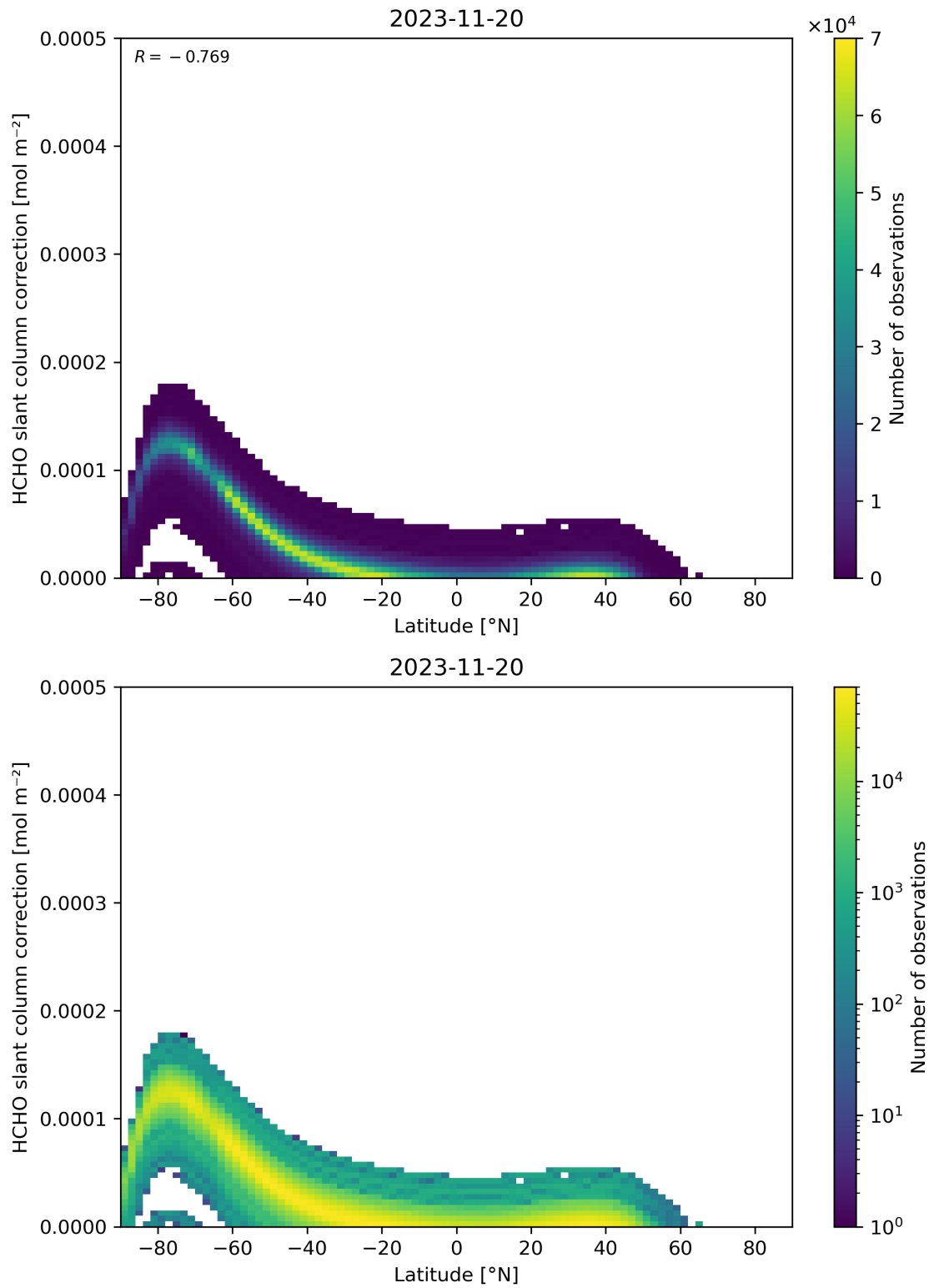
Figure 158: Scatter density plot of “Latitude” against “HCHO slant column correction” for 2023-11-19 to 2023-11-21.
