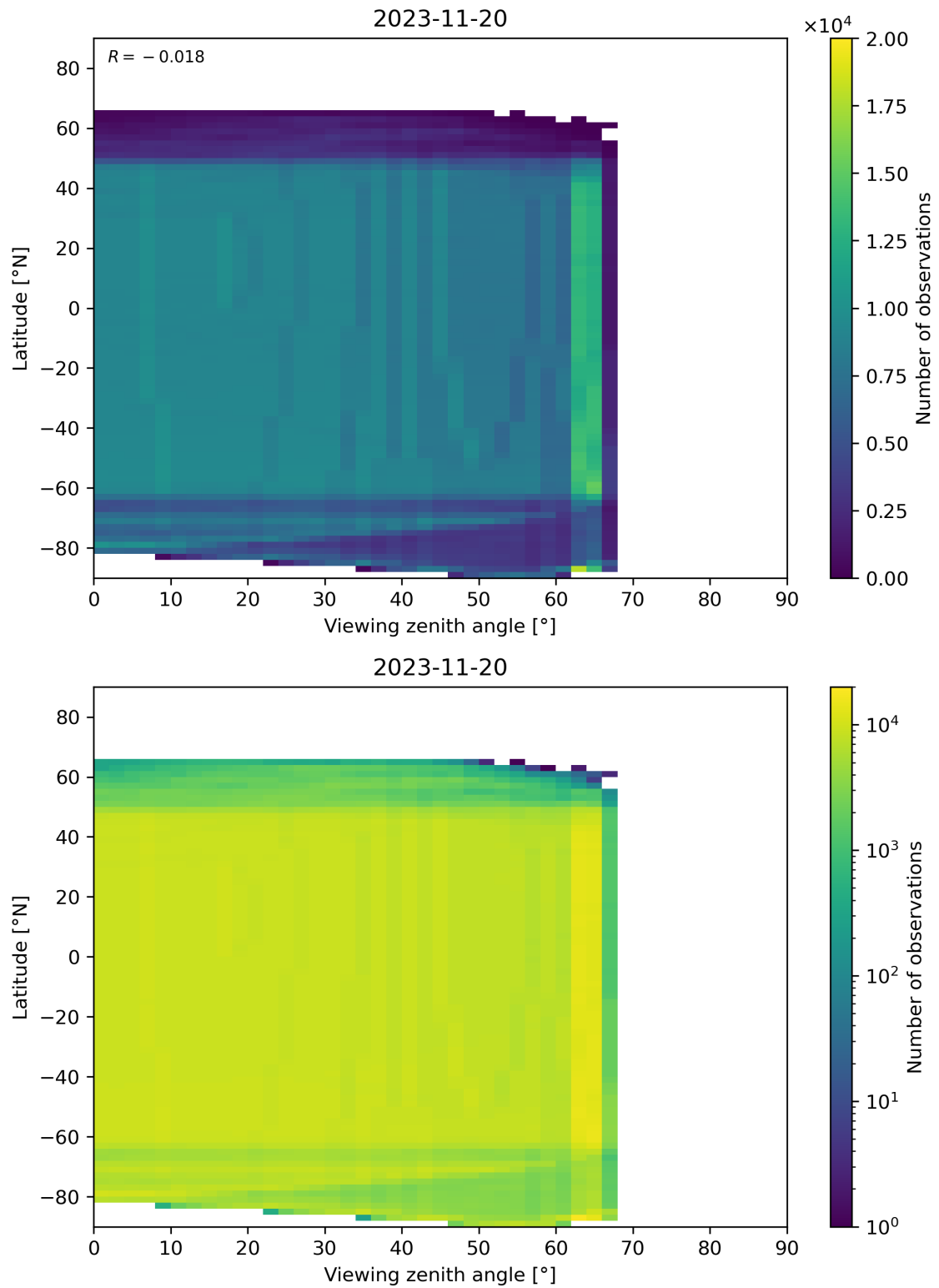
Figure 196: Scatter density plot of “Viewing zenith angle” against “Latitude” for 2023-11-19 to 2023-11-21.
