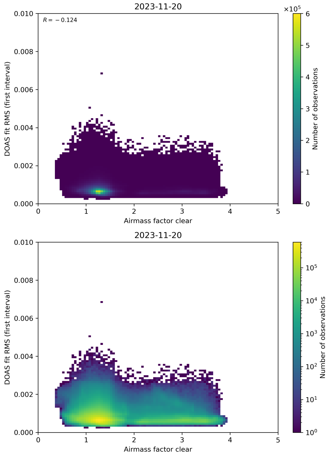
Figure 71: Scatter density plot of “Airmass factor clear” against “DOAS fit RMS (first interval)” for 2023-11-19 to 2023-11-21.
