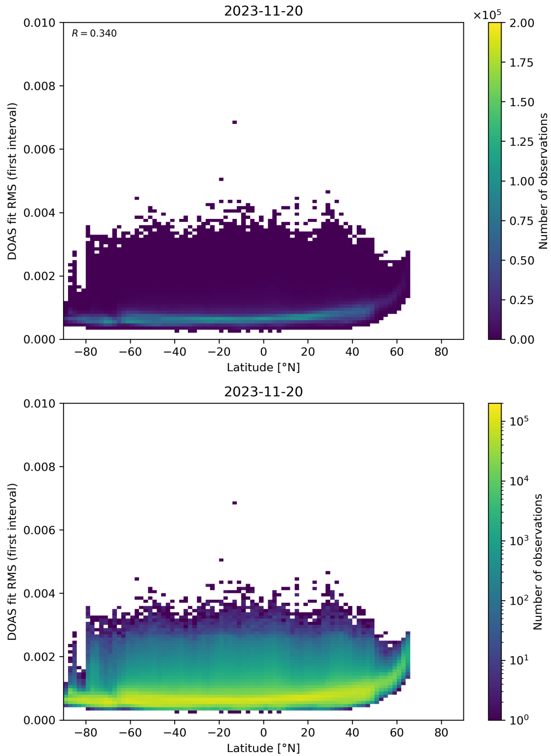
Figure 153: Scatter density plot of “Latitude” against “DOAS fit RMS (first interval)” for 2023-11-19 to 2023-11-21.
