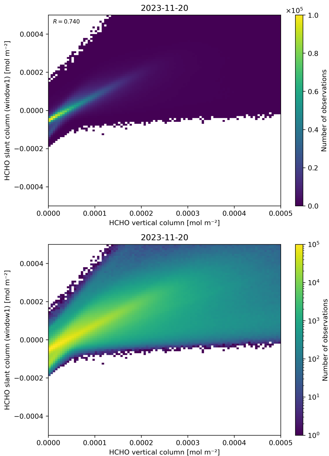
Figure 129: Scatter density plot of “HCHO vertical column” against “HCHO slant column (window1)” for 2023-11-19 to 2023-11-21.
