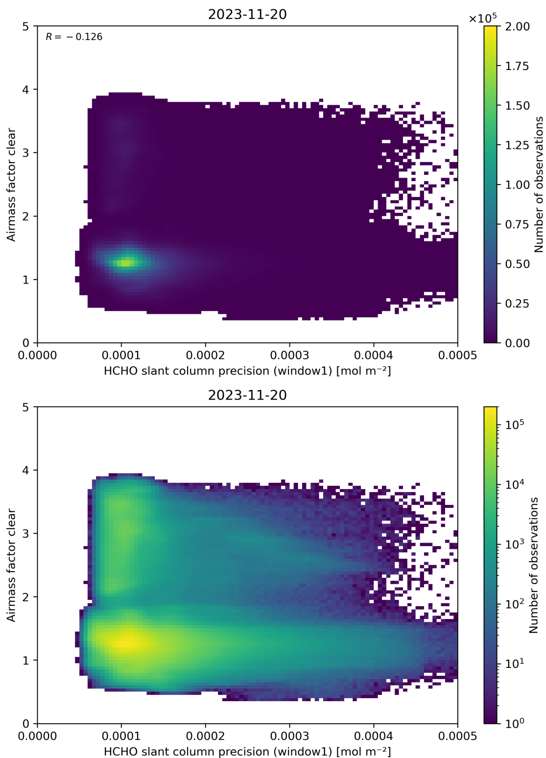
Figure 91: Scatter density plot of “HCHO slant column precision (window1)” against “Airmass factor clear” for 2023-11-19 to 2023-11-21.
