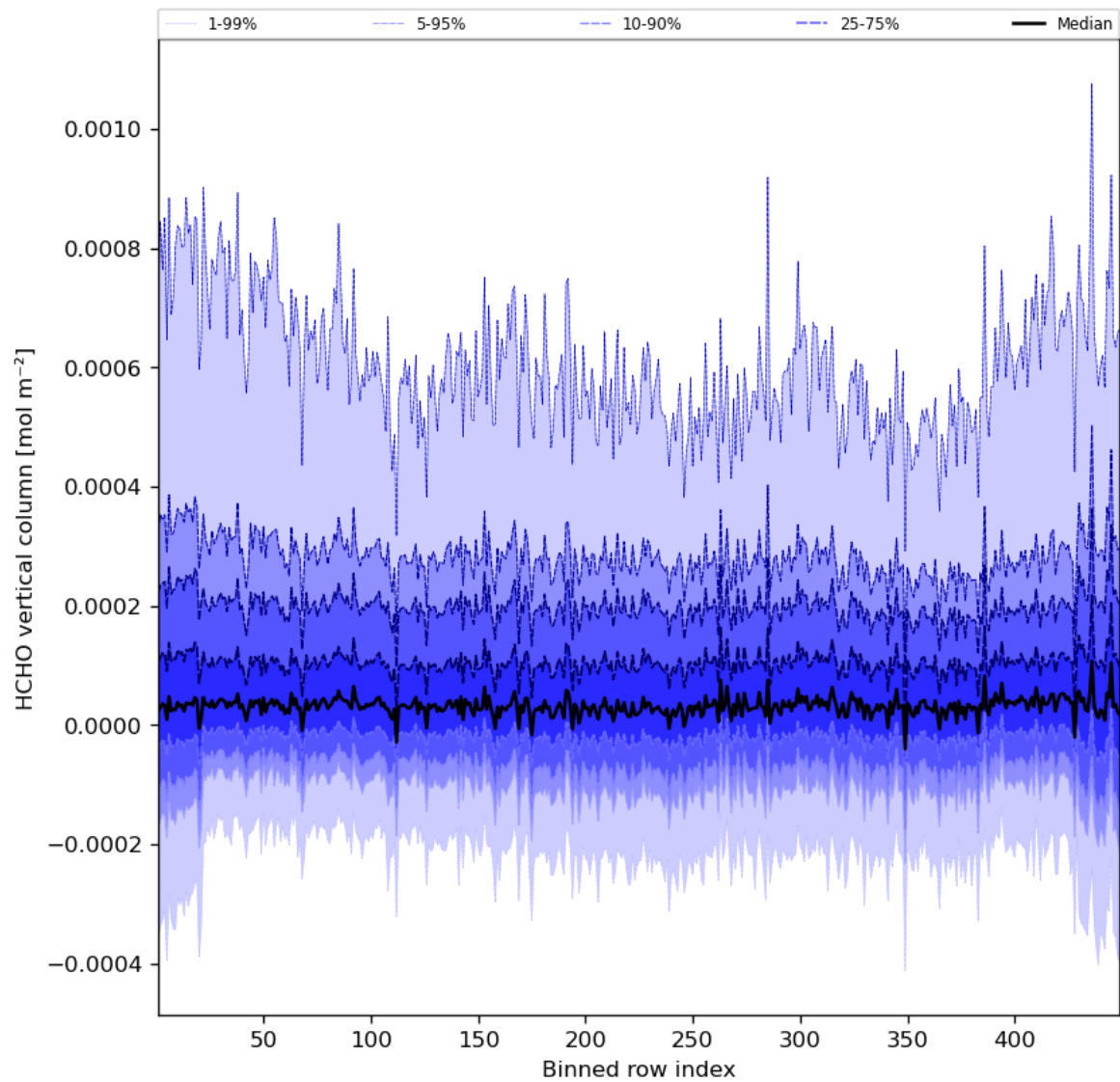
Figure 49: Along track statistics of “HCHO vertical column” for 2023-11-19 to 2023-11-21
