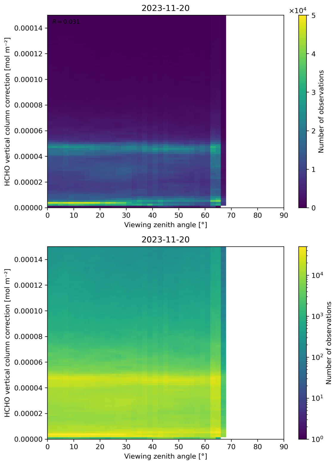
Figure 193: Scatter density plot of “Viewing zenith angle” against “HCHO vertical column correction” for 2023-11-19 to 2023-11-21.
