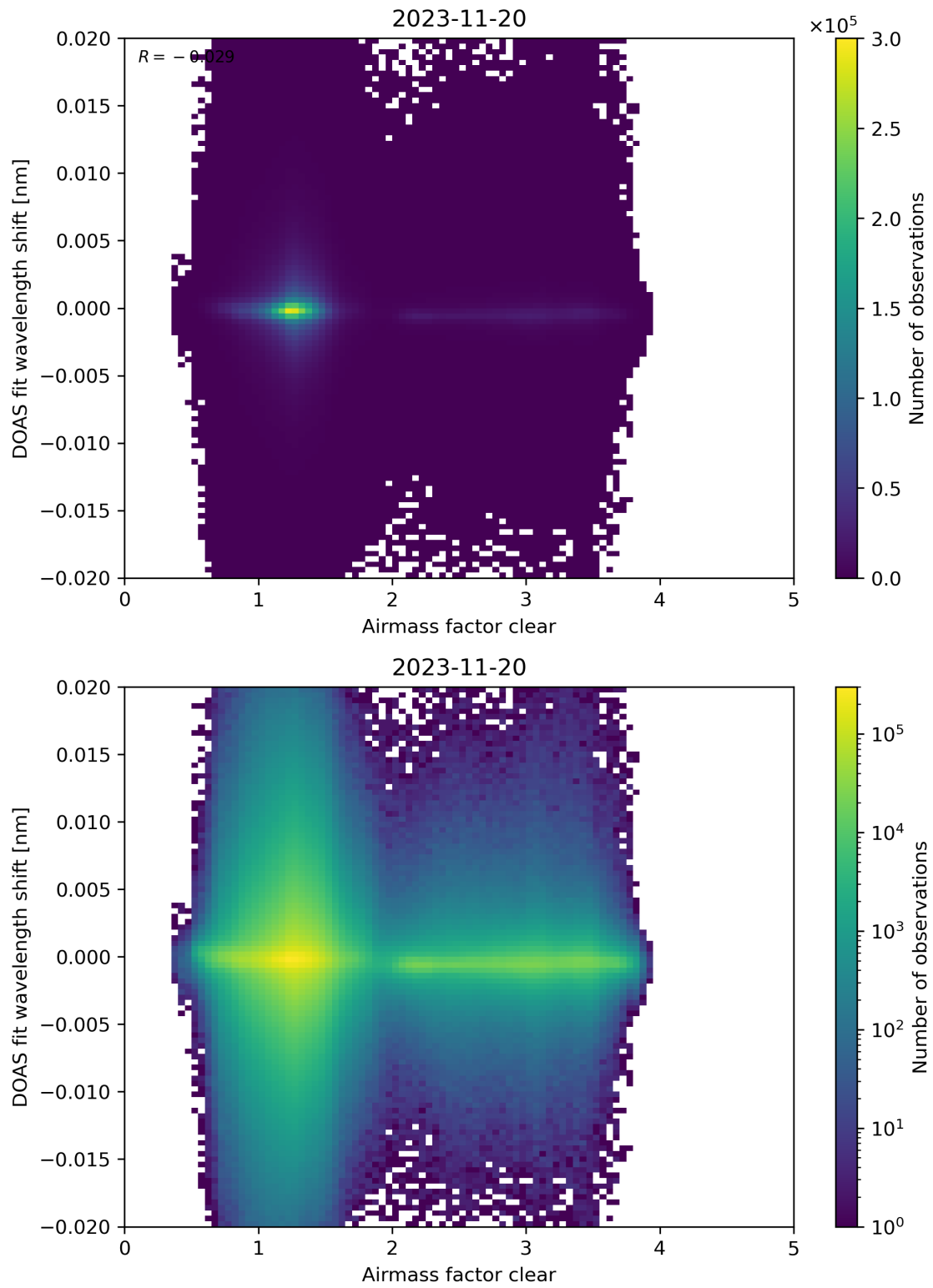
Figure 72: Scatter density plot of “Airmass factor clear” against “DOAS fit wavelength shift” for 2023-11-19 to 2023-11-21.
