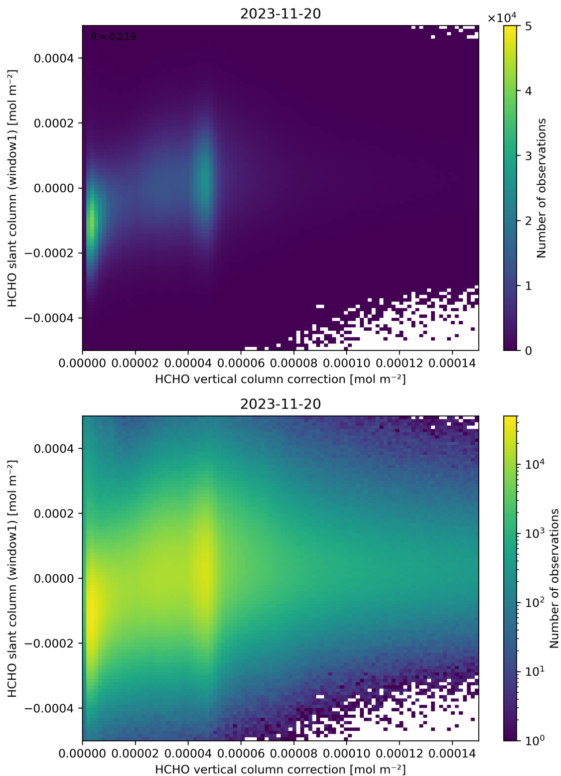
Figure 118: Scatter density plot of “HCHO vertical column correction” against “HCHO slant column (window1)” for 2023-11-19 to 2023-11-21.
