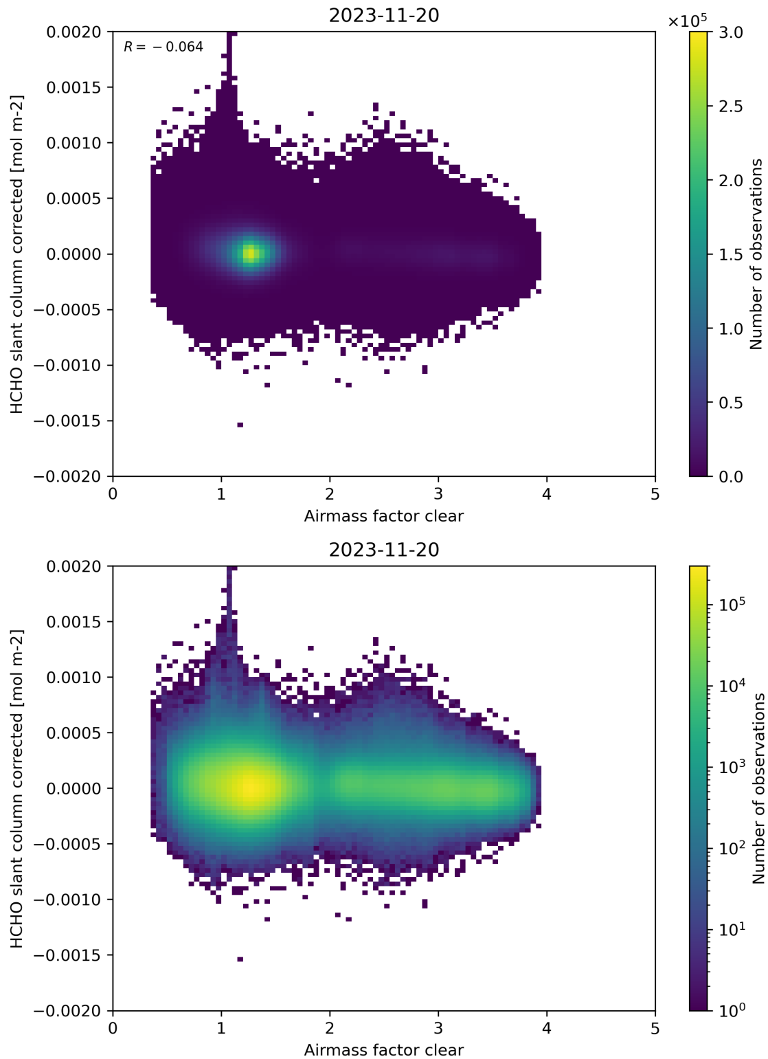
Figure 74: Scatter density plot of “Airmass factor clear” against “HCHO slant column corrected” for 2023-11-19 to 2023-11-21.
