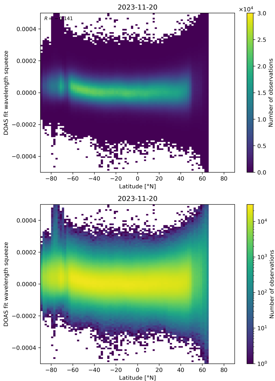
Figure 155: Scatter density plot of “Latitude” against “DOAS fit wavelength squeeze” for 2023-11-19 to 2023-11-21.
