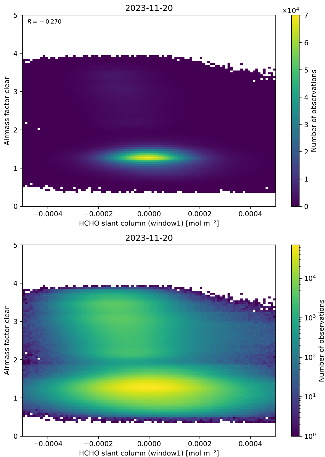
Figure 81: Scatter density plot of “HCHO slant column (window1)” against “Airmass factor clear” for 2023-11-19 to 2023-11-21.
