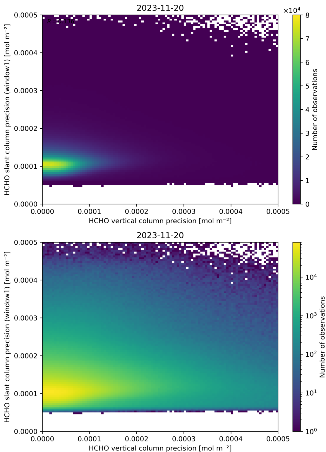
Figure 143: Scatter density plot of “HCHO vertical column precision” against “HCHO slant column precision (window1)” for 2023-11-19 to 2023-11-21.
