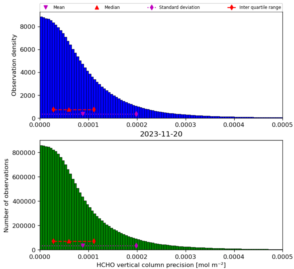
Figure 36: Histogram of “HCHO vertical column precision” for 2023-11-19 to 2023-11-21
