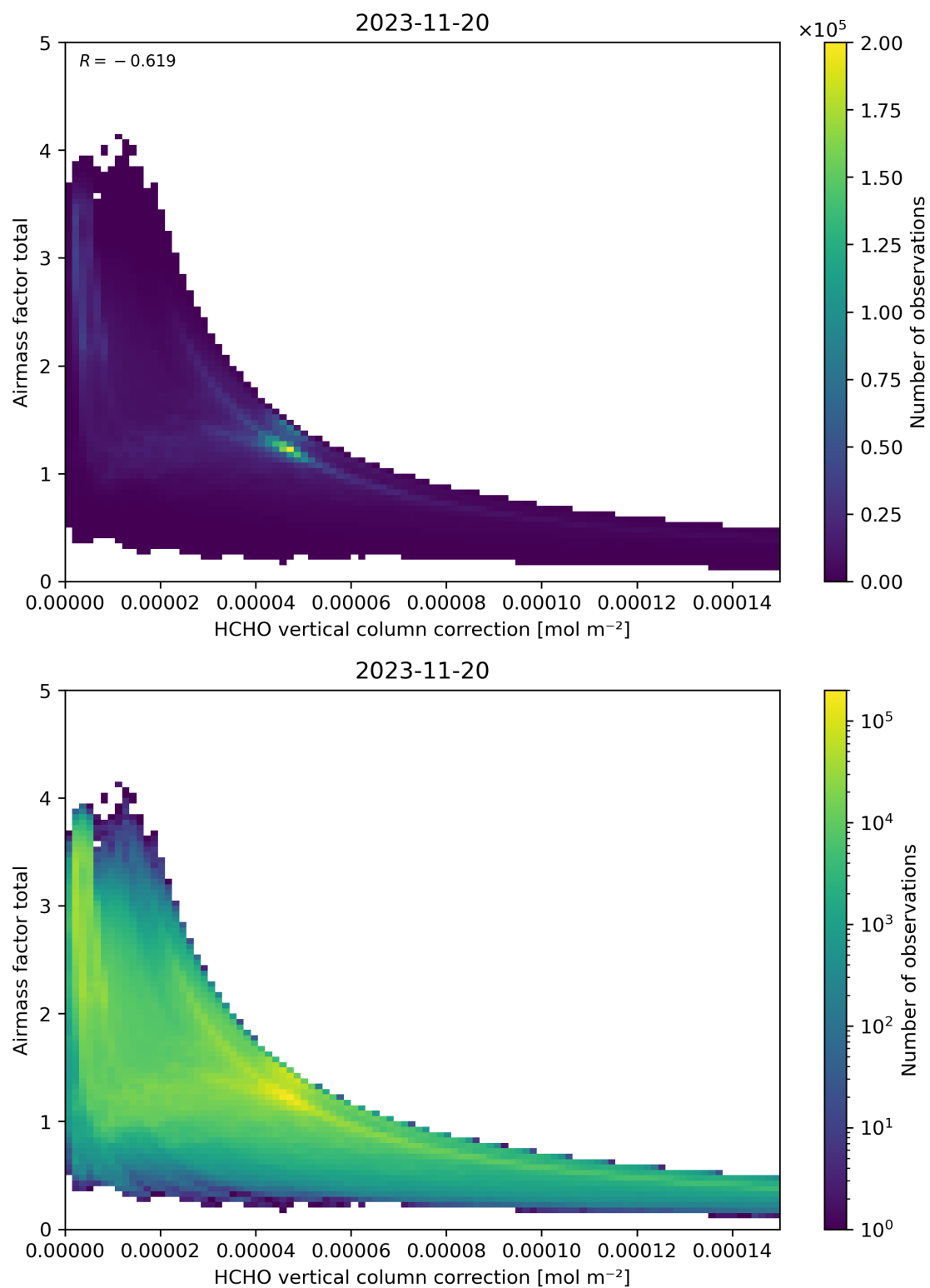
Figure 120: Scatter density plot of “HCHO vertical column correction” against “Airmass factor total” for 2023-11-19 to 2023-11-21.
