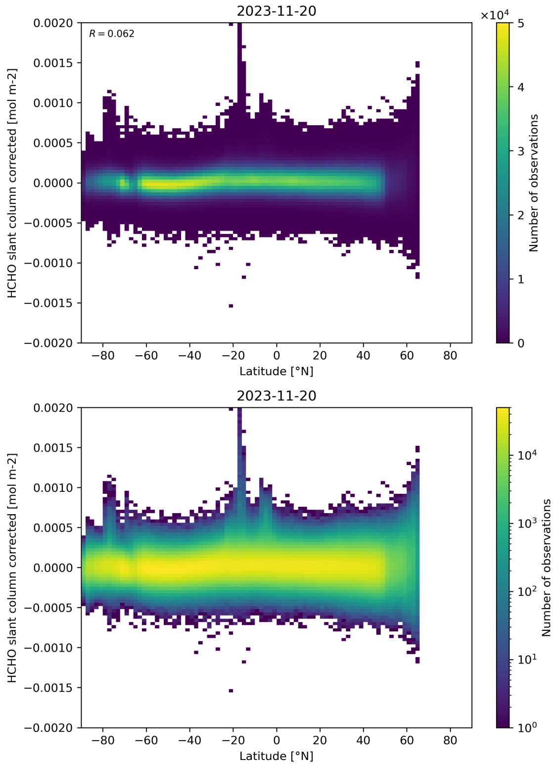
Figure 157: Scatter density plot of “Latitude” against “HCHO slant column corrected” for 2023-11-19 to 2023-11-21.
