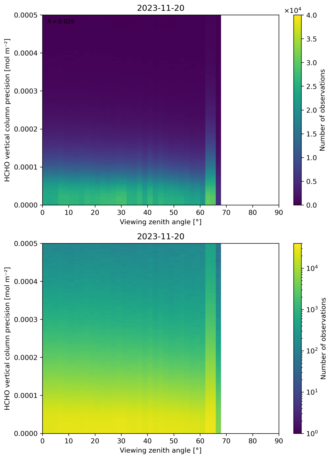
Figure 194: Scatter density plot of “Viewing zenith angle” against “HCHO vertical column precision” for 2023-11-19 to 2023-11-21.
