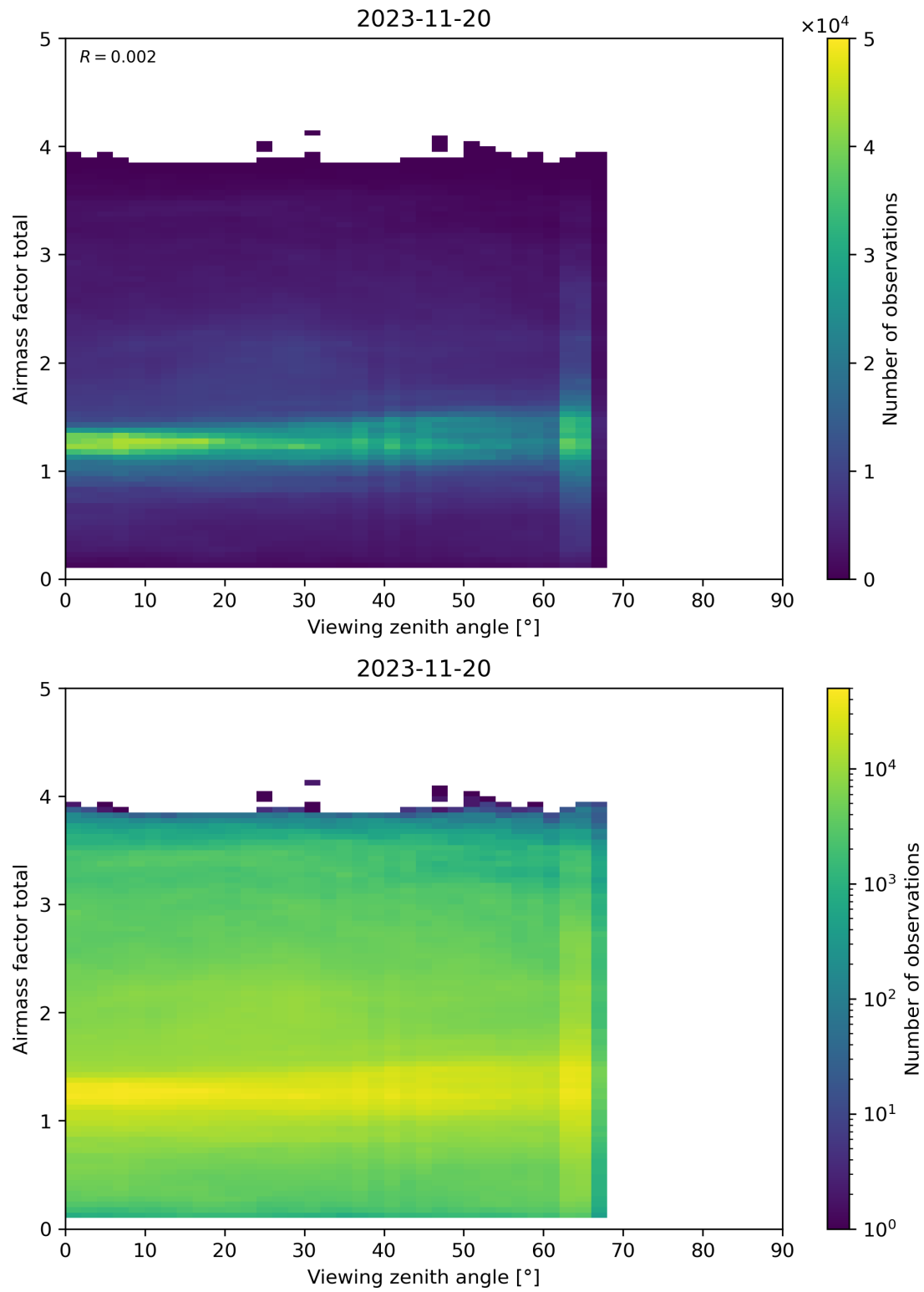
Figure 190: Scatter density plot of “Viewing zenith angle” against “Airmass factor total” for 2023-11-19 to 2023-11-21.
