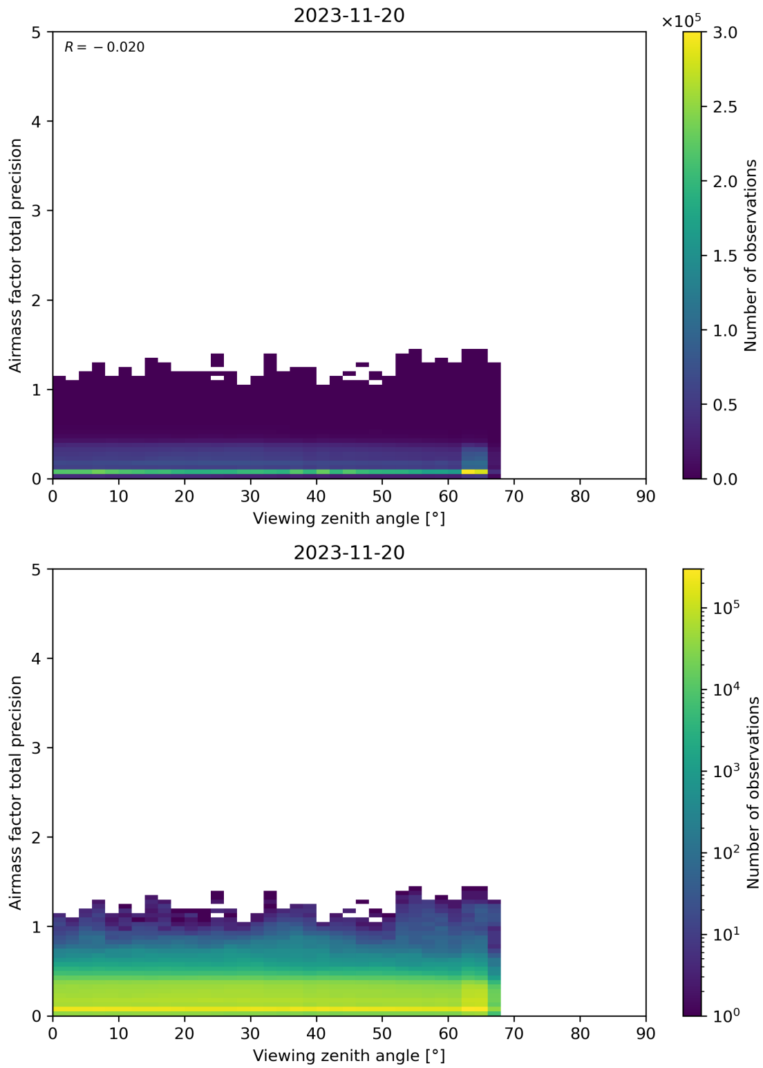
Figure 191: Scatter density plot of “Viewing zenith angle” against “Airmass factor total precision” for 2023-11-19 to 2023-11-21.
