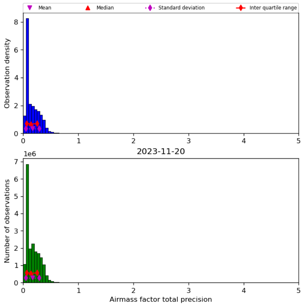
Figure 41: Histogram of “Airmass factor total precision” for 2023-11-19 to 2023-11-21
