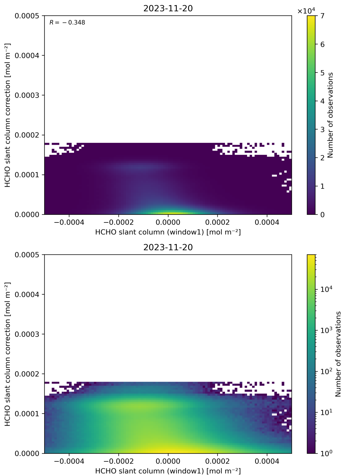
Figure 83: Scatter density plot of “HCHO slant column (window1)” against “HCHO slant column correction” for 2023-11-19 to 2023-11-21.
