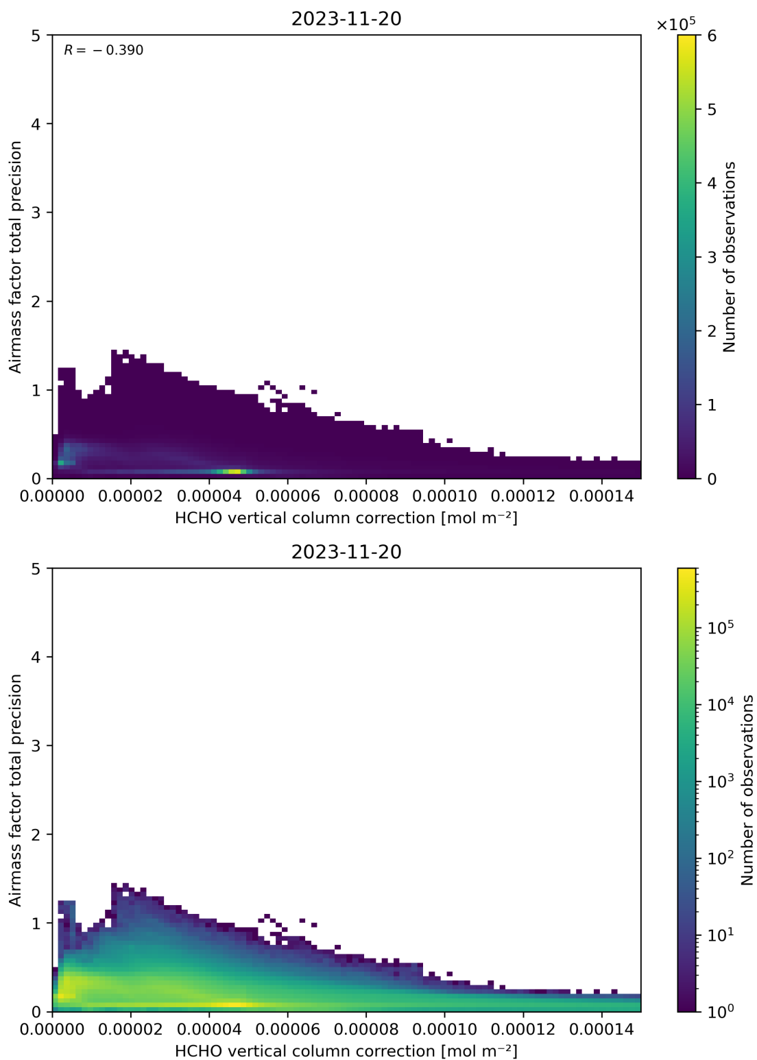
Figure 121: Scatter density plot of “HCHO vertical column correction” against “Airmass factor total precision” for 2023-11-19 to 2023-11-21.
