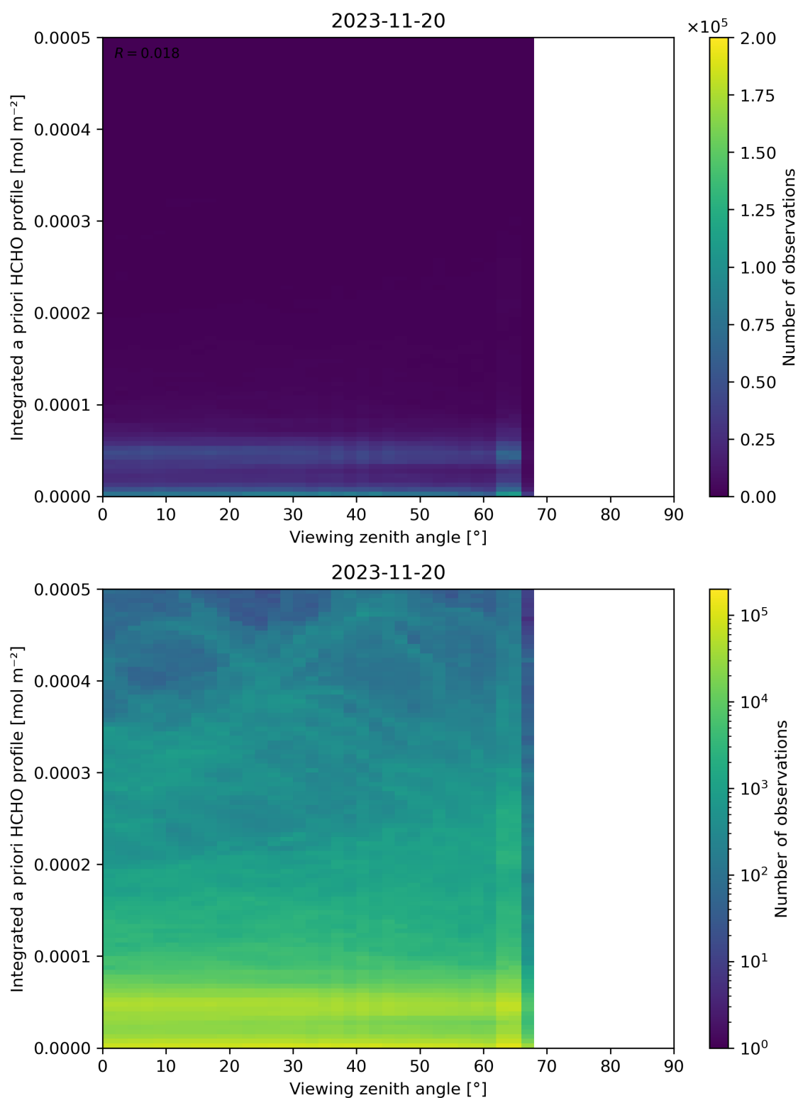
Figure 195: Scatter density plot of “Viewing zenith angle” against “Integrated a priori HCHO profile” for 2023-11-19 to 2023-11-21.
