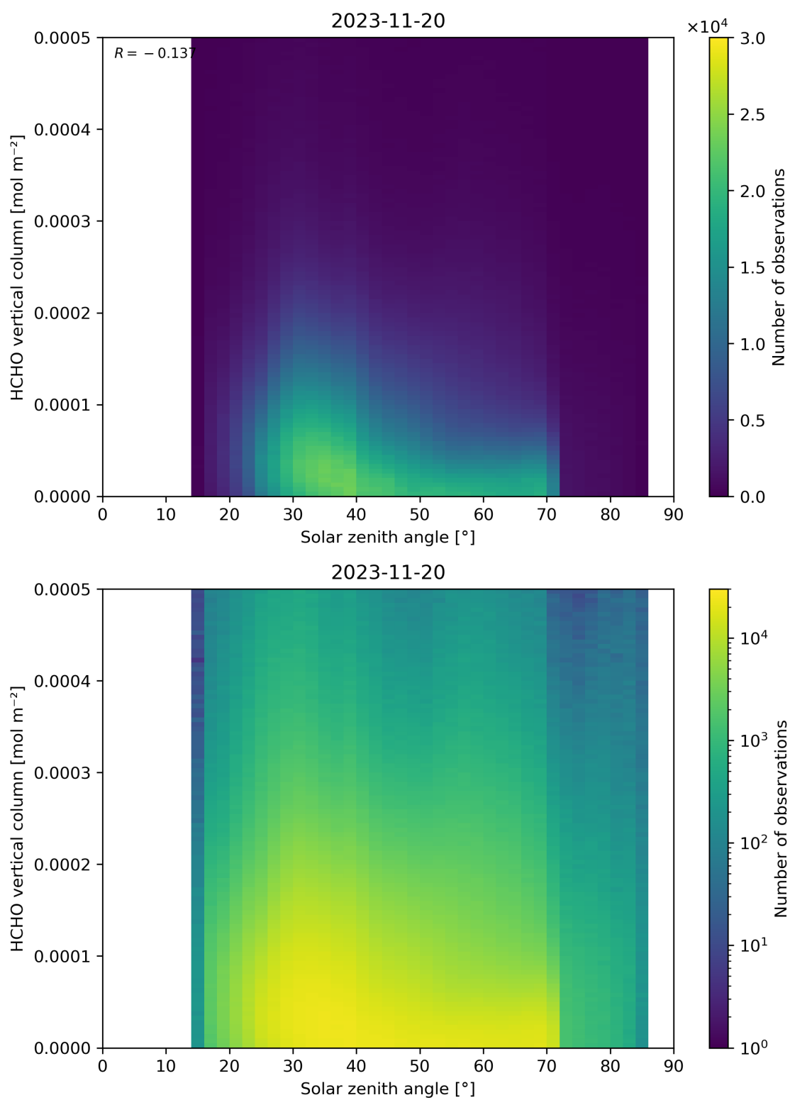
Figure 177: Scatter density plot of “Solar zenith angle” against “HCHO vertical column” for 2023-11-19 to 2023-11-21.
