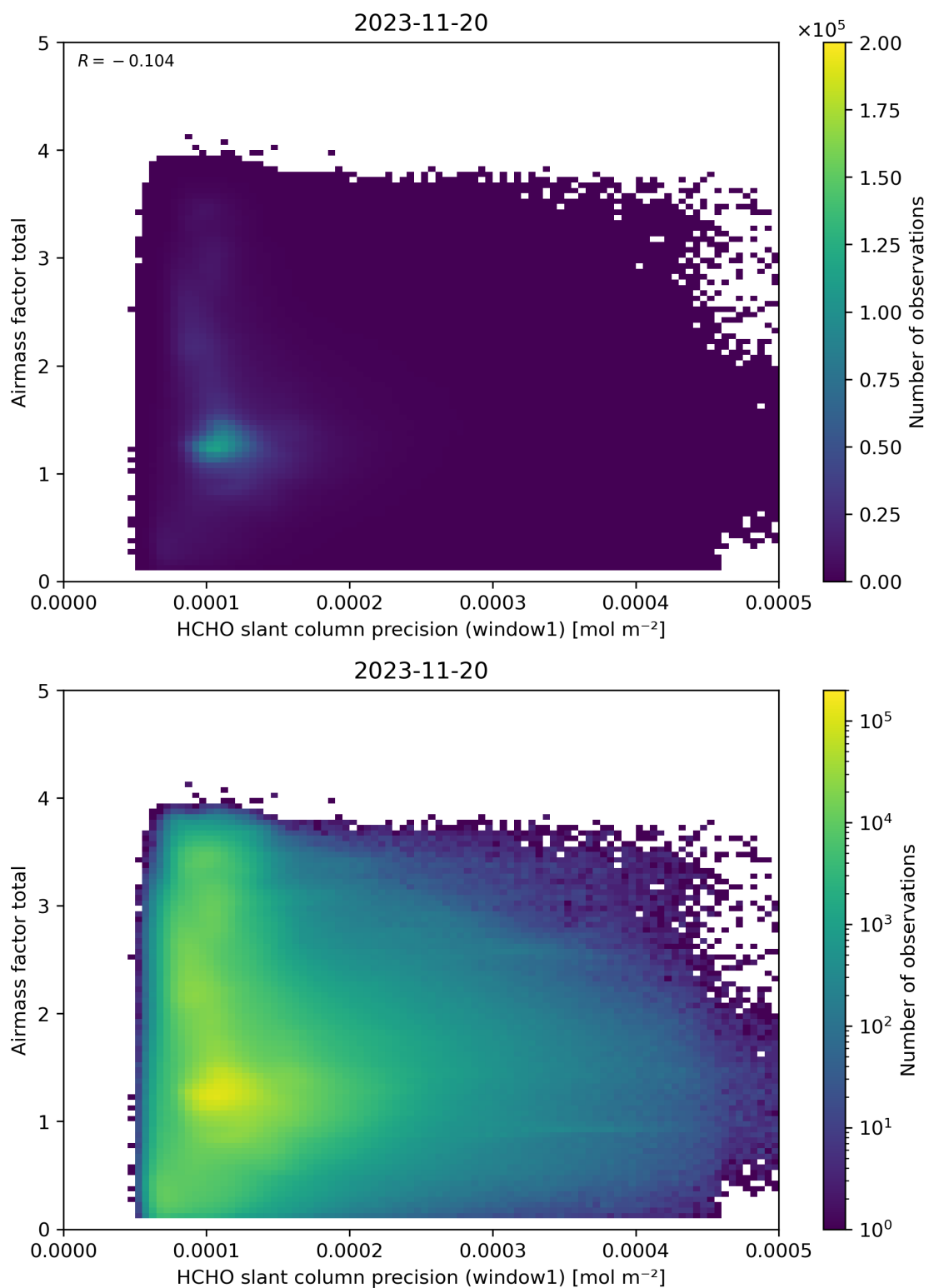
Figure 94: Scatter density plot of “HCHO slant column precision (window1)” against “Airmass factor total” for 2023-11-19 to 2023-11-21.
