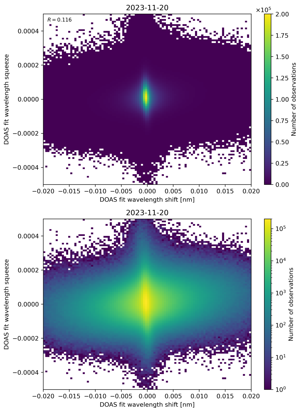
Figure 65: Scatter density plot of “DOAS fit wavelength shift” against “DOAS fit wavelength squeeze” for 2023-11-19 to 2023-11-21.
