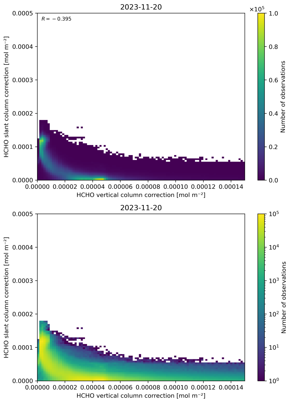
Figure 117: Scatter density plot of “HCHO vertical column correction” against “HCHO slant column correction” for 2023-11-19 to 2023-11-21.
