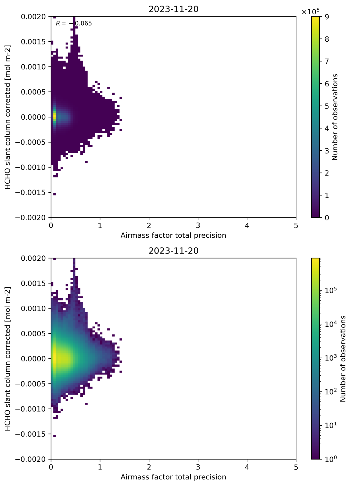
Figure 109: Scatter density plot of “Airmass factor total precision” against “HCHO slant column corrected” for 2023-11-19 to 2023-11-21.
