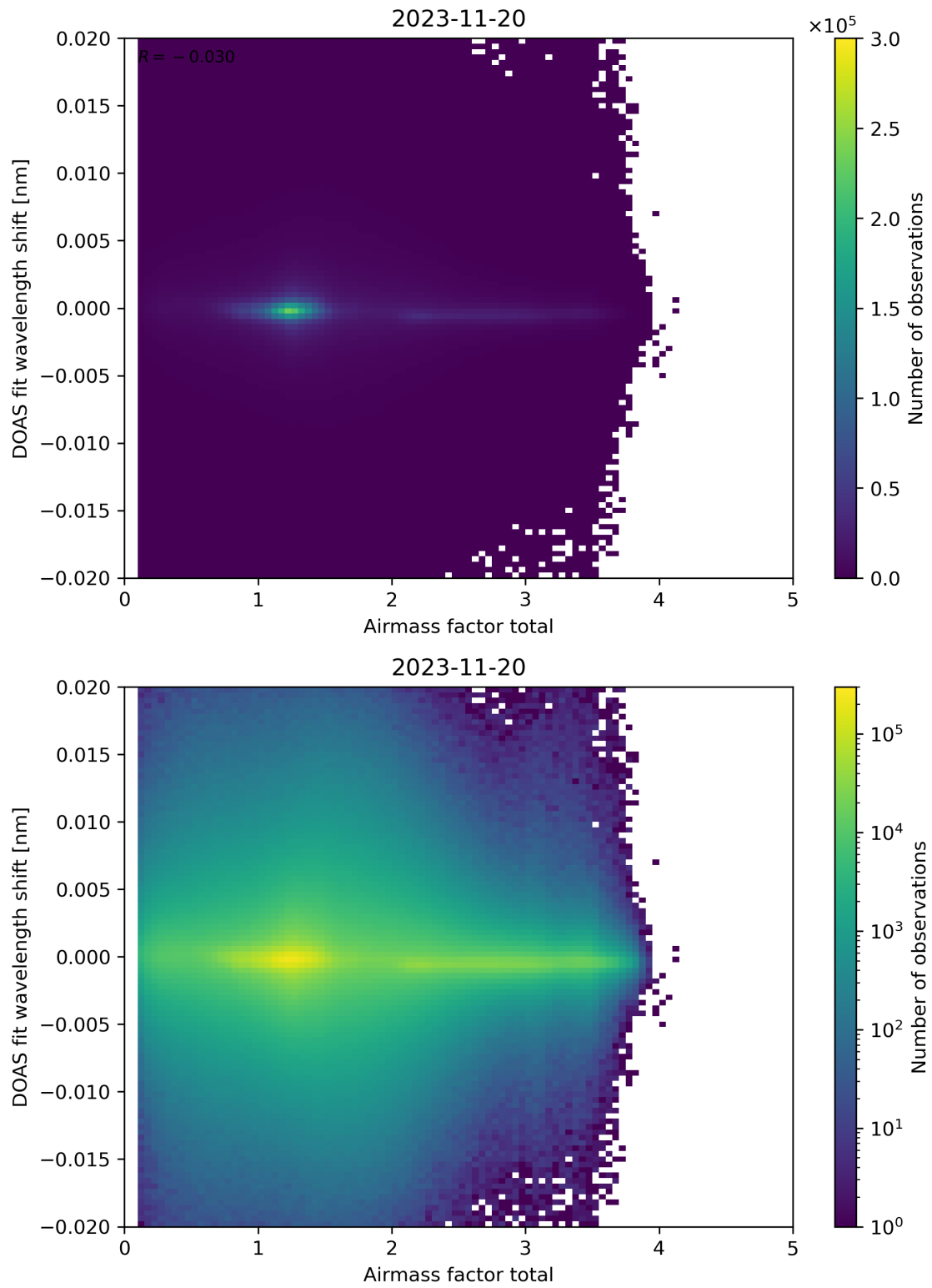
Figure 98: Scatter density plot of “Airmass factor total” against “DOAS fit wavelength shift” for 2023-11-19 to 2023-11-21.
