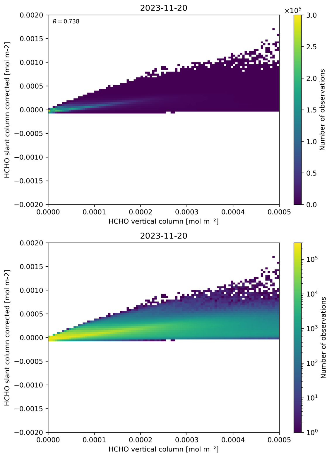
Figure 127: Scatter density plot of “HCHO vertical column” against “HCHO slant column corrected” for 2023-11-19 to 2023-11-21.
