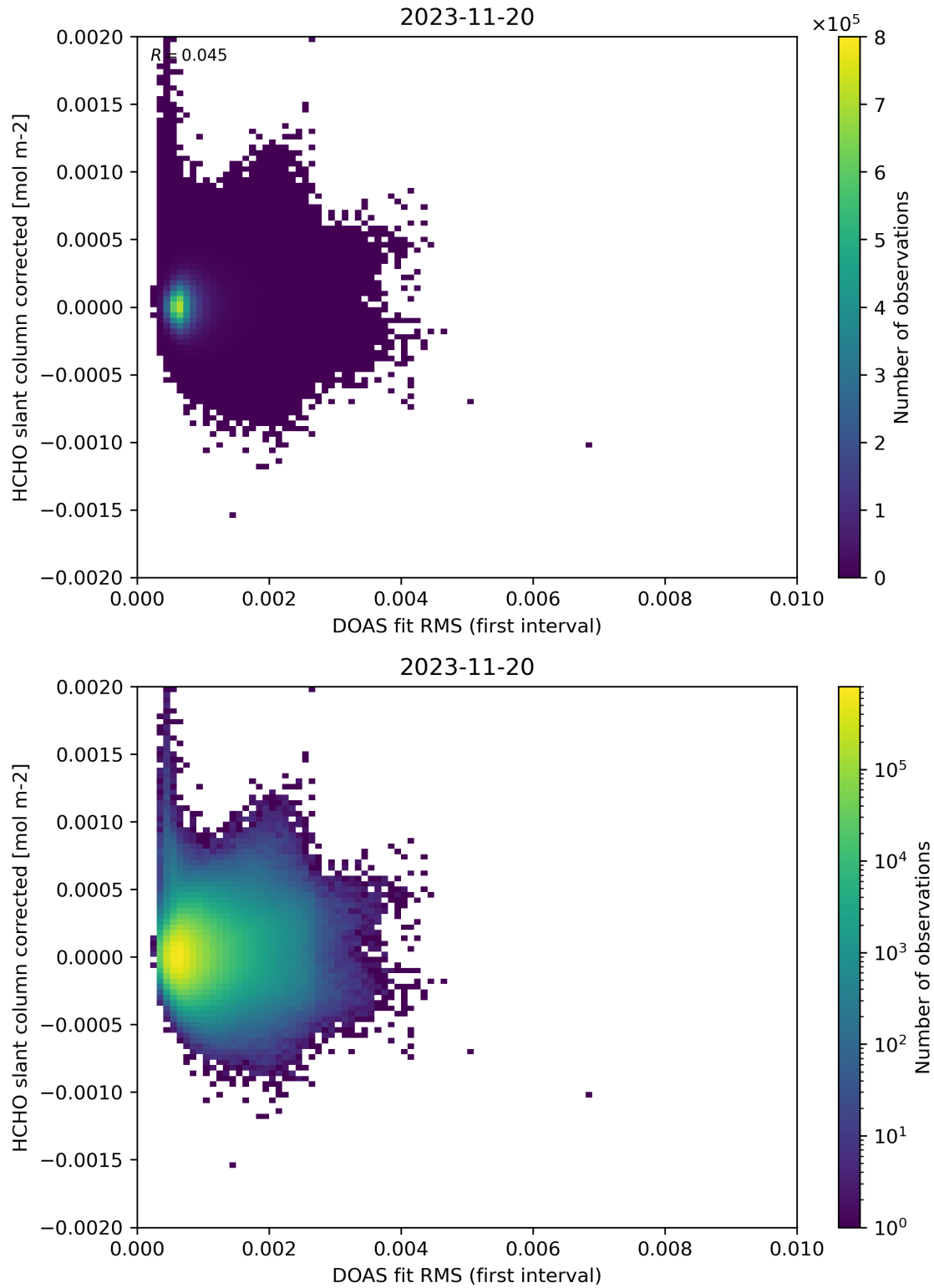
Figure 62: Scatter density plot of “DOAS fit RMS (first interval)” against “HCHO slant column corrected” for 2023-11-19 to 2023-11-21.
