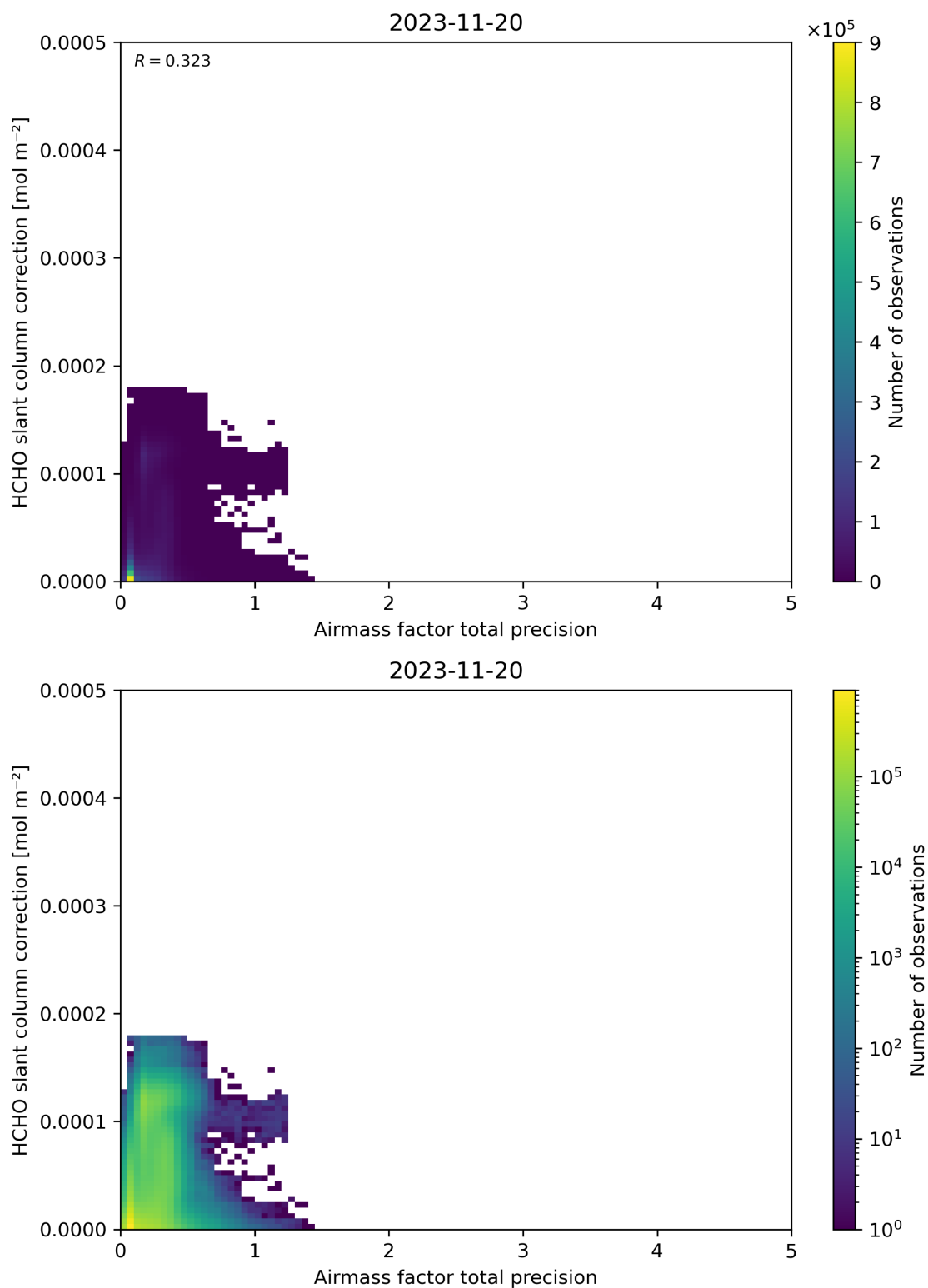
Figure 110: Scatter density plot of “Airmass factor total precision” against “HCHO slant column correction” for 2023-11-19 to 2023-11-21.
