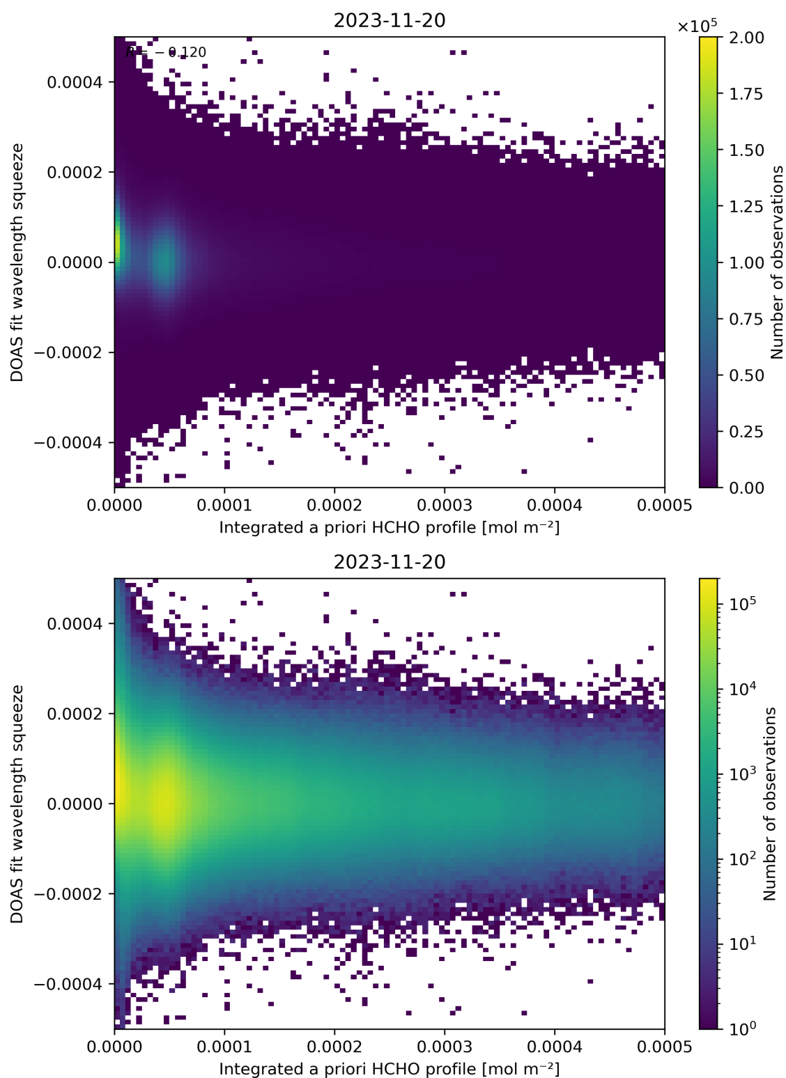
Figure 150: Scatter density plot of “Integrated a priori HCHO profile” against “DOAS fit wavelength squeeze” for 2023-11-19 to 2023-11-21.
