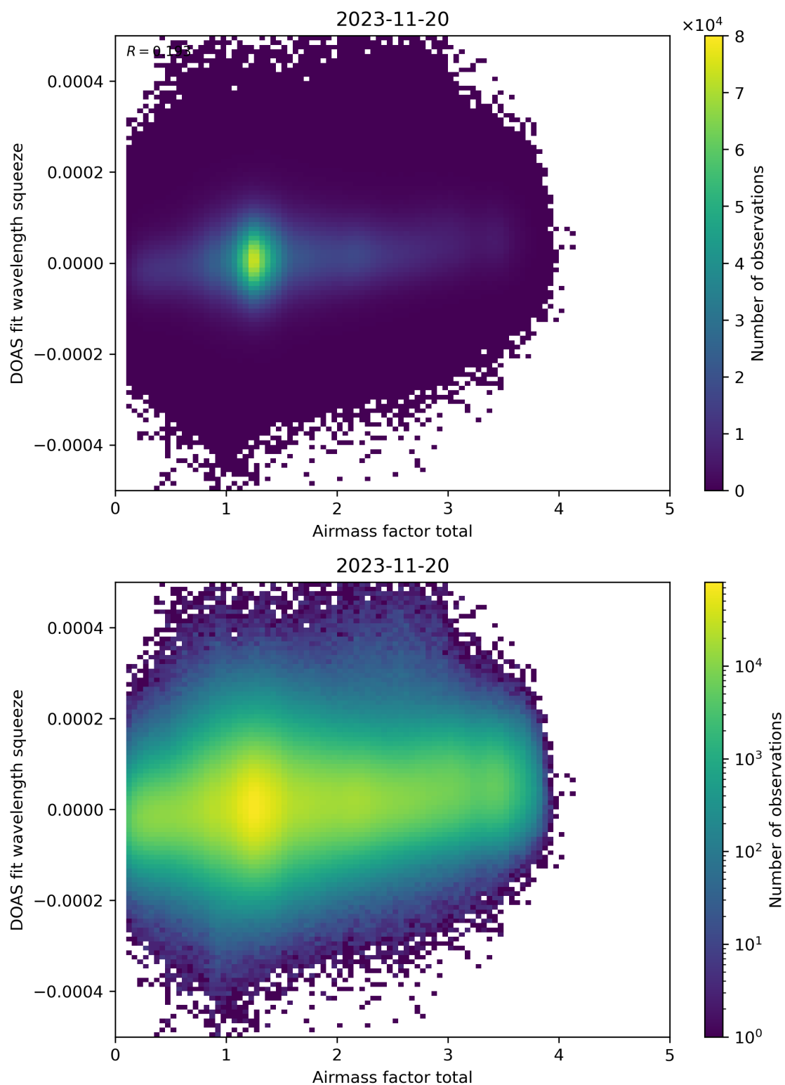
Figure 99: Scatter density plot of “Airmass factor total” against “DOAS fit wavelength squeeze” for 2023-11-19 to 2023-11-21.
