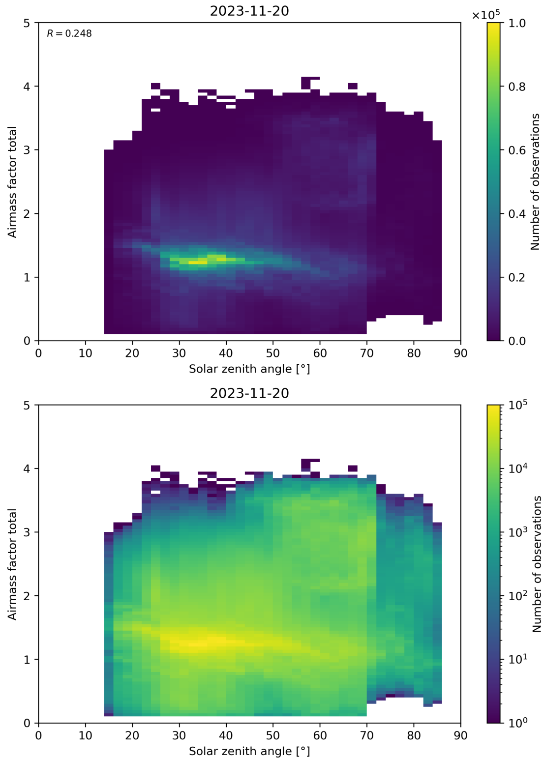
Figure 175: Scatter density plot of “Solar zenith angle” against “Airmass factor total” for 2023-11-19 to 2023-11-21.
