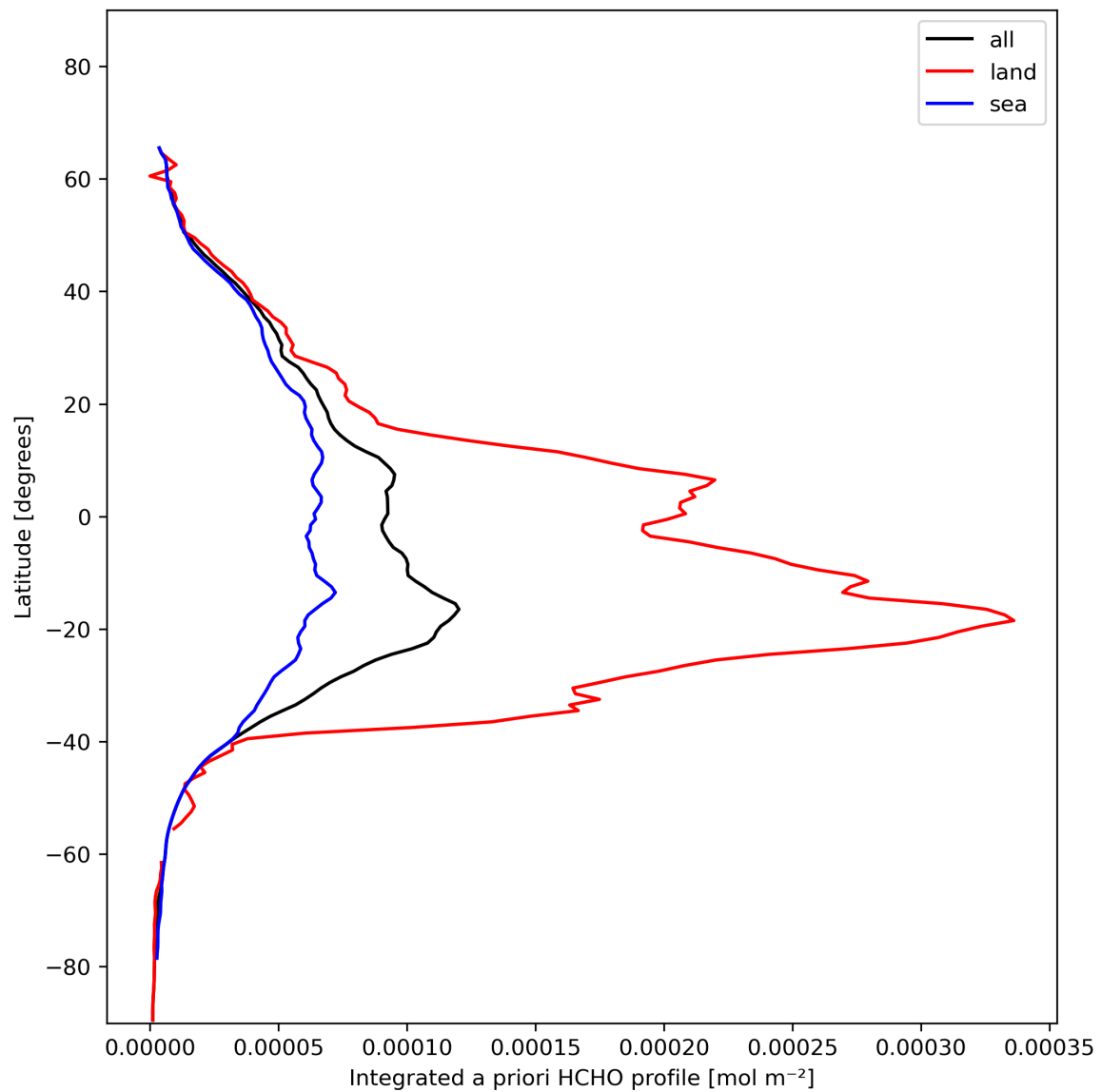
Figure 29: Zonal average of “Integrated a priori HCHO profile” for 2023-11-19 to 2023-11-21.
