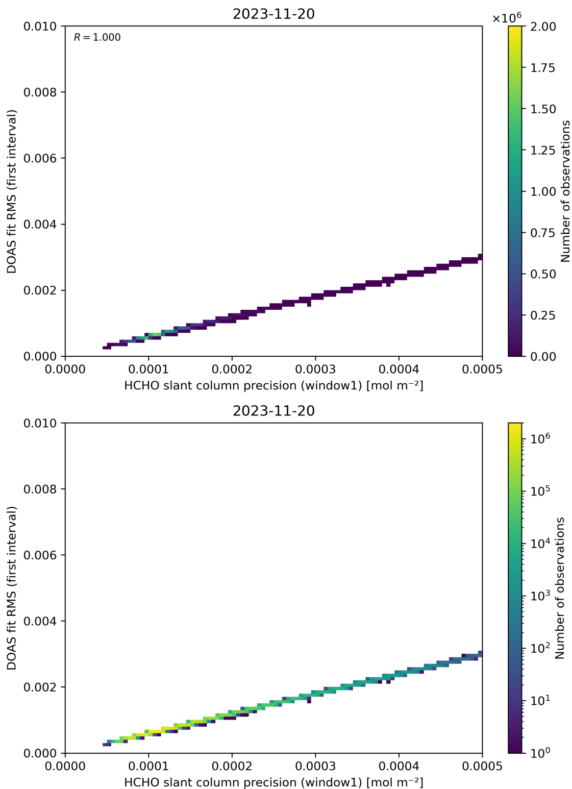
Figure 88: Scatter density plot of “HCHO slant column precision (window1)” against “DOAS fit RMS (first interval)” for 2023-11-19 to 2023-11-21.
