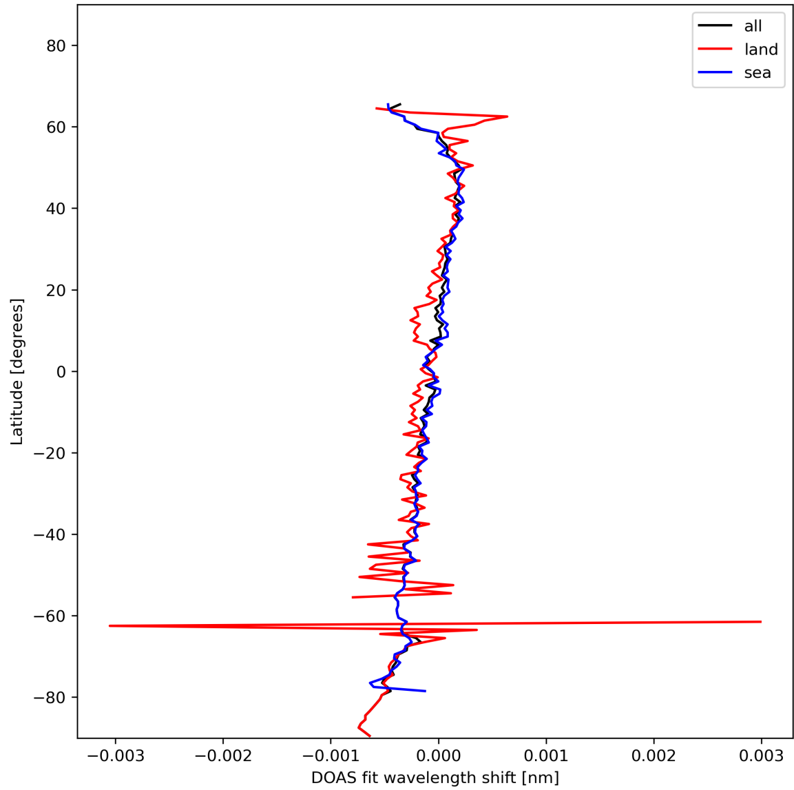
Figure 30: Zonal average of “DOAS fit wavelength shift” for 2023-11-19 to 2023-11-21.
