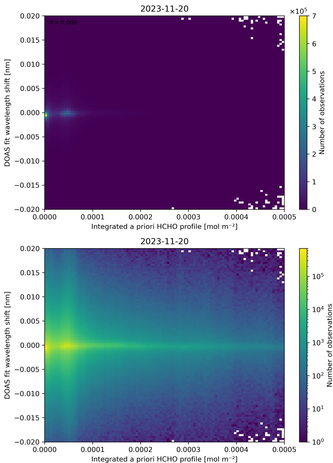
Figure 149: Scatter density plot of “Integrated a priori HCHO profile” against “DOAS fit wavelength shift” for 2023-11-19 to 2023-11-21.
