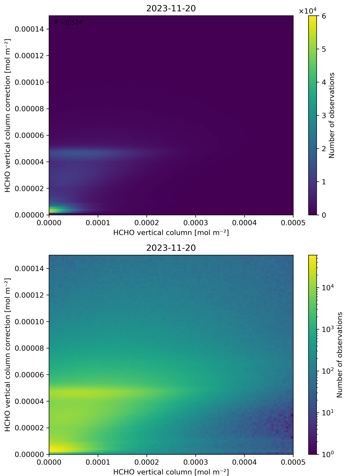
Figure 133: Scatter density plot of “HCHO vertical column” against “HCHO vertical column correction” for 2023-11-19 to 2023-11-21.
