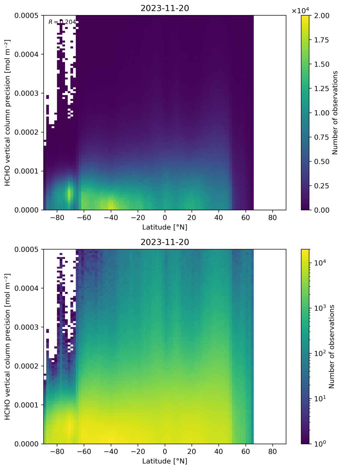
Figure 165: Scatter density plot of “Latitude” against “HCHO vertical column precision” for 2023-11-19 to 2023-11-21.
