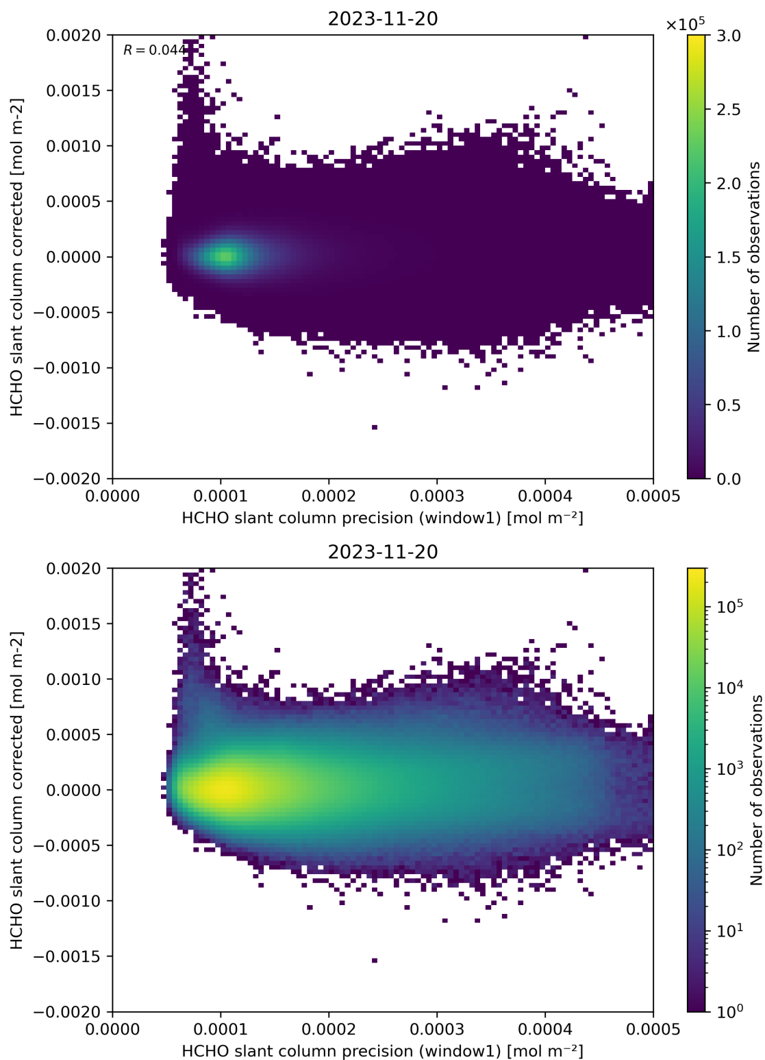
Figure 92: Scatter density plot of “HCHO slant column precision (window1)” against “HCHO slant column corrected” for 2023-11-19 to 2023-11-21.
