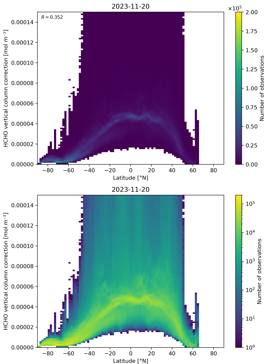
Figure 164: Scatter density plot of “Latitude” against “HCHO vertical column correction” for 2023-11-19 to 2023-11-21.
