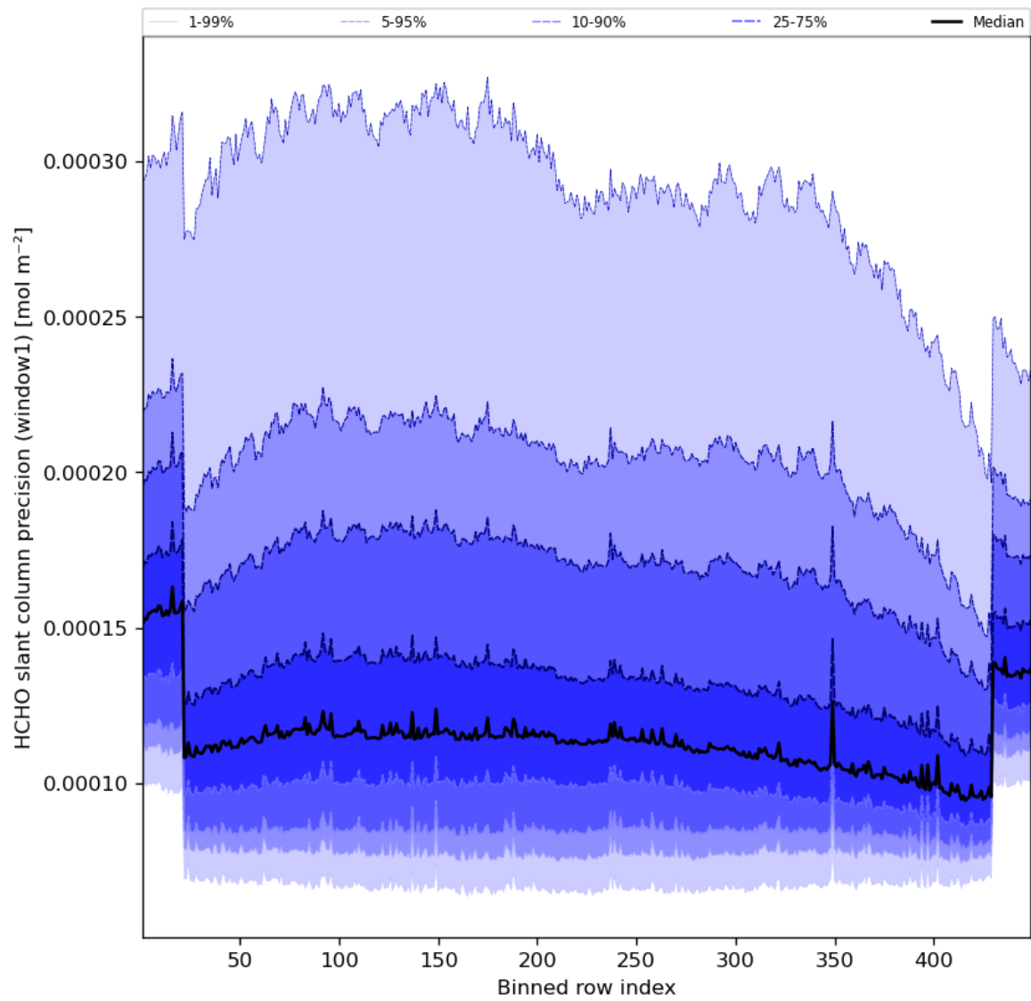
Figure 53: Along track statistics of “HCHO slant column precision (window1)” for 2023-11-19 to 2023-11-21
