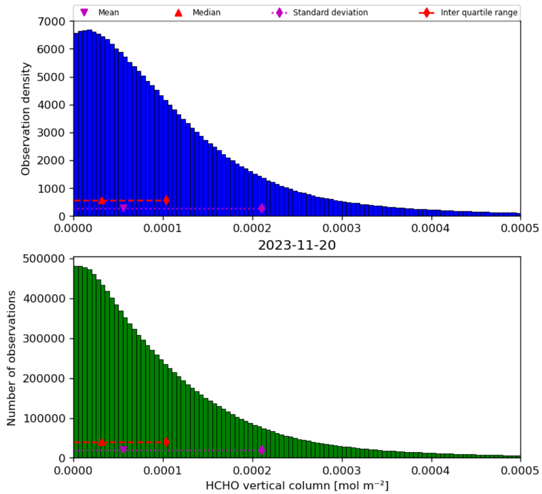
Figure 35: Histogram of “HCHO vertical column” for 2023-11-19 to 2023-11-21
