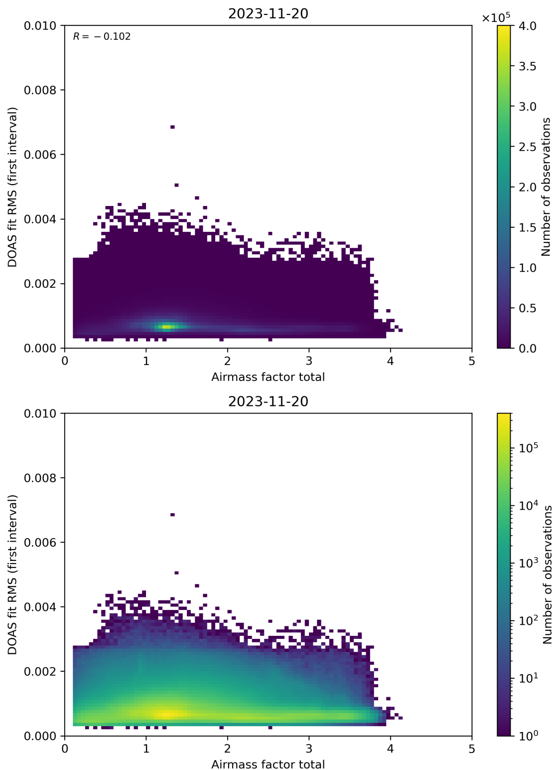
Figure 97: Scatter density plot of “Airmass factor total” against “DOAS fit RMS (first interval)” for 2023-11-19 to 2023-11-21.
