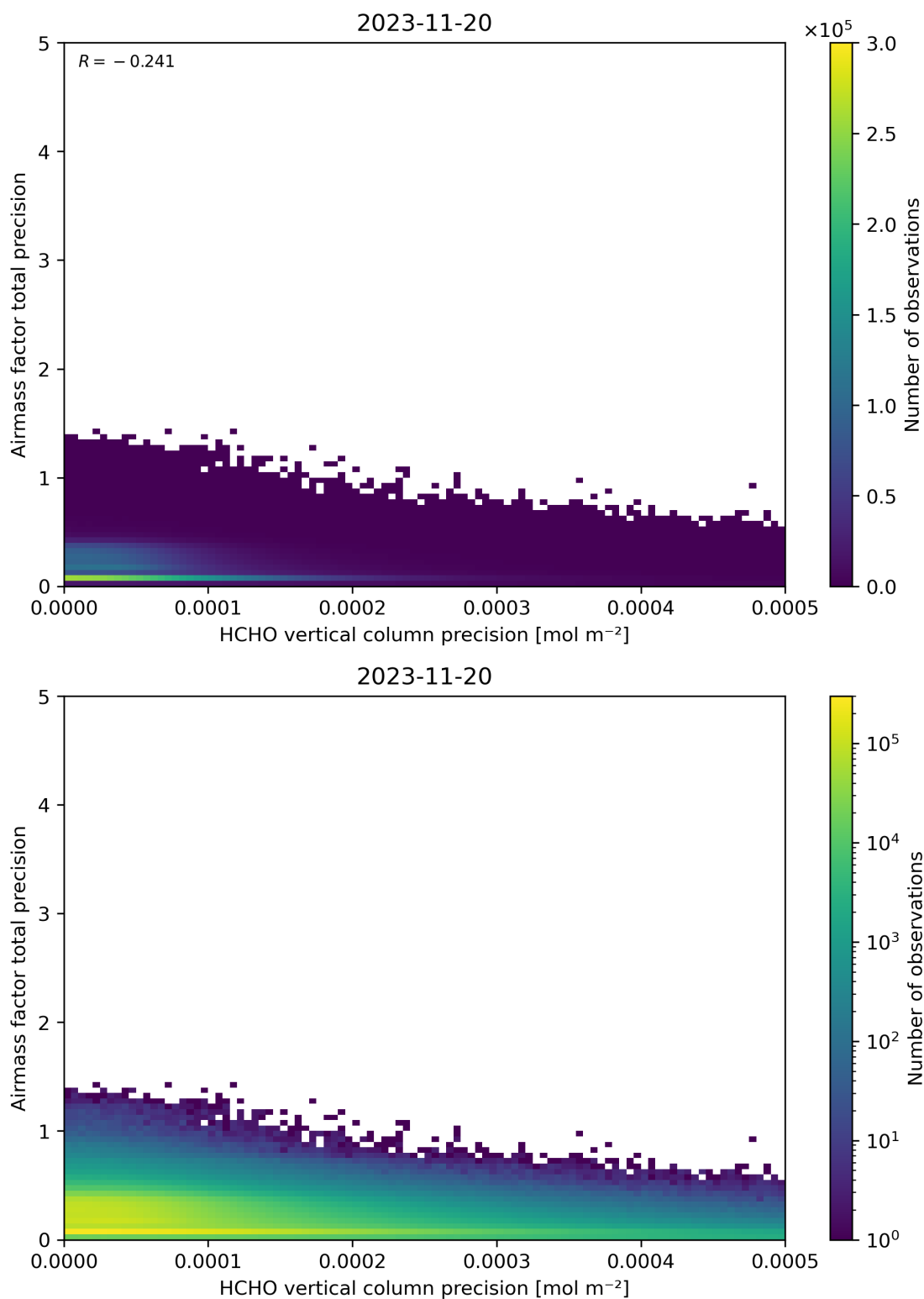
Figure 145: Scatter density plot of “HCHO vertical column precision” against “Airmass factor total precision” for 2023-11-19 to 2023-11-21.
