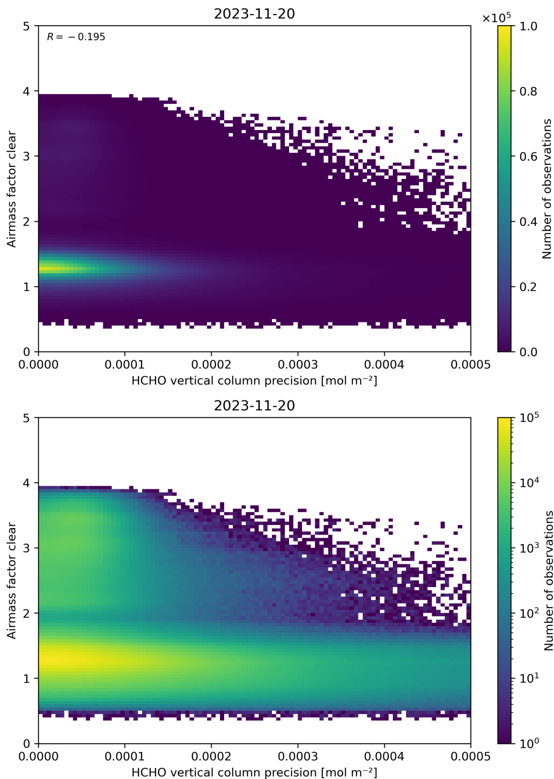
Figure 139: Scatter density plot of “HCHO vertical column precision” against “Airmass factor clear” for 2023-11-19 to 2023-11-21.
