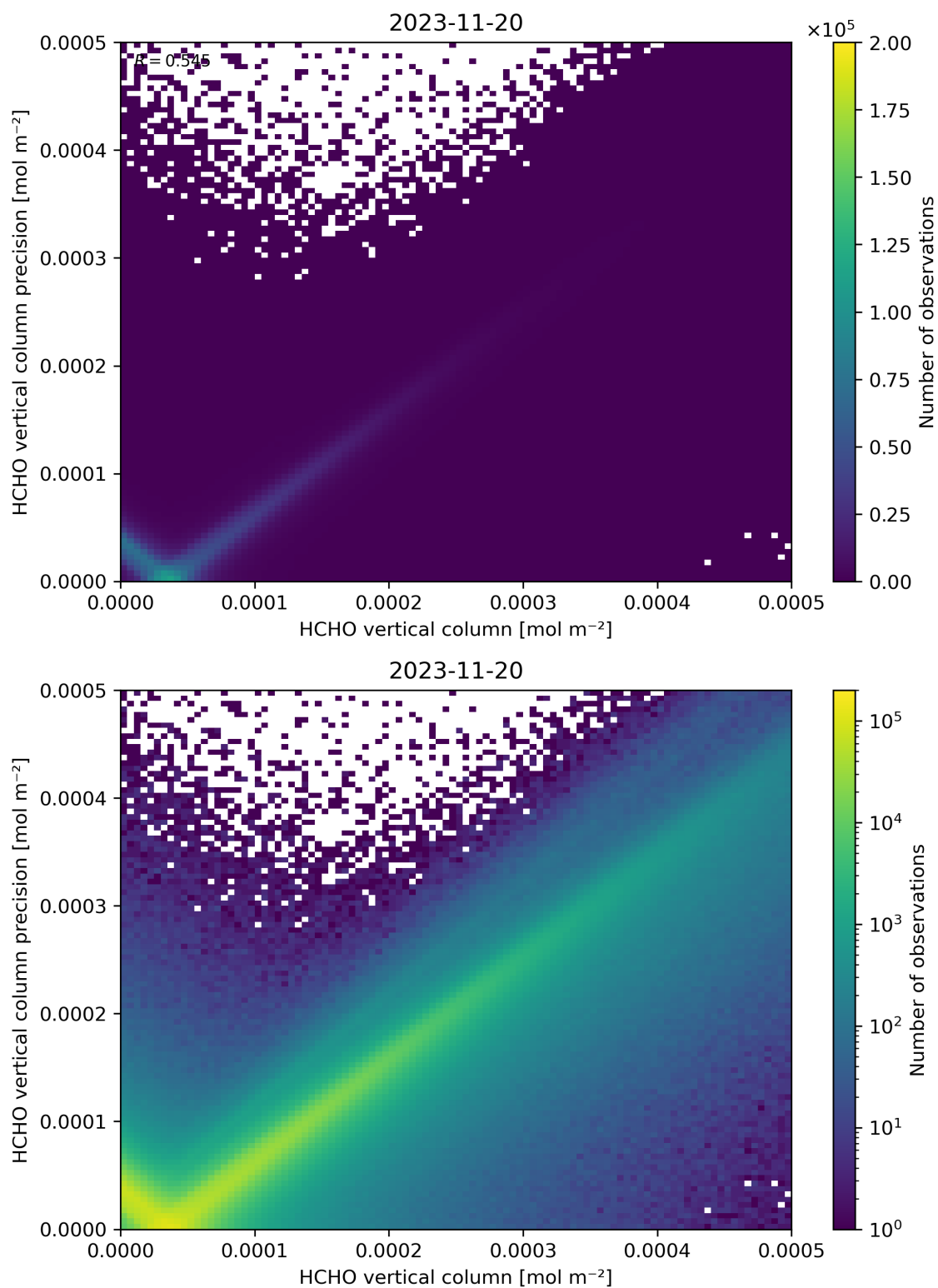
Figure 134: Scatter density plot of “HCHO vertical column” against “HCHO vertical column precision” for 2023-11-19 to 2023-11-21.
