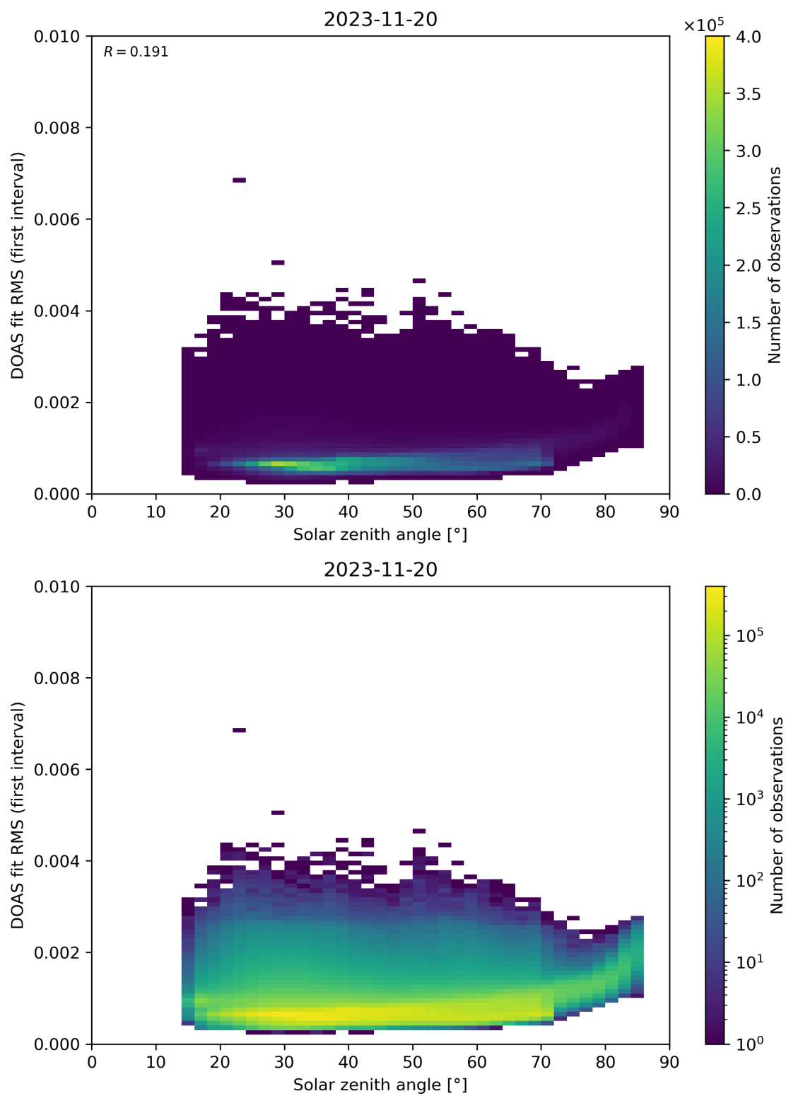
Figure 167: Scatter density plot of “Solar zenith angle” against “DOAS fit RMS (first interval)” for 2023-11-19 to 2023-11-21.
