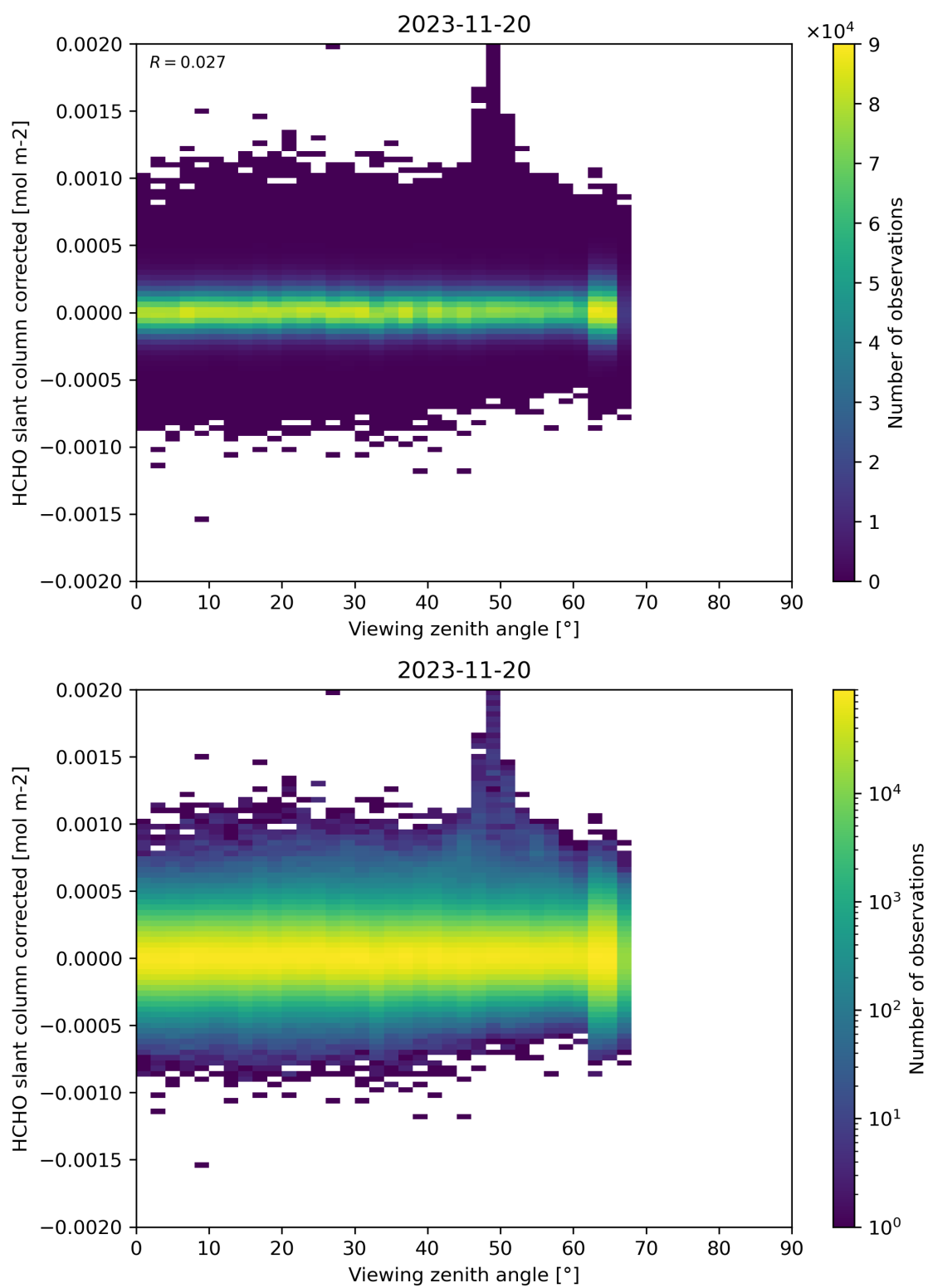
Figure 186: Scatter density plot of “Viewing zenith angle” against “HCHO slant column corrected” for 2023-11-19 to 2023-11-21.
