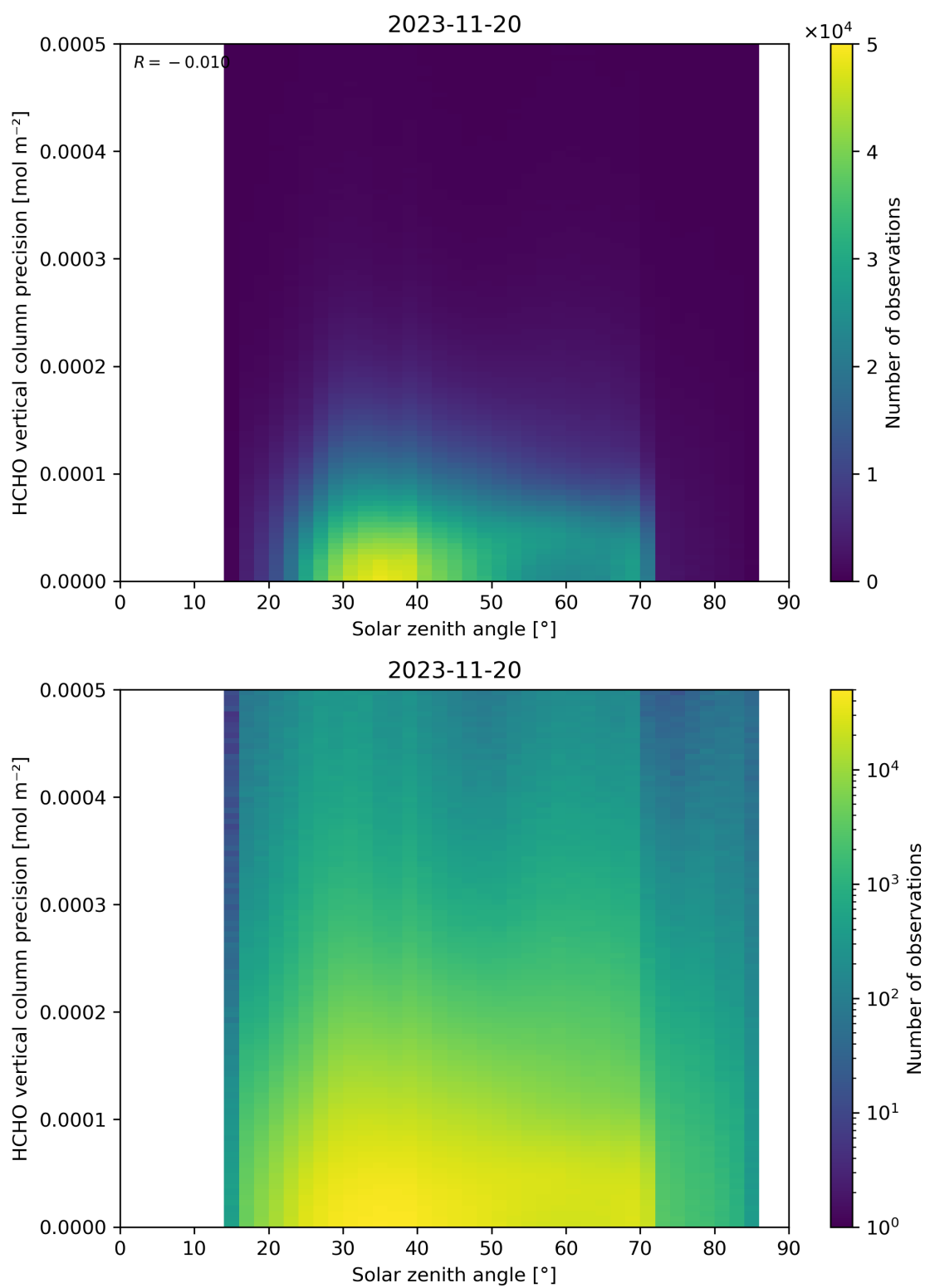
Figure 179: Scatter density plot of “Solar zenith angle” against “HCHO vertical column precision” for 2023-11-19 to 2023-11-21.
