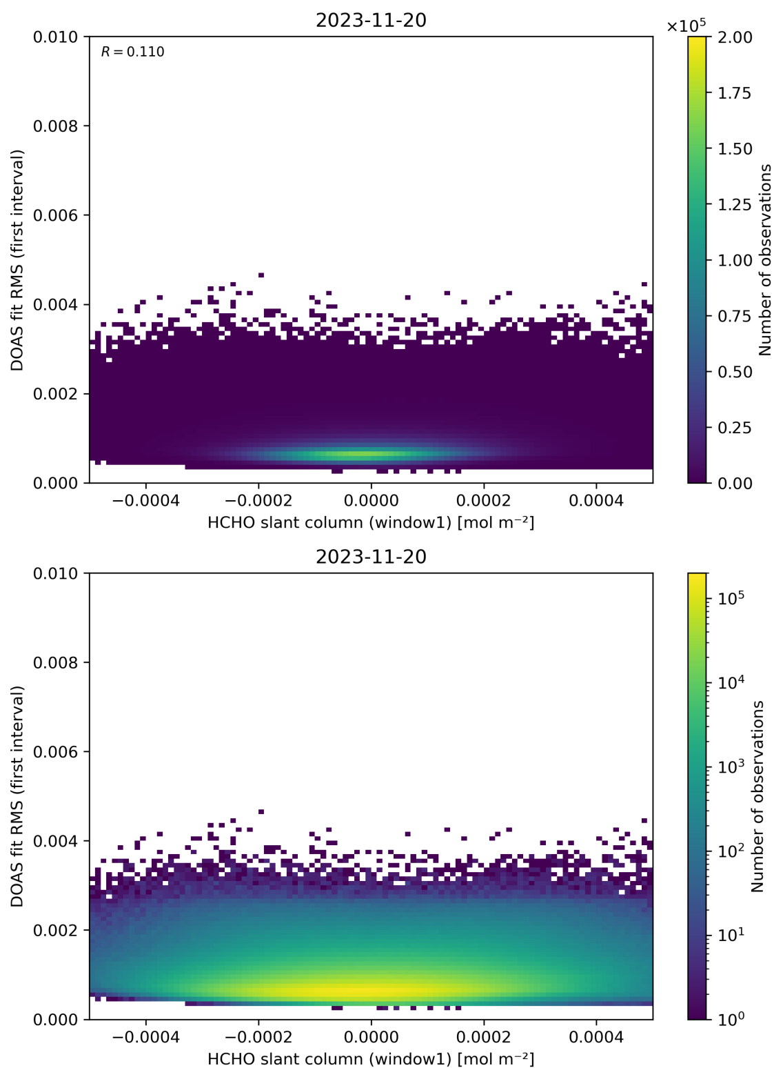
Figure 78: Scatter density plot of “HCHO slant column (window1)” against “DOAS fit RMS (first interval)” for 2023-11-19 to 2023-11-21.
