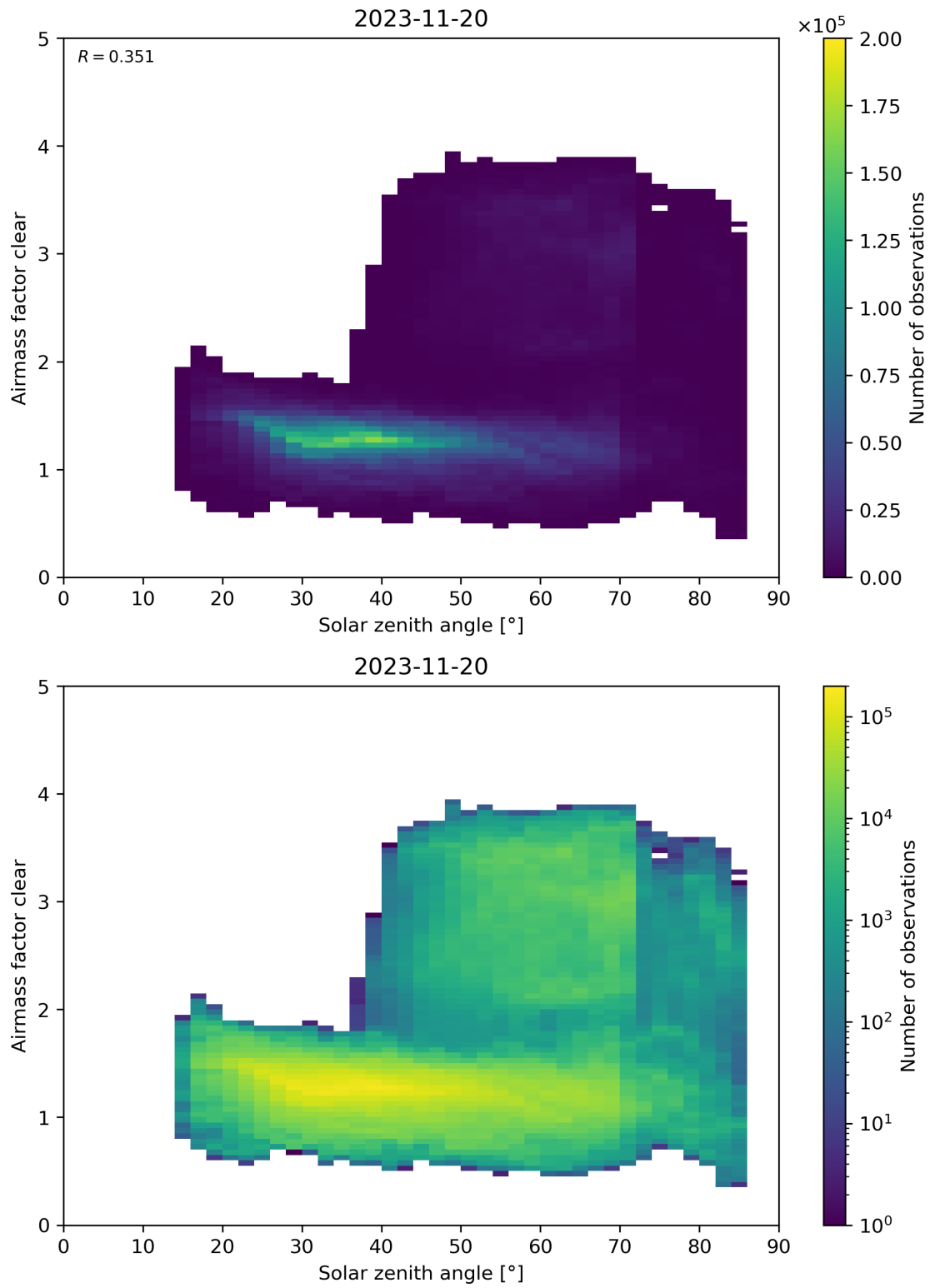
Figure 170: Scatter density plot of “Solar zenith angle” against “Airmass factor clear” for 2023-11-19 to 2023-11-21.
