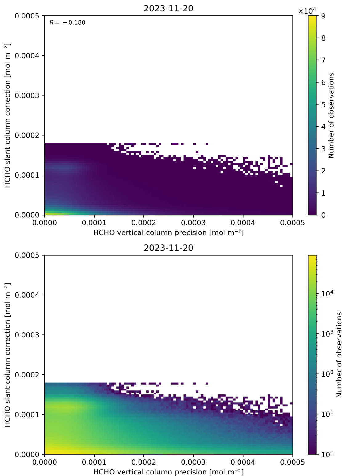
Figure 141: Scatter density plot of “HCHO vertical column precision” against “HCHO slant column correction” for 2023-11-19 to 2023-11-21.
