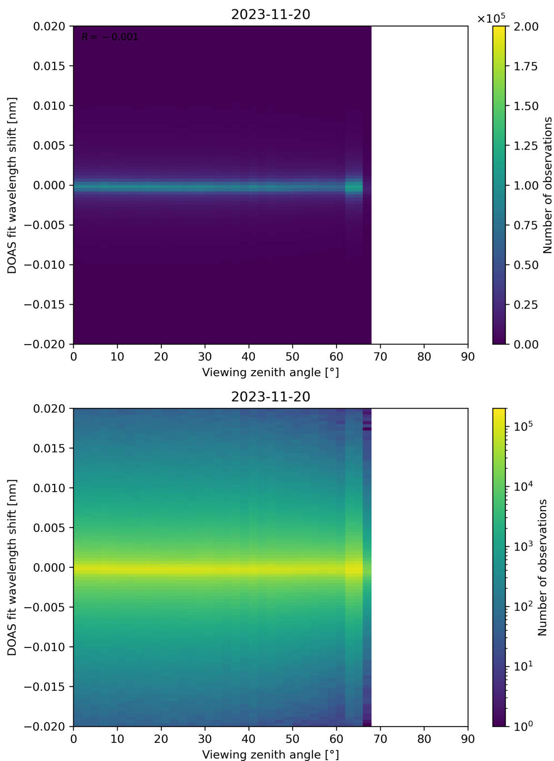
Figure 183: Scatter density plot of “Viewing zenith angle” against “DOAS fit wavelength shift” for 2023-11-19 to 2023-11-21.
