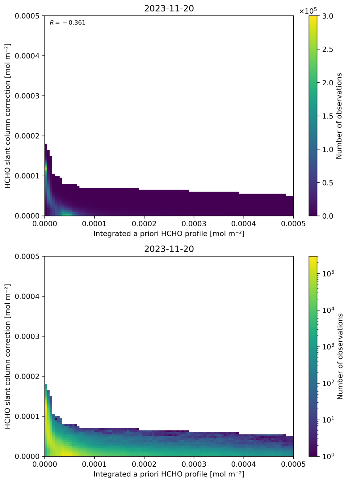
Figure 152: Scatter density plot of “Integrated a priori HCHO profile” against “HCHO slant column correction” for 2023-11-19 to 2023-11-21.
