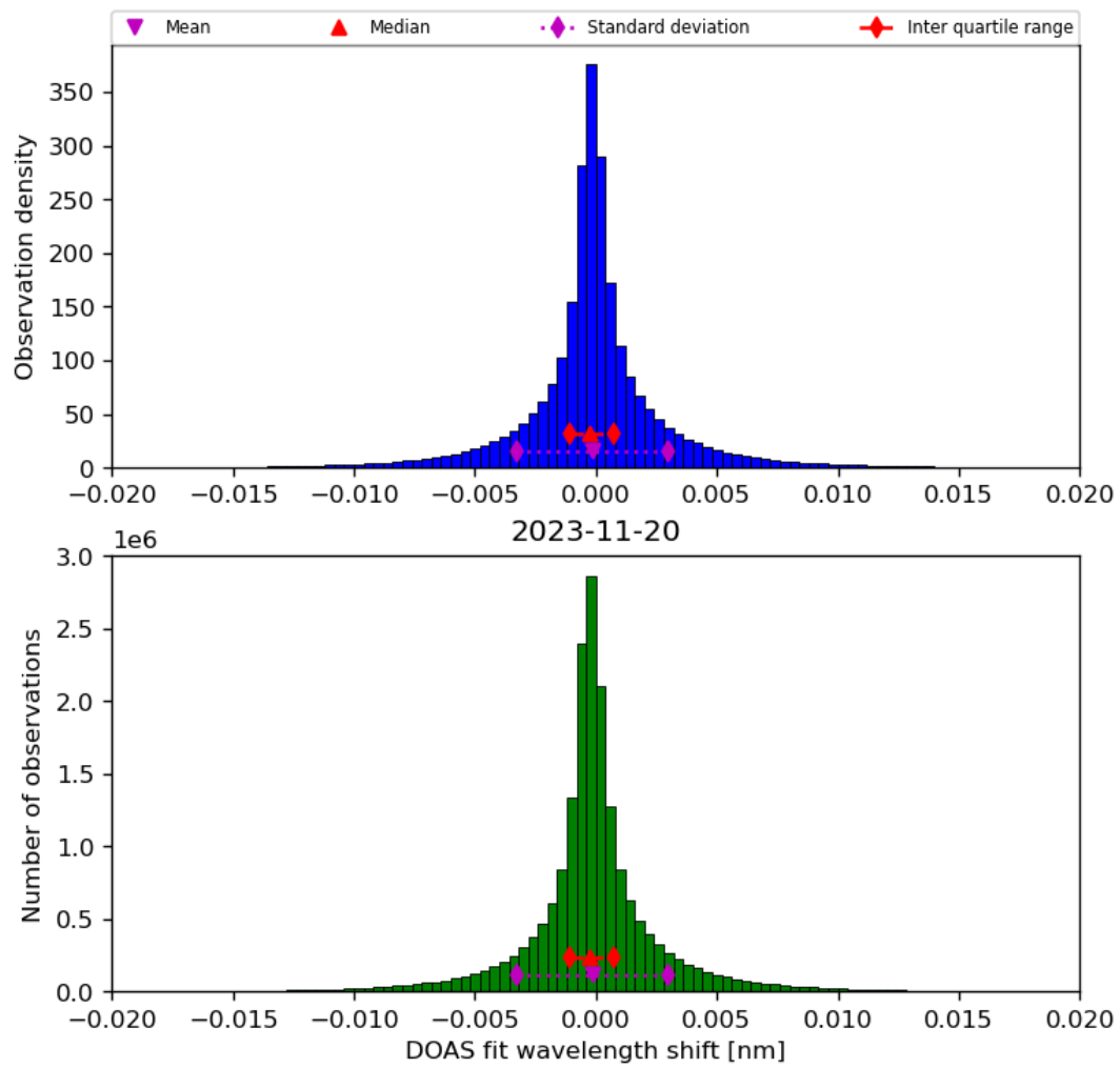
Figure 44: Histogram of “DOAS fit wavelength shift” for 2023-11-19 to 2023-11-21
