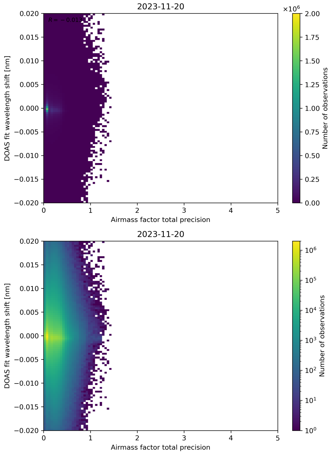
Figure 106: Scatter density plot of “Airmass factor total precision” against “DOAS fit wavelength shift” for 2023-11-19 to 2023-11-21.
