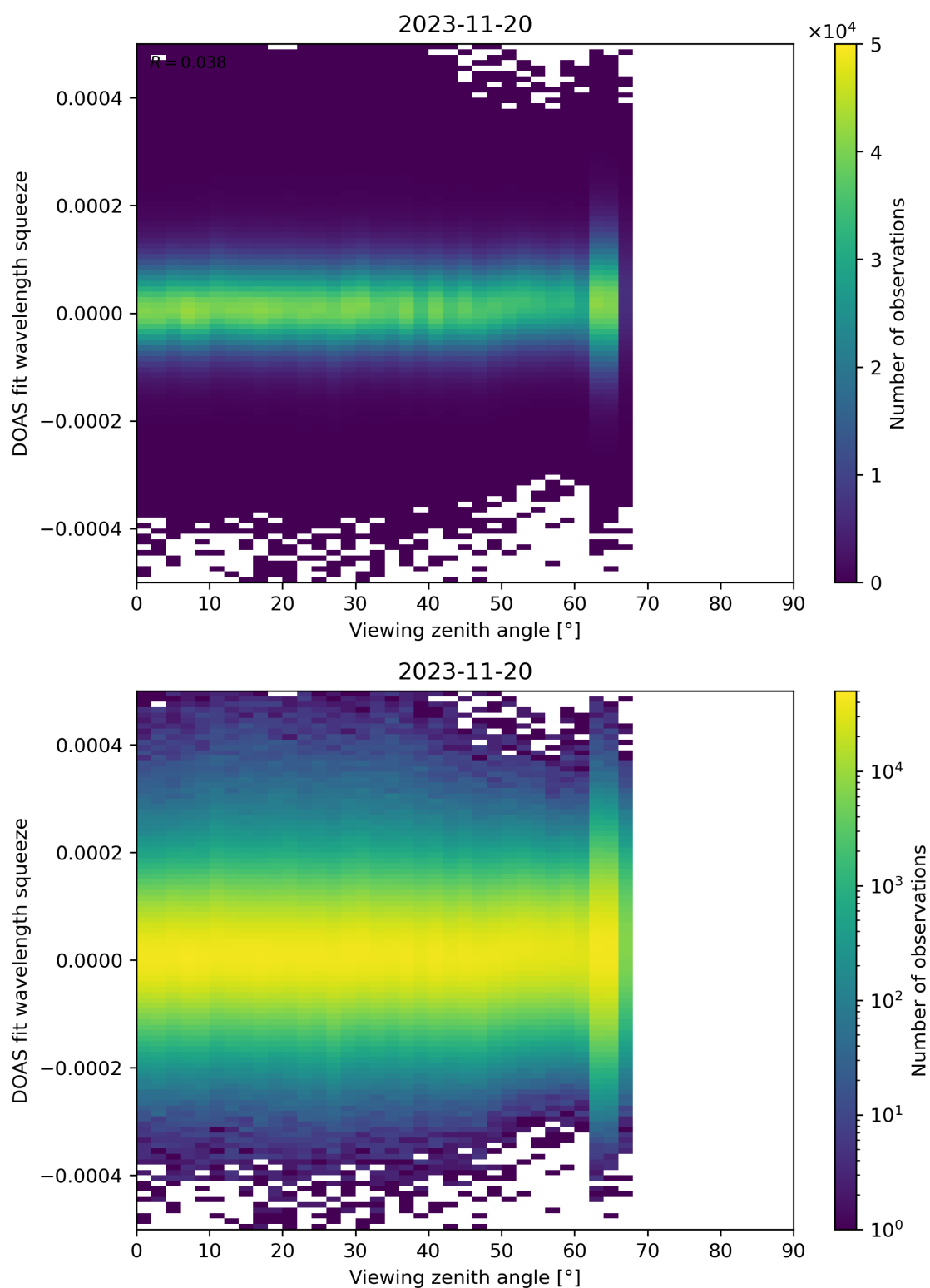
Figure 184: Scatter density plot of “Viewing zenith angle” against “DOAS fit wavelength squeeze” for 2023-11-19 to 2023-11-21.
