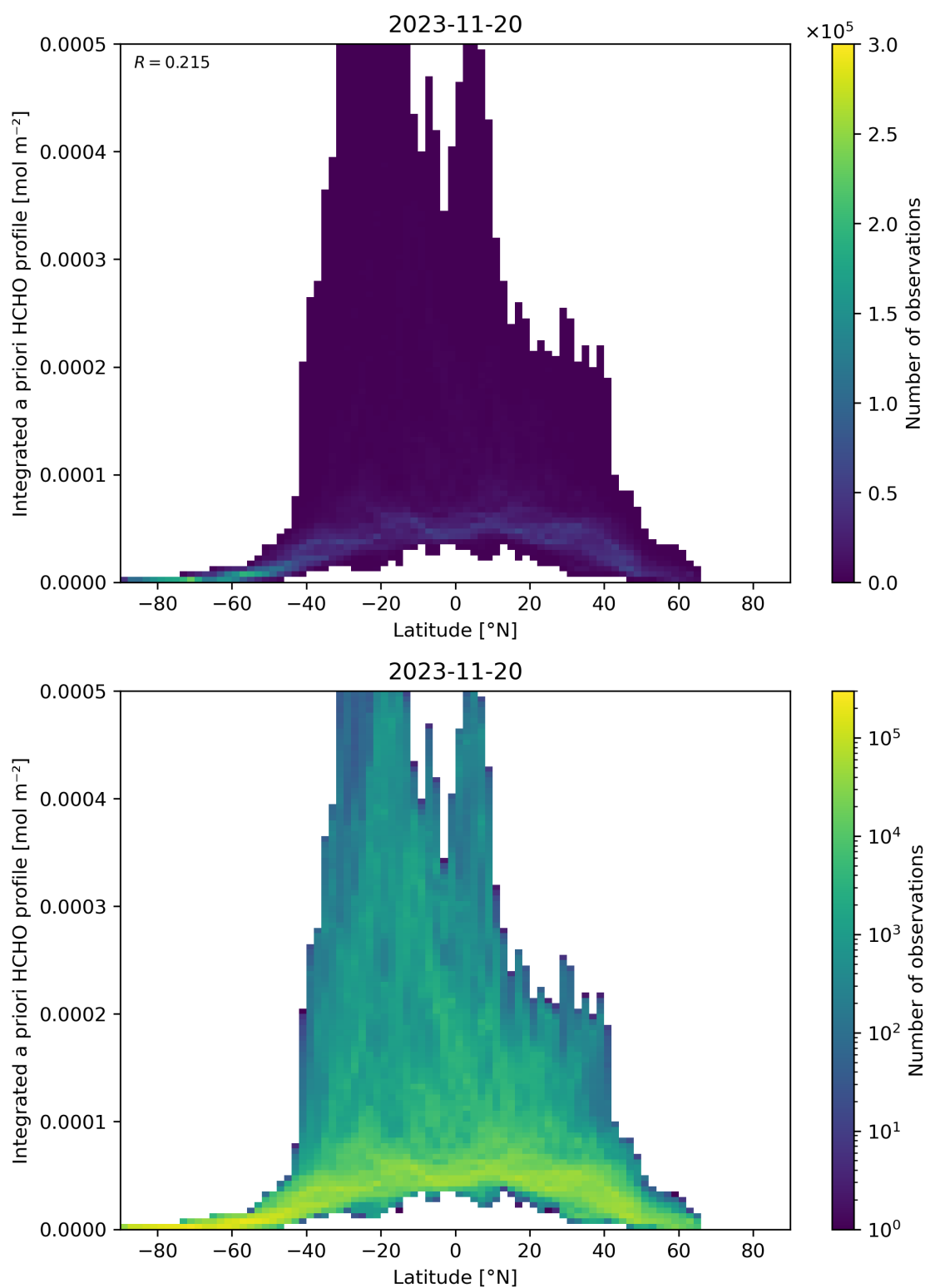
Figure 166: Scatter density plot of “Latitude” against “Integrated a priori HCHO profile” for 2023-11-19 to 2023-11-21.
