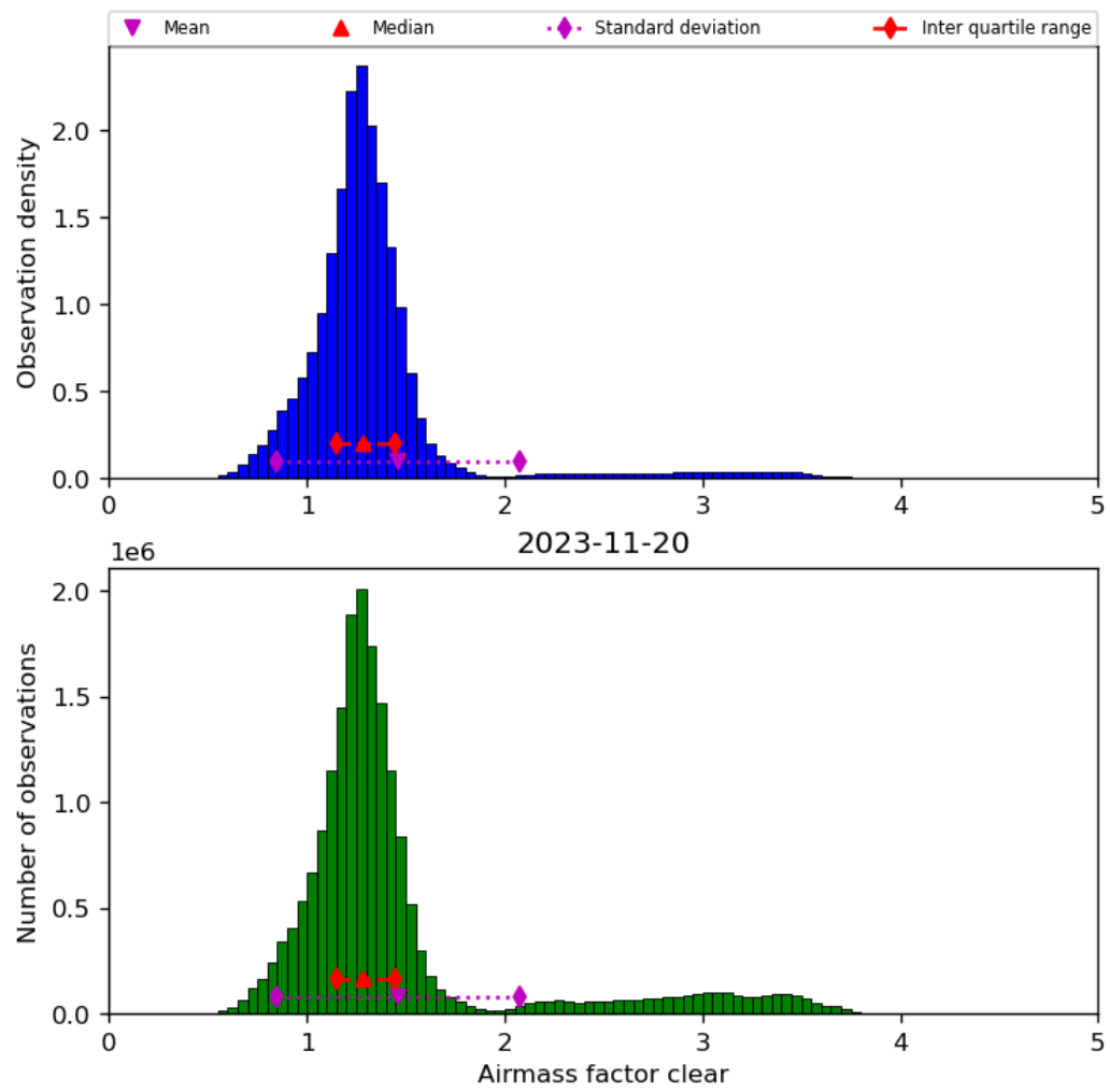
Figure 42: Histogram of “Airmass factor clear” for 2023-11-19 to 2023-11-21
