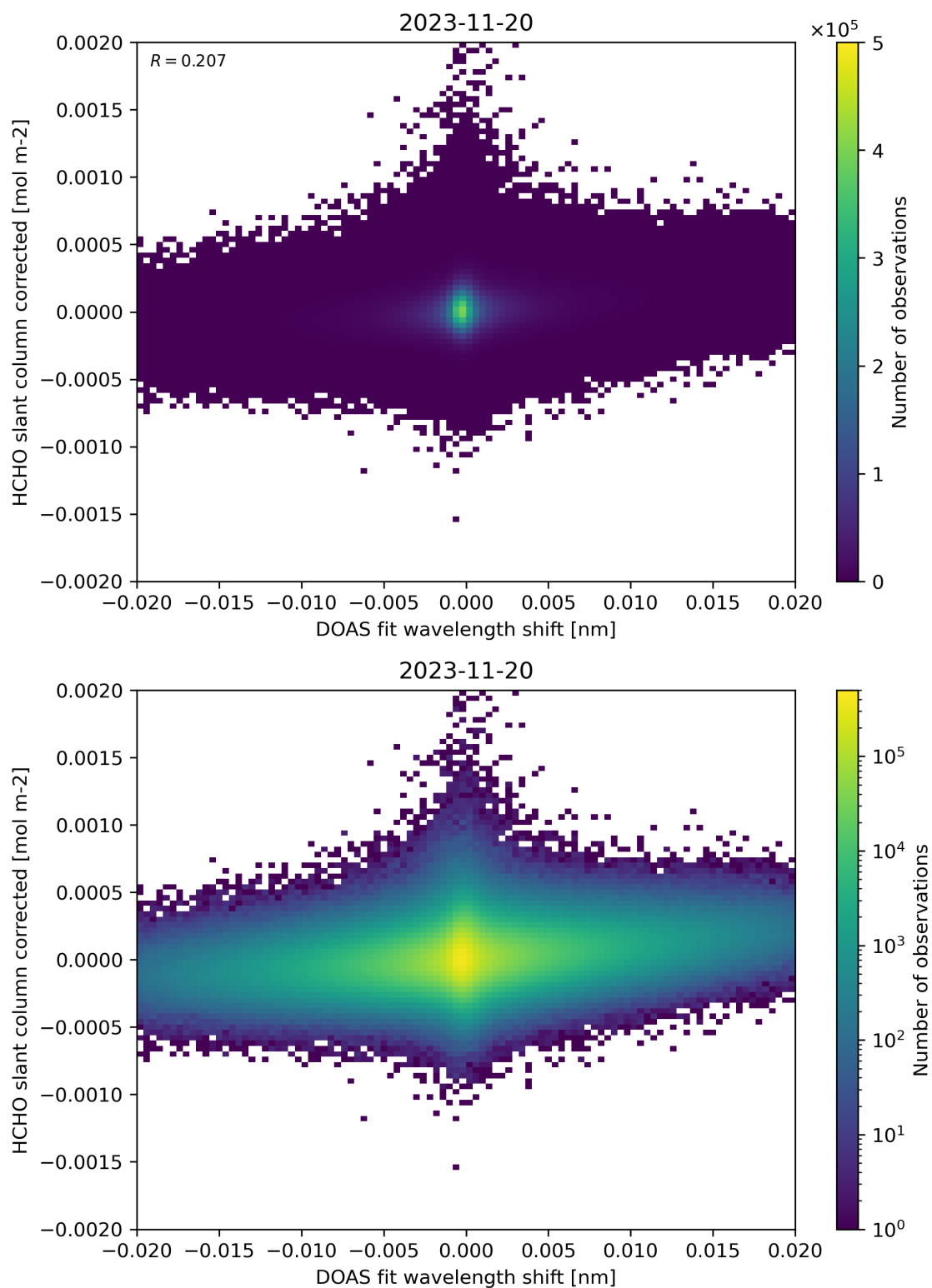
Figure 66: Scatter density plot of “DOAS fit wavelength shift” against “HCHO slant column corrected” for 2023-11-19 to 2023-11-21.
