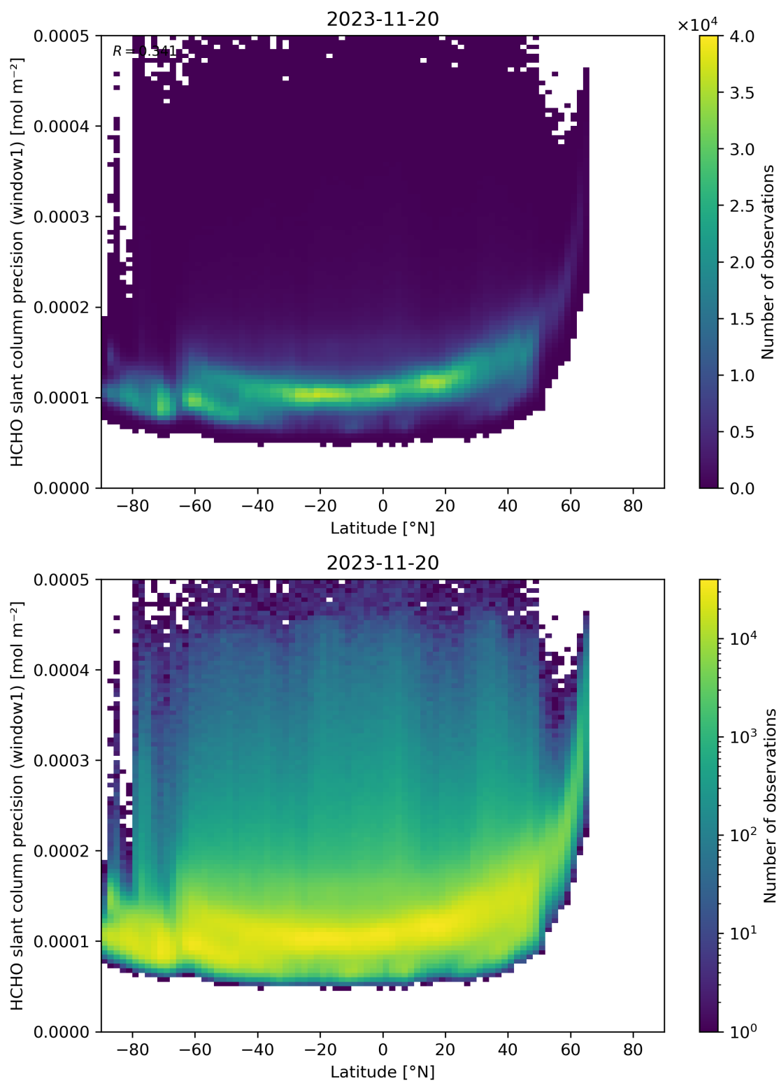
Figure 160: Scatter density plot of “Latitude” against “HCHO slant column precision (window1)” for 2023-11-19 to 2023-11-21.
