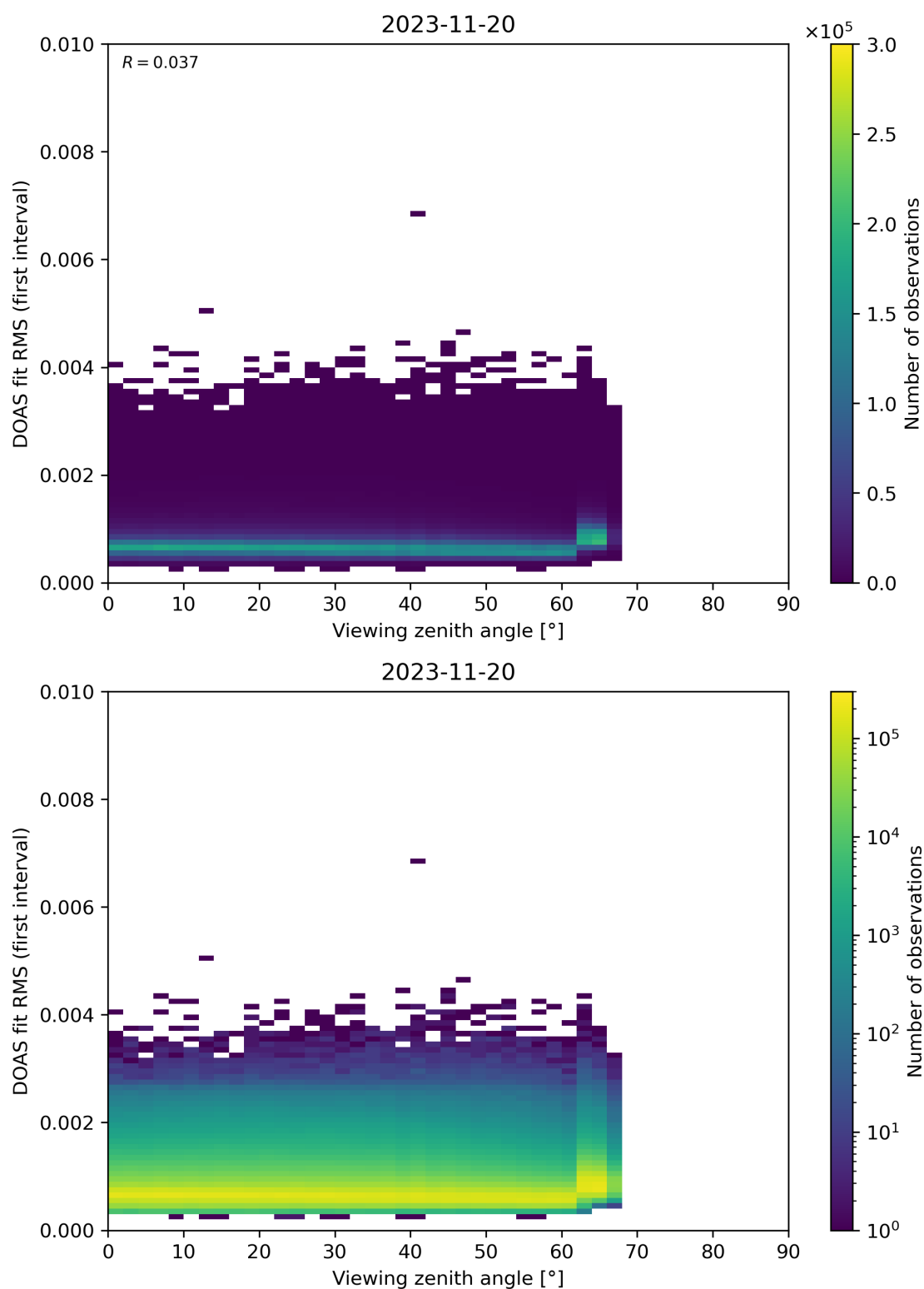
Figure 182: Scatter density plot of “Viewing zenith angle” against “DOAS fit RMS (first interval)” for 2023-11-19 to 2023-11-21.
