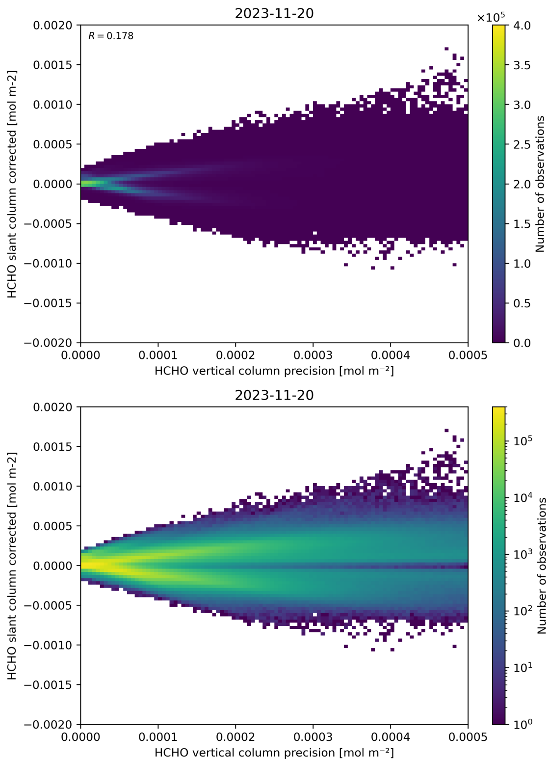
Figure 140: Scatter density plot of “HCHO vertical column precision” against “HCHO slant column corrected” for 2023-11-19 to 2023-11-21.
