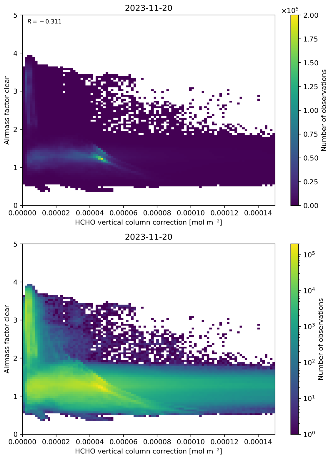
Figure 115: Scatter density plot of “HCHO vertical column correction” against “Airmass factor clear” for 2023-11-19 to 2023-11-21.
