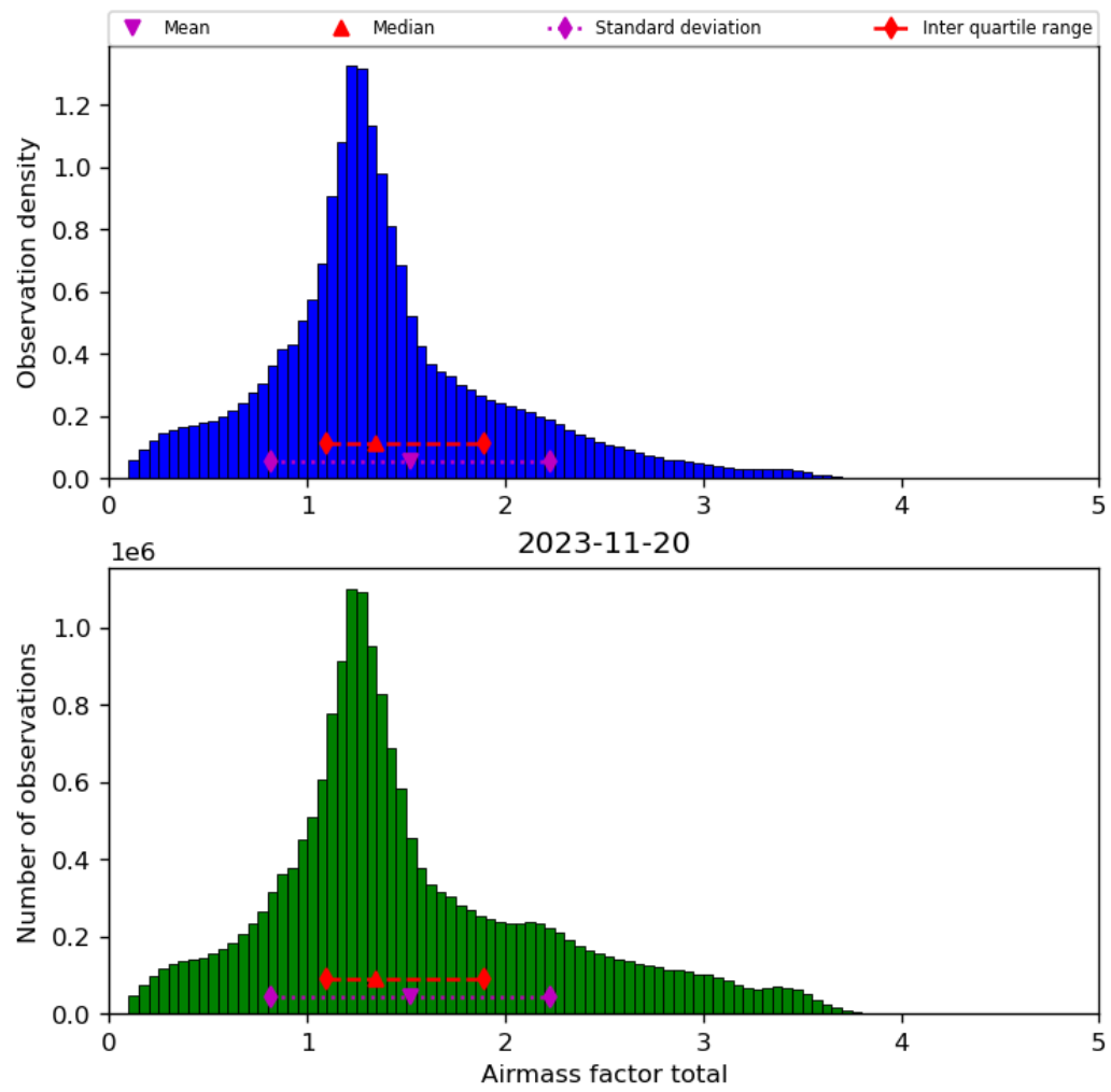
Figure 40: Histogram of “Airmass factor total” for 2023-11-19 to 2023-11-21
