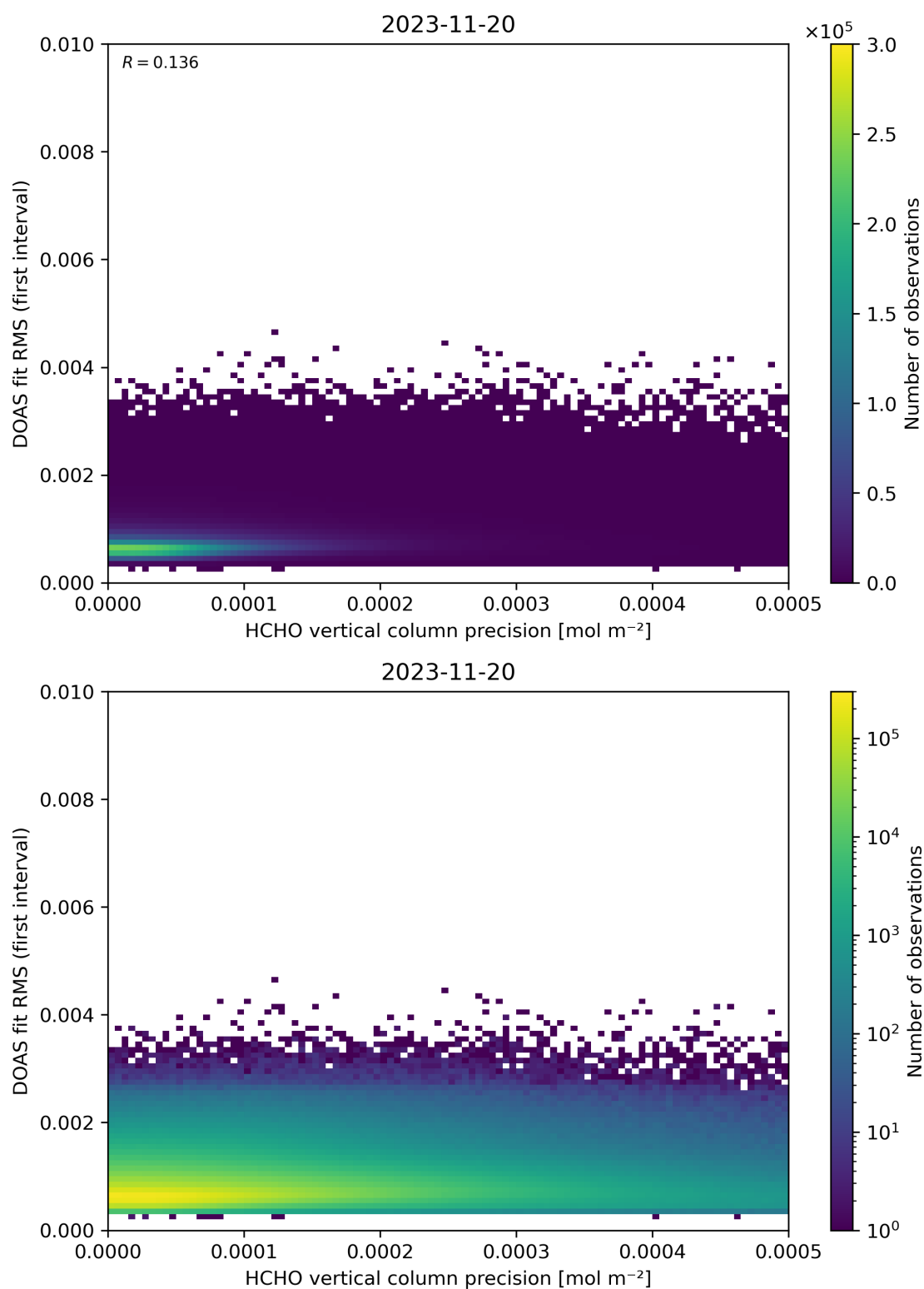
Figure 136: Scatter density plot of “HCHO vertical column precision” against “DOAS fit RMS (first interval)” for 2023-11-19 to 2023-11-21.
