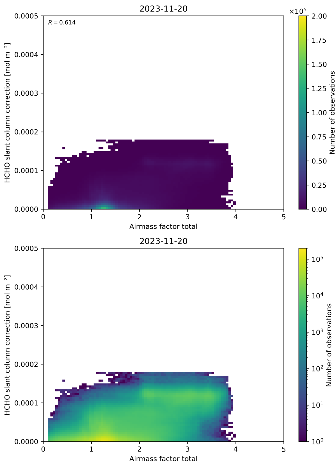
Figure 102: Scatter density plot of “Airmass factor total” against “HCHO slant column correction” for 2023-11-19 to 2023-11-21.
