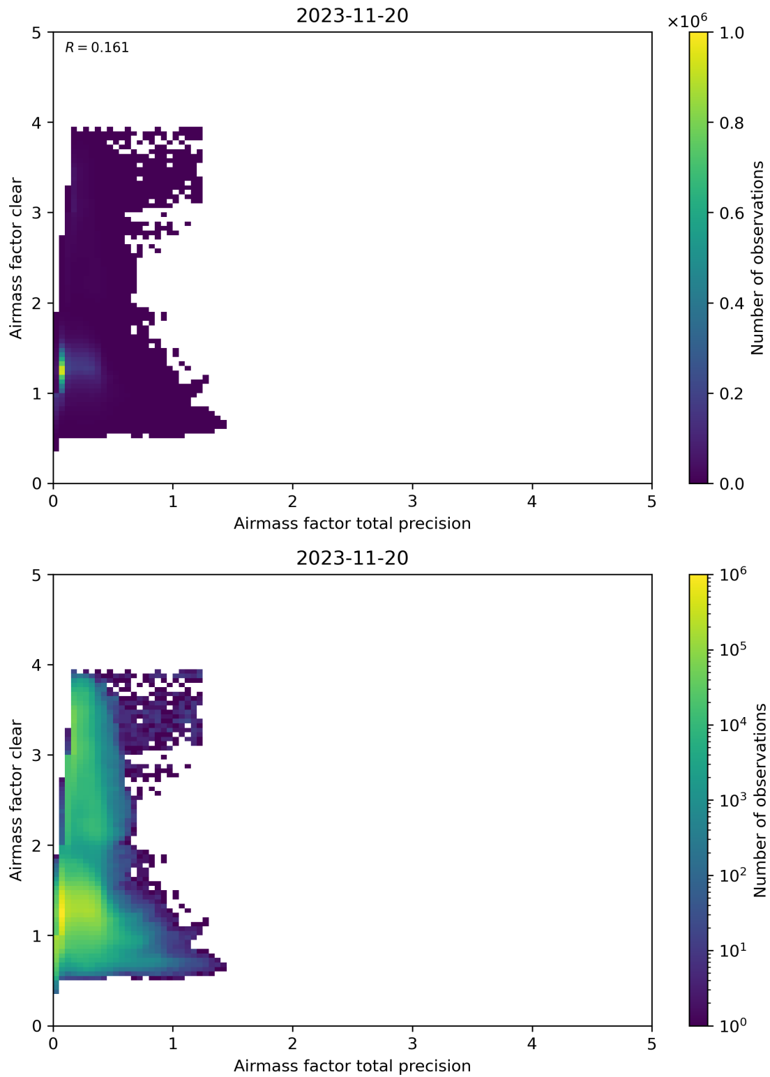
Figure 108: Scatter density plot of “Airmass factor total precision” against “Airmass factor clear” for 2023-11-19 to 2023-11-21.
