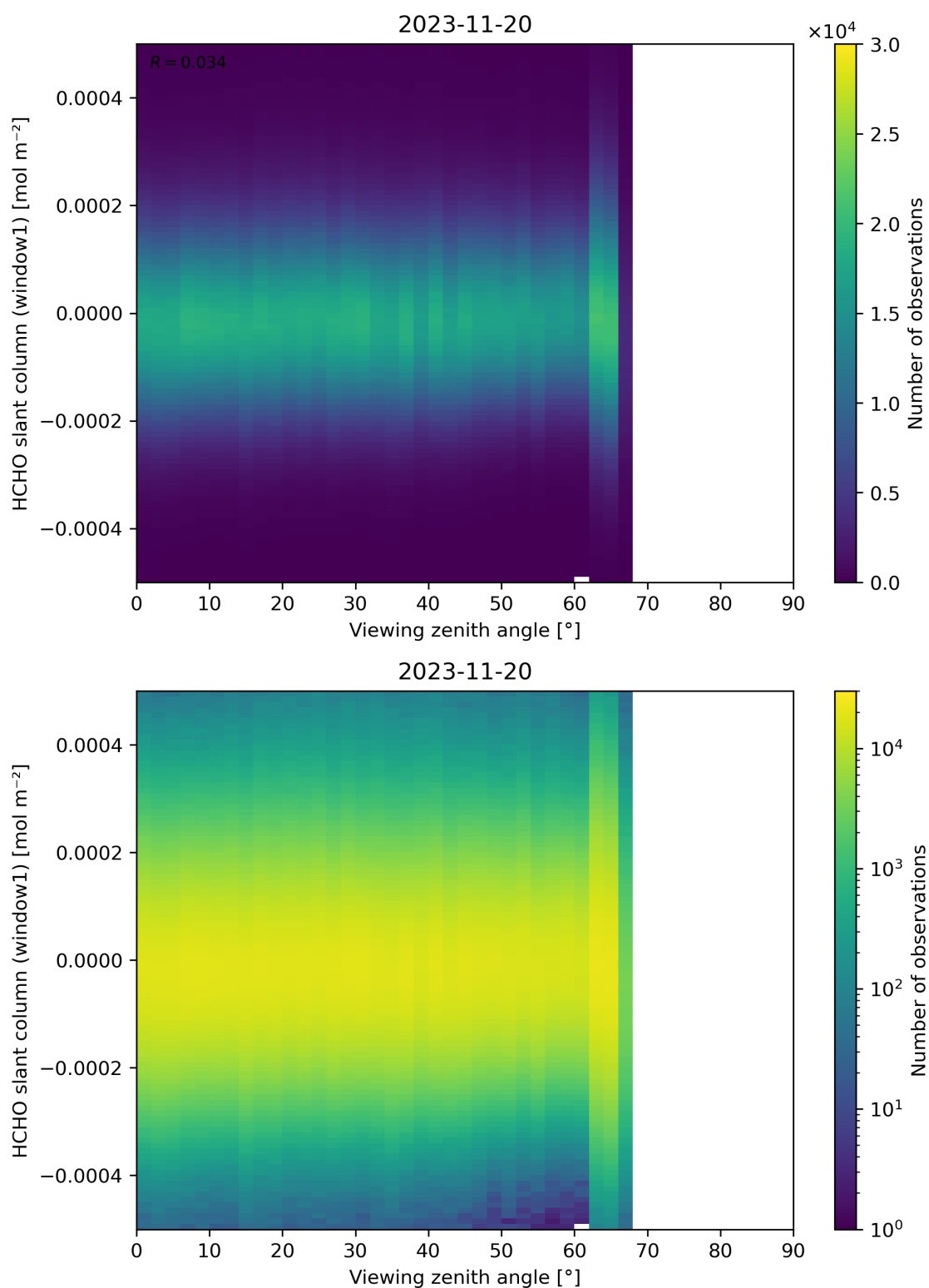
Figure 188: Scatter density plot of “Viewing zenith angle” against “HCHO slant column (window1)” for 2023-11-19 to 2023-11-21.
