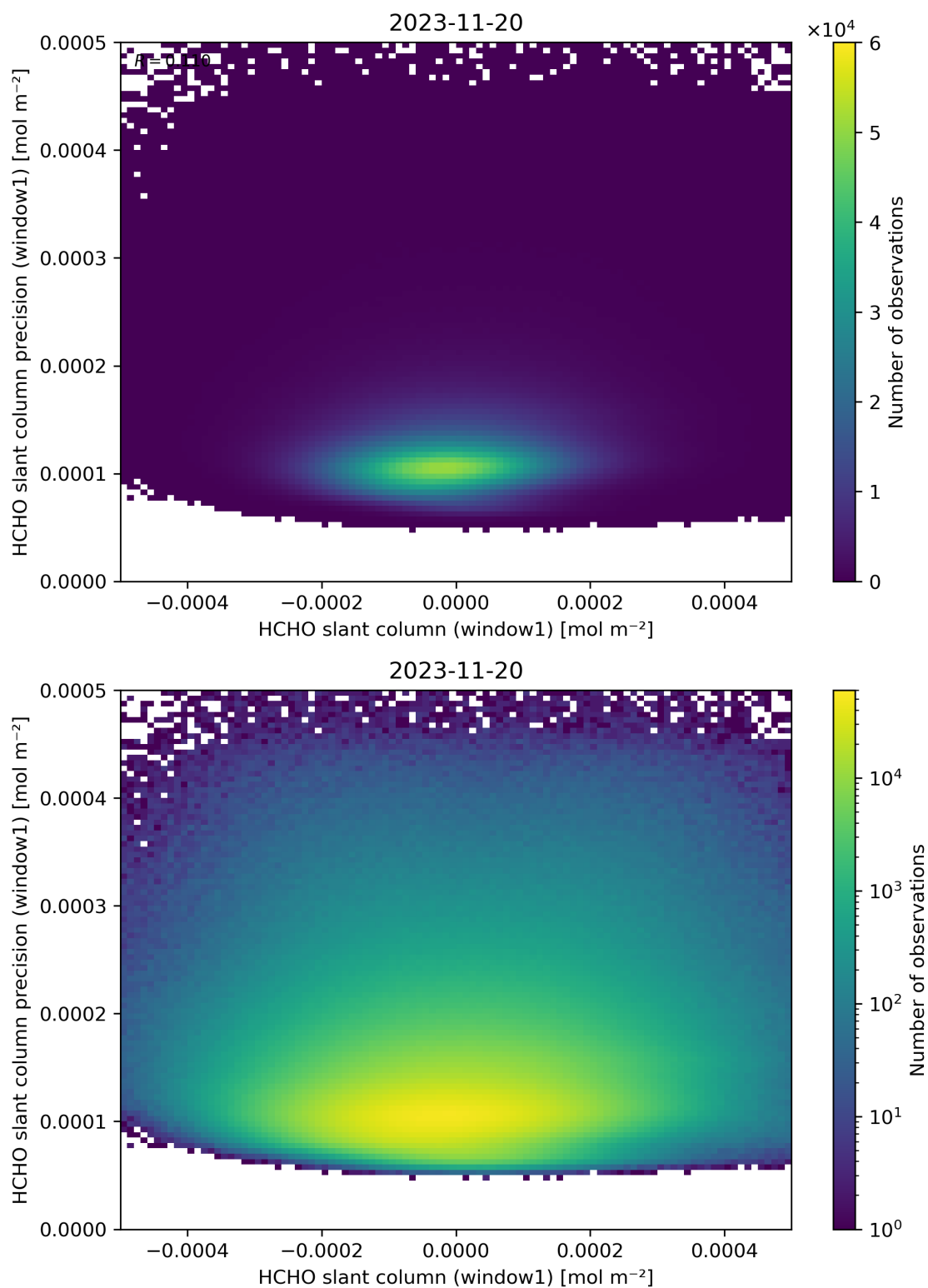
Figure 84: Scatter density plot of “HCHO slant column (window1)” against “HCHO slant column precision (window1)” for 2023-11-19 to 2023-11-21.
