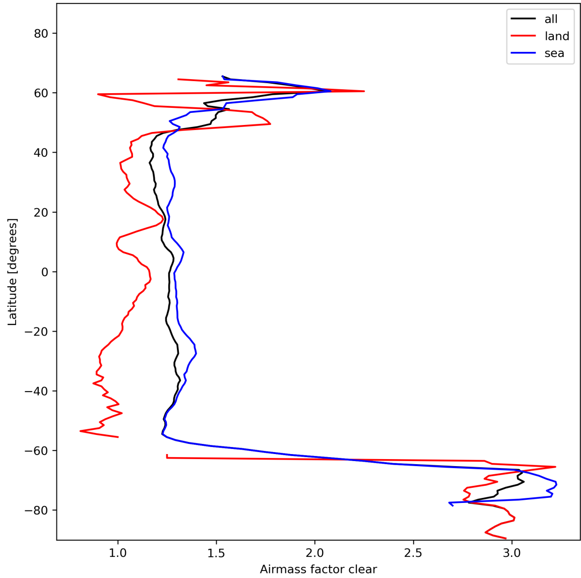
Figure 28: Zonal average of “Airmass factor clear” for 2023-11-19 to 2023-11-21.
