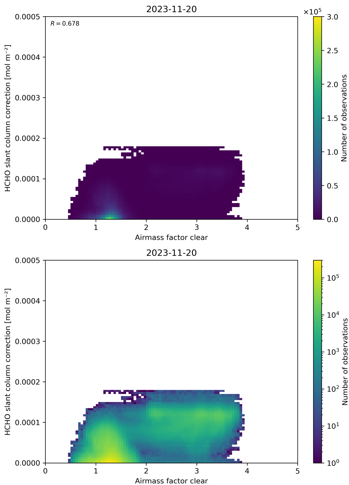
Figure 75: Scatter density plot of “Airmass factor clear” against “HCHO slant column correction” for 2023-11-19 to 2023-11-21.
