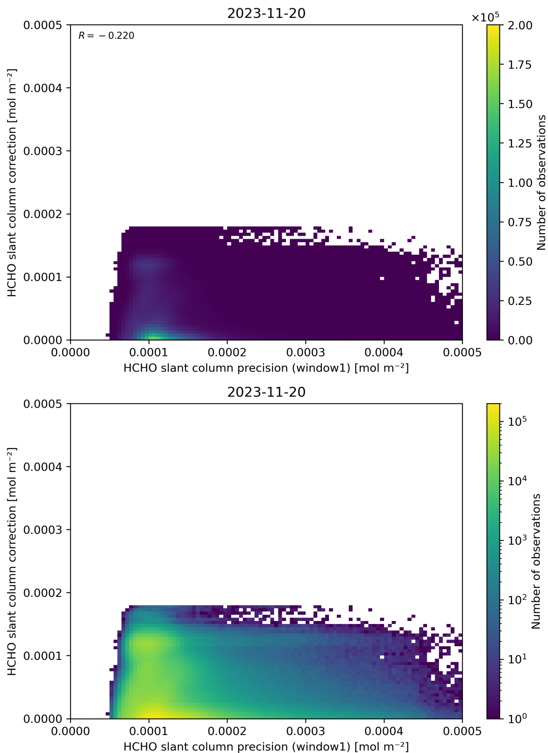
Figure 93: Scatter density plot of “HCHO slant column precision (window1)” against “HCHO slant column correction” for 2023-11-19 to 2023-11-21.
