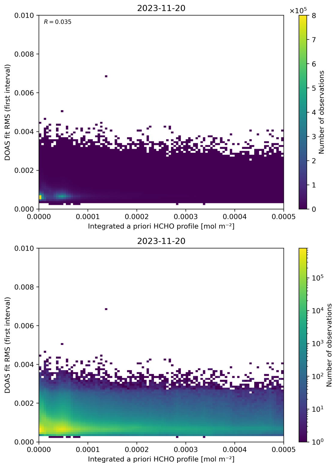
Figure 148: Scatter density plot of “Integrated a priori HCHO profile” against “DOAS fit RMS (first interval)” for 2023-11-19 to 2023-11-21.
