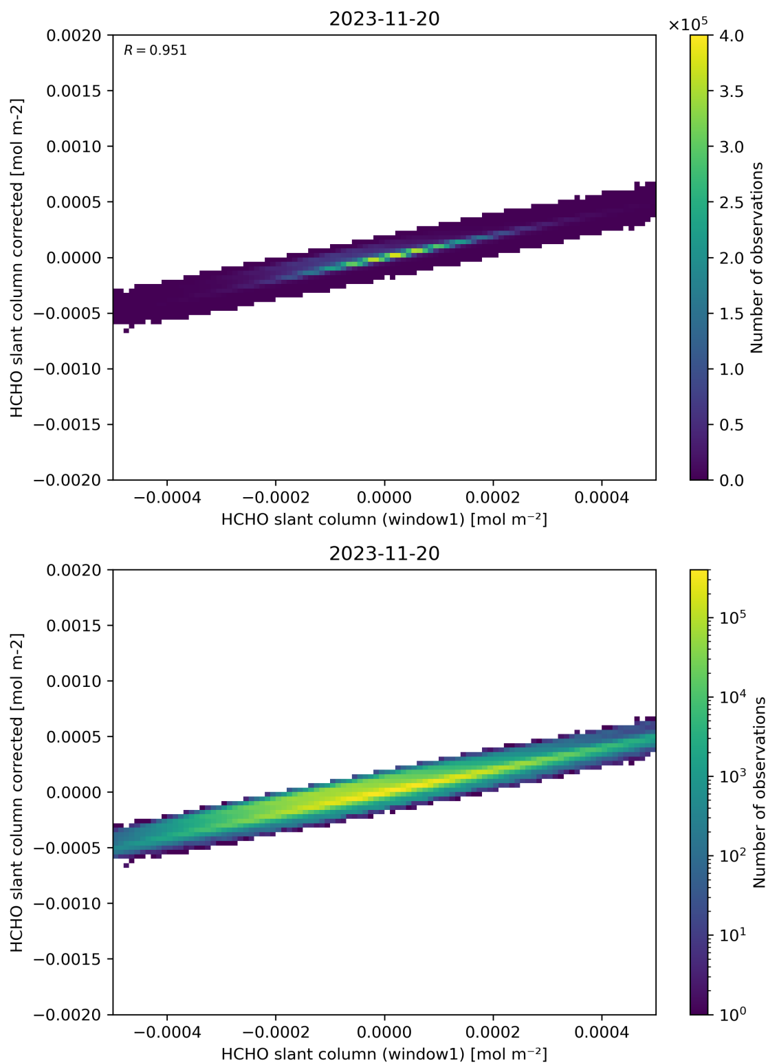
Figure 82: Scatter density plot of “HCHO slant column (window1)” against “HCHO slant column corrected” for 2023-11-19 to 2023-11-21.
