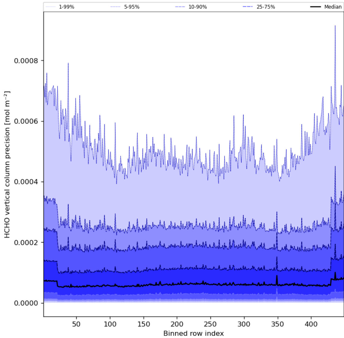
Figure 50: Along track statistics of “HCHO vertical column precision” for 2023-11-19 to 2023-11-21
