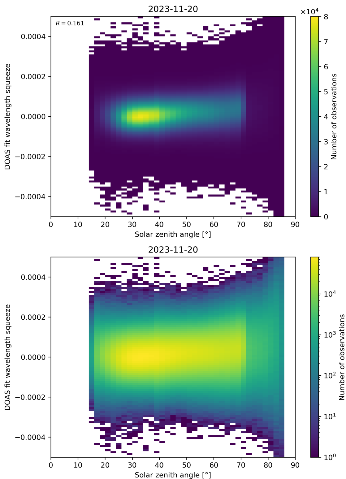
Figure 169: Scatter density plot of “Solar zenith angle” against “DOAS fit wavelength squeeze” for 2023-11-19 to 2023-11-21.
