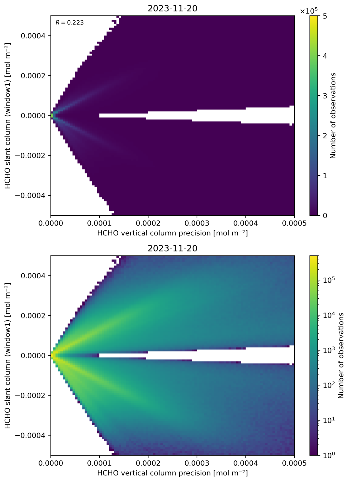
Figure 142: Scatter density plot of “HCHO vertical column precision” against “HCHO slant column (window1)” for 2023-11-19 to 2023-11-21.
