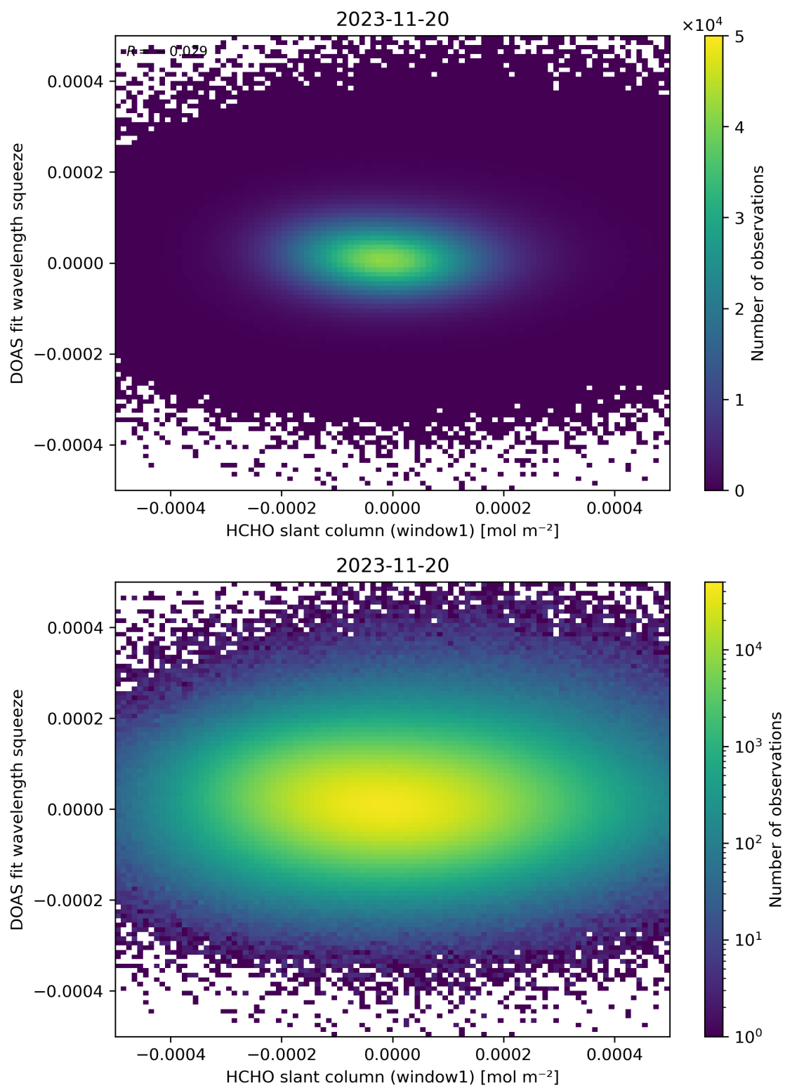
Figure 80: Scatter density plot of “HCHO slant column (window1)” against “DOAS fit wavelength squeeze” for 2023-11-19 to 2023-11-21.
