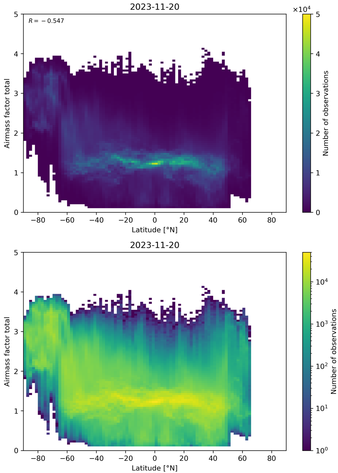
Figure 161: Scatter density plot of “Latitude” against “Airmass factor total” for 2023-11-19 to 2023-11-21.
