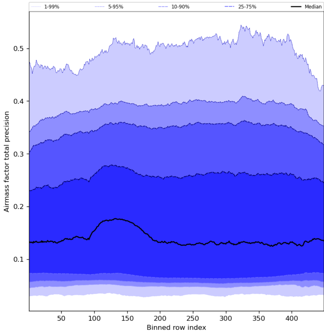
Figure 55: Along track statistics of “Airmass factor total precision” for 2023-11-19 to 2023-11-21
