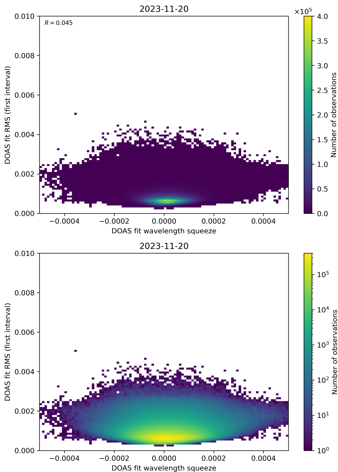
Figure 68: Scatter density plot of “DOAS fit wavelength squeeze” against “DOAS fit RMS (first interval)” for 2023-11-19 to 2023-11-21.
