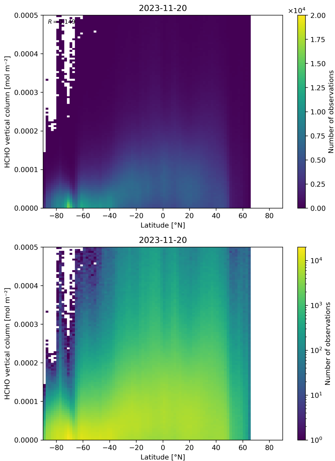
Figure 163: Scatter density plot of “Latitude” against “HCHO vertical column” for 2023-11-19 to 2023-11-21.
