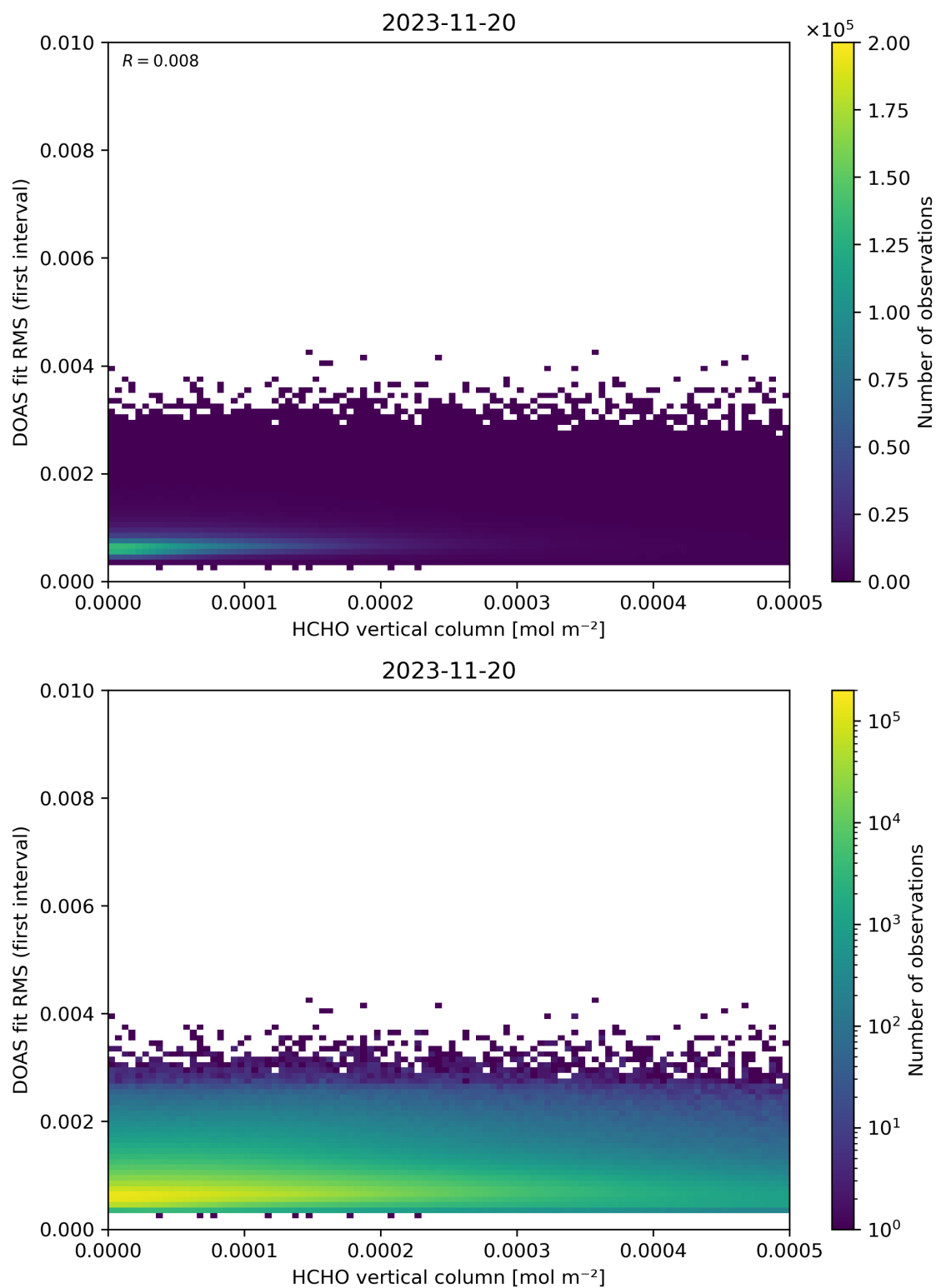
Figure 123: Scatter density plot of “HCHO vertical column” against “DOAS fit RMS (first interval)” for 2023-11-19 to 2023-11-21.
