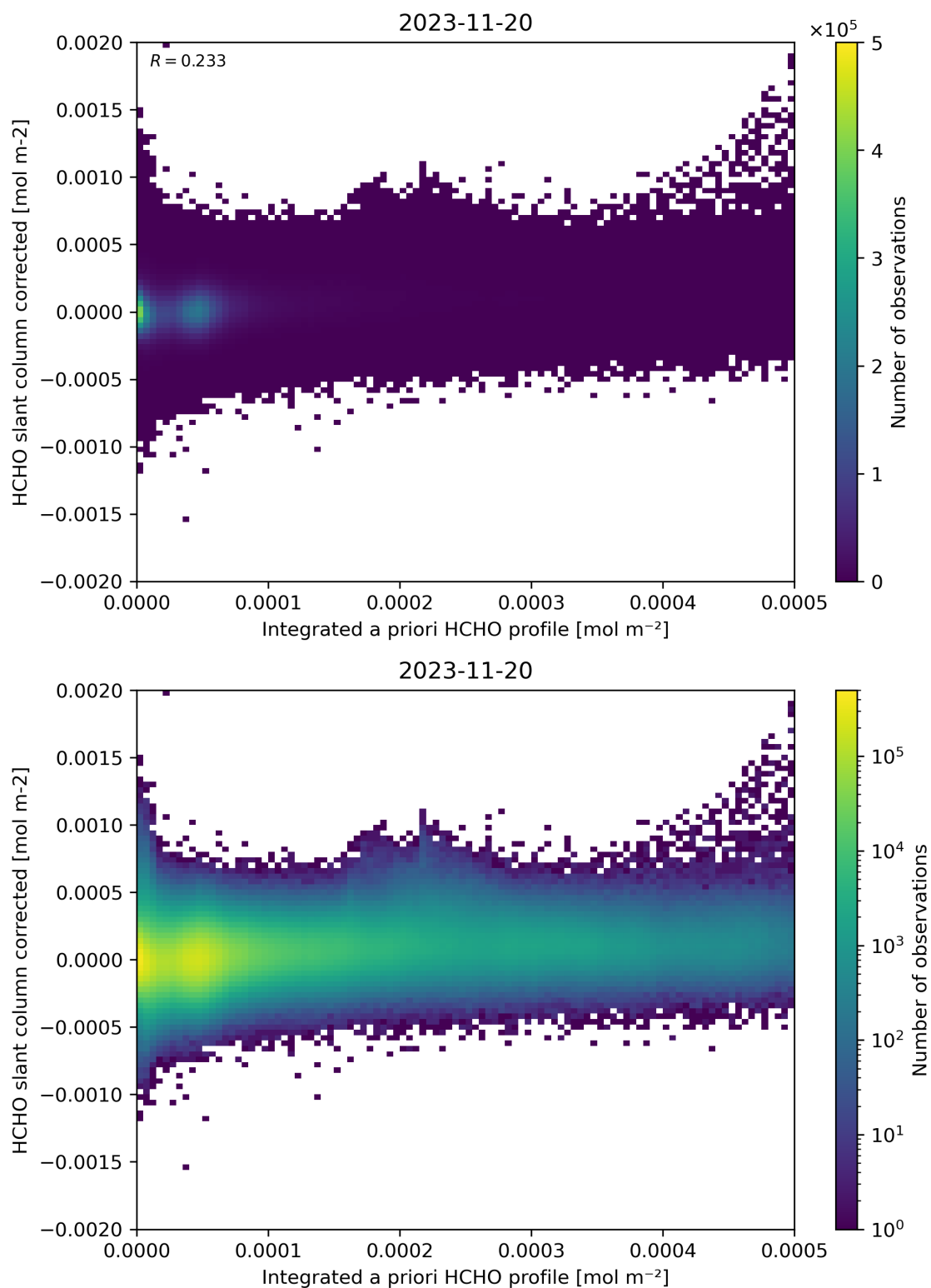
Figure 151: Scatter density plot of “Integrated a priori HCHO profile” against “HCHO slant column corrected” for 2023-11-19 to 2023-11-21.
