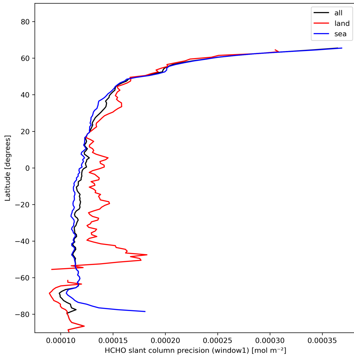
Figure 25: Zonal average of “HCHO slant column precision (window1)” for 2023-11-19 to 2023-11-21.
