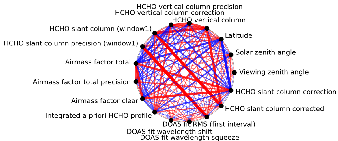
Figure 1: Map of correlation graph for 2023-11-19 to 2023-11-21.
