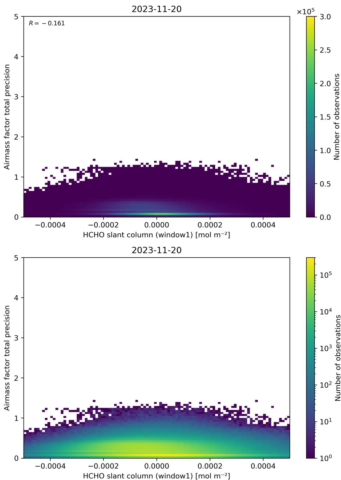
Figure 86: Scatter density plot of “HCHO slant column (window1)” against “Airmass factor total precision” for 2023-11-19 to 2023-11-21.
