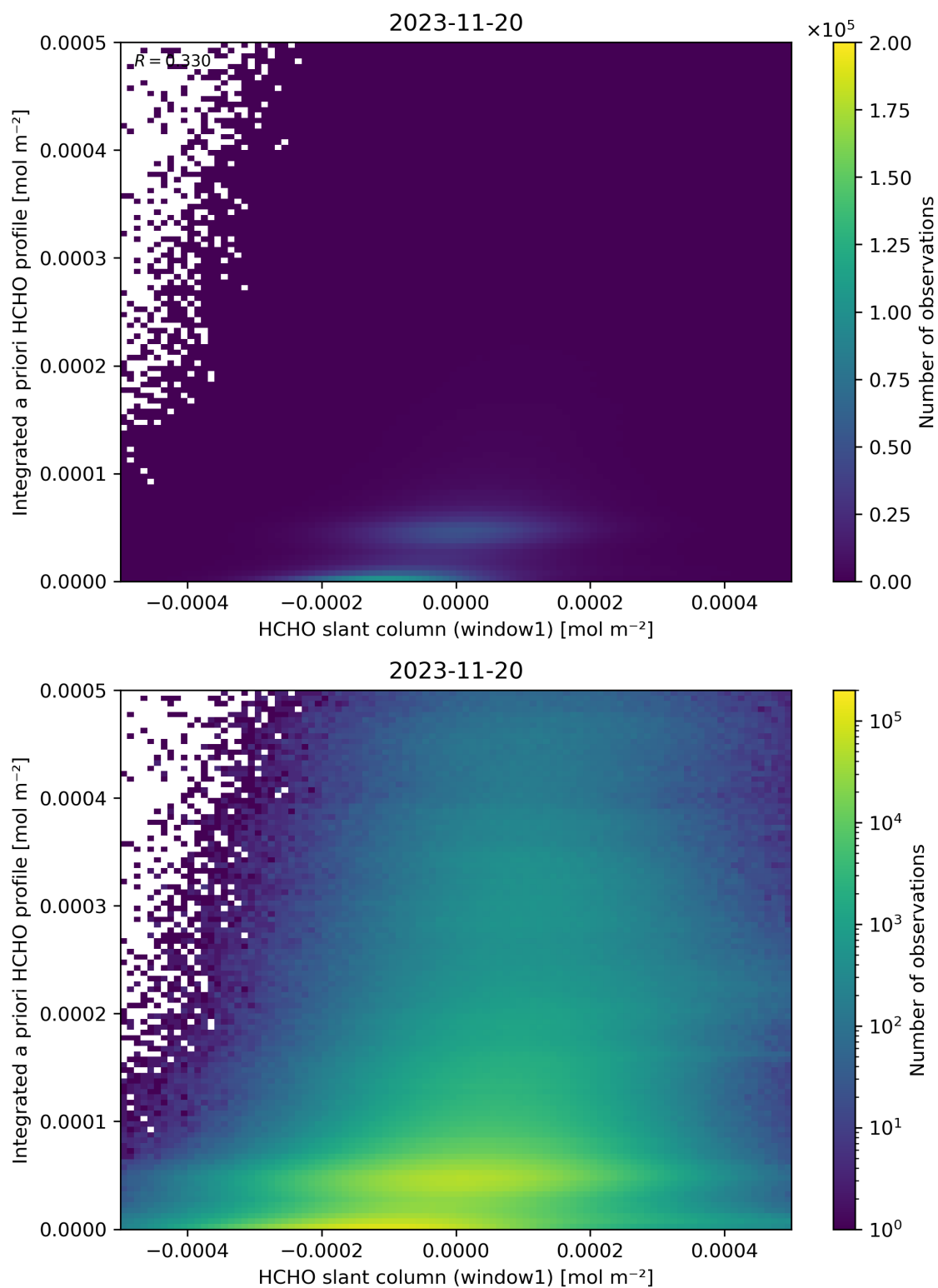
Figure 87: Scatter density plot of “HCHO slant column (window1)” against “Integrated a priori HCHO profile” for 2023-11-19 to 2023-11-21.
