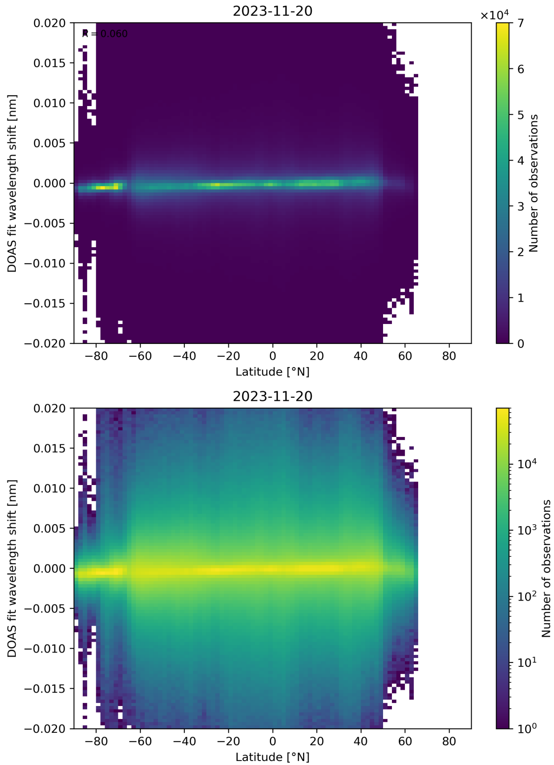
Figure 154: Scatter density plot of “Latitude” against “DOAS fit wavelength shift” for 2023-11-19 to 2023-11-21.
