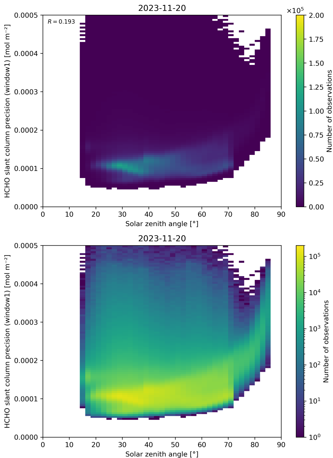
Figure 174: Scatter density plot of “Solar zenith angle” against “HCHO slant column precision (window1)” for 2023-11-19 to 2023-11-21.
