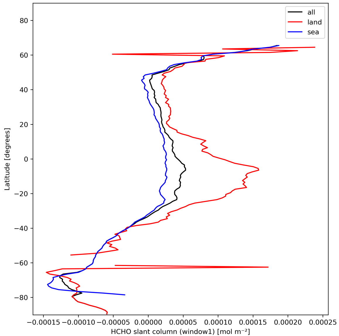
Figure 24: Zonal average of “HCHO slant column (window1)” for 2023-11-19 to 2023-11-21.
