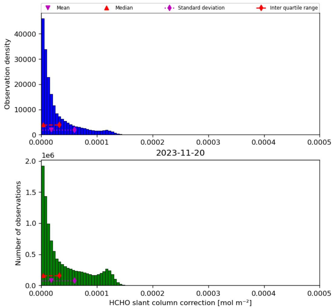
Figure 47: Histogram of “HCHO slant column correction” for 2023-11-19 to 2023-11-21
