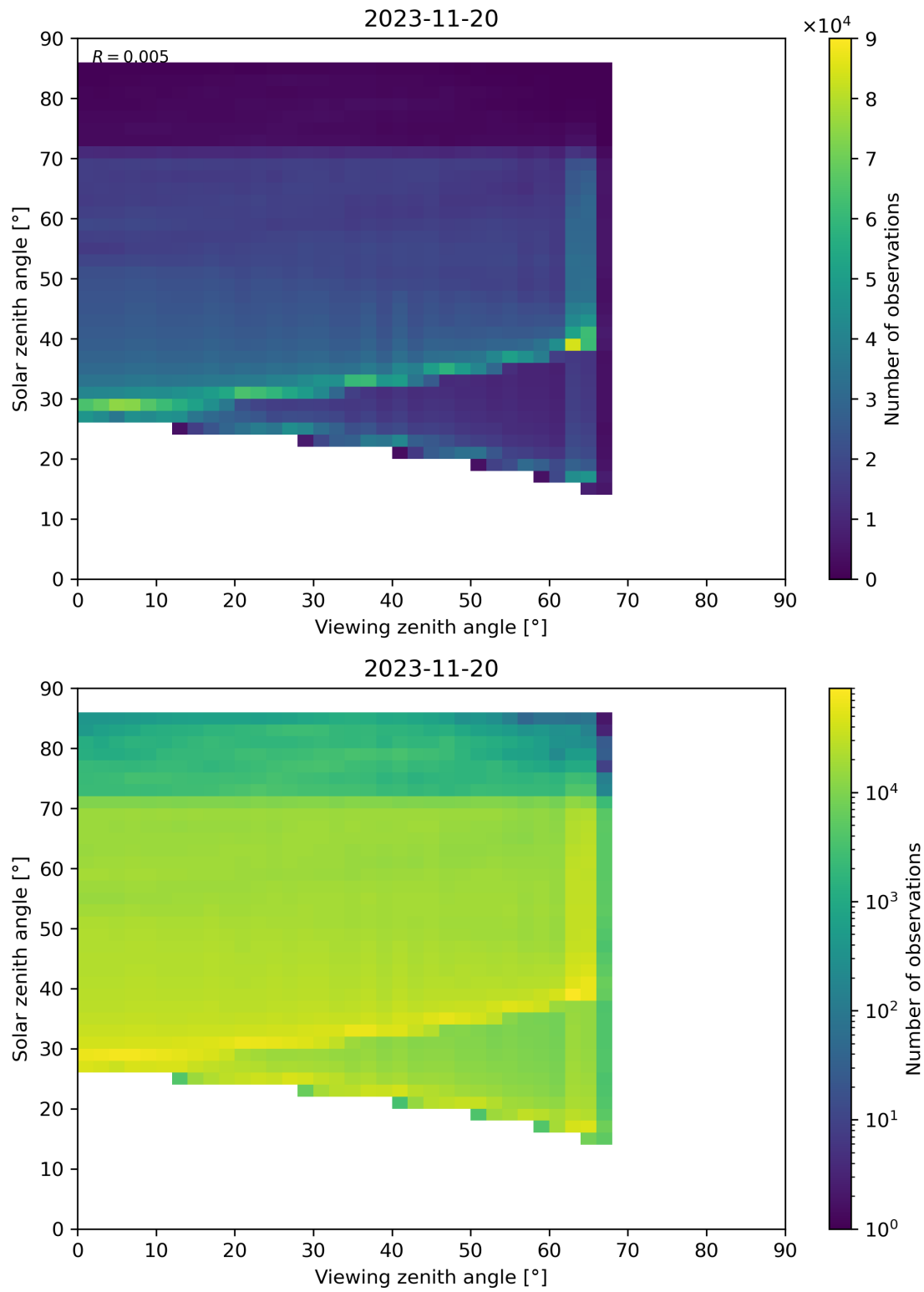
Figure 197: Scatter density plot of “Viewing zenith angle” against “Solar zenith angle” for 2023-11-19 to 2023-11-21.
