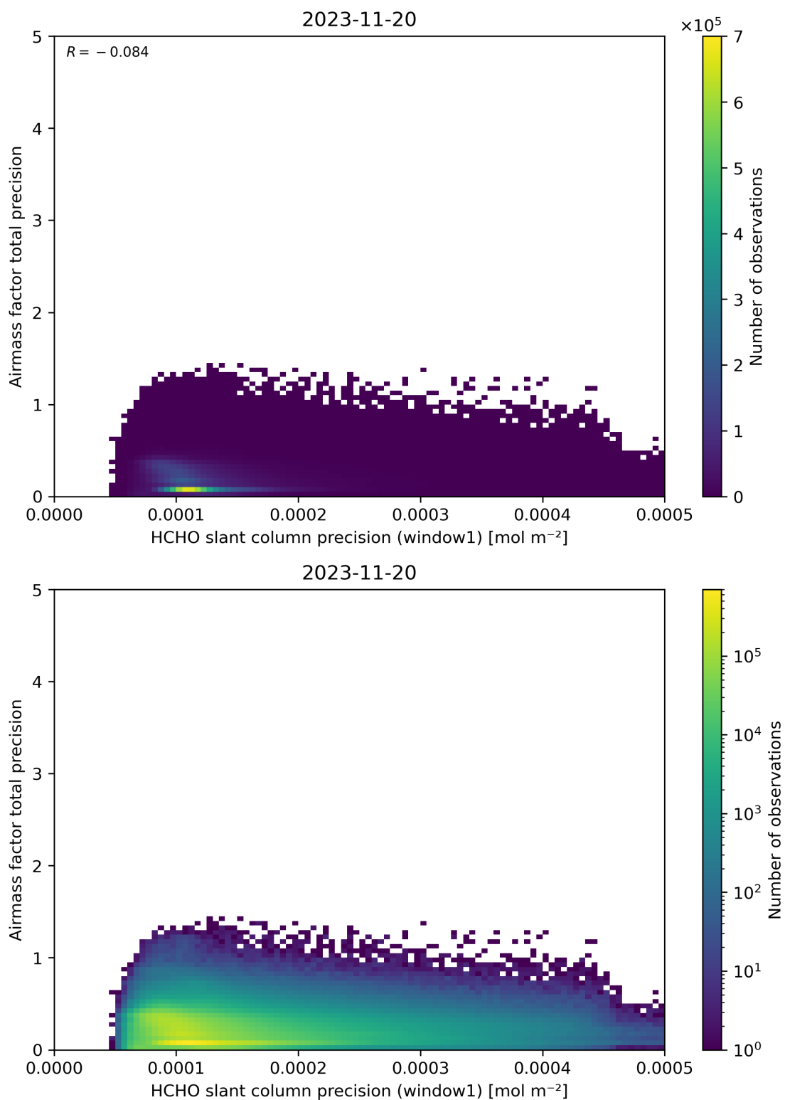
Figure 95: Scatter density plot of “HCHO slant column precision (window1)” against “Airmass factor total precision” for 2023-11-19 to 2023-11-21.
