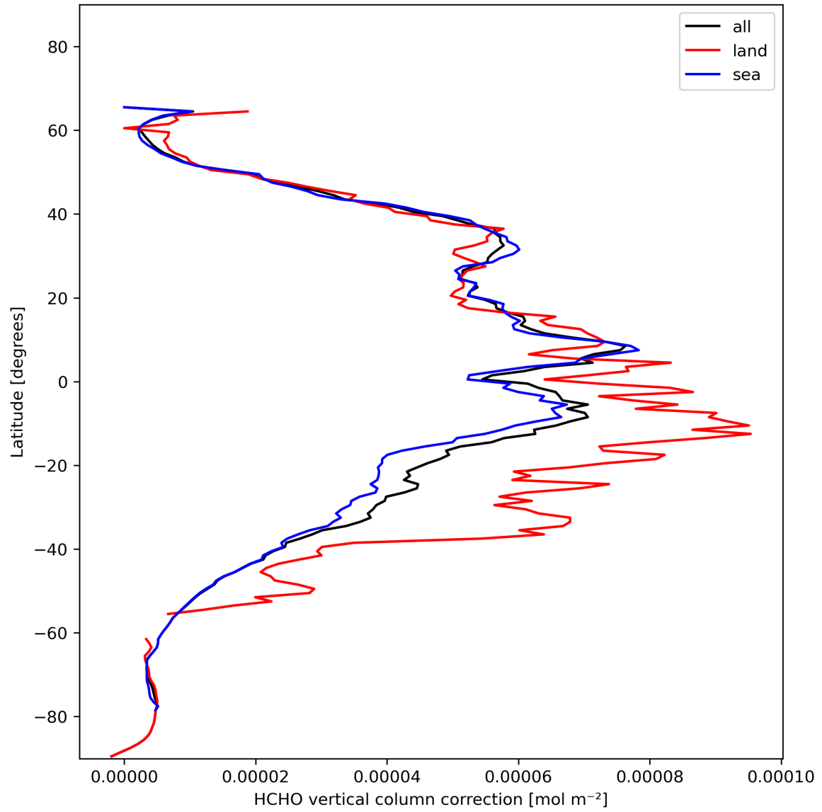
Figure 23: Zonal average of “HCHO vertical column correction” for 2023-11-19 to 2023-11-21.
