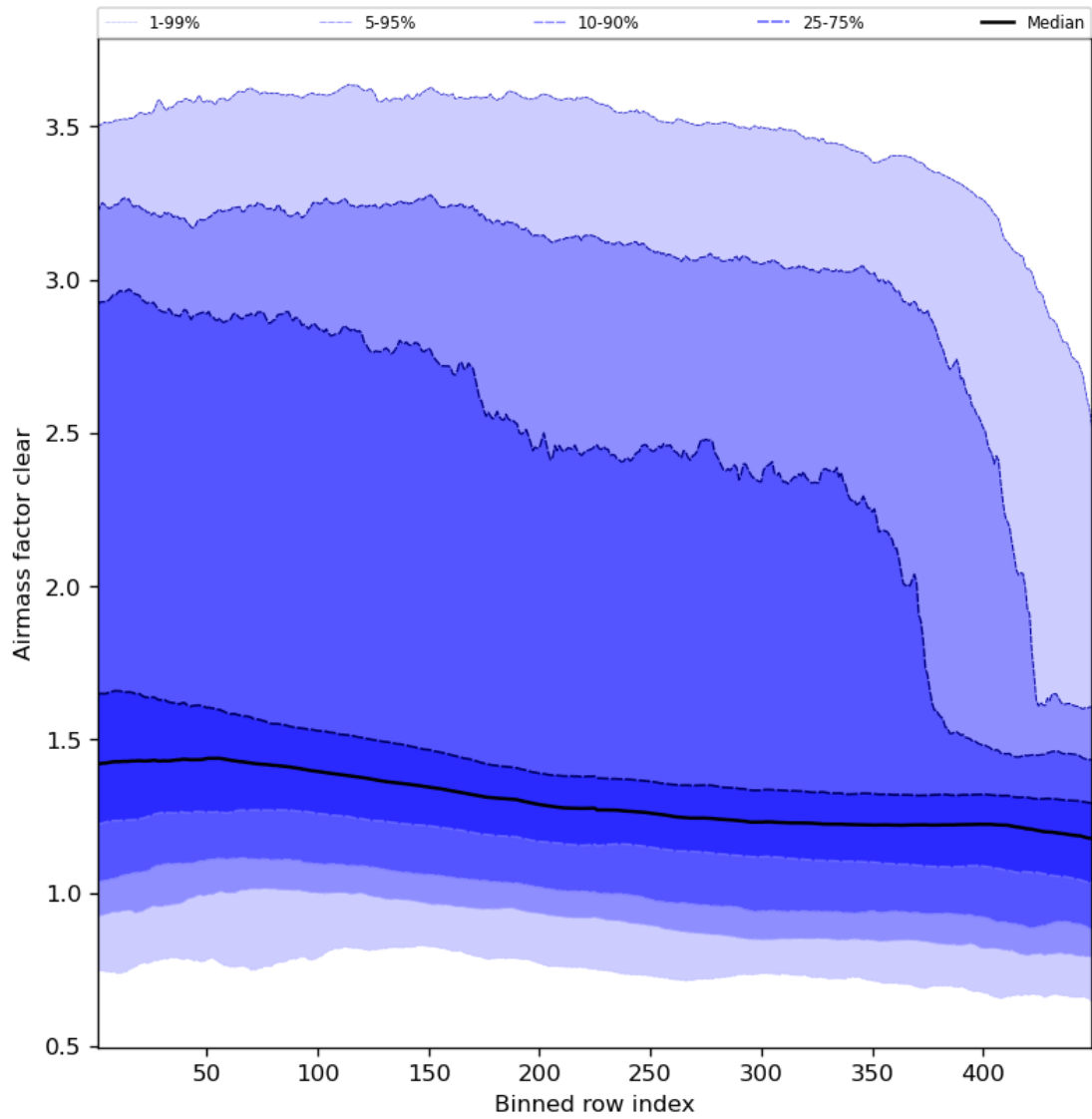
Figure 56: Along track statistics of “Airmass factor clear” for 2023-11-19 to 2023-11-21
