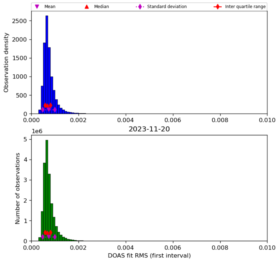
Figure 46: Histogram of “DOAS fit RMS (first interval)” for 2023-11-19 to 2023-11-21
