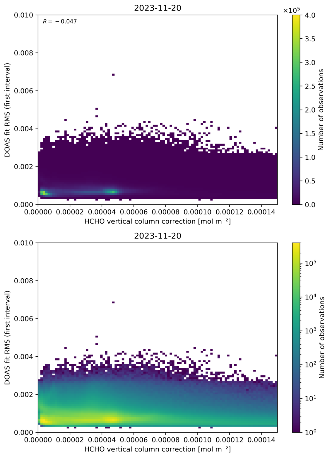
Figure 112: Scatter density plot of “HCHO vertical column correction” against “DOAS fit RMS (first interval)” for 2023-11-19 to 2023-11-21.
