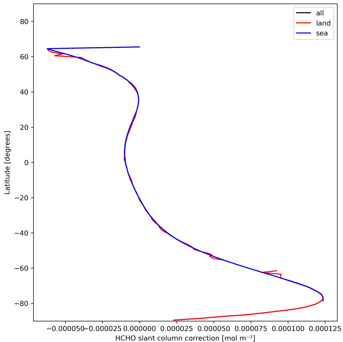
Figure 33: Zonal average of “HCHO slant column correction” for 2023-11-19 to 2023-11-21.
