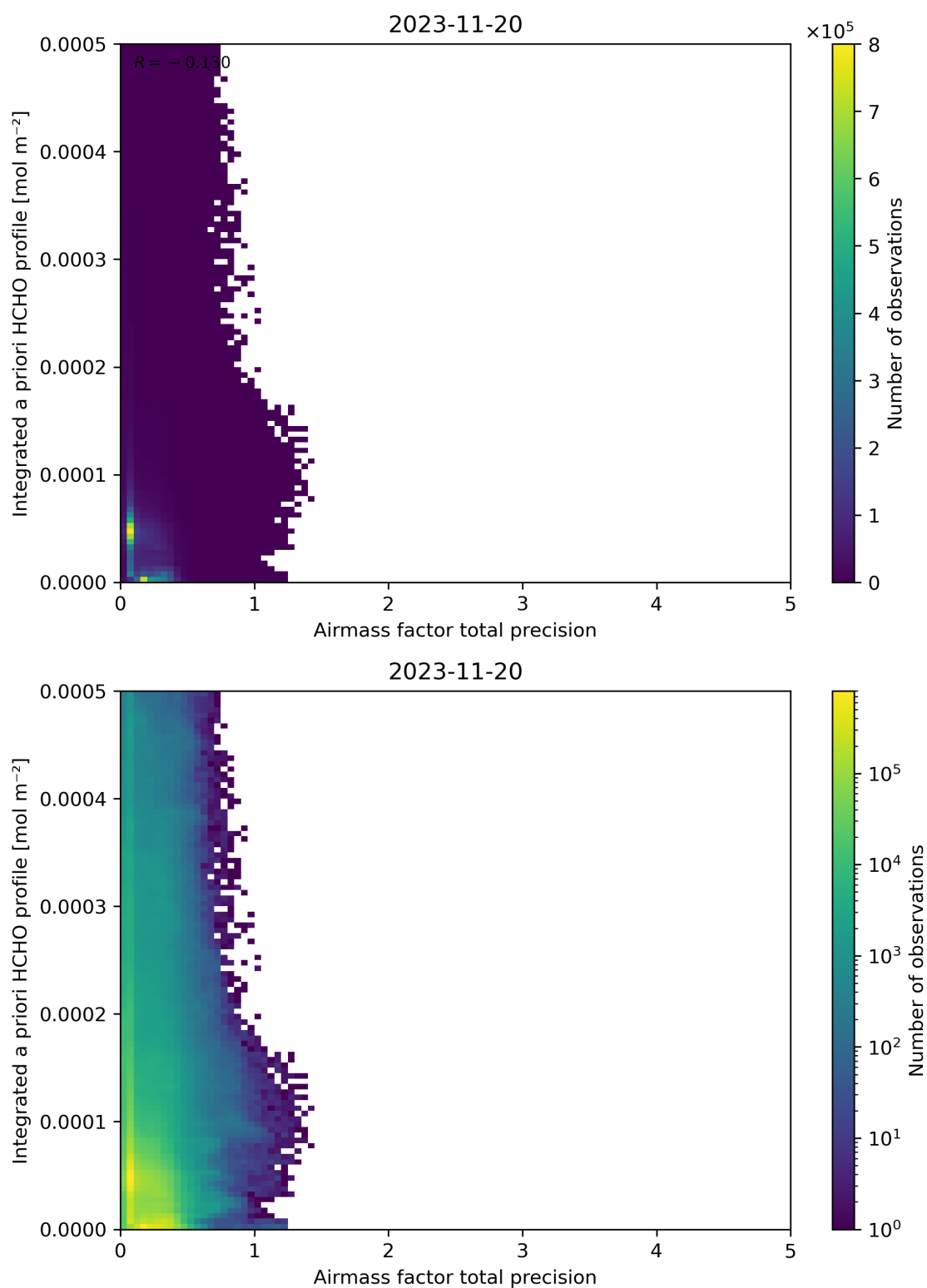
Figure 111: Scatter density plot of “Airmass factor total precision” against “Integrated a priori HCHO profile” for 2023-11-19 to 2023-11-21.
