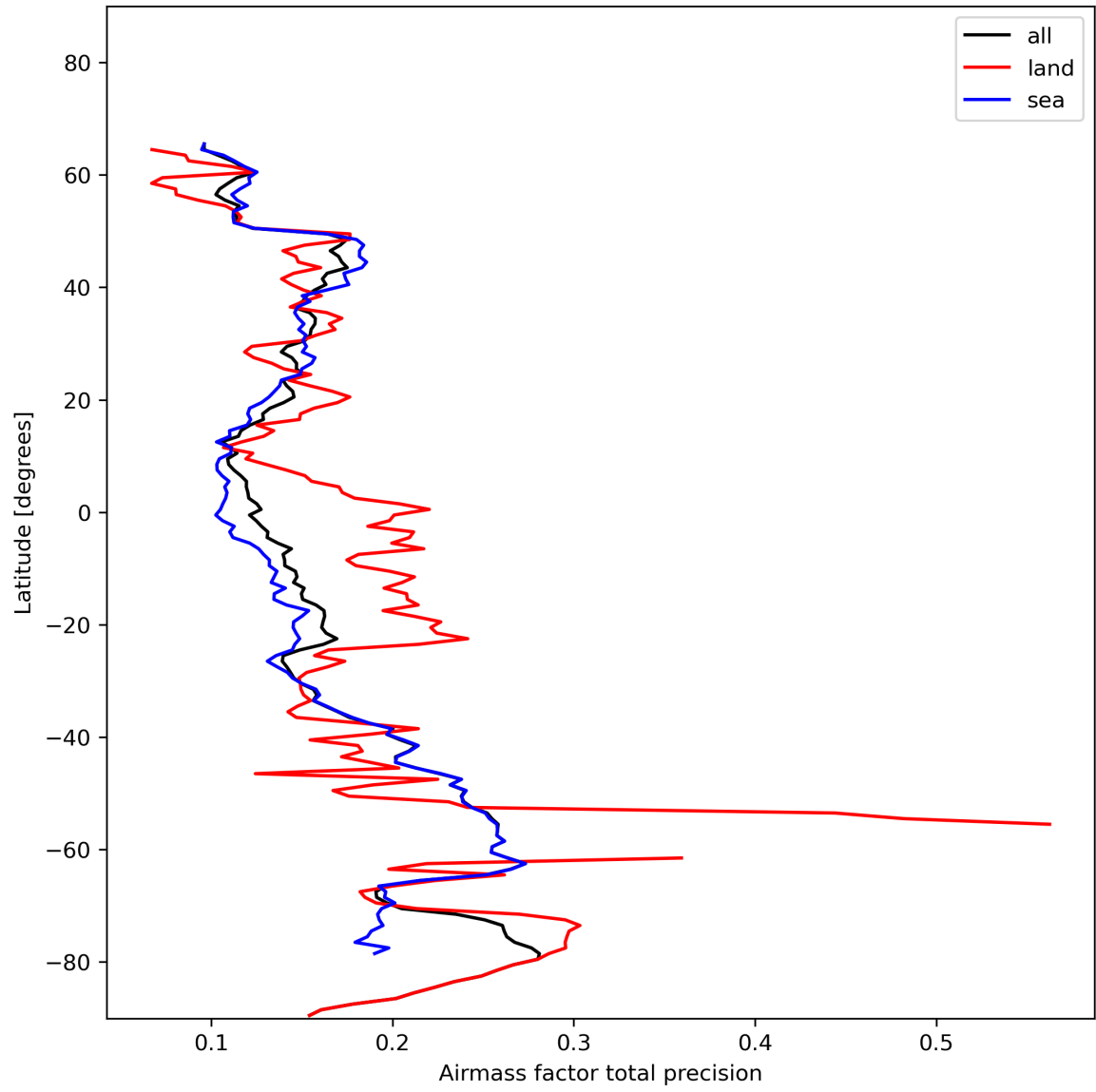
Figure 27: Zonal average of “Airmass factor total precision” for 2023-11-19 to 2023-11-21.
