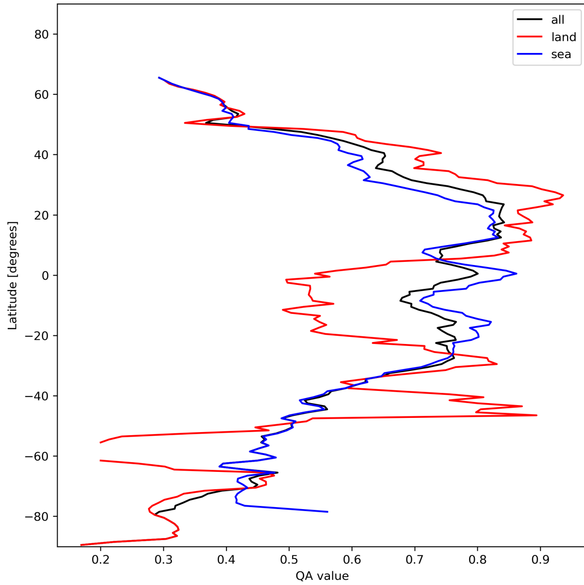
Figure 20: Zonal average of “QA value” for 2023-11-19 to 2023-11-21.
