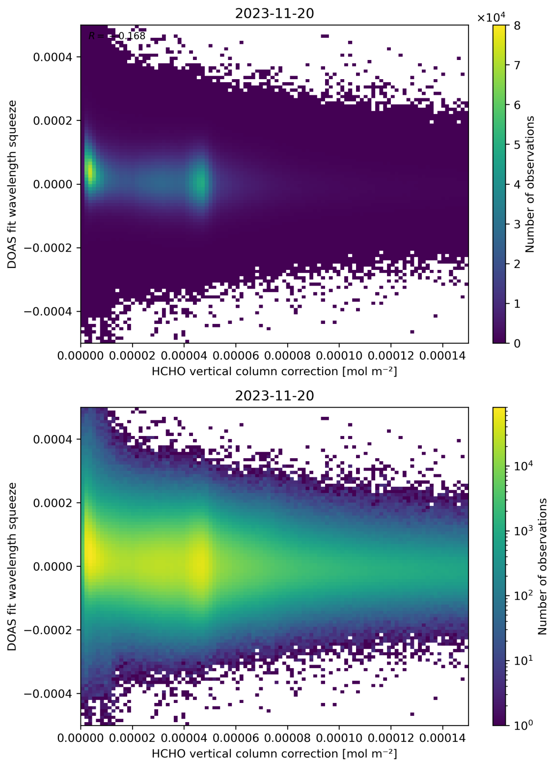
Figure 114: Scatter density plot of “HCHO vertical column correction” against “DOAS fit wavelength squeeze” for 2023-11-19 to 2023-11-21.
