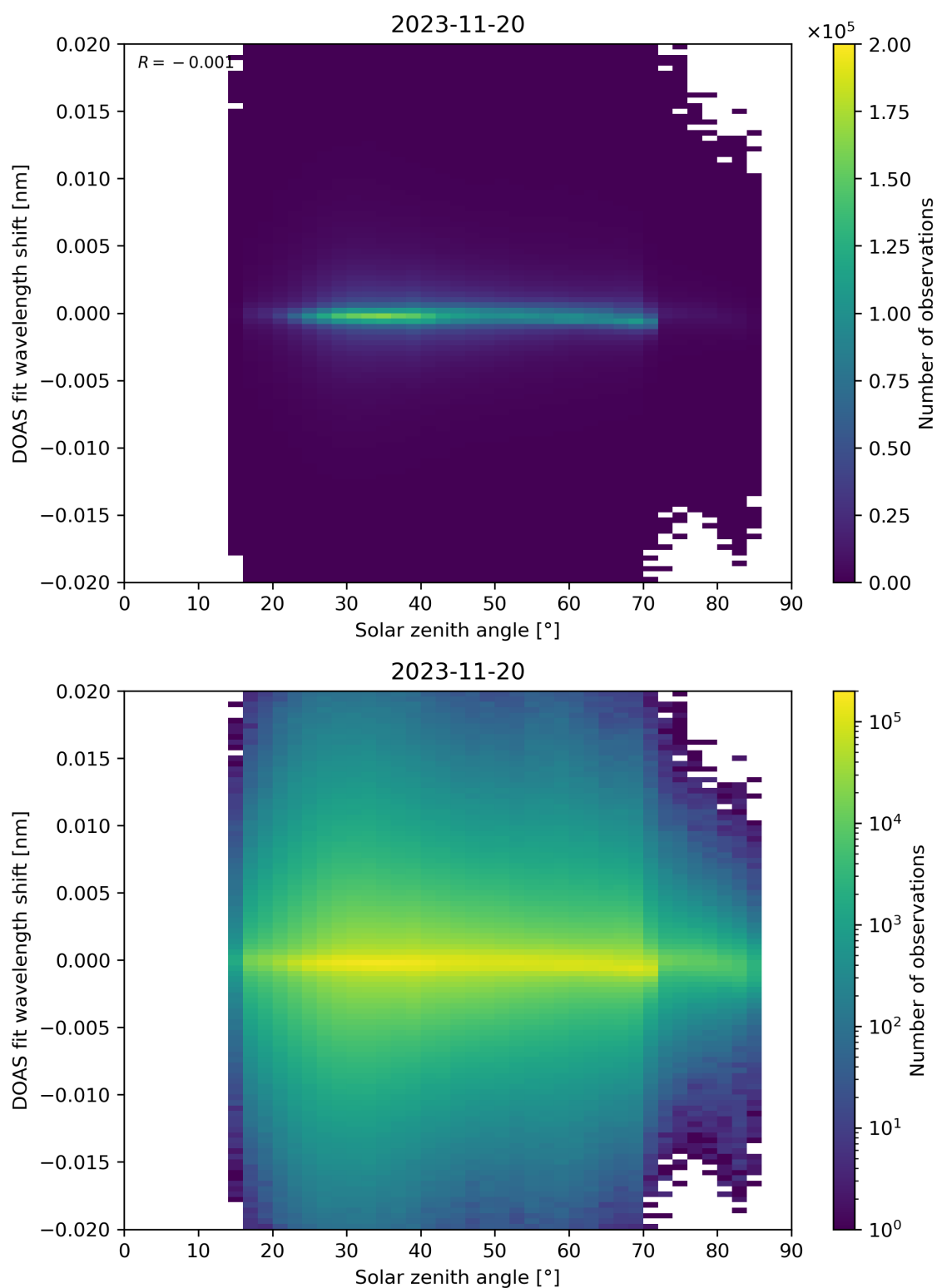
Figure 168: Scatter density plot of “Solar zenith angle” against “DOAS fit wavelength shift” for 2023-11-19 to 2023-11-21.
