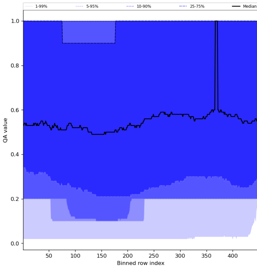
Figure 48: Along track statistics of “QA value” for 2023-11-19 to 2023-11-21
