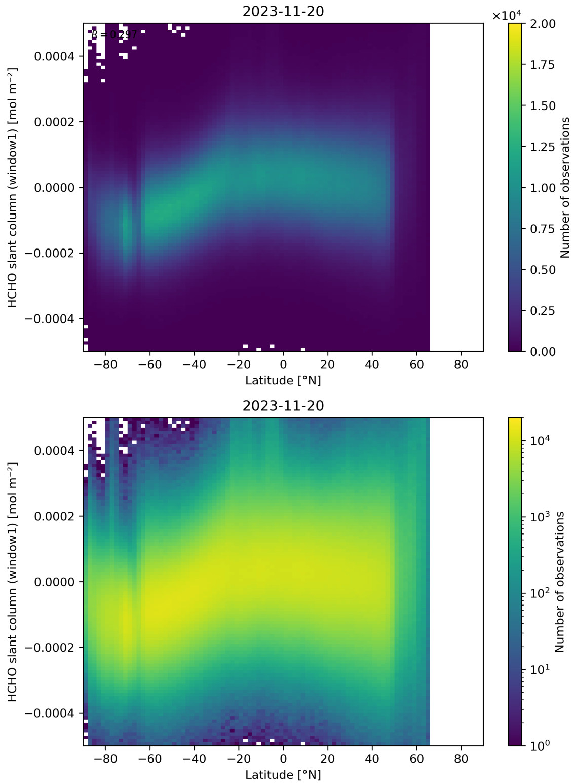
Figure 159: Scatter density plot of “Latitude” against “HCHO slant column (window1)” for 2023-11-19 to 2023-11-21.
