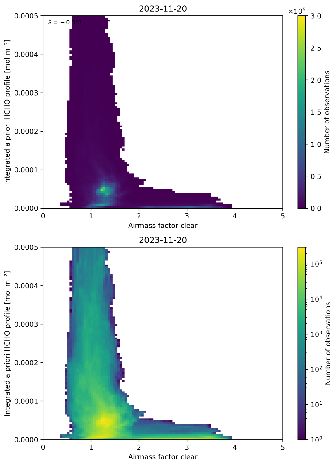
Figure 76: Scatter density plot of “Airmass factor clear” against “Integrated a priori HCHO profile” for 2023-11-19 to 2023-11-21.
