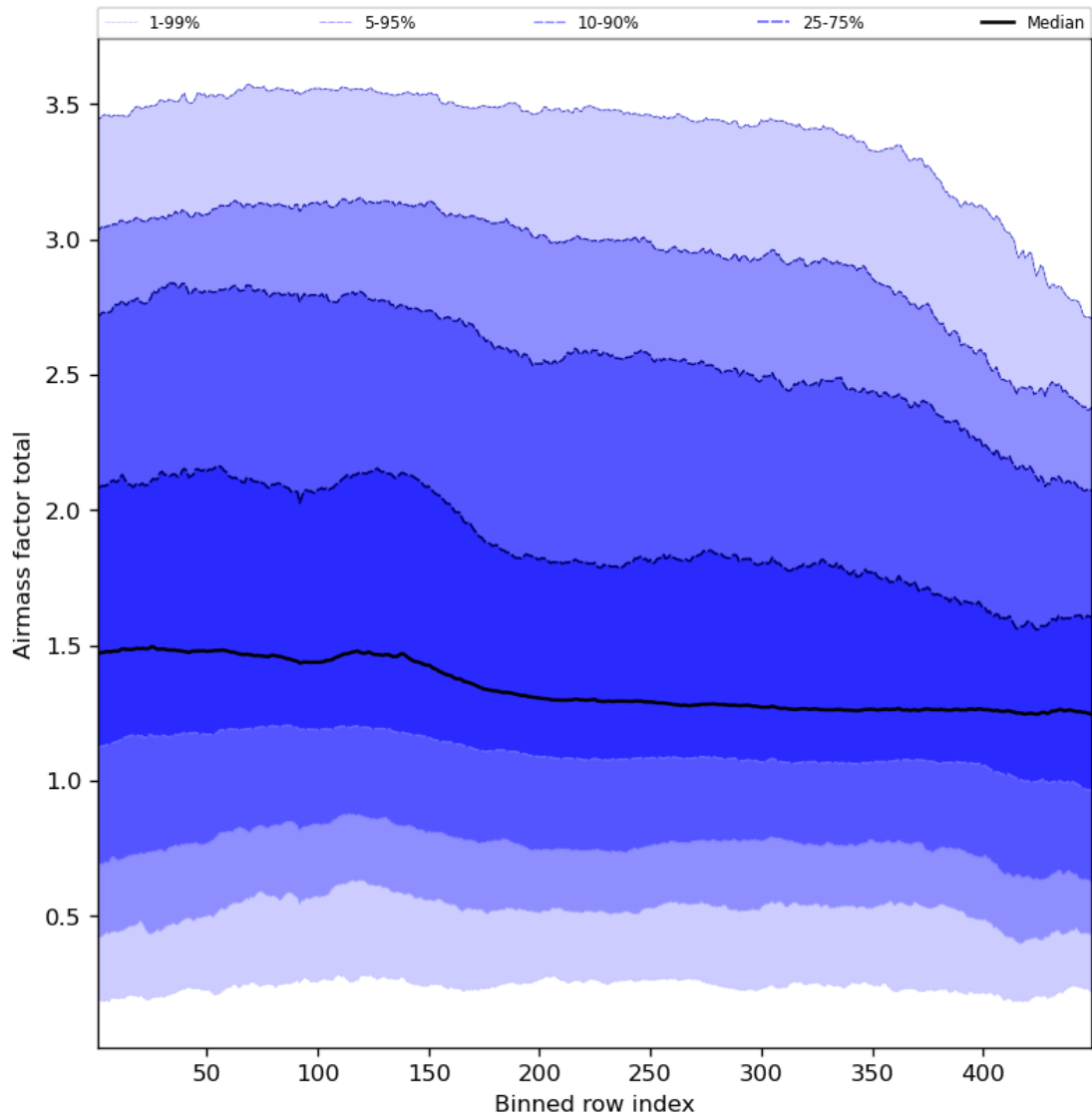
Figure 54: Along track statistics of “Airmass factor total” for 2023-11-19 to 2023-11-21
