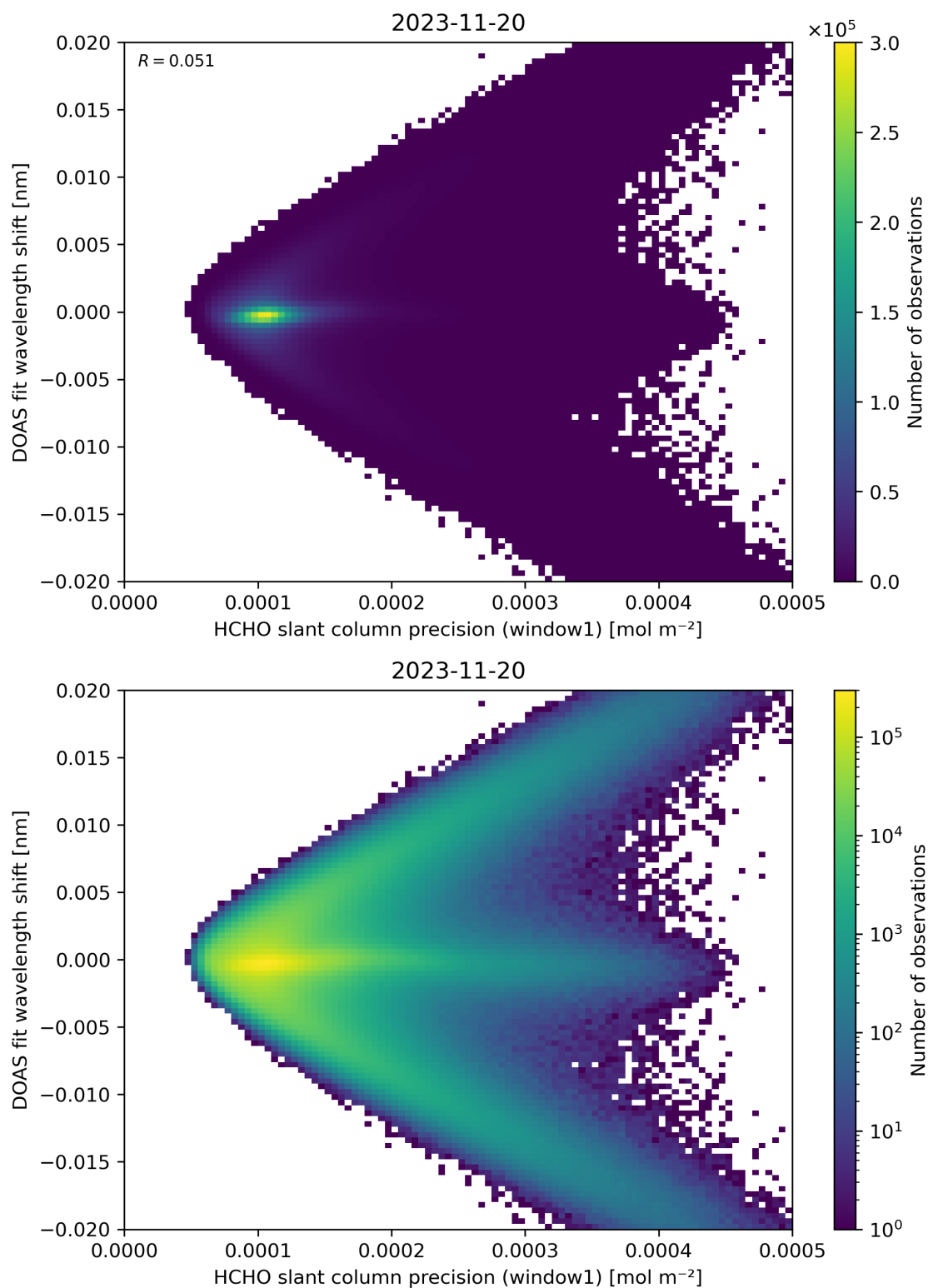
Figure 89: Scatter density plot of “HCHO slant column precision (window1)” against “DOAS fit wavelength shift” for 2023-11-19 to 2023-11-21.
