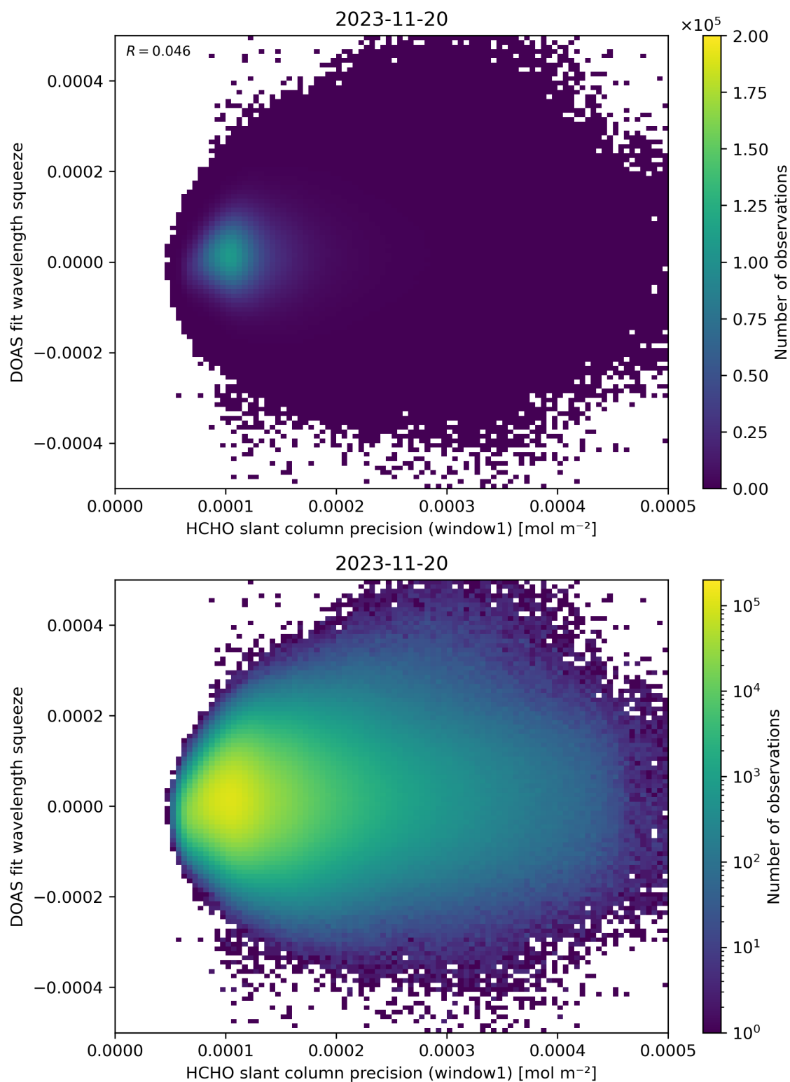
Figure 90: Scatter density plot of “HCHO slant column precision (window1)” against “DOAS fit wavelength squeeze” for 2023-11-19 to 2023-11-21.
