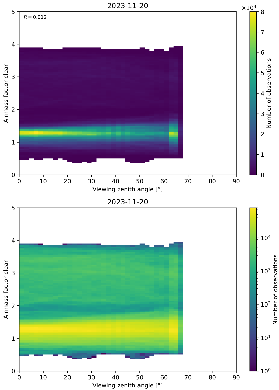
Figure 185: Scatter density plot of “Viewing zenith angle” against “Airmass factor clear” for 2023-11-19 to 2023-11-21.
