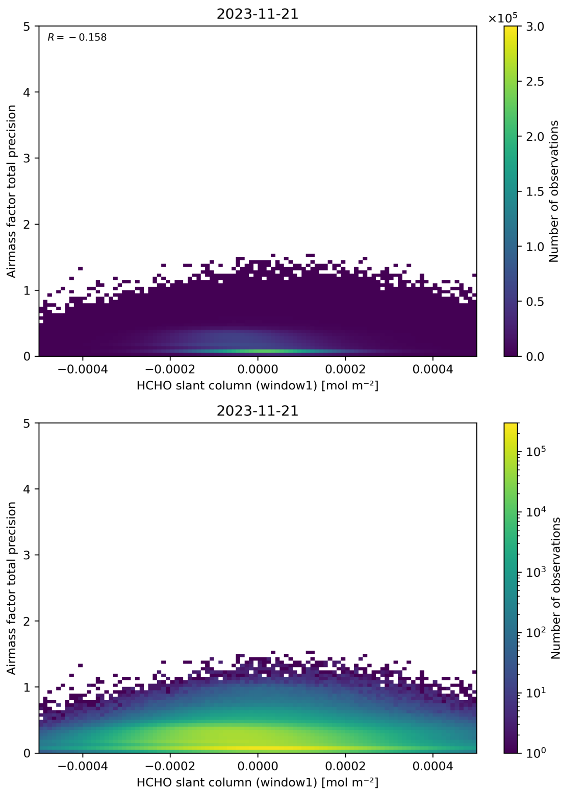
Figure 86: Scatter density plot of “HCHO slant column (window1)” against “Airmass factor total precision” for 2023-11-20 to 2023-11-22.
