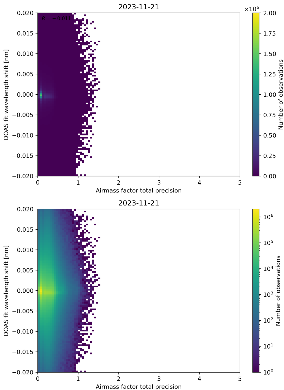
Figure 106: Scatter density plot of “Airmass factor total precision” against “DOAS fit wavelength shift” for 2023-11-20 to 2023-11-22.
