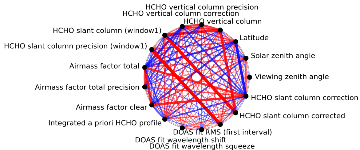
Figure 1: Map of correlation graph for 2023-11-20 to 2023-11-22.
