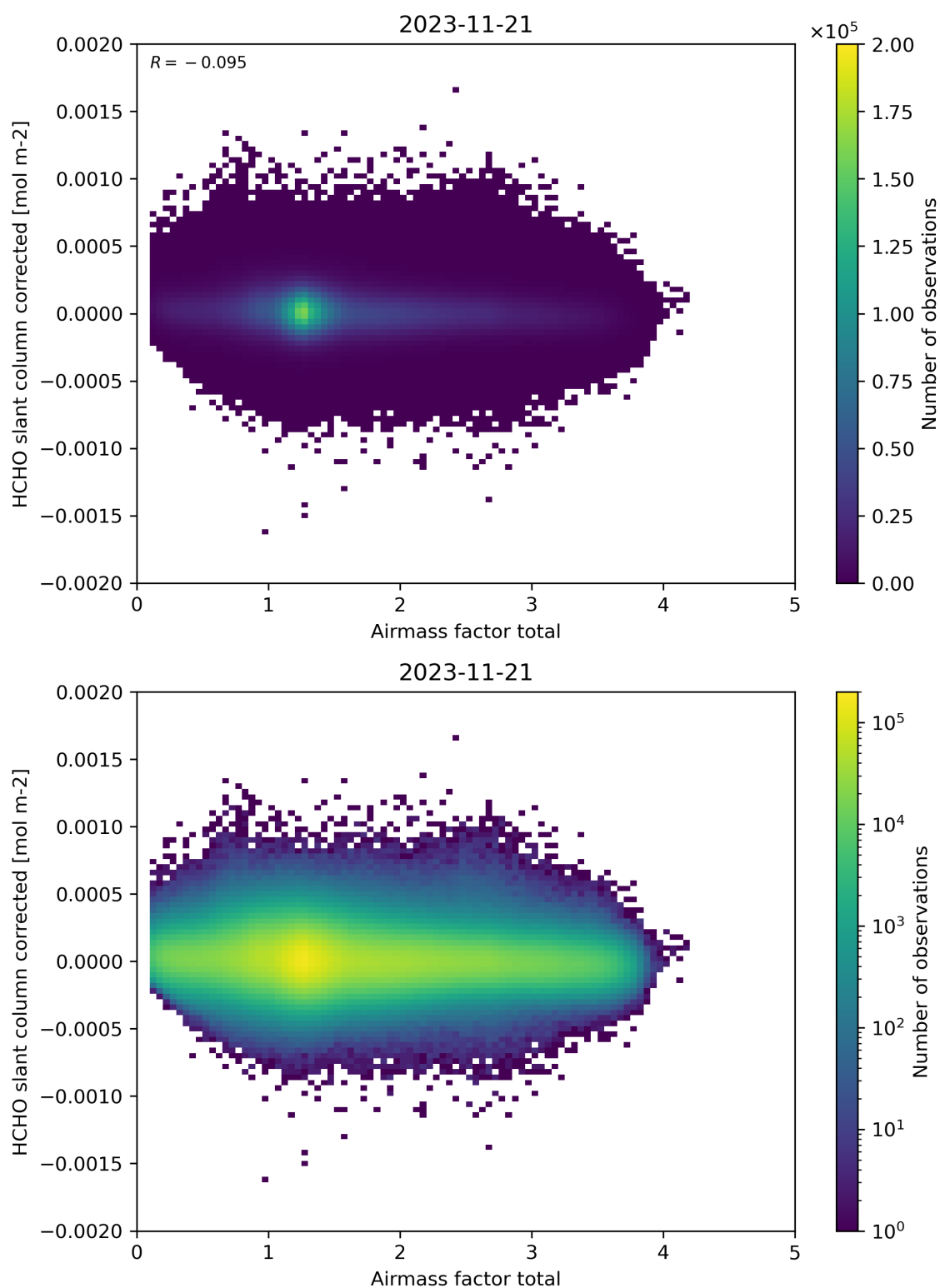
Figure 101: Scatter density plot of “Airmass factor total” against “HCHO slant column corrected” for 2023-11-20 to 2023-11-22.
