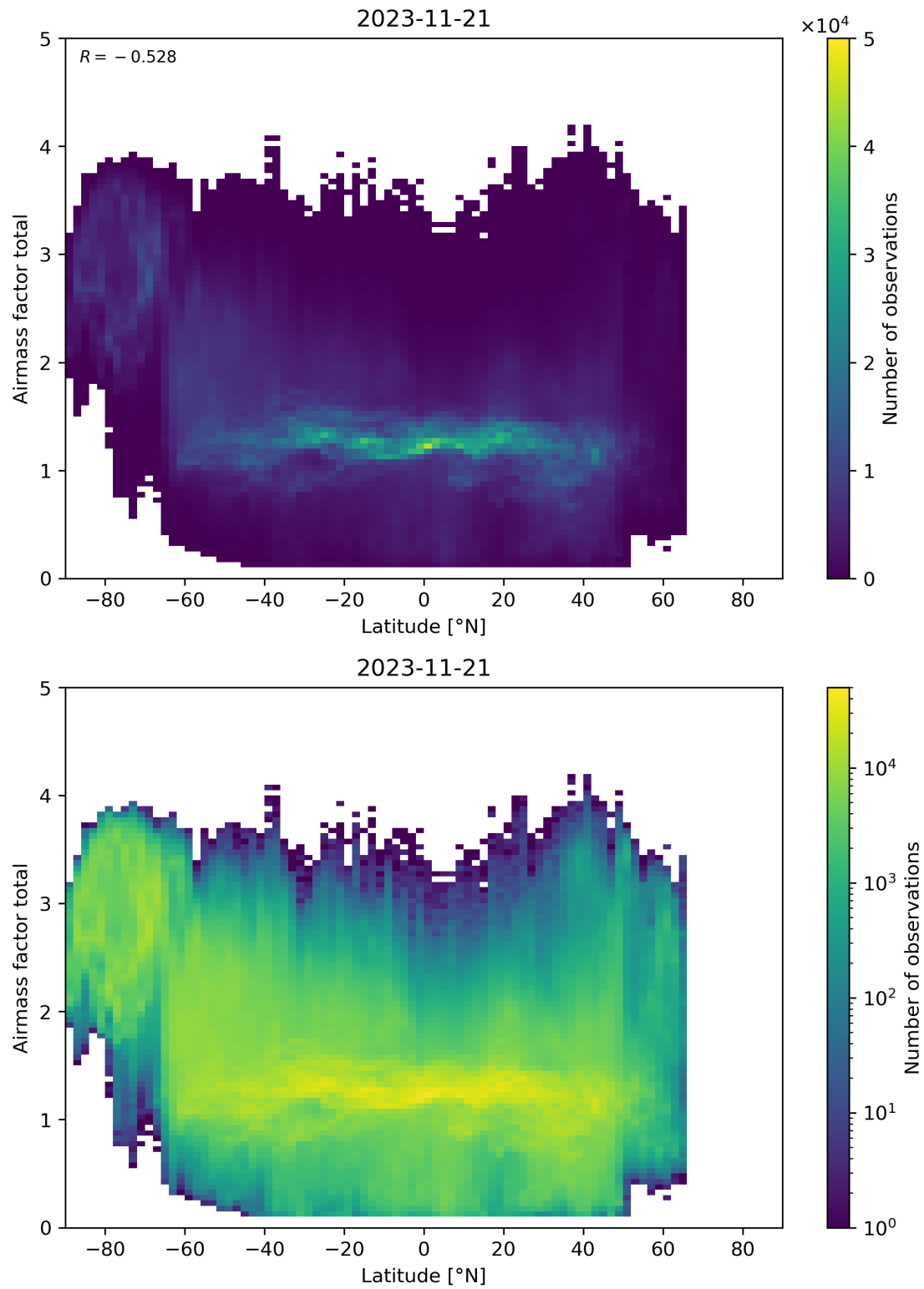
Figure 161: Scatter density plot of “Latitude” against “Airmass factor total” for 2023-11-20 to 2023-11-22.
