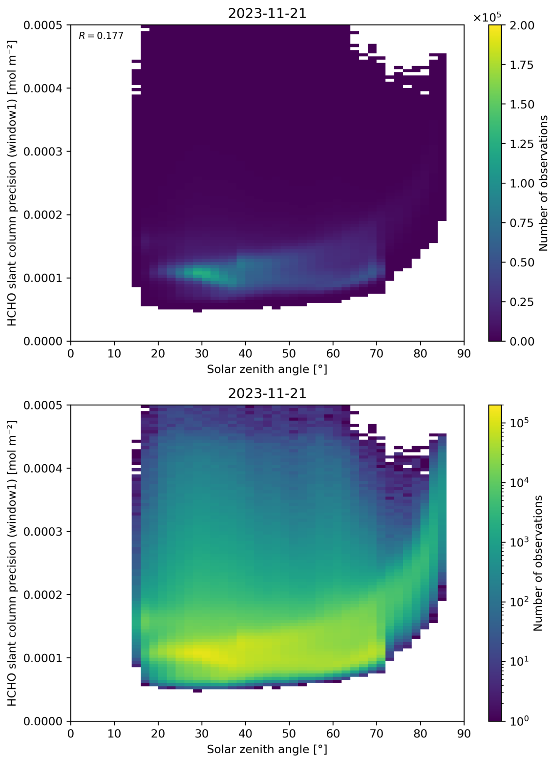
Figure 174: Scatter density plot of “Solar zenith angle” against “HCHO slant column precision (window1)” for 2023-11-20 to 2023-11-22.
