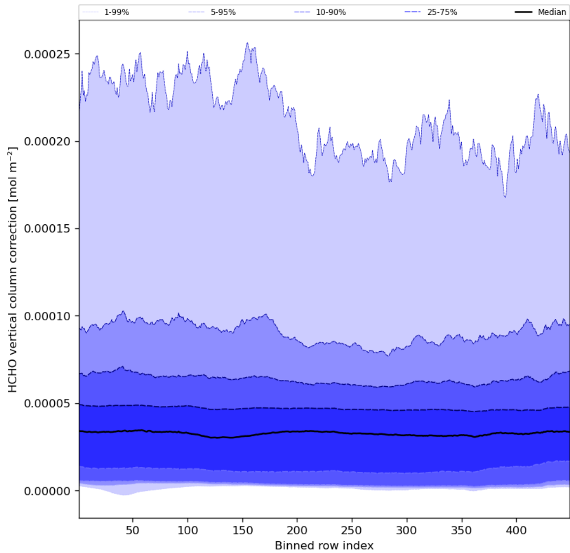
Figure 51: Along track statistics of “HCHO vertical column correction” for 2023-11-20 to 2023-11-22
