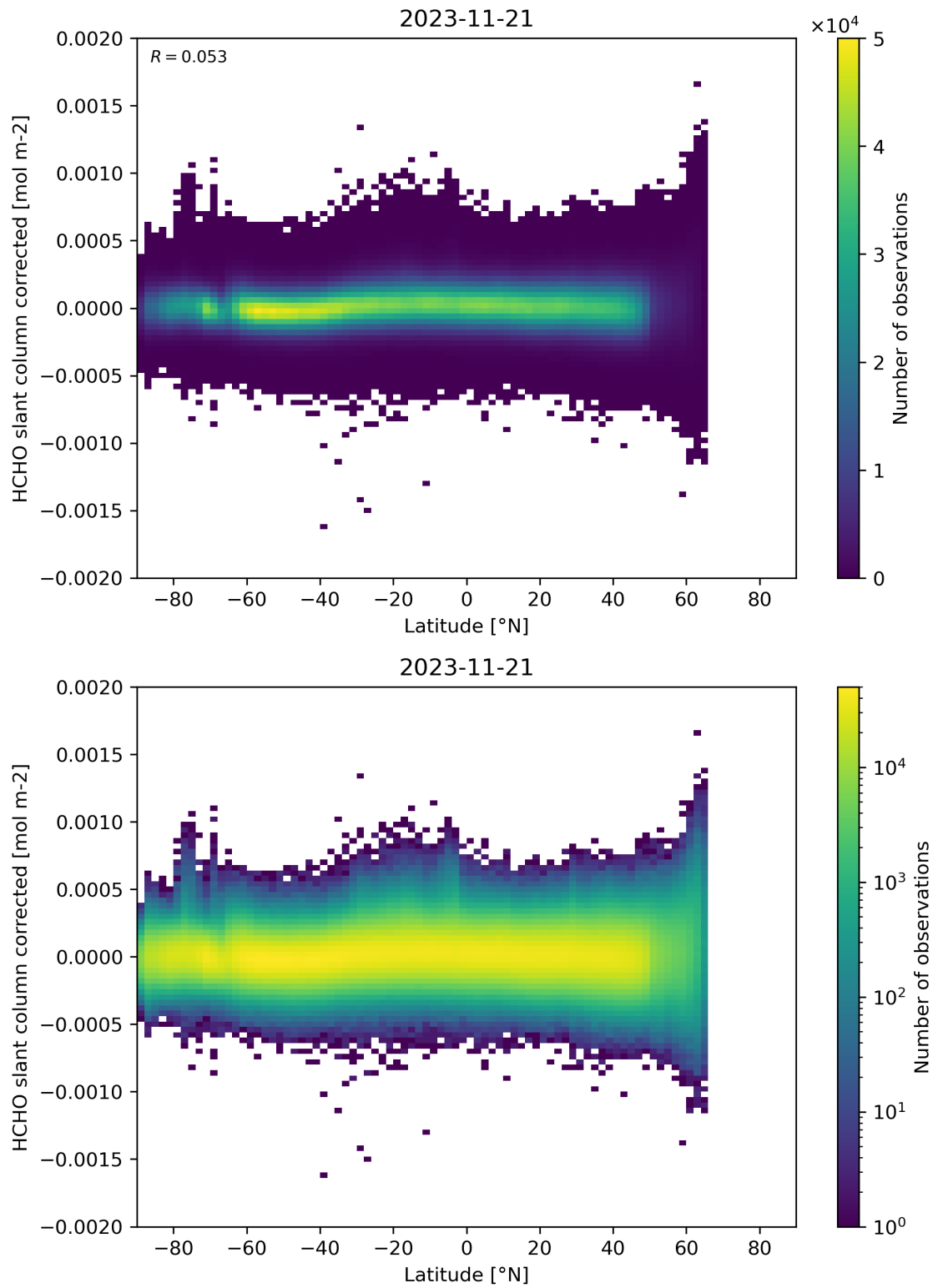
Figure 157: Scatter density plot of “Latitude” against “HCHO slant column corrected” for 2023-11-20 to 2023-11-22.
