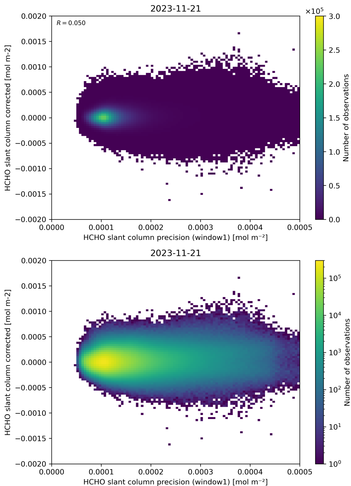
Figure 92: Scatter density plot of “HCHO slant column precision (window1)” against “HCHO slant column corrected” for 2023-11-20 to 2023-11-22.
