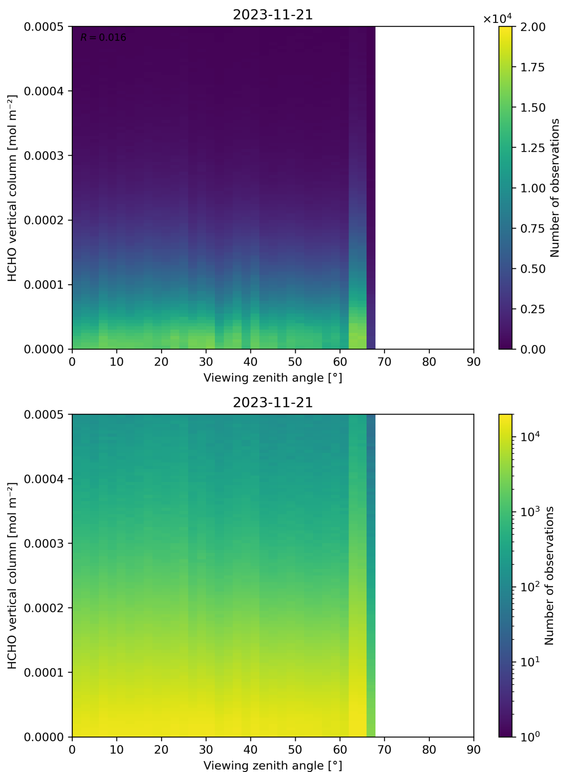
Figure 192: Scatter density plot of “Viewing zenith angle” against “HCHO vertical column” for 2023-11-20 to 2023-11-22.
