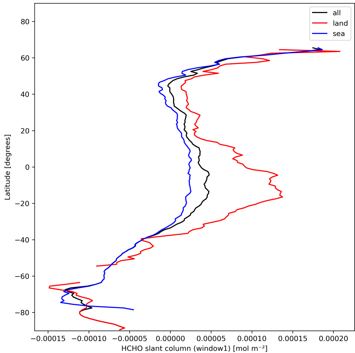
Figure 24: Zonal average of “HCHO slant column (window1)” for 2023-11-20 to 2023-11-22.
