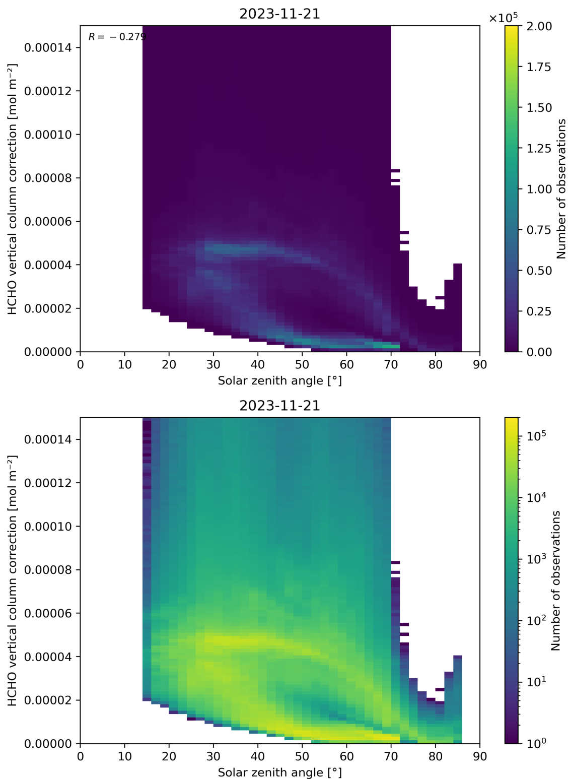
Figure 178: Scatter density plot of “Solar zenith angle” against “HCHO vertical column correction” for 2023-11-20 to 2023-11-22.
