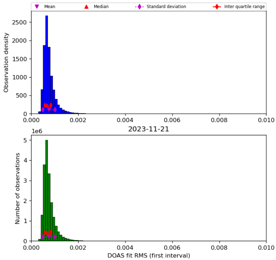
Figure 46: Histogram of “DOAS fit RMS (first interval)” for 2023-11-20 to 2023-11-22
