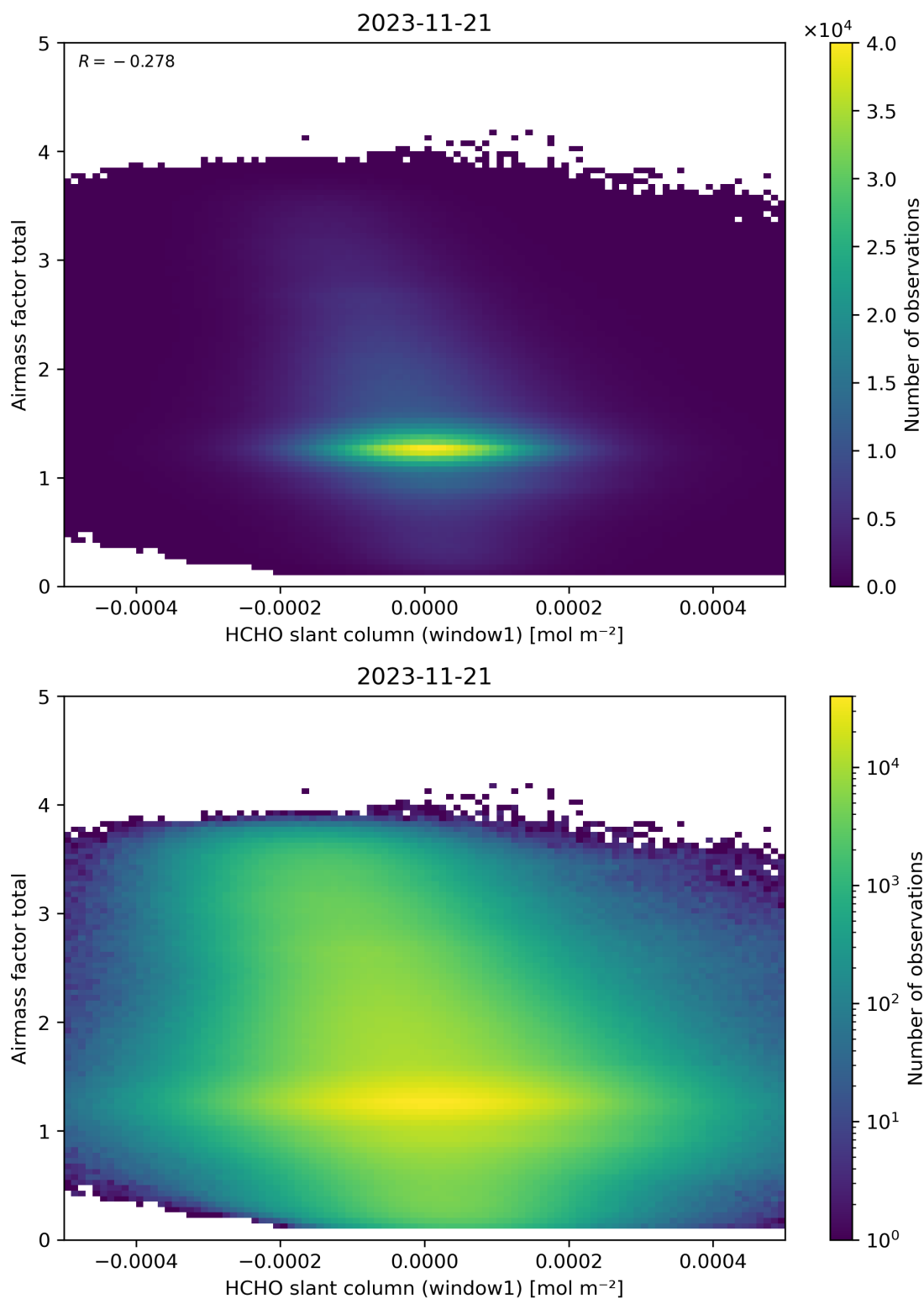
Figure 85: Scatter density plot of “HCHO slant column (window1)” against “Airmass factor total” for 2023-11-20 to 2023-11-22.
