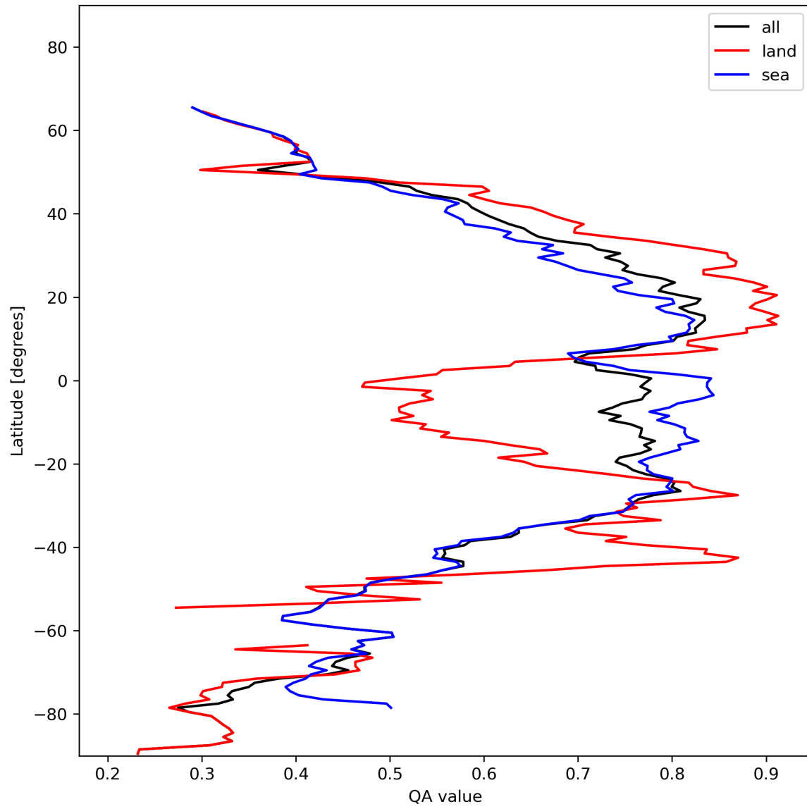
Figure 20: Zonal average of “QA value” for 2023-11-20 to 2023-11-22.
