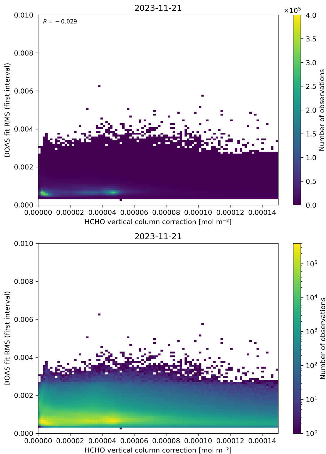
Figure 112: Scatter density plot of “HCHO vertical column correction” against “DOAS fit RMS (first interval)” for 2023-11-20 to 2023-11-22.
