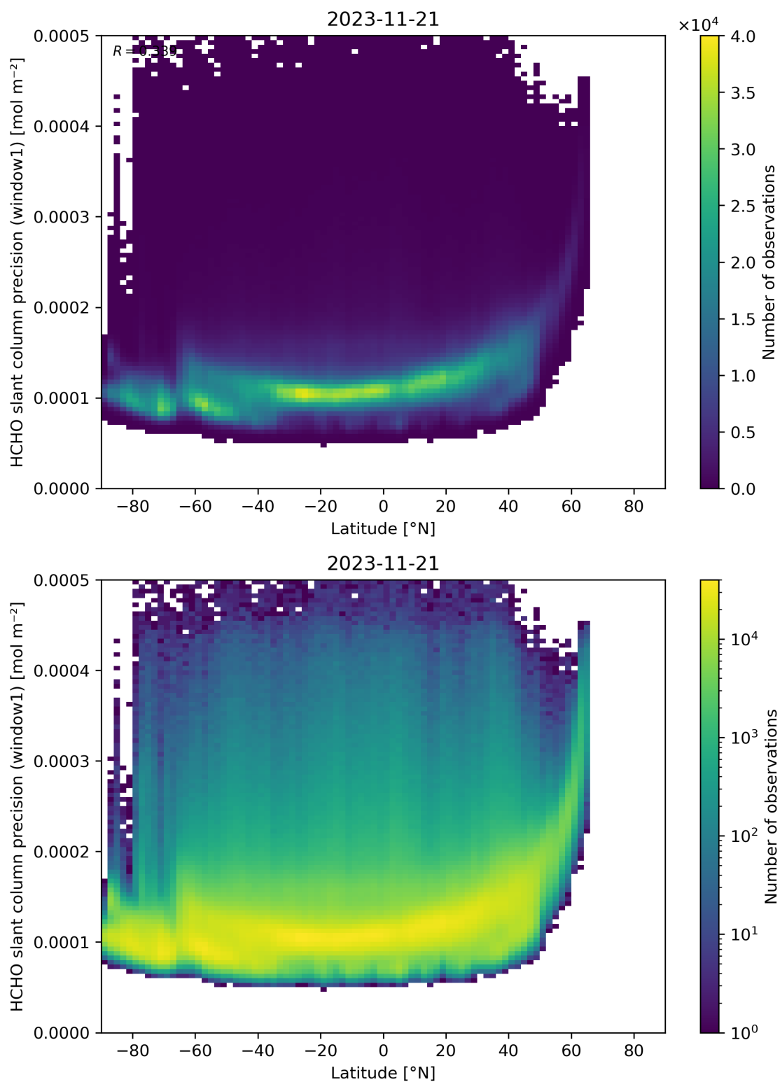
Figure 160: Scatter density plot of “Latitude” against “HCHO slant column precision (window1)” for 2023-11-20 to 2023-11-22.
