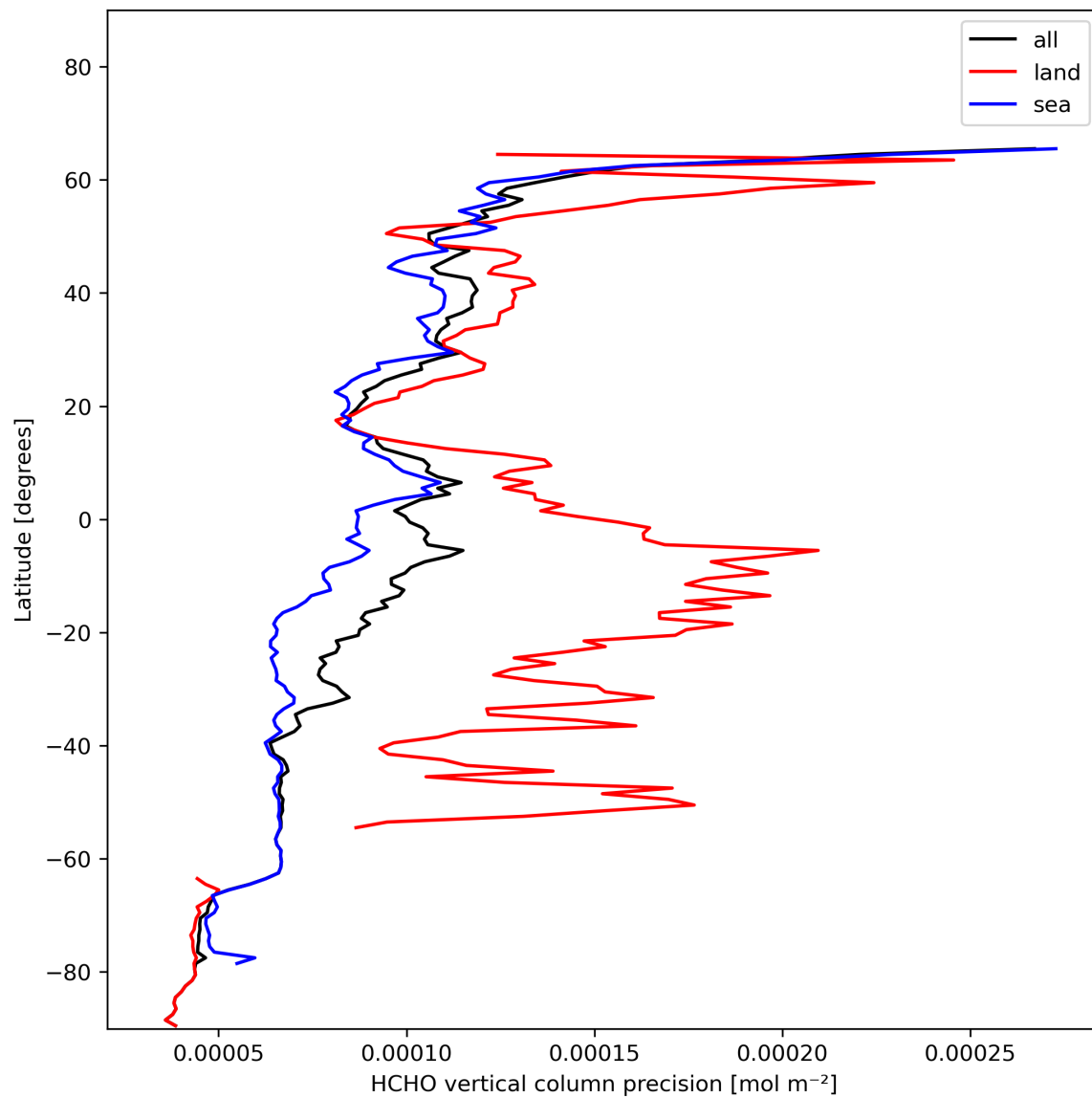
Figure 22: Zonal average of “HCHO vertical column precision” for 2023-11-20 to 2023-11-22.
