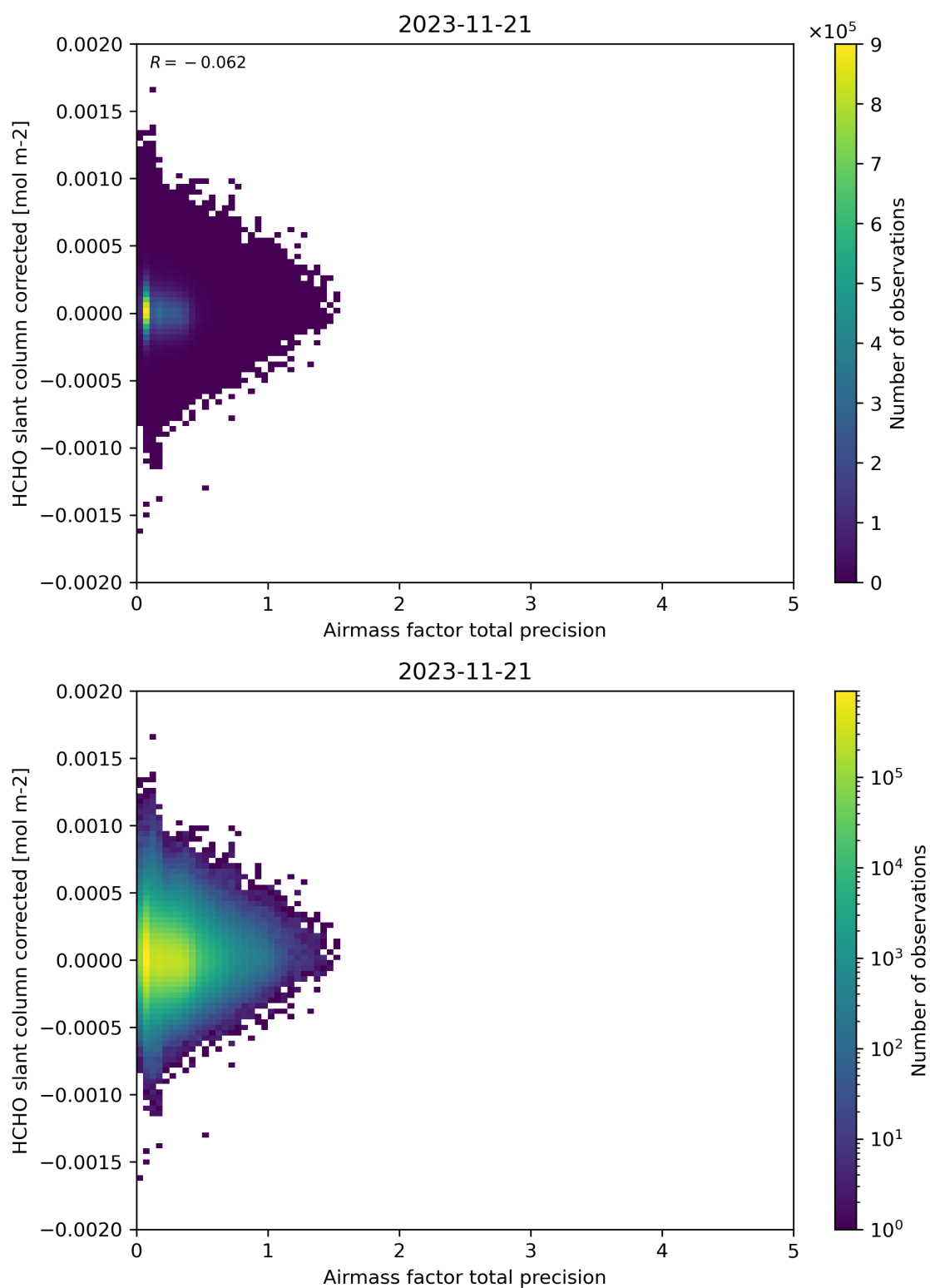
Figure 109: Scatter density plot of “Airmass factor total precision” against “HCHO slant column corrected” for 2023-11-20 to 2023-11-22.
