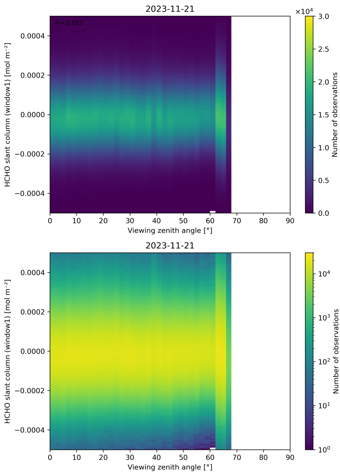
Figure 188: Scatter density plot of “Viewing zenith angle” against “HCHO slant column (window1)” for 2023-11-20 to 2023-11-22.
