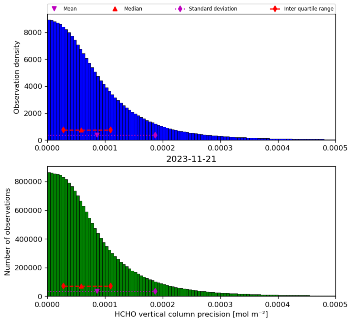
Figure 36: Histogram of “HCHO vertical column precision” for 2023-11-20 to 2023-11-22
