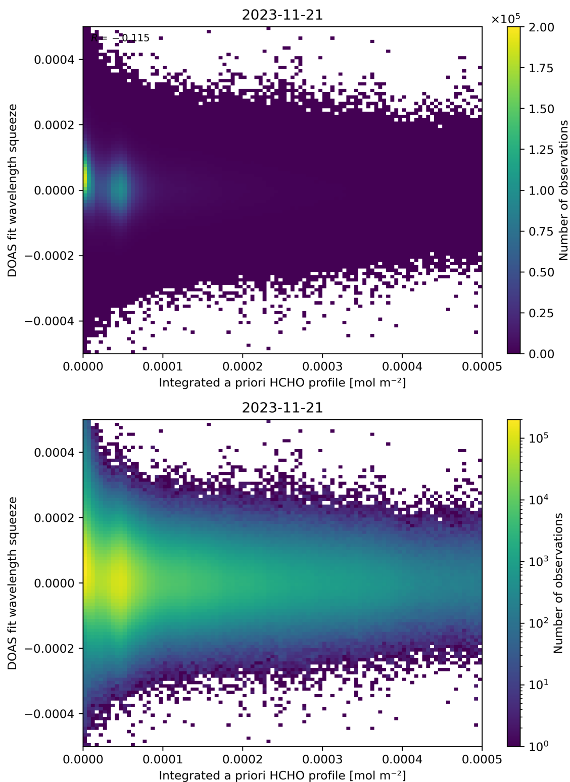
Figure 150: Scatter density plot of “Integrated a priori HCHO profile” against “DOAS fit wavelength squeeze” for 2023-11-20 to 2023-11-22.
