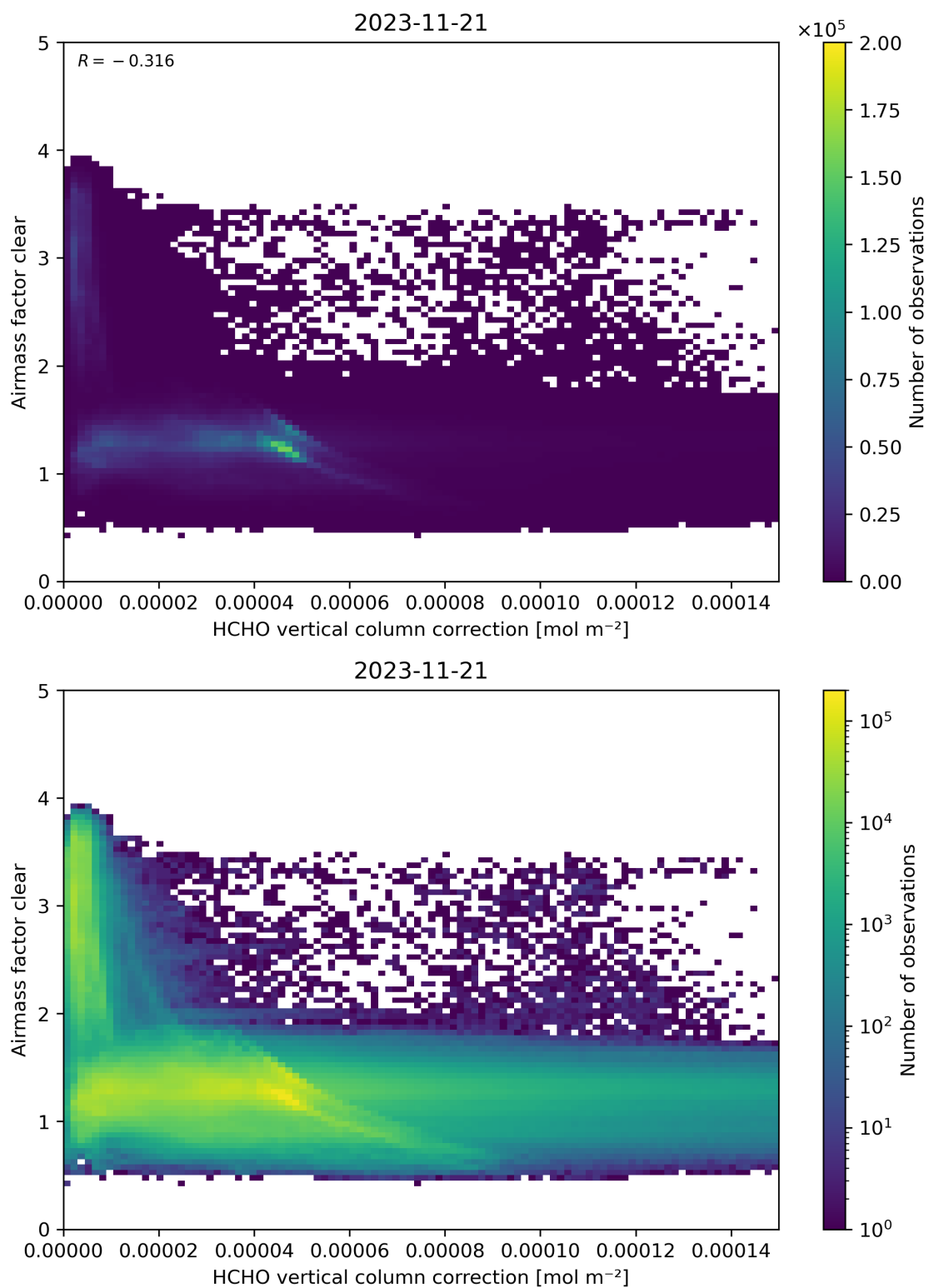
Figure 115: Scatter density plot of “HCHO vertical column correction” against “Airmass factor clear” for 2023-11-20 to 2023-11-22.
