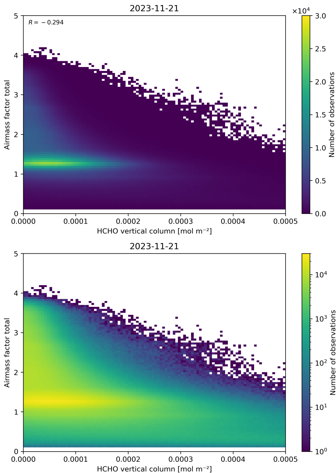
Figure 131: Scatter density plot of “HCHO vertical column” against “Airmass factor total” for 2023-11-20 to 2023-11-22.
