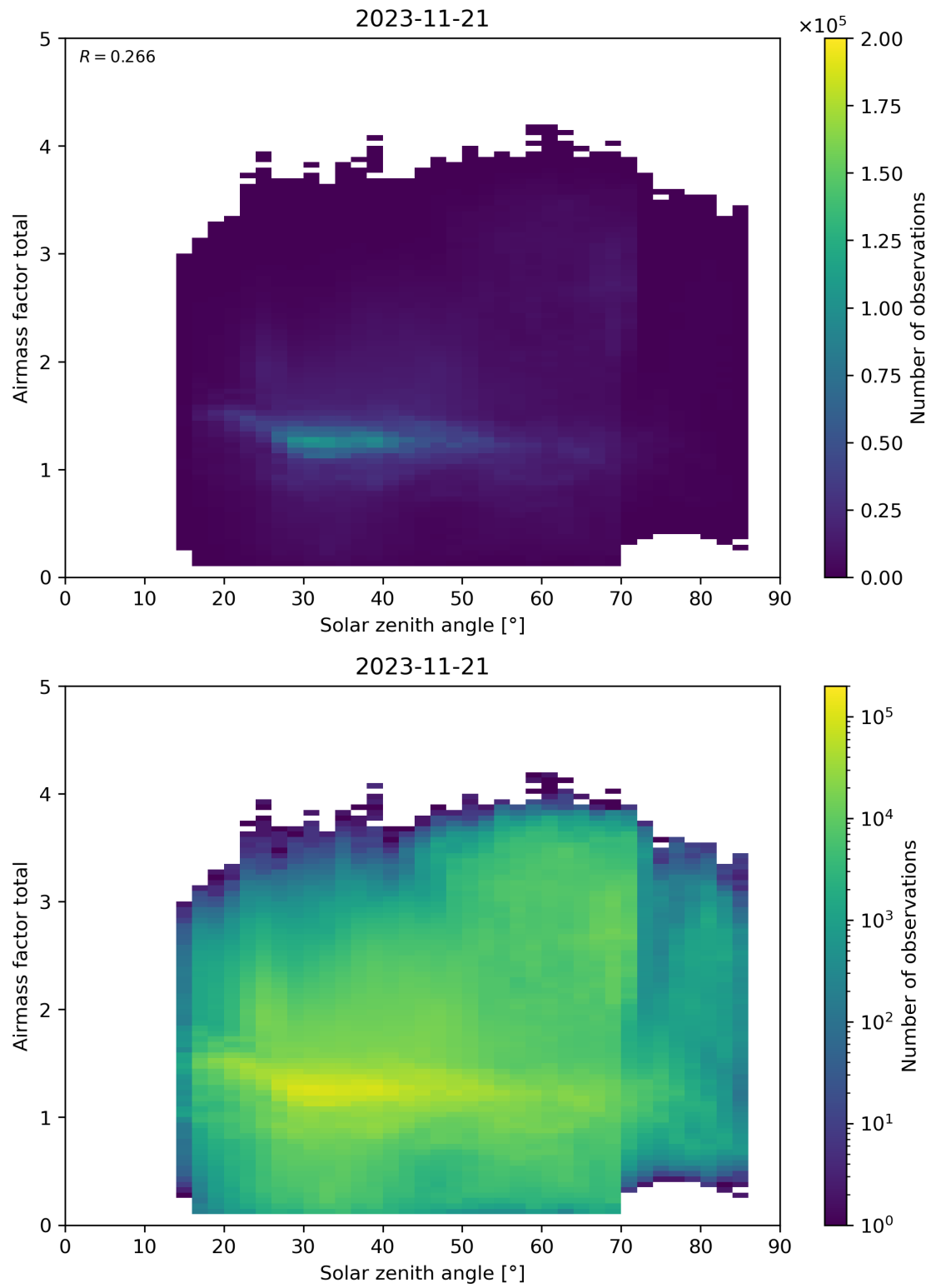
Figure 175: Scatter density plot of “Solar zenith angle” against “Airmass factor total” for 2023-11-20 to 2023-11-22.
