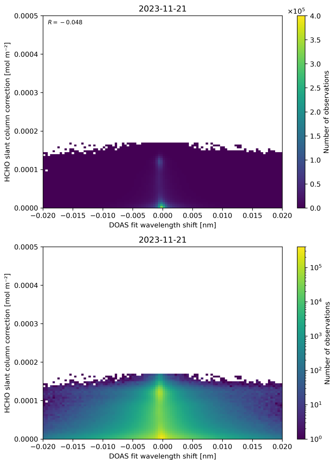
Figure 67: Scatter density plot of “DOAS fit wavelength shift” against “HCHO slant column correction” for 2023-11-20 to 2023-11-22.
