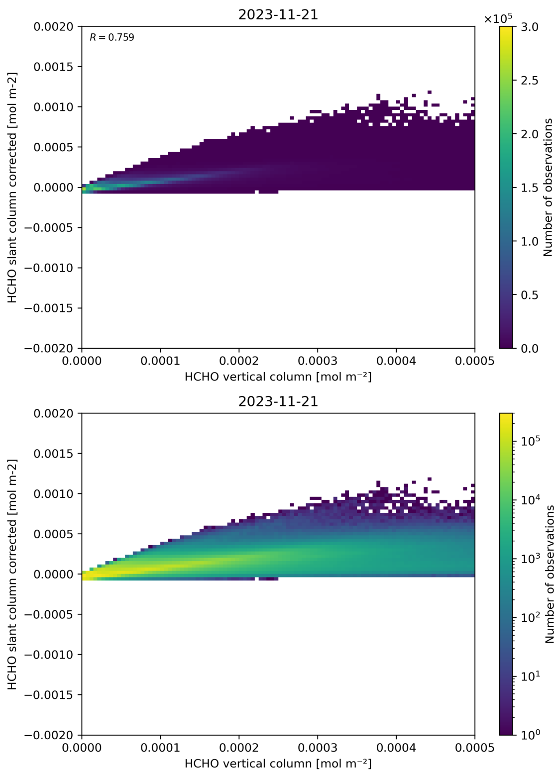
Figure 127: Scatter density plot of “HCHO vertical column” against “HCHO slant column corrected” for 2023-11-20 to 2023-11-22.
