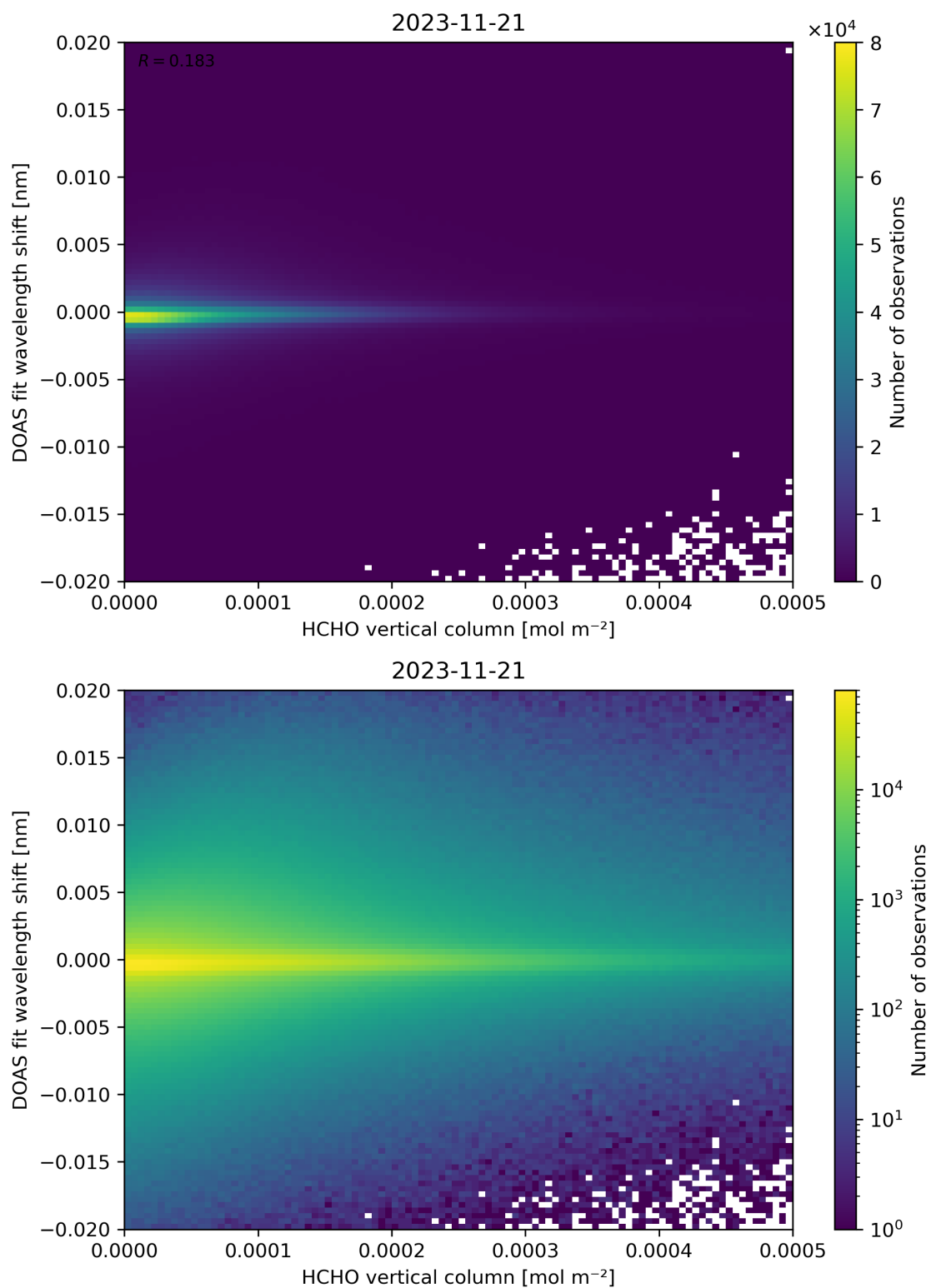
Figure 124: Scatter density plot of “HCHO vertical column” against “DOAS fit wavelength shift” for 2023-11-20 to 2023-11-22.
