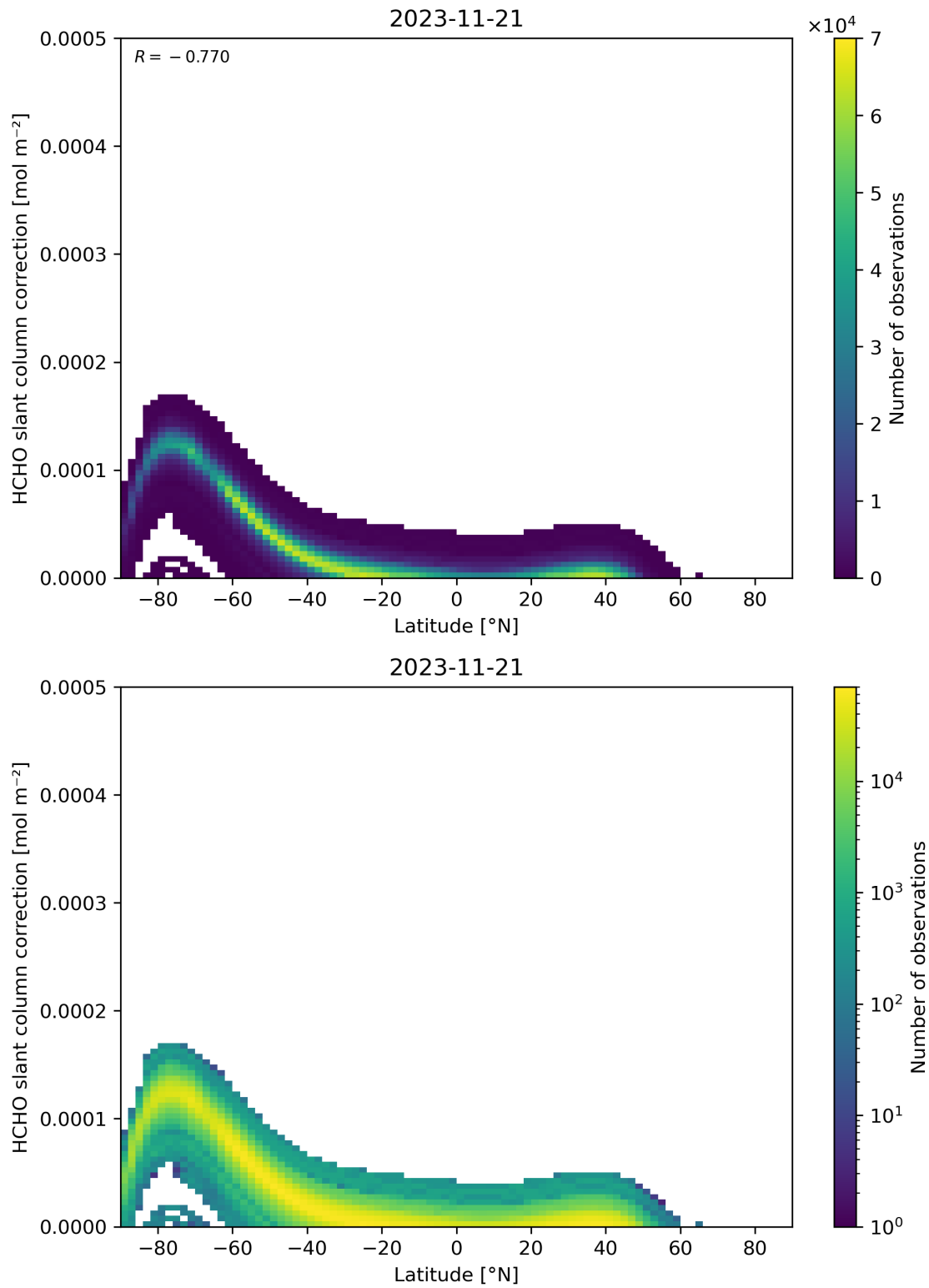
Figure 158: Scatter density plot of “Latitude” against “HCHO slant column correction” for 2023-11-20 to 2023-11-22.
