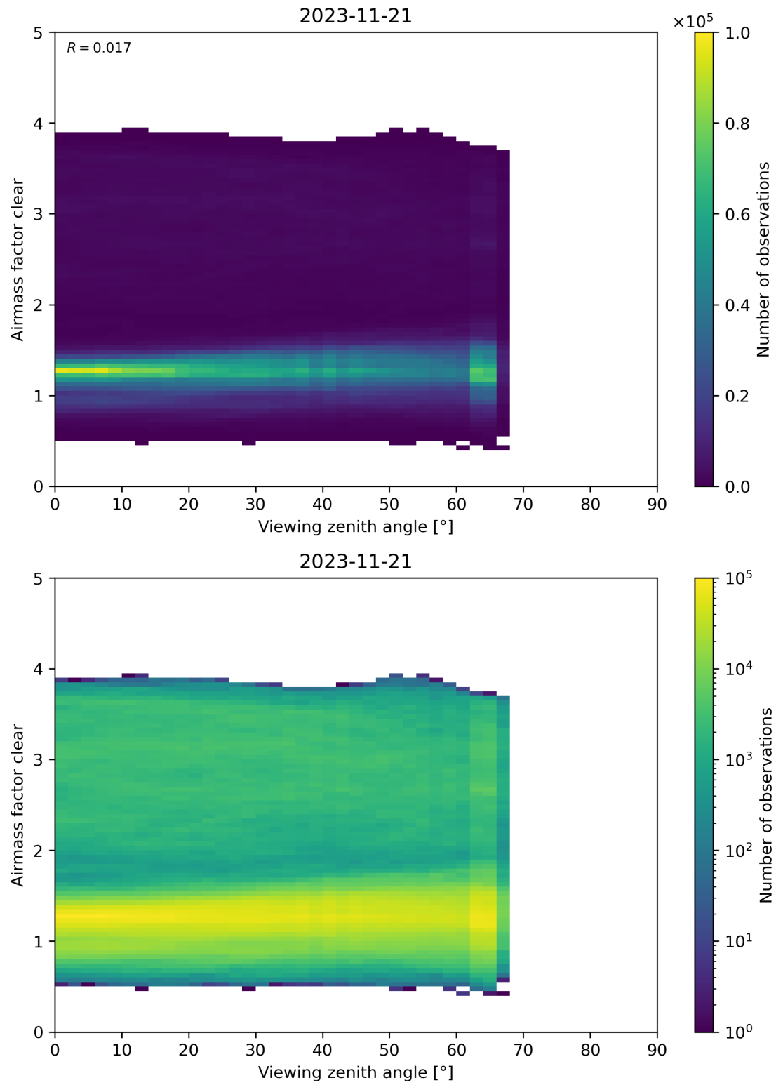
Figure 185: Scatter density plot of “Viewing zenith angle” against “Airmass factor clear” for 2023-11-20 to 2023-11-22.
