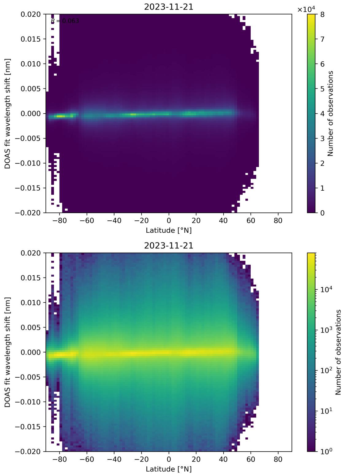
Figure 154: Scatter density plot of “Latitude” against “DOAS fit wavelength shift” for 2023-11-20 to 2023-11-22.
