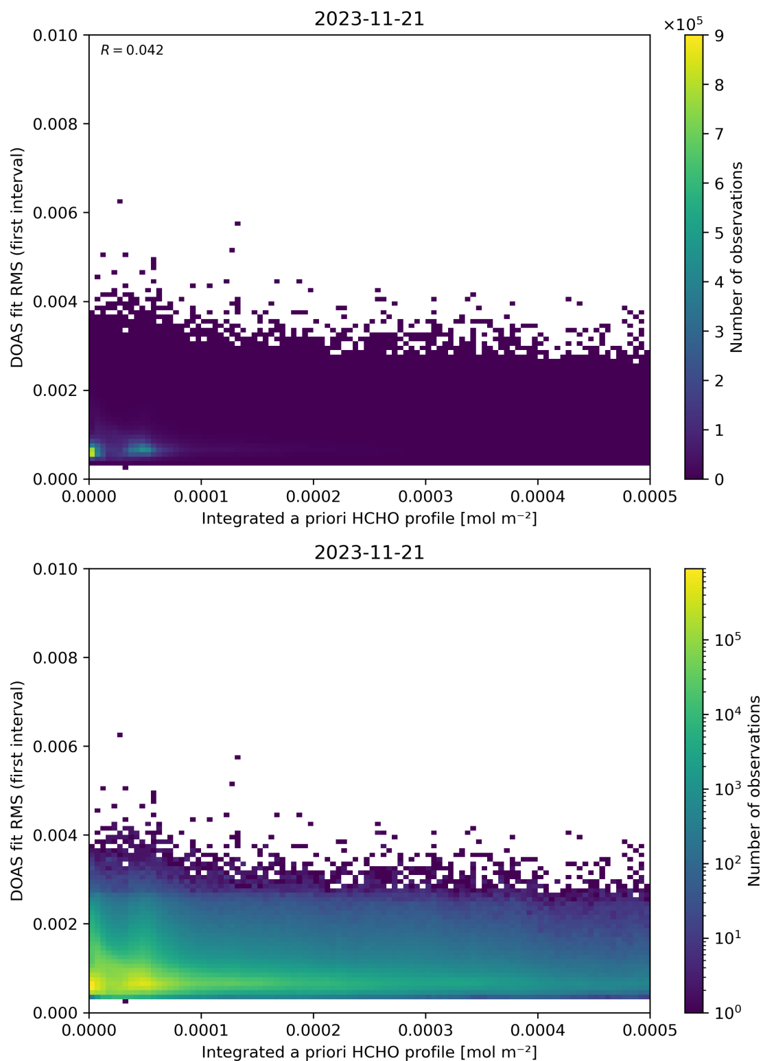
Figure 148: Scatter density plot of “Integrated a priori HCHO profile” against “DOAS fit RMS (first interval)” for 2023-11-20 to 2023-11-22.
