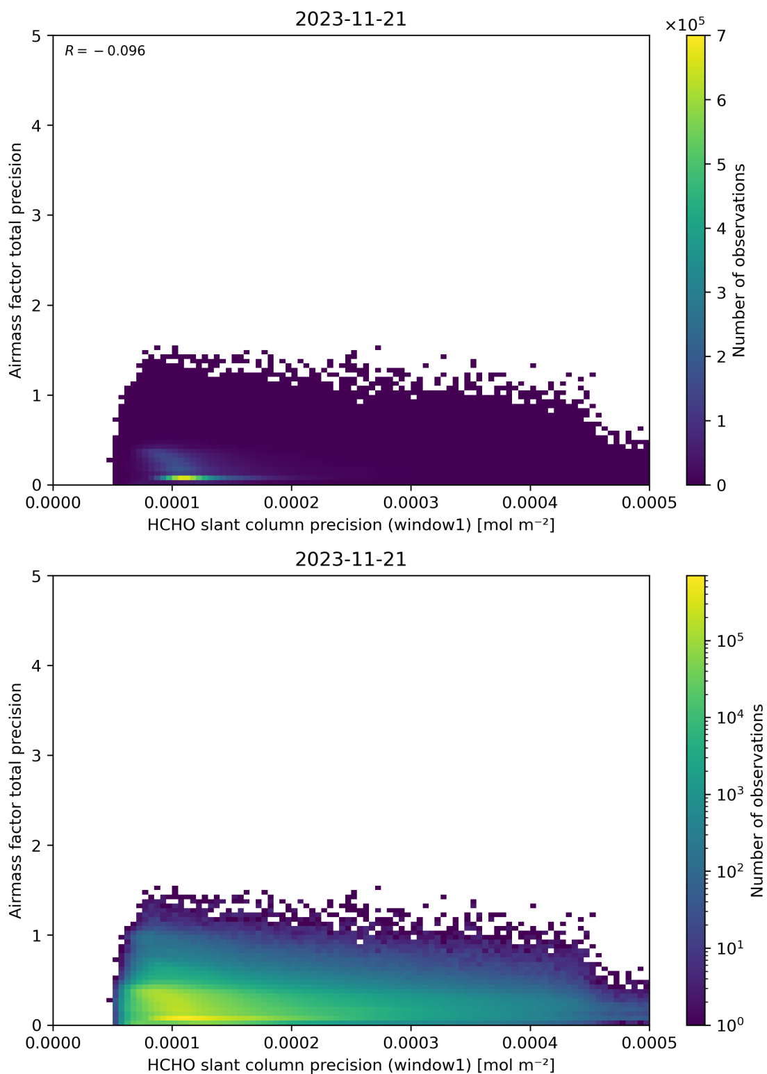
Figure 95: Scatter density plot of “HCHO slant column precision (window1)” against “Airmass factor total precision” for 2023-11-20 to 2023-11-22.
