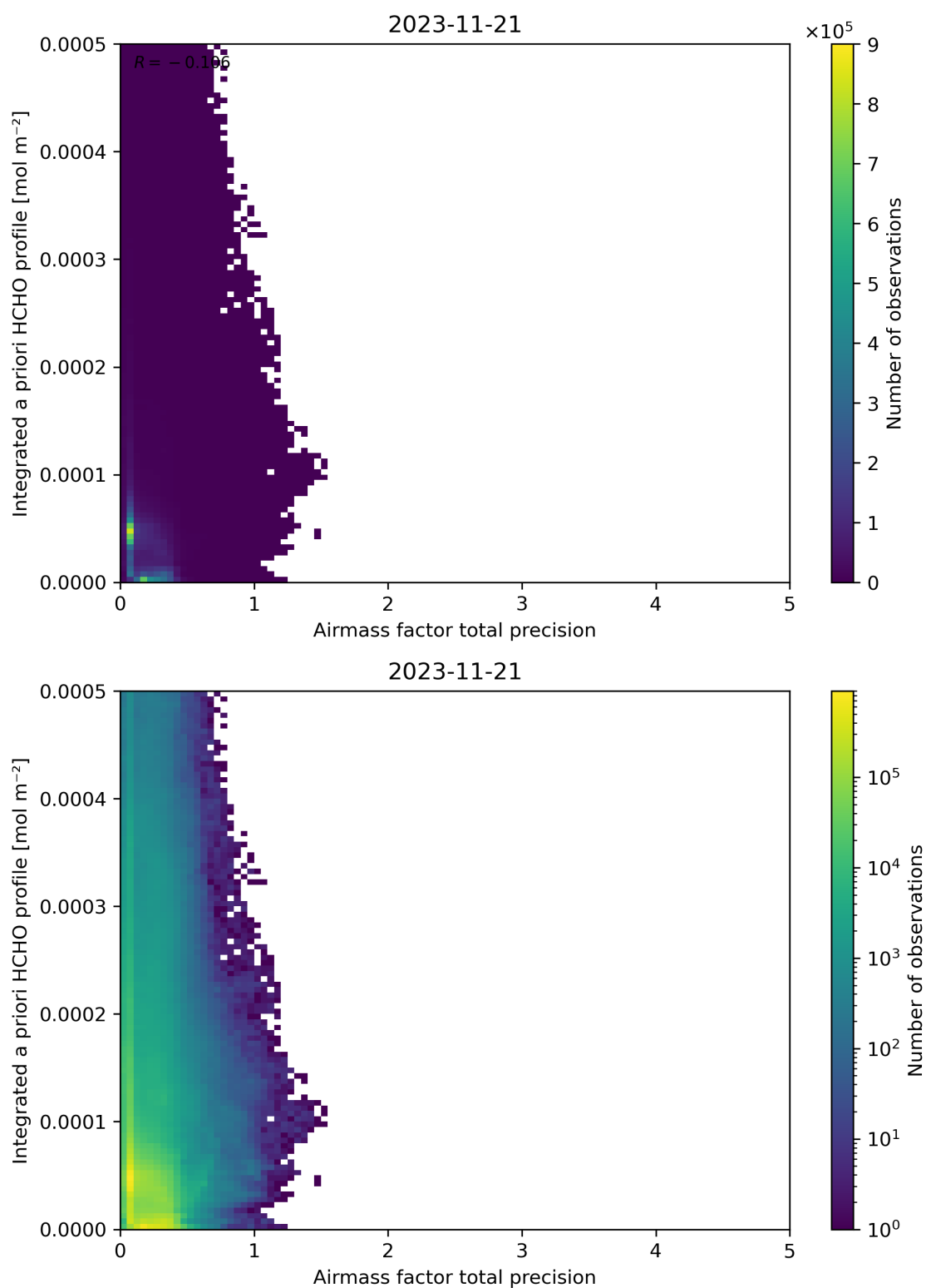
Figure 111: Scatter density plot of “Airmass factor total precision” against “Integrated a priori HCHO profile” for 2023-11-20 to 2023-11-22.
