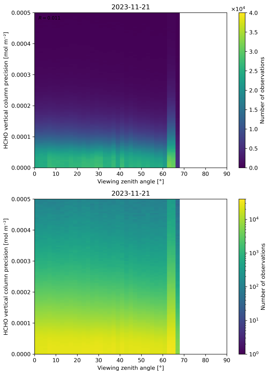
Figure 194: Scatter density plot of “Viewing zenith angle” against “HCHO vertical column precision” for 2023-11-20 to 2023-11-22.
