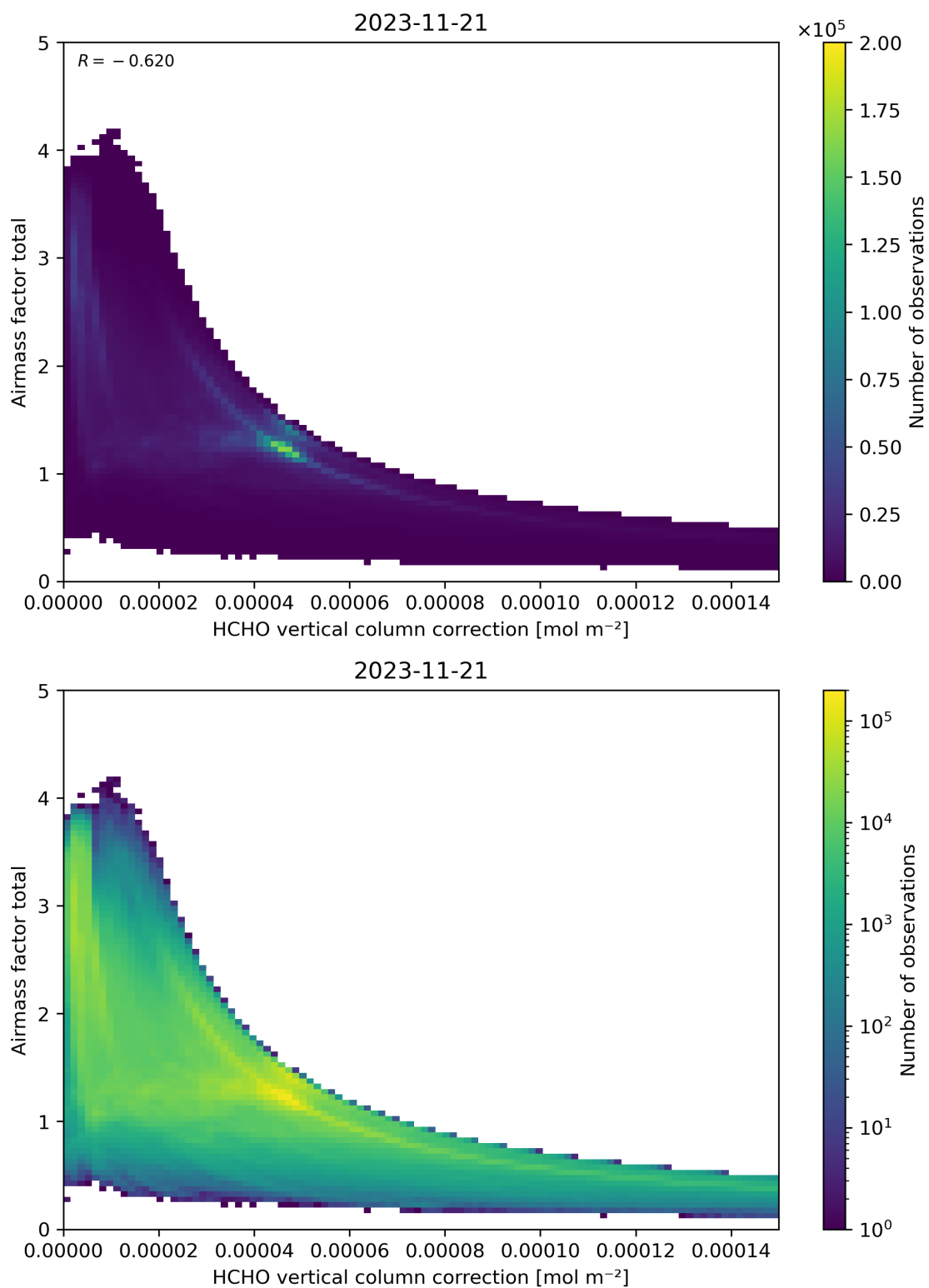
Figure 120: Scatter density plot of “HCHO vertical column correction” against “Airmass factor total” for 2023-11-20 to 2023-11-22.
