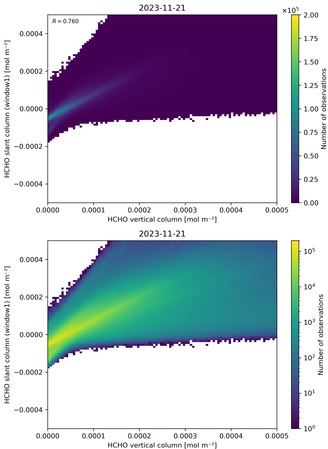
Figure 129: Scatter density plot of “HCHO vertical column” against “HCHO slant column (window1)” for 2023-11-20 to 2023-11-22.
