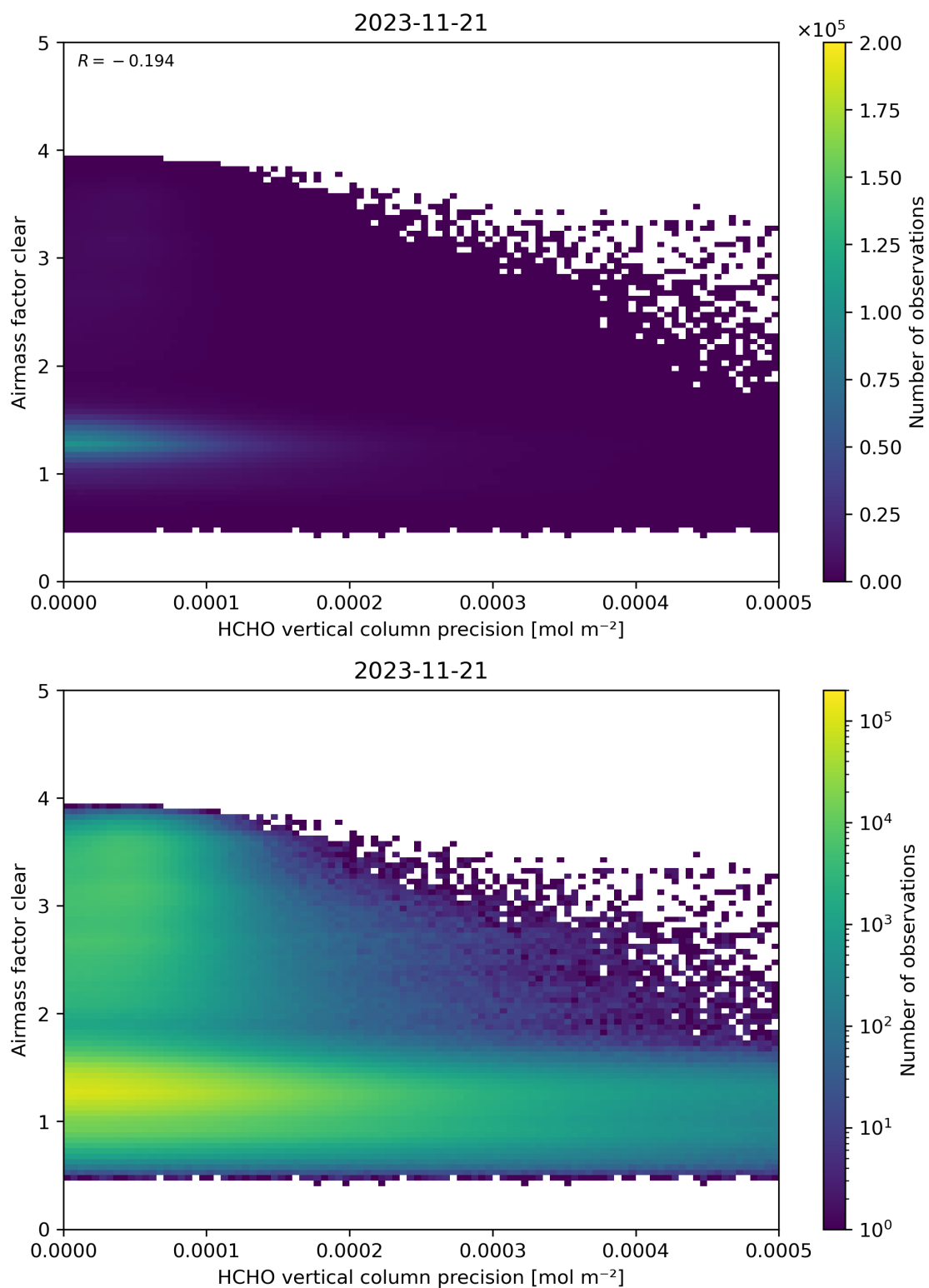
Figure 139: Scatter density plot of “HCHO vertical column precision” against “Airmass factor clear” for 2023-11-20 to 2023-11-22.
