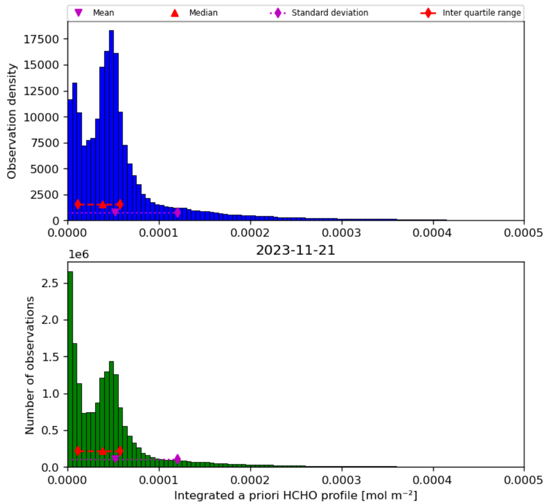
Figure 43: Histogram of “Integrated a priori HCHO profile” for 2023-11-20 to 2023-11-22
