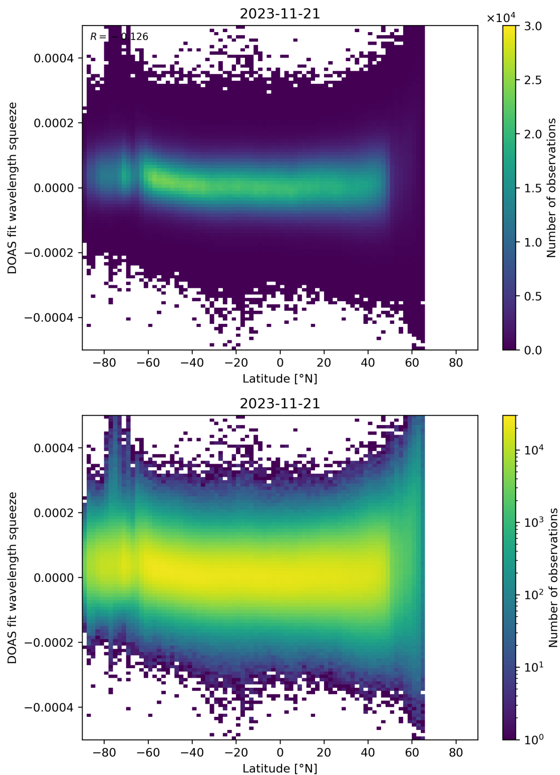
Figure 155: Scatter density plot of “Latitude” against “DOAS fit wavelength squeeze” for 2023-11-20 to 2023-11-22.
