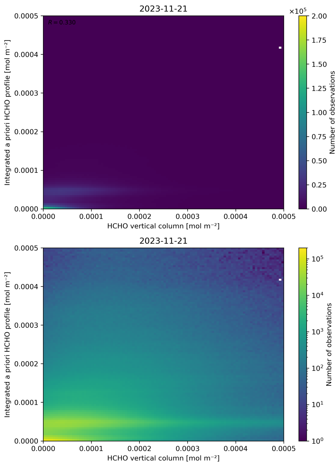
Figure 135: Scatter density plot of “HCHO vertical column” against “Integrated a priori HCHO profile” for 2023-11-20 to 2023-11-22.
