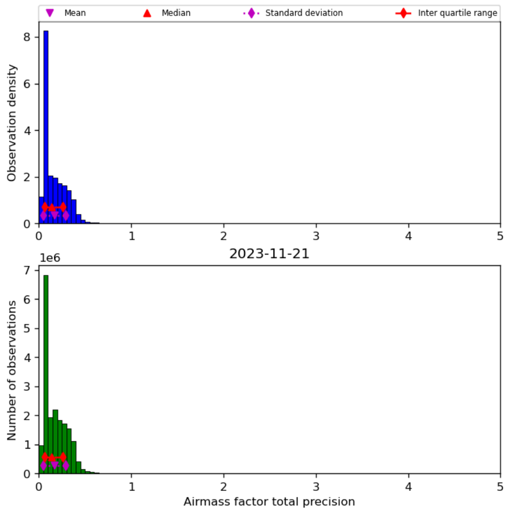
Figure 41: Histogram of “Airmass factor total precision” for 2023-11-20 to 2023-11-22
