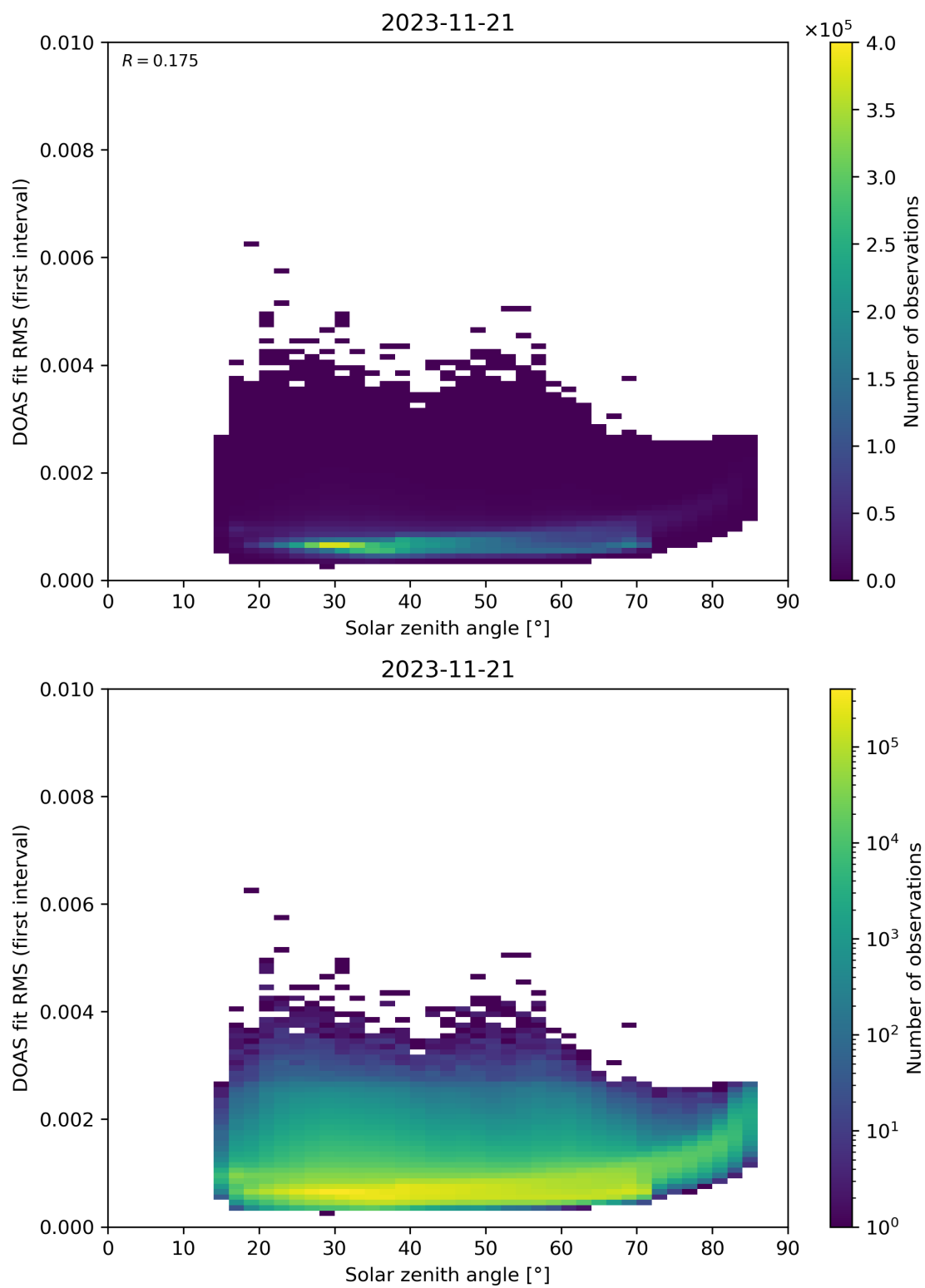
Figure 167: Scatter density plot of “Solar zenith angle” against “DOAS fit RMS (first interval)” for 2023-11-20 to 2023-11-22.
