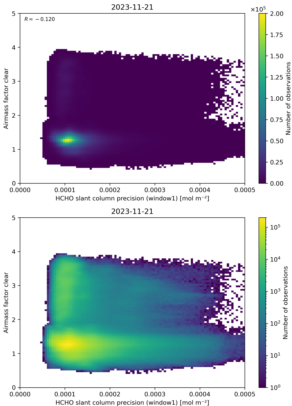
Figure 91: Scatter density plot of “HCHO slant column precision (window1)” against “Airmass factor clear” for 2023-11-20 to 2023-11-22.
