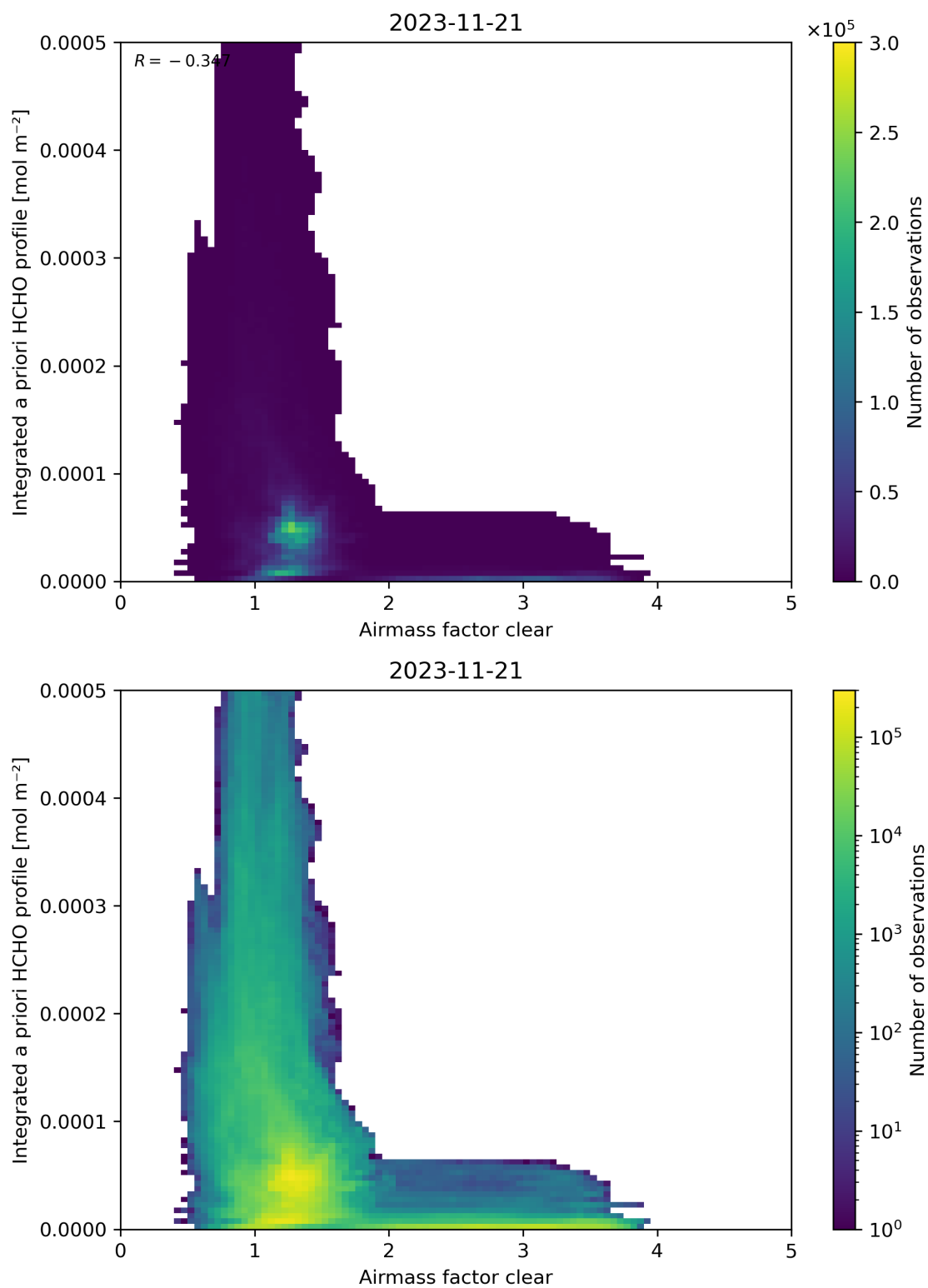
Figure 76: Scatter density plot of “Airmass factor clear” against “Integrated a priori HCHO profile” for 2023-11-20 to 2023-11-22.
