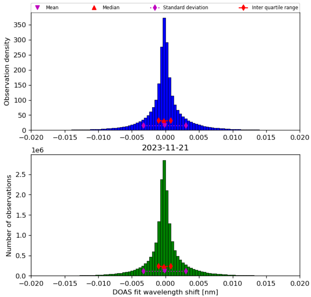
Figure 44: Histogram of “DOAS fit wavelength shift” for 2023-11-20 to 2023-11-22
