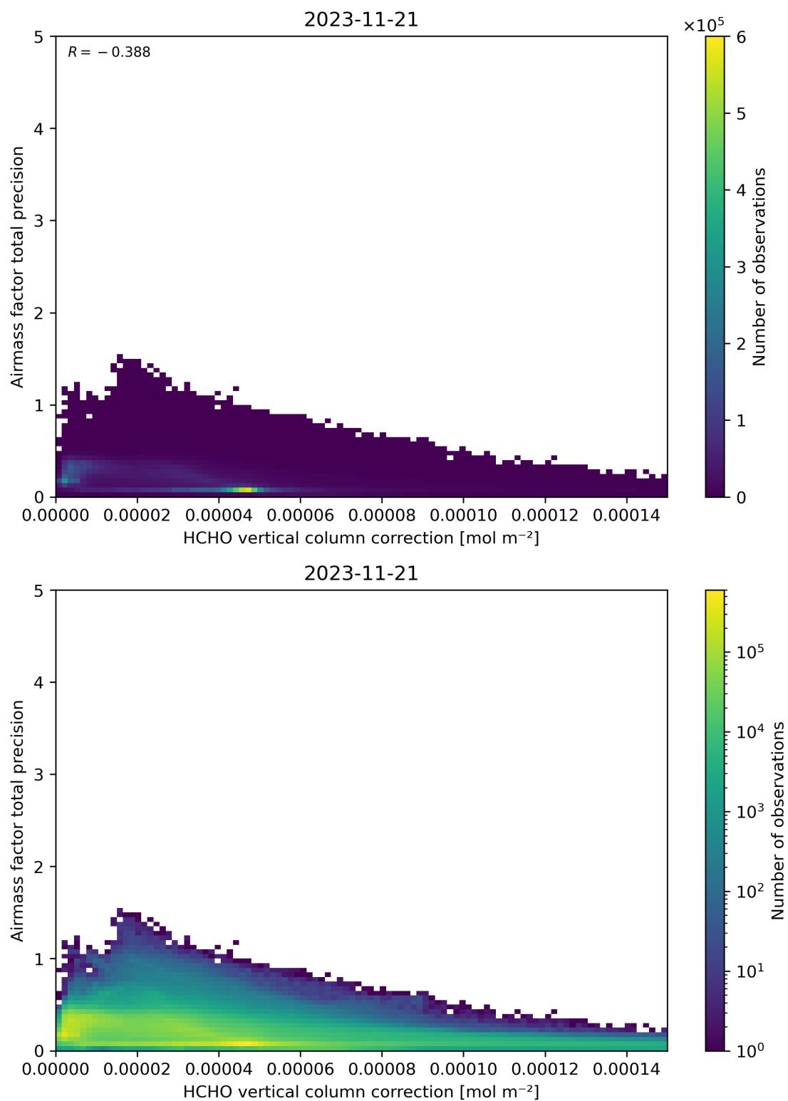
Figure 121: Scatter density plot of “HCHO vertical column correction” against “Airmass factor total precision” for 2023-11-20 to 2023-11-22.
