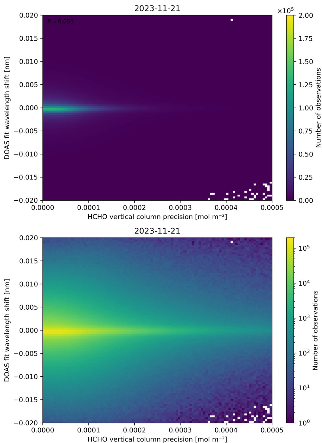
Figure 137: Scatter density plot of “HCHO vertical column precision” against “DOAS fit wavelength shift” for 2023-11-20 to 2023-11-22.
