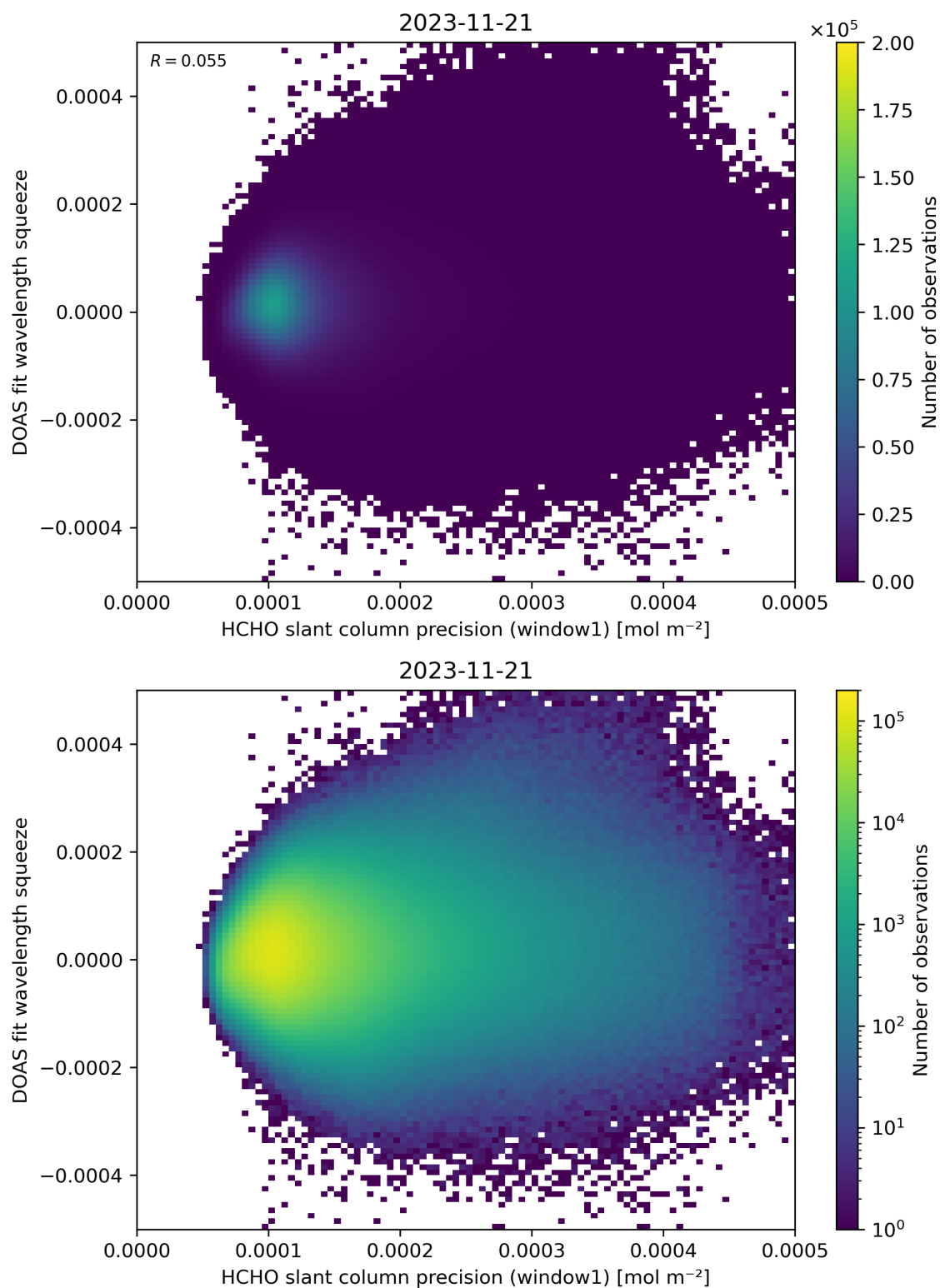
Figure 90: Scatter density plot of “HCHO slant column precision (window1)” against “DOAS fit wavelength squeeze” for 2023-11-20 to 2023-11-22.
