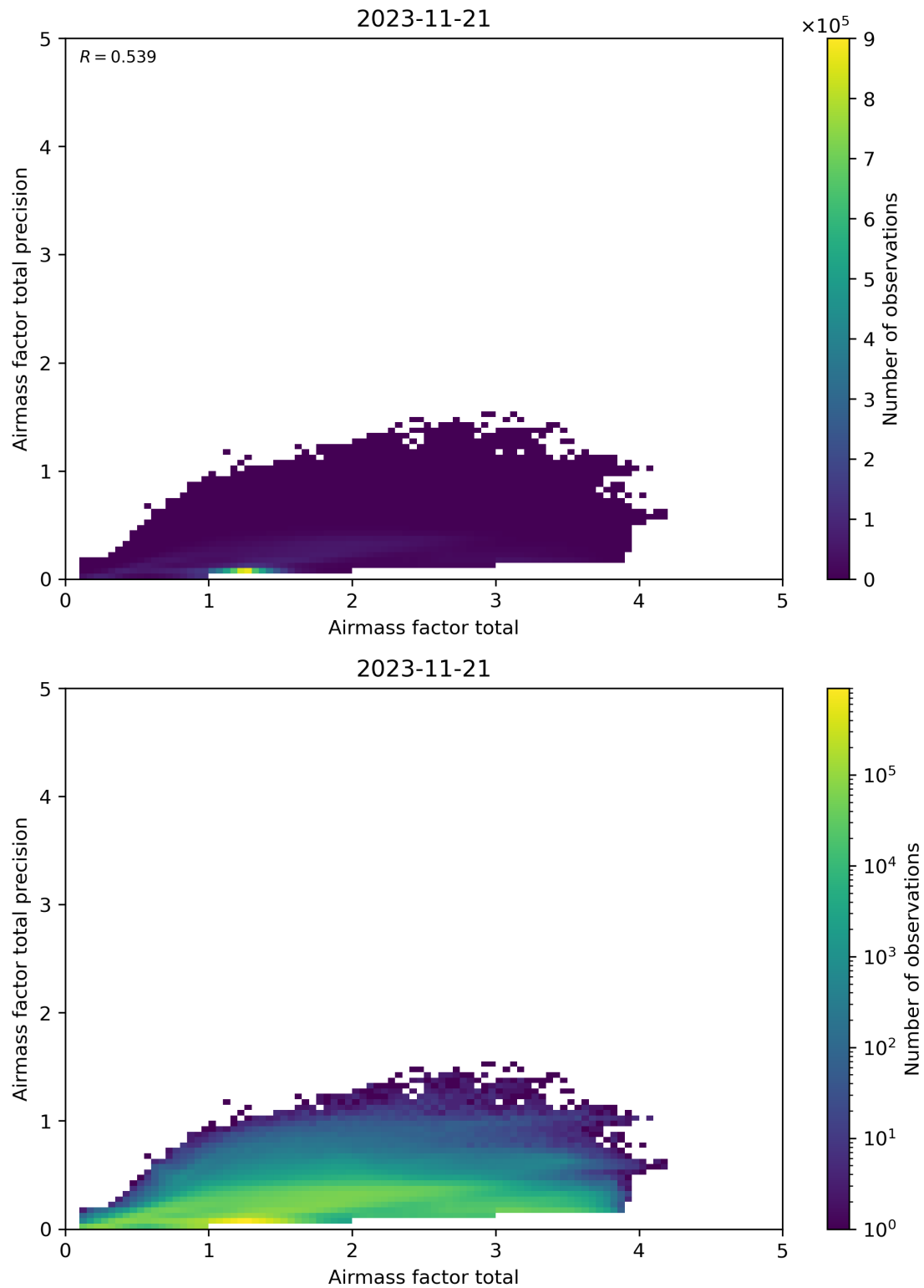
Figure 103: Scatter density plot of “Airmass factor total” against “Airmass factor total precision” for 2023-11-20 to 2023-11-22.
