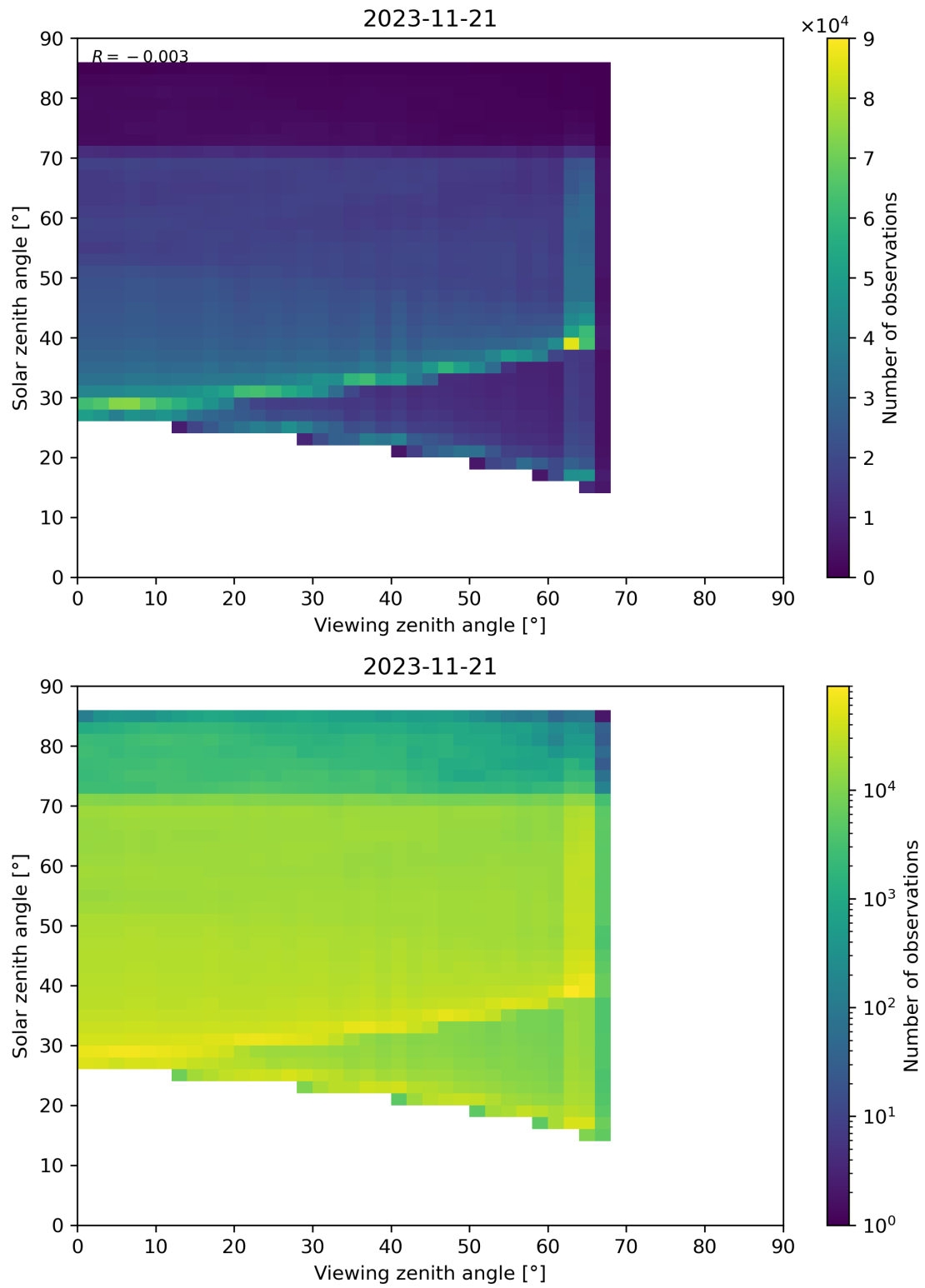
Figure 197: Scatter density plot of “Viewing zenith angle” against “Solar zenith angle” for 2023-11-20 to 2023-11-22.
