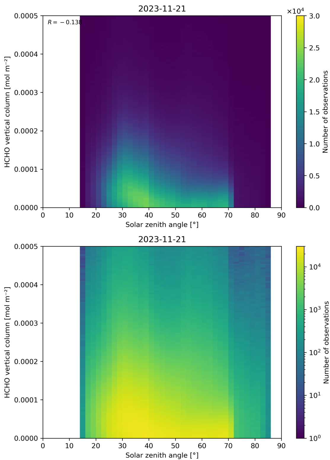
Figure 177: Scatter density plot of “Solar zenith angle” against “HCHO vertical column” for 2023-11-20 to 2023-11-22.
