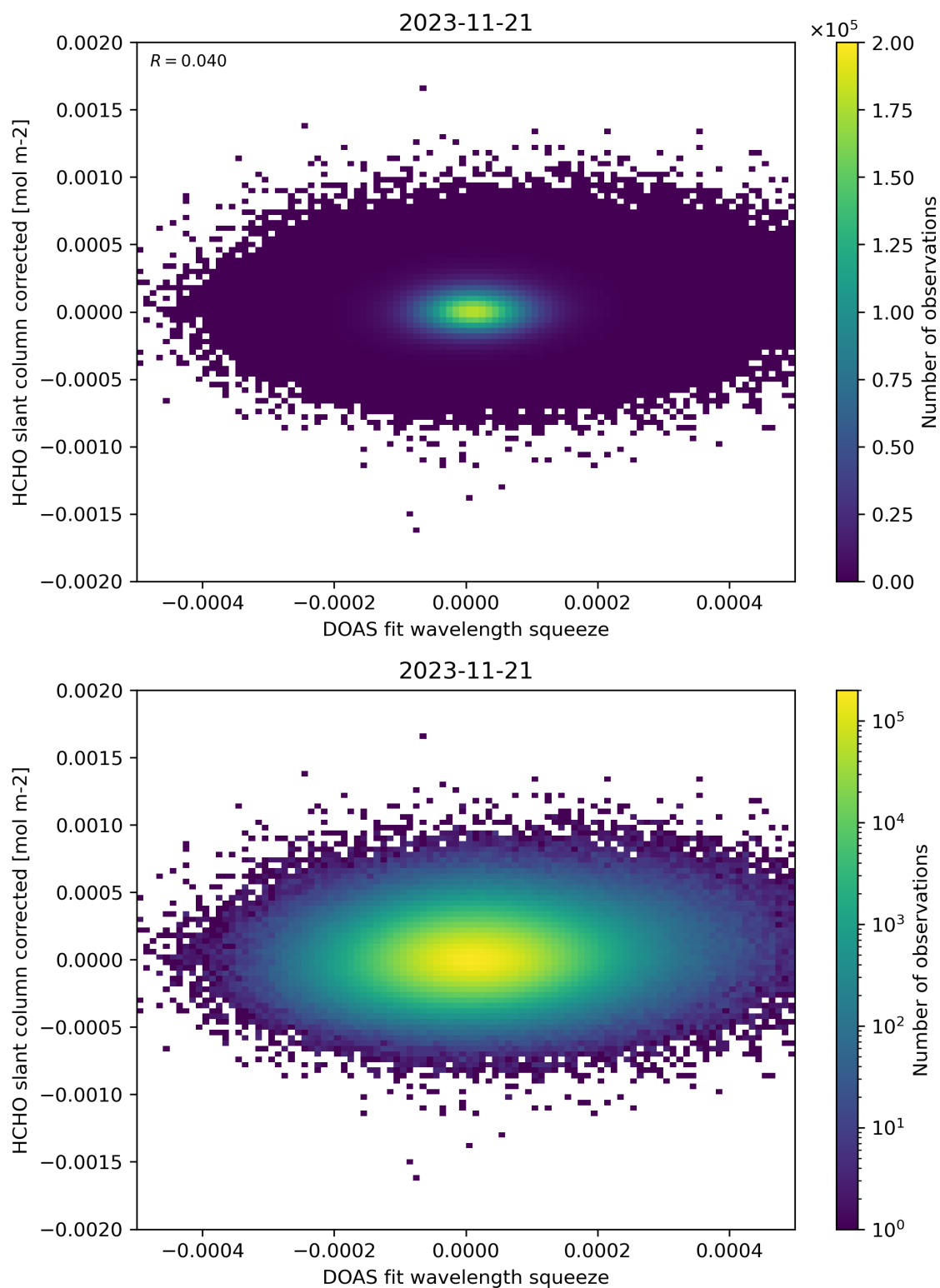
Figure 69: Scatter density plot of “DOAS fit wavelength squeeze” against “HCHO slant column corrected” for 2023-11-20 to 2023-11-22.
