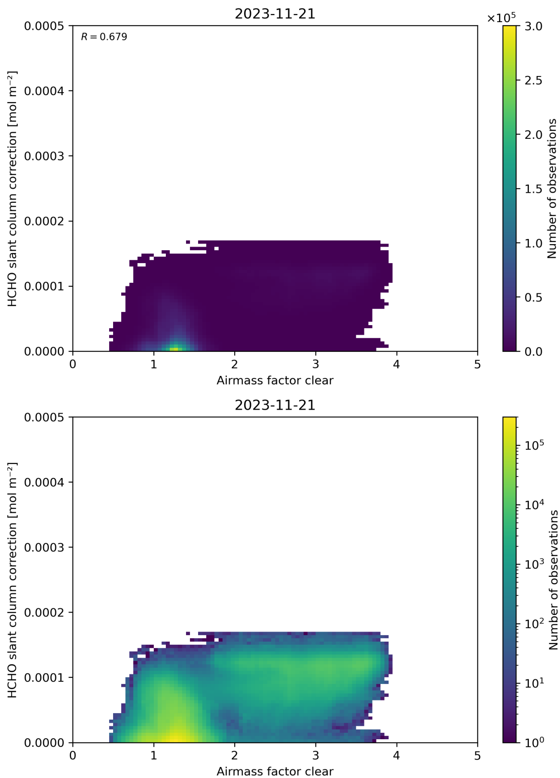
Figure 75: Scatter density plot of “Airmass factor clear” against “HCHO slant column correction” for 2023-11-20 to 2023-11-22.
