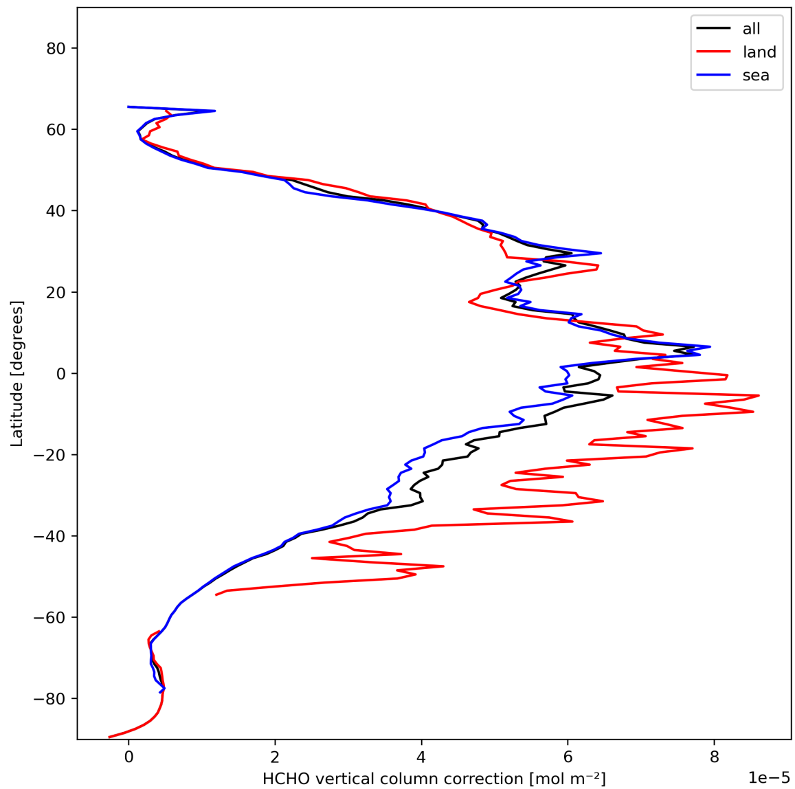
Figure 23: Zonal average of “HCHO vertical column correction” for 2023-11-20 to 2023-11-22.
