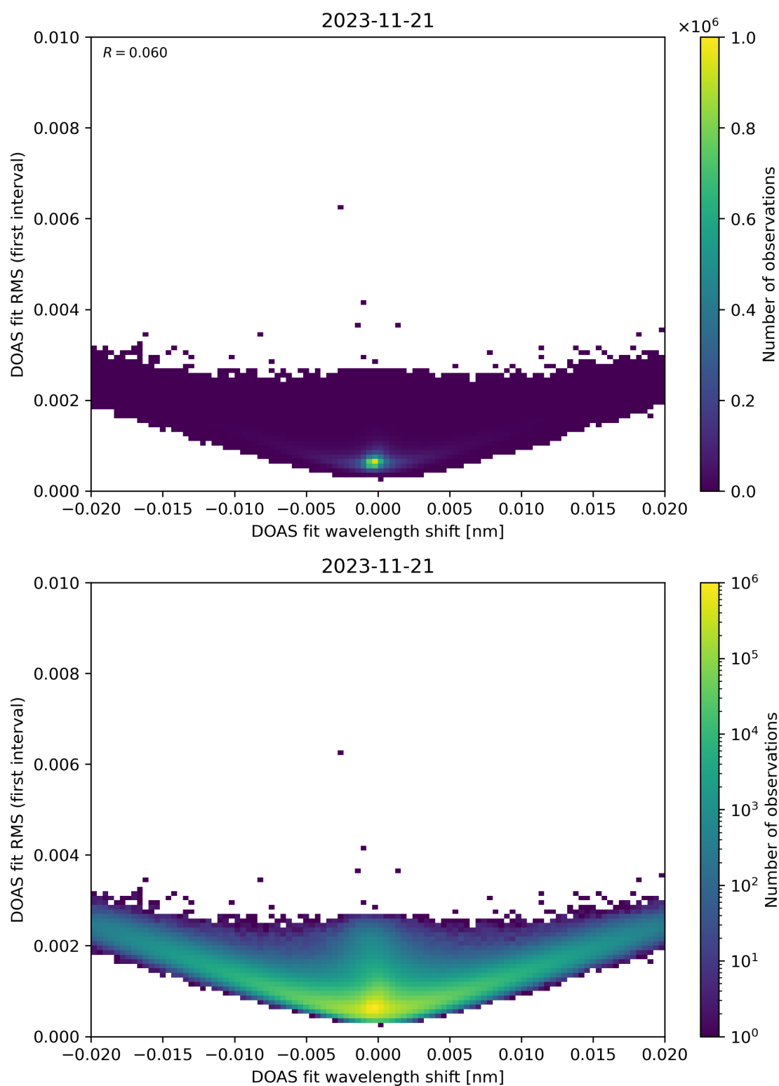
Figure 64: Scatter density plot of “DOAS fit wavelength shift” against “DOAS fit RMS (first interval)” for 2023-11-20 to 2023-11-22.
