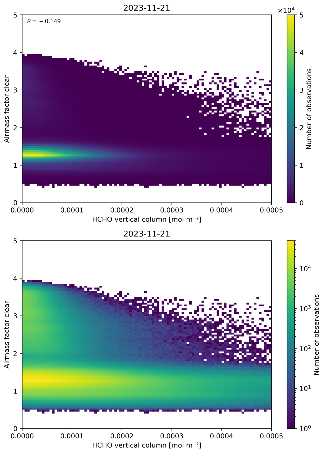
Figure 126: Scatter density plot of “HCHO vertical column” against “Airmass factor clear” for 2023-11-20 to 2023-11-22.
