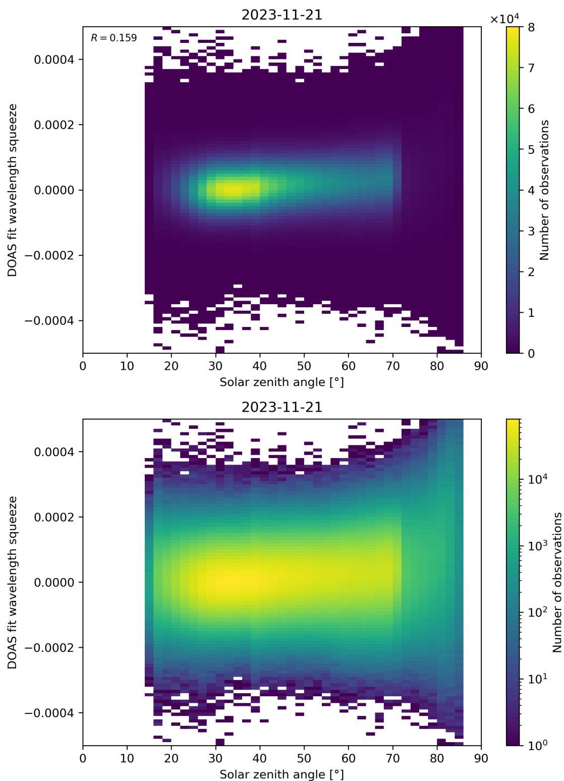
Figure 169: Scatter density plot of “Solar zenith angle” against “DOAS fit wavelength squeeze” for 2023-11-20 to 2023-11-22.
