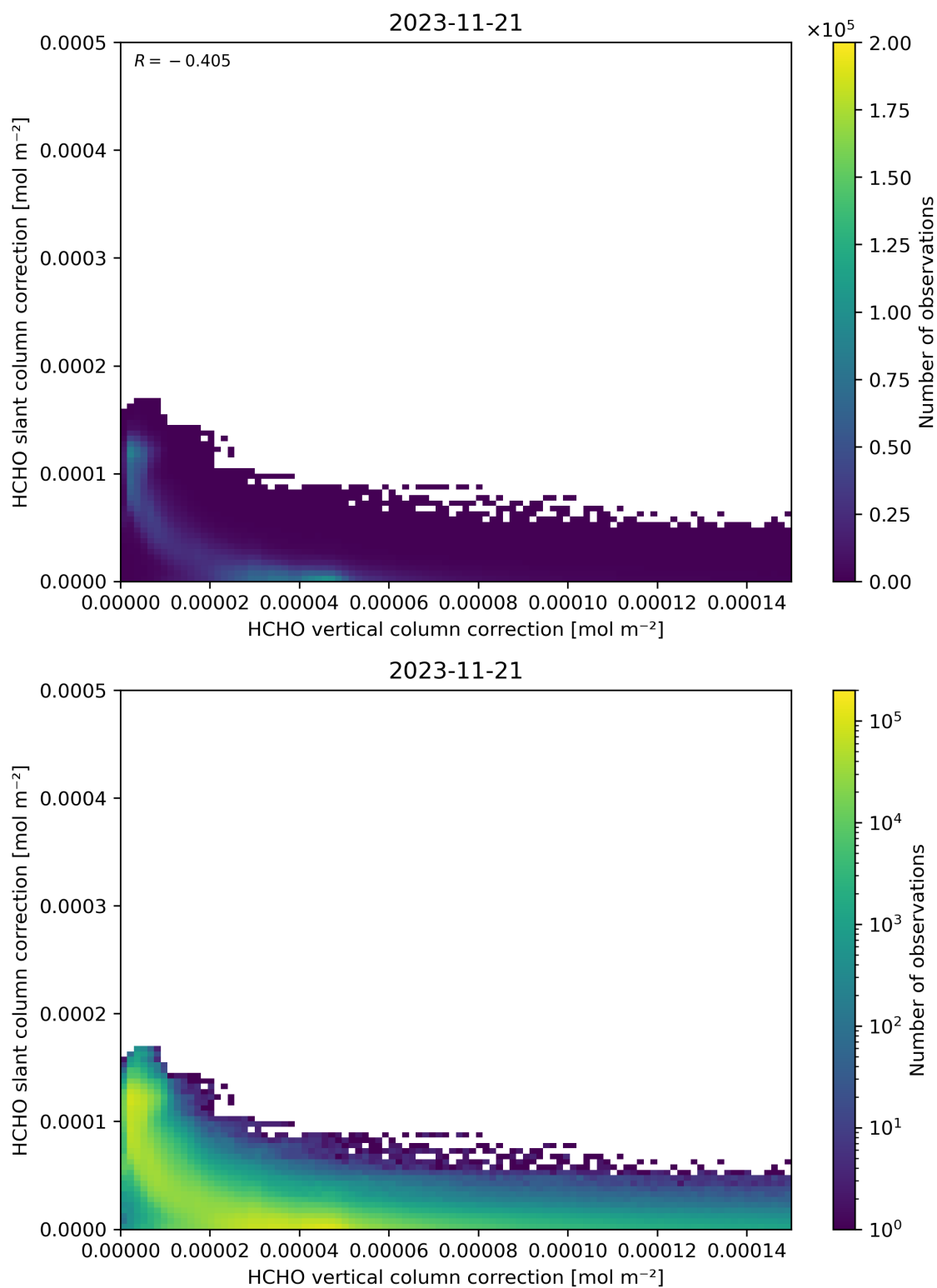
Figure 117: Scatter density plot of “HCHO vertical column correction” against “HCHO slant column correction” for 2023-11-20 to 2023-11-22.
