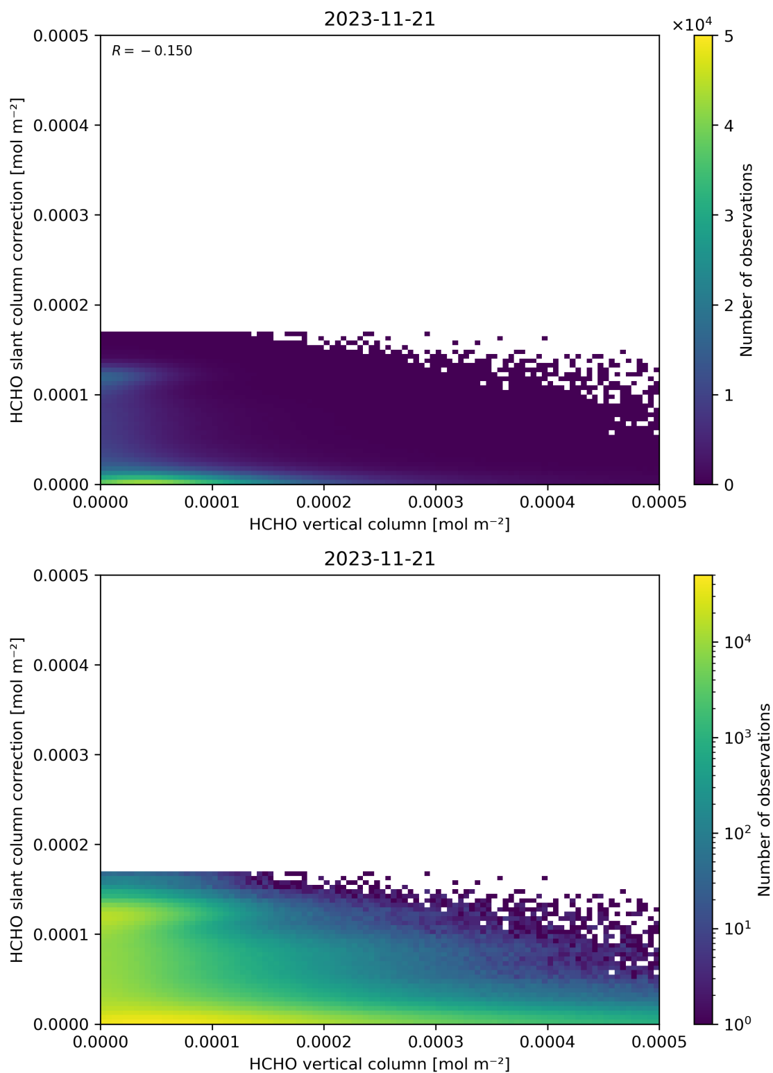
Figure 128: Scatter density plot of “HCHO vertical column” against “HCHO slant column correction” for 2023-11-20 to 2023-11-22.
