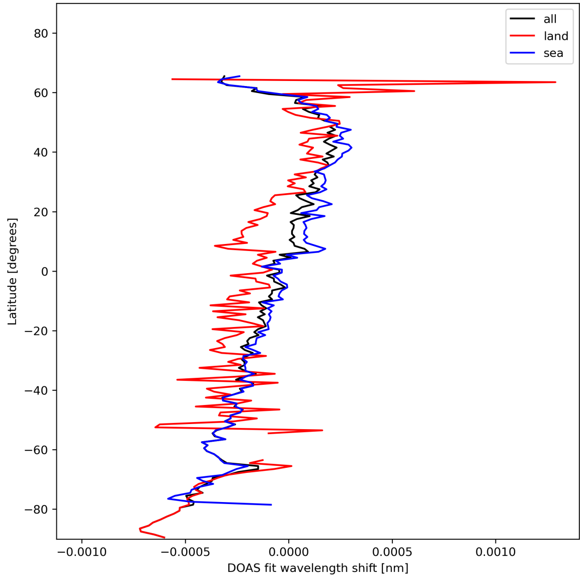
Figure 30: Zonal average of “DOAS fit wavelength shift” for 2023-11-20 to 2023-11-22.
