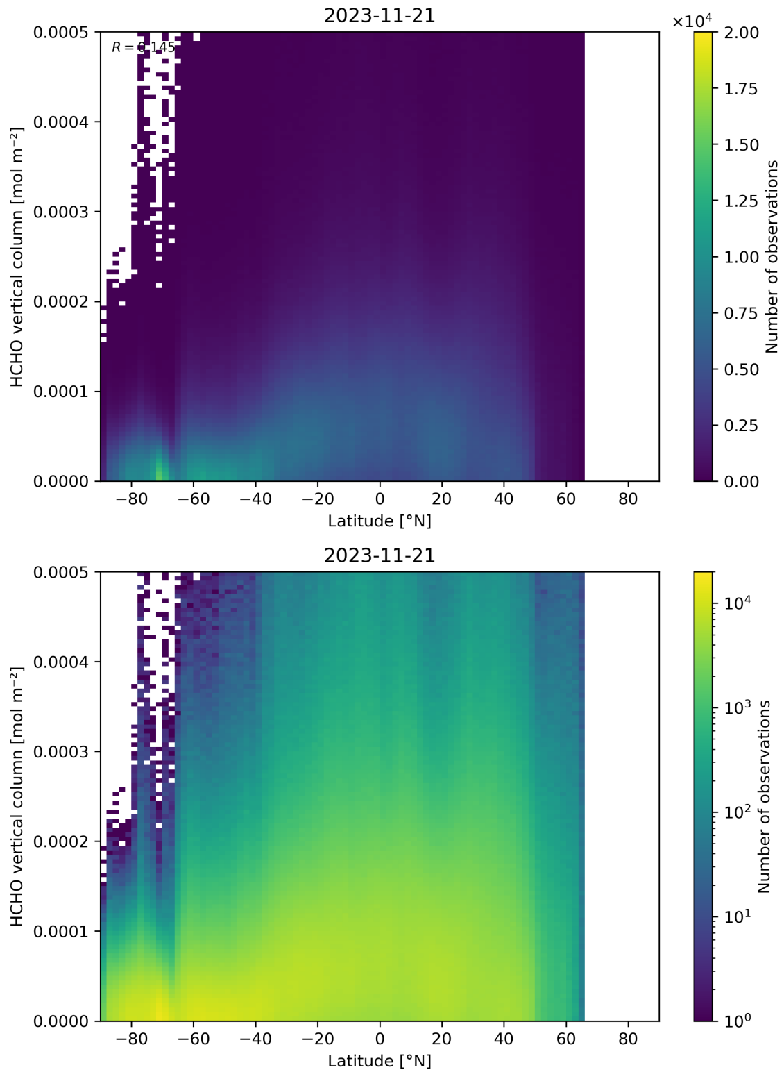
Figure 163: Scatter density plot of “Latitude” against “HCHO vertical column” for 2023-11-20 to 2023-11-22.
