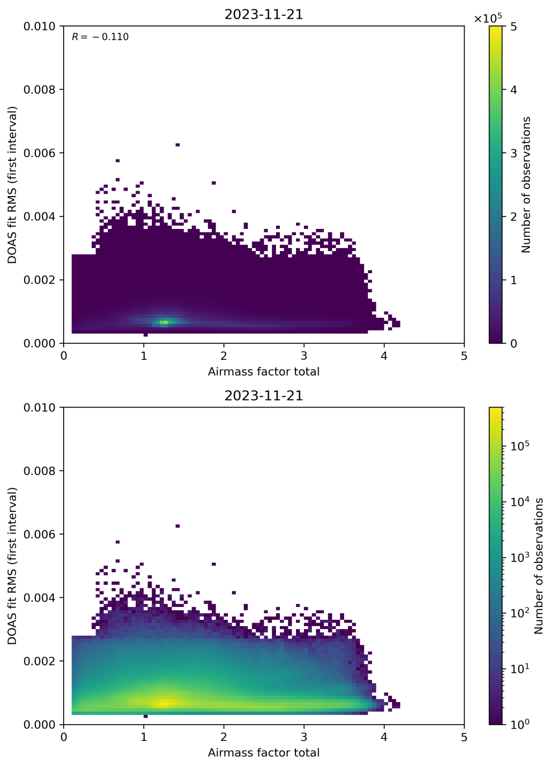
Figure 97: Scatter density plot of “Airmass factor total” against “DOAS fit RMS (first interval)” for 2023-11-20 to 2023-11-22.
