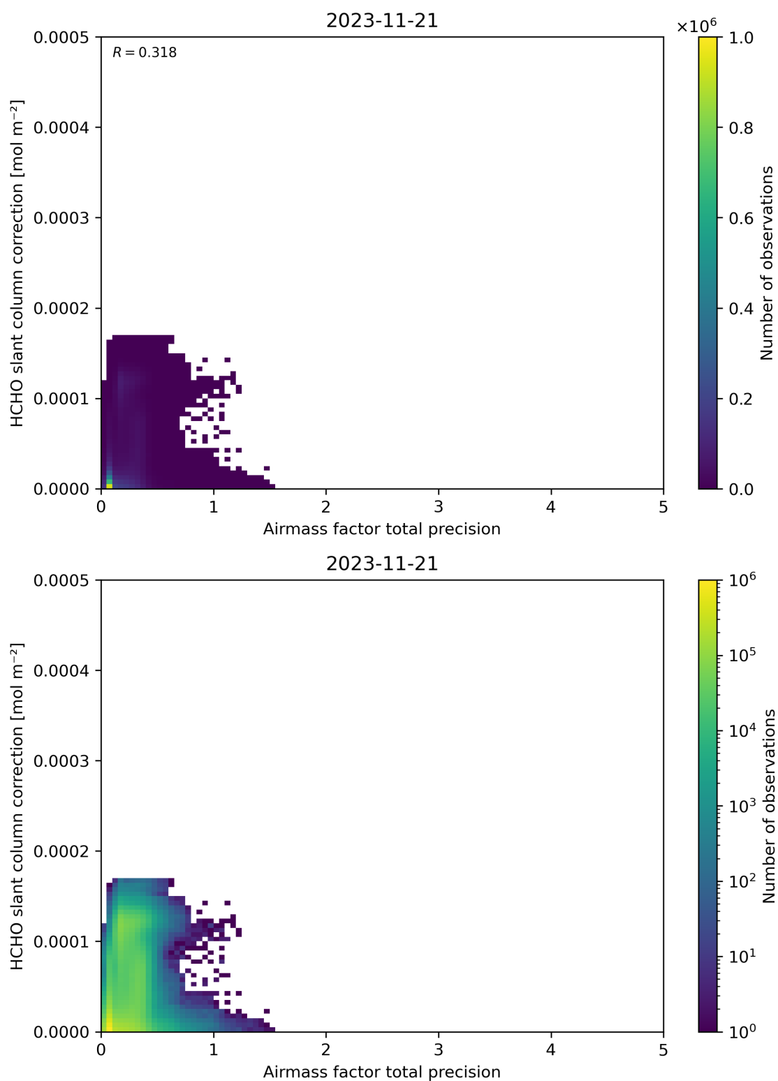
Figure 110: Scatter density plot of “Airmass factor total precision” against “HCHO slant column correction” for 2023-11-20 to 2023-11-22.
