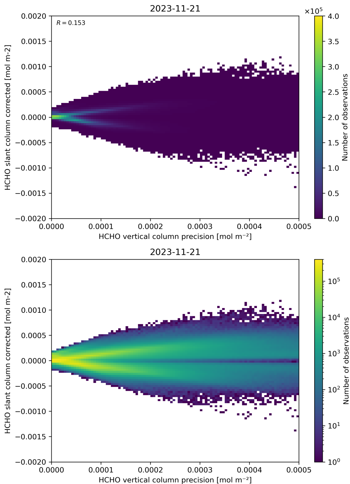
Figure 140: Scatter density plot of “HCHO vertical column precision” against “HCHO slant column corrected” for 2023-11-20 to 2023-11-22.
