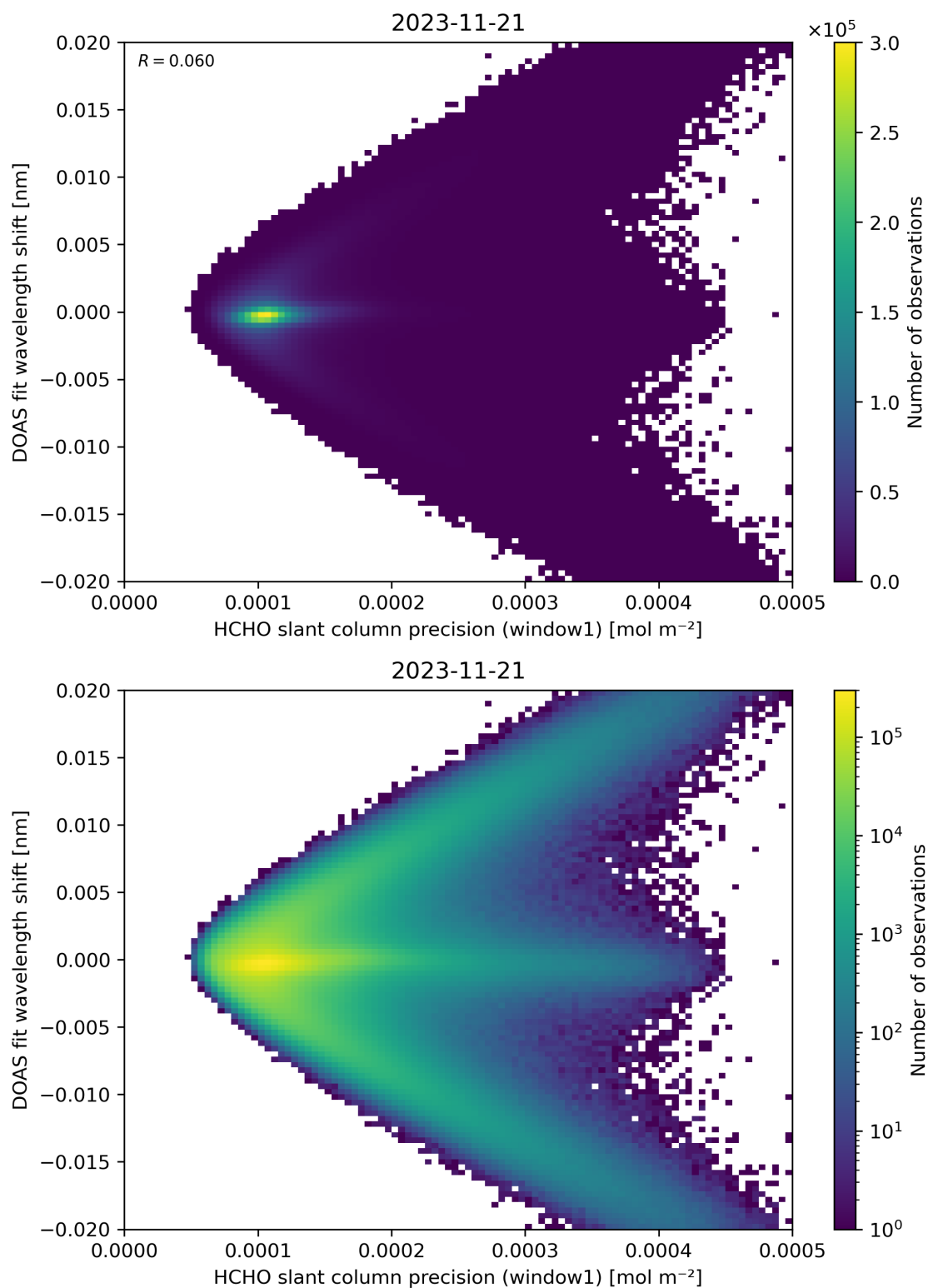
Figure 89: Scatter density plot of “HCHO slant column precision (window1)” against “DOAS fit wavelength shift” for 2023-11-20 to 2023-11-22.
