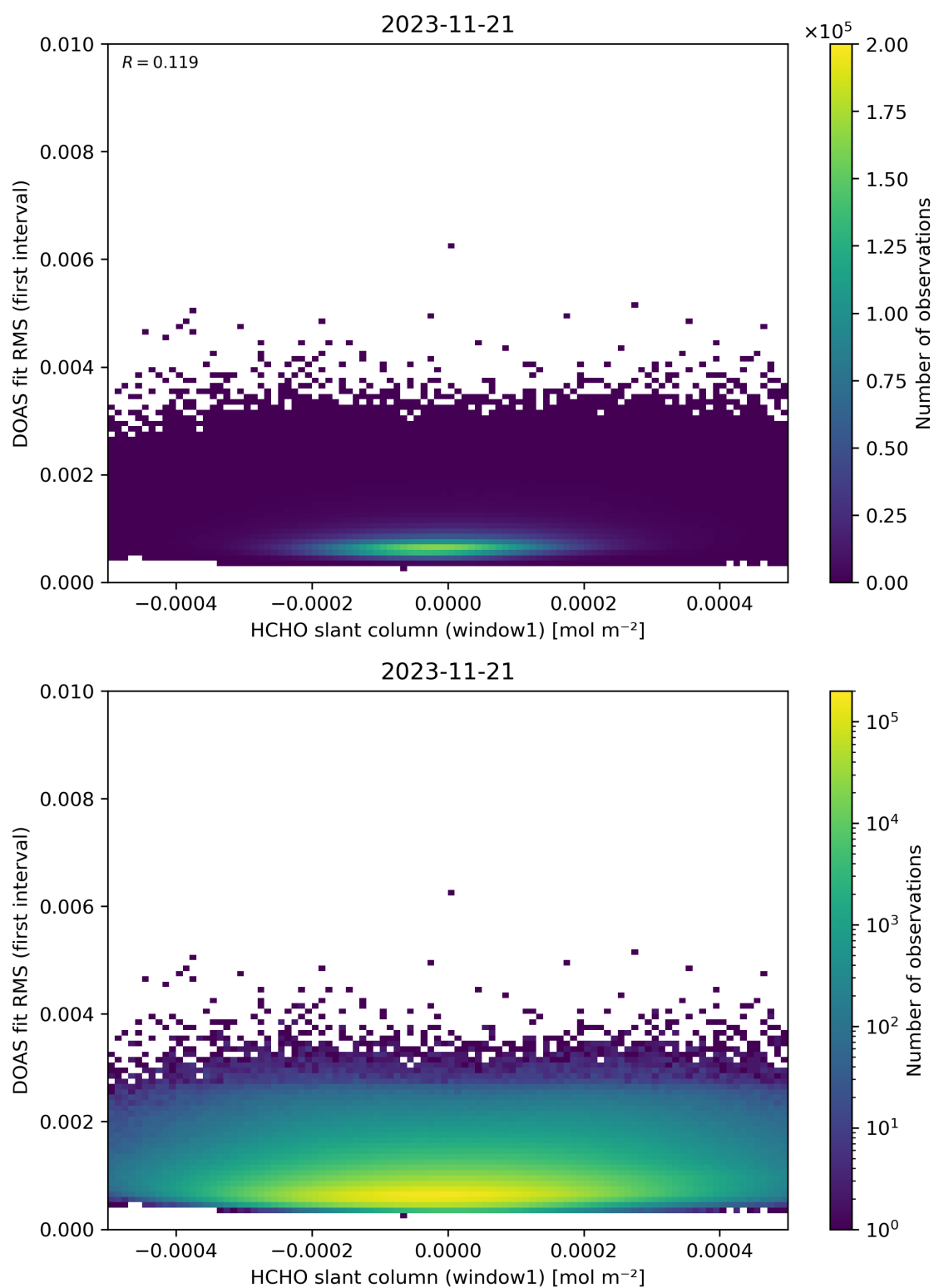
Figure 78: Scatter density plot of “HCHO slant column (window1)” against “DOAS fit RMS (first interval)” for 2023-11-20 to 2023-11-22.
