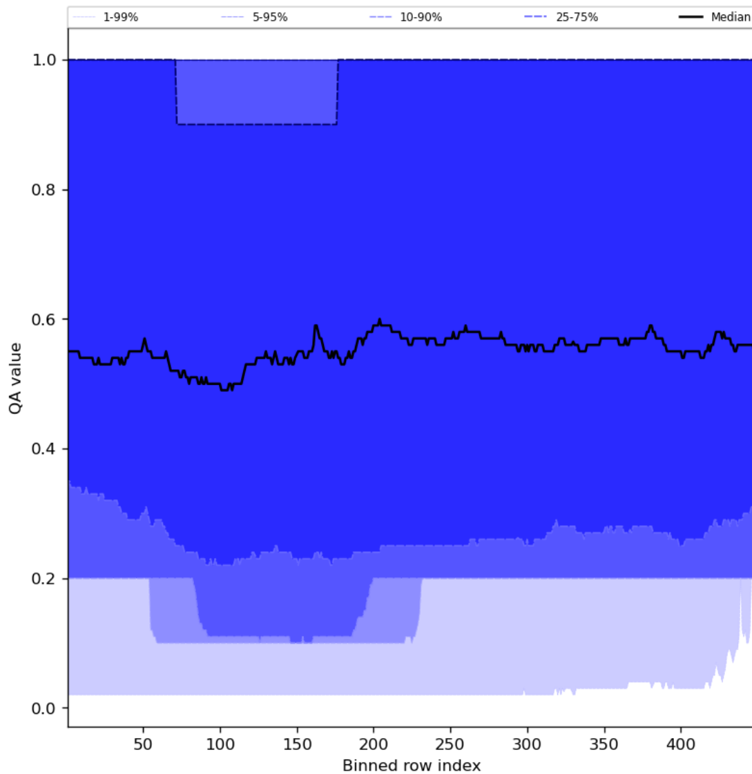
Figure 48: Along track statistics of “QA value” for 2023-11-20 to 2023-11-22
