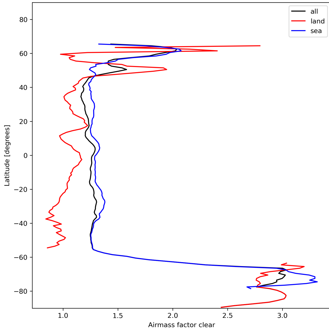
Figure 28: Zonal average of “Airmass factor clear” for 2023-11-20 to 2023-11-22.
