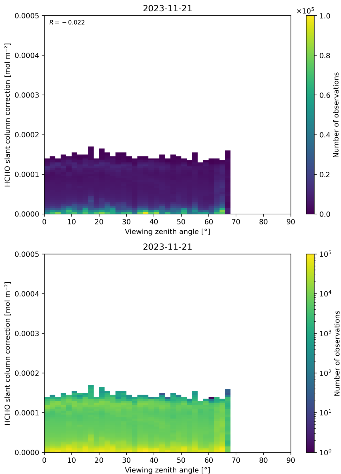
Figure 187: Scatter density plot of “Viewing zenith angle” against “HCHO slant column correction” for 2023-11-20 to 2023-11-22.
