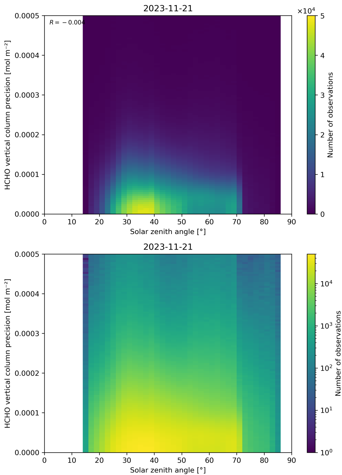
Figure 179: Scatter density plot of “Solar zenith angle” against “HCHO vertical column precision” for 2023-11-20 to 2023-11-22.
