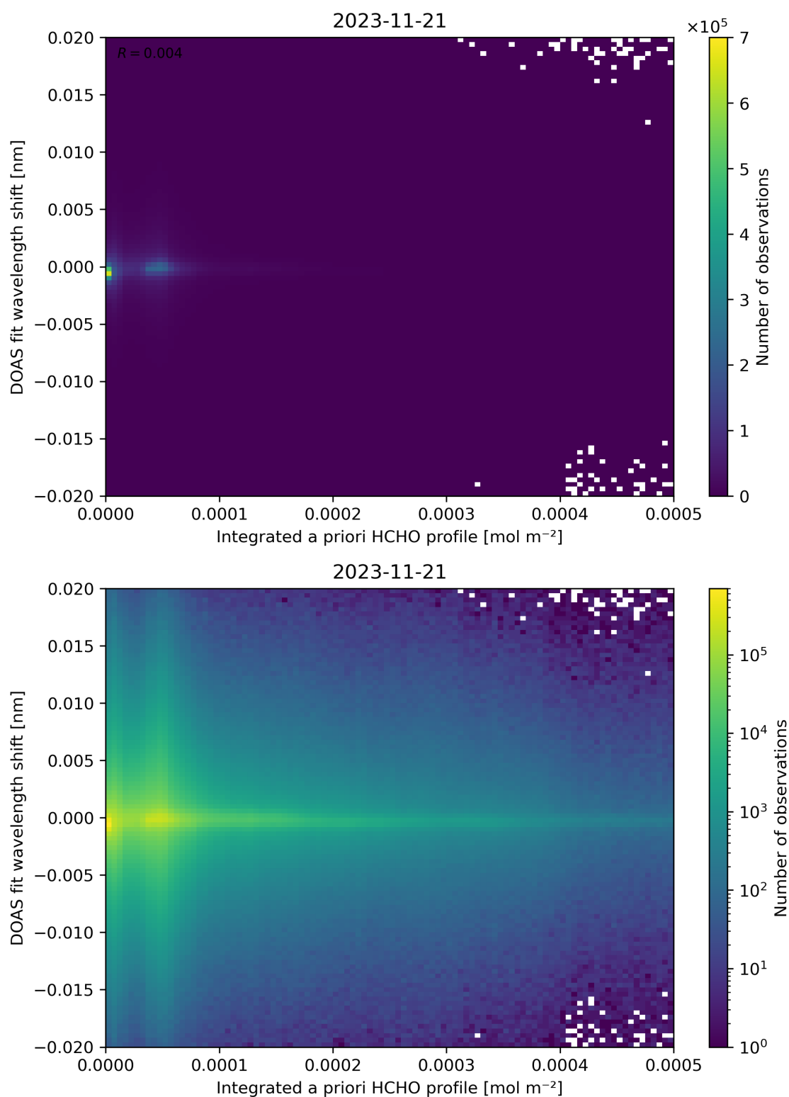
Figure 149: Scatter density plot of “Integrated a priori HCHO profile” against “DOAS fit wavelength shift” for 2023-11-20 to 2023-11-22.
