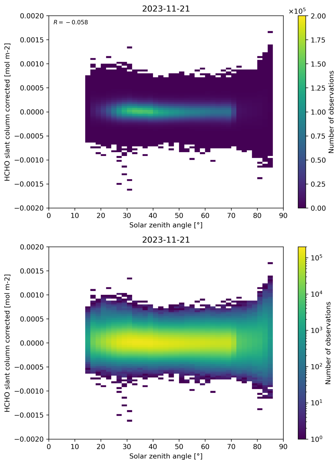
Figure 171: Scatter density plot of “Solar zenith angle” against “HCHO slant column corrected” for 2023-11-20 to 2023-11-22.
