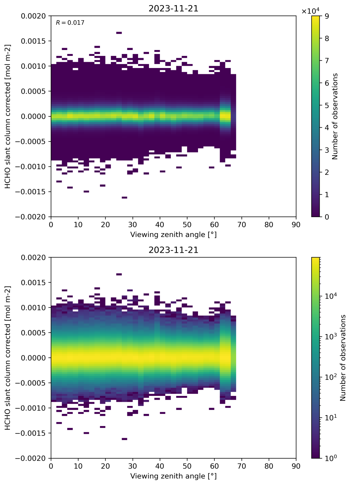
Figure 186: Scatter density plot of “Viewing zenith angle” against “HCHO slant column corrected” for 2023-11-20 to 2023-11-22.
