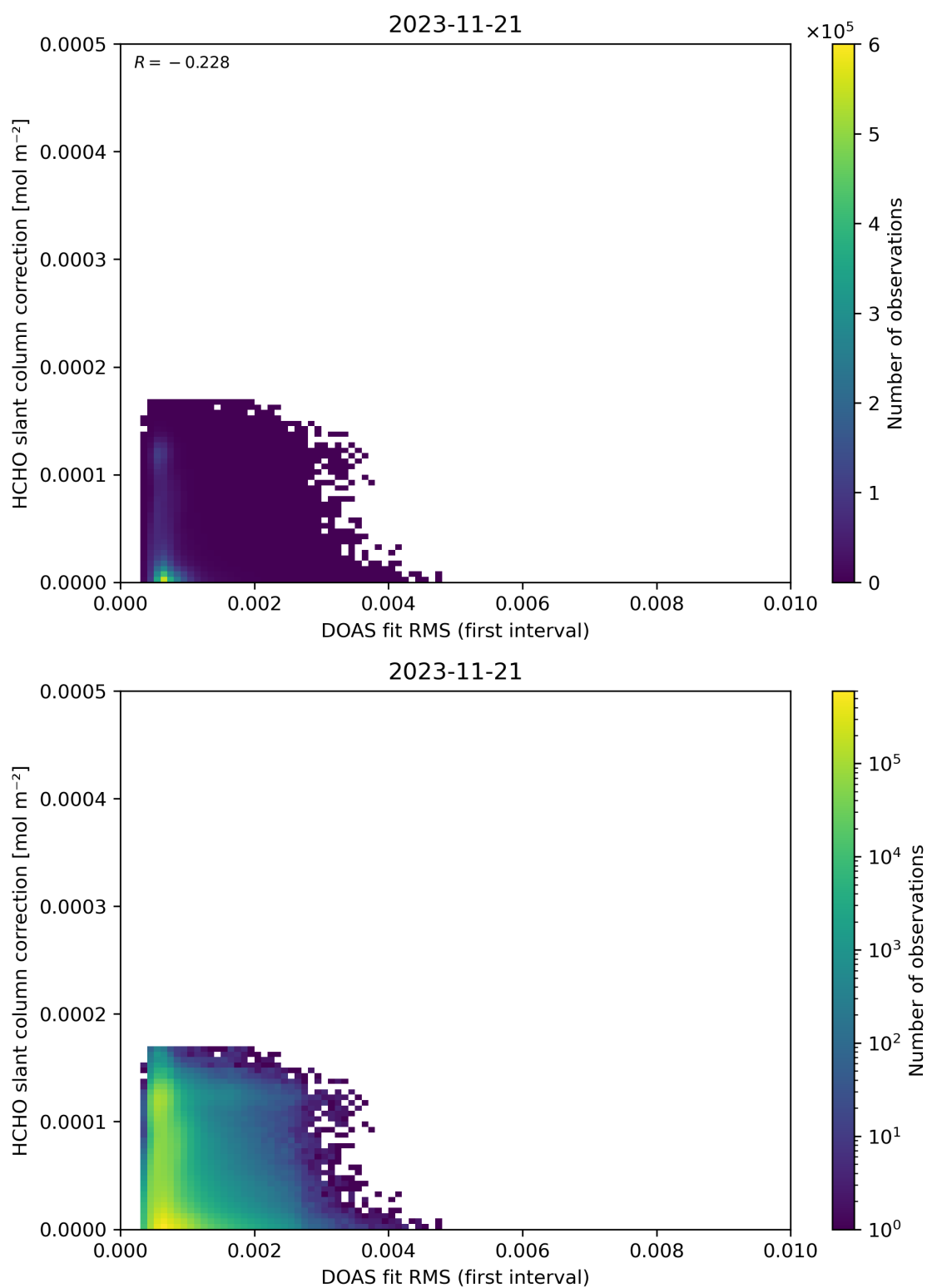
Figure 63: Scatter density plot of “DOAS fit RMS (first interval)” against “HCHO slant column correction” for 2023-11-20 to 2023-11-22.
