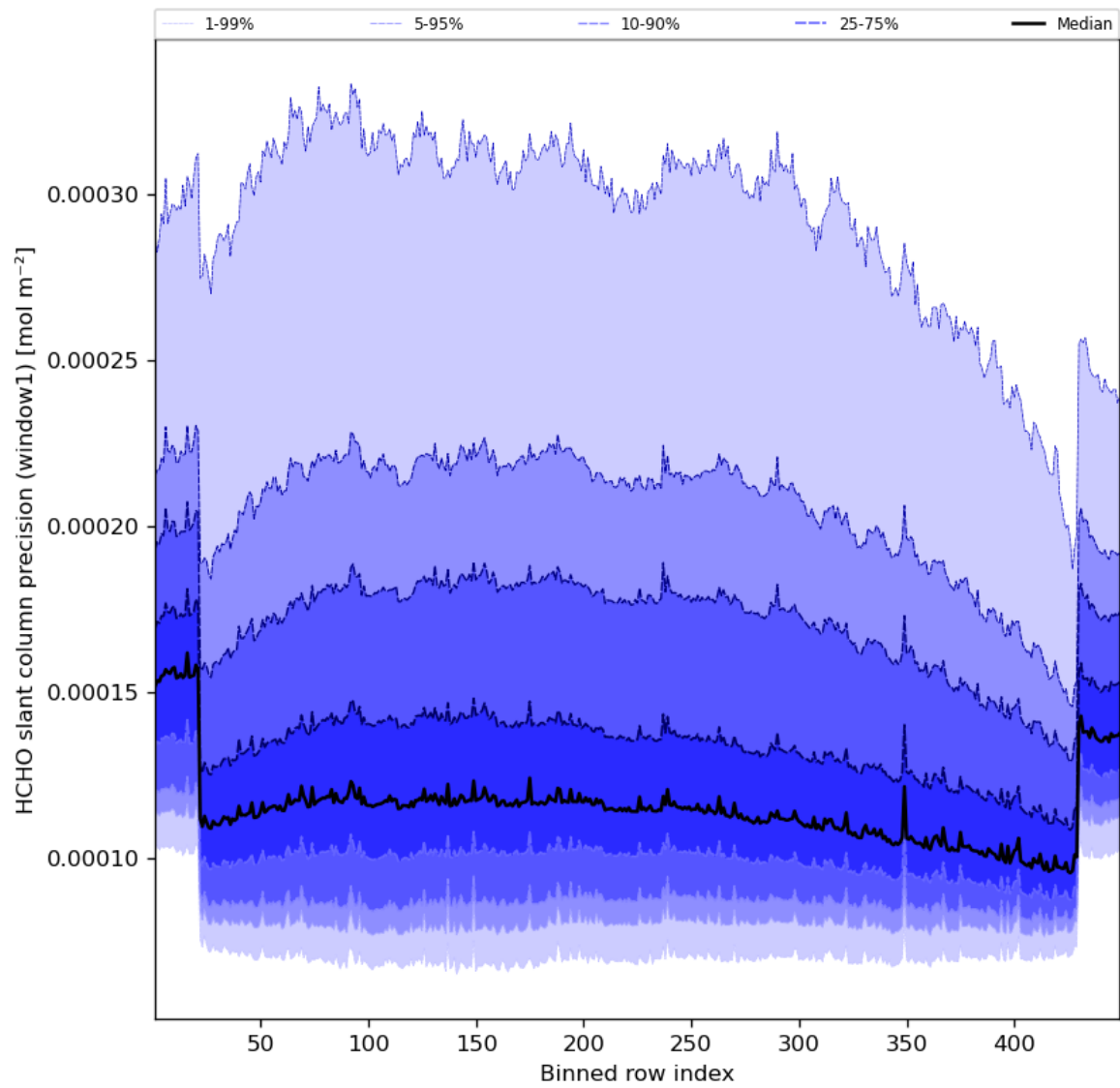
Figure 53: Along track statistics of “HCHO slant column precision (window1)” for 2023-11-20 to 2023-11-22
