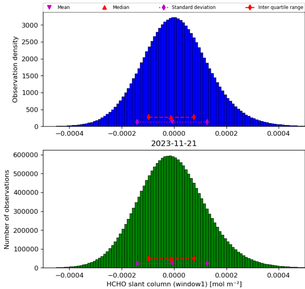
Figure 38: Histogram of “HCHO slant column (window1)” for 2023-11-20 to 2023-11-22
