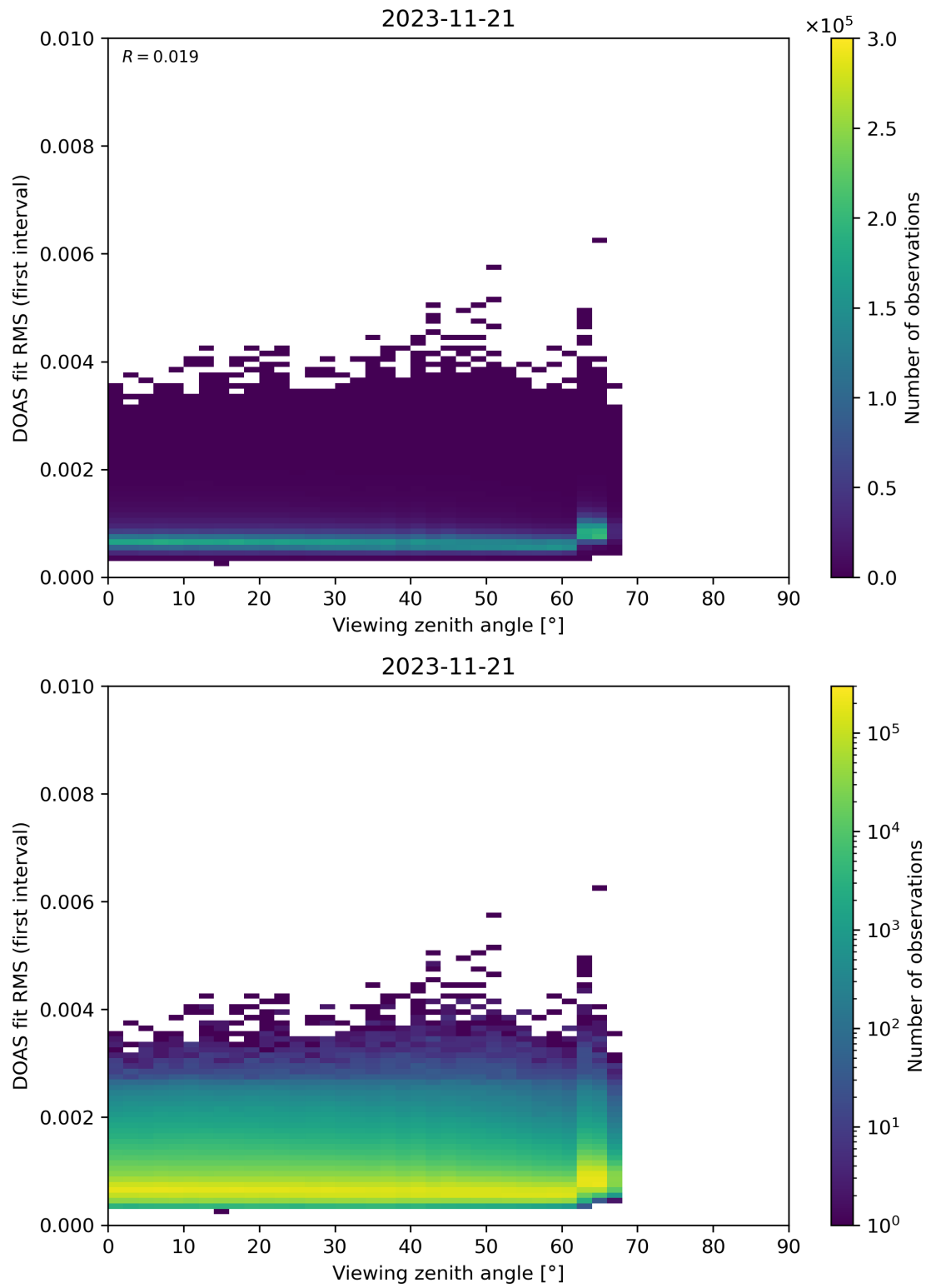
Figure 182: Scatter density plot of “Viewing zenith angle” against “DOAS fit RMS (first interval)” for 2023-11-20 to 2023-11-22.
