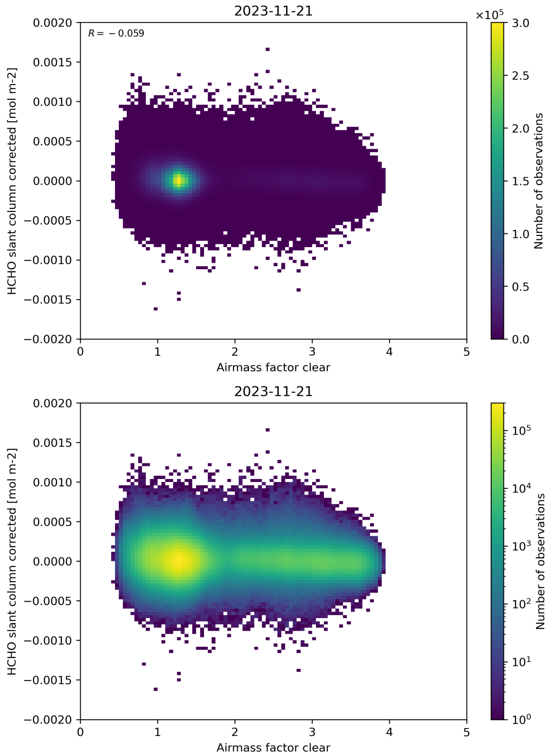
Figure 74: Scatter density plot of “Airmass factor clear” against “HCHO slant column corrected” for 2023-11-20 to 2023-11-22.
