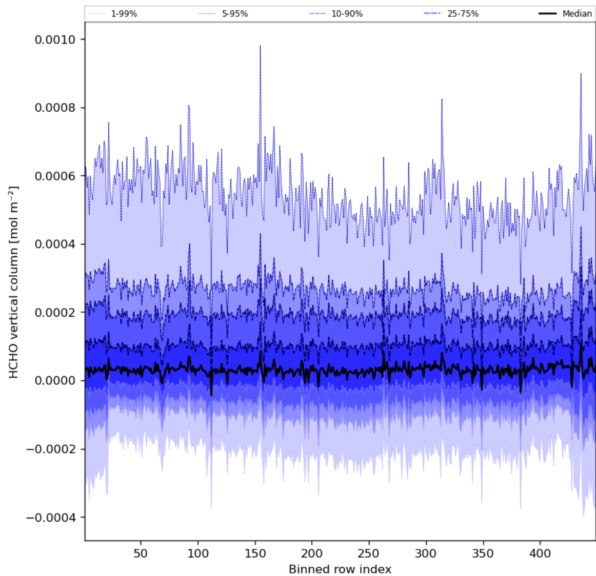
Figure 49: Along track statistics of “HCHO vertical column” for 2023-11-20 to 2023-11-22
