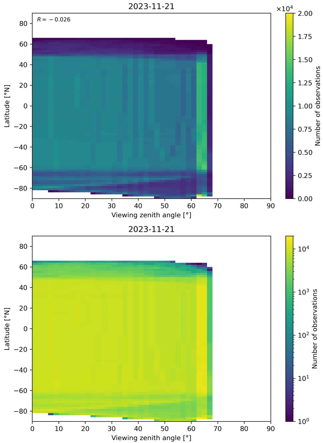
Figure 196: Scatter density plot of “Viewing zenith angle” against “Latitude” for 2023-11-20 to 2023-11-22.
