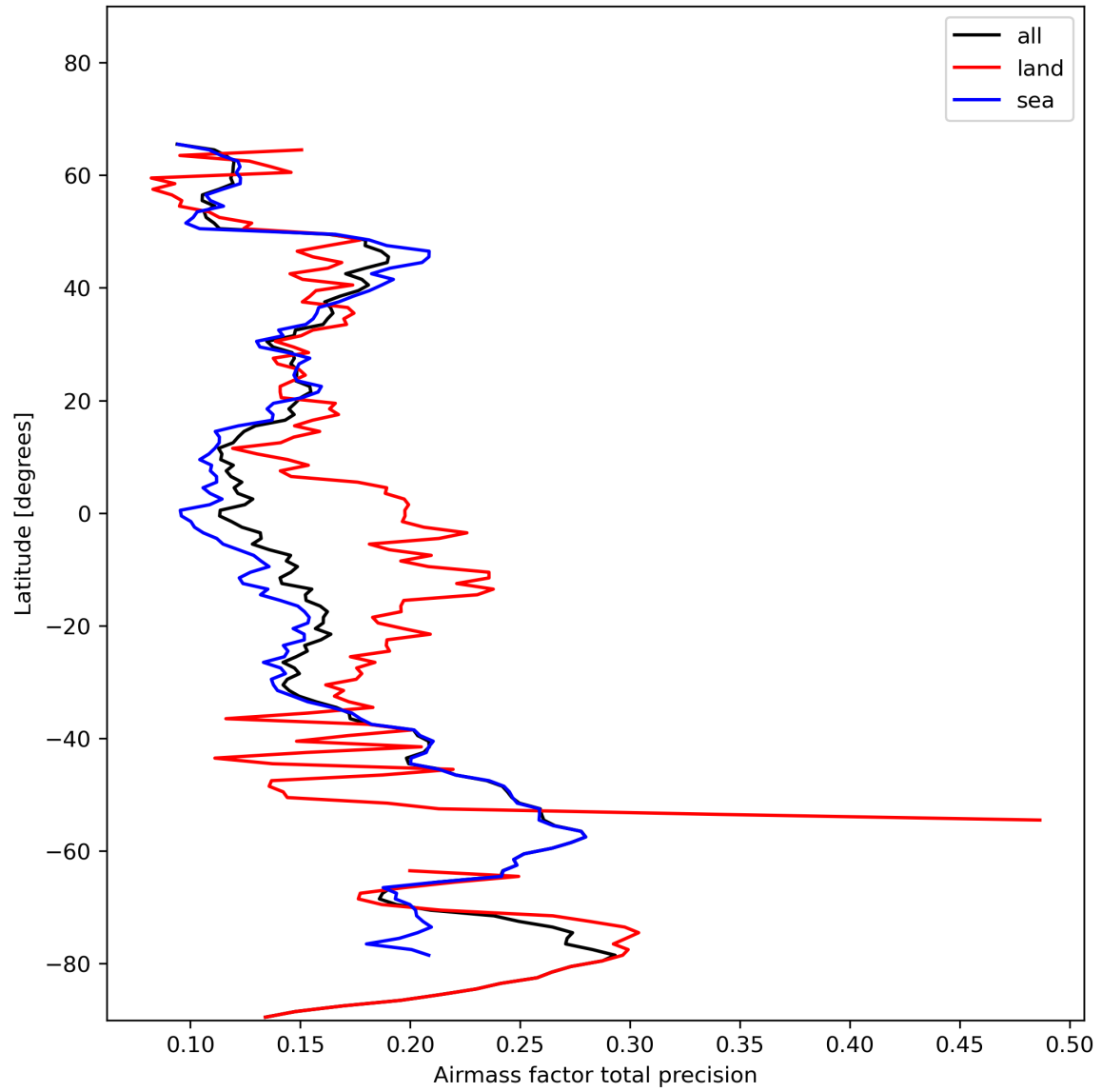
Figure 27: Zonal average of “Airmass factor total precision” for 2023-11-20 to 2023-11-22.
