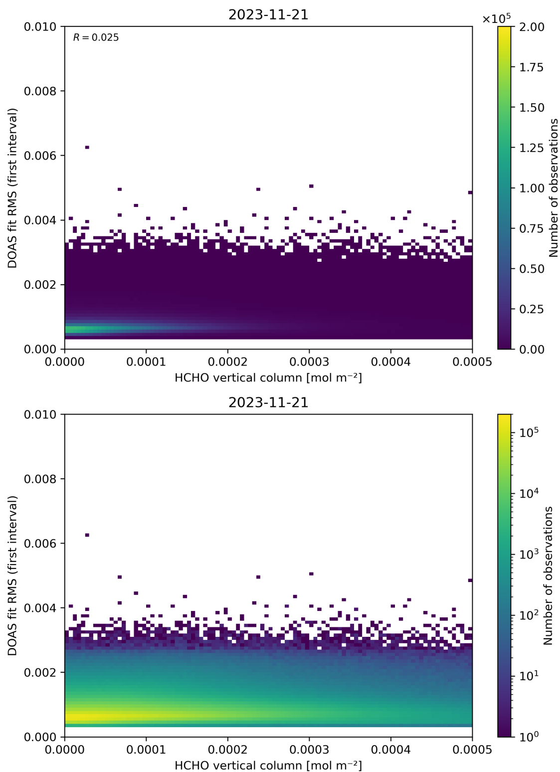
Figure 123: Scatter density plot of “HCHO vertical column” against “DOAS fit RMS (first interval)” for 2023-11-20 to 2023-11-22.
