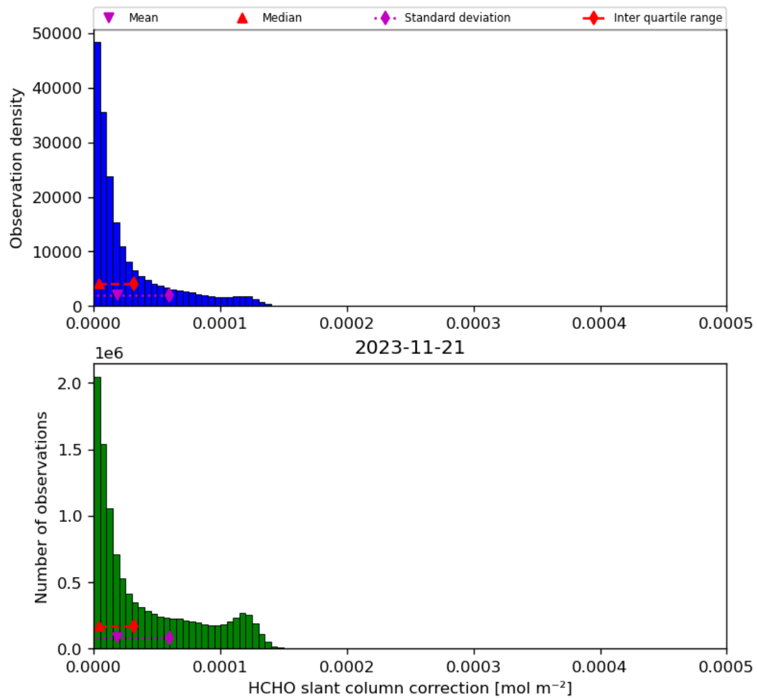
Figure 47: Histogram of “HCHO slant column correction” for 2023-11-20 to 2023-11-22
