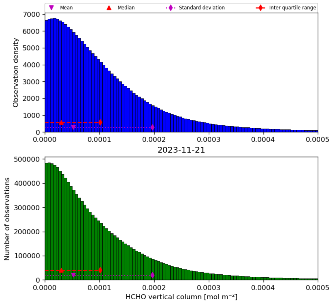
Figure 35: Histogram of “HCHO vertical column” for 2023-11-20 to 2023-11-22
