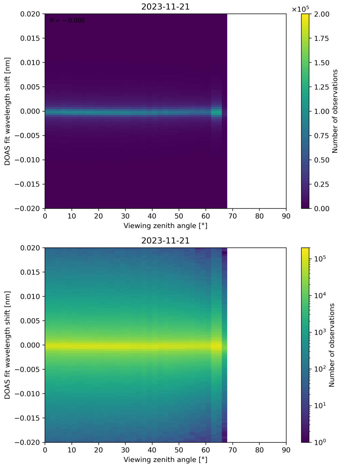
Figure 183: Scatter density plot of “Viewing zenith angle” against “DOAS fit wavelength shift” for 2023-11-20 to 2023-11-22.
