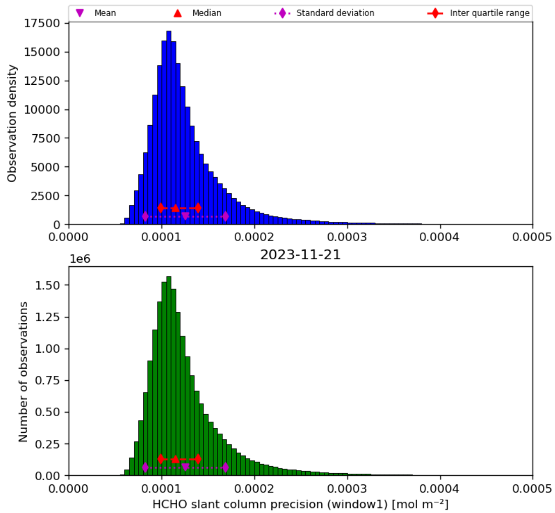
Figure 39: Histogram of “HCHO slant column precision (window1)” for 2023-11-20 to 2023-11-22
