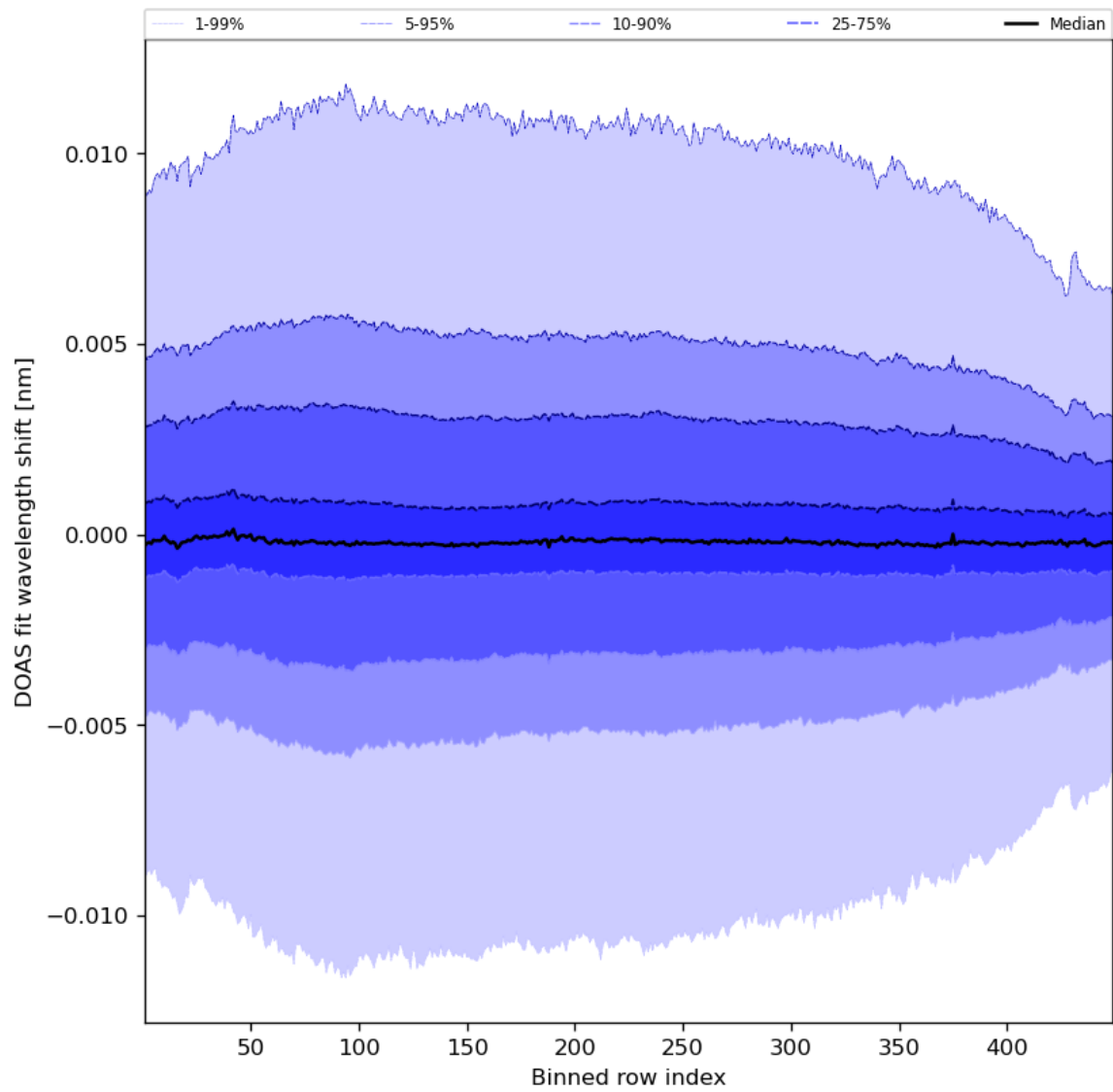
Figure 58: Along track statistics of “DOAS fit wavelength shift” for 2023-11-20 to 2023-11-22
