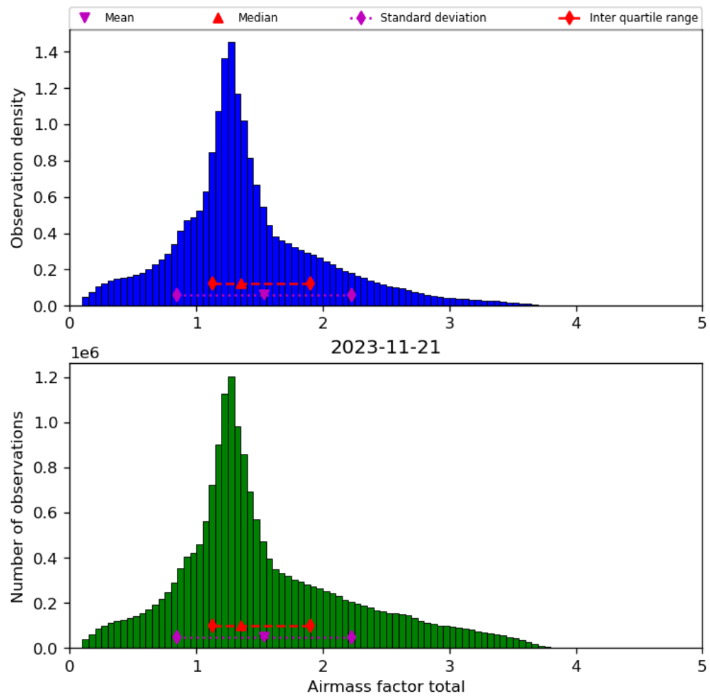
Figure 40: Histogram of “Airmass factor total” for 2023-11-20 to 2023-11-22
