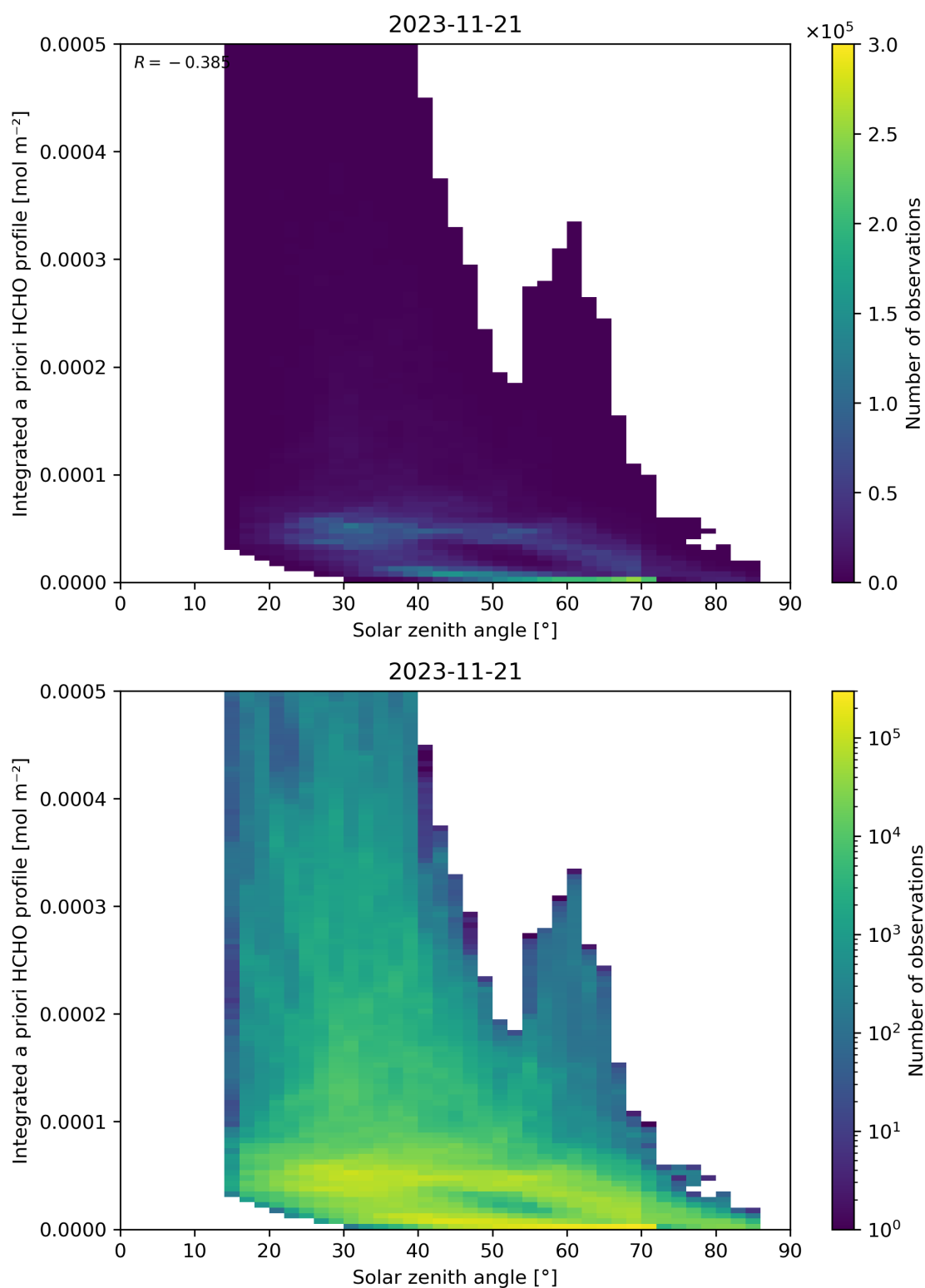
Figure 180: Scatter density plot of “Solar zenith angle” against “Integrated a priori HCHO profile” for 2023-11-20 to 2023-11-22.
