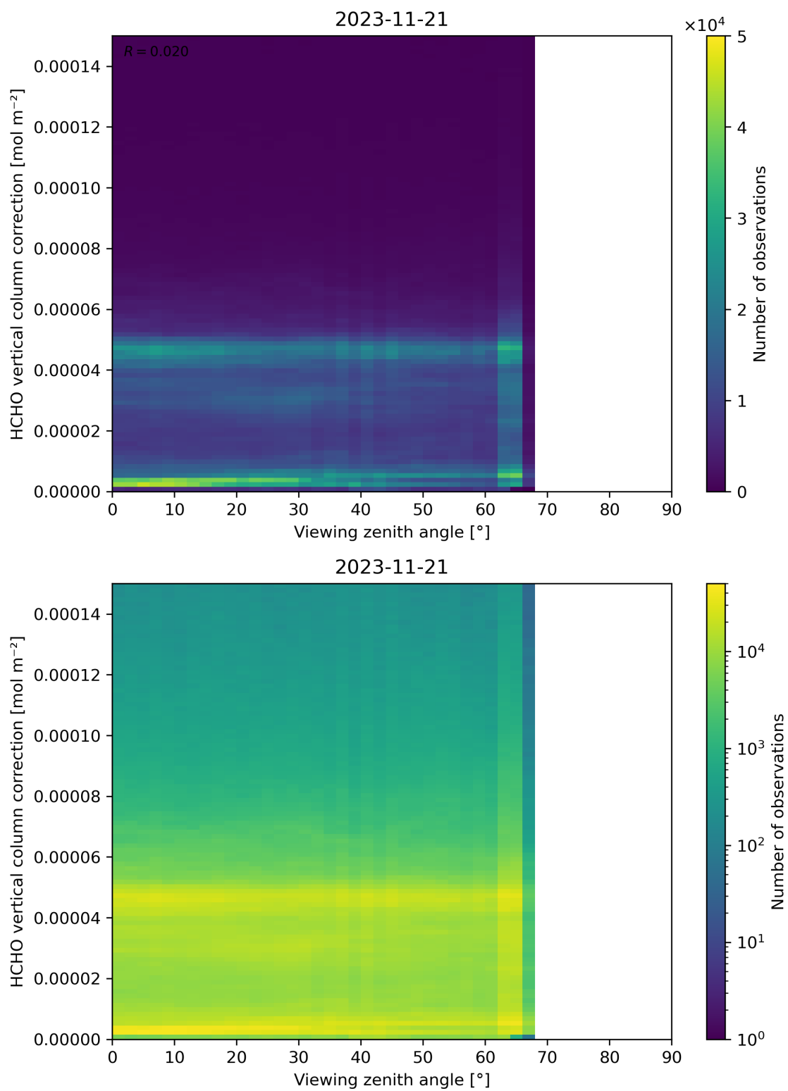
Figure 193: Scatter density plot of “Viewing zenith angle” against “HCHO vertical column correction” for 2023-11-20 to 2023-11-22.
