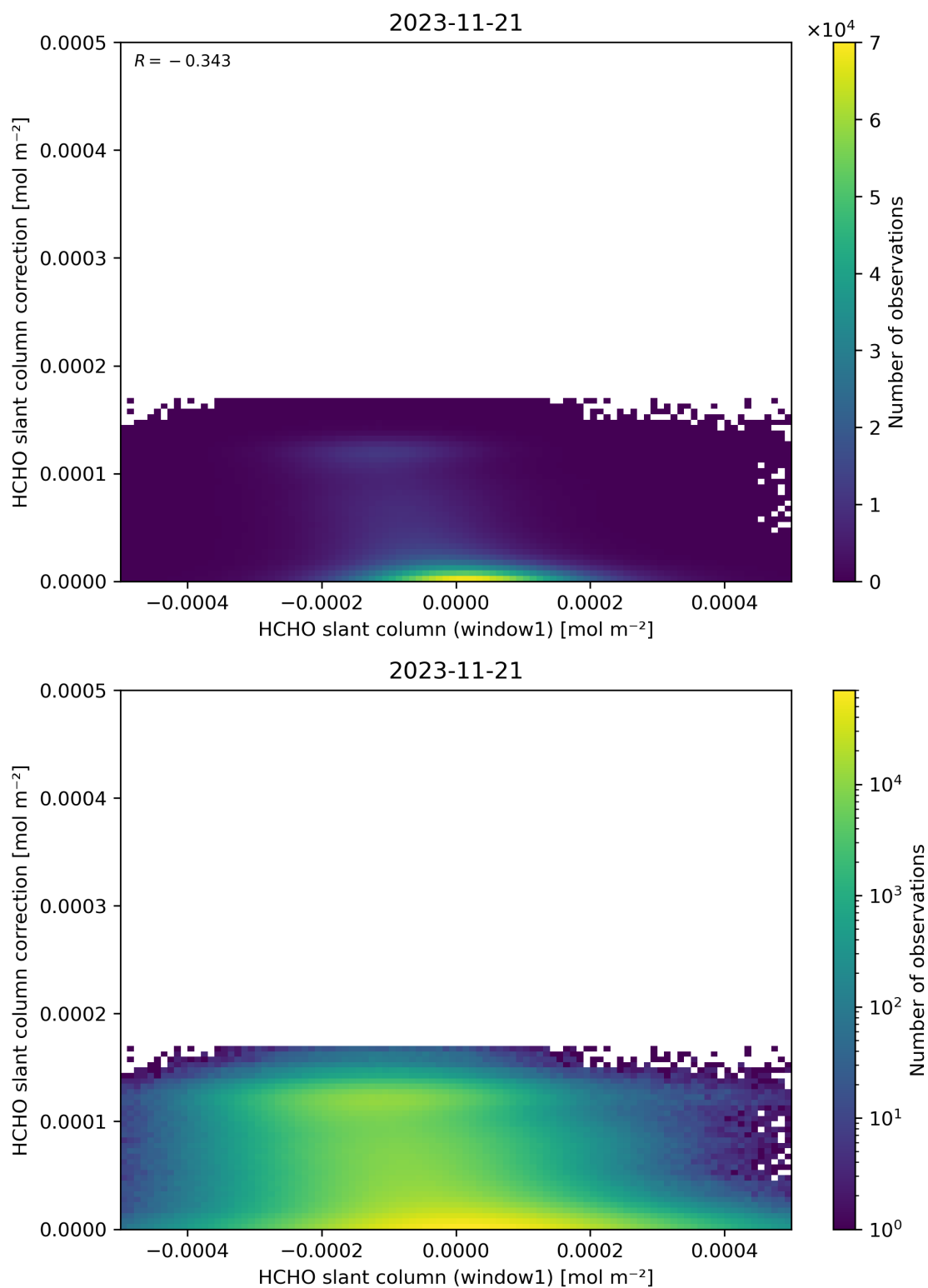
Figure 83: Scatter density plot of “HCHO slant column (window1)” against “HCHO slant column correction” for 2023-11-20 to 2023-11-22.
