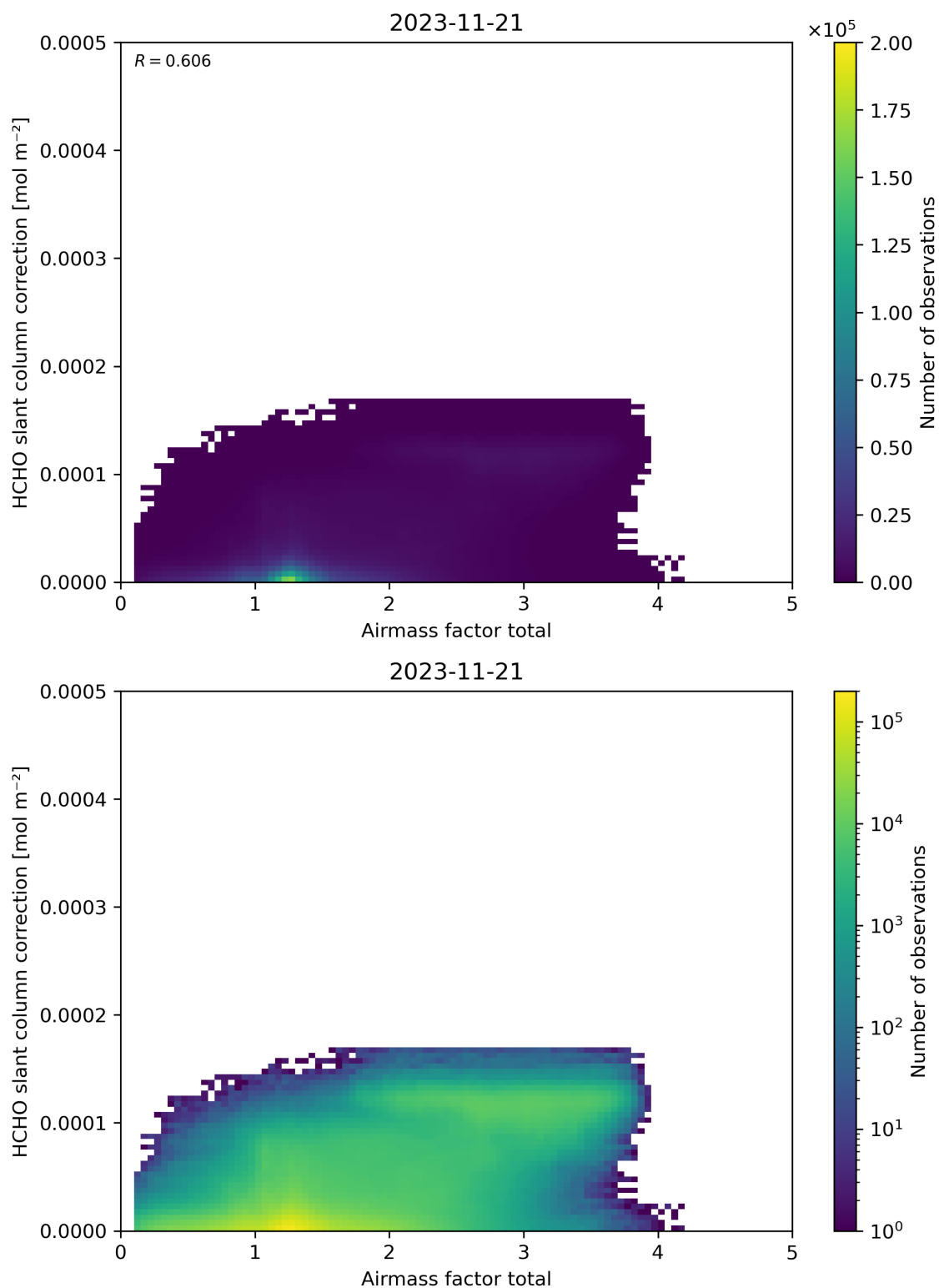
Figure 102: Scatter density plot of “Airmass factor total” against “HCHO slant column correction” for 2023-11-20 to 2023-11-22.
