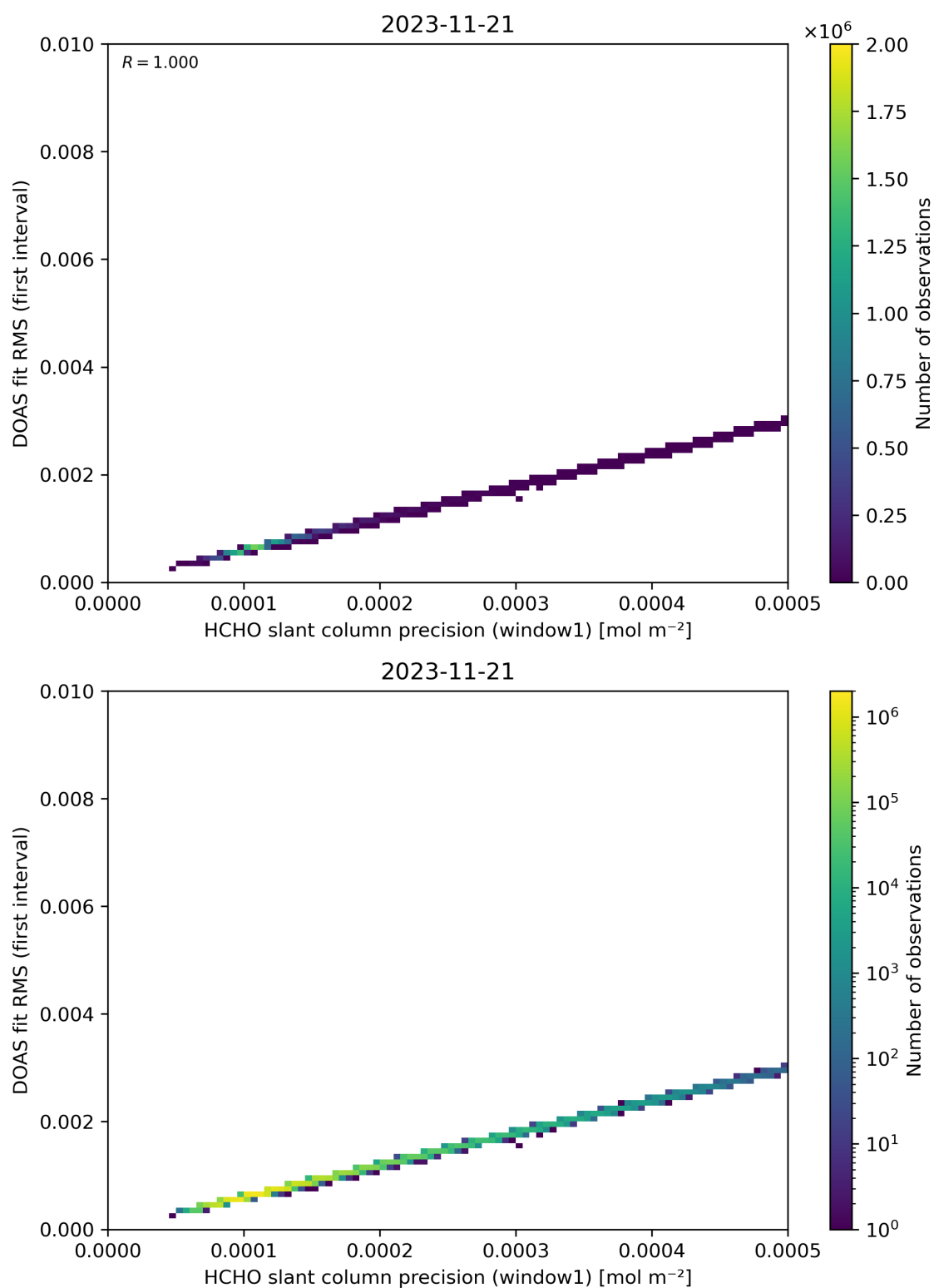
Figure 88: Scatter density plot of “HCHO slant column precision (window1)” against “DOAS fit RMS (first interval)” for 2023-11-20 to 2023-11-22.
