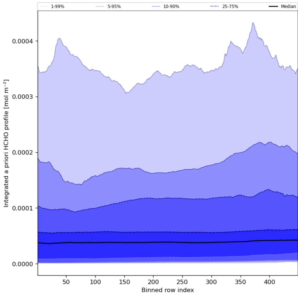
Figure 57: Along track statistics of “Integrated a priori HCHO profile” for 2023-11-20 to 2023-11-22
