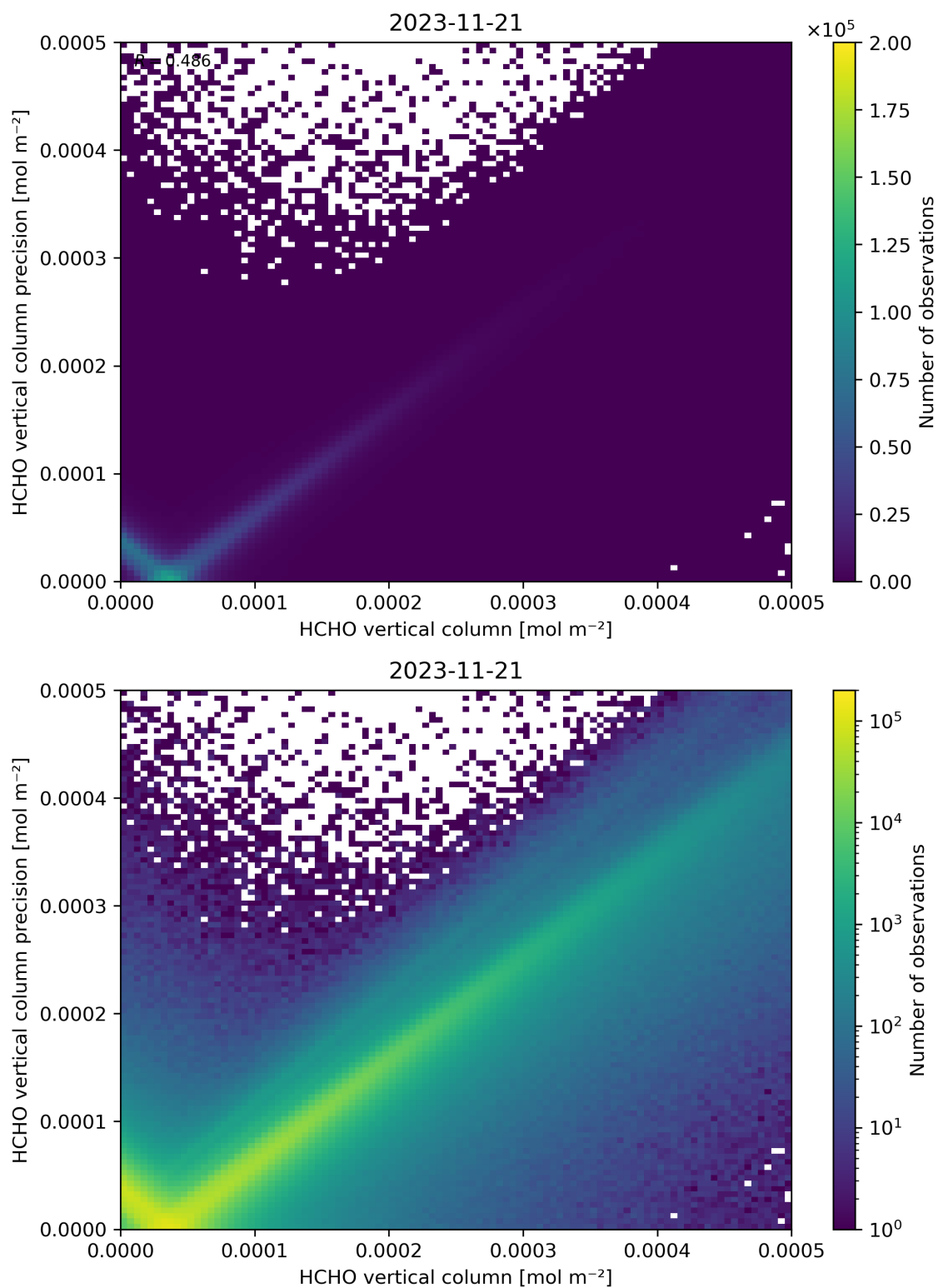
Figure 134: Scatter density plot of “HCHO vertical column” against “HCHO vertical column precision” for 2023-11-20 to 2023-11-22.
