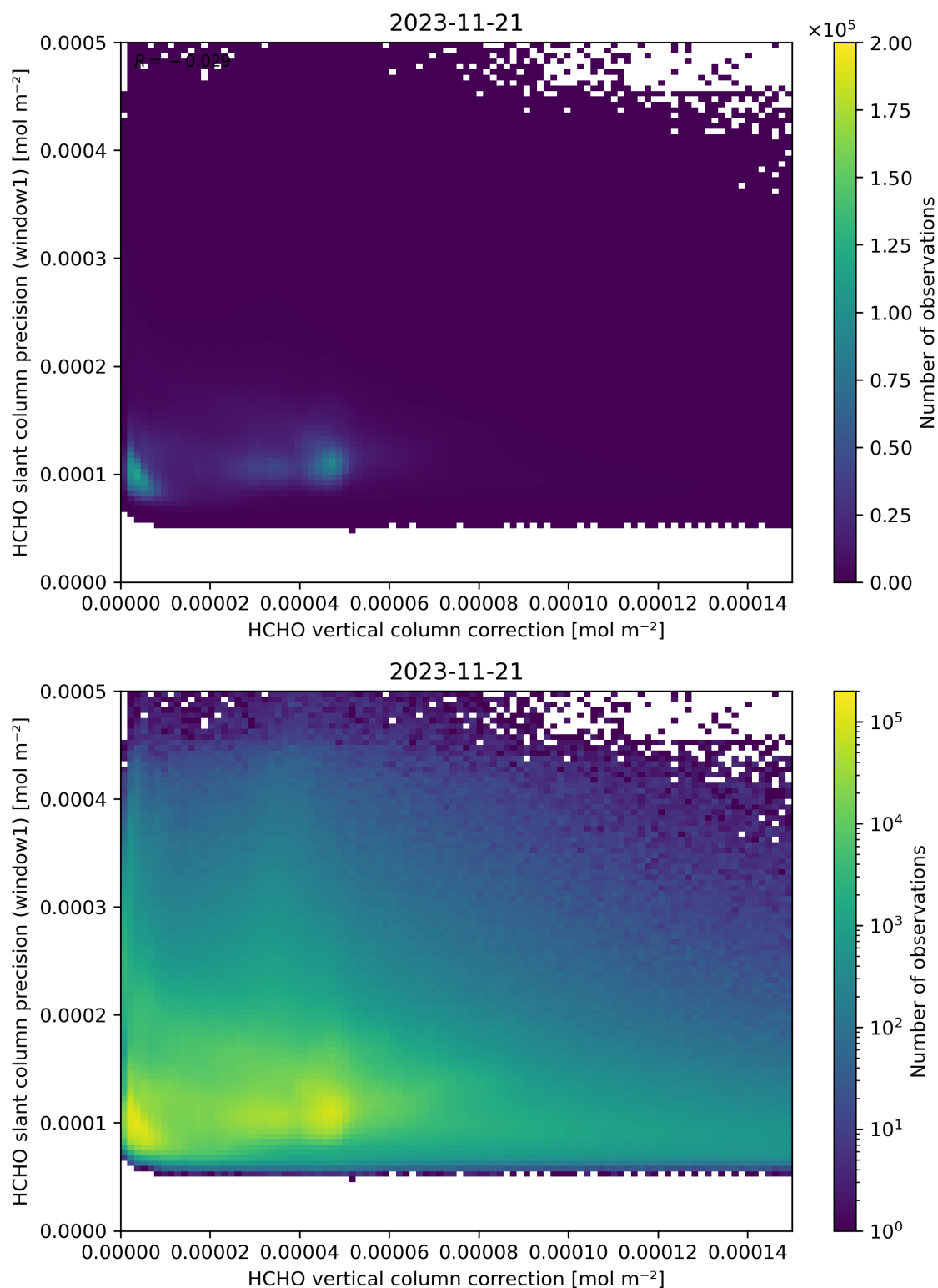
Figure 119: Scatter density plot of “HCHO vertical column correction” against “HCHO slant column precision (window1)” for 2023-11-20 to 2023-11-22.
