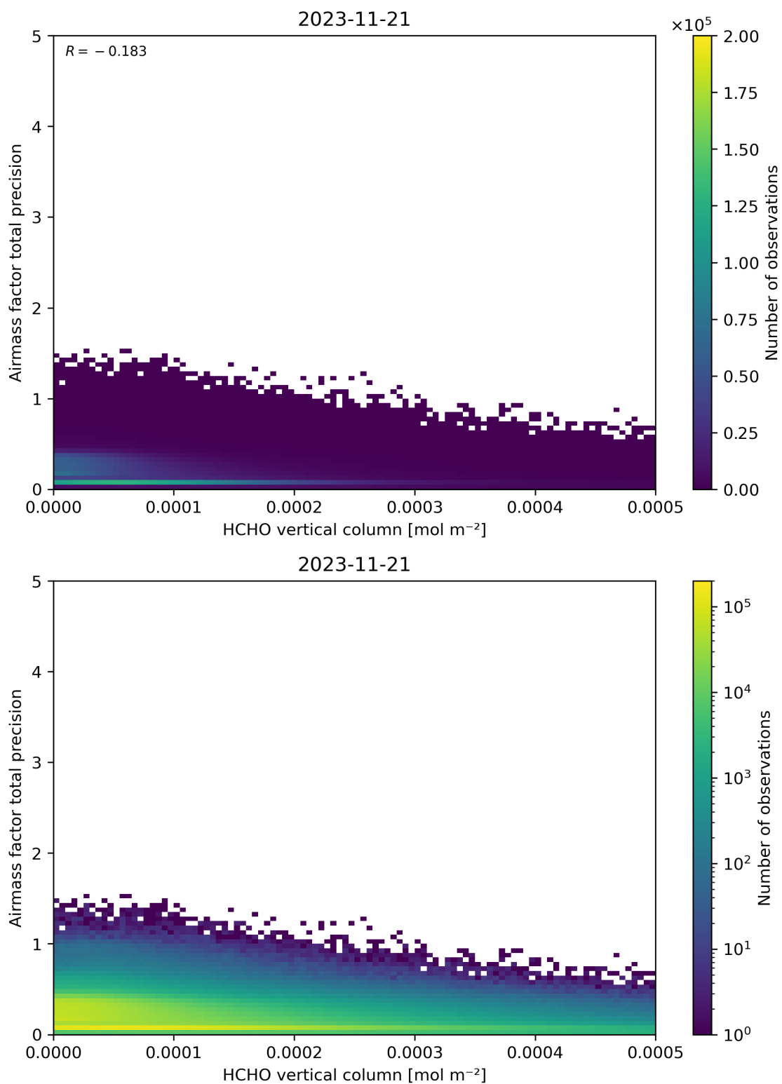
Figure 132: Scatter density plot of “HCHO vertical column” against “Airmass factor total precision” for 2023-11-20 to 2023-11-22.
