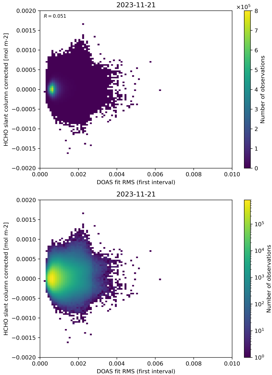
Figure 62: Scatter density plot of “DOAS fit RMS (first interval)” against “HCHO slant column corrected” for 2023-11-20 to 2023-11-22.
