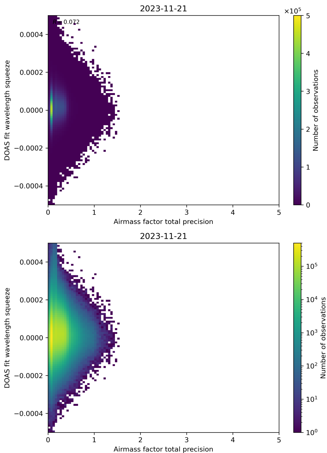
Figure 107: Scatter density plot of “Airmass factor total precision” against “DOAS fit wavelength squeeze” for 2023-11-20 to 2023-11-22.
