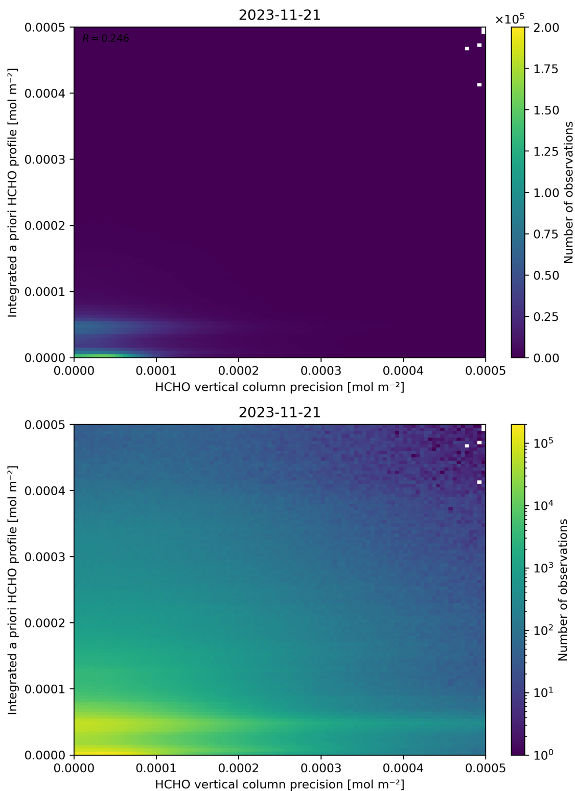
Figure 147: Scatter density plot of “HCHO vertical column precision” against “Integrated a priori HCHO profile” for 2023-11-20 to 2023-11-22.
