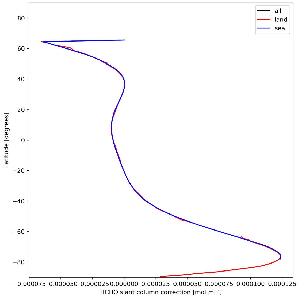
Figure 33: Zonal average of “HCHO slant column correction” for 2023-11-20 to 2023-11-22.
