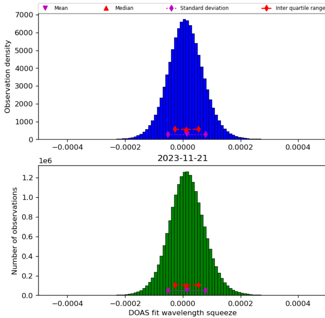
Figure 45: Histogram of “DOAS fit wavelength squeeze” for 2023-11-20 to 2023-11-22
