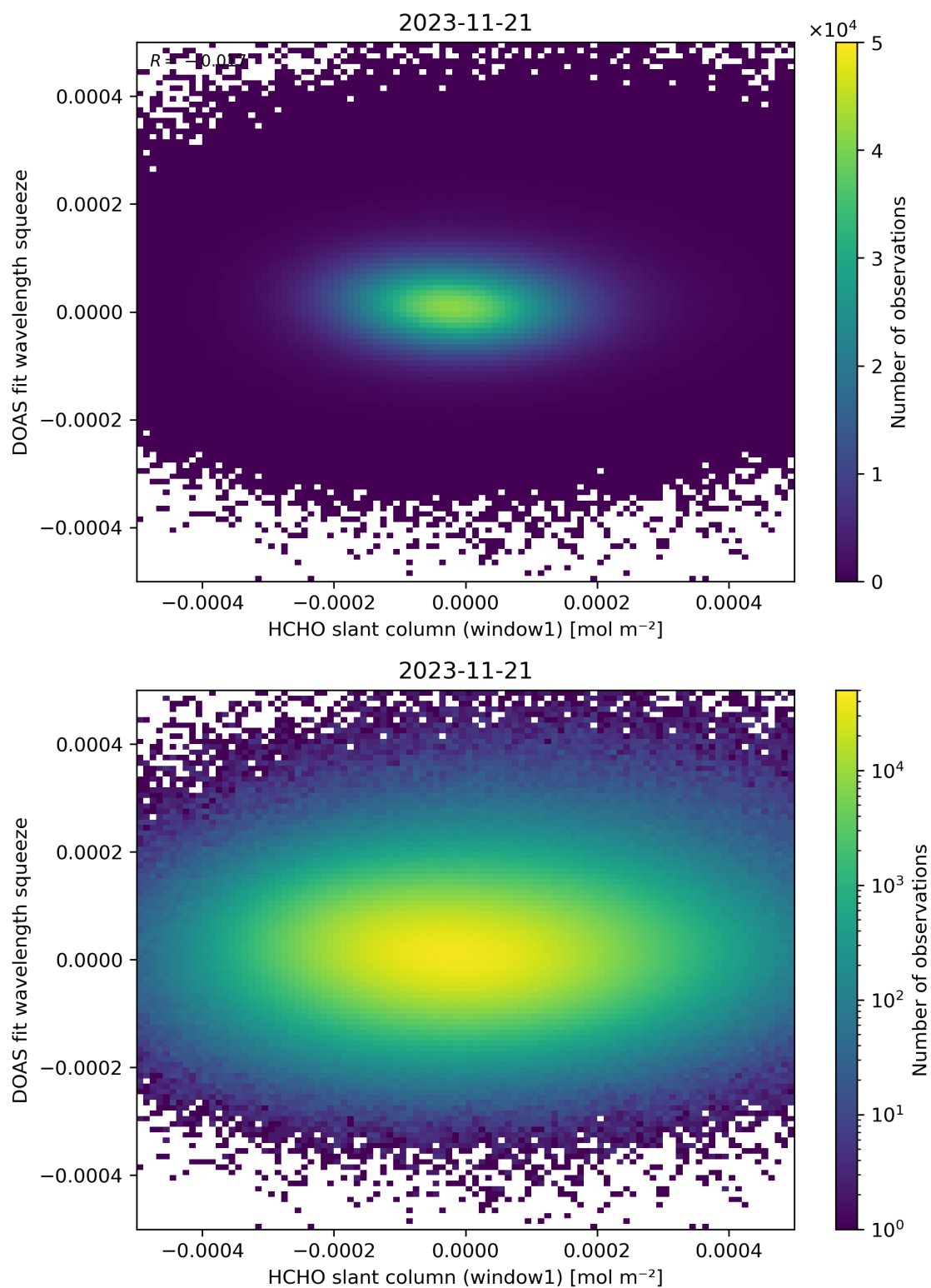
Figure 80: Scatter density plot of “HCHO slant column (window1)” against “DOAS fit wavelength squeeze” for 2023-11-20 to 2023-11-22.
