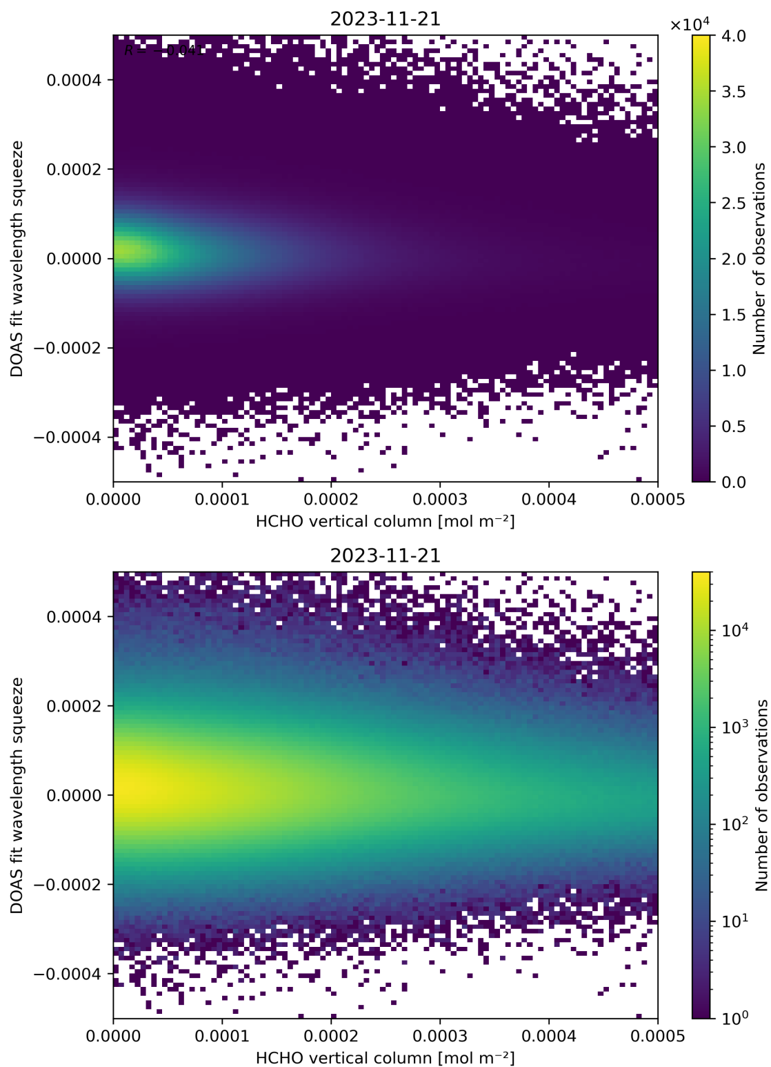
Figure 125: Scatter density plot of “HCHO vertical column” against “DOAS fit wavelength squeeze” for 2023-11-20 to 2023-11-22.
