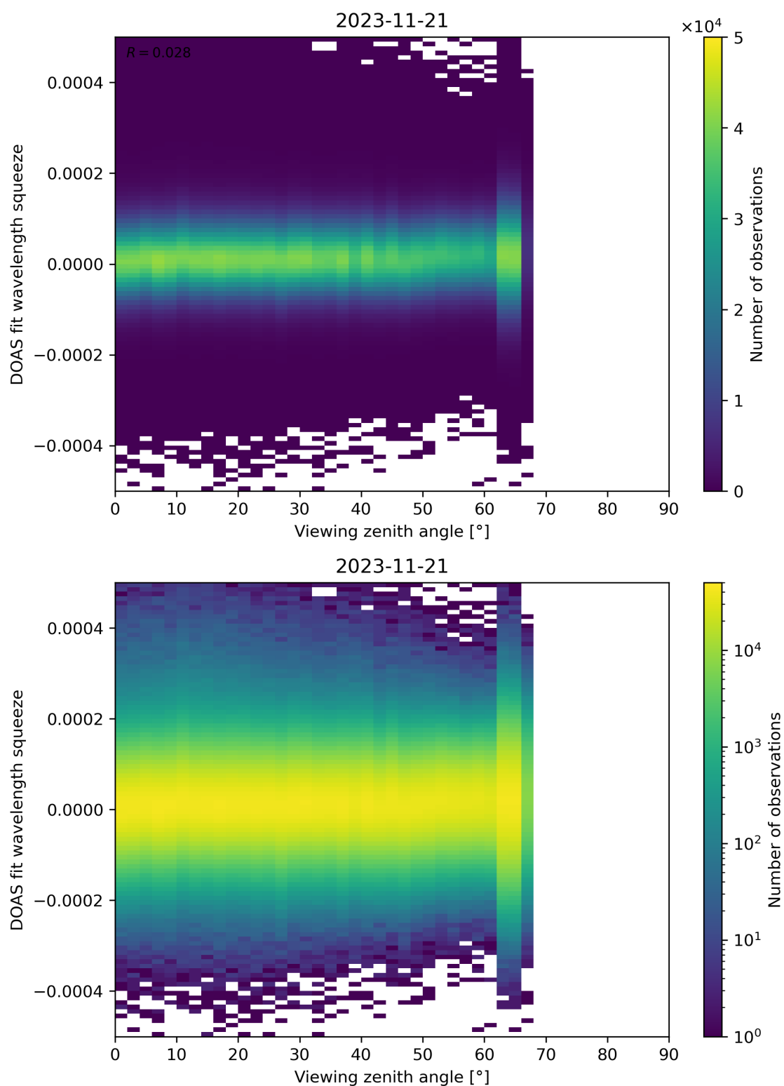
Figure 184: Scatter density plot of “Viewing zenith angle” against “DOAS fit wavelength squeeze” for 2023-11-20 to 2023-11-22.
