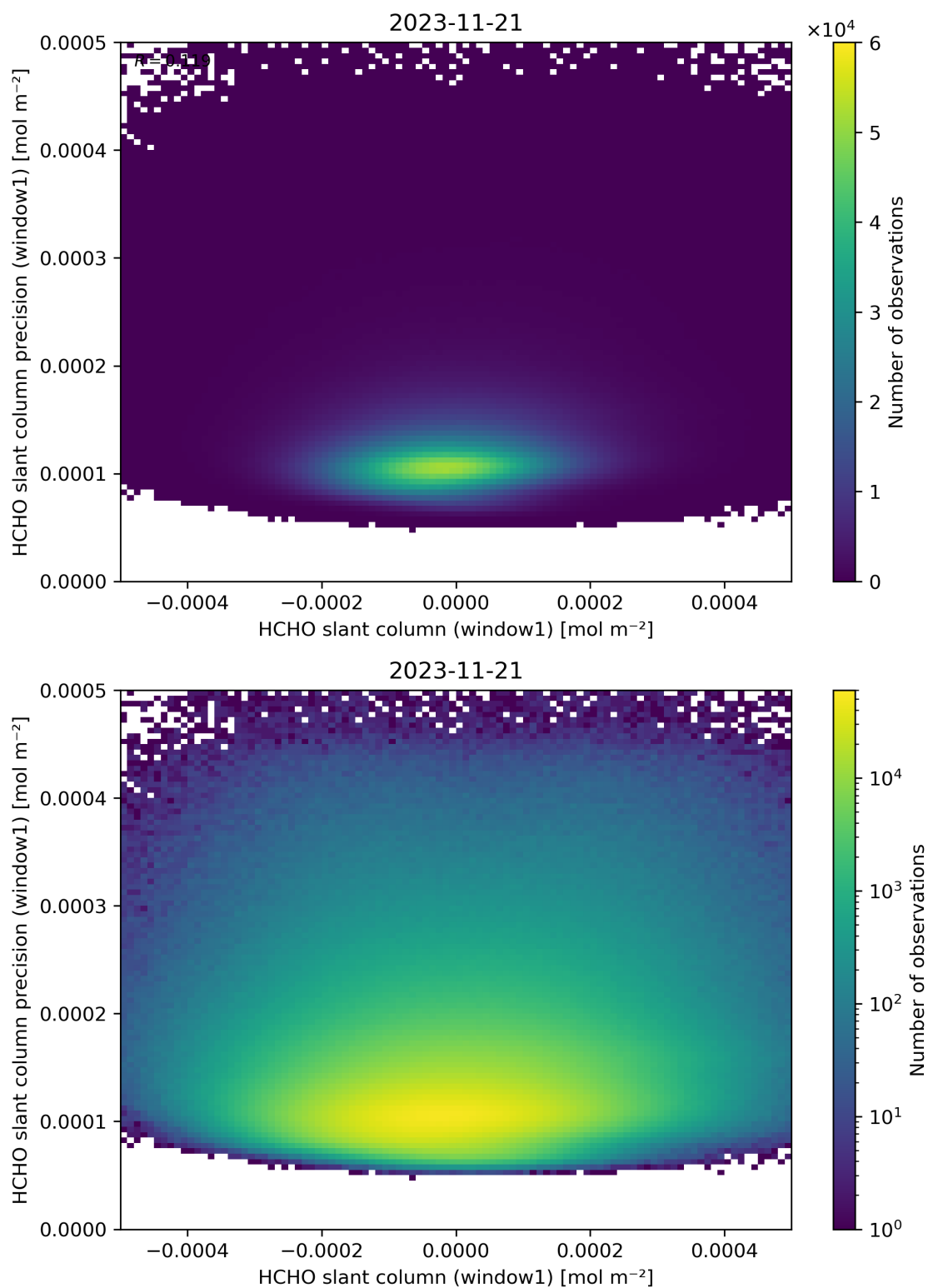
Figure 84: Scatter density plot of “HCHO slant column (window1)” against “HCHO slant column precision (window1)” for 2023-11-20 to 2023-11-22.
