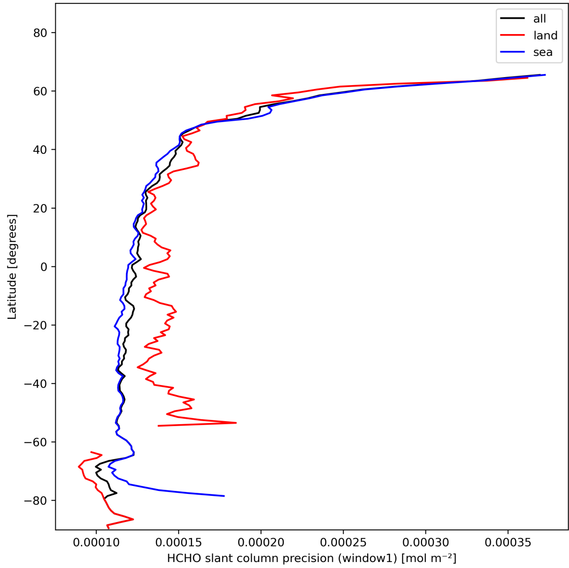
Figure 25: Zonal average of “HCHO slant column precision (window1)” for 2023-11-20 to 2023-11-22.
