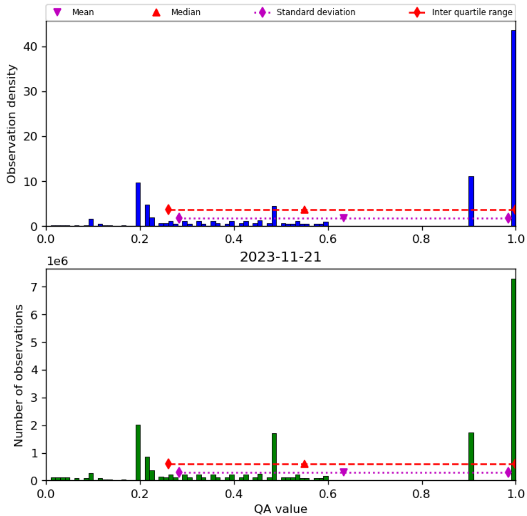
Figure 34: Histogram of “QA value” for 2023-11-20 to 2023-11-22
