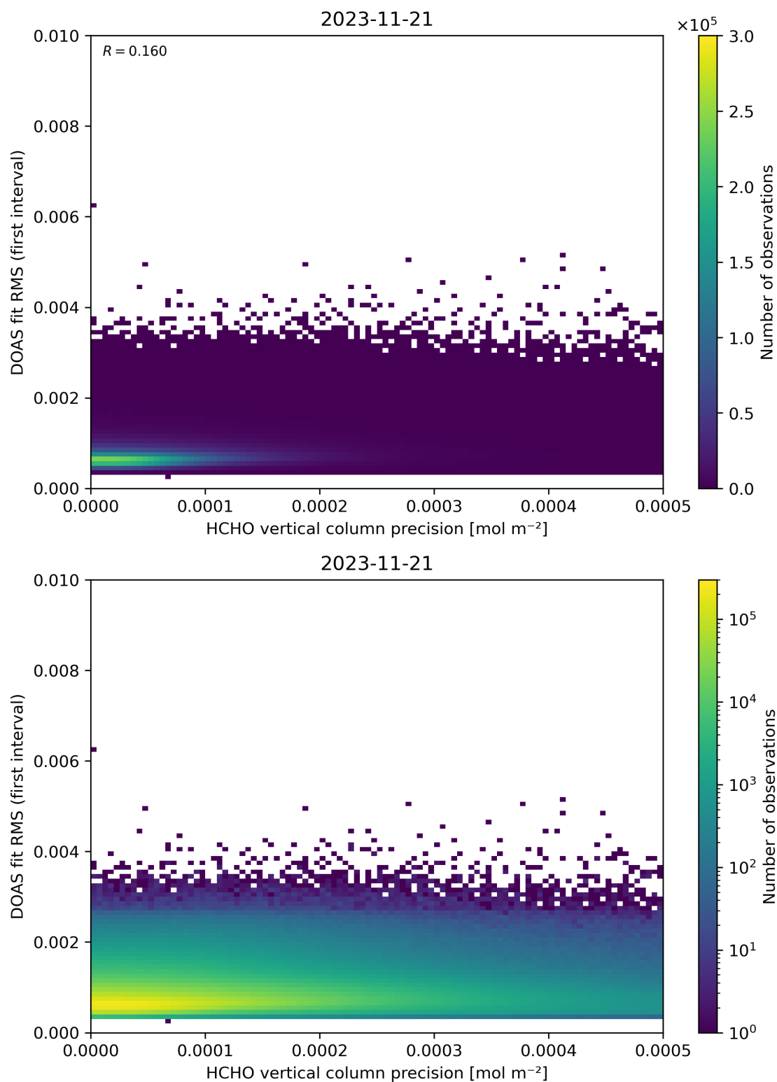
Figure 136: Scatter density plot of “HCHO vertical column precision” against “DOAS fit RMS (first interval)” for 2023-11-20 to 2023-11-22.
