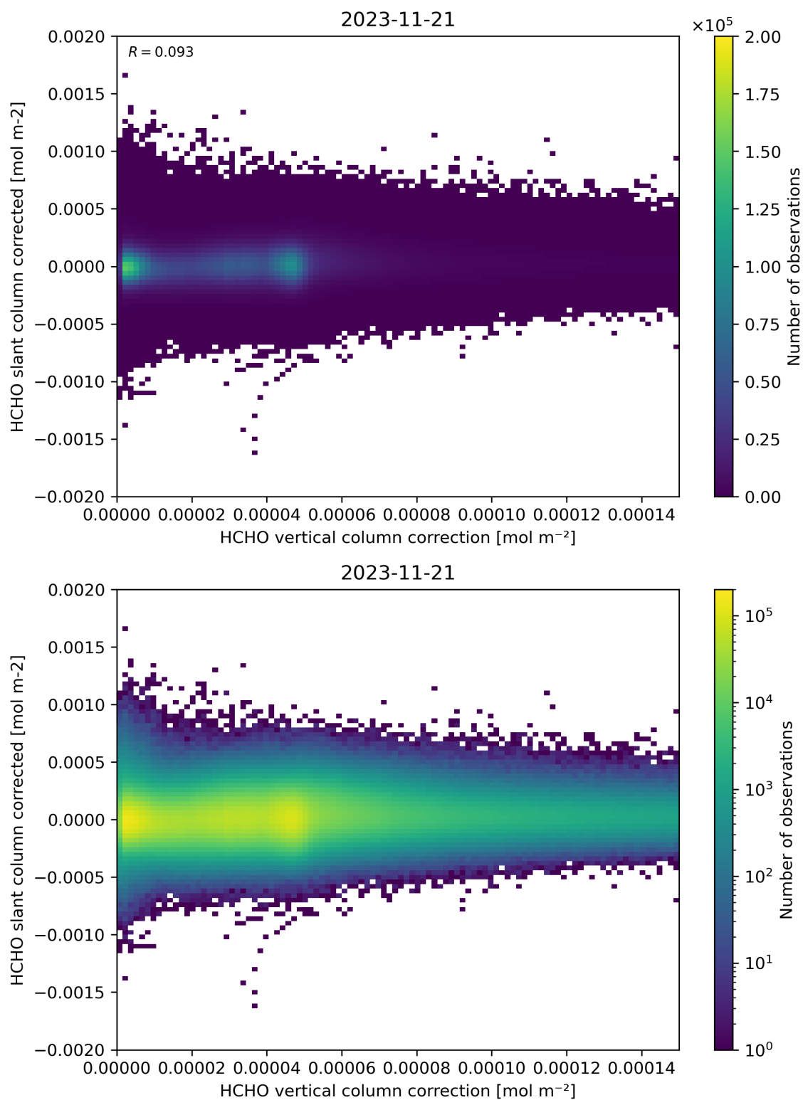
Figure 116: Scatter density plot of “HCHO vertical column correction” against “HCHO slant column corrected” for 2023-11-20 to 2023-11-22.
