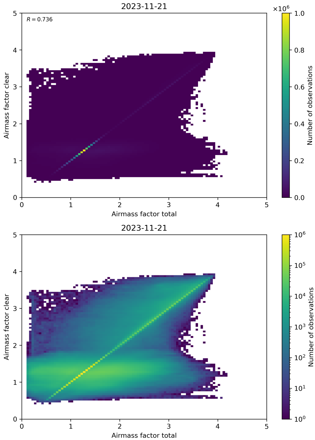
Figure 100: Scatter density plot of “Airmass factor total” against “Airmass factor clear” for 2023-11-20 to 2023-11-22.
