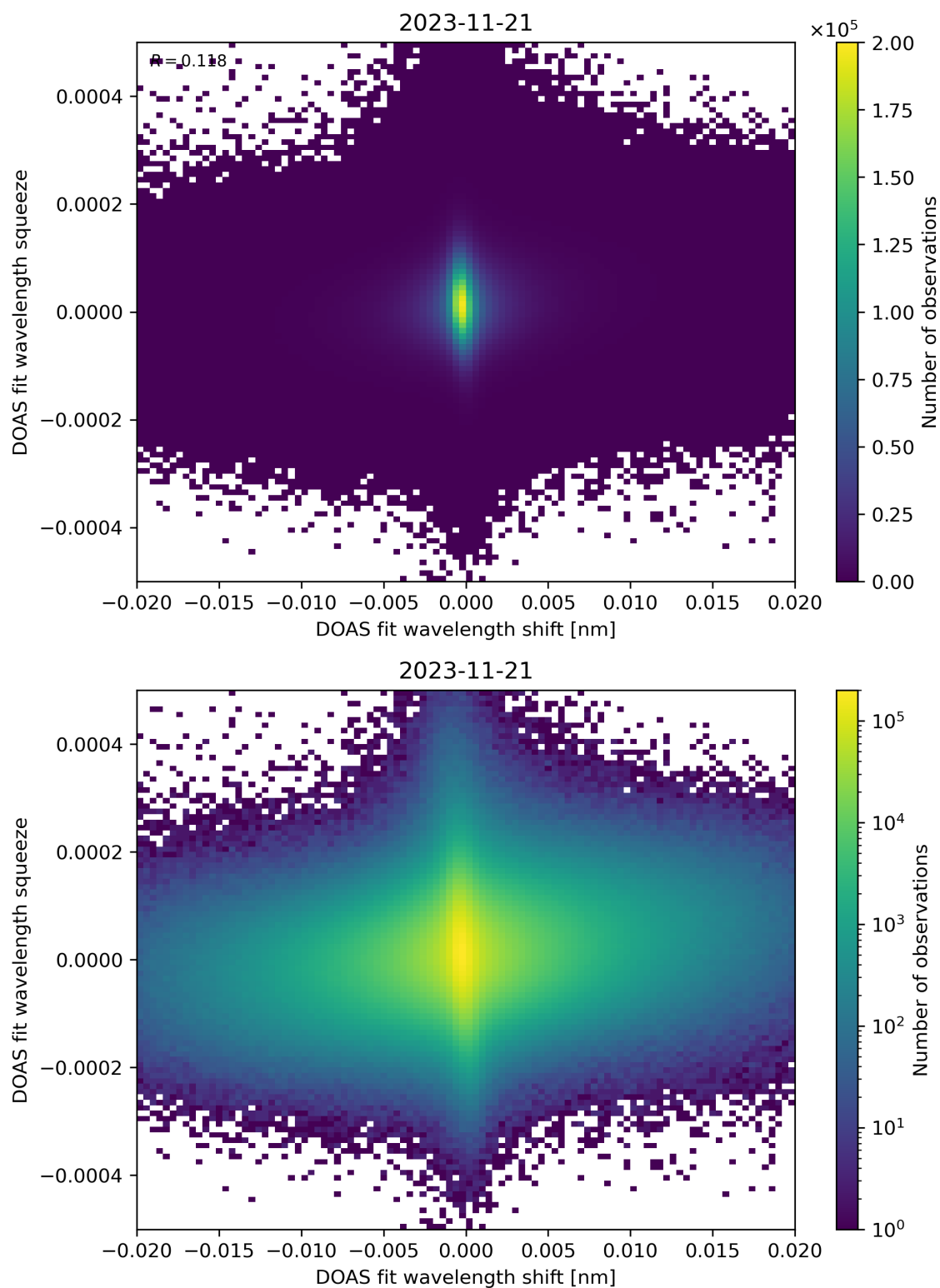
Figure 65: Scatter density plot of “DOAS fit wavelength shift” against “DOAS fit wavelength squeeze” for 2023-11-20 to 2023-11-22.
