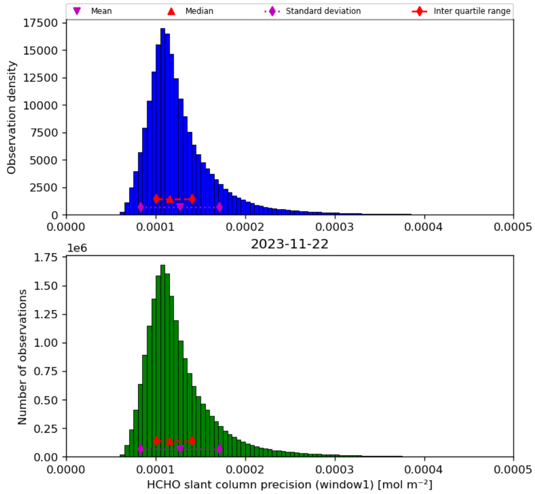
Figure 39: Histogram of “HCHO slant column precision (window1)” for 2023-11-21 to 2023-11-23
