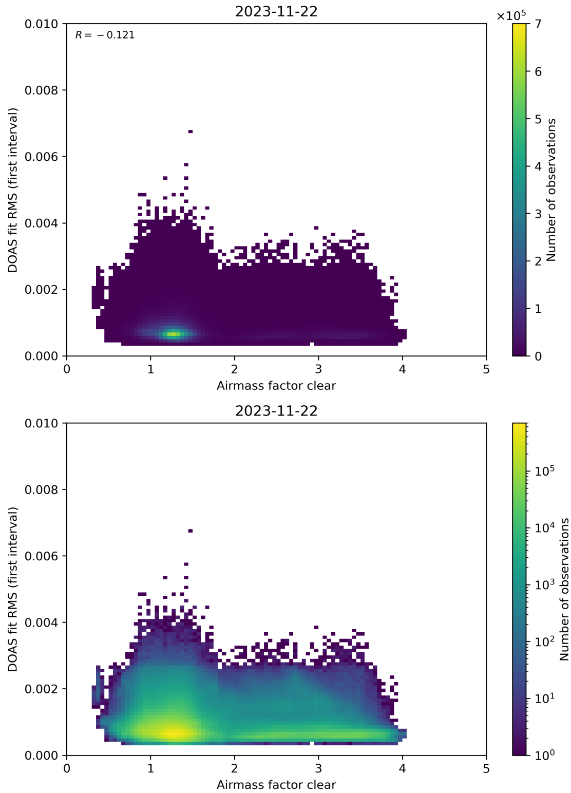
Figure 71: Scatter density plot of “Airmass factor clear” against “DOAS fit RMS (first interval)” for 2023-11-21 to 2023-11-23.
