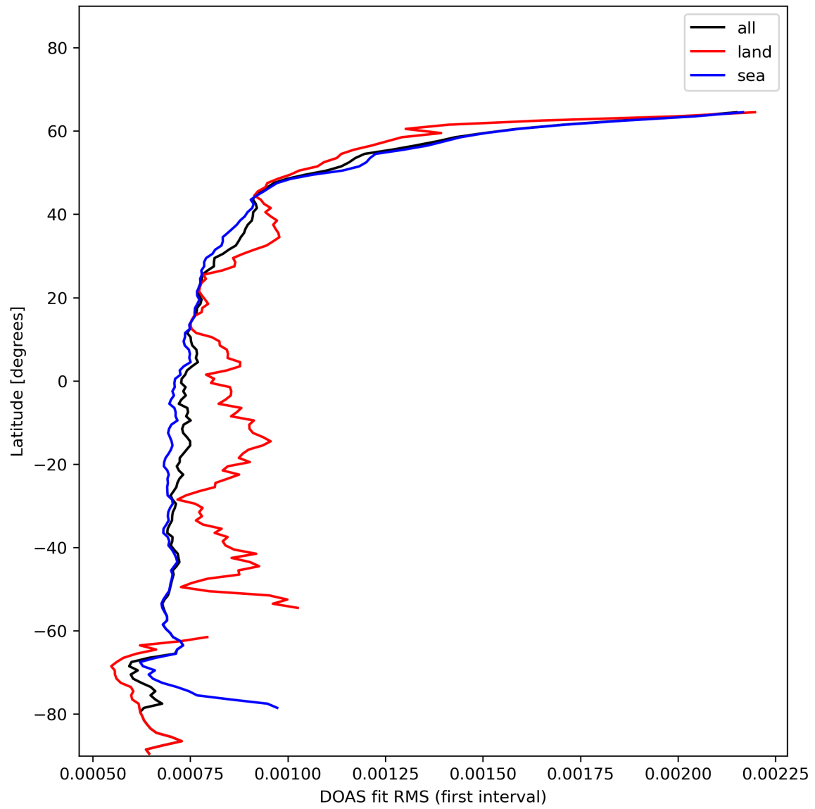
Figure 32: Zonal average of “DOAS fit RMS (first interval)” for 2023-11-21 to 2023-11-23.
