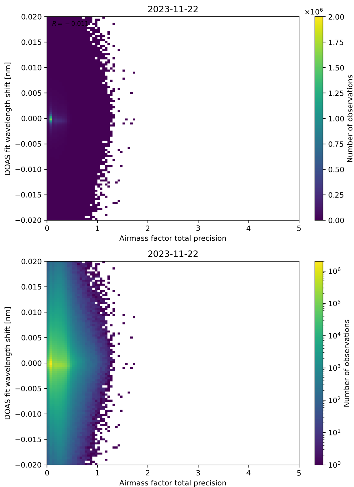
Figure 106: Scatter density plot of “Airmass factor total precision” against “DOAS fit wavelength shift” for 2023-11-21 to 2023-11-23.
