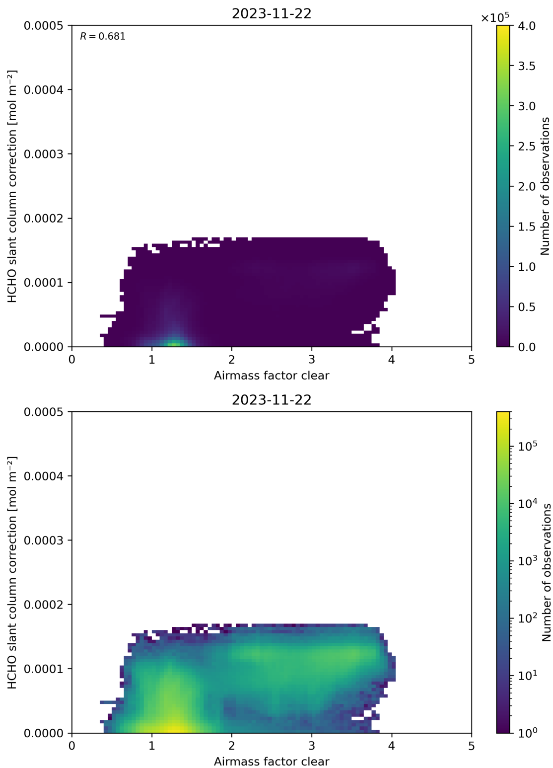
Figure 75: Scatter density plot of “Air mass factor clear” against “HCHO slant column correction” for 2023-11-21 to 2023-11-23.
