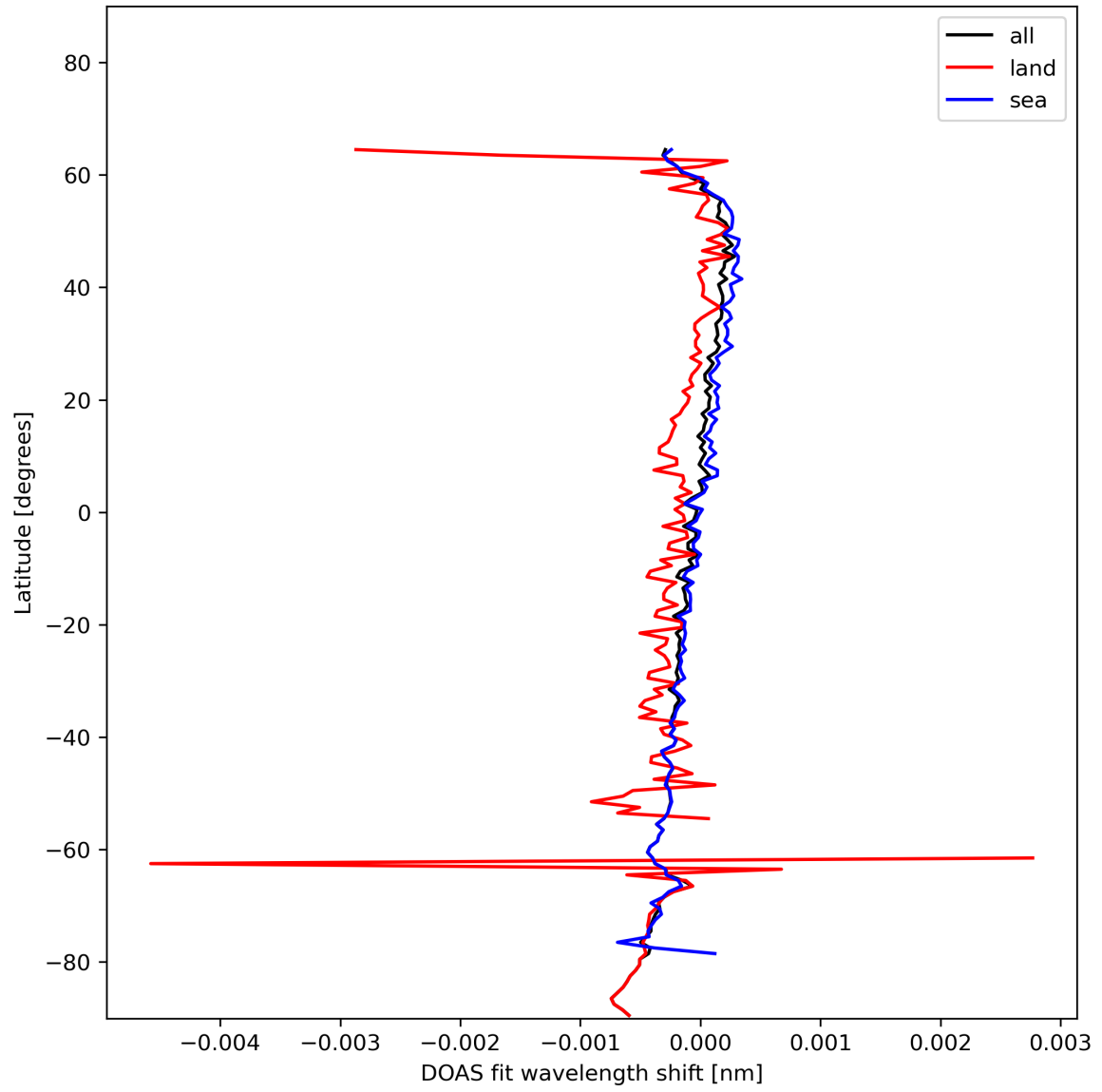
Figure 30: Zonal average of "DOAS fit wavelength shift" for 2023-11-21 to 2023-11-23.
