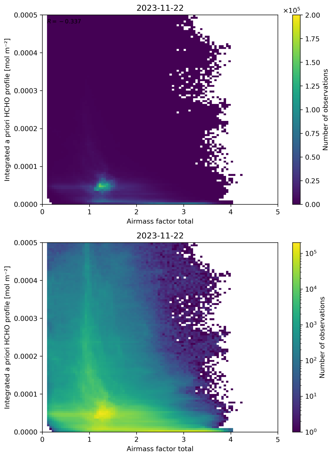
Figure 104: Scatter density plot of “Airmass factor total” against “Integrated a priori HCHO profile” for 2023-11-21 to 2023-11-23.
