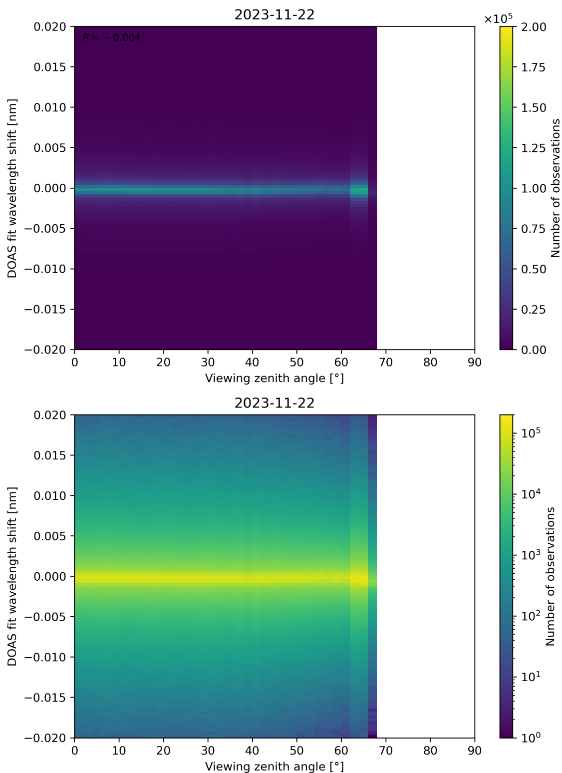
Figure 183: Scatter density plot of “Viewing zenith angle” against “DOAS fit wavelength shift” for 2023-11-21 to 2023-11-23.
