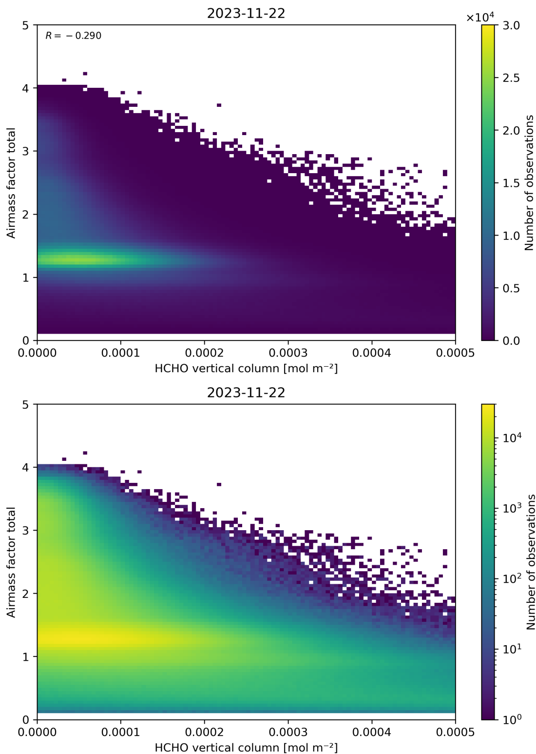
Figure 131: Scatter density plot of “HCHO vertical column” against “Airmass factor total” for 2023-11-21 to 2023-11-23.
