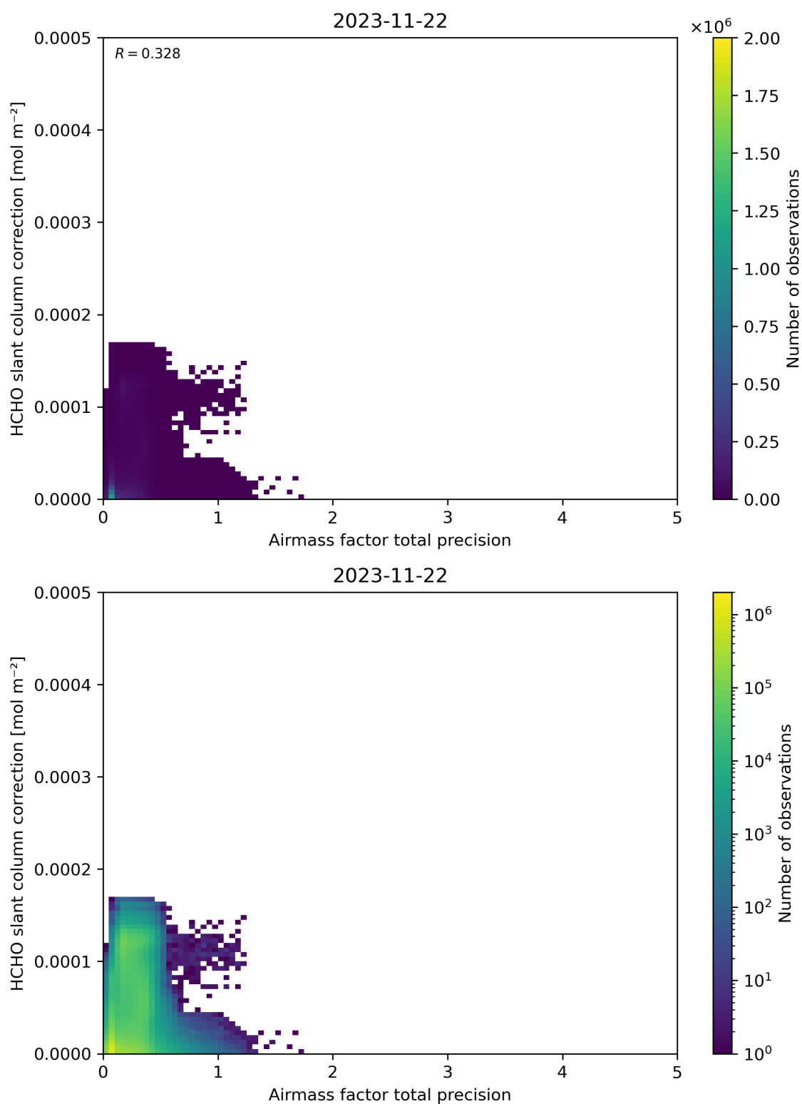
Figure 110: Scatter density plot of “Airmass factor total precision” against “HCHO slant column correction” for 2023-11-21 to 2023-11-23.
