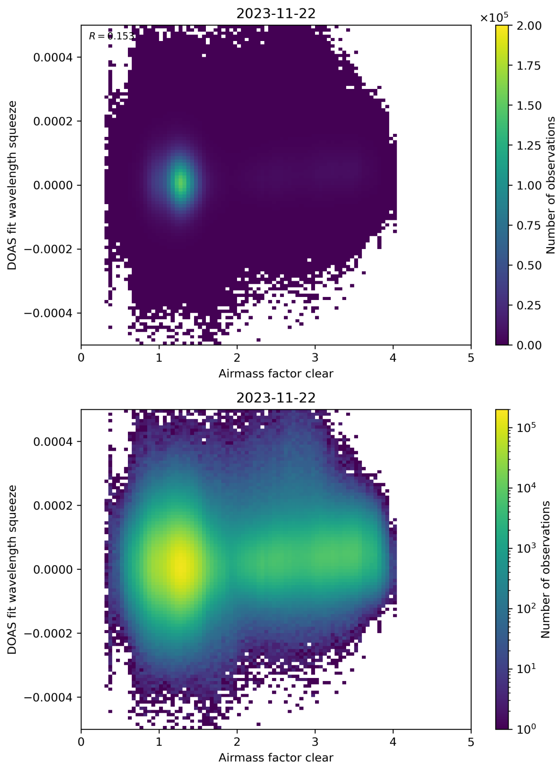
Figure 73: Scatter density plot of “Airmass factor clear” against “DOAS fit wavelength squeeze” for 2023-11-21 to 2023-11-23.
