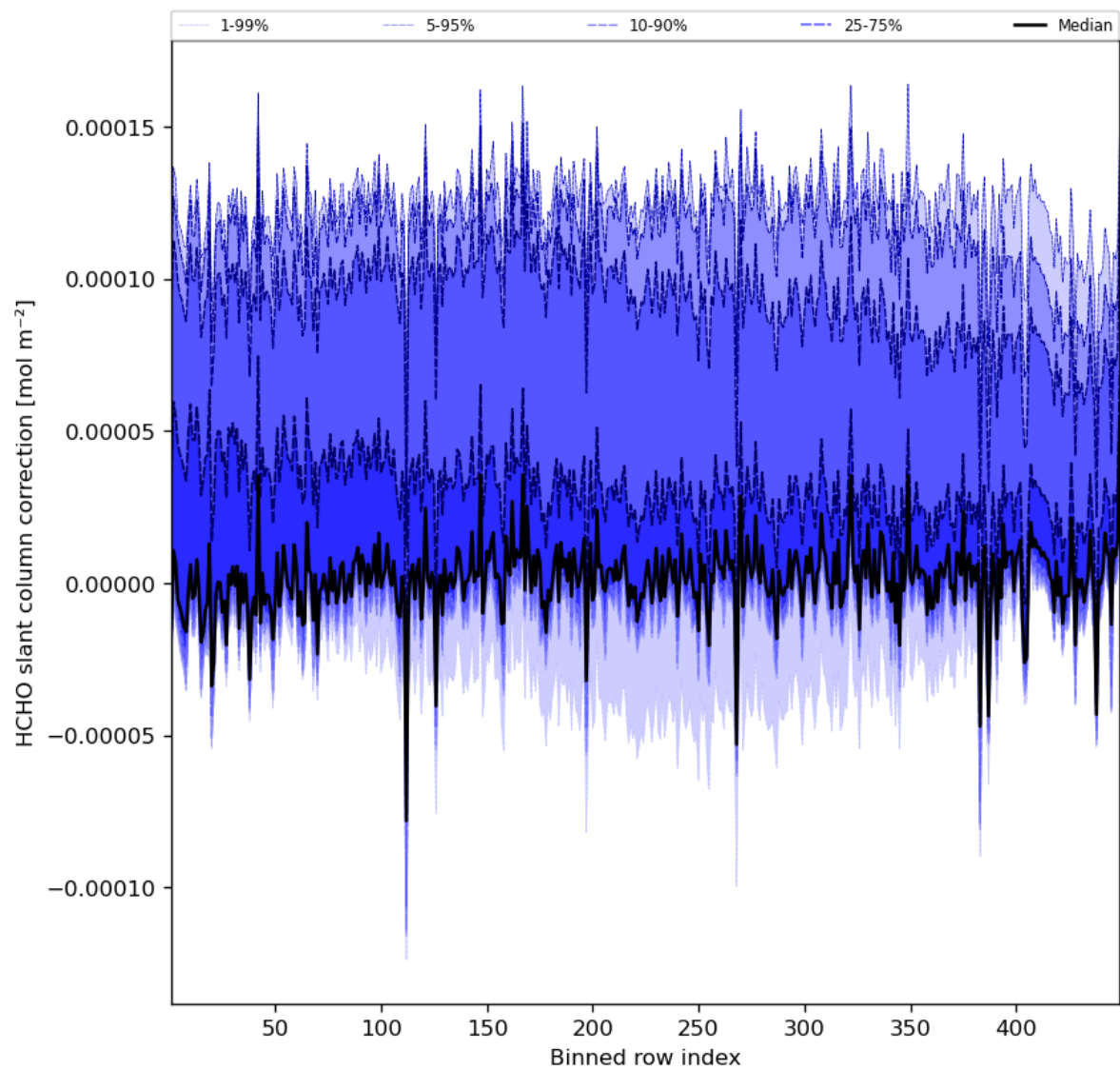
Figure 61: Along track statistics of “HCHO slant column correction” for 2023-11-21 to 2023-11-23
