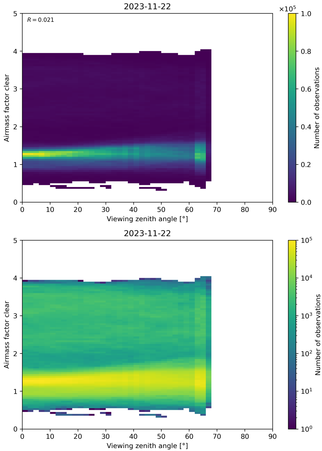
Figure 185: Scatter density plot of “Viewing zenith angle” against “Airmass factor clear” for 2023-11-21 to 2023-11-23.
