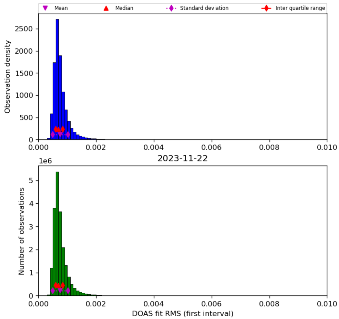
Figure 46: Histogram of “DOAS fit RMS (first interval)” for 2023-11-21 to 2023-11-23
