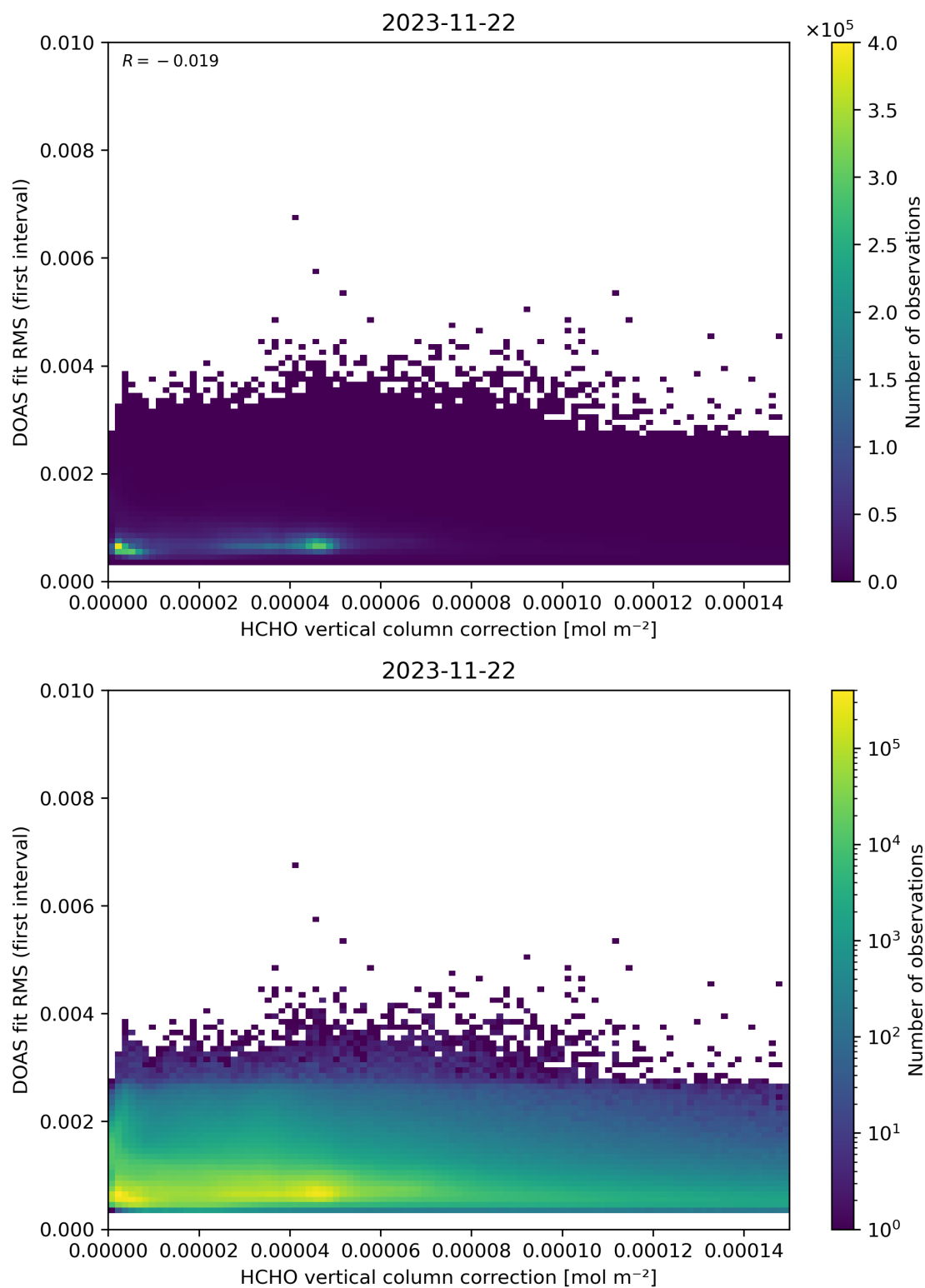
Figure 112: Scatter density plot of “HCHO vertical column correction” against “DOAS fit RMS (first interval)” for 2023-11-21 to 2023-11-23.
