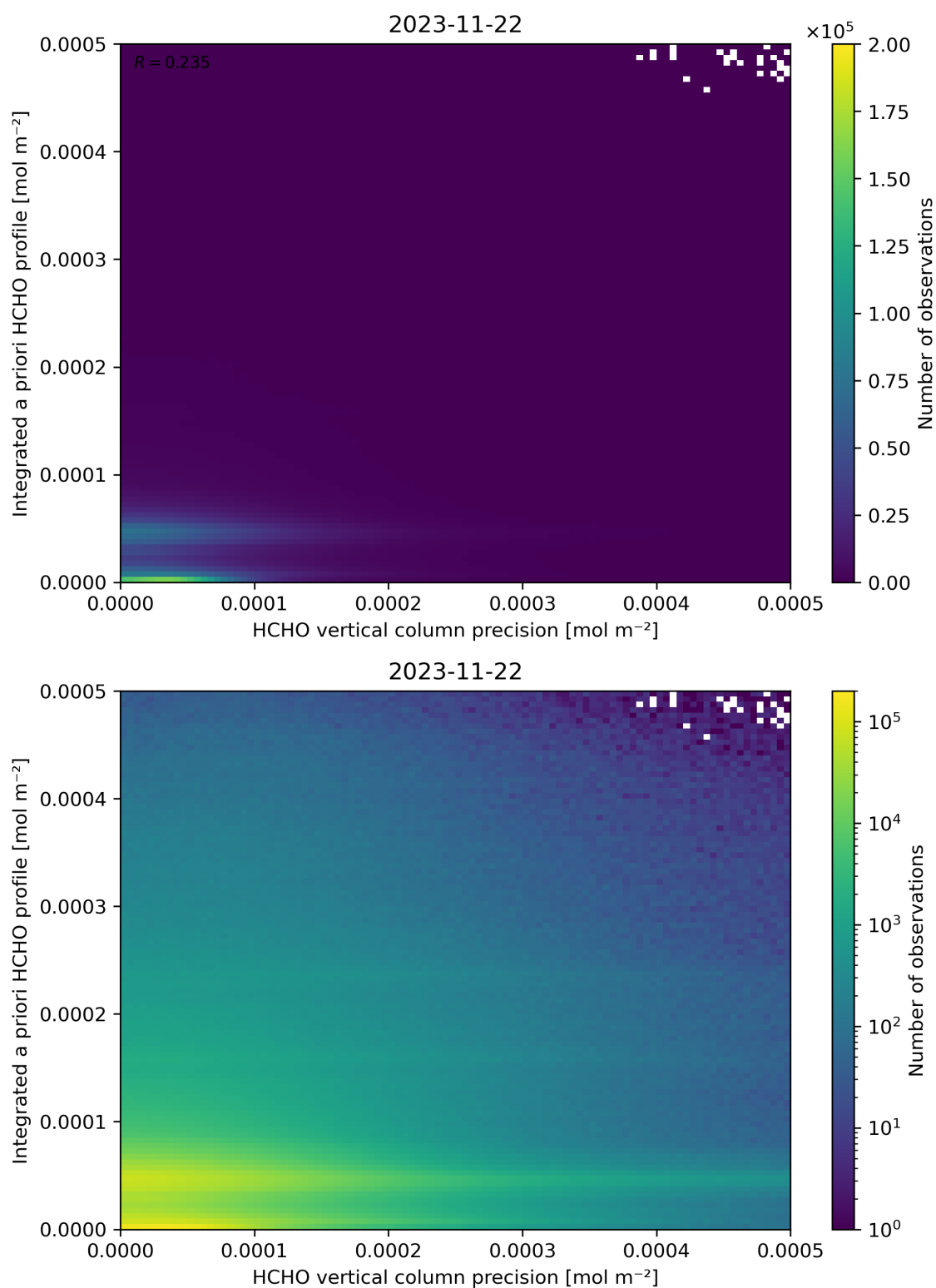
Figure 147: Scatter density plot of “HCHO vertical column precision” against “Integrated a priori HCHO profile” for 2023-11-21 to 2023-11-23.
