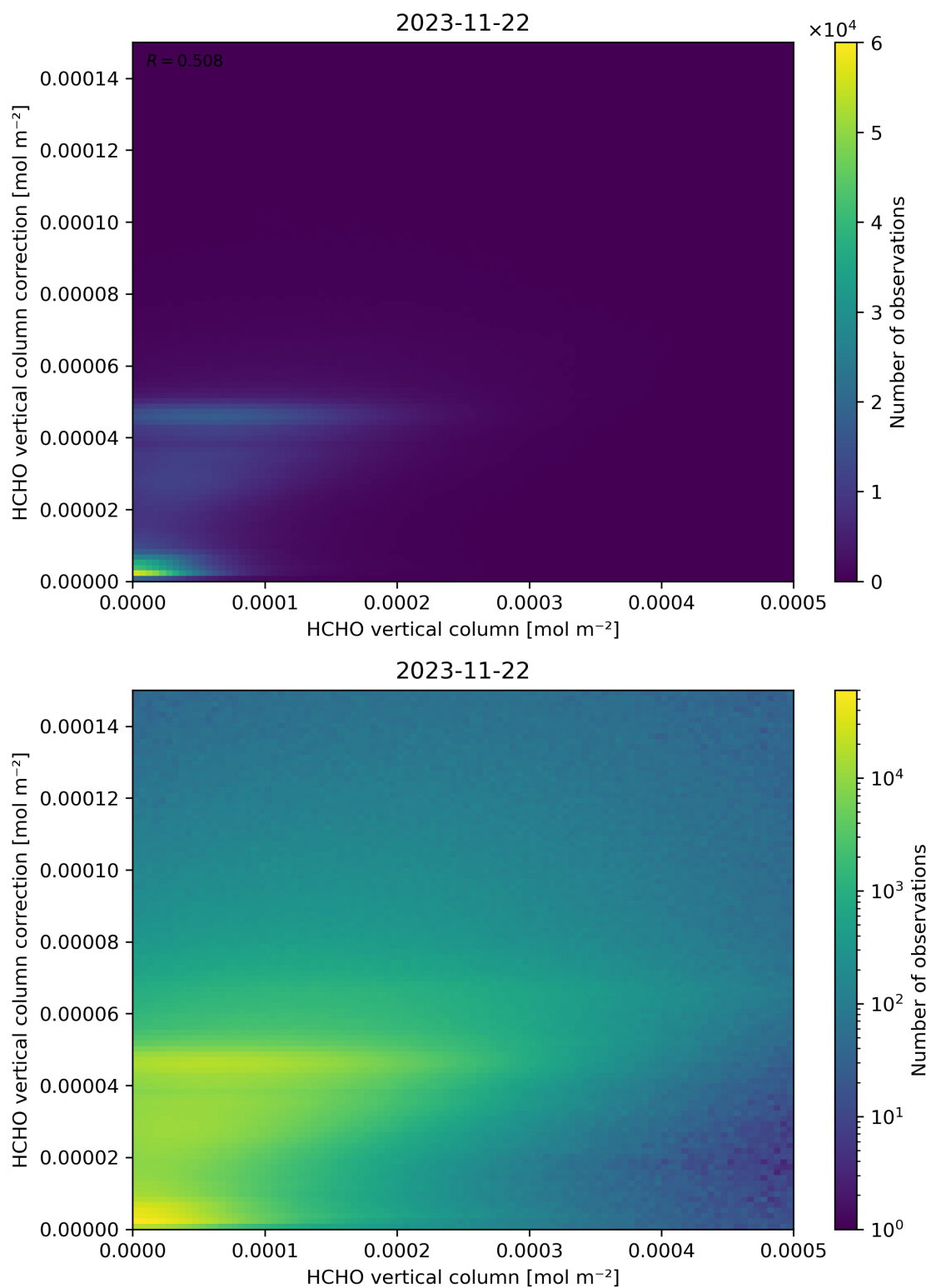
Figure 133: Scatter density plot of “HCHO vertical column” against “HCHO vertical column correction” for 2023-11-21 to 2023-11-23.
