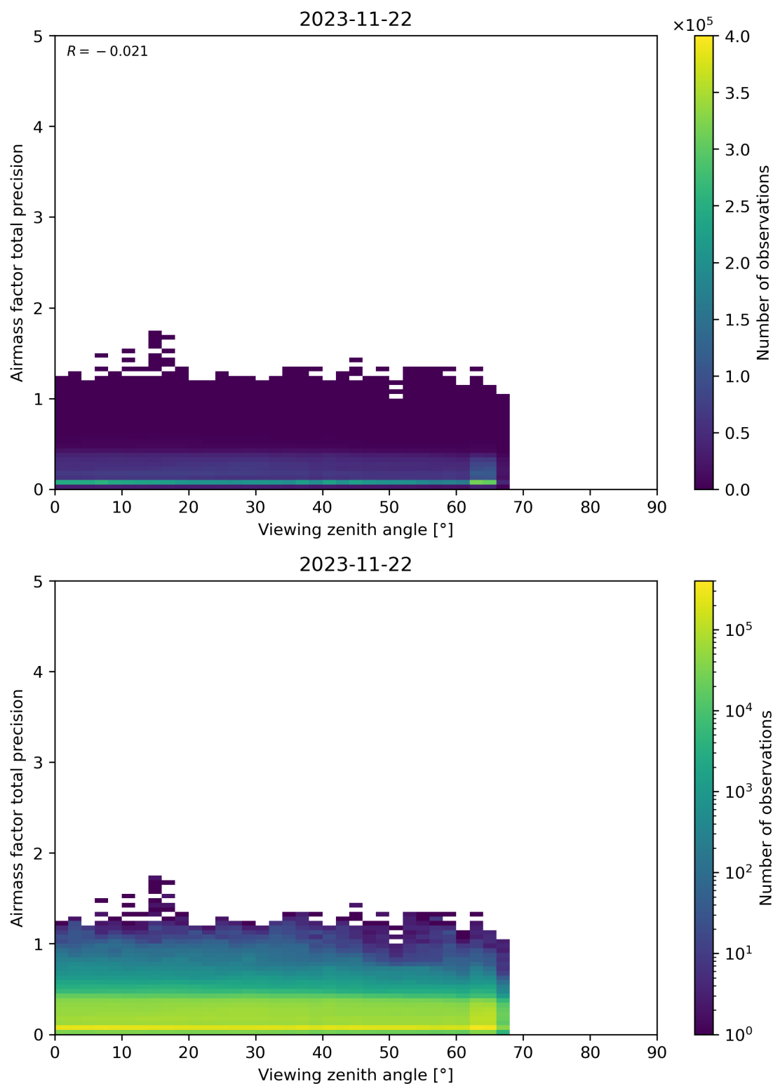
Figure 191: Scatter density plot of “Viewing zenith angle” against “Airmass factor total precision” for 2023-11-21 to 2023-11-23.
