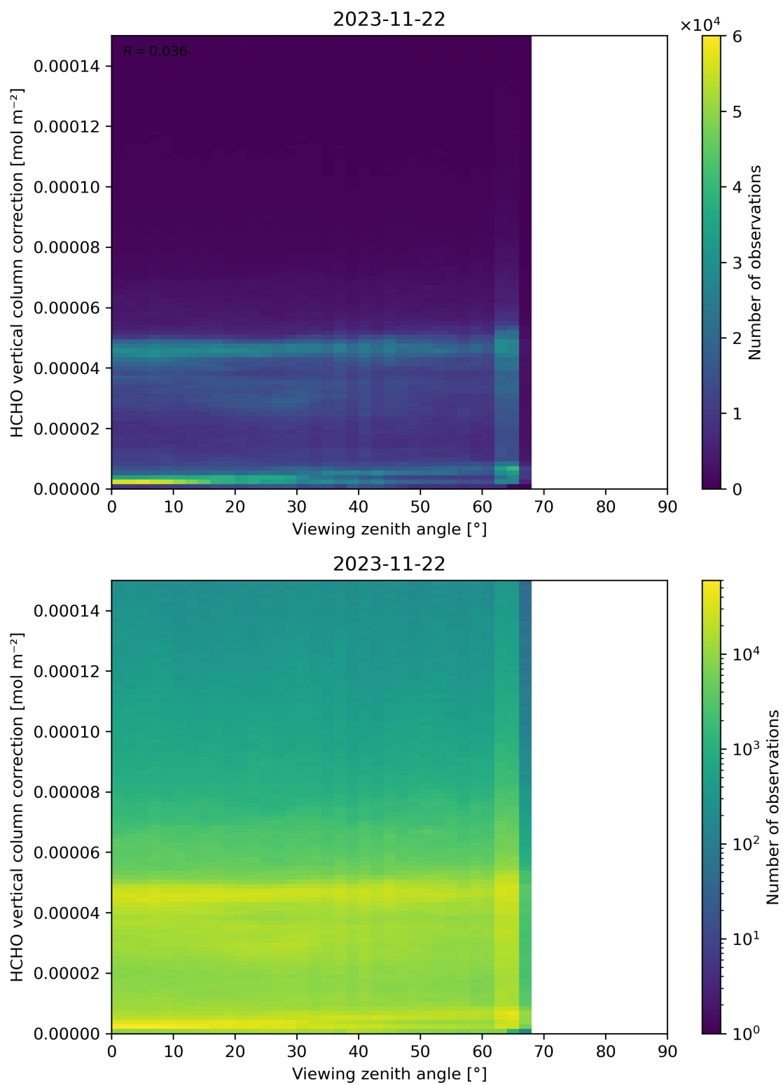
Figure 193: Scatter density plot of “Viewing zenith angle” against “HCHO vertical column correction” for 2023-11-21 to 2023-11-23.
