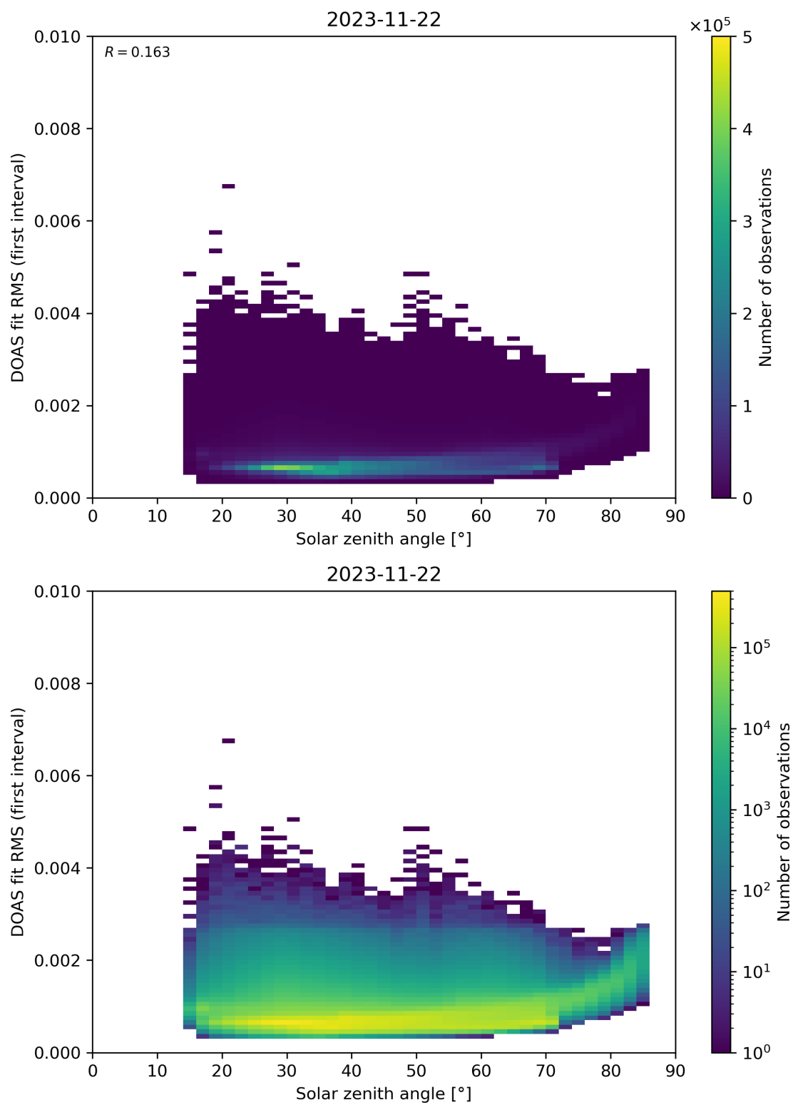
Figure 167: Scatter density plot of “Solar zenith angle” against “DOAS fit RMS (first interval)” for 2023-11-21 to 2023-11-23.
