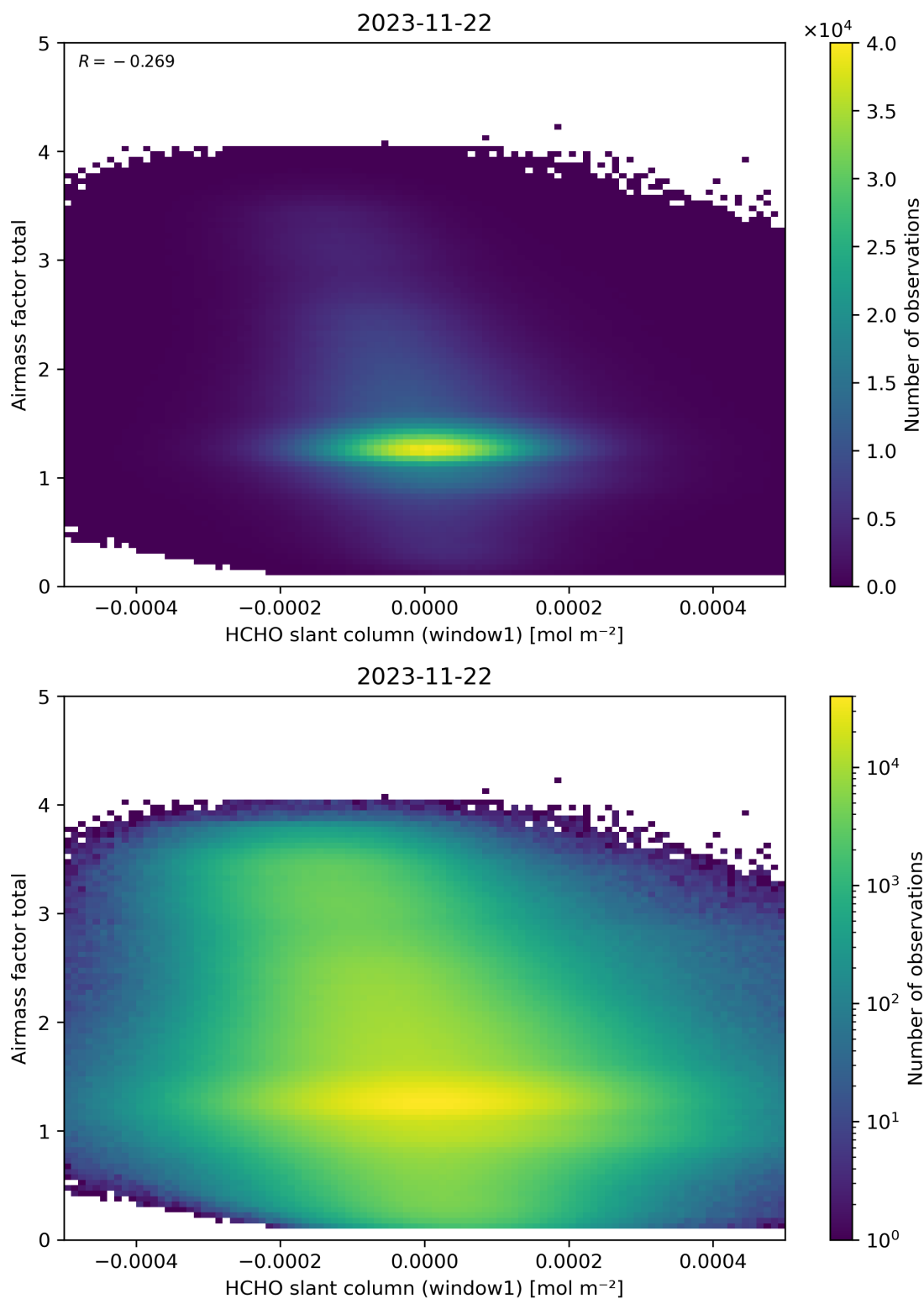
Figure 85: Scatter density plot of “HCHO slant column (window1)” against “Airmass factor total” for 2023-11-21 to 2023-11-23.
