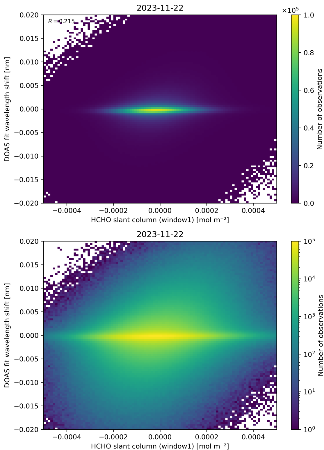
Figure 79: Scatter density plot of “HCHO slant column (window1)” against “DOAS fit wavelength shift” for 2023-11-21 to 2023-11-23.
