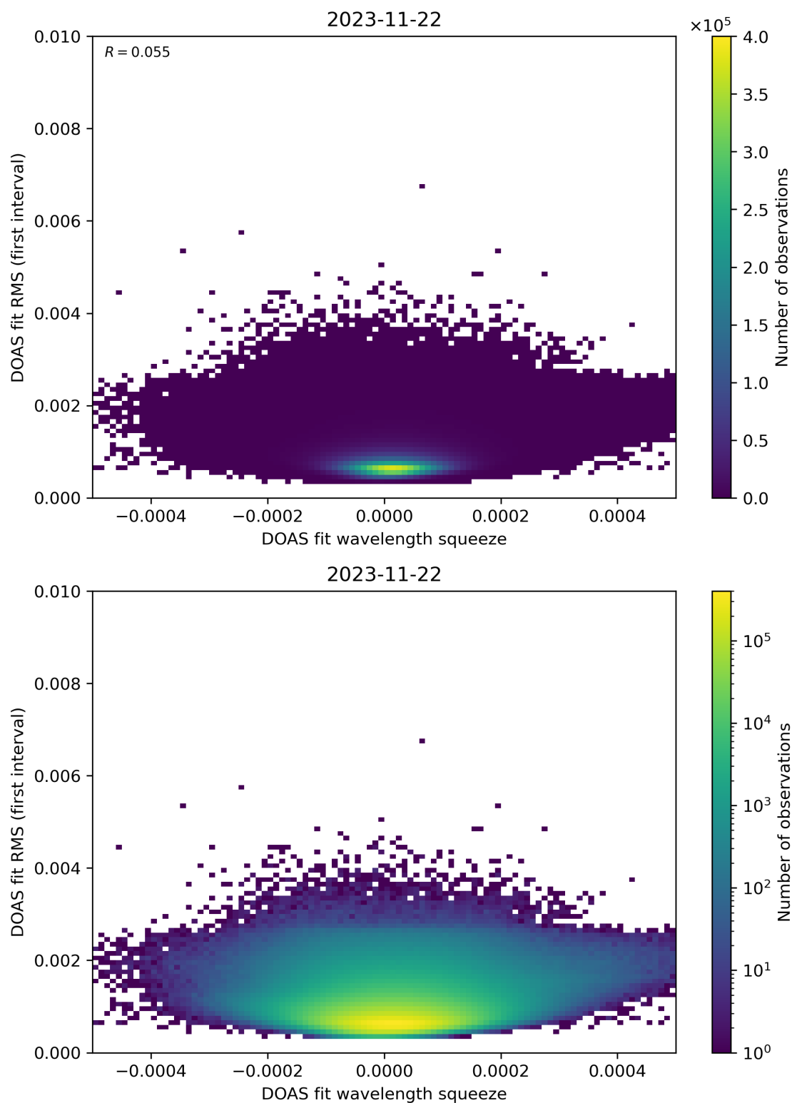
Figure 68: Scatter density plot of “DOAS fit wavelength squeeze” against “DOAS fit RMS (first interval)” for 2023-11-21 to 2023-11-23.
