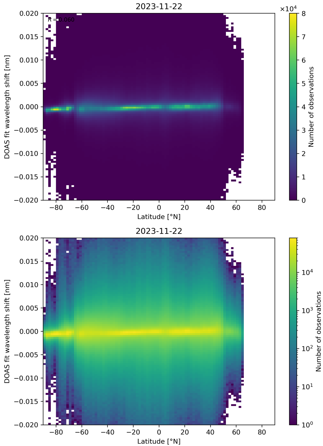
Figure 154: Scatter density plot of “Latitude” against “DOAS fit wavelength shift” for 2023-11-21 to 2023-11-23.
