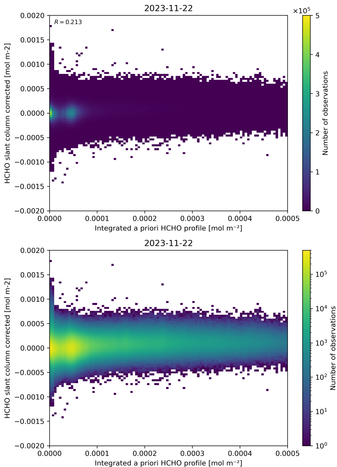
Figure 151: Scatter density plot of “Integrated a priori HCHO profile” against “HCHO slant column corrected” for 2023-11-21 to 2023-11-23.
