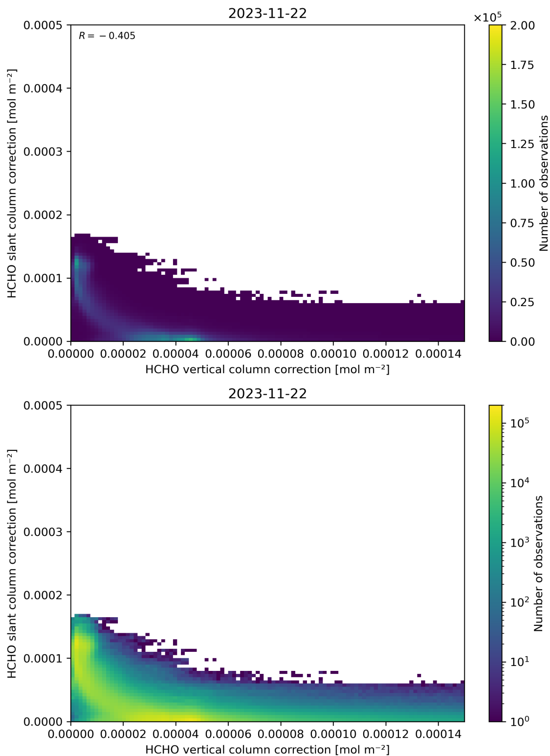
Figure 117: Scatter density plot of “HCHO vertical column correction” against “HCHO slant column correction” for 2023-11-21 to 2023-11-23.
