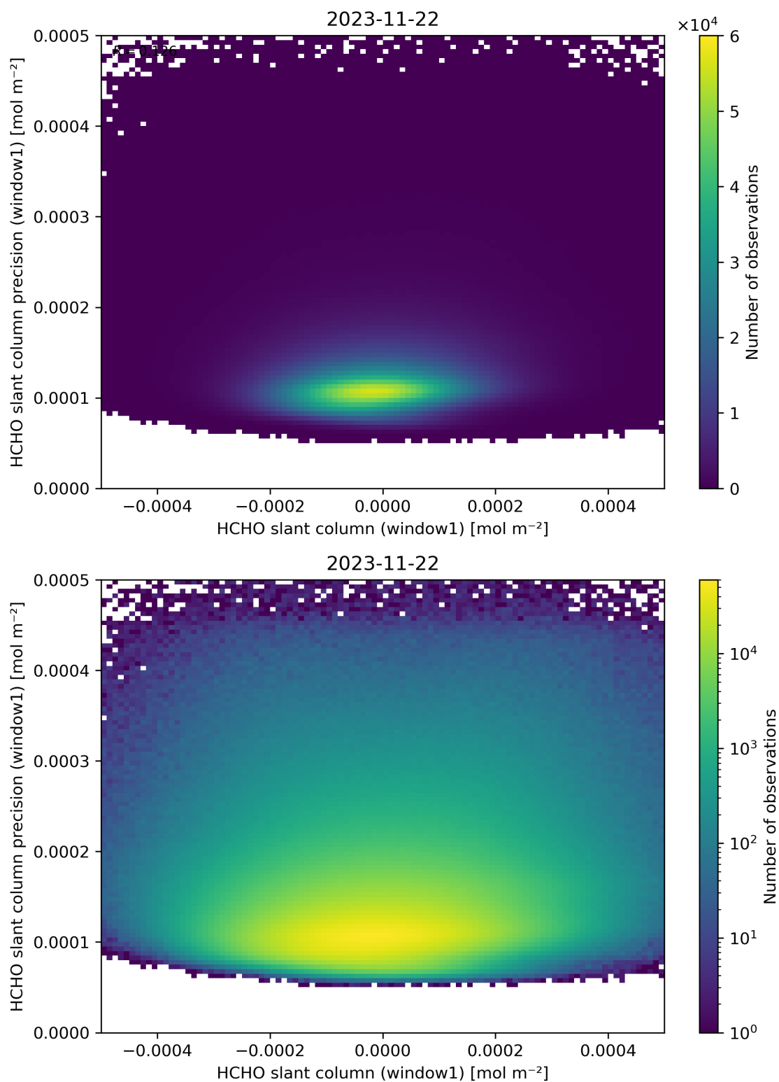
Figure 84: Scatter density plot of “HCHO slant column (window1)” against “HCHO slant column precision (window1)” for 2023-11-21 to 2023-11-23.
