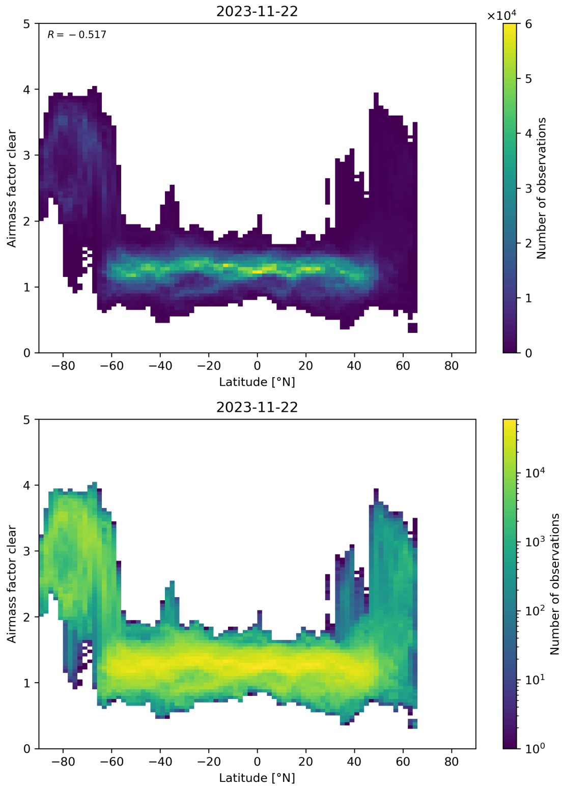
Figure 156: Scatter density plot of “Latitude” against “Airmass factor clear” for 2023-11-21 to 2023-11-23.
