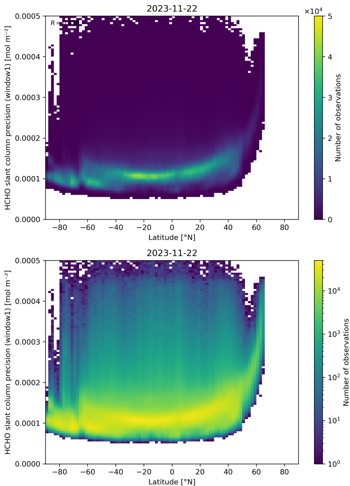
Figure 160: Scatter density plot of “Latitude” against “HCHO slant column precision (window1)” for 2023-11-21 to 2023-11-23.
