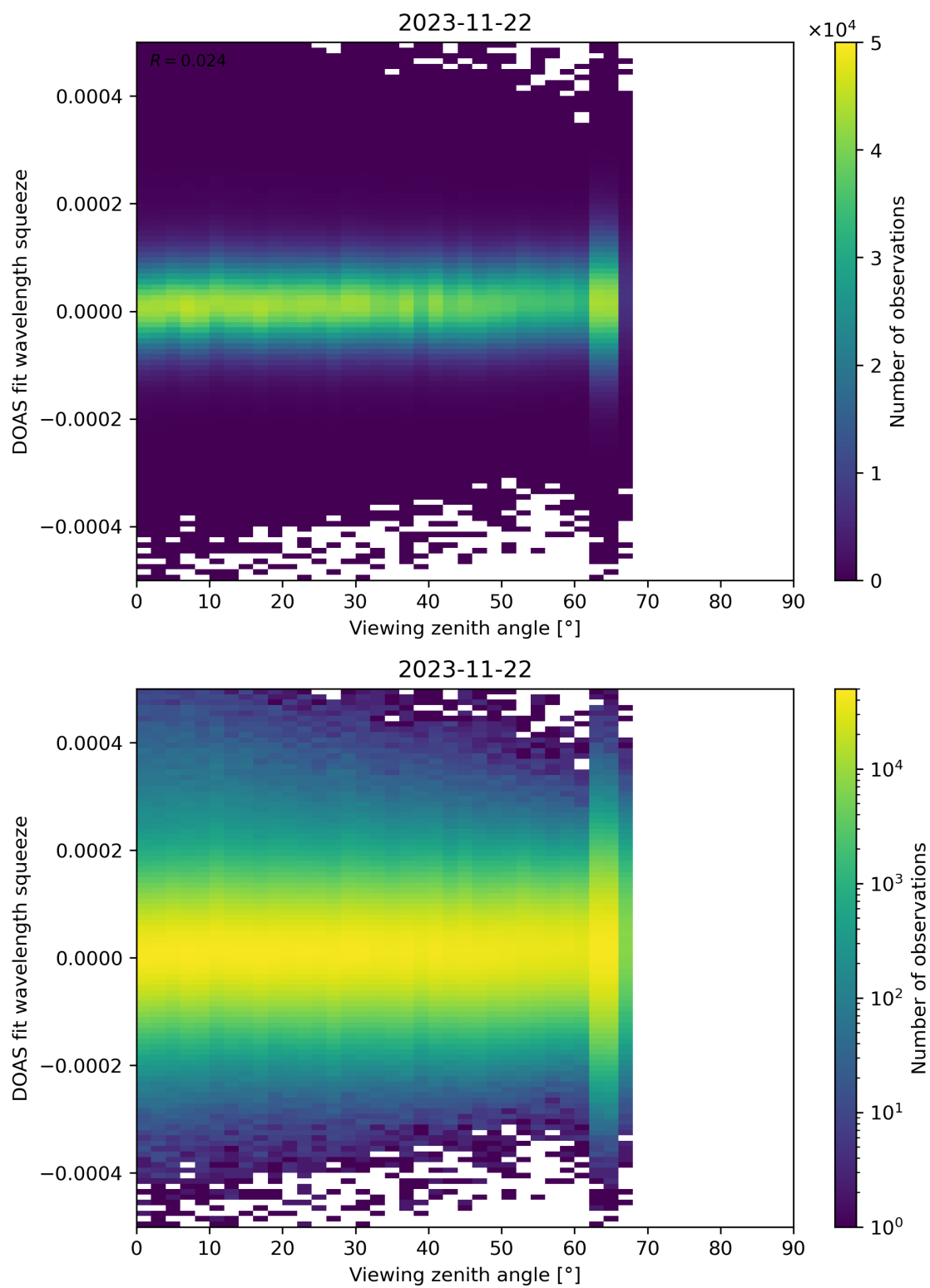
Figure 184: Scatter density plot of “Viewing zenith angle” against “DOAS fit wavelength squeeze” for 2023-11-21 to 2023-11-23.
