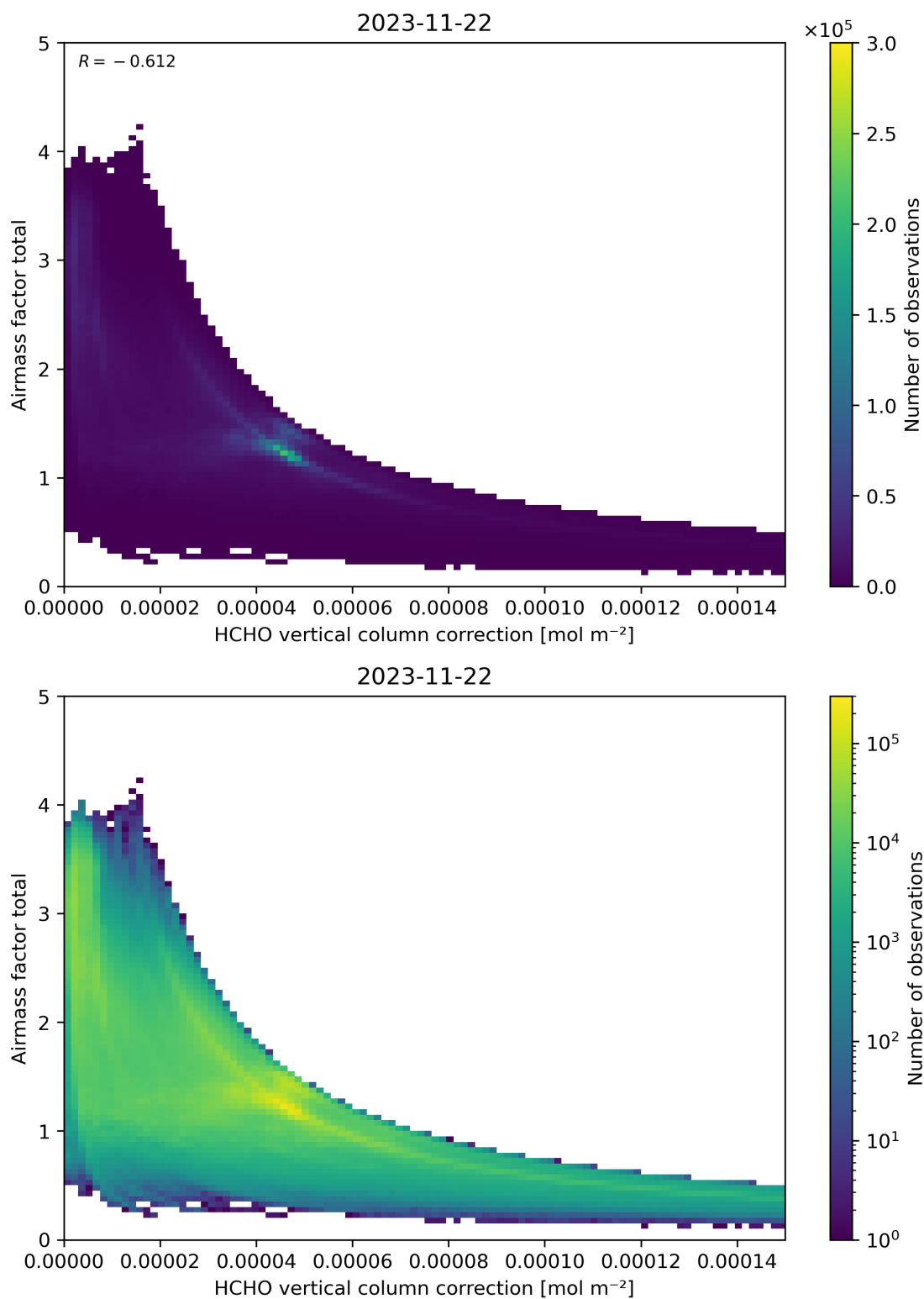
Figure 120: Scatter density plot of “HCHO vertical column correction” against “Airmass factor total” for 2023-11-21 to 2023-11-23.
