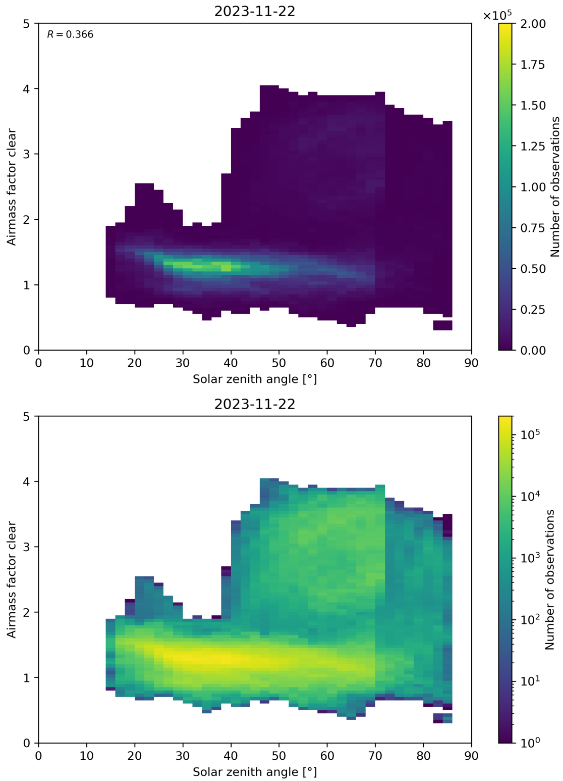
Figure 170: Scatter density plot of “Solar zenith angle” against “Airmass factor clear” for 2023-11-21 to 2023-11-23.
