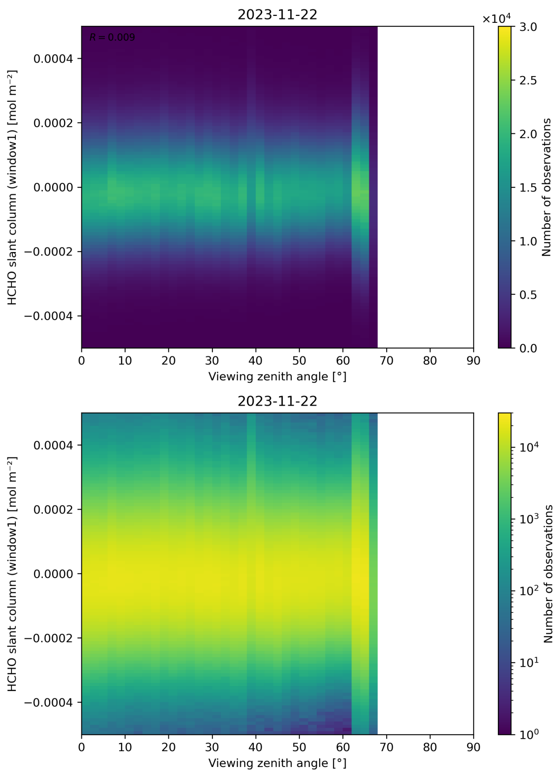
Figure 188: Scatter density plot of “Viewing zenith angle” against “HCHO slant column (window1)” for 2023-11-21 to 2023-11-23.
