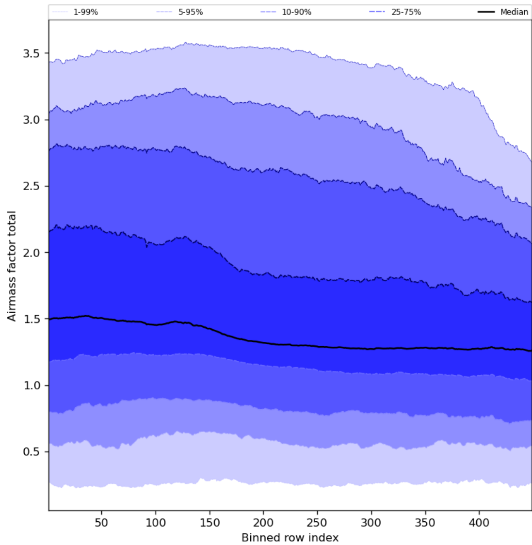
Figure 54: Along track statistics of “Airmass factor total” for 2023-11-21 to 2023-11-23
