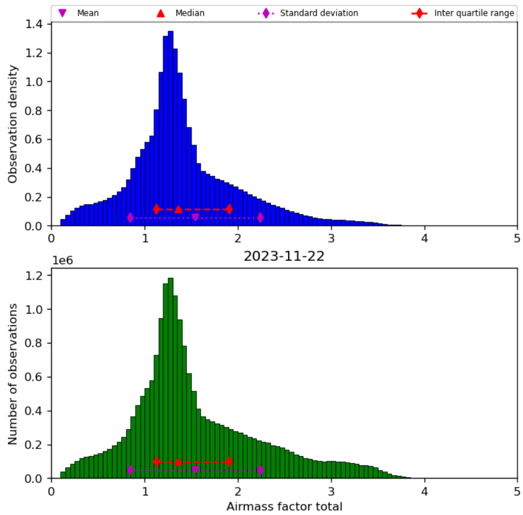
Figure 40: Histogram of “Airmass factor total” for 2023-11-21 to 2023-11-23
