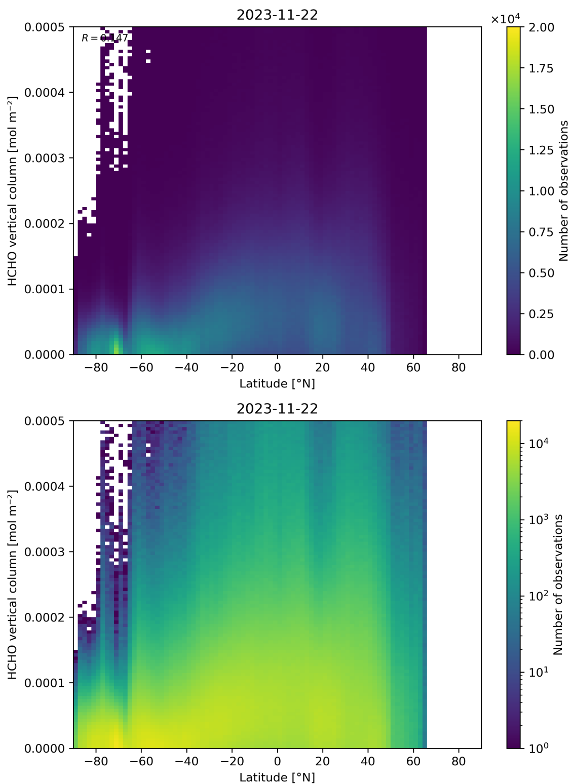
Figure 163: Scatter density plot of “Latitude” against “HCHO vertical column” for 2023-11-21 to 2023-11-23.
