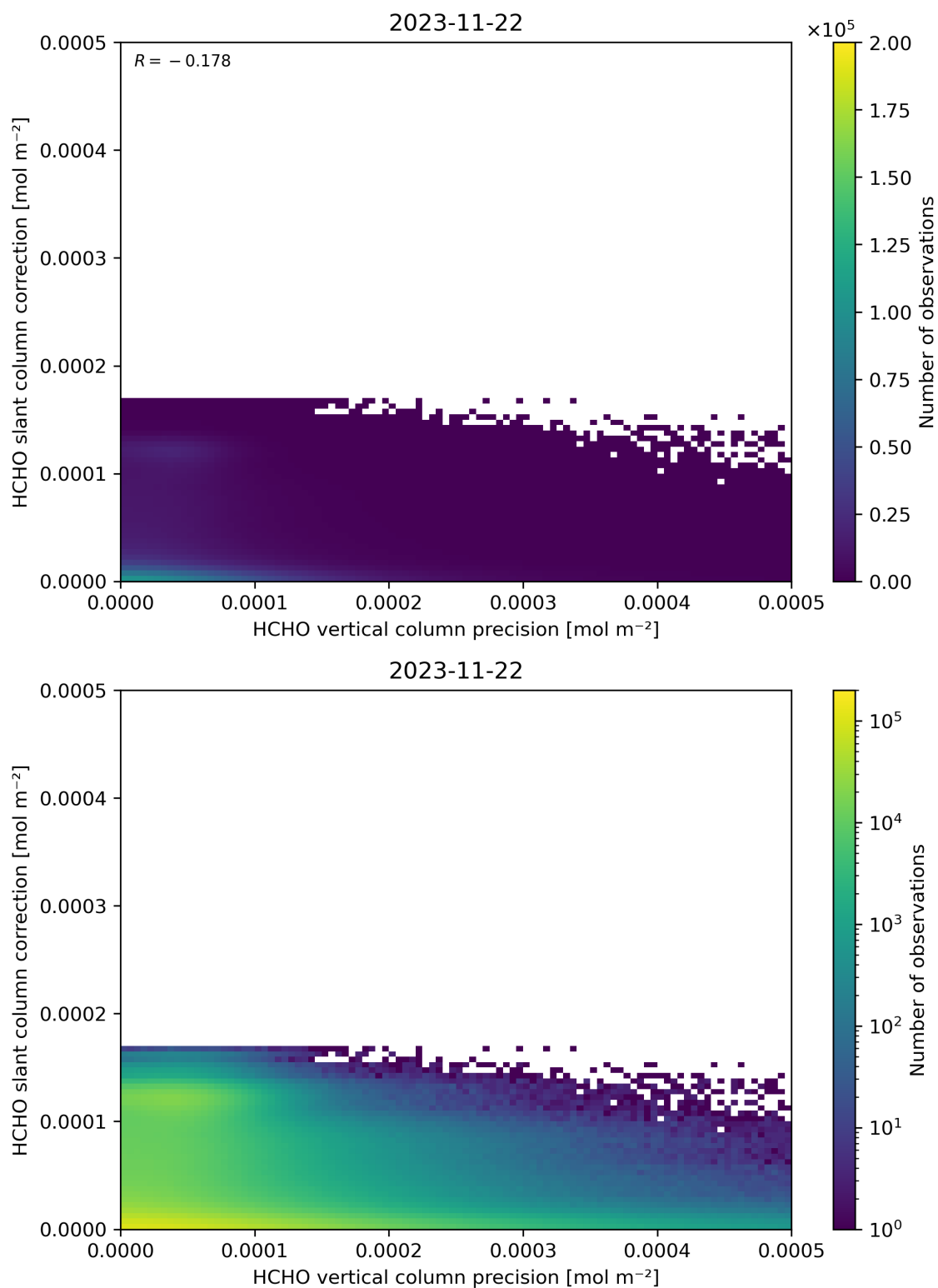
Figure 141: Scatter density plot of “HCHO vertical column precision” against “HCHO slant column correction” for 2023-11-21 to 2023-11-23.
