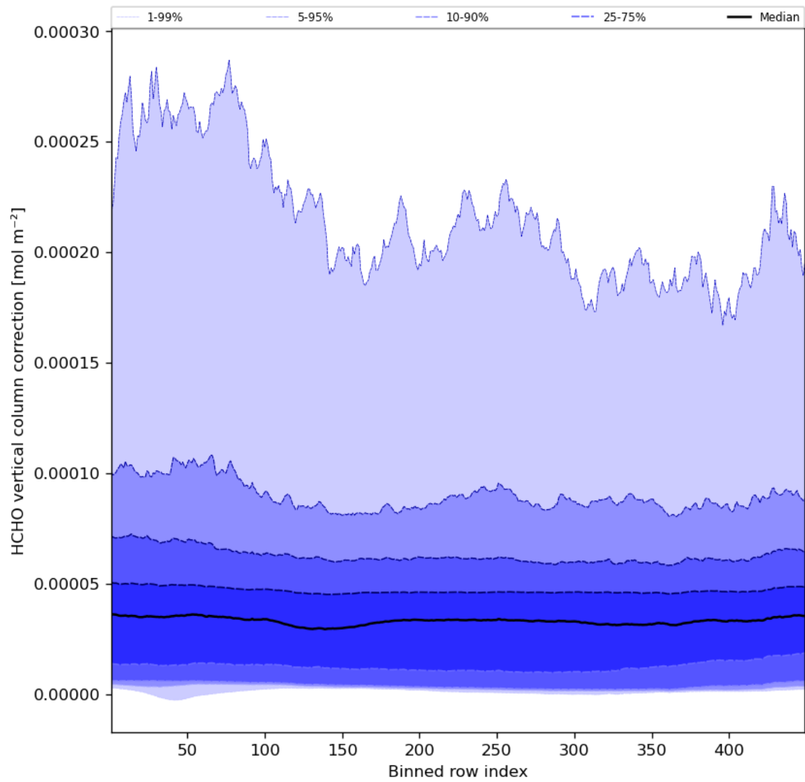
Figure 51: Along track statistics of “HCHO vertical column correction” for 2023-11-21 to 2023-11-23
