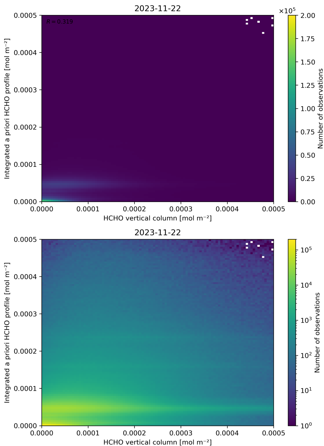
Figure 135: Scatter density plot of “HCHO vertical column” against “Integrated a priori HCHO profile” for 2023-11-21 to 2023-11-23.
