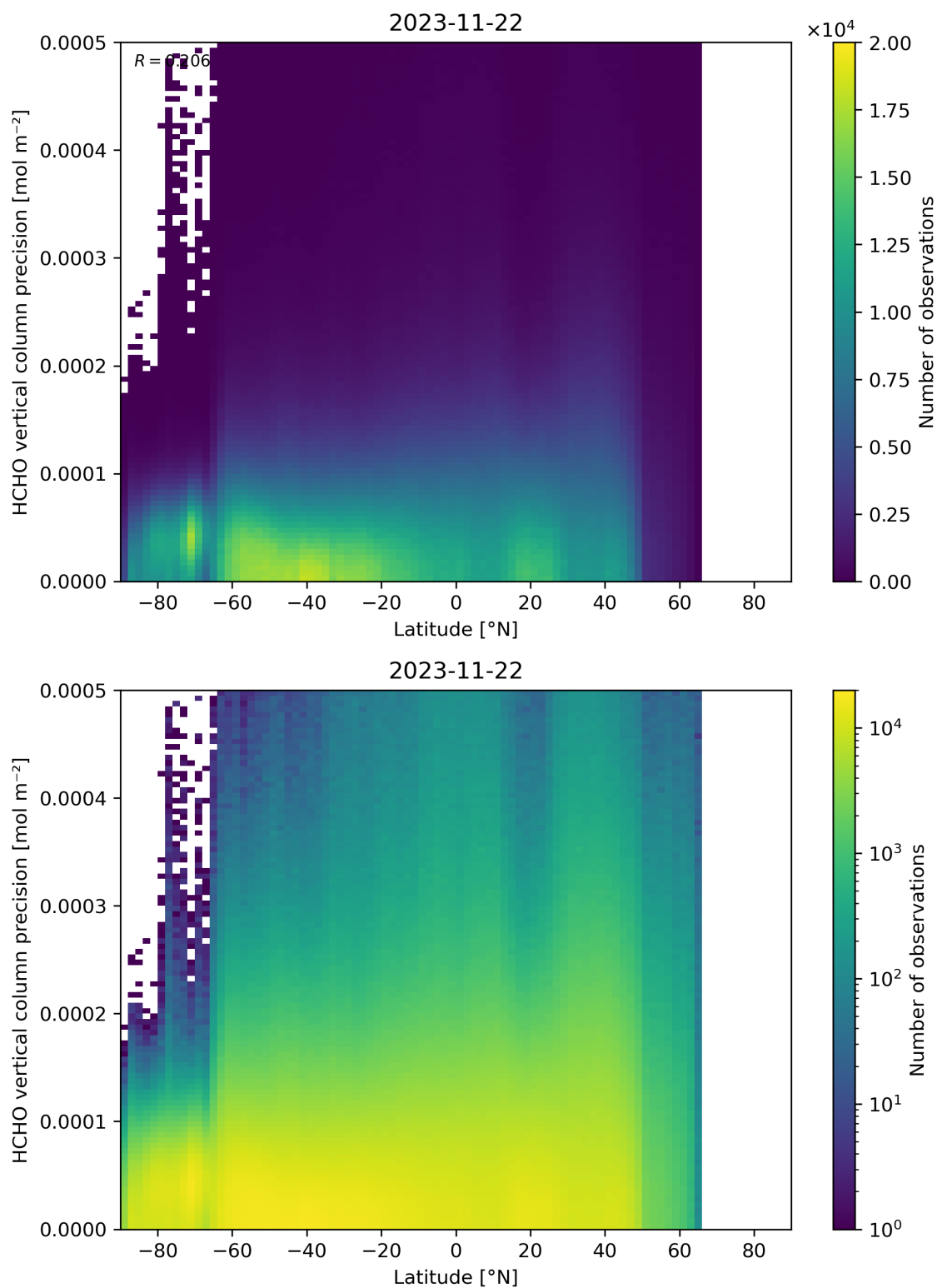
Figure 165: Scatter density plot of “Latitude” against “HCHO vertical column precision” for 2023-11-21 to 2023-11-23.
