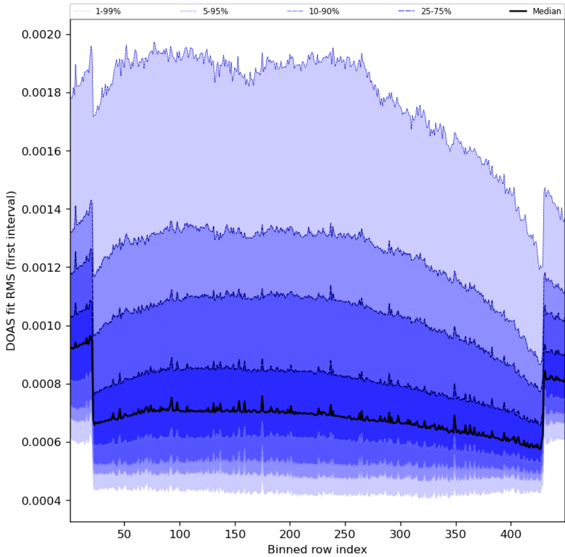
Figure 60: Along track statistics of “DOAS fit RMS (first interval)” for 2023-11-21 to 2023-11-23
