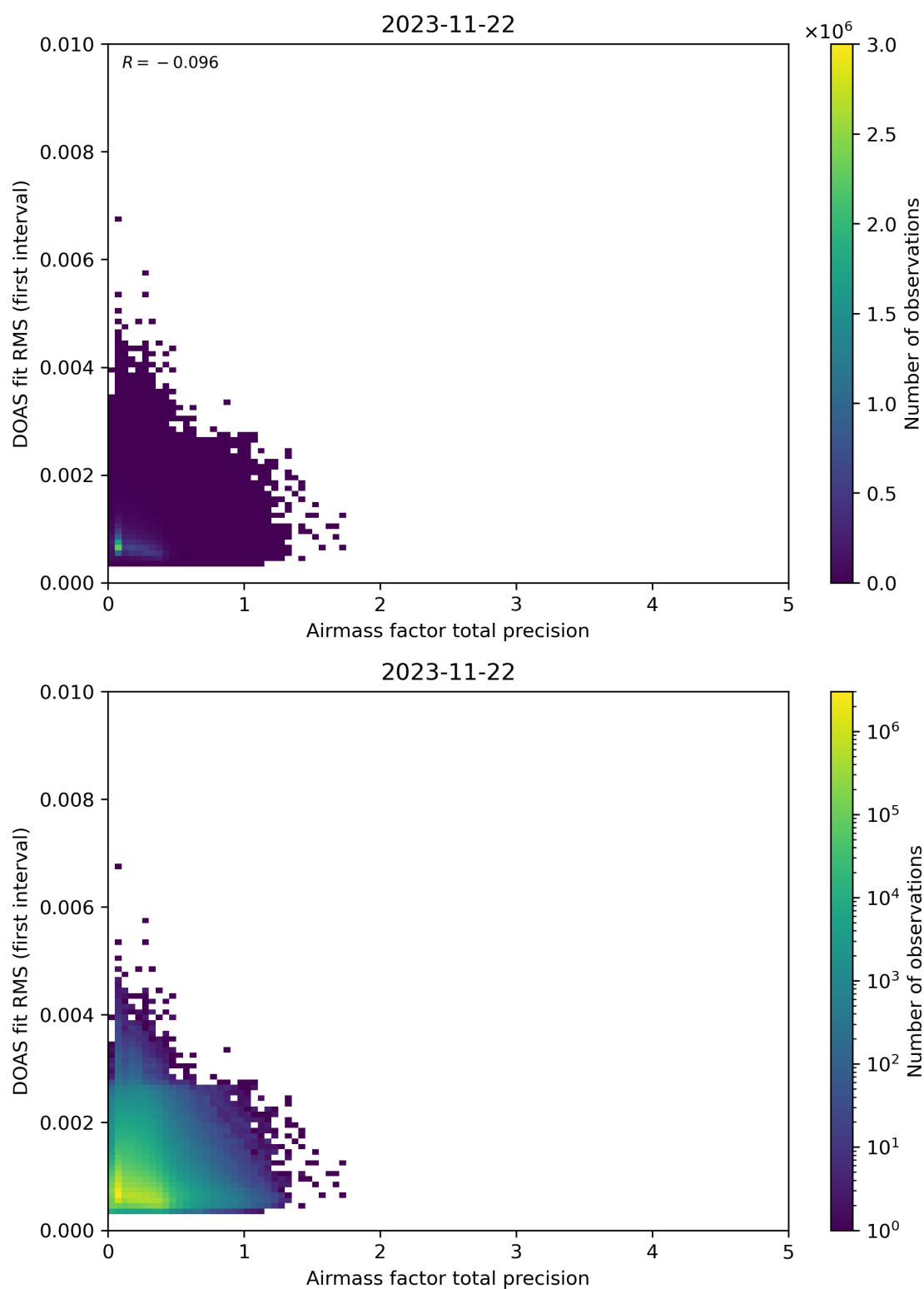
Figure 105: Scatter density plot of “Airmass factor total precision” against “DOAS fit RMS (first interval)” for 2023-11-21 to 2023-11-23.
