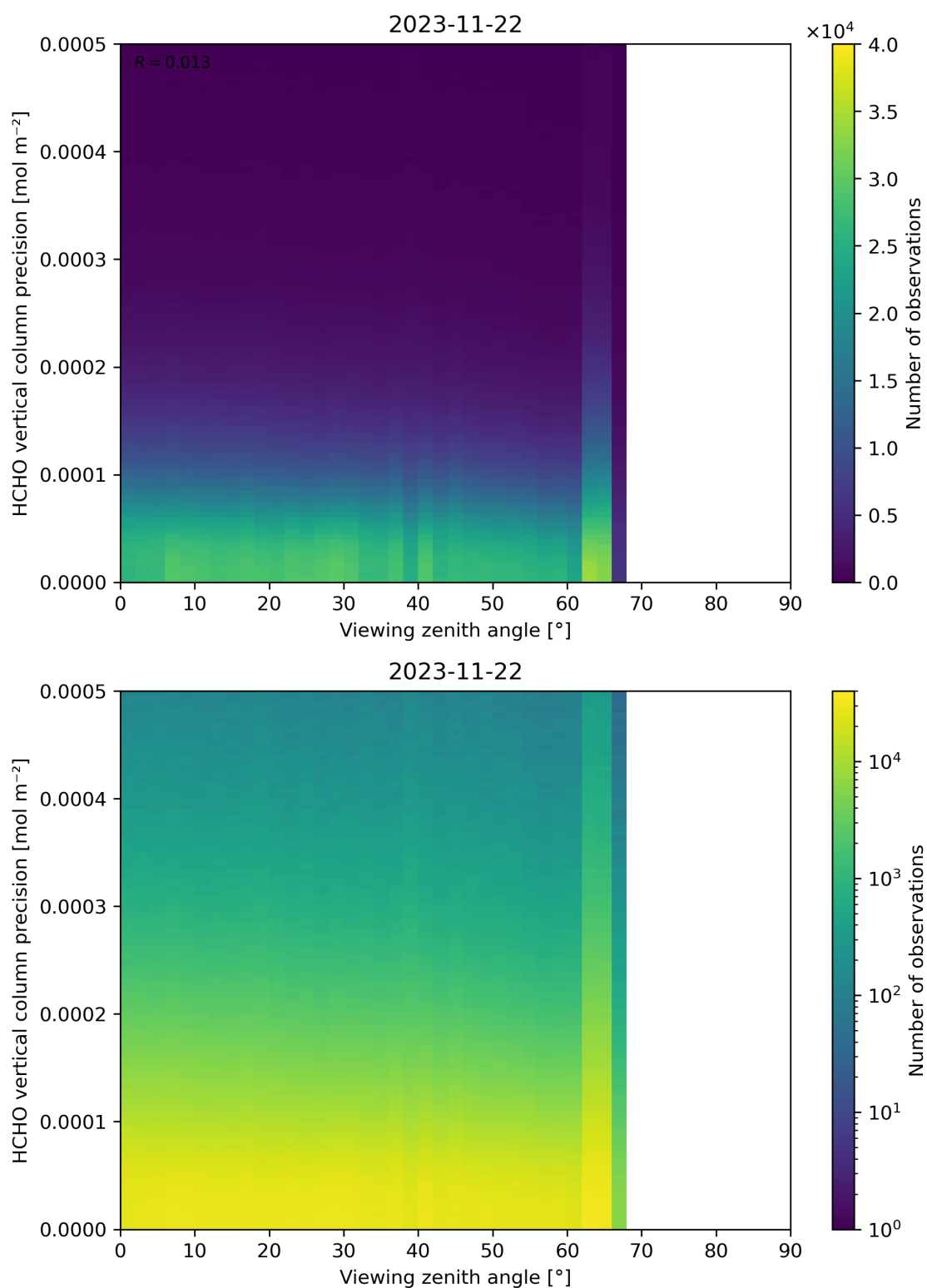
Figure 194: Scatter density plot of “Viewing zenith angle” against “HCHO vertical column precision” for 2023-11-21 to 2023-11-23.
