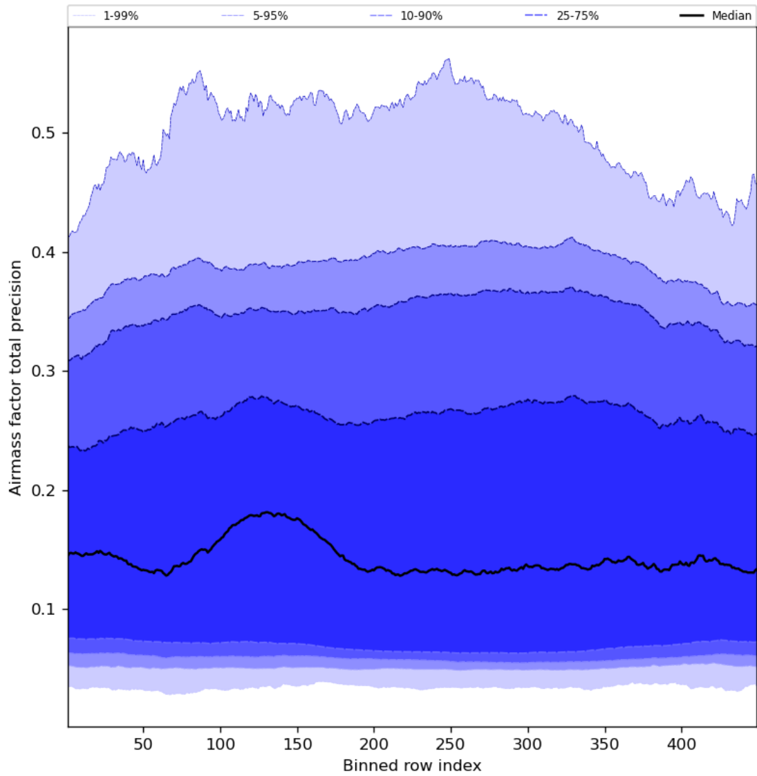
Figure 55: Along track statistics of “Airmass factor total precision” for 2023-11-21 to 2023-11-23
