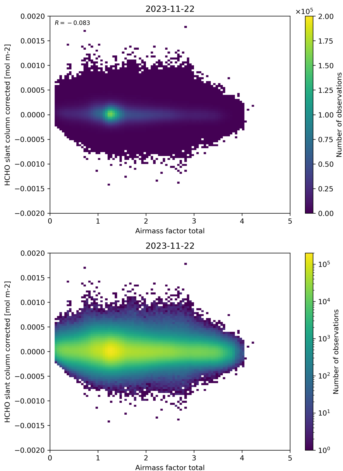
Figure 101: Scatter density plot of “Airmass factor total” against “HCHO slant column corrected” for 2023-11-21 to 2023-11-23.
