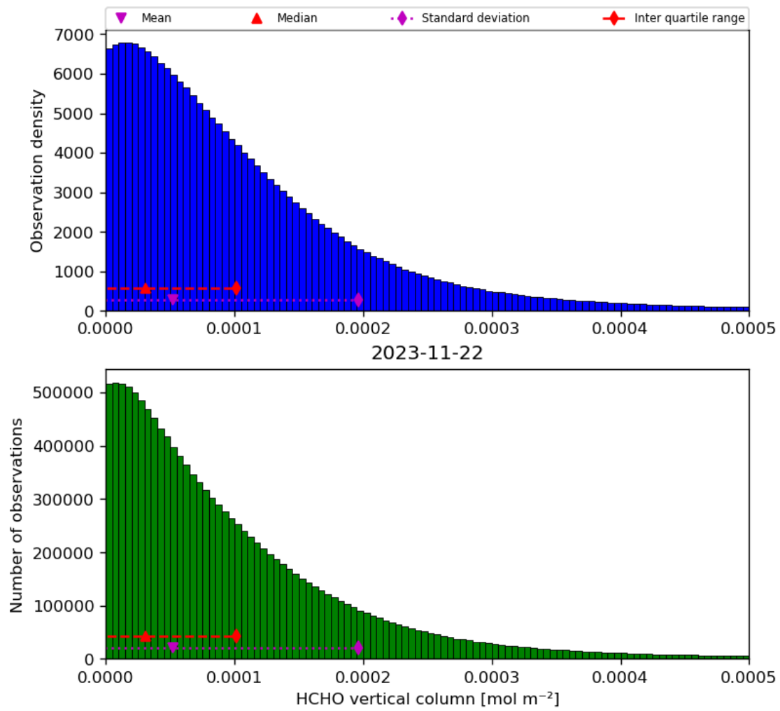
Figure 35: Histogram of “HCHO vertical column” for 2023-11-21 to 2023-11-23
