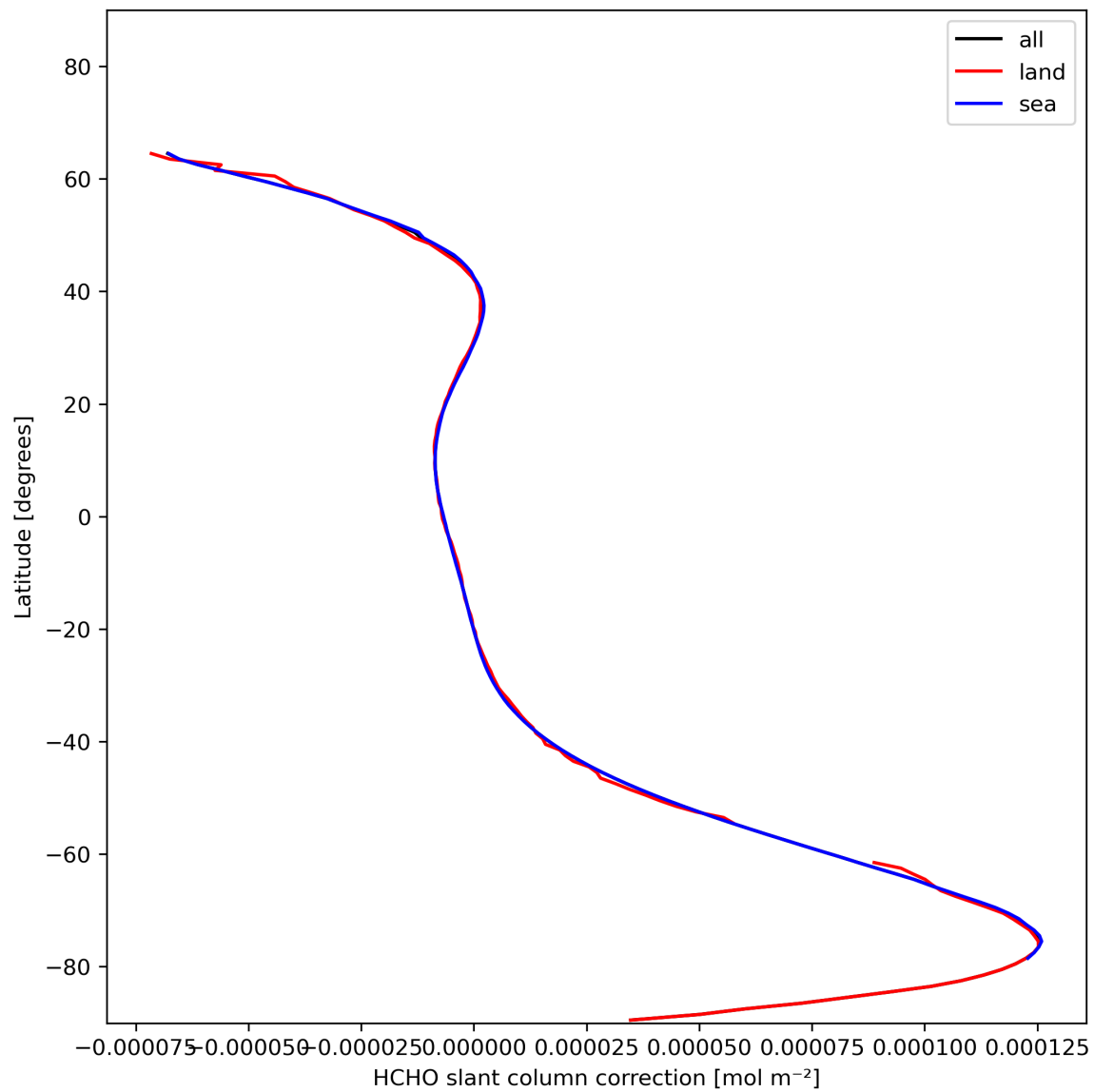
Figure 33: Zonal average of “HCHO slant column correction” for 2023-11-21 to 2023-11-23.
