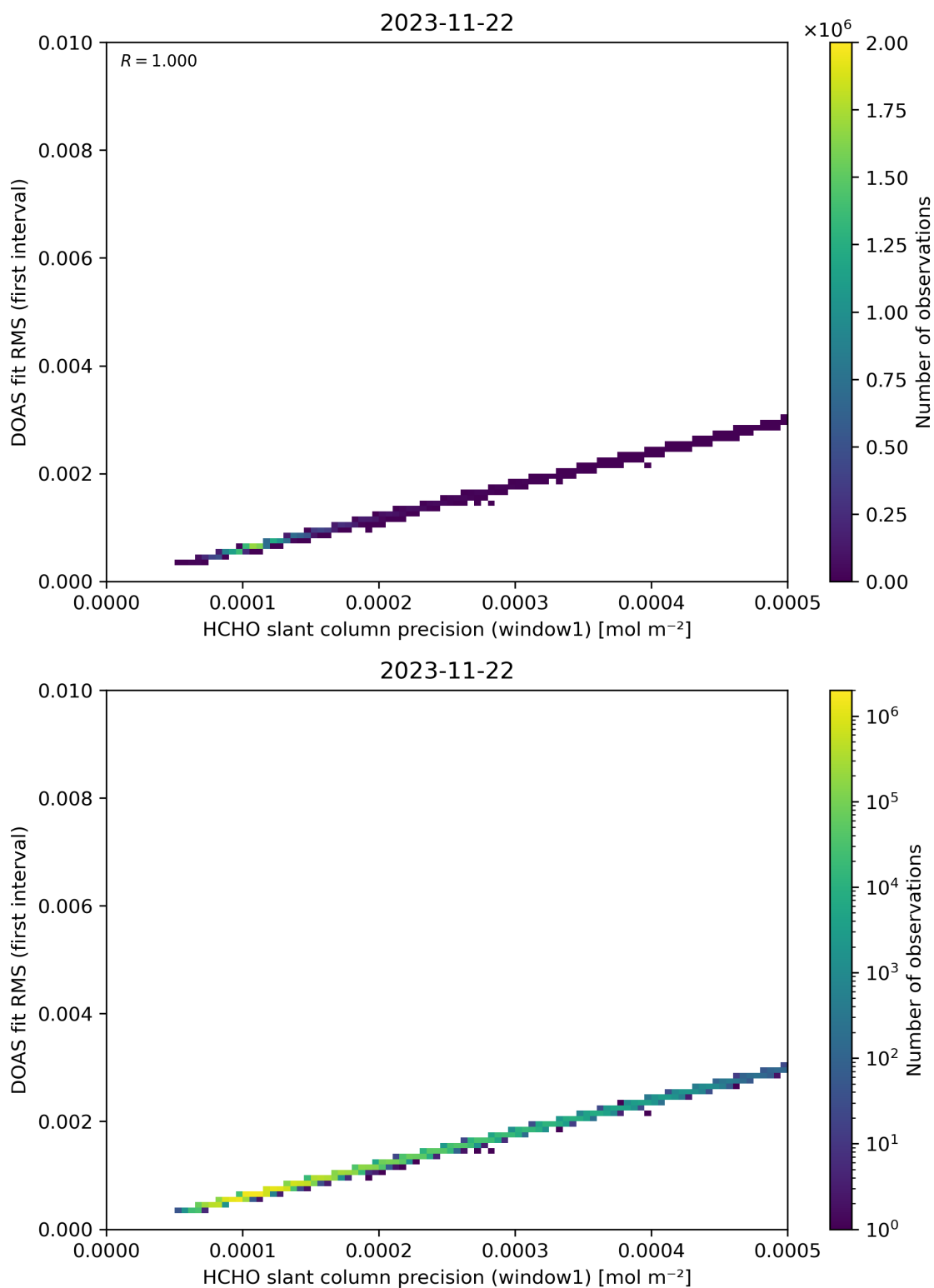
Figure 88: Scatter density plot of “HCHO slant column precision (window1)” against “DOAS fit RMS (first interval)” for 2023-11-21 to 2023-11-23.
