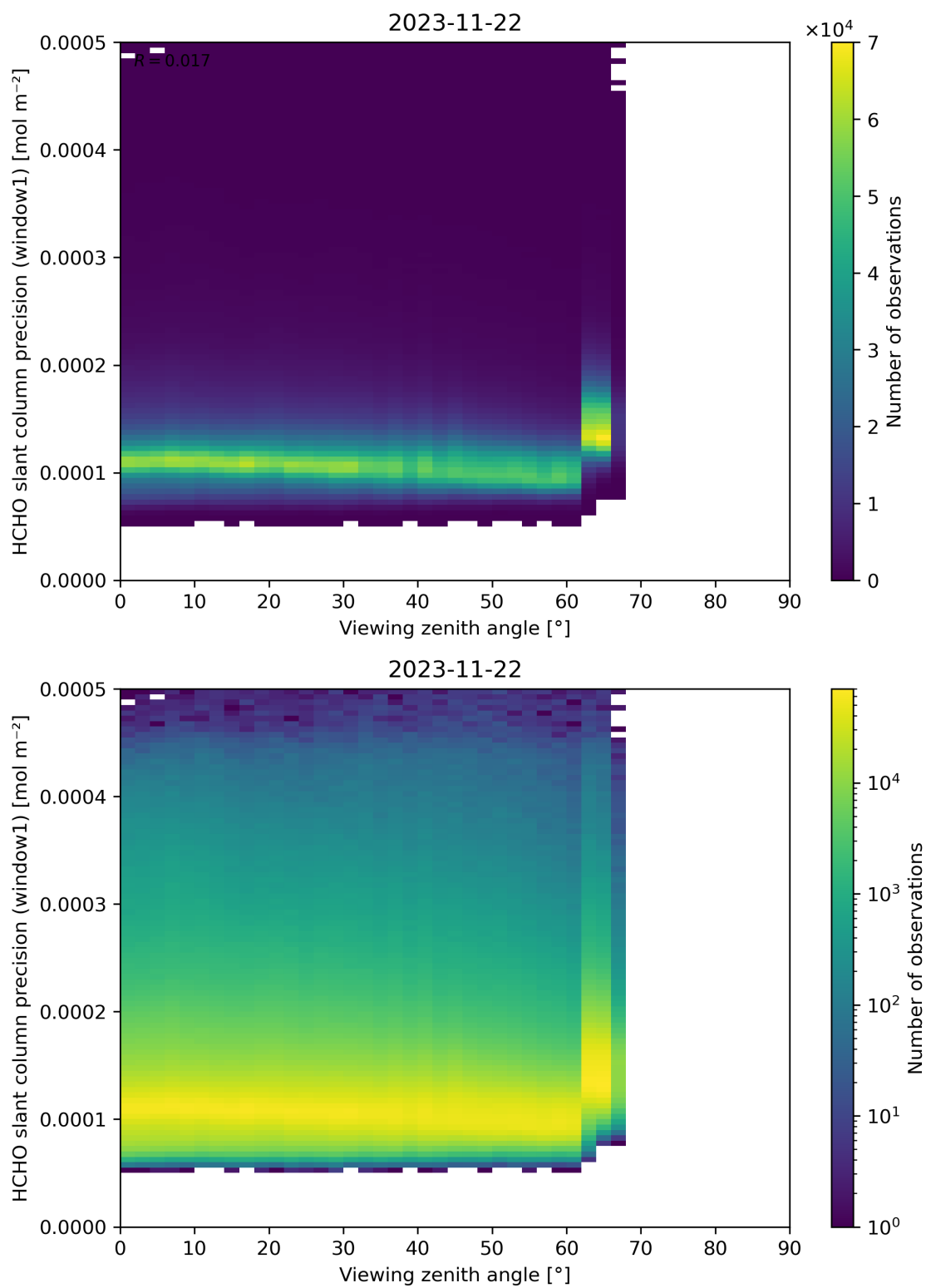
Figure 189: Scatter density plot of “Viewing zenith angle” against “HCHO slant column precision (window1)” for 2023-11-21 to 2023-11-23.
