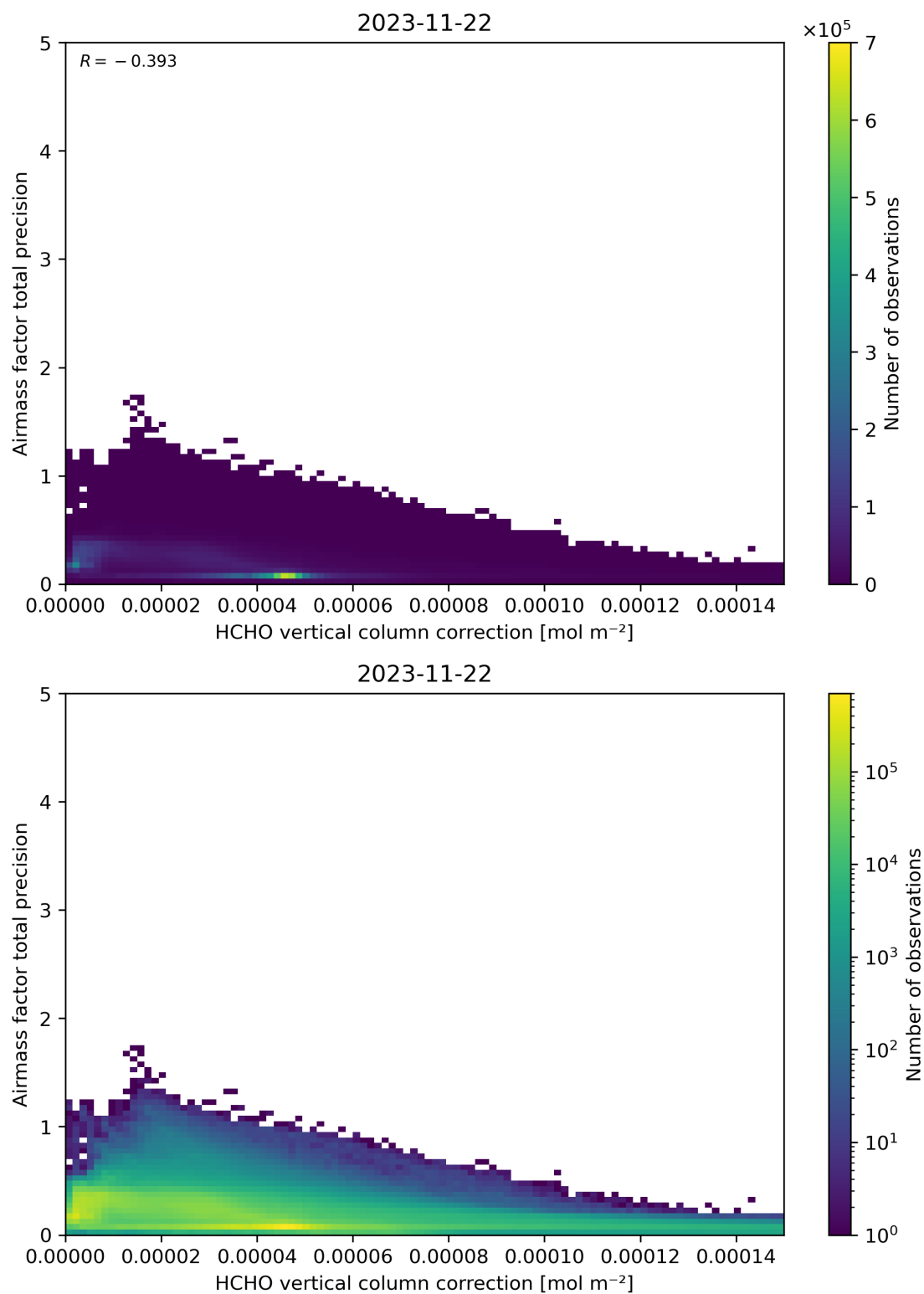
Figure 121: Scatter density plot of “HCHO vertical column correction” against “Airmass factor total precision” for 2023-11-21 to 2023-11-23.
