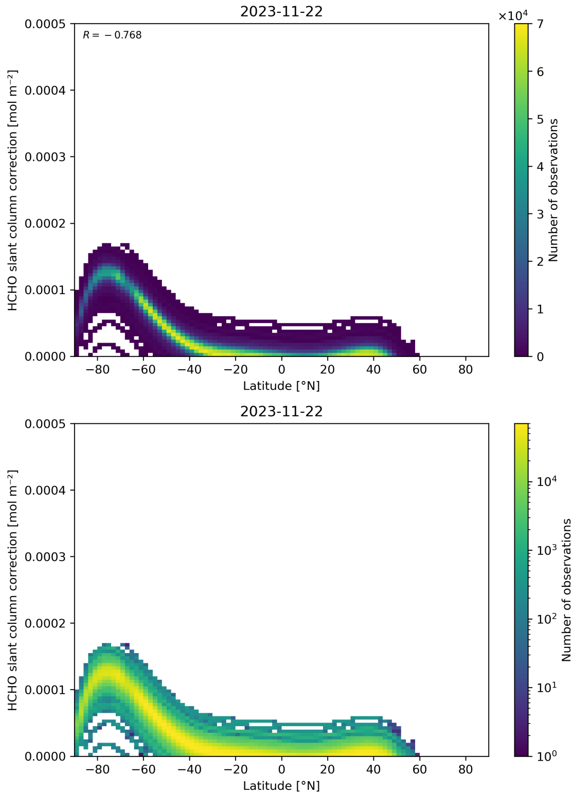
Figure 158: Scatter density plot of “Latitude” against “HCHO slant column correction” for 2023-11-21 to 2023-11-23.
