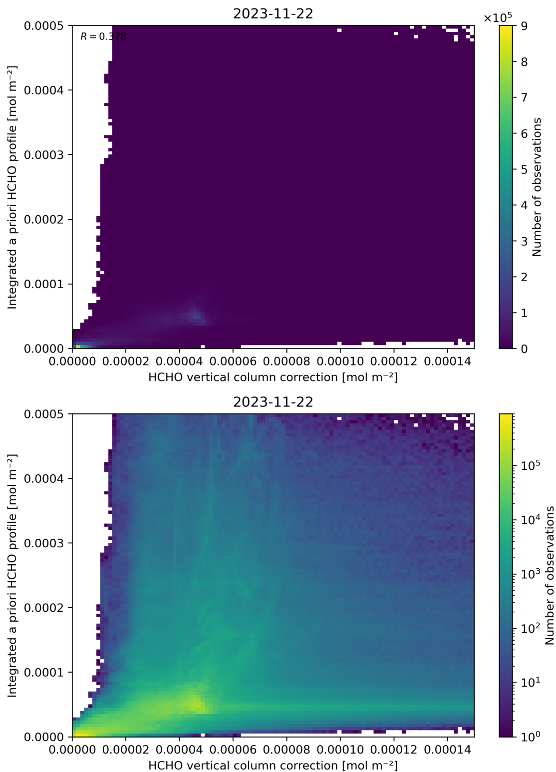
Figure 122: Scatter density plot of “HCHO vertical column correction” against “Integrated a priori HCHO profile” for 2023-11-21 to 2023-11-23.
