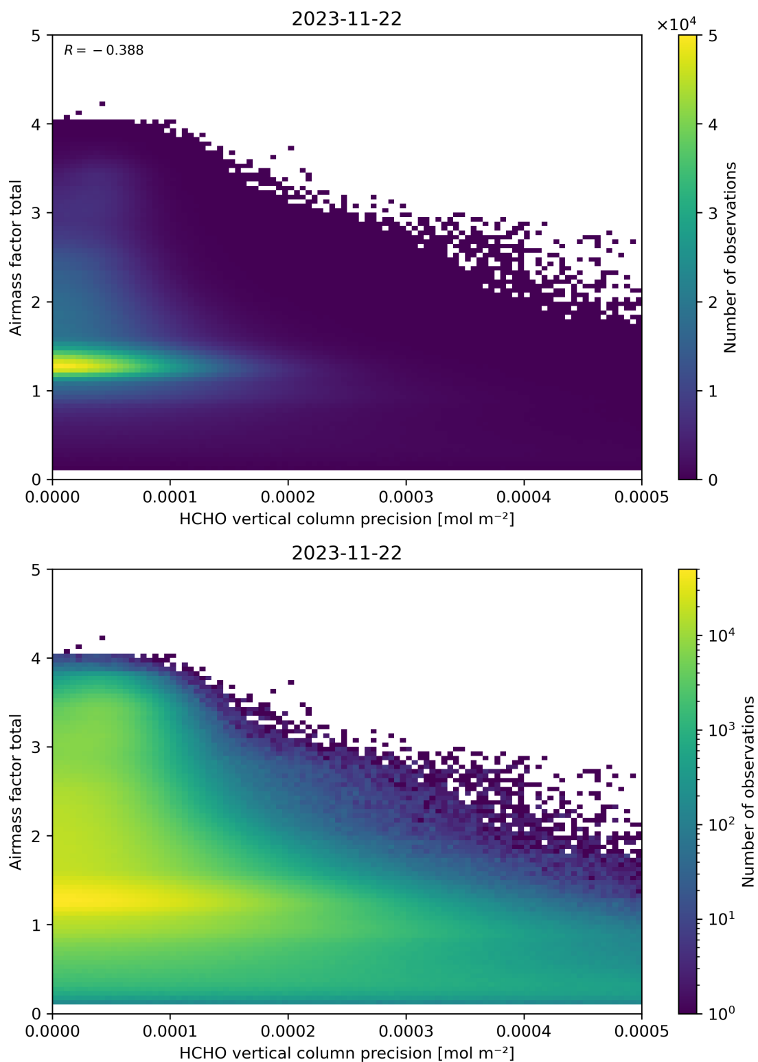
Figure 144: Scatter density plot of “HCHO vertical column precision” against “Airmass factor total” for 2023-11-21 to 2023-11-23.
