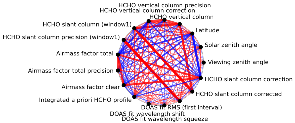
Figure 1: Map of correlation graph for 2023-11-21 to 2023-11-23.
