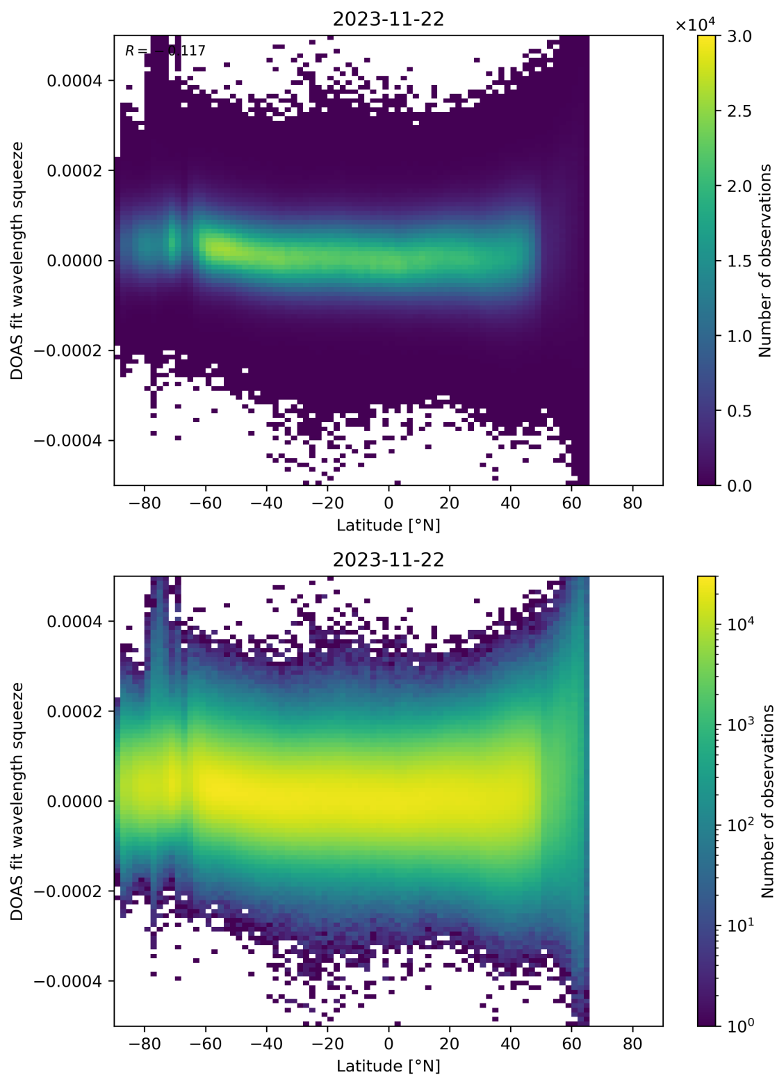
Figure 155: Scatter density plot of “Latitude” against “DOAS fit wavelength squeeze” for 2023-11-21 to 2023-11-23.
