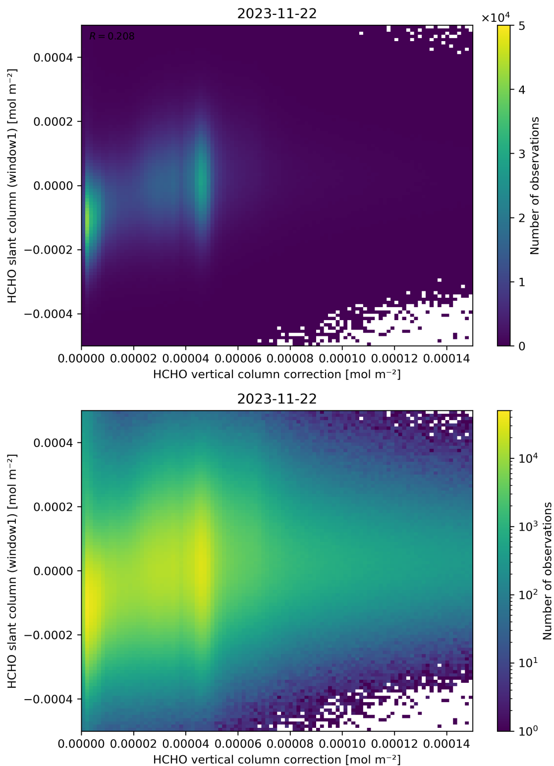
Figure 118: Scatter density plot of “HCHO vertical column correction” against “HCHO slant column (window1)” for 2023-11-21 to 2023-11-23.
