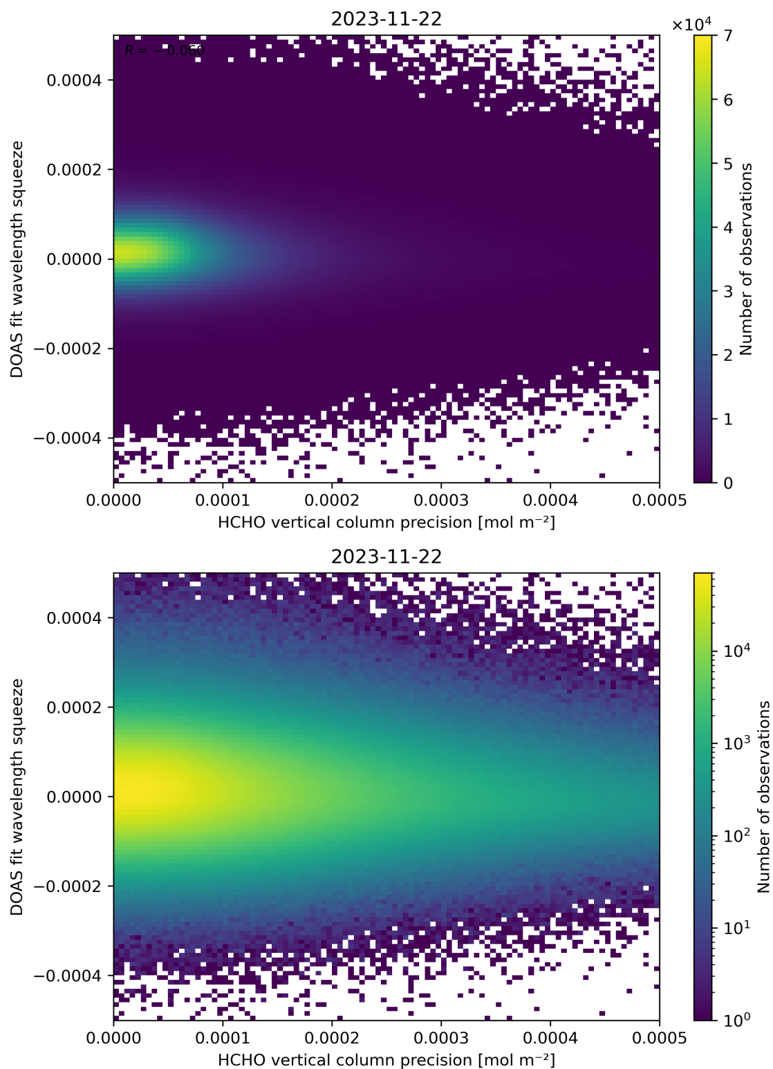
Figure 138: Scatter density plot of “HCHO vertical column precision” against “DOAS fit wavelength squeeze” for 2023-11-21 to 2023-11-23.
