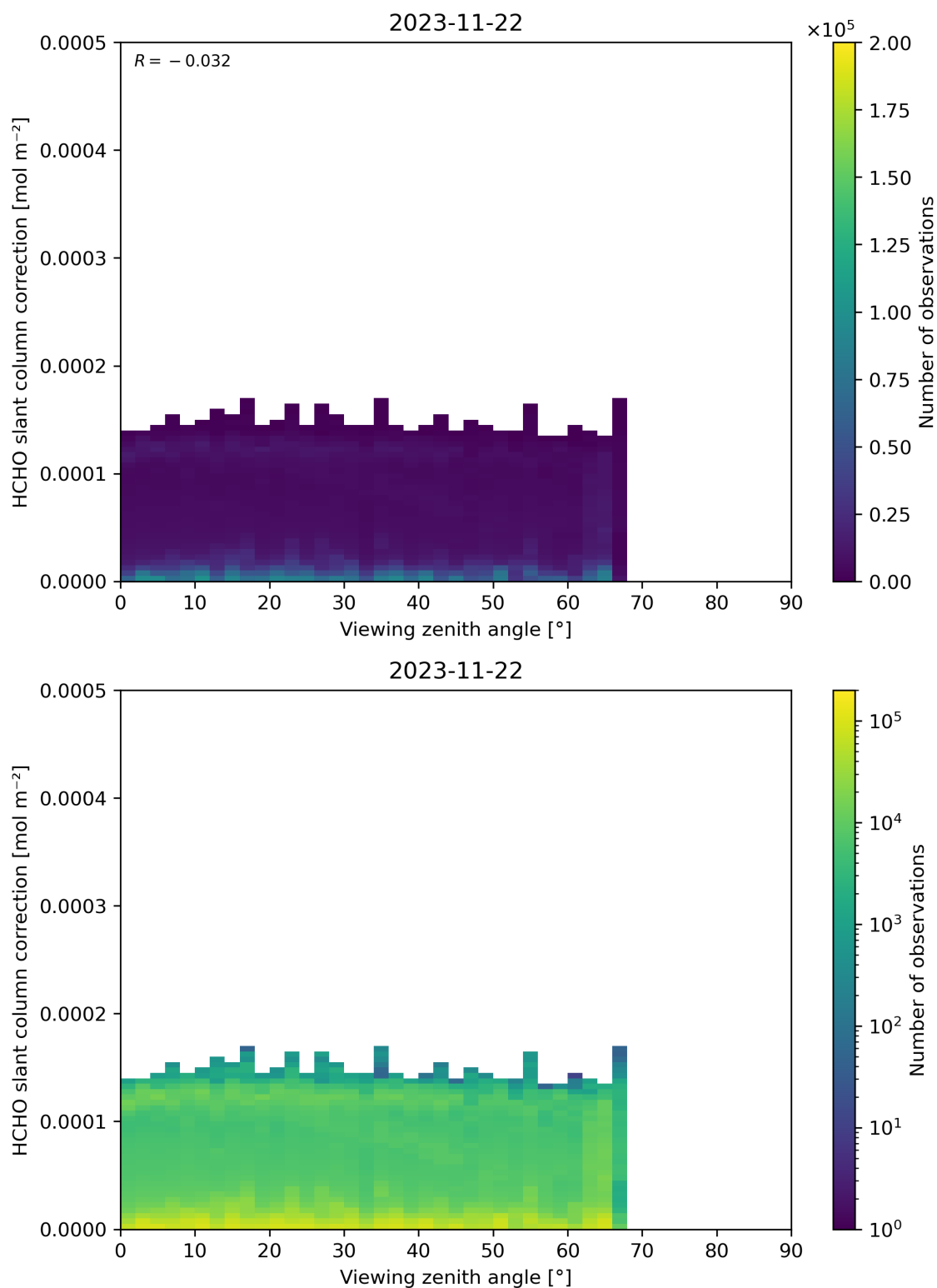
Figure 187: Scatter density plot of “Viewing zenith angle” against “HCHO slant column correction” for 2023-11-21 to 2023-11-23.
