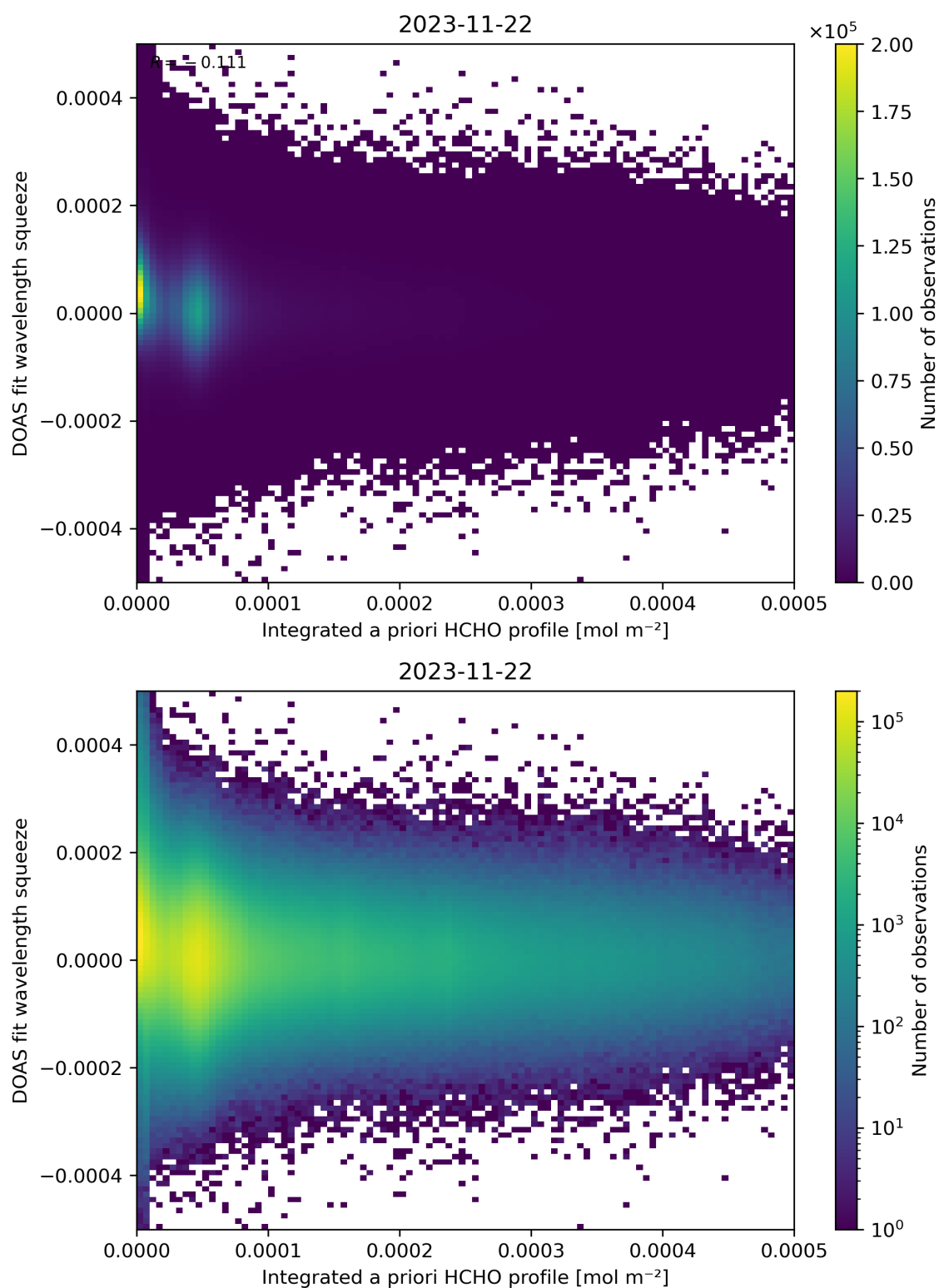
Figure 150: Scatter density plot of “Integrated a priori HCHO profile” against “DOAS fit wavelength squeeze” for 2023-11-21 to 2023-11-23.
