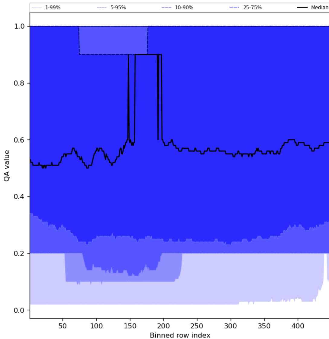
Figure 48: Along track statistics of “QA value” for 2023-11-21 to 2023-11-23
