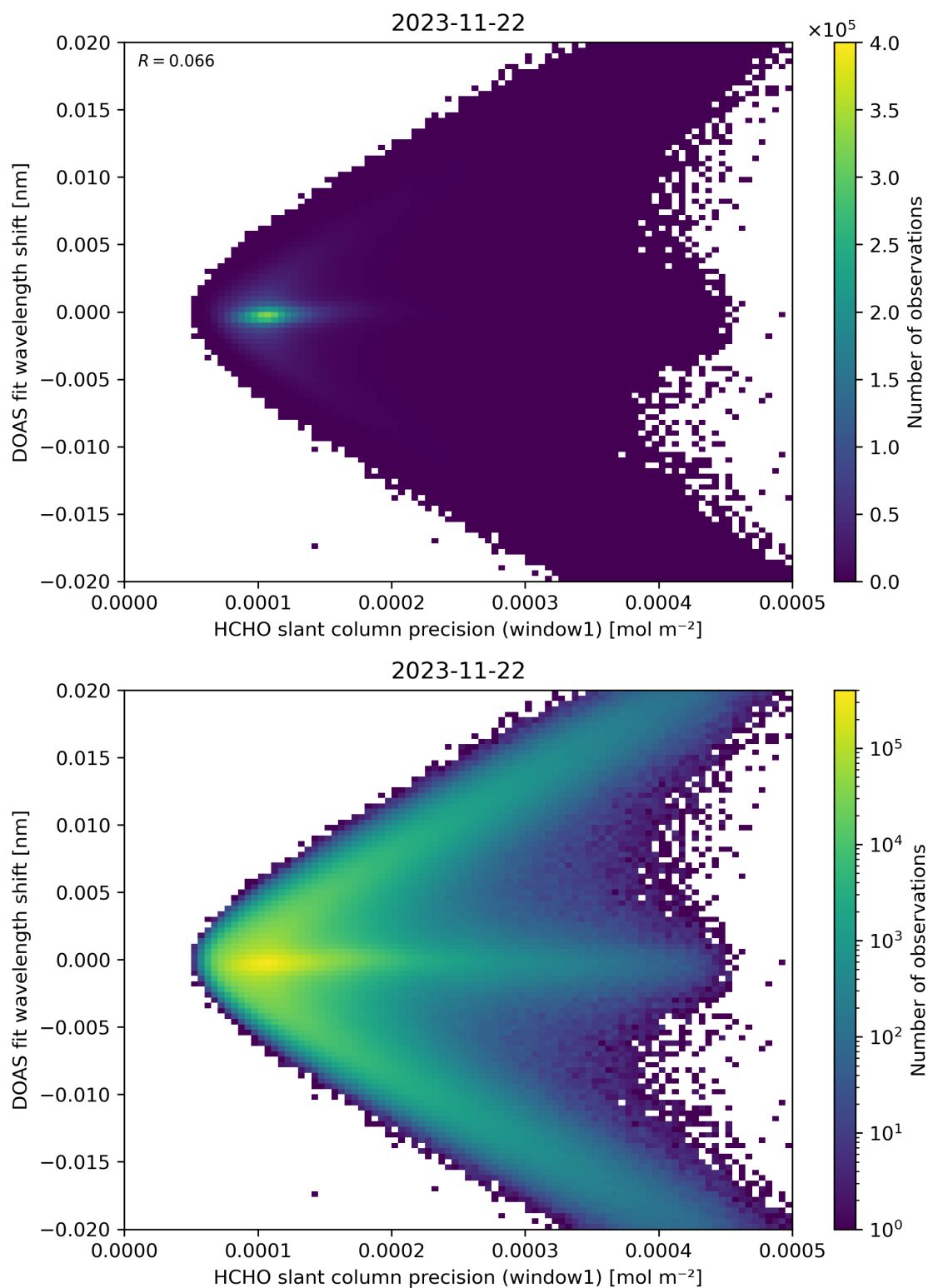
Figure 89: Scatter density plot of “HCHO slant column precision (window1)” against “DOAS fit wavelength shift” for 2023-11-21 to 2023-11-23.
