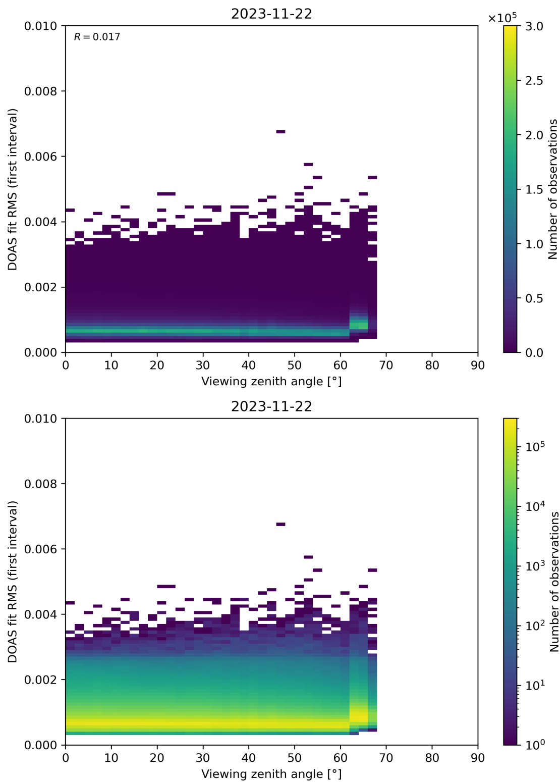
Figure 182: Scatter density plot of “Viewing zenith angle” against “DOAS fit RMS (first interval)” for 2023-11-21 to 2023-11-23.
