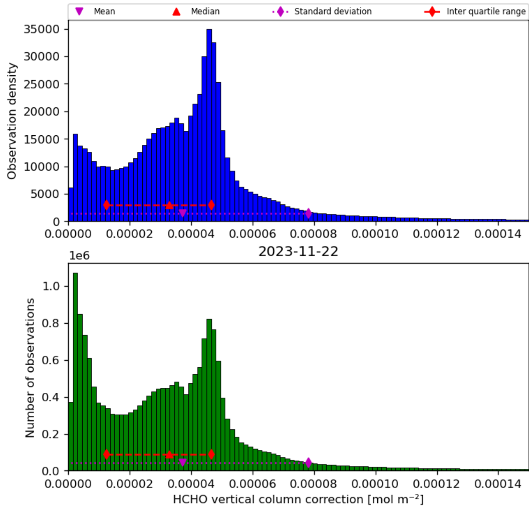
Figure 37: Histogram of “HCHO vertical column correction” for 2023-11-21 to 2023-11-23
