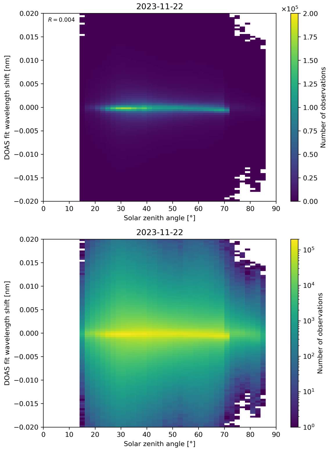
Figure 168: Scatter density plot of “Solar zenith angle” against “DOAS fit wavelength shift” for 2023-11-21 to 2023-11-23.
