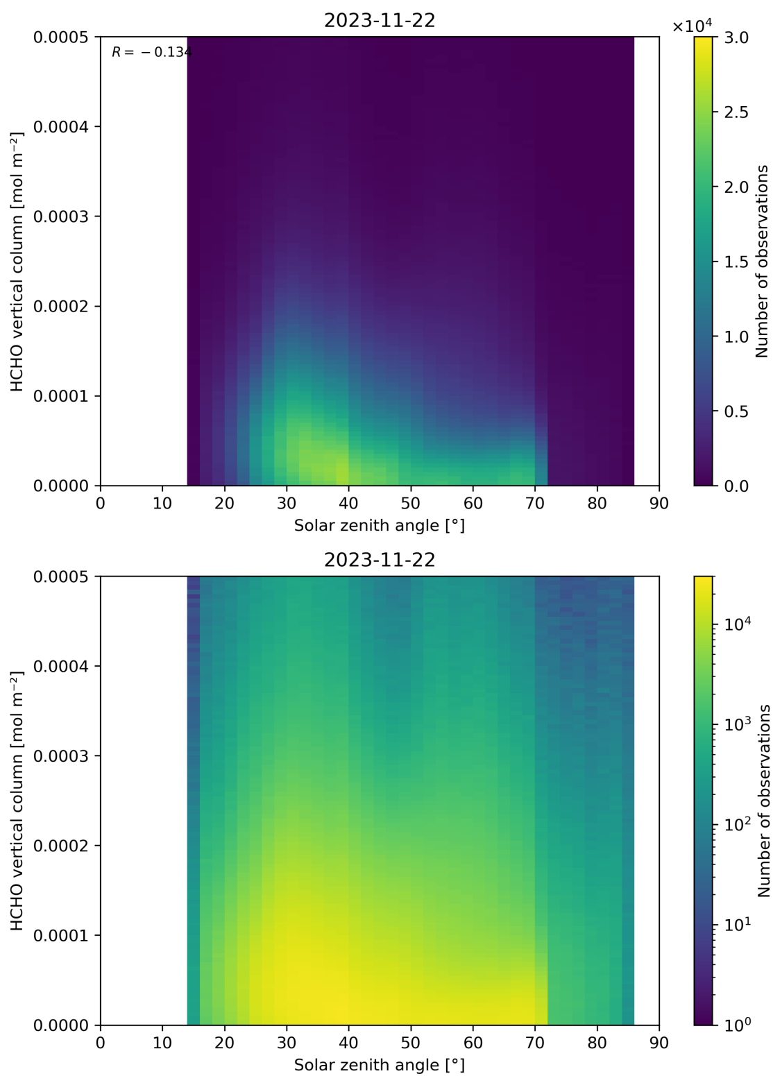
Figure 177: Scatter density plot of “Solar zenith angle” against “HCHO vertical column” for 2023-11-21 to 2023-11-23.
