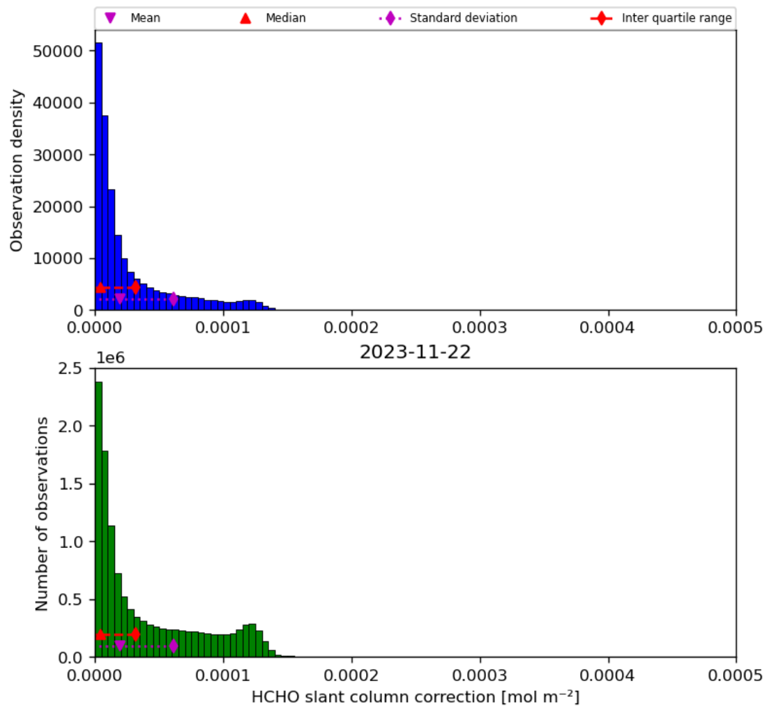
Figure 47: Histogram of “HCHO slant column correction” for 2023-11-21 to 2023-11-23
