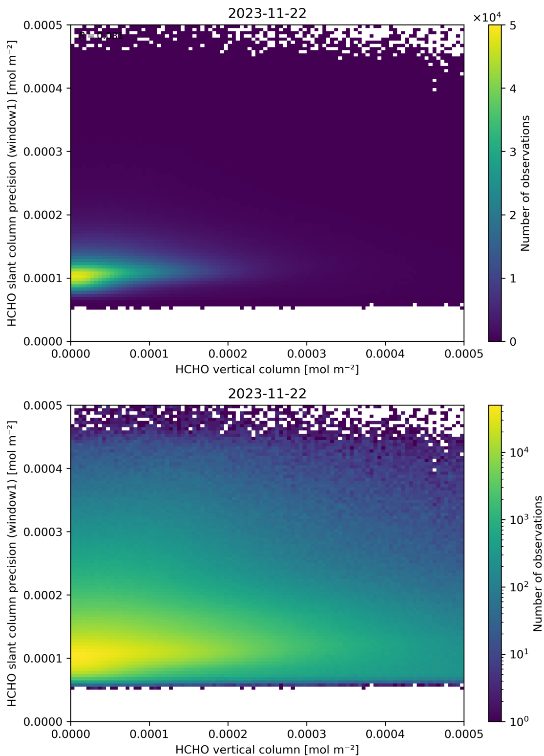
Figure 130: Scatter density plot of “HCHO vertical column” against “HCHO slant column precision (window1)” for 2023-11-21 to 2023-11-23.
