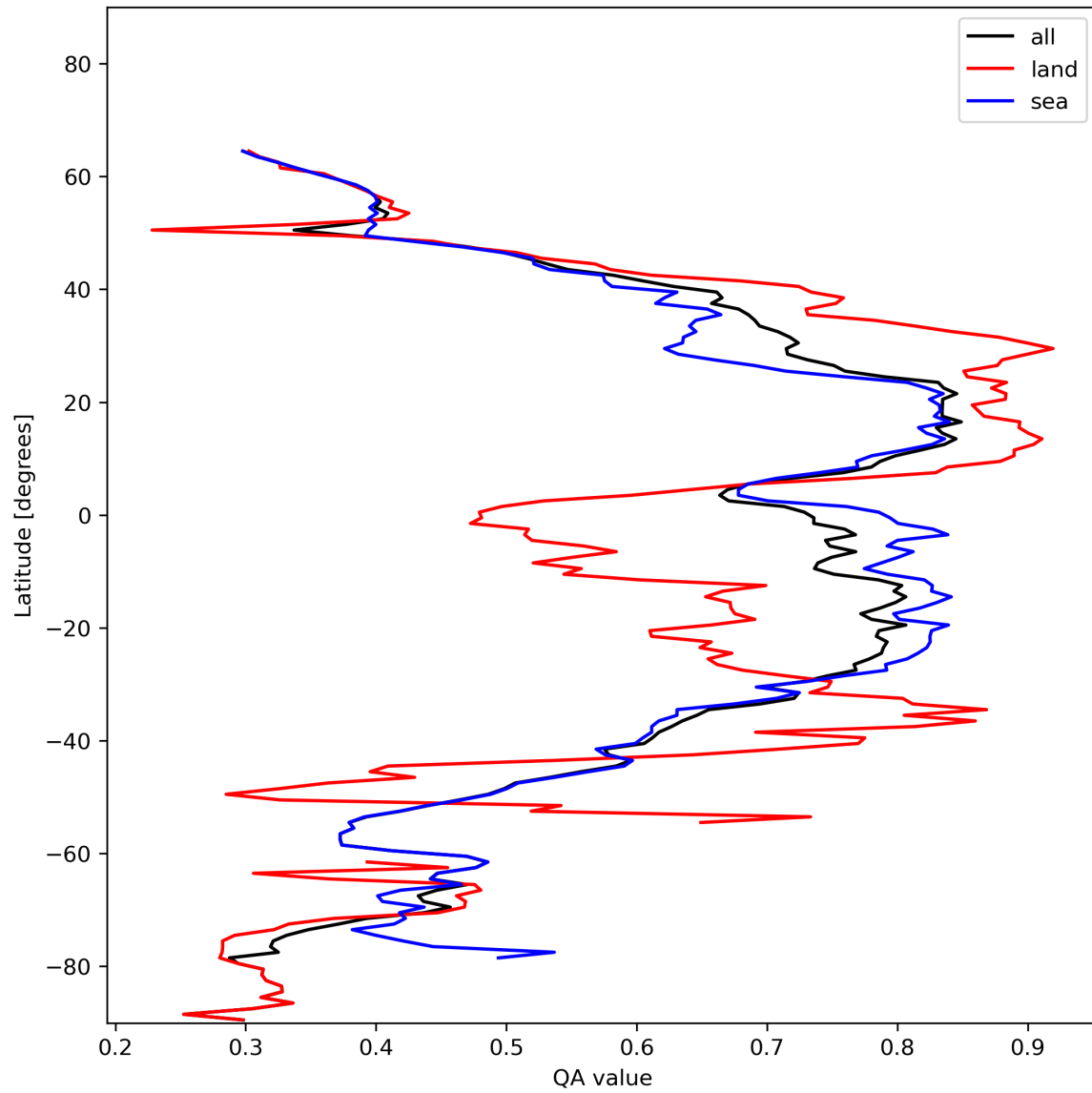
Figure 20: Zonal average of “QA value” for 2023-11-21 to 2023-11-23.
