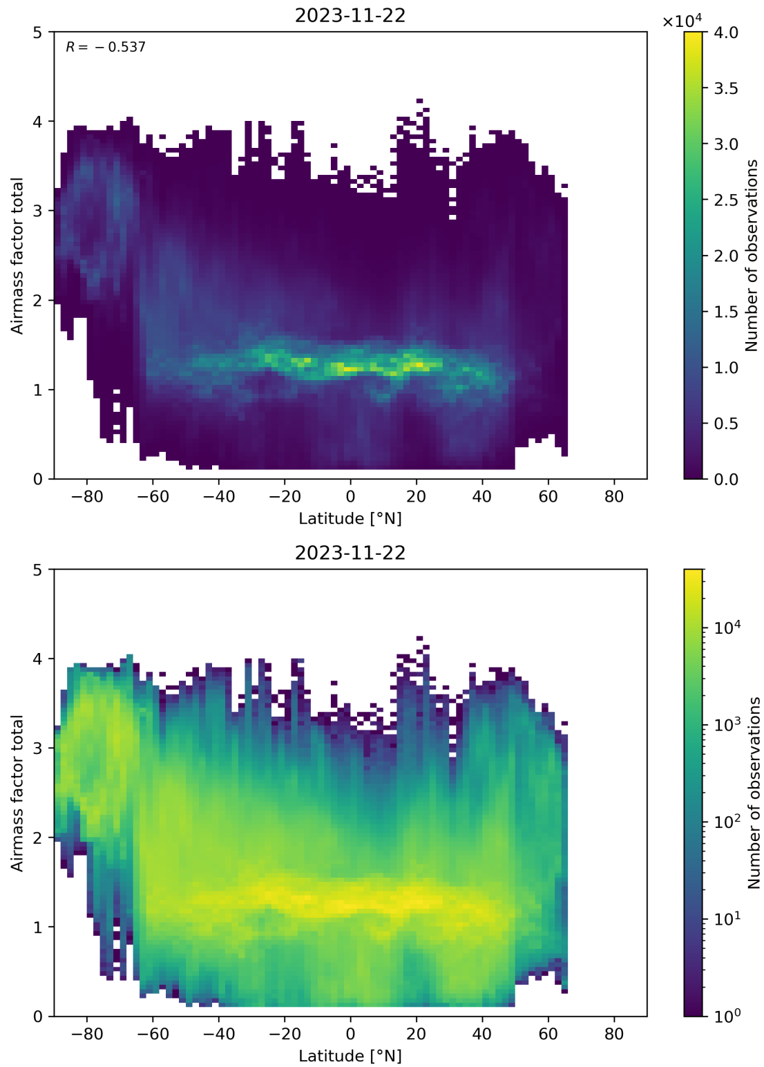
Figure 161: Scatter density plot of “Latitude” against “Airmass factor total” for 2023-11-21 to 2023-11-23.
