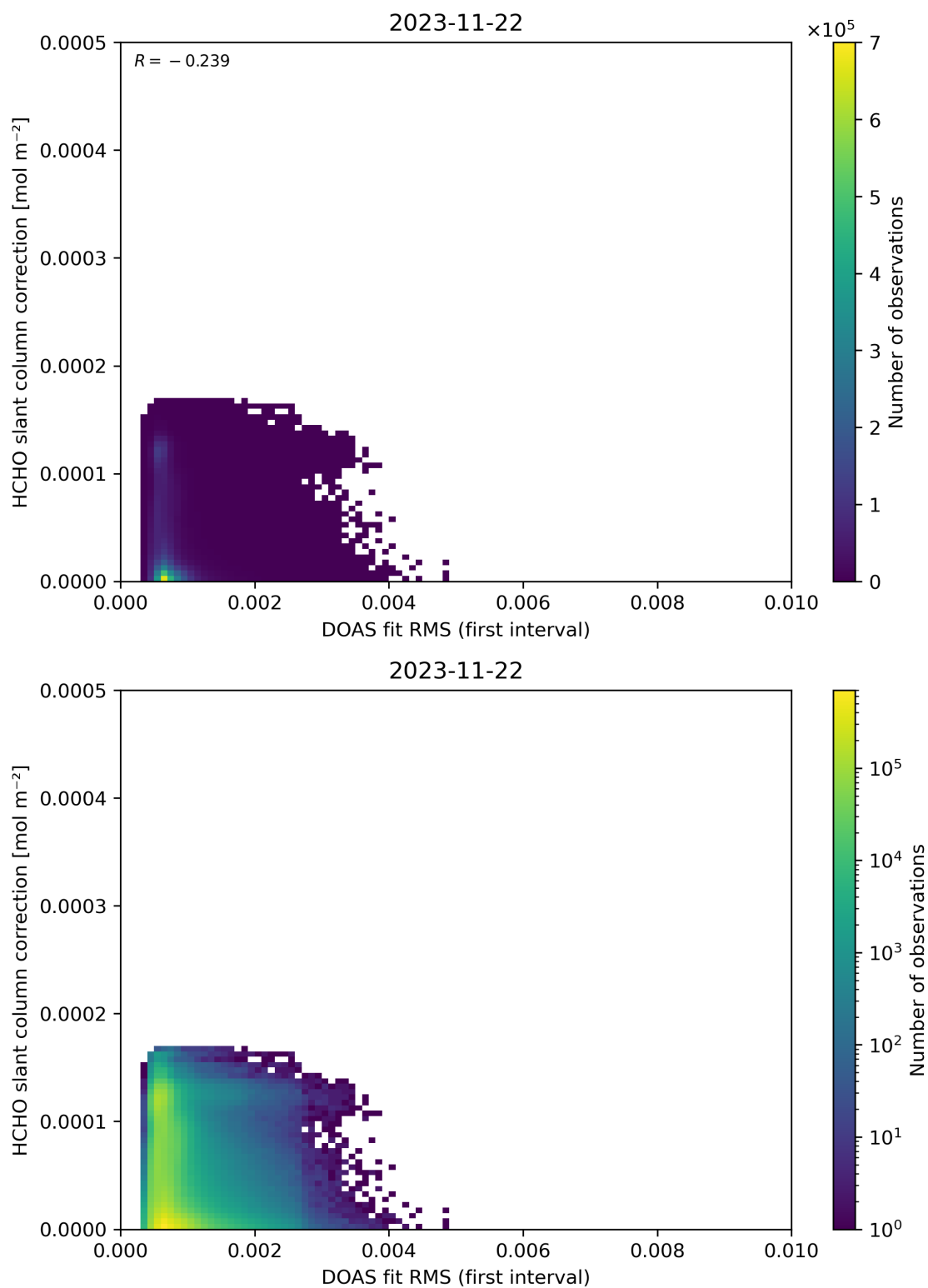
Figure 63: Scatter density plot of “DOAS fit RMS (first interval)” against “HCHO slant column correction” for 2023-11-21 to 2023-11-23.
