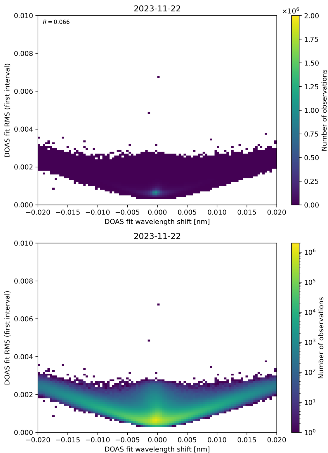
Figure 64: Scatter density plot of “DOAS fit wavelength shift” against “DOAS fit RMS (first interval)” for 2023-11-21 to 2023-11-23.
