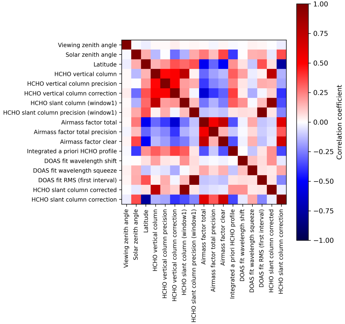
Figure 2: Map of correlation matrix for 2023-11-21 to 2023-11-23.
