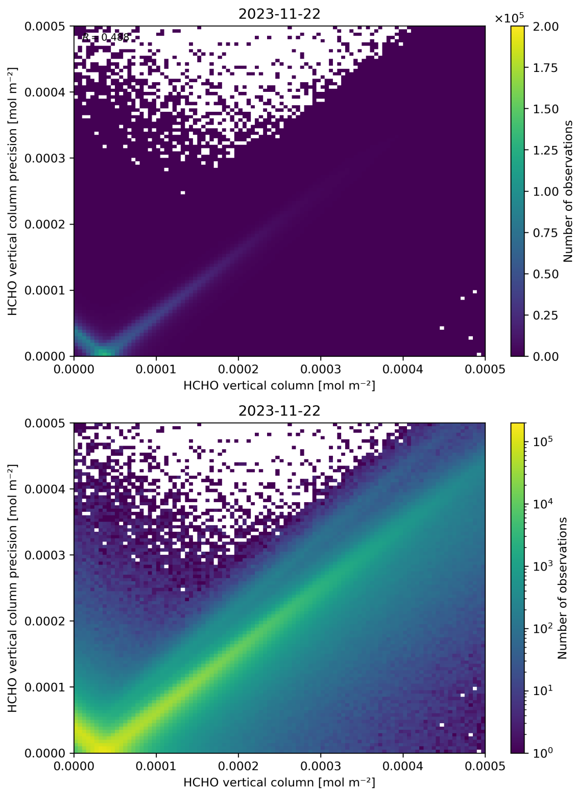
Figure 134: Scatter density plot of “HCHO vertical column” against “HCHO vertical column precision” for 2023-11-21 to 2023-11-23.
