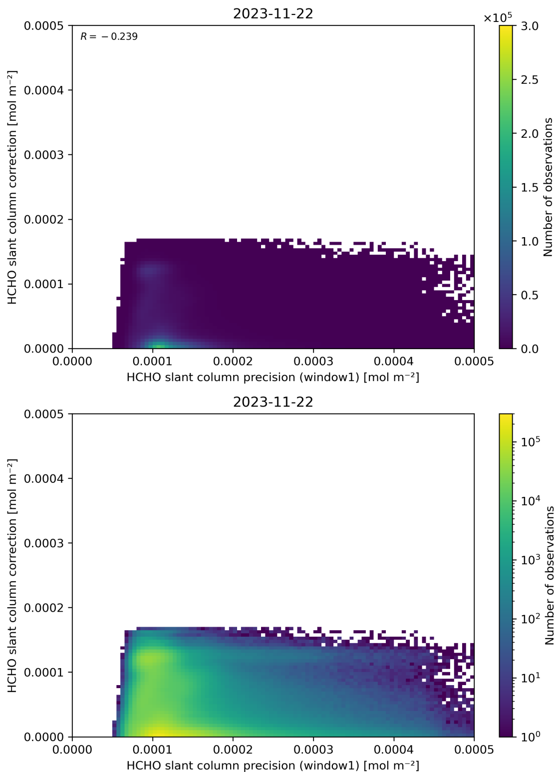
Figure 93: Scatter density plot of “HCHO slant column precision (window1)” against “HCHO slant column correction” for 2023-11-21 to 2023-11-23.
