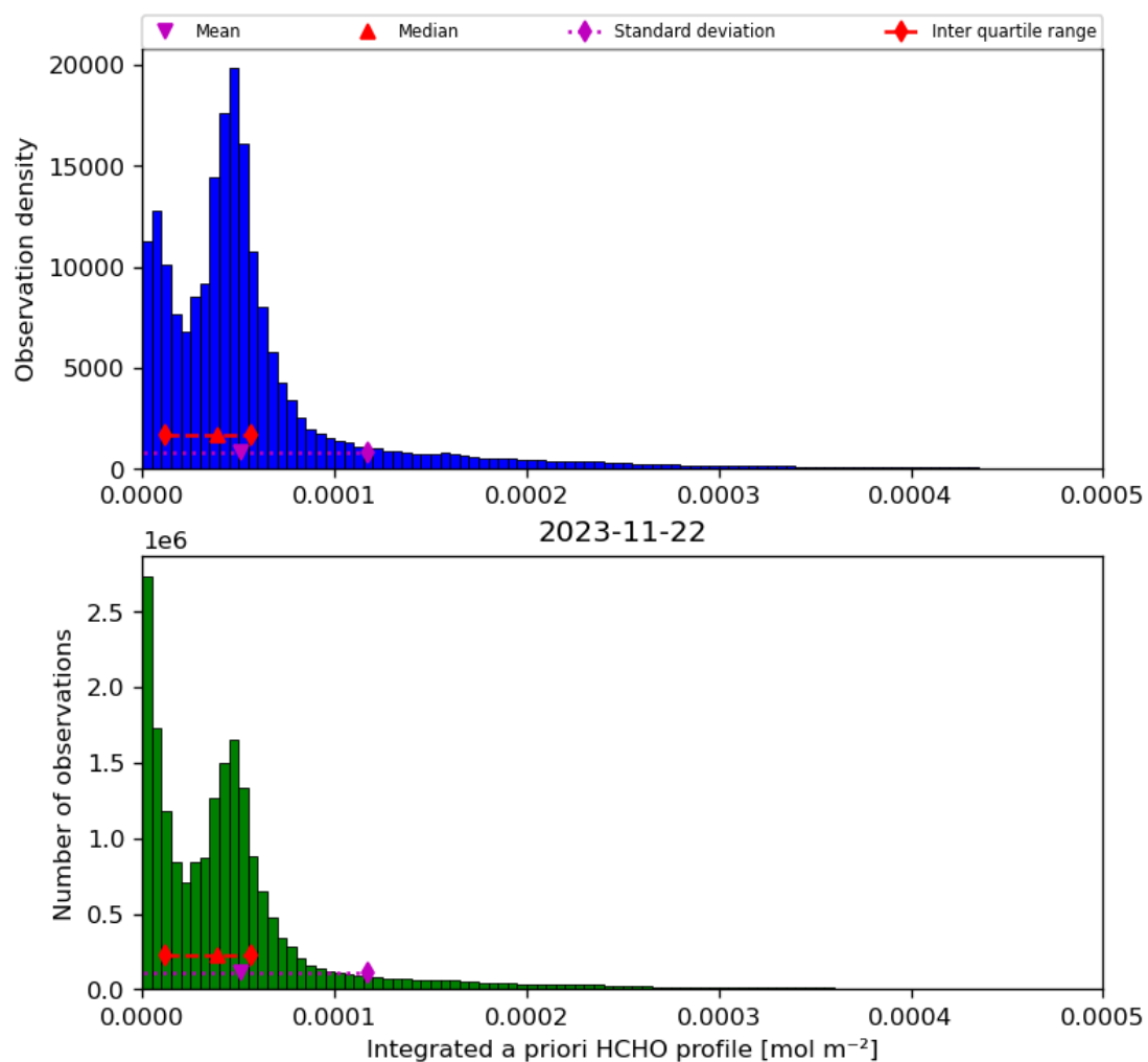
Figure 43: Histogram of “Integrated a priori HCHO profile” for 2023-11-21 to 2023-11-23
