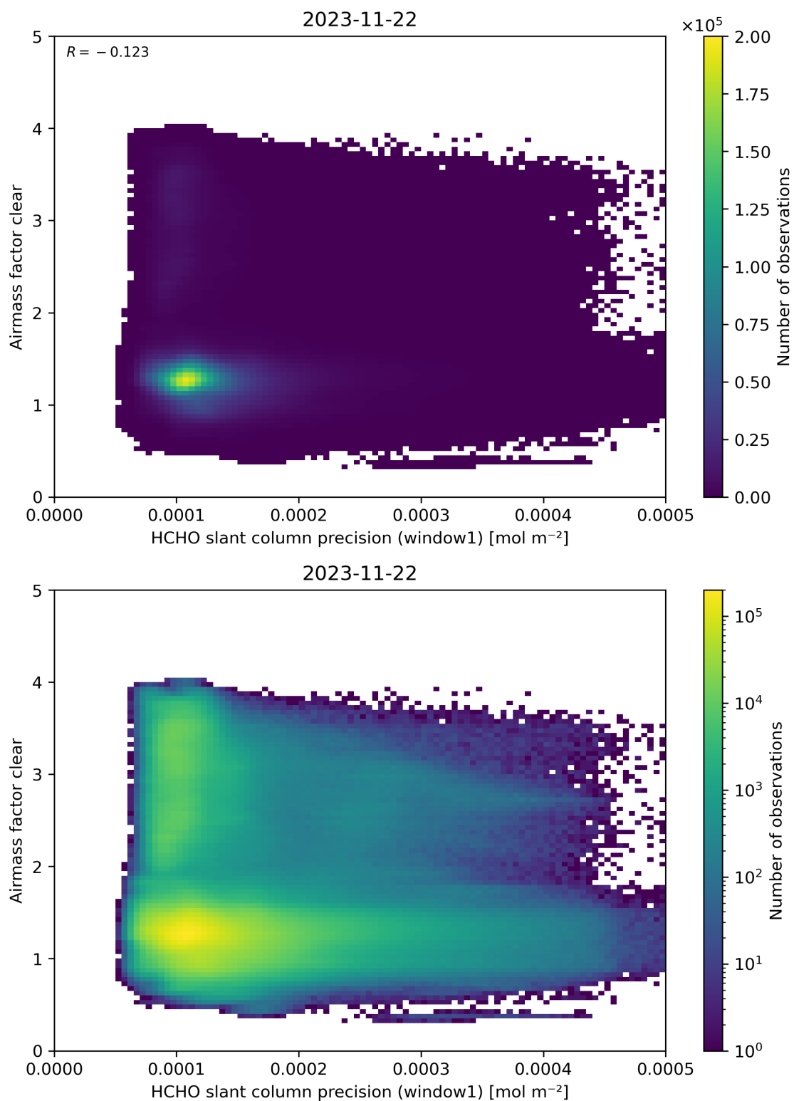
Figure 91: Scatter density plot of “HCHO slant column precision (window1)” against “Airmass factor clear” for 2023-11-21 to 2023-11-23.
