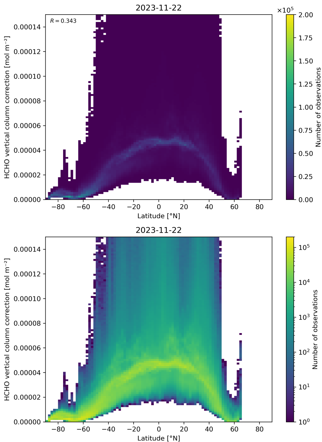
Figure 164: Scatter density plot of “Latitude” against “HCHO vertical column correction” for 2023-11-21 to 2023-11-23.
