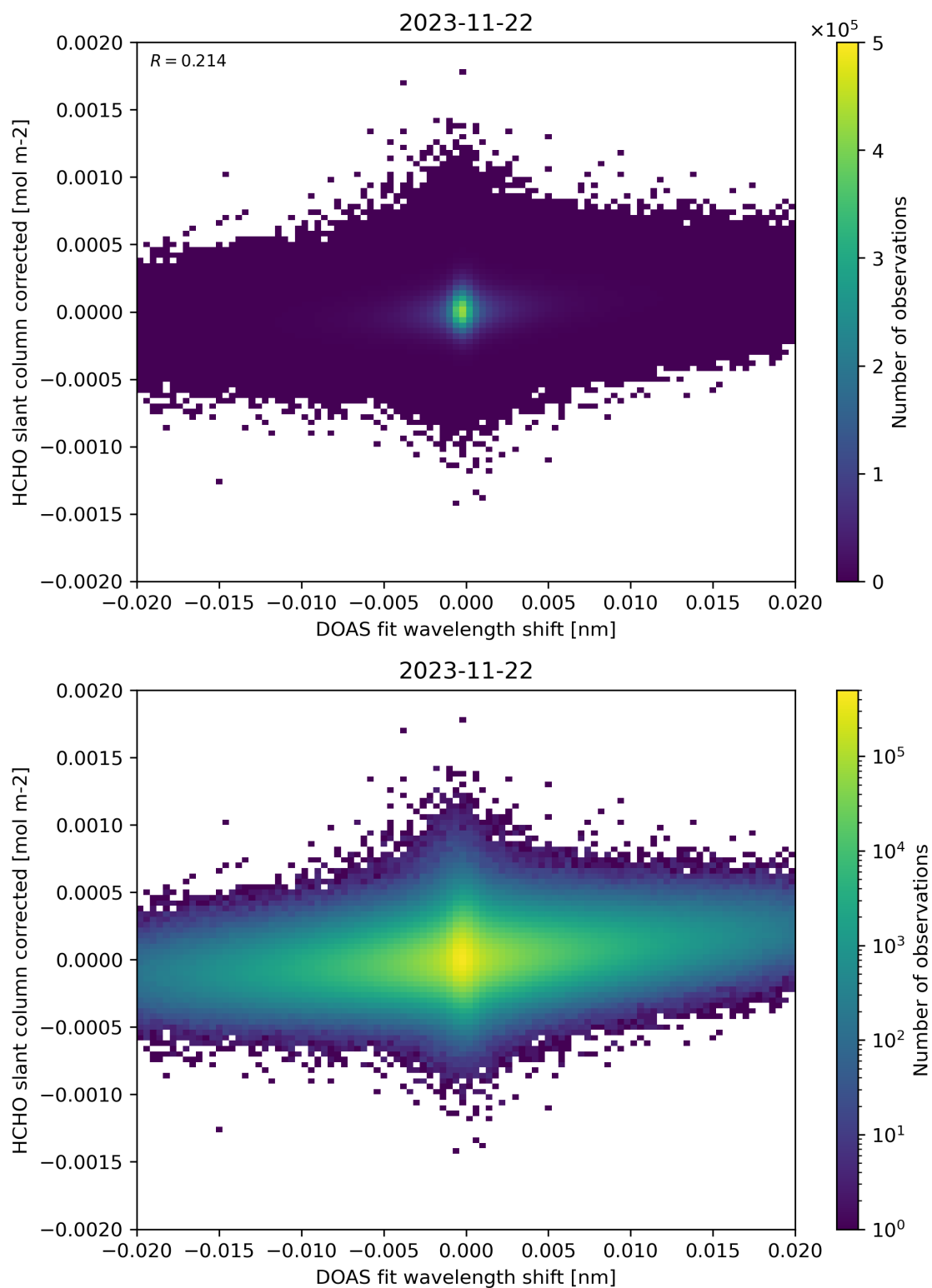
Figure 66: Scatter density plot of “DOAS fit wavelength shift” against “HCHO slant column corrected” for 2023-11-21 to 2023-11-23.
