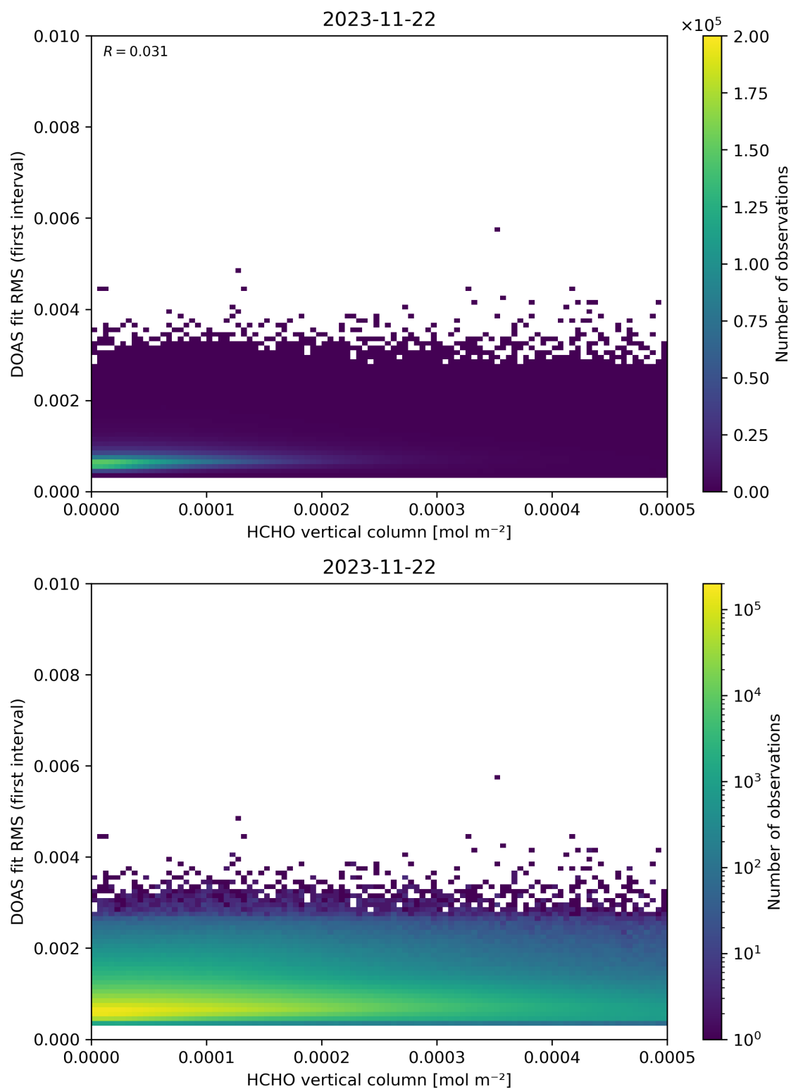
Figure 123: Scatter density plot of “HCHO vertical column” against “DOAS fit RMS (first interval)” for 2023-11-21 to 2023-11-23.
