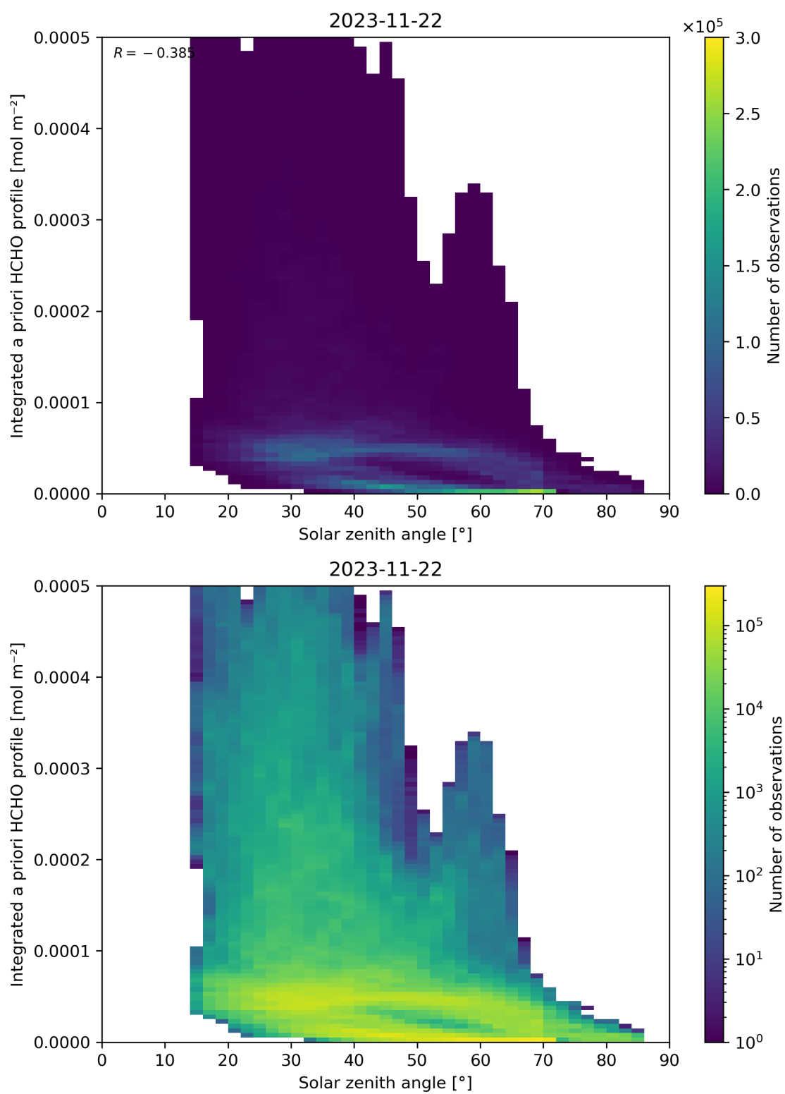
Figure 180: Scatter density plot of “Solar zenith angle” against “Integrated a priori HCHO profile” for 2023-11-21 to 2023-11-23.
