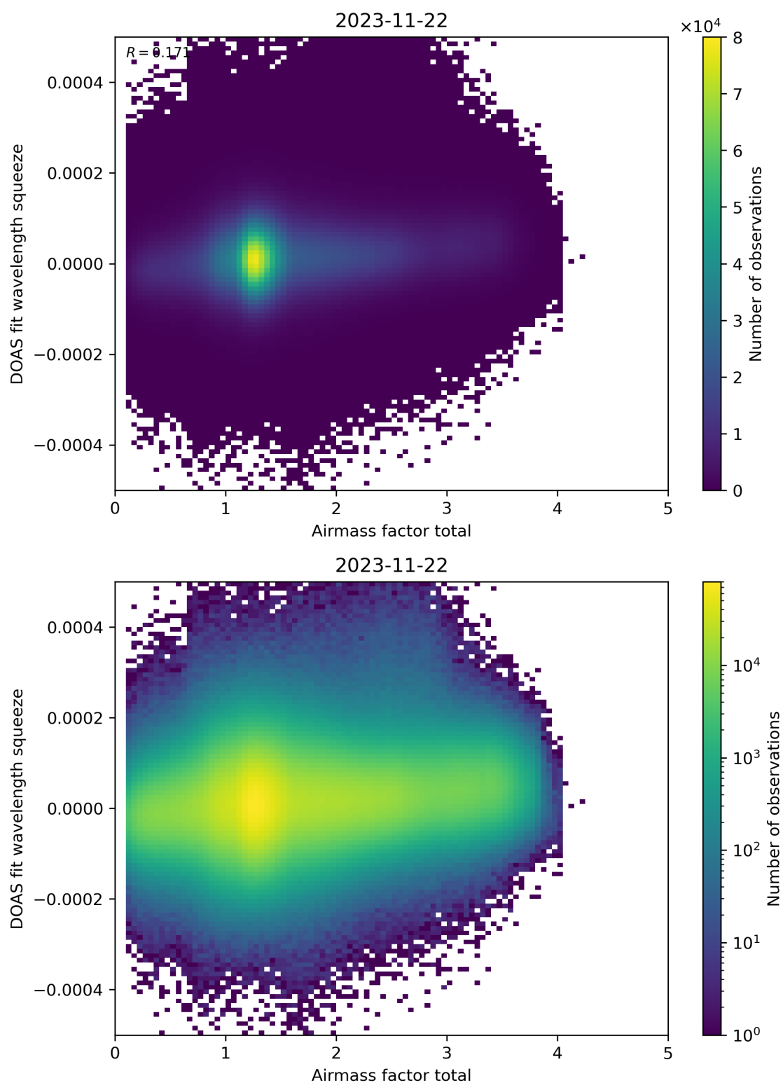
Figure 99: Scatter density plot of “Airmass factor total” against “DOAS fit wavelength squeeze” for 2023-11-21 to 2023-11-23.
