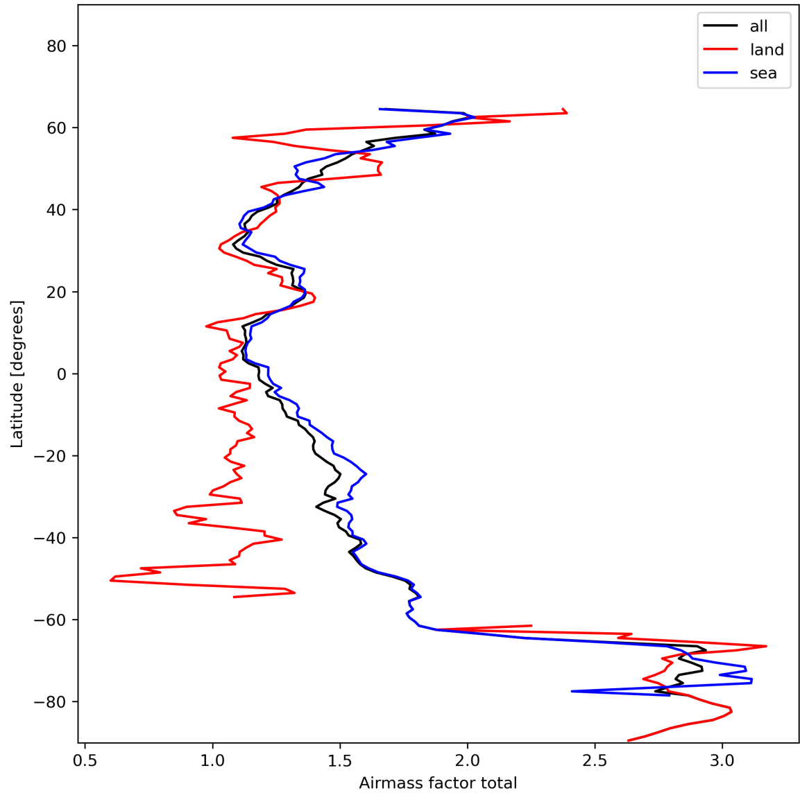
Figure 26: Zonal average of “Airmass factor total” for 2023-11-21 to 2023-11-23.
