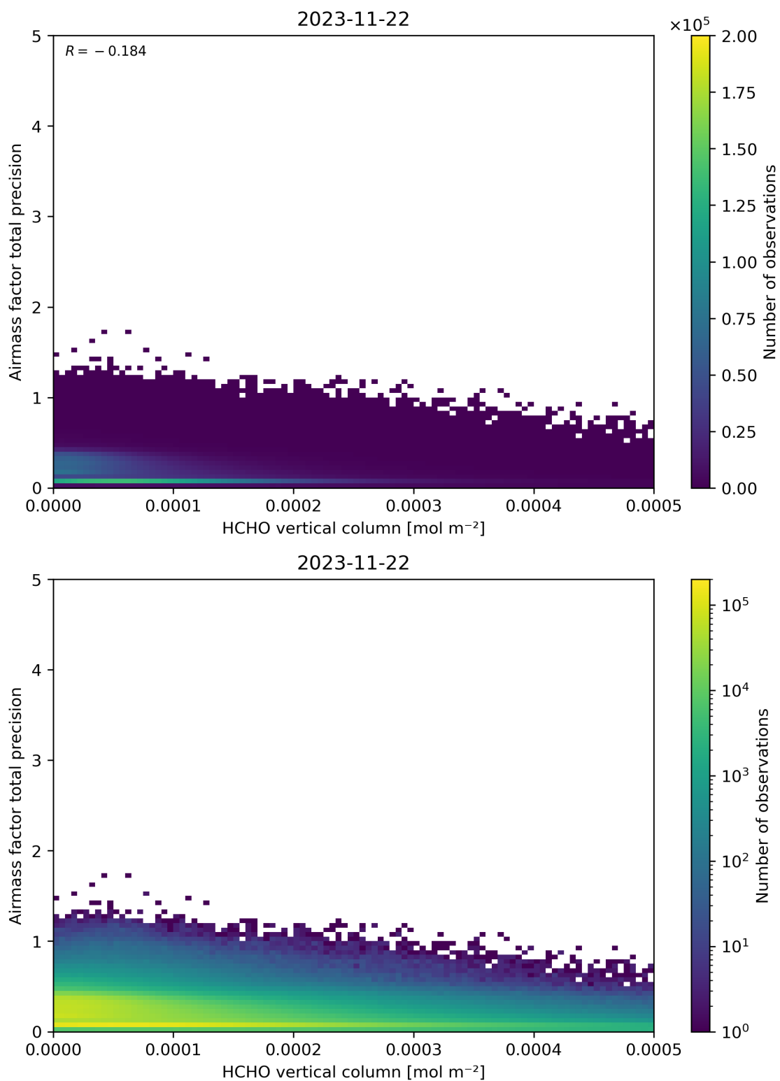
Figure 132: Scatter density plot of “HCHO vertical column” against “Airmass factor total precision” for 2023-11-21 to 2023-11-23.
