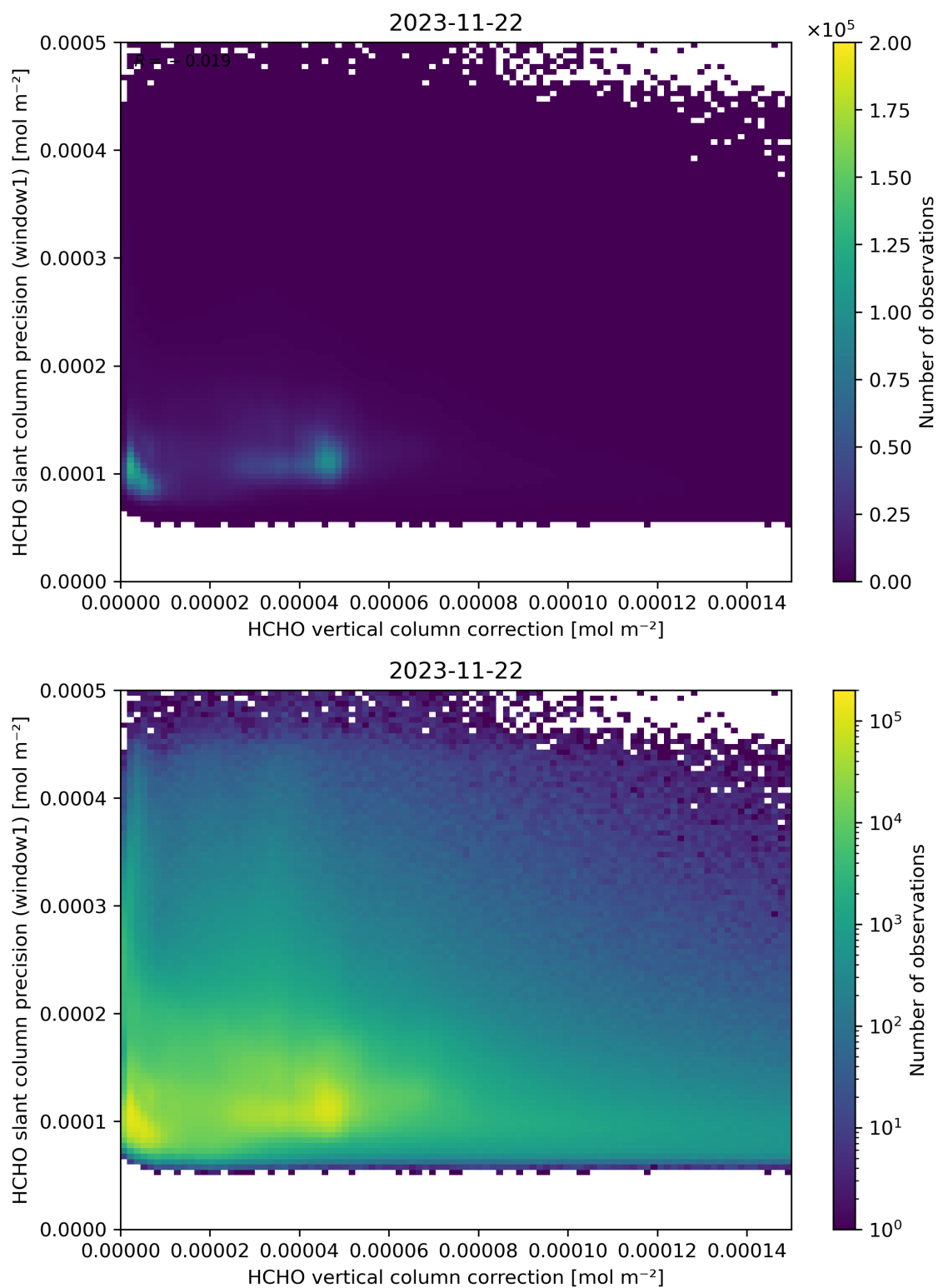
Figure 119: Scatter density plot of “HCHO vertical column correction” against “HCHO slant column precision (window1)” for 2023-11-21 to 2023-11-23.
