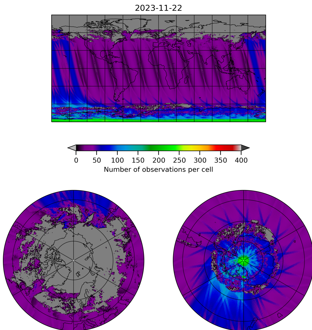
Figure 19: Map of the number of observations for 2023-11-21 to 2023-11-23
