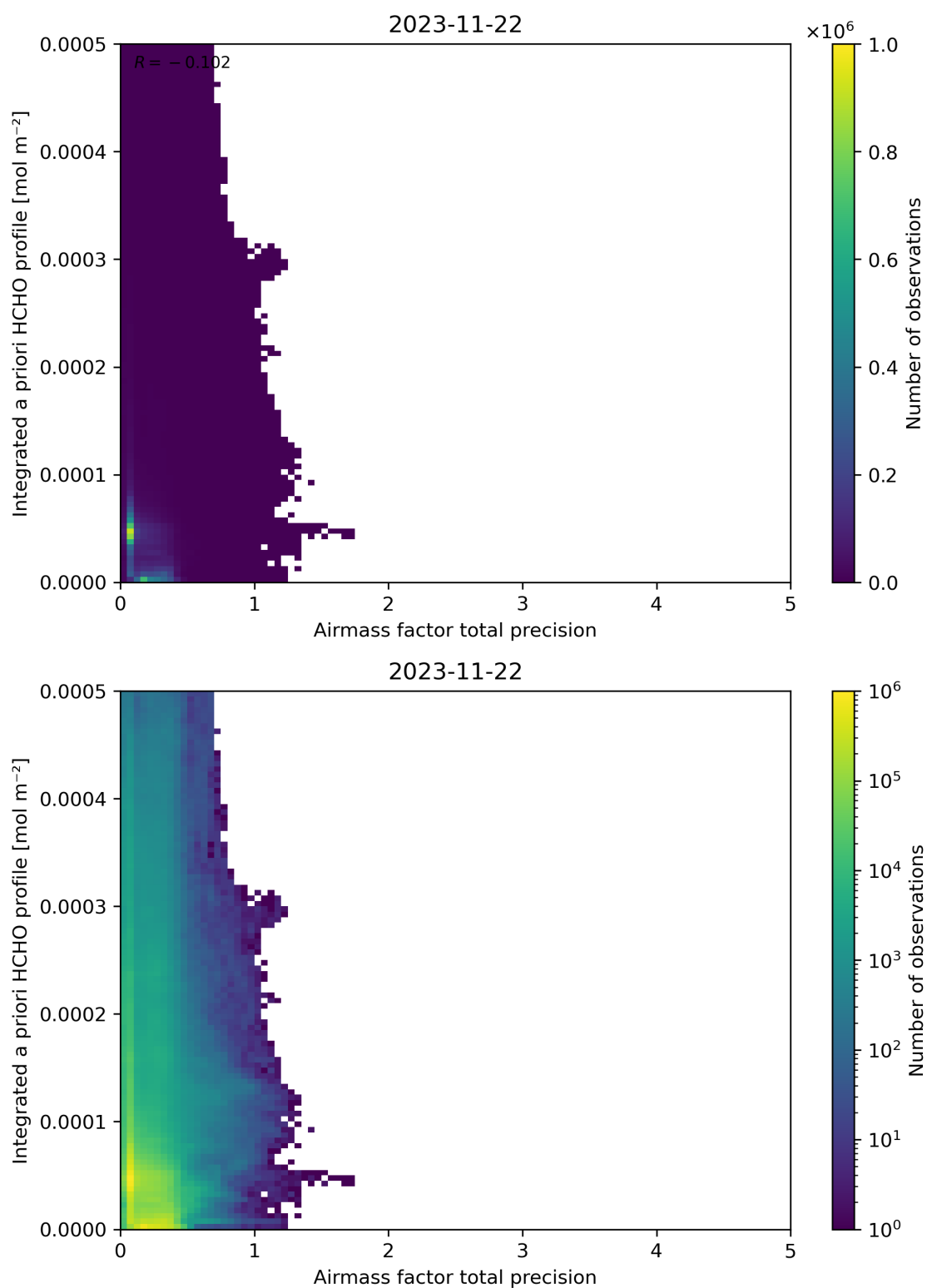
Figure 111: Scatter density plot of “Airmass factor total precision” against “Integrated a priori HCHO profile” for 2023-11-21 to 2023-11-23.
