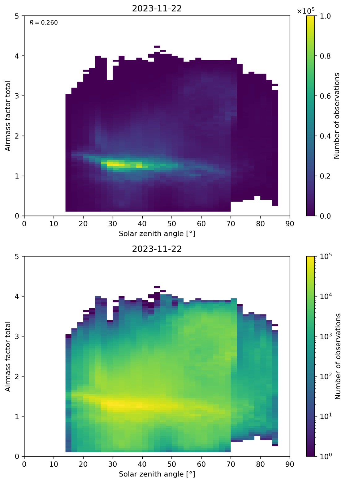
Figure 175: Scatter density plot of “Solar zenith angle” against “Airmass factor total” for 2023-11-21 to 2023-11-23.
