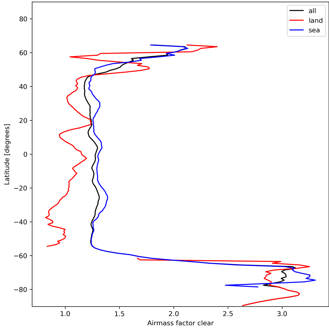
Figure 28: Zonal average of “Airmass factor clear” for 2023-11-21 to 2023-11-23.
