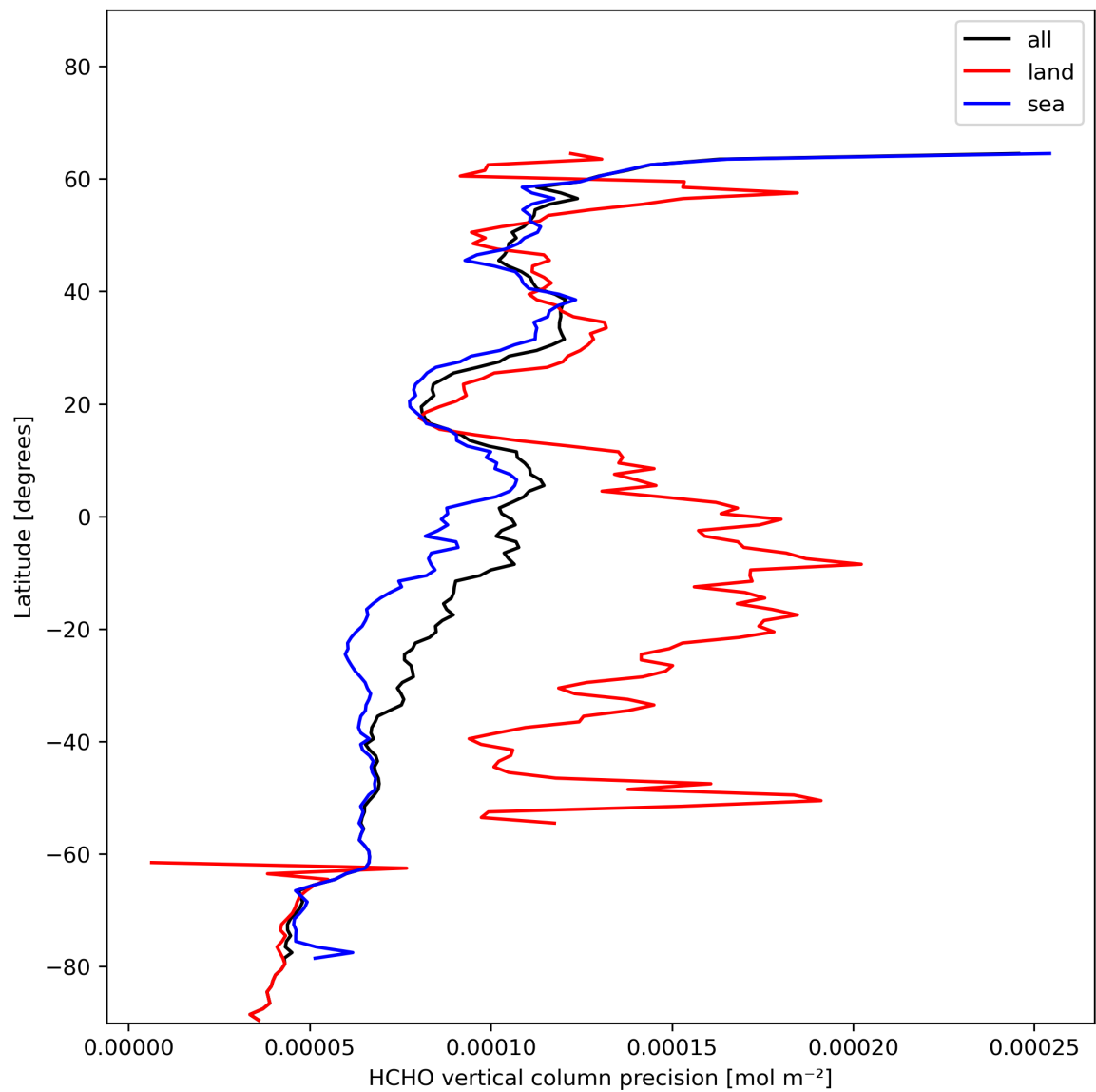
Figure 22: Zonal average of “HCHO vertical column precision” for 2023-11-21 to 2023-11-23.
