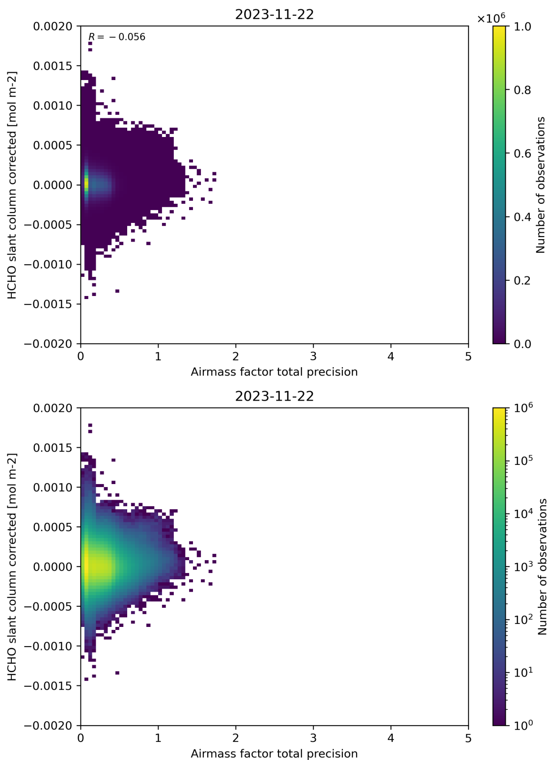
Figure 109: Scatter density plot of “Airmass factor total precision” against “HCHO slant column corrected” for 2023-11-21 to 2023-11-23.
