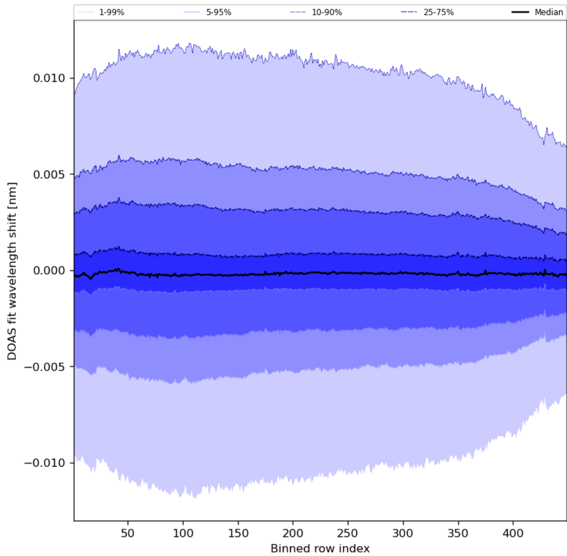
Figure 58: Along track statistics of “DOAS fit wavelength shift” for 2023-11-21 to 2023-11-23
