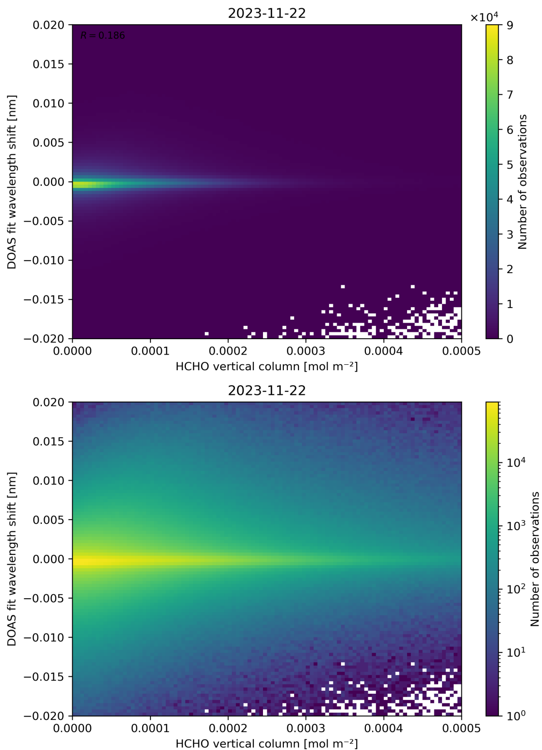
Figure 124: Scatter density plot of “HCHO vertical column” against “DOAS fit wavelength shift” for 2023-11-21 to 2023-11-23.
