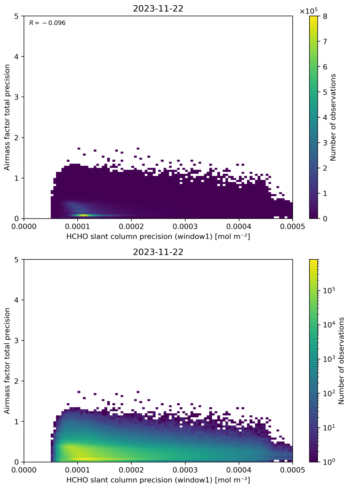
Figure 95: Scatter density plot of “HCHO slant column precision (window1)” against “Airmass factor total precision” for 2023-11-21 to 2023-11-23.
