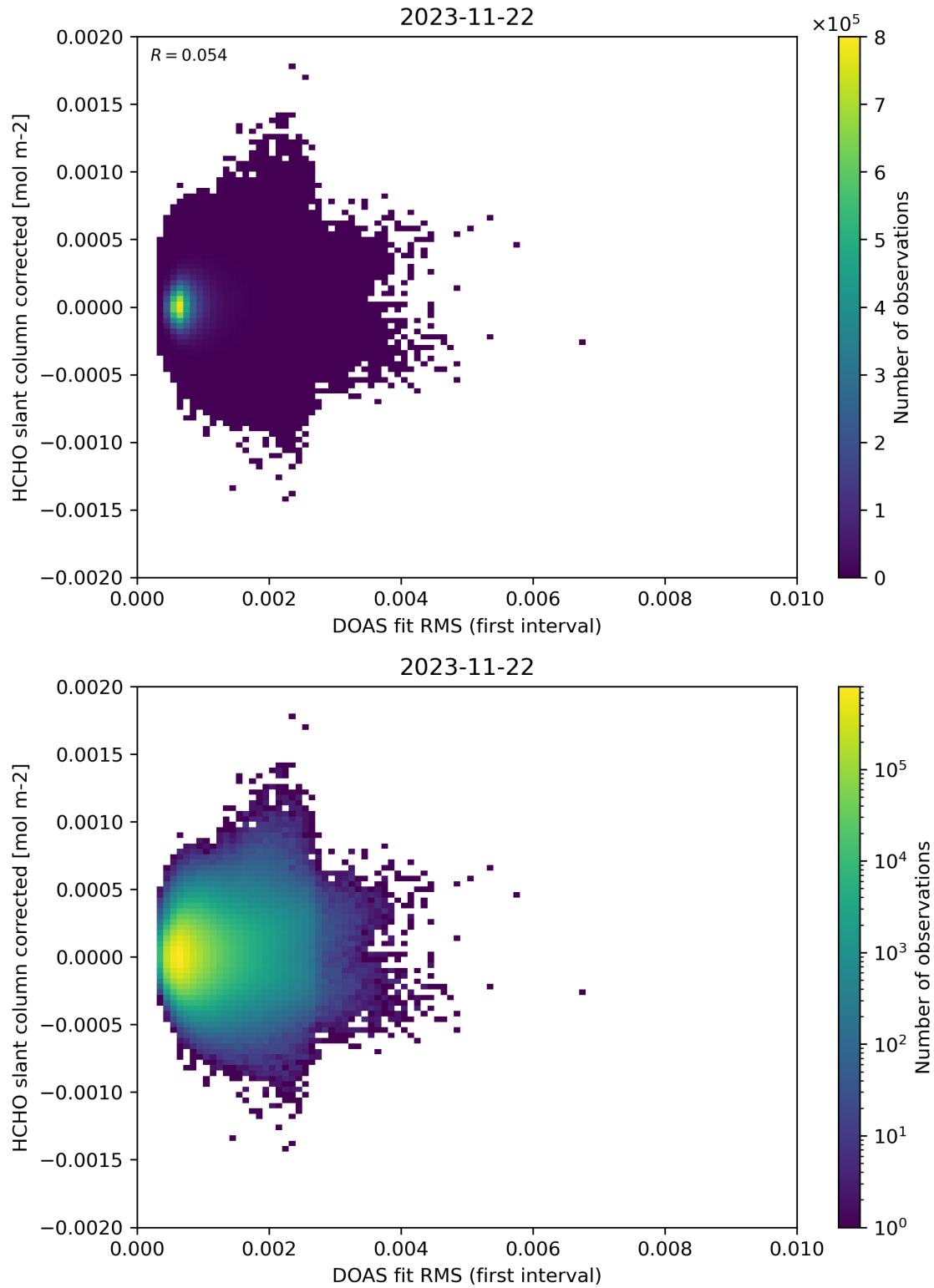
Figure 62: Scatter density plot of “DOAS fit RMS (first interval)” against “HCHO slant column corrected” for 2023-11-21 to 2023-11-23.
