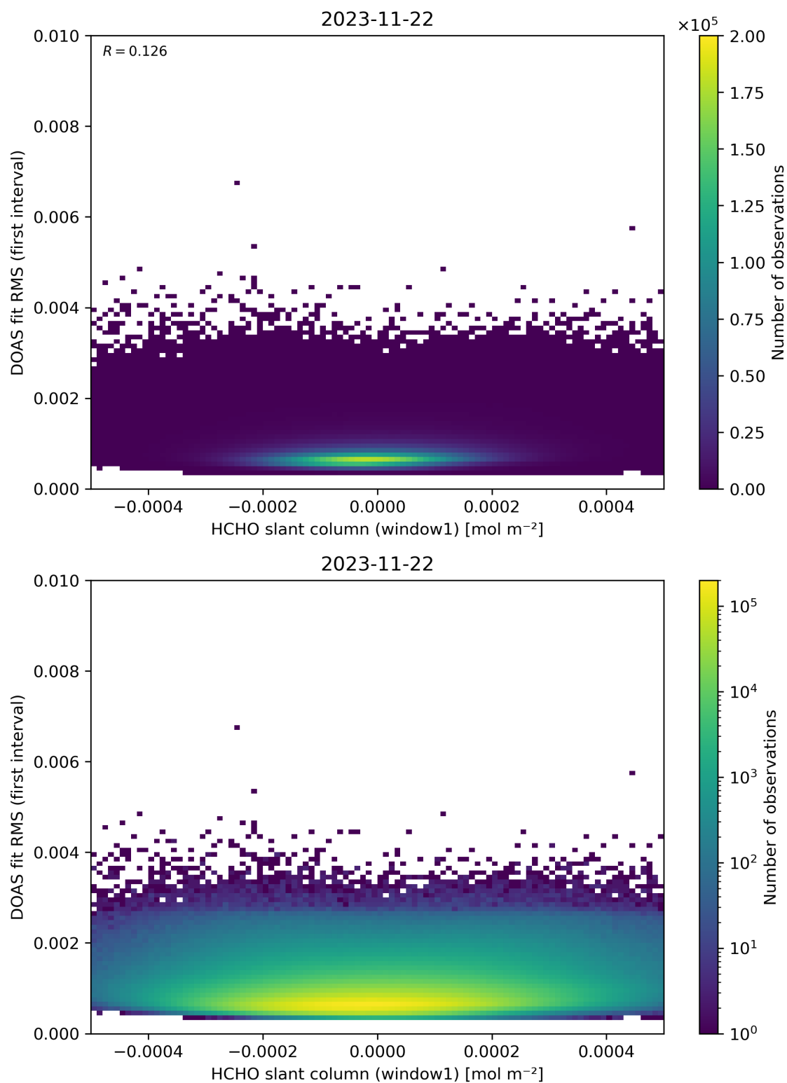
Figure 78: Scatter density plot of “HCHO slant column (window1)” against “DOAS fit RMS (first interval)” for 2023-11-21 to 2023-11-23.
