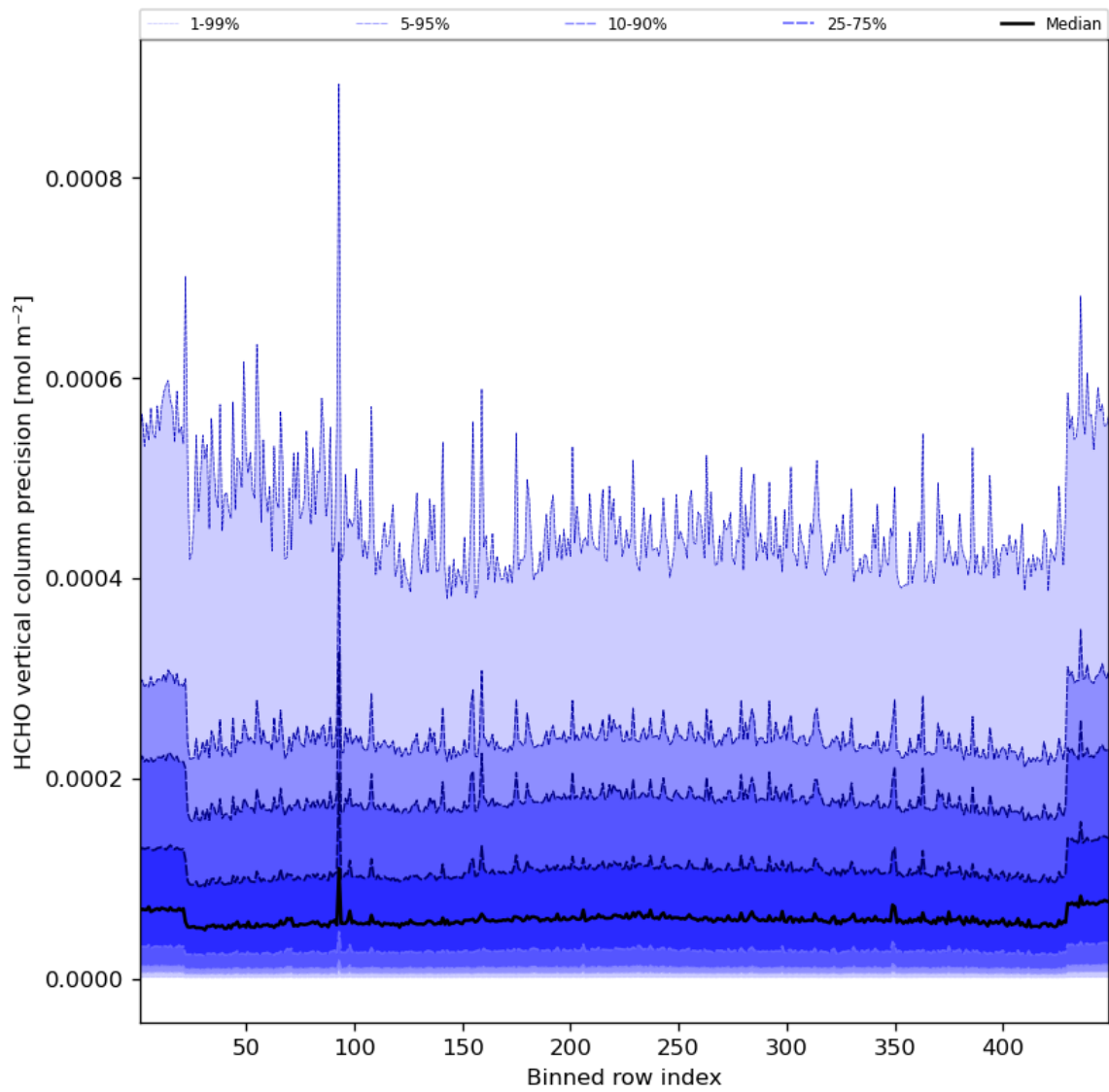
Figure 50: Along track statistics of “HCHO vertical column precision” for 2023-11-21 to 2023-11-23
