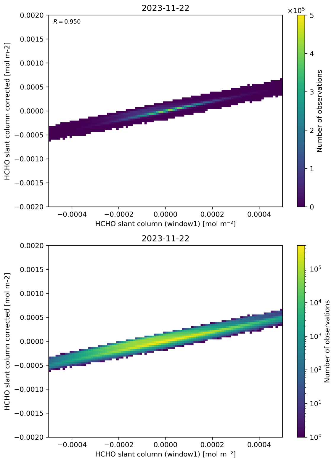
Figure 82: Scatter density plot of “HCHO slant column (window1)” against “HCHO slant column corrected” for 2023-11-21 to 2023-11-23.
