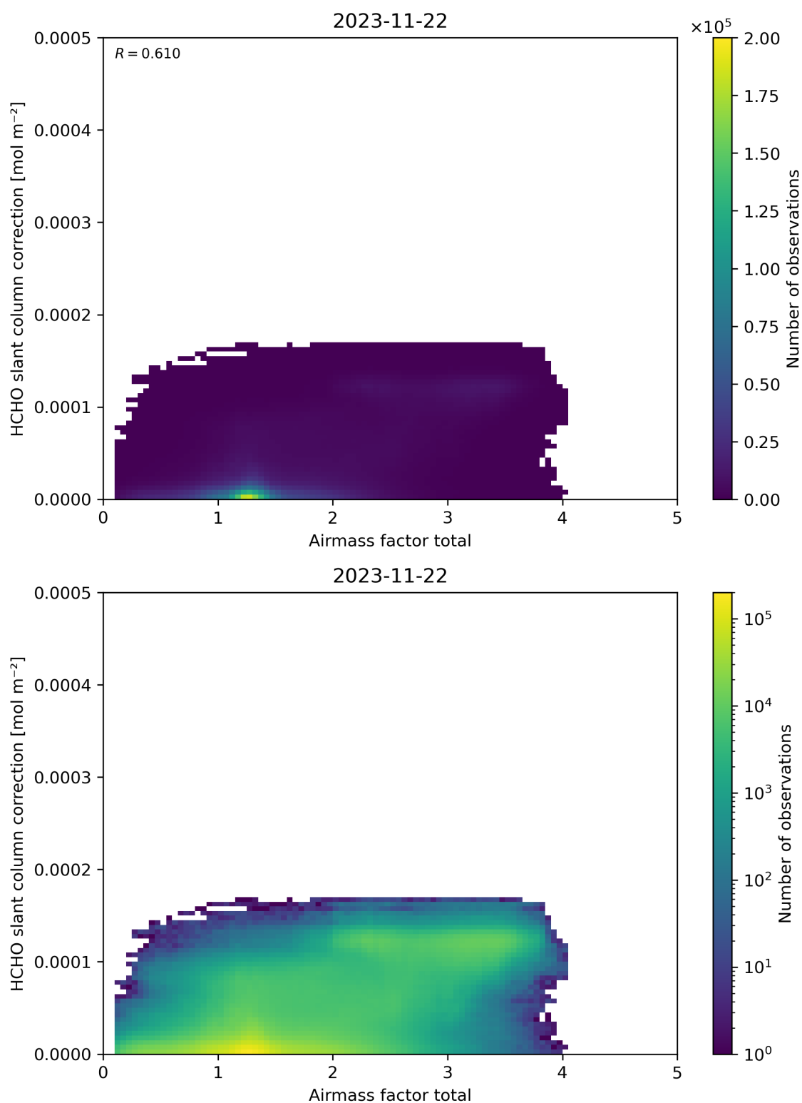
Figure 102: Scatter density plot of “Airmass factor total” against “HCHO slant column correction” for 2023-11-21 to 2023-11-23.
