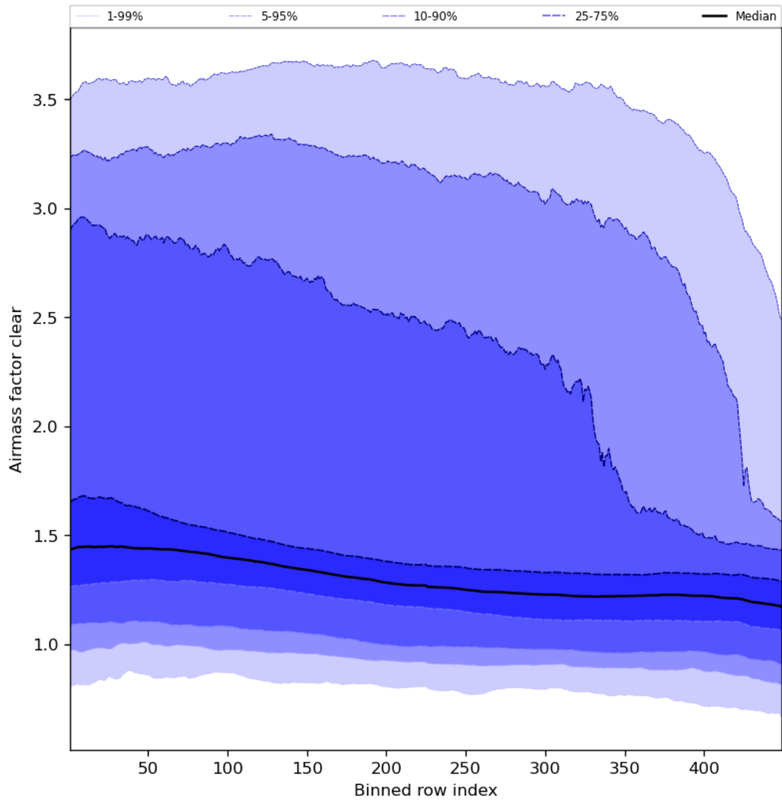
Figure 56: Along track statistics of “Airmass factor clear” for 2023-11-21 to 2023-11-23
