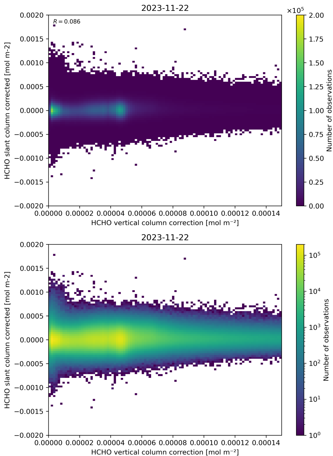
Figure 116: Scatter density plot of “HCHO vertical column correction” against “HCHO slant column corrected” for 2023-11-21 to 2023-11-23.
