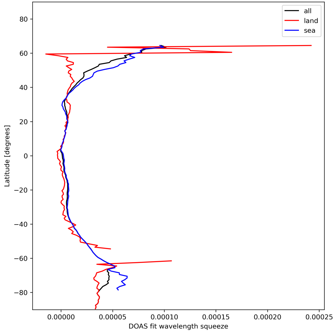
Figure 31: Zonal average of “DOAS fit wavelength squeeze” for 2023-11-21 to 2023-11-23.
