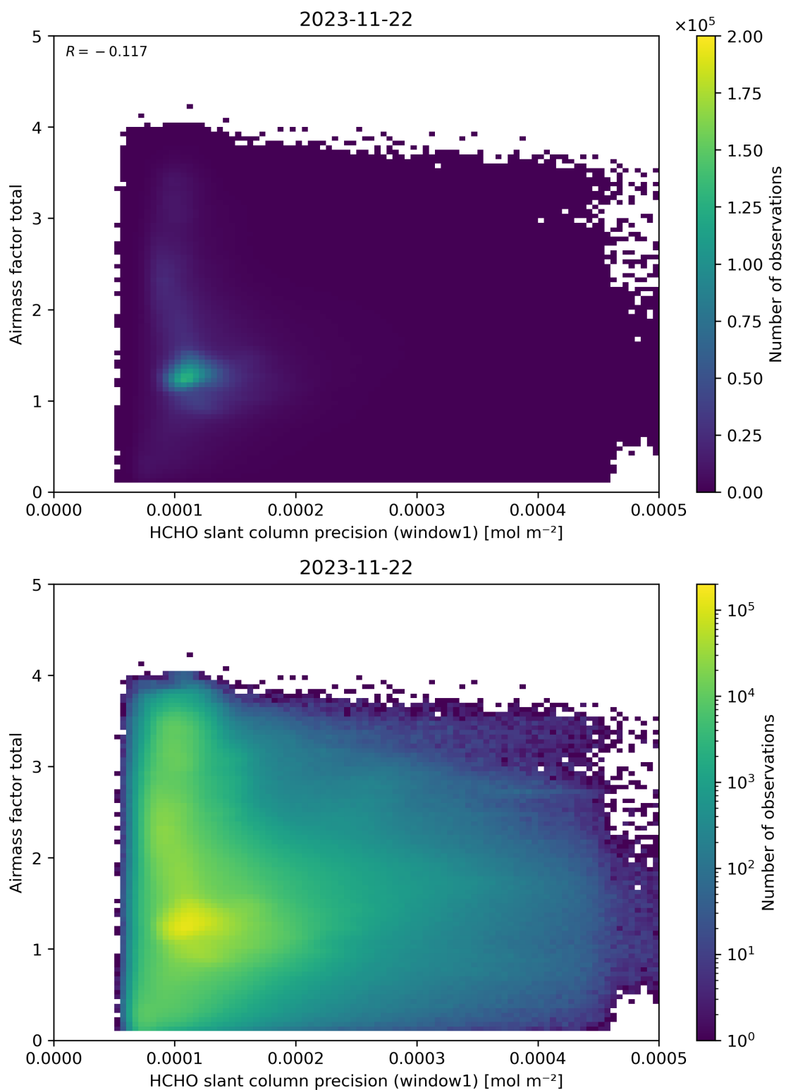
Figure 94: Scatter density plot of “HCHO slant column precision (window1)” against “Airmass factor total” for 2023-11-21 to 2023-11-23.
