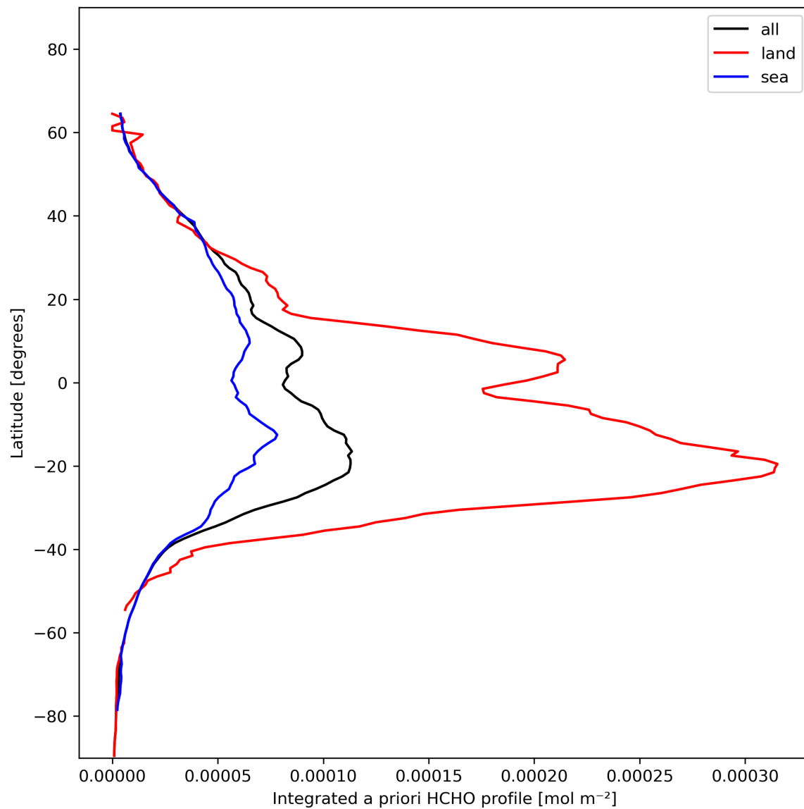
Figure 29: Zonal average of “Integrated a priori HCHO profile” for 2023-11-21 to 2023-11-23.
