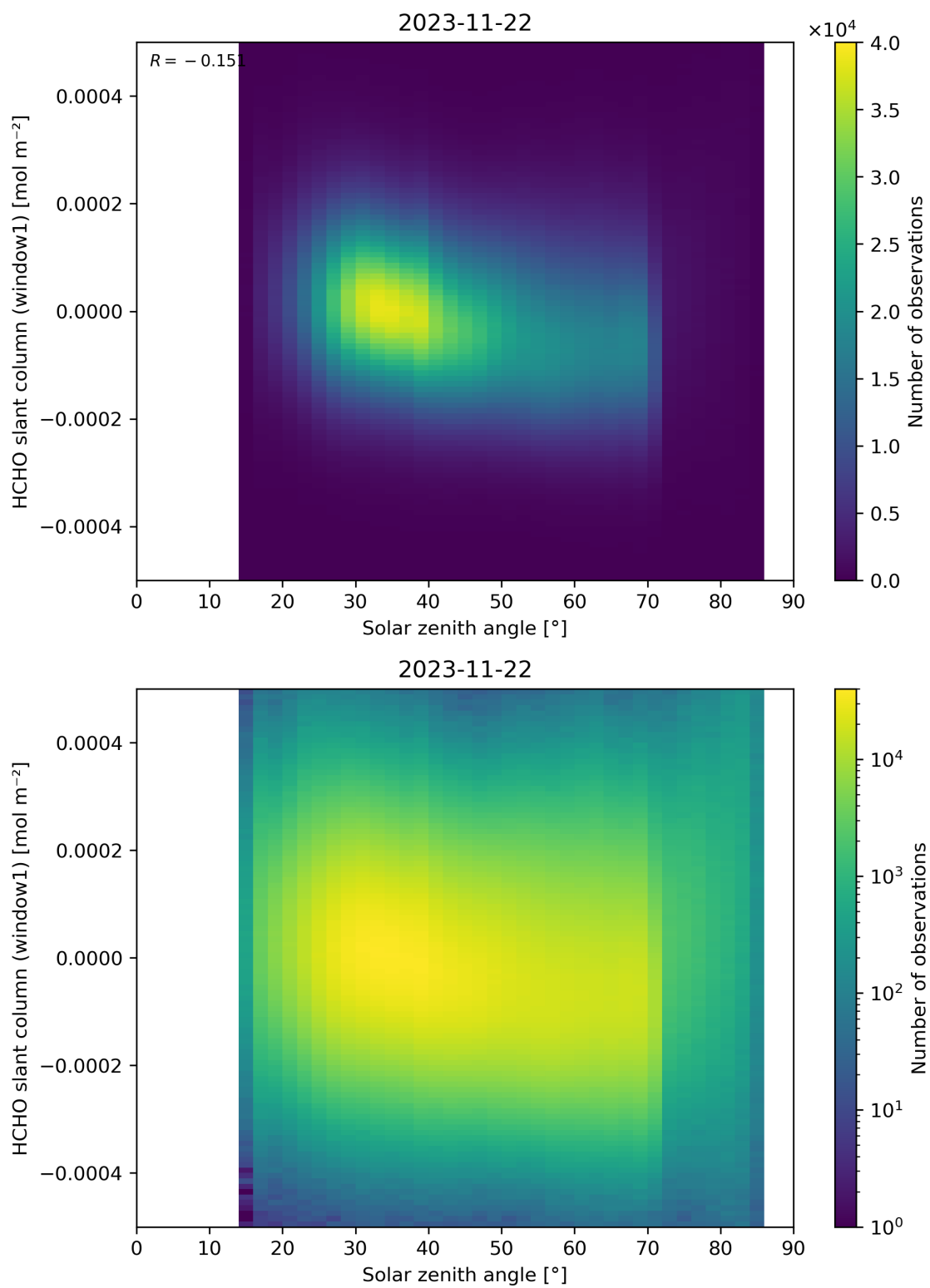
Figure 173: Scatter density plot of “Solar zenith angle” against “HCHO slant column (window1)” for 2023-11-21 to 2023-11-23.
