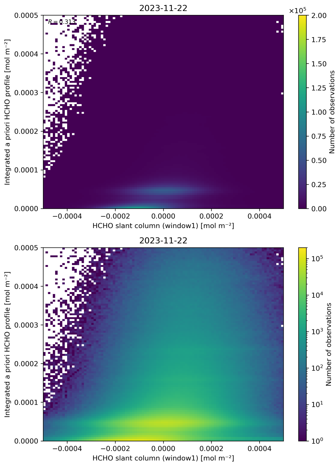
Figure 87: Scatter density plot of “HCHO slant column (window1)” against “Integrated a priori HCHO profile” for 2023-11-21 to 2023-11-23.
