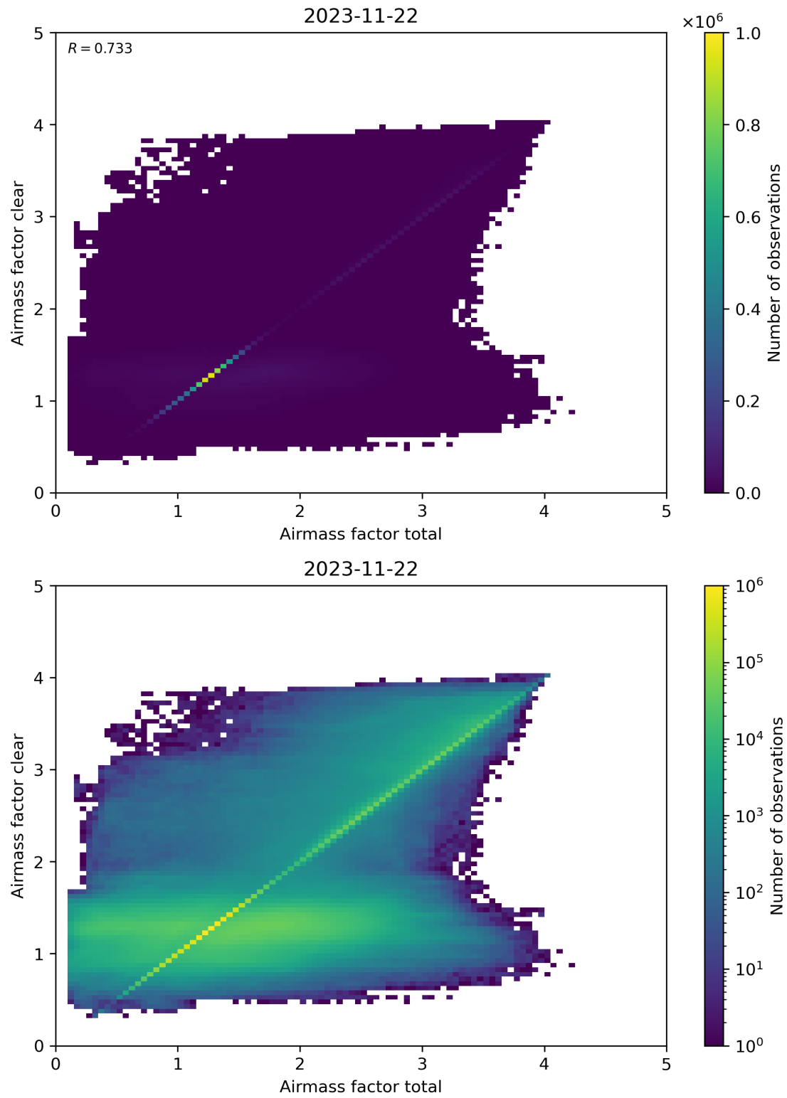
Figure 100: Scatter density plot of “Airmass factor total” against “Airmass factor clear” for 2023-11-21 to 2023-11-23.
