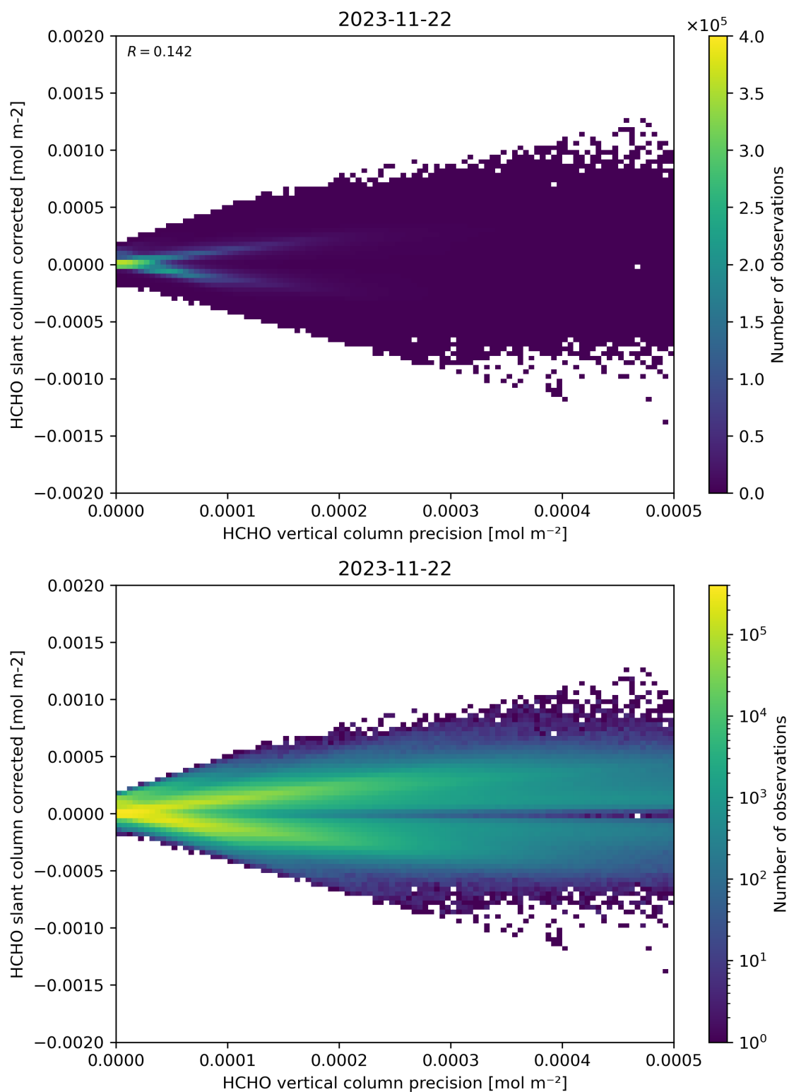
Figure 140: Scatter density plot of “HCHO vertical column precision” against “HCHO slant column corrected” for 2023-11-21 to 2023-11-23.
