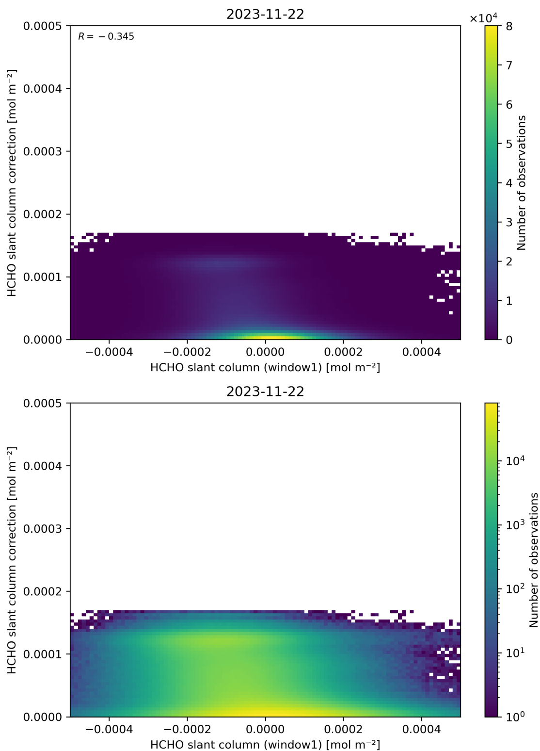
Figure 83: Scatter density plot of “HCHO slant column (window1)” against “HCHO slant column correction” for 2023-11-21 to 2023-11-23.
