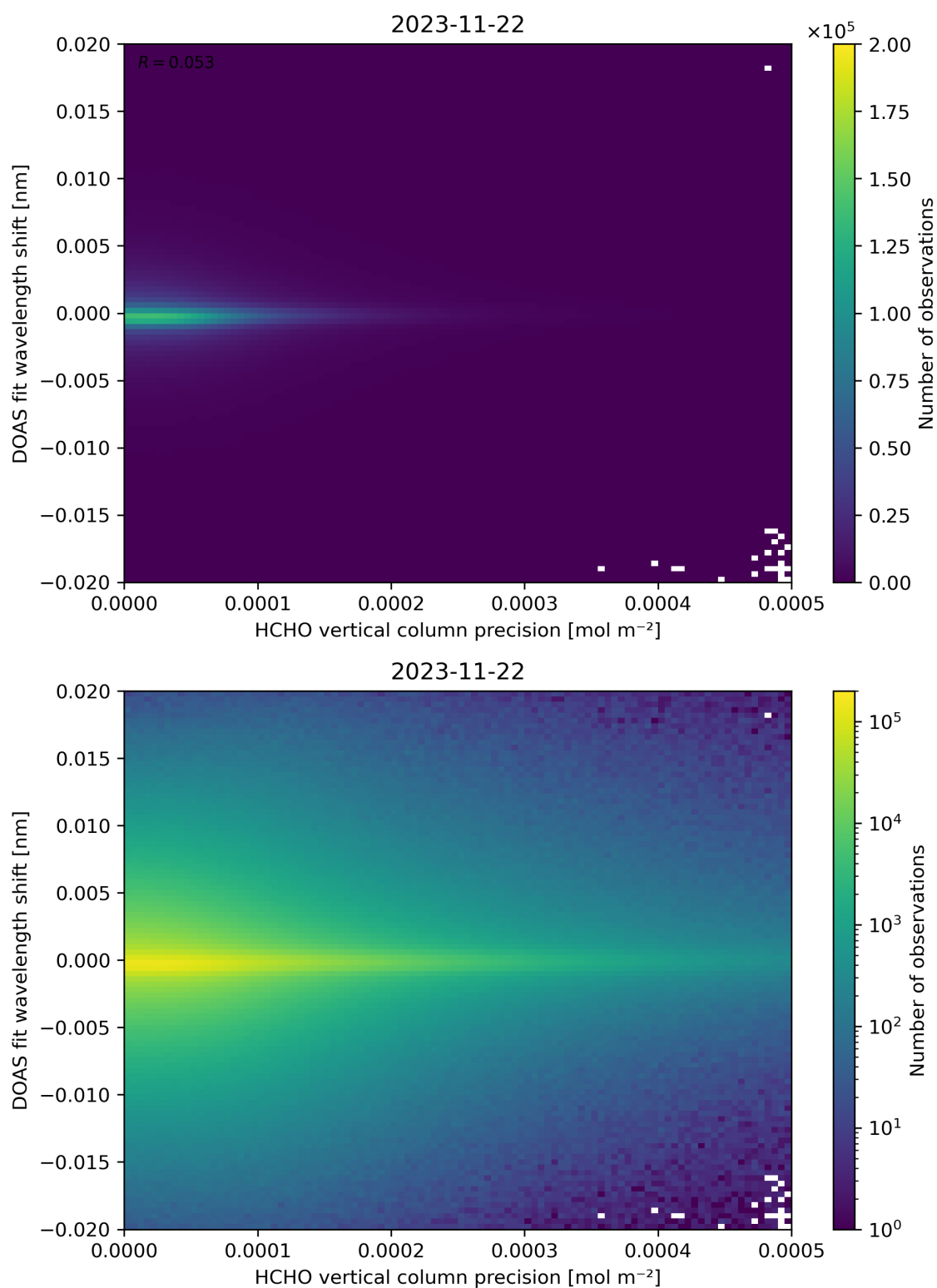
Figure 137: Scatter density plot of “HCHO vertical column precision” against “DOAS fit wavelength shift” for 2023-11-21 to 2023-11-23.
