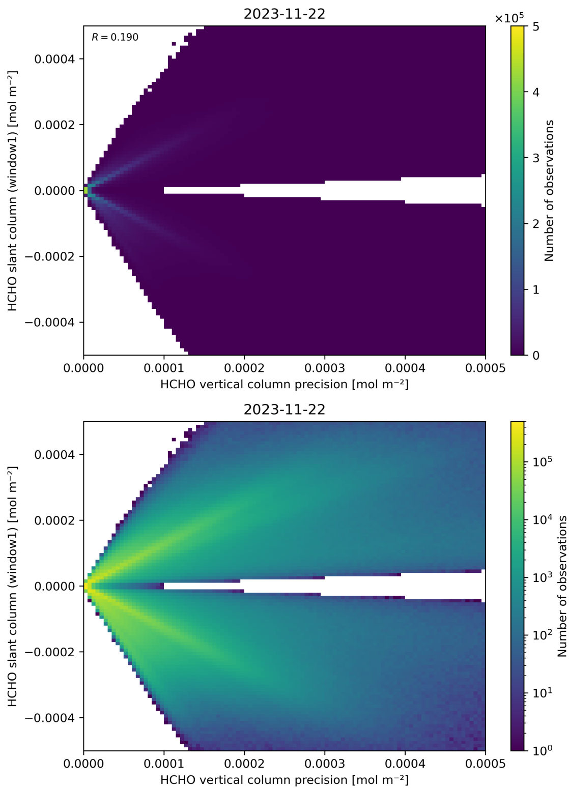
Figure 142: Scatter density plot of “HCHO vertical column precision” against “HCHO slant column (window1)” for 2023-11-21 to 2023-11-23.
