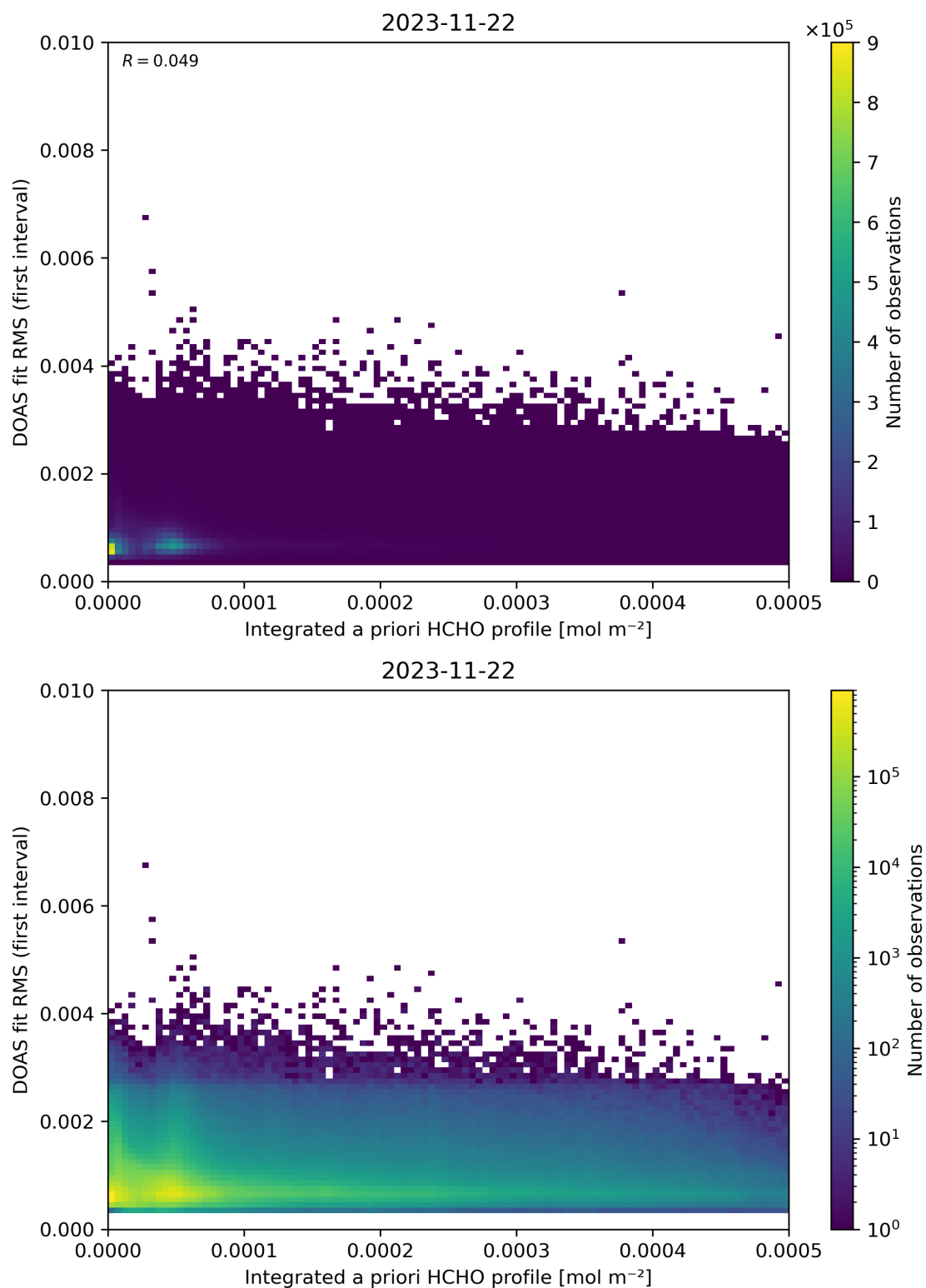
Figure 148: Scatter density plot of “Integrated a priori HCHO profile” against “DOAS fit RMS (first interval)” for 2023-11-21 to 2023-11-23.
