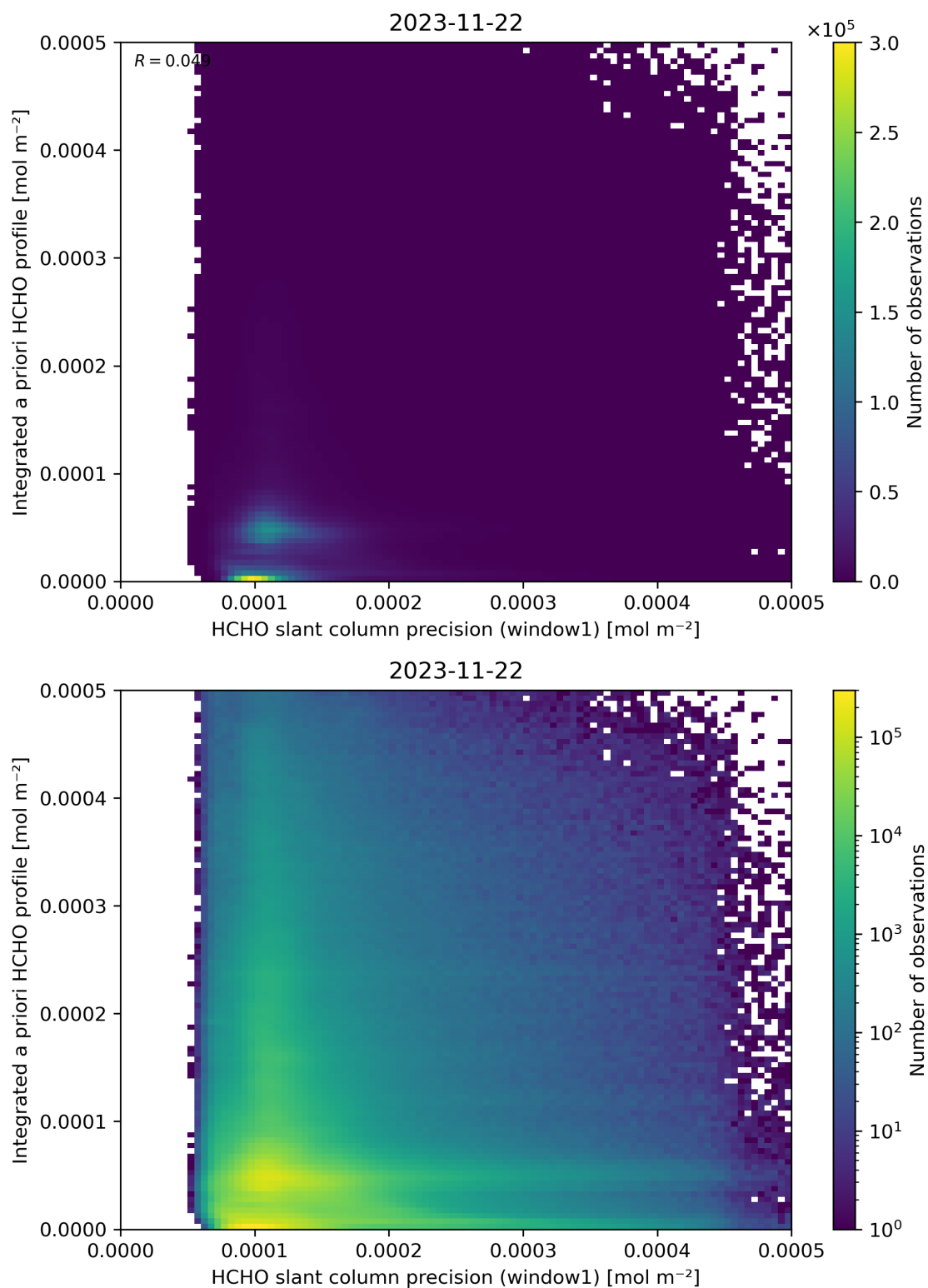
Figure 96: Scatter density plot of “HCHO slant column precision (window1)” against “Integrated a priori HCHO profile” for 2023-11-21 to 2023-11-23.
