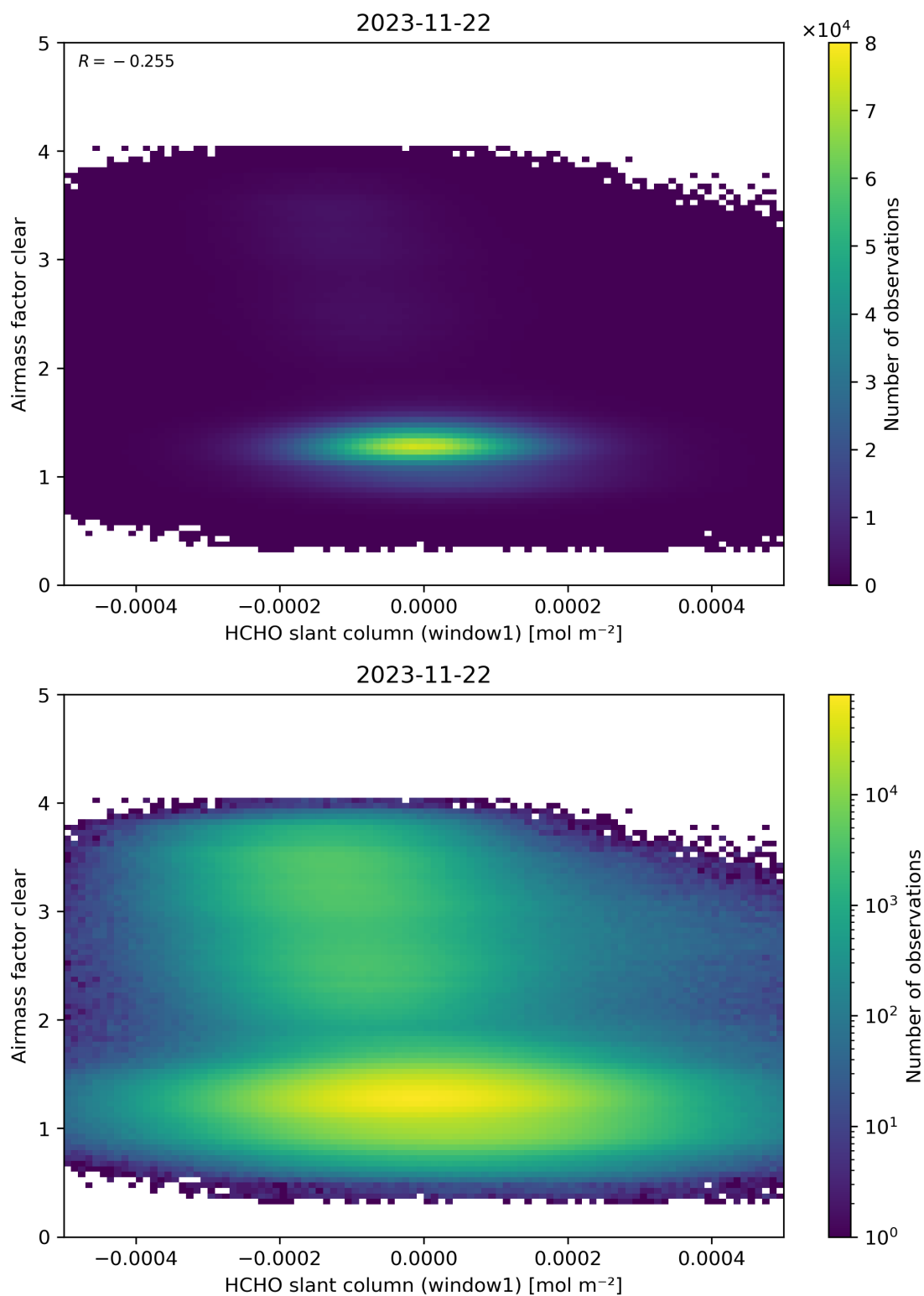
Figure 81: Scatter density plot of “HCHO slant column (window1)” against “Airmass factor clear” for 2023-11-21 to 2023-11-23.
