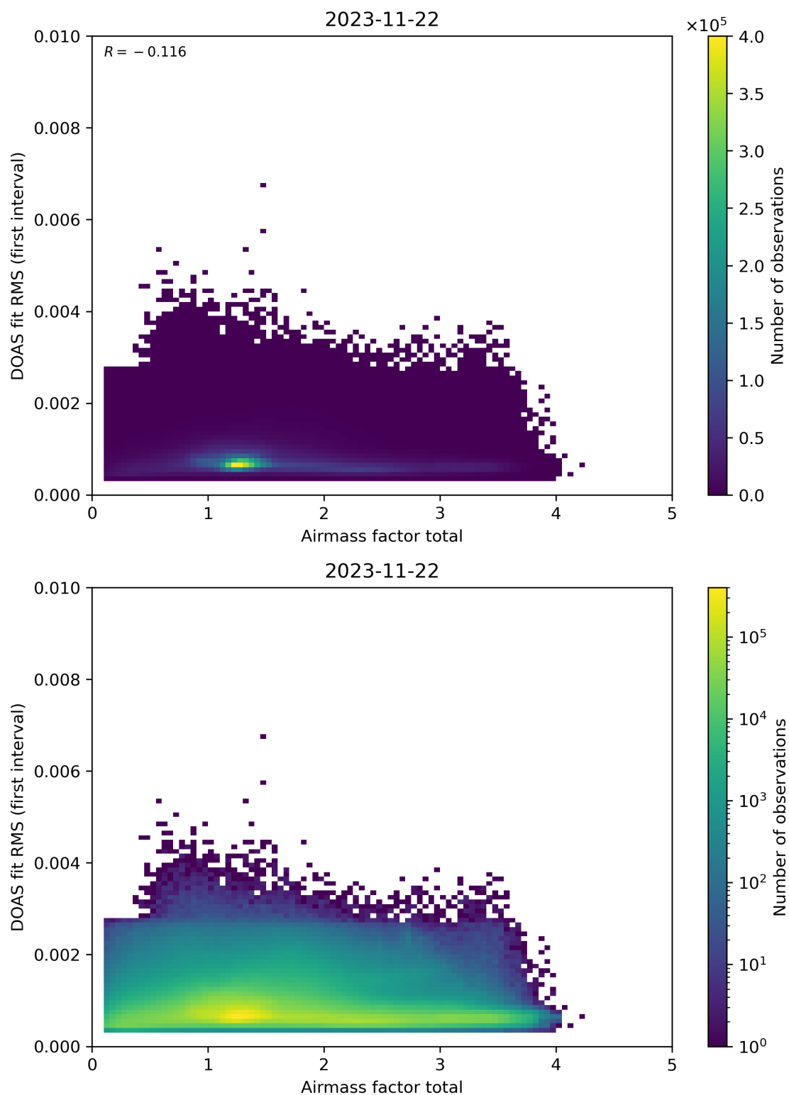
Figure 97: Scatter density plot of “Airmass factor total” against “DOAS fit RMS (first interval)” for 2023-11-21 to 2023-11-23.
