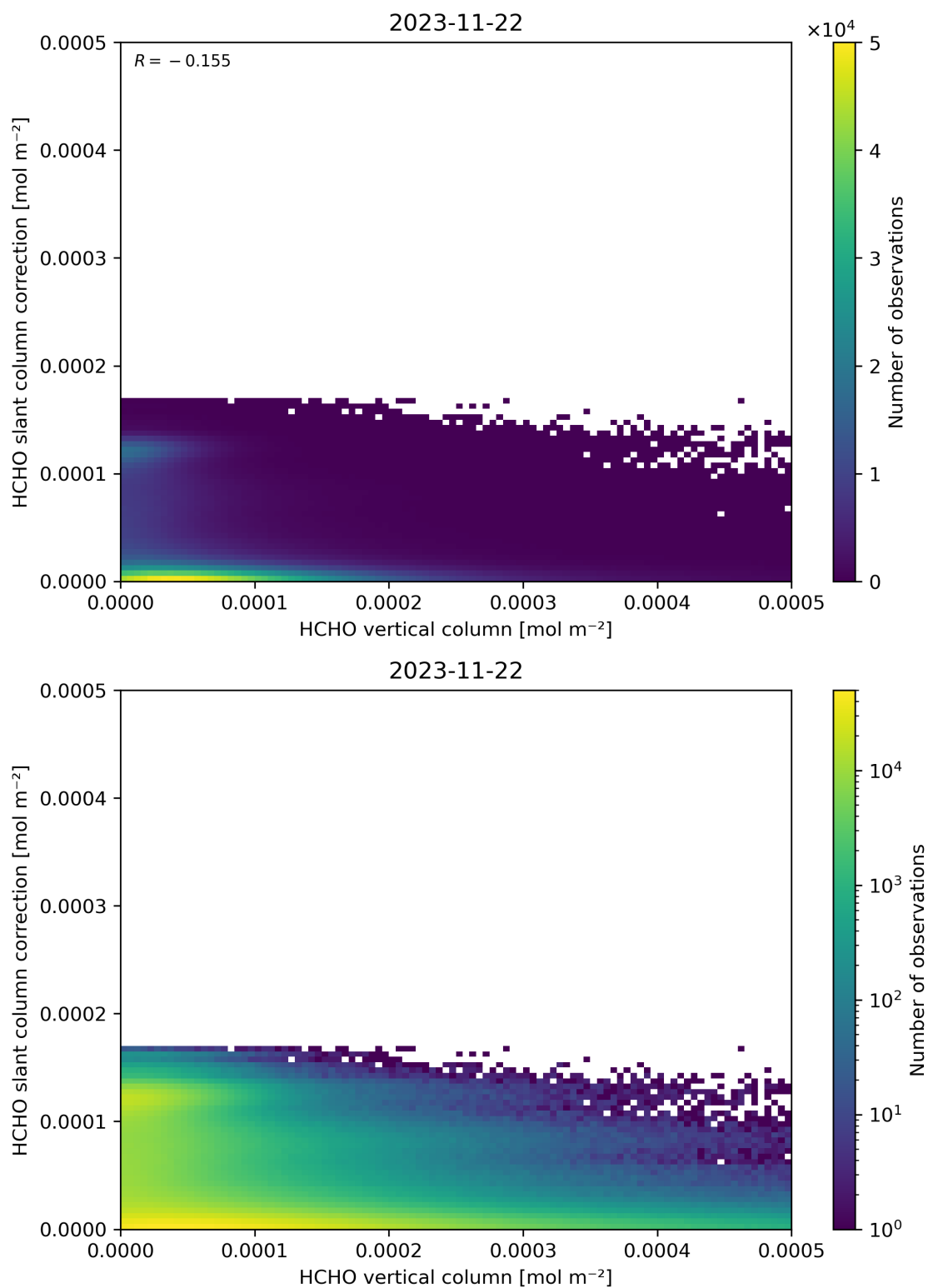
Figure 128: Scatter density plot of “HCHO vertical column” against “HCHO slant column correction” for 2023-11-21 to 2023-11-23.
