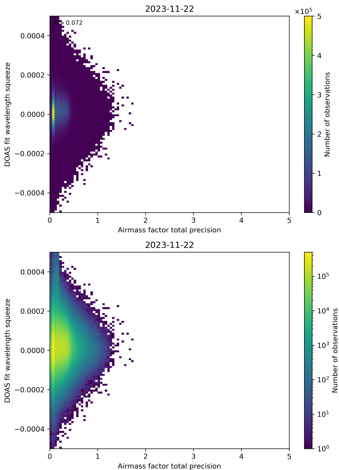
Figure 107: Scatter density plot of “Airmass factor total precision” against “DOAS fit wavelength squeeze” for 2023-11-21 to 2023-11-23.
