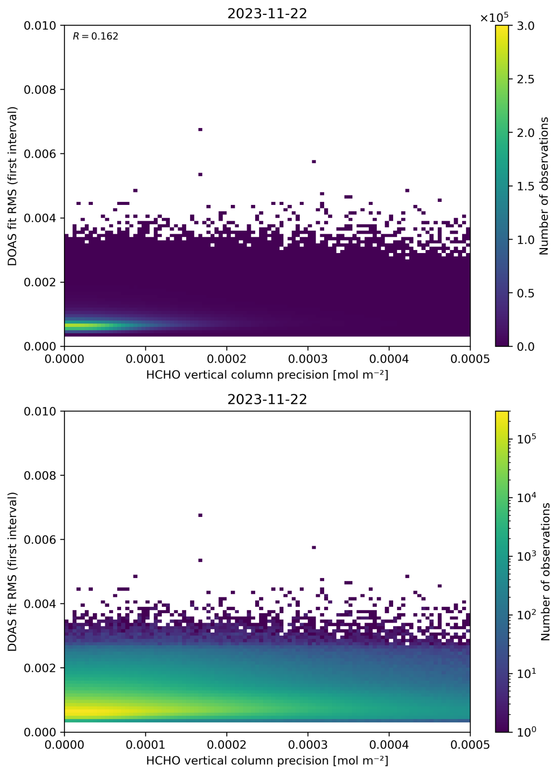
Figure 136: Scatter density plot of “HCHO vertical column precision” against “DOAS fit RMS (first interval)” for 2023-11-21 to 2023-11-23.
