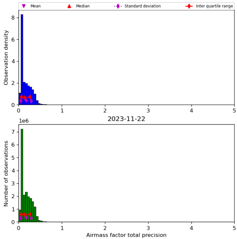
Figure 41: Histogram of “Airmass factor total precision” for 2023-11-21 to 2023-11-23
