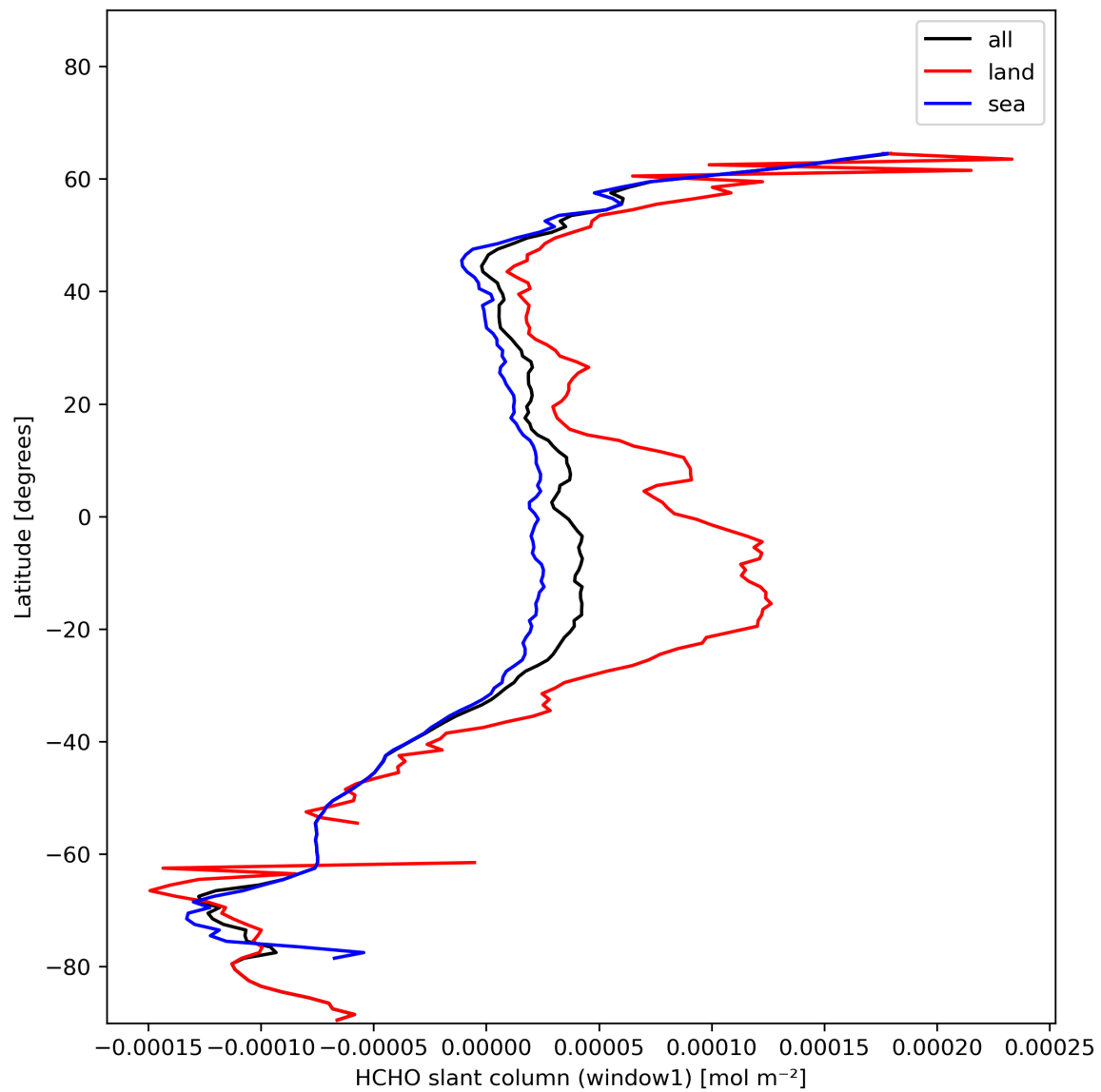
Figure 24: Zonal average of “HCHO slant column (window1)” for 2023-11-21 to 2023-11-23.
