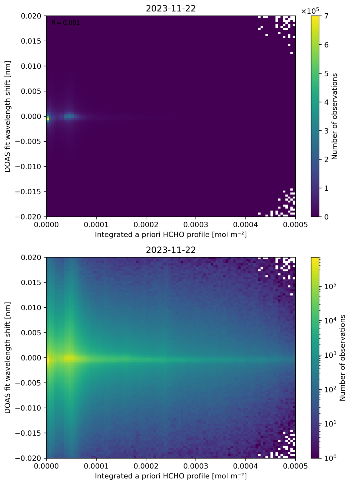
Figure 149: Scatter density plot of “Integrated a priori HCHO profile” against “DOAS fit wavelength shift” for 2023-11-21 to 2023-11-23.
