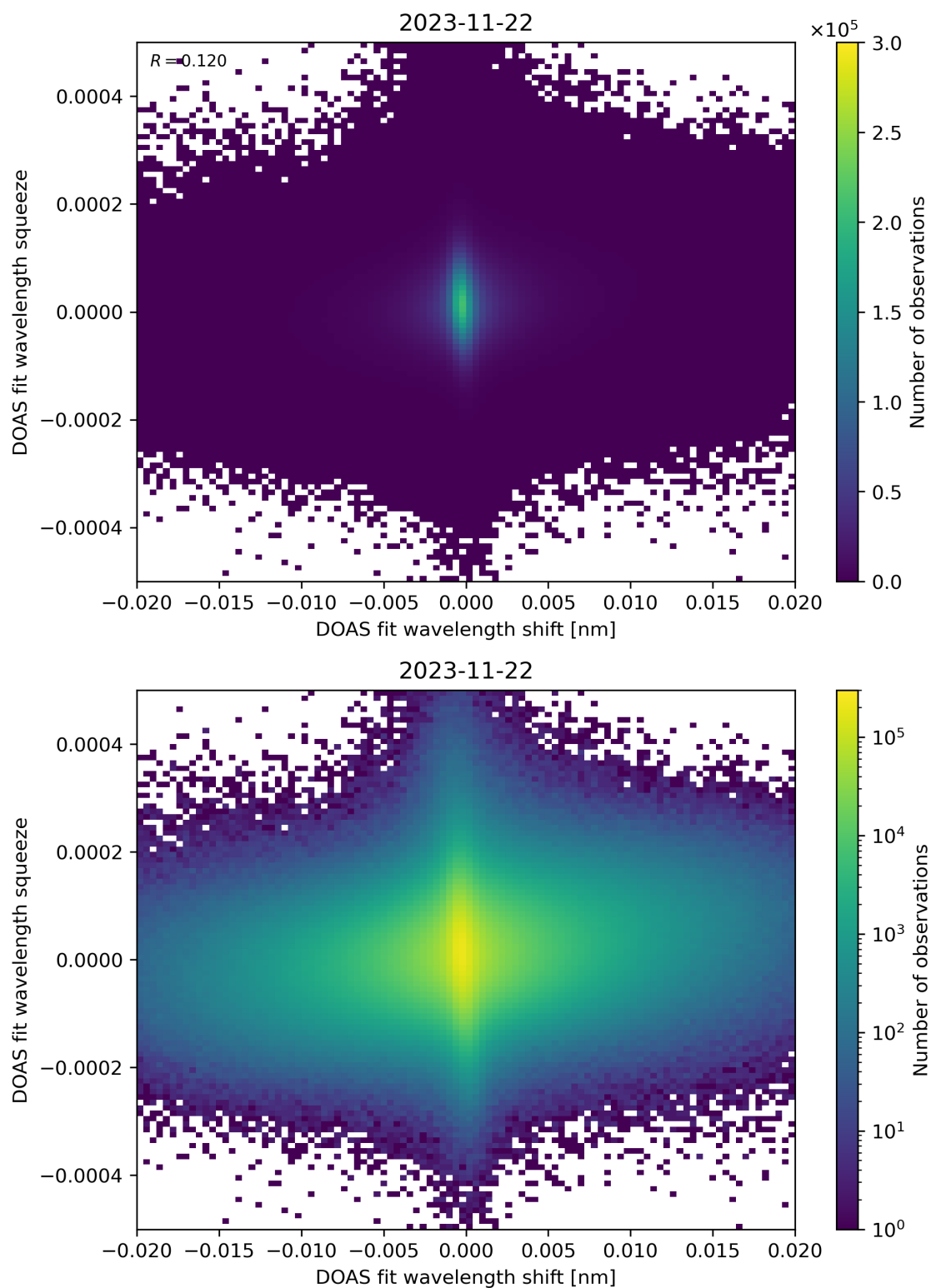
Figure 65: Scatter density plot of “DOAS fit wavelength shift” against “DOAS fit wavelength squeeze” for 2023-11-21 to 2023-11-23.
