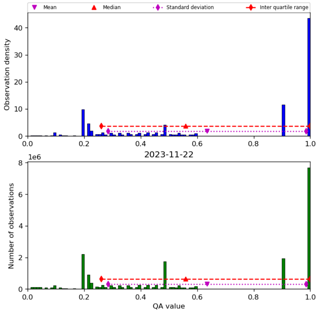
Figure 34: Histogram of “QA value” for 2023-11-21 to 2023-11-23
