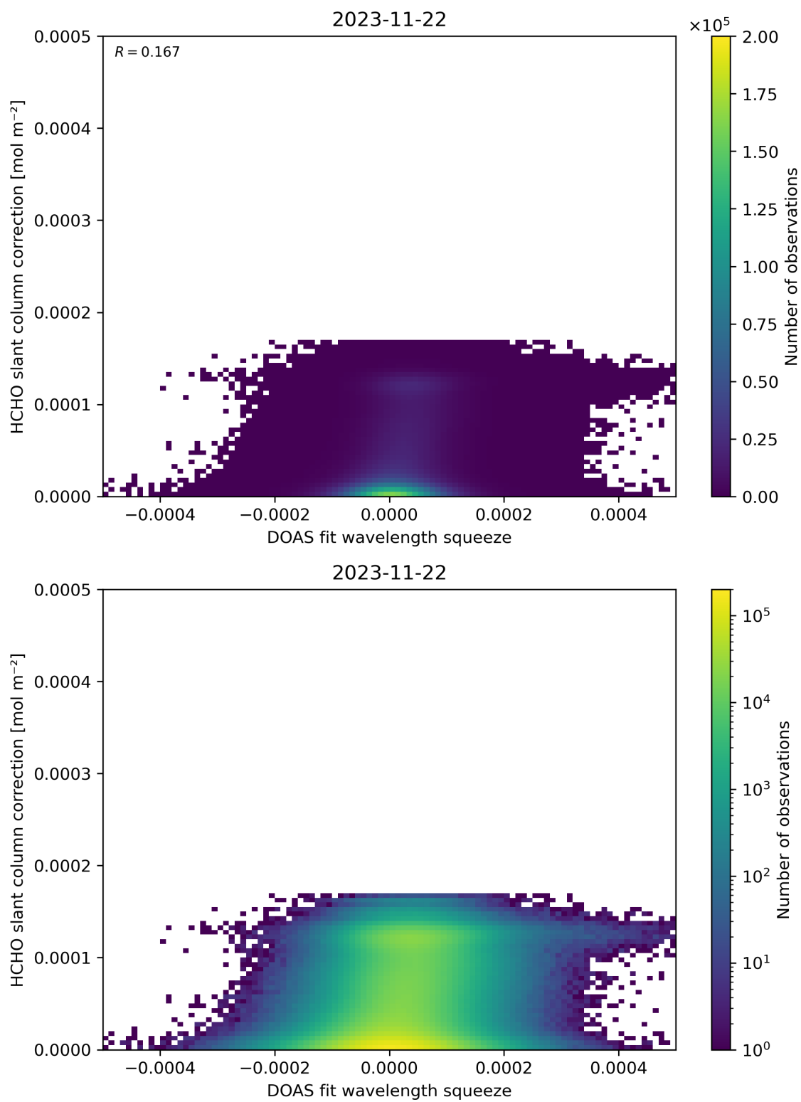
Figure 70: Scatter density plot of “DOAS fit wavelength squeeze” against “HCHO slant column correction” for 2023-11-21 to 2023-11-23.
