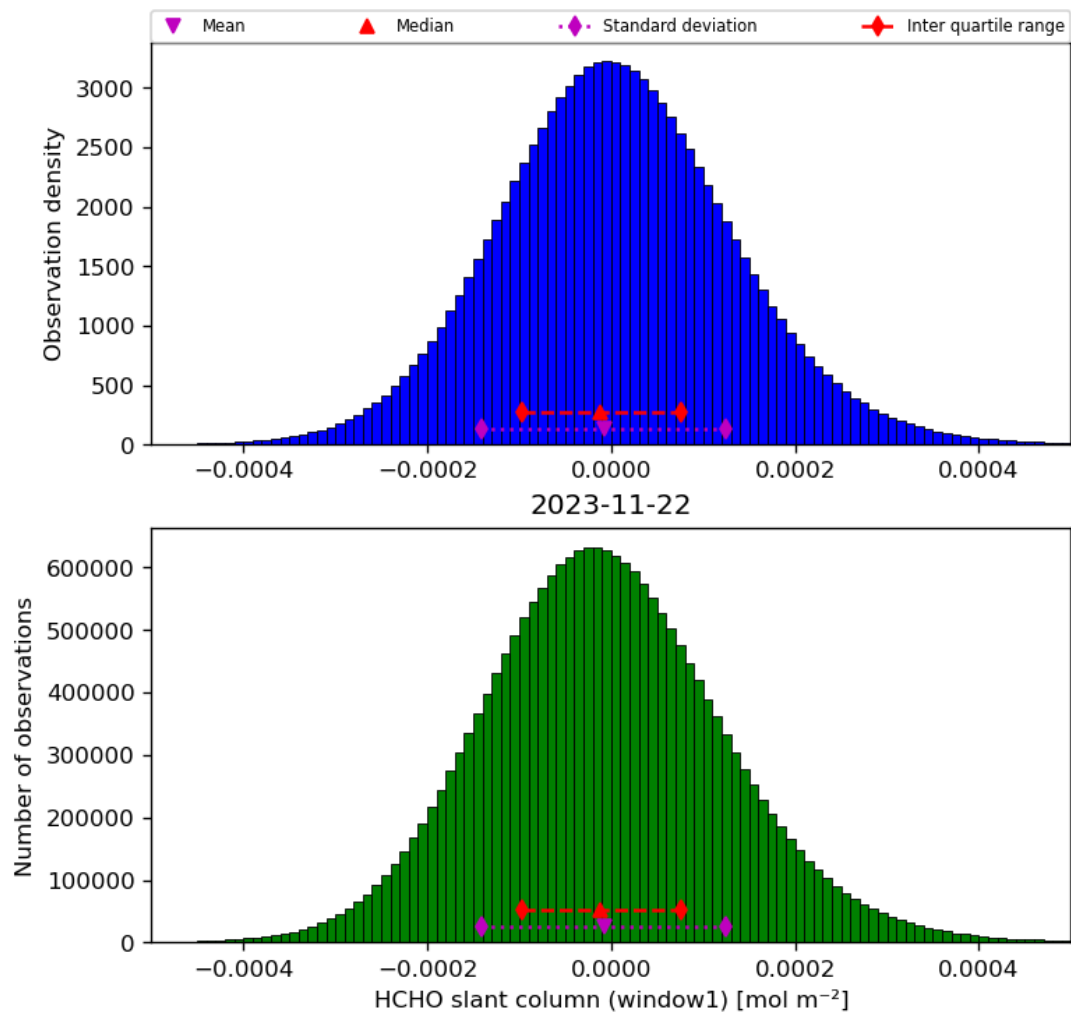
Figure 38: Histogram of “HCHO slant column (window1)” for 2023-11-21 to 2023-11-23
