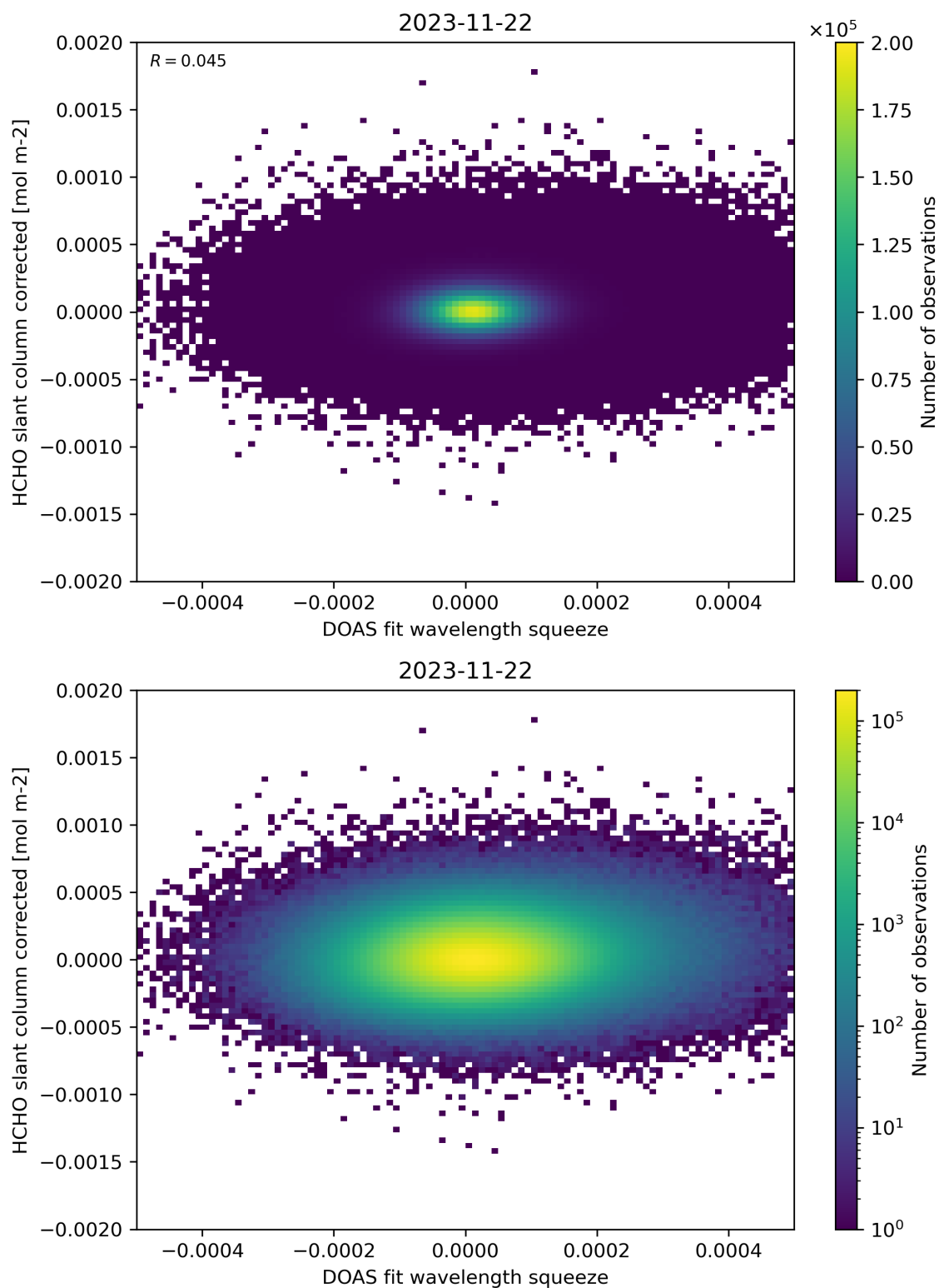
Figure 69: Scatter density plot of “DOAS fit wavelength squeeze” against “HCHO slant column corrected” for 2023-11-21 to 2023-11-23.
