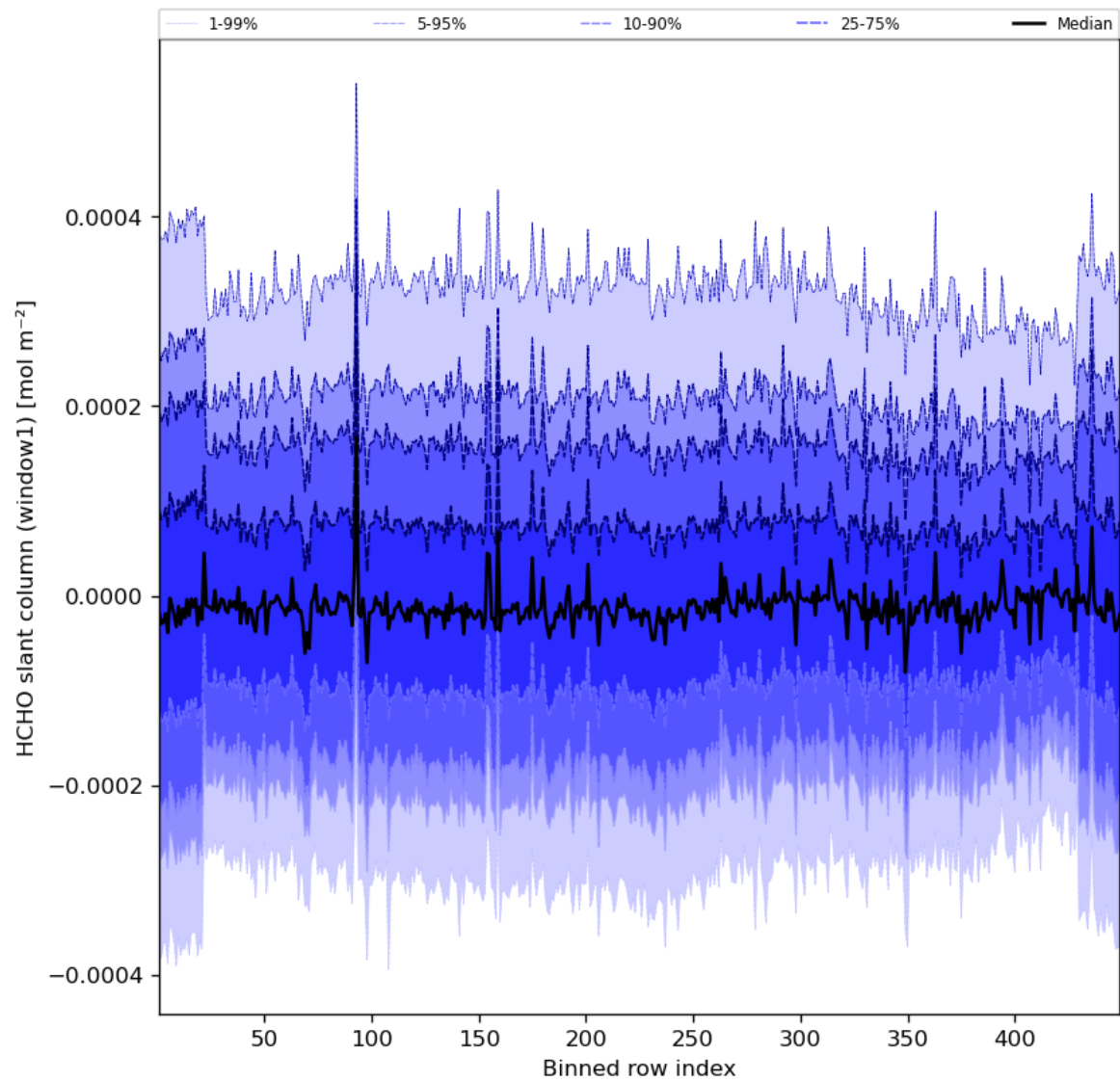
Figure 52: Along track statistics of “HCHO slant column (window1)” for 2023-11-21 to 2023-11-23
