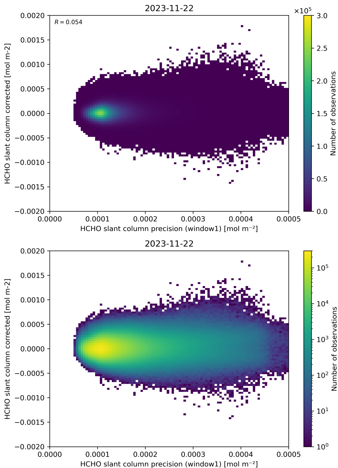
Figure 92: Scatter density plot of “HCHO slant column precision (window1)” against “HCHO slant column corrected” for 2023-11-21 to 2023-11-23.
