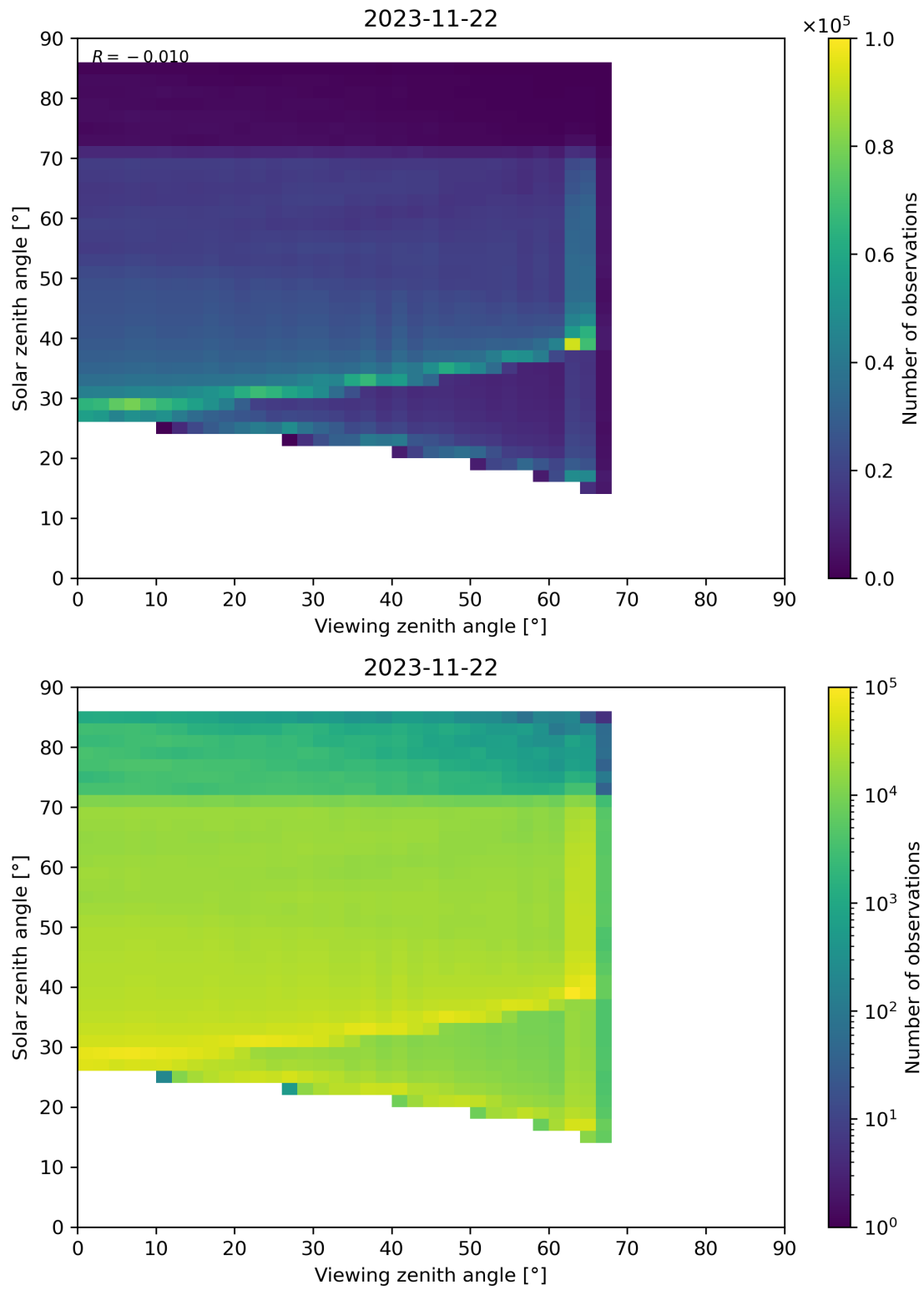
Figure 197: Scatter density plot of “Viewing zenith angle” against “Solar zenith angle” for 2023-11-21 to 2023-11-23.
