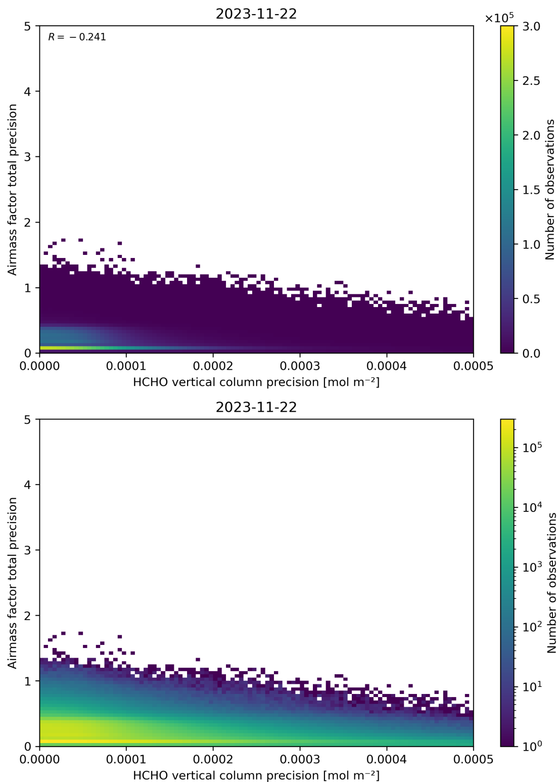
Figure 145: Scatter density plot of “HCHO vertical column precision” against “Airmass factor total precision” for 2023-11-21 to 2023-11-23.
