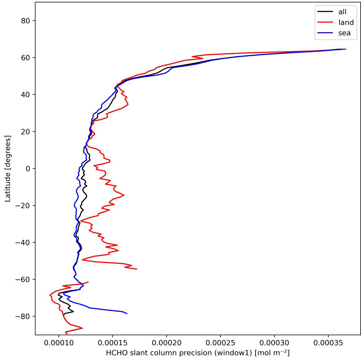
Figure 25: Zonal average of “HCHO slant column precision (window1)” for 2023-11-21 to 2023-11-23.
