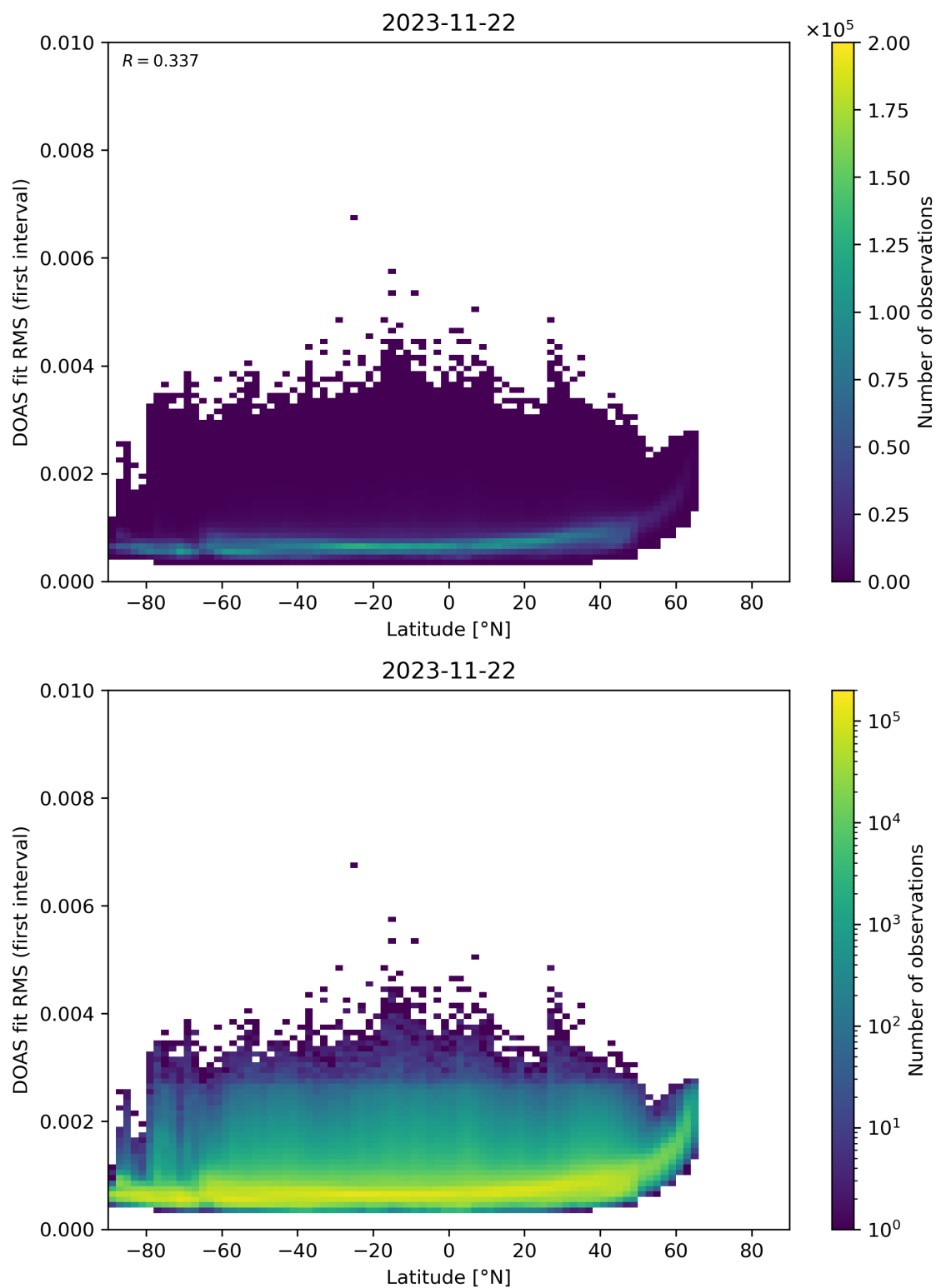
Figure 153: Scatter density plot of “Latitude” against “DOAS fit RMS (first interval)” for 2023-11-21 to 2023-11-23.
