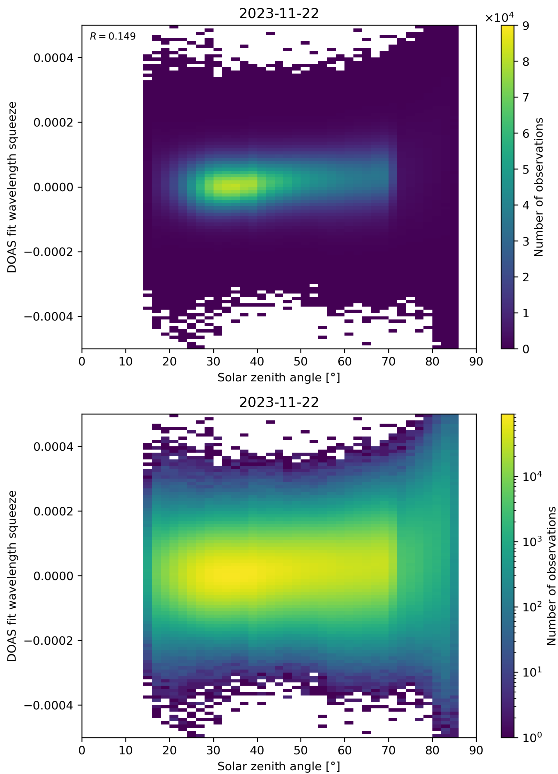
Figure 169: Scatter density plot of “Solar zenith angle” against “DOAS fit wavelength squeeze” for 2023-11-21 to 2023-11-23.
