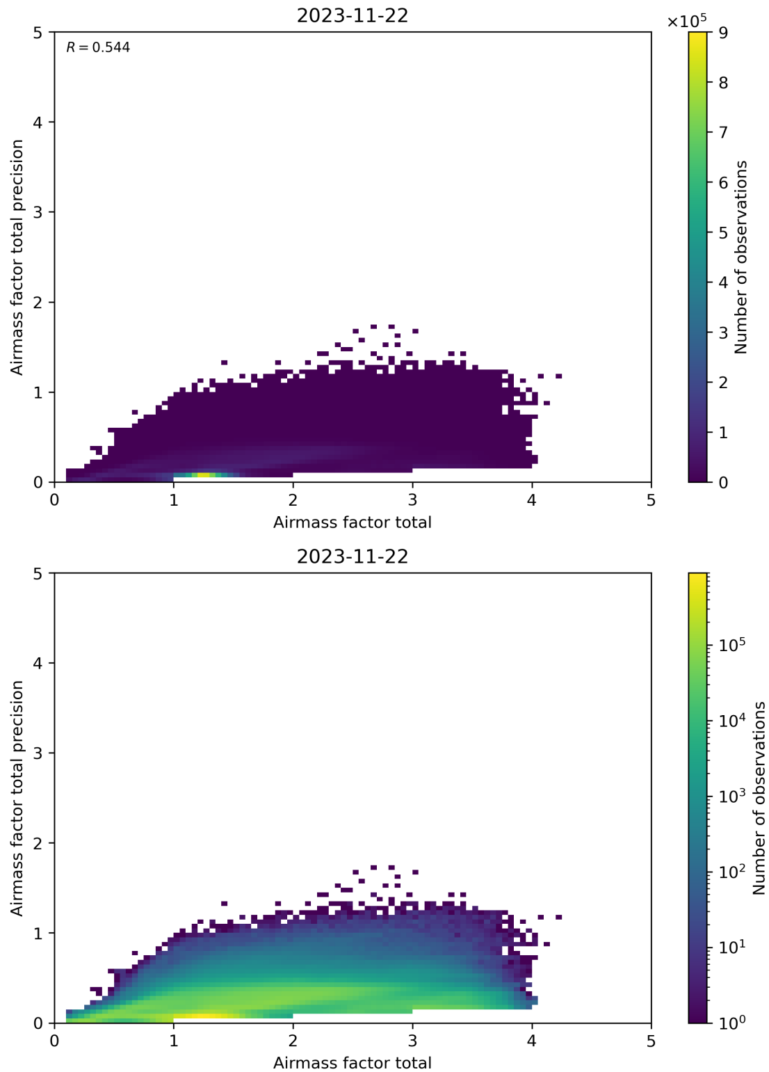
Figure 103: Scatter density plot of “Airmass factor total” against “Airmass factor total precision” for 2023-11-21 to 2023-11-23.
