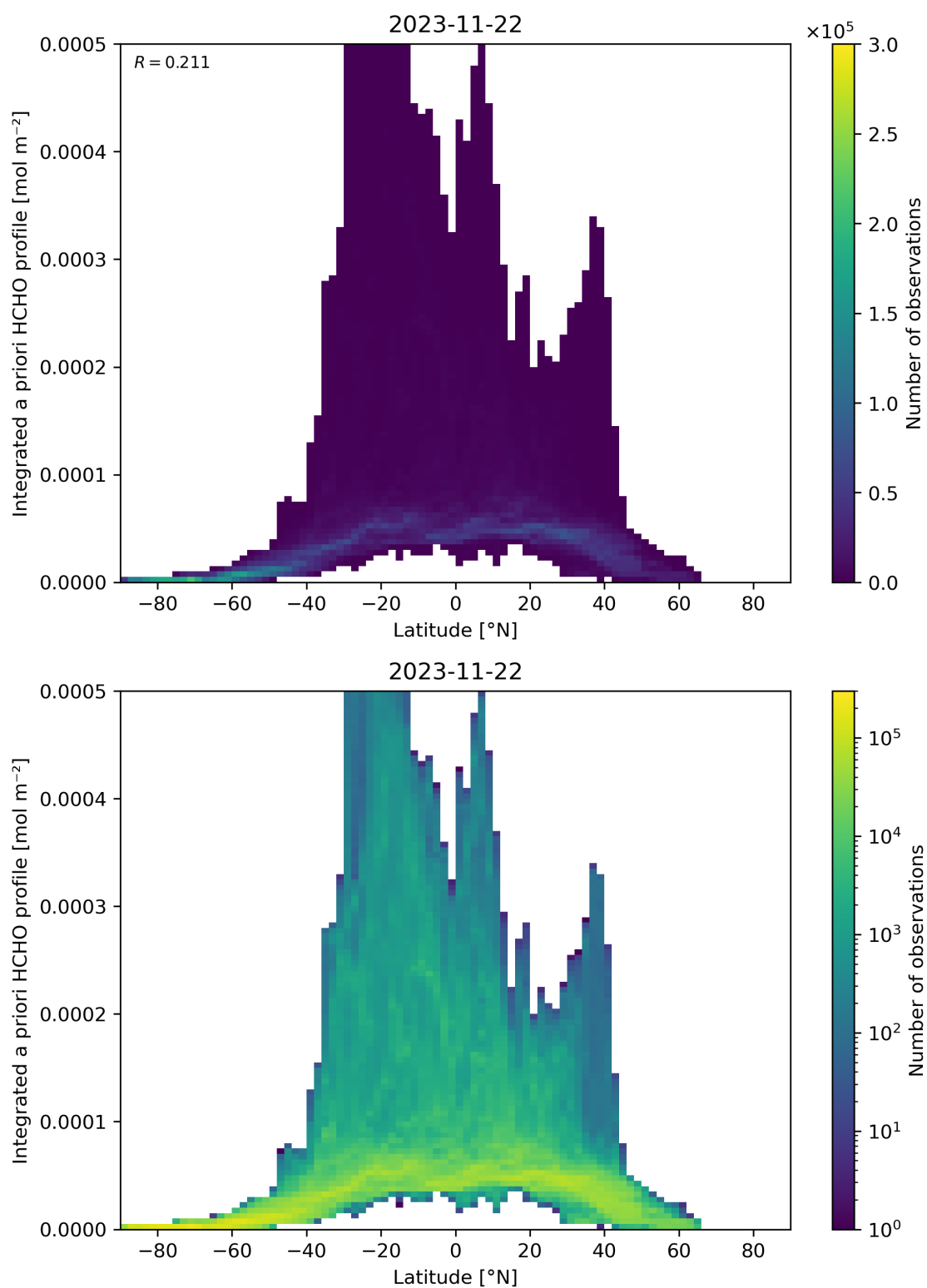
Figure 166: Scatter density plot of “Latitude” against “Integrated a priori HCHO profile” for 2023-11-21 to 2023-11-23.
