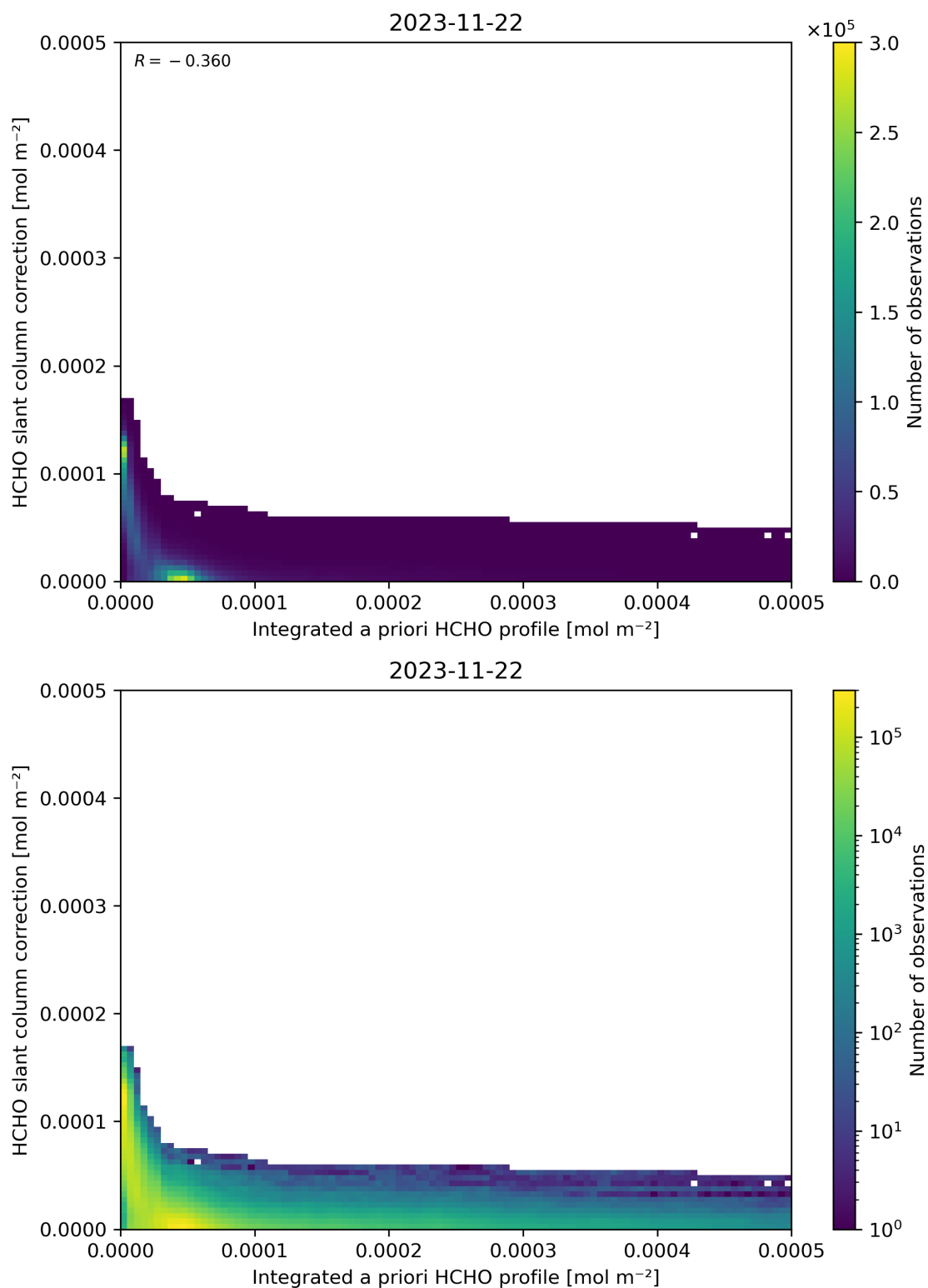
Figure 152: Scatter density plot of “Integrated a priori HCHO profile” against “HCHO slant column correction” for 2023-11-21 to 2023-11-23.
