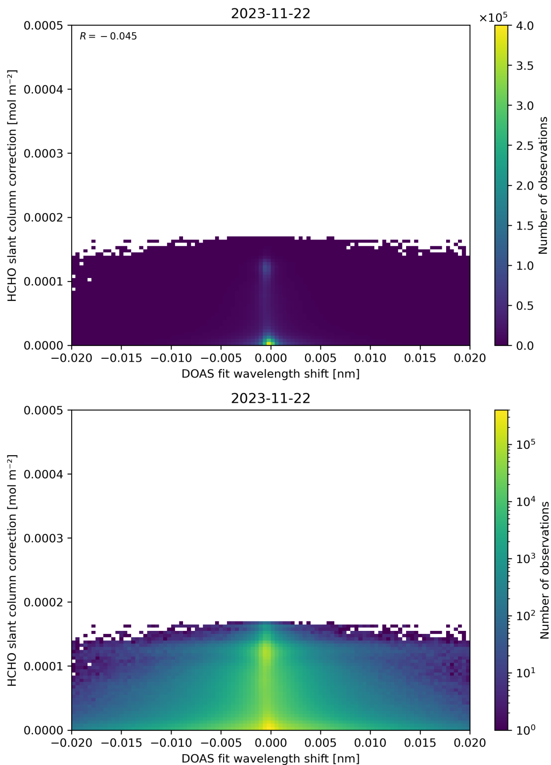
Figure 67: Scatter density plot of “DOAS fit wavelength shift” against “HCHO slant column correction” for 2023-11-21 to 2023-11-23.
