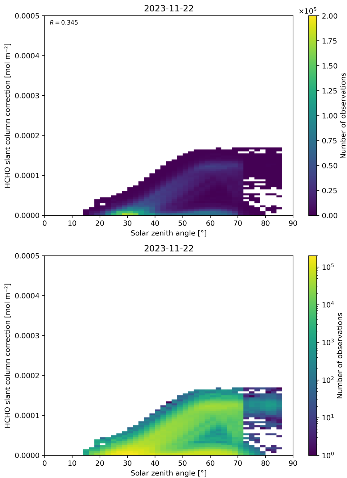
Figure 172: Scatter density plot of “Solar zenith angle” against “HCHO slant column correction” for 2023-11-21 to 2023-11-23.
