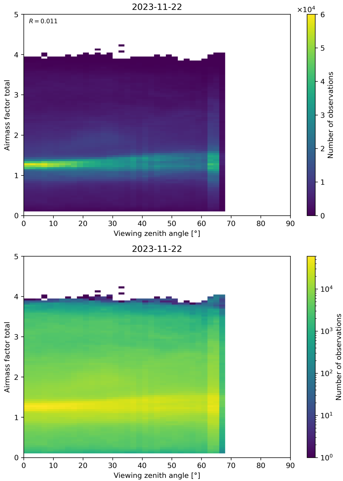
Figure 190: Scatter density plot of “Viewing zenith angle” against “Airmass factor total” for 2023-11-21 to 2023-11-23.
