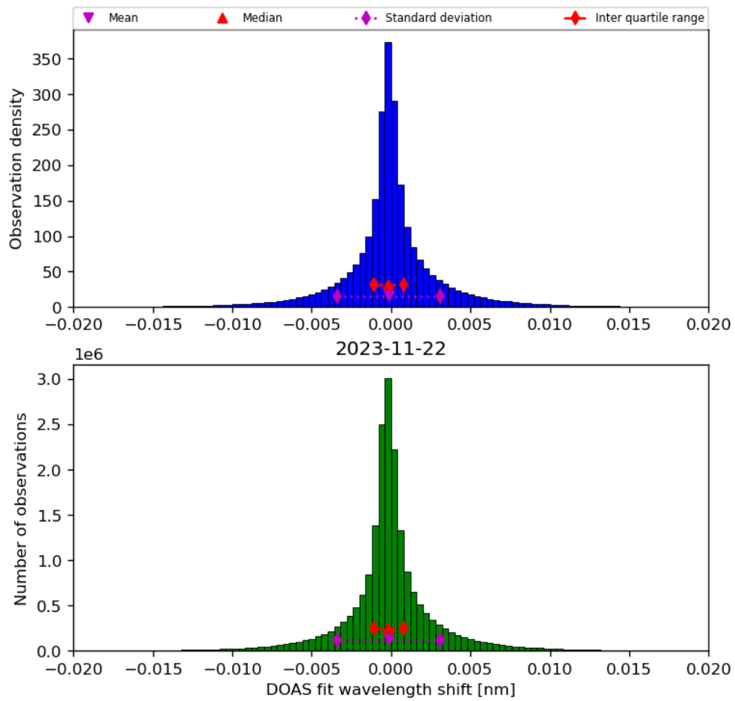
Figure 44: Histogram of “DOAS fit wavelength shift” for 2023-11-21 to 2023-11-23
