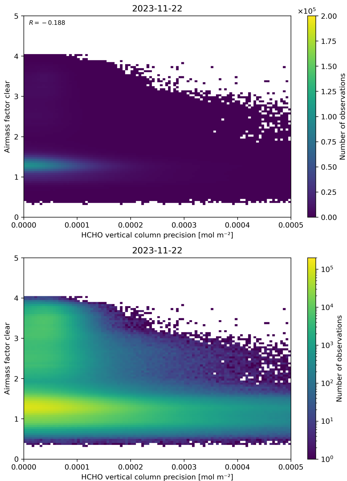
Figure 139: Scatter density plot of “HCHO vertical column precision” against “Airmass factor clear” for 2023-11-21 to 2023-11-23.
