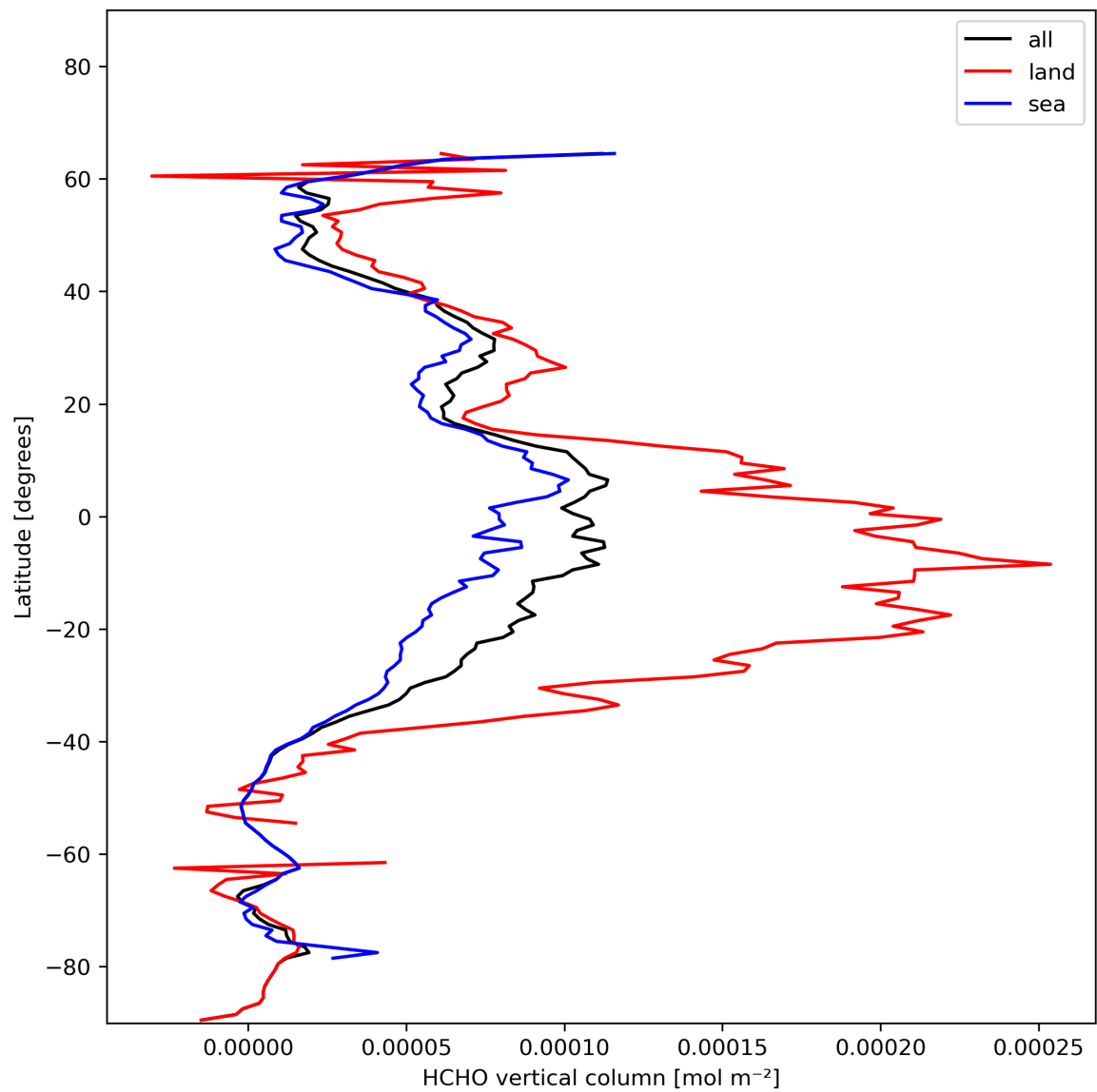
Figure 21: Zonal average of “HCHO vertical column” for 2023-11-21 to 2023-11-23.
