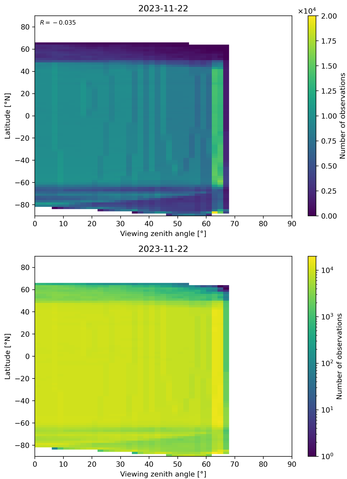
Figure 196: Scatter density plot of “Viewing zenith angle” against “Latitude” for 2023-11-21 to 2023-11-23.
