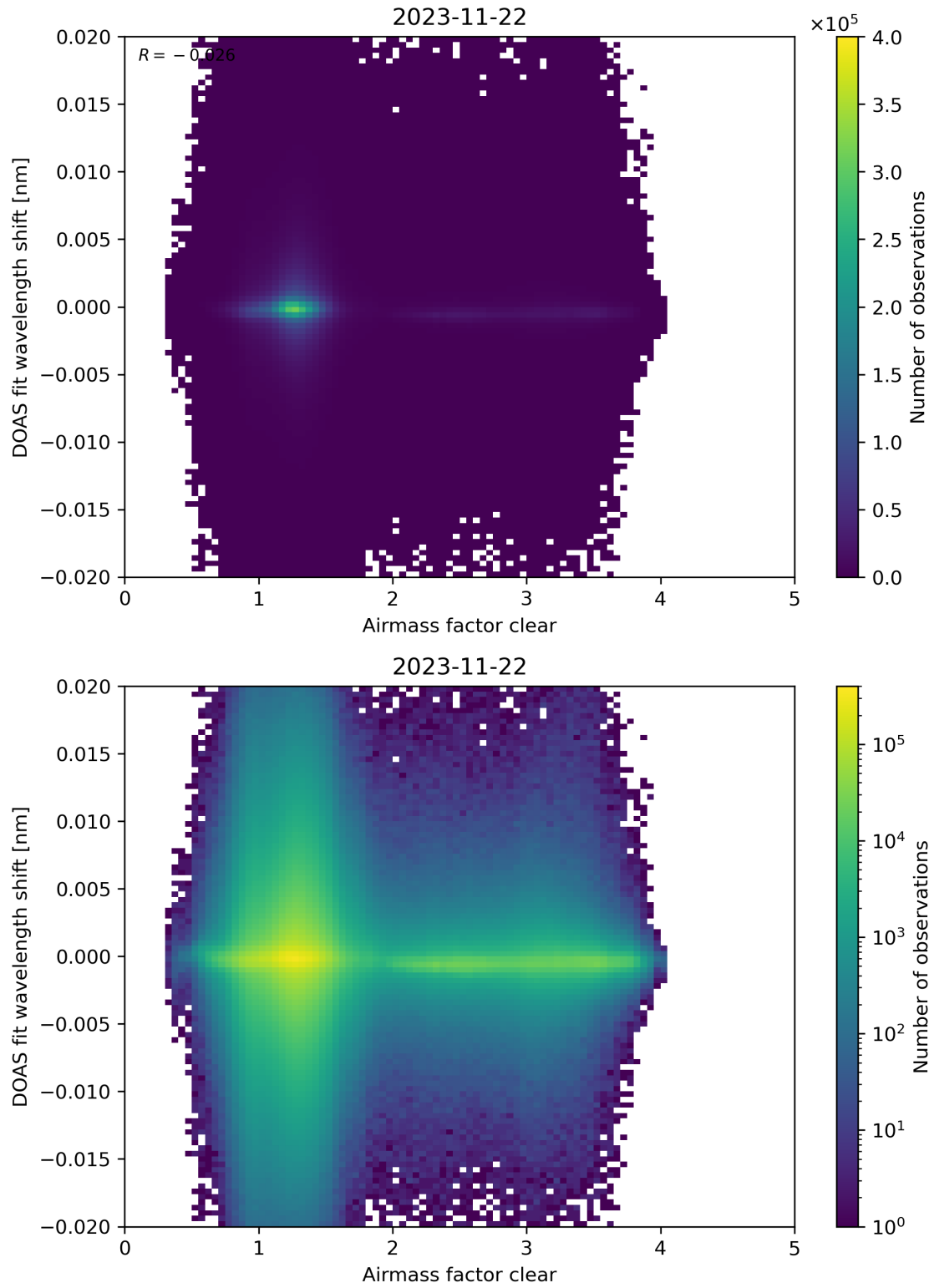
Figure 72: Scatter density plot of “Airmass factor clear” against “DOAS fit wavelength shift” for 2023-11-21 to 2023-11-23.
