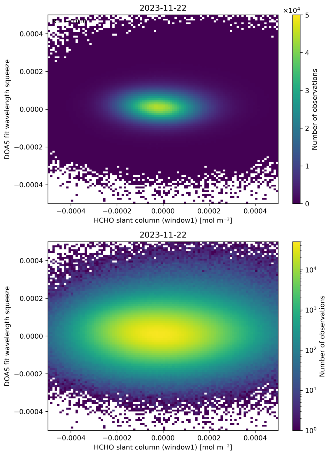
Figure 80: Scatter density plot of “HCHO slant column (window1)” against “DOAS fit wavelength squeeze” for 2023-11-21 to 2023-11-23.
