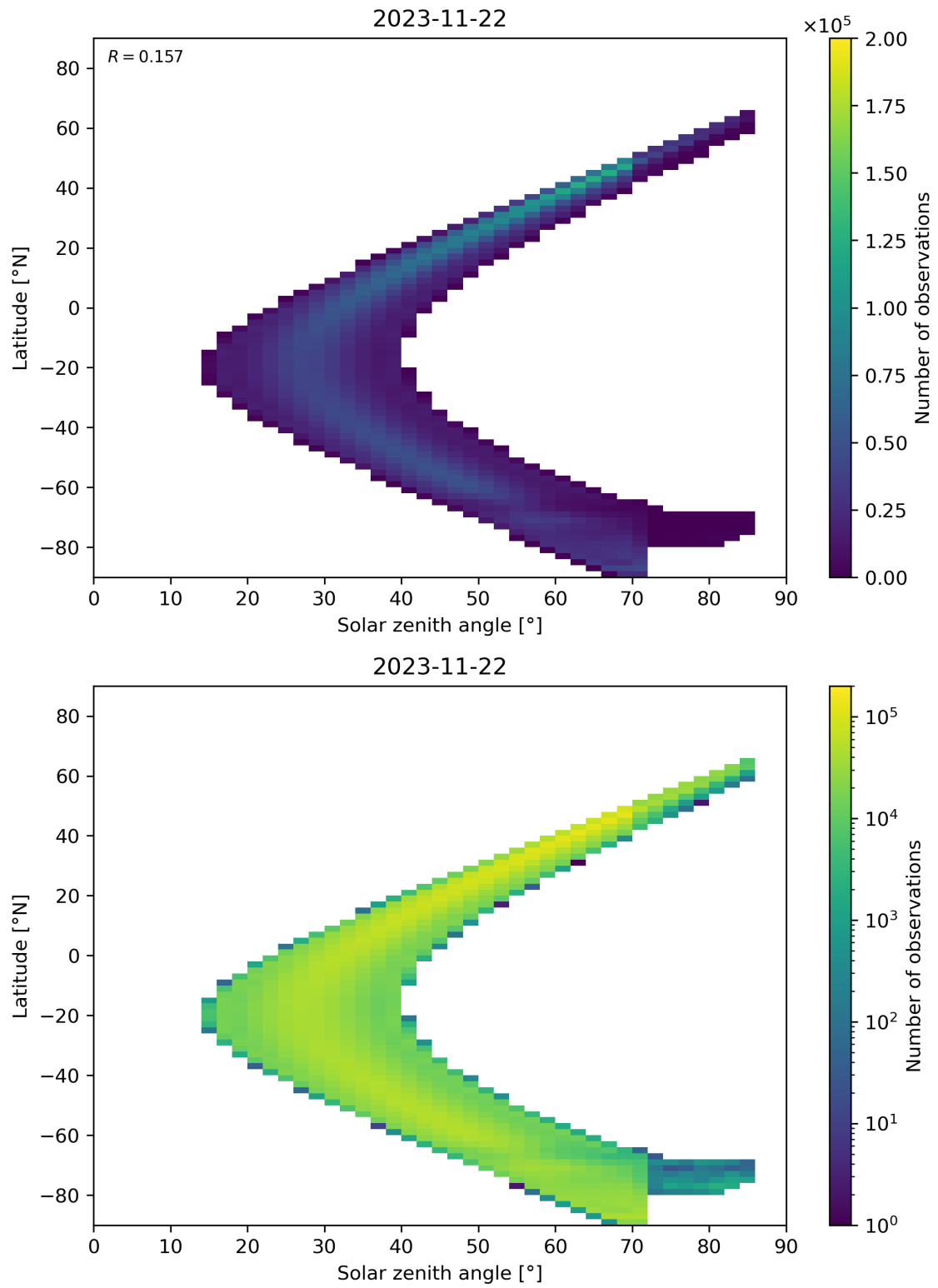
Figure 181: Scatter density plot of “Solar zenith angle” against “Latitude” for 2023-11-21 to 2023-11-23.
