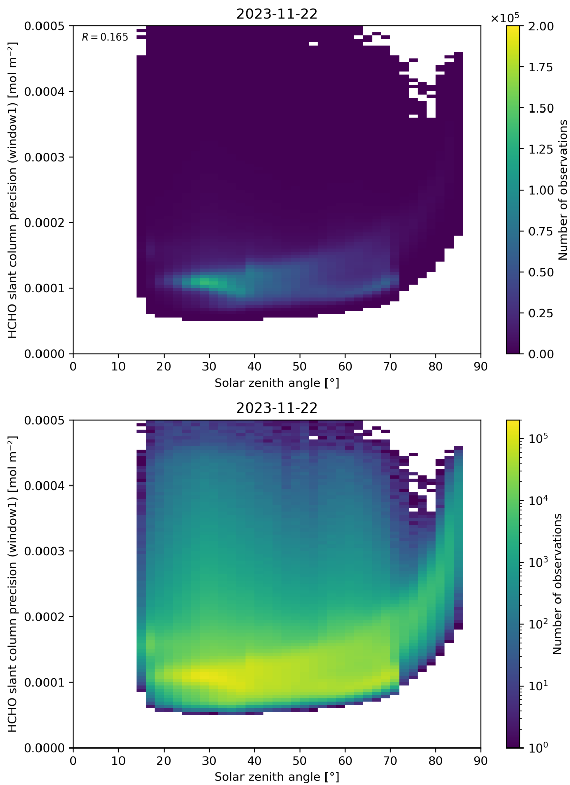
Figure 174: Scatter density plot of “Solar zenith angle” against “HCHO slant column precision (window1)” for 2023-11-21 to 2023-11-23.
