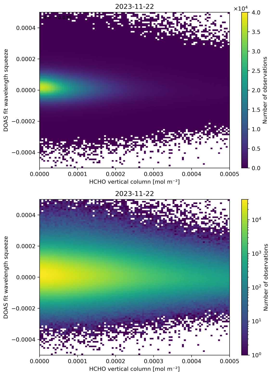
Figure 125: Scatter density plot of “HCHO vertical column” against “DOAS fit wavelength squeeze” for 2023-11-21 to 2023-11-23.
