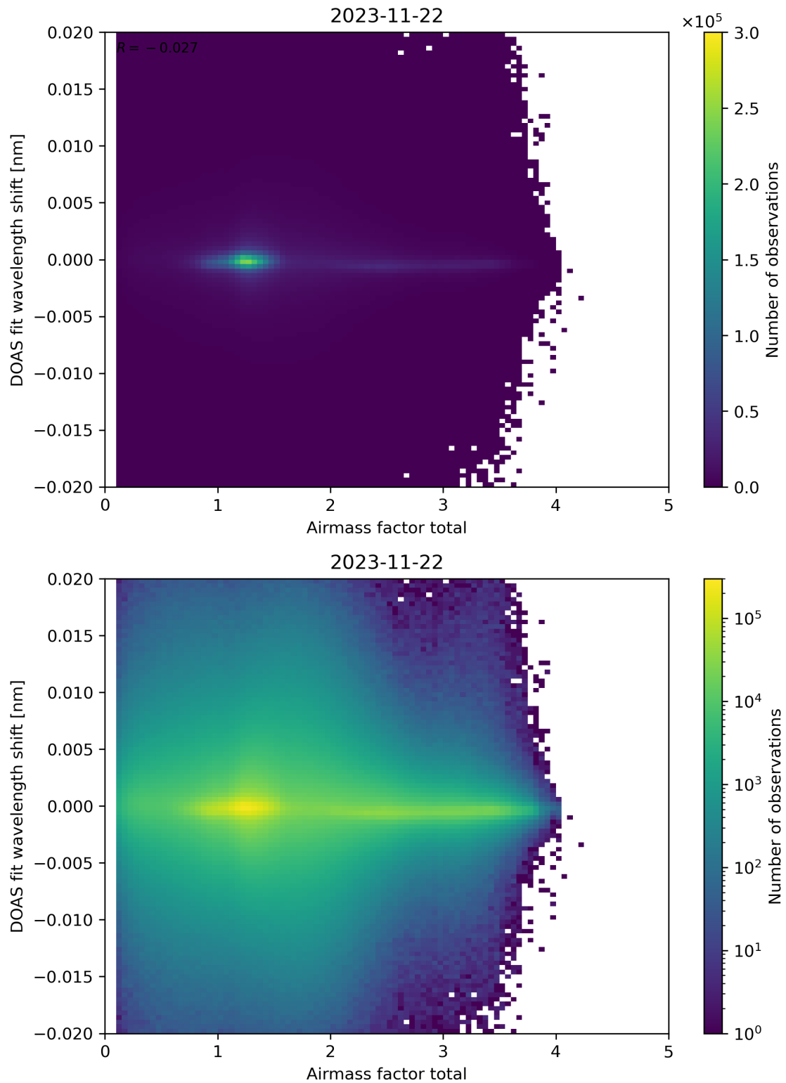
Figure 98: Scatter density plot of “Airmass factor total” against “DOAS fit wavelength shift” for 2023-11-21 to 2023-11-23.
