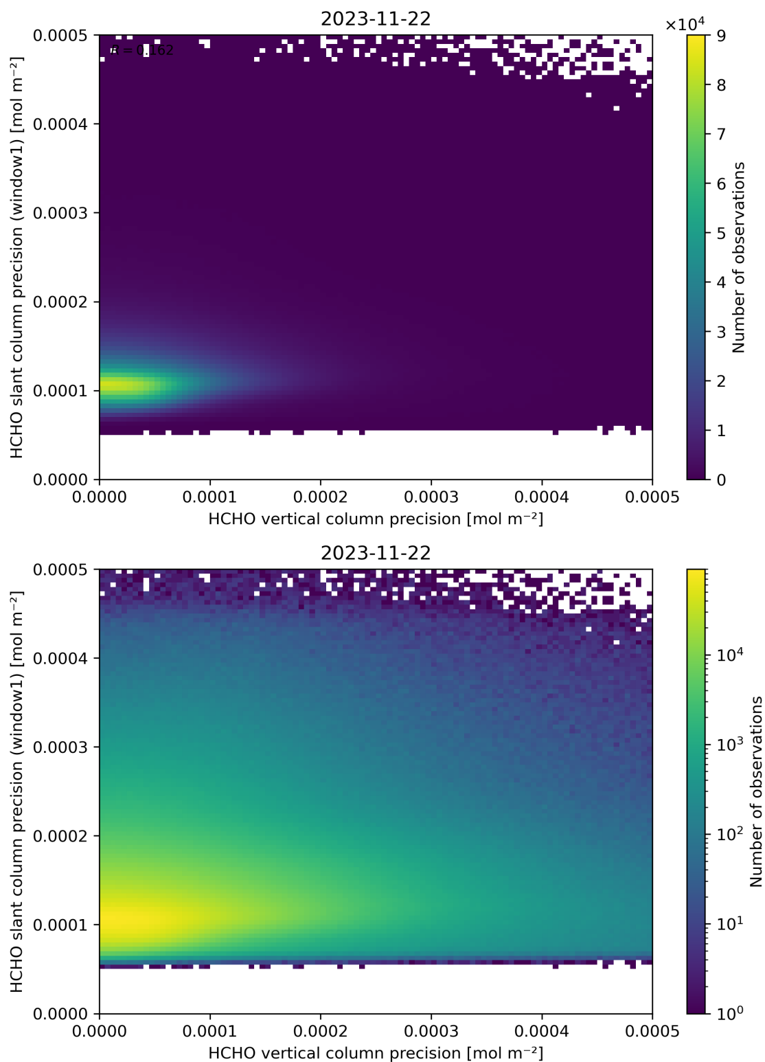
Figure 143: Scatter density plot of “HCHO vertical column precision” against “HCHO slant column precision (window1)” for 2023-11-21 to 2023-11-23.
