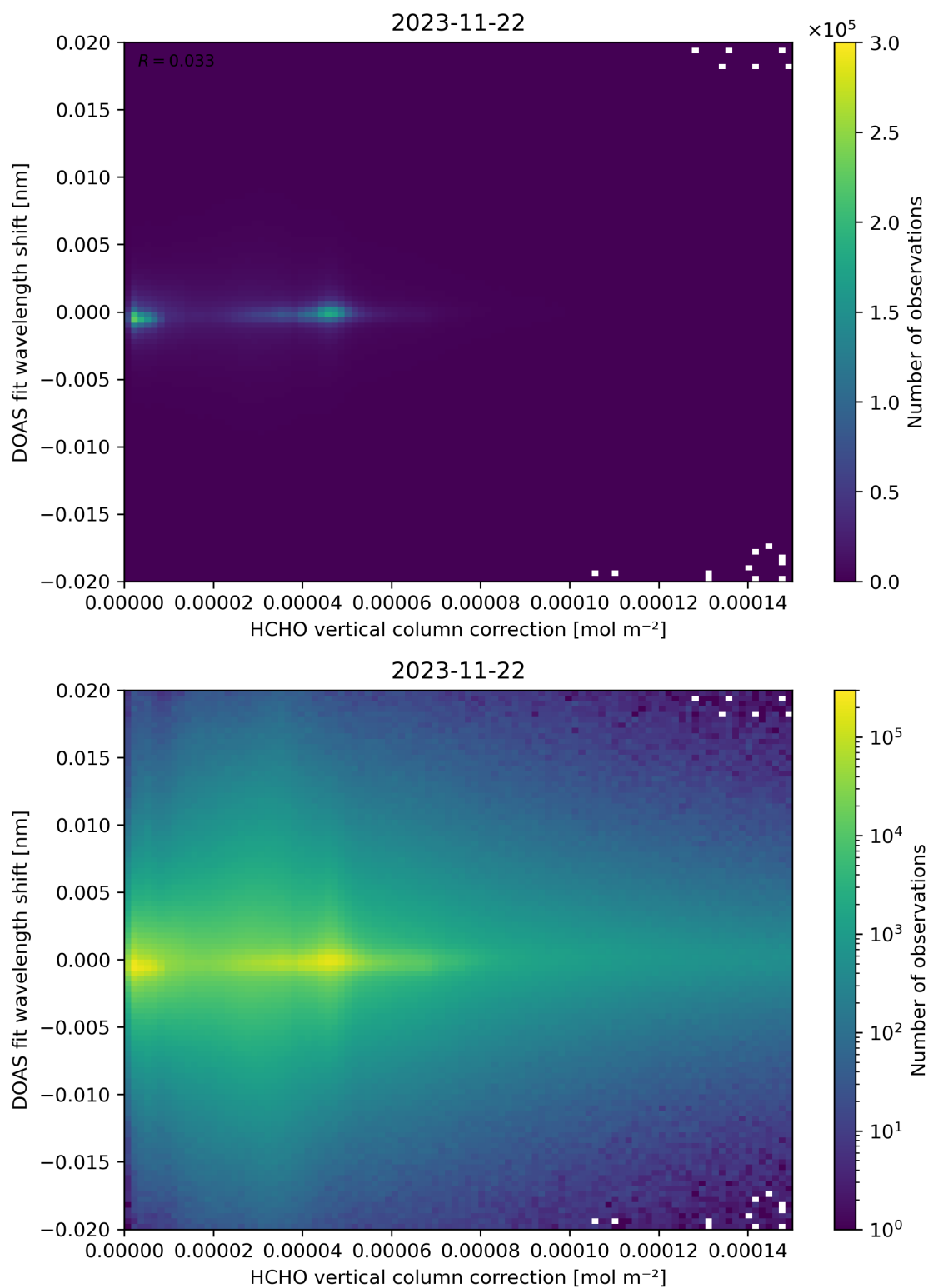
Figure 113: Scatter density plot of “HCHO vertical column correction” against “DOAS fit wavelength shift” for 2023-11-21 to 2023-11-23.
