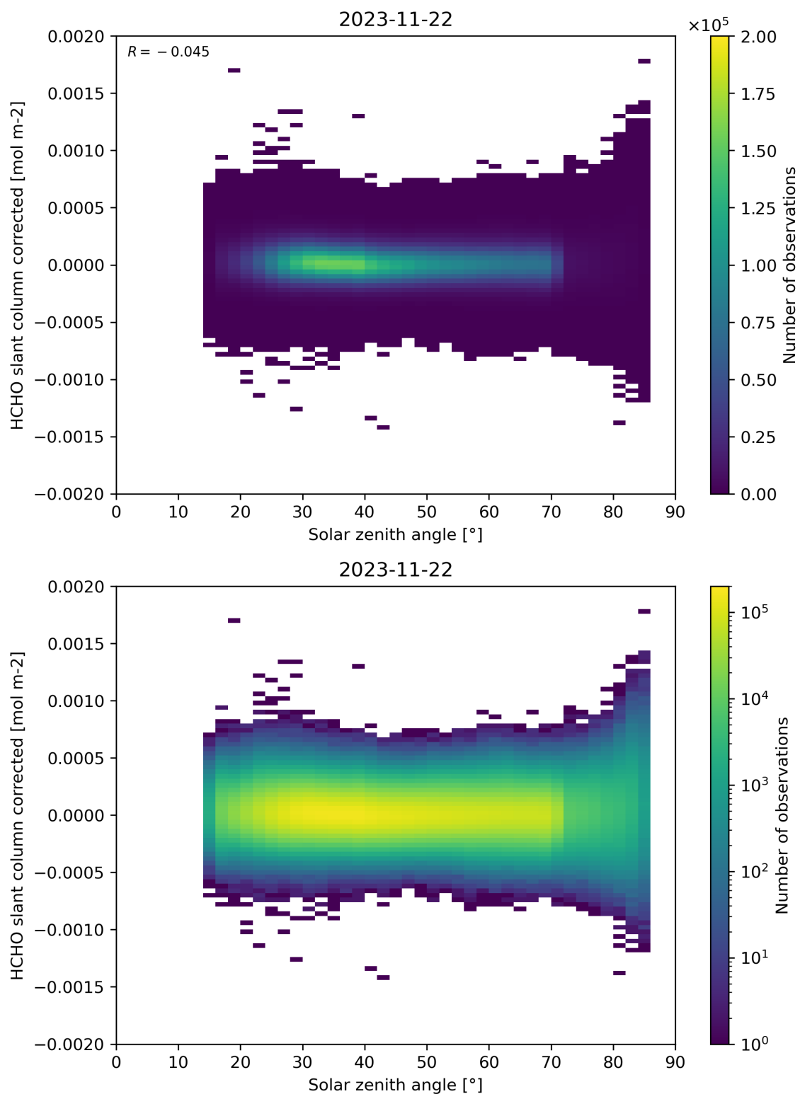
Figure 171: Scatter density plot of “Solar zenith angle” against “HCHO slant column corrected” for 2023-11-21 to 2023-11-23.
