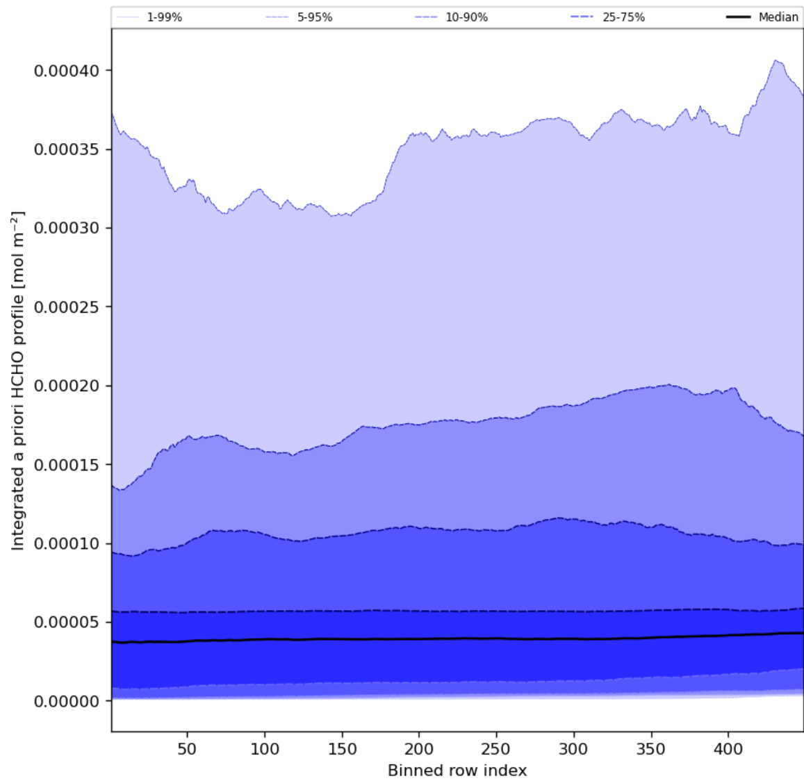
Figure 57: Along track statistics of "Integrated a priori HCHO profile" for 2023-11-21 to 2023-11-23
