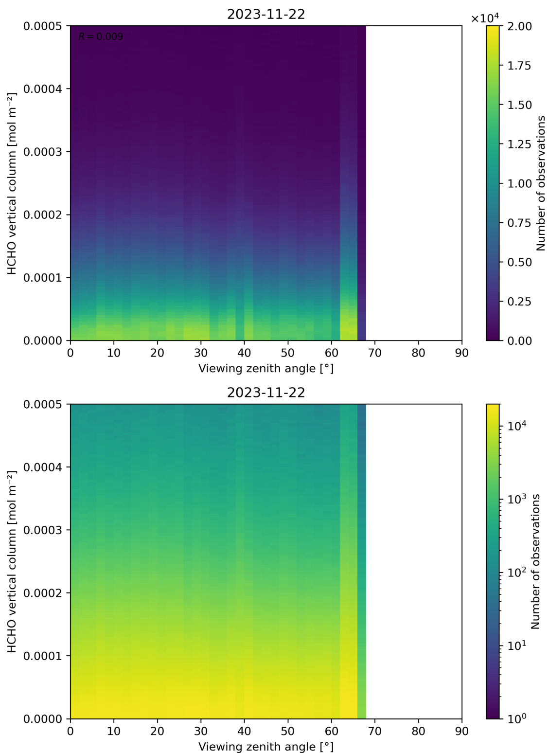
Figure 192: Scatter density plot of “Viewing zenith angle” against “HCHO vertical column” for 2023-11-21 to 2023-11-23.
