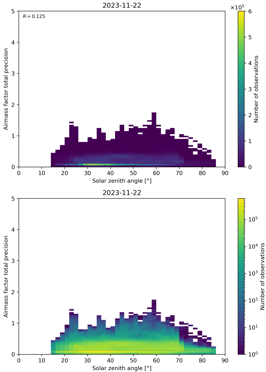
Figure 176: Scatter density plot of “Solar zenith angle” against “Airmass factor total precision” for 2023-11-21 to 2023-11-23.
