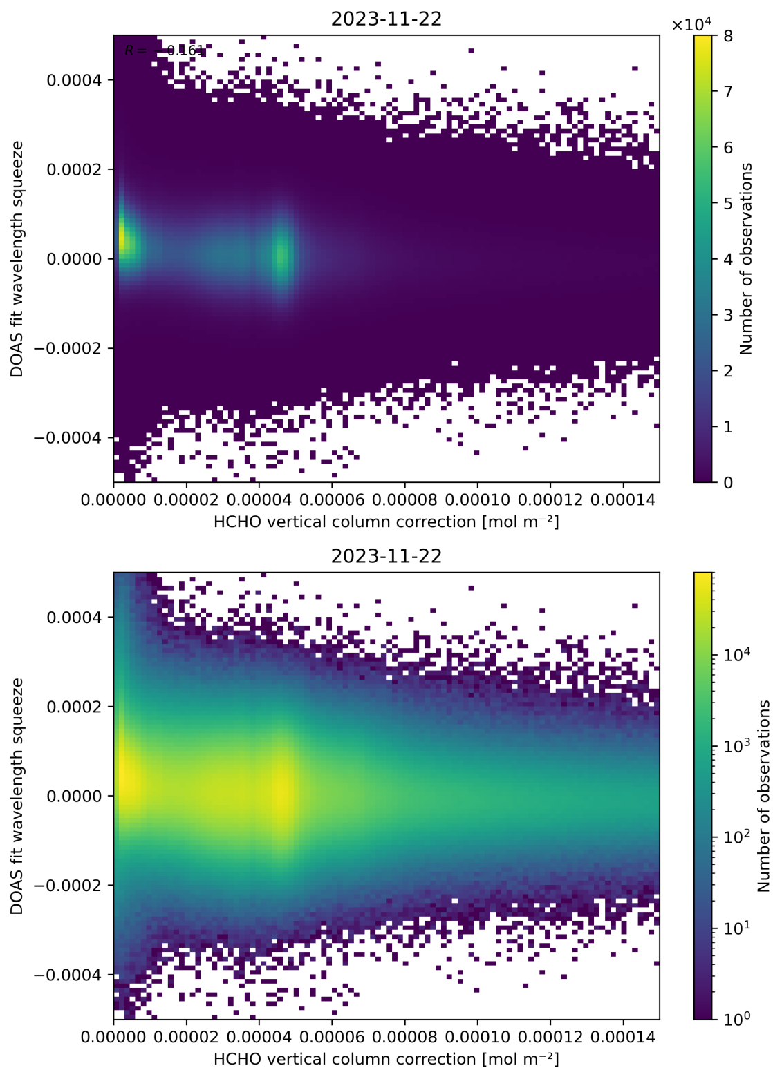
Figure 114: Scatter density plot of “HCHO vertical column correction” against “DOAS fit wavelength squeeze” for 2023-11-21 to 2023-11-23.
