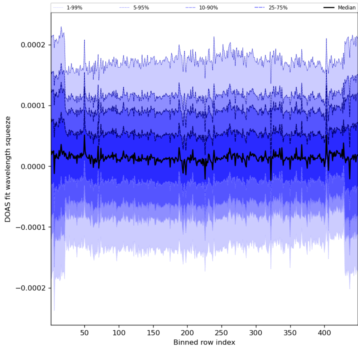
Figure 59: Along track statistics of “DOAS fit wavelength squeeze” for 2023-11-21 to 2023-11-23
