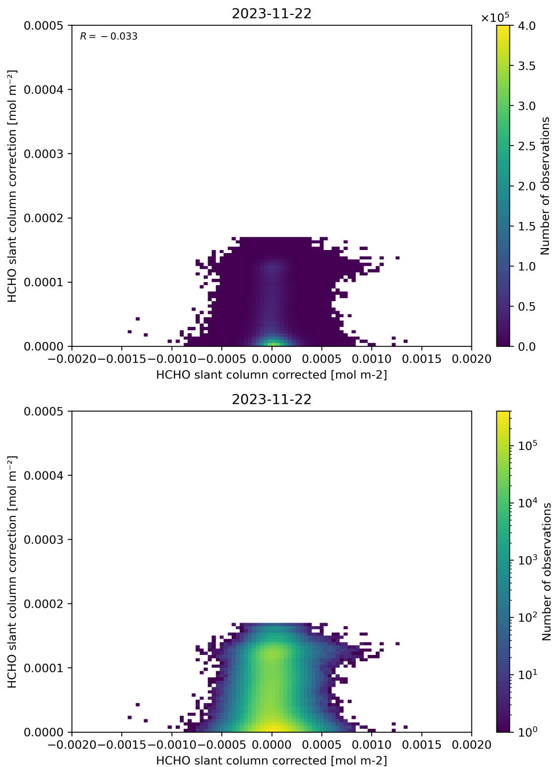
Figure 77: Scatter density plot of “HCHO slant column corrected” against “HCHO slant column correction” for 2023-11-21 to 2023-11-23.
