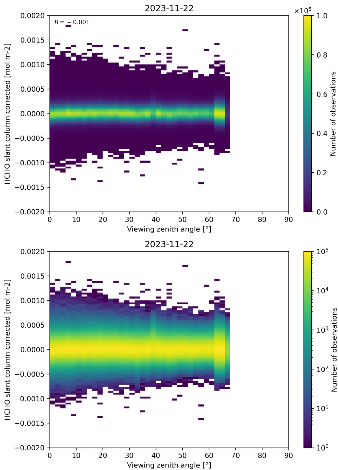
Figure 186: Scatter density plot of “Viewing zenith angle” against “HCHO slant column corrected” for 2023-11-21 to 2023-11-23.
