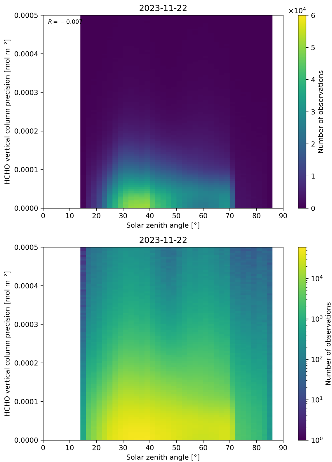
Figure 179: Scatter density plot of “Solar zenith angle” against “HCHO vertical column precision” for 2023-11-21 to 2023-11-23.
