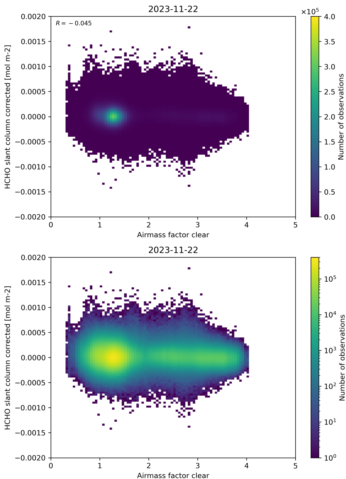
Figure 74: Scatter density plot of “Airmass factor clear” against “HCHO slant column corrected” for 2023-11-21 to 2023-11-23.
