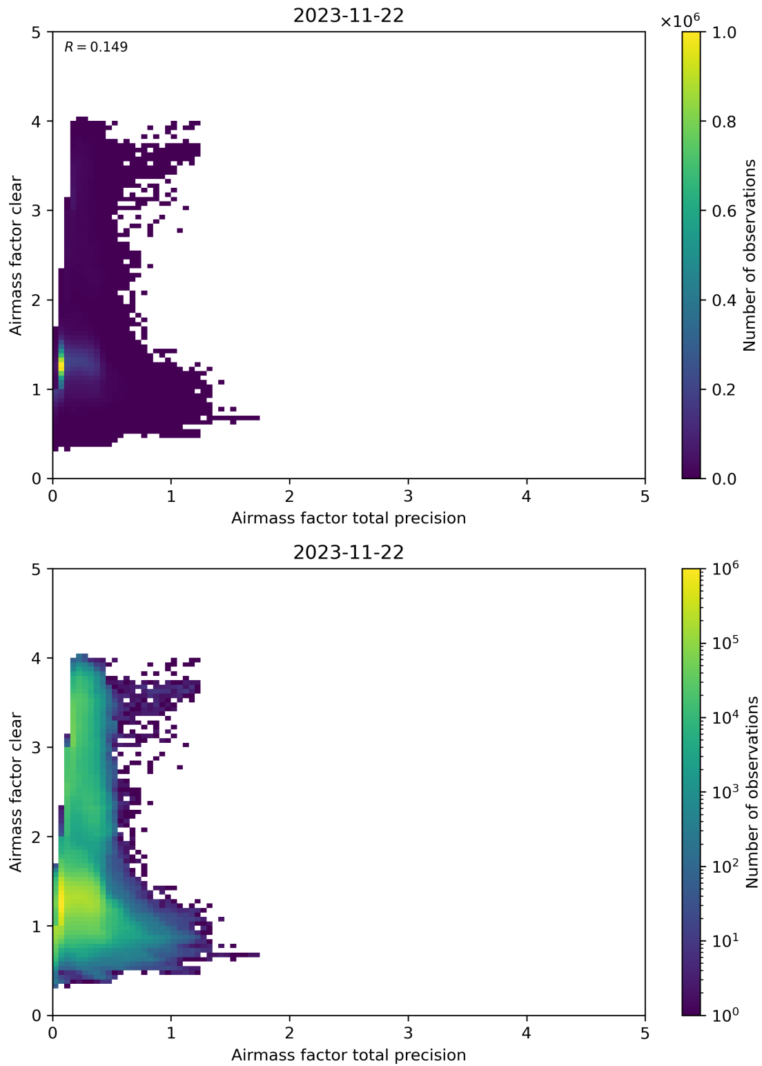
Figure 108: Scatter density plot of “Airmass factor total precision” against “Airmass factor clear” for 2023-11-21 to 2023-11-23.
