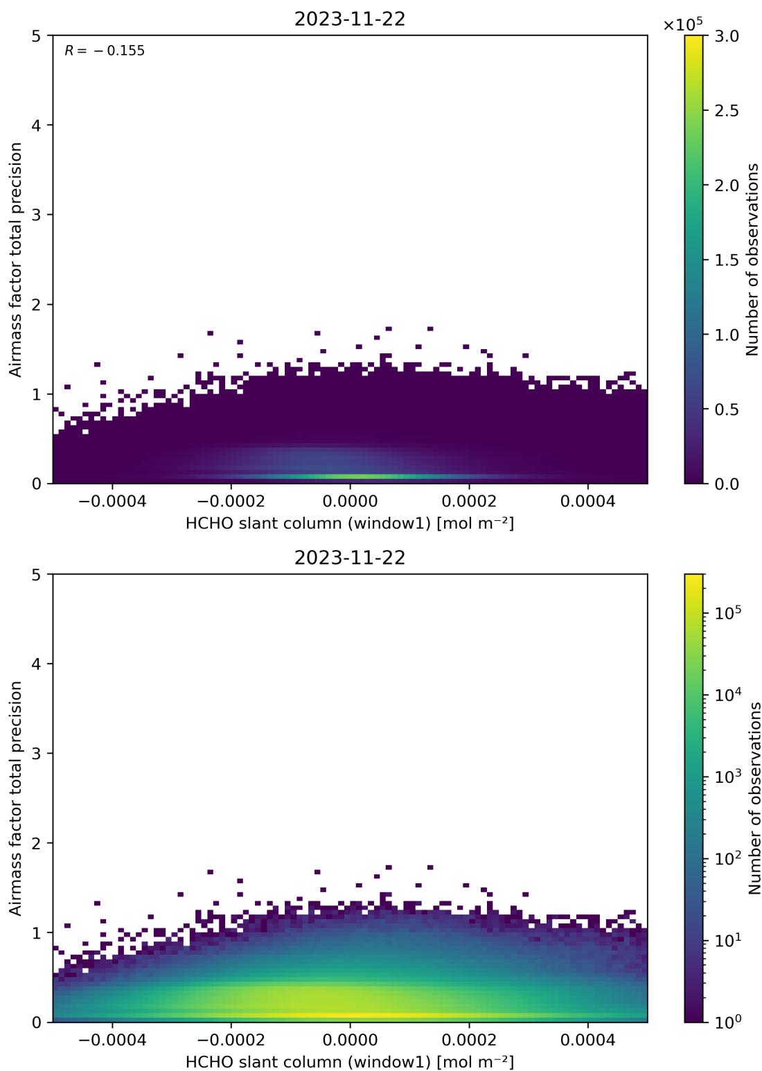
Figure 86: Scatter density plot of “HCHO slant column (window1)” against “Airmass factor total precision” for 2023-11-21 to 2023-11-23.
