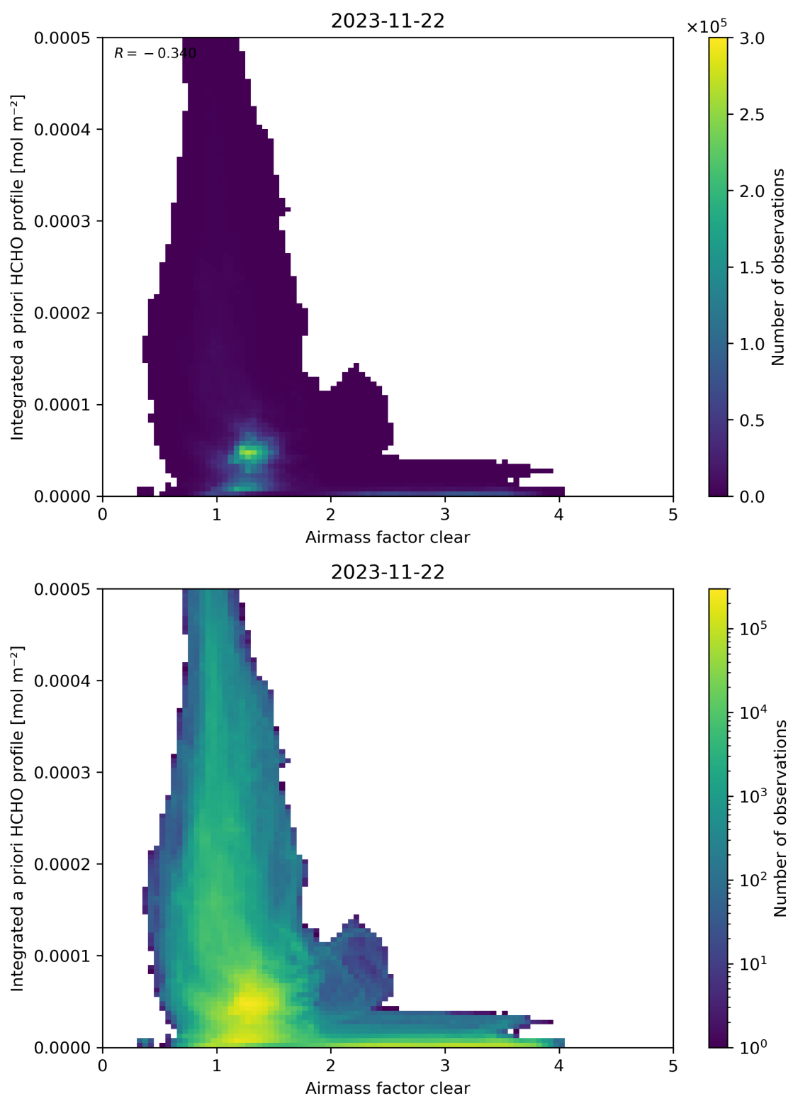
Figure 76: Scatter density plot of “Airmass factor clear” against “Integrated a priori HCHO profile” for 2023-11-21 to 2023-11-23.
