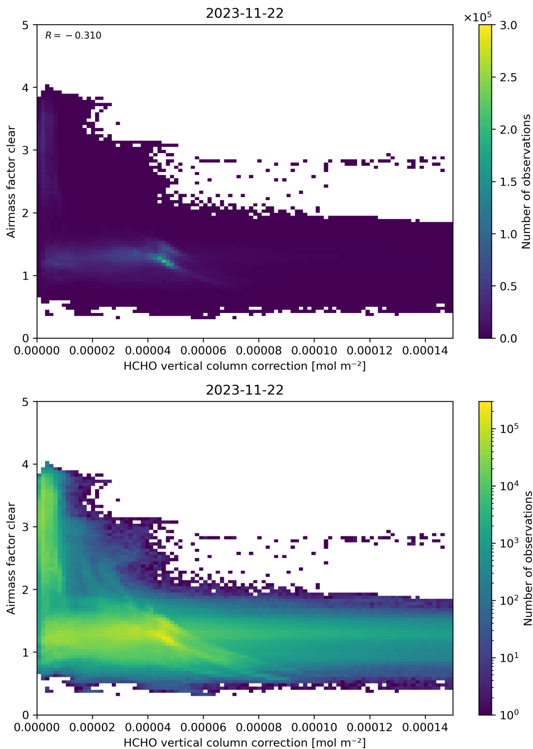
Figure 115: Scatter density plot of “HCHO vertical column correction” against “Airmass factor clear” for 2023-11-21 to 2023-11-23.
