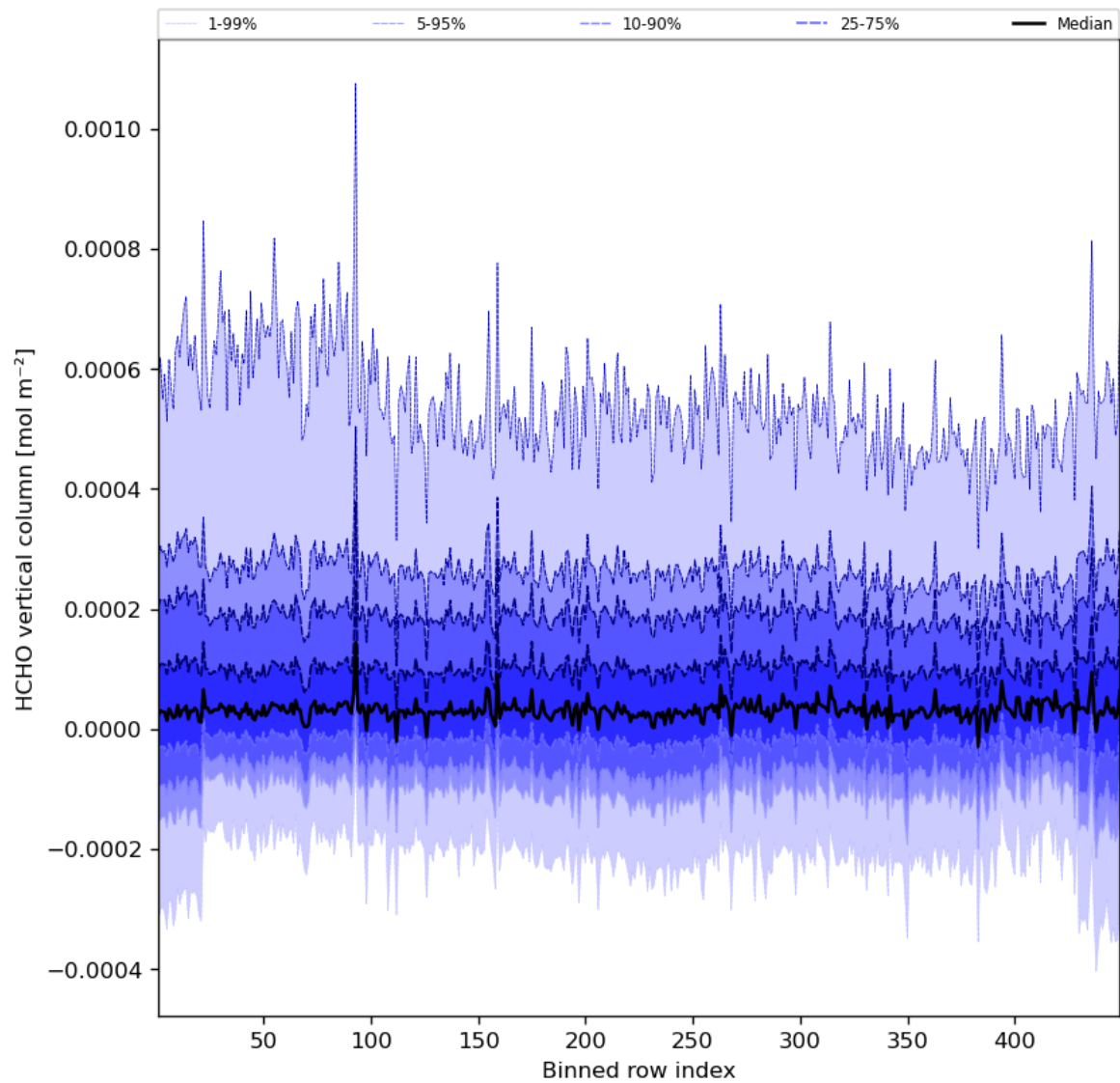
Figure 49: Along track statistics of “HCHO vertical column” for 2023-11-21 to 2023-11-23
