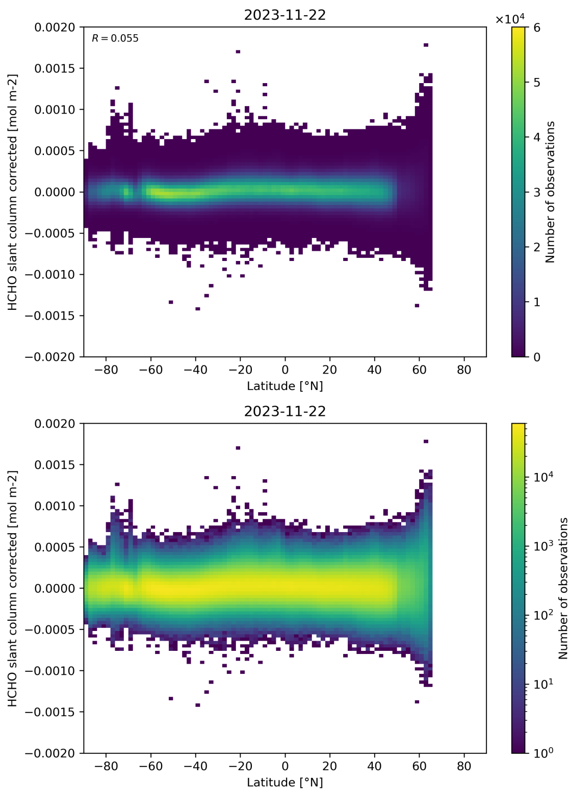
Figure 157: Scatter density plot of “Latitude” against “HCHO slant column corrected” for 2023-11-21 to 2023-11-23.
