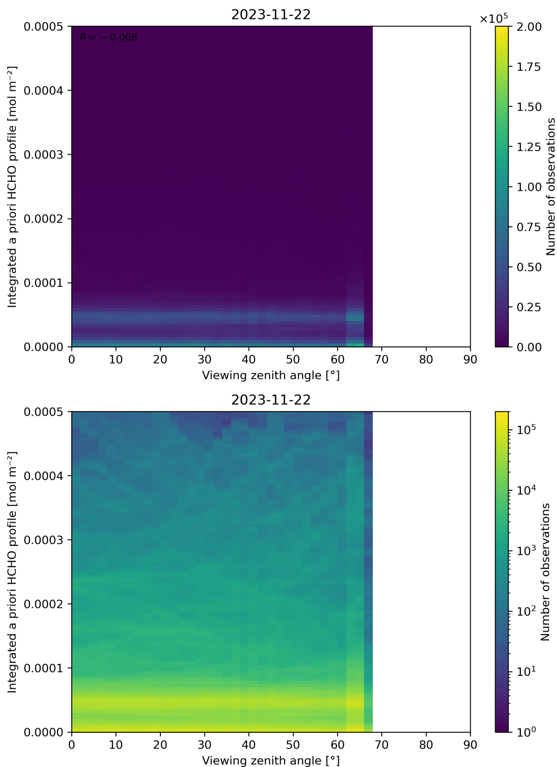
Figure 195: Scatter density plot of “Viewing zenith angle” against “Integrated a priori HCHO profile” for 2023-11-21 to 2023-11-23.
