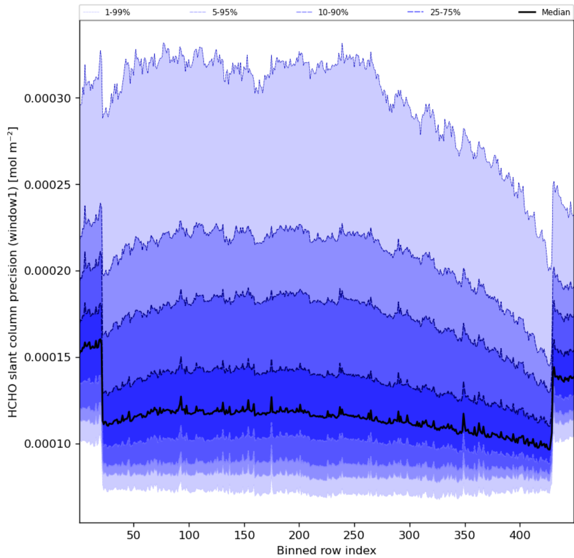
Figure 53: Along track statistics of “HCHO slant column precision (window1)” for 2023-11-21 to 2023-11-23
