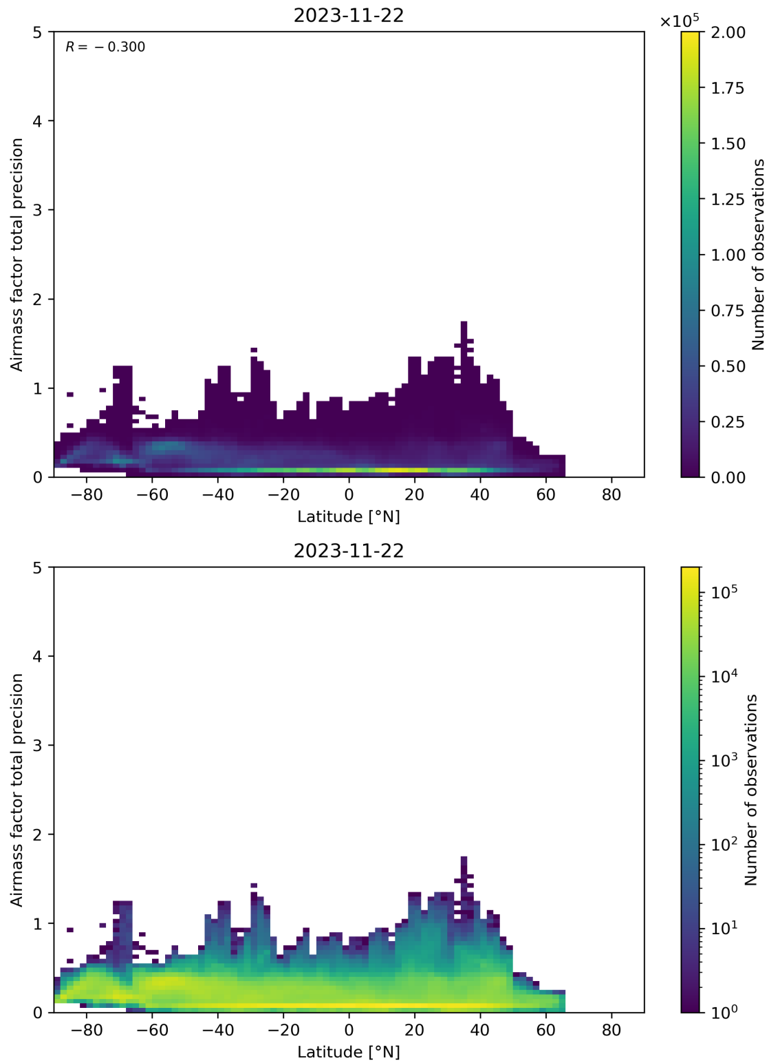
Figure 162: Scatter density plot of “Latitude” against “Airmass factor total precision” for 2023-11-21 to 2023-11-23.
