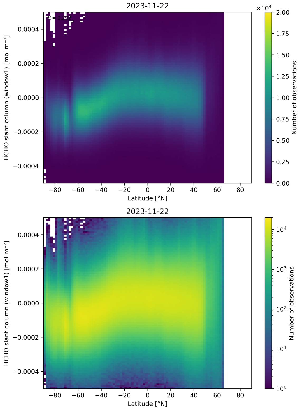
Figure 159: Scatter density plot of “Latitude” against “HCHO slant column (window1)” for 2023-11-21 to 2023-11-23.
