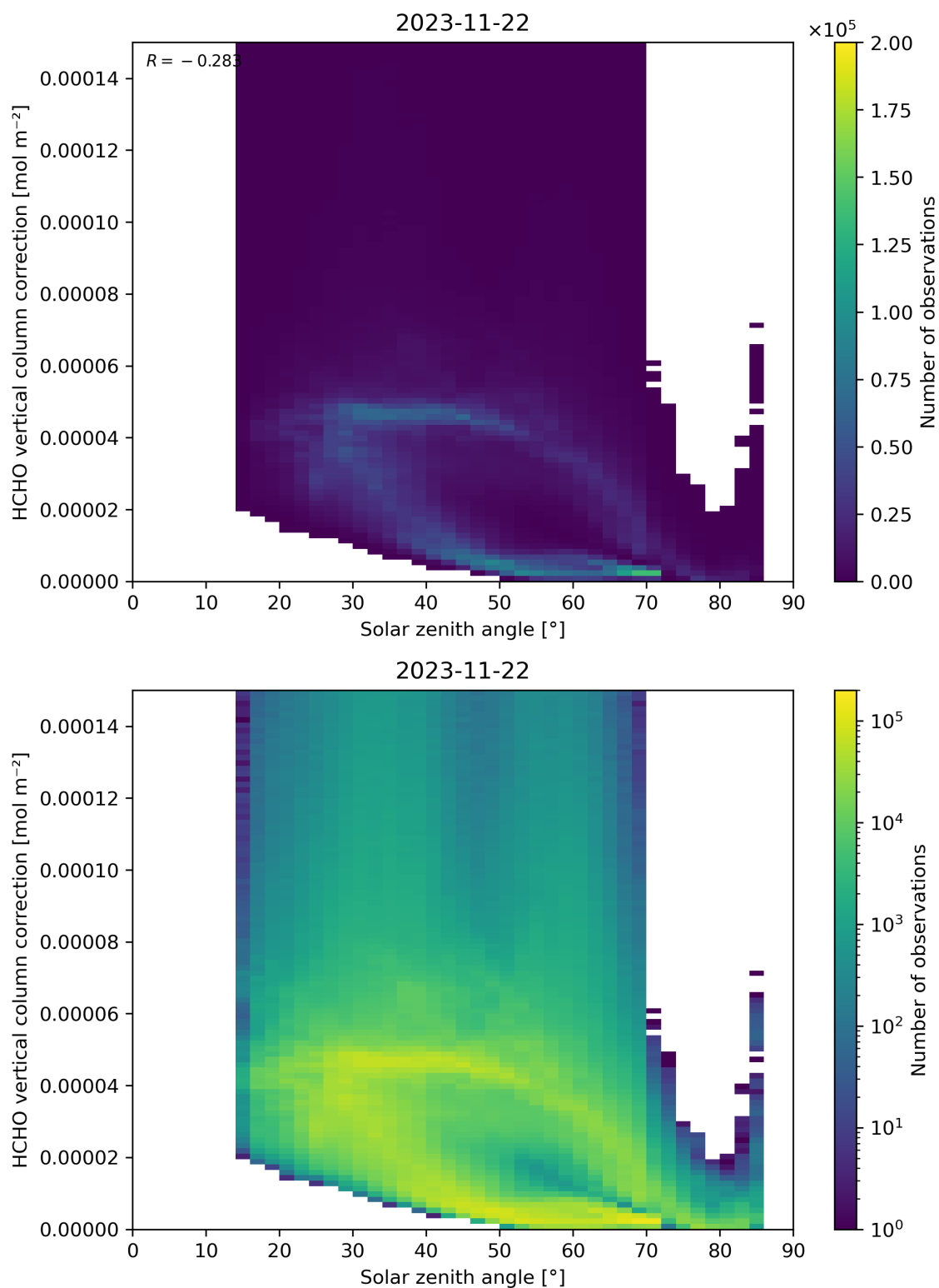
Figure 178: Scatter density plot of “Solar zenith angle” against “HCHO vertical column correction” for 2023-11-21 to 2023-11-23.
