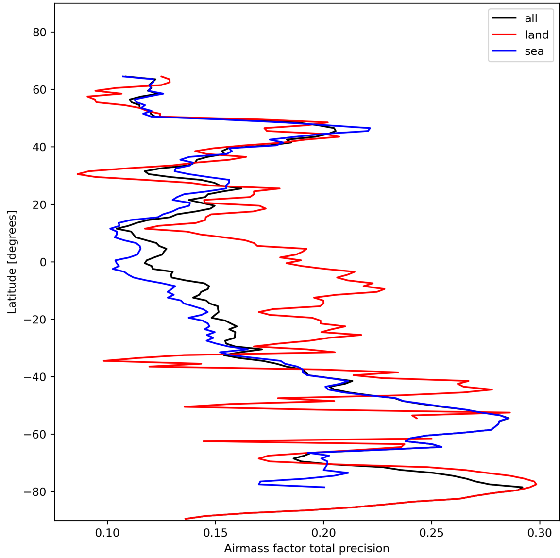
Figure 27: Zonal average of “Airmass factor total precision” for 2023-11-21 to 2023-11-23.
