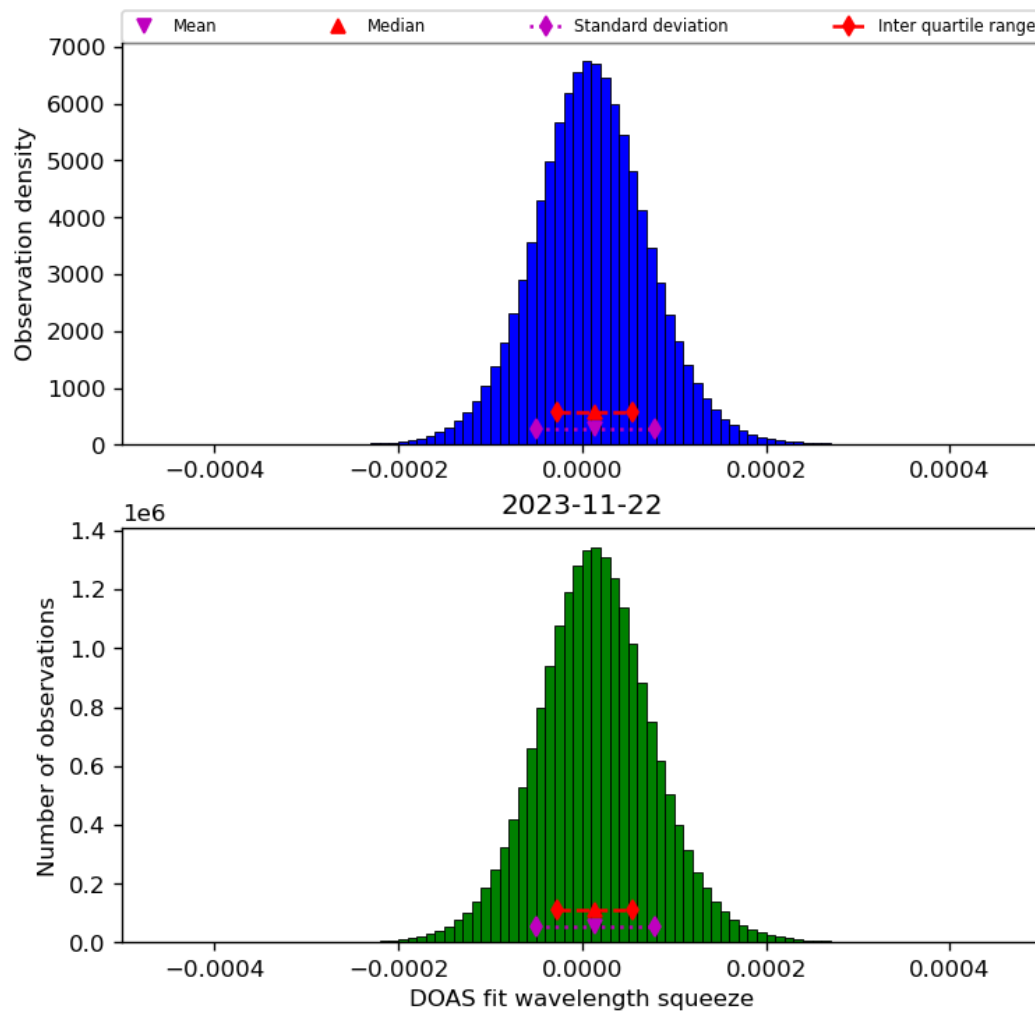
Figure 45: Histogram of “DOAS fit wavelength squeeze” for 2023-11-21 to 2023-11-23
