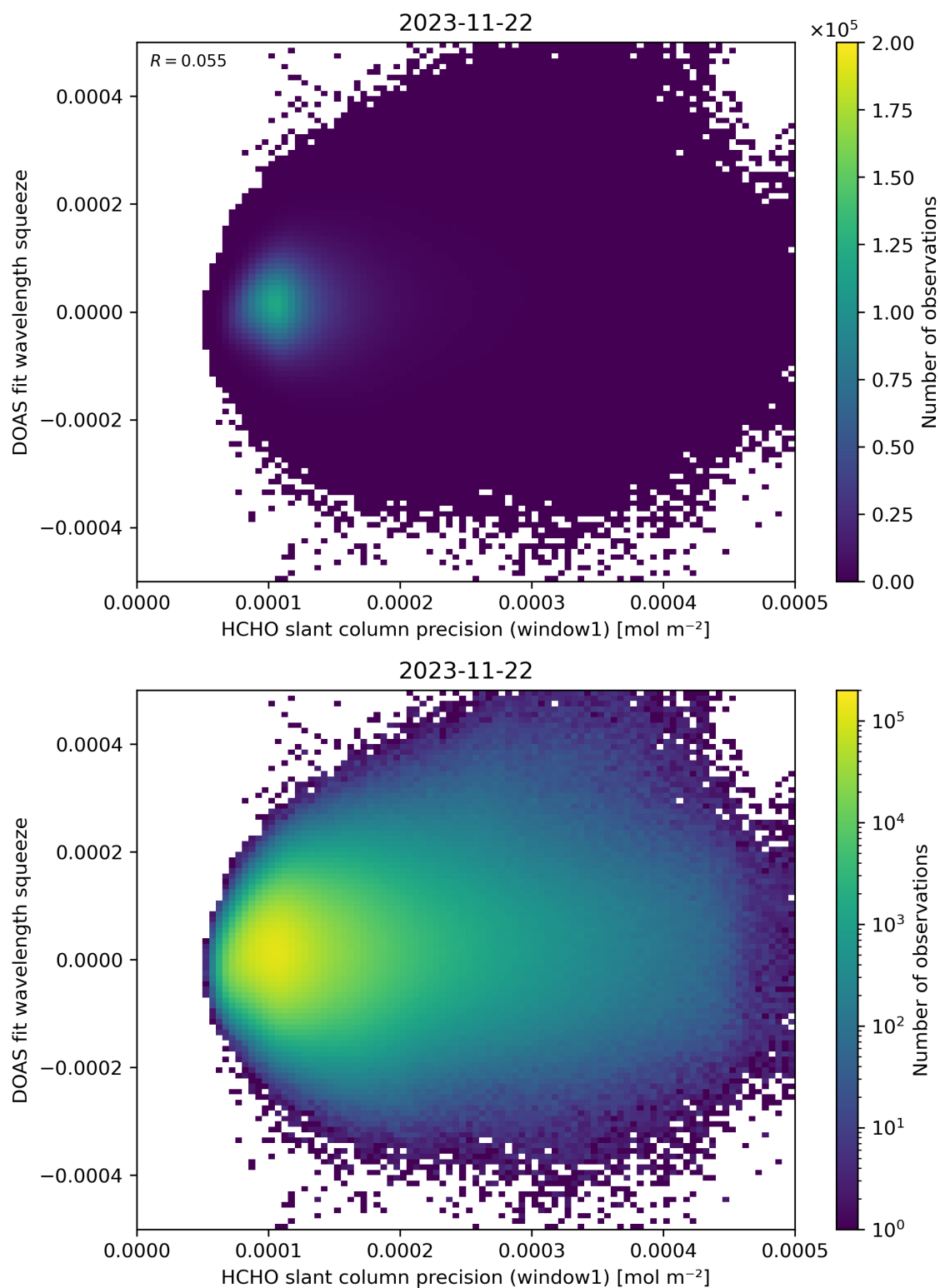
Figure 90: Scatter density plot of “HCHO slant column precision (window1)” against “DOAS fit wavelength squeeze” for 2023-11-21 to 2023-11-23.
