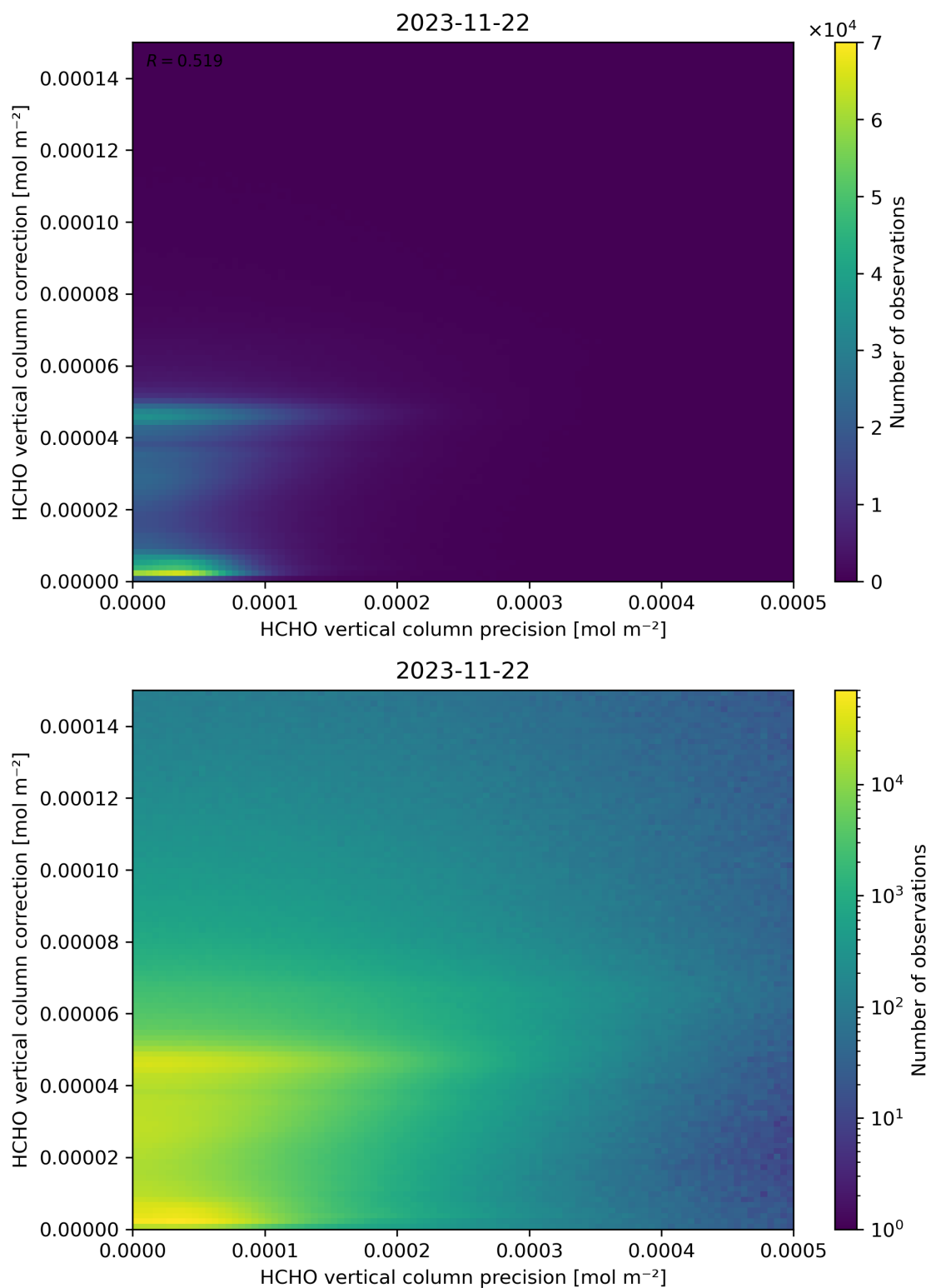
Figure 146: Scatter density plot of “HCHO vertical column precision” against “HCHO vertical column correction” for 2023-11-21 to 2023-11-23.
