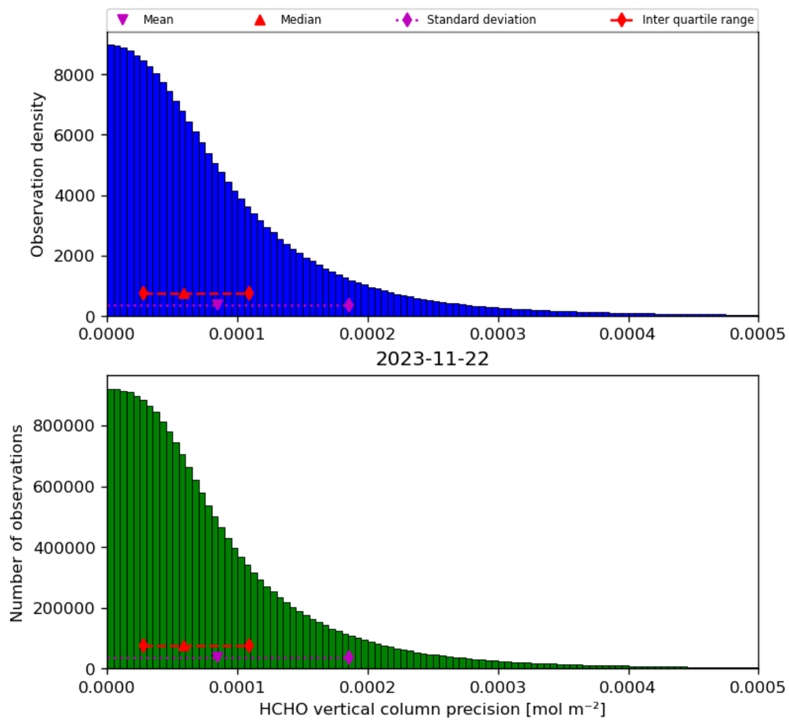
Figure 36: Histogram of “HCHO vertical column precision” for 2023-11-21 to 2023-11-23
