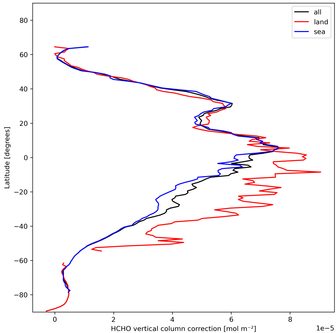
Figure 23: Zonal average of “HCHO vertical column correction” for 2023-11-21 to 2023-11-23.
