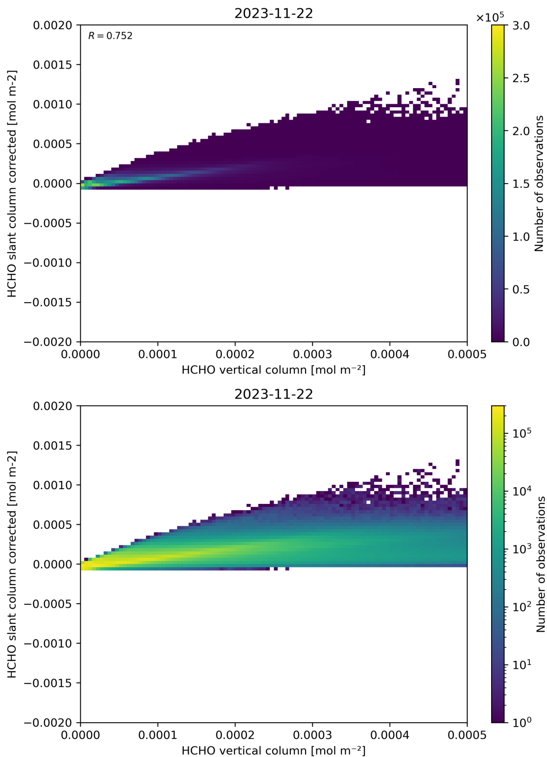
Figure 127: Scatter density plot of “HCHO vertical column” against “HCHO slant column corrected” for 2023-11-21 to 2023-11-23.
