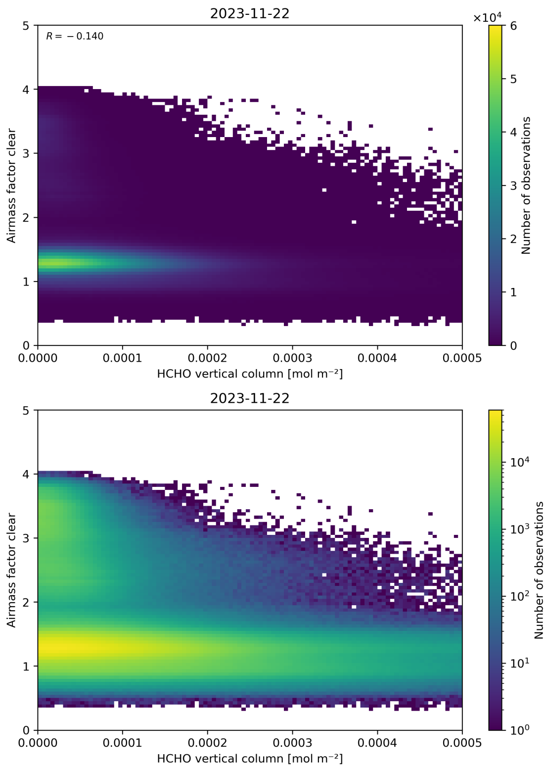
Figure 126: Scatter density plot of “HCHO vertical column” against “Airmass factor clear” for 2023-11-21 to 2023-11-23.
