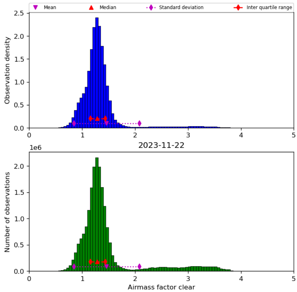
Figure 42: Histogram of “Airmass factor clear” for 2023-11-21 to 2023-11-23
