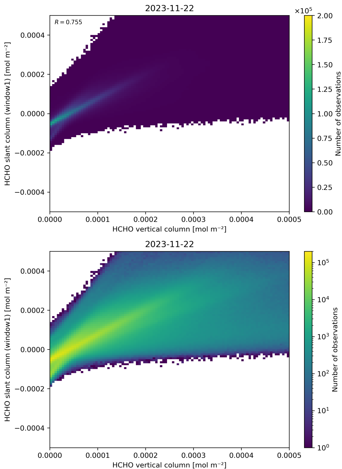
Figure 129: Scatter density plot of “HCHO vertical column” against “HCHO slant column (window1)” for 2023-11-21 to 2023-11-23.
