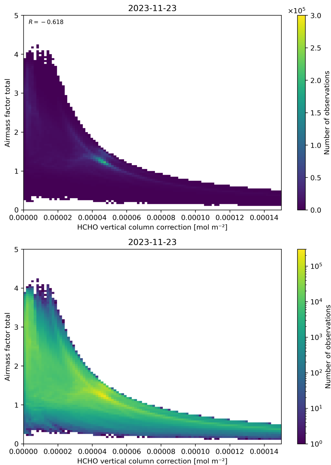
Figure 120: Scatter density plot of “HCHO vertical column correction” against “Airmass factor total” for 2023-11-23 to 2023-11-24.
