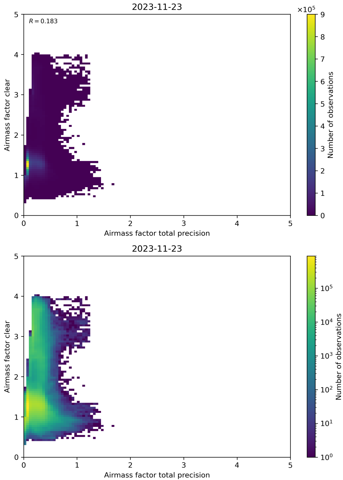
Figure 108: Scatter density plot of “Airmass factor total precision” against “Airmass factor clear” for 2023-11-23 to 2023-11-24.
