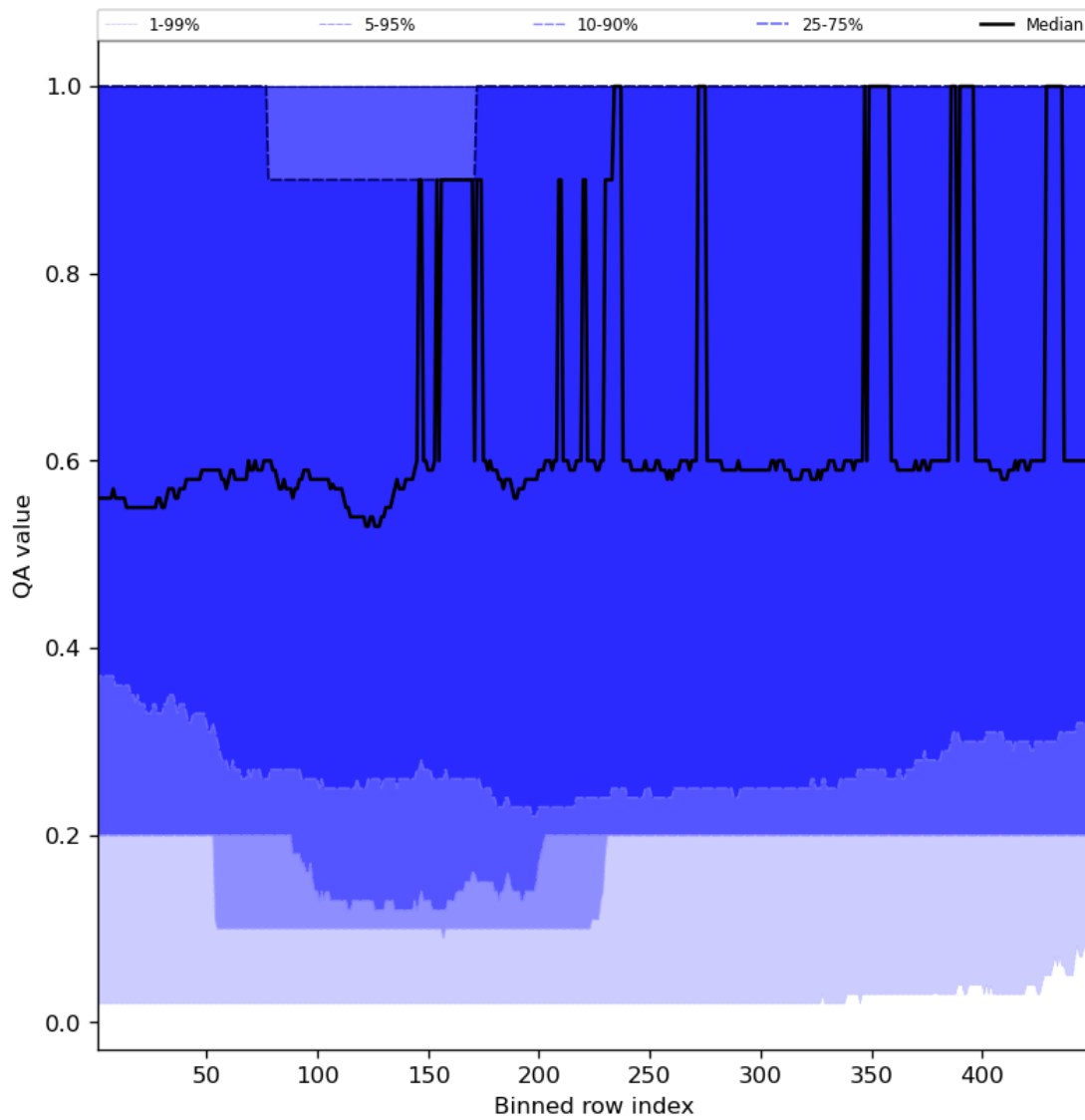
Figure 48: Along track statistics of “QA value” for 2023-11-23 to 2023-11-24
