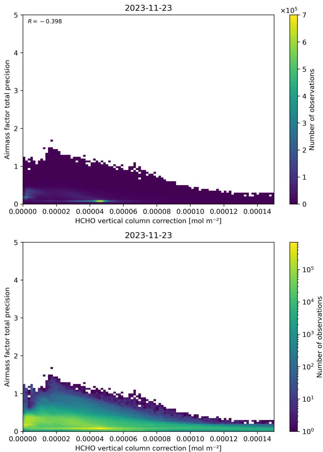
Figure 121: Scatter density plot of “HCHO vertical column correction” against “Airmass factor total precision” for 2023-11-23 to 2023-11-24.
