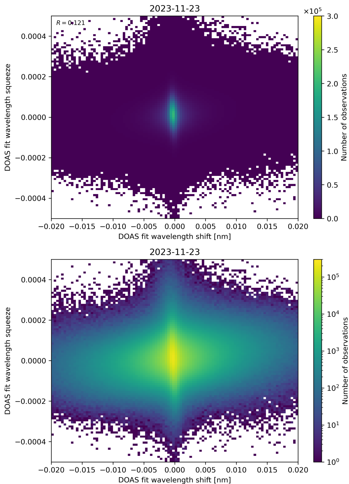
Figure 65: Scatter density plot of “DOAS fit wavelength shift” against “DOAS fit wavelength squeeze” for 2023-11-23 to 2023-11-24.
