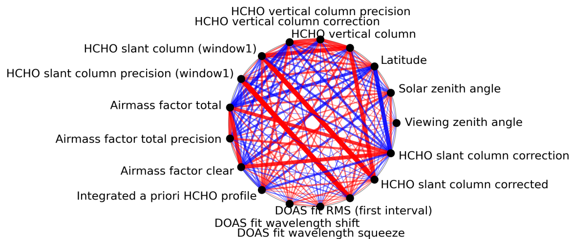
Figure 1: Map of correlation graph for 2023-11-23 to 2023-11-24.
