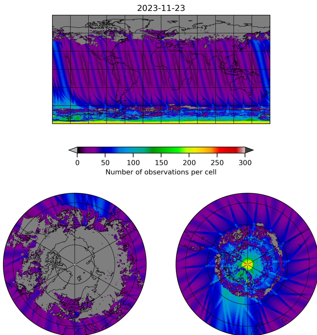
Figure 19: Map of the number of observations for 2023-11-23 to 2023-11-24
