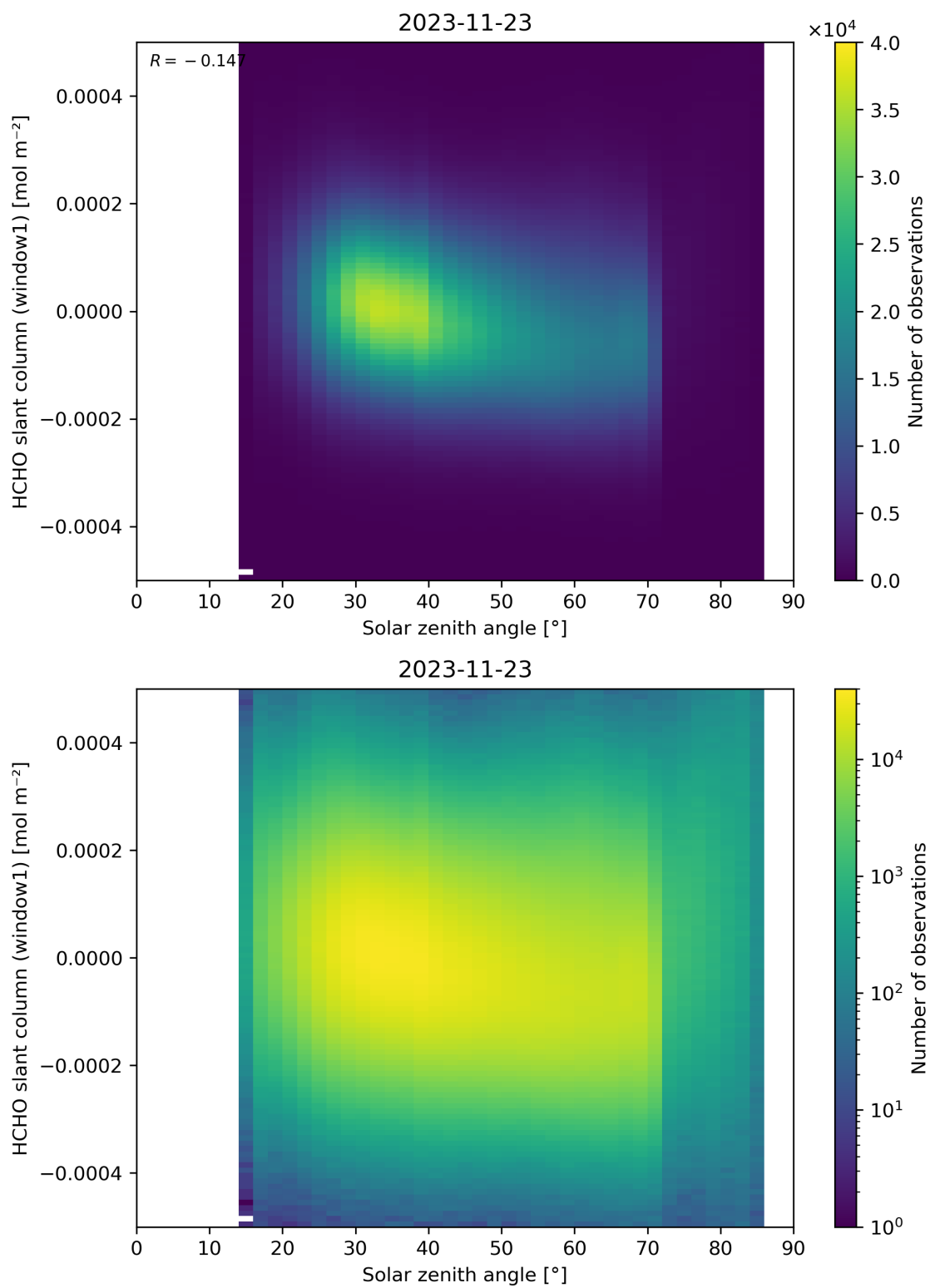
Figure 173: Scatter density plot of “Solar zenith angle” against “HCHO slant column (window1)” for 2023-11-23 to 2023-11-24.
