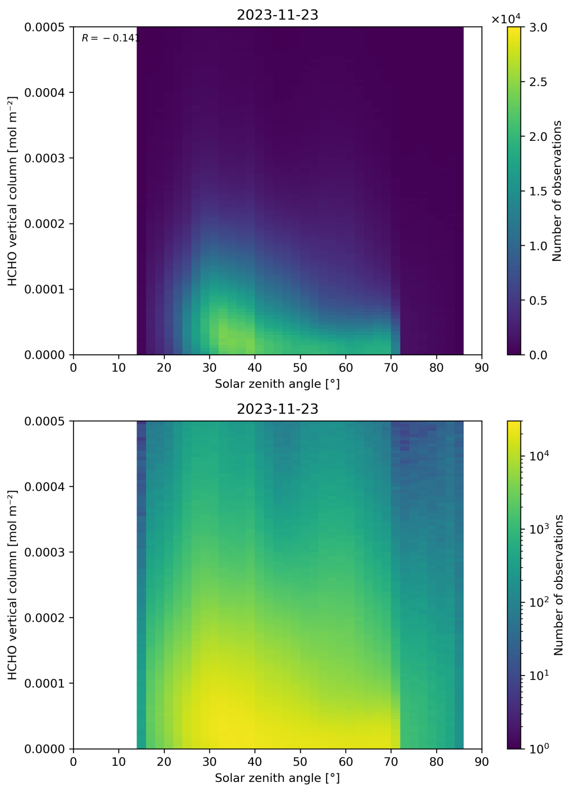
Figure 177: Scatter density plot of “Solar zenith angle” against “HCHO vertical column” for 2023-11-23 to 2023-11-24.
