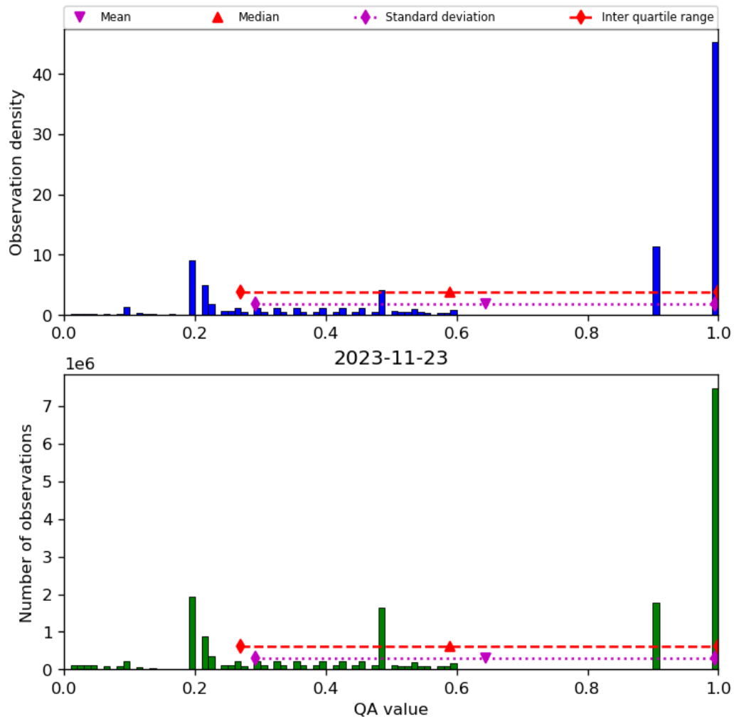
Figure 34: Histogram of “QA value” for 2023-11-23 to 2023-11-24
