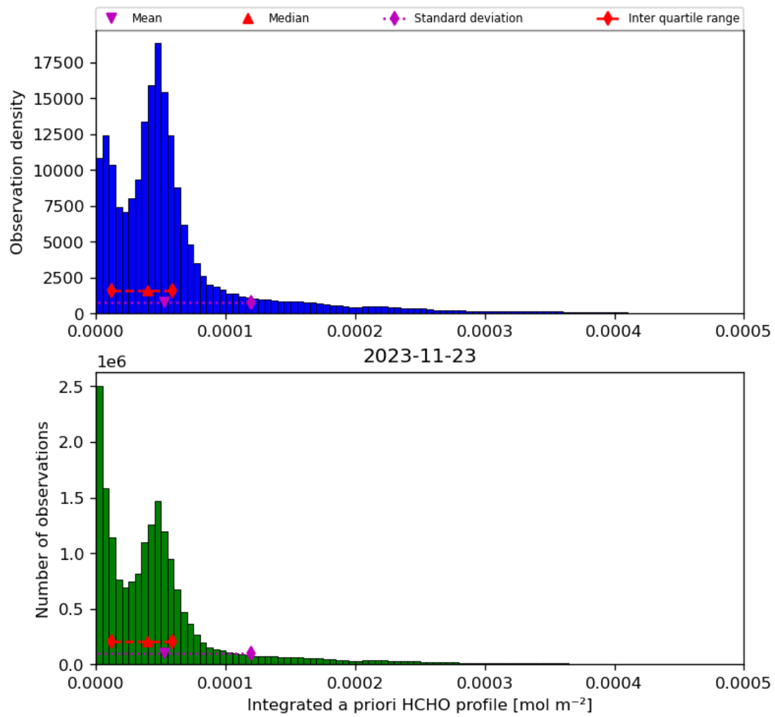
Figure 43: Histogram of “Integrated a priori HCHO profile” for 2023-11-23 to 2023-11-24
