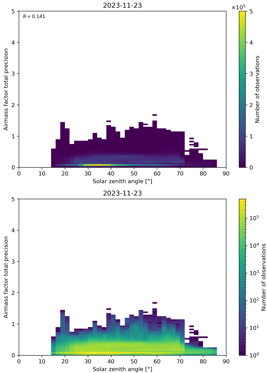
Figure 176: Scatter density plot of “Solar zenith angle” against “Airmass factor total precision” for 2023-11-23 to 2023-11-24.
