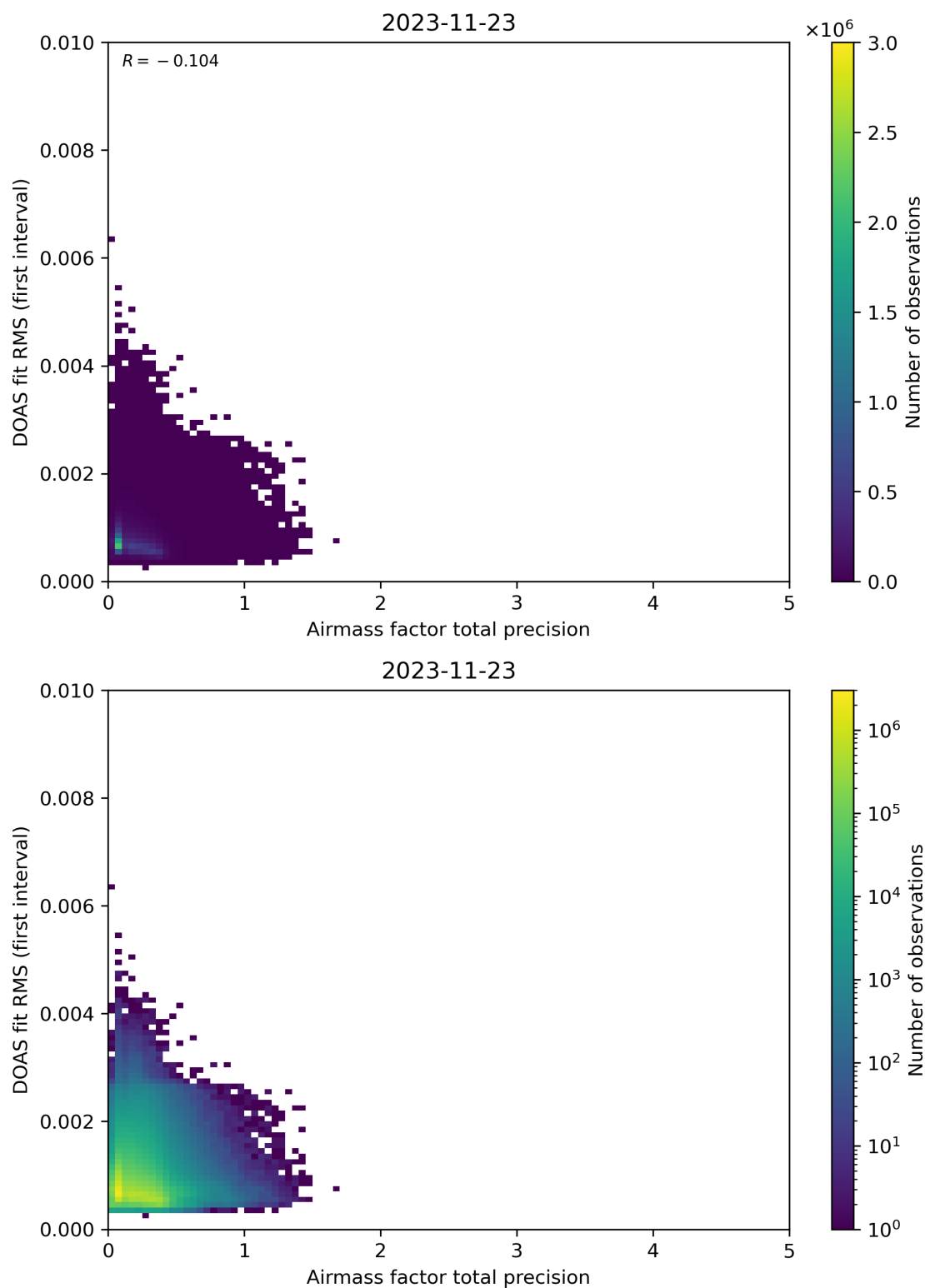
Figure 105: Scatter density plot of “Airmass factor total precision” against “DOAS fit RMS (first interval)” for 2023-11-23 to 2023-11-24.
