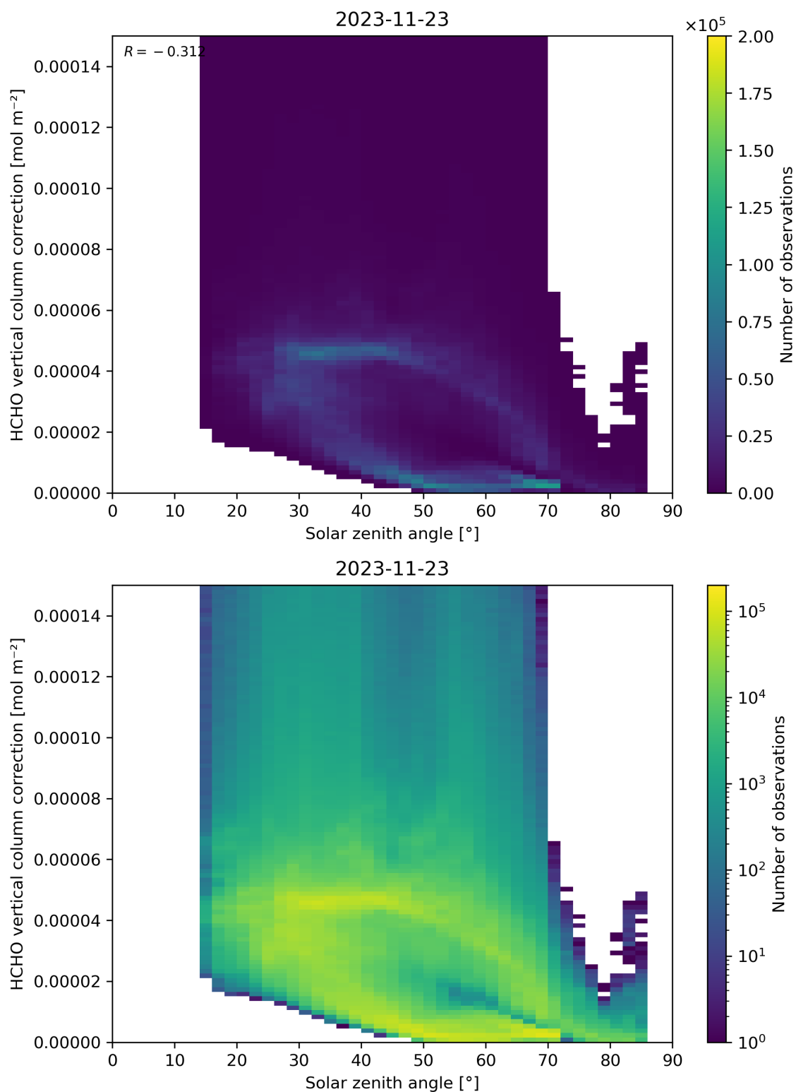
Figure 178: Scatter density plot of “Solar zenith angle” against “HCHO vertical column correction” for 2023-11-23 to 2023-11-24.
