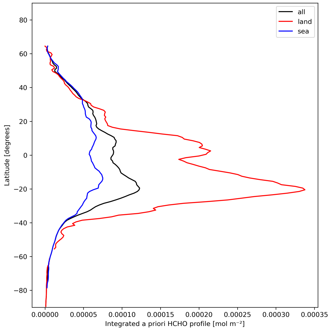
Figure 29: Zonal average of “Integrated a priori HCHO profile” for 2023-11-23 to 2023-11-24.
