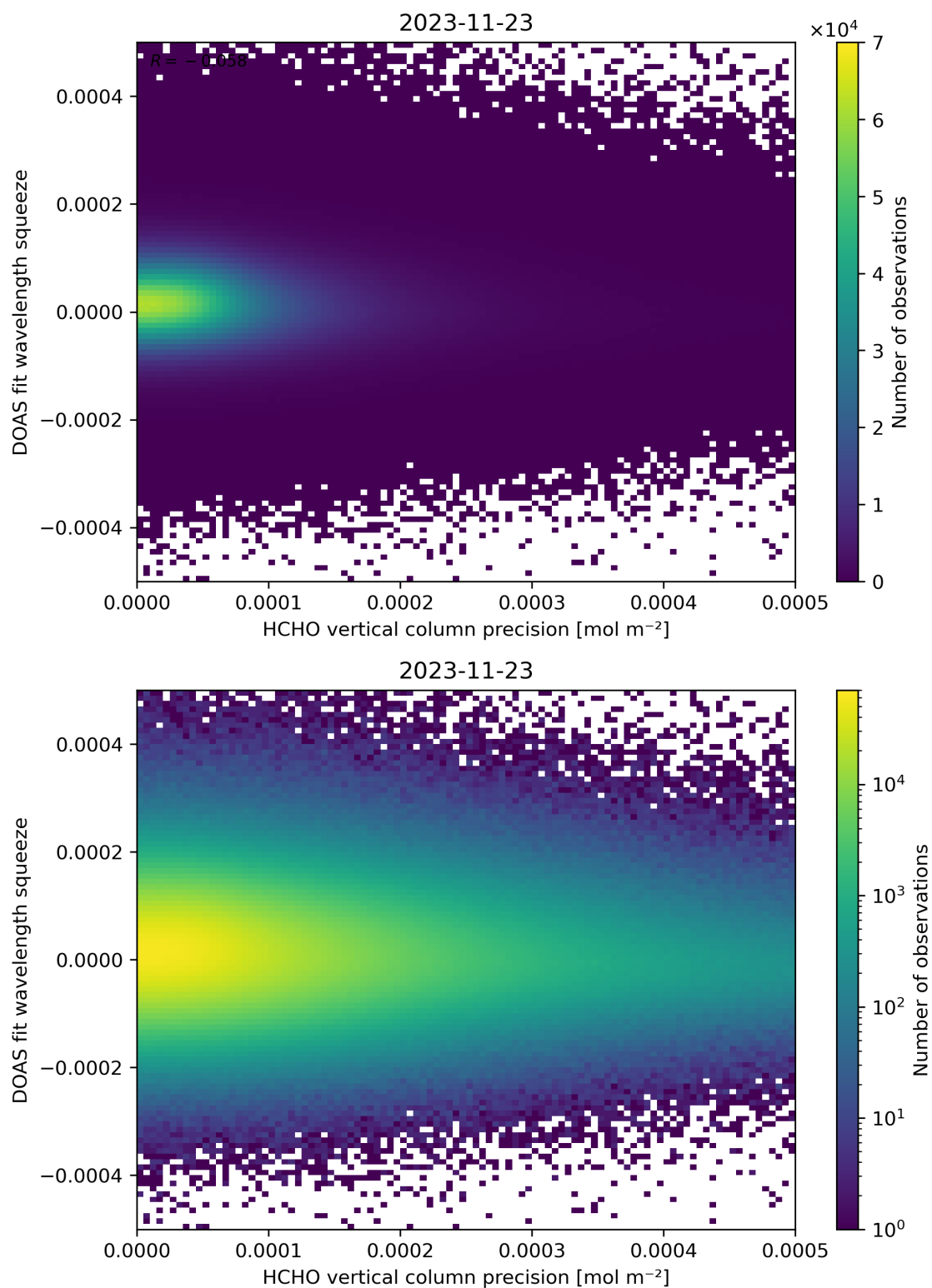
Figure 138: Scatter density plot of “HCHO vertical column precision” against “DOAS fit wavelength squeeze” for 2023-11-23 to 2023-11-24.
