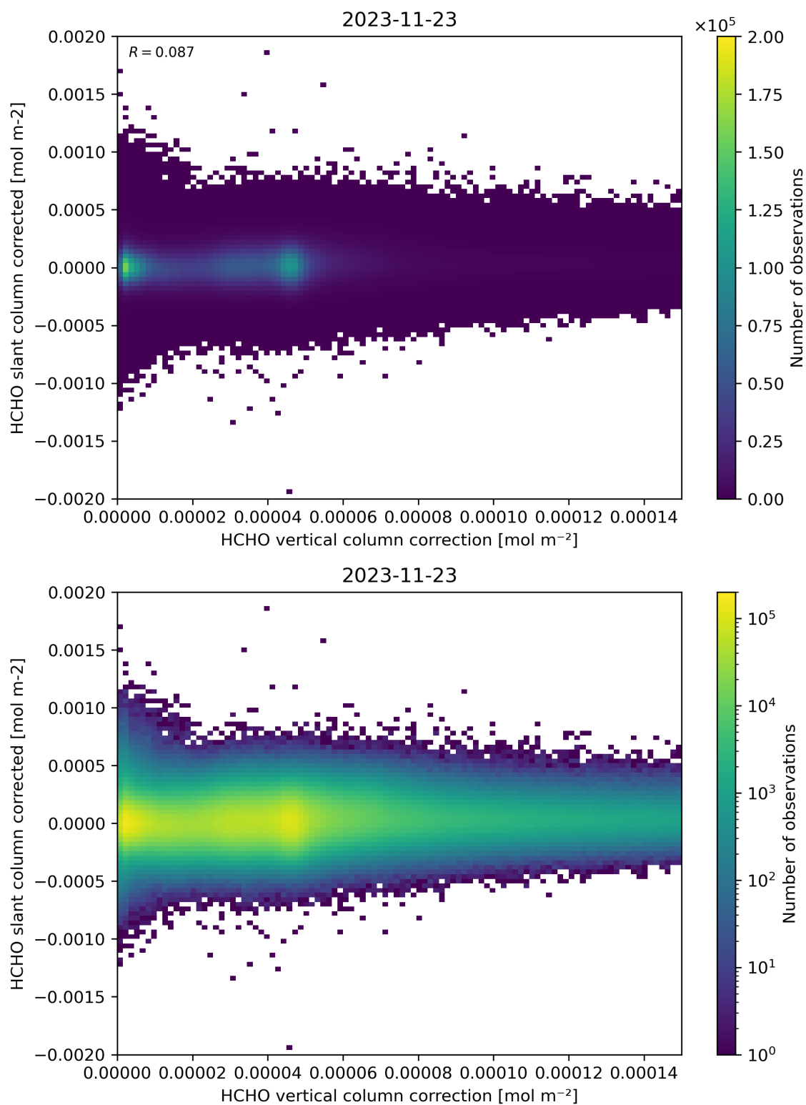
Figure 116: Scatter density plot of “HCHO vertical column correction” against “HCHO slant column corrected” for 2023-11-23 to 2023-11-24.
