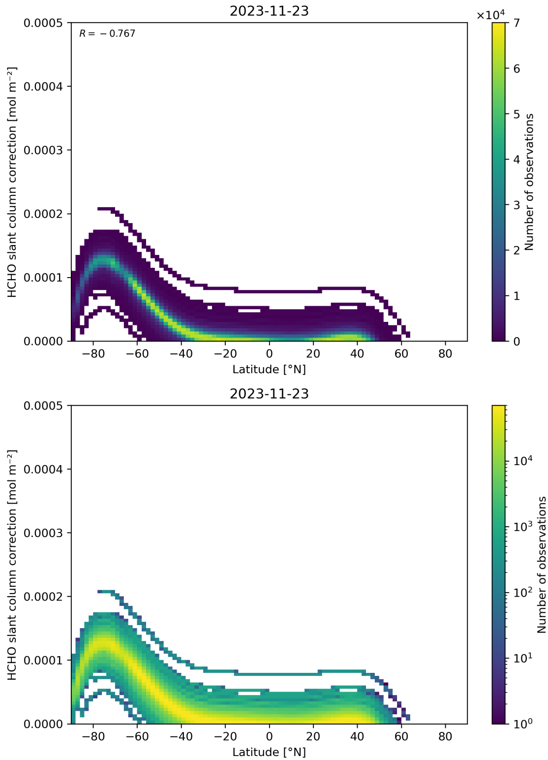
Figure 158: Scatter density plot of “Latitude” against “HCHO slant column correction” for 2023-11-23 to 2023-11-24.
