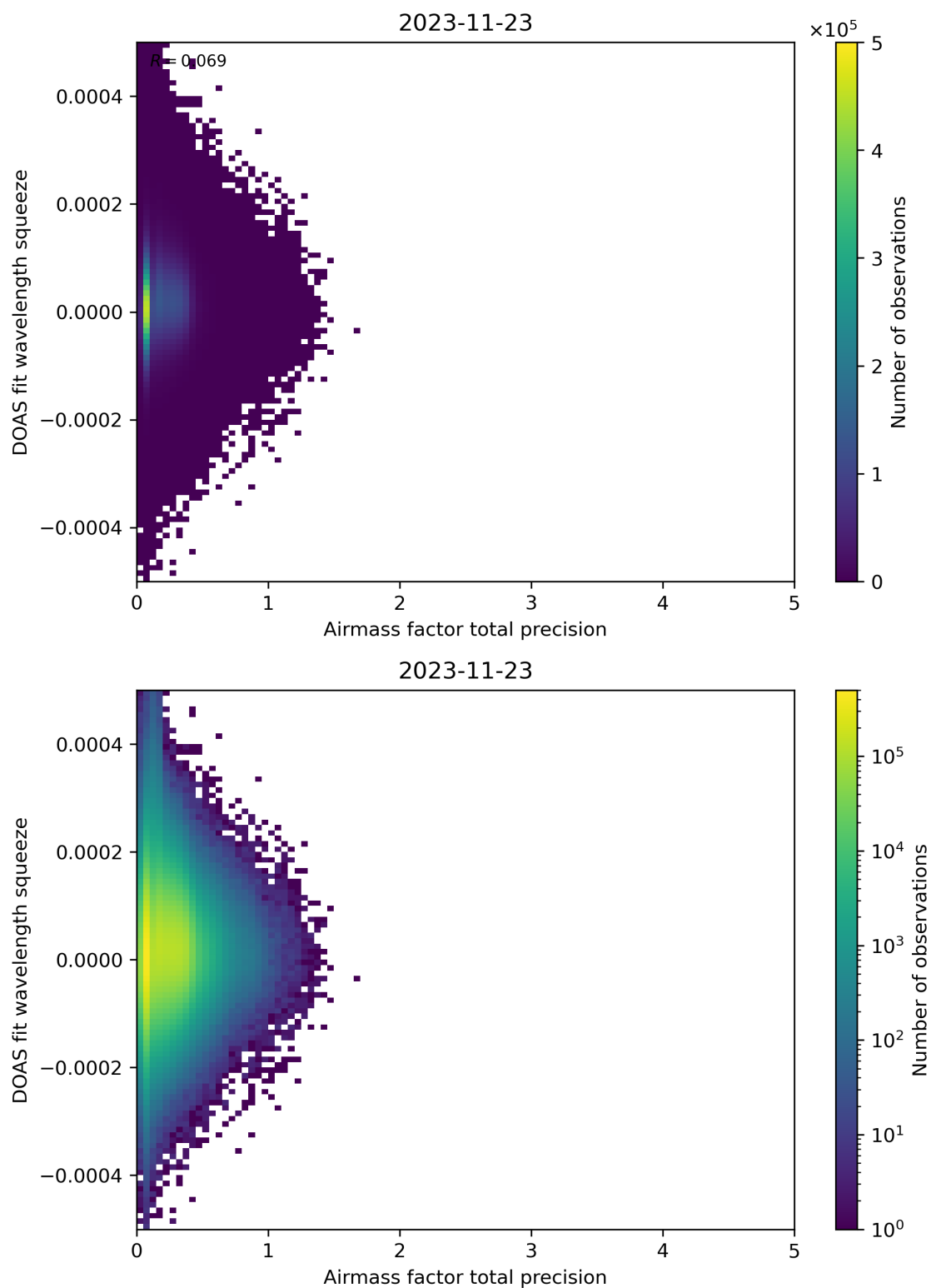
Figure 107: Scatter density plot of “Airmass factor total precision” against “DOAS fit wavelength squeeze” for 2023-11-23 to 2023-11-24.
