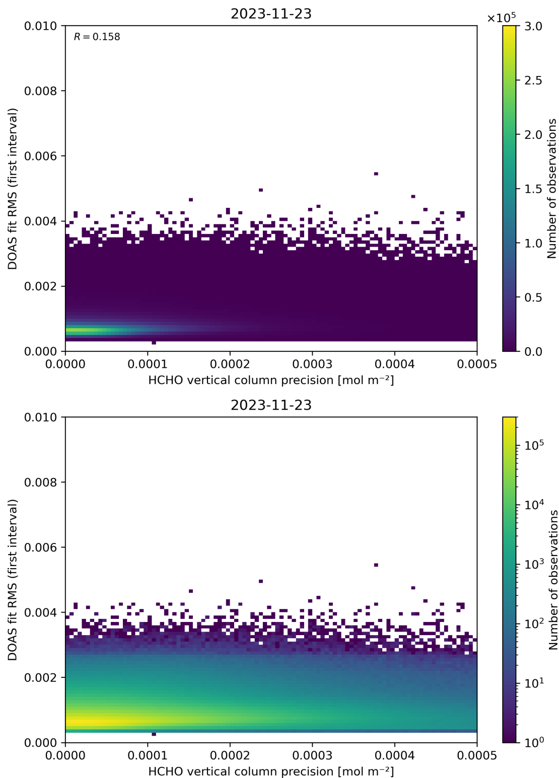
Figure 136: Scatter density plot of “HCHO vertical column precision” against “DOAS fit RMS (first interval)” for 2023-11-23 to 2023-11-24.
