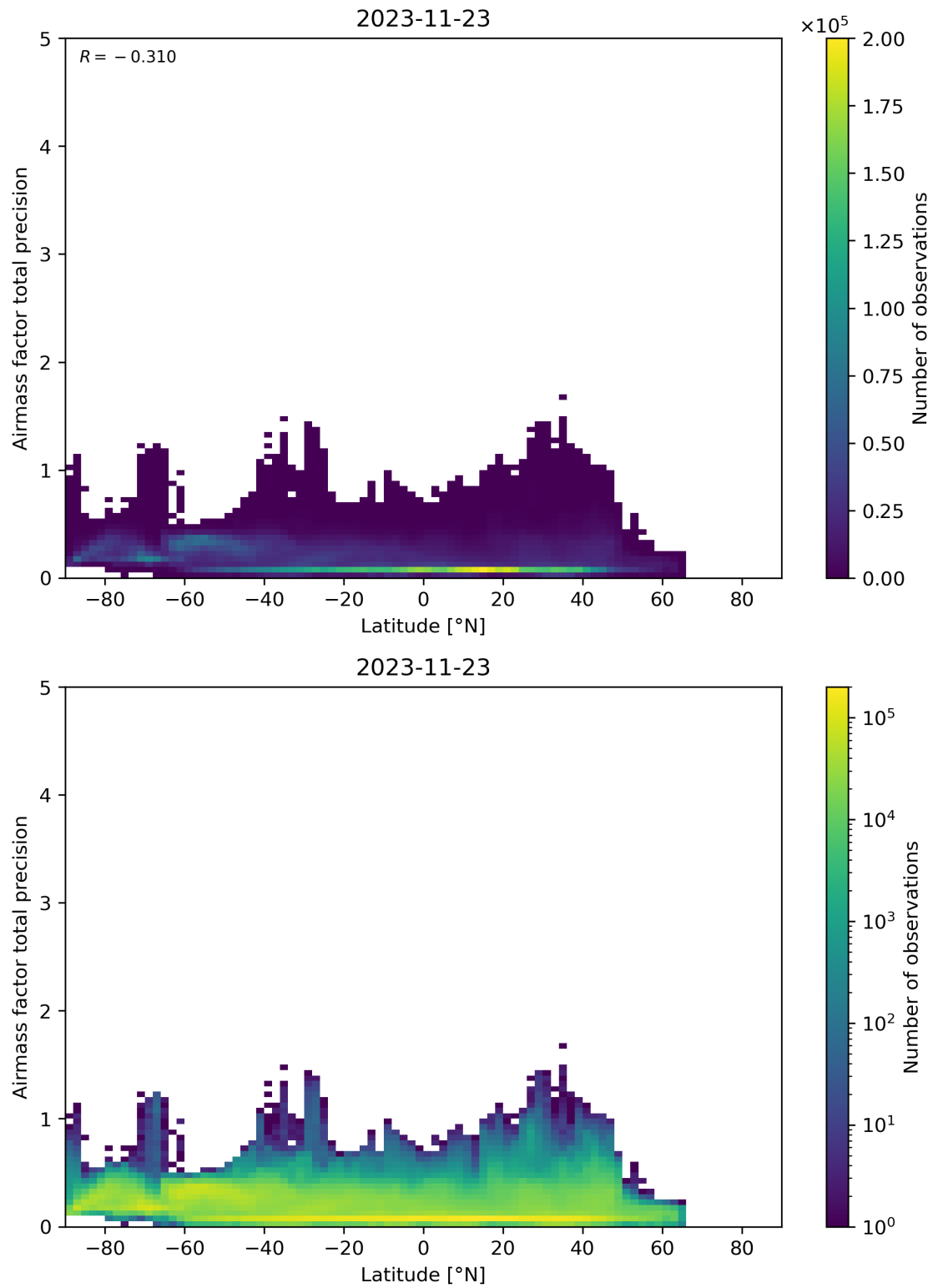
Figure 162: Scatter density plot of “Latitude” against “Airmass factor total precision” for 2023-11-23 to 2023-11-24.
