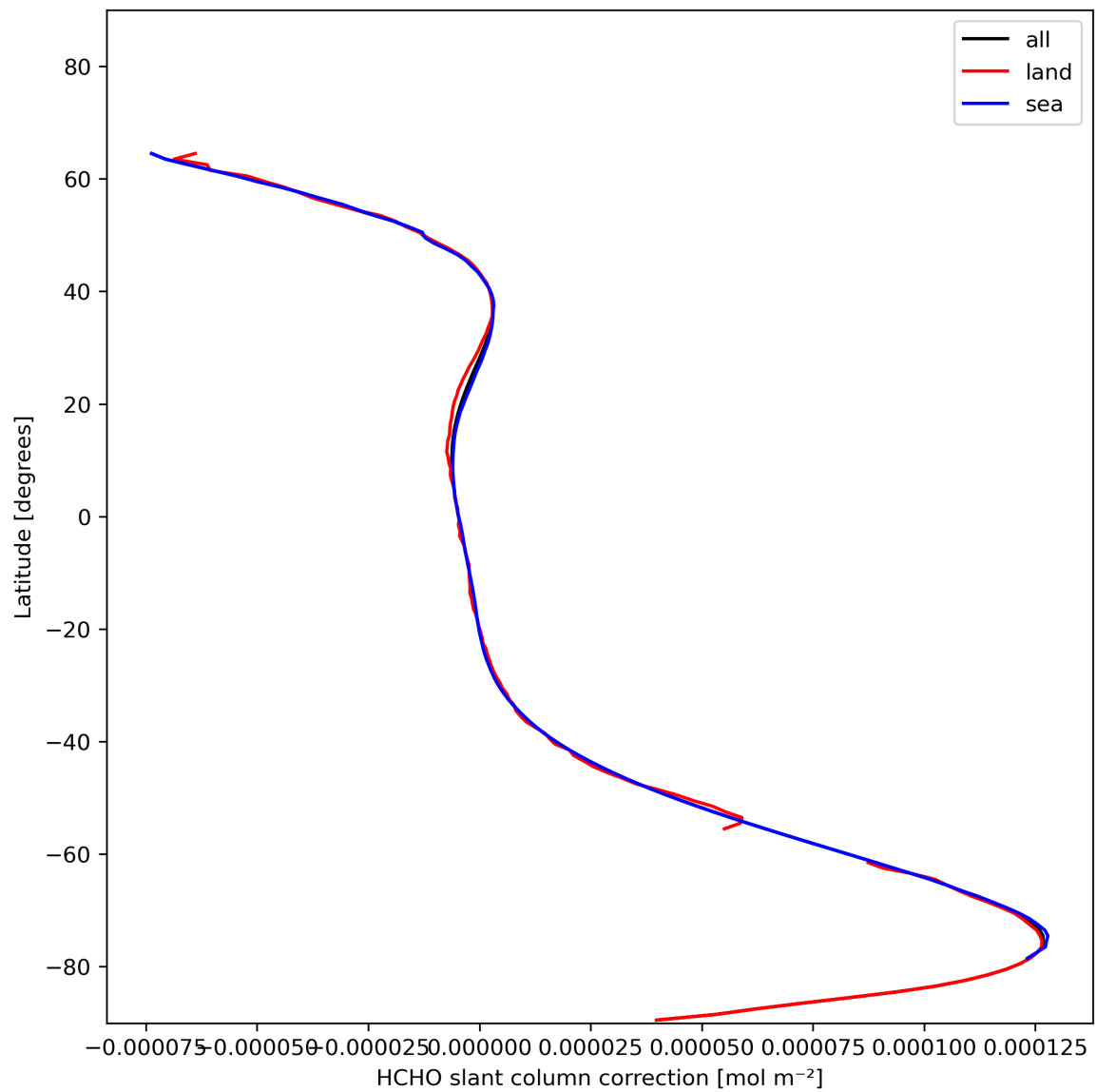
Figure 33: Zonal average of “HCHO slant column correction” for 2023-11-23 to 2023-11-24.
