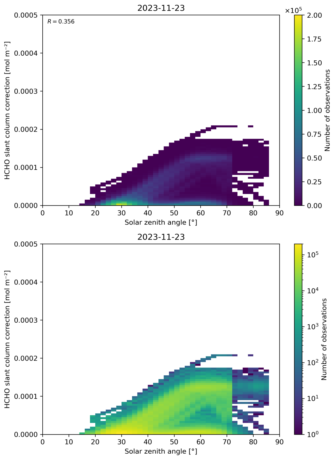
Figure 172: Scatter density plot of “Solar zenith angle” against “HCHO slant column correction” for 2023-11-23 to 2023-11-24.
