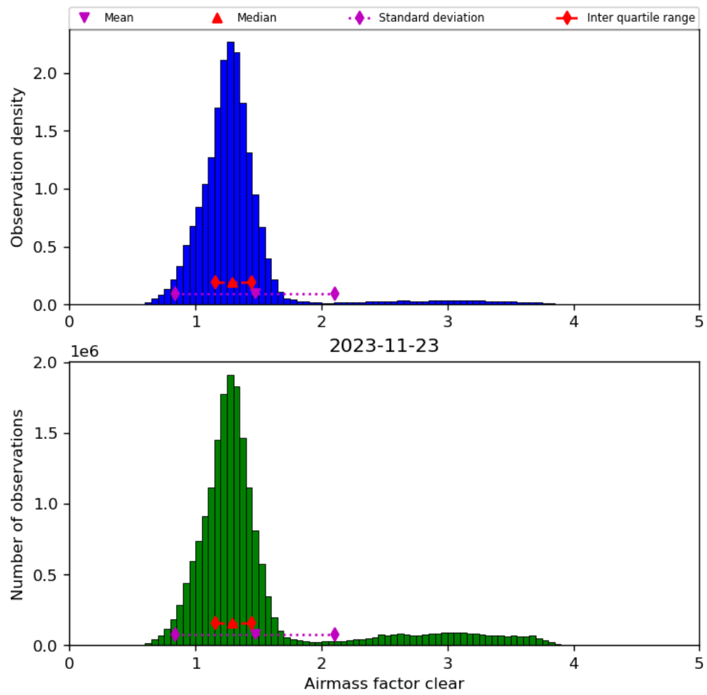
Figure 42: Histogram of “Airmass factor clear” for 2023-11-23 to 2023-11-24
