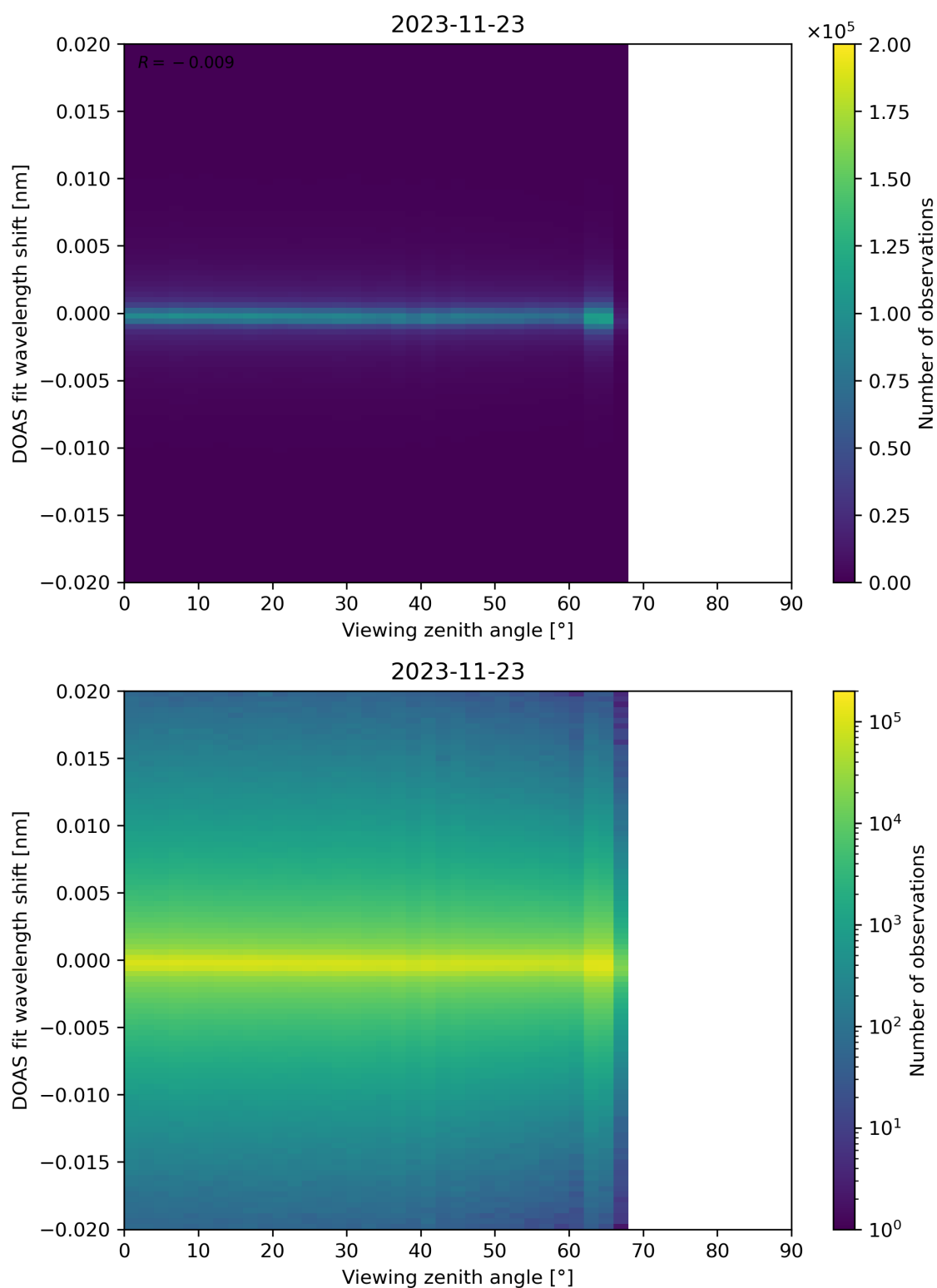
Figure 183: Scatter density plot of “Viewing zenith angle” against “DOAS fit wavelength shift” for 2023-11-23 to 2023-11-24.
