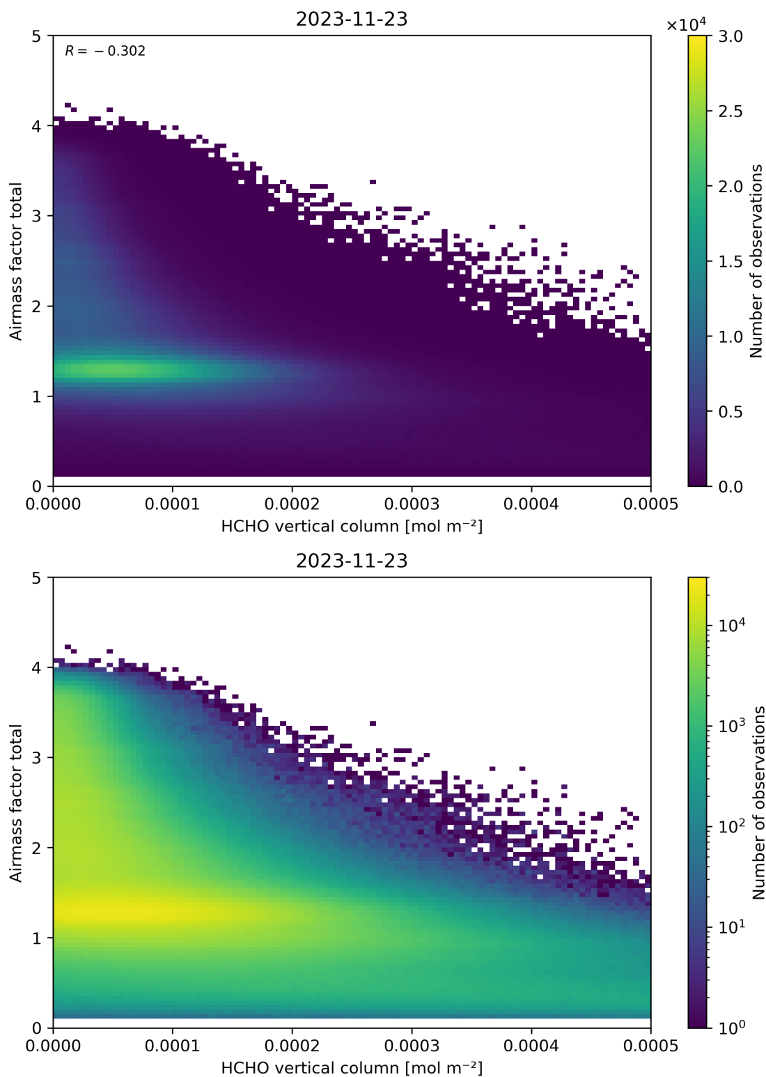
Figure 131: Scatter density plot of “HCHO vertical column” against “Airmass factor total” for 2023-11-23 to 2023-11-24.
