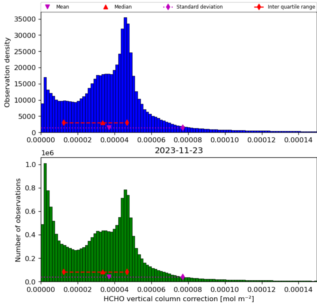
Figure 37: Histogram of “HCHO vertical column correction” for 2023-11-23 to 2023-11-24
