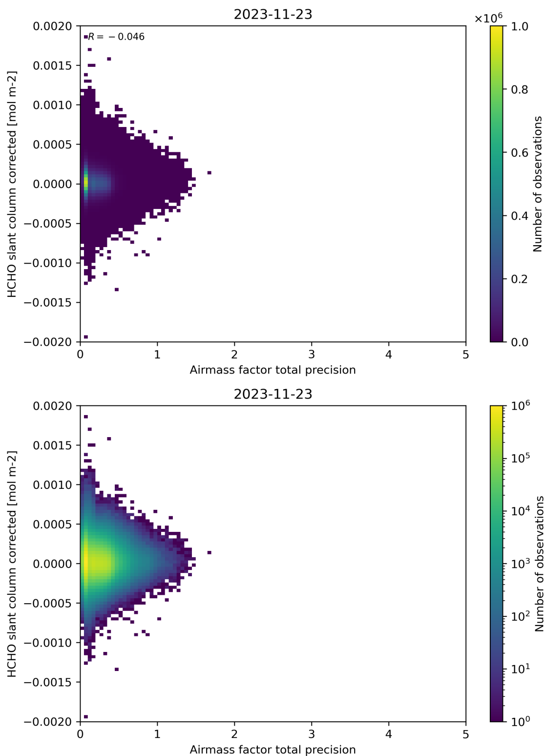
Figure 109: Scatter density plot of “Airmass factor total precision” against “HCHO slant column corrected” for 2023-11-23 to 2023-11-24.
