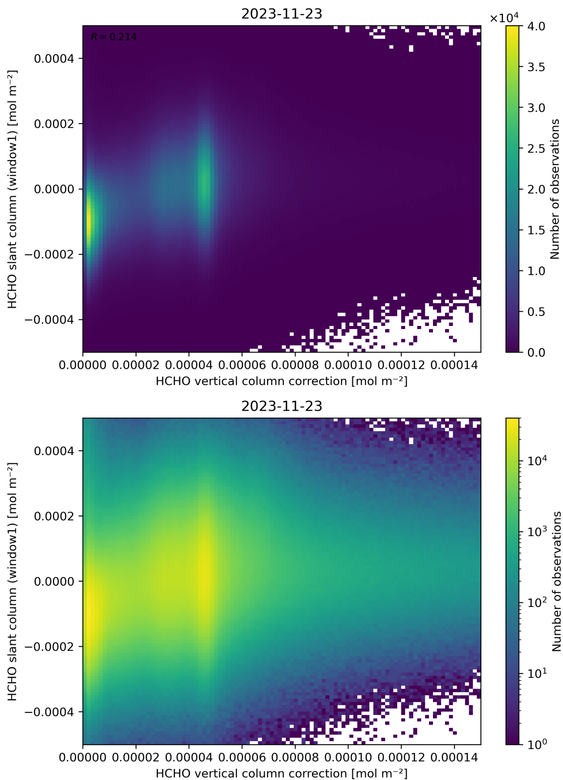
Figure 118: Scatter density plot of “HCHO vertical column correction” against “HCHO slant column (window1)” for 2023-11-23 to 2023-11-24.
