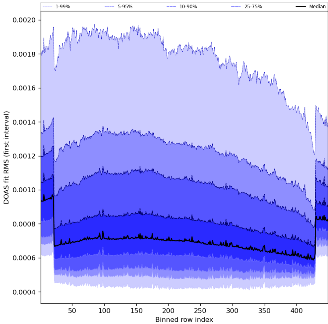
Figure 60: Along track statistics of “DOAS fit RMS (first interval)” for 2023-11-23 to 2023-11-24
