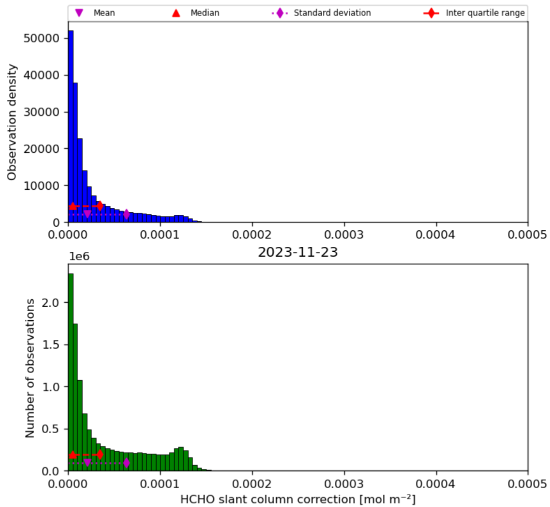
Figure 47: Histogram of “HCHO slant column correction” for 2023-11-23 to 2023-11-24
