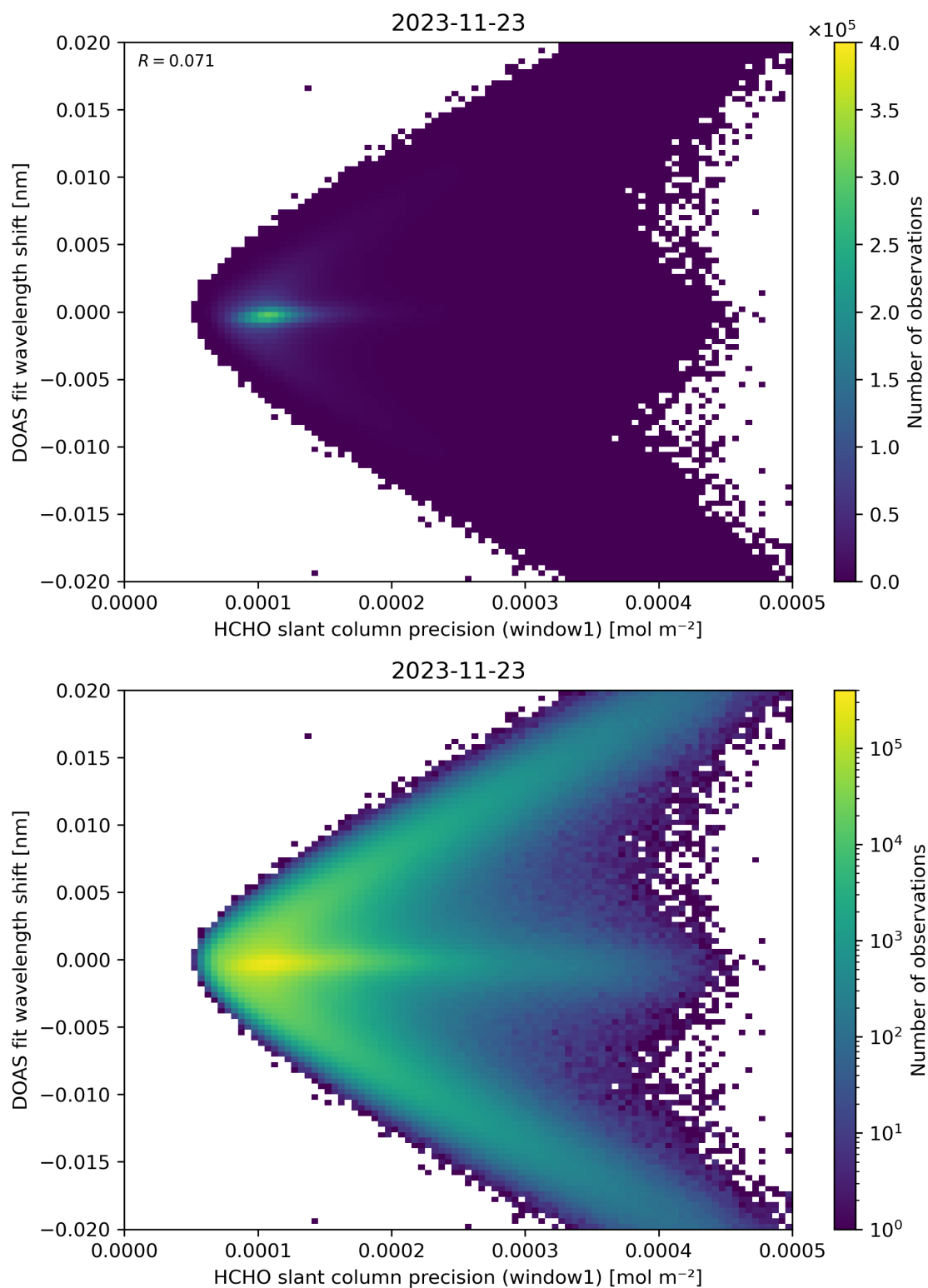
Figure 89: Scatter density plot of “HCHO slant column precision (window1)” against “DOAS fit wavelength shift” for 2023-11-23 to 2023-11-24.
