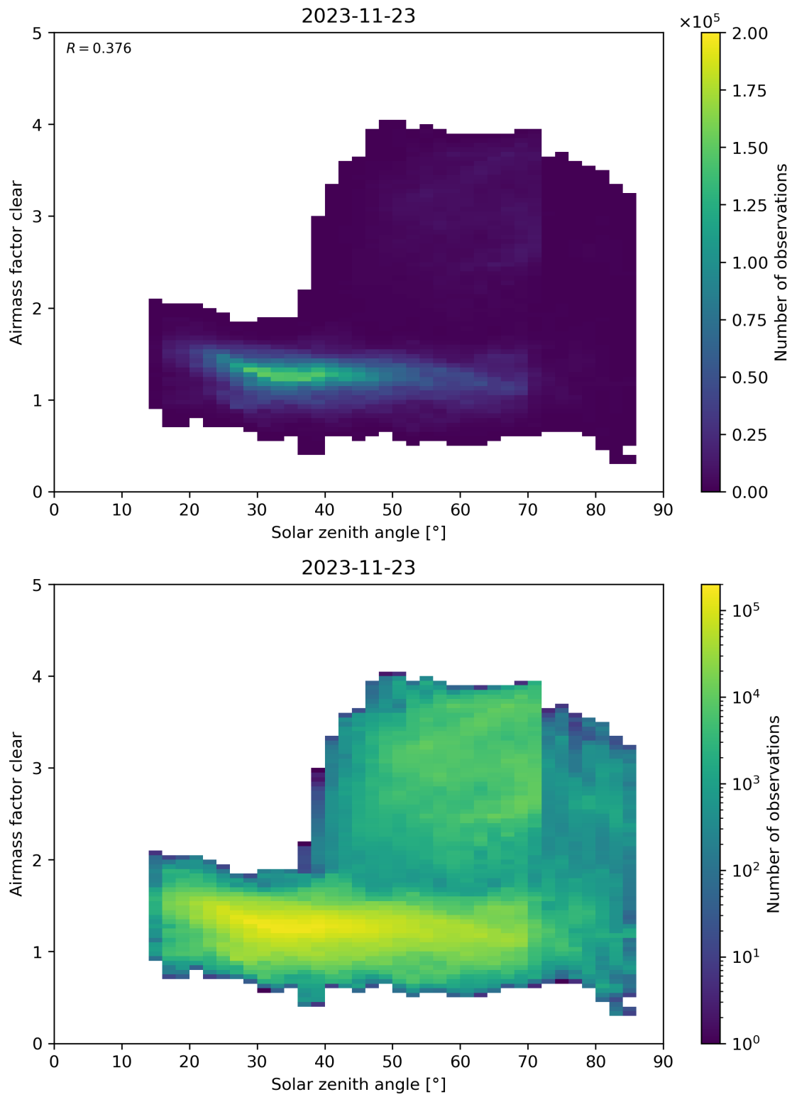
Figure 170: Scatter density plot of “Solar zenith angle” against “Airmass factor clear” for 2023-11-23 to 2023-11-24.
