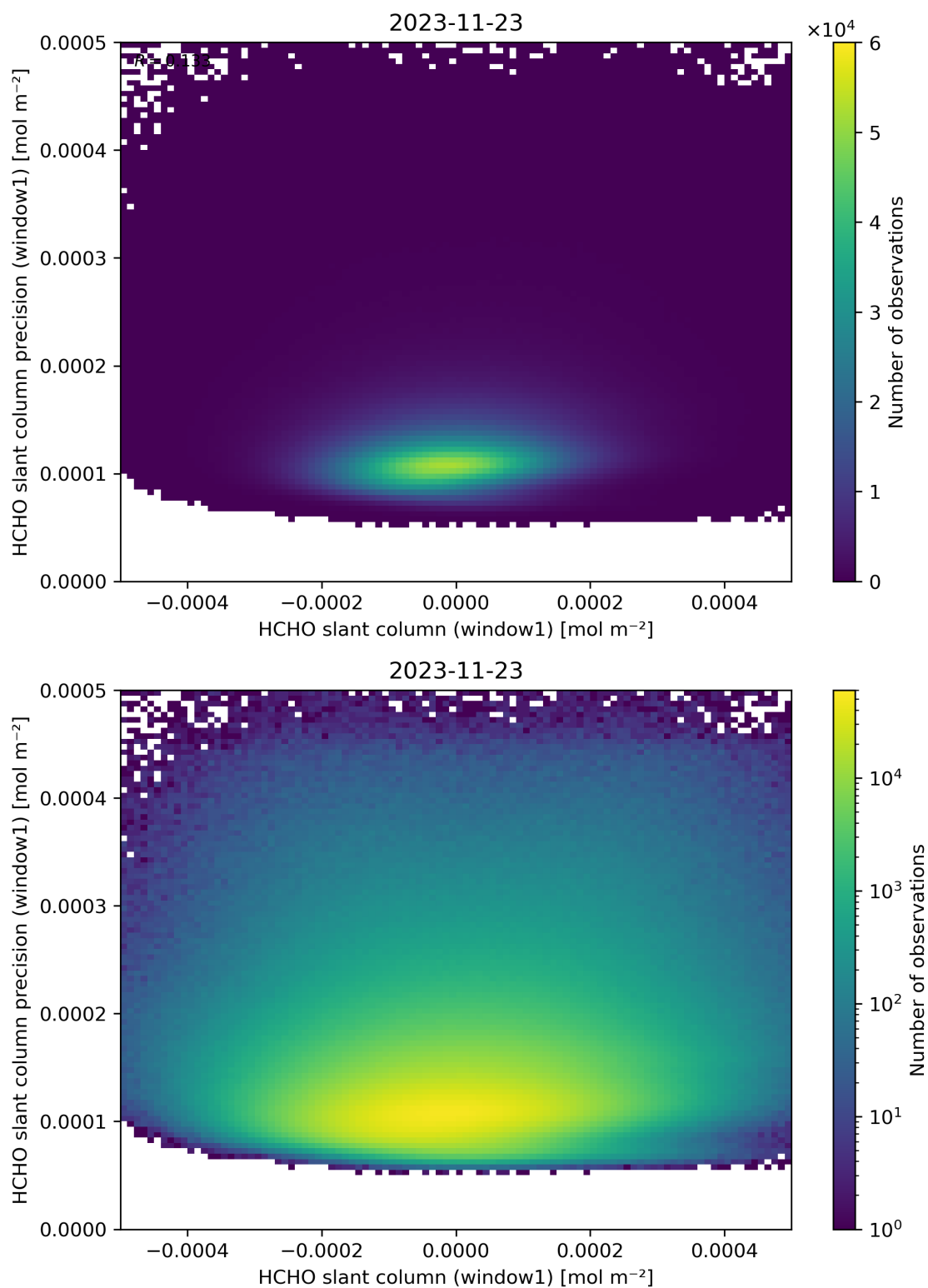
Figure 84: Scatter density plot of “HCHO slant column (window1)” against “HCHO slant column precision (window1)” for 2023-11-23 to 2023-11-24.
