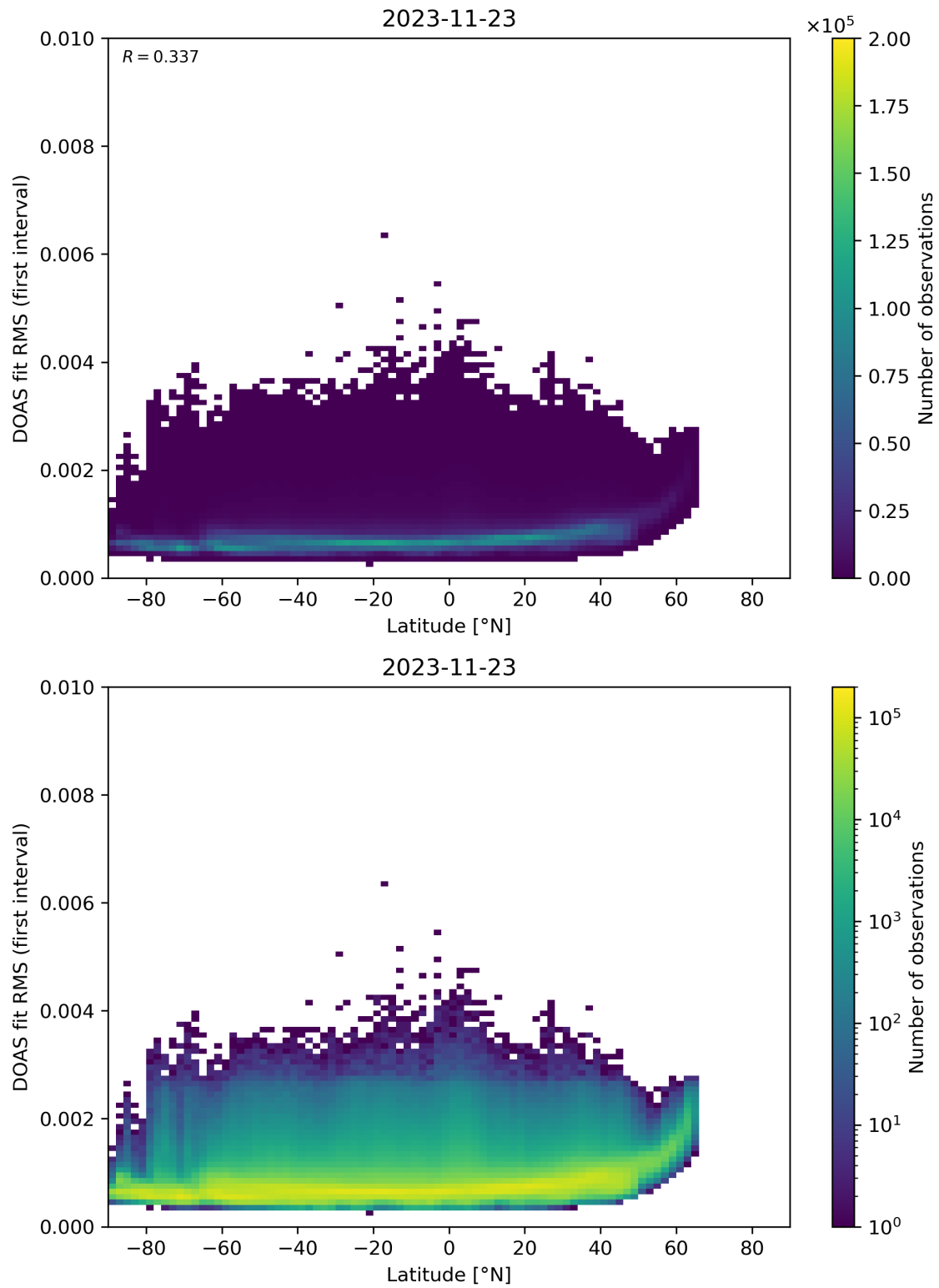
Figure 153: Scatter density plot of “Latitude” against “DOAS fit RMS (first interval)” for 2023-11-23 to 2023-11-24.
