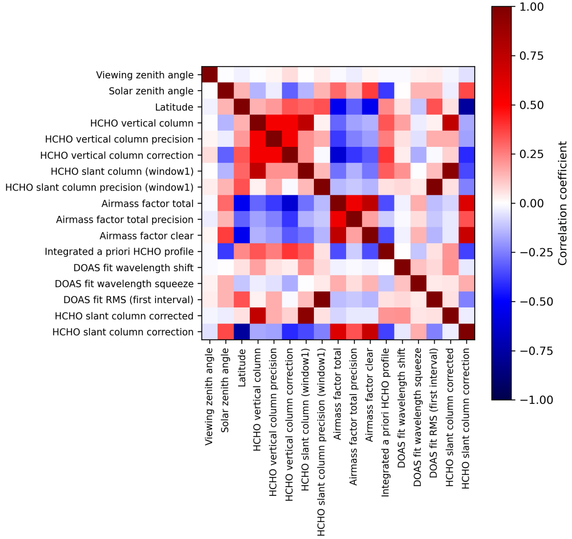
Figure 2: Map of correlation matrix for 2023-11-23 to 2023-11-24.
