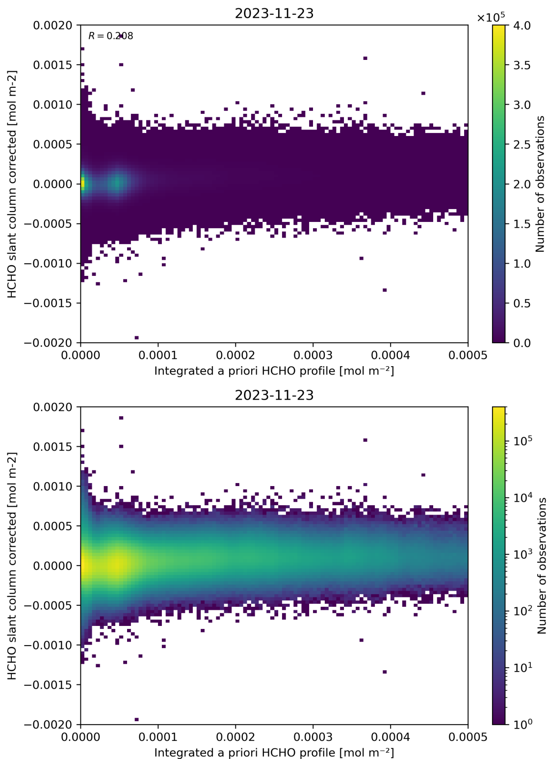
Figure 151: Scatter density plot of “Integrated a priori HCHO profile” against “HCHO slant column corrected” for 2023-11-23 to 2023-11-24.
