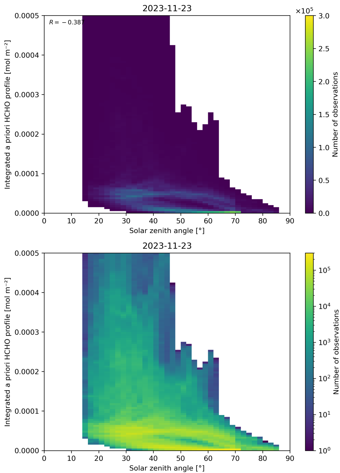
Figure 180: Scatter density plot of “Solar zenith angle” against “Integrated a priori HCHO profile” for 2023-11-23 to 2023-11-24.
