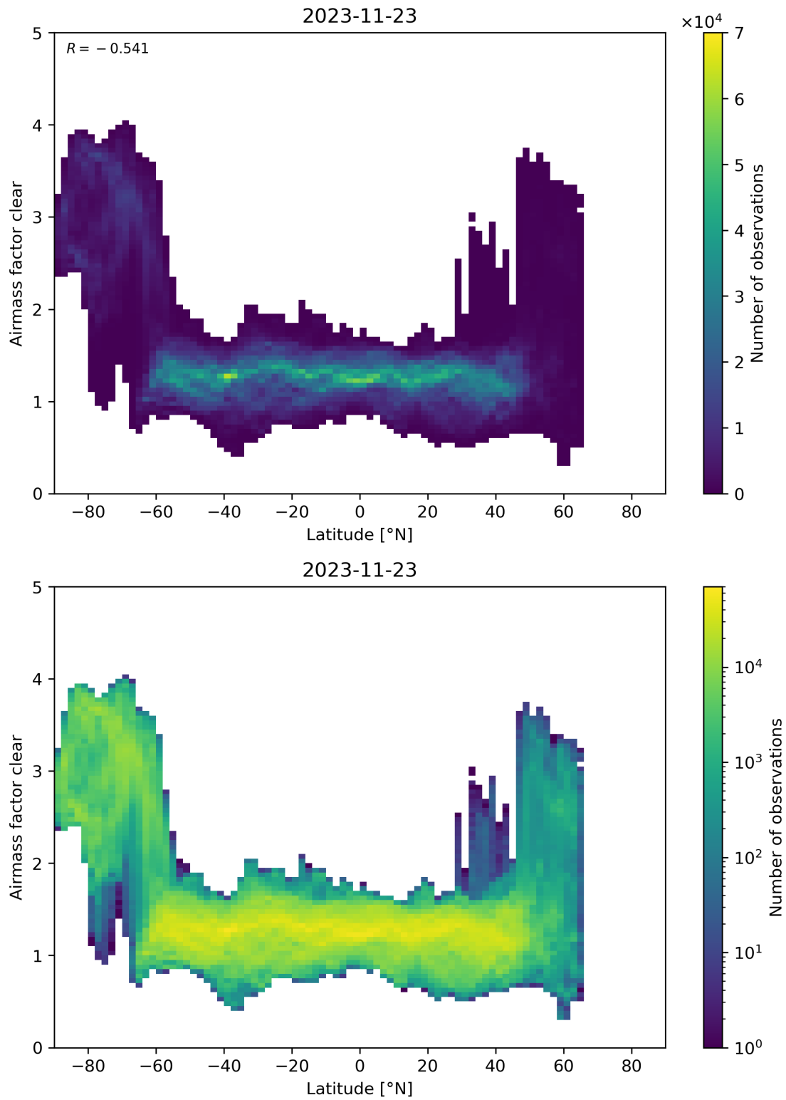
Figure 156: Scatter density plot of “Latitude” against “Airmass factor clear” for 2023-11-23 to 2023-11-24.
