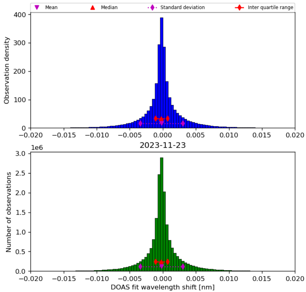
Figure 44: Histogram of “DOAS fit wavelength shift” for 2023-11-23 to 2023-11-24
