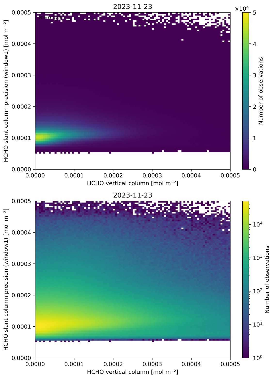
Figure 130: Scatter density plot of “HCHO vertical column” against “HCHO slant column precision (window1)” for 2023-11-23 to 2023-11-24.
