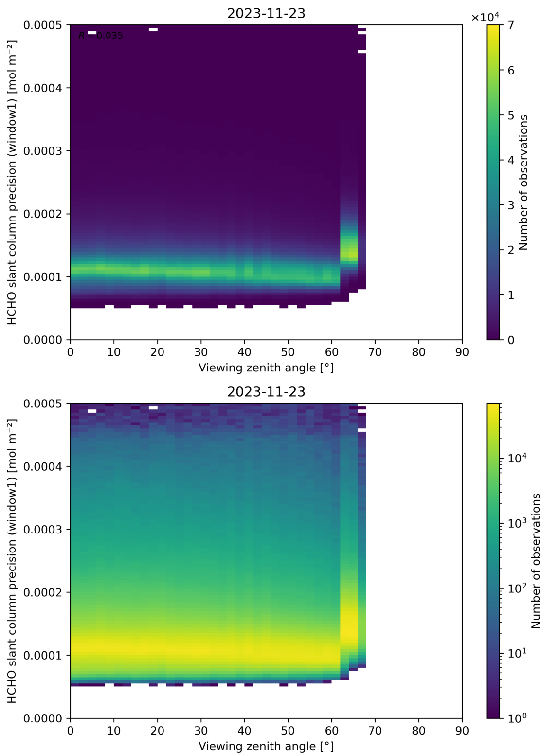
Figure 189: Scatter density plot of “Viewing zenith angle” against “HCHO slant column precision (window1)” for 2023-11-23 to 2023-11-24.
