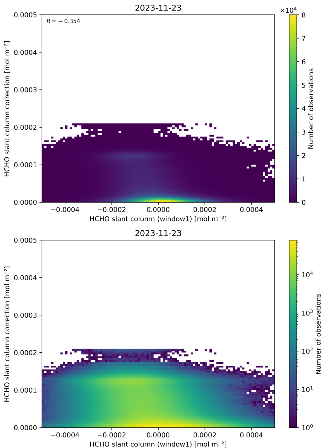
Figure 83: Scatter density plot of “HCHO slant column (window1)” against “HCHO slant column correction” for 2023-11-23 to 2023-11-24.
