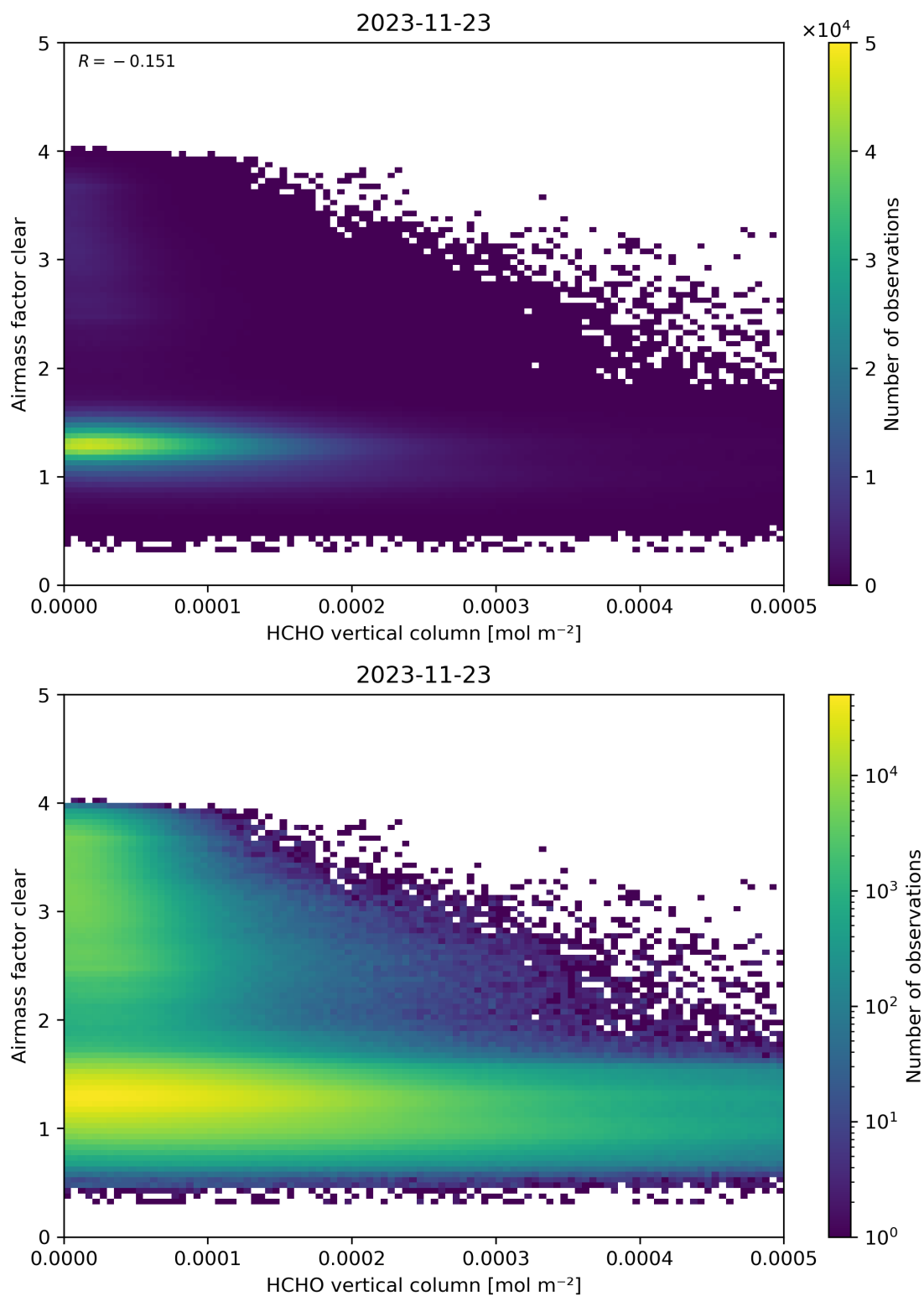
Figure 126: Scatter density plot of “HCHO vertical column” against “Airmass factor clear” for 2023-11-23 to 2023-11-24.
