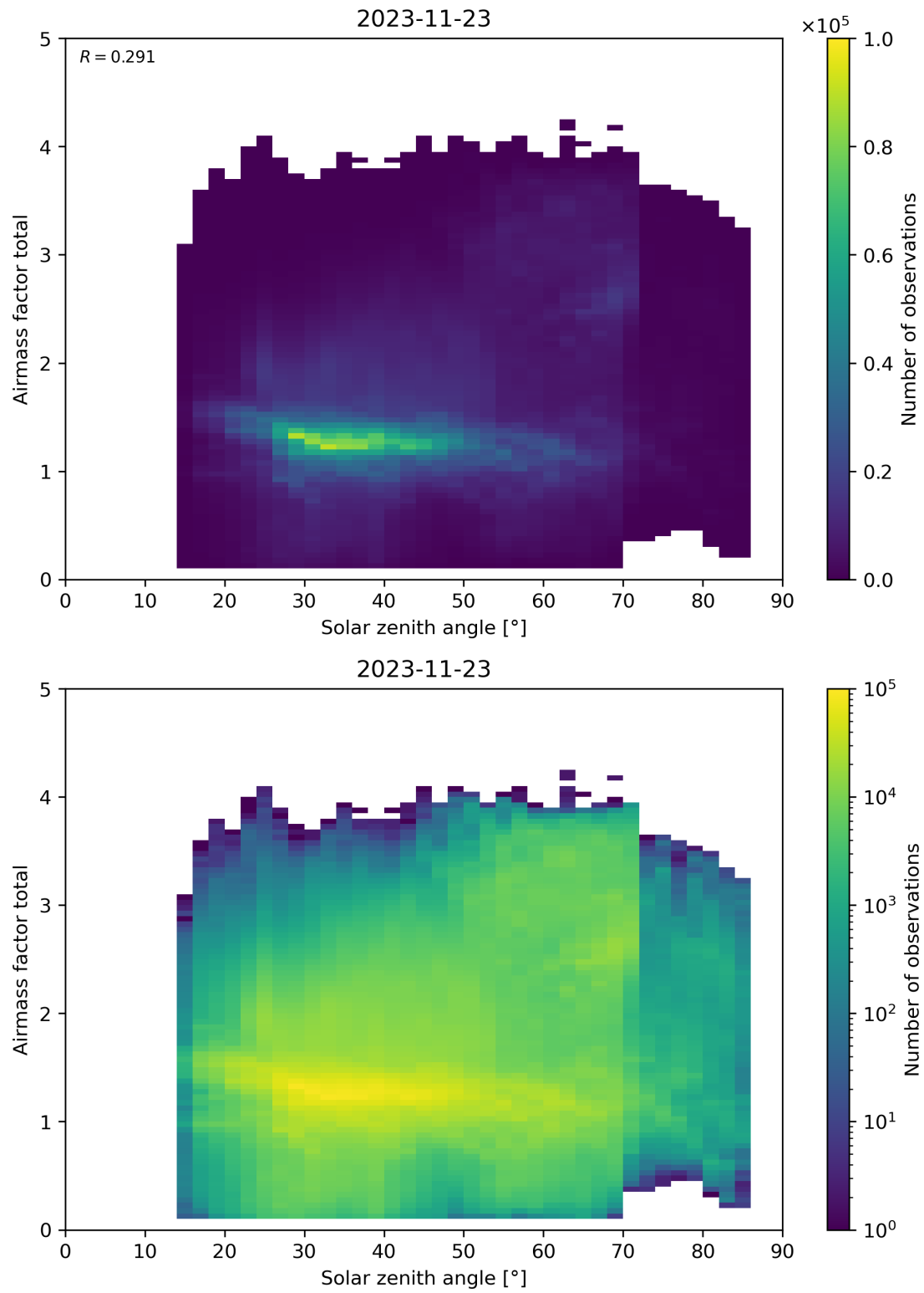
Figure 175: Scatter density plot of “Solar zenith angle” against “Airmass factor total” for 2023-11-23 to 2023-11-24.
