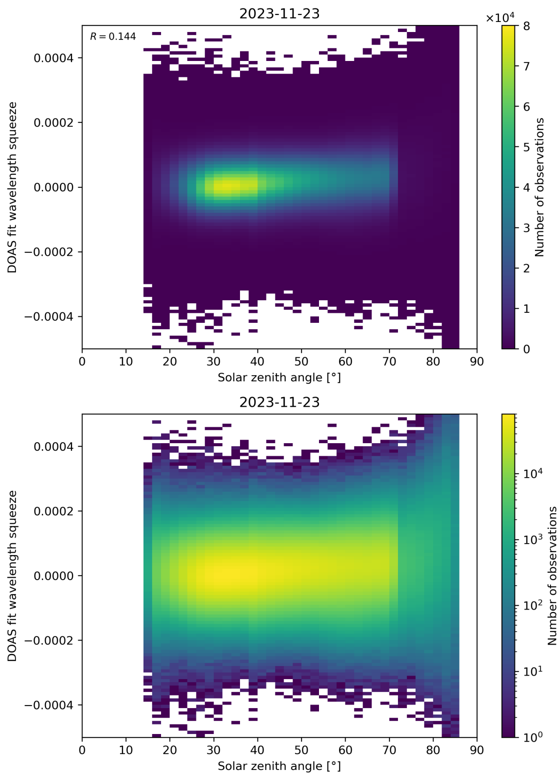
Figure 169: Scatter density plot of “Solar zenith angle” against “DOAS fit wavelength squeeze” for 2023-11-23 to 2023-11-24.
