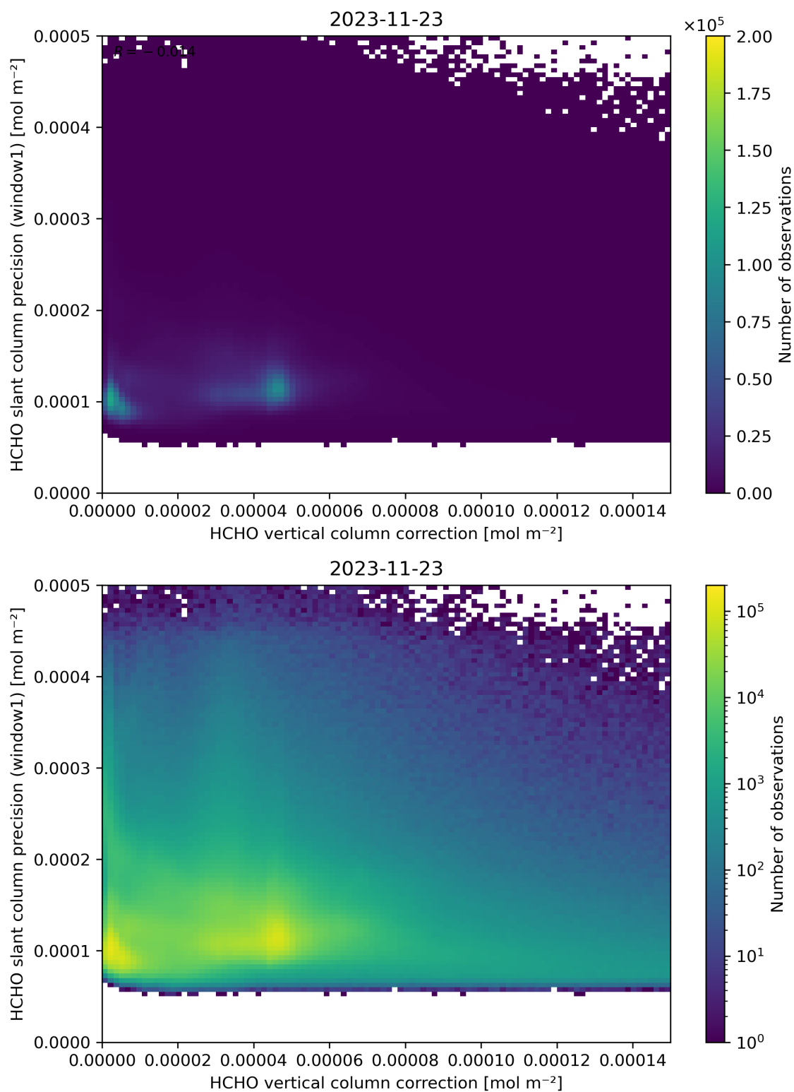
Figure 119: Scatter density plot of “HCHO vertical column correction” against “HCHO slant column precision (window1)” for 2023-11-23 to 2023-11-24.
