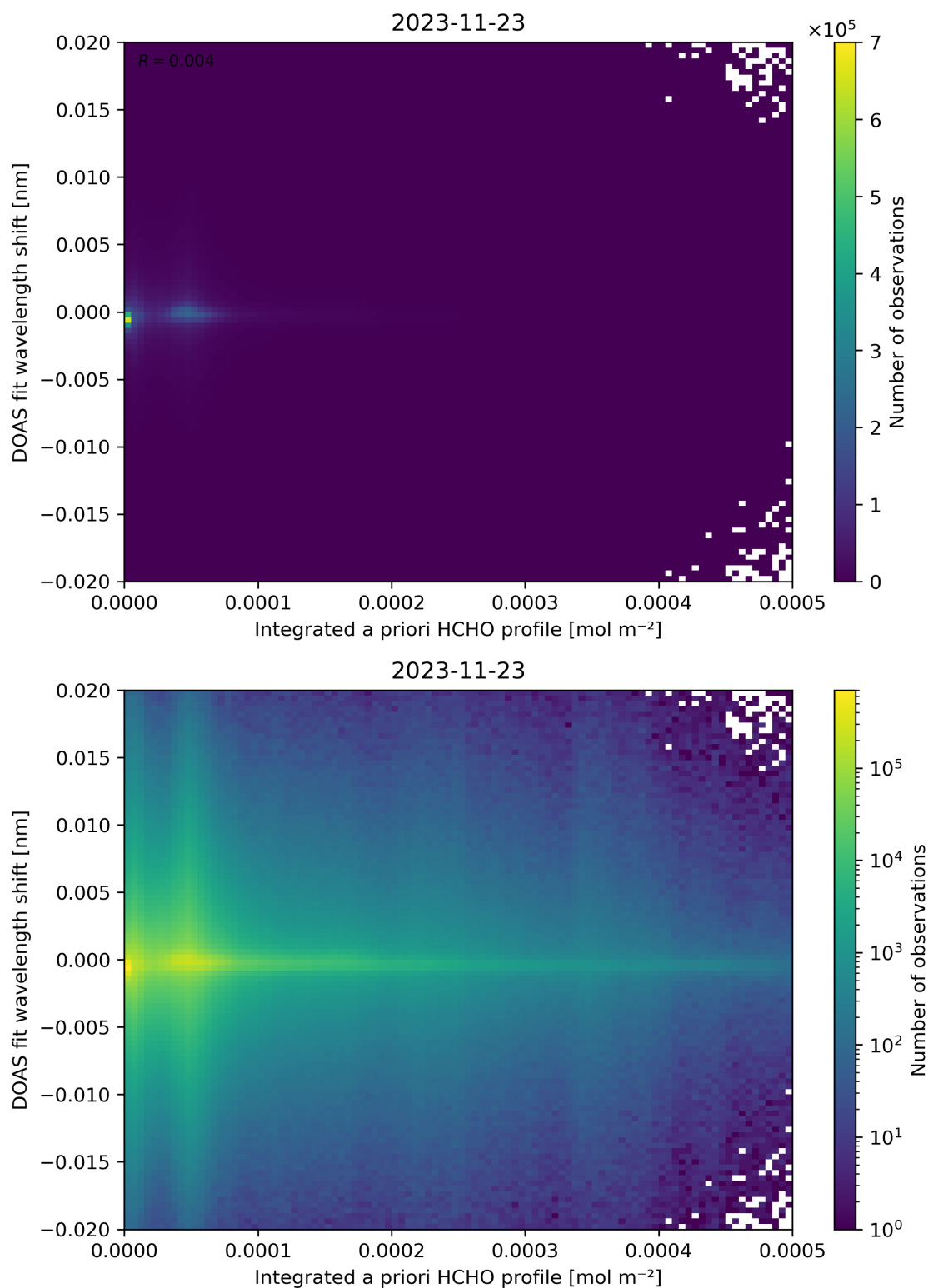
Figure 149: Scatter density plot of “Integrated a priori HCHO profile” against “DOAS fit wavelength shift” for 2023-11-23 to 2023-11-24.
