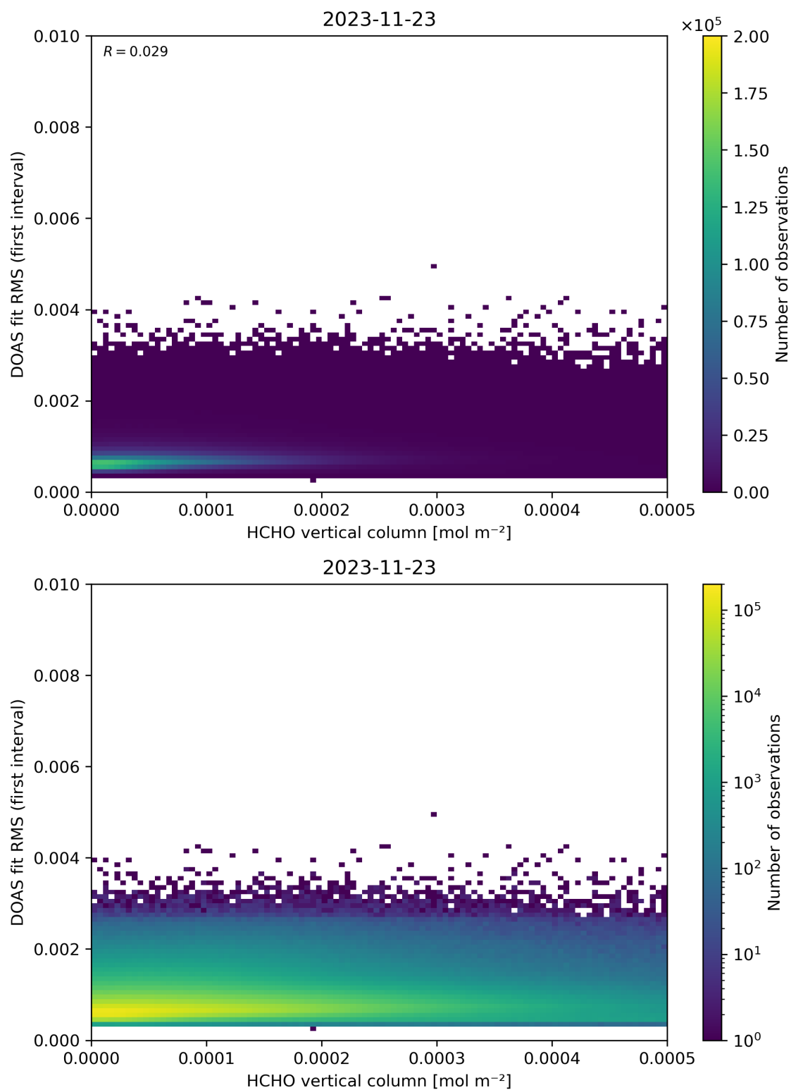
Figure 123: Scatter density plot of “HCHO vertical column” against “DOAS fit RMS (first interval)” for 2023-11-23 to 2023-11-24.
