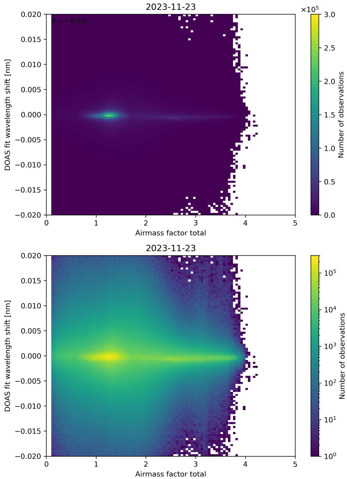
Figure 98: Scatter density plot of “Airmass factor total” against “DOAS fit wavelength shift” for 2023-11-23 to 2023-11-24.
