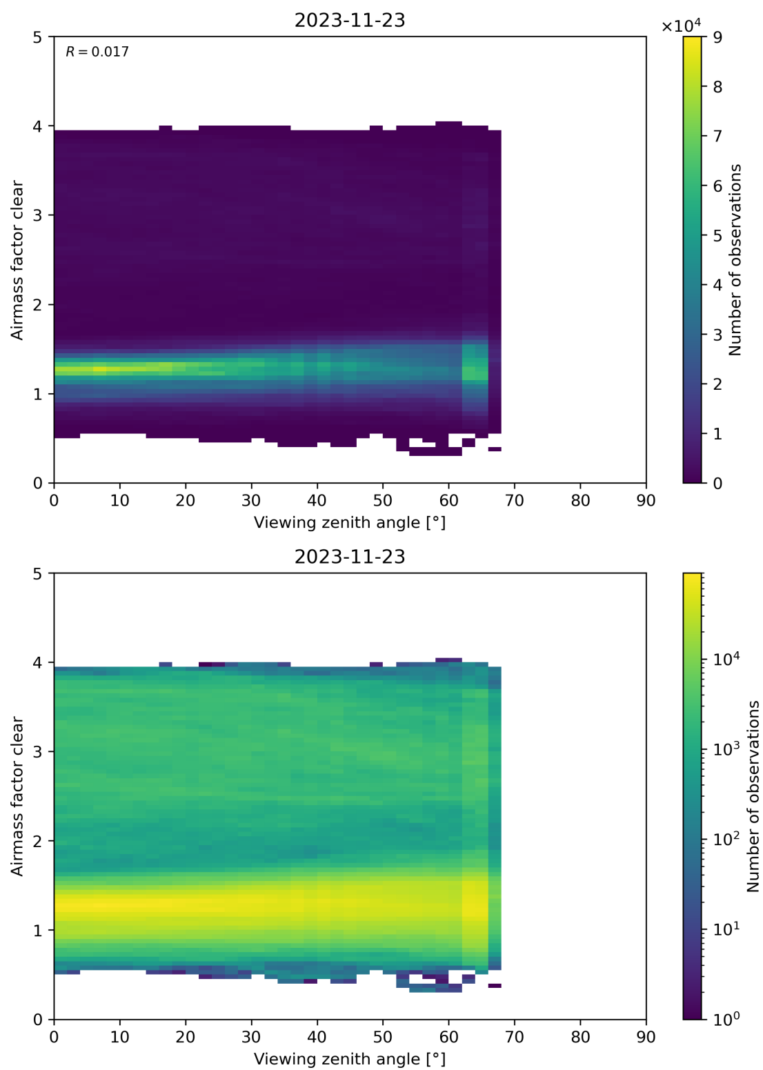
Figure 185: Scatter density plot of “Viewing zenith angle” against “Airmass factor clear” for 2023-11-23 to 2023-11-24.
