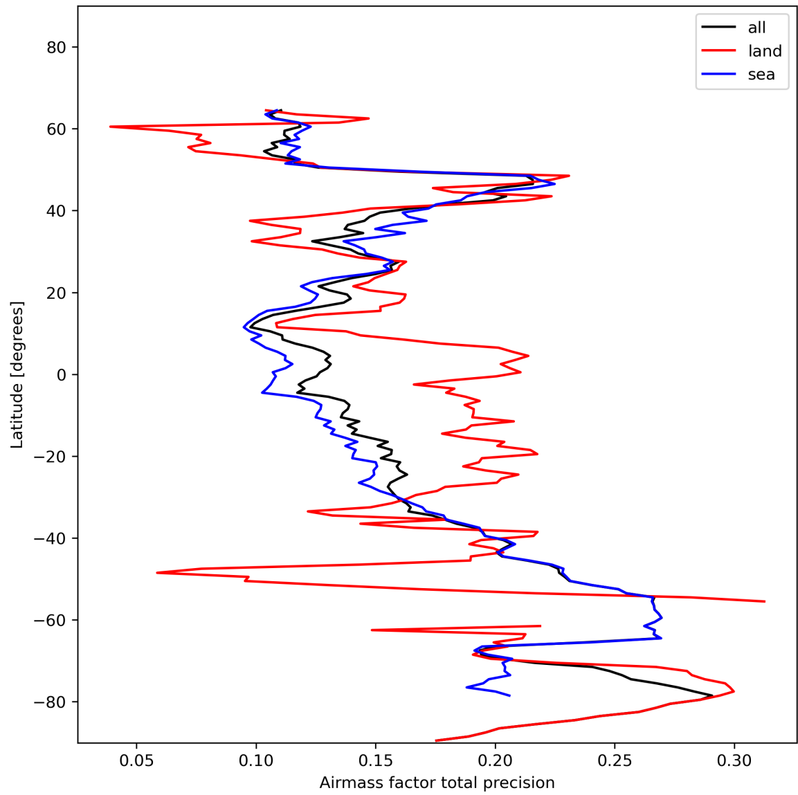
Figure 27: Zonal average of “Airmass factor total precision” for 2023-11-23 to 2023-11-24.
