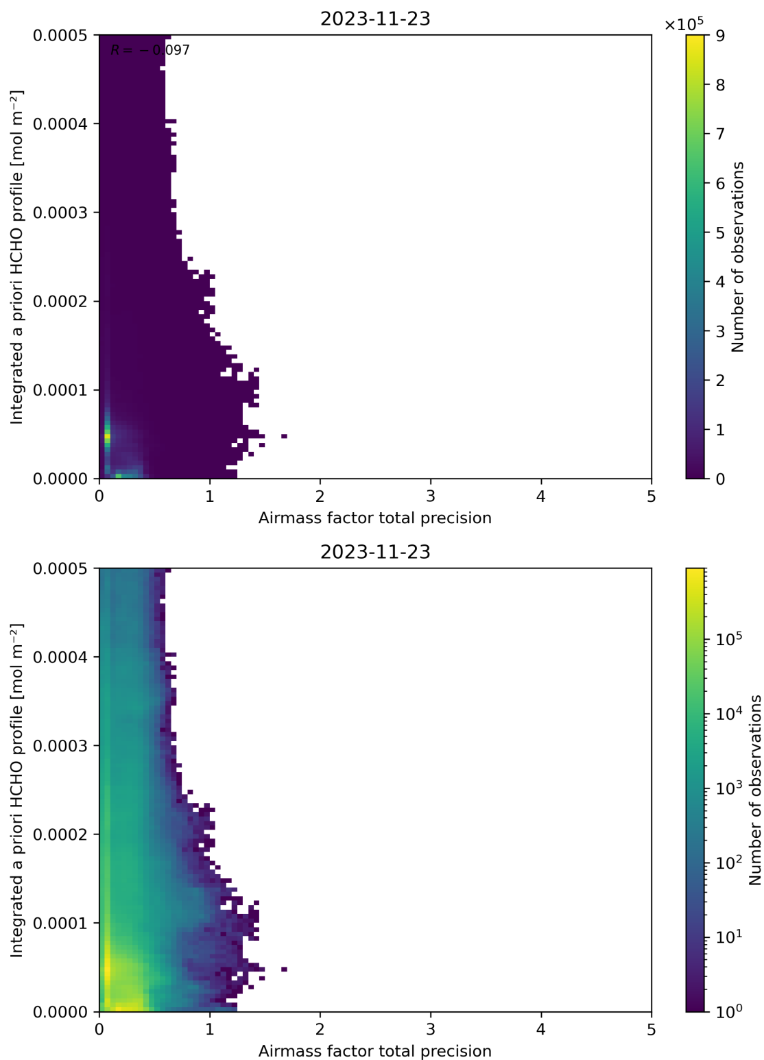
Figure 111: Scatter density plot of “Airmass factor total precision” against “Integrated a priori HCHO profile” for 2023-11-23 to 2023-11-24.
