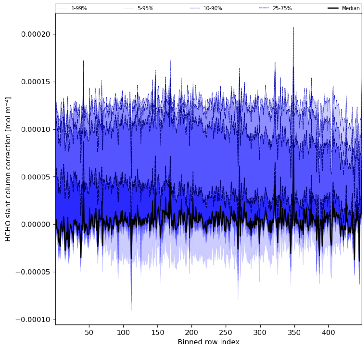
Figure 61: Along track statistics of “HCHO slant column correction” for 2023-11-23 to 2023-11-24
