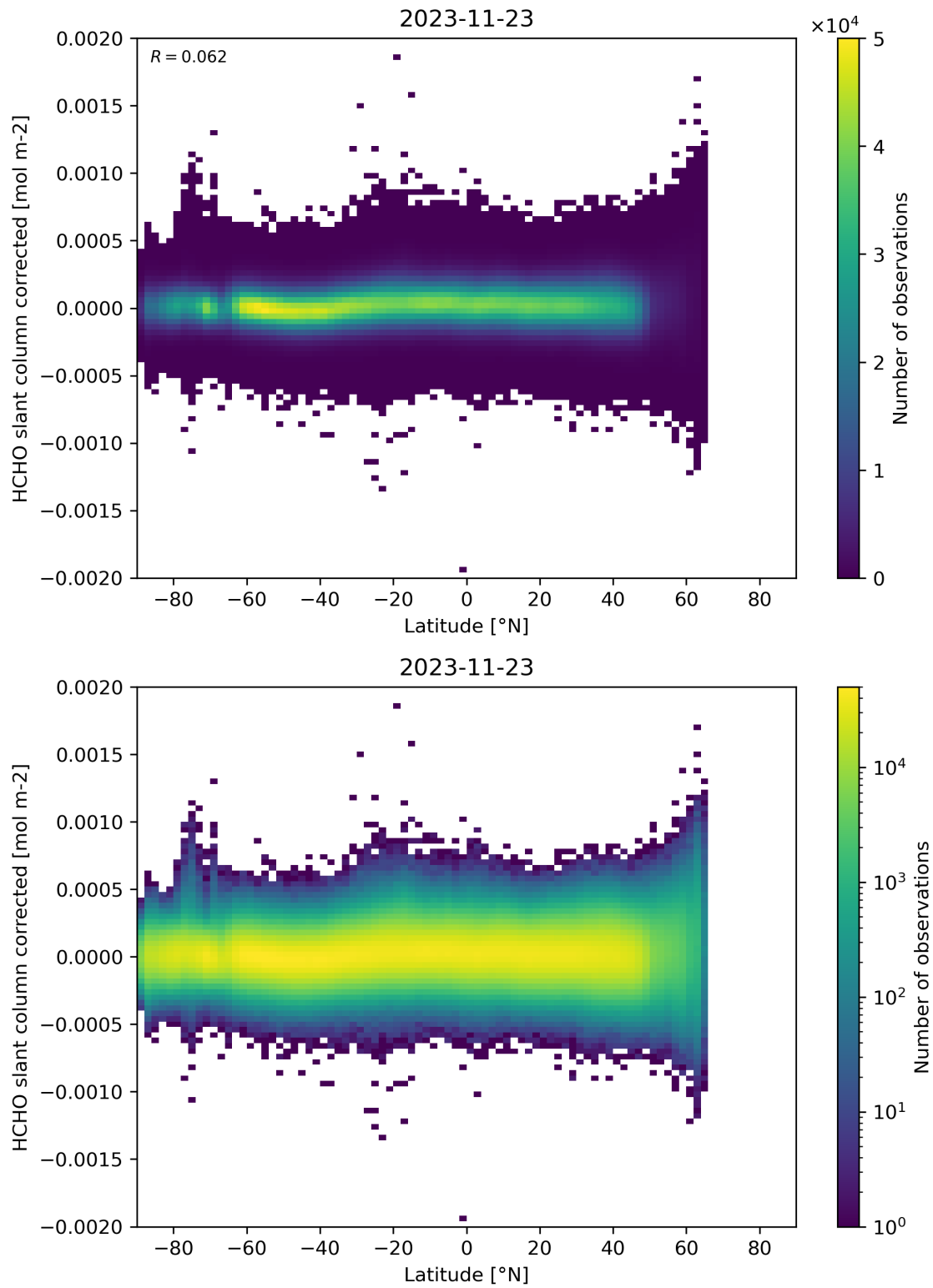
Figure 157: Scatter density plot of “Latitude” against “HCHO slant column corrected” for 2023-11-23 to 2023-11-24.
