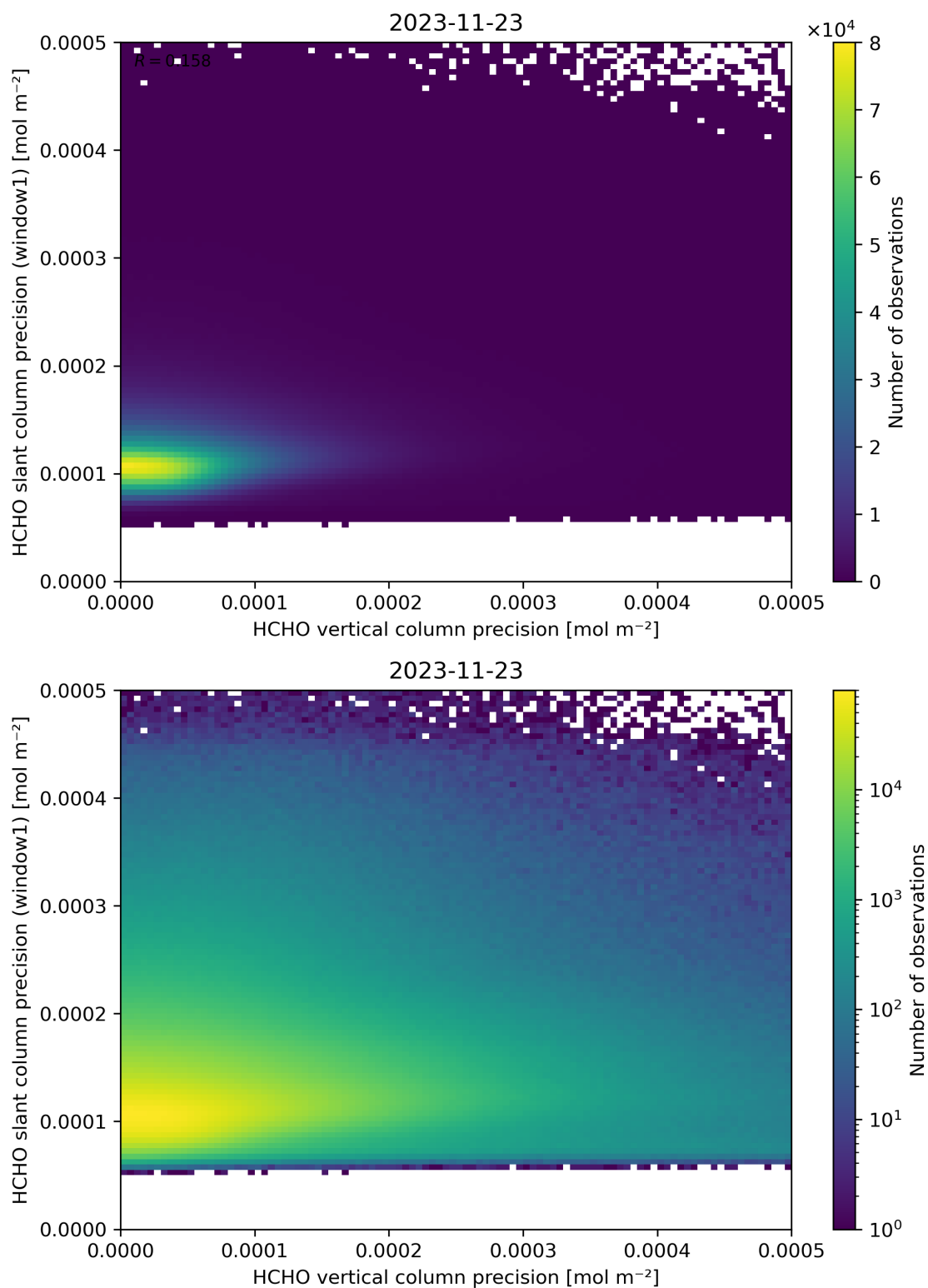
Figure 143: Scatter density plot of “HCHO vertical column precision” against “HCHO slant column precision (window1)” for 2023-11-23 to 2023-11-24.
