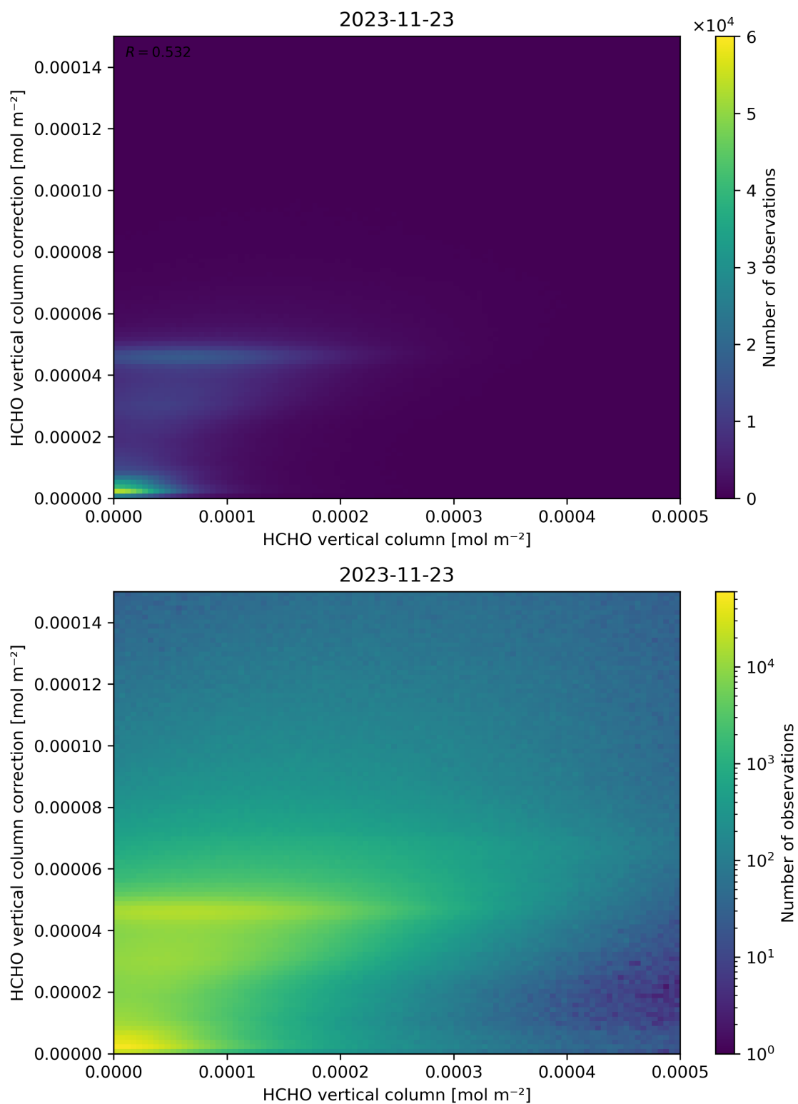
Figure 133: Scatter density plot of “HCHO vertical column” against “HCHO vertical column correction” for 2023-11-23 to 2023-11-24.
