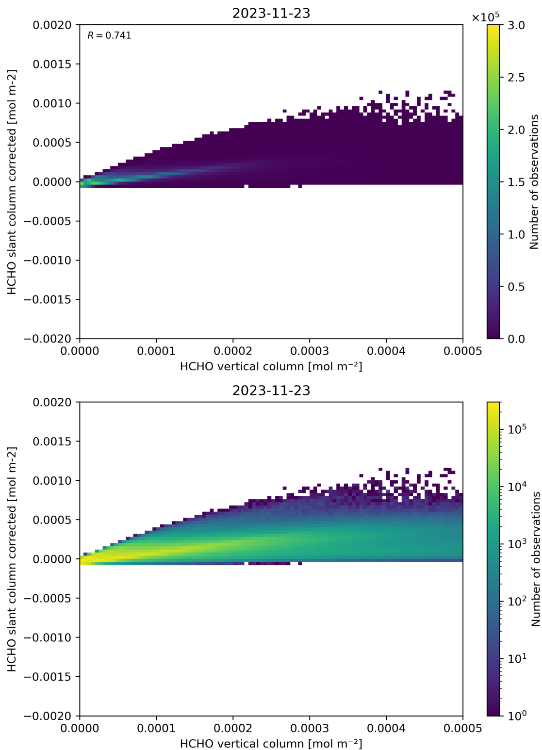
Figure 127: Scatter density plot of “HCHO vertical column” against “HCHO slant column corrected” for 2023-11-23 to 2023-11-24.
