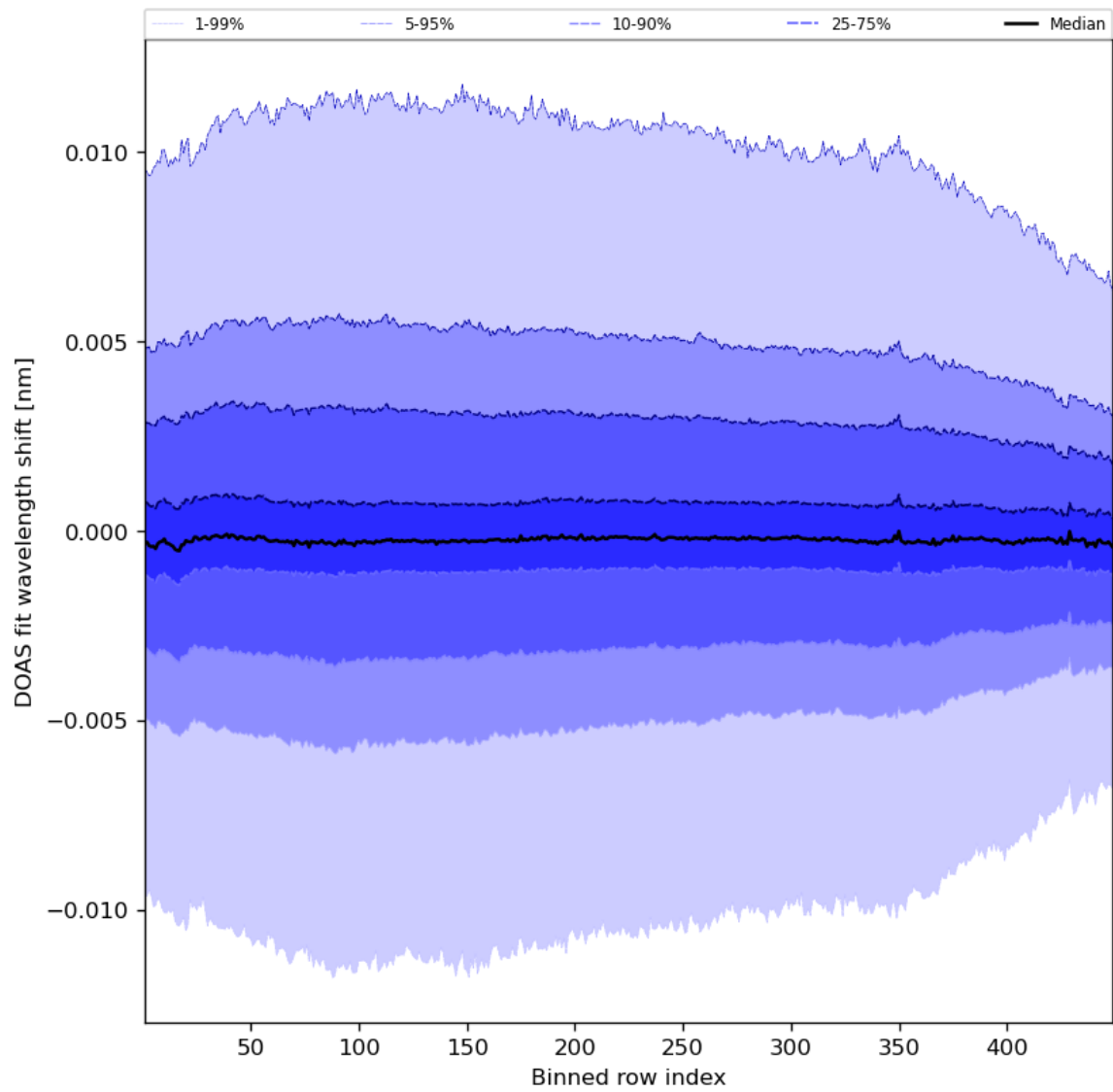
Figure 58: Along track statistics of “DOAS fit wavelength shift” for 2023-11-23 to 2023-11-24
