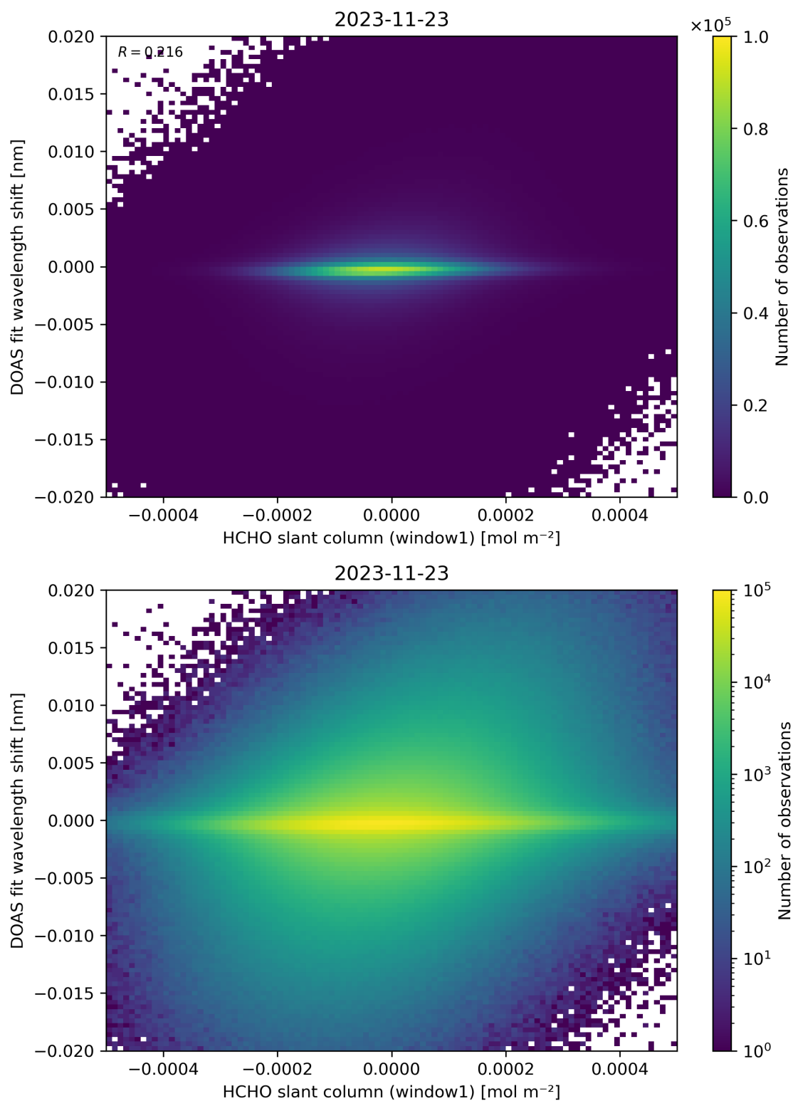
Figure 79: Scatter density plot of “HCHO slant column (window1)” against “DOAS fit wavelength shift” for 2023-11-23 to 2023-11-24.
