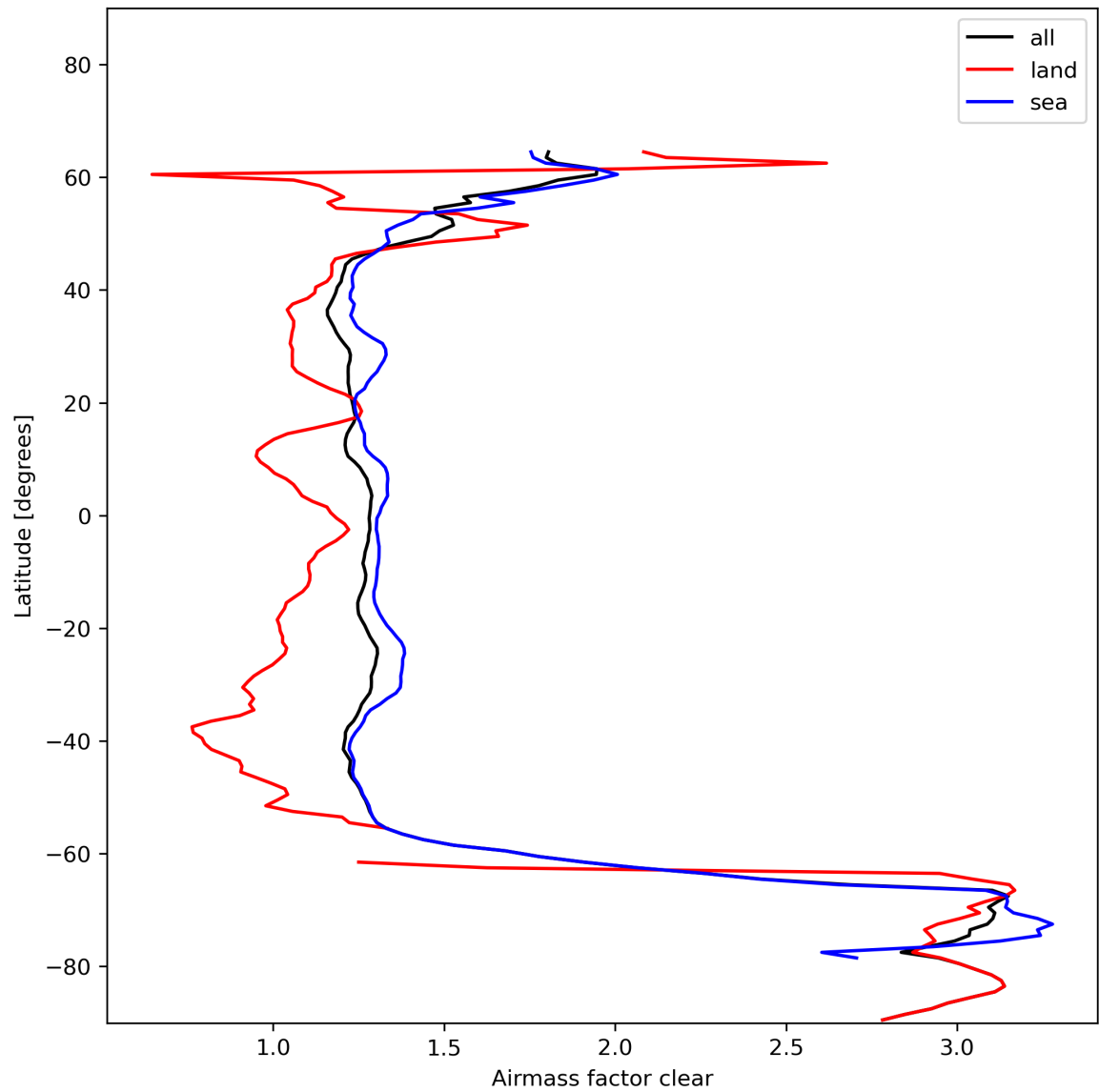
Figure 28: Zonal average of “Airmass factor clear” for 2023-11-23 to 2023-11-24.
