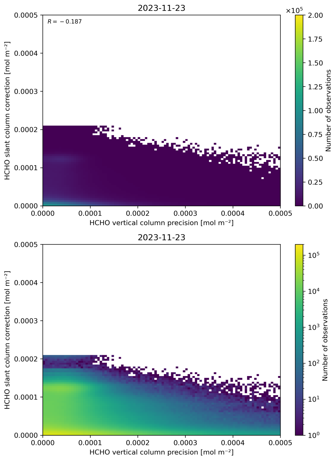
Figure 141: Scatter density plot of “HCHO vertical column precision” against “HCHO slant column correction” for 2023-11-23 to 2023-11-24.
