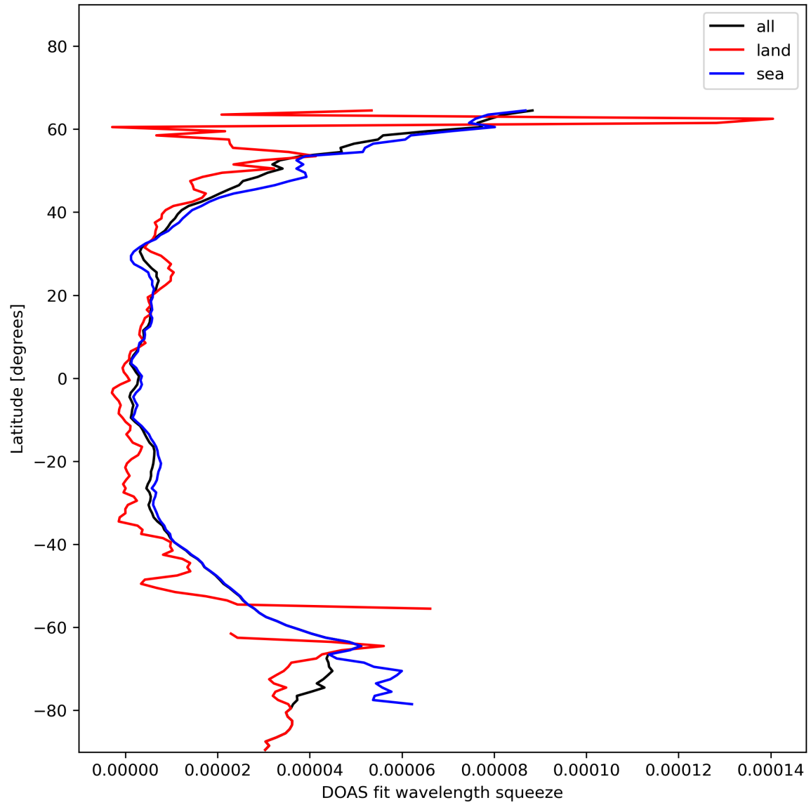
Figure 31: Zonal average of “DOAS fit wavelength squeeze” for 2023-11-23 to 2023-11-24.
