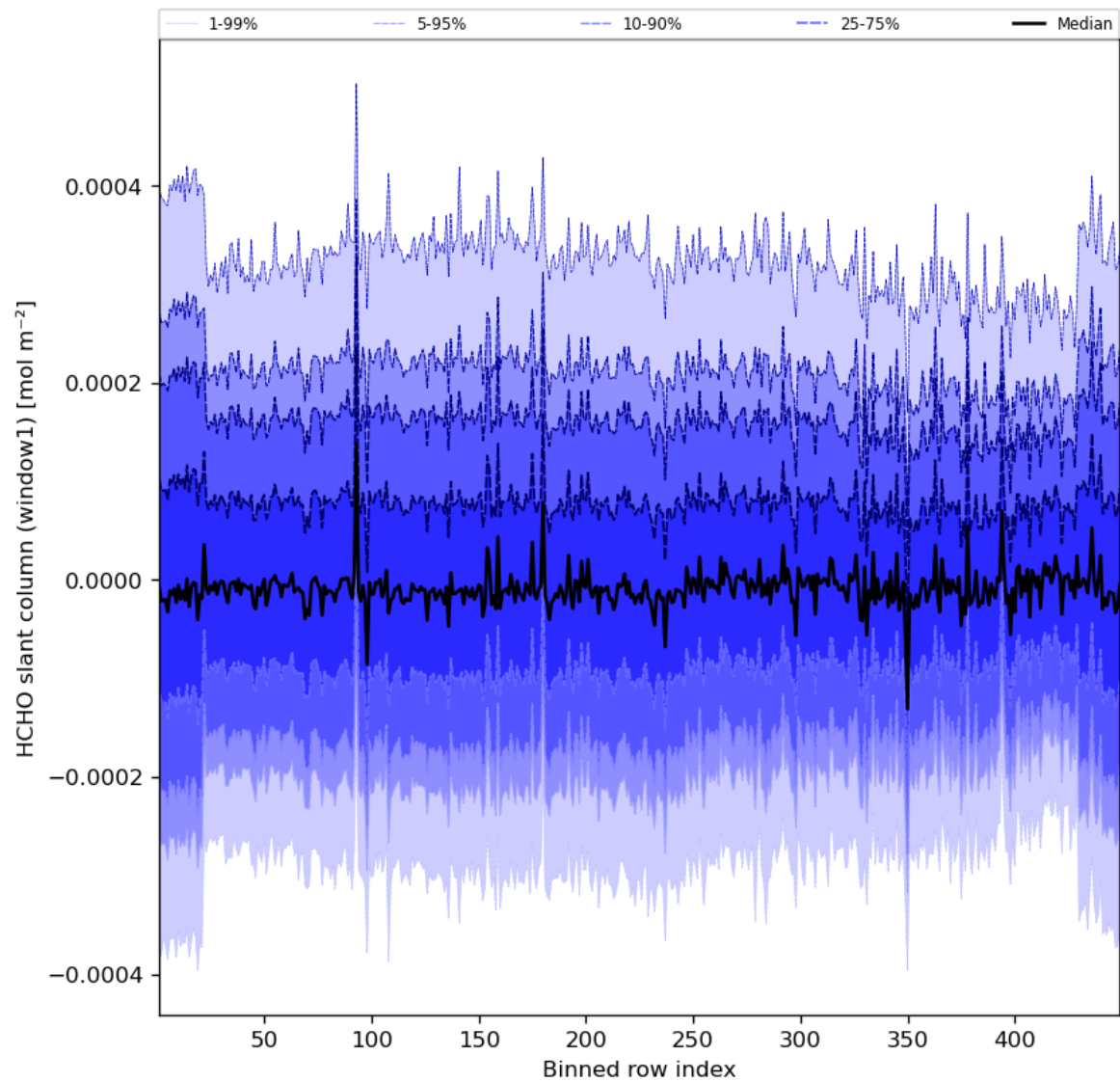
Figure 52: Along track statistics of “HCHO slant column (window1)” for 2023-11-23 to 2023-11-24
