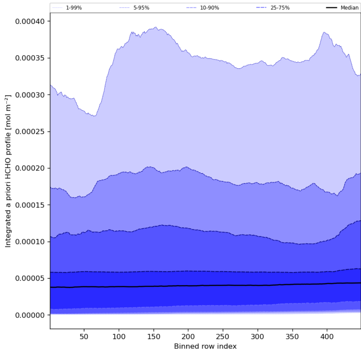
Figure 57: Along track statistics of “Integrated a priori HCHO profile” for 2023-11-23 to 2023-11-24
