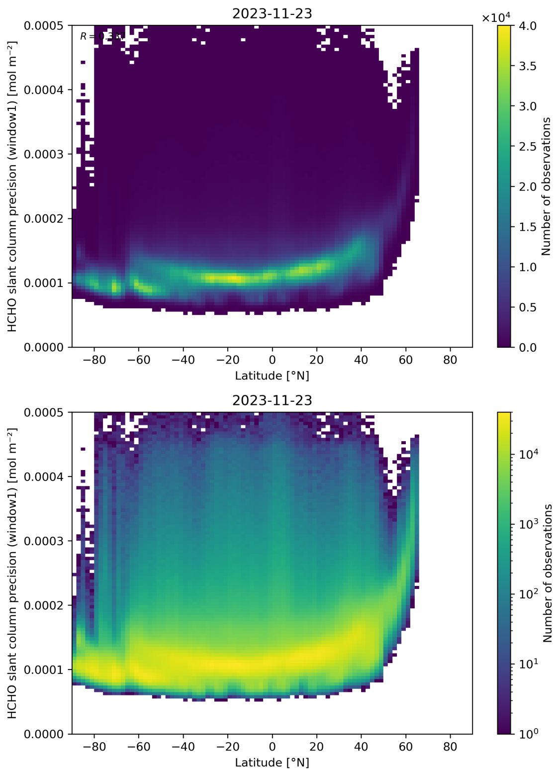
Figure 160: Scatter density plot of “Latitude” against “HCHO slant column precision (window1)” for 2023-11-23 to 2023-11-24.
