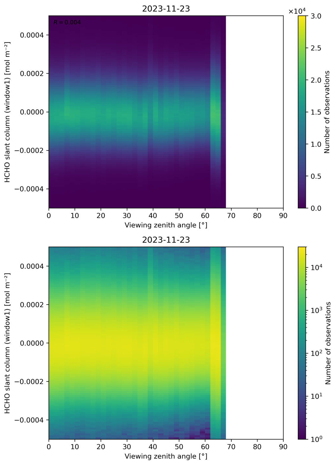
Figure 188: Scatter density plot of “Viewing zenith angle” against “HCHO slant column (window1)” for 2023-11-23 to 2023-11-24.
