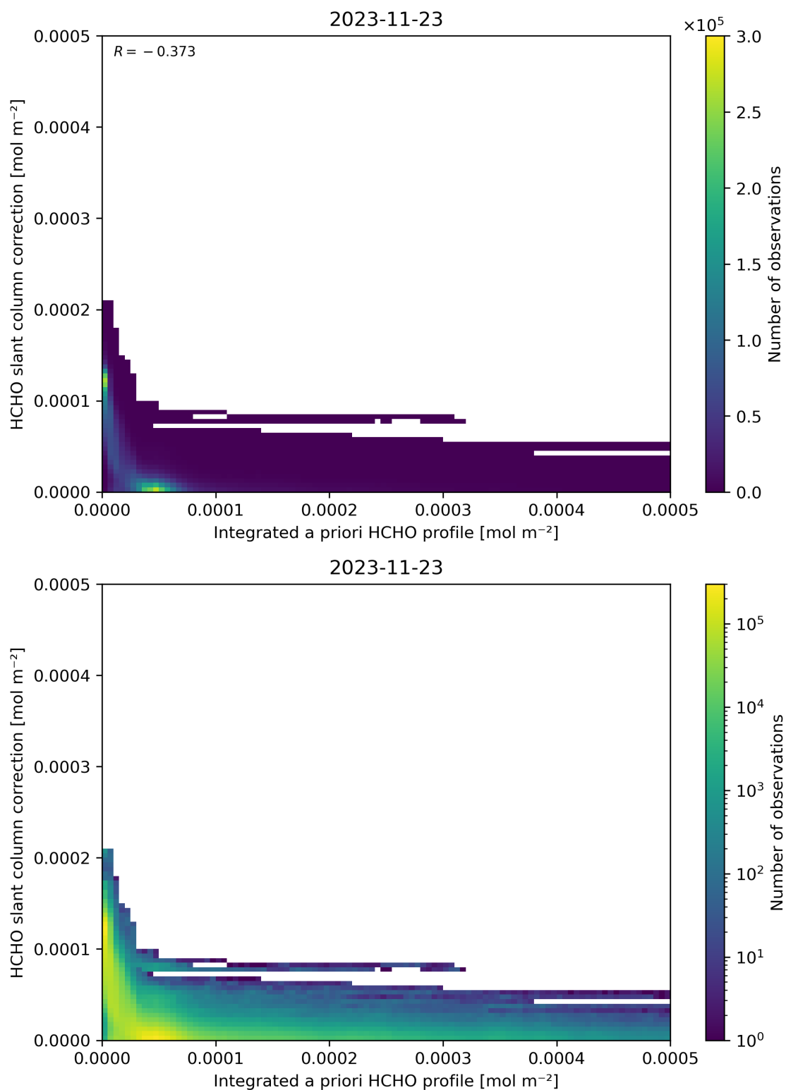
Figure 152: Scatter density plot of “Integrated a priori HCHO profile” against “HCHO slant column correction” for 2023-11-23 to 2023-11-24.
