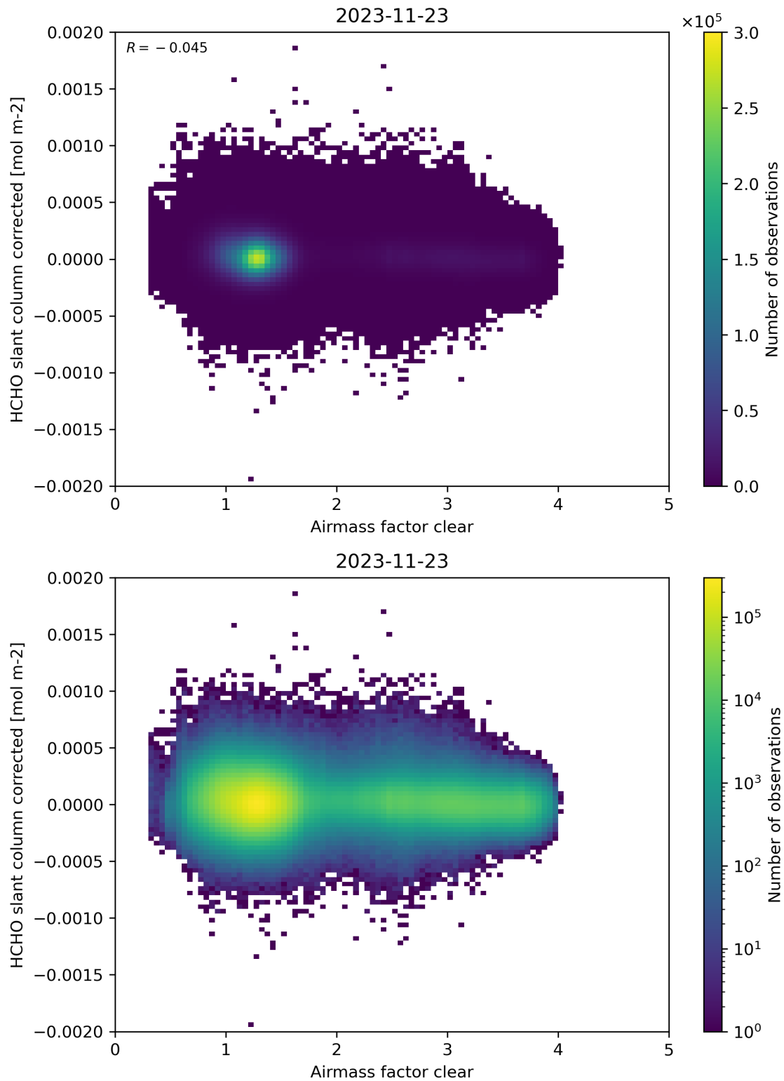
Figure 74: Scatter density plot of “Airmass factor clear” against “HCHO slant column corrected” for 2023-11-23 to 2023-11-24.
