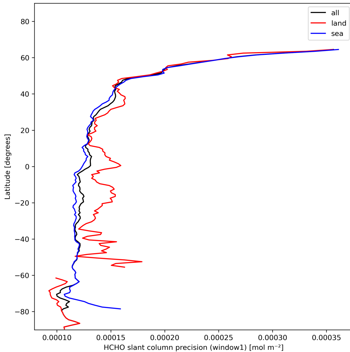
Figure 25: Zonal average of “HCHO slant column precision (window1)” for 2023-11-23 to 2023-11-24.
