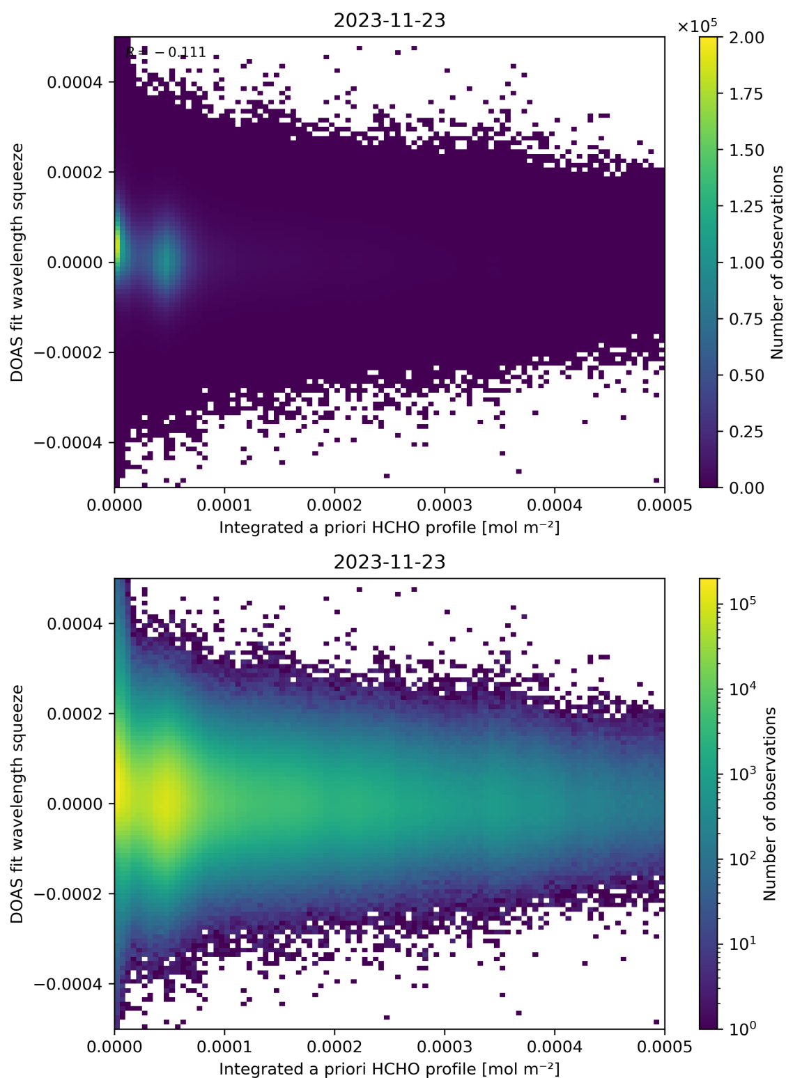
Figure 150: Scatter density plot of “Integrated a priori HCHO profile” against “DOAS fit wavelength squeeze” for 2023-11-23 to 2023-11-24.
