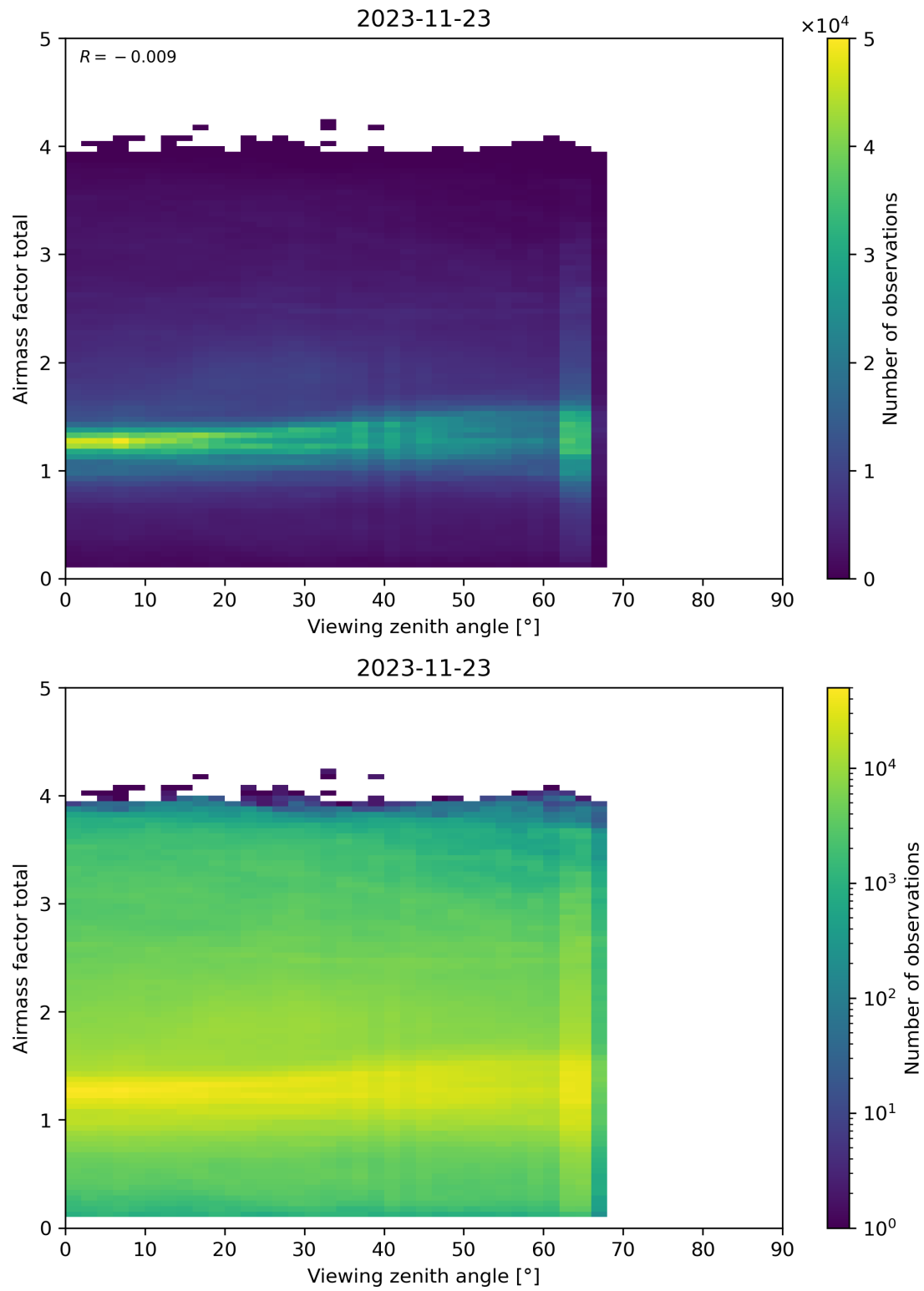
Figure 190: Scatter density plot of “Viewing zenith angle” against “Airmass factor total” for 2023-11-23 to 2023-11-24.
