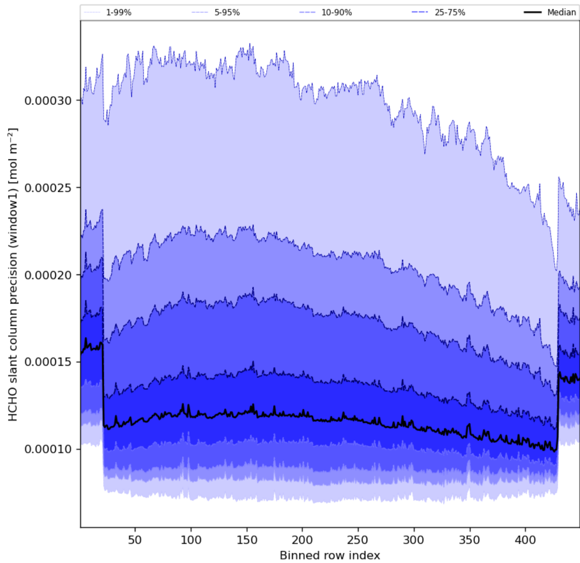
Figure 53: Along track statistics of “HCHO slant column precision (window1)” for 2023-11-23 to 2023-11-24
