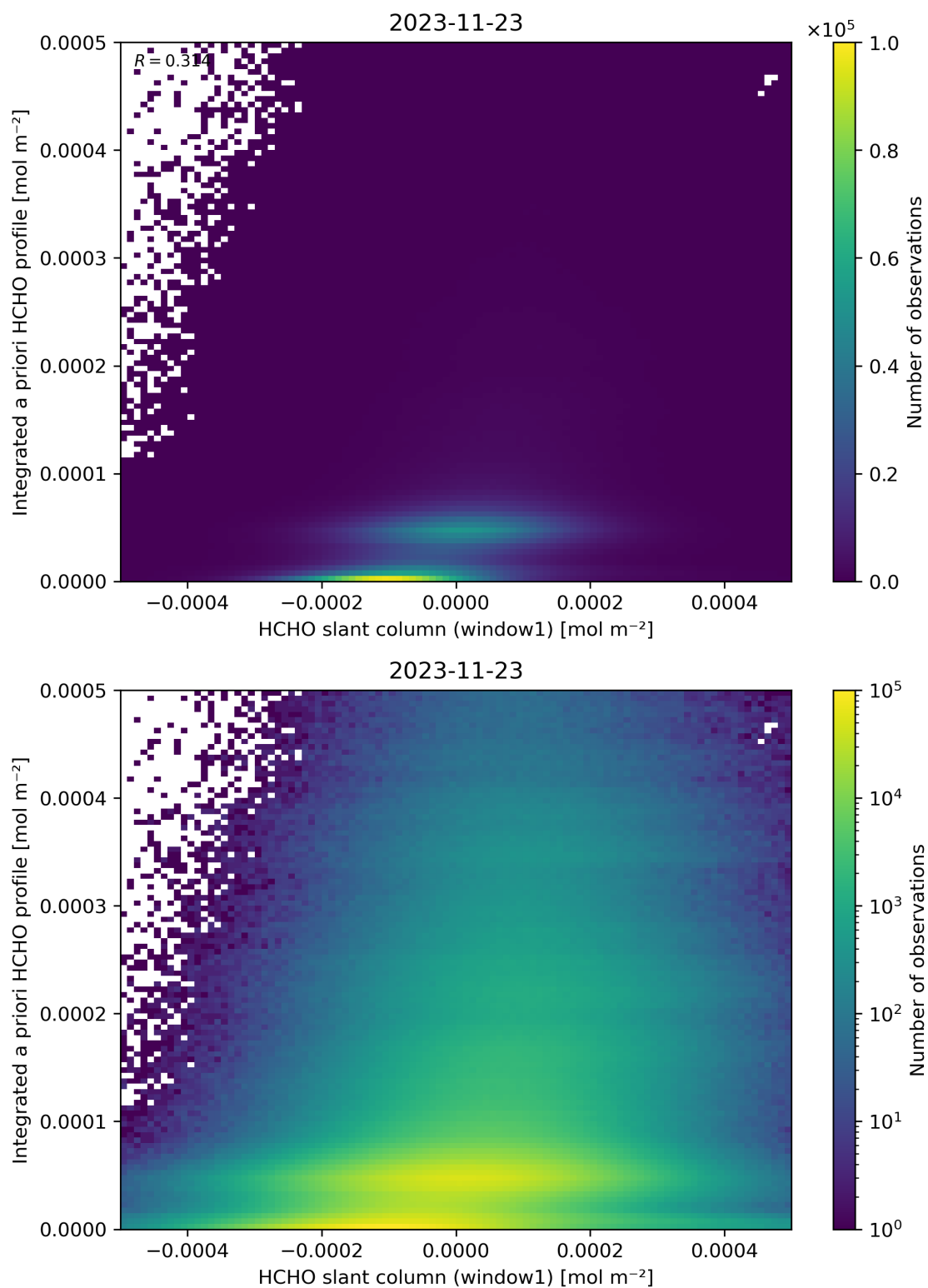
Figure 87: Scatter density plot of “HCHO slant column (window1)” against “Integrated a priori HCHO profile” for 2023-11-23 to 2023-11-24.
