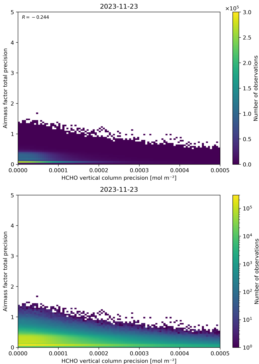
Figure 145: Scatter density plot of “HCHO vertical column precision” against “Airmass factor total precision” for 2023-11-23 to 2023-11-24.
