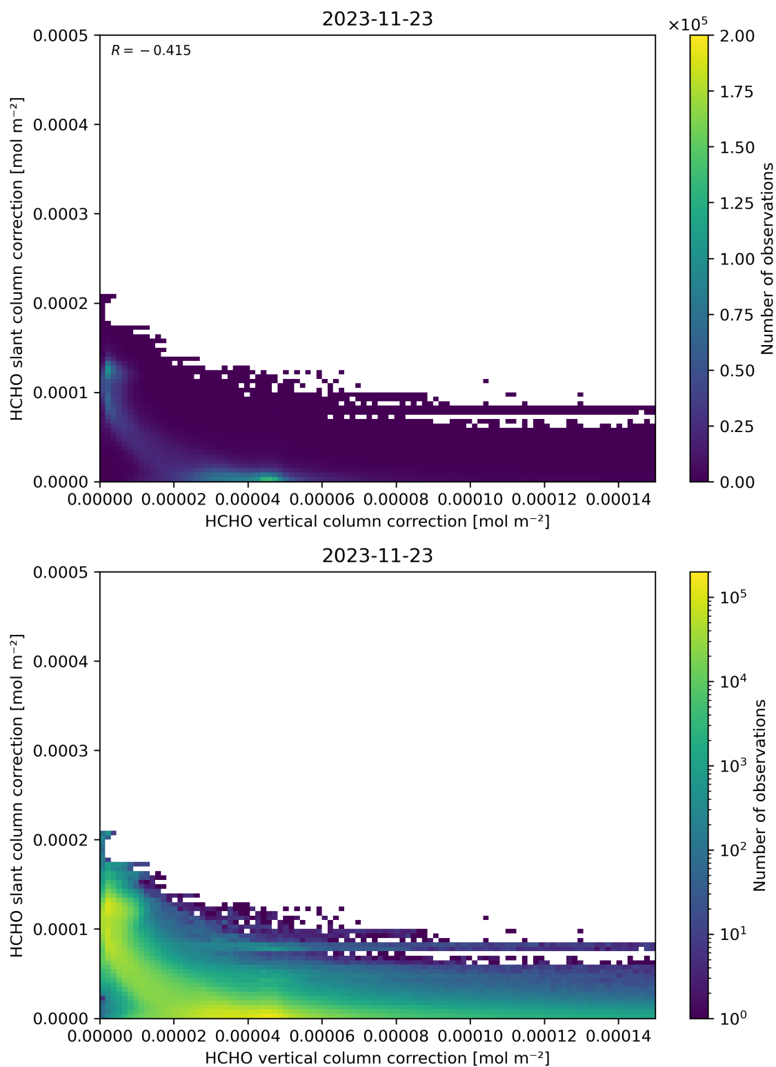
Figure 117: Scatter density plot of “HCHO vertical column correction” against “HCHO slant column correction” for 2023-11-23 to 2023-11-24.
