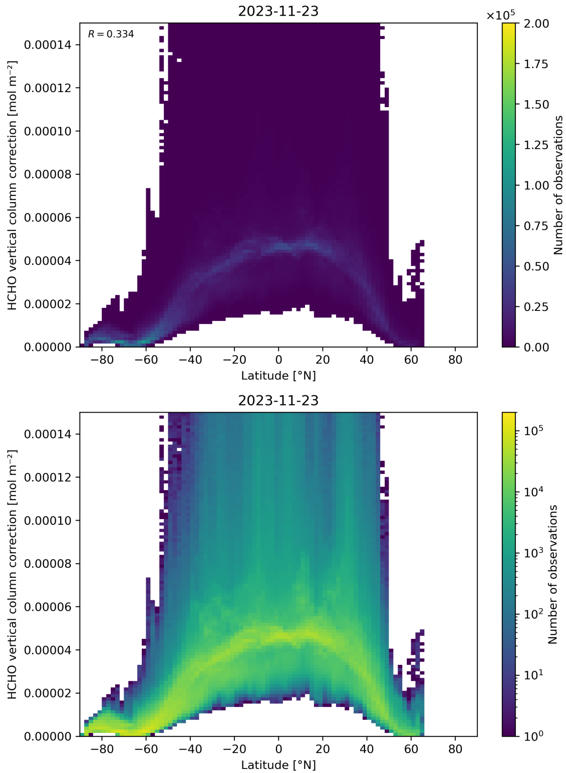
Figure 164: Scatter density plot of “Latitude” against “HCHO vertical column correction” for 2023-11-23 to 2023-11-24.
