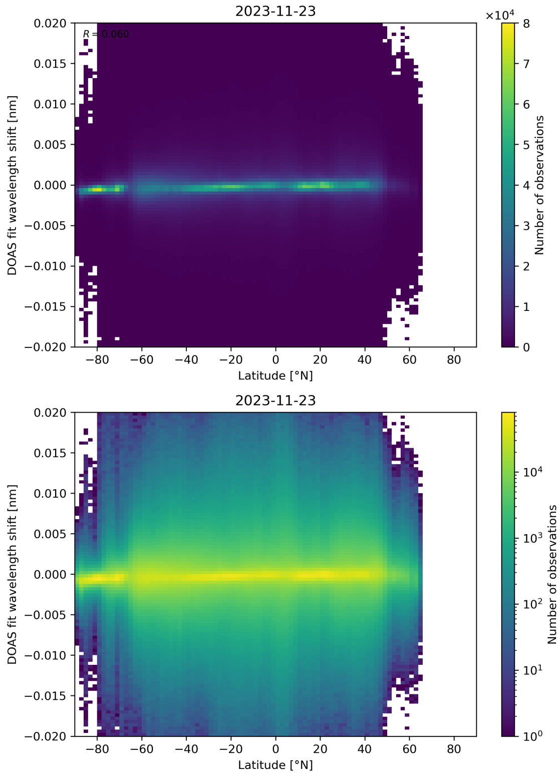
Figure 154: Scatter density plot of “Latitude” against “DOAS fit wavelength shift” for 2023-11-23 to 2023-11-24.
