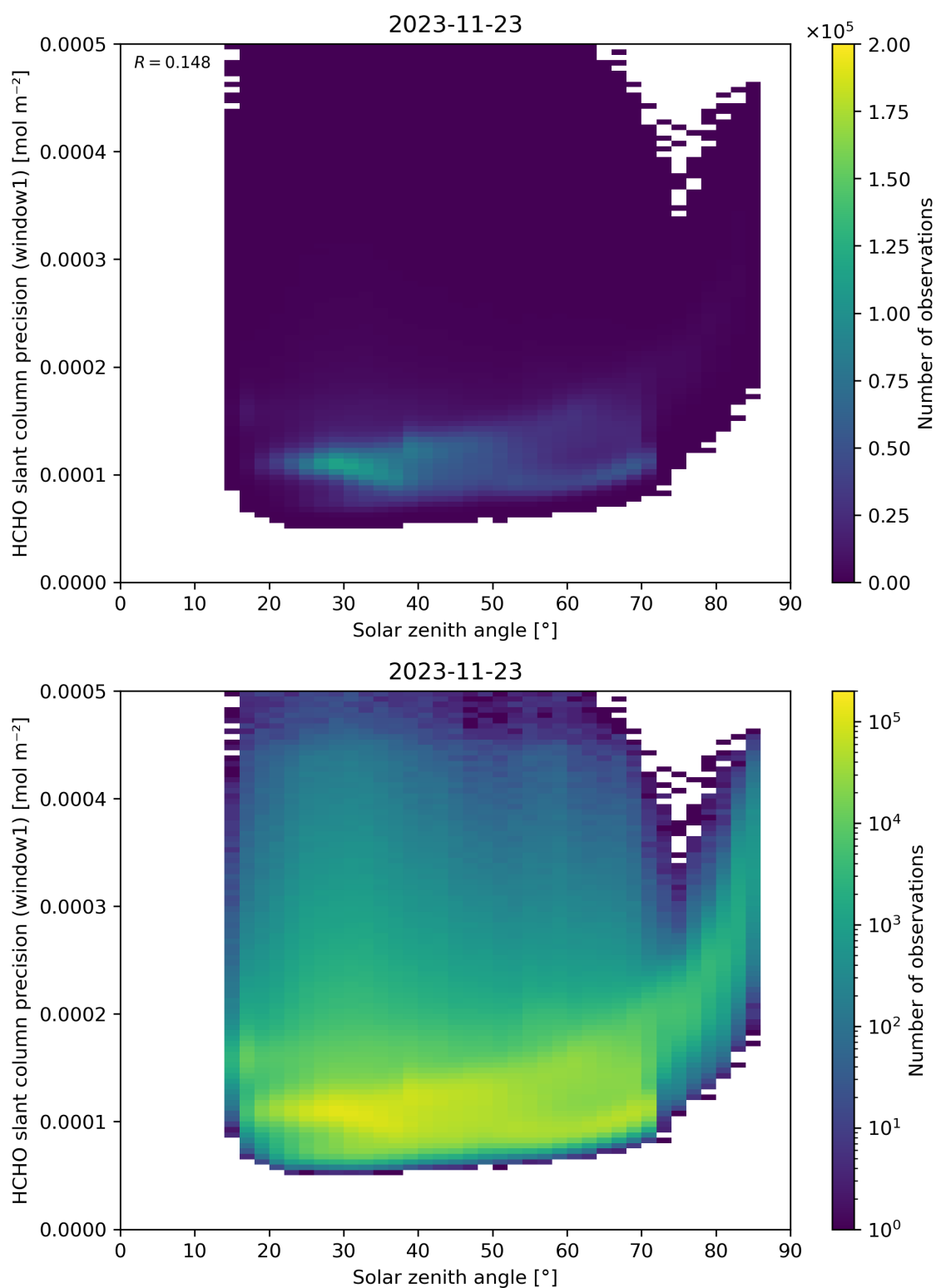
Figure 174: Scatter density plot of “Solar zenith angle” against “HCHO slant column precision (window1)” for 2023-11-23 to 2023-11-24.
