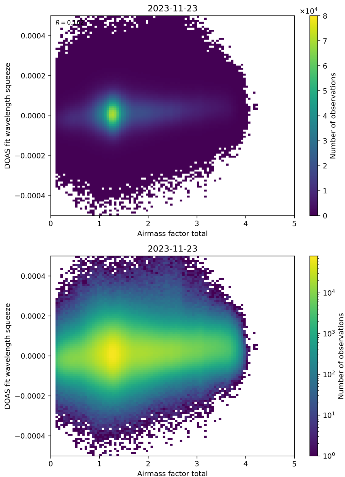
Figure 99: Scatter density plot of “Airmass factor total” against “DOAS fit wavelength squeeze” for 2023-11-23 to 2023-11-24.
