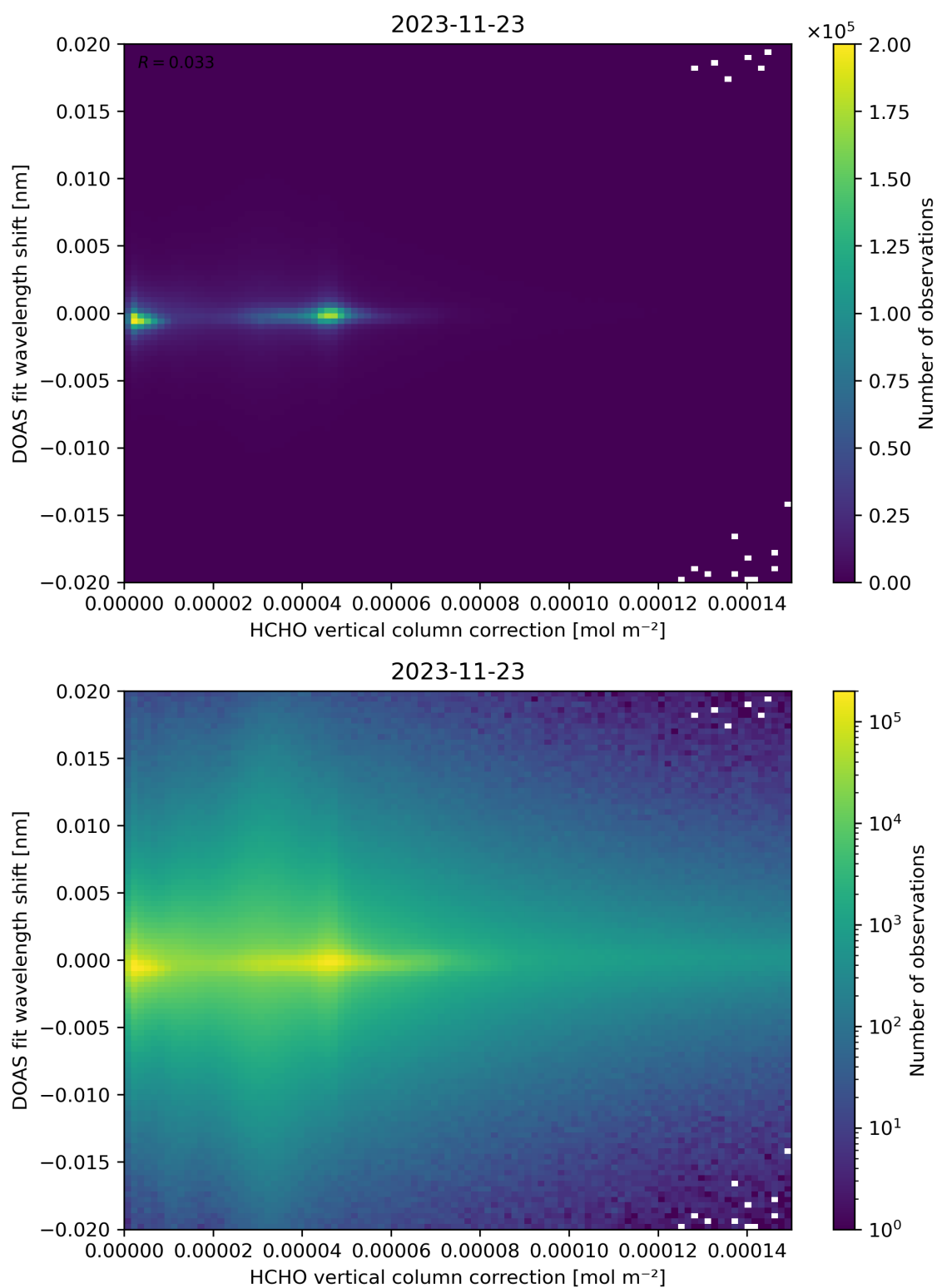
Figure 113: Scatter density plot of “HCHO vertical column correction” against “DOAS fit wavelength shift” for 2023-11-23 to 2023-11-24.
