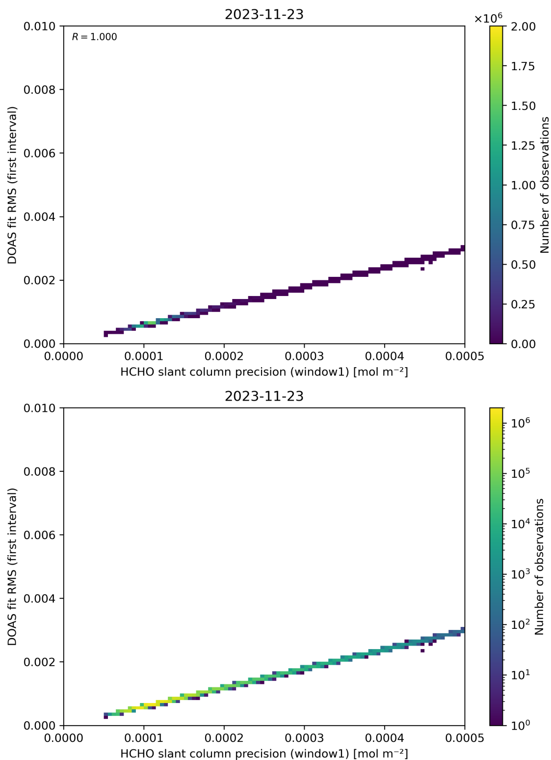
Figure 88: Scatter density plot of “HCHO slant column precision (window1)” against “DOAS fit RMS (first interval)” for 2023-11-23 to 2023-11-24.
