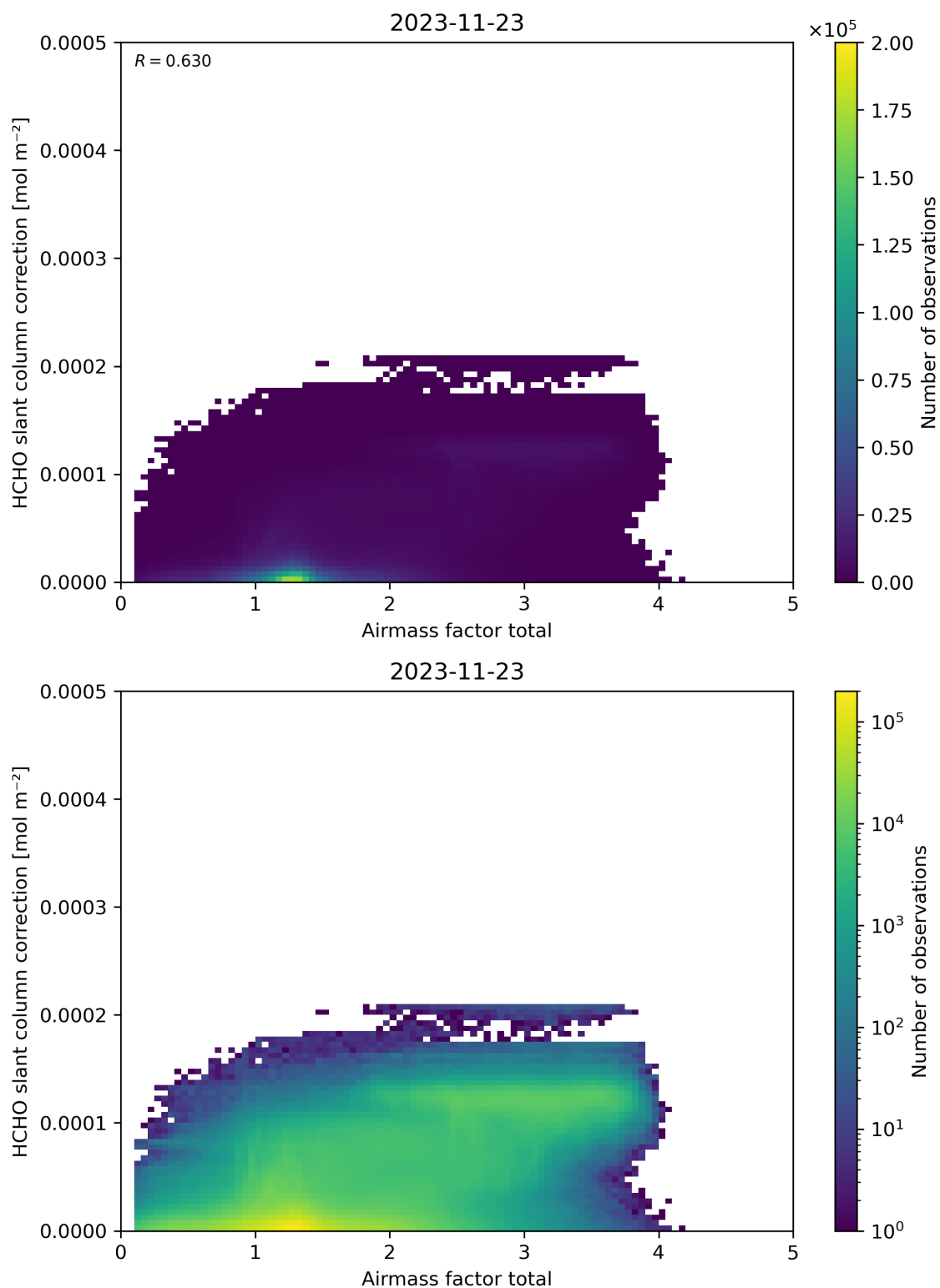
Figure 102: Scatter density plot of “Airmass factor total” against “HCHO slant column correction” for 2023-11-23 to 2023-11-24.
