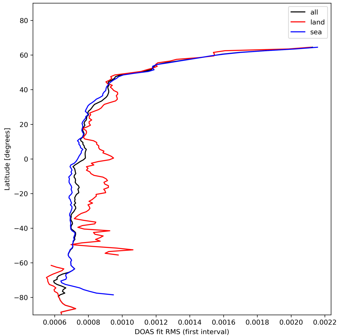
Figure 32: Zonal average of “DOAS fit RMS (first interval)” for 2023-11-23 to 2023-11-24.
