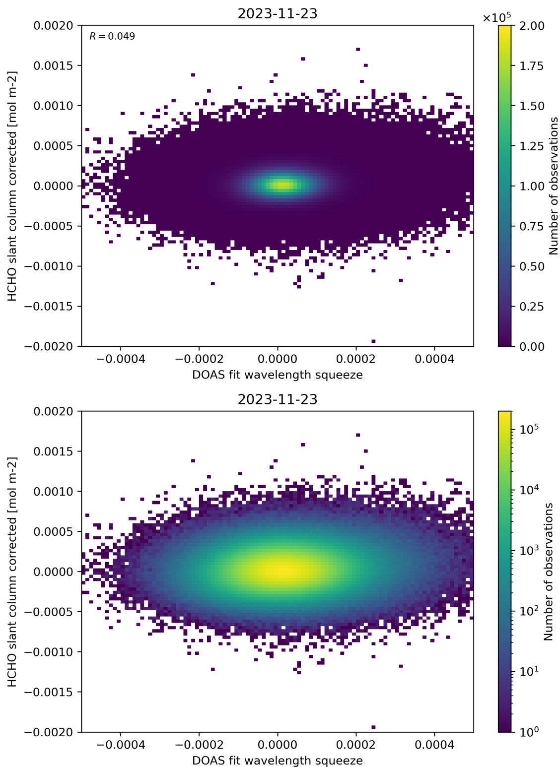
Figure 69: Scatter density plot of “DOAS fit wavelength squeeze” against “HCHO slant column corrected” for 2023-11-23 to 2023-11-24.
