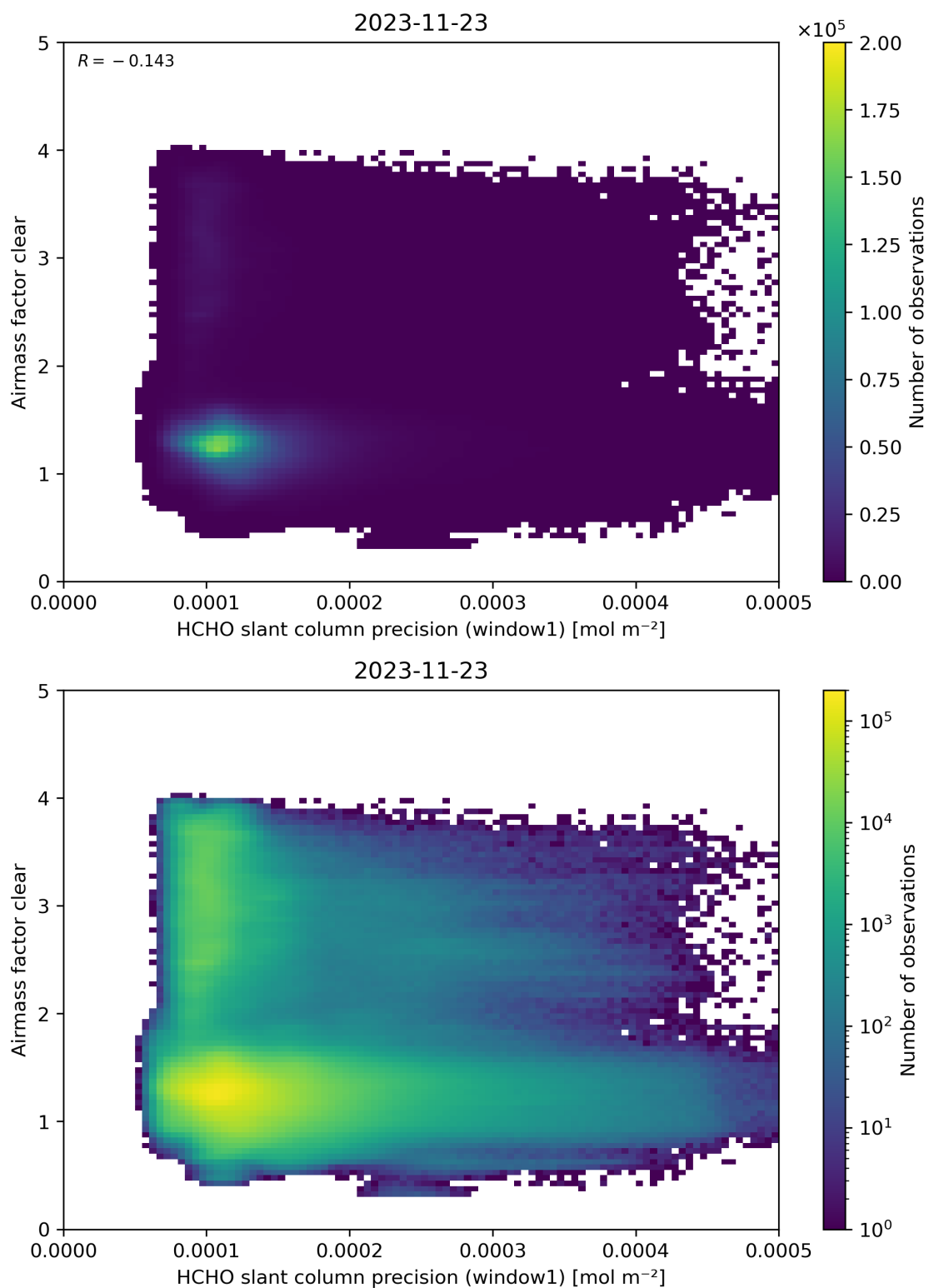
Figure 91: Scatter density plot of “HCHO slant column precision (window1)” against “Airmass factor clear” for 2023-11-23 to 2023-11-24.
