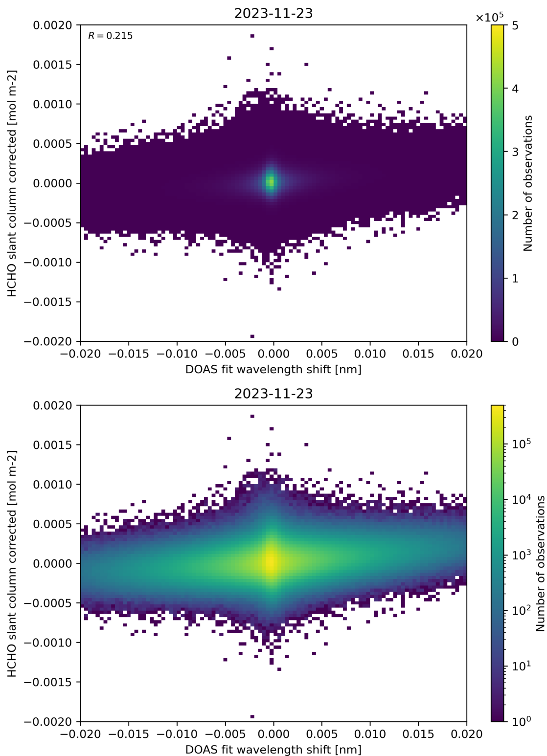
Figure 66: Scatter density plot of “DOAS fit wavelength shift” against “HCHO slant column corrected” for 2023-11-23 to 2023-11-24.
