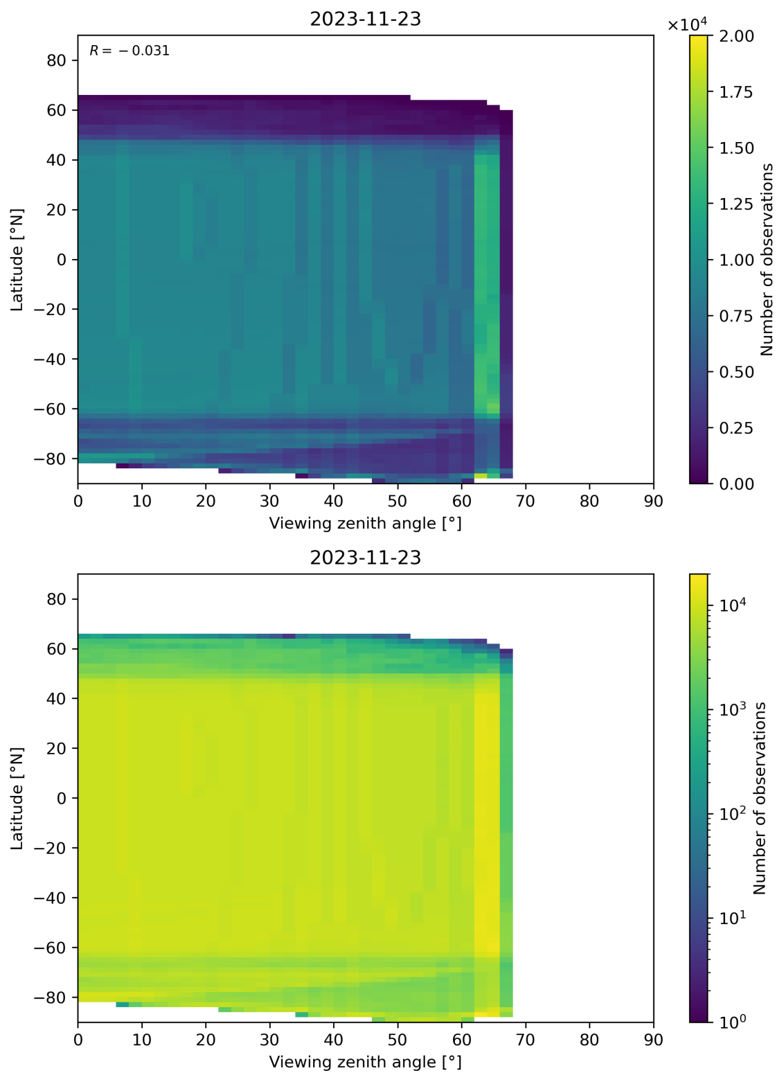
Figure 196: Scatter density plot of “Viewing zenith angle” against “Latitude” for 2023-11-23 to 2023-11-24.
