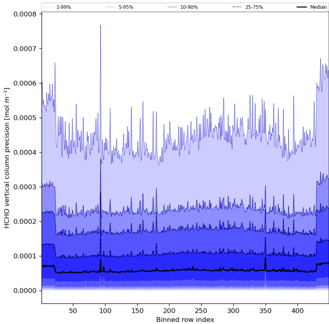
Figure 50: Along track statistics of “HCHO vertical column precision” for 2023-11-23 to 2023-11-24
