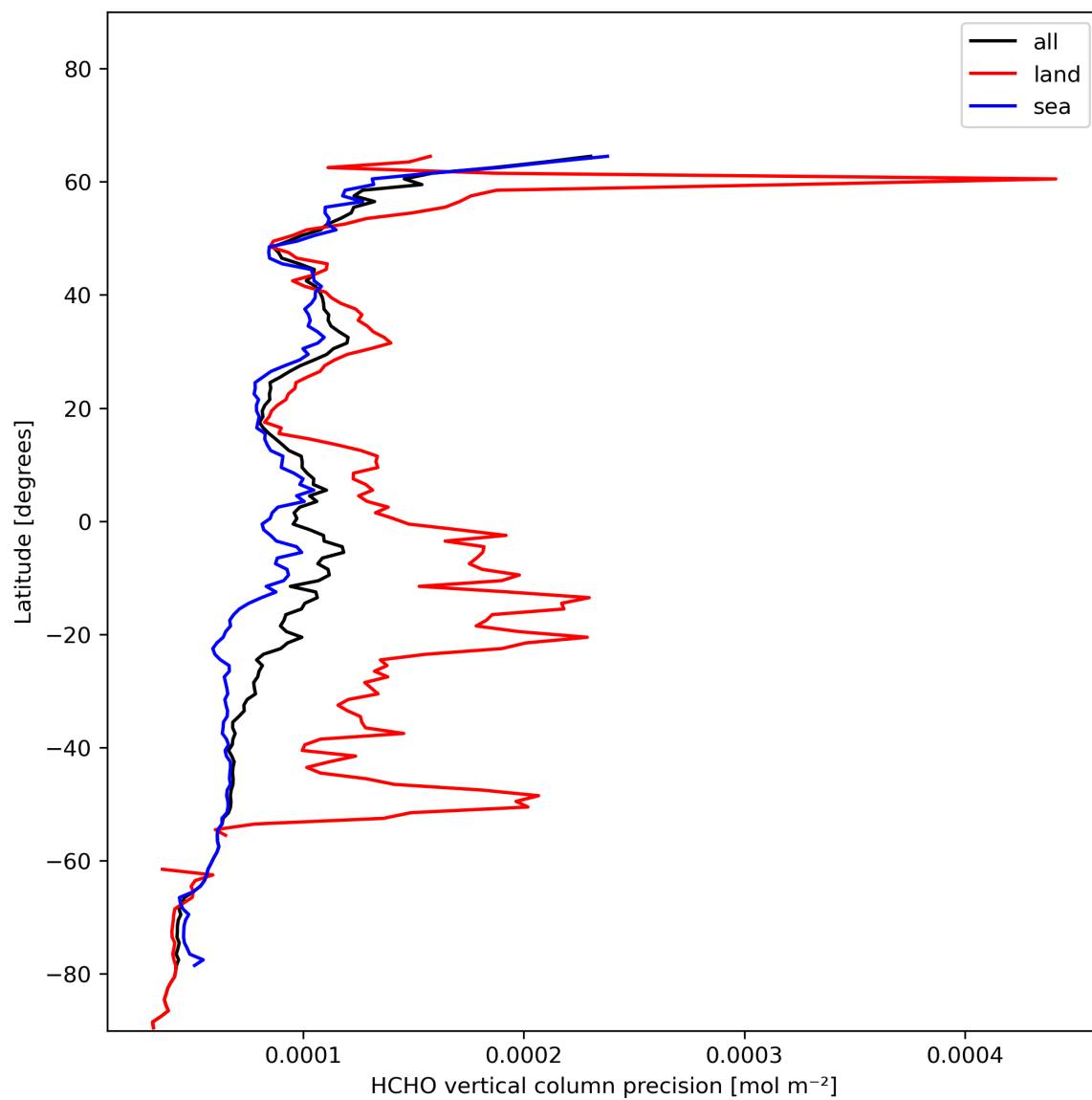
Figure 22: Zonal average of “HCHO vertical column precision” for 2023-11-23 to 2023-11-24.
