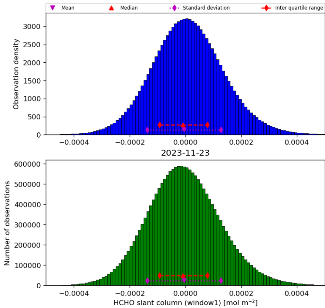
Figure 38: Histogram of “HCHO slant column (window1)” for 2023-11-23 to 2023-11-24
