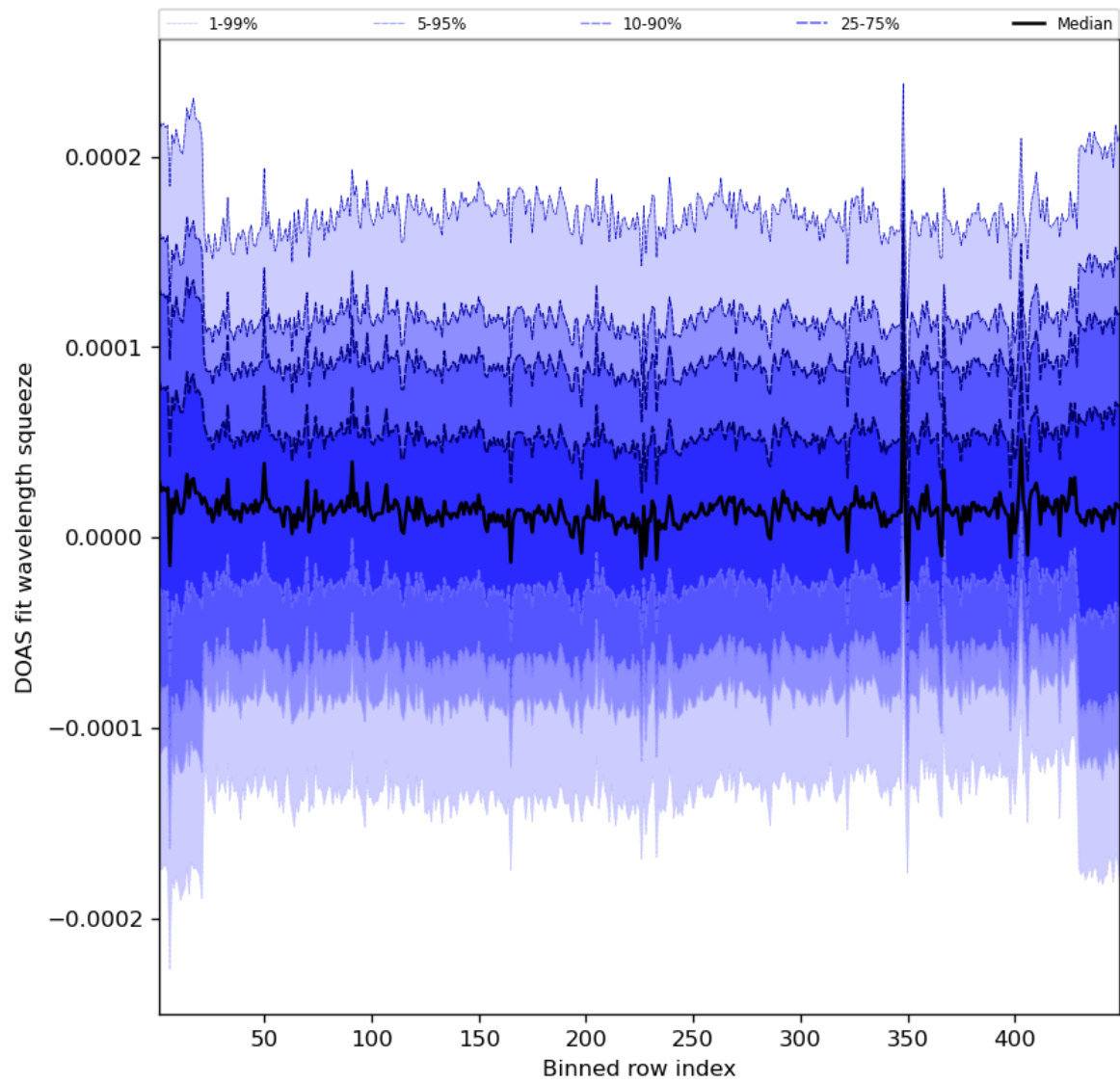
Figure 59: Along track statistics of “DOAS fit wavelength squeeze” for 2023-11-23 to 2023-11-24
