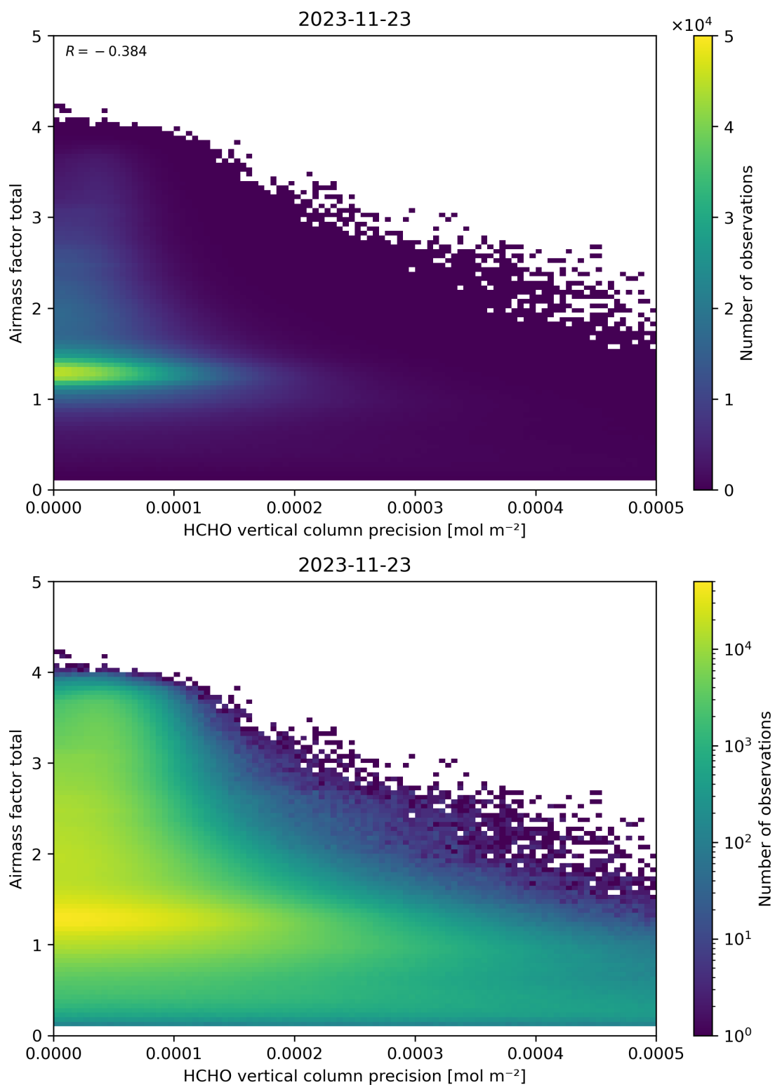
Figure 144: Scatter density plot of “HCHO vertical column precision” against “Airmass factor total” for 2023-11-23 to 2023-11-24.
