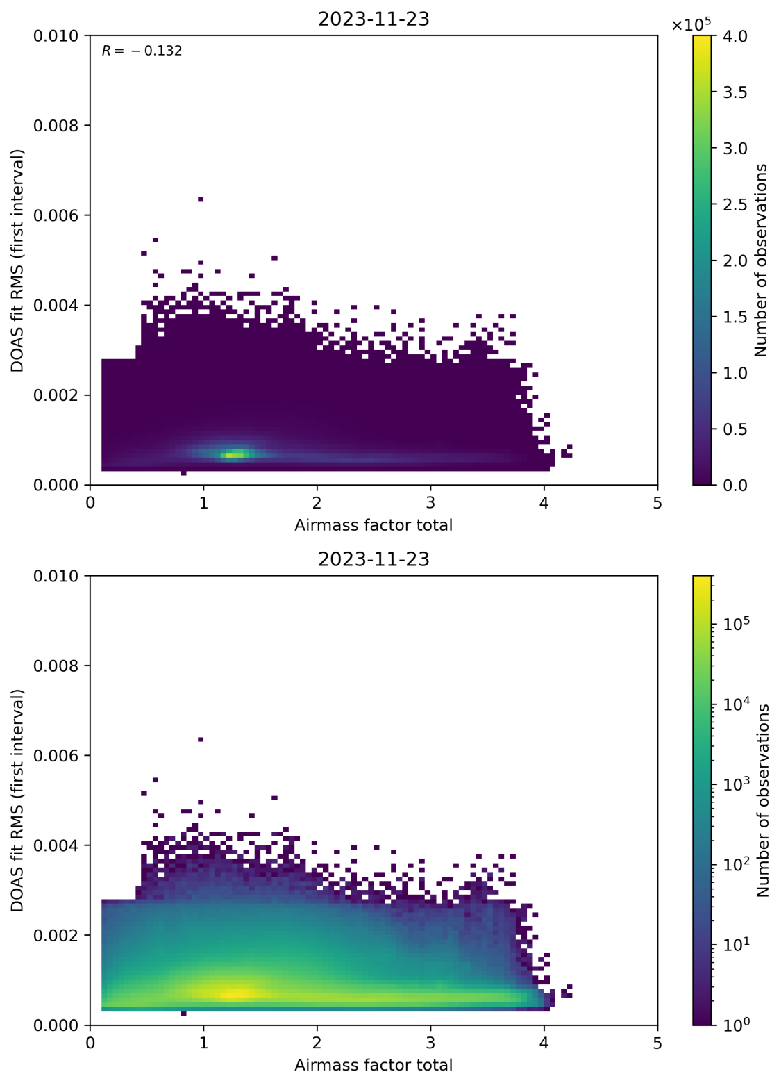
Figure 97: Scatter density plot of “Airmass factor total” against “DOAS fit RMS (first interval)” for 2023-11-23 to 2023-11-24.
