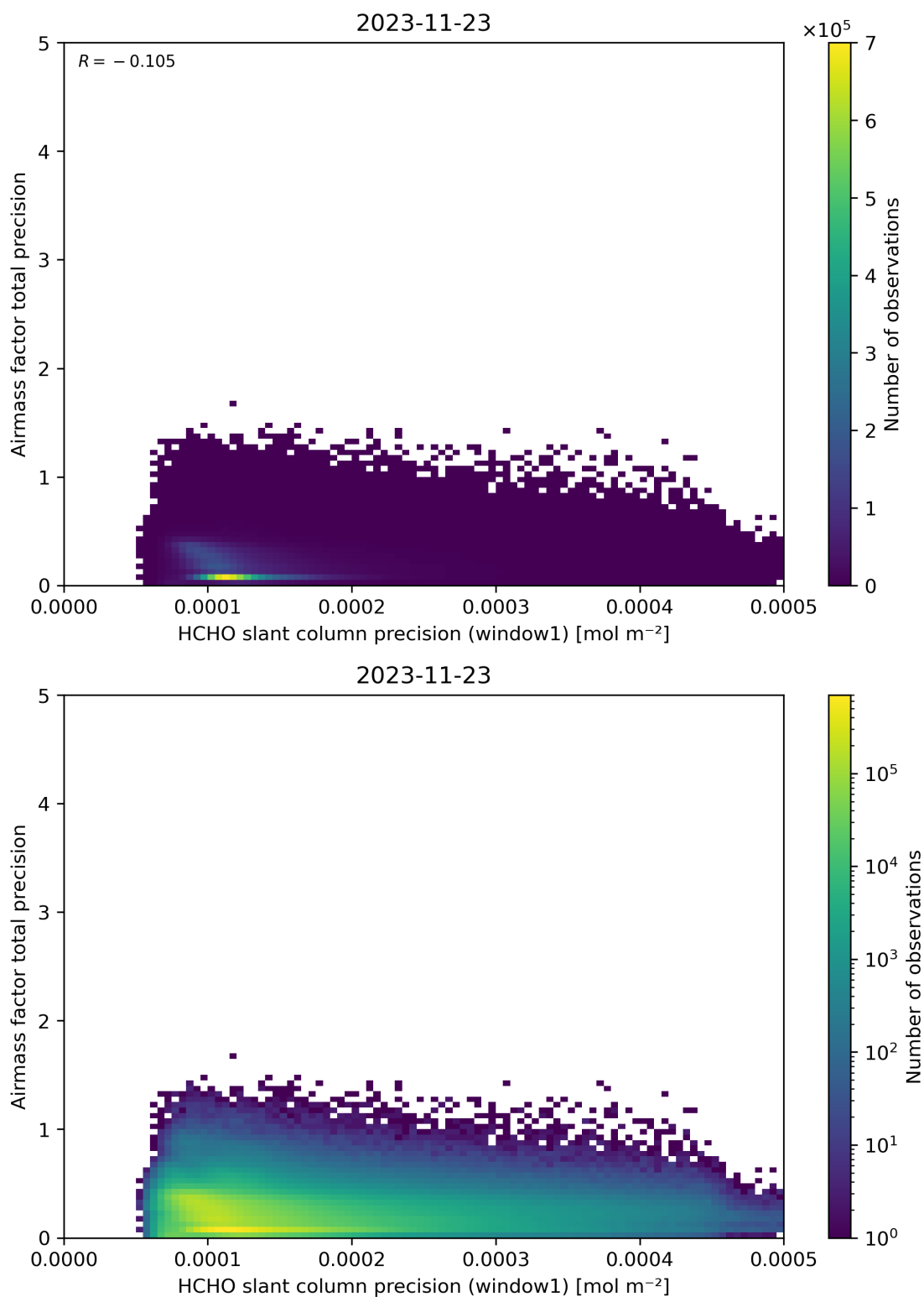
Figure 95: Scatter density plot of “HCHO slant column precision (window1)” against “Airmass factor total precision” for 2023-11-23 to 2023-11-24.
