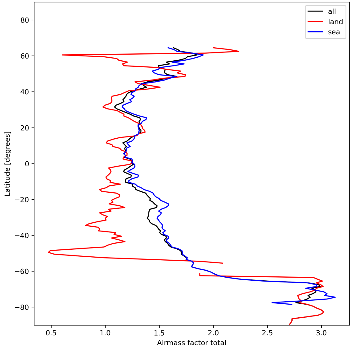
Figure 26: Zonal average of “Airmass factor total” for 2023-11-23 to 2023-11-24.
