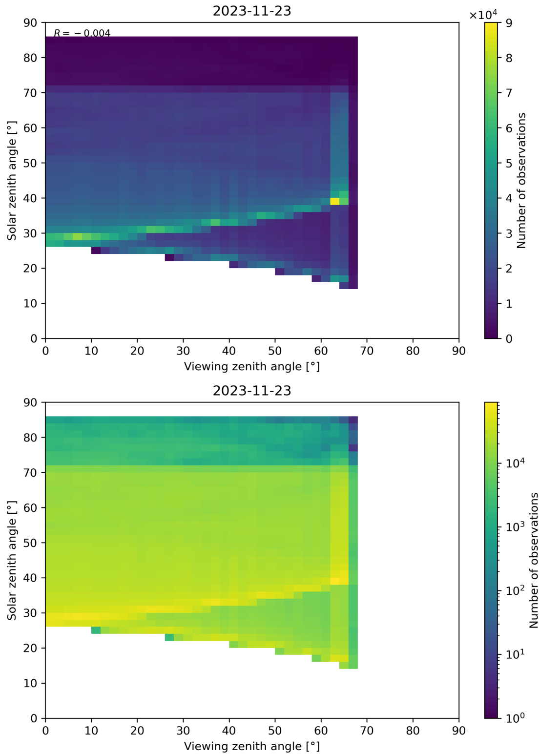
Figure 197: Scatter density plot of “Viewing zenith angle” against “Solar zenith angle” for 2023-11-23 to 2023-11-24.
