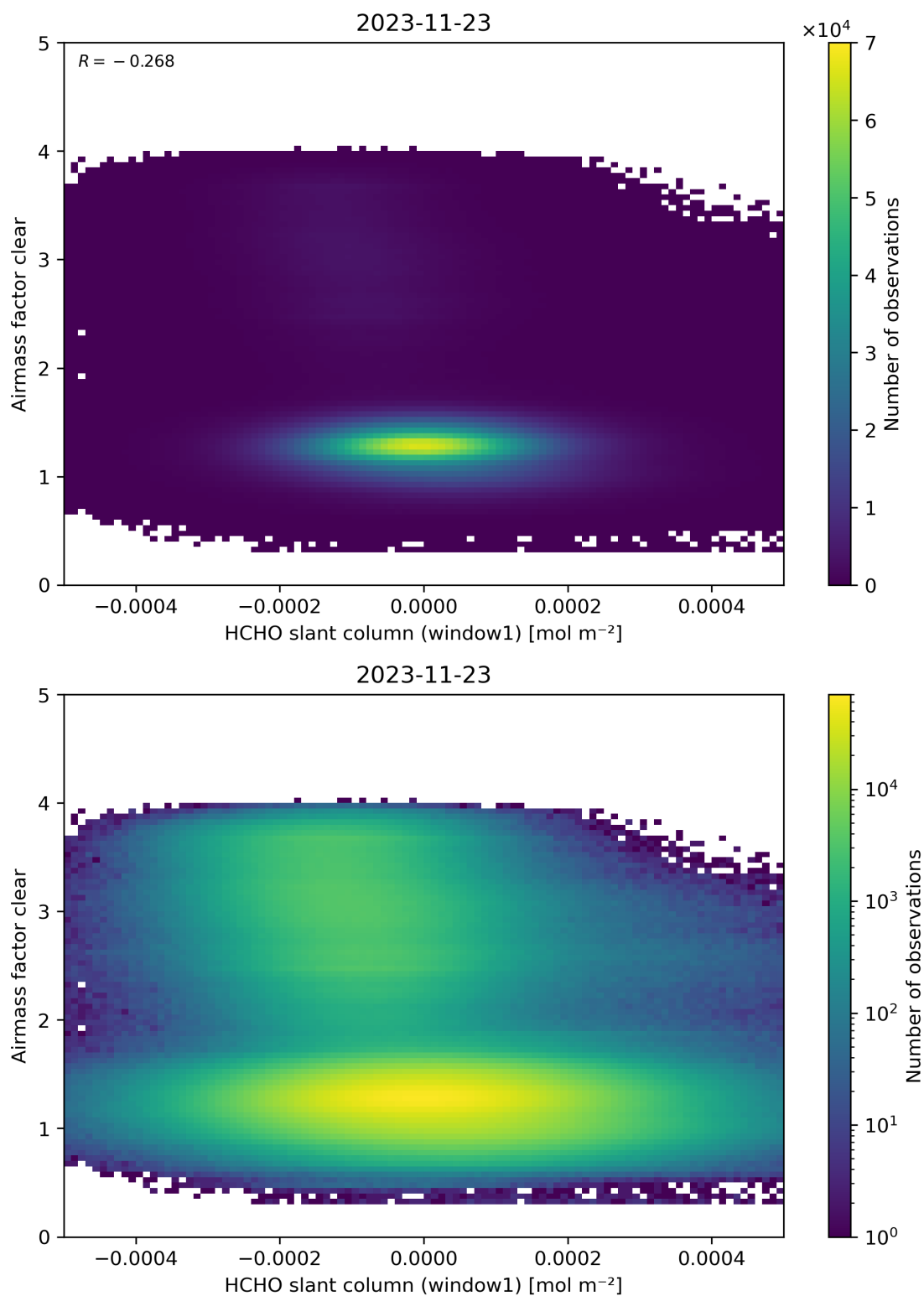
Figure 81: Scatter density plot of “HCHO slant column (window1)” against “Airmass factor clear” for 2023-11-23 to 2023-11-24.
