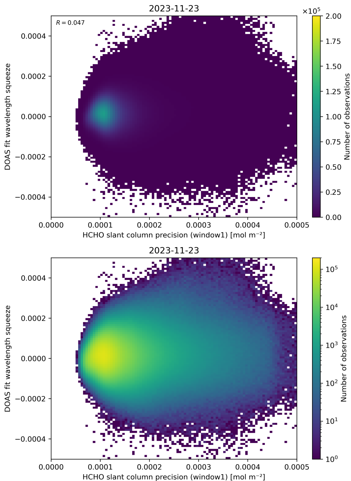
Figure 90: Scatter density plot of “HCHO slant column precision (window1)” against “DOAS fit wavelength squeeze” for 2023-11-23 to 2023-11-24.
