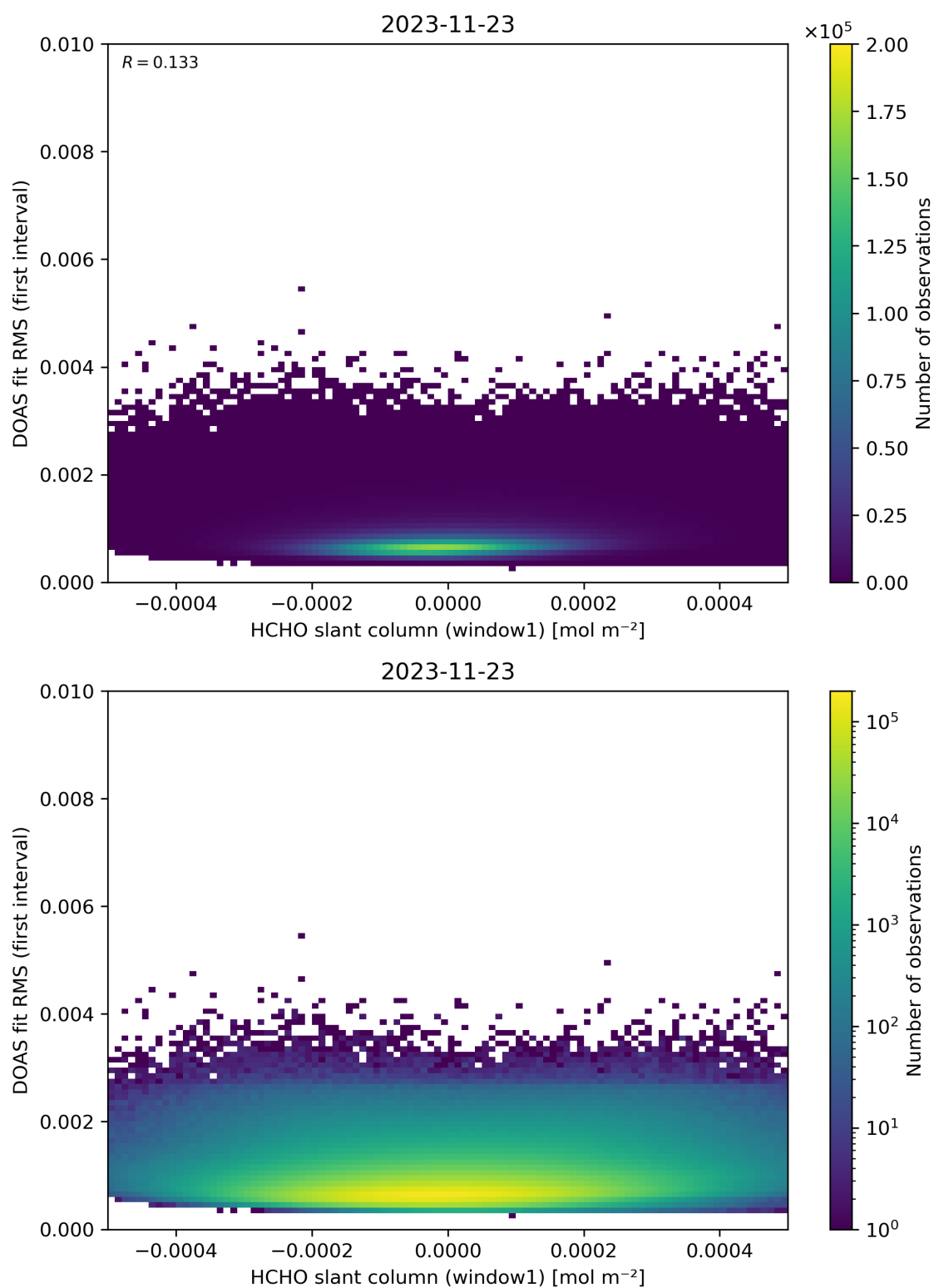
Figure 78: Scatter density plot of “HCHO slant column (window1)” against “DOAS fit RMS (first interval)” for 2023-11-23 to 2023-11-24.
