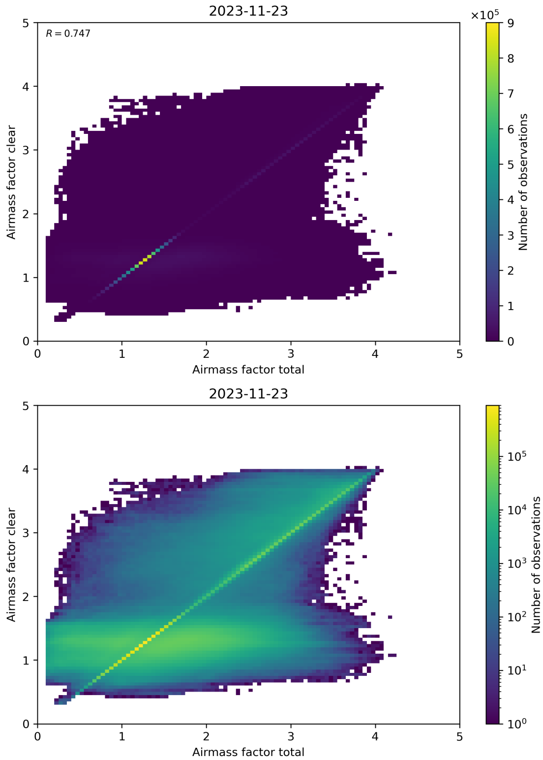
Figure 100: Scatter density plot of “Airmass factor total” against “Airmass factor clear” for 2023-11-23 to 2023-11-24.
