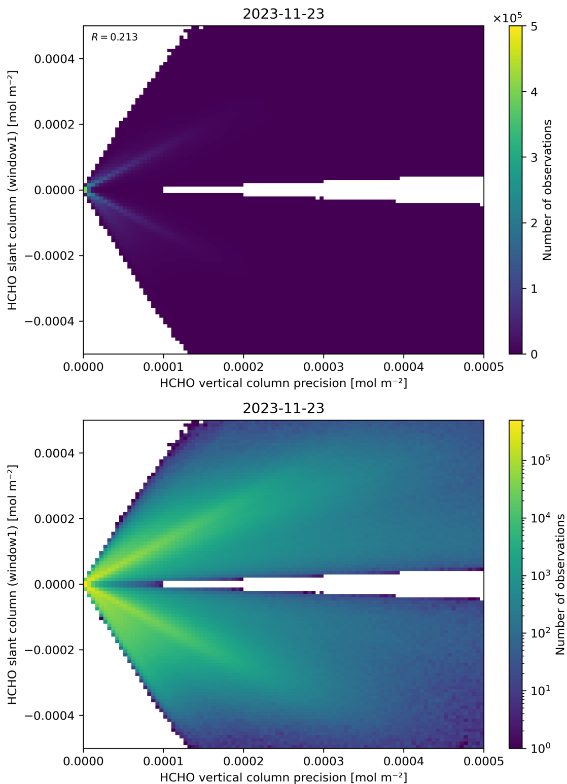
Figure 142: Scatter density plot of “HCHO vertical column precision” against “HCHO slant column (window1)” for 2023-11-23 to 2023-11-24.
