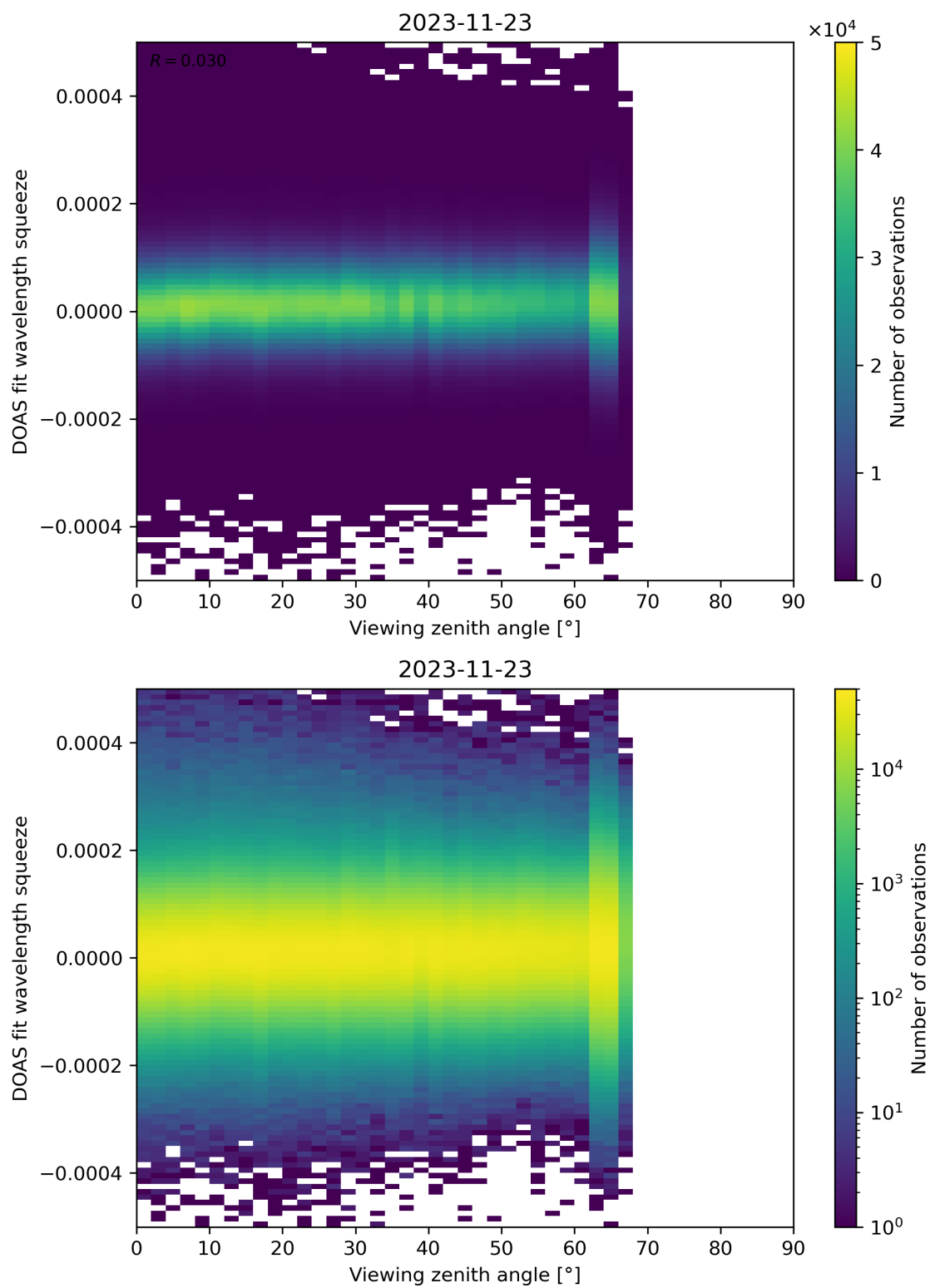
Figure 184: Scatter density plot of “Viewing zenith angle” against “DOAS fit wavelength squeeze” for 2023-11-23 to 2023-11-24.
