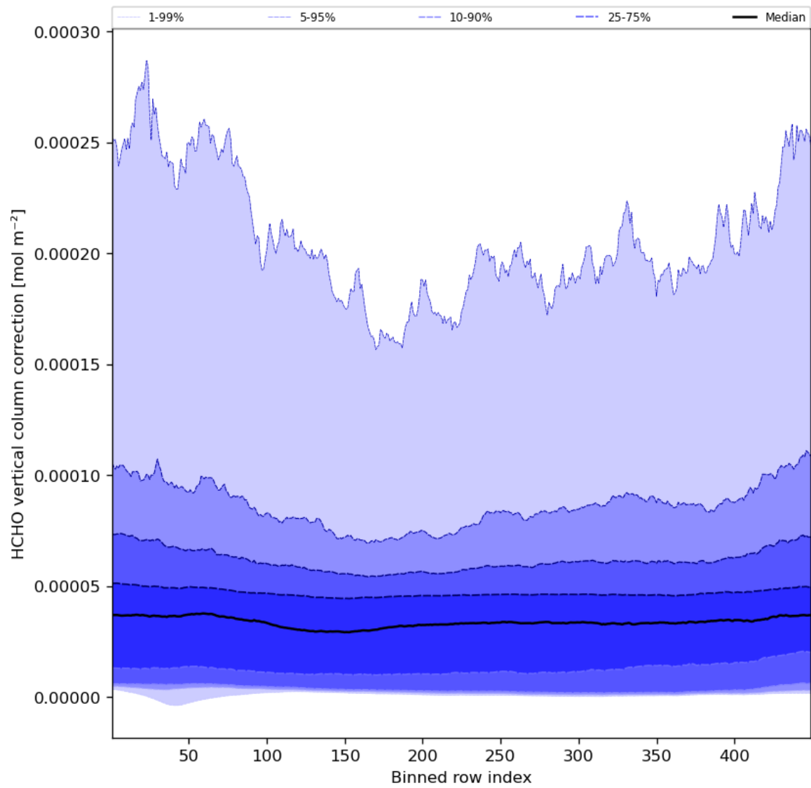
Figure 51: Along track statistics of “HCHO vertical column correction” for 2023-11-23 to 2023-11-24
