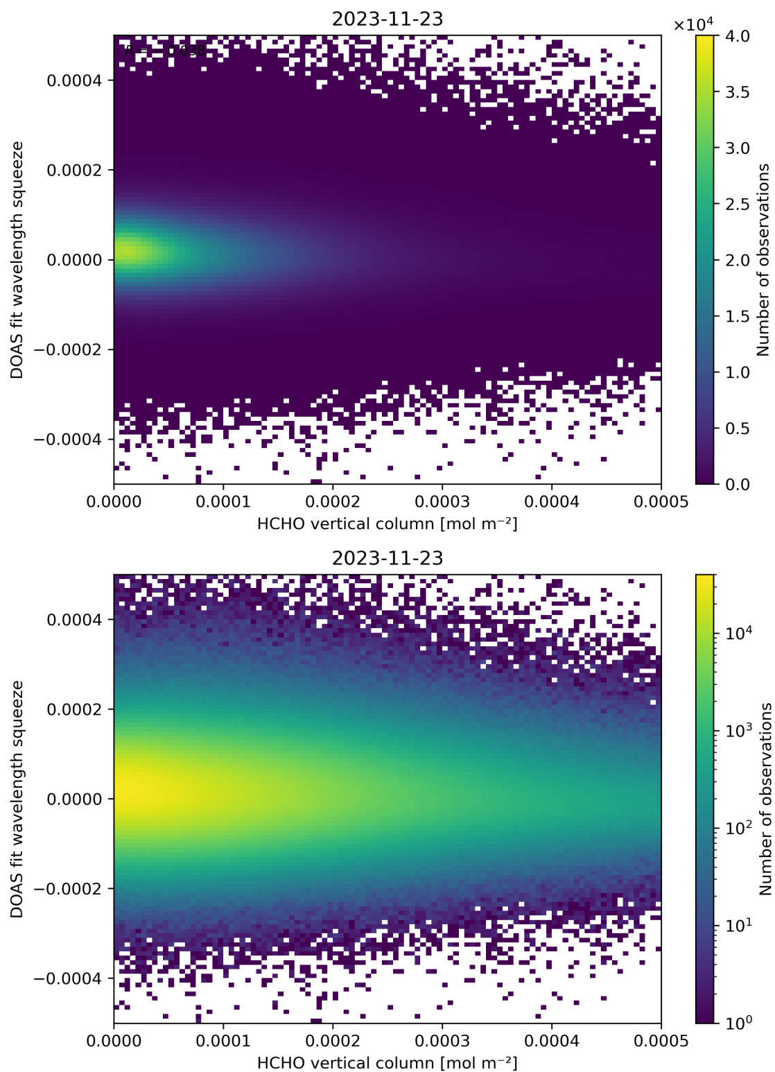
Figure 125: Scatter density plot of “HCHO vertical column” against “DOAS fit wavelength squeeze” for 2023-11-23 to 2023-11-24.
