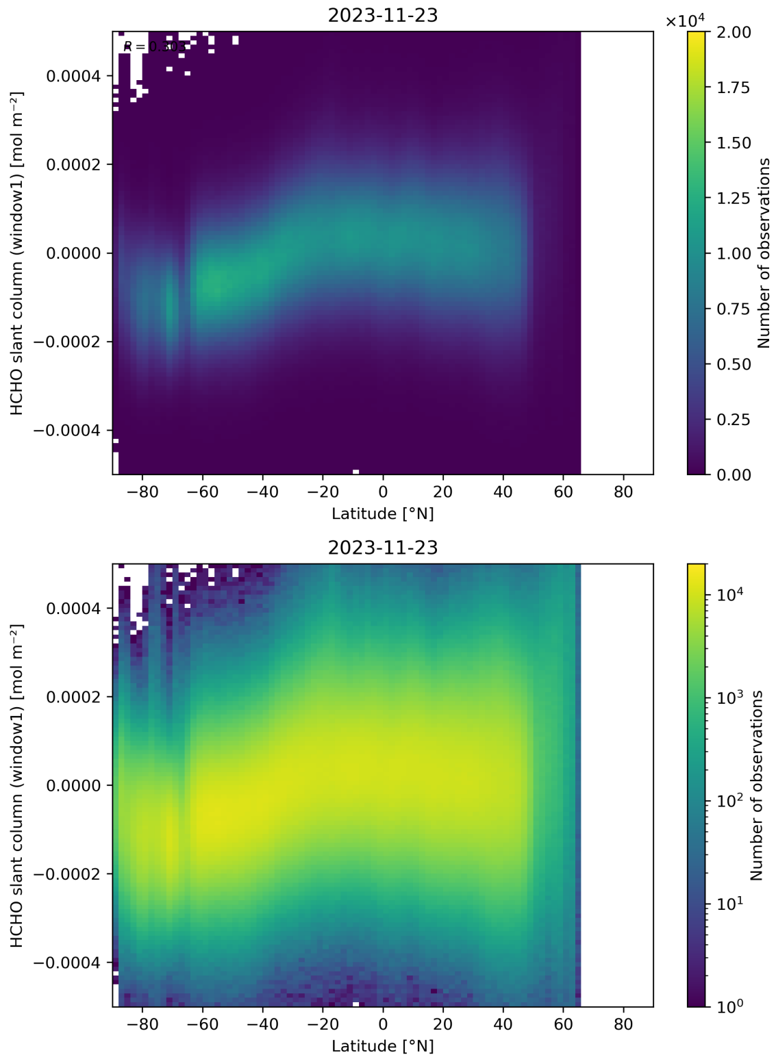
Figure 159: Scatter density plot of “Latitude” against “HCHO slant column (window1)” for 2023-11-23 to 2023-11-24.
