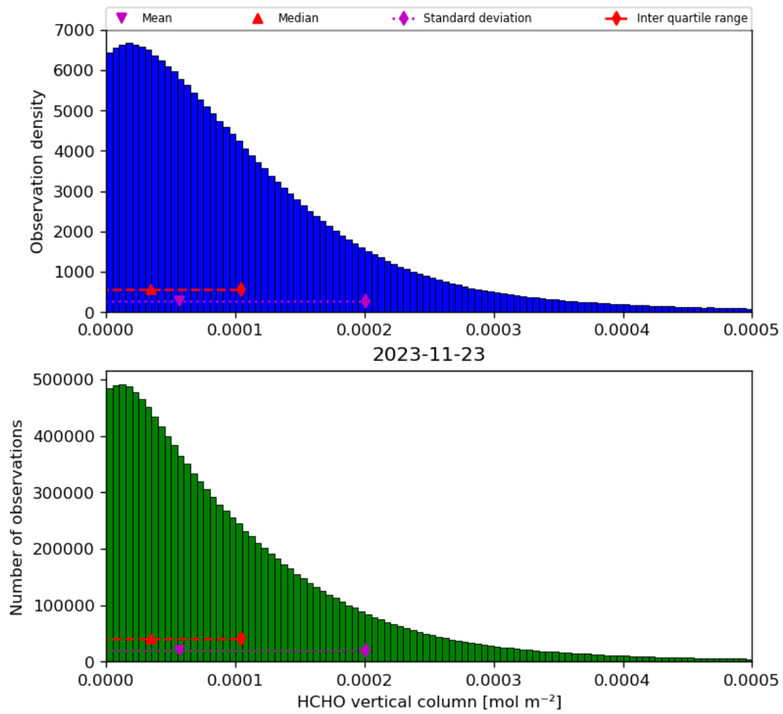
Figure 35: Histogram of “HCHO vertical column” for 2023-11-23 to 2023-11-24
