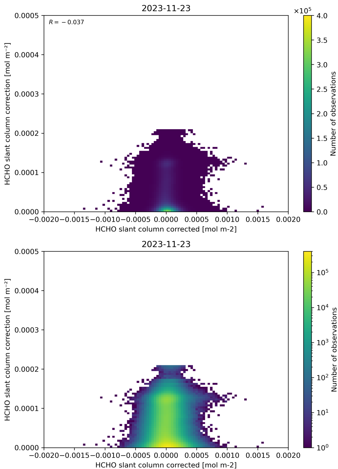
Figure 77: Scatter density plot of “HCHO slant column corrected” against “HCHO slant column correction” for 2023-11-23 to 2023-11-24.
