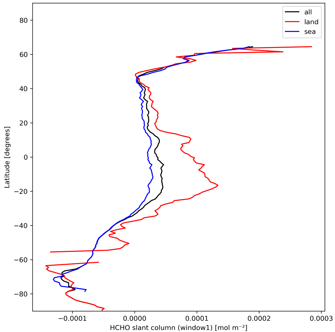
Figure 24: Zonal average of “HCHO slant column (window1)” for 2023-11-23 to 2023-11-24.
