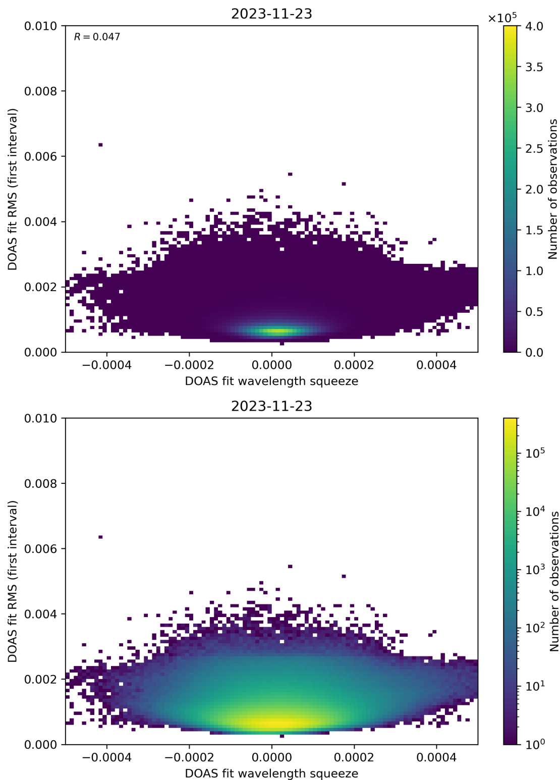
Figure 68: Scatter density plot of “DOAS fit wavelength squeeze” against “DOAS fit RMS (first interval)” for 2023-11-23 to 2023-11-24.
