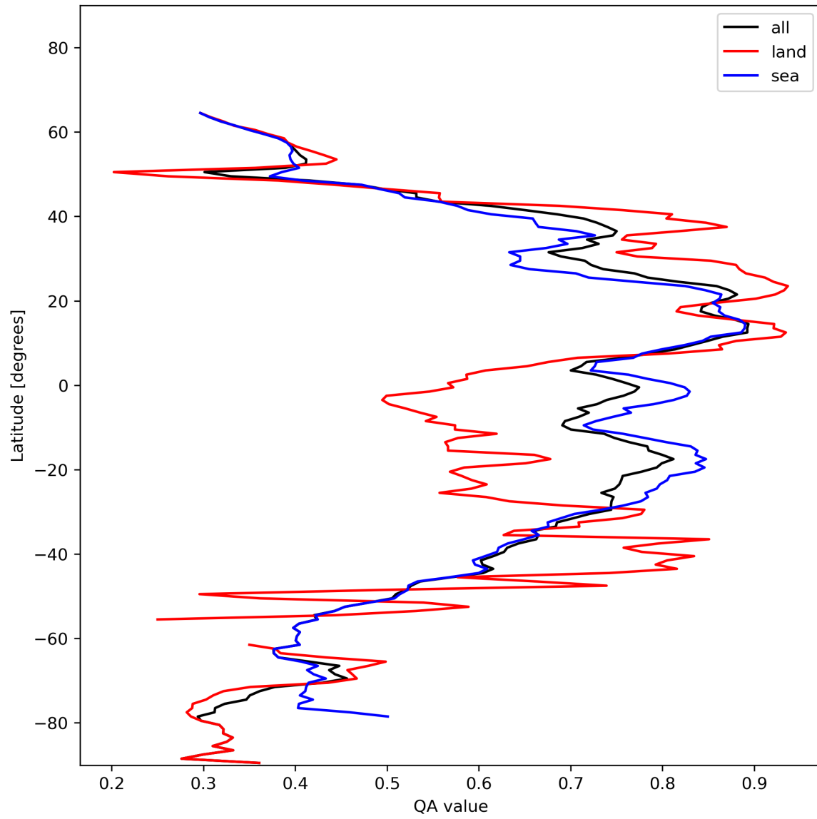
Figure 20: Zonal average of “QA value” for 2023-11-23 to 2023-11-24.
