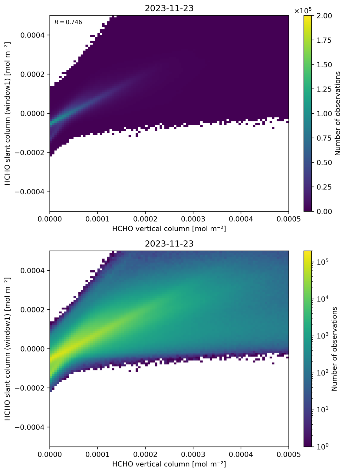
Figure 129: Scatter density plot of “HCHO vertical column” against “HCHO slant column (window1)” for 2023-11-23 to 2023-11-24.
