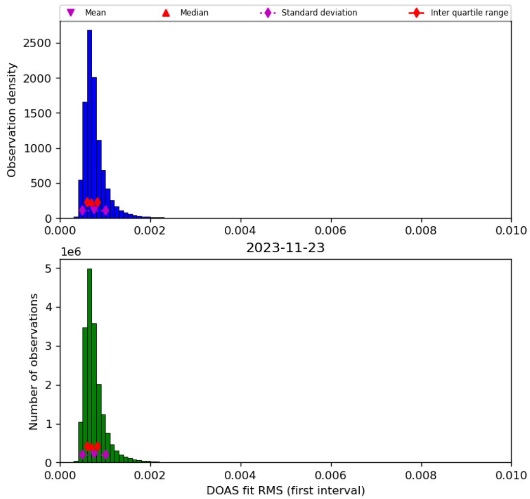
Figure 46: Histogram of “DOAS fit RMS (first interval)” for 2023-11-23 to 2023-11-24
