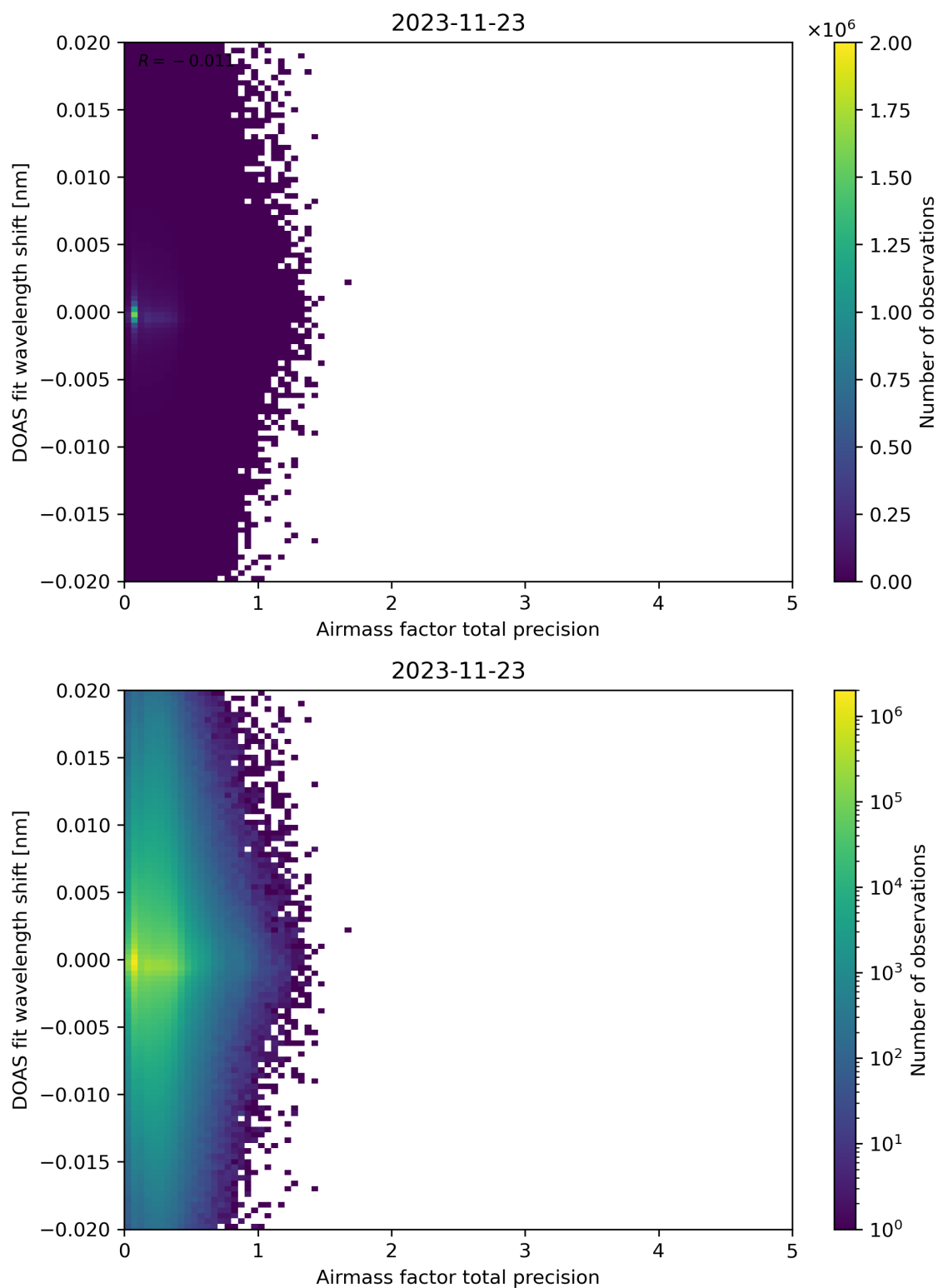
Figure 106: Scatter density plot of “Airmass factor total precision” against “DOAS fit wavelength shift” for 2023-11-23 to 2023-11-24.
