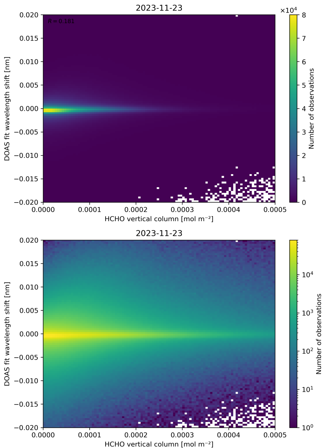
Figure 124: Scatter density plot of “HCHO vertical column” against “DOAS fit wavelength shift” for 2023-11-23 to 2023-11-24.
