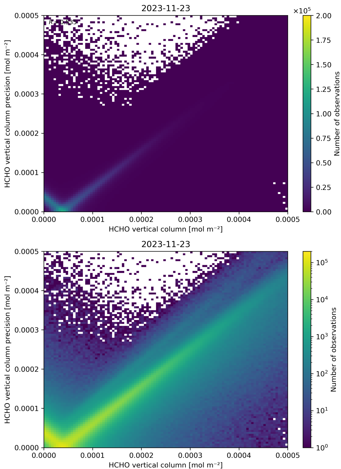
Figure 134: Scatter density plot of “HCHO vertical column” against “HCHO vertical column precision” for 2023-11-23 to 2023-11-24.
