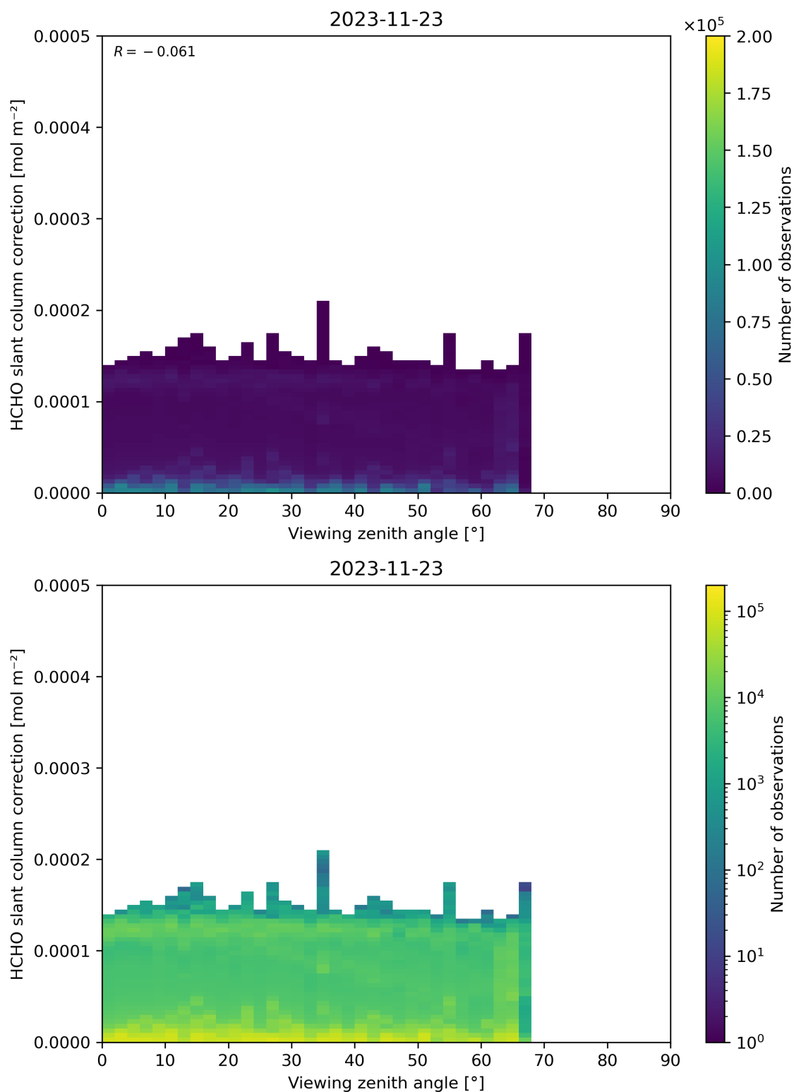
Figure 187: Scatter density plot of “Viewing zenith angle” against “HCHO slant column correction” for 2023-11-23 to 2023-11-24.
