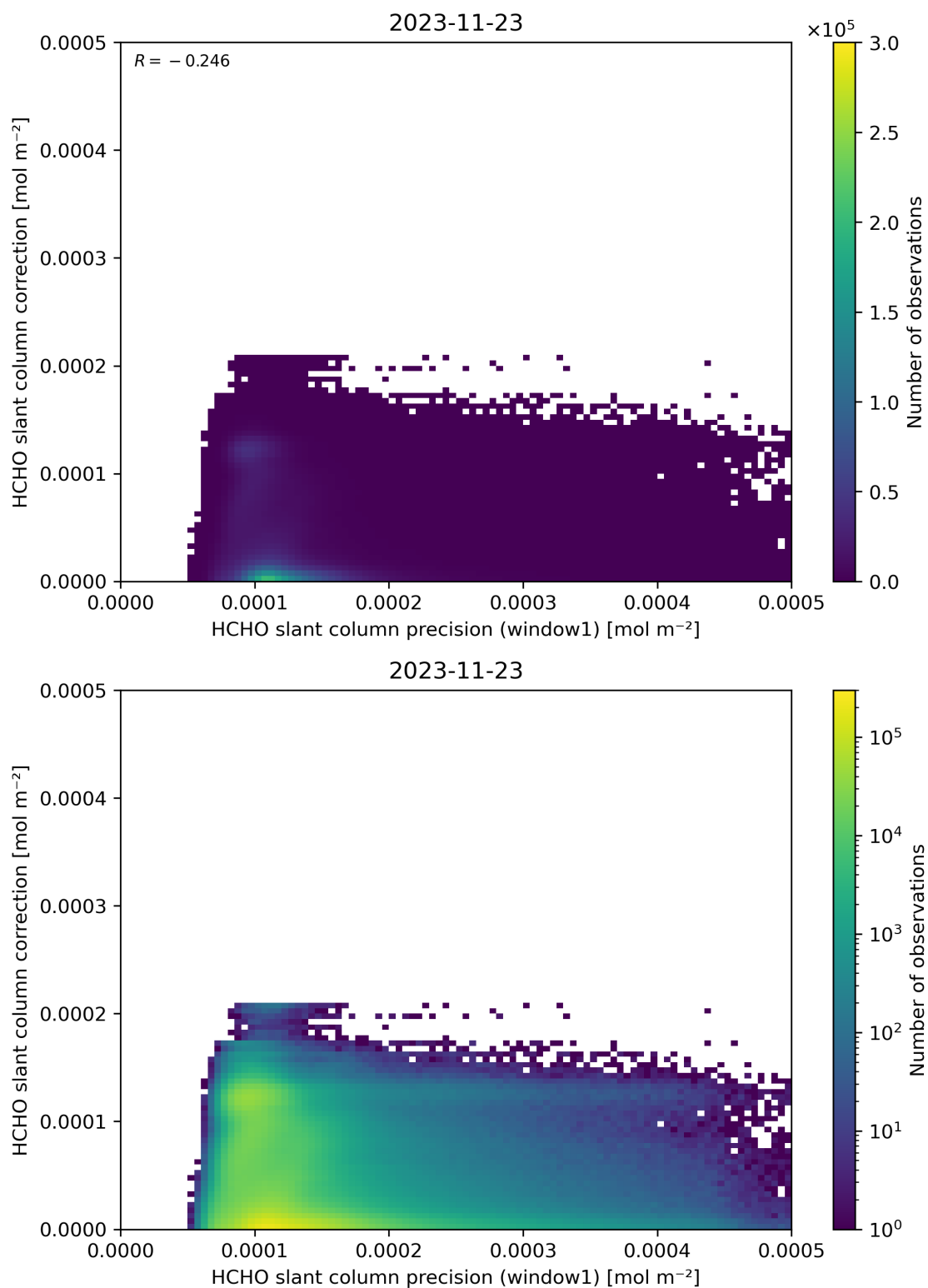
Figure 93: Scatter density plot of “HCHO slant column precision (window1)” against “HCHO slant column correction” for 2023-11-23 to 2023-11-24.
