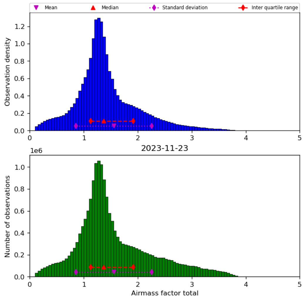
Figure 40: Histogram of “Airmass factor total” for 2023-11-23 to 2023-11-24
