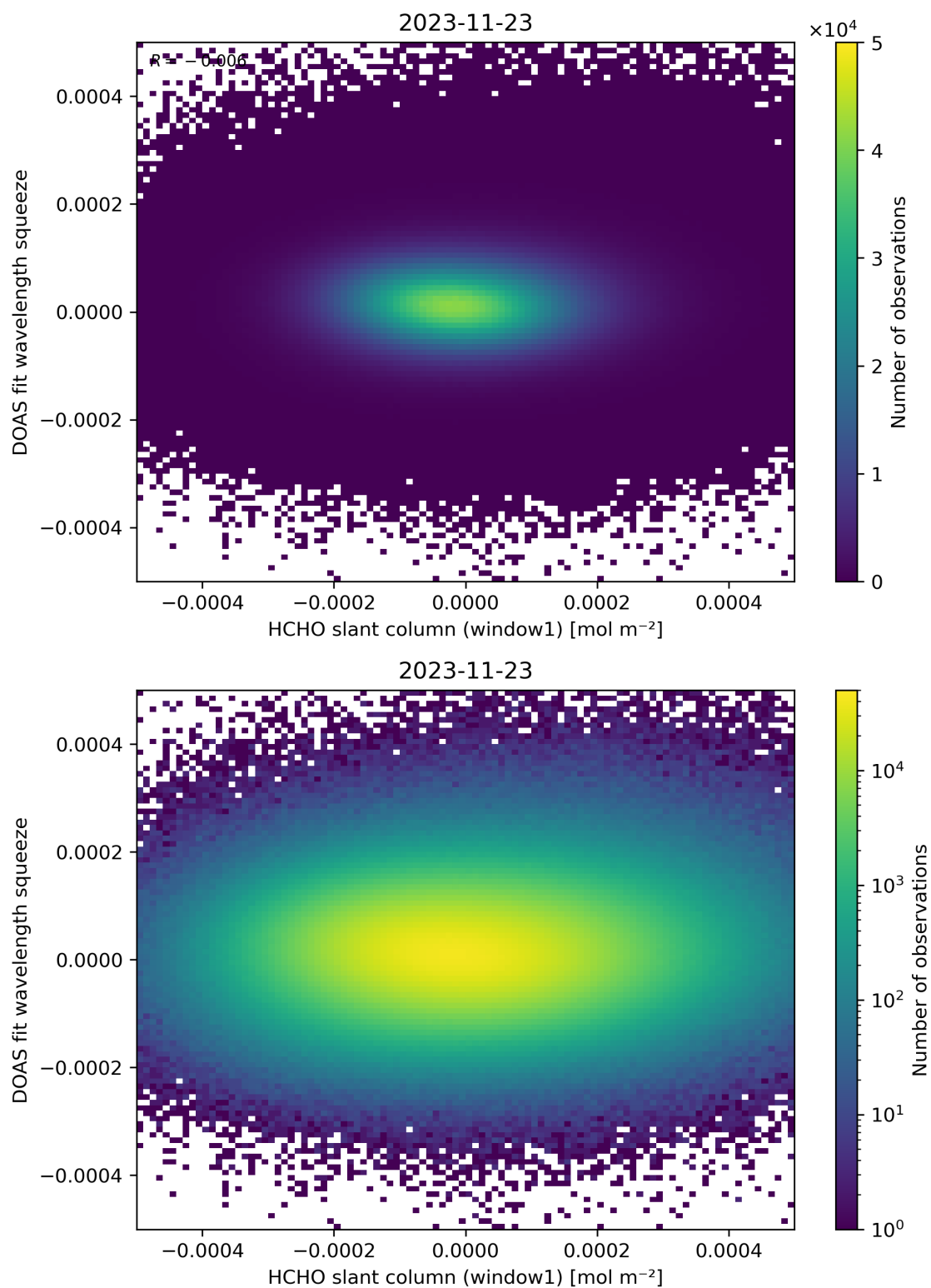
Figure 80: Scatter density plot of “HCHO slant column (window1)” against “DOAS fit wavelength squeeze” for 2023-11-23 to 2023-11-24.
