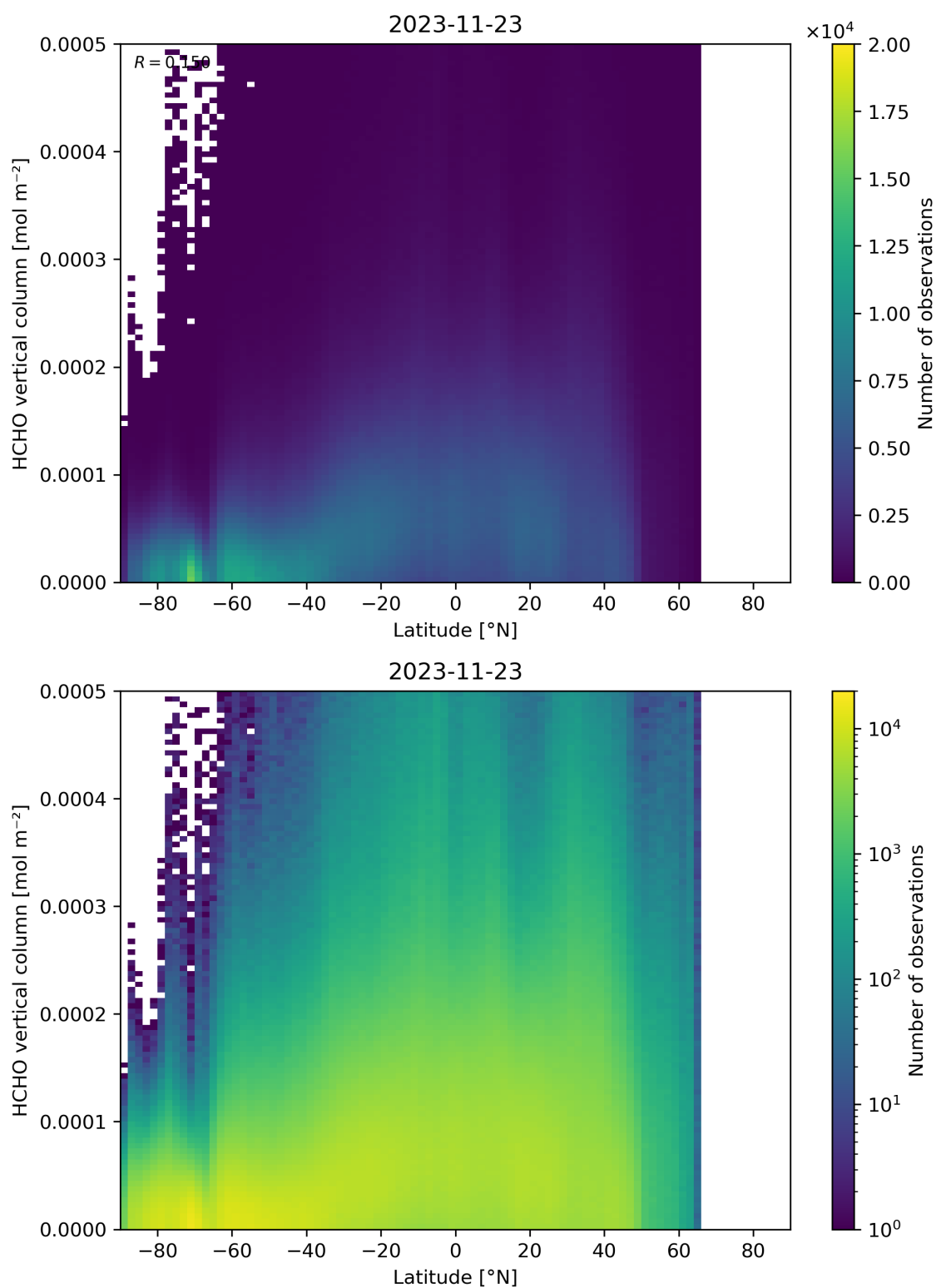
Figure 163: Scatter density plot of “Latitude” against “HCHO vertical column” for 2023-11-23 to 2023-11-24.
