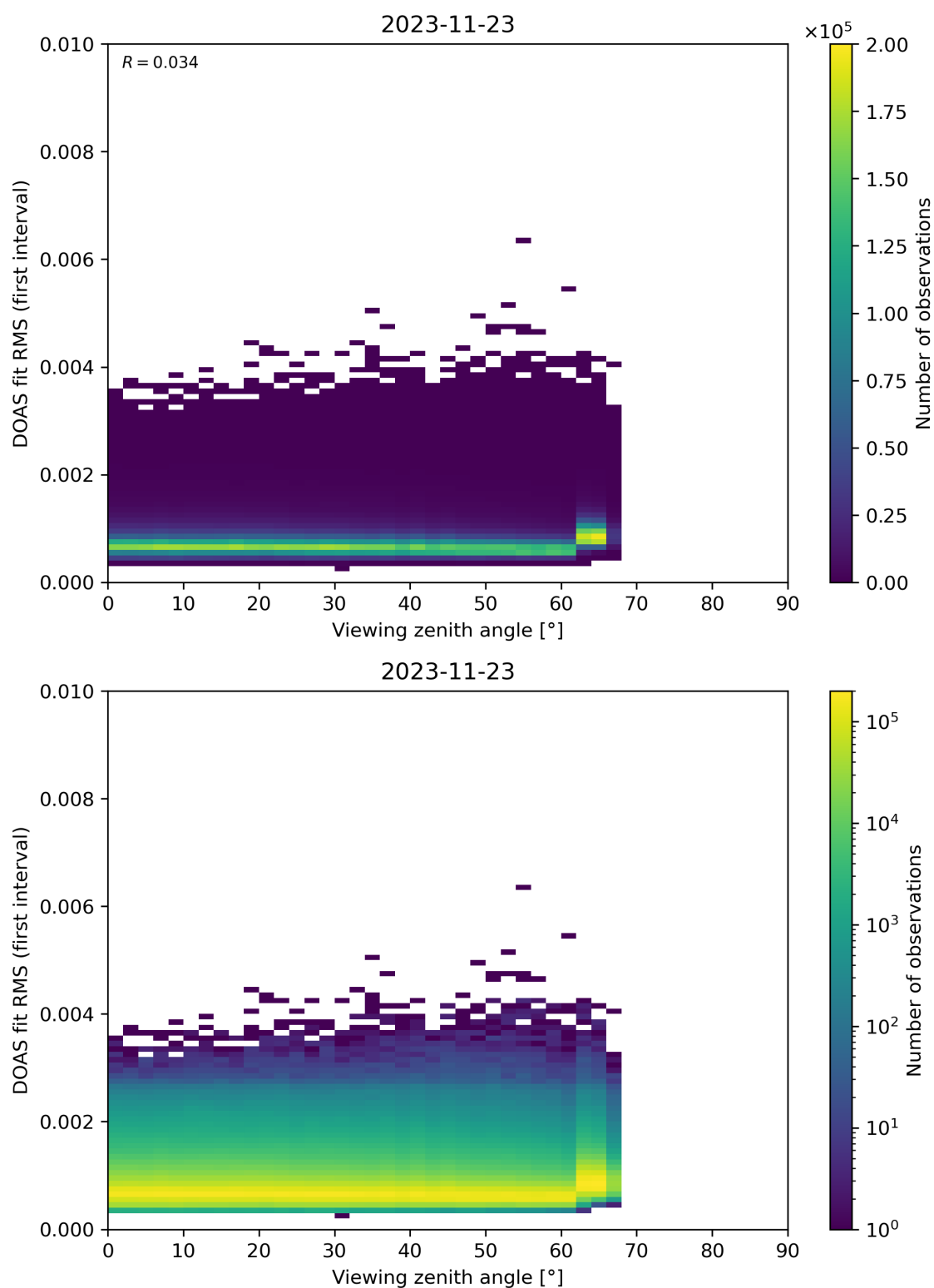
Figure 182: Scatter density plot of “Viewing zenith angle” against “DOAS fit RMS (first interval)” for 2023-11-23 to 2023-11-24.
