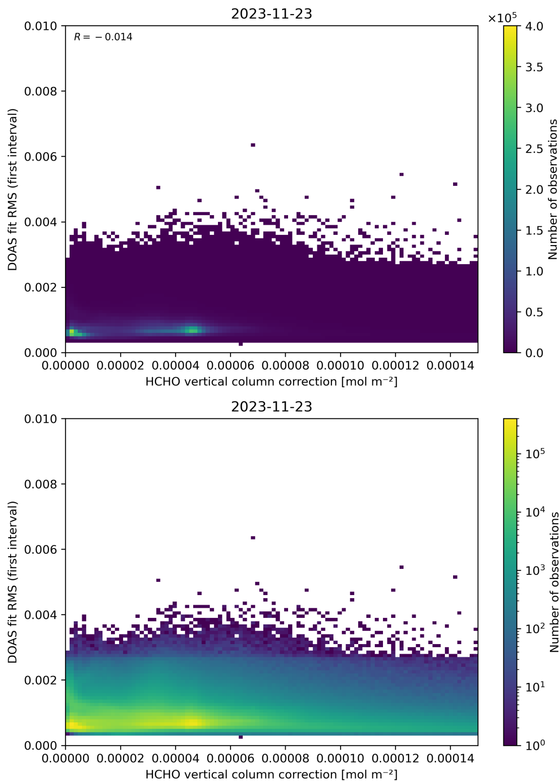
Figure 112: Scatter density plot of “HCHO vertical column correction” against “DOAS fit RMS (first interval)” for 2023-11-23 to 2023-11-24.
