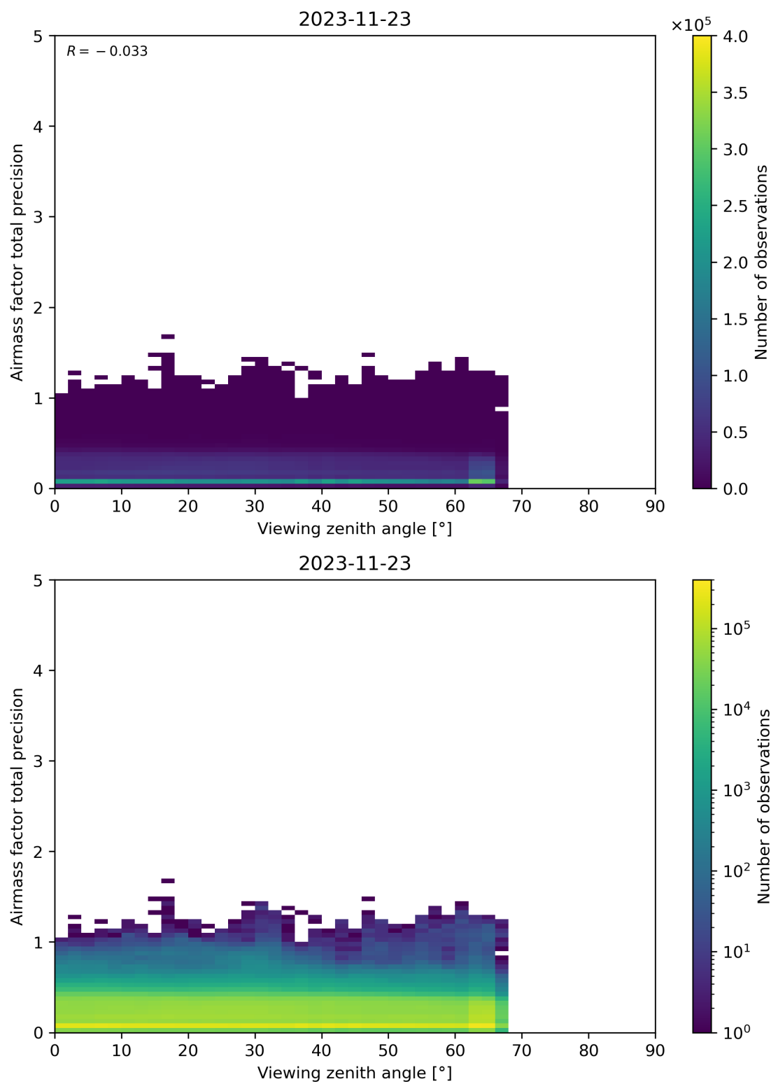
Figure 191: Scatter density plot of “Viewing zenith angle” against “Airmass factor total precision” for 2023-11-23 to 2023-11-24.
