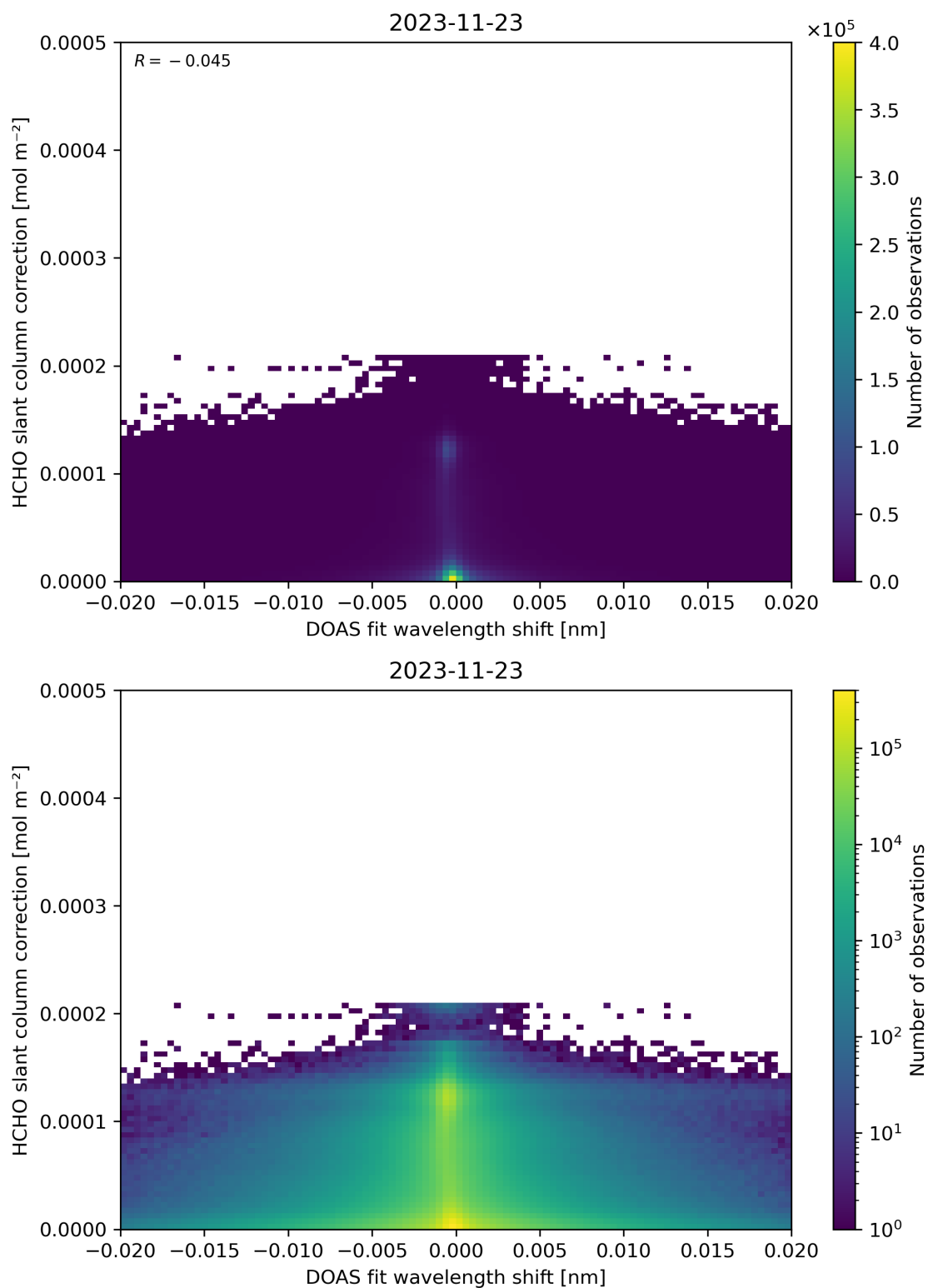
Figure 67: Scatter density plot of “DOAS fit wavelength shift” against “HCHO slant column correction” for 2023-11-23 to 2023-11-24.
