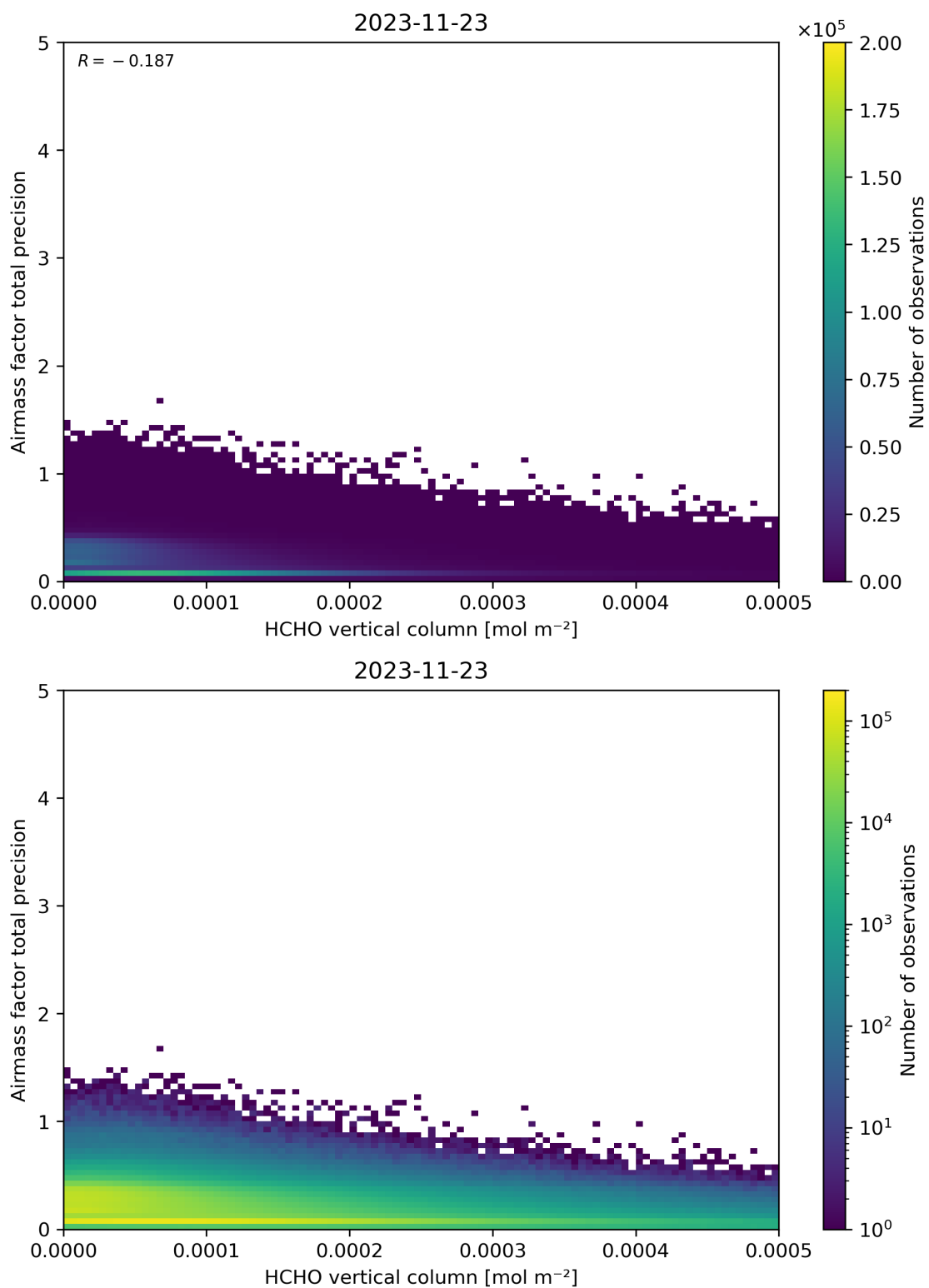
Figure 132: Scatter density plot of “HCHO vertical column” against “Airmass factor total precision” for 2023-11-23 to 2023-11-24.
