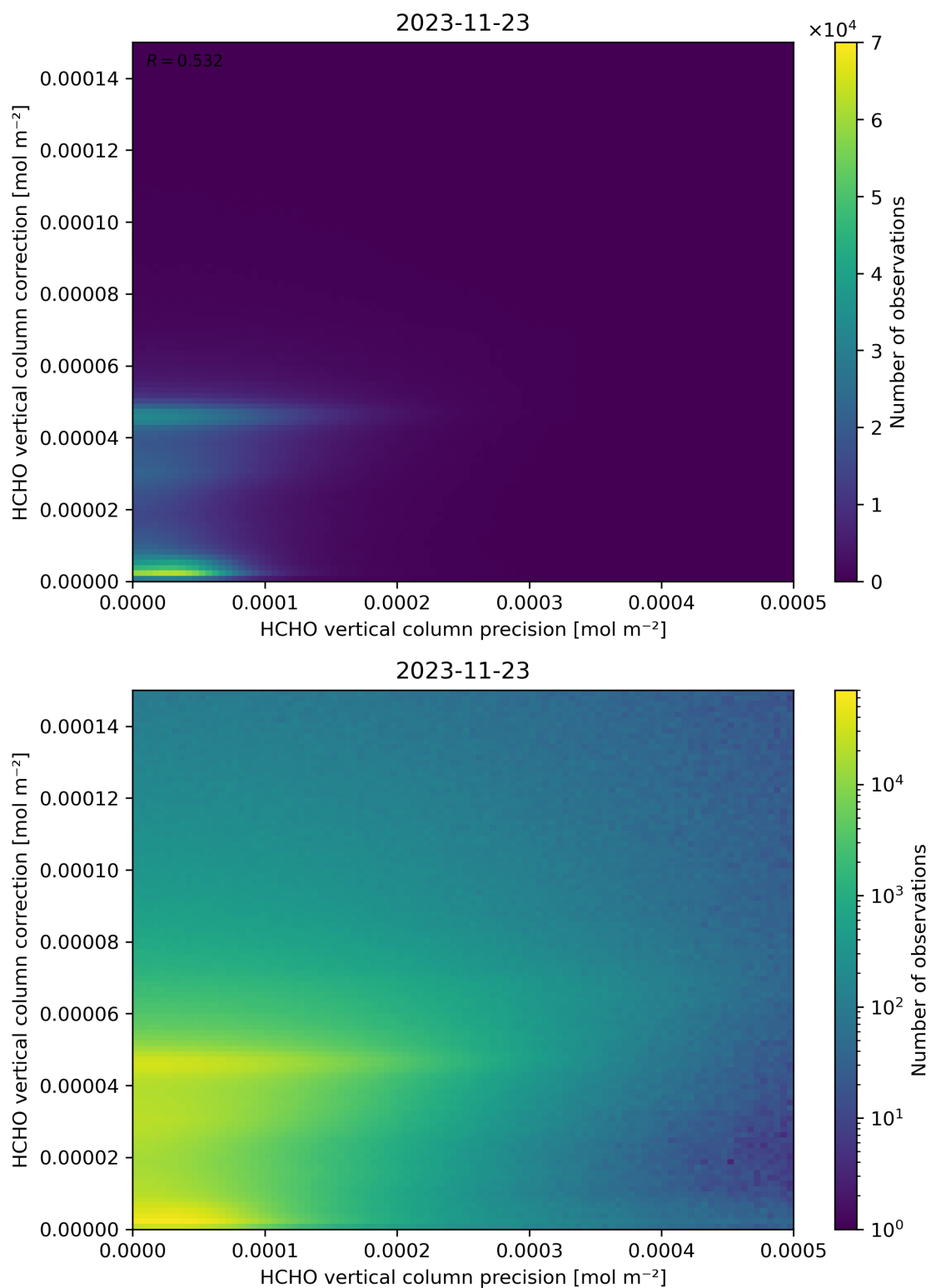
Figure 146: Scatter density plot of “HCHO vertical column precision” against “HCHO vertical column correction” for 2023-11-23 to 2023-11-24.
