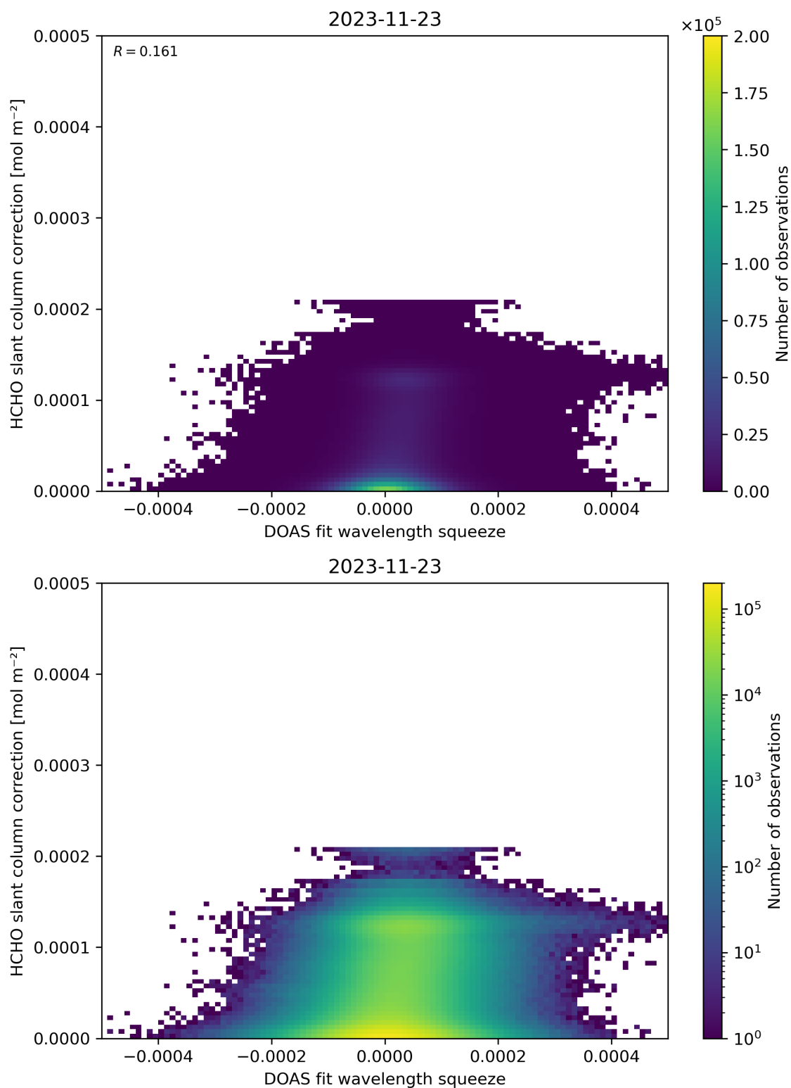
Figure 70: Scatter density plot of “DOAS fit wavelength squeeze” against “HCHO slant column correction” for 2023-11-23 to 2023-11-24.
