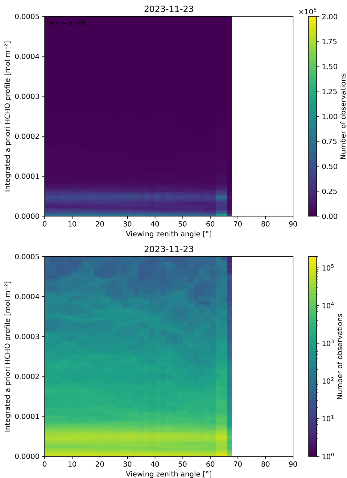
Figure 195: Scatter density plot of “Viewing zenith angle” against “Integrated a priori HCHO profile” for 2023-11-23 to 2023-11-24.
