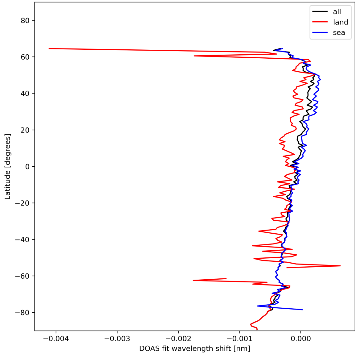
Figure 30: Zonal average of “DOAS fit wavelength shift” for 2023-11-23 to 2023-11-24.
