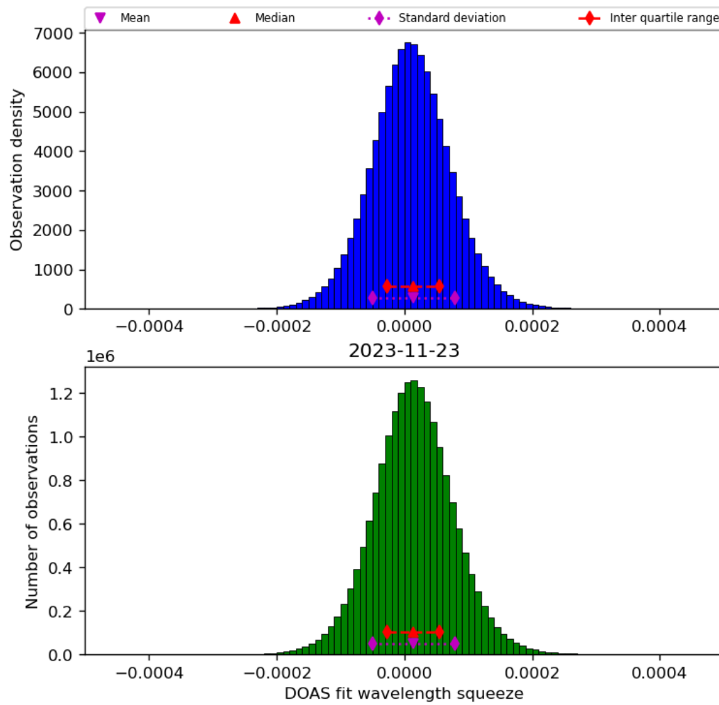
Figure 45: Histogram of “DOAS fit wavelength squeeze” for 2023-11-23 to 2023-11-24
