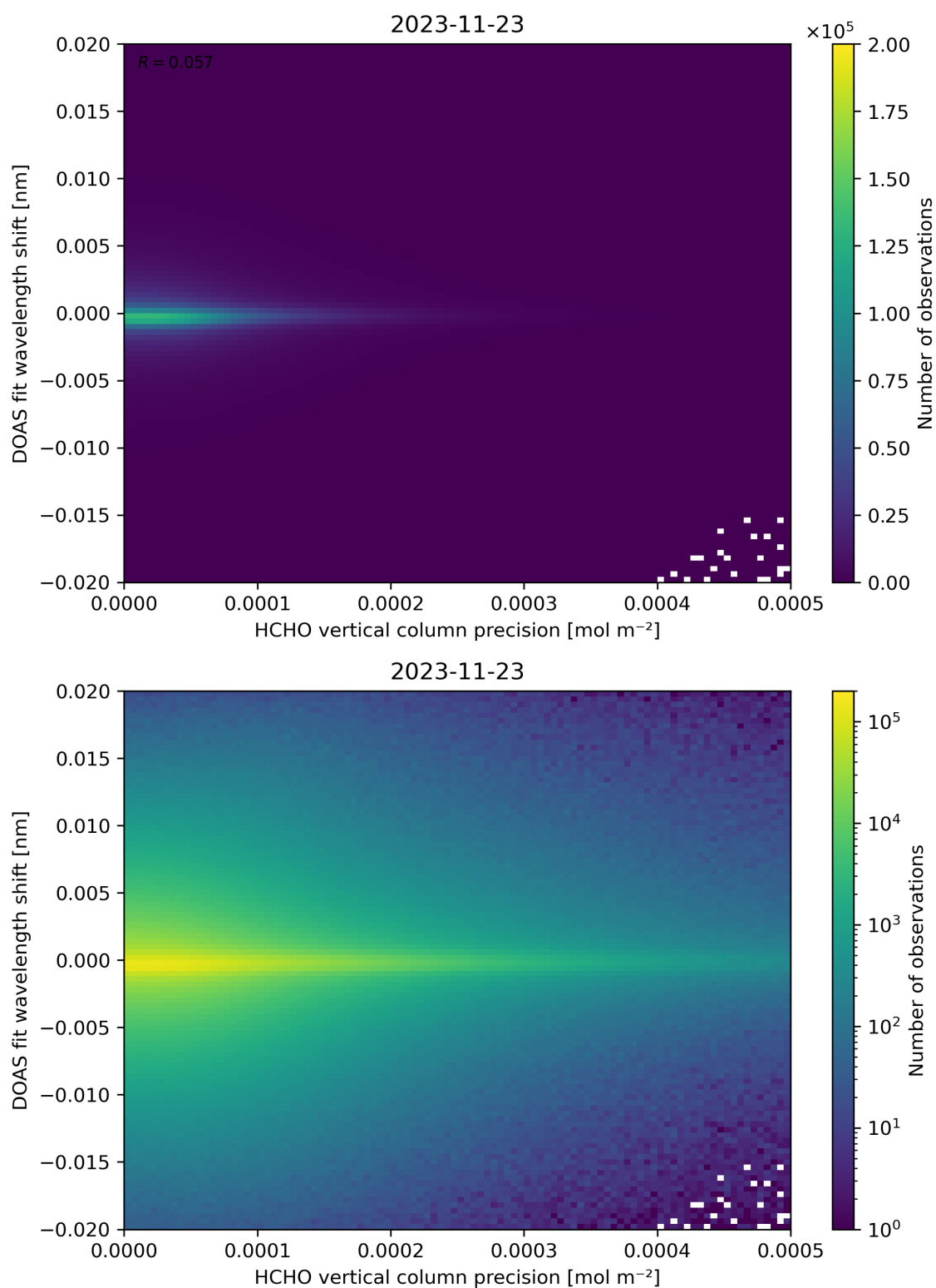
Figure 137: Scatter density plot of “HCHO vertical column precision” against “DOAS fit wavelength shift” for 2023-11-23 to 2023-11-24.
