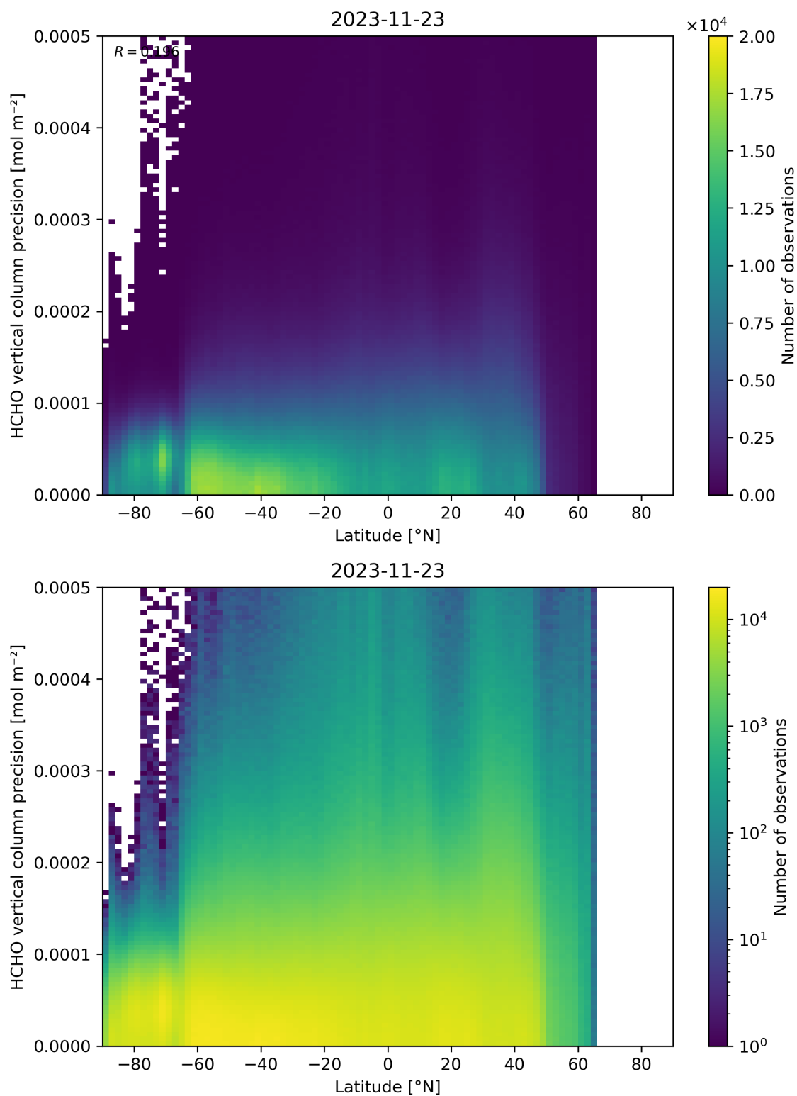
Figure 165: Scatter density plot of “Latitude” against “HCHO vertical column precision” for 2023-11-23 to 2023-11-24.
