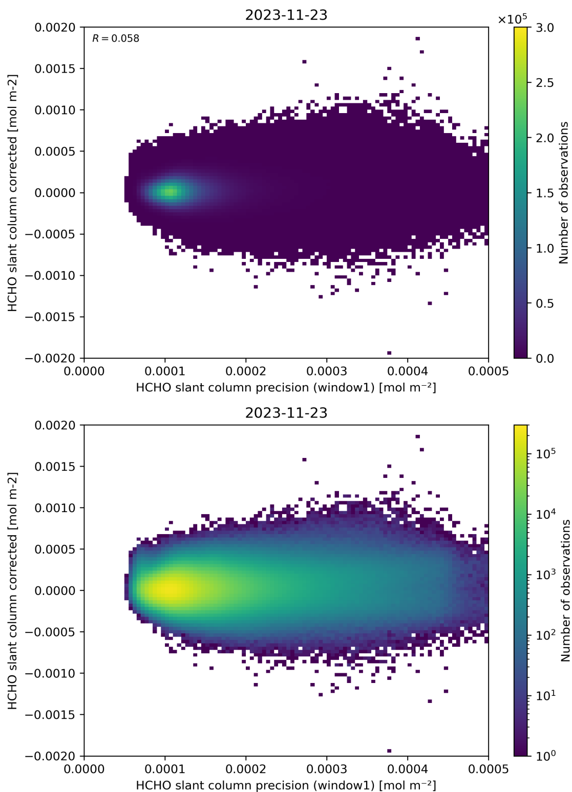
Figure 92: Scatter density plot of “HCHO slant column precision (window1)” against “HCHO slant column corrected” for 2023-11-23 to 2023-11-24.
