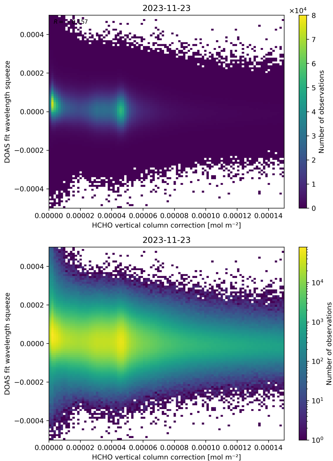
Figure 114: Scatter density plot of “HCHO vertical column correction” against “DOAS fit wavelength squeeze” for 2023-11-23 to 2023-11-24.
