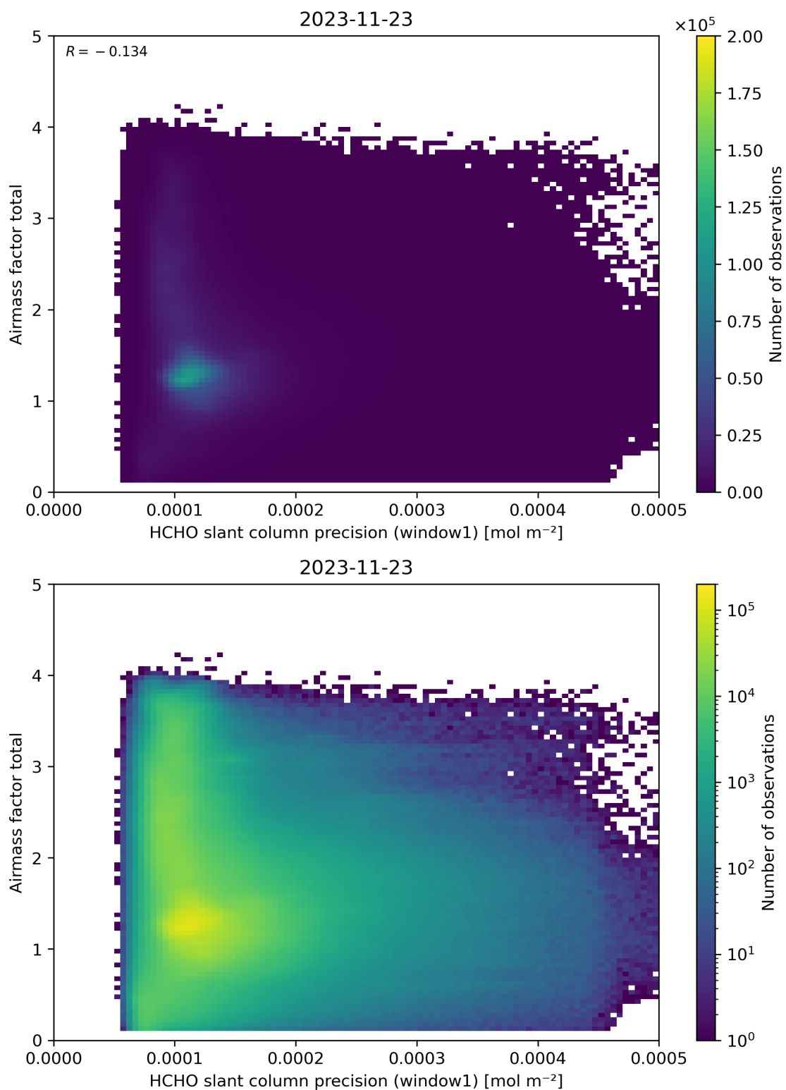
Figure 94: Scatter density plot of “HCHO slant column precision (window1)” against “Airmass factor total” for 2023-11-23 to 2023-11-24.
