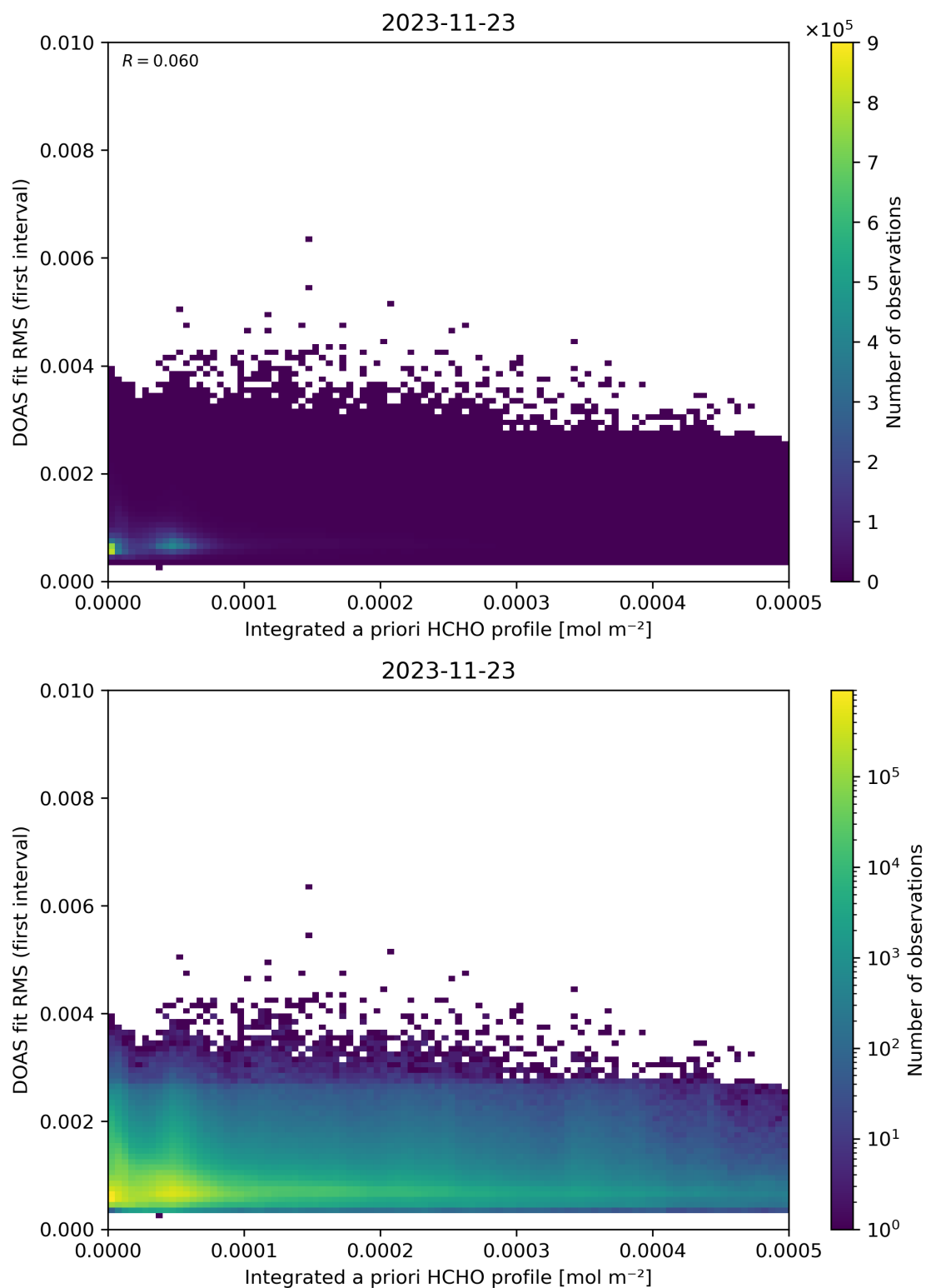
Figure 148: Scatter density plot of “Integrated a priori HCHO profile” against “DOAS fit RMS (first interval)” for 2023-11-23 to 2023-11-24.
