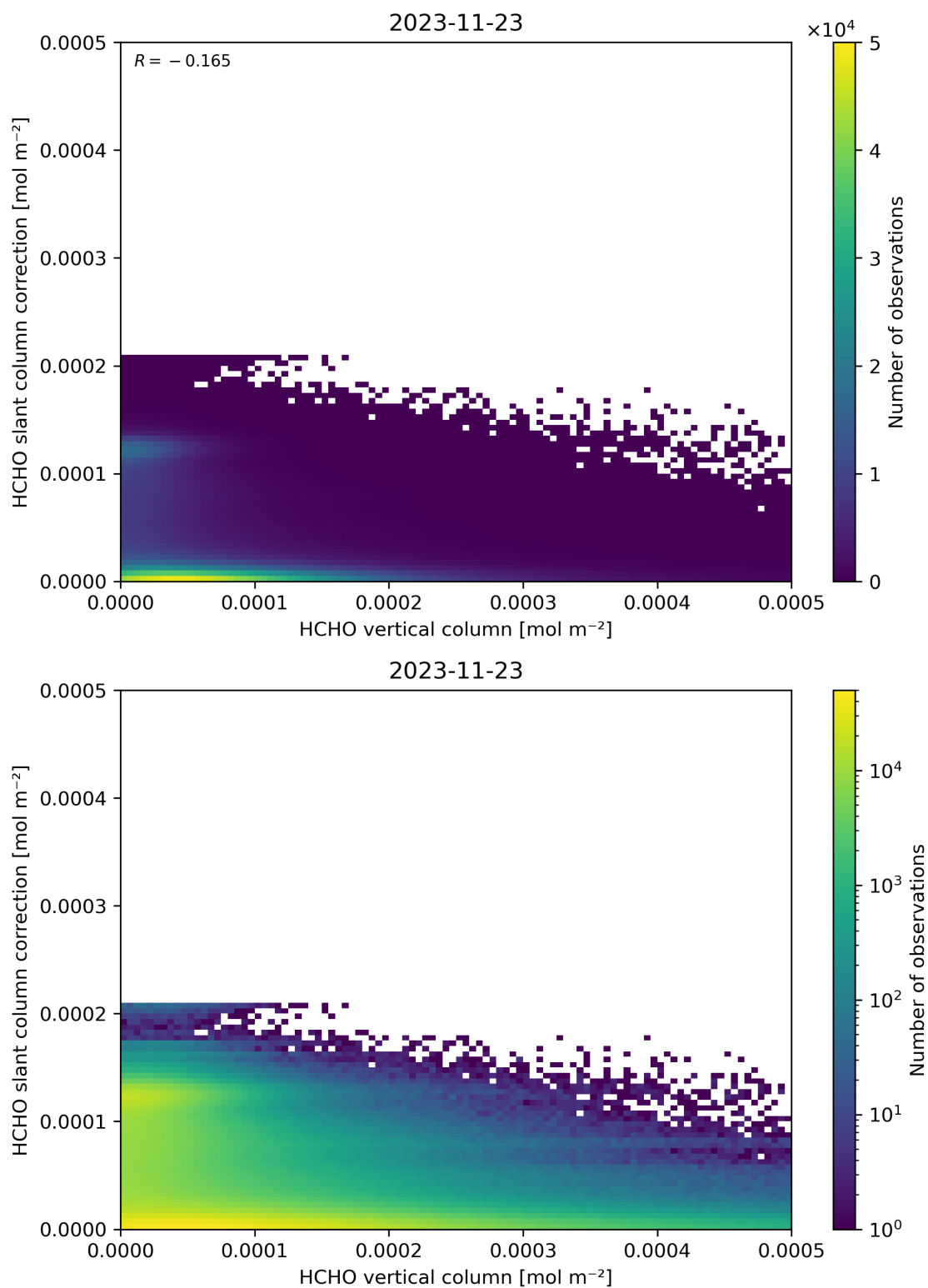
Figure 128: Scatter density plot of “HCHO vertical column” against “HCHO slant column correction” for 2023-11-23 to 2023-11-24.
