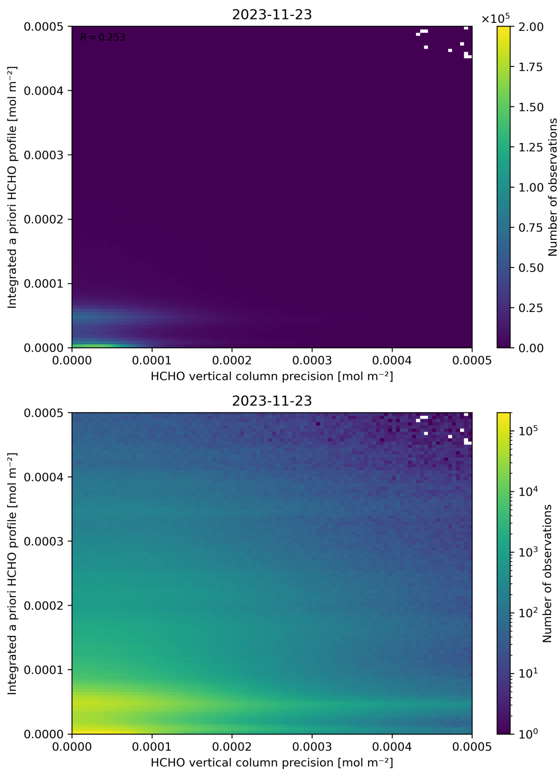
Figure 147: Scatter density plot of “HCHO vertical column precision” against “Integrated a priori HCHO profile” for 2023-11-23 to 2023-11-24.
