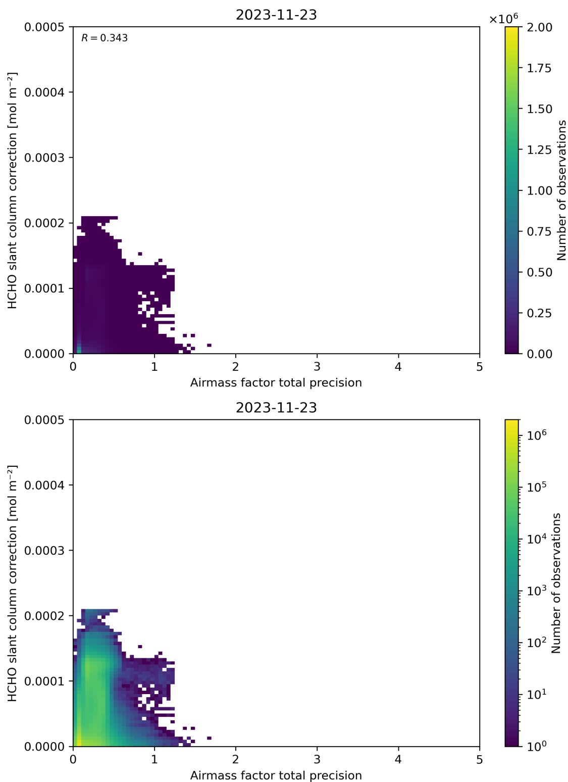
Figure 110: Scatter density plot of “Airmass factor total precision” against “HCHO slant column correction” for 2023-11-23 to 2023-11-24.
