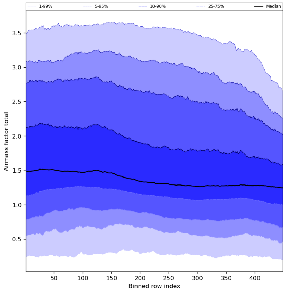
Figure 54: Along track statistics of “Airmass factor total” for 2023-11-23 to 2023-11-24
