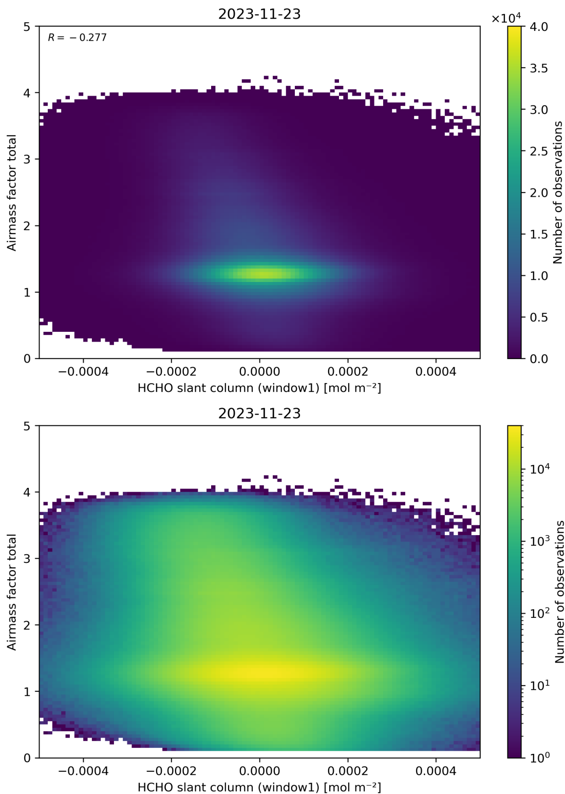
Figure 85: Scatter density plot of “HCHO slant column (window1)” against “Airmass factor total” for 2023-11-23 to 2023-11-24.
