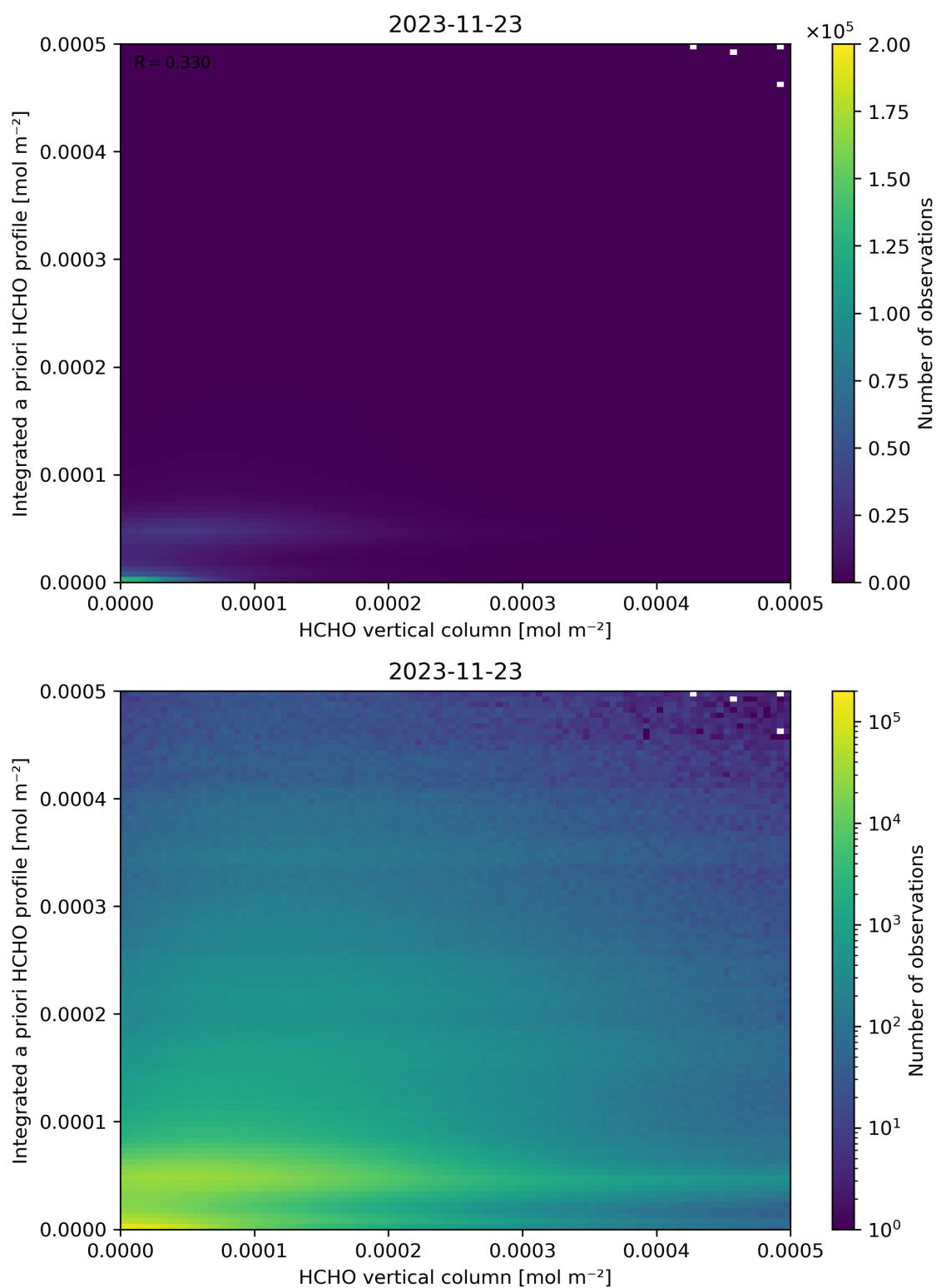
Figure 135: Scatter density plot of “HCHO vertical column” against “Integrated a priori HCHO profile” for 2023-11-23 to 2023-11-24.
