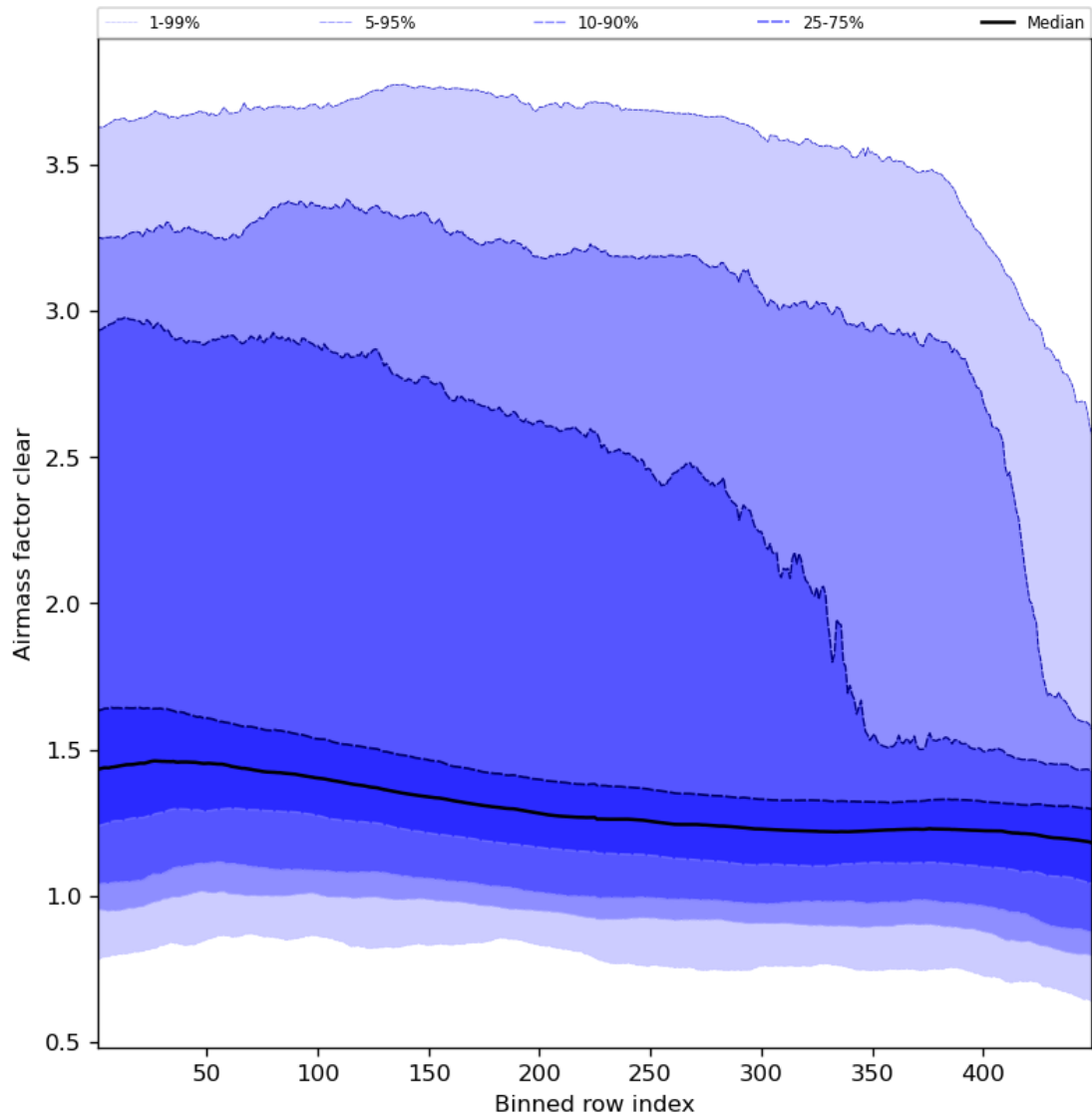
Figure 56: Along track statistics of “Airmass factor clear” for 2023-11-23 to 2023-11-24
