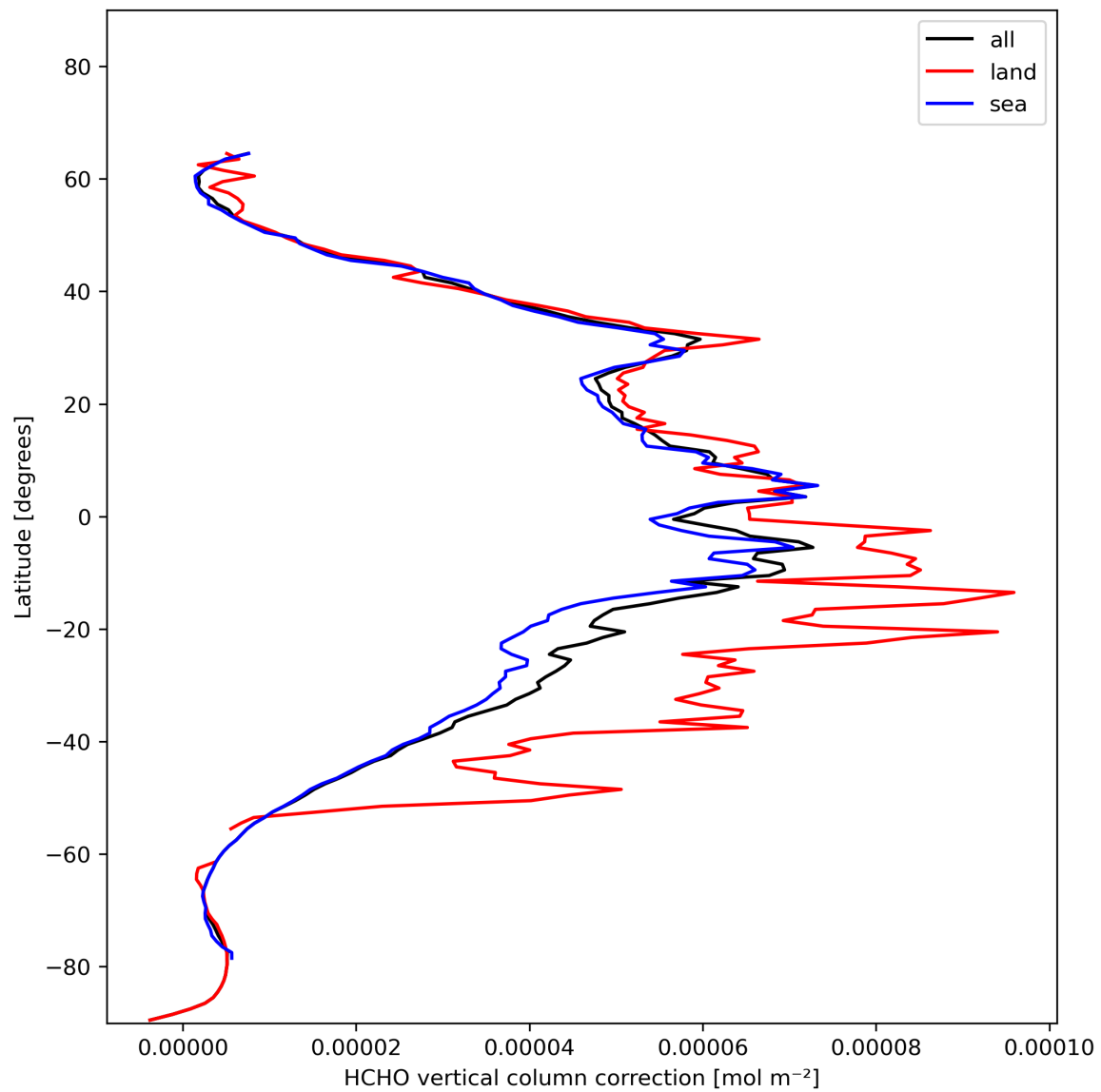
Figure 23: Zonal average of “HCHO vertical column correction” for 2023-11-23 to 2023-11-24.
