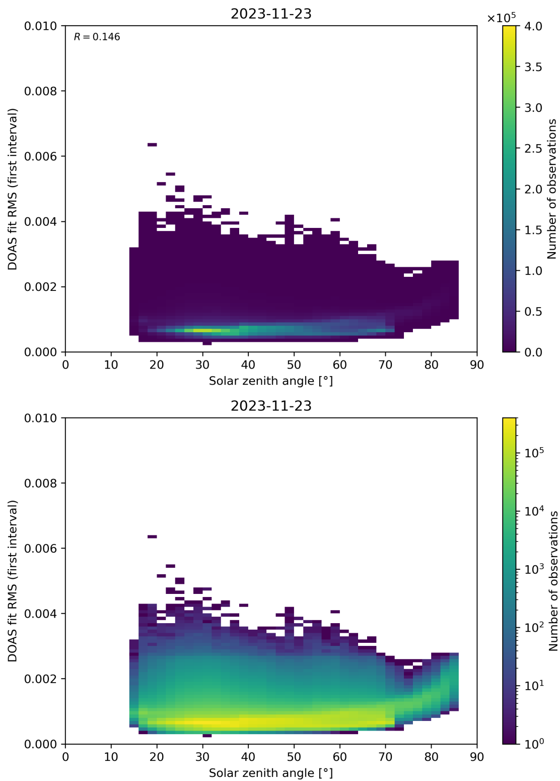
Figure 167: Scatter density plot of “Solar zenith angle” against “DOAS fit RMS (first interval)” for 2023-11-23 to 2023-11-24.
