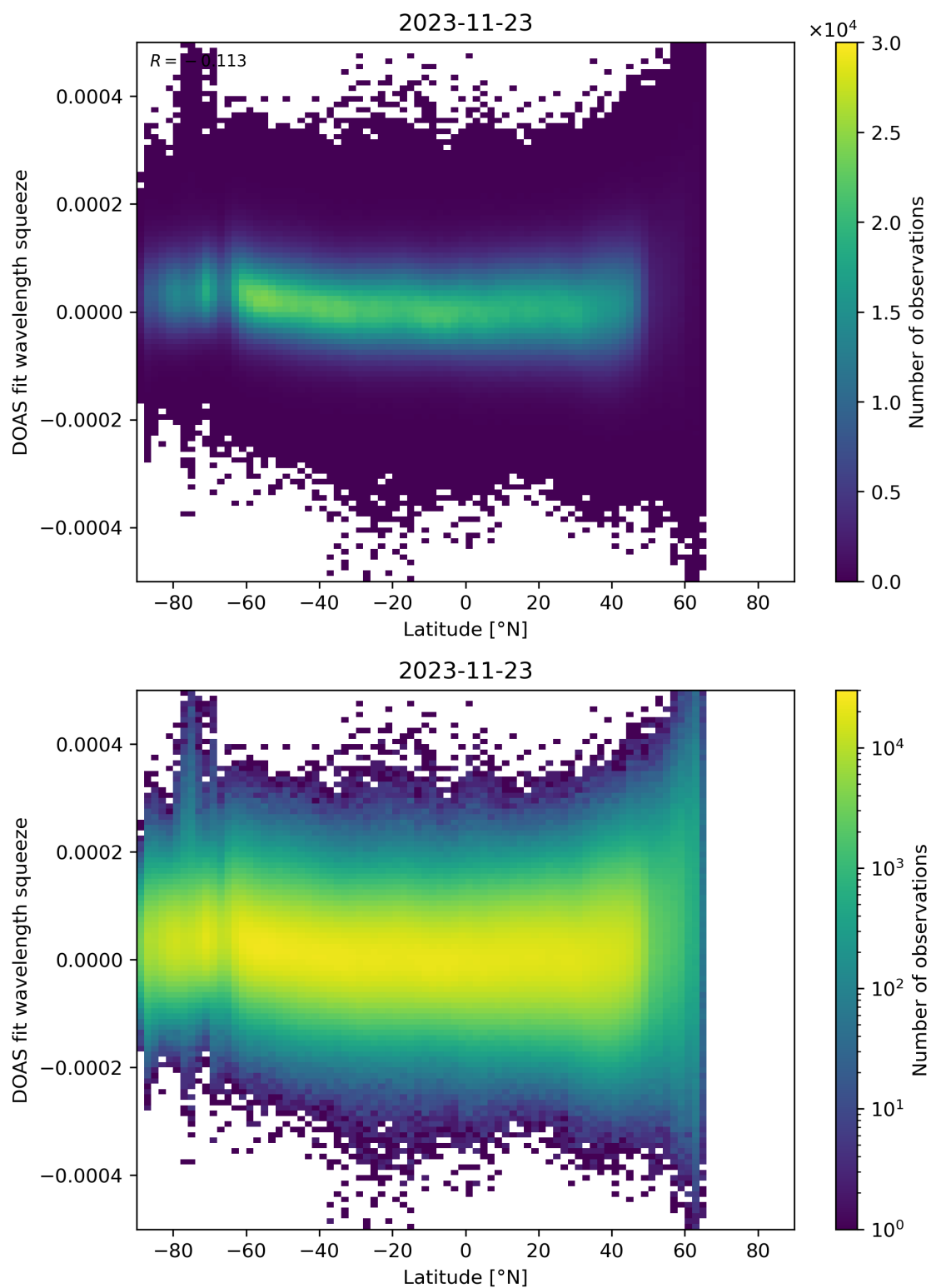
Figure 155: Scatter density plot of “Latitude” against “DOAS fit wavelength squeeze” for 2023-11-23 to 2023-11-24.
