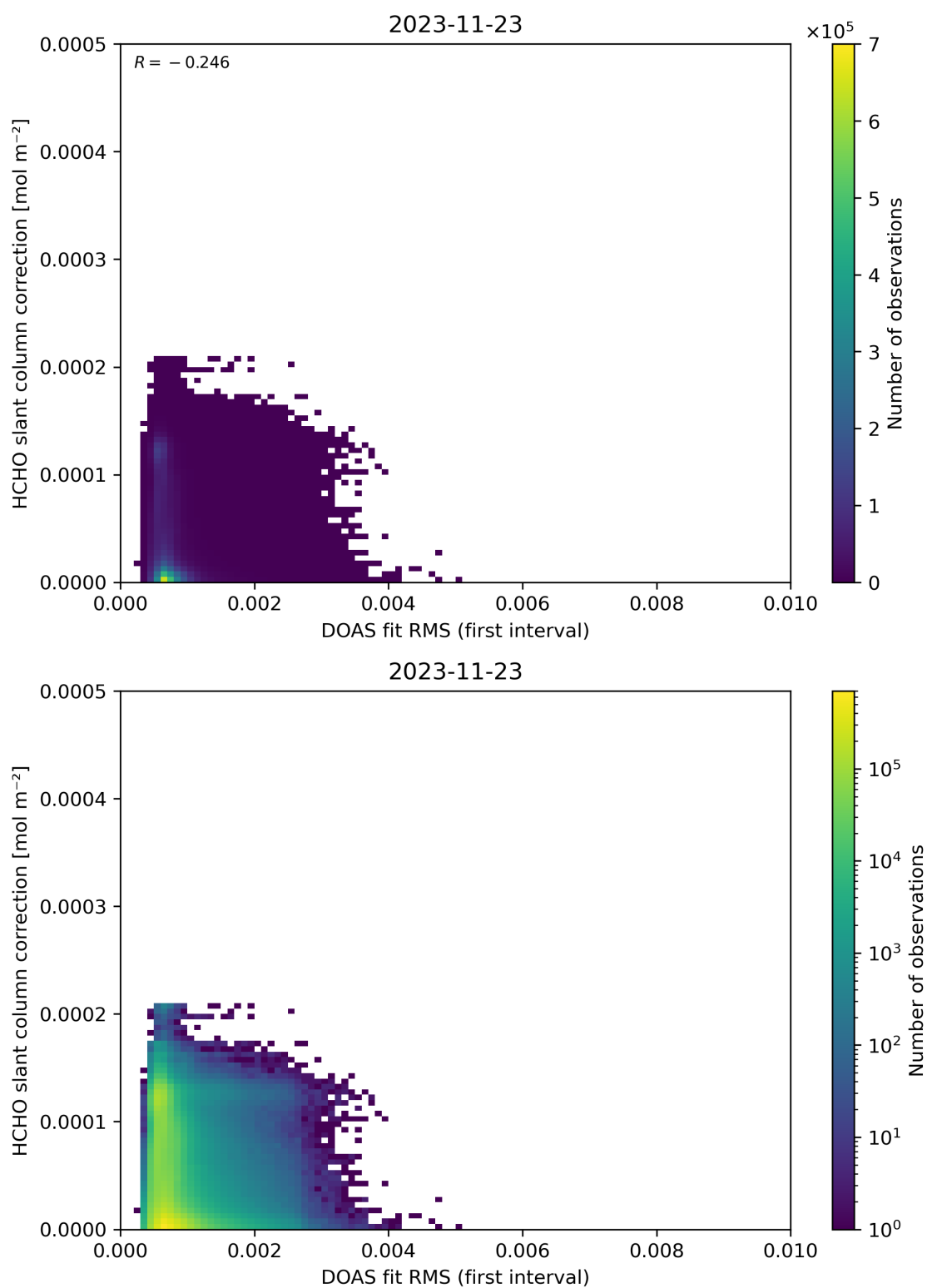
Figure 63: Scatter density plot of “DOAS fit RMS (first interval)” against “HCHO slant column correction” for 2023-11-23 to 2023-11-24.
