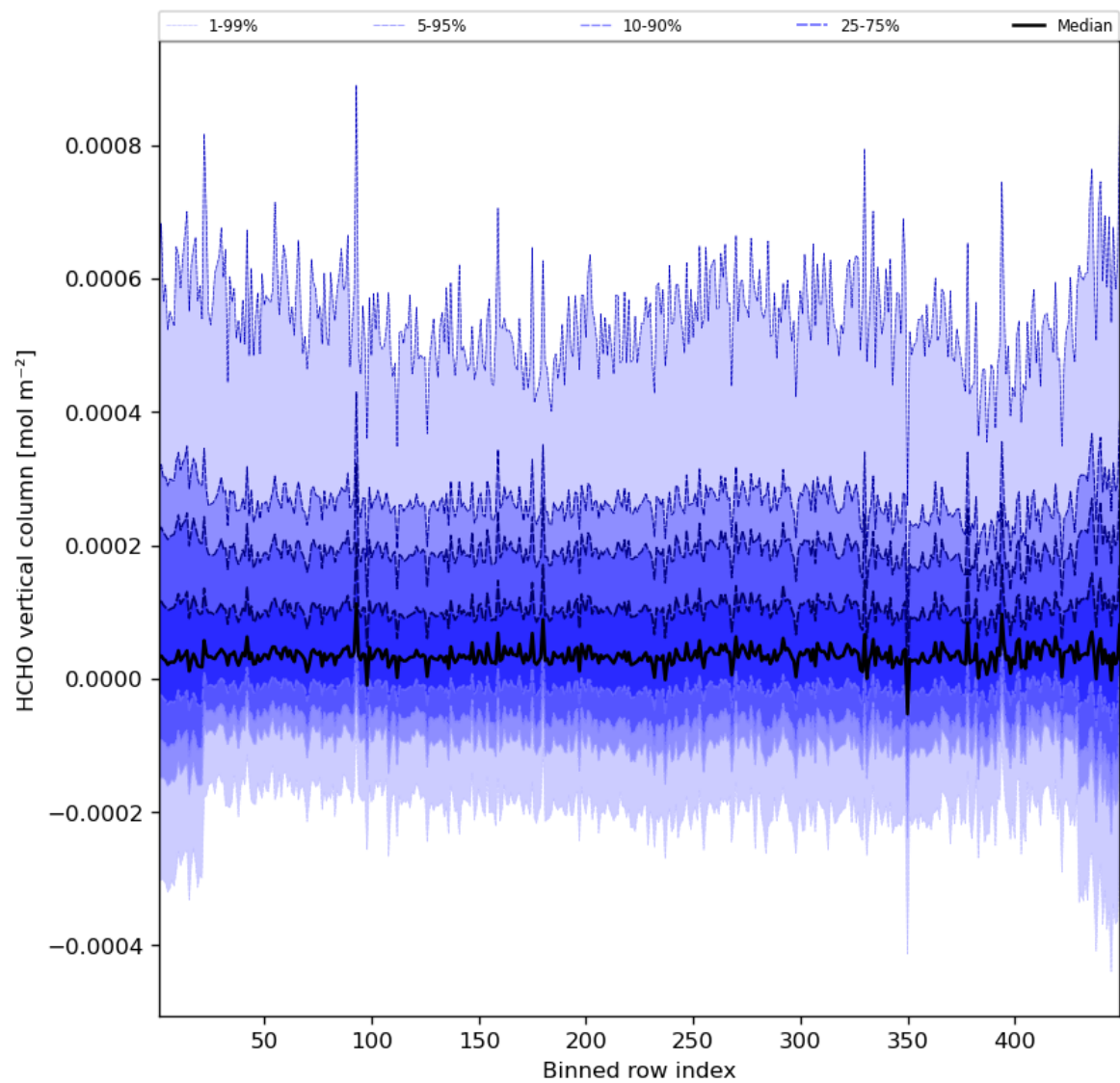
Figure 49: Along track statistics of “HCHO vertical column” for 2023-11-23 to 2023-11-24
