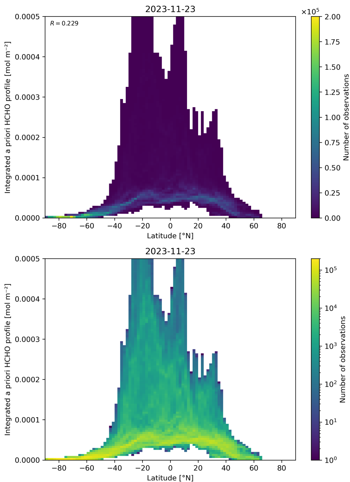
Figure 166: Scatter density plot of “Latitude” against “Integrated a priori HCHO profile” for 2023-11-23 to 2023-11-24.
