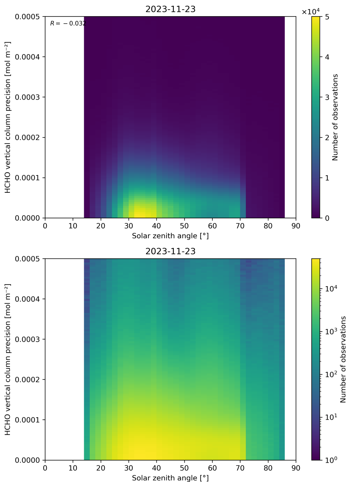
Figure 179: Scatter density plot of “Solar zenith angle” against “HCHO vertical column precision” for 2023-11-23 to 2023-11-24.
