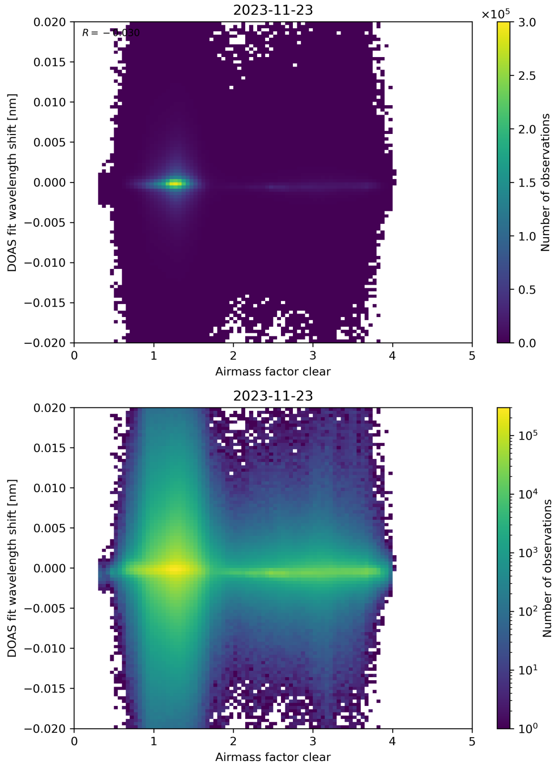
Figure 72: Scatter density plot of “Airmass factor clear” against “DOAS fit wavelength shift” for 2023-11-23 to 2023-11-24.
