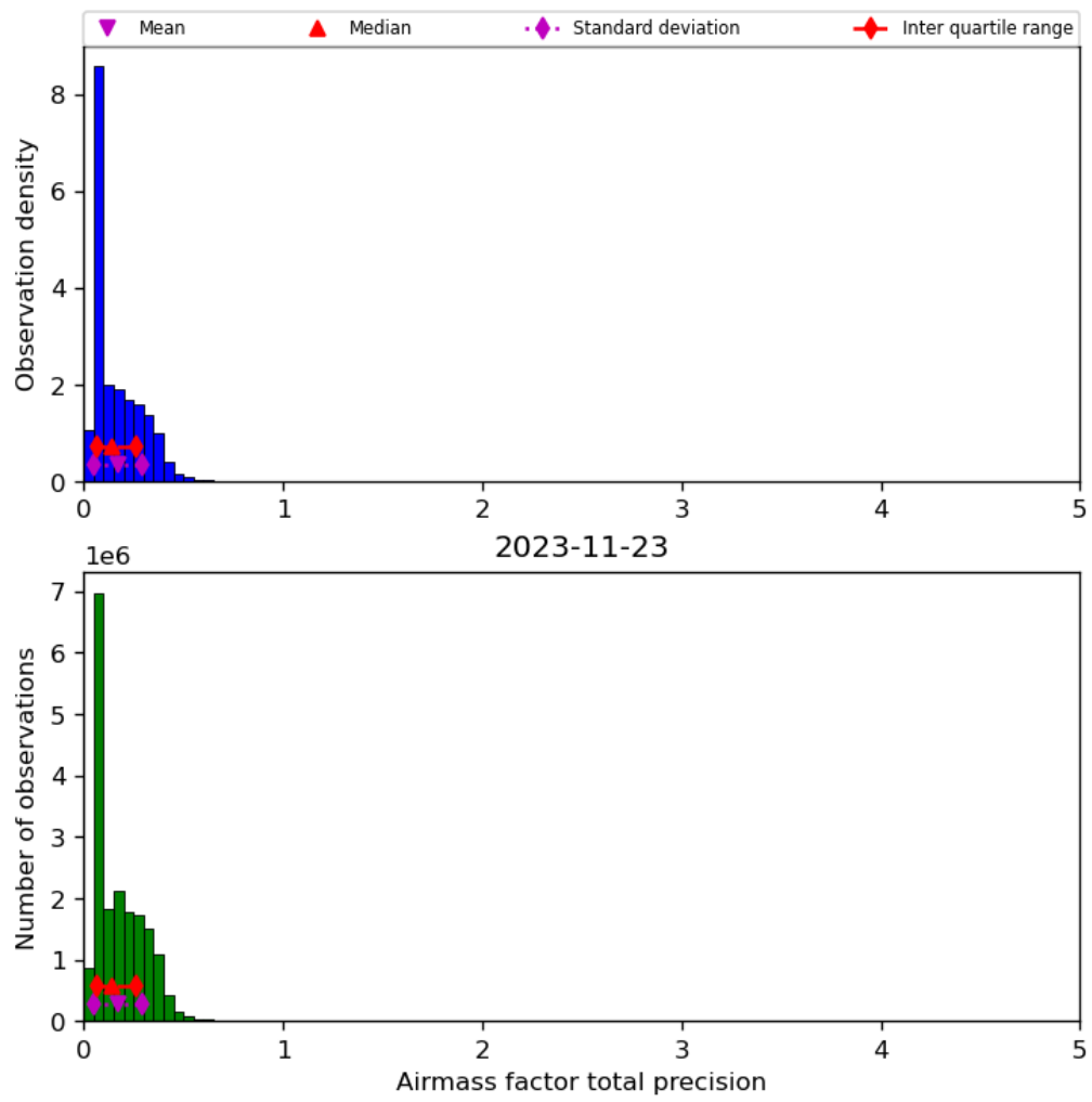
Figure 41: Histogram of “Airmass factor total precision” for 2023-11-23 to 2023-11-24
