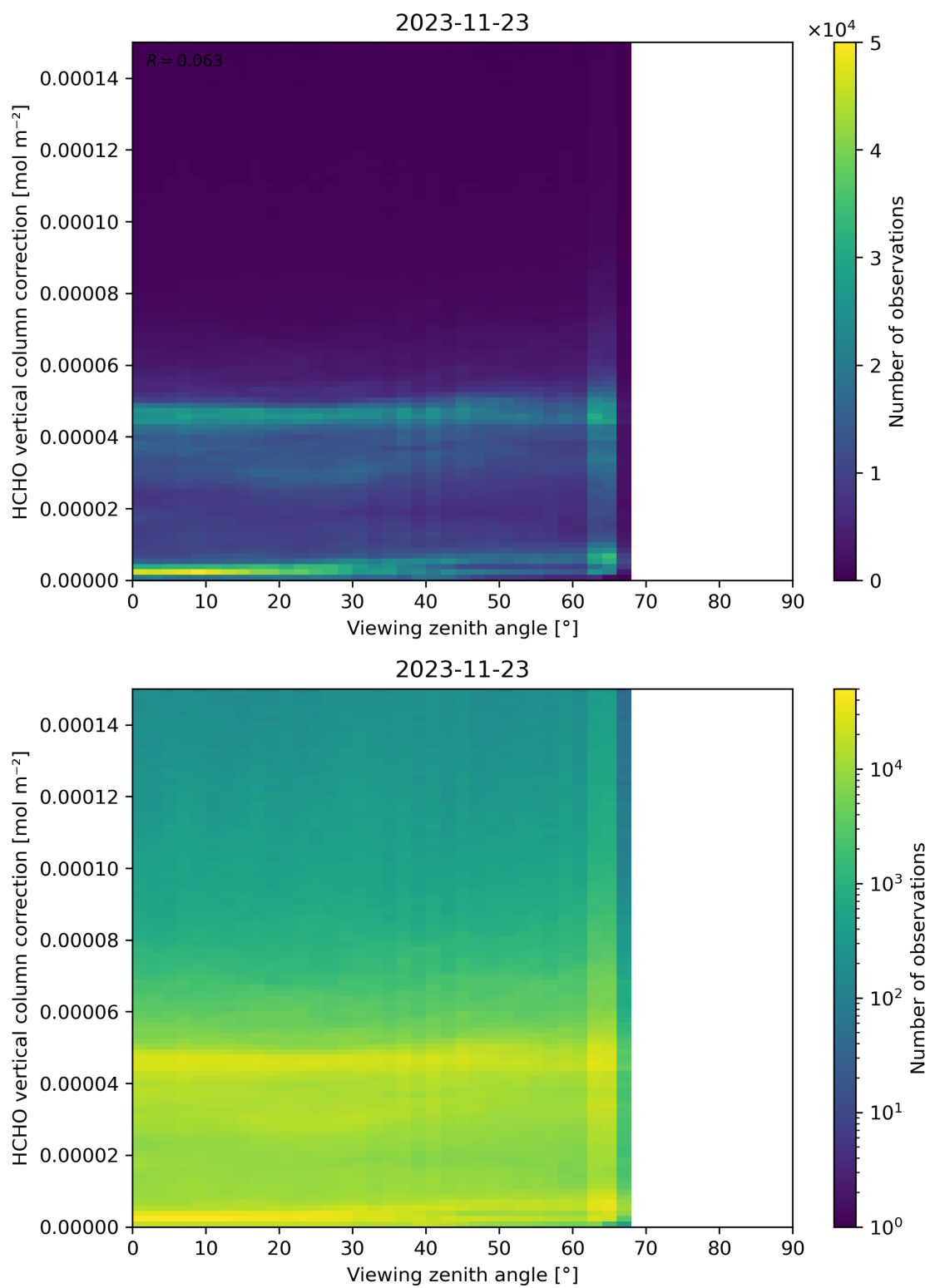
Figure 193: Scatter density plot of “Viewing zenith angle” against “HCHO vertical column correction” for 2023-11-23 to 2023-11-24.
