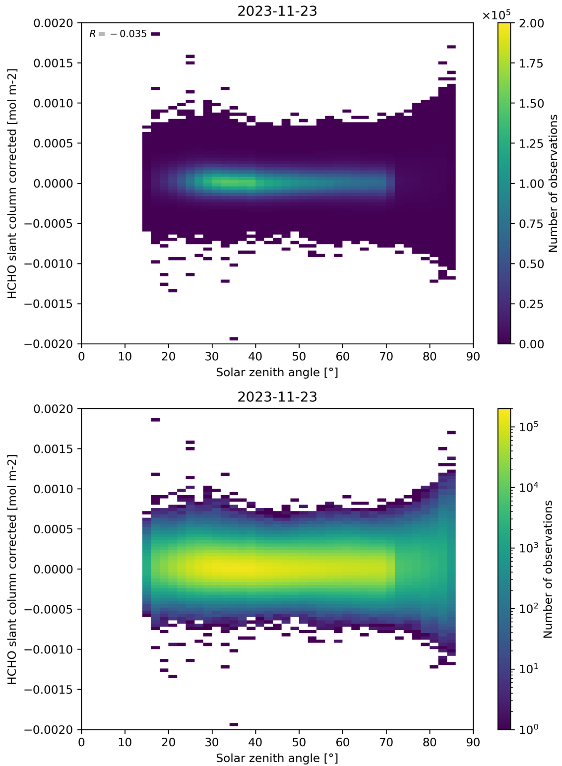
Figure 171: Scatter density plot of “Solar zenith angle” against “HCHO slant column corrected” for 2023-11-23 to 2023-11-24.
