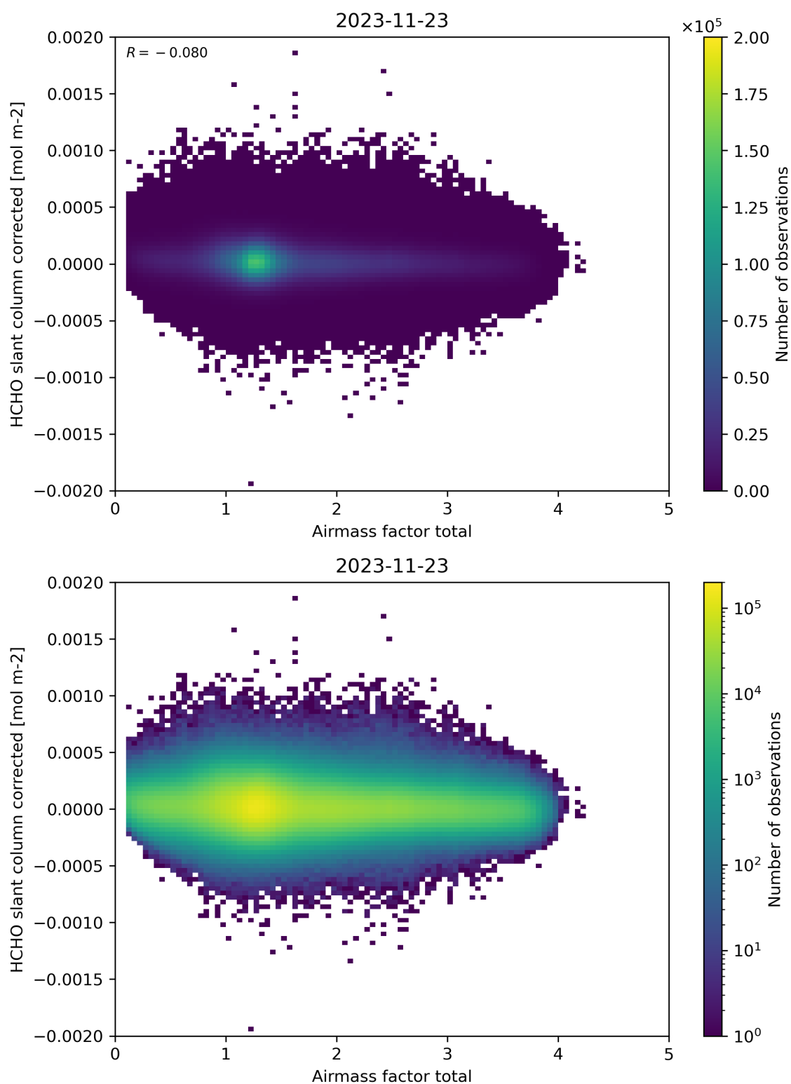
Figure 101: Scatter density plot of “Airmass factor total” against “HCHO slant column corrected” for 2023-11-23 to 2023-11-24.
