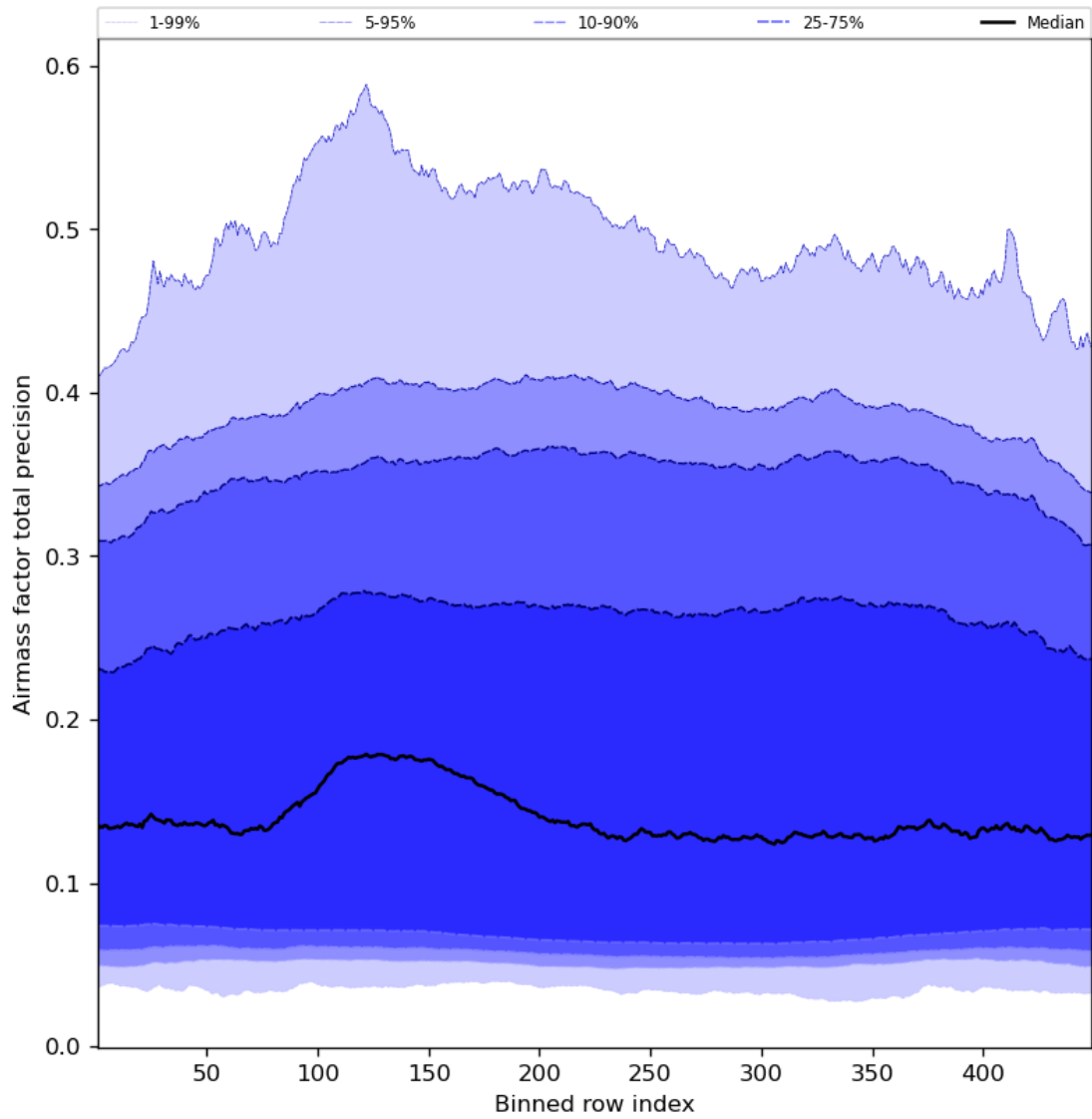
Figure 55: Along track statistics of “Airmass factor total precision” for 2023-11-23 to 2023-11-24
