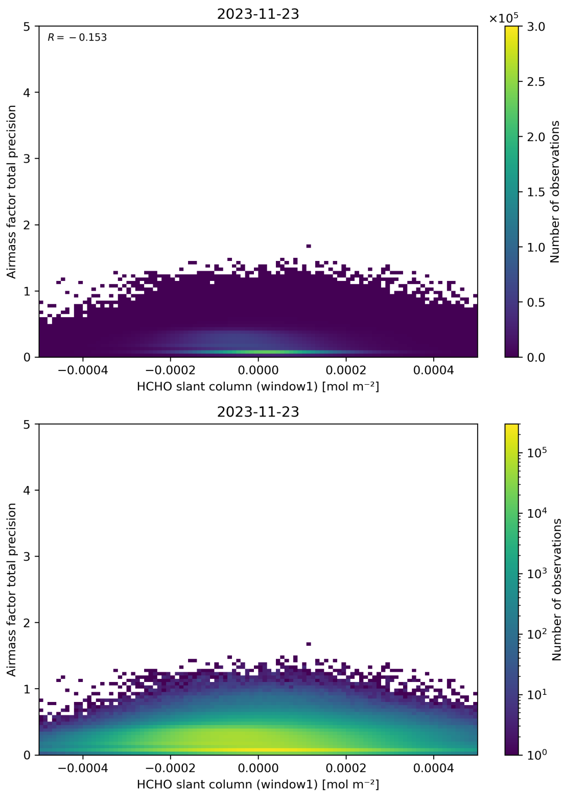
Figure 86: Scatter density plot of “HCHO slant column (window1)” against “Airmass factor total precision” for 2023-11-23 to 2023-11-24.
