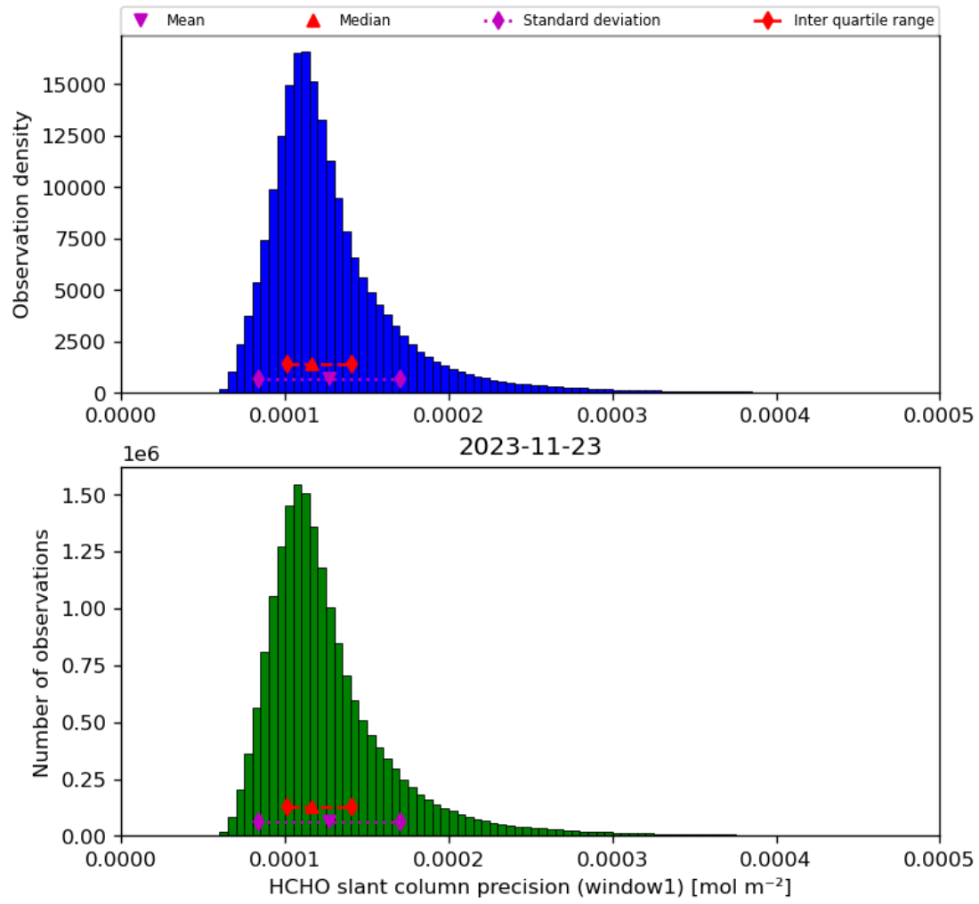
Figure 39: Histogram of “HCHO slant column precision (window1)” for 2023-11-23 to 2023-11-24
