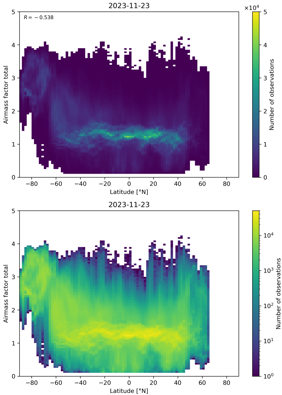
Figure 161: Scatter density plot of “Latitude” against “Airmass factor total” for 2023-11-23 to 2023-11-24.
