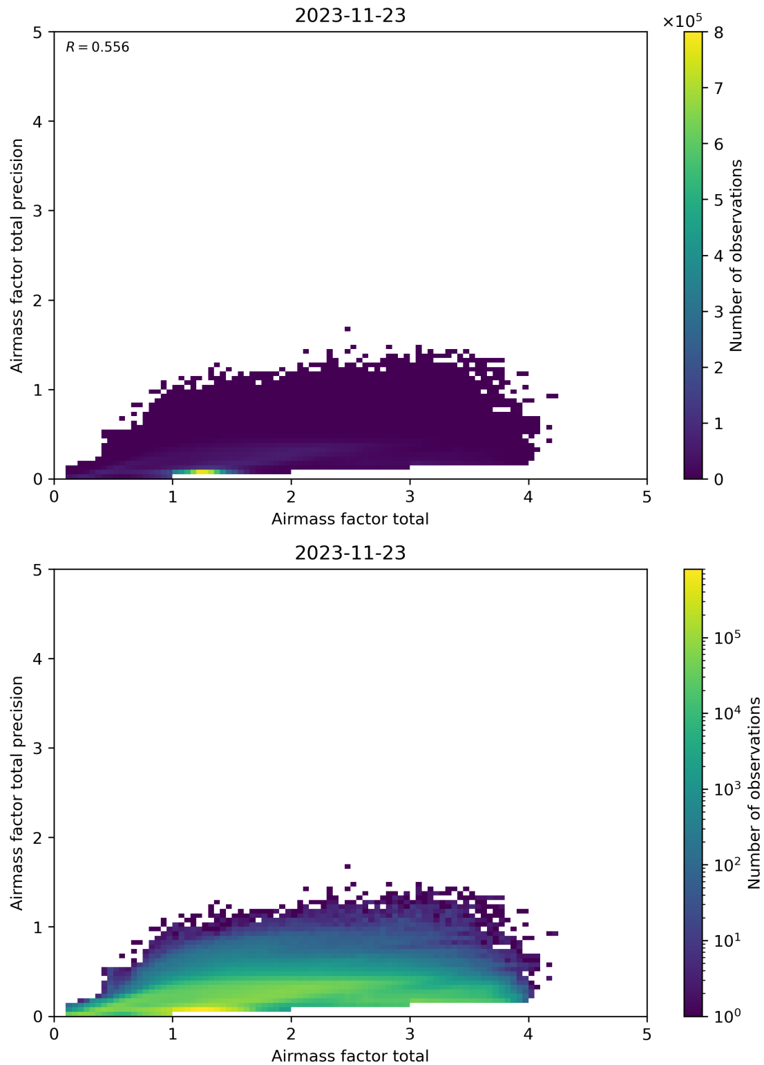
Figure 103: Scatter density plot of “Airmass factor total” against “Airmass factor total precision” for 2023-11-23 to 2023-11-24.
