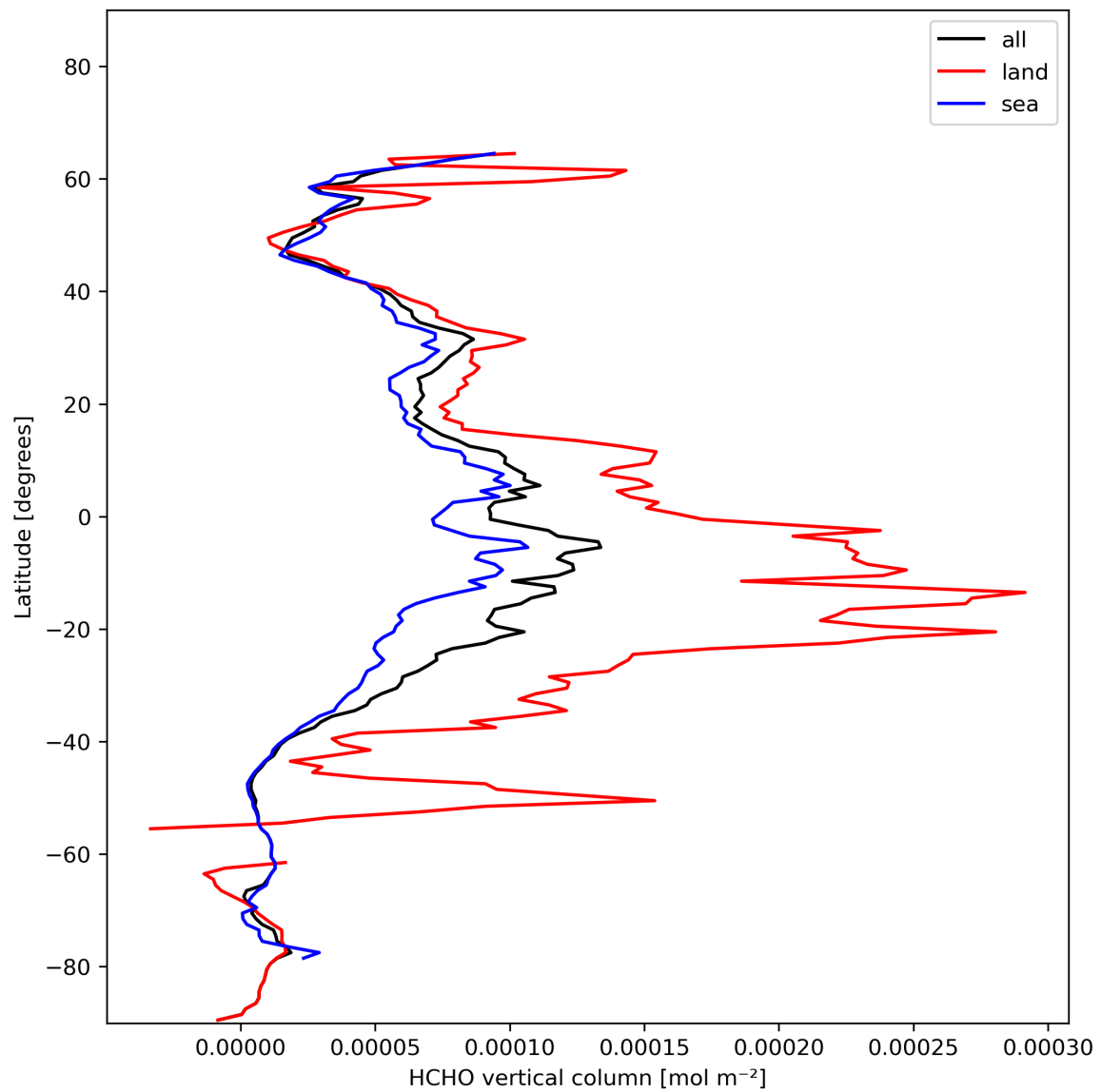
Figure 21: Zonal average of “HCHO vertical column” for 2023-11-23 to 2023-11-24.
