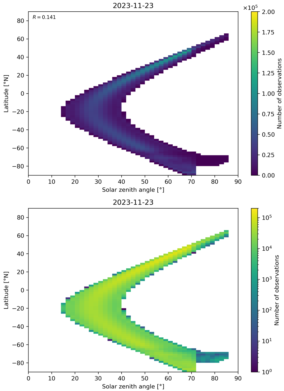
Figure 181: Scatter density plot of “Solar zenith angle” against “Latitude” for 2023-11-23 to 2023-11-24.
