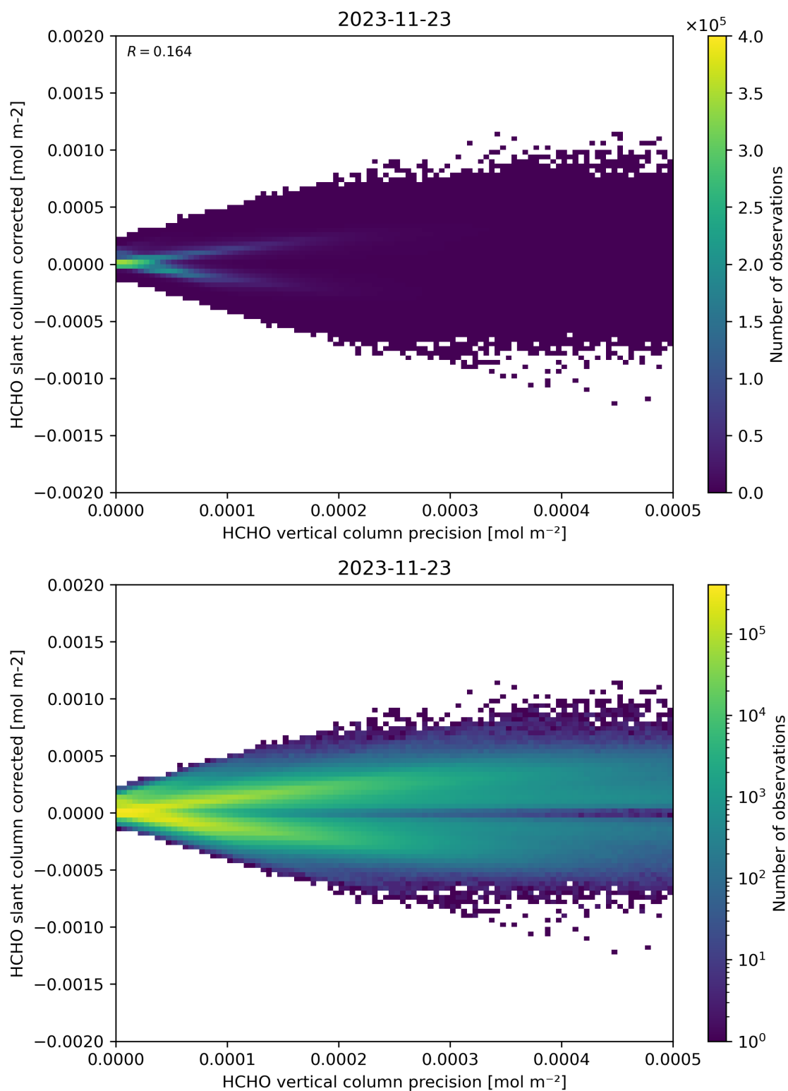
Figure 140: Scatter density plot of “HCHO vertical column precision” against “HCHO slant column corrected” for 2023-11-23 to 2023-11-24.
