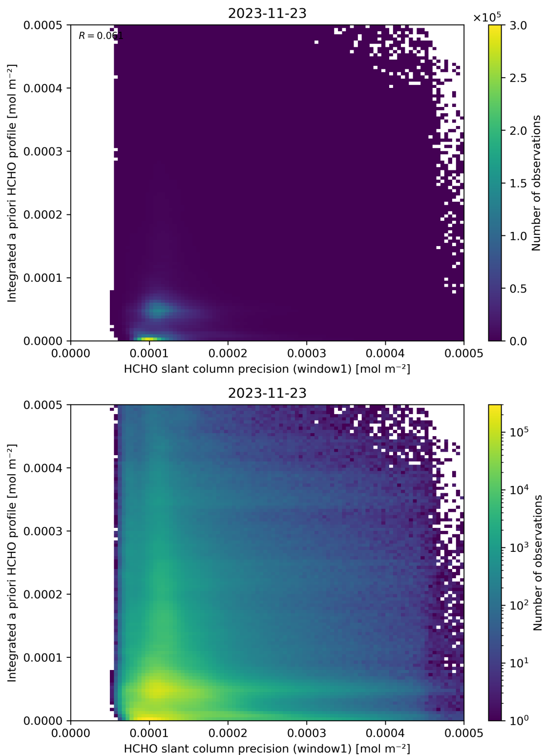
Figure 96: Scatter density plot of “HCHO slant column precision (window1)” against “Integrated a priori HCHO profile” for 2023-11-23 to 2023-11-24.
