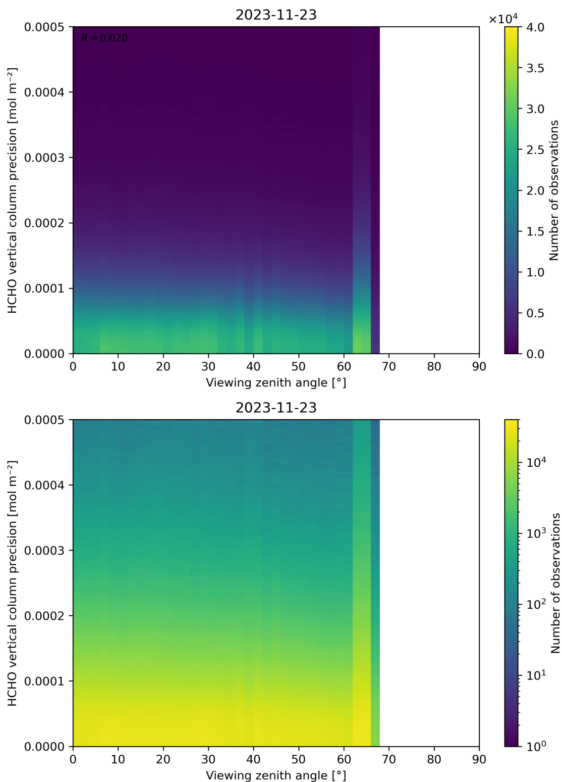
Figure 194: Scatter density plot of “Viewing zenith angle” against “HCHO vertical column precision” for 2023-11-23 to 2023-11-24.
