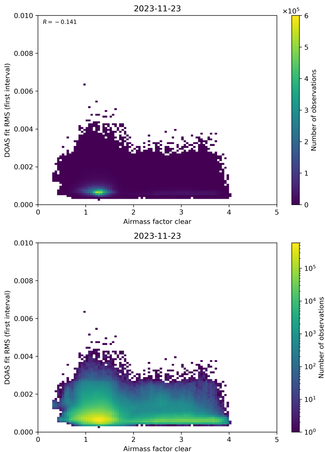
Figure 71: Scatter density plot of “Airmass factor clear” against “DOAS fit RMS (first interval)” for 2023-11-23 to 2023-11-24.
