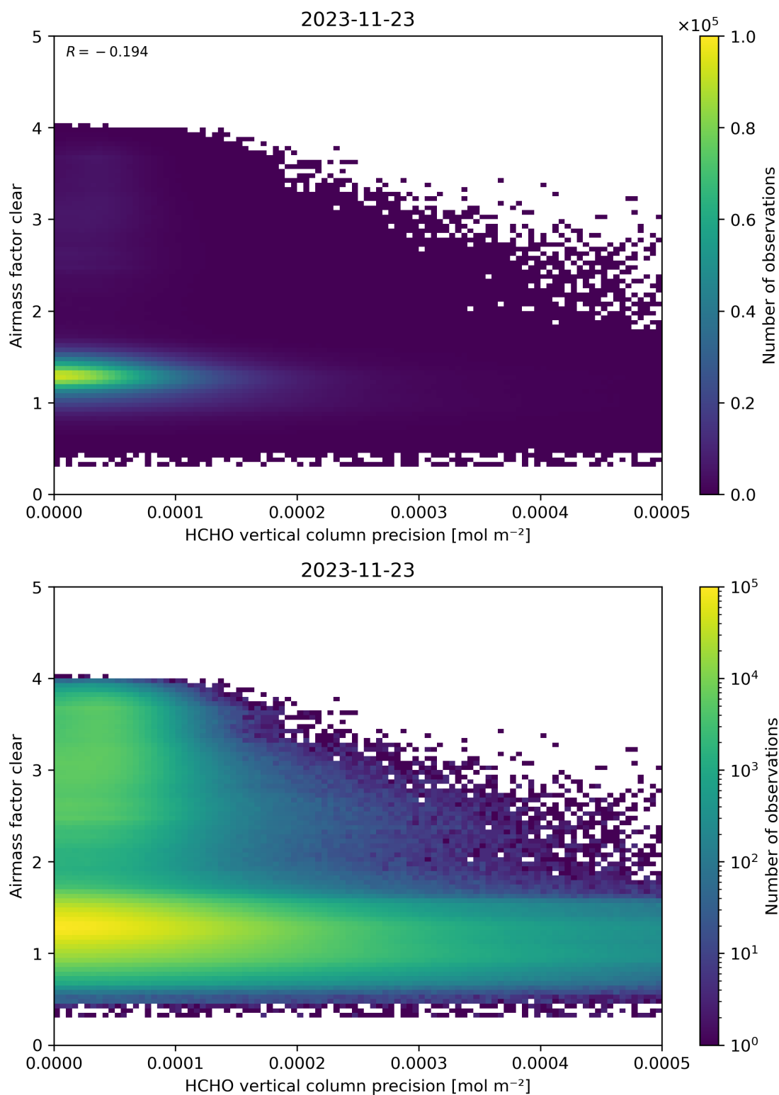
Figure 139: Scatter density plot of “HCHO vertical column precision” against “Airmass factor clear” for 2023-11-23 to 2023-11-24.
