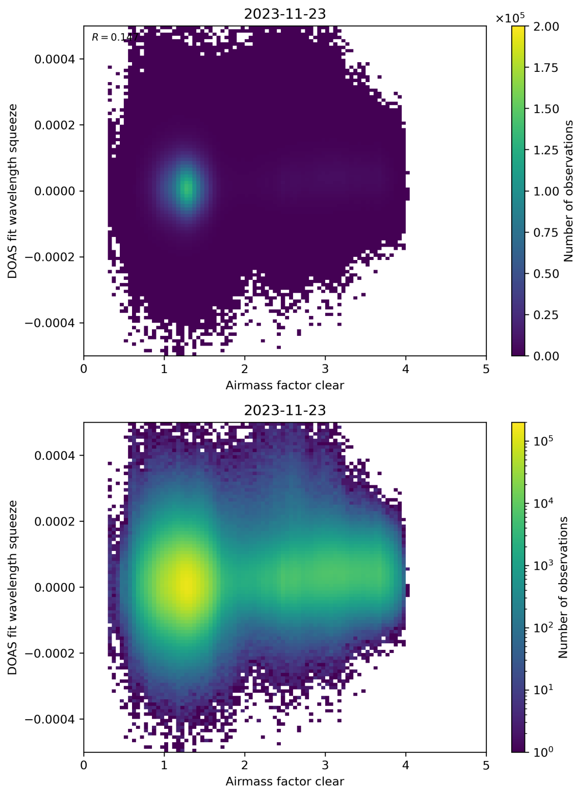
Figure 73: Scatter density plot of “Airmass factor clear” against “DOAS fit wavelength squeeze” for 2023-11-23 to 2023-11-24.
