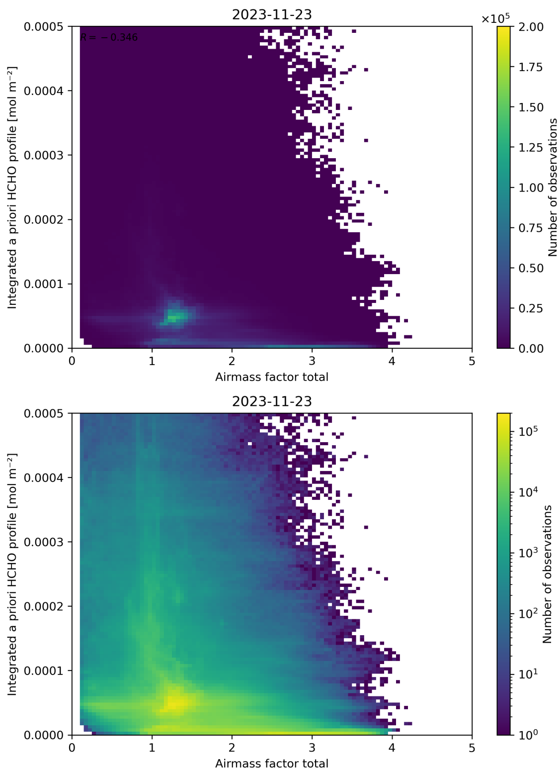
Figure 104: Scatter density plot of “Airmass factor total” against “Integrated a priori HCHO profile” for 2023-11-23 to 2023-11-24.
