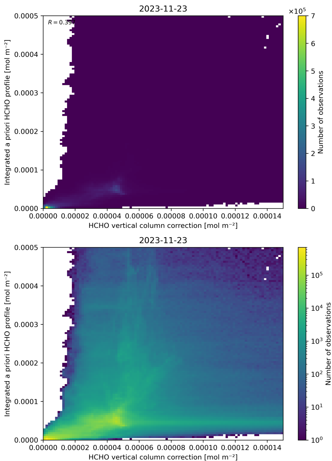
Figure 122: Scatter density plot of “HCHO vertical column correction” against “Integrated a priori HCHO profile” for 2023-11-23 to 2023-11-24.
