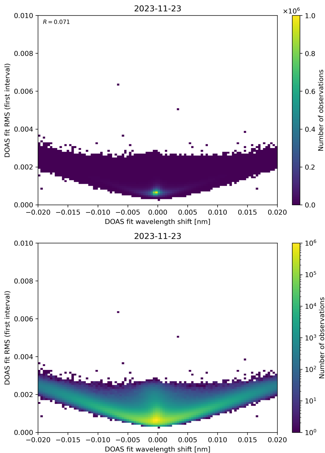
Figure 64: Scatter density plot of “DOAS fit wavelength shift” against “DOAS fit RMS (first interval)” for 2023-11-23 to 2023-11-24.
