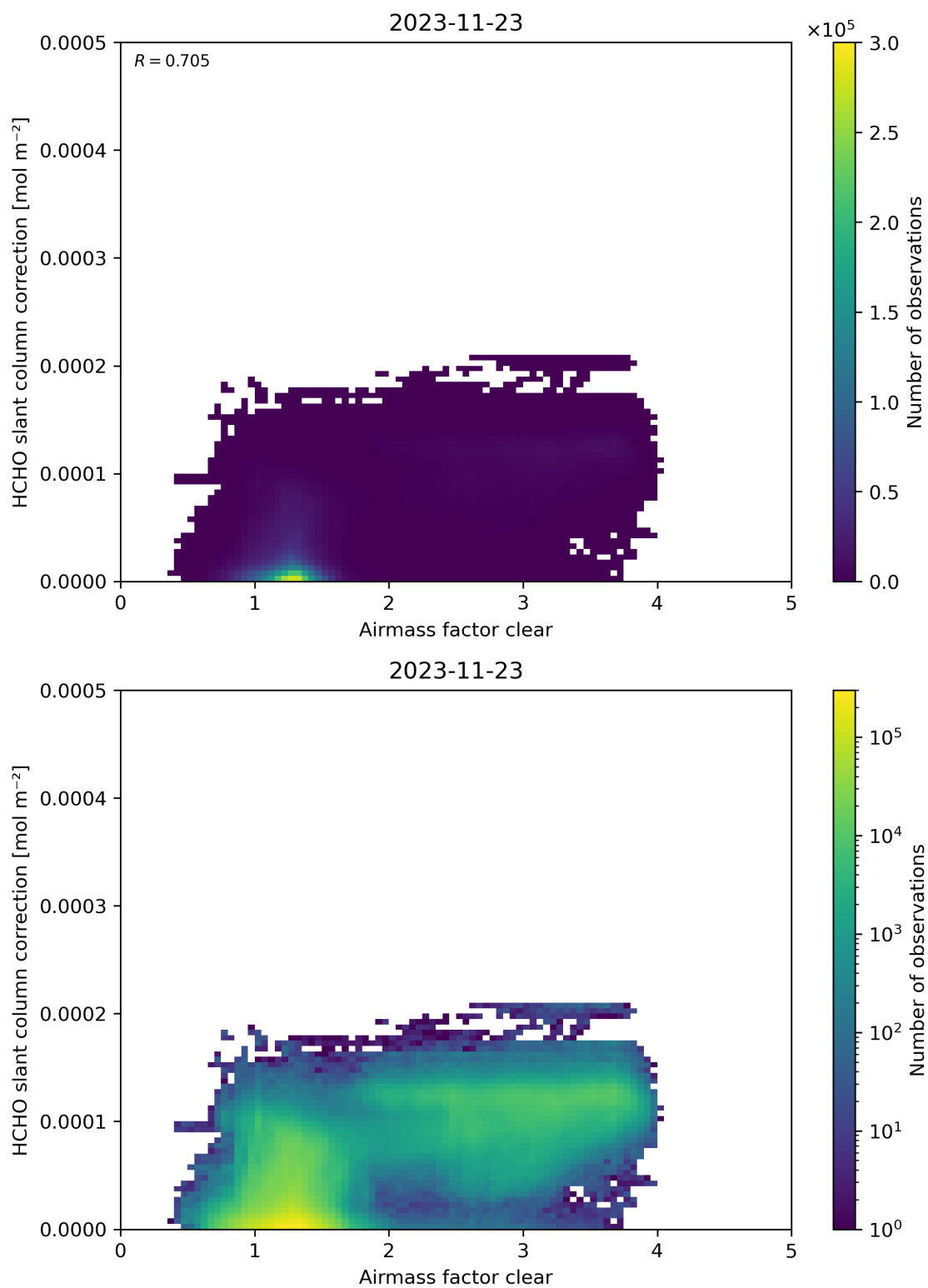
Figure 75: Scatter density plot of “Airmass factor clear” against “HCHO slant column correction” for 2023-11-23 to 2023-11-24.
