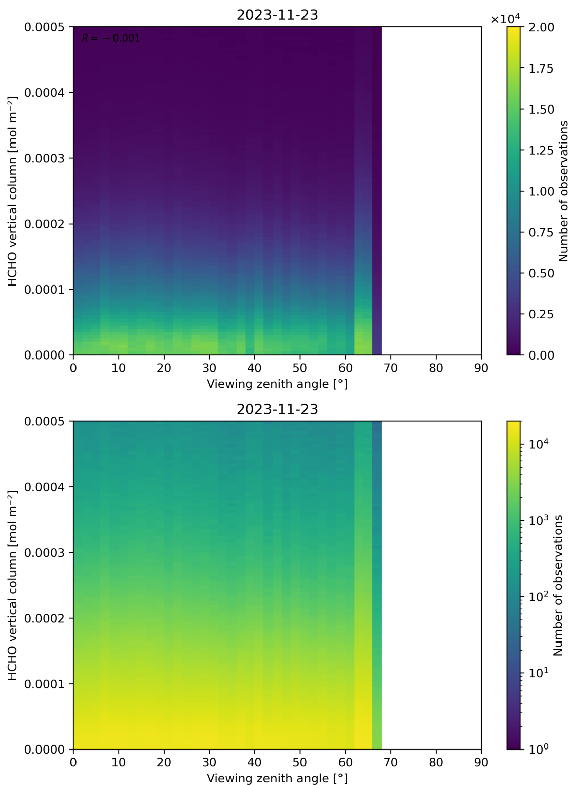
Figure 192: Scatter density plot of “Viewing zenith angle” against “HCHO vertical column” for 2023-11-23 to 2023-11-24.
