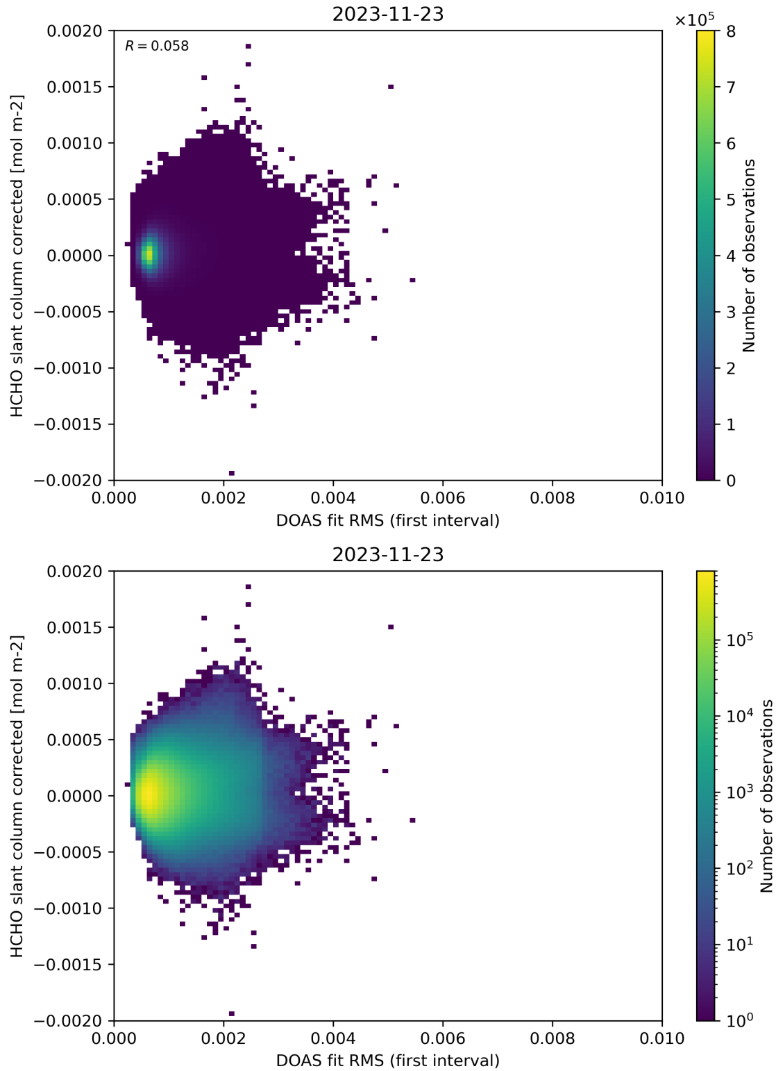
Figure 62: Scatter density plot of “DOAS fit RMS (first interval)” against “HCHO slant column corrected” for 2023-11-23 to 2023-11-24.
