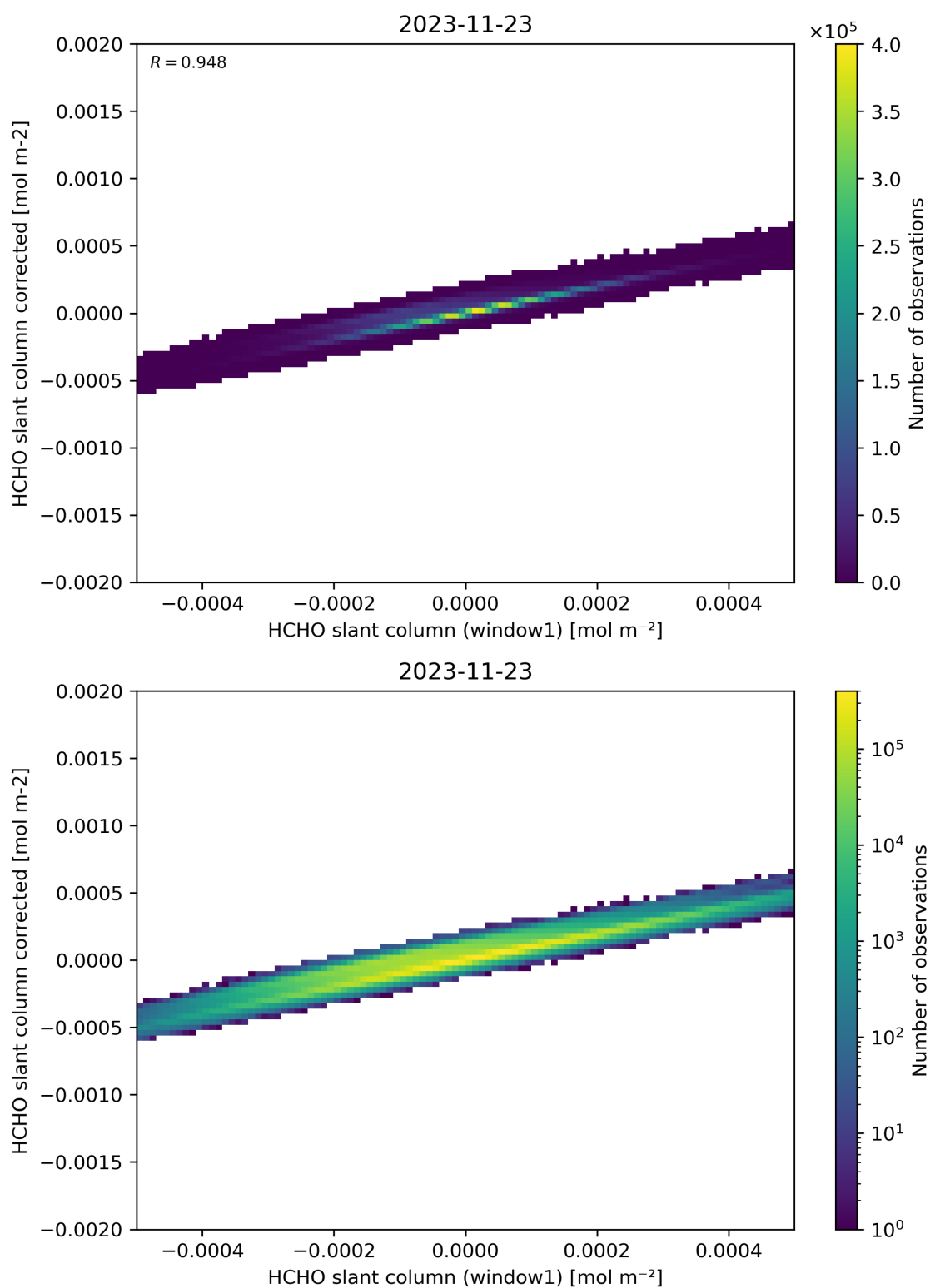
Figure 82: Scatter density plot of “HCHO slant column (window1)” against “HCHO slant column corrected” for 2023-11-23 to 2023-11-24.
