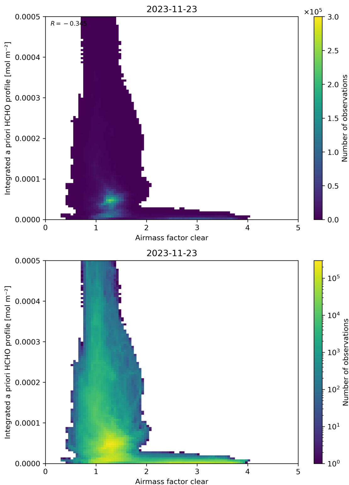
Figure 76: Scatter density plot of “Airmass factor clear” against “Integrated a priori HCHO profile” for 2023-11-23 to 2023-11-24.
