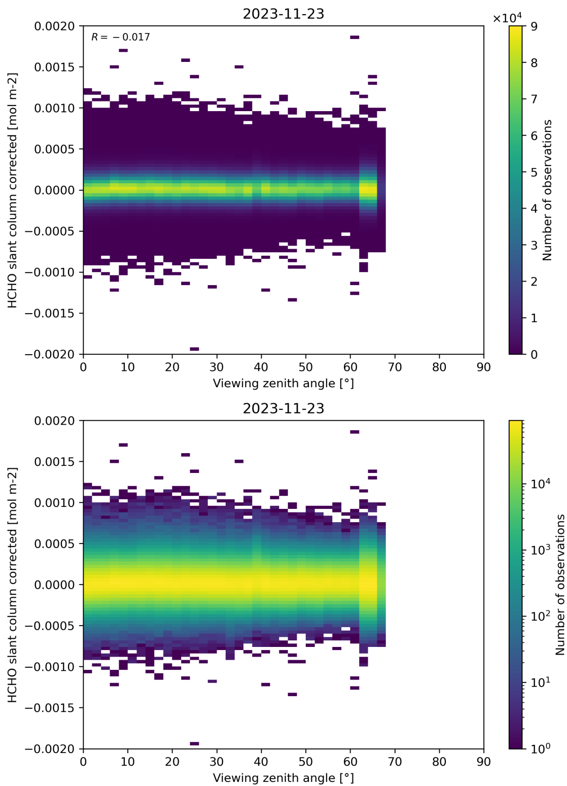
Figure 186: Scatter density plot of “Viewing zenith angle” against “HCHO slant column corrected” for 2023-11-23 to 2023-11-24.
