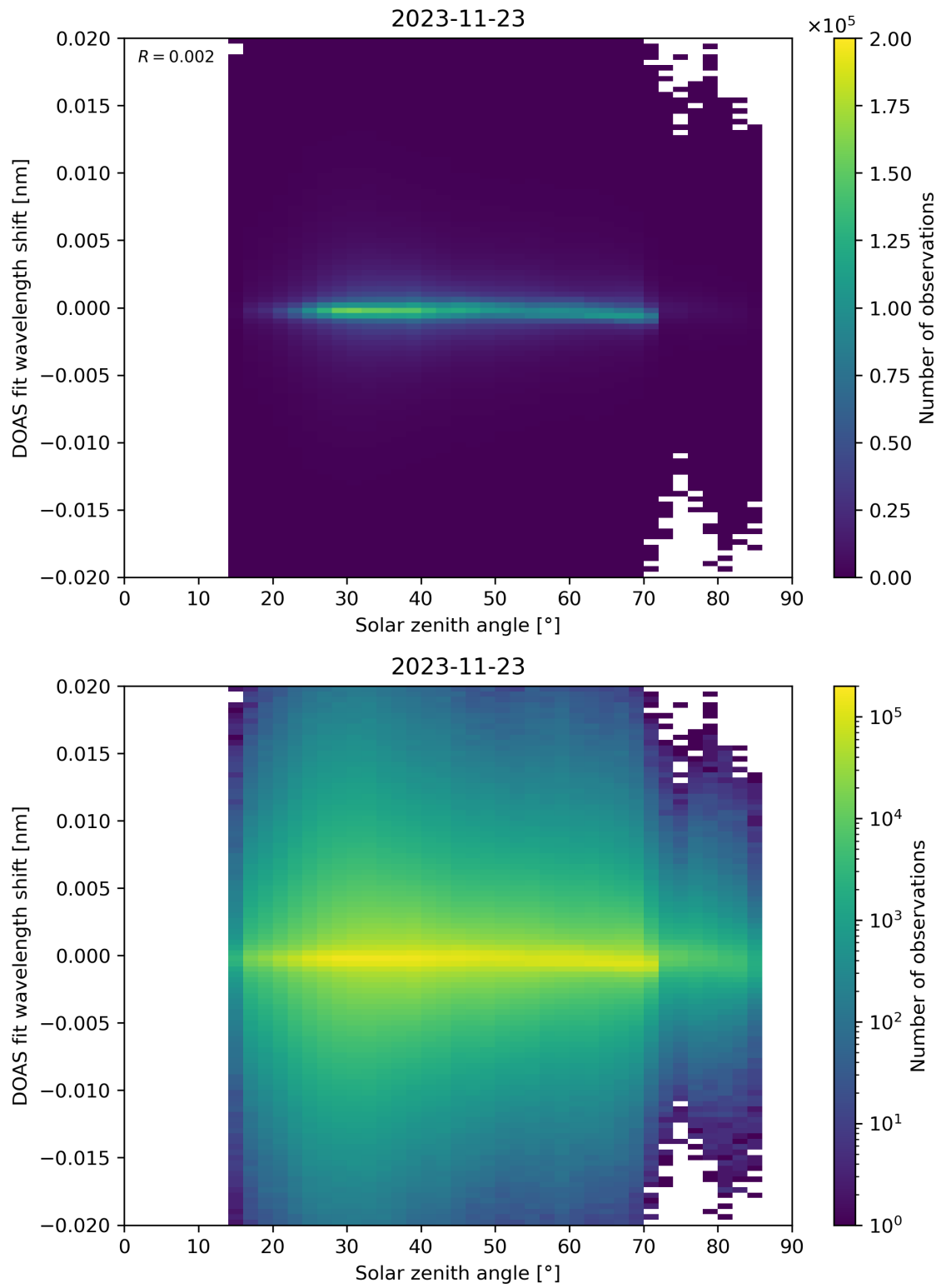
Figure 168: Scatter density plot of “Solar zenith angle” against “DOAS fit wavelength shift” for 2023-11-23 to 2023-11-24.
