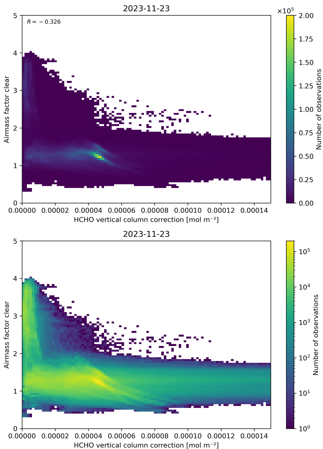
Figure 115: Scatter density plot of “HCHO vertical column correction” against “Airmass factor clear” for 2023-11-23 to 2023-11-24.
