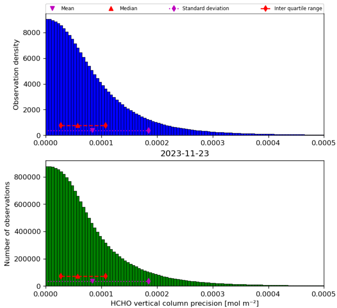
Figure 36: Histogram of “HCHO vertical column precision” for 2023-11-23 to 2023-11-24
