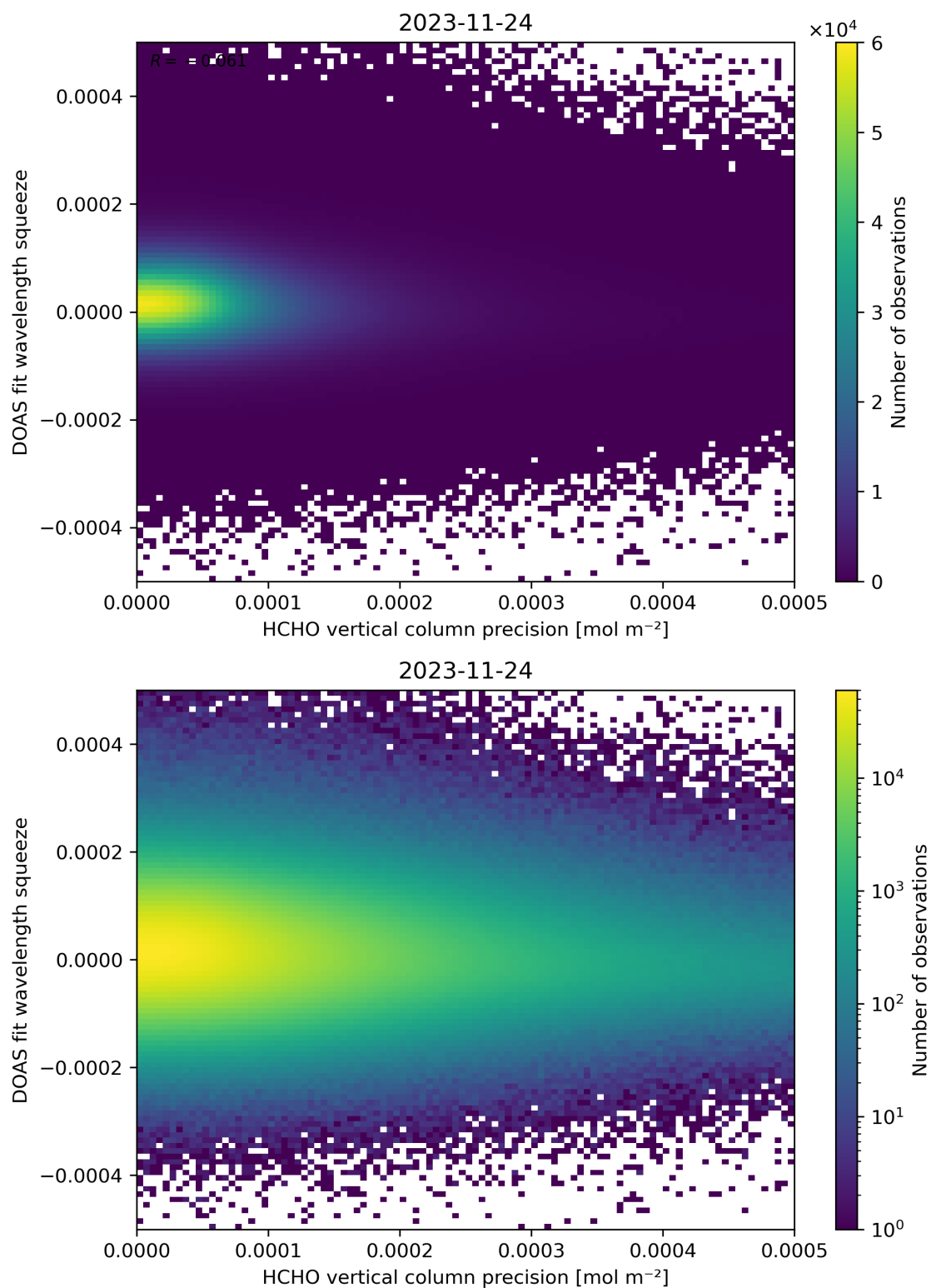
Figure 138: Scatter density plot of “HCHO vertical column precision” against “DOAS fit wavelength squeeze” for 2023-11-23 to 2023-11-25.
