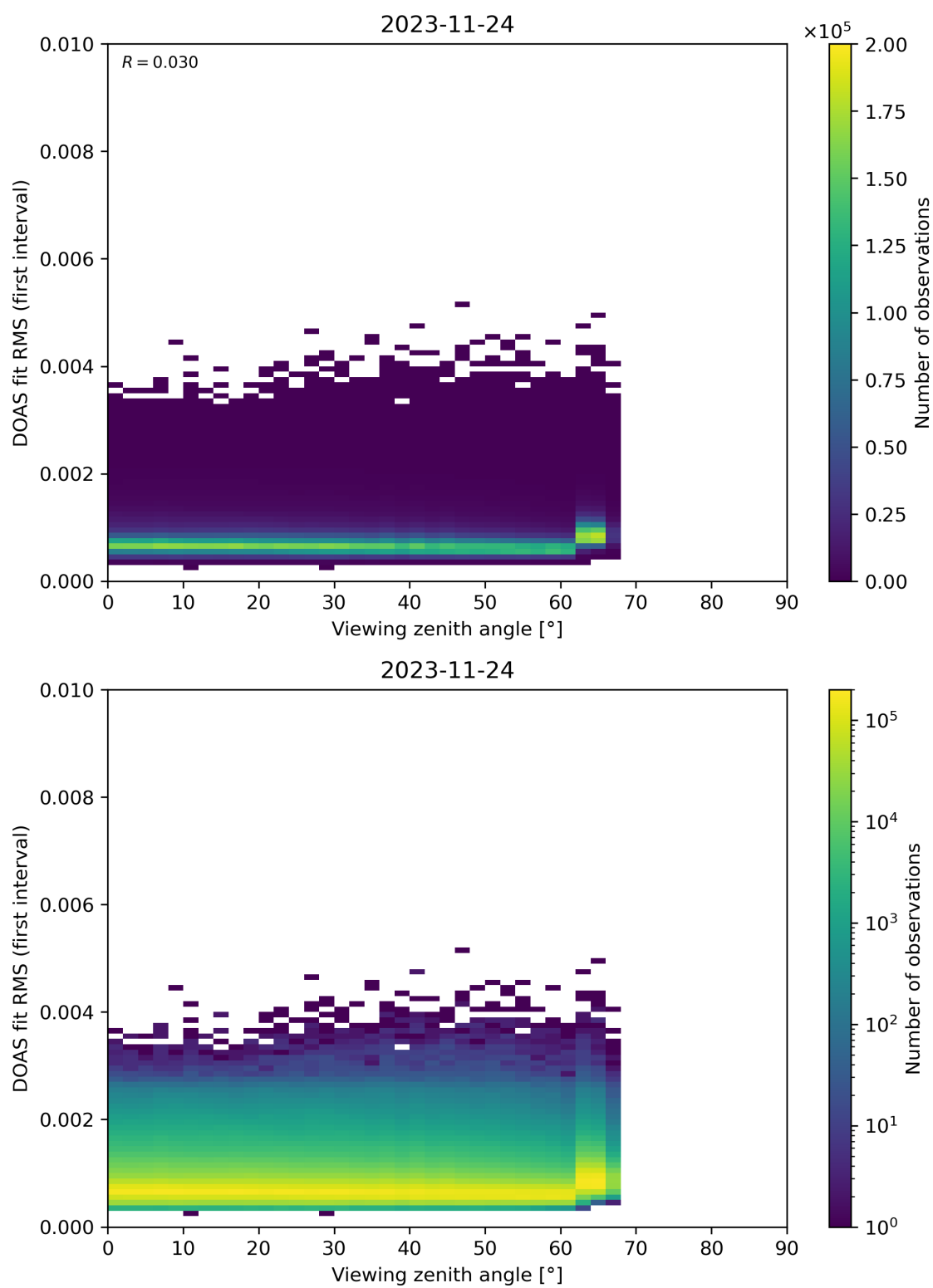
Figure 182: Scatter density plot of “Viewing zenith angle” against “DOAS fit RMS (first interval)” for 2023-11-23 to 2023-11-25.
