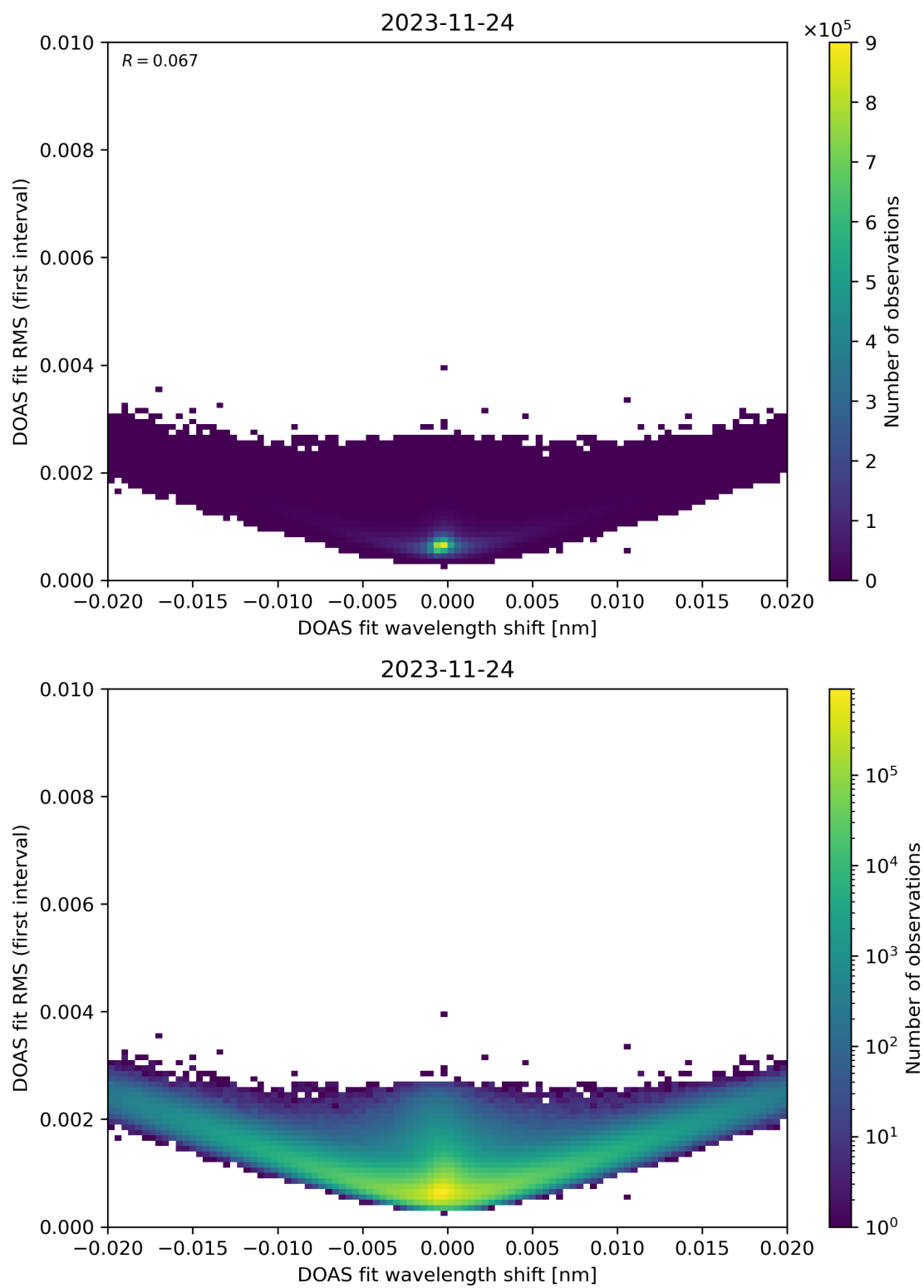
Figure 64: Scatter density plot of “DOAS fit wavelength shift” against “DOAS fit RMS (first interval)” for 2023-11-23 to 2023-11-25.
