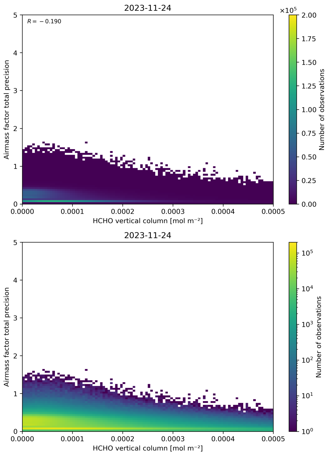
Figure 132: Scatter density plot of “HCHO vertical column” against “Airmass factor total precision” for 2023-11-23 to 2023-11-25.
