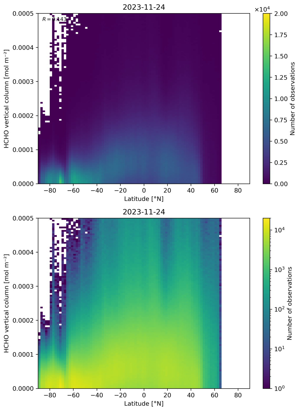
Figure 163: Scatter density plot of “Latitude” against “HCHO vertical column” for 2023-11-23 to 2023-11-25.
