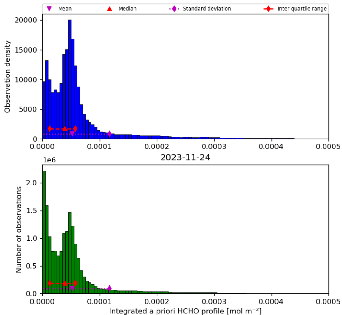
Figure 43: Histogram of “Integrated a priori HCHO profile” for 2023-11-23 to 2023-11-25
