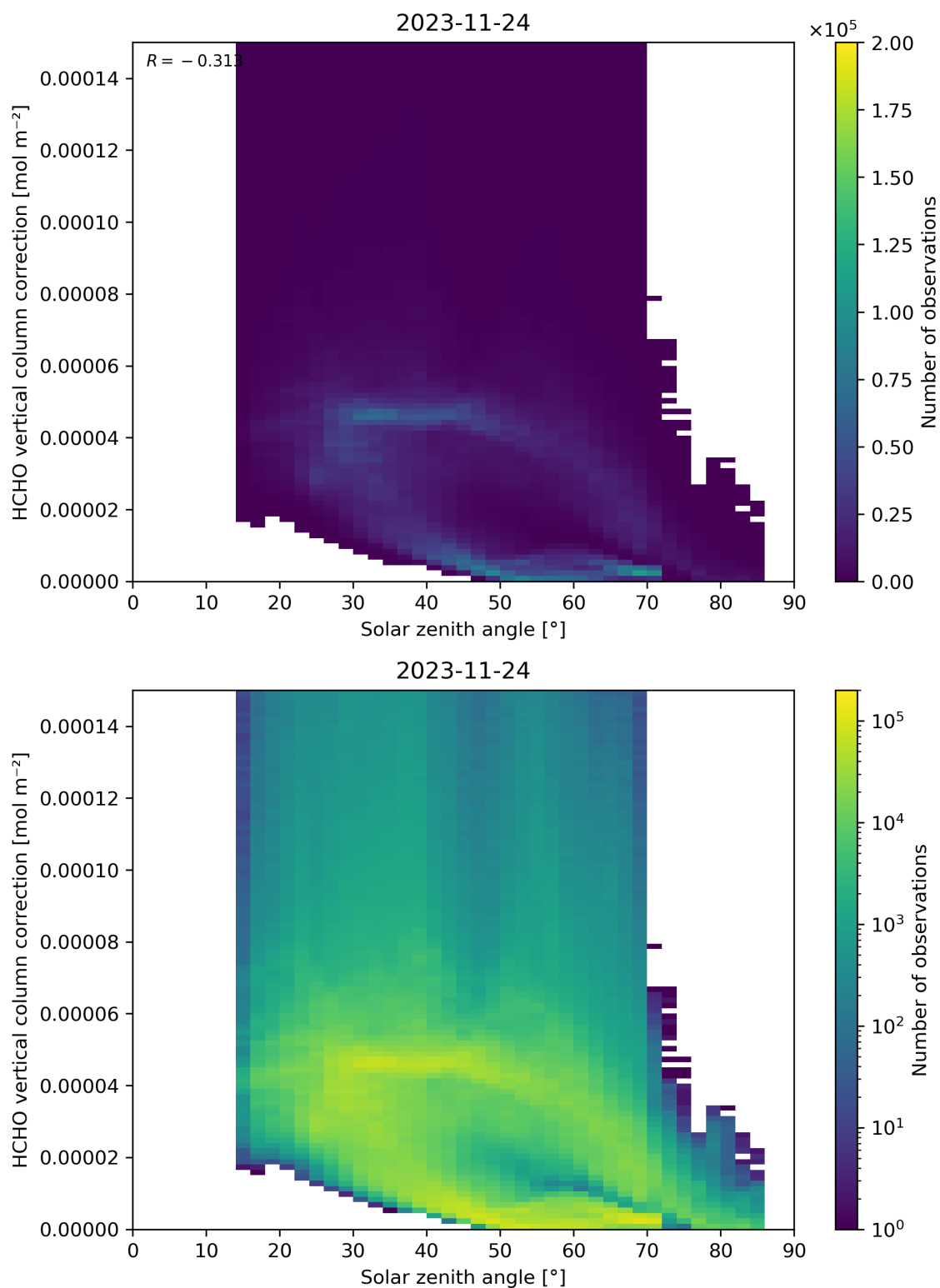
Figure 178: Scatter density plot of “Solar zenith angle” against “HCHO vertical column correction” for 2023-11-23 to 2023-11-25.
