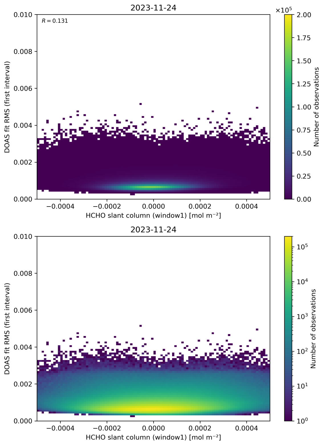
Figure 78: Scatter density plot of “HCHO slant column (window1)” against “DOAS fit RMS (first interval)” for 2023-11-23 to 2023-11-25.
