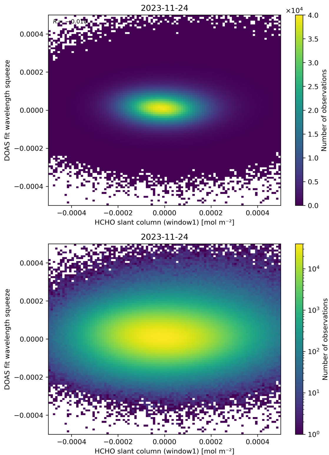
Figure 80: Scatter density plot of “HCHO slant column (window1)” against “DOAS fit wavelength squeeze” for 2023-11-23 to 2023-11-25.
