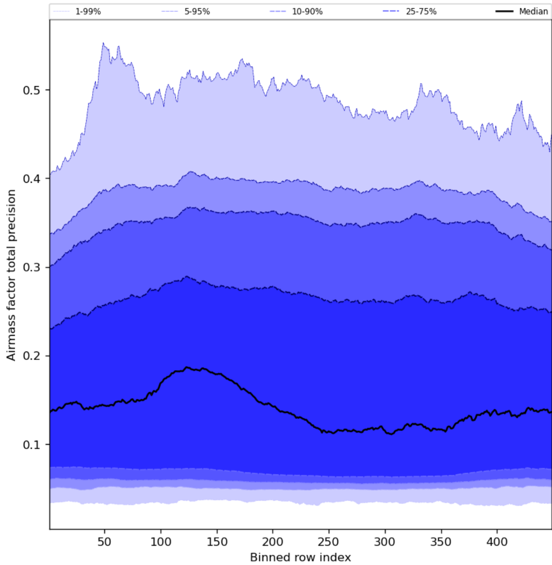
Figure 55: Along track statistics of “Airmass factor total precision” for 2023-11-23 to 2023-11-25
