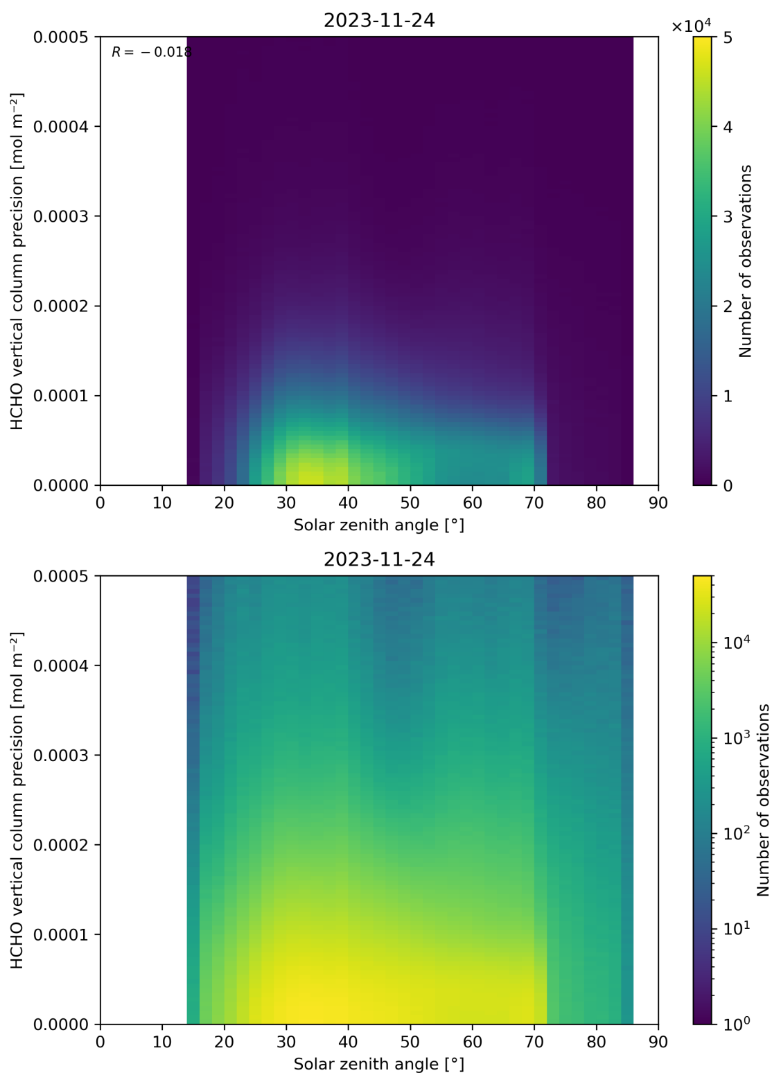
Figure 179: Scatter density plot of “Solar zenith angle” against “HCHO vertical column precision” for 2023-11-23 to 2023-11-25.
