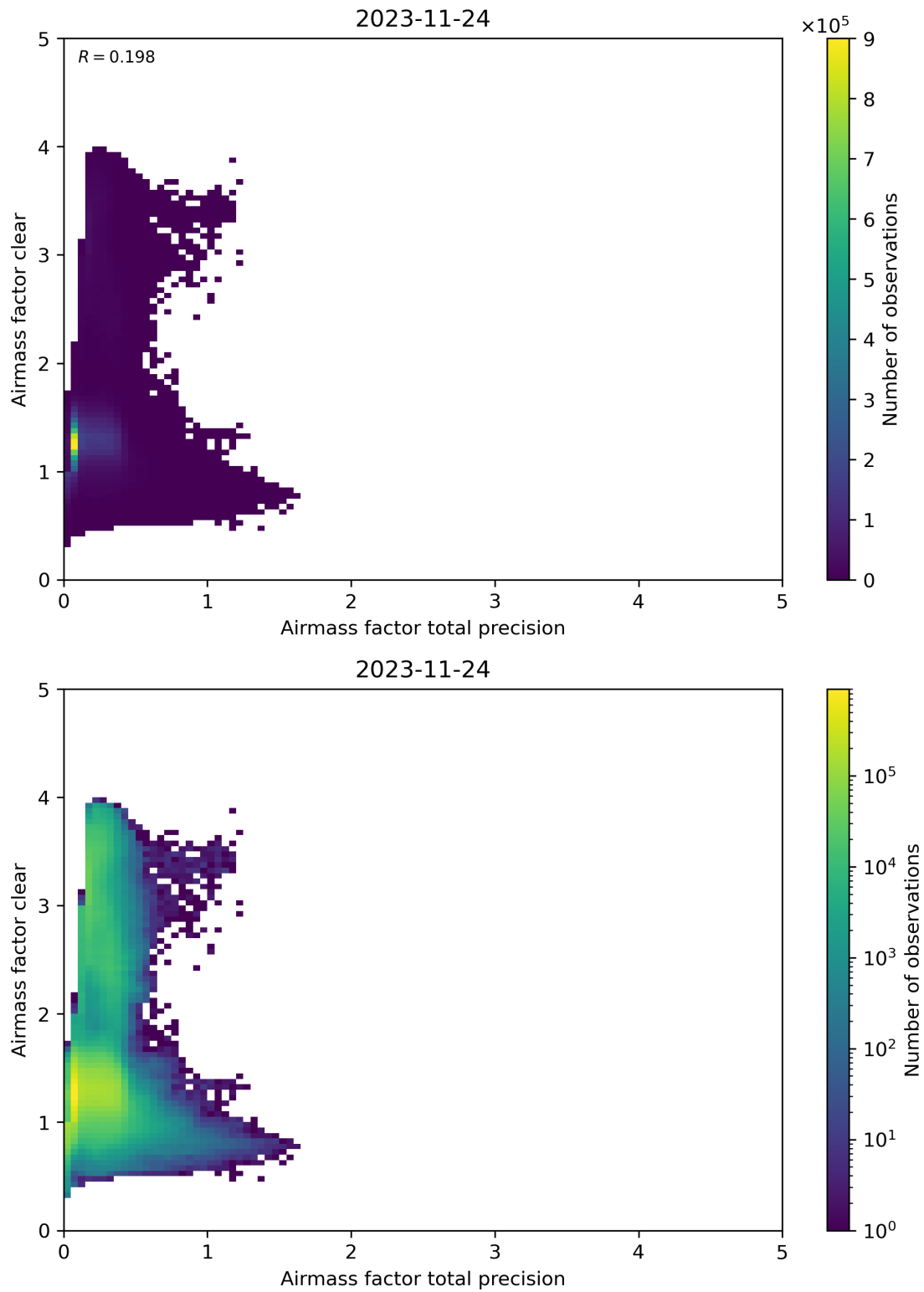
Figure 108: Scatter density plot of “Airmass factor total precision” against “Airmass factor clear” for 2023-11-23 to 2023-11-25.
