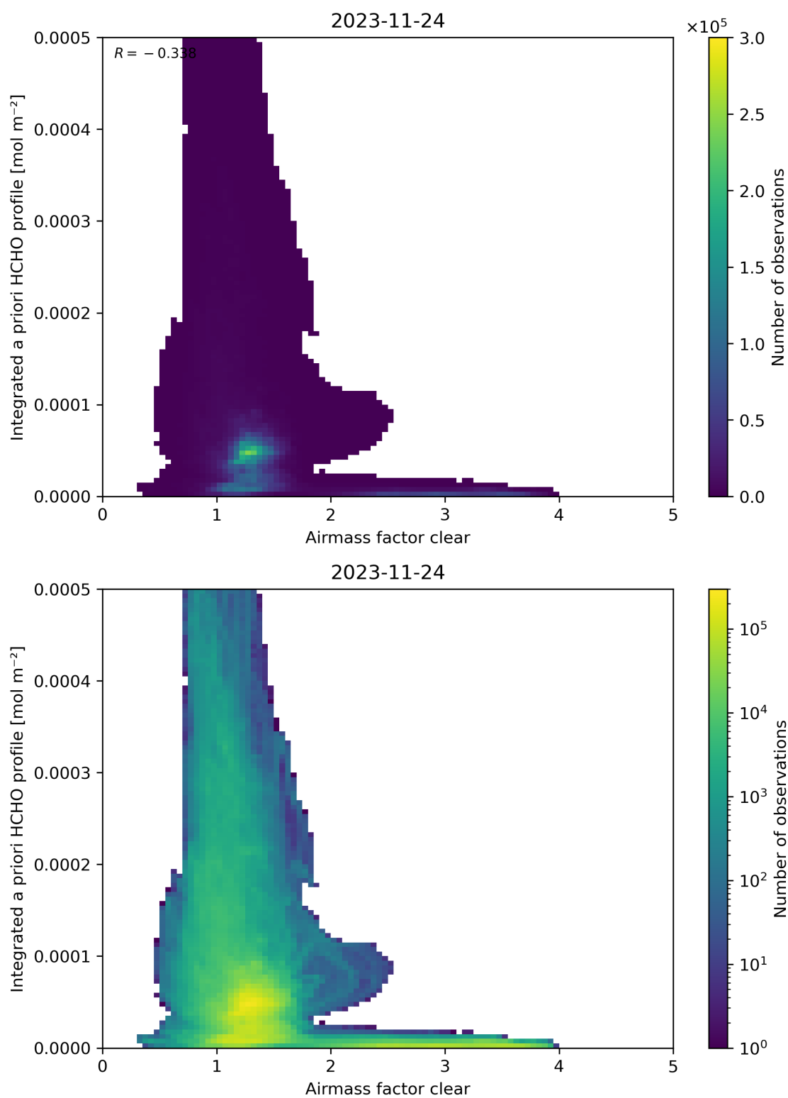
Figure 76: Scatter density plot of “Airmass factor clear” against “Integrated a priori HCHO profile” for 2023-11-23 to 2023-11-25.
