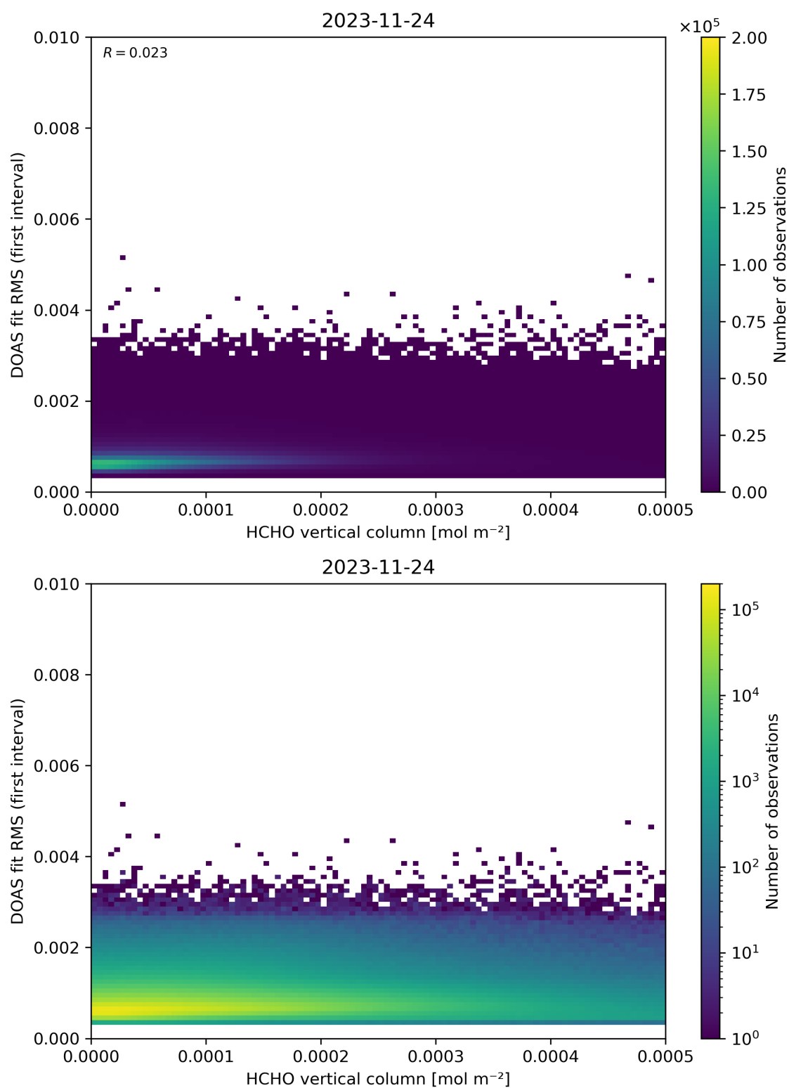
Figure 123: Scatter density plot of “HCHO vertical column” against “DOAS fit RMS (first interval)” for 2023-11-23 to 2023-11-25.
