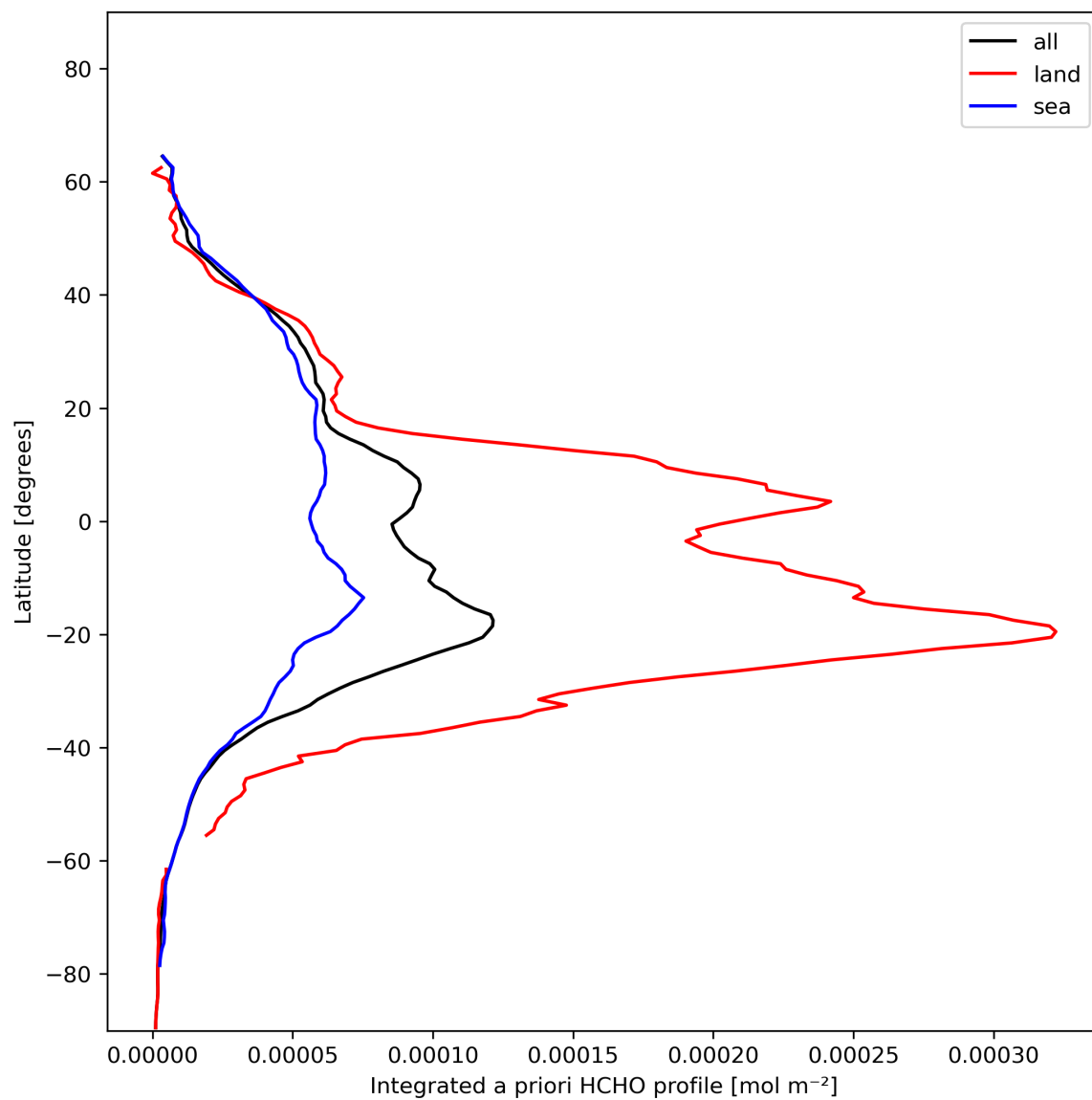
Figure 29: Zonal average of “Integrated a priori HCHO profile” for 2023-11-23 to 2023-11-25.
