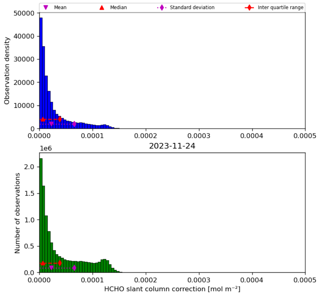
Figure 47: Histogram of “HCHO slant column correction” for 2023-11-23 to 2023-11-25
