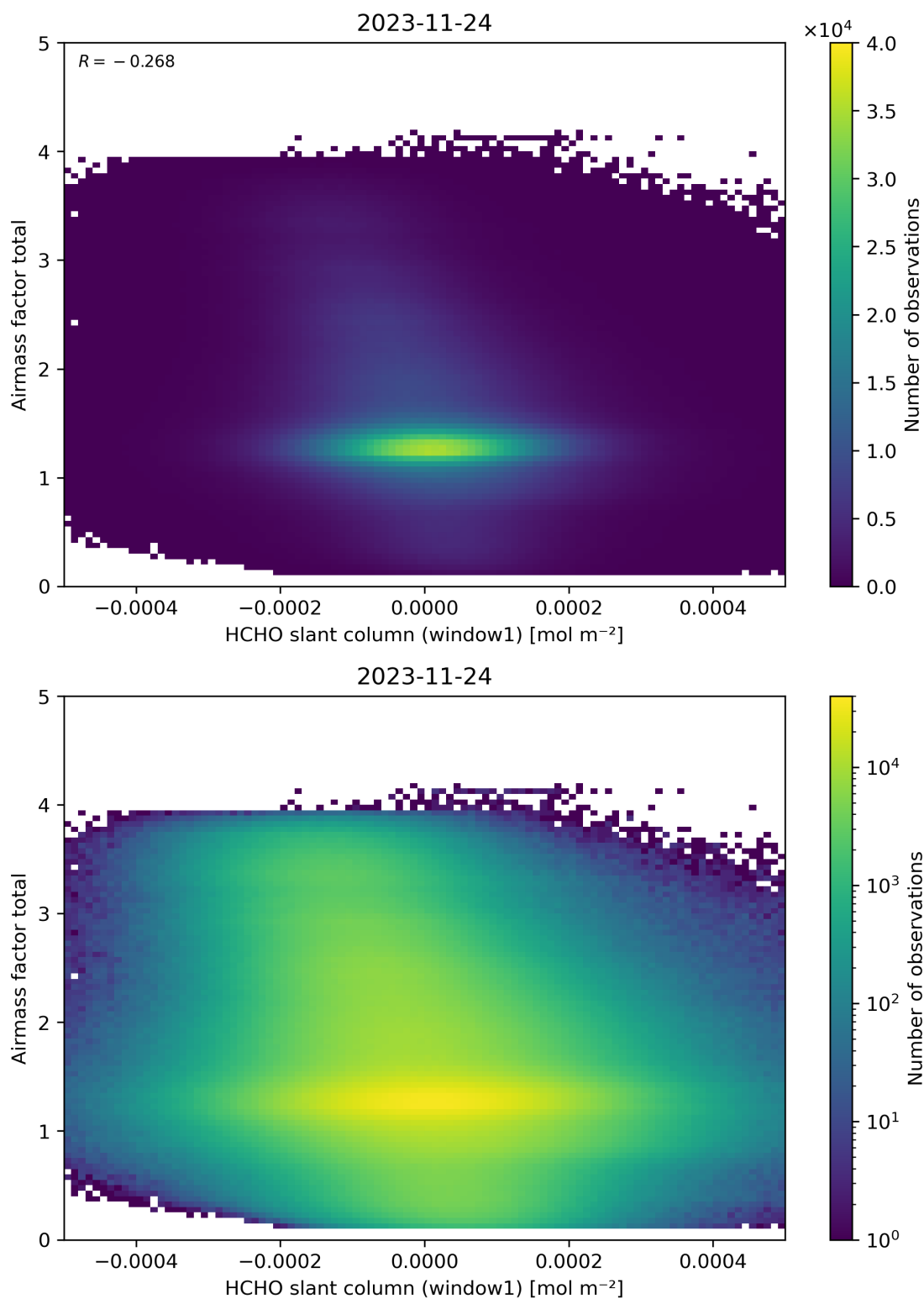
Figure 85: Scatter density plot of “HCHO slant column (window1)” against “Airmass factor total” for 2023-11-23 to 2023-11-25.
