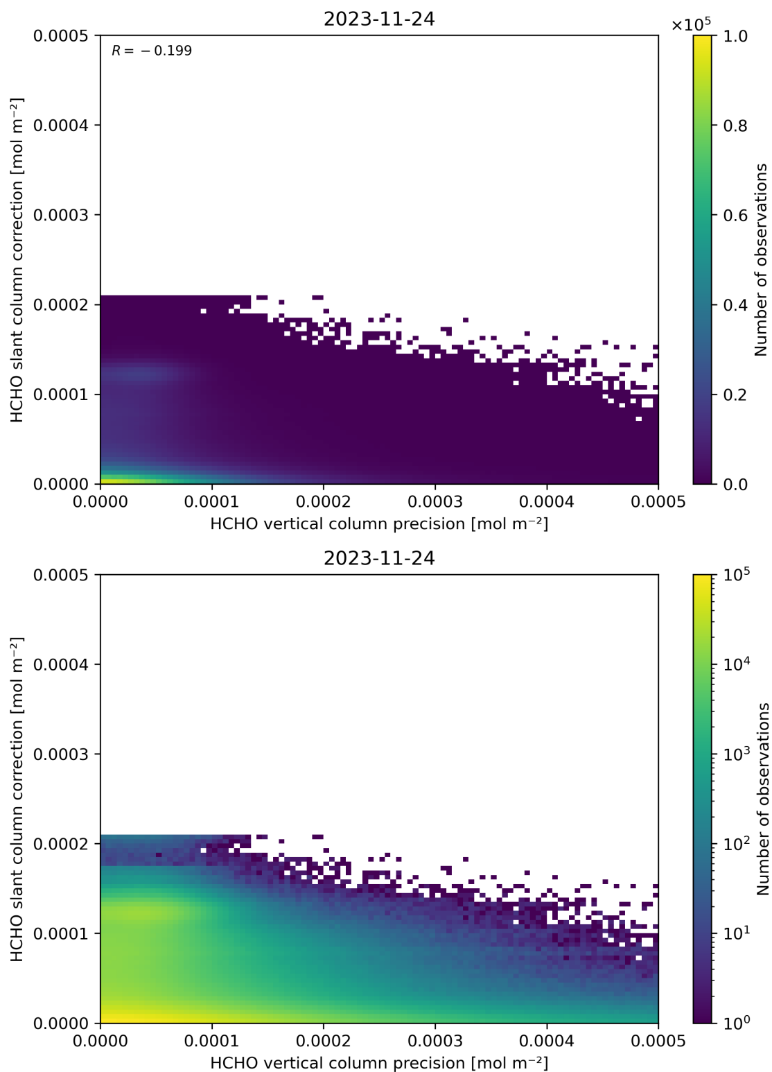
Figure 141: Scatter density plot of “HCHO vertical column precision” against “HCHO slant column correction” for 2023-11-23 to 2023-11-25.
