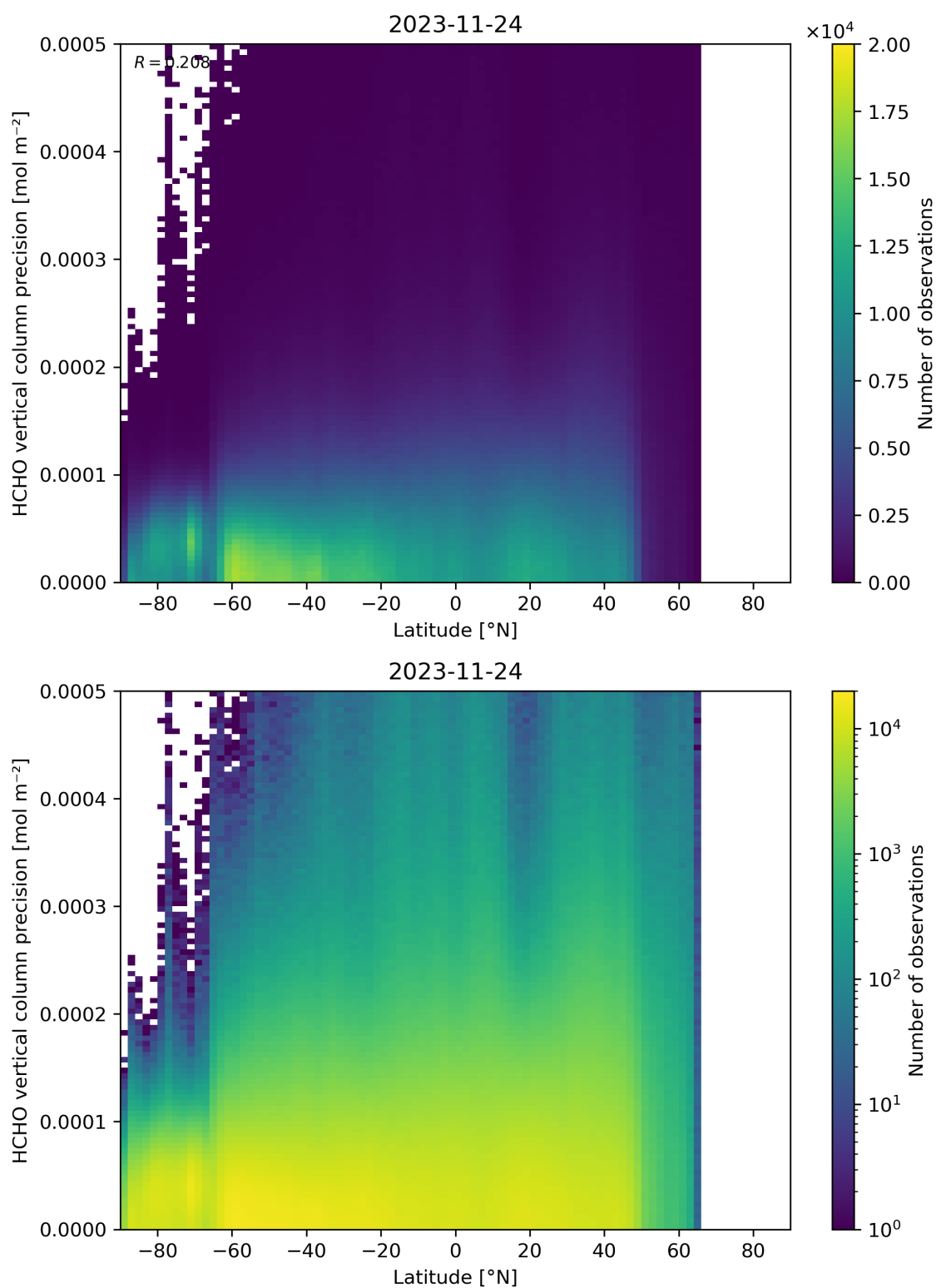
Figure 165: Scatter density plot of “Latitude” against “HCHO vertical column precision” for 2023-11-23 to 2023-11-25.
