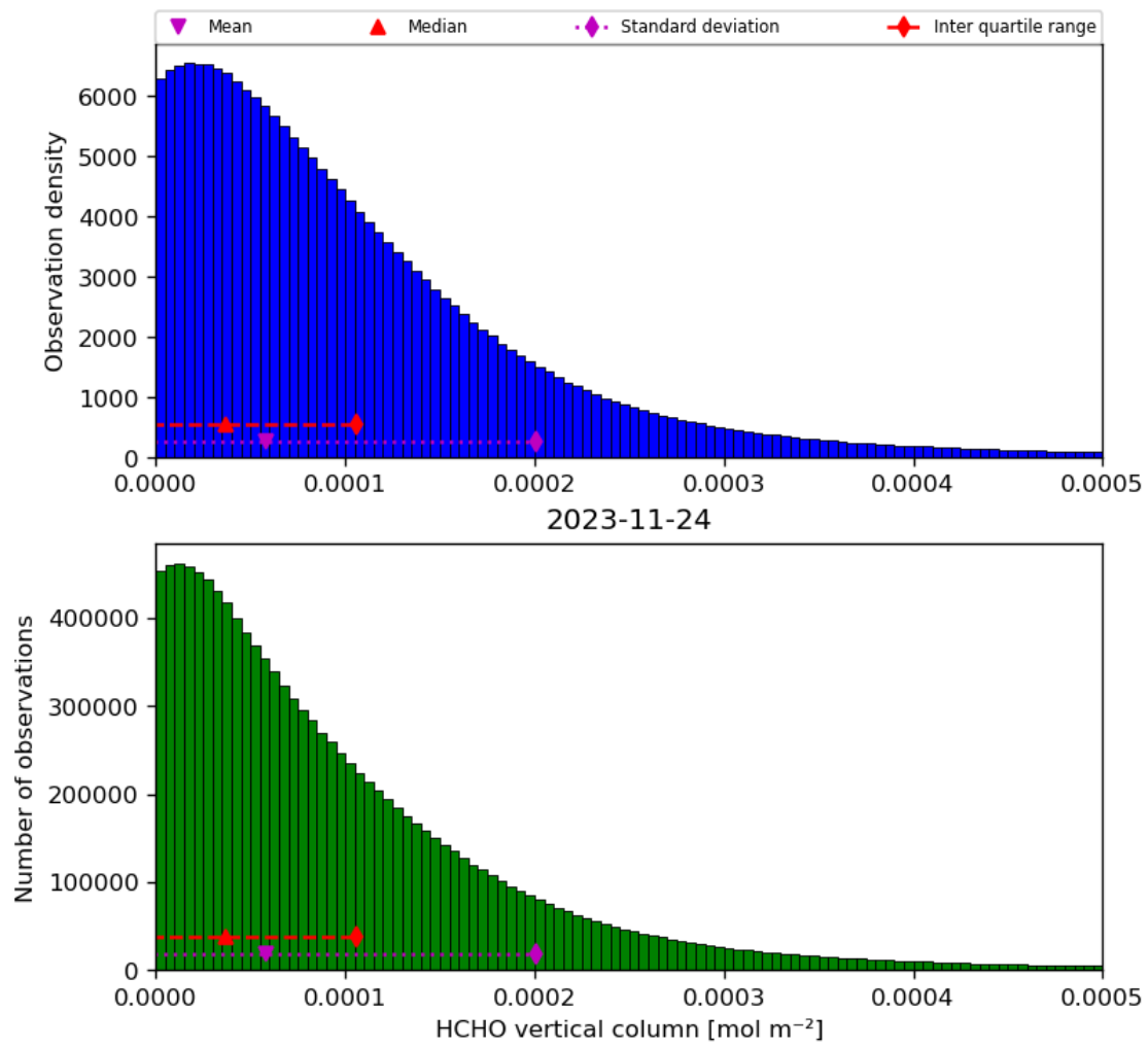
Figure 35: Histogram of “HCHO vertical column” for 2023-11-23 to 2023-11-25
