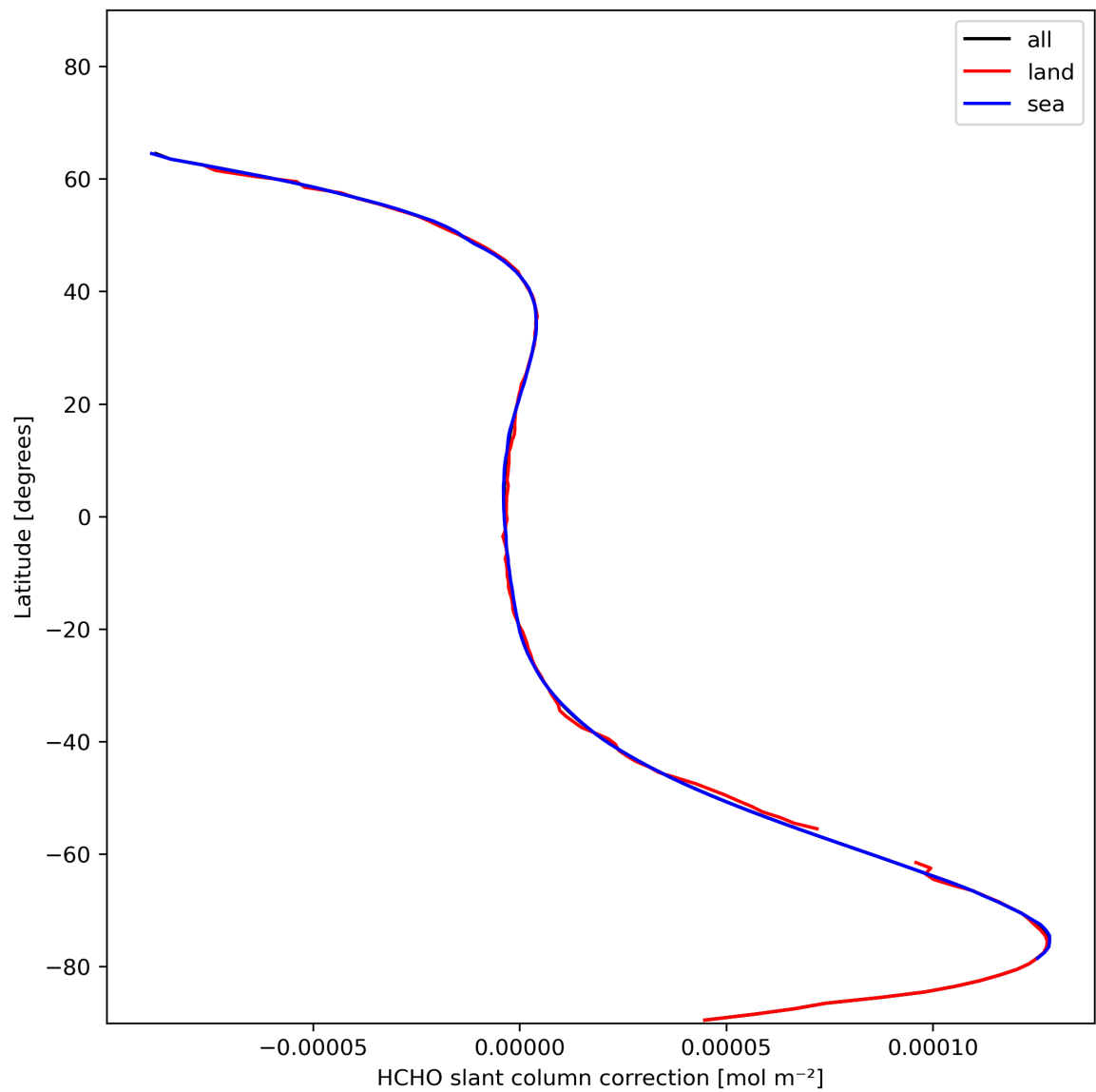
Figure 33: Zonal average of “HCHO slant column correction” for 2023-11-23 to 2023-11-25.
