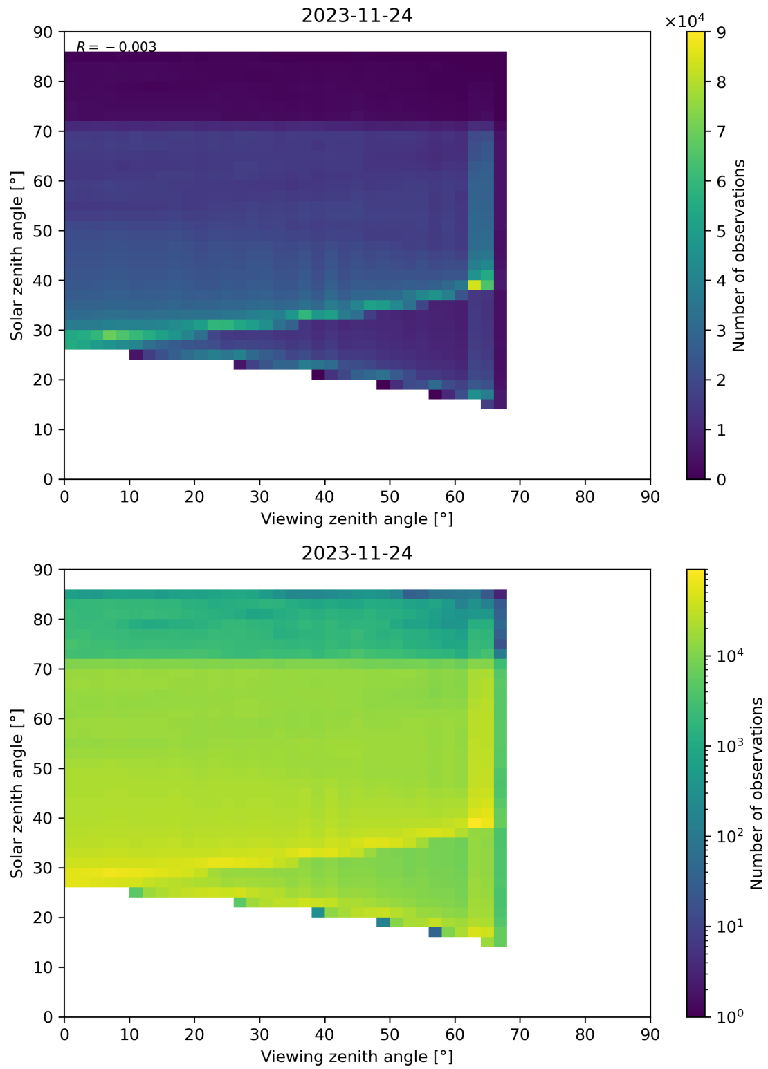
Figure 197: Scatter density plot of “Viewing zenith angle” against “Solar zenith angle” for 2023-11-23 to 2023-11-25.
