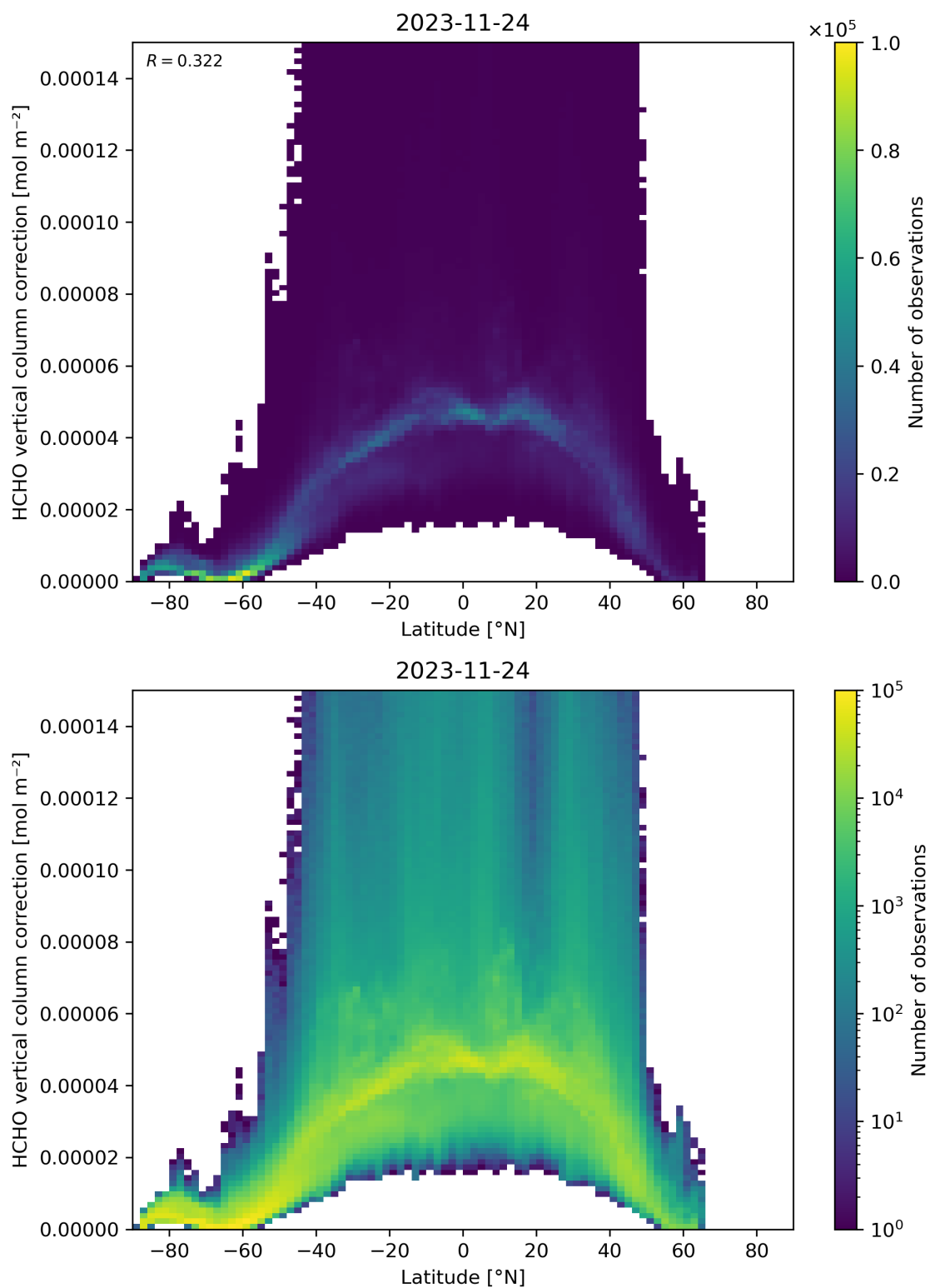
Figure 164: Scatter density plot of “Latitude” against “HCHO vertical column correction” for 2023-11-23 to 2023-11-25.
