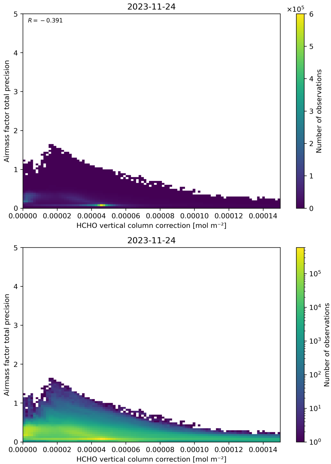
Figure 121: Scatter density plot of “HCHO vertical column correction” against “Airmass factor total precision” for 2023-11-23 to 2023-11-25.
