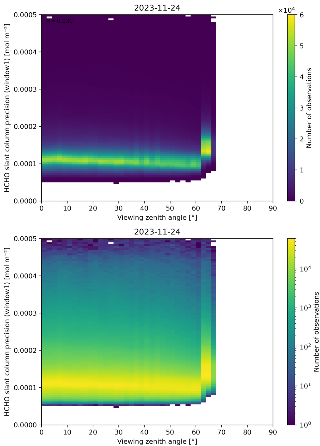
Figure 189: Scatter density plot of “Viewing zenith angle” against “HCHO slant column precision (window1)” for 2023-11-23 to 2023-11-25.
