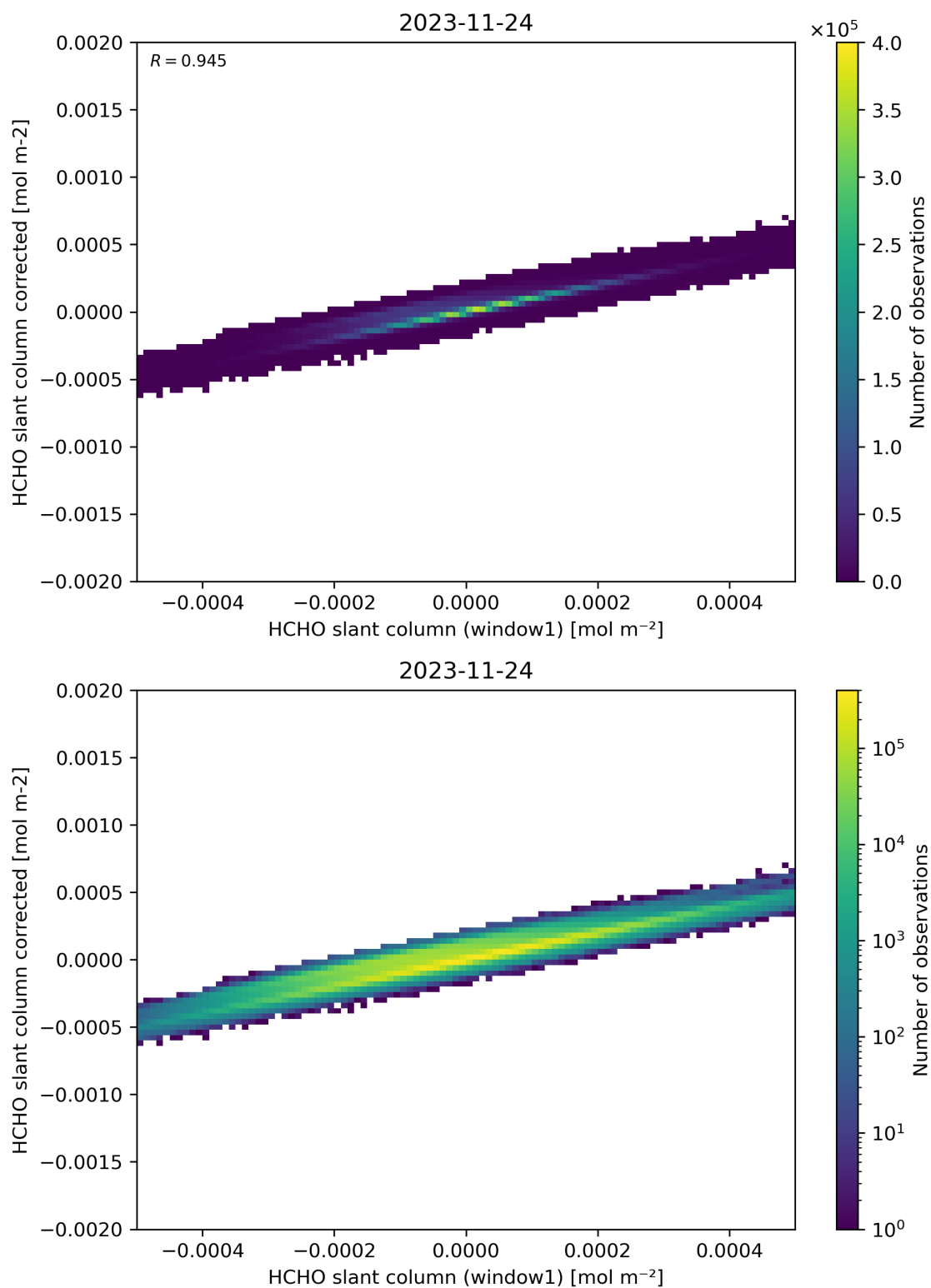
Figure 82: Scatter density plot of “HCHO slant column (window1)” against “HCHO slant column corrected” for 2023-11-23 to 2023-11-25.
