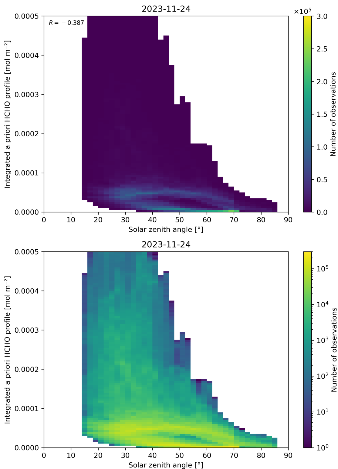
Figure 180: Scatter density plot of “Solar zenith angle” against “Integrated a priori HCHO profile” for 2023-11-23 to 2023-11-25.
