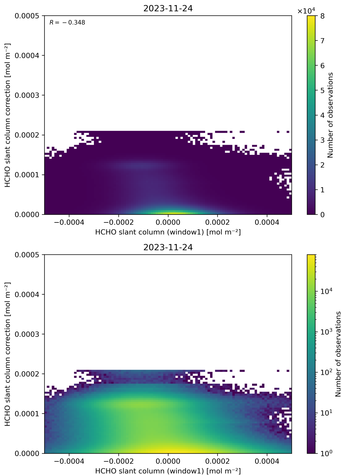
Figure 83: Scatter density plot of “HCHO slant column (window1)” against “HCHO slant column correction” for 2023-11-23 to 2023-11-25.
