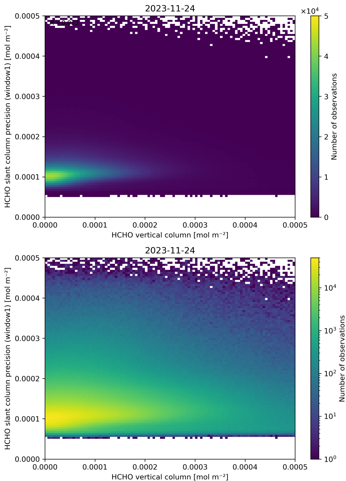
Figure 130: Scatter density plot of “HCHO vertical column” against “HCHO slant column precision (window1)” for 2023-11-23 to 2023-11-25.
