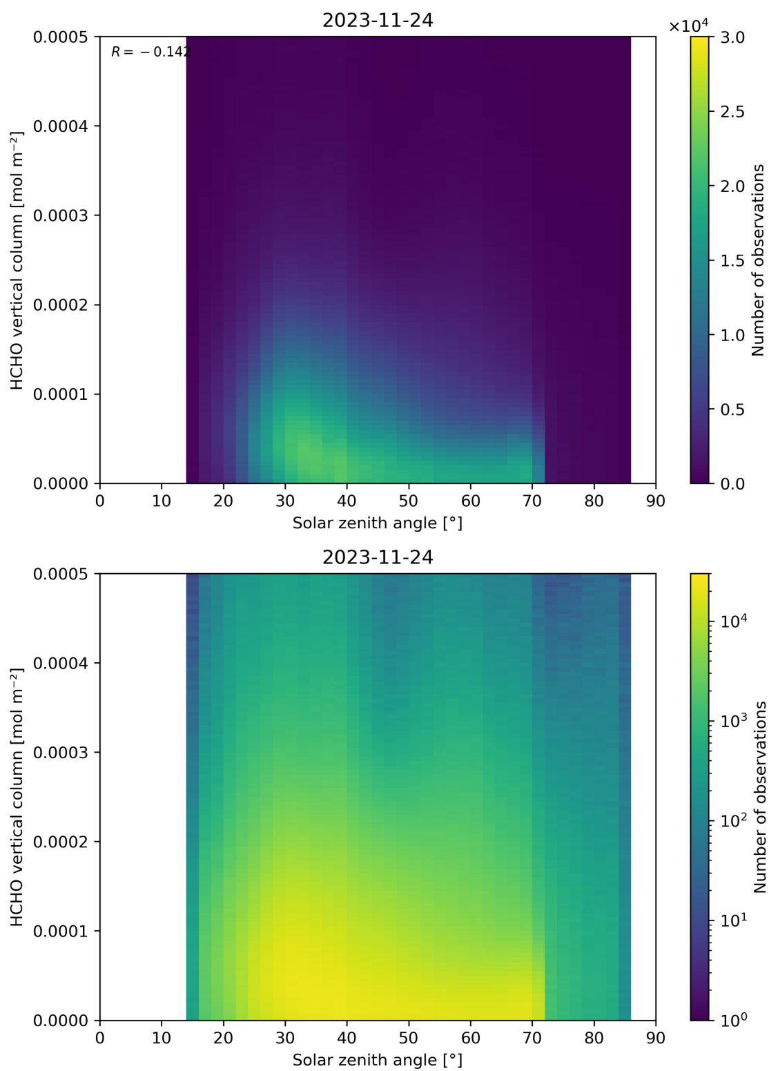
Figure 177: Scatter density plot of “Solar zenith angle” against “HCHO vertical column” for 2023-11-23 to 2023-11-25.
