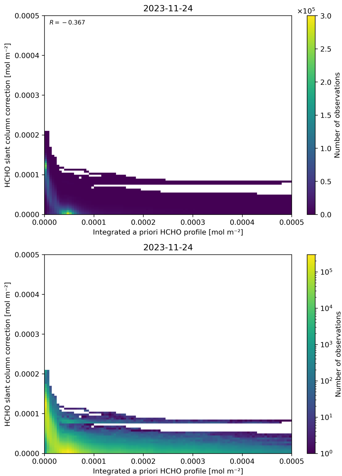
Figure 152: Scatter density plot of “Integrated a priori HCHO profile” against “HCHO slant column correction” for 2023-11-23 to 2023-11-25.
