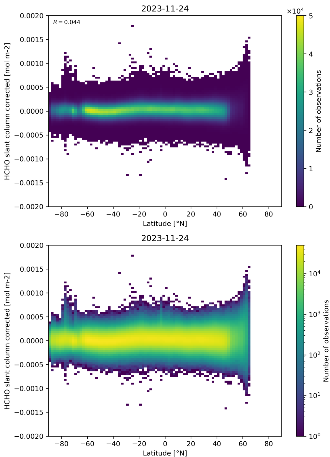
Figure 157: Scatter density plot of “Latitude” against “HCHO slant column corrected” for 2023-11-23 to 2023-11-25.
