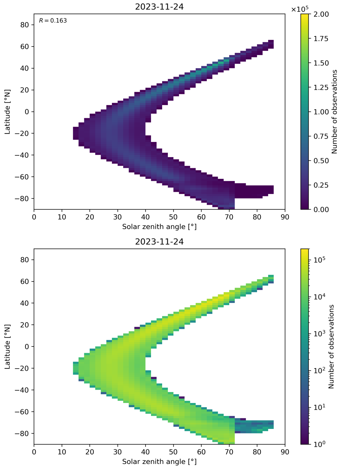
Figure 181: Scatter density plot of “Solar zenith angle” against “Latitude” for 2023-11-23 to 2023-11-25.
