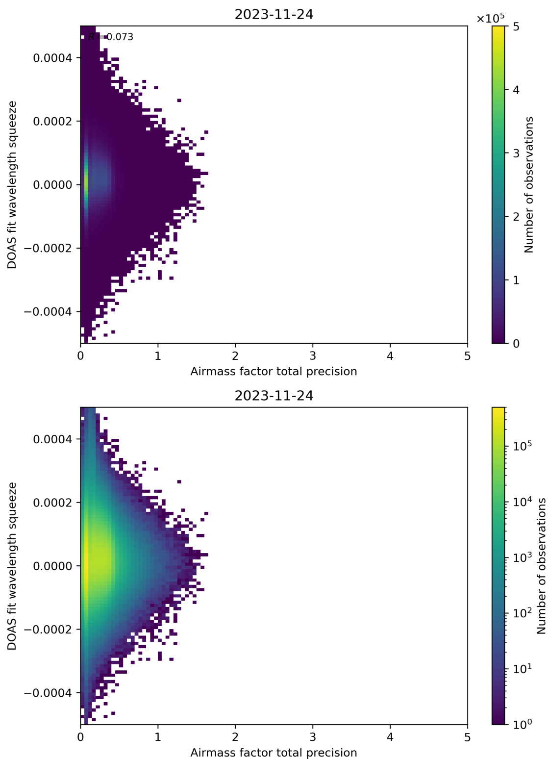
Figure 107: Scatter density plot of “Airmass factor total precision” against “DOAS fit wavelength squeeze” for 2023-11-23 to 2023-11-25.
