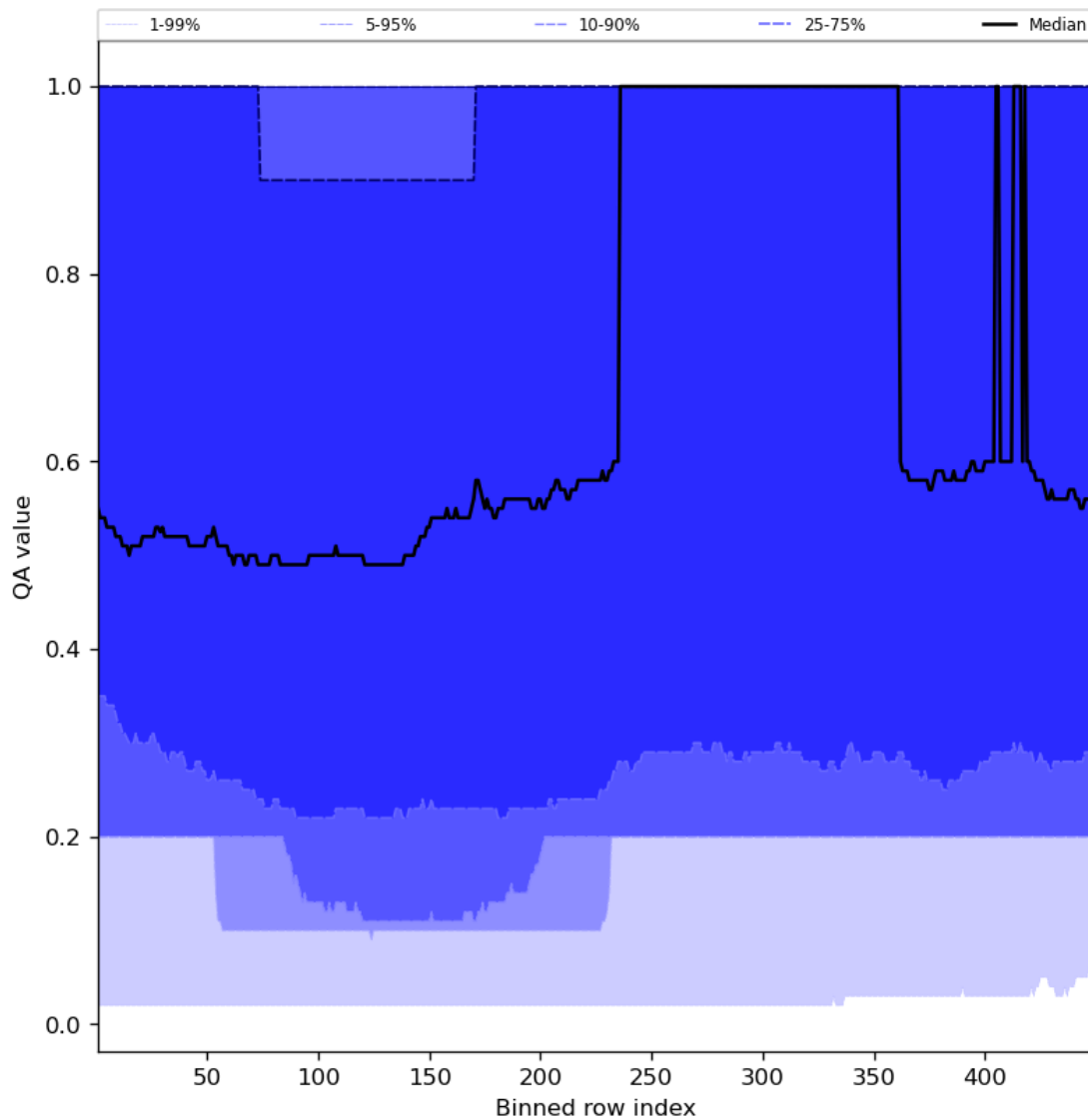
Figure 48: Along track statistics of “QA value” for 2023-11-23 to 2023-11-25
