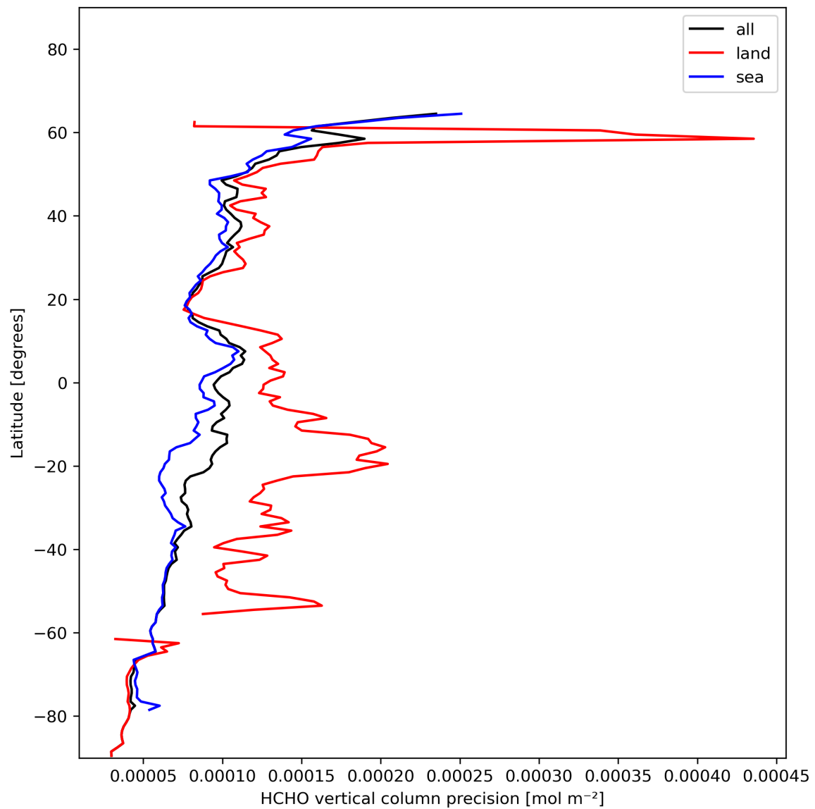
Figure 22: Zonal average of “HCHO vertical column precision” for 2023-11-23 to 2023-11-25.
