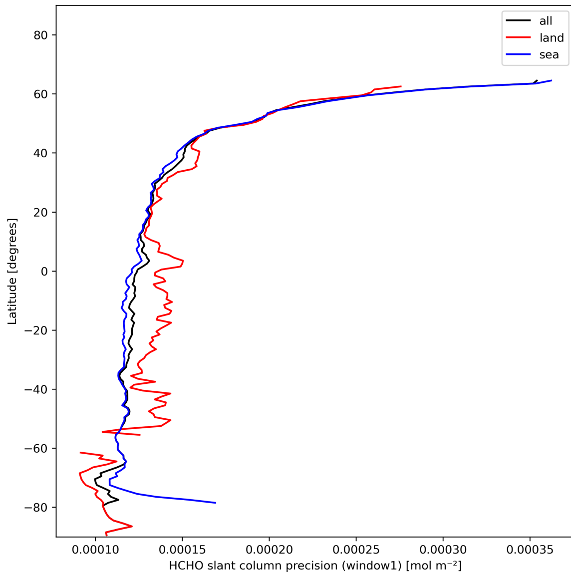
Figure 25: Zonal average of “HCHO slant column precision (window1)” for 2023-11-23 to 2023-11-25.
