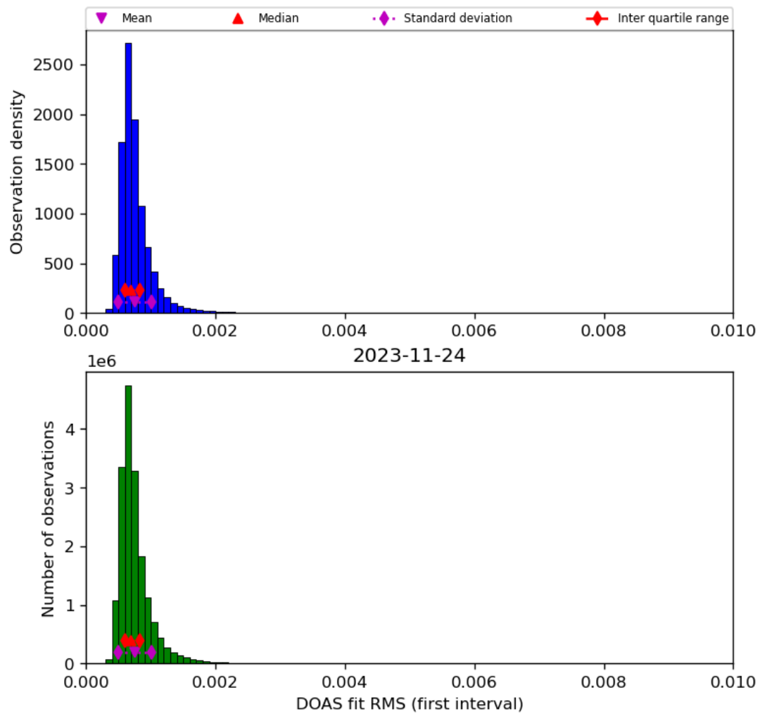
Figure 46: Histogram of “DOAS fit RMS (first interval)” for 2023-11-23 to 2023-11-25
