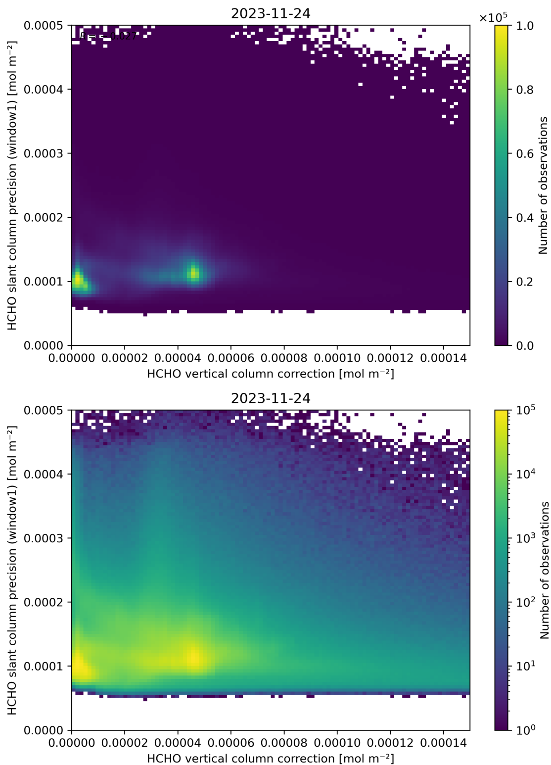
Figure 119: Scatter density plot of “HCHO vertical column correction” against “HCHO slant column precision (window1)” for 2023-11-23 to 2023-11-25.
