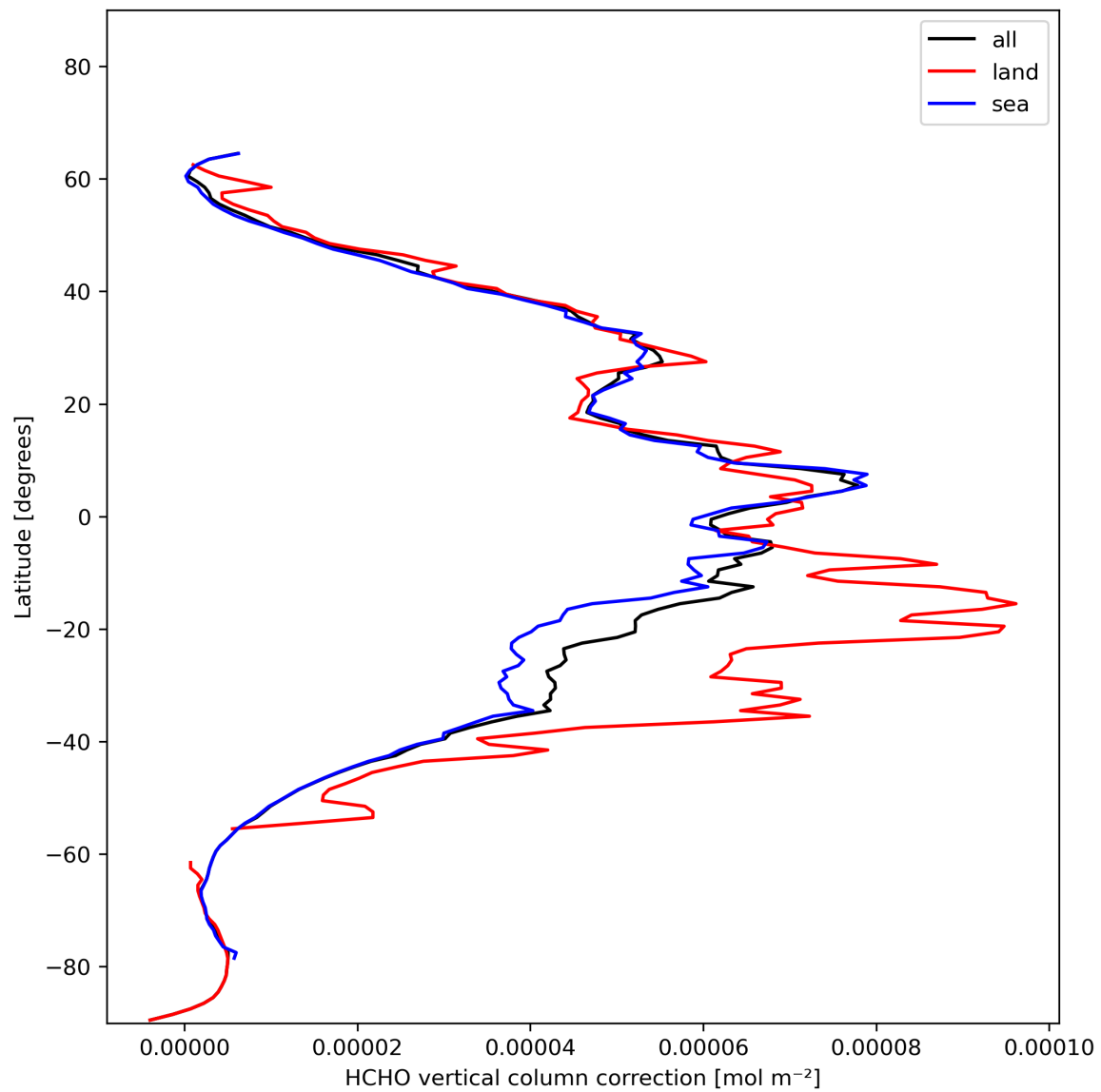
Figure 23: Zonal average of “HCHO vertical column correction” for 2023-11-23 to 2023-11-25.
