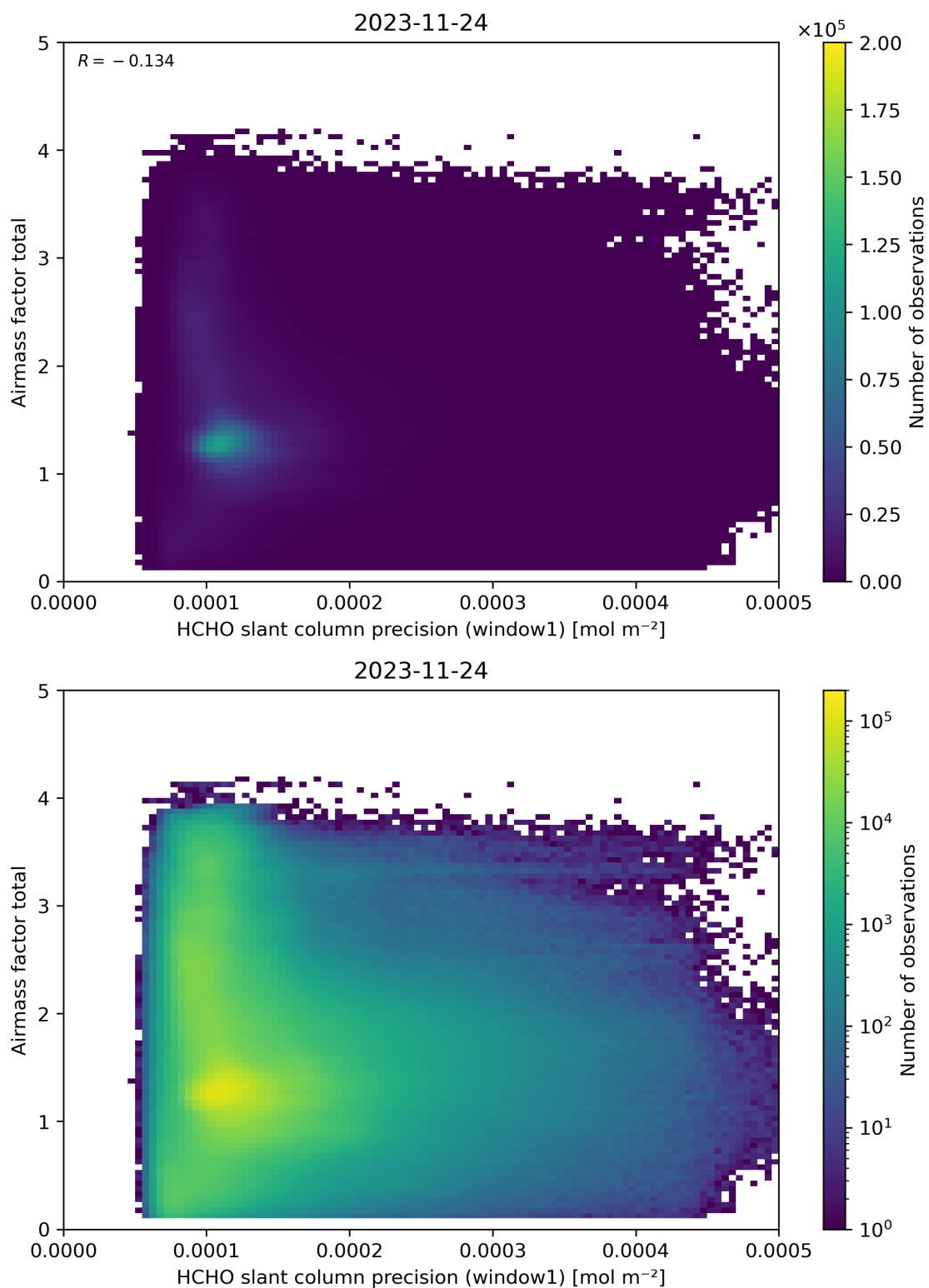
Figure 94: Scatter density plot of “HCHO slant column precision (window1)” against “Airmass factor total” for 2023-11-23 to 2023-11-25.
