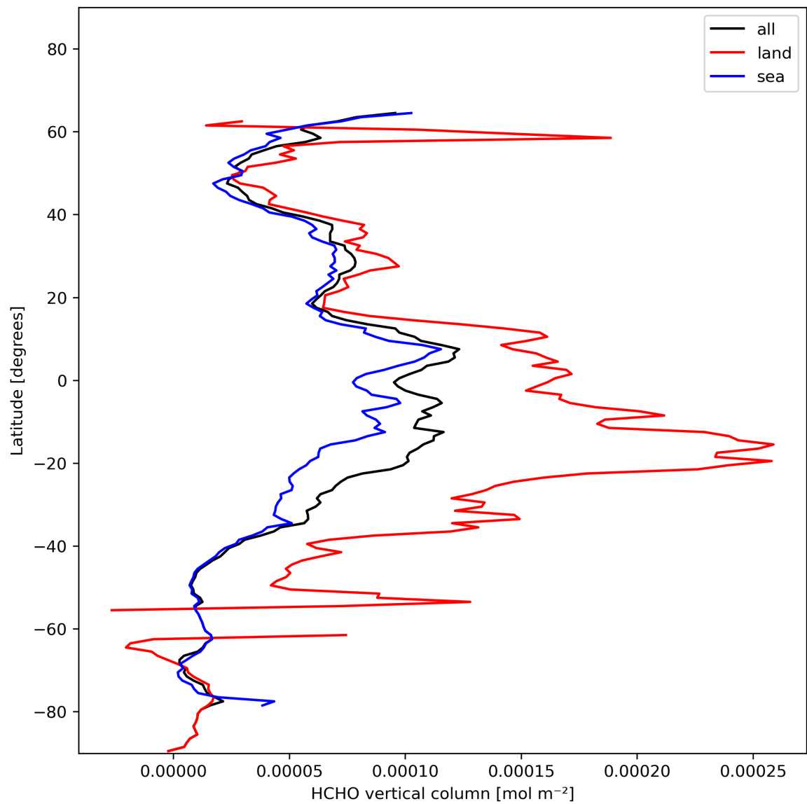
Figure 21: Zonal average of “HCHO vertical column” for 2023-11-23 to 2023-11-25.
