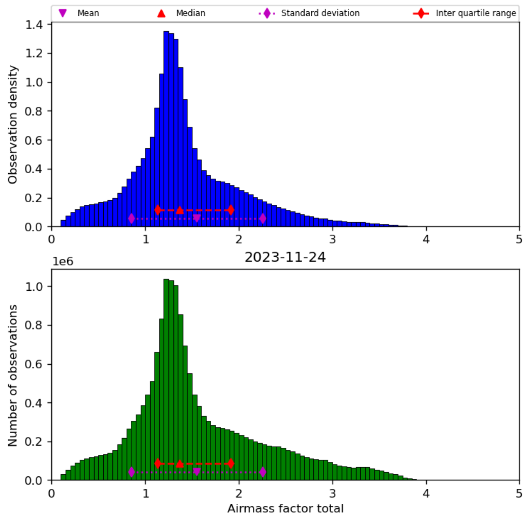
Figure 40: Histogram of “Airmass factor total” for 2023-11-23 to 2023-11-25
