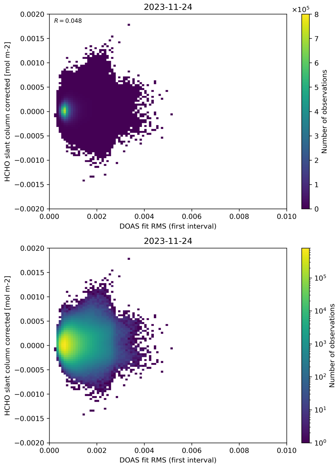
Figure 62: Scatter density plot of “DOAS fit RMS (first interval)” against “HCHO slant column corrected” for 2023-11-23 to 2023-11-25.
