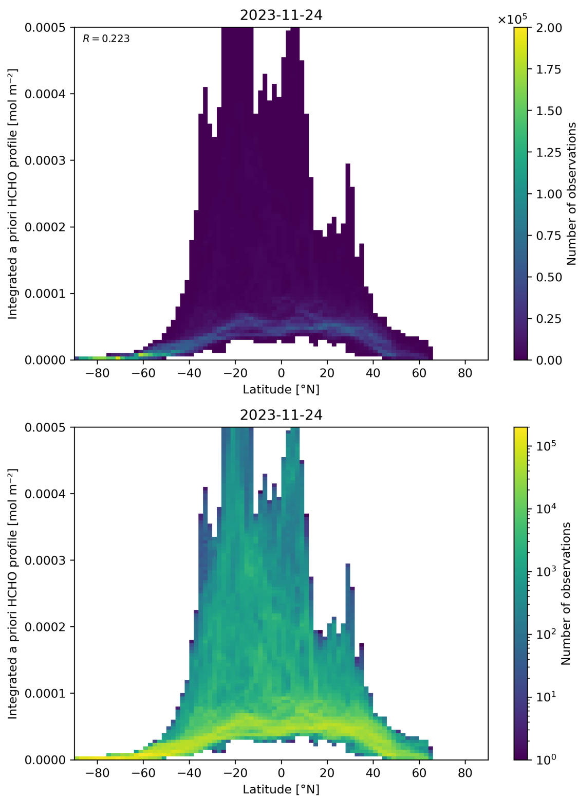
Figure 166: Scatter density plot of “Latitude” against “Integrated a priori HCHO profile” for 2023-11-23 to 2023-11-25.
