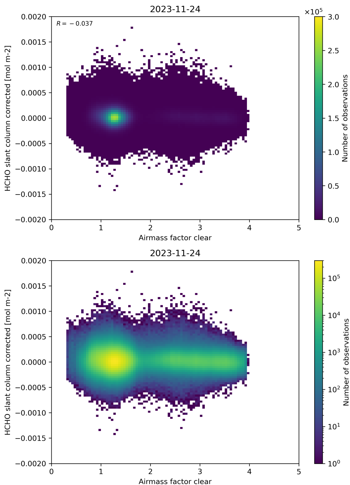
Figure 74: Scatter density plot of “Airmass factor clear” against “HCHO slant column corrected” for 2023-11-23 to 2023-11-25.
