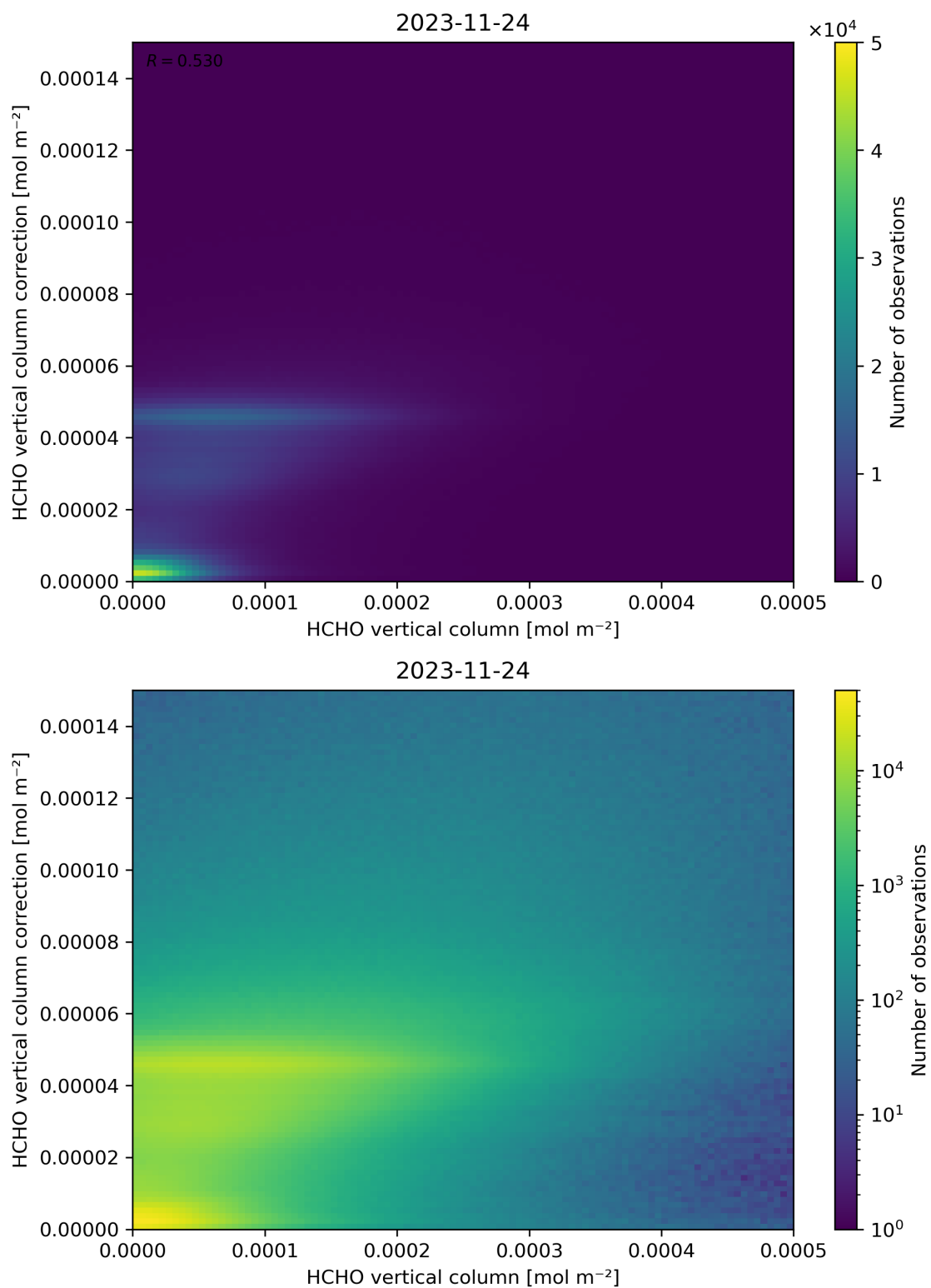
Figure 133: Scatter density plot of “HCHO vertical column” against “HCHO vertical column correction” for 2023-11-23 to 2023-11-25.
