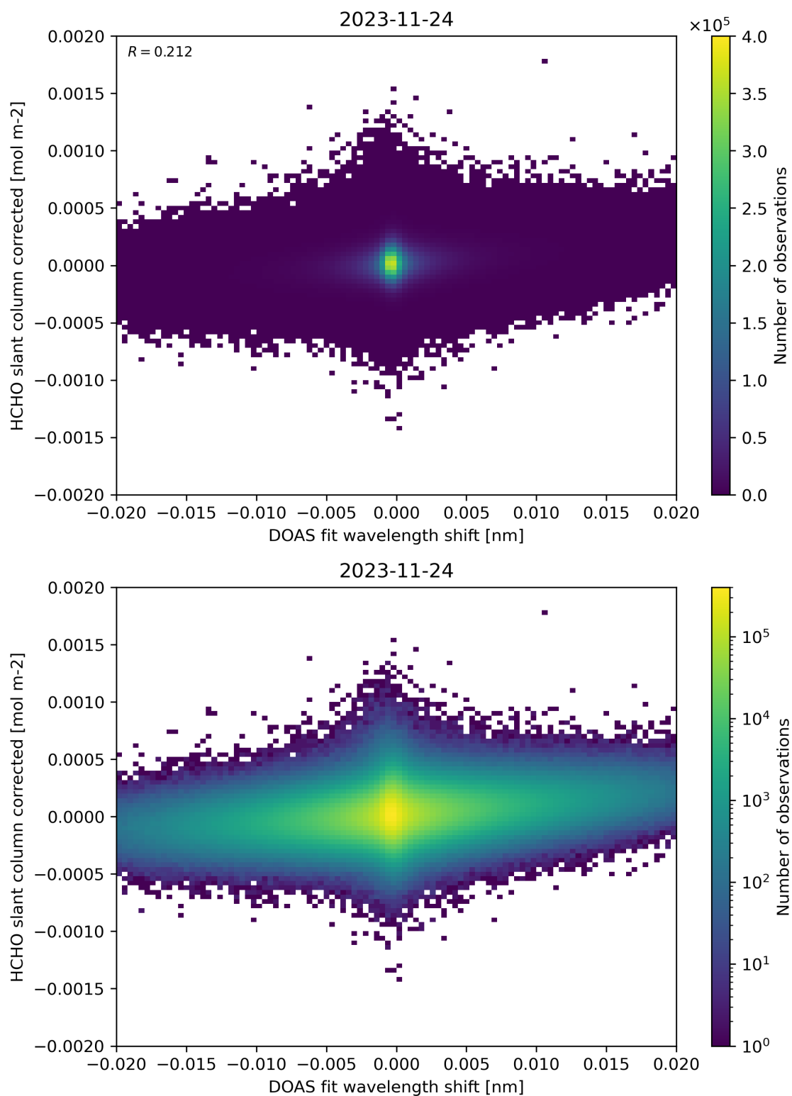
Figure 66: Scatter density plot of “DOAS fit wavelength shift” against “HCHO slant column corrected” for 2023-11-23 to 2023-11-25.
