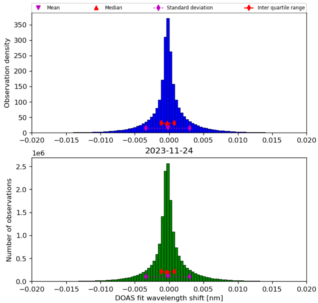
Figure 44: Histogram of “DOAS fit wavelength shift” for 2023-11-23 to 2023-11-25
