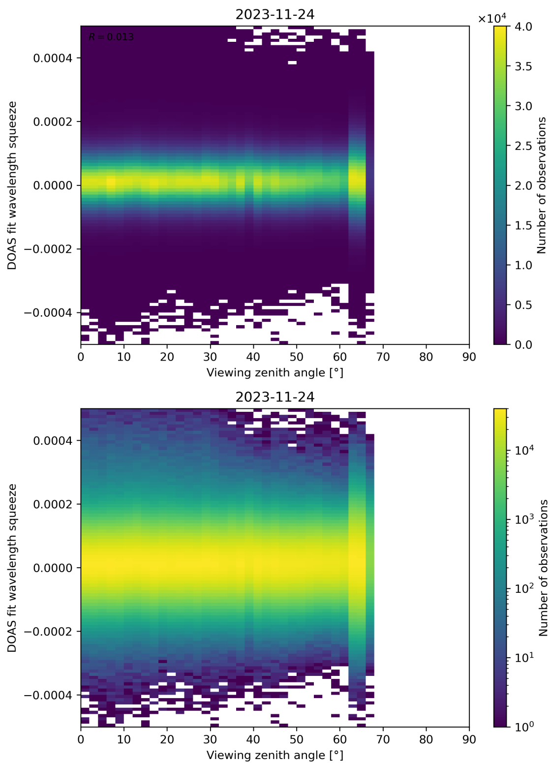
Figure 184: Scatter density plot of “Viewing zenith angle” against “DOAS fit wavelength squeeze” for 2023-11-23 to 2023-11-25.
