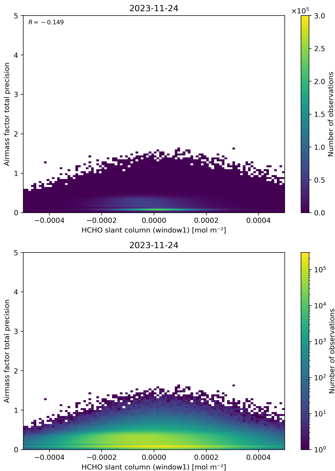
Figure 86: Scatter density plot of “HCHO slant column (window1)” against “Airmass factor total precision” for 2023-11-23 to 2023-11-25.
