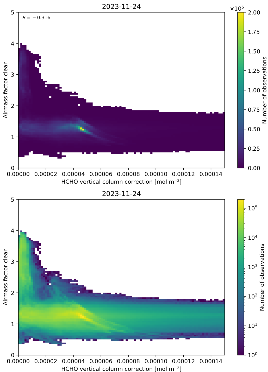
Figure 115: Scatter density plot of “HCHO vertical column correction” against “Airmass factor clear” for 2023-11-23 to 2023-11-25.
