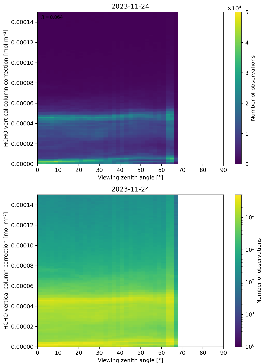
Figure 193: Scatter density plot of “Viewing zenith angle” against “HCHO vertical column correction” for 2023-11-23 to 2023-11-25.
