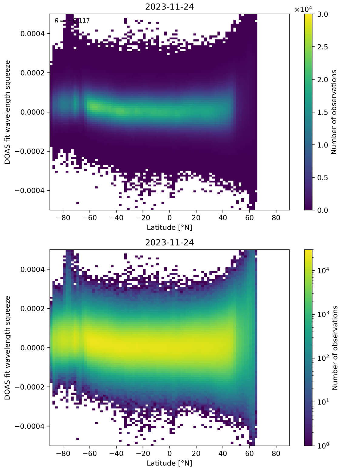
Figure 155: Scatter density plot of “Latitude” against “DOAS fit wavelength squeeze” for 2023-11-23 to 2023-11-25.
