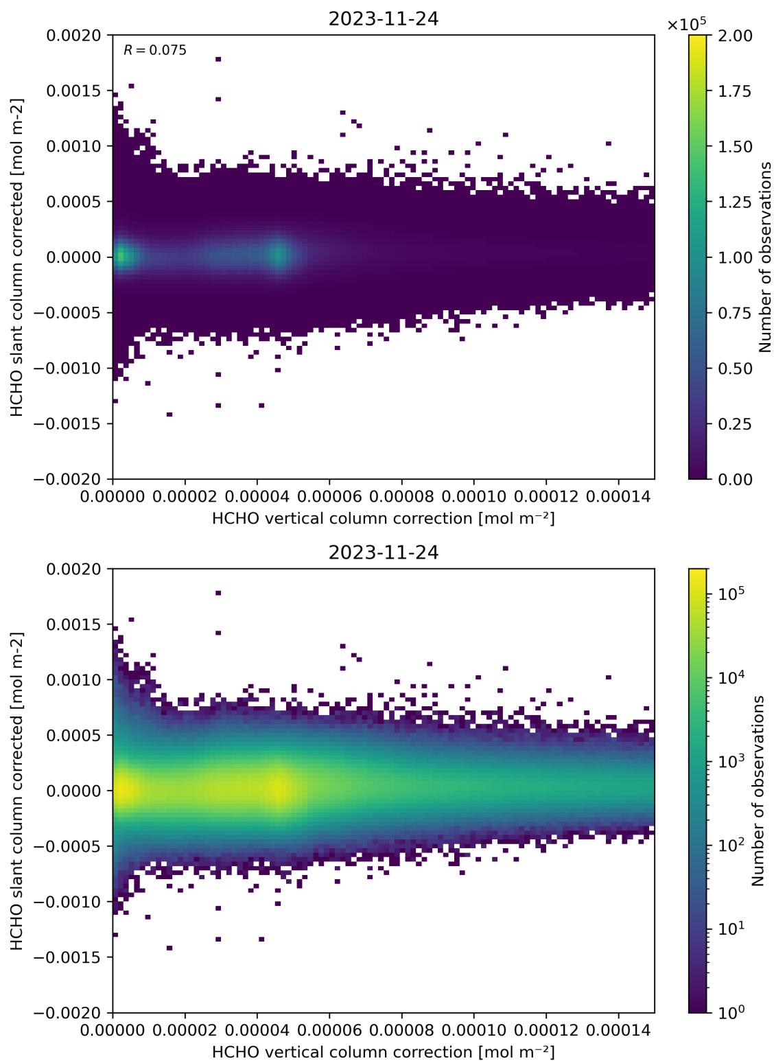
Figure 116: Scatter density plot of “HCHO vertical column correction” against “HCHO slant column corrected” for 2023-11-23 to 2023-11-25.
