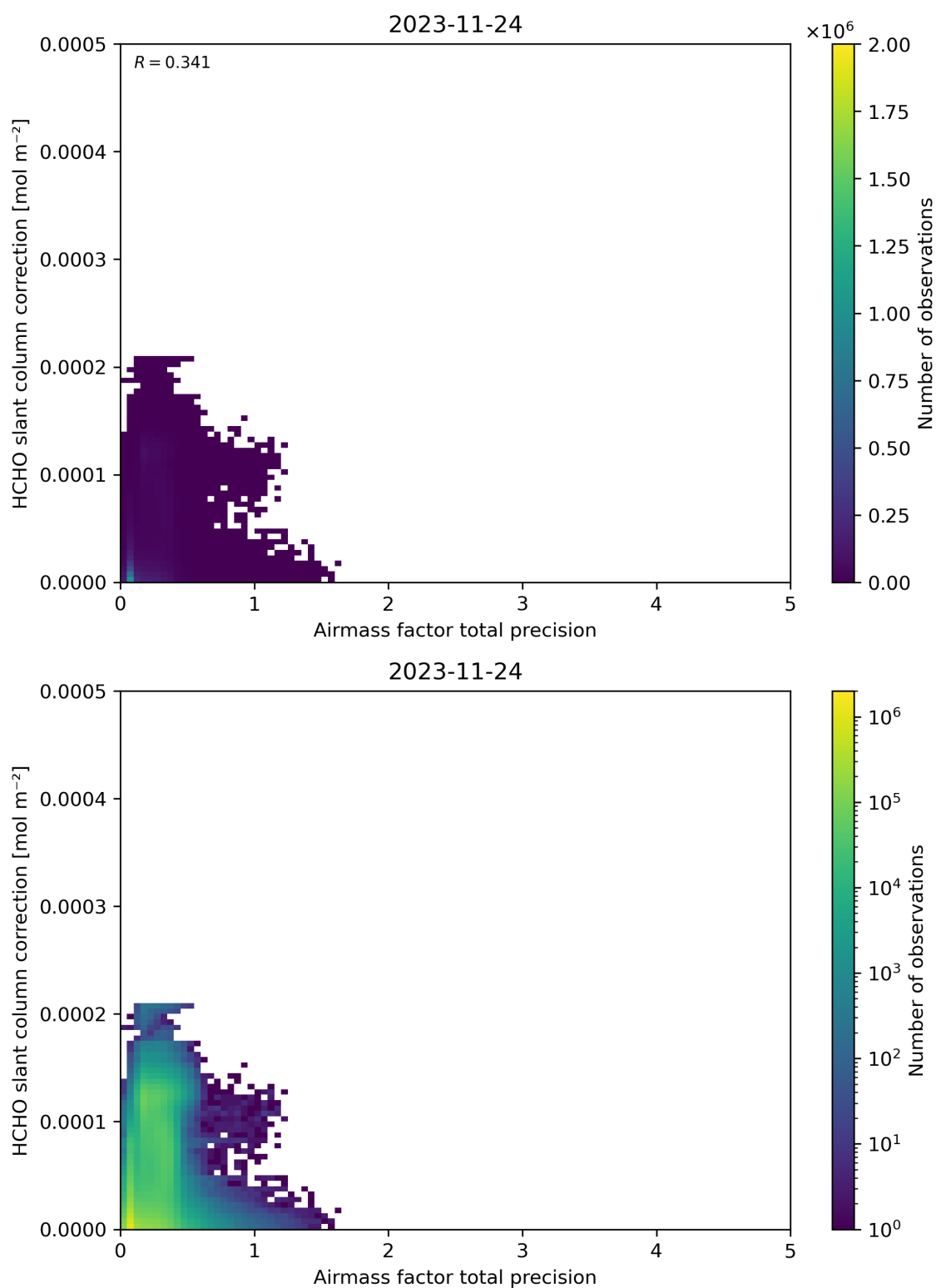
Figure 110: Scatter density plot of “Airmass factor total precision” against “HCHO slant column correction” for 2023-11-23 to 2023-11-25.
