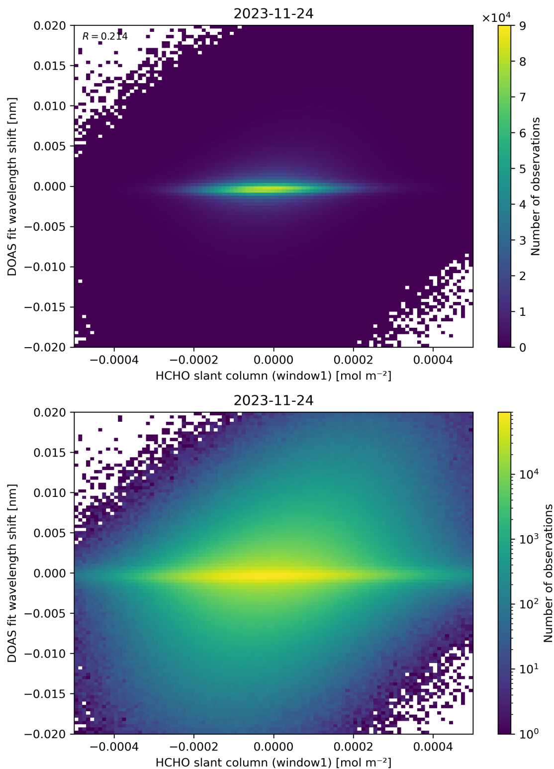
Figure 79: Scatter density plot of “HCHO slant column (window1)” against “DOAS fit wavelength shift” for 2023-11-23 to 2023-11-25.
