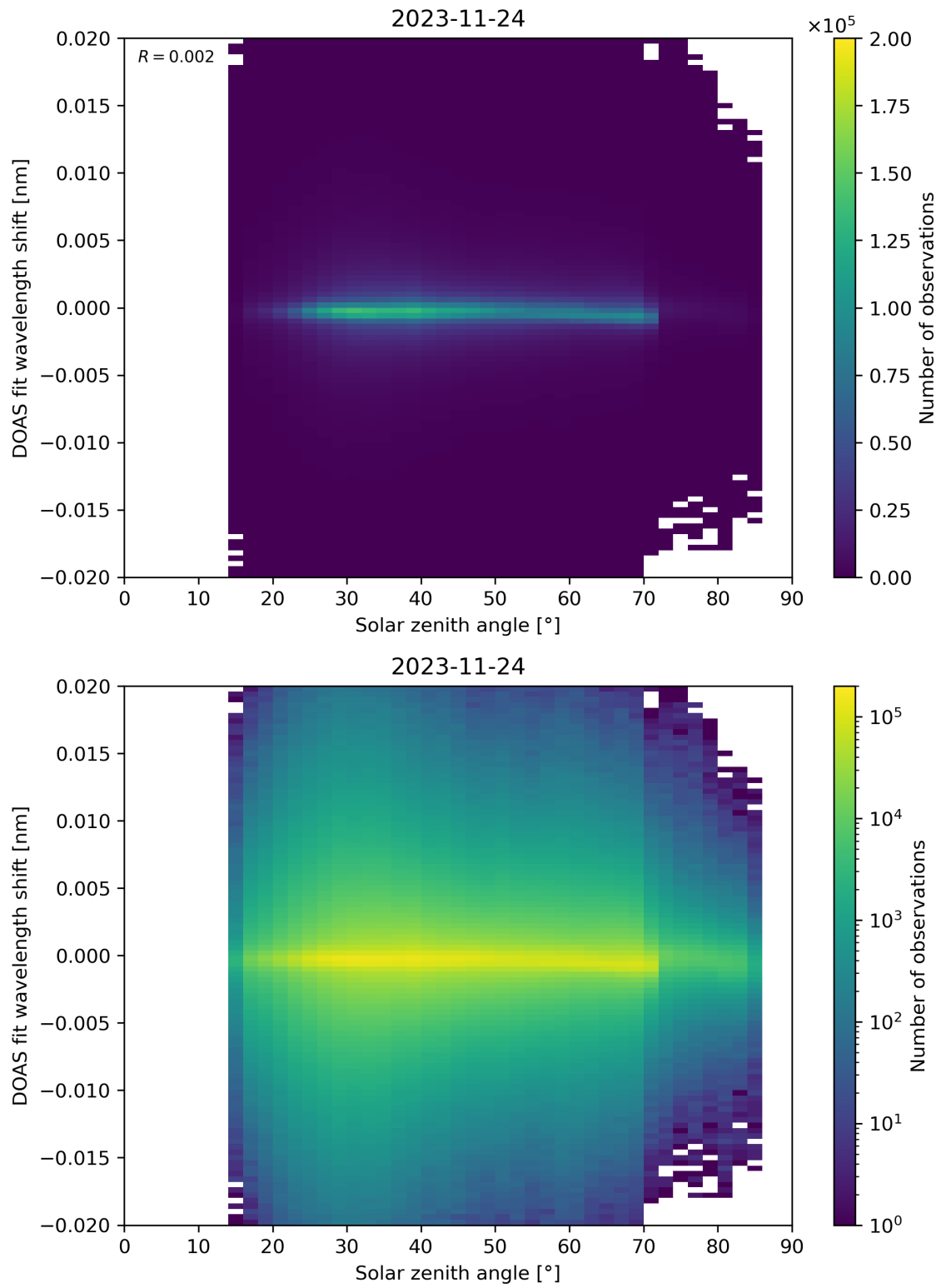
Figure 168: Scatter density plot of “Solar zenith angle” against “DOAS fit wavelength shift” for 2023-11-23 to 2023-11-25.
