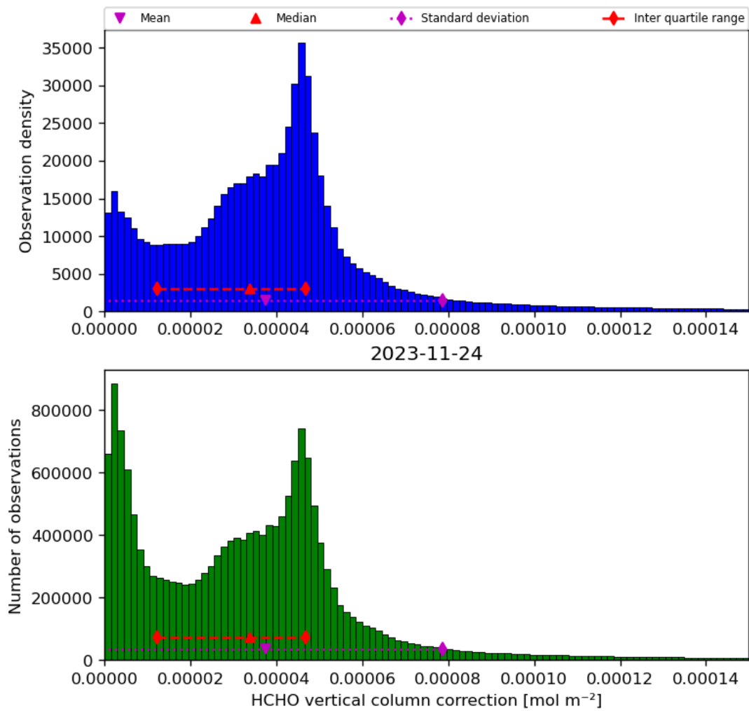
Figure 37: Histogram of “HCHO vertical column correction” for 2023-11-23 to 2023-11-25
