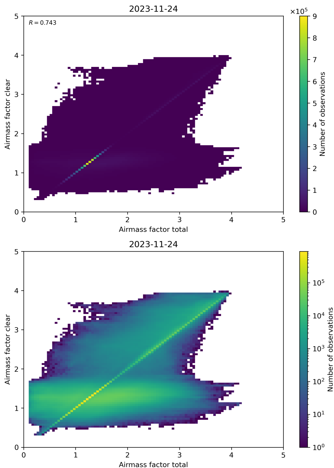
Figure 100: Scatter density plot of “Airmass factor total” against “Airmass factor clear” for 2023-11-23 to 2023-11-25.
