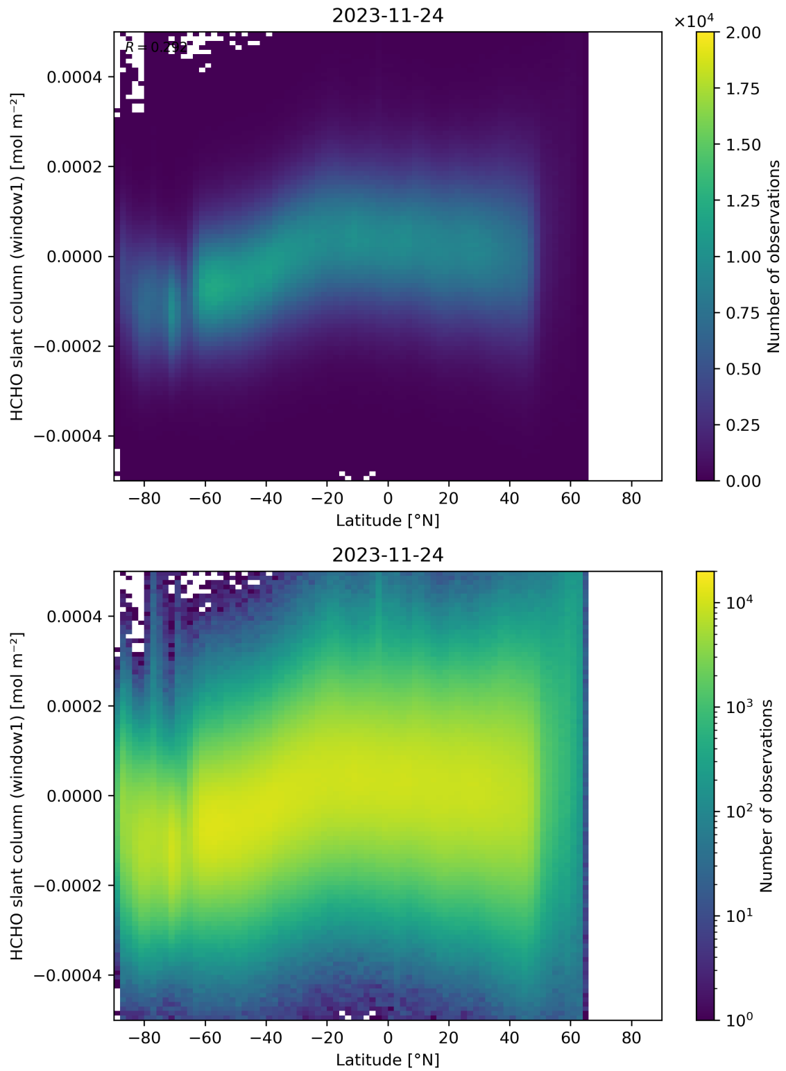
Figure 159: Scatter density plot of “Latitude” against “HCHO slant column (window1)” for 2023-11-23 to 2023-11-25.
