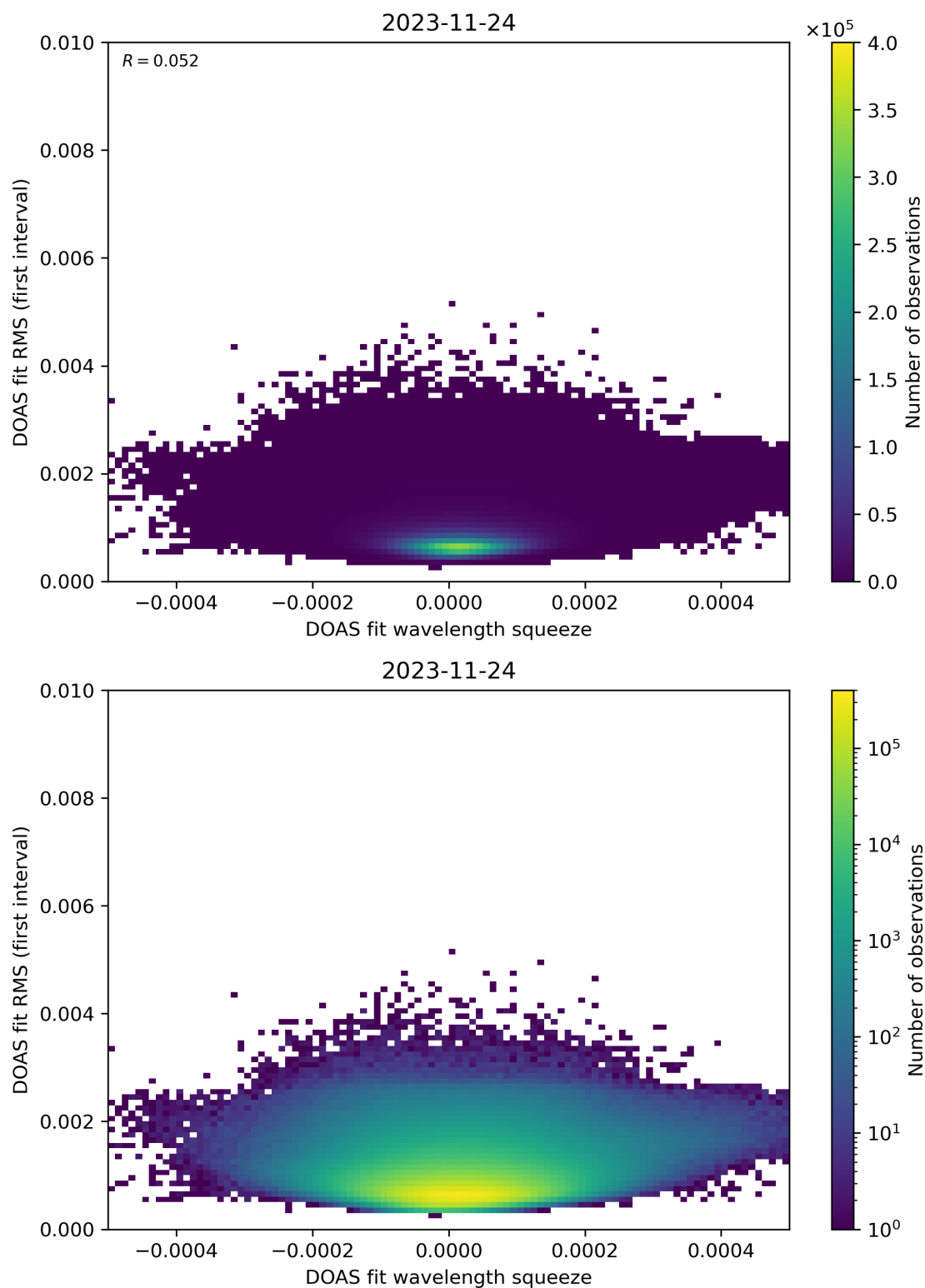
Figure 68: Scatter density plot of “DOAS fit wavelength squeeze” against “DOAS fit RMS (first interval)” for 2023-11-23 to 2023-11-25.
