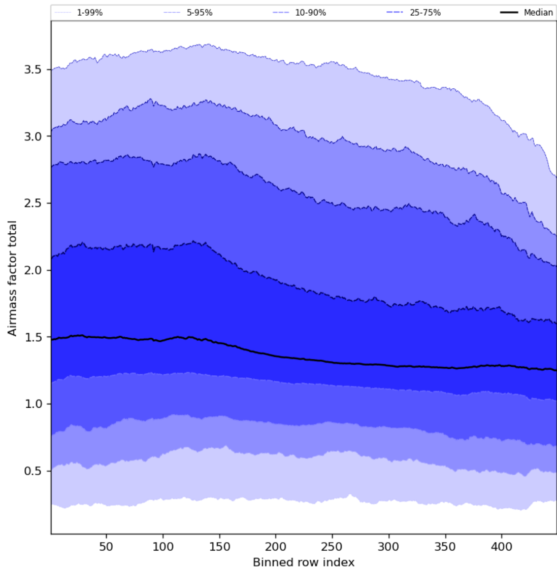
Figure 54: Along track statistics of “Airmass factor total” for 2023-11-23 to 2023-11-25
