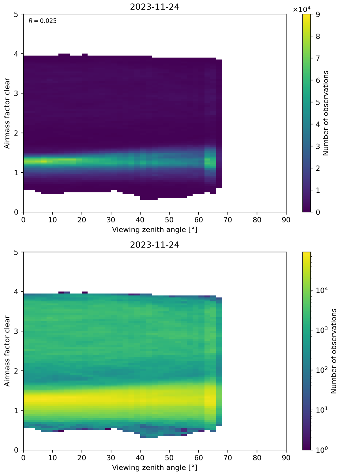
Figure 185: Scatter density plot of “Viewing zenith angle” against “Airmass factor clear” for 2023-11-23 to 2023-11-25.
