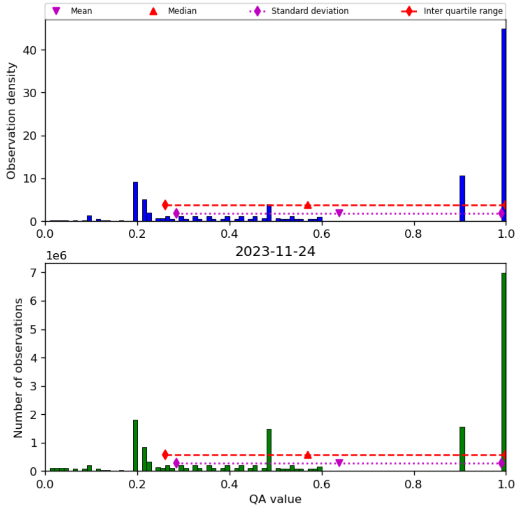
Figure 34: Histogram of “QA value” for 2023-11-23 to 2023-11-25
