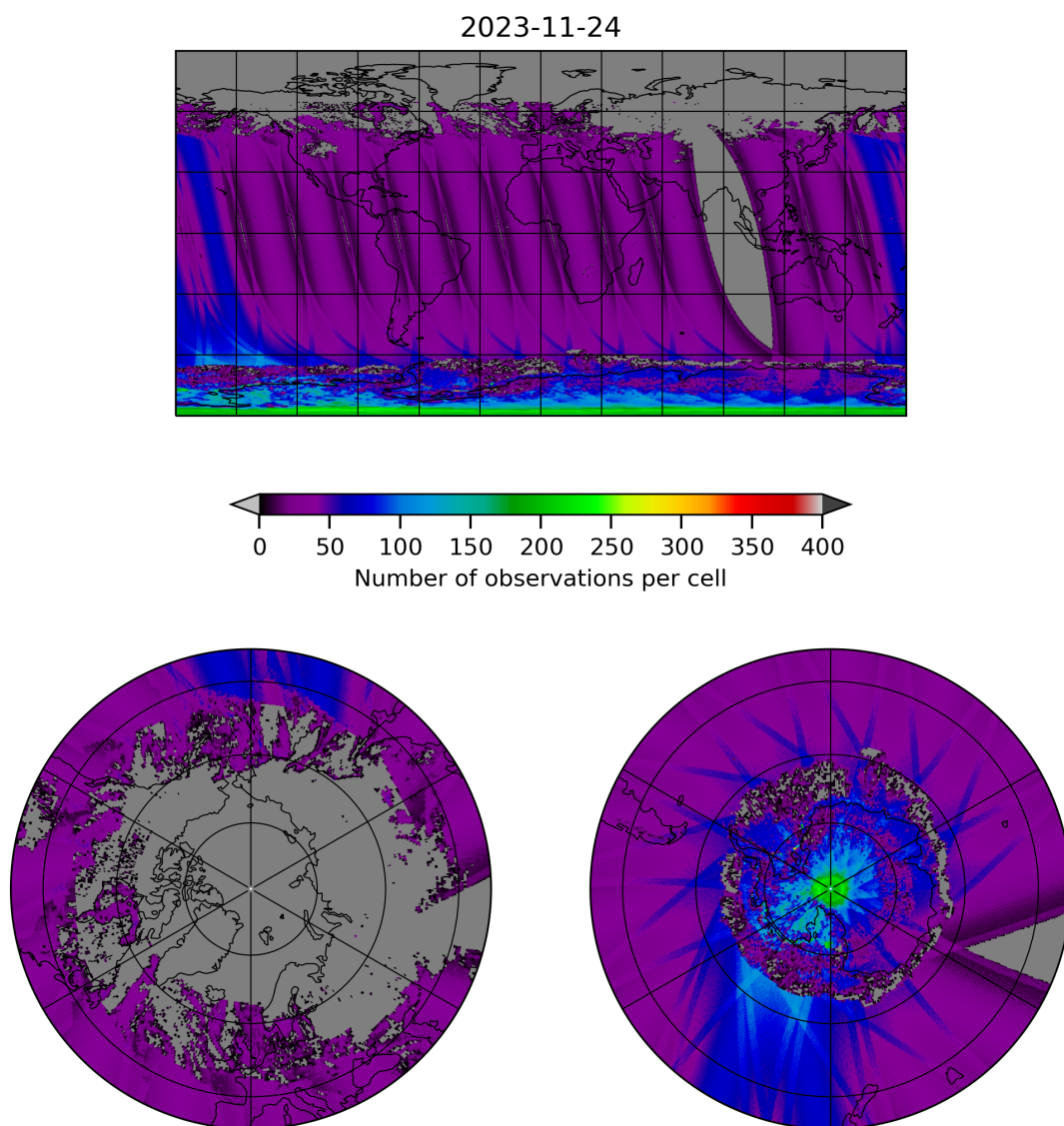
Figure 19: Map of the number of observations for 2023-11-23 to 2023-11-25
