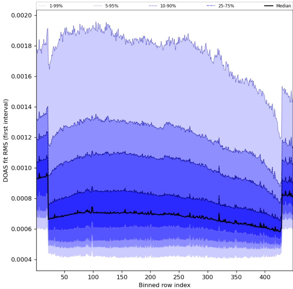
Figure 60: Along track statistics of “DOAS fit RMS (first interval)” for 2023-11-23 to 2023-11-25
