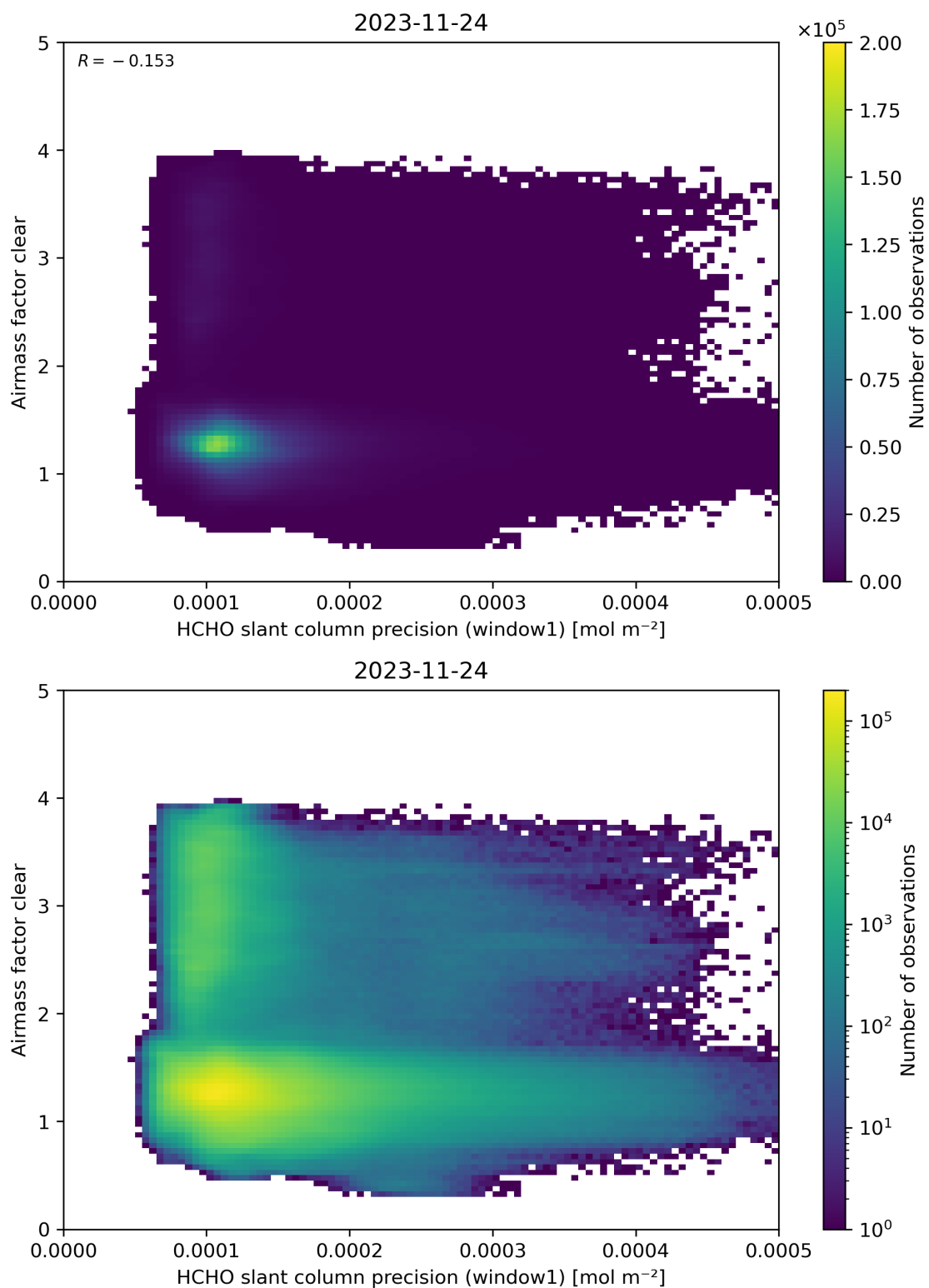
Figure 91: Scatter density plot of “HCHO slant column precision (window1)” against “Airmass factor clear” for 2023-11-23 to 2023-11-25.
