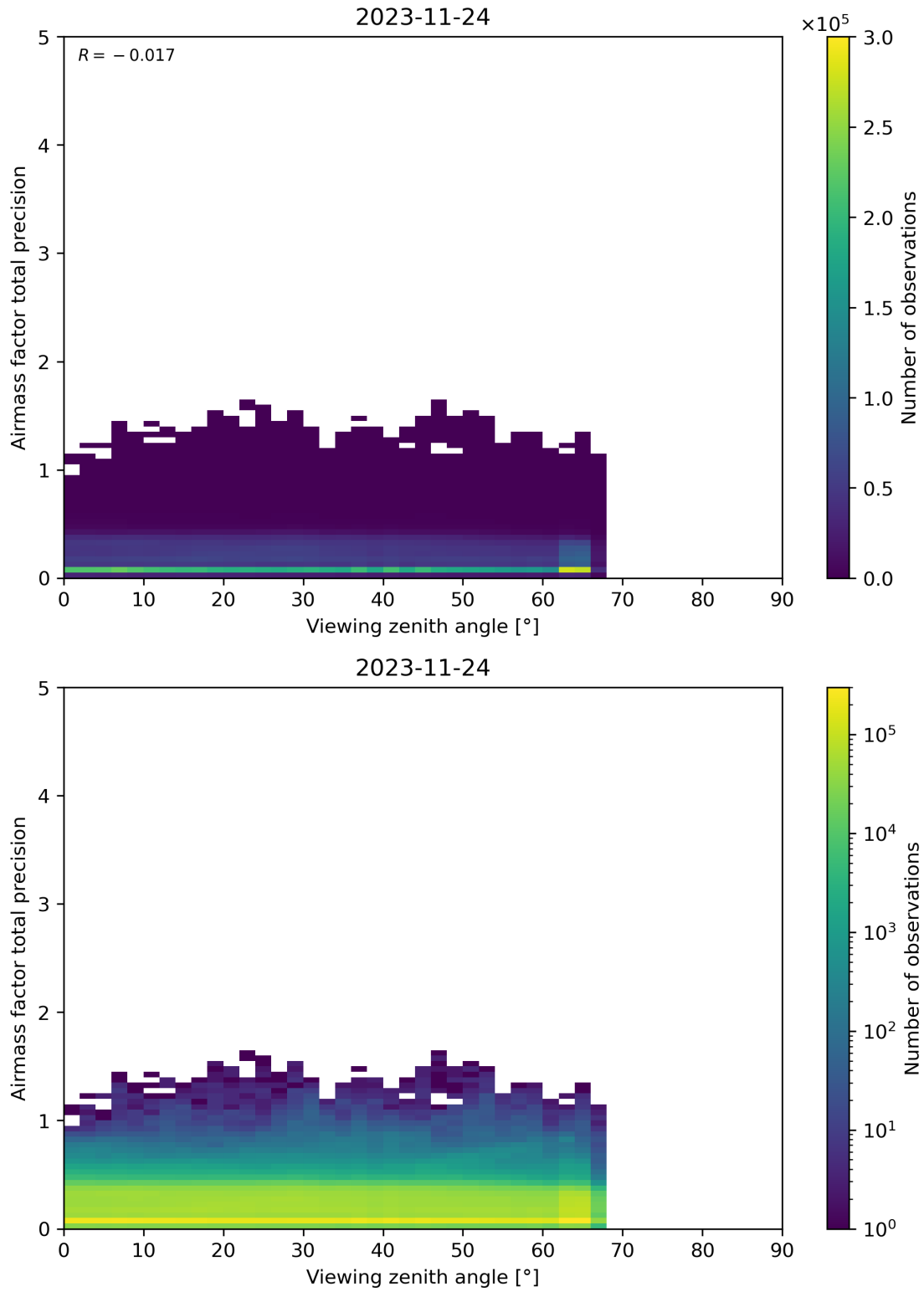
Figure 191: Scatter density plot of “Viewing zenith angle” against “Airmass factor total precision” for 2023-11-23 to 2023-11-25.
