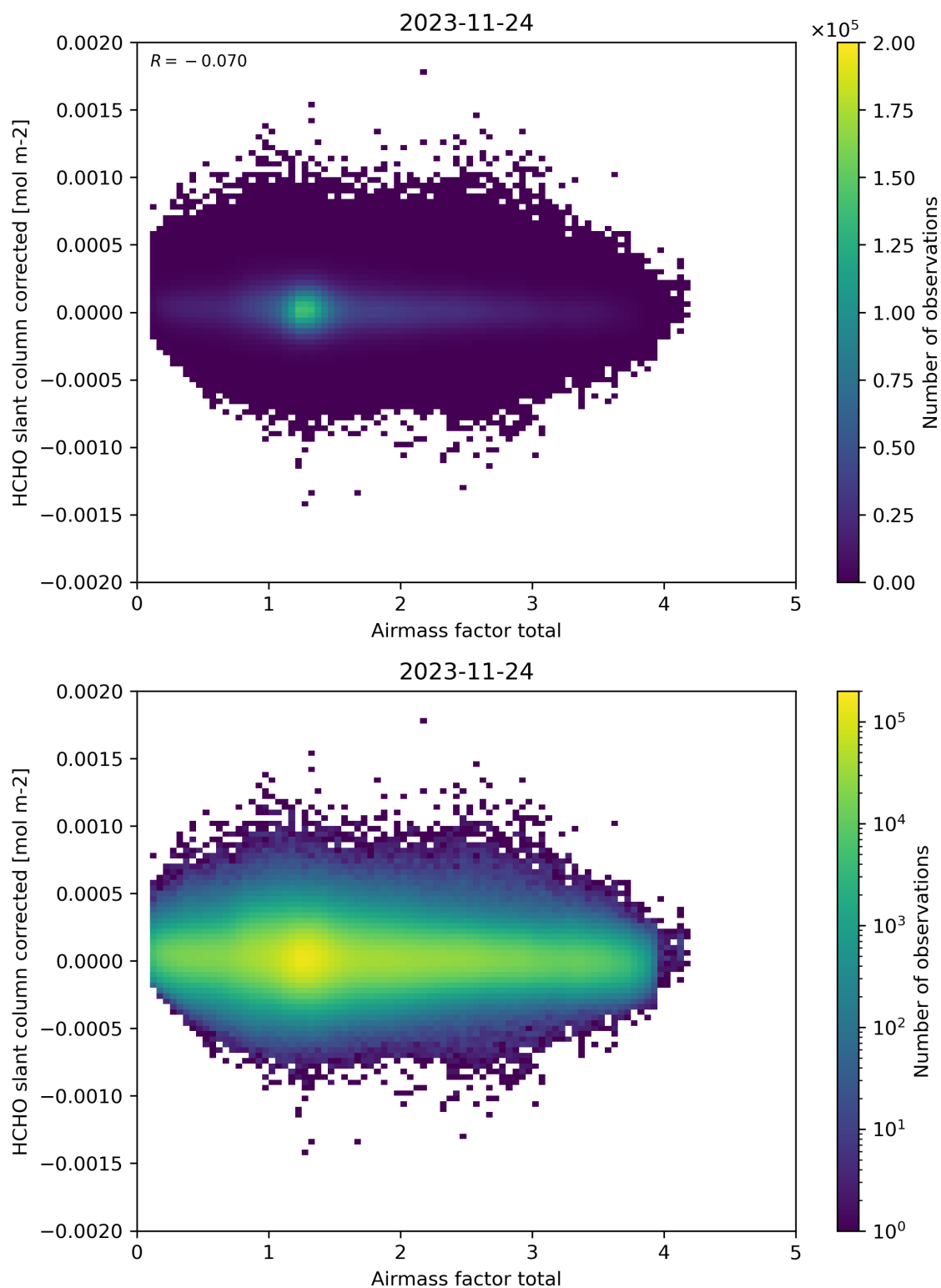
Figure 101: Scatter density plot of “Airmass factor total” against “HCHO slant column corrected” for 2023-11-23 to 2023-11-25.
