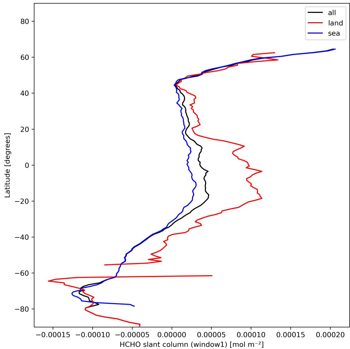
Figure 24: Zonal average of “HCHO slant column (window1)” for 2023-11-23 to 2023-11-25.
