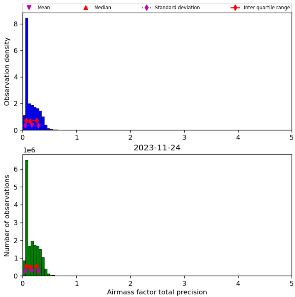
Figure 41: Histogram of “Airmass factor total precision” for 2023-11-23 to 2023-11-25
