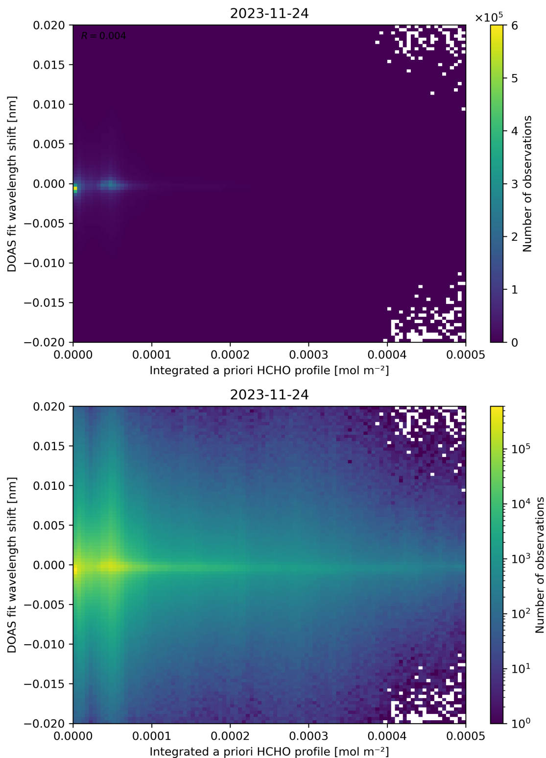
Figure 149: Scatter density plot of “Integrated a priori HCHO profile” against “DOAS fit wavelength shift” for 2023-11-23 to 2023-11-25.
