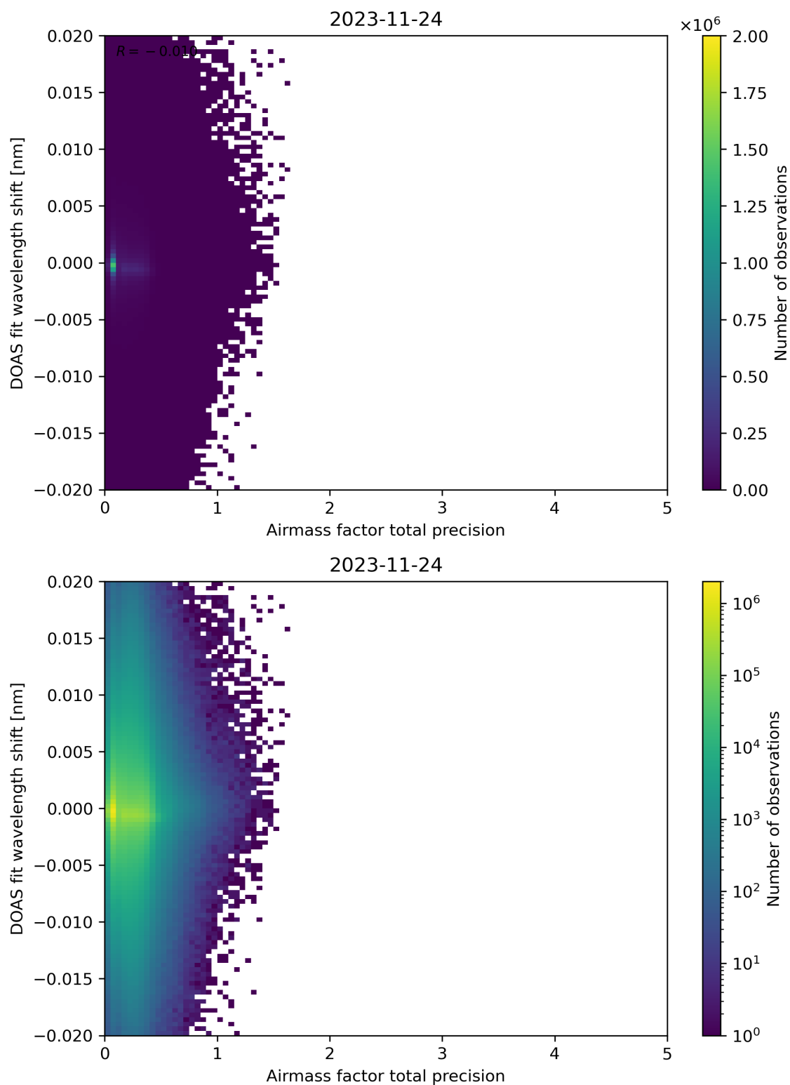
Figure 106: Scatter density plot of “Airmass factor total precision” against “DOAS fit wavelength shift” for 2023-11-23 to 2023-11-25.
