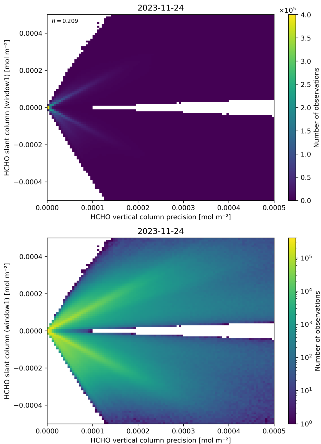
Figure 142: Scatter density plot of “HCHO vertical column precision” against “HCHO slant column (window1)” for 2023-11-23 to 2023-11-25.
