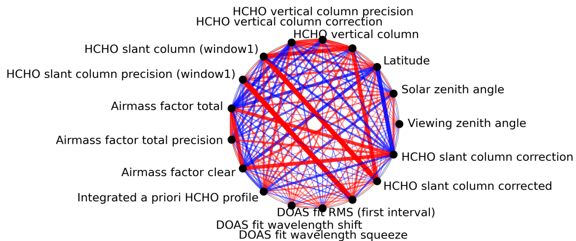
Figure 1: Map of correlation graph for 2023-11-23 to 2023-11-25.
