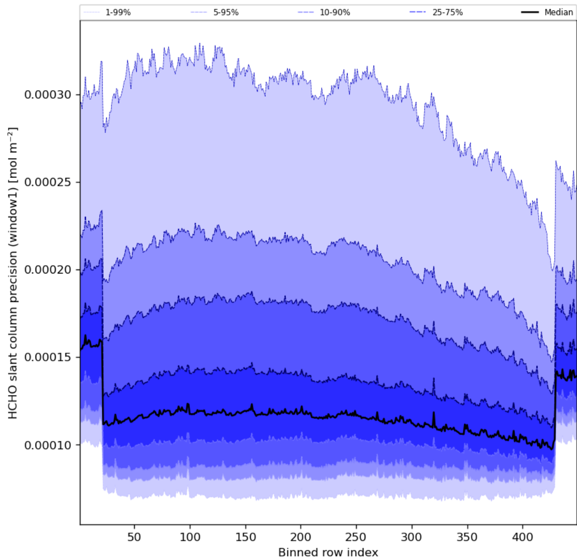
Figure 53: Along track statistics of “HCHO slant column precision (window1)” for 2023-11-23 to 2023-11-25
