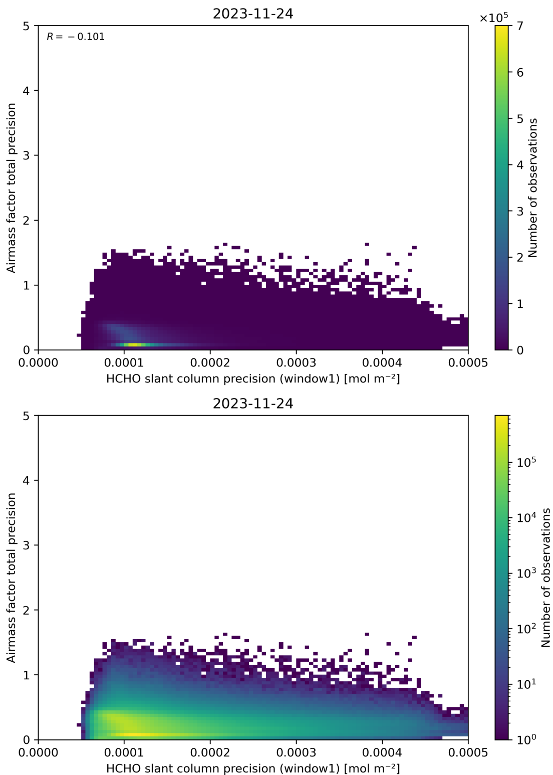
Figure 95: Scatter density plot of “HCHO slant column precision (window1)” against “Airmass factor total precision” for 2023-11-23 to 2023-11-25.
