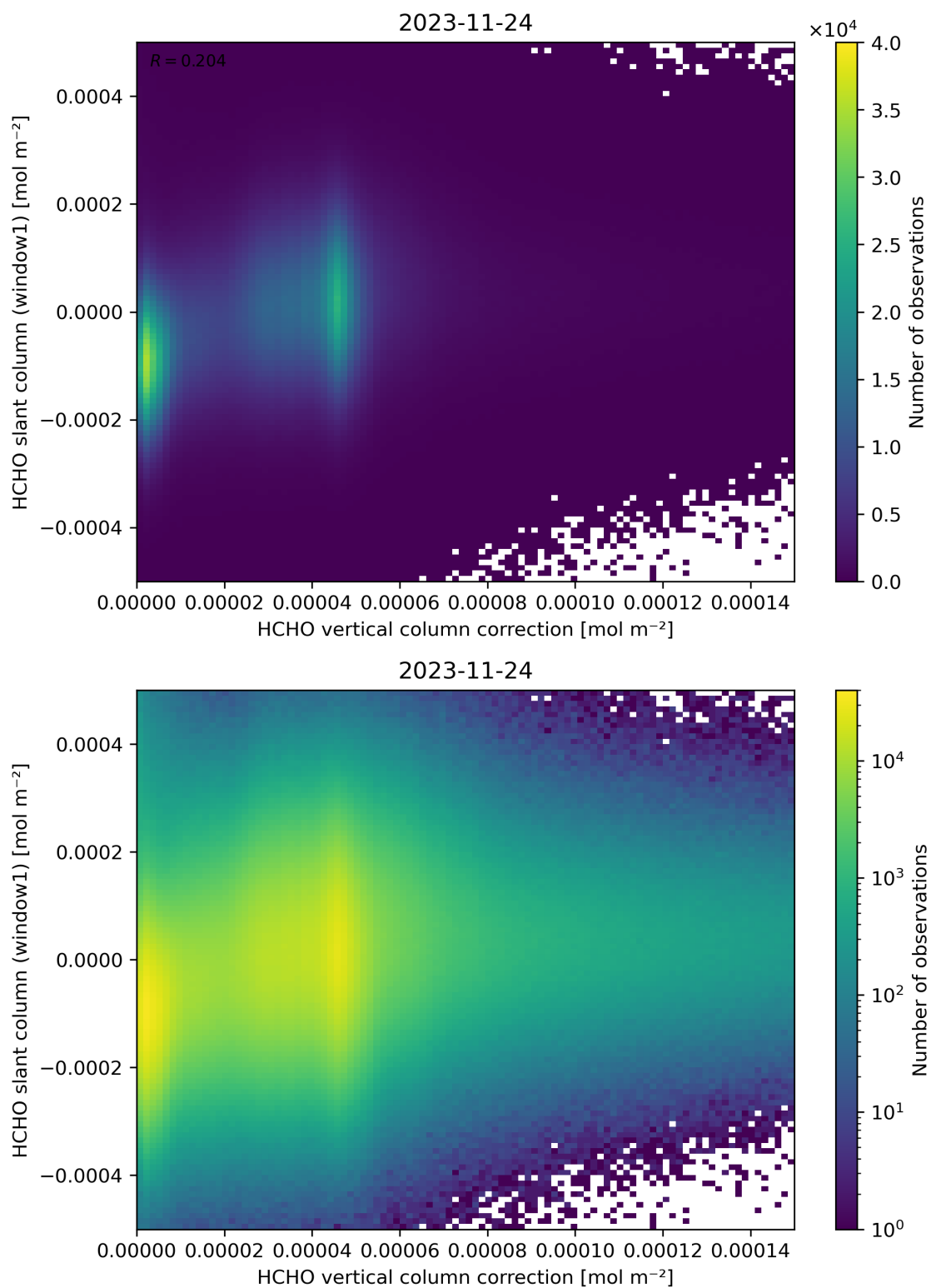
Figure 118: Scatter density plot of “HCHO vertical column correction” against “HCHO slant column (window1)” for 2023-11-23 to 2023-11-25.
