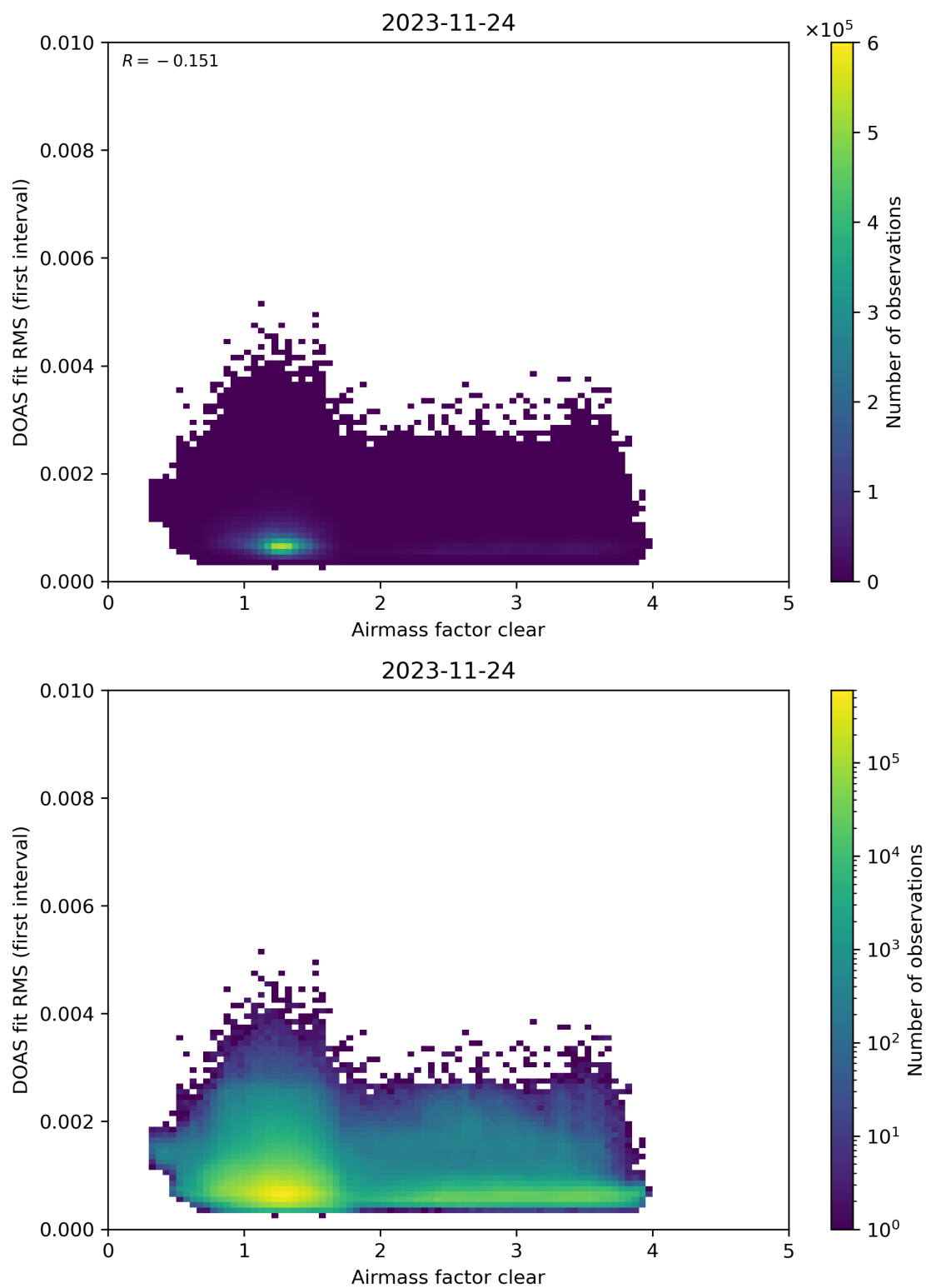
Figure 71: Scatter density plot of “Airmass factor clear” against “DOAS fit RMS (first interval)” for 2023-11-23 to 2023-11-25.
