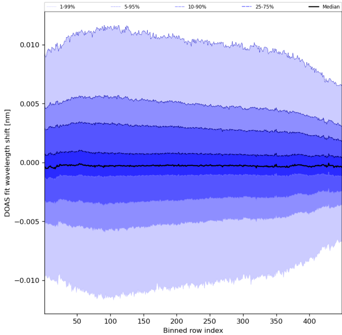
Figure 58: Along track statistics of “DOAS fit wavelength shift” for 2023-11-23 to 2023-11-25
