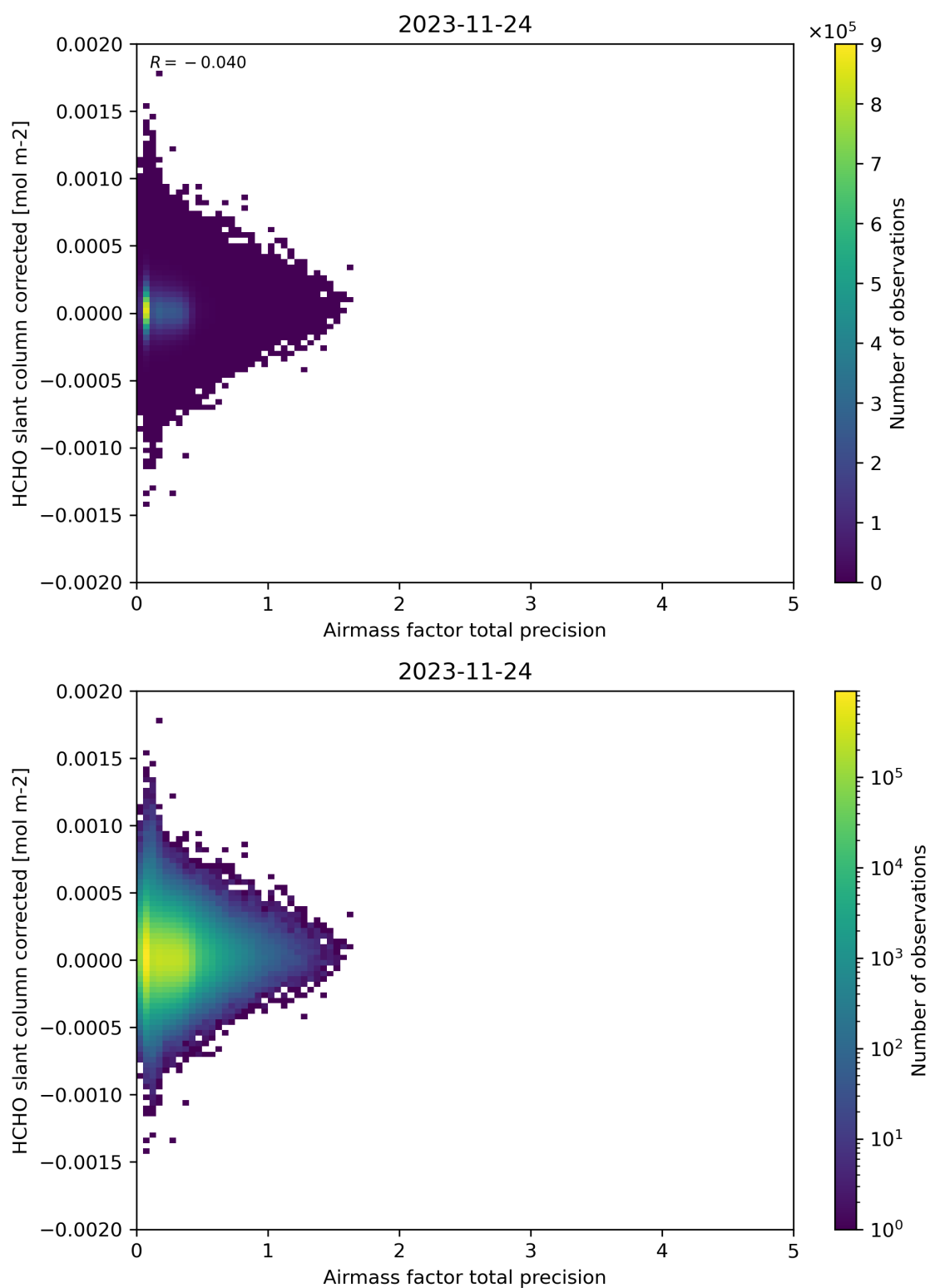
Figure 109: Scatter density plot of “Airmass factor total precision” against “HCHO slant column corrected” for 2023-11-23 to 2023-11-25.
