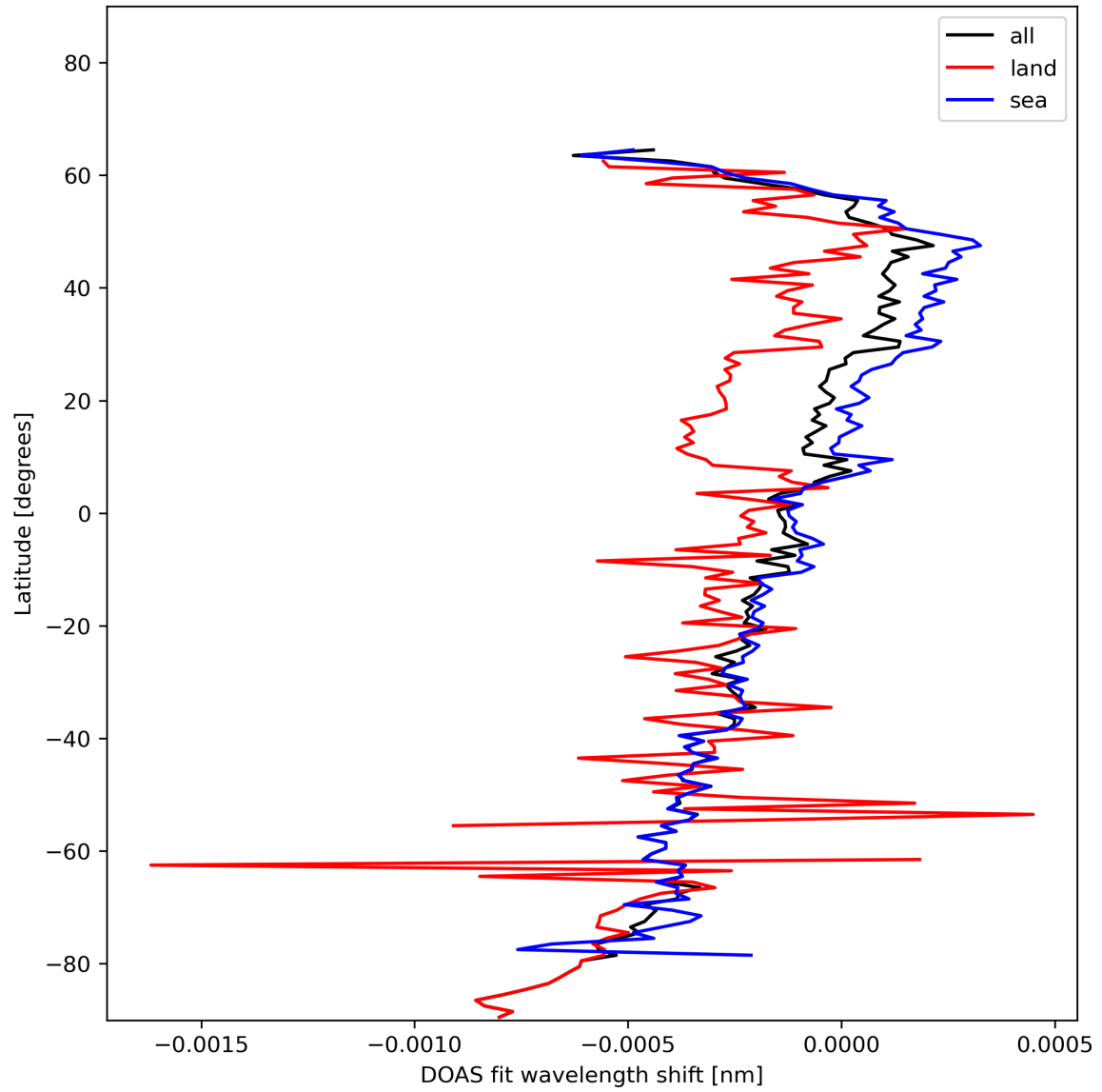
Figure 30: Zonal average of “DOAS fit wavelength shift” for 2023-11-23 to 2023-11-25.
