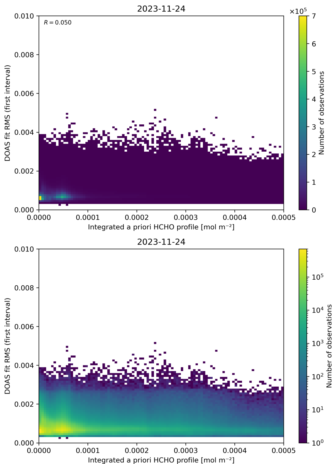
Figure 148: Scatter density plot of “Integrated a priori HCHO profile” against “DOAS fit RMS (first interval)” for 2023-11-23 to 2023-11-25.
