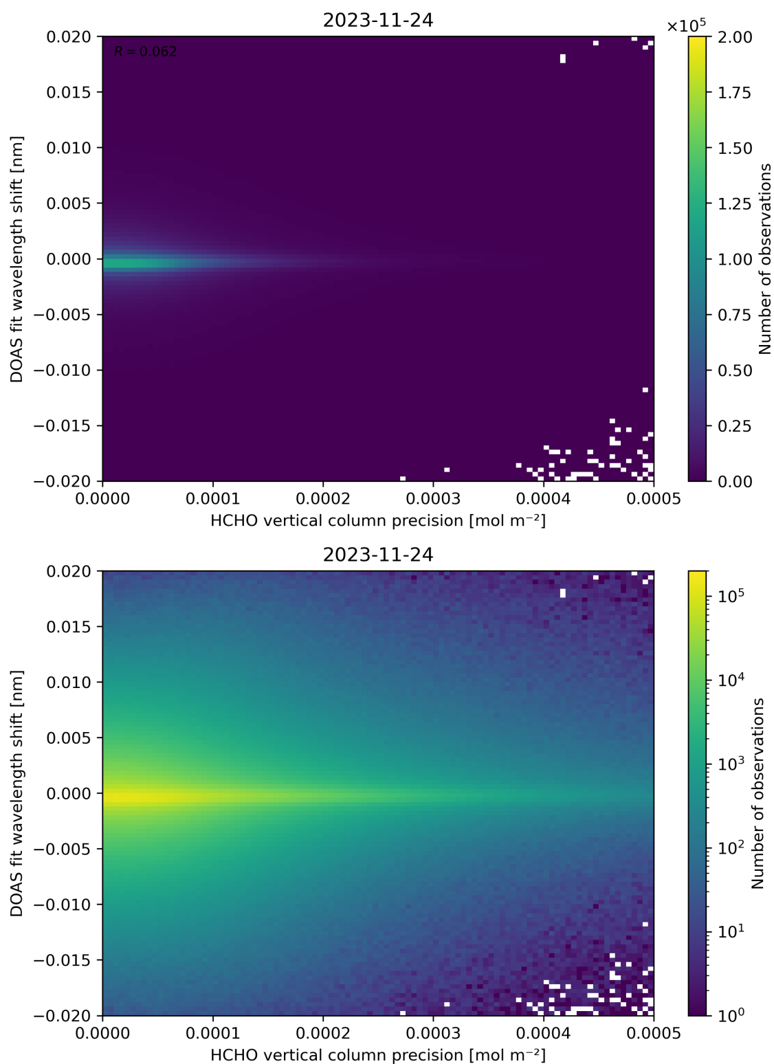
Figure 137: Scatter density plot of “HCHO vertical column precision” against “DOAS fit wavelength shift” for 2023-11-23 to 2023-11-25.
