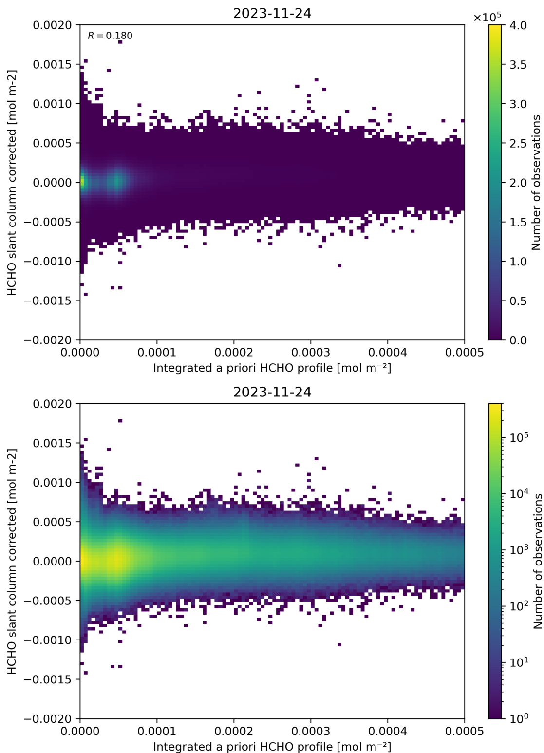
Figure 151: Scatter density plot of “Integrated a priori HCHO profile” against “HCHO slant column corrected” for 2023-11-23 to 2023-11-25.
