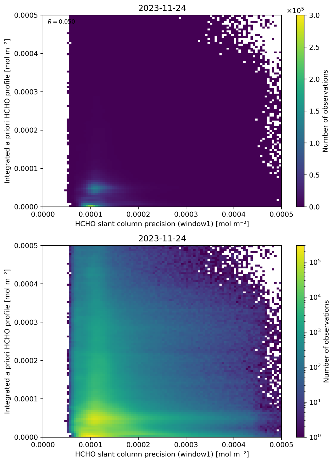
Figure 96: Scatter density plot of “HCHO slant column precision (window1)” against “Integrated a priori HCHO profile” for 2023-11-23 to 2023-11-25.
