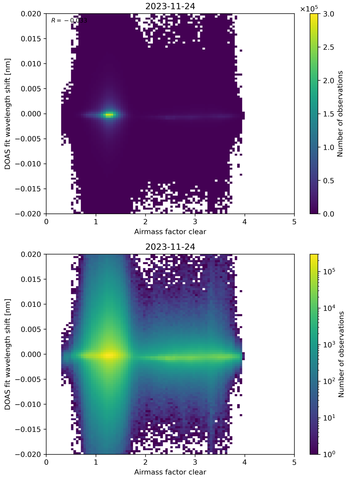
Figure 72: Scatter density plot of “Airmass factor clear” against “DOAS fit wavelength shift” for 2023-11-23 to 2023-11-25.
