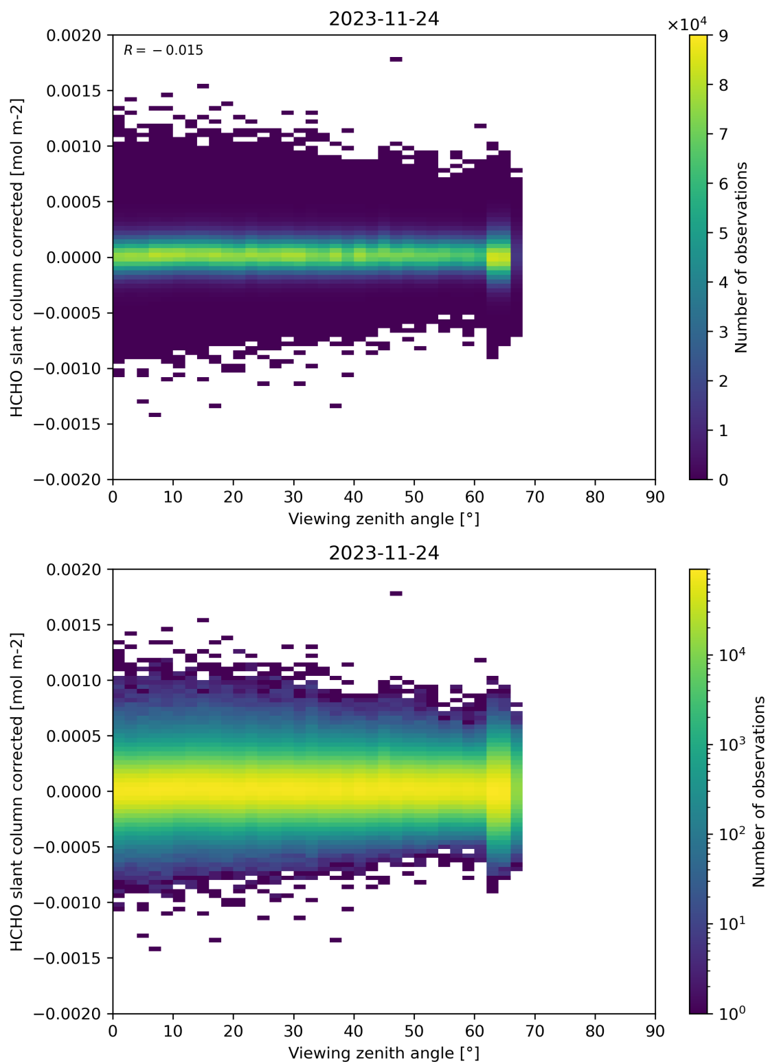
Figure 186: Scatter density plot of “Viewing zenith angle” against “HCHO slant column corrected” for 2023-11-23 to 2023-11-25.
