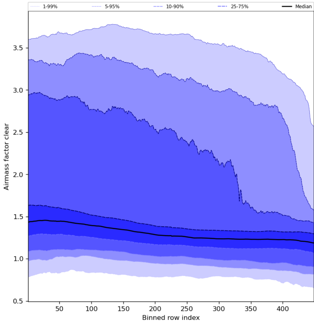
Figure 56: Along track statistics of “Airmass factor clear” for 2023-11-23 to 2023-11-25
