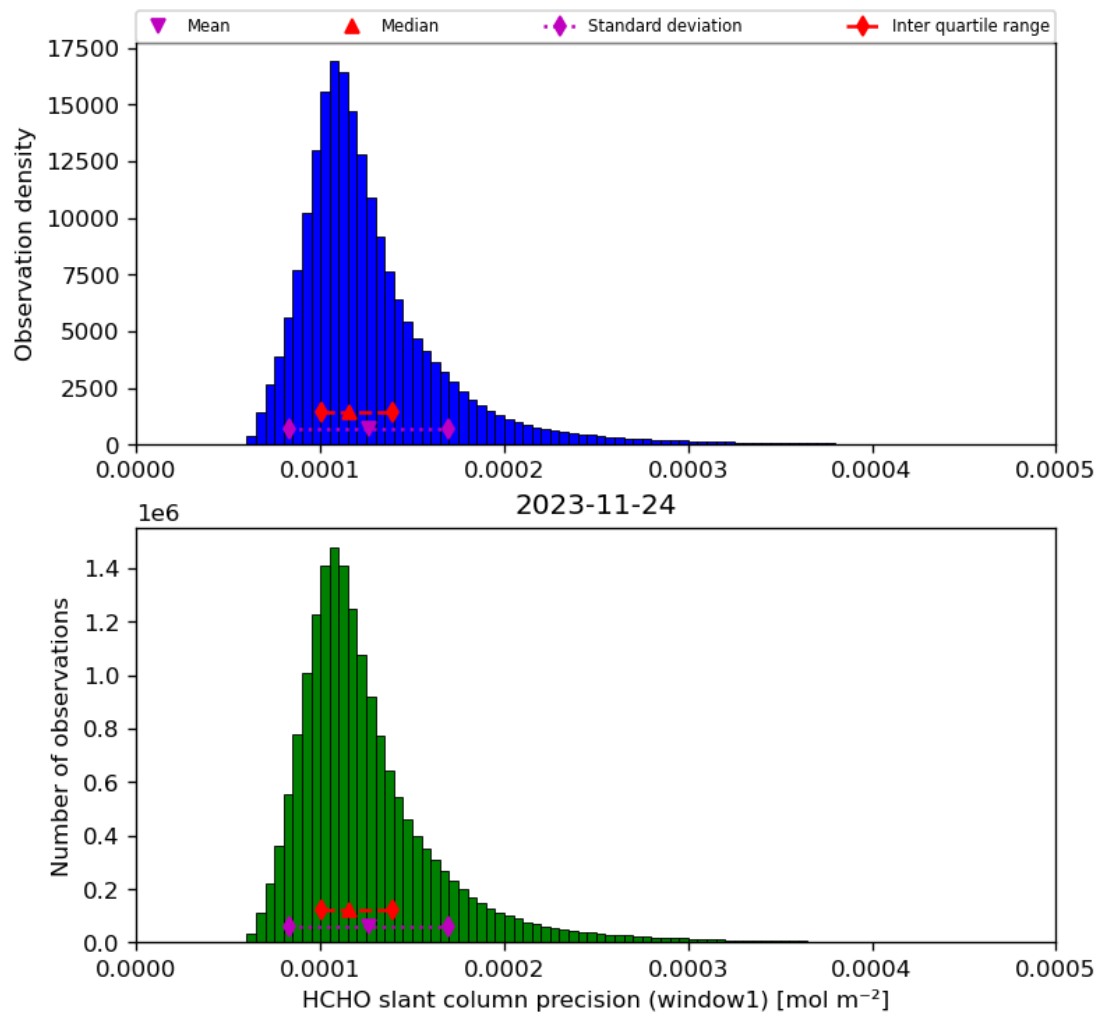
Figure 39: Histogram of “HCHO slant column precision (window1)” for 2023-11-23 to 2023-11-25
