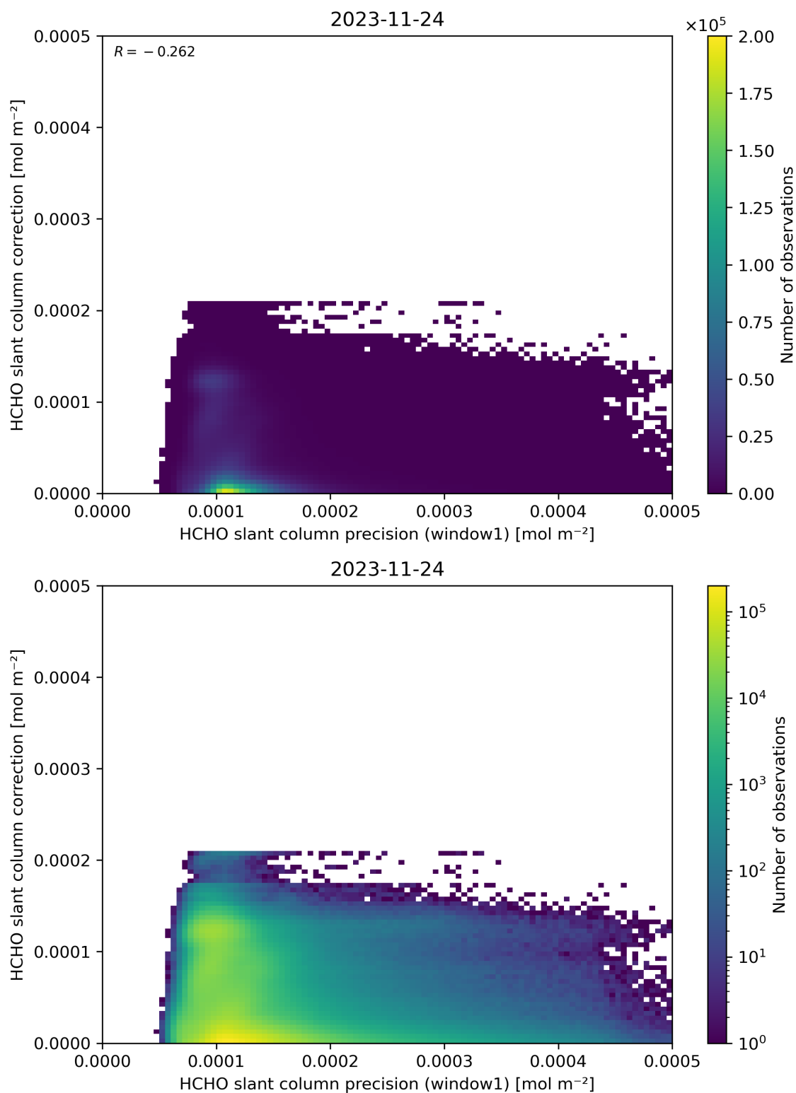
Figure 93: Scatter density plot of “HCHO slant column precision (window1)” against “HCHO slant column correction” for 2023-11-23 to 2023-11-25.
