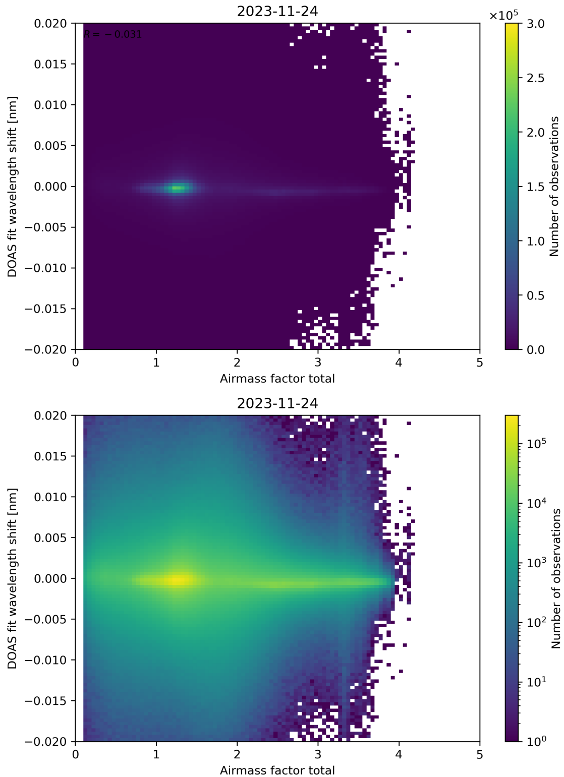
Figure 98: Scatter density plot of “Airmass factor total” against “DOAS fit wavelength shift” for 2023-11-23 to 2023-11-25.
