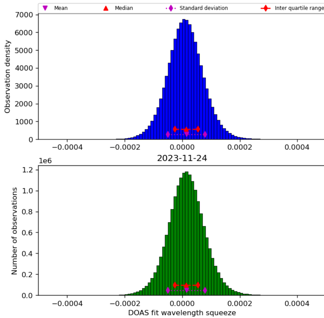
Figure 45: Histogram of “DOAS fit wavelength squeeze” for 2023-11-23 to 2023-11-25
