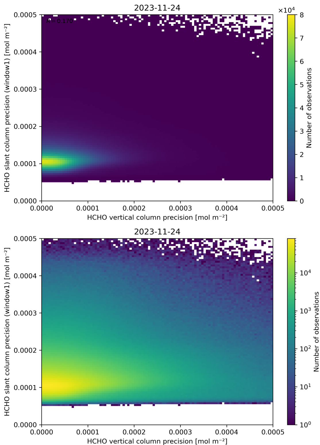
Figure 143: Scatter density plot of “HCHO vertical column precision” against “HCHO slant column precision (window1)” for 2023-11-23 to 2023-11-25.
