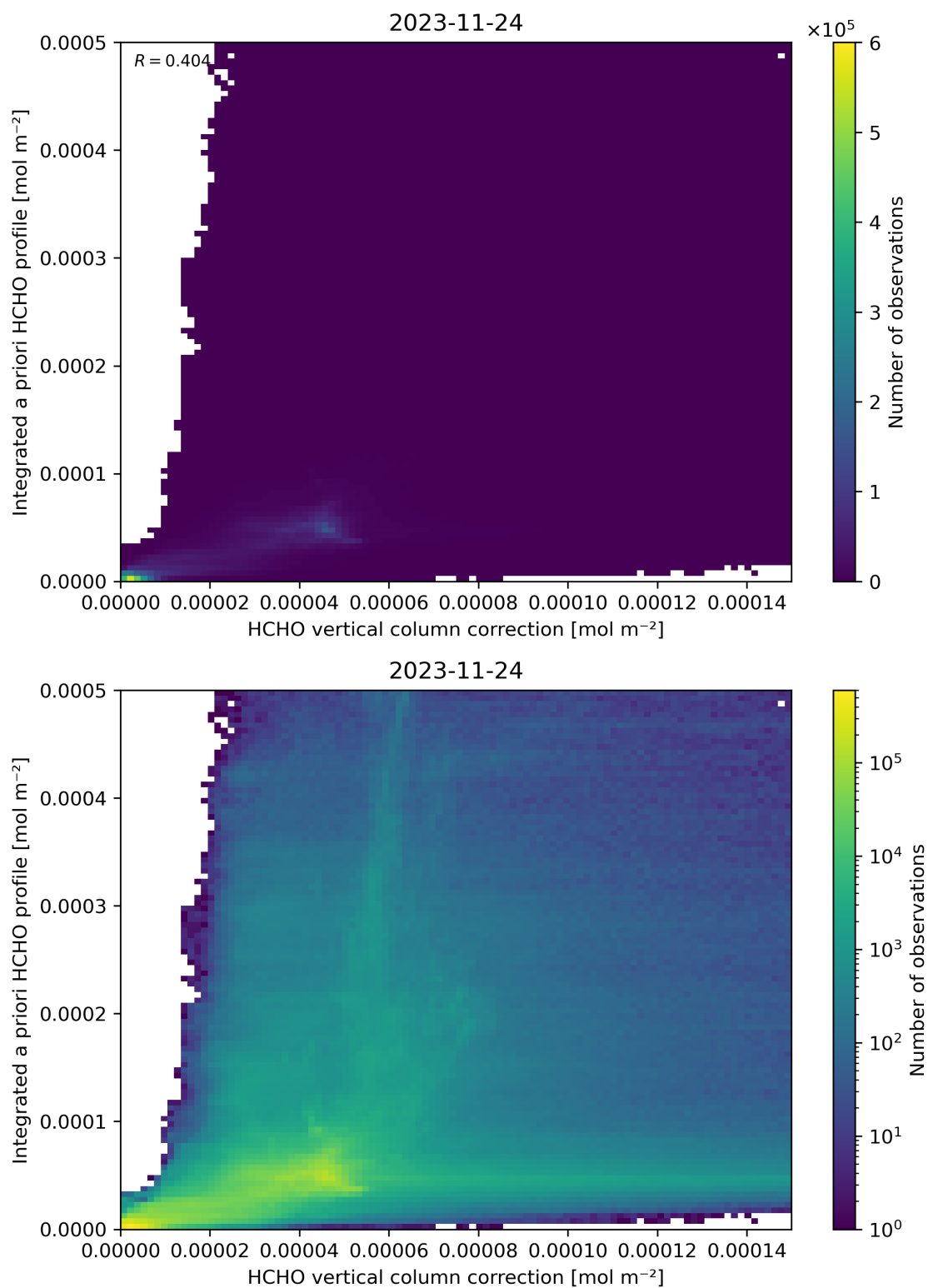
Figure 122: Scatter density plot of “HCHO vertical column correction” against “Integrated a priori HCHO profile” for 2023-11-23 to 2023-11-25.
