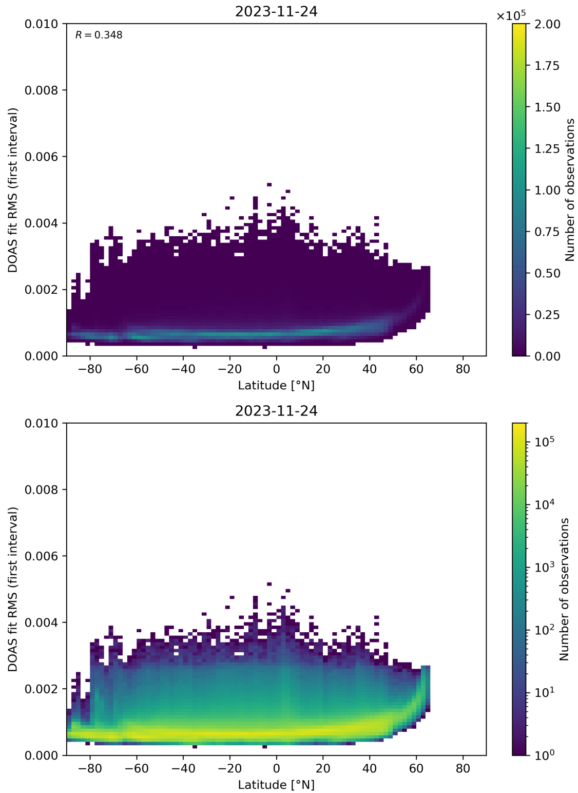
Figure 153: Scatter density plot of “Latitude” against “DOAS fit RMS (first interval)” for 2023-11-23 to 2023-11-25.
