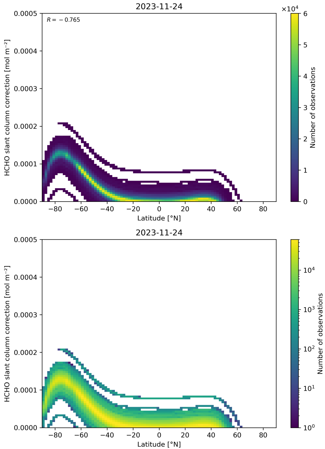
Figure 158: Scatter density plot of “Latitude” against “HCHO slant column correction” for 2023-11-23 to 2023-11-25.
