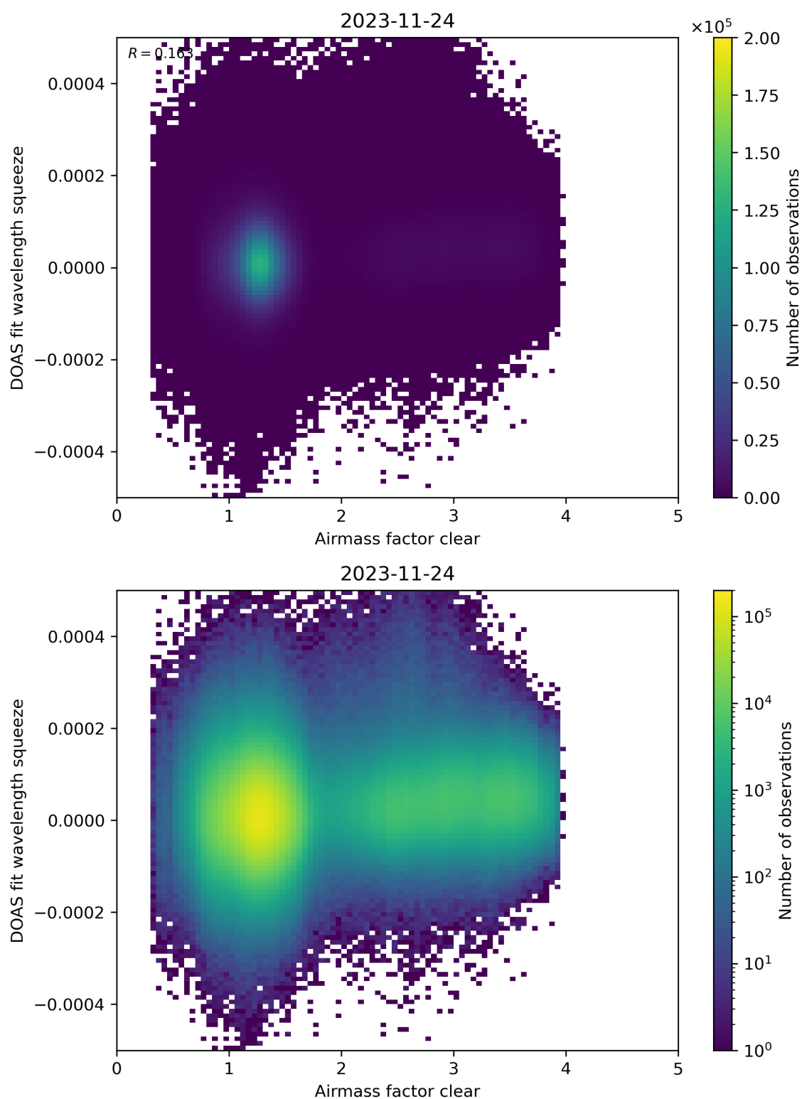
Figure 73: Scatter density plot of “Airmass factor clear” against “DOAS fit wavelength squeeze” for 2023-11-23 to 2023-11-25.
