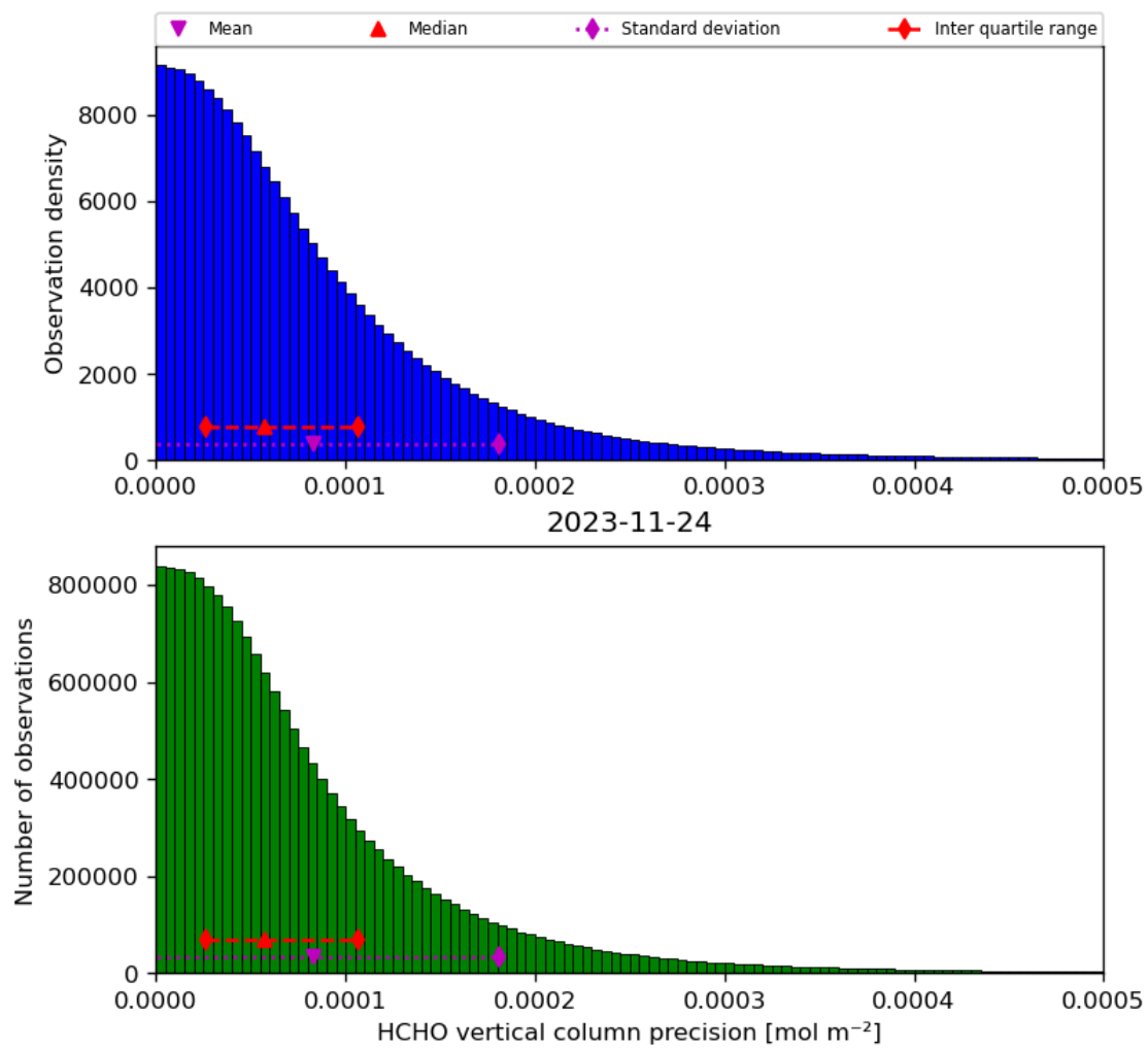
Figure 36: Histogram of “HCHO vertical column precision” for 2023-11-23 to 2023-11-25
