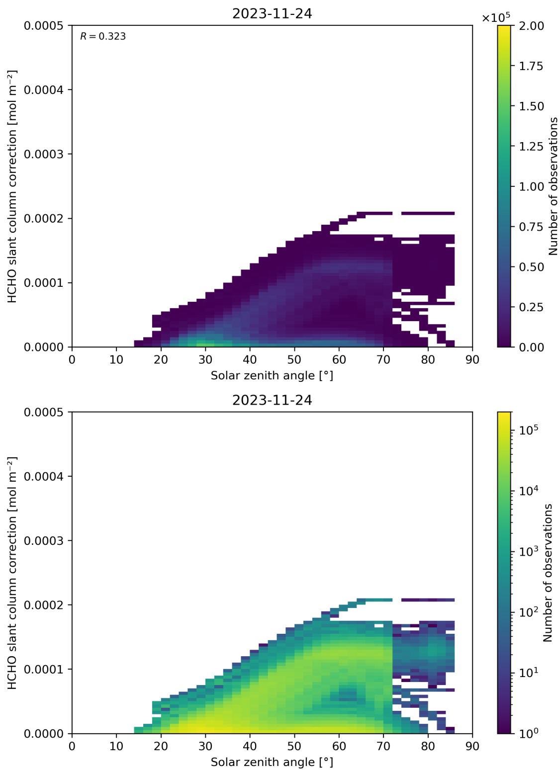
Figure 172: Scatter density plot of “Solar zenith angle” against “HCHO slant column correction” for 2023-11-23 to 2023-11-25.
