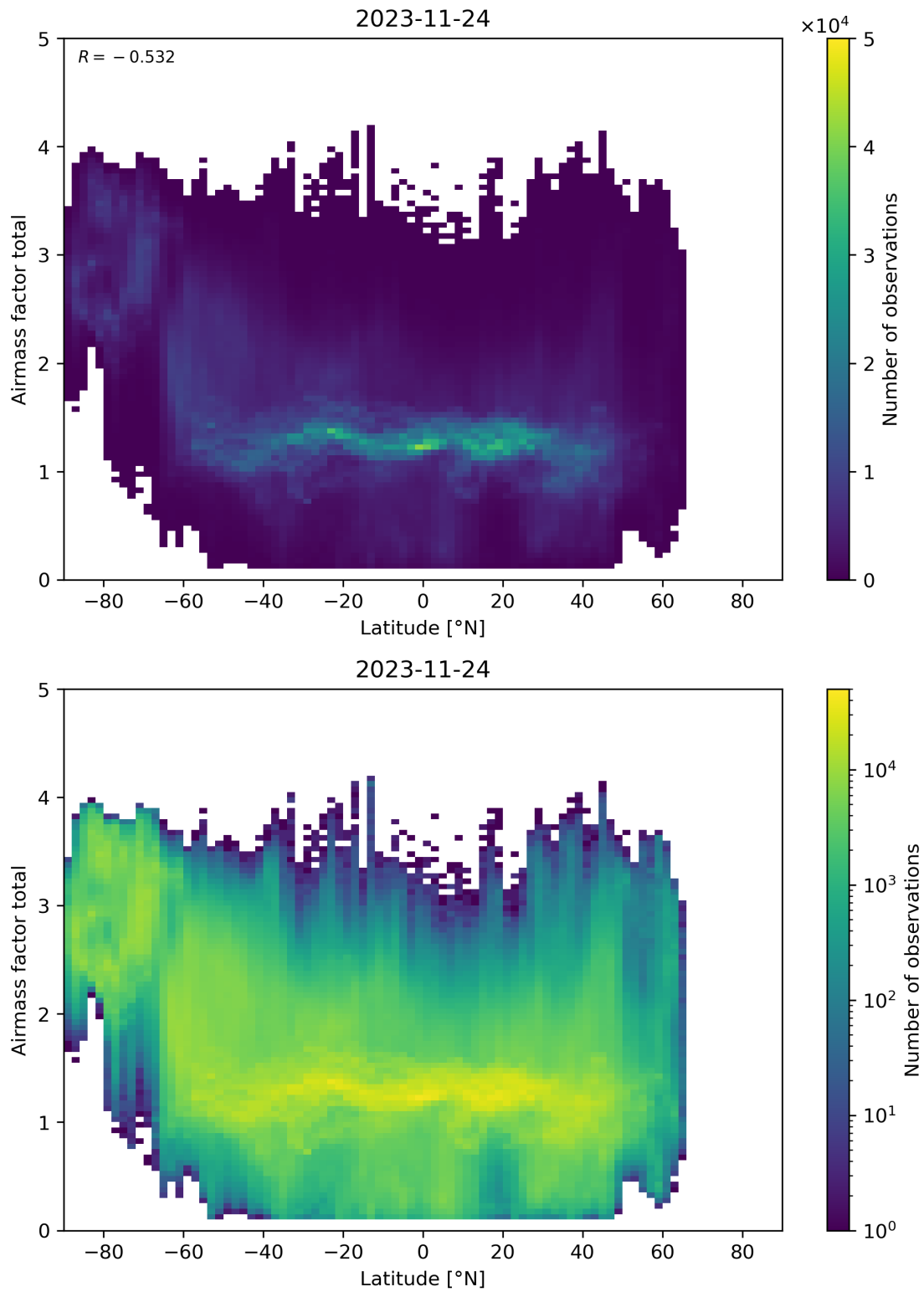
Figure 161: Scatter density plot of “Latitude” against “Airmass factor total” for 2023-11-23 to 2023-11-25.
