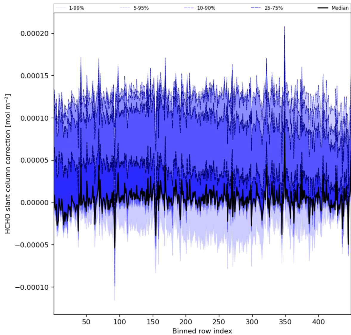
Figure 61: Along track statistics of “HCHO slant column correction” for 2023-11-23 to 2023-11-25
