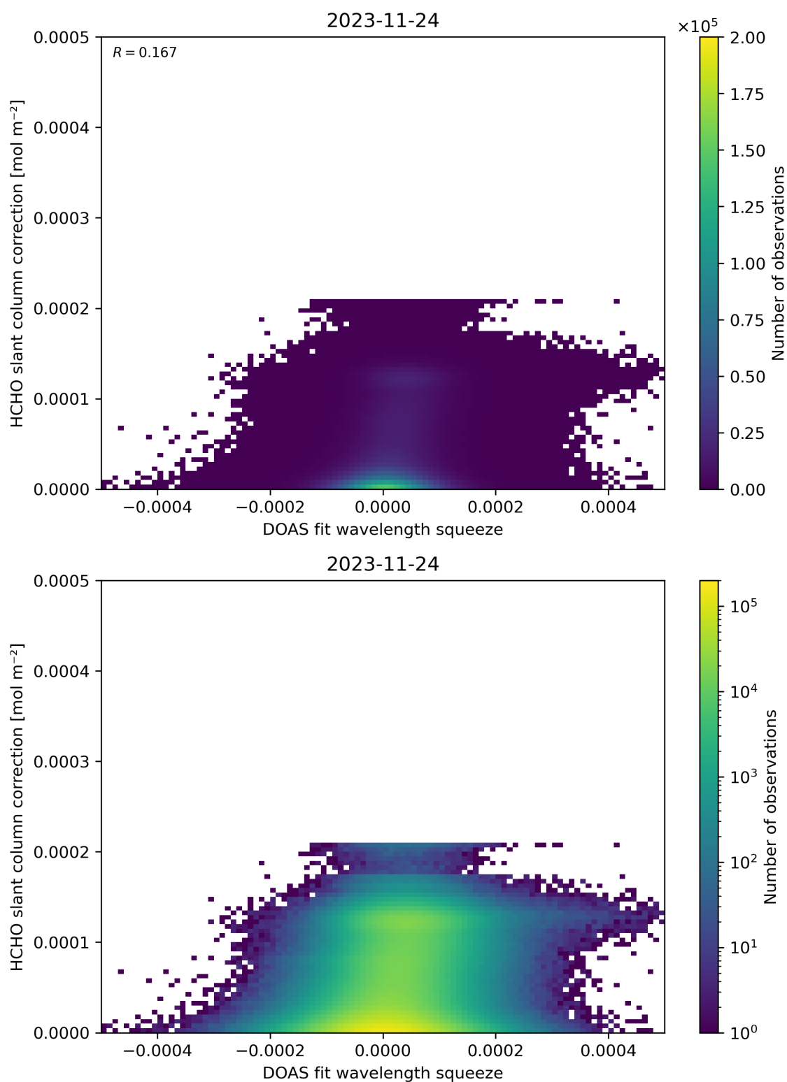
Figure 70: Scatter density plot of “DOAS fit wavelength squeeze” against “HCHO slant column correction” for 2023-11-23 to 2023-11-25.
