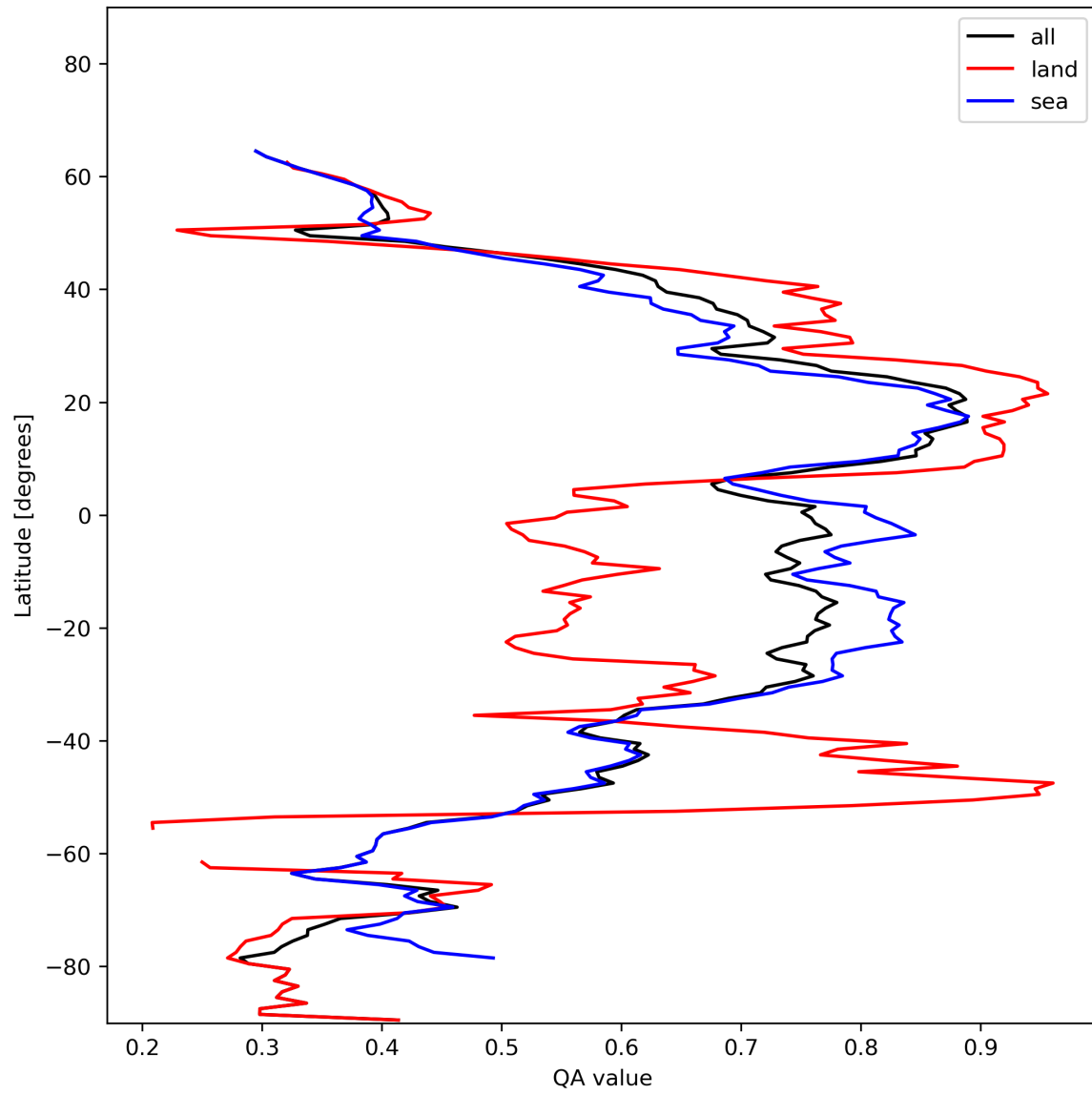
Figure 20: Zonal average of “QA value” for 2023-11-23 to 2023-11-25.
