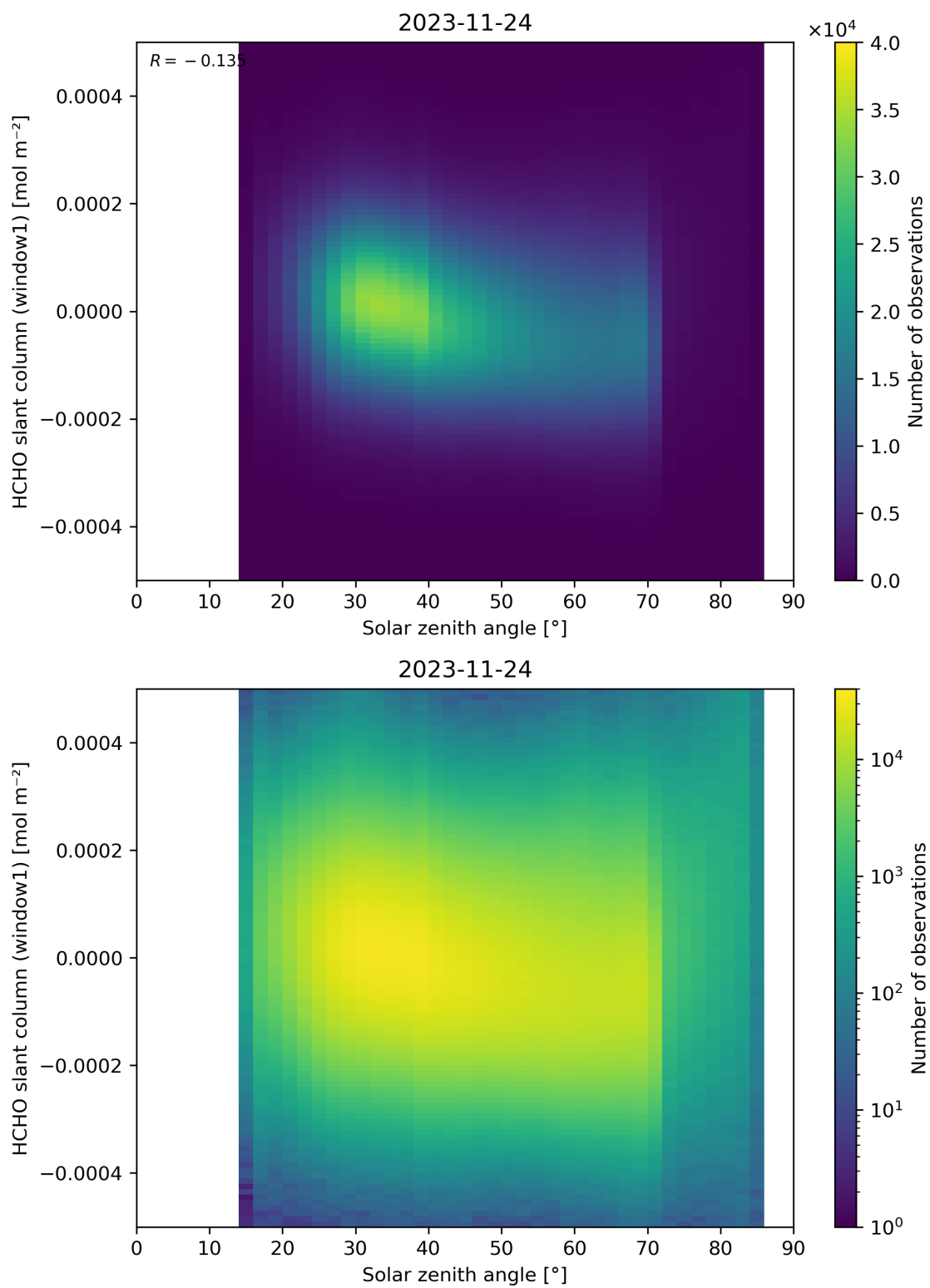
Figure 173: Scatter density plot of “Solar zenith angle” against “HCHO slant column (window1)” for 2023-11-23 to 2023-11-25.
