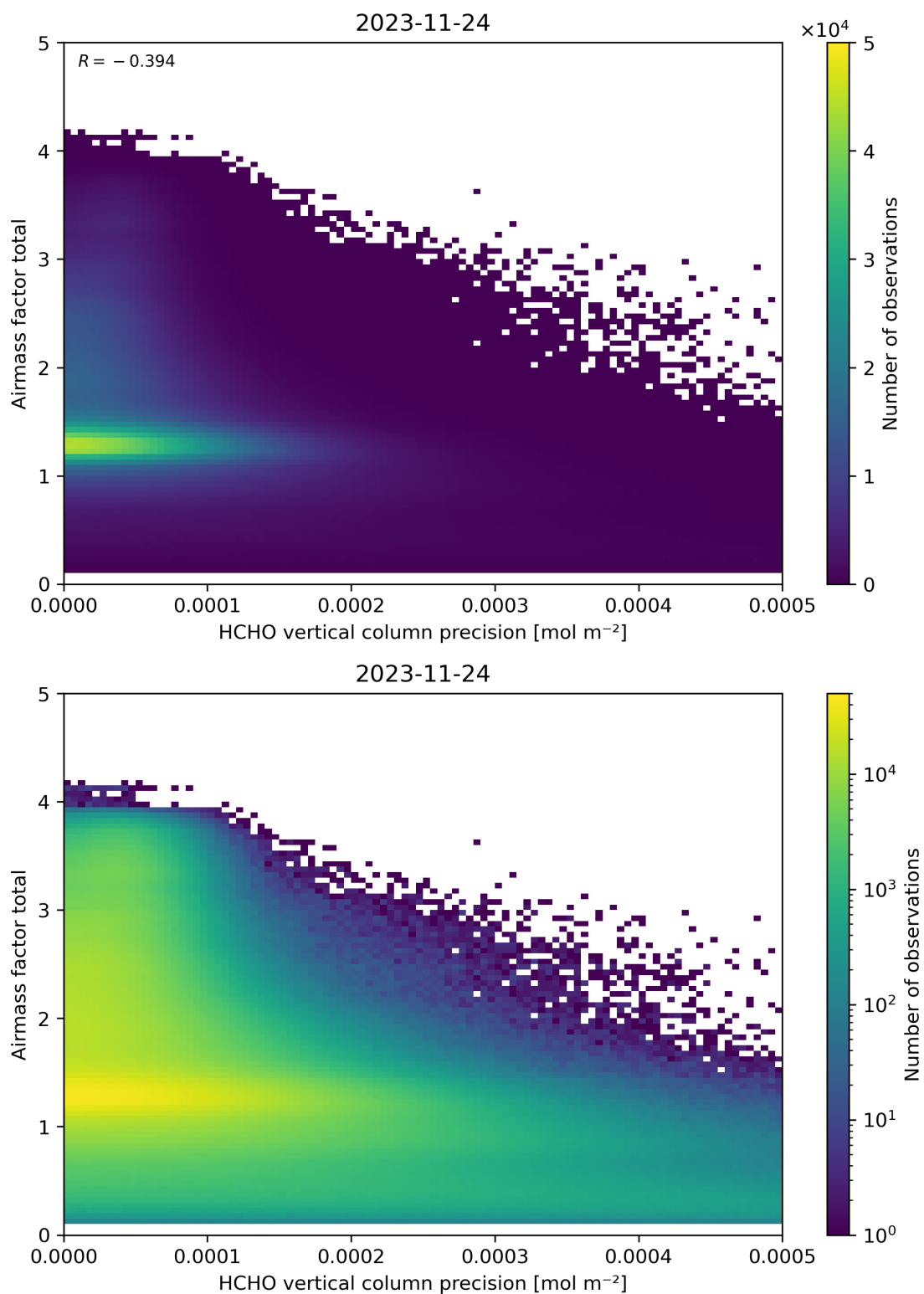
Figure 144: Scatter density plot of “HCHO vertical column precision” against “Airmass factor total” for 2023-11-23 to 2023-11-25.
