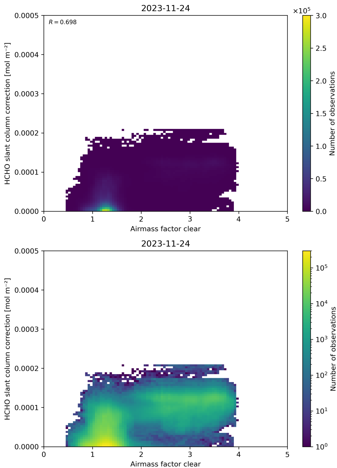
Figure 75: Scatter density plot of “Airmass factor clear” against “HCHO slant column correction” for 2023-11-23 to 2023-11-25.
