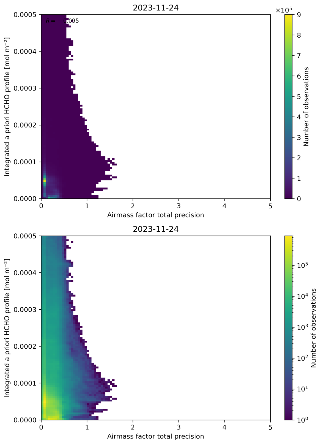
Figure 111: Scatter density plot of “Airmass factor total precision” against “Integrated a priori HCHO profile” for 2023-11-23 to 2023-11-25.
