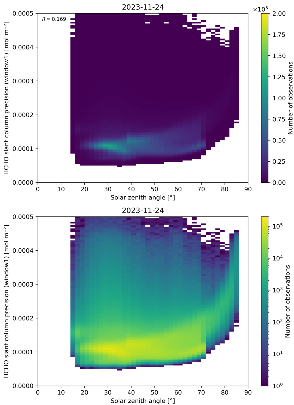
Figure 174: Scatter density plot of “Solar zenith angle” against “HCHO slant column precision (window1)” for 2023-11-23 to 2023-11-25.
