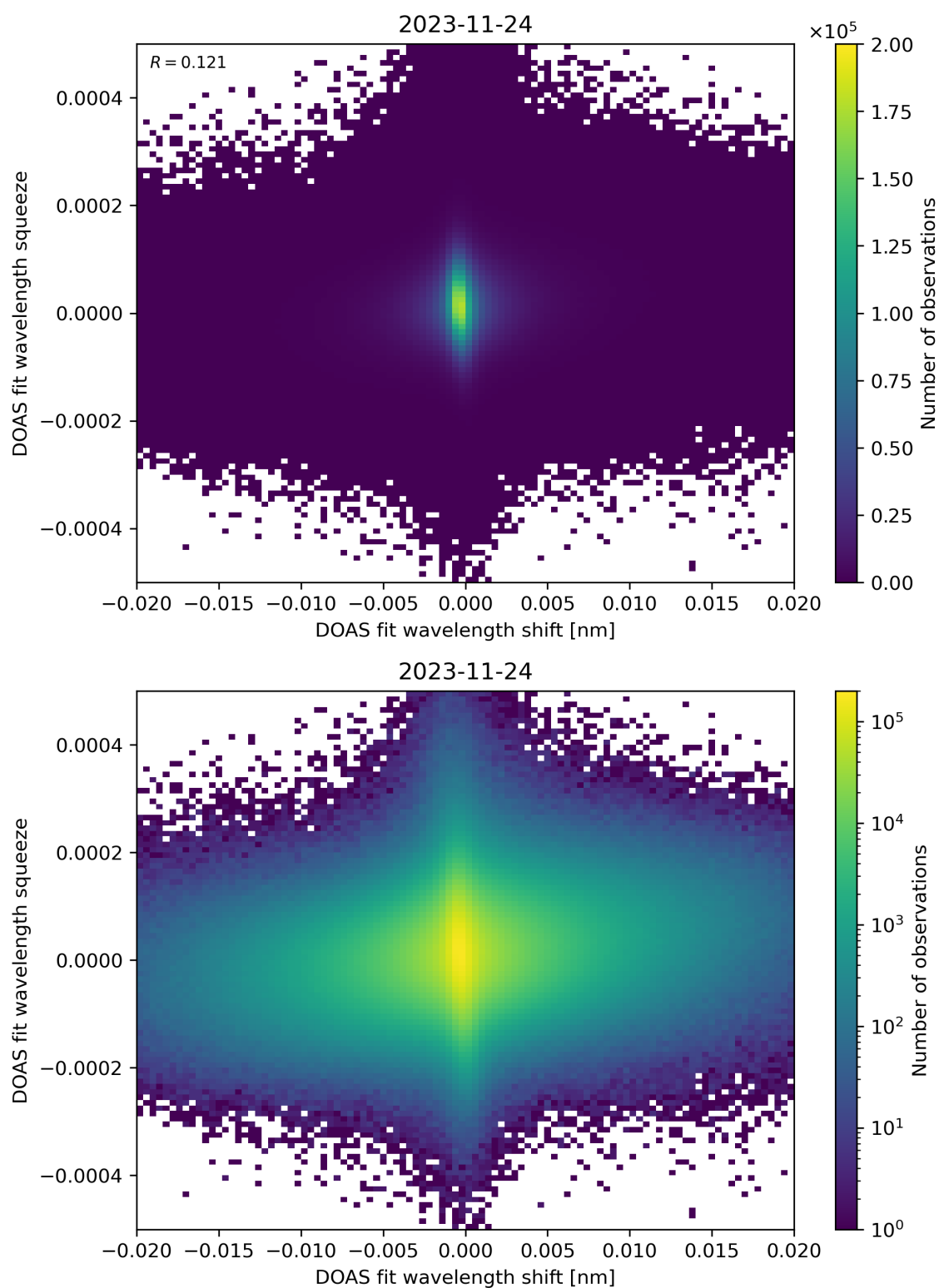
Figure 65: Scatter density plot of “DOAS fit wavelength shift” against “DOAS fit wavelength squeeze” for 2023-11-23 to 2023-11-25.
