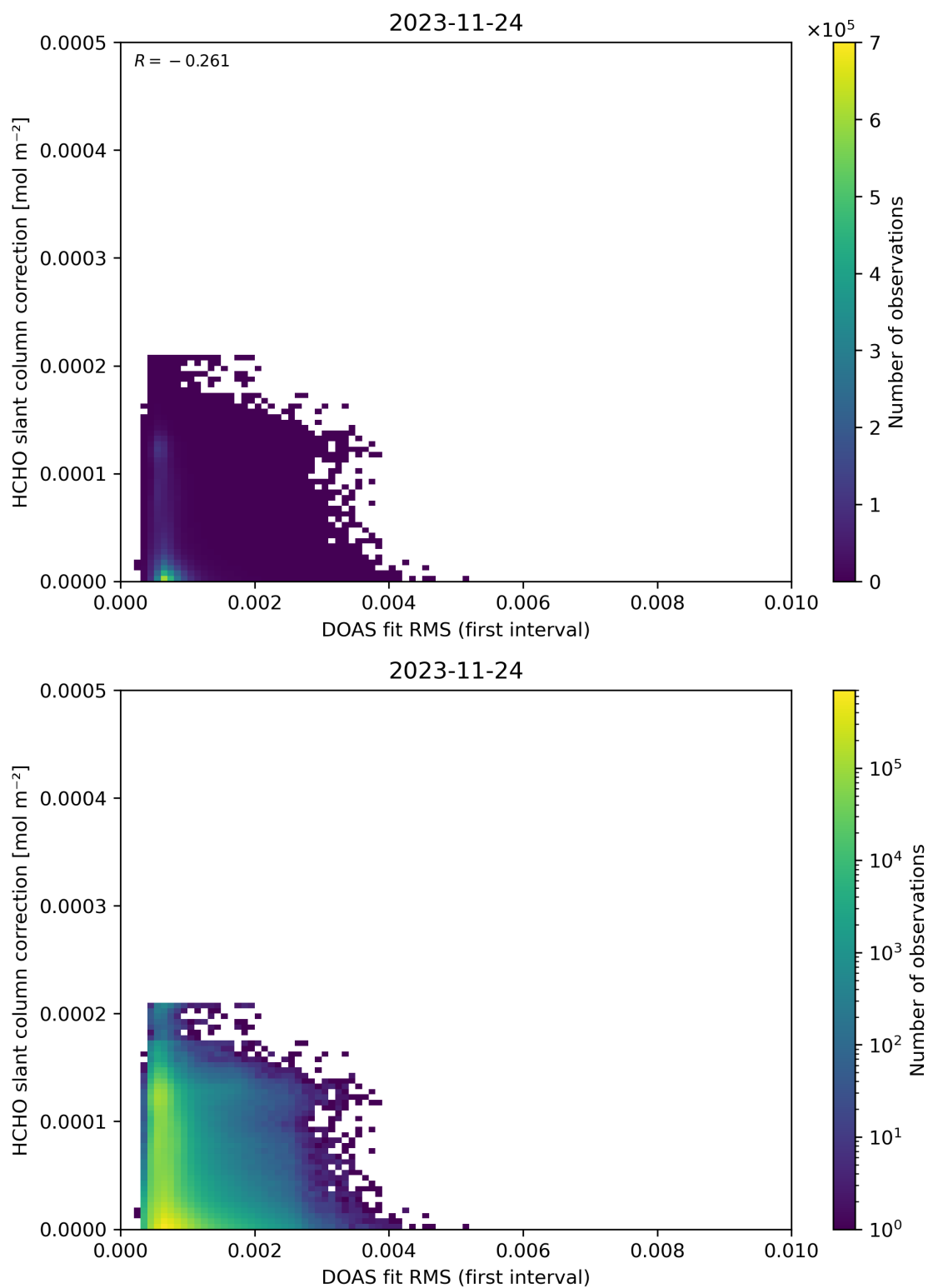
Figure 63: Scatter density plot of “DOAS fit RMS (first interval)” against “HCHO slant column correction” for 2023-11-23 to 2023-11-25.
