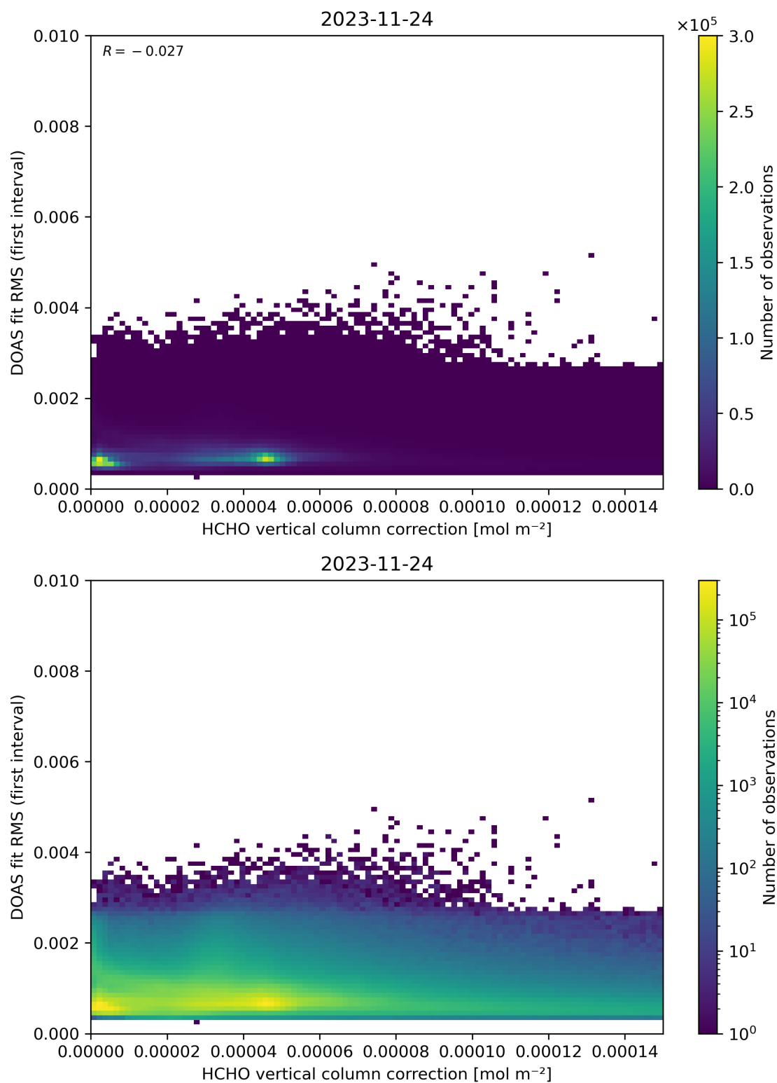
Figure 112: Scatter density plot of “HCHO vertical column correction” against “DOAS fit RMS (first interval)” for 2023-11-23 to 2023-11-25.
