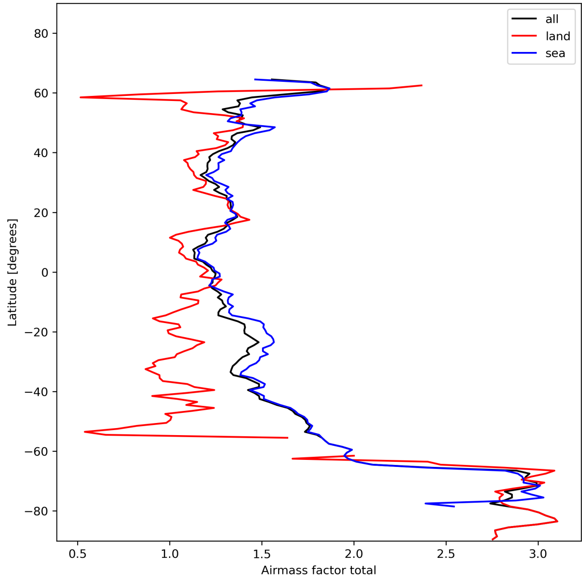
Figure 26: Zonal average of “Airmass factor total” for 2023-11-23 to 2023-11-25.
