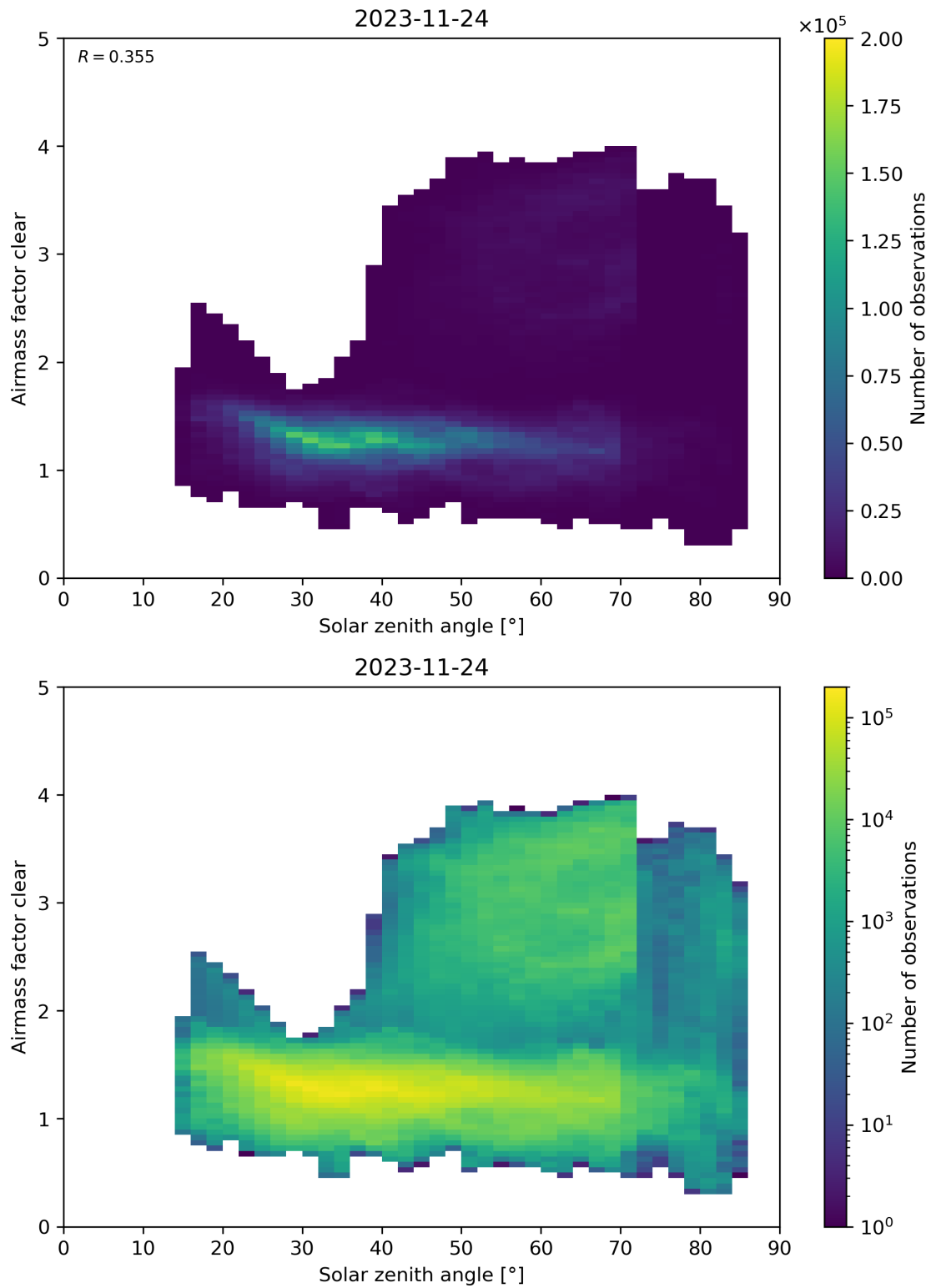
Figure 170: Scatter density plot of “Solar zenith angle” against “Airmass factor clear” for 2023-11-23 to 2023-11-25.
