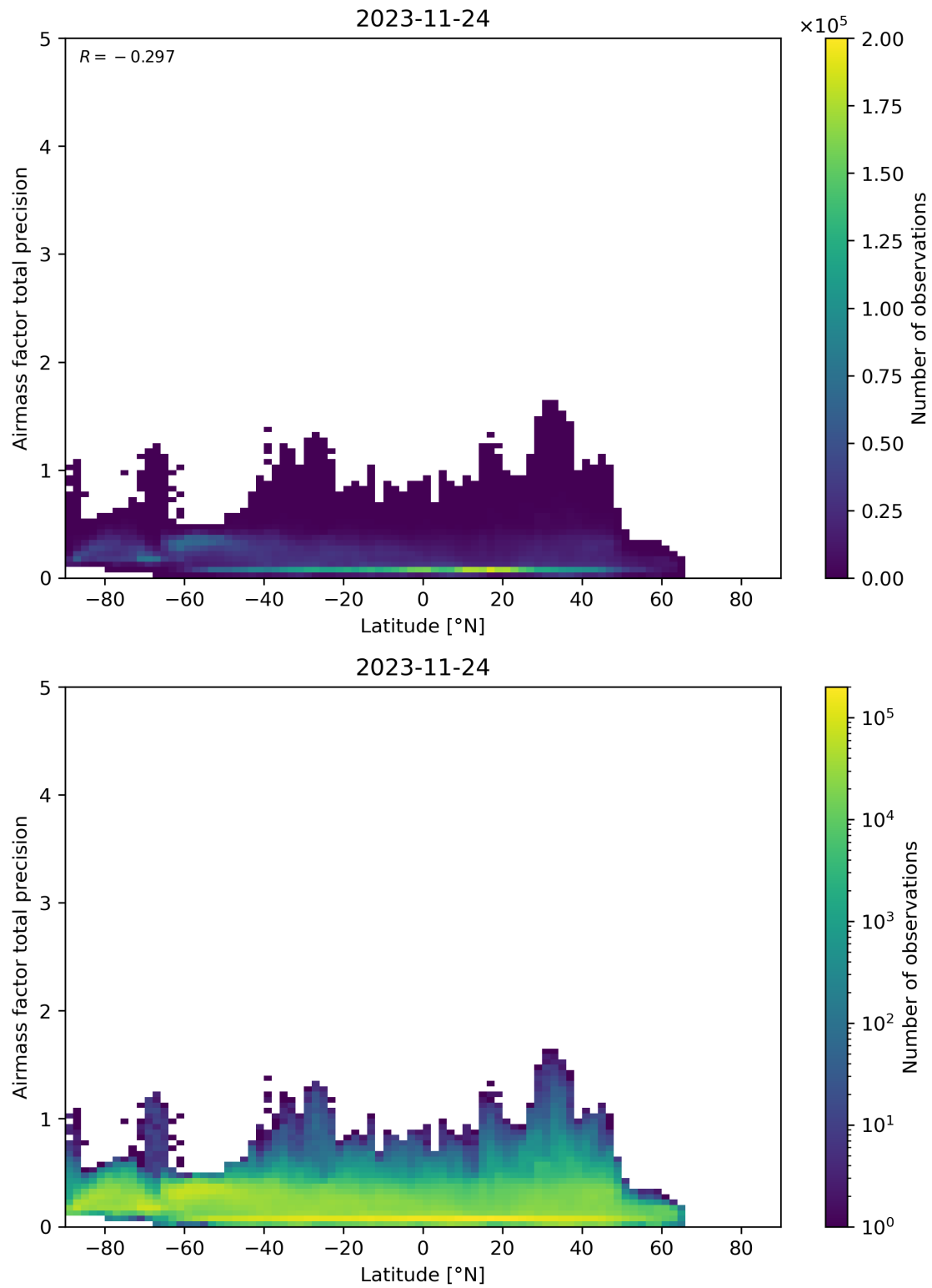
Figure 162: Scatter density plot of “Latitude” against “Airmass factor total precision” for 2023-11-23 to 2023-11-25.
