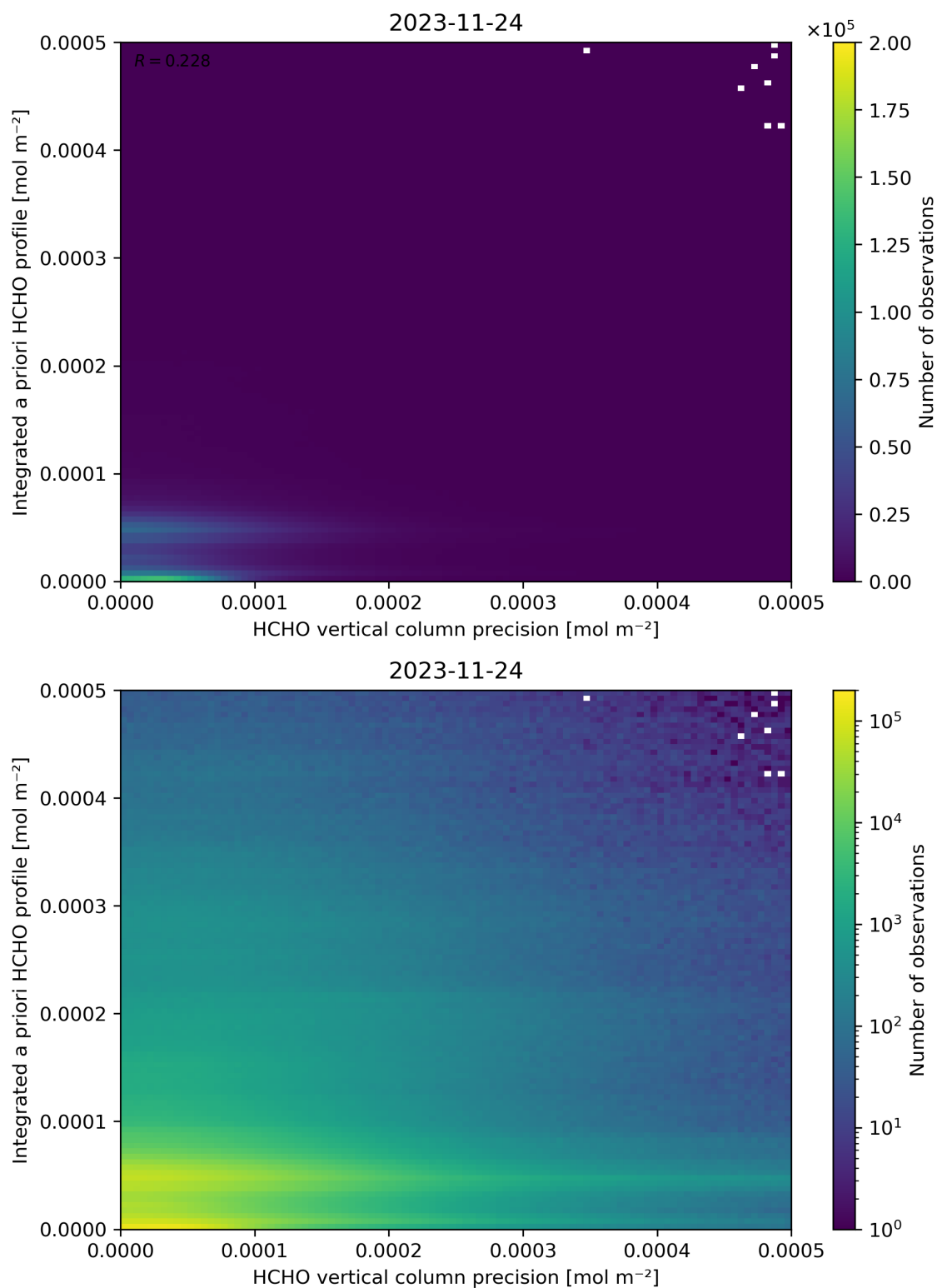
Figure 147: Scatter density plot of “HCHO vertical column precision” against “Integrated a priori HCHO profile” for 2023-11-23 to 2023-11-25.
