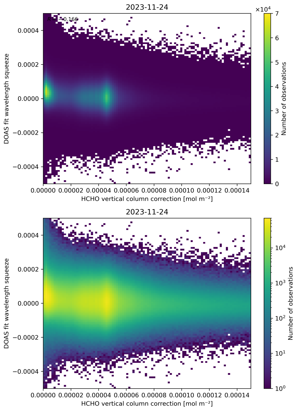
Figure 114: Scatter density plot of “HCHO vertical column correction” against “DOAS fit wavelength squeeze” for 2023-11-23 to 2023-11-25.
