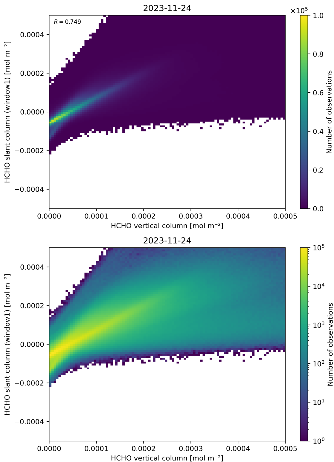
Figure 129: Scatter density plot of “HCHO vertical column” against “HCHO slant column (window1)” for 2023-11-23 to 2023-11-25.
