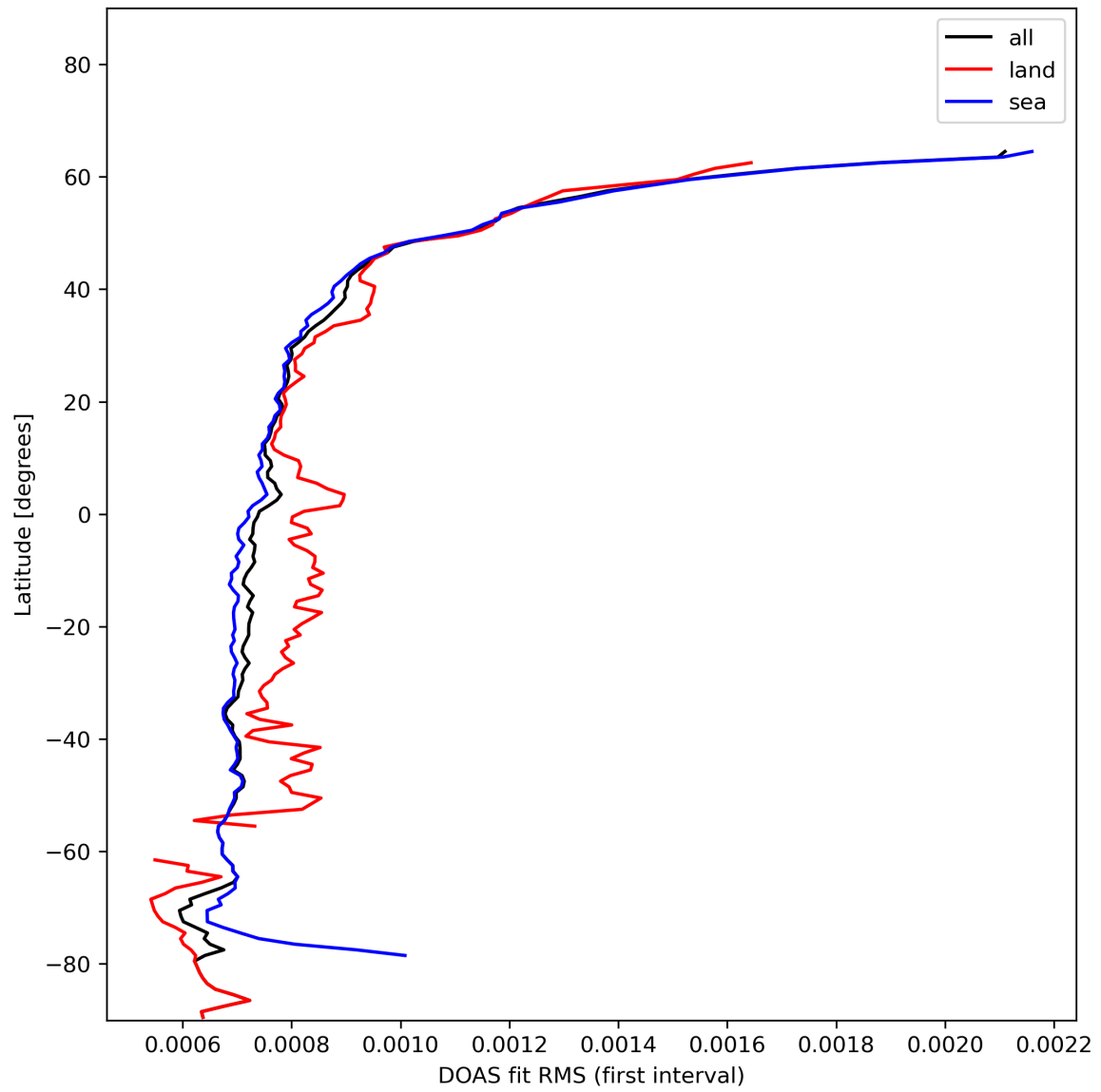
Figure 32: Zonal average of “DOAS fit RMS (first interval)” for 2023-11-23 to 2023-11-25.
