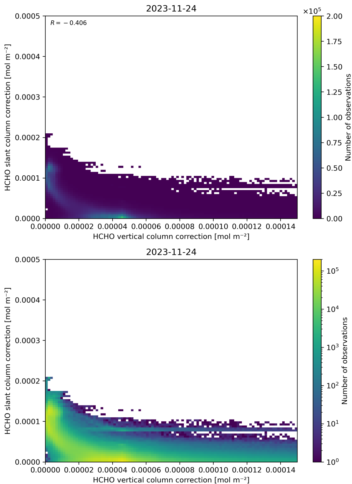
Figure 117: Scatter density plot of “HCHO vertical column correction” against “HCHO slant column correction” for 2023-11-23 to 2023-11-25.
