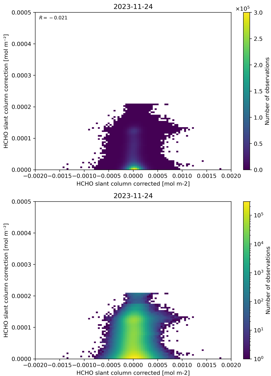
Figure 77: Scatter density plot of “HCHO slant column corrected” against “HCHO slant column correction” for 2023-11-23 to 2023-11-25.
