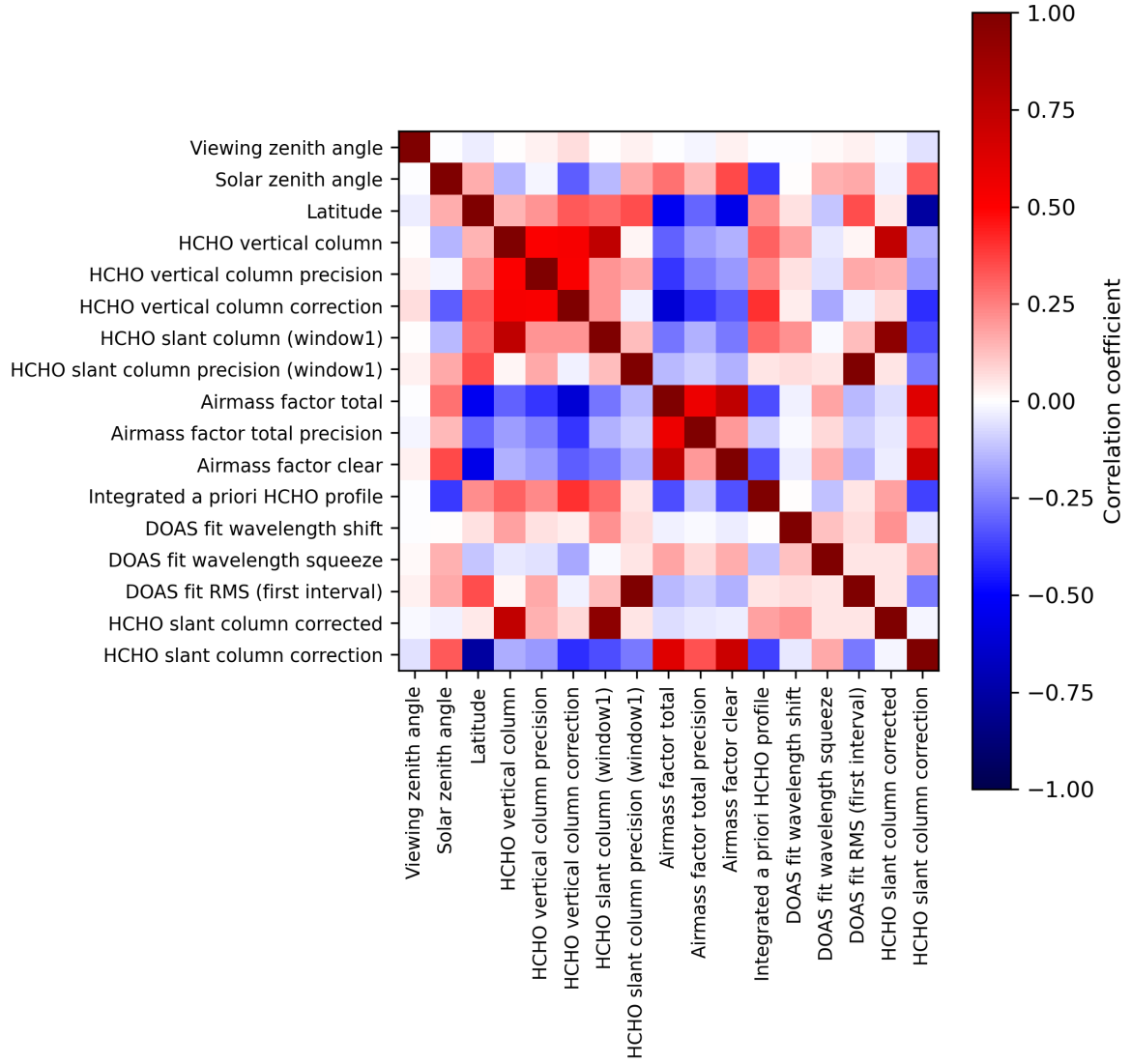
Figure 2: Map of correlation matrix for 2023-11-23 to 2023-11-25.
