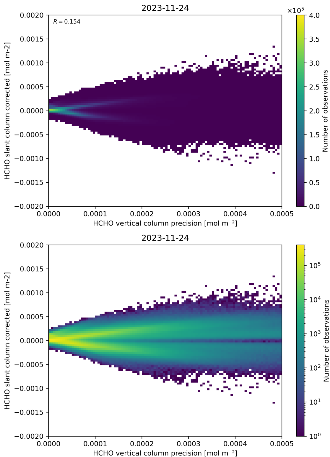
Figure 140: Scatter density plot of “HCHO vertical column precision” against “HCHO slant column corrected” for 2023-11-23 to 2023-11-25.
