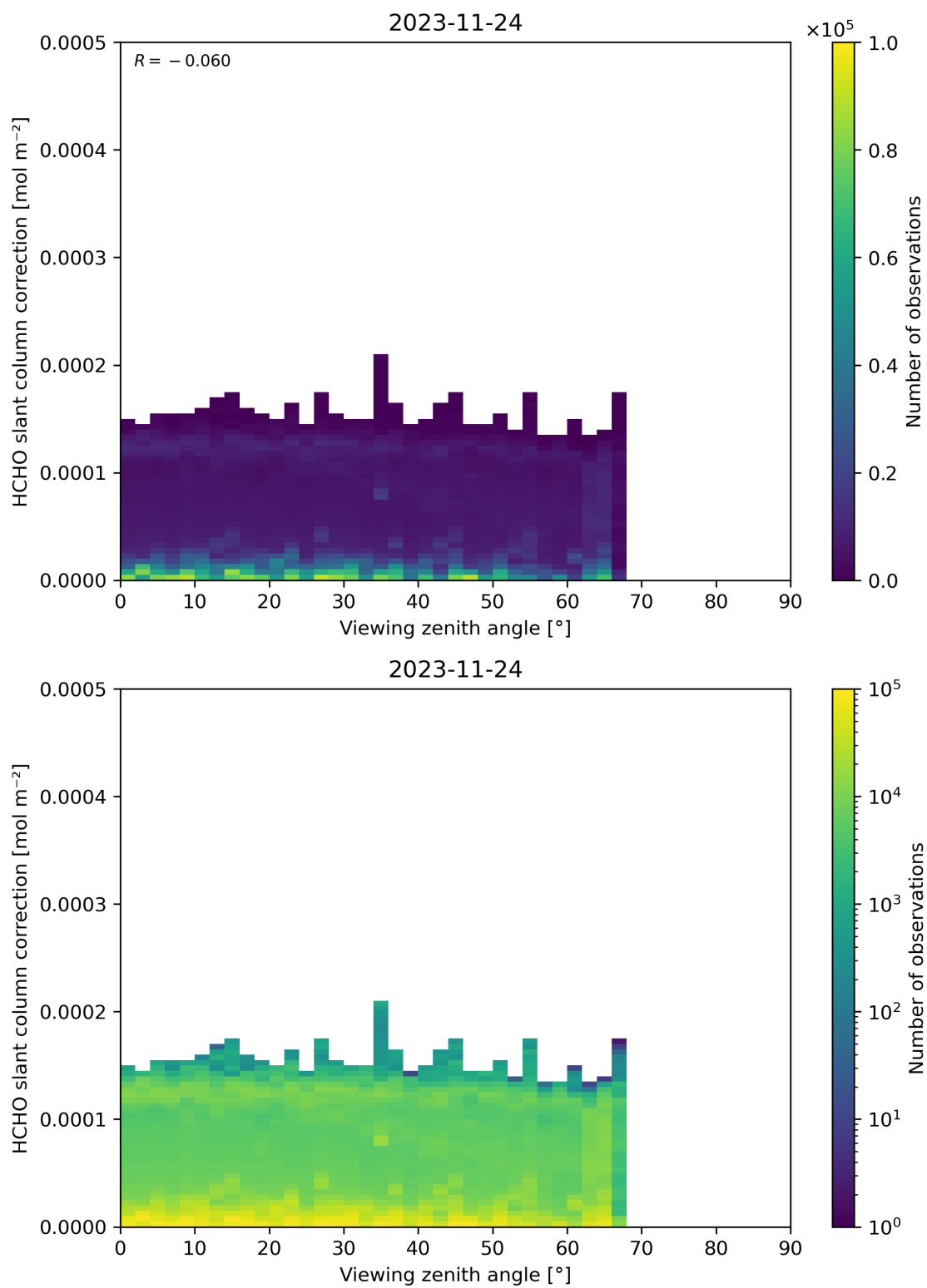
Figure 187: Scatter density plot of “Viewing zenith angle” against “HCHO slant column correction” for 2023-11-23 to 2023-11-25.
