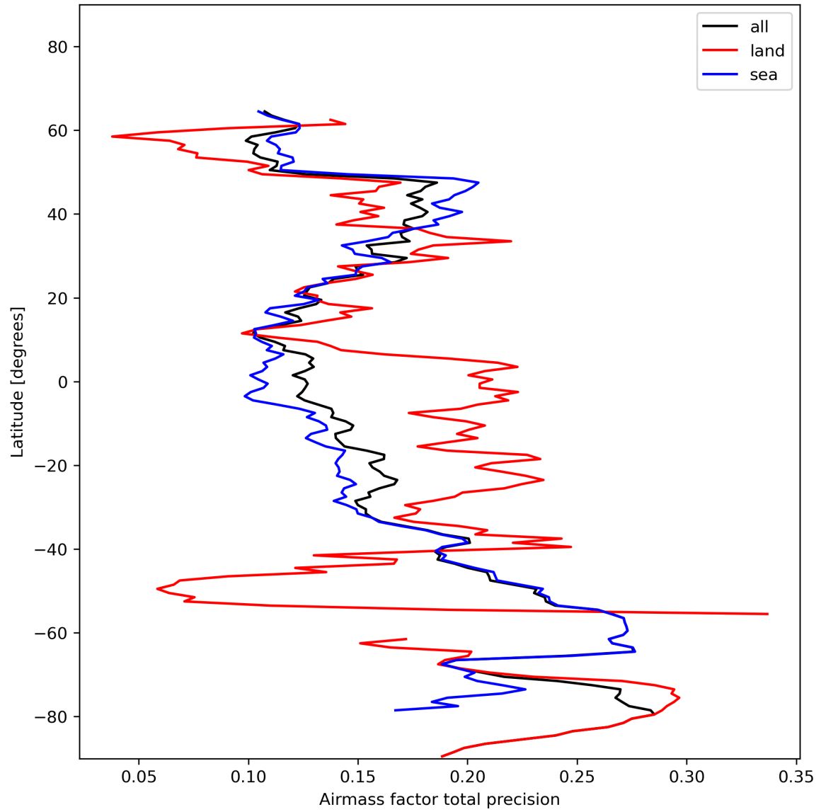
Figure 27: Zonal average of “Airmass factor total precision” for 2023-11-23 to 2023-11-25.
