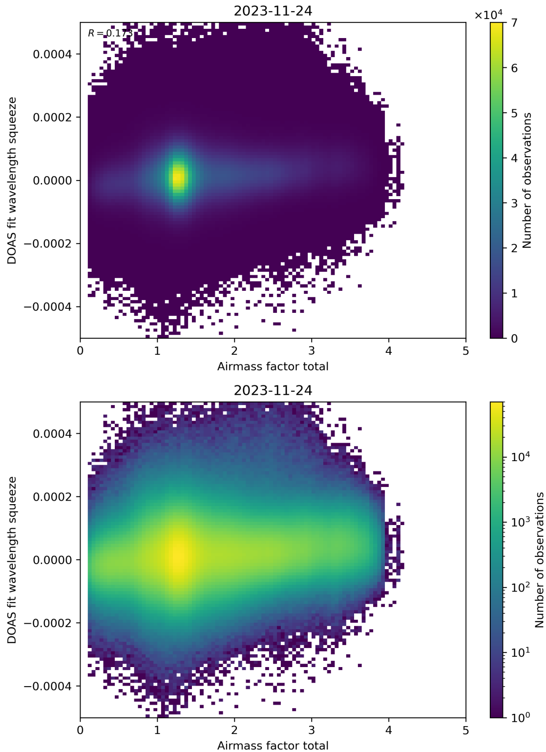
Figure 99: Scatter density plot of “Airmass factor total” against “DOAS fit wavelength squeeze” for 2023-11-23 to 2023-11-25.
