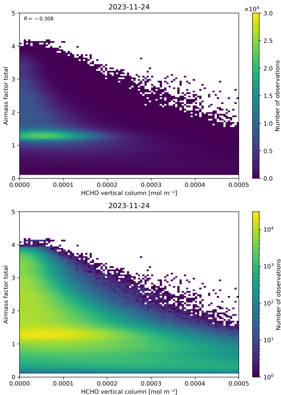
Figure 131: Scatter density plot of “HCHO vertical column” against “Airmass factor total” for 2023-11-23 to 2023-11-25.
