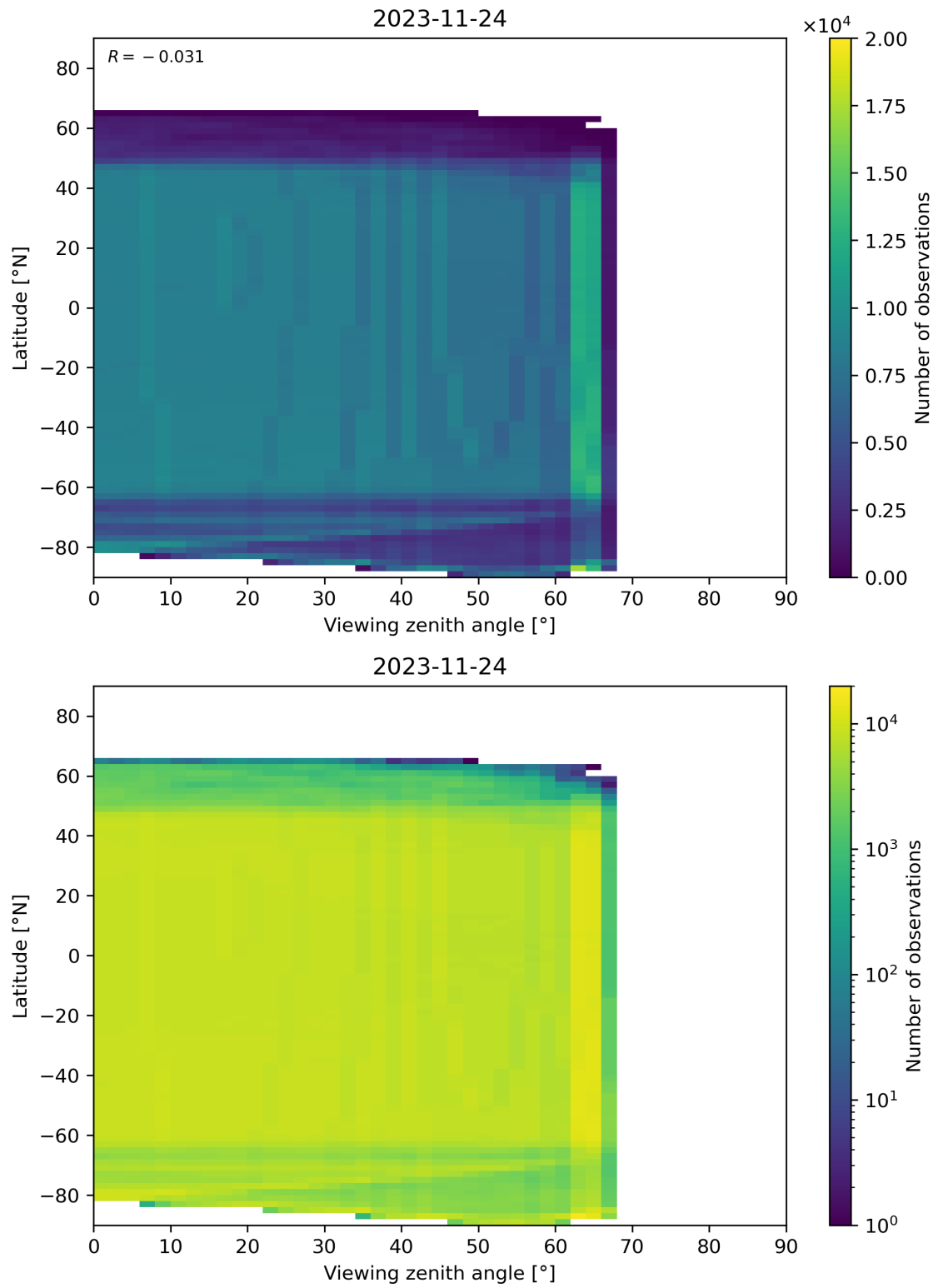
Figure 196: Scatter density plot of “Viewing zenith angle” against “Latitude” for 2023-11-23 to 2023-11-25.
