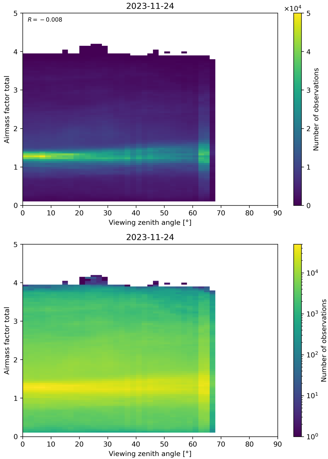
Figure 190: Scatter density plot of “Viewing zenith angle” against “Airmass factor total” for 2023-11-23 to 2023-11-25.
