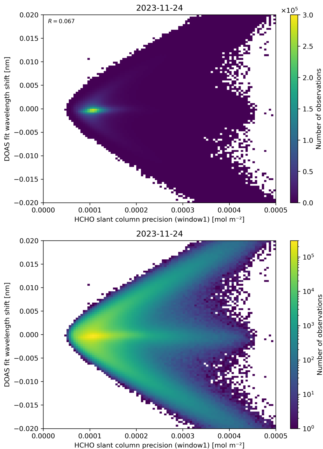
Figure 89: Scatter density plot of “HCHO slant column precision (window1)” against “DOAS fit wavelength shift” for 2023-11-23 to 2023-11-25.
