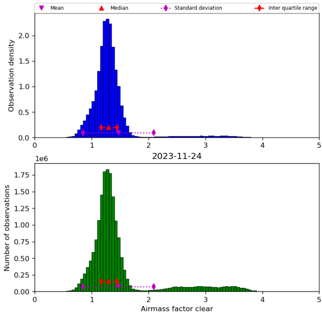
Figure 42: Histogram of “Airmass factor clear” for 2023-11-23 to 2023-11-25
