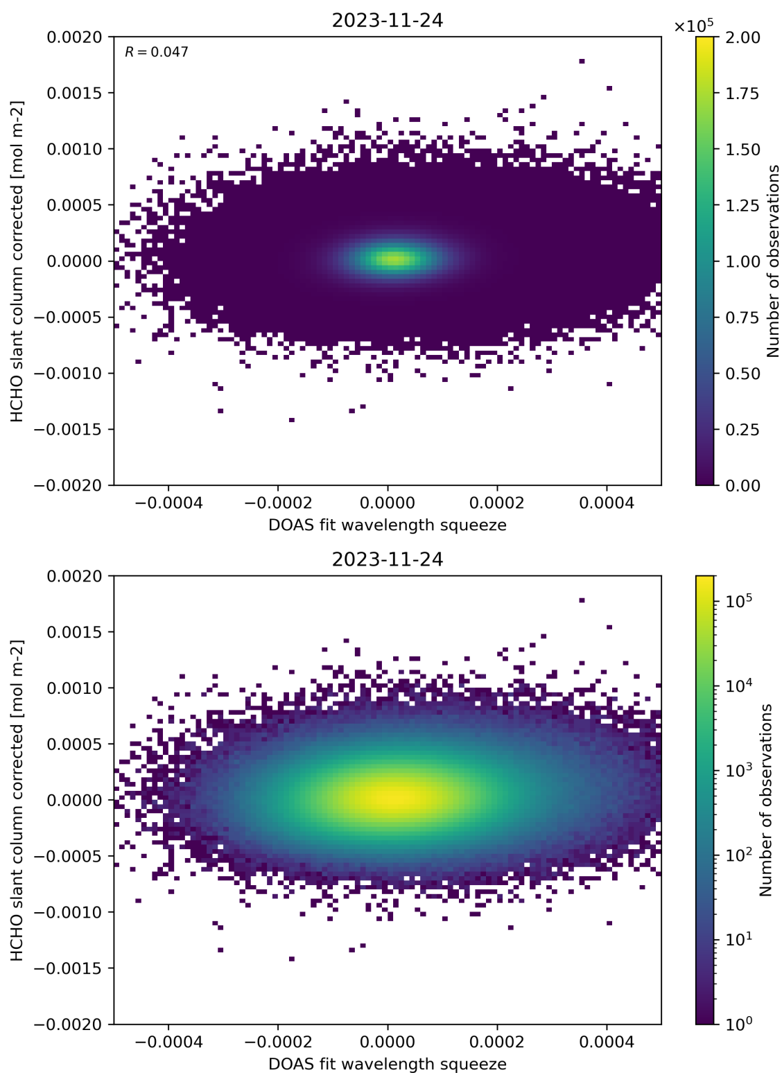
Figure 69: Scatter density plot of “DOAS fit wavelength squeeze” against “HCHO slant column corrected” for 2023-11-23 to 2023-11-25.
