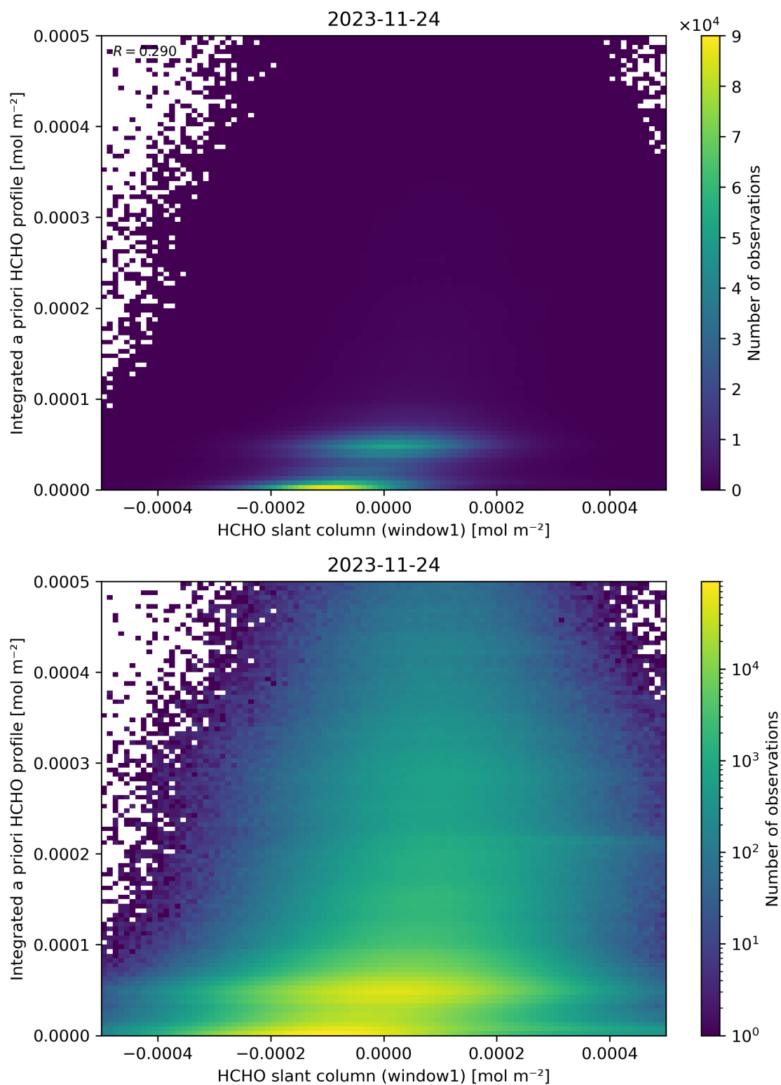
Figure 87: Scatter density plot of “HCHO slant column (window1)” against “Integrated a priori HCHO profile” for 2023-11-23 to 2023-11-25.
