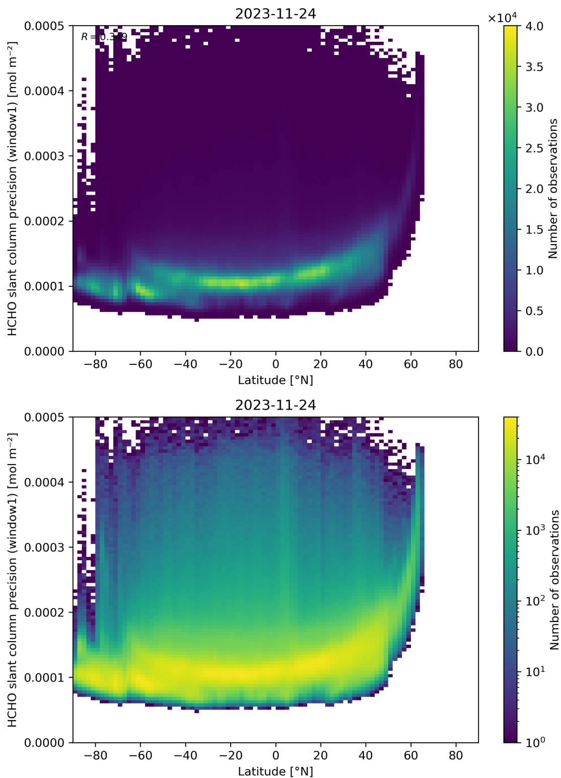
Figure 160: Scatter density plot of “Latitude” against “HCHO slant column precision (window1)” for 2023-11-23 to 2023-11-25.
