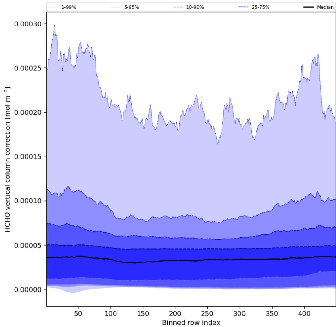
Figure 51: Along track statistics of “HCHO vertical column correction” for 2023-11-23 to 2023-11-25
