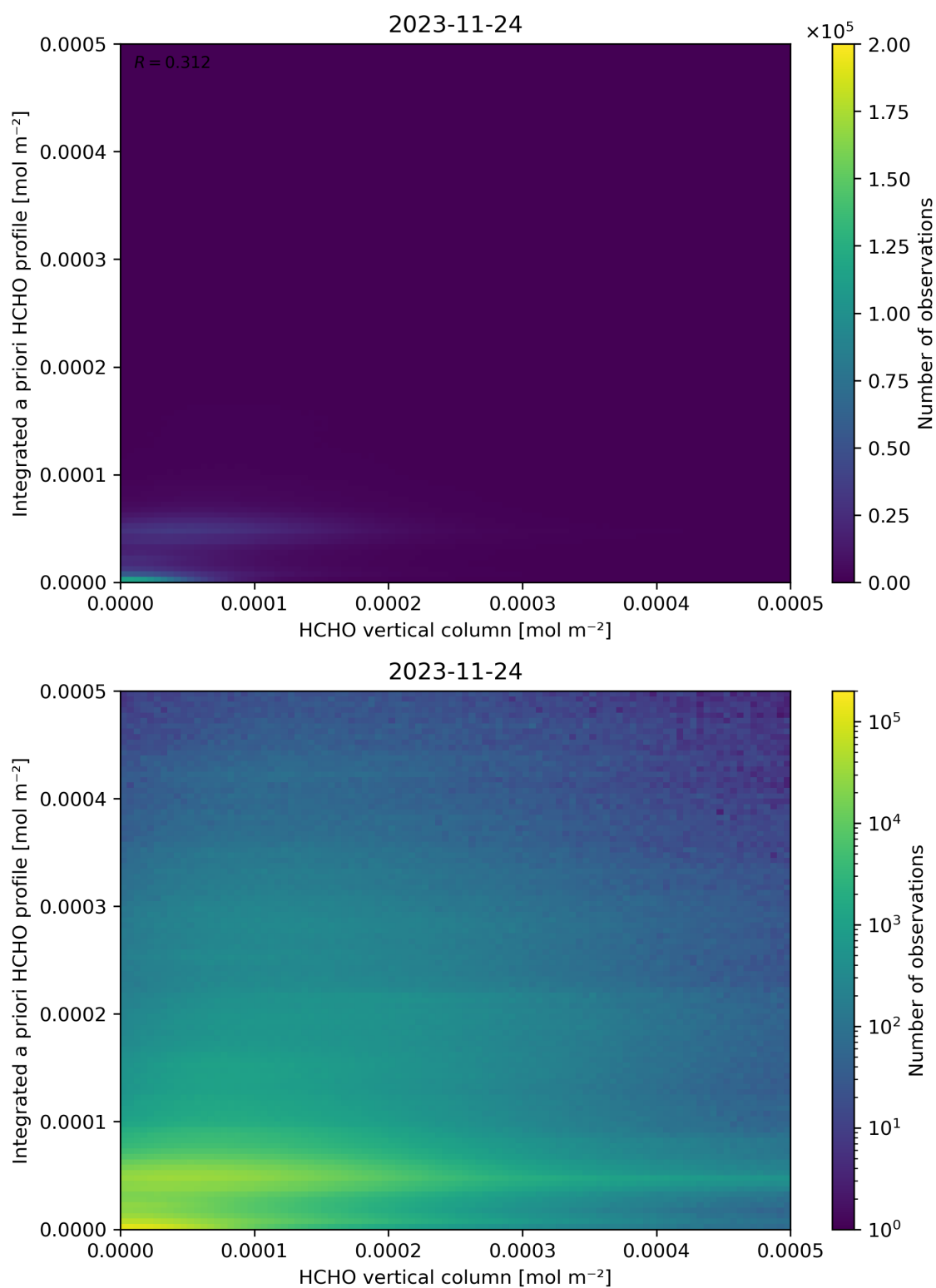
Figure 135: Scatter density plot of “HCHO vertical column” against “Integrated a priori HCHO profile” for 2023-11-23 to 2023-11-25.
