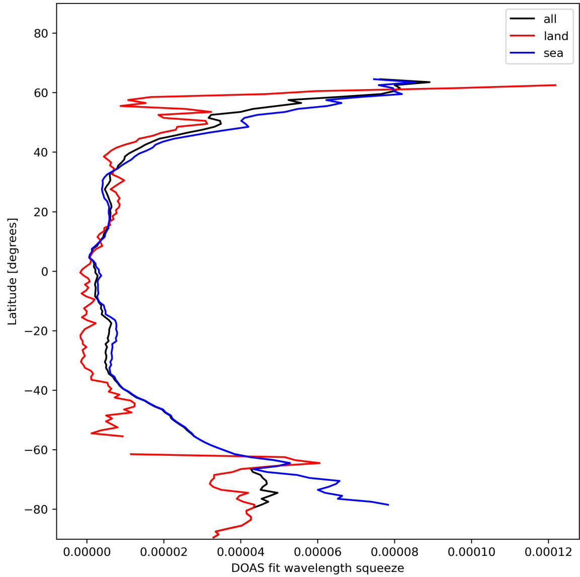
Figure 31: Zonal average of “DOAS fit wavelength squeeze” for 2023-11-23 to 2023-11-25.
