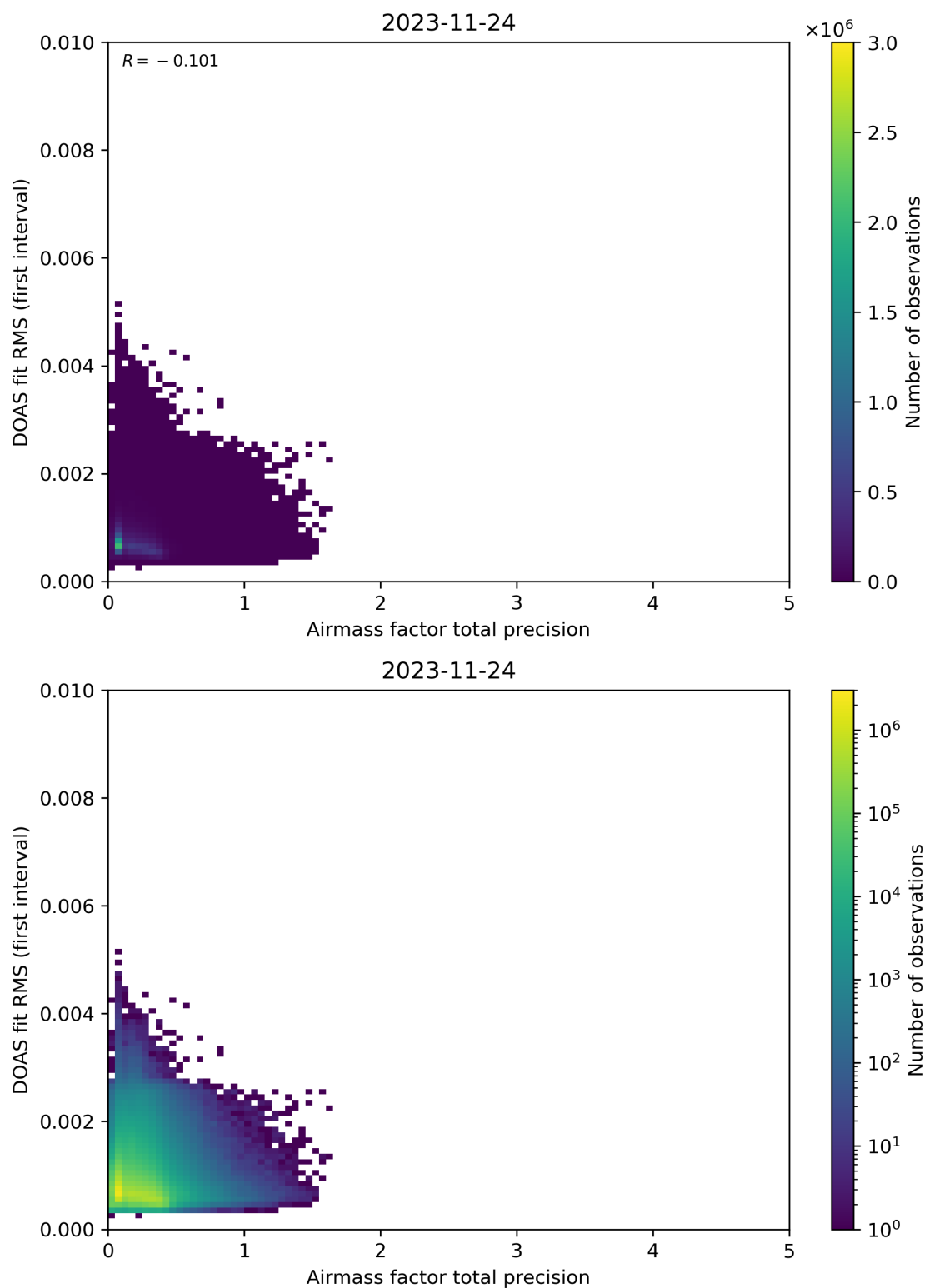
Figure 105: Scatter density plot of “Airmass factor total precision” against “DOAS fit RMS (first interval)” for 2023-11-23 to 2023-11-25.
