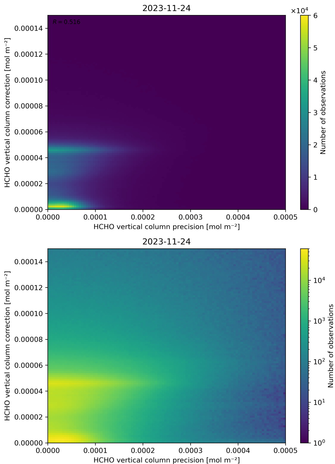
Figure 146: Scatter density plot of “HCHO vertical column precision” against “HCHO vertical column correction” for 2023-11-23 to 2023-11-25.
