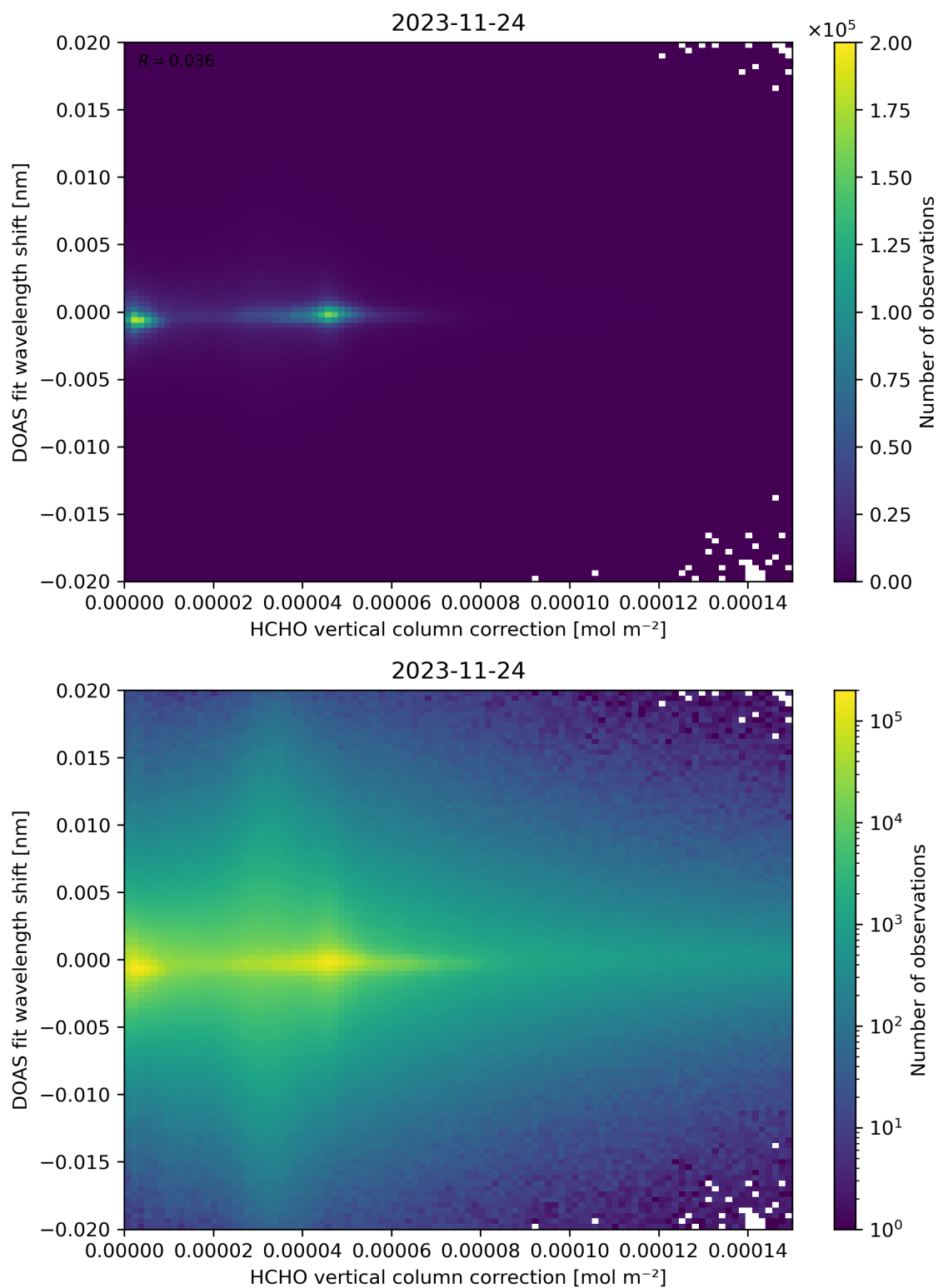
Figure 113: Scatter density plot of “HCHO vertical column correction” against “DOAS fit wavelength shift” for 2023-11-23 to 2023-11-25.
