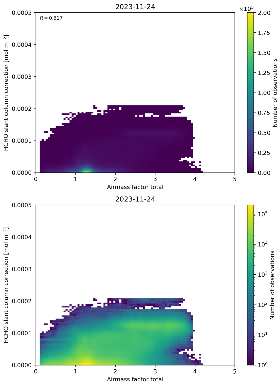
Figure 102: Scatter density plot of “Airmass factor total” against “HCHO slant column correction” for 2023-11-23 to 2023-11-25.
