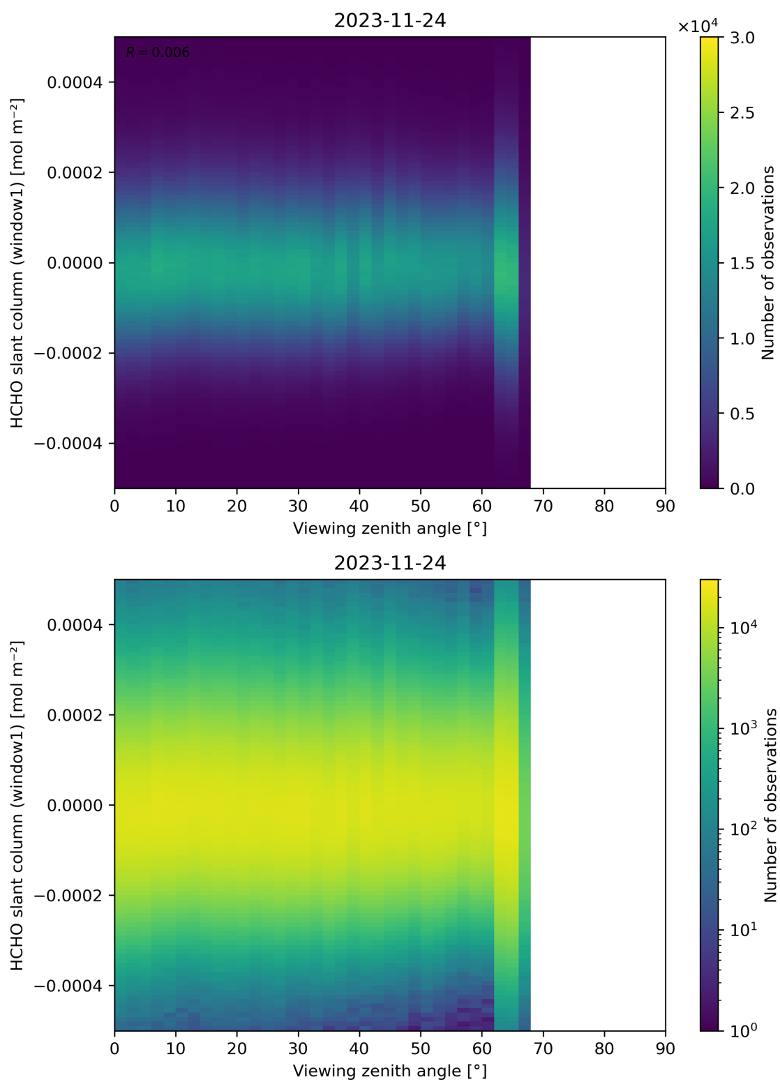
Figure 188: Scatter density plot of “Viewing zenith angle” against “HCHO slant column (window1)” for 2023-11-23 to 2023-11-25.
