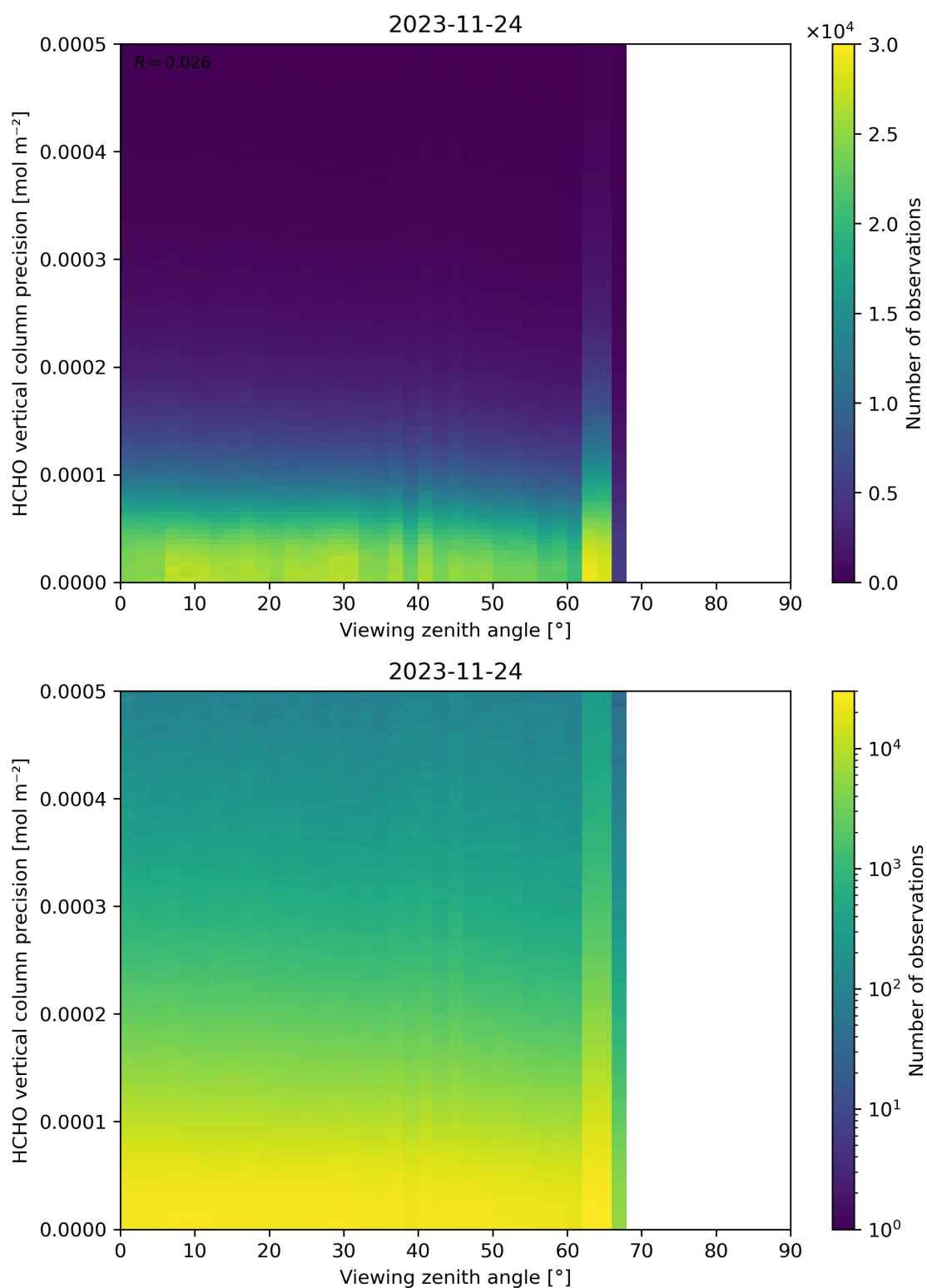
Figure 194: Scatter density plot of “Viewing zenith angle” against “HCHO vertical column precision” for 2023-11-23 to 2023-11-25.
