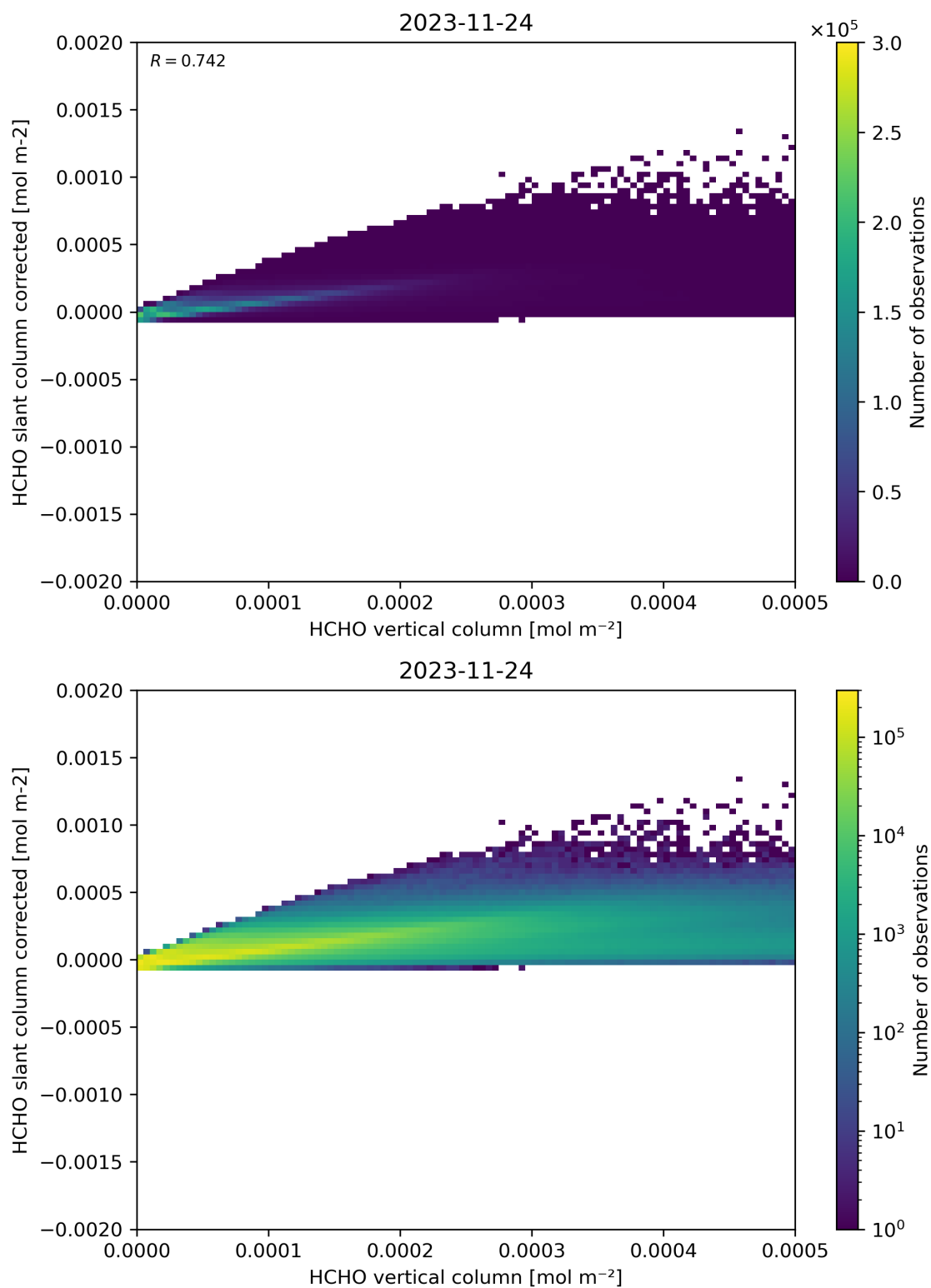
Figure 127: Scatter density plot of “HCHO vertical column” against “HCHO slant column corrected” for 2023-11-23 to 2023-11-25.
