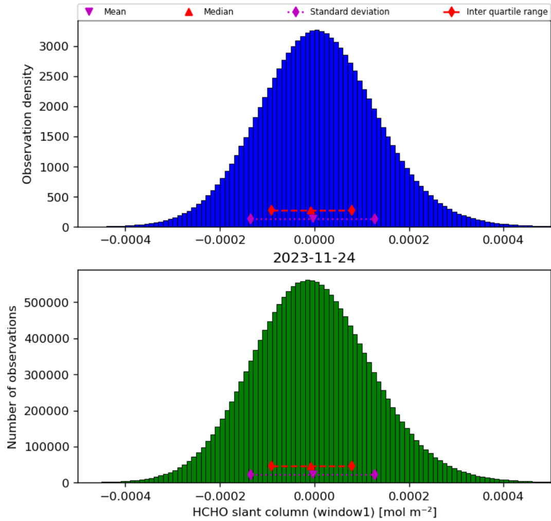
Figure 38: Histogram of “HCHO slant column (window1)” for 2023-11-23 to 2023-11-25
