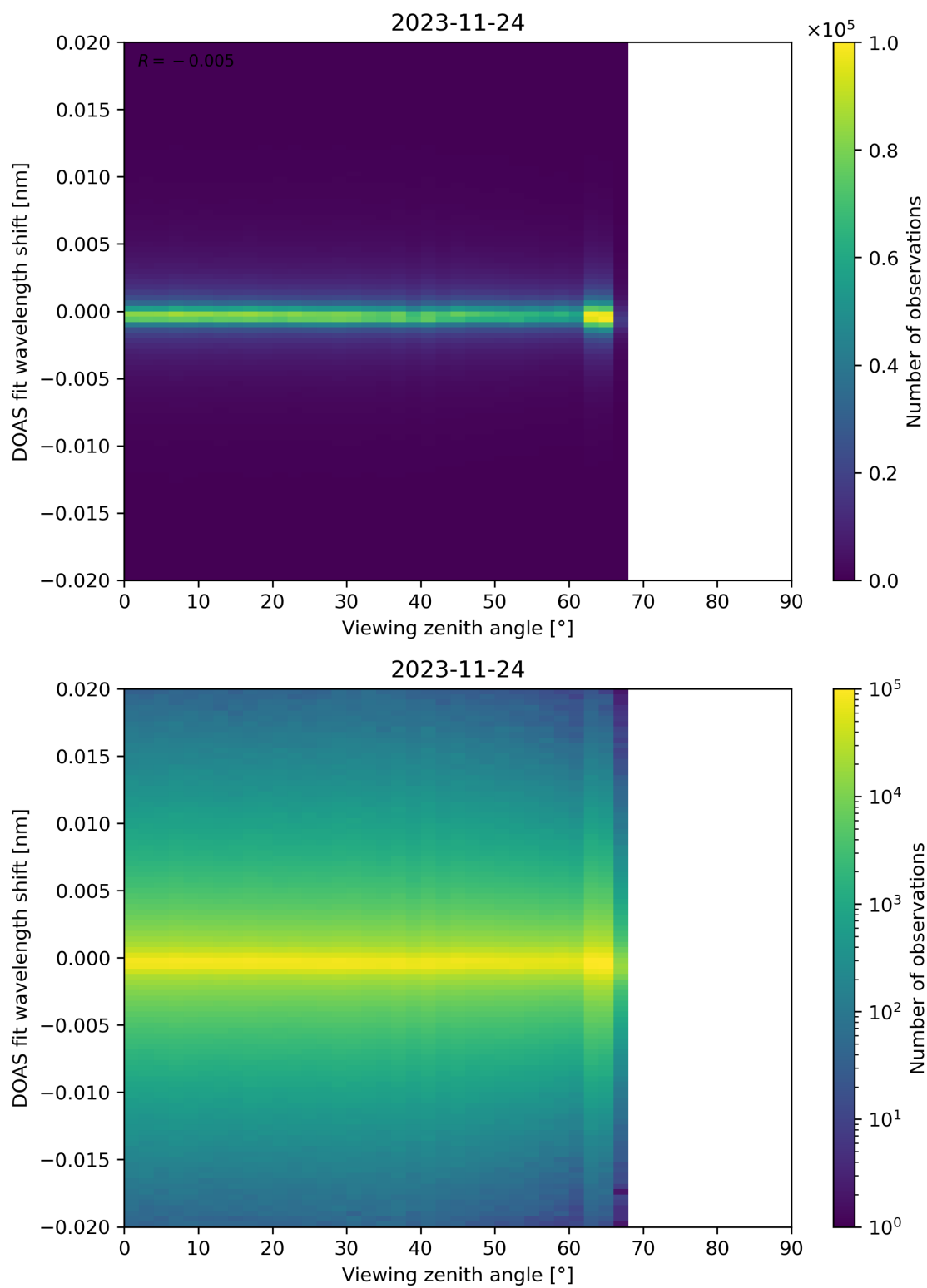
Figure 183: Scatter density plot of “Viewing zenith angle” against “DOAS fit wavelength shift” for 2023-11-23 to 2023-11-25.
