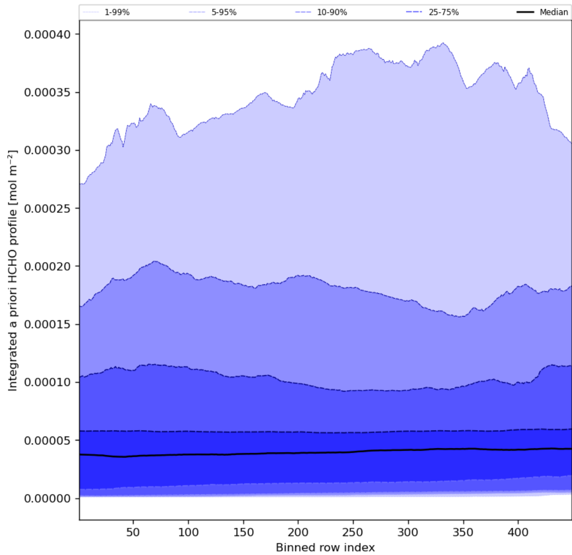
Figure 57: Along track statistics of “Integrated a priori HCHO profile” for 2023-11-23 to 2023-11-25
