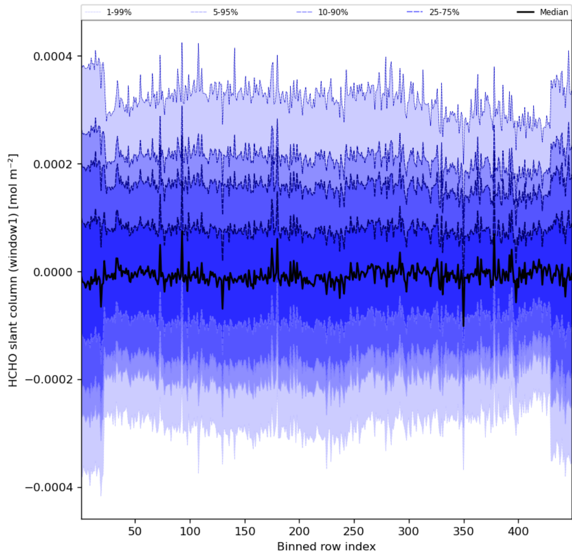
Figure 52: Along track statistics of “HCHO slant column (window1)” for 2023-11-23 to 2023-11-25
