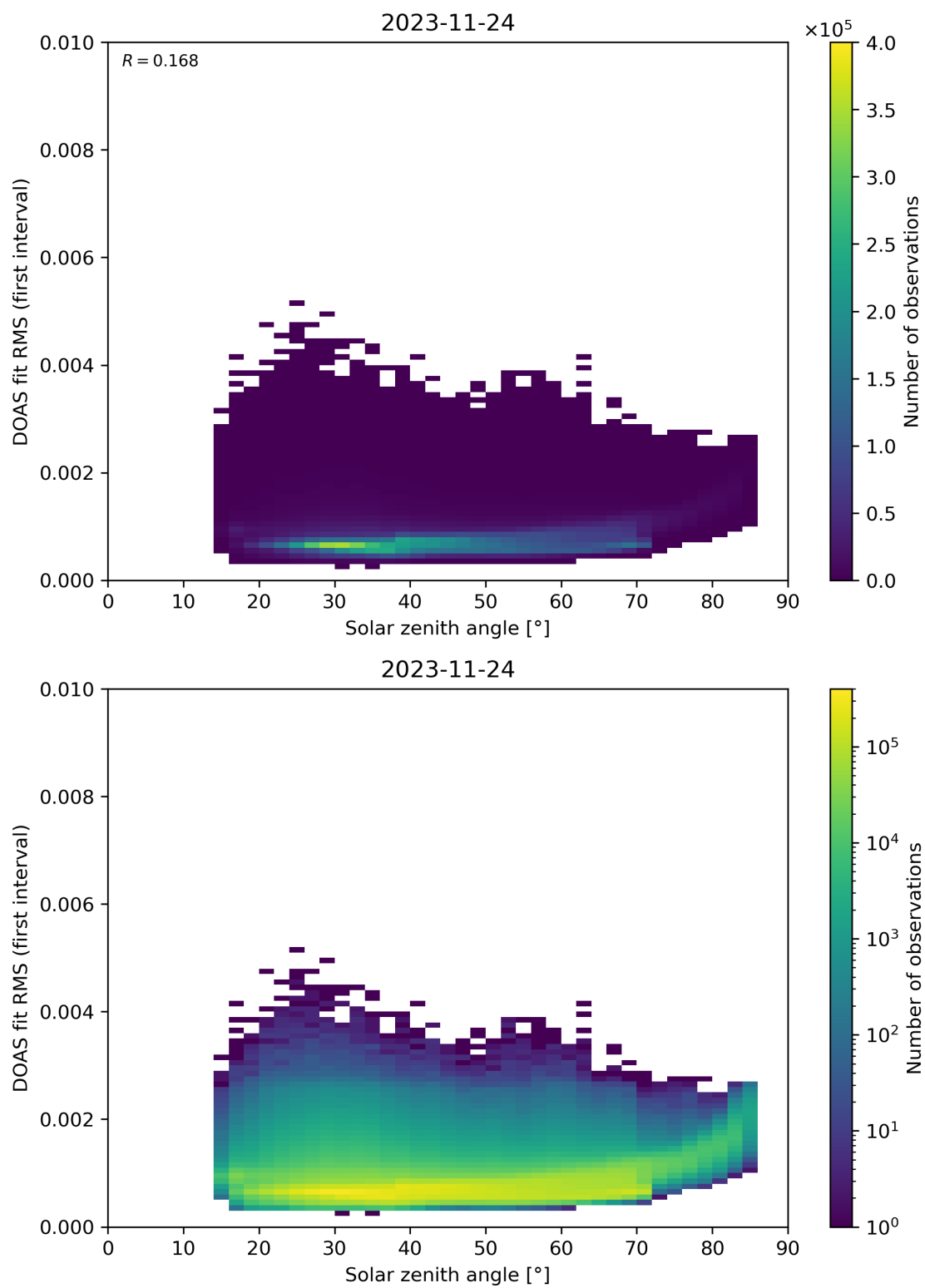
Figure 167: Scatter density plot of “Solar zenith angle” against “DOAS fit RMS (first interval)” for 2023-11-23 to 2023-11-25.
