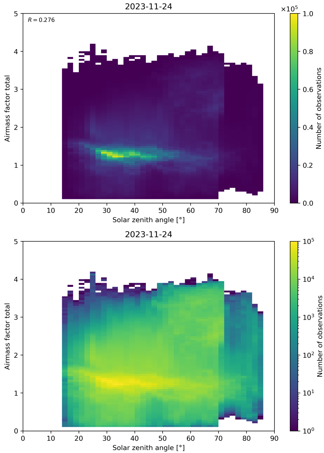
Figure 175: Scatter density plot of “Solar zenith angle” against “Airmass factor total” for 2023-11-23 to 2023-11-25.
