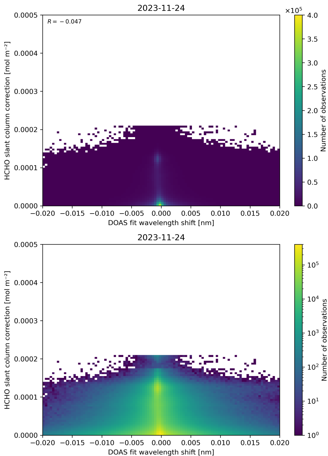
Figure 67: Scatter density plot of “DOAS fit wavelength shift” against “HCHO slant column correction” for 2023-11-23 to 2023-11-25.
