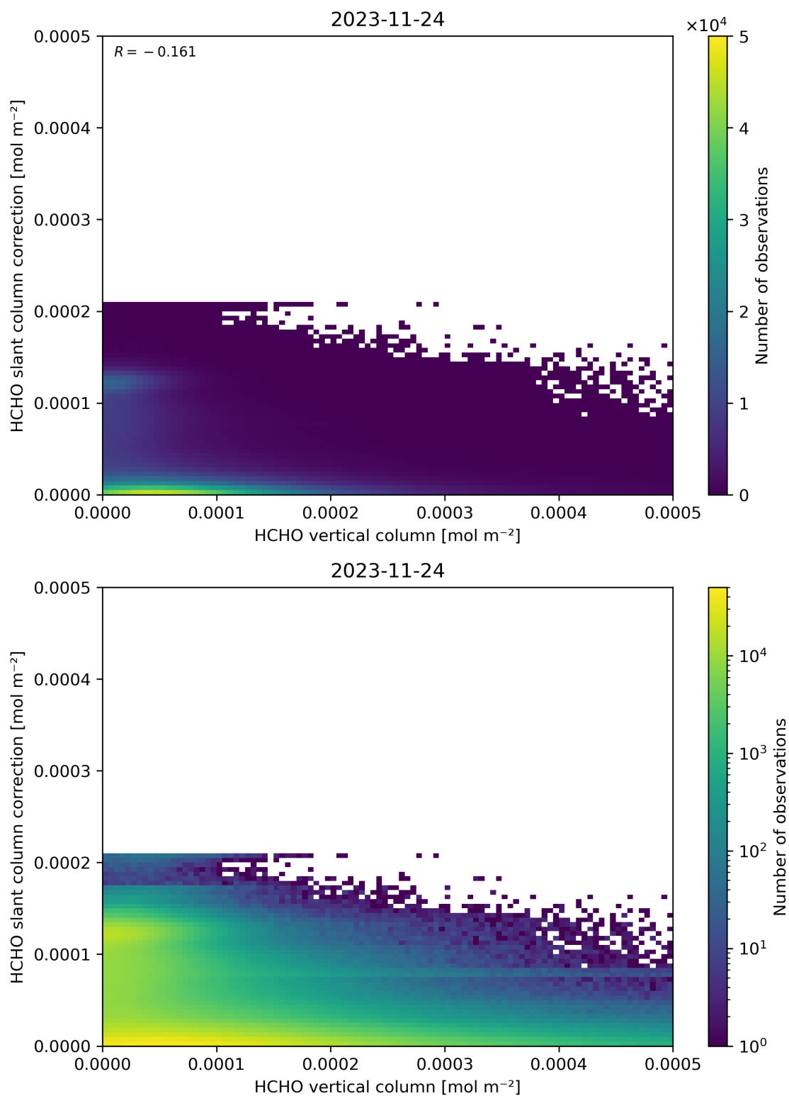
Figure 128: Scatter density plot of “HCHO vertical column” against “HCHO slant column correction” for 2023-11-23 to 2023-11-25.
