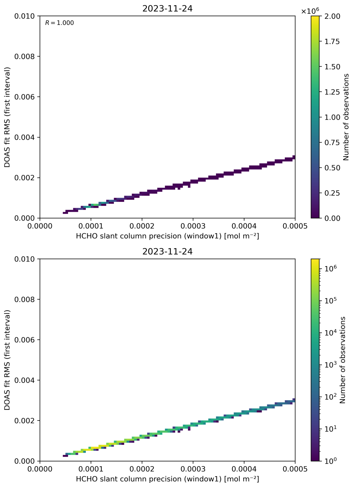
Figure 88: Scatter density plot of “HCHO slant column precision (window1)” against “DOAS fit RMS (first interval)” for 2023-11-23 to 2023-11-25.
