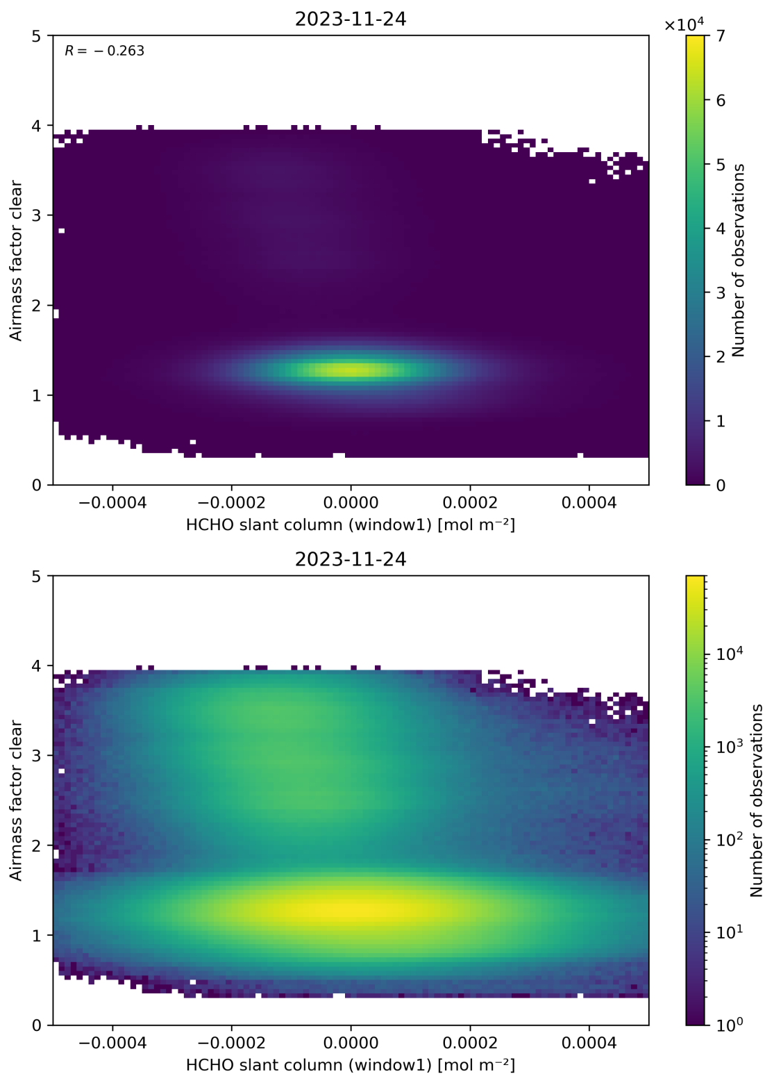
Figure 81: Scatter density plot of “HCHO slant column (window1)” against “Airmass factor clear” for 2023-11-23 to 2023-11-25.
