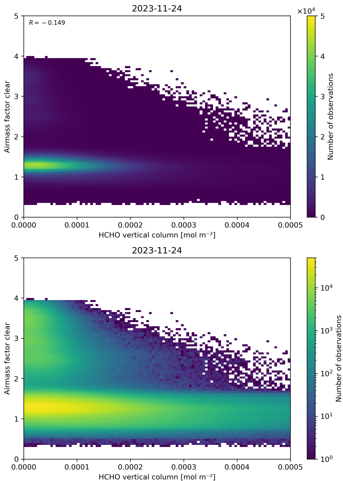
Figure 126: Scatter density plot of “HCHO vertical column” against “Airmass factor clear” for 2023-11-23 to 2023-11-25.
