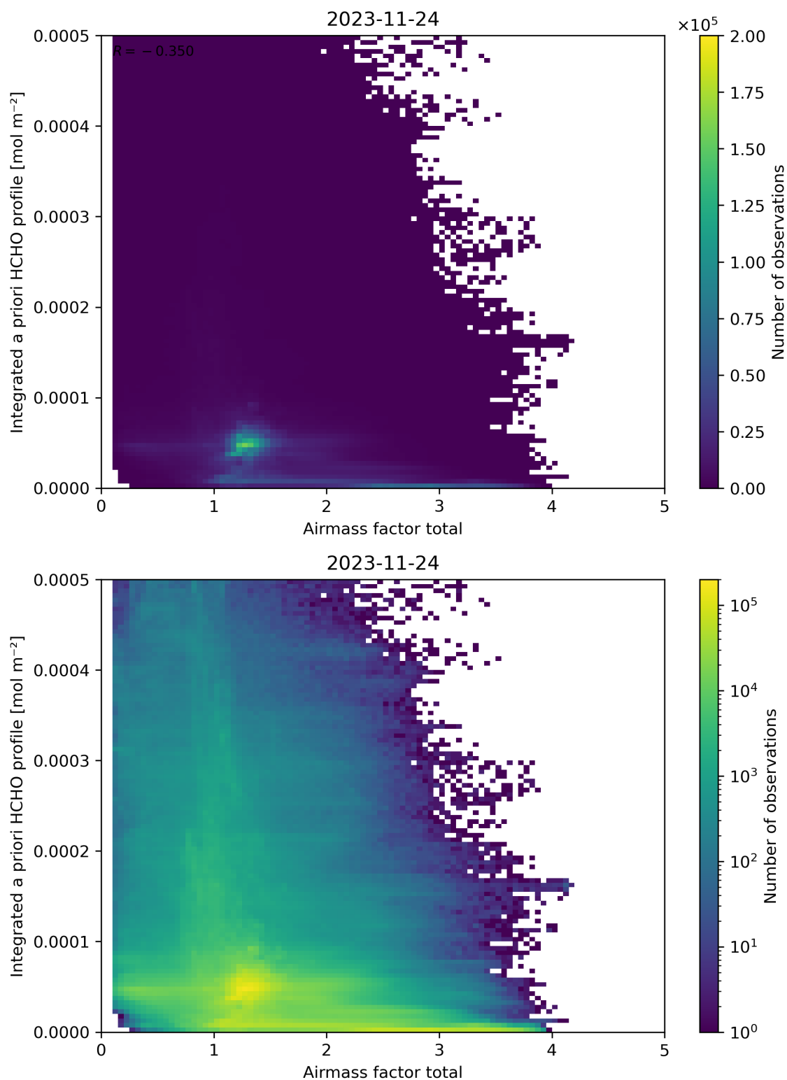
Figure 104: Scatter density plot of “Airmass factor total” against “Integrated a priori HCHO profile” for 2023-11-23 to 2023-11-25.
