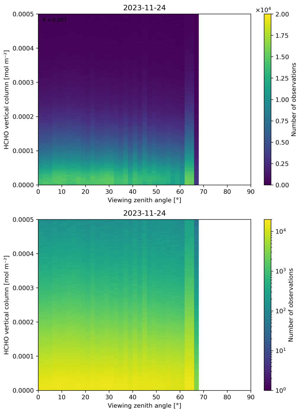
Figure 192: Scatter density plot of “Viewing zenith angle” against “HCHO vertical column” for 2023-11-23 to 2023-11-25.
