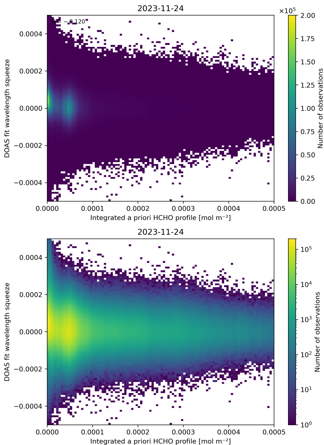
Figure 150: Scatter density plot of “Integrated a priori HCHO profile” against “DOAS fit wavelength squeeze” for 2023-11-23 to 2023-11-25.
