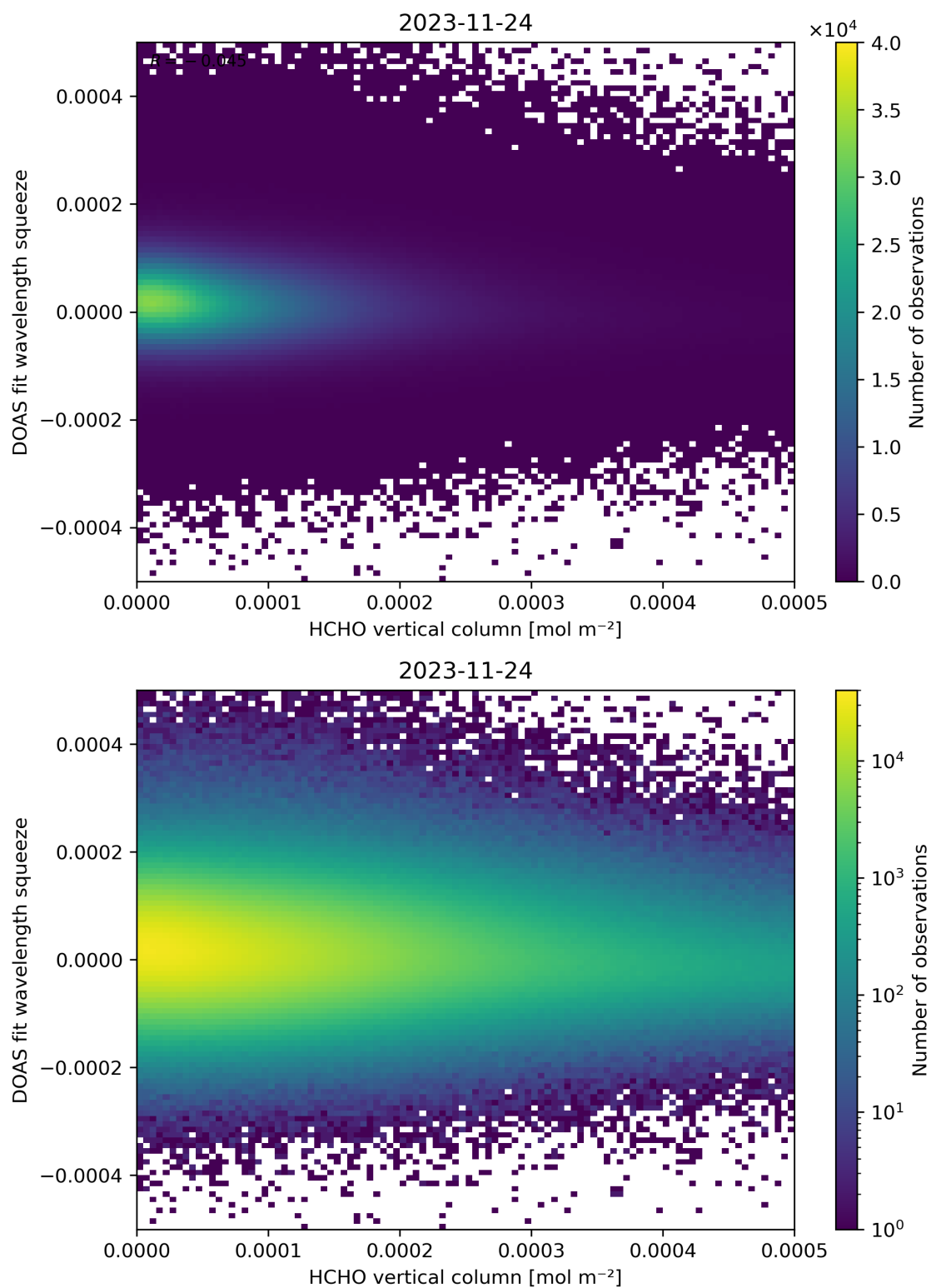
Figure 125: Scatter density plot of “HCHO vertical column” against “DOAS fit wavelength squeeze” for 2023-11-23 to 2023-11-25.
