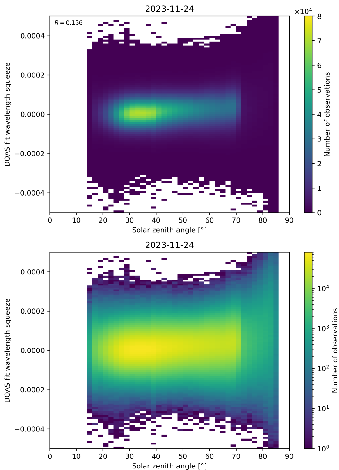
Figure 169: Scatter density plot of “Solar zenith angle” against “DOAS fit wavelength squeeze” for 2023-11-23 to 2023-11-25.
