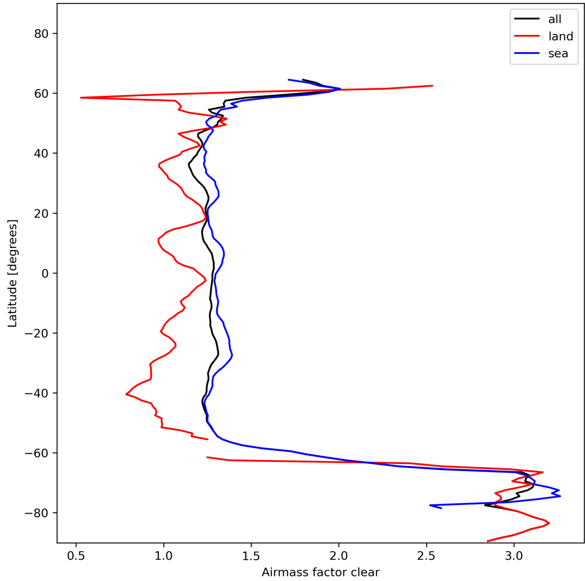
Figure 28: Zonal average of “Airmass factor clear” for 2023-11-23 to 2023-11-25.
