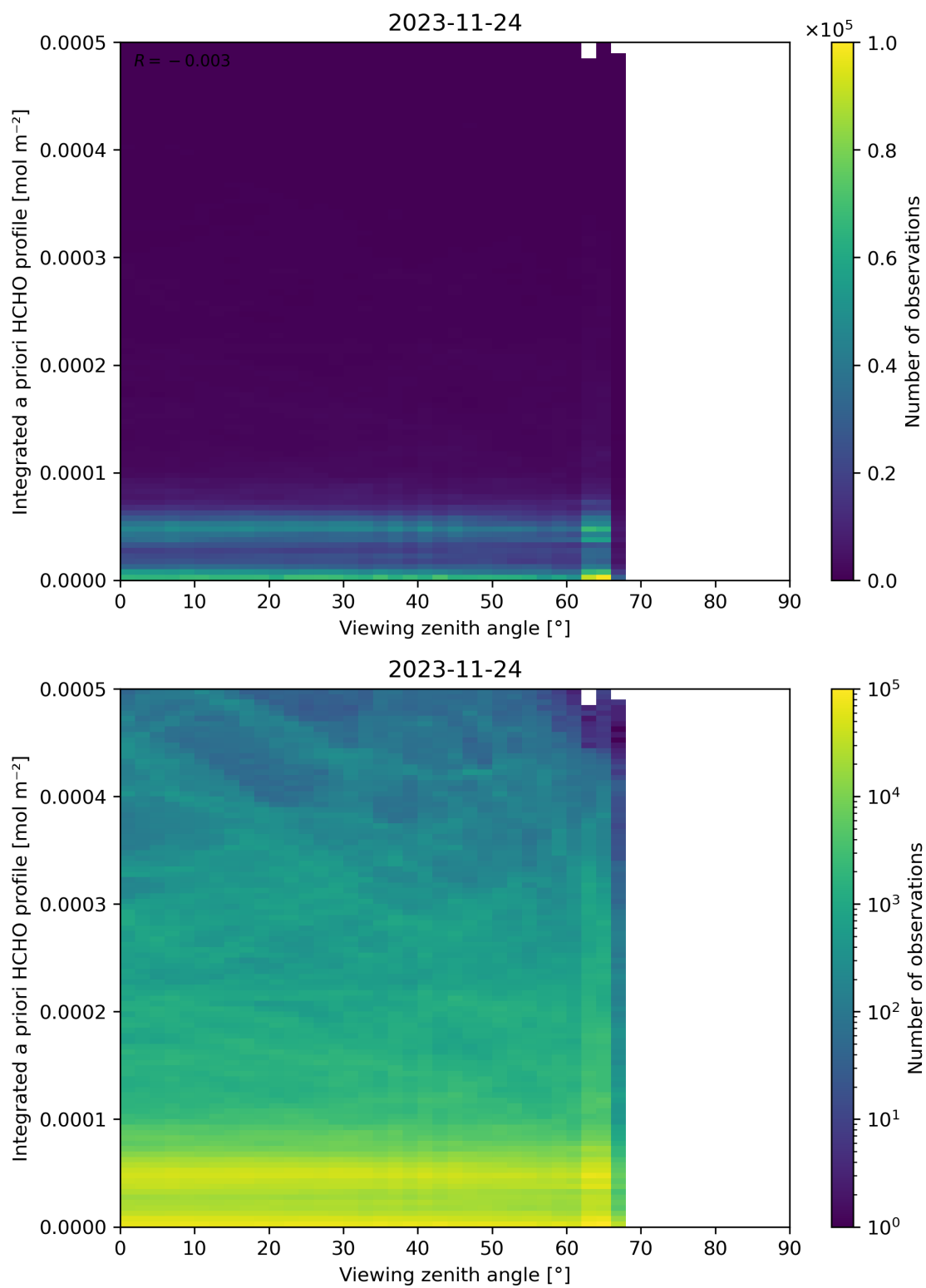
Figure 195: Scatter density plot of “Viewing zenith angle” against “Integrated a priori HCHO profile” for 2023-11-23 to 2023-11-25.
