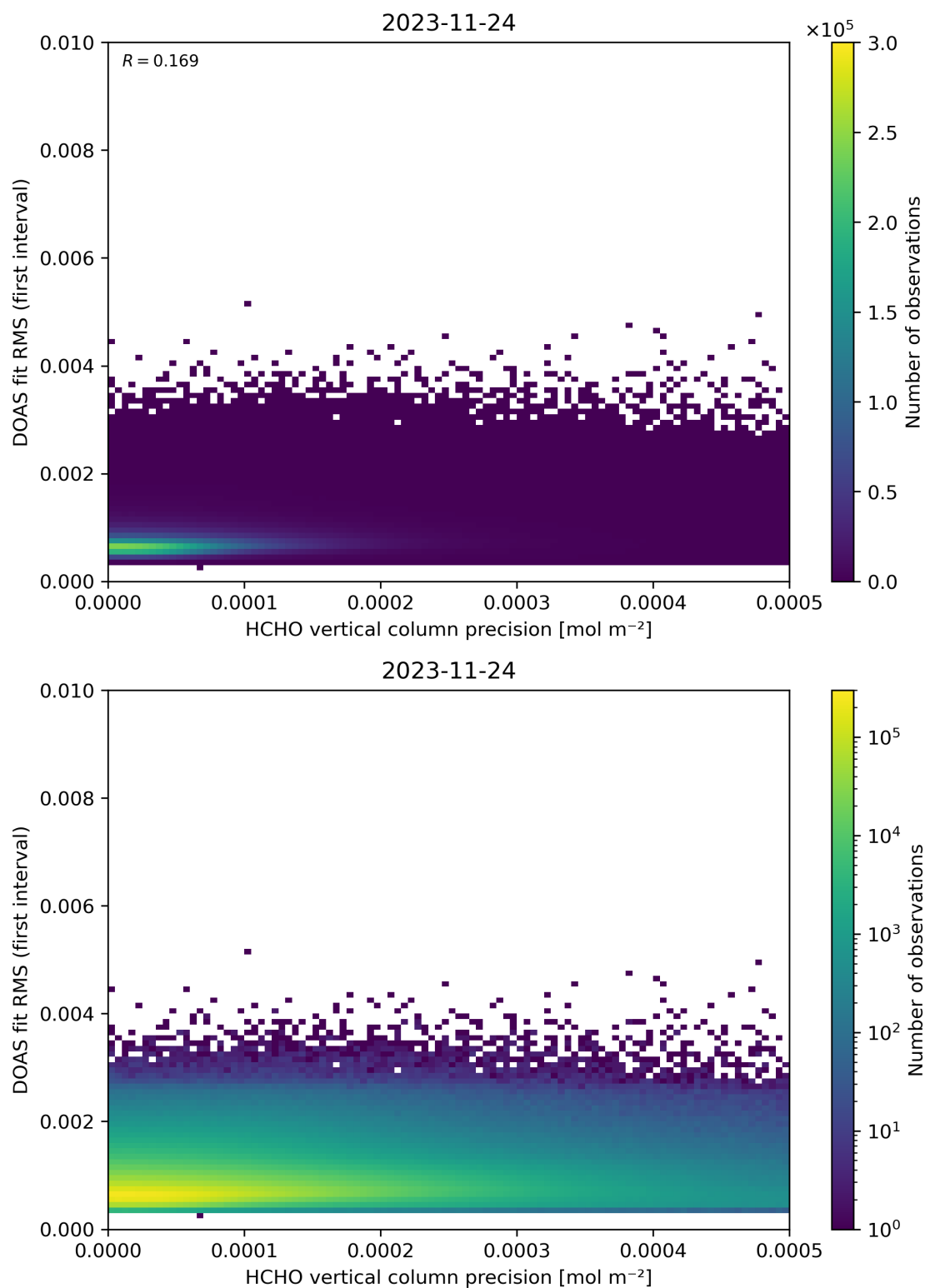
Figure 136: Scatter density plot of “HCHO vertical column precision” against “DOAS fit RMS (first interval)” for 2023-11-23 to 2023-11-25.
