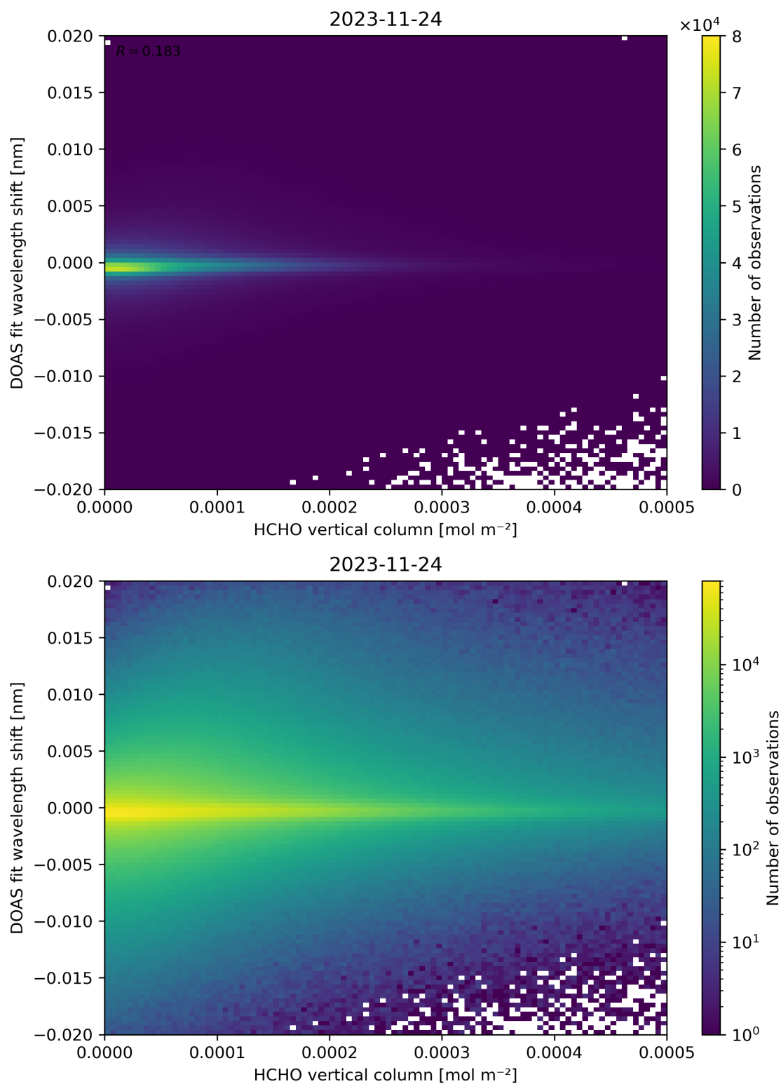
Figure 124: Scatter density plot of “HCHO vertical column” against “DOAS fit wavelength shift” for 2023-11-23 to 2023-11-25.
