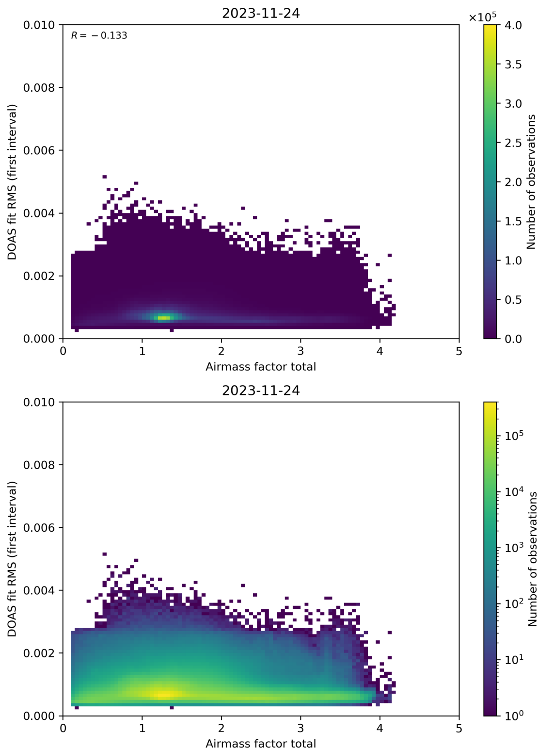
Figure 97: Scatter density plot of “Airmass factor total” against “DOAS fit RMS (first interval)” for 2023-11-23 to 2023-11-25.
