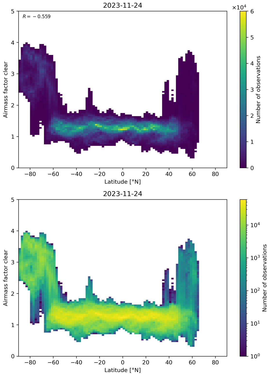
Figure 156: Scatter density plot of “Latitude” against “Airmass factor clear” for 2023-11-23 to 2023-11-25.
