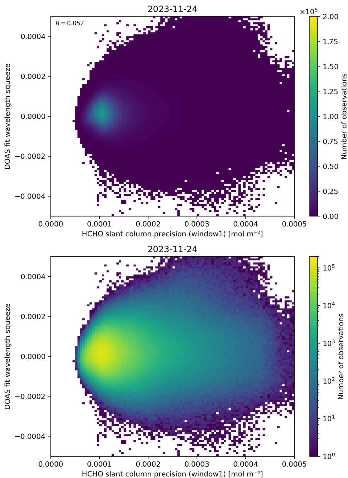
Figure 90: Scatter density plot of “HCHO slant column precision (window1)” against “DOAS fit wavelength squeeze” for 2023-11-23 to 2023-11-25.
