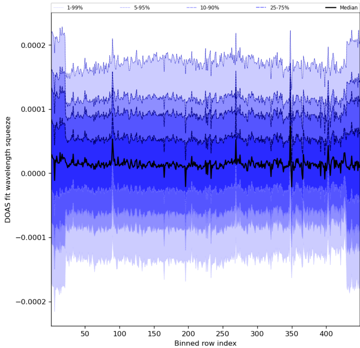
Figure 59: Along track statistics of “DOAS fit wavelength squeeze” for 2023-11-23 to 2023-11-25
