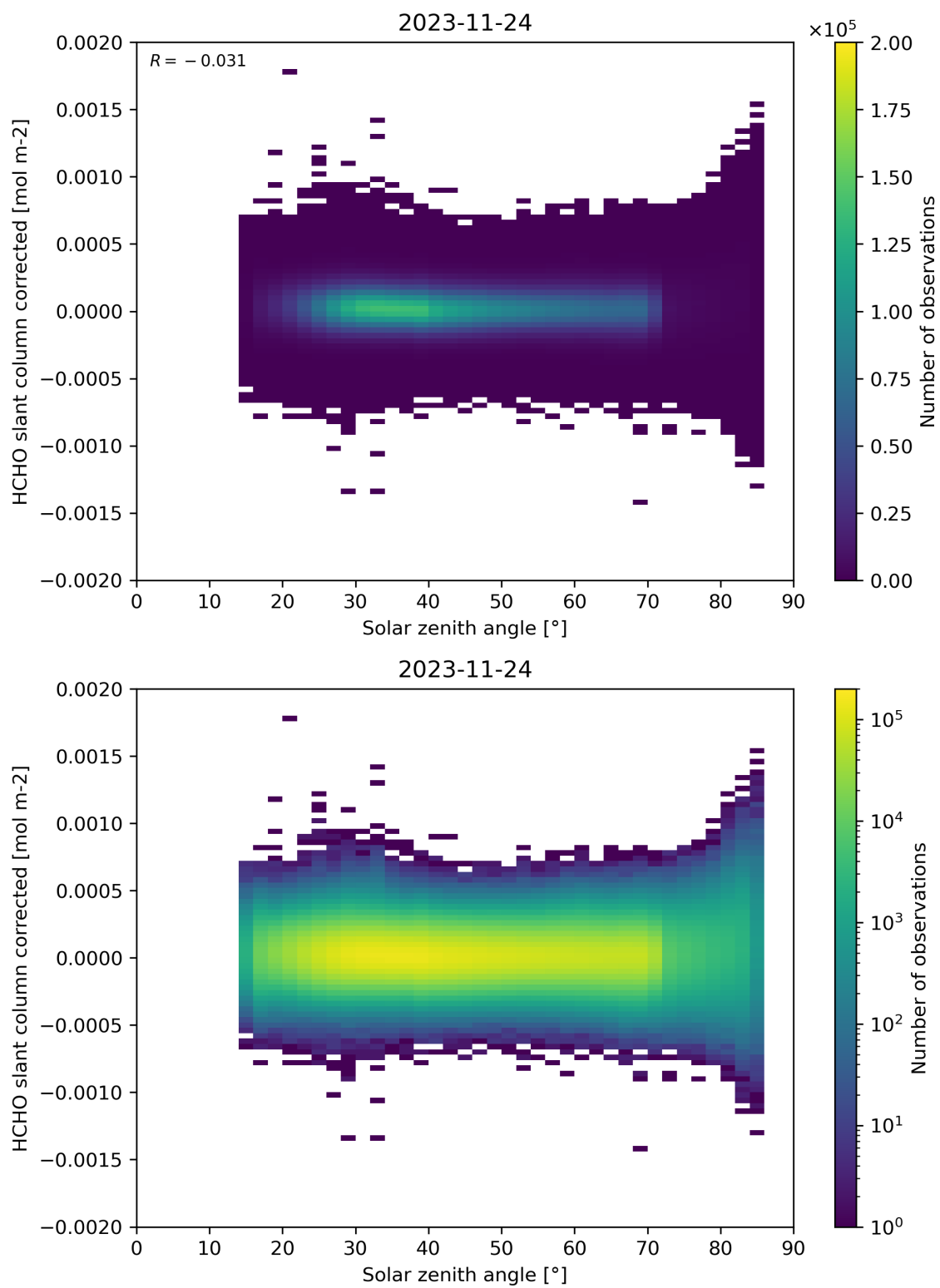
Figure 171: Scatter density plot of “Solar zenith angle” against “HCHO slant column corrected” for 2023-11-23 to 2023-11-25.
