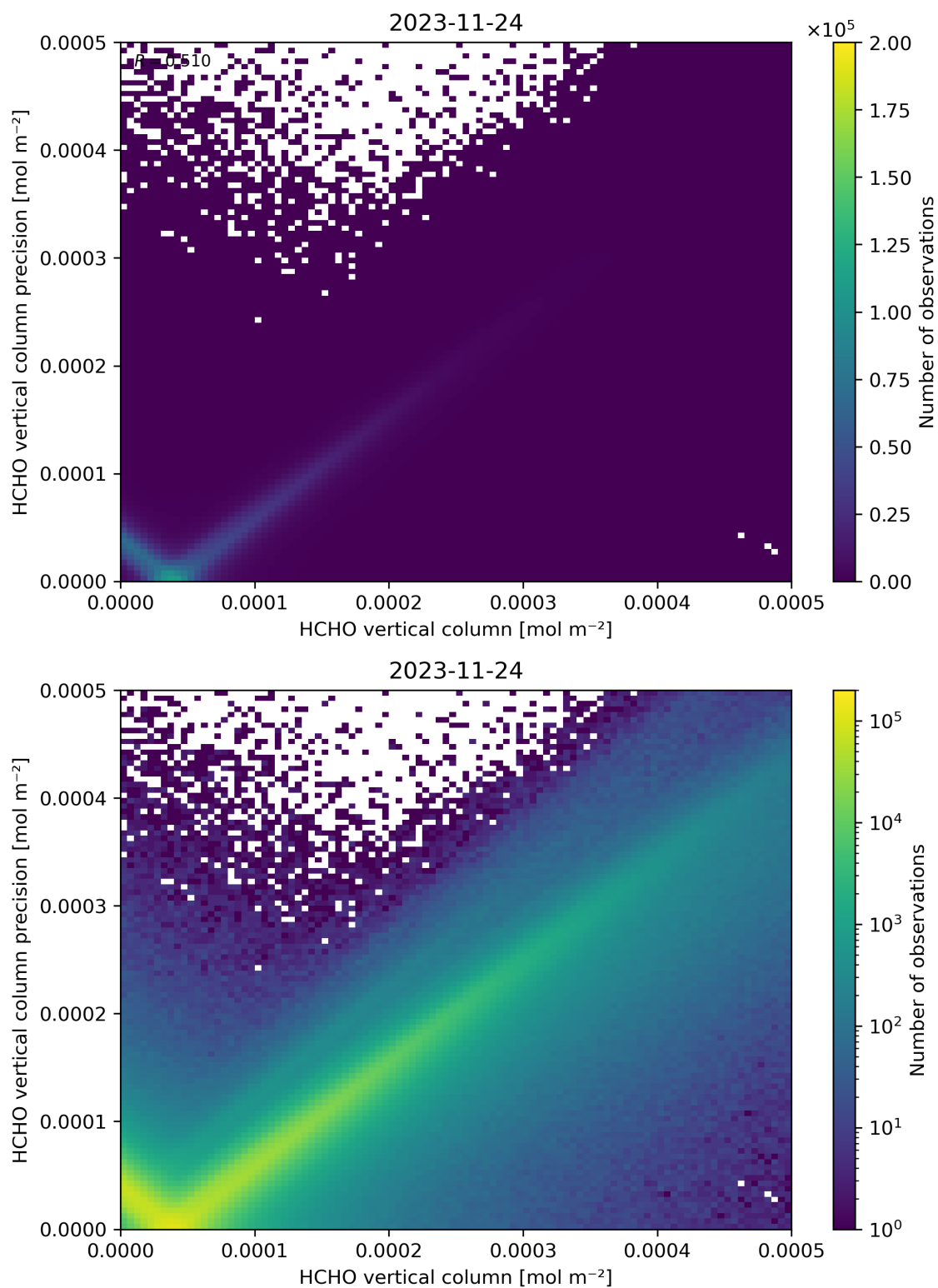
Figure 134: Scatter density plot of “HCHO vertical column” against “HCHO vertical column precision” for 2023-11-23 to 2023-11-25.
