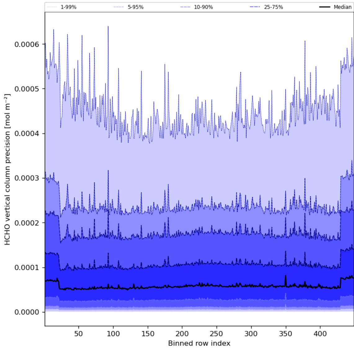
Figure 50: Along track statistics of “HCHO vertical column precision” for 2023-11-23 to 2023-11-25
