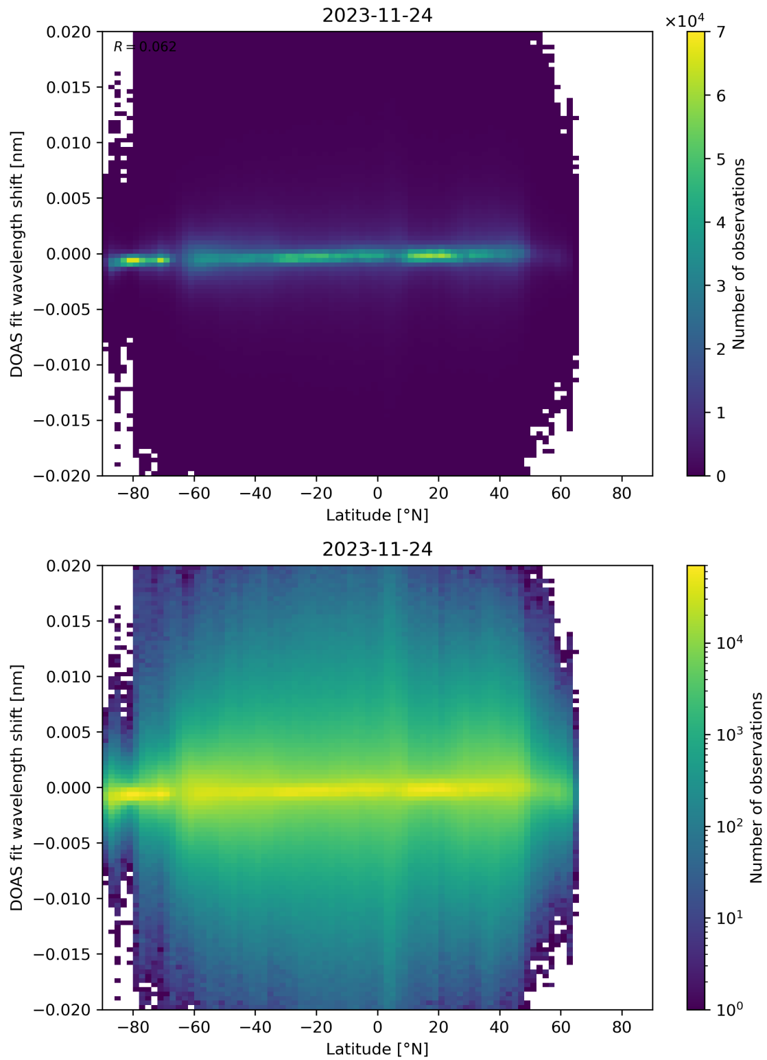
Figure 154: Scatter density plot of “Latitude” against “DOAS fit wavelength shift” for 2023-11-23 to 2023-11-25.
