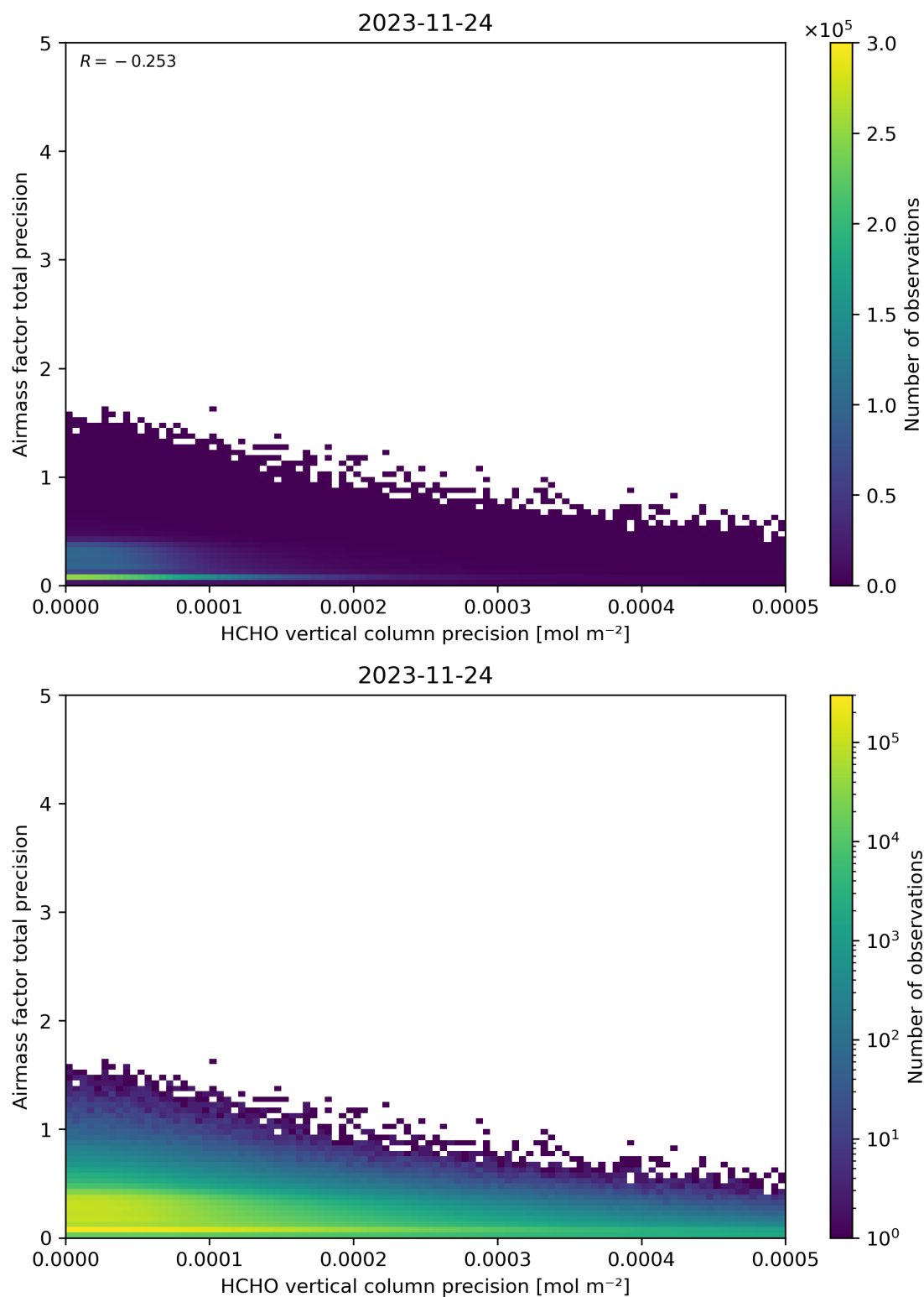
Figure 145: Scatter density plot of “HCHO vertical column precision” against “Airmass factor total precision” for 2023-11-23 to 2023-11-25.
