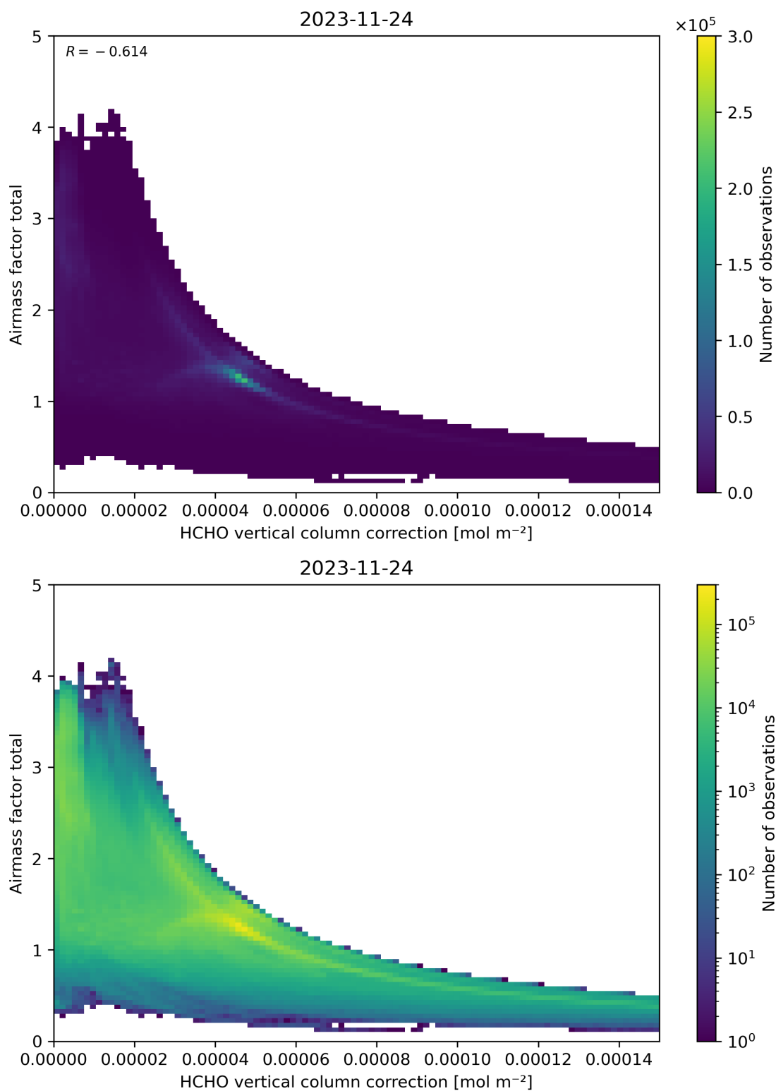
Figure 120: Scatter density plot of “HCHO vertical column correction” against “Airmass factor total” for 2023-11-23 to 2023-11-25.
