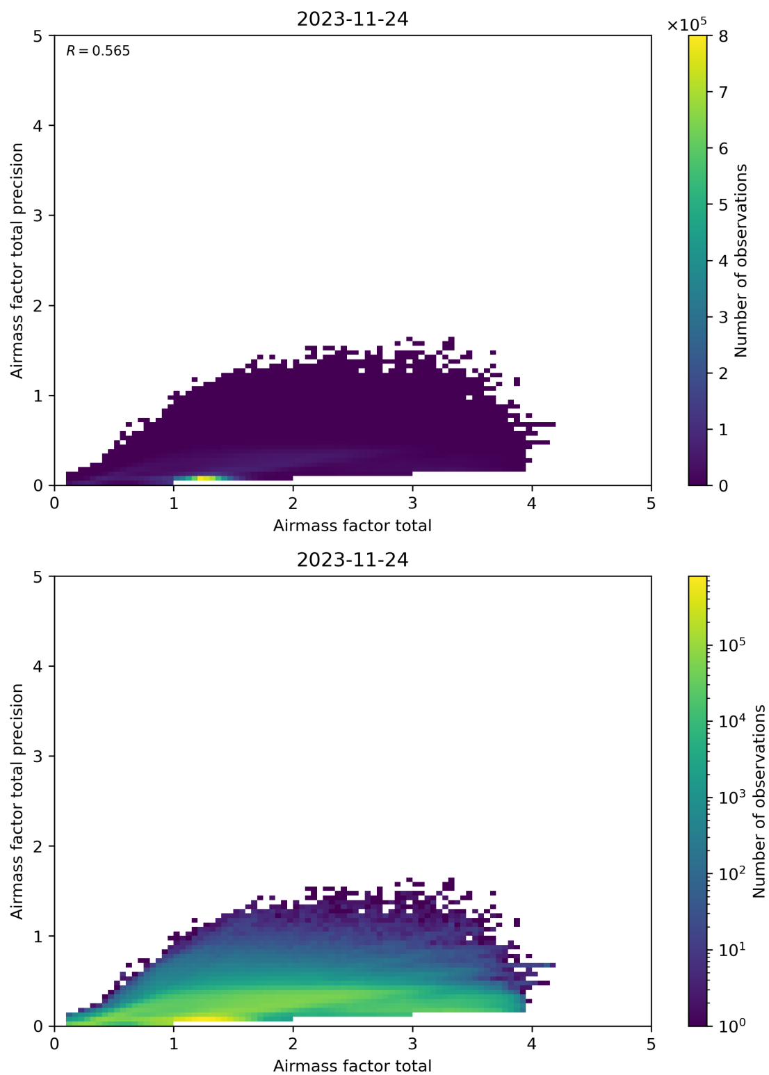
Figure 103: Scatter density plot of “Airmass factor total” against “Airmass factor total precision” for 2023-11-23 to 2023-11-25.
