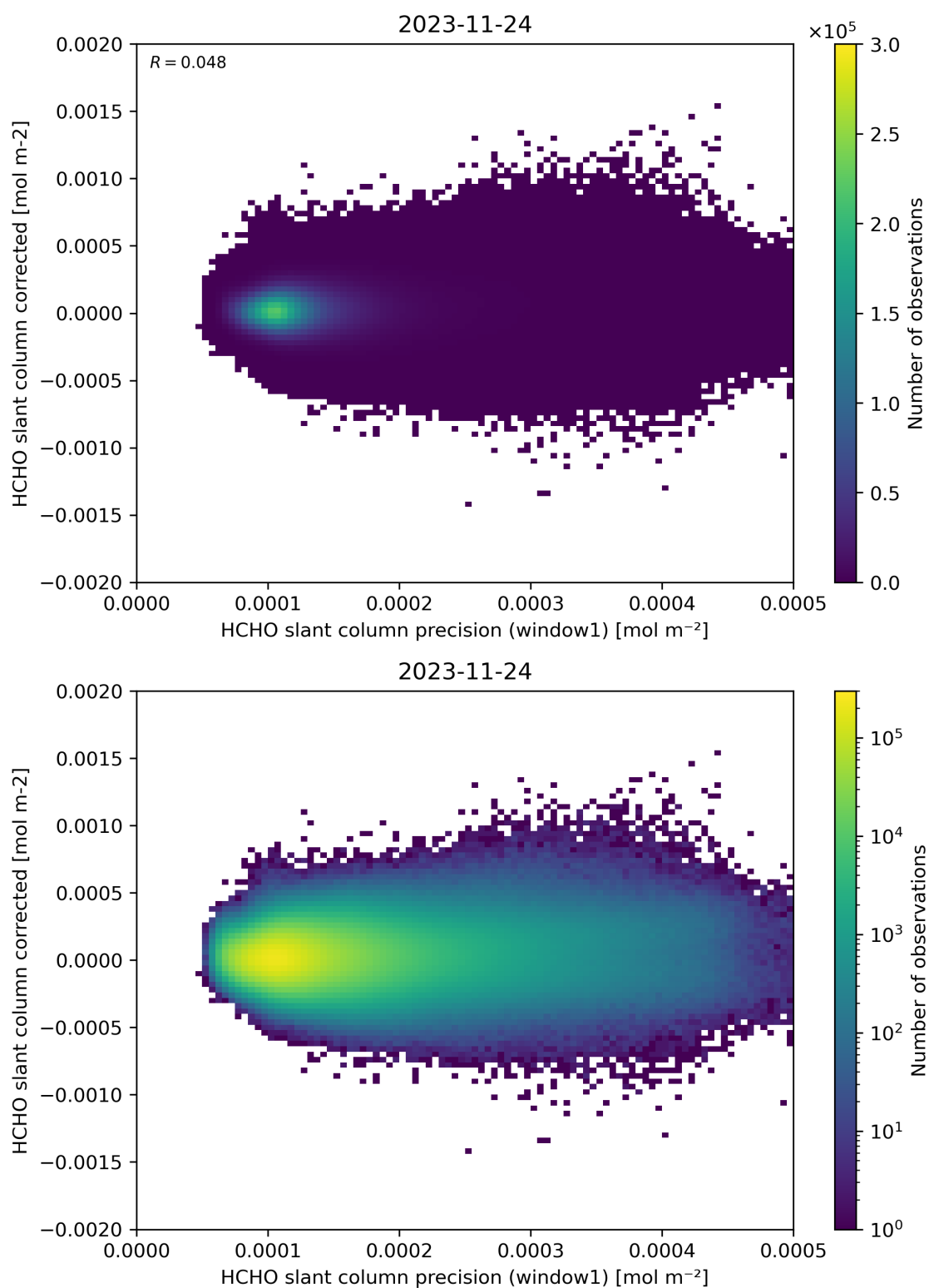
Figure 92: Scatter density plot of “HCHO slant column precision (window1)” against “HCHO slant column corrected” for 2023-11-23 to 2023-11-25.
