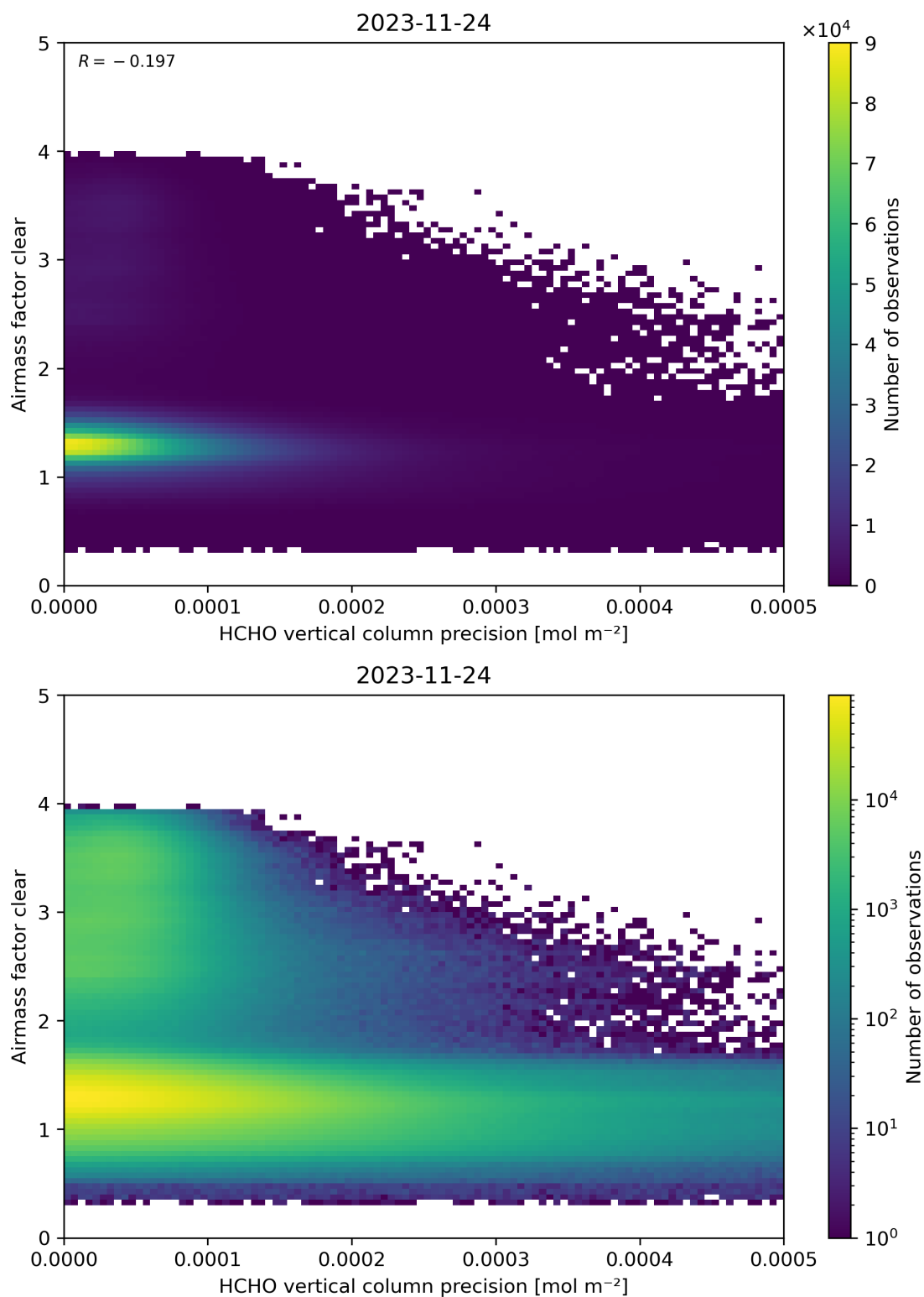
Figure 139: Scatter density plot of “HCHO vertical column precision” against “Airmass factor clear” for 2023-11-23 to 2023-11-25.
