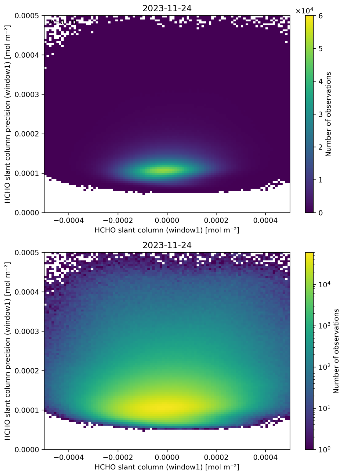
Figure 84: Scatter density plot of “HCHO slant column (window1)” against “HCHO slant column precision (window1)” for 2023-11-23 to 2023-11-25.
