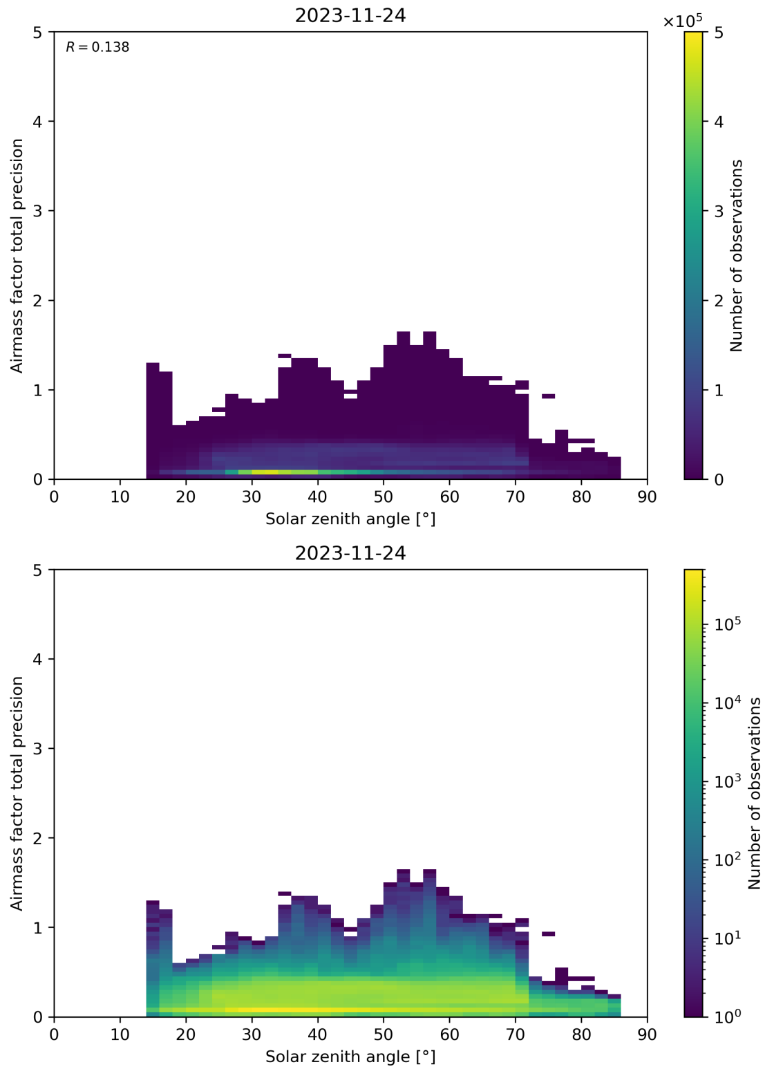
Figure 176: Scatter density plot of “Solar zenith angle” against “Airmass factor total precision” for 2023-11-23 to 2023-11-25.
