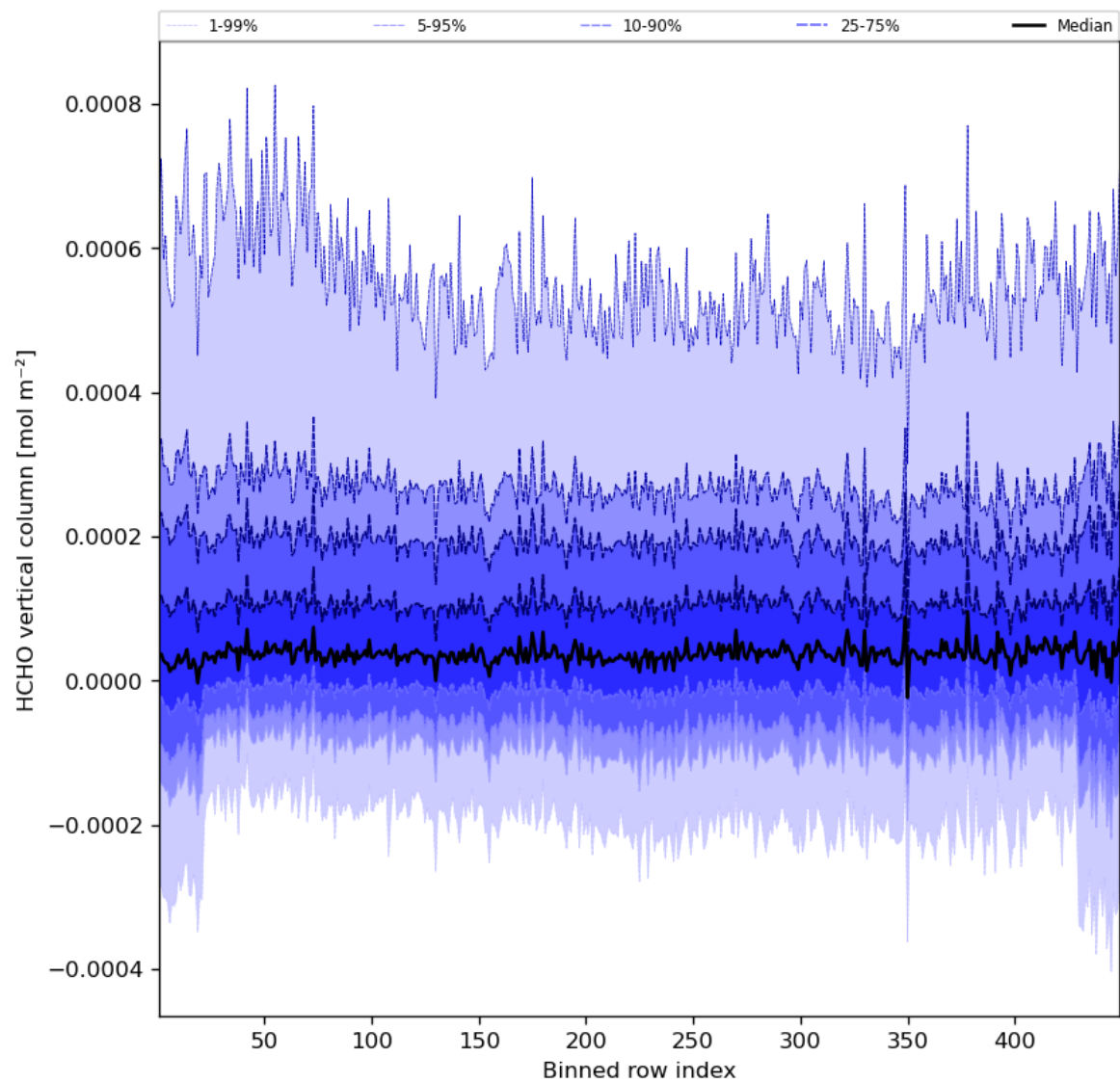
Figure 49: Along track statistics of “HCHO vertical column” for 2023-11-23 to 2023-11-25
