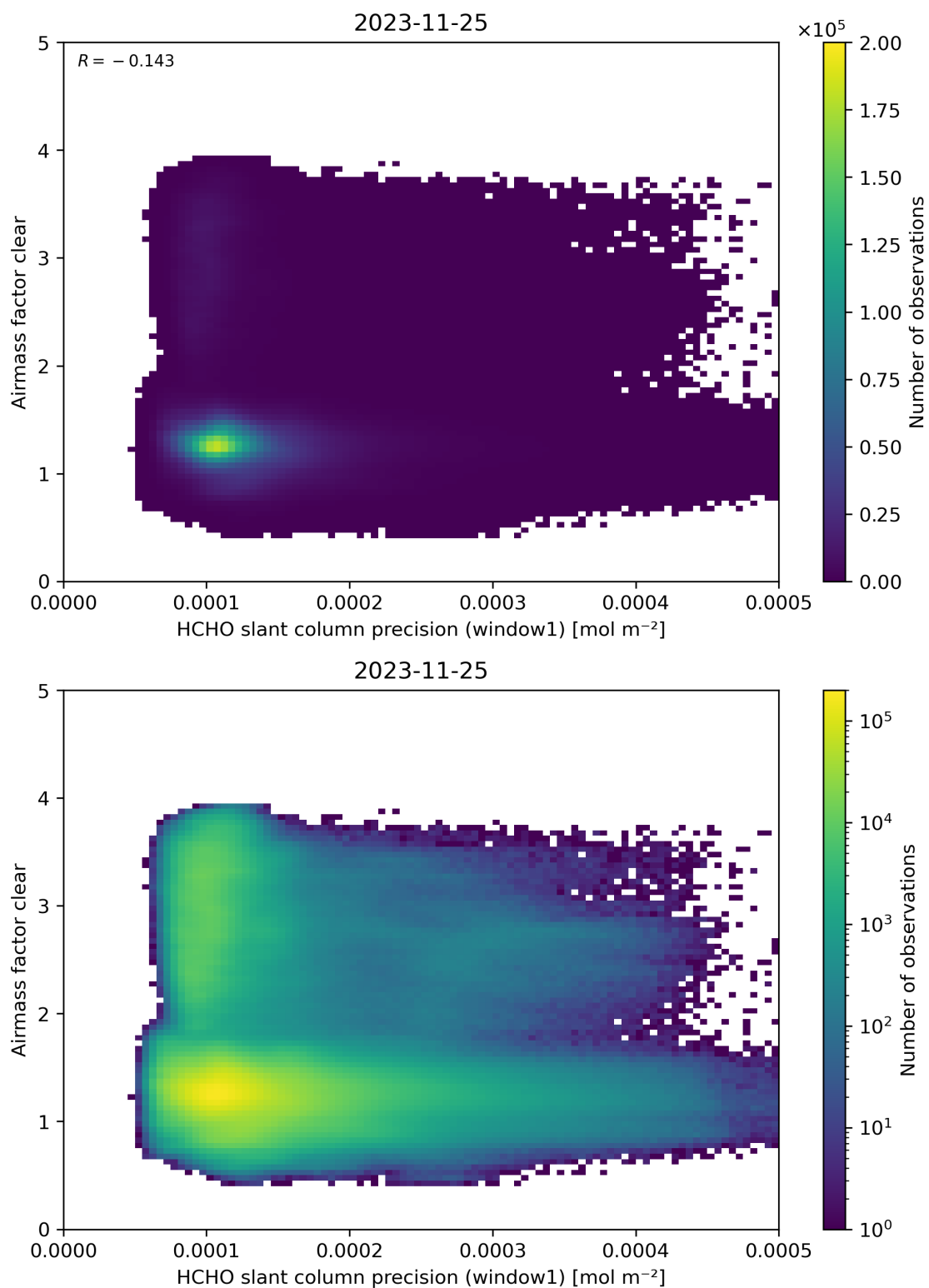
Figure 91: Scatter density plot of “HCHO slant column precision (window1)” against “Airmass factor clear” for 2023-11-24 to 2023-11-26.
