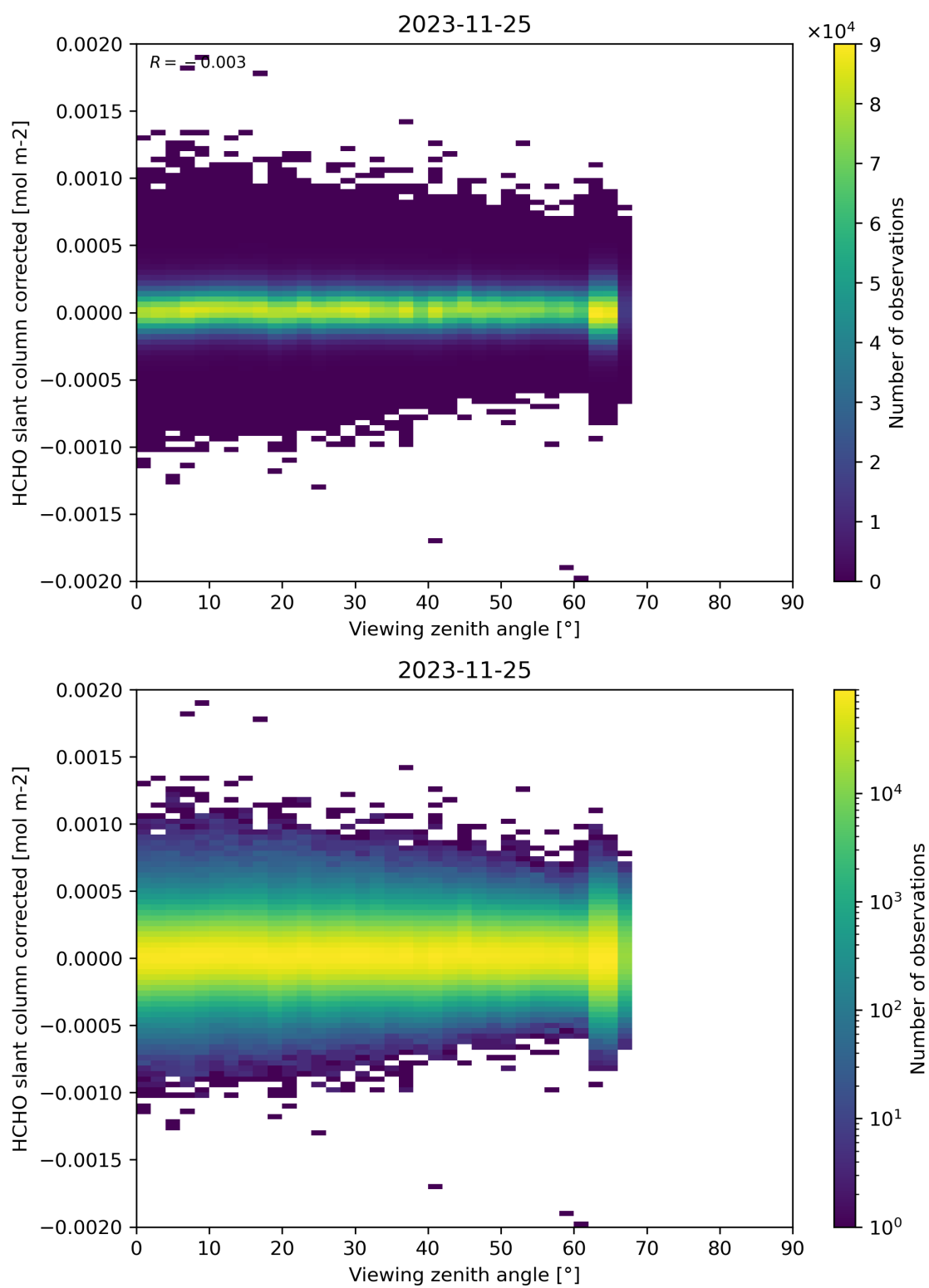
Figure 186: Scatter density plot of “Viewing zenith angle” against “HCHO slant column corrected” for 2023-11-24 to 2023-11-26.
