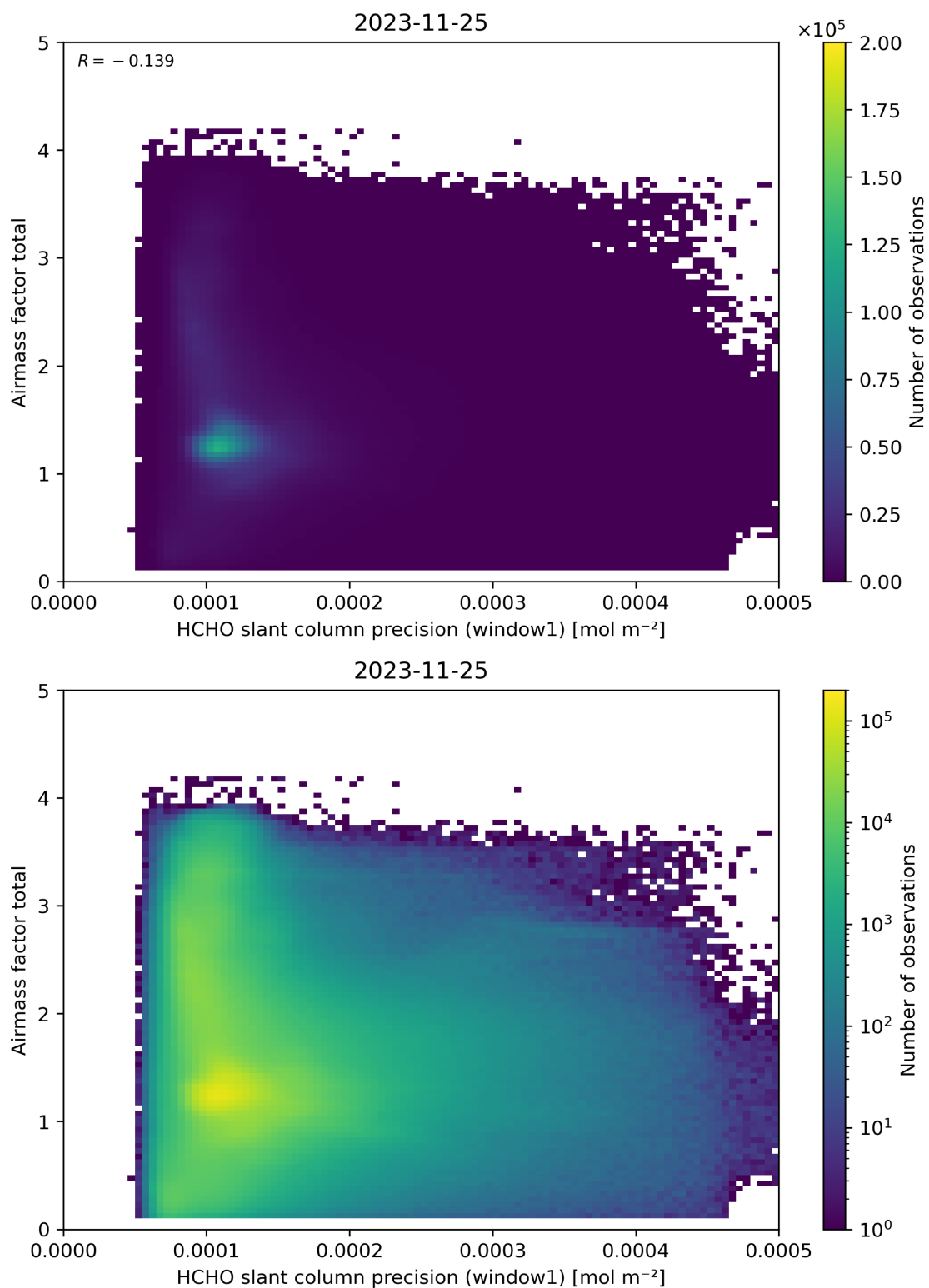
Figure 94: Scatter density plot of “HCHO slant column precision (window1)” against “Airmass factor total” for 2023-11-24 to 2023-11-26.
