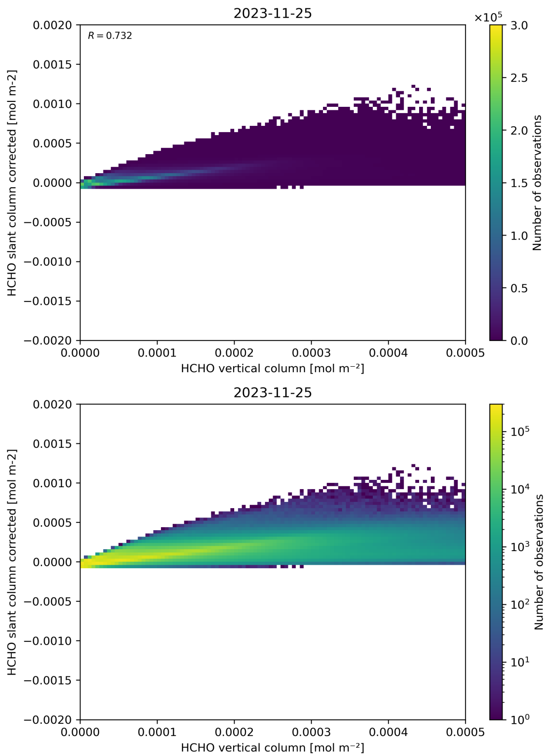
Figure 127: Scatter density plot of “HCHO vertical column” against “HCHO slant column corrected” for 2023-11-24 to 2023-11-26.
