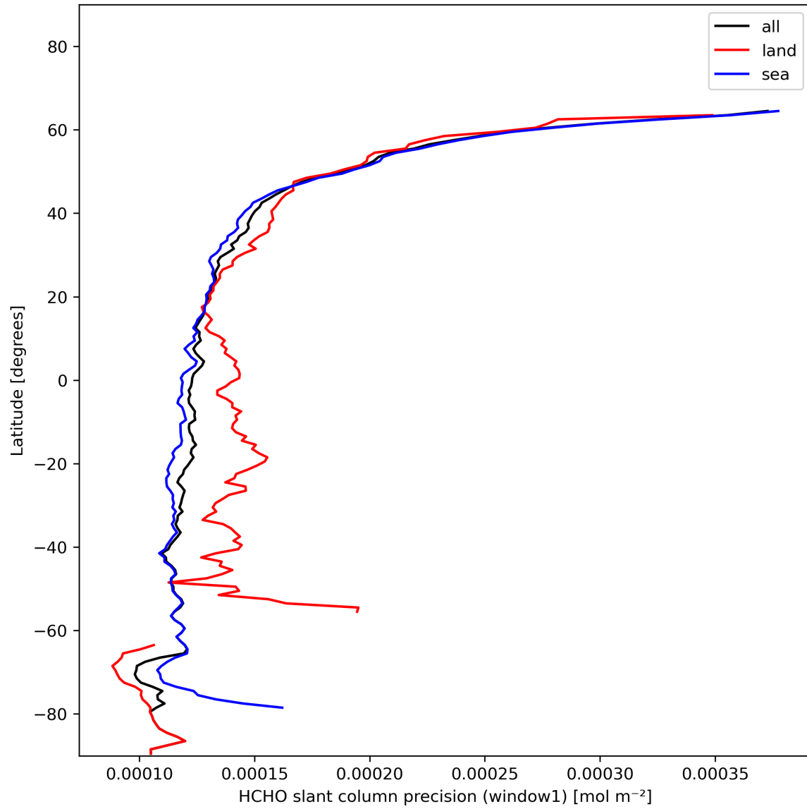
Figure 25: Zonal average of “HCHO slant column precision (window1)” for 2023-11-24 to 2023-11-26.
