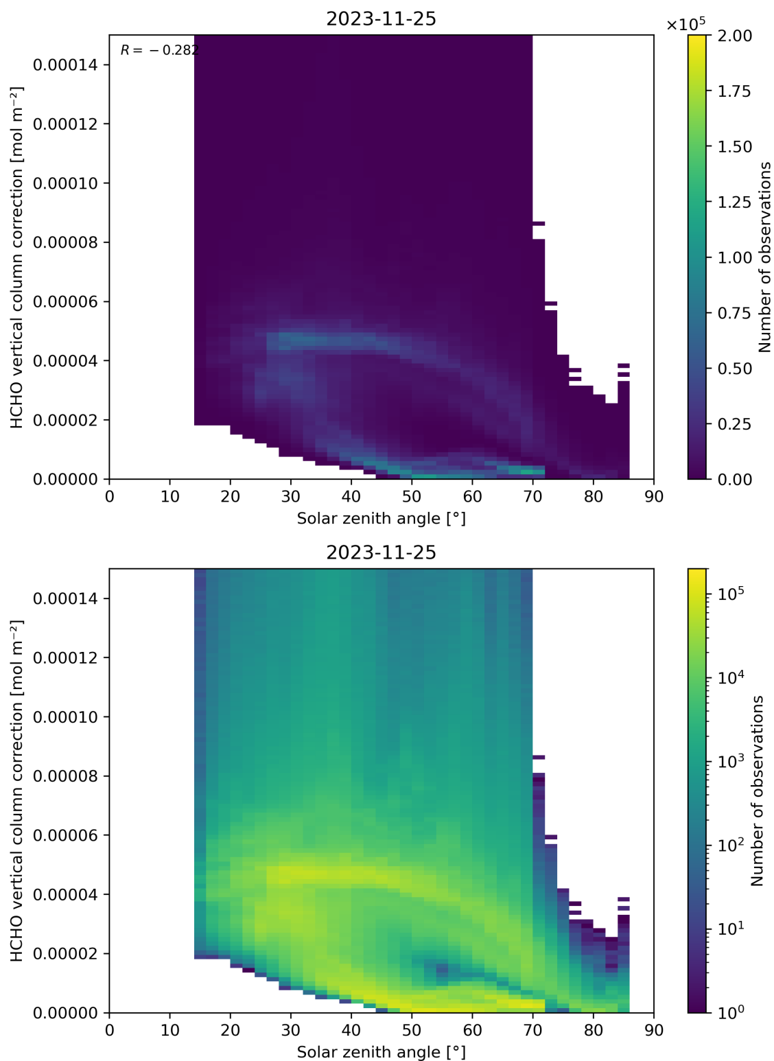
Figure 178: Scatter density plot of “Solar zenith angle” against “HCHO vertical column correction” for 2023-11-24 to 2023-11-26.
