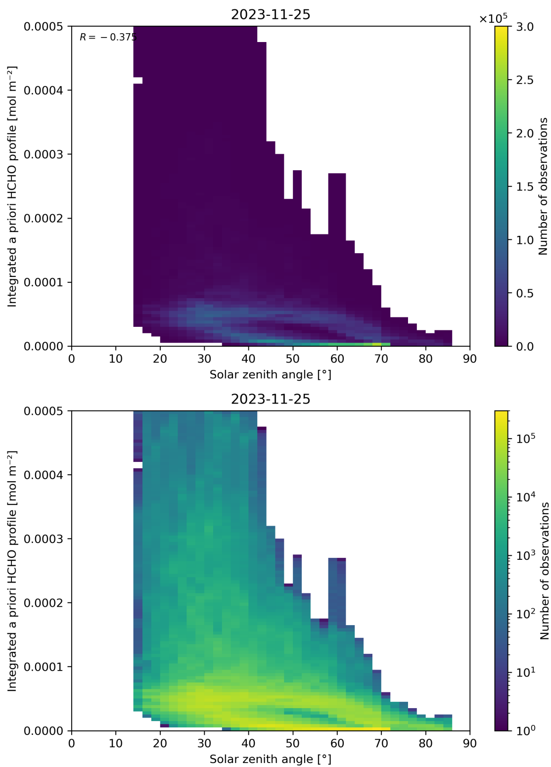
Figure 180: Scatter density plot of “Solar zenith angle” against “Integrated a priori HCHO profile” for 2023-11-24 to 2023-11-26.
