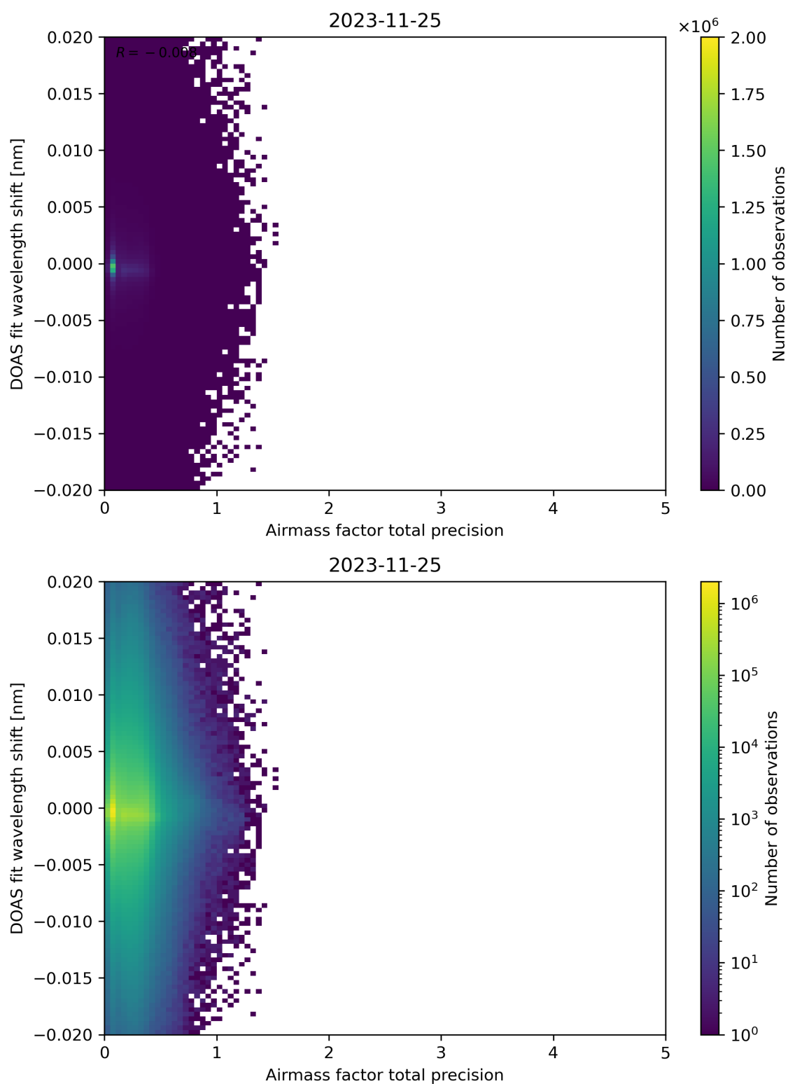
Figure 106: Scatter density plot of “Airmass factor total precision” against “DOAS fit wavelength shift” for 2023-11-24 to 2023-11-26.
