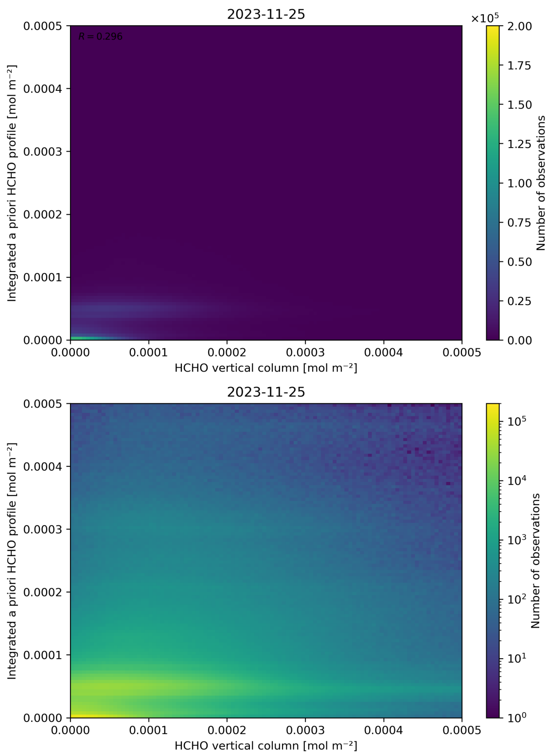
Figure 135: Scatter density plot of “HCHO vertical column” against “Integrated a priori HCHO profile” for 2023-11-24 to 2023-11-26.
