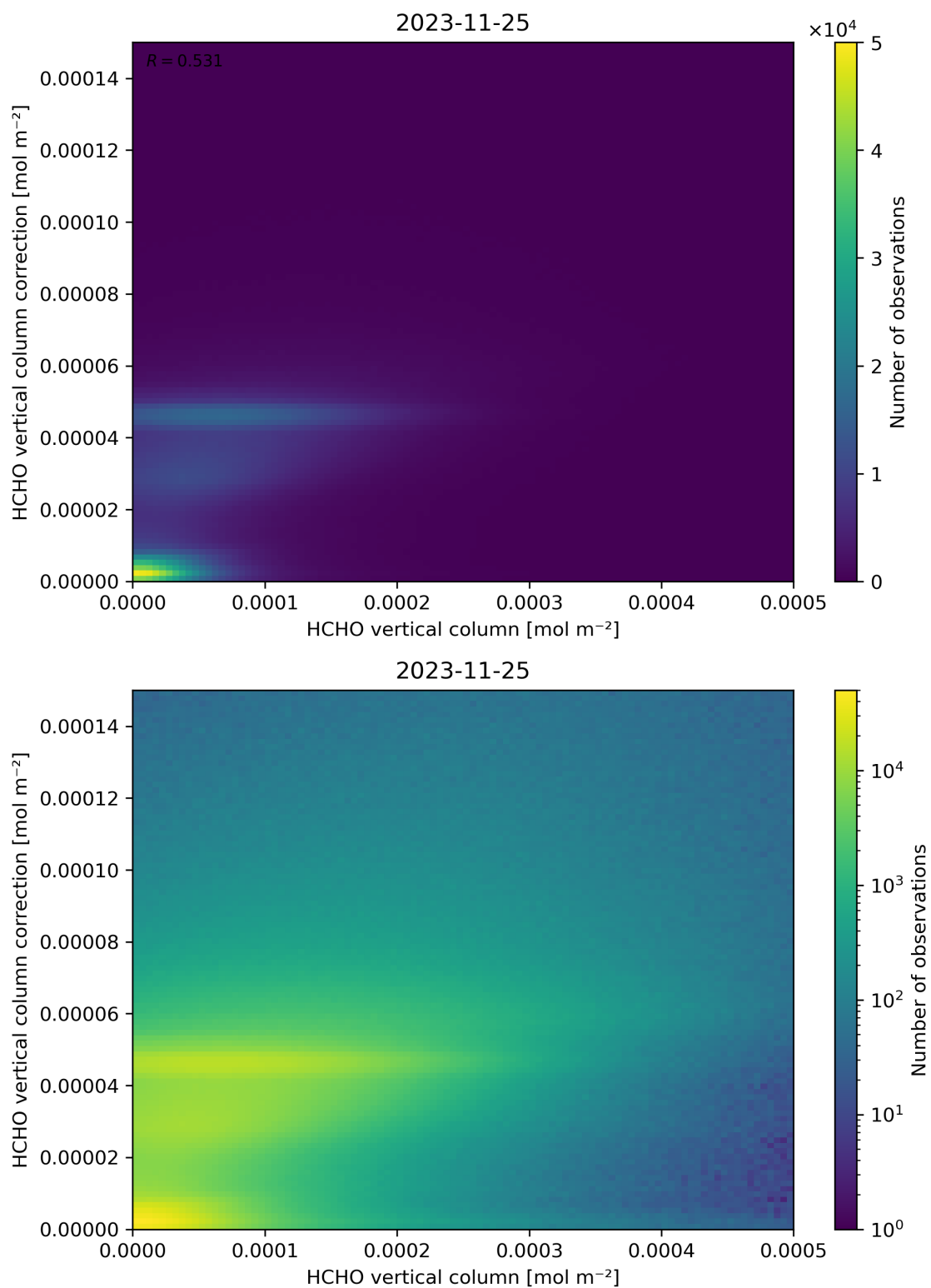
Figure 133: Scatter density plot of “HCHO vertical column” against “HCHO vertical column correction” for 2023-11-24 to 2023-11-26.
