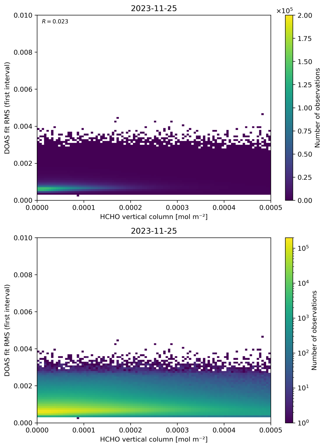
Figure 123: Scatter density plot of “HCHO vertical column” against “DOAS fit RMS (first interval)” for 2023-11-24 to 2023-11-26.
