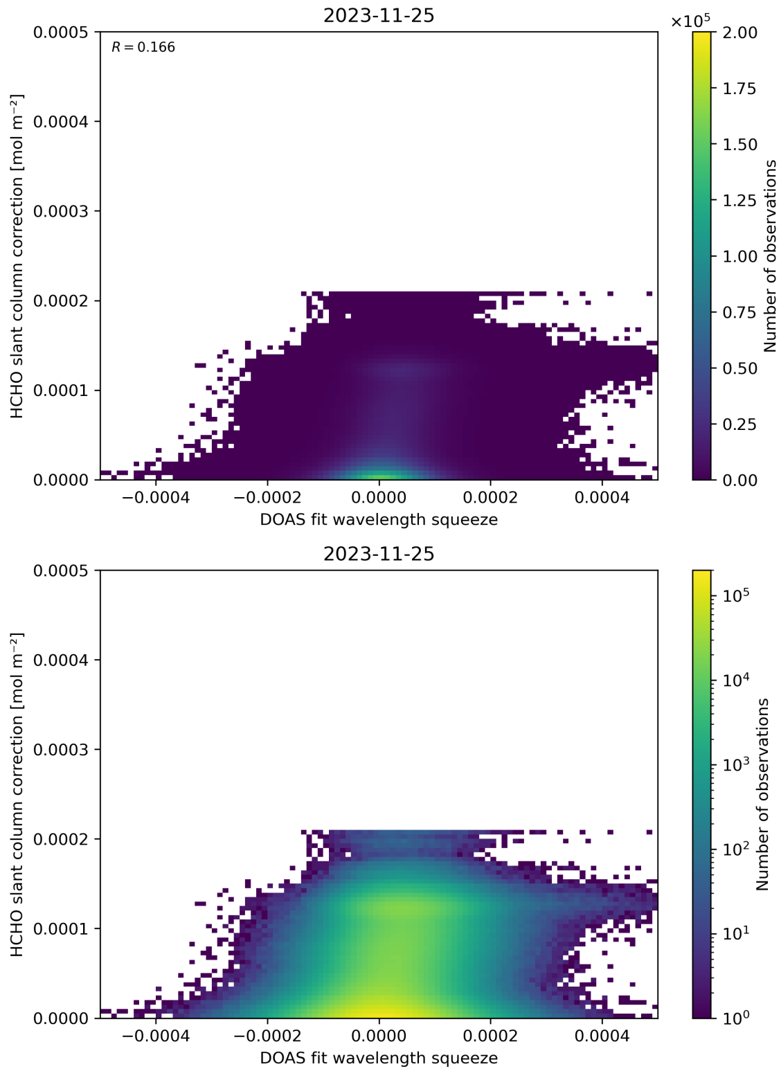
Figure 70: Scatter density plot of “DOAS fit wavelength squeeze” against “HCHO slant column correction” for 2023-11-24 to 2023-11-26.
