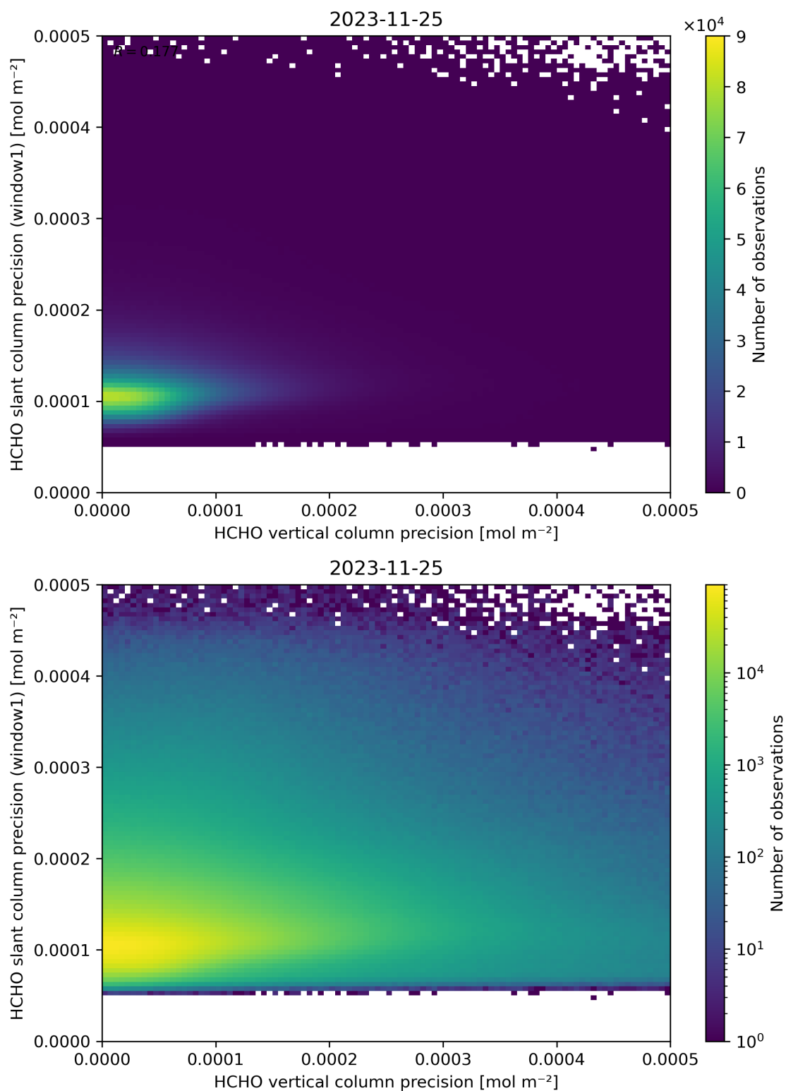
Figure 143: Scatter density plot of “HCHO vertical column precision” against “HCHO slant column precision (window1)” for 2023-11-24 to 2023-11-26.
