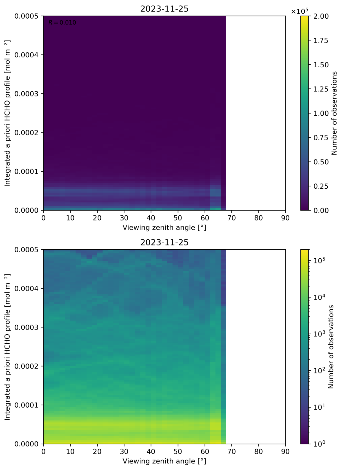
Figure 195: Scatter density plot of “Viewing zenith angle” against “Integrated a priori HCHO profile” for 2023-11-24 to 2023-11-26.
