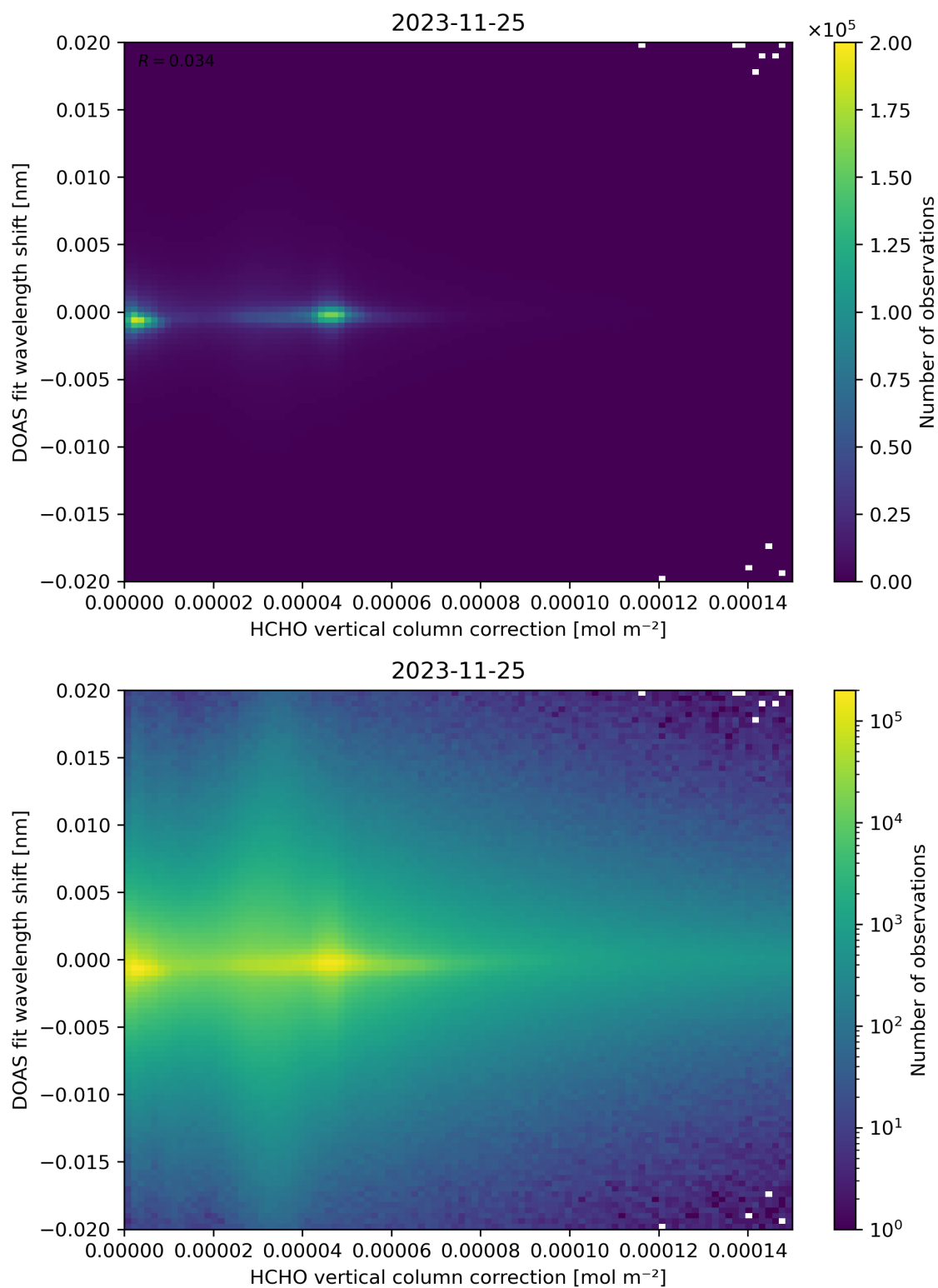
Figure 113: Scatter density plot of “HCHO vertical column correction” against “DOAS fit wavelength shift” for 2023-11-24 to 2023-11-26.
