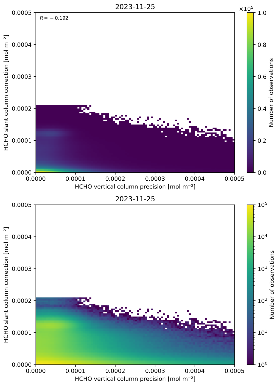
Figure 141: Scatter density plot of “HCHO vertical column precision” against “HCHO slant column correction” for 2023-11-24 to 2023-11-26.
