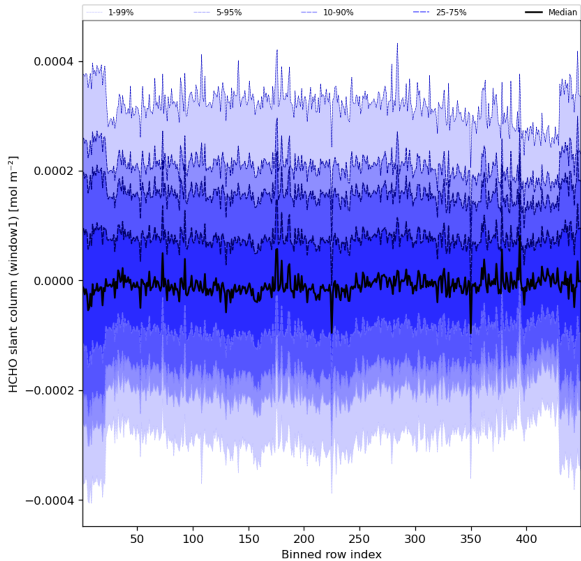
Figure 52: Along track statistics of “HCHO slant column (window1)” for 2023-11-24 to 2023-11-26
