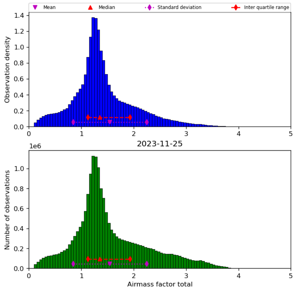
Figure 40: Histogram of “Airmass factor total” for 2023-11-24 to 2023-11-26
