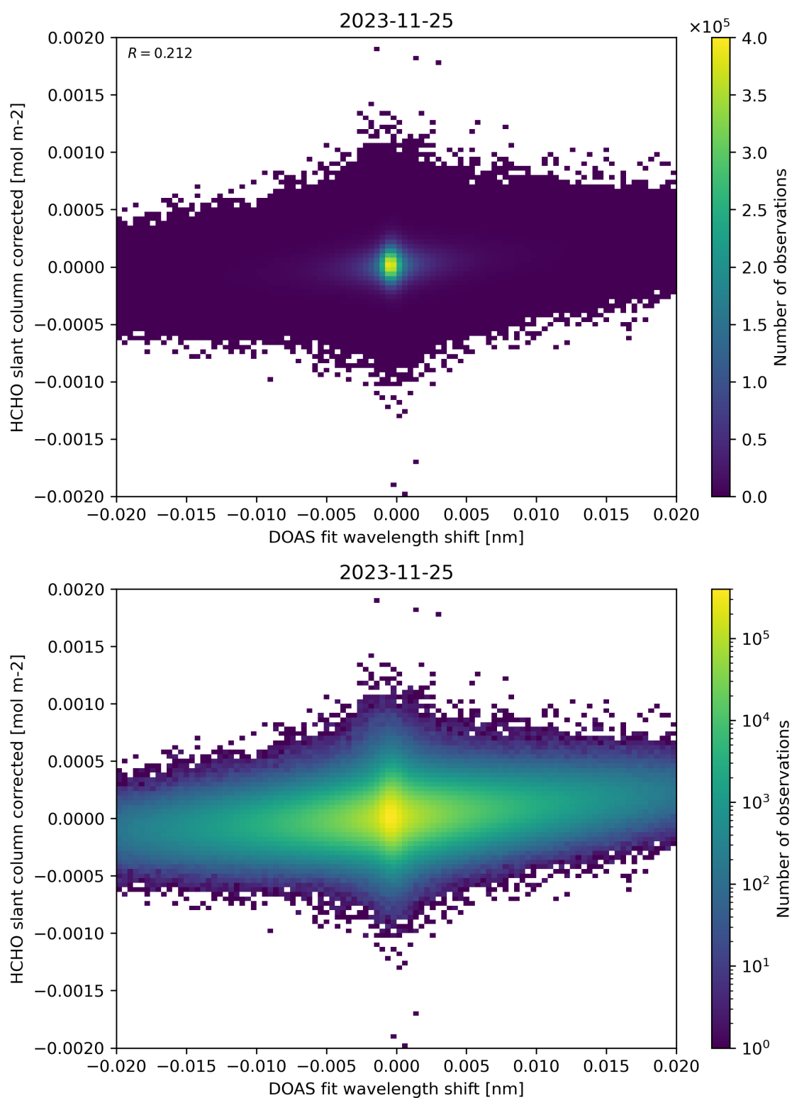
Figure 66: Scatter density plot of “DOAS fit wavelength shift” against “HCHO slant column corrected” for 2023-11-24 to 2023-11-26.
