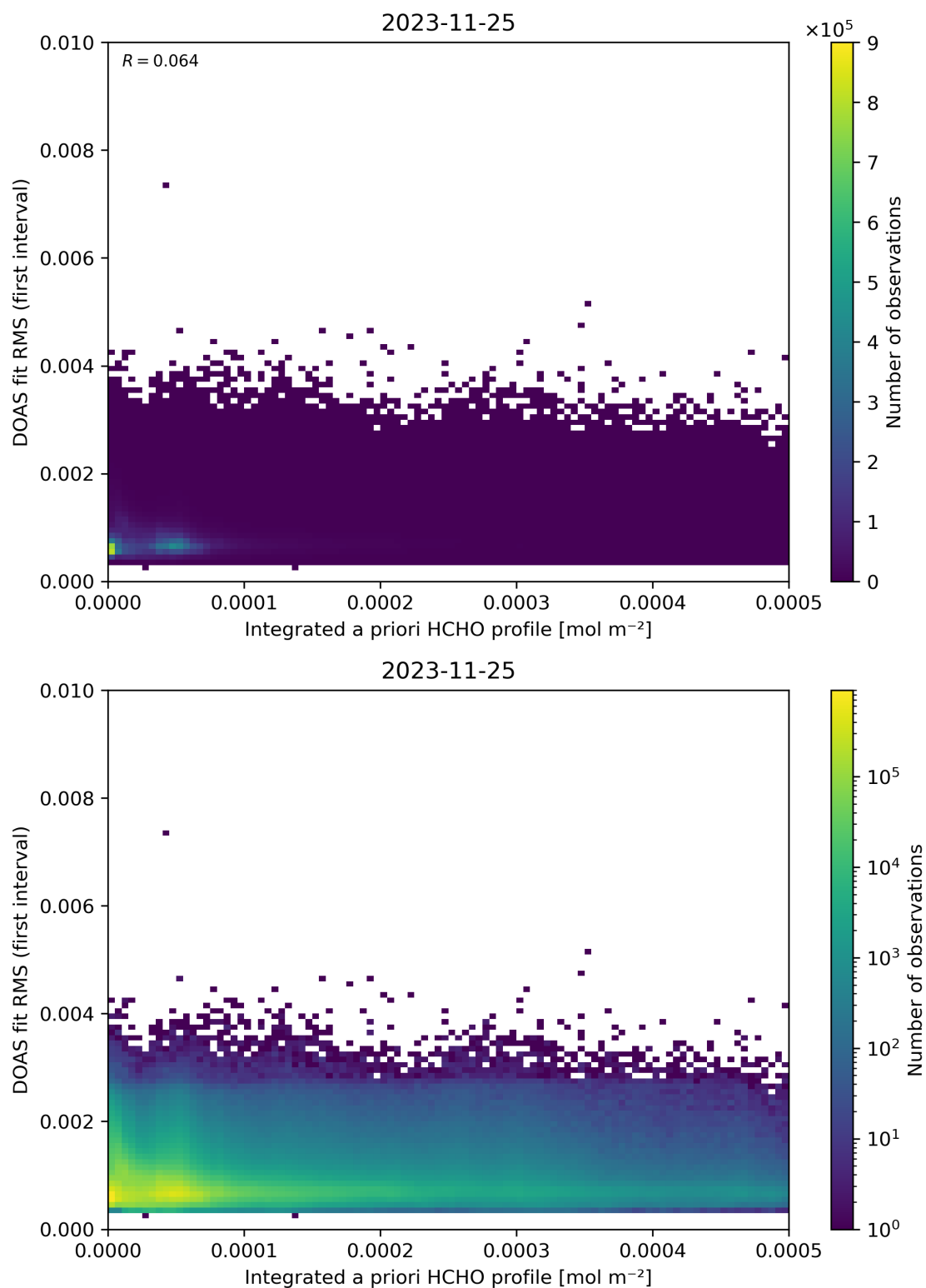
Figure 148: Scatter density plot of “Integrated a priori HCHO profile” against “DOAS fit RMS (first interval)” for 2023-11-24 to 2023-11-26.
