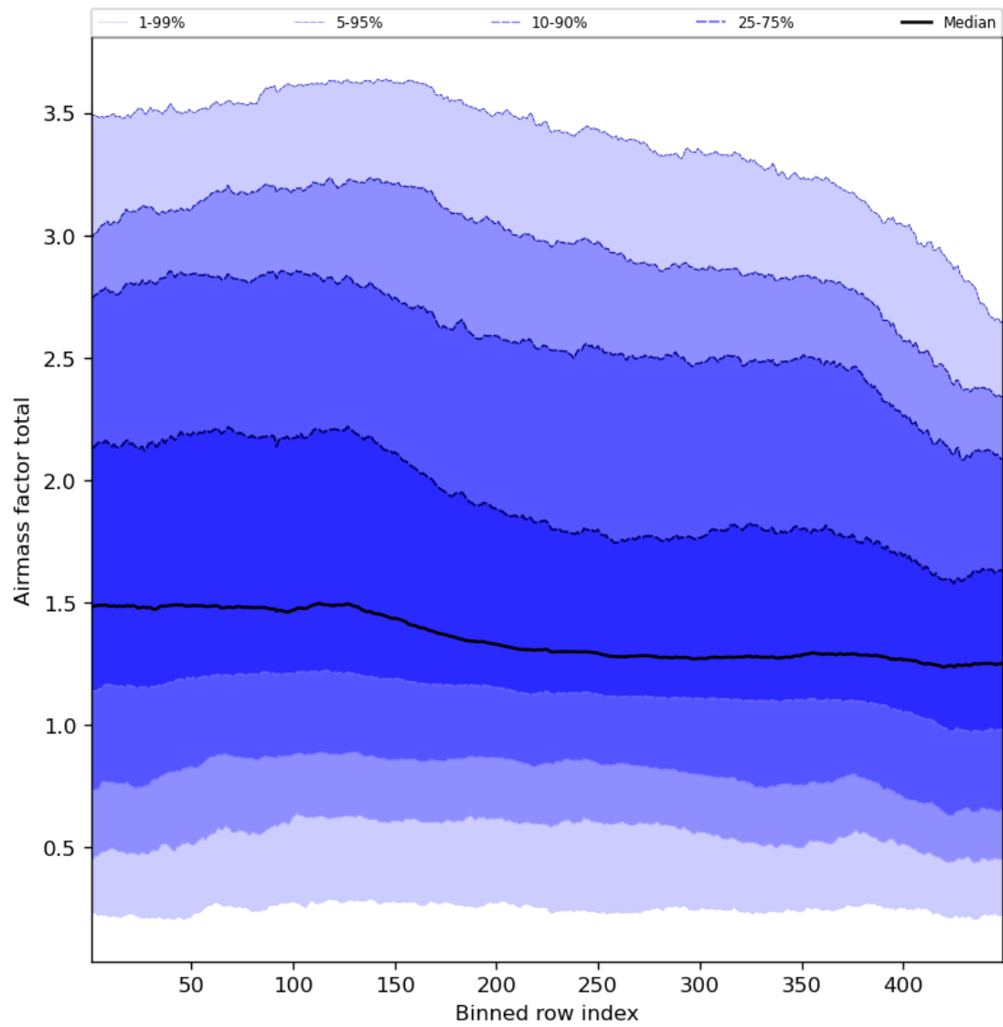
Figure 54: Along track statistics of “Airmass factor total” for 2023-11-24 to 2023-11-26
