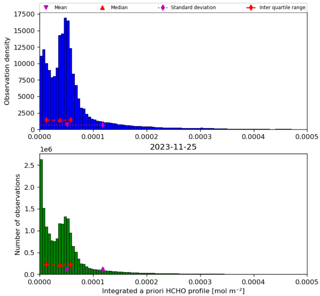
Figure 43: Histogram of “Integrated a priori HCHO profile” for 2023-11-24 to 2023-11-26
