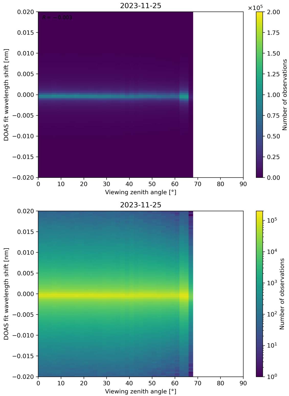
Figure 183: Scatter density plot of “Viewing zenith angle” against “DOAS fit wavelength shift” for 2023-11-24 to 2023-11-26.
