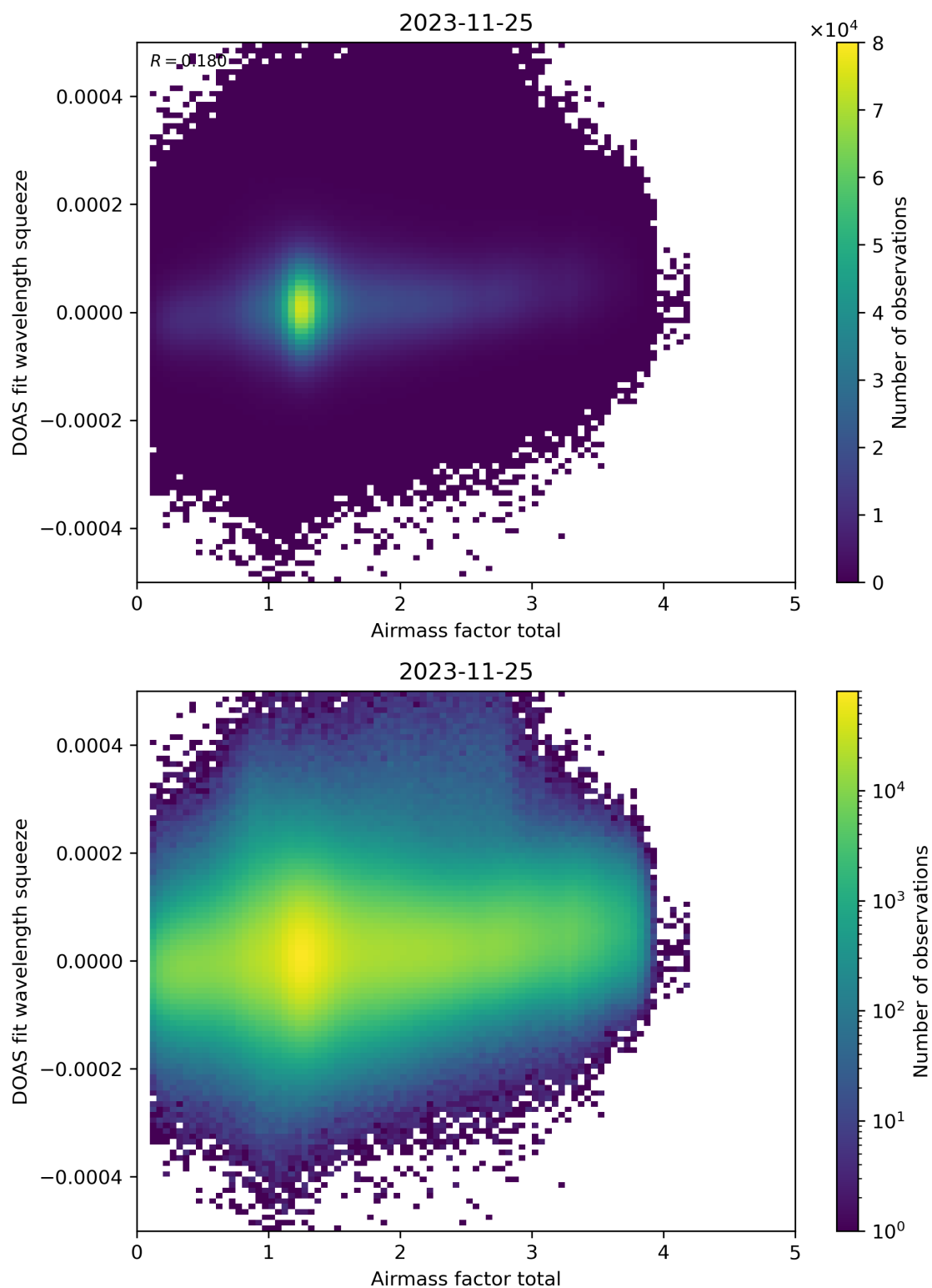
Figure 99: Scatter density plot of “Airmass factor total” against “DOAS fit wavelength squeeze” for 2023-11-24 to 2023-11-26.
