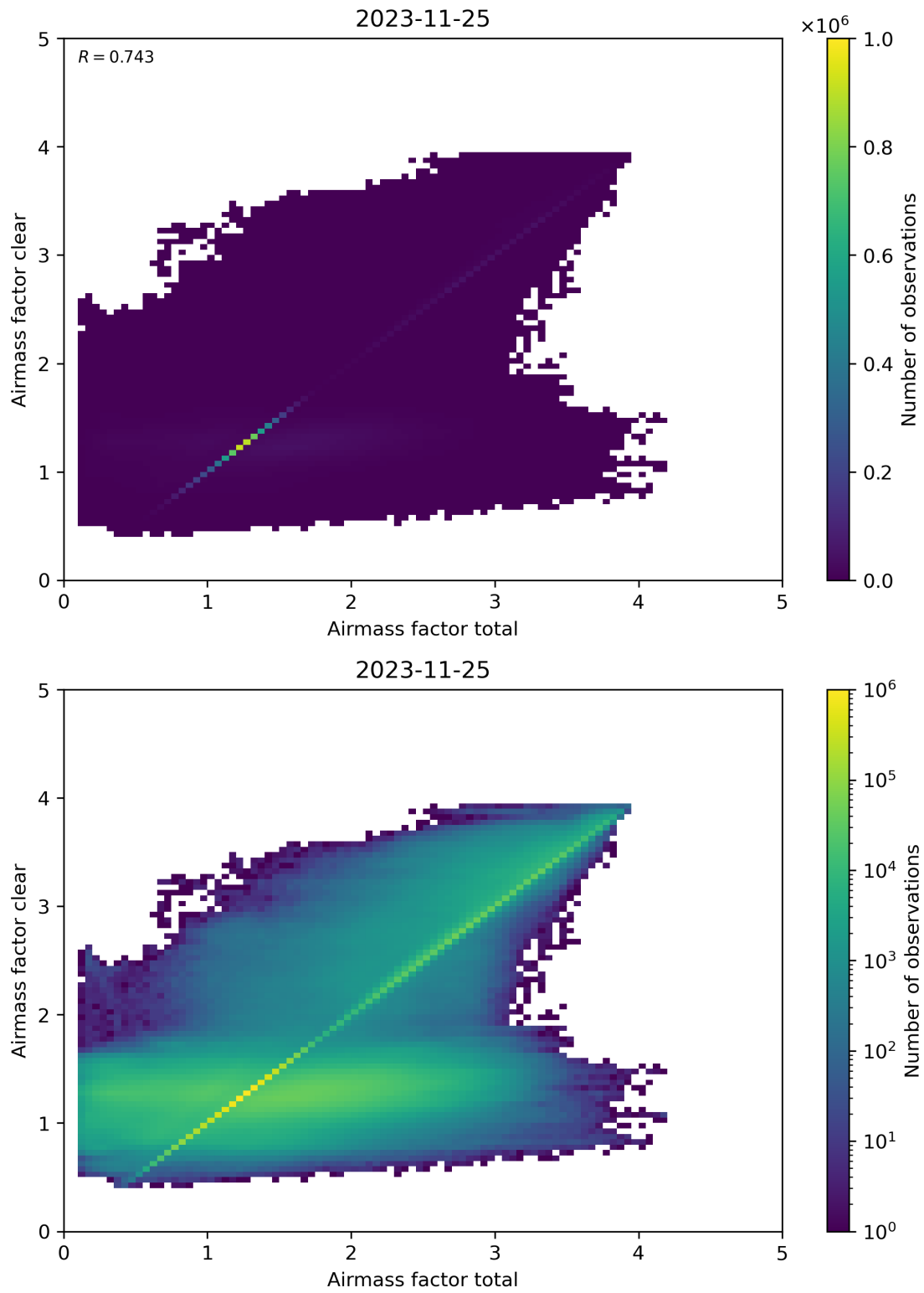
Figure 100: Scatter density plot of “Airmass factor total” against “Airmass factor clear” for 2023-11-24 to 2023-11-26.
