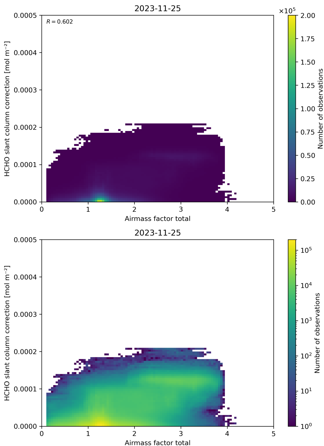
Figure 102: Scatter density plot of “Airmass factor total” against “HCHO slant column correction” for 2023-11-24 to 2023-11-26.
