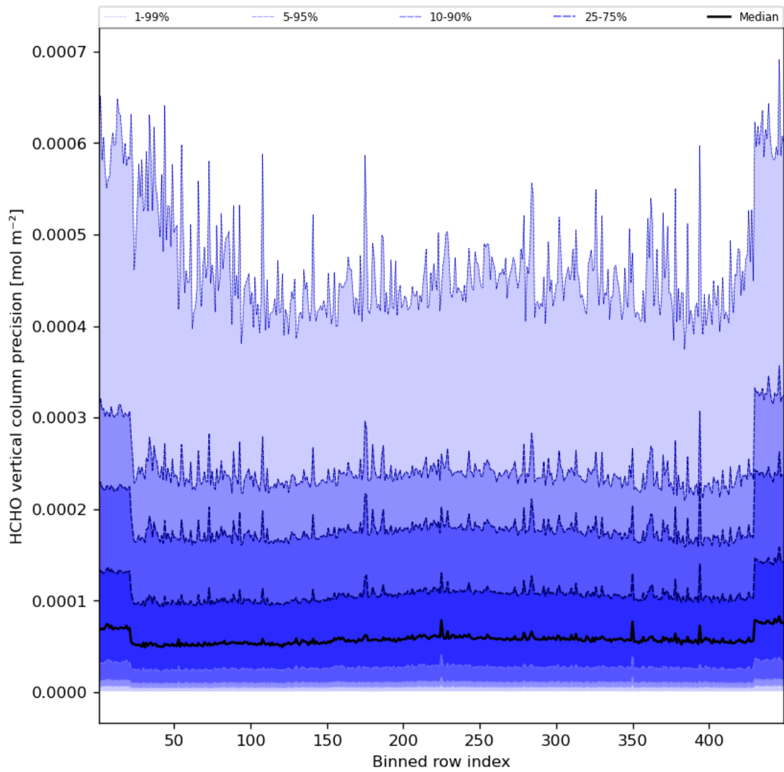
Figure 50: Along track statistics of “HCHO vertical column precision” for 2023-11-24 to 2023-11-26
