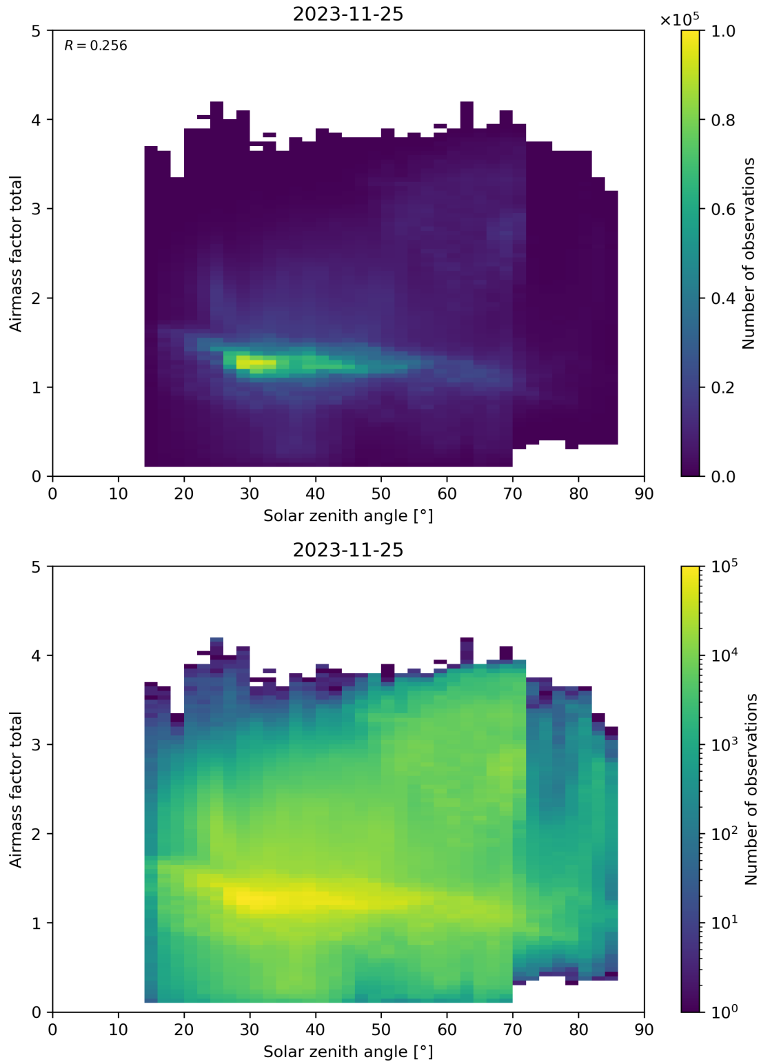
Figure 175: Scatter density plot of “Solar zenith angle” against “Airmass factor total” for 2023-11-24 to 2023-11-26.
