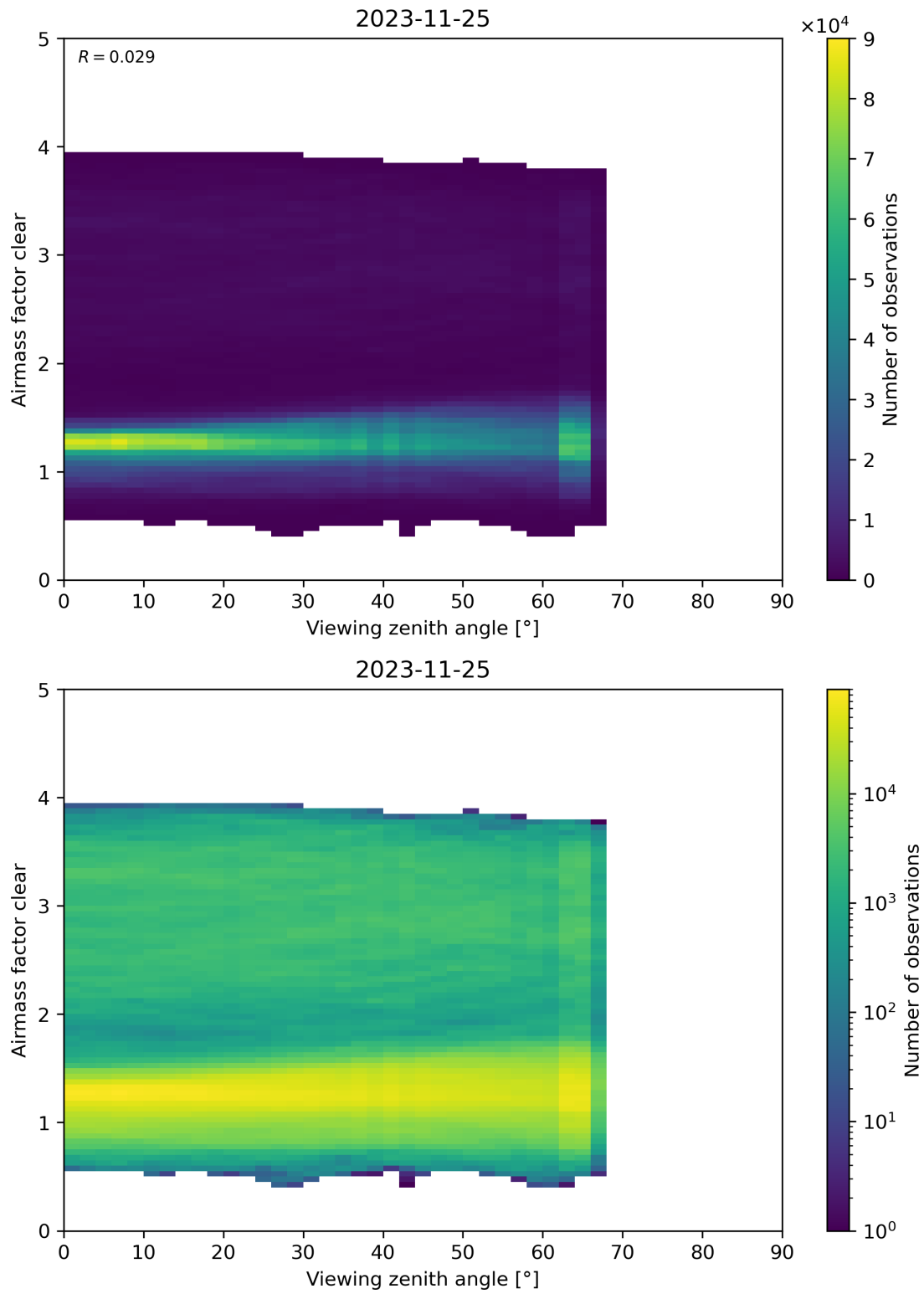
Figure 185: Scatter density plot of “Viewing zenith angle” against “Airmass factor clear” for 2023-11-24 to 2023-11-26.
