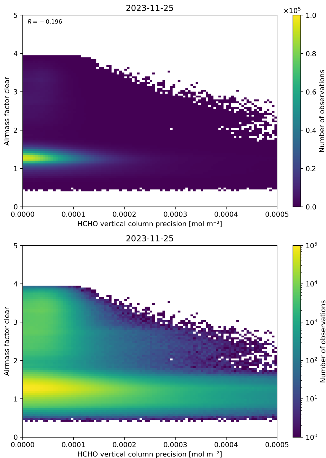
Figure 139: Scatter density plot of “HCHO vertical column precision” against “Airmass factor clear” for 2023-11-24 to 2023-11-26.
