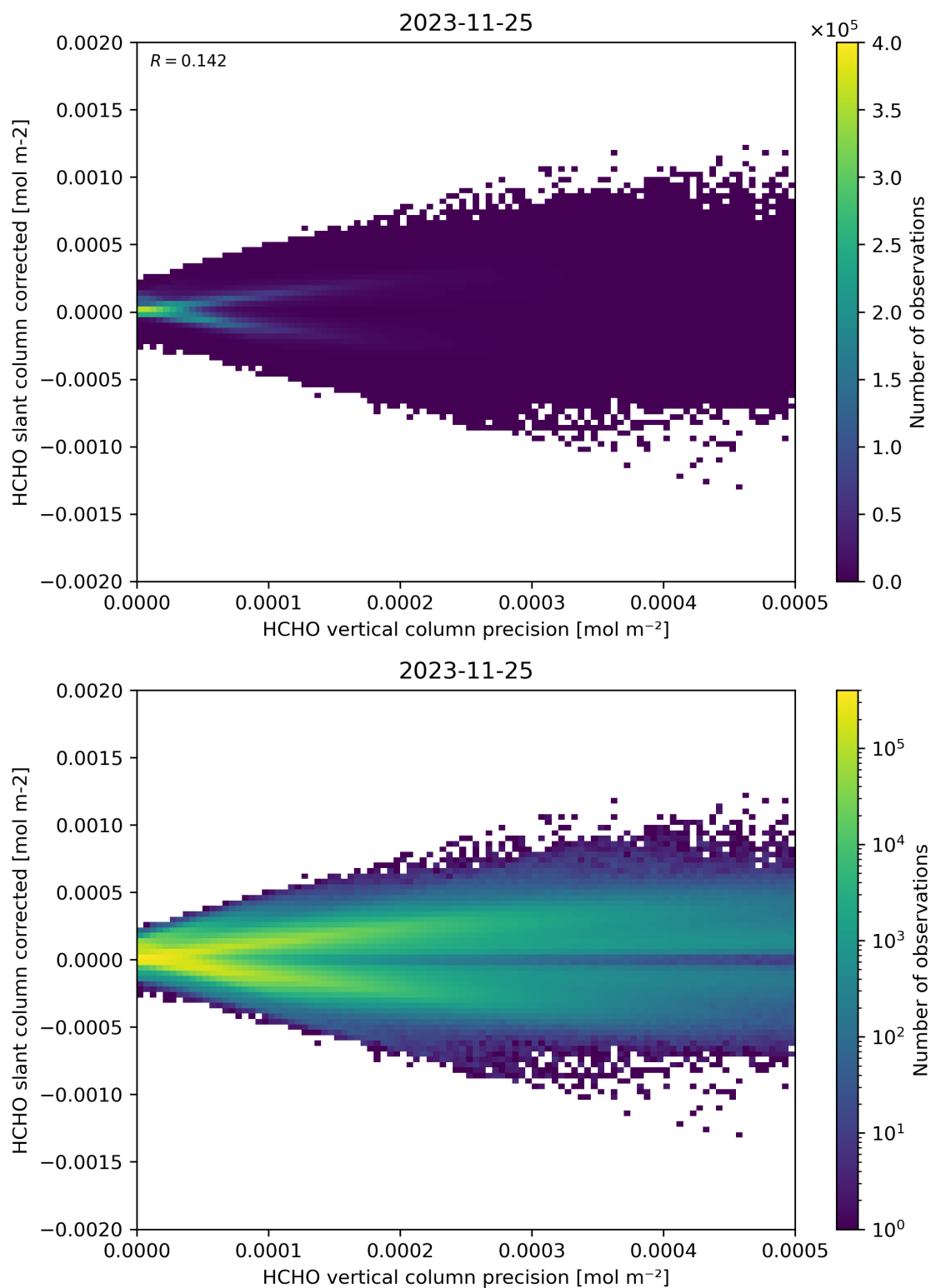
Figure 140: Scatter density plot of “HCHO vertical column precision” against “HCHO slant column corrected” for 2023-11-24 to 2023-11-26.
