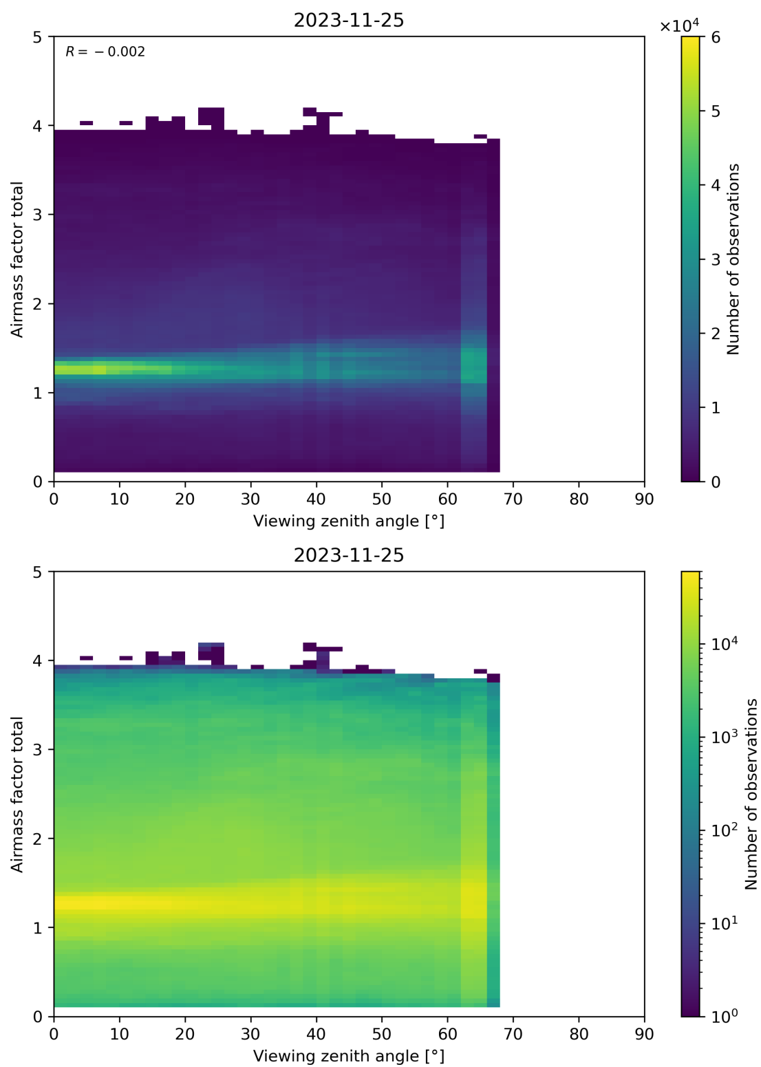
Figure 190: Scatter density plot of “Viewing zenith angle” against “Airmass factor total” for 2023-11-24 to 2023-11-26.
