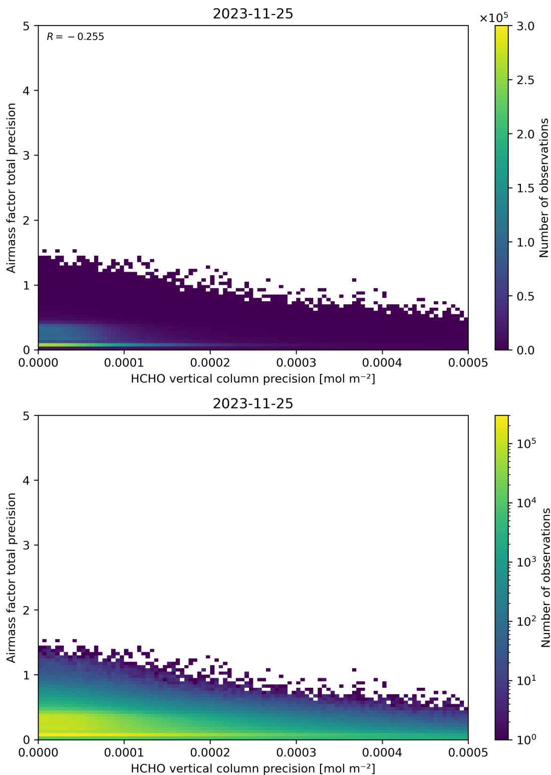
Figure 145: Scatter density plot of “HCHO vertical column precision” against “Airmass factor total precision” for 2023-11-24 to 2023-11-26.
