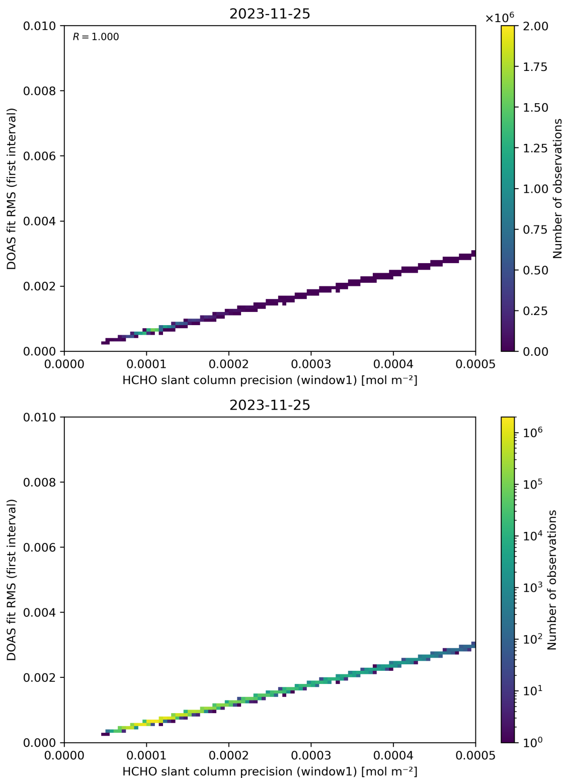
Figure 88: Scatter density plot of “HCHO slant column precision (window1)” against “DOAS fit RMS (first interval)” for 2023-11-24 to 2023-11-26.
