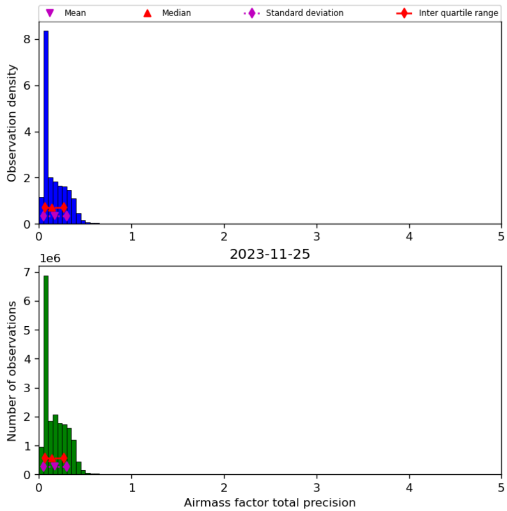
Figure 41: Histogram of “Airmass factor total precision” for 2023-11-24 to 2023-11-26
