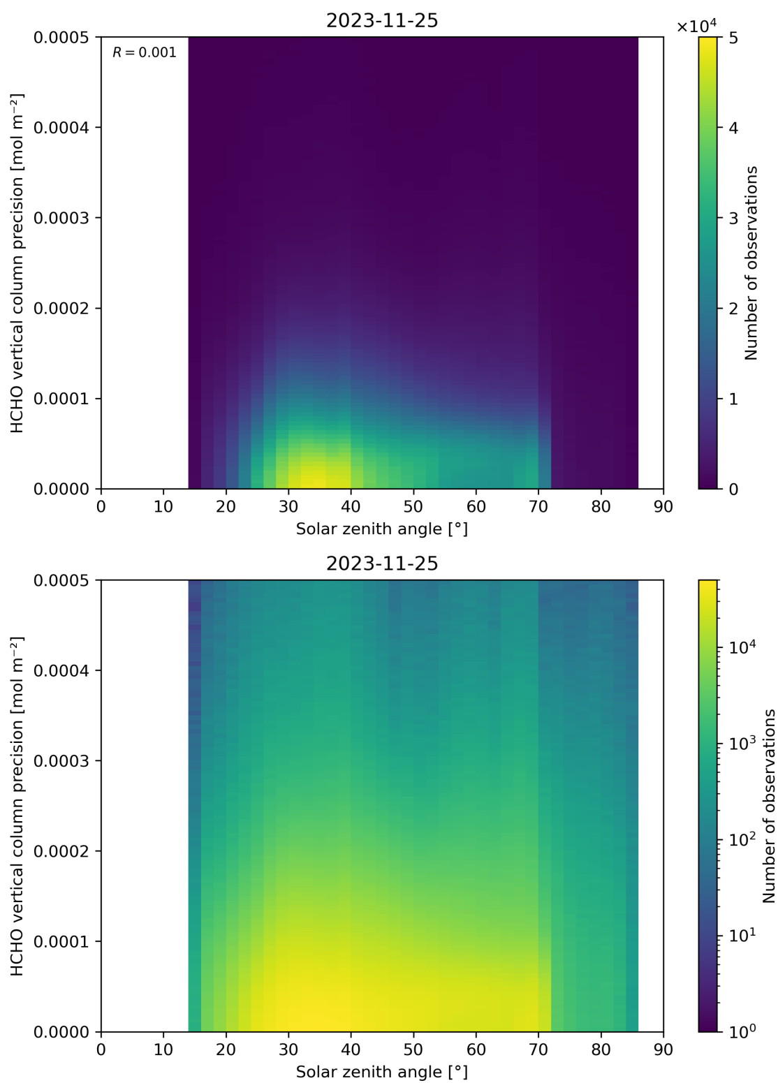
Figure 179: Scatter density plot of “Solar zenith angle” against “HCHO vertical column precision” for 2023-11-24 to 2023-11-26.
