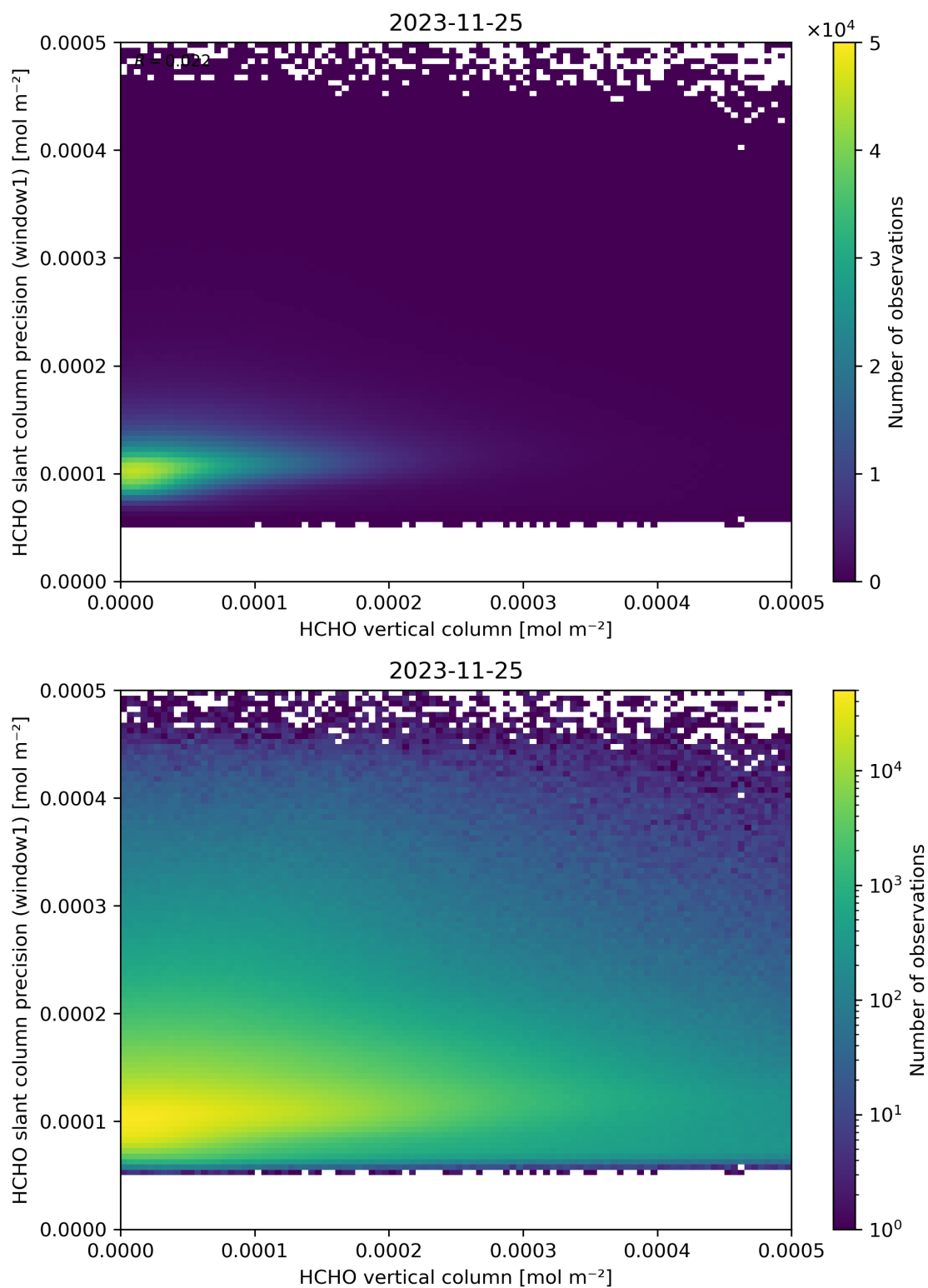
Figure 130: Scatter density plot of “HCHO vertical column” against “HCHO slant column precision (window1)” for 2023-11-24 to 2023-11-26.
