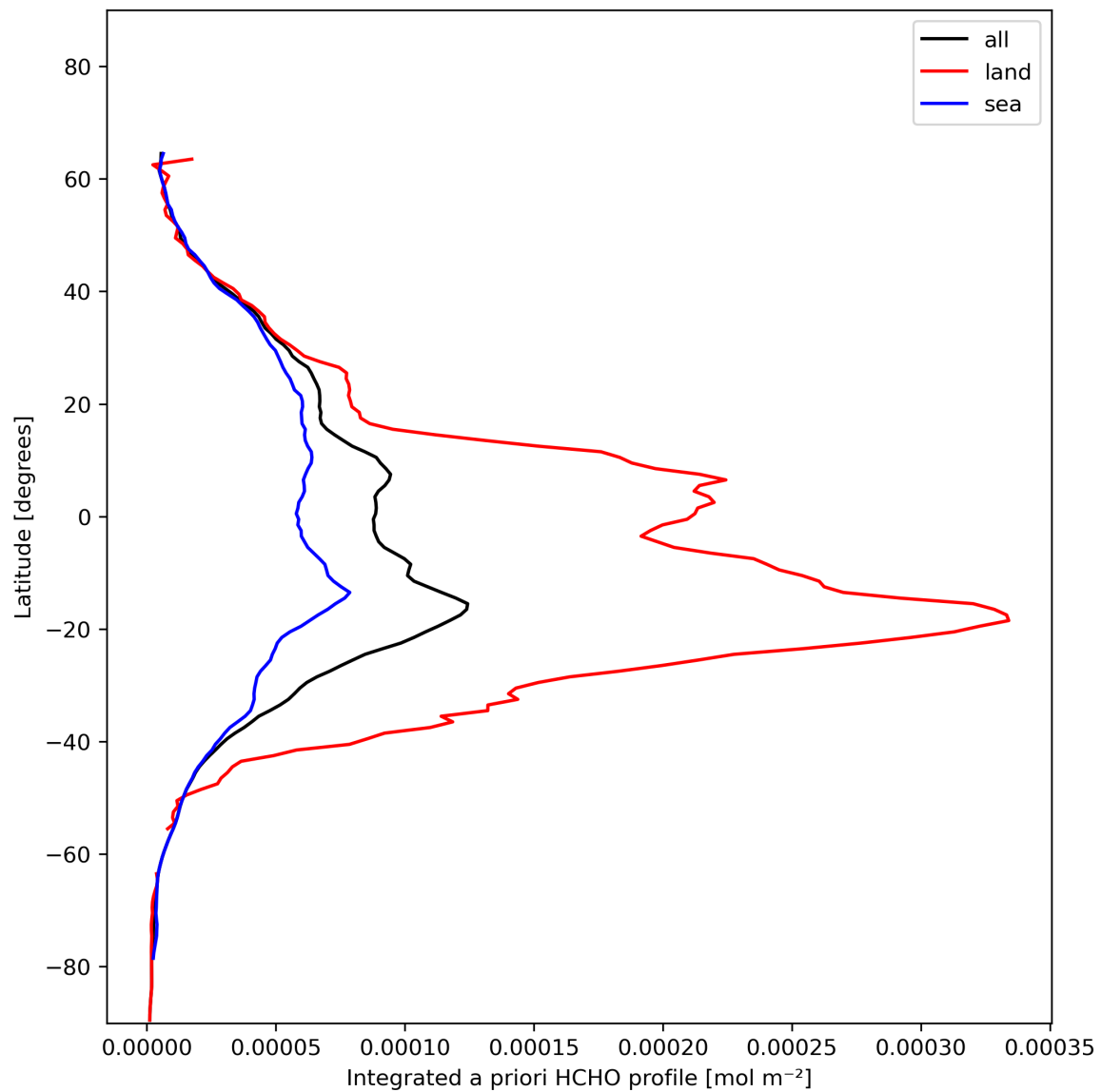
Figure 29: Zonal average of “Integrated a priori HCHO profile” for 2023-11-24 to 2023-11-26.
