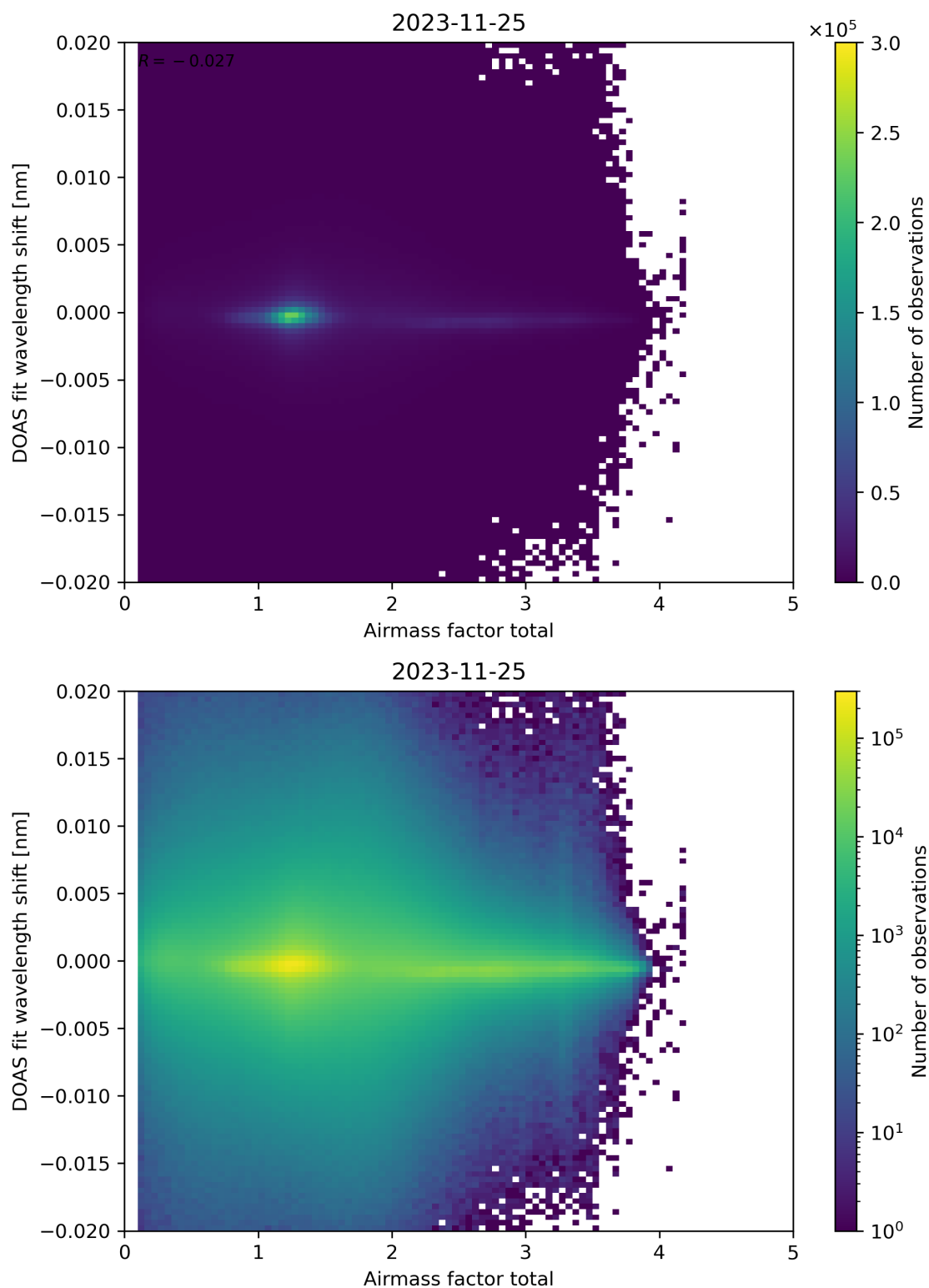
Figure 98: Scatter density plot of “Airmass factor total” against “DOAS fit wavelength shift” for 2023-11-24 to 2023-11-26.
