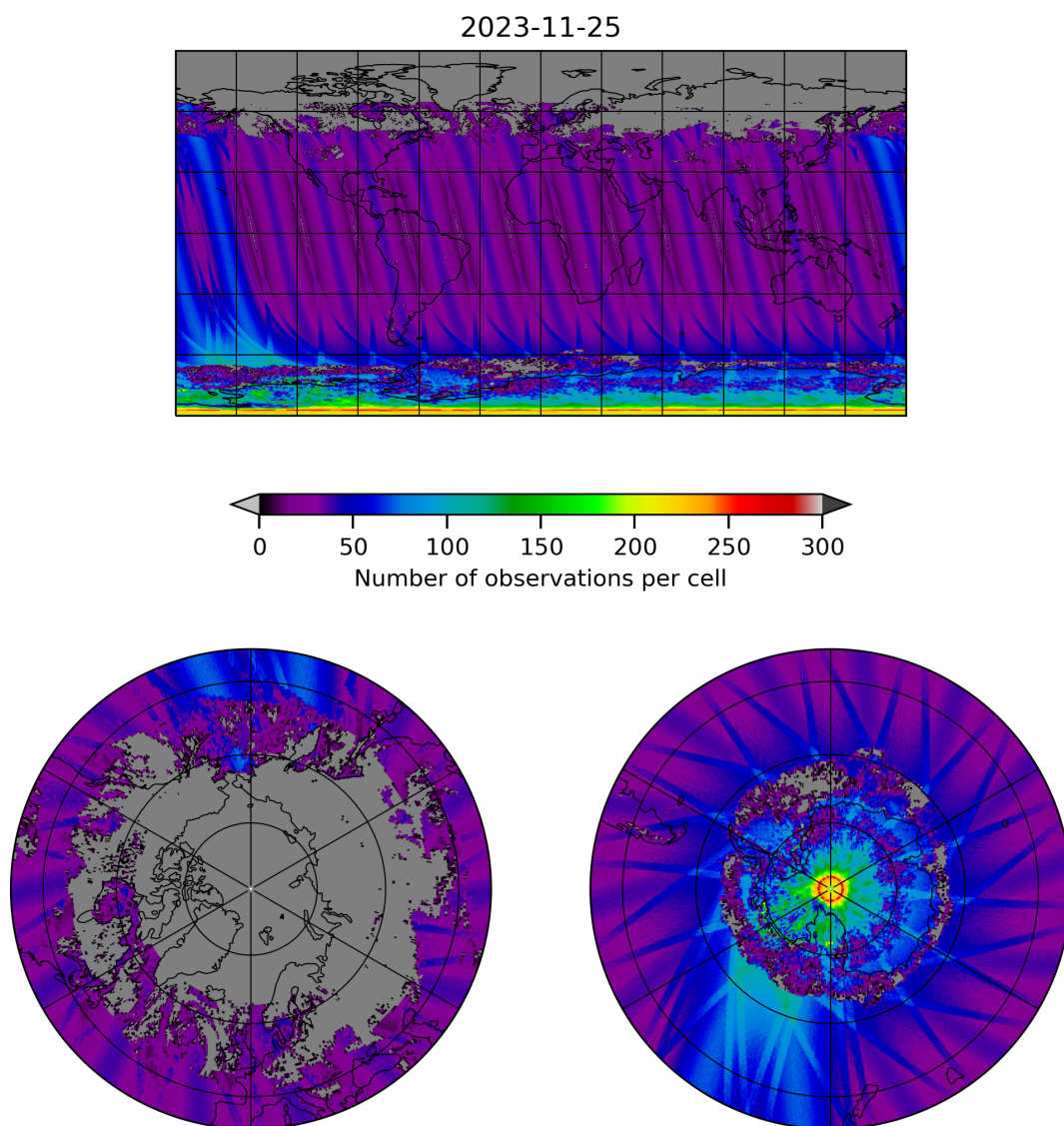
Figure 19: Map of the number of observations for 2023-11-24 to 2023-11-26
