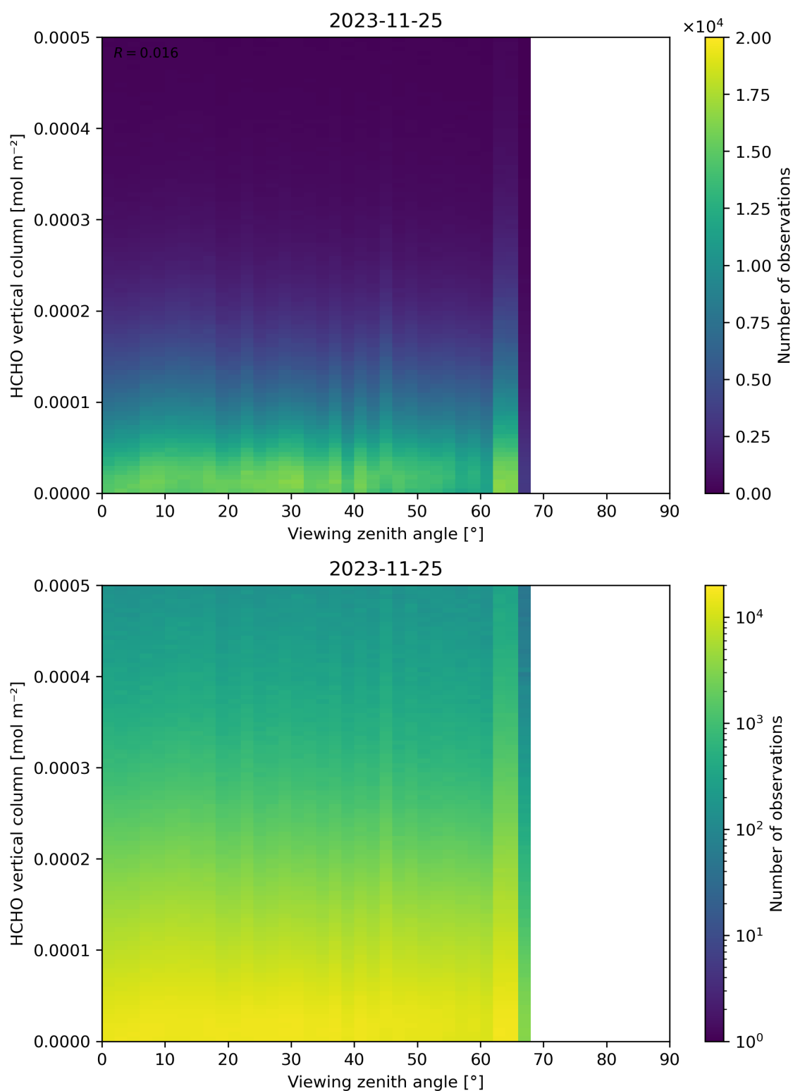
Figure 192: Scatter density plot of “Viewing zenith angle” against “HCHO vertical column” for 2023-11-24 to 2023-11-26.
