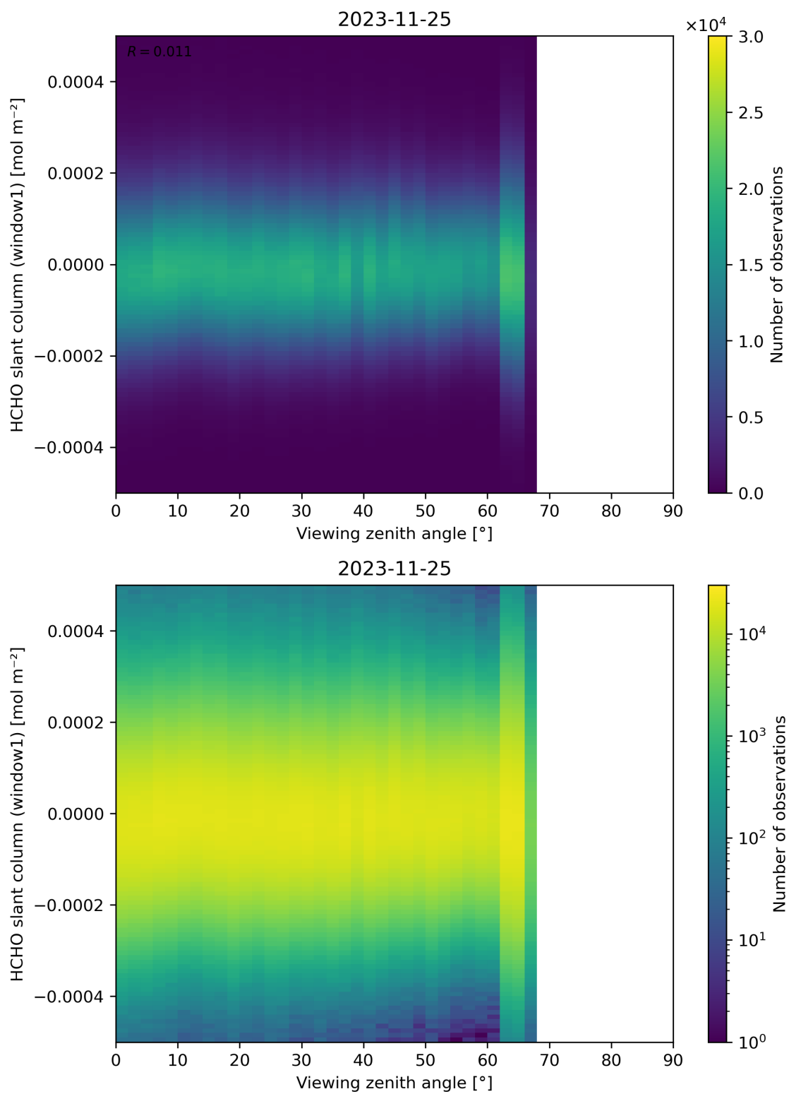
Figure 188: Scatter density plot of “Viewing zenith angle” against “HCHO slant column (window1)” for 2023-11-24 to 2023-11-26.
