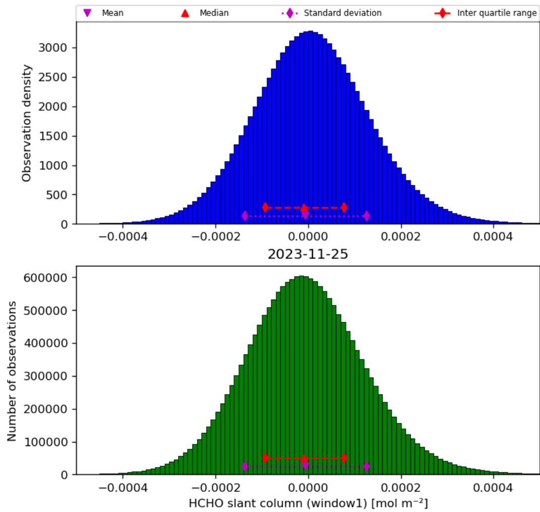
Figure 38: Histogram of “HCHO slant column (window1)” for 2023-11-24 to 2023-11-26
