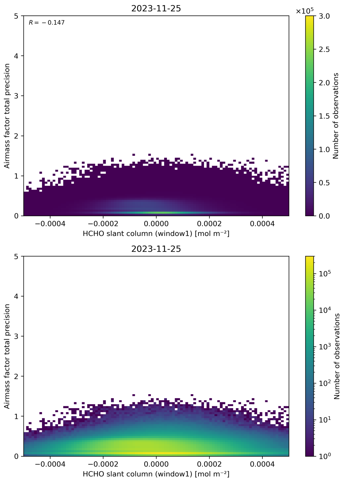
Figure 86: Scatter density plot of “HCHO slant column (window1)” against “Airmass factor total precision” for 2023-11-24 to 2023-11-26.
