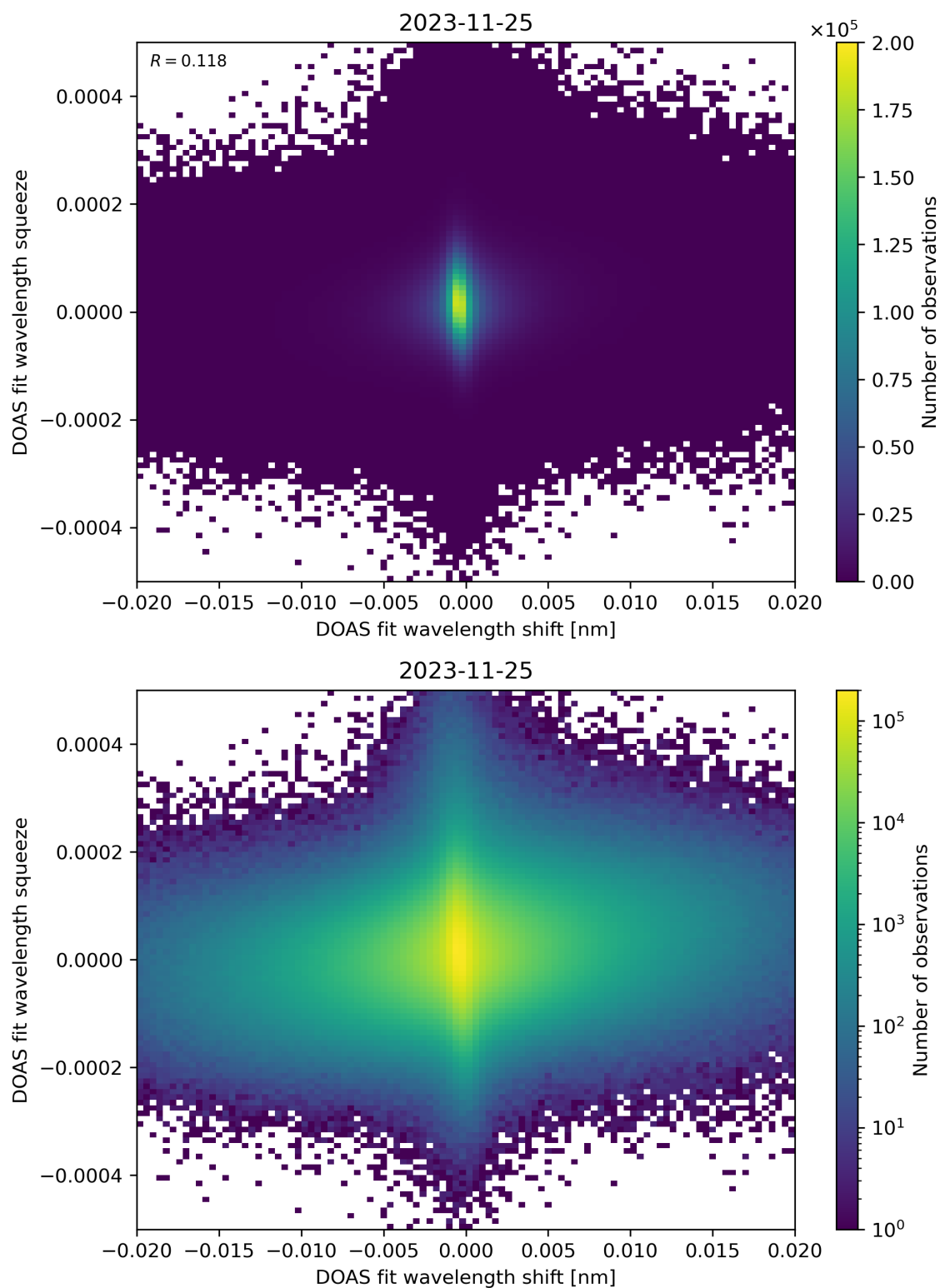
Figure 65: Scatter density plot of “DOAS fit wavelength shift” against “DOAS fit wavelength squeeze” for 2023-11-24 to 2023-11-26.
