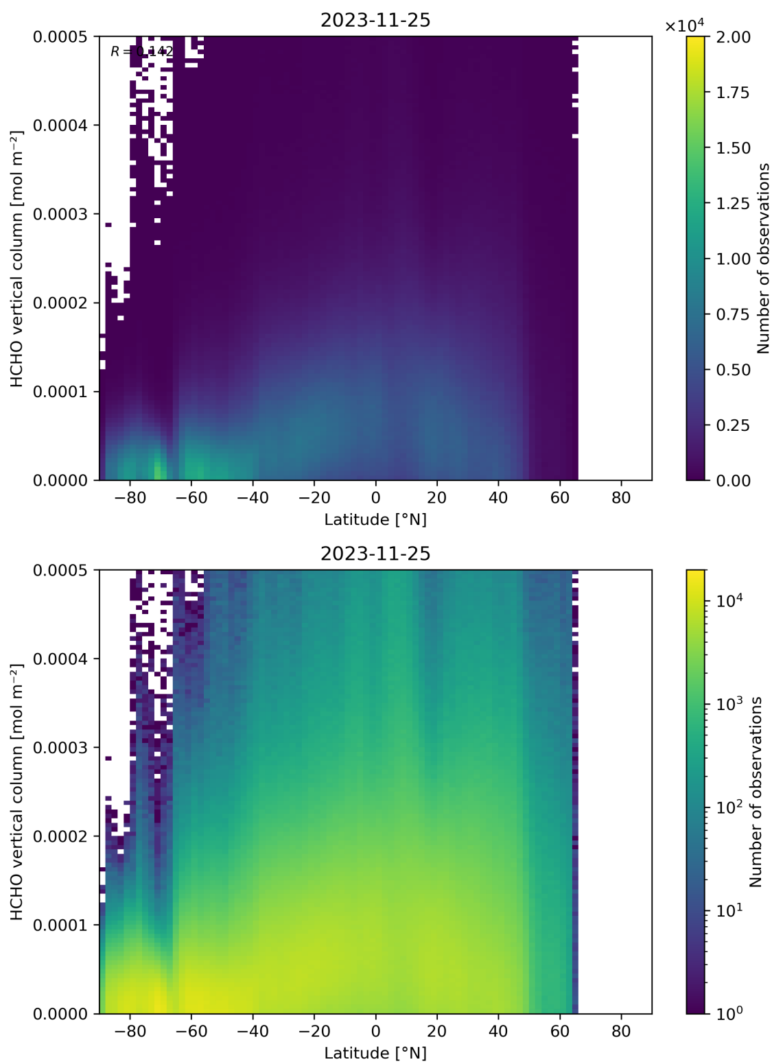
Figure 163: Scatter density plot of “Latitude” against “HCHO vertical column” for 2023-11-24 to 2023-11-26.
