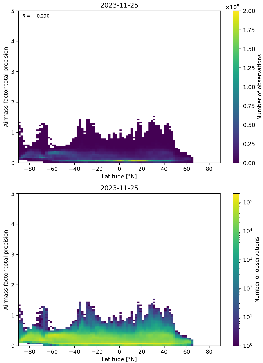
Figure 162: Scatter density plot of “Latitude” against “Airmass factor total precision” for 2023-11-24 to 2023-11-26.
