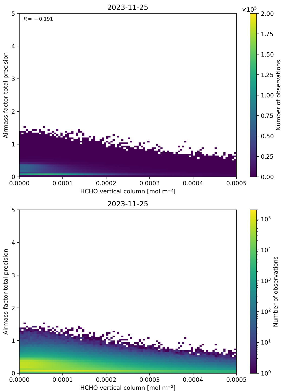
Figure 132: Scatter density plot of “HCHO vertical column” against “Airmass factor total precision” for 2023-11-24 to 2023-11-26.
