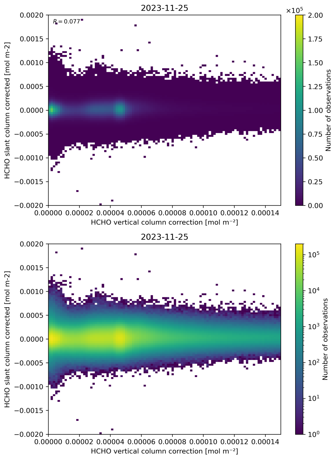
Figure 116: Scatter density plot of “HCHO vertical column correction” against “HCHO slant column corrected” for 2023-11-24 to 2023-11-26.
