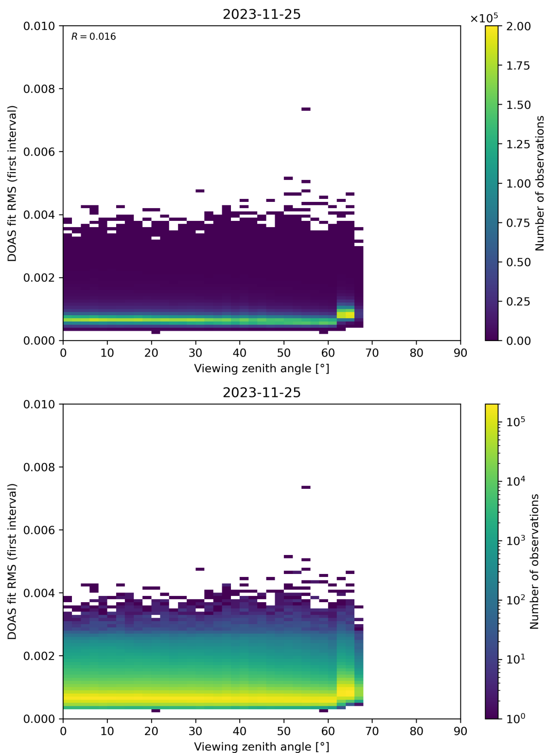
Figure 182: Scatter density plot of “Viewing zenith angle” against “DOAS fit RMS (first interval)” for 2023-11-24 to 2023-11-26.
