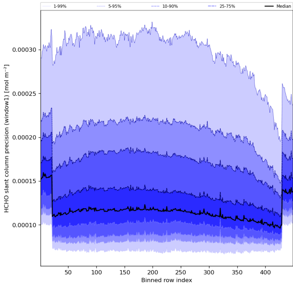
Figure 53: Along track statistics of “HCHO slant column precision (window1)” for 2023-11-24 to 2023-11-26
