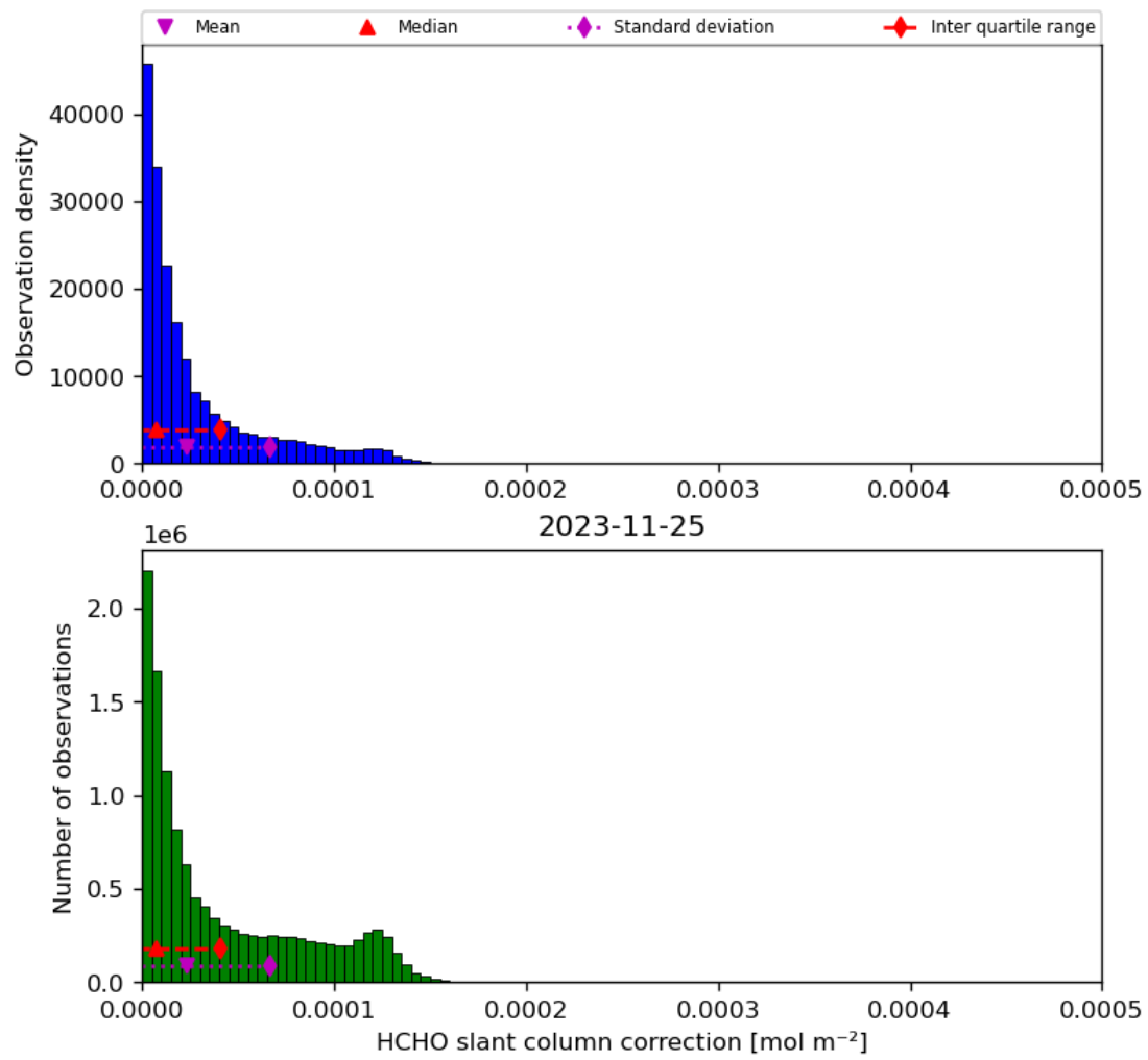
Figure 47: Histogram of “HCHO slant column correction” for 2023-11-24 to 2023-11-26
