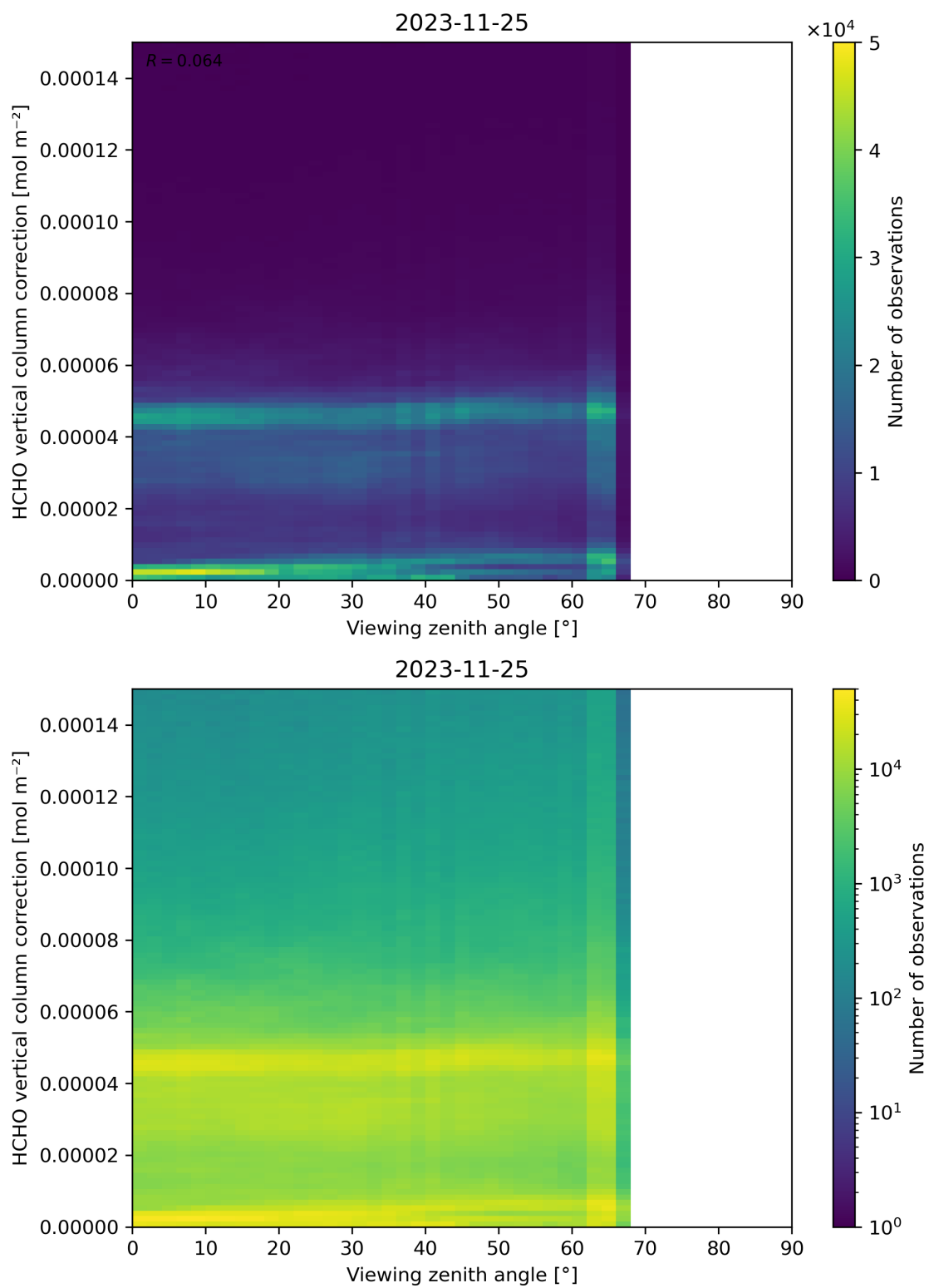
Figure 193: Scatter density plot of “Viewing zenith angle” against “HCHO vertical column correction” for 2023-11-24 to 2023-11-26.
