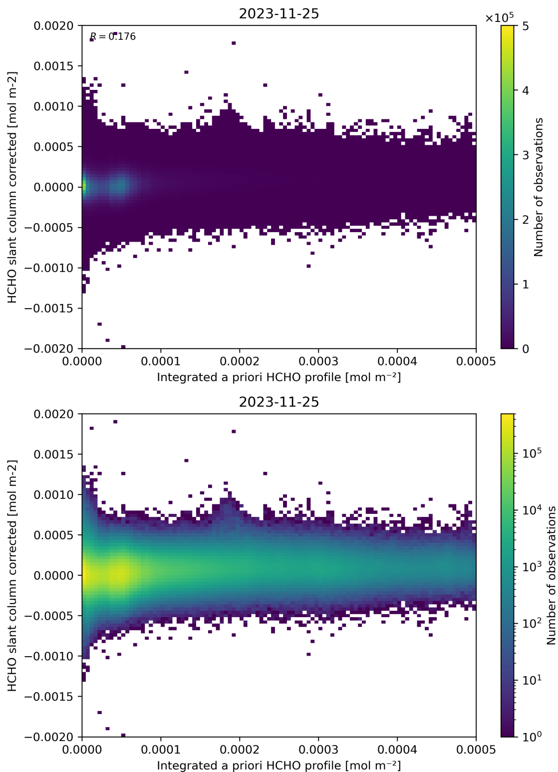
Figure 151: Scatter density plot of “Integrated a priori HCHO profile” against “HCHO slant column corrected” for 2023-11-24 to 2023-11-26.
