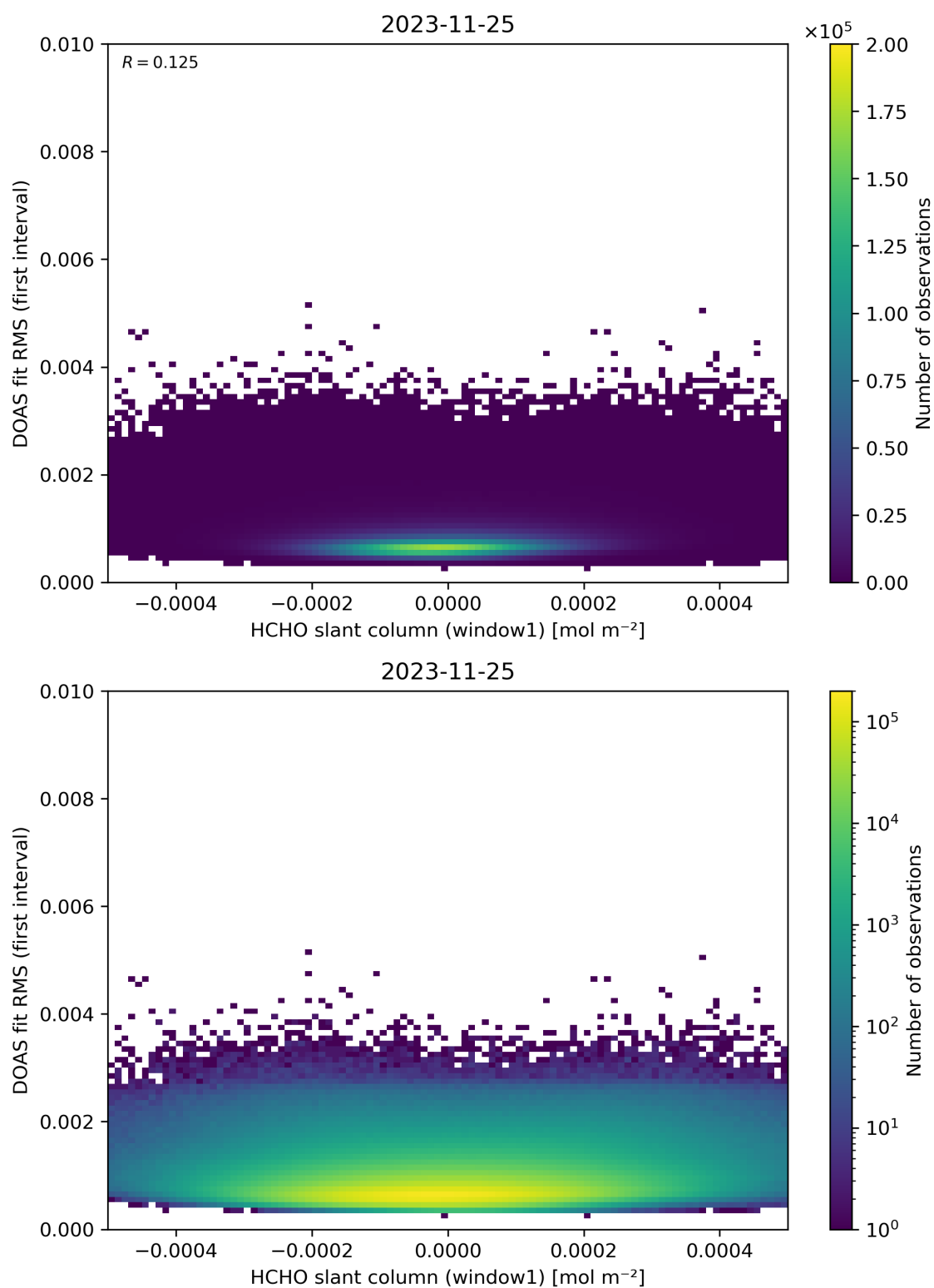
Figure 78: Scatter density plot of “HCHO slant column (window1)” against “DOAS fit RMS (first interval)” for 2023-11-24 to 2023-11-26.
