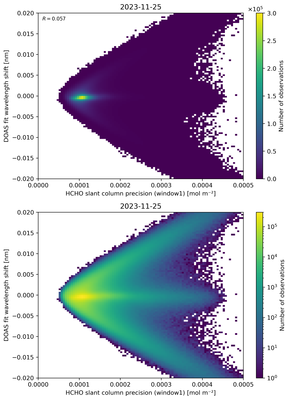
Figure 89: Scatter density plot of “HCHO slant column precision (window1)” against “DOAS fit wavelength shift” for 2023-11-24 to 2023-11-26.
