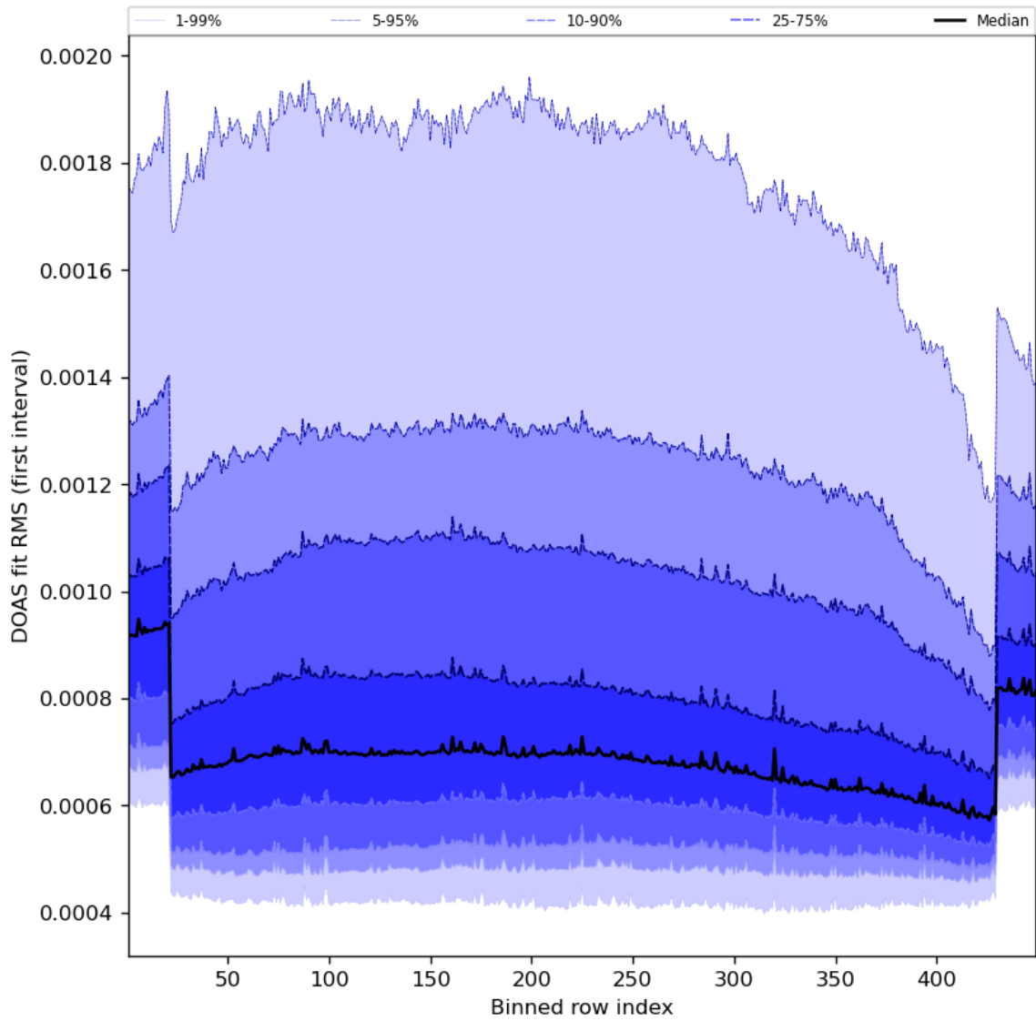
Figure 60: Along track statistics of “DOAS fit RMS (first interval)” for 2023-11-24 to 2023-11-26
