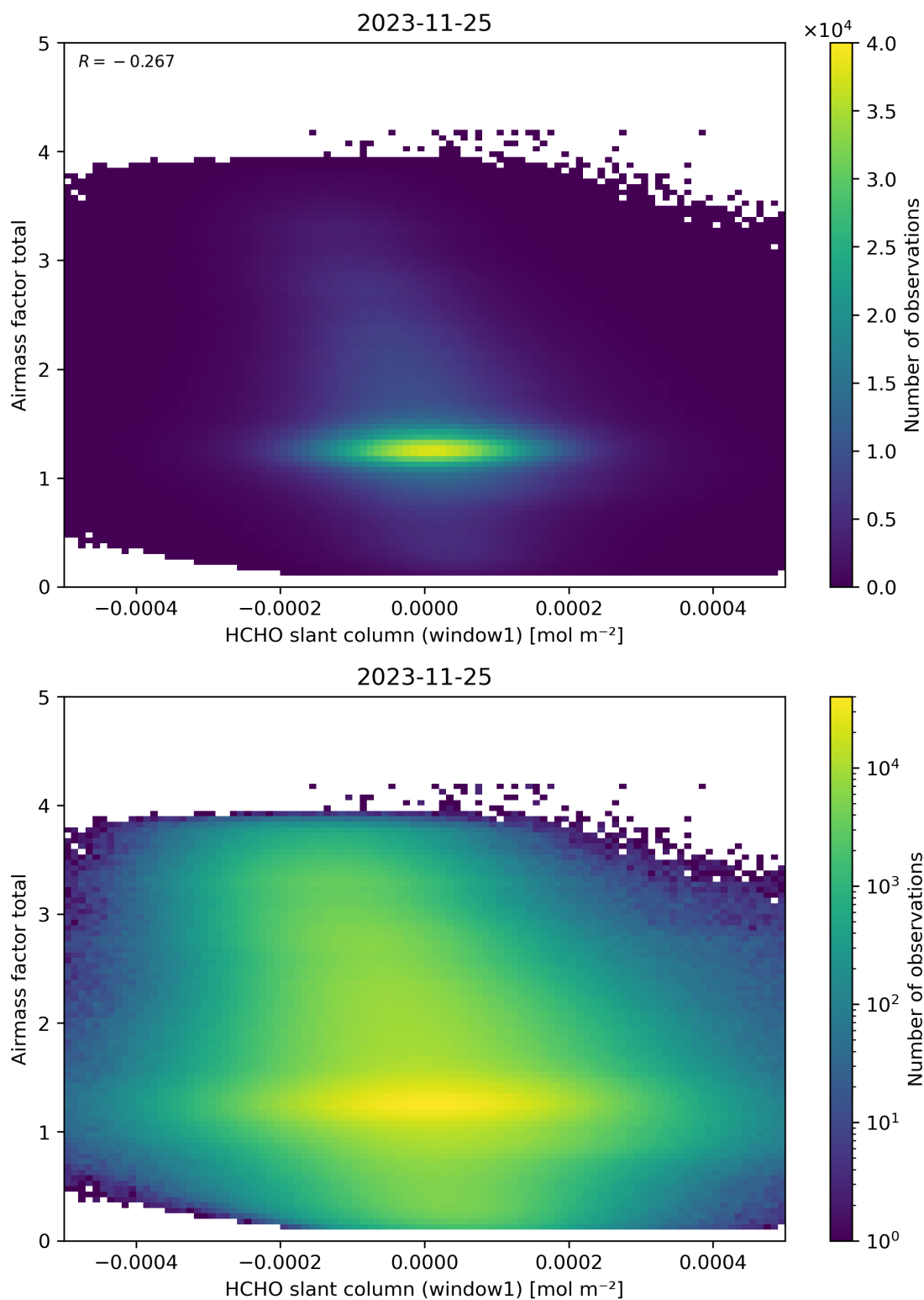
Figure 85: Scatter density plot of “HCHO slant column (window1)” against “Airmass factor total” for 2023-11-24 to 2023-11-26.
