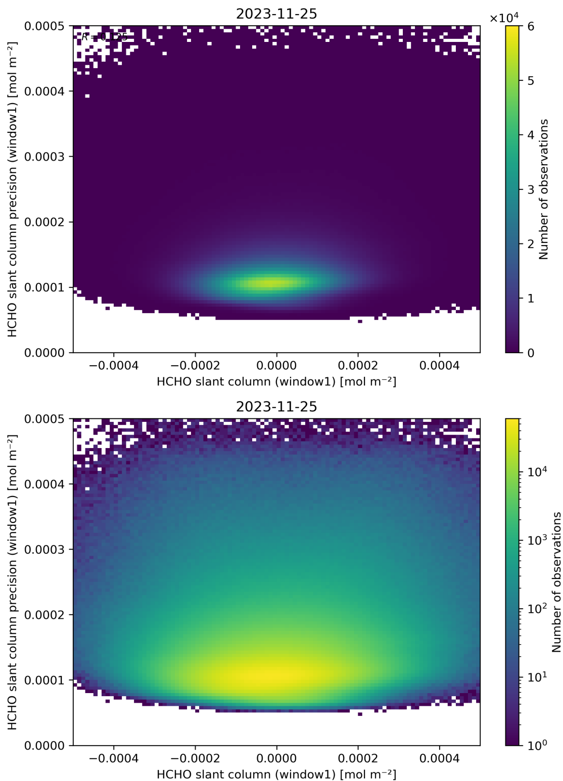
Figure 84: Scatter density plot of “HCHO slant column (window1)” against “HCHO slant column precision (window1)” for 2023-11-24 to 2023-11-26.
