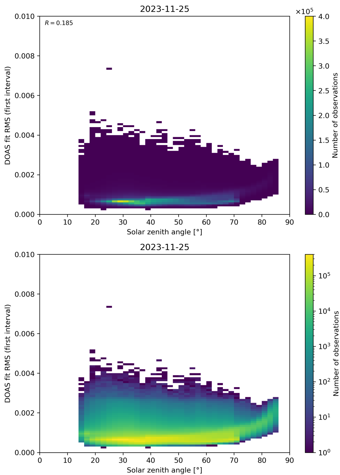
Figure 167: Scatter density plot of “Solar zenith angle” against “DOAS fit RMS (first interval)” for 2023-11-24 to 2023-11-26.
