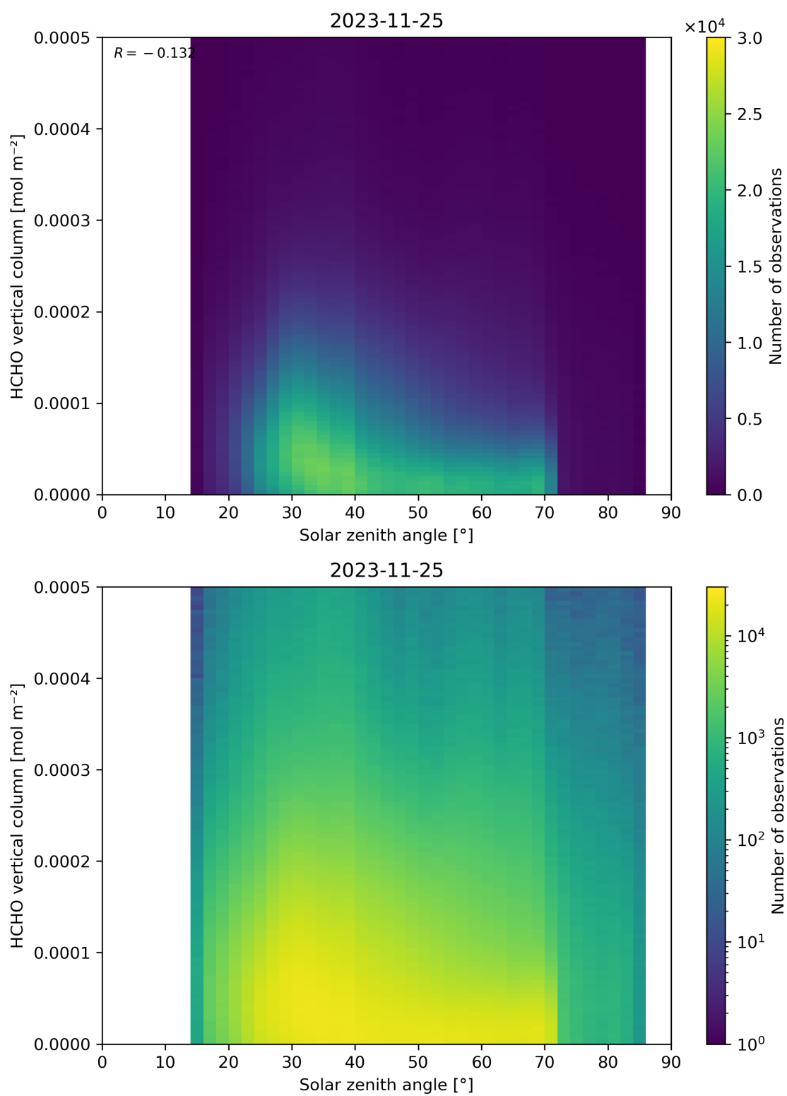
Figure 177: Scatter density plot of “Solar zenith angle” against “HCHO vertical column” for 2023-11-24 to 2023-11-26.
