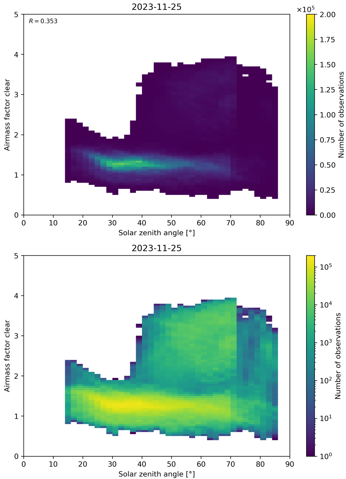
Figure 170: Scatter density plot of “Solar zenith angle” against “Airmass factor clear” for 2023-11-24 to 2023-11-26.
