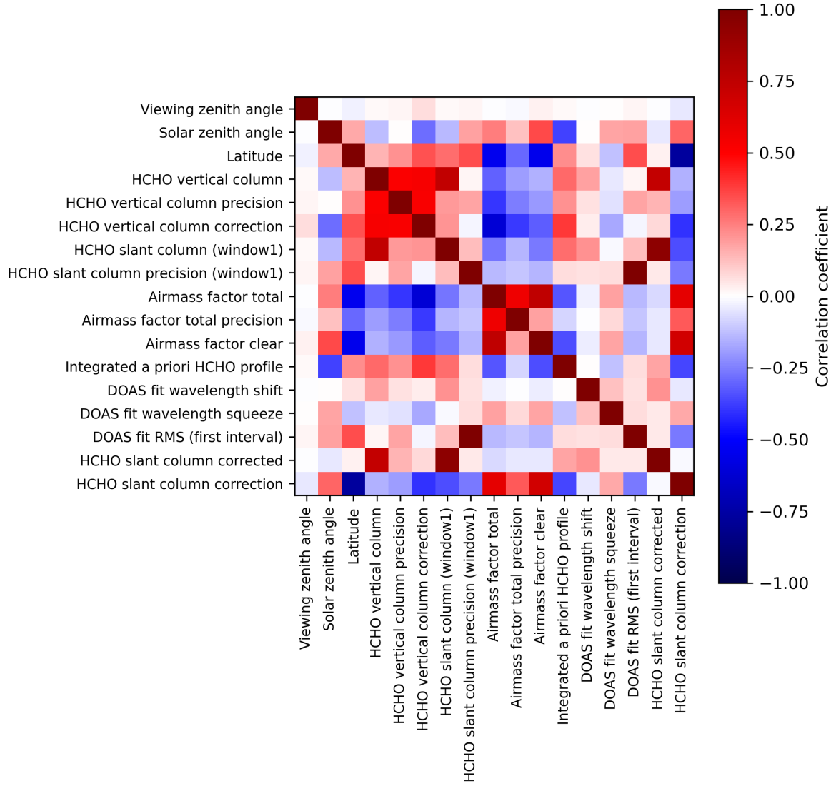
Figure 2: Map of correlation matrix for 2023-11-24 to 2023-11-26.
