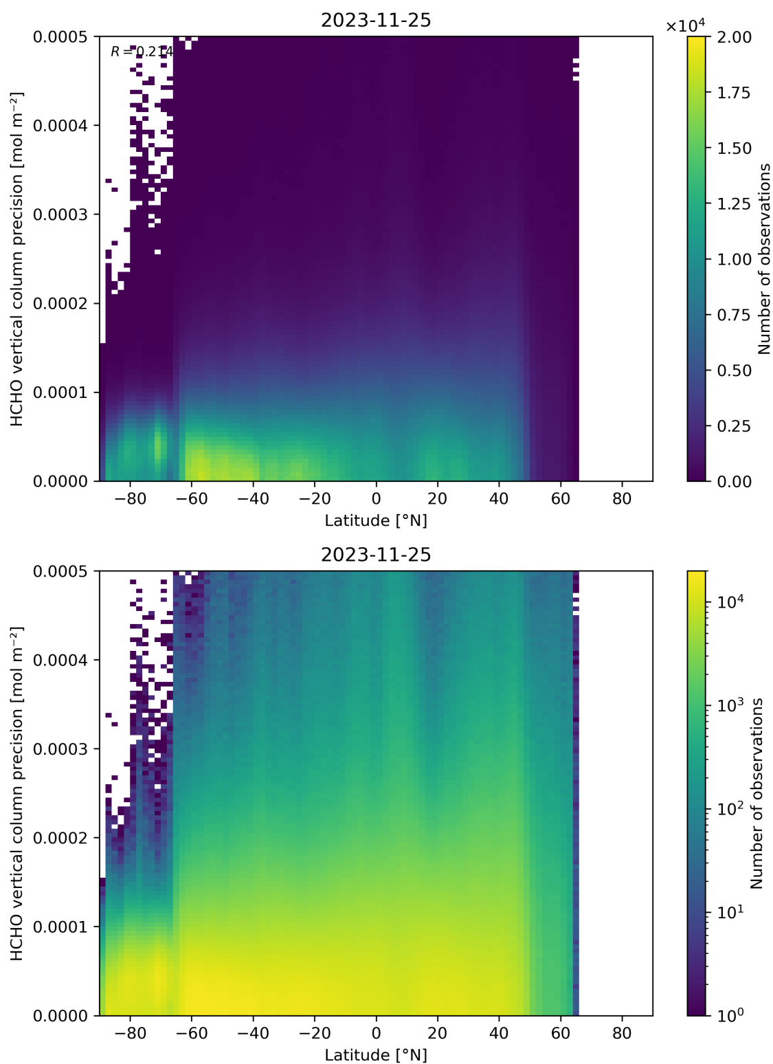
Figure 165: Scatter density plot of “Latitude” against “HCHO vertical column precision” for 2023-11-24 to 2023-11-26.
