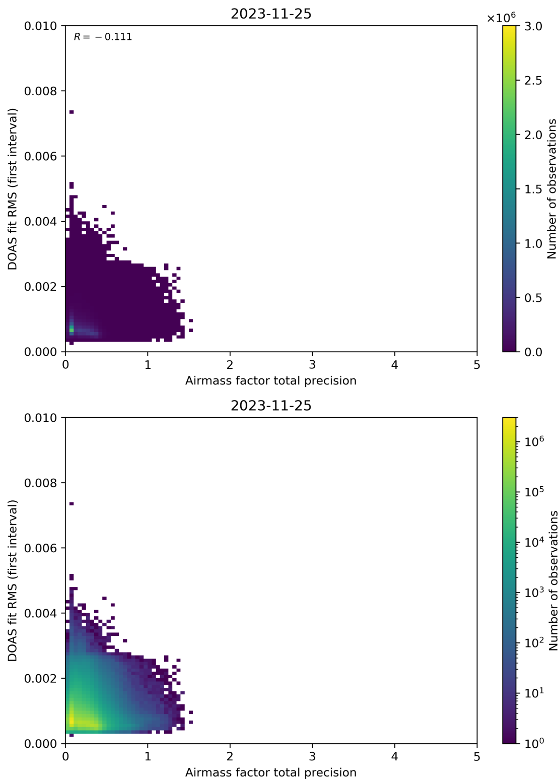
Figure 105: Scatter density plot of “Airmass factor total precision” against “DOAS fit RMS (first interval)” for 2023-11-24 to 2023-11-26.
