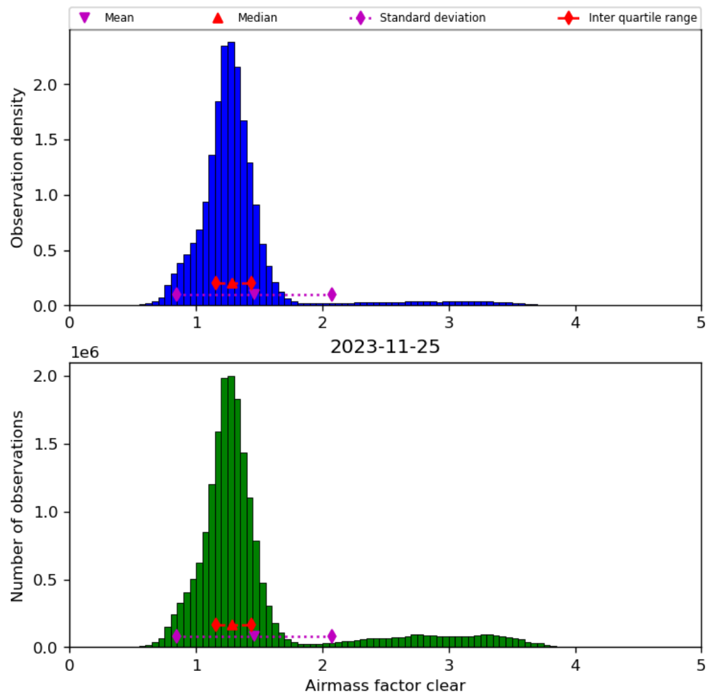
Figure 42: Histogram of “Airmass factor clear” for 2023-11-24 to 2023-11-26
