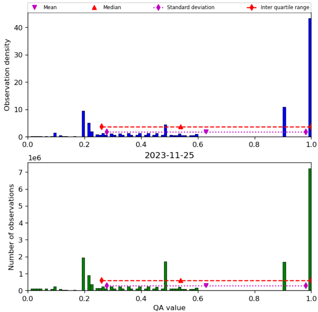
Figure 34: Histogram of “QA value” for 2023-11-24 to 2023-11-26
