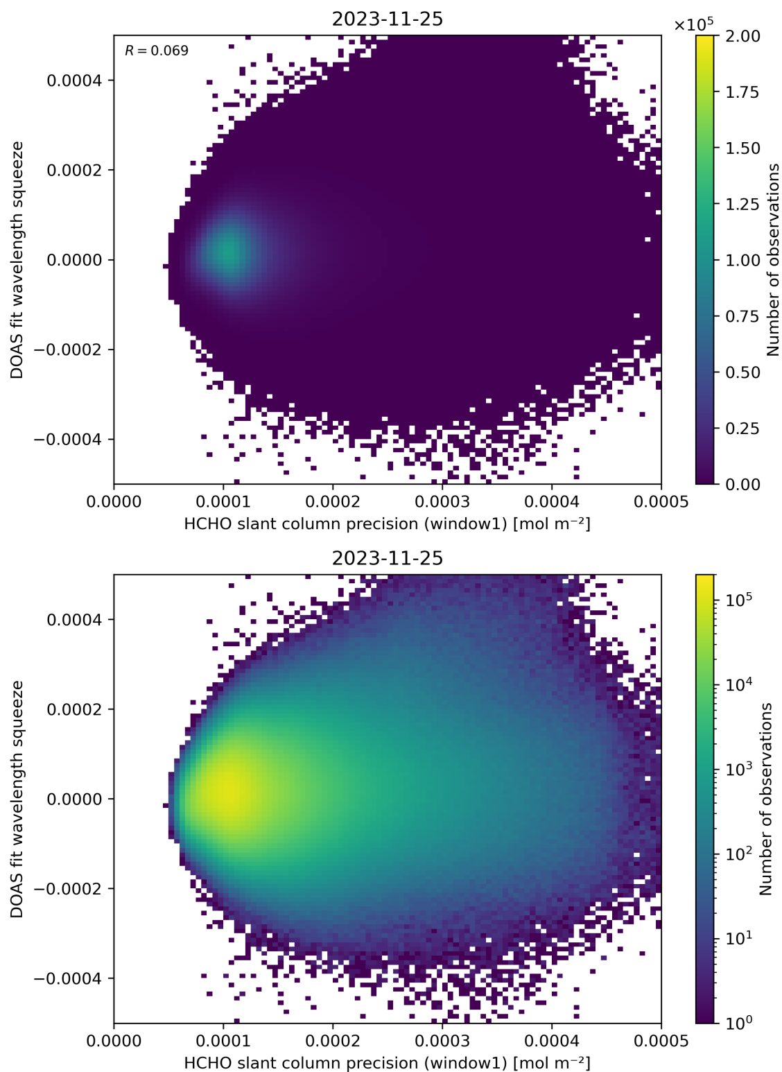
Figure 90: Scatter density plot of “HCHO slant column precision (window1)” against “DOAS fit wavelength squeeze” for 2023-11-24 to 2023-11-26.
