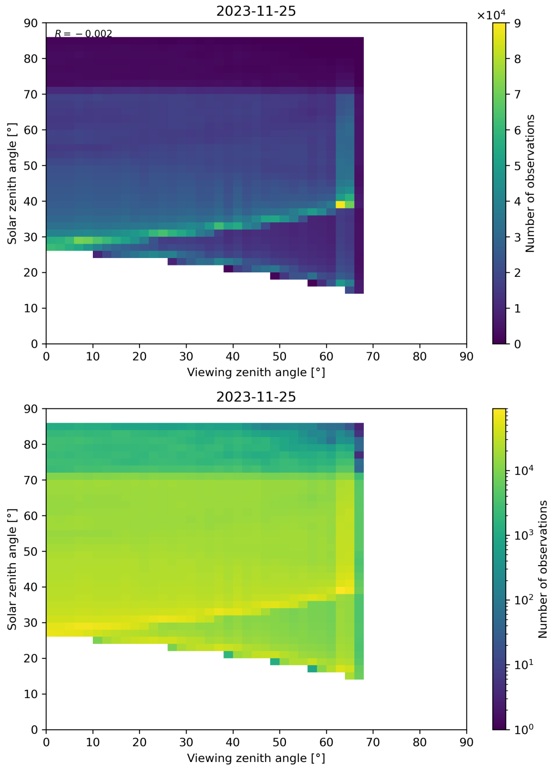
Figure 197: Scatter density plot of “Viewing zenith angle” against “Solar zenith angle” for 2023-11-24 to 2023-11-26.
