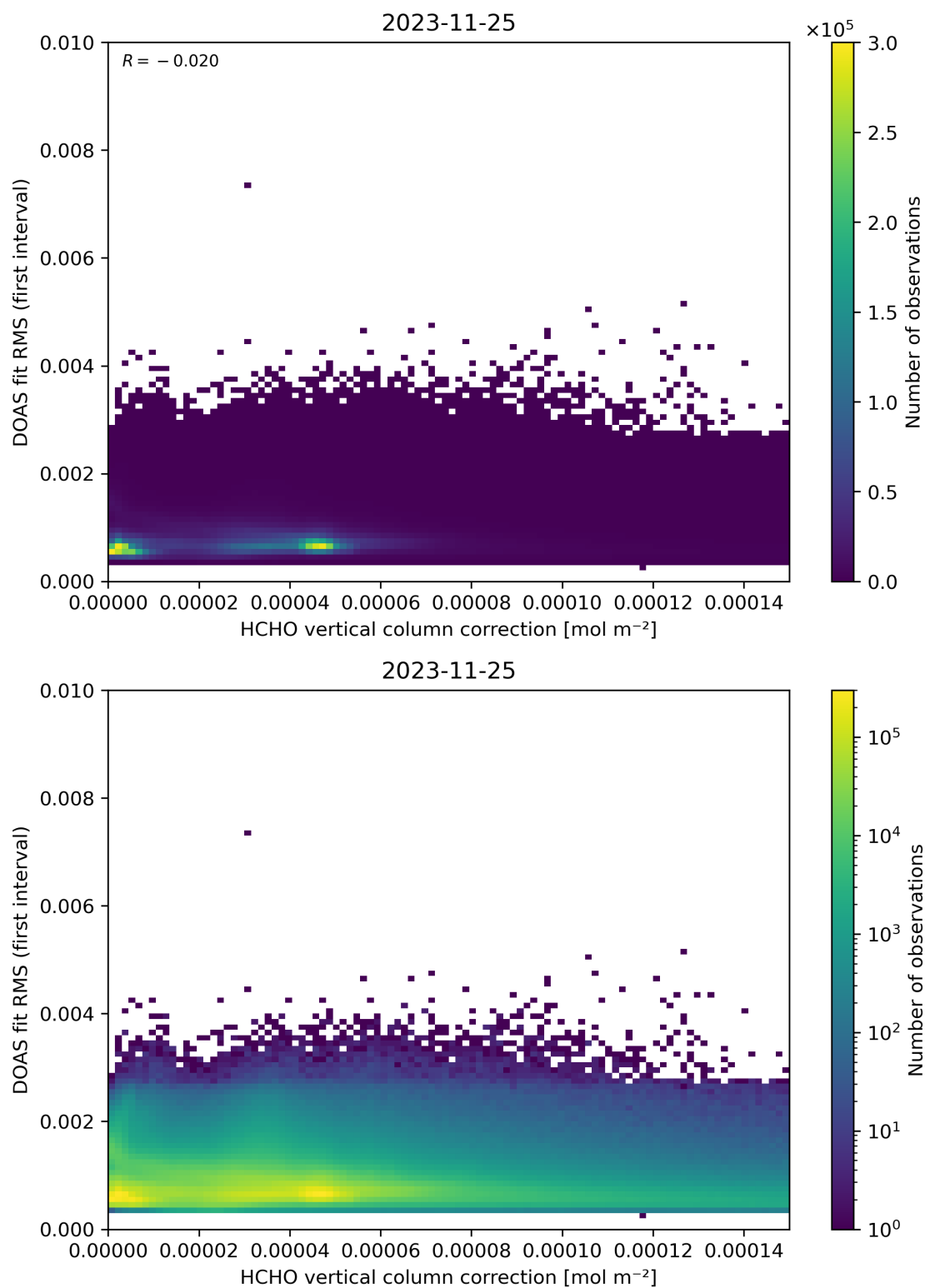
Figure 112: Scatter density plot of “HCHO vertical column correction” against “DOAS fit RMS (first interval)” for 2023-11-24 to 2023-11-26.
