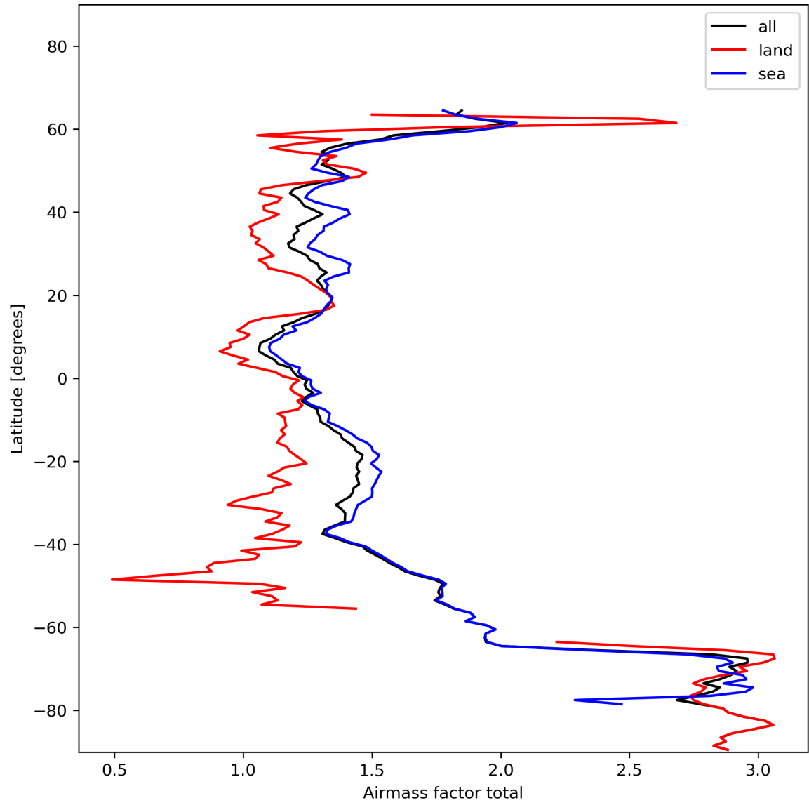
Figure 26: Zonal average of “Airmass factor total” for 2023-11-24 to 2023-11-26.
