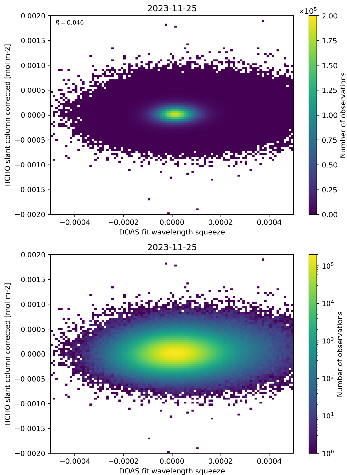
Figure 69: Scatter density plot of “DOAS fit wavelength squeeze” against “HCHO slant column corrected” for 2023-11-24 to 2023-11-26.
