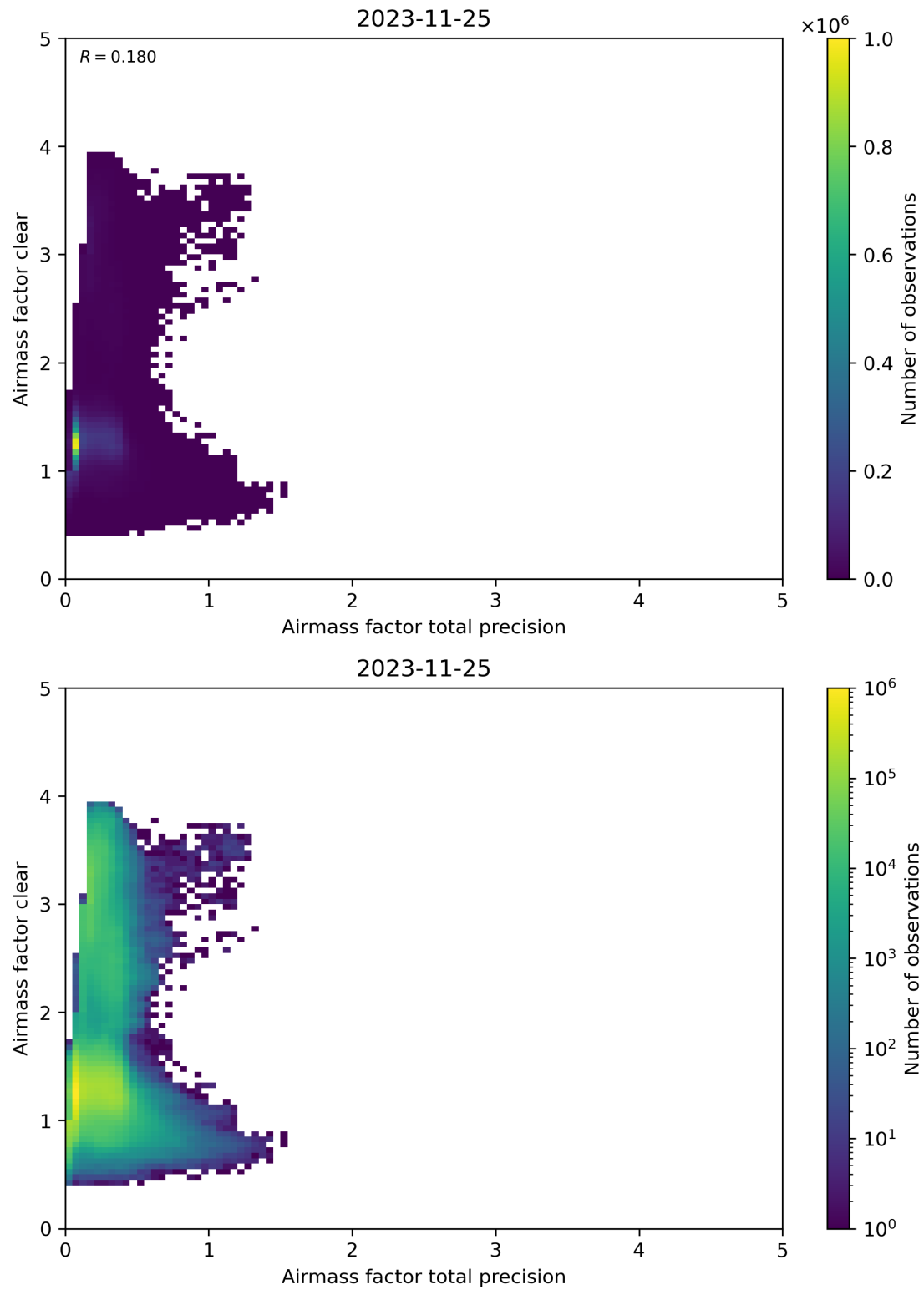
Figure 108: Scatter density plot of “Airmass factor total precision” against “Airmass factor clear” for 2023-11-24 to 2023-11-26.
