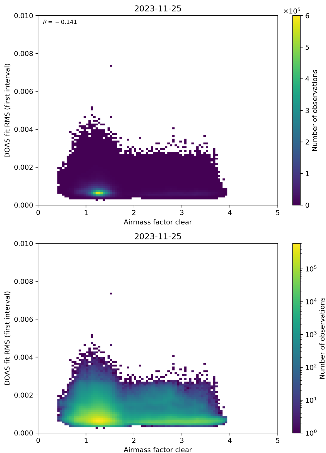
Figure 71: Scatter density plot of “Airmass factor clear” against “DOAS fit RMS (first interval)” for 2023-11-24 to 2023-11-26.
