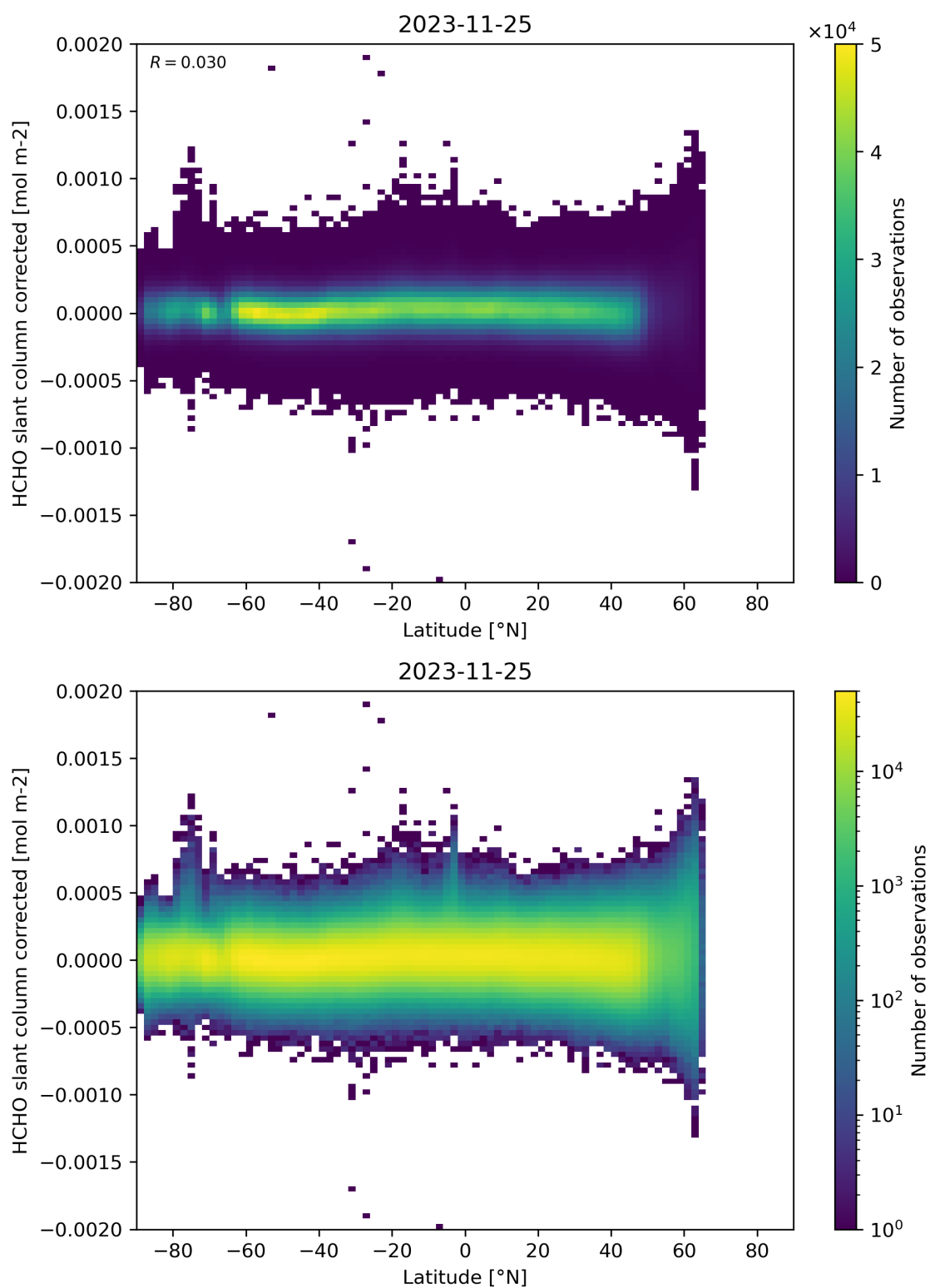
Figure 157: Scatter density plot of “Latitude” against “HCHO slant column corrected” for 2023-11-24 to 2023-11-26.
