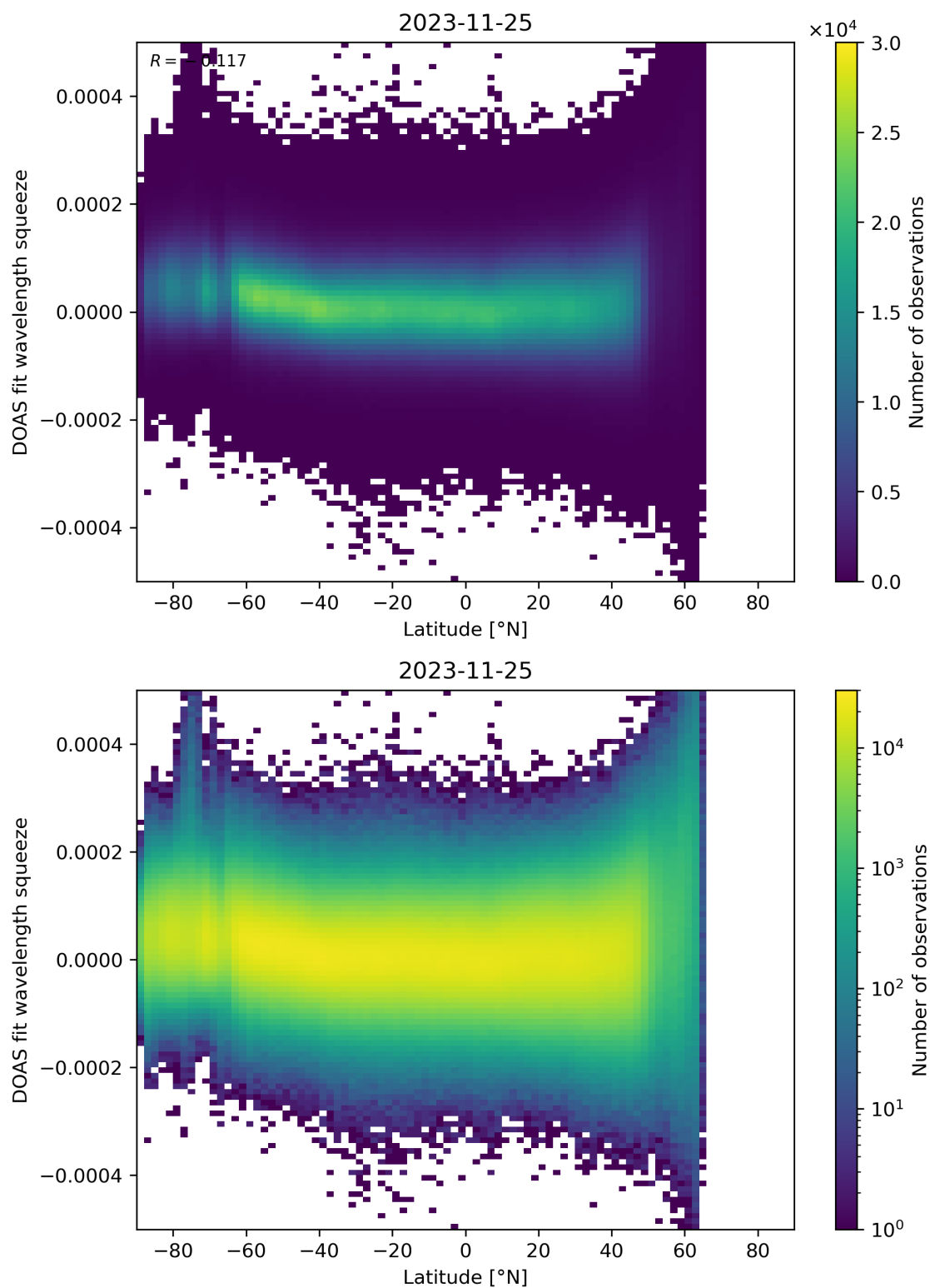
Figure 155: Scatter density plot of “Latitude” against “DOAS fit wavelength squeeze” for 2023-11-24 to 2023-11-26.
