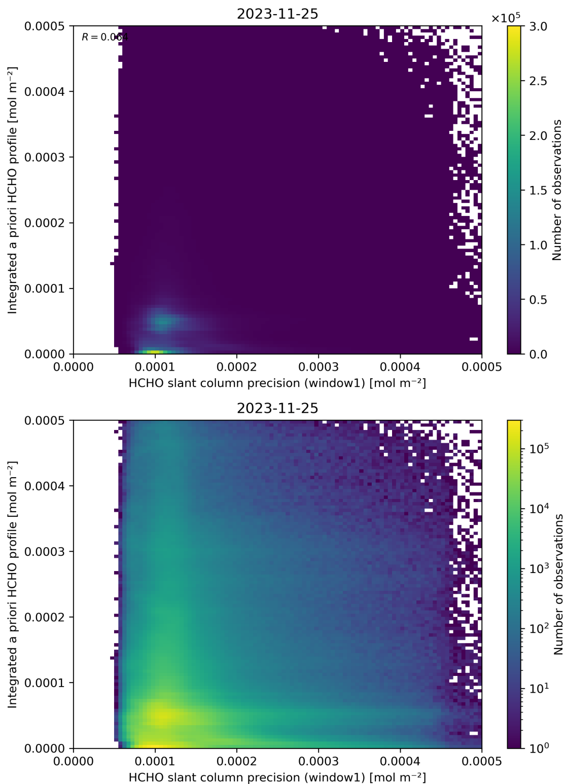
Figure 96: Scatter density plot of “HCHO slant column precision (window1)” against “Integrated a priori HCHO profile” for 2023-11-24 to 2023-11-26.
