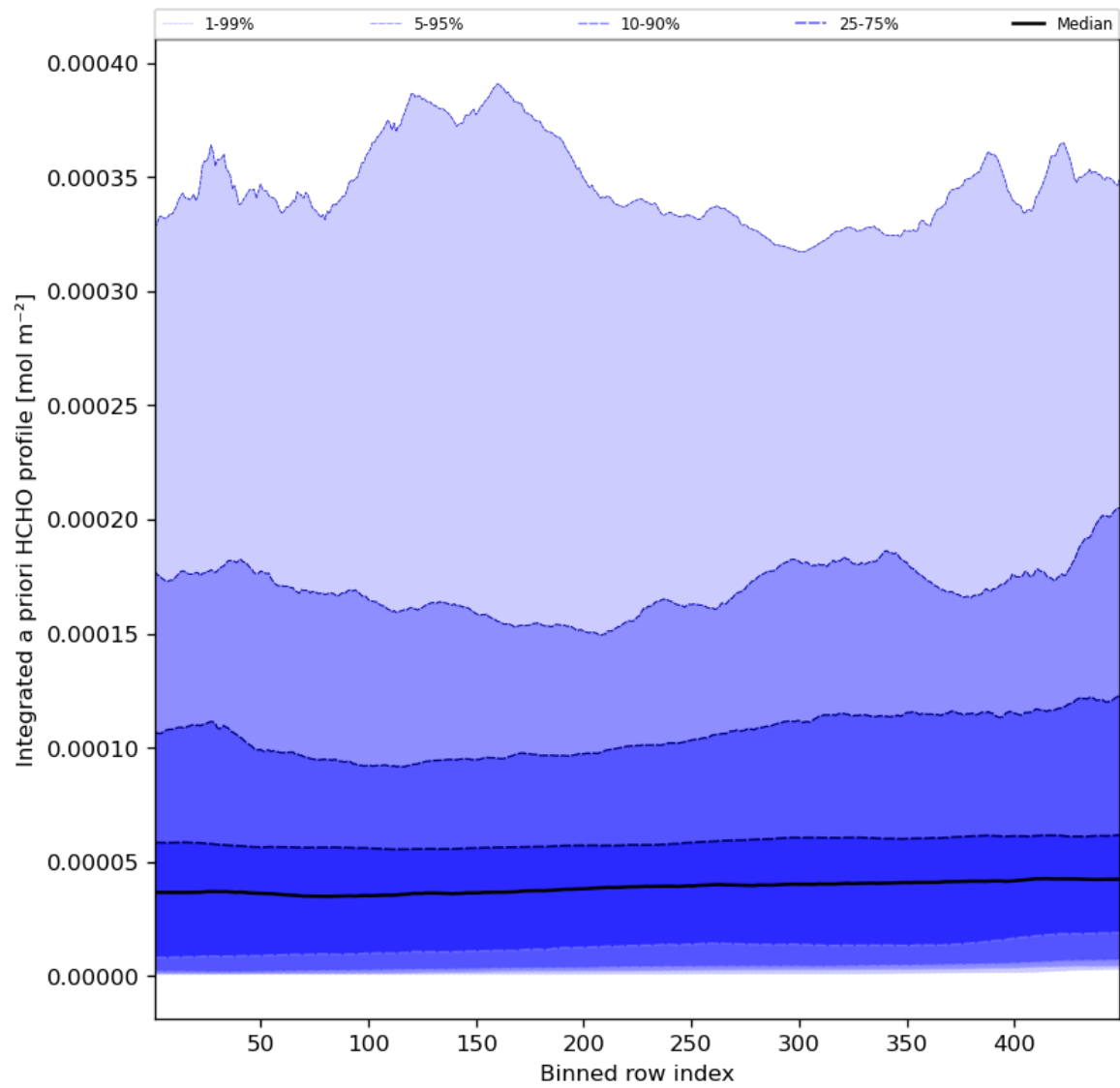
Figure 57: Along track statistics of “Integrated a priori HCHO profile” for 2023-11-24 to 2023-11-26
