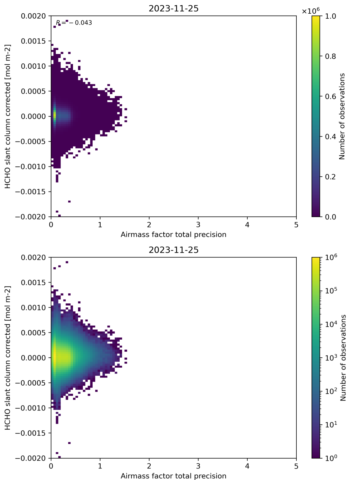
Figure 109: Scatter density plot of “Airmass factor total precision” against “HCHO slant column corrected” for 2023-11-24 to 2023-11-26.
