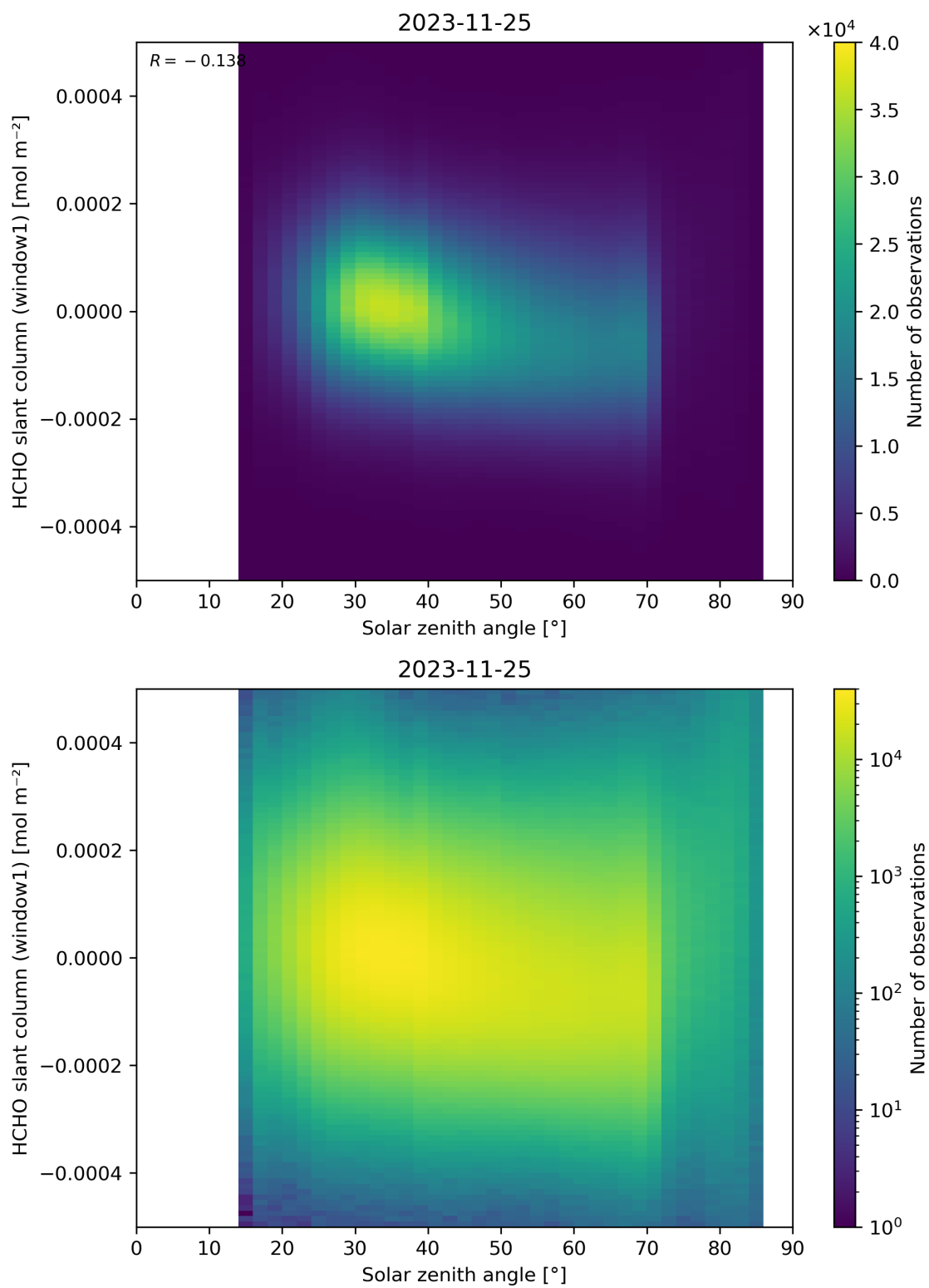
Figure 173: Scatter density plot of “Solar zenith angle” against “HCHO slant column (window1)” for 2023-11-24 to 2023-11-26.
