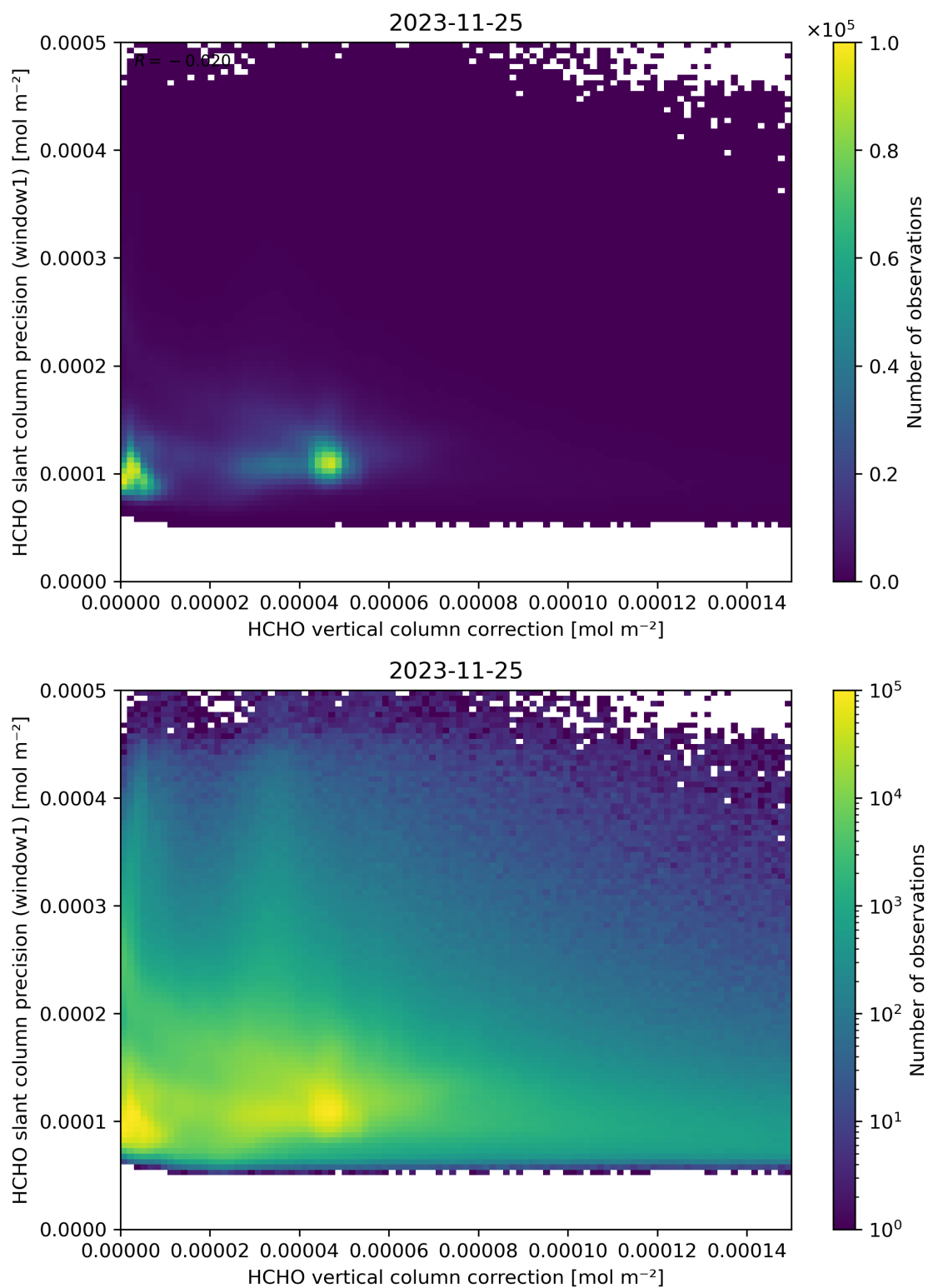
Figure 119: Scatter density plot of “HCHO vertical column correction” against “HCHO slant column precision (window1)” for 2023-11-24 to 2023-11-26.
