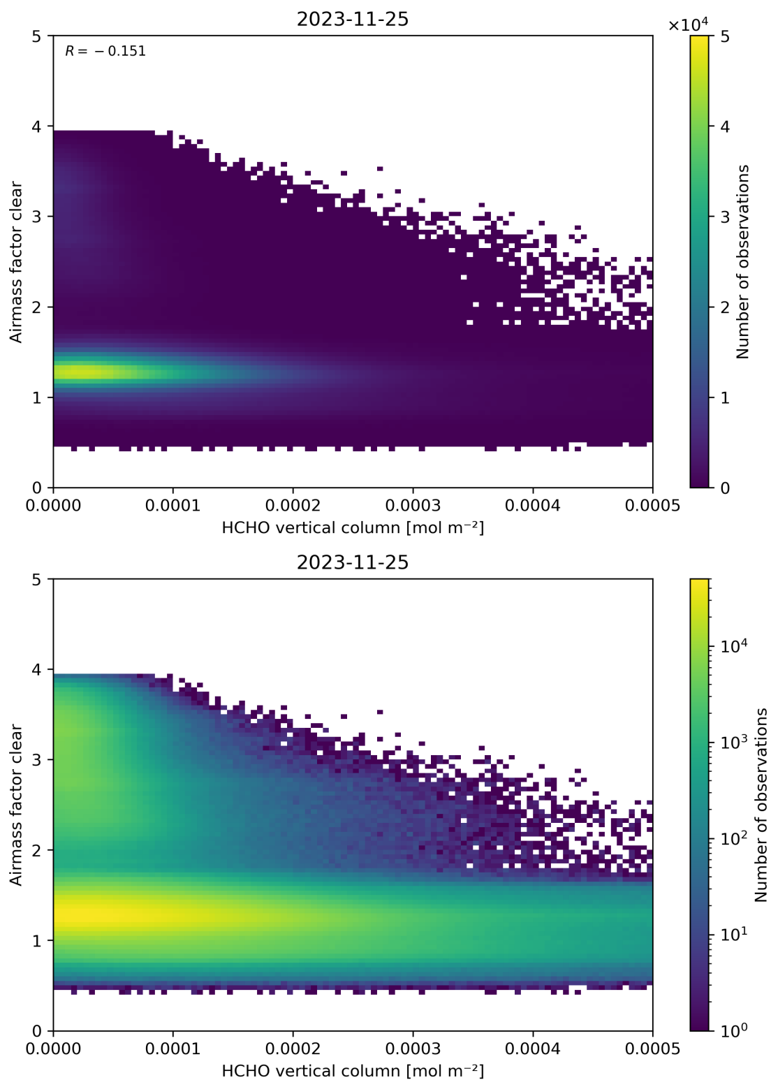
Figure 126: Scatter density plot of “HCHO vertical column” against “Airmass factor clear” for 2023-11-24 to 2023-11-26.
