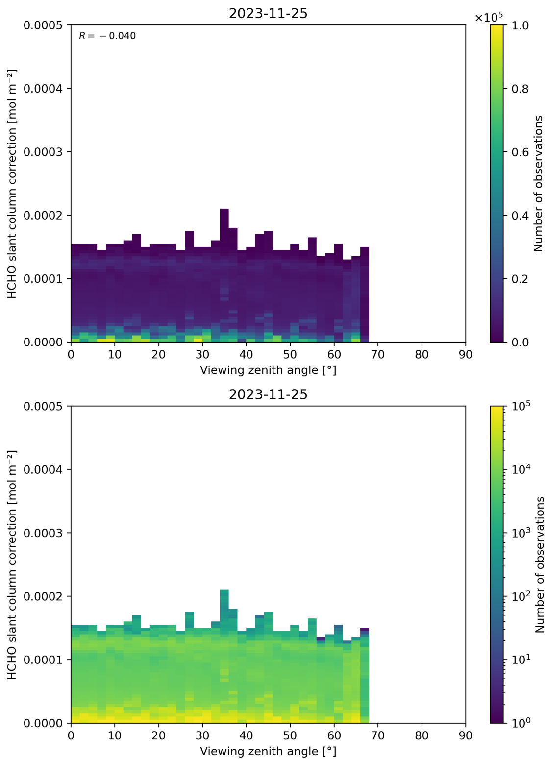
Figure 187: Scatter density plot of “Viewing zenith angle” against “HCHO slant column correction” for 2023-11-24 to 2023-11-26.
