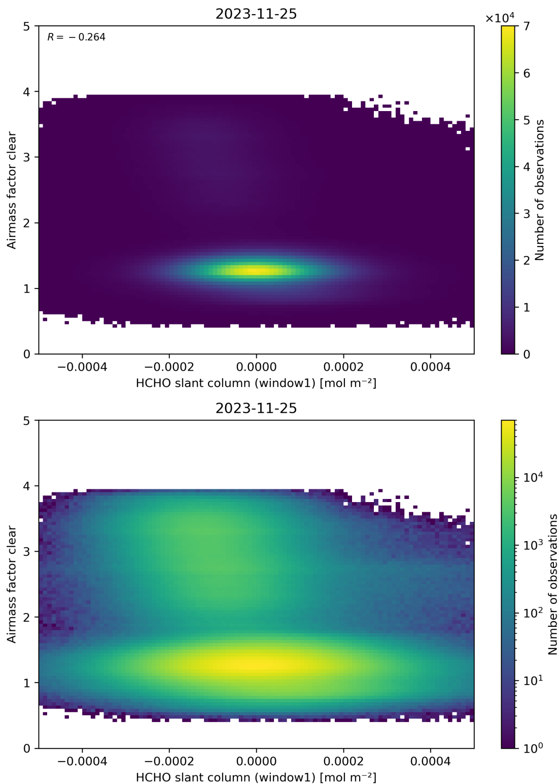
Figure 81: Scatter density plot of “HCHO slant column (window1)” against “Airmass factor clear” for 2023-11-24 to 2023-11-26.
