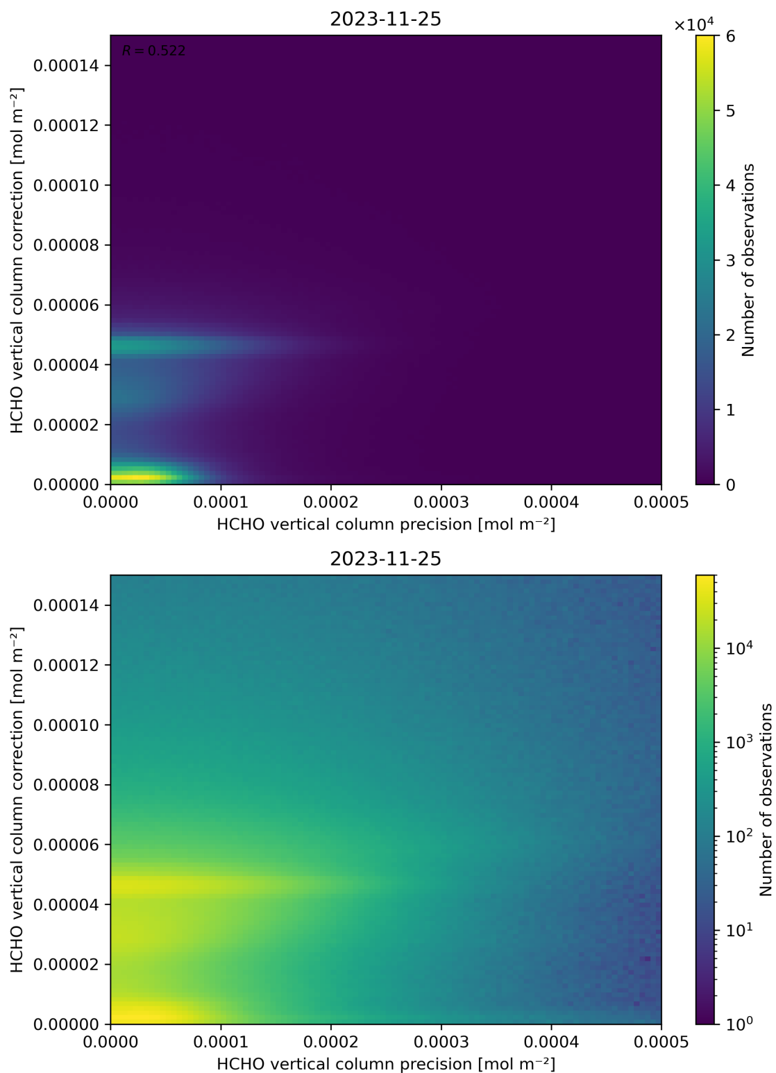
Figure 146: Scatter density plot of “HCHO vertical column precision” against “HCHO vertical column correction” for 2023-11-24 to 2023-11-26.
