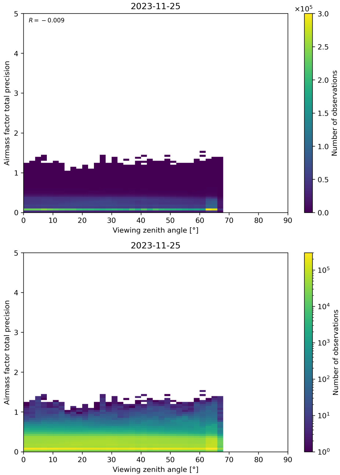
Figure 191: Scatter density plot of “Viewing zenith angle” against “Airmass factor total precision” for 2023-11-24 to 2023-11-26.
