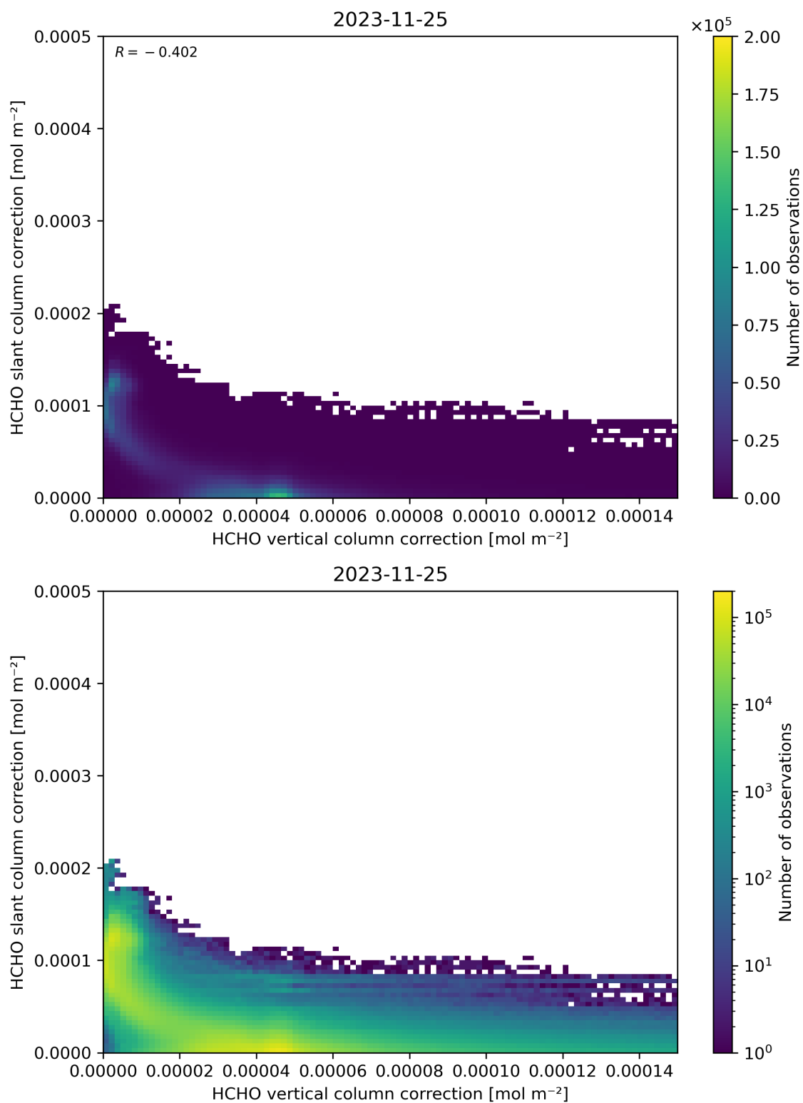
Figure 117: Scatter density plot of “HCHO vertical column correction” against “HCHO slant column correction” for 2023-11-24 to 2023-11-26.
