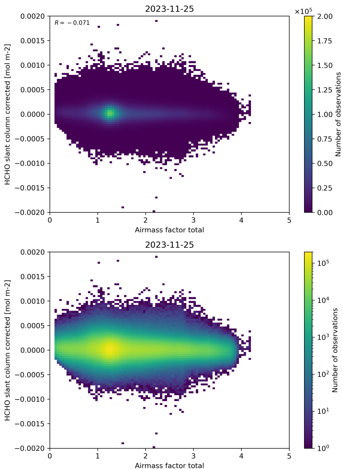
Figure 101: Scatter density plot of “Airmass factor total” against “HCHO slant column corrected” for 2023-11-24 to 2023-11-26.
