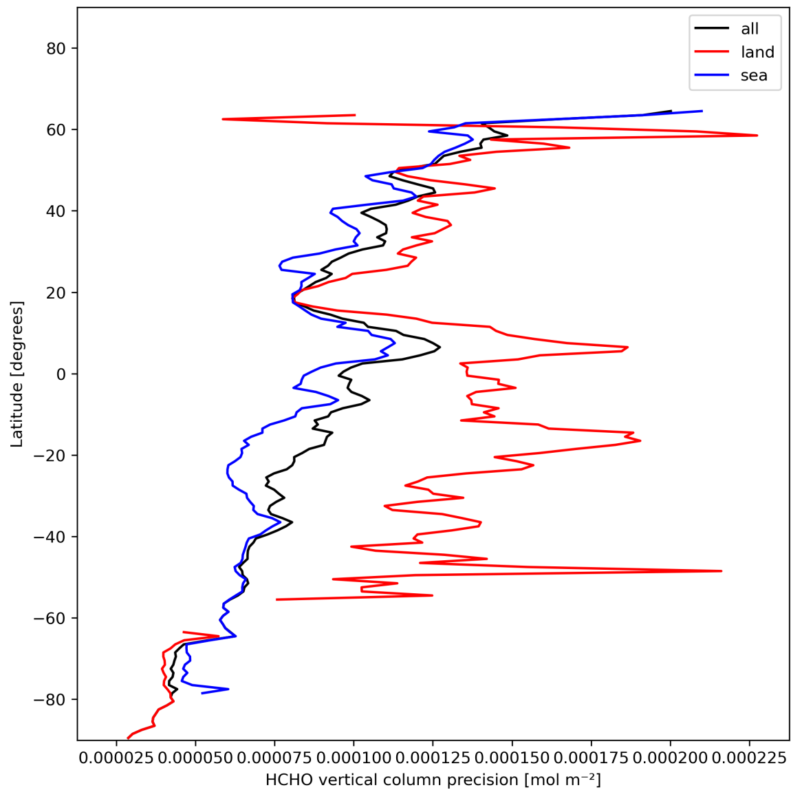
Figure 22: Zonal average of “HCHO vertical column precision” for 2023-11-24 to 2023-11-26.
