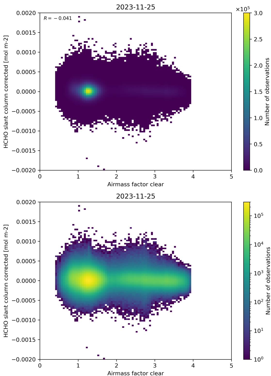
Figure 74: Scatter density plot of “Airmass factor clear” against “HCHO slant column corrected” for 2023-11-24 to 2023-11-26.
