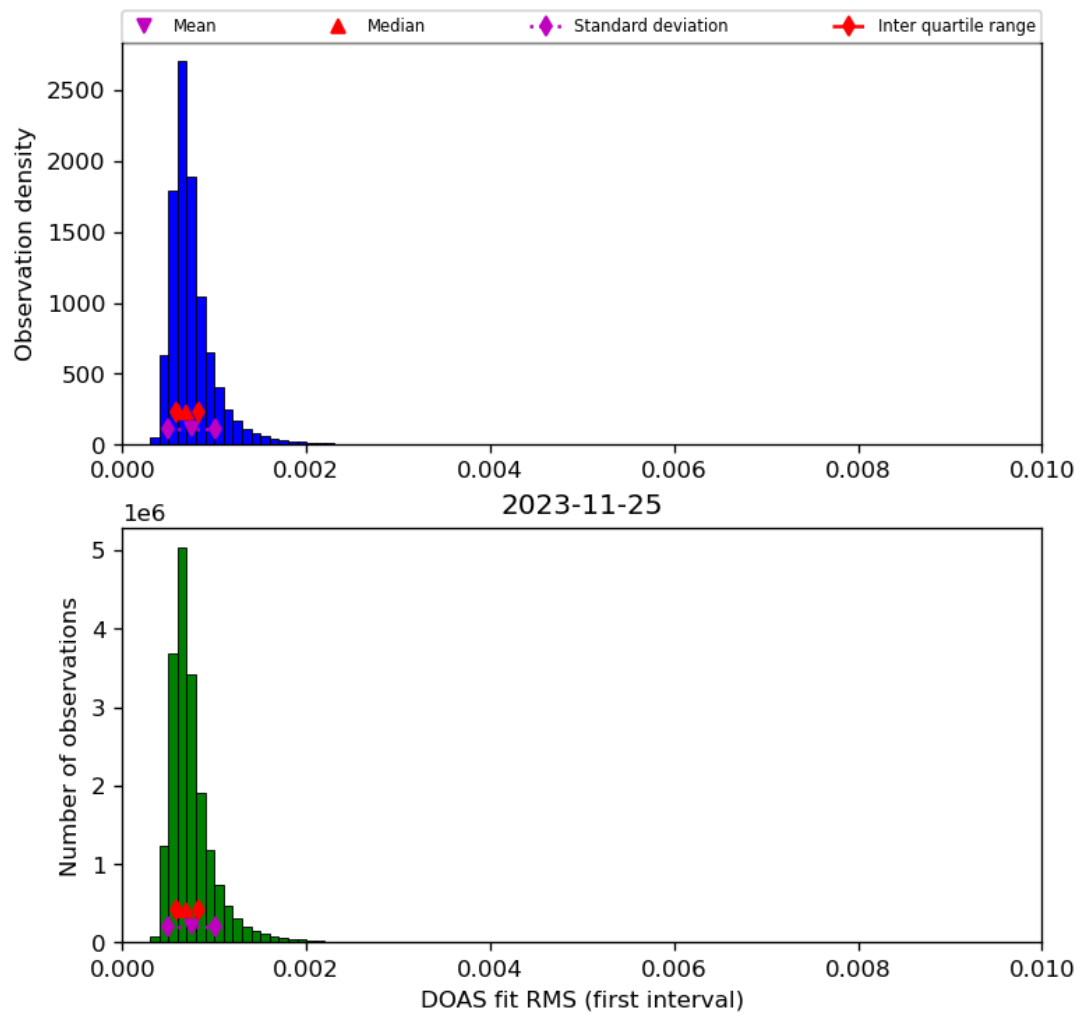
Figure 46: Histogram of “DOAS fit RMS (first interval)” for 2023-11-24 to 2023-11-26
