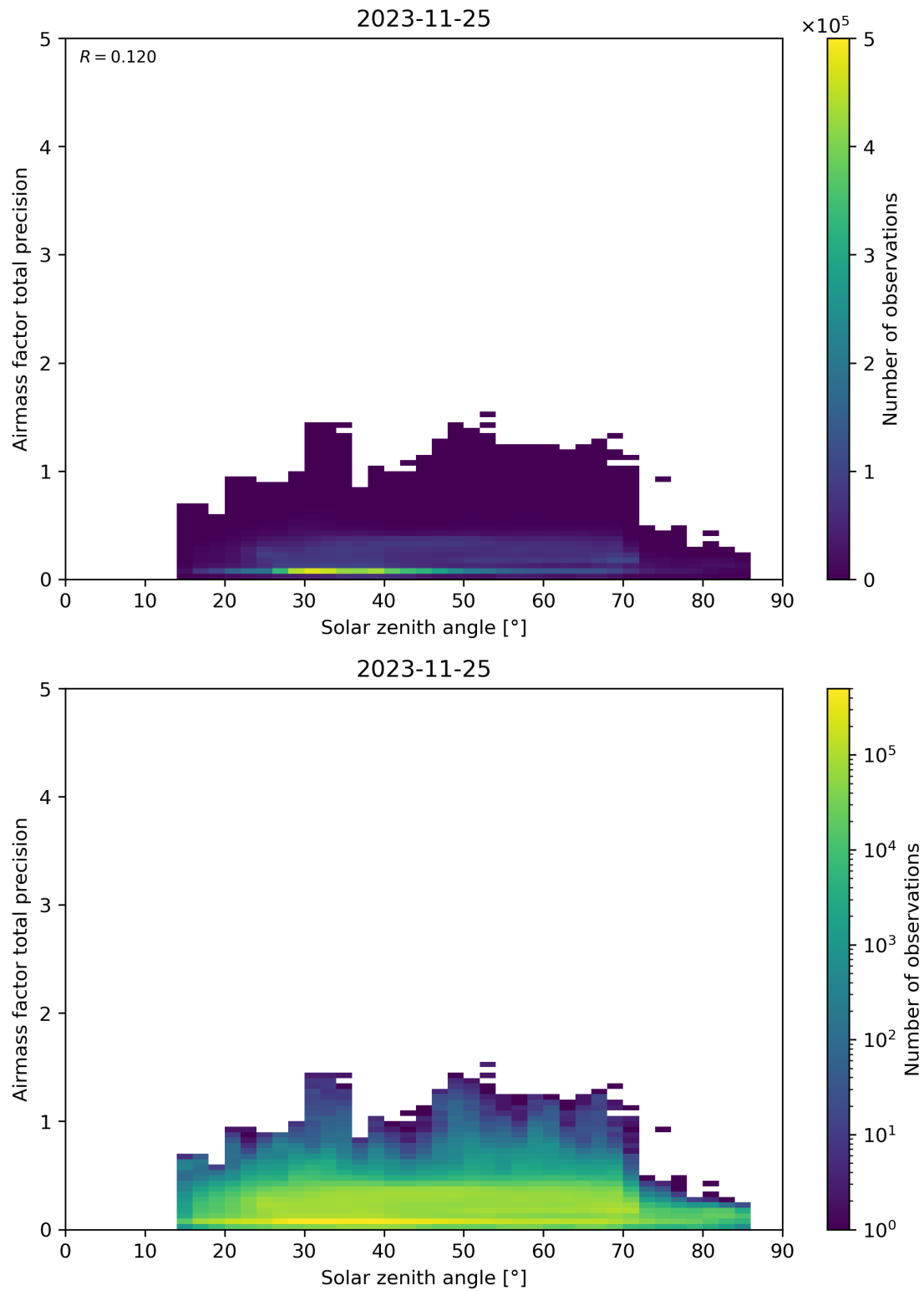
Figure 176: Scatter density plot of “Solar zenith angle” against “Airmass factor total precision” for 2023-11-24 to 2023-11-26.
