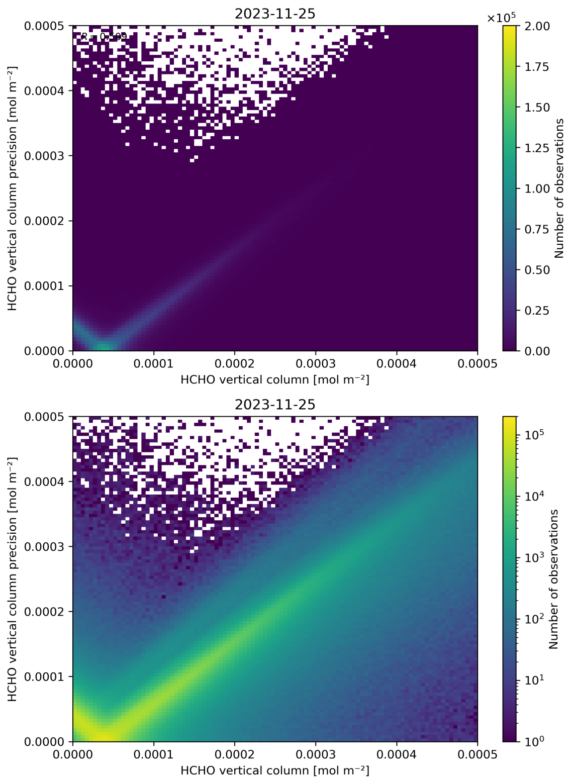
Figure 134: Scatter density plot of “HCHO vertical column” against “HCHO vertical column precision” for 2023-11-24 to 2023-11-26.
