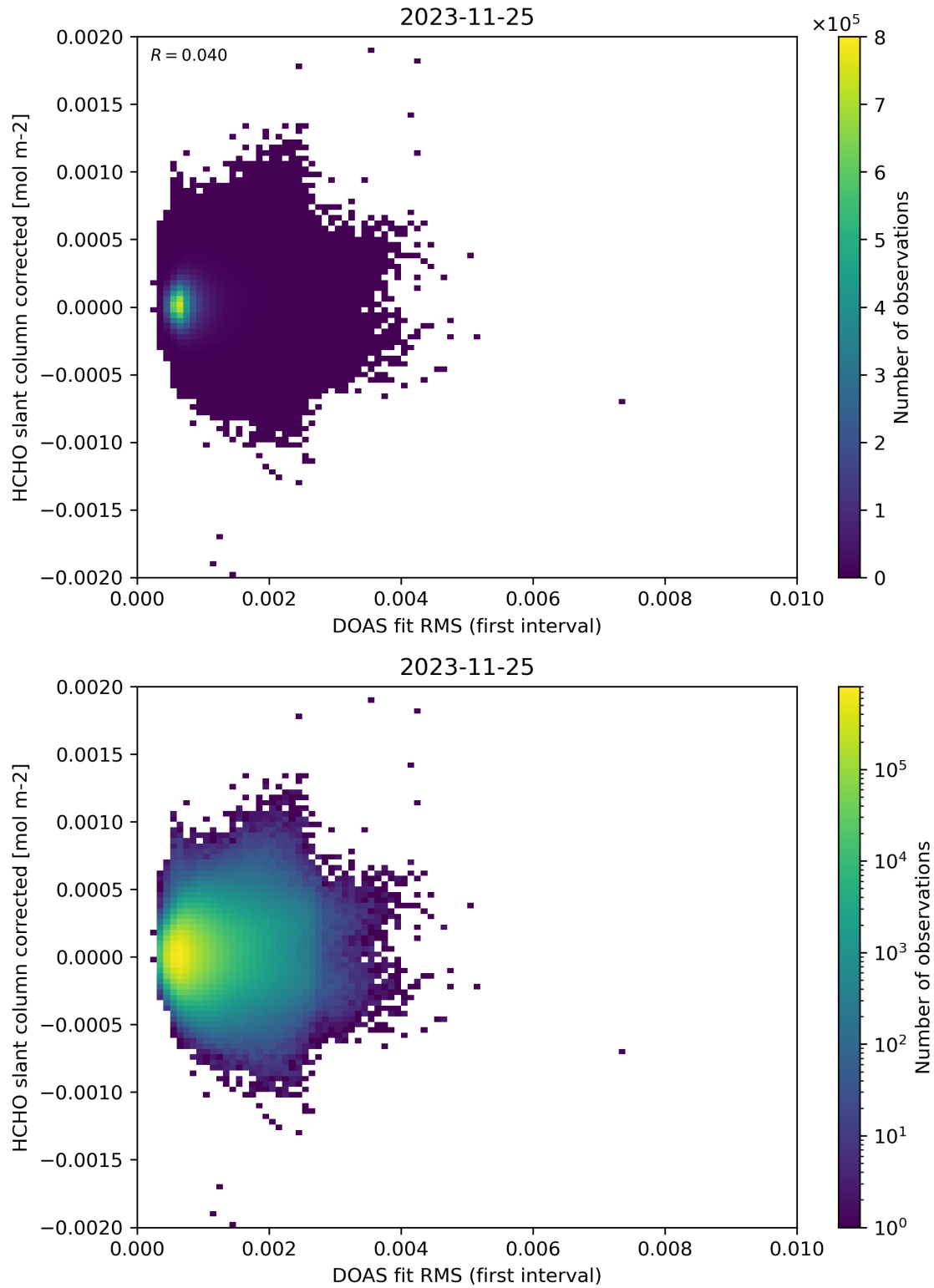
Figure 62: Scatter density plot of “DOAS fit RMS (first interval)” against “HCHO slant column corrected” for 2023-11-24 to 2023-11-26.
