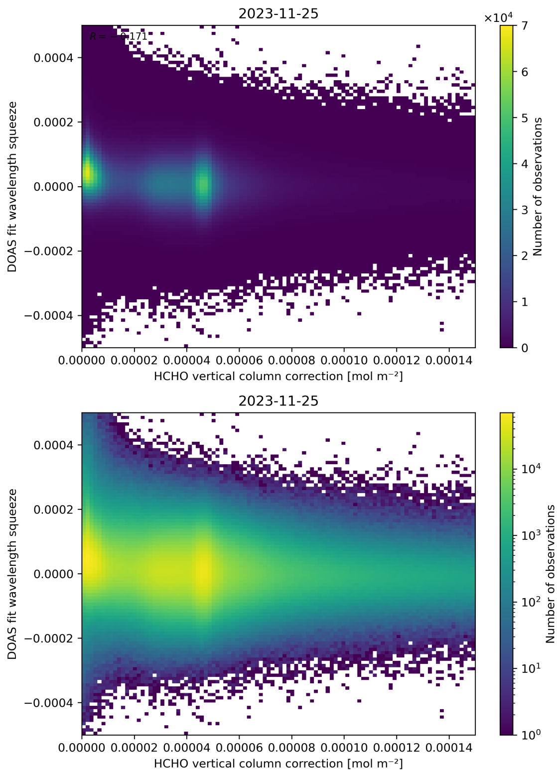
Figure 114: Scatter density plot of “HCHO vertical column correction” against “DOAS fit wavelength squeeze” for 2023-11-24 to 2023-11-26.
