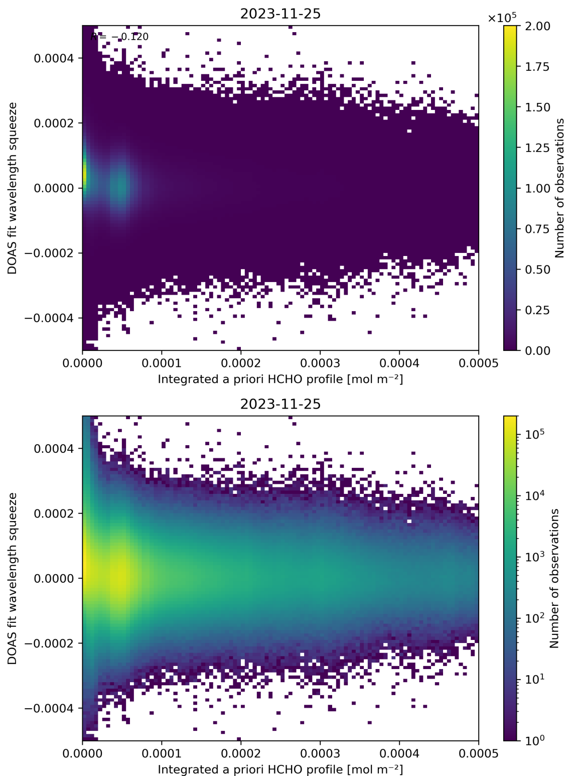
Figure 150: Scatter density plot of “Integrated a priori HCHO profile” against “DOAS fit wavelength squeeze” for 2023-11-24 to 2023-11-26.
