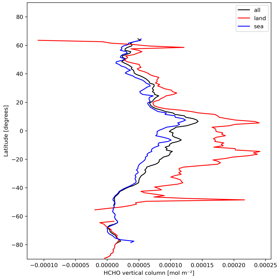
Figure 21: Zonal average of “HCHO vertical column” for 2023-11-24 to 2023-11-26.
