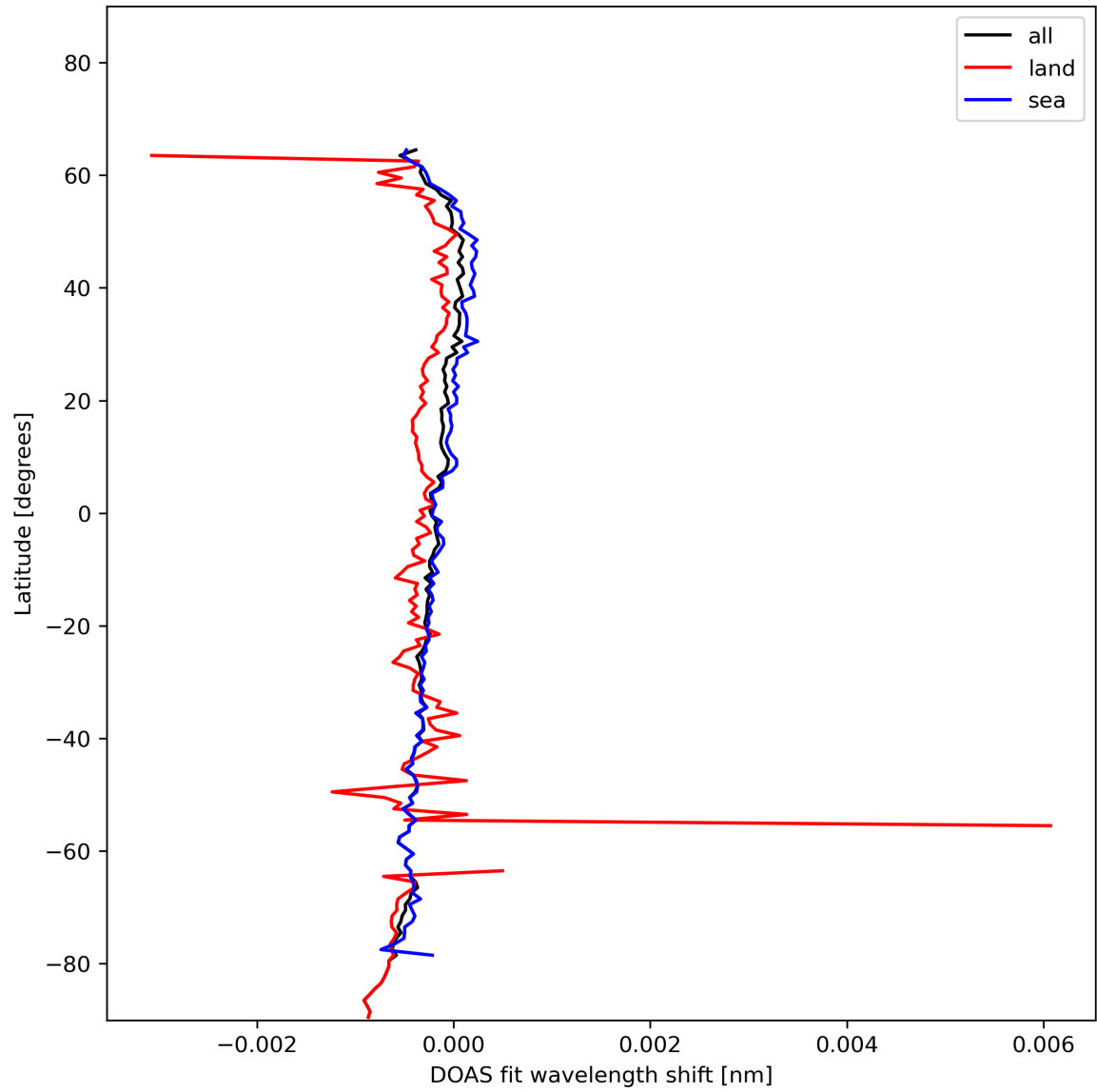
Figure 30: Zonal average of “DOAS fit wavelength shift” for 2023-11-24 to 2023-11-26.
