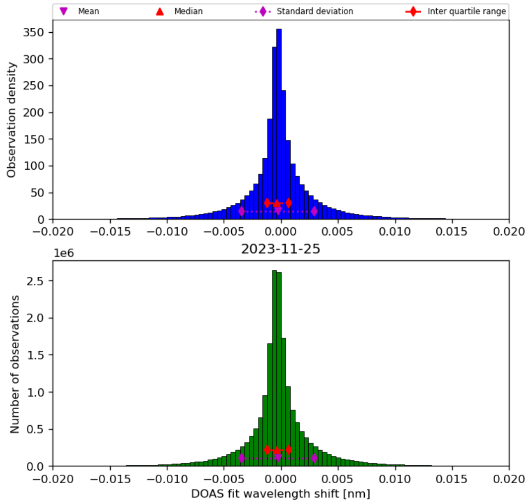
Figure 44: Histogram of “DOAS fit wavelength shift” for 2023-11-24 to 2023-11-26
