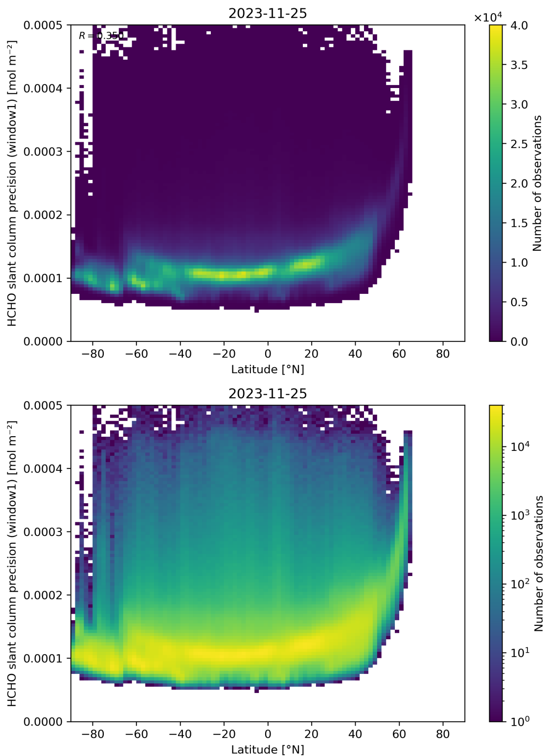
Figure 160: Scatter density plot of “Latitude” against “HCHO slant column precision (window1)” for 2023-11-24 to 2023-11-26.
