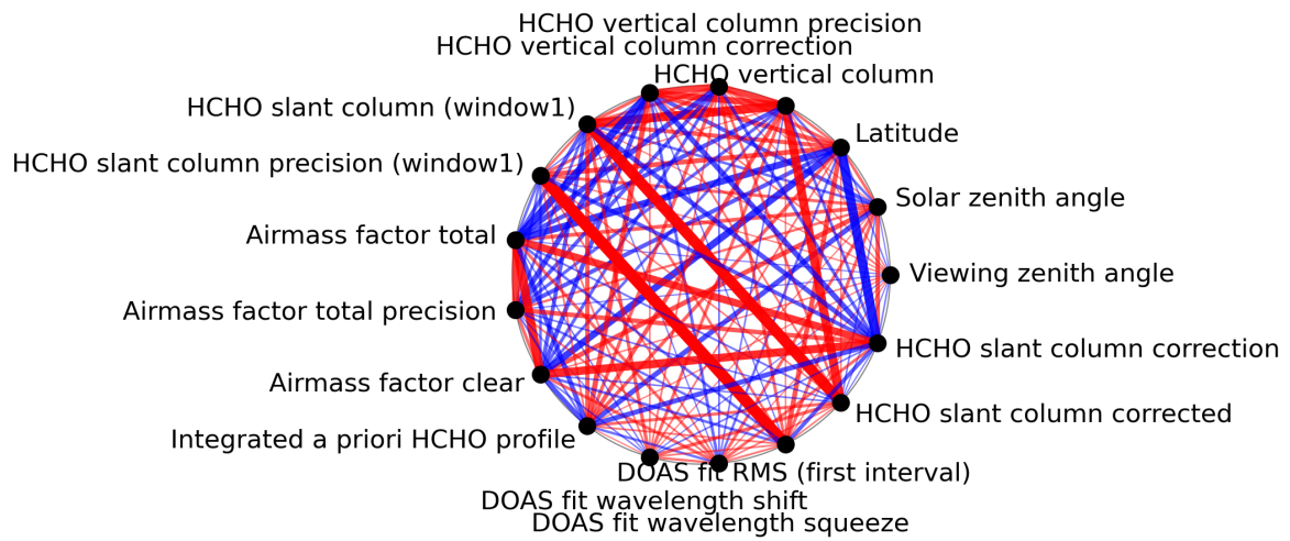
Figure 1: Map of correlation graph for 2023-11-24 to 2023-11-26.
