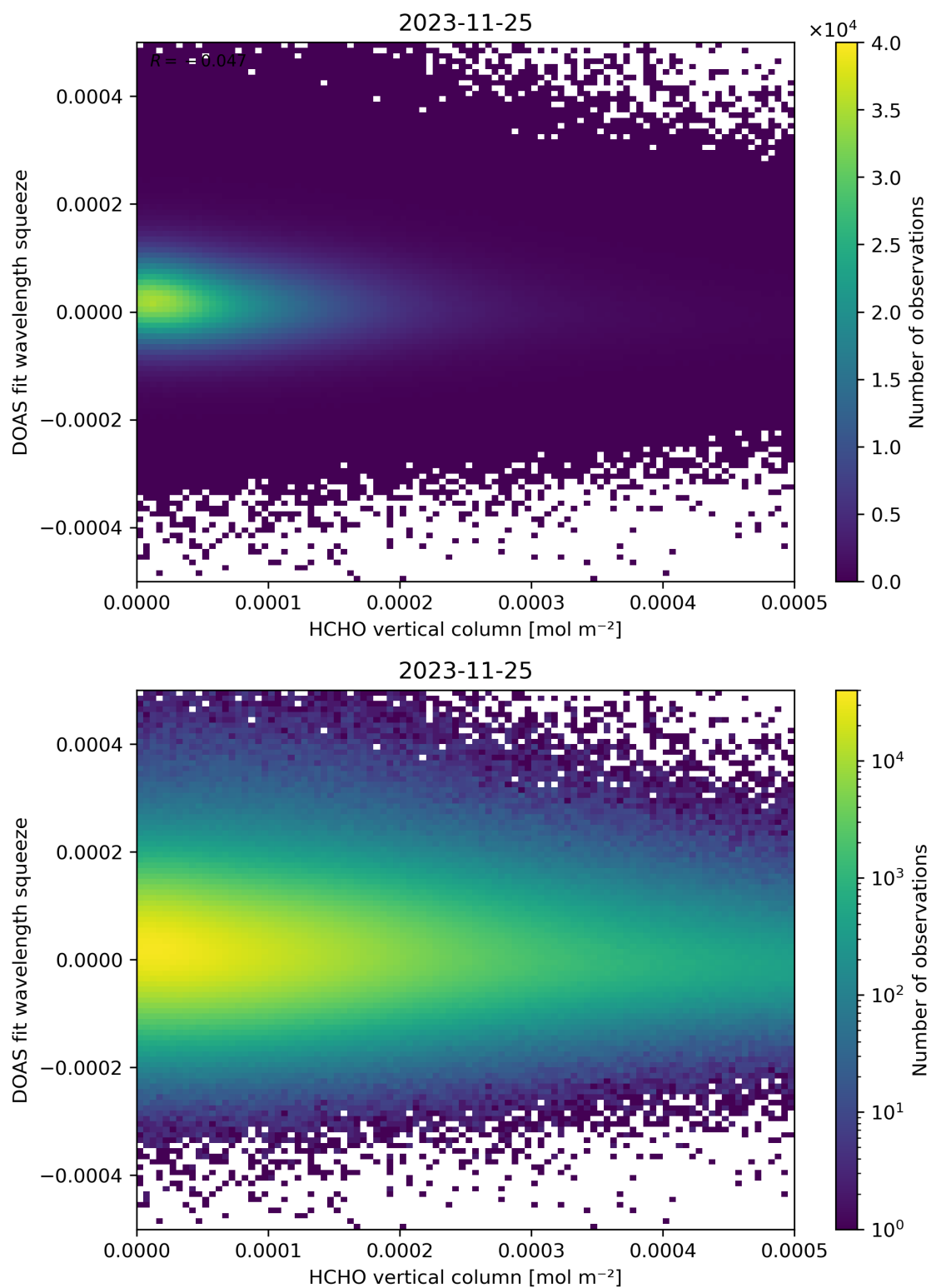
Figure 125: Scatter density plot of “HCHO vertical column” against “DOAS fit wavelength squeeze” for 2023-11-24 to 2023-11-26.
