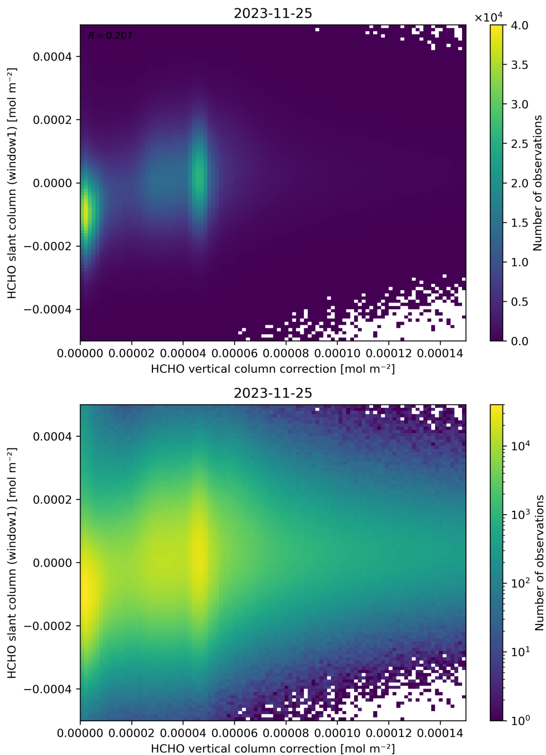
Figure 118: Scatter density plot of “HCHO vertical column correction” against “HCHO slant column (window1)” for 2023-11-24 to 2023-11-26.
