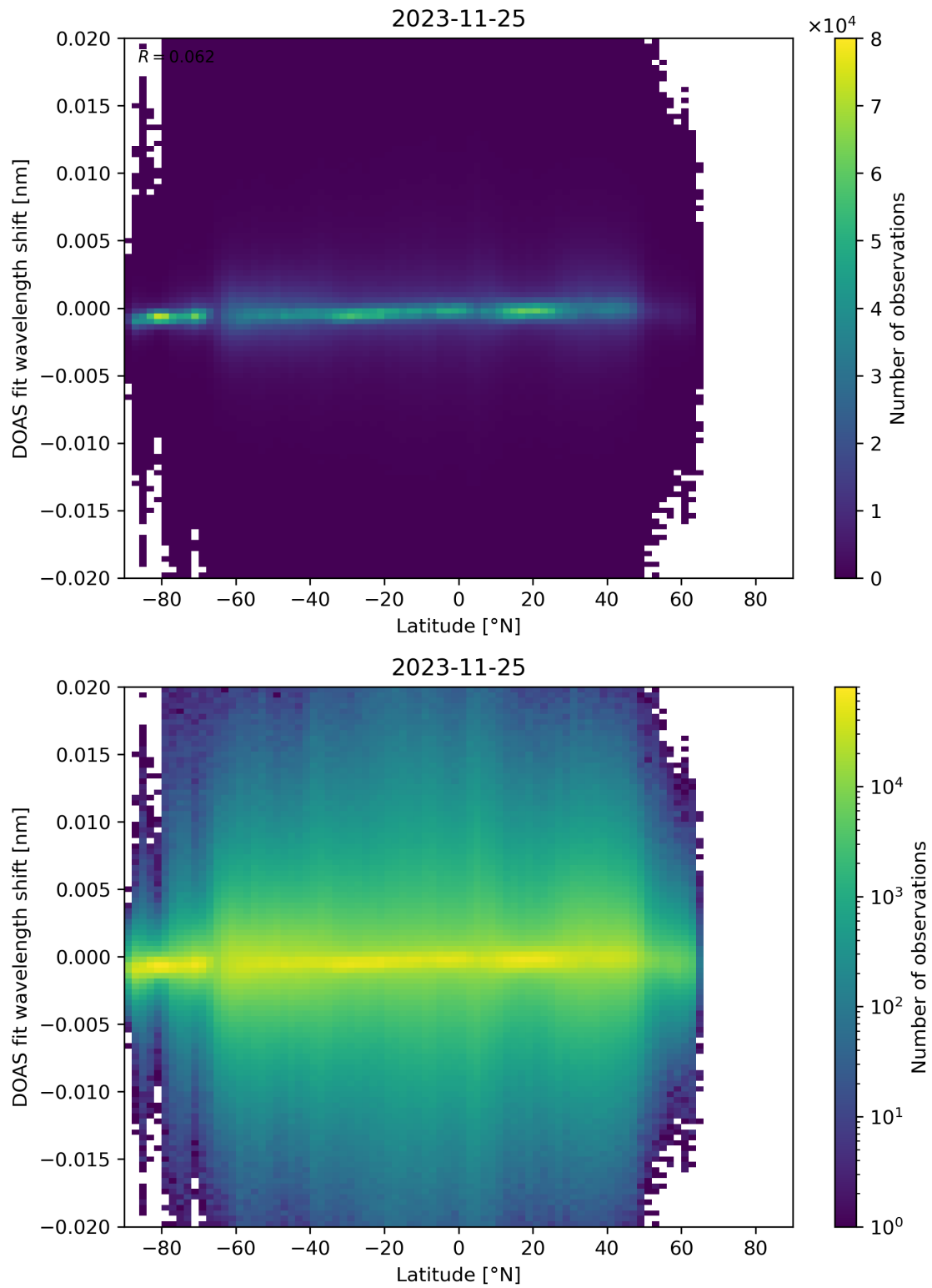
Figure 154: Scatter density plot of “Latitude” against “DOAS fit wavelength shift” for 2023-11-24 to 2023-11-26.
