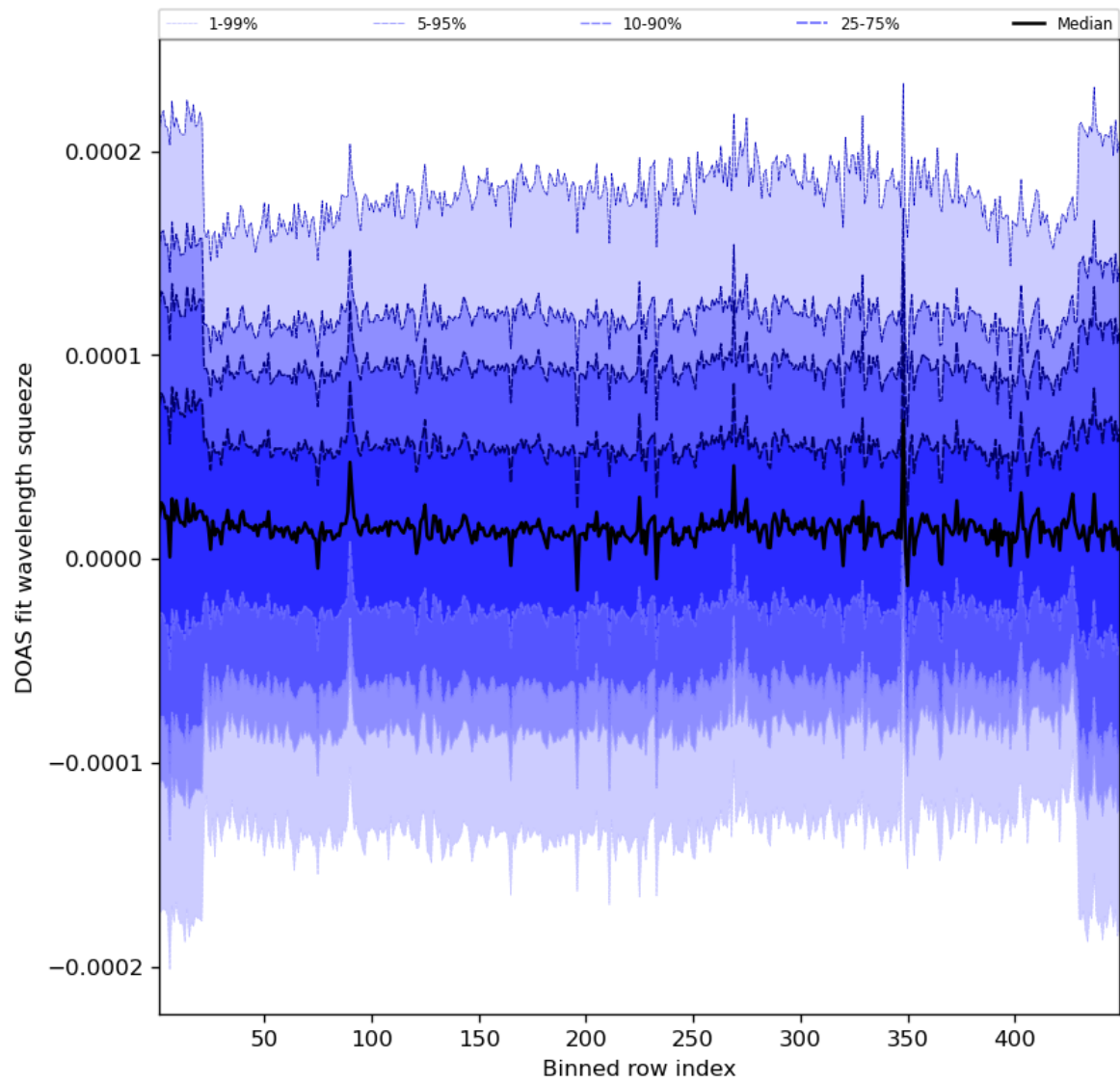
Figure 59: Along track statistics of “DOAS fit wavelength squeeze” for 2023-11-24 to 2023-11-26
