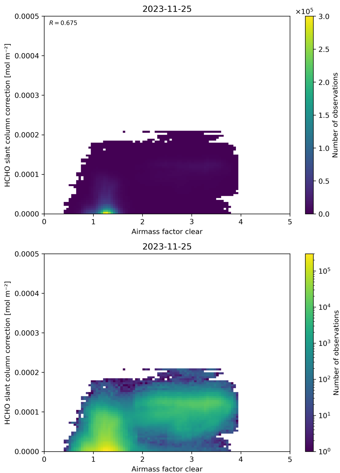
Figure 75: Scatter density plot of “Airmass factor clear” against “HCHO slant column correction” for 2023-11-24 to 2023-11-26.
