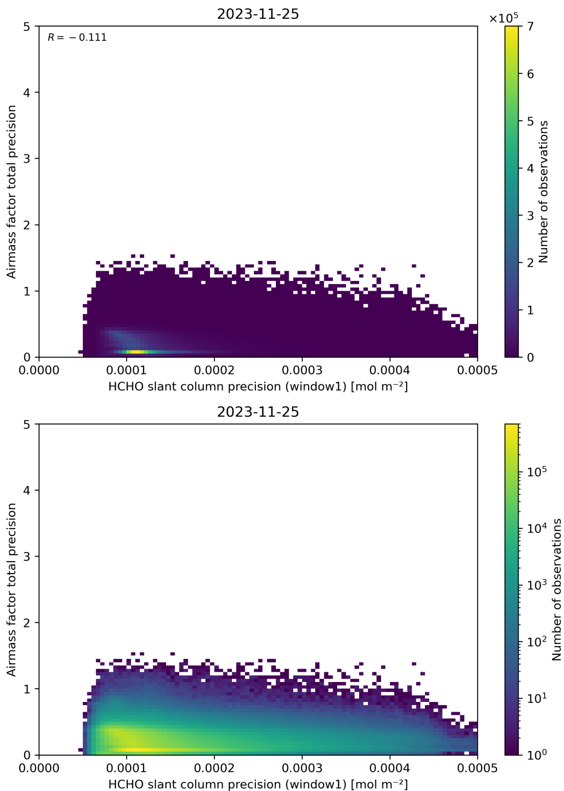
Figure 95: Scatter density plot of “HCHO slant column precision (window1)” against “Airmass factor total precision” for 2023-11-24 to 2023-11-26.
