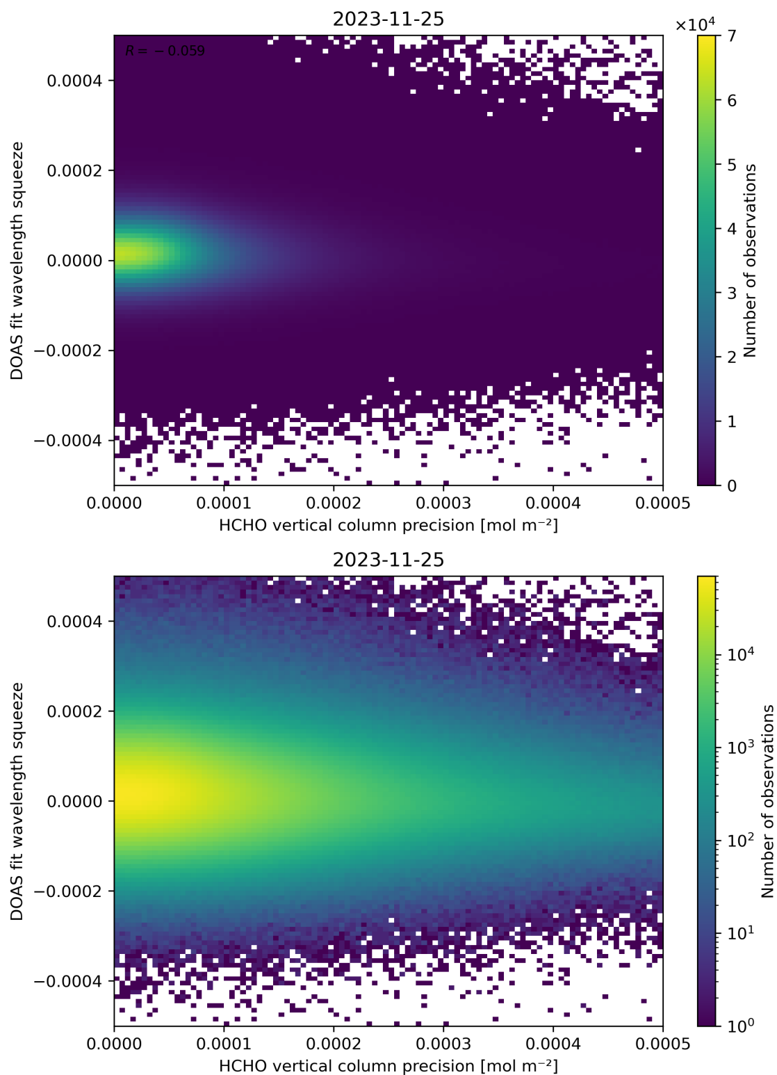
Figure 138: Scatter density plot of “HCHO vertical column precision” against “DOAS fit wavelength squeeze” for 2023-11-24 to 2023-11-26.
