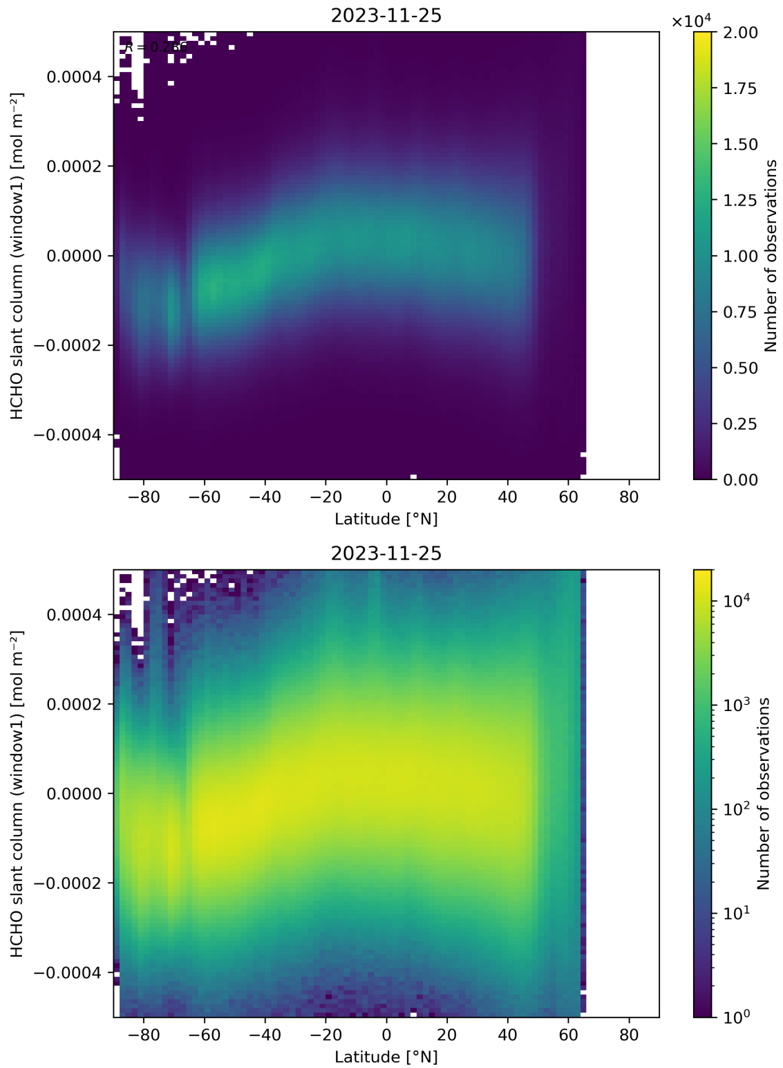
Figure 159: Scatter density plot of “Latitude” against “HCHO slant column (window1)” for 2023-11-24 to 2023-11-26.
