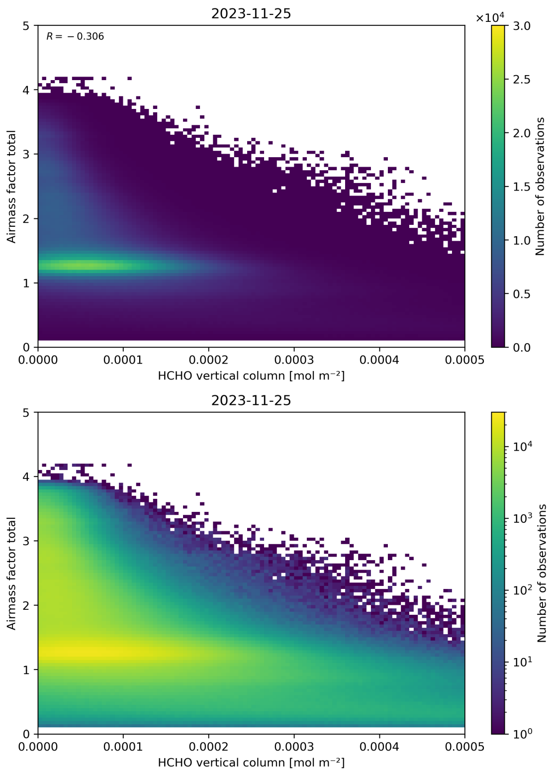
Figure 131: Scatter density plot of “HCHO vertical column” against “Airmass factor total” for 2023-11-24 to 2023-11-26.
