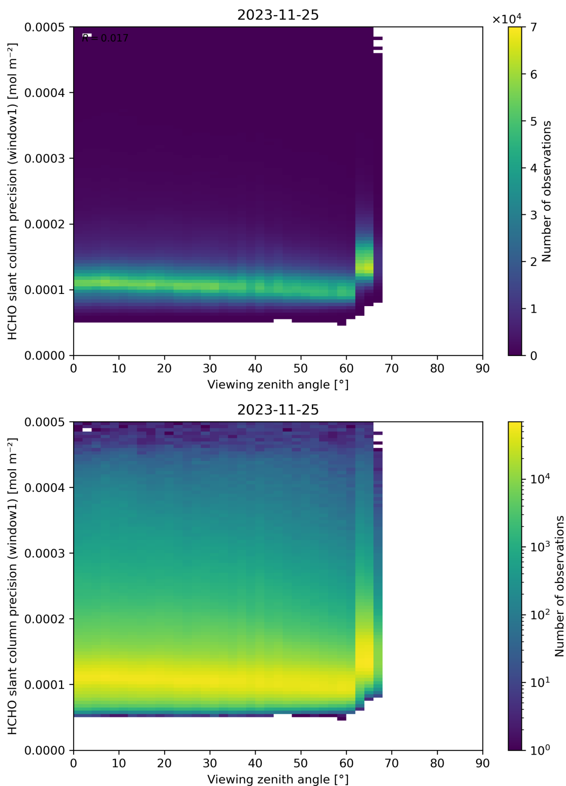
Figure 189: Scatter density plot of “Viewing zenith angle” against “HCHO slant column precision (window1)” for 2023-11-24 to 2023-11-26.
