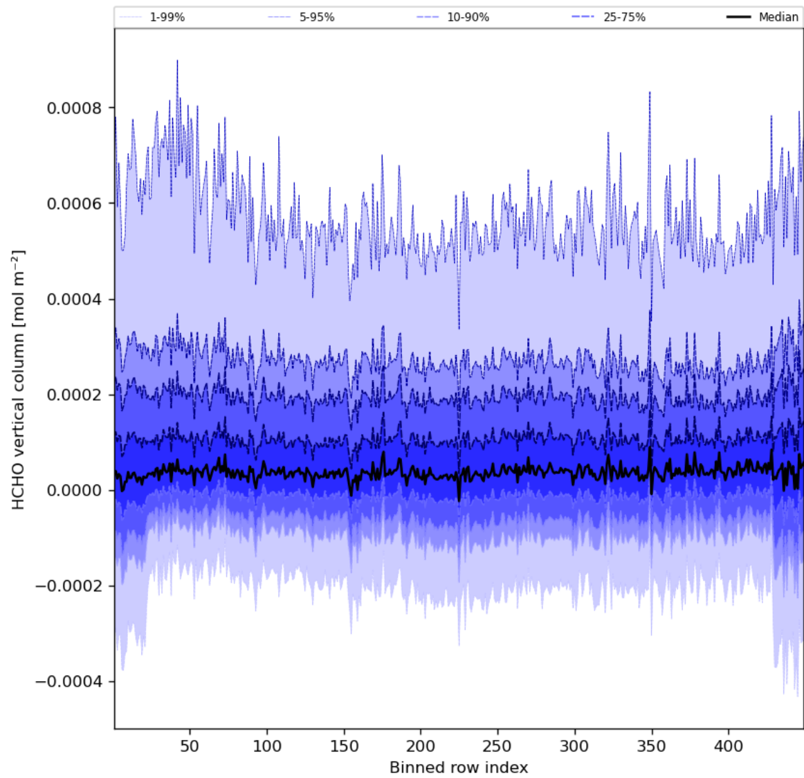
Figure 49: Along track statistics of “HCHO vertical column” for 2023-11-24 to 2023-11-26
