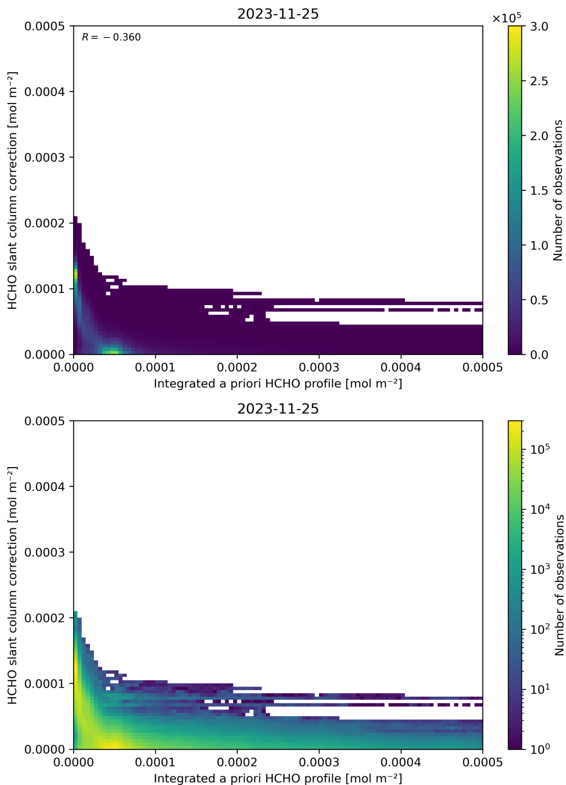
Figure 152: Scatter density plot of “Integrated a priori HCHO profile” against “HCHO slant column correction” for 2023-11-24 to 2023-11-26.
