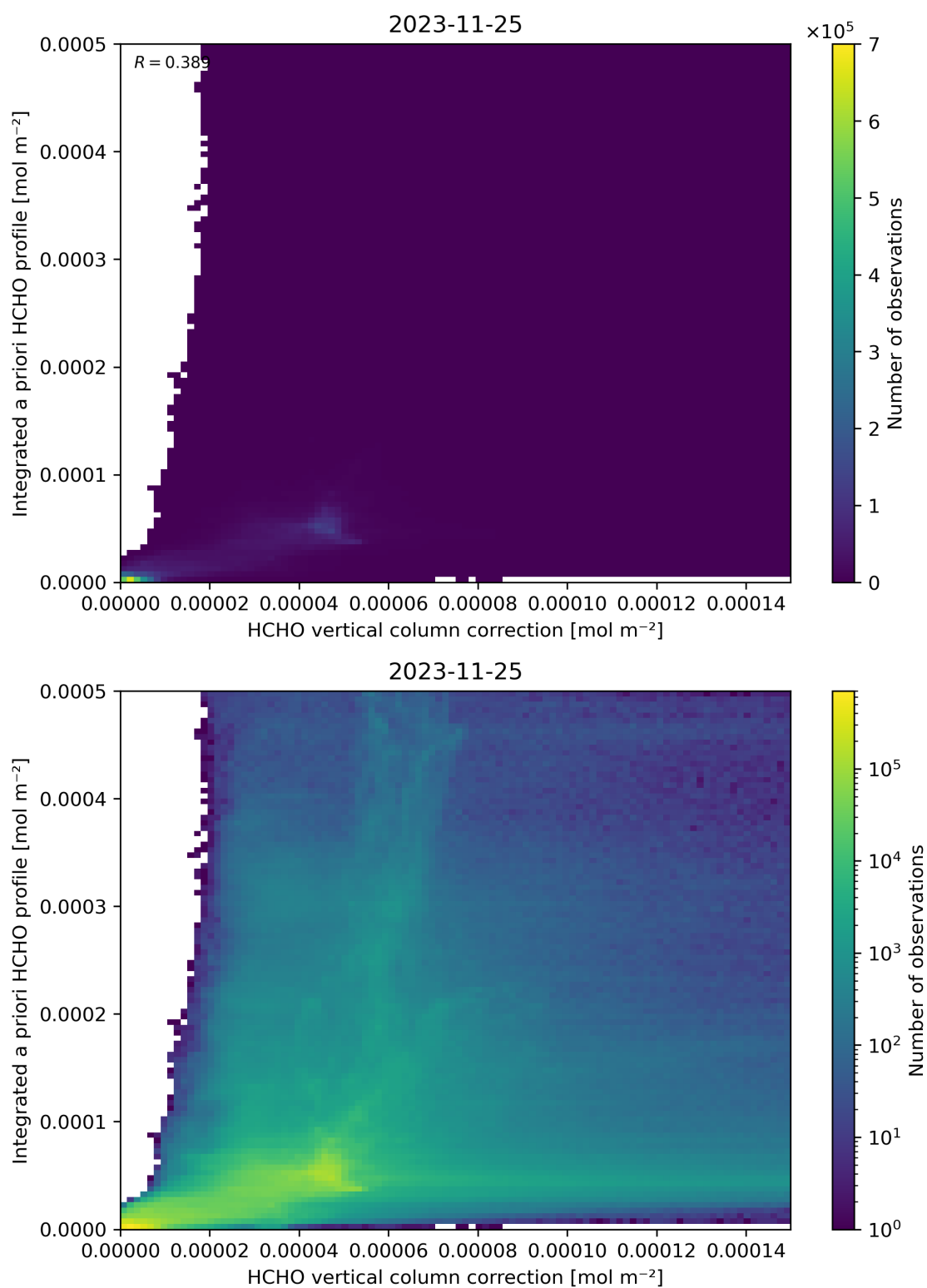
Figure 122: Scatter density plot of “HCHO vertical column correction” against “Integrated a priori HCHO profile” for 2023-11-24 to 2023-11-26.
