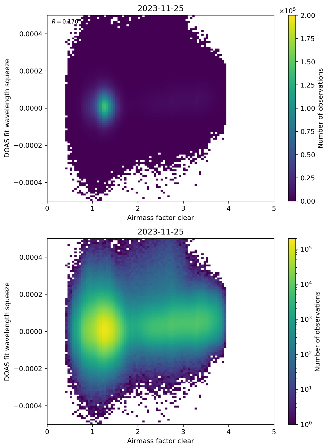
Figure 73: Scatter density plot of “Airmass factor clear” against “DOAS fit wavelength squeeze” for 2023-11-24 to 2023-11-26.
