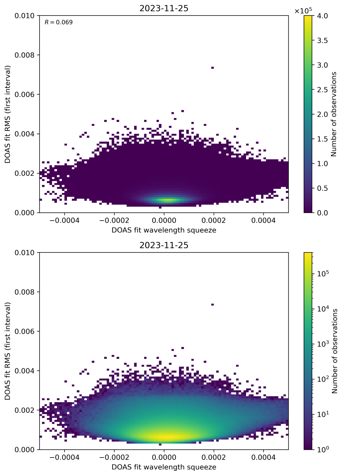
Figure 68: Scatter density plot of “DOAS fit wavelength squeeze” against “DOAS fit RMS (first interval)” for 2023-11-24 to 2023-11-26.
