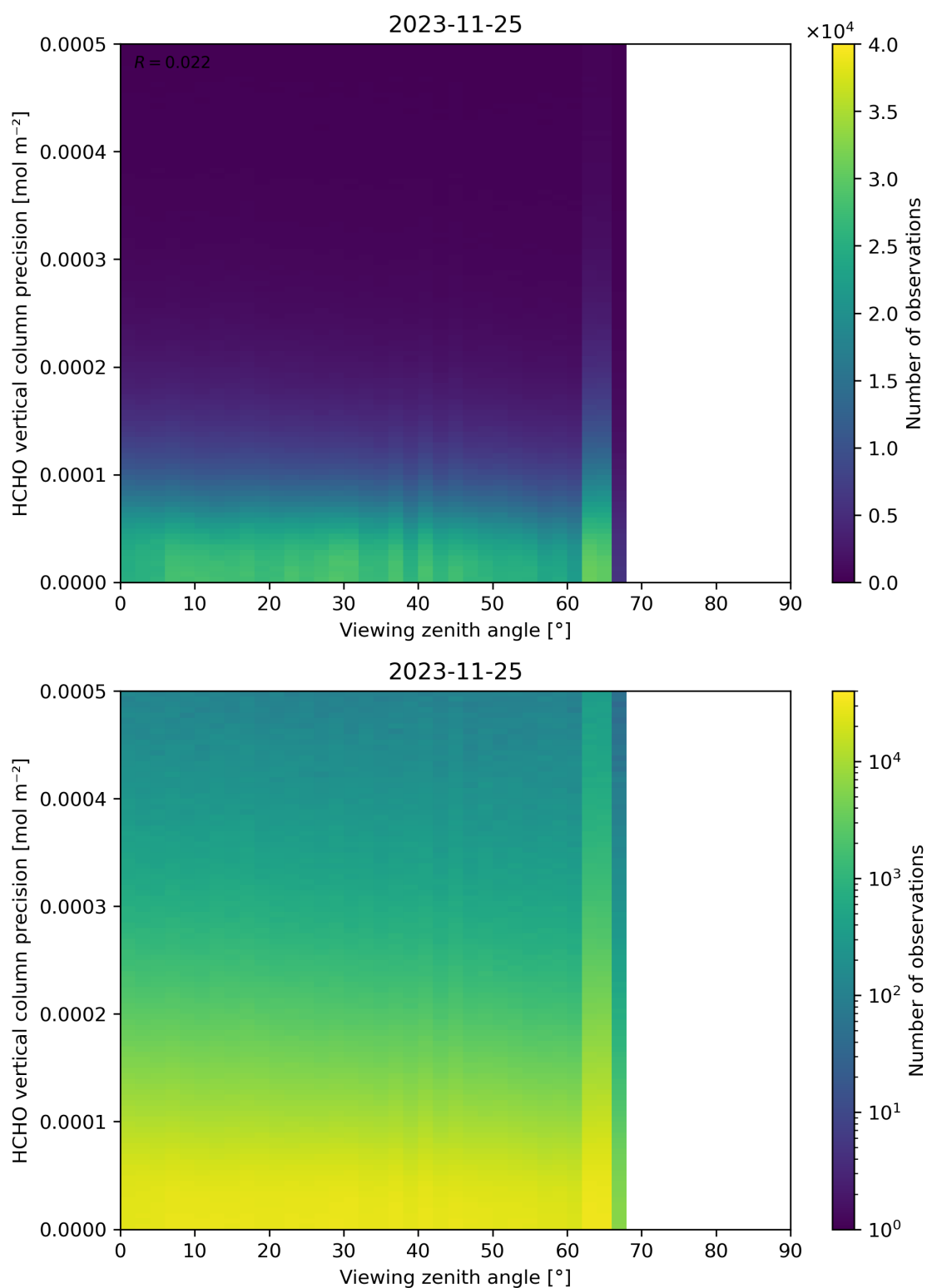
Figure 194: Scatter density plot of “Viewing zenith angle” against “HCHO vertical column precision” for 2023-11-24 to 2023-11-26.
