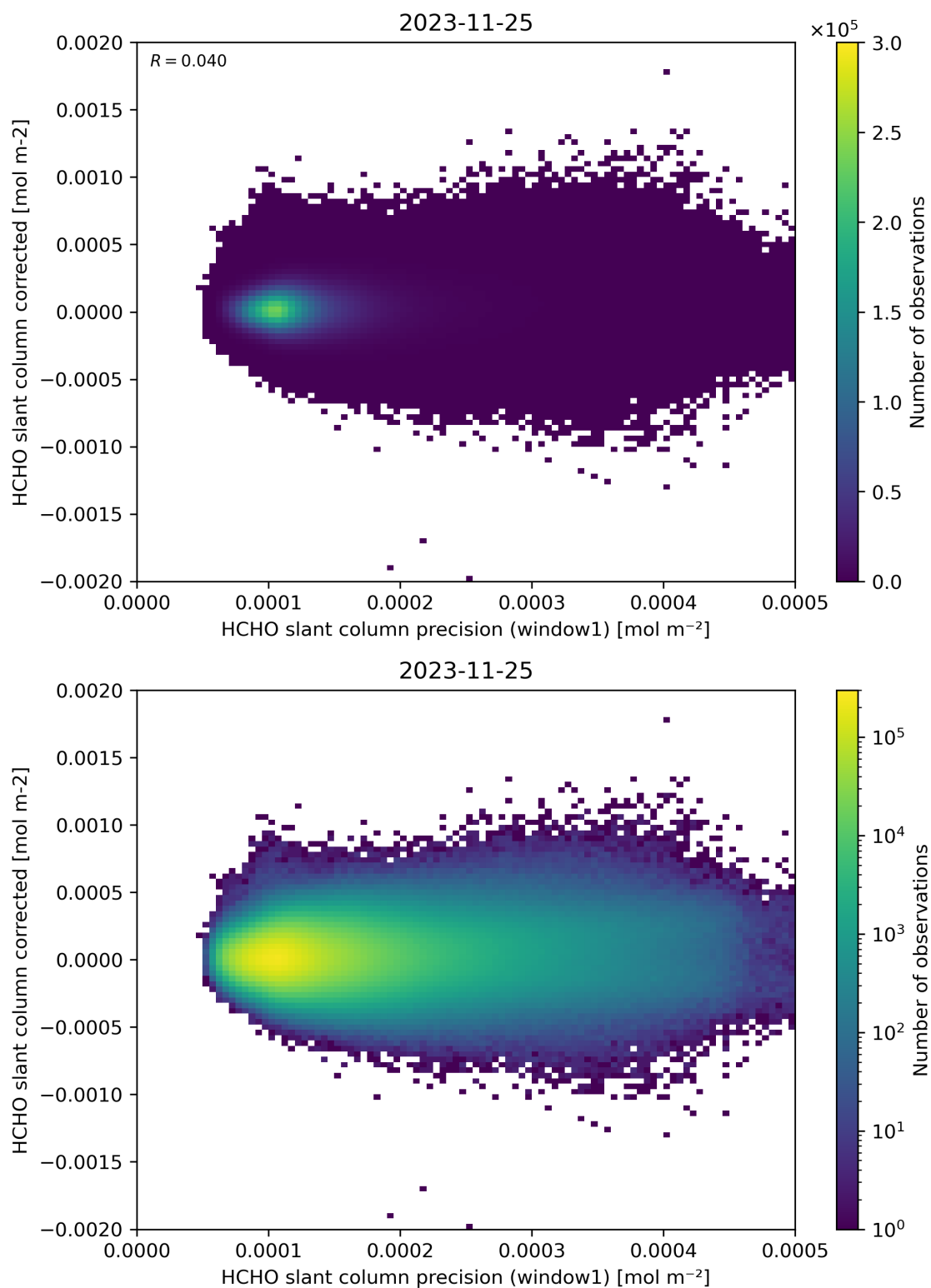
Figure 92: Scatter density plot of “HCHO slant column precision (window1)” against “HCHO slant column corrected” for 2023-11-24 to 2023-11-26.
