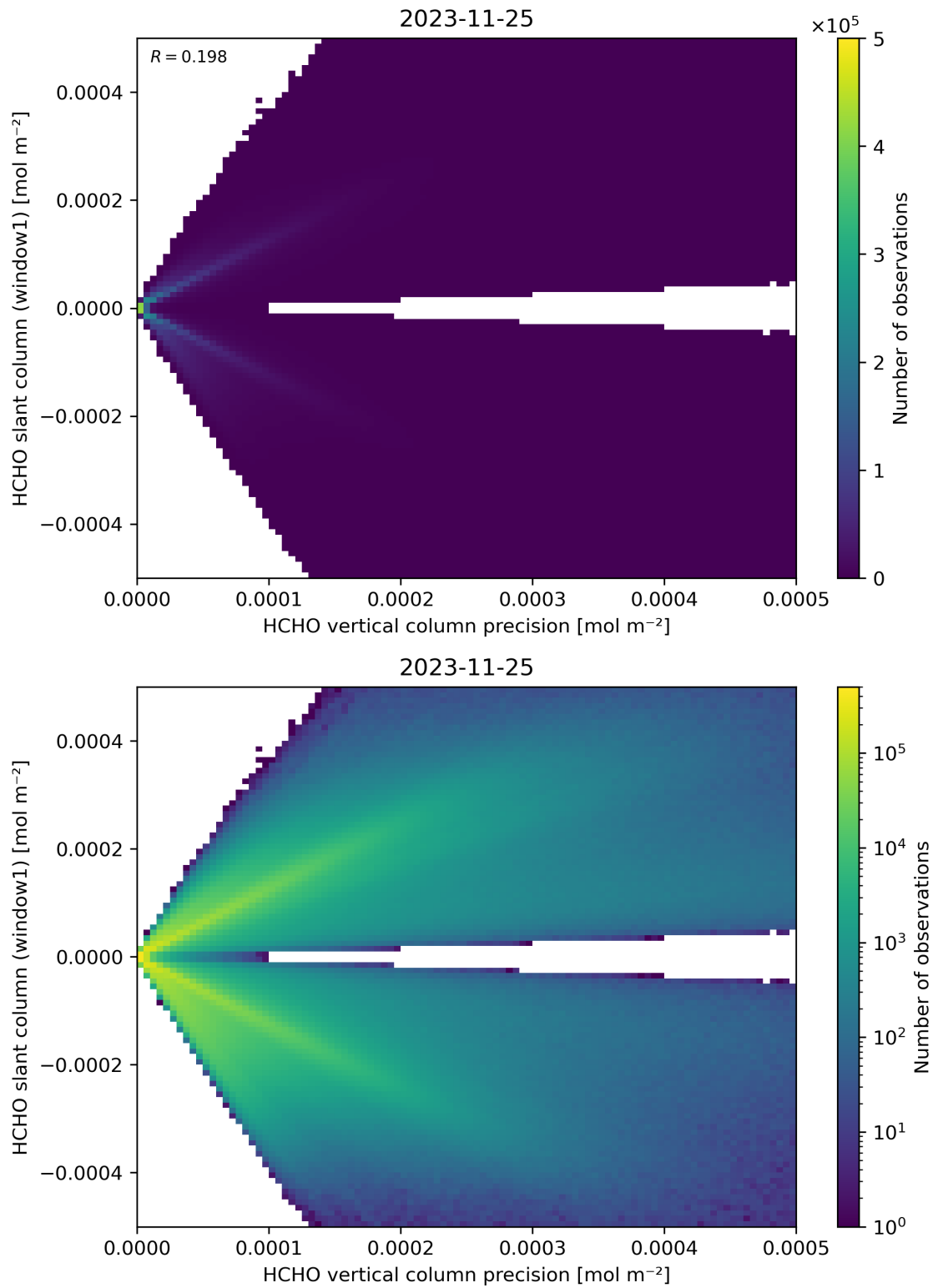
Figure 142: Scatter density plot of “HCHO vertical column precision” against “HCHO slant column (window1)” for 2023-11-24 to 2023-11-26.
