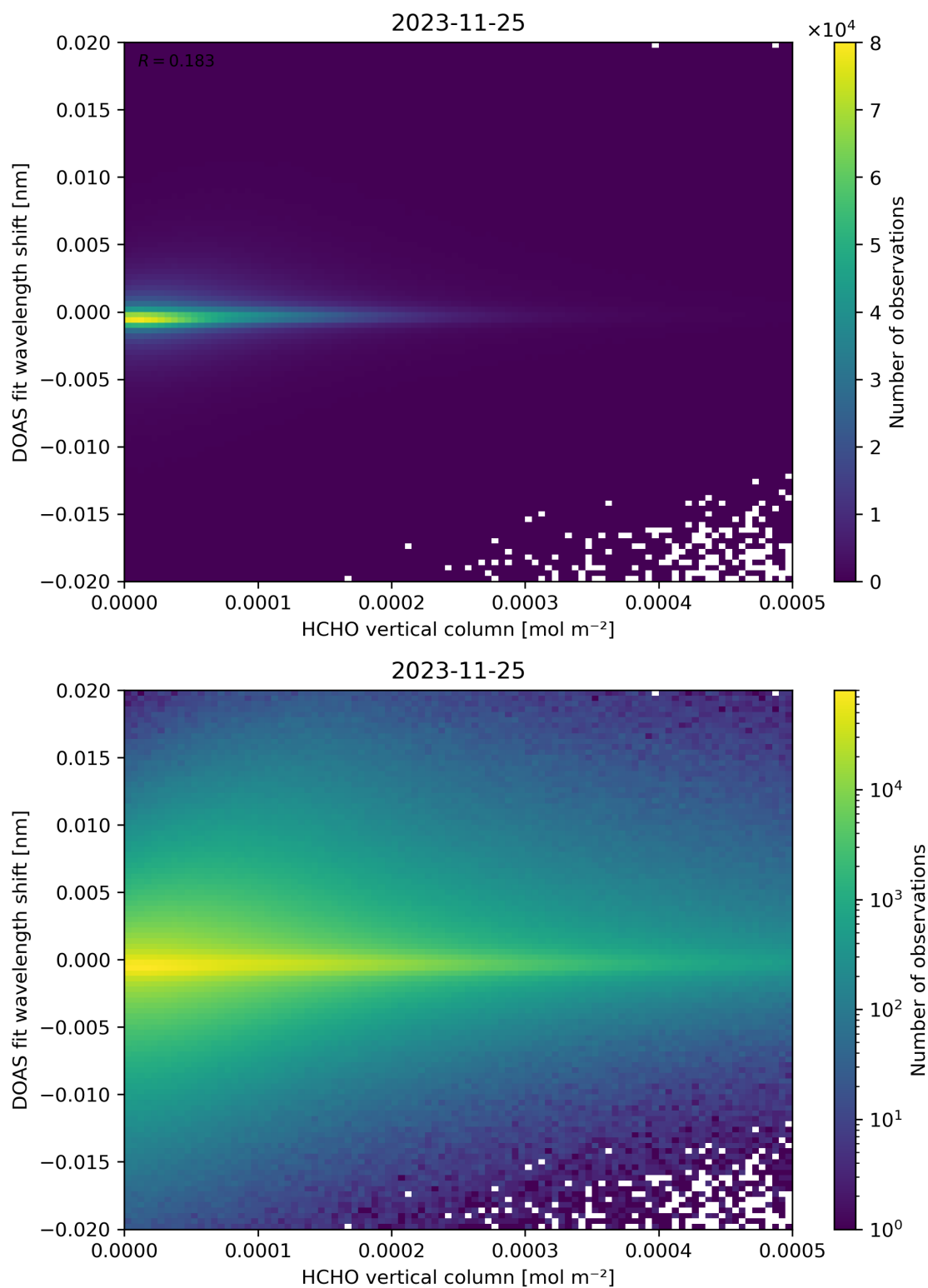
Figure 124: Scatter density plot of “HCHO vertical column” against “DOAS fit wavelength shift” for 2023-11-24 to 2023-11-26.
