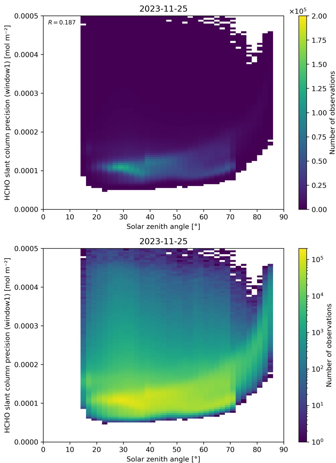
Figure 174: Scatter density plot of “Solar zenith angle” against “HCHO slant column precision (window1)” for 2023-11-24 to 2023-11-26.
