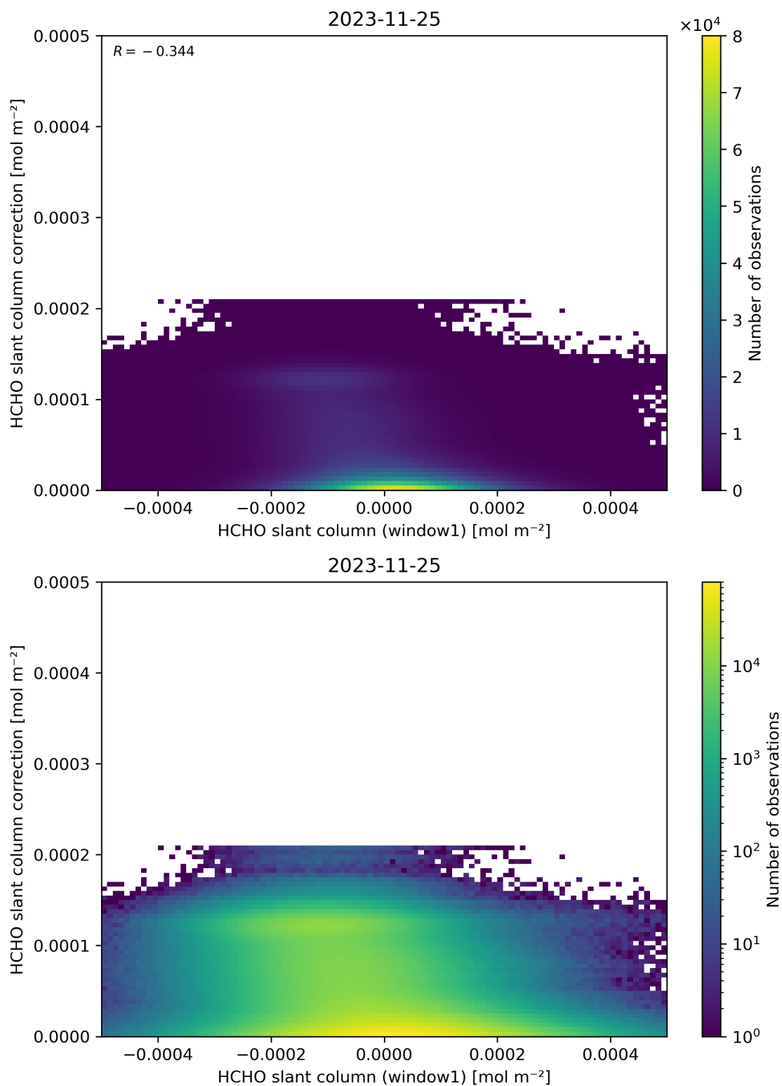
Figure 83: Scatter density plot of “HCHO slant column (window1)” against “HCHO slant column correction” for 2023-11-24 to 2023-11-26.
