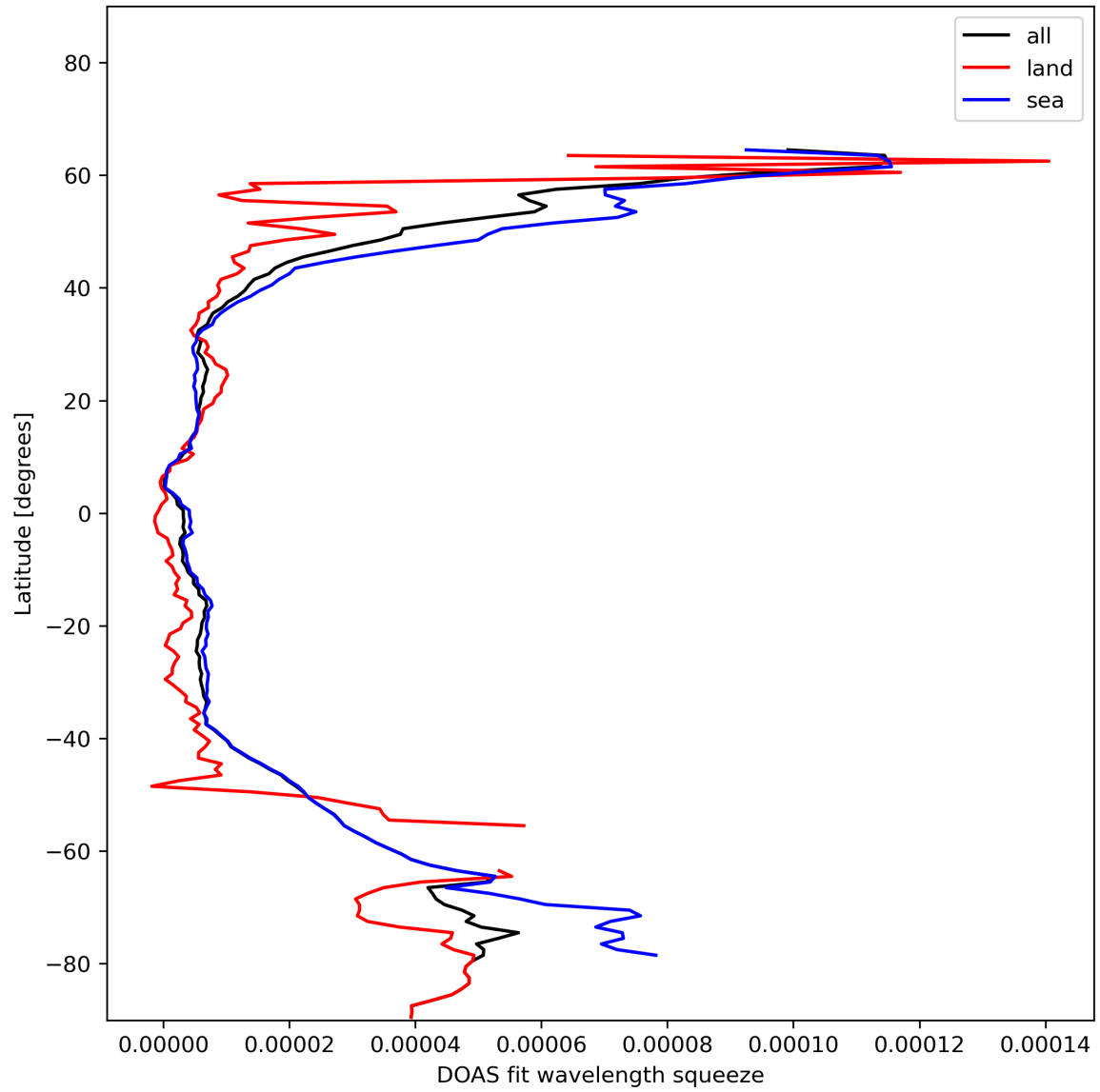
Figure 31: Zonal average of “DOAS fit wavelength squeeze” for 2023-11-24 to 2023-11-26.
