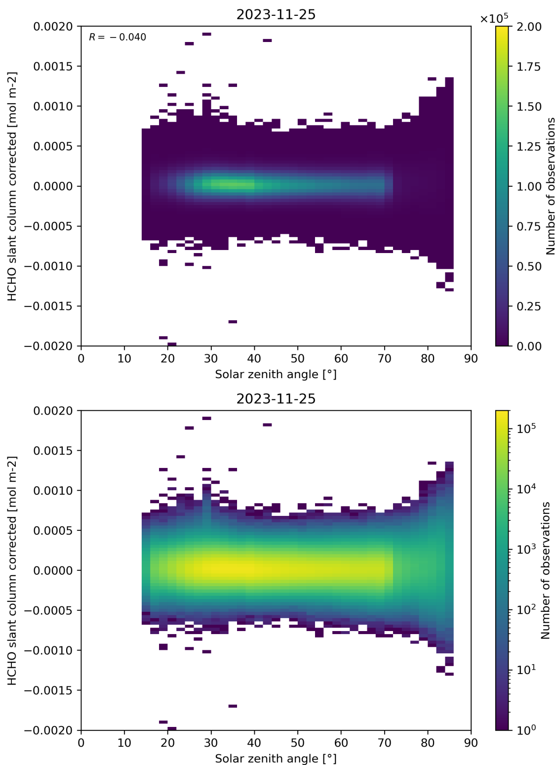
Figure 171: Scatter density plot of “Solar zenith angle” against “HCHO slant column corrected” for 2023-11-24 to 2023-11-26.
