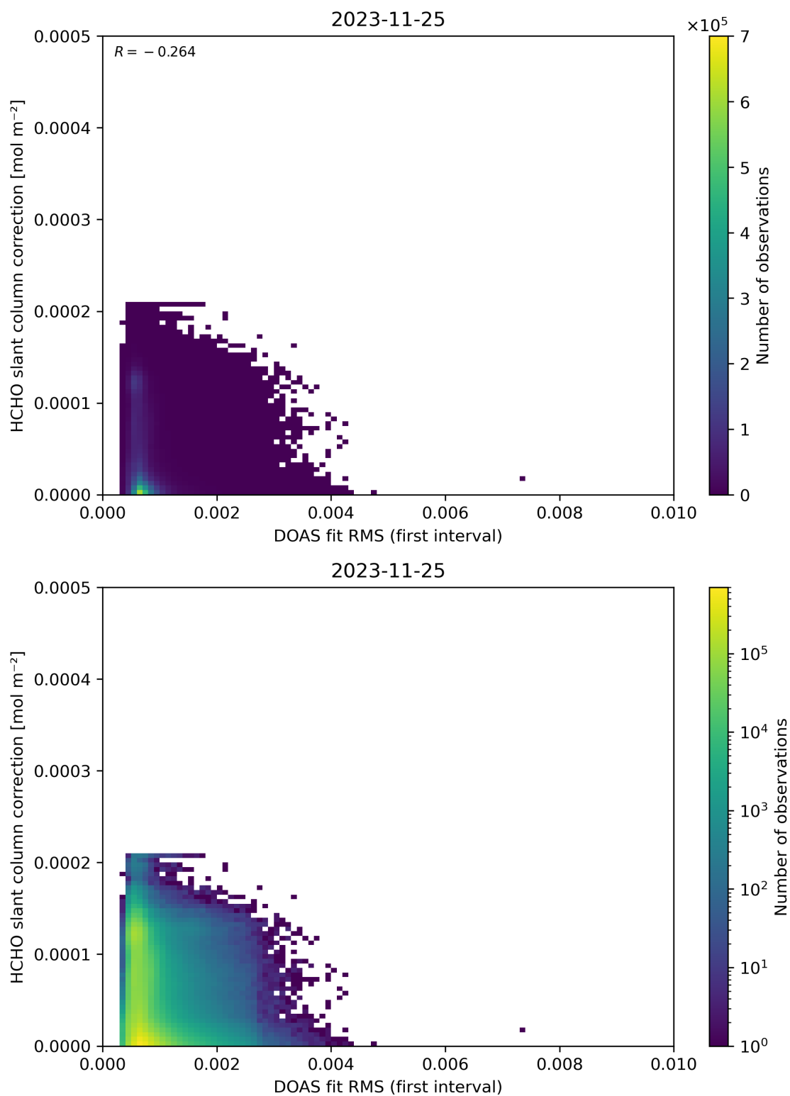
Figure 63: Scatter density plot of “DOAS fit RMS (first interval)” against “HCHO slant column correction” for 2023-11-24 to 2023-11-26.
