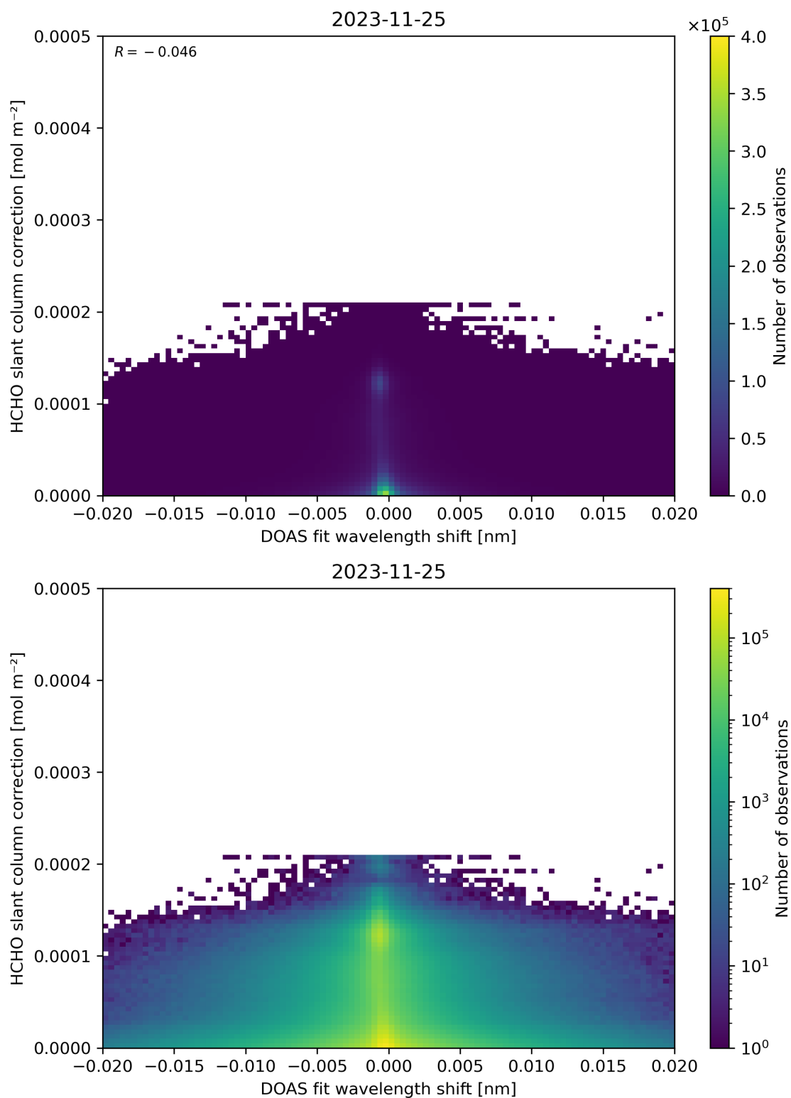
Figure 67: Scatter density plot of “DOAS fit wavelength shift” against “HCHO slant column correction” for 2023-11-24 to 2023-11-26.
