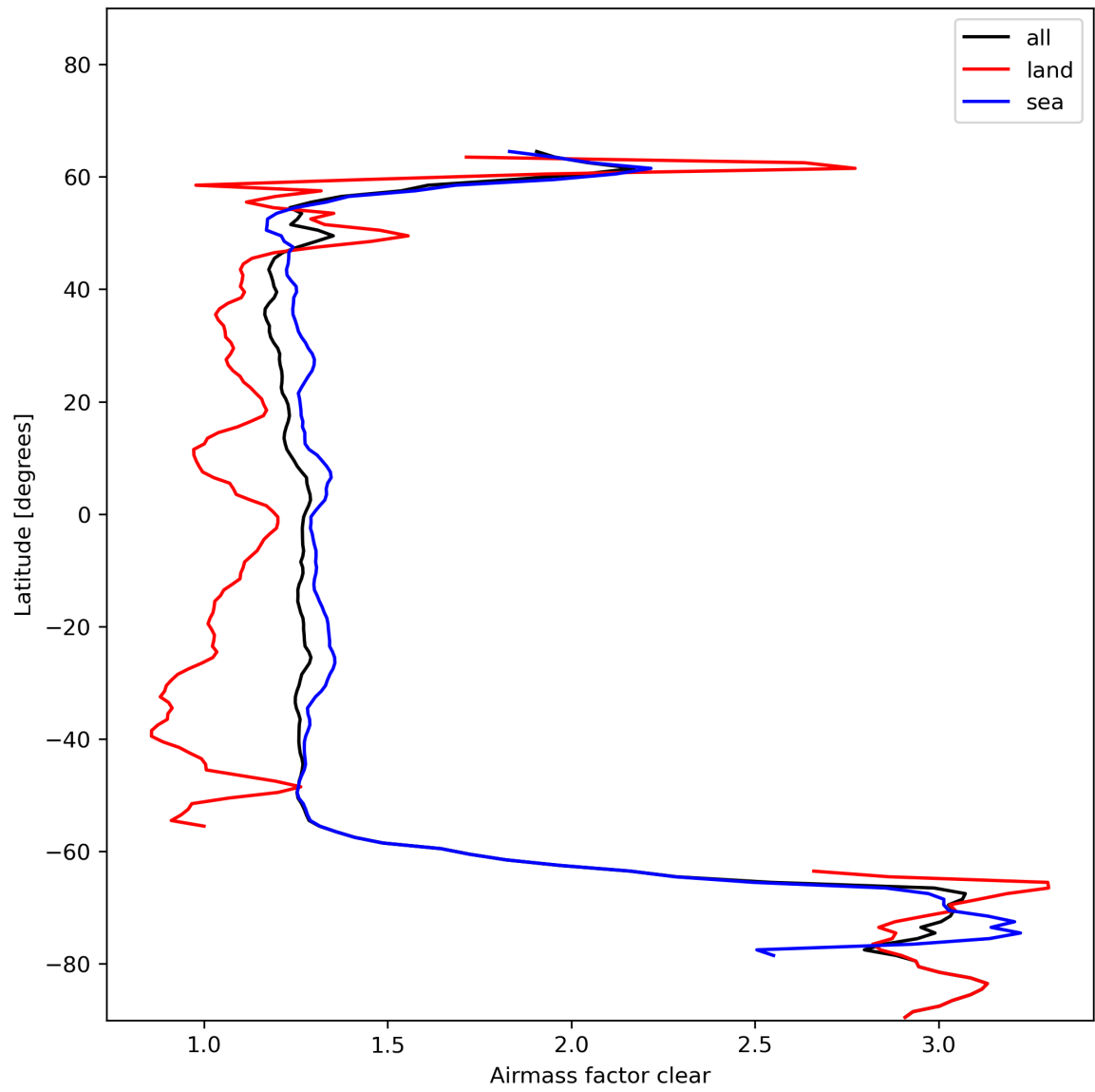
Figure 28: Zonal average of “Airmass factor clear” for 2023-11-24 to 2023-11-26.
