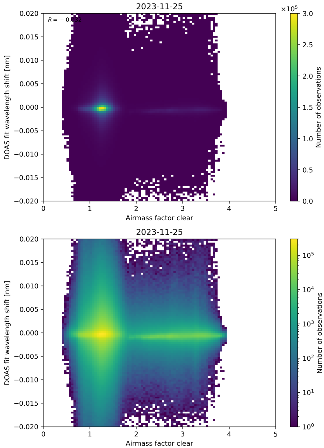
Figure 72: Scatter density plot of “Airmass factor clear” against “DOAS fit wavelength shift” for 2023-11-24 to 2023-11-26.
