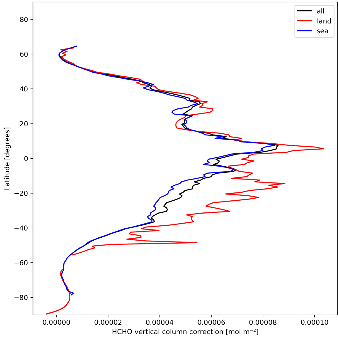
Figure 23: Zonal average of “HCHO vertical column correction” for 2023-11-24 to 2023-11-26.
