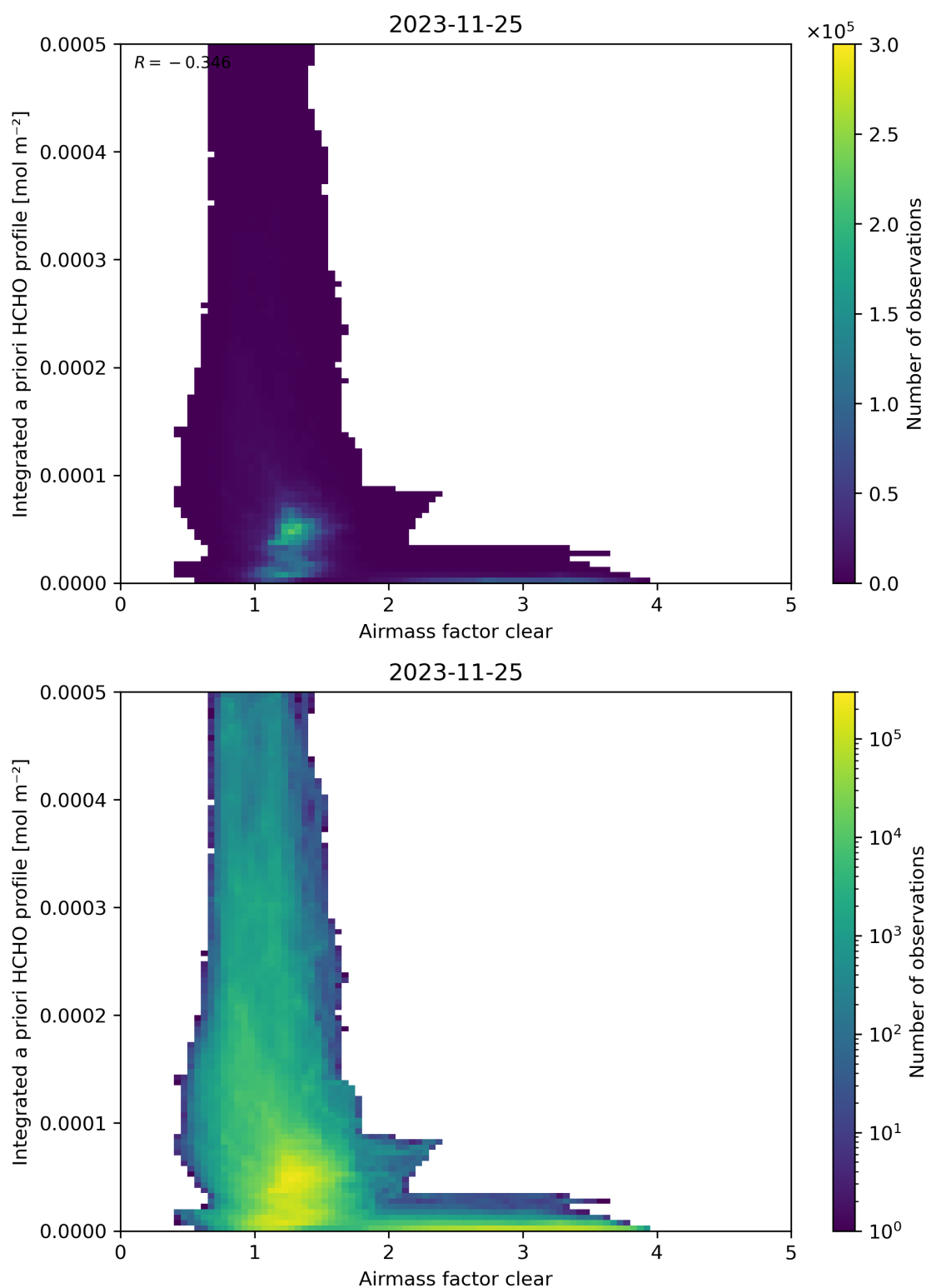
Figure 76: Scatter density plot of “Airmass factor clear” against “Integrated a priori HCHO profile” for 2023-11-24 to 2023-11-26.
