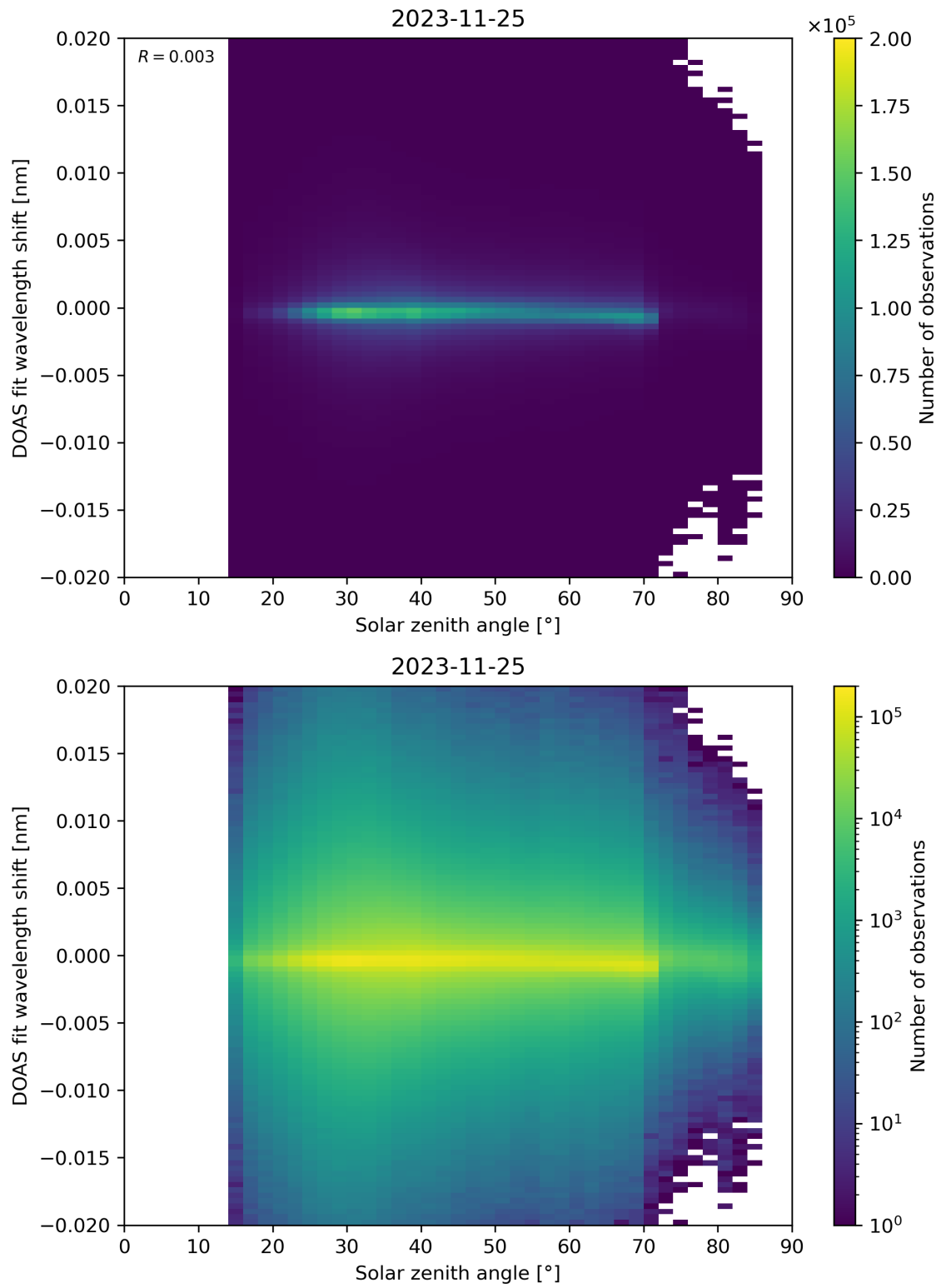
Figure 168: Scatter density plot of “Solar zenith angle” against “DOAS fit wavelength shift” for 2023-11-24 to 2023-11-26.
