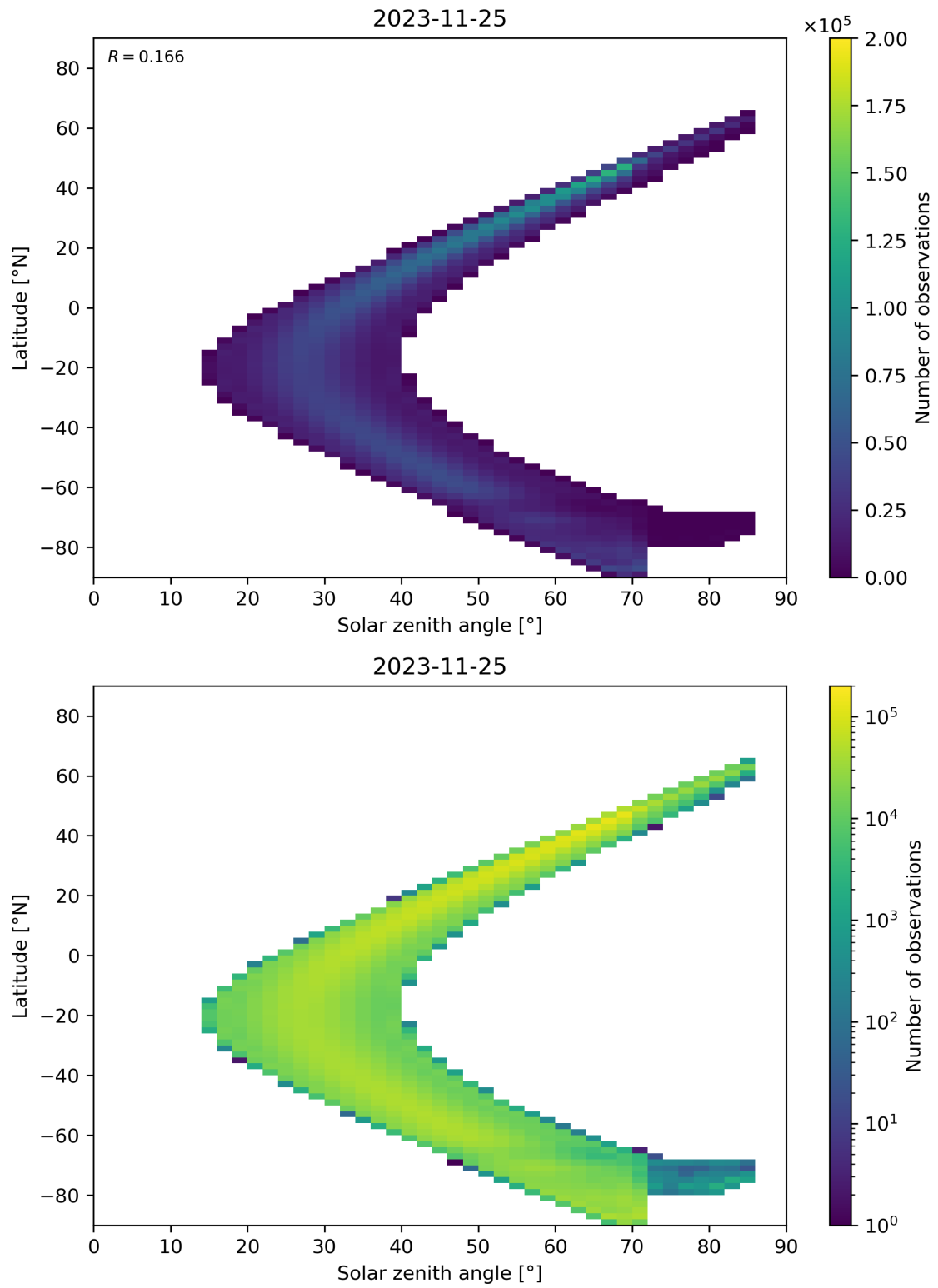
Figure 181: Scatter density plot of “Solar zenith angle” against “Latitude” for 2023-11-24 to 2023-11-26.
