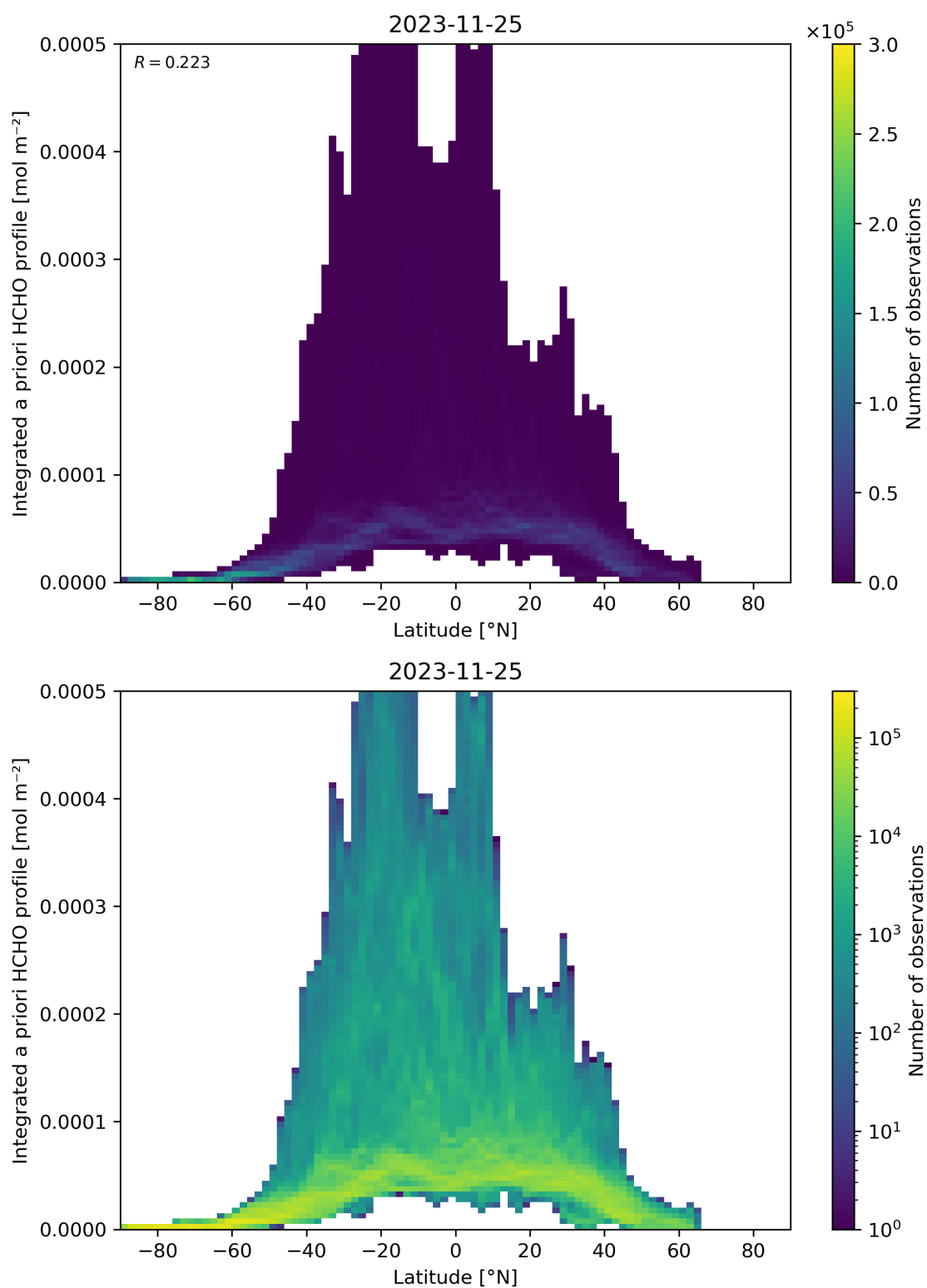
Figure 166: Scatter density plot of “Latitude” against “Integrated a priori HCHO profile” for 2023-11-24 to 2023-11-26.
