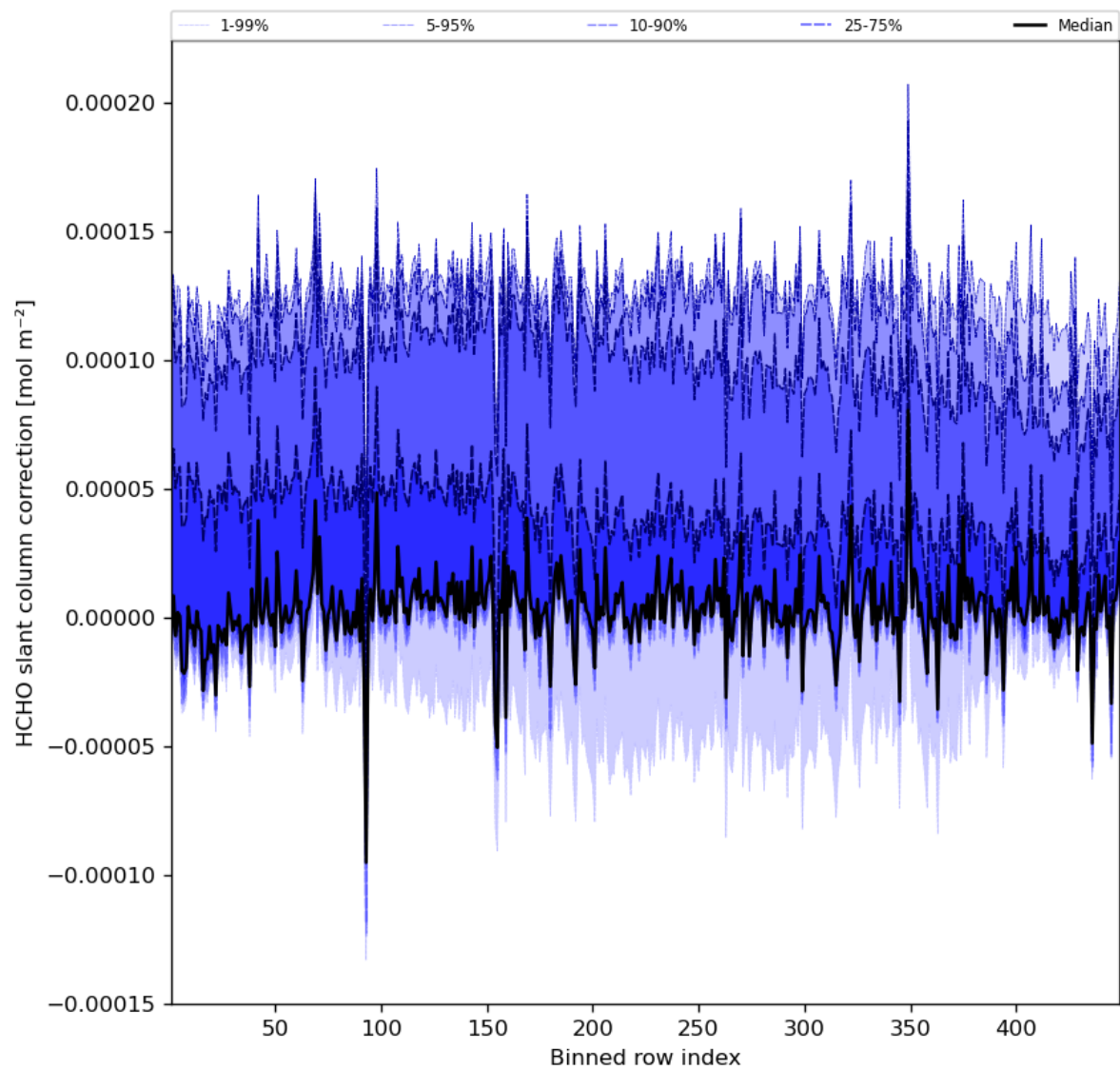
Figure 61: Along track statistics of “HCHO slant column correction” for 2023-11-24 to 2023-11-26
