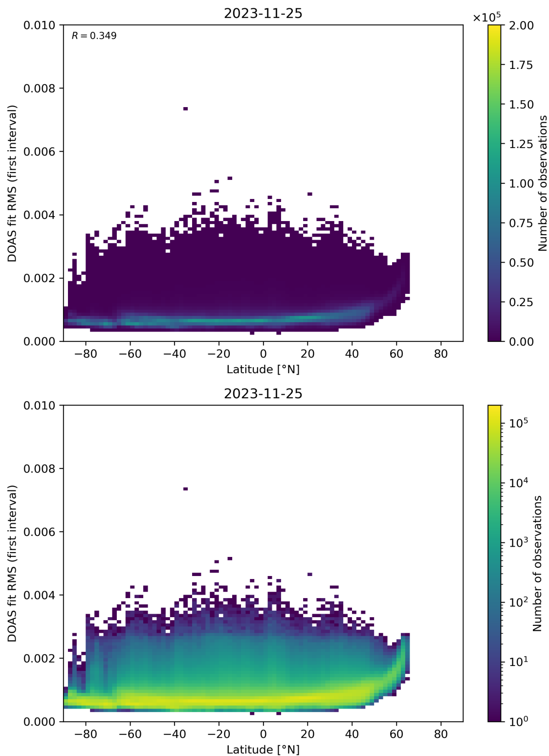
Figure 153: Scatter density plot of “Latitude” against “DOAS fit RMS (first interval)” for 2023-11-24 to 2023-11-26.
