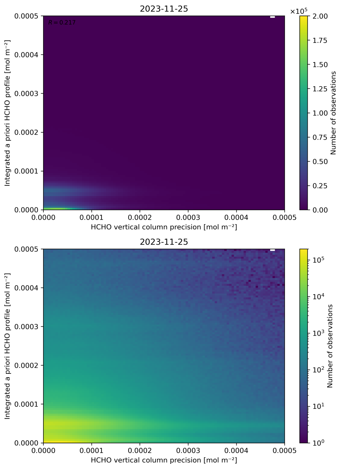
Figure 147: Scatter density plot of “HCHO vertical column precision” against “Integrated a priori HCHO profile” for 2023-11-24 to 2023-11-26.
