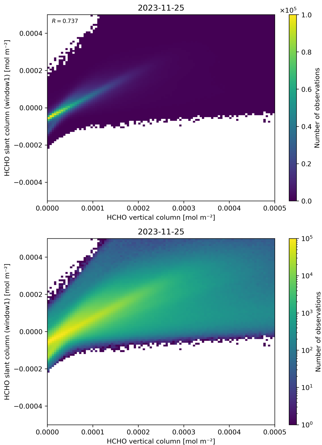
Figure 129: Scatter density plot of “HCHO vertical column” against “HCHO slant column (window1)” for 2023-11-24 to 2023-11-26.
