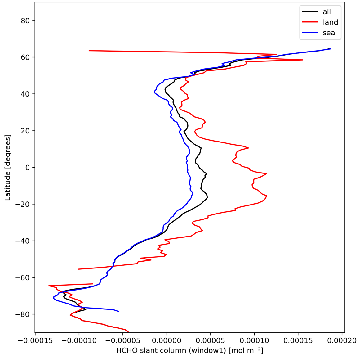
Figure 24: Zonal average of “HCHO slant column (window1)” for 2023-11-24 to 2023-11-26.
