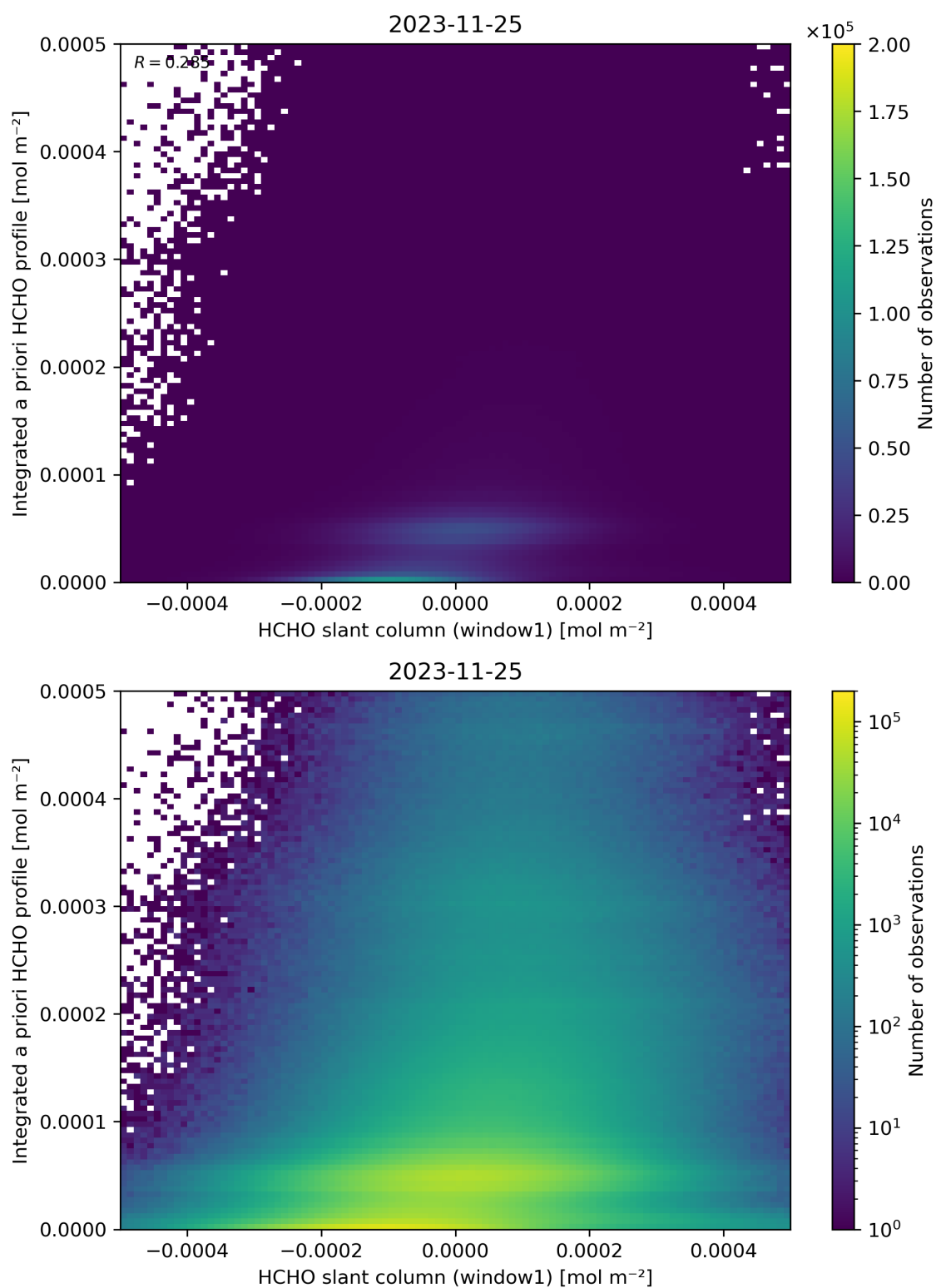
Figure 87: Scatter density plot of “HCHO slant column (window1)” against “Integrated a priori HCHO profile” for 2023-11-24 to 2023-11-26.
