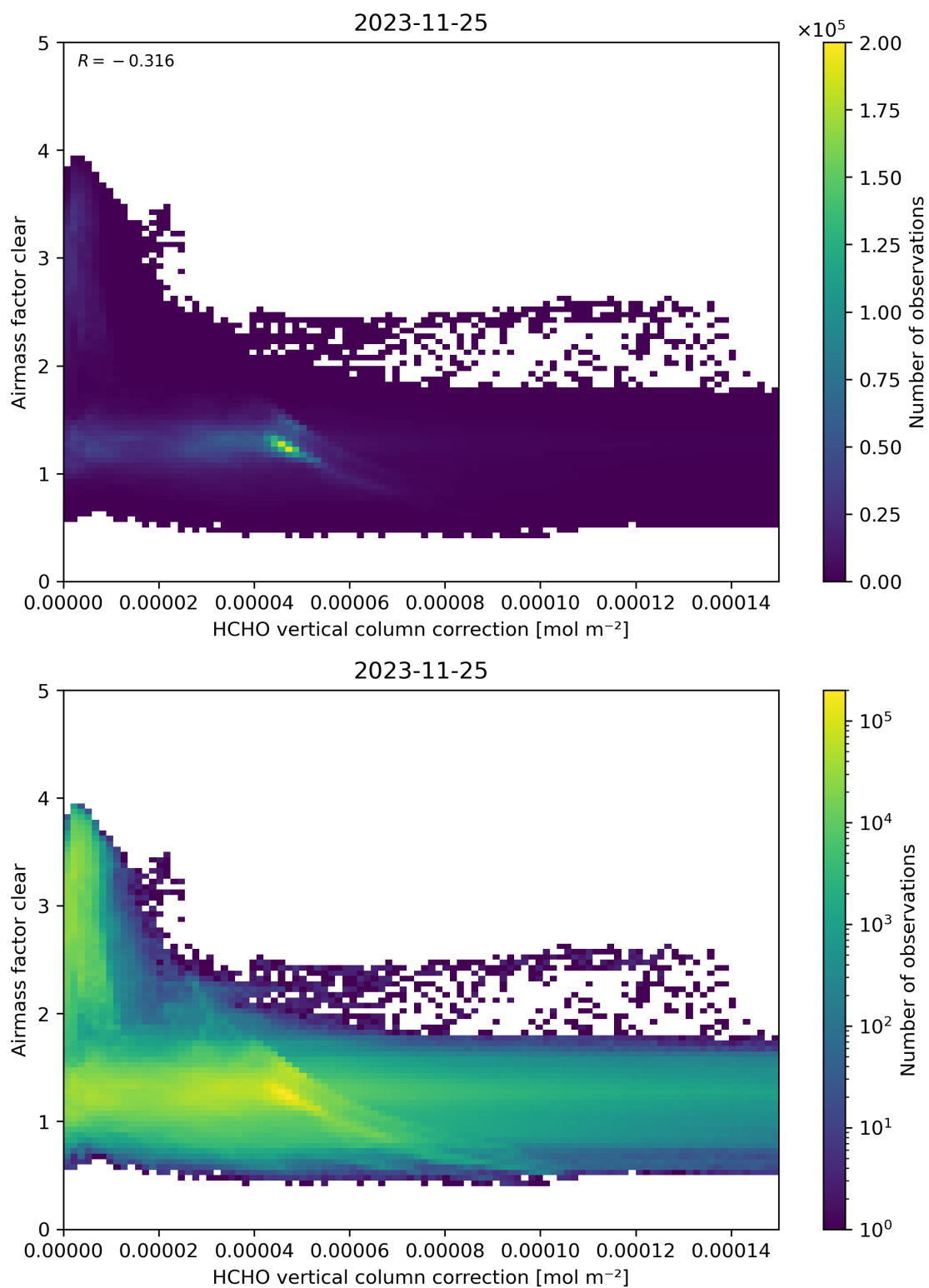
Figure 115: Scatter density plot of “HCHO vertical column correction” against “Airmass factor clear” for 2023-11-24 to 2023-11-26.
