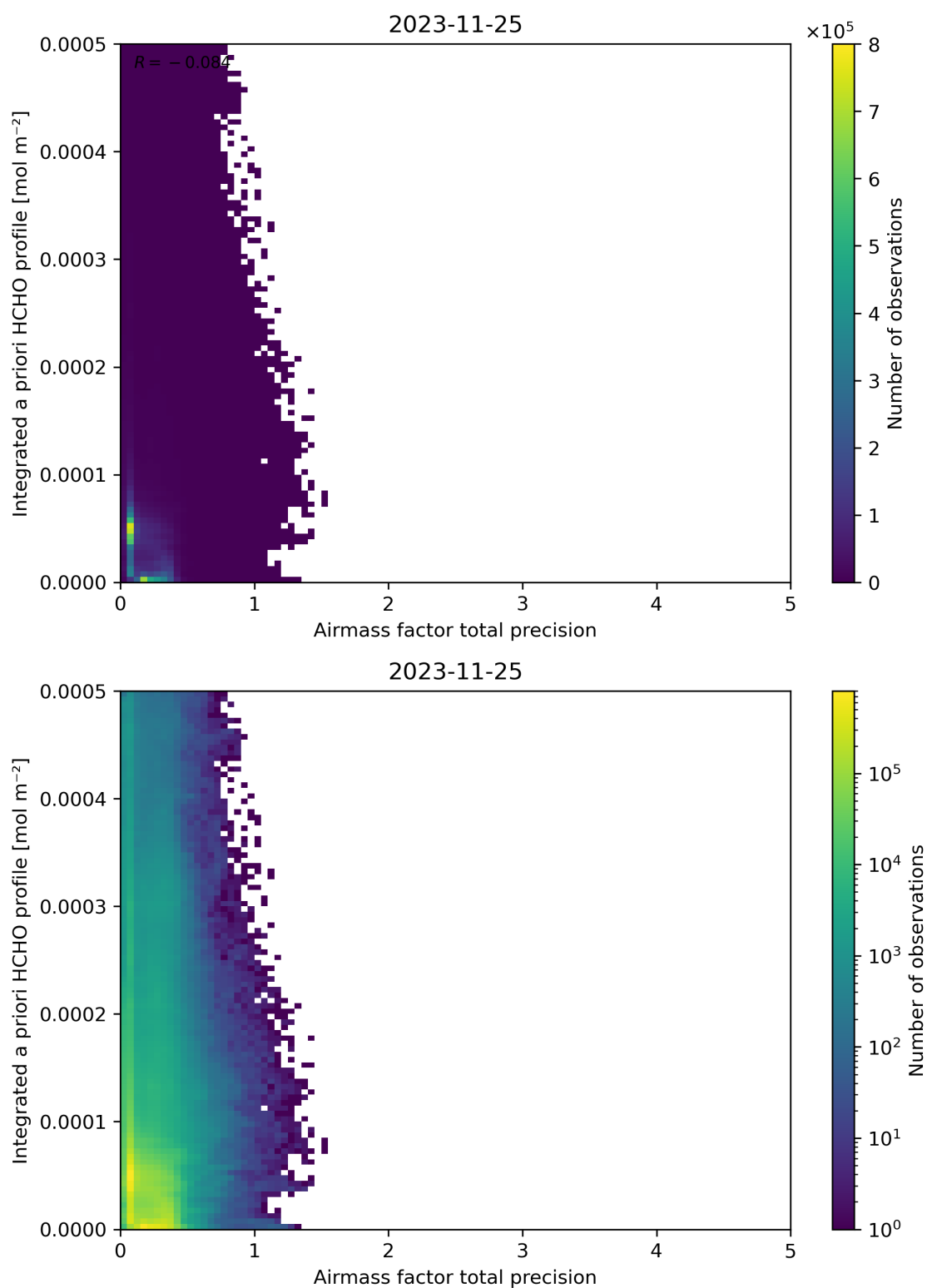
Figure 111: Scatter density plot of “Airmass factor total precision” against “Integrated a priori HCHO profile” for 2023-11-24 to 2023-11-26.
