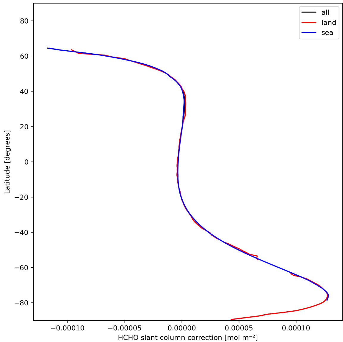
Figure 33: Zonal average of “HCHO slant column correction” for 2023-11-24 to 2023-11-26.
