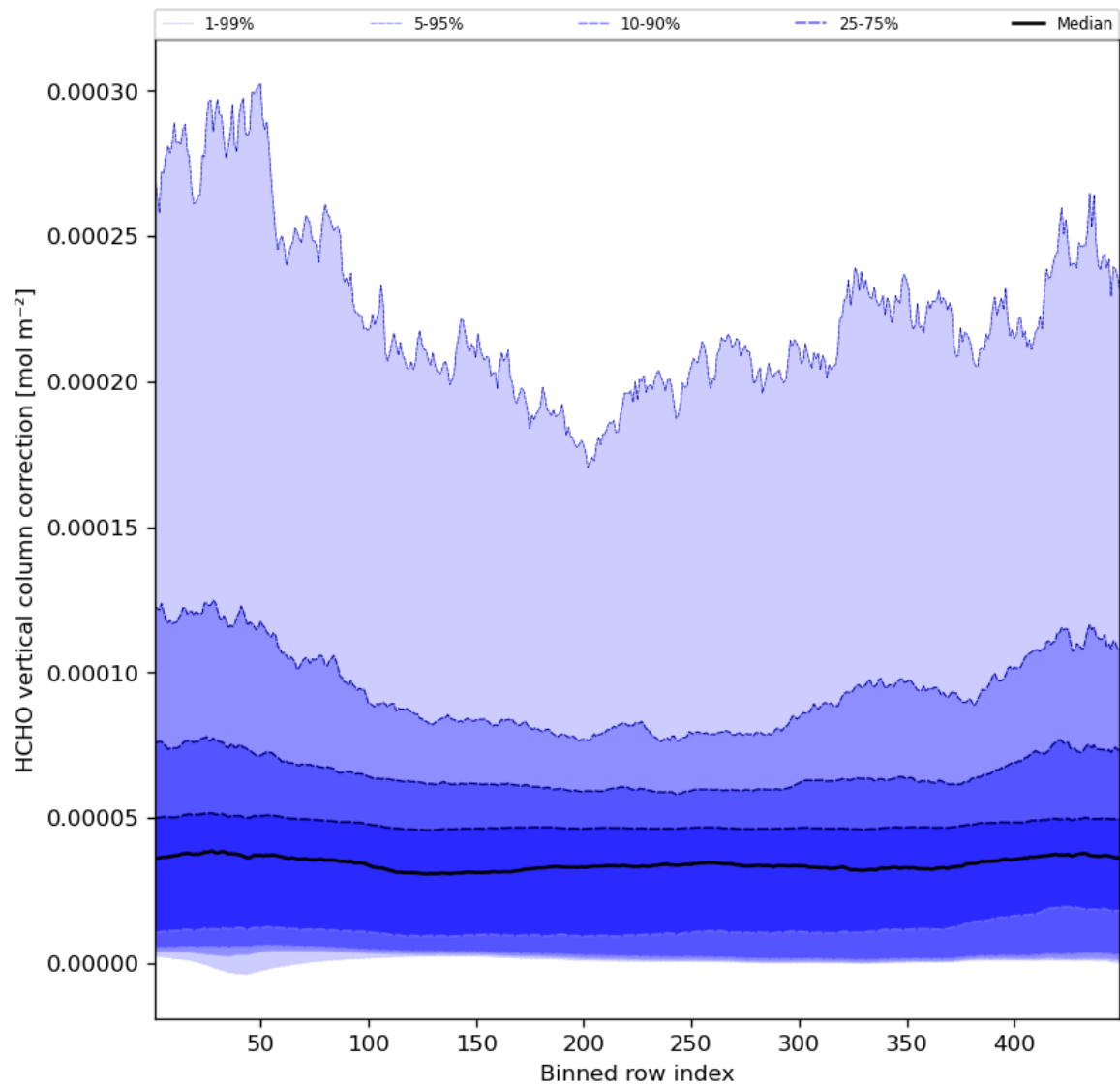
Figure 51: Along track statistics of “HCHO vertical column correction” for 2023-11-24 to 2023-11-26
