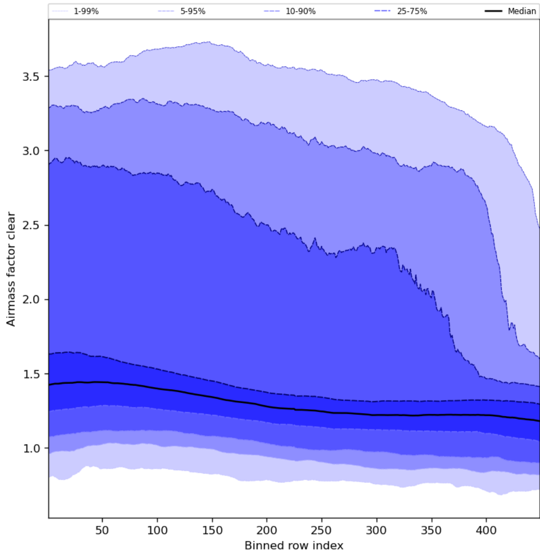
Figure 56: Along track statistics of “Airmass factor clear” for 2023-11-24 to 2023-11-26
