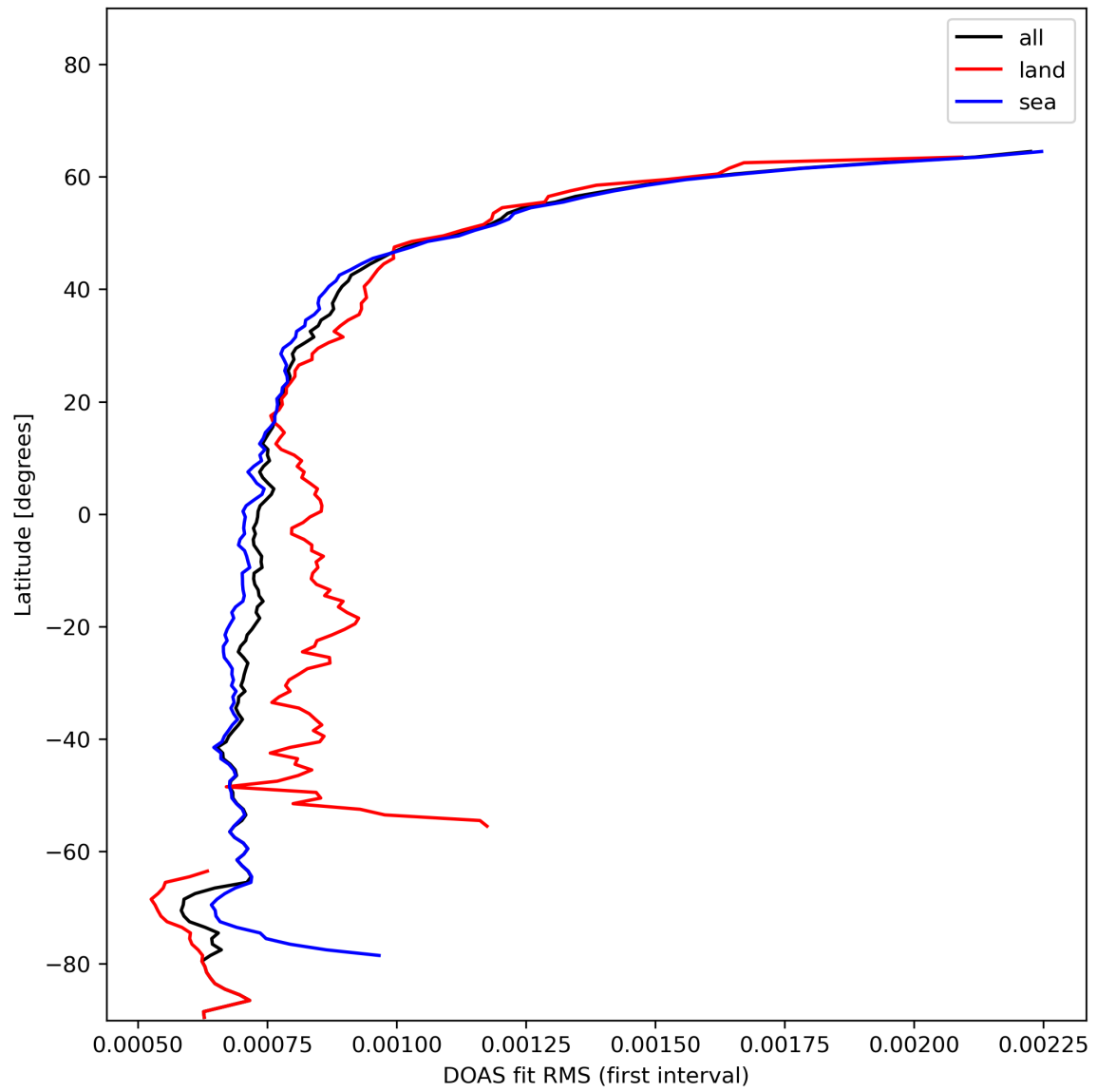
Figure 32: Zonal average of “DOAS fit RMS (first interval)” for 2023-11-24 to 2023-11-26.
