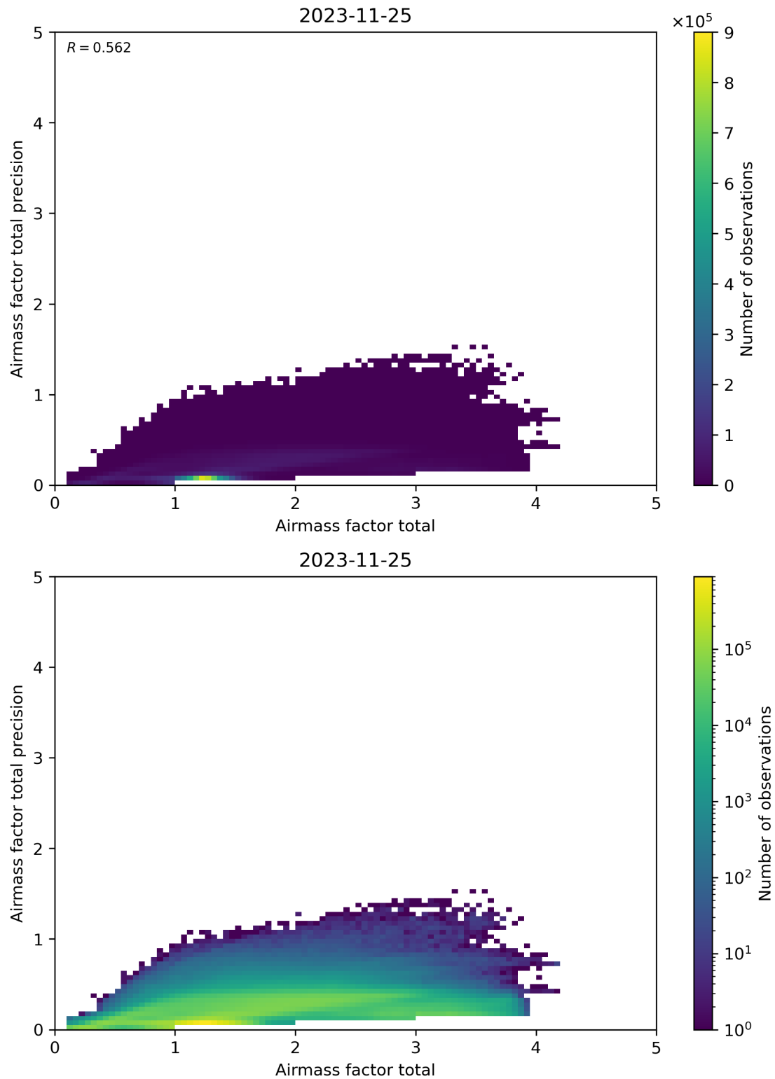
Figure 103: Scatter density plot of “Airmass factor total” against “Airmass factor total precision” for 2023-11-24 to 2023-11-26.
