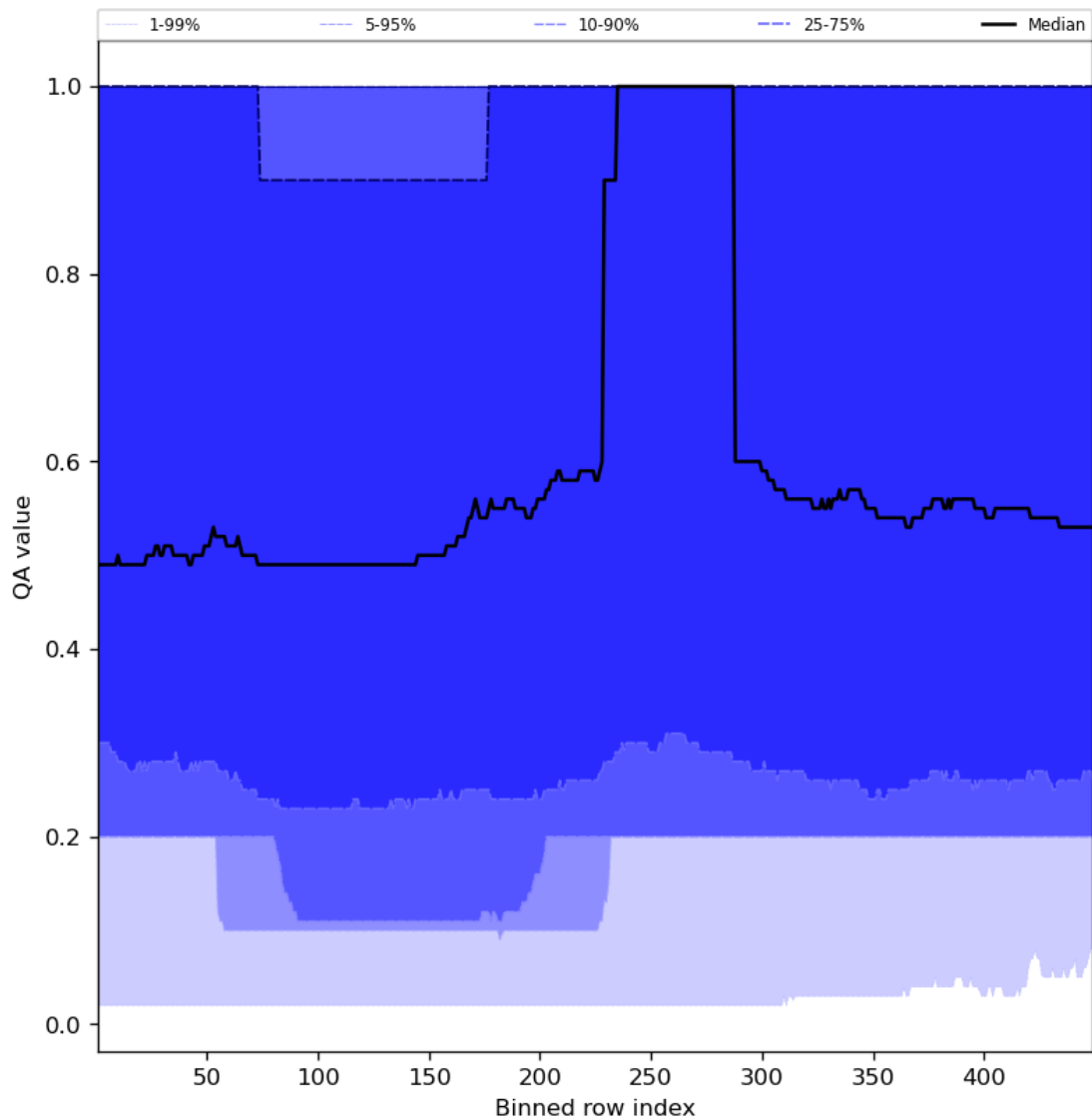
Figure 48: Along track statistics of “QA value” for 2023-11-24 to 2023-11-26
