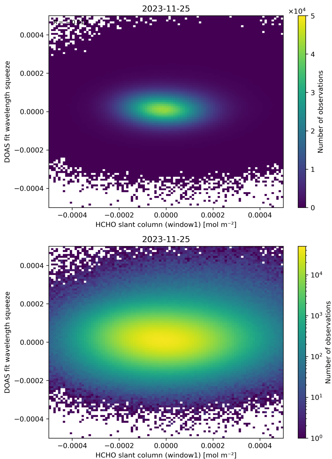
Figure 80: Scatter density plot of “HCHO slant column (window1)” against “DOAS fit wavelength squeeze” for 2023-11-24 to 2023-11-26.
