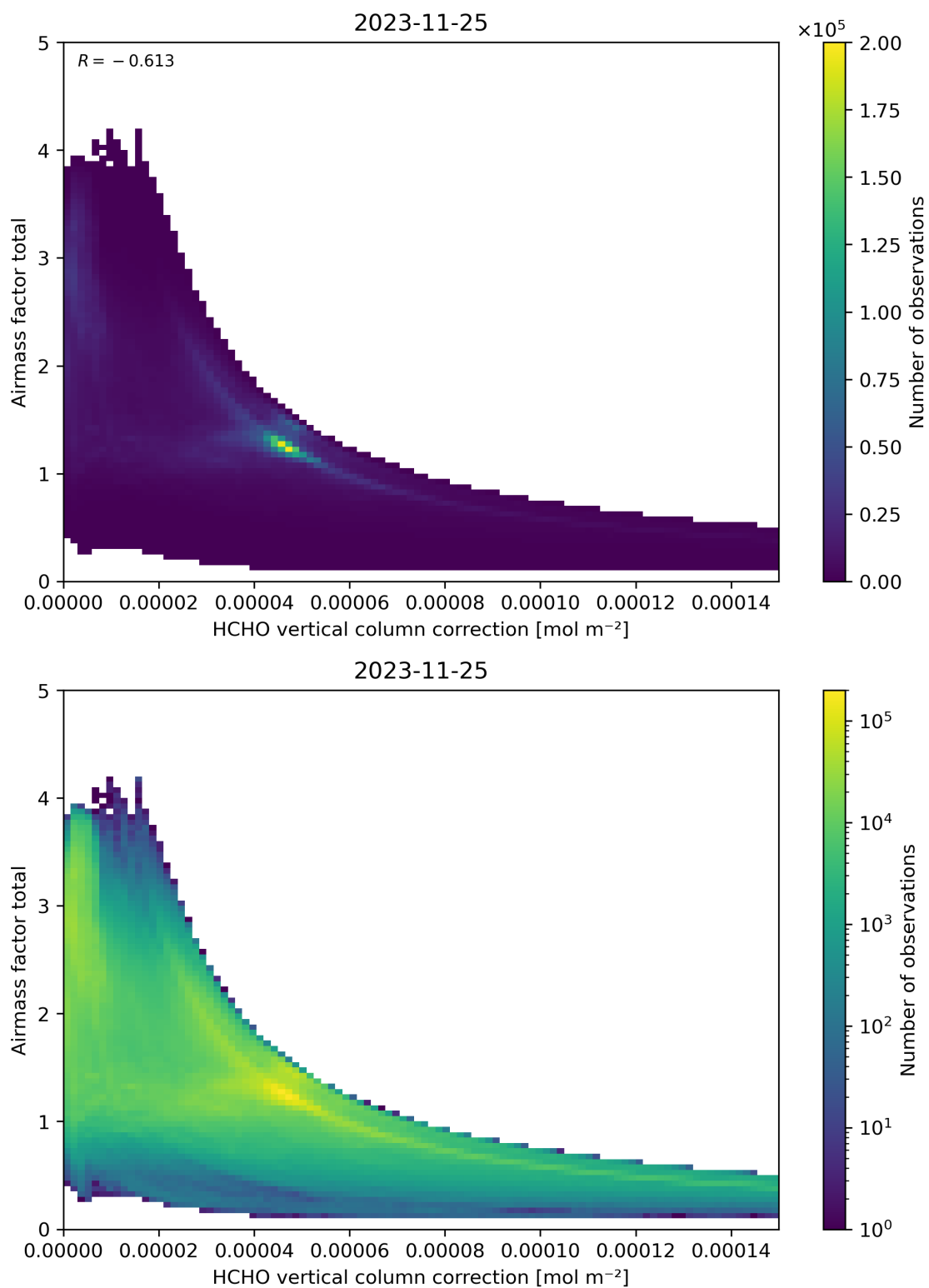
Figure 120: Scatter density plot of “HCHO vertical column correction” against “Airmass factor total” for 2023-11-24 to 2023-11-26.
