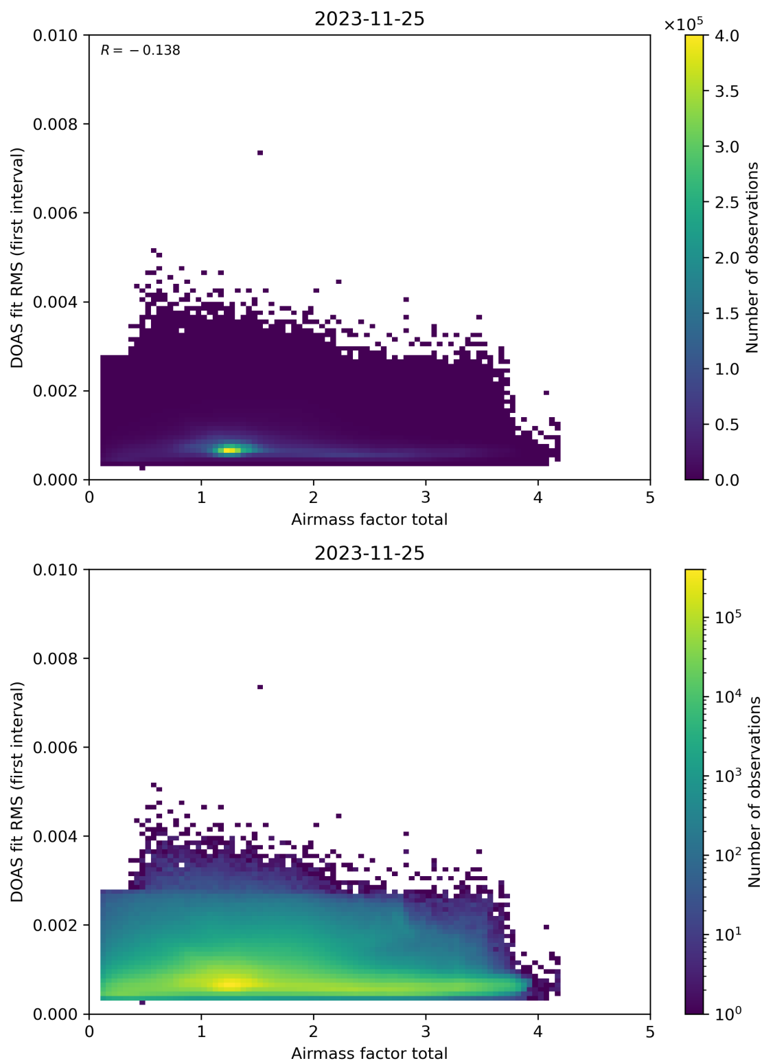
Figure 97: Scatter density plot of “Airmass factor total” against “DOAS fit RMS (first interval)” for 2023-11-24 to 2023-11-26.
