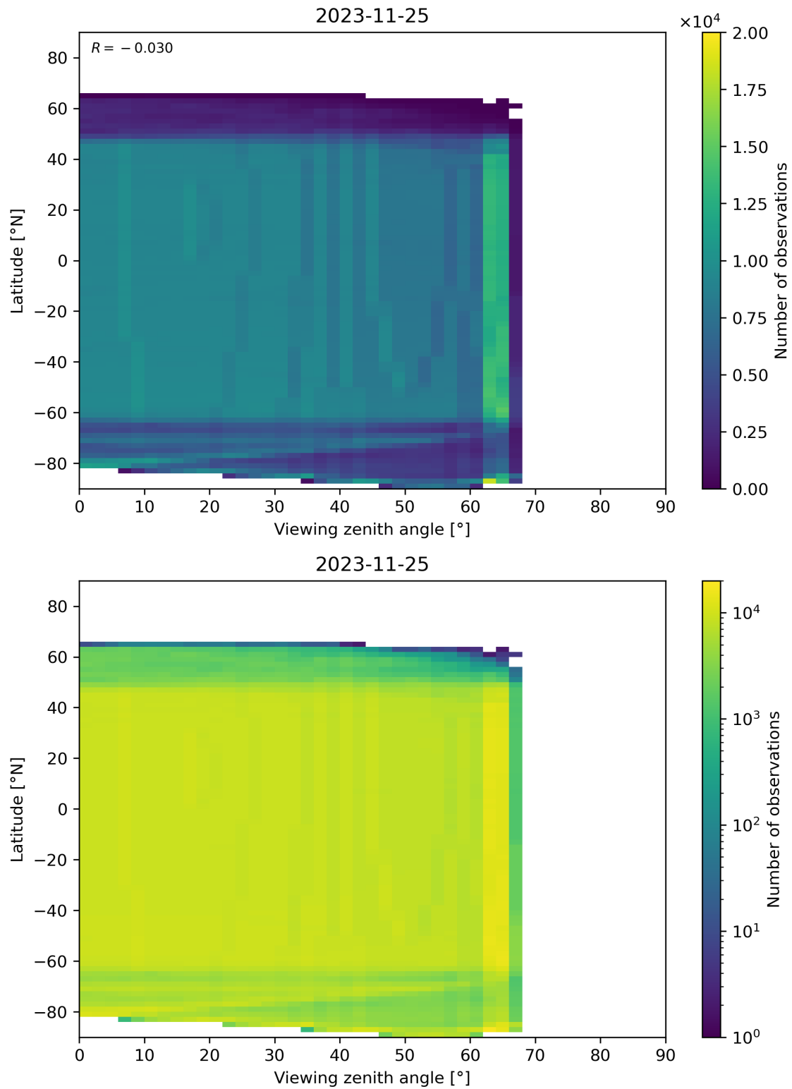
Figure 196: Scatter density plot of “Viewing zenith angle” against “Latitude” for 2023-11-24 to 2023-11-26.
