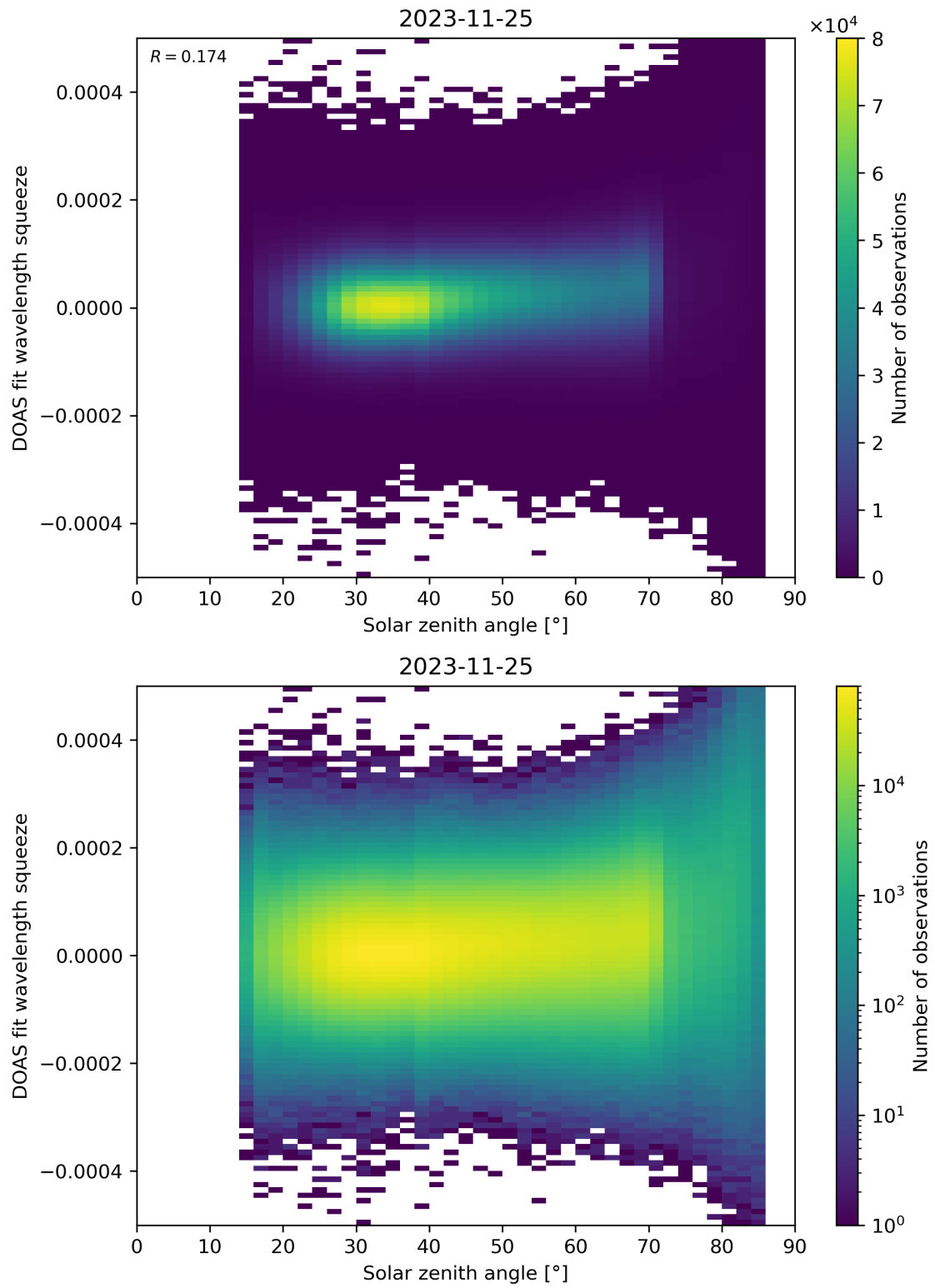
Figure 169: Scatter density plot of “Solar zenith angle” against “DOAS fit wavelength squeeze” for 2023-11-24 to 2023-11-26.
