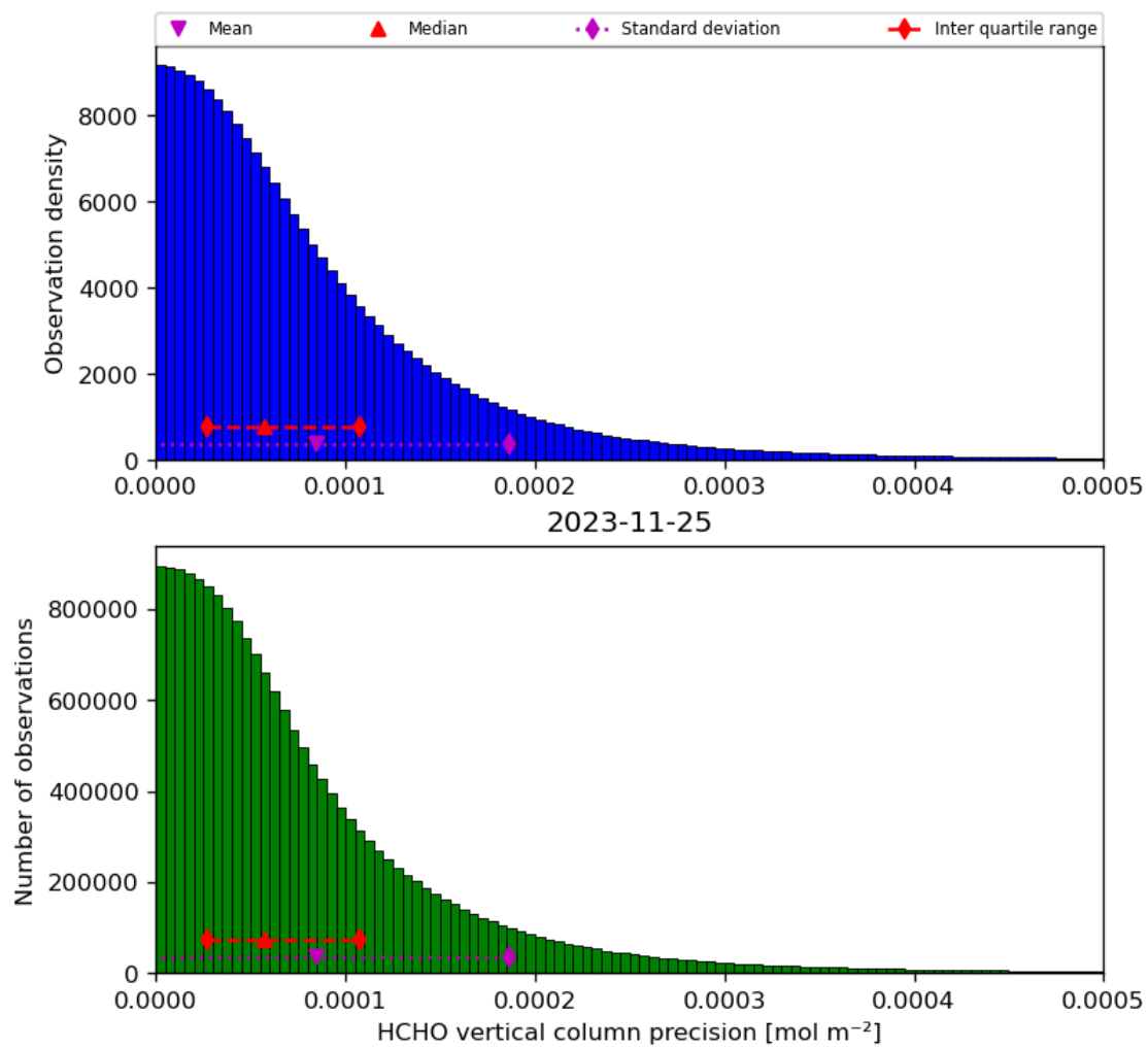
Figure 36: Histogram of “HCHO vertical column precision” for 2023-11-24 to 2023-11-26
