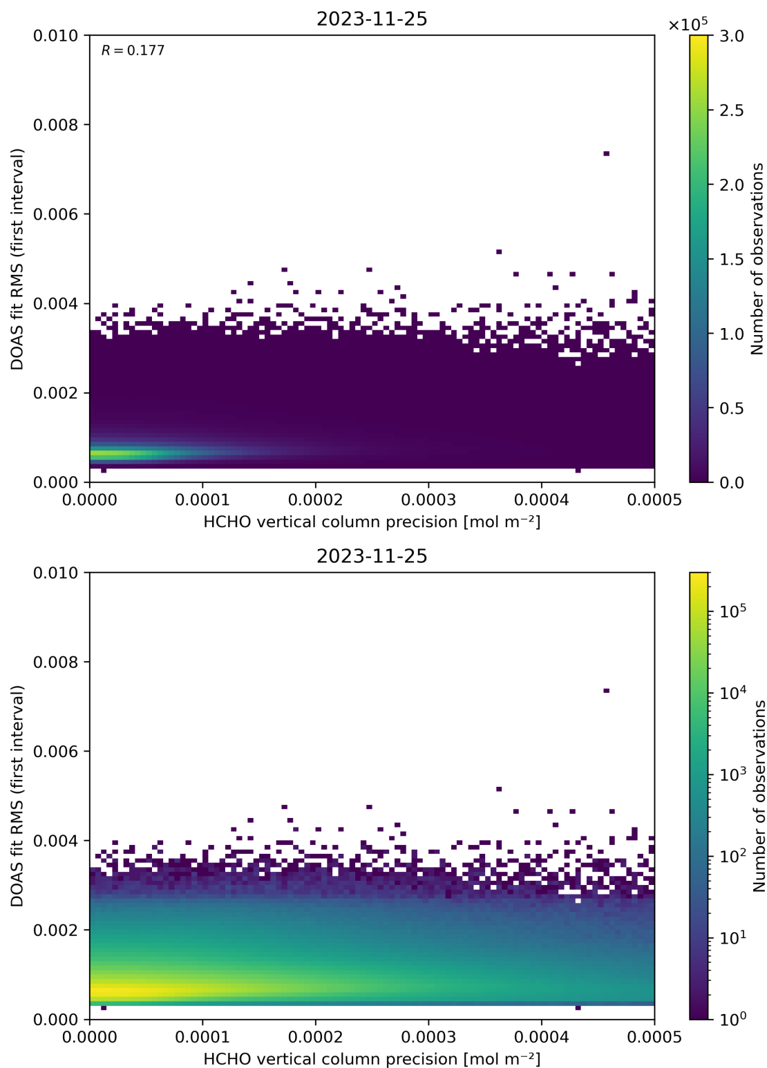
Figure 136: Scatter density plot of “HCHO vertical column precision” against “DOAS fit RMS (first interval)” for 2023-11-24 to 2023-11-26.
