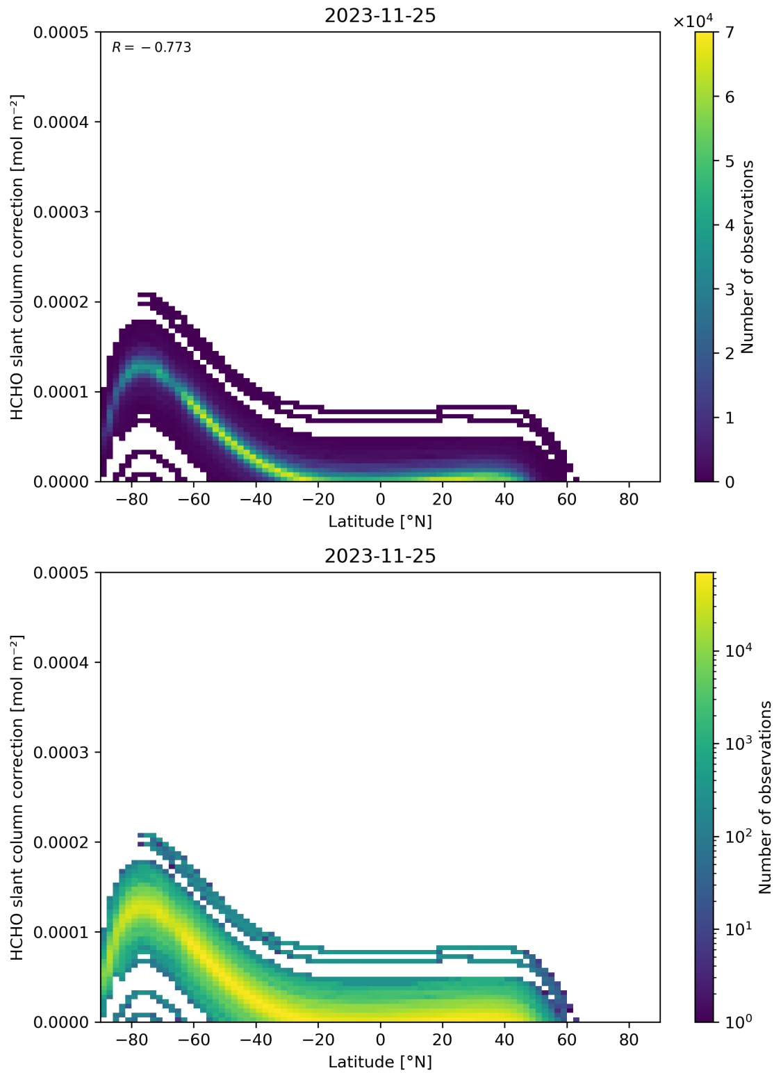
Figure 158: Scatter density plot of “Latitude” against “HCHO slant column correction” for 2023-11-24 to 2023-11-26.
