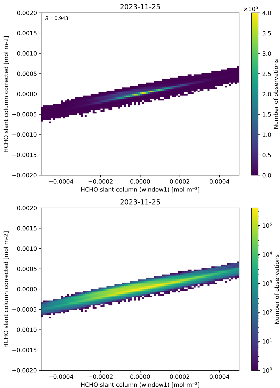
Figure 82: Scatter density plot of “HCHO slant column (window1)” against “HCHO slant column corrected” for 2023-11-24 to 2023-11-26.
