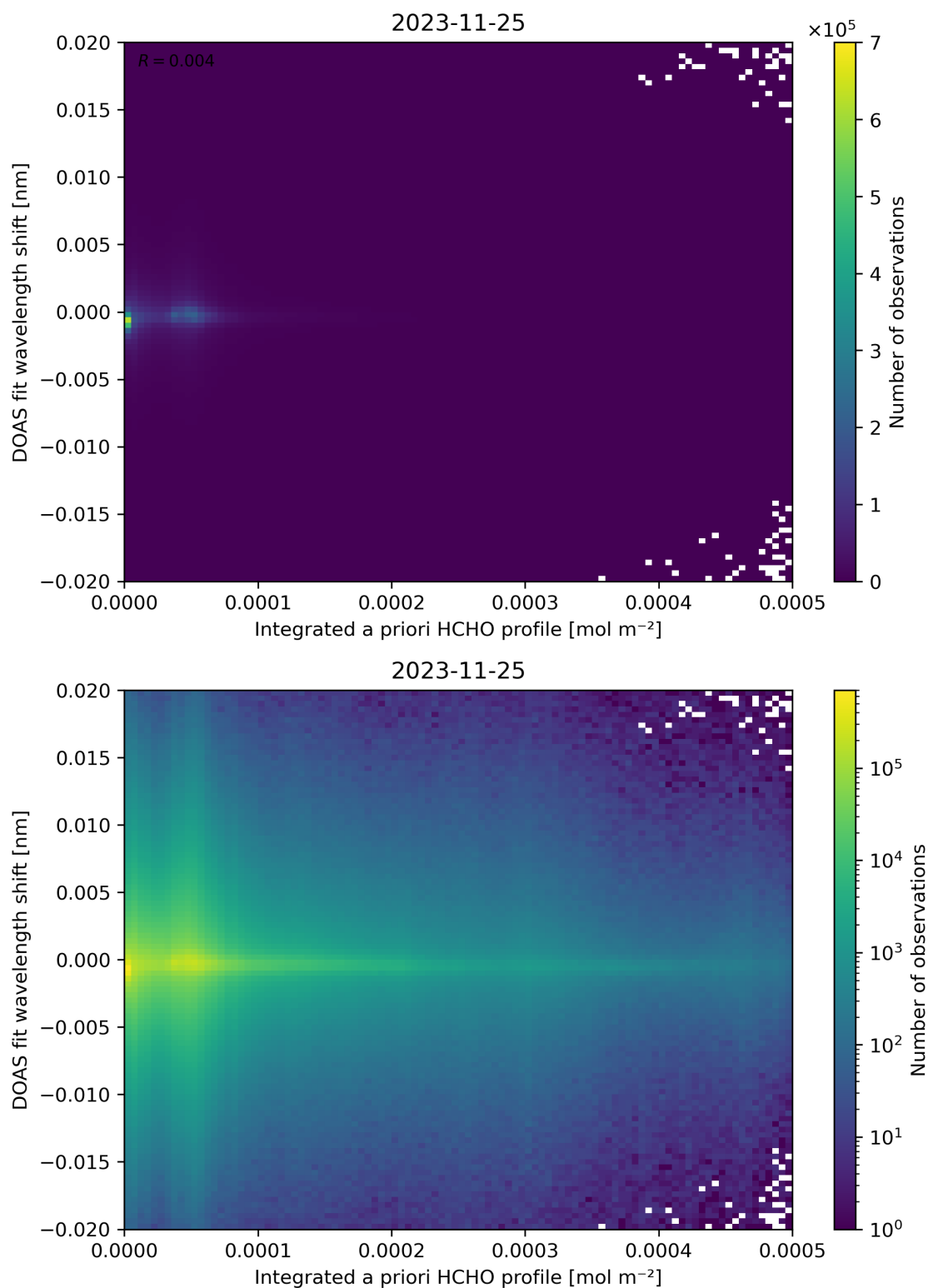
Figure 149: Scatter density plot of “Integrated a priori HCHO profile” against “DOAS fit wavelength shift” for 2023-11-24 to 2023-11-26.
