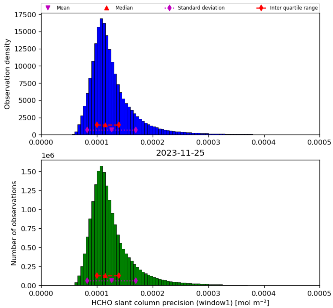
Figure 39: Histogram of “HCHO slant column precision (window1)” for 2023-11-24 to 2023-11-26
