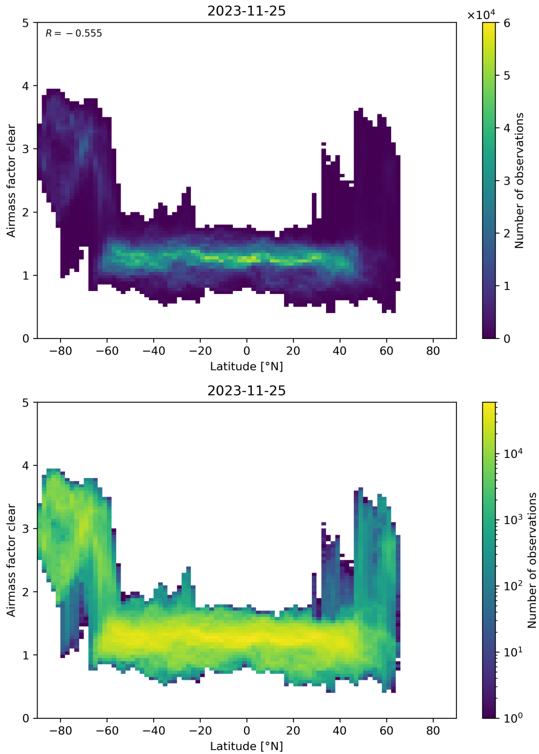
Figure 156: Scatter density plot of “Latitude” against “Airmass factor clear” for 2023-11-24 to 2023-11-26.
