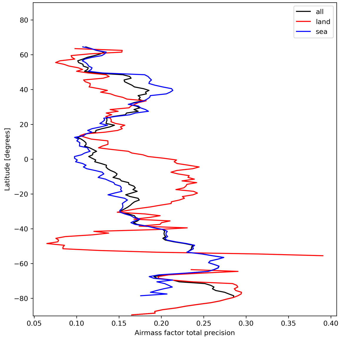
Figure 27: Zonal average of “Airmass factor total precision” for 2023-11-24 to 2023-11-26.
