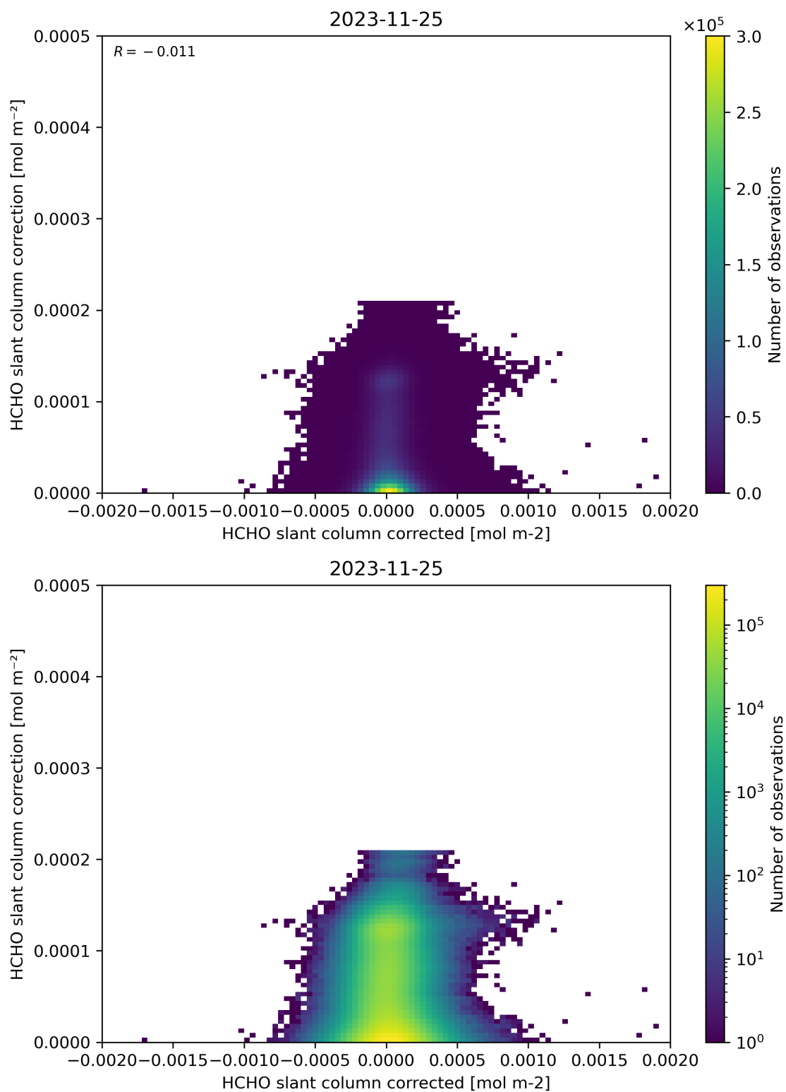
Figure 77: Scatter density plot of “HCHO slant column corrected” against “HCHO slant column correction” for 2023-11-24 to 2023-11-26.
