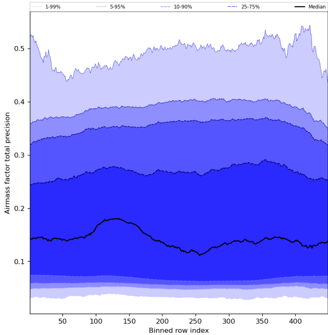
Figure 55: Along track statistics of “Airmass factor total precision” for 2023-11-24 to 2023-11-26
