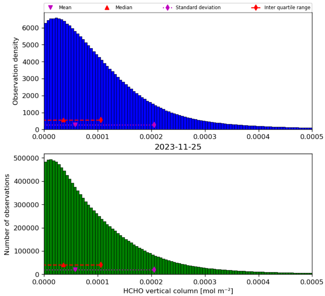
Figure 35: Histogram of “HCHO vertical column” for 2023-11-24 to 2023-11-26
