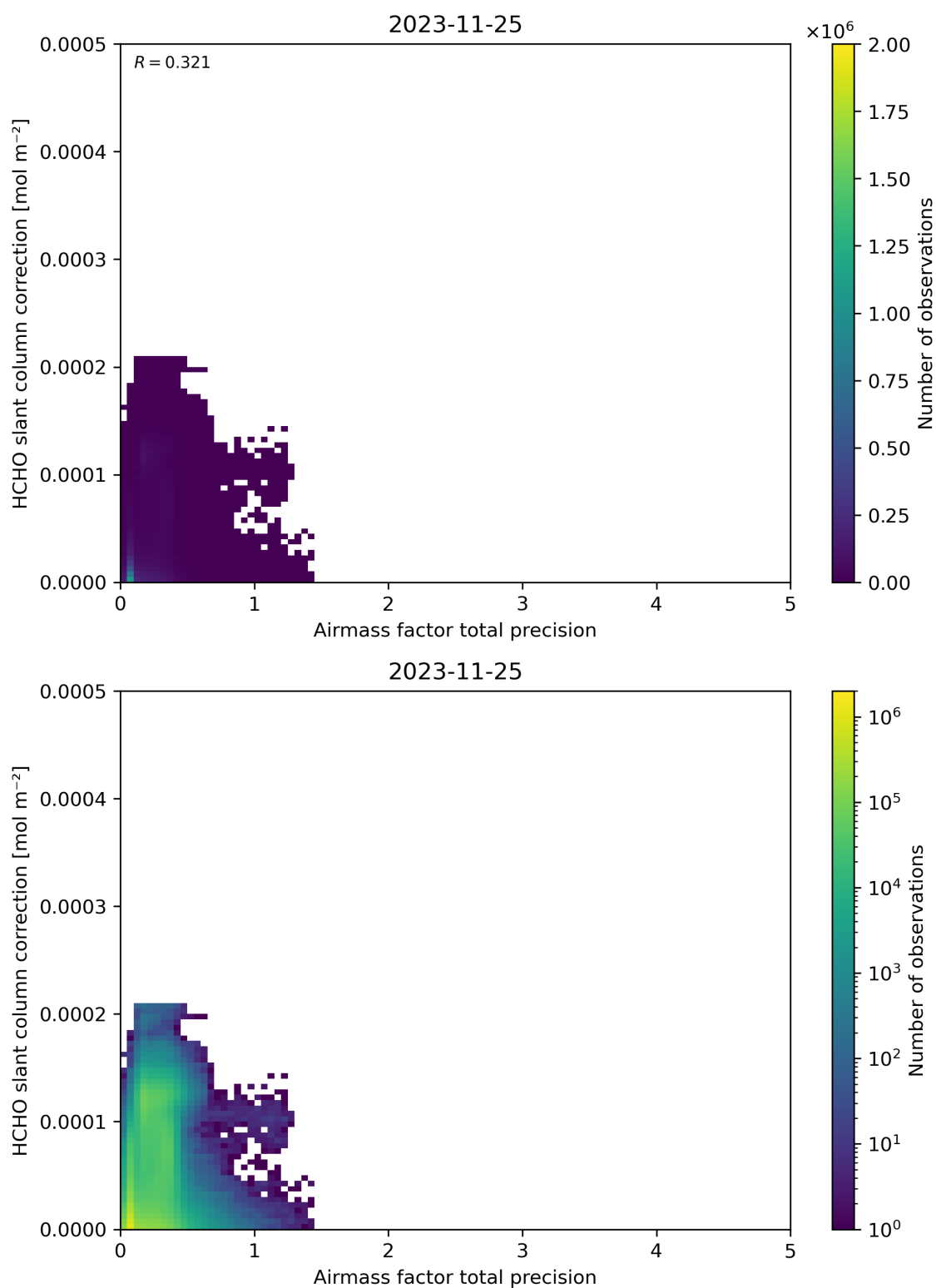
Figure 110: Scatter density plot of “Airmass factor total precision” against “HCHO slant column correction” for 2023-11-24 to 2023-11-26.
