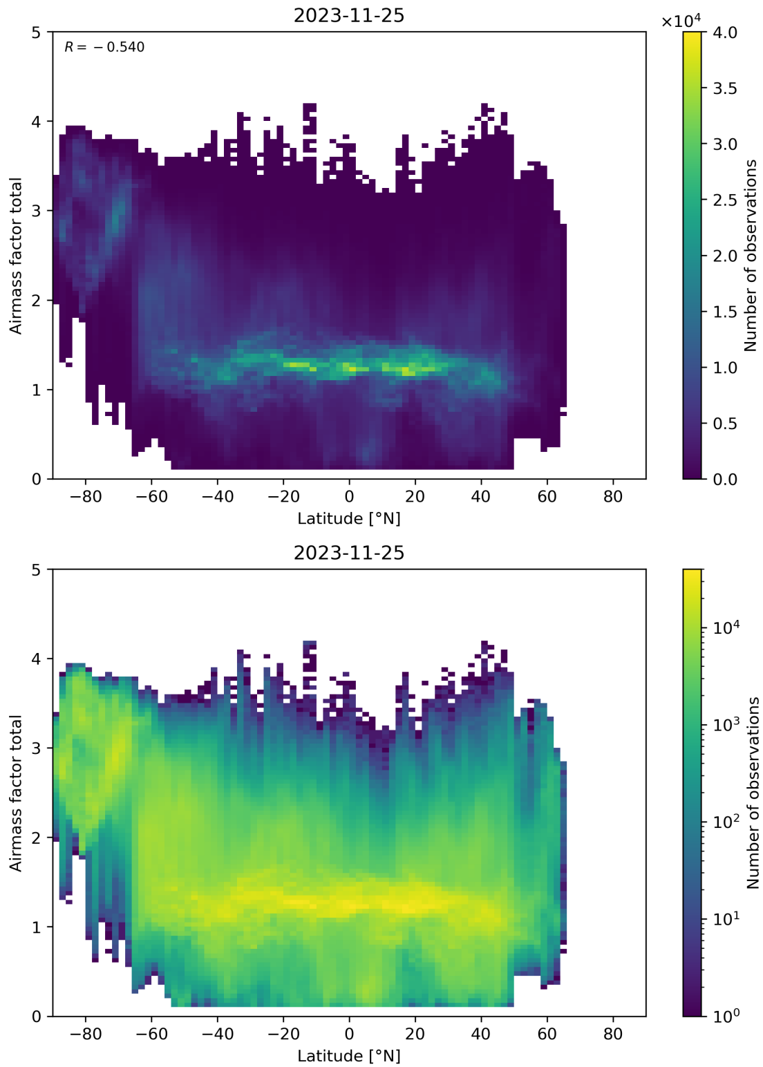
Figure 161: Scatter density plot of “Latitude” against “Airmass factor total” for 2023-11-24 to 2023-11-26.
