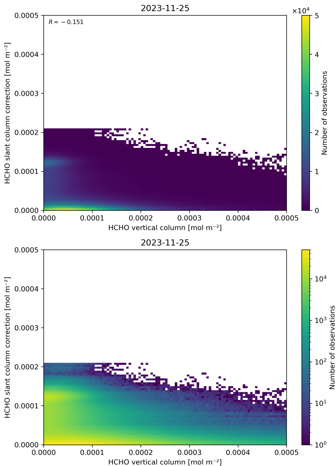
Figure 128: Scatter density plot of “HCHO vertical column” against “HCHO slant column correction” for 2023-11-24 to 2023-11-26.
