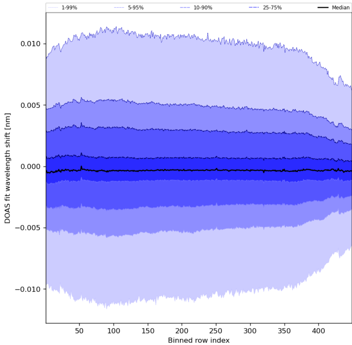
Figure 58: Along track statistics of “DOAS fit wavelength shift” for 2023-11-24 to 2023-11-26
