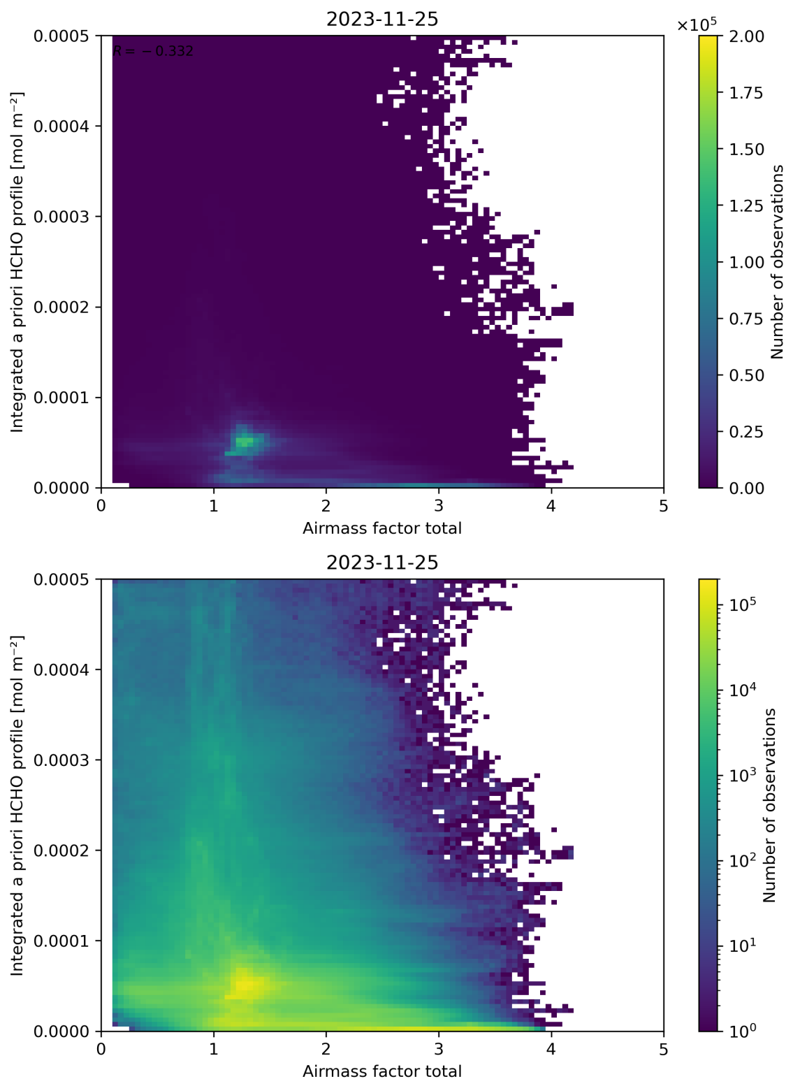
Figure 104: Scatter density plot of “Airmass factor total” against “Integrated a priori HCHO profile” for 2023-11-24 to 2023-11-26.
