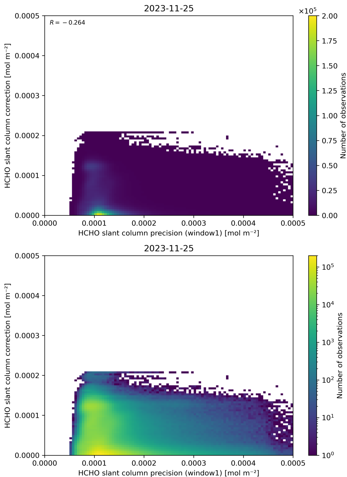
Figure 93: Scatter density plot of “HCHO slant column precision (window1)” against “HCHO slant column correction” for 2023-11-24 to 2023-11-26.
