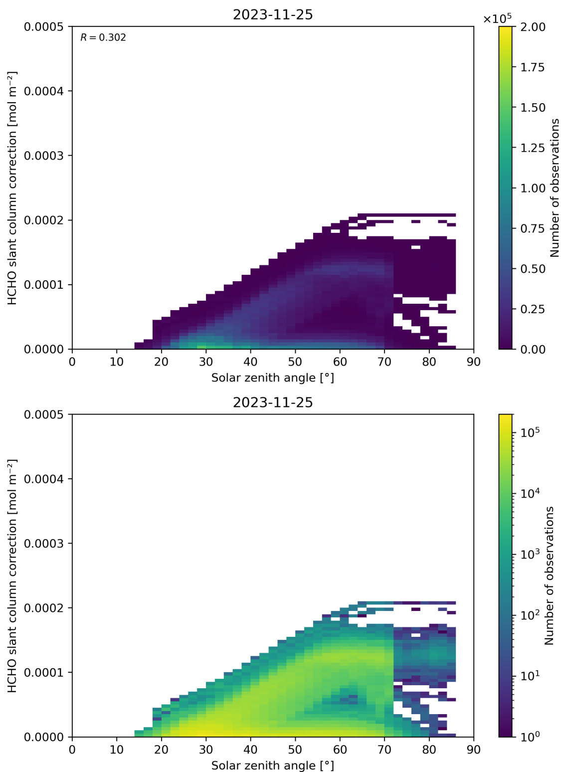
Figure 172: Scatter density plot of “Solar zenith angle” against “HCHO slant column correction” for 2023-11-24 to 2023-11-26.
