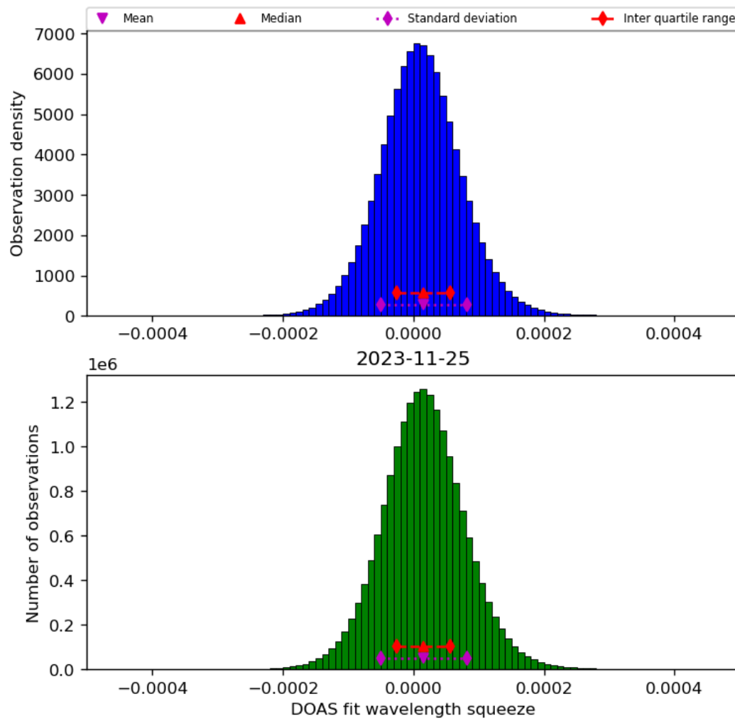
Figure 45: Histogram of “DOAS fit wavelength squeeze” for 2023-11-24 to 2023-11-26
