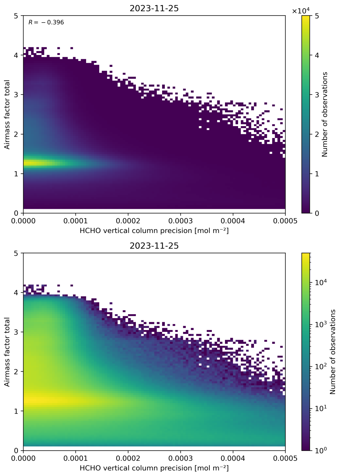
Figure 144: Scatter density plot of “HCHO vertical column precision” against “Airmass factor total” for 2023-11-24 to 2023-11-26.
