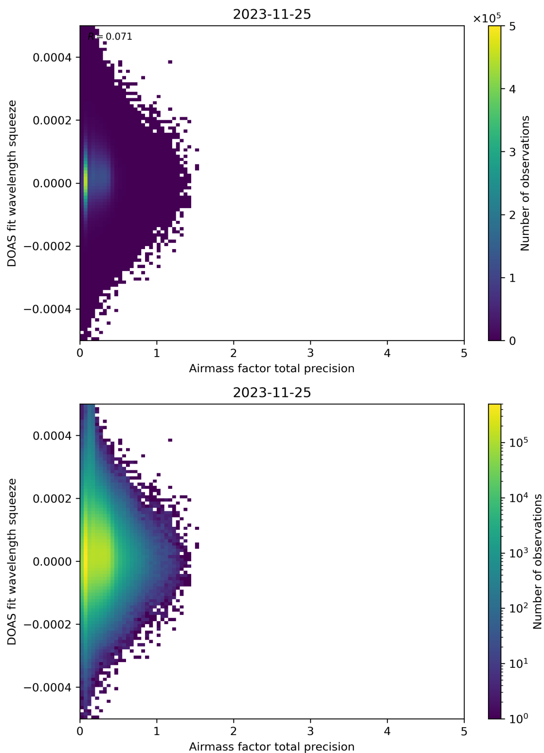
Figure 107: Scatter density plot of “Airmass factor total precision” against “DOAS fit wavelength squeeze” for 2023-11-24 to 2023-11-26.
