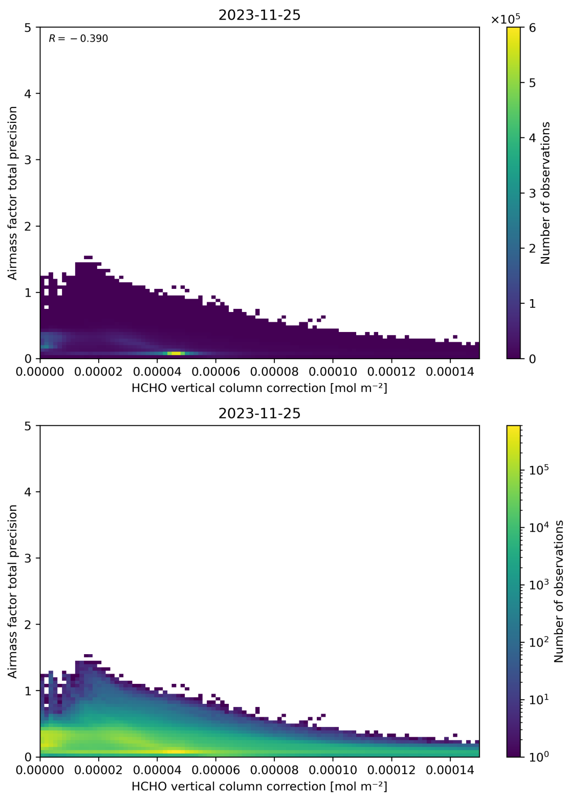
Figure 121: Scatter density plot of “HCHO vertical column correction” against “Airmass factor total precision” for 2023-11-24 to 2023-11-26.
