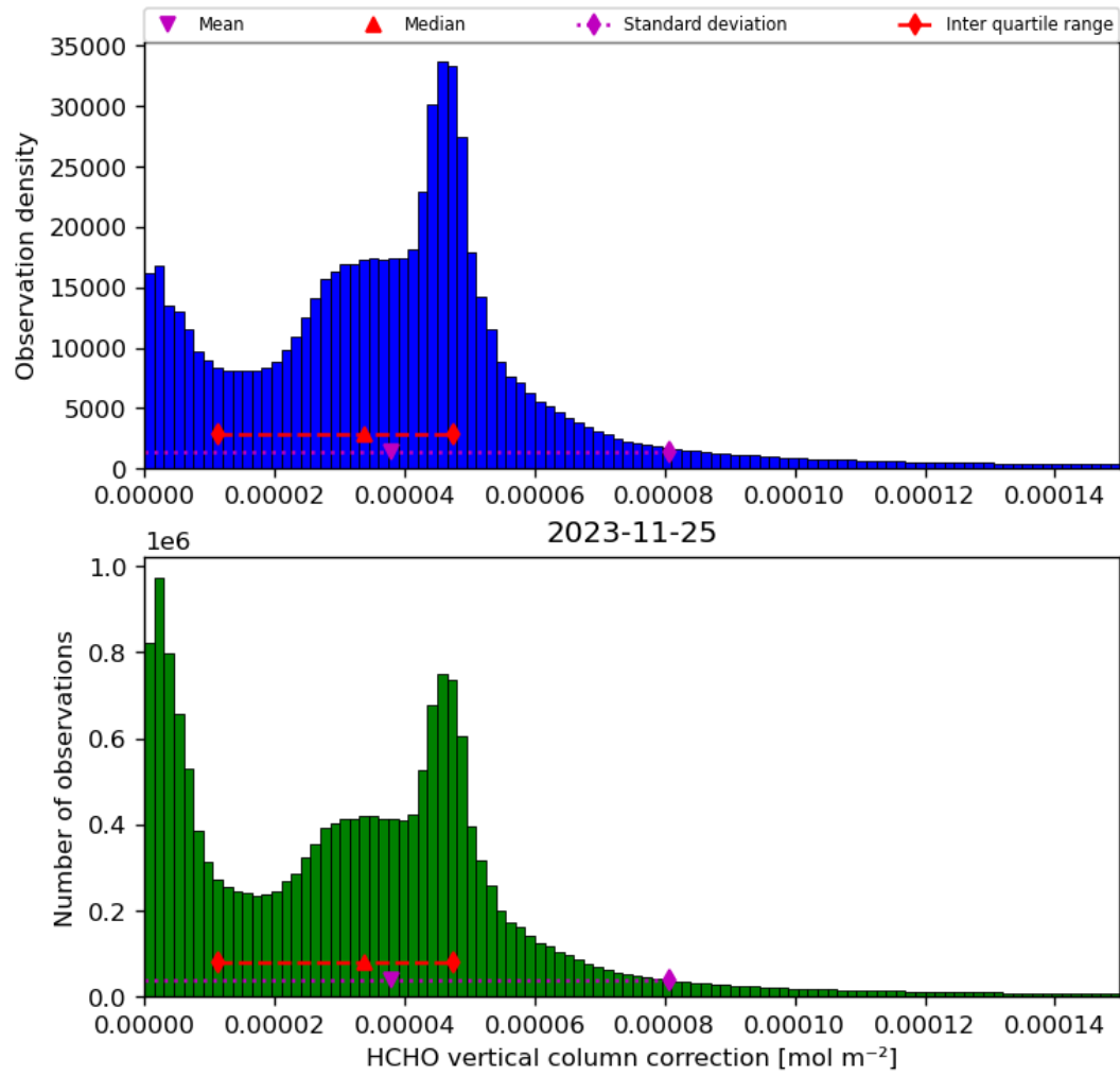
Figure 37: Histogram of “HCHO vertical column correction” for 2023-11-24 to 2023-11-26
