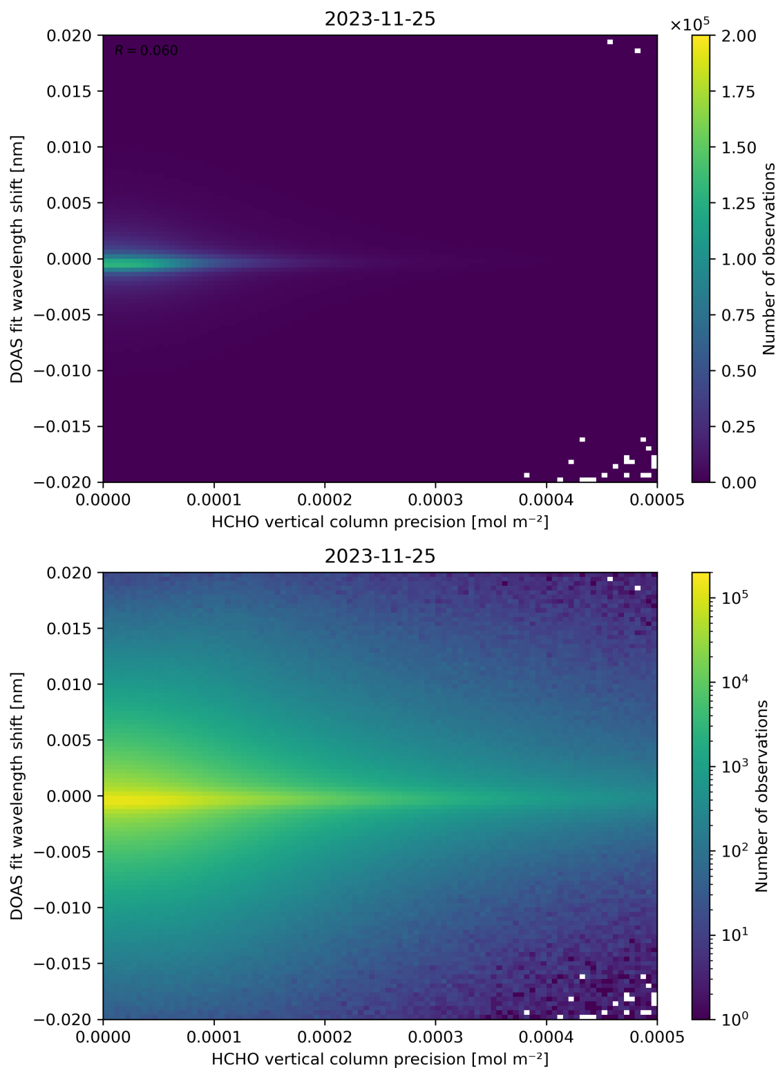
Figure 137: Scatter density plot of “HCHO vertical column precision” against “DOAS fit wavelength shift” for 2023-11-24 to 2023-11-26.
