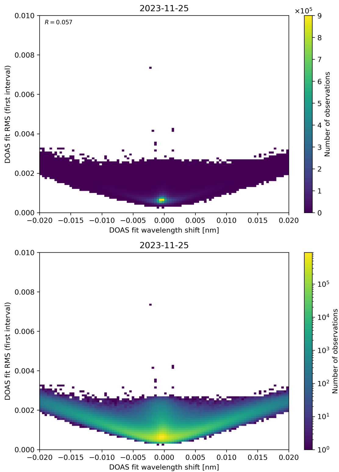
Figure 64: Scatter density plot of “DOAS fit wavelength shift” against “DOAS fit RMS (first interval)” for 2023-11-24 to 2023-11-26.
