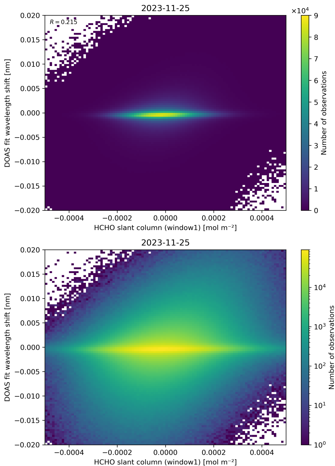
Figure 79: Scatter density plot of “HCHO slant column (window1)” against “DOAS fit wavelength shift” for 2023-11-24 to 2023-11-26.
