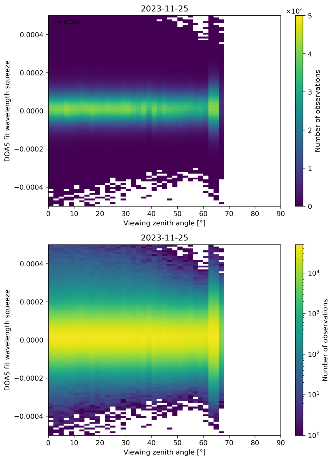
Figure 184: Scatter density plot of “Viewing zenith angle” against “DOAS fit wavelength squeeze” for 2023-11-24 to 2023-11-26.
