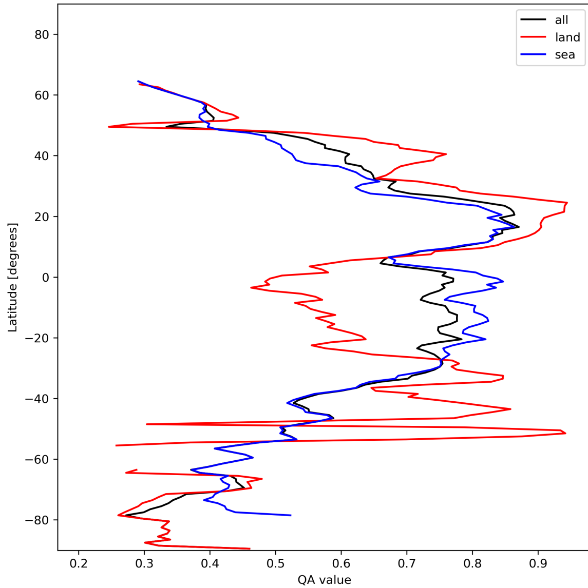
Figure 20: Zonal average of “QA value” for 2023-11-24 to 2023-11-26.
