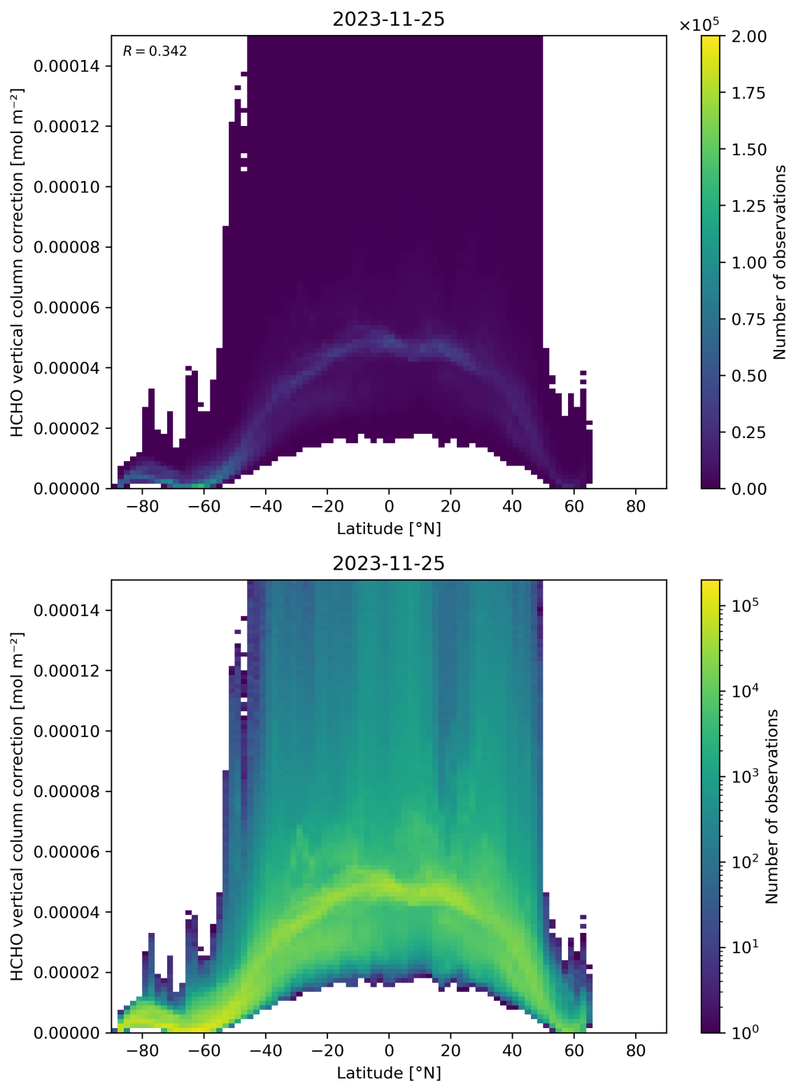
Figure 164: Scatter density plot of “Latitude” against “HCHO vertical column correction” for 2023-11-24 to 2023-11-26.
