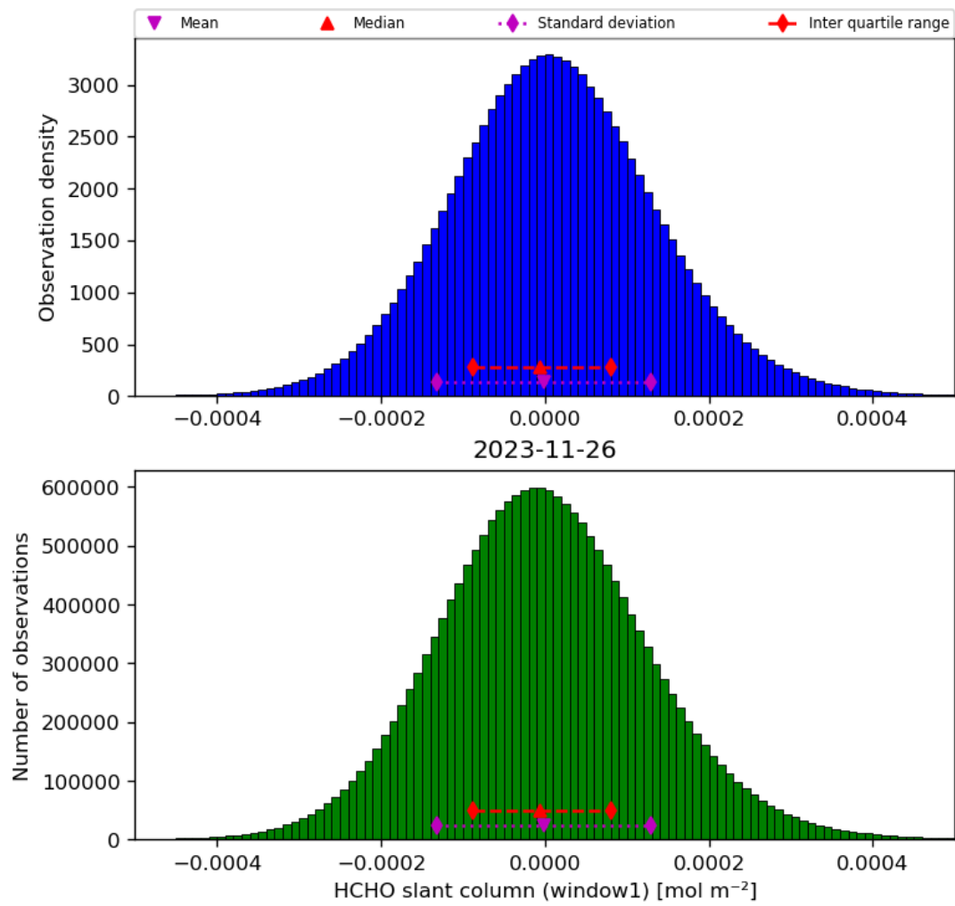
Figure 38: Histogram of “HCHO slant column (window1)” for 2023-11-25 to 2023-11-27
