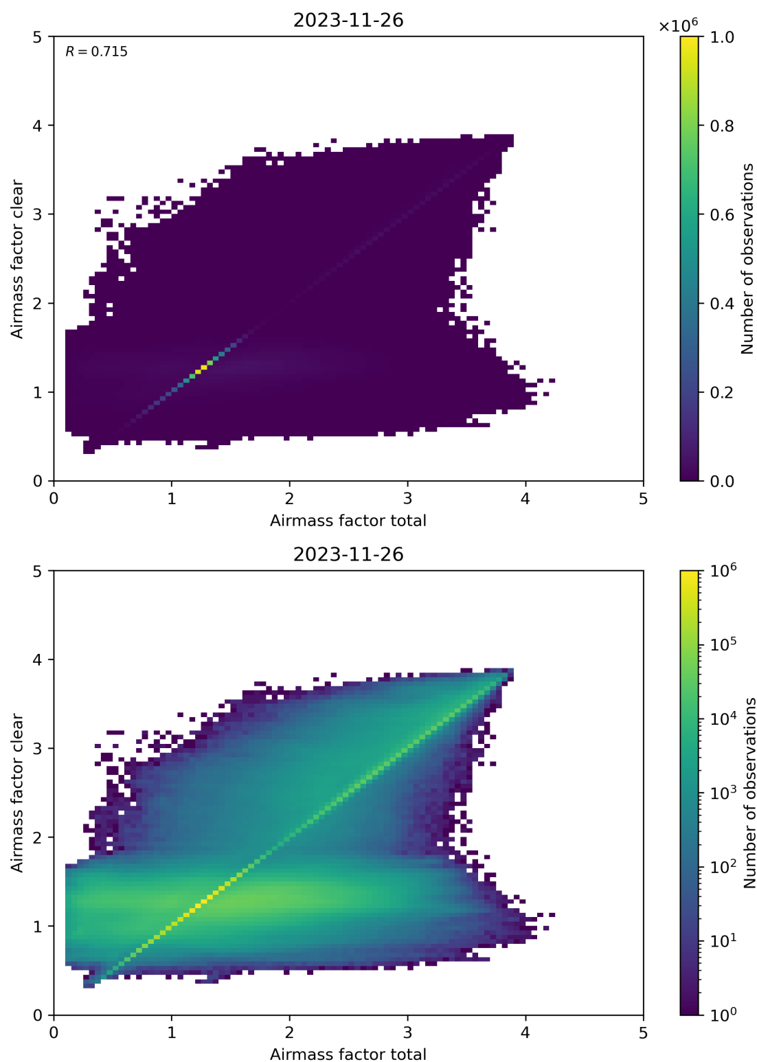
Figure 100: Scatter density plot of “Airmass factor total” against “Airmass factor clear” for 2023-11-25 to 2023-11-27.
