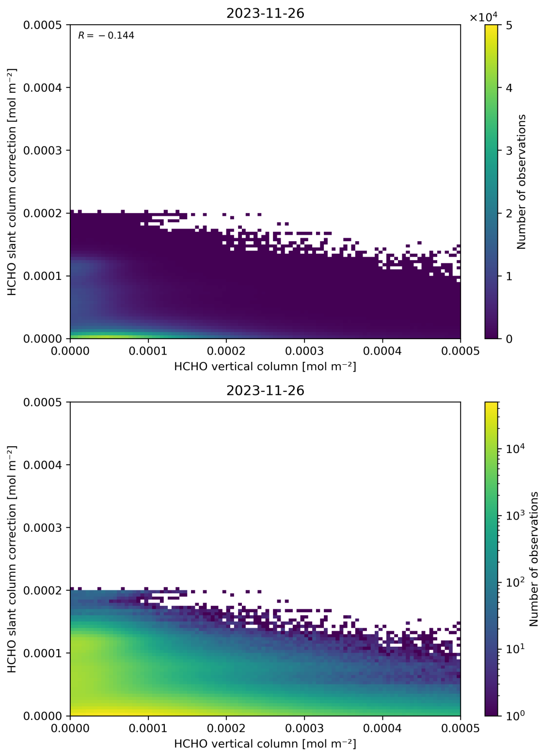
Figure 128: Scatter density plot of “HCHO vertical column” against “HCHO slant column correction” for 2023-11-25 to 2023-11-27.
