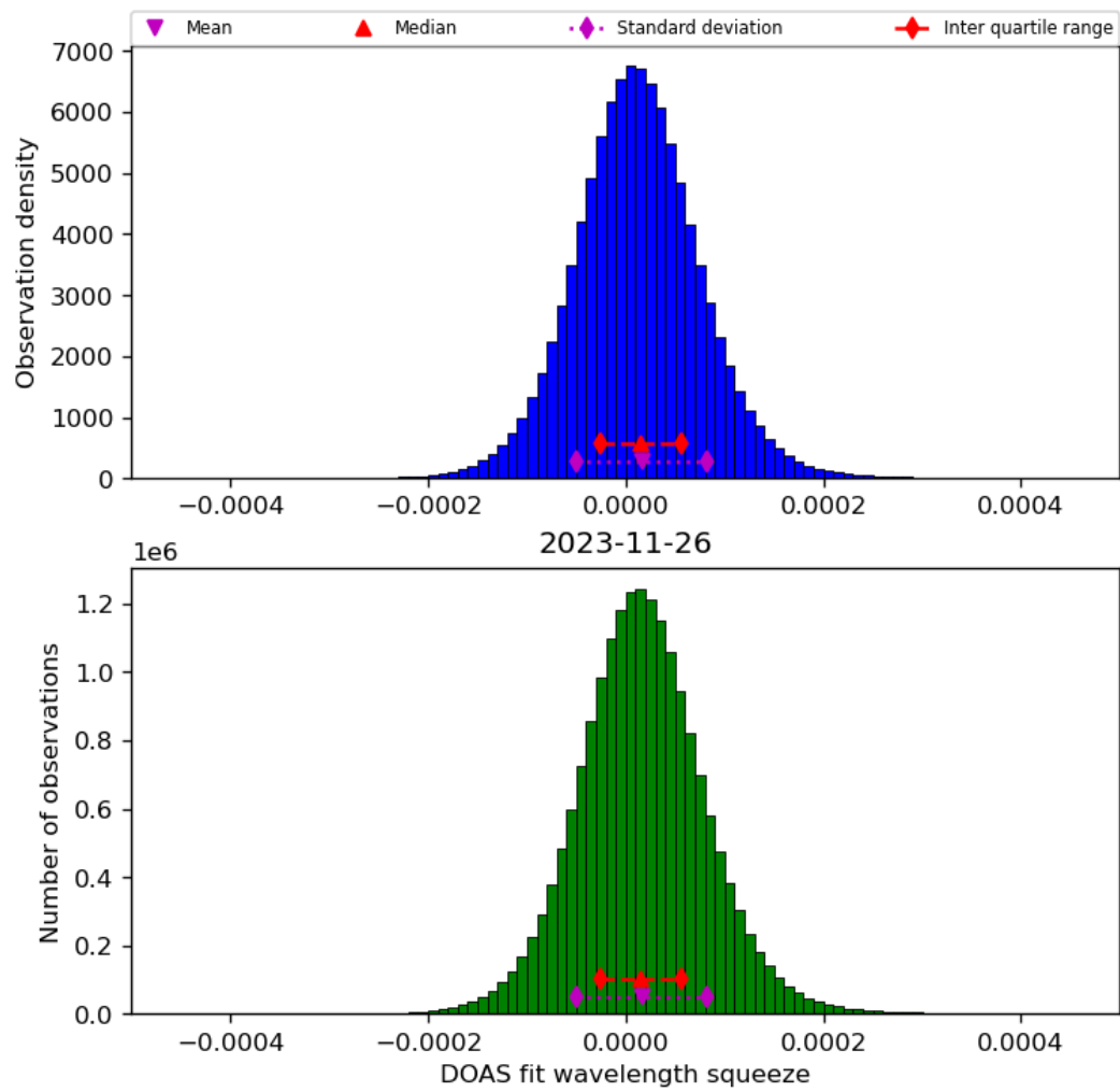
Figure 45: Histogram of “DOAS fit wavelength squeeze” for 2023-11-25 to 2023-11-27
