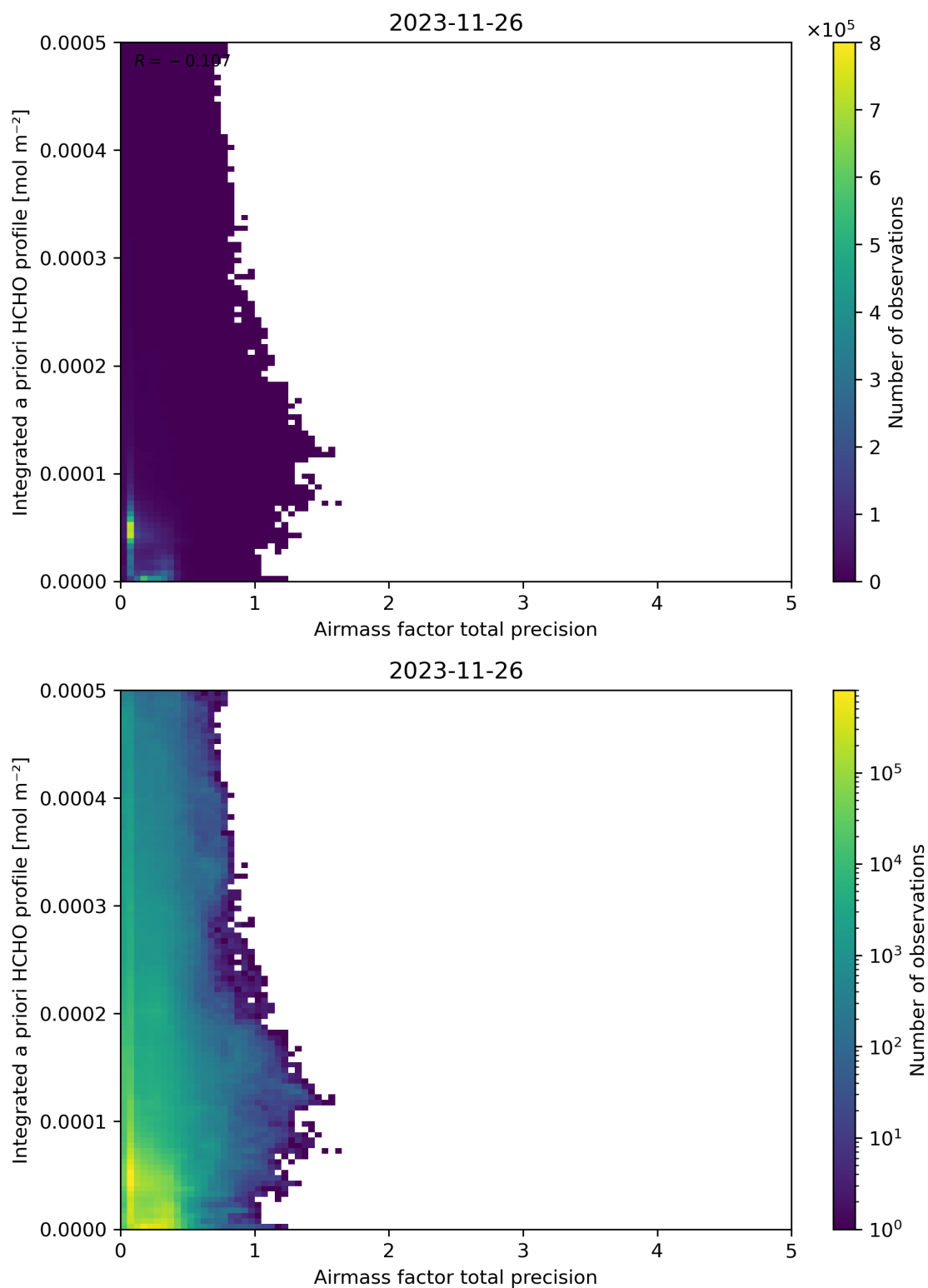
Figure 111: Scatter density plot of “Airmass factor total precision” against “Integrated a priori HCHO profile” for 2023-11-25 to 2023-11-27.
