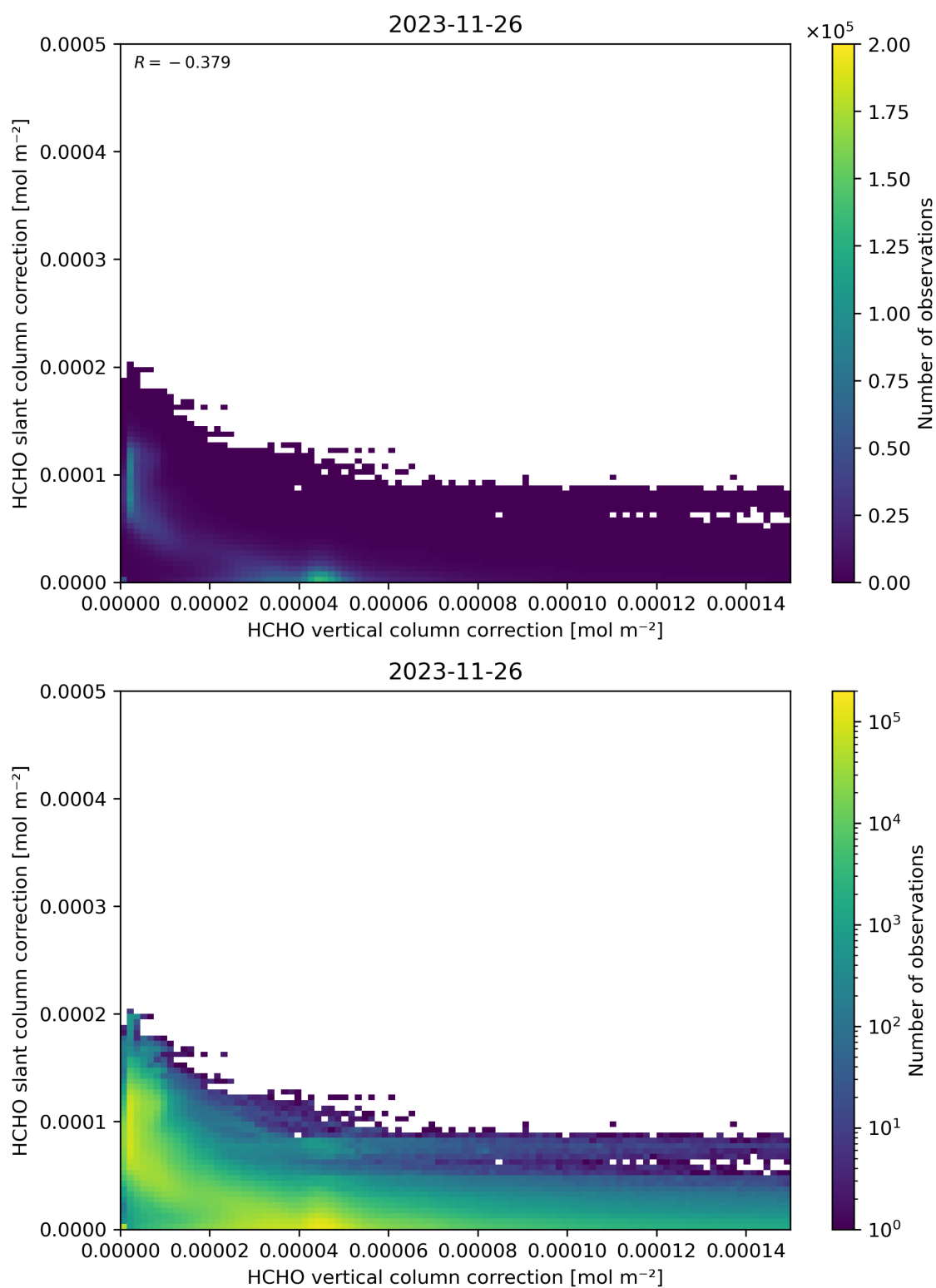
Figure 117: Scatter density plot of “HCHO vertical column correction” against “HCHO slant column correction” for 2023-11-25 to 2023-11-27.
