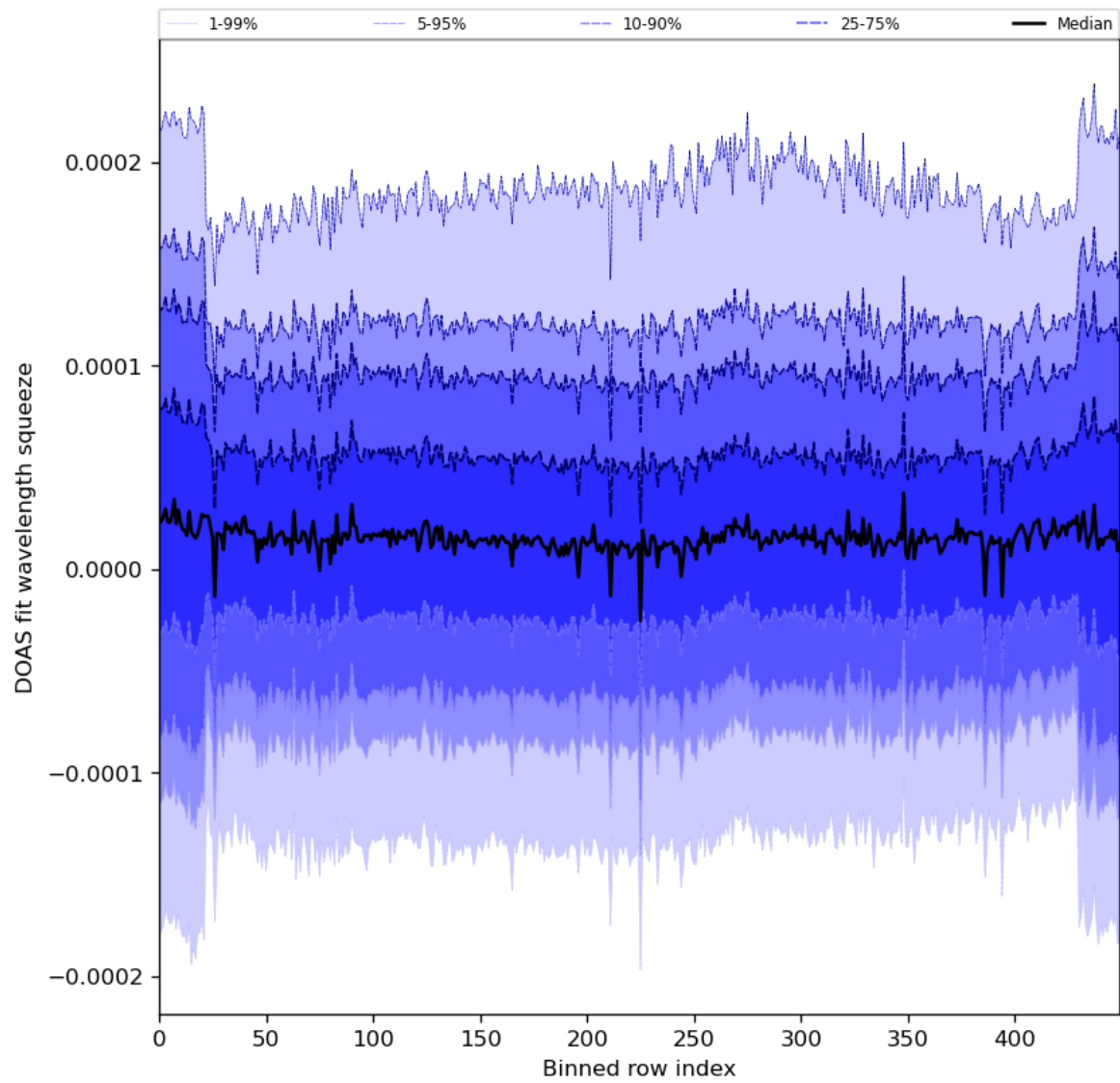
Figure 59: Along track statistics of “DOAS fit wavelength squeeze” for 2023-11-25 to 2023-11-27
