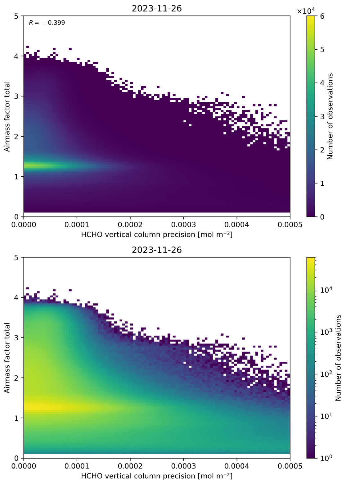
Figure 144: Scatter density plot of “HCHO vertical column precision” against “Airmass factor total” for 2023-11-25 to 2023-11-27.
