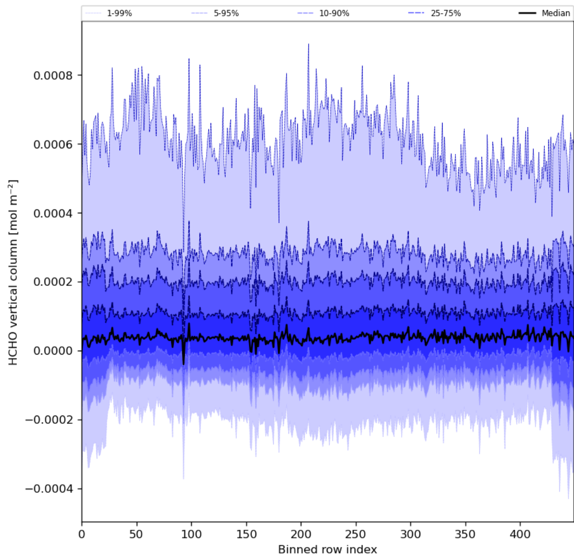
Figure 49: Along track statistics of “HCHO vertical column” for 2023-11-25 to 2023-11-27
