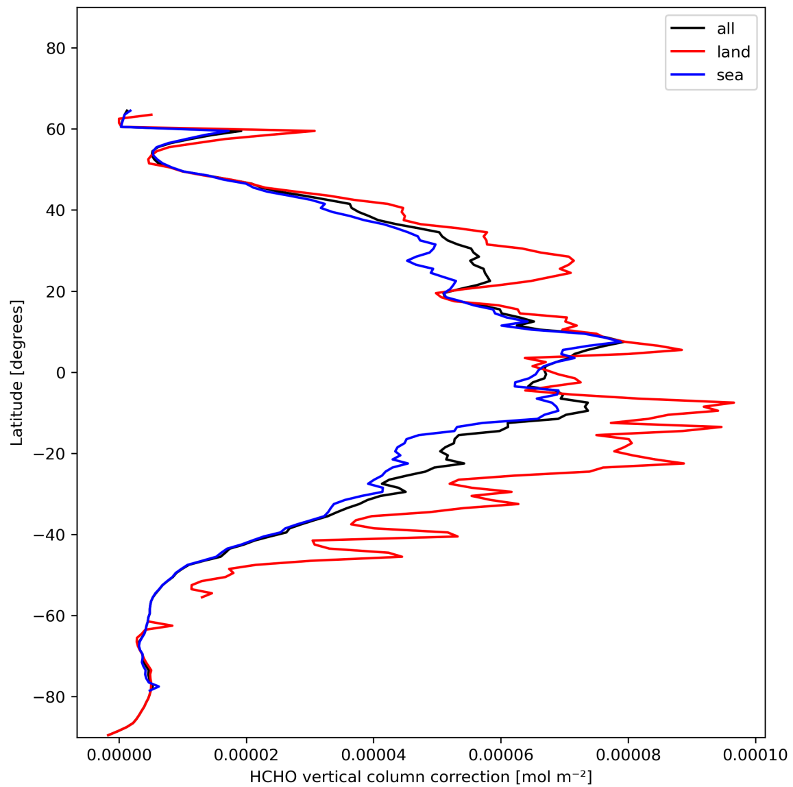
Figure 23: Zonal average of “HCHO vertical column correction” for 2023-11-25 to 2023-11-27.
