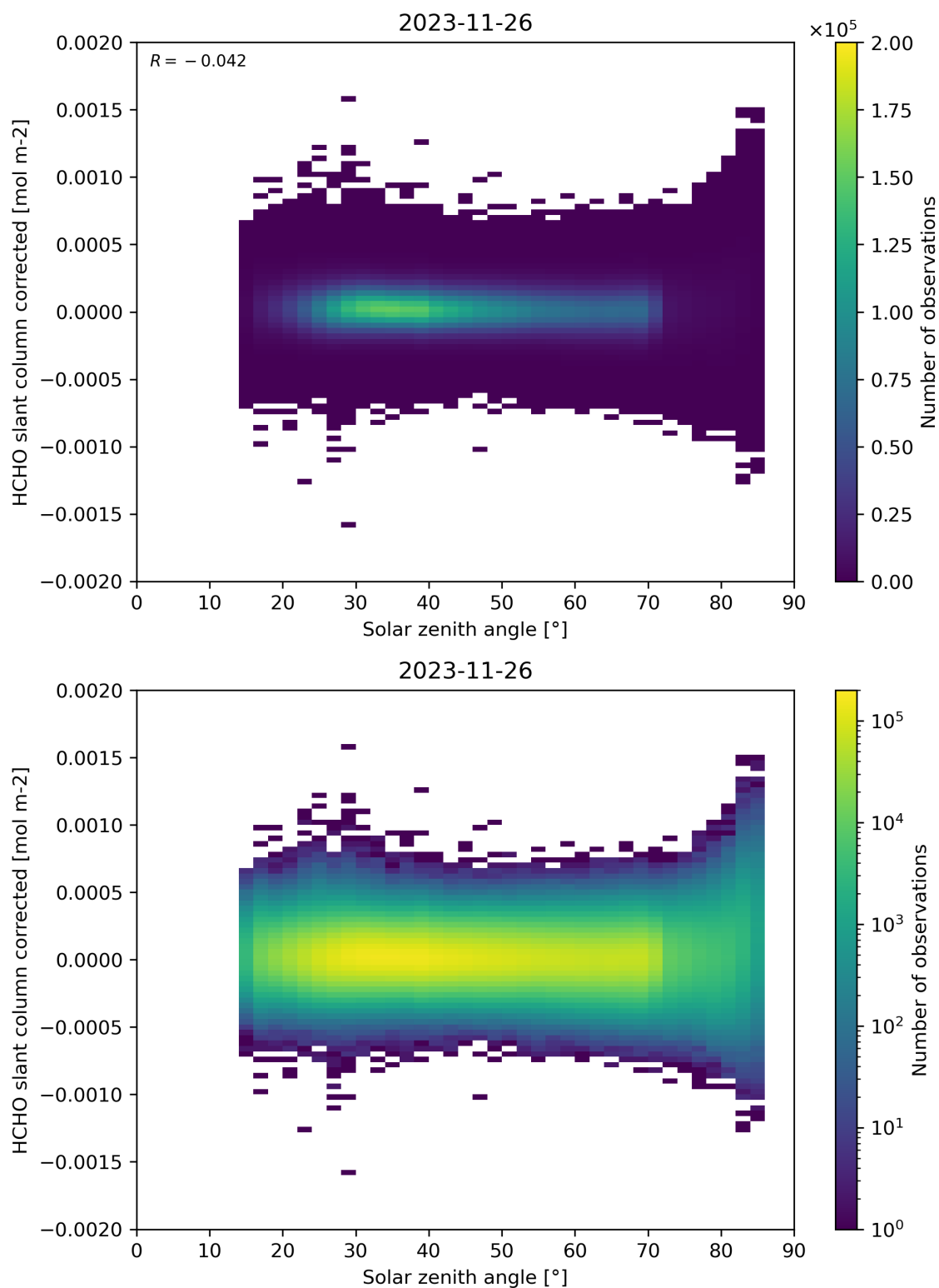
Figure 171: Scatter density plot of “Solar zenith angle” against “HCHO slant column corrected” for 2023-11-25 to 2023-11-27.
