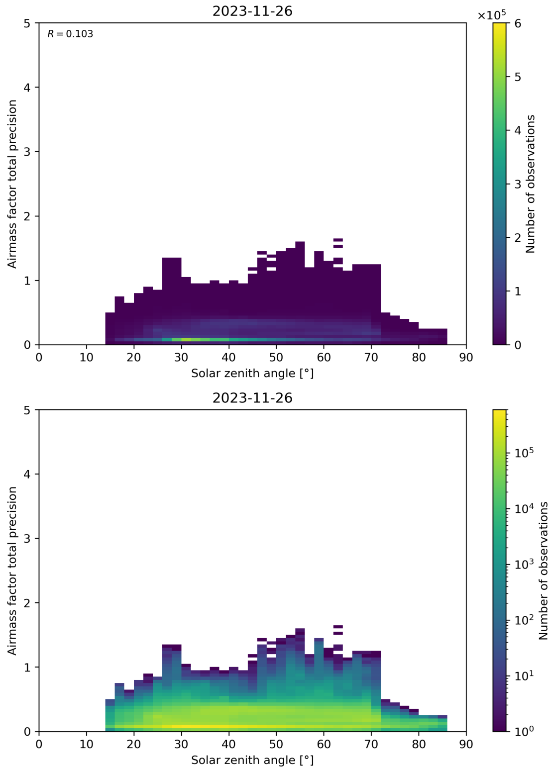
Figure 176: Scatter density plot of “Solar zenith angle” against “Airmass factor total precision” for 2023-11-25 to 2023-11-27.
