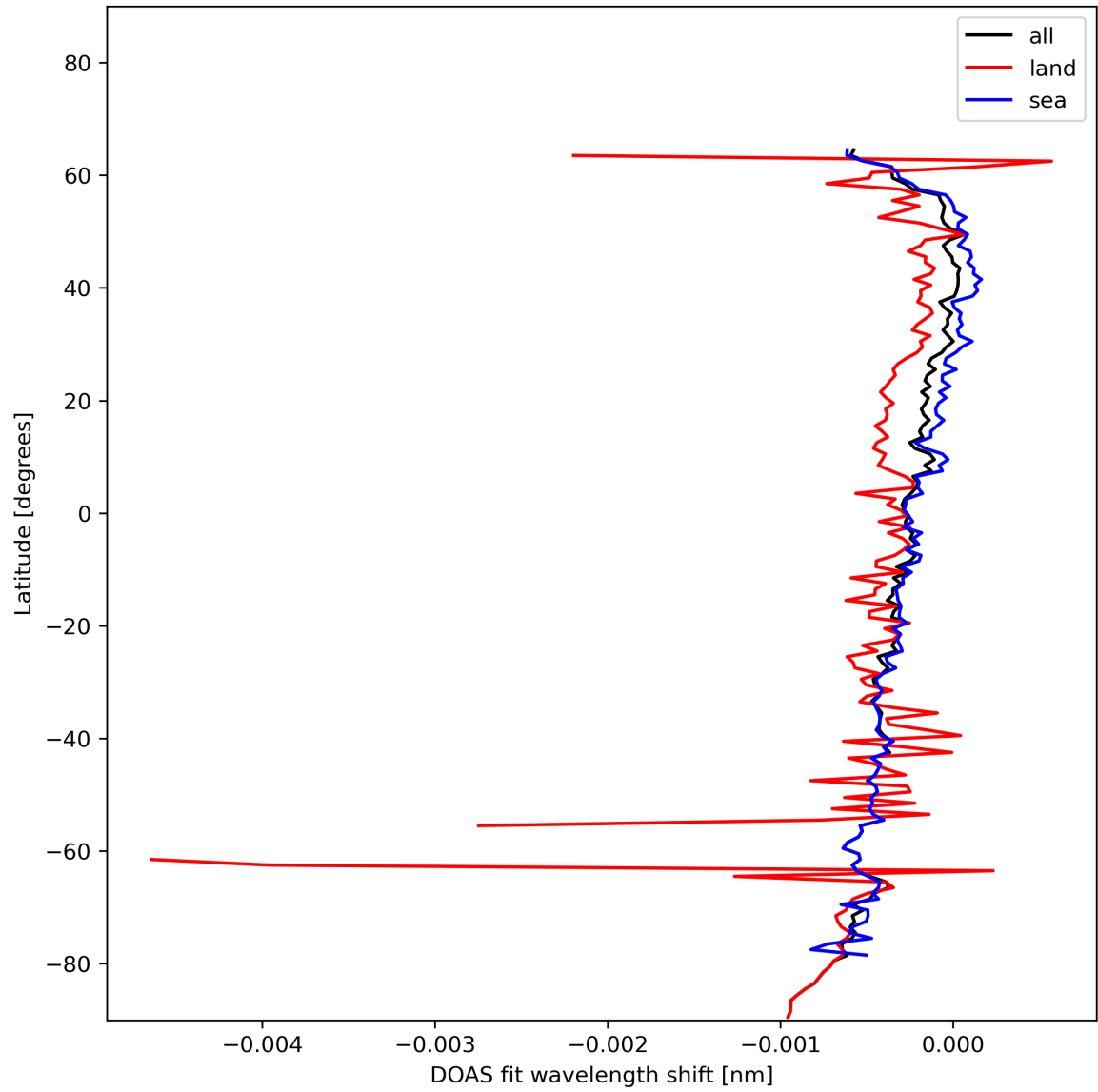
Figure 30: Zonal average of “DOAS fit wavelength shift” for 2023-11-25 to 2023-11-27.
