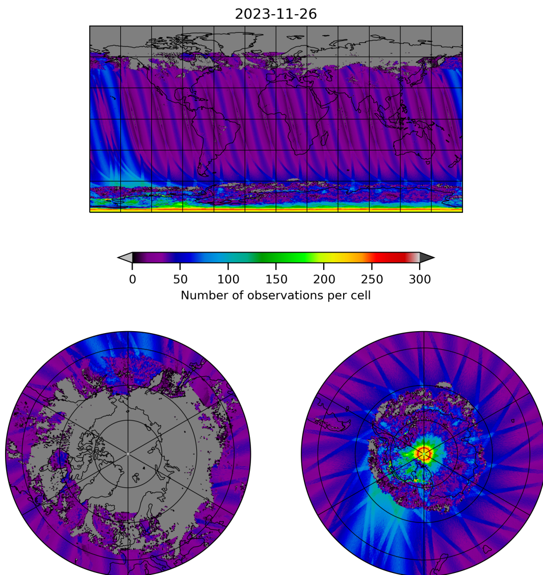
Figure 19: Map of the number of observations for 2023-11-25 to 2023-11-27
