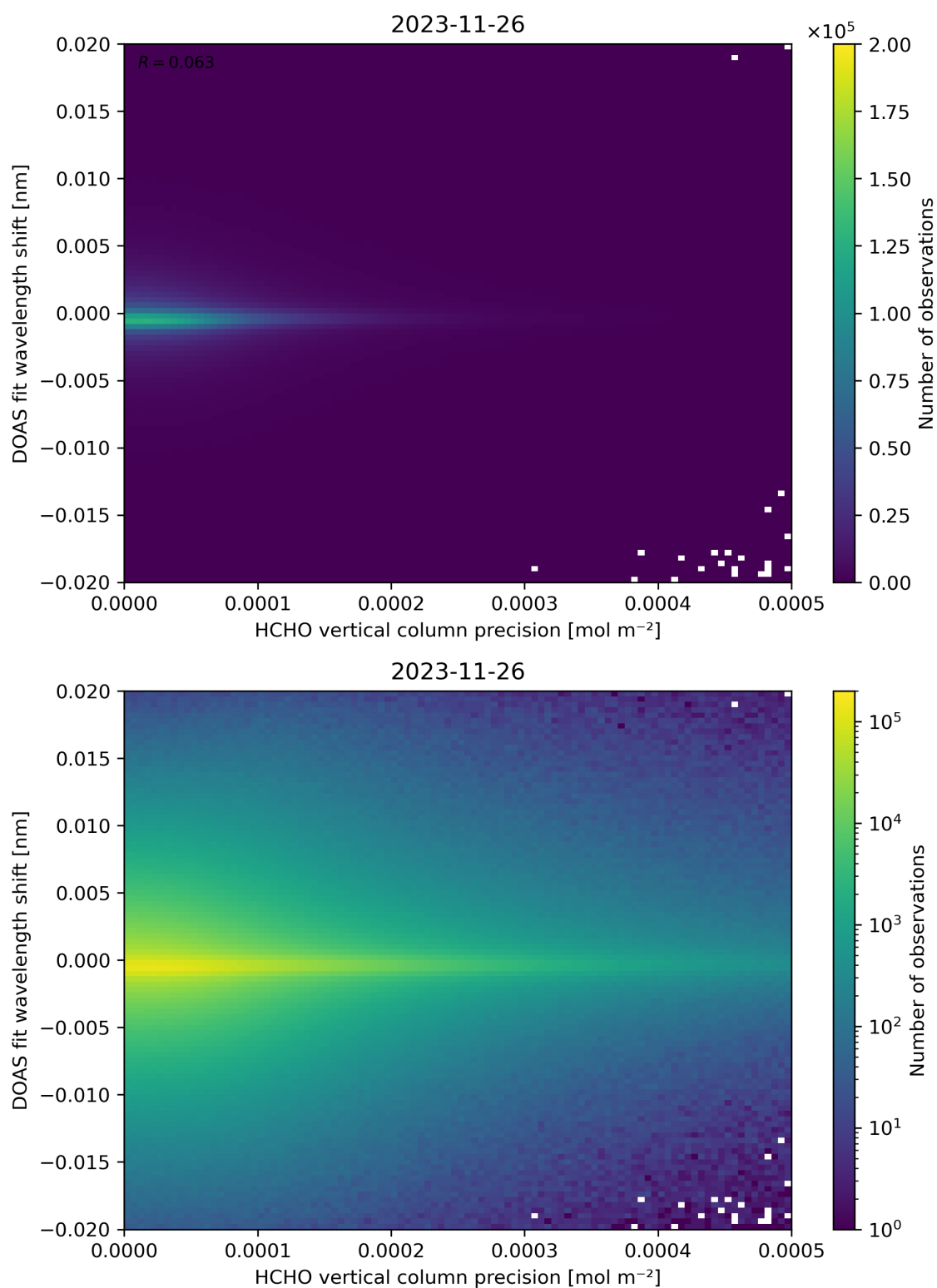
Figure 137: Scatter density plot of “HCHO vertical column precision” against “DOAS fit wavelength shift” for 2023-11-25 to 2023-11-27.
