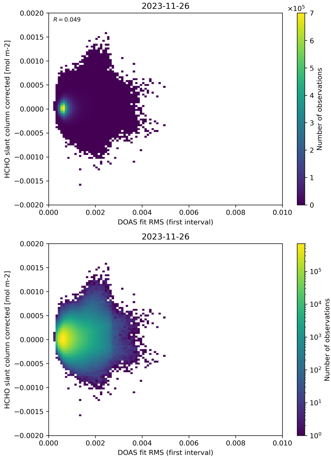
Figure 62: Scatter density plot of “DOAS fit RMS (first interval)” against “HCHO slant column corrected” for 2023-11-25 to 2023-11-27.
