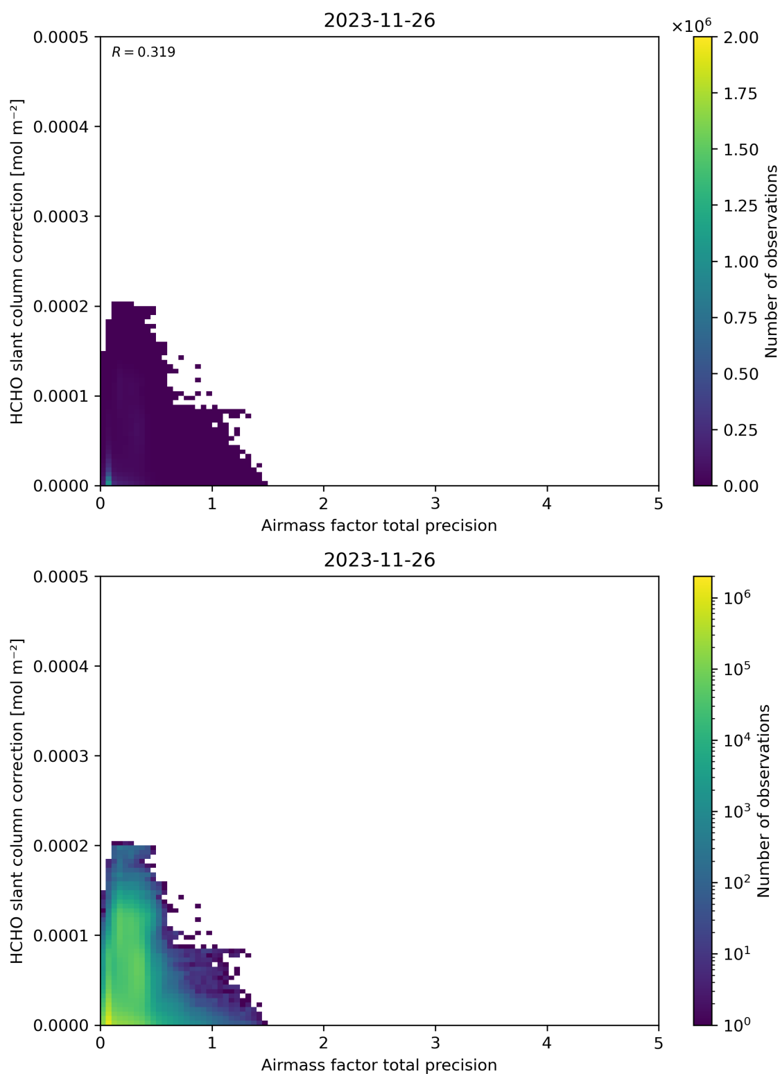
Figure 110: Scatter density plot of “Airmass factor total precision” against “HCHO slant column correction” for 2023-11-25 to 2023-11-27.
