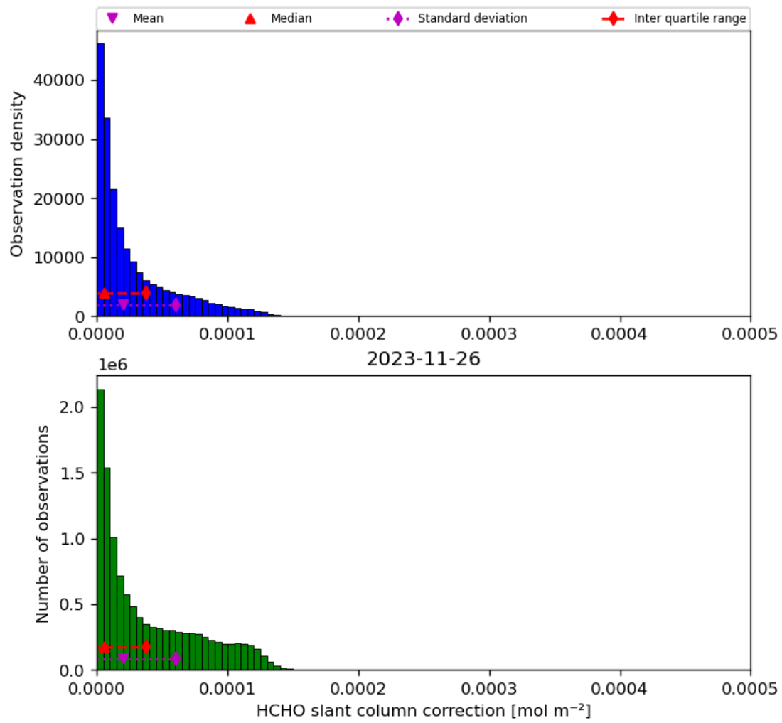
Figure 47: Histogram of “HCHO slant column correction” for 2023-11-25 to 2023-11-27
