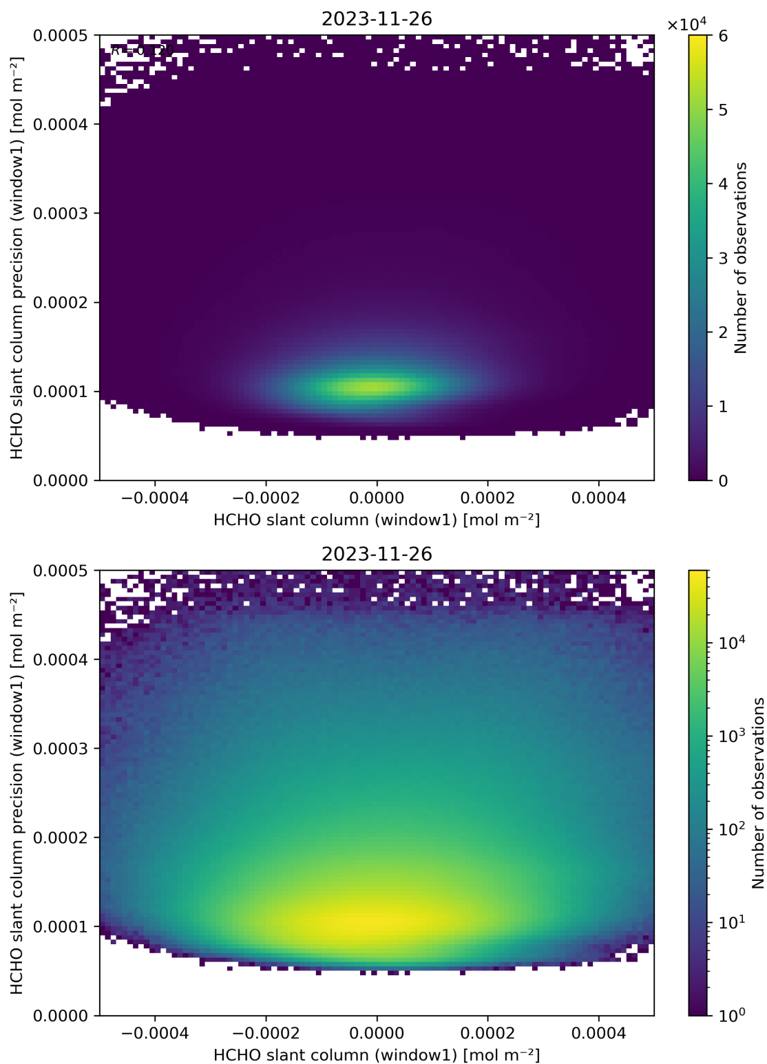
Figure 84: Scatter density plot of “HCHO slant column (window1)” against “HCHO slant column precision (window1)” for 2023-11-25 to 2023-11-27.
