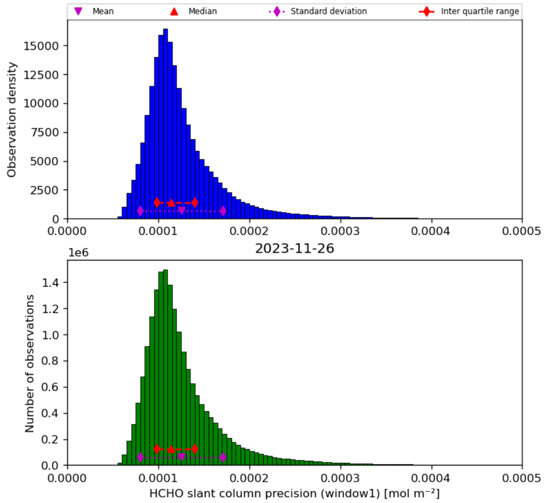
Figure 39: Histogram of “HCHO slant column precision (window1)” for 2023-11-25 to 2023-11-27
