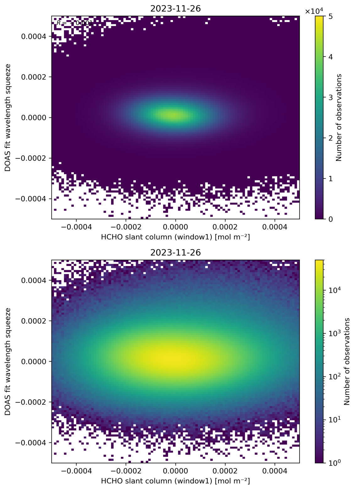
Figure 80: Scatter density plot of “HCHO slant column (window1)” against “DOAS fit wavelength squeeze” for 2023-11-25 to 2023-11-27.
