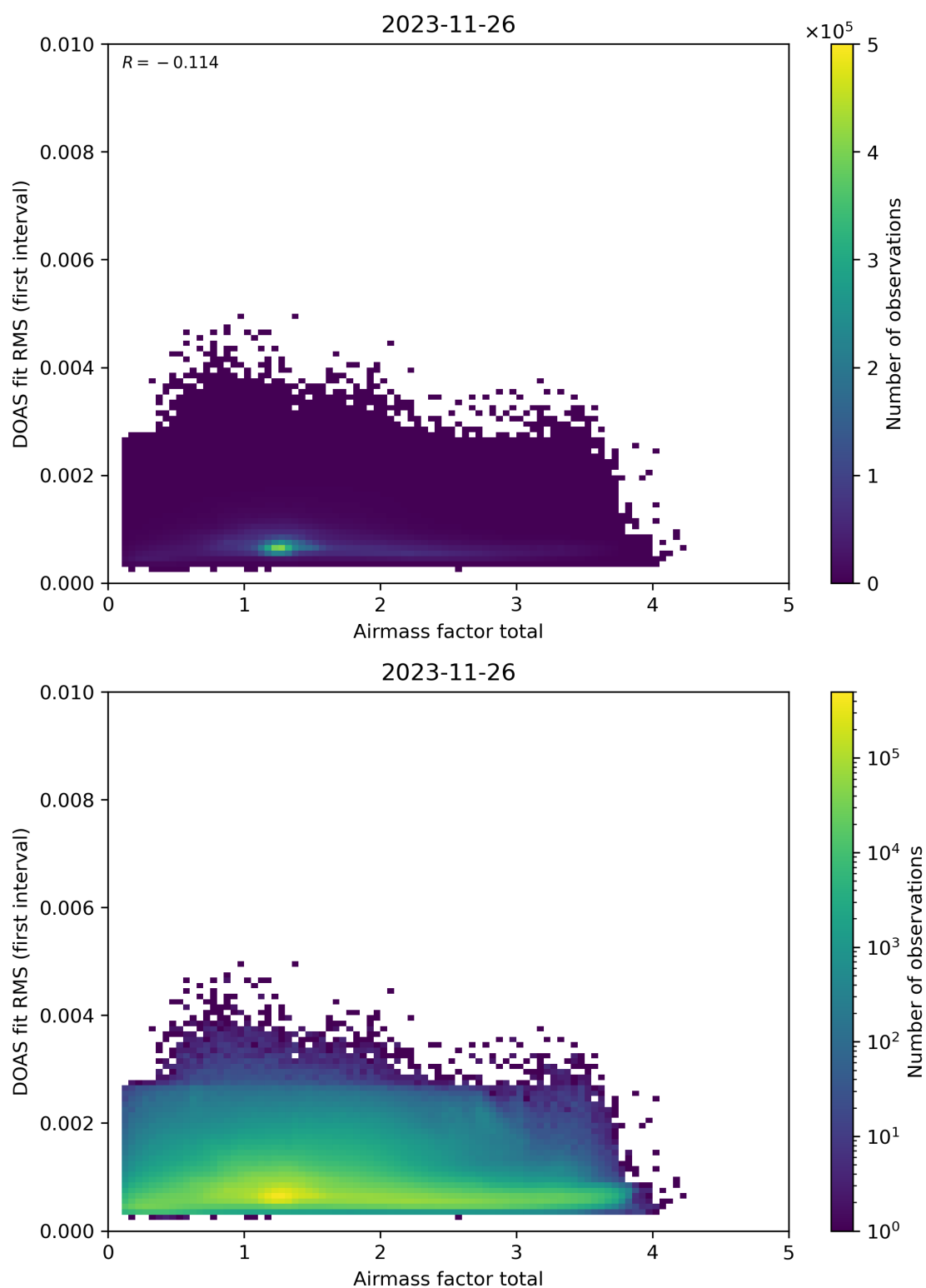
Figure 97: Scatter density plot of “Airmass factor total” against “DOAS fit RMS (first interval)” for 2023-11-25 to 2023-11-27.
