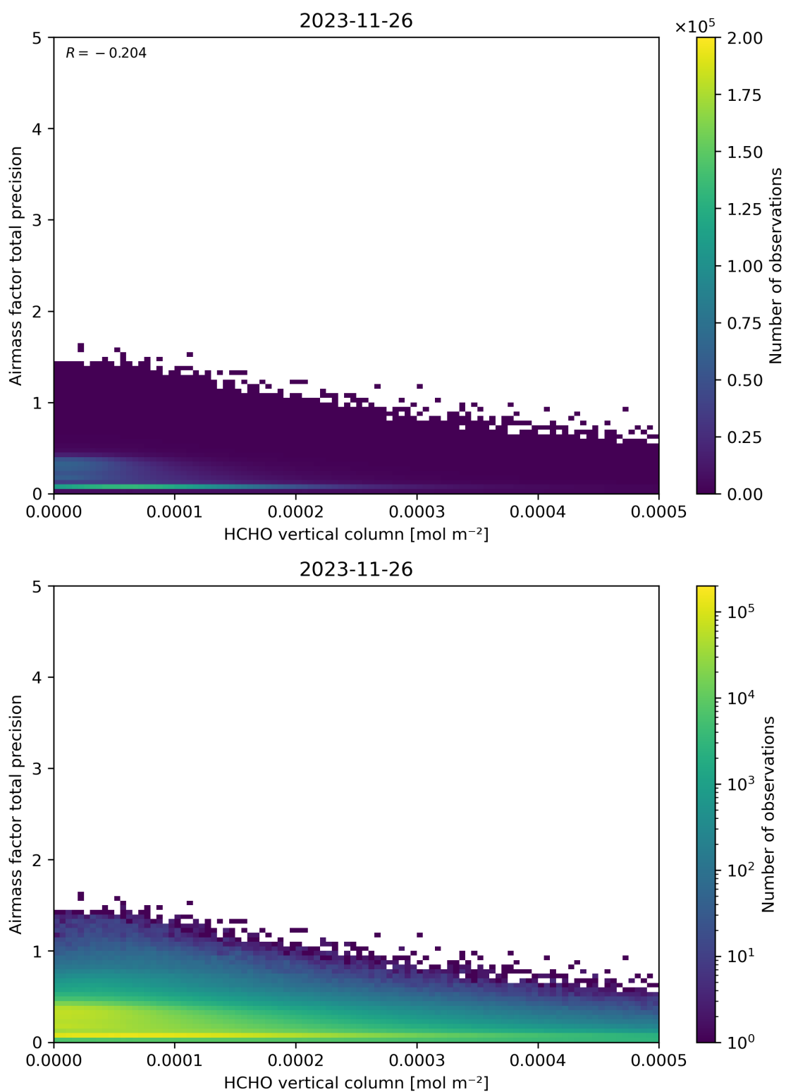
Figure 132: Scatter density plot of “HCHO vertical column” against “Airmass factor total precision” for 2023-11-25 to 2023-11-27.
