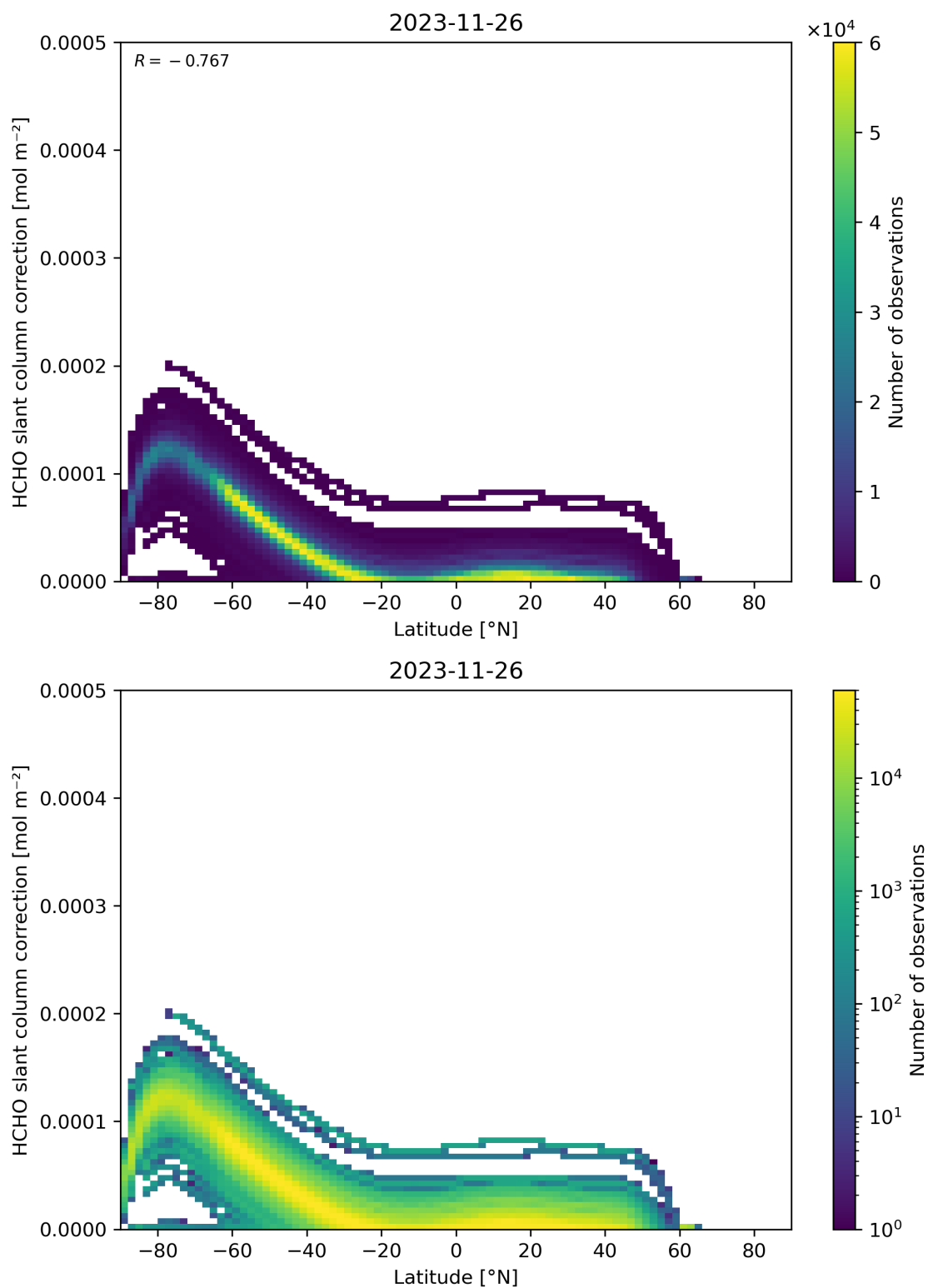
Figure 158: Scatter density plot of “Latitude” against “HCHO slant column correction” for 2023-11-25 to 2023-11-27.
