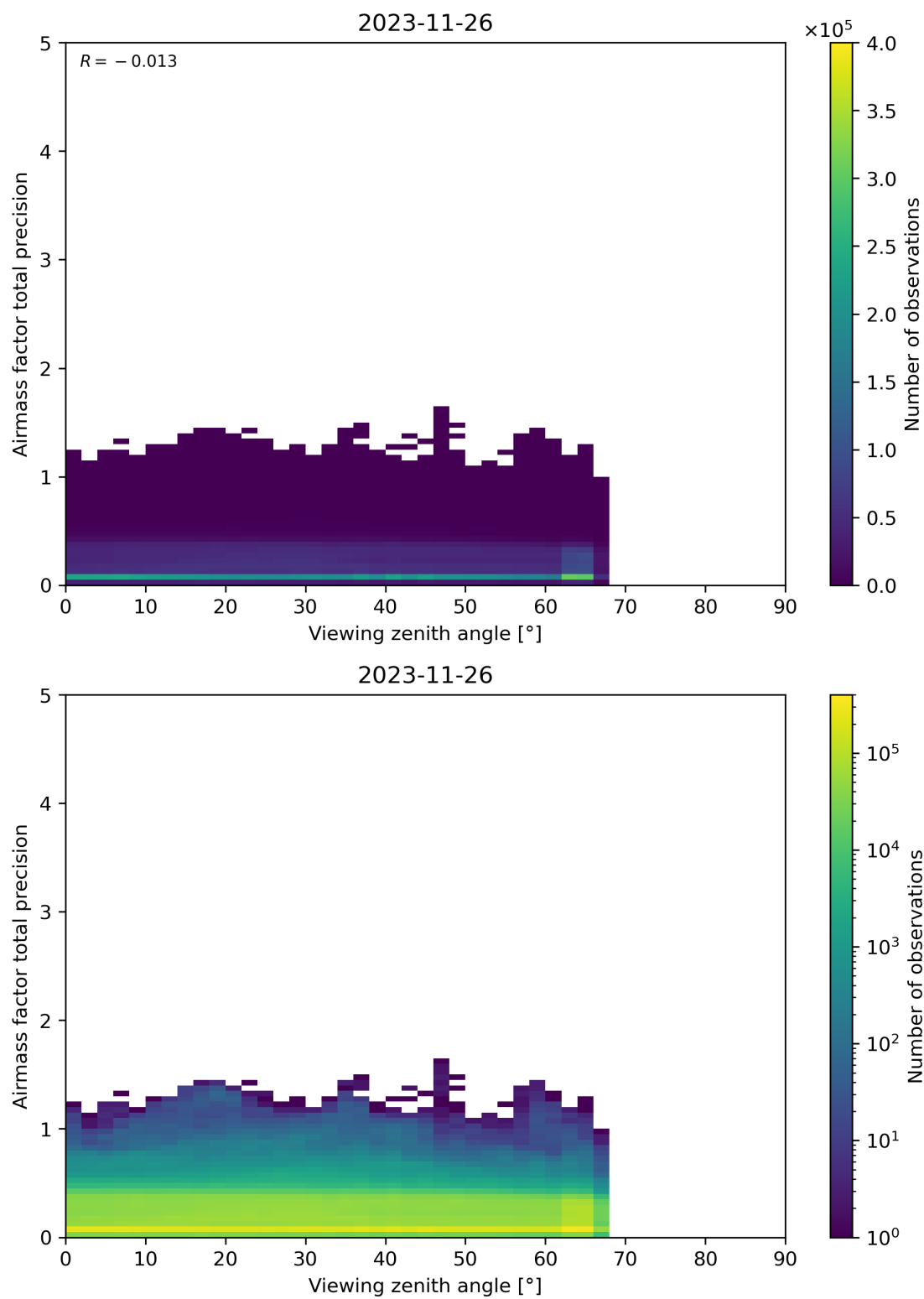
Figure 191: Scatter density plot of “Viewing zenith angle” against “Airmass factor total precision” for 2023-11-25 to 2023-11-27.
