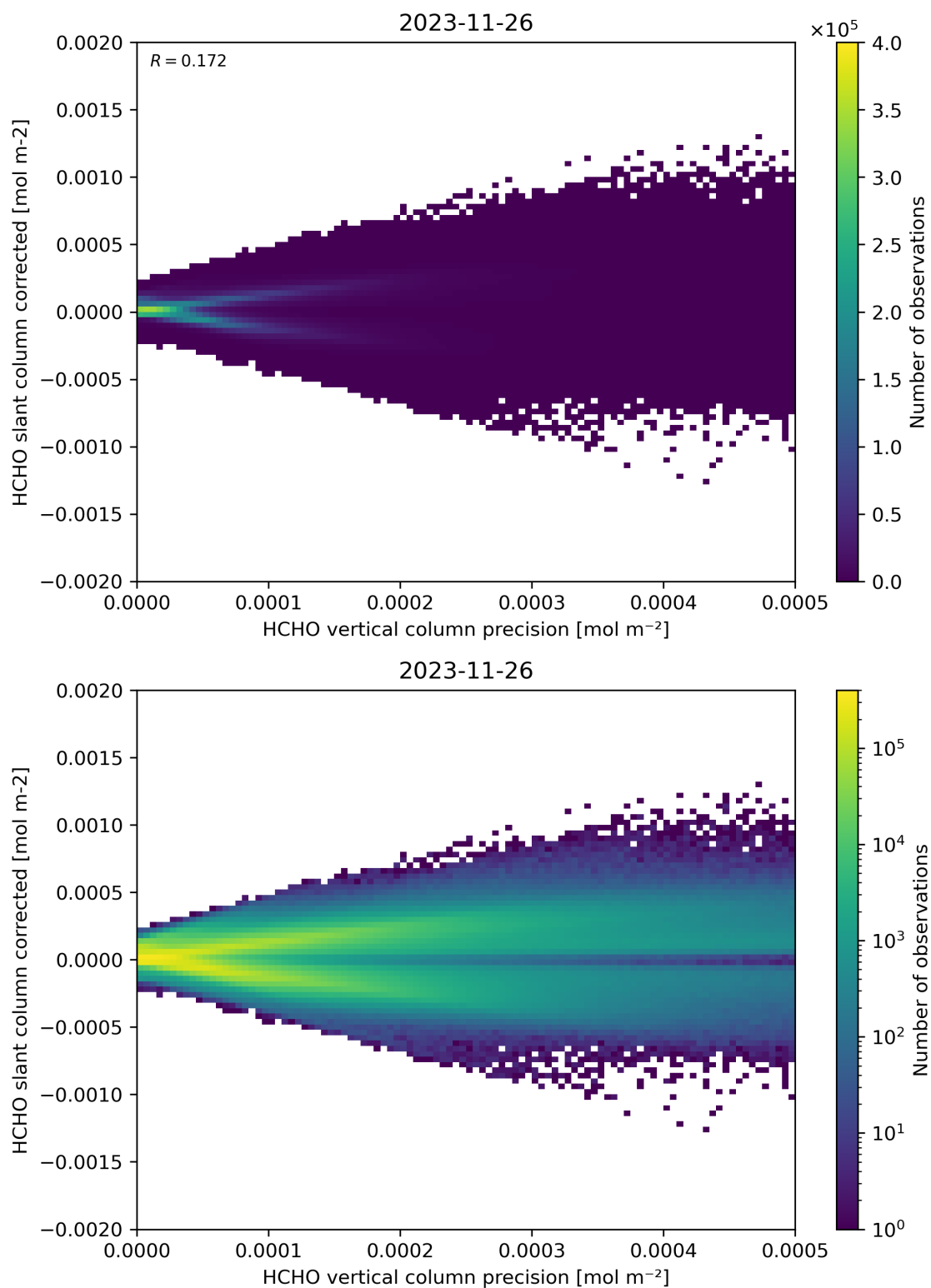
Figure 140: Scatter density plot of “HCHO vertical column precision” against “HCHO slant column corrected” for 2023-11-25 to 2023-11-27.
