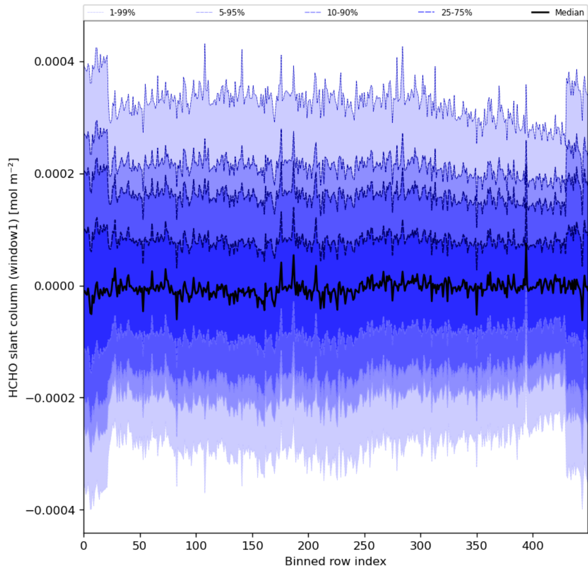
Figure 52: Along track statistics of “HCHO slant column (window1)” for 2023-11-25 to 2023-11-27
