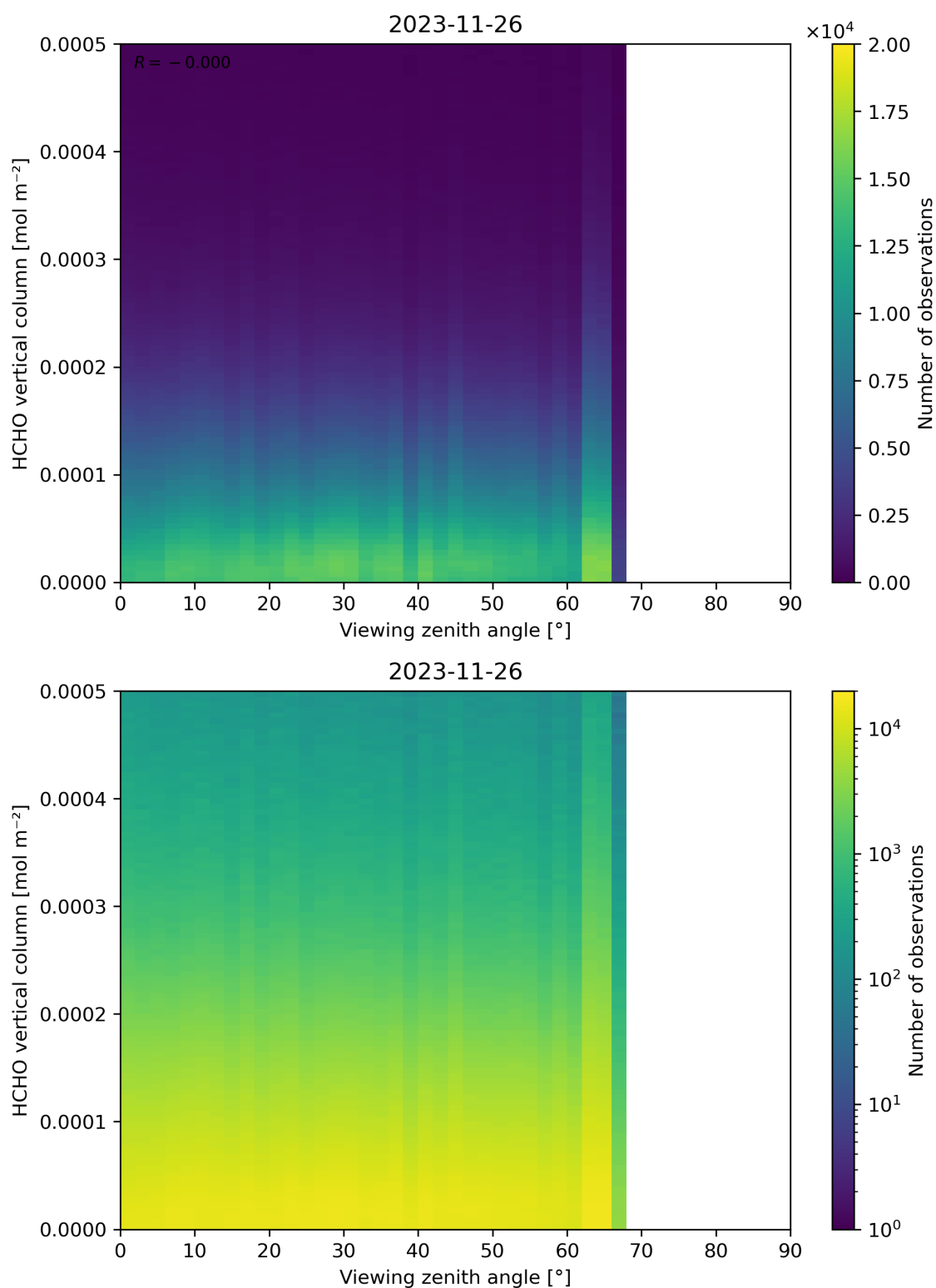
Figure 192: Scatter density plot of “Viewing zenith angle” against “HCHO vertical column” for 2023-11-25 to 2023-11-27.
