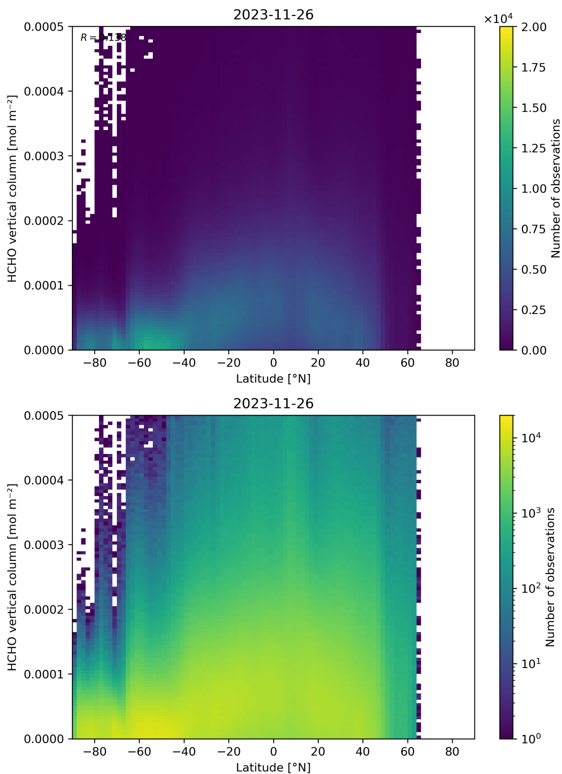
Figure 163: Scatter density plot of “Latitude” against “HCHO vertical column” for 2023-11-25 to 2023-11-27.
