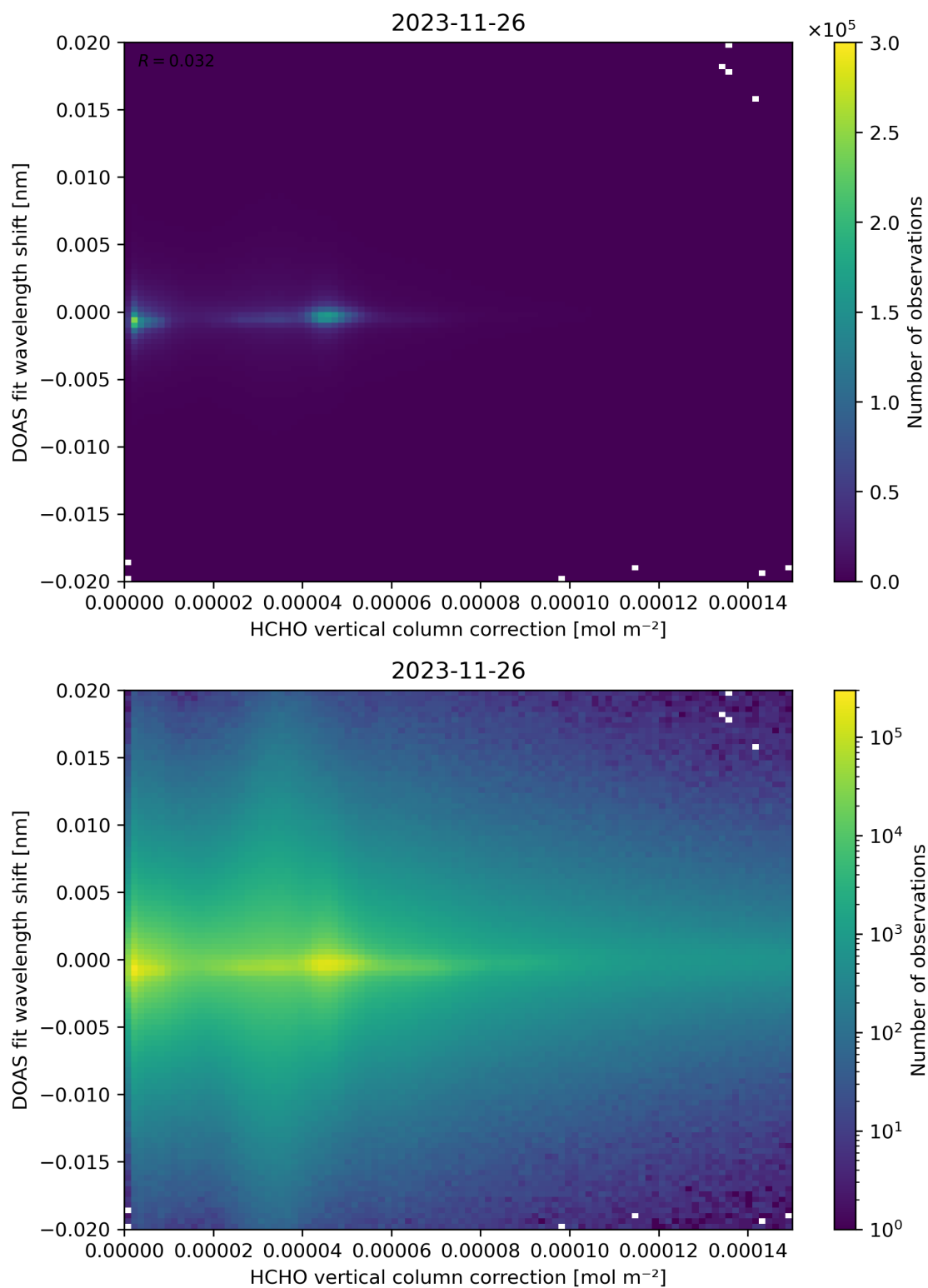
Figure 113: Scatter density plot of “HCHO vertical column correction” against “DOAS fit wavelength shift” for 2023-11-25 to 2023-11-27.
