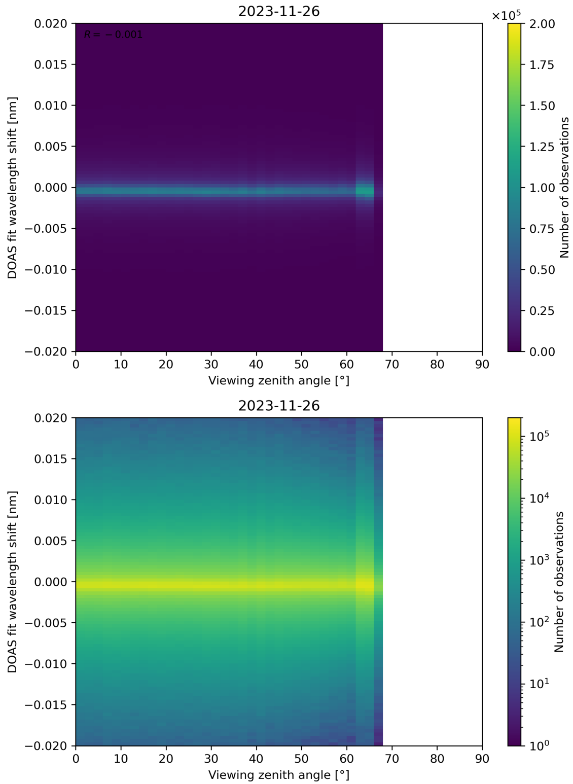
Figure 183: Scatter density plot of “Viewing zenith angle” against “DOAS fit wavelength shift” for 2023-11-25 to 2023-11-27.
