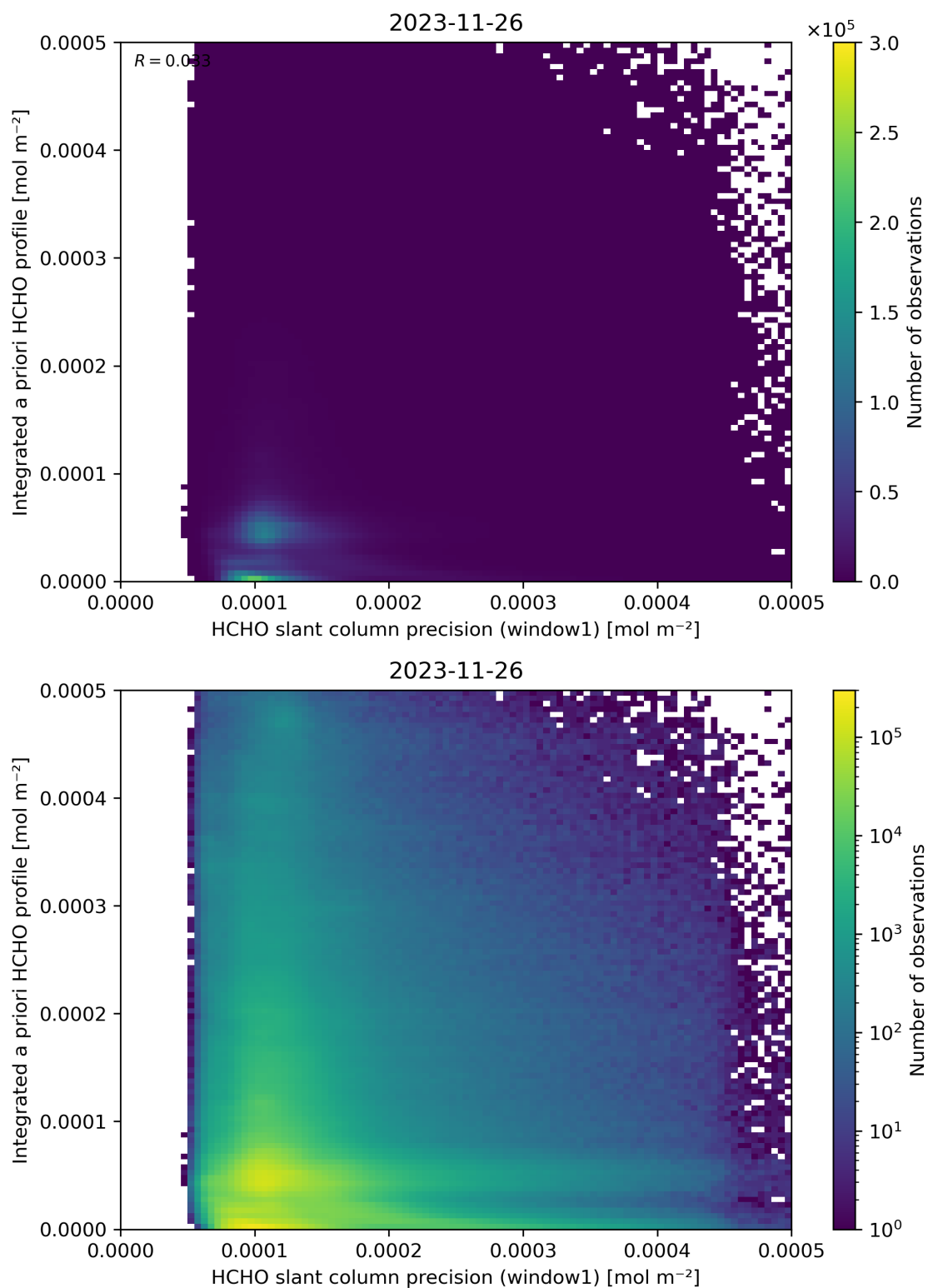
Figure 96: Scatter density plot of “HCHO slant column precision (window1)” against “Integrated a priori HCHO profile” for 2023-11-25 to 2023-11-27.
