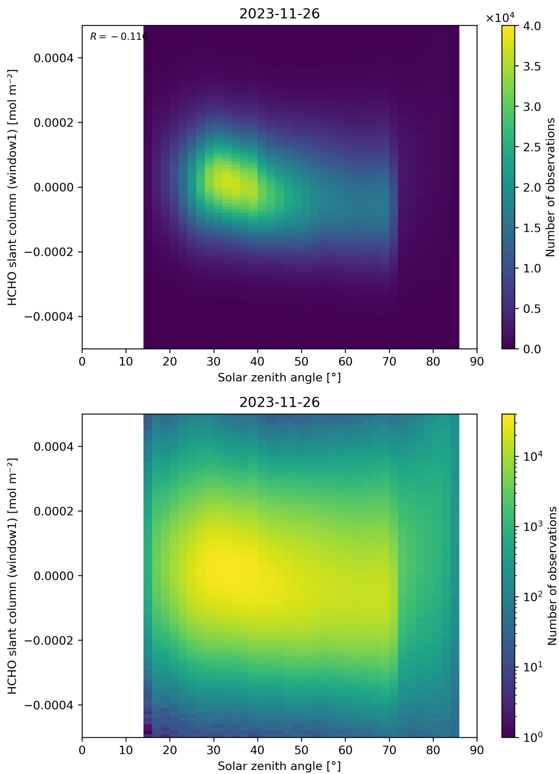
Figure 173: Scatter density plot of “Solar zenith angle” against “HCHO slant column (window1)” for 2023-11-25 to 2023-11-27.
