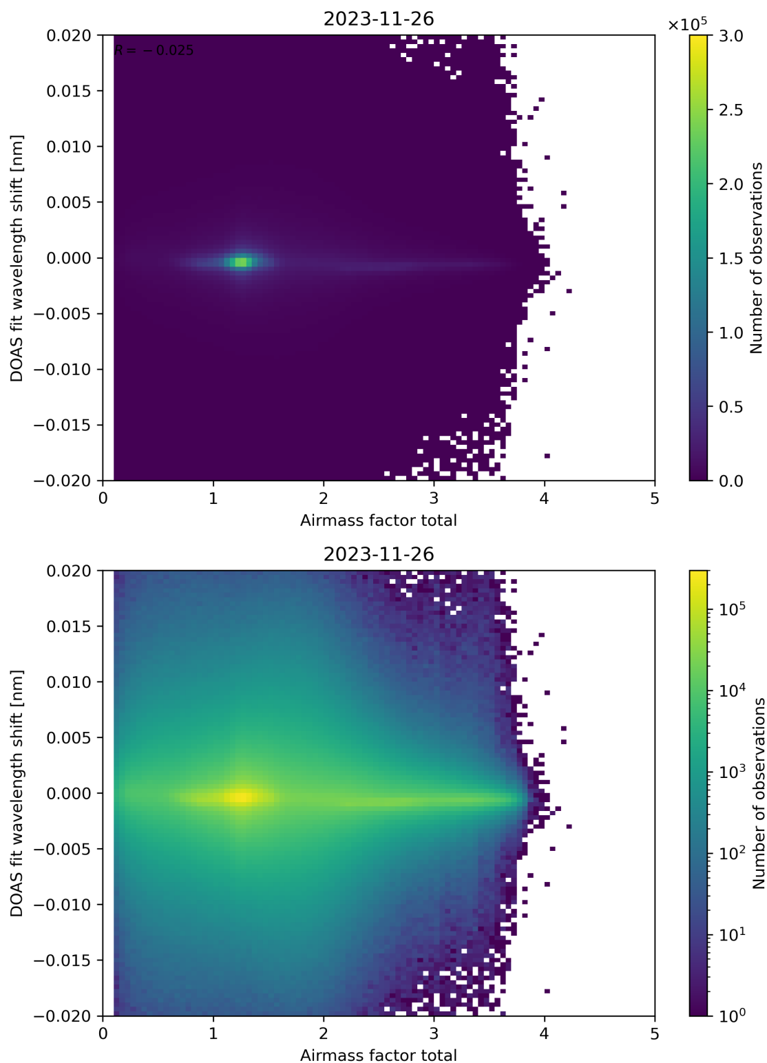
Figure 98: Scatter density plot of “Airmass factor total” against “DOAS fit wavelength shift” for 2023-11-25 to 2023-11-27.
