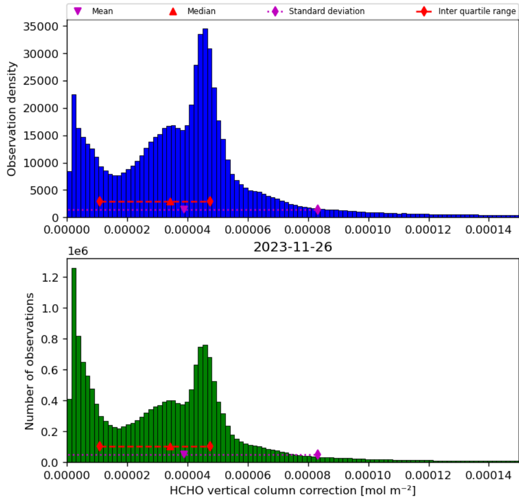
Figure 37: Histogram of “HCHO vertical column correction” for 2023-11-25 to 2023-11-27
