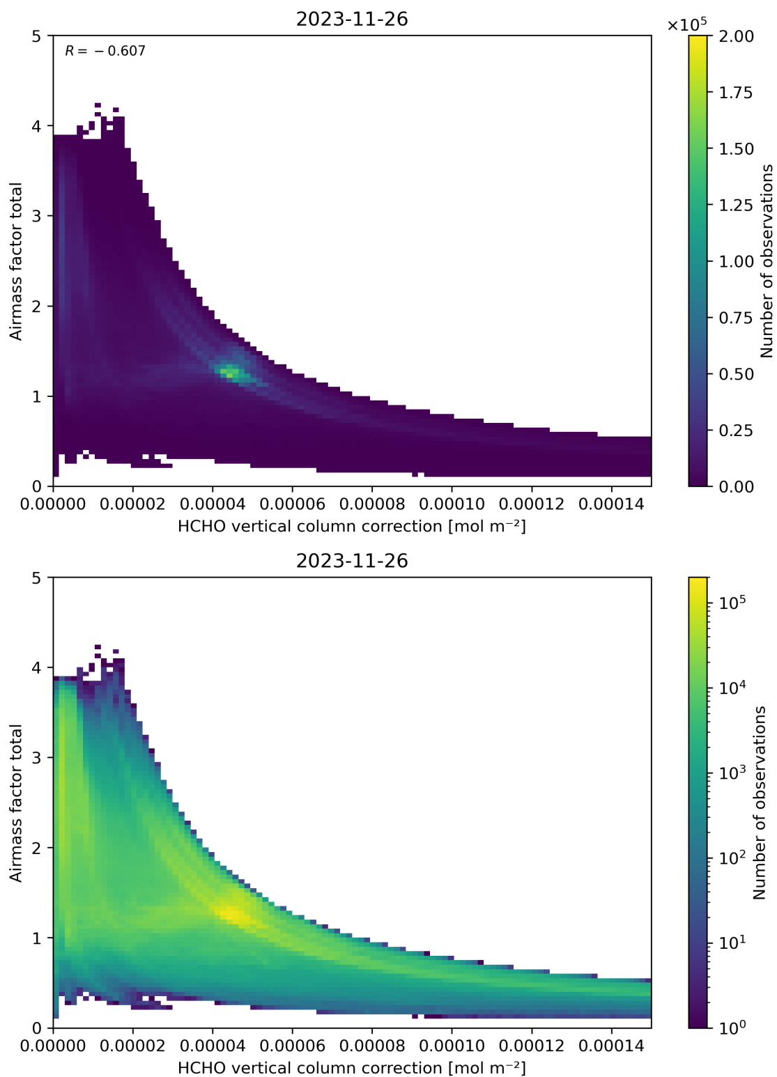
Figure 120: Scatter density plot of “HCHO vertical column correction” against “Airmass factor total” for 2023-11-25 to 2023-11-27.
