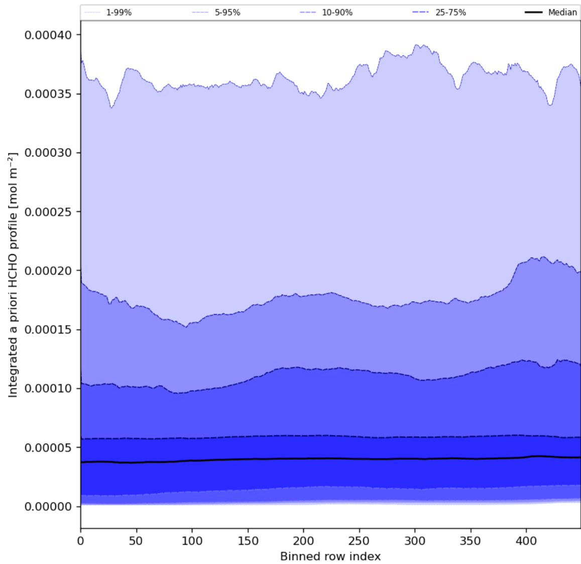
Figure 57: Along track statistics of “Integrated a priori HCHO profile” for 2023-11-25 to 2023-11-27
