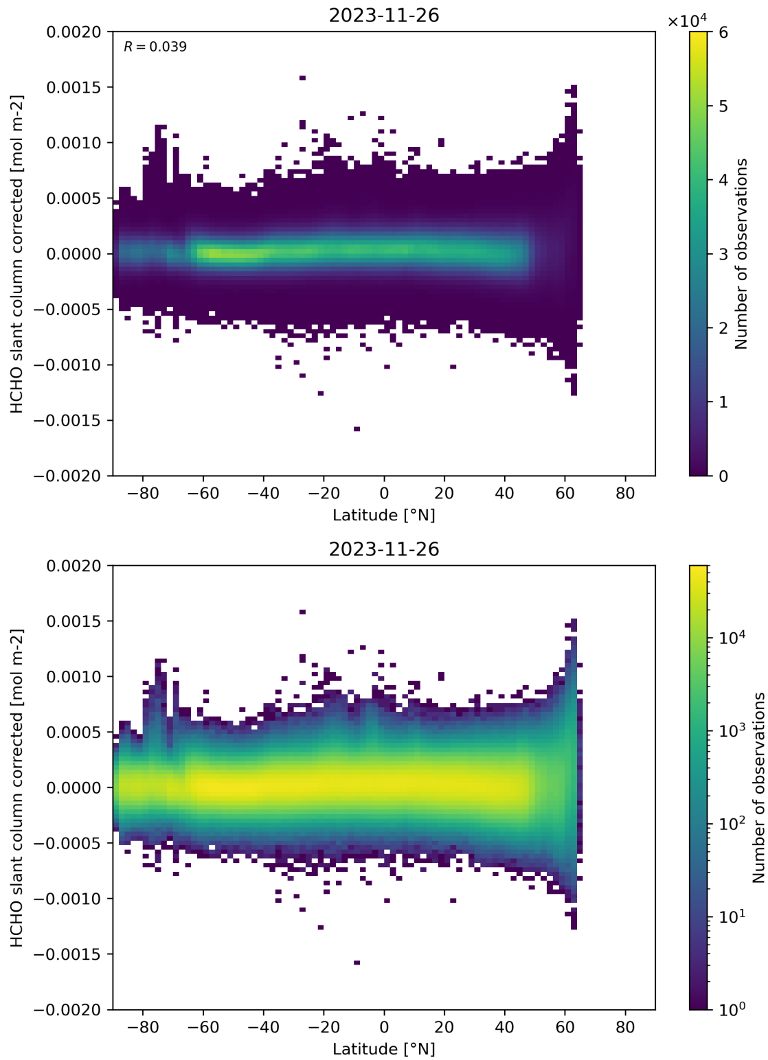
Figure 157: Scatter density plot of “Latitude” against “HCHO slant column corrected” for 2023-11-25 to 2023-11-27.
