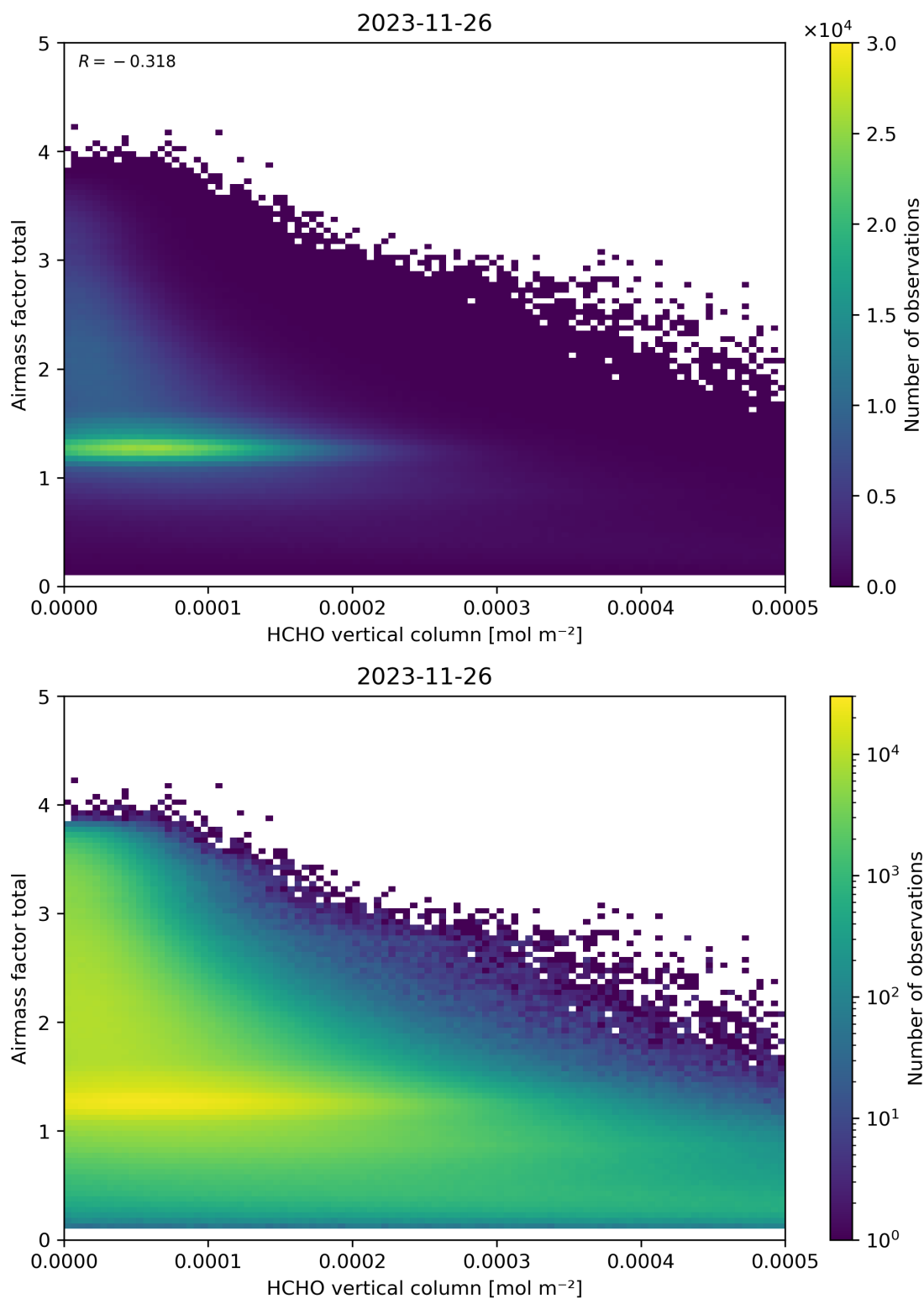
Figure 131: Scatter density plot of “HCHO vertical column” against “Airmass factor total” for 2023-11-25 to 2023-11-27.
