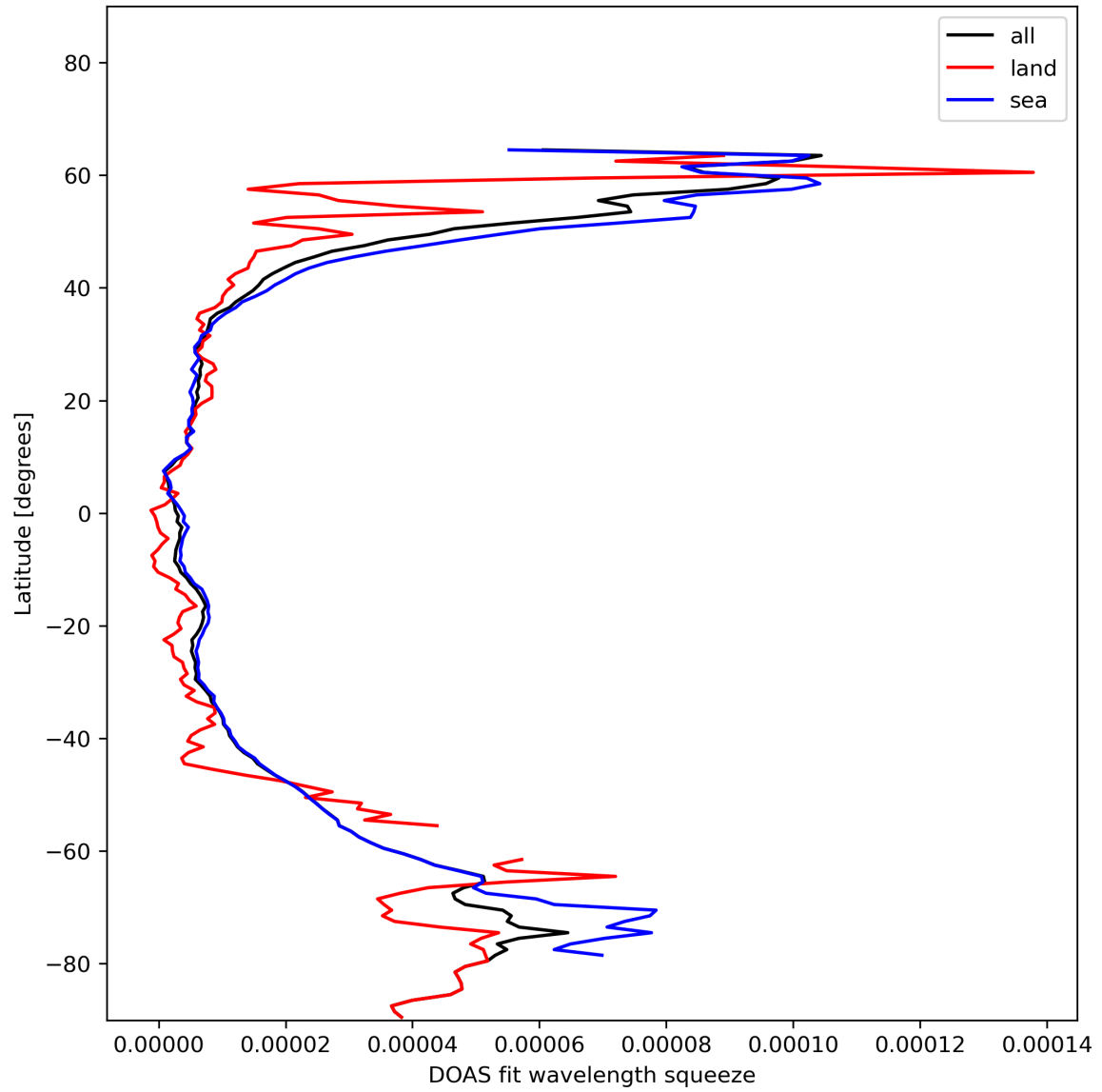
Figure 31: Zonal average of “DOAS fit wavelength squeeze” for 2023-11-25 to 2023-11-27.
