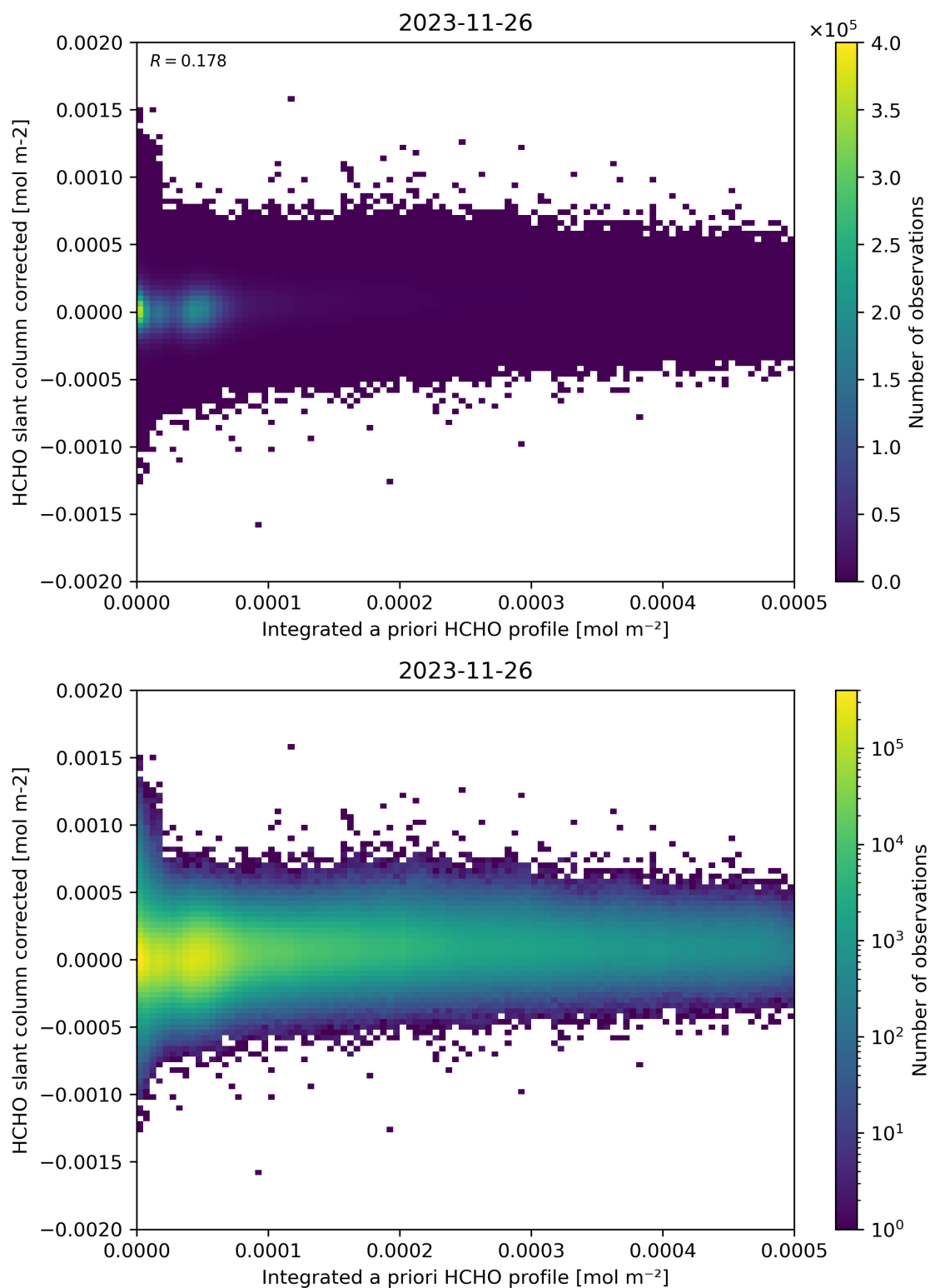
Figure 151: Scatter density plot of “Integrated a priori HCHO profile” against “HCHO slant column corrected” for 2023-11-25 to 2023-11-27.
