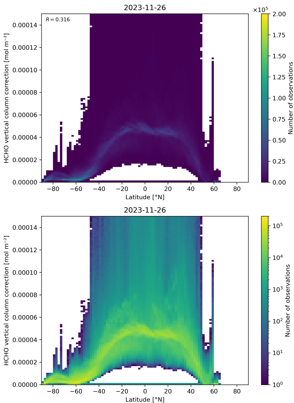
Figure 164: Scatter density plot of “Latitude” against “HCHO vertical column correction” for 2023-11-25 to 2023-11-27.
