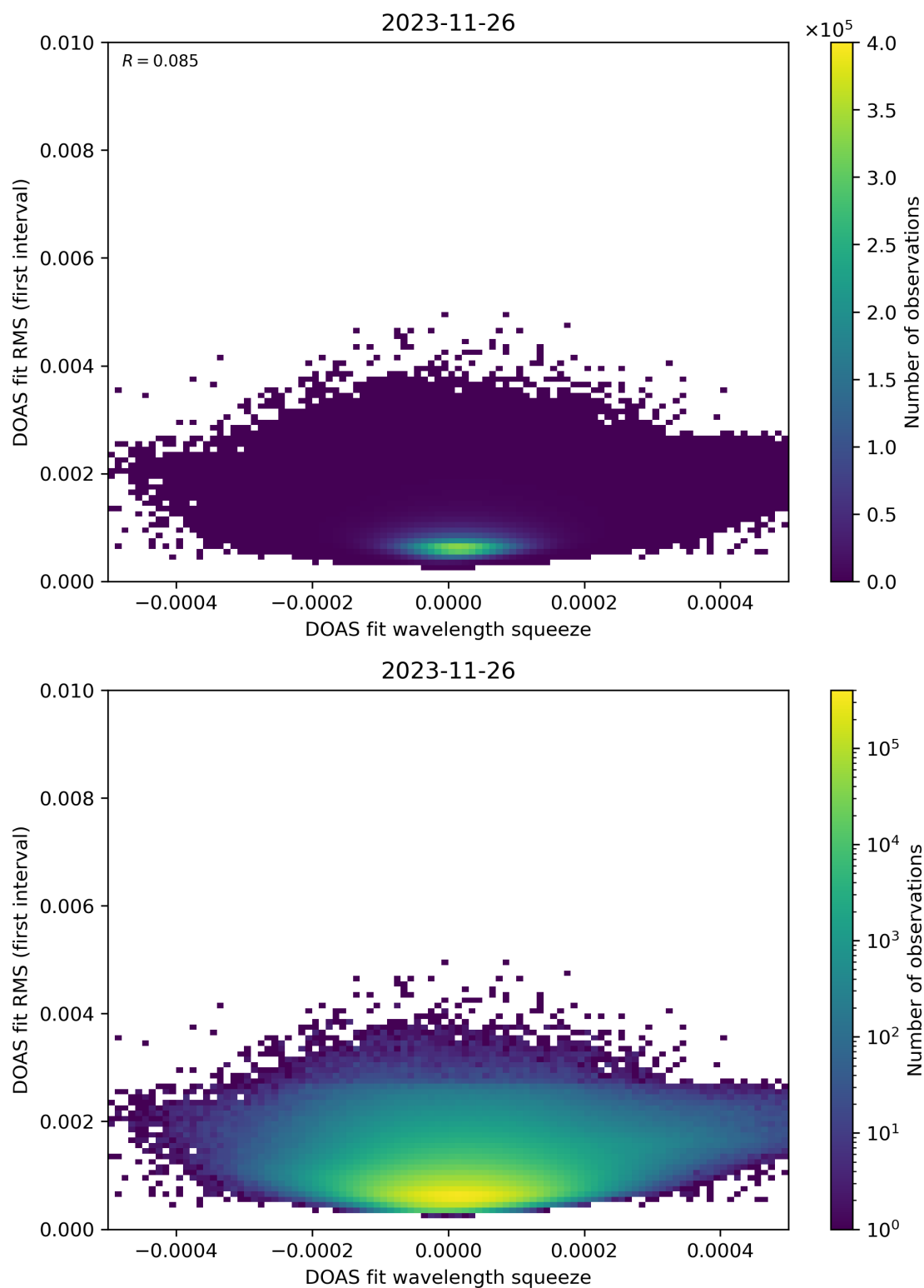
Figure 68: Scatter density plot of “DOAS fit wavelength squeeze” against “DOAS fit RMS (first interval)” for 2023-11-25 to 2023-11-27.
