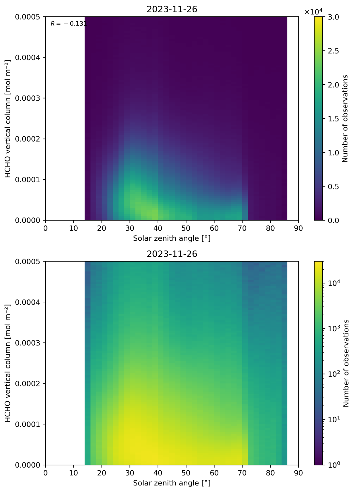
Figure 177: Scatter density plot of “Solar zenith angle” against “HCHO vertical column” for 2023-11-25 to 2023-11-27.
