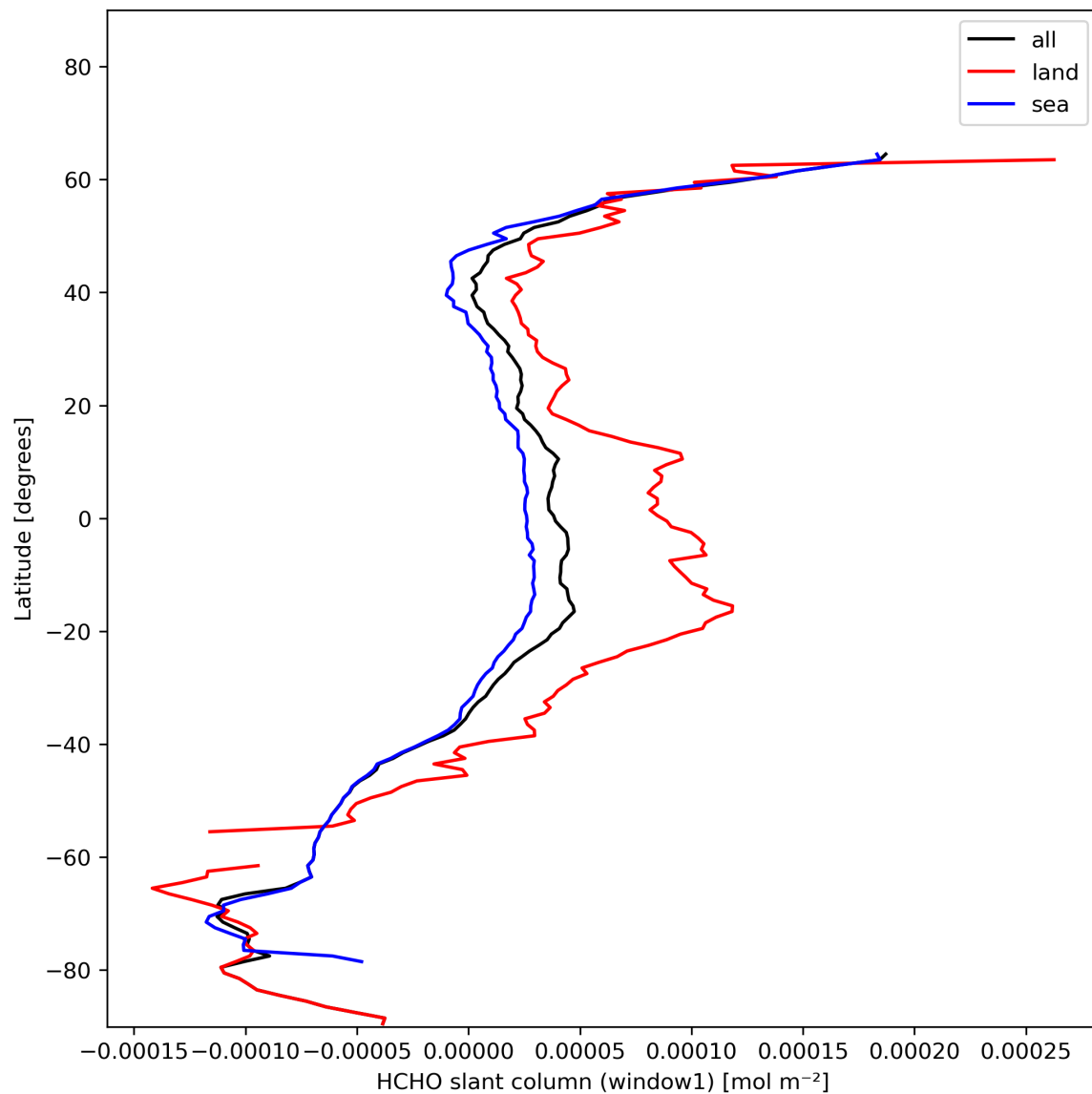
Figure 24: Zonal average of “HCHO slant column (window1)” for 2023-11-25 to 2023-11-27.
