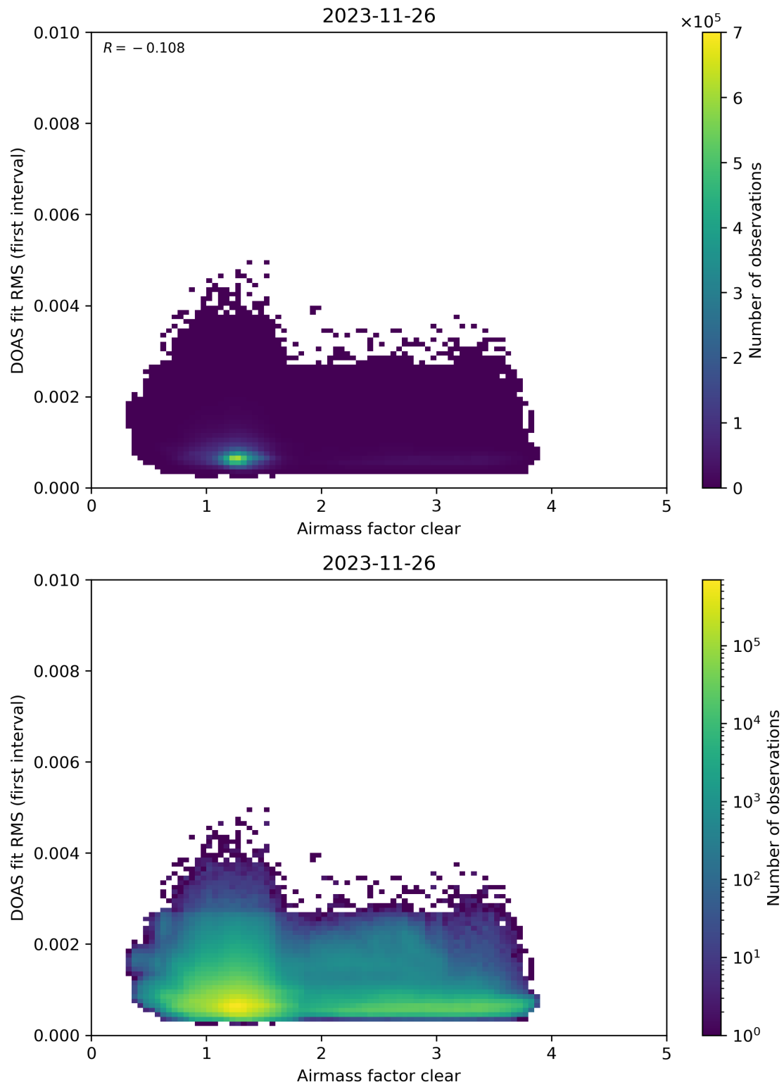
Figure 71: Scatter density plot of “Airmass factor clear” against “DOAS fit RMS (first interval)” for 2023-11-25 to 2023-11-27.
