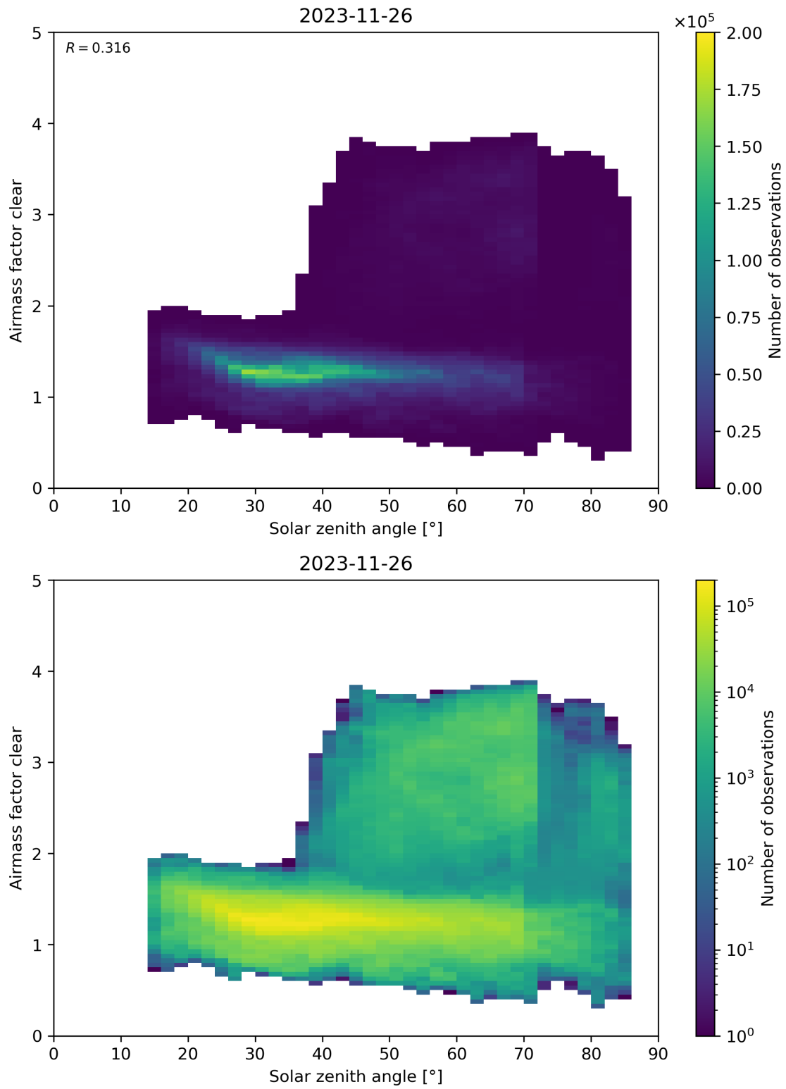
Figure 170: Scatter density plot of “Solar zenith angle” against “Airmass factor clear” for 2023-11-25 to 2023-11-27.
