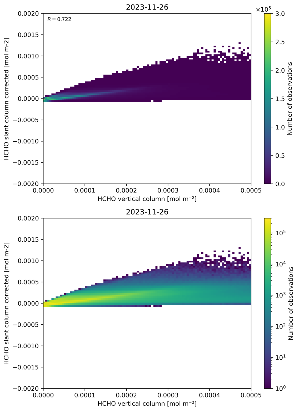
Figure 127: Scatter density plot of “HCHO vertical column” against “HCHO slant column corrected” for 2023-11-25 to 2023-11-27.
