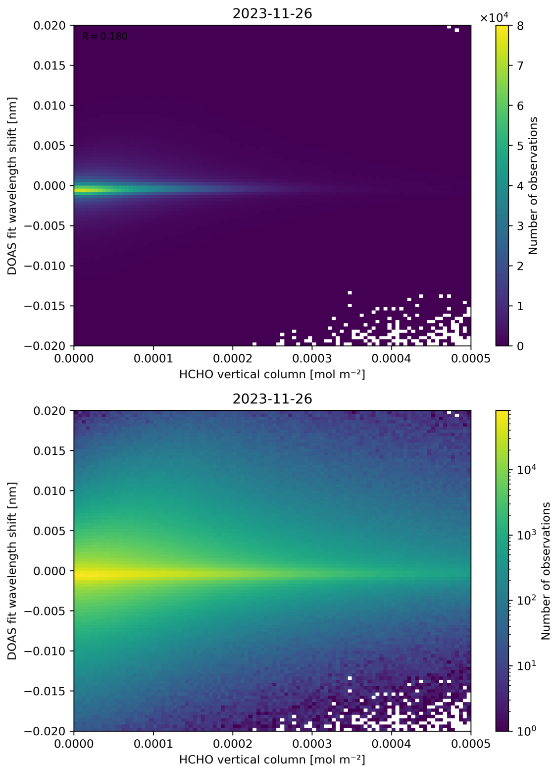
Figure 124: Scatter density plot of “HCHO vertical column” against “DOAS fit wavelength shift” for 2023-11-25 to 2023-11-27.
