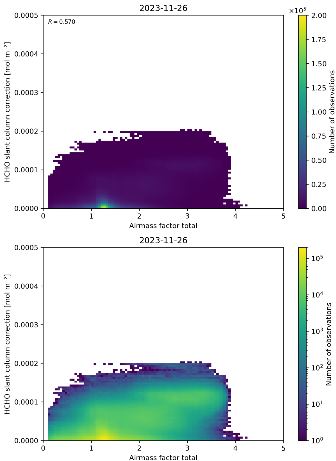
Figure 102: Scatter density plot of “Airmass factor total” against “HCHO slant column correction” for 2023-11-25 to 2023-11-27.
