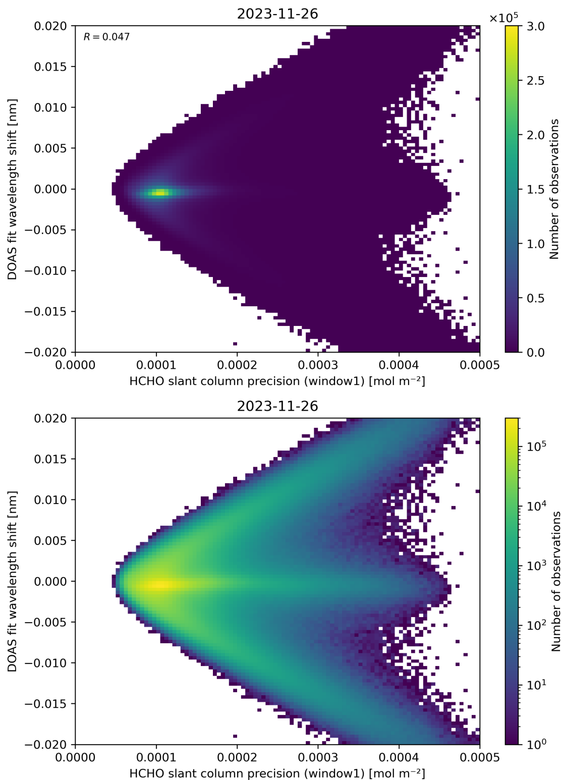
Figure 89: Scatter density plot of “HCHO slant column precision (window1)” against “DOAS fit wavelength shift” for 2023-11-25 to 2023-11-27.
