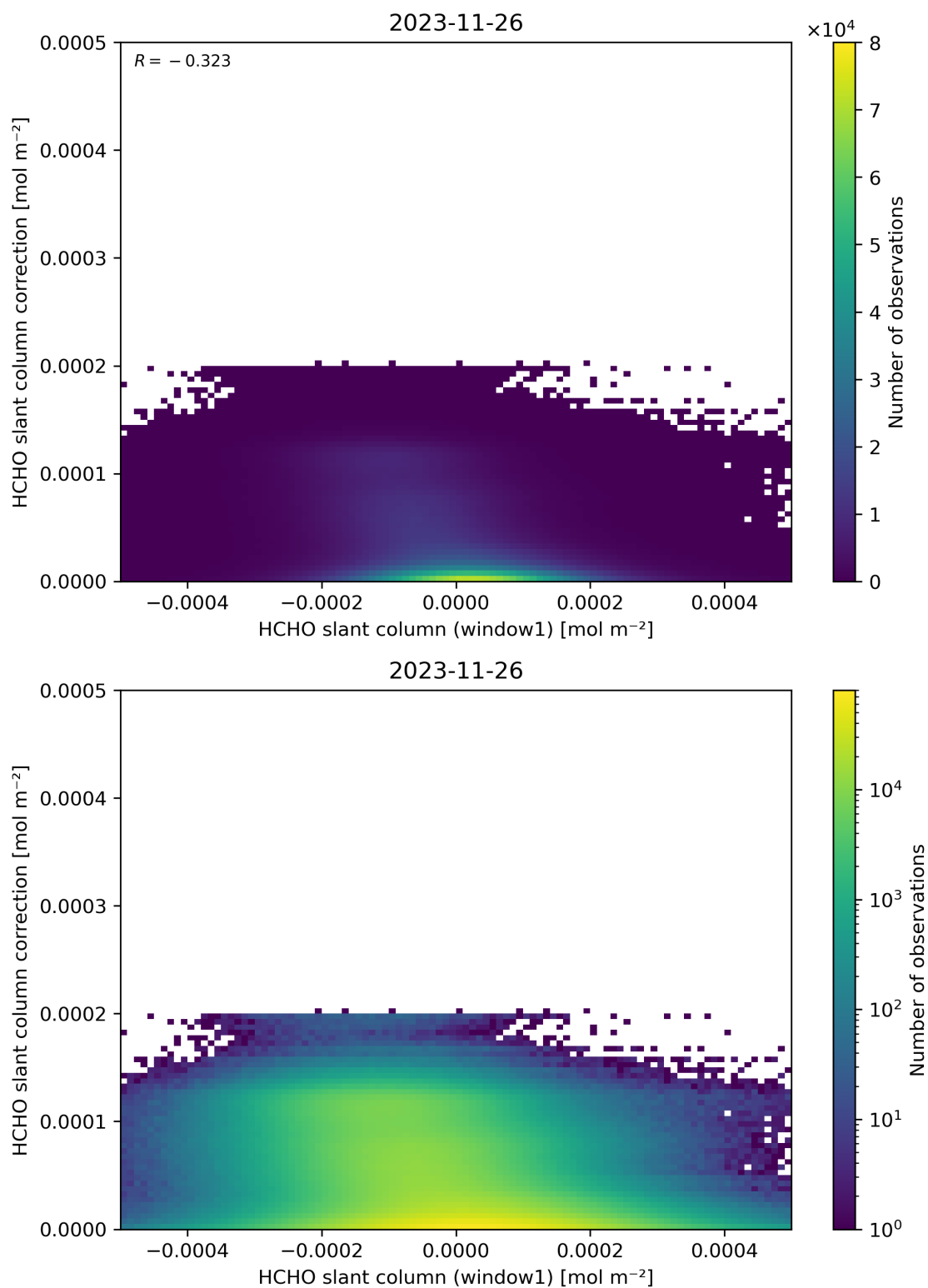
Figure 83: Scatter density plot of “HCHO slant column (window1)” against “HCHO slant column correction” for 2023-11-25 to 2023-11-27.
