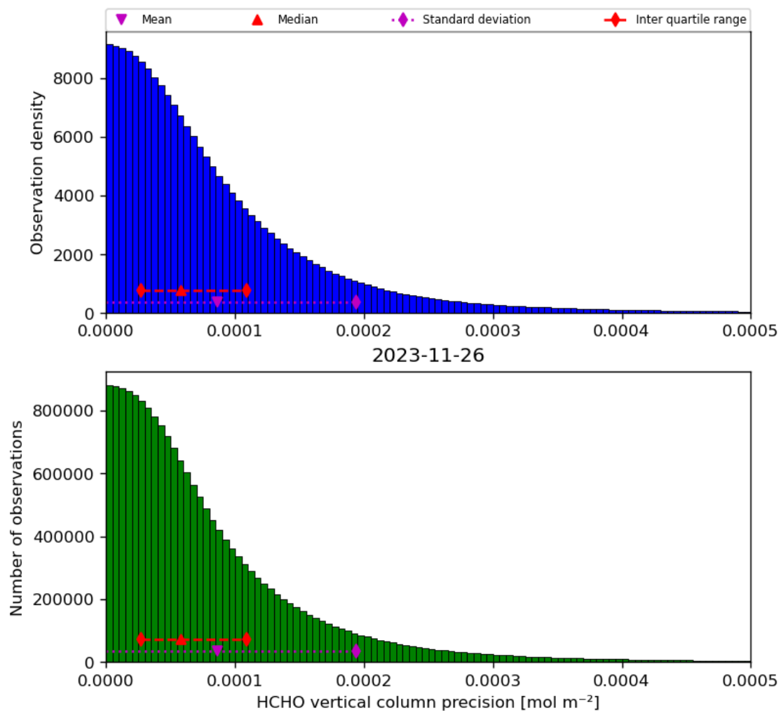
Figure 36: Histogram of “HCHO vertical column precision” for 2023-11-25 to 2023-11-27
