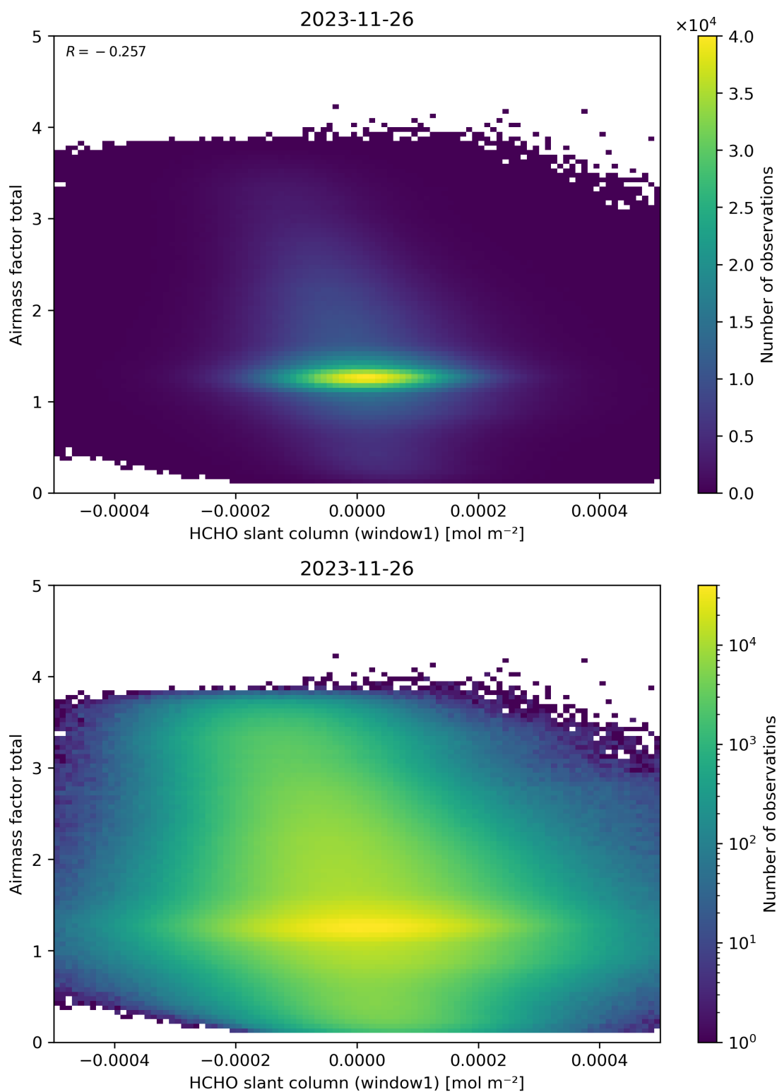
Figure 85: Scatter density plot of “HCHO slant column (window1)” against “Airmass factor total” for 2023-11-25 to 2023-11-27.
