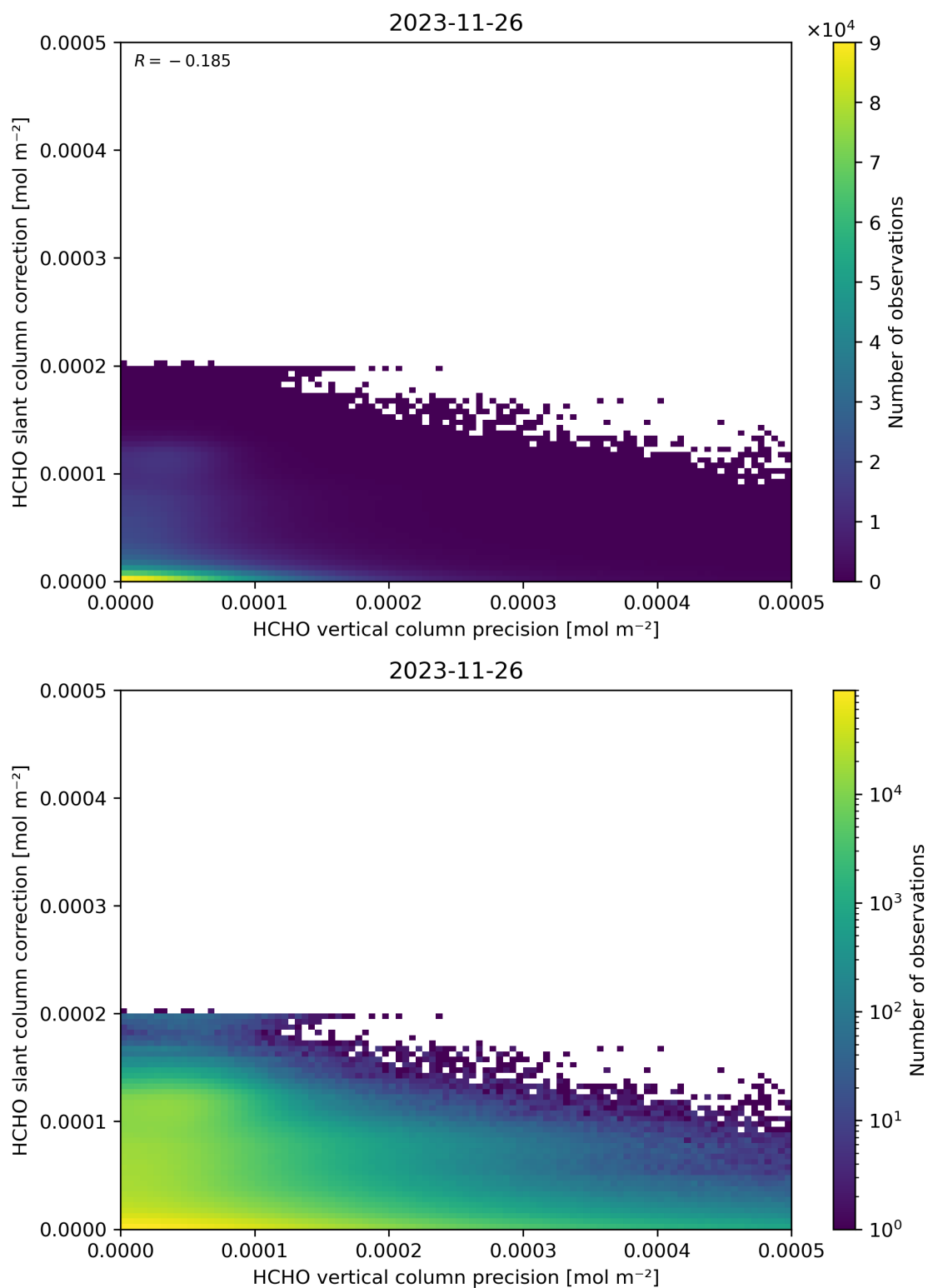
Figure 141: Scatter density plot of “HCHO vertical column precision” against “HCHO slant column correction” for 2023-11-25 to 2023-11-27.
