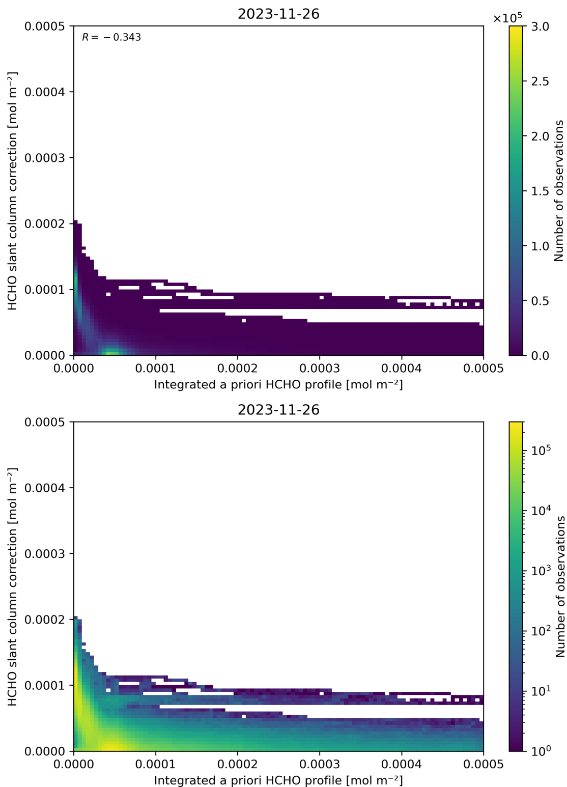
Figure 152: Scatter density plot of “Integrated a priori HCHO profile” against “HCHO slant column correction” for 2023-11-25 to 2023-11-27.
