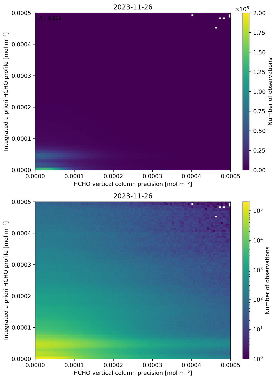
Figure 147: Scatter density plot of “HCHO vertical column precision” against “Integrated a priori HCHO profile” for 2023-11-25 to 2023-11-27.
