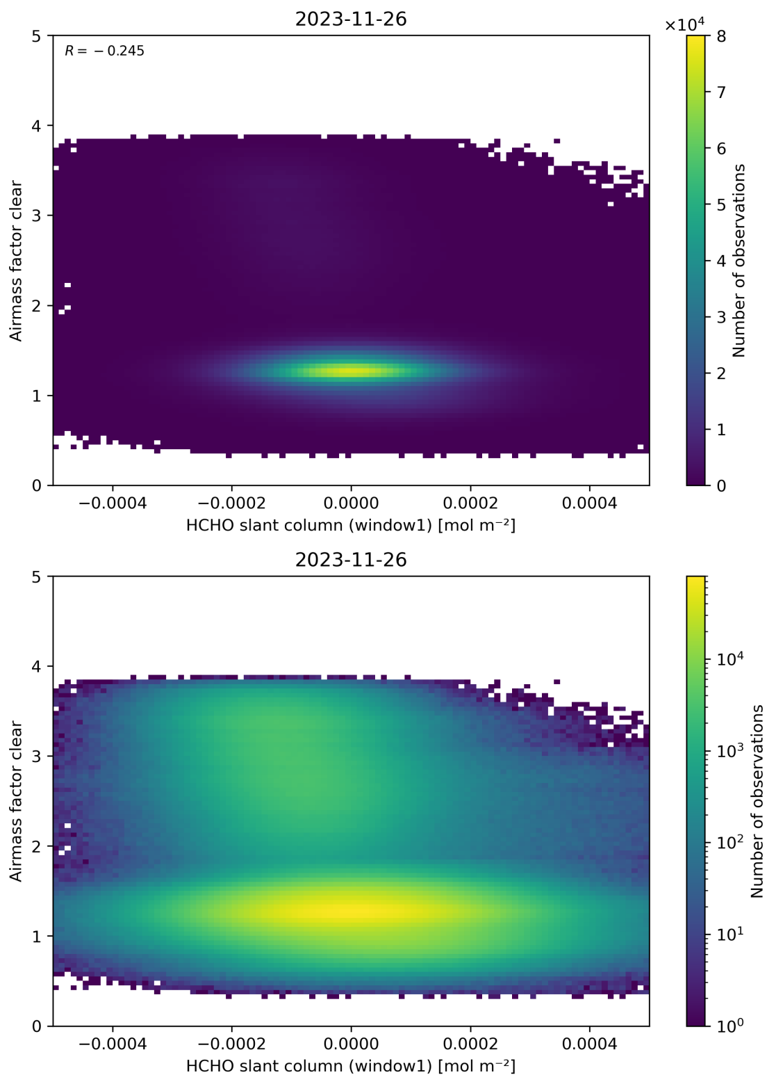
Figure 81: Scatter density plot of “HCHO slant column (window1)” against “Airmass factor clear” for 2023-11-25 to 2023-11-27.
