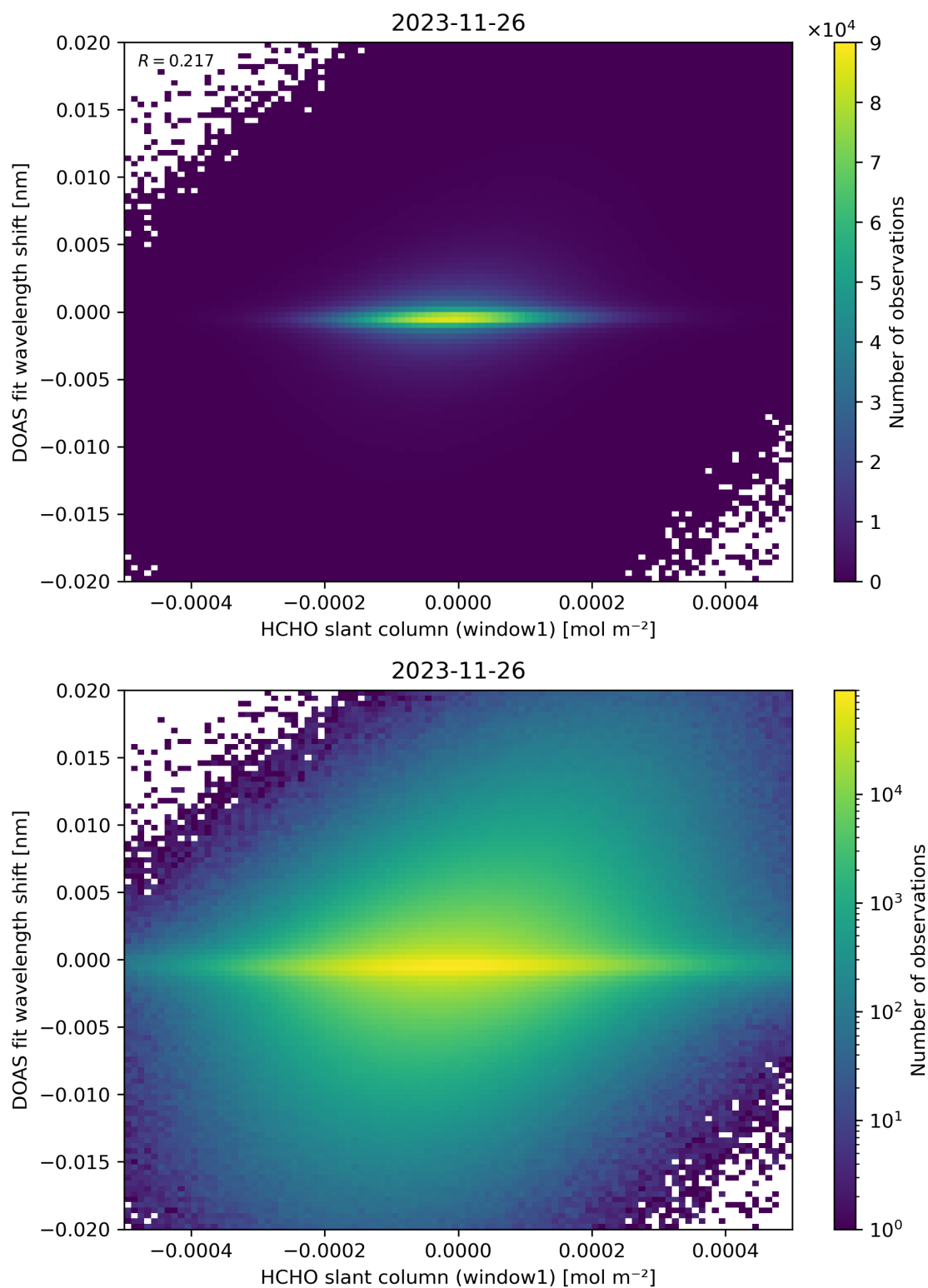
Figure 79: Scatter density plot of “HCHO slant column (window1)” against “DOAS fit wavelength shift” for 2023-11-25 to 2023-11-27.
