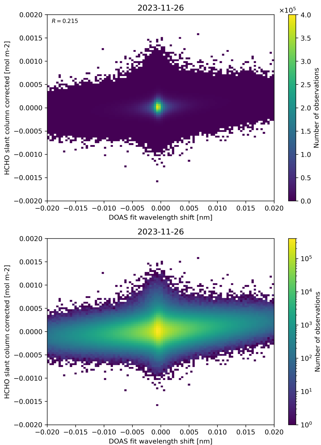
Figure 66: Scatter density plot of “DOAS fit wavelength shift” against “HCHO slant column corrected” for 2023-11-25 to 2023-11-27.
