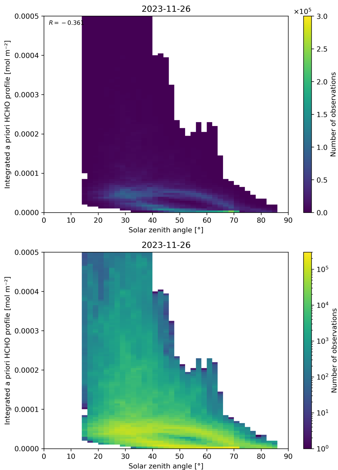
Figure 180: Scatter density plot of “Solar zenith angle” against “Integrated a priori HCHO profile” for 2023-11-25 to 2023-11-27.
