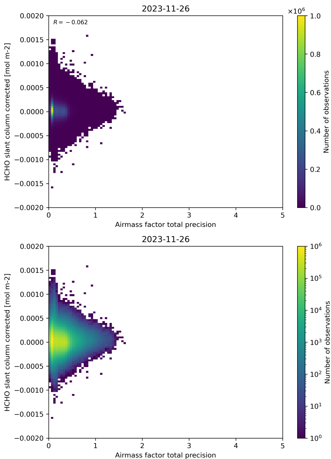
Figure 109: Scatter density plot of “Airmass factor total precision” against “HCHO slant column corrected” for 2023-11-25 to 2023-11-27.
