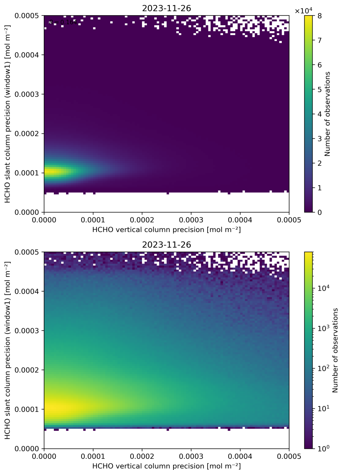
Figure 143: Scatter density plot of “HCHO vertical column precision” against “HCHO slant column precision (window1)” for 2023-11-25 to 2023-11-27.
