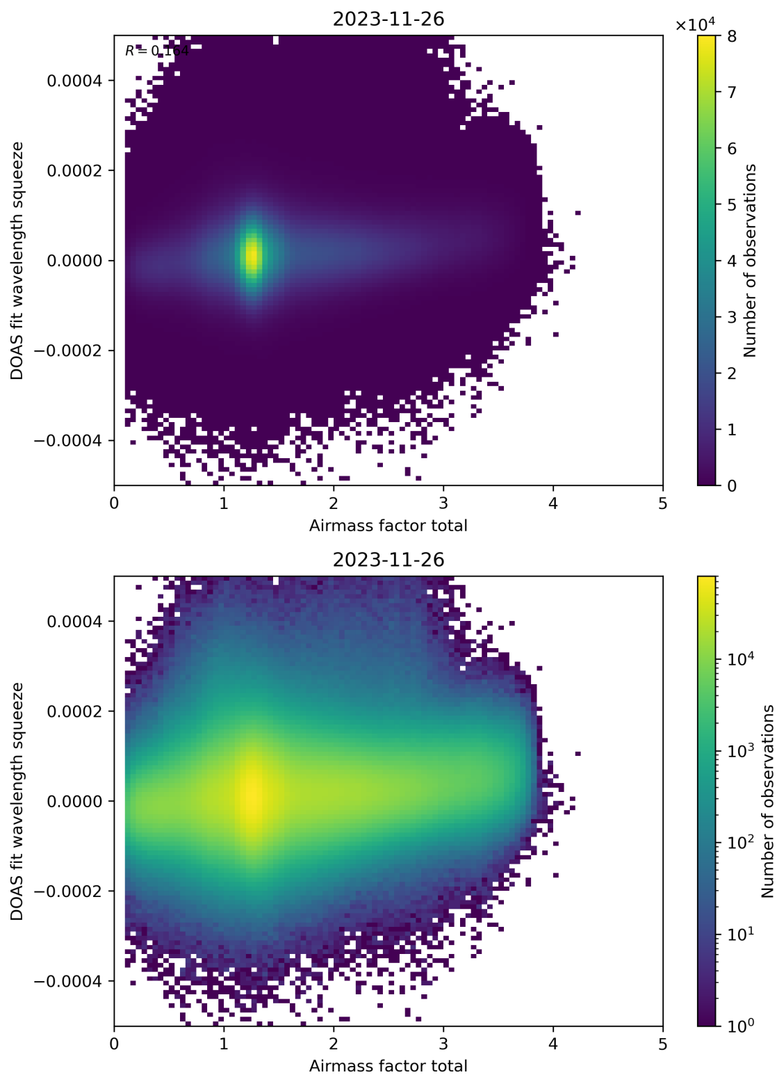
Figure 99: Scatter density plot of “Airmass factor total” against “DOAS fit wavelength squeeze” for 2023-11-25 to 2023-11-27.
