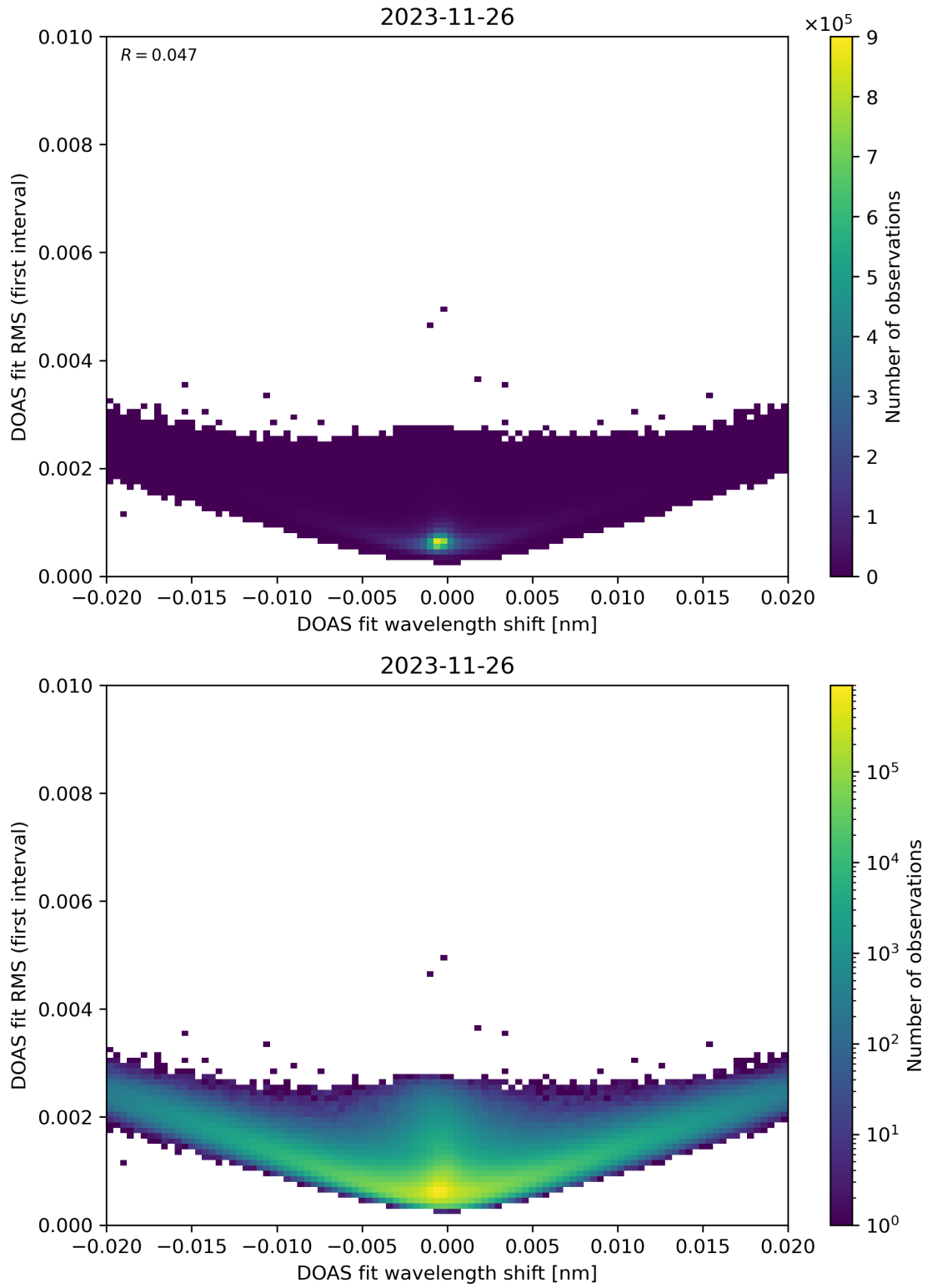
Figure 64: Scatter density plot of “DOAS fit wavelength shift” against “DOAS fit RMS (first interval)” for 2023-11-25 to 2023-11-27.
