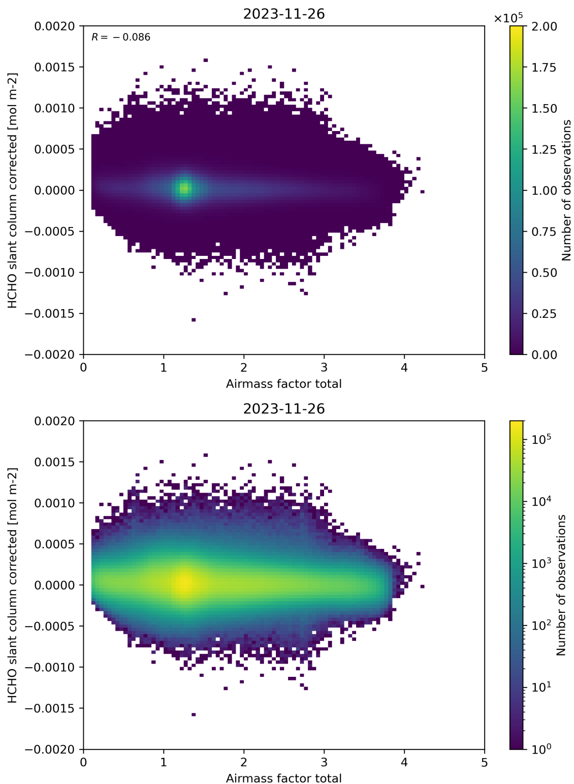
Figure 101: Scatter density plot of “Airmass factor total” against “HCHO slant column corrected” for 2023-11-25 to 2023-11-27.
