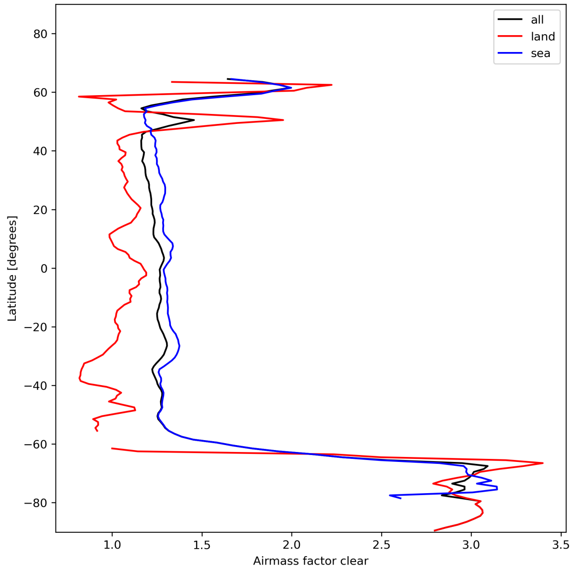
Figure 28: Zonal average of “Airmass factor clear” for 2023-11-25 to 2023-11-27.
