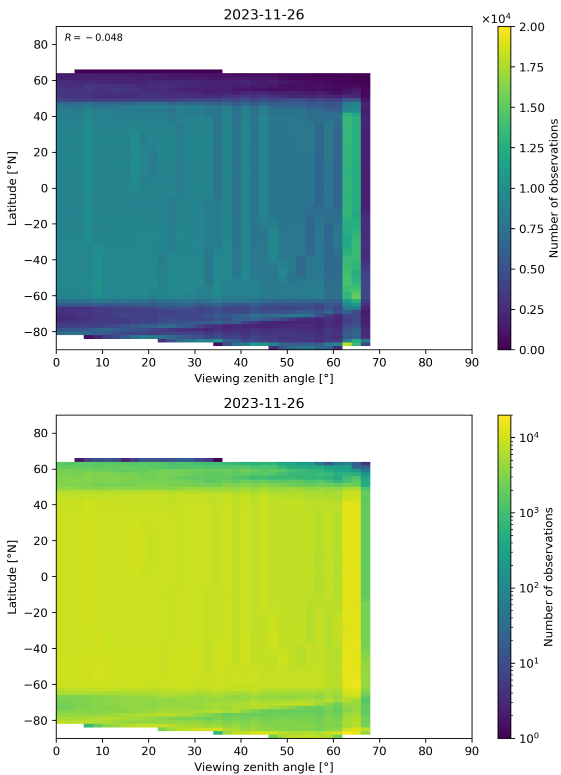
Figure 196: Scatter density plot of “Viewing zenith angle” against “Latitude” for 2023-11-25 to 2023-11-27.
