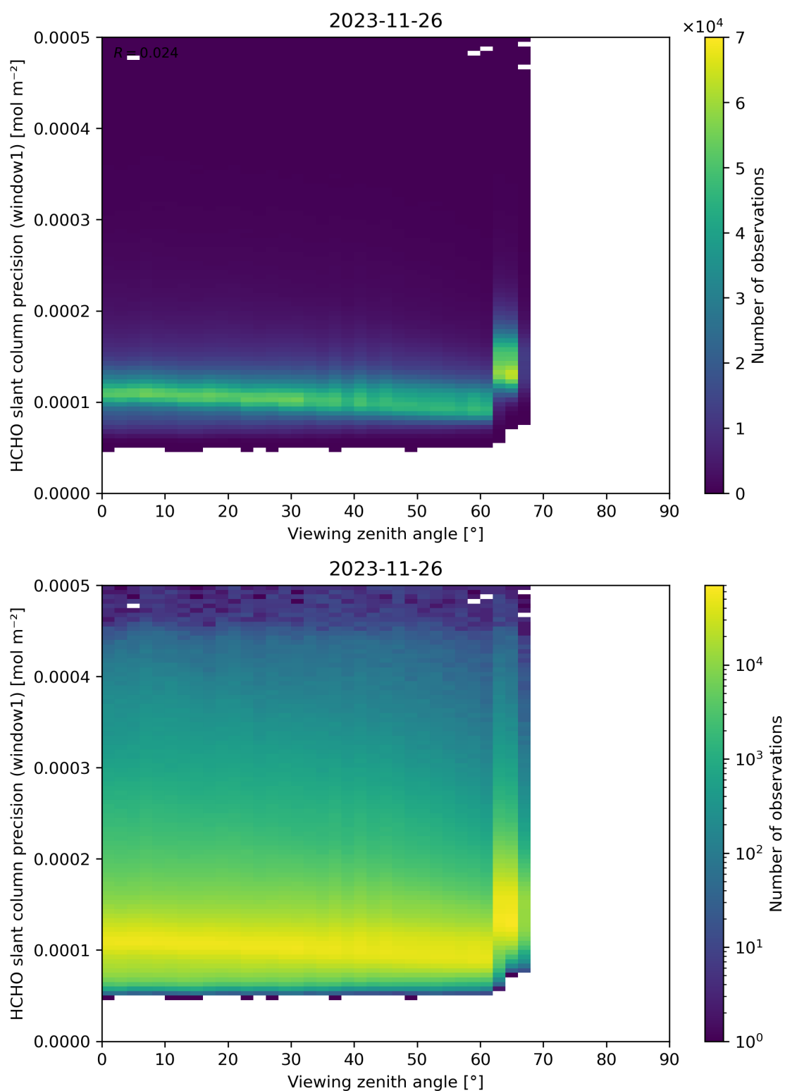
Figure 189: Scatter density plot of “Viewing zenith angle” against “HCHO slant column precision (window1)” for 2023-11-25 to 2023-11-27.
