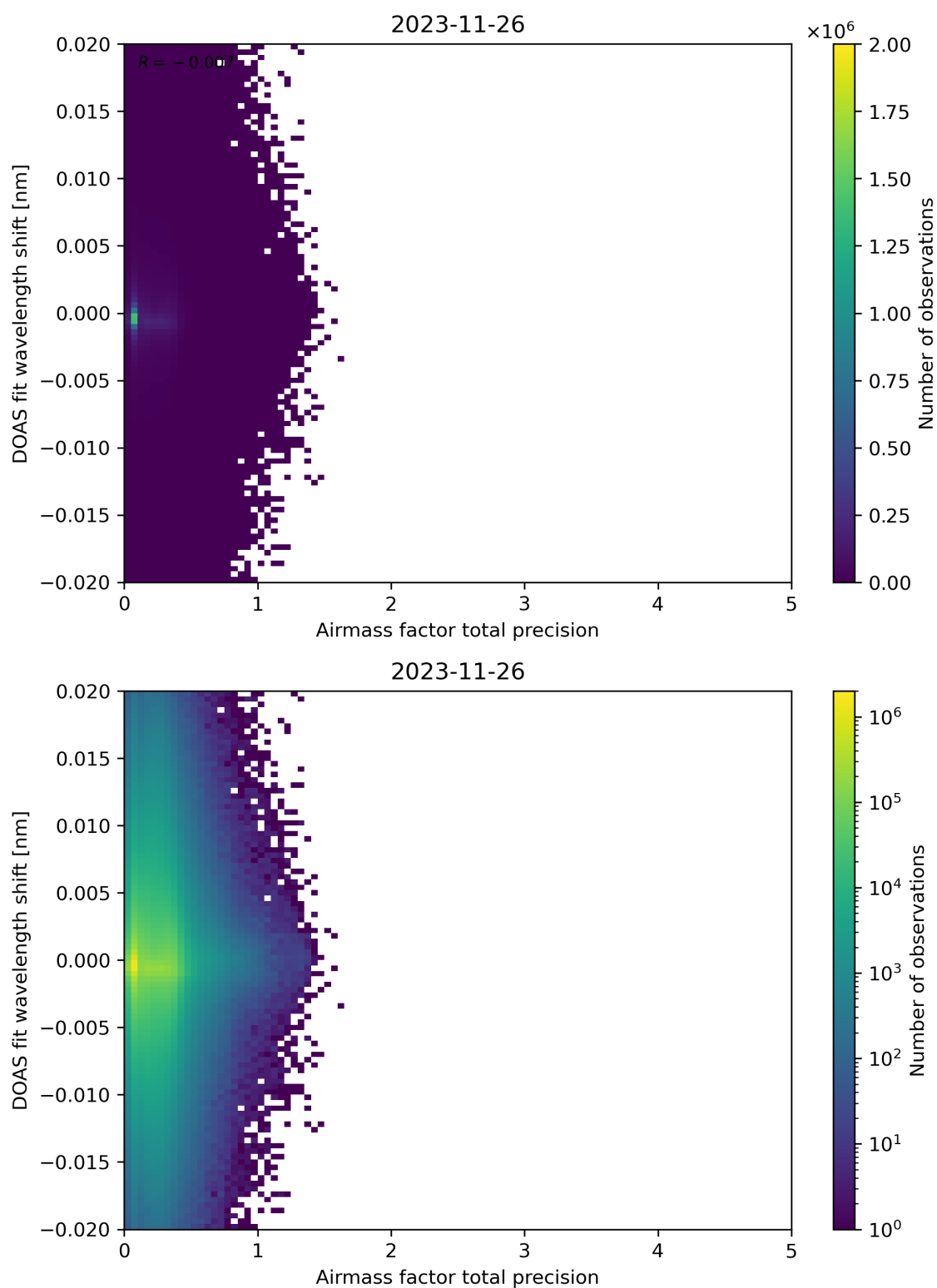
Figure 106: Scatter density plot of “Airmass factor total precision” against “DOAS fit wavelength shift” for 2023-11-25 to 2023-11-27.
