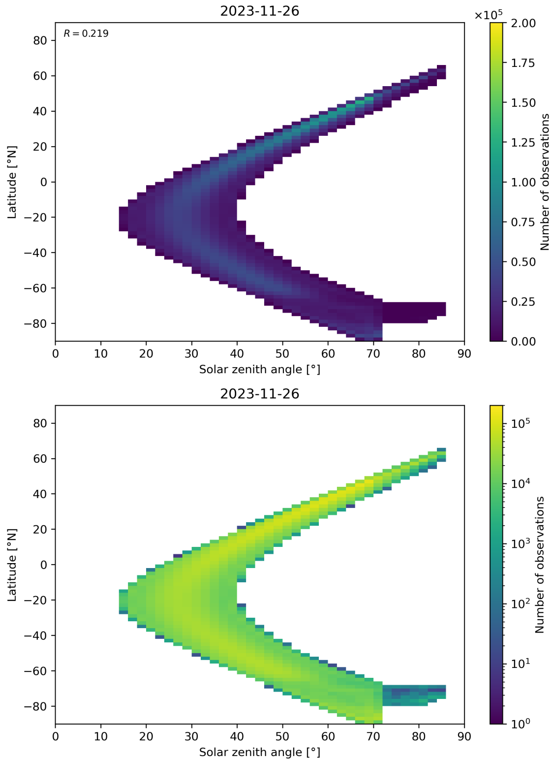
Figure 181: Scatter density plot of “Solar zenith angle” against “Latitude” for 2023-11-25 to 2023-11-27.
