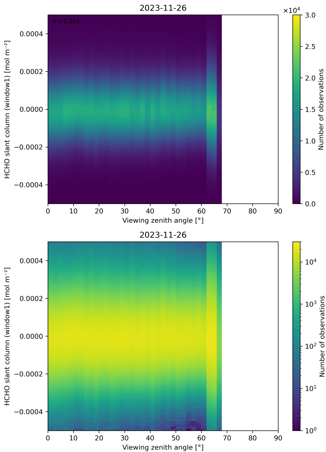
Figure 188: Scatter density plot of “Viewing zenith angle” against “HCHO slant column (window1)” for 2023-11-25 to 2023-11-27.
