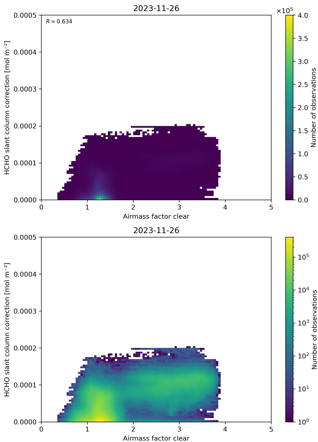
Figure 75: Scatter density plot of “Airmass factor clear” against “HCHO slant column correction” for 2023-11-25 to 2023-11-27.
