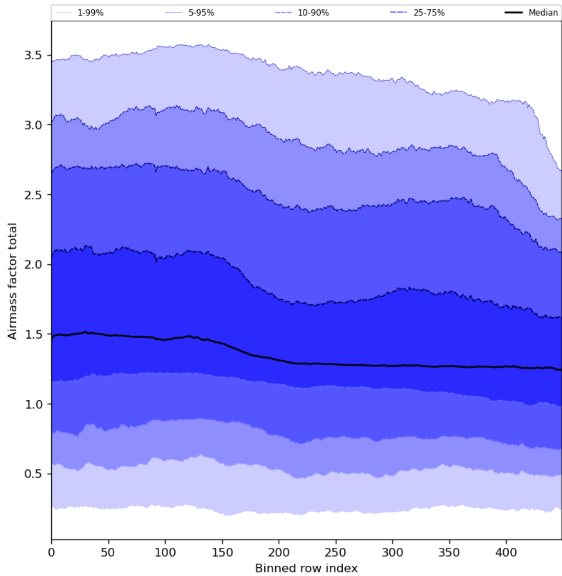
Figure 54: Along track statistics of “Airmass factor total” for 2023-11-25 to 2023-11-27
