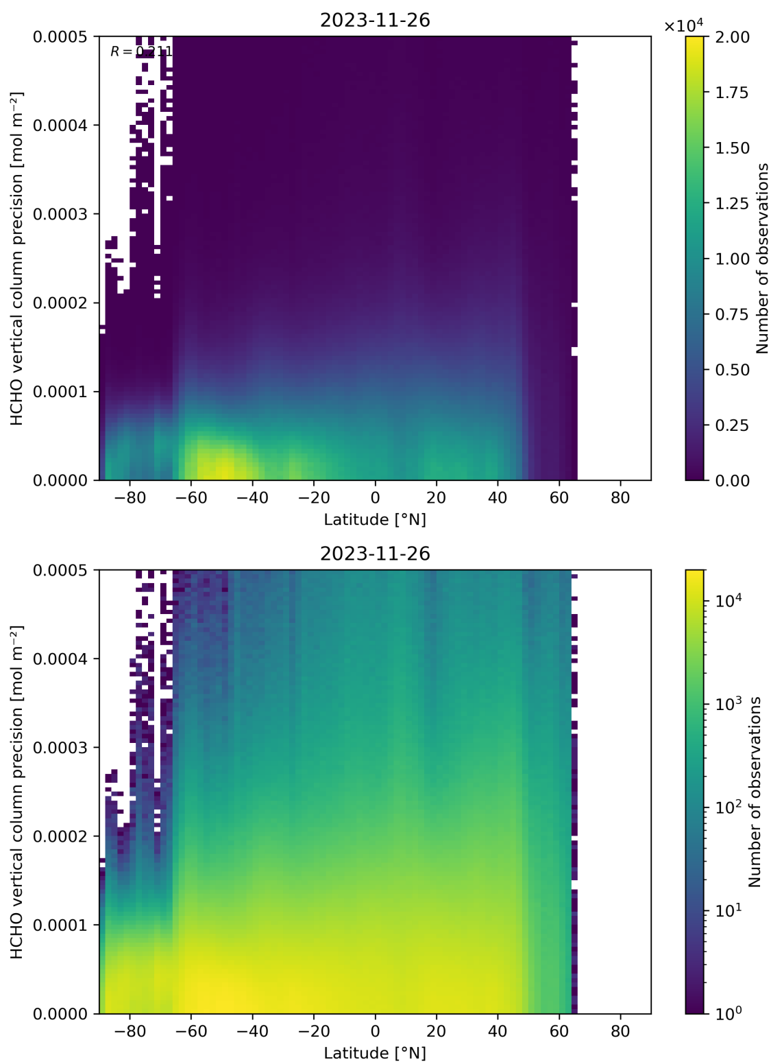
Figure 165: Scatter density plot of “Latitude” against “HCHO vertical column precision” for 2023-11-25 to 2023-11-27.
