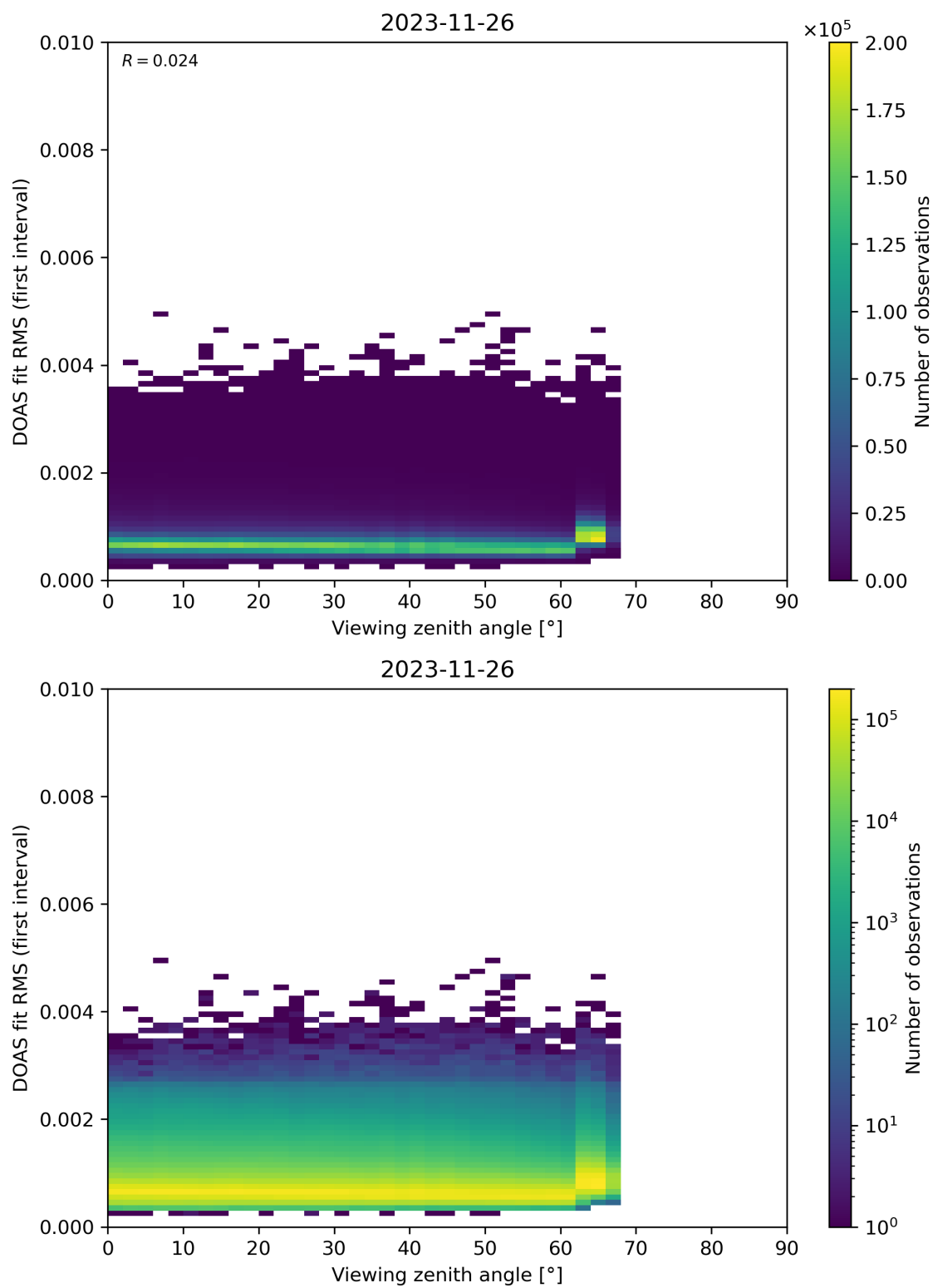
Figure 182: Scatter density plot of “Viewing zenith angle” against “DOAS fit RMS (first interval)” for 2023-11-25 to 2023-11-27.
