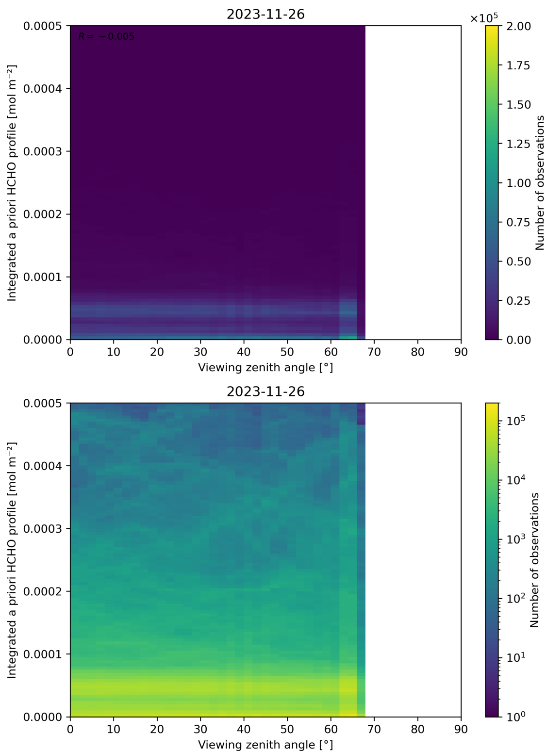
Figure 195: Scatter density plot of “Viewing zenith angle” against “Integrated a priori HCHO profile” for 2023-11-25 to 2023-11-27.
