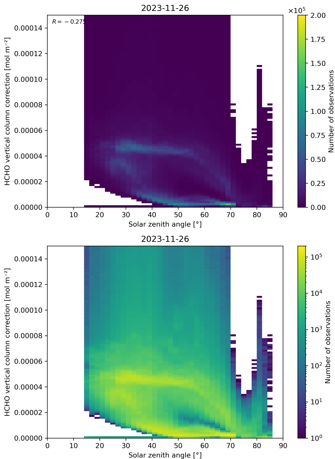
Figure 178: Scatter density plot of “Solar zenith angle” against “HCHO vertical column correction” for 2023-11-25 to 2023-11-27.
