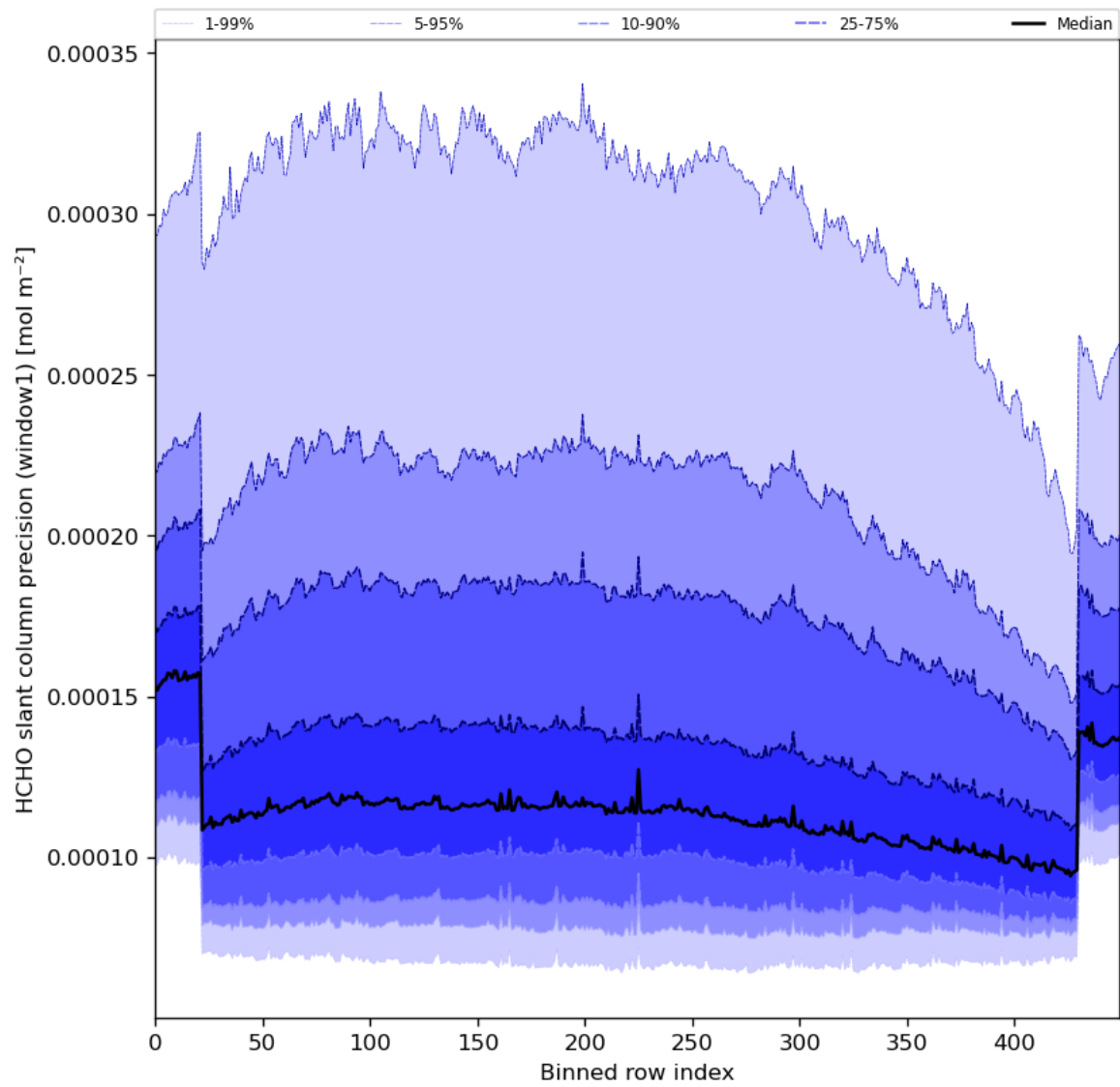
Figure 53: Along track statistics of “HCHO slant column precision (window1)” for 2023-11-25 to 2023-11-27
