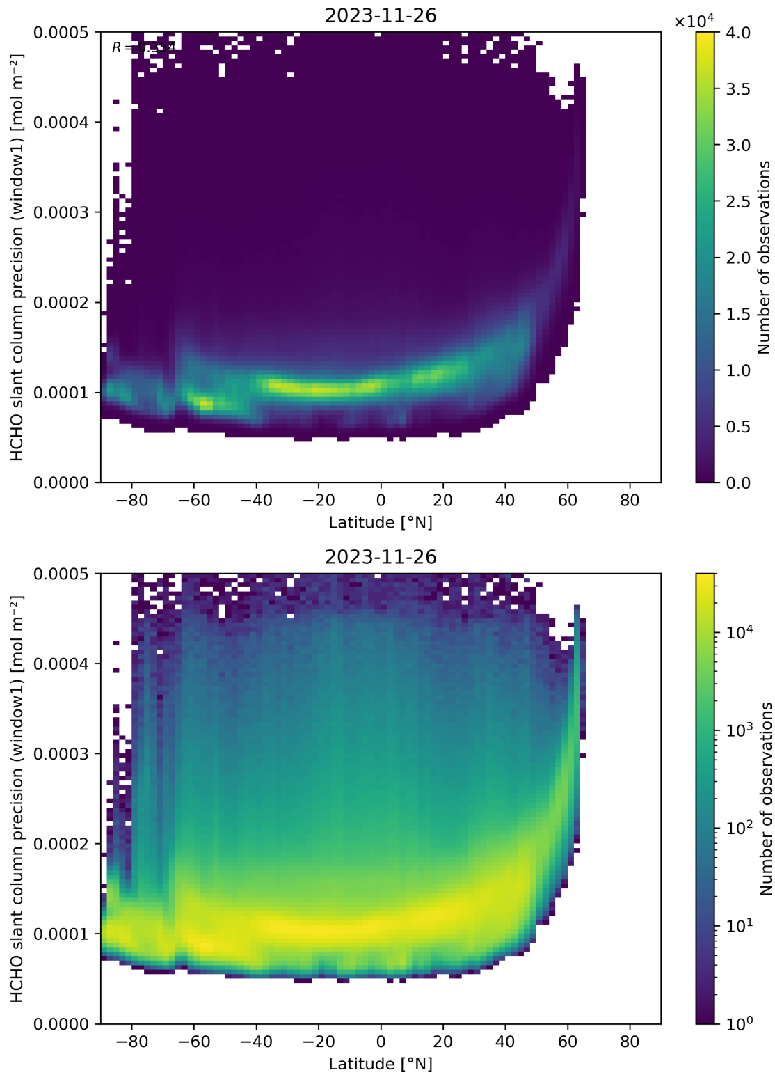
Figure 160: Scatter density plot of “Latitude” against “HCHO slant column precision (window1)” for 2023-11-25 to 2023-11-27.
