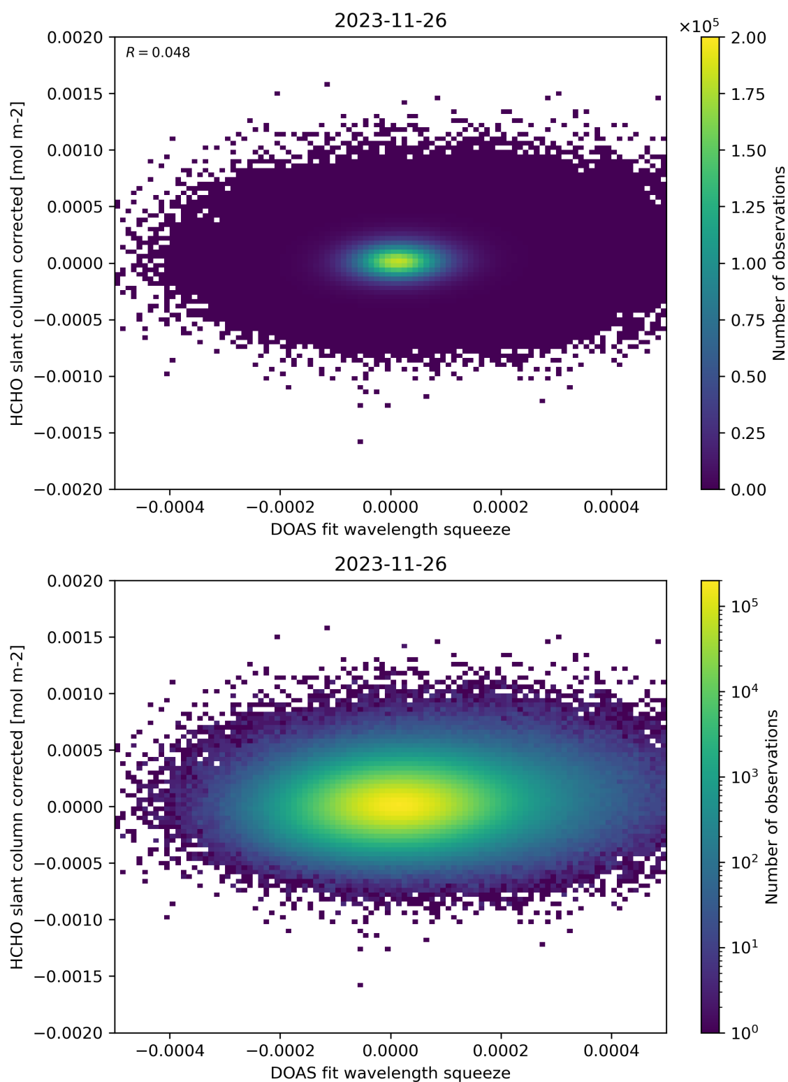
Figure 69: Scatter density plot of “DOAS fit wavelength squeeze” against “HCHO slant column corrected” for 2023-11-25 to 2023-11-27.
