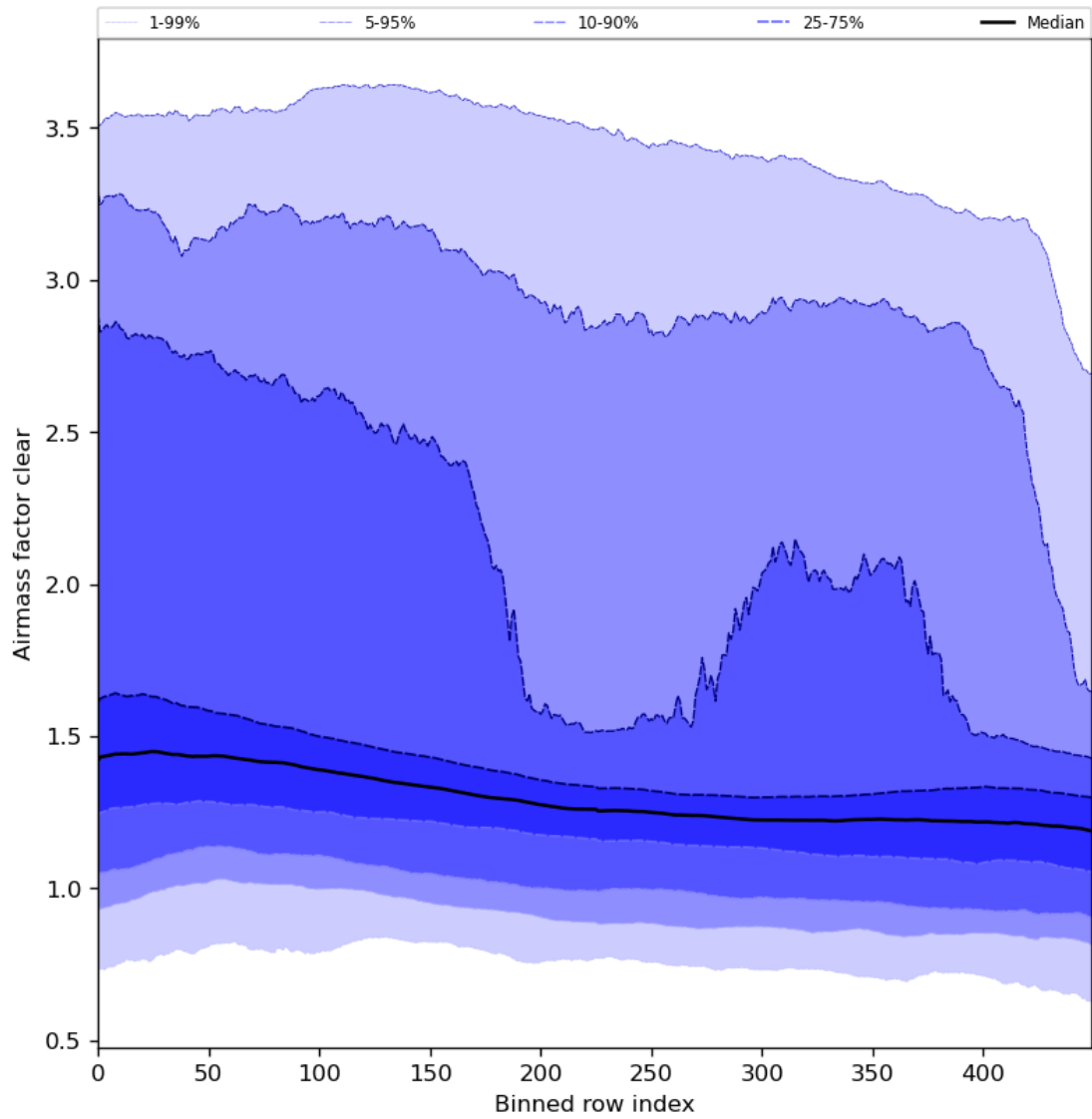
Figure 56: Along track statistics of “Airmass factor clear” for 2023-11-25 to 2023-11-27
