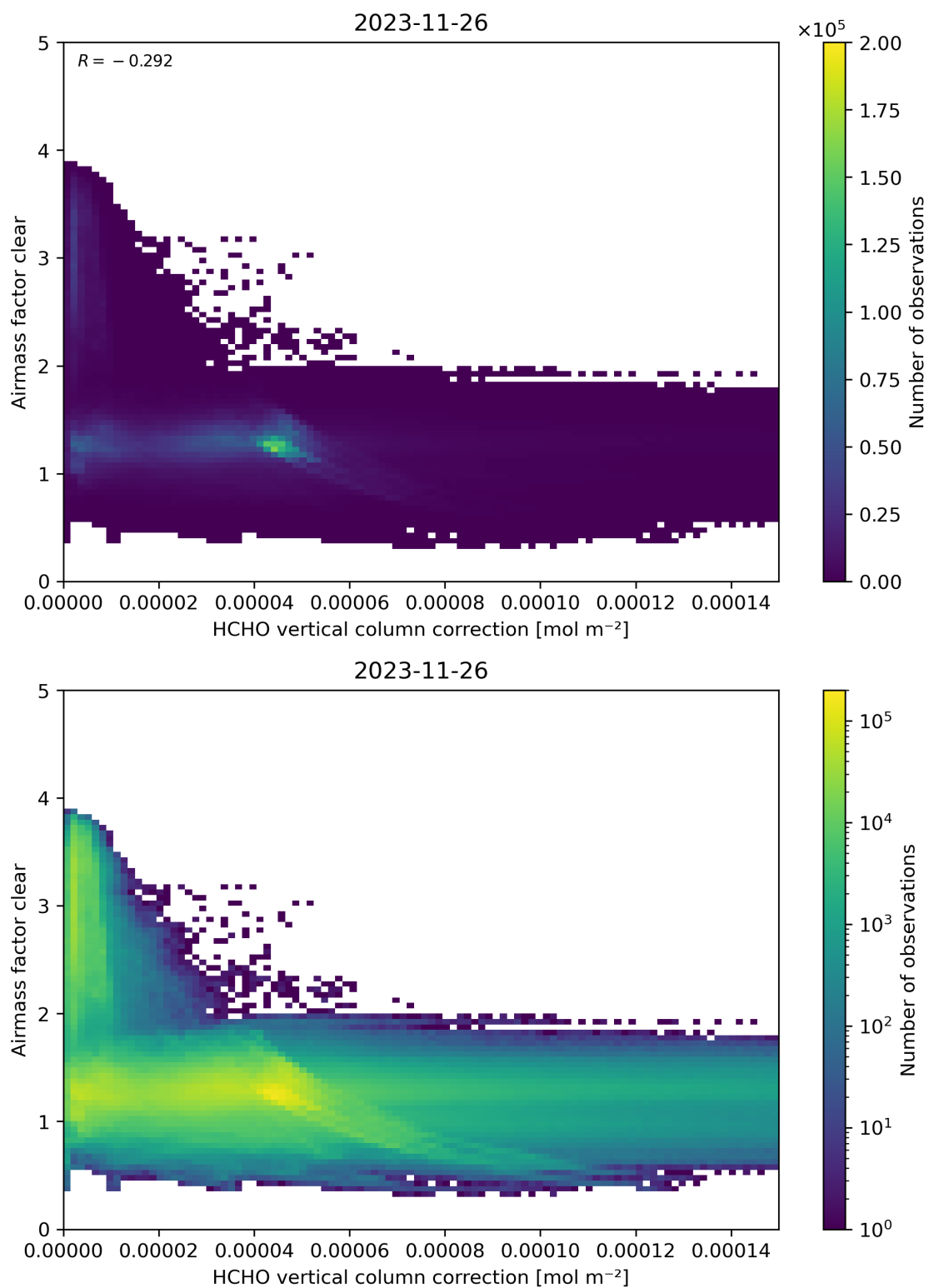
Figure 115: Scatter density plot of “HCHO vertical column correction” against “Airmass factor clear” for 2023-11-25 to 2023-11-27.
