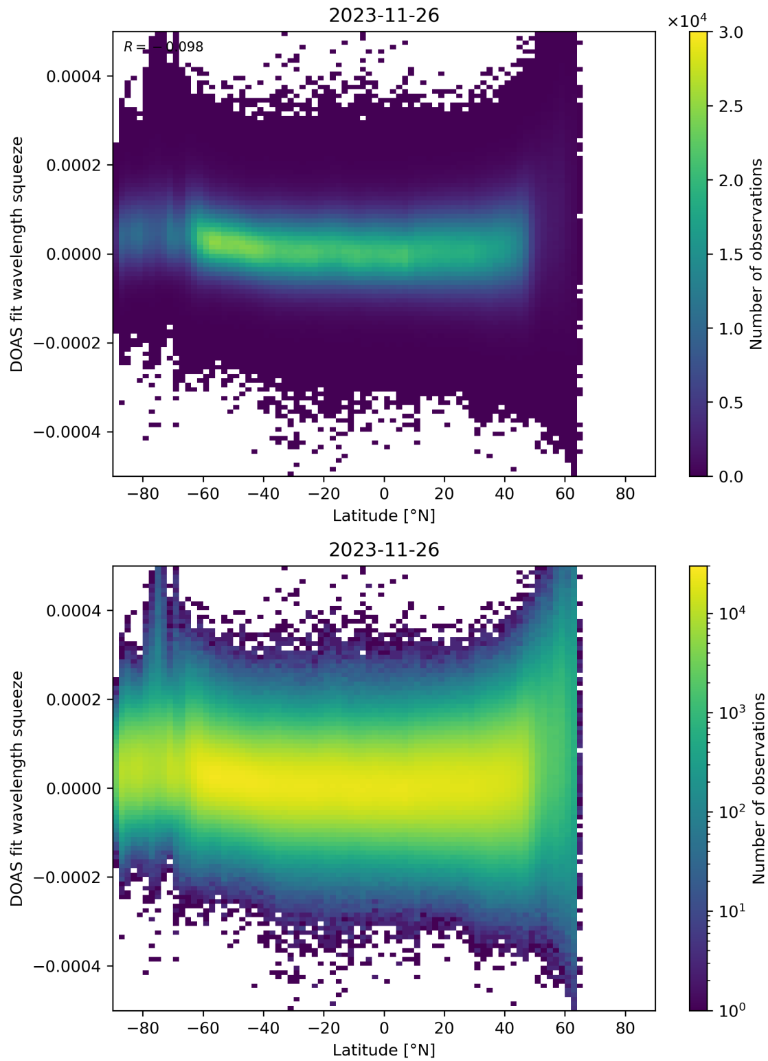
Figure 155: Scatter density plot of “Latitude” against “DOAS fit wavelength squeeze” for 2023-11-25 to 2023-11-27.
