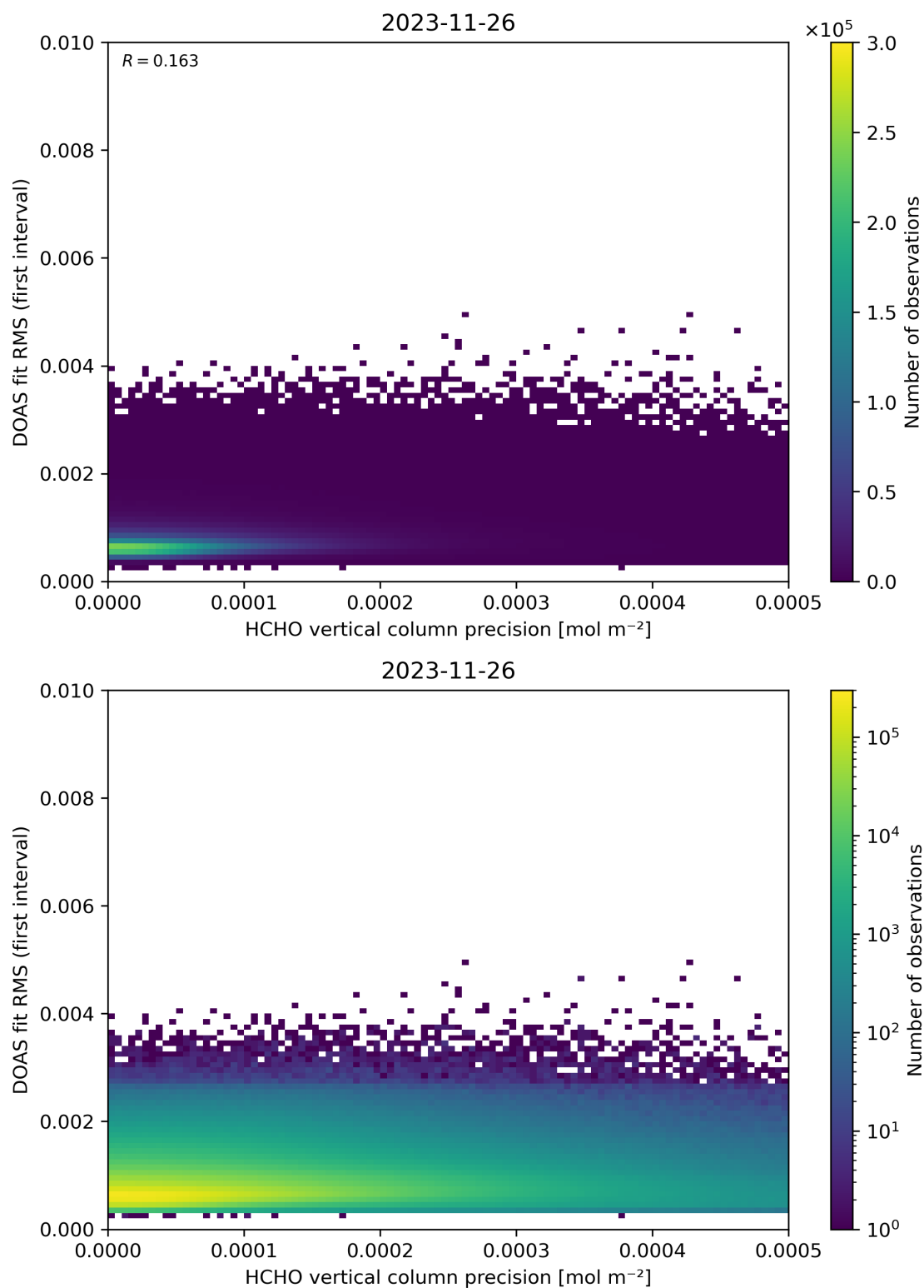
Figure 136: Scatter density plot of “HCHO vertical column precision” against “DOAS fit RMS (first interval)” for 2023-11-25 to 2023-11-27.
