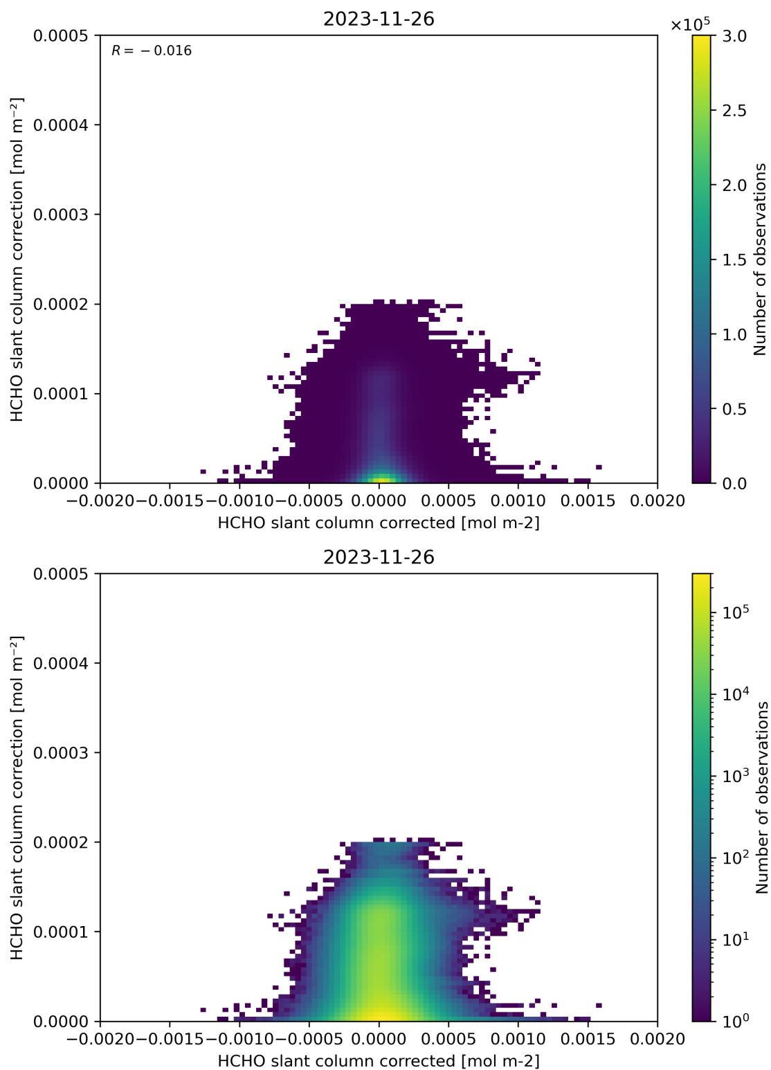
Figure 77: Scatter density plot of “HCHO slant column corrected” against “HCHO slant column correction” for 2023-11-25 to 2023-11-27.
