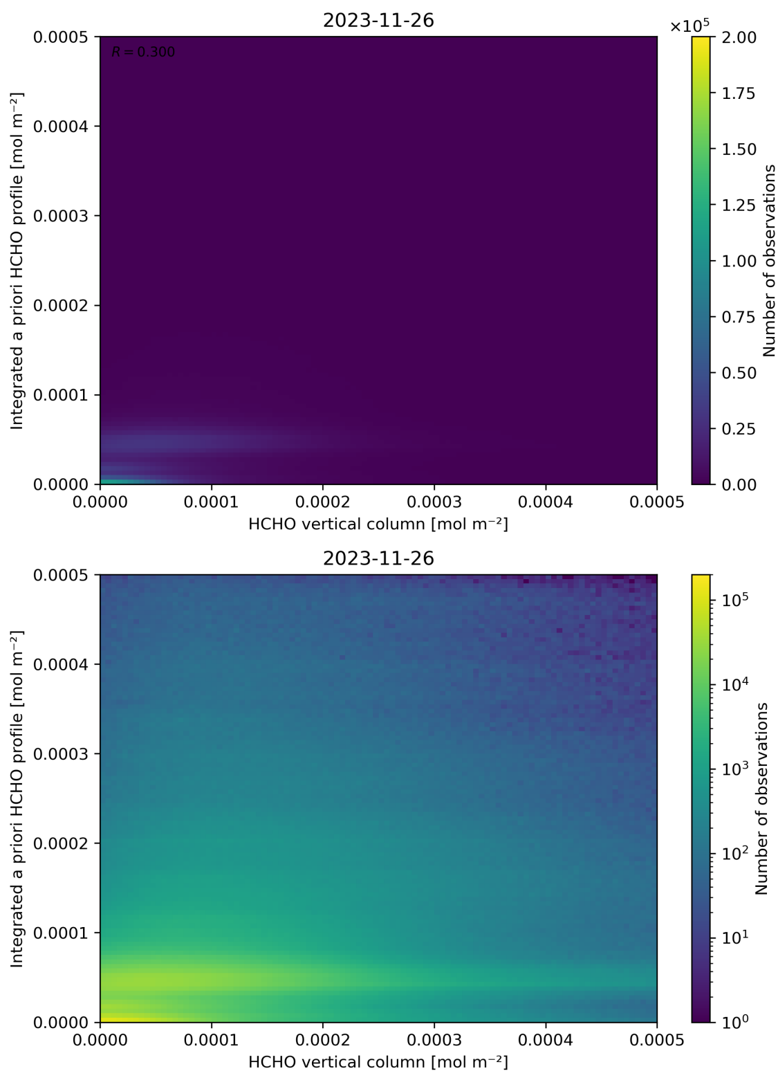
Figure 135: Scatter density plot of “HCHO vertical column” against “Integrated a priori HCHO profile” for 2023-11-25 to 2023-11-27.
