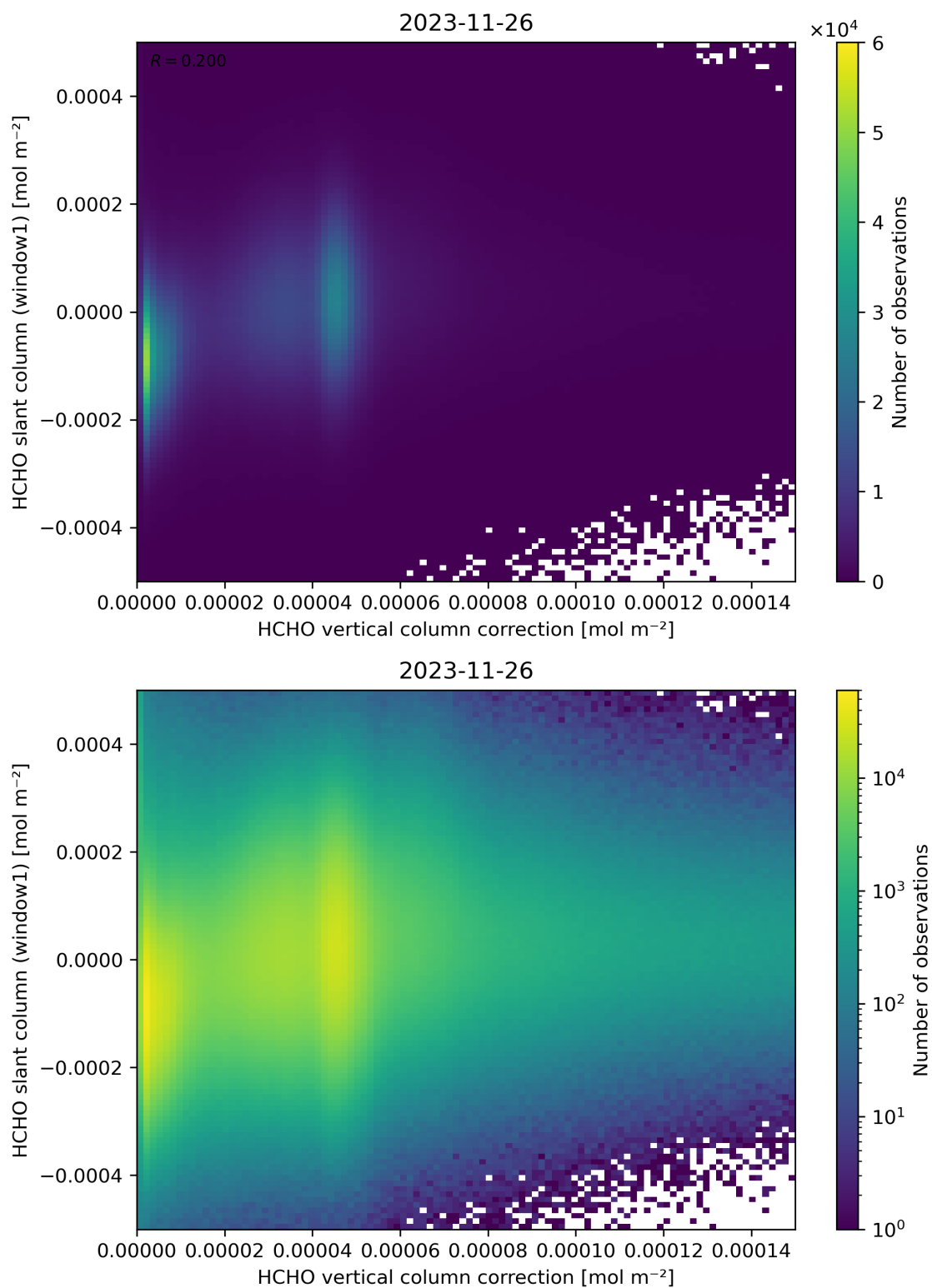
Figure 118: Scatter density plot of “HCHO vertical column correction” against “HCHO slant column (window1)” for 2023-11-25 to 2023-11-27.
