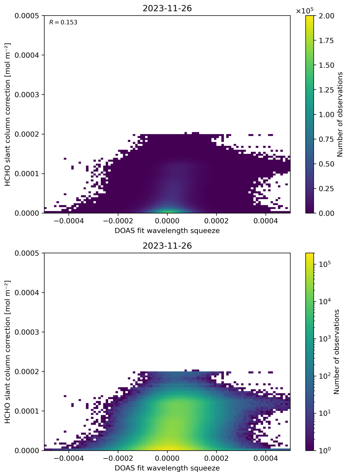
Figure 70: Scatter density plot of “DOAS fit wavelength squeeze” against “HCHO slant column correction” for 2023-11-25 to 2023-11-27.
