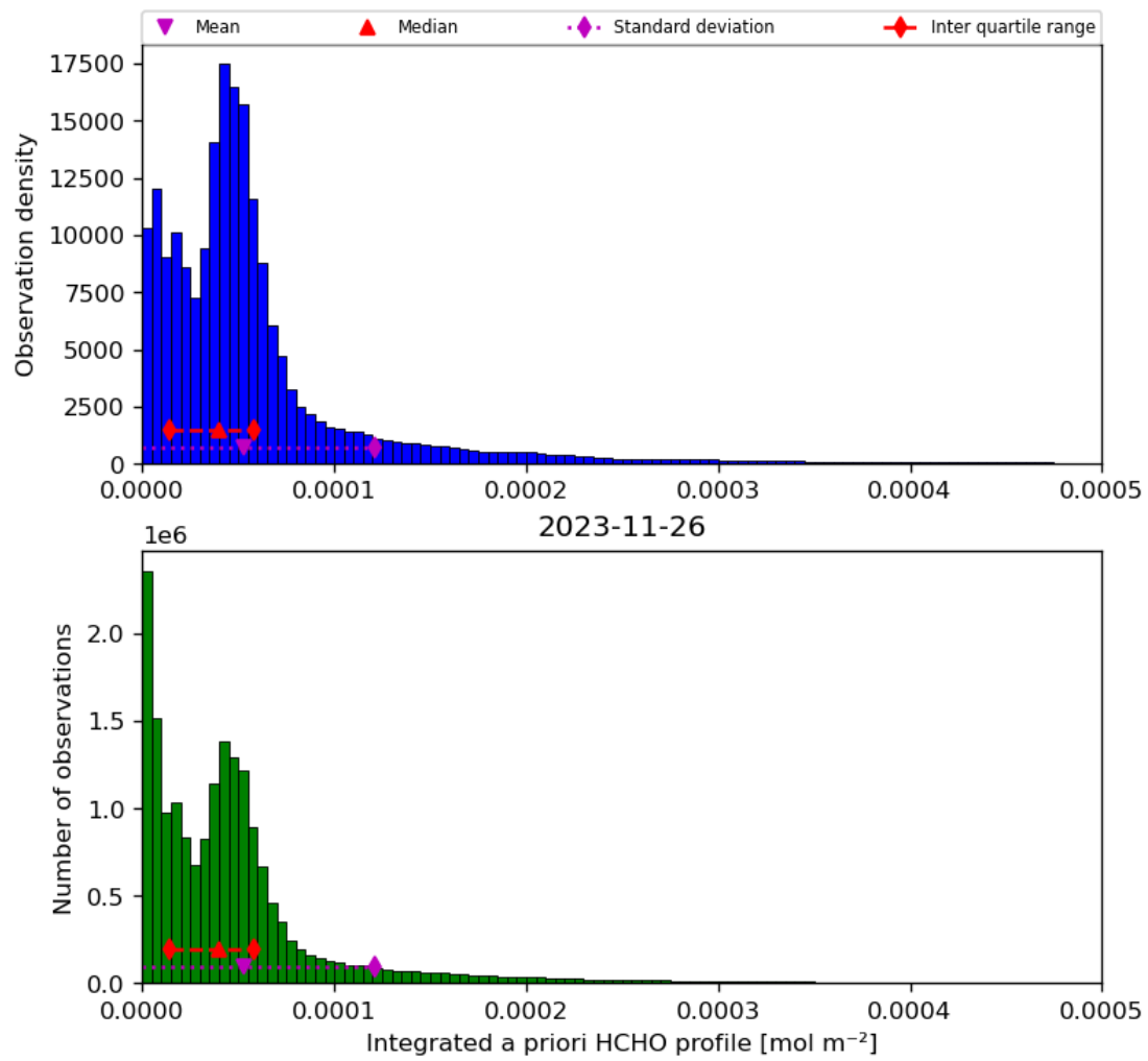
Figure 43: Histogram of “Integrated a priori HCHO profile” for 2023-11-25 to 2023-11-27
