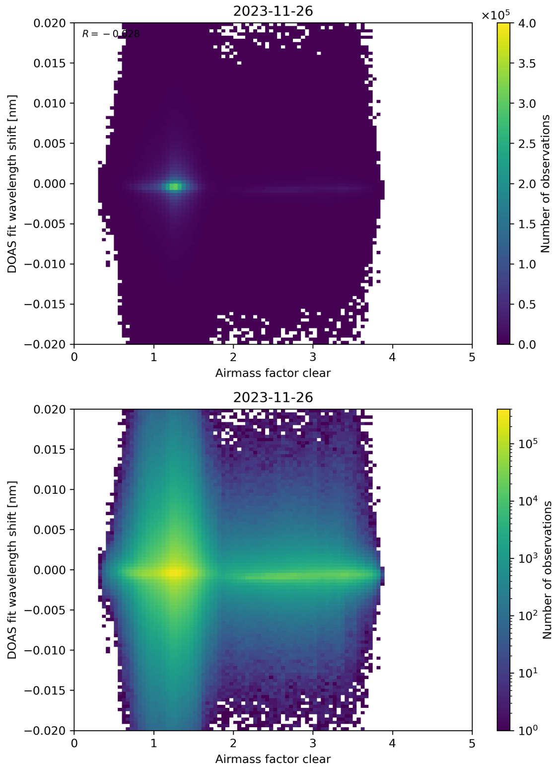
Figure 72: Scatter density plot of “Airmass factor clear” against “DOAS fit wavelength shift” for 2023-11-25 to 2023-11-27.
