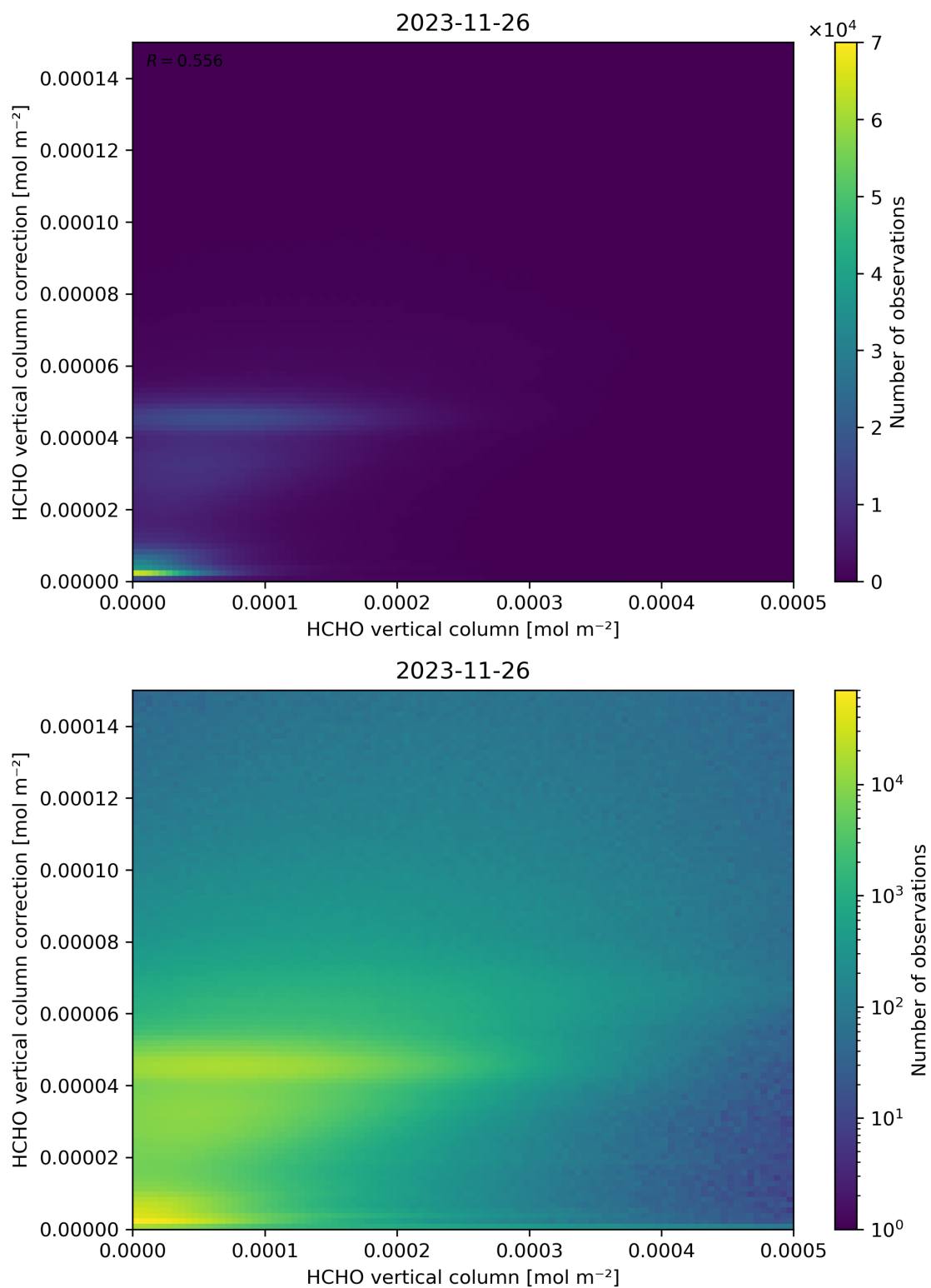
Figure 133: Scatter density plot of “HCHO vertical column” against “HCHO vertical column correction” for 2023-11-25 to 2023-11-27.
