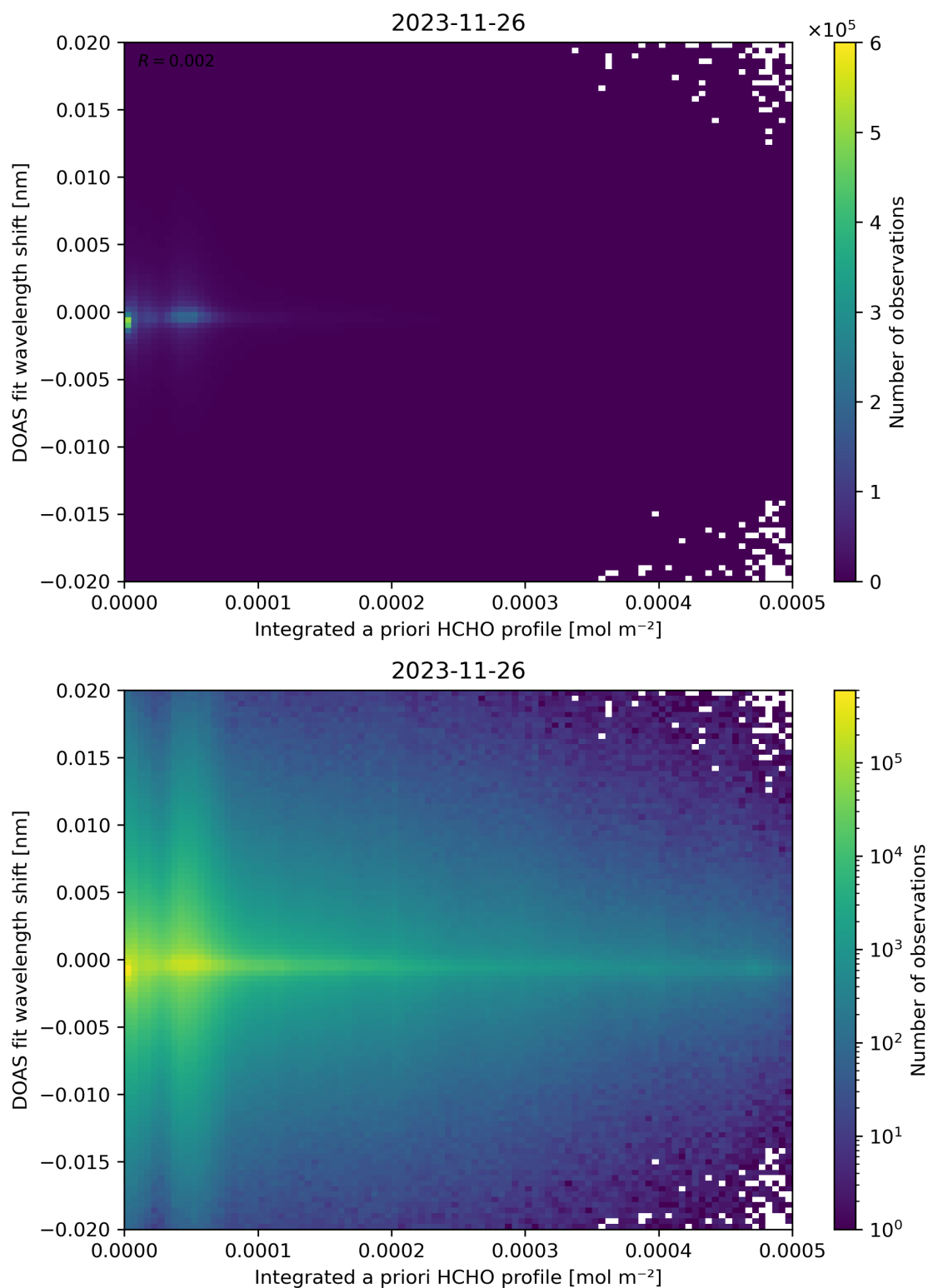
Figure 149: Scatter density plot of “Integrated a priori HCHO profile” against “DOAS fit wavelength shift” for 2023-11-25 to 2023-11-27.
