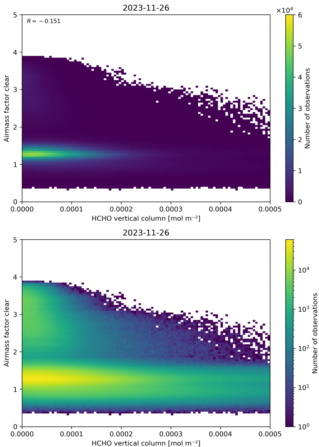
Figure 126: Scatter density plot of “HCHO vertical column” against “Airmass factor clear” for 2023-11-25 to 2023-11-27.
