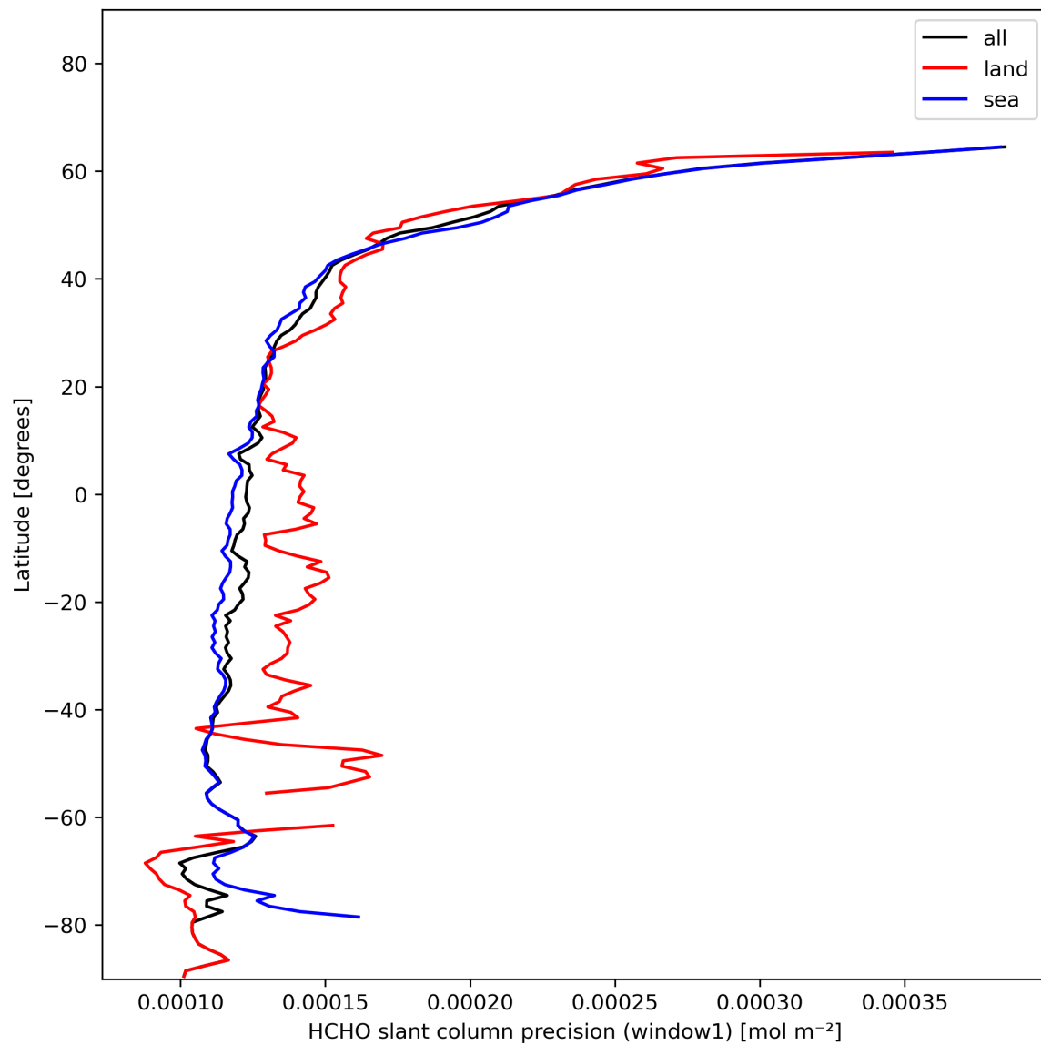
Figure 25: Zonal average of “HCHO slant column precision (window1)” for 2023-11-25 to 2023-11-27.
