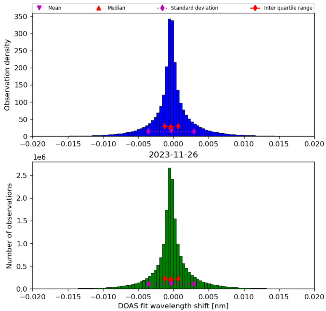
Figure 44: Histogram of “DOAS fit wavelength shift” for 2023-11-25 to 2023-11-27
