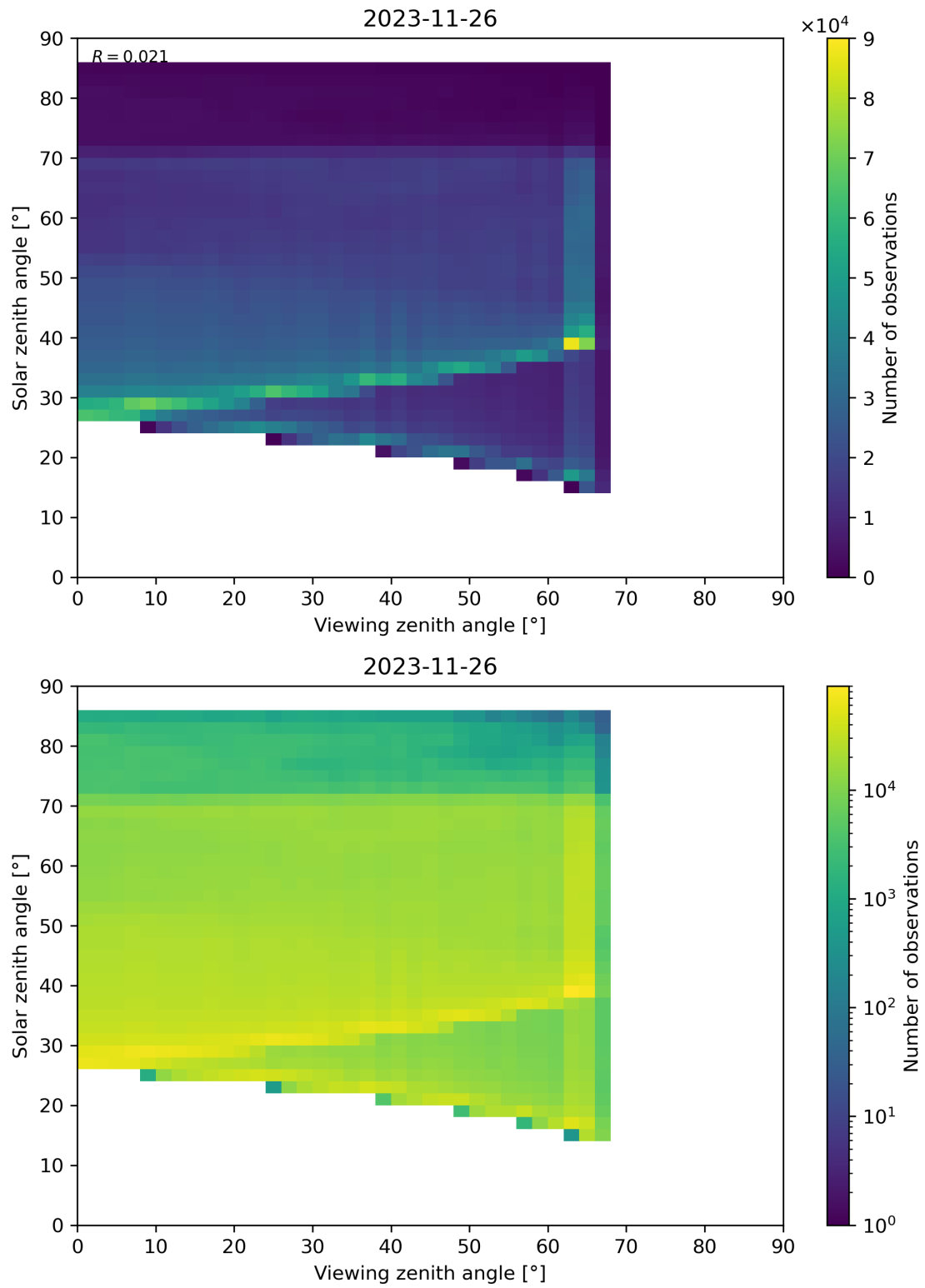
Figure 197: Scatter density plot of “Viewing zenith angle” against “Solar zenith angle” for 2023-11-25 to 2023-11-27.
