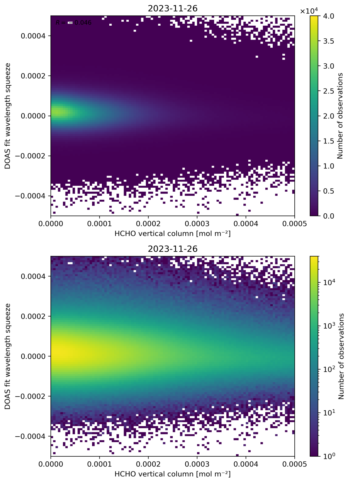
Figure 125: Scatter density plot of “HCHO vertical column” against “DOAS fit wavelength squeeze” for 2023-11-25 to 2023-11-27.
