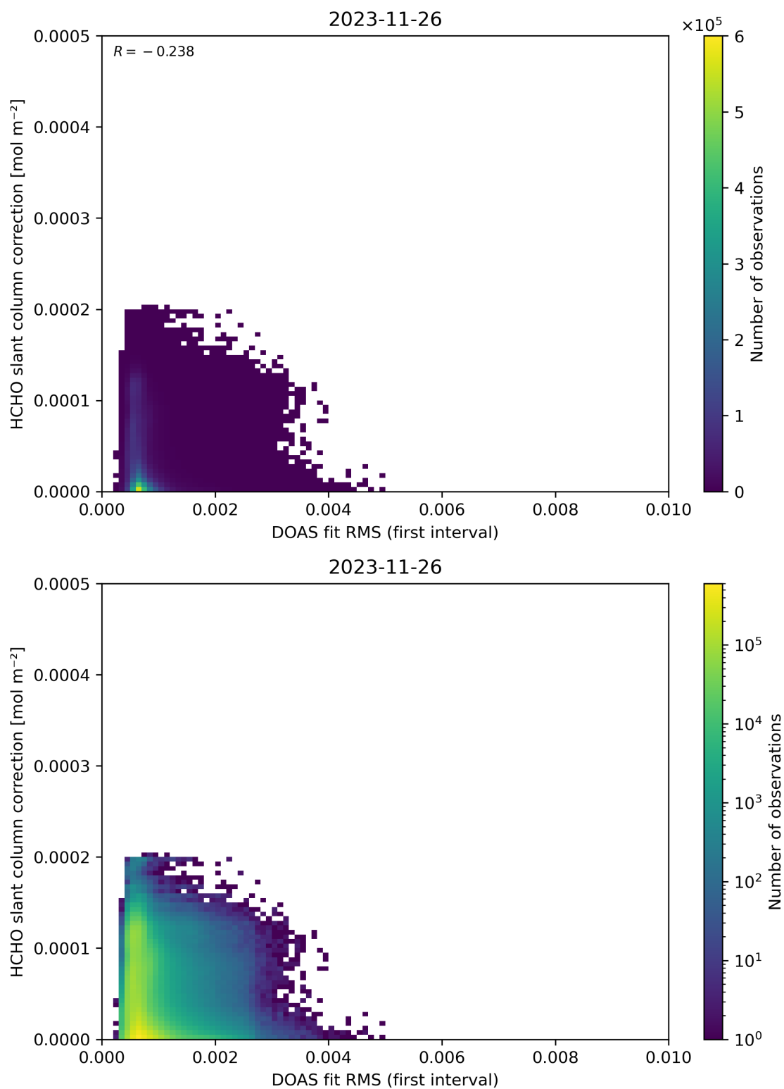
Figure 63: Scatter density plot of “DOAS fit RMS (first interval)” against “HCHO slant column correction” for 2023-11-25 to 2023-11-27.
