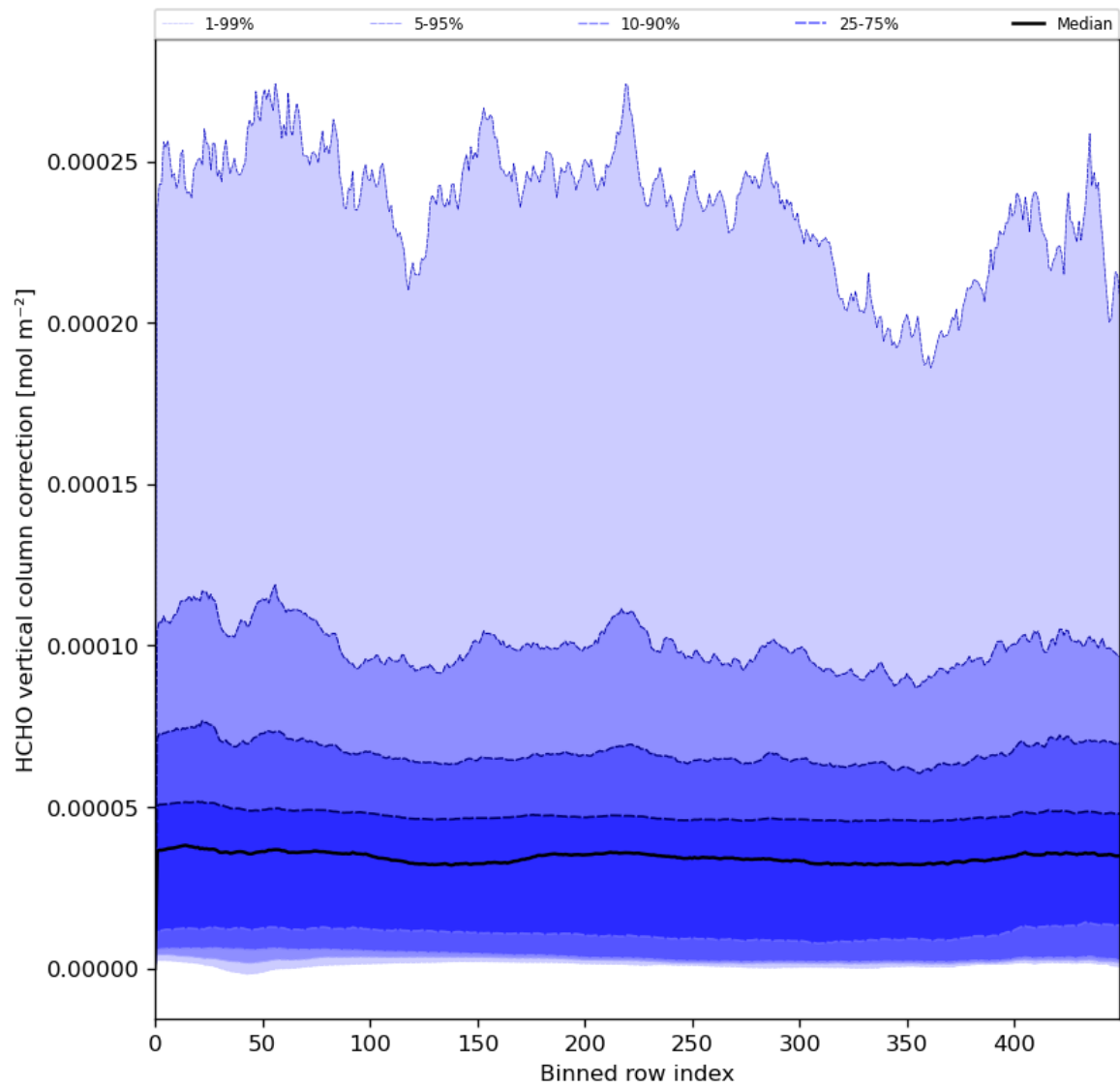
Figure 51: Along track statistics of “HCHO vertical column correction” for 2023-11-25 to 2023-11-27
