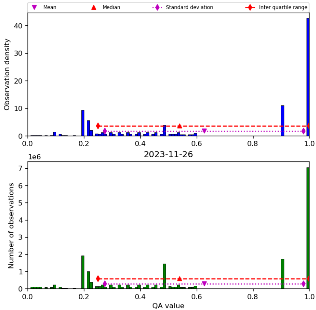
Figure 34: Histogram of “QA value” for 2023-11-25 to 2023-11-27
