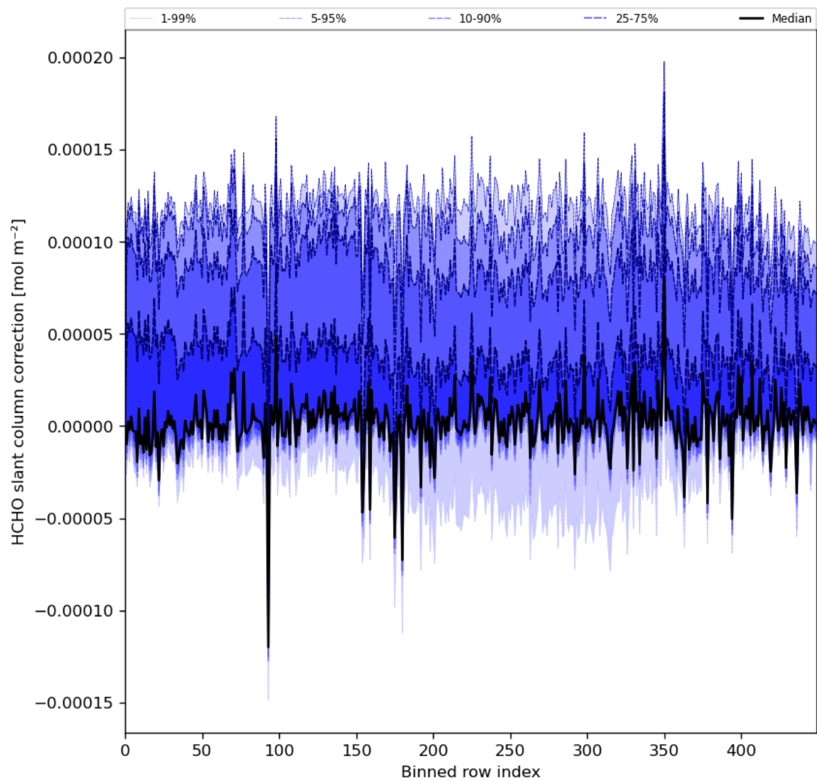
Figure 61: Along track statistics of “HCHO slant column correction” for 2023-11-25 to 2023-11-27
