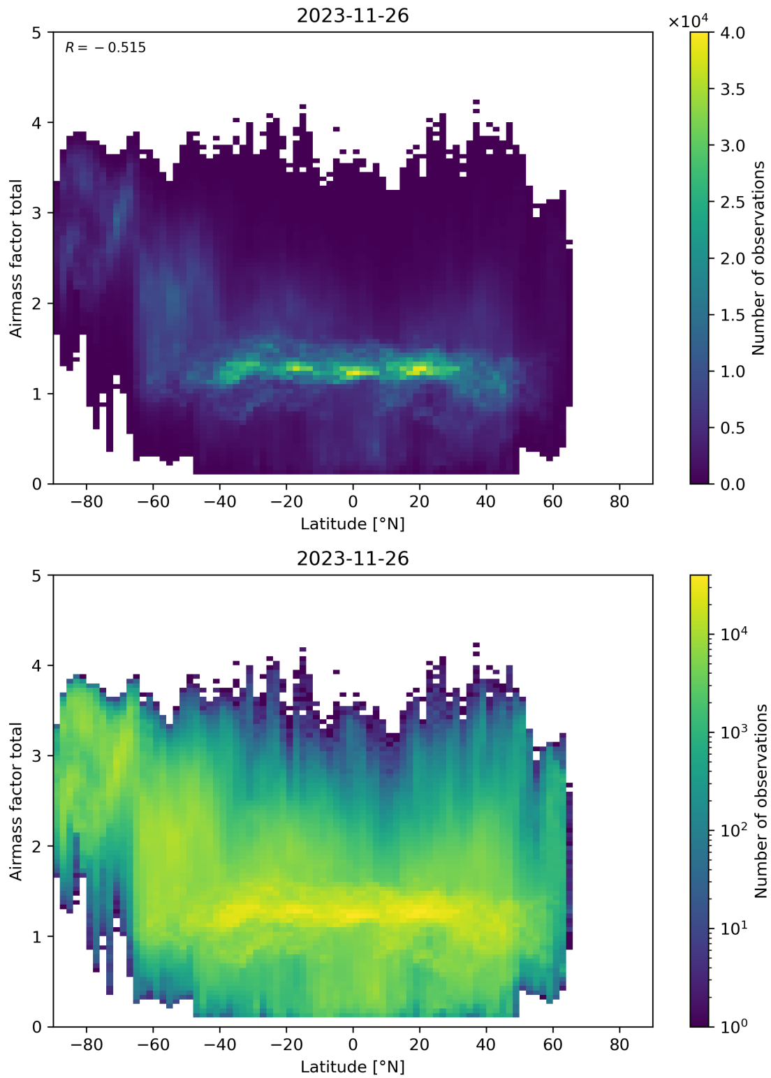
Figure 161: Scatter density plot of “Latitude” against “Airmass factor total” for 2023-11-25 to 2023-11-27.
