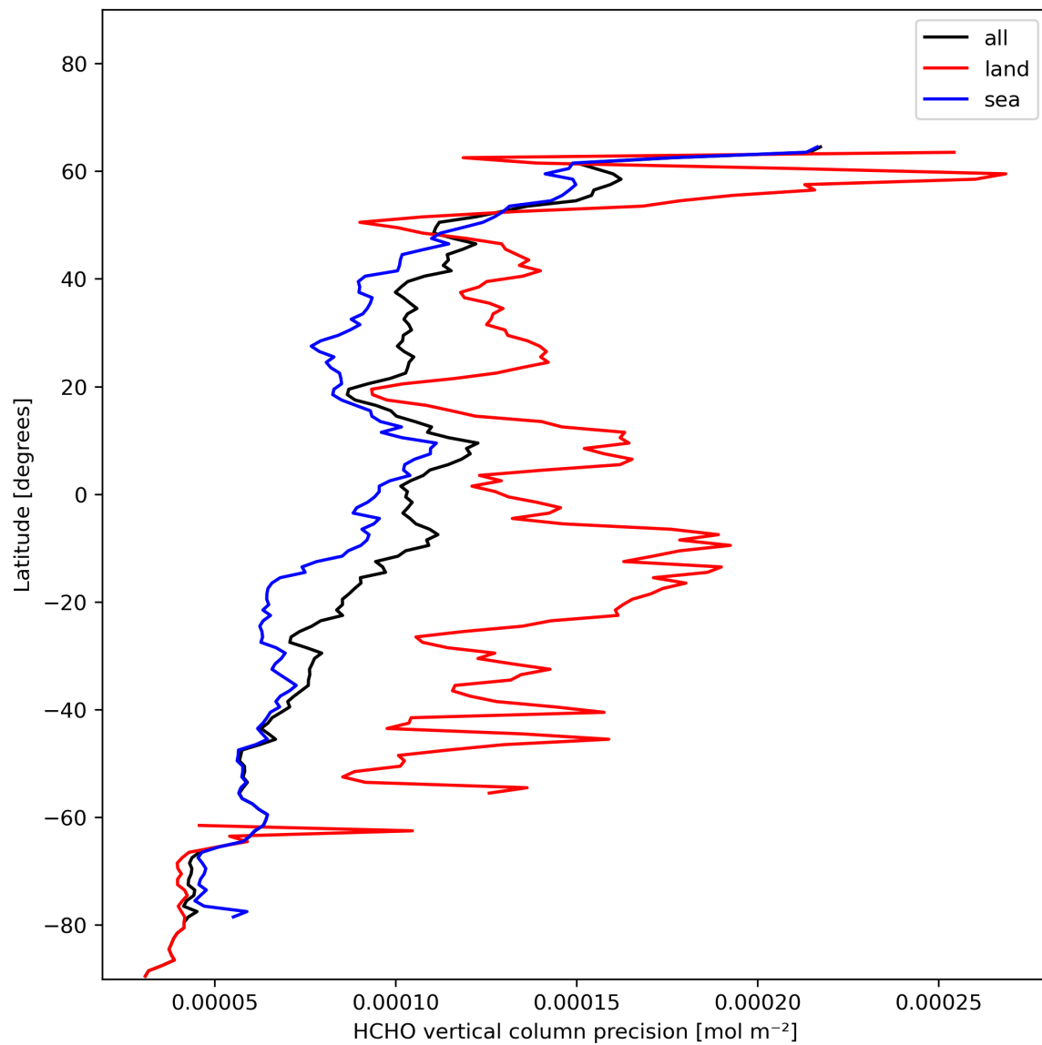
Figure 22: Zonal average of “HCHO vertical column precision” for 2023-11-25 to 2023-11-27.
