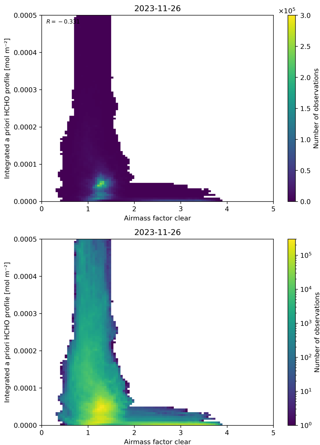
Figure 76: Scatter density plot of “Airmass factor clear” against “Integrated a priori HCHO profile” for 2023-11-25 to 2023-11-27.
