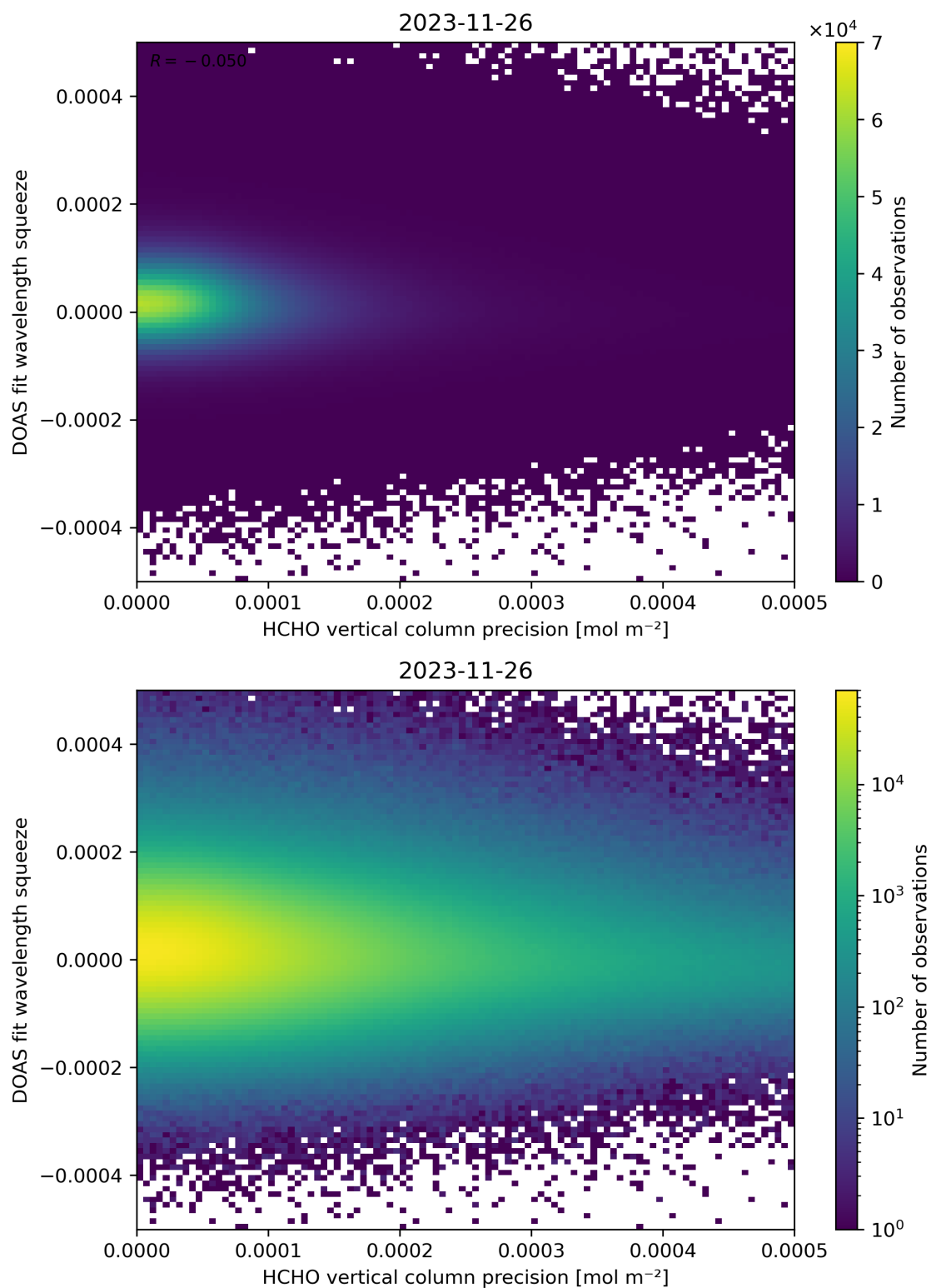
Figure 138: Scatter density plot of “HCHO vertical column precision” against “DOAS fit wavelength squeeze” for 2023-11-25 to 2023-11-27.
