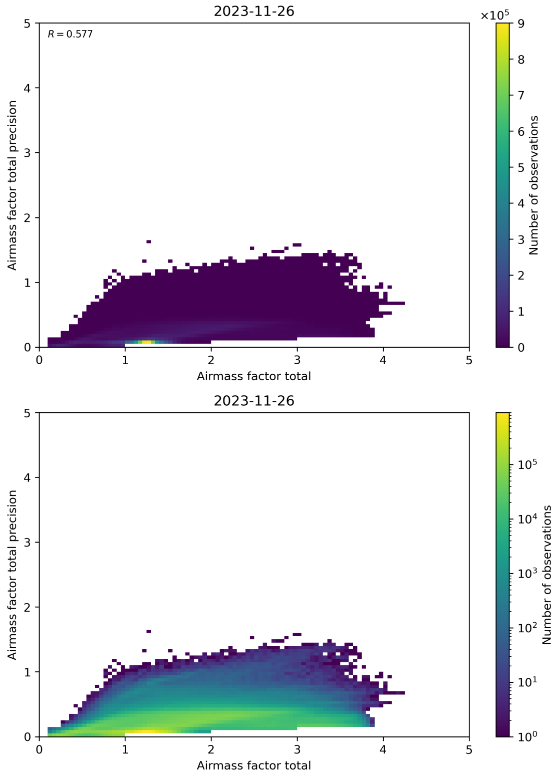
Figure 103: Scatter density plot of “Airmass factor total” against “Airmass factor total precision” for 2023-11-25 to 2023-11-27.
