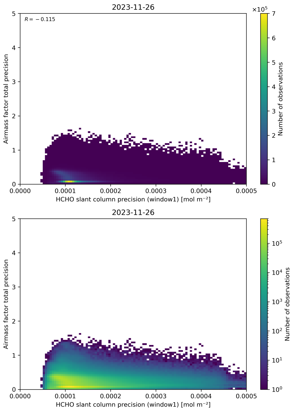
Figure 95: Scatter density plot of “HCHO slant column precision (window1)” against “Airmass factor total precision” for 2023-11-25 to 2023-11-27.
