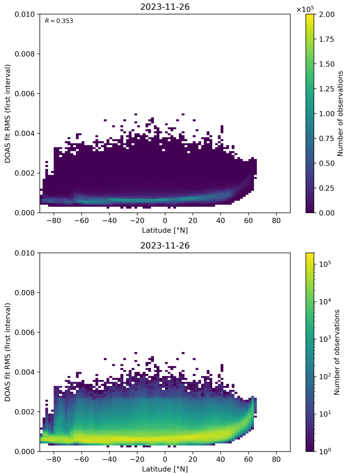
Figure 153: Scatter density plot of “Latitude” against “DOAS fit RMS (first interval)” for 2023-11-25 to 2023-11-27.
