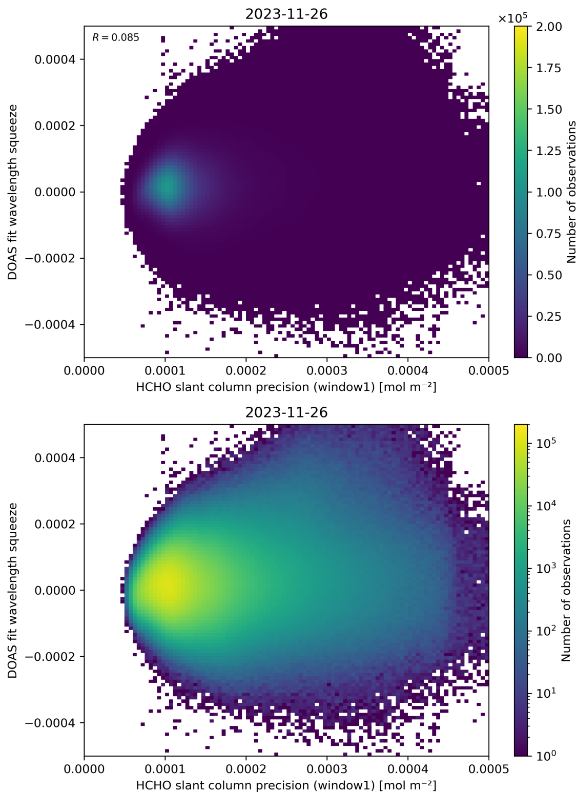
Figure 90: Scatter density plot of “HCHO slant column precision (window1)” against “DOAS fit wavelength squeeze” for 2023-11-25 to 2023-11-27.
