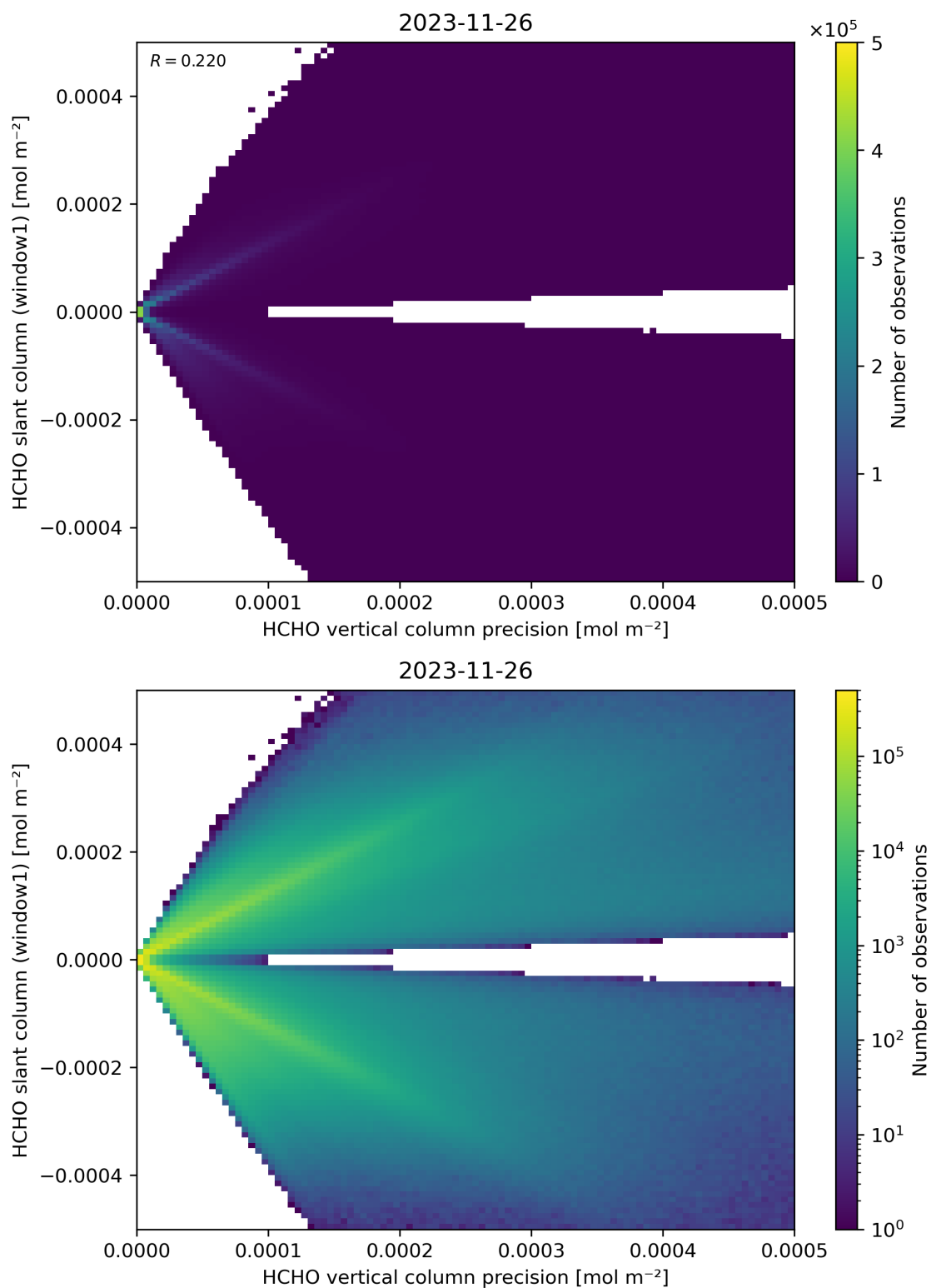
Figure 142: Scatter density plot of “HCHO vertical column precision” against “HCHO slant column (window1)” for 2023-11-25 to 2023-11-27.
