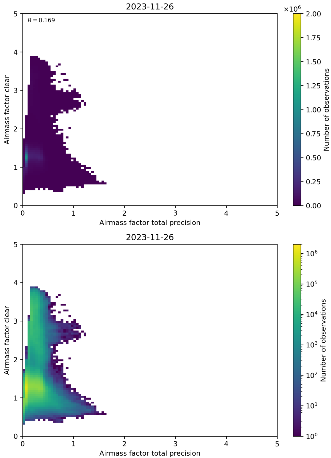
Figure 108: Scatter density plot of “Airmass factor total precision” against “Airmass factor clear” for 2023-11-25 to 2023-11-27.
