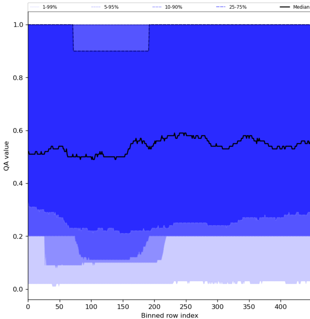
Figure 48: Along track statistics of “QA value” for 2023-11-25 to 2023-11-27
