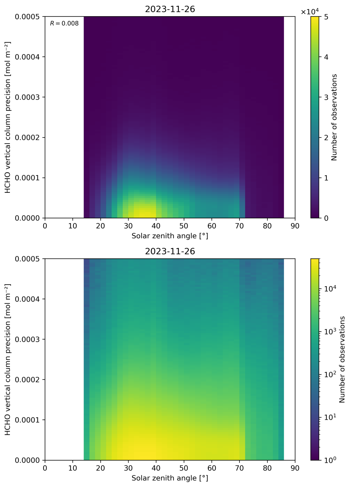
Figure 179: Scatter density plot of “Solar zenith angle” against “HCHO vertical column precision” for 2023-11-25 to 2023-11-27.
