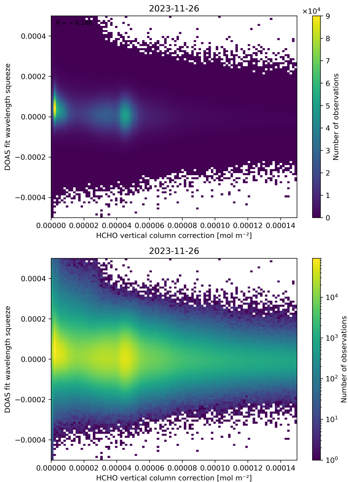
Figure 114: Scatter density plot of “HCHO vertical column correction” against “DOAS fit wavelength squeeze” for 2023-11-25 to 2023-11-27.
