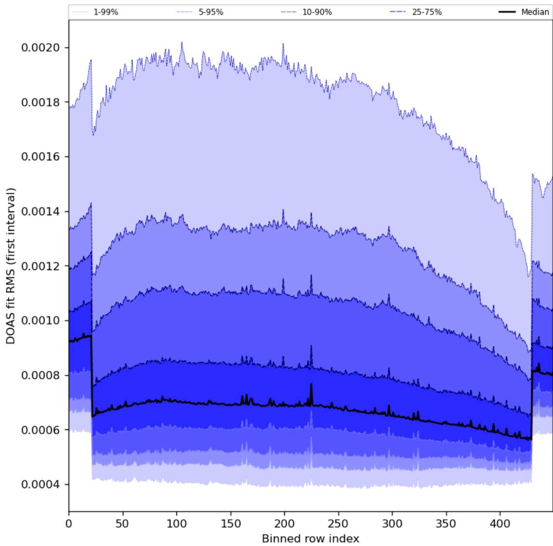
Figure 60: Along track statistics of “DOAS fit RMS (first interval)” for 2023-11-25 to 2023-11-27
