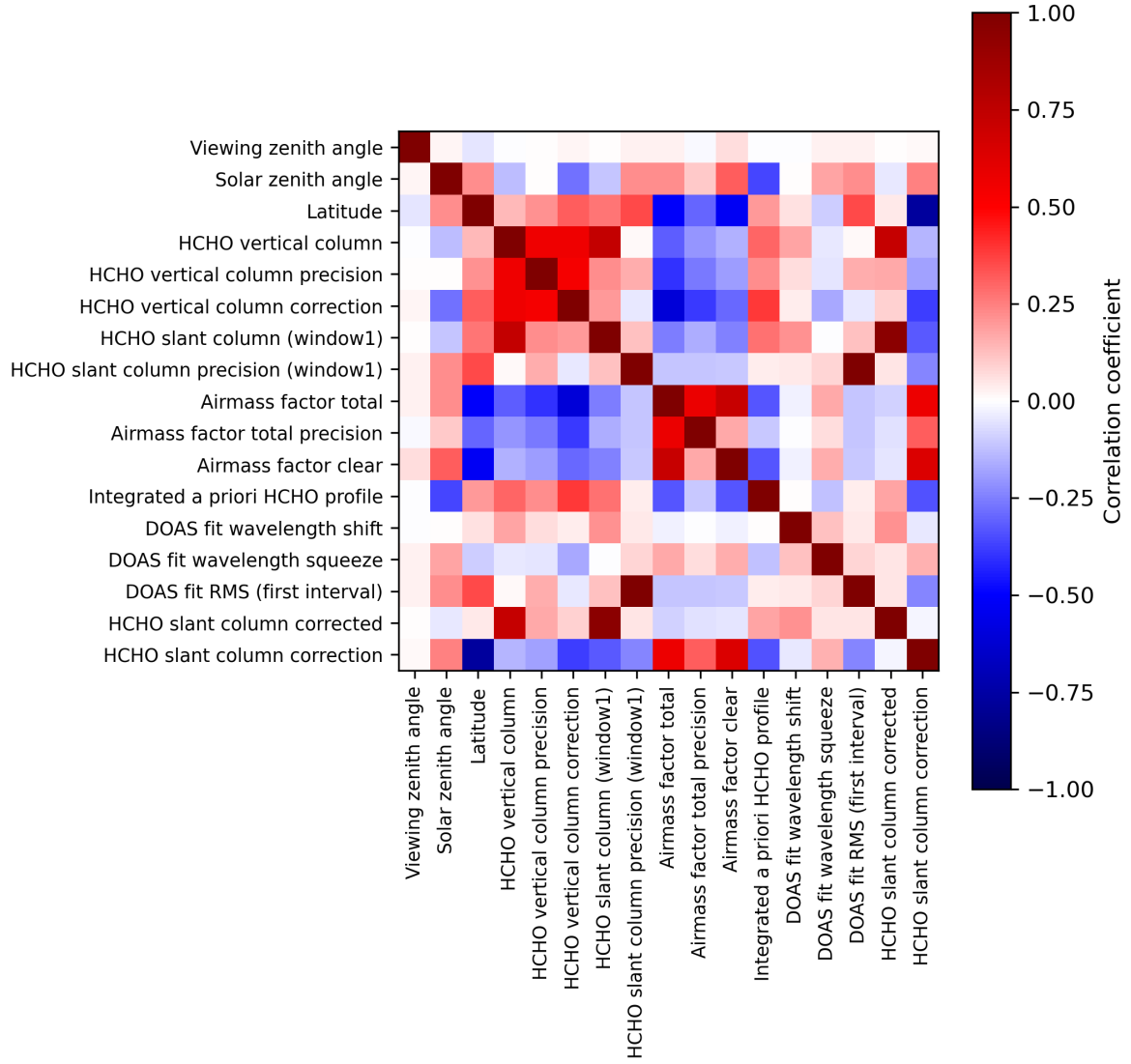
Figure 2: Map of correlation matrix for 2023-11-25 to 2023-11-27.
