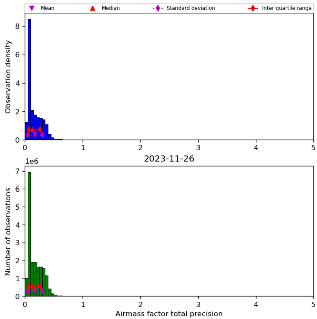
Figure 41: Histogram of “Airmass factor total precision” for 2023-11-25 to 2023-11-27
