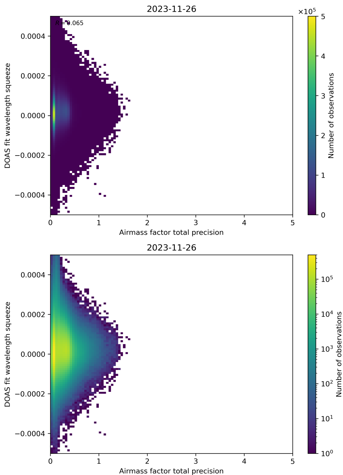
Figure 107: Scatter density plot of “Airmass factor total precision” against “DOAS fit wavelength squeeze” for 2023-11-25 to 2023-11-27.
