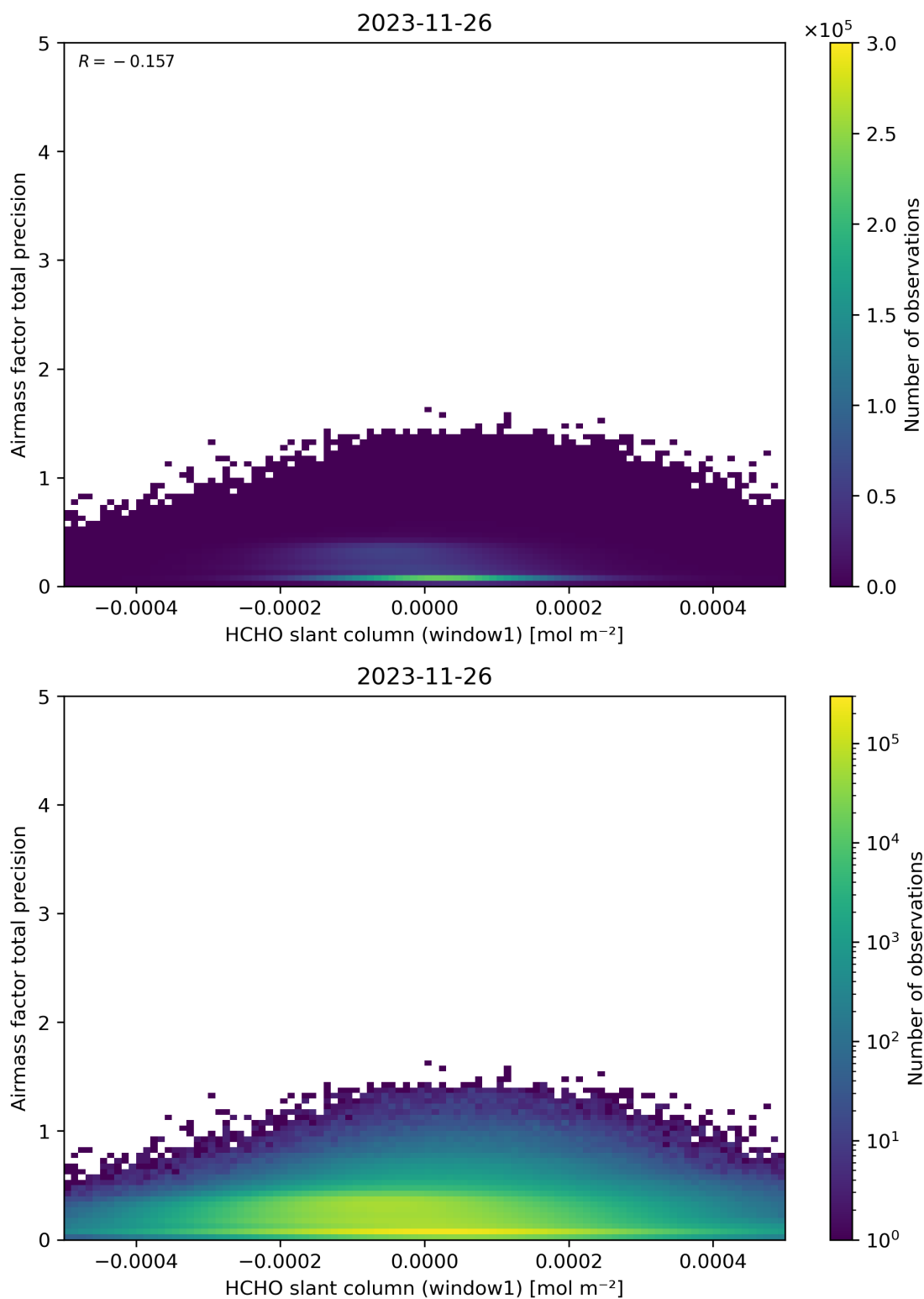
Figure 86: Scatter density plot of “HCHO slant column (window1)” against “Airmass factor total precision” for 2023-11-25 to 2023-11-27.
