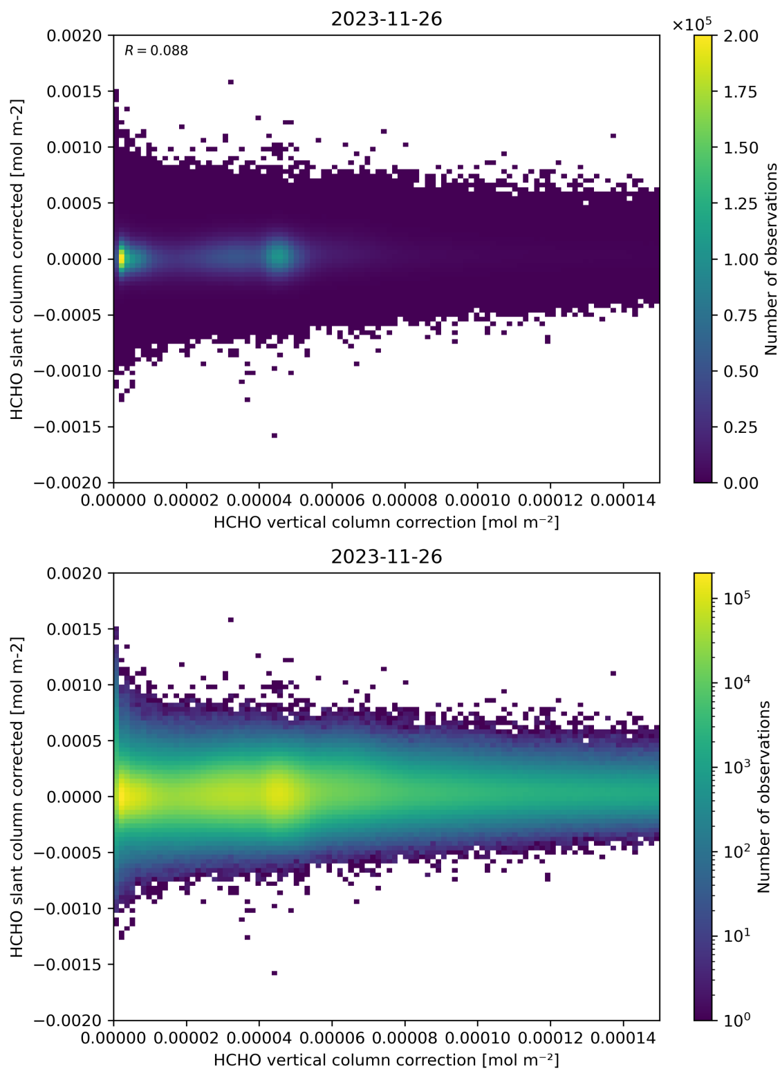
Figure 116: Scatter density plot of “HCHO vertical column correction” against “HCHO slant column corrected” for 2023-11-25 to 2023-11-27.
