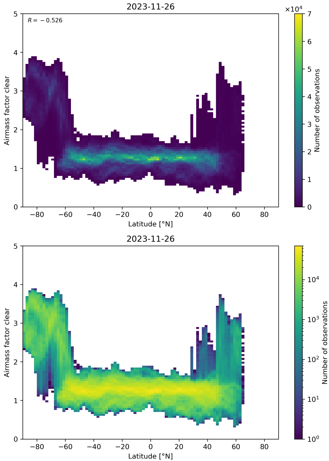
Figure 156: Scatter density plot of “Latitude” against “Airmass factor clear” for 2023-11-25 to 2023-11-27.
