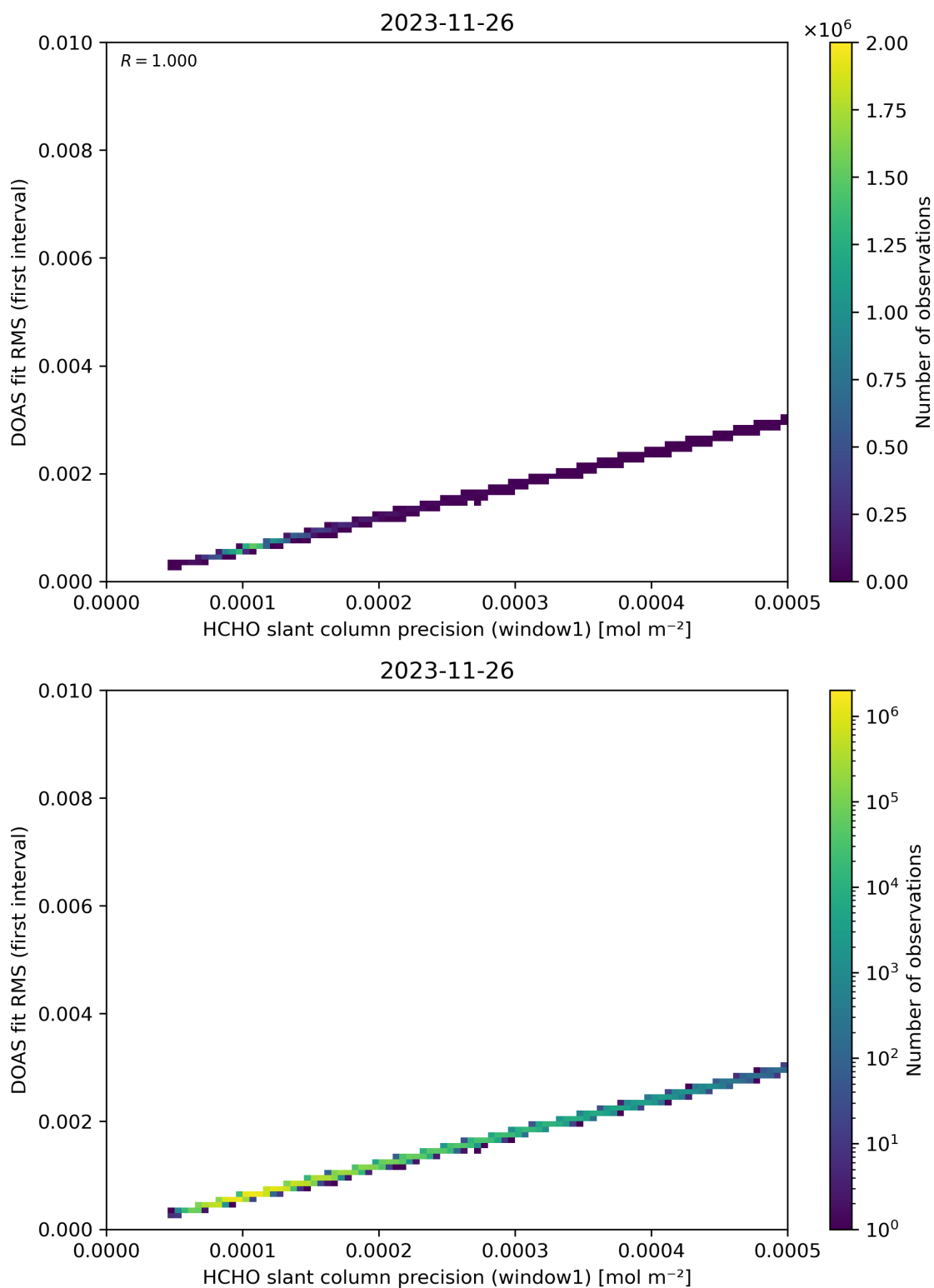
Figure 88: Scatter density plot of “HCHO slant column precision (window1)” against “DOAS fit RMS (first interval)” for 2023-11-25 to 2023-11-27.
