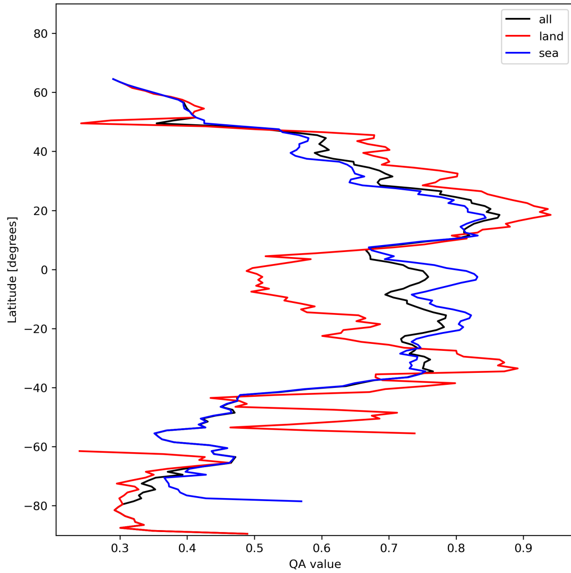
Figure 20: Zonal average of “QA value” for 2023-11-25 to 2023-11-27.
