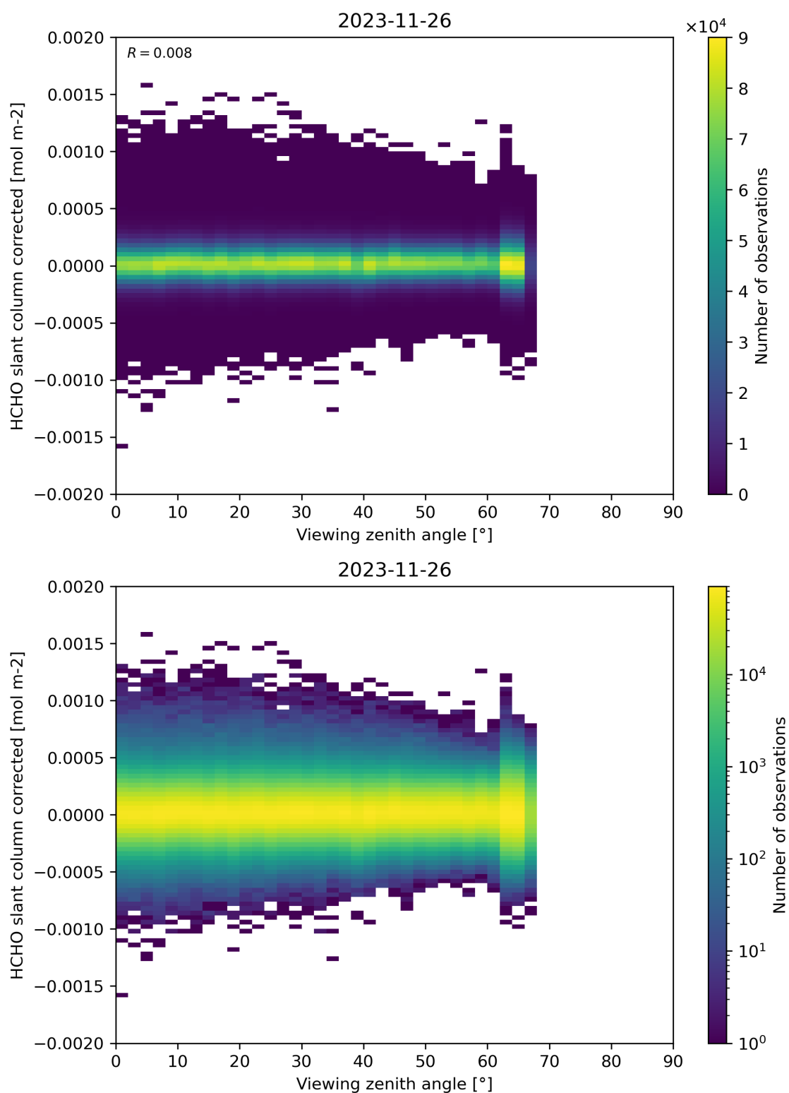
Figure 186: Scatter density plot of “Viewing zenith angle” against “HCHO slant column corrected” for 2023-11-25 to 2023-11-27.
