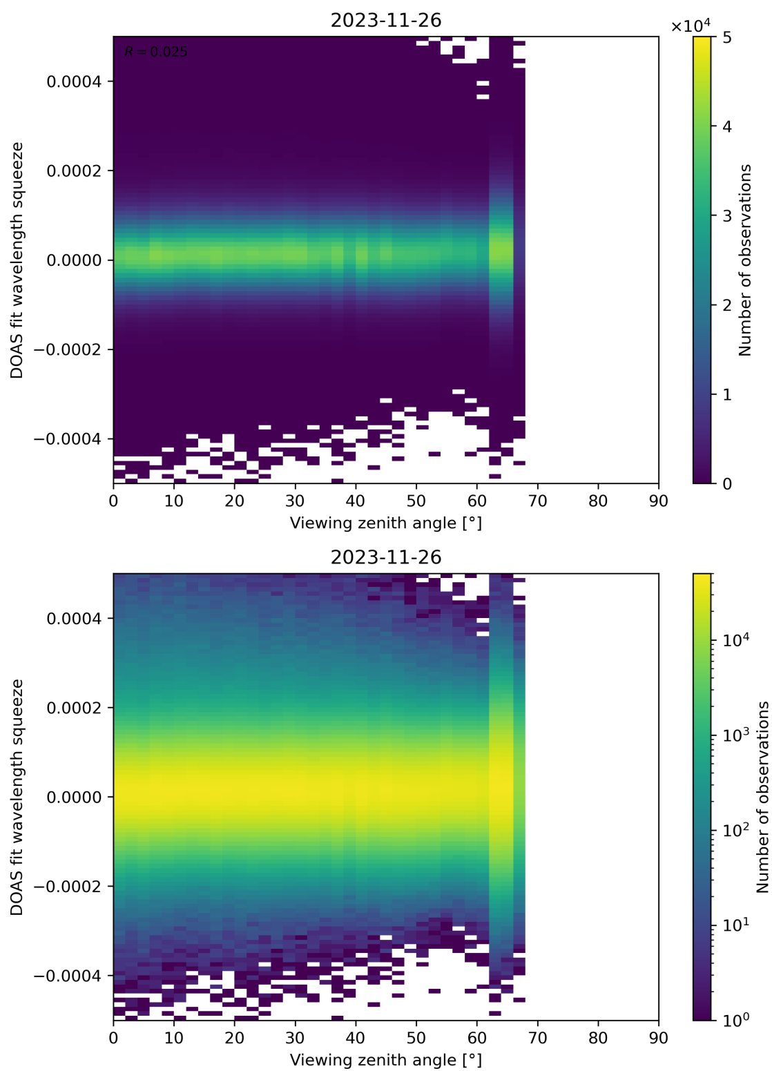
Figure 184: Scatter density plot of “Viewing zenith angle” against “DOAS fit wavelength squeeze” for 2023-11-25 to 2023-11-27.
