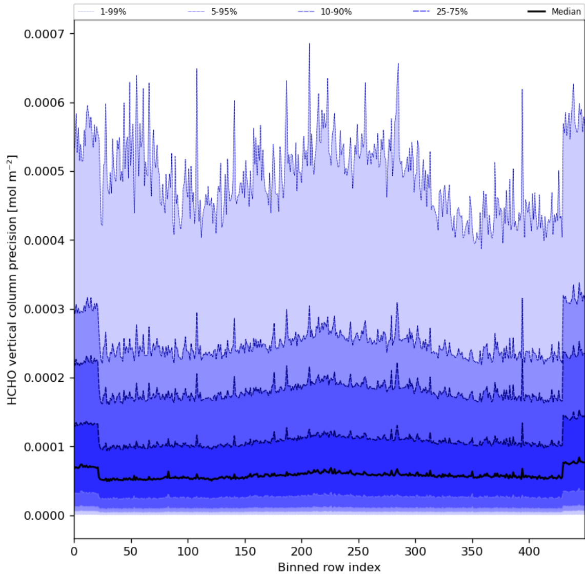
Figure 50: Along track statistics of “HCHO vertical column precision” for 2023-11-25 to 2023-11-27
