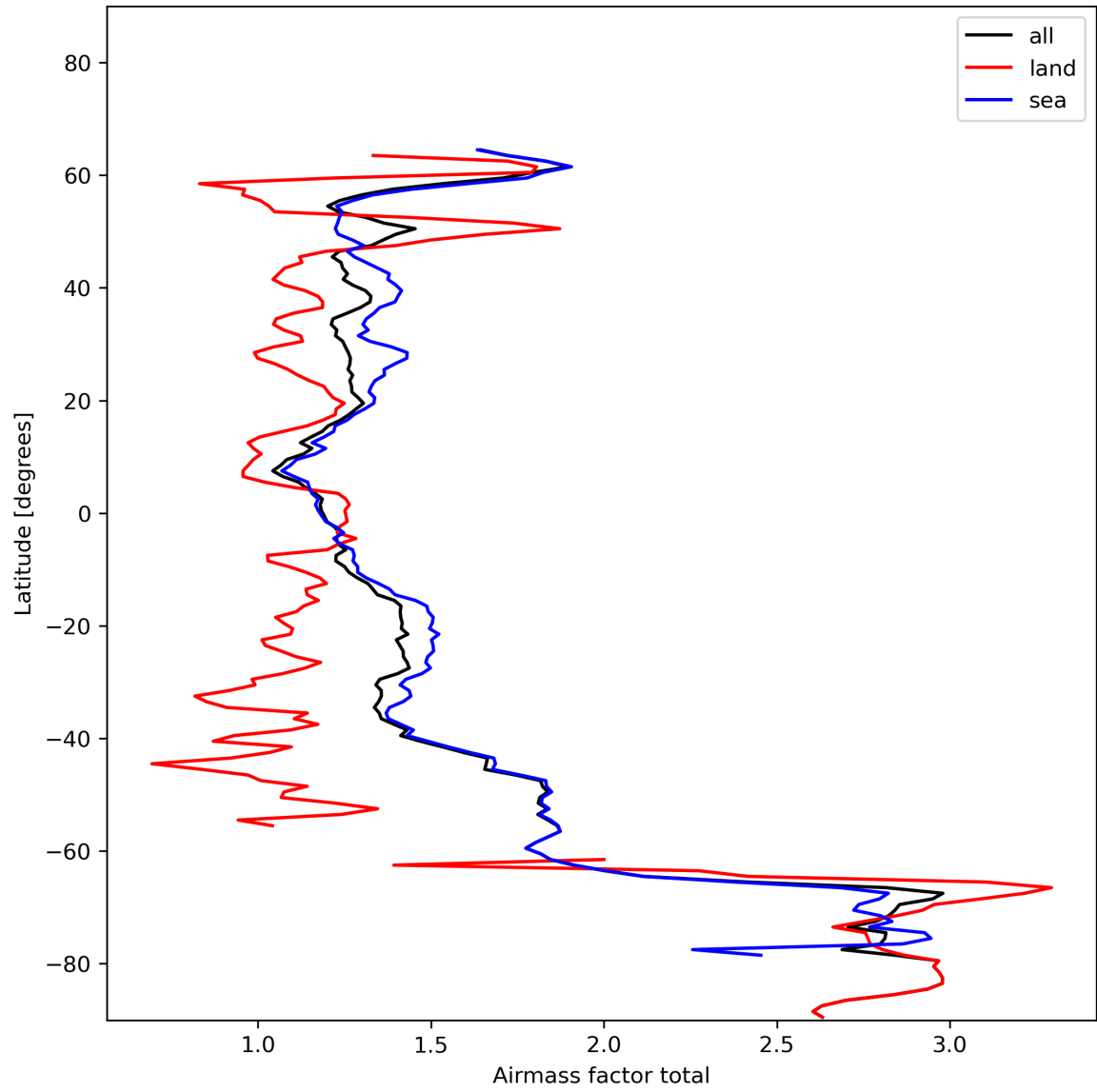
Figure 26: Zonal average of “Airmass factor total” for 2023-11-25 to 2023-11-27.
