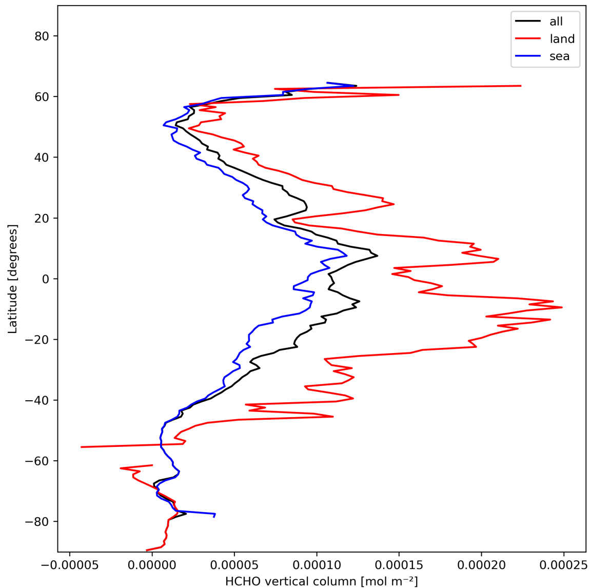
Figure 21: Zonal average of “HCHO vertical column” for 2023-11-25 to 2023-11-27.
