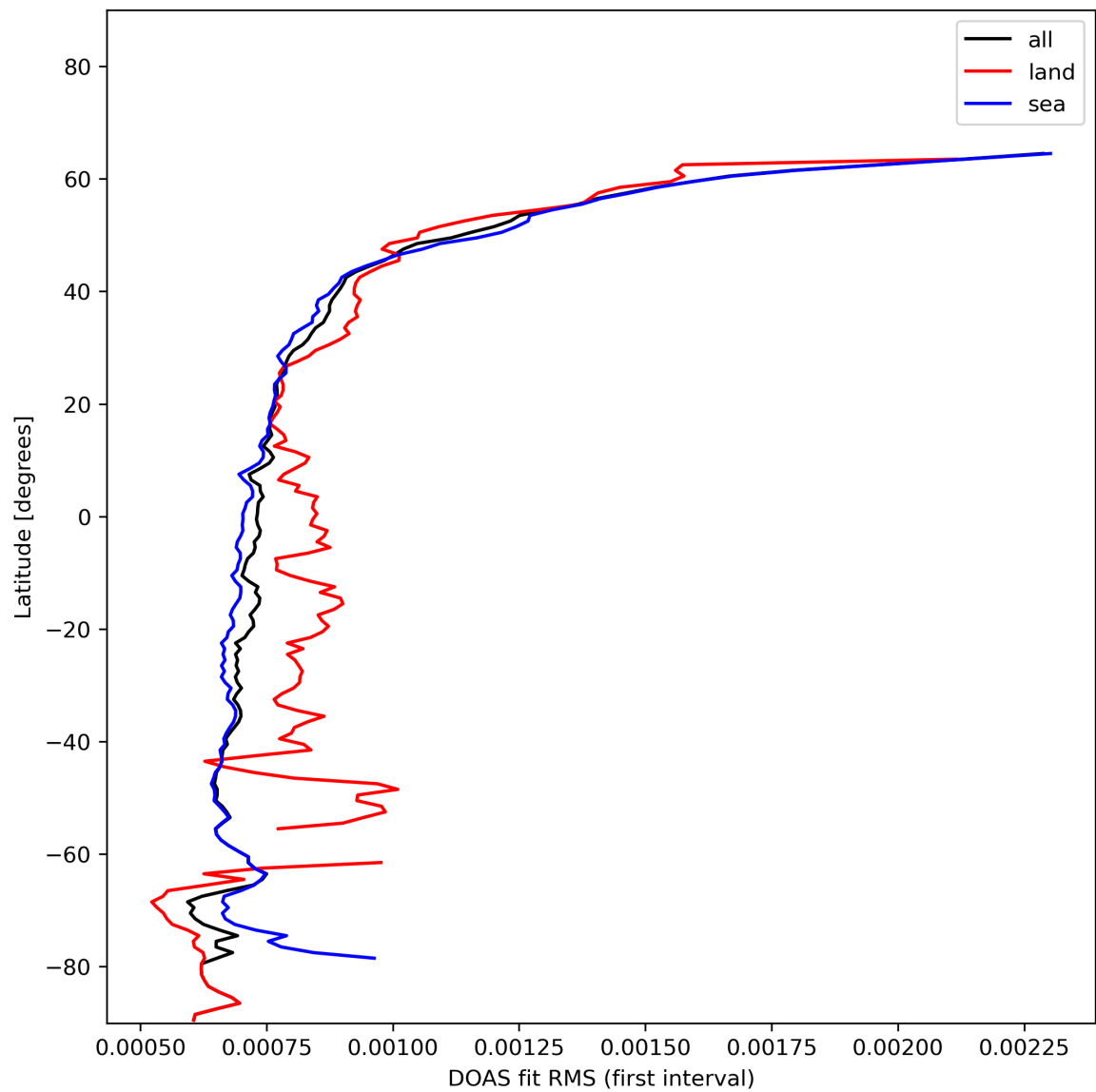
Figure 32: Zonal average of “DOAS fit RMS (first interval)” for 2023-11-25 to 2023-11-27.
