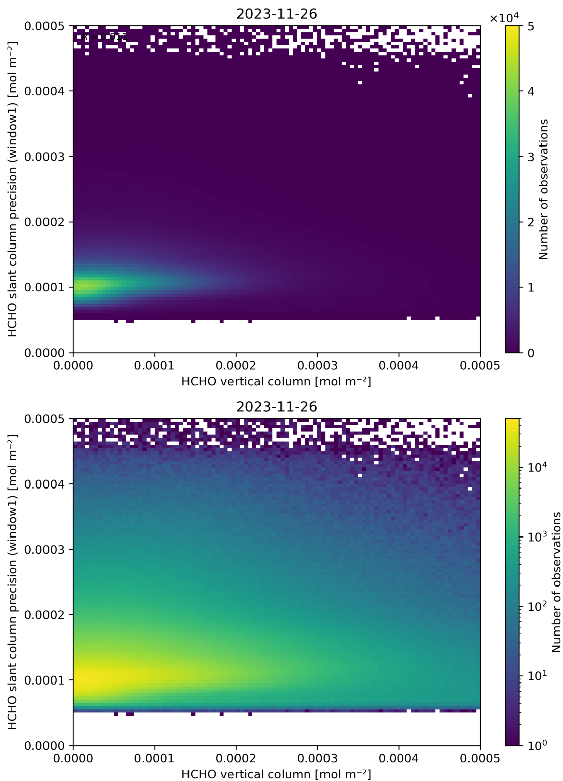
Figure 130: Scatter density plot of “HCHO vertical column” against “HCHO slant column precision (window1)” for 2023-11-25 to 2023-11-27.
