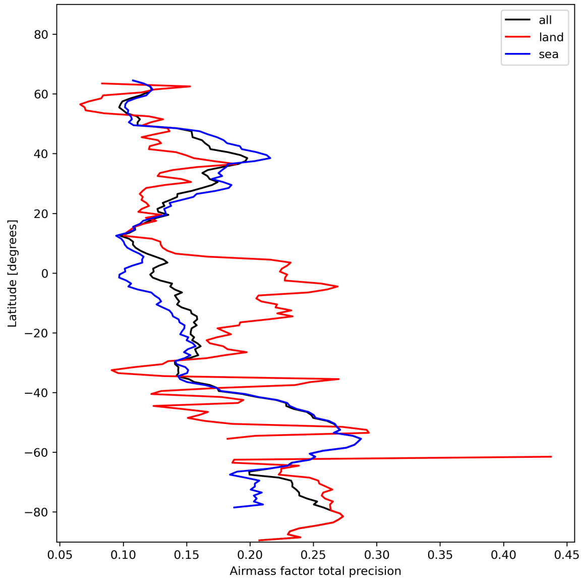
Figure 27: Zonal average of “Airmass factor total precision” for 2023-11-25 to 2023-11-27.
