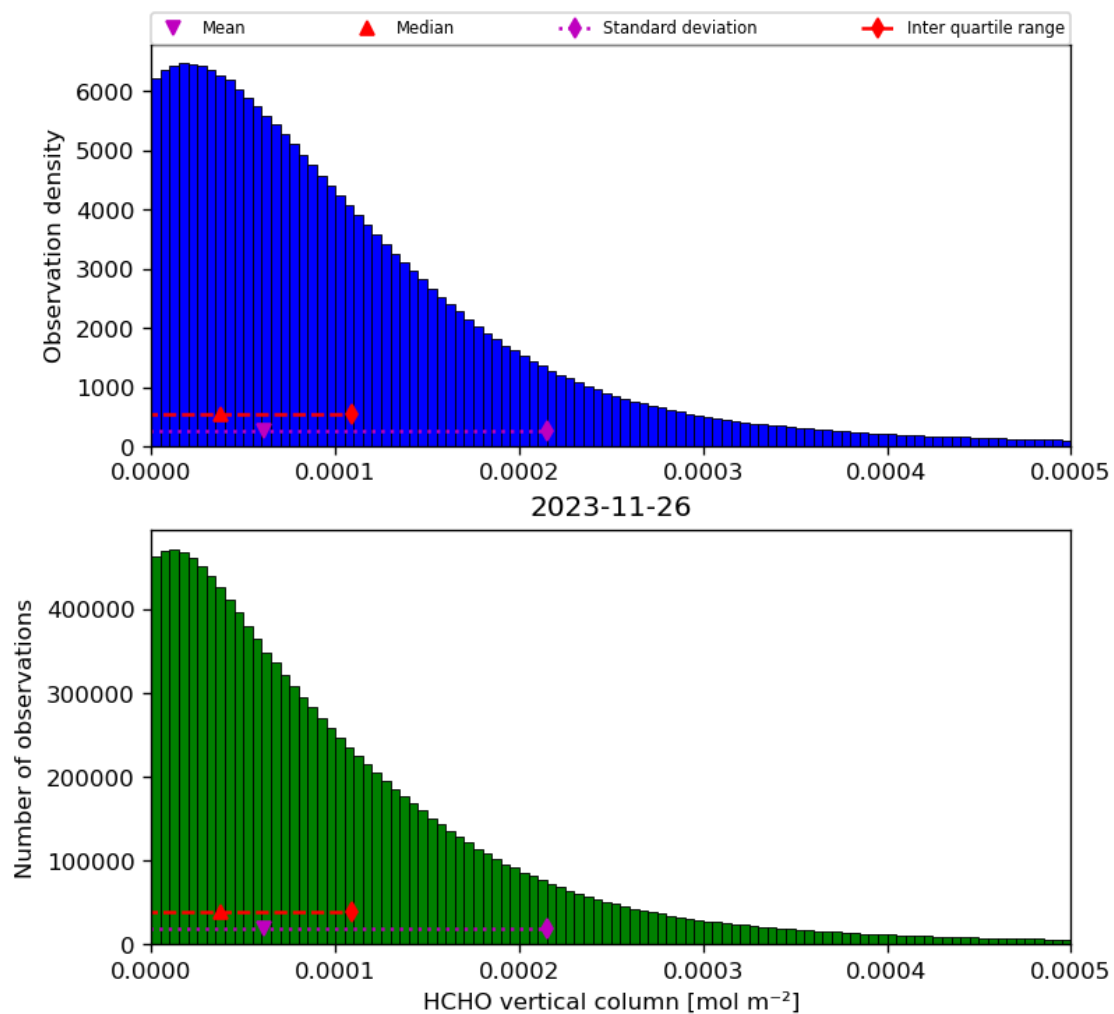
Figure 35: Histogram of “HCHO vertical column” for 2023-11-25 to 2023-11-27
