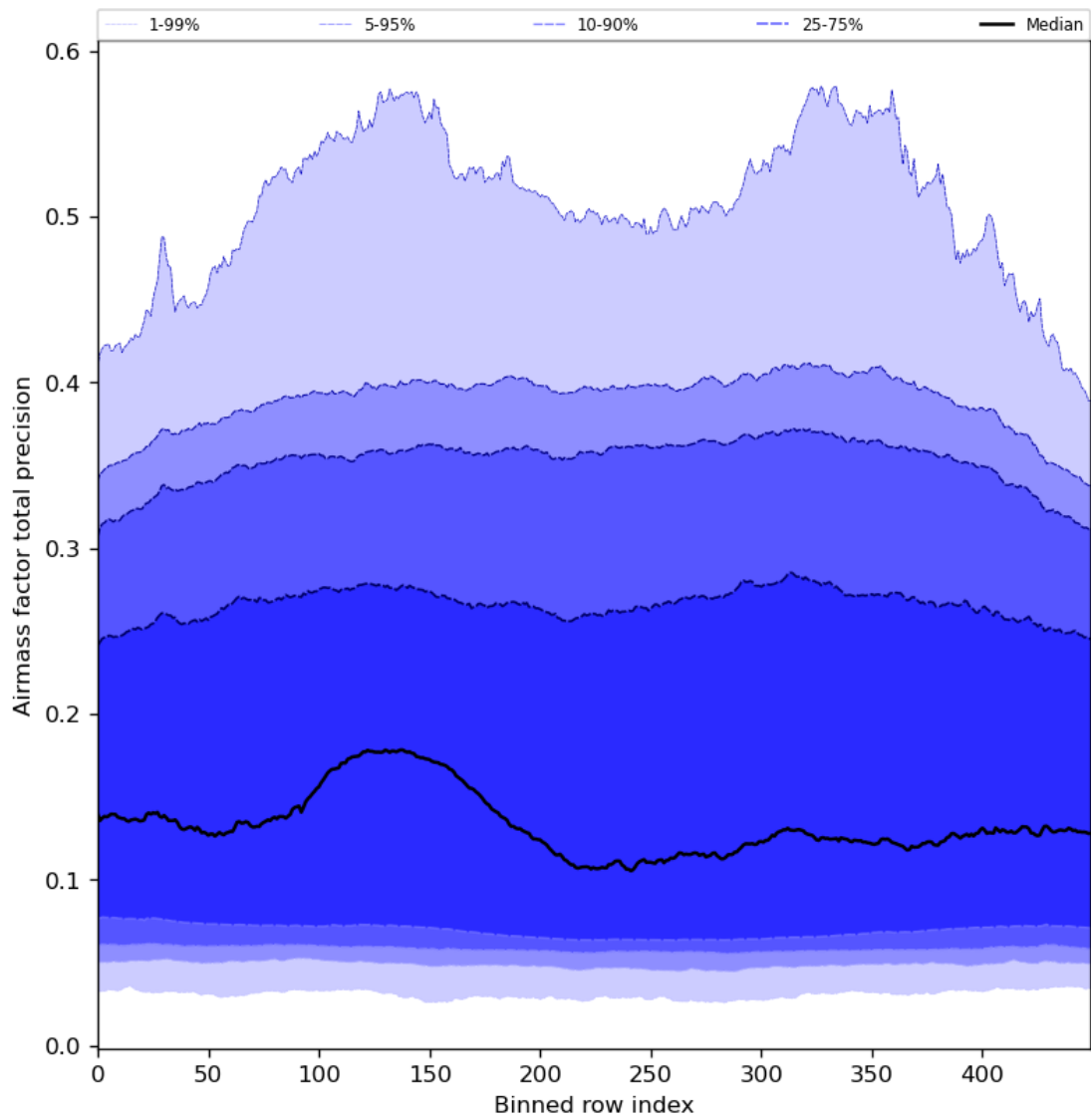
Figure 55: Along track statistics of “Airmass factor total precision” for 2023-11-25 to 2023-11-27
