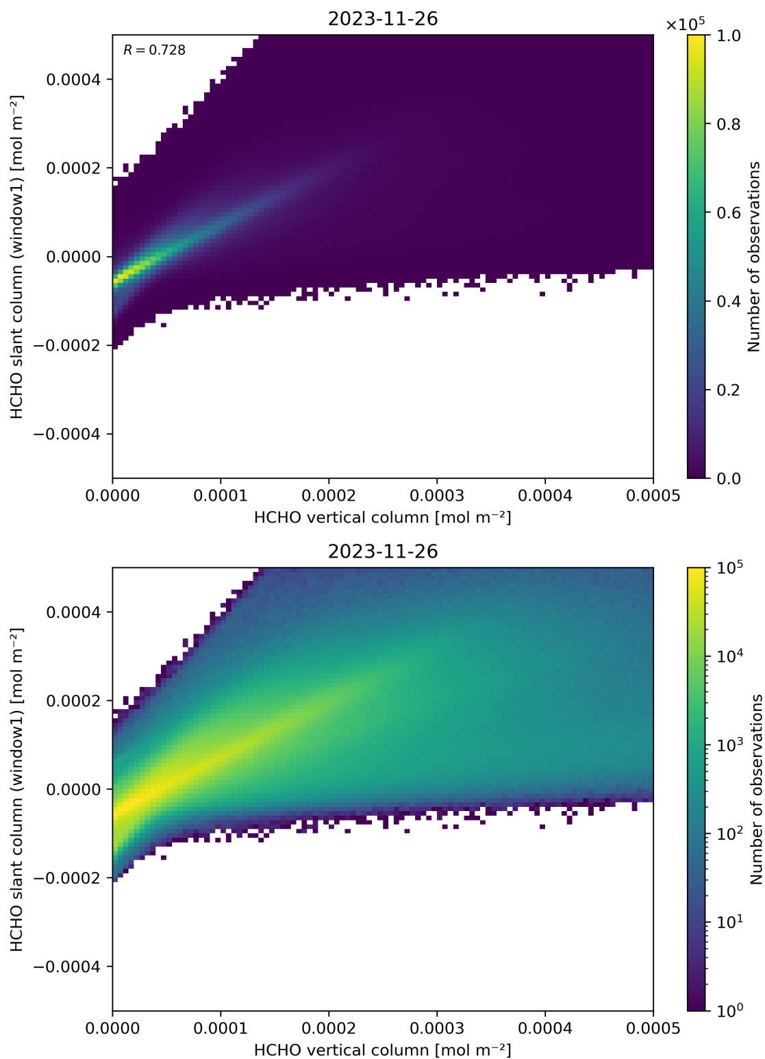
Figure 129: Scatter density plot of “HCHO vertical column” against “HCHO slant column (window1)” for 2023-11-25 to 2023-11-27.
