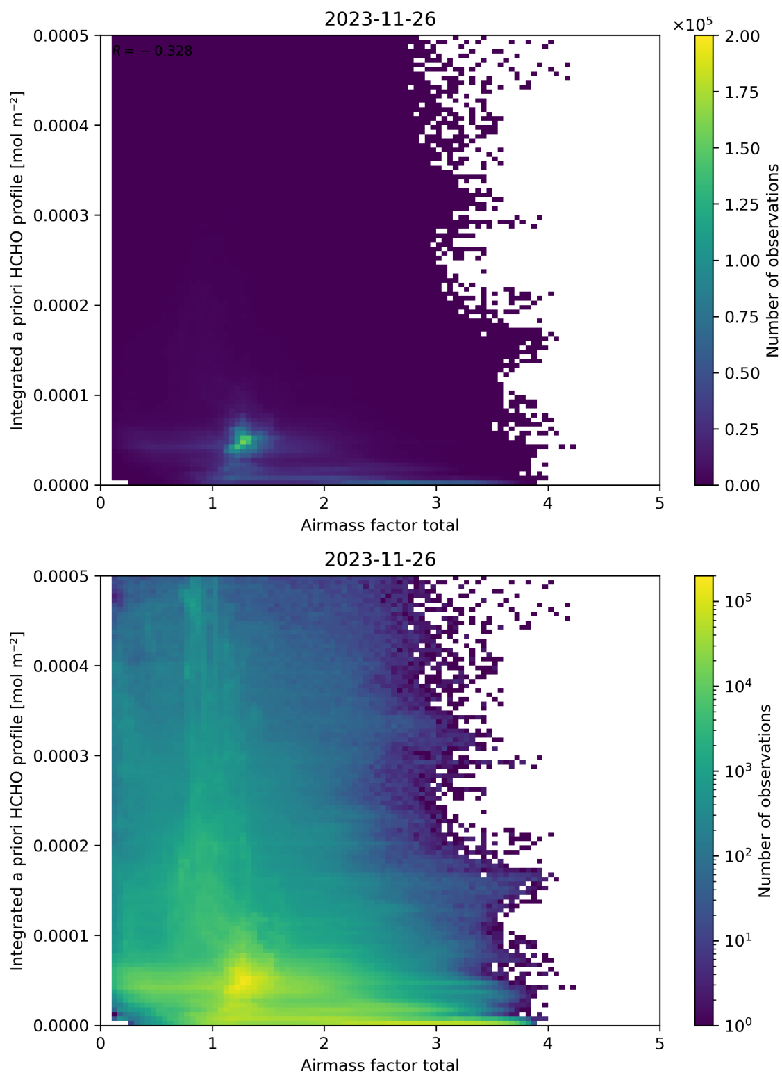
Figure 104: Scatter density plot of “Airmass factor total” against “Integrated a priori HCHO profile” for 2023-11-25 to 2023-11-27.
