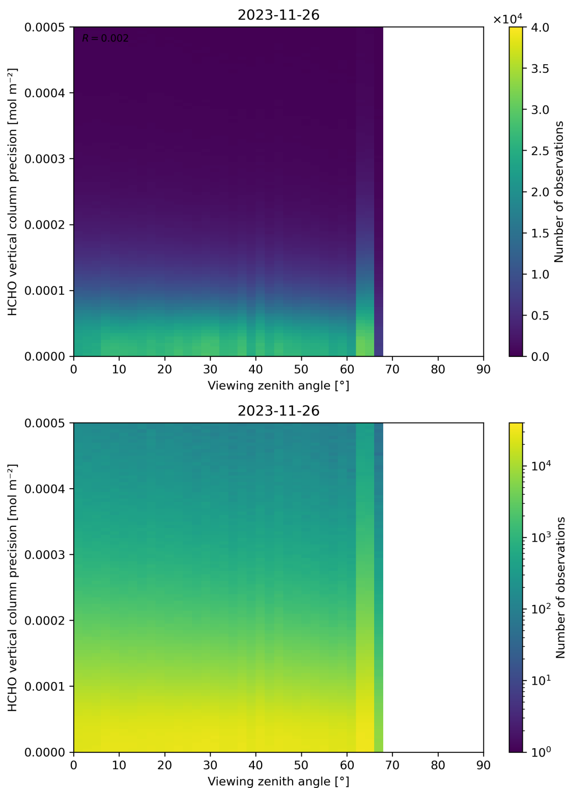
Figure 194: Scatter density plot of “Viewing zenith angle” against “HCHO vertical column precision” for 2023-11-25 to 2023-11-27.
