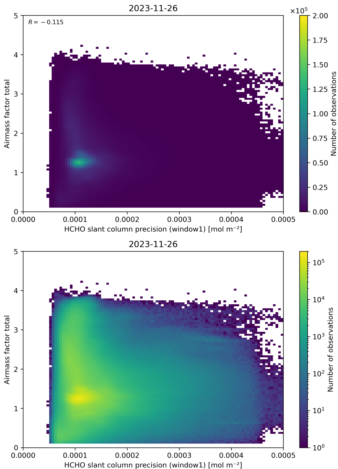
Figure 94: Scatter density plot of “HCHO slant column precision (window1)” against “Airmass factor total” for 2023-11-25 to 2023-11-27.
