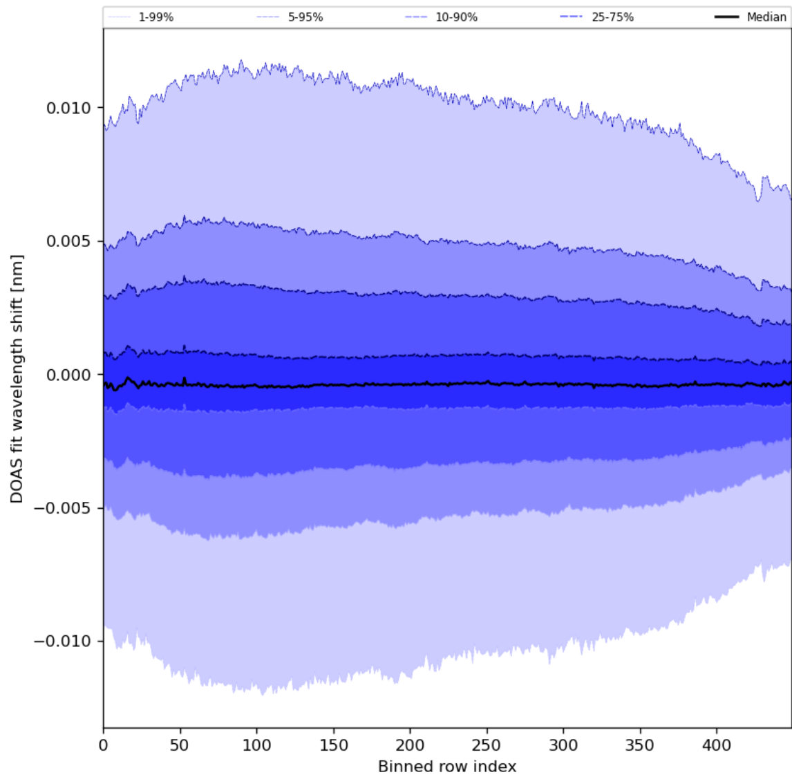
Figure 58: Along track statistics of “DOAS fit wavelength shift” for 2023-11-25 to 2023-11-27
