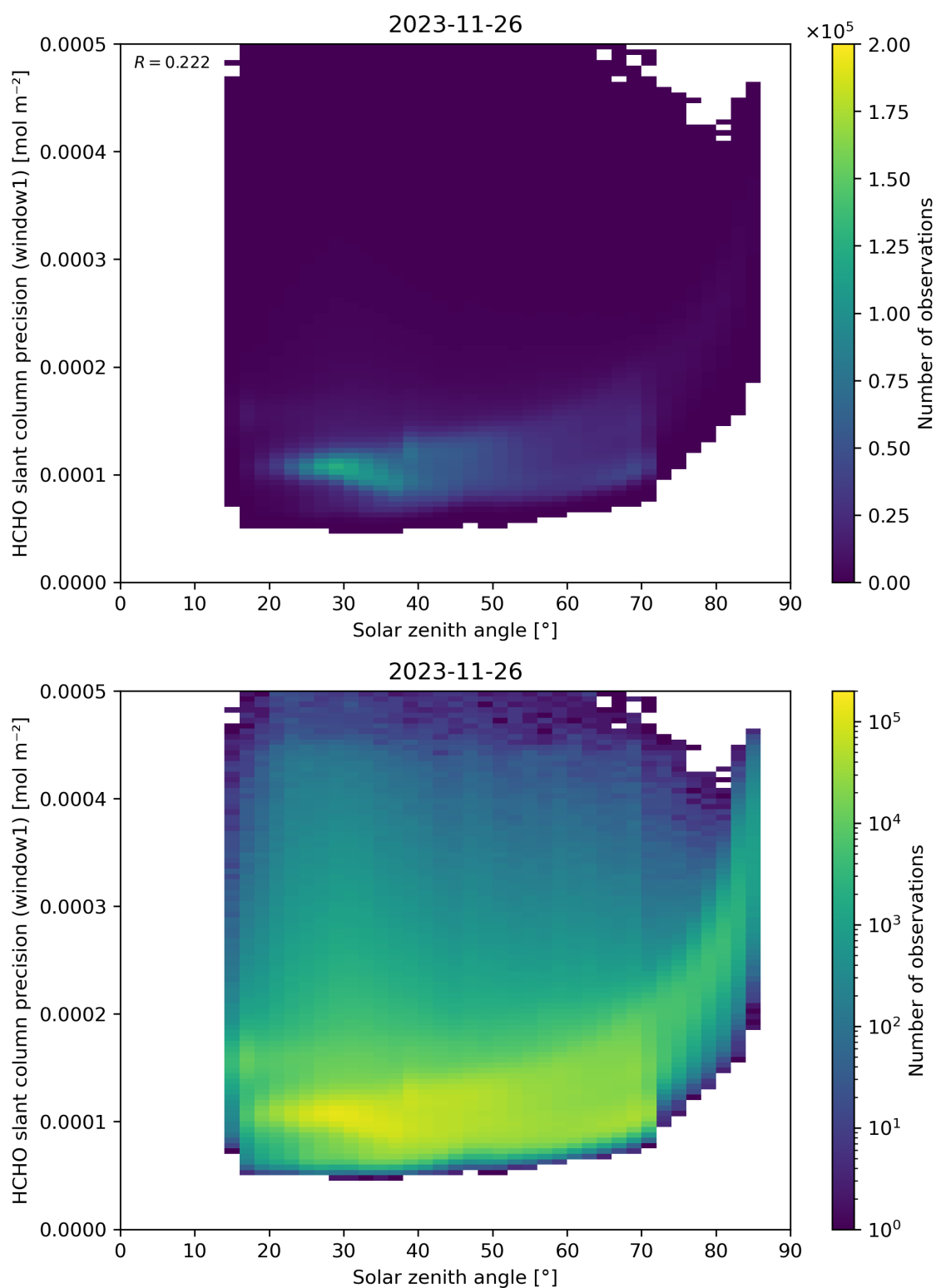
Figure 174: Scatter density plot of “Solar zenith angle” against “HCHO slant column precision (window1)” for 2023-11-25 to 2023-11-27.
