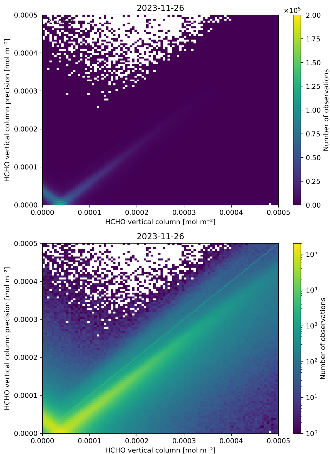
Figure 134: Scatter density plot of “HCHO vertical column” against “HCHO vertical column precision” for 2023-11-25 to 2023-11-27.
