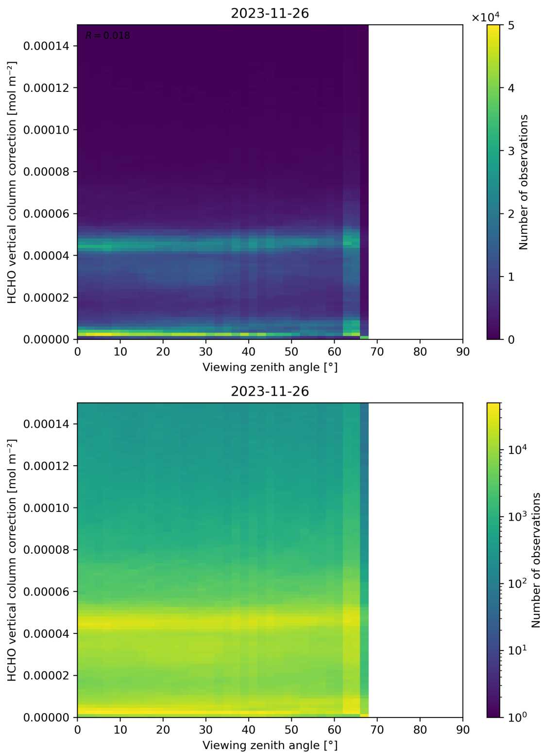
Figure 193: Scatter density plot of “Viewing zenith angle” against “HCHO vertical column correction” for 2023-11-25 to 2023-11-27.
