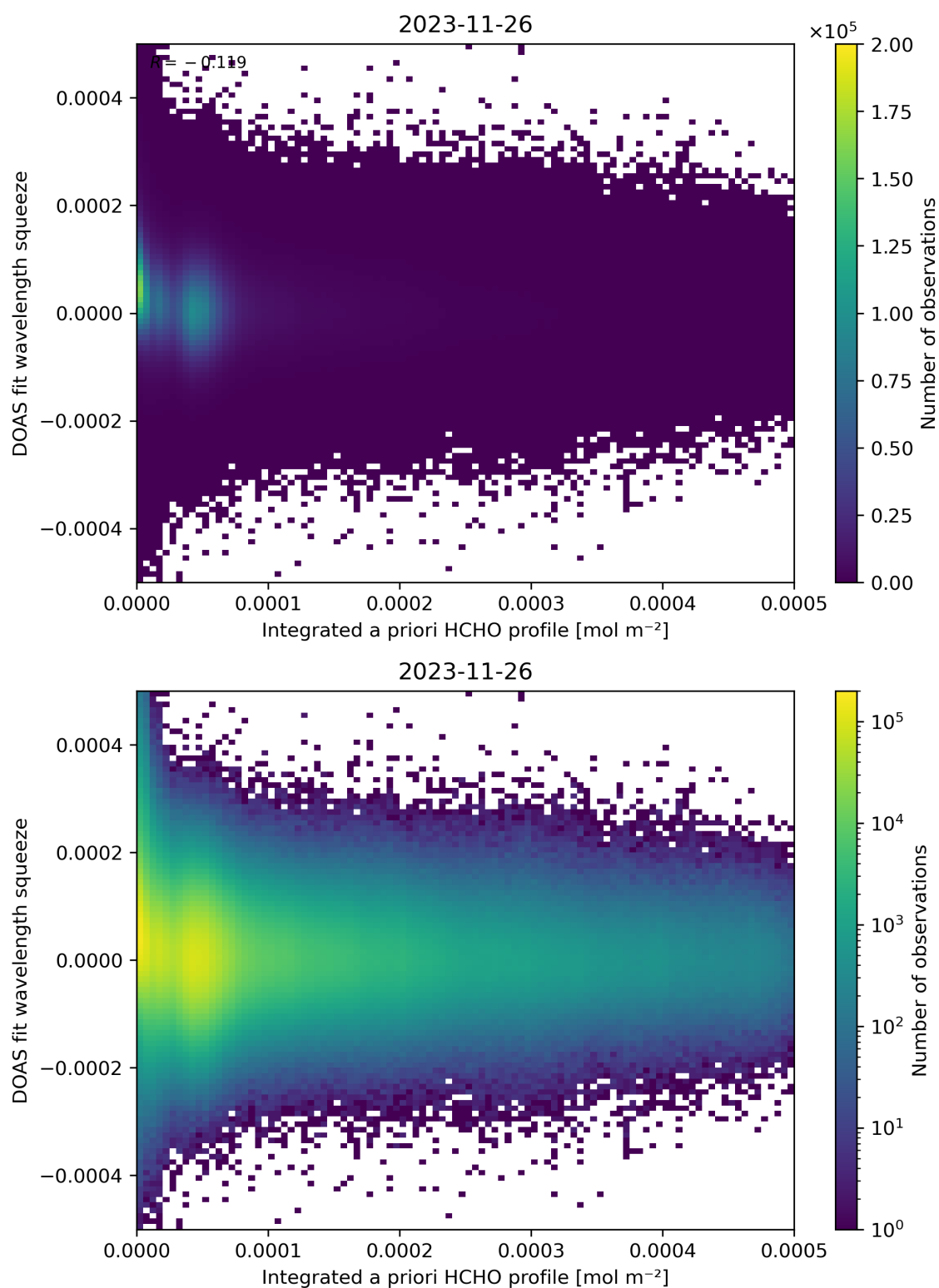
Figure 150: Scatter density plot of “Integrated a priori HCHO profile” against “DOAS fit wavelength squeeze” for 2023-11-25 to 2023-11-27.
