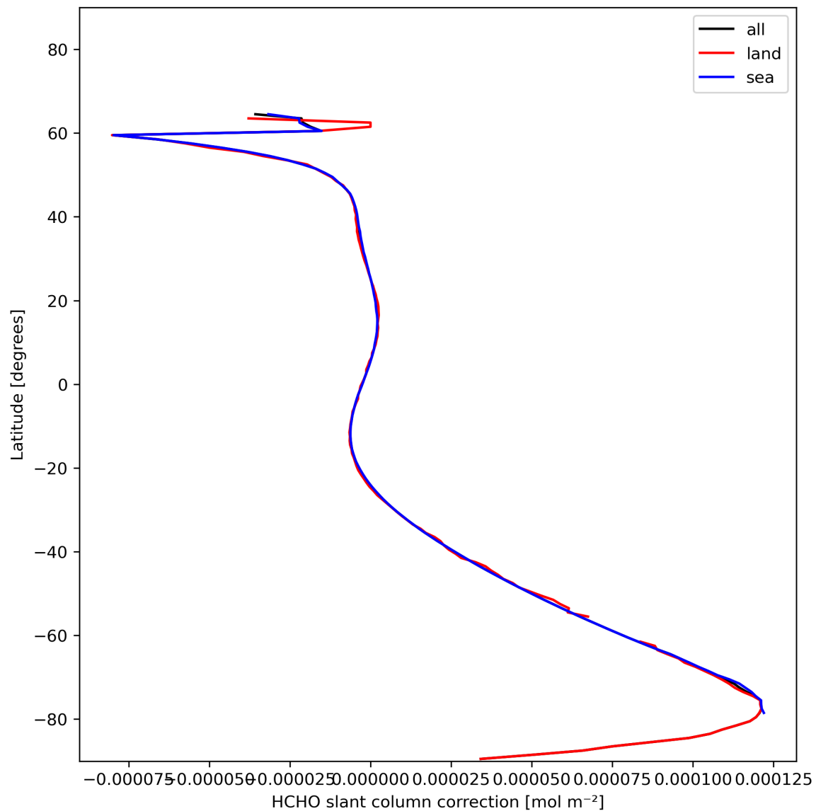
Figure 33: Zonal average of “HCHO slant column correction” for 2023-11-25 to 2023-11-27.
