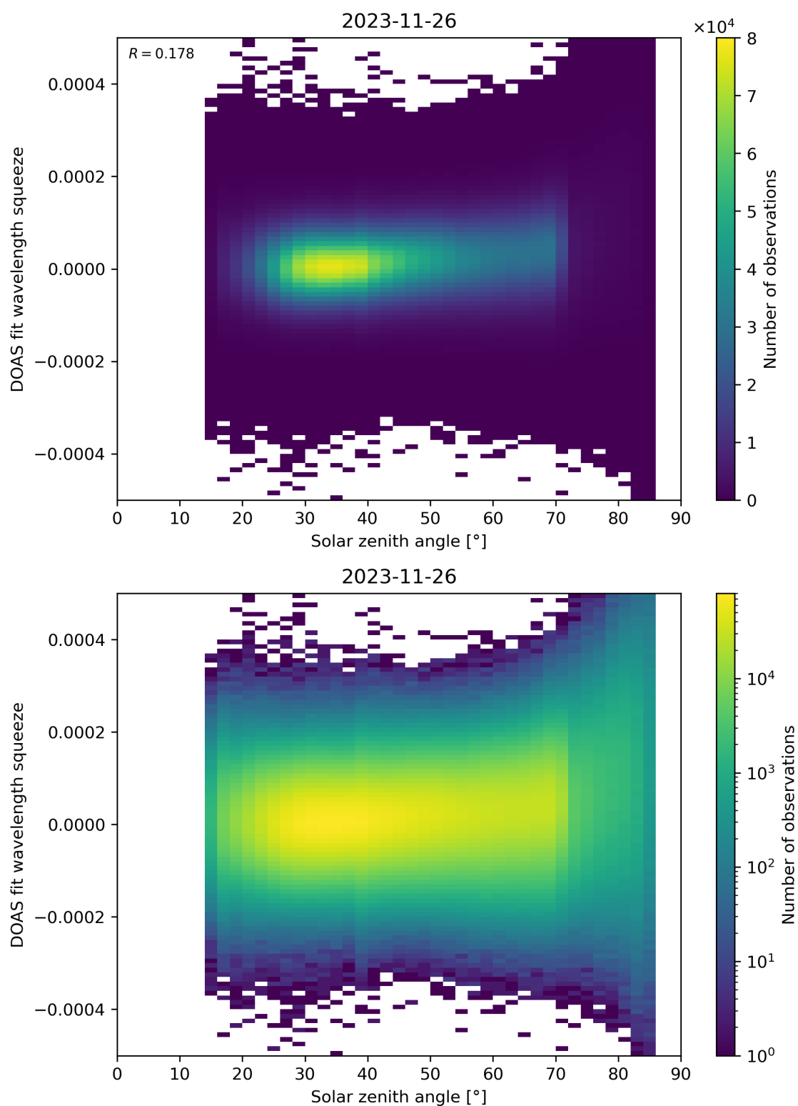
Figure 169: Scatter density plot of “Solar zenith angle” against “DOAS fit wavelength squeeze” for 2023-11-25 to 2023-11-27.
