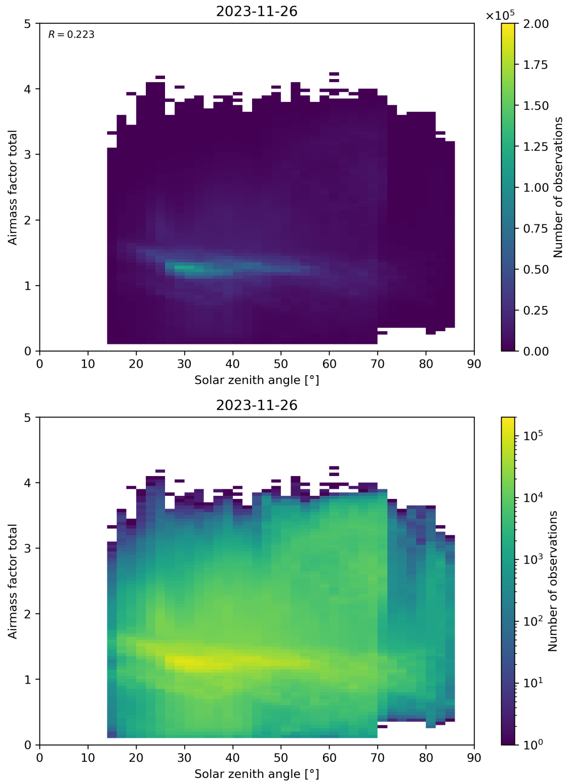
Figure 175: Scatter density plot of “Solar zenith angle” against “Airmass factor total” for 2023-11-25 to 2023-11-27.
