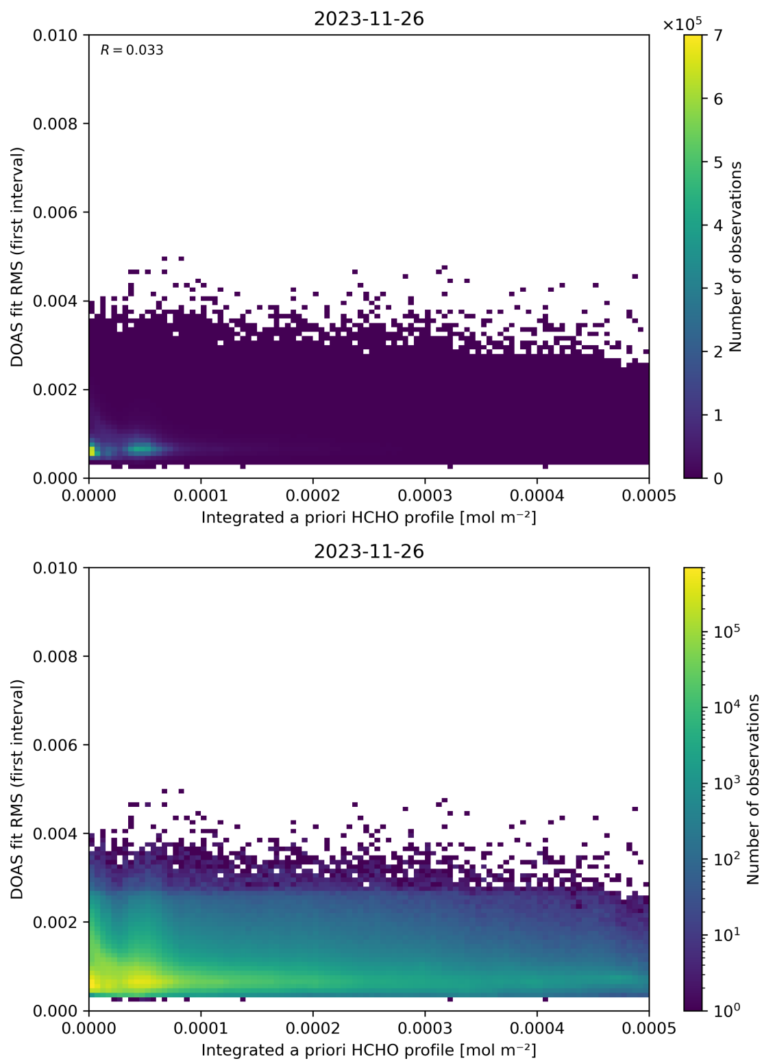
Figure 148: Scatter density plot of “Integrated a priori HCHO profile” against “DOAS fit RMS (first interval)” for 2023-11-25 to 2023-11-27.
