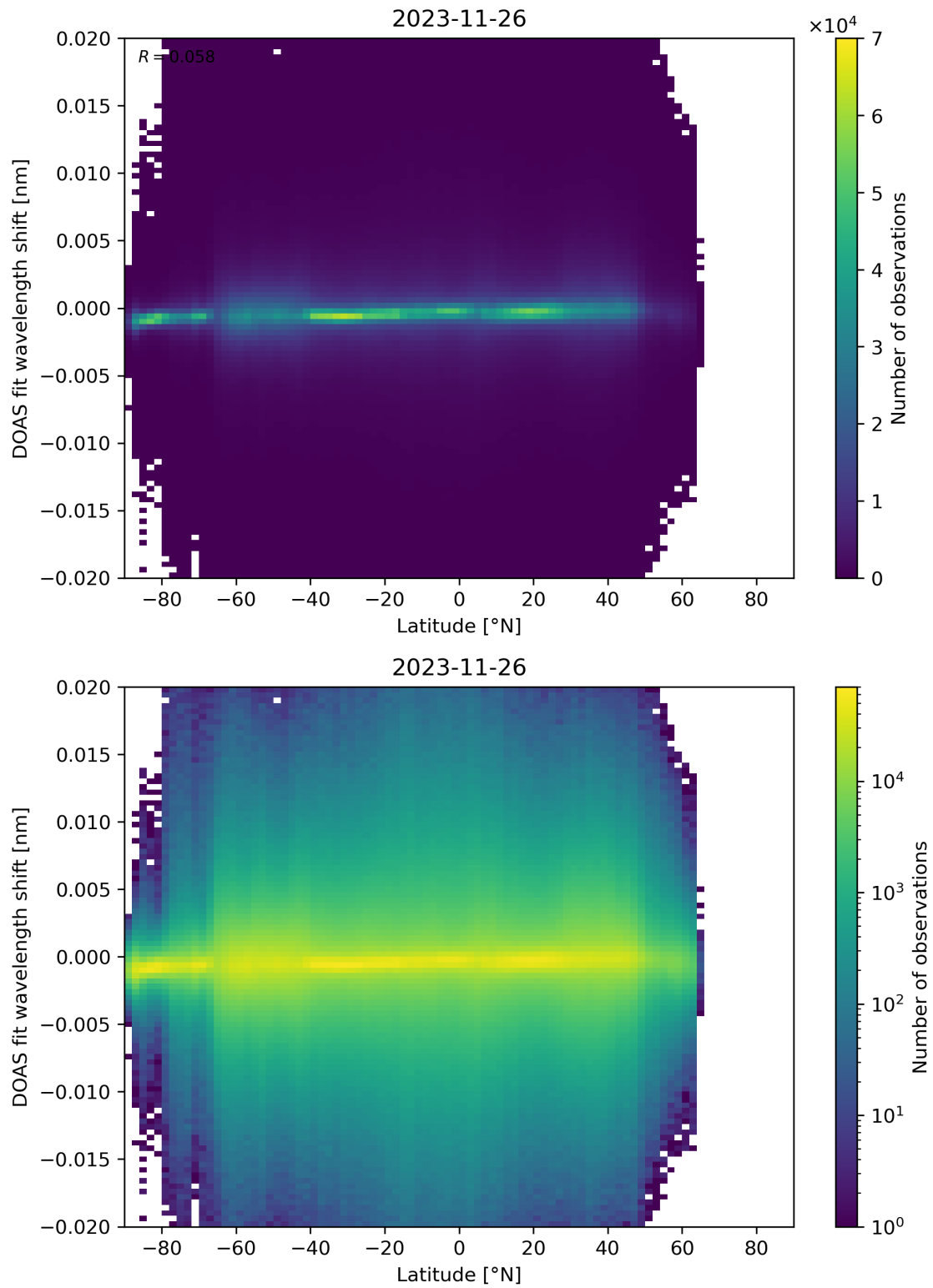
Figure 154: Scatter density plot of “Latitude” against “DOAS fit wavelength shift” for 2023-11-25 to 2023-11-27.
