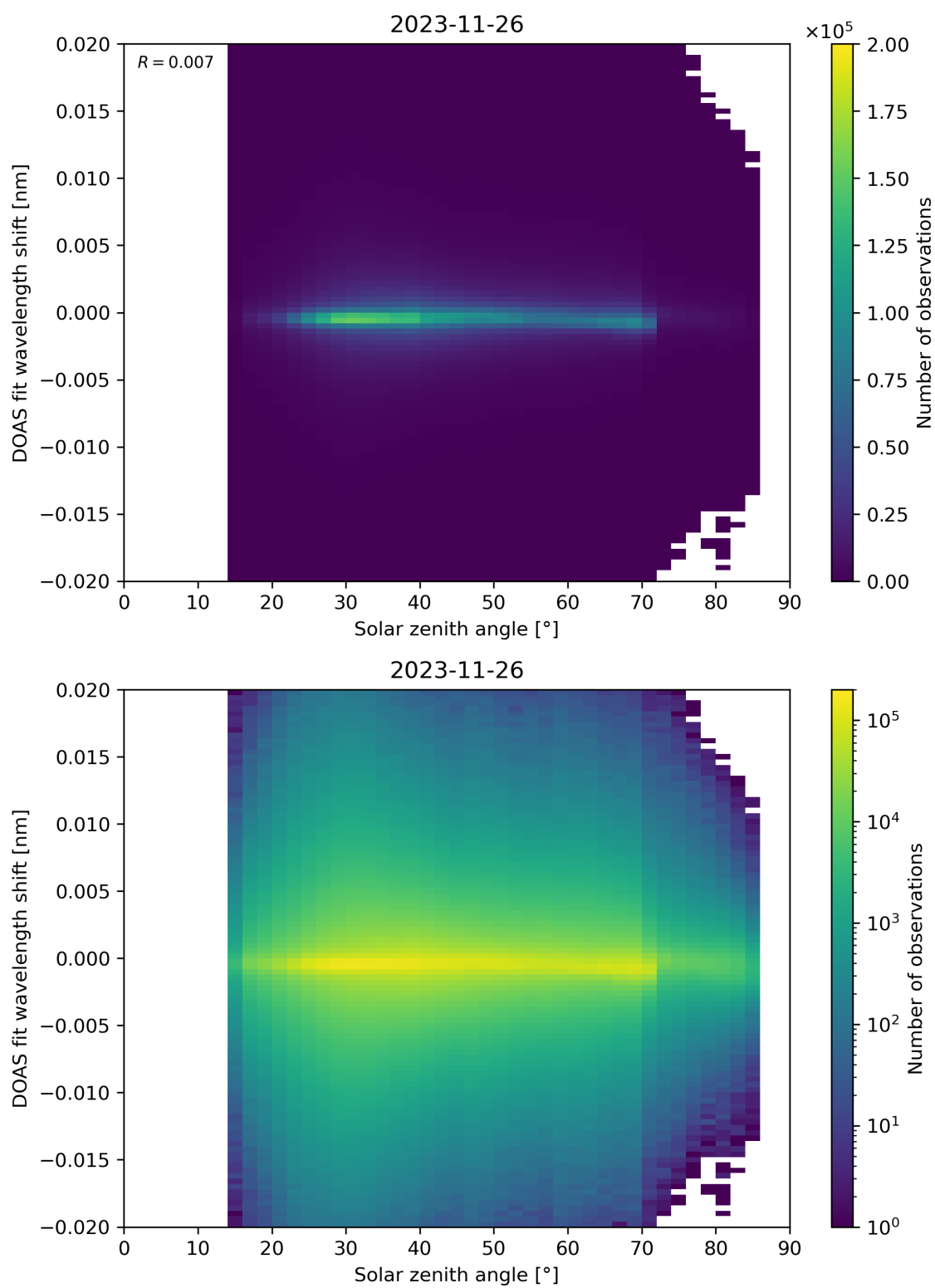
Figure 168: Scatter density plot of “Solar zenith angle” against “DOAS fit wavelength shift” for 2023-11-25 to 2023-11-27.
