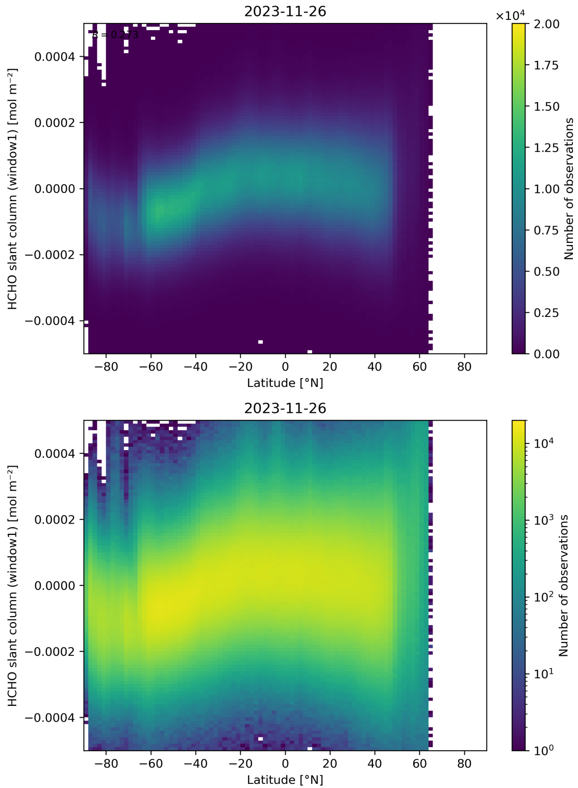
Figure 159: Scatter density plot of “Latitude” against “HCHO slant column (window1)” for 2023-11-25 to 2023-11-27.
