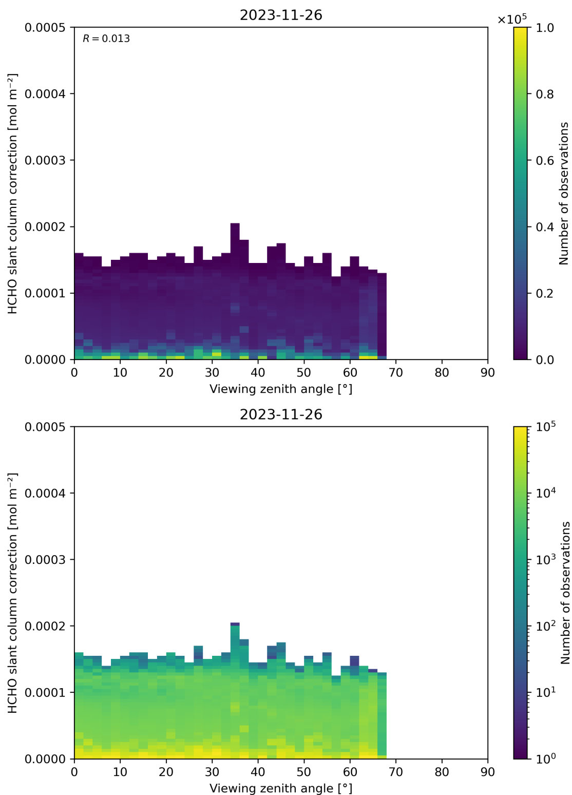
Figure 187: Scatter density plot of “Viewing zenith angle” against “HCHO slant column correction” for 2023-11-25 to 2023-11-27.
