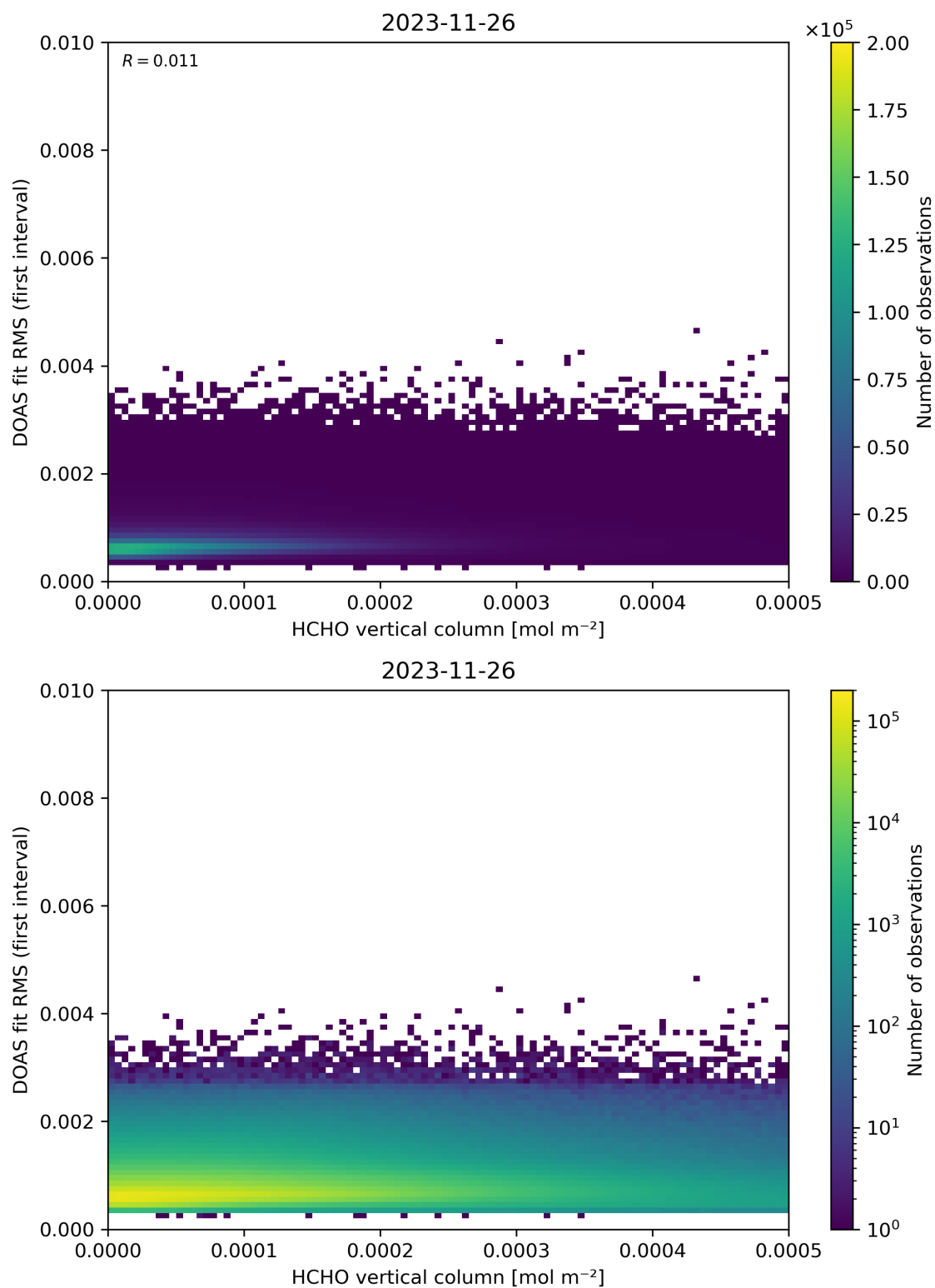
Figure 123: Scatter density plot of “HCHO vertical column” against “DOAS fit RMS (first interval)” for 2023-11-25 to 2023-11-27.
