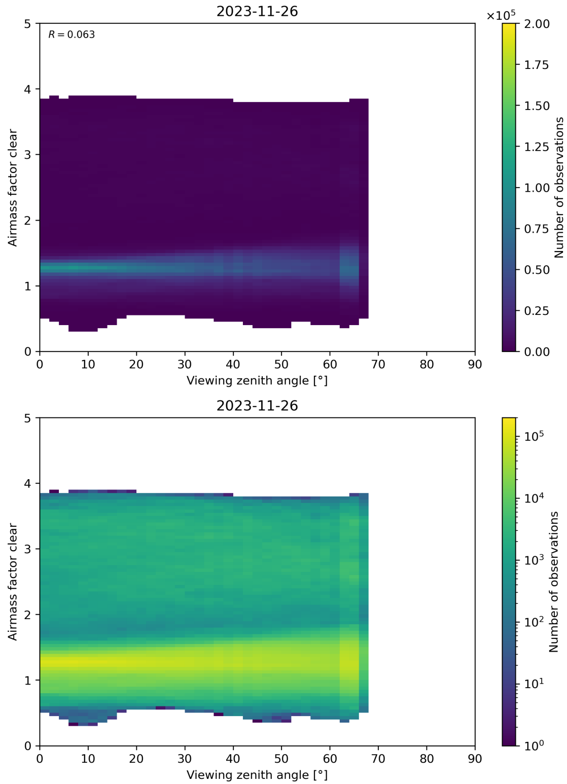
Figure 185: Scatter density plot of “Viewing zenith angle” against “Airmass factor clear” for 2023-11-25 to 2023-11-27.
