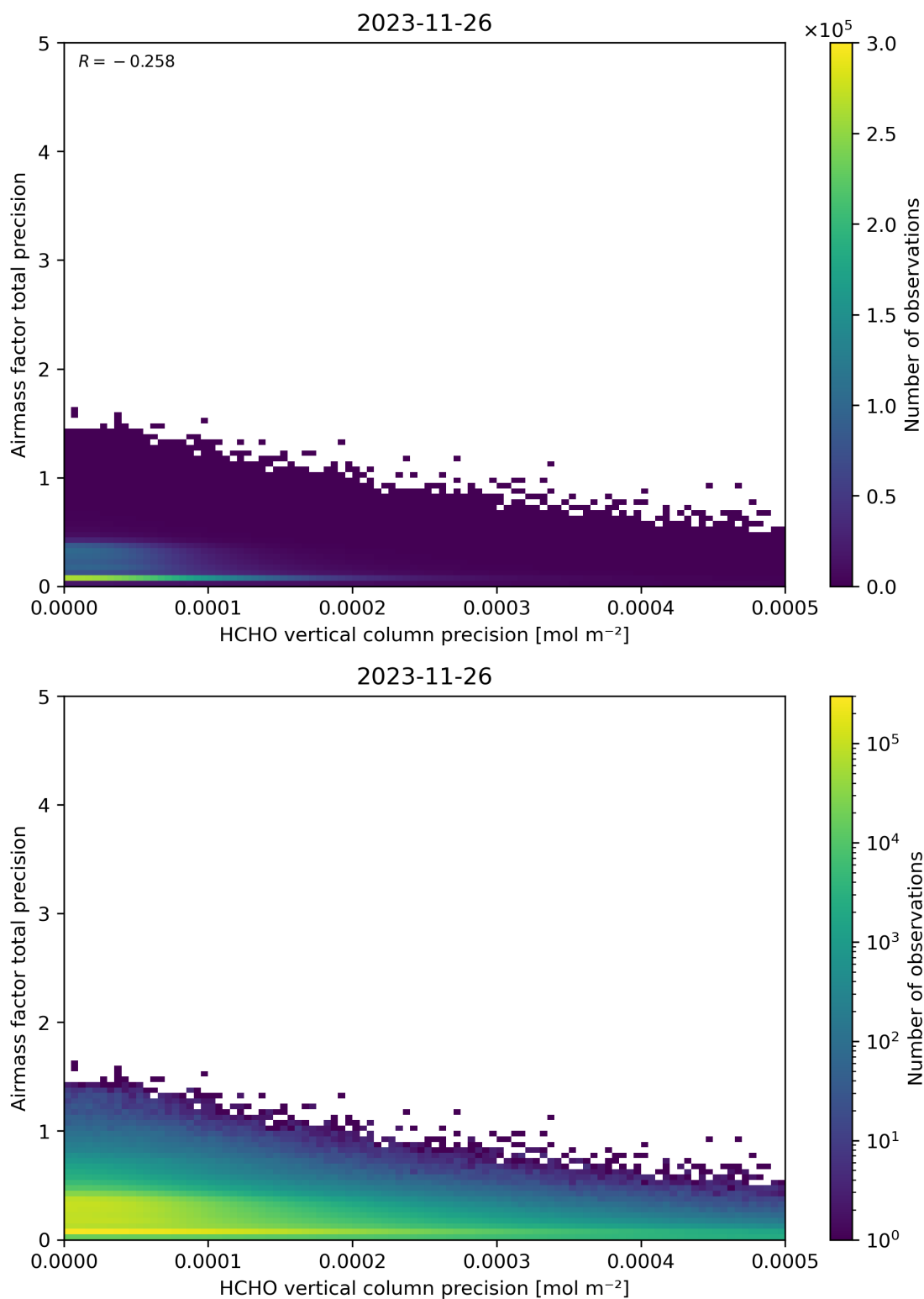
Figure 145: Scatter density plot of “HCHO vertical column precision” against “Airmass factor total precision” for 2023-11-25 to 2023-11-27.
