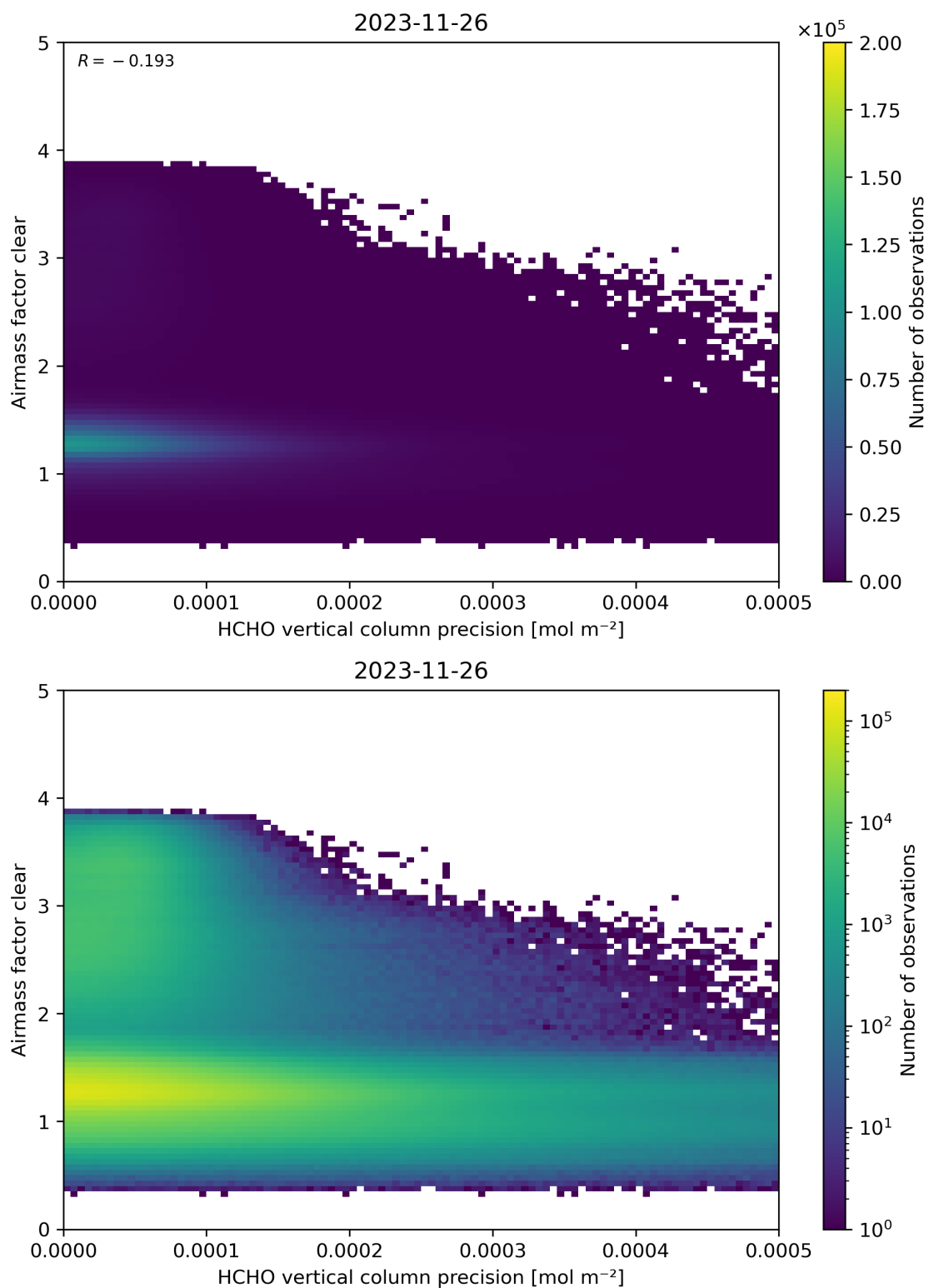
Figure 139: Scatter density plot of “HCHO vertical column precision” against “Airmass factor clear” for 2023-11-25 to 2023-11-27.
