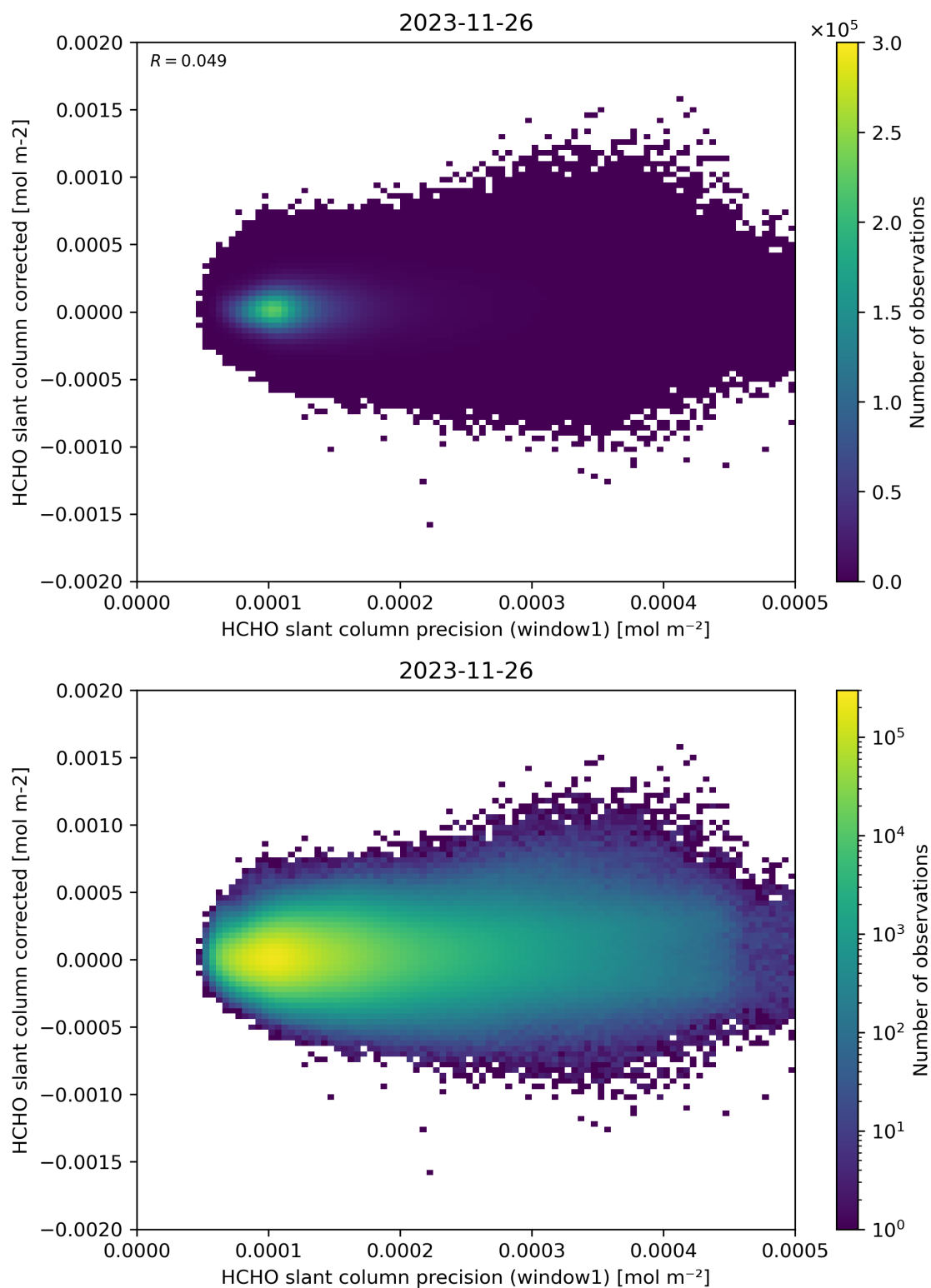
Figure 92: Scatter density plot of “HCHO slant column precision (window1)” against “HCHO slant column corrected” for 2023-11-25 to 2023-11-27.
