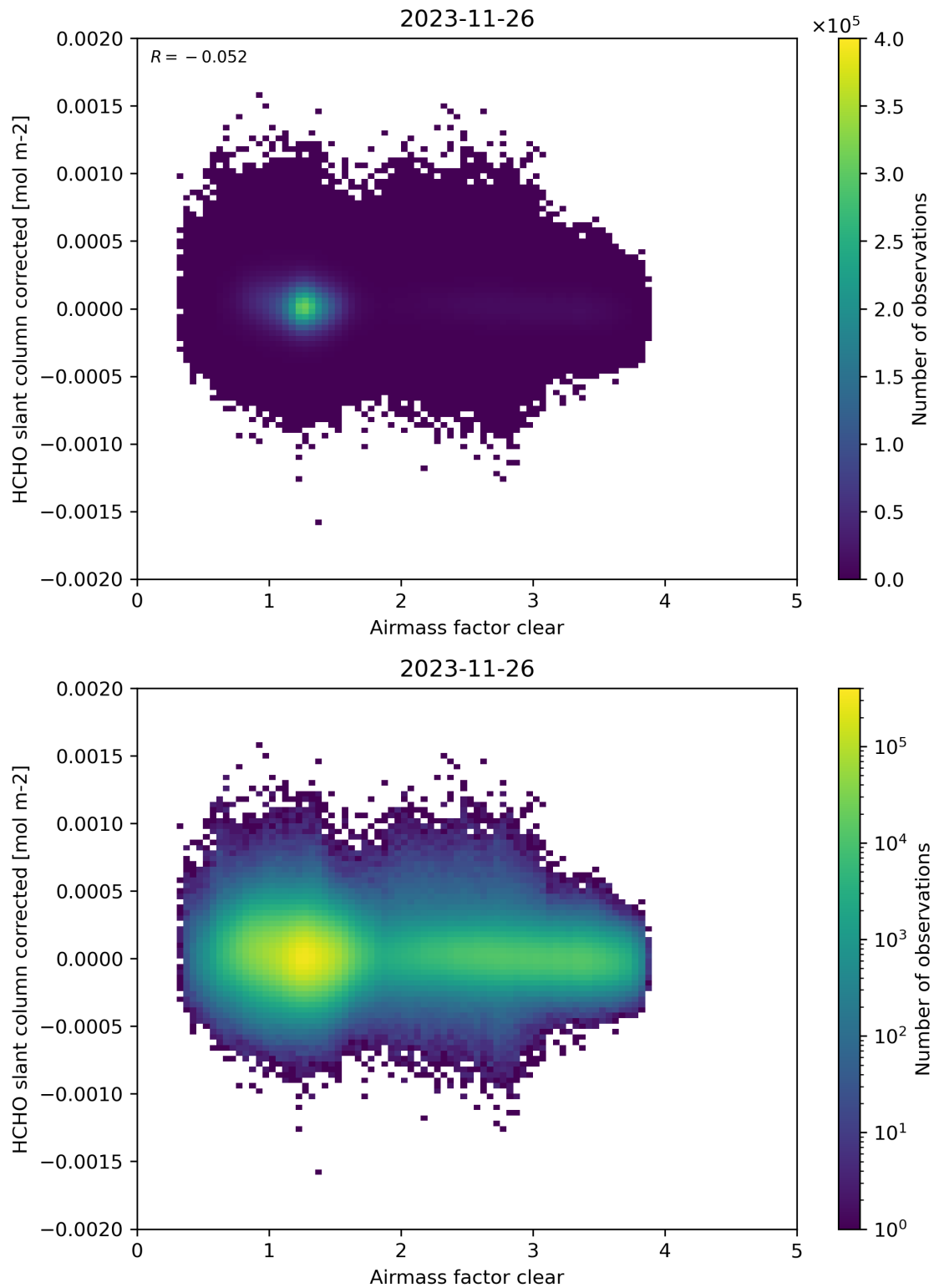
Figure 74: Scatter density plot of “Airmass factor clear” against “HCHO slant column corrected” for 2023-11-25 to 2023-11-27.
