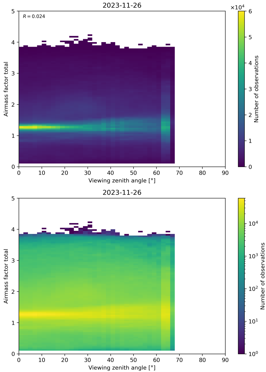
Figure 190: Scatter density plot of “Viewing zenith angle” against “Airmass factor total” for 2023-11-25 to 2023-11-27.
