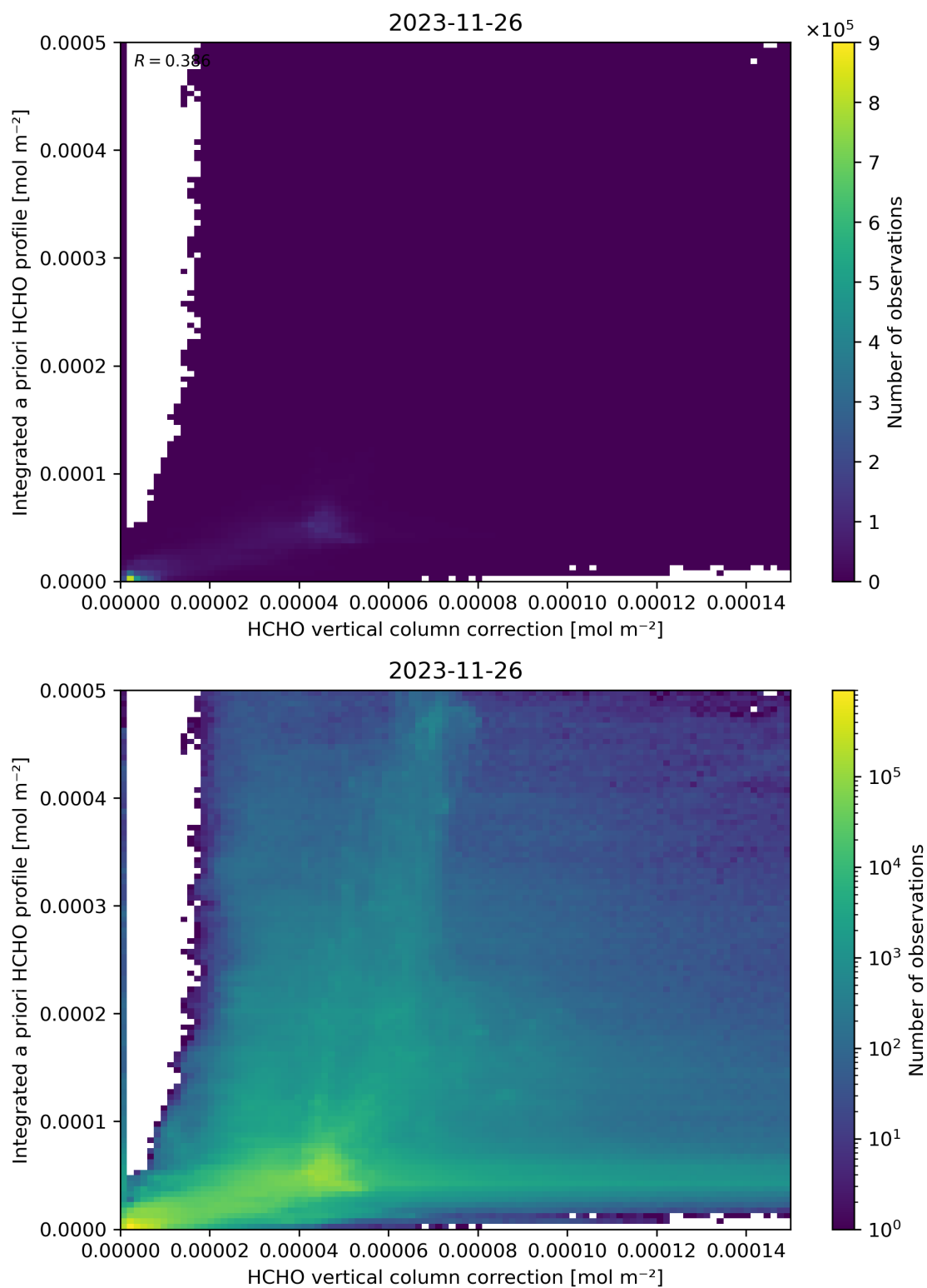
Figure 122: Scatter density plot of “HCHO vertical column correction” against “Integrated a priori HCHO profile” for 2023-11-25 to 2023-11-27.
