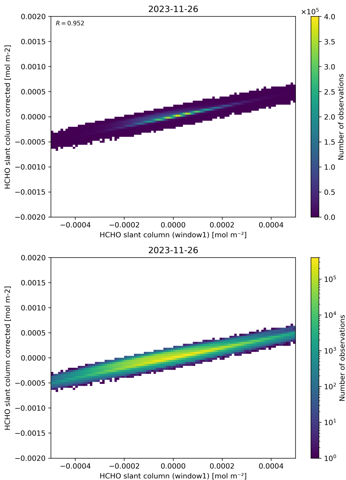
Figure 82: Scatter density plot of “HCHO slant column (window1)” against “HCHO slant column corrected” for 2023-11-25 to 2023-11-27.
