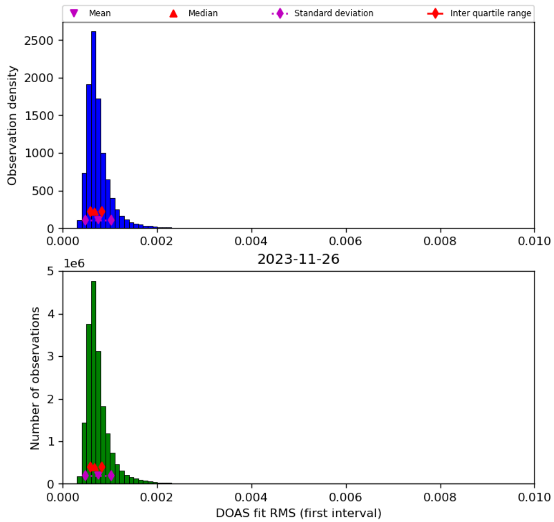
Figure 46: Histogram of “DOAS fit RMS (first interval)” for 2023-11-25 to 2023-11-27
