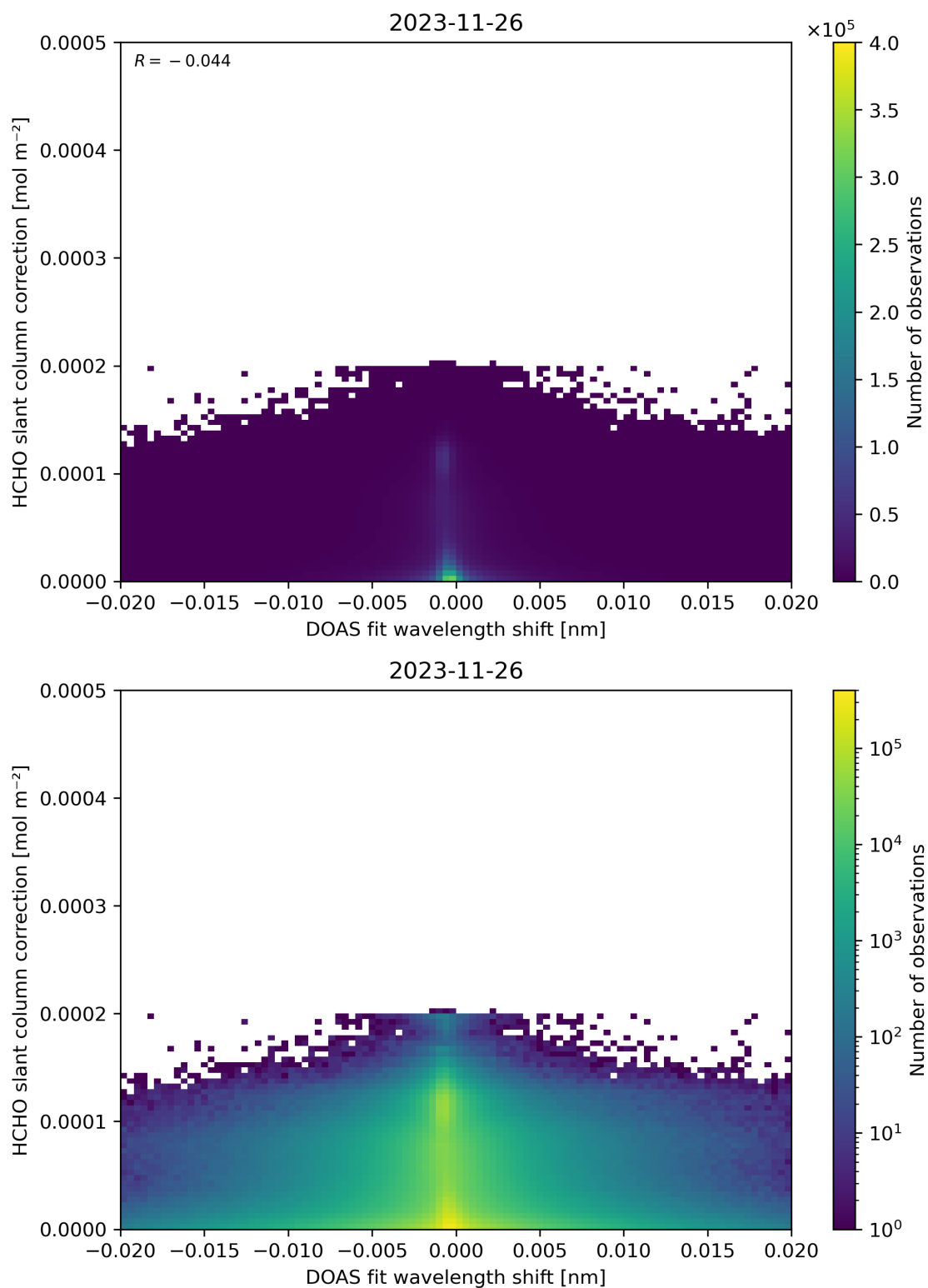
Figure 67: Scatter density plot of “DOAS fit wavelength shift” against “HCHO slant column correction” for 2023-11-25 to 2023-11-27.
