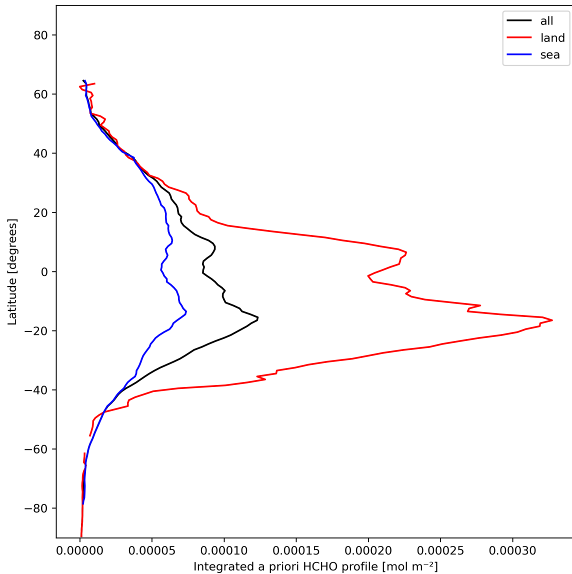
Figure 29: Zonal average of “Integrated a priori HCHO profile” for 2023-11-25 to 2023-11-27.
