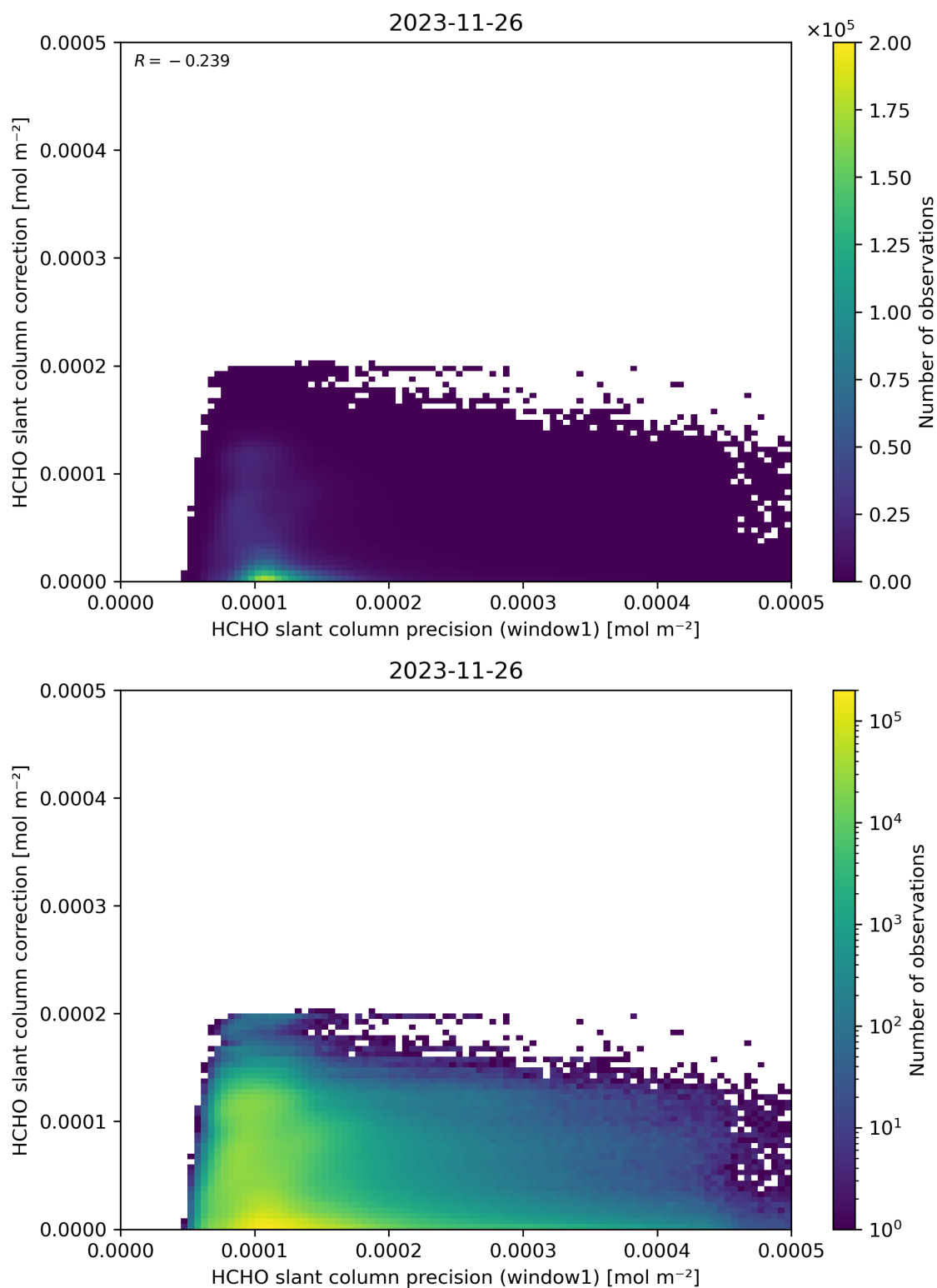
Figure 93: Scatter density plot of “HCHO slant column precision (window1)” against “HCHO slant column correction” for 2023-11-25 to 2023-11-27.
