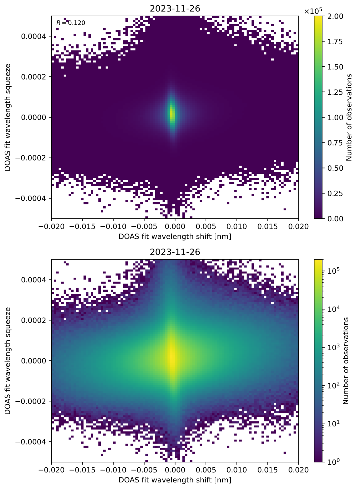
Figure 65: Scatter density plot of “DOAS fit wavelength shift” against “DOAS fit wavelength squeeze” for 2023-11-25 to 2023-11-27.
