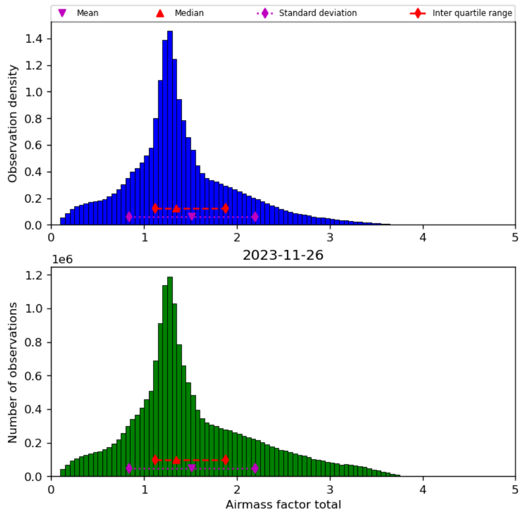
Figure 40: Histogram of “Airmass factor total” for 2023-11-25 to 2023-11-27
