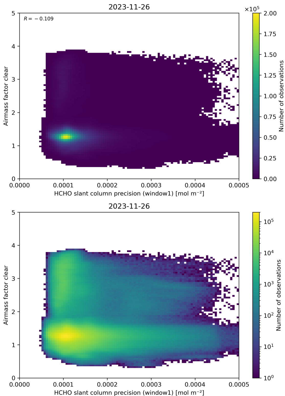
Figure 91: Scatter density plot of “HCHO slant column precision (window1)” against “Airmass factor clear” for 2023-11-25 to 2023-11-27.
