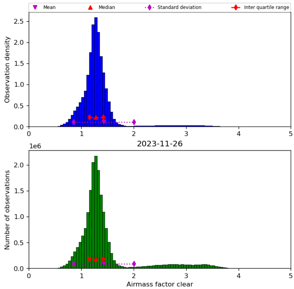
Figure 42: Histogram of “Airmass factor clear” for 2023-11-25 to 2023-11-27
