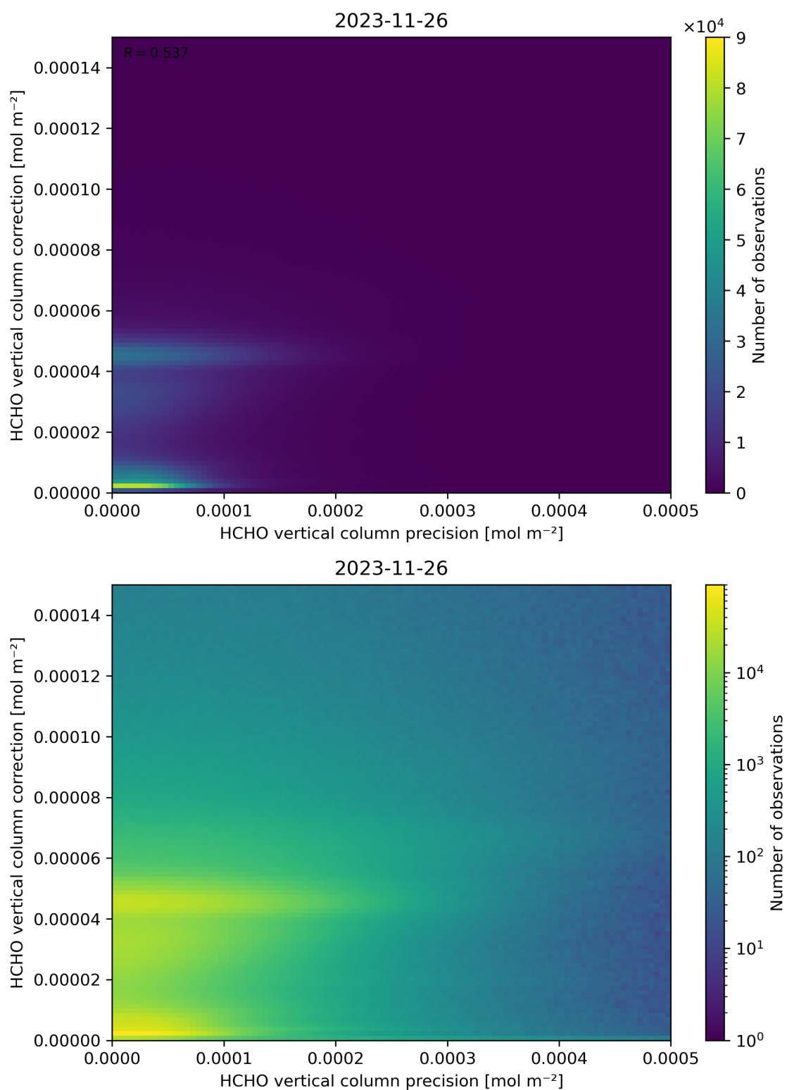
Figure 146: Scatter density plot of “HCHO vertical column precision” against “HCHO vertical column correction” for 2023-11-25 to 2023-11-27.
