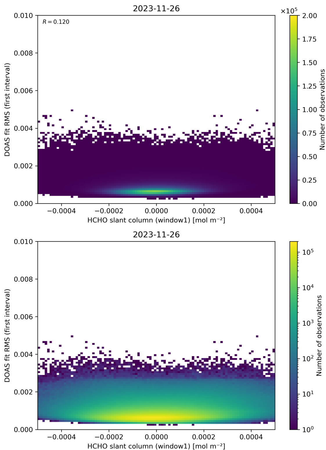
Figure 78: Scatter density plot of “HCHO slant column (window1)” against “DOAS fit RMS (first interval)” for 2023-11-25 to 2023-11-27.
