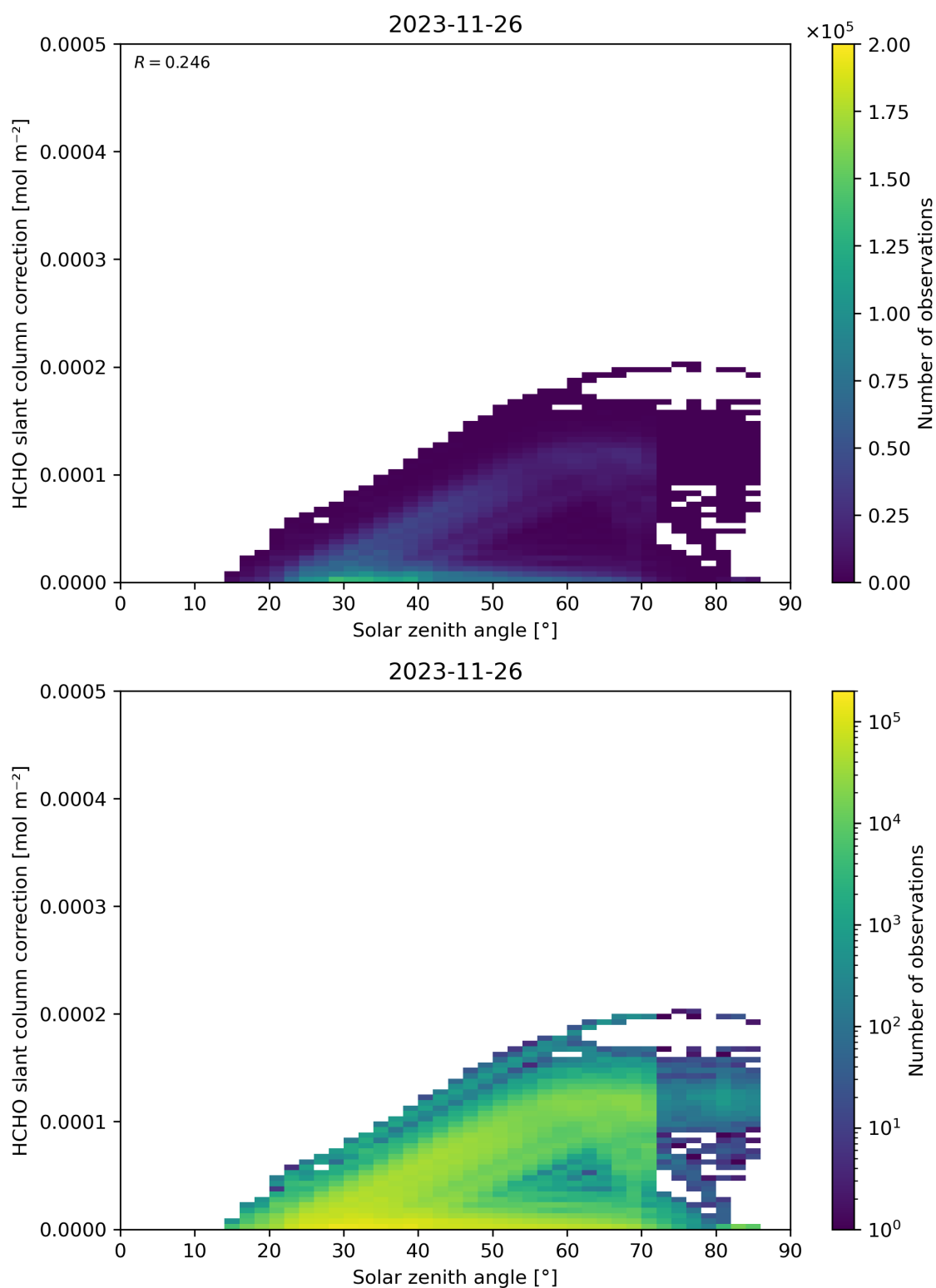
Figure 172: Scatter density plot of “Solar zenith angle” against “HCHO slant column correction” for 2023-11-25 to 2023-11-27.
