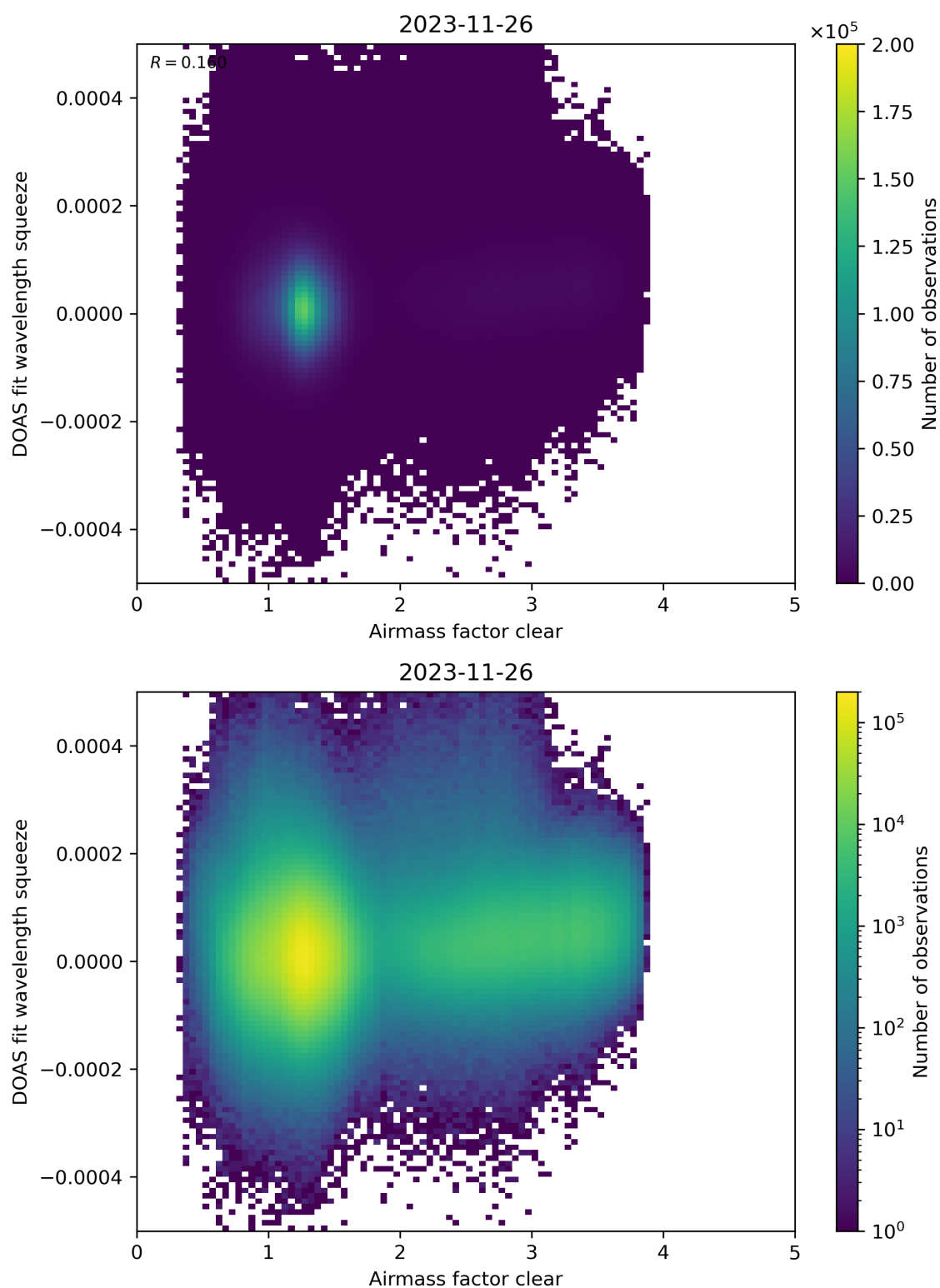
Figure 73: Scatter density plot of “Airmass factor clear” against “DOAS fit wavelength squeeze” for 2023-11-25 to 2023-11-27.
