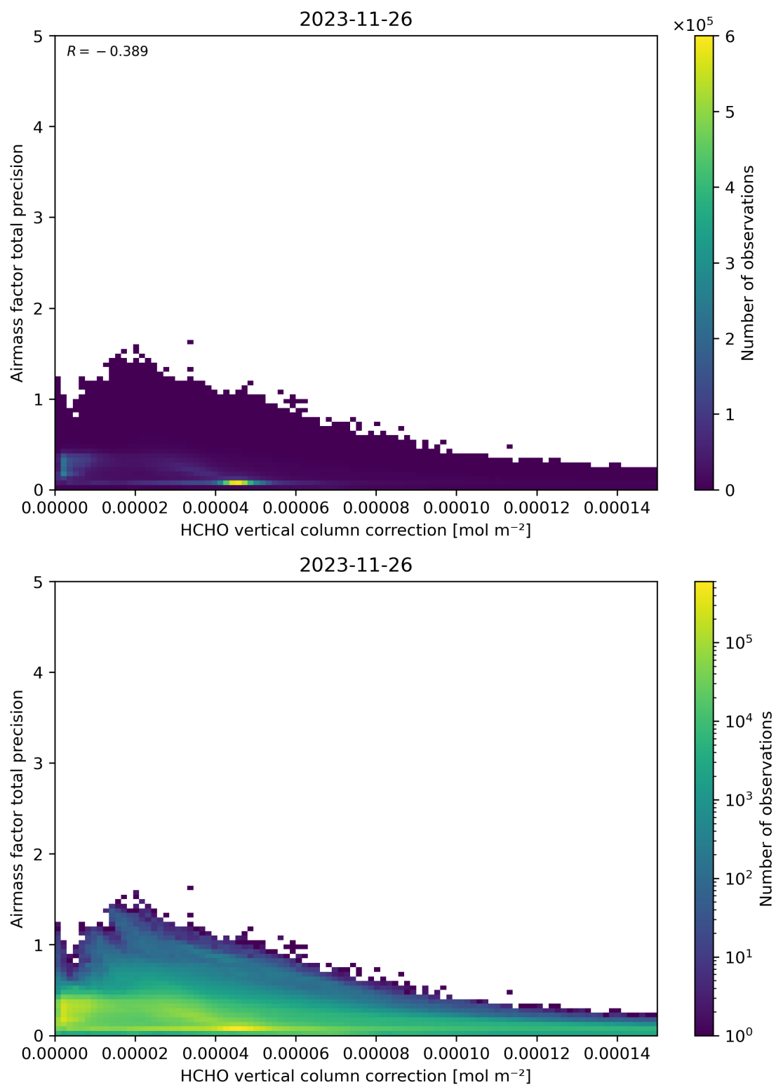
Figure 121: Scatter density plot of “HCHO vertical column correction” against “Airmass factor total precision” for 2023-11-25 to 2023-11-27.
