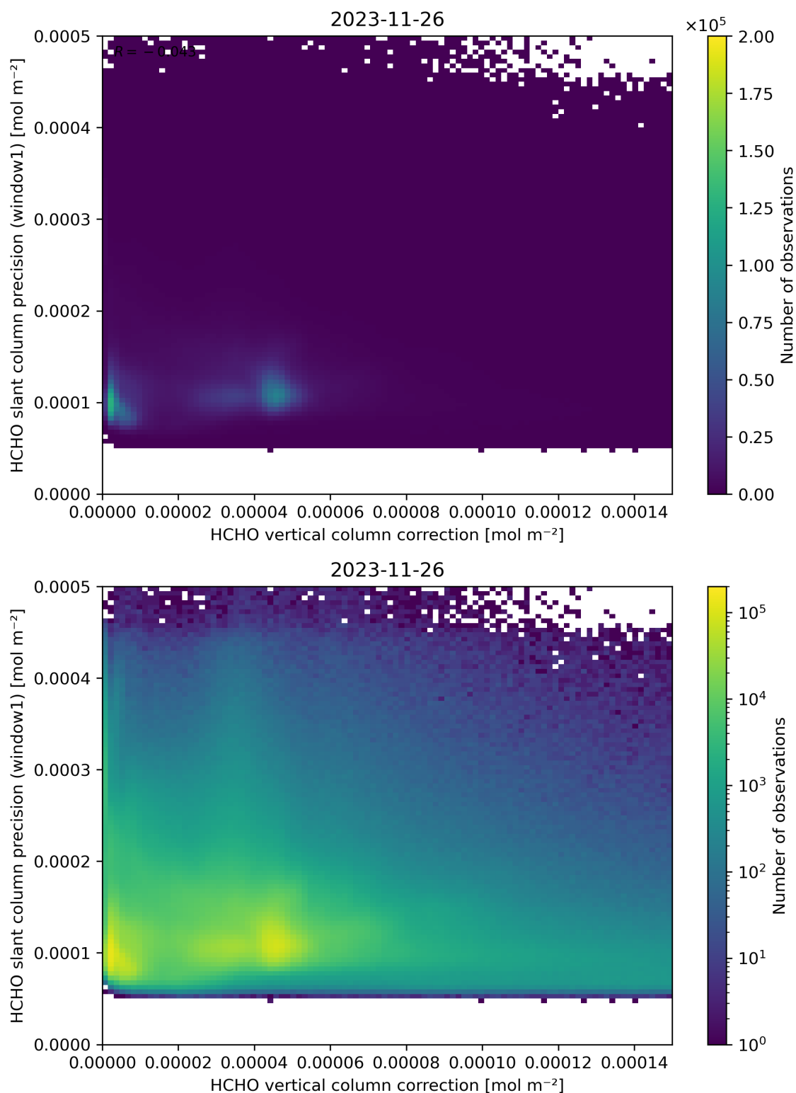
Figure 119: Scatter density plot of “HCHO vertical column correction” against “HCHO slant column precision (window1)” for 2023-11-25 to 2023-11-27.
