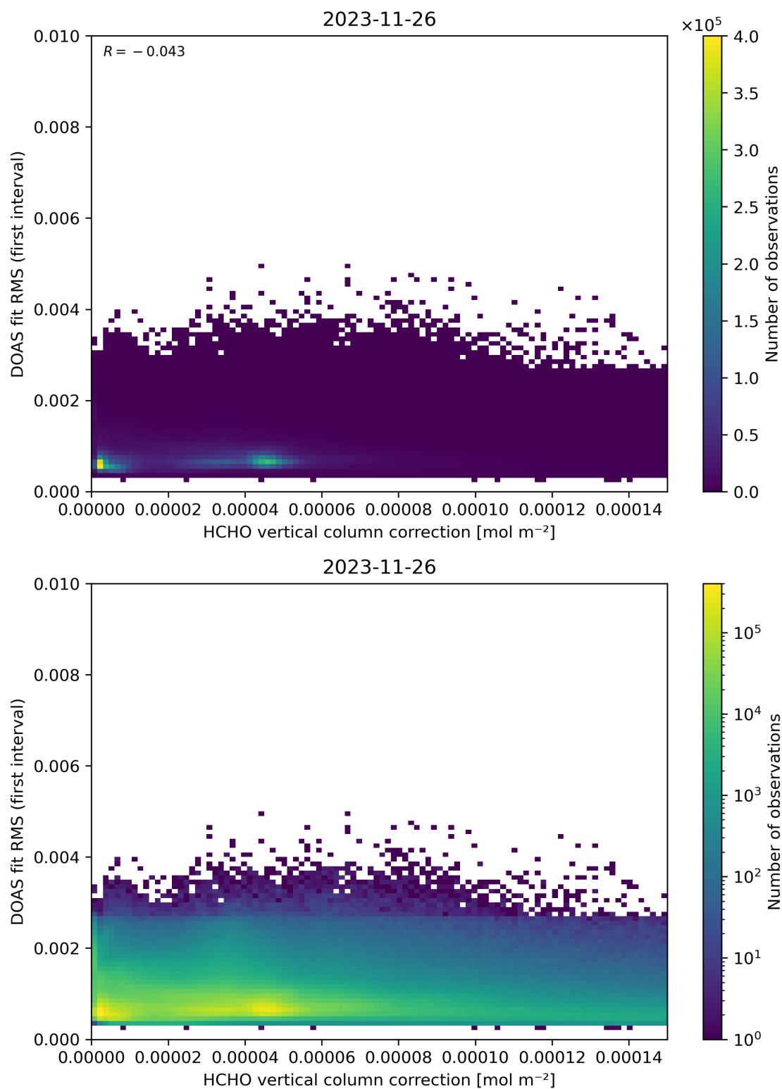
Figure 112: Scatter density plot of “HCHO vertical column correction” against “DOAS fit RMS (first interval)” for 2023-11-25 to 2023-11-27.
