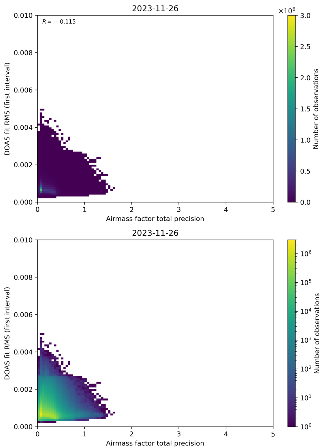
Figure 105: Scatter density plot of “Airmass factor total precision” against “DOAS fit RMS (first interval)” for 2023-11-25 to 2023-11-27.
