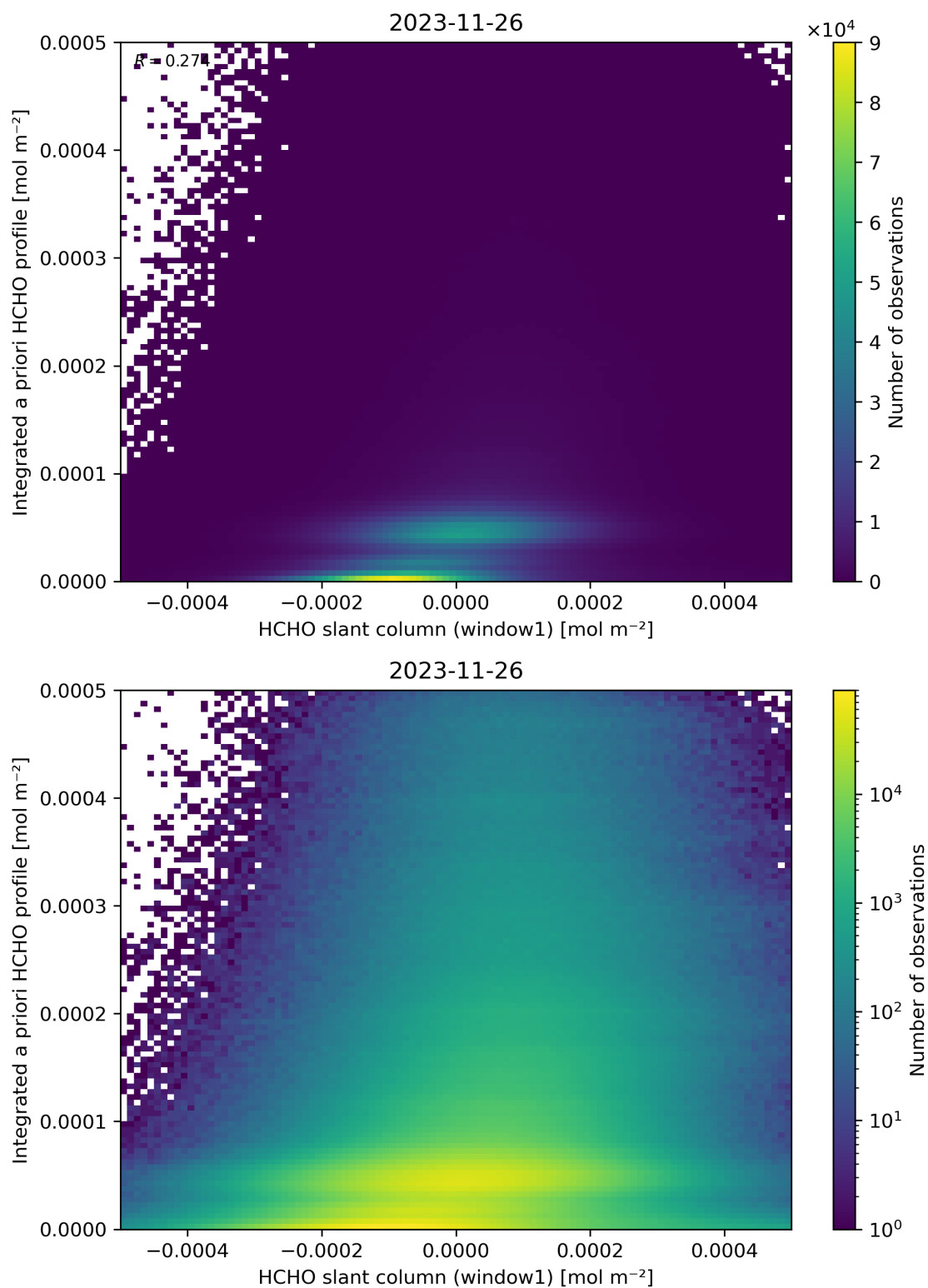
Figure 87: Scatter density plot of “HCHO slant column (window1)” against “Integrated a priori HCHO profile” for 2023-11-25 to 2023-11-27.
