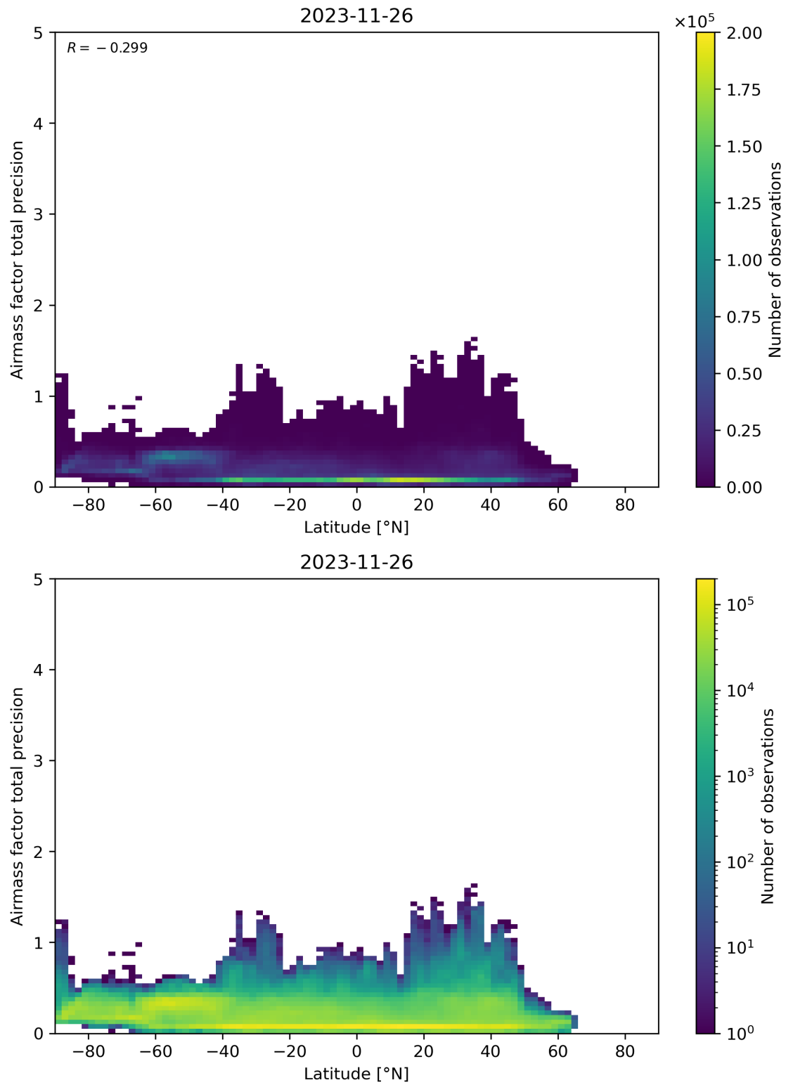
Figure 162: Scatter density plot of “Latitude” against “Airmass factor total precision” for 2023-11-25 to 2023-11-27.
