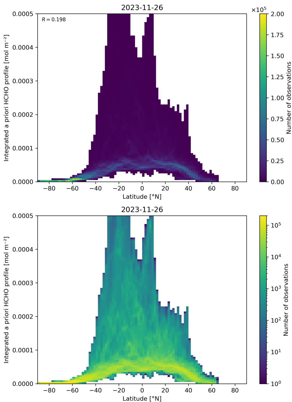
Figure 166: Scatter density plot of “Latitude” against “Integrated a priori HCHO profile” for 2023-11-25 to 2023-11-27.
