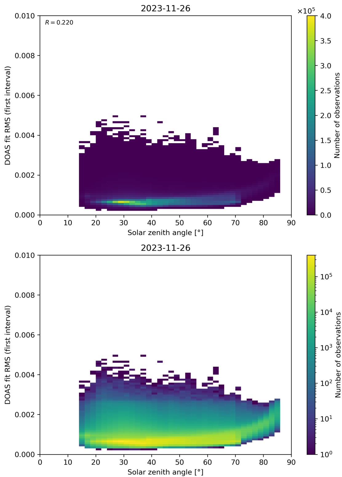
Figure 167: Scatter density plot of “Solar zenith angle” against “DOAS fit RMS (first interval)” for 2023-11-25 to 2023-11-27.
