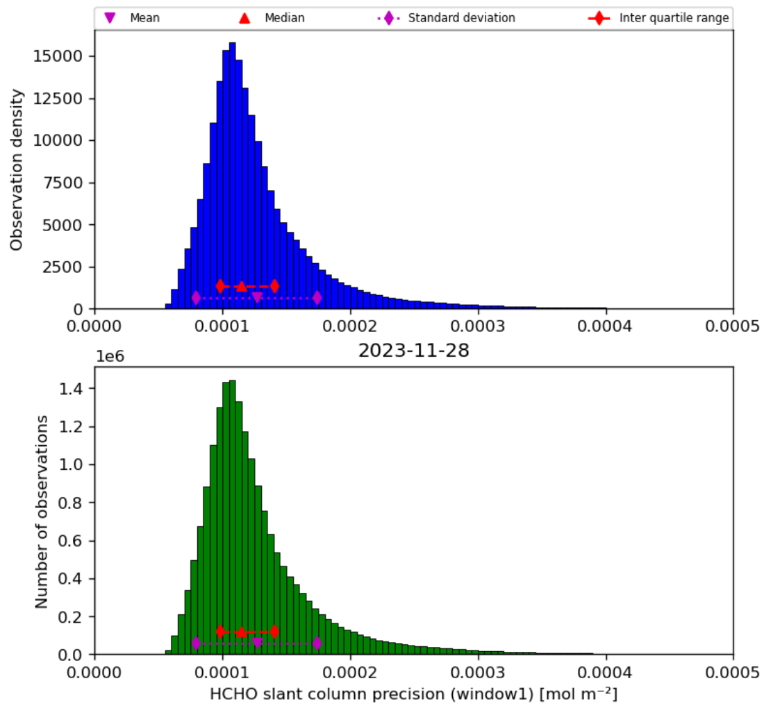
Figure 39: Histogram of “HCHO slant column precision (window1)” for 2023-11-28 to 2023-11-29
