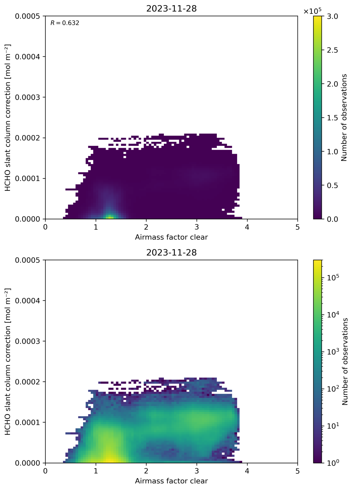
Figure 75: Scatter density plot of “Airmass factor clear” against “HCHO slant column correction” for 2023-11-28 to 2023-11-29.
