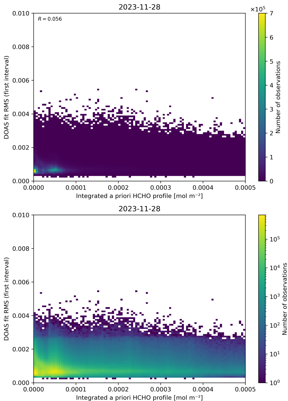
Figure 148: Scatter density plot of “Integrated a priori HCHO profile” against “DOAS fit RMS (first interval)” for 2023-11-28 to 2023-11-29.
