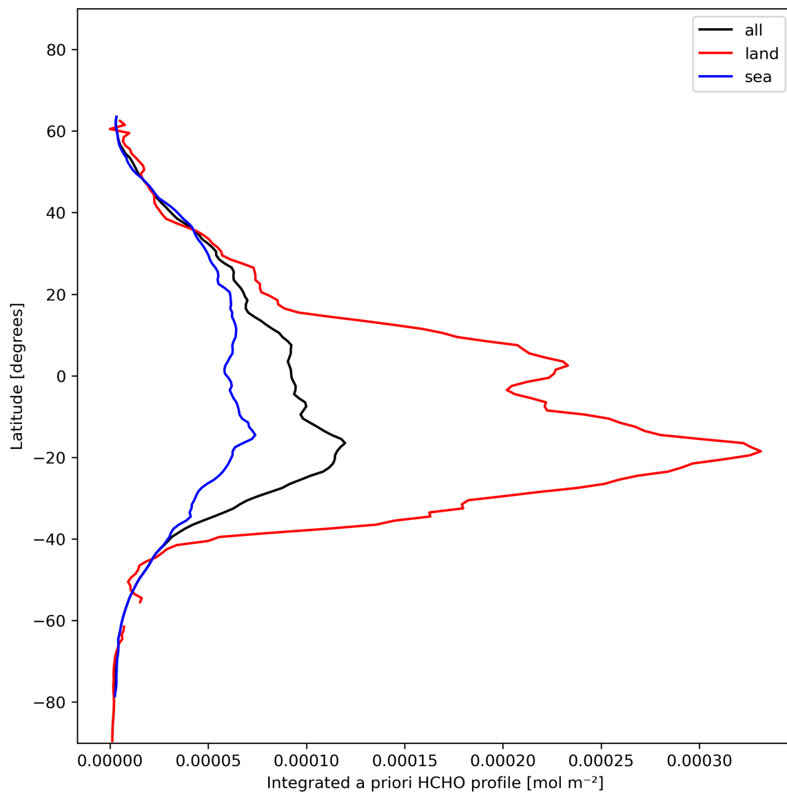
Figure 29: Zonal average of “Integrated a priori HCHO profile” for 2023-11-28 to 2023-11-29.
