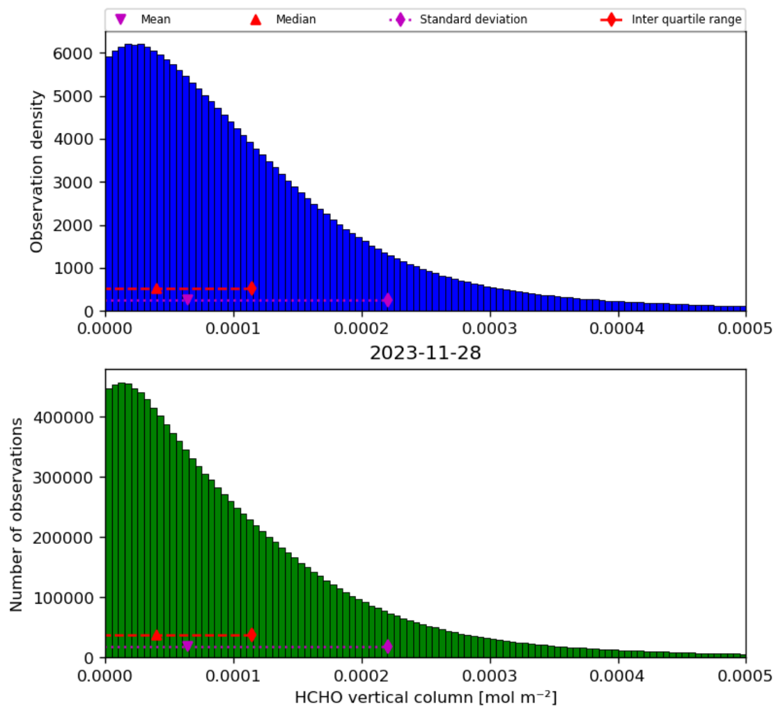
Figure 35: Histogram of “HCHO vertical column” for 2023-11-28 to 2023-11-29
