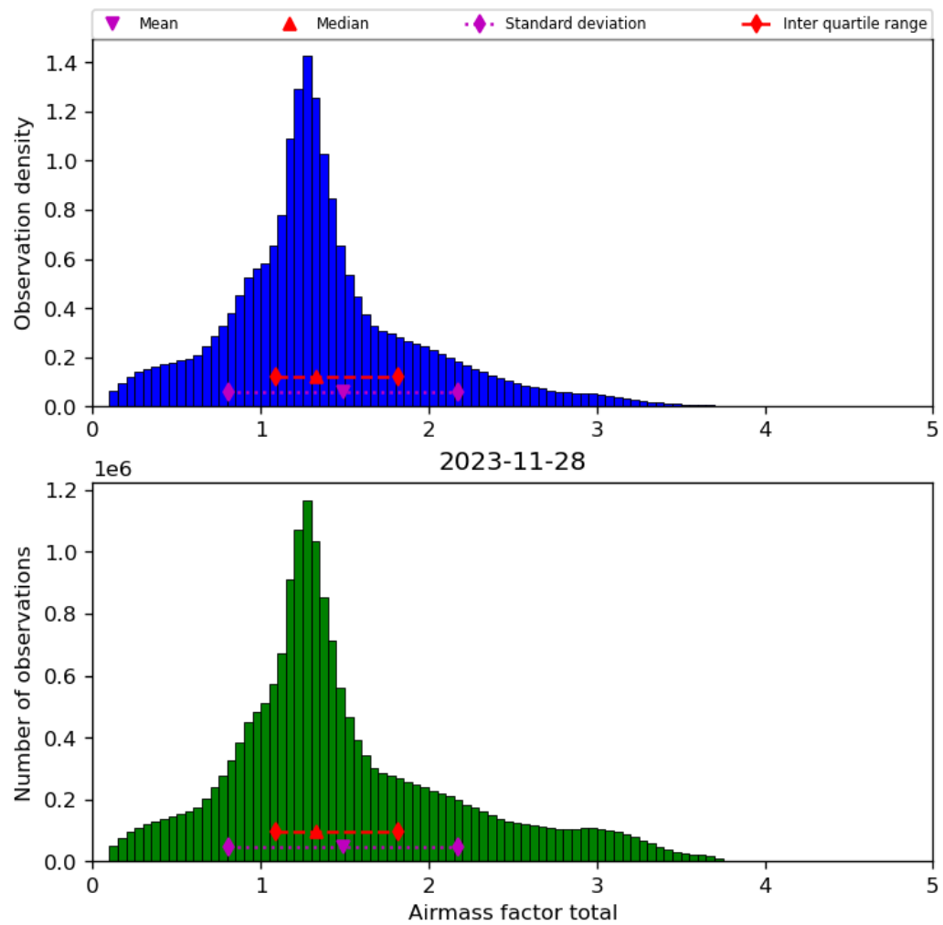
Figure 40: Histogram of “Airmass factor total” for 2023-11-28 to 2023-11-29
