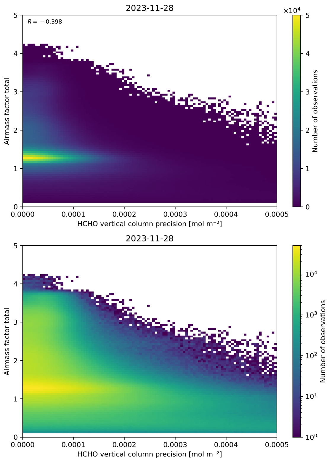
Figure 144: Scatter density plot of “HCHO vertical column precision” against “Airmass factor total” for 2023-11-28 to 2023-11-29.
