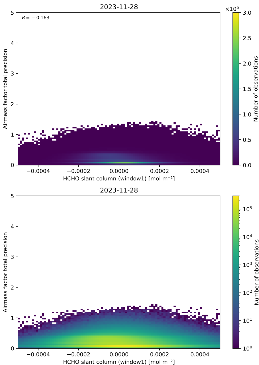
Figure 86: Scatter density plot of “HCHO slant column (window1)” against “Airmass factor total precision” for 2023-11-28 to 2023-11-29.
