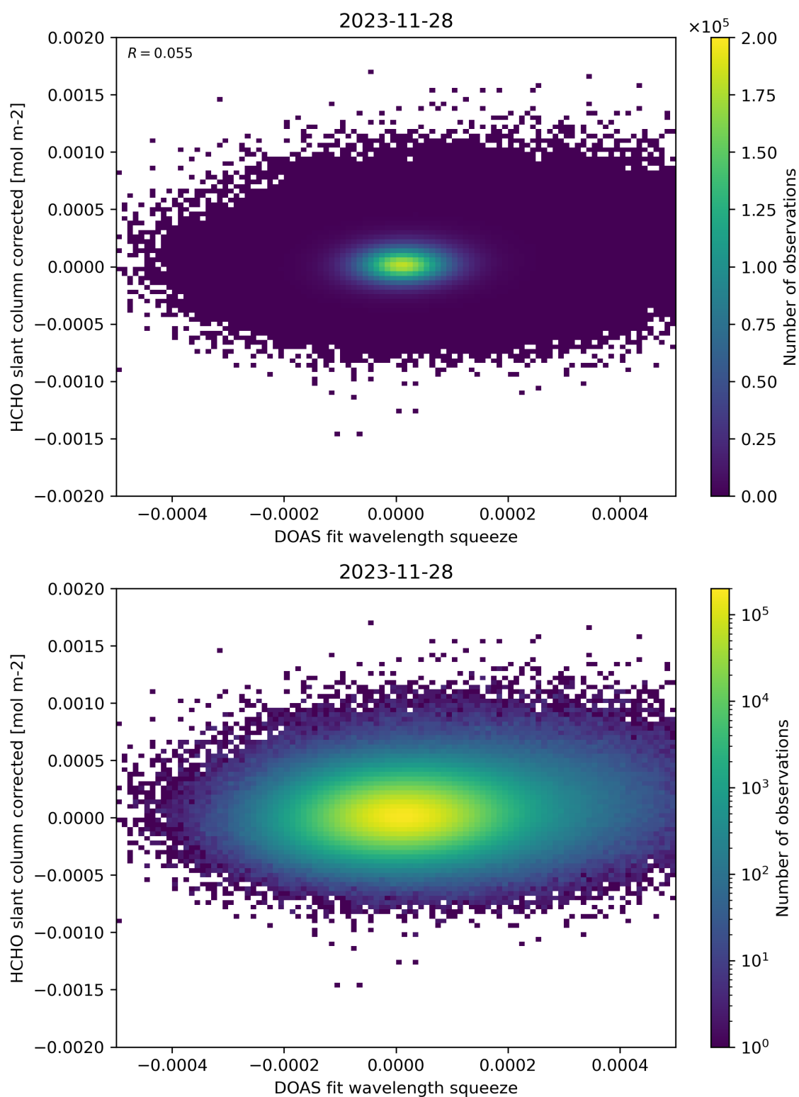
Figure 69: Scatter density plot of “DOAS fit wavelength squeeze” against “HCHO slant column corrected” for 2023-11-28 to 2023-11-29.
