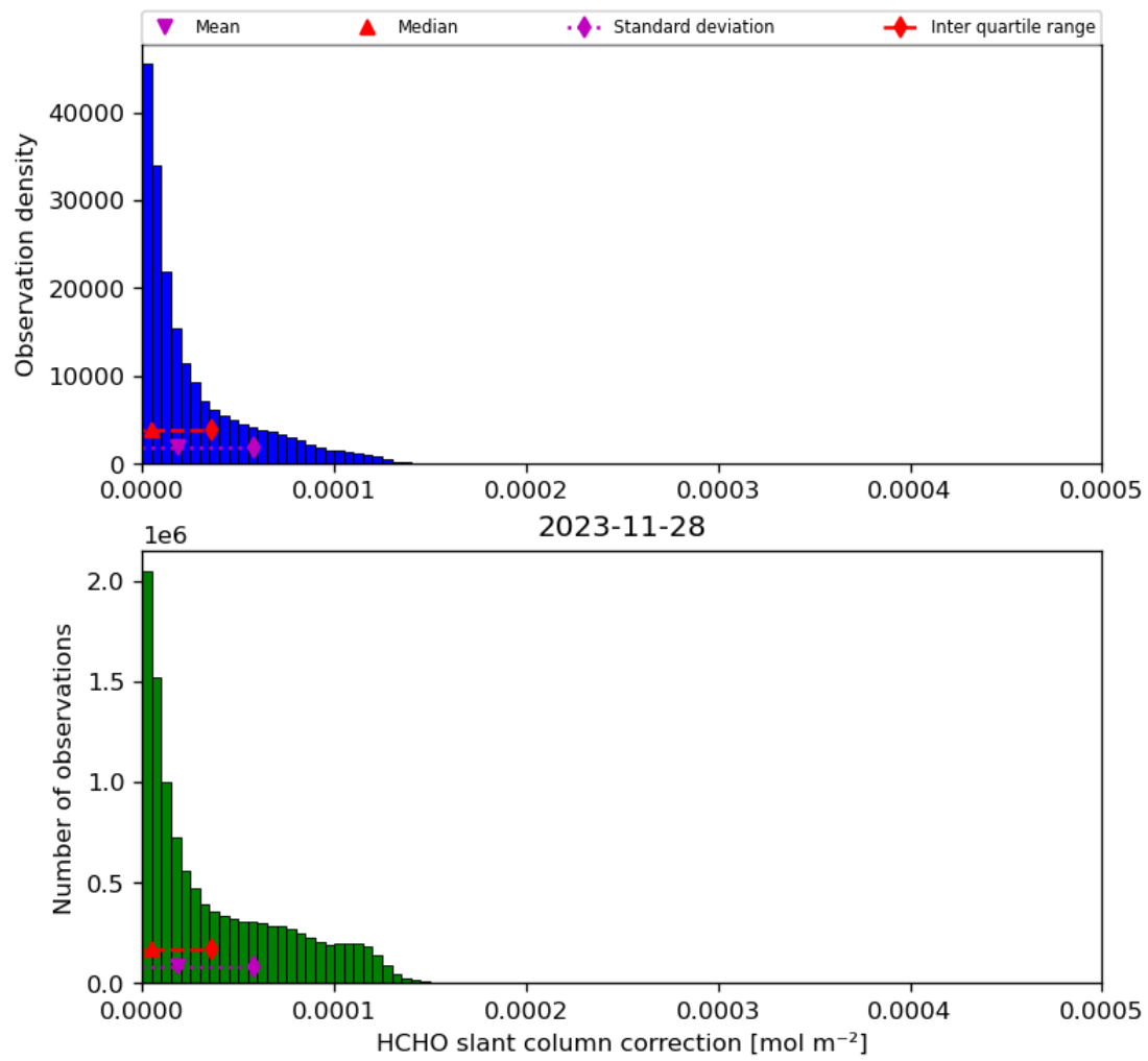
Figure 47: Histogram of “HCHO slant column correction” for 2023-11-28 to 2023-11-29
