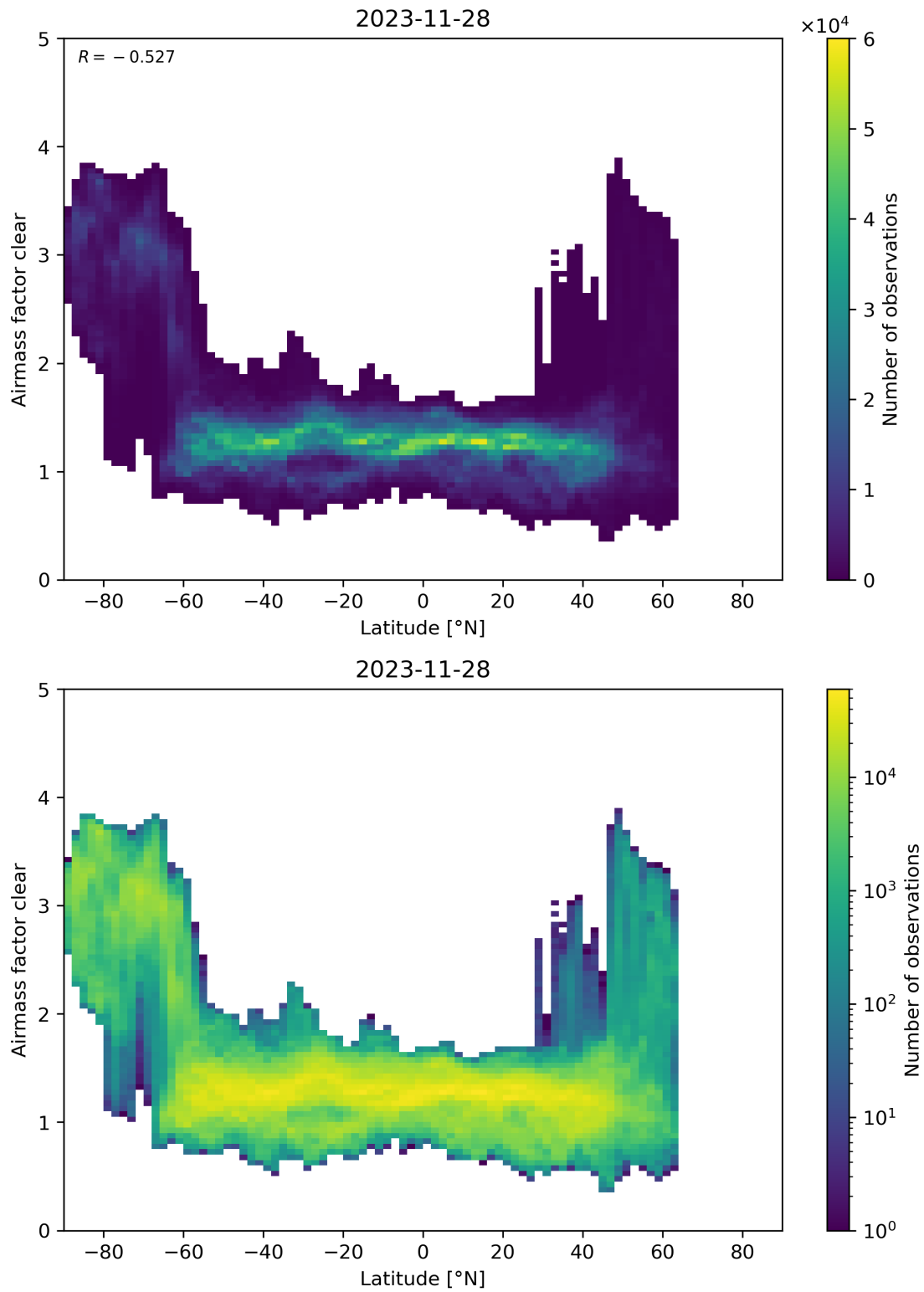
Figure 156: Scatter density plot of “Latitude” against “Airmass factor clear” for 2023-11-28 to 2023-11-29.
