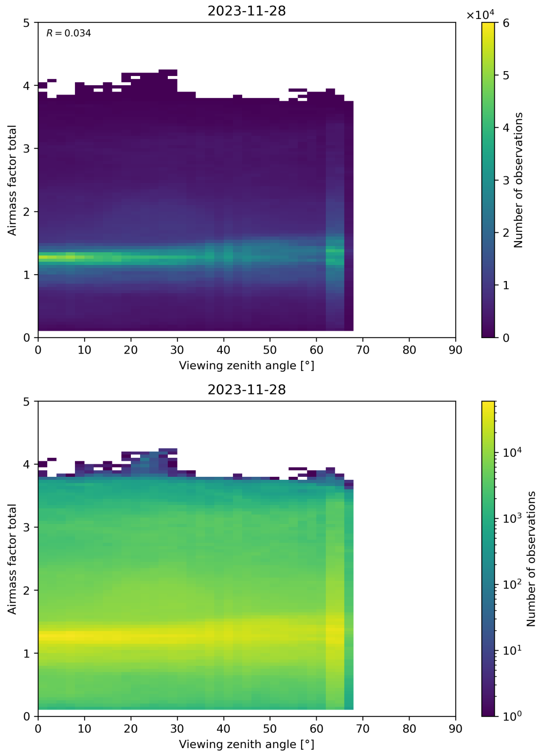
Figure 190: Scatter density plot of “Viewing zenith angle” against “Airmass factor total” for 2023-11-28 to 2023-11-29.
