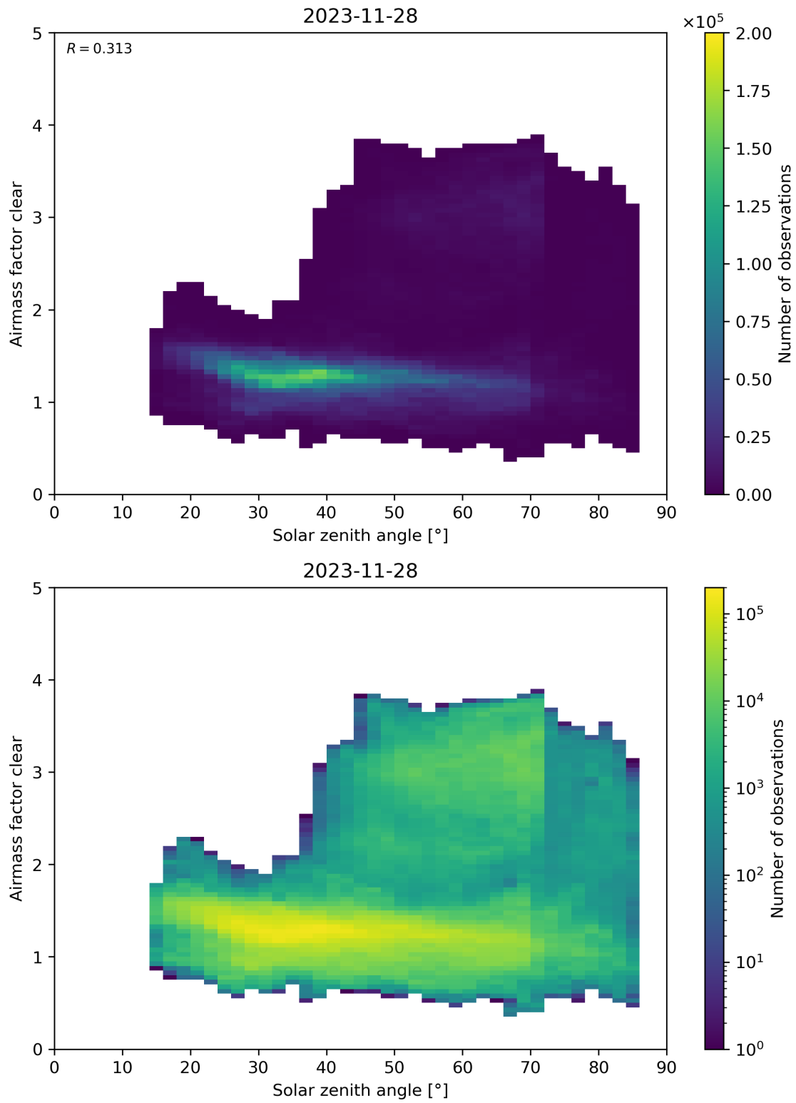
Figure 170: Scatter density plot of “Solar zenith angle” against “Airmass factor clear” for 2023-11-28 to 2023-11-29.
