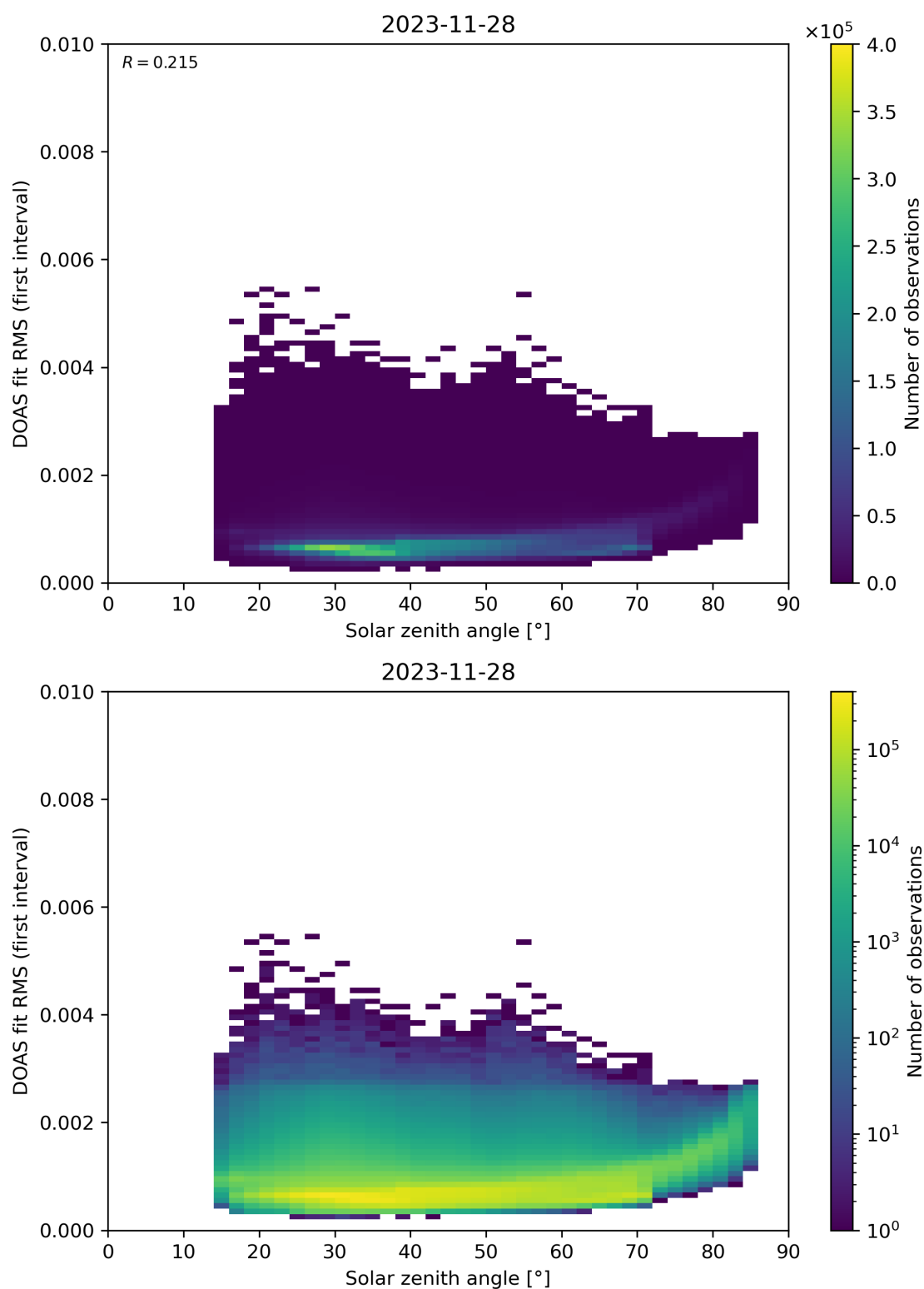
Figure 167: Scatter density plot of “Solar zenith angle” against “DOAS fit RMS (first interval)” for 2023-11-28 to 2023-11-29.
