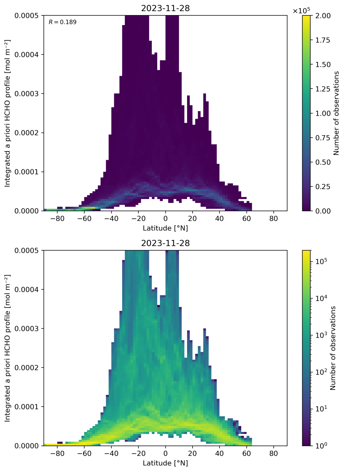
Figure 166: Scatter density plot of “Latitude” against “Integrated a priori HCHO profile” for 2023-11-28 to 2023-11-29.
