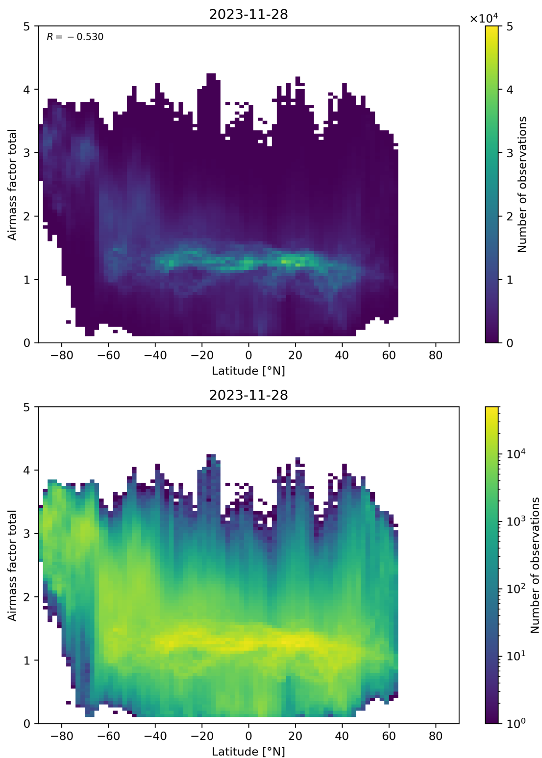
Figure 161: Scatter density plot of “Latitude” against “Airmass factor total” for 2023-11-28 to 2023-11-29.
