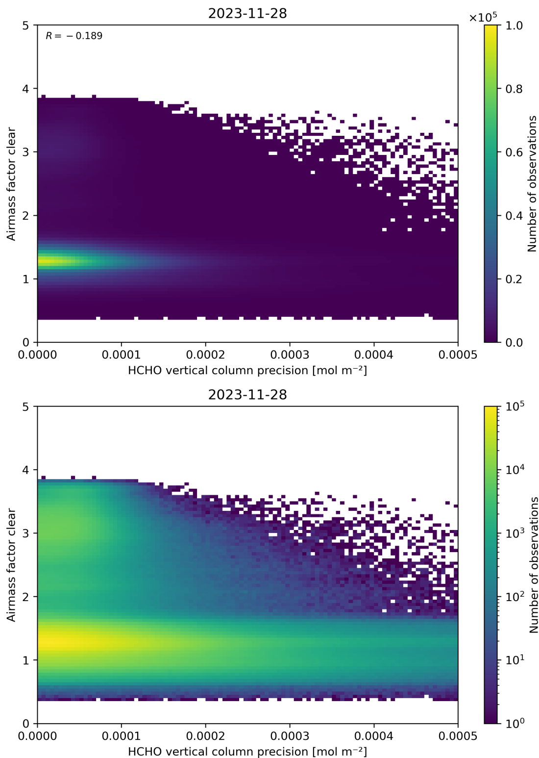
Figure 139: Scatter density plot of “HCHO vertical column precision” against “Airmass factor clear” for 2023-11-28 to 2023-11-29.
