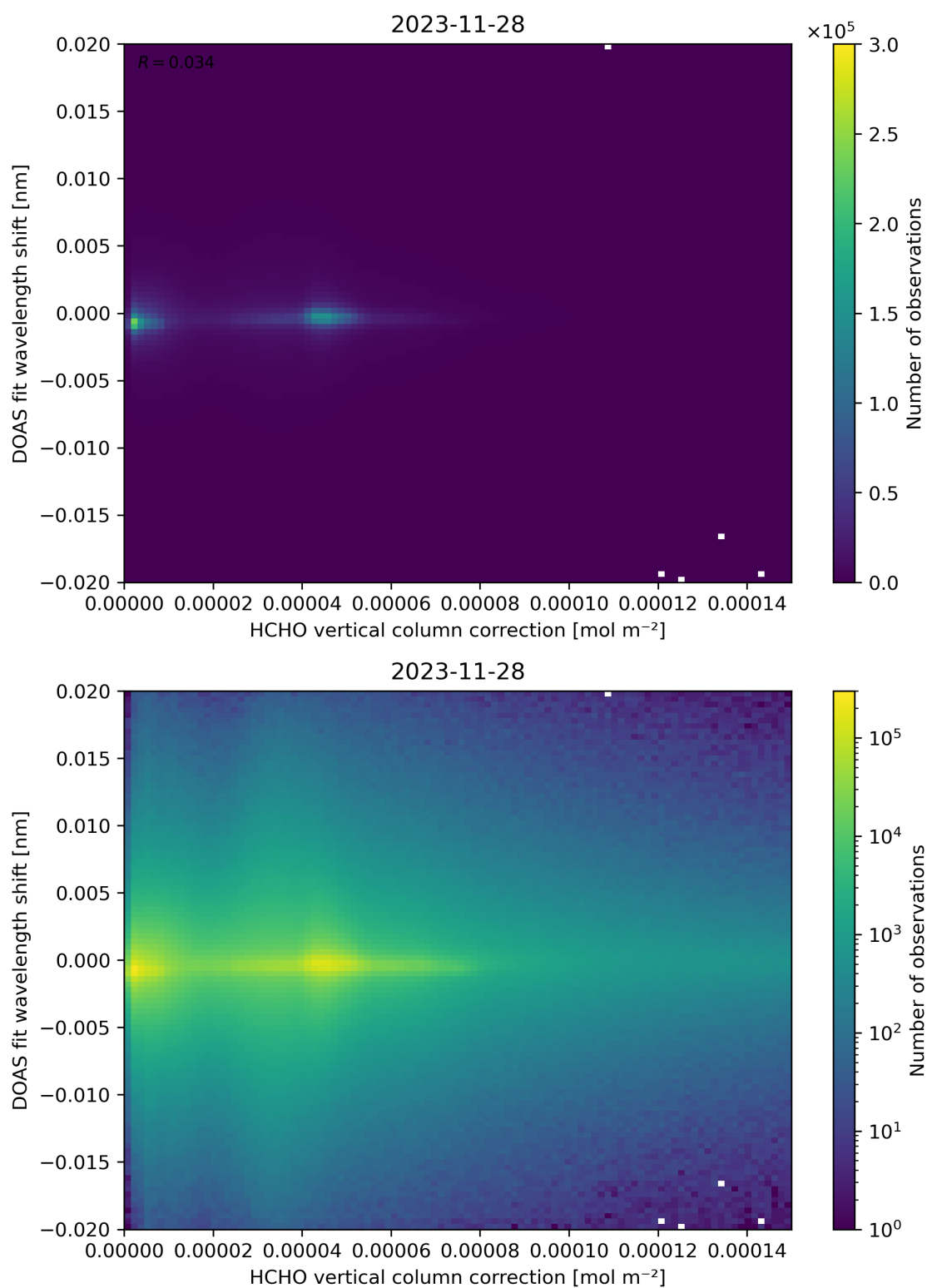
Figure 113: Scatter density plot of “HCHO vertical column correction” against “DOAS fit wavelength shift” for 2023-11-28 to 2023-11-29.
