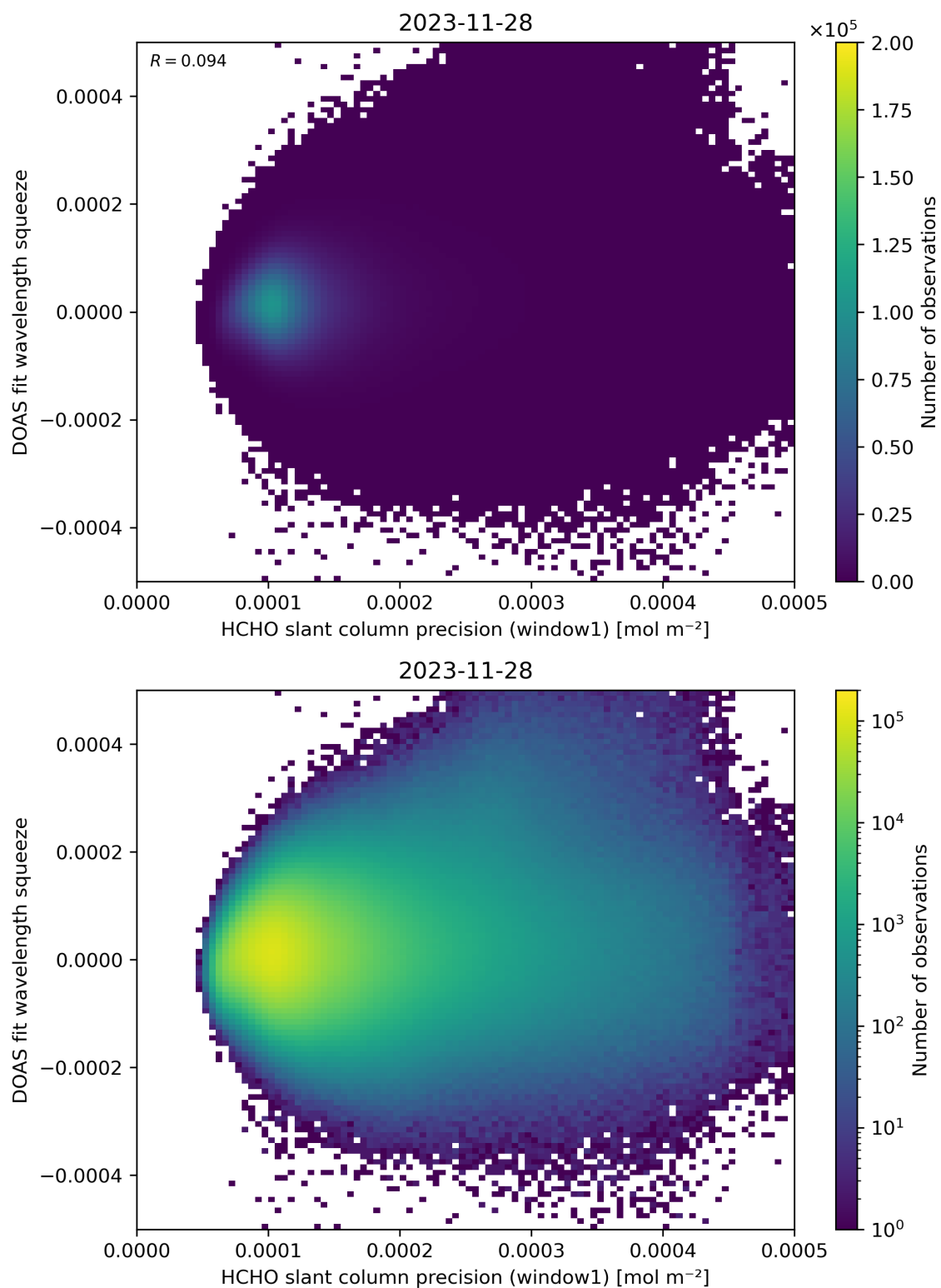
Figure 90: Scatter density plot of “HCHO slant column precision (window1)” against “DOAS fit wavelength squeeze” for 2023-11-28 to 2023-11-29.
