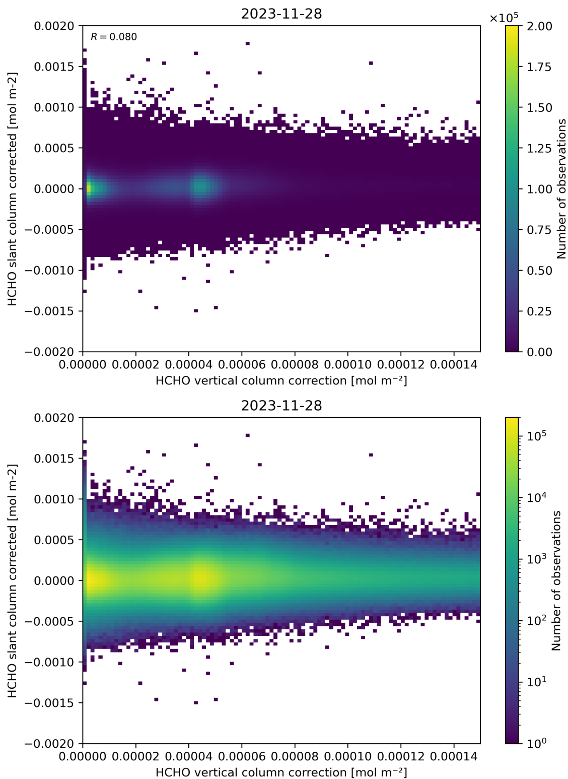
Figure 116: Scatter density plot of “HCHO vertical column correction” against “HCHO slant column corrected” for 2023-11-28 to 2023-11-29.
