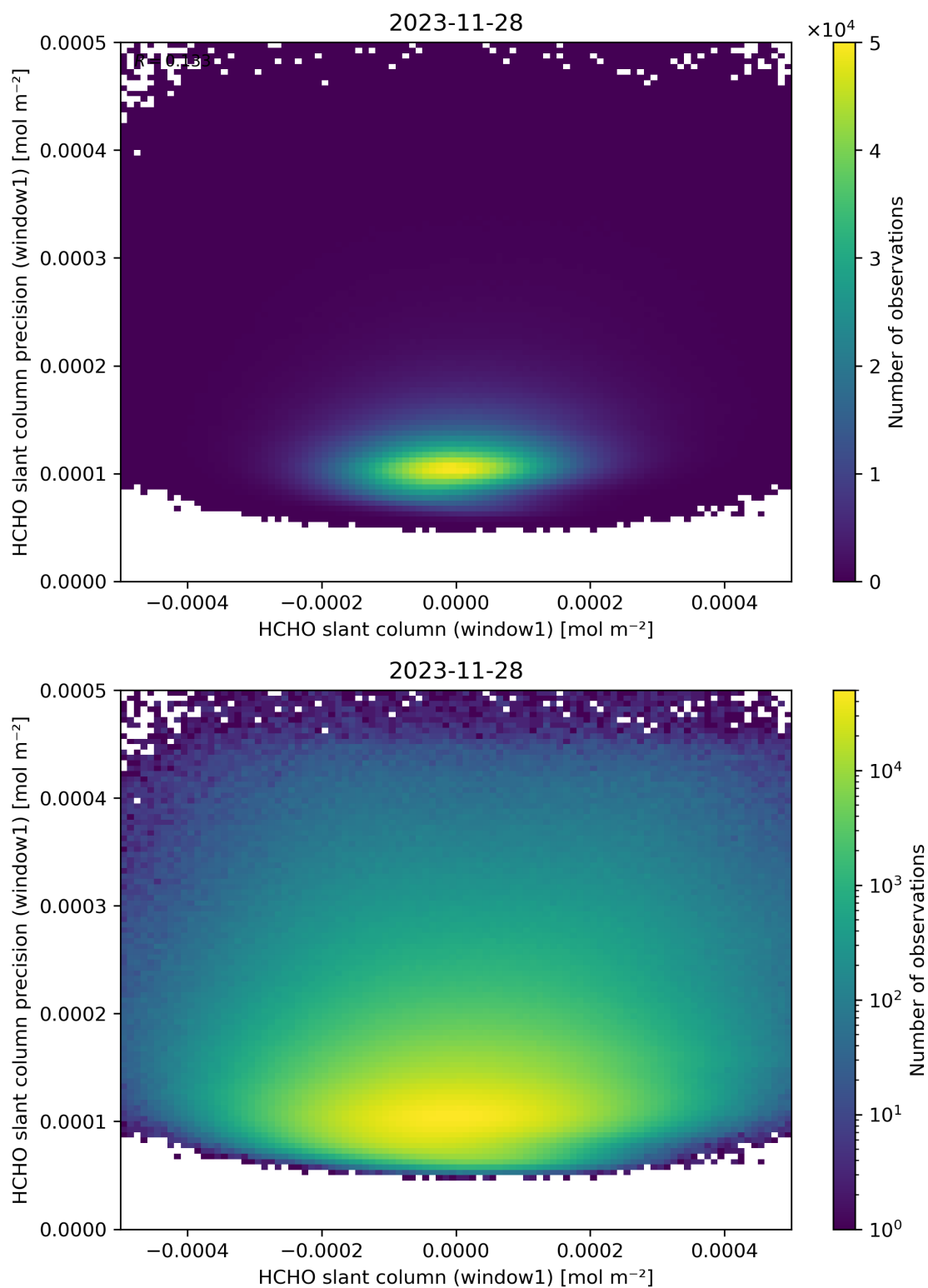
Figure 84: Scatter density plot of “HCHO slant column (window1)” against “HCHO slant column precision (window1)” for 2023-11-28 to 2023-11-29.
