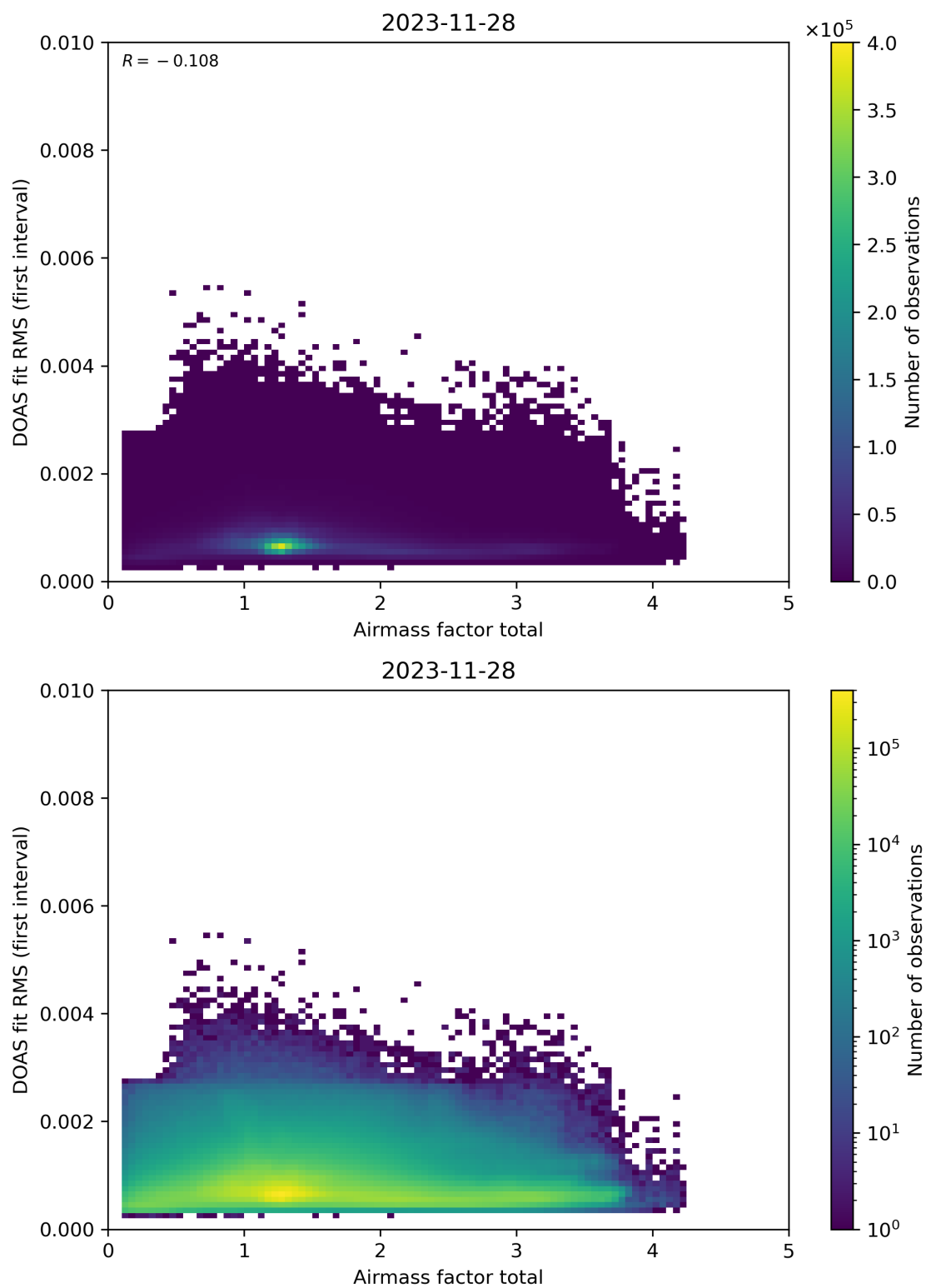
Figure 97: Scatter density plot of “Airmass factor total” against “DOAS fit RMS (first interval)” for 2023-11-28 to 2023-11-29.
