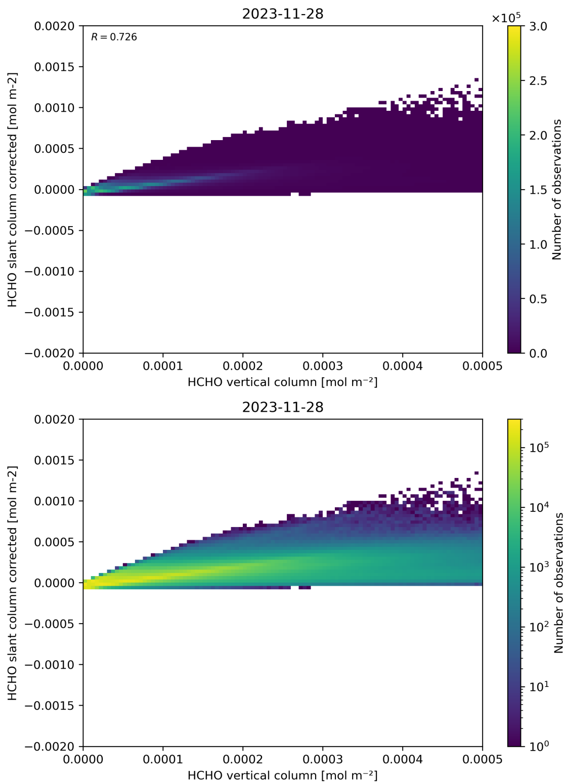
Figure 127: Scatter density plot of “HCHO vertical column” against “HCHO slant column corrected” for 2023-11-28 to 2023-11-29.
