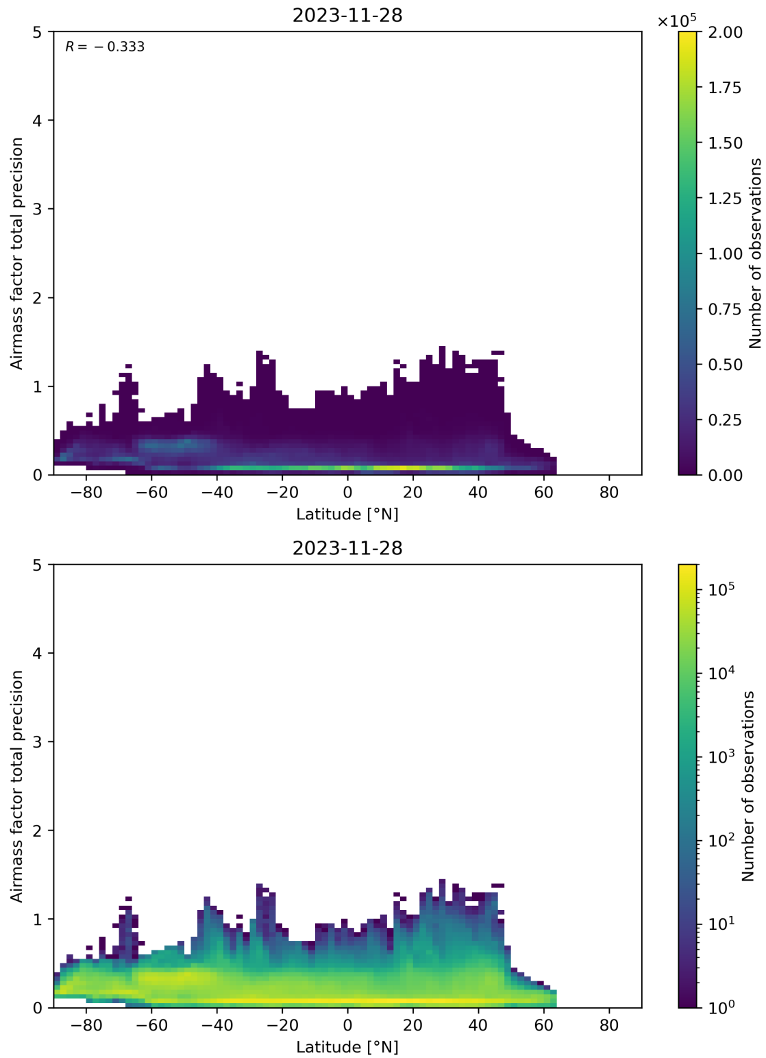
Figure 162: Scatter density plot of “Latitude” against “Airmass factor total precision” for 2023-11-28 to 2023-11-29.
