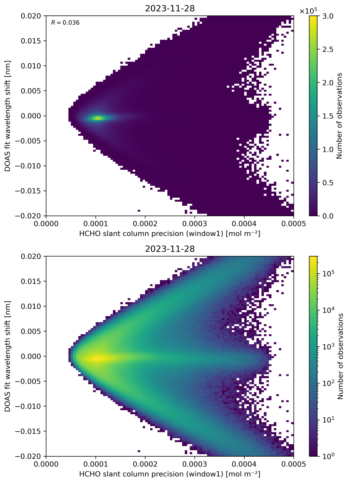
Figure 89: Scatter density plot of “HCHO slant column precision (window1)” against “DOAS fit wavelength shift” for 2023-11-28 to 2023-11-29.
