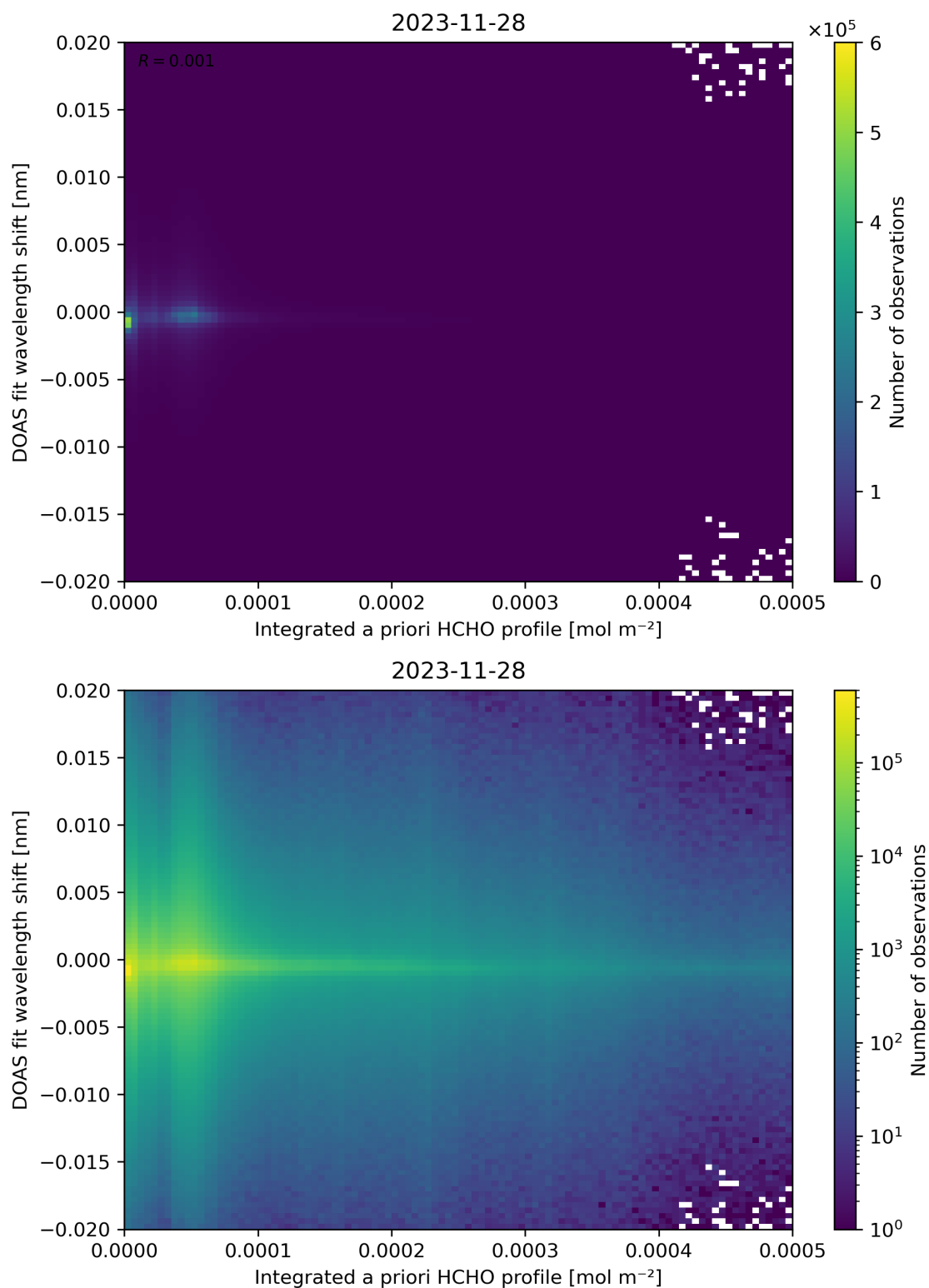
Figure 149: Scatter density plot of “Integrated a priori HCHO profile” against “DOAS fit wavelength shift” for 2023-11-28 to 2023-11-29.
