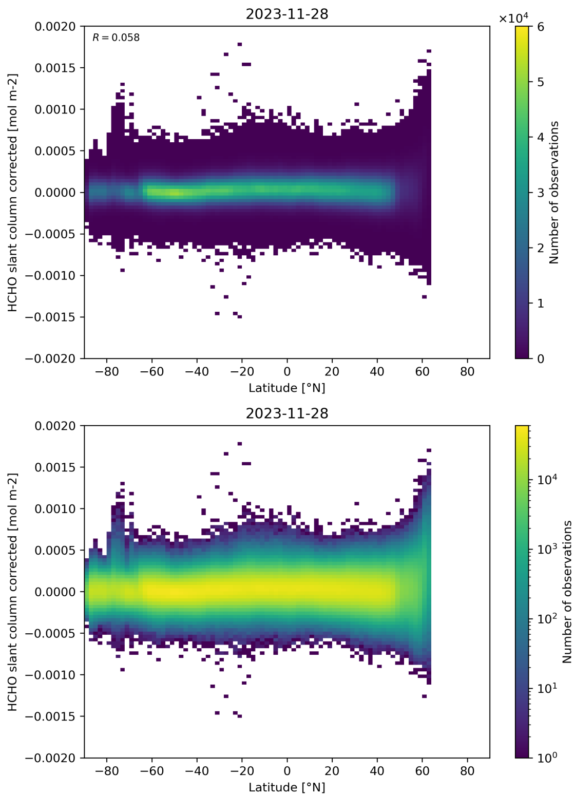
Figure 157: Scatter density plot of “Latitude” against “HCHO slant column corrected” for 2023-11-28 to 2023-11-29.
