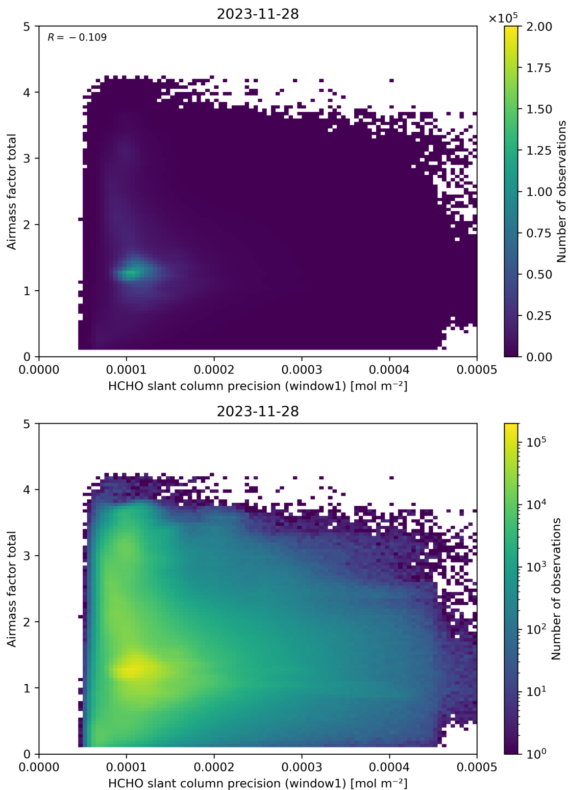
Figure 94: Scatter density plot of “HCHO slant column precision (window1)” against “Airmass factor total” for 2023-11-28 to 2023-11-29.
