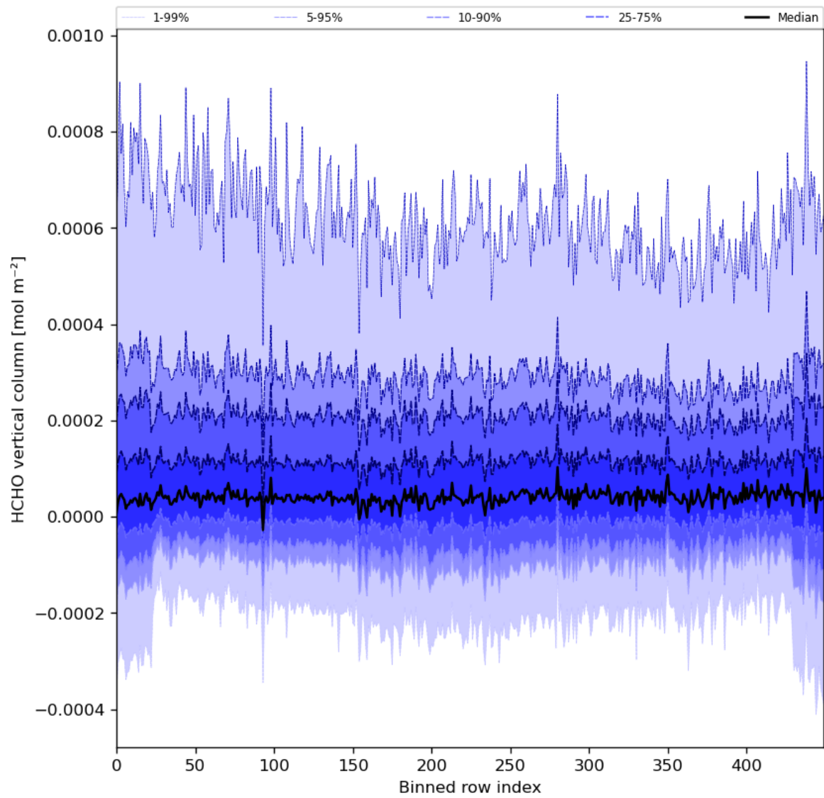
Figure 49: Along track statistics of “HCHO vertical column” for 2023-11-28 to 2023-11-29
