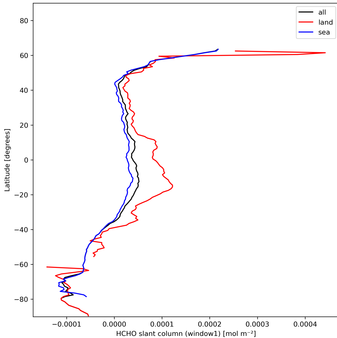
Figure 24: Zonal average of “HCHO slant column (window1)” for 2023-11-28 to 2023-11-29.
