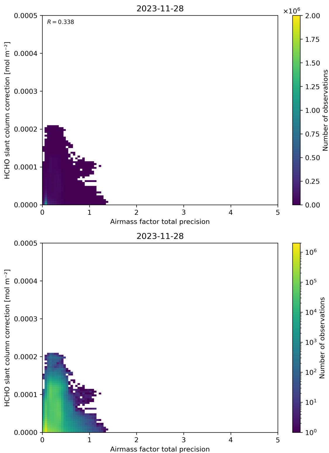
Figure 110: Scatter density plot of “Airmass factor total precision” against “HCHO slant column correction” for 2023-11-28 to 2023-11-29.
