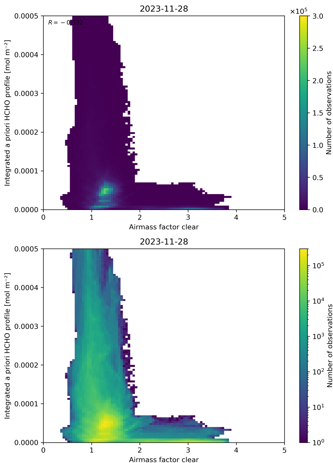
Figure 76: Scatter density plot of “Airmass factor clear” against “Integrated a priori HCHO profile” for 2023-11-28 to 2023-11-29.
