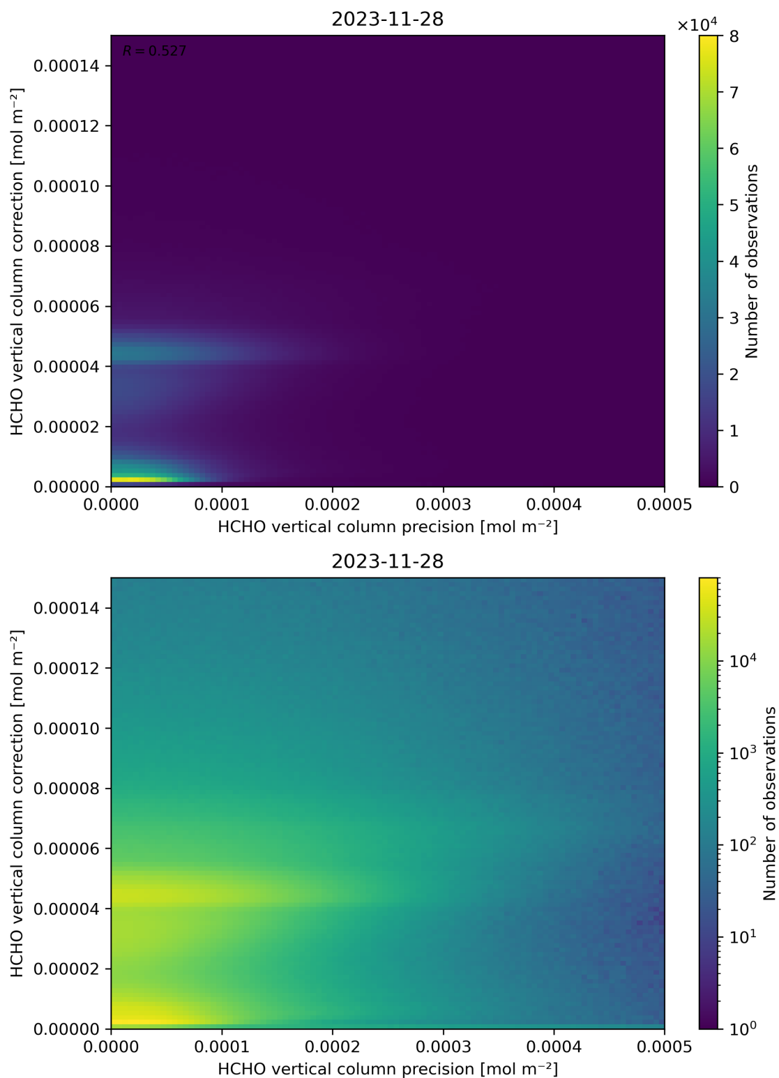
Figure 146: Scatter density plot of “HCHO vertical column precision” against “HCHO vertical column correction” for 2023-11-28 to 2023-11-29.
