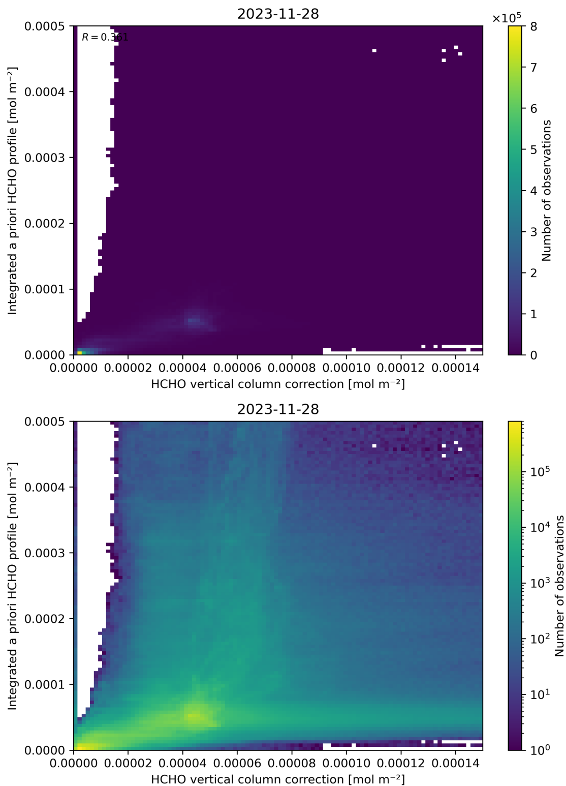
Figure 122: Scatter density plot of “HCHO vertical column correction” against “Integrated a priori HCHO profile” for 2023-11-28 to 2023-11-29.
