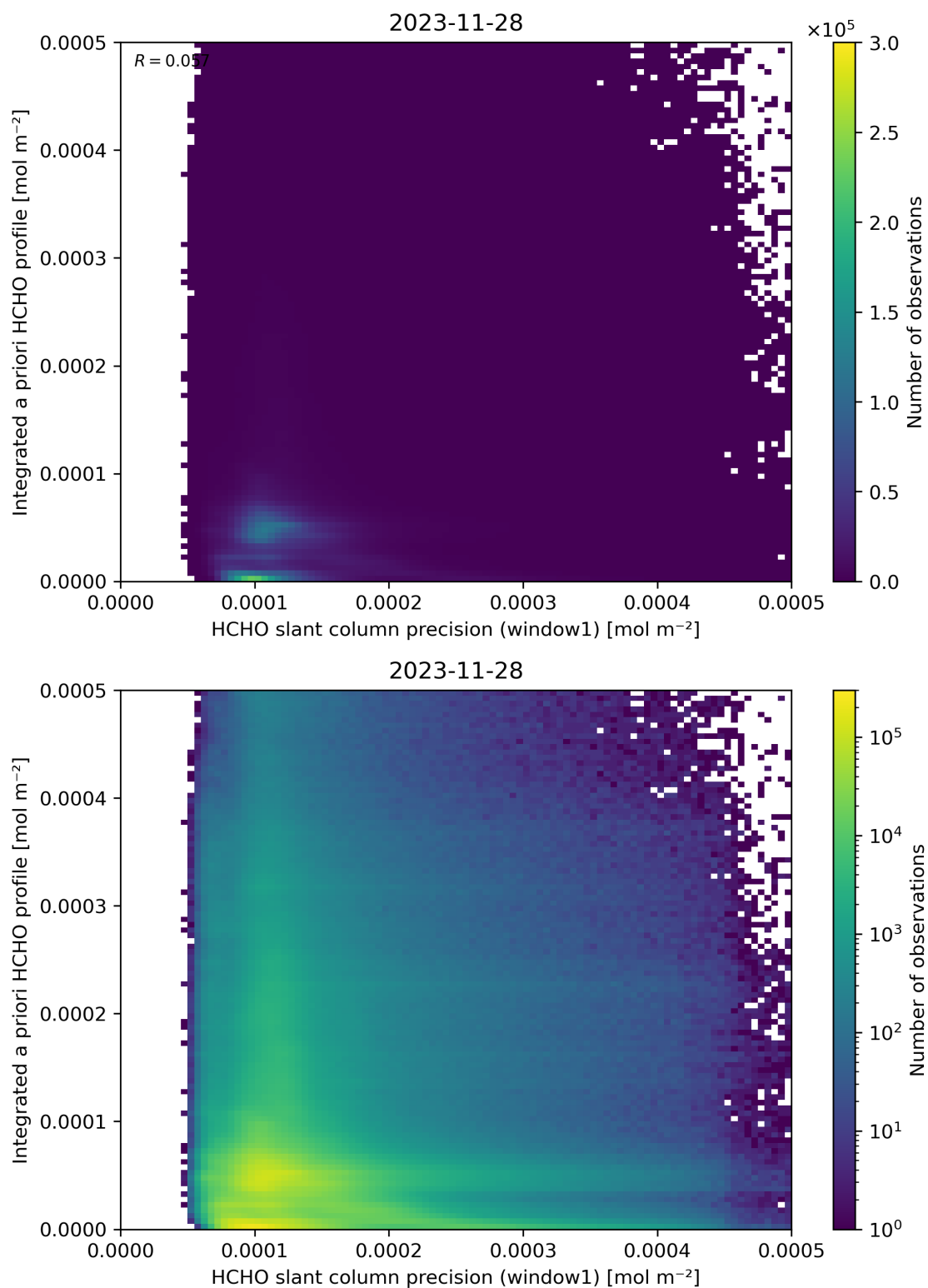
Figure 96: Scatter density plot of “HCHO slant column precision (window1)” against “Integrated a priori HCHO profile” for 2023-11-28 to 2023-11-29.
