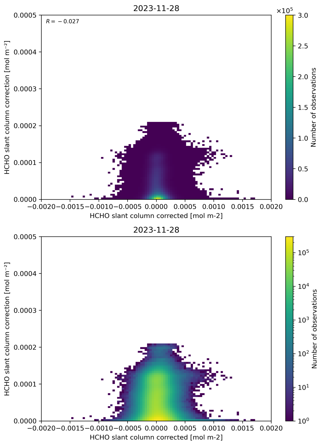
Figure 77: Scatter density plot of “HCHO slant column corrected” against “HCHO slant column correction” for 2023-11-28 to 2023-11-29.
