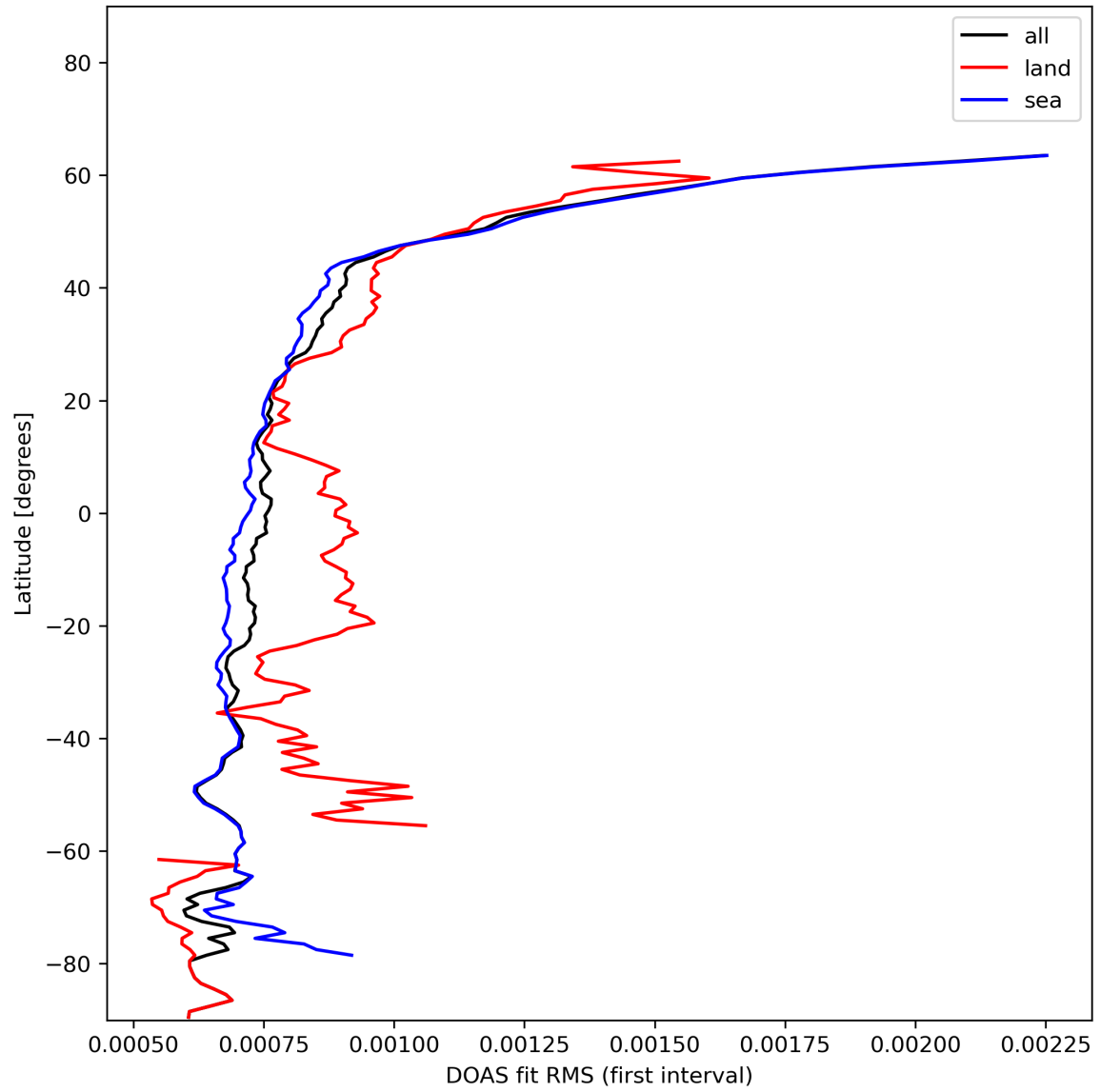
Figure 32: Zonal average of “DOAS fit RMS (first interval)” for 2023-11-28 to 2023-11-29.
