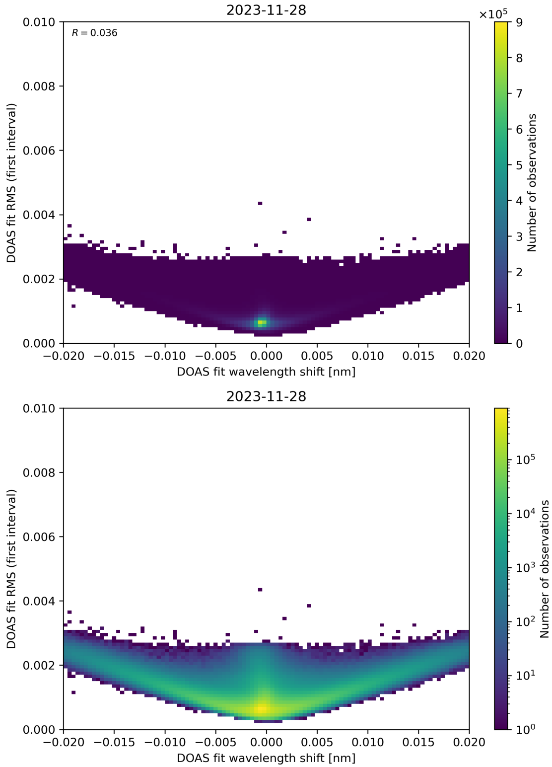
Figure 64: Scatter density plot of “DOAS fit wavelength shift” against “DOAS fit RMS (first interval)” for 2023-11-28 to 2023-11-29.
