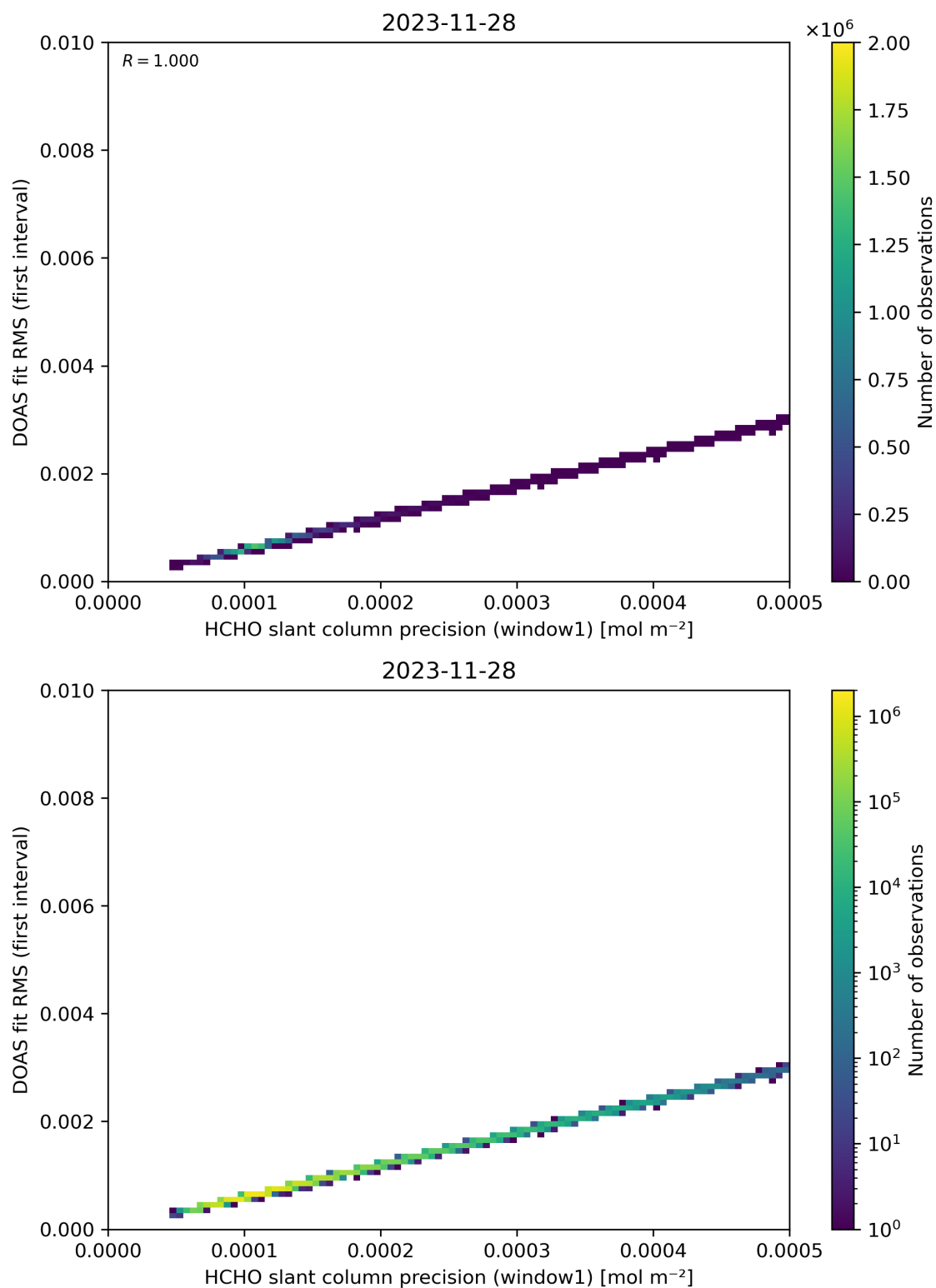
Figure 88: Scatter density plot of “HCHO slant column precision (window1)” against “DOAS fit RMS (first interval)” for 2023-11-28 to 2023-11-29.
