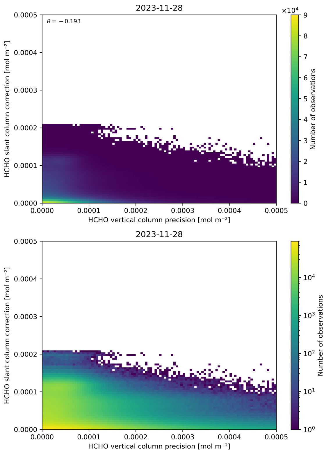
Figure 141: Scatter density plot of “HCHO vertical column precision” against “HCHO slant column correction” for 2023-11-28 to 2023-11-29.
