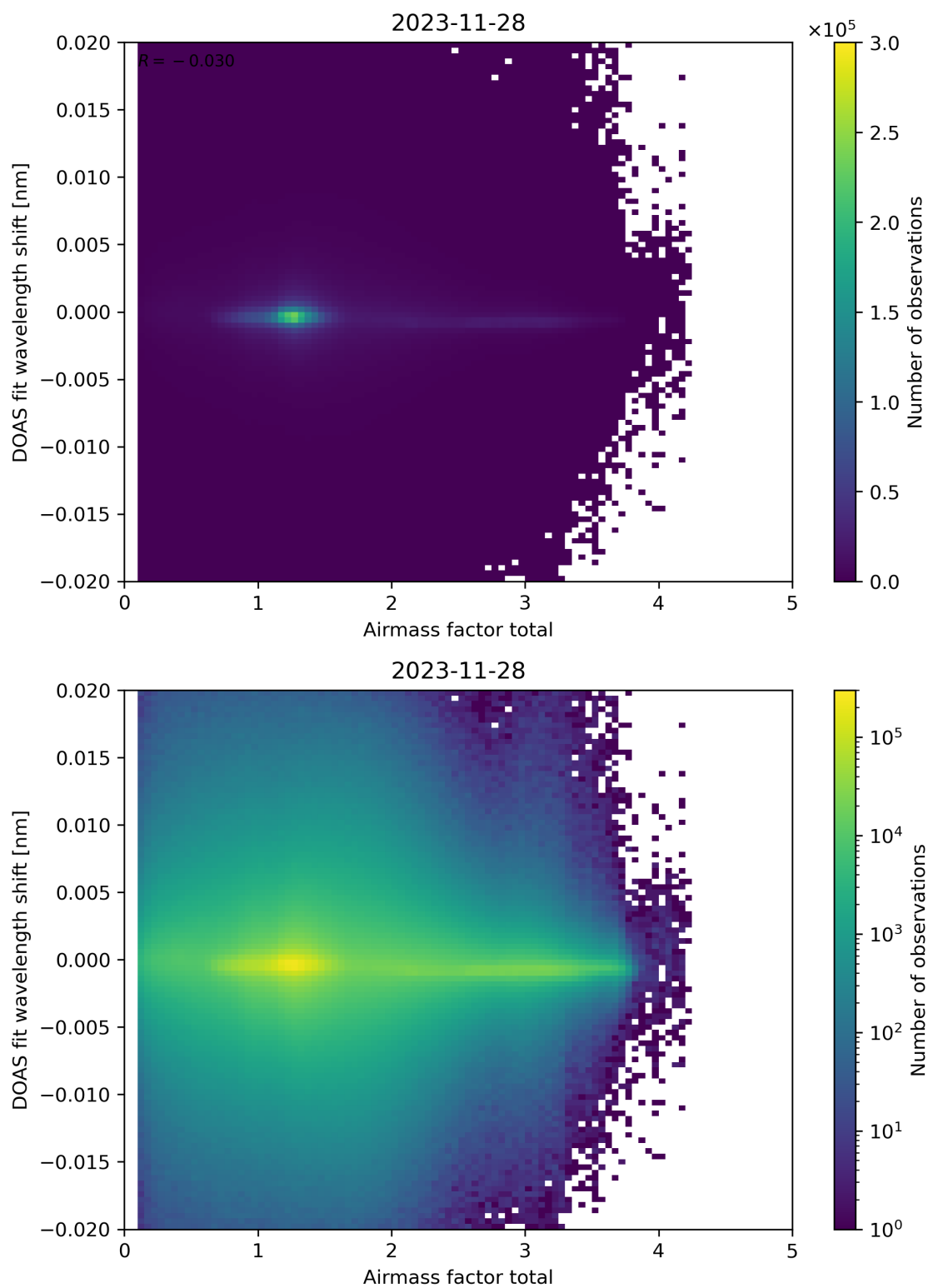
Figure 98: Scatter density plot of “Airmass factor total” against “DOAS fit wavelength shift” for 2023-11-28 to 2023-11-29.
