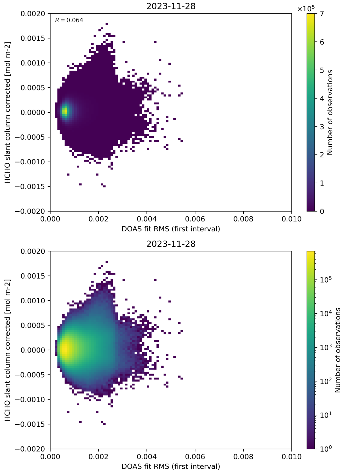
Figure 62: Scatter density plot of “DOAS fit RMS (first interval)” against “HCHO slant column corrected” for 2023-11-28 to 2023-11-29.
