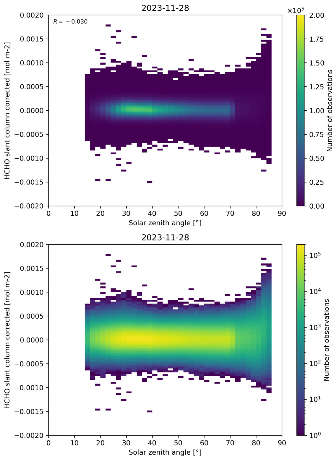
Figure 171: Scatter density plot of “Solar zenith angle” against “HCHO slant column corrected” for 2023-11-28 to 2023-11-29.
