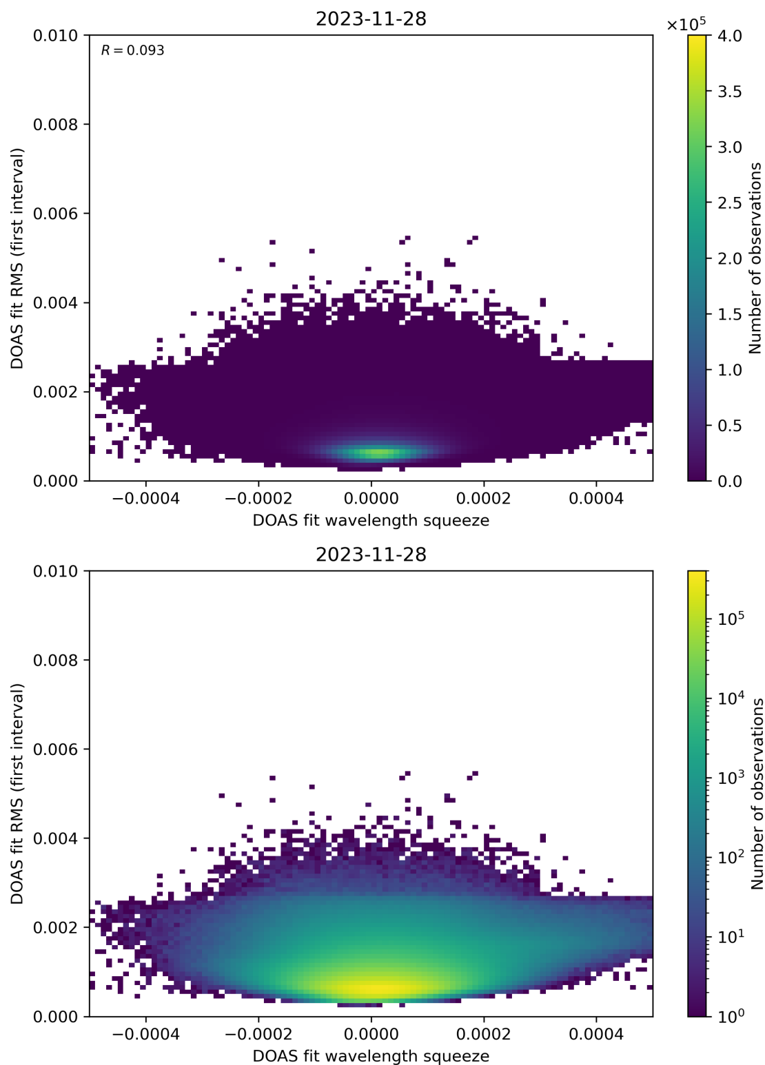
Figure 68: Scatter density plot of “DOAS fit wavelength squeeze” against “DOAS fit RMS (first interval)” for 2023-11-28 to 2023-11-29.
