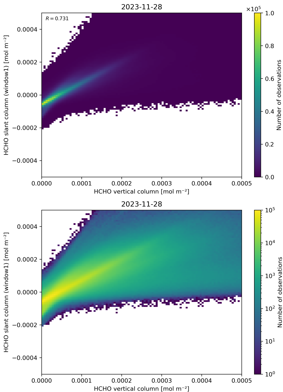
Figure 129: Scatter density plot of “HCHO vertical column” against “HCHO slant column (window1)” for 2023-11-28 to 2023-11-29.
