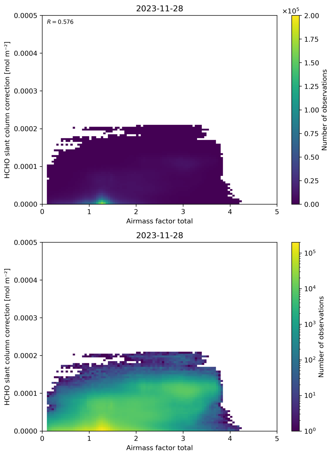
Figure 102: Scatter density plot of “Airmass factor total” against “HCHO slant column correction” for 2023-11-28 to 2023-11-29.
