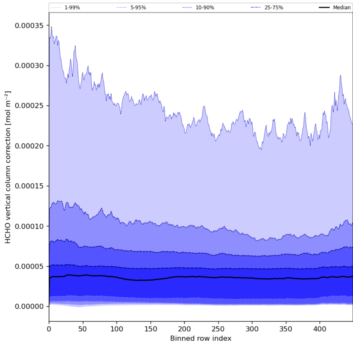
Figure 51: Along track statistics of “HCHO vertical column correction” for 2023-11-28 to 2023-11-29
