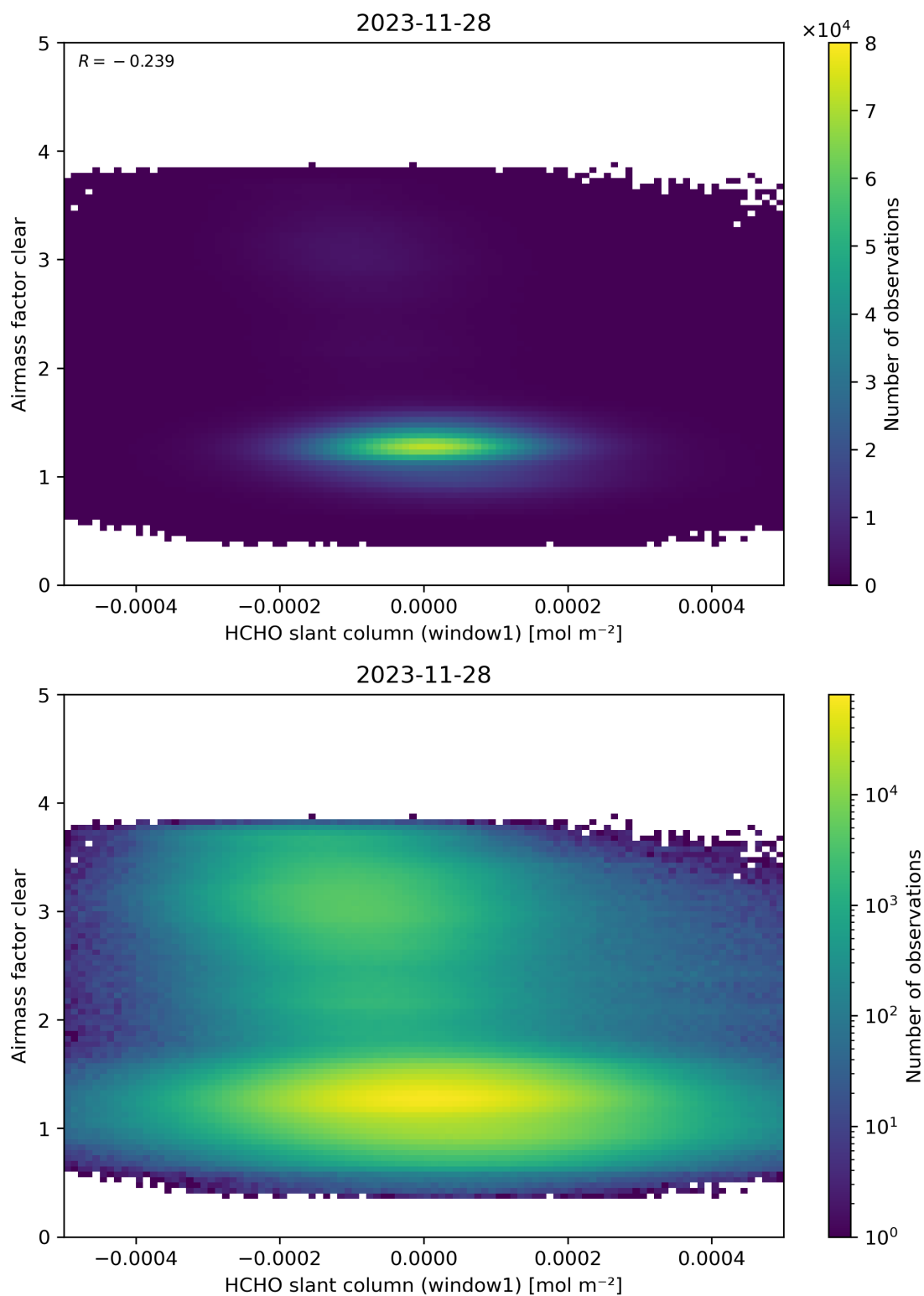
Figure 81: Scatter density plot of “HCHO slant column (window1)” against “Airmass factor clear” for 2023-11-28 to 2023-11-29.
