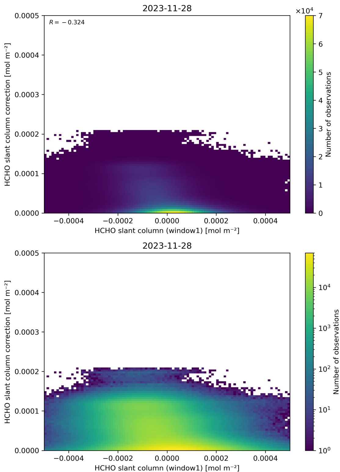
Figure 83: Scatter density plot of “HCHO slant column (window1)” against “HCHO slant column correction” for 2023-11-28 to 2023-11-29.
