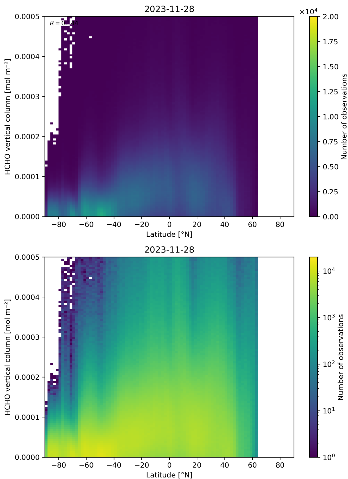
Figure 163: Scatter density plot of “Latitude” against “HCHO vertical column” for 2023-11-28 to 2023-11-29.
