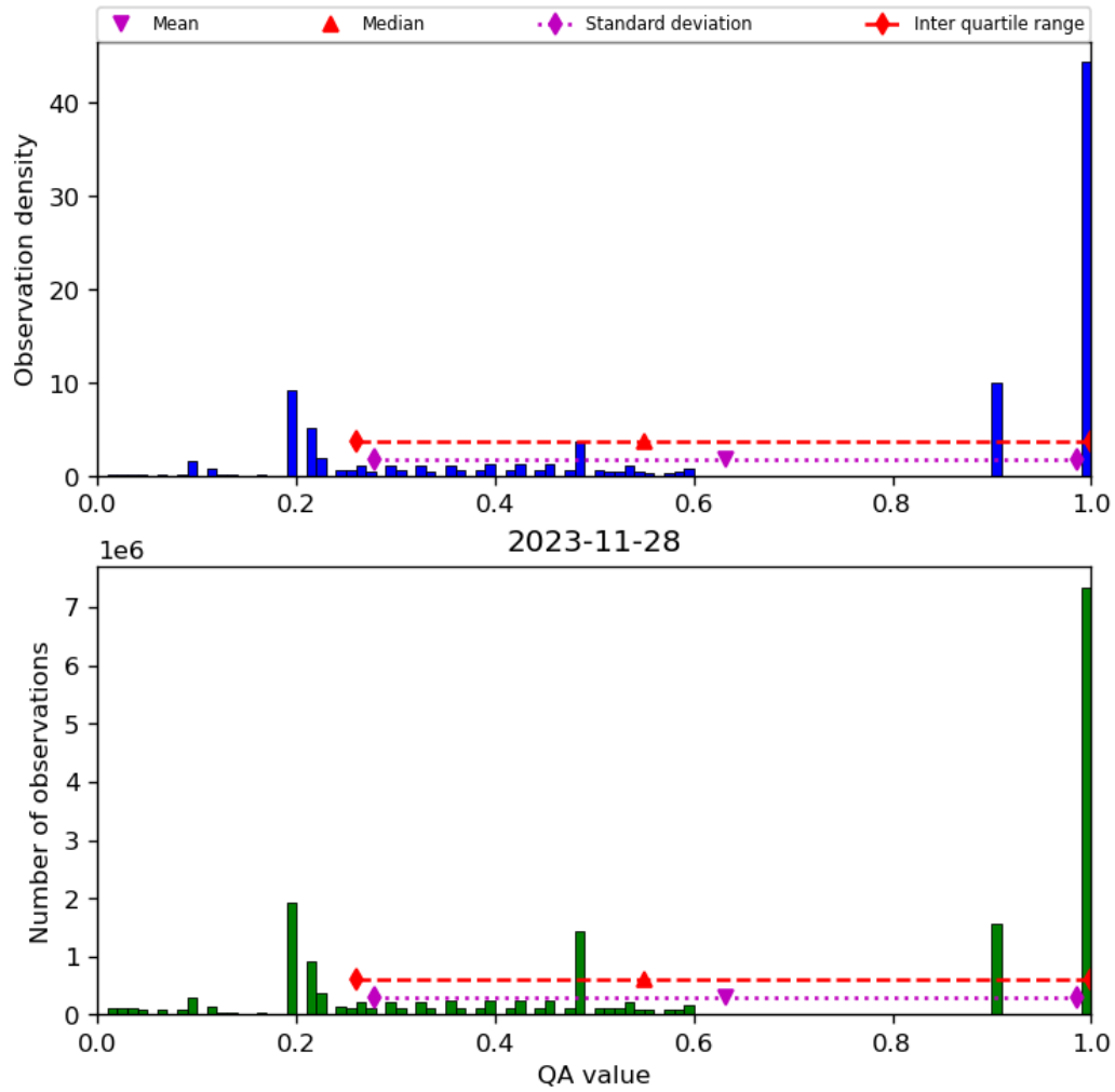
Figure 34: Histogram of “QA value” for 2023-11-28 to 2023-11-29
