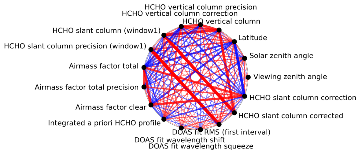
Figure 1: Map of correlation graph for 2023-11-28 to 2023-11-29.
