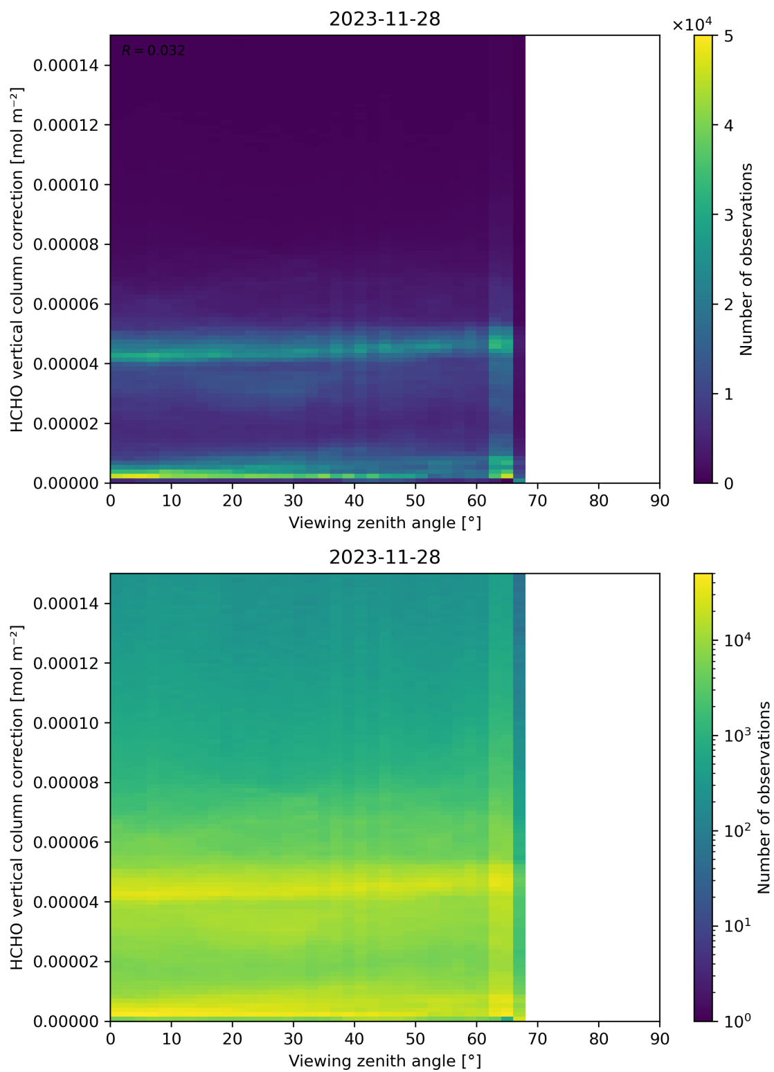
Figure 193: Scatter density plot of “Viewing zenith angle” against “HCHO vertical column correction” for 2023-11-28 to 2023-11-29.
