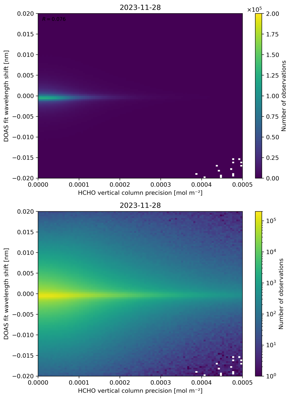
Figure 137: Scatter density plot of “HCHO vertical column precision” against “DOAS fit wavelength shift” for 2023-11-28 to 2023-11-29.
