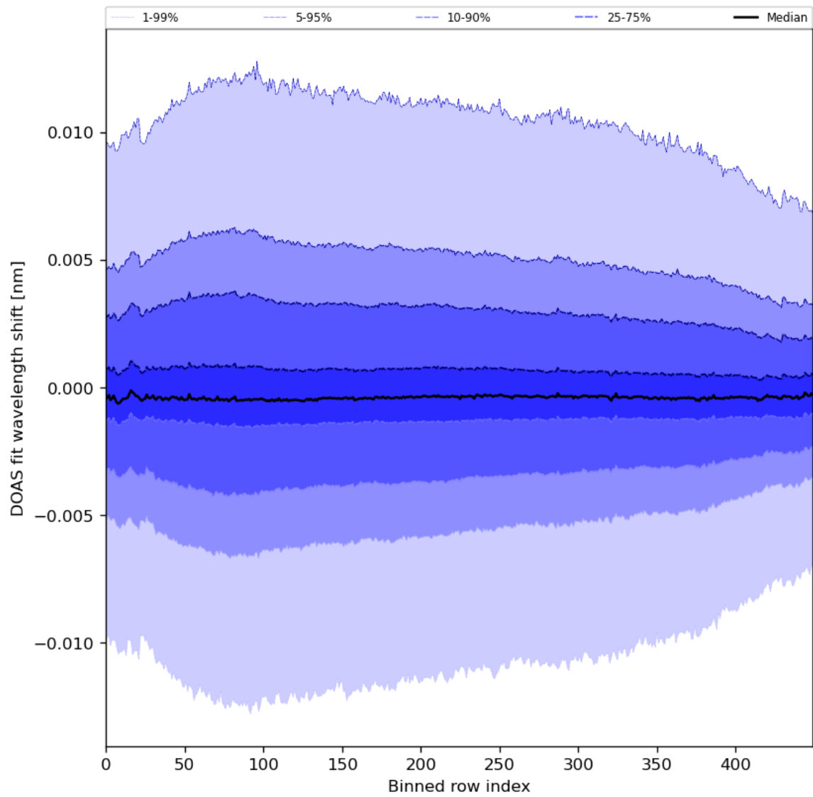
Figure 58: Along track statistics of “DOAS fit wavelength shift” for 2023-11-28 to 2023-11-29
