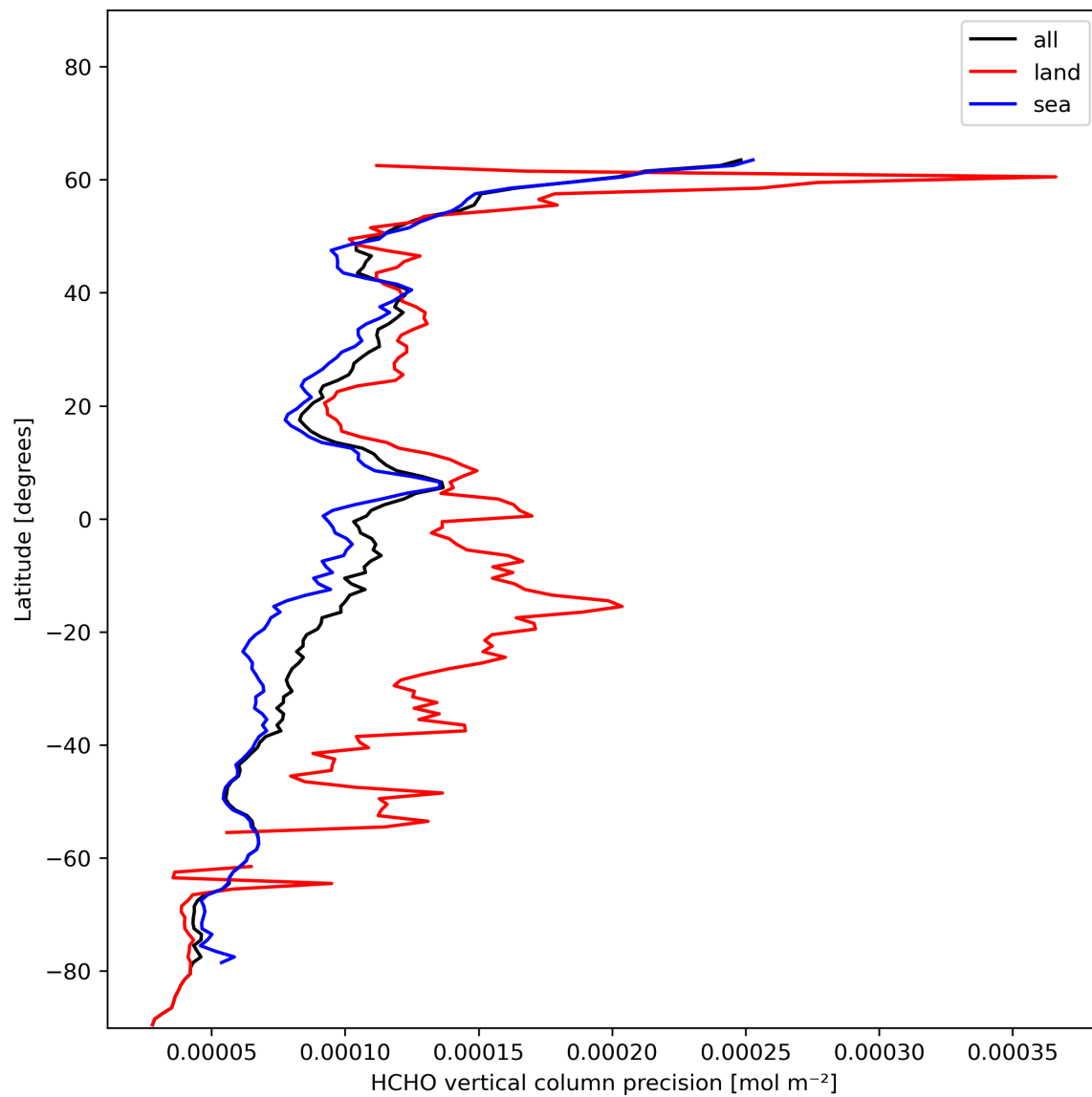
Figure 22: Zonal average of “HCHO vertical column precision” for 2023-11-28 to 2023-11-29.
