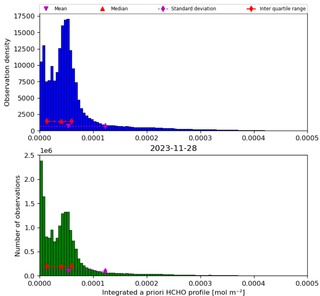
Figure 43: Histogram of “Integrated a priori HCHO profile” for 2023-11-28 to 2023-11-29
