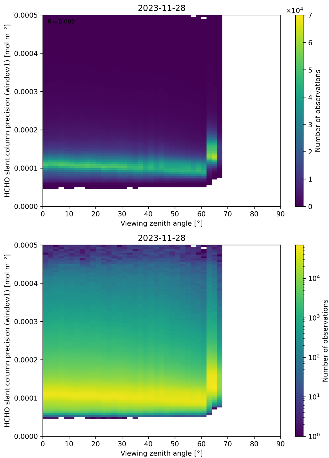
Figure 189: Scatter density plot of “Viewing zenith angle” against “HCHO slant column precision (window1)” for 2023-11-28 to 2023-11-29.
