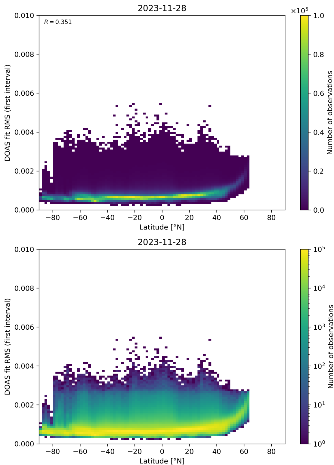
Figure 153: Scatter density plot of “Latitude” against “DOAS fit RMS (first interval)” for 2023-11-28 to 2023-11-29.
