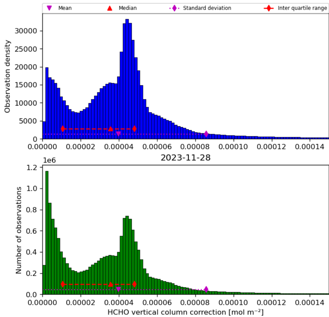
Figure 37: Histogram of “HCHO vertical column correction” for 2023-11-28 to 2023-11-29
