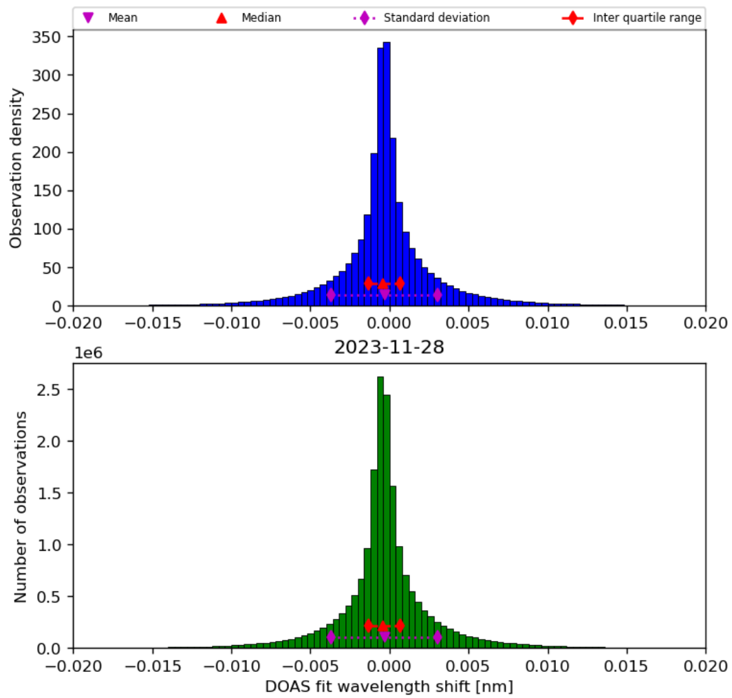
Figure 44: Histogram of “DOAS fit wavelength shift” for 2023-11-28 to 2023-11-29
