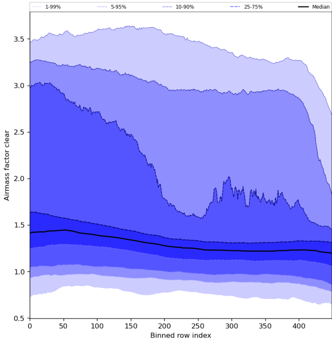
Figure 56: Along track statistics of “Airmass factor clear” for 2023-11-28 to 2023-11-29
