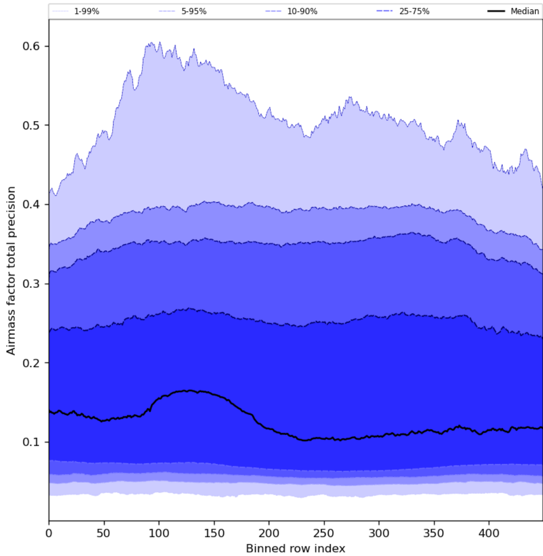
Figure 55: Along track statistics of “Airmass factor total precision” for 2023-11-28 to 2023-11-29
