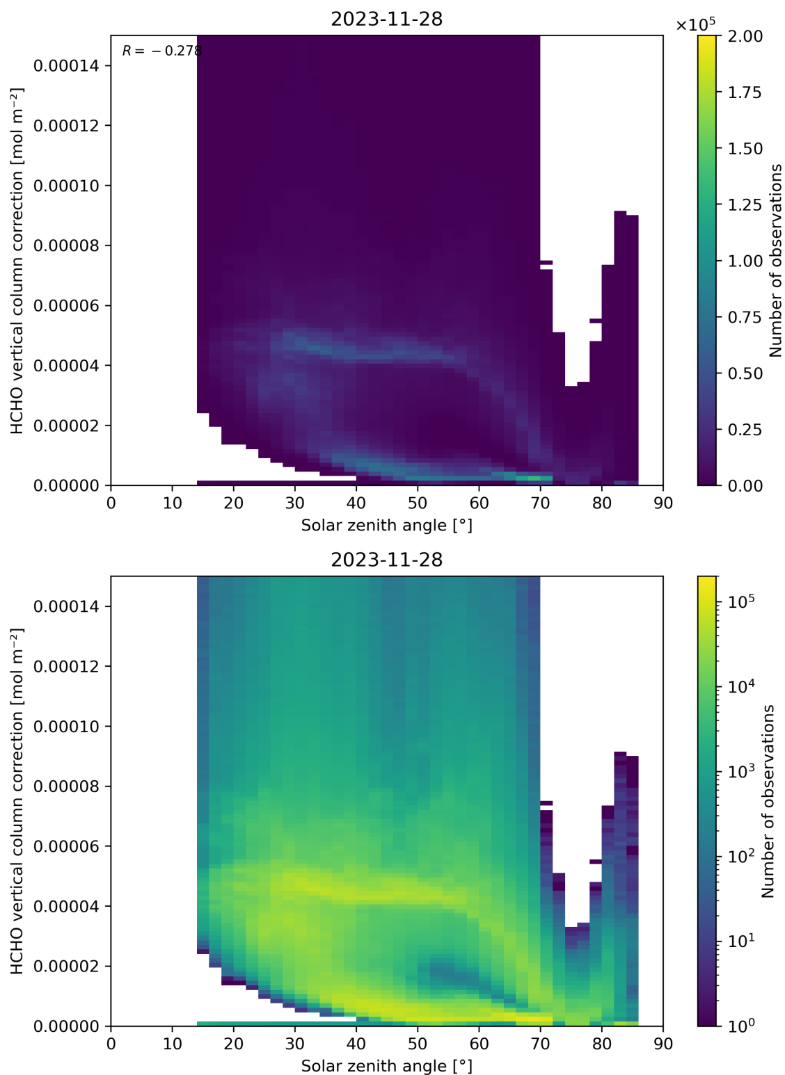
Figure 178: Scatter density plot of “Solar zenith angle” against “HCHO vertical column correction” for 2023-11-28 to 2023-11-29.
