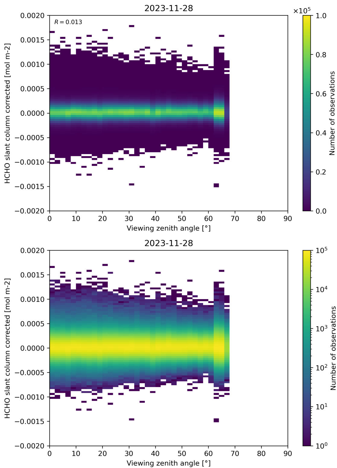
Figure 186: Scatter density plot of “Viewing zenith angle” against “HCHO slant column corrected” for 2023-11-28 to 2023-11-29.
