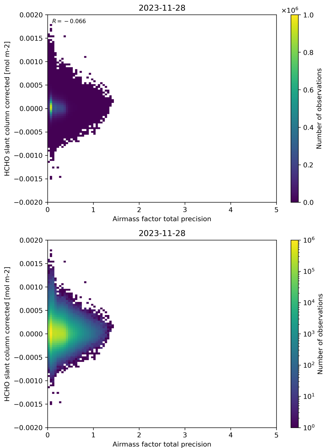
Figure 109: Scatter density plot of “Airmass factor total precision” against “HCHO slant column corrected” for 2023-11-28 to 2023-11-29.
