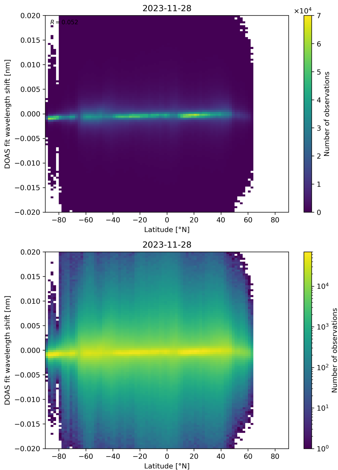
Figure 154: Scatter density plot of “Latitude” against “DOAS fit wavelength shift” for 2023-11-28 to 2023-11-29.
