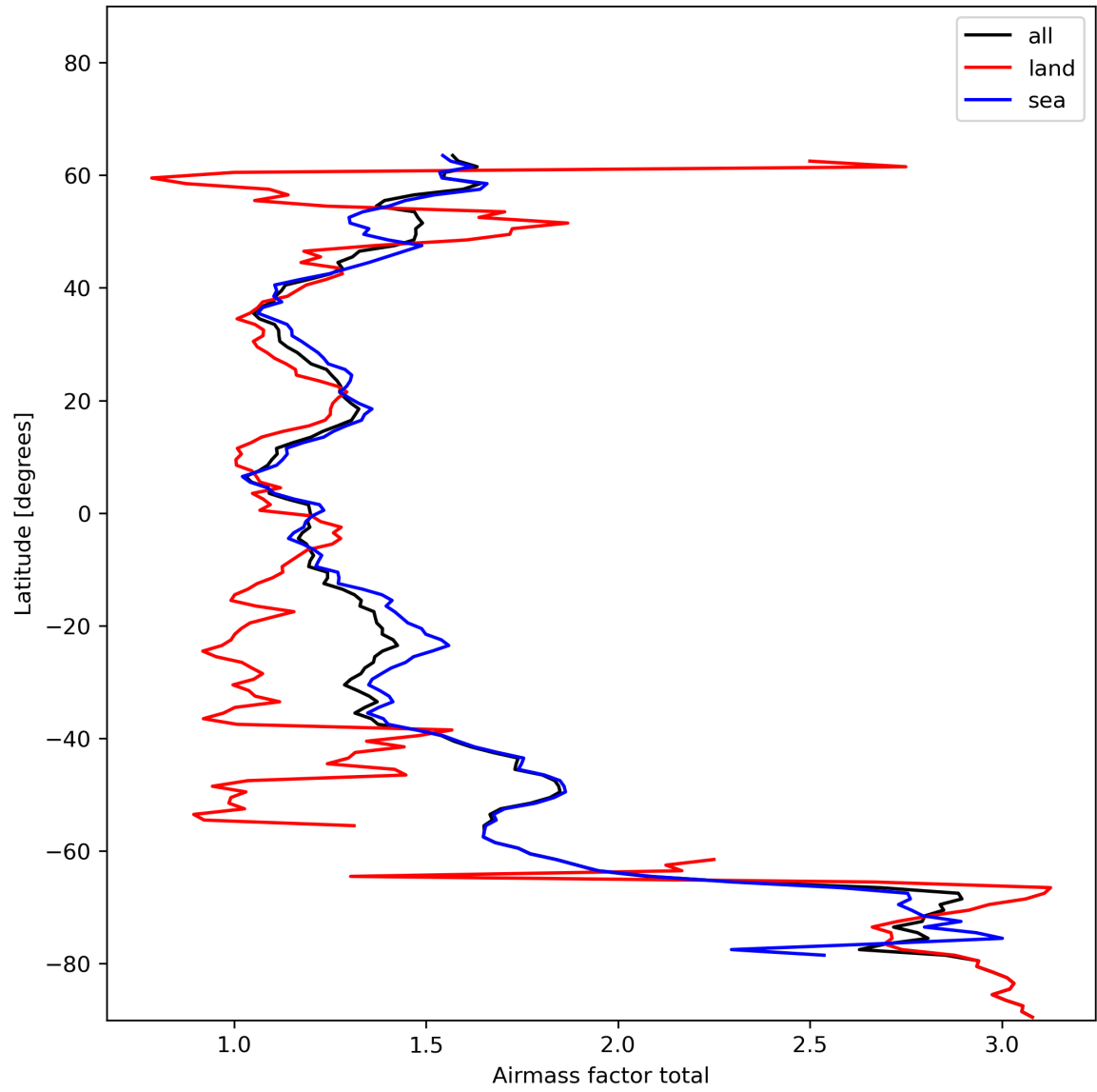
Figure 26: Zonal average of “Airmass factor total” for 2023-11-28 to 2023-11-29.
