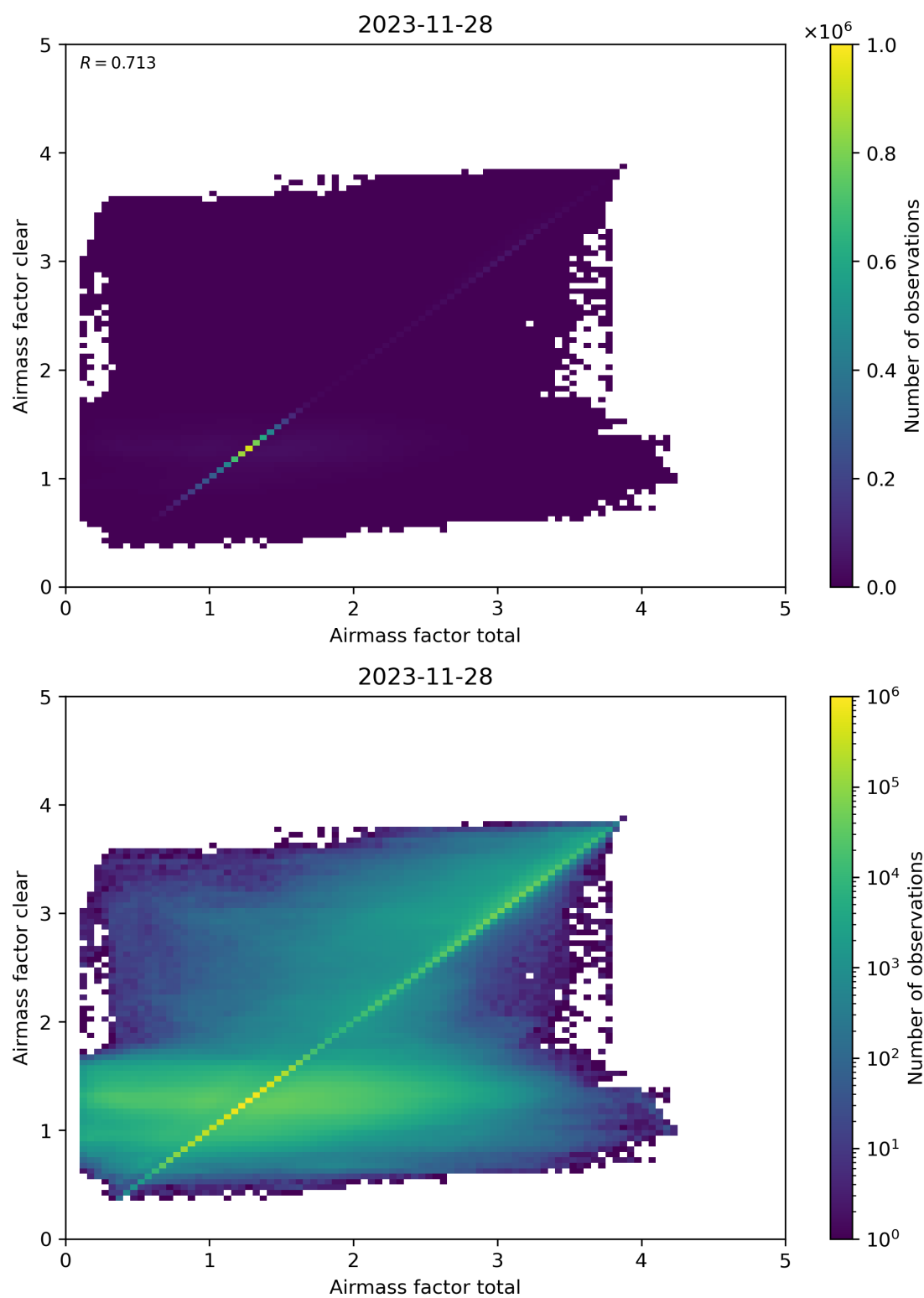
Figure 100: Scatter density plot of “Airmass factor total” against “Airmass factor clear” for 2023-11-28 to 2023-11-29.
