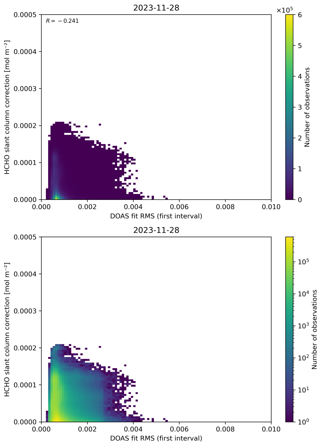
Figure 63: Scatter density plot of “DOAS fit RMS (first interval)” against “HCHO slant column correction” for 2023-11-28 to 2023-11-29.
