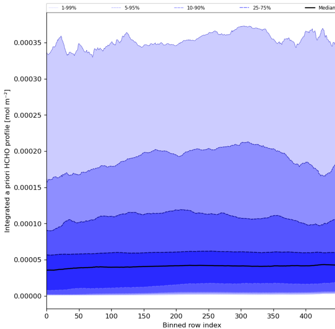
Figure 57: Along track statistics of "Integrated a priori HCHO profile" for 2023-11-28 to 2023-11-29
