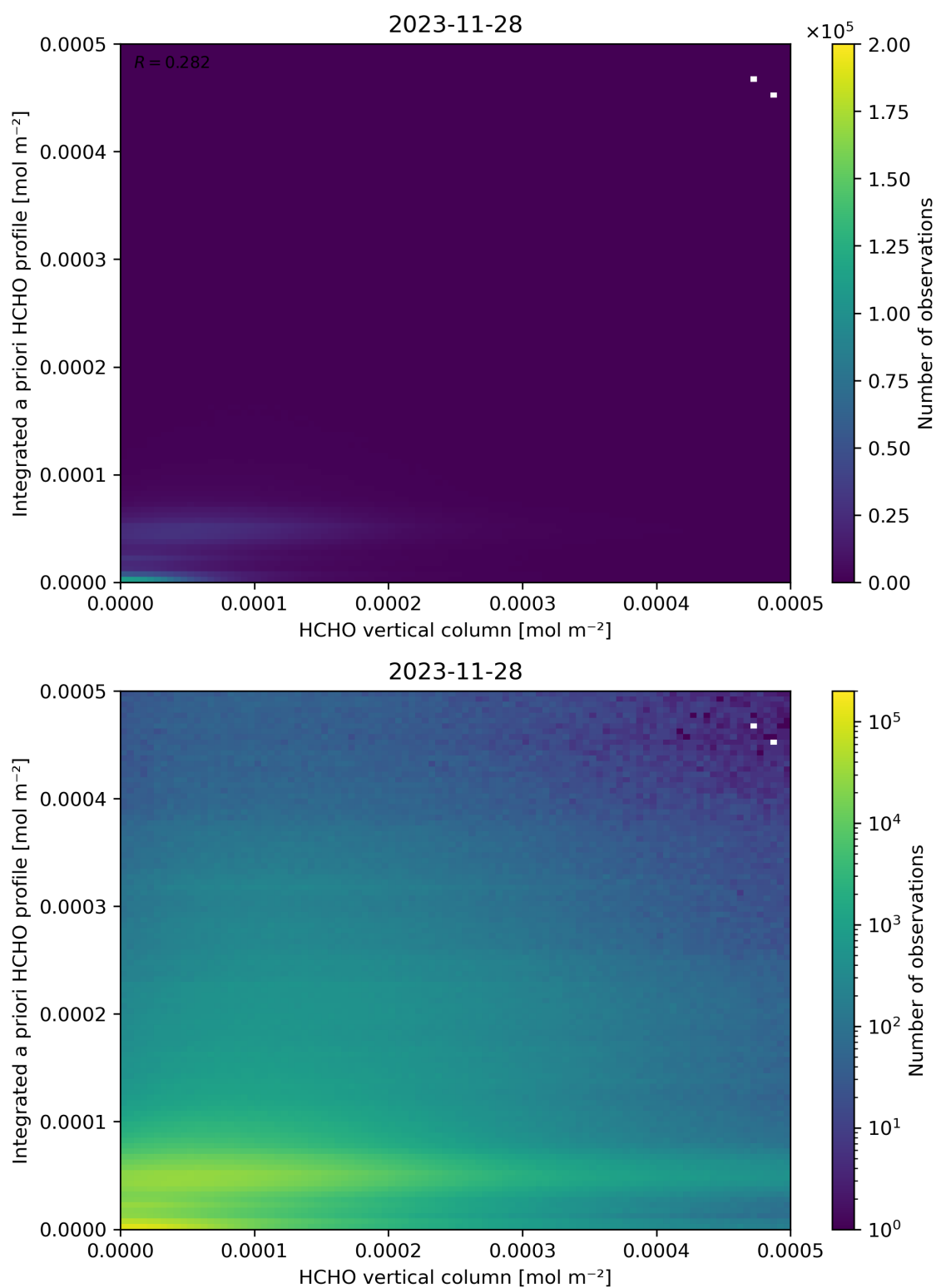
Figure 135: Scatter density plot of “HCHO vertical column” against “Integrated a priori HCHO profile” for 2023-11-28 to 2023-11-29.
