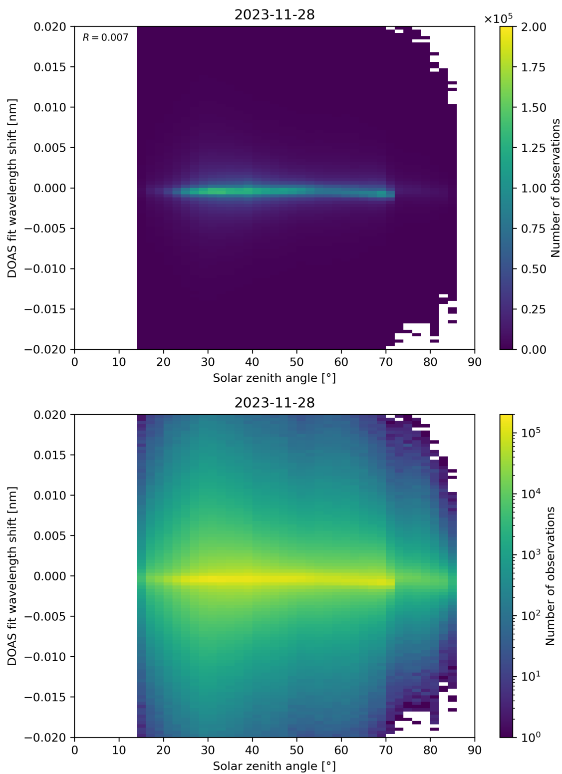
Figure 168: Scatter density plot of “Solar zenith angle” against “DOAS fit wavelength shift” for 2023-11-28 to 2023-11-29.
