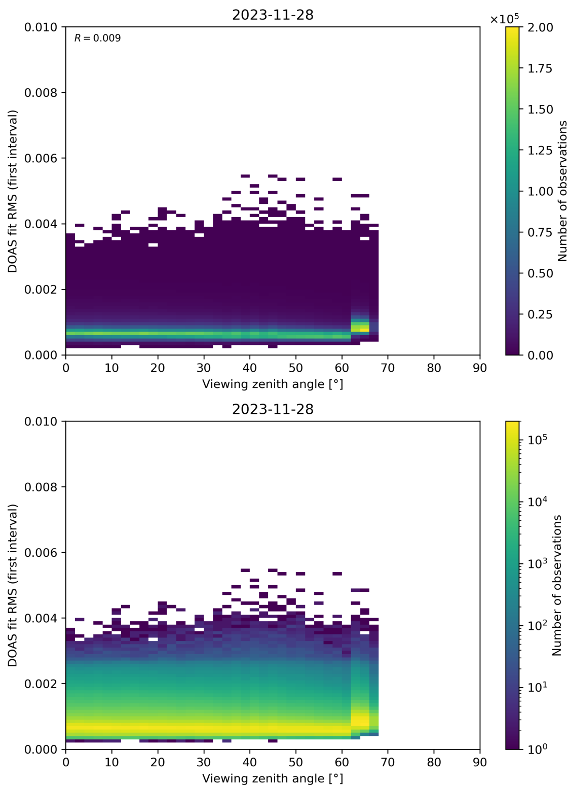
Figure 182: Scatter density plot of “Viewing zenith angle” against “DOAS fit RMS (first interval)” for 2023-11-28 to 2023-11-29.
