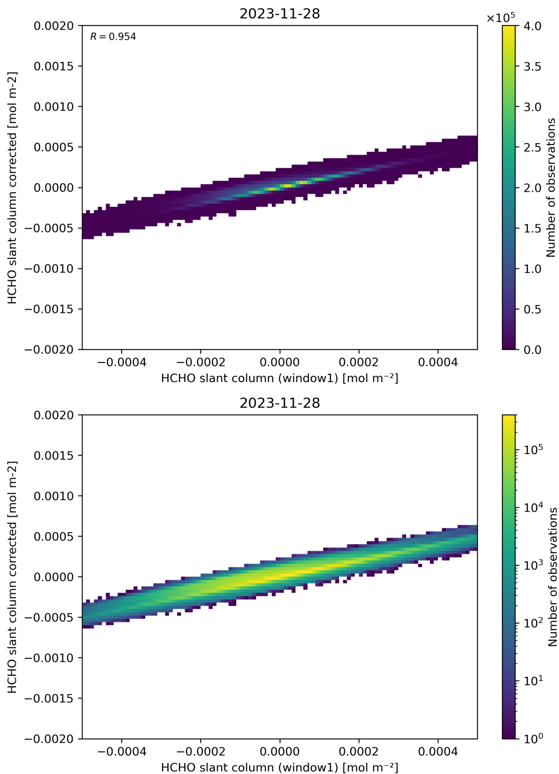
Figure 82: Scatter density plot of “HCHO slant column (window1)” against “HCHO slant column corrected” for 2023-11-28 to 2023-11-29.
