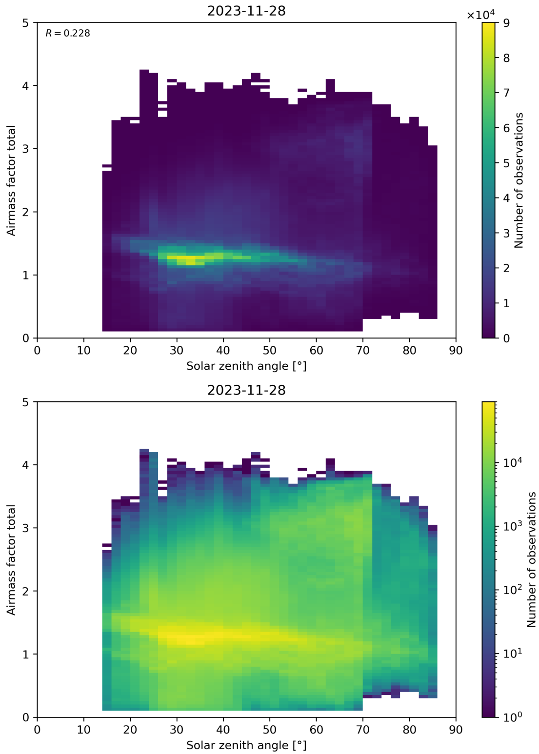
Figure 175: Scatter density plot of “Solar zenith angle” against “Airmass factor total” for 2023-11-28 to 2023-11-29.
