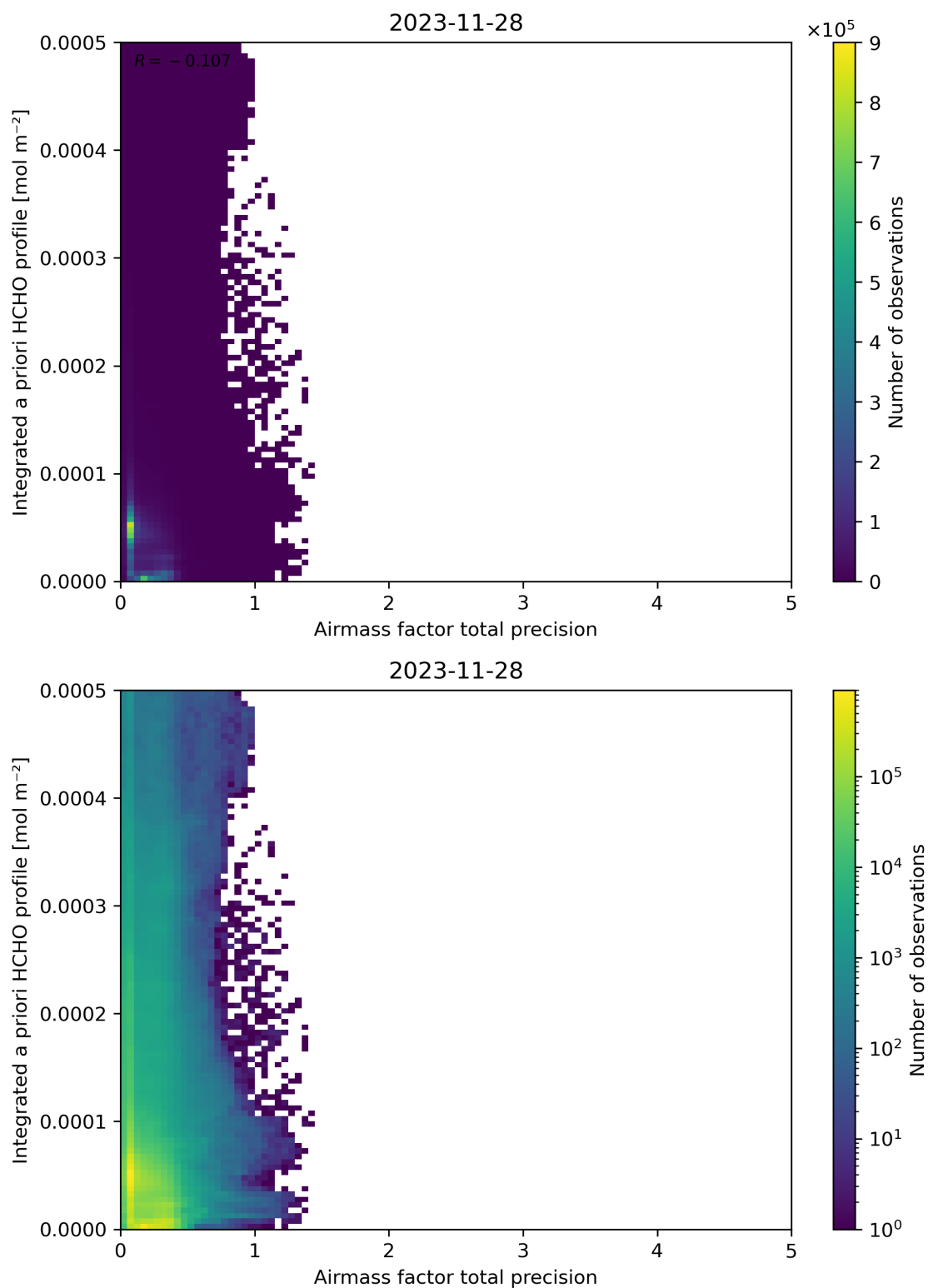
Figure 111: Scatter density plot of “Airmass factor total precision” against “Integrated a priori HCHO profile” for 2023-11-28 to 2023-11-29.
