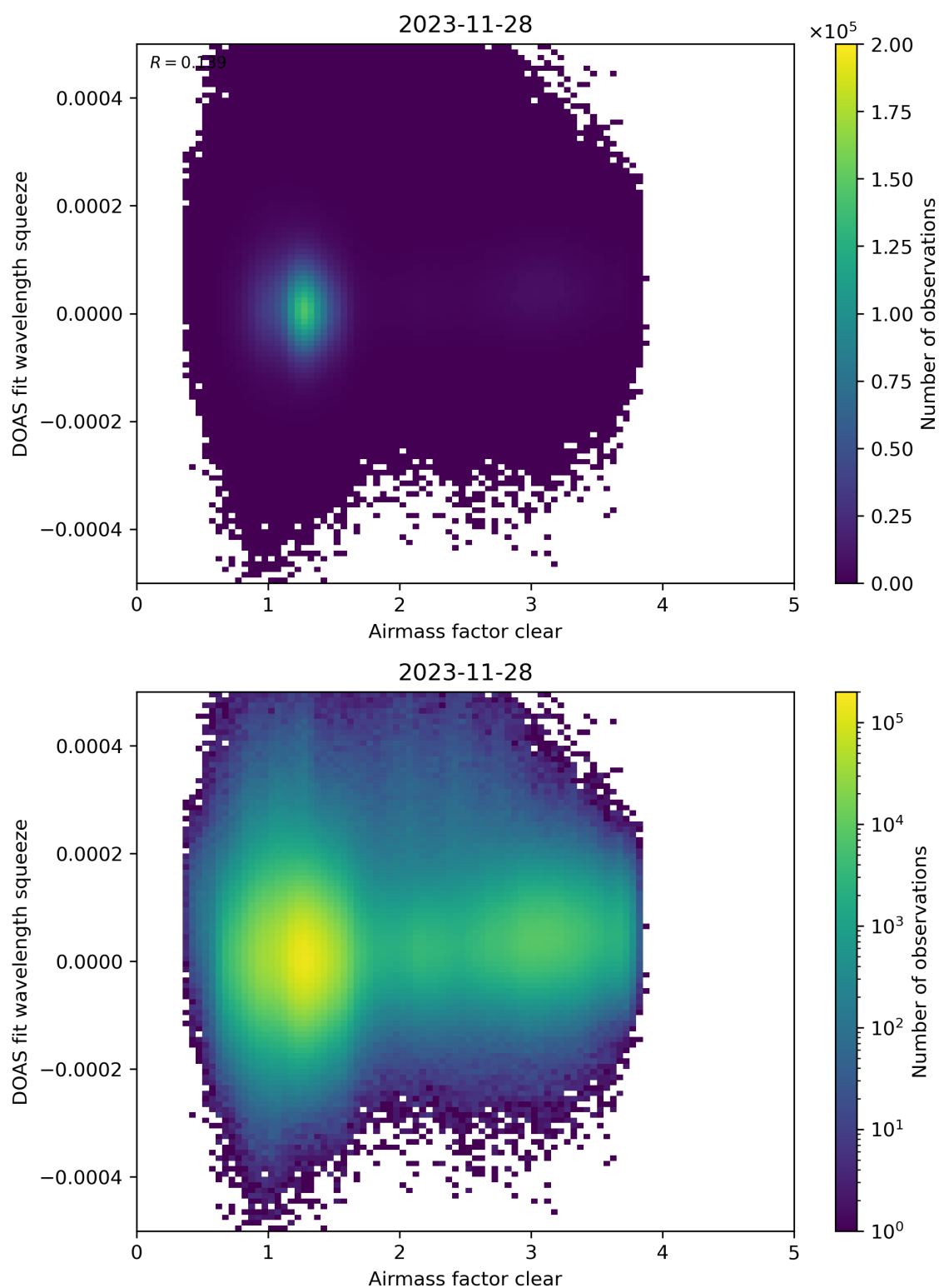
Figure 73: Scatter density plot of “Airmass factor clear” against “DOAS fit wavelength squeeze” for 2023-11-28 to 2023-11-29.
