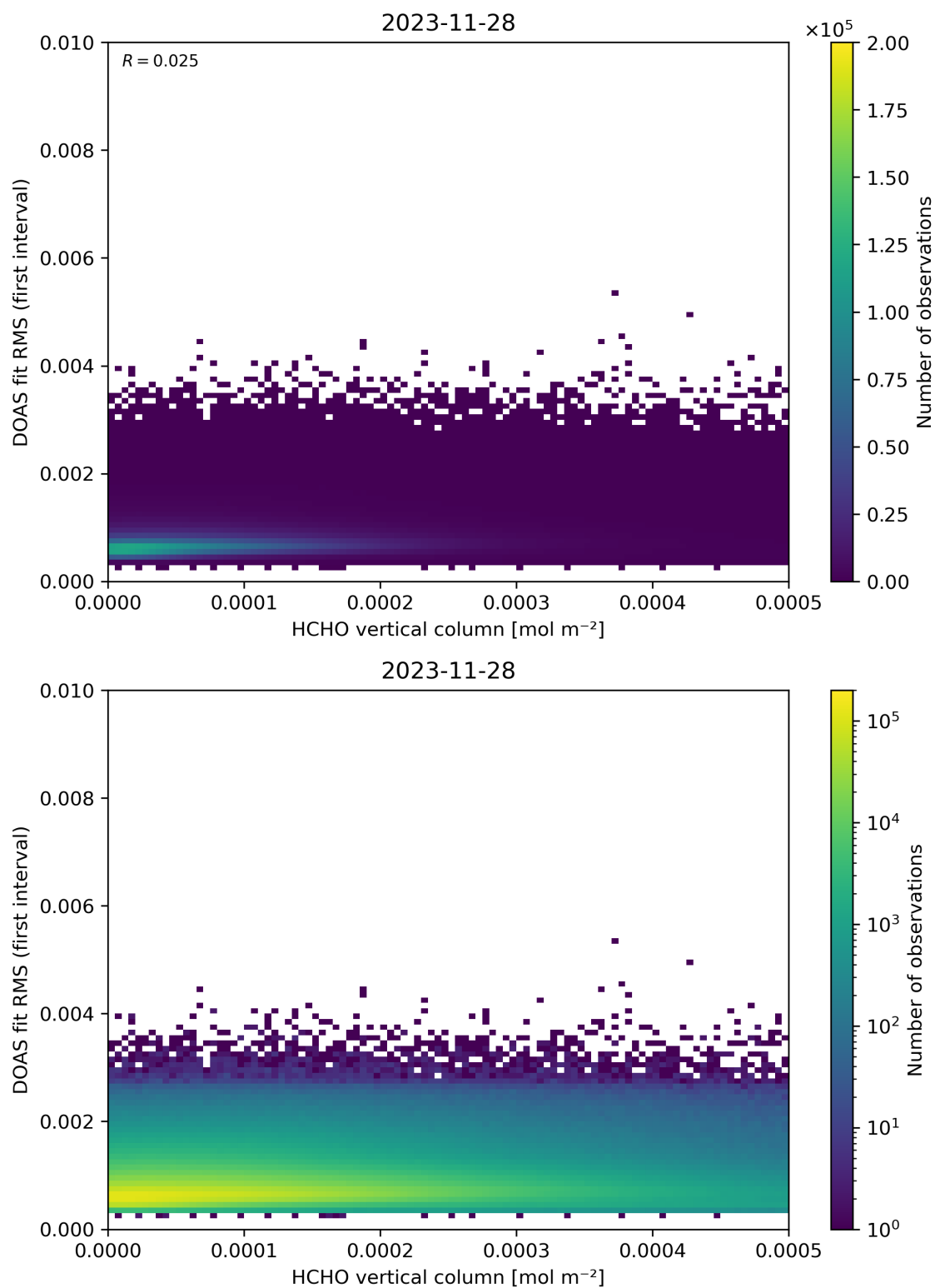
Figure 123: Scatter density plot of “HCHO vertical column” against “DOAS fit RMS (first interval)” for 2023-11-28 to 2023-11-29.
