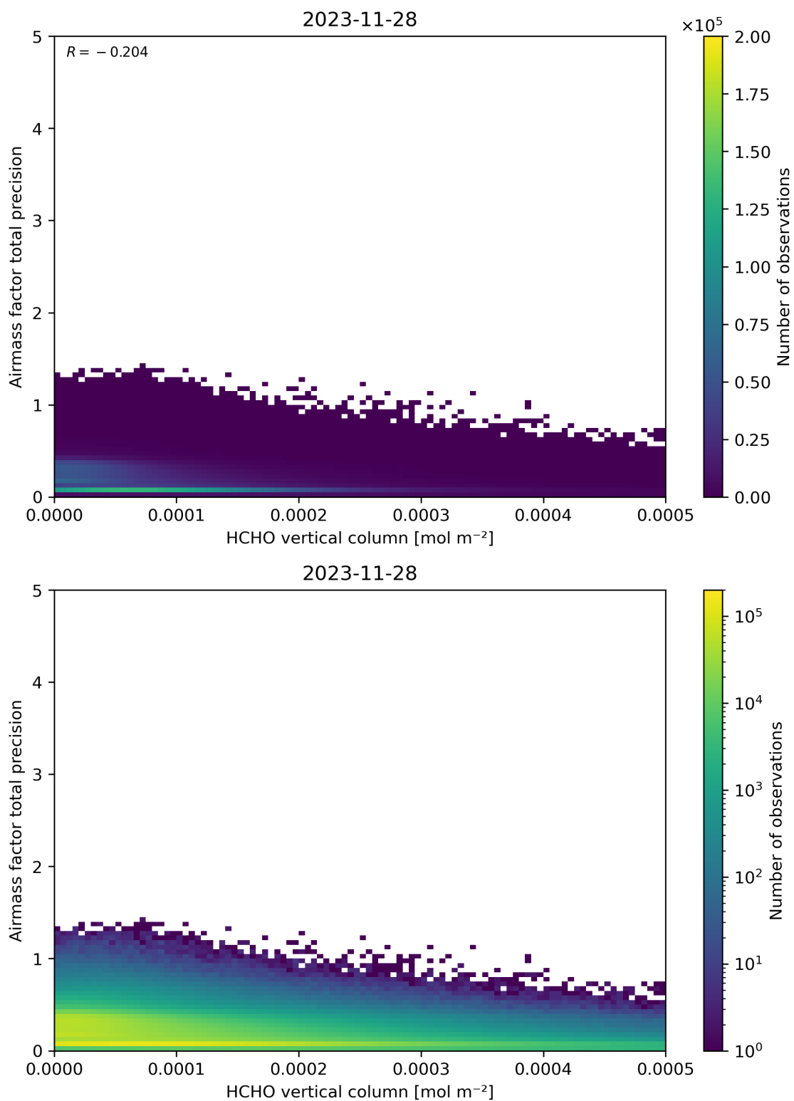
Figure 132: Scatter density plot of “HCHO vertical column” against “Airmass factor total precision” for 2023-11-28 to 2023-11-29.
