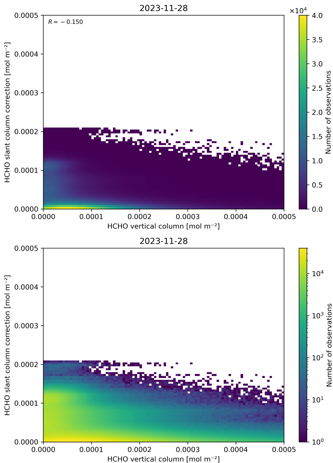
Figure 128: Scatter density plot of “HCHO vertical column” against “HCHO slant column correction” for 2023-11-28 to 2023-11-29.
