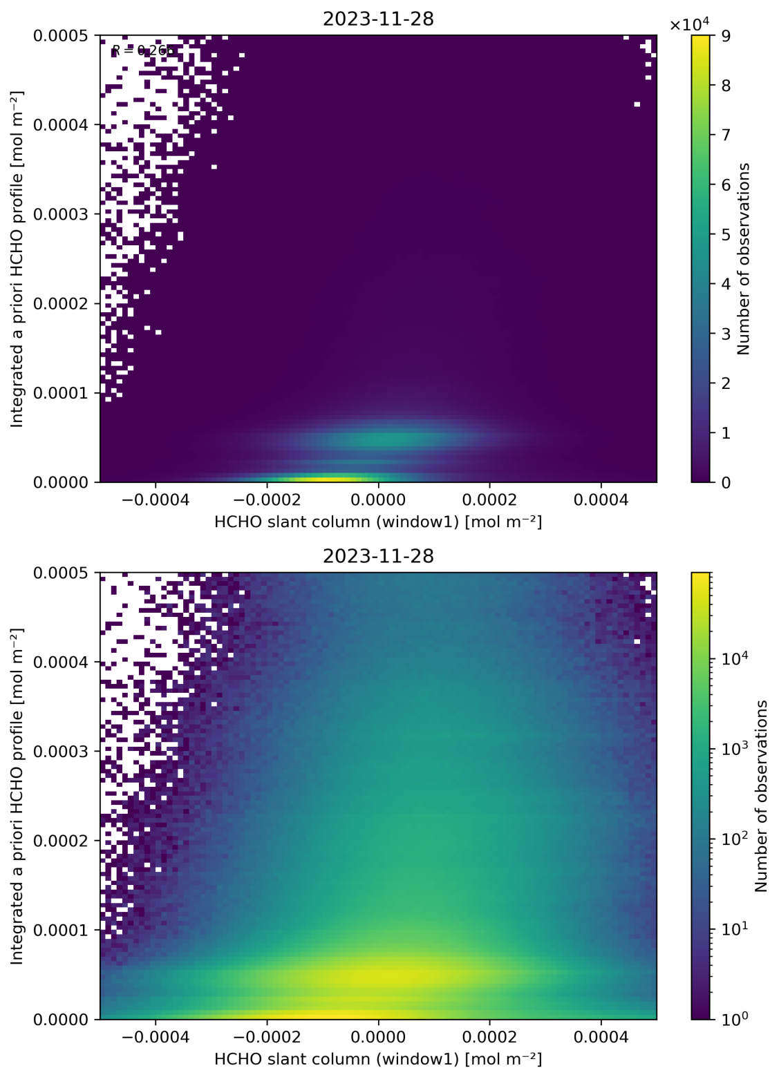
Figure 87: Scatter density plot of “HCHO slant column (window1)” against “Integrated a priori HCHO profile” for 2023-11-28 to 2023-11-29.
