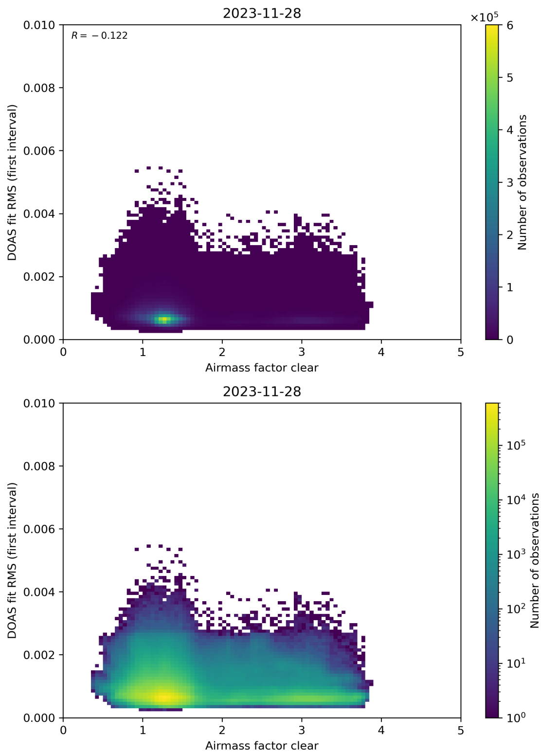
Figure 71: Scatter density plot of “Airmass factor clear” against “DOAS fit RMS (first interval)” for 2023-11-28 to 2023-11-29.
