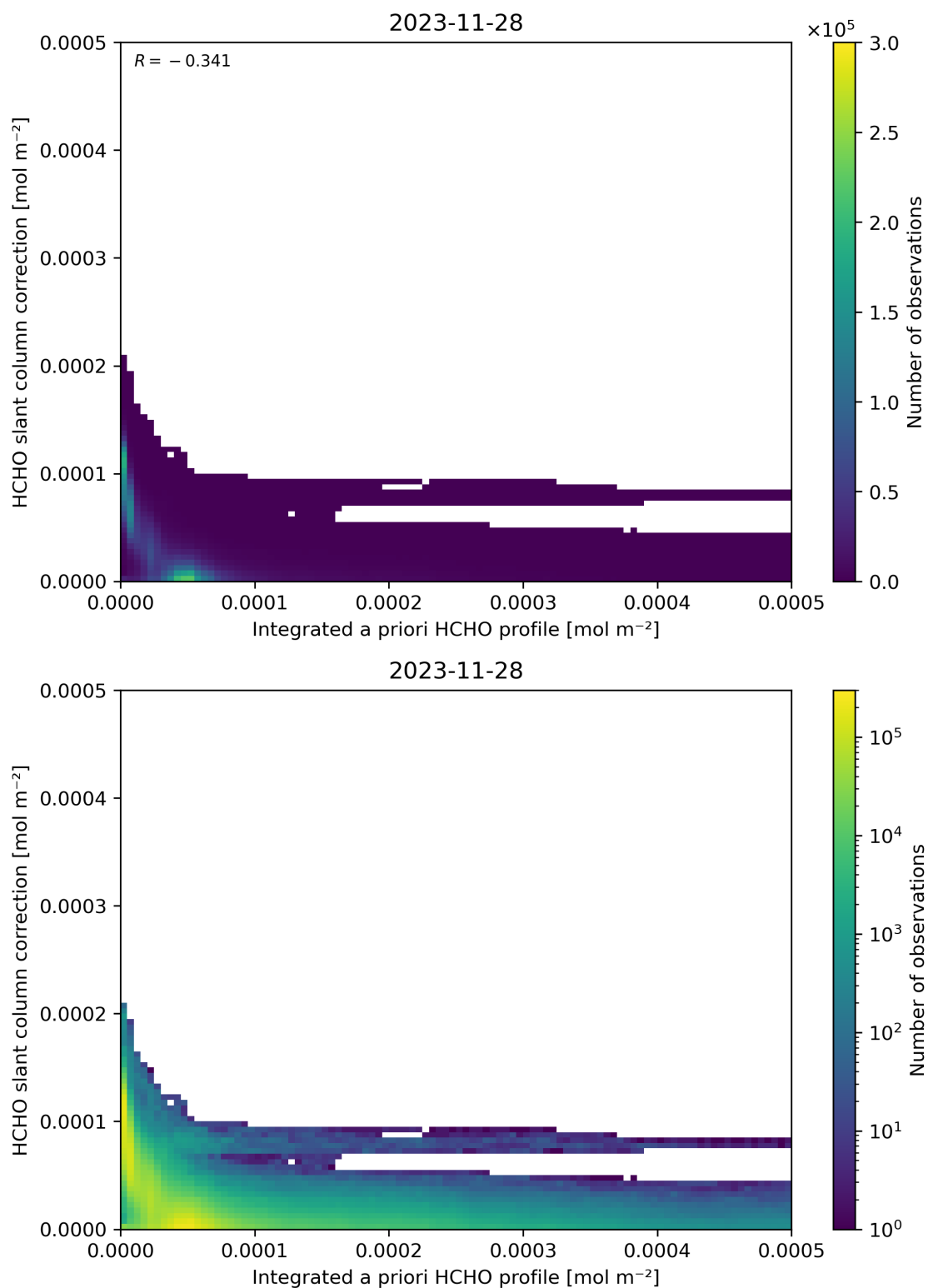
Figure 152: Scatter density plot of “Integrated a priori HCHO profile” against “HCHO slant column correction” for 2023-11-28 to 2023-11-29.
