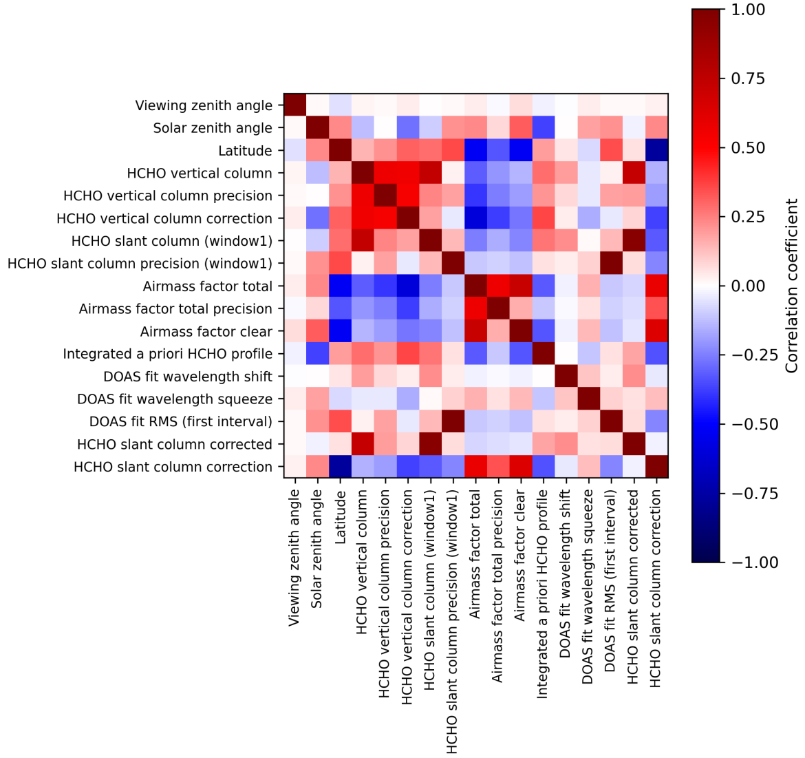
Figure 2: Map of correlation matrix for 2023-11-28 to 2023-11-29.
