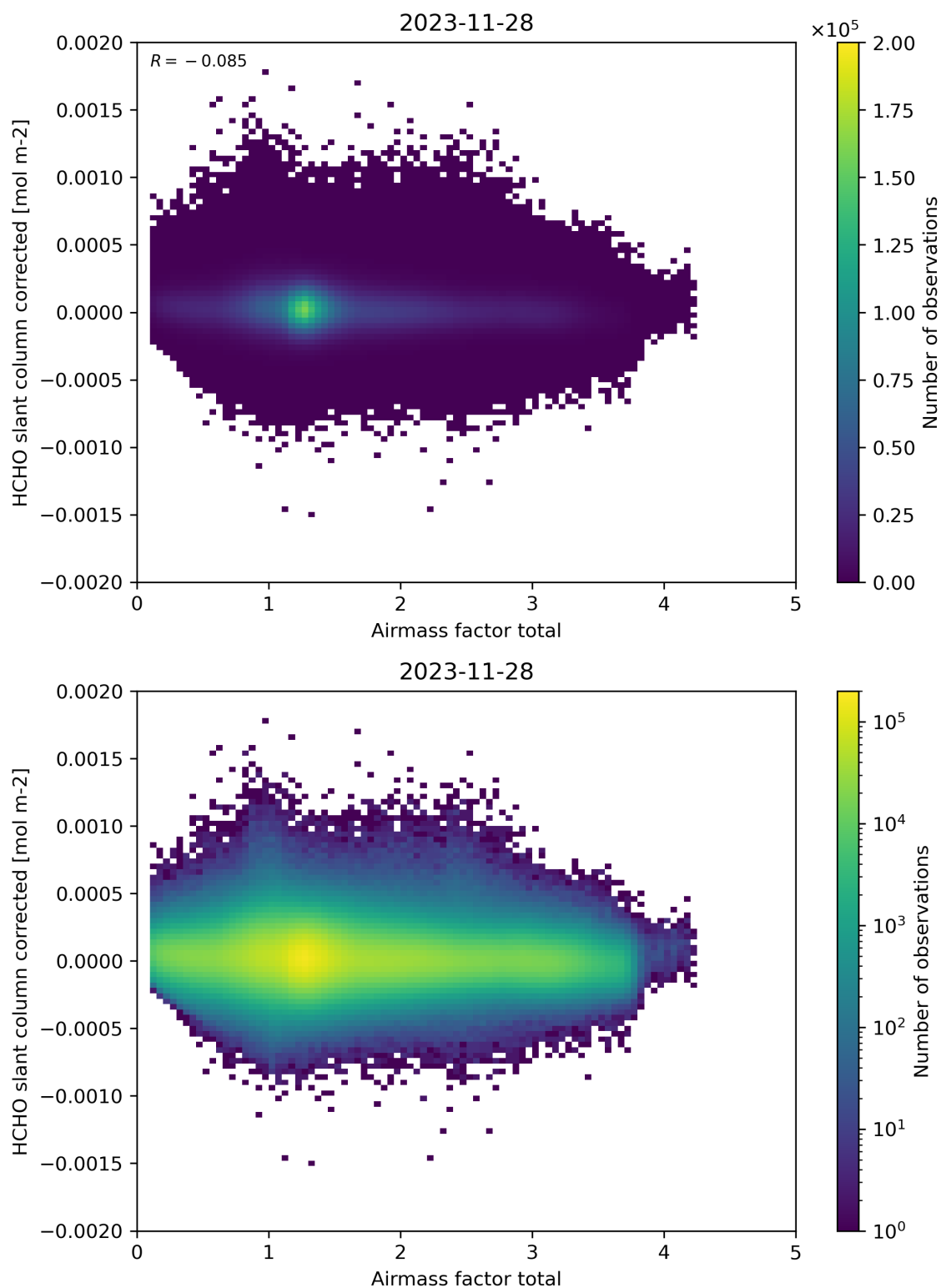
Figure 101: Scatter density plot of “Airmass factor total” against “HCHO slant column corrected” for 2023-11-28 to 2023-11-29.
