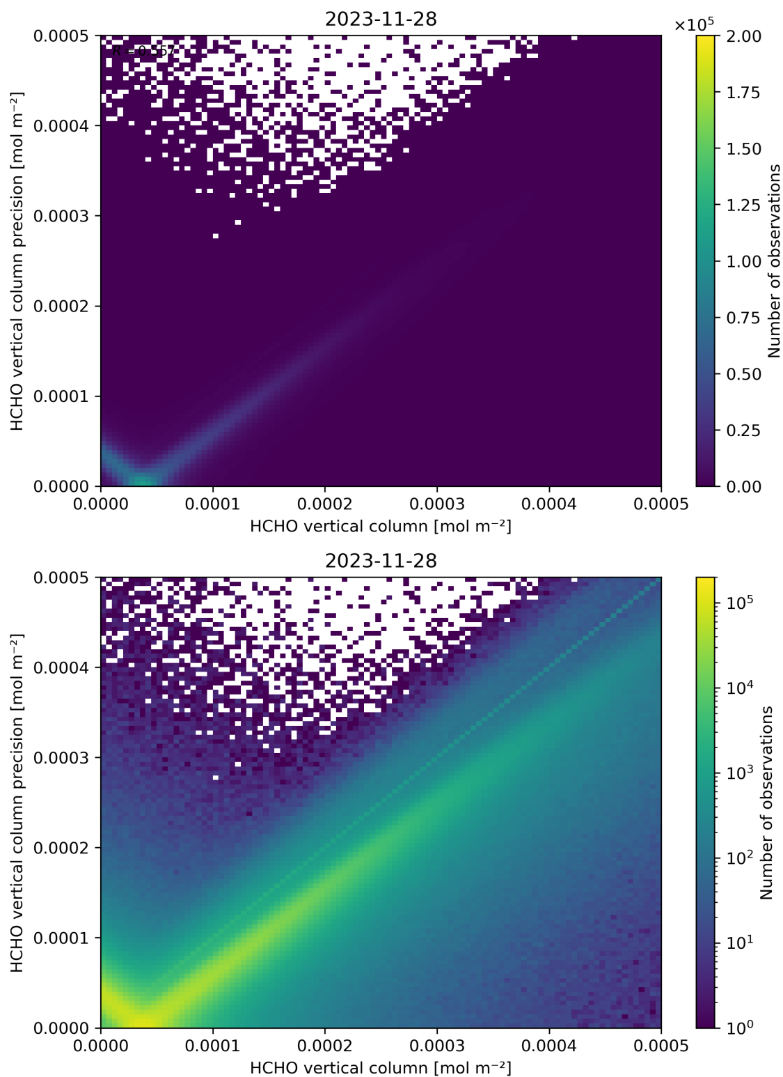
Figure 134: Scatter density plot of “HCHO vertical column” against “HCHO vertical column precision” for 2023-11-28 to 2023-11-29.
