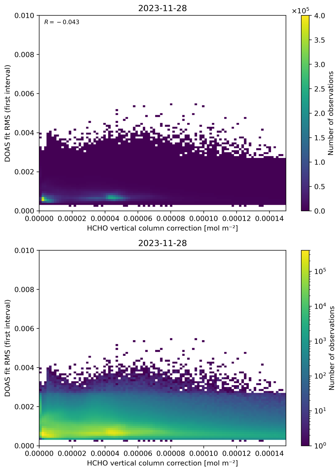
Figure 112: Scatter density plot of “HCHO vertical column correction” against “DOAS fit RMS (first interval)” for 2023-11-28 to 2023-11-29.
