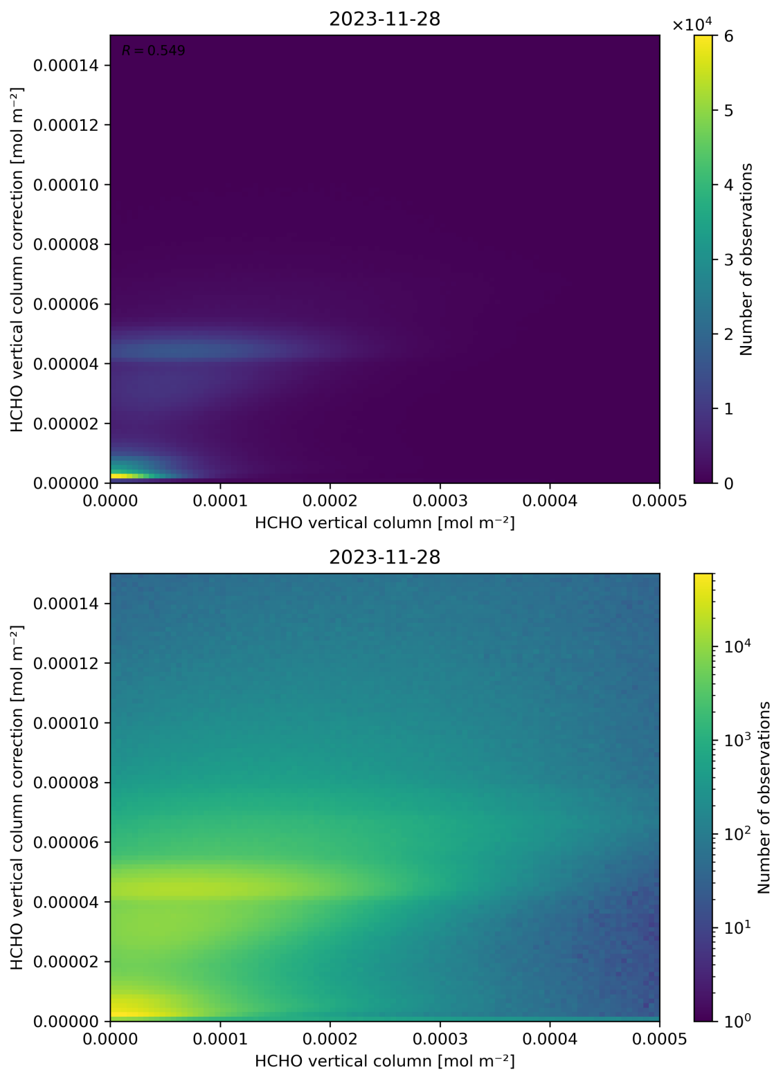
Figure 133: Scatter density plot of “HCHO vertical column” against “HCHO vertical column correction” for 2023-11-28 to 2023-11-29.
