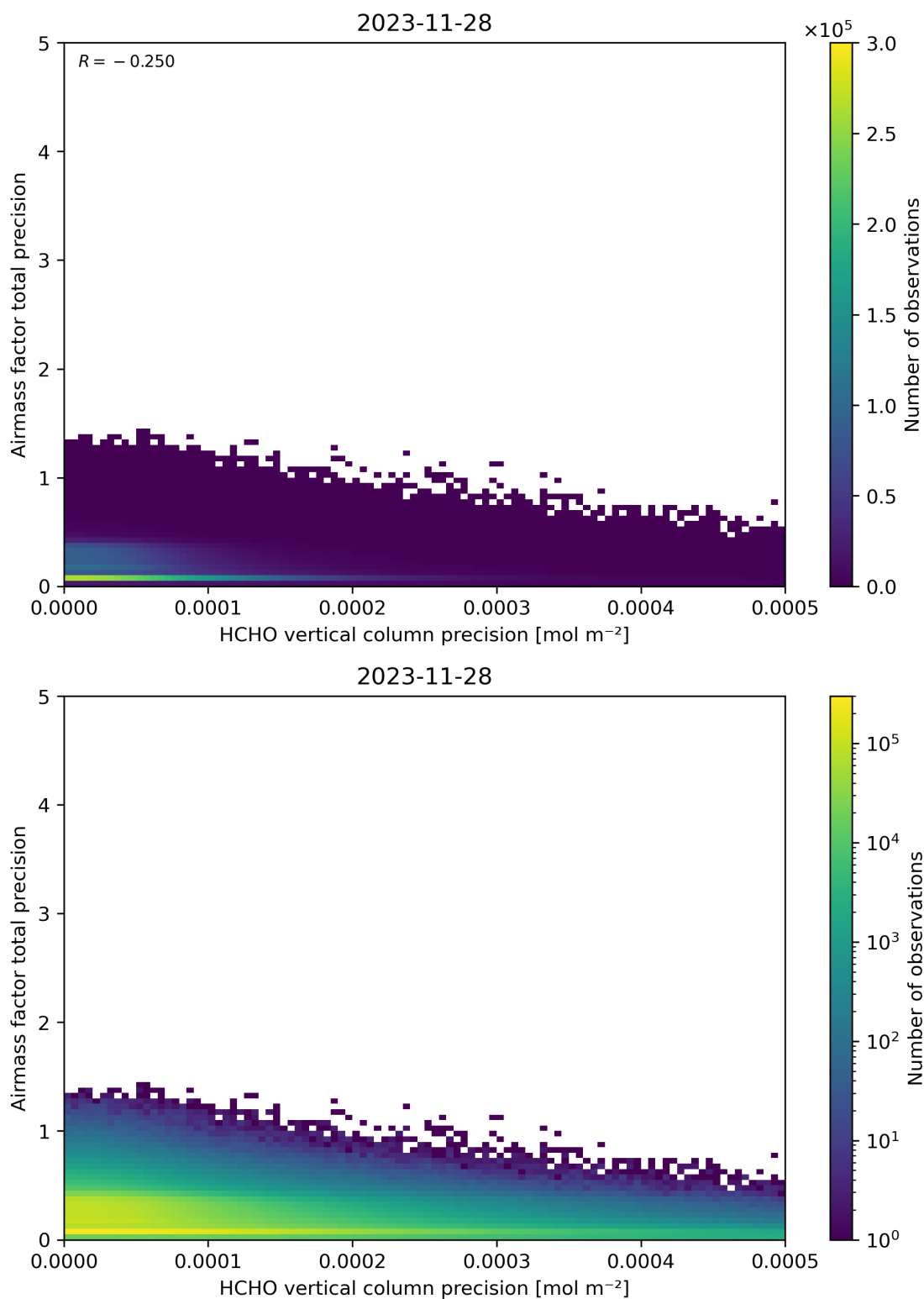
Figure 145: Scatter density plot of “HCHO vertical column precision” against “Airmass factor total precision” for 2023-11-28 to 2023-11-29.
