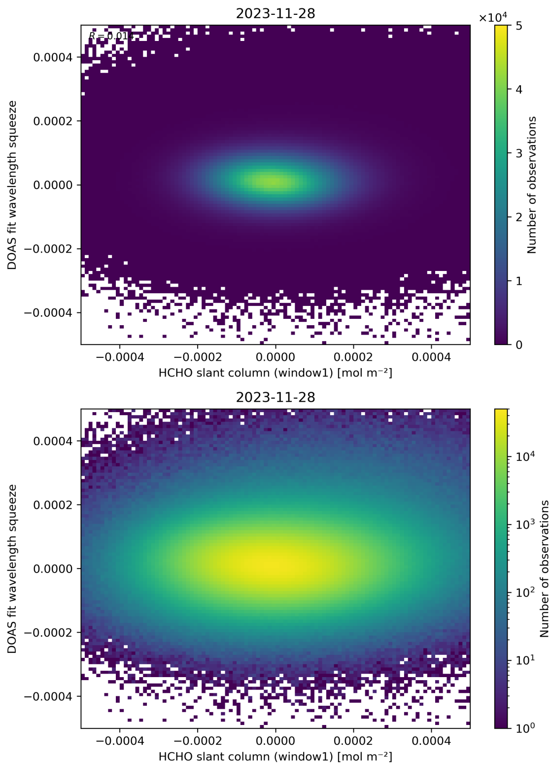
Figure 80: Scatter density plot of “HCHO slant column (window1)” against “DOAS fit wavelength squeeze” for 2023-11-28 to 2023-11-29.
