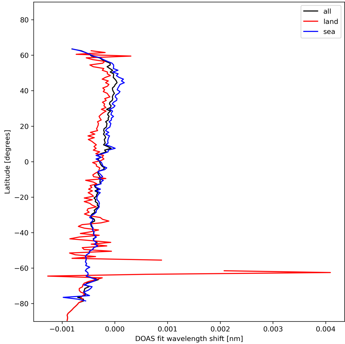
Figure 30: Zonal average of “DOAS fit wavelength shift” for 2023-11-28 to 2023-11-29.
