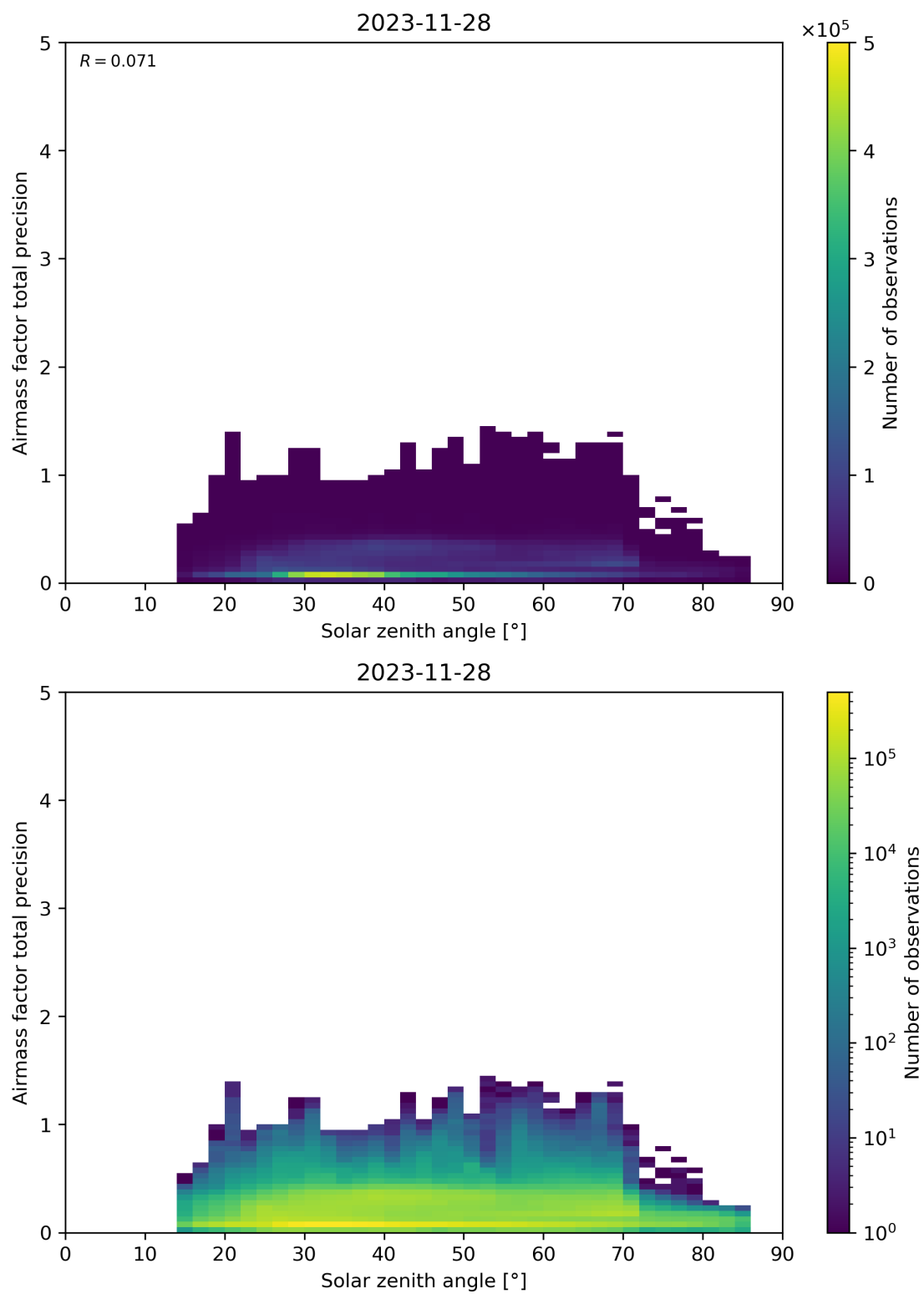
Figure 176: Scatter density plot of “Solar zenith angle” against “Airmass factor total precision” for 2023-11-28 to 2023-11-29.
