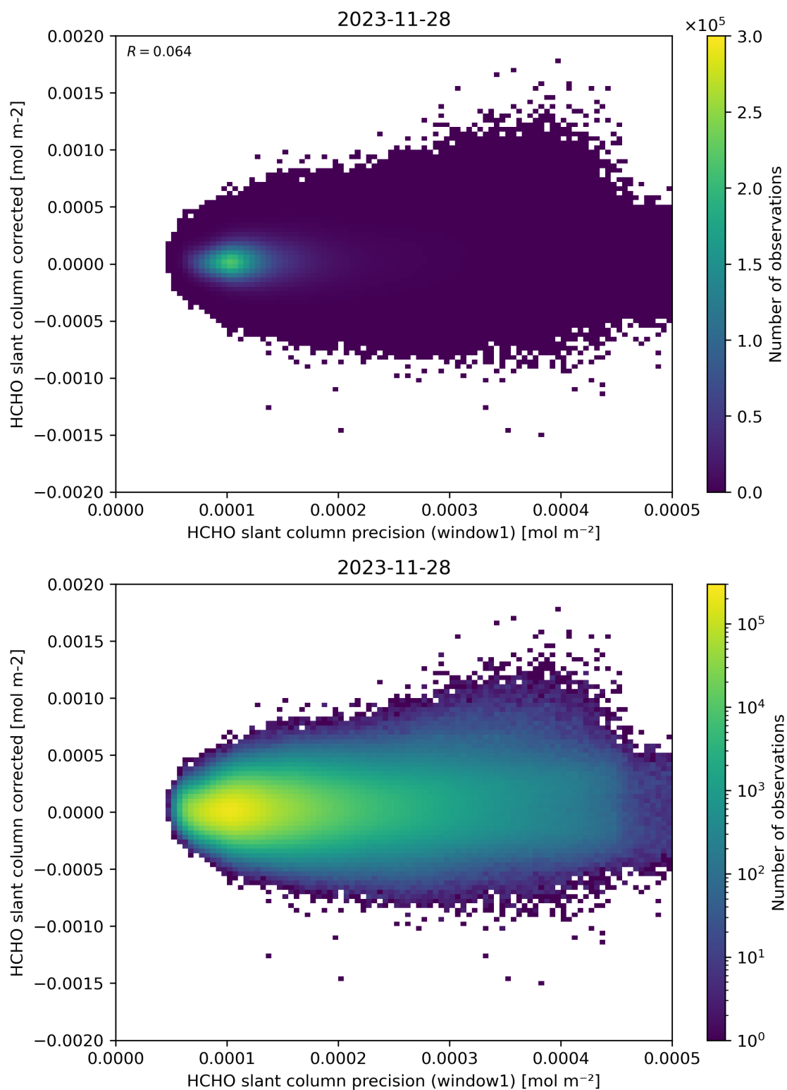
Figure 92: Scatter density plot of “HCHO slant column precision (window1)” against “HCHO slant column corrected” for 2023-11-28 to 2023-11-29.
