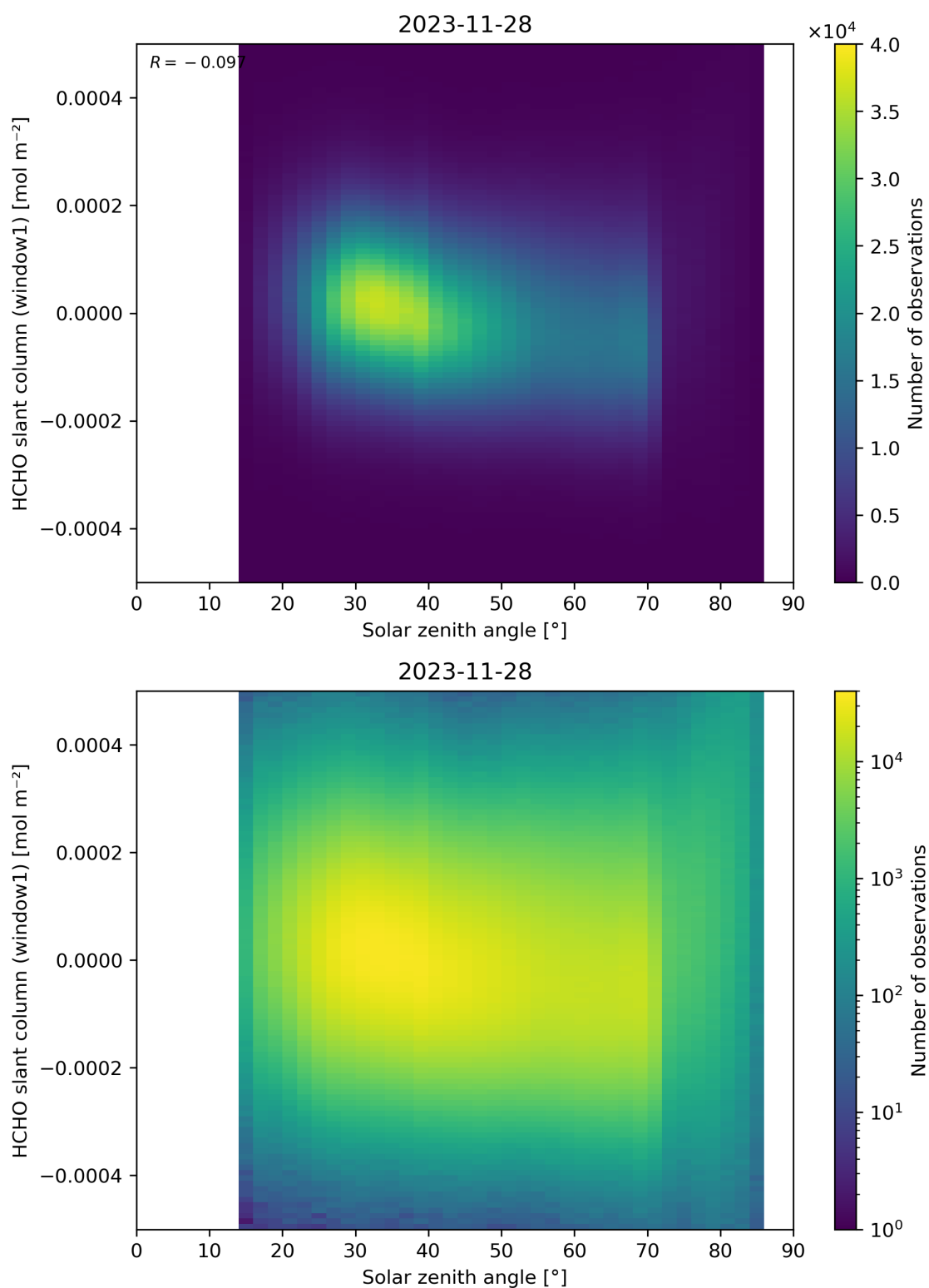
Figure 173: Scatter density plot of “Solar zenith angle” against “HCHO slant column (window1)” for 2023-11-28 to 2023-11-29.
