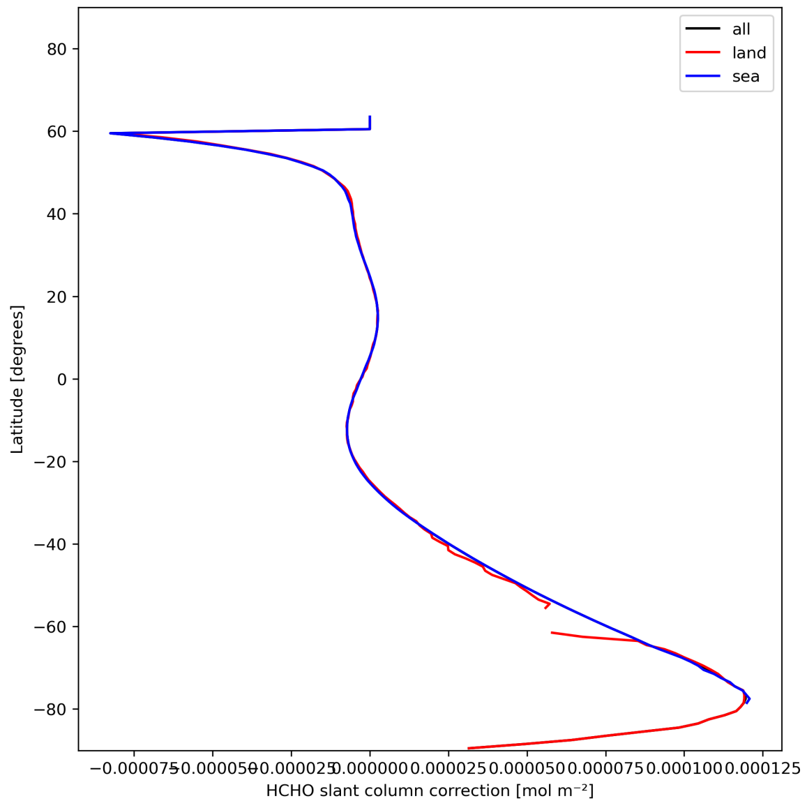
Figure 33: Zonal average of “HCHO slant column correction” for 2023-11-28 to 2023-11-29.
