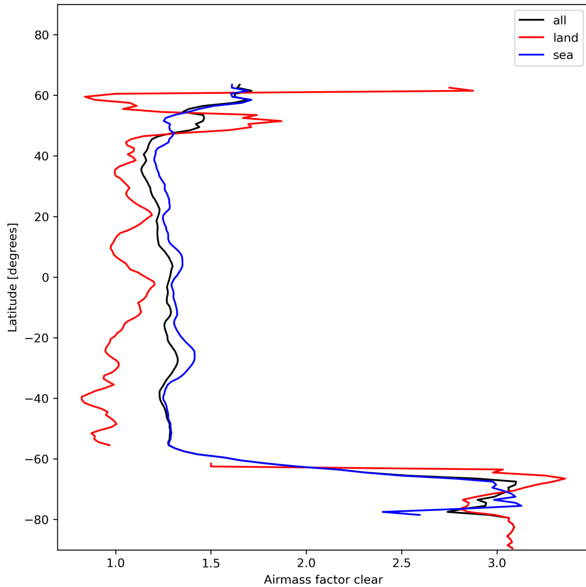
Figure 28: Zonal average of “Airmass factor clear” for 2023-11-28 to 2023-11-29.
