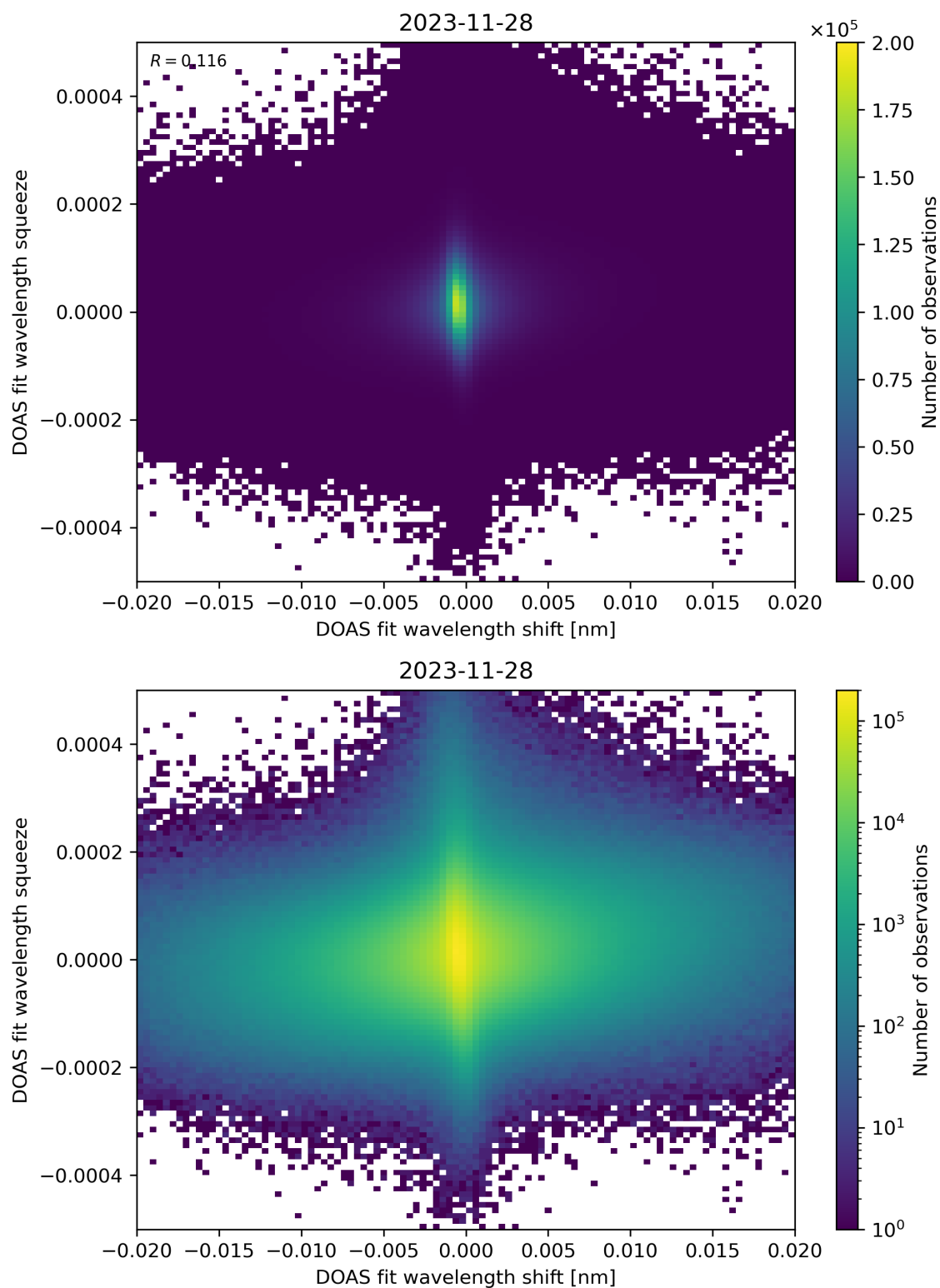
Figure 65: Scatter density plot of “DOAS fit wavelength shift” against “DOAS fit wavelength squeeze” for 2023-11-28 to 2023-11-29.
