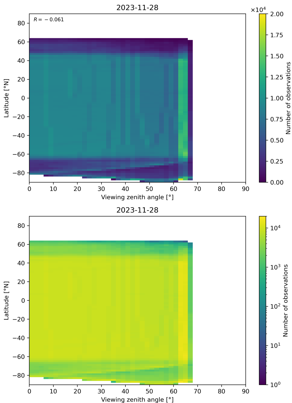
Figure 196: Scatter density plot of “Viewing zenith angle” against “Latitude” for 2023-11-28 to 2023-11-29.
