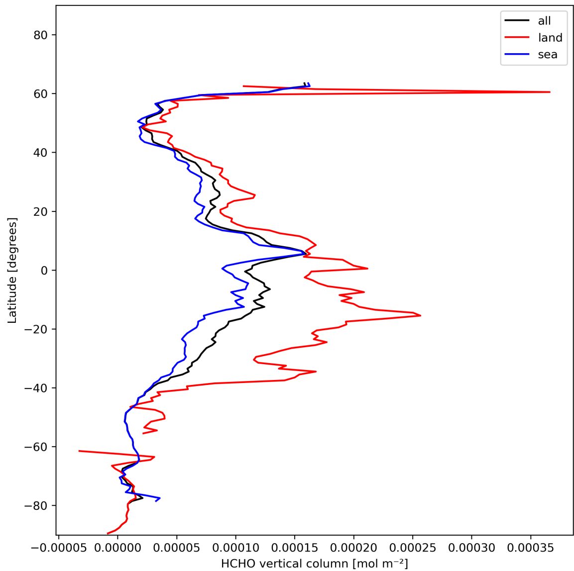
Figure 21: Zonal average of “HCHO vertical column” for 2023-11-28 to 2023-11-29.
