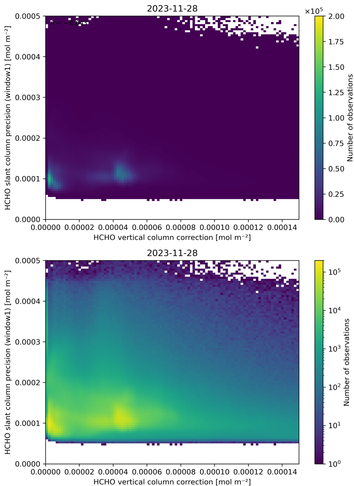
Figure 119: Scatter density plot of “HCHO vertical column correction” against “HCHO slant column precision (window1)” for 2023-11-28 to 2023-11-29.
