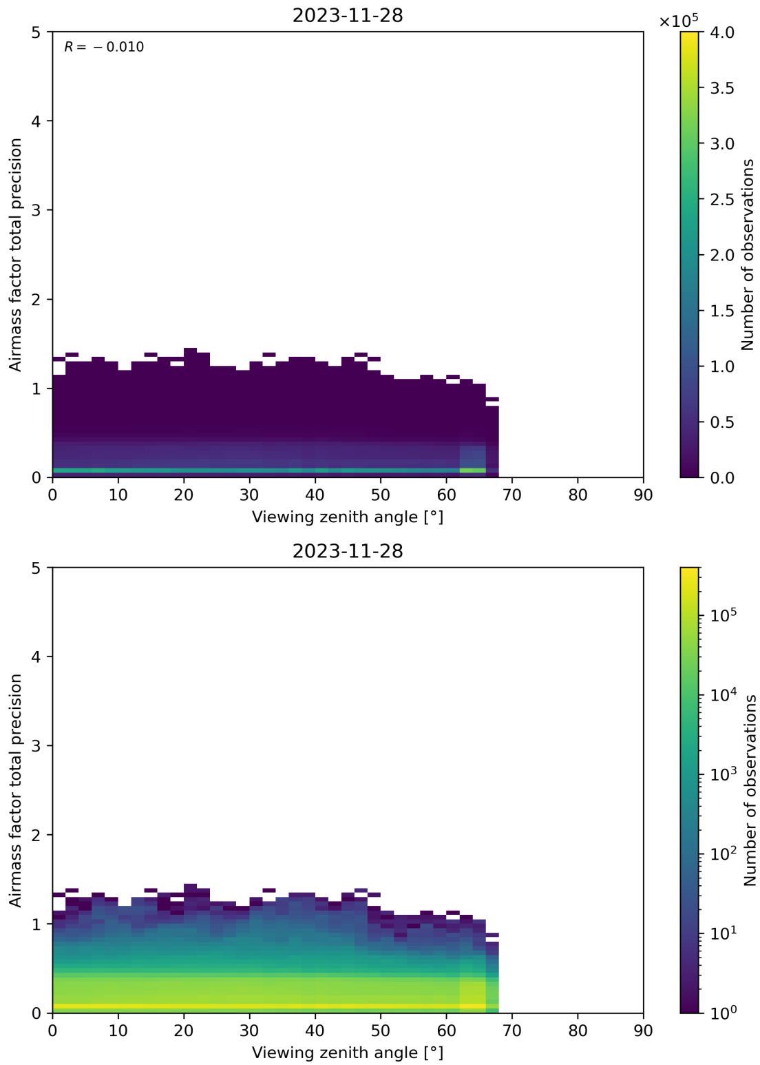
Figure 191: Scatter density plot of “Viewing zenith angle” against “Airmass factor total precision” for 2023-11-28 to 2023-11-29.
