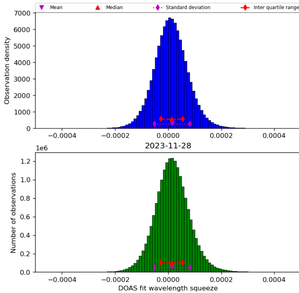
Figure 45: Histogram of “DOAS fit wavelength squeeze” for 2023-11-28 to 2023-11-29
