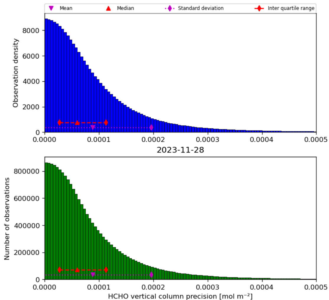
Figure 36: Histogram of “HCHO vertical column precision” for 2023-11-28 to 2023-11-29
