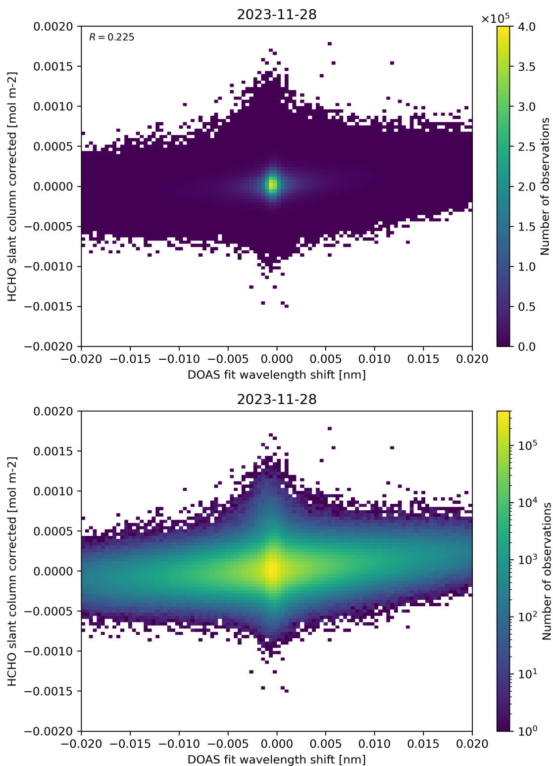
Figure 66: Scatter density plot of “DOAS fit wavelength shift” against “HCHO slant column corrected” for 2023-11-28 to 2023-11-29.
