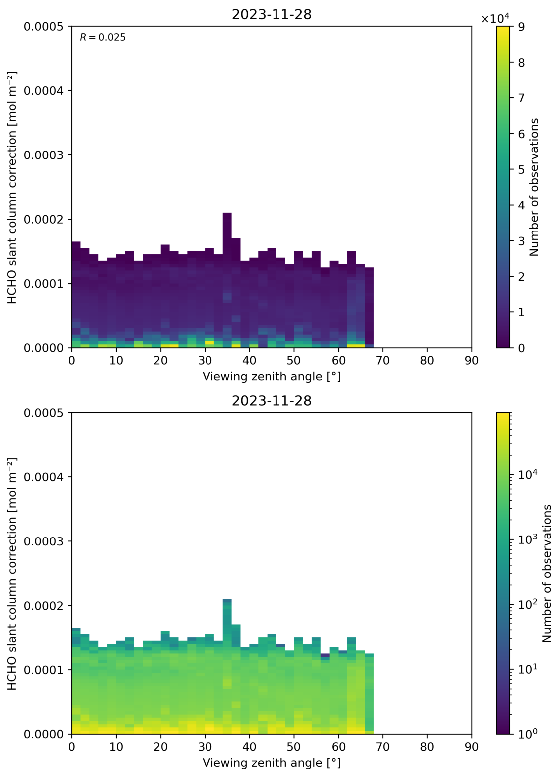
Figure 187: Scatter density plot of “Viewing zenith angle” against “HCHO slant column correction” for 2023-11-28 to 2023-11-29.
