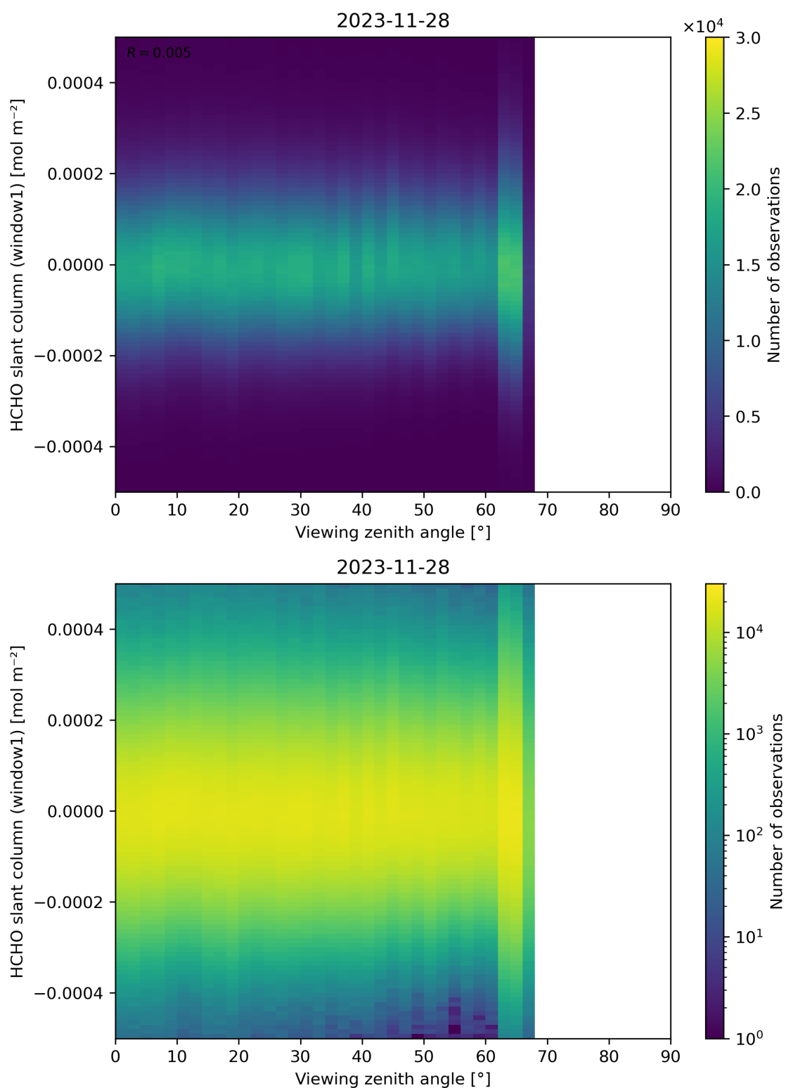
Figure 188: Scatter density plot of “Viewing zenith angle” against “HCHO slant column (window1)” for 2023-11-28 to 2023-11-29.
