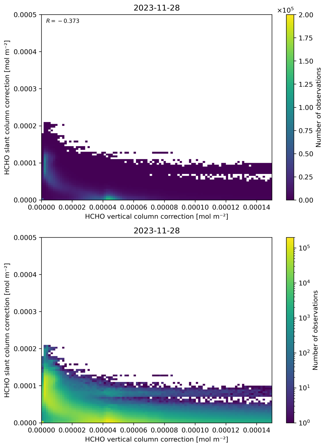
Figure 117: Scatter density plot of “HCHO vertical column correction” against “HCHO slant column correction” for 2023-11-28 to 2023-11-29.
