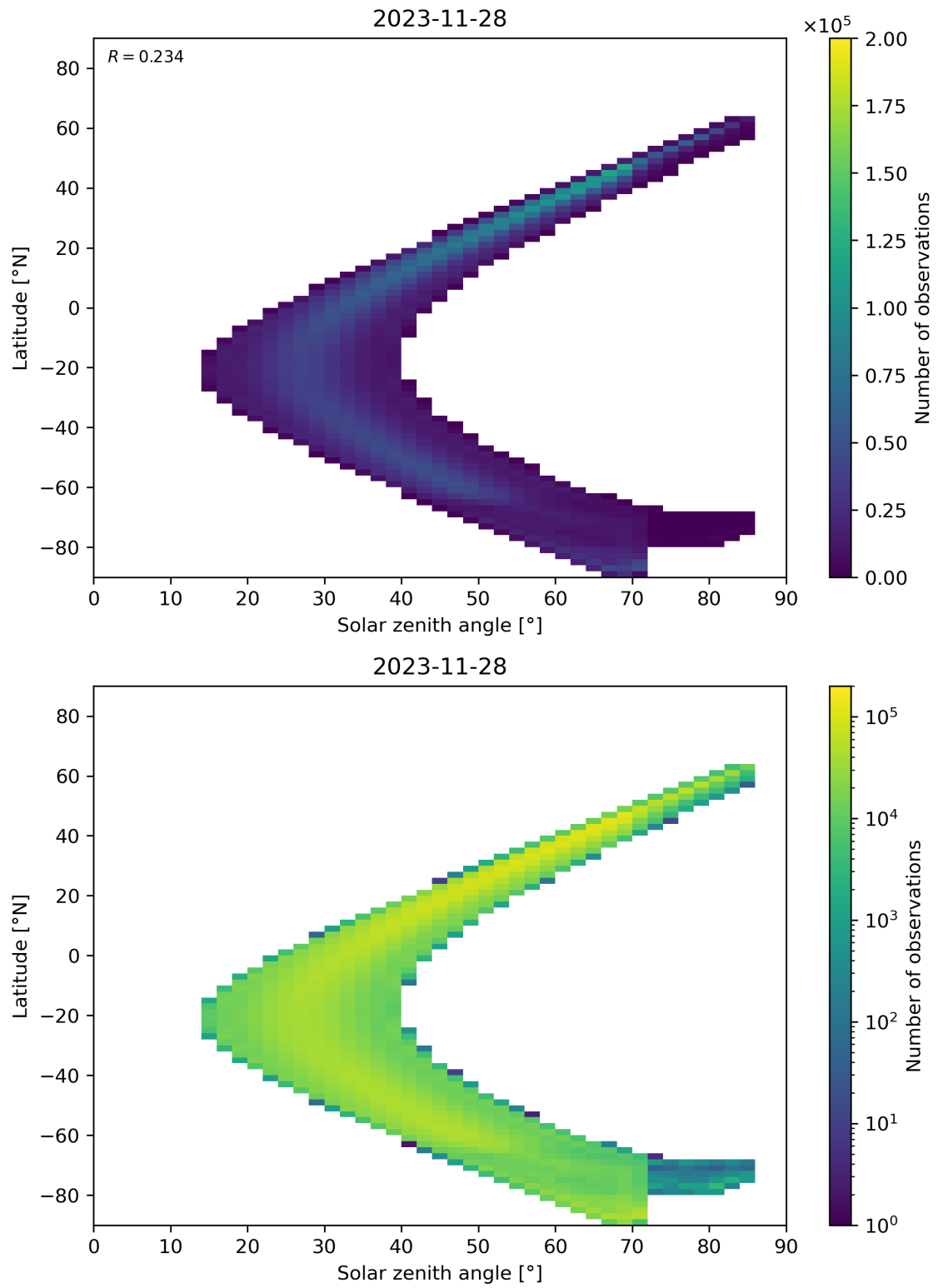
Figure 181: Scatter density plot of “Solar zenith angle” against “Latitude” for 2023-11-28 to 2023-11-29.
