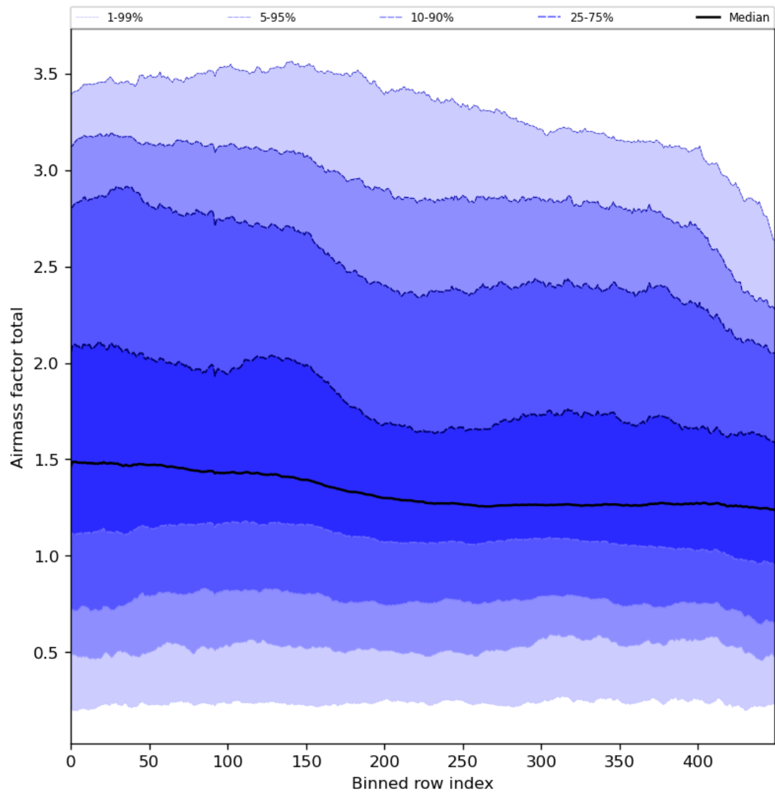
Figure 54: Along track statistics of “Airmass factor total” for 2023-11-28 to 2023-11-29
