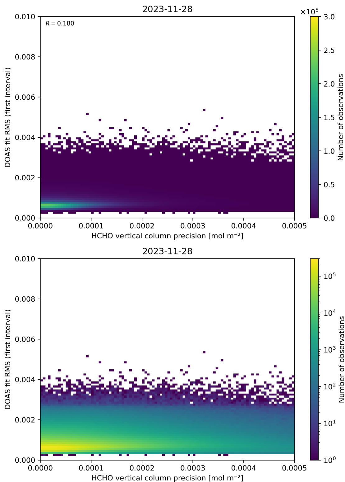
Figure 136: Scatter density plot of “HCHO vertical column precision” against “DOAS fit RMS (first interval)” for 2023-11-28 to 2023-11-29.
