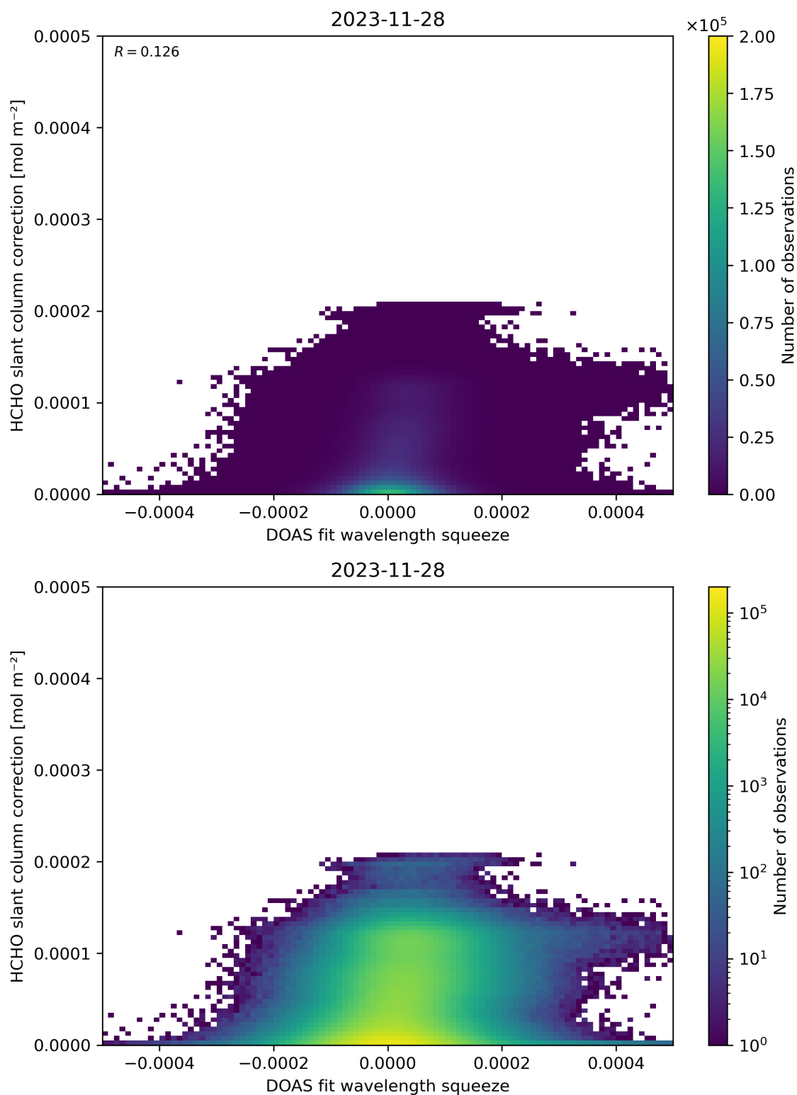
Figure 70: Scatter density plot of “DOAS fit wavelength squeeze” against “HCHO slant column correction” for 2023-11-28 to 2023-11-29.
