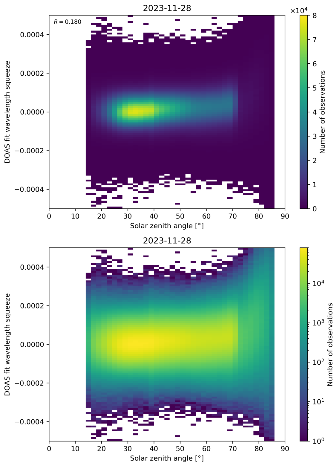
Figure 169: Scatter density plot of “Solar zenith angle” against “DOAS fit wavelength squeeze” for 2023-11-28 to 2023-11-29.
