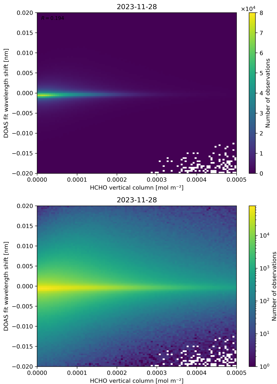
Figure 124: Scatter density plot of “HCHO vertical column” against “DOAS fit wavelength shift” for 2023-11-28 to 2023-11-29.
