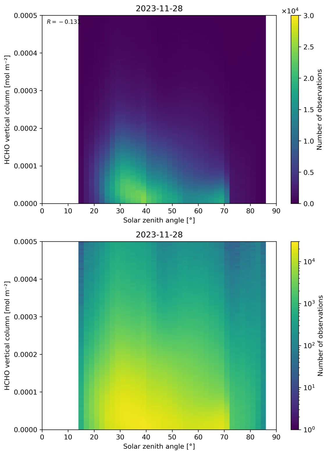
Figure 177: Scatter density plot of “Solar zenith angle” against “HCHO vertical column” for 2023-11-28 to 2023-11-29.
