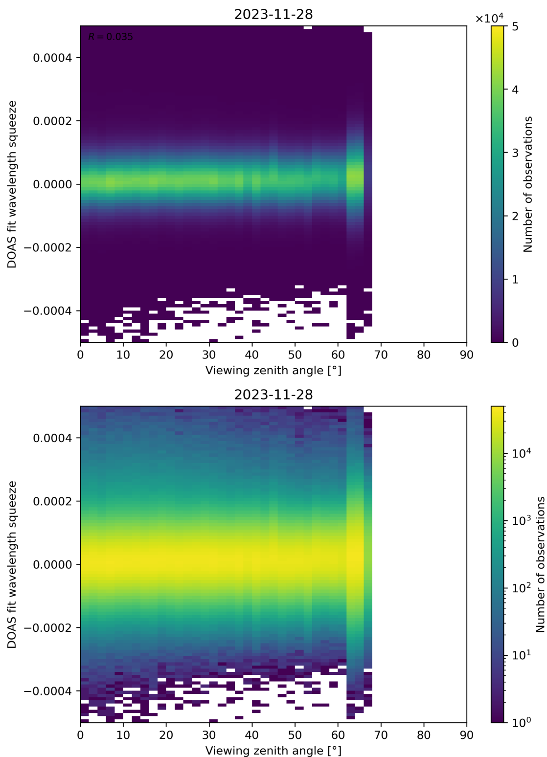
Figure 184: Scatter density plot of “Viewing zenith angle” against “DOAS fit wavelength squeeze” for 2023-11-28 to 2023-11-29.
