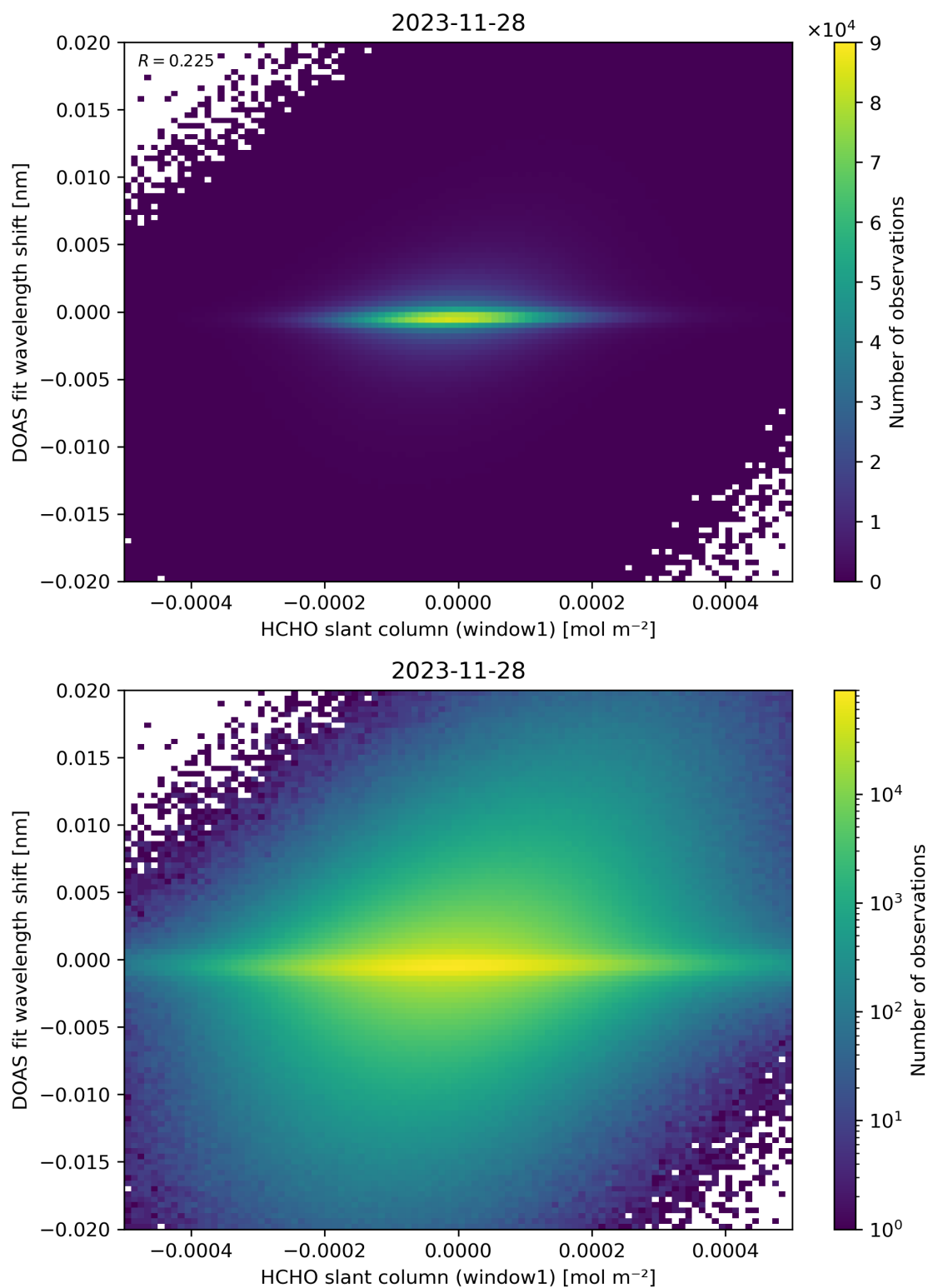
Figure 79: Scatter density plot of “HCHO slant column (window1)” against “DOAS fit wavelength shift” for 2023-11-28 to 2023-11-29.
