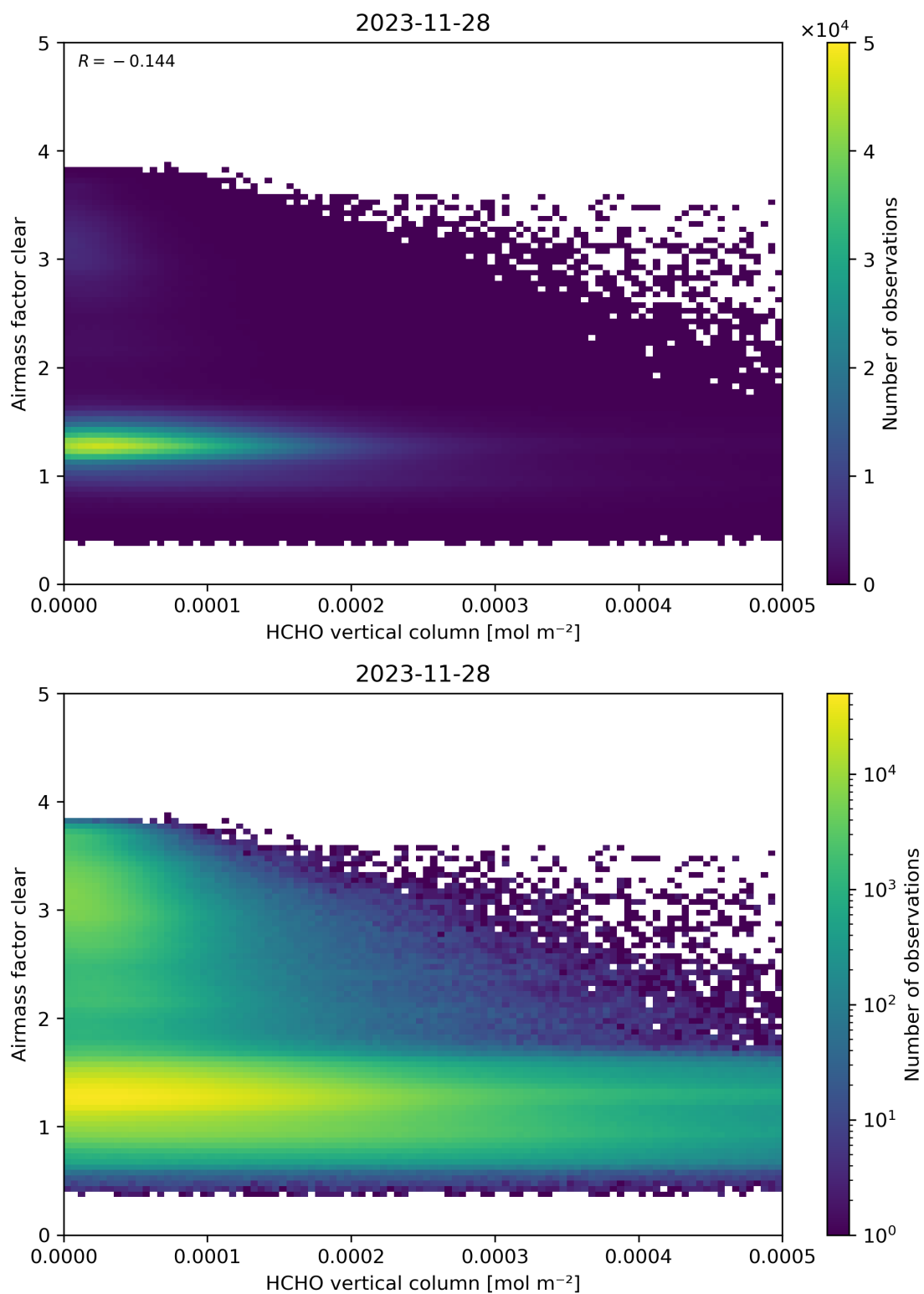
Figure 126: Scatter density plot of “HCHO vertical column” against “Airmass factor clear” for 2023-11-28 to 2023-11-29.
