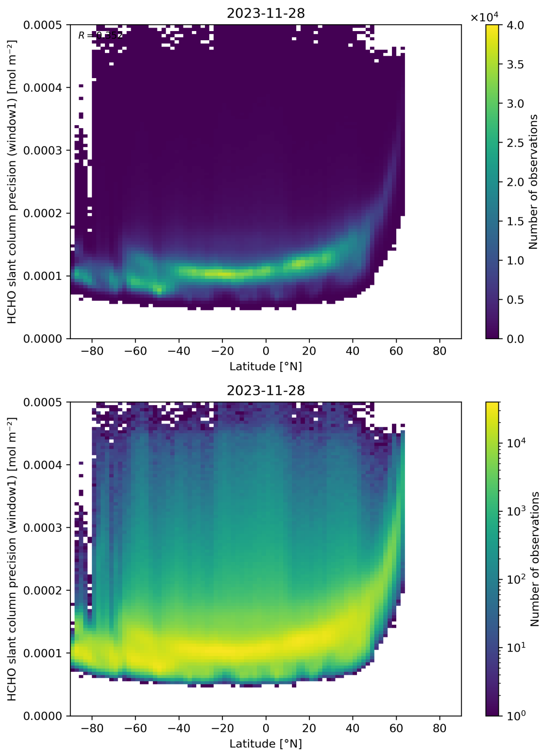
Figure 160: Scatter density plot of “Latitude” against “HCHO slant column precision (window1)” for 2023-11-28 to 2023-11-29.
