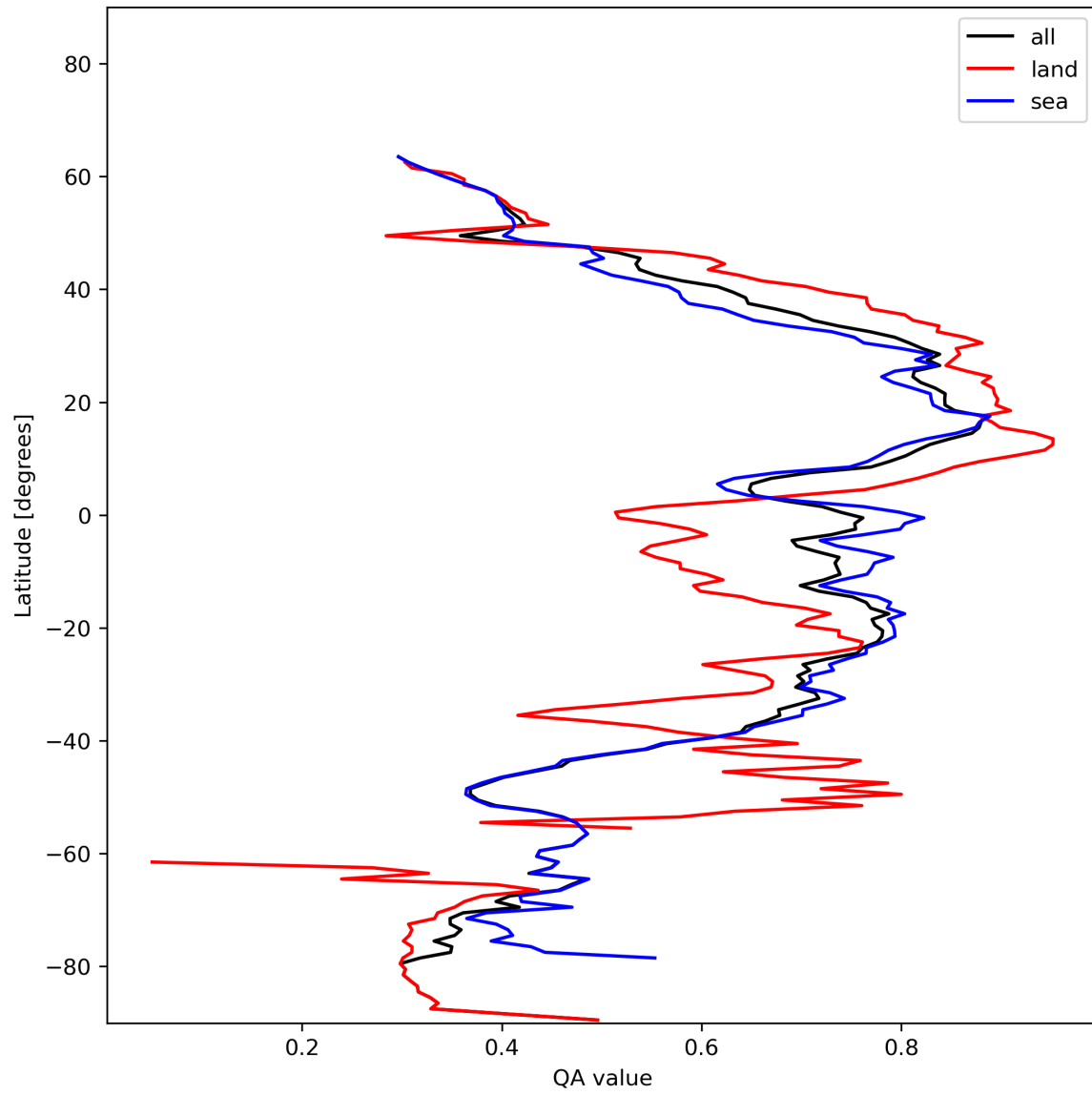
Figure 20: Zonal average of “QA value” for 2023-11-28 to 2023-11-29.
