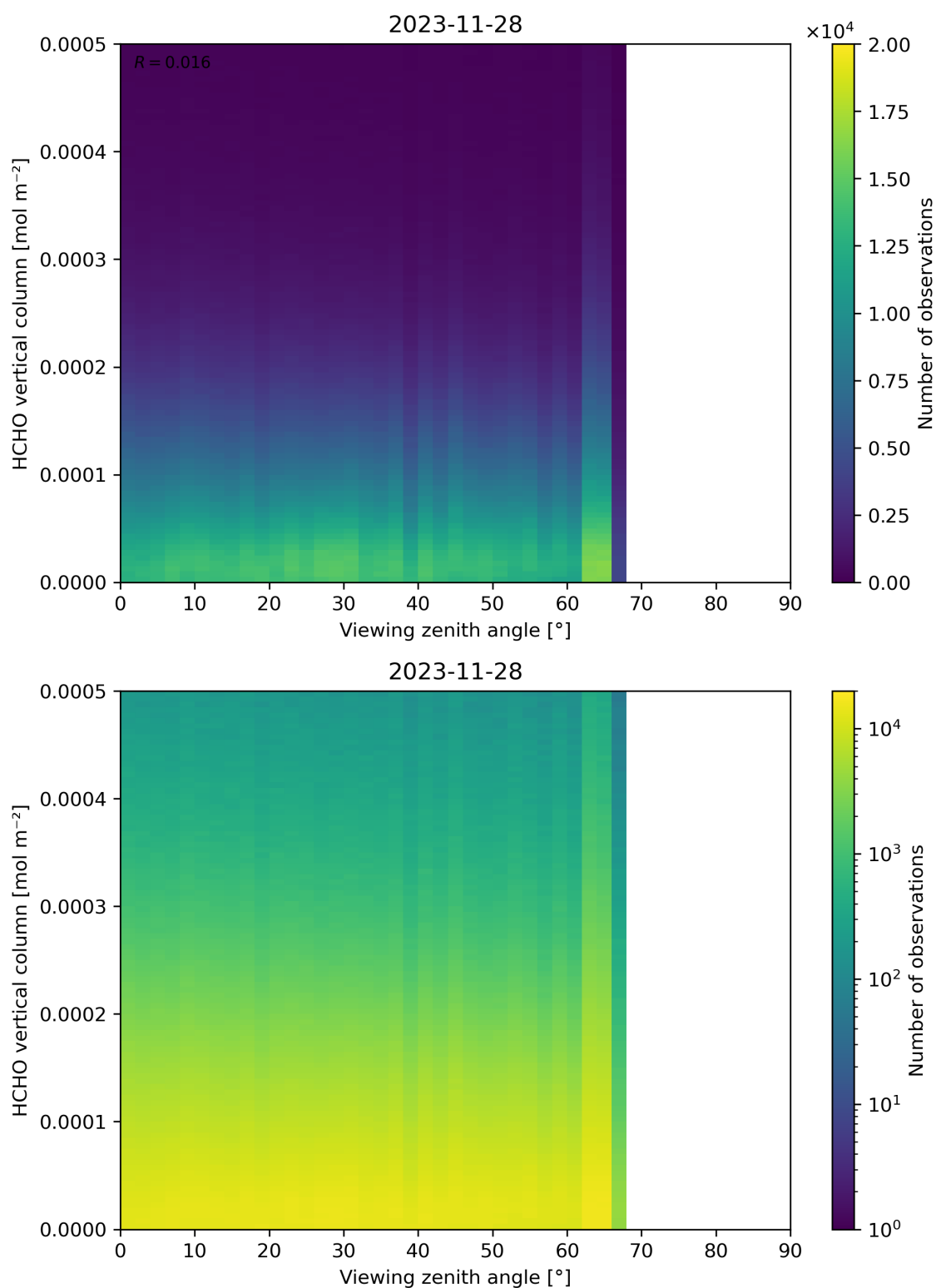
Figure 192: Scatter density plot of “Viewing zenith angle” against “HCHO vertical column” for 2023-11-28 to 2023-11-29.
