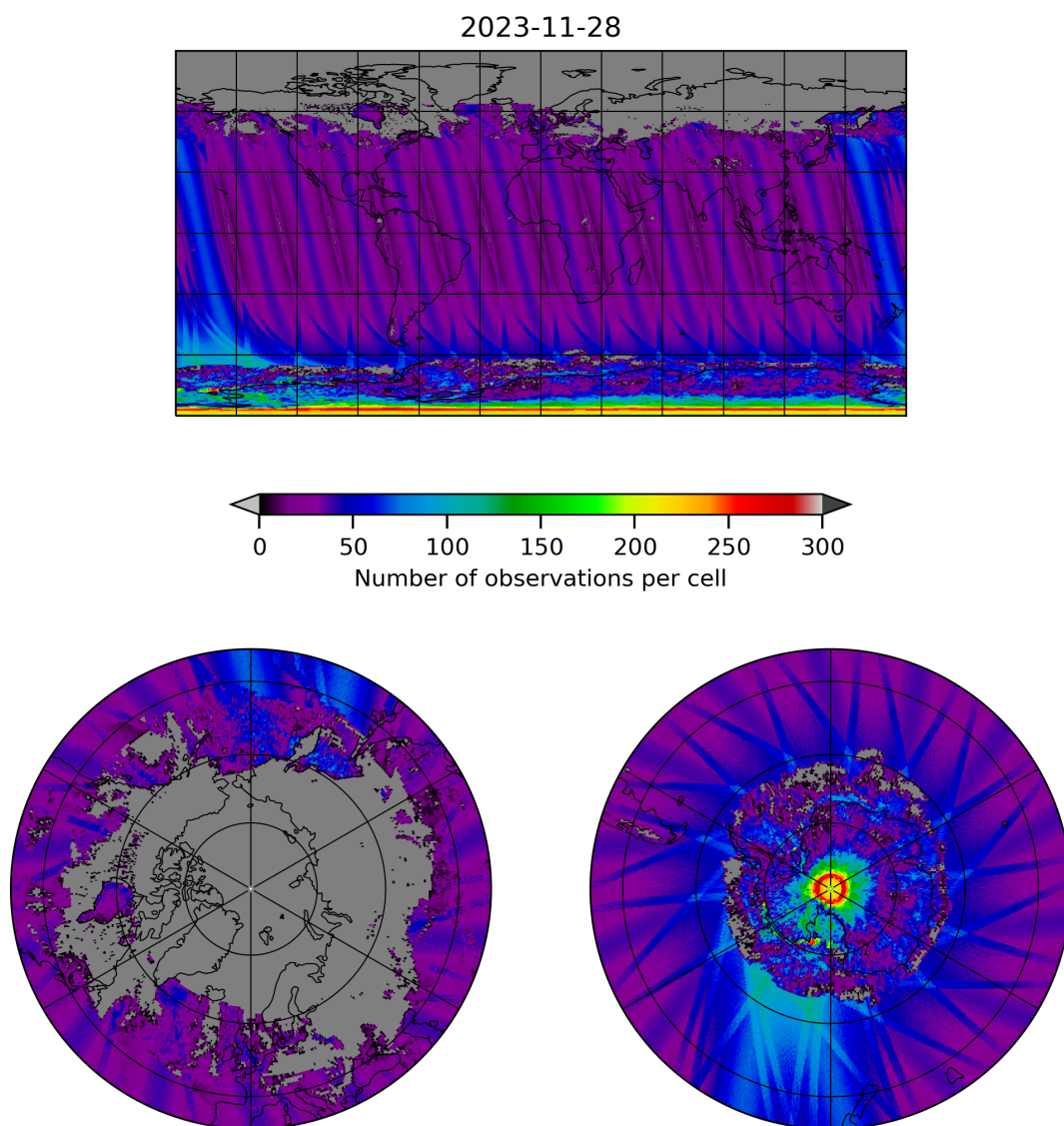
Figure 19: Map of the number of observations for 2023-11-28 to 2023-11-29
