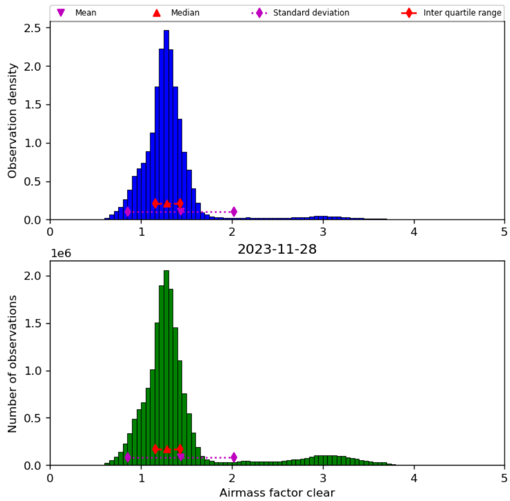
Figure 42: Histogram of “Airmass factor clear” for 2023-11-28 to 2023-11-29
