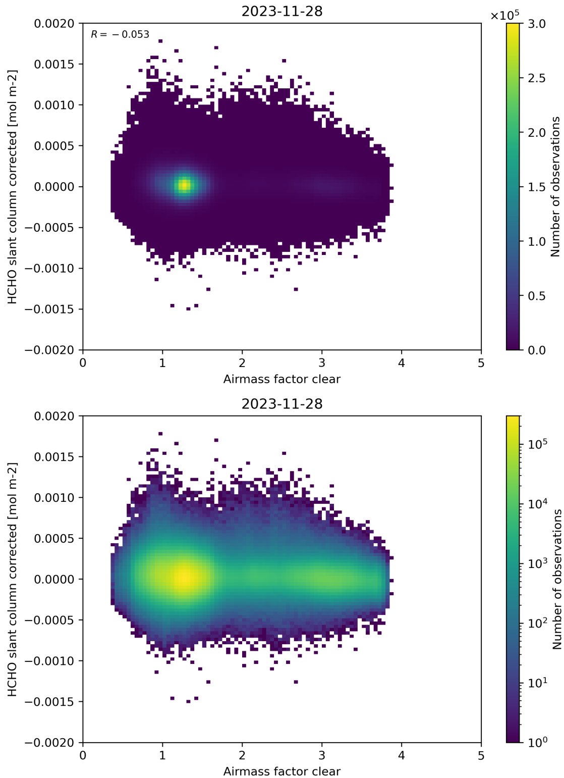
Figure 74: Scatter density plot of “Airmass factor clear” against “HCHO slant column corrected” for 2023-11-28 to 2023-11-29.
