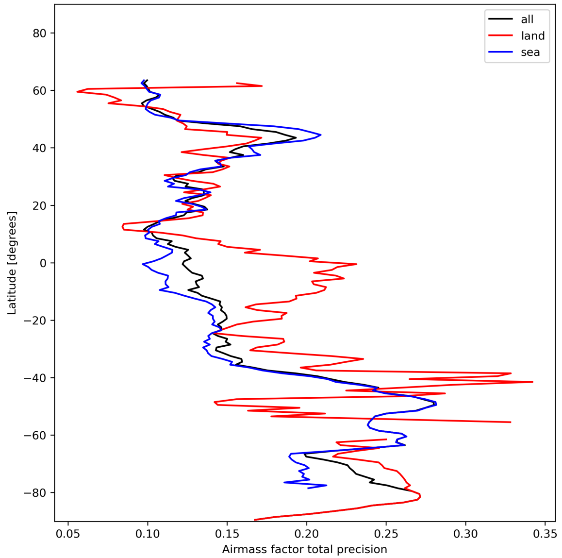
Figure 27: Zonal average of “Airmass factor total precision” for 2023-11-28 to 2023-11-29.
