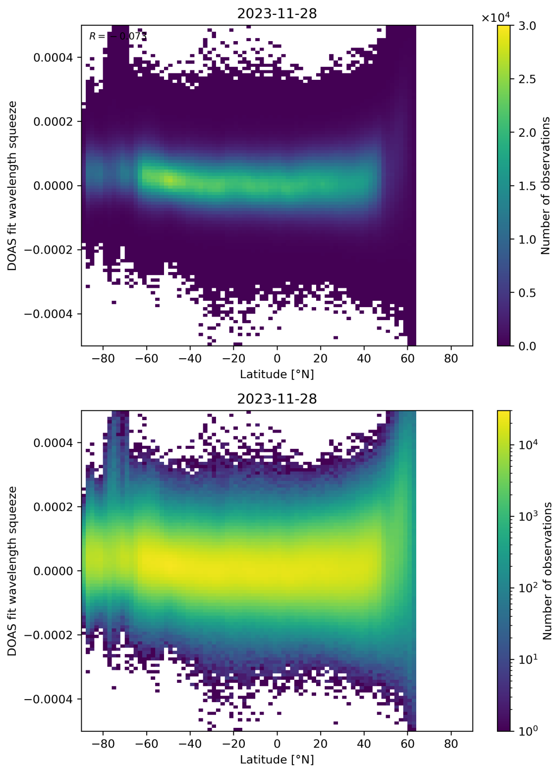
Figure 155: Scatter density plot of “Latitude” against “DOAS fit wavelength squeeze” for 2023-11-28 to 2023-11-29.
