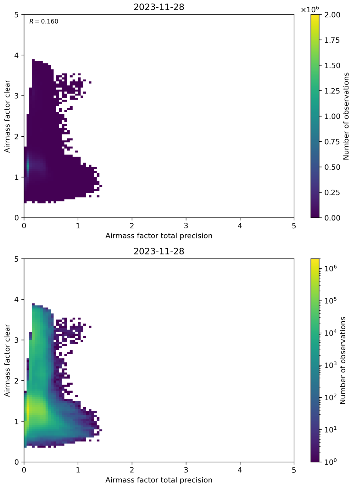
Figure 108: Scatter density plot of “Airmass factor total precision” against “Airmass factor clear” for 2023-11-28 to 2023-11-29.
