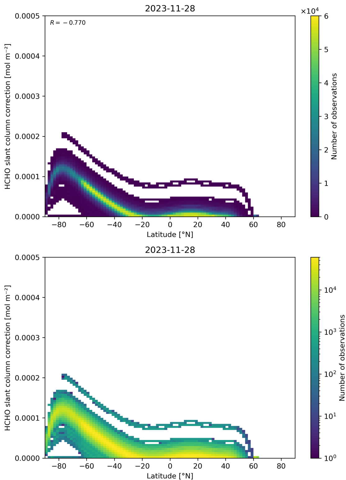
Figure 158: Scatter density plot of “Latitude” against “HCHO slant column correction” for 2023-11-28 to 2023-11-29.
