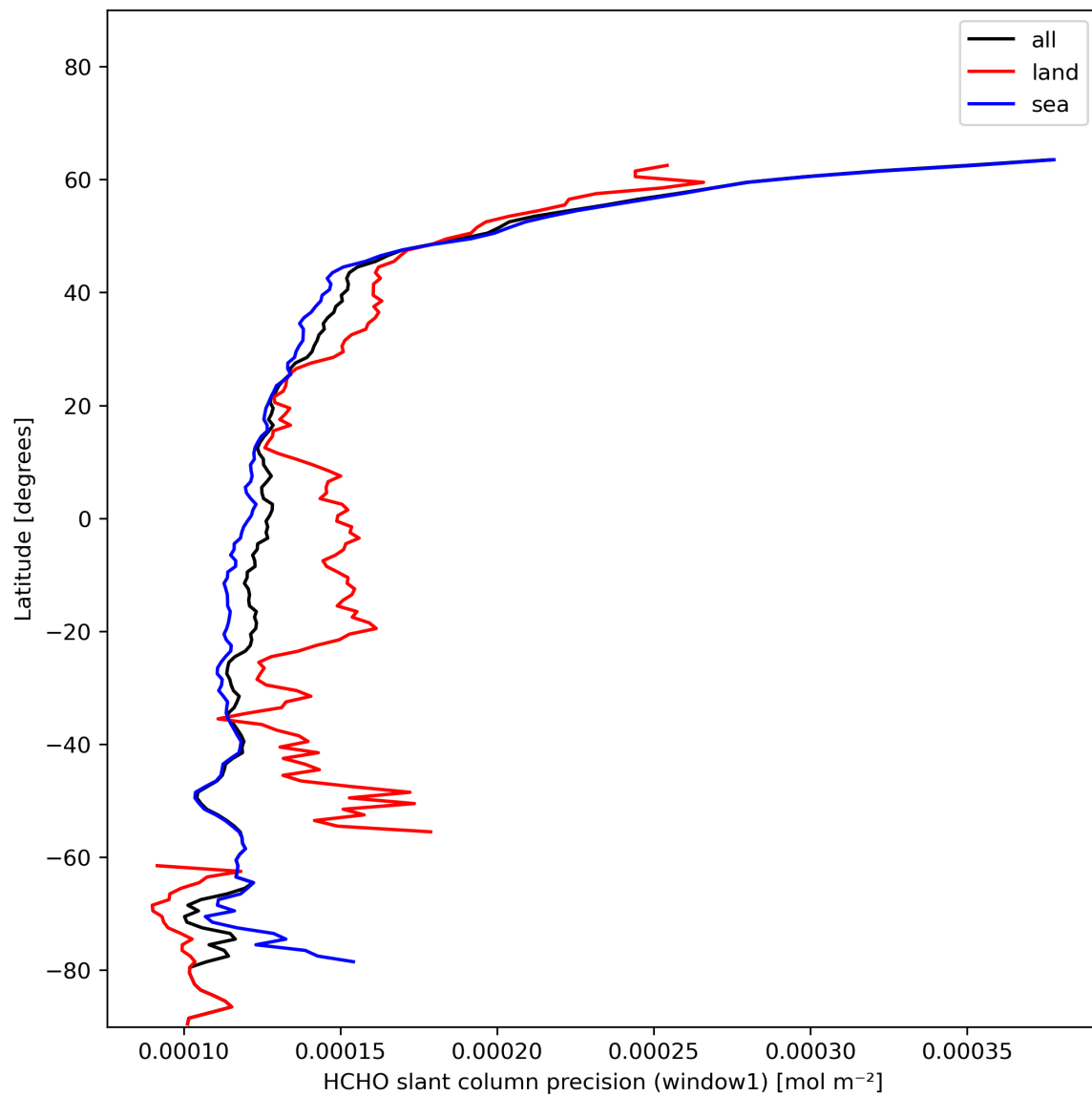
Figure 25: Zonal average of “HCHO slant column precision (window1)” for 2023-11-28 to 2023-11-29.
