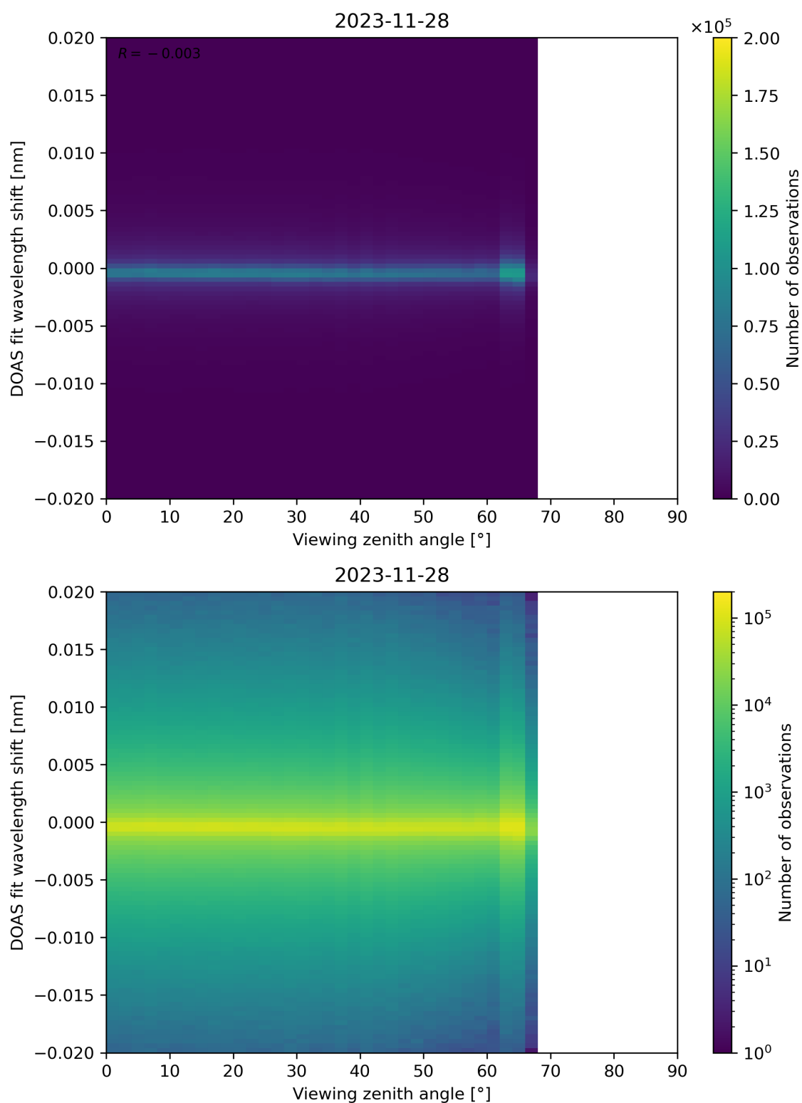
Figure 183: Scatter density plot of “Viewing zenith angle” against “DOAS fit wavelength shift” for 2023-11-28 to 2023-11-29.
