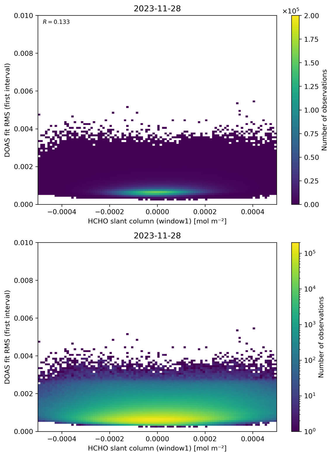
Figure 78: Scatter density plot of “HCHO slant column (window1)” against “DOAS fit RMS (first interval)” for 2023-11-28 to 2023-11-29.
