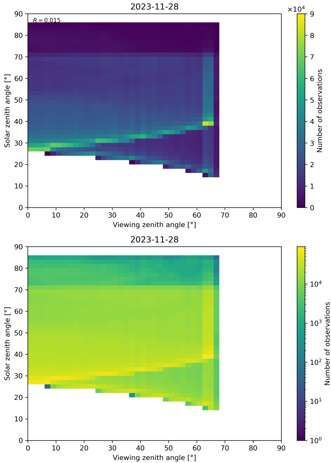
Figure 197: Scatter density plot of “Viewing zenith angle” against “Solar zenith angle” for 2023-11-28 to 2023-11-29.
