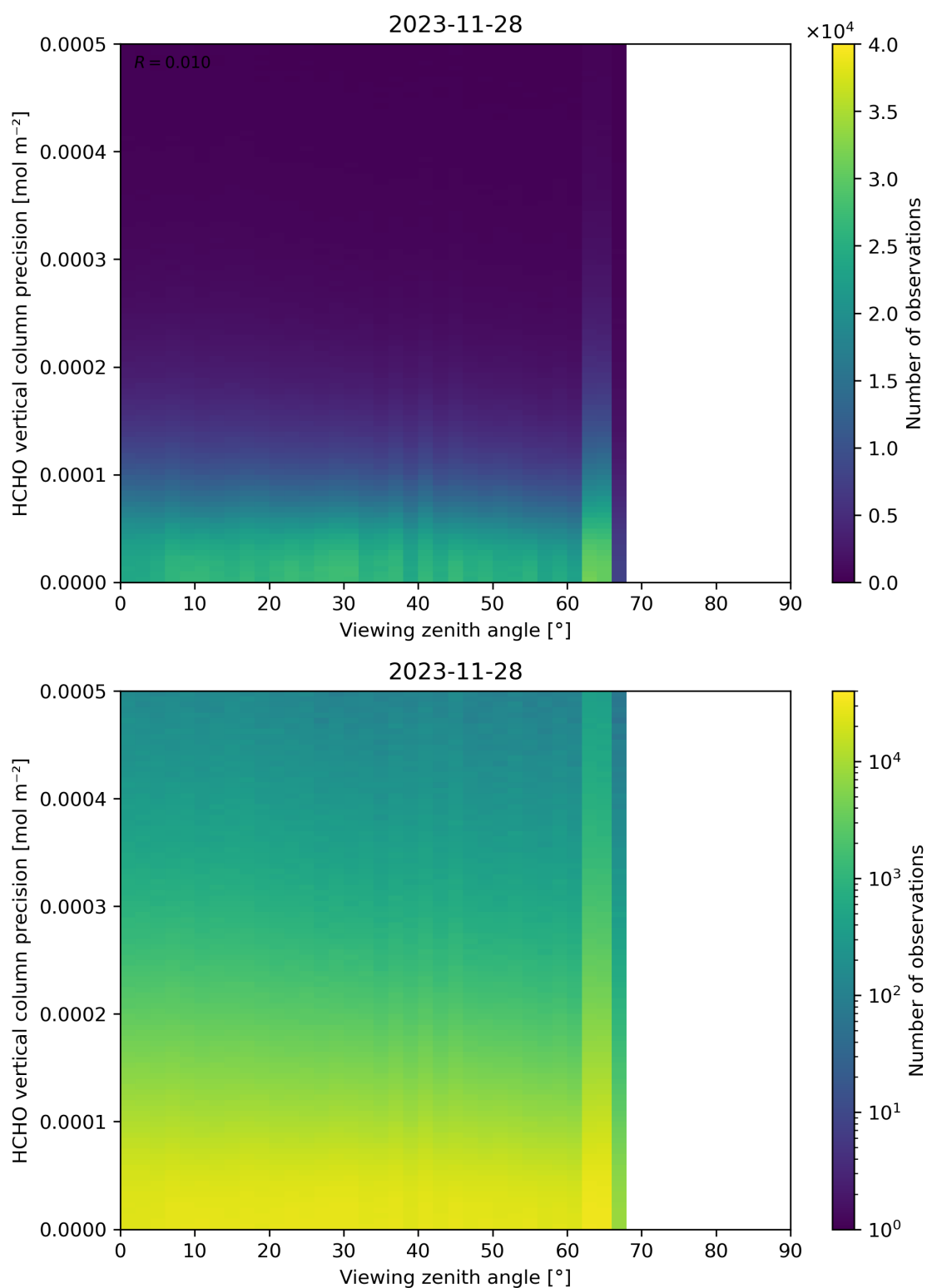
Figure 194: Scatter density plot of “Viewing zenith angle” against “HCHO vertical column precision” for 2023-11-28 to 2023-11-29.
