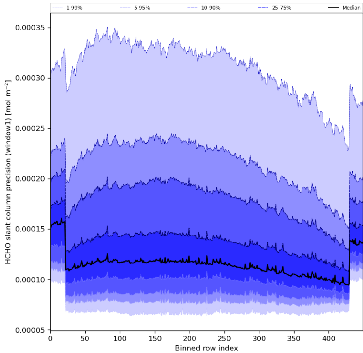
Figure 53: Along track statistics of “HCHO slant column precision (window1)” for 2023-11-28 to 2023-11-29
