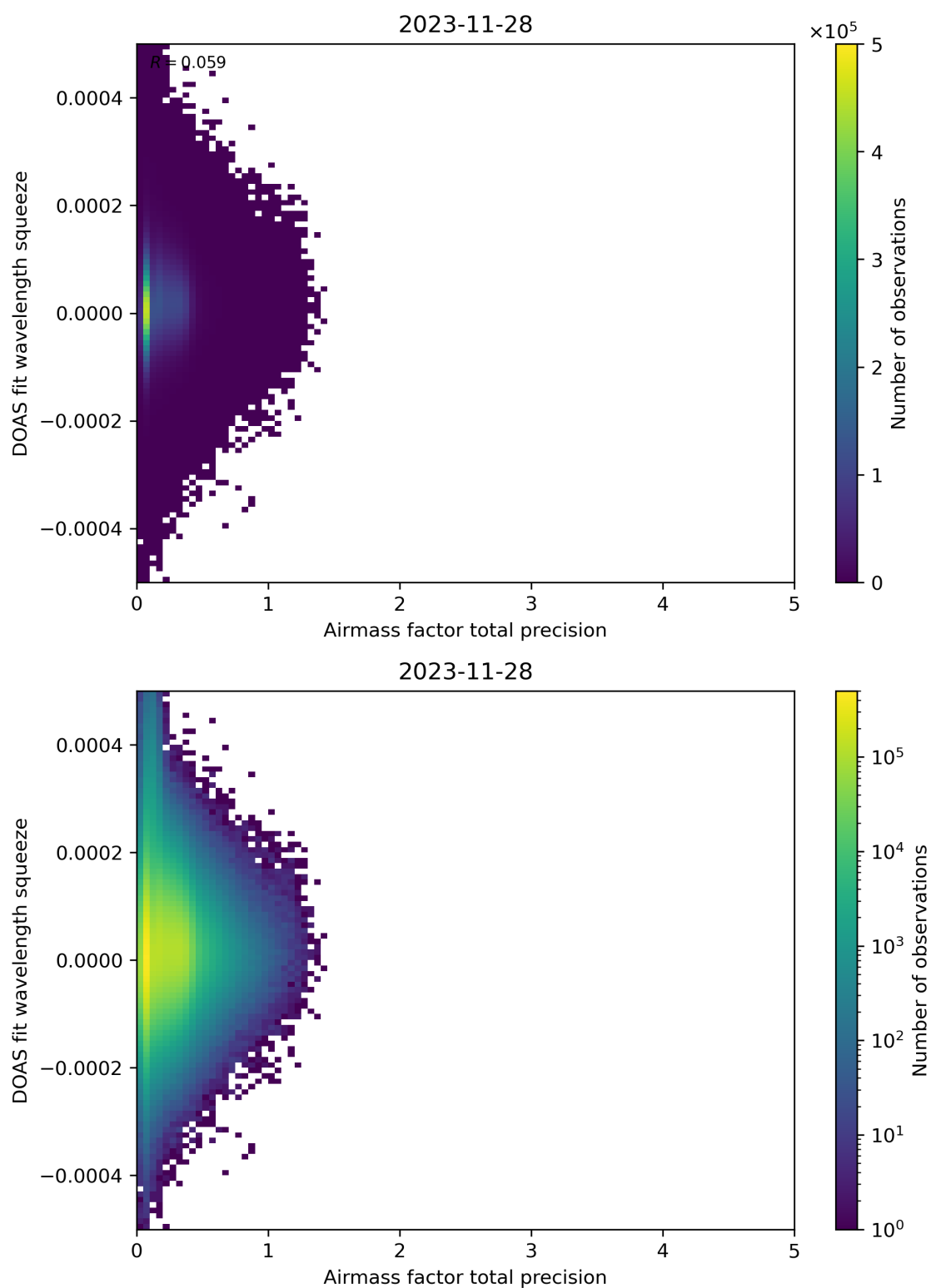
Figure 107: Scatter density plot of “Airmass factor total precision” against “DOAS fit wavelength squeeze” for 2023-11-28 to 2023-11-29.
