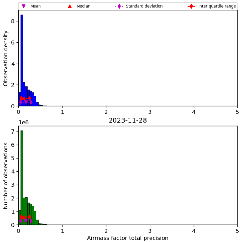
Figure 41: Histogram of “Airmass factor total precision” for 2023-11-28 to 2023-11-29
