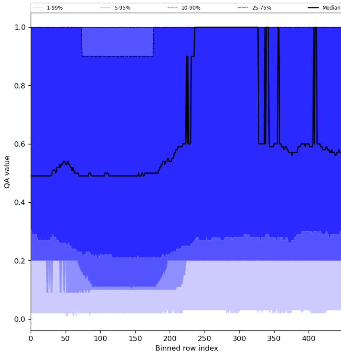
Figure 48: Along track statistics of “QA value” for 2023-11-28 to 2023-11-29
