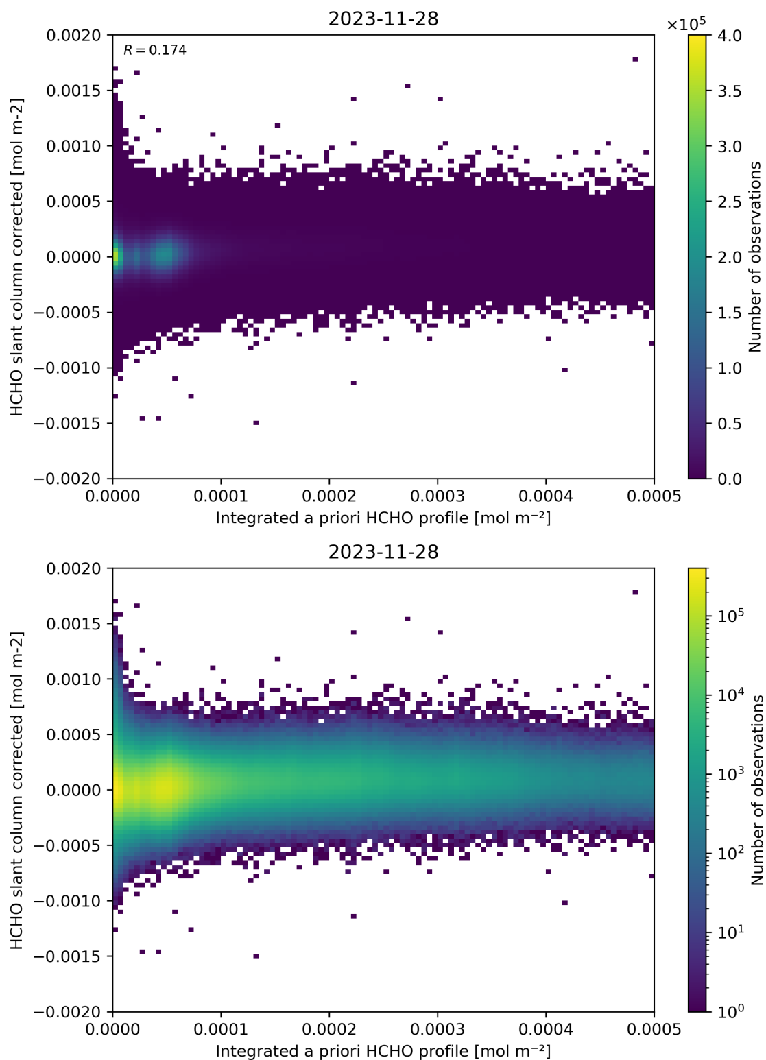
Figure 151: Scatter density plot of “Integrated a priori HCHO profile” against “HCHO slant column corrected” for 2023-11-28 to 2023-11-29.
