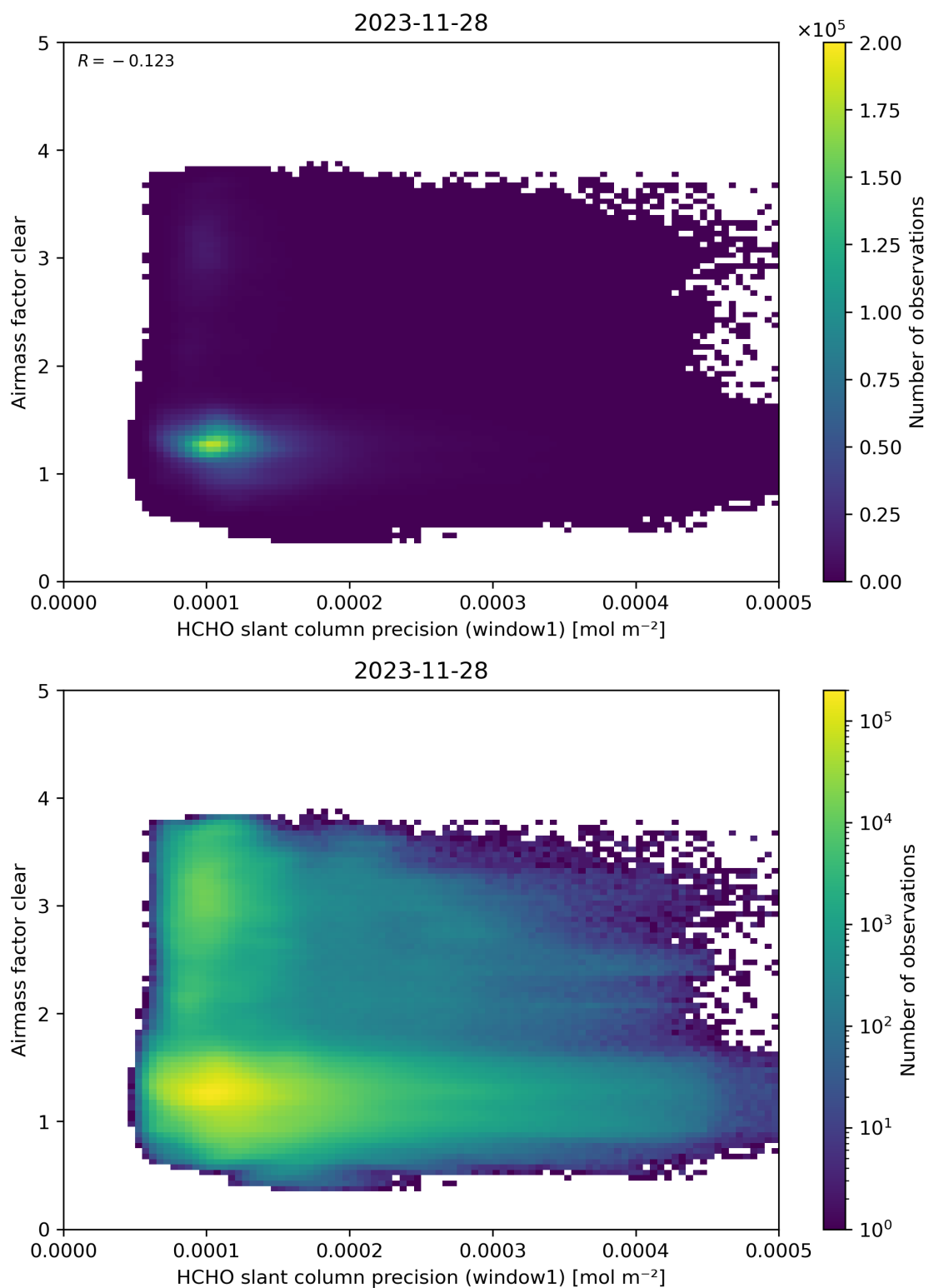
Figure 91: Scatter density plot of “HCHO slant column precision (window1)” against “Airmass factor clear” for 2023-11-28 to 2023-11-29.
