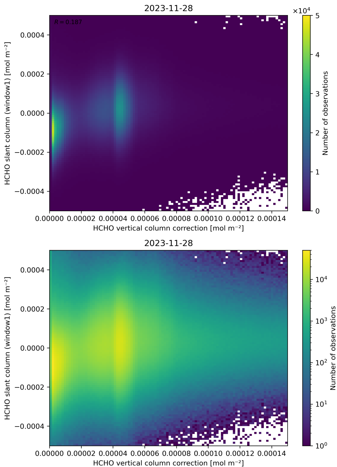
Figure 118: Scatter density plot of “HCHO vertical column correction” against “HCHO slant column (window1)” for 2023-11-28 to 2023-11-29.
