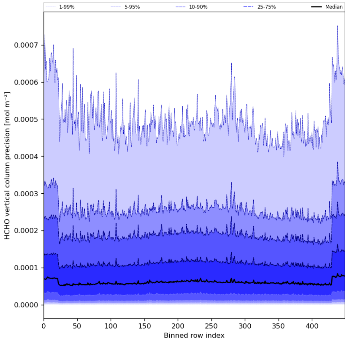
Figure 50: Along track statistics of "HCHO vertical column precision" for 2023-11-28 to 2023-11-29
