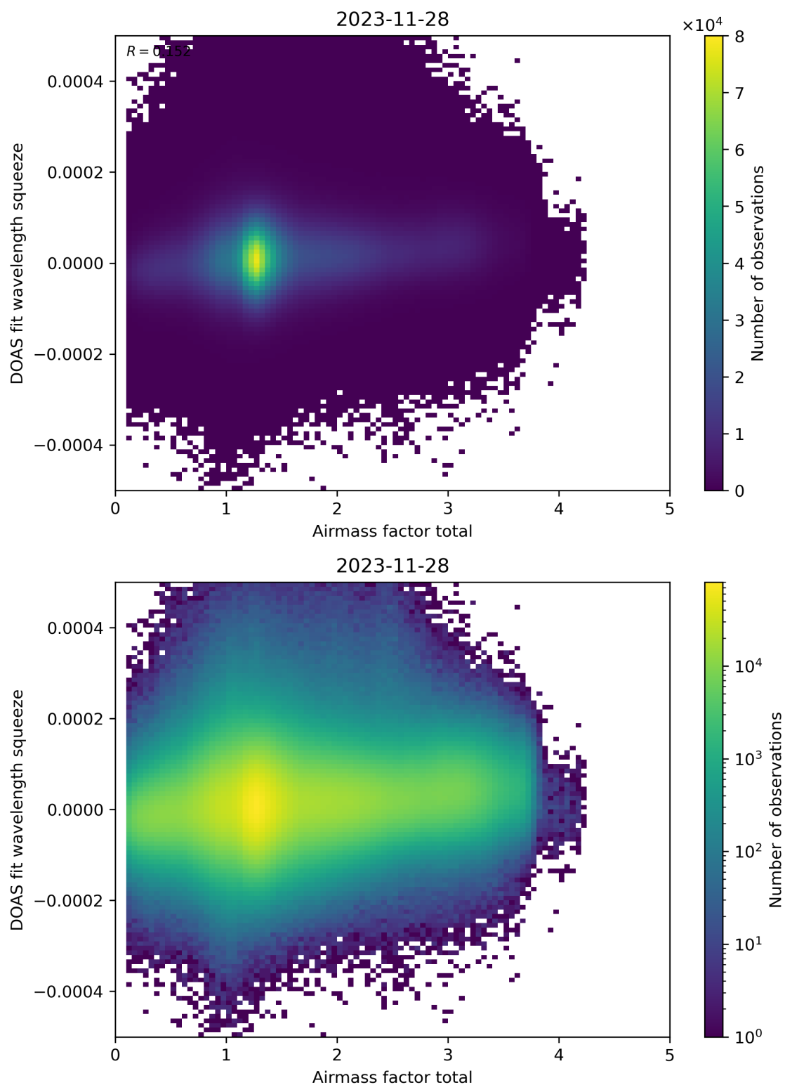
Figure 99: Scatter density plot of “Airmass factor total” against “DOAS fit wavelength squeeze” for 2023-11-28 to 2023-11-29.
