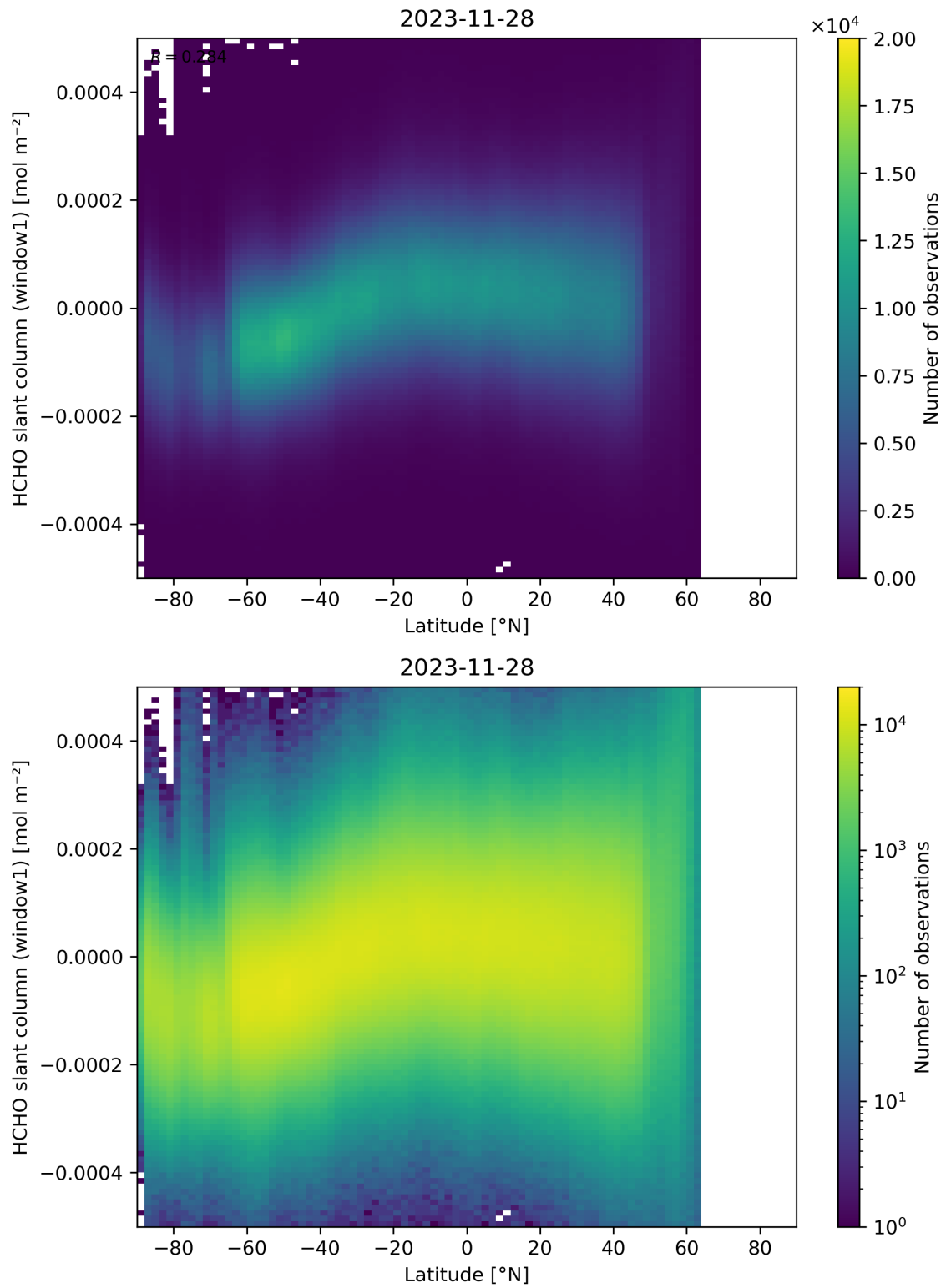
Figure 159: Scatter density plot of “Latitude” against “HCHO slant column (window1)” for 2023-11-28 to 2023-11-29.
