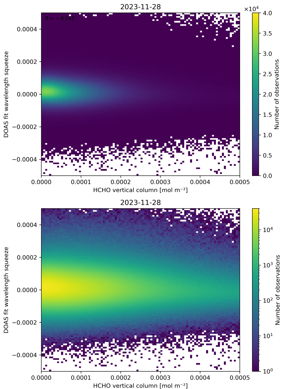
Figure 125: Scatter density plot of “HCHO vertical column” against “DOAS fit wavelength squeeze” for 2023-11-28 to 2023-11-29.
