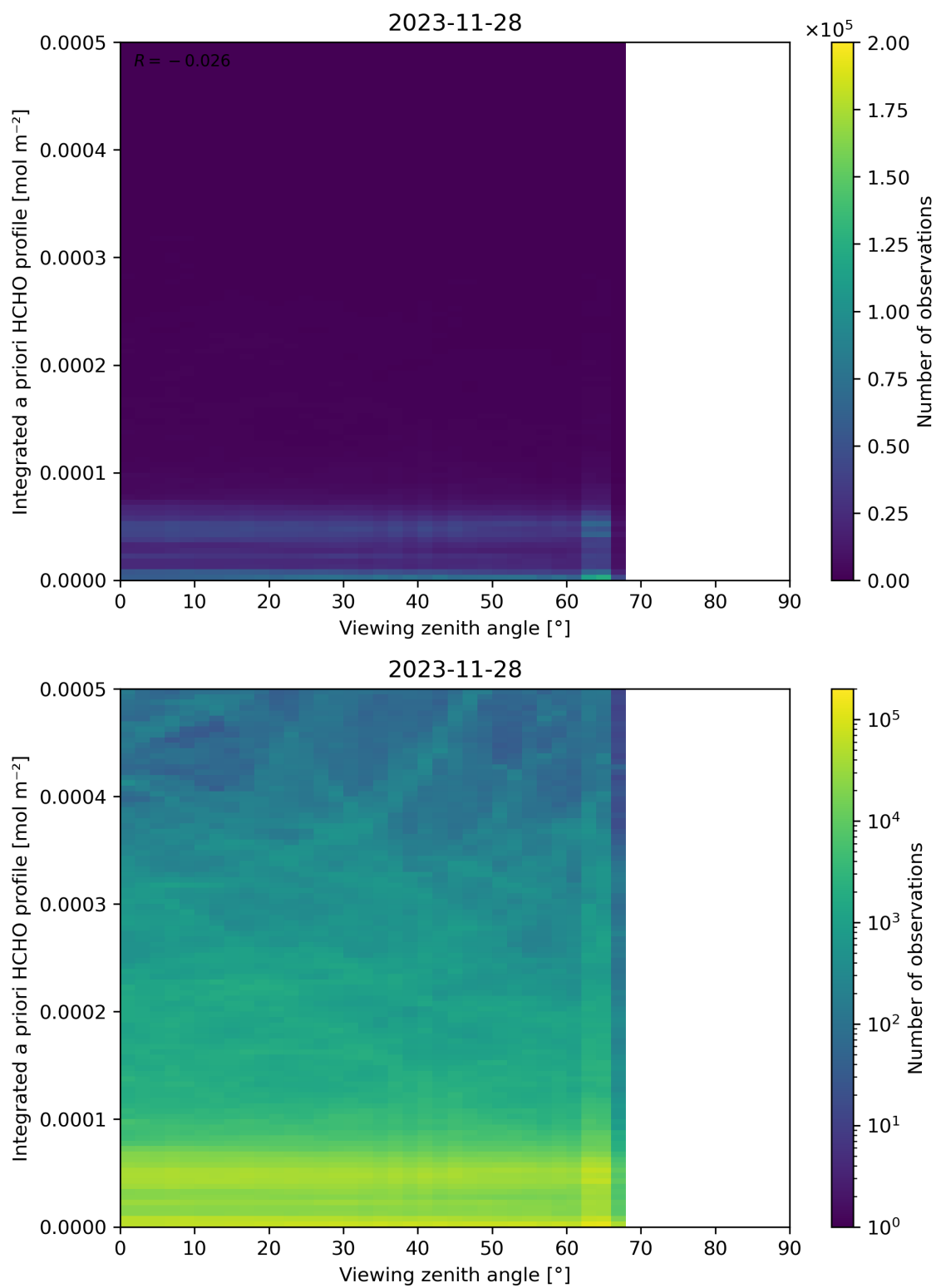
Figure 195: Scatter density plot of “Viewing zenith angle” against “Integrated a priori HCHO profile” for 2023-11-28 to 2023-11-29.
