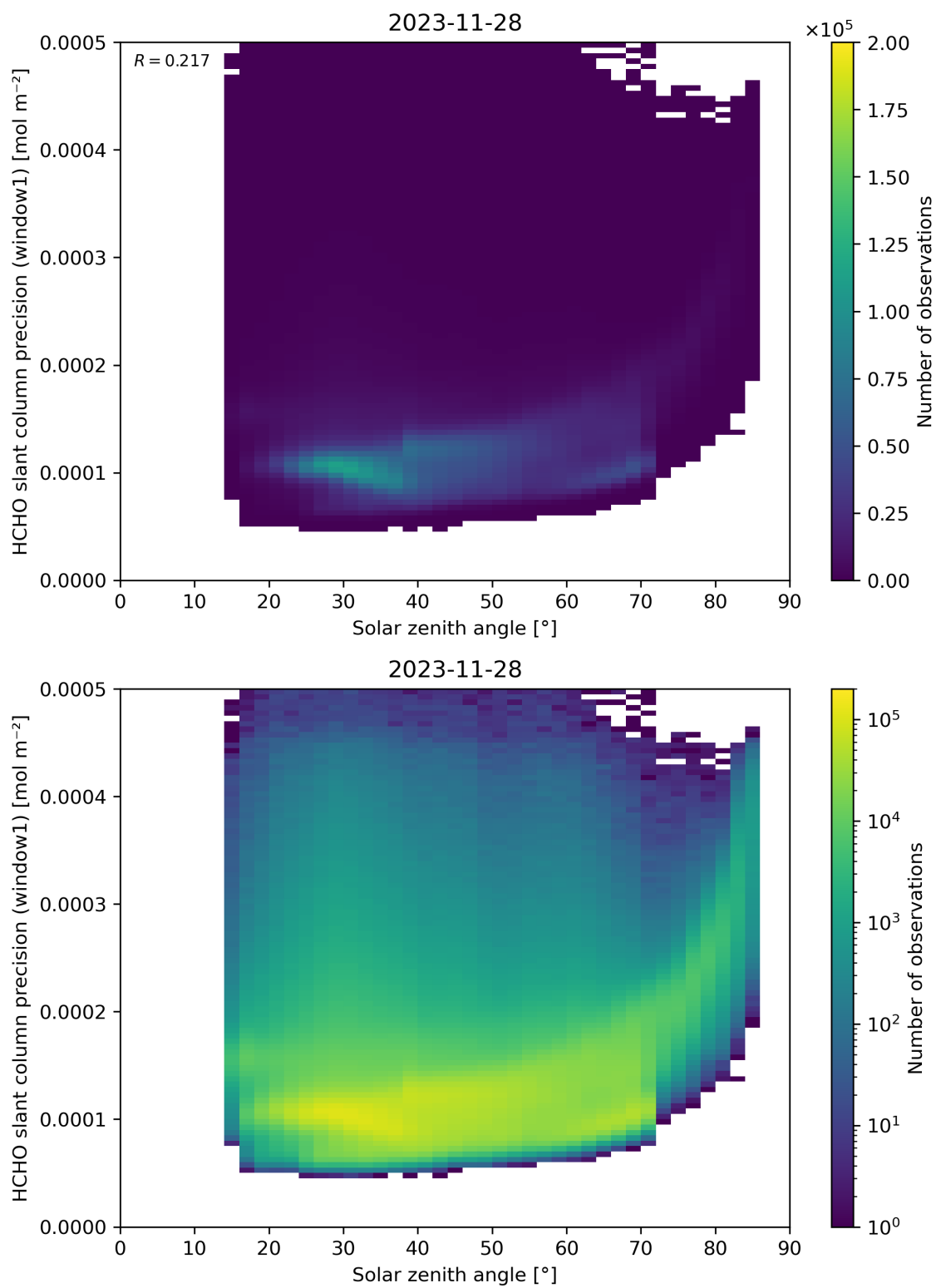
Figure 174: Scatter density plot of “Solar zenith angle” against “HCHO slant column precision (window1)” for 2023-11-28 to 2023-11-29.
