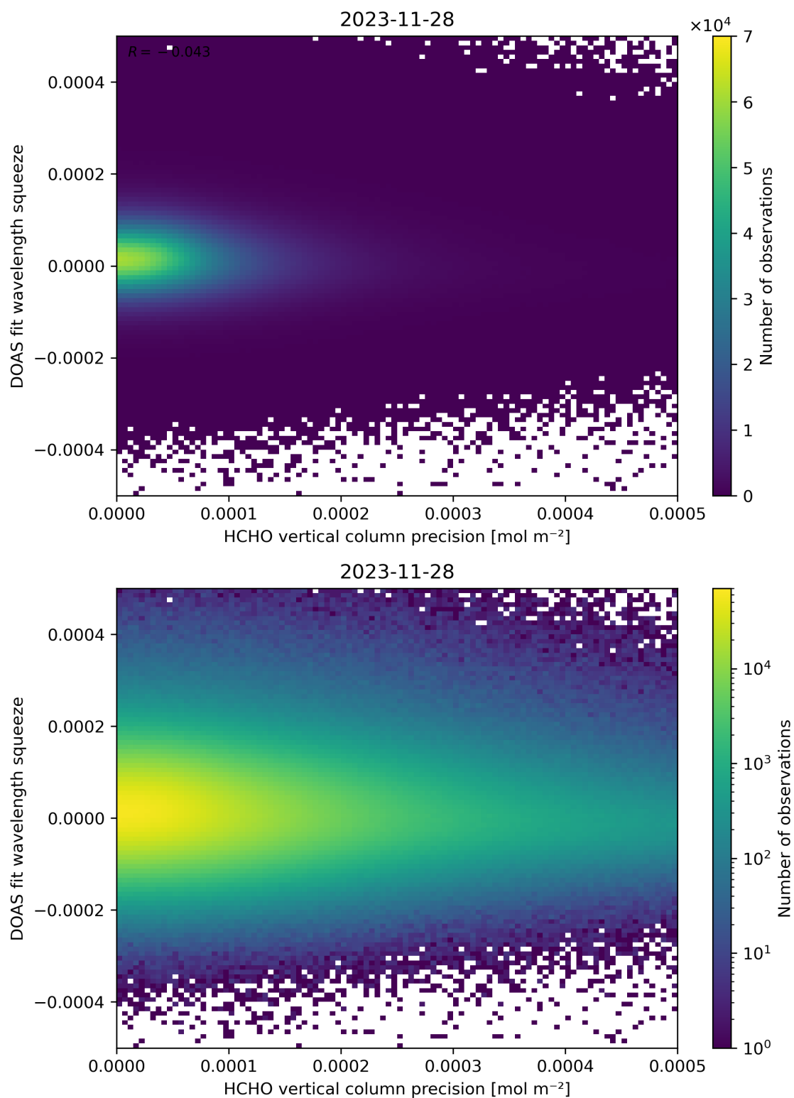
Figure 138: Scatter density plot of “HCHO vertical column precision” against “DOAS fit wavelength squeeze” for 2023-11-28 to 2023-11-29.
