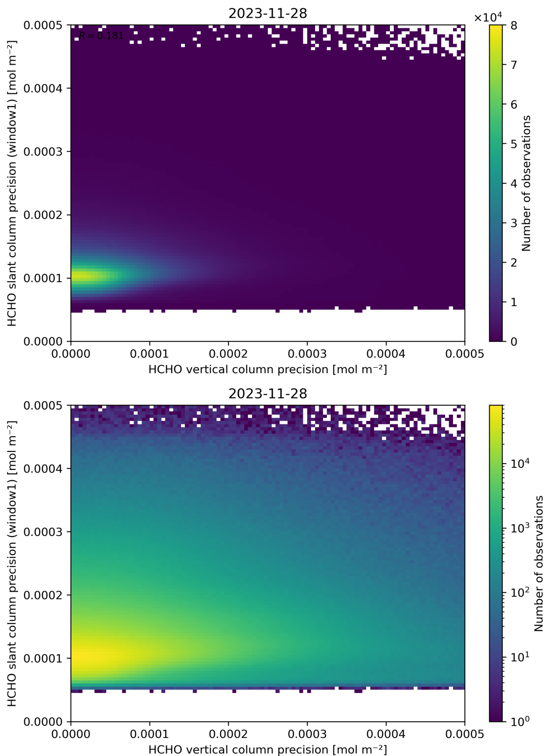
Figure 143: Scatter density plot of “HCHO vertical column precision” against “HCHO slant column precision (window1)” for 2023-11-28 to 2023-11-29.
