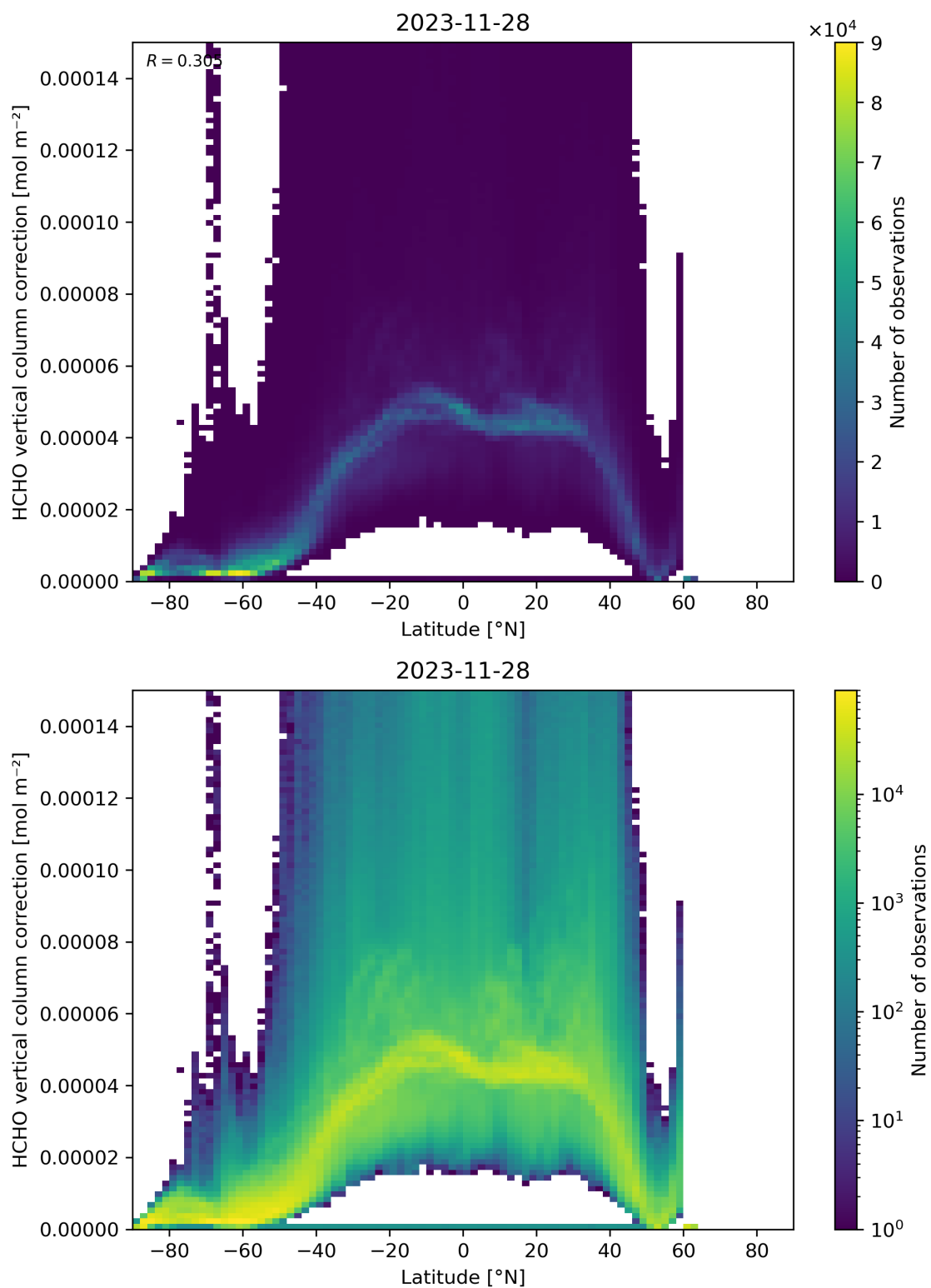
Figure 164: Scatter density plot of “Latitude” against “HCHO vertical column correction” for 2023-11-28 to 2023-11-29.
