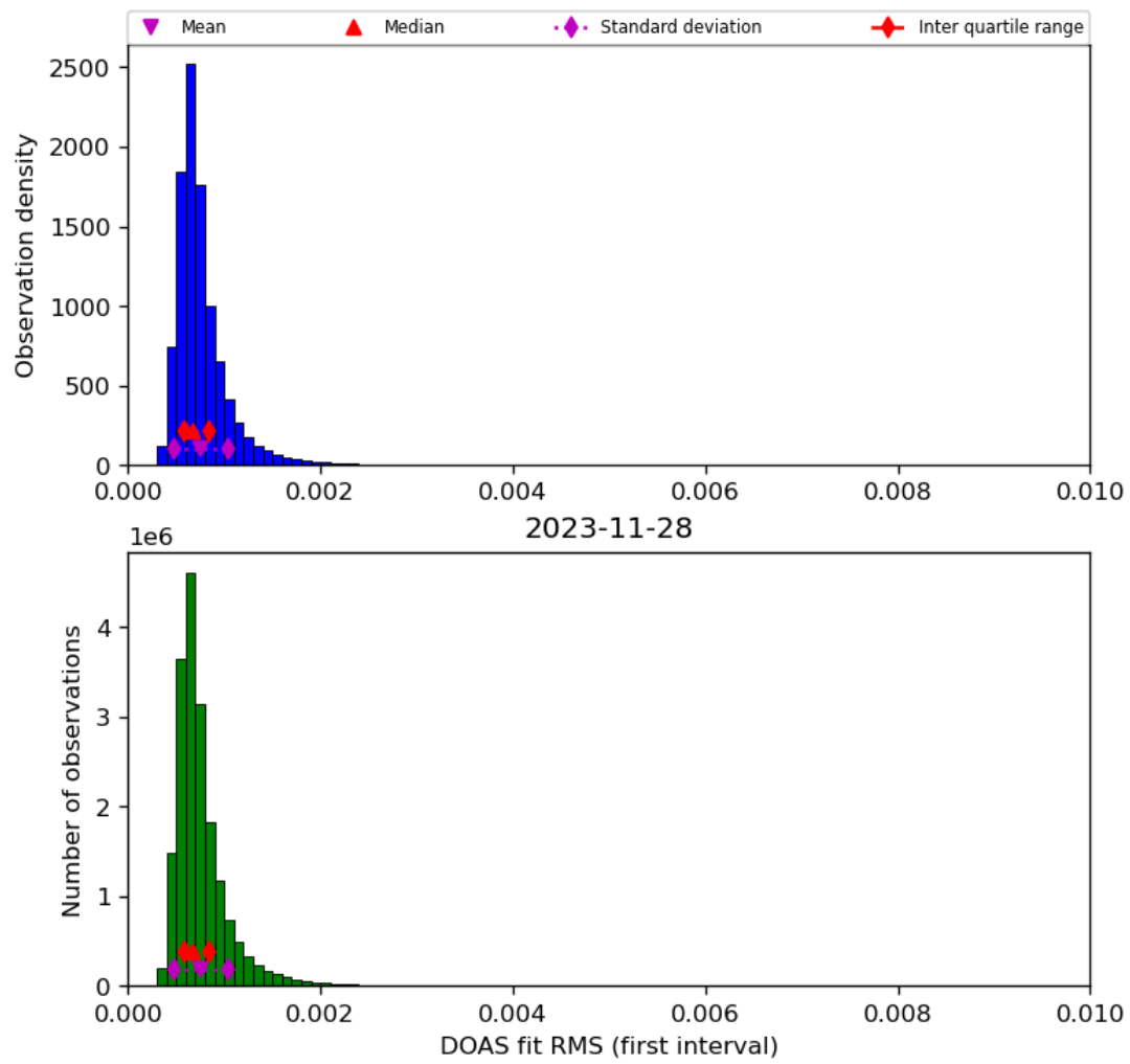
Figure 46: Histogram of “DOAS fit RMS (first interval)” for 2023-11-28 to 2023-11-29
