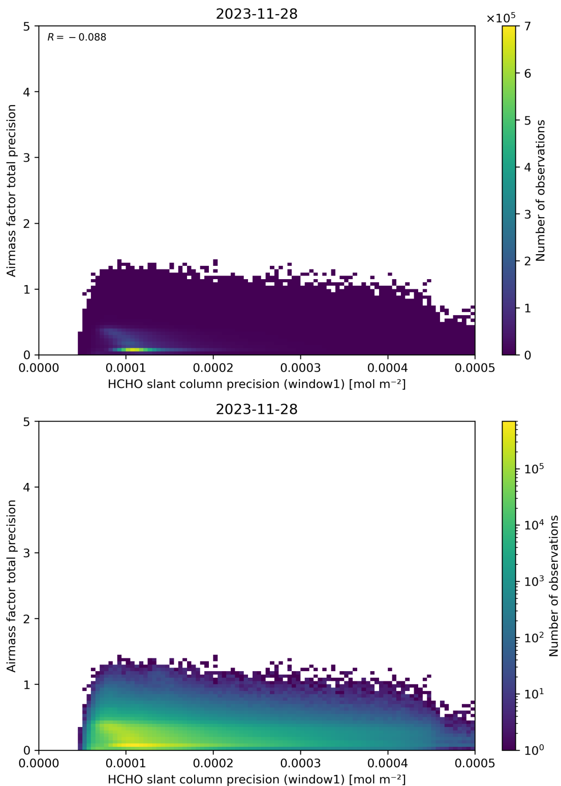
Figure 95: Scatter density plot of “HCHO slant column precision (window1)” against “Airmass factor total precision” for 2023-11-28 to 2023-11-29.
