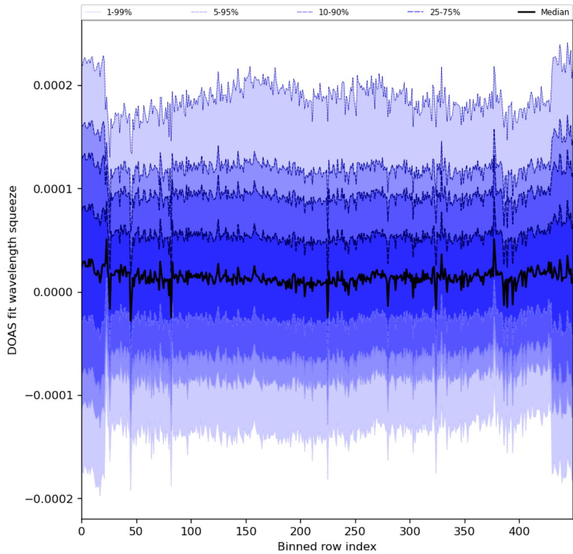
Figure 59: Along track statistics of “DOAS fit wavelength squeeze” for 2023-11-28 to 2023-11-29
