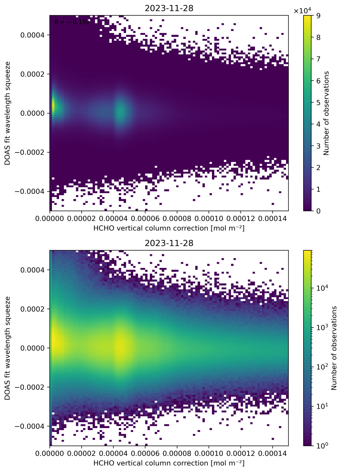
Figure 114: Scatter density plot of “HCHO vertical column correction” against “DOAS fit wavelength squeeze” for 2023-11-28 to 2023-11-29.
