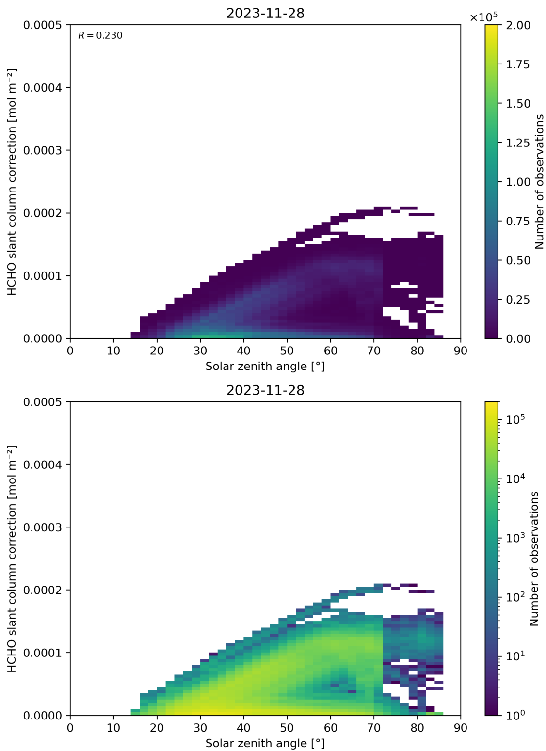
Figure 172: Scatter density plot of “Solar zenith angle” against “HCHO slant column correction” for 2023-11-28 to 2023-11-29.
