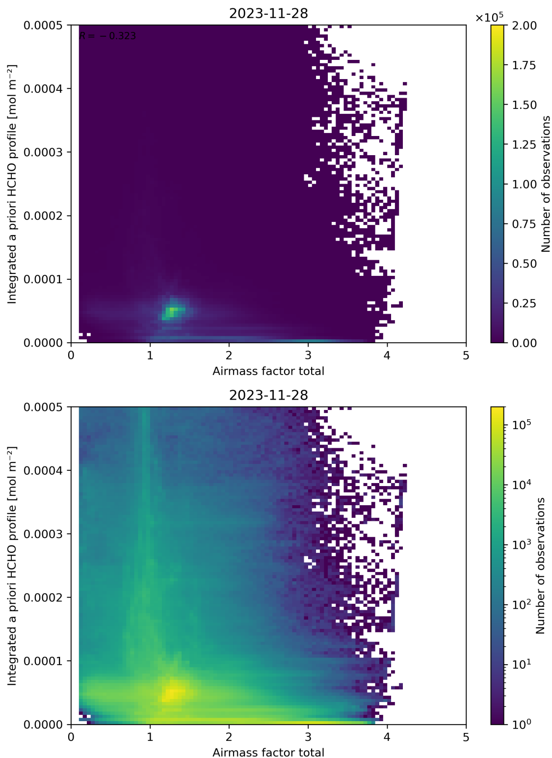
Figure 104: Scatter density plot of “Airmass factor total” against “Integrated a priori HCHO profile” for 2023-11-28 to 2023-11-29.
