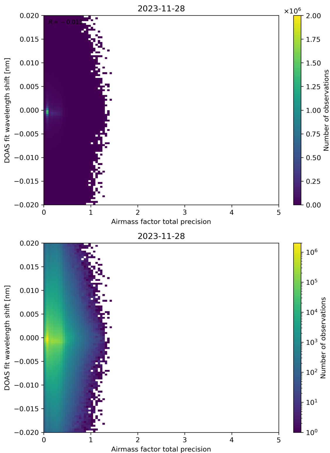
Figure 106: Scatter density plot of “Airmass factor total precision” against “DOAS fit wavelength shift” for 2023-11-28 to 2023-11-29.
