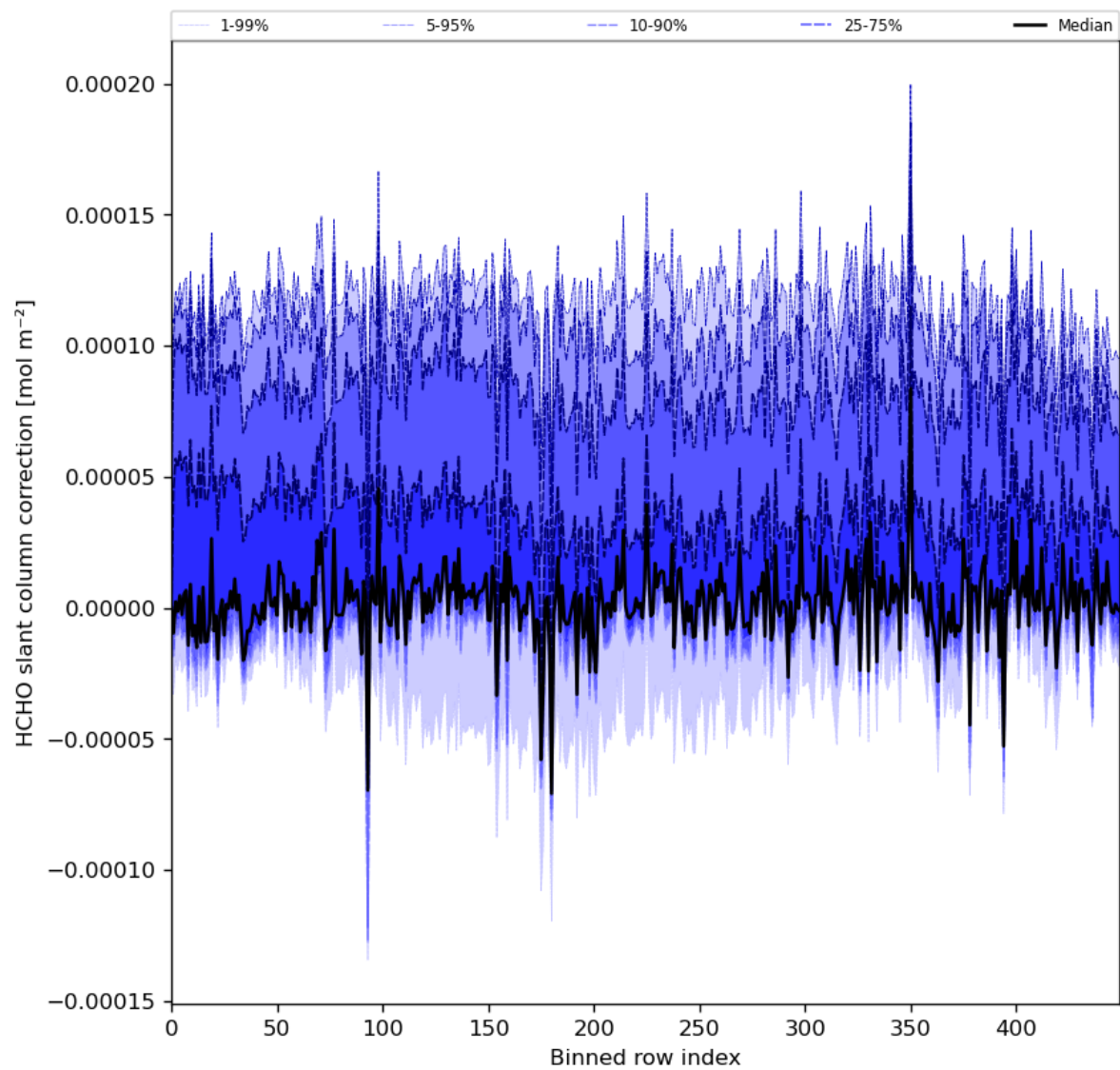
Figure 61: Along track statistics of “HCHO slant column correction” for 2023-11-28 to 2023-11-29
