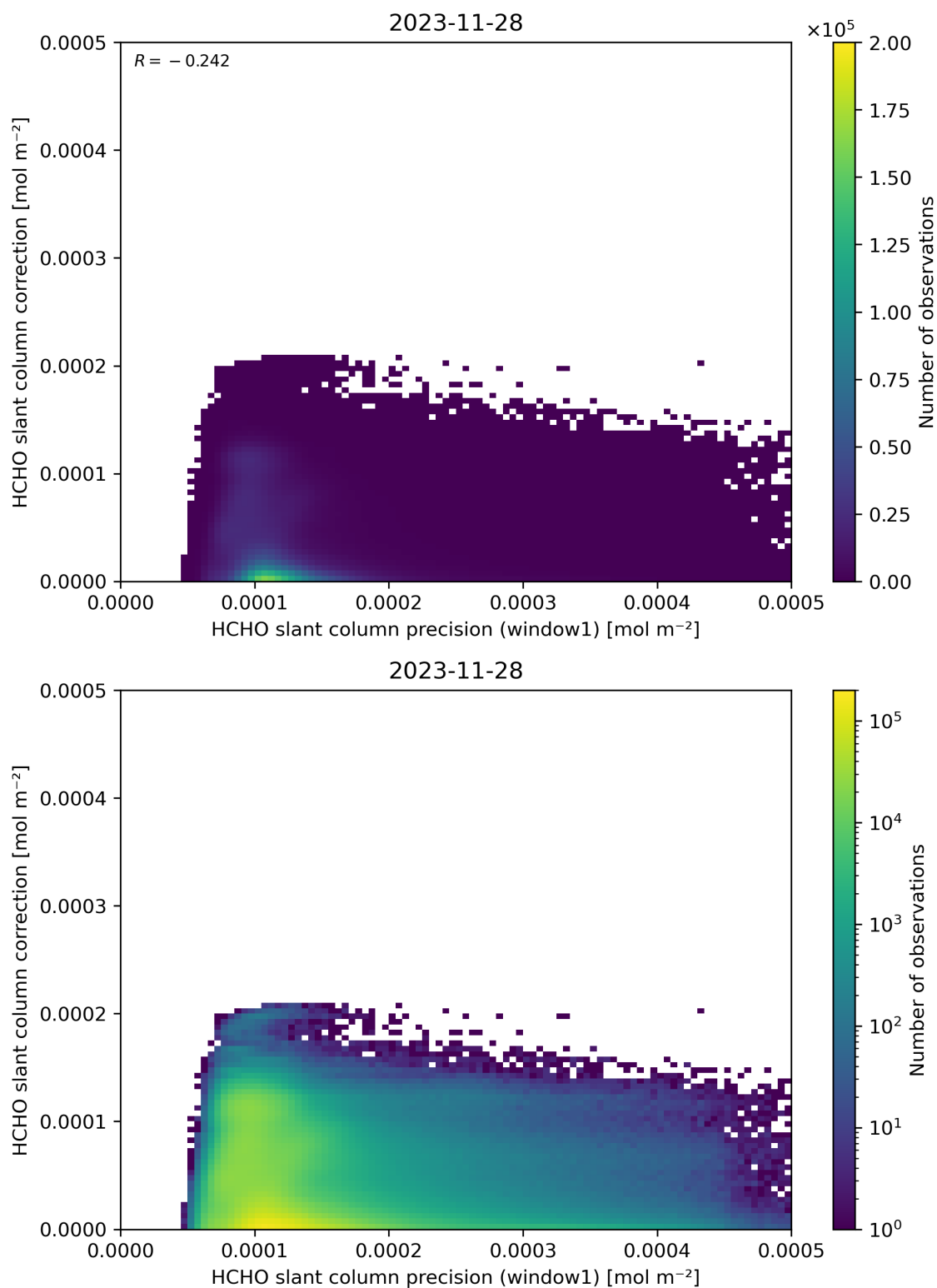
Figure 93: Scatter density plot of “HCHO slant column precision (window1)” against “HCHO slant column correction” for 2023-11-28 to 2023-11-29.
