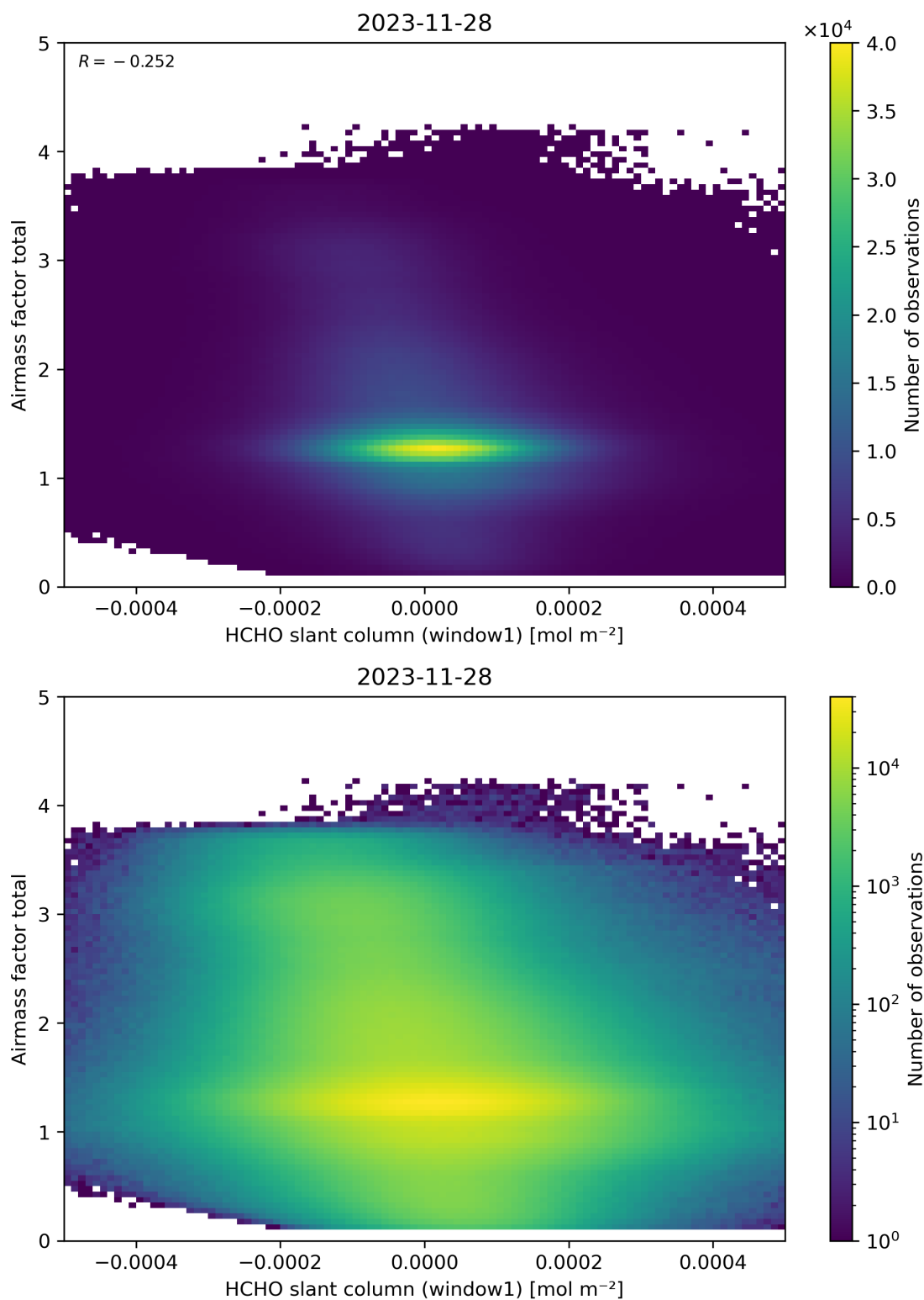
Figure 85: Scatter density plot of “HCHO slant column (window1)” against “Airmass factor total” for 2023-11-28 to 2023-11-29.
