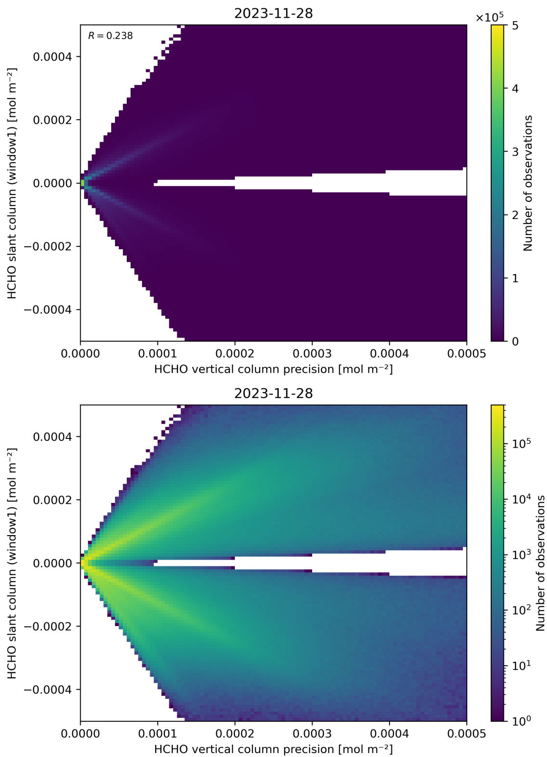
Figure 142: Scatter density plot of “HCHO vertical column precision” against “HCHO slant column (window1)” for 2023-11-28 to 2023-11-29.
