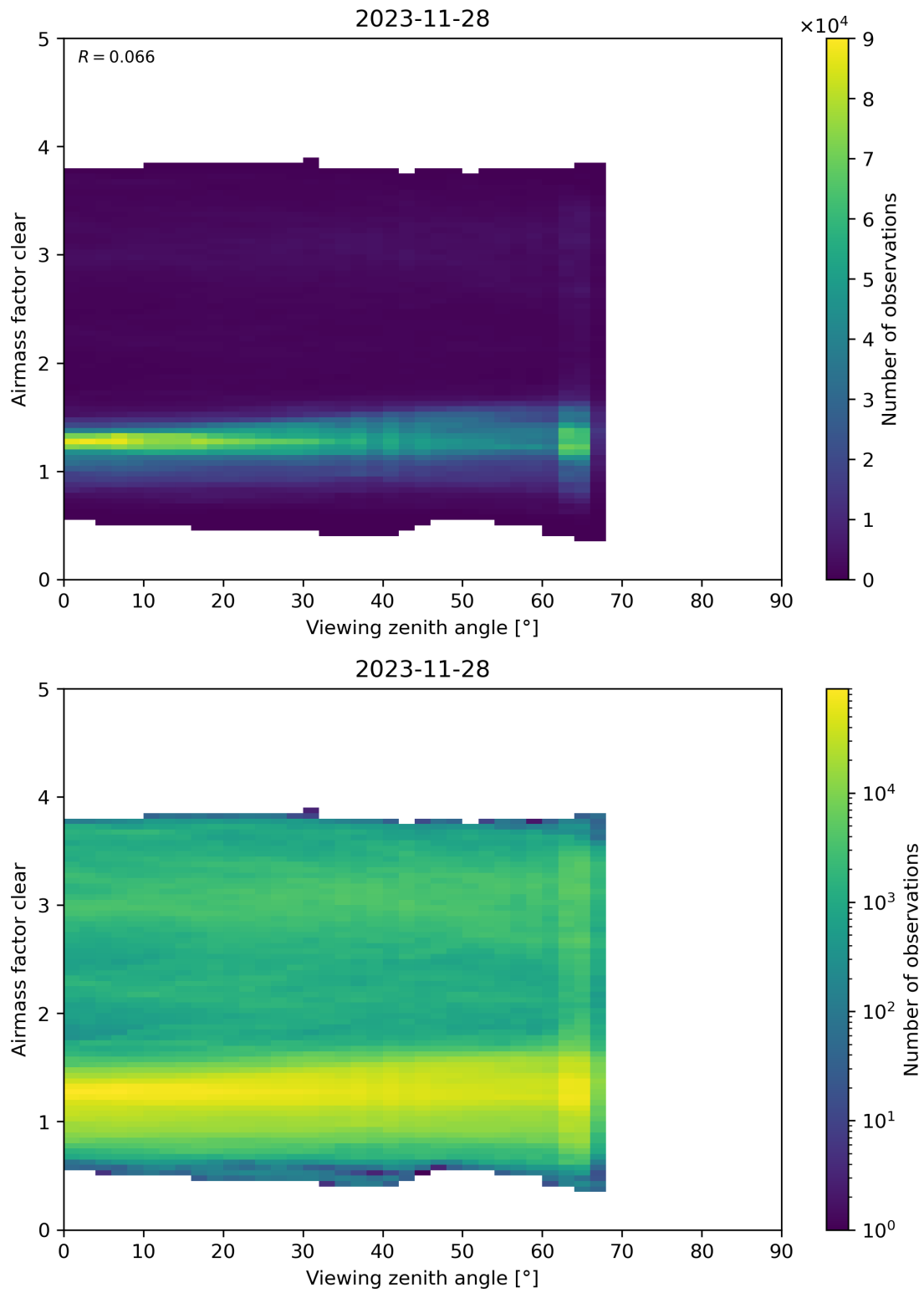
Figure 185: Scatter density plot of “Viewing zenith angle” against “Airmass factor clear” for 2023-11-28 to 2023-11-29.
