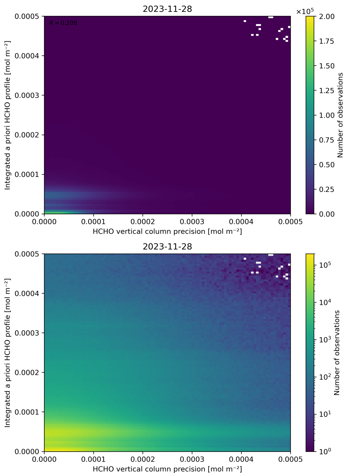
Figure 147: Scatter density plot of “HCHO vertical column precision” against “Integrated a priori HCHO profile” for 2023-11-28 to 2023-11-29.
