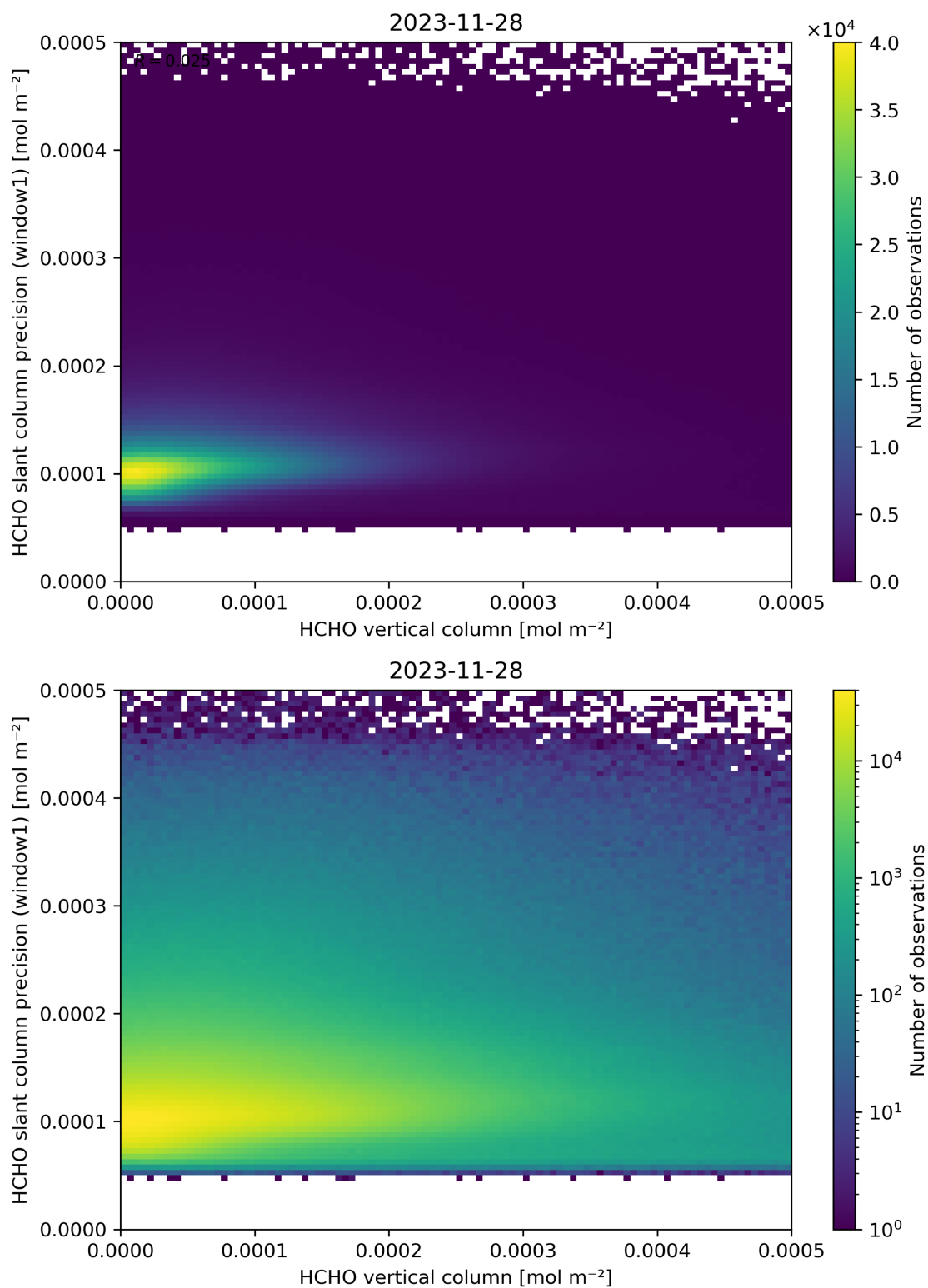
Figure 130: Scatter density plot of “HCHO vertical column” against “HCHO slant column precision (window1)” for 2023-11-28 to 2023-11-29.
