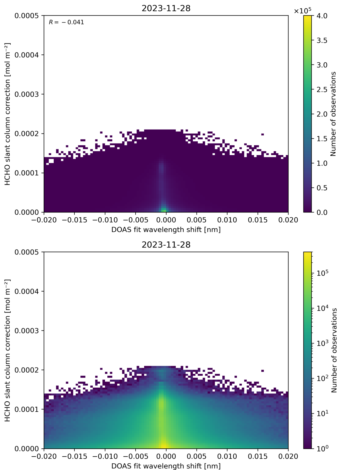
Figure 67: Scatter density plot of “DOAS fit wavelength shift” against “HCHO slant column correction” for 2023-11-28 to 2023-11-29.
