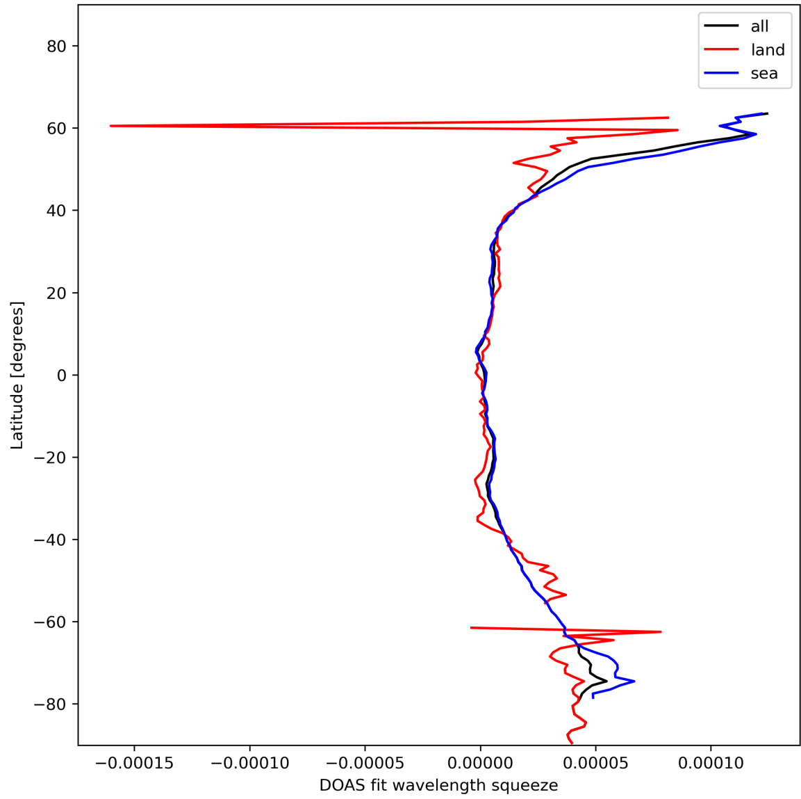
Figure 31: Zonal average of "DOAS fit wavelength squeeze" for 2023-11-28 to 2023-11-29.
