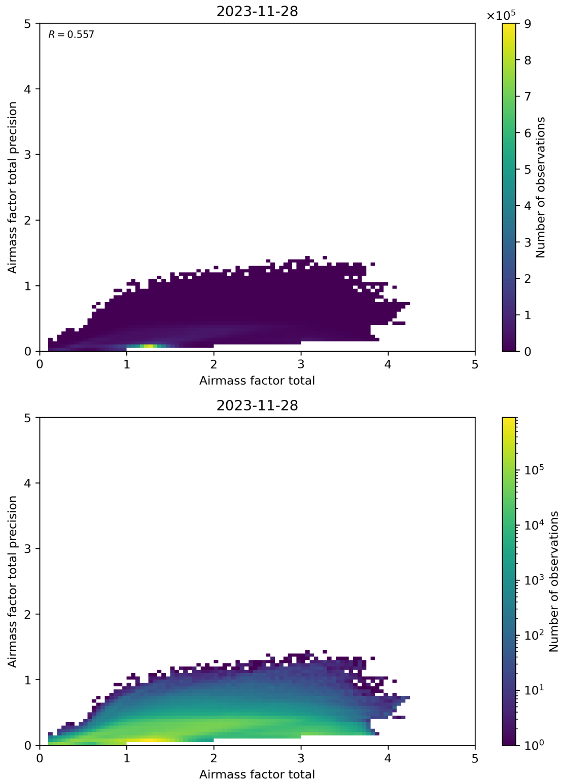
Figure 103: Scatter density plot of “Airmass factor total” against “Airmass factor total precision” for 2023-11-28 to 2023-11-29.
