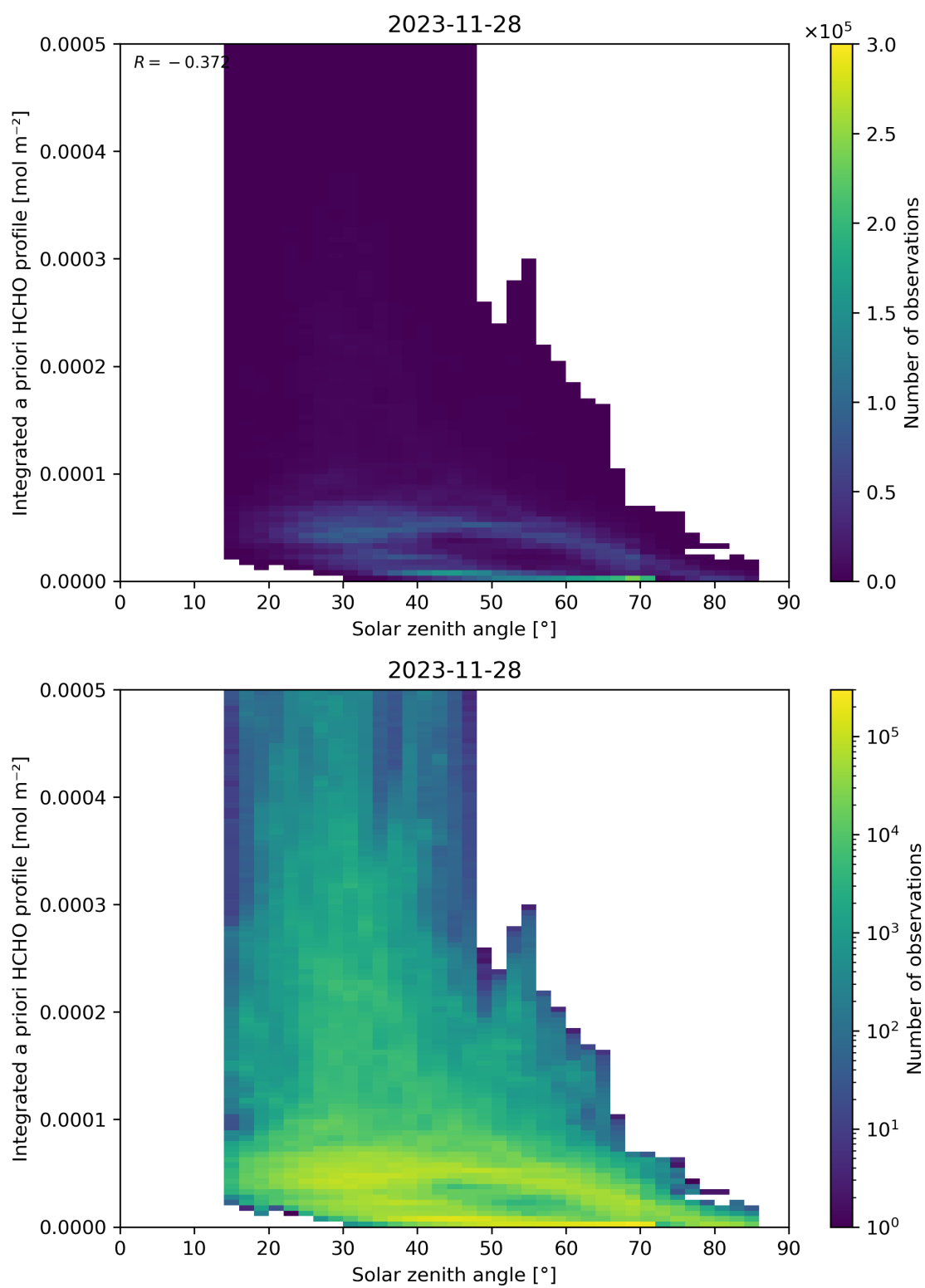
Figure 180: Scatter density plot of “Solar zenith angle” against “Integrated a priori HCHO profile” for 2023-11-28 to 2023-11-29.
