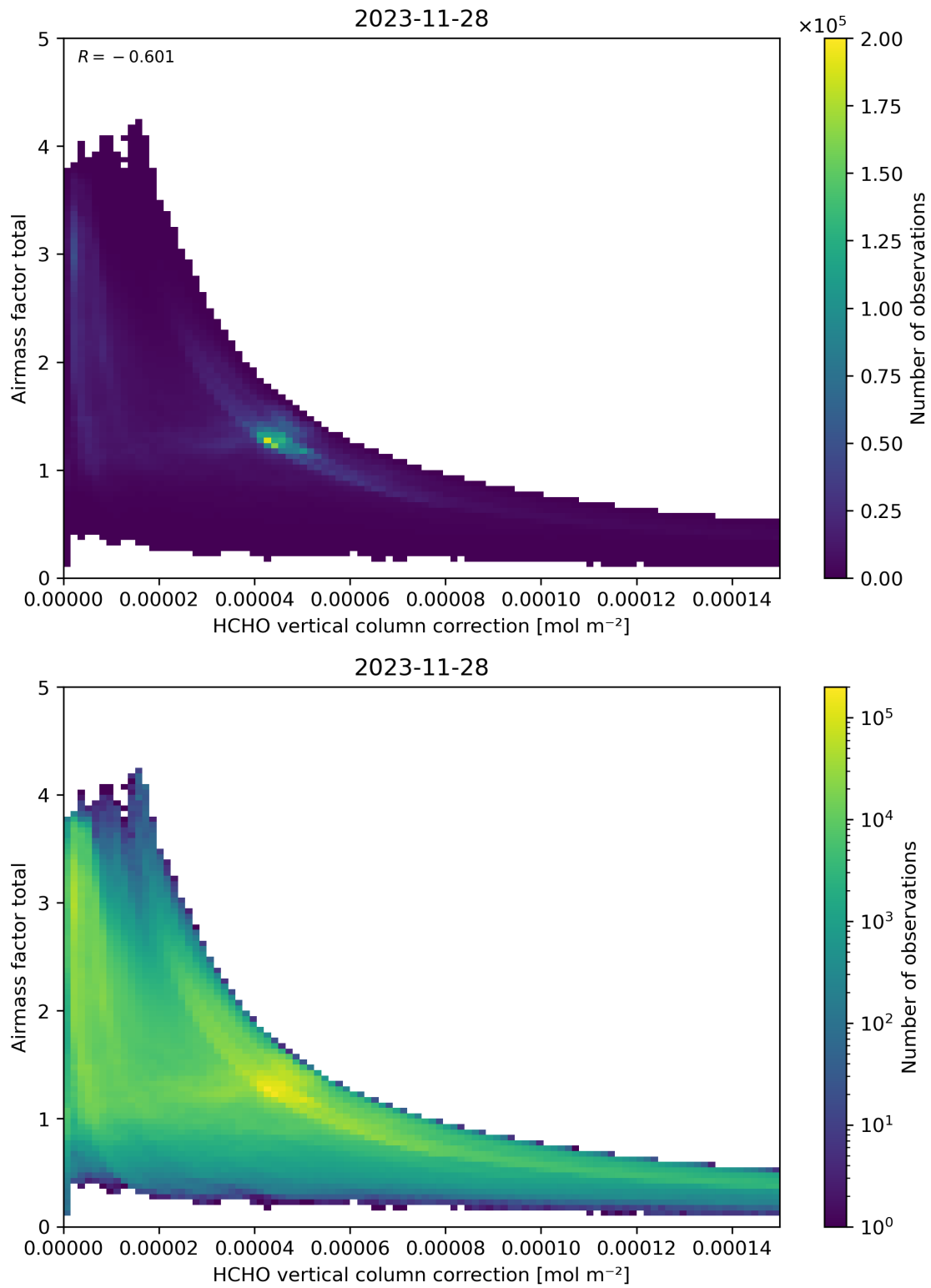
Figure 120: Scatter density plot of “HCHO vertical column correction” against “Airmass factor total” for 2023-11-28 to 2023-11-29.
