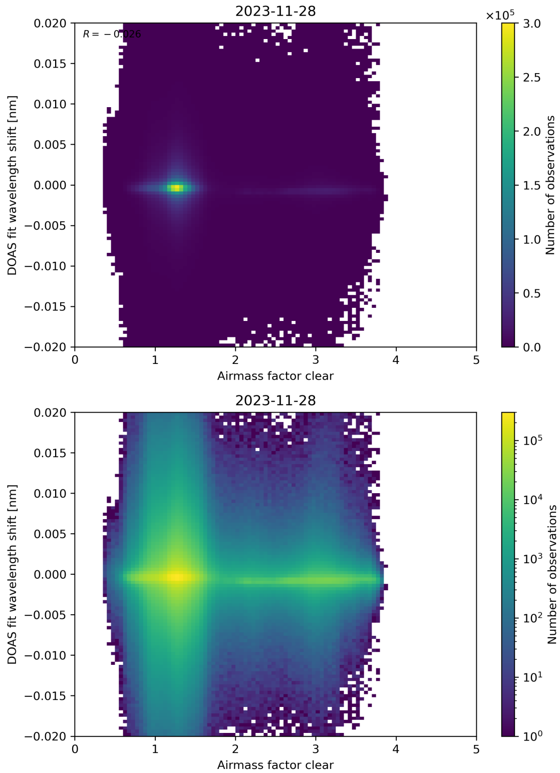
Figure 72: Scatter density plot of “Airmass factor clear” against “DOAS fit wavelength shift” for 2023-11-28 to 2023-11-29.
