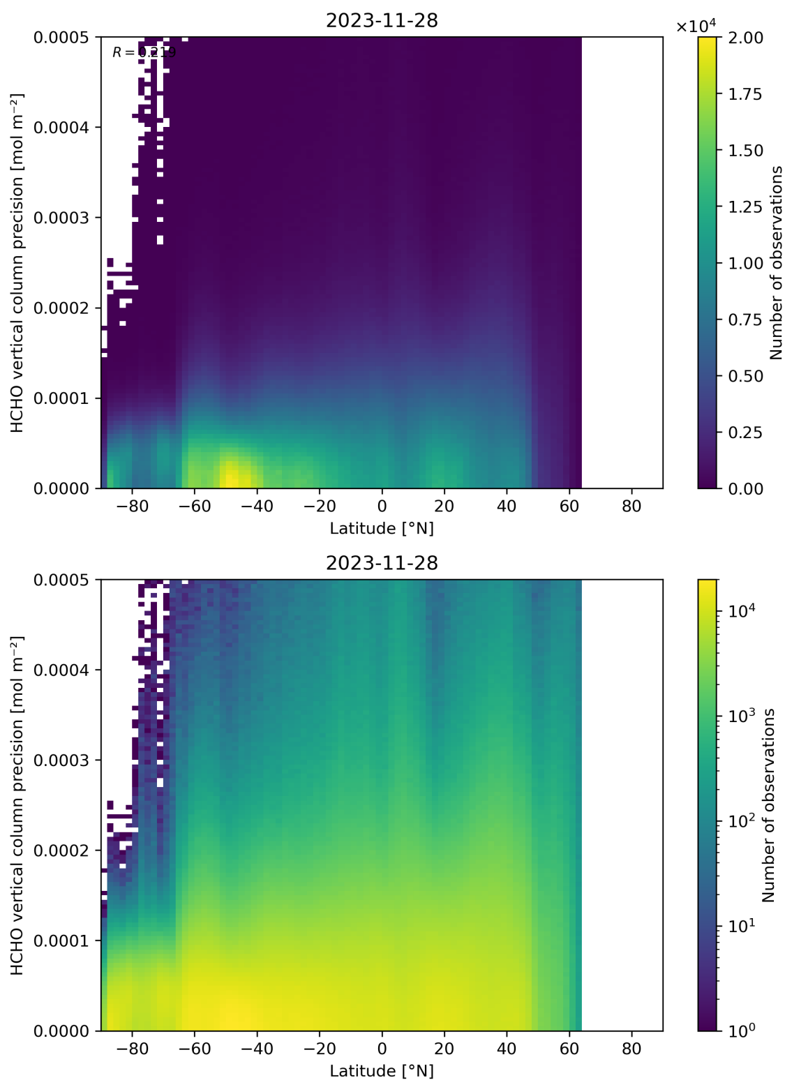
Figure 165: Scatter density plot of “Latitude” against “HCHO vertical column precision” for 2023-11-28 to 2023-11-29.
