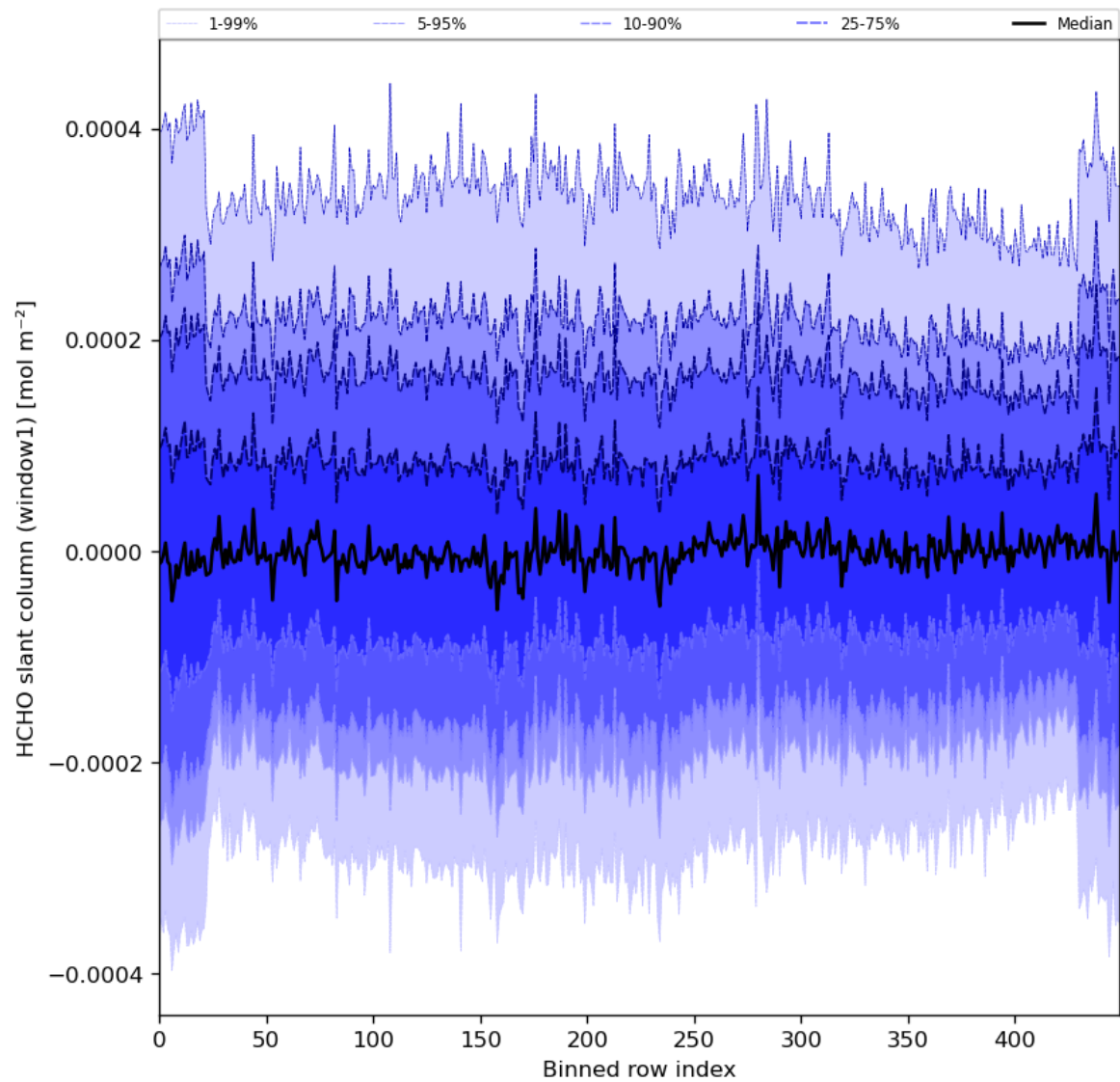
Figure 52: Along track statistics of “HCHO slant column (window1)” for 2023-11-28 to 2023-11-29
