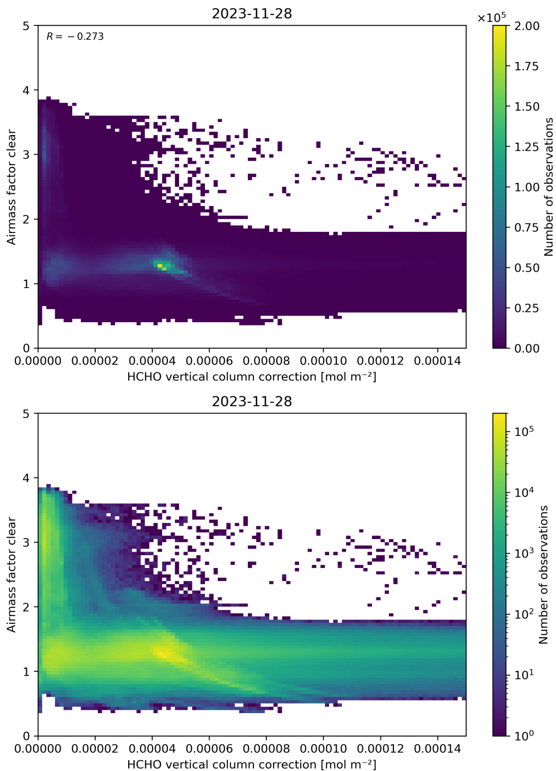
Figure 115: Scatter density plot of “HCHO vertical column correction” against “Airmass factor clear” for 2023-11-28 to 2023-11-29.
