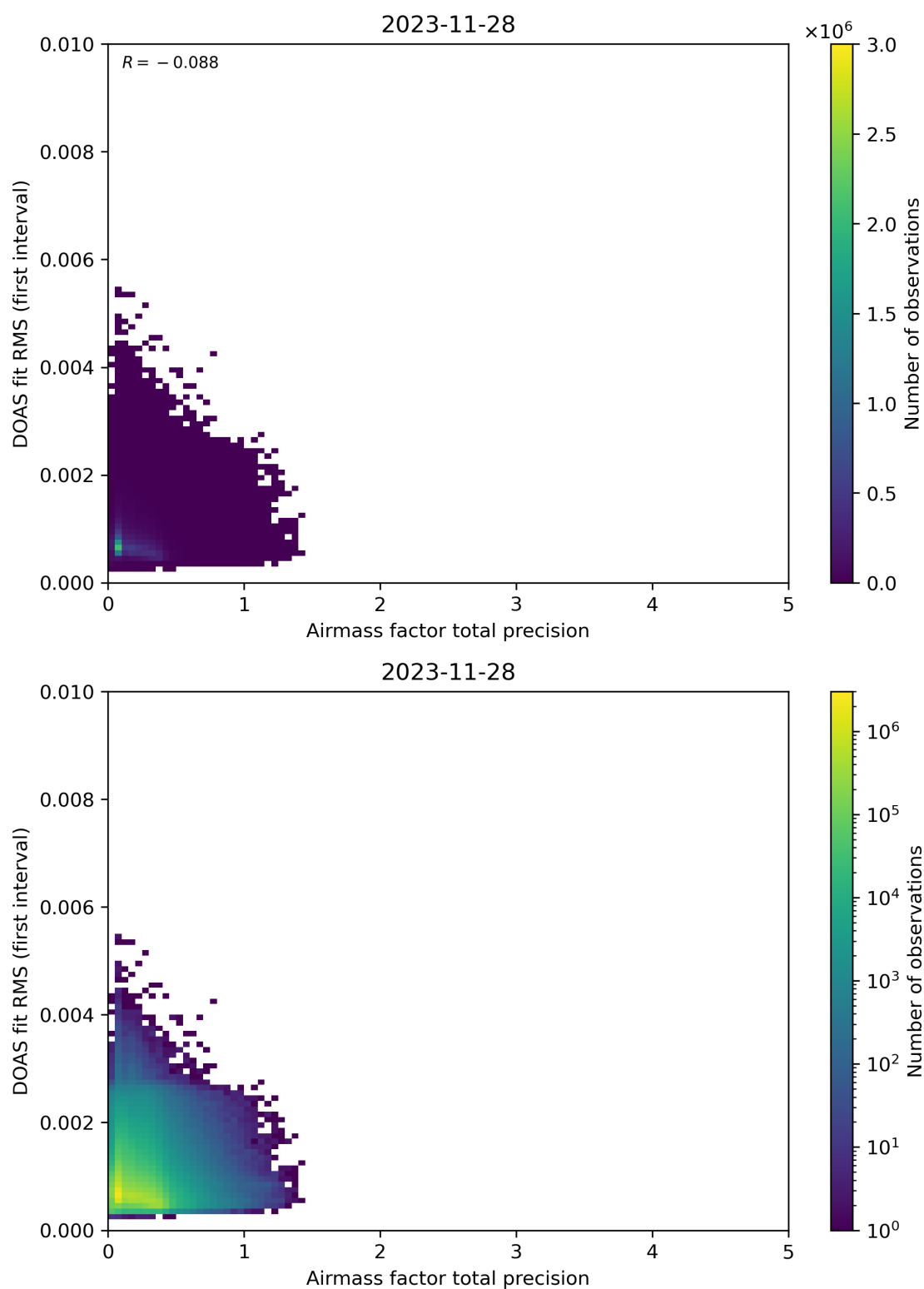
Figure 105: Scatter density plot of “Airmass factor total precision” against “DOAS fit RMS (first interval)” for 2023-11-28 to 2023-11-29.
