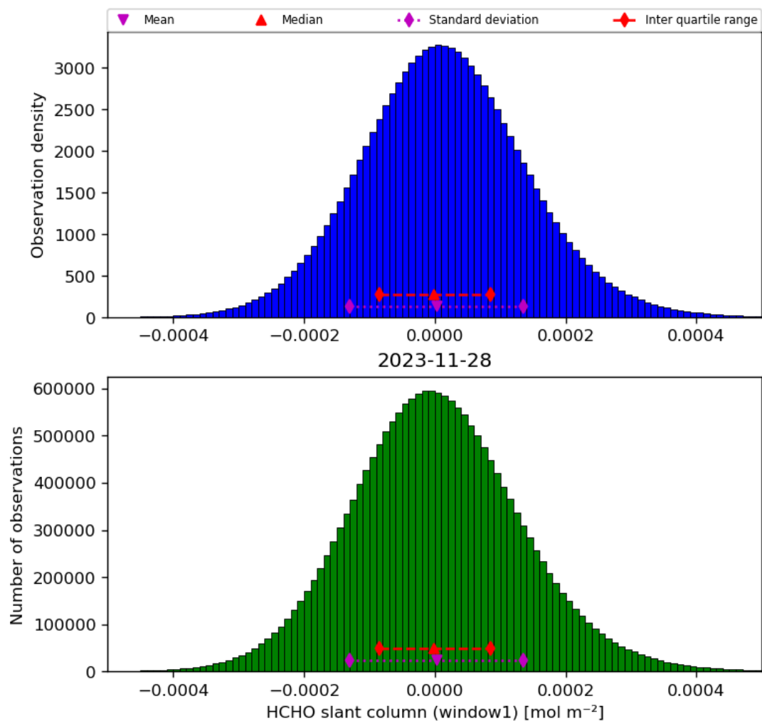
Figure 38: Histogram of “HCHO slant column (window1)” for 2023-11-28 to 2023-11-29
