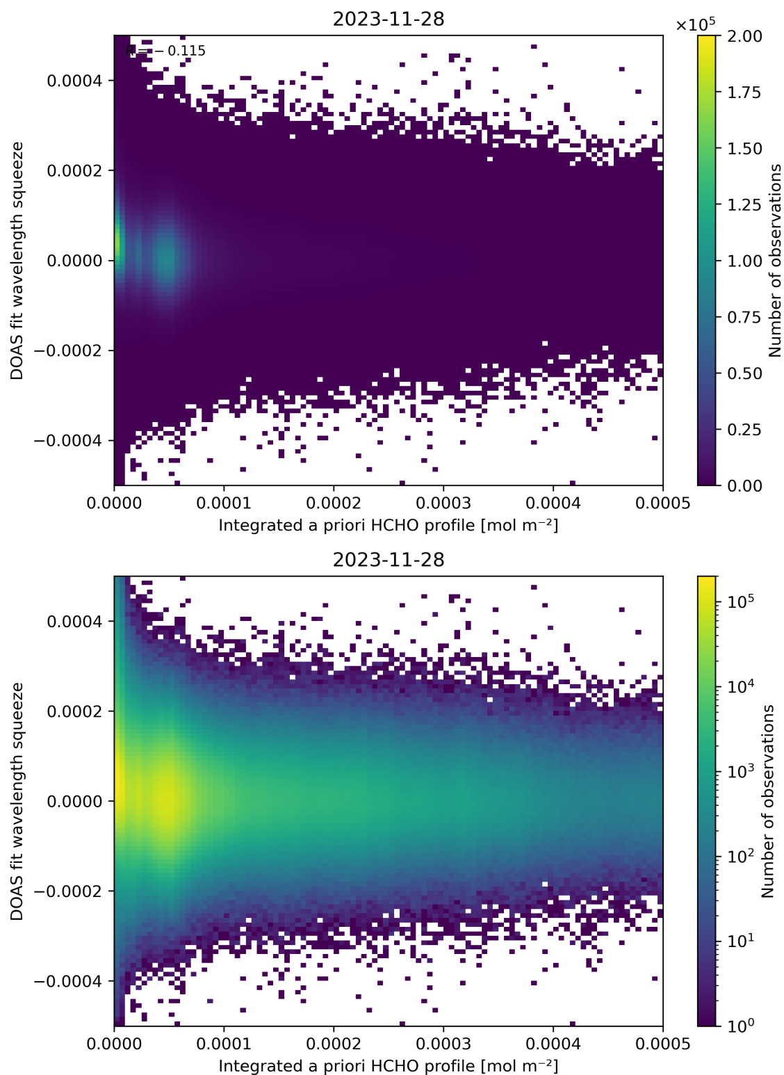
Figure 150: Scatter density plot of “Integrated a priori HCHO profile” against “DOAS fit wavelength squeeze” for 2023-11-28 to 2023-11-29.
