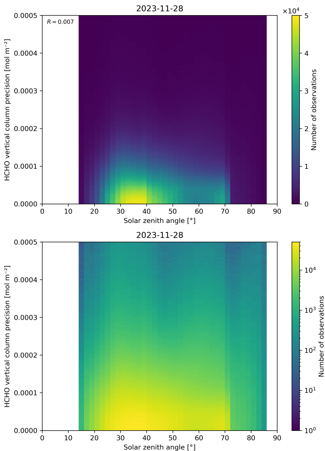
Figure 179: Scatter density plot of “Solar zenith angle” against “HCHO vertical column precision” for 2023-11-28 to 2023-11-29.
