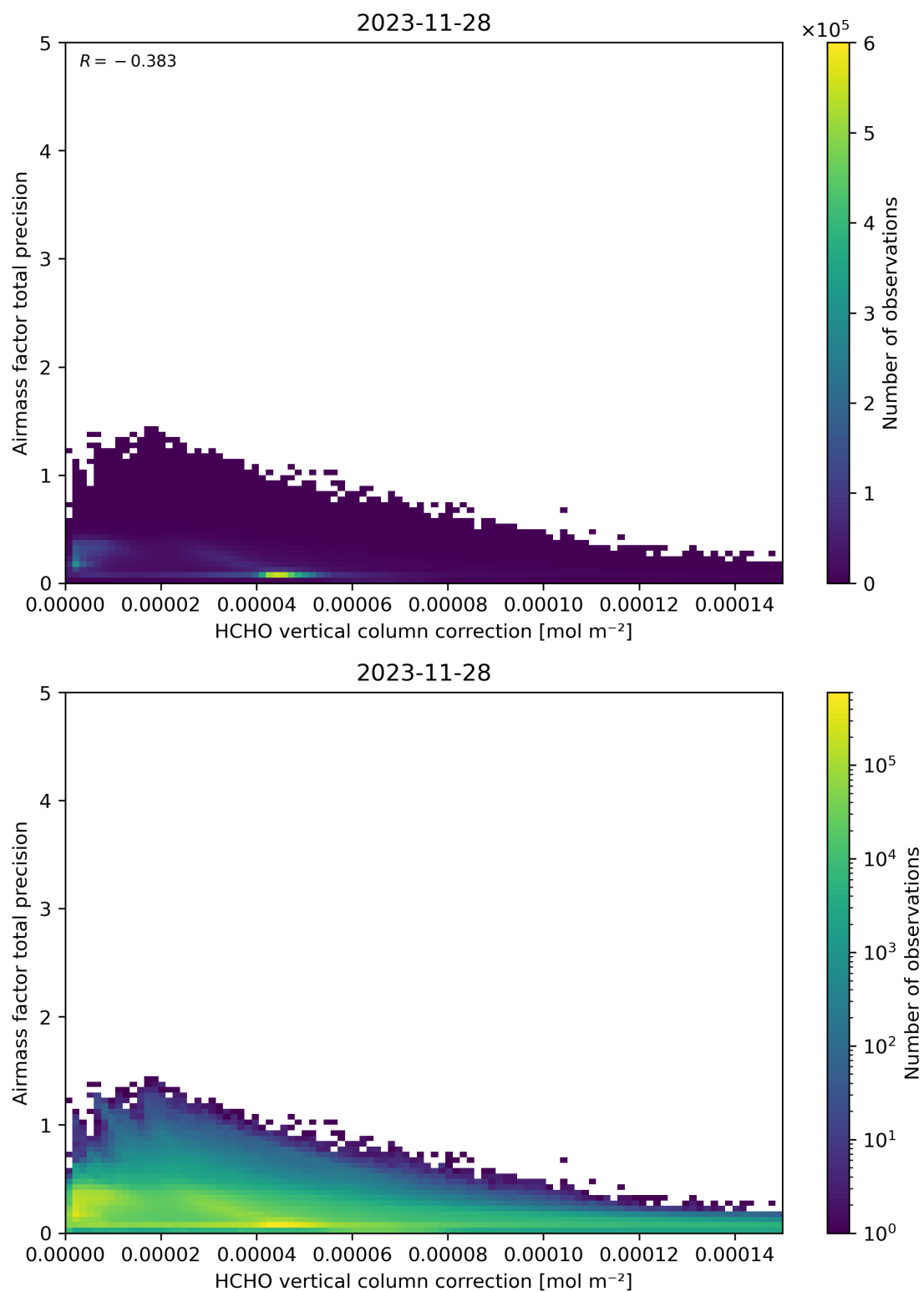
Figure 121: Scatter density plot of “HCHO vertical column correction” against “Airmass factor total precision” for 2023-11-28 to 2023-11-29.
