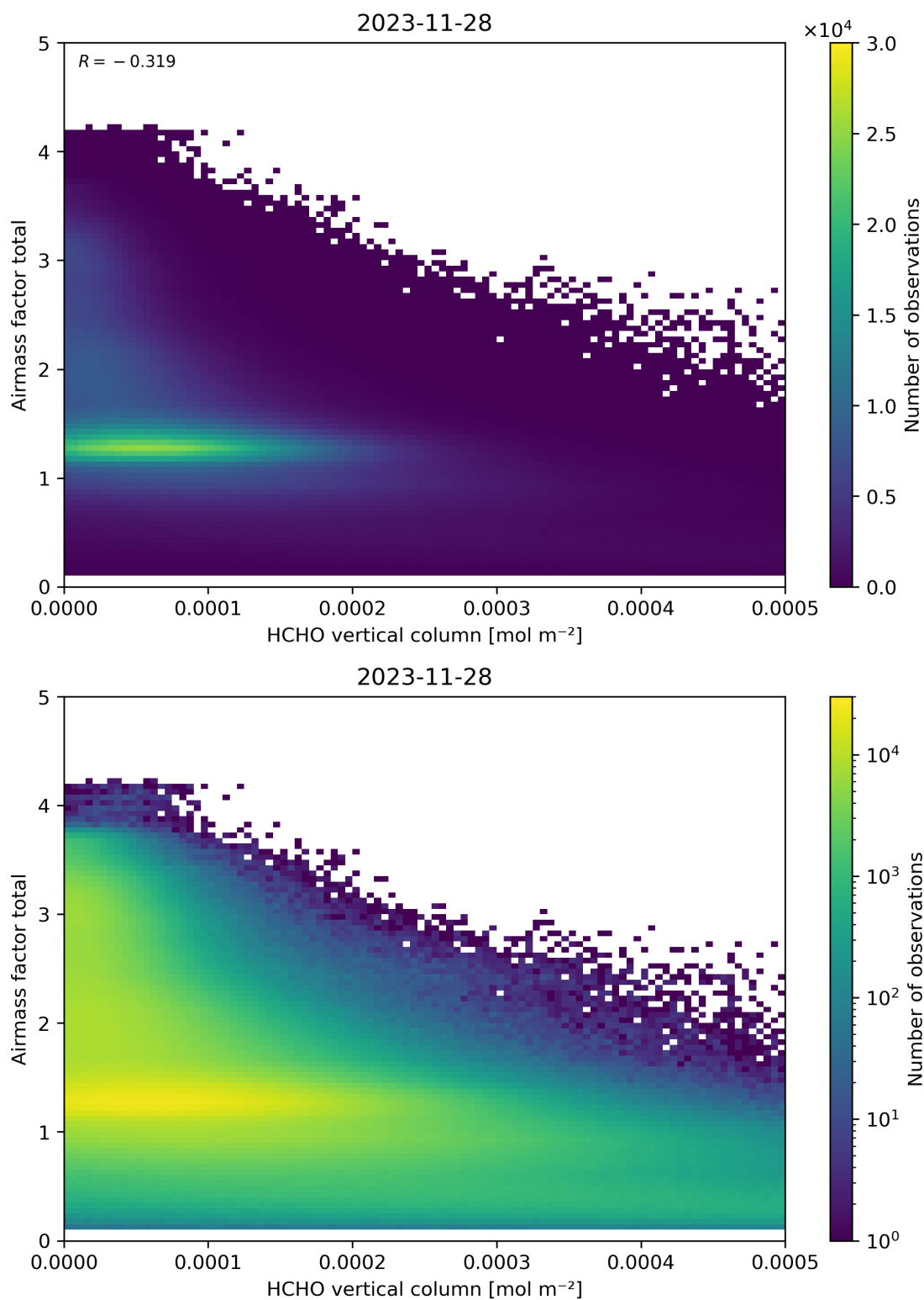
Figure 131: Scatter density plot of “HCHO vertical column” against “Airmass factor total” for 2023-11-28 to 2023-11-29.
