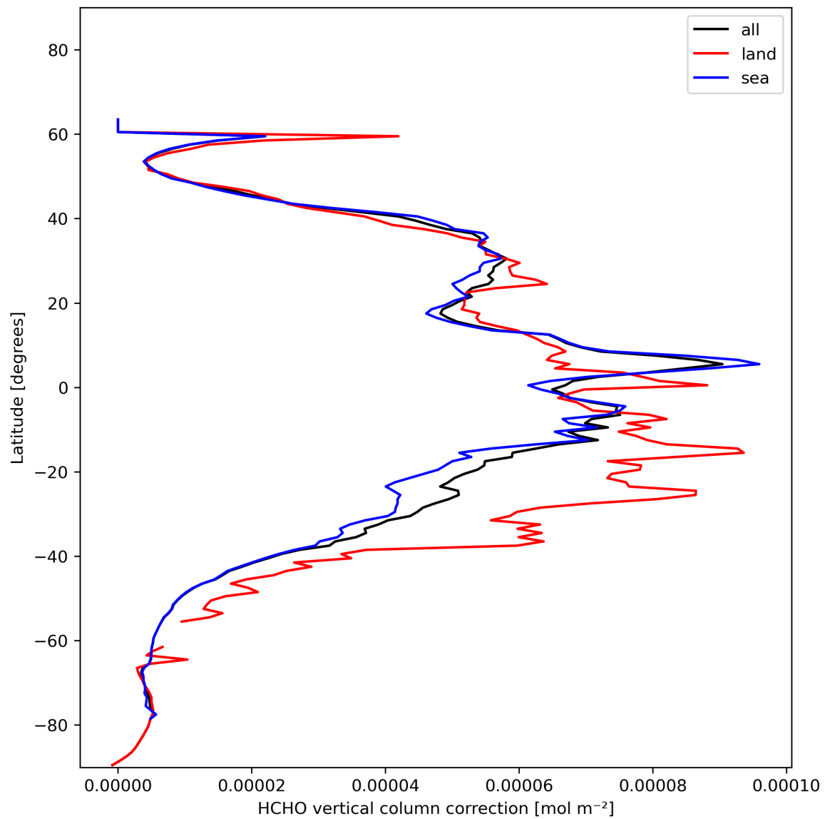
Figure 23: Zonal average of “HCHO vertical column correction” for 2023-11-28 to 2023-11-29.
