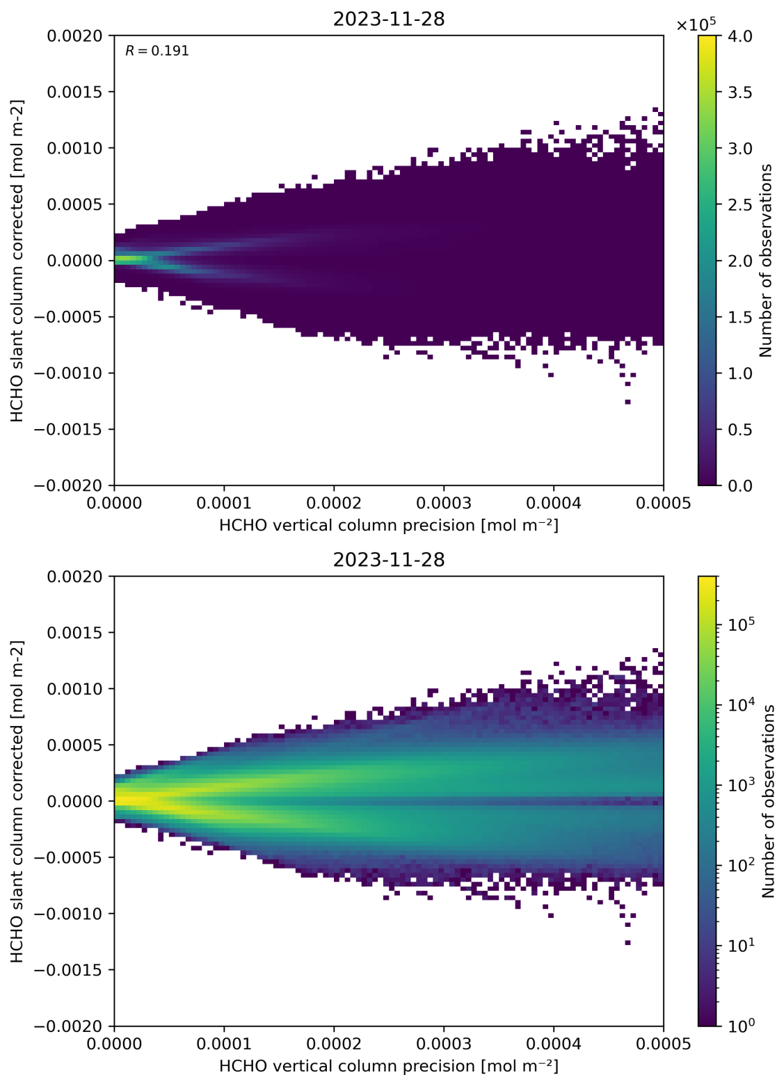
Figure 140: Scatter density plot of “HCHO vertical column precision” against “HCHO slant column corrected” for 2023-11-28 to 2023-11-29.
