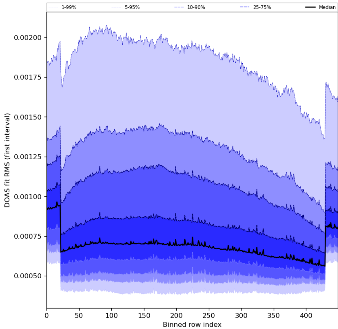
Figure 60: Along track statistics of “DOAS fit RMS (first interval)” for 2023-11-28 to 2023-11-29
