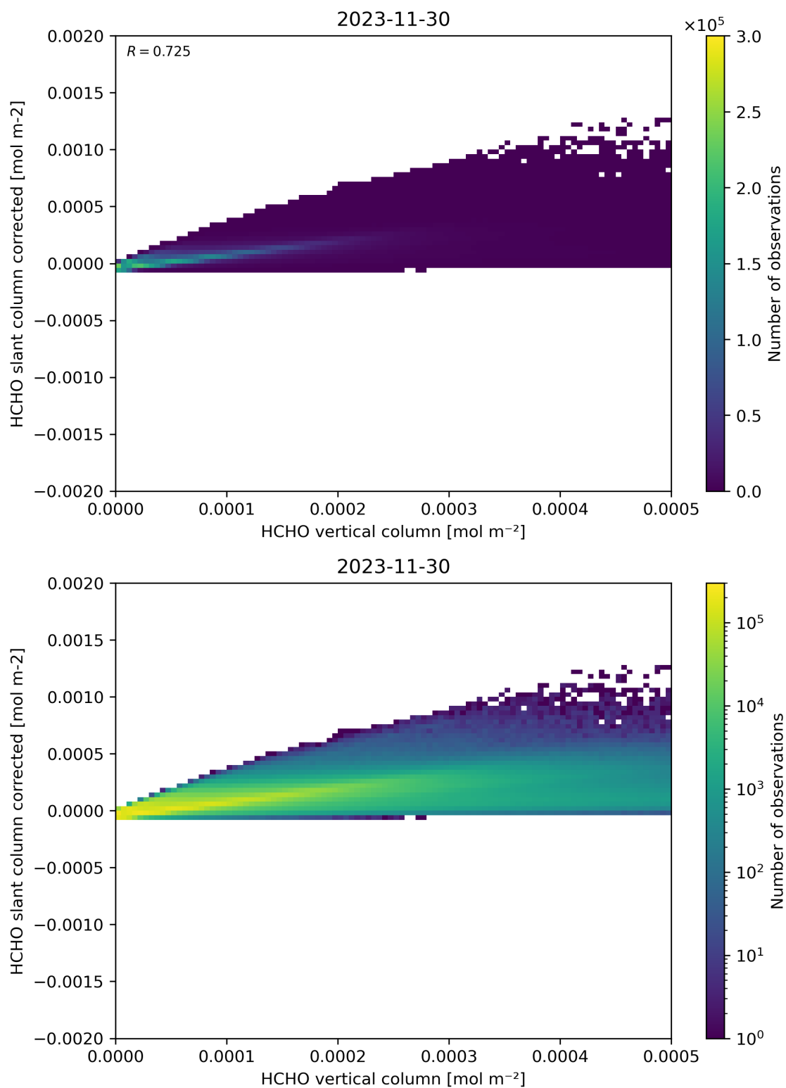
Figure 127: Scatter density plot of “HCHO vertical column” against “HCHO slant column corrected” for 2023-11-29 to 2023-12-01.
