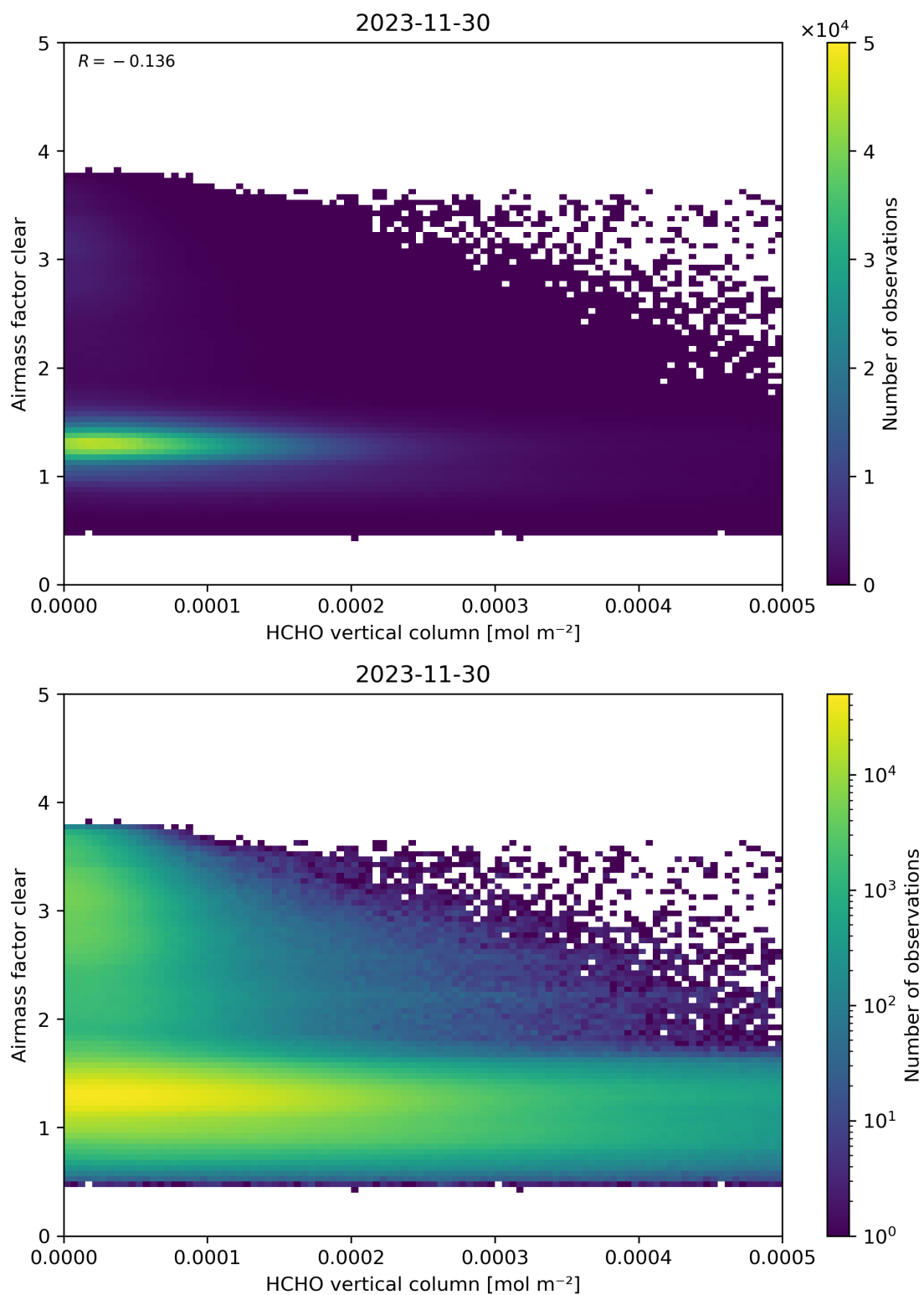
Figure 126: Scatter density plot of “HCHO vertical column” against “Airmass factor clear” for 2023-11-29 to 2023-12-01.
