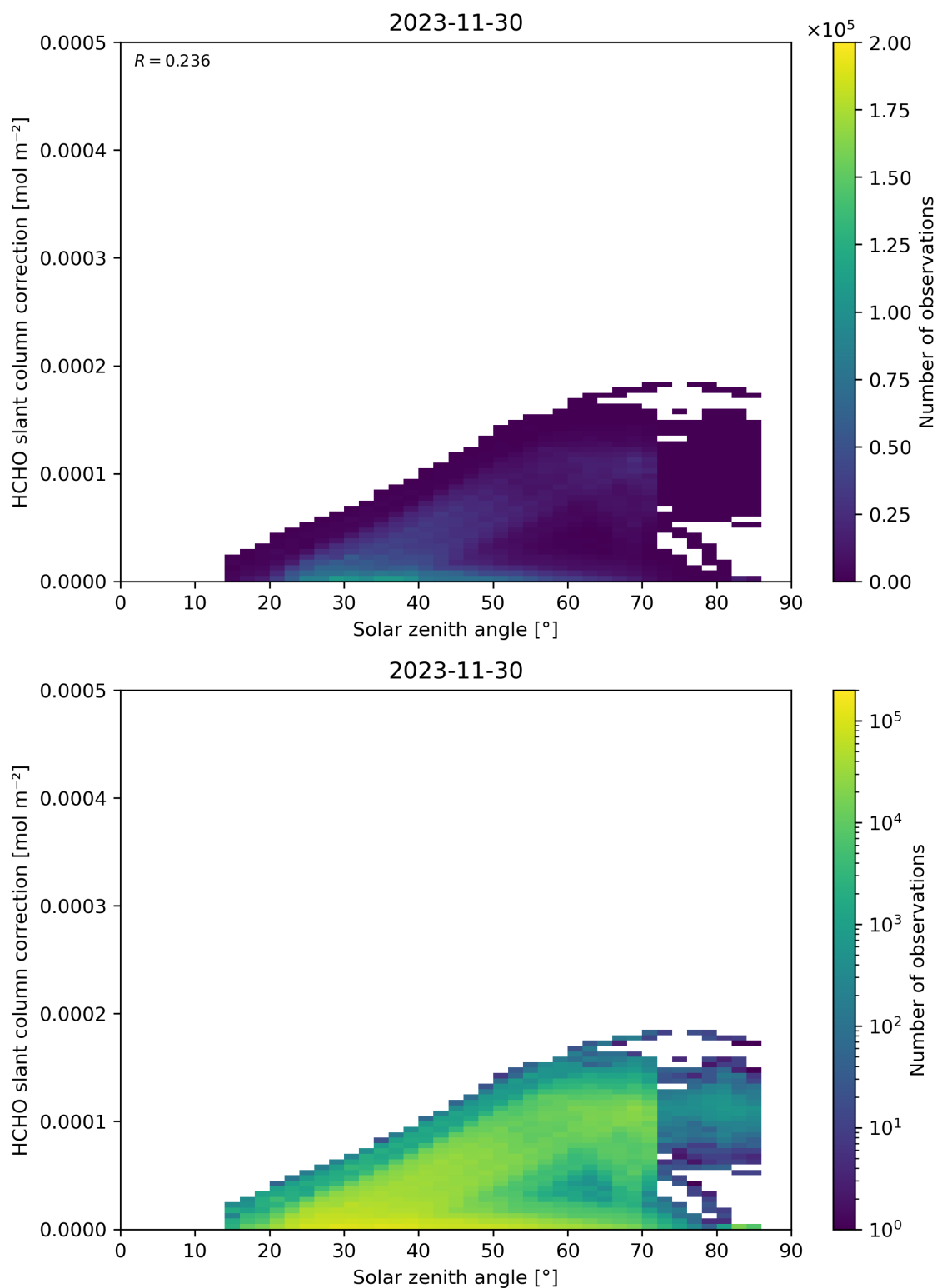
Figure 172: Scatter density plot of “Solar zenith angle” against “HCHO slant column correction” for 2023-11-29 to 2023-12-01.
