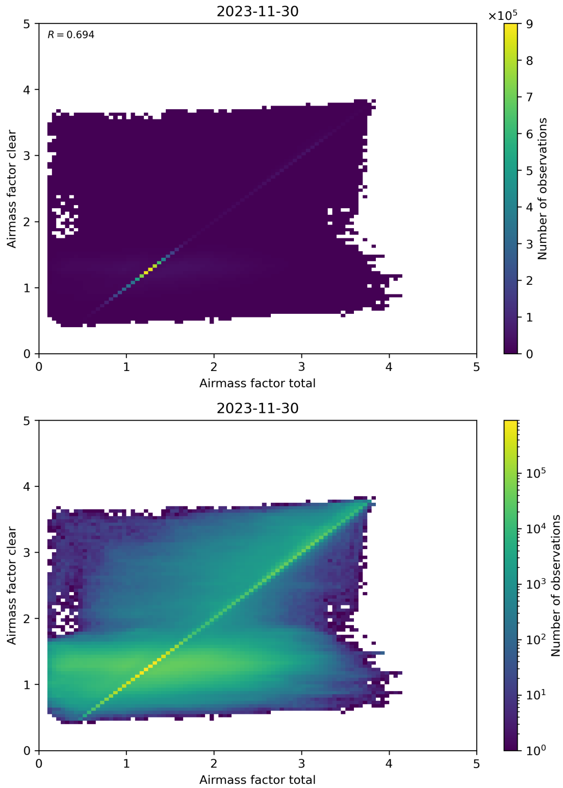
Figure 100: Scatter density plot of “Airmass factor total” against “Airmass factor clear” for 2023-11-29 to 2023-12-01.
