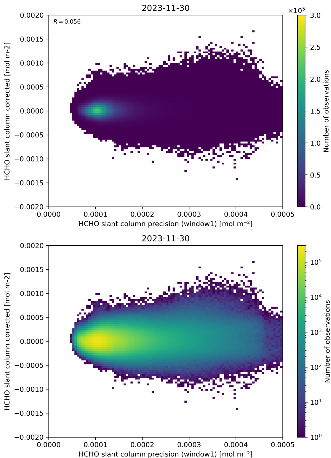
Figure 92: Scatter density plot of “HCHO slant column precision (window1)” against “HCHO slant column corrected” for 2023-11-29 to 2023-12-01.
