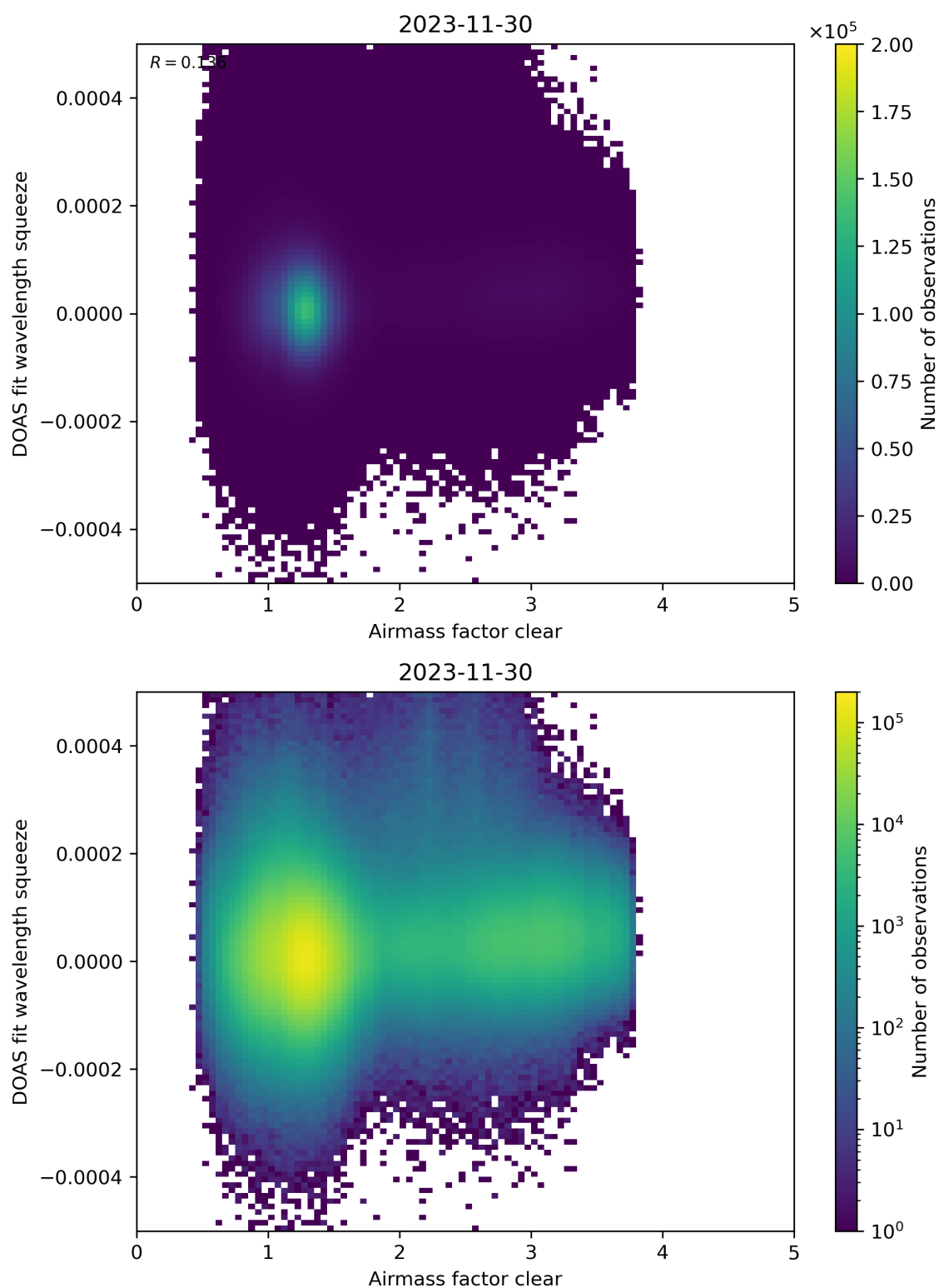
Figure 73: Scatter density plot of “Airmass factor clear” against “DOAS fit wavelength squeeze” for 2023-11-29 to 2023-12-01.
