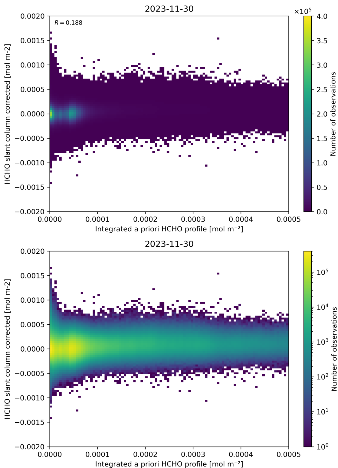
Figure 151: Scatter density plot of “Integrated a priori HCHO profile” against “HCHO slant column corrected” for 2023-11-29 to 2023-12-01.
