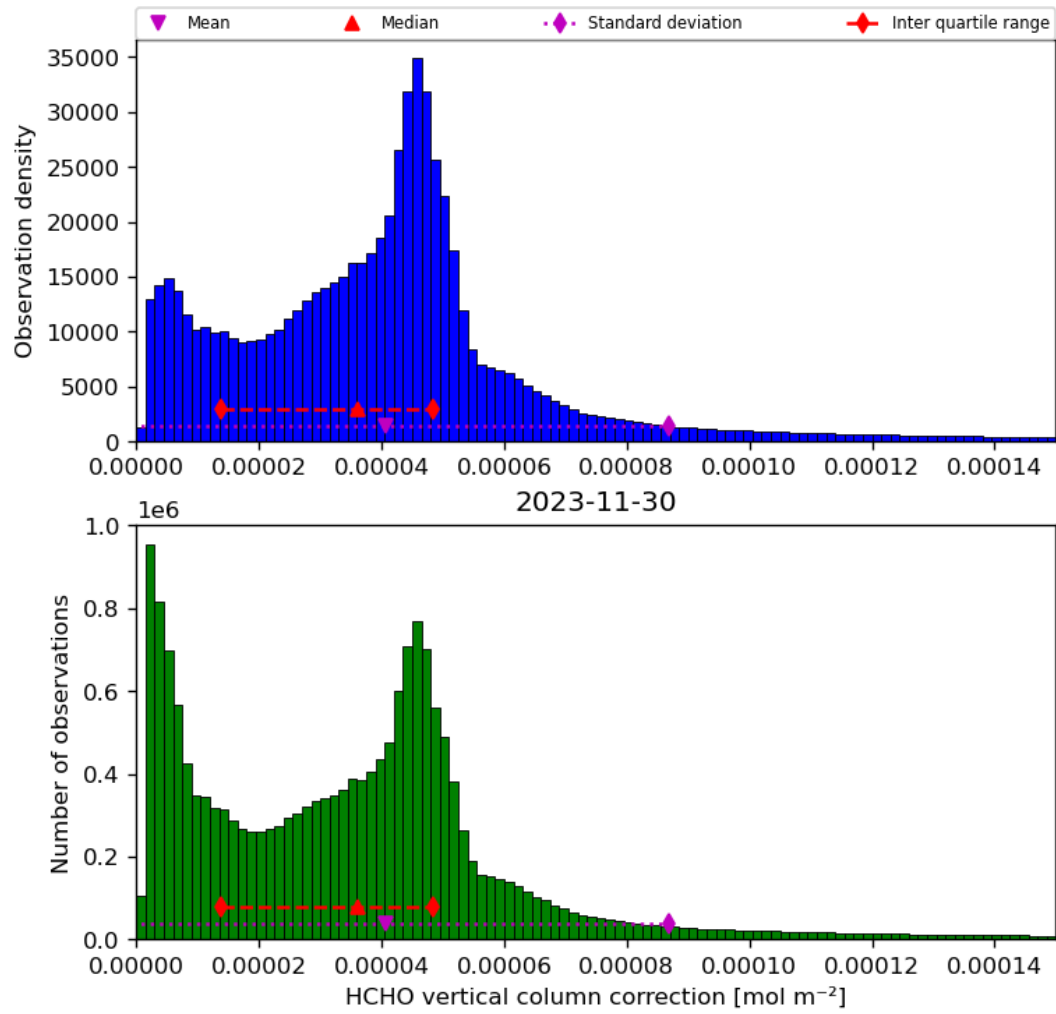
Figure 37: Histogram of “HCHO vertical column correction” for 2023-11-29 to 2023-12-01
