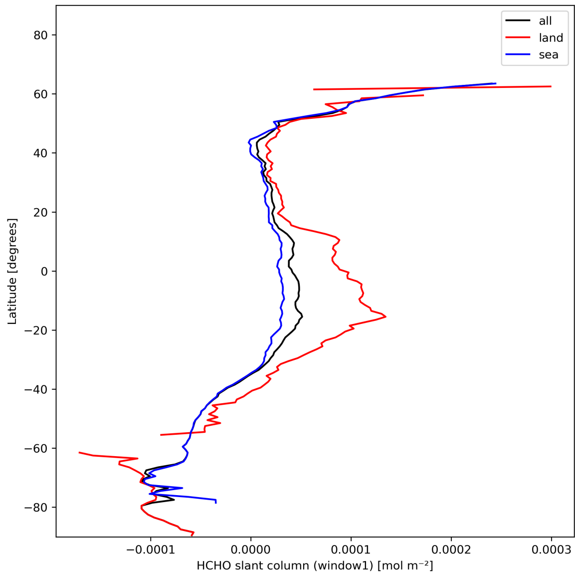
Figure 24: Zonal average of “HCHO slant column (window1)” for 2023-11-29 to 2023-12-01.
