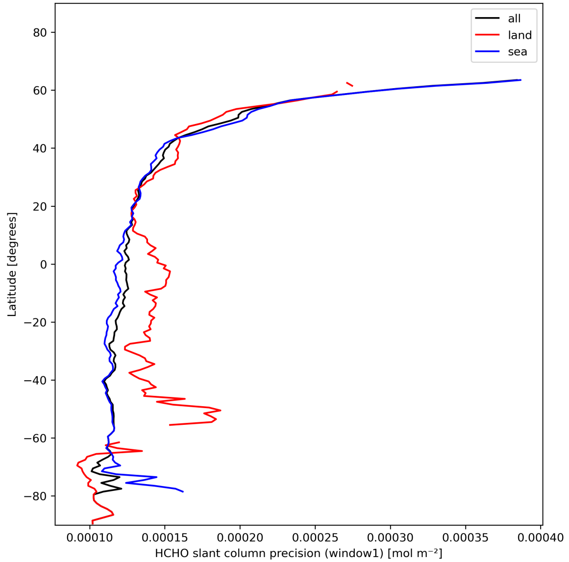
Figure 25: Zonal average of “HCHO slant column precision (window1)” for 2023-11-29 to 2023-12-01.
