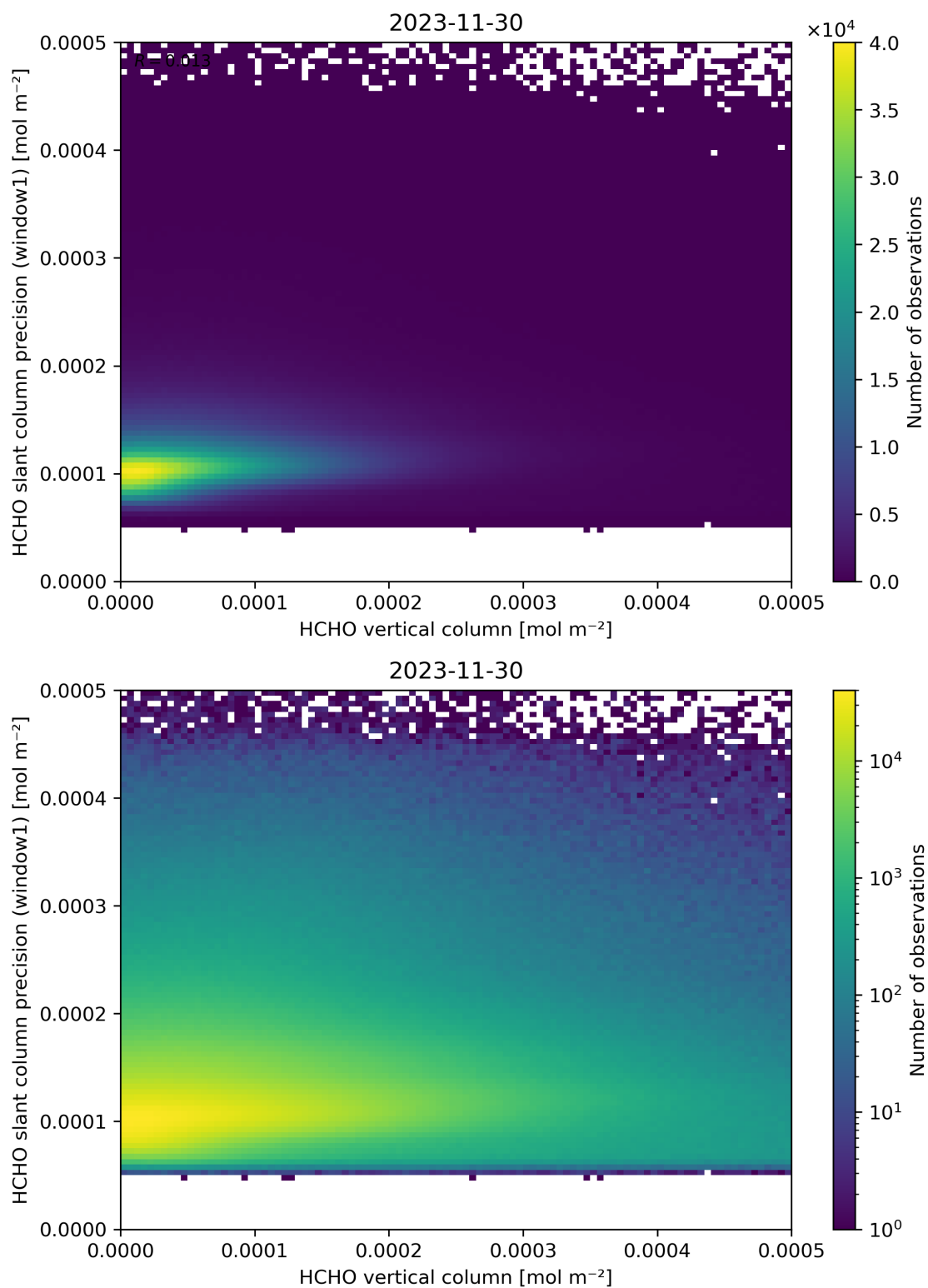
Figure 130: Scatter density plot of “HCHO vertical column” against “HCHO slant column precision (window1)” for 2023-11-29 to 2023-12-01.
