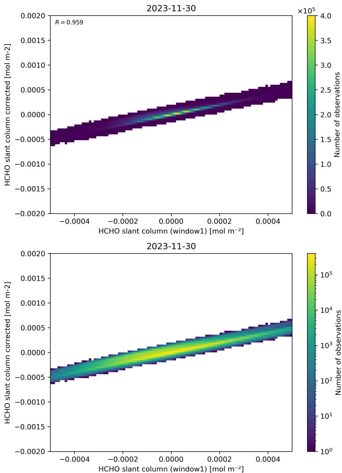
Figure 82: Scatter density plot of “HCHO slant column (window1)” against “HCHO slant column corrected” for 2023-11-29 to 2023-12-01.
