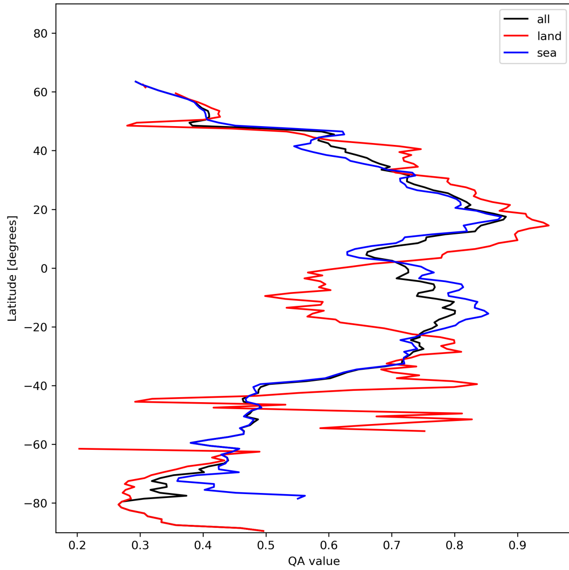
Figure 20: Zonal average of “QA value” for 2023-11-29 to 2023-12-01.
