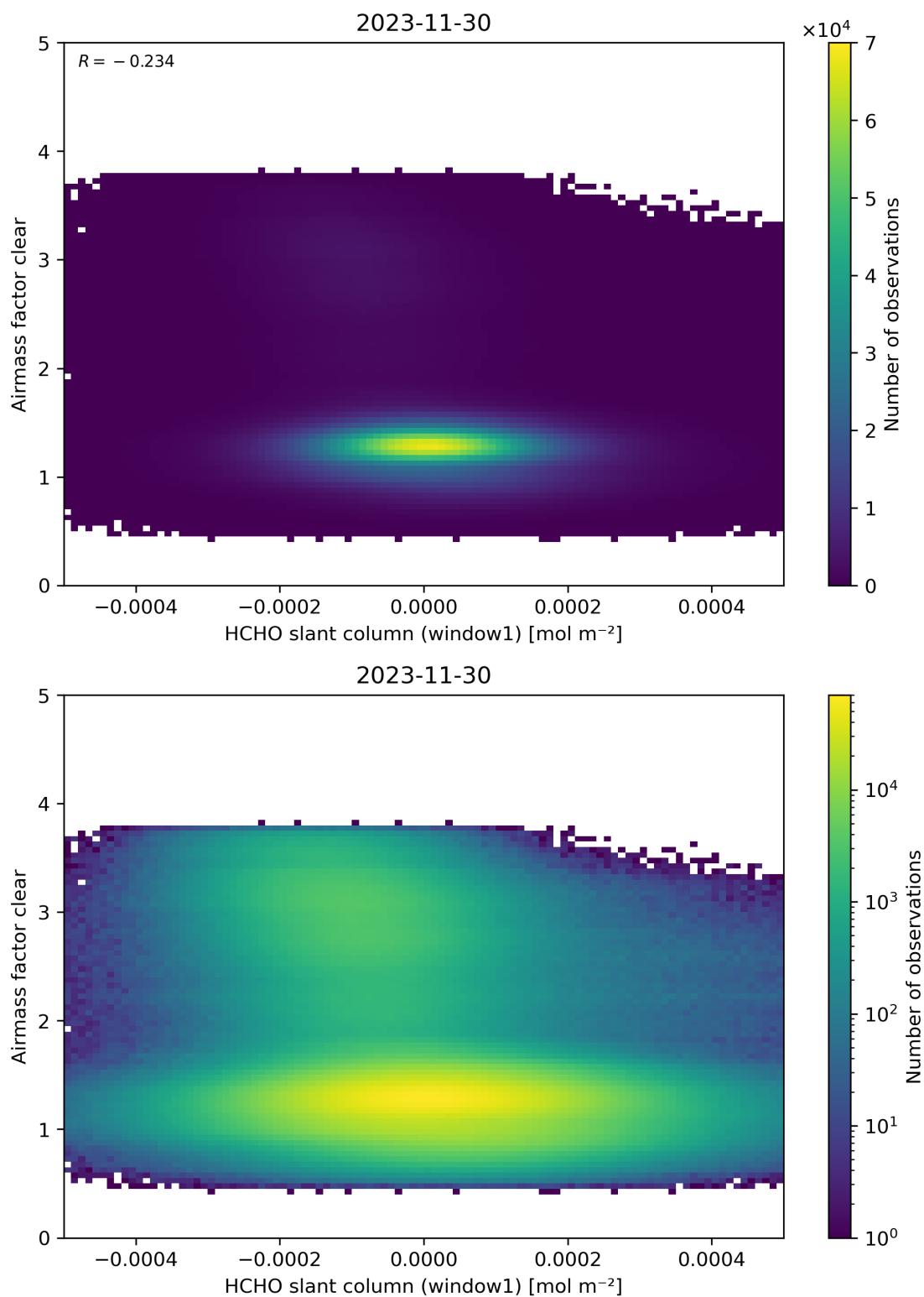
Figure 81: Scatter density plot of “HCHO slant column (window1)” against “Airmass factor clear” for 2023-11-29 to 2023-12-01.
