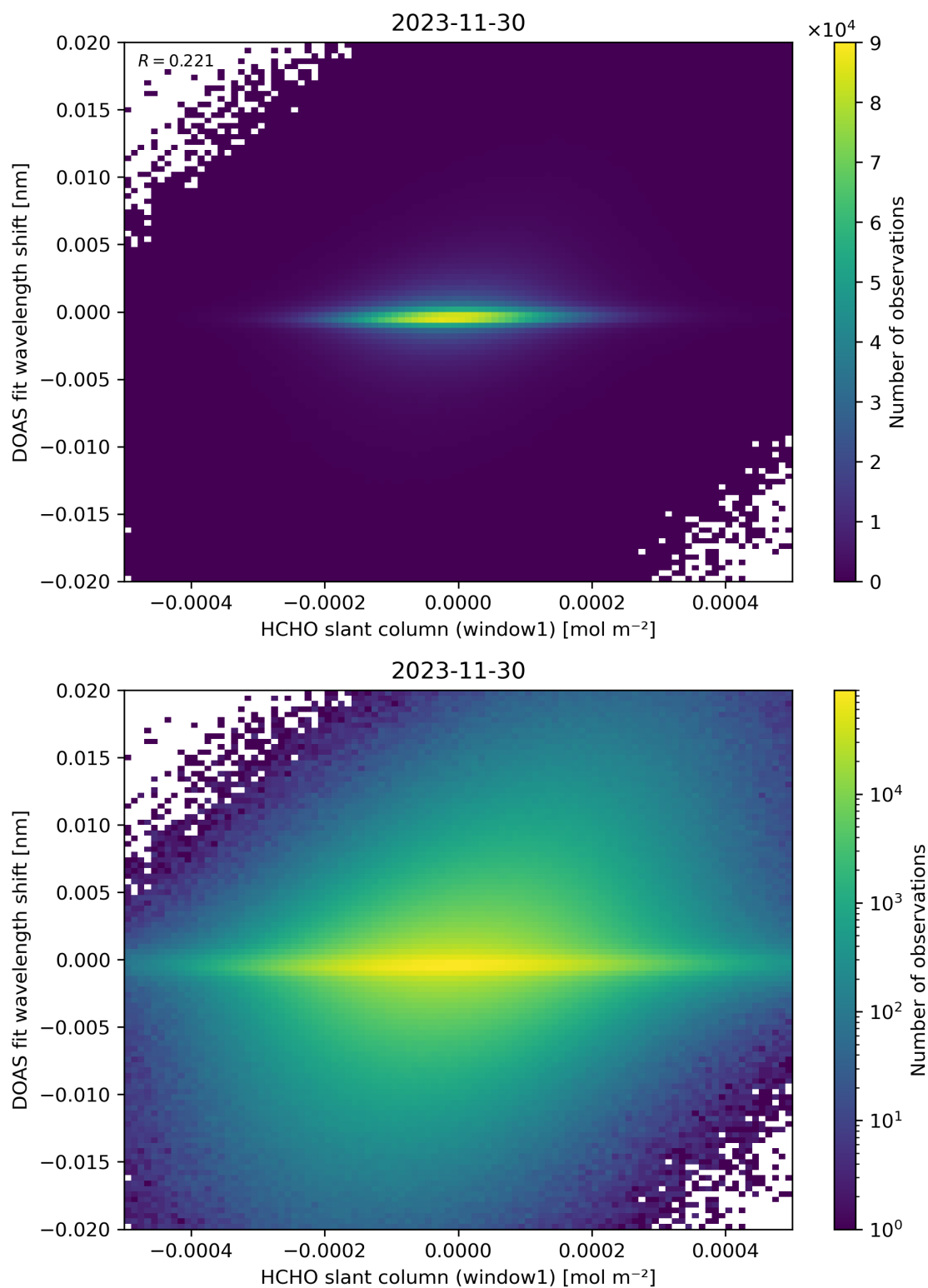
Figure 79: Scatter density plot of “HCHO slant column (window1)” against “DOAS fit wavelength shift” for 2023-11-29 to 2023-12-01.
