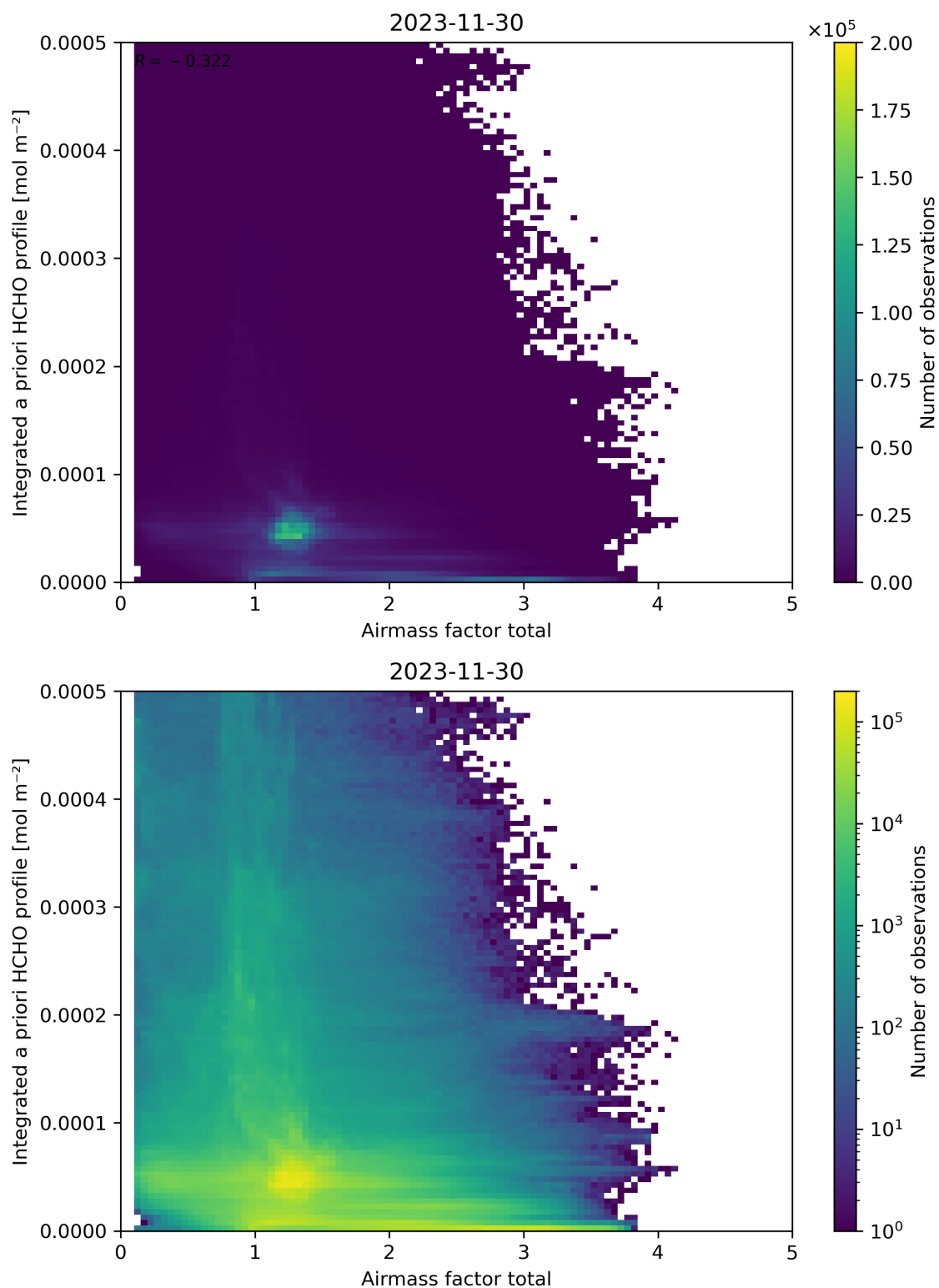
Figure 104: Scatter density plot of “Airmass factor total” against “Integrated a priori HCHO profile” for 2023-11-29 to 2023-12-01.
