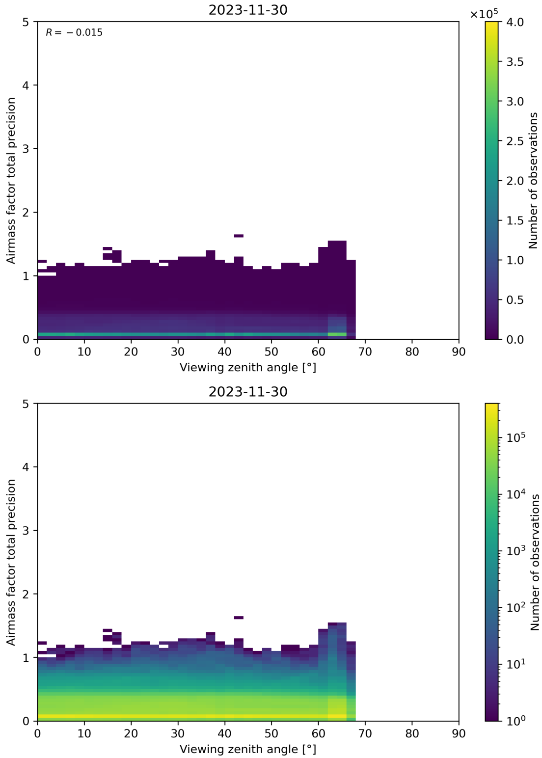
Figure 191: Scatter density plot of “Viewing zenith angle” against “Airmass factor total precision” for 2023-11-29 to 2023-12-01.
