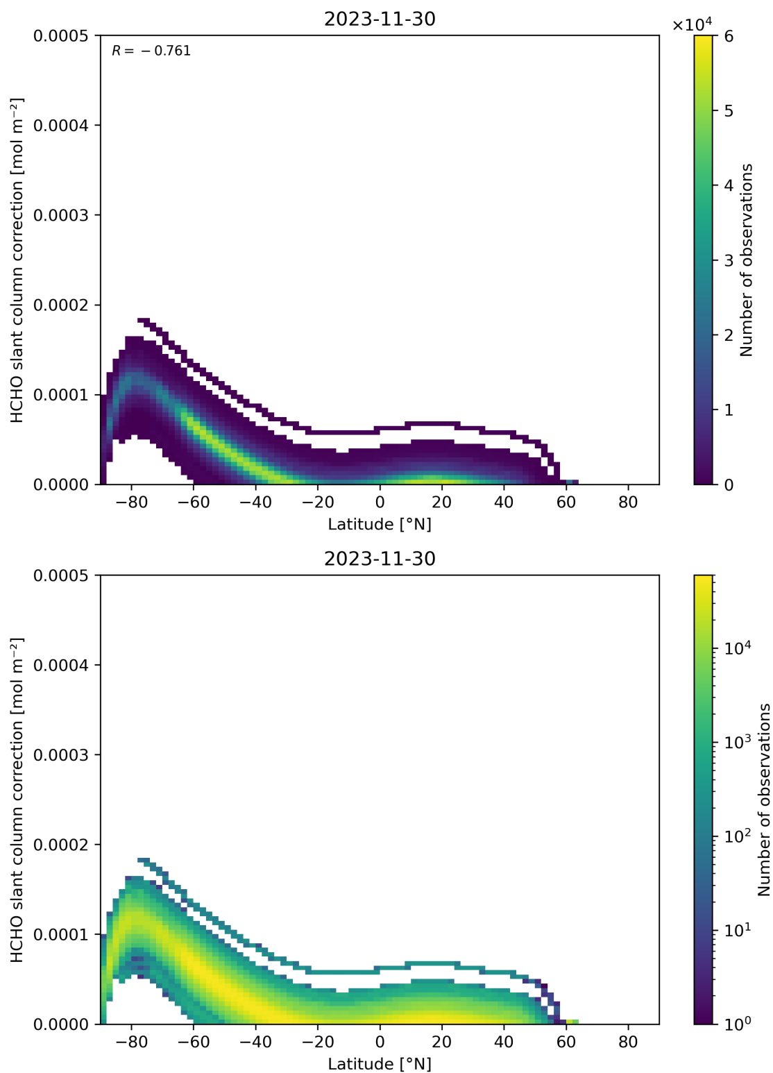
Figure 158: Scatter density plot of “Latitude” against “HCHO slant column correction” for 2023-11-29 to 2023-12-01.
