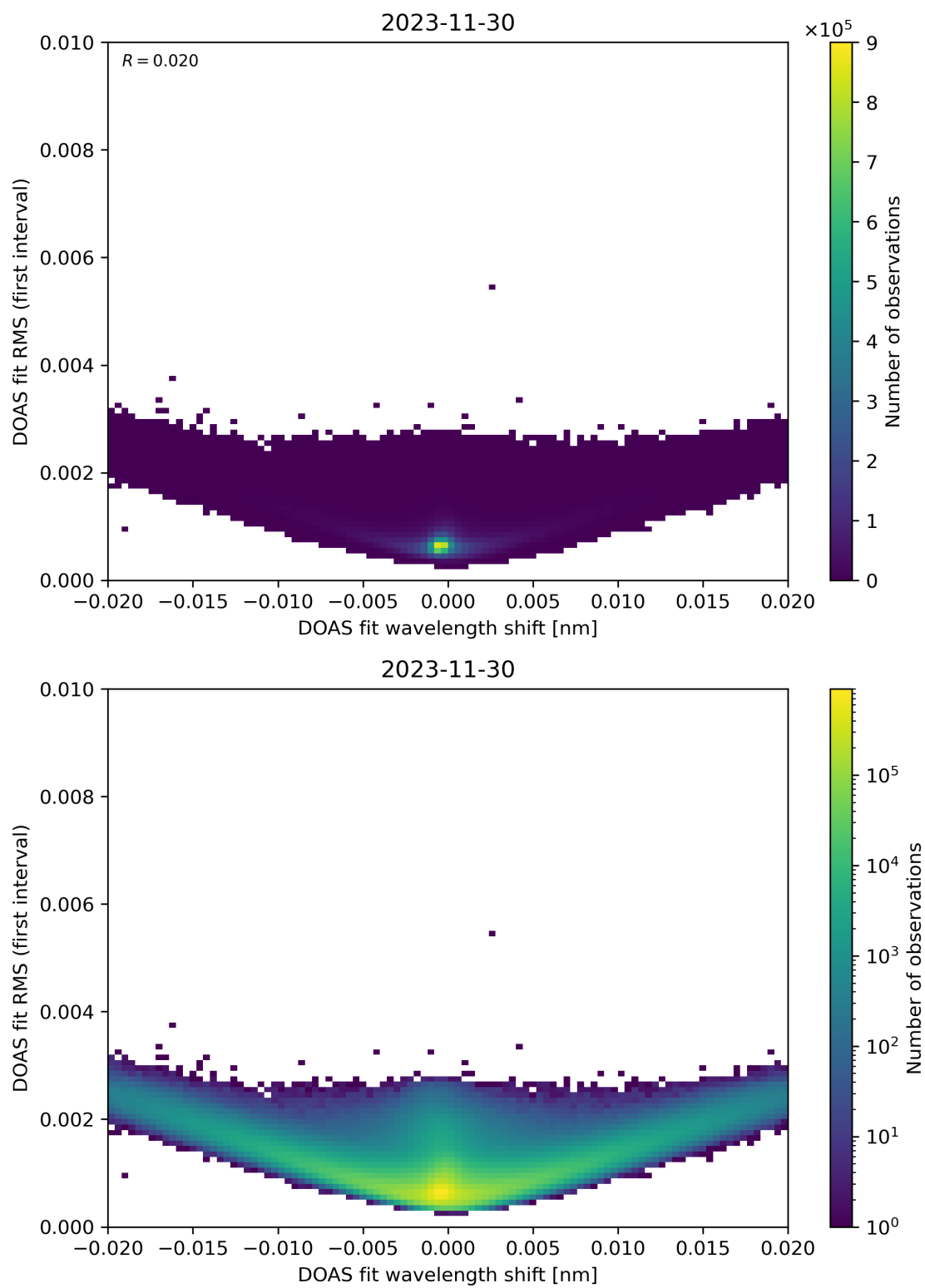
Figure 64: Scatter density plot of “DOAS fit wavelength shift” against “DOAS fit RMS (first interval)” for 2023-11-29 to 2023-12-01.
