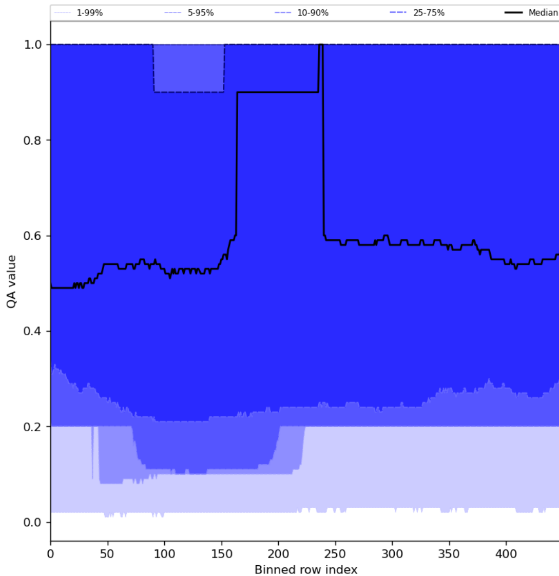
Figure 48: Along track statistics of “QA value” for 2023-11-29 to 2023-12-01
