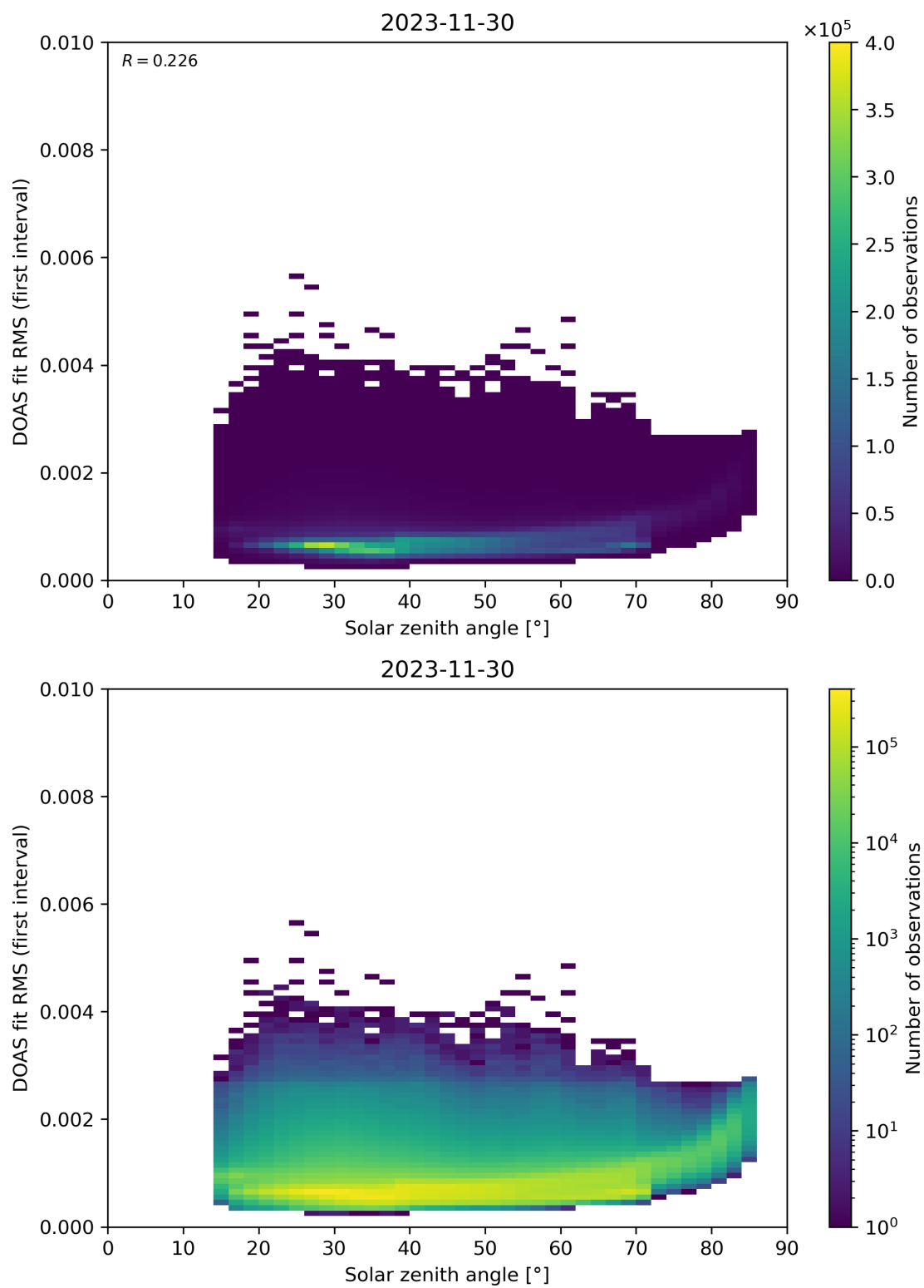
Figure 167: Scatter density plot of “Solar zenith angle” against “DOAS fit RMS (first interval)” for 2023-11-29 to 2023-12-01.
