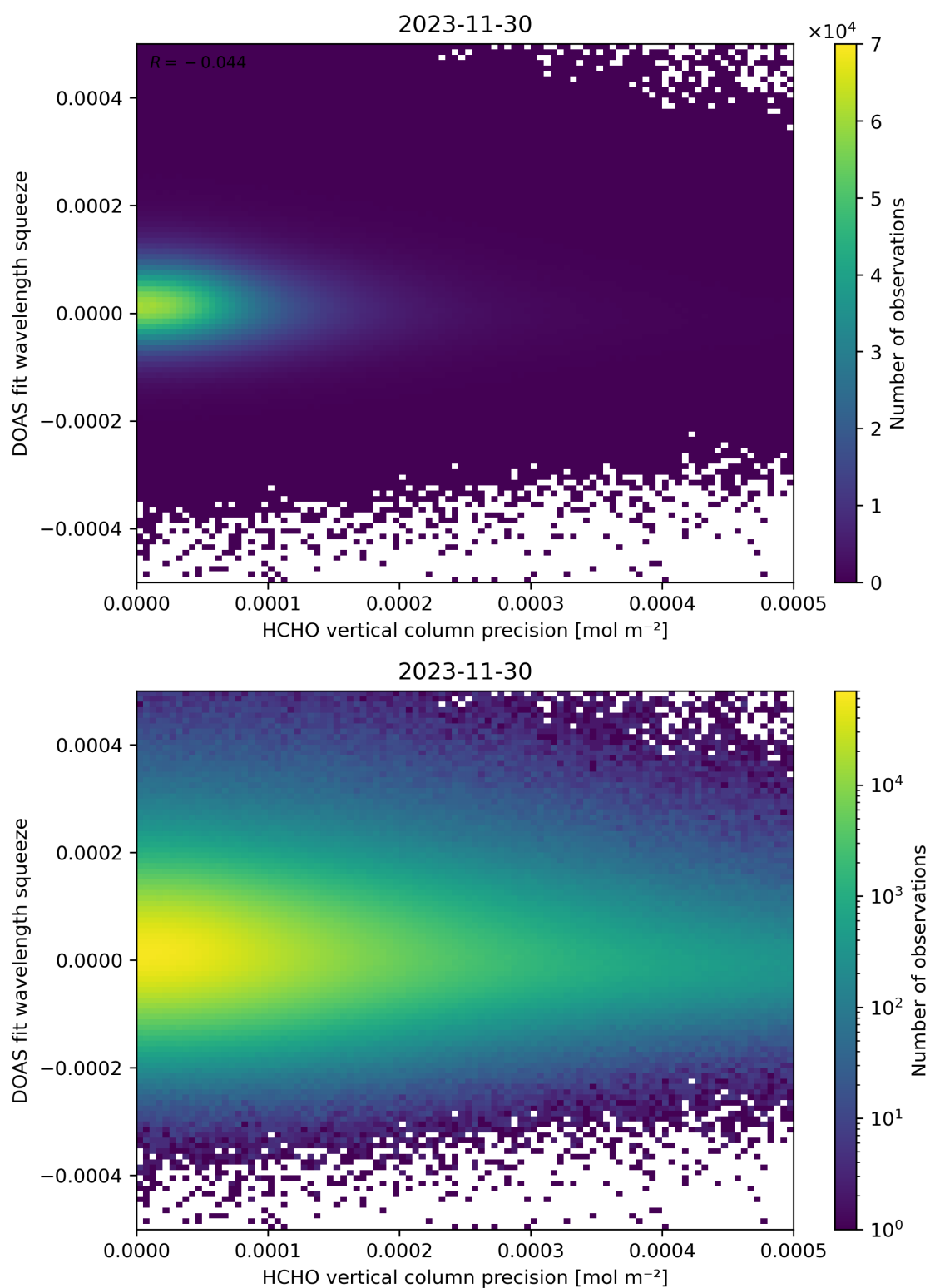
Figure 138: Scatter density plot of “HCHO vertical column precision” against “DOAS fit wavelength squeeze” for 2023-11-29 to 2023-12-01.
