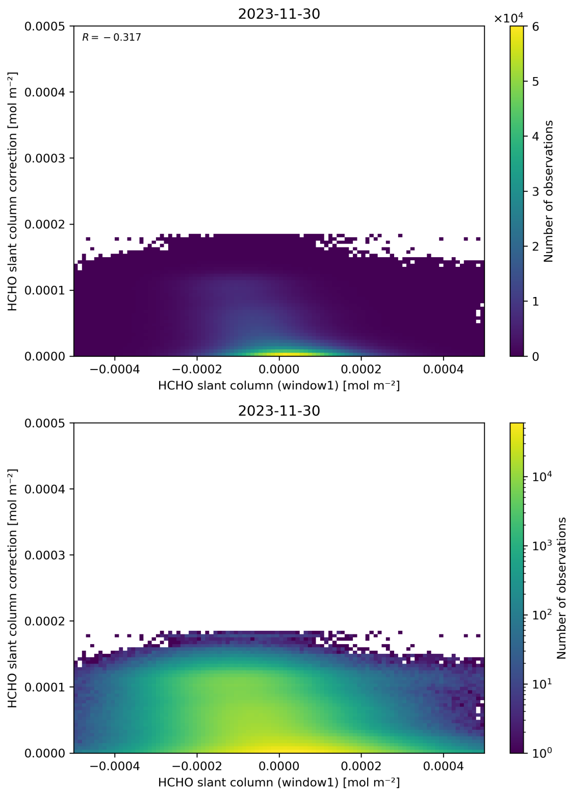
Figure 83: Scatter density plot of “HCHO slant column (window1)” against “HCHO slant column correction” for 2023-11-29 to 2023-12-01.
