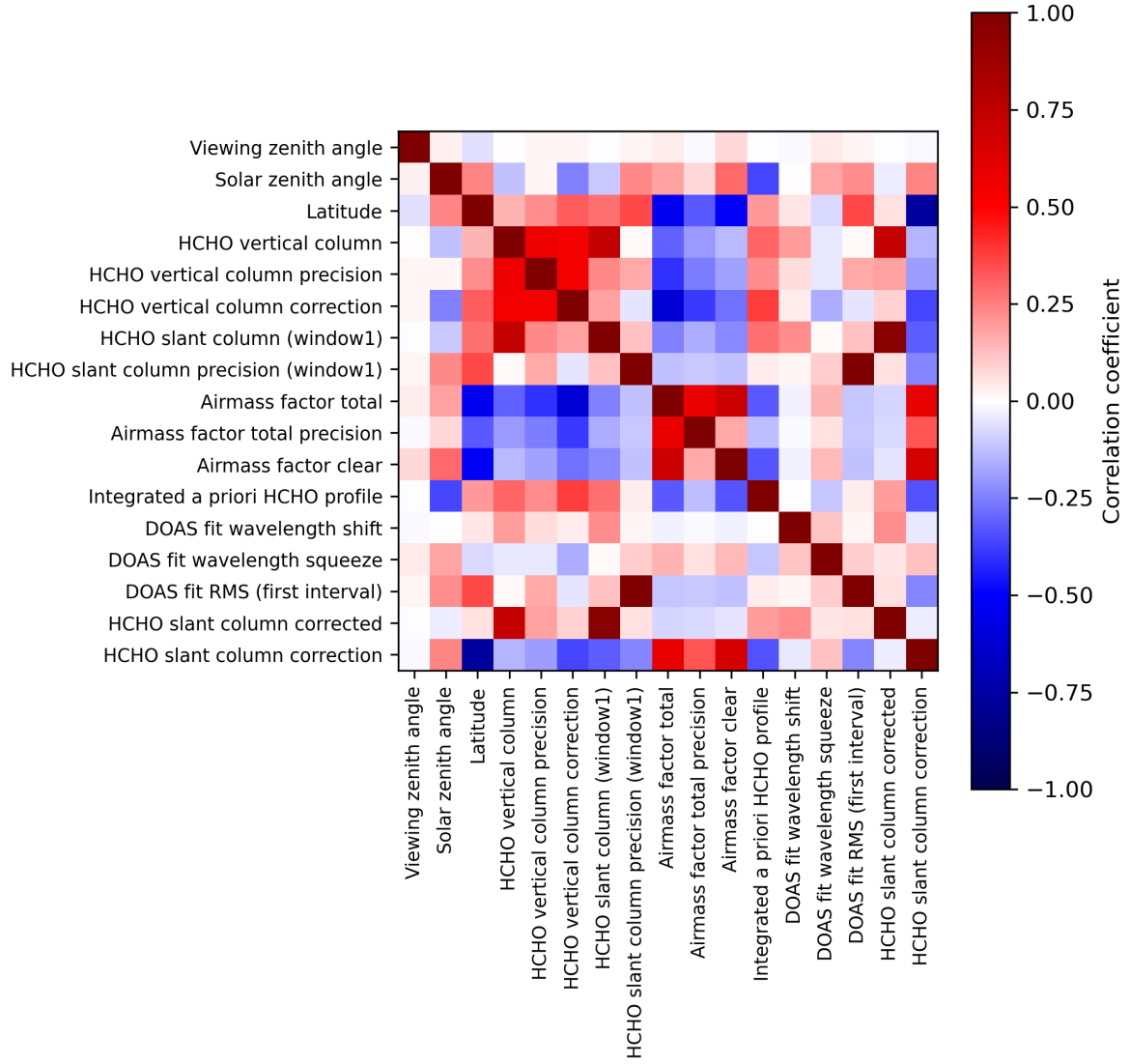
Figure 2: Map of correlation matrix for 2023-11-29 to 2023-12-01.
