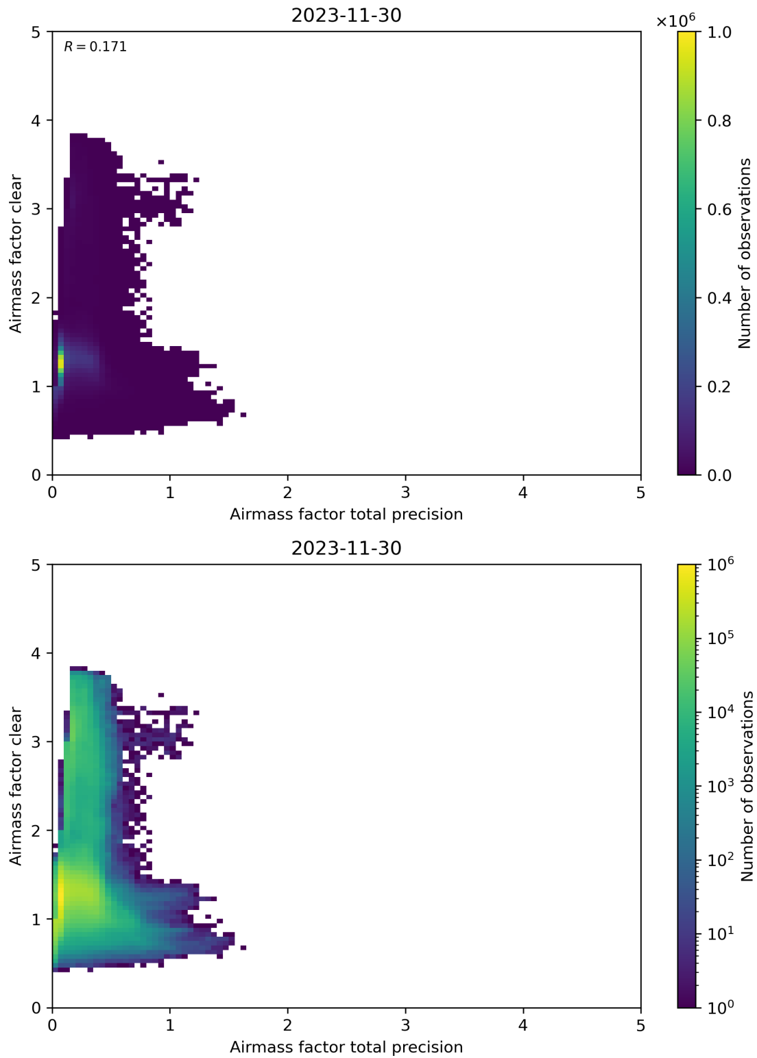
Figure 108: Scatter density plot of “Airmass factor total precision” against “Airmass factor clear” for 2023-11-29 to 2023-12-01.
