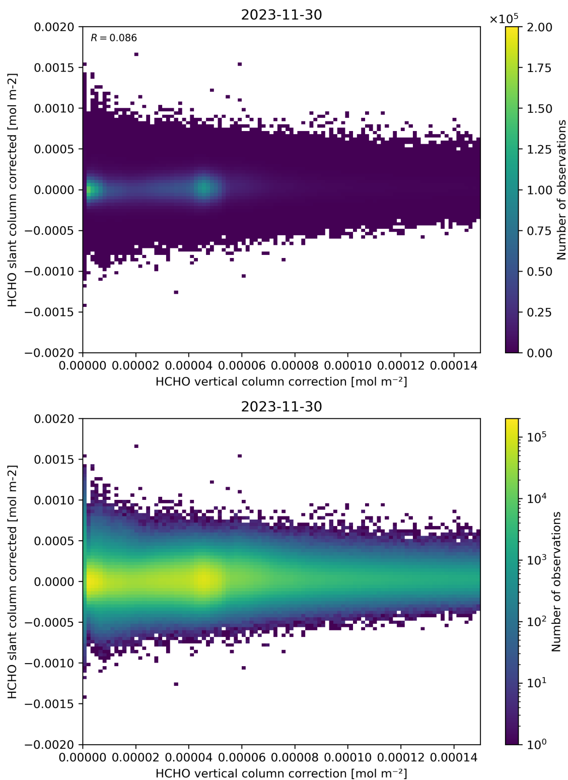
Figure 116: Scatter density plot of “HCHO vertical column correction” against “HCHO slant column corrected” for 2023-11-29 to 2023-12-01.
