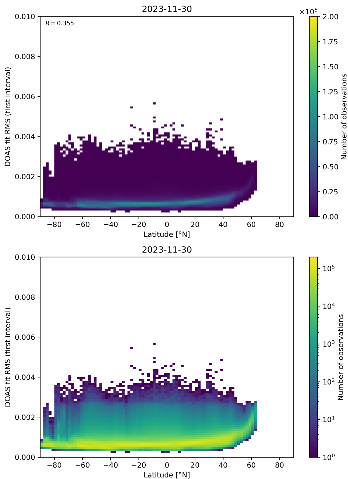
Figure 153: Scatter density plot of “Latitude” against “DOAS fit RMS (first interval)” for 2023-11-29 to 2023-12-01.
