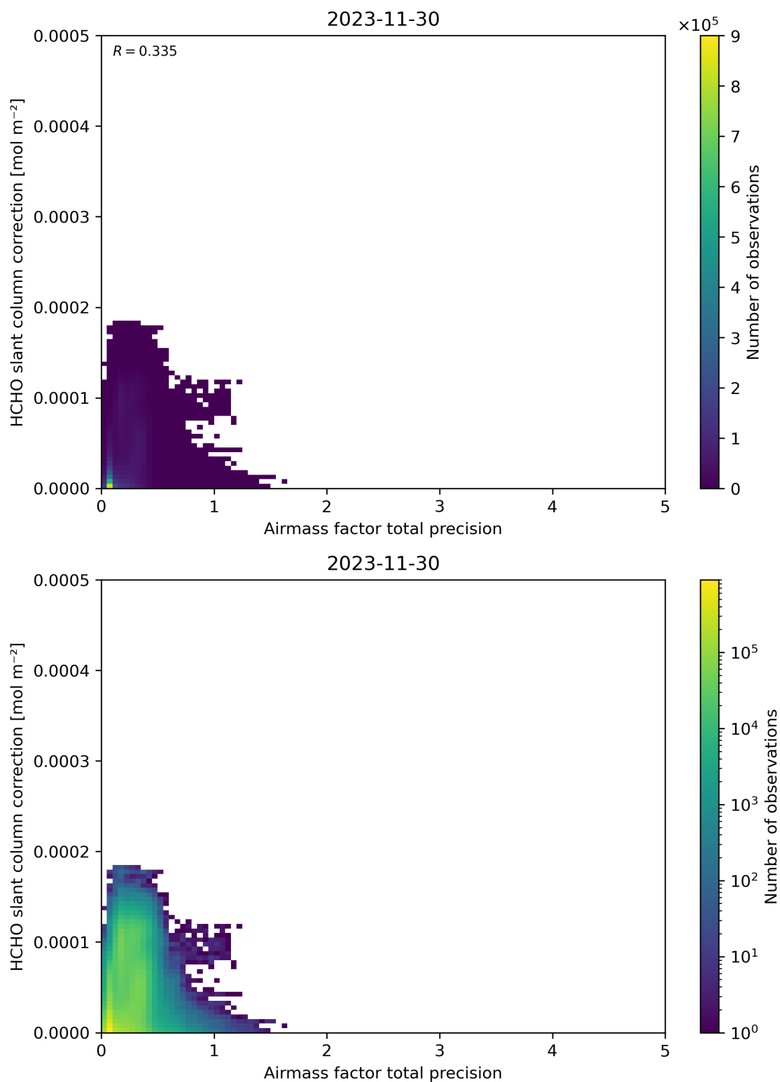
Figure 110: Scatter density plot of “Airmass factor total precision” against “HCHO slant column correction” for 2023-11-29 to 2023-12-01.
