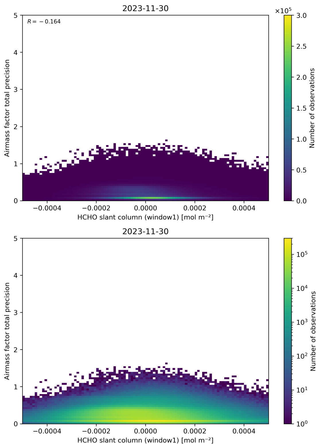
Figure 86: Scatter density plot of “HCHO slant column (window1)” against “Airmass factor total precision” for 2023-11-29 to 2023-12-01.
