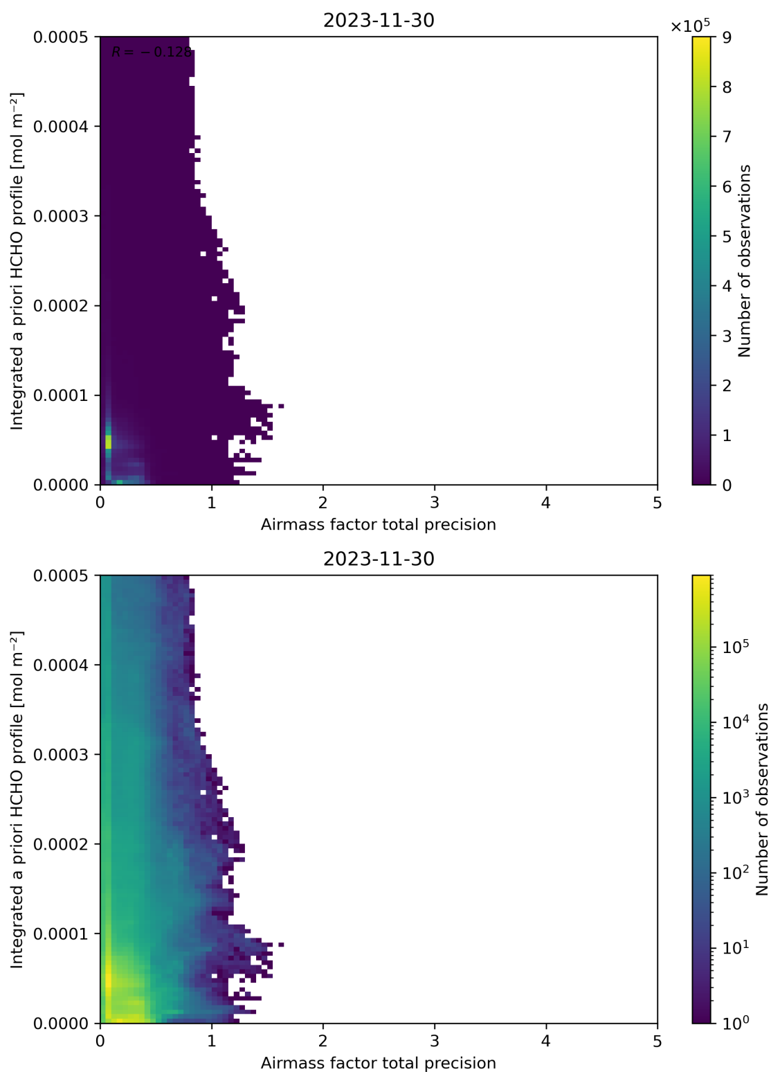
Figure 111: Scatter density plot of “Airmass factor total precision” against “Integrated a priori HCHO profile” for 2023-11-29 to 2023-12-01.
