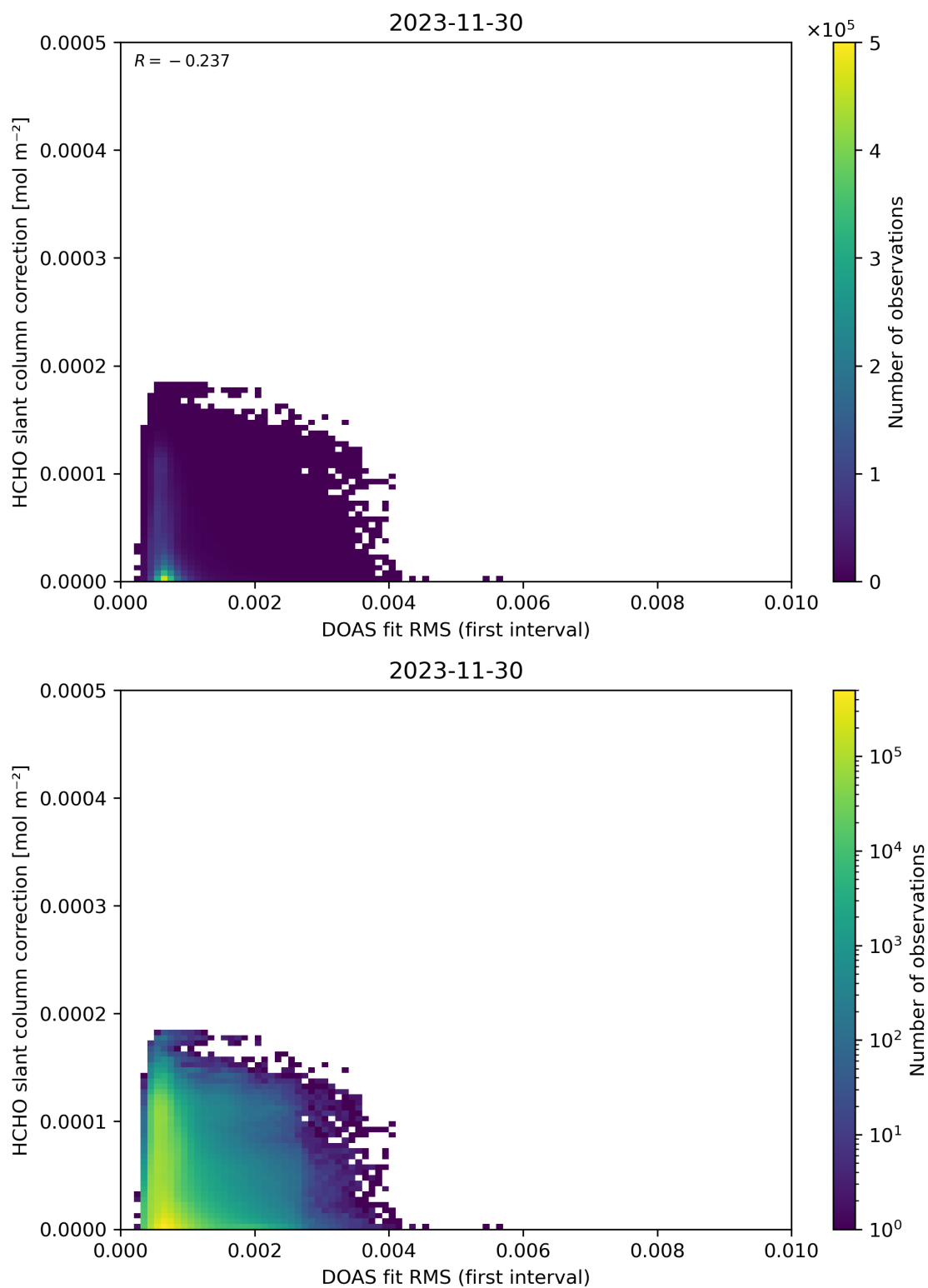
Figure 63: Scatter density plot of “DOAS fit RMS (first interval)” against “HCHO slant column correction” for 2023-11-29 to 2023-12-01.
