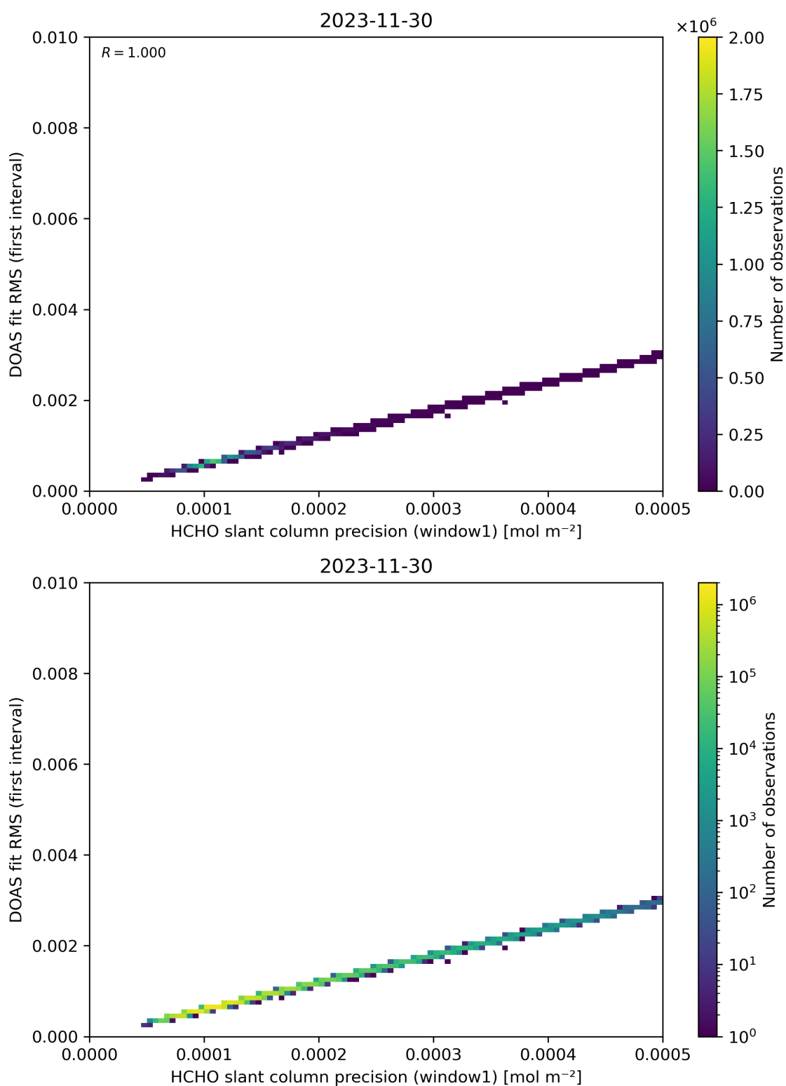
Figure 88: Scatter density plot of “HCHO slant column precision (window1)” against “DOAS fit RMS (first interval)” for 2023-11-29 to 2023-12-01.
