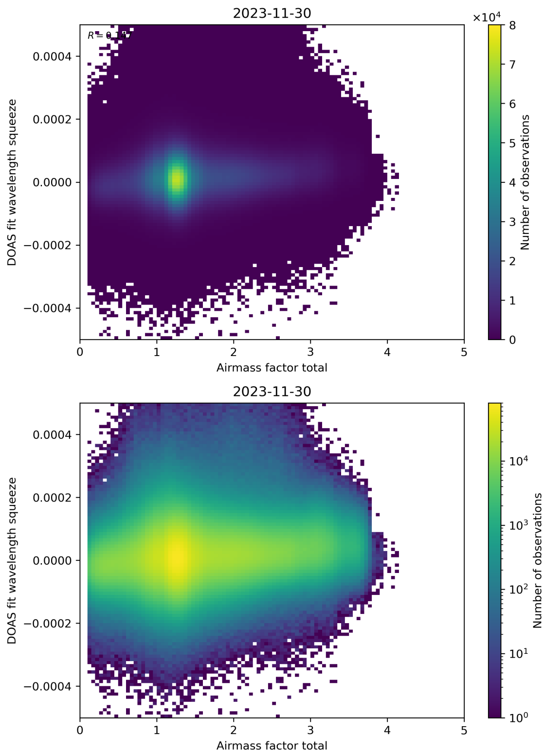
Figure 99: Scatter density plot of “Airmass factor total” against “DOAS fit wavelength squeeze” for 2023-11-29 to 2023-12-01.
