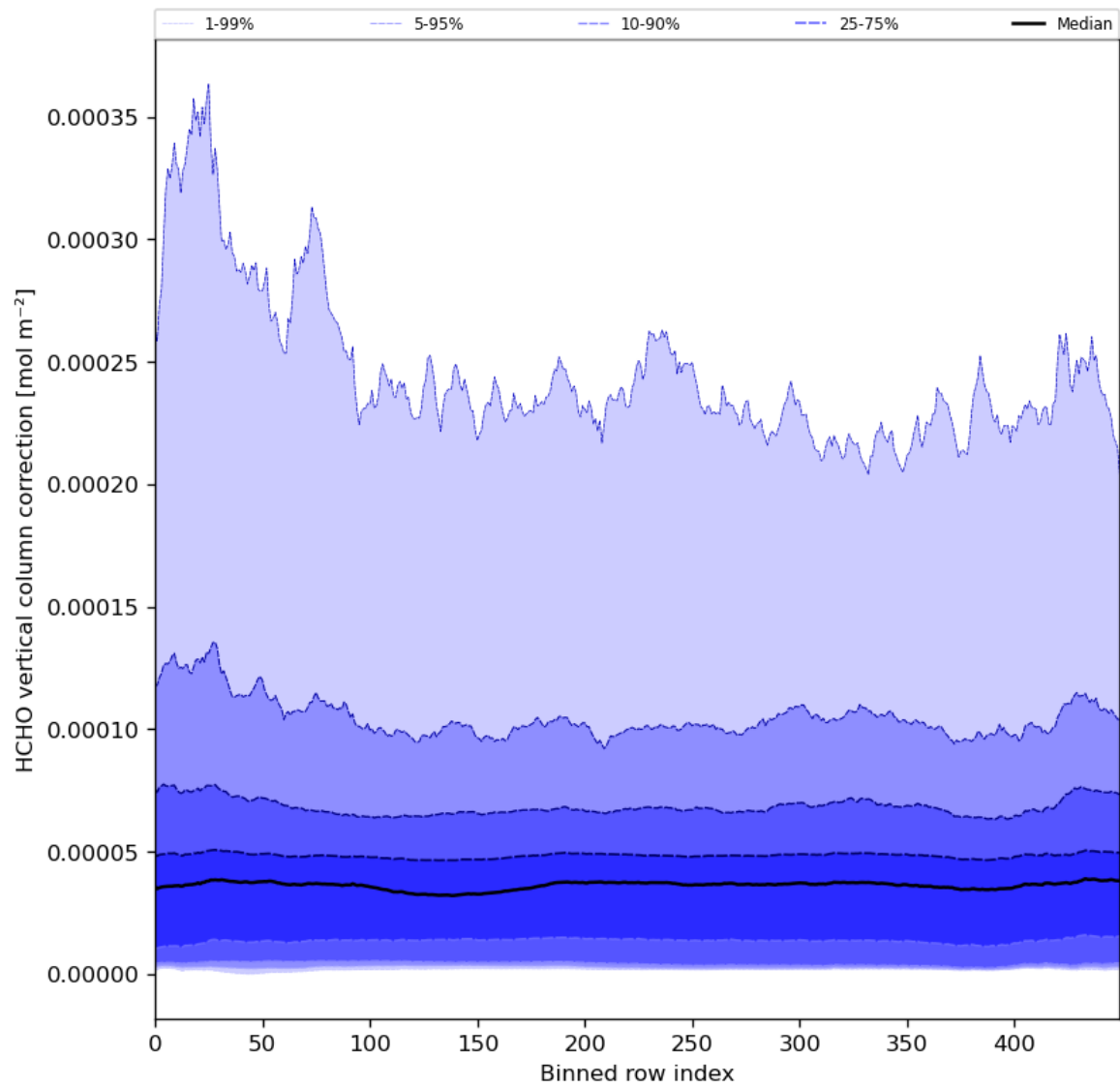
Figure 51: Along track statistics of “HCHO vertical column correction” for 2023-11-29 to 2023-12-01
