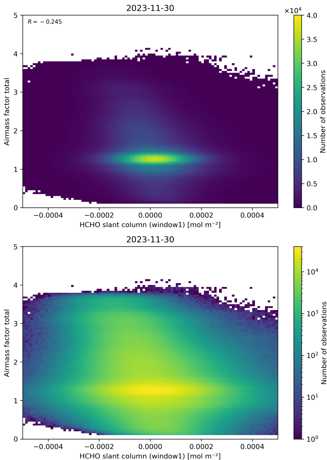
Figure 85: Scatter density plot of “HCHO slant column (window1)” against “Airmass factor total” for 2023-11-29 to 2023-12-01.
