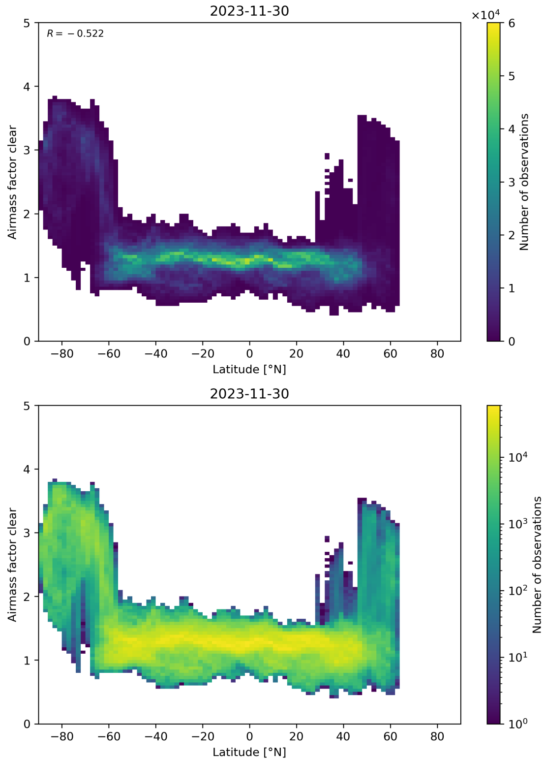
Figure 156: Scatter density plot of “Latitude” against “Airmass factor clear” for 2023-11-29 to 2023-12-01.
