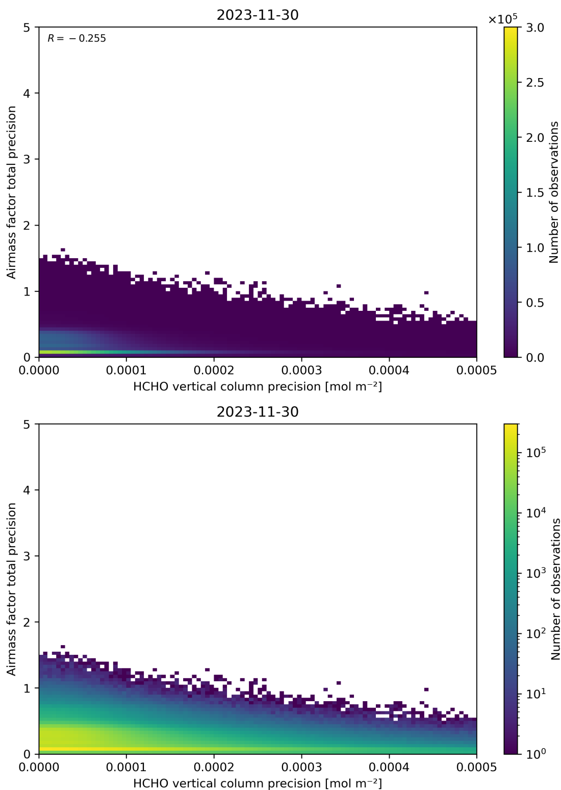
Figure 145: Scatter density plot of “HCHO vertical column precision” against “Airmass factor total precision” for 2023-11-29 to 2023-12-01.
