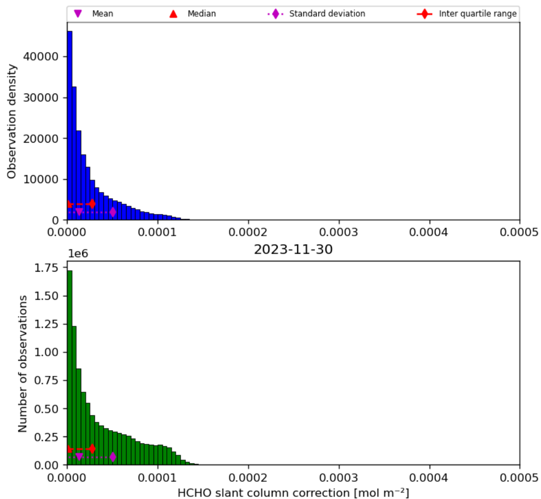
Figure 47: Histogram of “HCHO slant column correction” for 2023-11-29 to 2023-12-01
