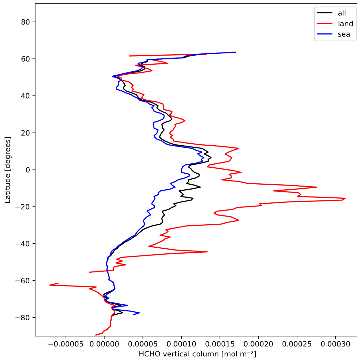
Figure 21: Zonal average of “HCHO vertical column” for 2023-11-29 to 2023-12-01.
