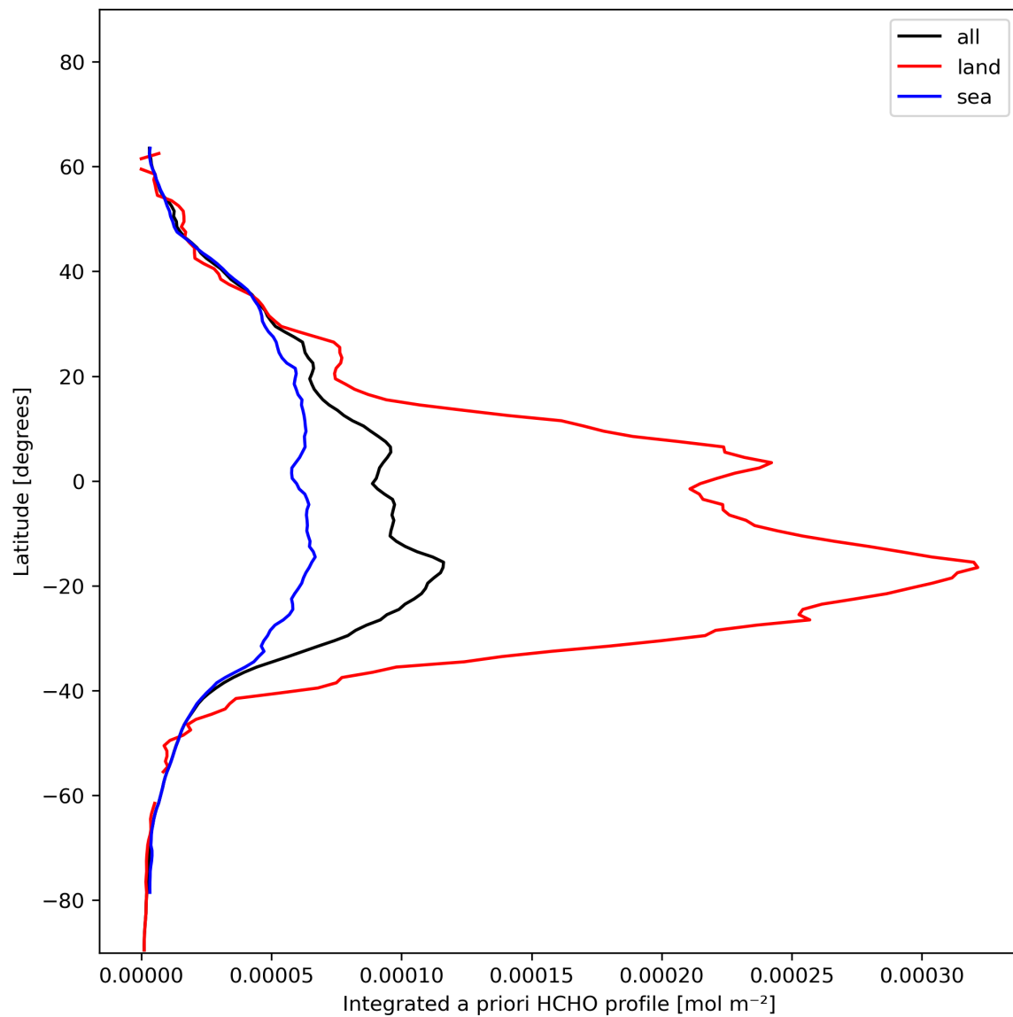
Figure 29: Zonal average of “Integrated a priori HCHO profile” for 2023-11-29 to 2023-12-01.
