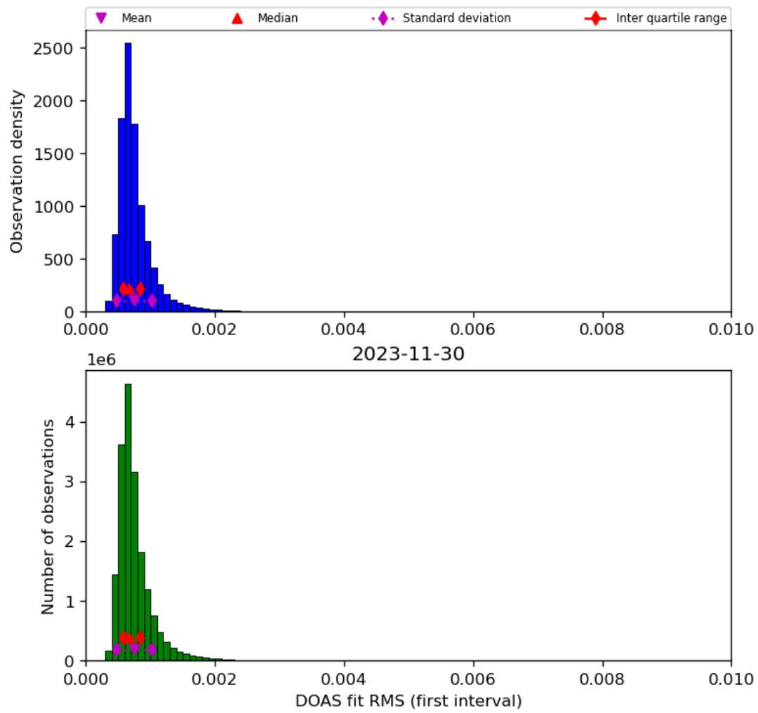
Figure 46: Histogram of “DOAS fit RMS (first interval)” for 2023-11-29 to 2023-12-01
