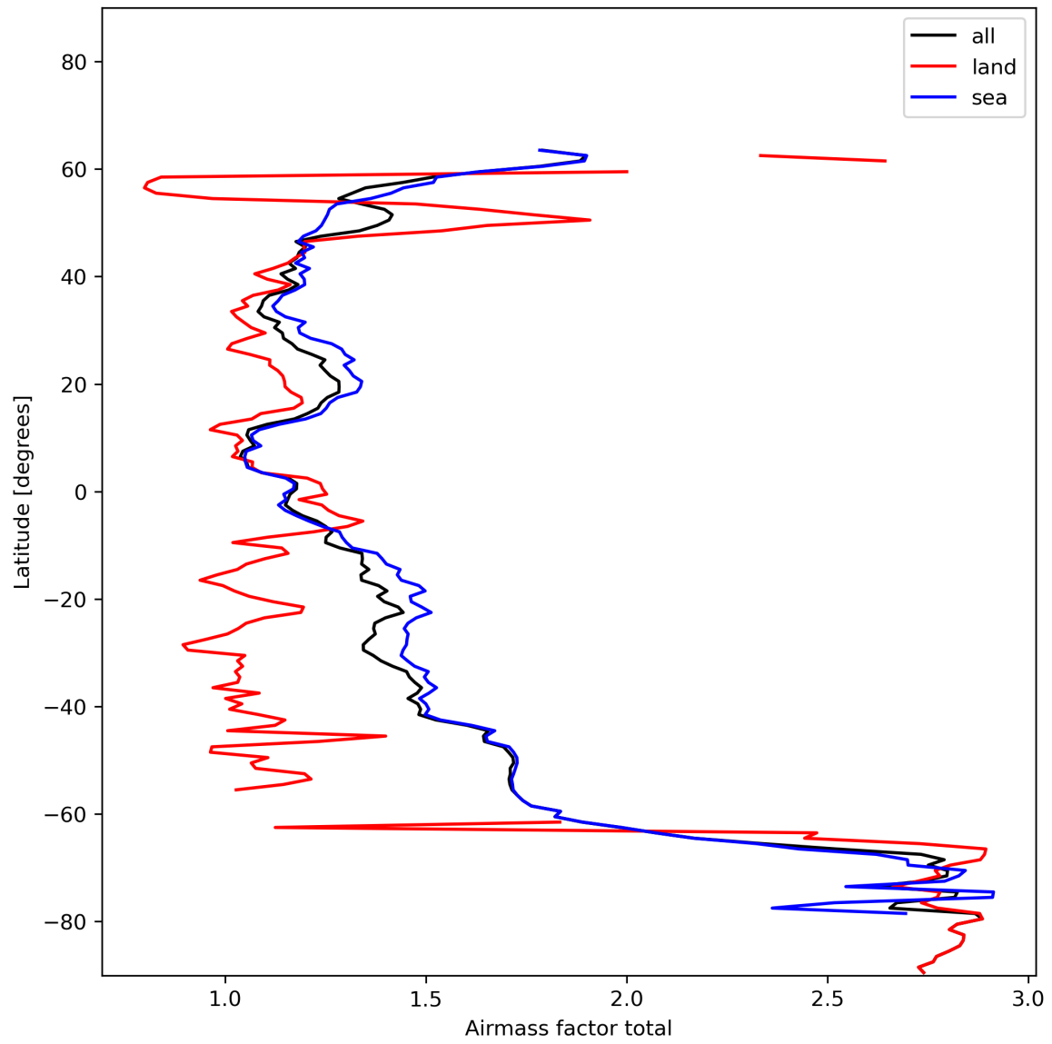
Figure 26: Zonal average of “Airmass factor total” for 2023-11-29 to 2023-12-01.
