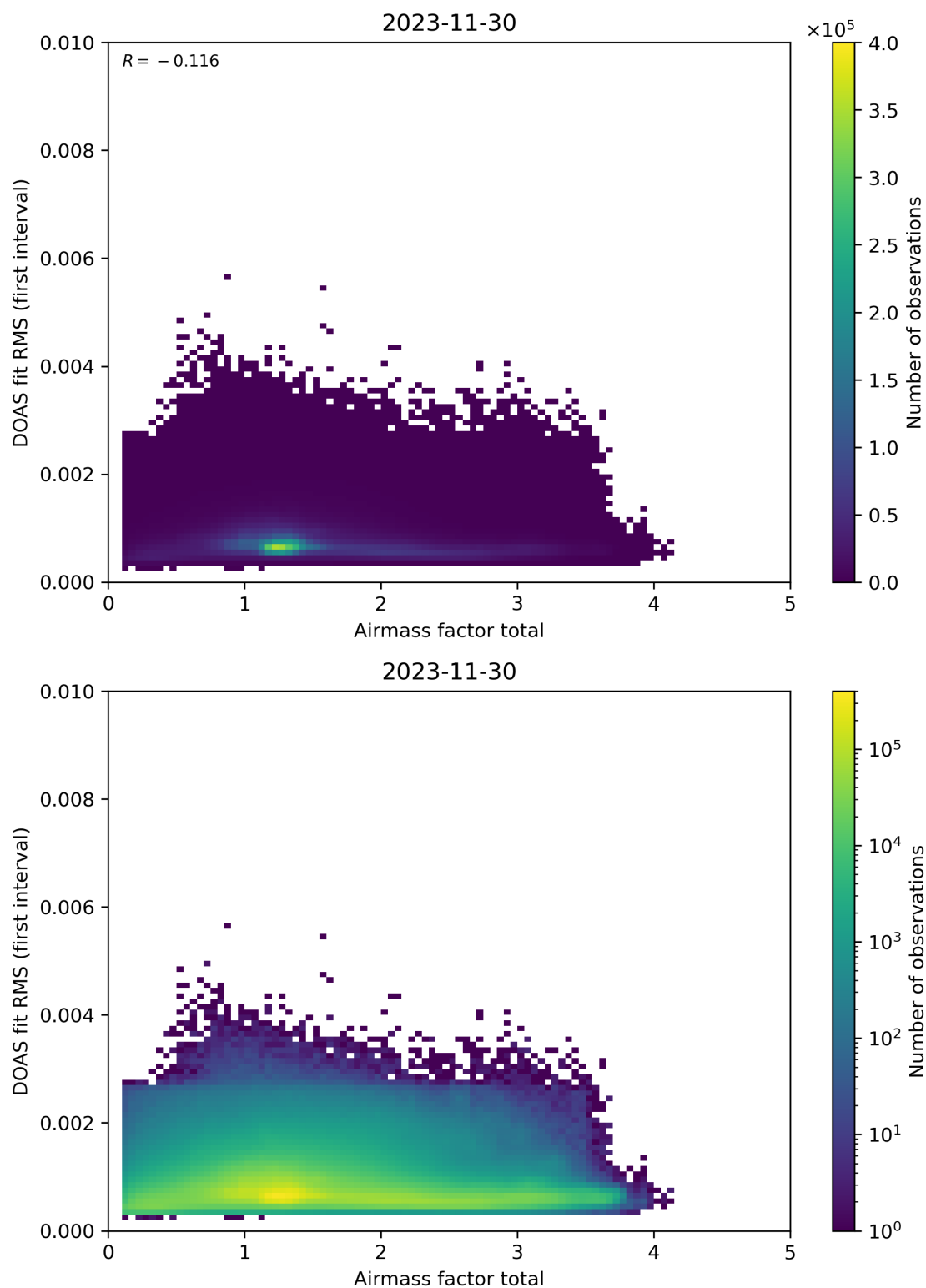
Figure 97: Scatter density plot of “Airmass factor total” against “DOAS fit RMS (first interval)” for 2023-11-29 to 2023-12-01.
