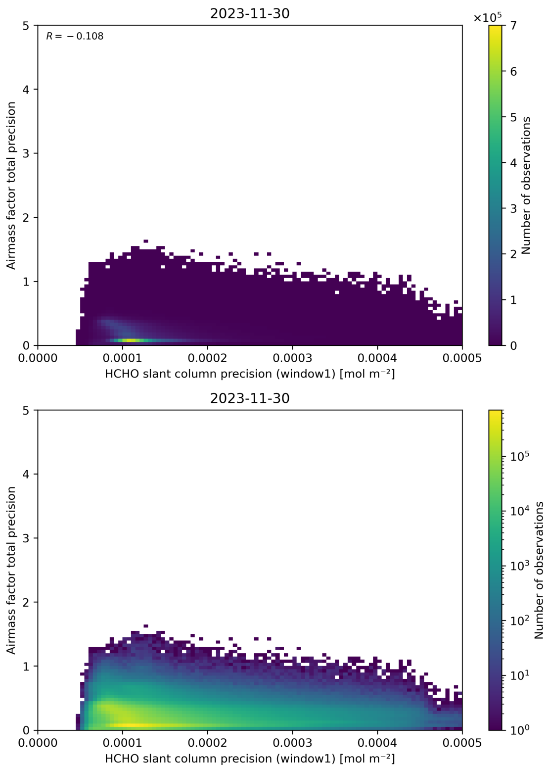
Figure 95: Scatter density plot of “HCHO slant column precision (window1)” against “Airmass factor total precision” for 2023-11-29 to 2023-12-01.
