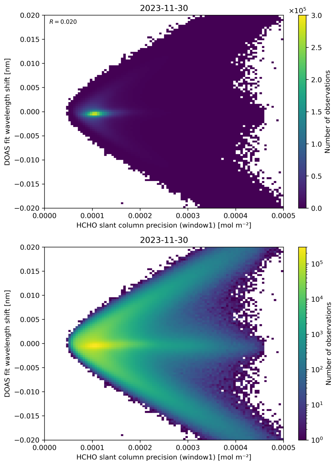
Figure 89: Scatter density plot of “HCHO slant column precision (window1)” against “DOAS fit wavelength shift” for 2023-11-29 to 2023-12-01.
