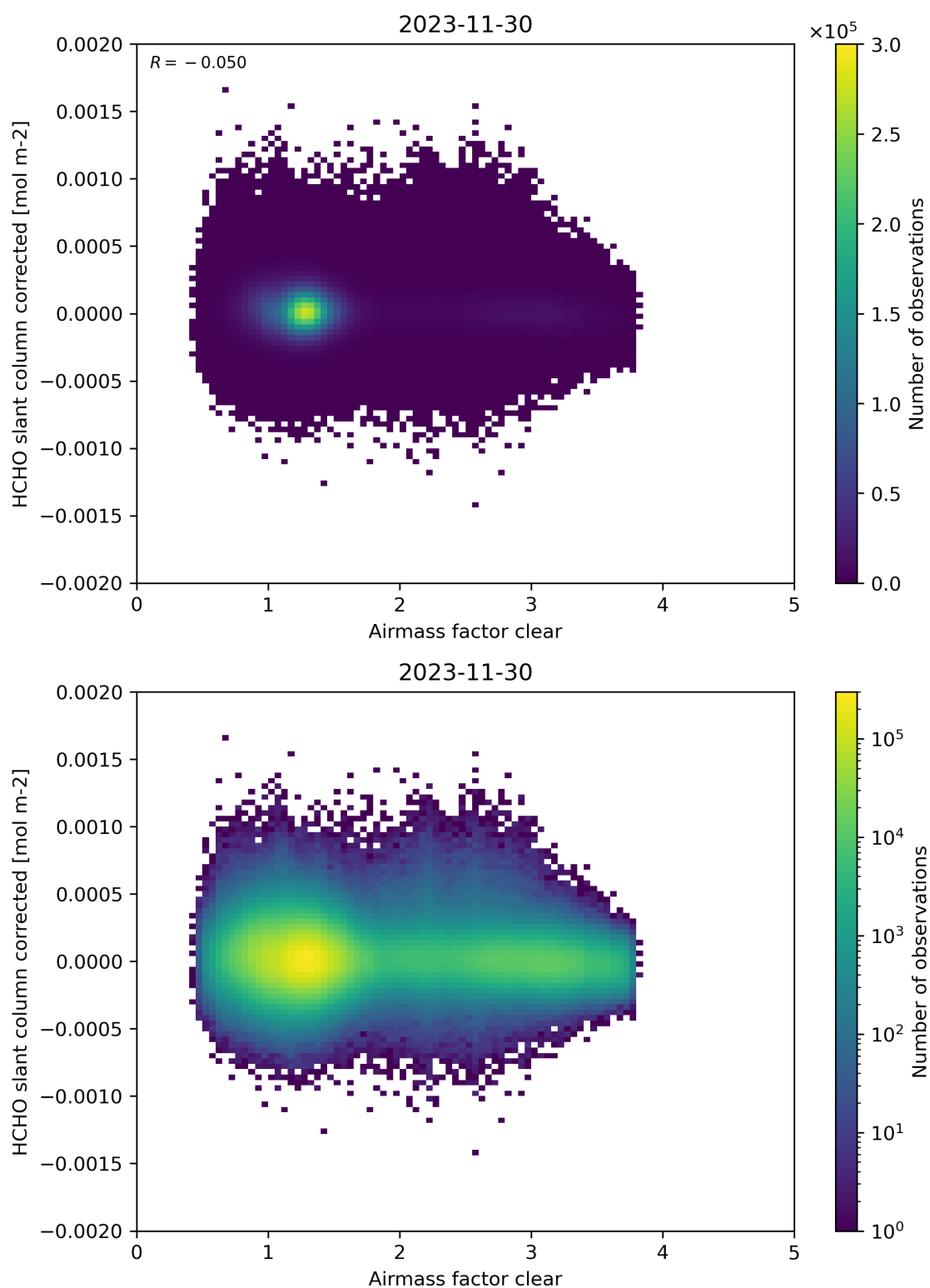
Figure 74: Scatter density plot of “Airmass factor clear” against “HCHO slant column corrected” for 2023-11-29 to 2023-12-01.
