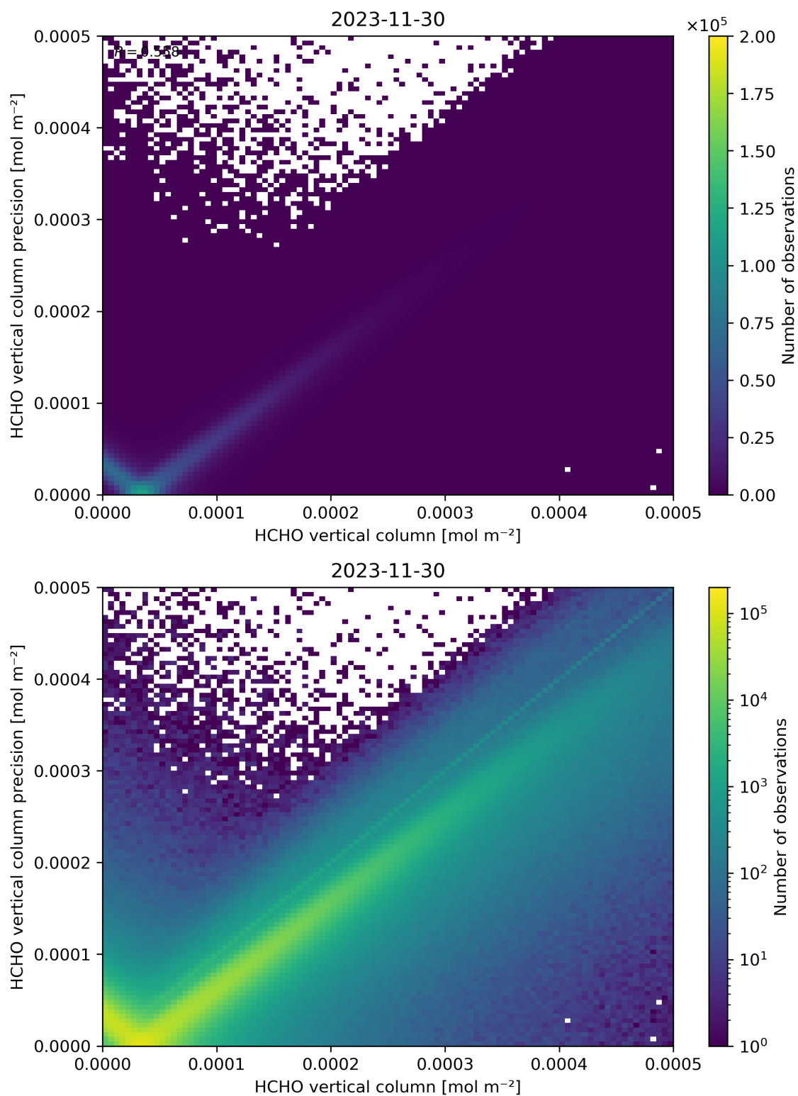
Figure 134: Scatter density plot of “HCHO vertical column” against “HCHO vertical column precision” for 2023-11-29 to 2023-12-01.
