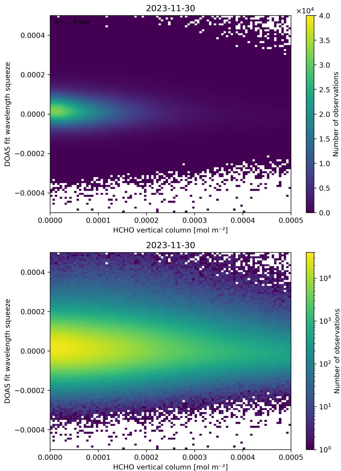
Figure 125: Scatter density plot of “HCHO vertical column” against “DOAS fit wavelength squeeze” for 2023-11-29 to 2023-12-01.
