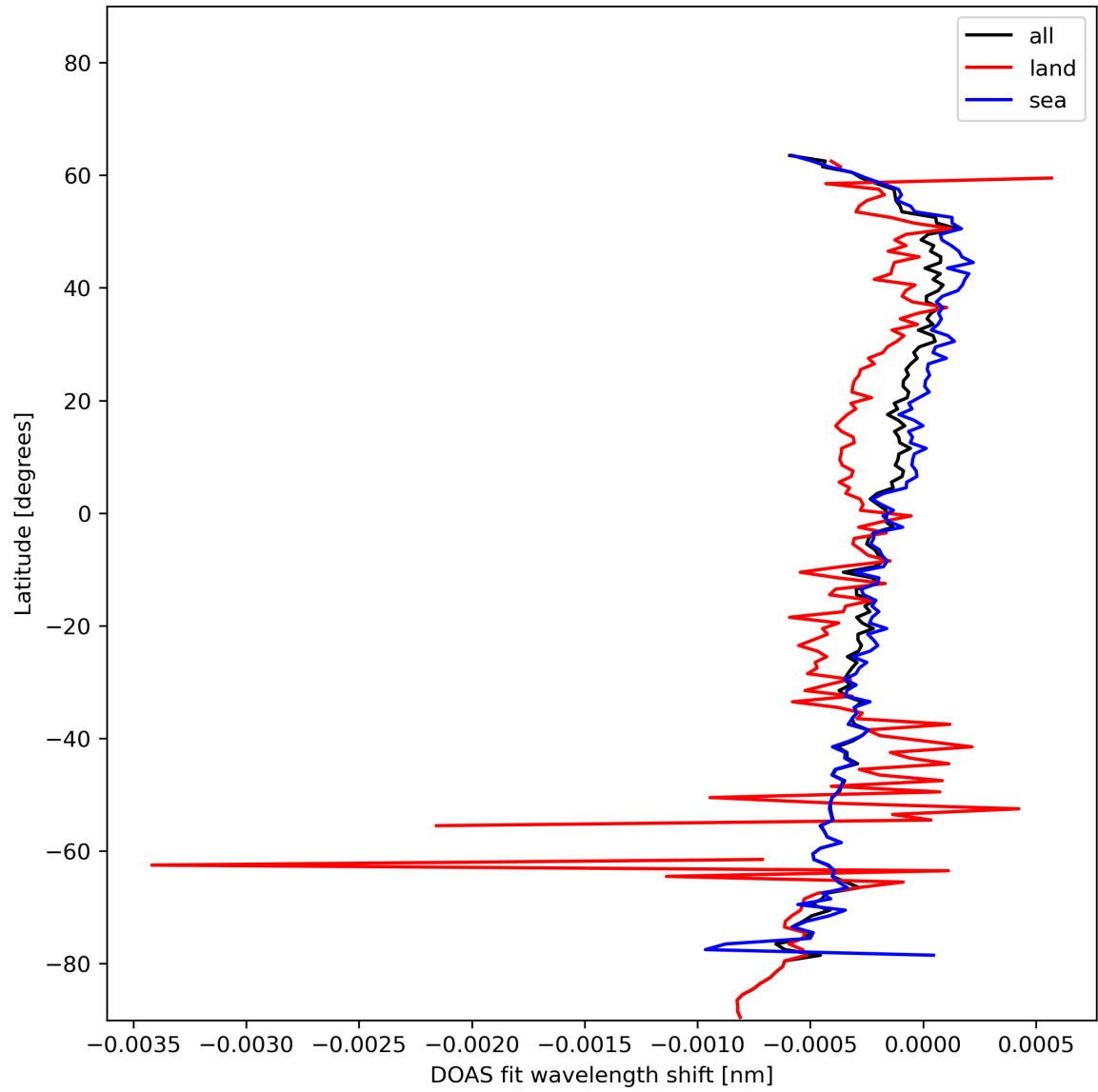
Figure 30: Zonal average of “DOAS fit wavelength shift” for 2023-11-29 to 2023-12-01.
