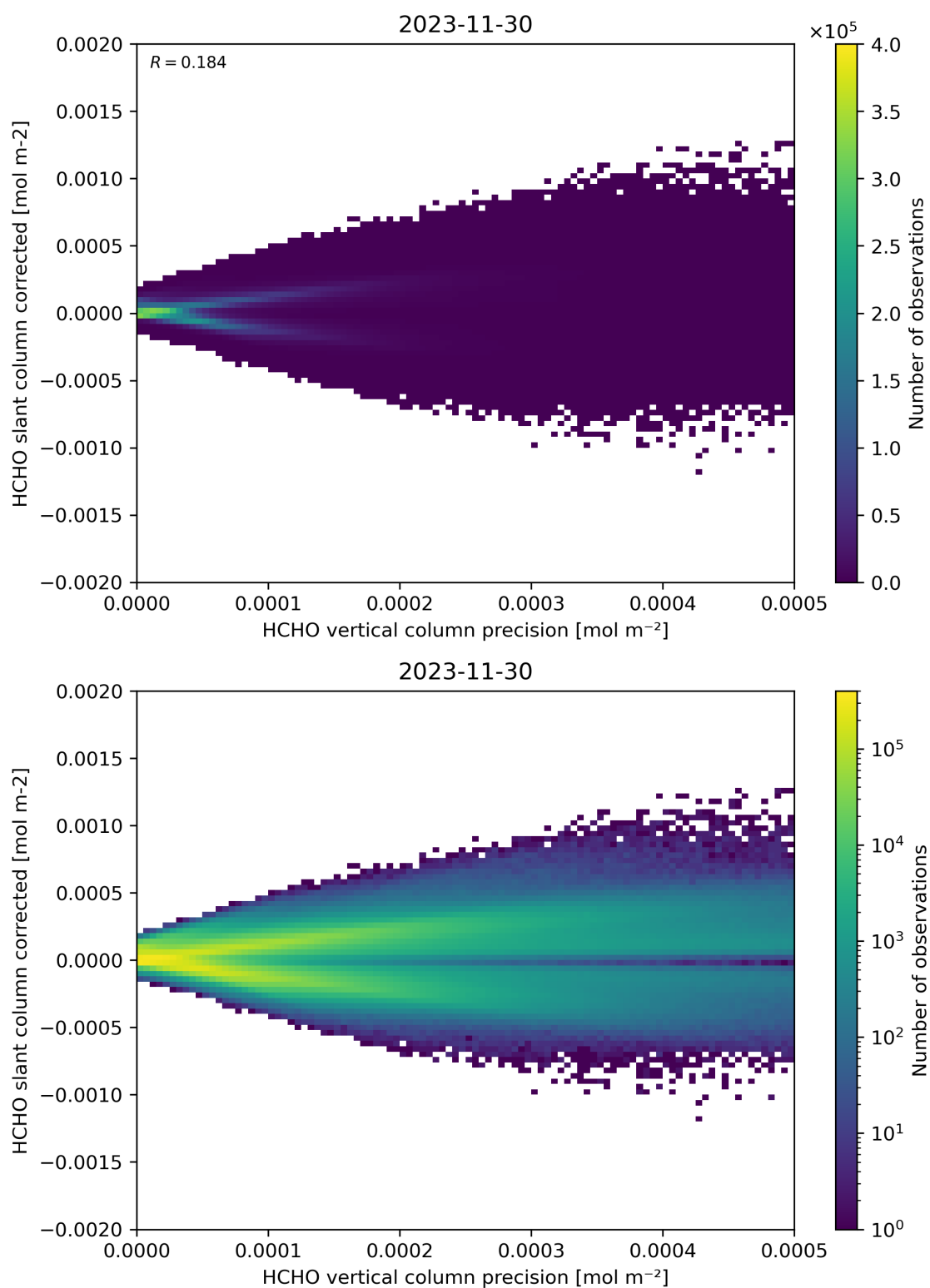
Figure 140: Scatter density plot of “HCHO vertical column precision” against “HCHO slant column corrected” for 2023-11-29 to 2023-12-01.
