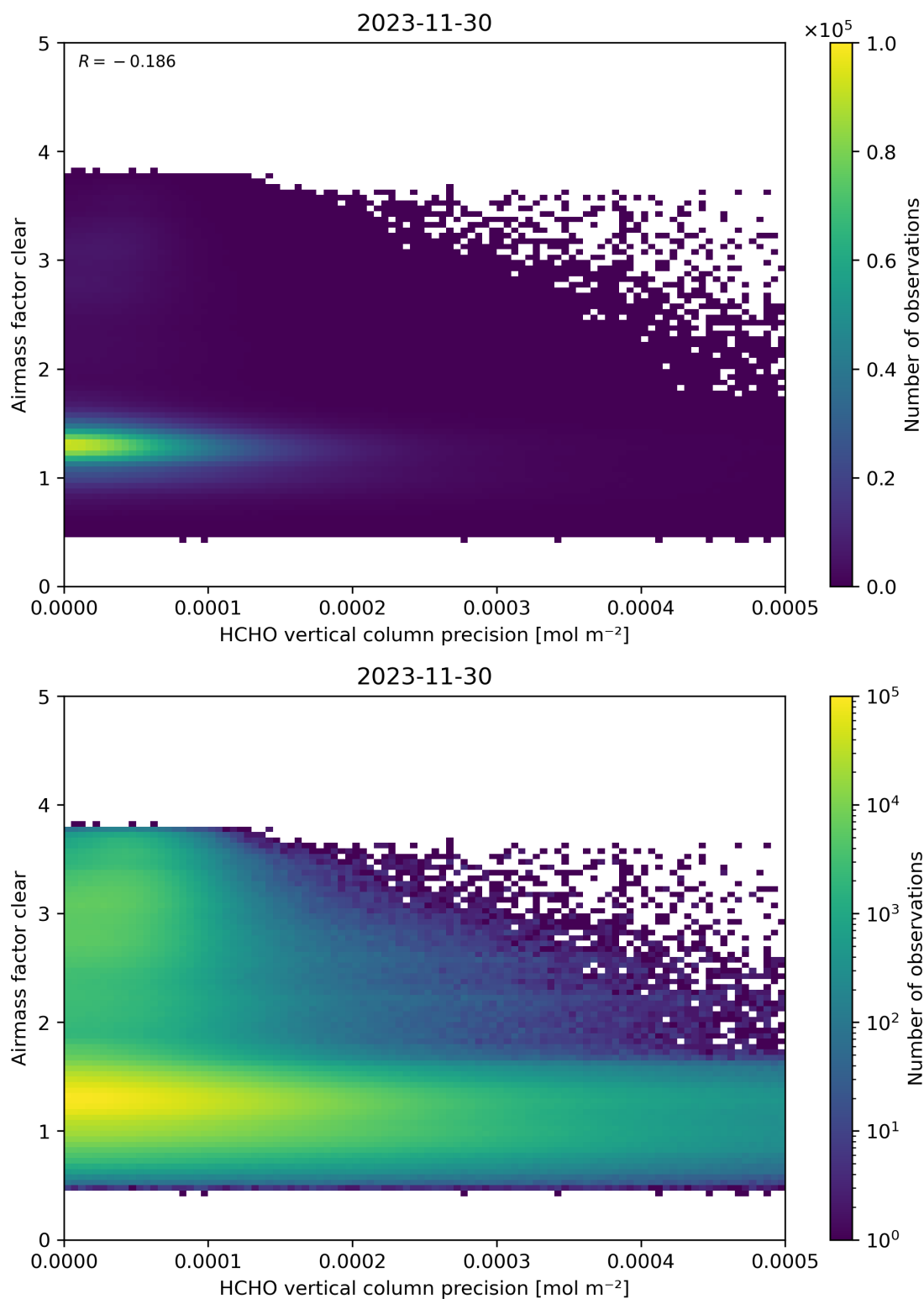
Figure 139: Scatter density plot of “HCHO vertical column precision” against “Airmass factor clear” for 2023-11-29 to 2023-12-01.
