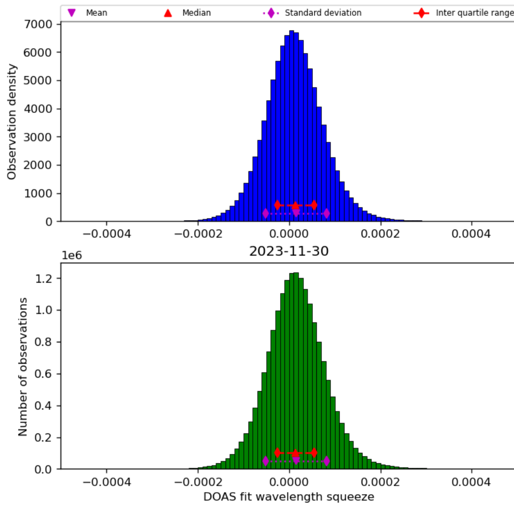
Figure 45: Histogram of “DOAS fit wavelength squeeze” for 2023-11-29 to 2023-12-01
