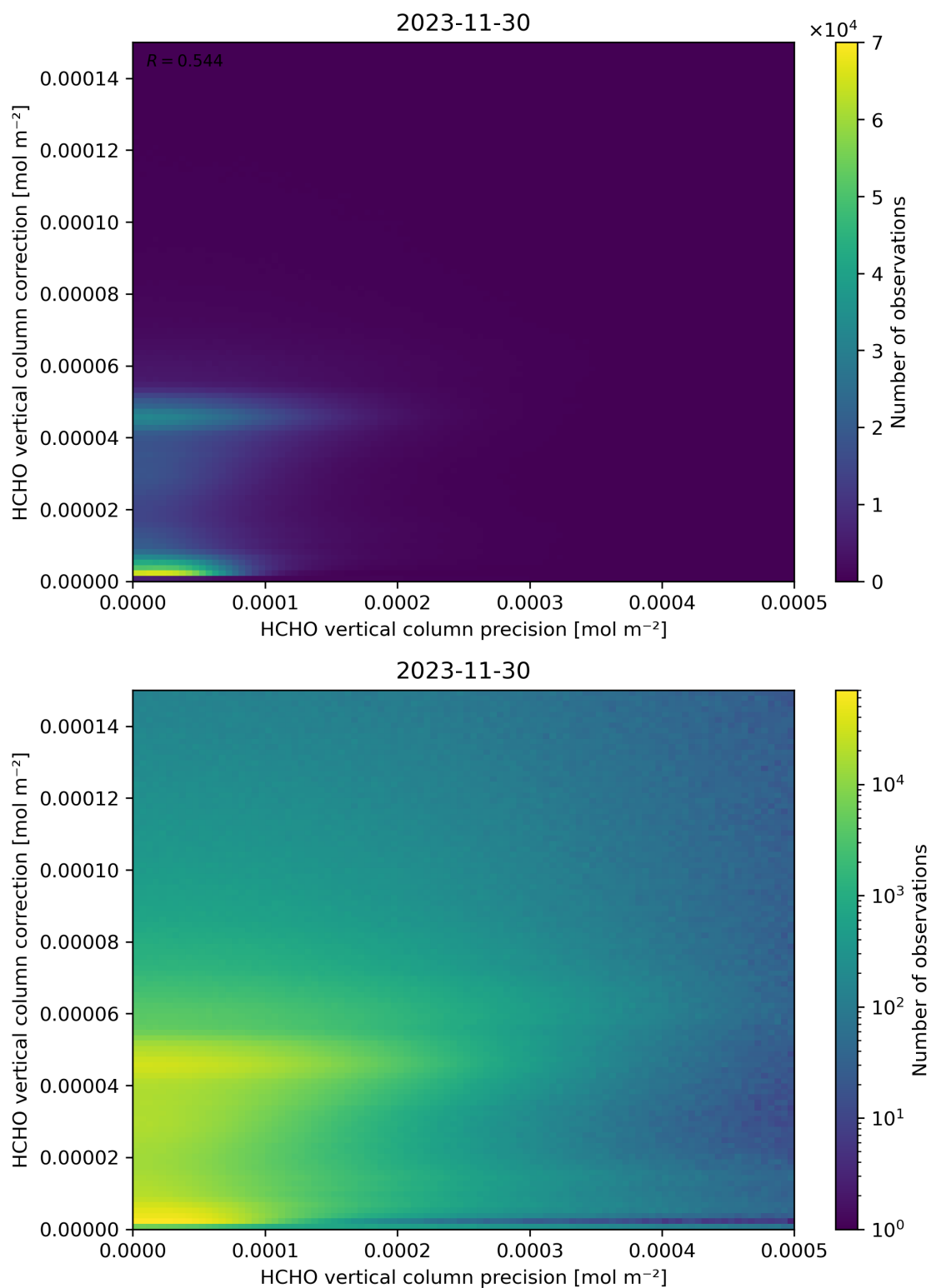
Figure 146: Scatter density plot of “HCHO vertical column precision” against “HCHO vertical column correction” for 2023-11-29 to 2023-12-01.
