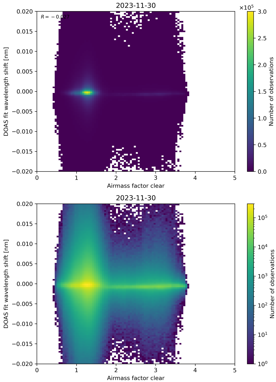
Figure 72: Scatter density plot of “Airmass factor clear” against “DOAS fit wavelength shift” for 2023-11-29 to 2023-12-01.
