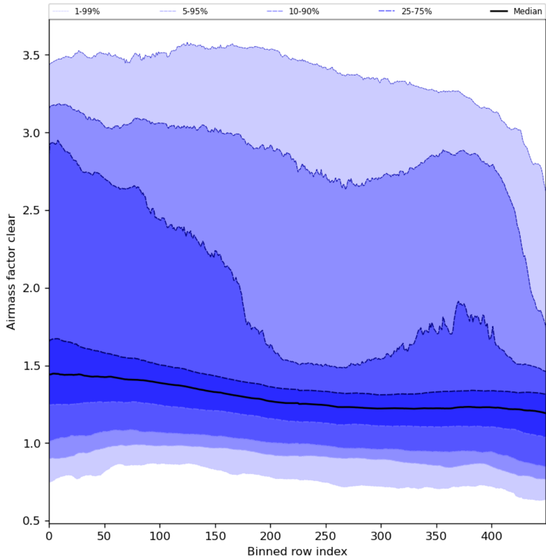
Figure 56: Along track statistics of “Airmass factor clear” for 2023-11-29 to 2023-12-01
