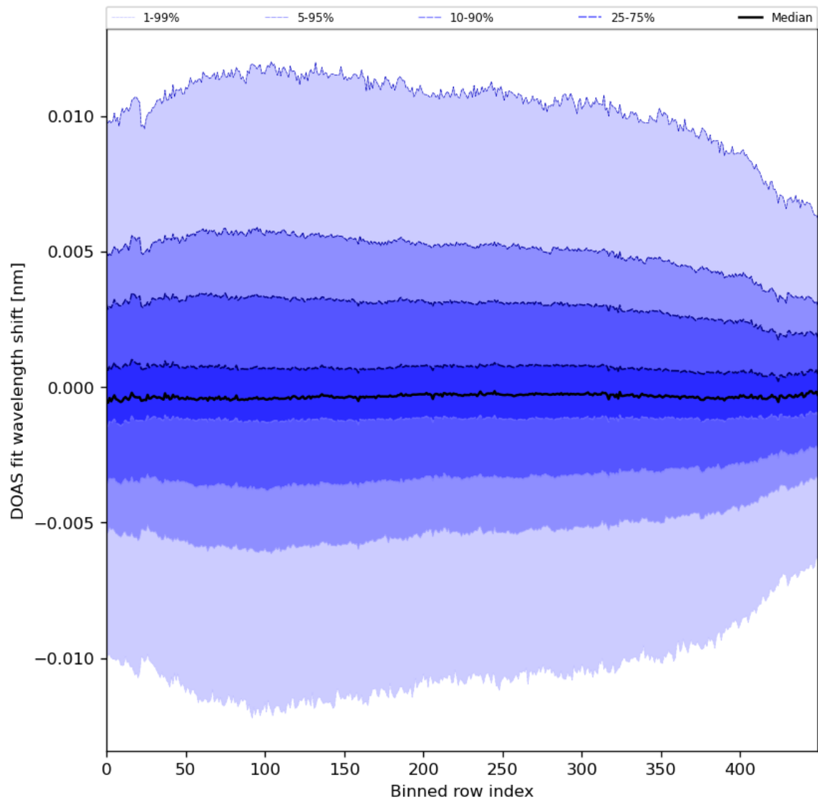
Figure 58: Along track statistics of “DOAS fit wavelength shift” for 2023-11-29 to 2023-12-01
