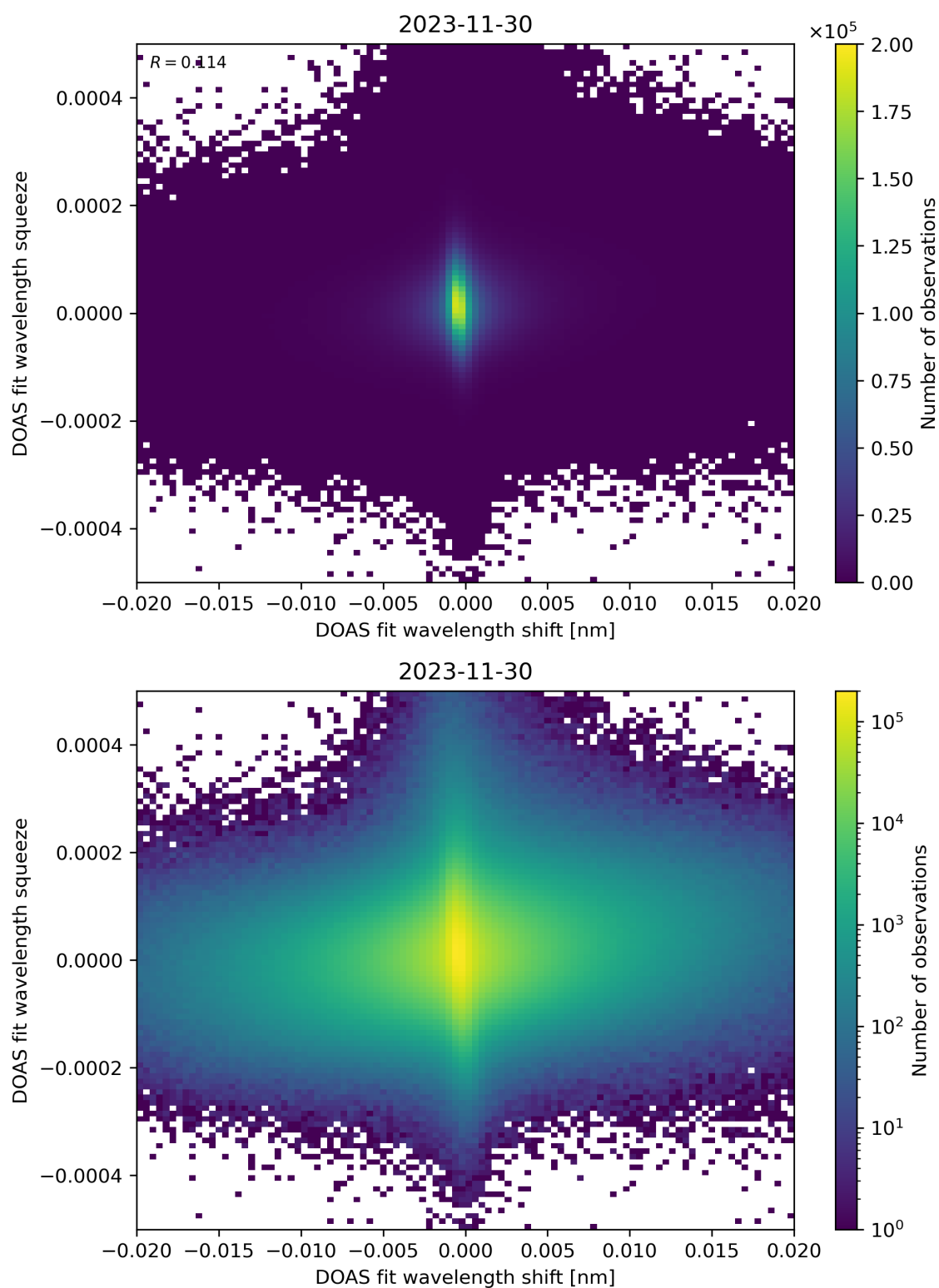
Figure 65: Scatter density plot of “DOAS fit wavelength shift” against “DOAS fit wavelength squeeze” for 2023-11-29 to 2023-12-01.
