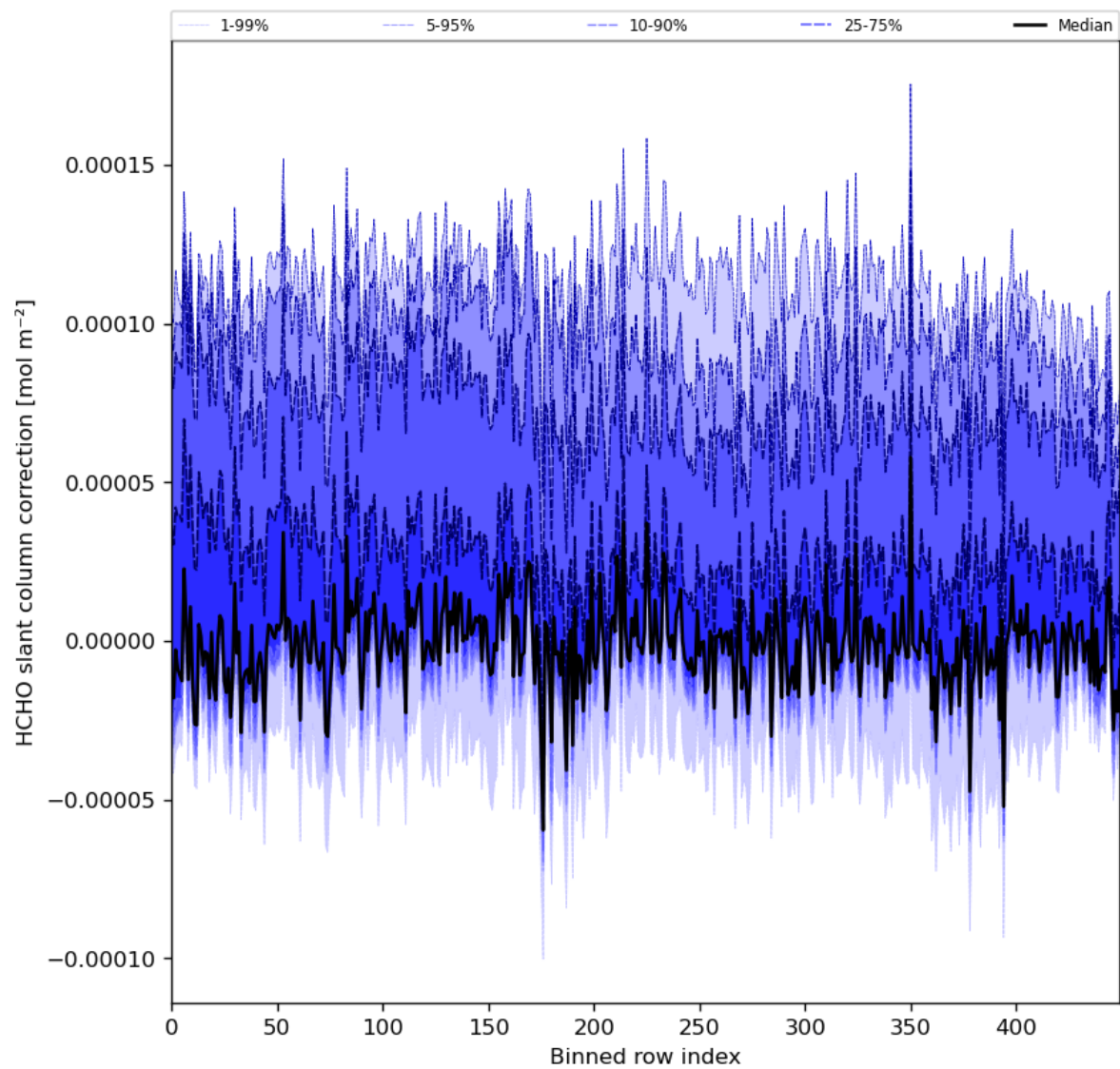
Figure 61: Along track statistics of “HCHO slant column correction” for 2023-11-29 to 2023-12-01
