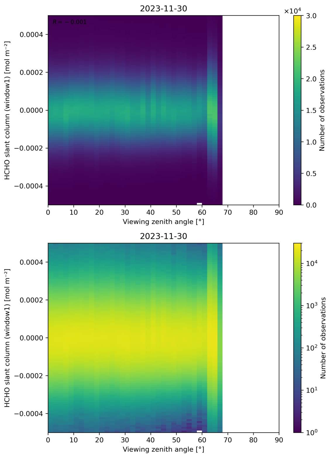
Figure 188: Scatter density plot of “Viewing zenith angle” against “HCHO slant column (window1)” for 2023-11-29 to 2023-12-01.
