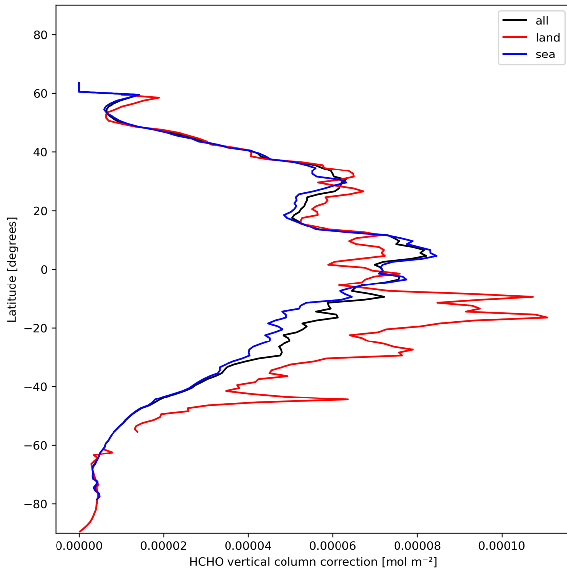
Figure 23: Zonal average of “HCHO vertical column correction” for 2023-11-29 to 2023-12-01.
