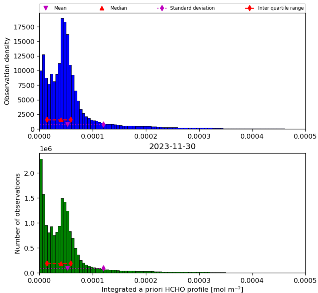
Figure 43: Histogram of “Integrated a priori HCHO profile” for 2023-11-29 to 2023-12-01
