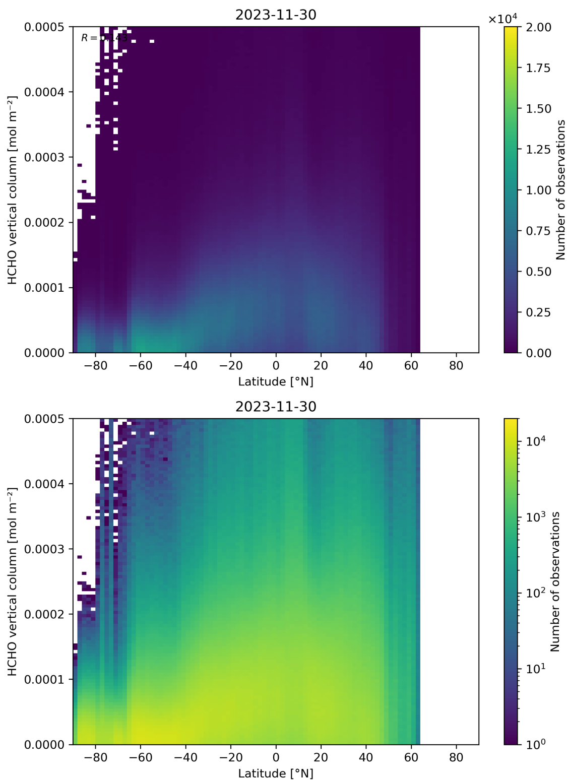
Figure 163: Scatter density plot of “Latitude” against “HCHO vertical column” for 2023-11-29 to 2023-12-01.
