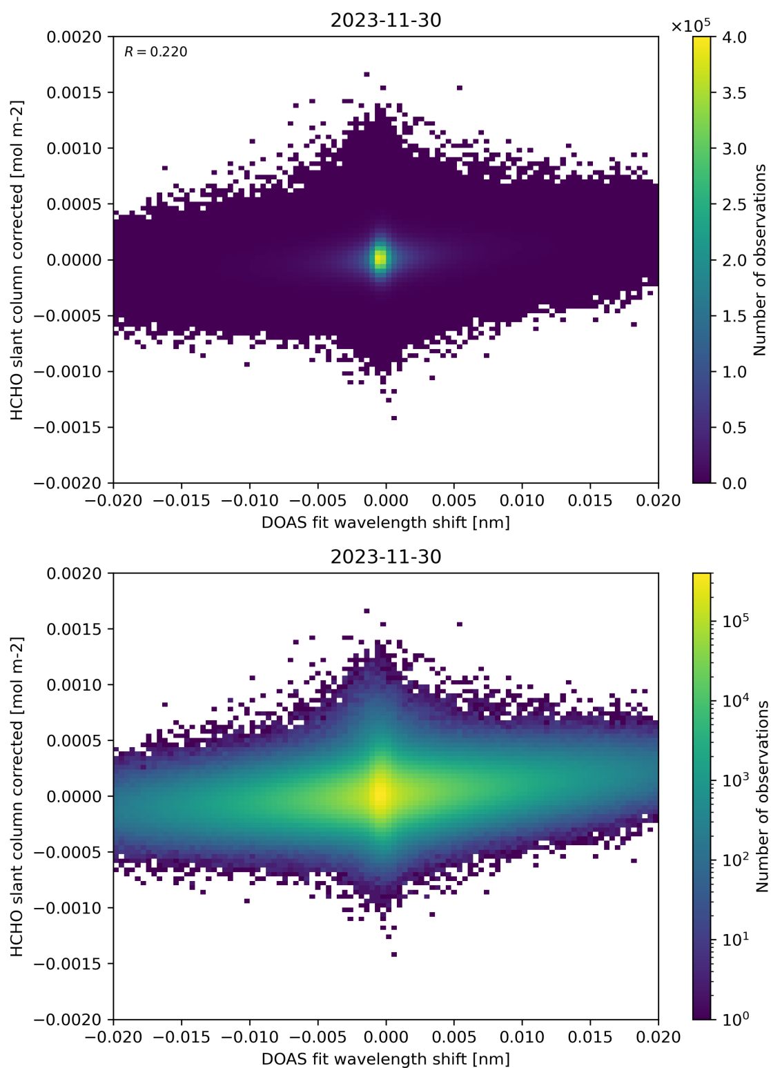
Figure 66: Scatter density plot of “DOAS fit wavelength shift” against “HCHO slant column corrected” for 2023-11-29 to 2023-12-01.
