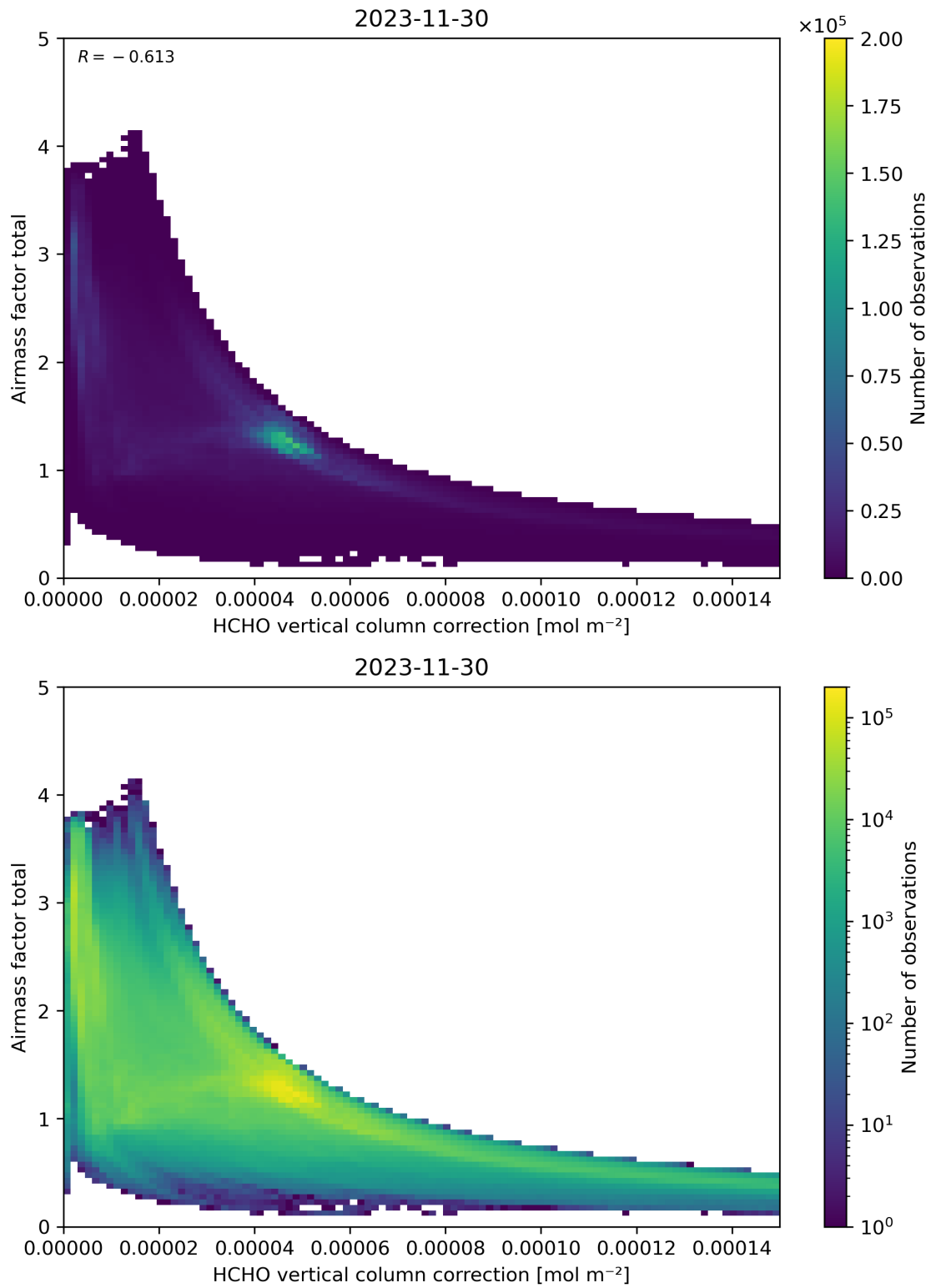
Figure 120: Scatter density plot of “HCHO vertical column correction” against “Airmass factor total” for 2023-11-29 to 2023-12-01.
