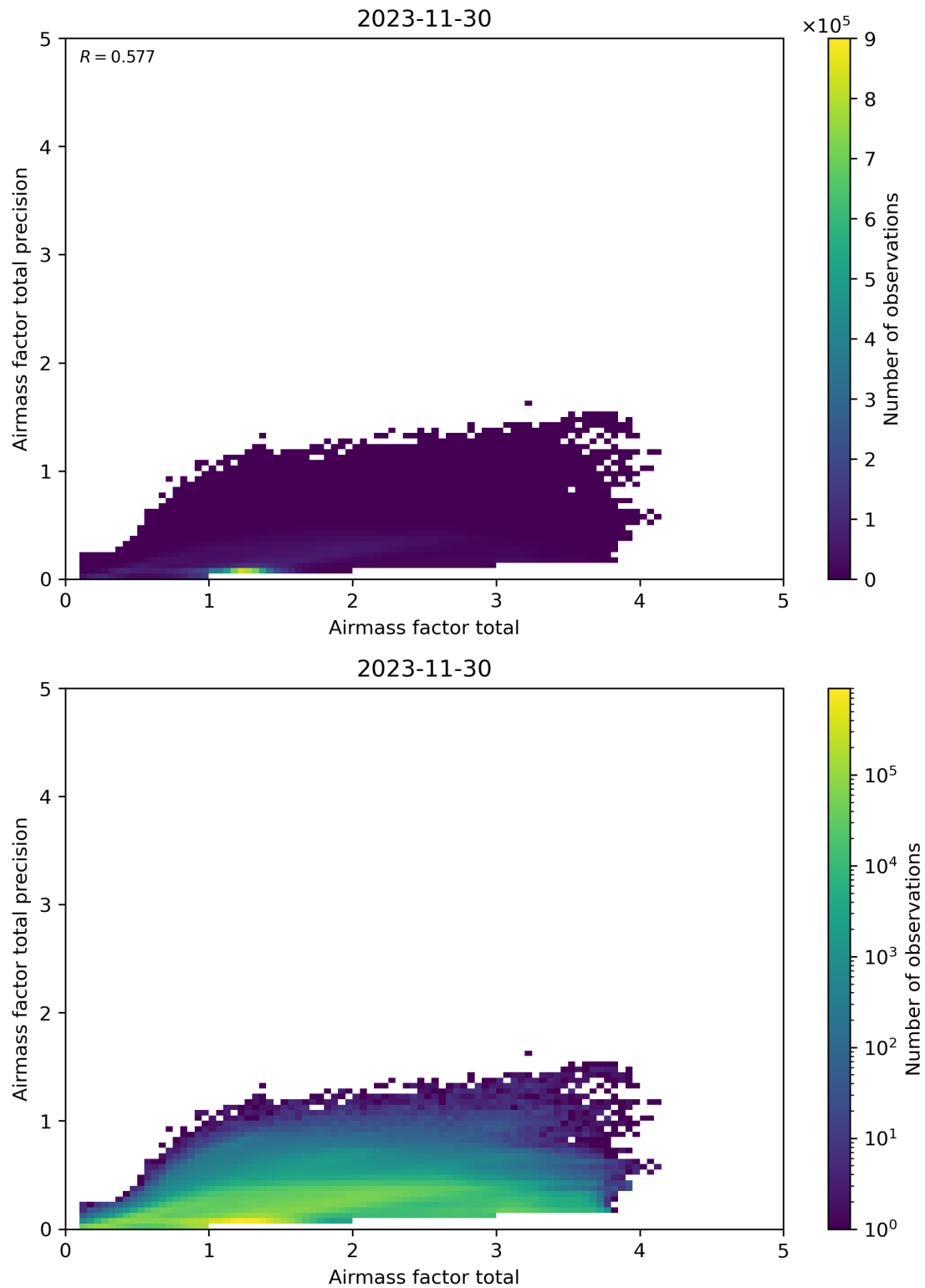
Figure 103: Scatter density plot of “Airmass factor total” against “Airmass factor total precision” for 2023-11-29 to 2023-12-01.
