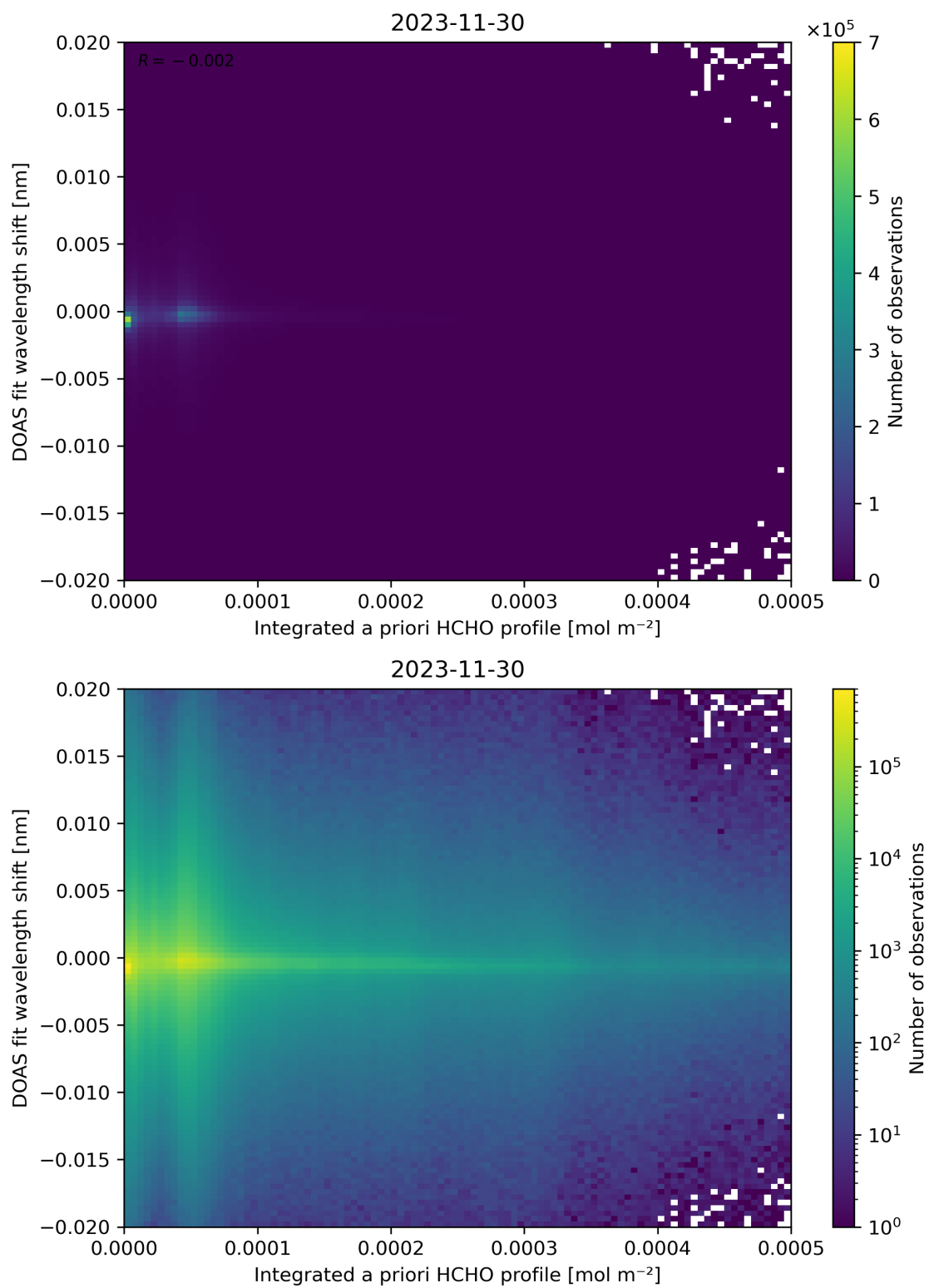
Figure 149: Scatter density plot of “Integrated a priori HCHO profile” against “DOAS fit wavelength shift” for 2023-11-29 to 2023-12-01.
