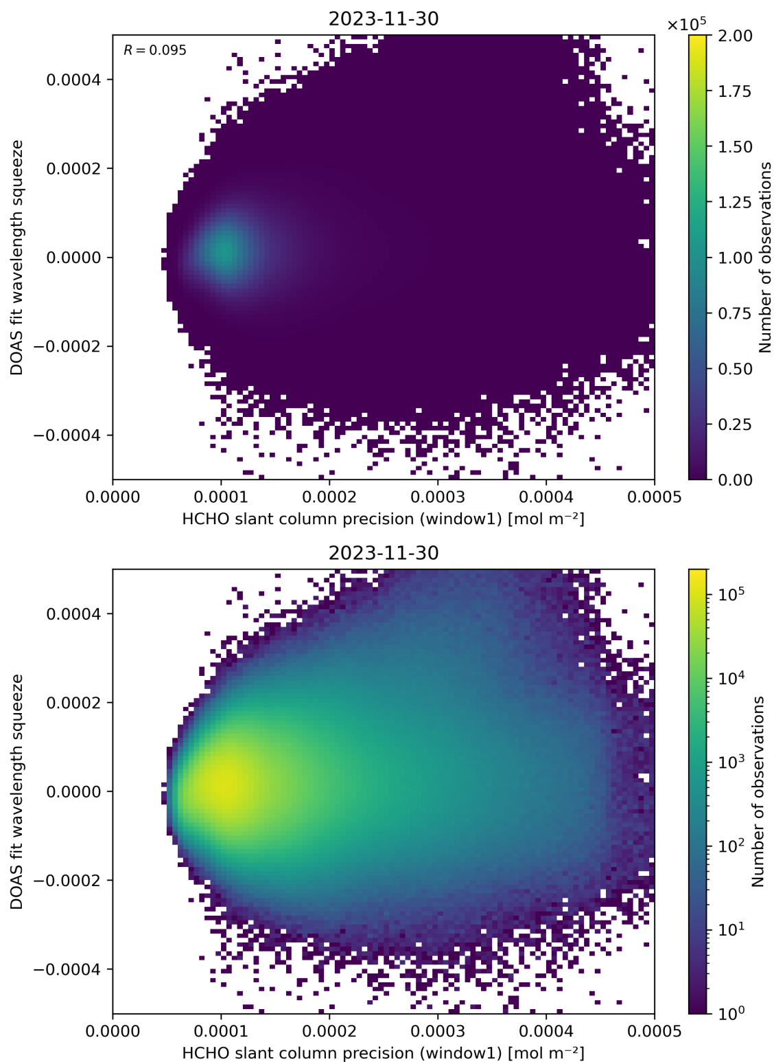
Figure 90: Scatter density plot of “HCHO slant column precision (window1)” against “DOAS fit wavelength squeeze” for 2023-11-29 to 2023-12-01.
