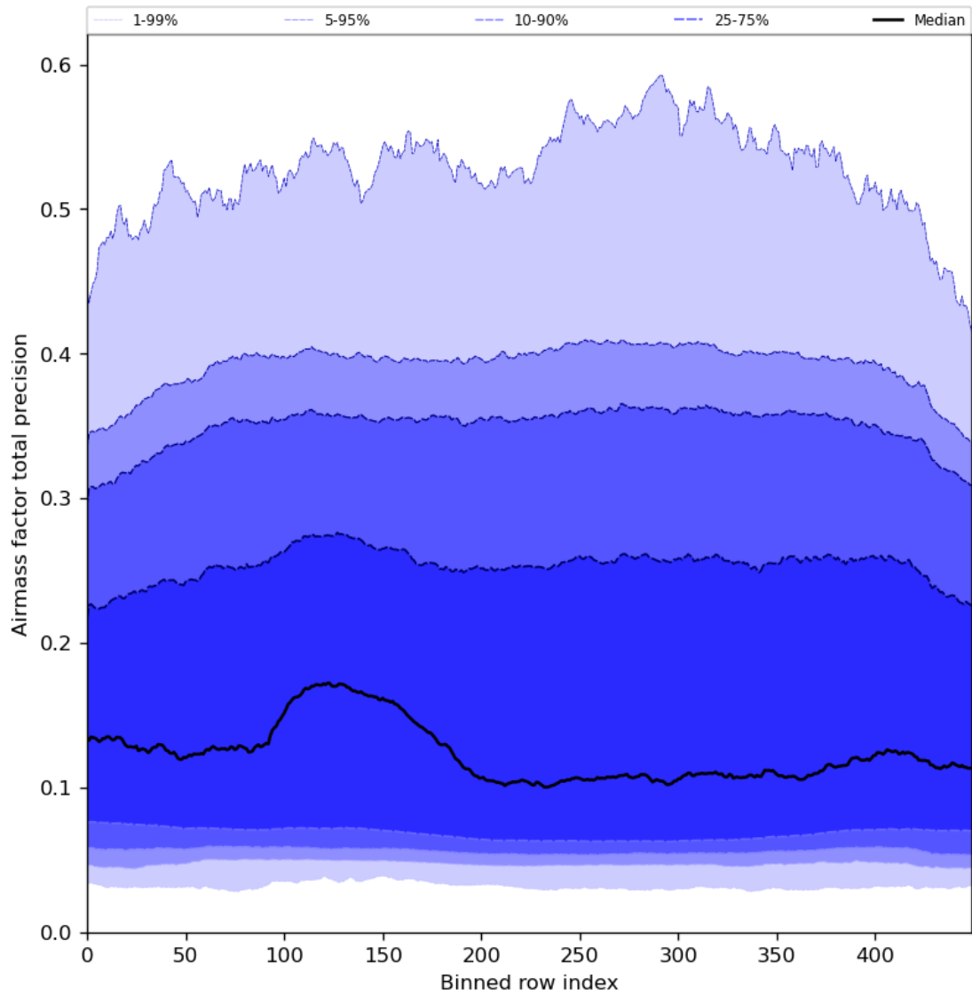
Figure 55: Along track statistics of “Airmass factor total precision” for 2023-11-29 to 2023-12-01
