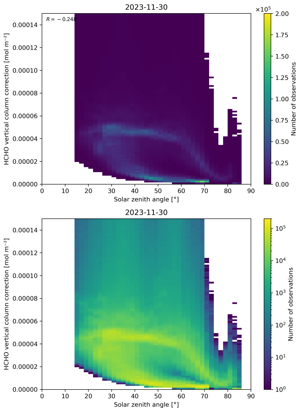
Figure 178: Scatter density plot of “Solar zenith angle” against “HCHO vertical column correction” for 2023-11-29 to 2023-12-01.
