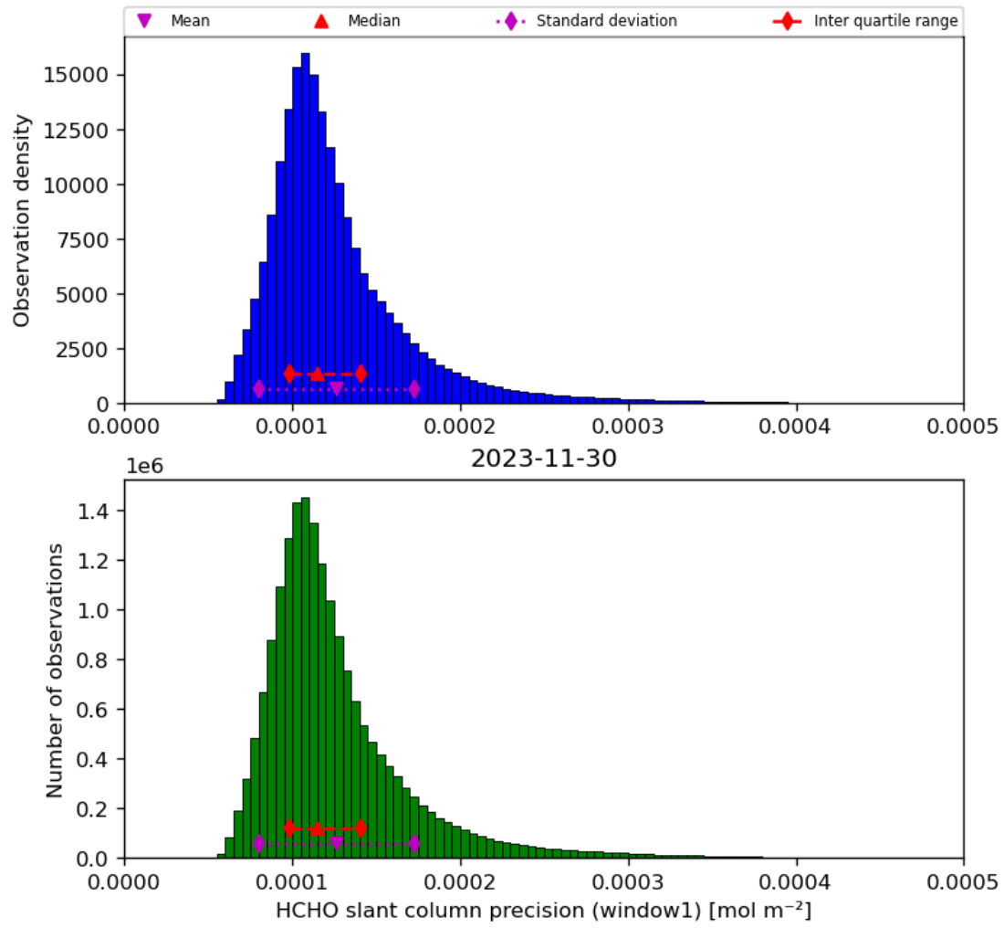
Figure 39: Histogram of “HCHO slant column precision (window1)” for 2023-11-29 to 2023-12-01
