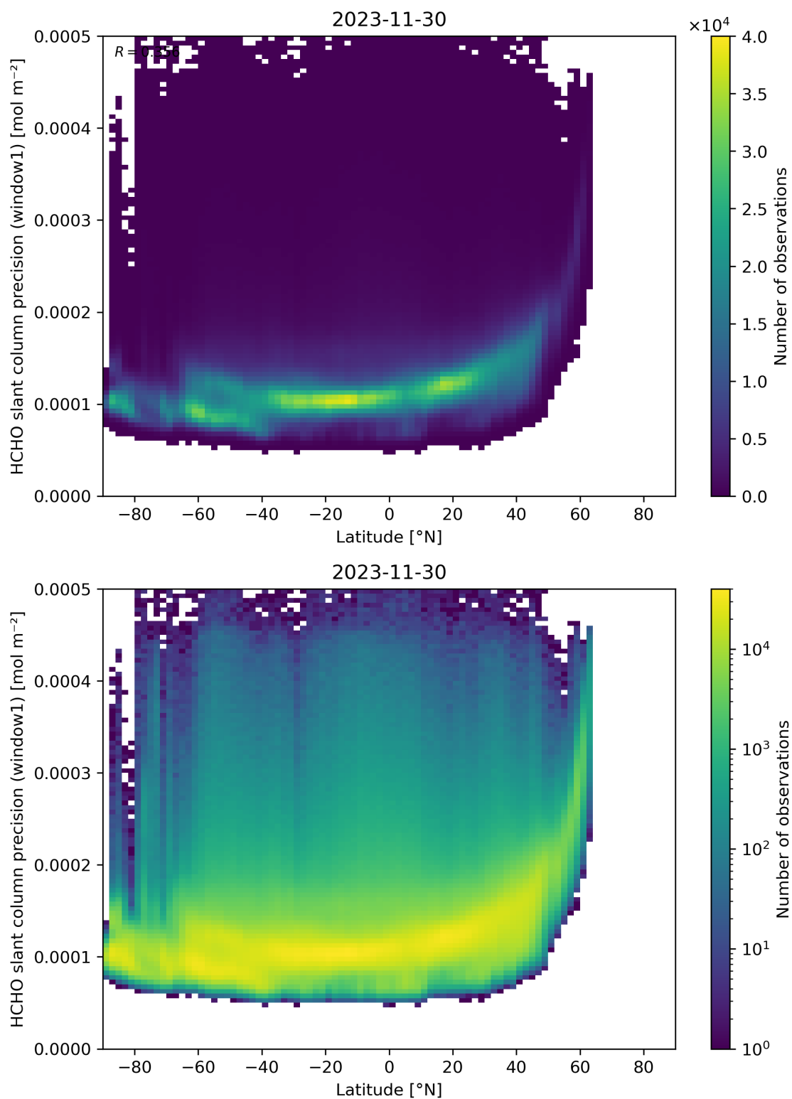
Figure 160: Scatter density plot of “Latitude” against “HCHO slant column precision (window1)” for 2023-11-29 to 2023-12-01.
