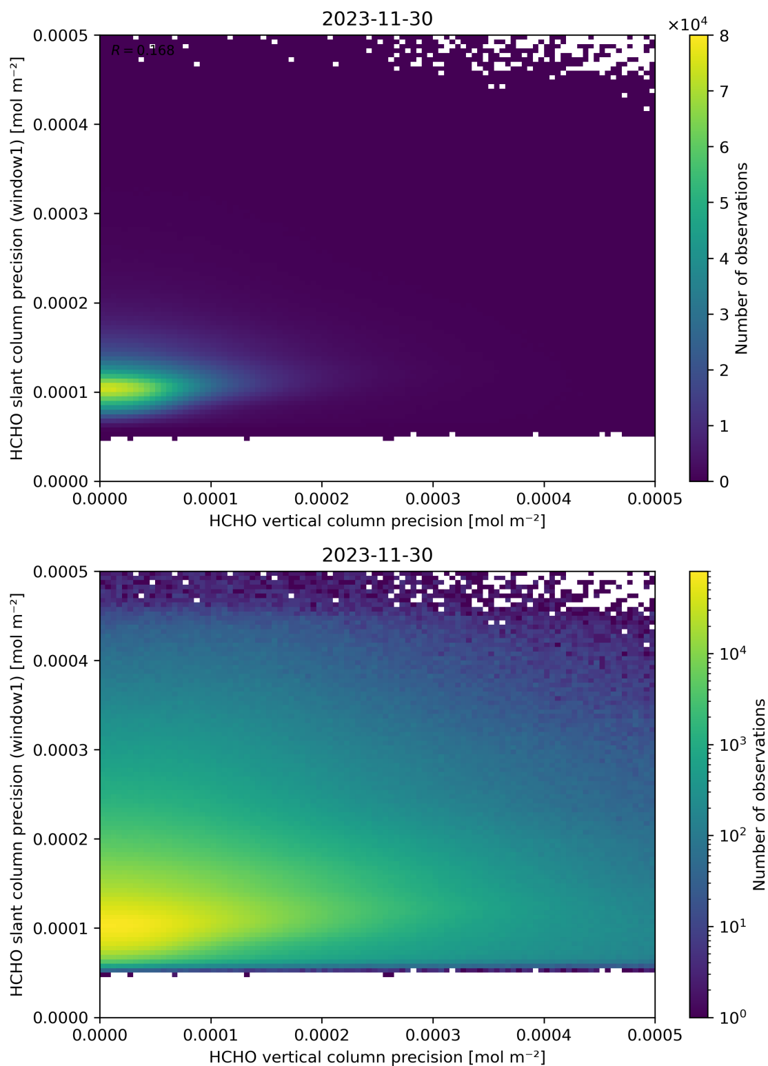
Figure 143: Scatter density plot of “HCHO vertical column precision” against “HCHO slant column precision (window1)” for 2023-11-29 to 2023-12-01.
