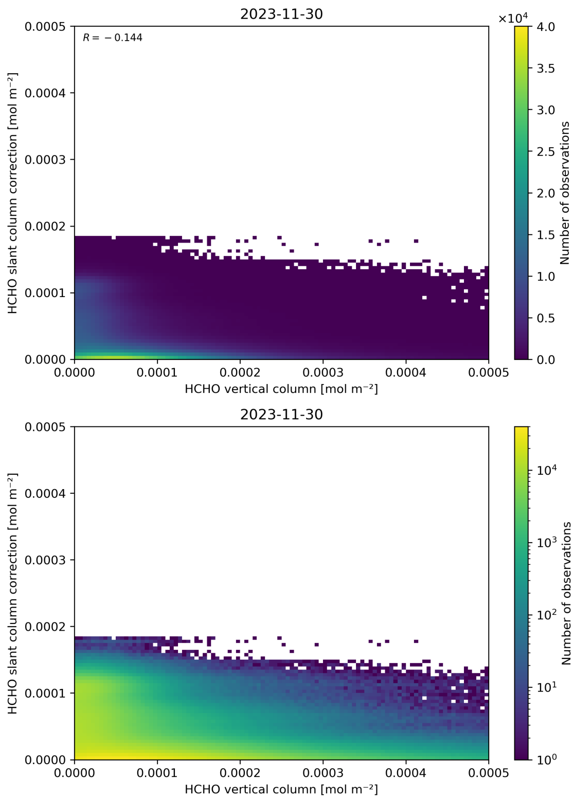
Figure 128: Scatter density plot of “HCHO vertical column” against “HCHO slant column correction” for 2023-11-29 to 2023-12-01.
