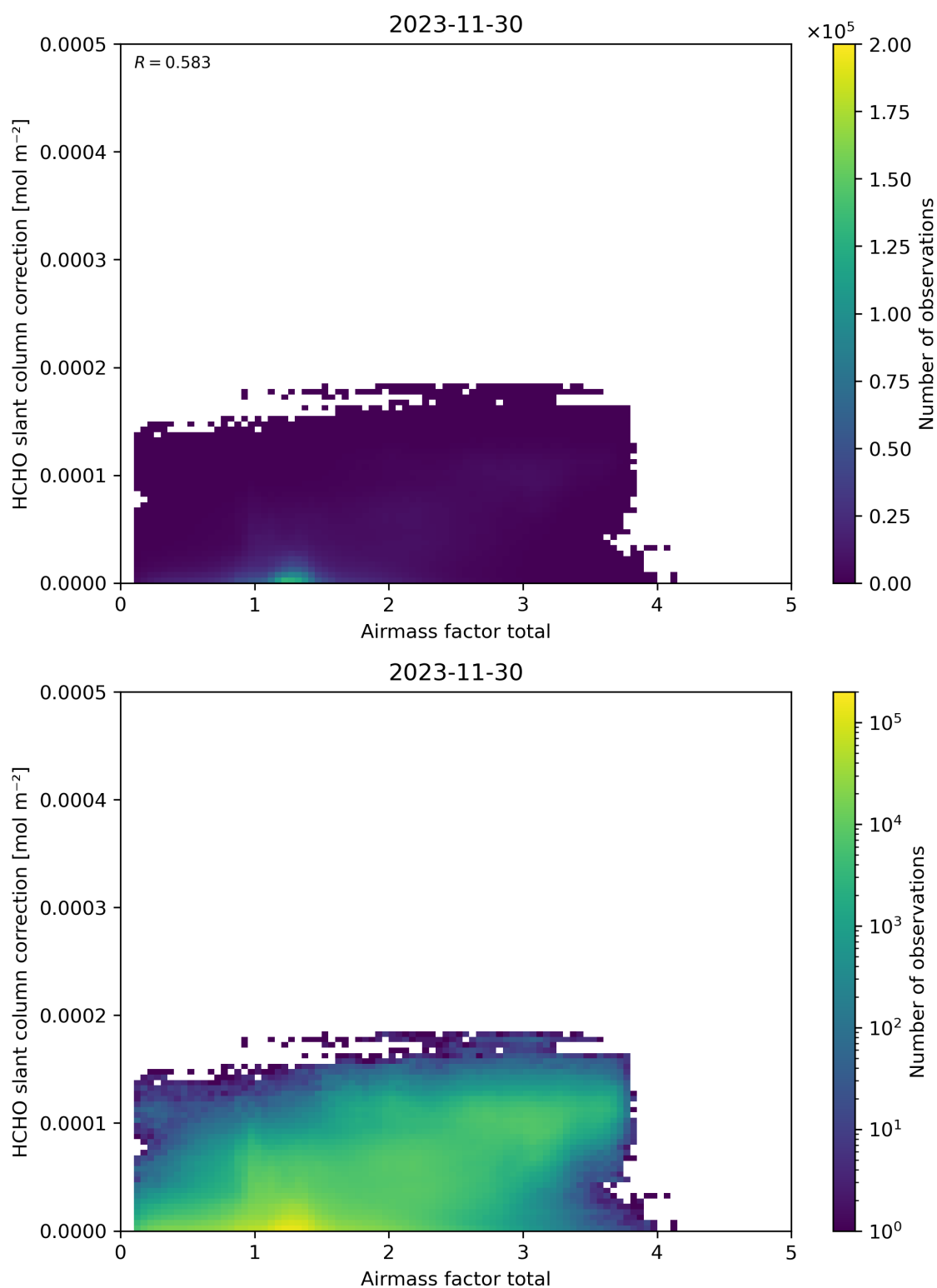
Figure 102: Scatter density plot of “Airmass factor total” against “HCHO slant column correction” for 2023-11-29 to 2023-12-01.
