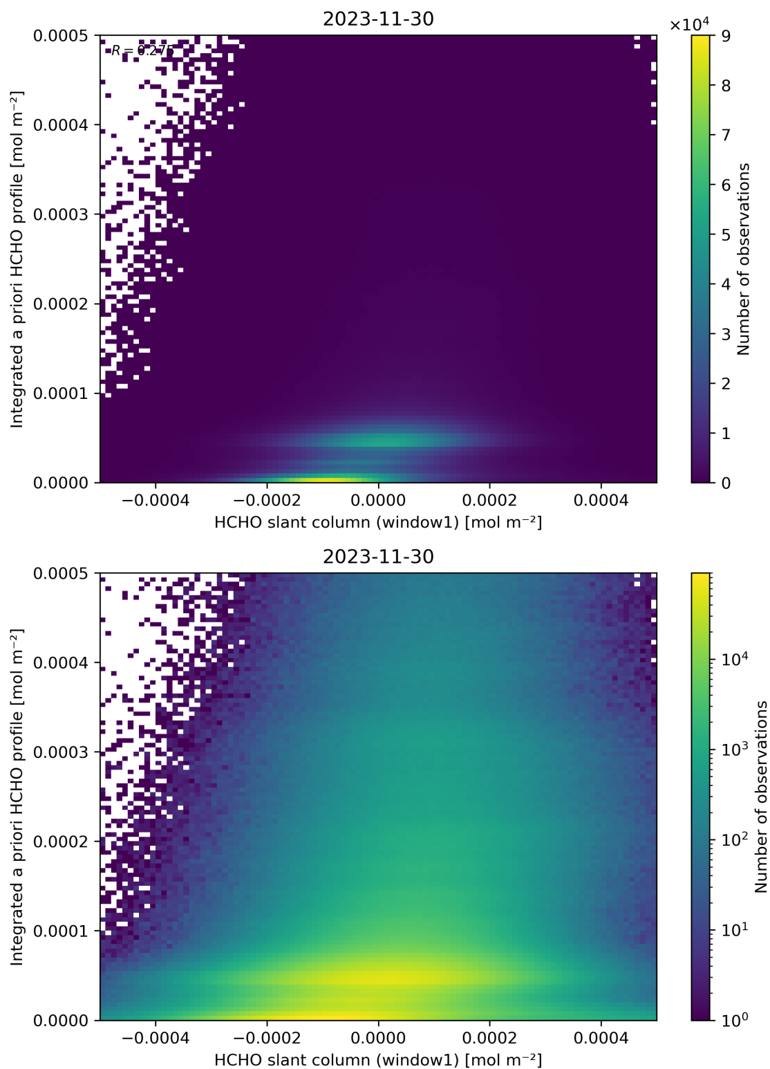
Figure 87: Scatter density plot of “HCHO slant column (window1)” against “Integrated a priori HCHO profile” for 2023-11-29 to 2023-12-01.
