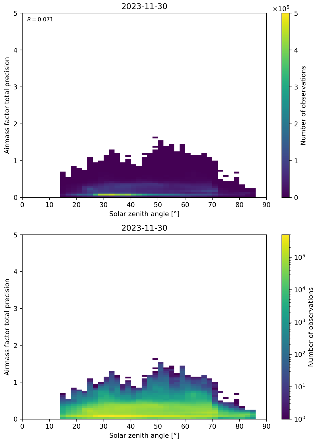
Figure 176: Scatter density plot of “Solar zenith angle” against “Airmass factor total precision” for 2023-11-29 to 2023-12-01.
