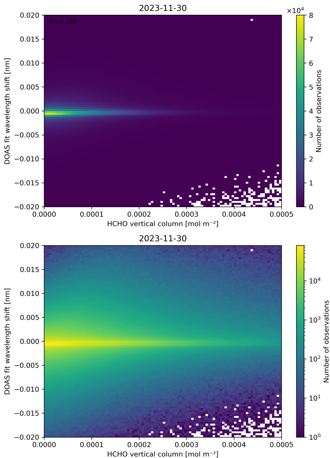
Figure 124: Scatter density plot of “HCHO vertical column” against “DOAS fit wavelength shift” for 2023-11-29 to 2023-12-01.
