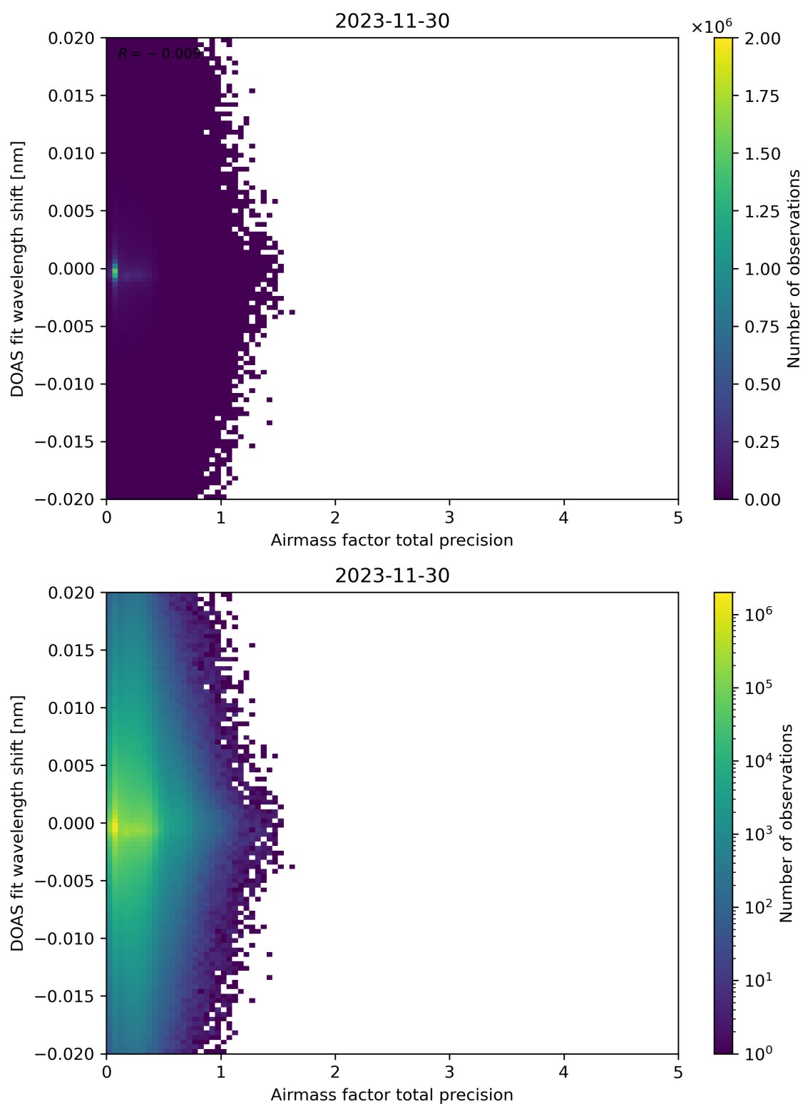
Figure 106: Scatter density plot of “Airmass factor total precision” against “DOAS fit wavelength shift” for 2023-11-29 to 2023-12-01.
