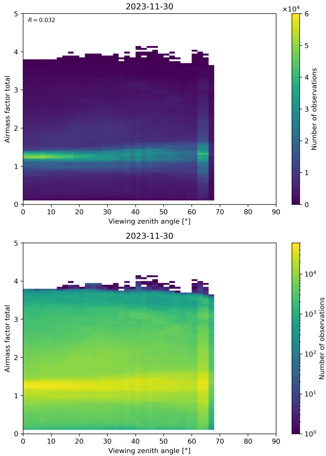
Figure 190: Scatter density plot of “Viewing zenith angle” against “Airmass factor total” for 2023-11-29 to 2023-12-01.
