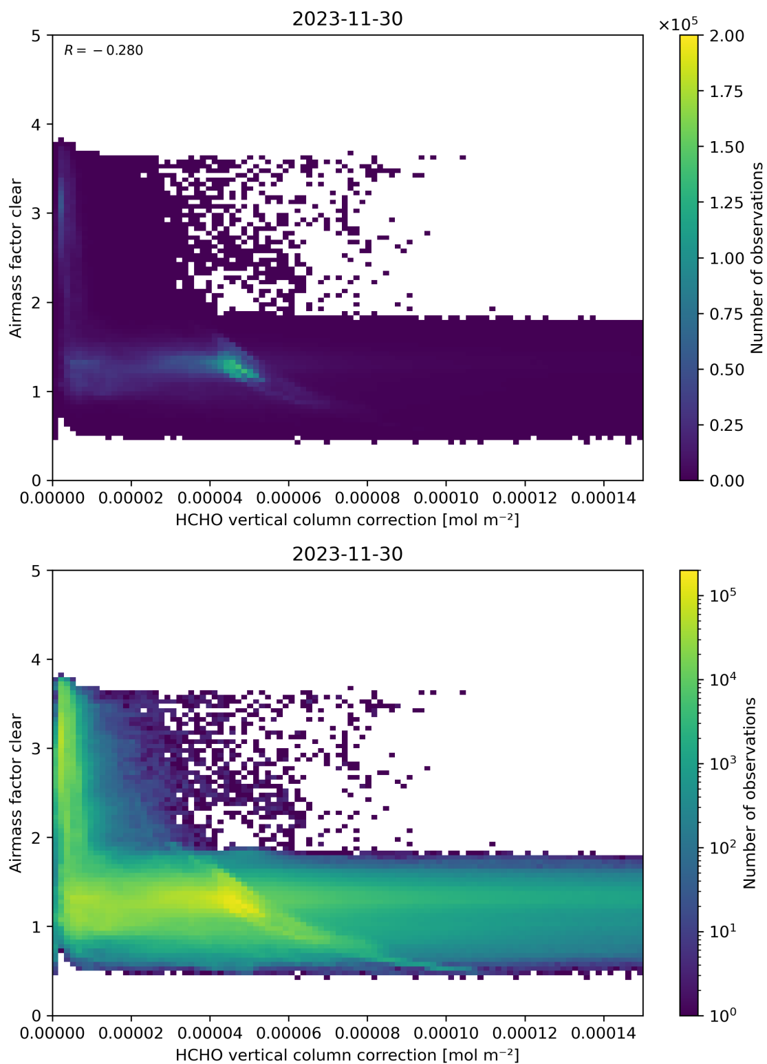
Figure 115: Scatter density plot of “HCHO vertical column correction” against “Airmass factor clear” for 2023-11-29 to 2023-12-01.
