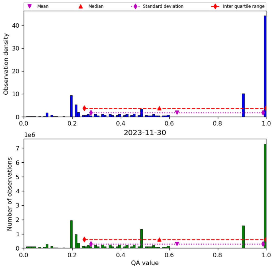
Figure 34: Histogram of “QA value” for 2023-11-29 to 2023-12-01
