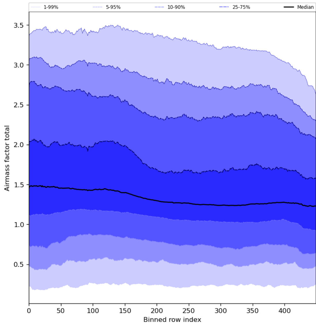
Figure 54: Along track statistics of “Airmass factor total” for 2023-11-29 to 2023-12-01
