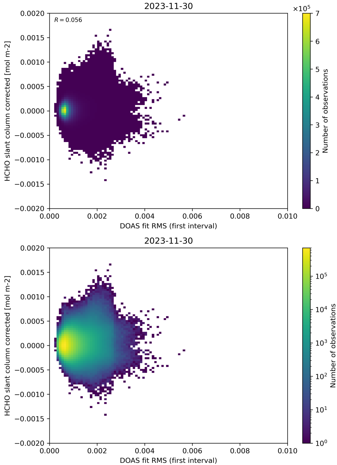
Figure 62: Scatter density plot of “DOAS fit RMS (first interval)” against “HCHO slant column corrected” for 2023-11-29 to 2023-12-01.
