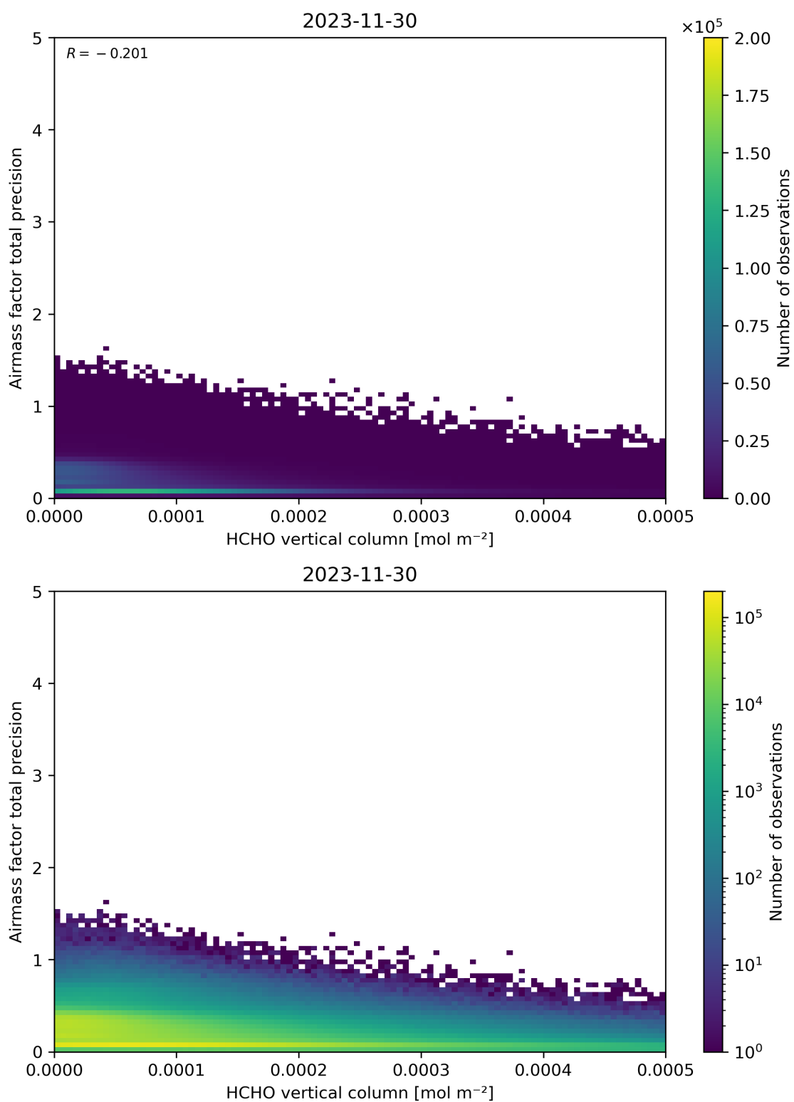
Figure 132: Scatter density plot of “HCHO vertical column” against “Airmass factor total precision” for 2023-11-29 to 2023-12-01.
