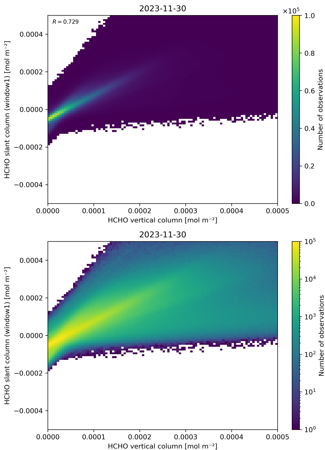
Figure 129: Scatter density plot of “HCHO vertical column” against “HCHO slant column (window1)” for 2023-11-29 to 2023-12-01.
