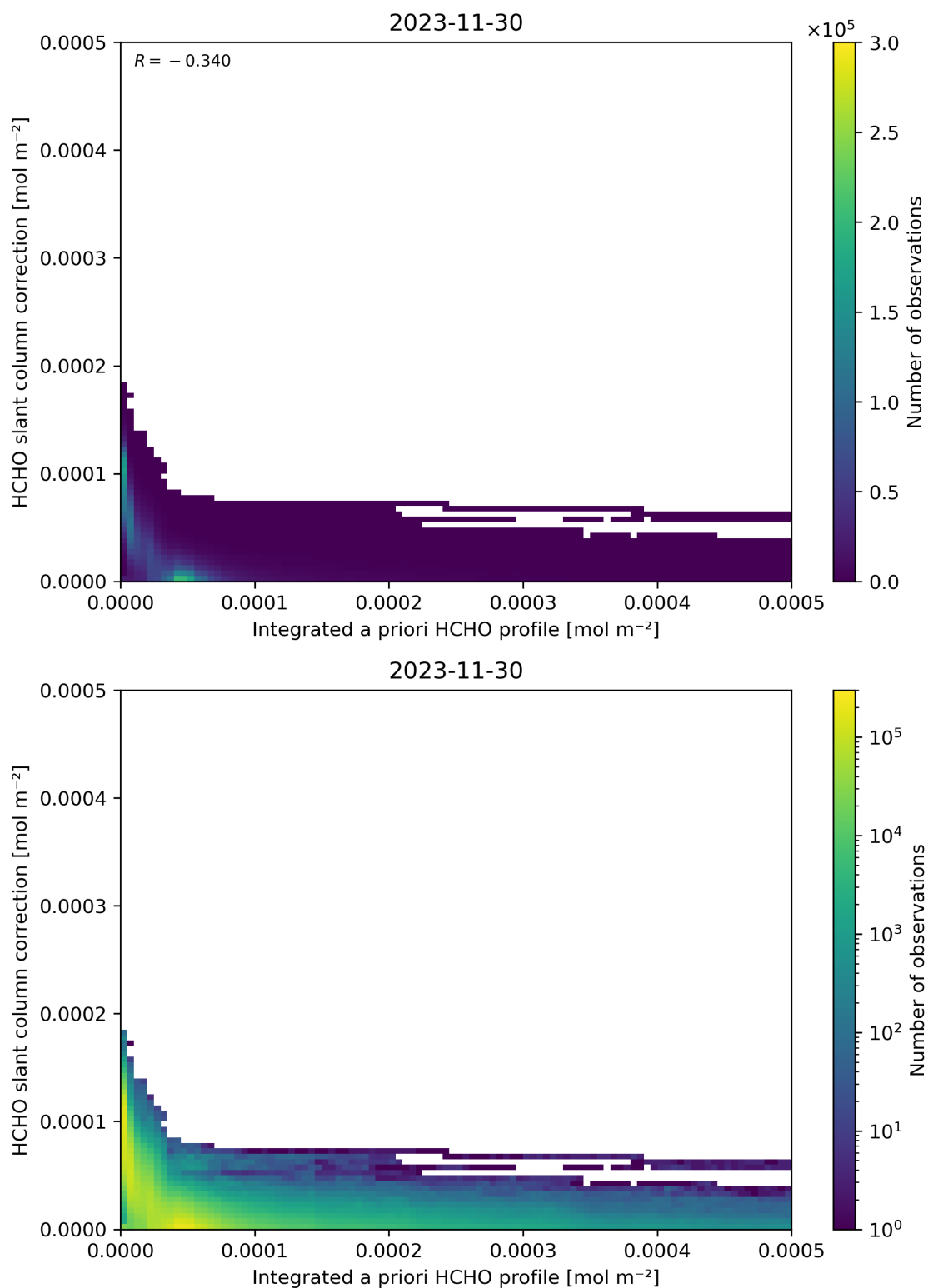
Figure 152: Scatter density plot of “Integrated a priori HCHO profile” against “HCHO slant column correction” for 2023-11-29 to 2023-12-01.
