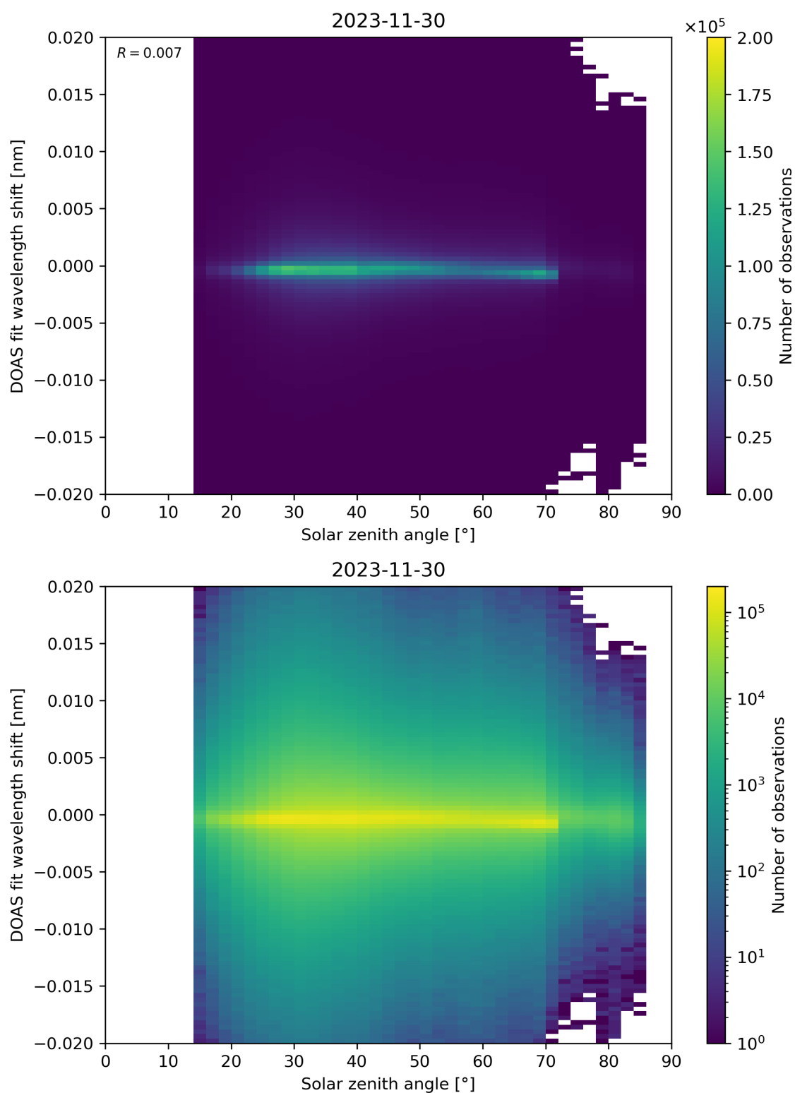
Figure 168: Scatter density plot of “Solar zenith angle” against “DOAS fit wavelength shift” for 2023-11-29 to 2023-12-01.
