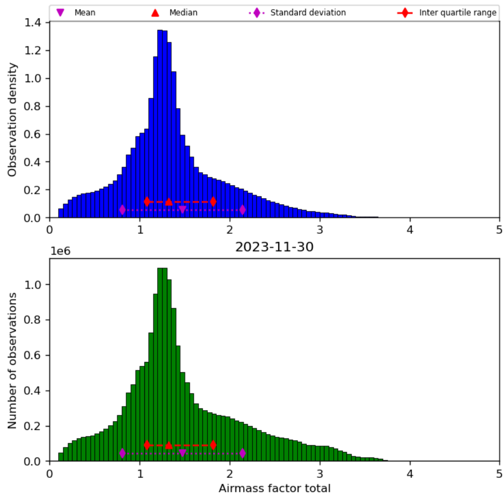
Figure 40: Histogram of “Airmass factor total” for 2023-11-29 to 2023-12-01
