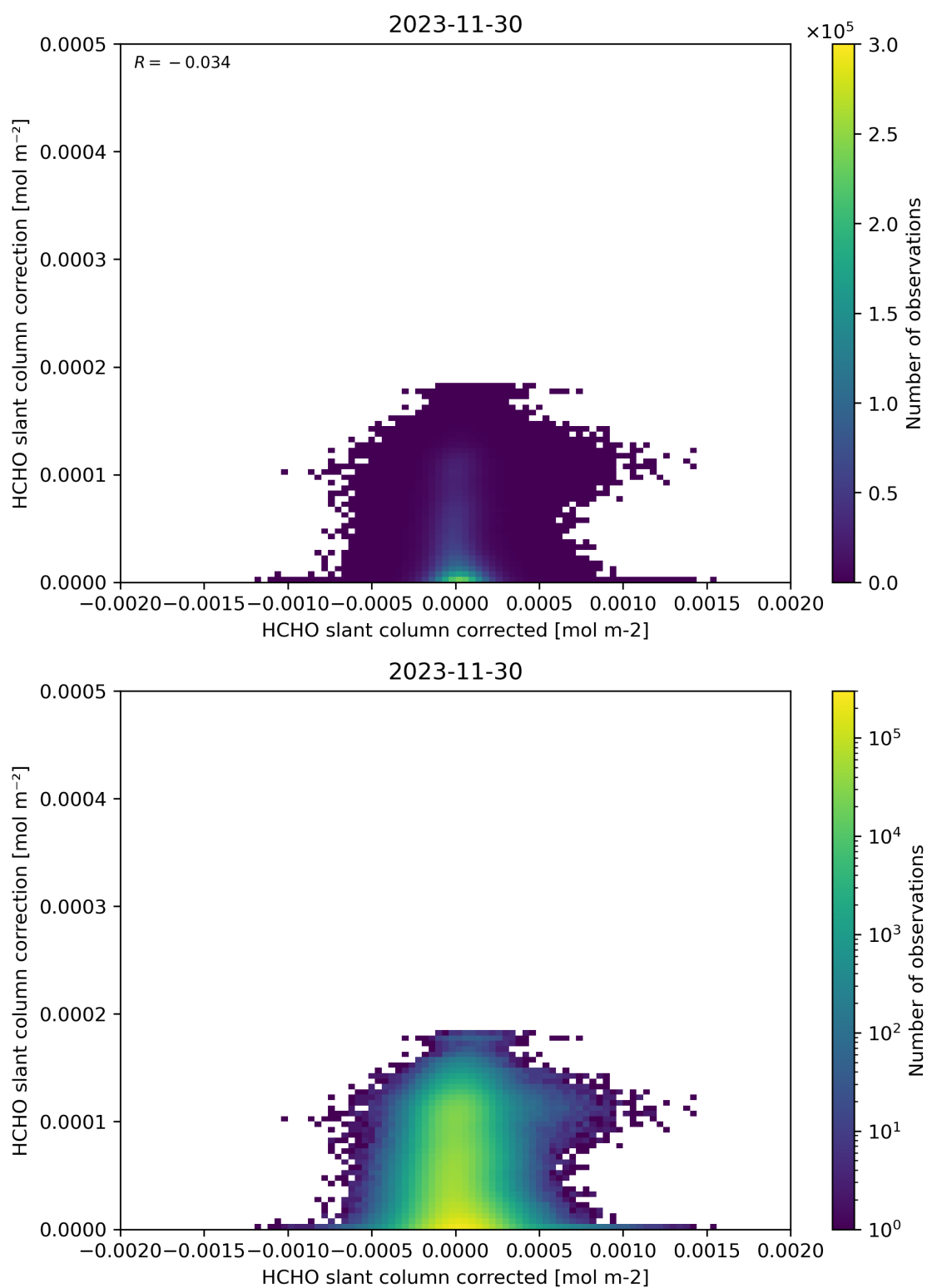
Figure 77: Scatter density plot of “HCHO slant column corrected” against “HCHO slant column correction” for 2023-11-29 to 2023-12-01.
