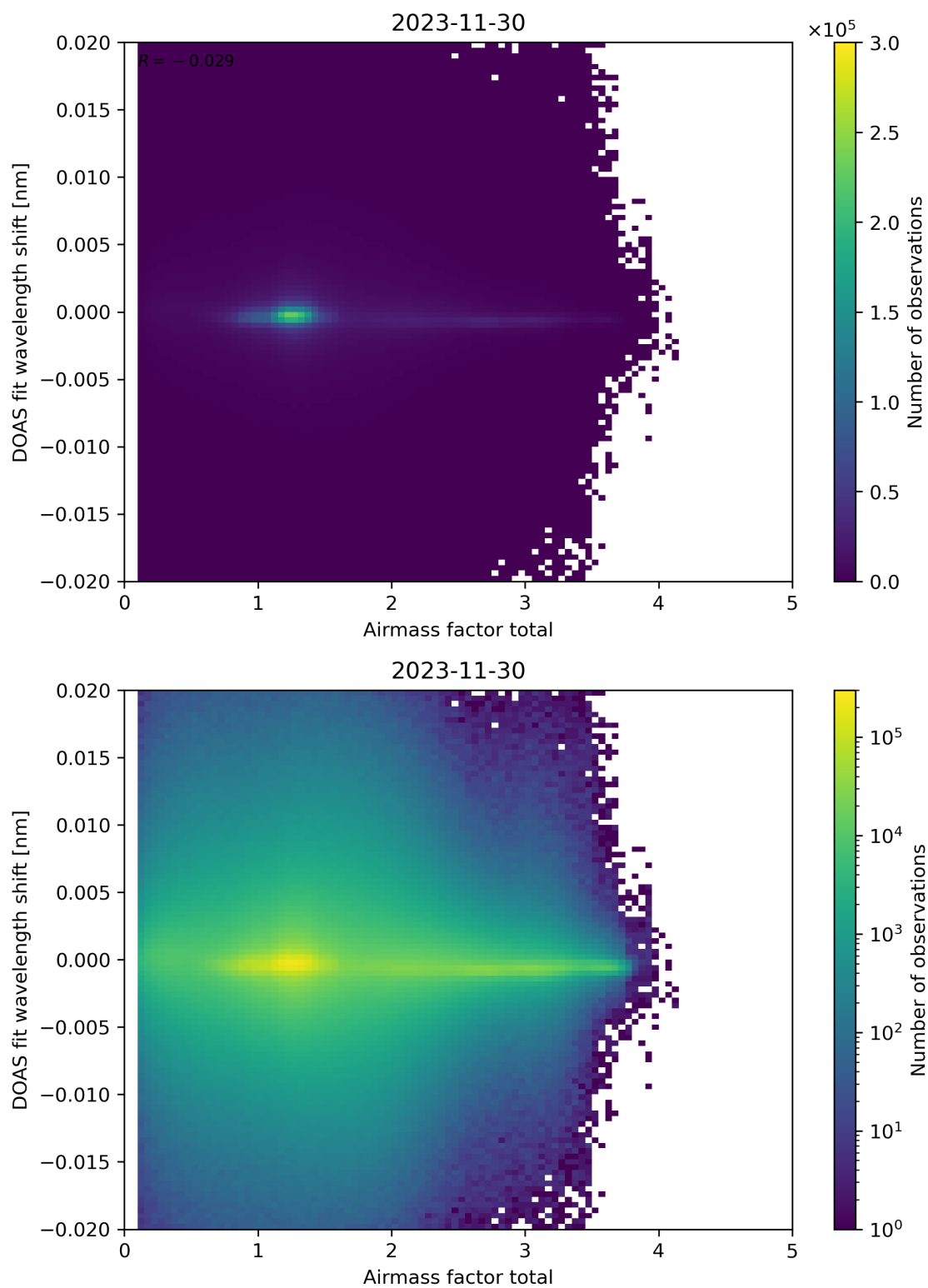
Figure 98: Scatter density plot of “Airmass factor total” against “DOAS fit wavelength shift” for 2023-11-29 to 2023-12-01.
