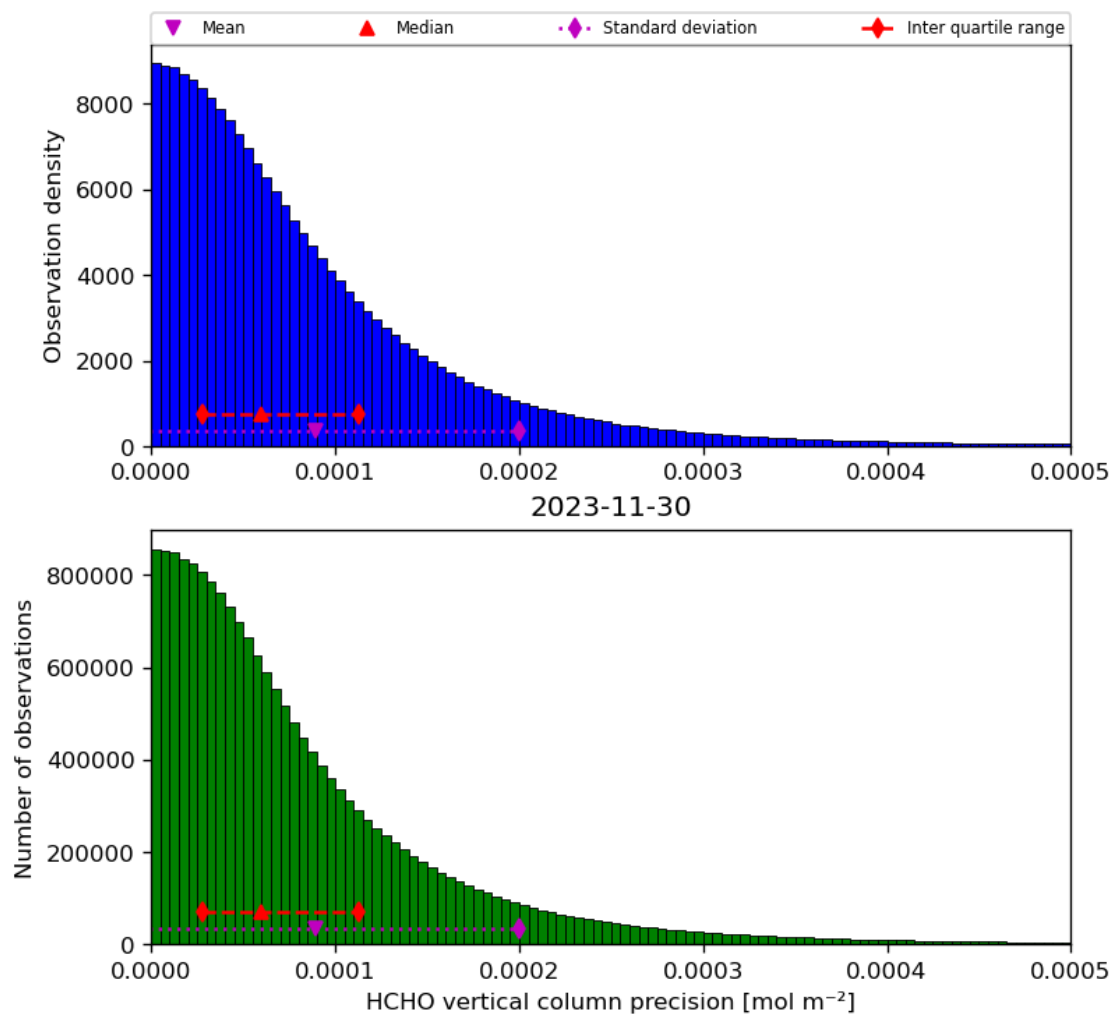
Figure 36: Histogram of “HCHO vertical column precision” for 2023-11-29 to 2023-12-01
