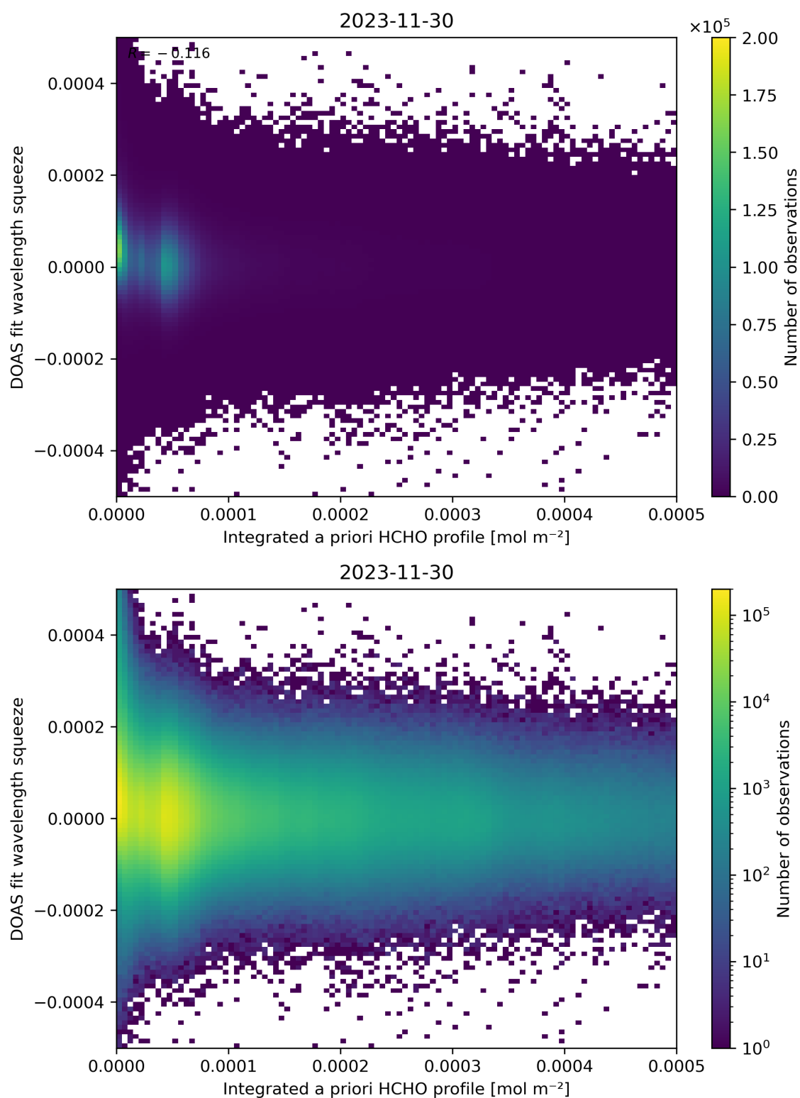
Figure 150: Scatter density plot of “Integrated a priori HCHO profile” against “DOAS fit wavelength squeeze” for 2023-11-29 to 2023-12-01.
