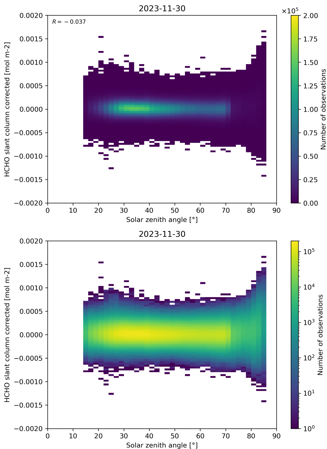
Figure 171: Scatter density plot of “Solar zenith angle” against “HCHO slant column corrected” for 2023-11-29 to 2023-12-01.
