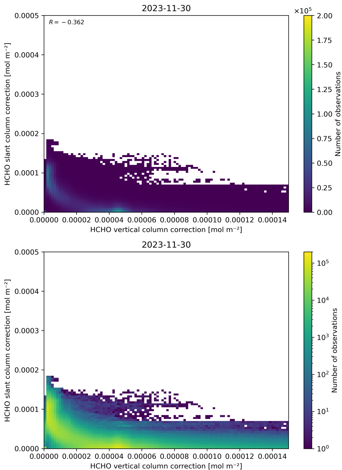
Figure 117: Scatter density plot of “HCHO vertical column correction” against “HCHO slant column correction” for 2023-11-29 to 2023-12-01.
