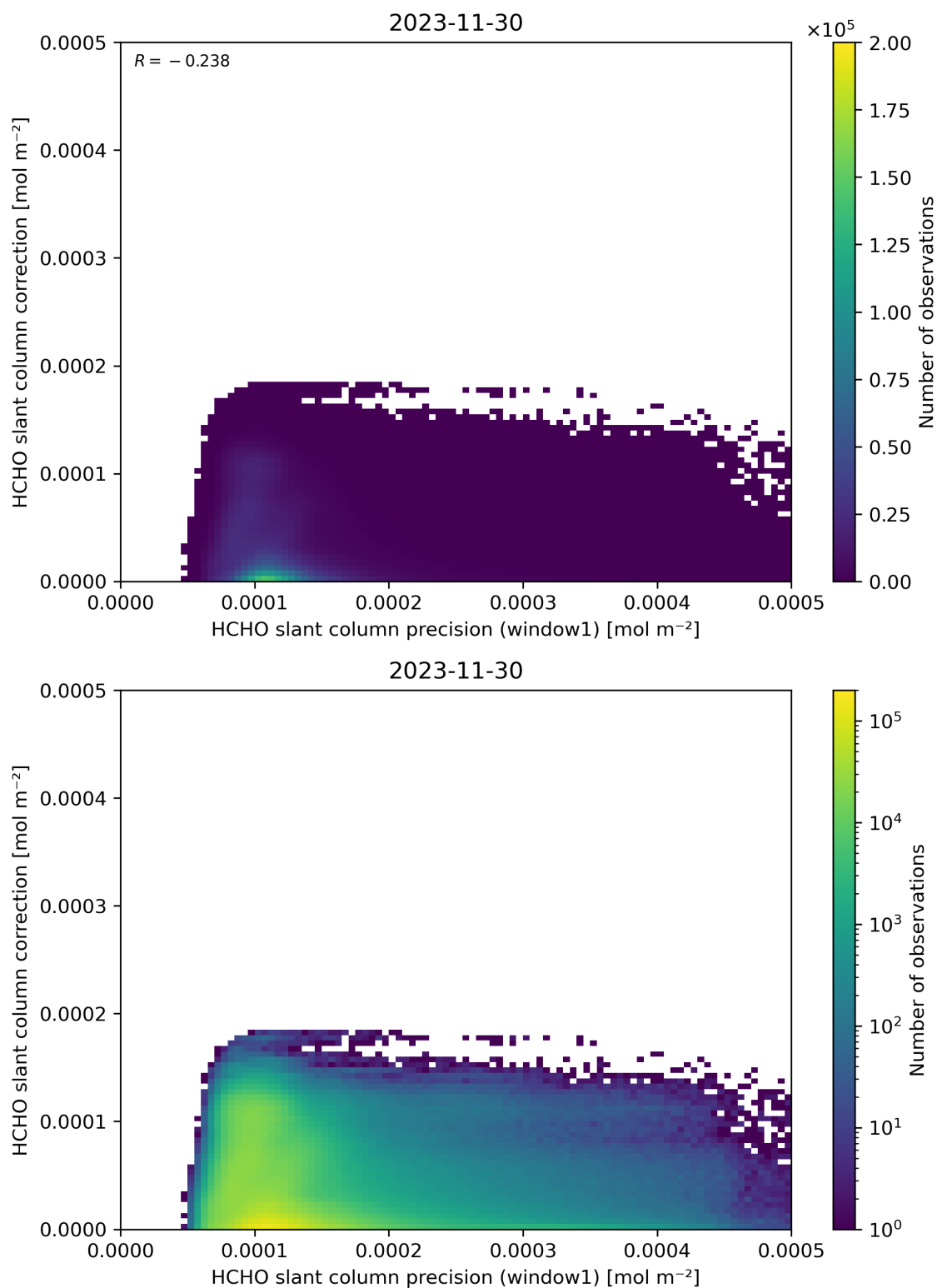
Figure 93: Scatter density plot of “HCHO slant column precision (window1)” against “HCHO slant column correction” for 2023-11-29 to 2023-12-01.
