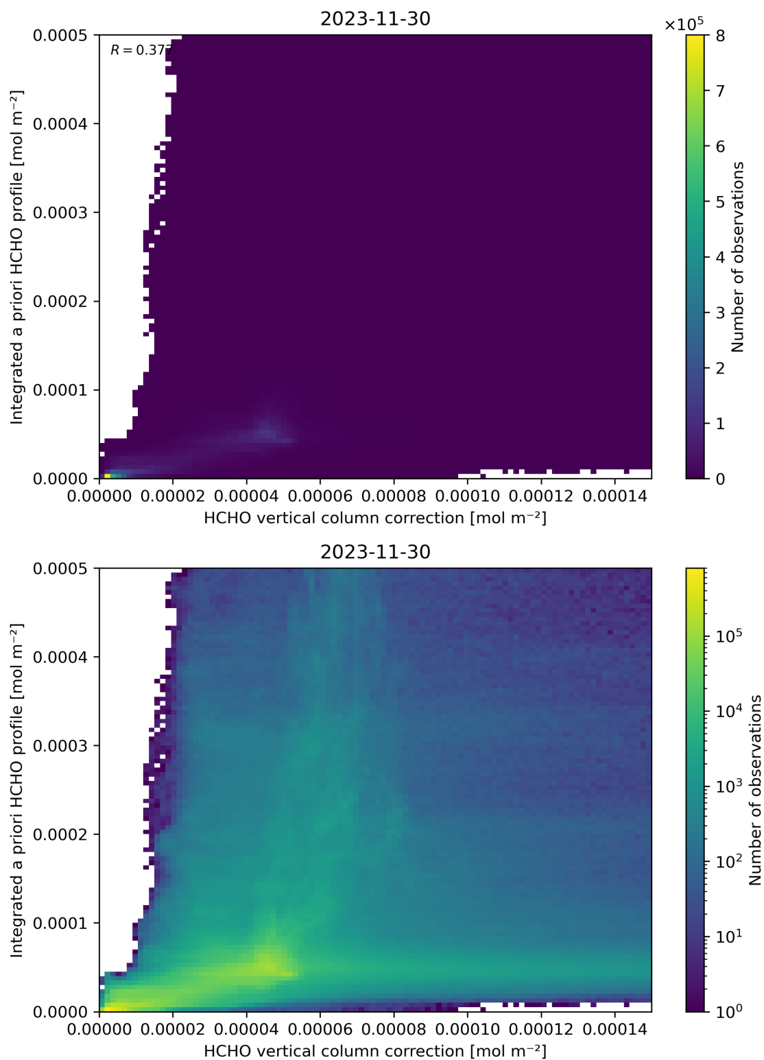
Figure 122: Scatter density plot of “HCHO vertical column correction” against “Integrated a priori HCHO profile” for 2023-11-29 to 2023-12-01.
