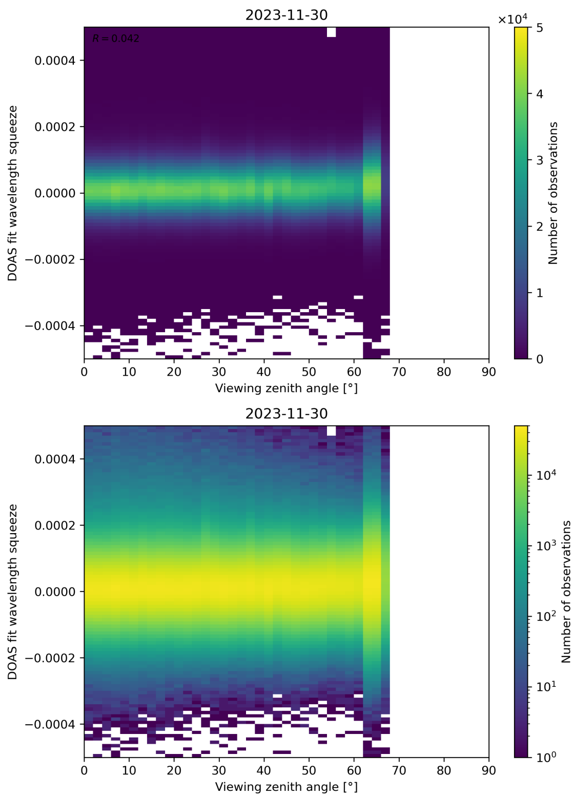
Figure 184: Scatter density plot of “Viewing zenith angle” against “DOAS fit wavelength squeeze” for 2023-11-29 to 2023-12-01.
