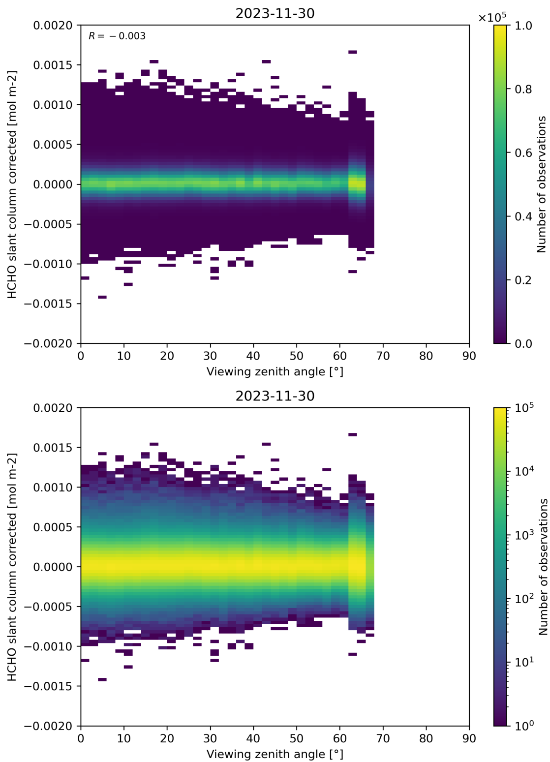
Figure 186: Scatter density plot of “Viewing zenith angle” against “HCHO slant column corrected” for 2023-11-29 to 2023-12-01.
