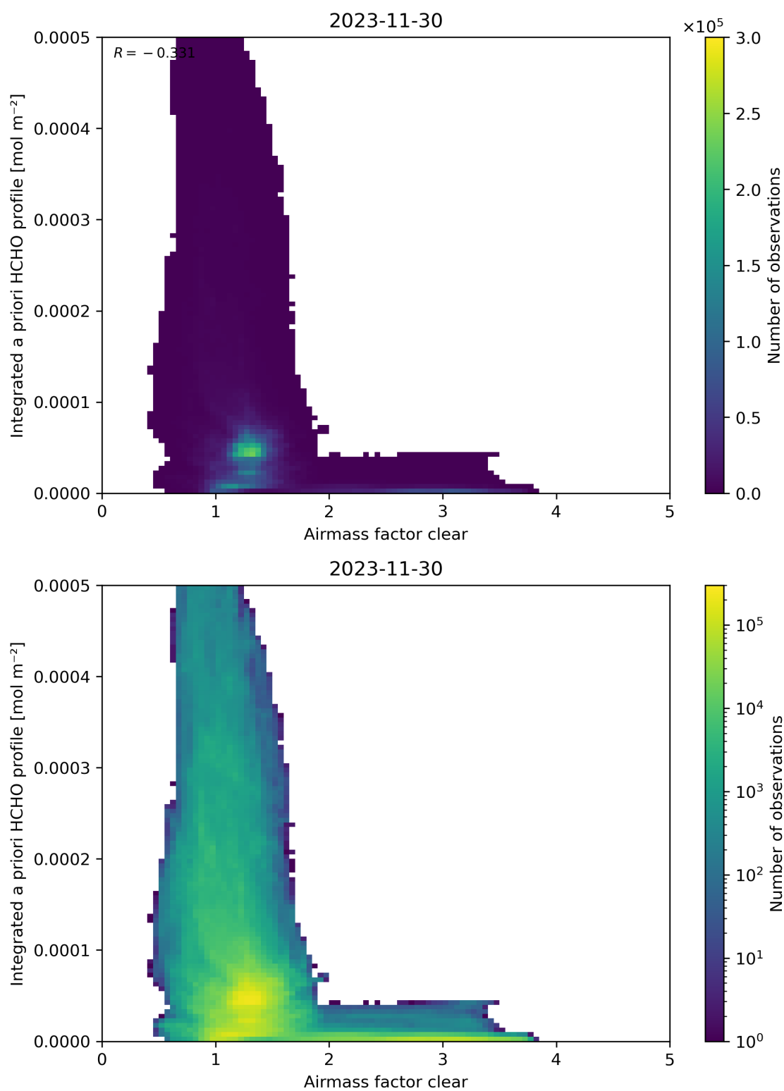
Figure 76: Scatter density plot of “Airmass factor clear” against “Integrated a priori HCHO profile” for 2023-11-29 to 2023-12-01.
