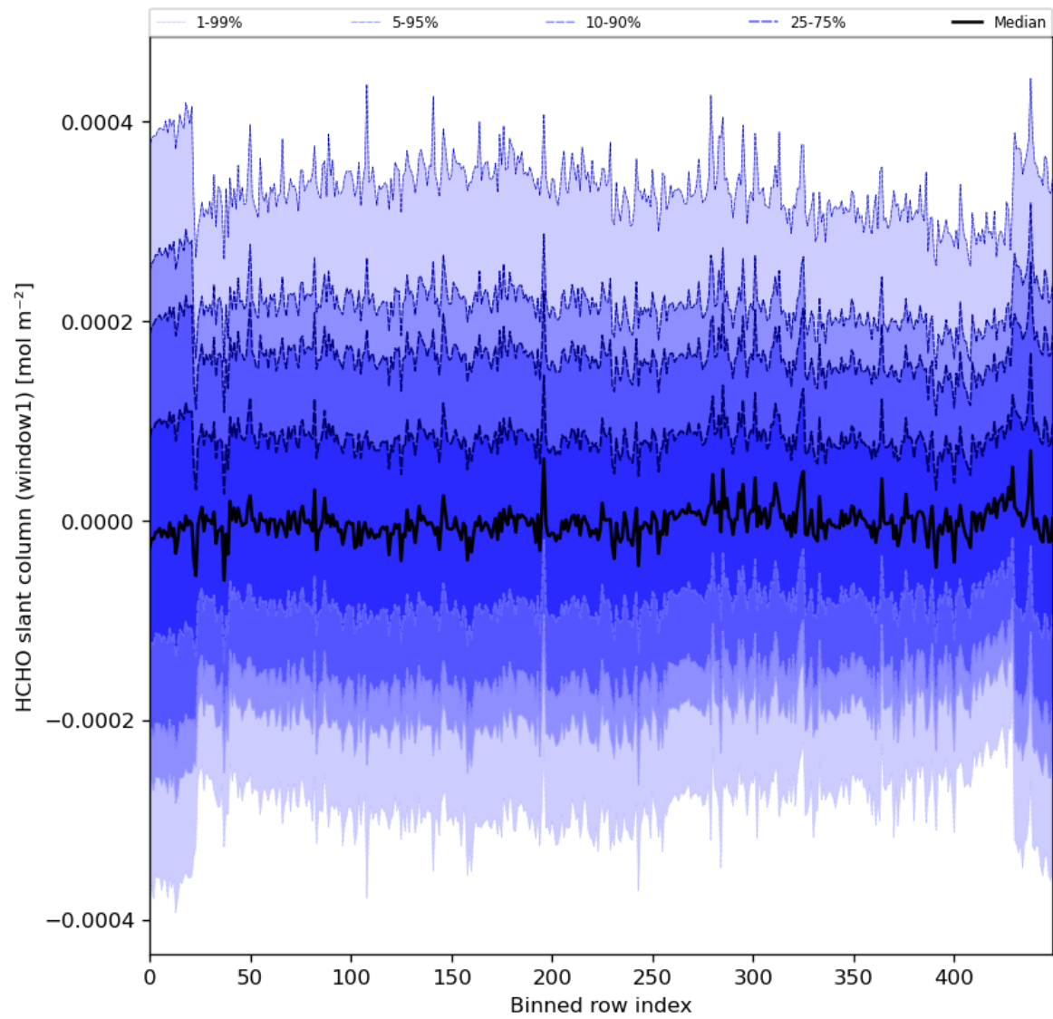
Figure 52: Along track statistics of “HCHO slant column (window1)” for 2023-11-29 to 2023-12-01
