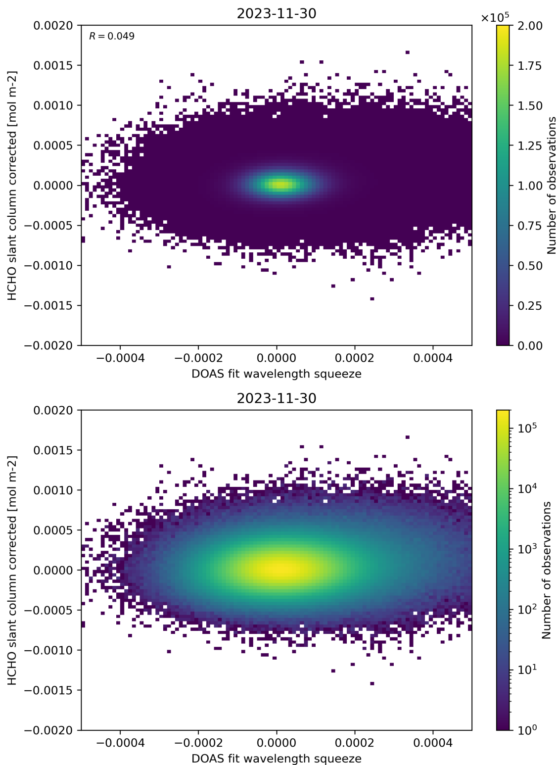
Figure 69: Scatter density plot of “DOAS fit wavelength squeeze” against “HCHO slant column corrected” for 2023-11-29 to 2023-12-01.
