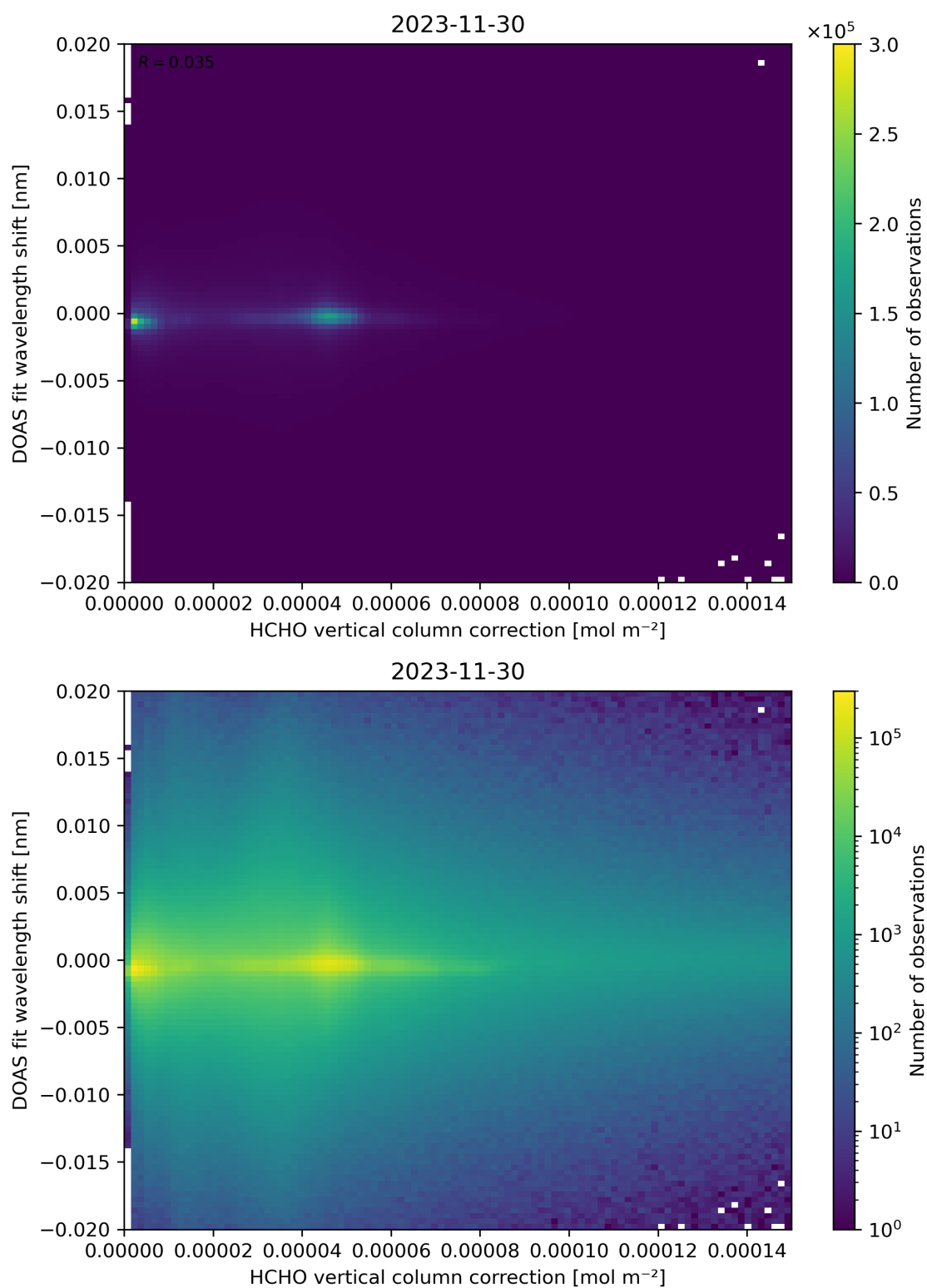
Figure 113: Scatter density plot of “HCHO vertical column correction” against “DOAS fit wavelength shift” for 2023-11-29 to 2023-12-01.
