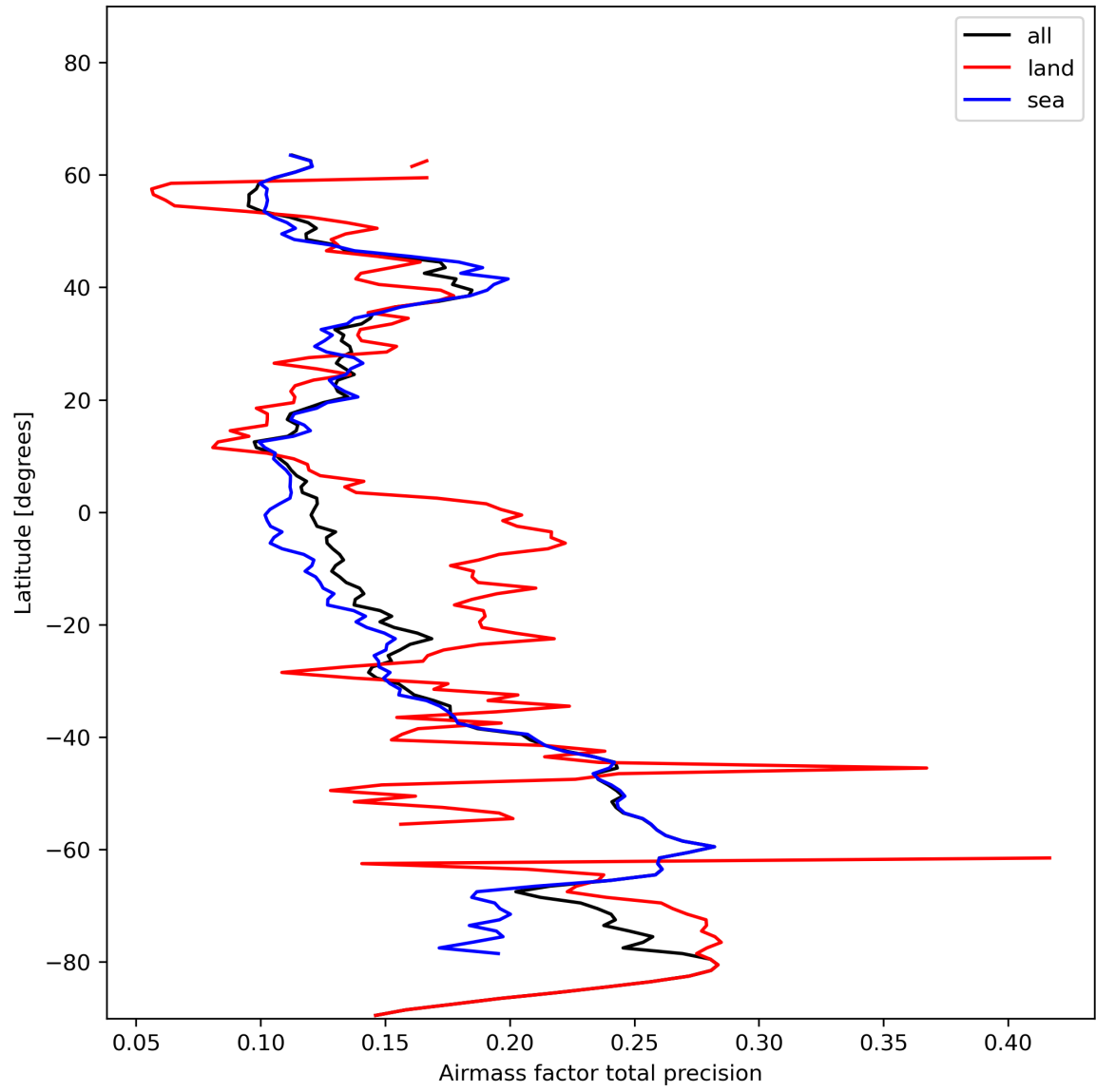
Figure 27: Zonal average of “Airmass factor total precision” for 2023-11-29 to 2023-12-01.
