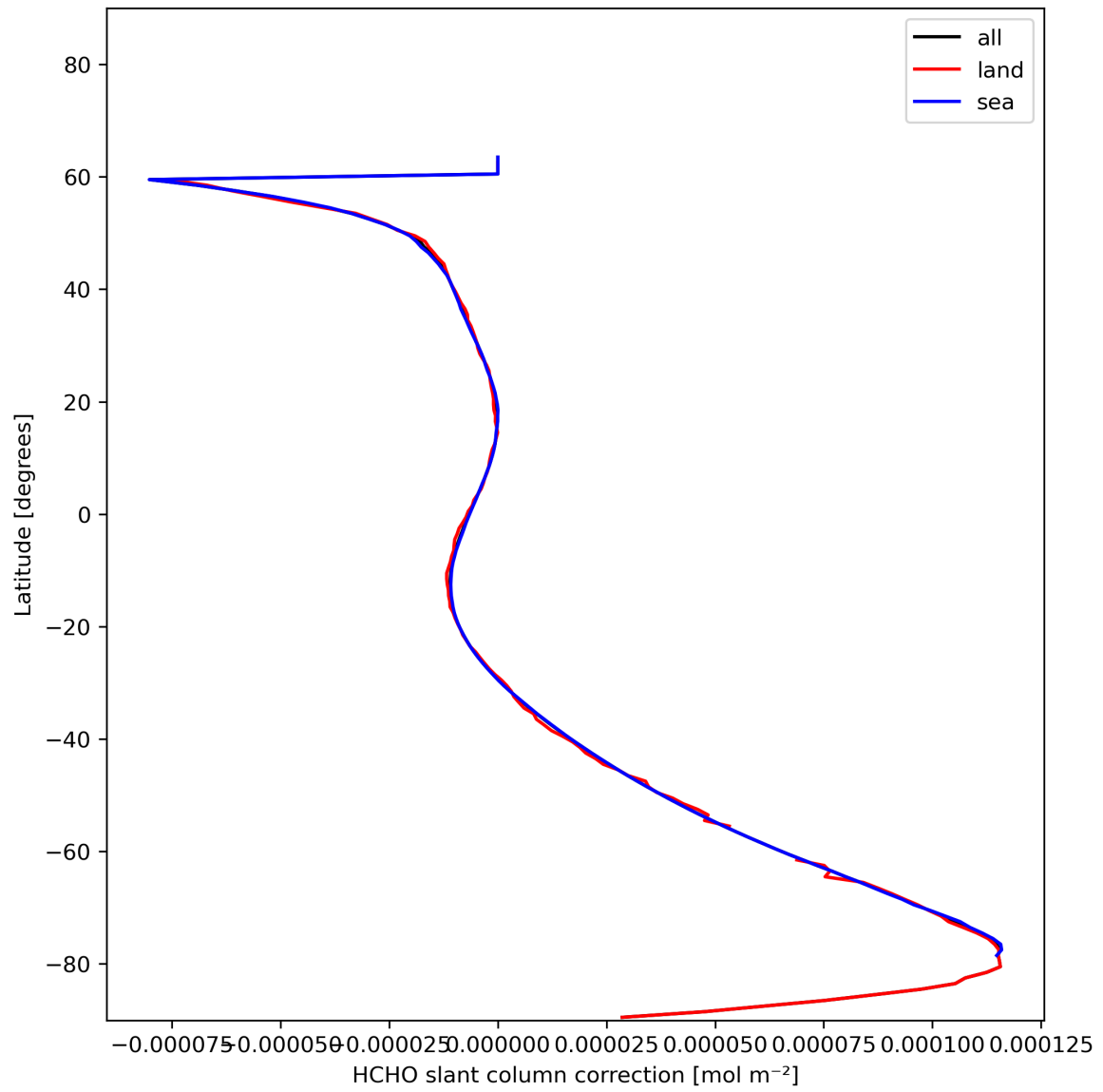
Figure 33: Zonal average of “HCHO slant column correction” for 2023-11-29 to 2023-12-01.
