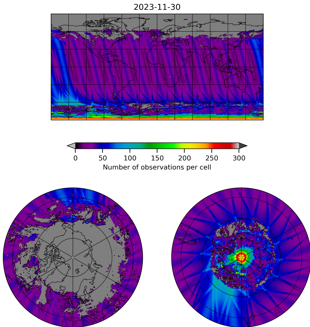
Figure 19: Map of the number of observations for 2023-11-29 to 2023-12-01
