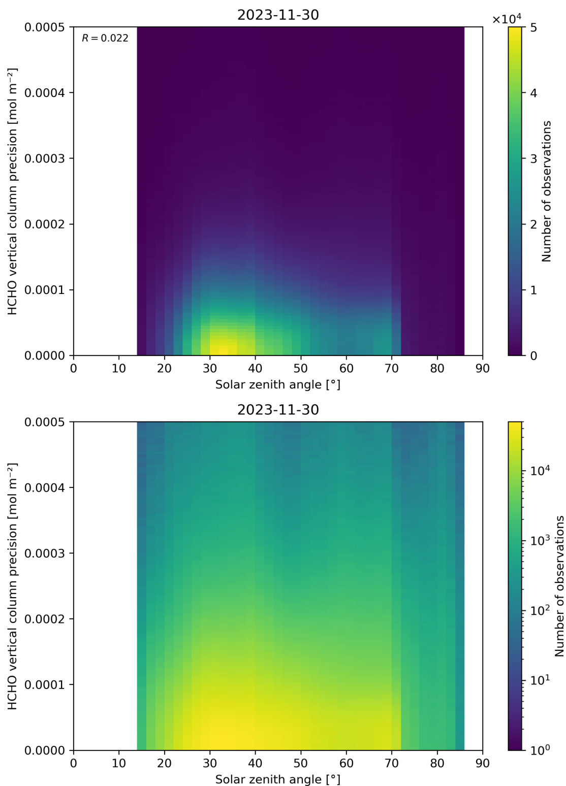
Figure 179: Scatter density plot of “Solar zenith angle” against “HCHO vertical column precision” for 2023-11-29 to 2023-12-01.
