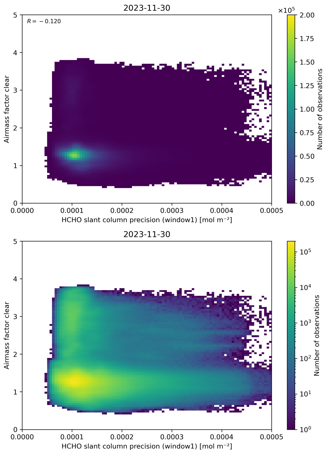
Figure 91: Scatter density plot of “HCHO slant column precision (window1)” against “Airmass factor clear” for 2023-11-29 to 2023-12-01.
