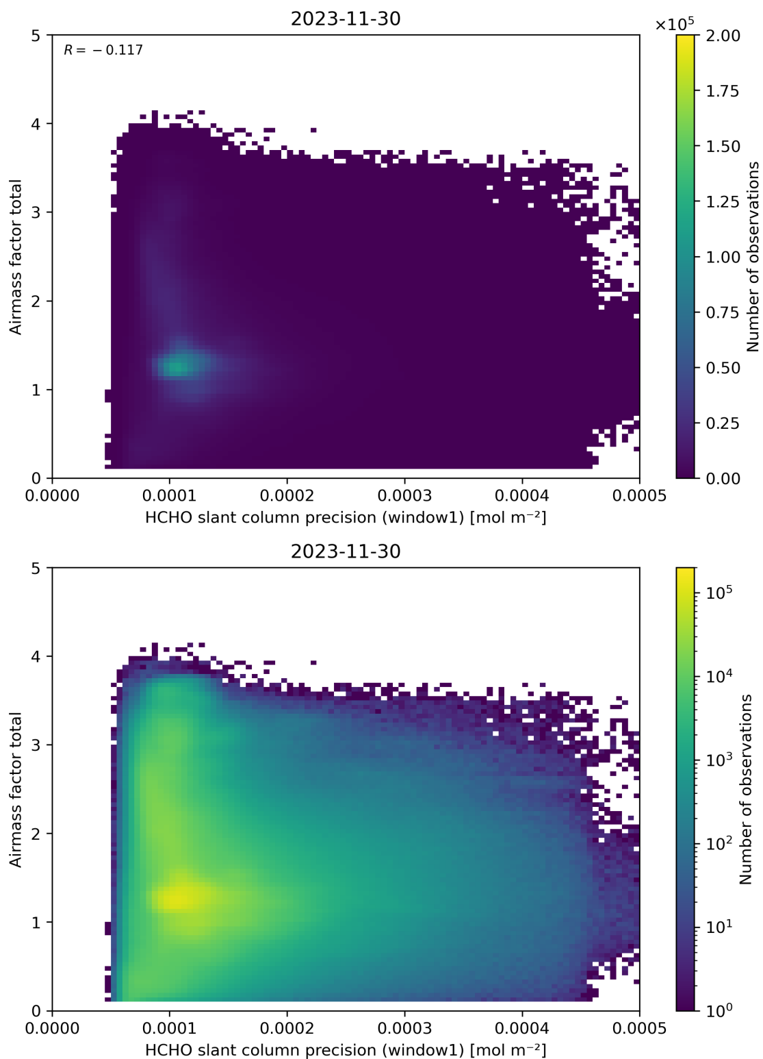
Figure 94: Scatter density plot of “HCHO slant column precision (window1)” against “Airmass factor total” for 2023-11-29 to 2023-12-01.
