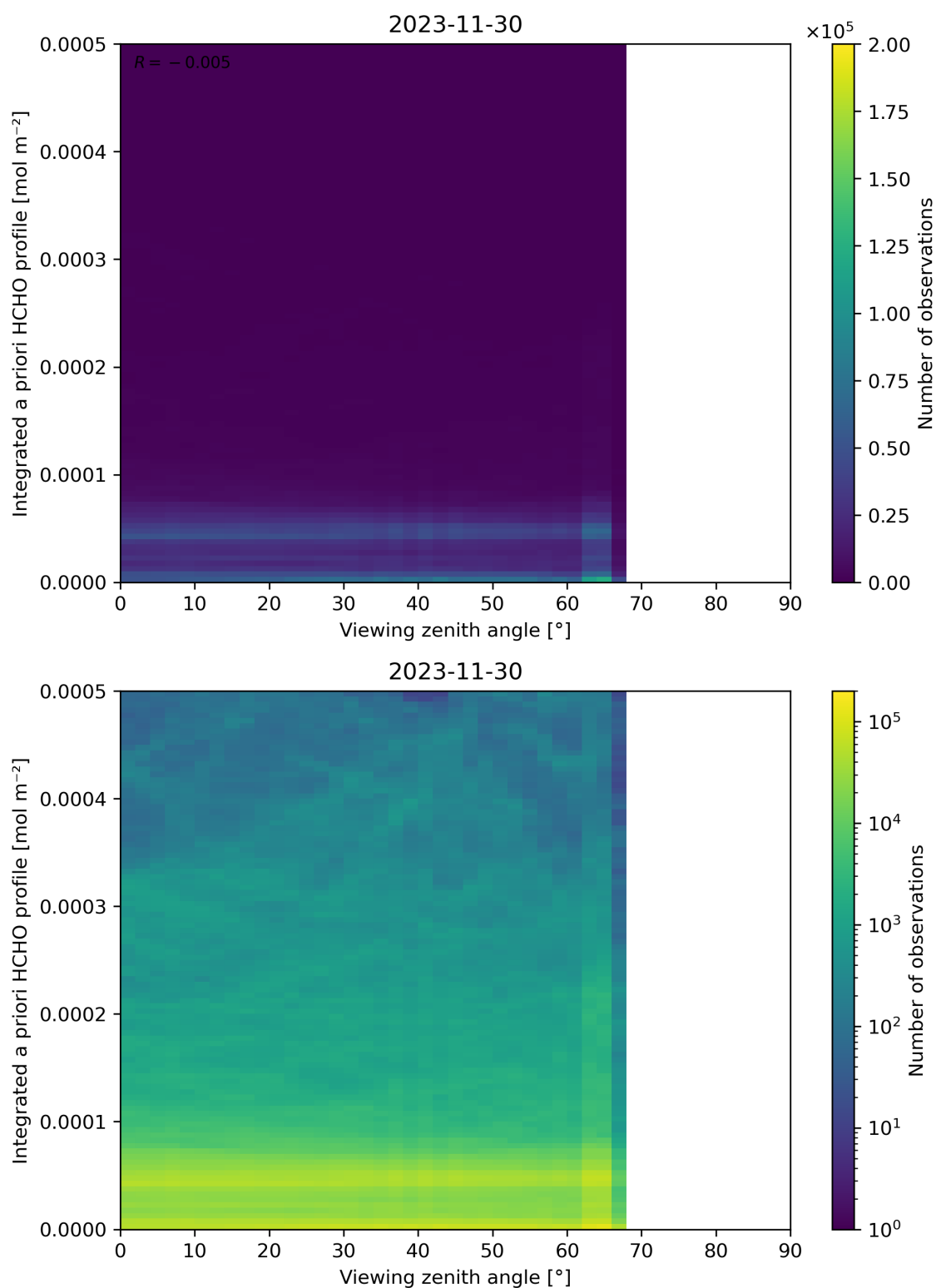
Figure 195: Scatter density plot of “Viewing zenith angle” against “Integrated a priori HCHO profile” for 2023-11-29 to 2023-12-01.
