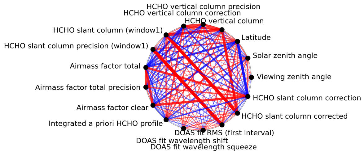
Figure 1: Map of correlation graph for 2023-11-29 to 2023-12-01.
