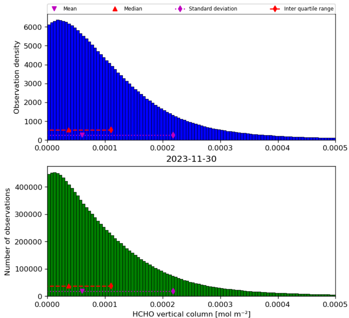
Figure 35: Histogram of “HCHO vertical column” for 2023-11-29 to 2023-12-01
