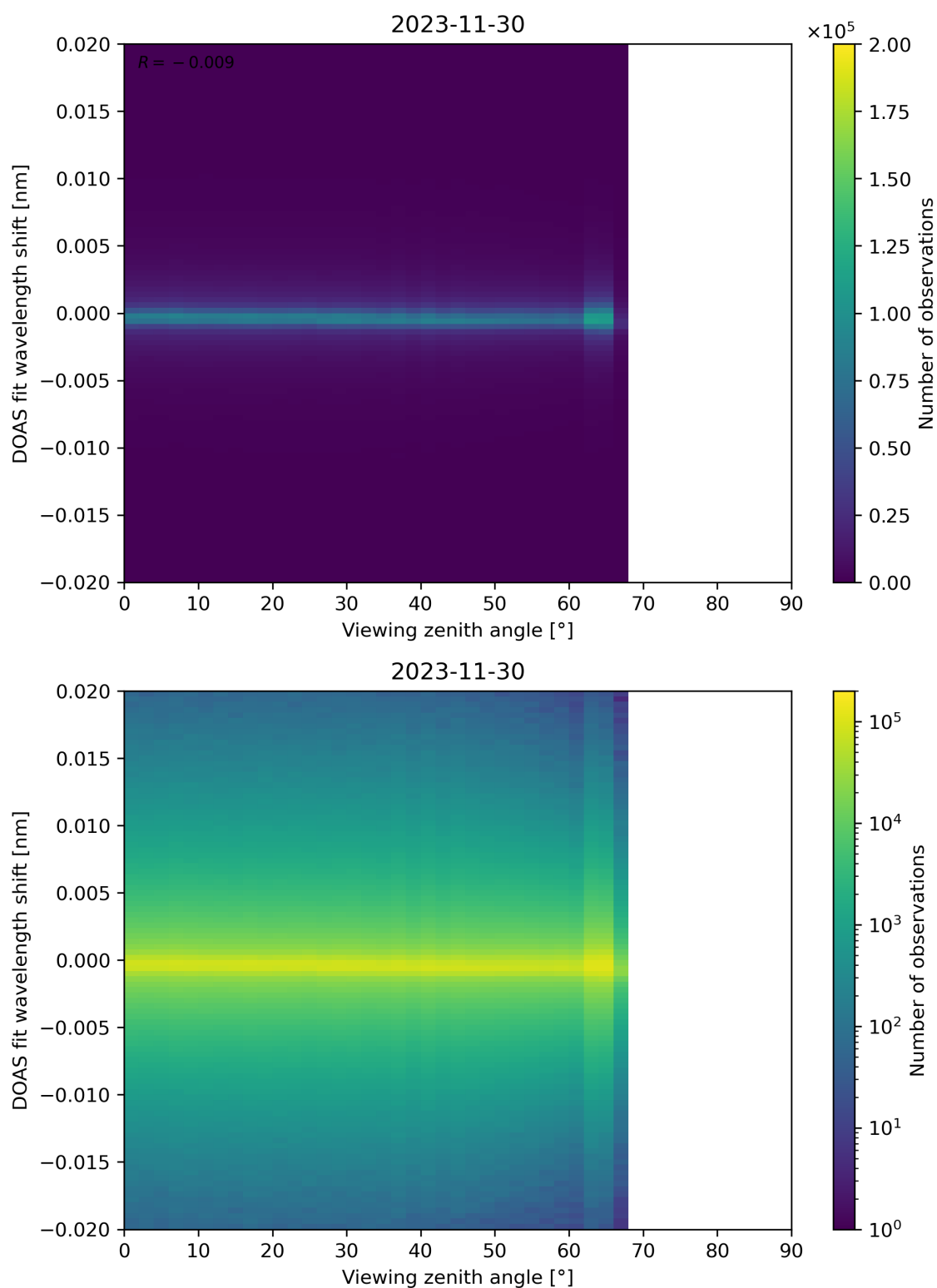
Figure 183: Scatter density plot of “Viewing zenith angle” against “DOAS fit wavelength shift” for 2023-11-29 to 2023-12-01.
