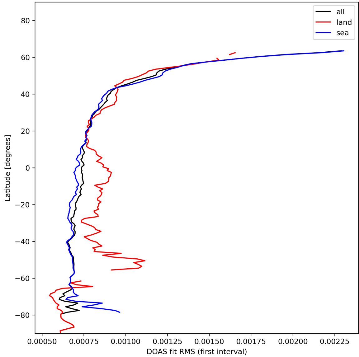
Figure 32: Zonal average of “DOAS fit RMS (first interval)” for 2023-11-29 to 2023-12-01.
