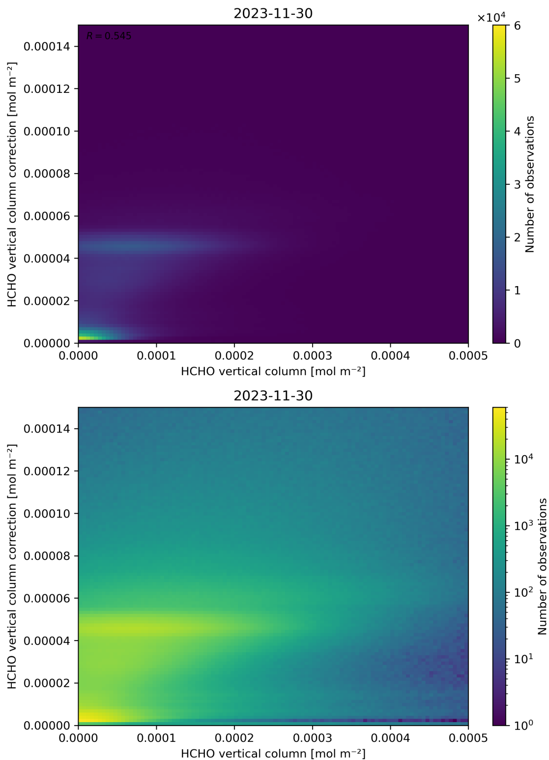
Figure 133: Scatter density plot of “HCHO vertical column” against “HCHO vertical column correction” for 2023-11-29 to 2023-12-01.
