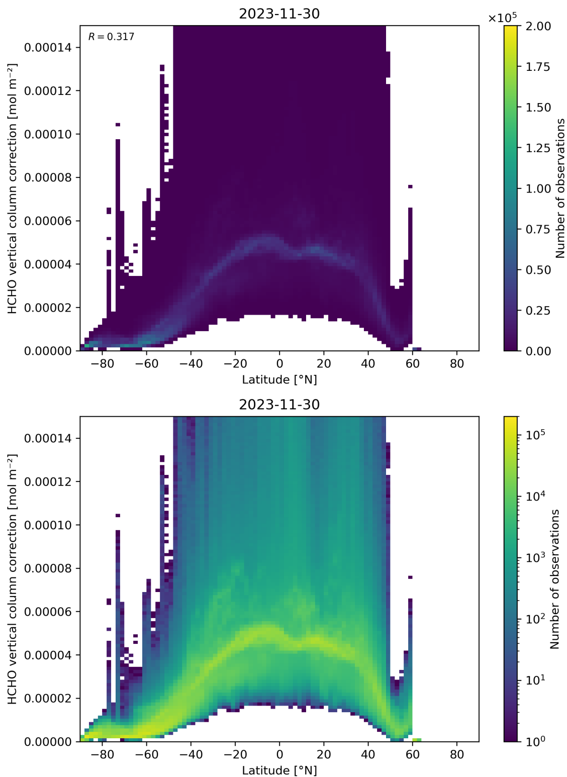
Figure 164: Scatter density plot of “Latitude” against “HCHO vertical column correction” for 2023-11-29 to 2023-12-01.
