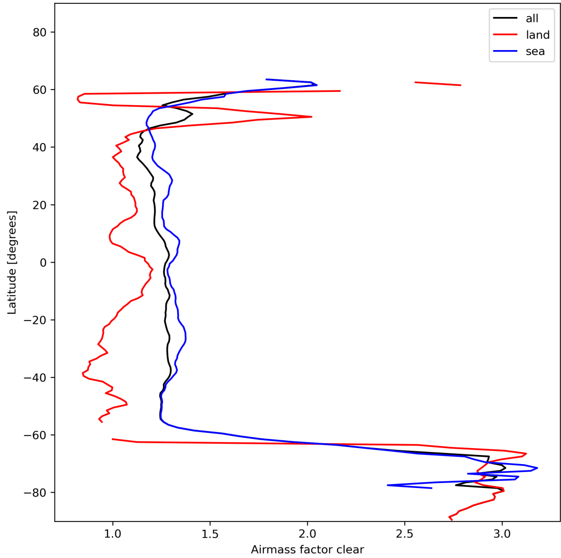
Figure 28: Zonal average of “Airmass factor clear” for 2023-11-29 to 2023-12-01.
