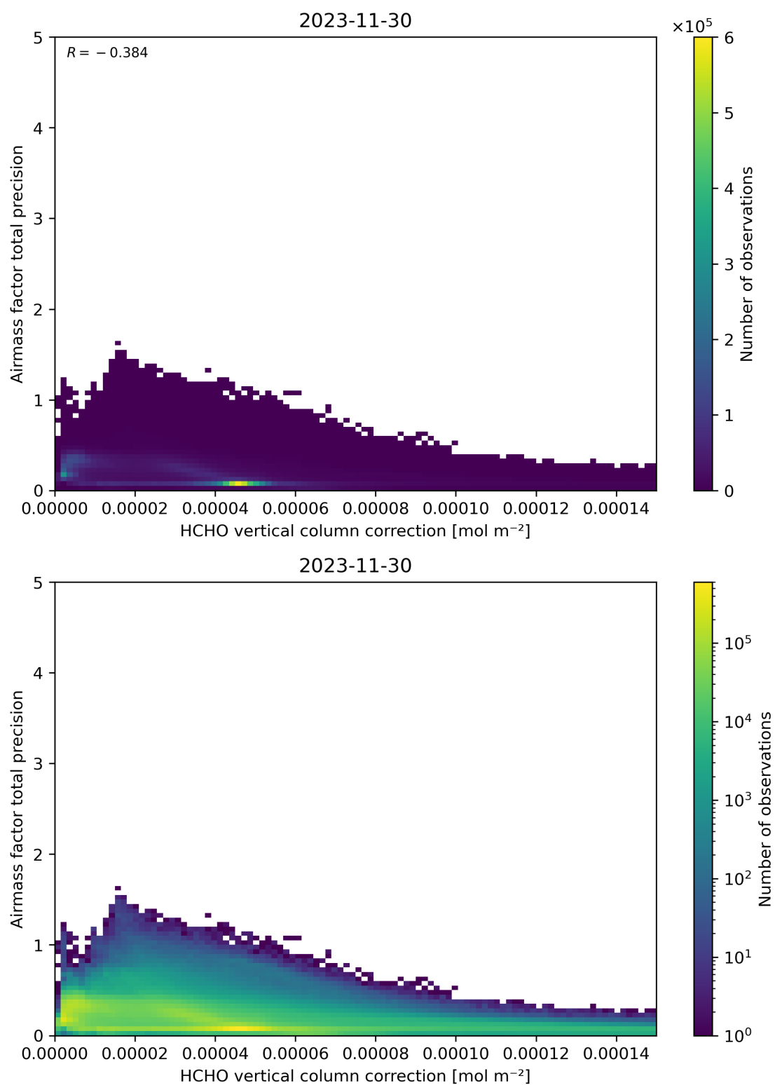
Figure 121: Scatter density plot of “HCHO vertical column correction” against “Airmass factor total precision” for 2023-11-29 to 2023-12-01.
