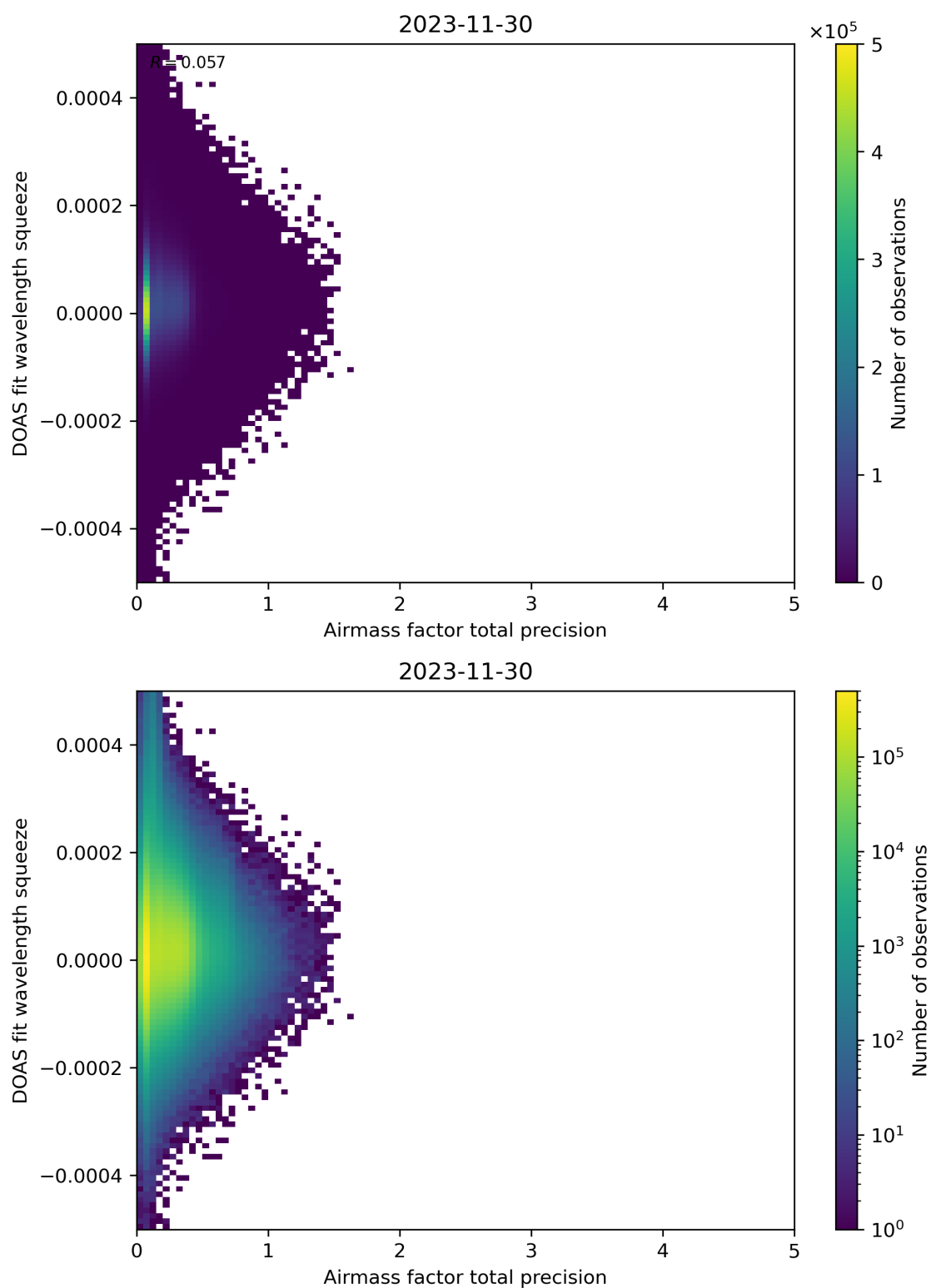
Figure 107: Scatter density plot of “Airmass factor total precision” against “DOAS fit wavelength squeeze” for 2023-11-29 to 2023-12-01.
