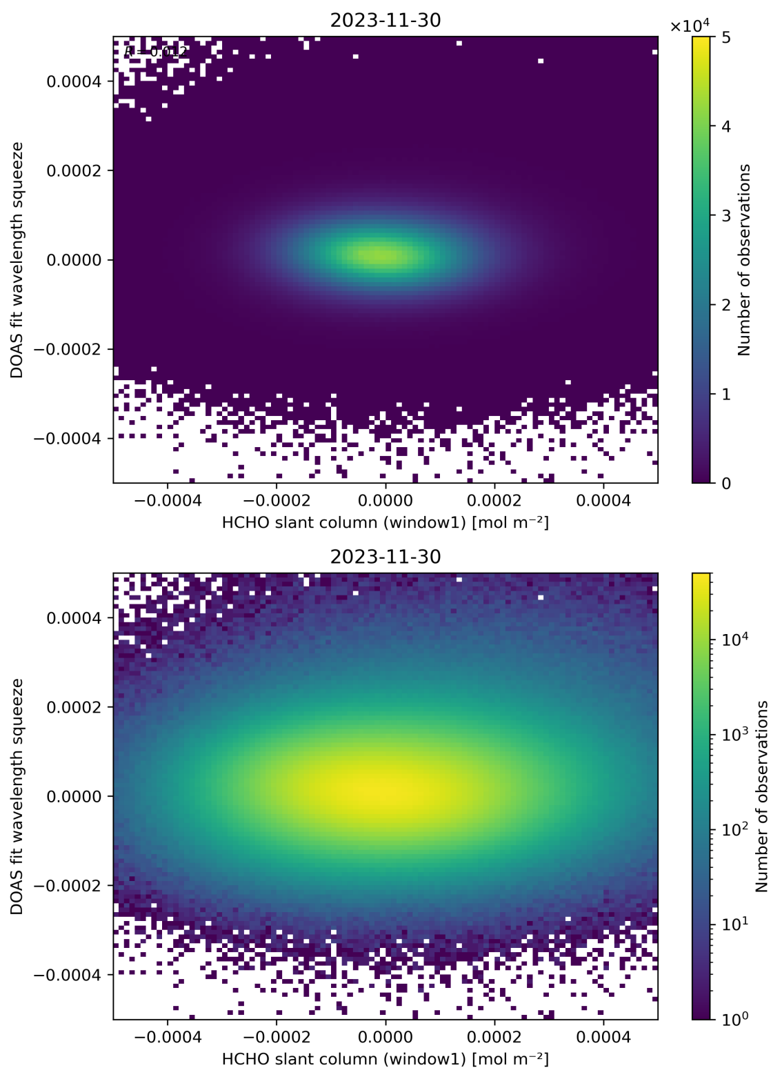
Figure 80: Scatter density plot of “HCHO slant column (window1)” against “DOAS fit wavelength squeeze” for 2023-11-29 to 2023-12-01.
