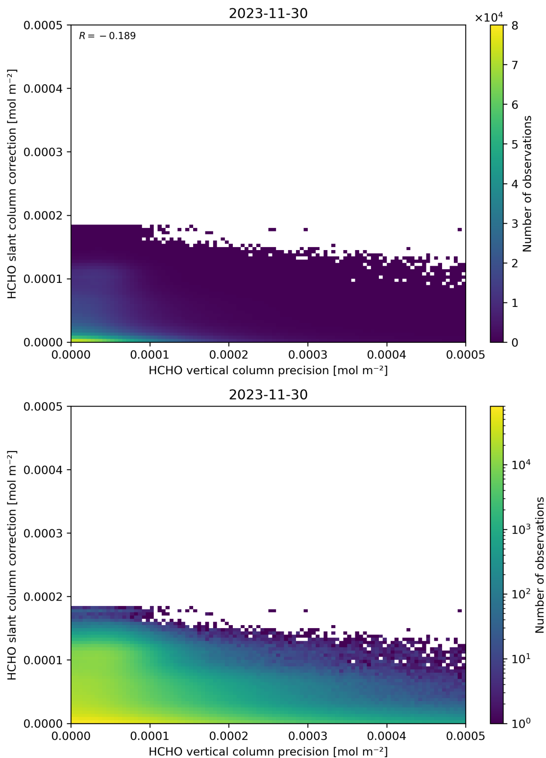
Figure 141: Scatter density plot of “HCHO vertical column precision” against “HCHO slant column correction” for 2023-11-29 to 2023-12-01.
