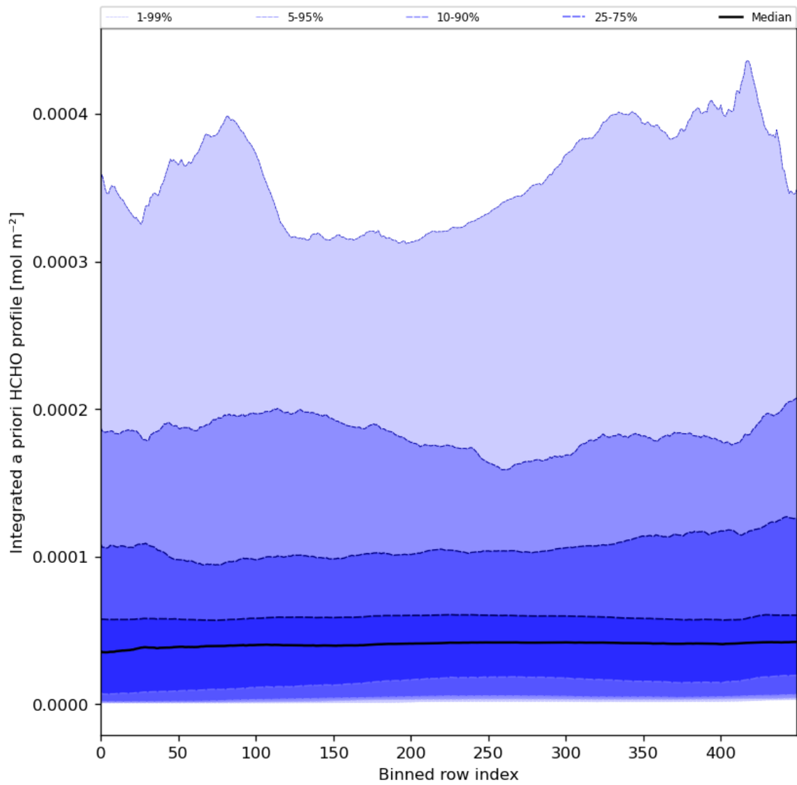
Figure 57: Along track statistics of “Integrated a priori HCHO profile” for 2023-11-29 to 2023-12-01
