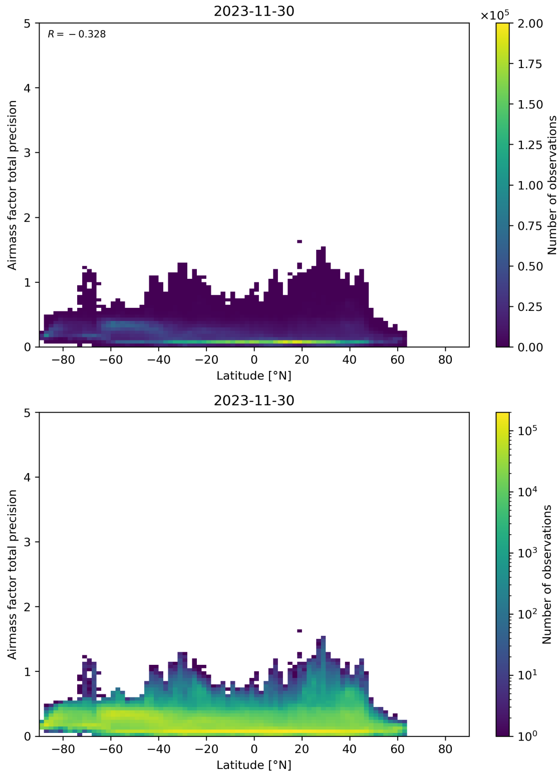
Figure 162: Scatter density plot of “Latitude” against “Airmass factor total precision” for 2023-11-29 to 2023-12-01.
