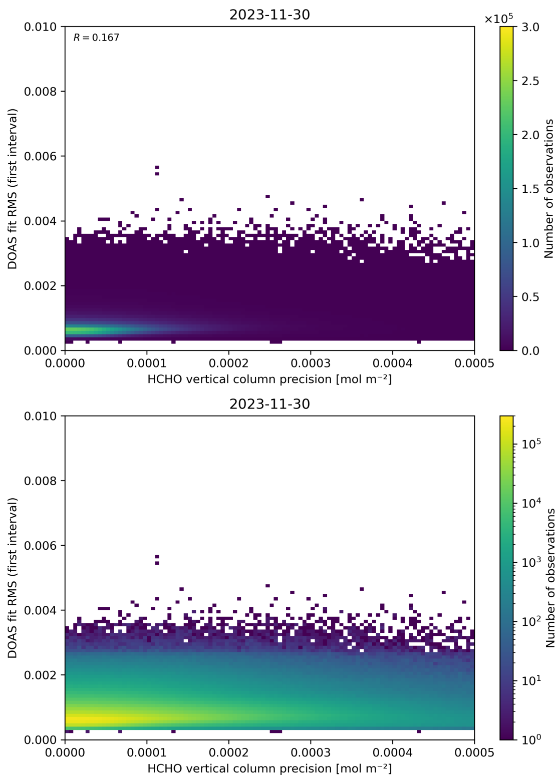
Figure 136: Scatter density plot of “HCHO vertical column precision” against “DOAS fit RMS (first interval)” for 2023-11-29 to 2023-12-01.
