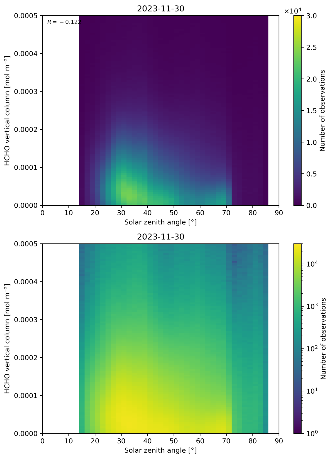
Figure 177: Scatter density plot of “Solar zenith angle” against “HCHO vertical column” for 2023-11-29 to 2023-12-01.
