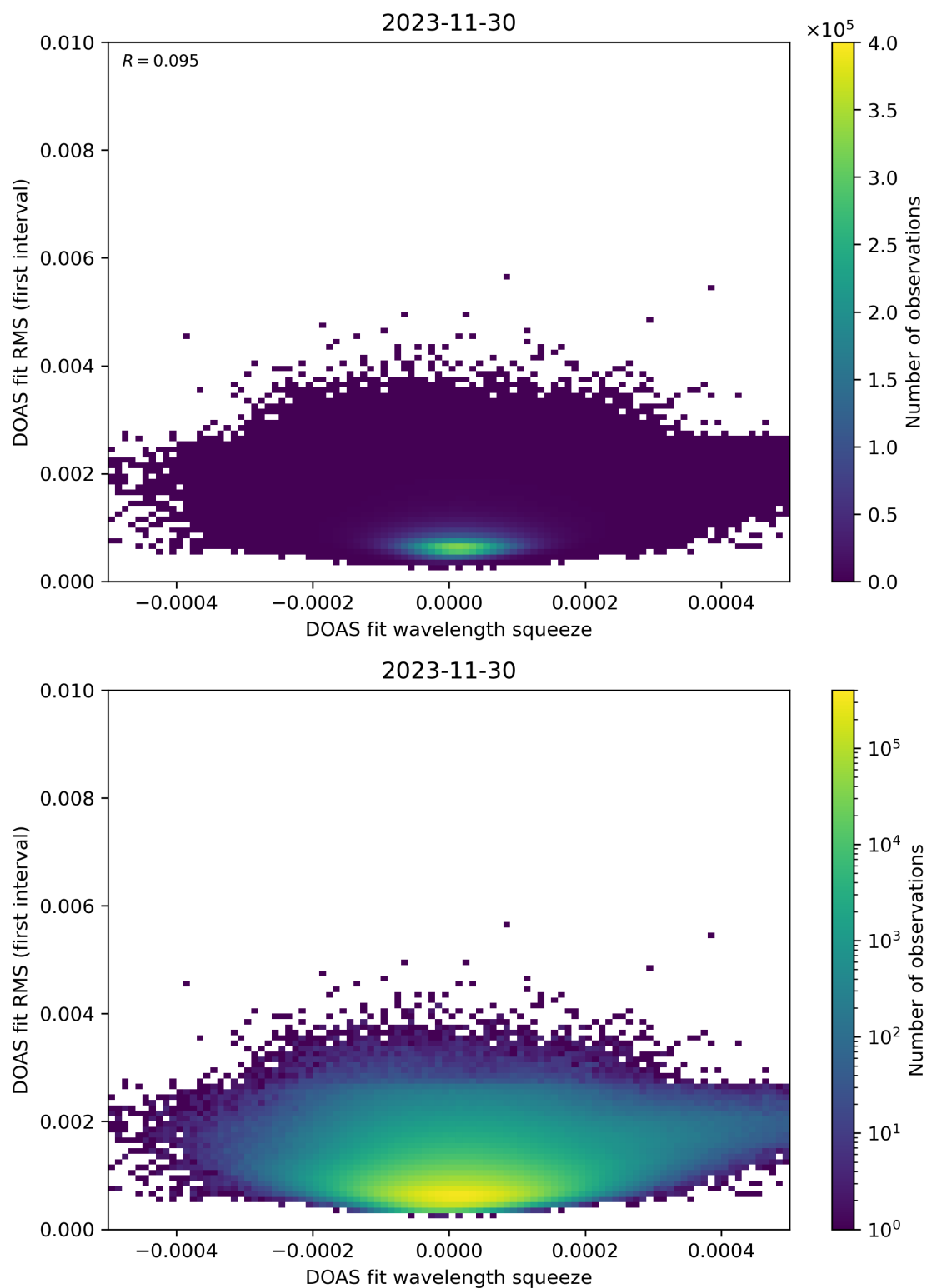
Figure 68: Scatter density plot of “DOAS fit wavelength squeeze” against “DOAS fit RMS (first interval)” for 2023-11-29 to 2023-12-01.
