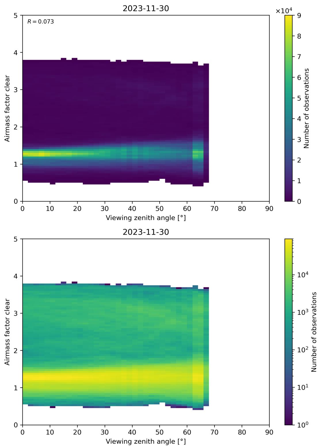
Figure 185: Scatter density plot of “Viewing zenith angle” against “Airmass factor clear” for 2023-11-29 to 2023-12-01.
