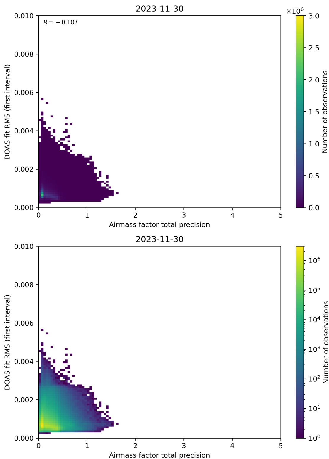
Figure 105: Scatter density plot of “Airmass factor total precision” against “DOAS fit RMS (first interval)” for 2023-11-29 to 2023-12-01.
