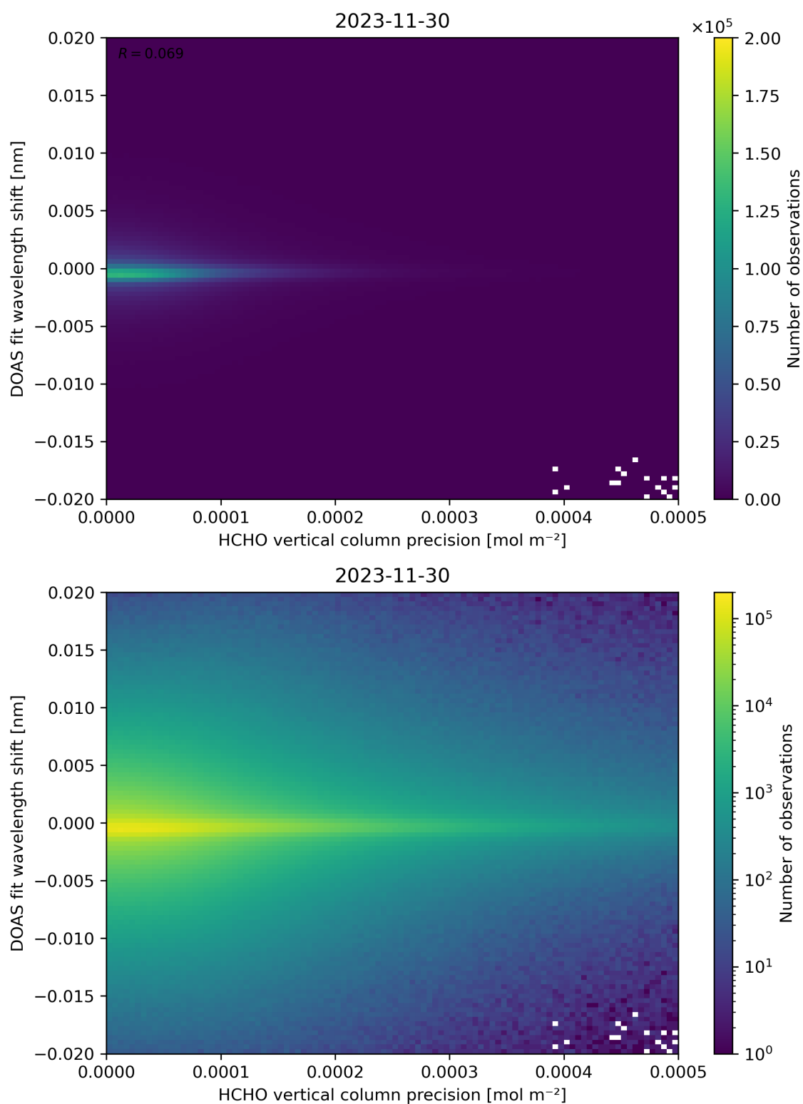
Figure 137: Scatter density plot of “HCHO vertical column precision” against “DOAS fit wavelength shift” for 2023-11-29 to 2023-12-01.
