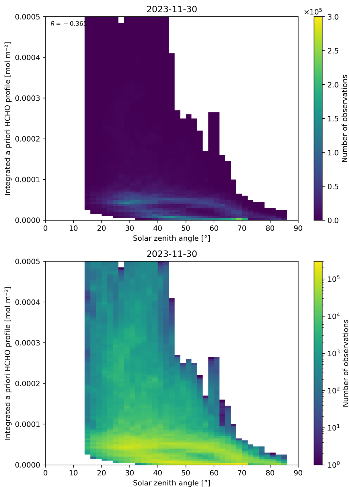
Figure 180: Scatter density plot of “Solar zenith angle” against “Integrated a priori HCHO profile” for 2023-11-29 to 2023-12-01.
