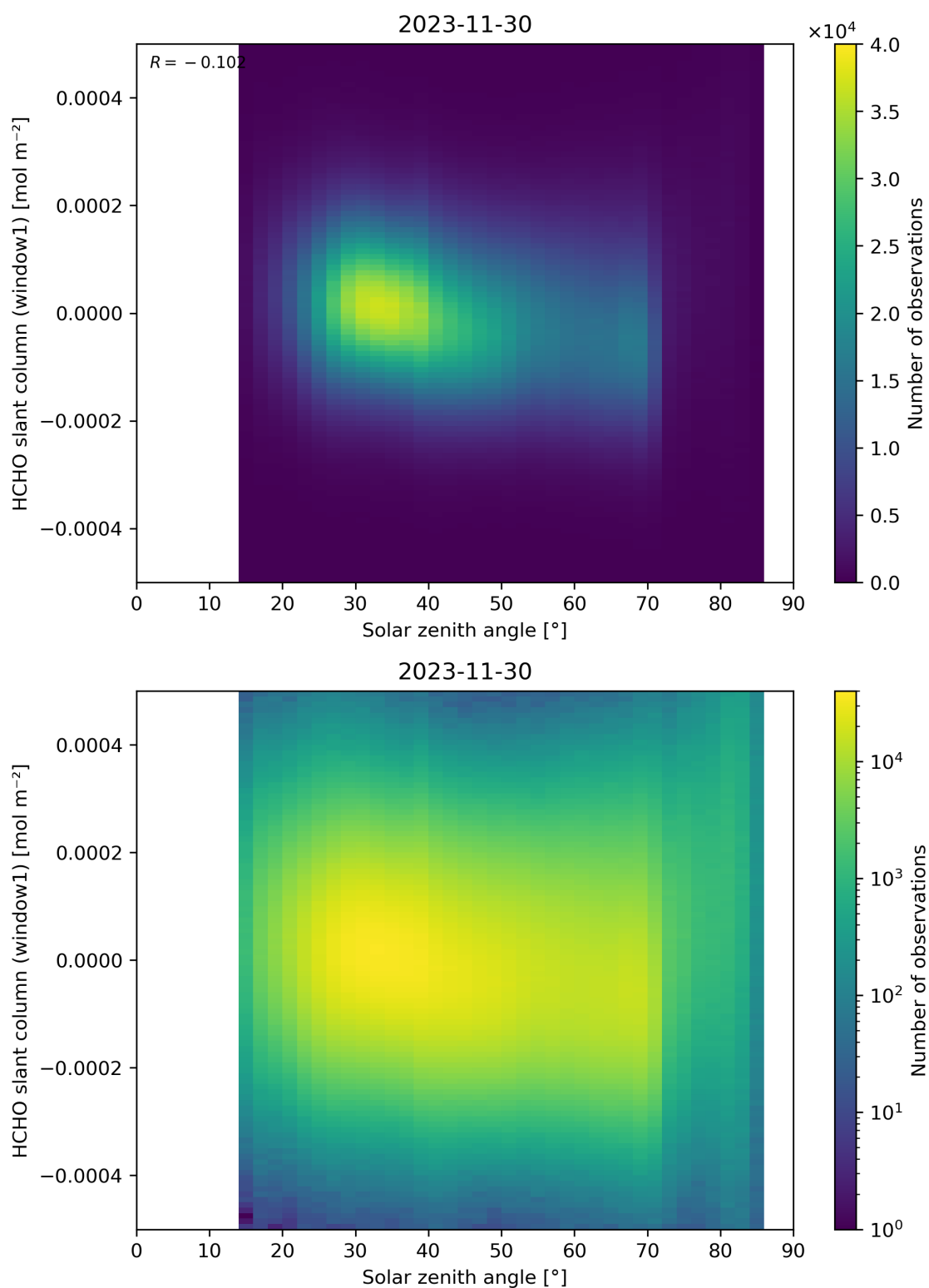
Figure 173: Scatter density plot of “Solar zenith angle” against “HCHO slant column (window1)” for 2023-11-29 to 2023-12-01.
