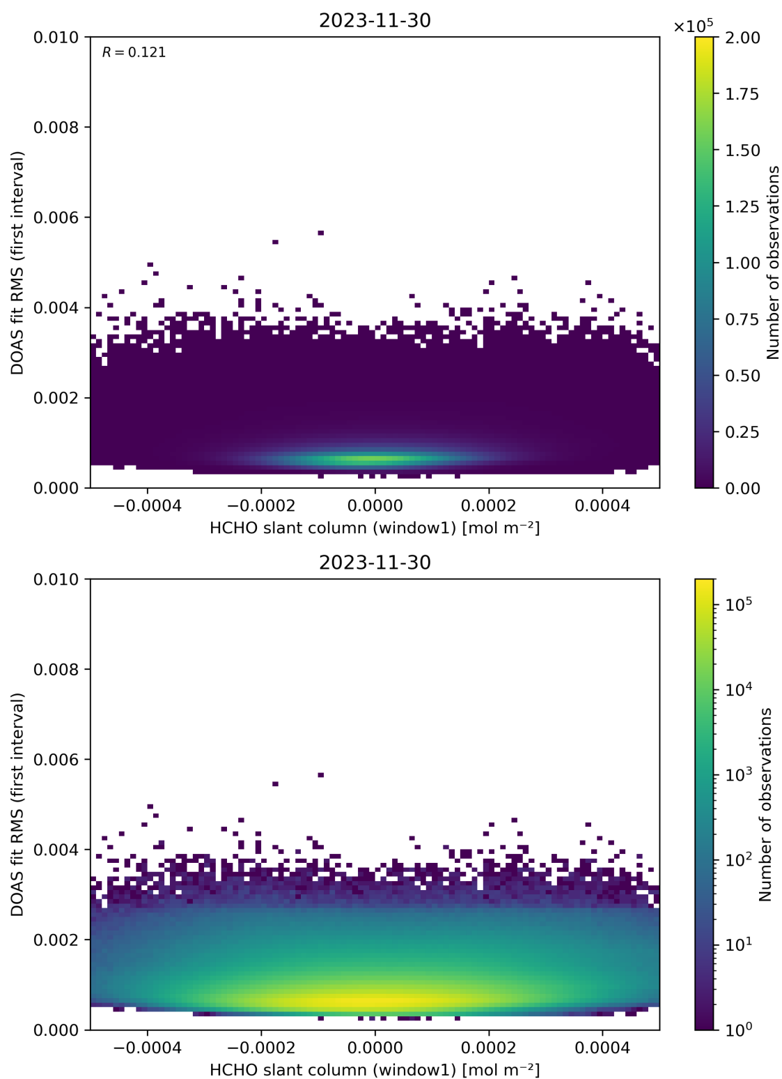
Figure 78: Scatter density plot of “HCHO slant column (window1)” against “DOAS fit RMS (first interval)” for 2023-11-29 to 2023-12-01.
