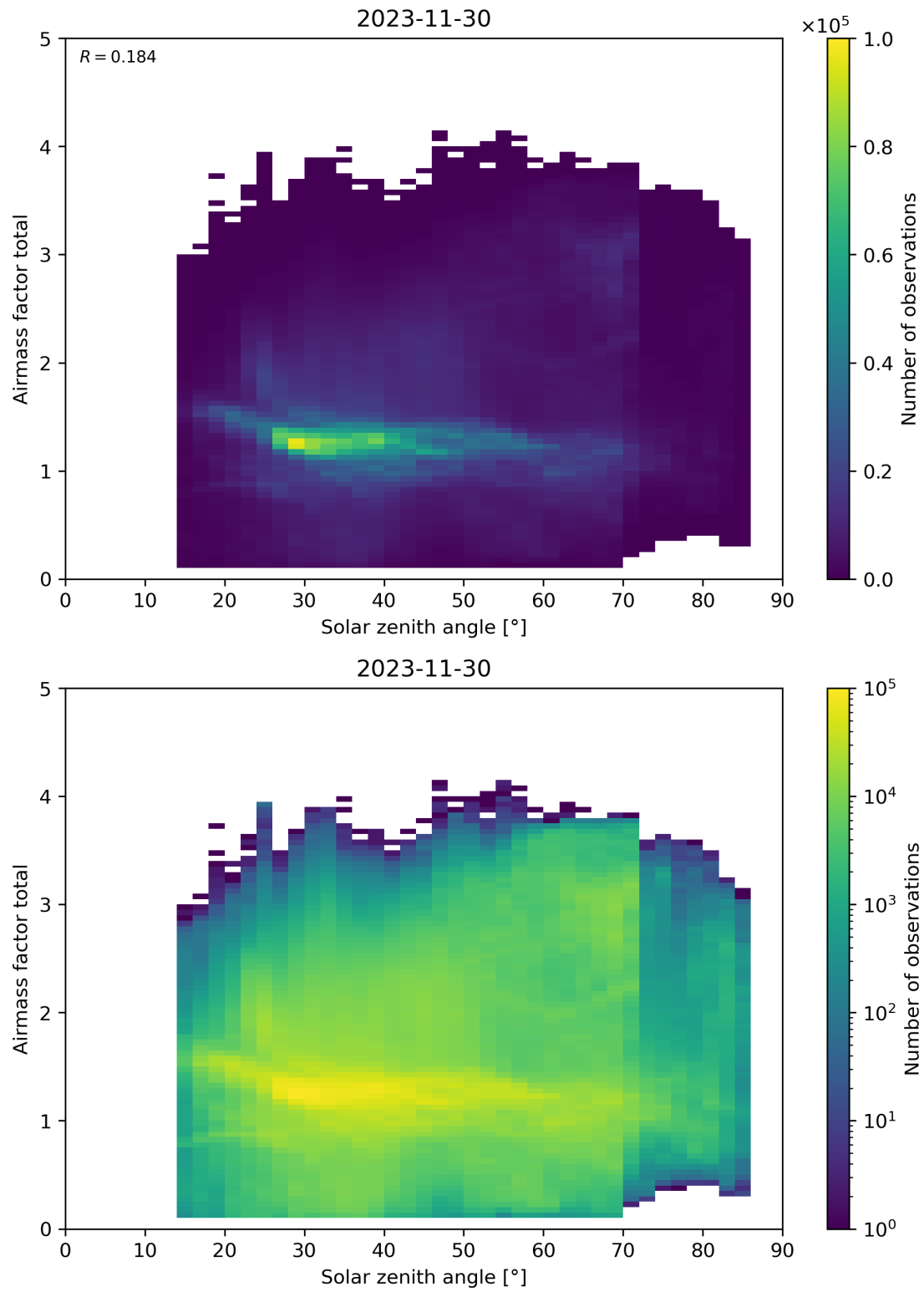
Figure 175: Scatter density plot of “Solar zenith angle” against “Airmass factor total” for 2023-11-29 to 2023-12-01.
