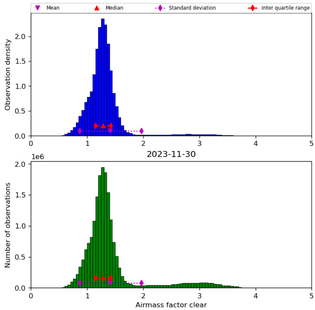
Figure 42: Histogram of “Airmass factor clear” for 2023-11-29 to 2023-12-01
