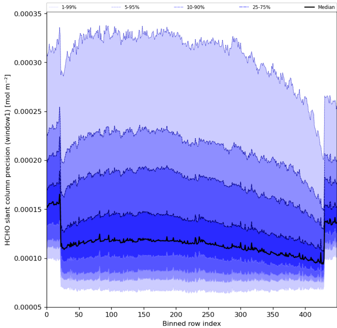
Figure 53: Along track statistics of “HCHO slant column precision (window1)” for 2023-11-29 to 2023-12-01
