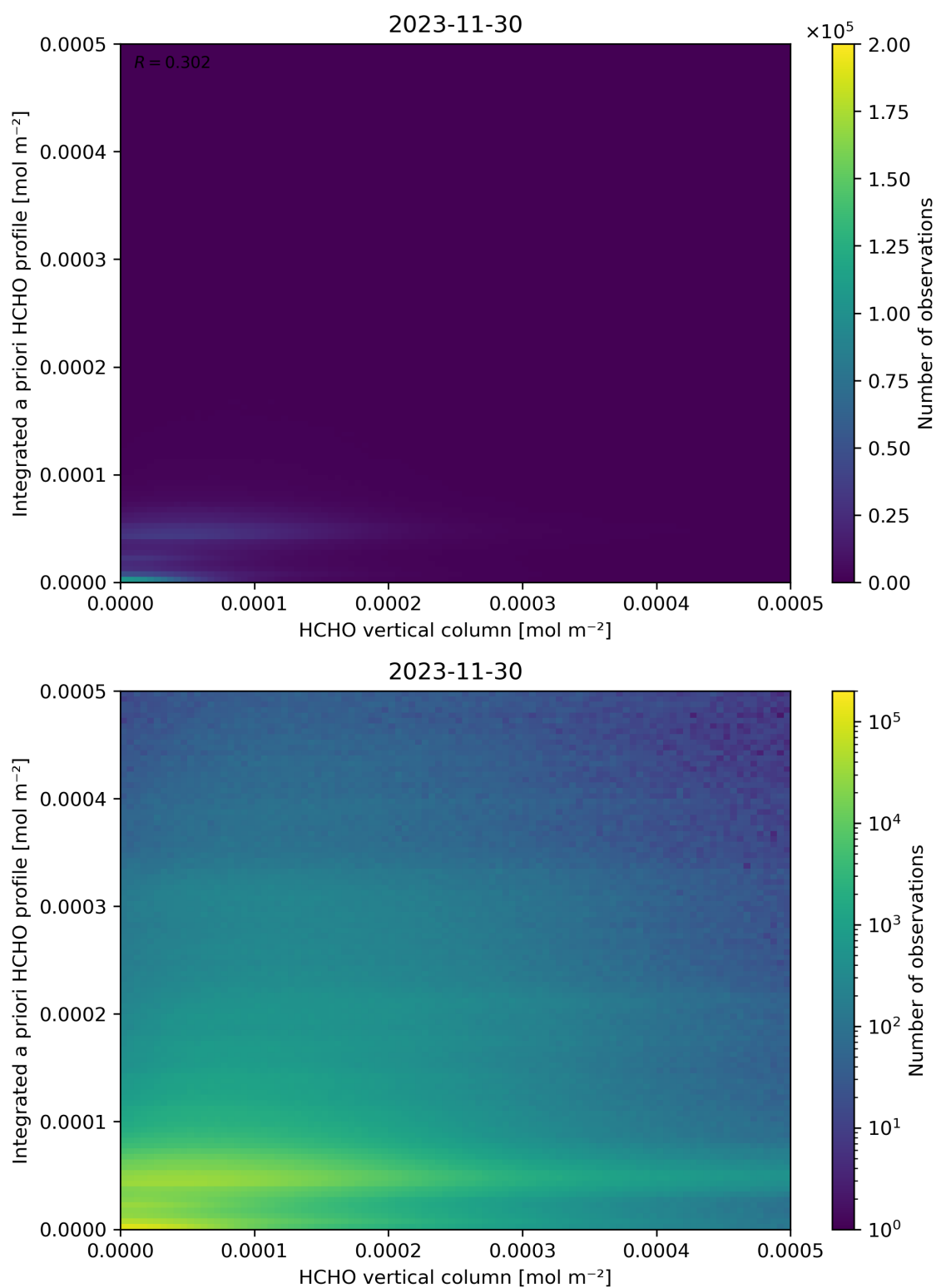
Figure 135: Scatter density plot of “HCHO vertical column” against “Integrated a priori HCHO profile” for 2023-11-29 to 2023-12-01.
