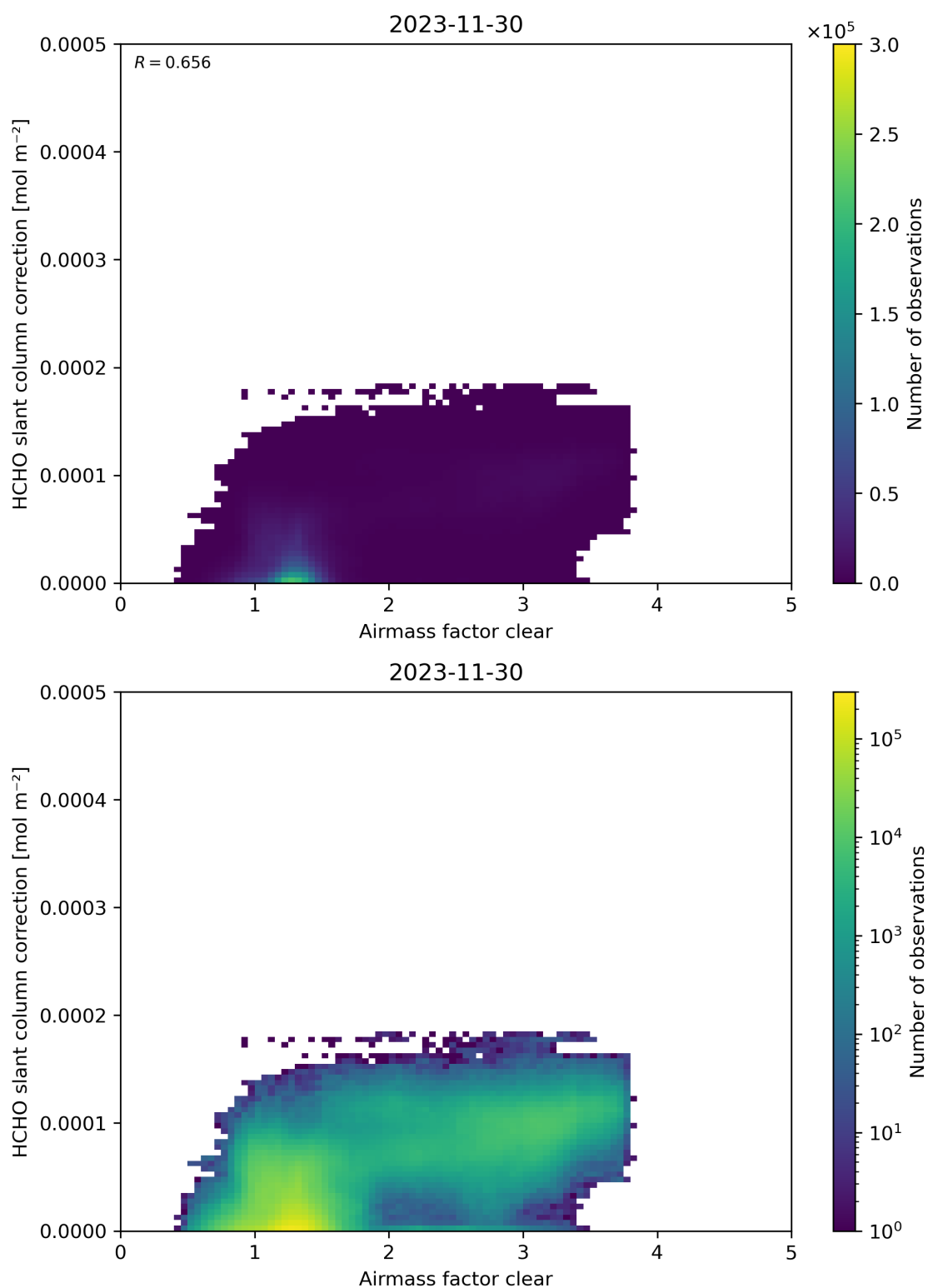
Figure 75: Scatter density plot of “Airmass factor clear” against “HCHO slant column correction” for 2023-11-29 to 2023-12-01.
