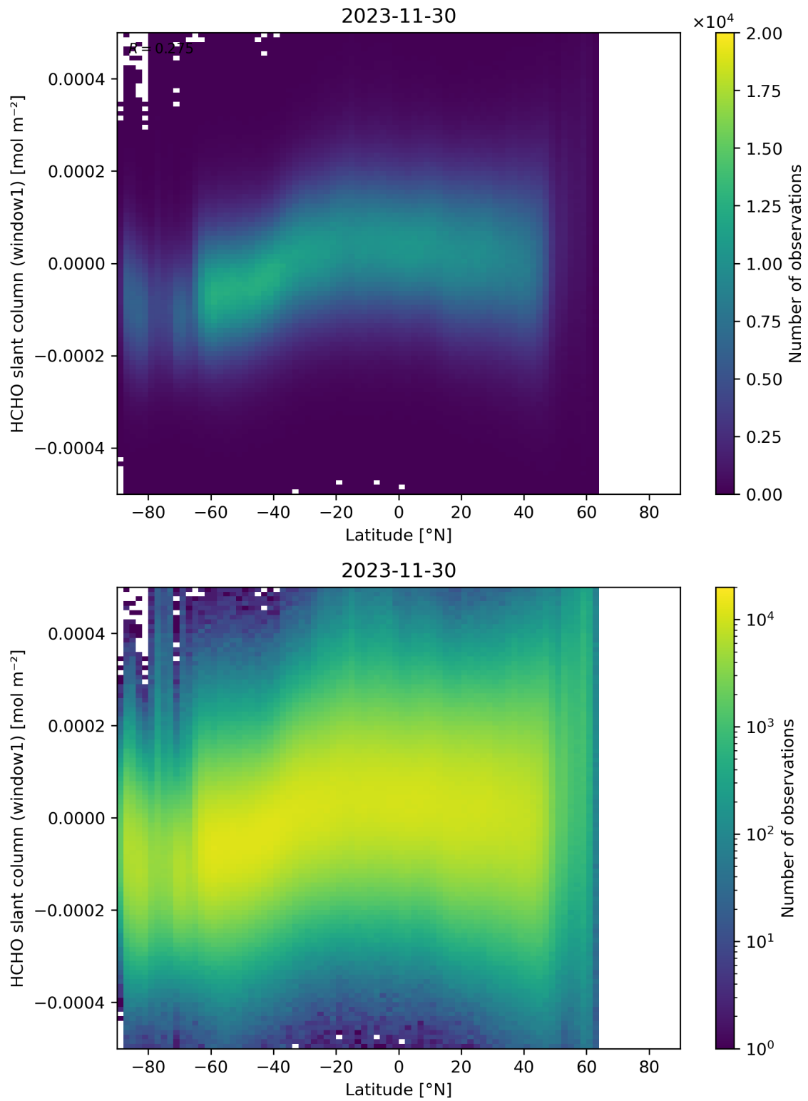
Figure 159: Scatter density plot of “Latitude” against “HCHO slant column (window1)” for 2023-11-29 to 2023-12-01.
