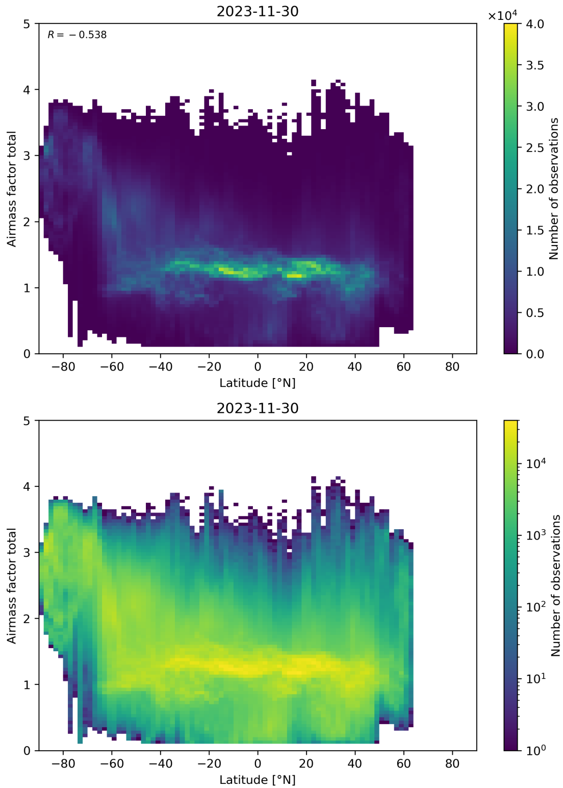
Figure 161: Scatter density plot of “Latitude” against “Airmass factor total” for 2023-11-29 to 2023-12-01.
