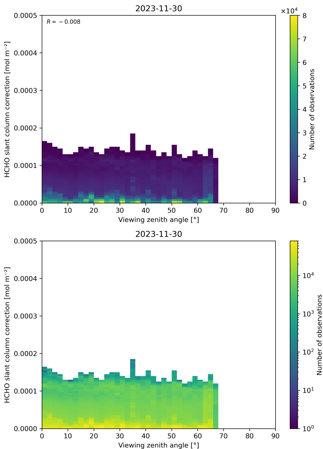
Figure 187: Scatter density plot of “Viewing zenith angle” against “HCHO slant column correction” for 2023-11-29 to 2023-12-01.
