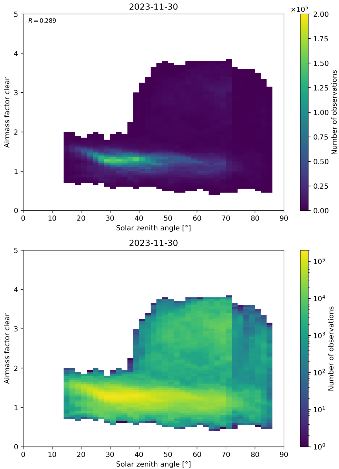
Figure 170: Scatter density plot of “Solar zenith angle” against “Airmass factor clear” for 2023-11-29 to 2023-12-01.
