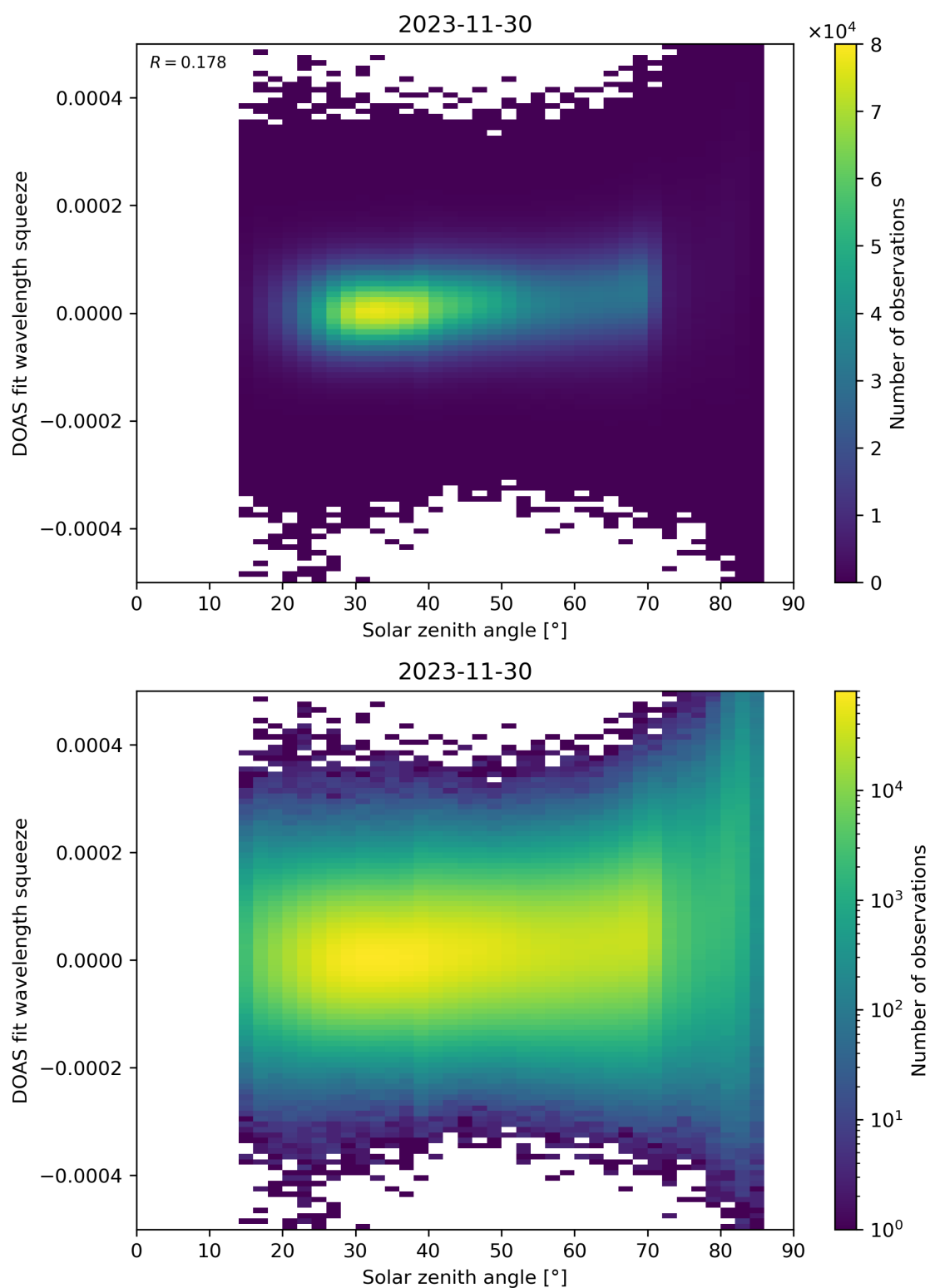
Figure 169: Scatter density plot of “Solar zenith angle” against “DOAS fit wavelength squeeze” for 2023-11-29 to 2023-12-01.
