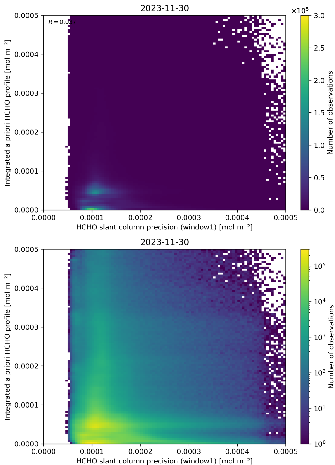
Figure 96: Scatter density plot of “HCHO slant column precision (window1)” against “Integrated a priori HCHO profile” for 2023-11-29 to 2023-12-01.
