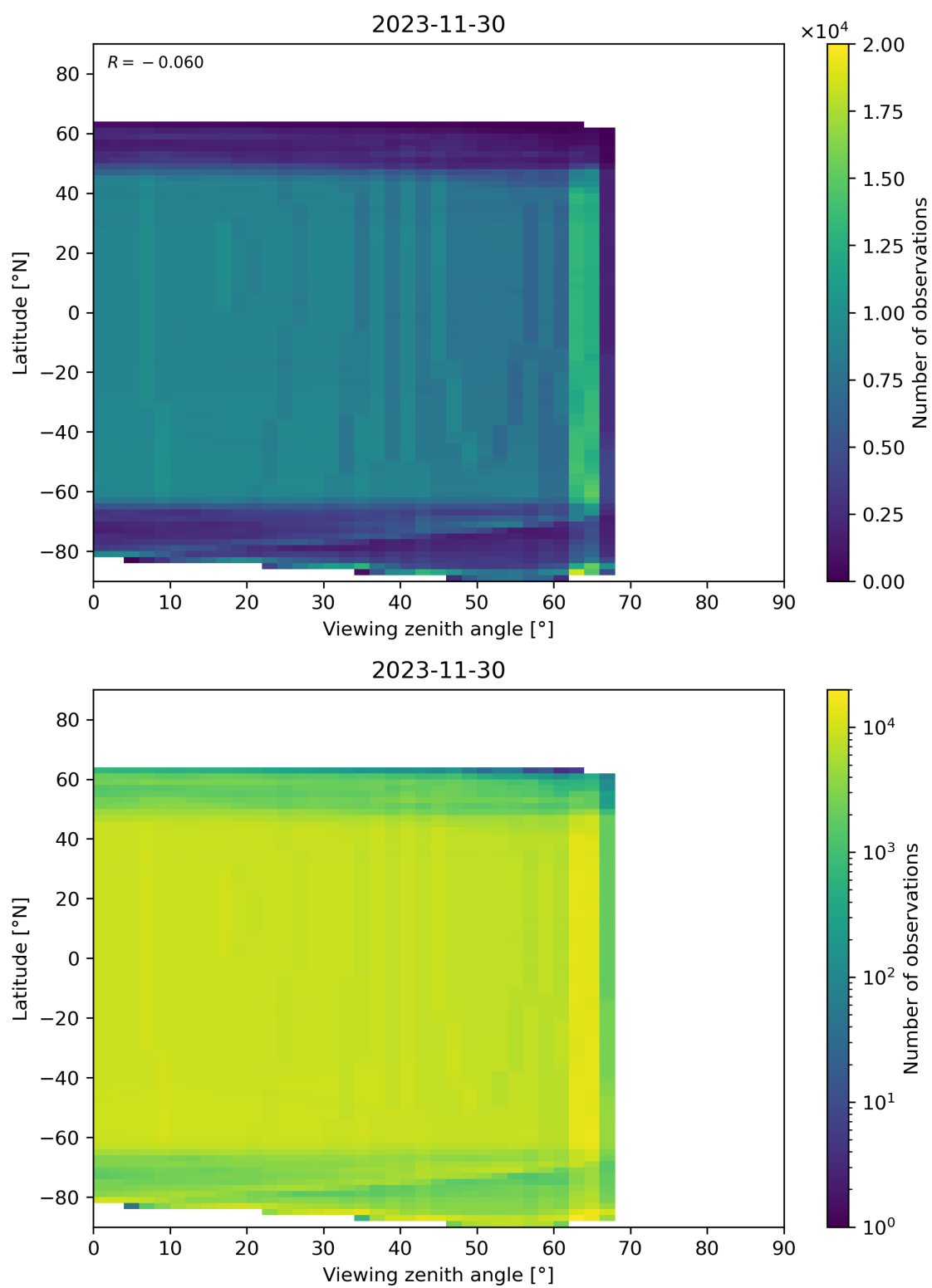
Figure 196: Scatter density plot of “Viewing zenith angle” against “Latitude” for 2023-11-29 to 2023-12-01.
