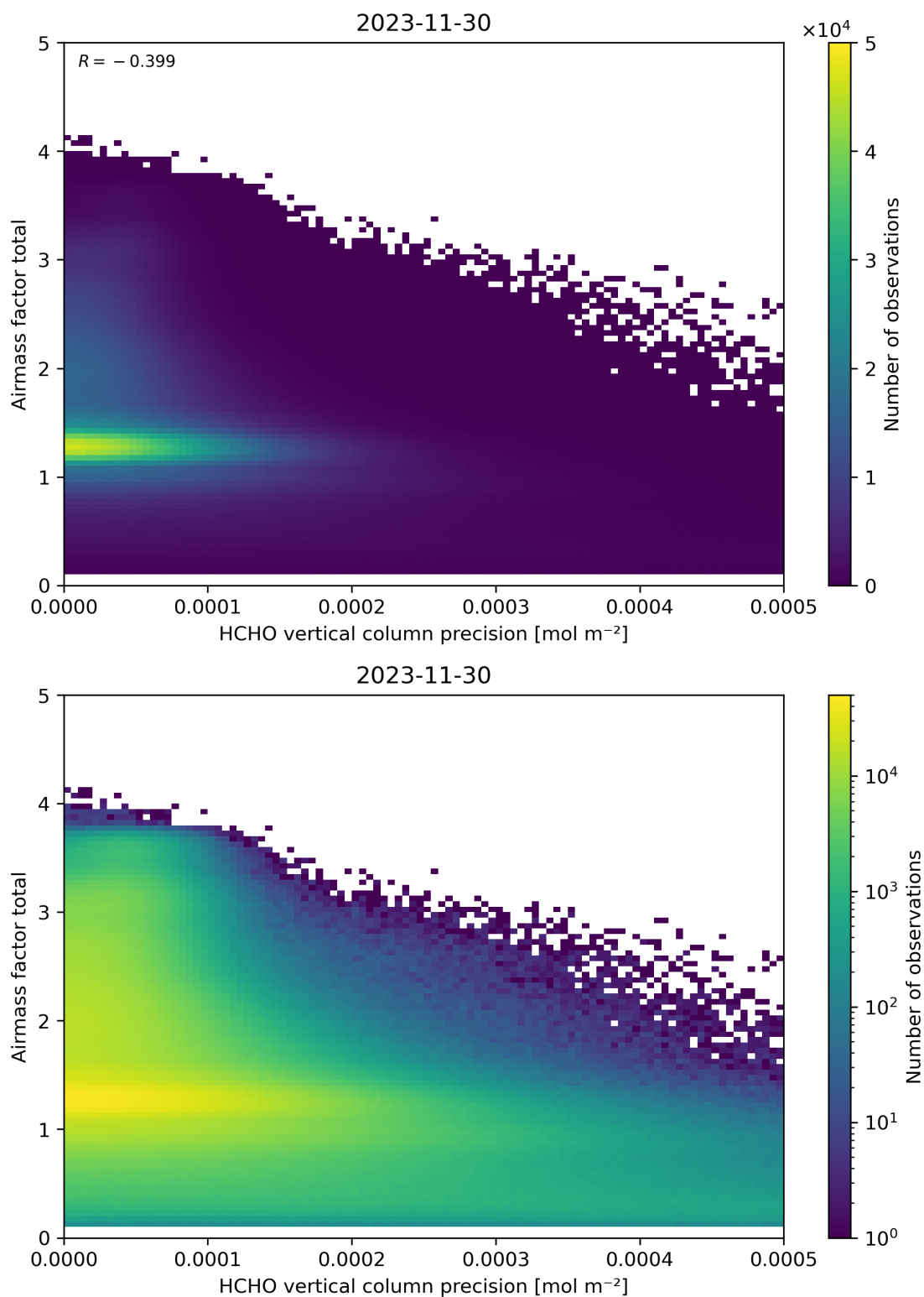
Figure 144: Scatter density plot of “HCHO vertical column precision” against “Airmass factor total” for 2023-11-29 to 2023-12-01.
