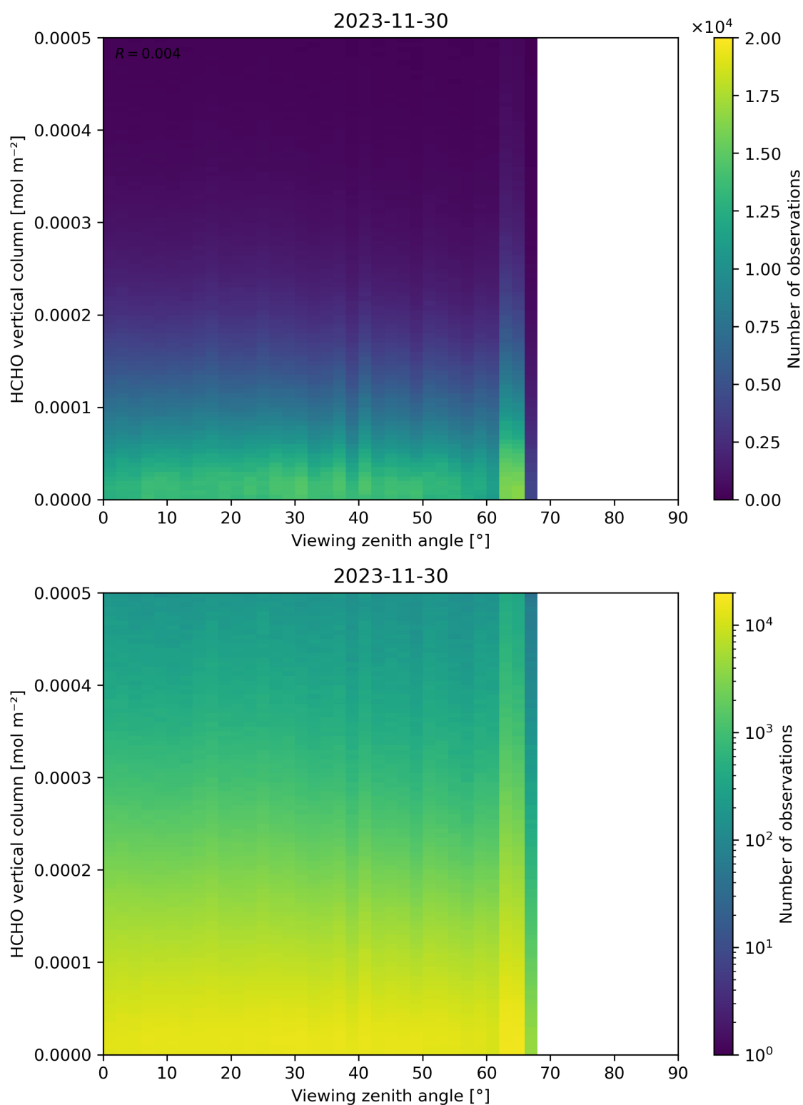
Figure 192: Scatter density plot of “Viewing zenith angle” against “HCHO vertical column” for 2023-11-29 to 2023-12-01.
