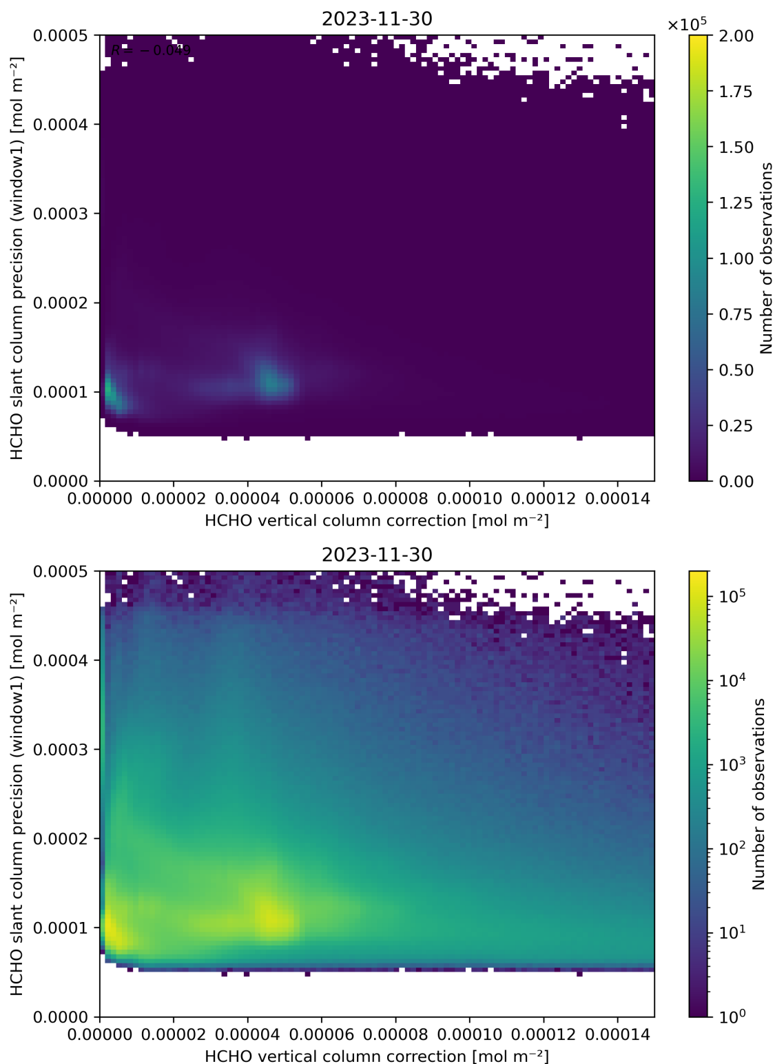
Figure 119: Scatter density plot of “HCHO vertical column correction” against “HCHO slant column precision (window1)” for 2023-11-29 to 2023-12-01.
