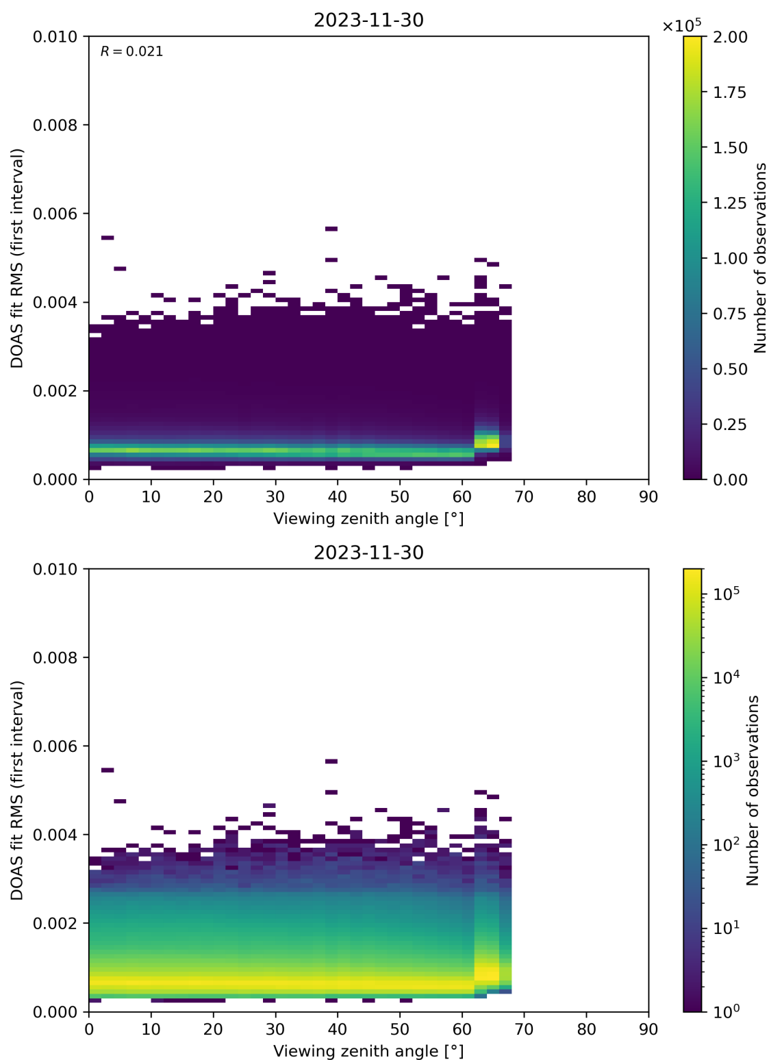
Figure 182: Scatter density plot of “Viewing zenith angle” against “DOAS fit RMS (first interval)” for 2023-11-29 to 2023-12-01.
