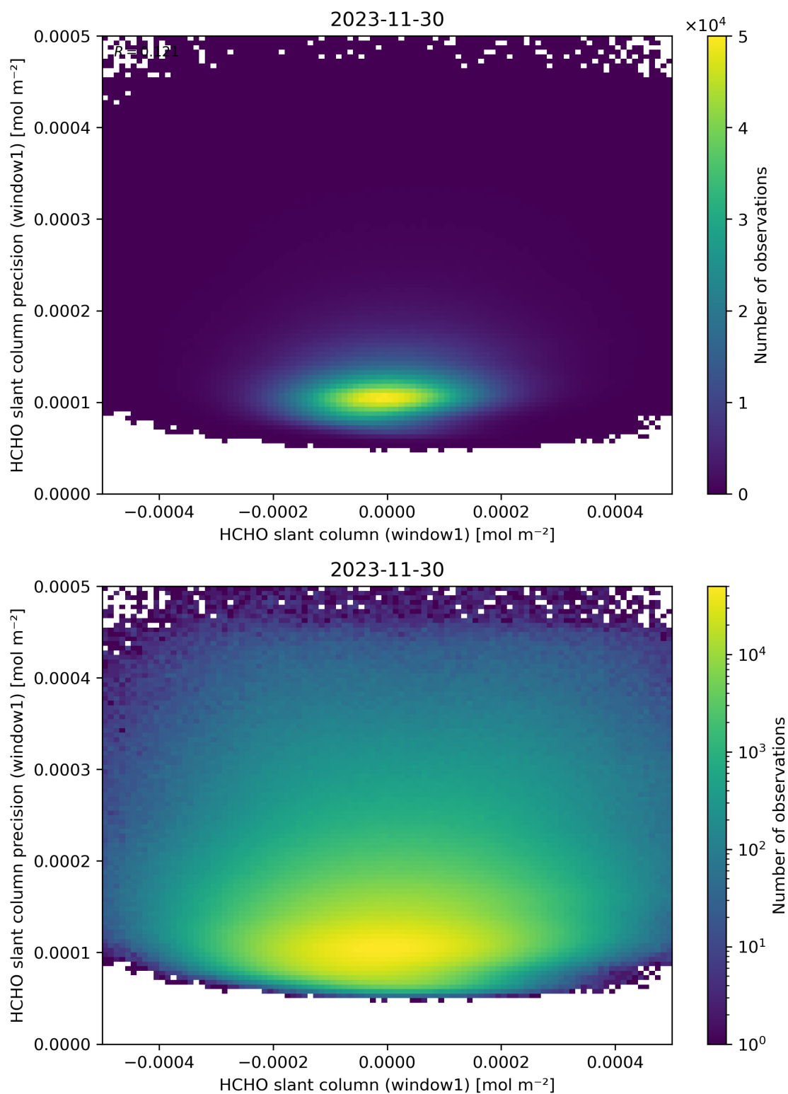
Figure 84: Scatter density plot of “HCHO slant column (window1)” against “HCHO slant column precision (window1)” for 2023-11-29 to 2023-12-01.
