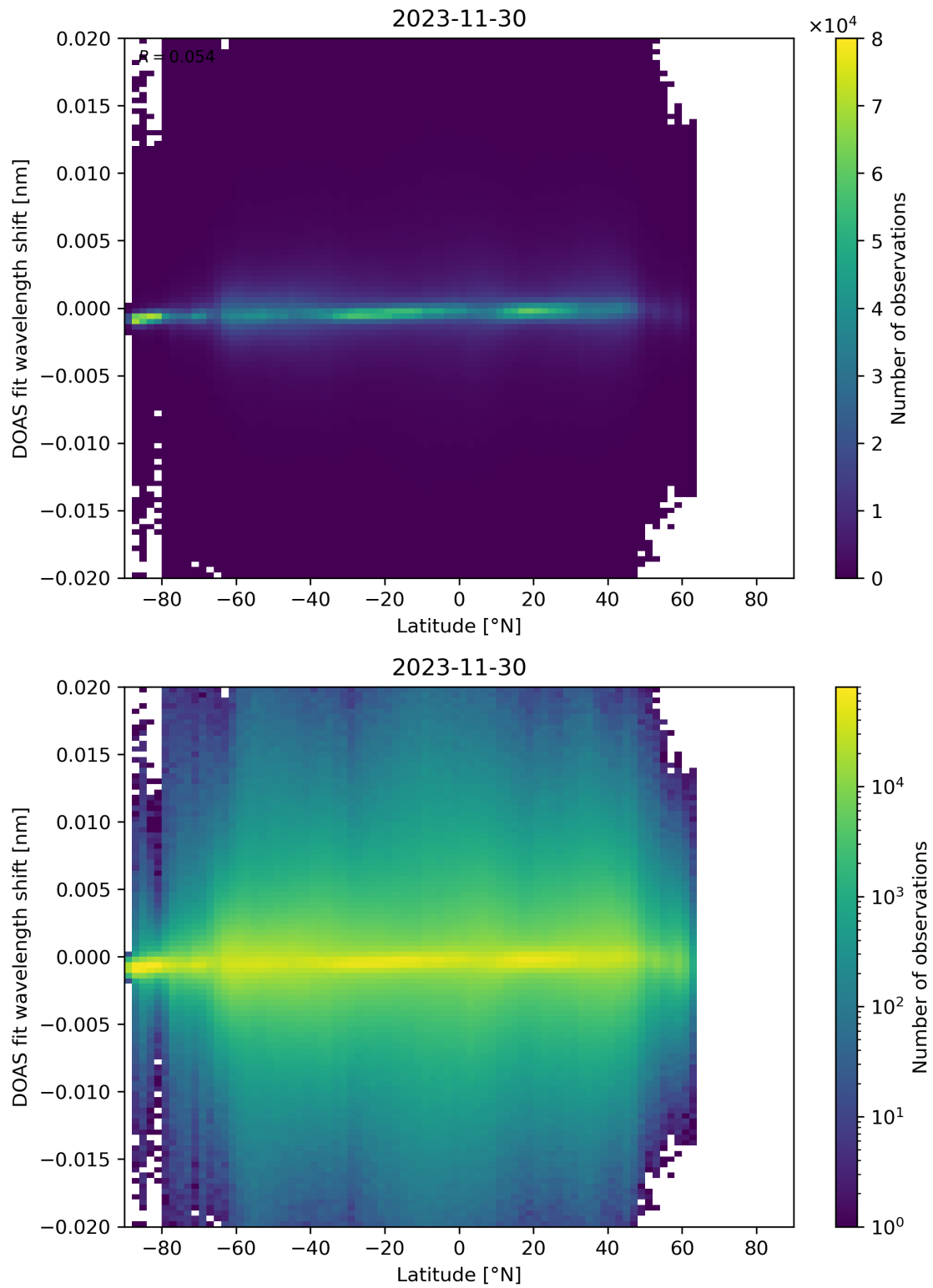
Figure 154: Scatter density plot of “Latitude” against “DOAS fit wavelength shift” for 2023-11-29 to 2023-12-01.
