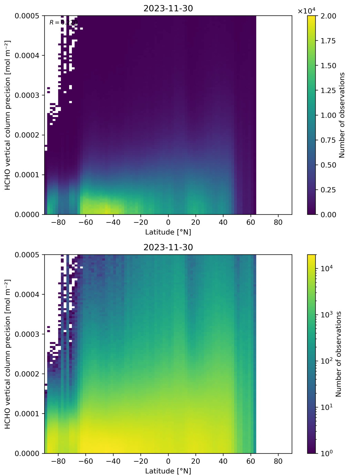
Figure 165: Scatter density plot of “Latitude” against “HCHO vertical column precision” for 2023-11-29 to 2023-12-01.
