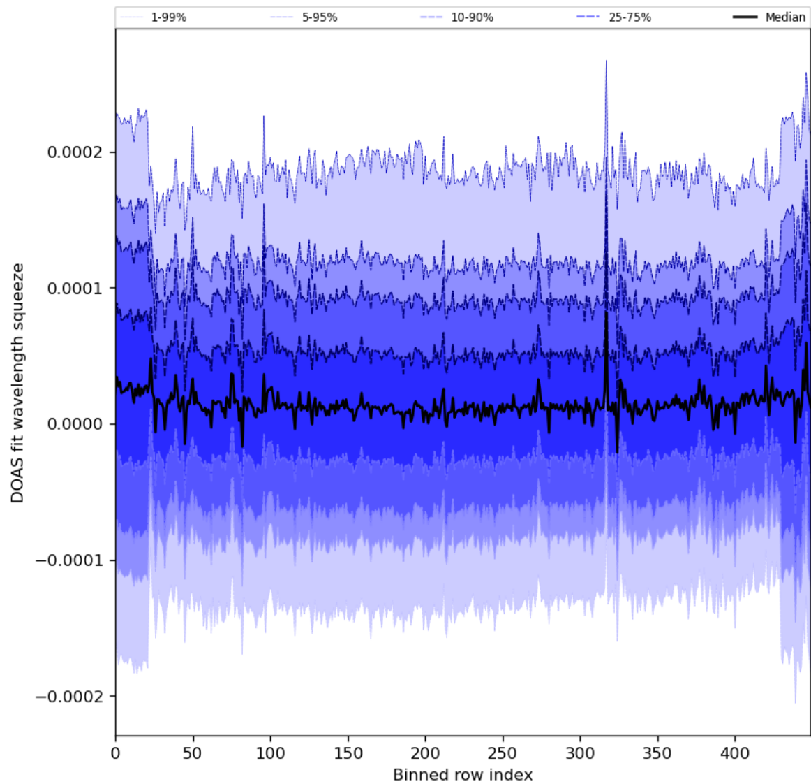
Figure 59: Along track statistics of “DOAS fit wavelength squeeze” for 2023-11-29 to 2023-12-01
