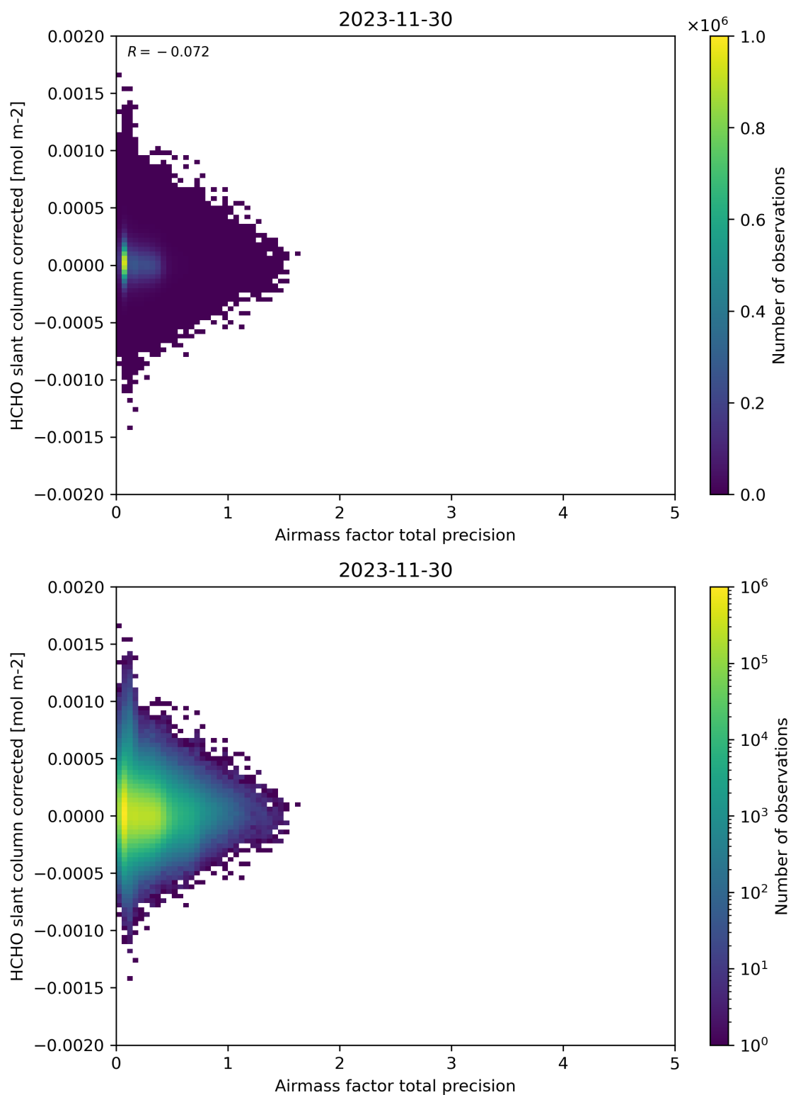
Figure 109: Scatter density plot of “Airmass factor total precision” against “HCHO slant column corrected” for 2023-11-29 to 2023-12-01.
