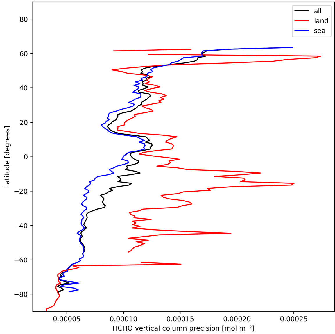
Figure 22: Zonal average of “HCHO vertical column precision” for 2023-11-29 to 2023-12-01.
