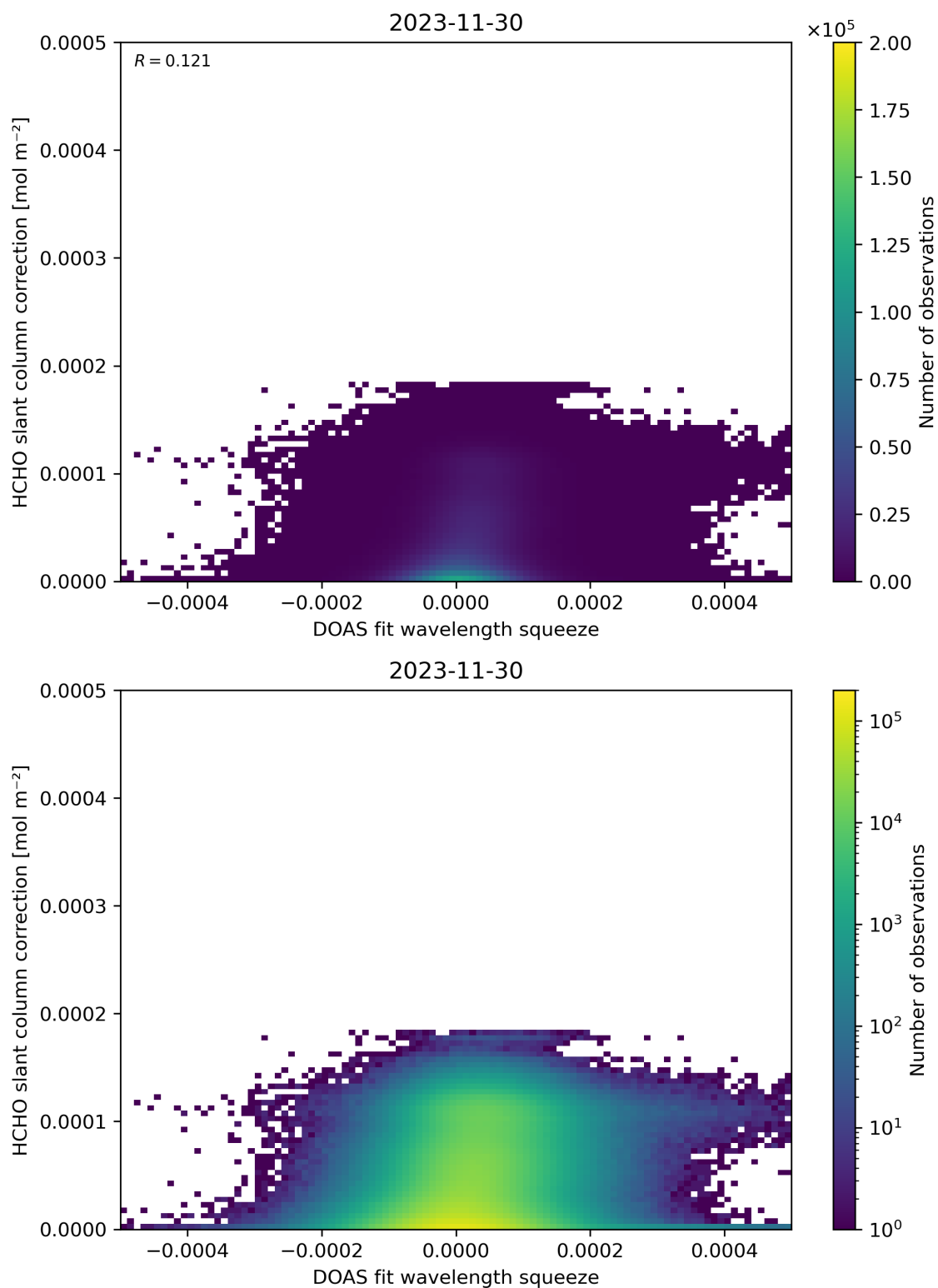
Figure 70: Scatter density plot of “DOAS fit wavelength squeeze” against “HCHO slant column correction” for 2023-11-29 to 2023-12-01.
