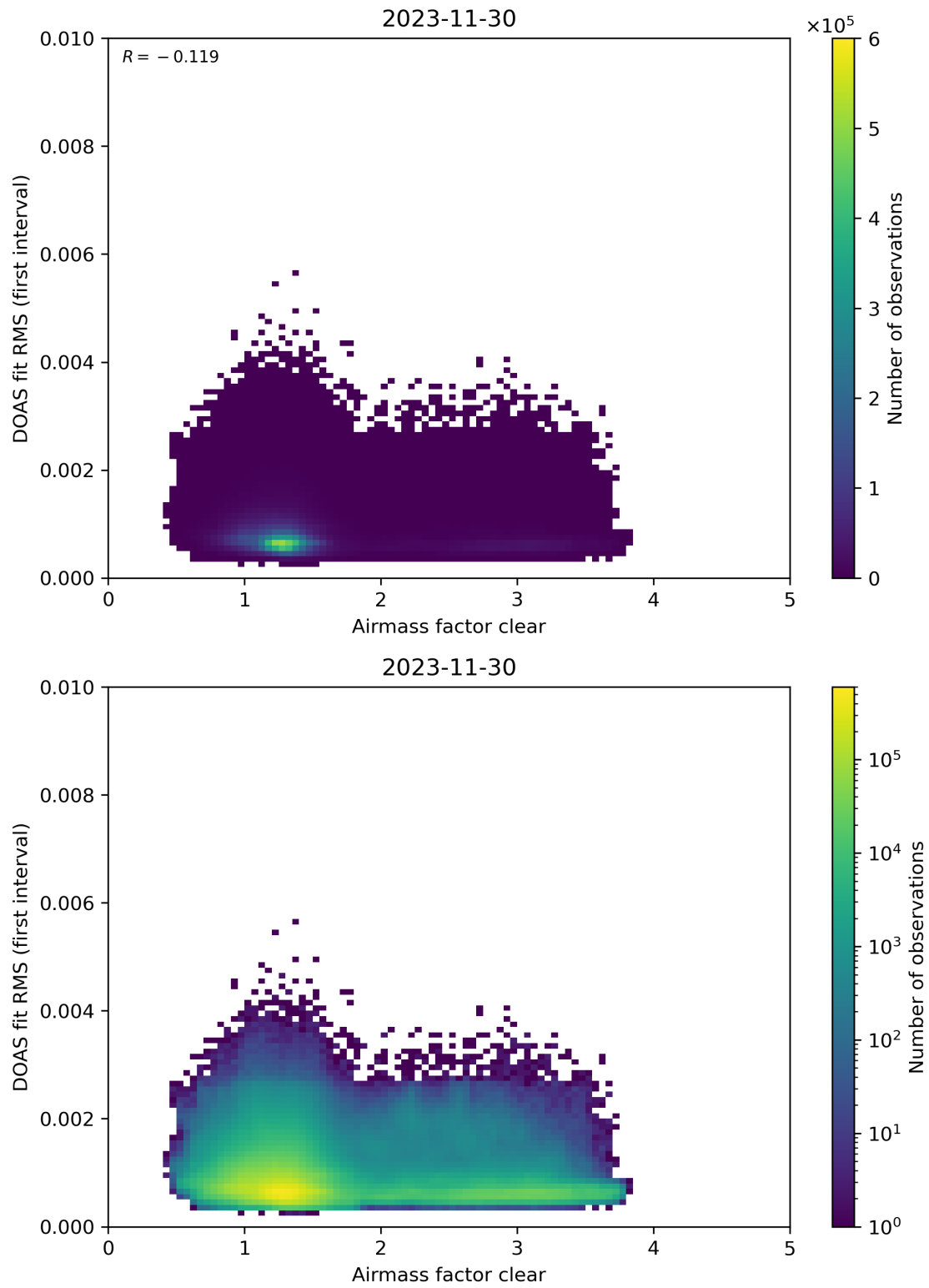
Figure 71: Scatter density plot of “Airmass factor clear” against “DOAS fit RMS (first interval)” for 2023-11-29 to 2023-12-01.
