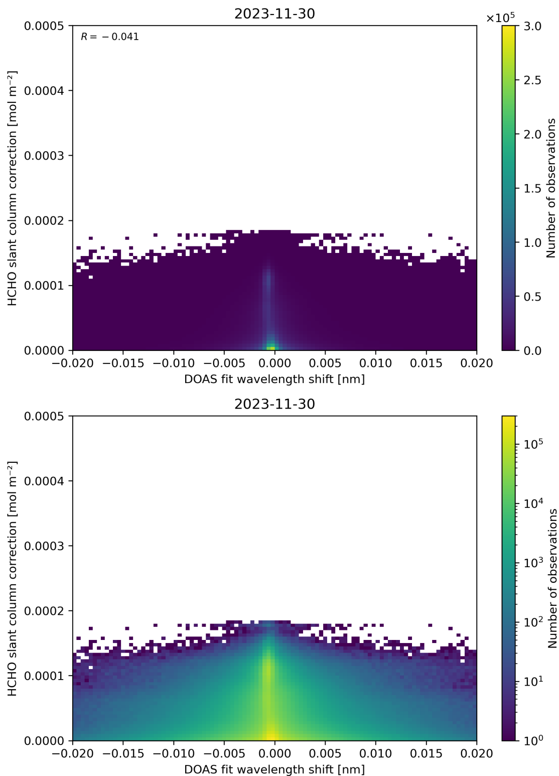
Figure 67: Scatter density plot of “DOAS fit wavelength shift” against “HCHO slant column correction” for 2023-11-29 to 2023-12-01.
