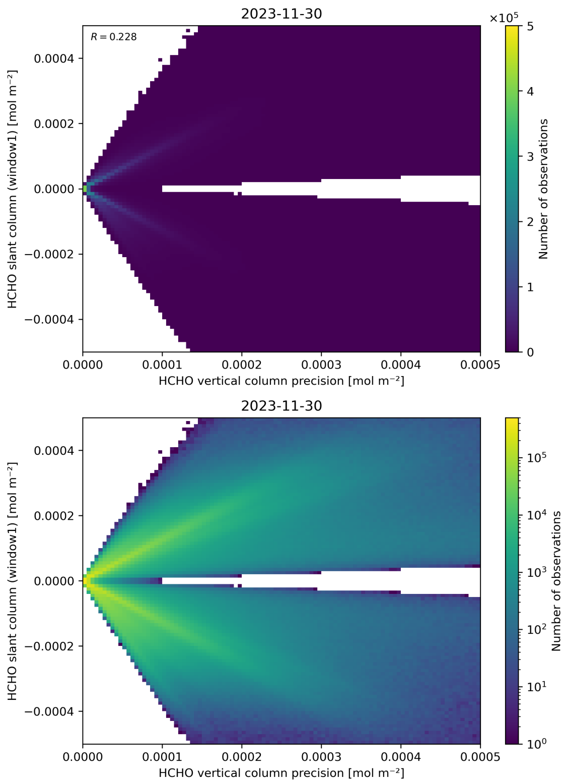
Figure 142: Scatter density plot of “HCHO vertical column precision” against “HCHO slant column (window1)” for 2023-11-29 to 2023-12-01.
