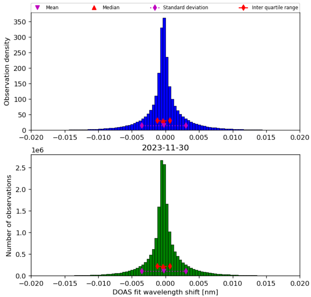
Figure 44: Histogram of “DOAS fit wavelength shift” for 2023-11-29 to 2023-12-01
