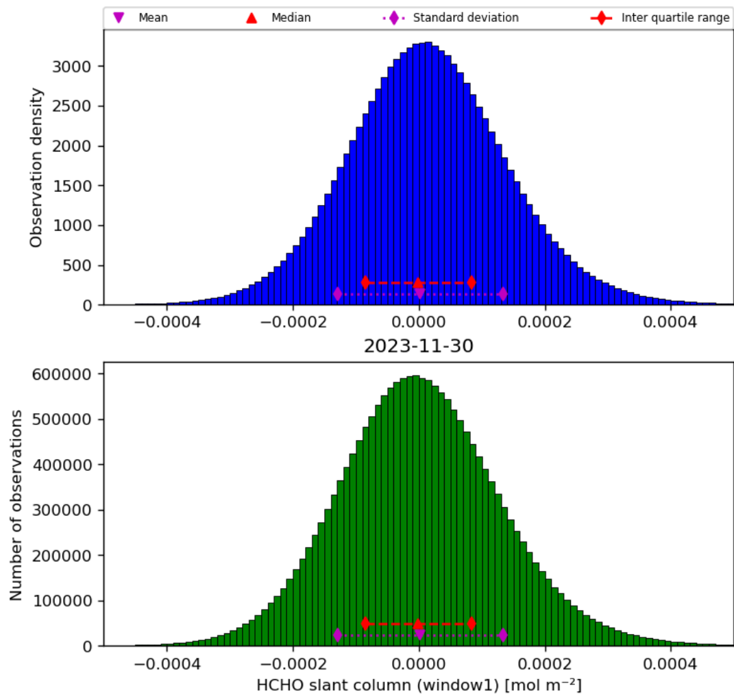
Figure 38: Histogram of “HCHO slant column (window1)” for 2023-11-29 to 2023-12-01
