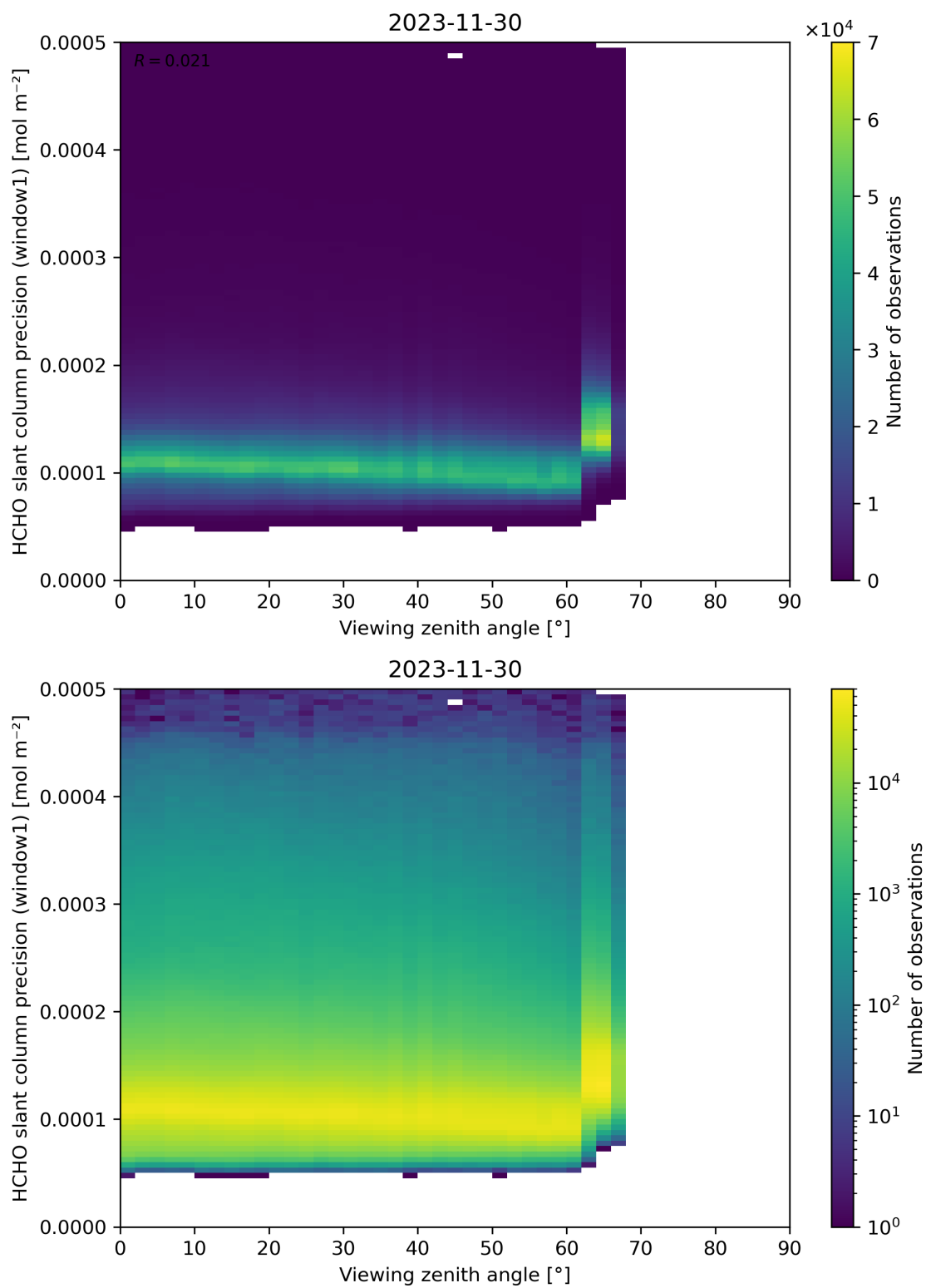
Figure 189: Scatter density plot of “Viewing zenith angle” against “HCHO slant column precision (window1)” for 2023-11-29 to 2023-12-01.
