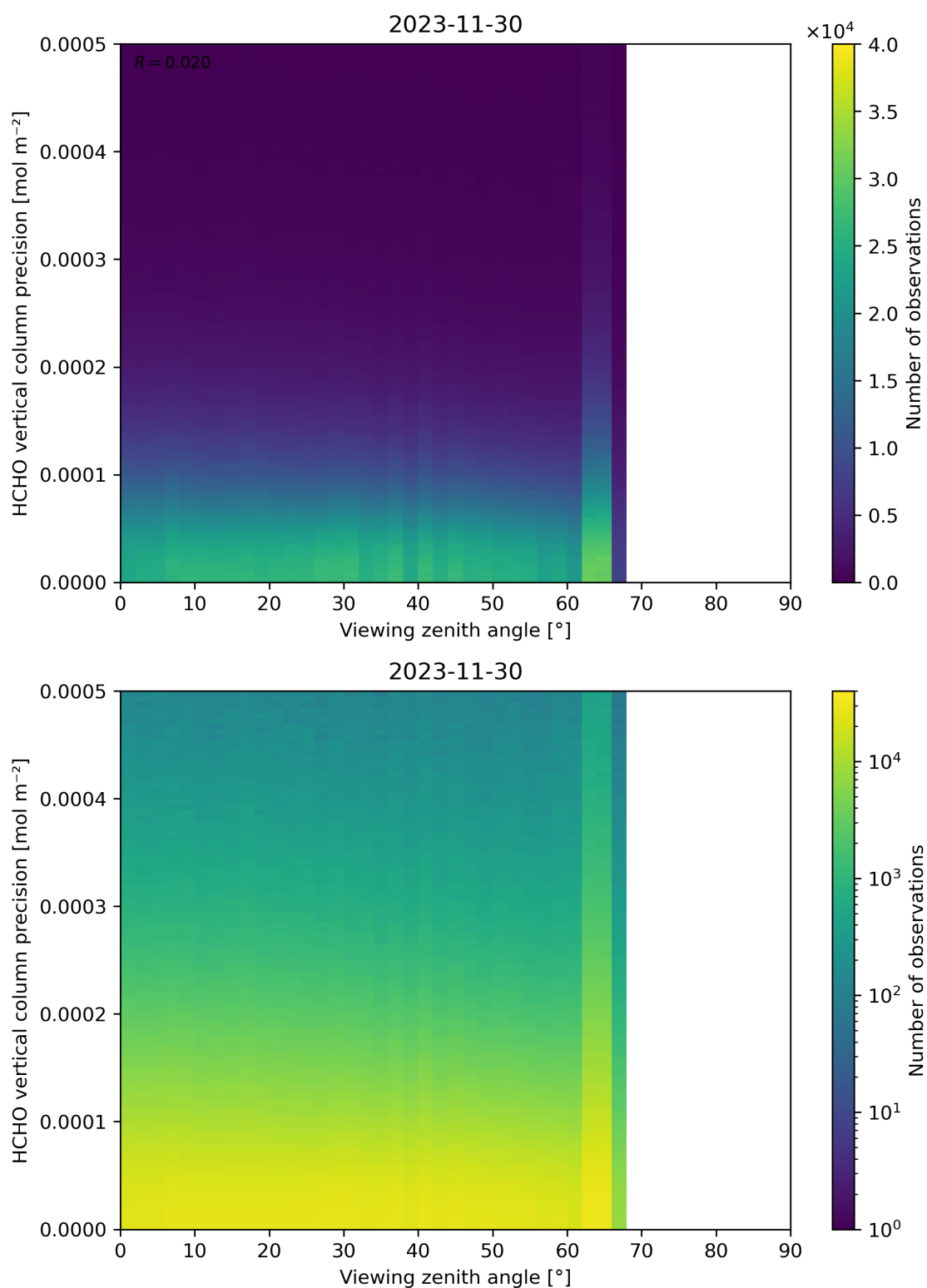
Figure 194: Scatter density plot of “Viewing zenith angle” against “HCHO vertical column precision” for 2023-11-29 to 2023-12-01.
