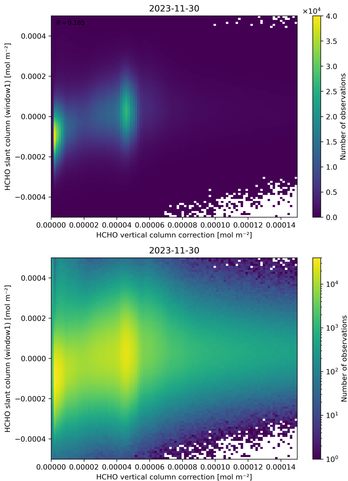
Figure 118: Scatter density plot of “HCHO vertical column correction” against “HCHO slant column (window1)” for 2023-11-29 to 2023-12-01.
