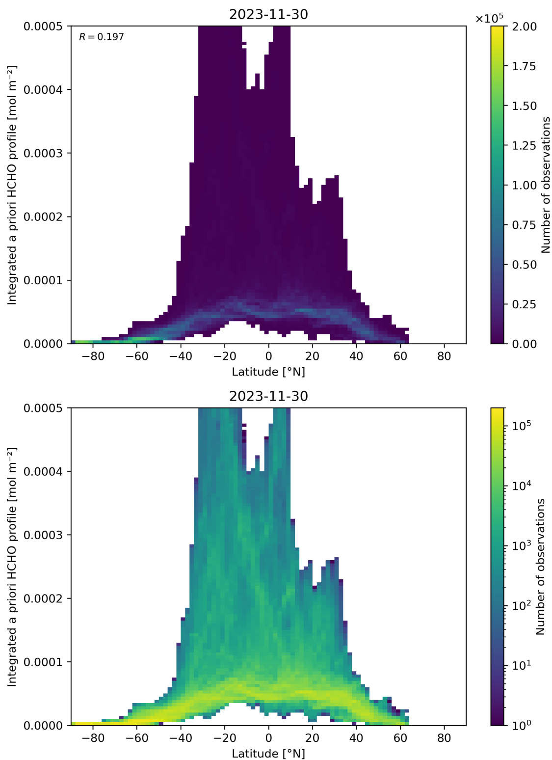
Figure 166: Scatter density plot of “Latitude” against “Integrated a priori HCHO profile” for 2023-11-29 to 2023-12-01.
