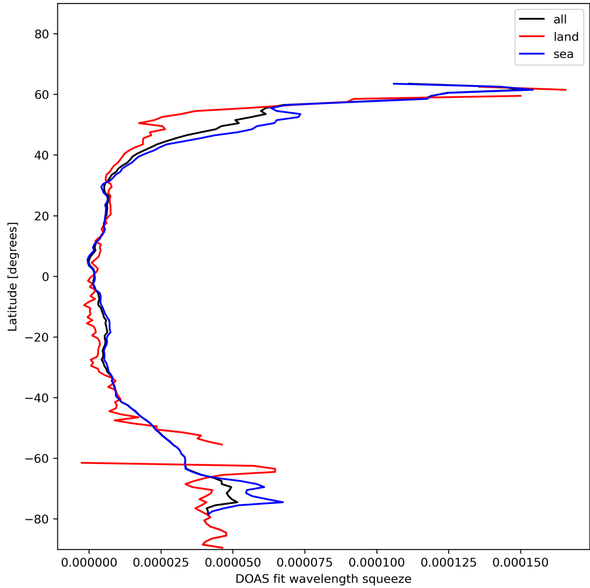
Figure 31: Zonal average of “DOAS fit wavelength squeeze” for 2023-11-29 to 2023-12-01.
