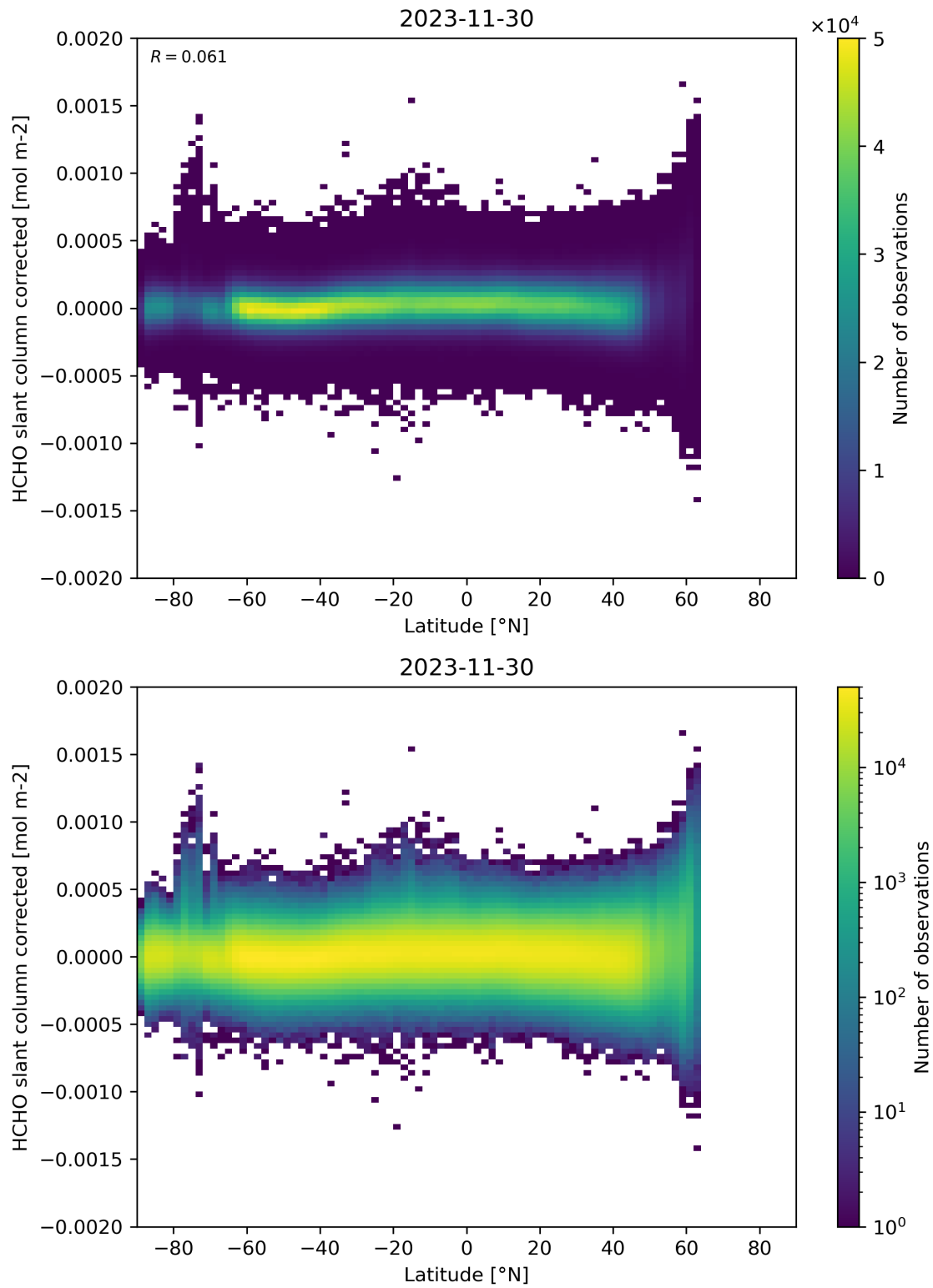
Figure 157: Scatter density plot of “Latitude” against “HCHO slant column corrected” for 2023-11-29 to 2023-12-01.
