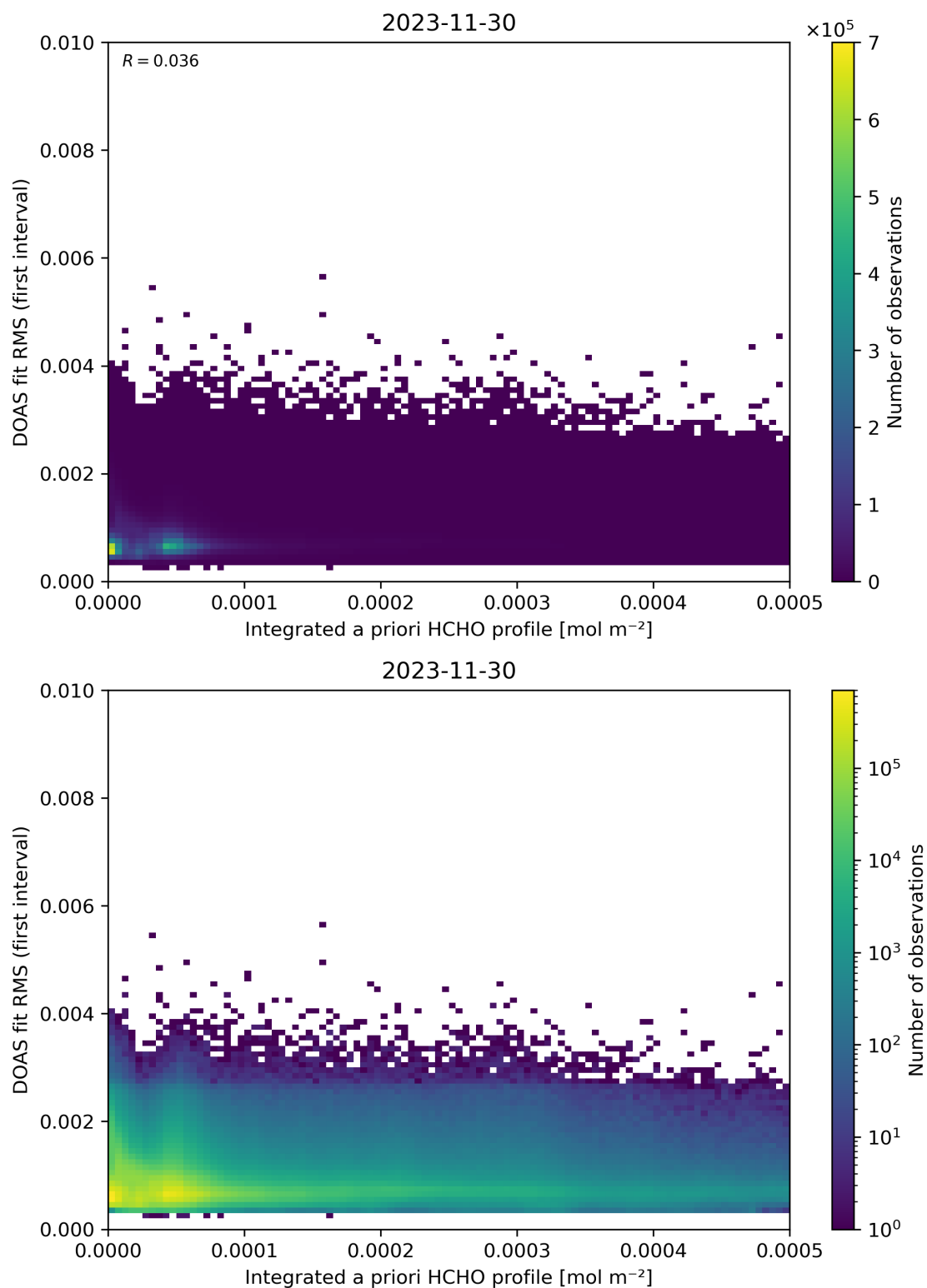
Figure 148: Scatter density plot of “Integrated a priori HCHO profile” against “DOAS fit RMS (first interval)” for 2023-11-29 to 2023-12-01.
