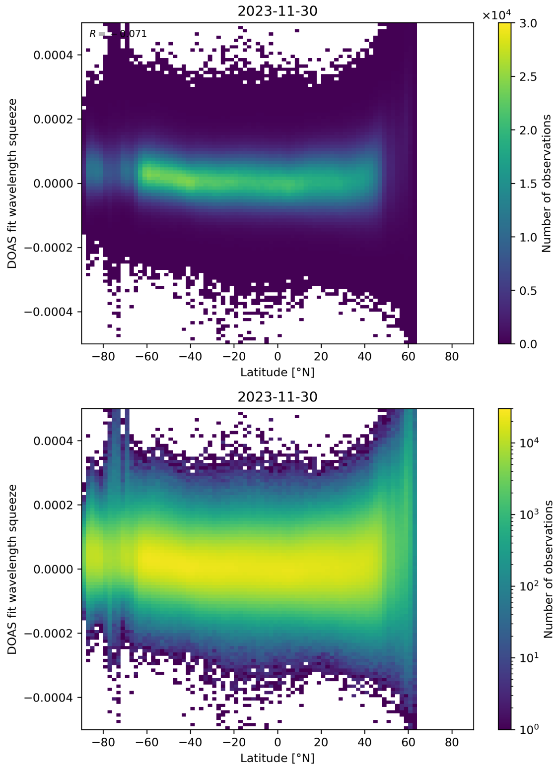
Figure 155: Scatter density plot of “Latitude” against “DOAS fit wavelength squeeze” for 2023-11-29 to 2023-12-01.
