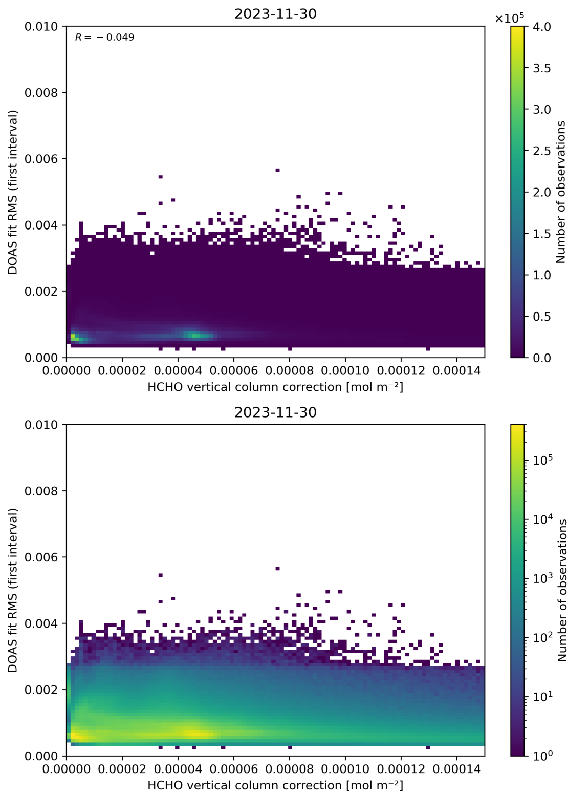
Figure 112: Scatter density plot of “HCHO vertical column correction” against “DOAS fit RMS (first interval)” for 2023-11-29 to 2023-12-01.
