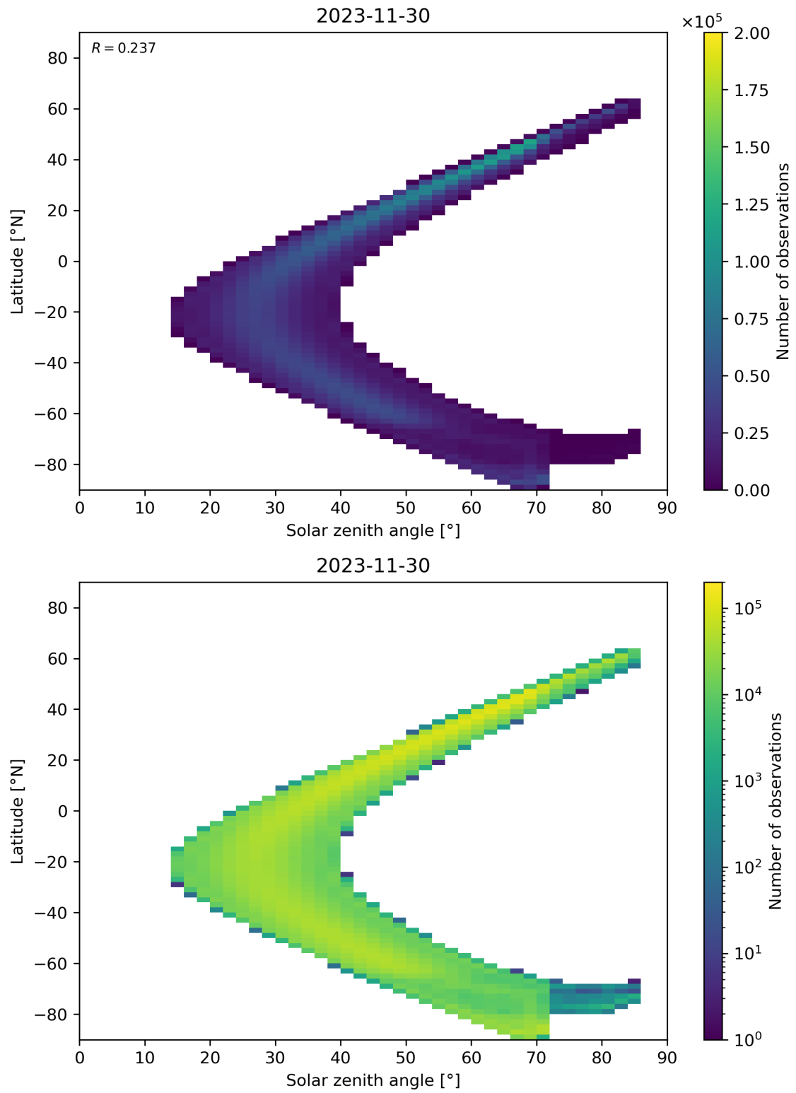
Figure 181: Scatter density plot of “Solar zenith angle” against “Latitude” for 2023-11-29 to 2023-12-01.
