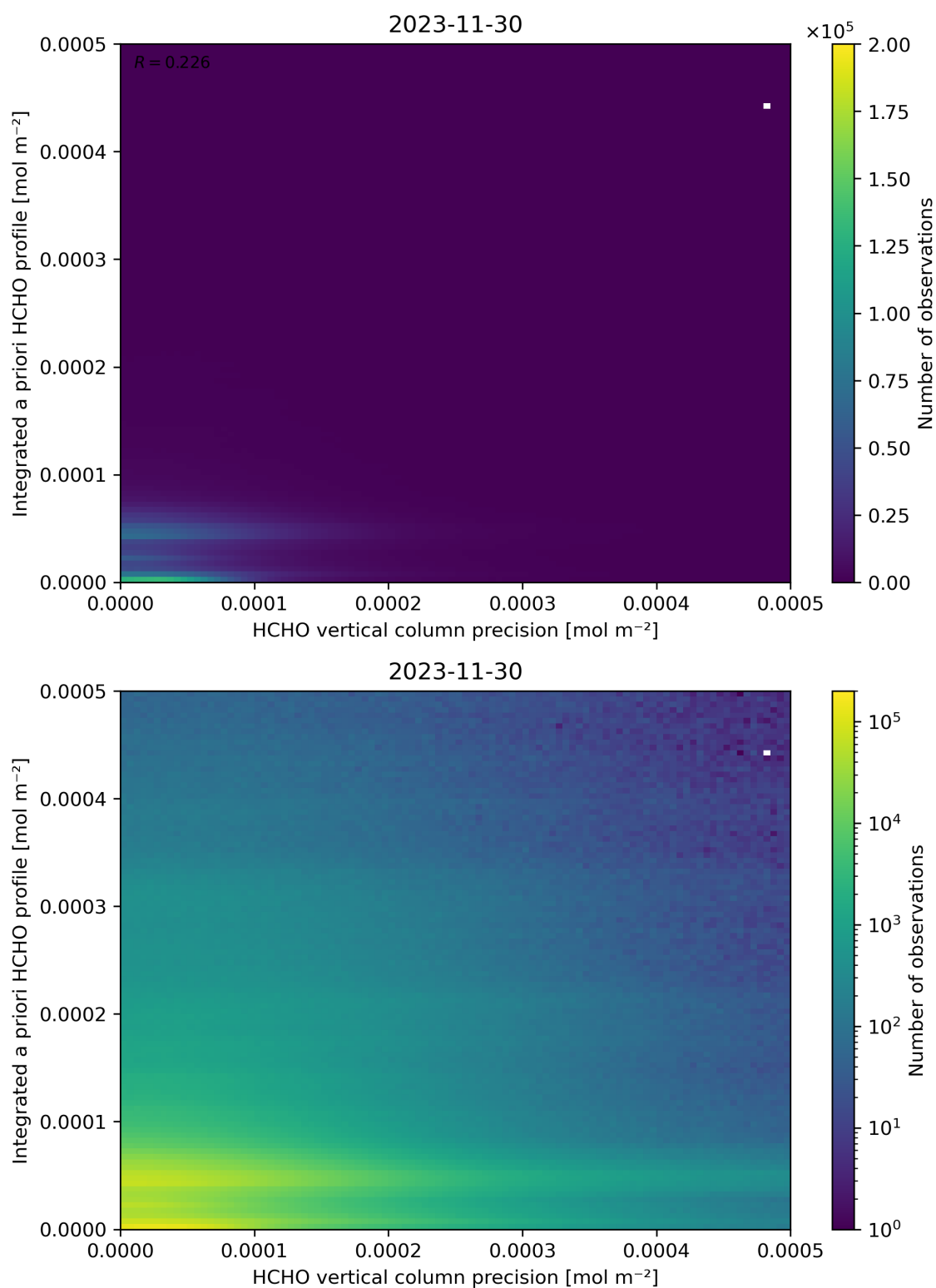
Figure 147: Scatter density plot of “HCHO vertical column precision” against “Integrated a priori HCHO profile” for 2023-11-29 to 2023-12-01.
