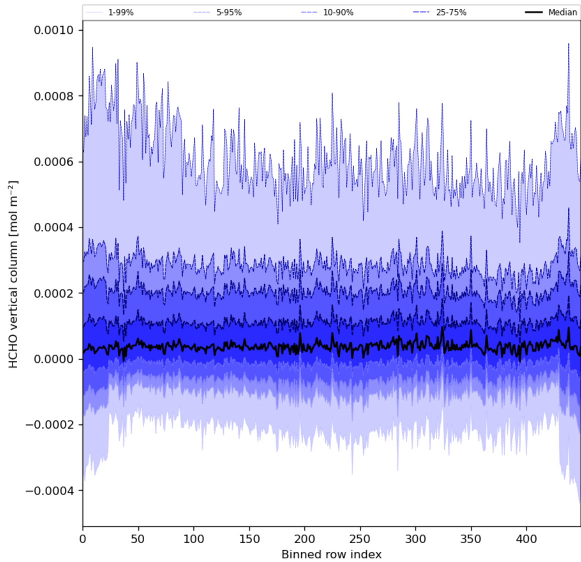
Figure 49: Along track statistics of “HCHO vertical column” for 2023-11-29 to 2023-12-01
