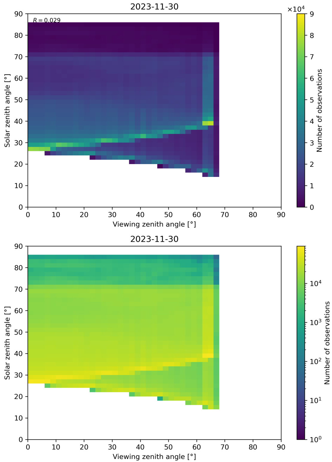
Figure 197: Scatter density plot of “Viewing zenith angle” against “Solar zenith angle” for 2023-11-29 to 2023-12-01.
