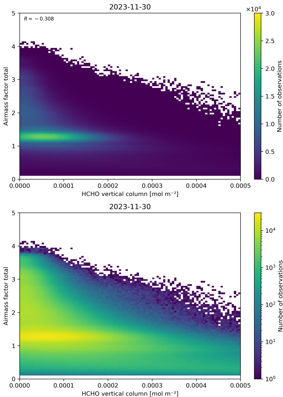
Figure 131: Scatter density plot of “HCHO vertical column” against “Airmass factor total” for 2023-11-29 to 2023-12-01.
