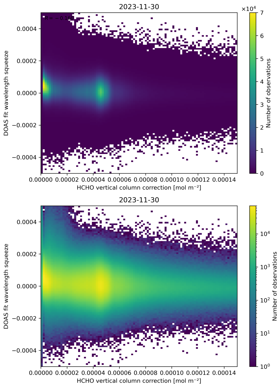
Figure 114: Scatter density plot of “HCHO vertical column correction” against “DOAS fit wavelength squeeze” for 2023-11-29 to 2023-12-01.
