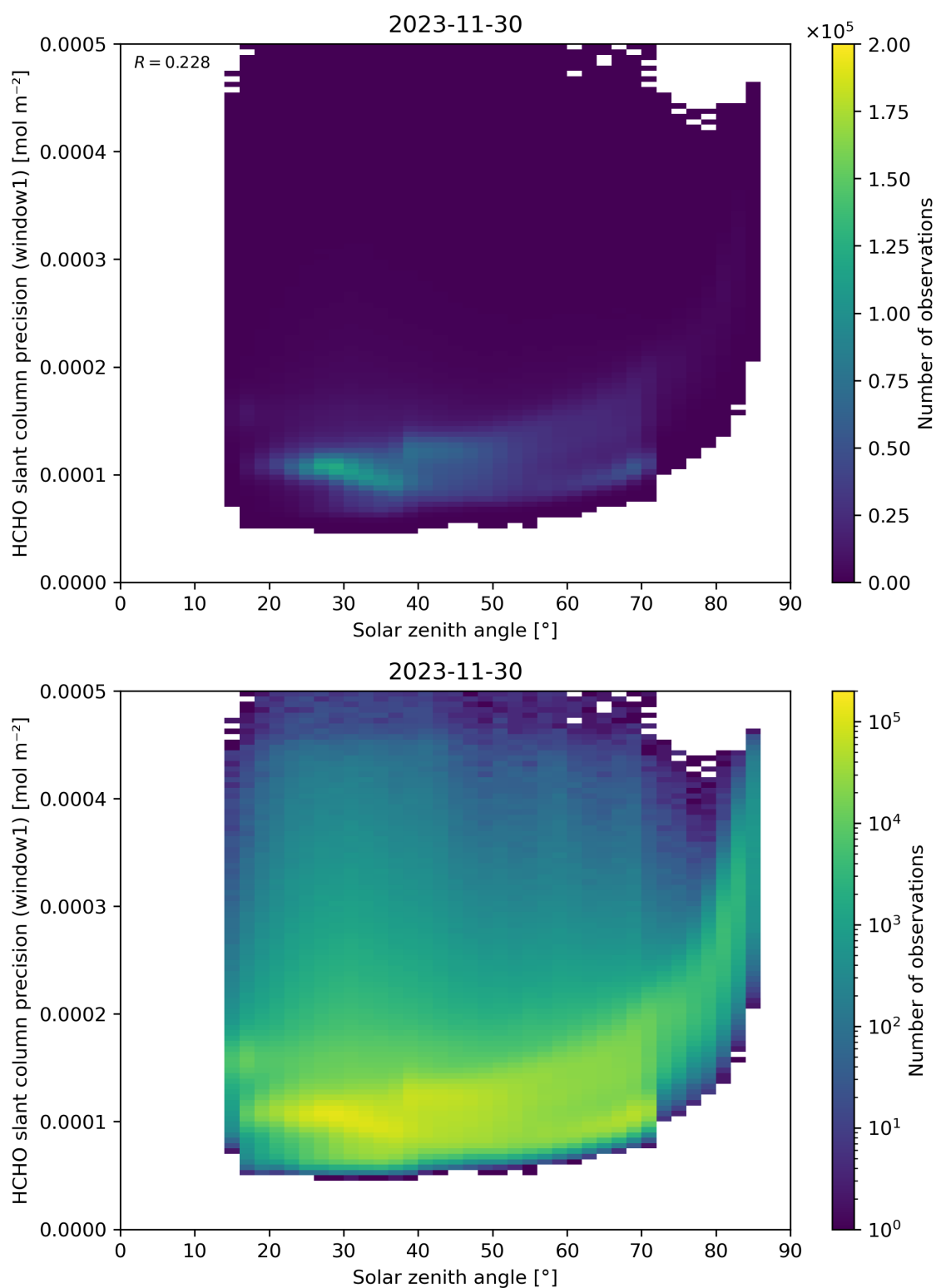
Figure 174: Scatter density plot of “Solar zenith angle” against “HCHO slant column precision (window1)” for 2023-11-29 to 2023-12-01.
