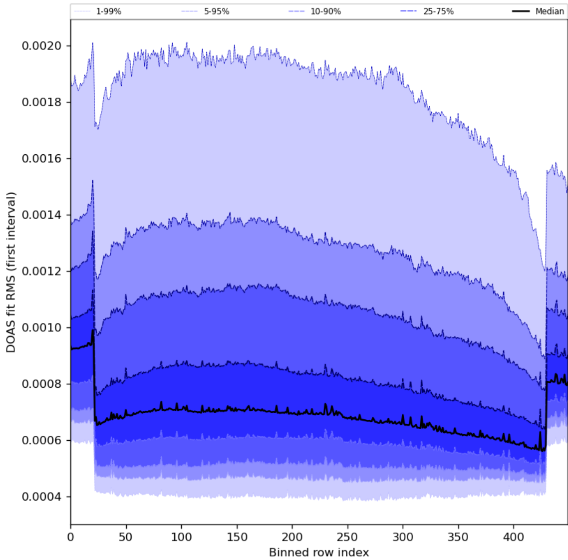
Figure 60: Along track statistics of “DOAS fit RMS (first interval)” for 2023-11-29 to 2023-12-01
