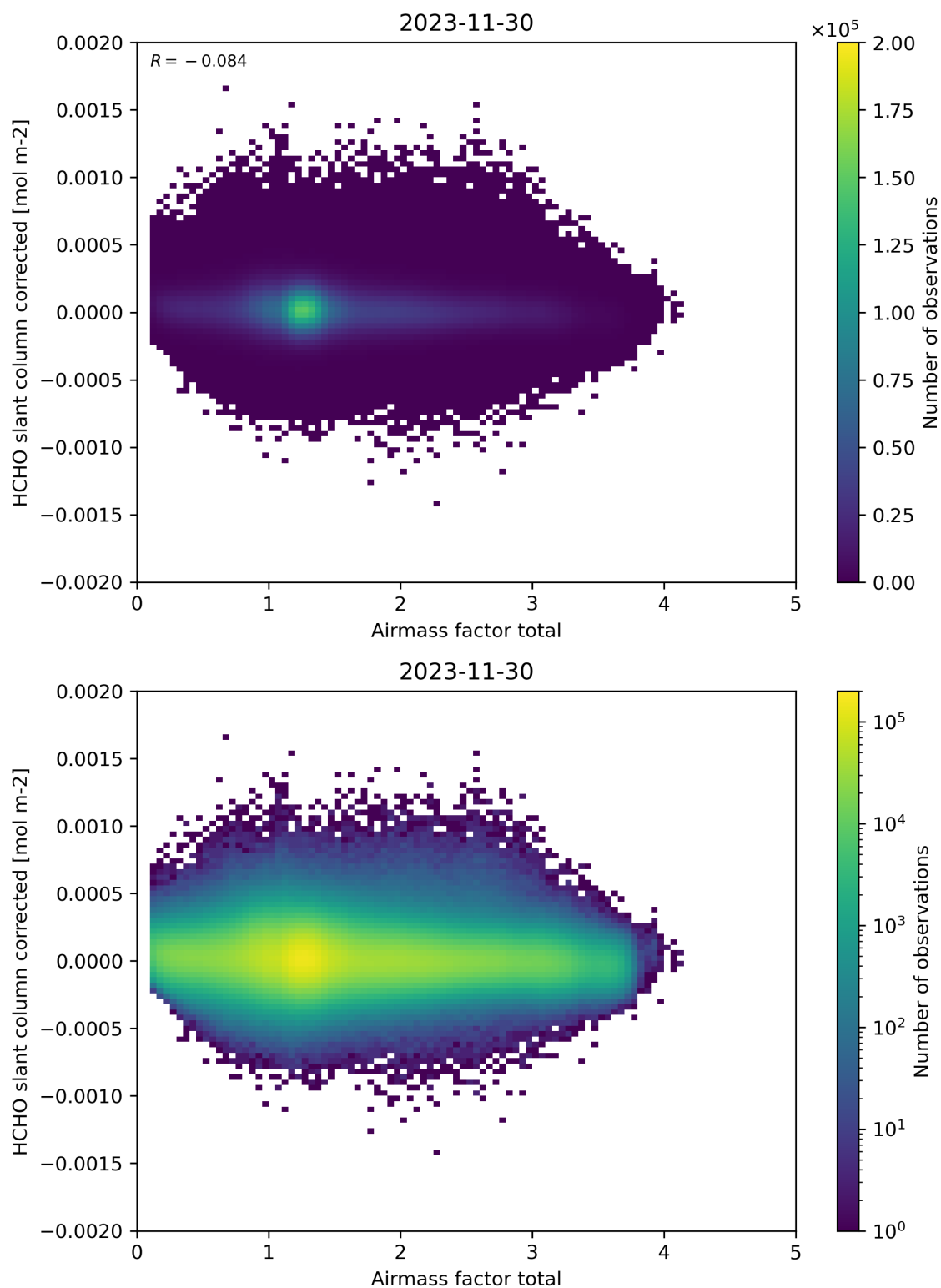
Figure 101: Scatter density plot of “Airmass factor total” against “HCHO slant column corrected” for 2023-11-29 to 2023-12-01.
