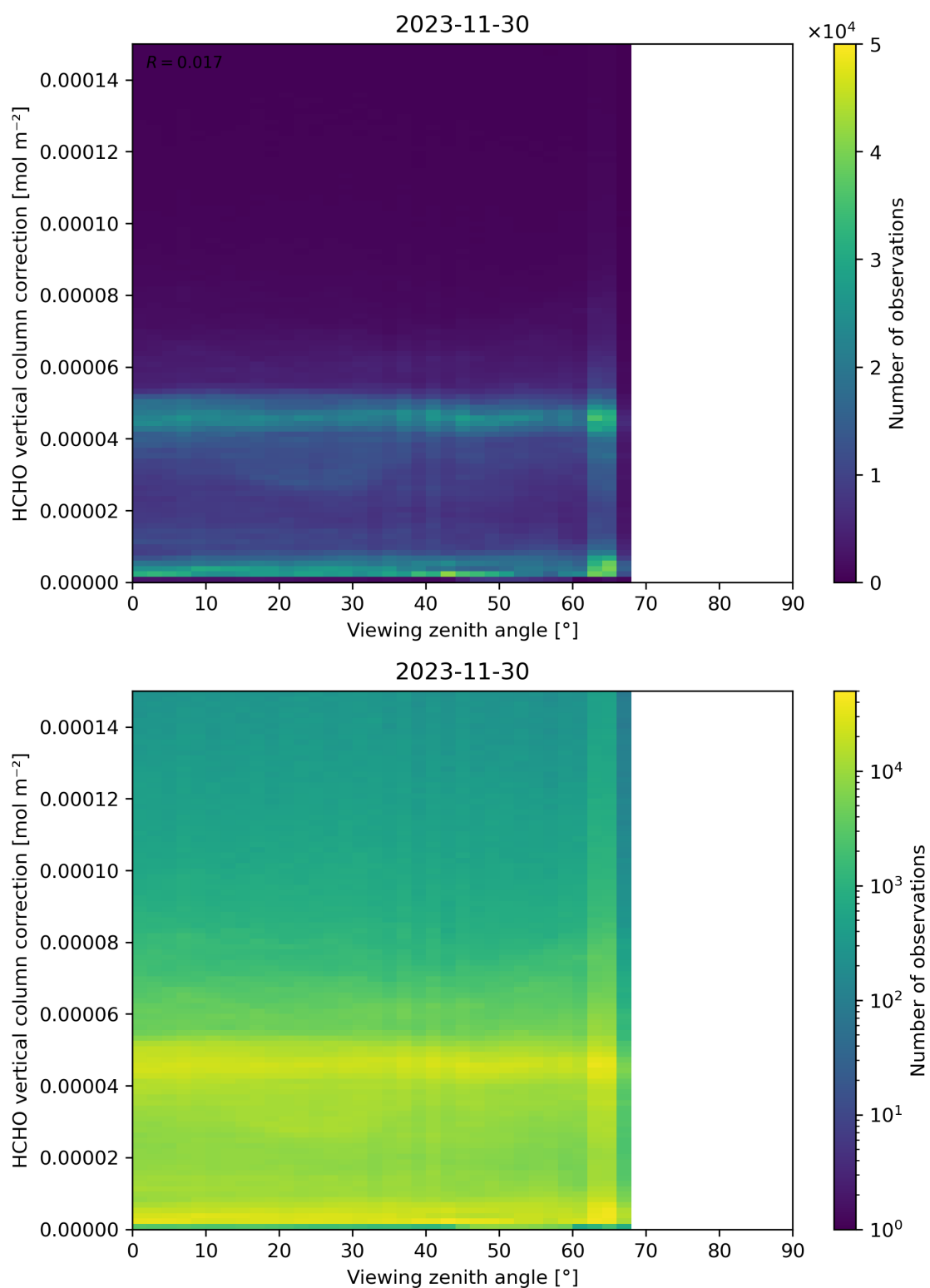
Figure 193: Scatter density plot of “Viewing zenith angle” against “HCHO vertical column correction” for 2023-11-29 to 2023-12-01.
