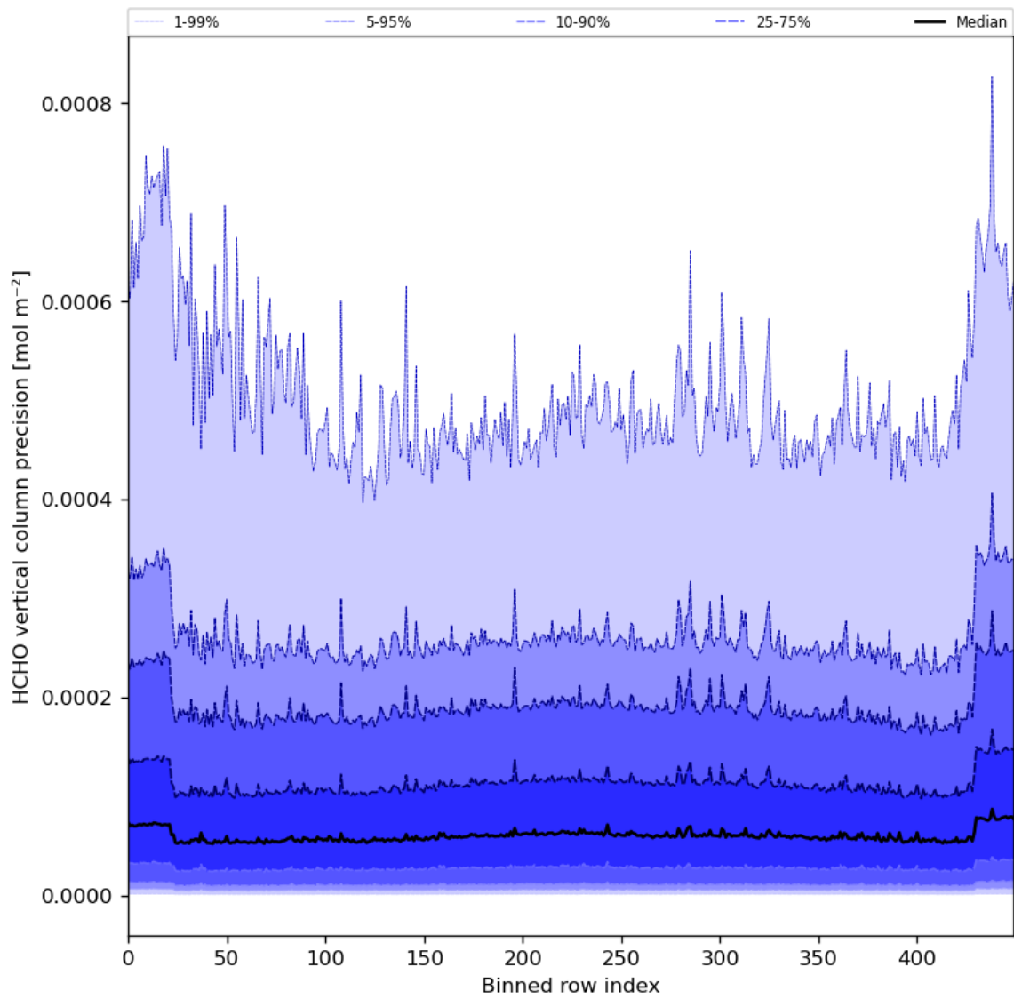
Figure 50: Along track statistics of “HCHO vertical column precision” for 2023-11-29 to 2023-12-01
