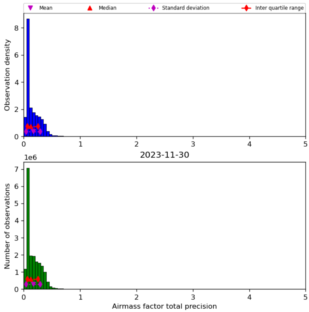
Figure 41: Histogram of “Airmass factor total precision” for 2023-11-29 to 2023-12-01
