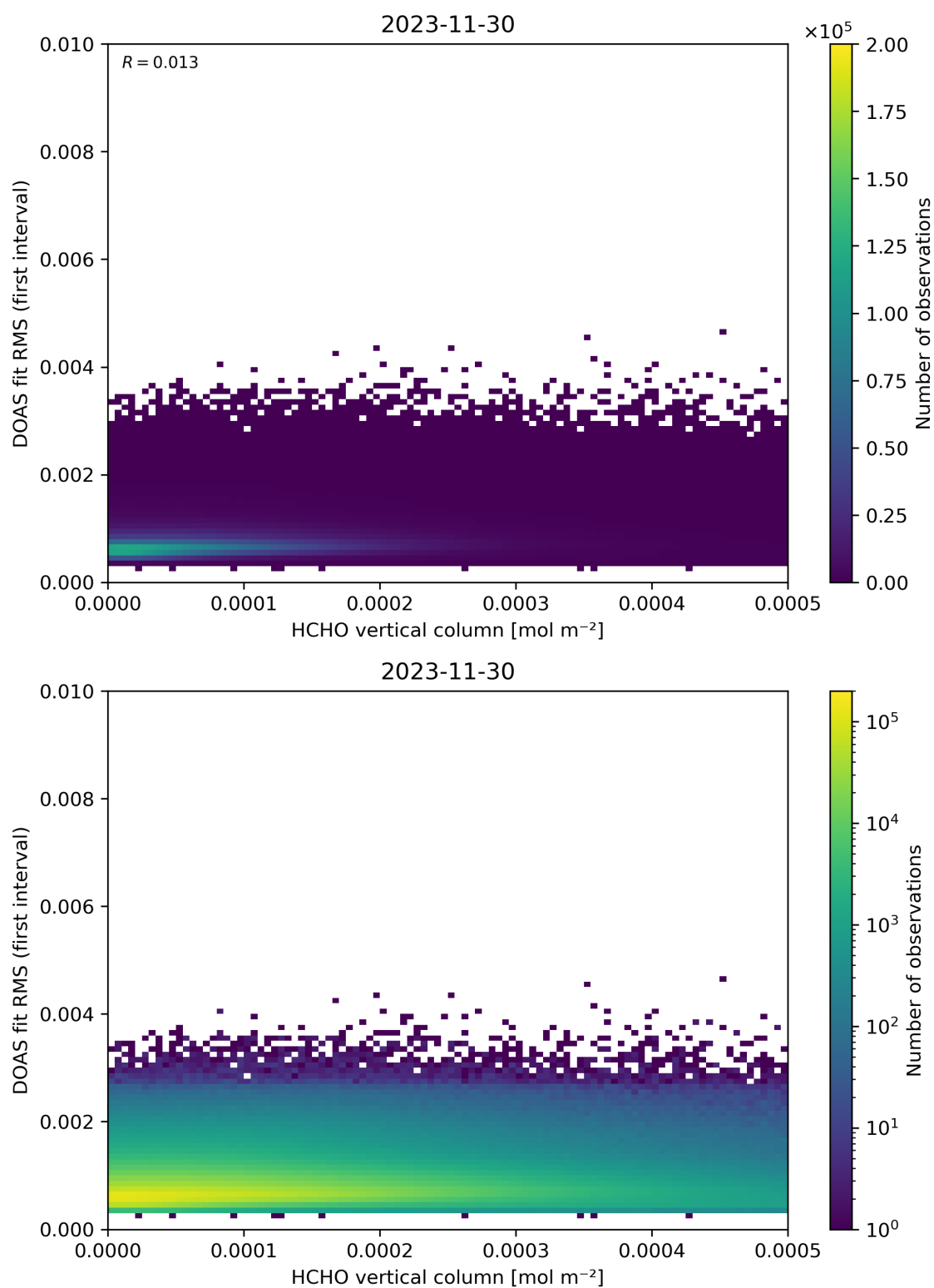
Figure 123: Scatter density plot of “HCHO vertical column” against “DOAS fit RMS (first interval)” for 2023-11-29 to 2023-12-01.
