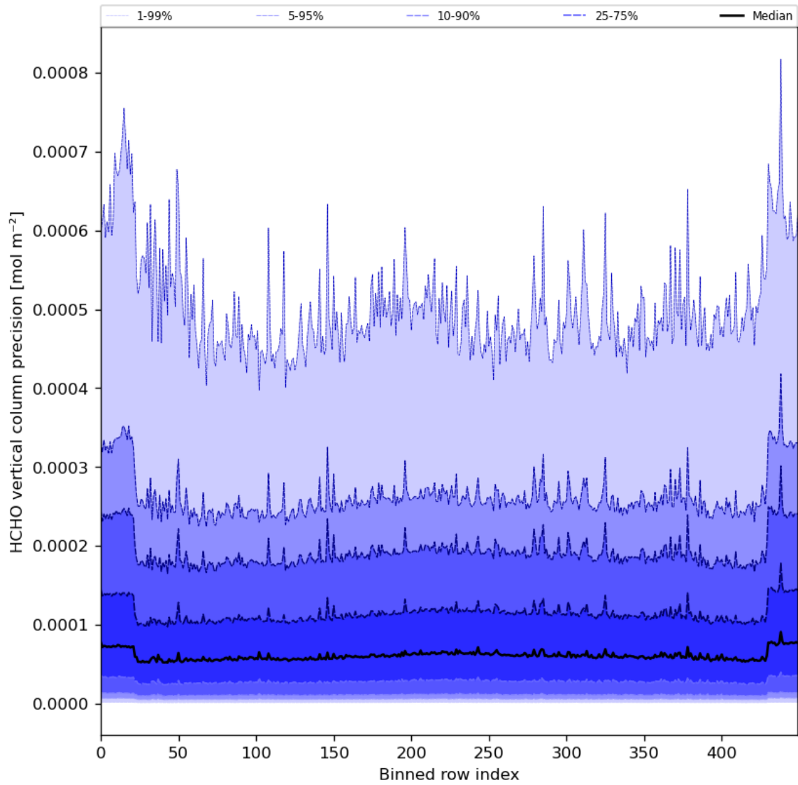
Figure 50: Along track statistics of “HCHO vertical column precision” for 2023-11-30 to 2023-12-02
