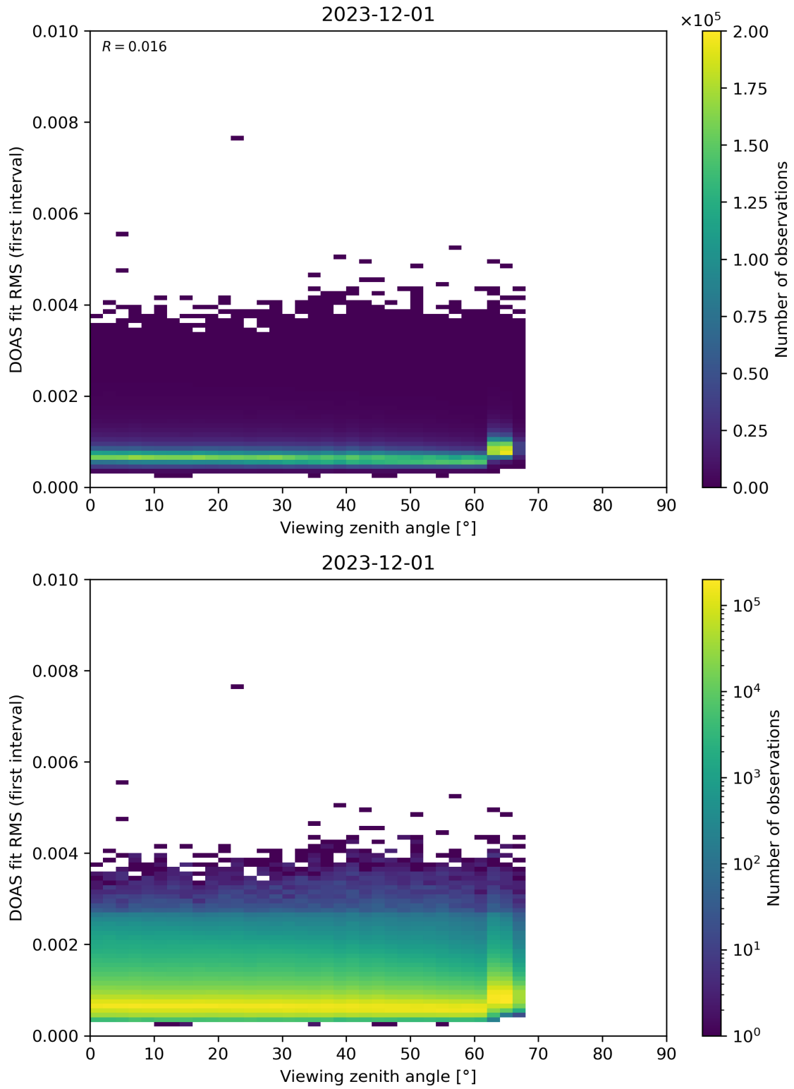
Figure 182: Scatter density plot of “Viewing zenith angle” against “DOAS fit RMS (first interval)” for 2023-11-30 to 2023-12-02.
