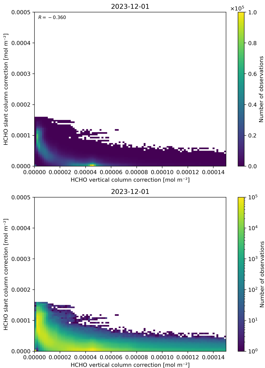
Figure 117: Scatter density plot of “HCHO vertical column correction” against “HCHO slant column correction” for 2023-11-30 to 2023-12-02.
