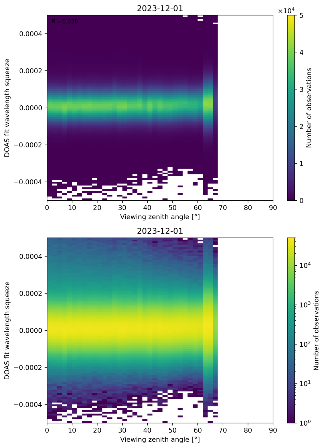
Figure 184: Scatter density plot of “Viewing zenith angle” against “DOAS fit wavelength squeeze” for 2023-11-30 to 2023-12-02.
