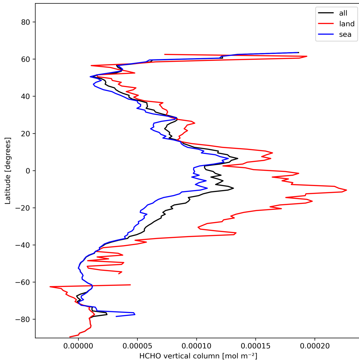
Figure 21: Zonal average of “HCHO vertical column” for 2023-11-30 to 2023-12-02.
