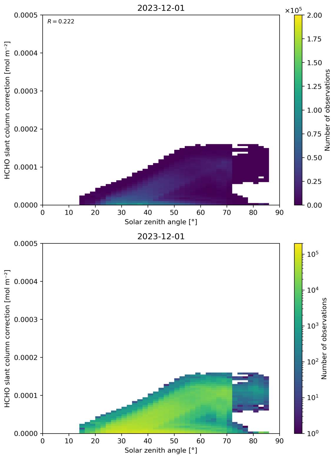
Figure 172: Scatter density plot of “Solar zenith angle” against “HCHO slant column correction” for 2023-11-30 to 2023-12-02.
