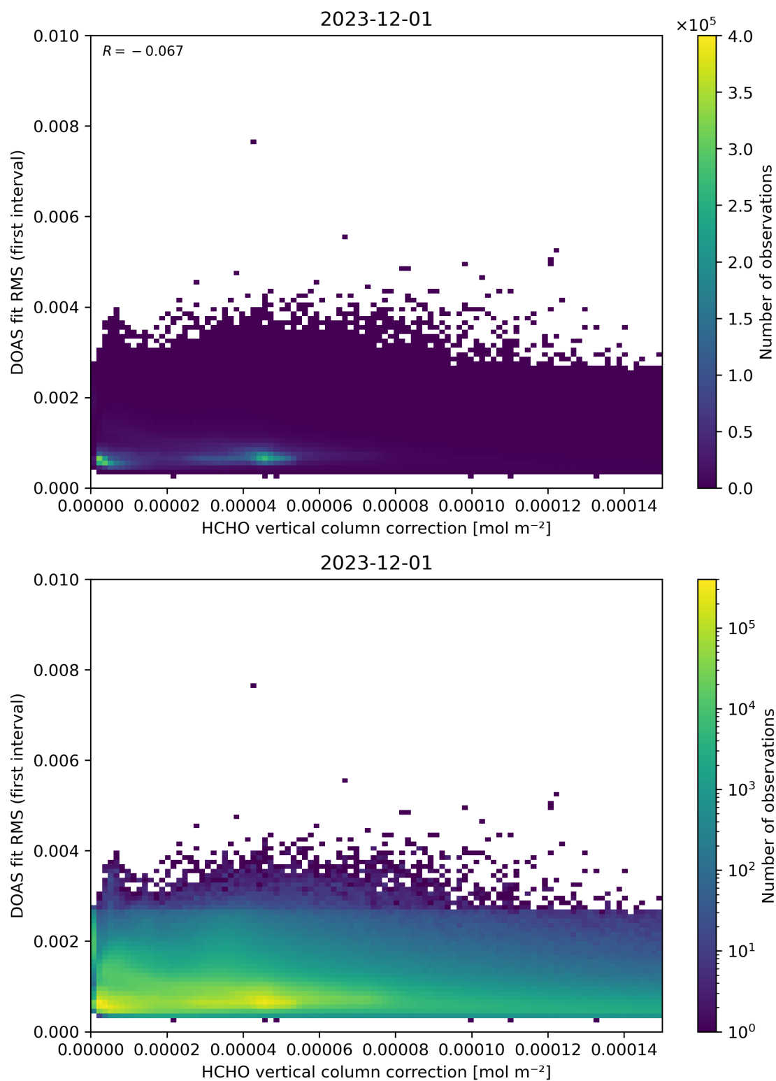
Figure 112: Scatter density plot of “HCHO vertical column correction” against “DOAS fit RMS (first interval)” for 2023-11-30 to 2023-12-02.
