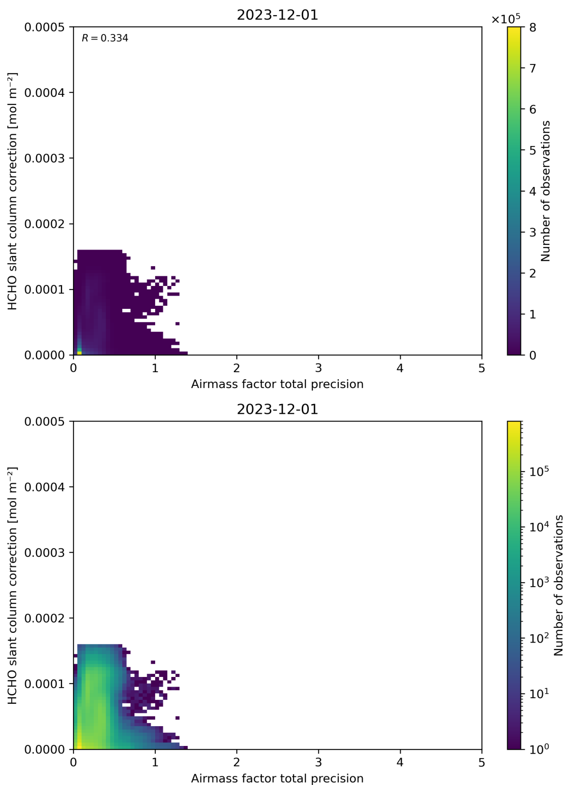
Figure 110: Scatter density plot of “Airmass factor total precision” against “HCHO slant column correction” for 2023-11-30 to 2023-12-02.
