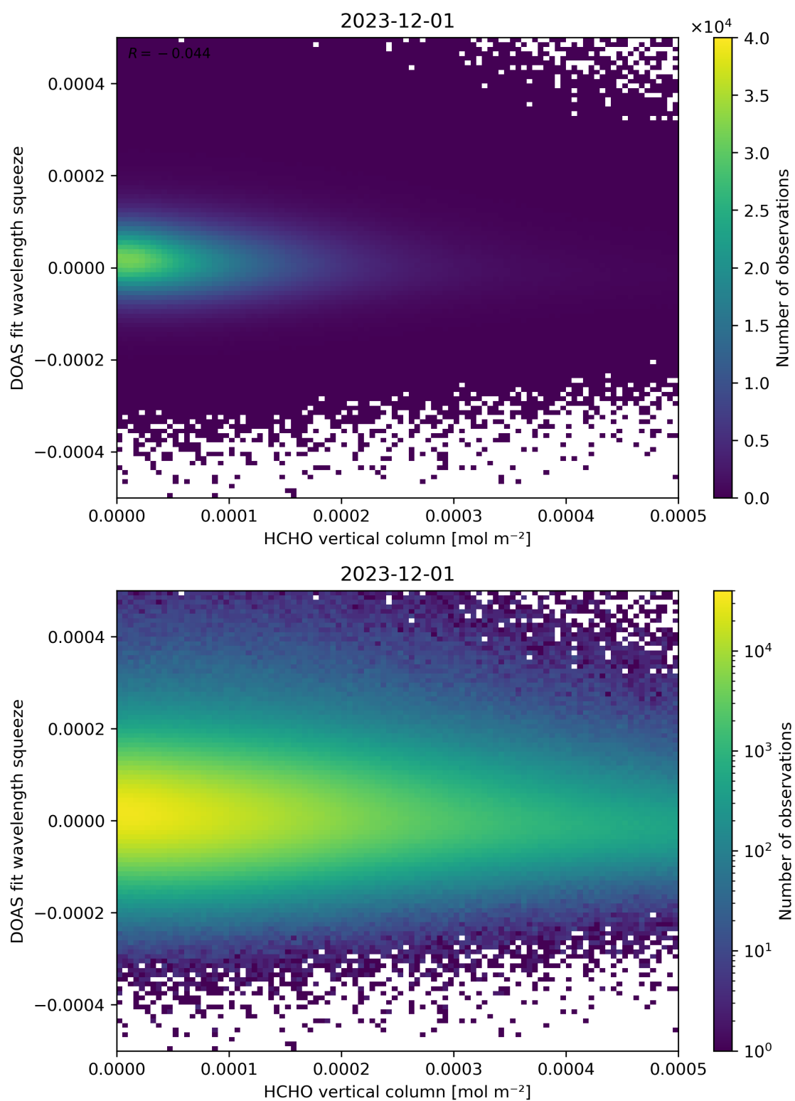
Figure 125: Scatter density plot of “HCHO vertical column” against “DOAS fit wavelength squeeze” for 2023-11-30 to 2023-12-02.
