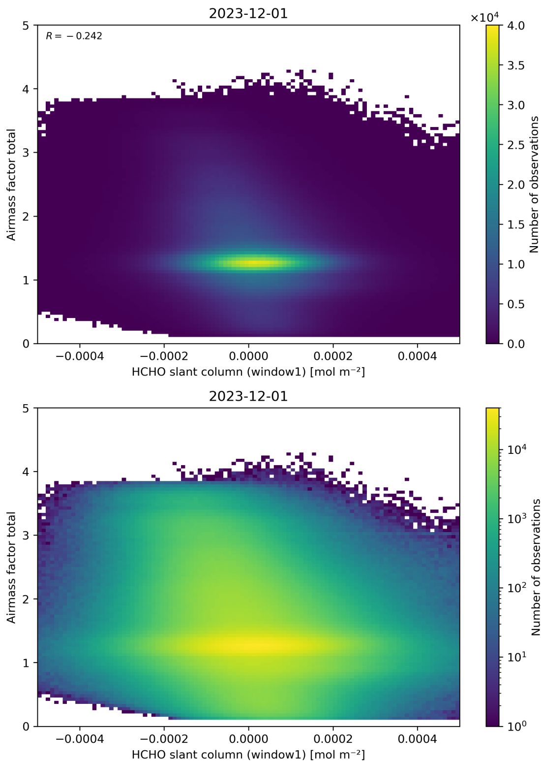
Figure 85: Scatter density plot of “HCHO slant column (window1)” against “Airmass factor total” for 2023-11-30 to 2023-12-02.
