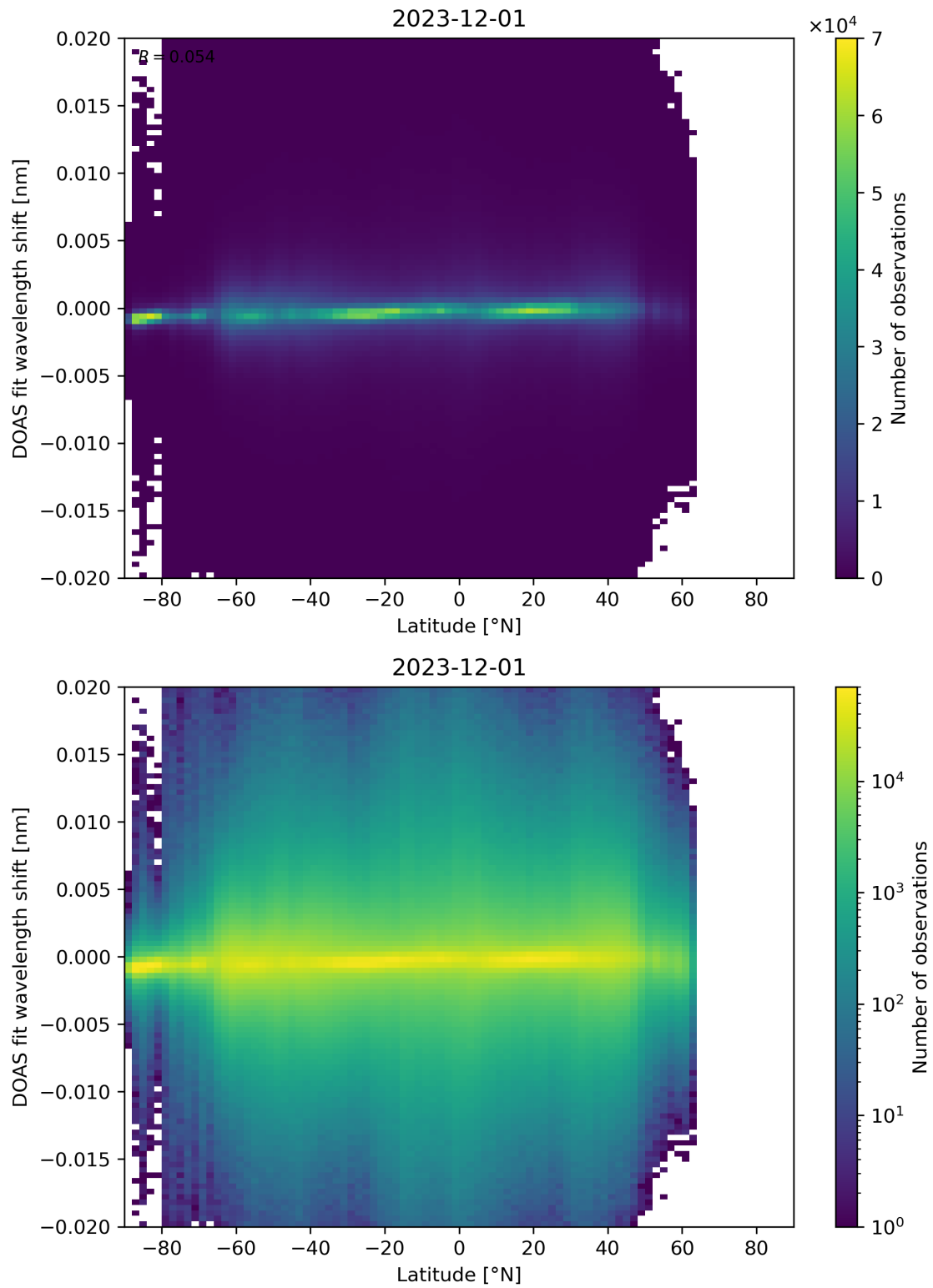
Figure 154: Scatter density plot of “Latitude” against “DOAS fit wavelength shift” for 2023-11-30 to 2023-12-02.
