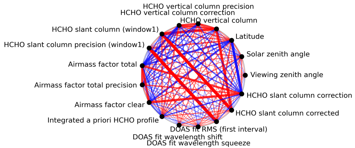
Figure 1: Map of correlation graph for 2023-11-30 to 2023-12-02.
