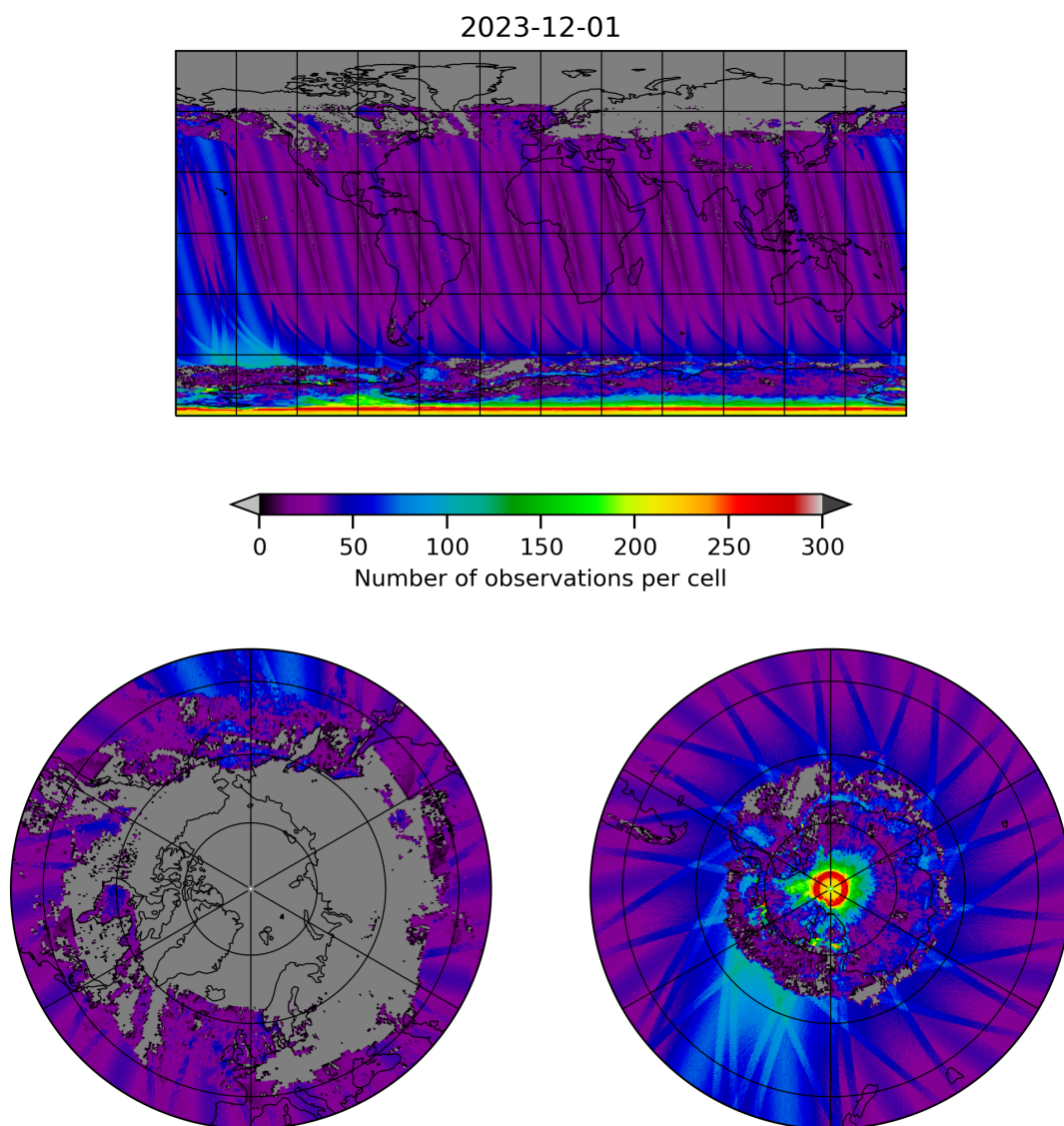
Figure 19: Map of the number of observations for 2023-11-30 to 2023-12-02
