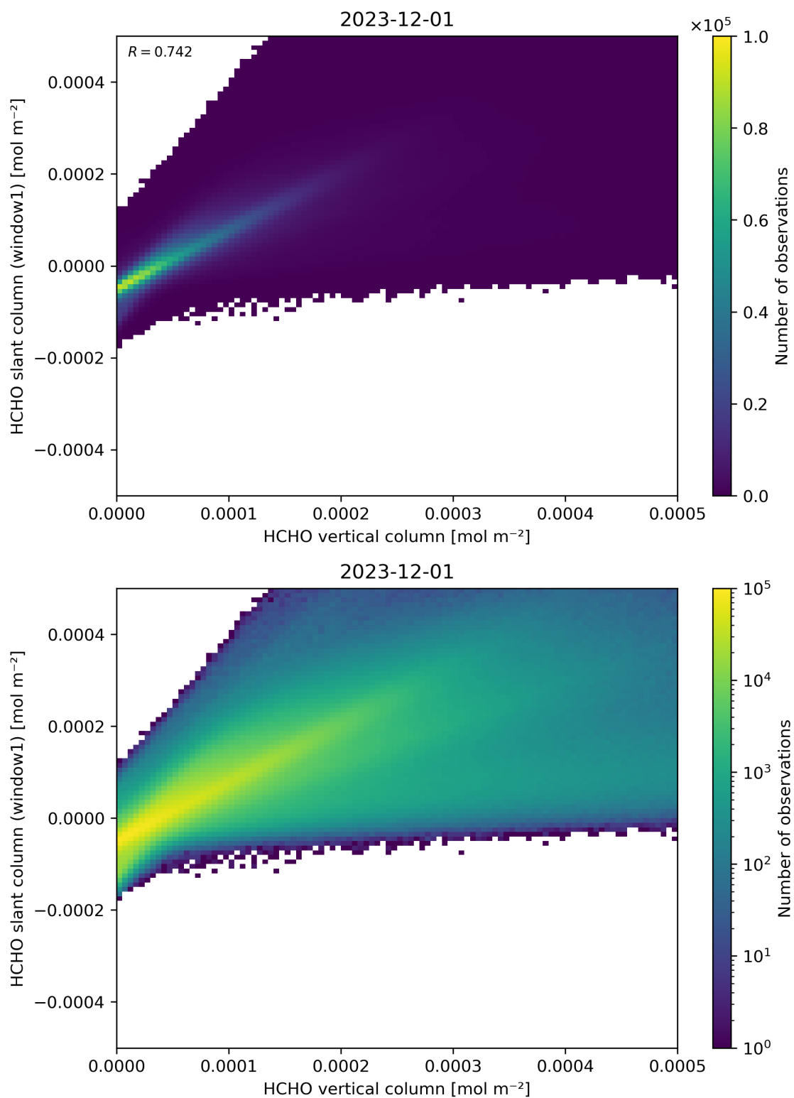
Figure 129: Scatter density plot of “HCHO vertical column” against “HCHO slant column (window1)” for 2023-11-30 to 2023-12-02.
