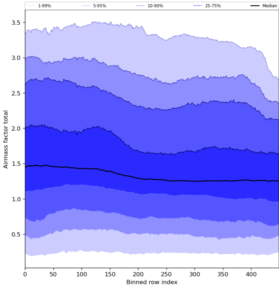
Figure 54: Along track statistics of “Airmass factor total” for 2023-11-30 to 2023-12-02
