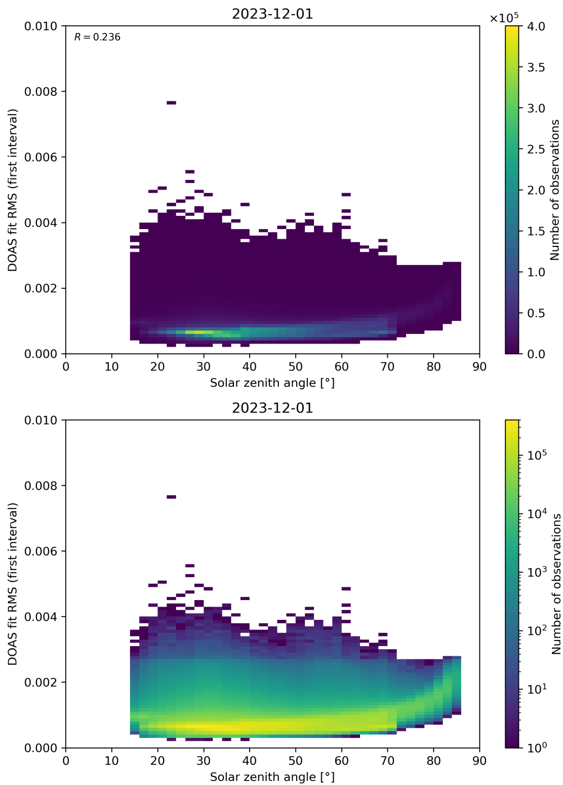
Figure 167: Scatter density plot of “Solar zenith angle” against “DOAS fit RMS (first interval)” for 2023-11-30 to 2023-12-02.
