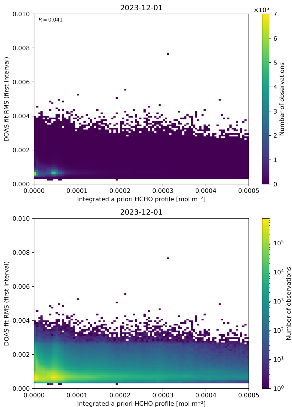
Figure 148: Scatter density plot of “Integrated a priori HCHO profile” against “DOAS fit RMS (first interval)” for 2023-11-30 to 2023-12-02.
