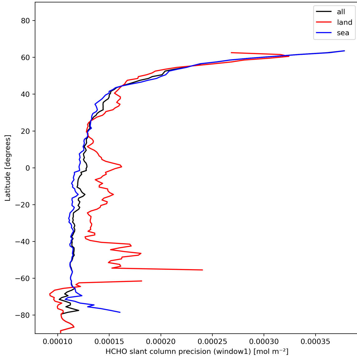
Figure 25: Zonal average of "HCHO slant column precision (window1)" for 2023-11-30 to 2023-12-02.
