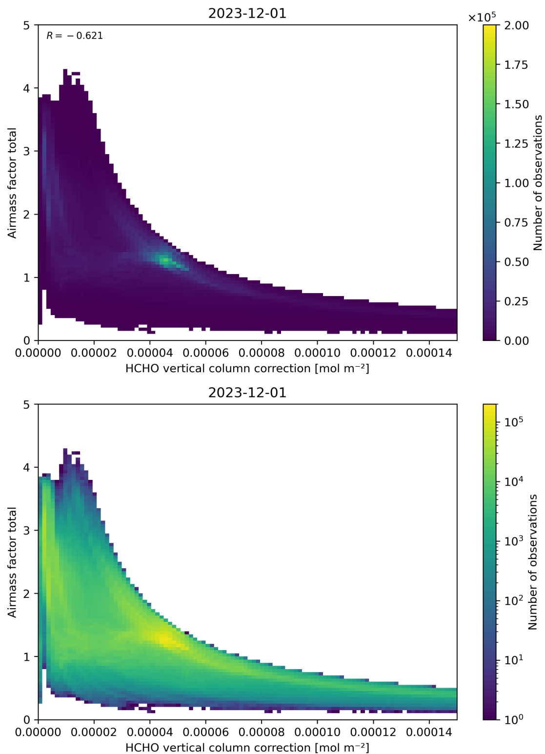
Figure 120: Scatter density plot of “HCHO vertical column correction” against “Airmass factor total” for 2023-11-30 to 2023-12-02.
