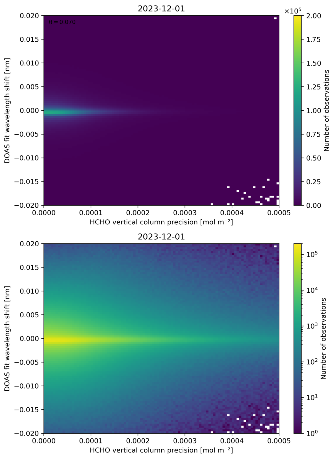
Figure 137: Scatter density plot of “HCHO vertical column precision” against “DOAS fit wavelength shift” for 2023-11-30 to 2023-12-02.
