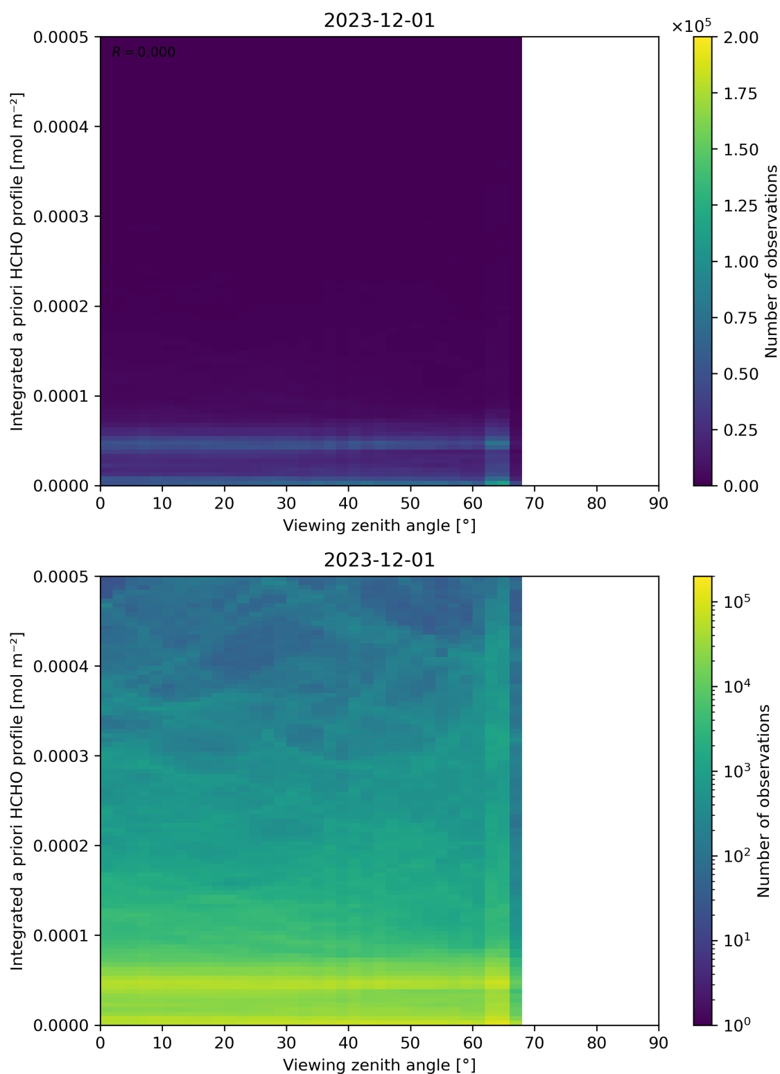
Figure 195: Scatter density plot of “Viewing zenith angle” against “Integrated a priori HCHO profile” for 2023-11-30 to 2023-12-02.
