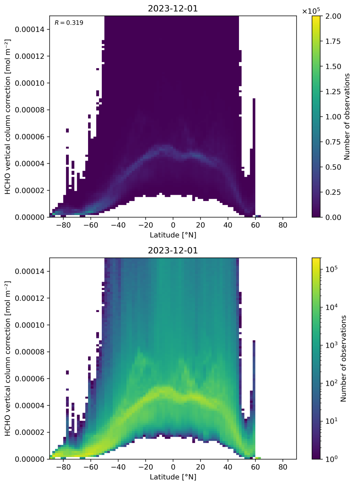
Figure 164: Scatter density plot of “Latitude” against “HCHO vertical column correction” for 2023-11-30 to 2023-12-02.
