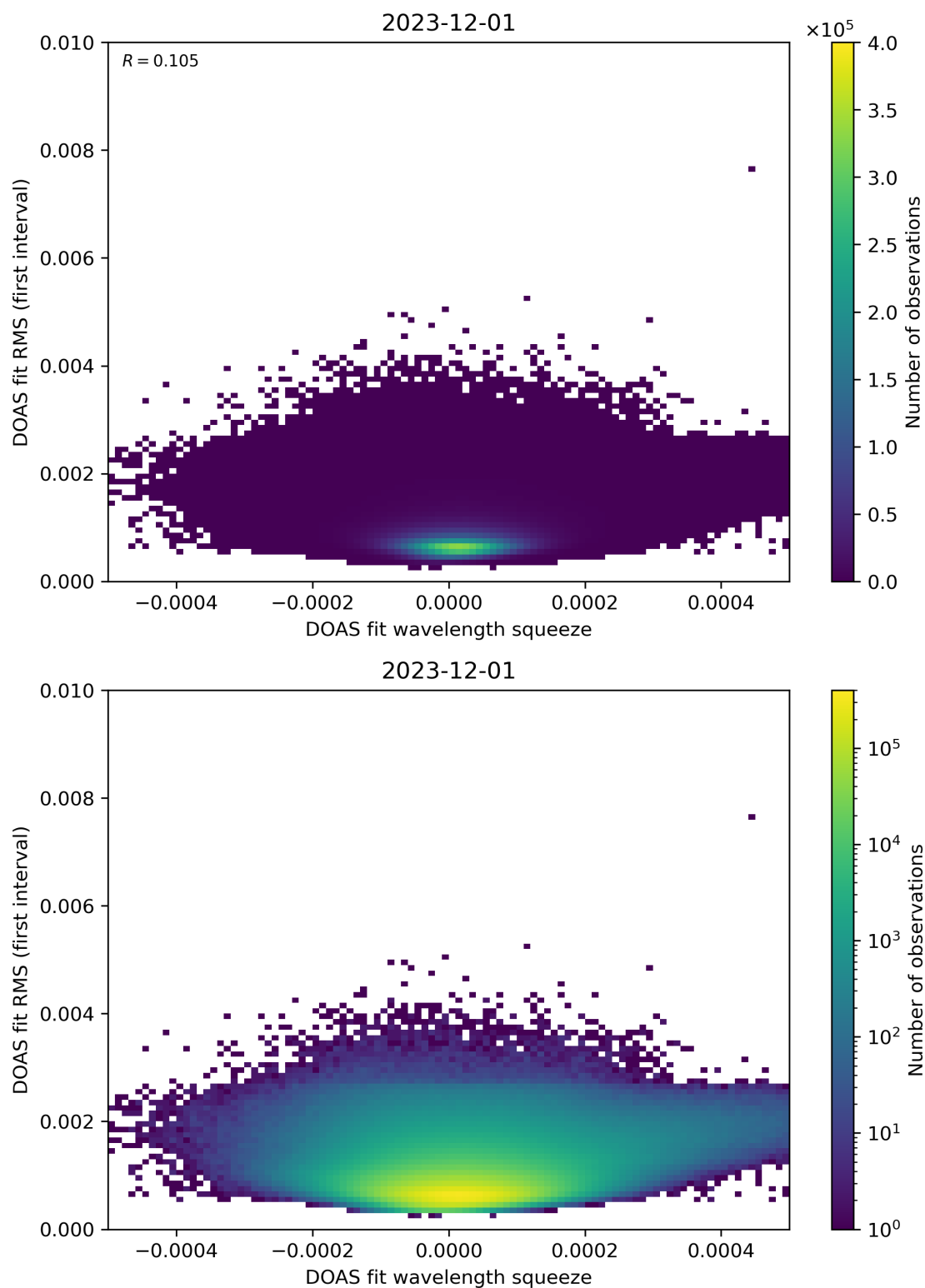
Figure 68: Scatter density plot of “DOAS fit wavelength squeeze” against “DOAS fit RMS (first interval)” for 2023-11-30 to 2023-12-02.
