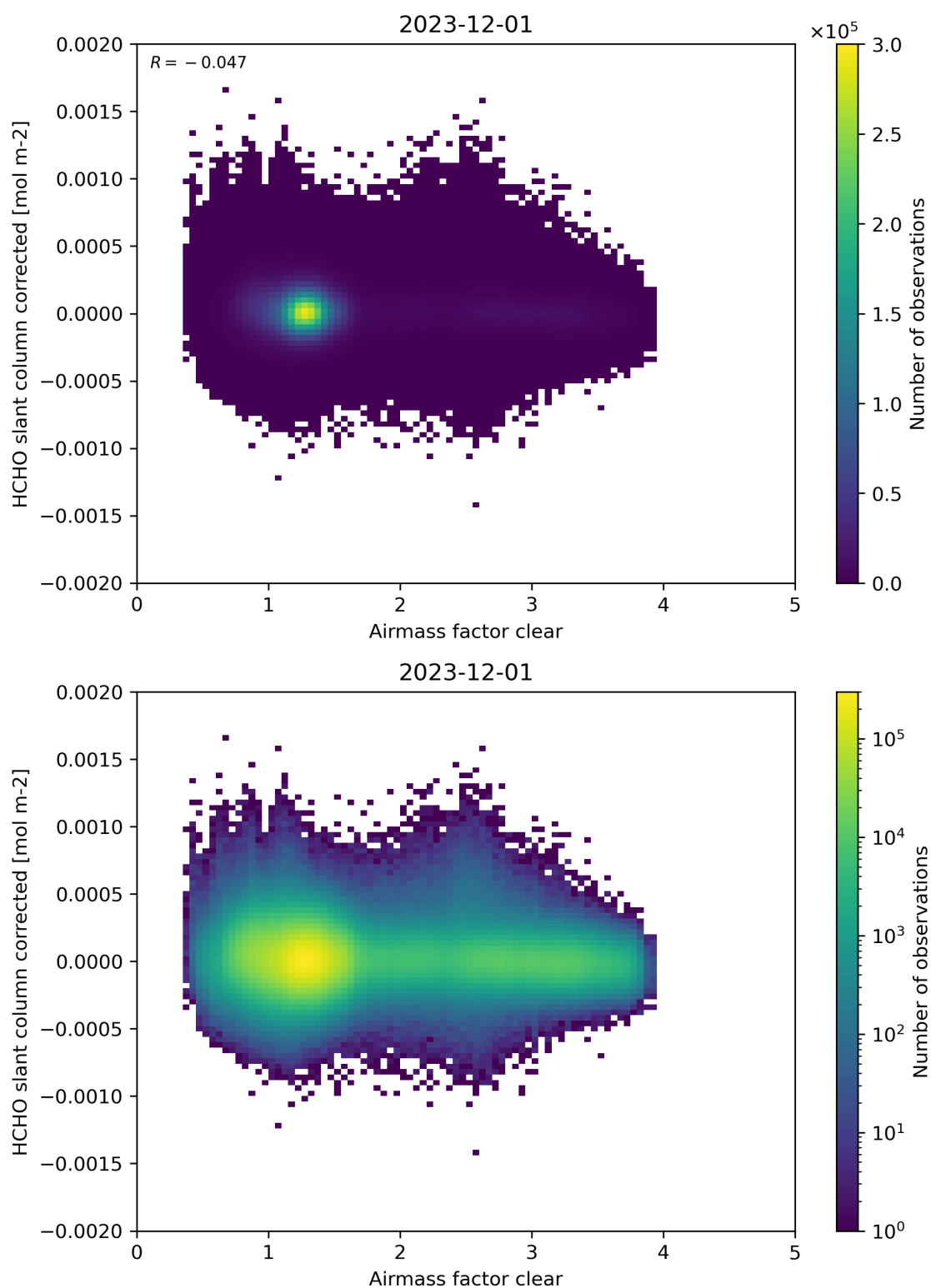
Figure 74: Scatter density plot of “Airmass factor clear” against “HCHO slant column corrected” for 2023-11-30 to 2023-12-02.
