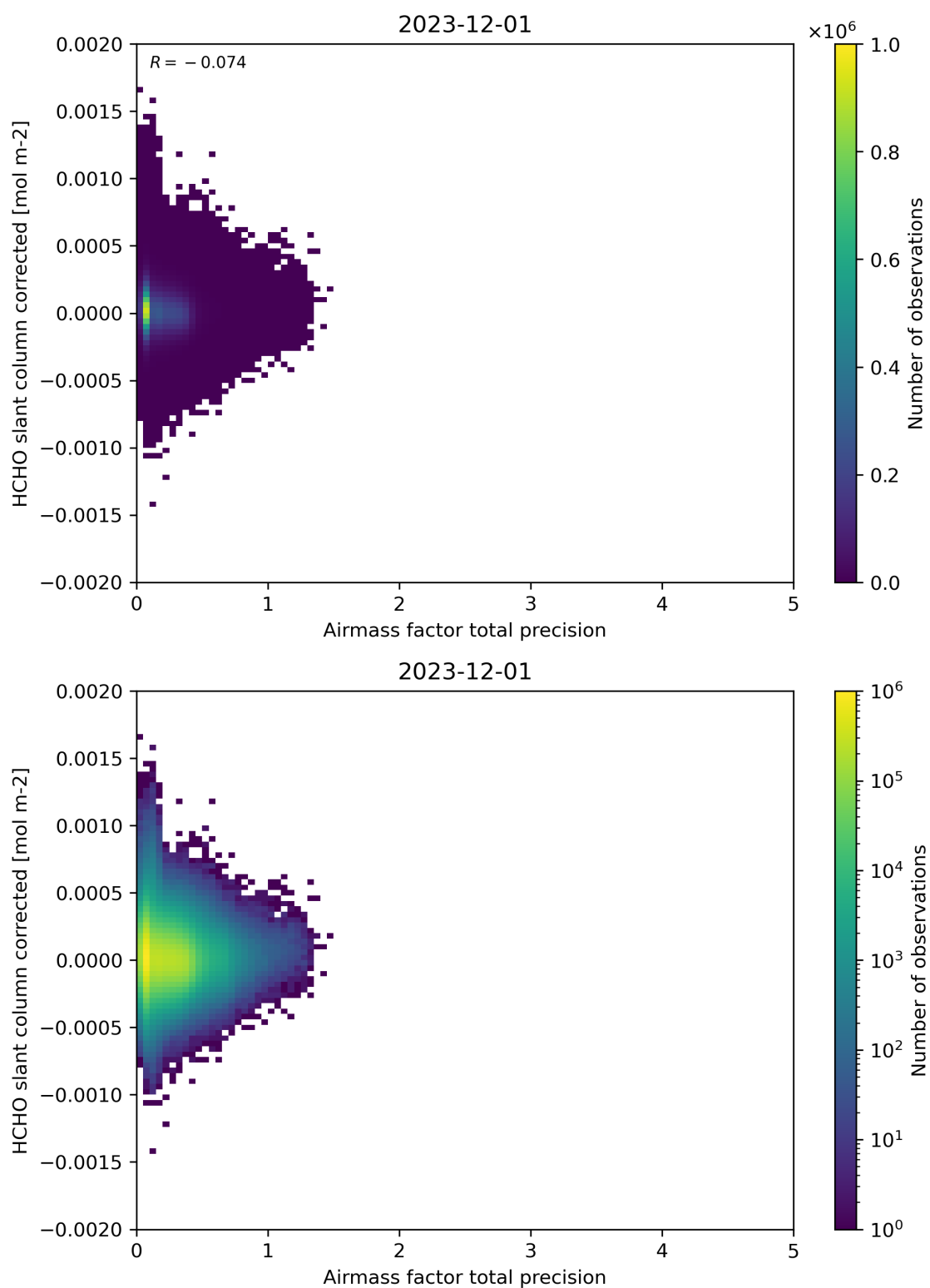
Figure 109: Scatter density plot of “Airmass factor total precision” against “HCHO slant column corrected” for 2023-11-30 to 2023-12-02.
