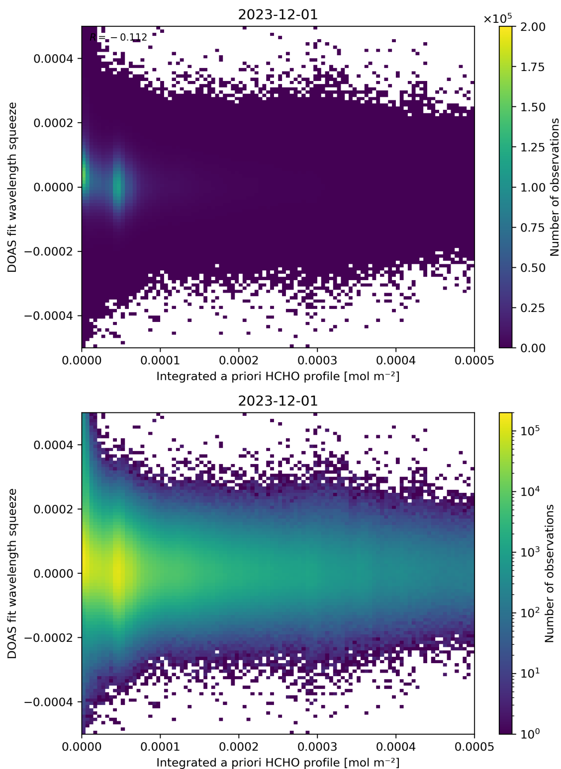
Figure 150: Scatter density plot of “Integrated a priori HCHO profile” against “DOAS fit wavelength squeeze” for 2023-11-30 to 2023-12-02.
