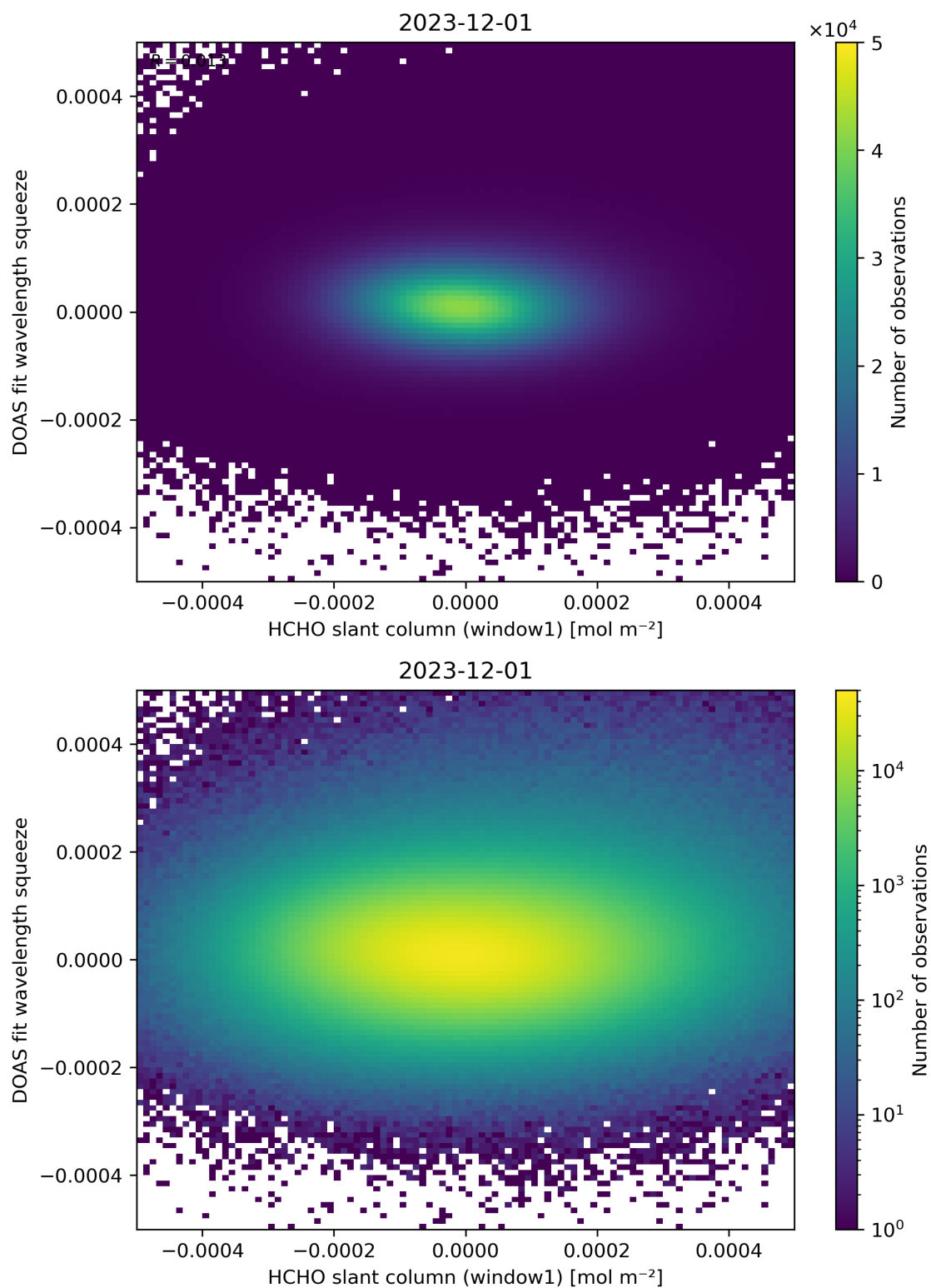
Figure 80: Scatter density plot of “HCHO slant column (window1)” against “DOAS fit wavelength squeeze” for 2023-11-30 to 2023-12-02.
