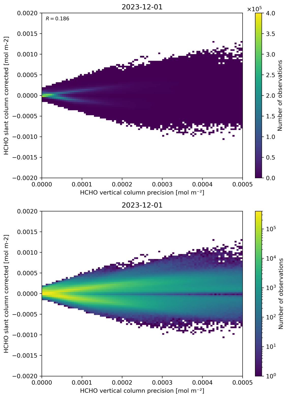
Figure 140: Scatter density plot of “HCHO vertical column precision” against “HCHO slant column corrected” for 2023-11-30 to 2023-12-02.
