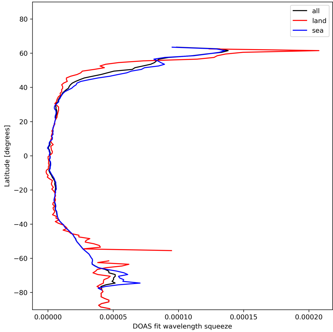
Figure 31: Zonal average of “DOAS fit wavelength squeeze” for 2023-11-30 to 2023-12-02.
