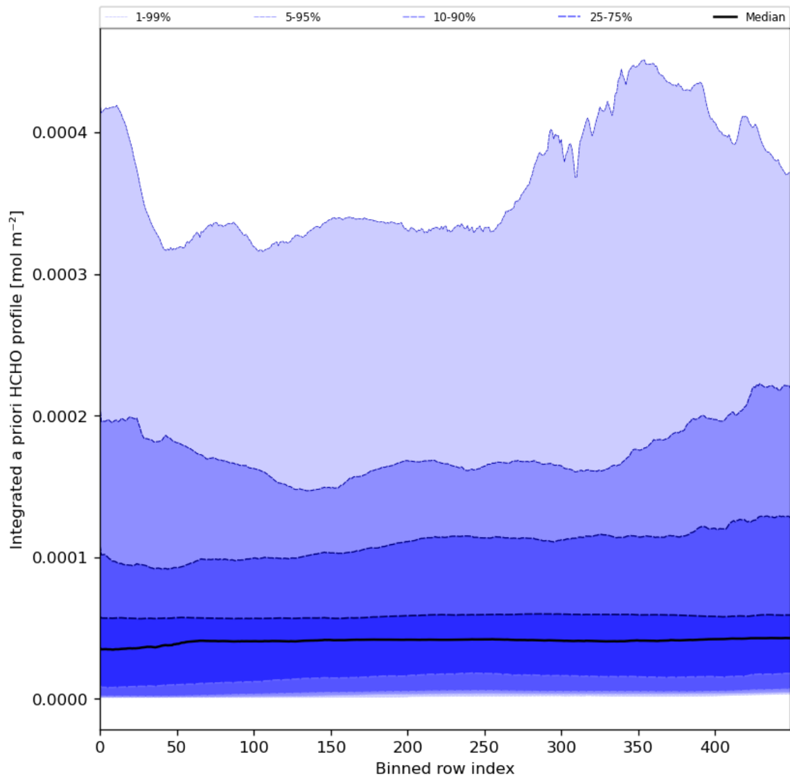
Figure 57: Along track statistics of "Integrated a priori HCHO profile" for 2023-11-30 to 2023-12-02
