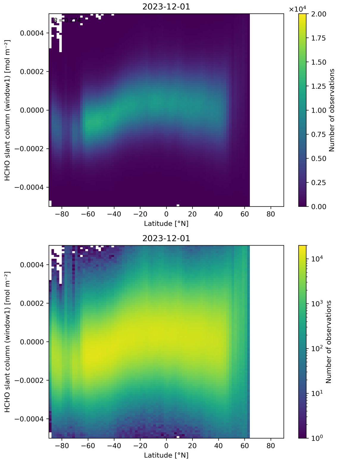
Figure 159: Scatter density plot of “Latitude” against “HCHO slant column (window1)” for 2023-11-30 to 2023-12-02.
