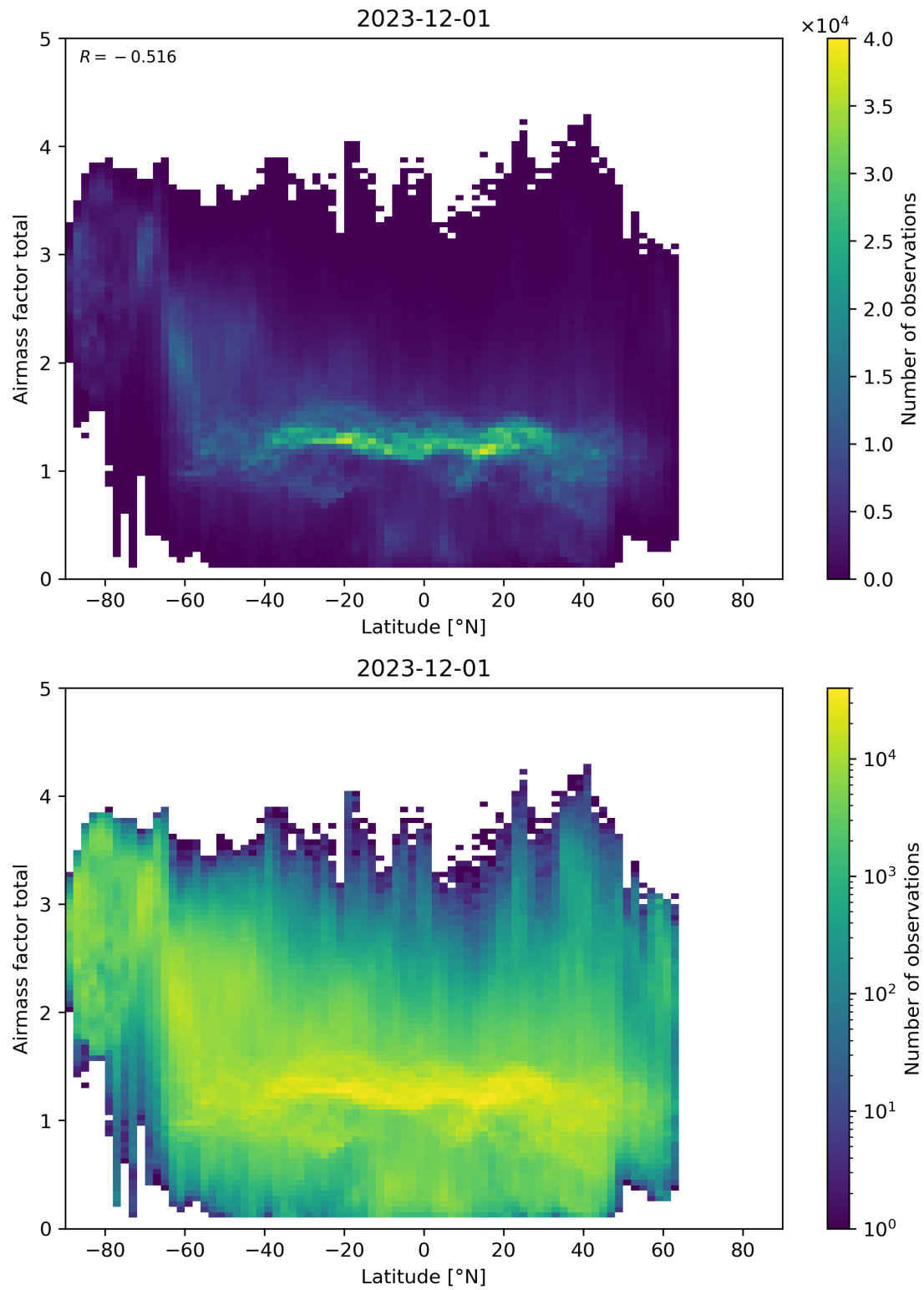
Figure 161: Scatter density plot of “Latitude” against “Airmass factor total” for 2023-11-30 to 2023-12-02.
