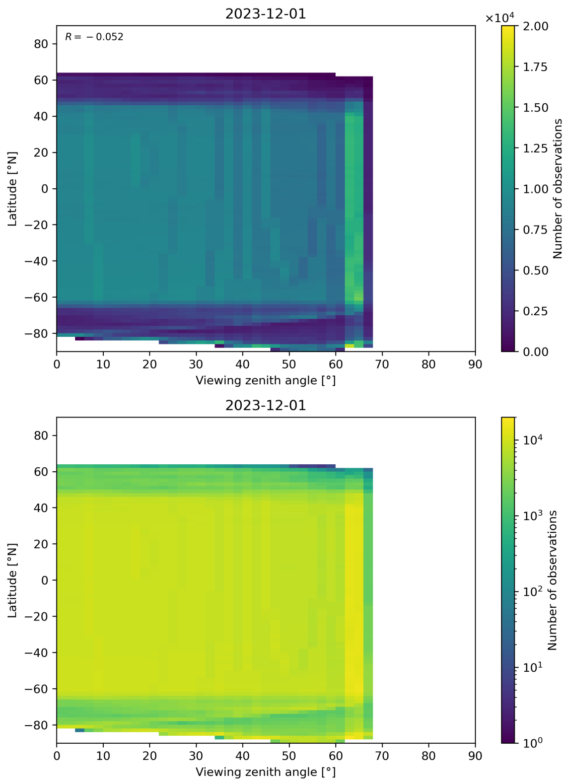
Figure 196: Scatter density plot of “Viewing zenith angle” against “Latitude” for 2023-11-30 to 2023-12-02.
