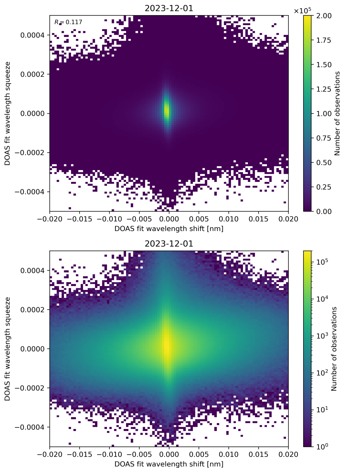
Figure 65: Scatter density plot of “DOAS fit wavelength shift” against “DOAS fit wavelength squeeze” for 2023-11-30 to 2023-12-02.
