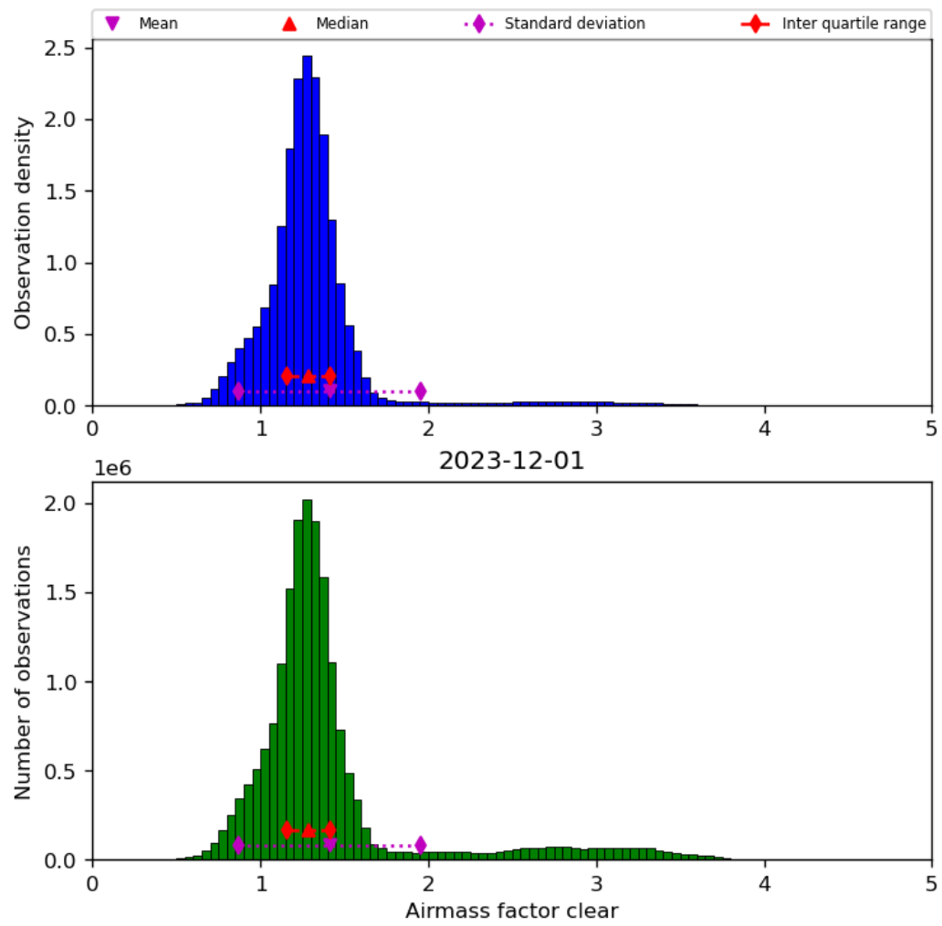
Figure 42: Histogram of “Airmass factor clear” for 2023-11-30 to 2023-12-02
