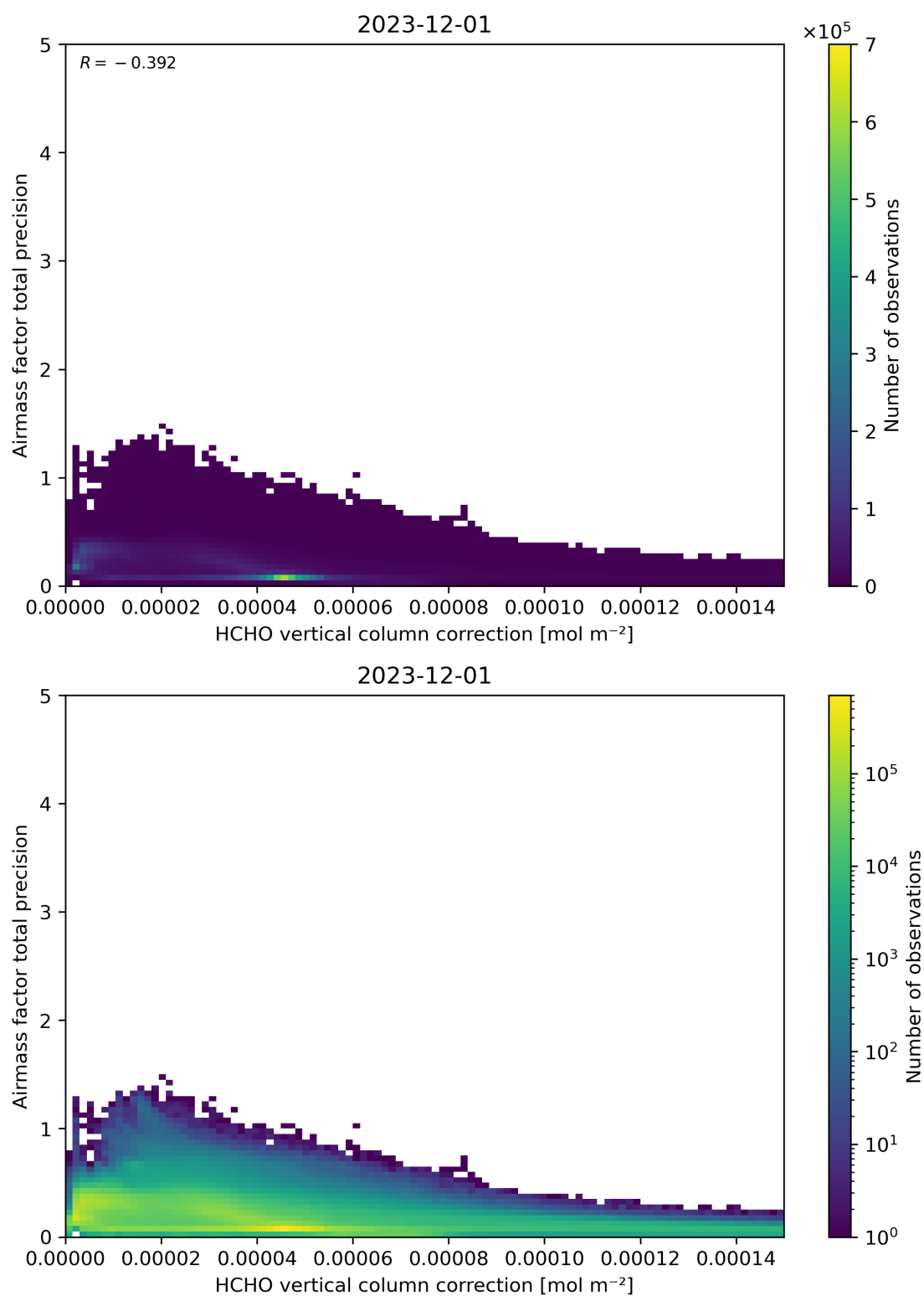
Figure 121: Scatter density plot of “HCHO vertical column correction” against “Airmass factor total precision” for 2023-11-30 to 2023-12-02.
