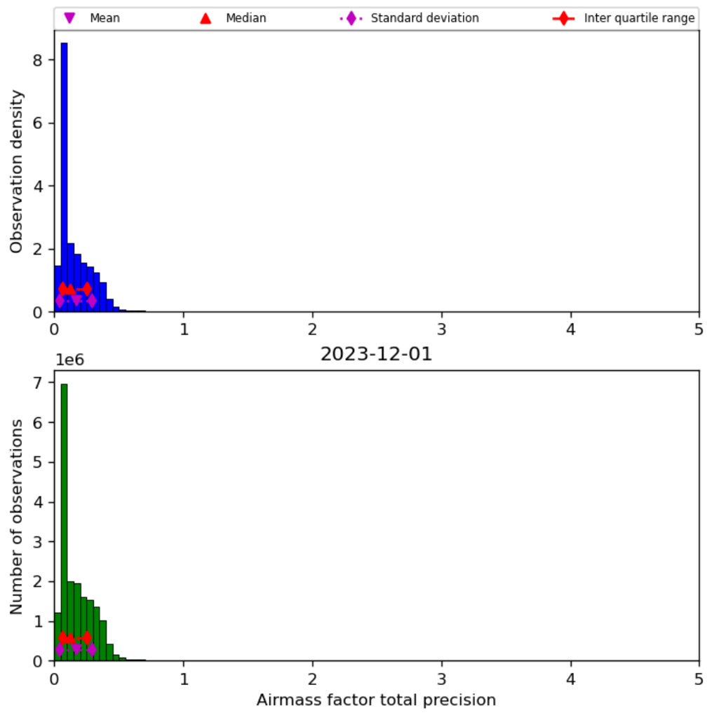
Figure 41: Histogram of “Airmass factor total precision” for 2023-11-30 to 2023-12-02
