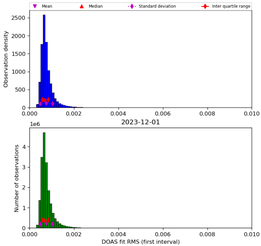
Figure 46: Histogram of “DOAS fit RMS (first interval)” for 2023-11-30 to 2023-12-02
