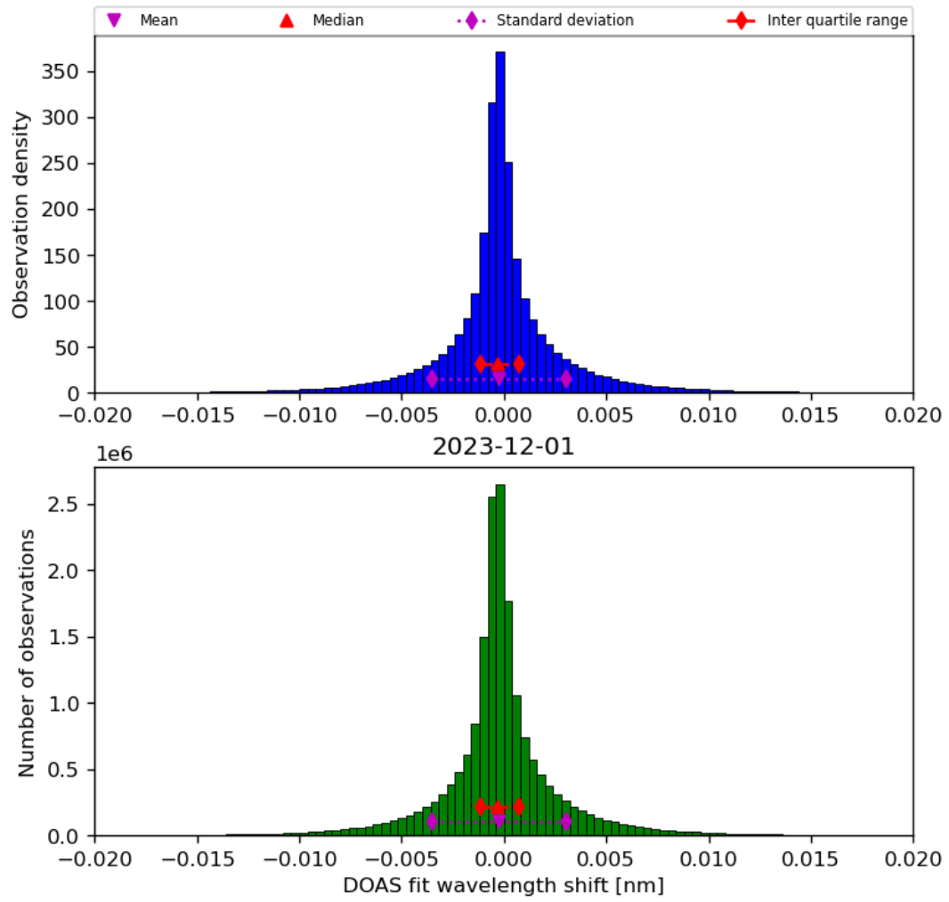
Figure 44: Histogram of “DOAS fit wavelength shift” for 2023-11-30 to 2023-12-02
