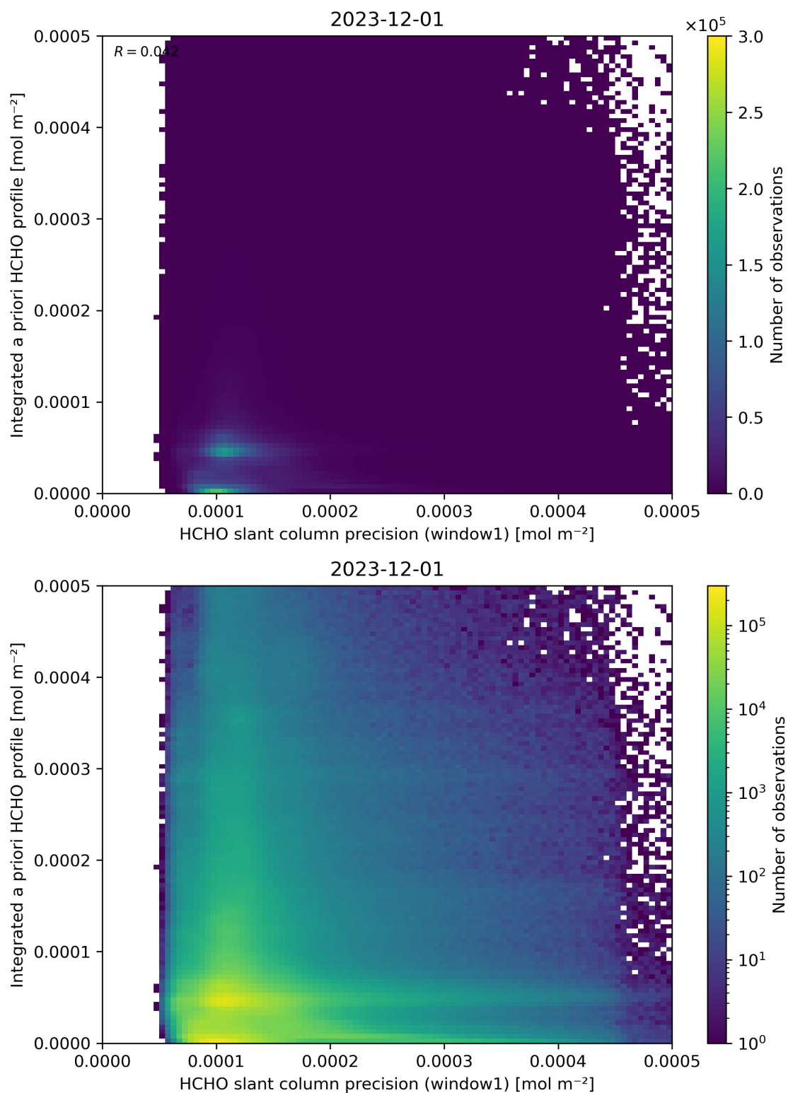
Figure 96: Scatter density plot of “HCHO slant column precision (window1)” against “Integrated a priori HCHO profile” for 2023-11-30 to 2023-12-02.
