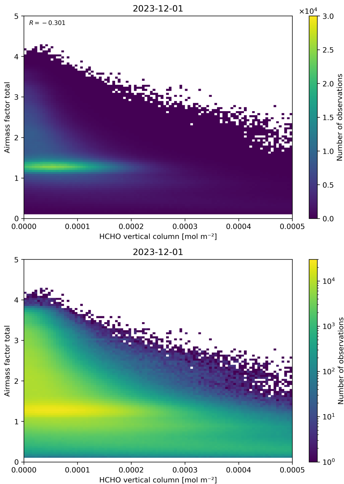
Figure 131: Scatter density plot of “HCHO vertical column” against “Airmass factor total” for 2023-11-30 to 2023-12-02.
