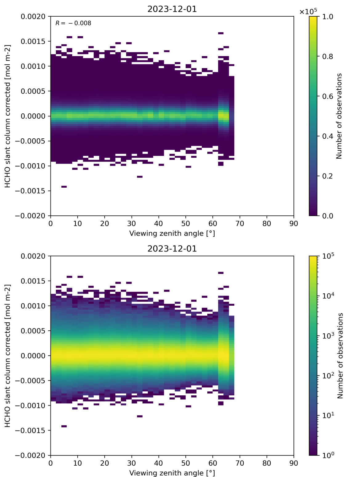
Figure 186: Scatter density plot of “Viewing zenith angle” against “HCHO slant column corrected” for 2023-11-30 to 2023-12-02.
