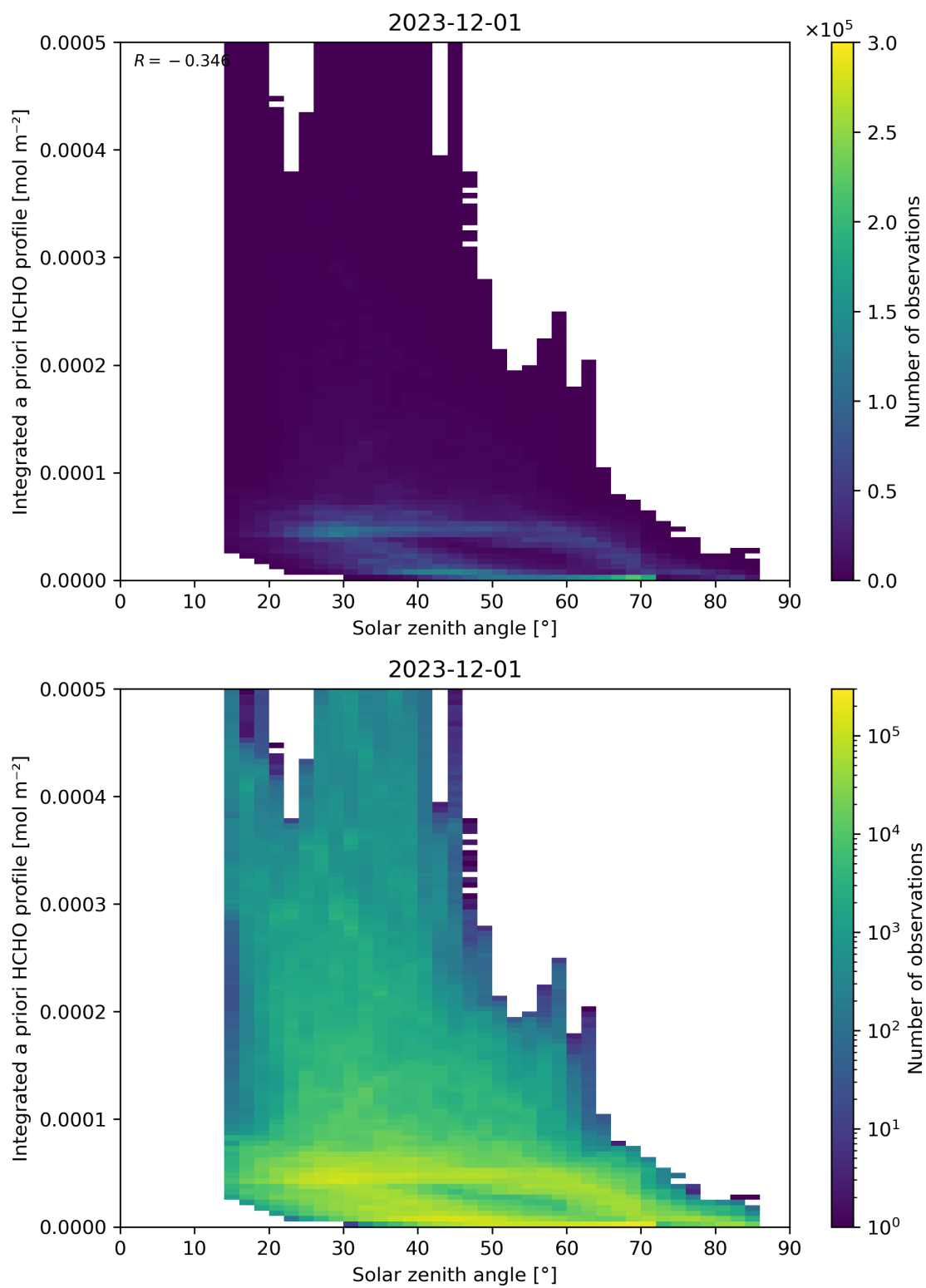
Figure 180: Scatter density plot of “Solar zenith angle” against “Integrated a priori HCHO profile” for 2023-11-30 to 2023-12-02.
