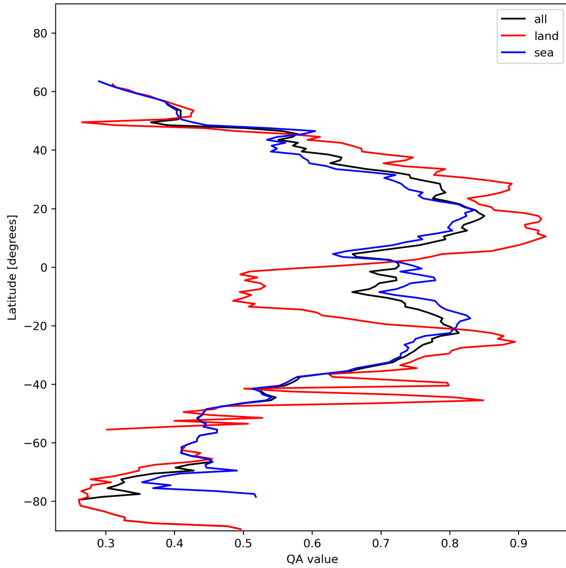
Figure 20: Zonal average of “QA value” for 2023-11-30 to 2023-12-02.
