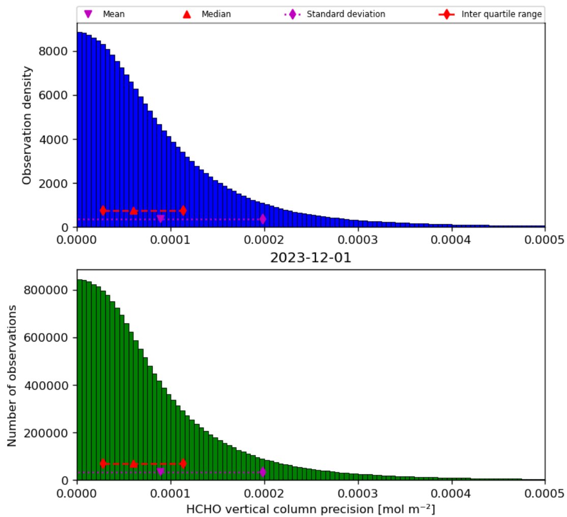
Figure 36: Histogram of “HCHO vertical column precision” for 2023-11-30 to 2023-12-02
