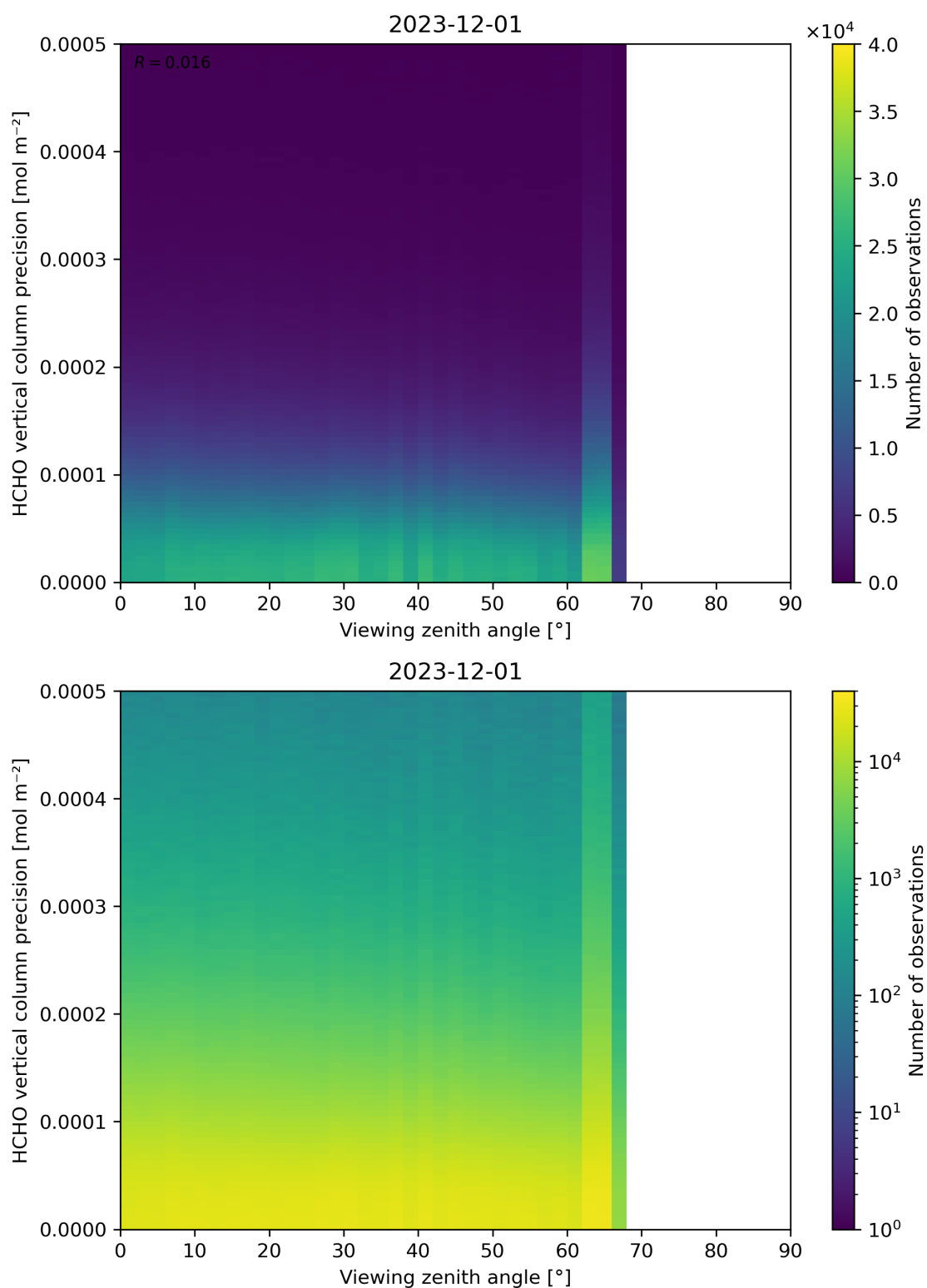
Figure 194: Scatter density plot of “Viewing zenith angle” against “HCHO vertical column precision” for 2023-11-30 to 2023-12-02.
