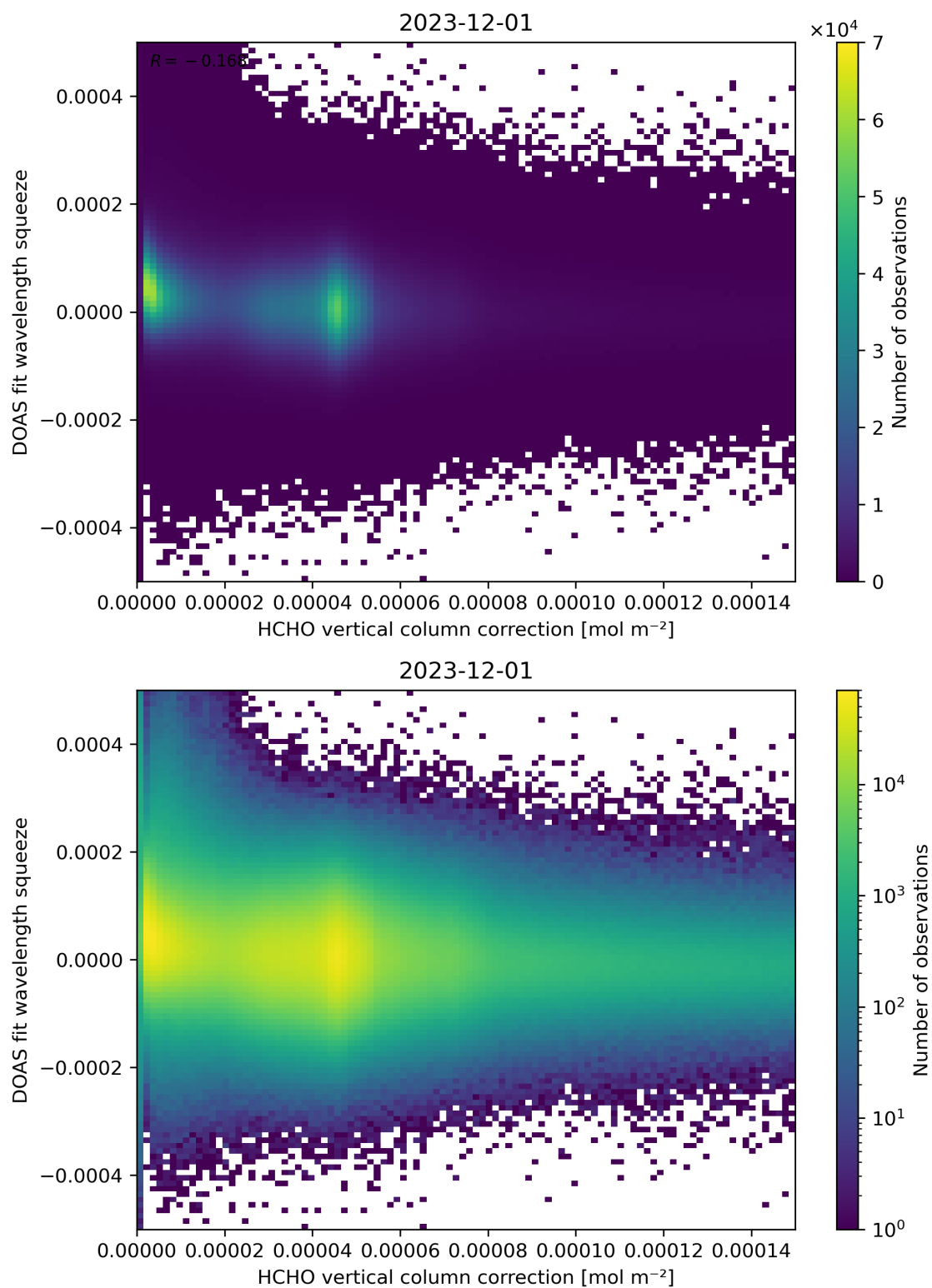
Figure 114: Scatter density plot of “HCHO vertical column correction” against “DOAS fit wavelength squeeze” for 2023-11-30 to 2023-12-02.
