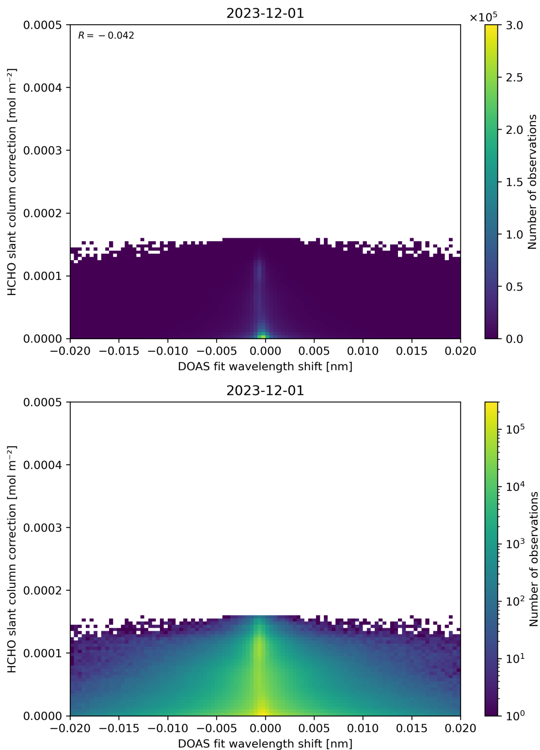
Figure 67: Scatter density plot of “DOAS fit wavelength shift” against “HCHO slant column correction” for 2023-11-30 to 2023-12-02.
