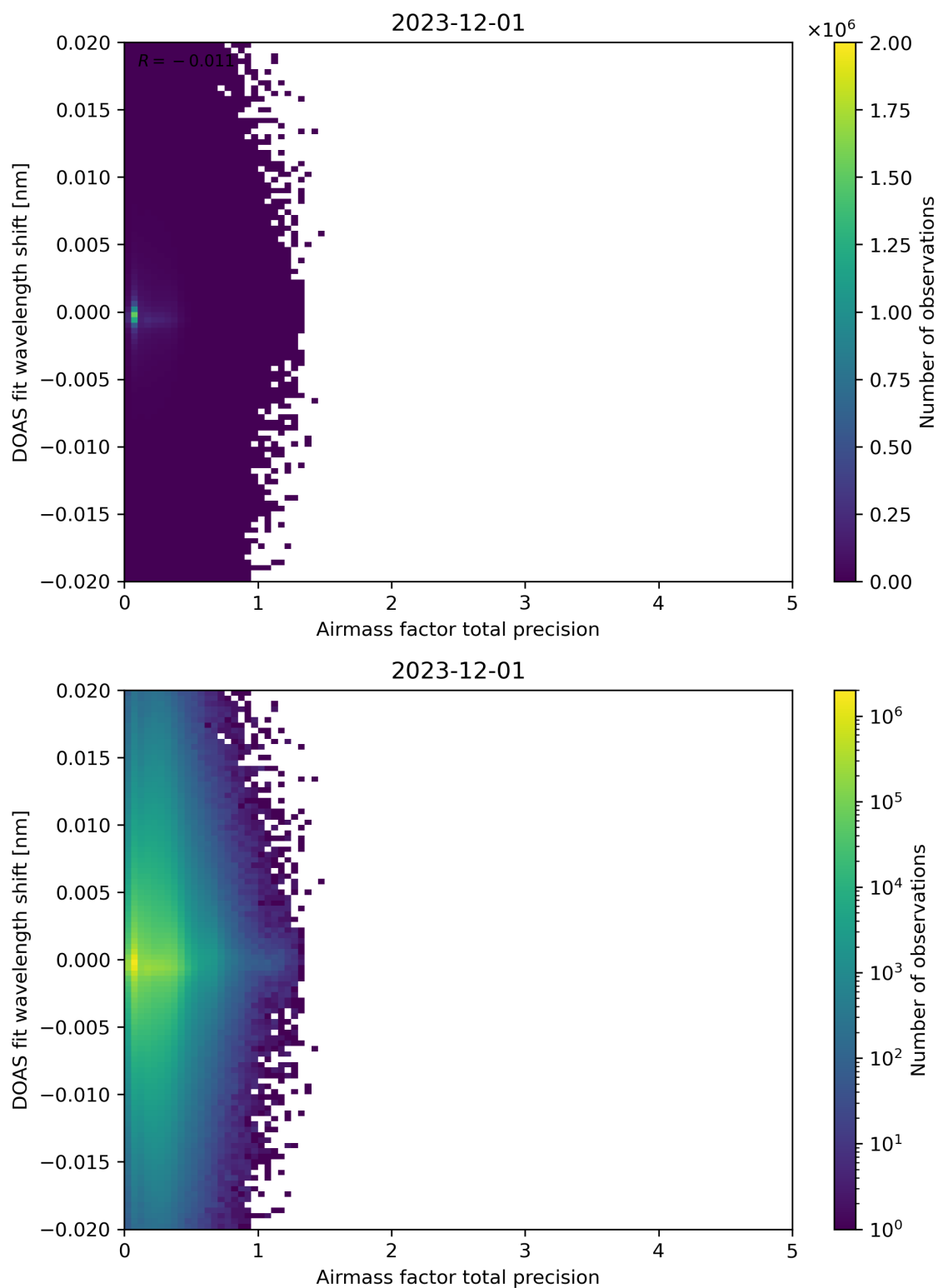
Figure 106: Scatter density plot of “Airmass factor total precision” against “DOAS fit wavelength shift” for 2023-11-30 to 2023-12-02.
