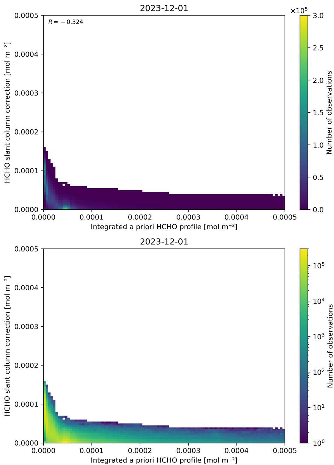
Figure 152: Scatter density plot of “Integrated a priori HCHO profile” against “HCHO slant column correction” for 2023-11-30 to 2023-12-02.
