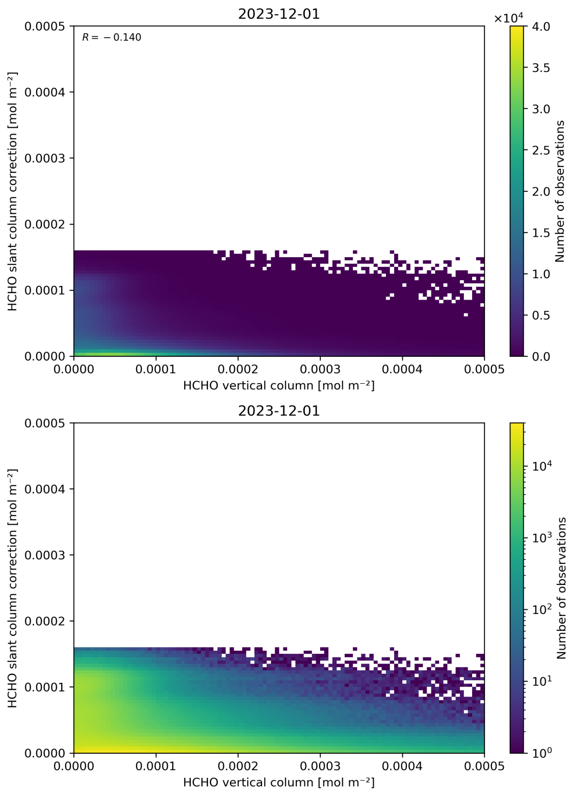
Figure 128: Scatter density plot of “HCHO vertical column” against “HCHO slant column correction” for 2023-11-30 to 2023-12-02.
