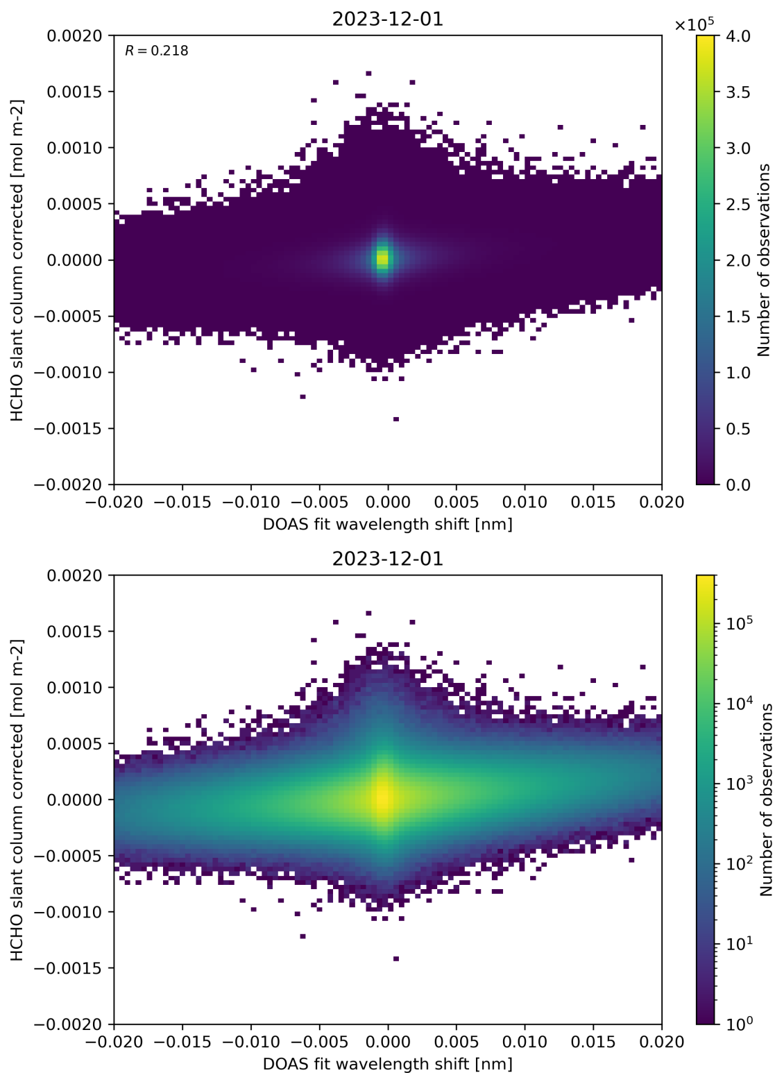
Figure 66: Scatter density plot of “DOAS fit wavelength shift” against “HCHO slant column corrected” for 2023-11-30 to 2023-12-02.
