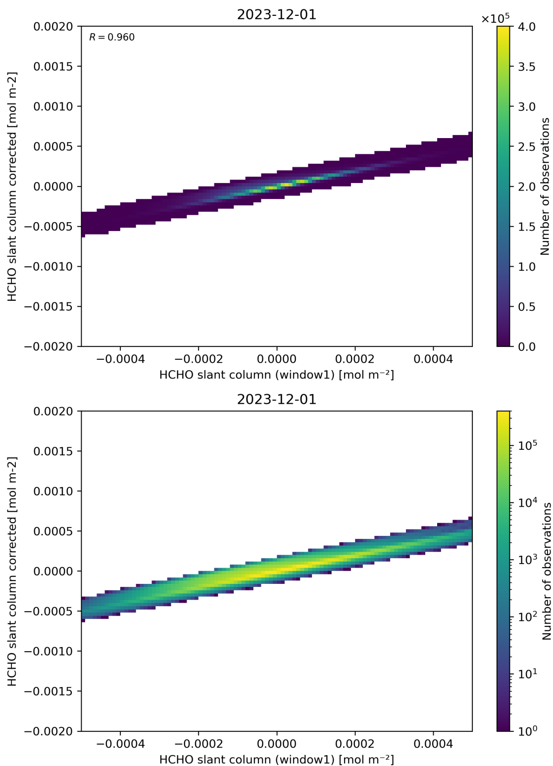
Figure 82: Scatter density plot of “HCHO slant column (window1)” against “HCHO slant column corrected” for 2023-11-30 to 2023-12-02.
