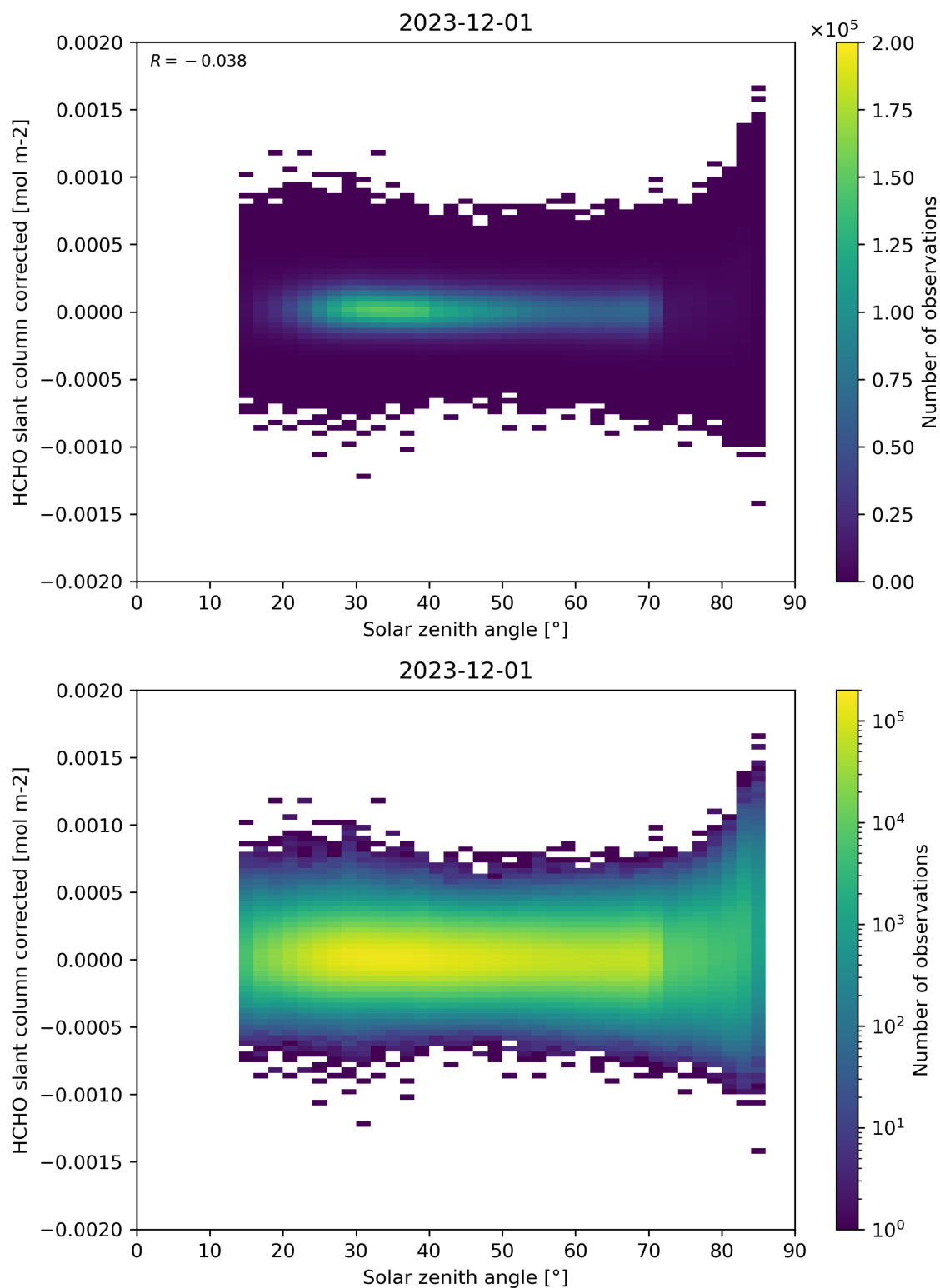
Figure 171: Scatter density plot of “Solar zenith angle” against “HCHO slant column corrected” for 2023-11-30 to 2023-12-02.
