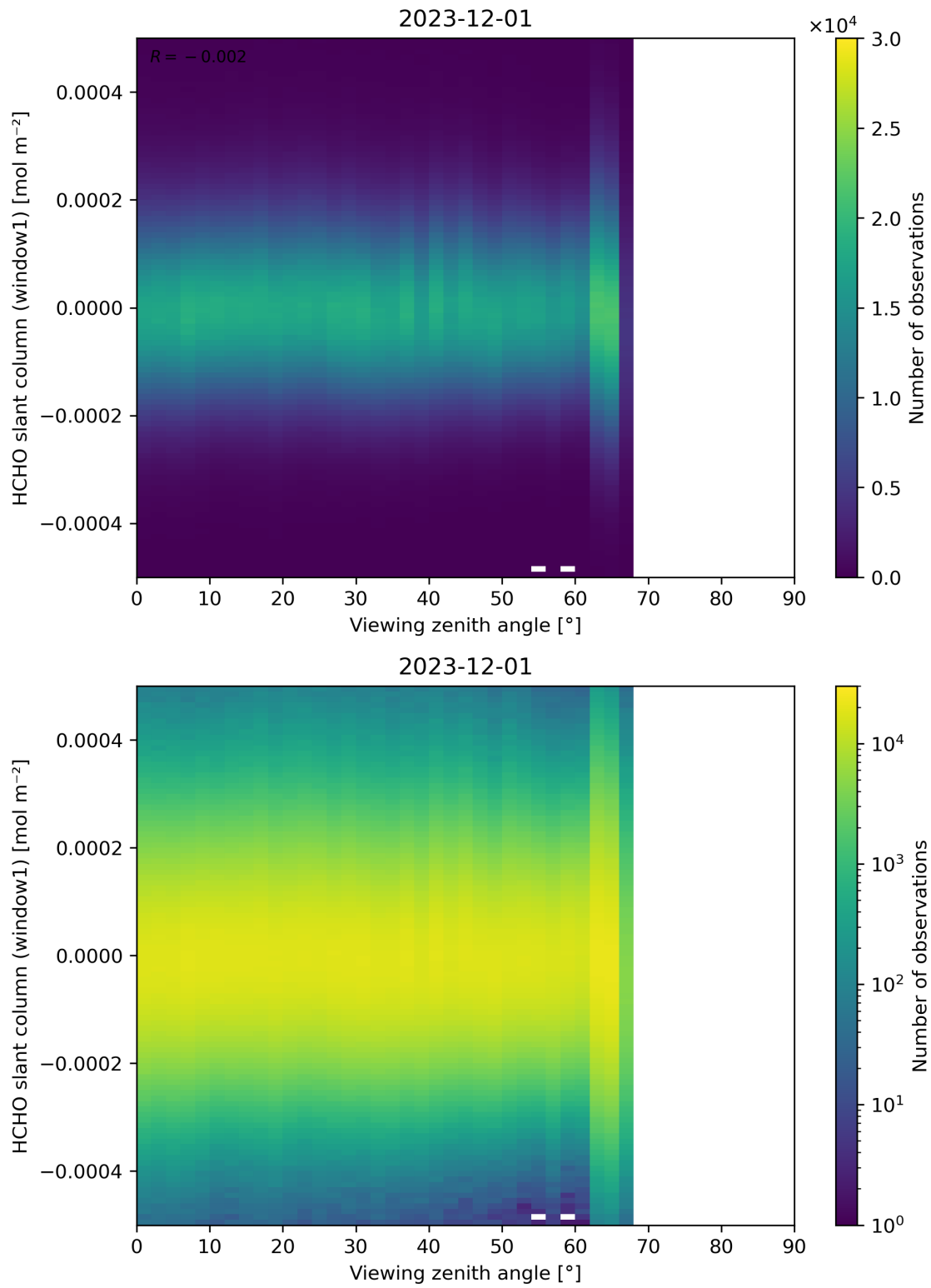
Figure 188: Scatter density plot of “Viewing zenith angle” against “HCHO slant column (window1)” for 2023-11-30 to 2023-12-02.
