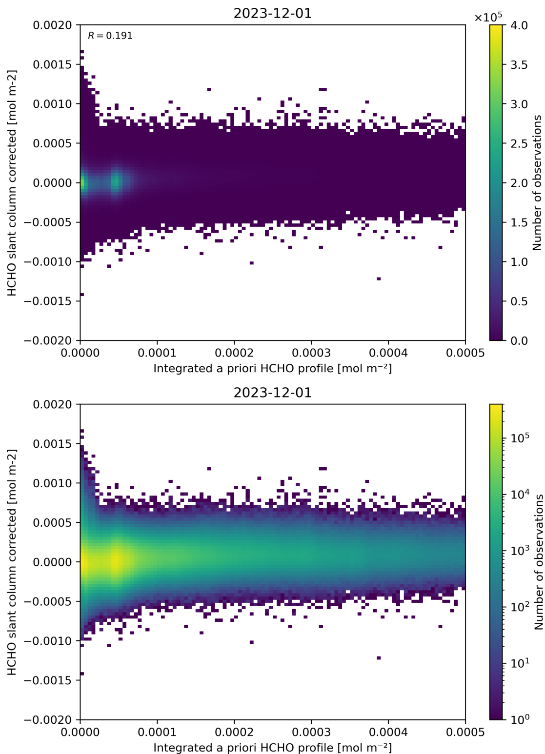
Figure 151: Scatter density plot of “Integrated a priori HCHO profile” against “HCHO slant column corrected” for 2023-11-30 to 2023-12-02.
