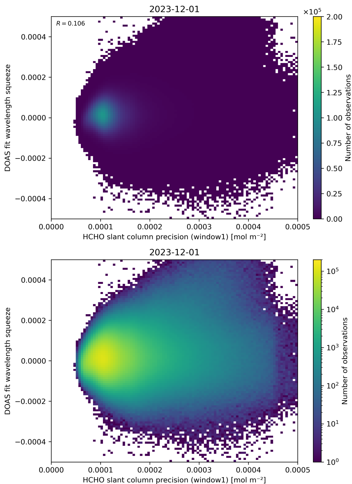
Figure 90: Scatter density plot of “HCHO slant column precision (window1)” against “DOAS fit wavelength squeeze” for 2023-11-30 to 2023-12-02.
