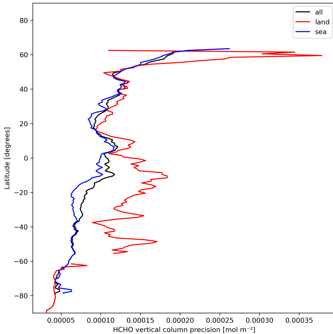
Figure 22: Zonal average of “HCHO vertical column precision” for 2023-11-30 to 2023-12-02.
