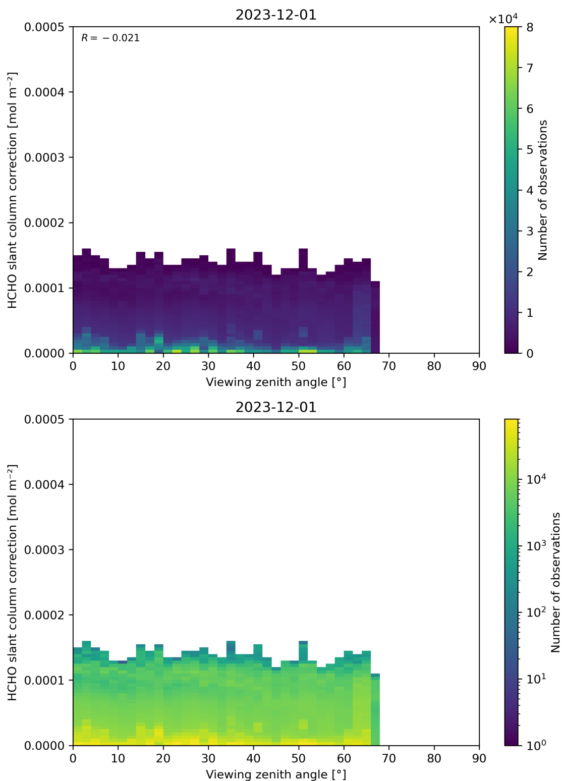
Figure 187: Scatter density plot of “Viewing zenith angle” against “HCHO slant column correction” for 2023-11-30 to 2023-12-02.
