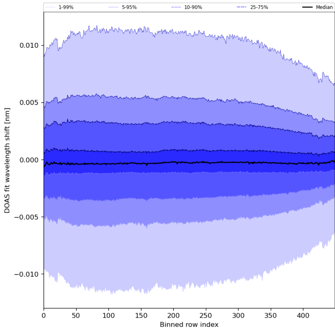
Figure 58: Along track statistics of “DOAS fit wavelength shift” for 2023-11-30 to 2023-12-02
