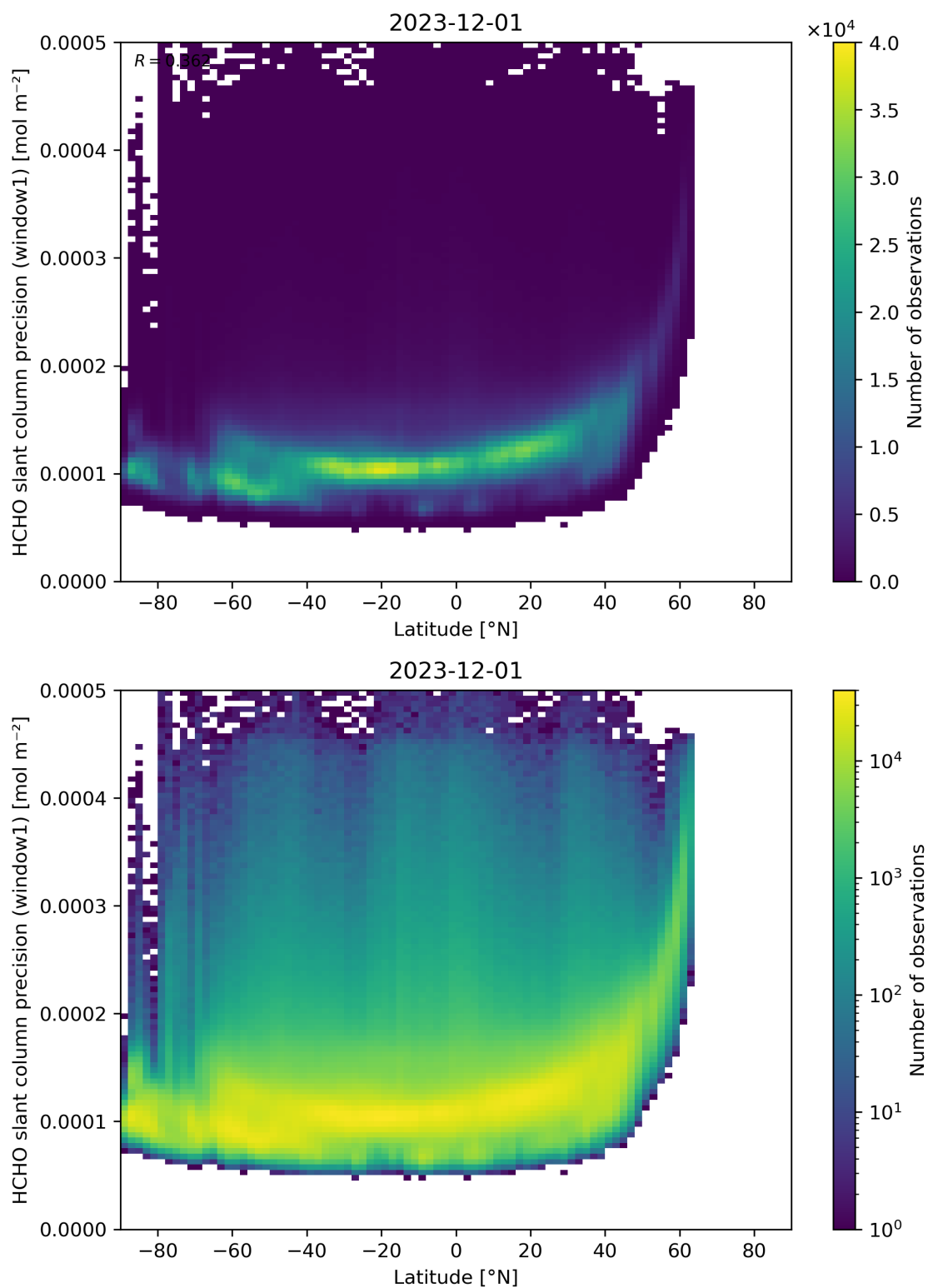
Figure 160: Scatter density plot of “Latitude” against “HCHO slant column precision (window1)” for 2023-11-30 to 2023-12-02.
