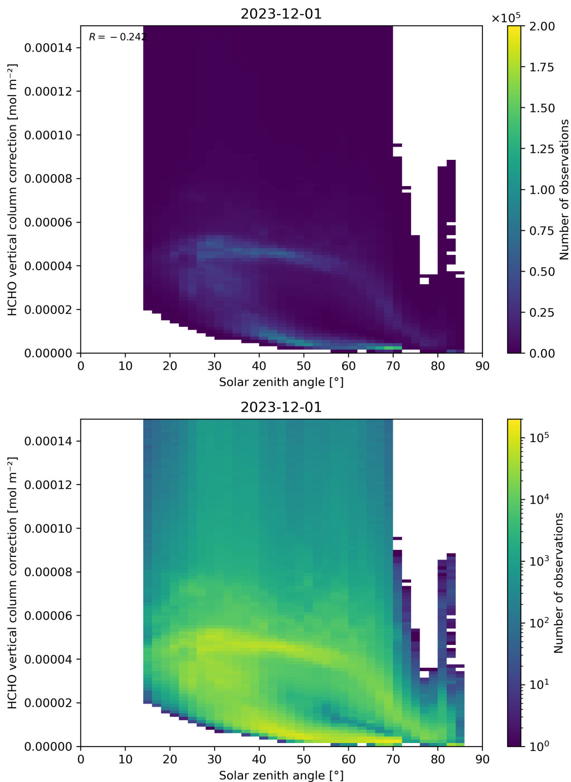
Figure 178: Scatter density plot of “Solar zenith angle” against “HCHO vertical column correction” for 2023-11-30 to 2023-12-02.
