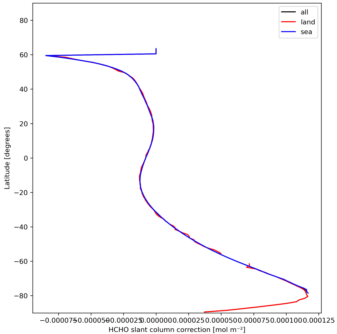
Figure 33: Zonal average of “HCHO slant column correction” for 2023-11-30 to 2023-12-02.
