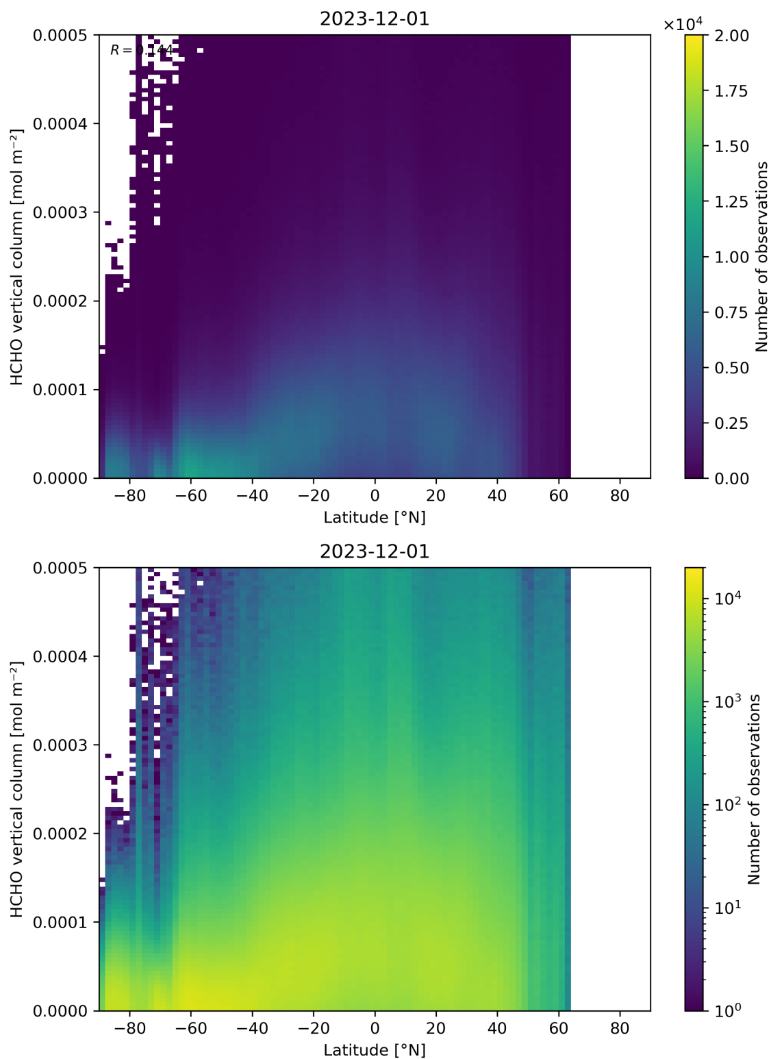
Figure 163: Scatter density plot of “Latitude” against “HCHO vertical column” for 2023-11-30 to 2023-12-02.
