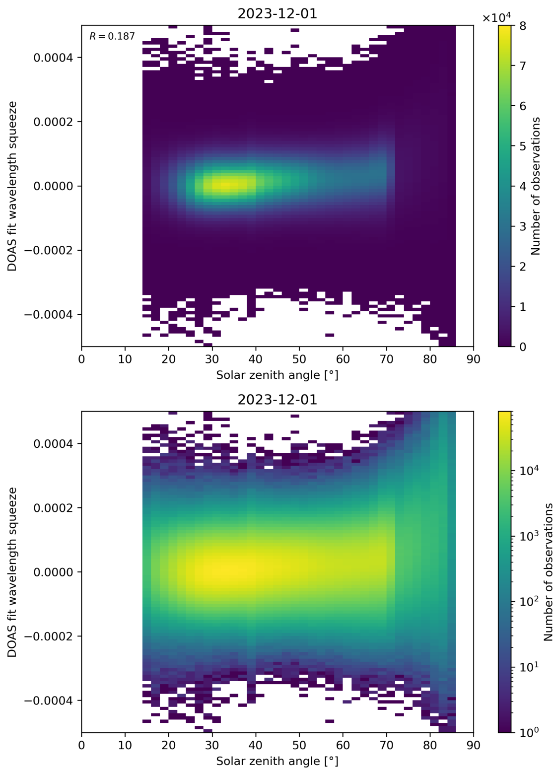
Figure 169: Scatter density plot of “Solar zenith angle” against “DOAS fit wavelength squeeze” for 2023-11-30 to 2023-12-02.
