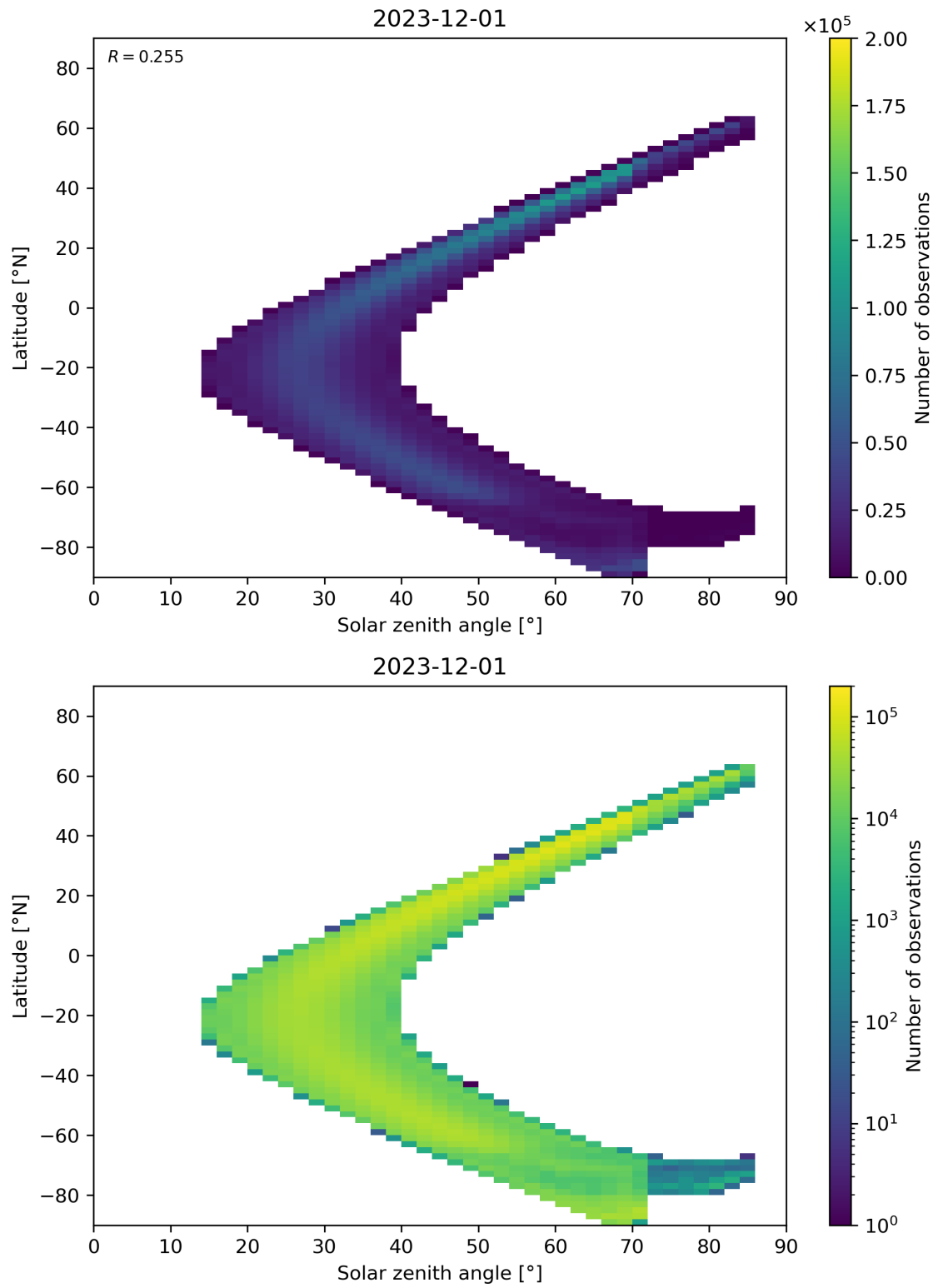
Figure 181: Scatter density plot of “Solar zenith angle” against “Latitude” for 2023-11-30 to 2023-12-02.
