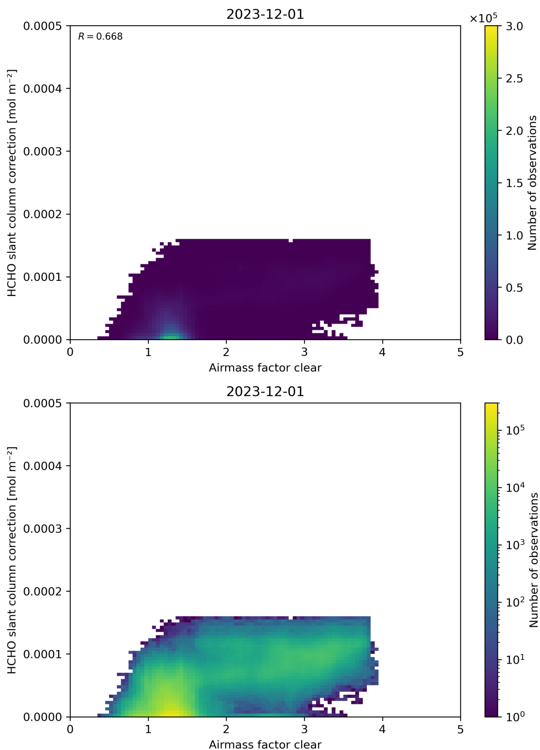
Figure 75: Scatter density plot of “Airmass factor clear” against “HCHO slant column correction” for 2023-11-30 to 2023-12-02.
