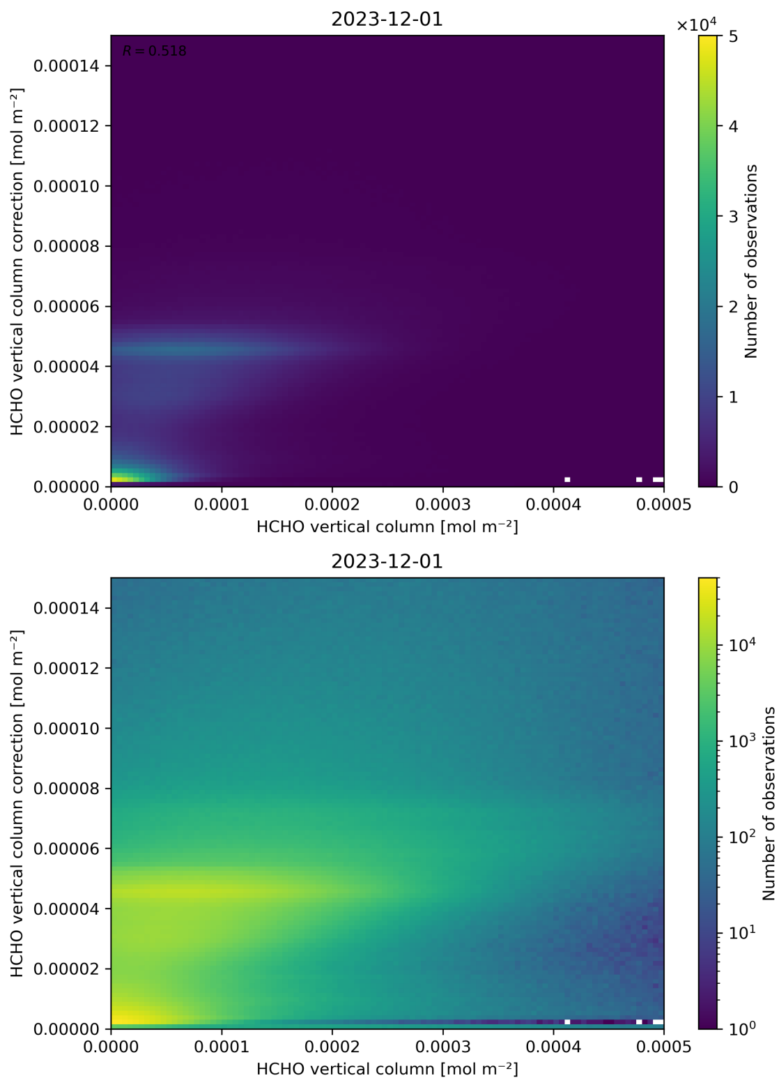
Figure 133: Scatter density plot of “HCHO vertical column” against “HCHO vertical column correction” for 2023-11-30 to 2023-12-02.
