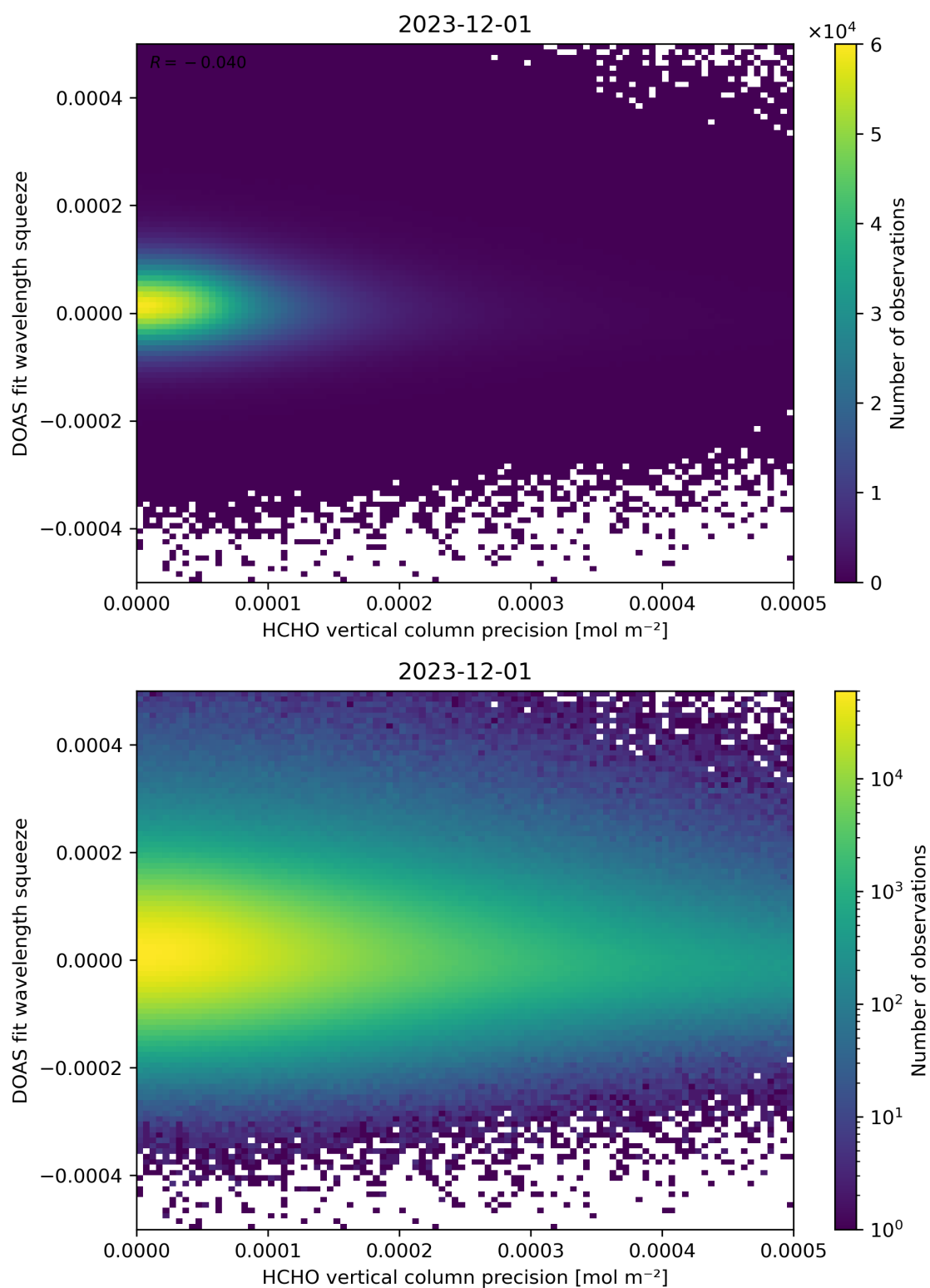
Figure 138: Scatter density plot of “HCHO vertical column precision” against “DOAS fit wavelength squeeze” for 2023-11-30 to 2023-12-02.
