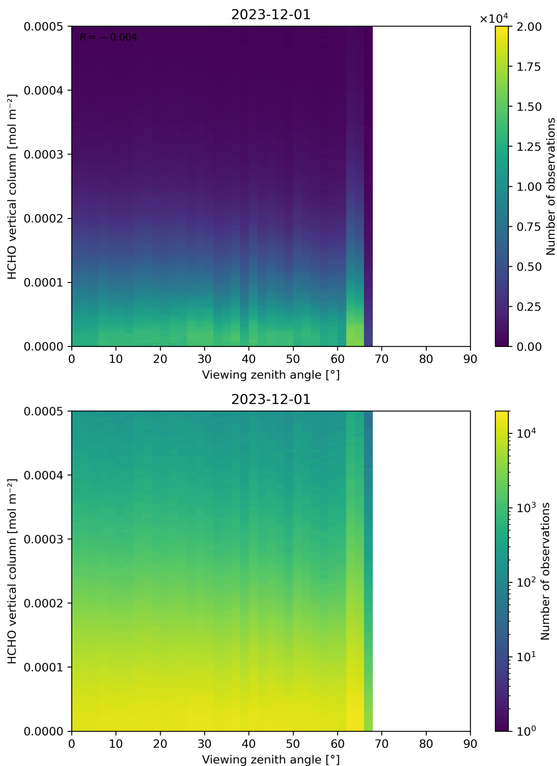
Figure 192: Scatter density plot of “Viewing zenith angle” against “HCHO vertical column” for 2023-11-30 to 2023-12-02.
