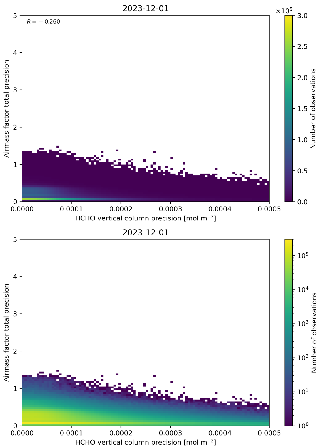
Figure 145: Scatter density plot of “HCHO vertical column precision” against “Airmass factor total precision” for 2023-11-30 to 2023-12-02.
