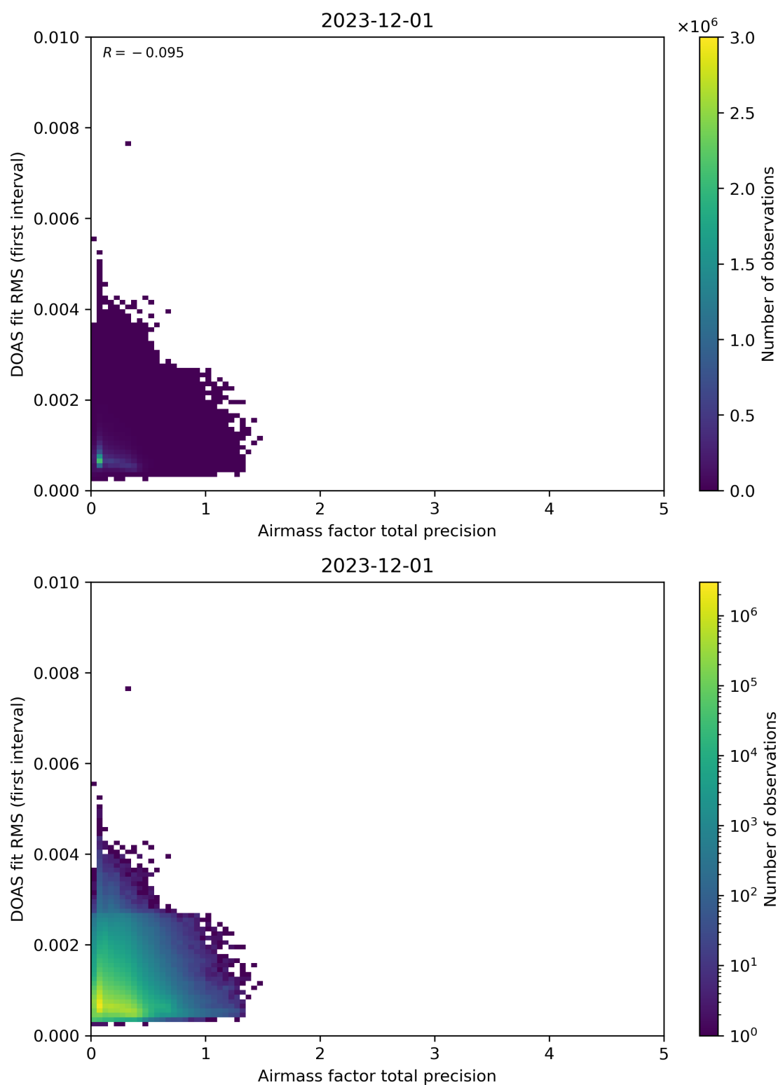
Figure 105: Scatter density plot of “Airmass factor total precision” against “DOAS fit RMS (first interval)” for 2023-11-30 to 2023-12-02.
