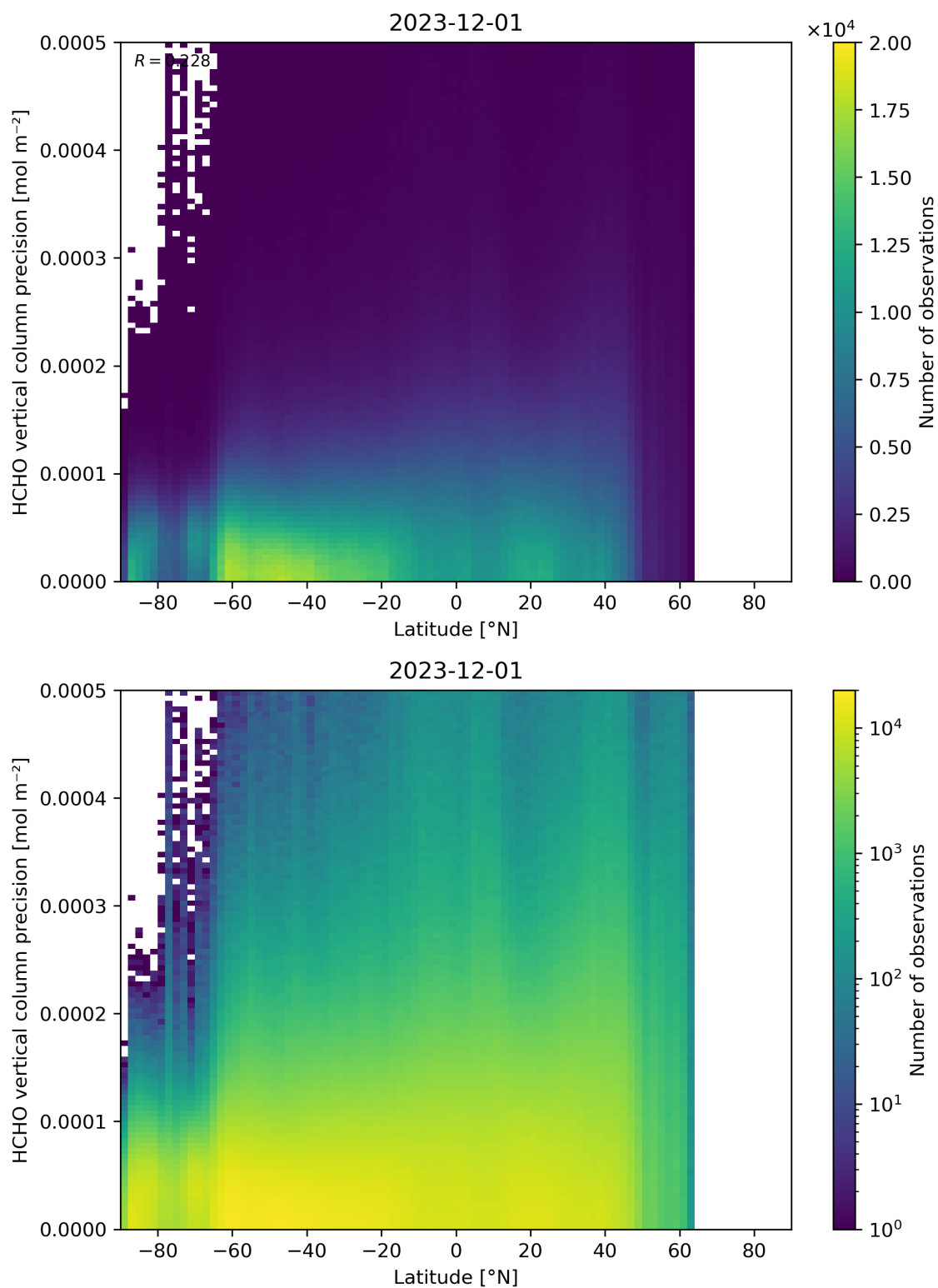
Figure 165: Scatter density plot of “Latitude” against “HCHO vertical column precision” for 2023-11-30 to 2023-12-02.
