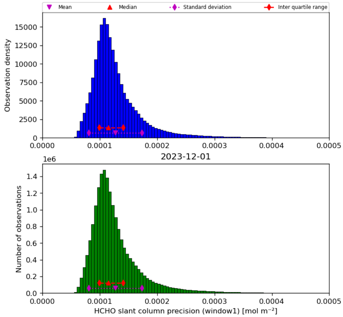
Figure 39: Histogram of “HCHO slant column precision (window1)” for 2023-11-30 to 2023-12-02
