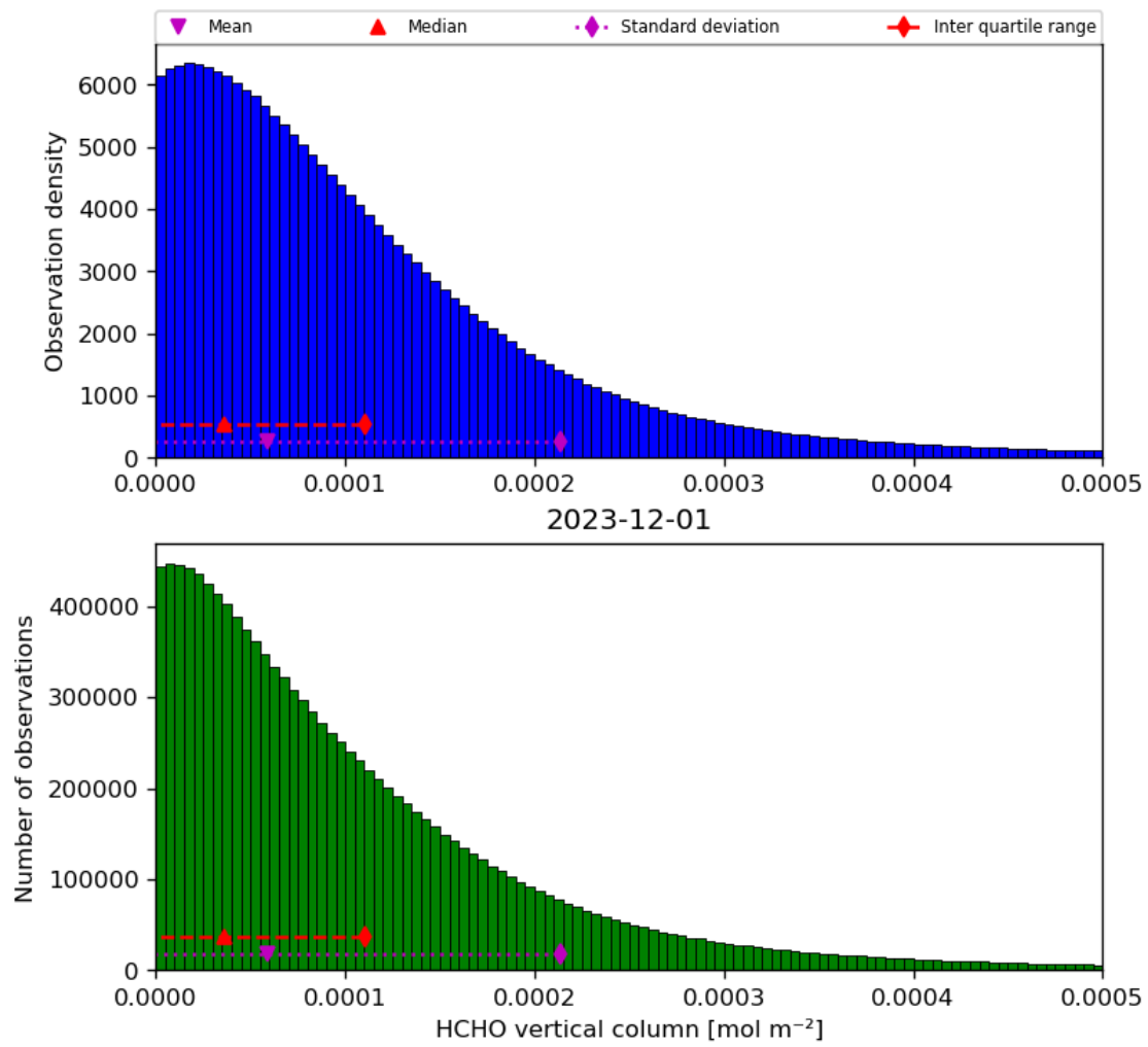
Figure 35: Histogram of “HCHO vertical column” for 2023-11-30 to 2023-12-02
