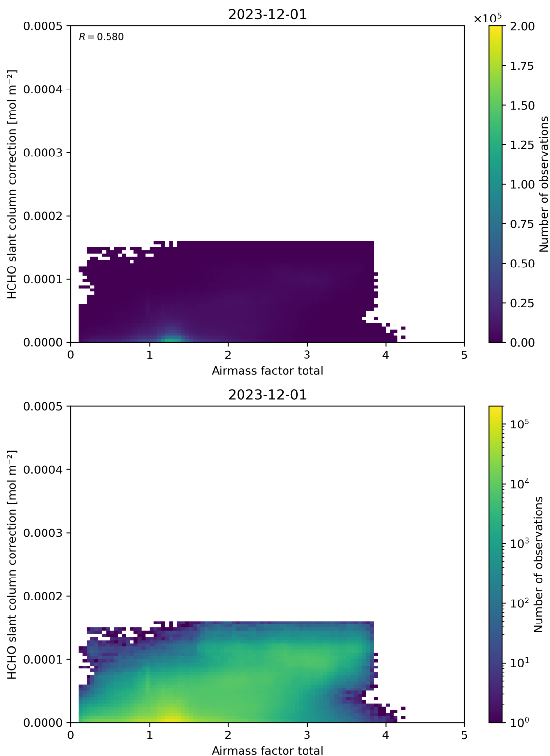
Figure 102: Scatter density plot of “Airmass factor total” against “HCHO slant column correction” for 2023-11-30 to 2023-12-02.
