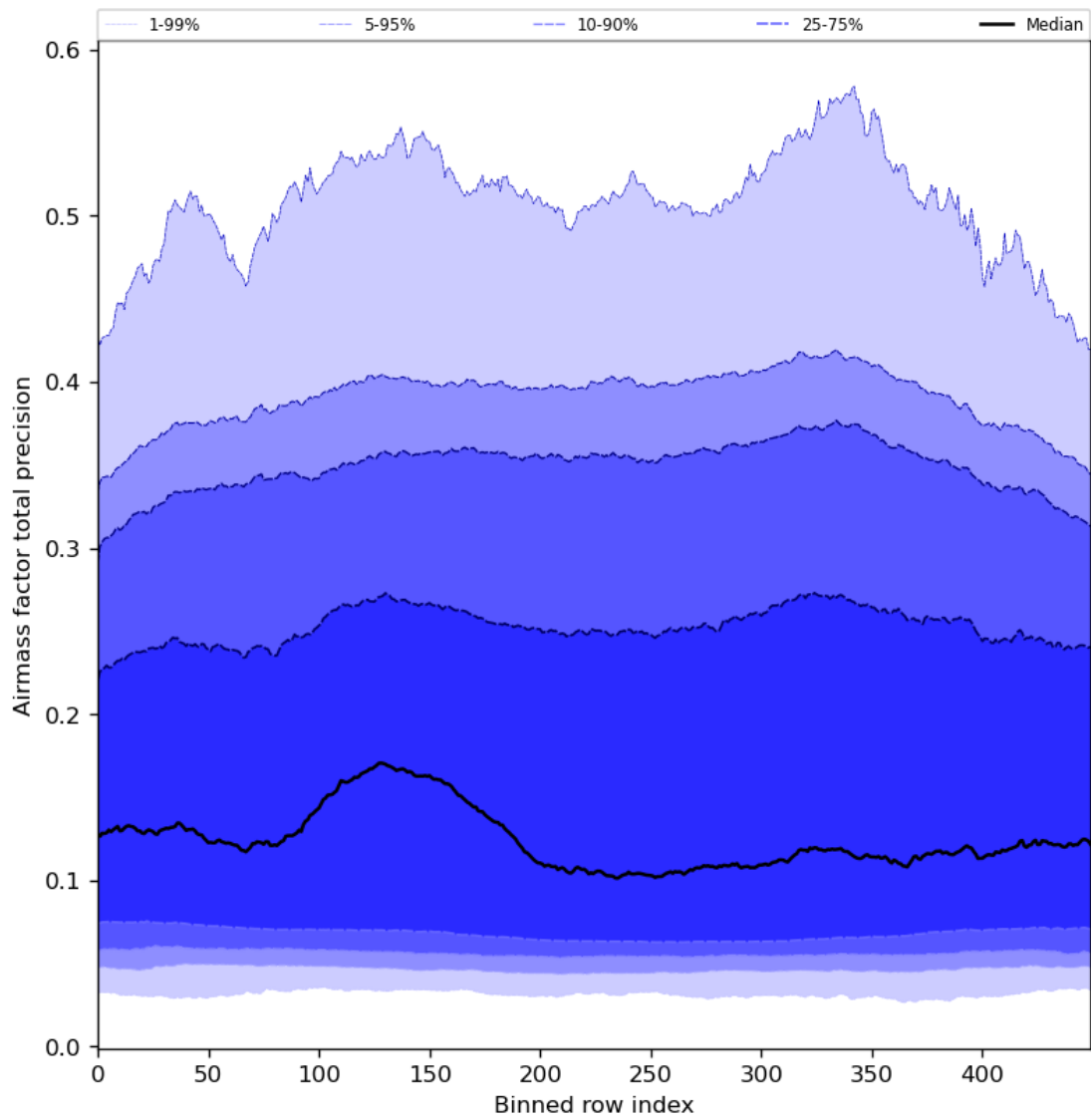
Figure 55: Along track statistics of “Airmass factor total precision” for 2023-11-30 to 2023-12-02
