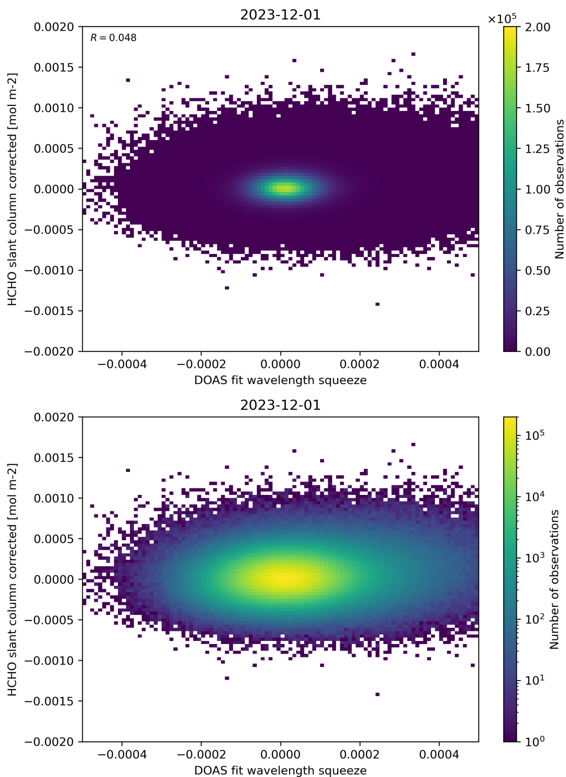
Figure 69: Scatter density plot of “DOAS fit wavelength squeeze” against “HCHO slant column corrected” for 2023-11-30 to 2023-12-02.
