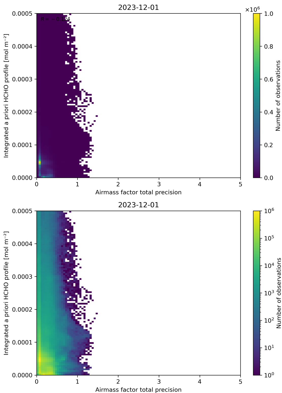
Figure 111: Scatter density plot of “Airmass factor total precision” against “Integrated a priori HCHO profile” for 2023-11-30 to 2023-12-02.
