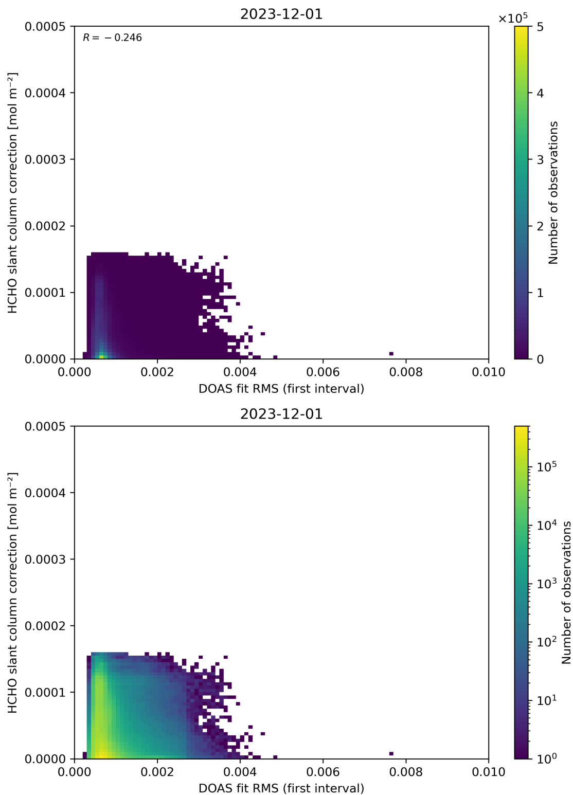
Figure 63: Scatter density plot of “DOAS fit RMS (first interval)” against “HCHO slant column correction” for 2023-11-30 to 2023-12-02.
