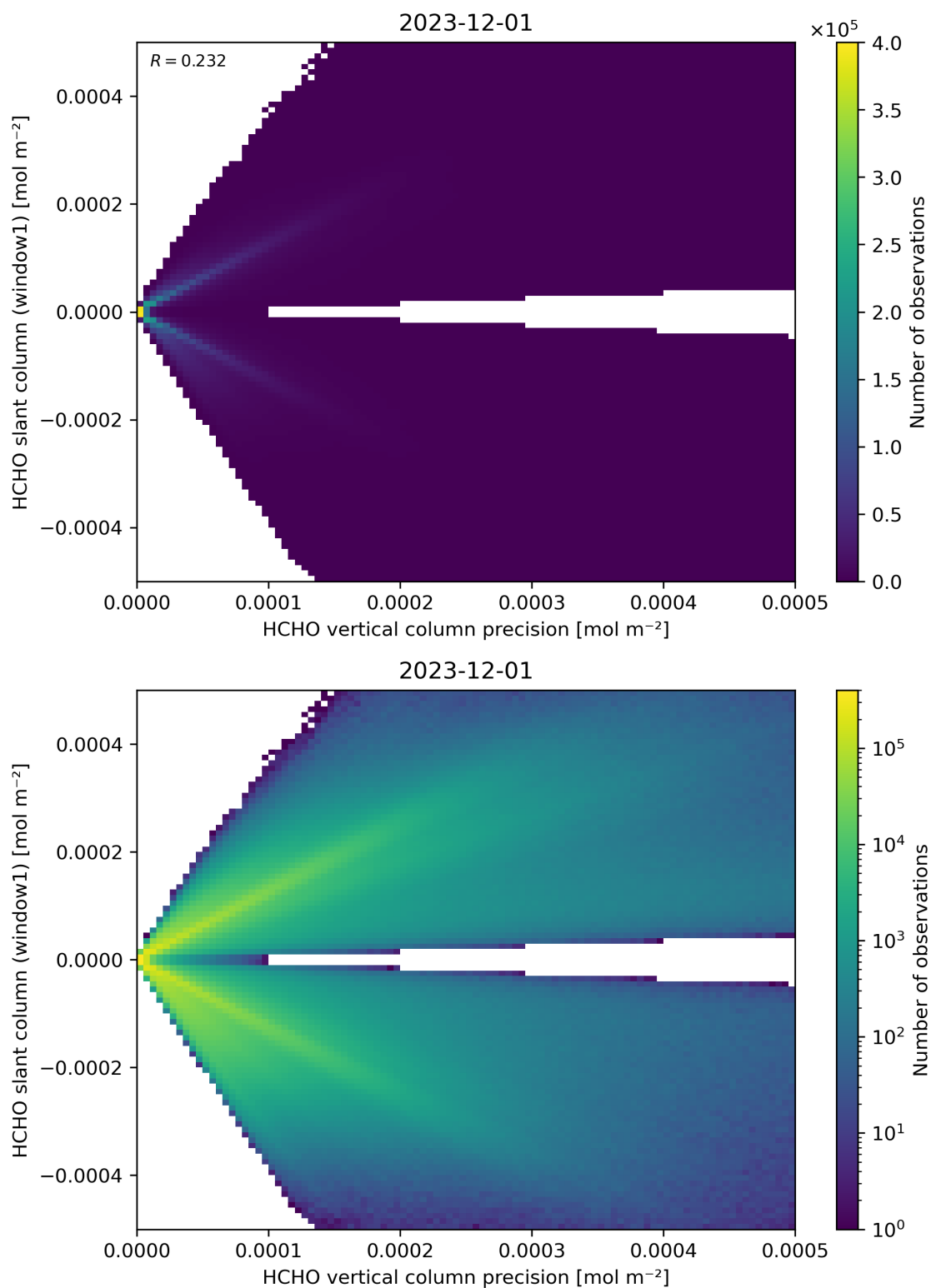
Figure 142: Scatter density plot of “HCHO vertical column precision” against “HCHO slant column (window1)” for 2023-11-30 to 2023-12-02.
