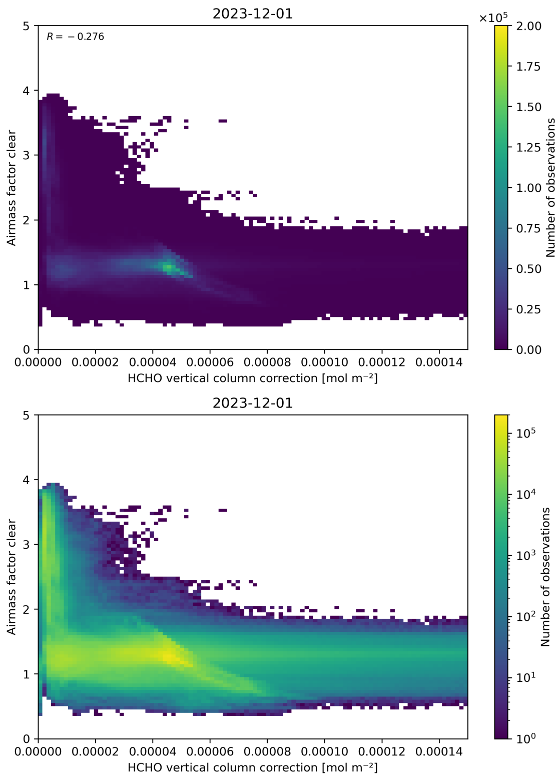
Figure 115: Scatter density plot of “HCHO vertical column correction” against “Airmass factor clear” for 2023-11-30 to 2023-12-02.
