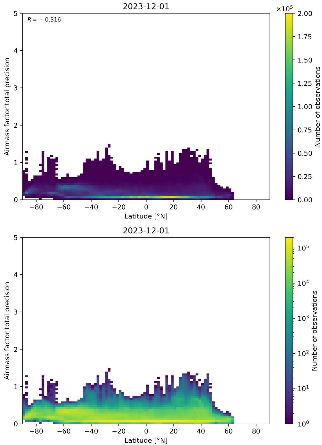
Figure 162: Scatter density plot of “Latitude” against “Airmass factor total precision” for 2023-11-30 to 2023-12-02.
