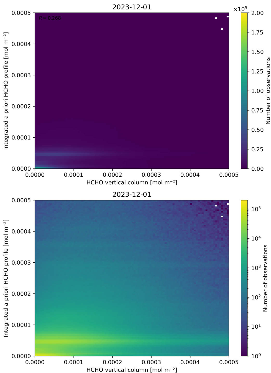
Figure 135: Scatter density plot of “HCHO vertical column” against “Integrated a priori HCHO profile” for 2023-11-30 to 2023-12-02.
