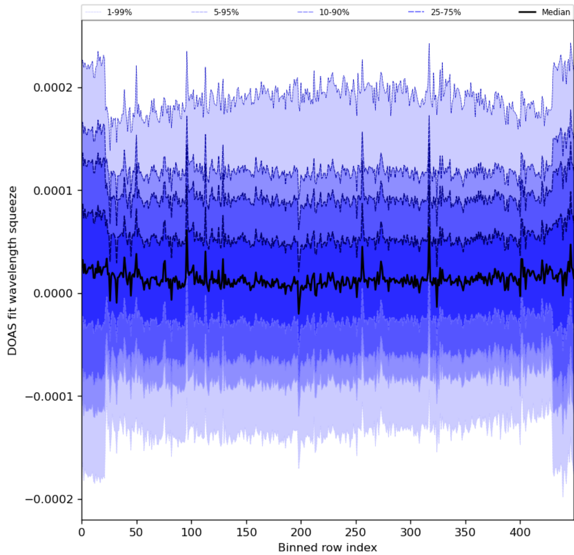
Figure 59: Along track statistics of “DOAS fit wavelength squeeze” for 2023-11-30 to 2023-12-02
