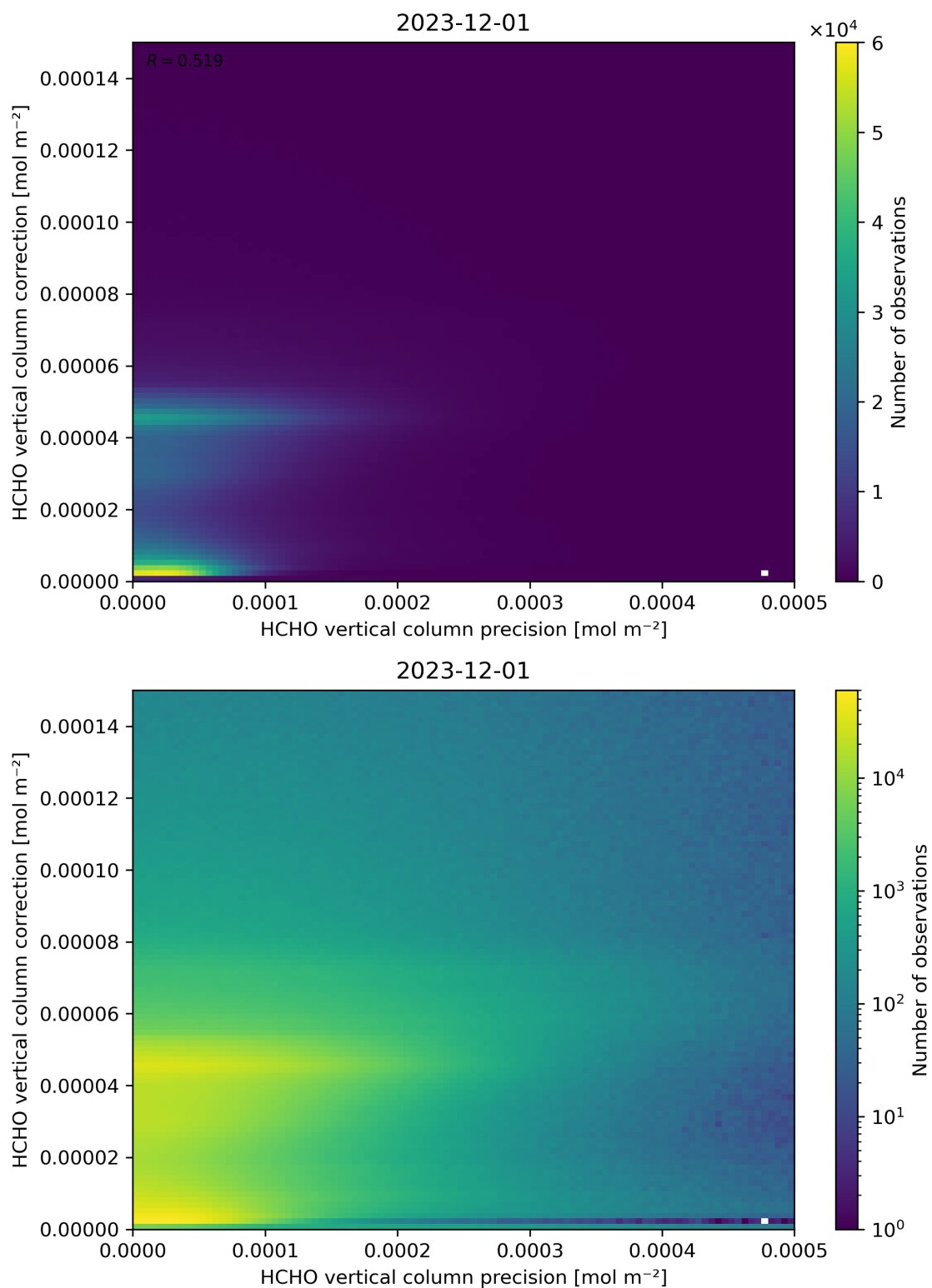
Figure 146: Scatter density plot of “HCHO vertical column precision” against “HCHO vertical column correction” for 2023-11-30 to 2023-12-02.
