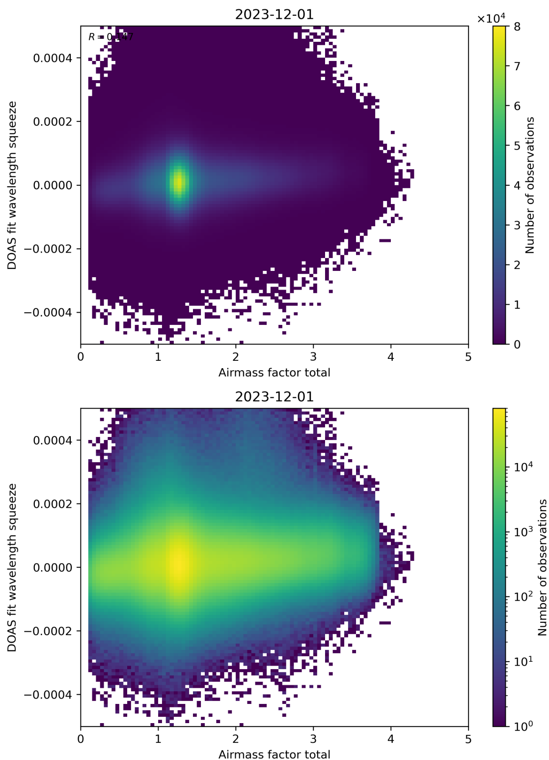
Figure 99: Scatter density plot of “Airmass factor total” against “DOAS fit wavelength squeeze” for 2023-11-30 to 2023-12-02.
