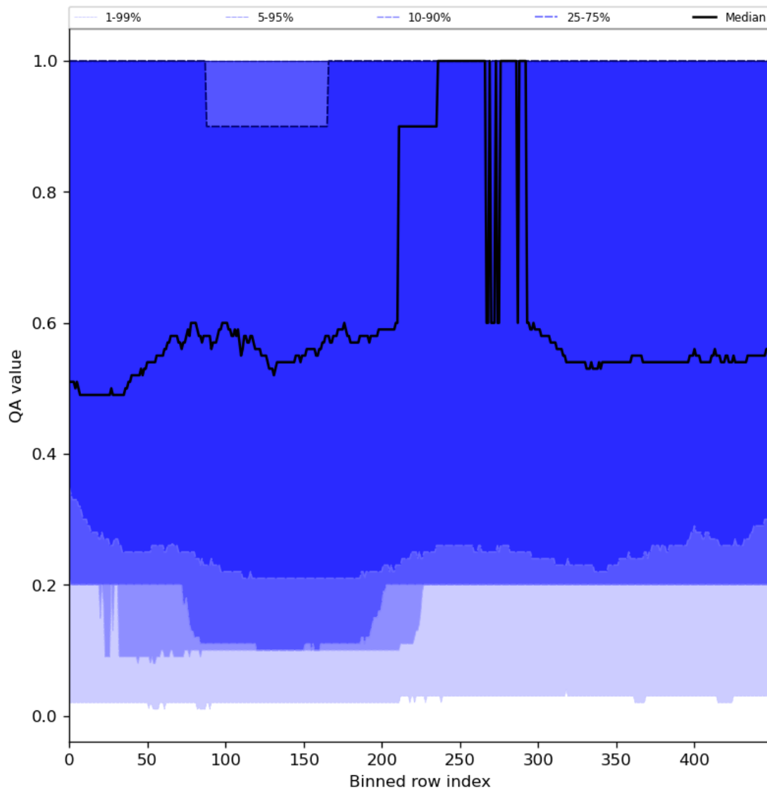
Figure 48: Along track statistics of “QA value” for 2023-11-30 to 2023-12-02
