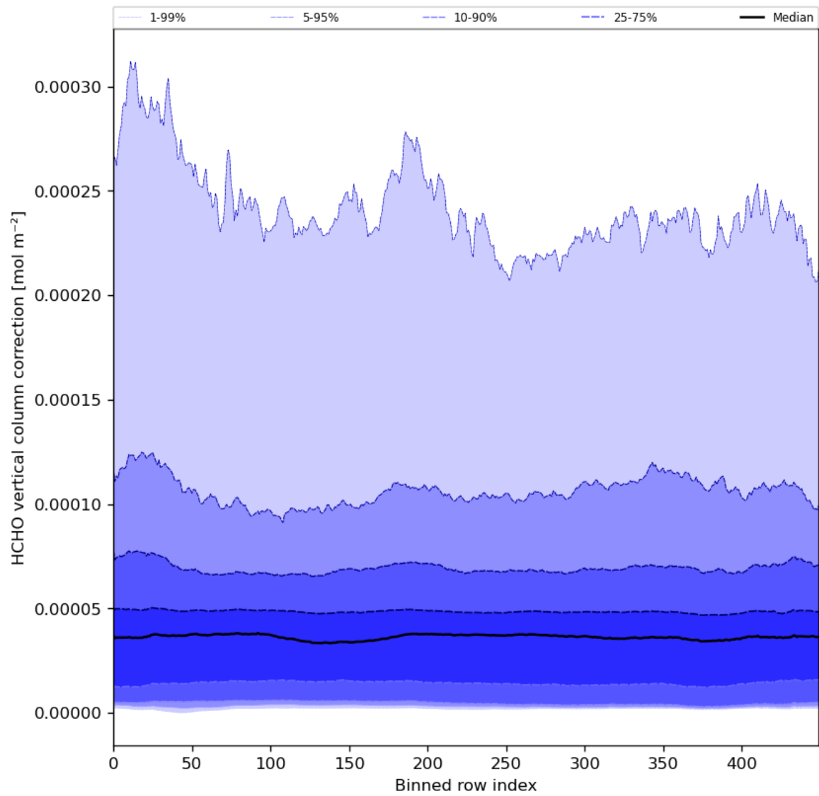
Figure 51: Along track statistics of “HCHO vertical column correction” for 2023-11-30 to 2023-12-02
