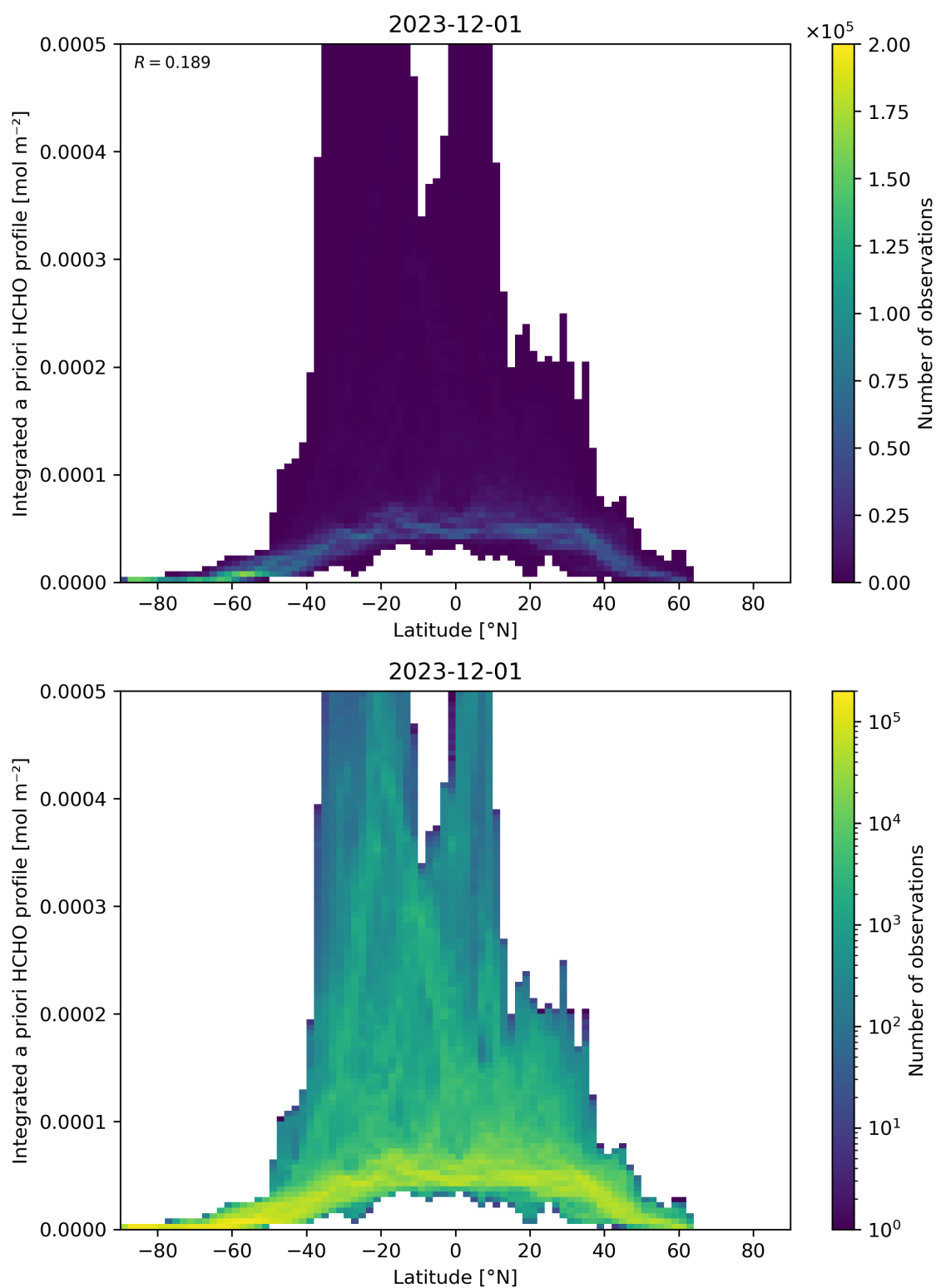
Figure 166: Scatter density plot of “Latitude” against “Integrated a priori HCHO profile” for 2023-11-30 to 2023-12-02.
