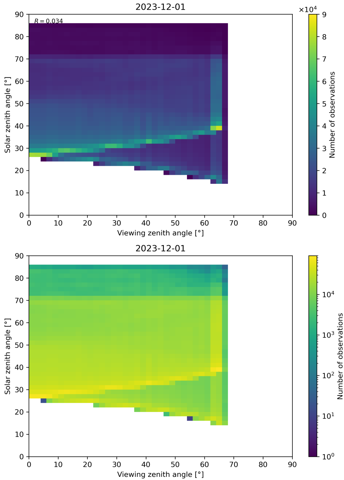
Figure 197: Scatter density plot of “Viewing zenith angle” against “Solar zenith angle” for 2023-11-30 to 2023-12-02.
