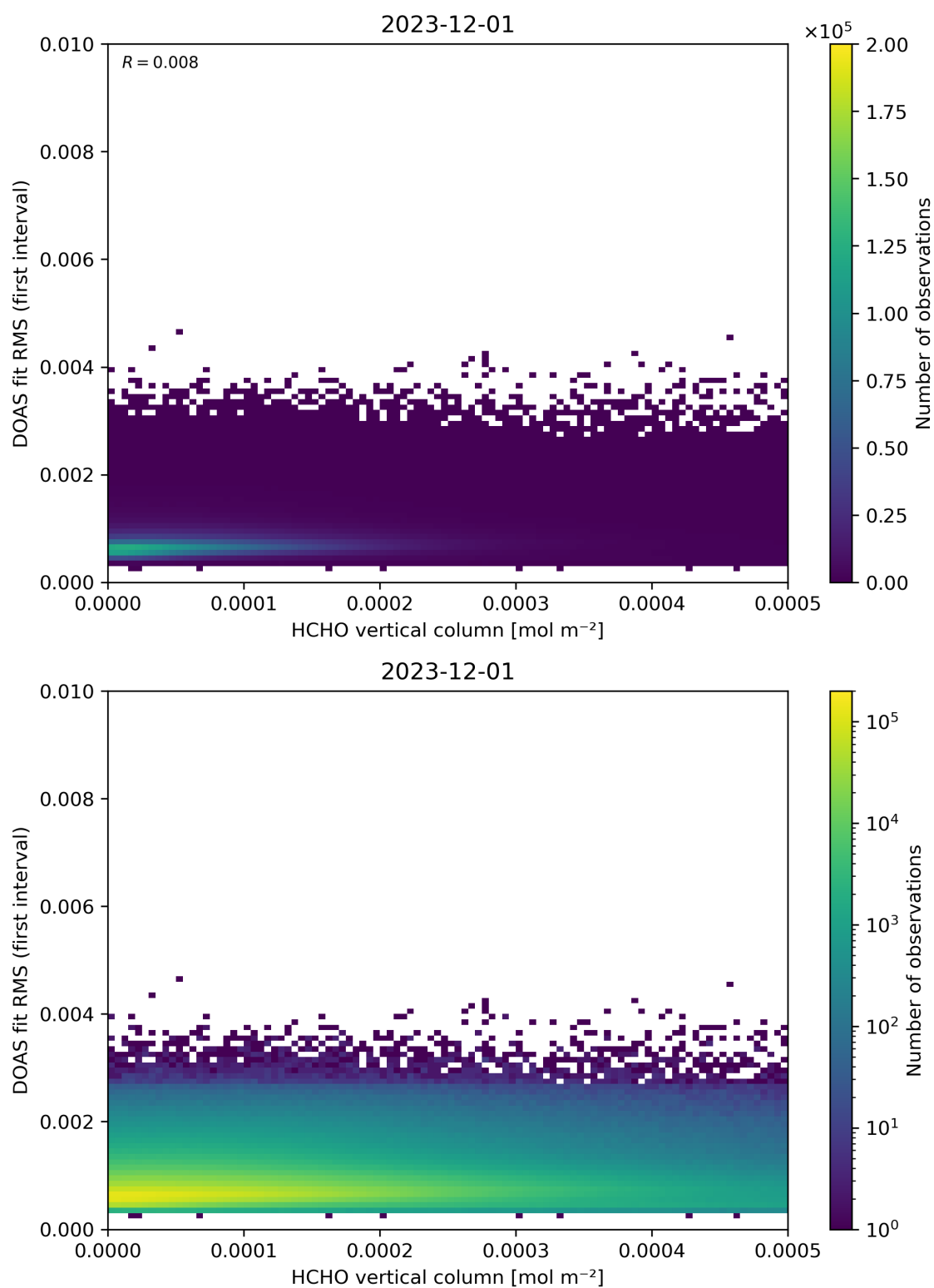
Figure 123: Scatter density plot of “HCHO vertical column” against “DOAS fit RMS (first interval)” for 2023-11-30 to 2023-12-02.
