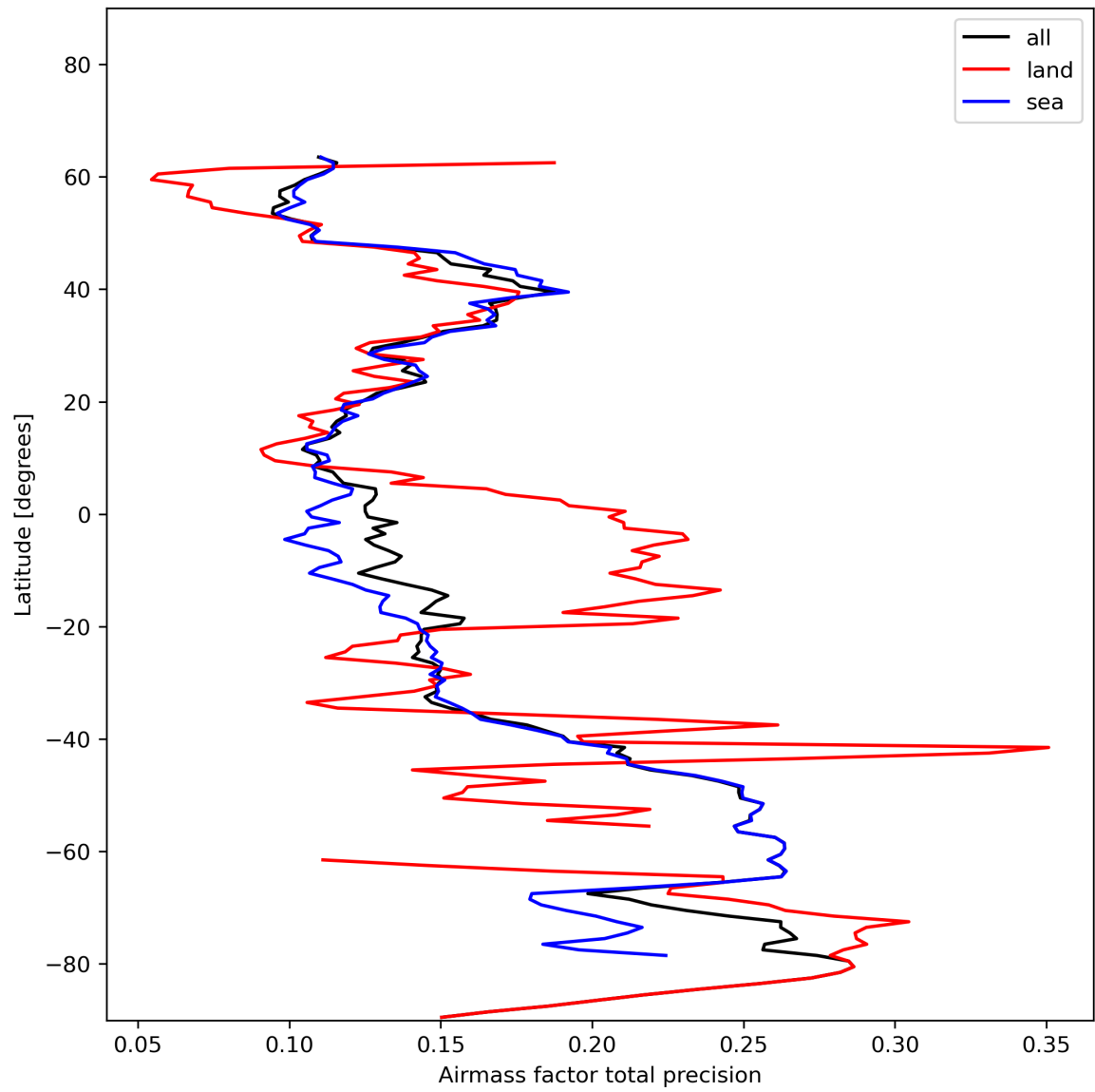
Figure 27: Zonal average of “Airmass factor total precision” for 2023-11-30 to 2023-12-02.
