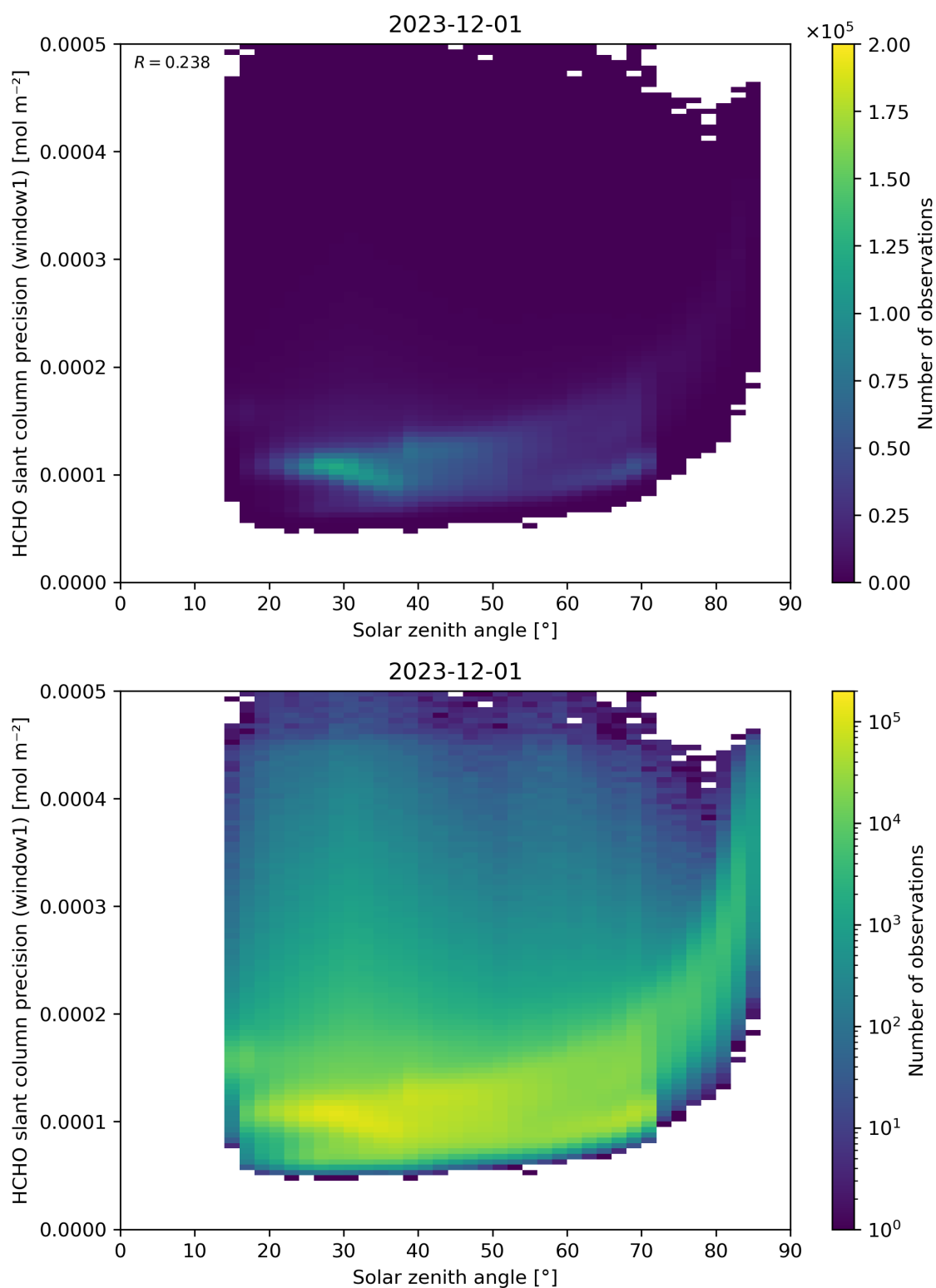
Figure 174: Scatter density plot of “Solar zenith angle” against “HCHO slant column precision (window1)” for 2023-11-30 to 2023-12-02.
