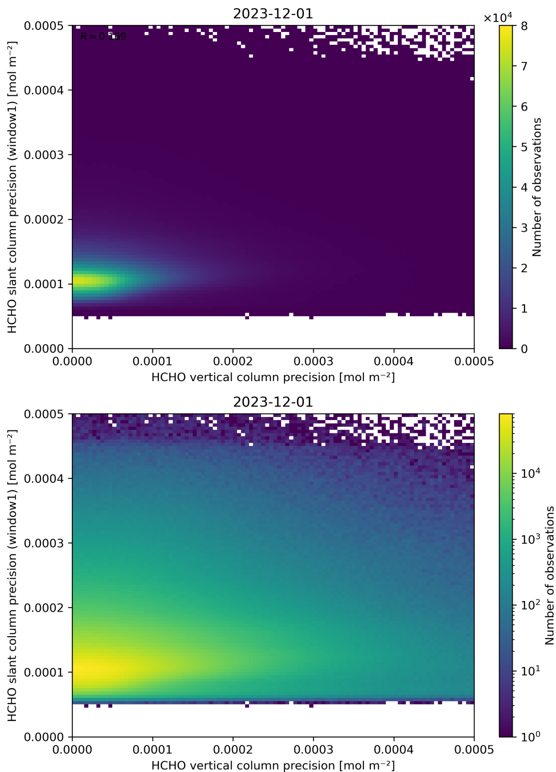
Figure 143: Scatter density plot of “HCHO vertical column precision” against “HCHO slant column precision (window1)” for 2023-11-30 to 2023-12-02.
