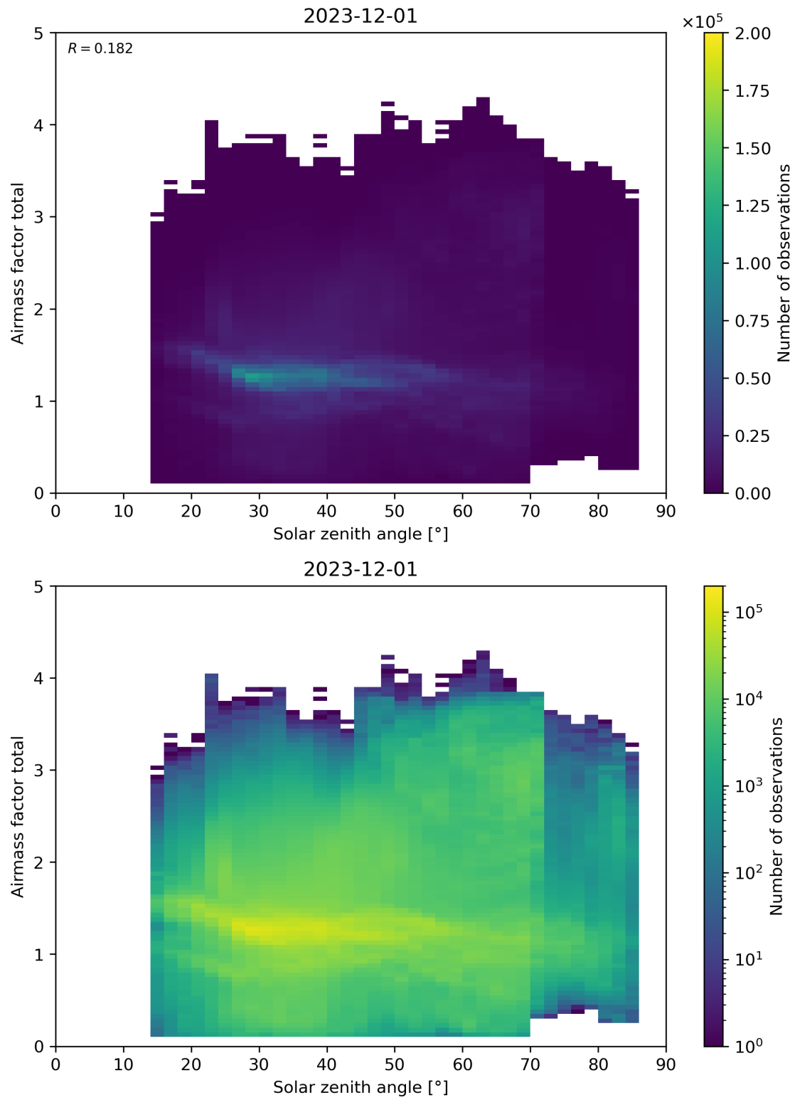
Figure 175: Scatter density plot of “Solar zenith angle” against “Airmass factor total” for 2023-11-30 to 2023-12-02.
