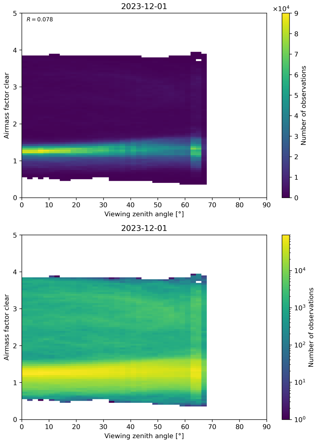
Figure 185: Scatter density plot of “Viewing zenith angle” against “Airmass factor clear” for 2023-11-30 to 2023-12-02.
