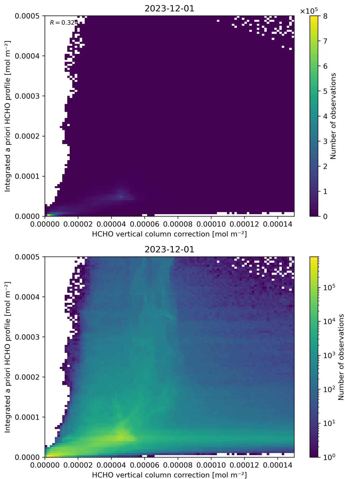
Figure 122: Scatter density plot of “HCHO vertical column correction” against “Integrated a priori HCHO profile” for 2023-11-30 to 2023-12-02.
