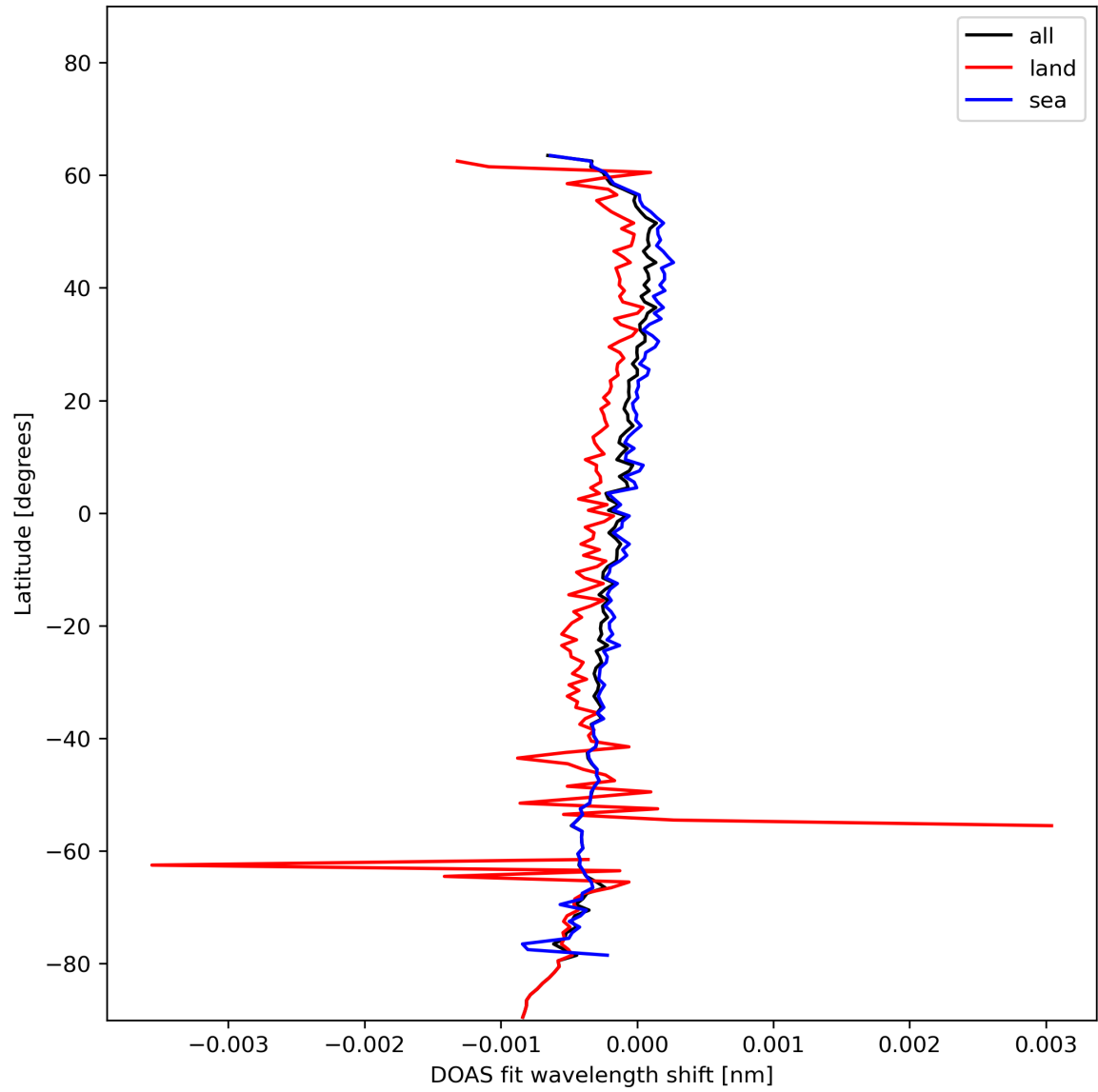
Figure 30: Zonal average of “DOAS fit wavelength shift” for 2023-11-30 to 2023-12-02.
