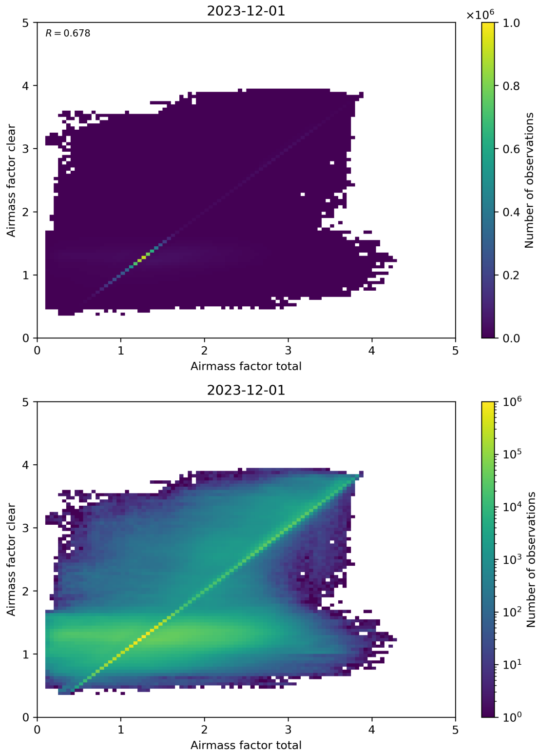
Figure 100: Scatter density plot of “Airmass factor total” against “Airmass factor clear” for 2023-11-30 to 2023-12-02.
