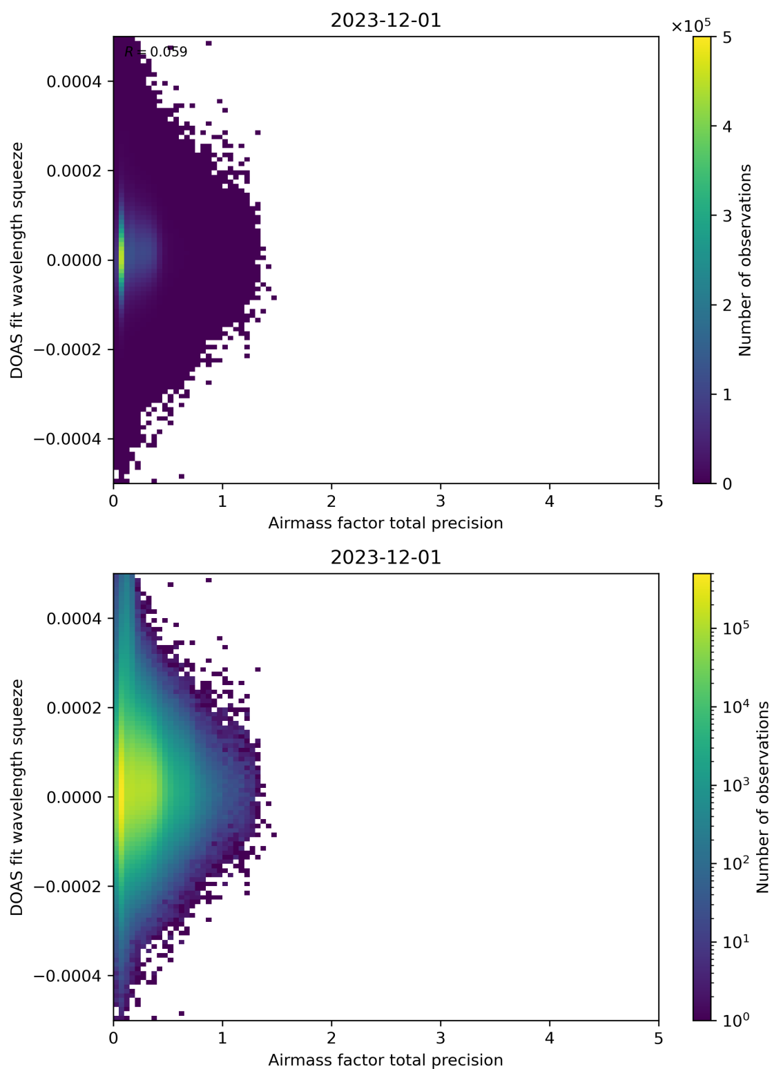
Figure 107: Scatter density plot of “Airmass factor total precision” against “DOAS fit wavelength squeeze” for 2023-11-30 to 2023-12-02.
