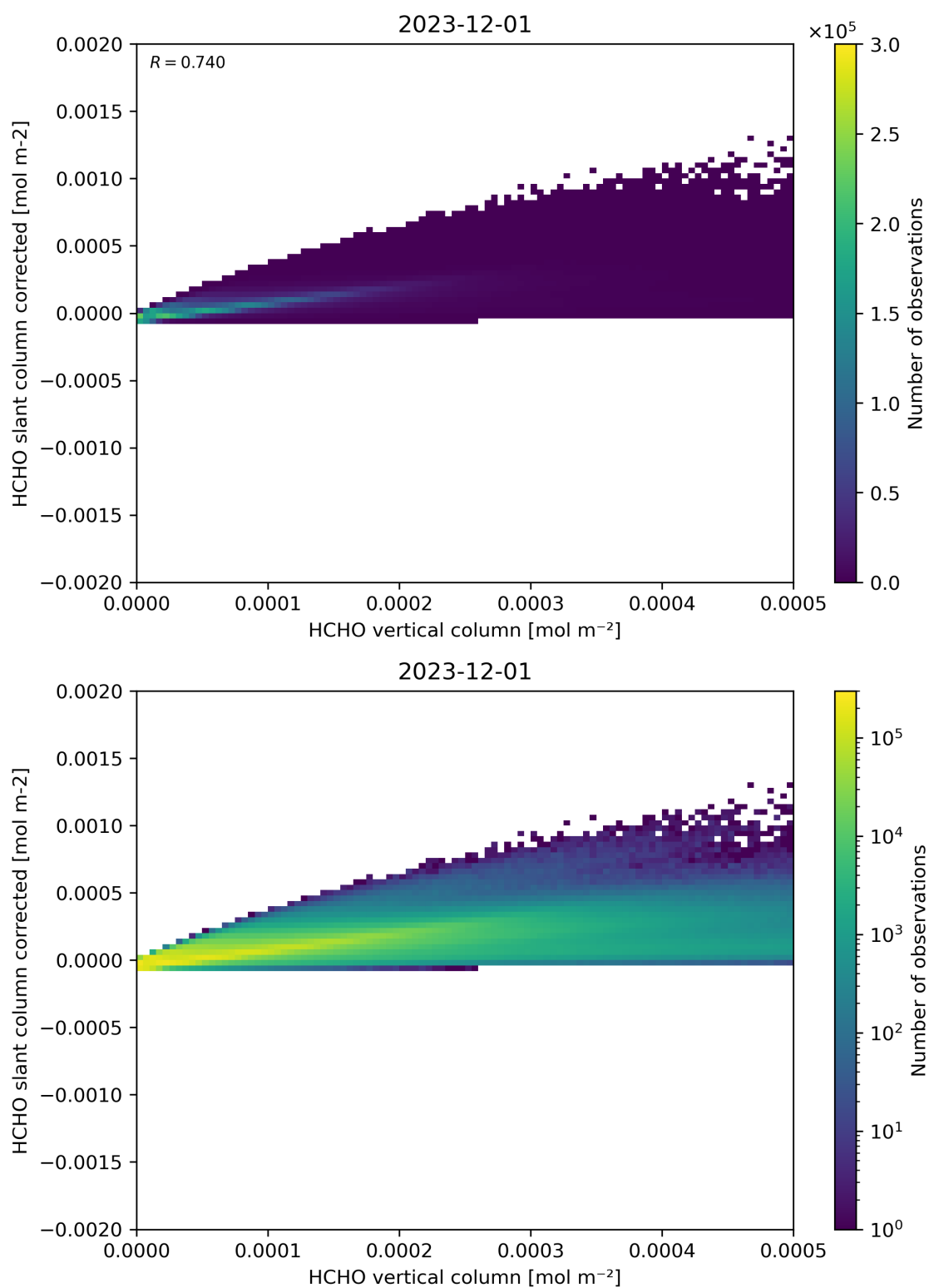
Figure 127: Scatter density plot of “HCHO vertical column” against “HCHO slant column corrected” for 2023-11-30 to 2023-12-02.
