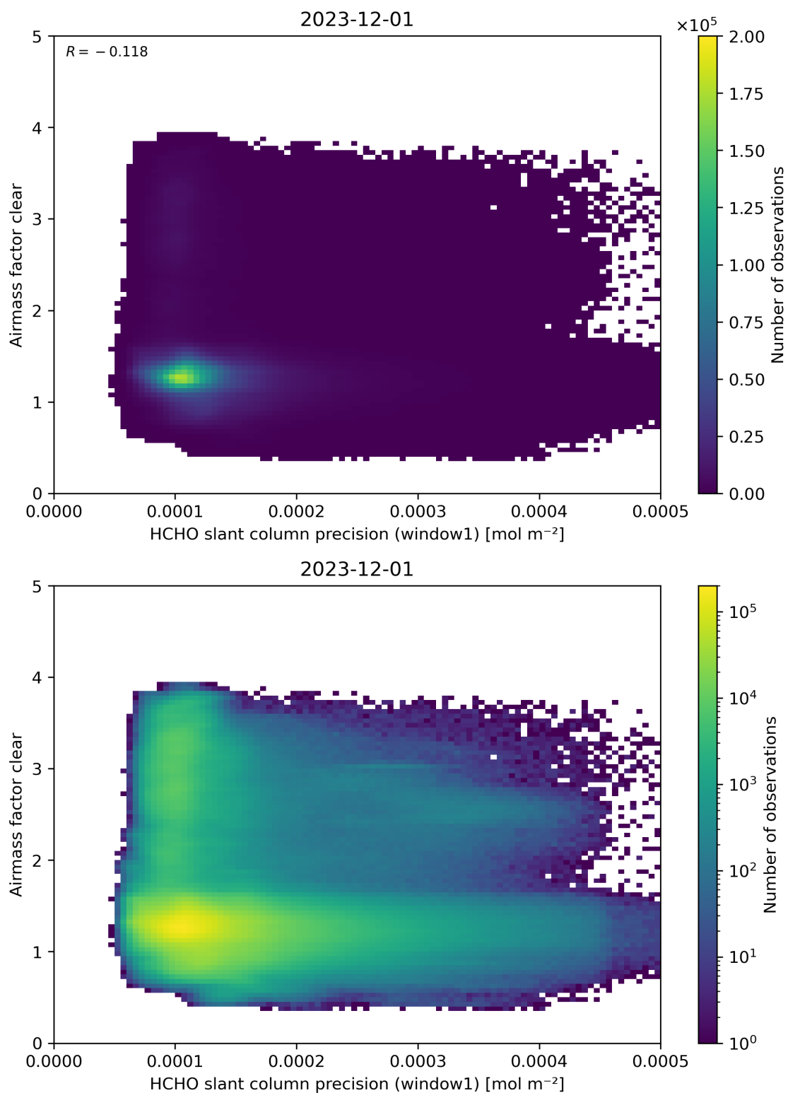
Figure 91: Scatter density plot of “HCHO slant column precision (window1)” against “Airmass factor clear” for 2023-11-30 to 2023-12-02.
