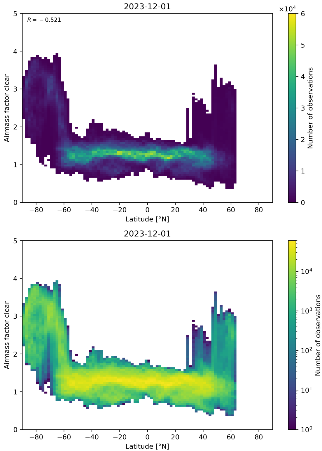
Figure 156: Scatter density plot of “Latitude” against “Airmass factor clear” for 2023-11-30 to 2023-12-02.
