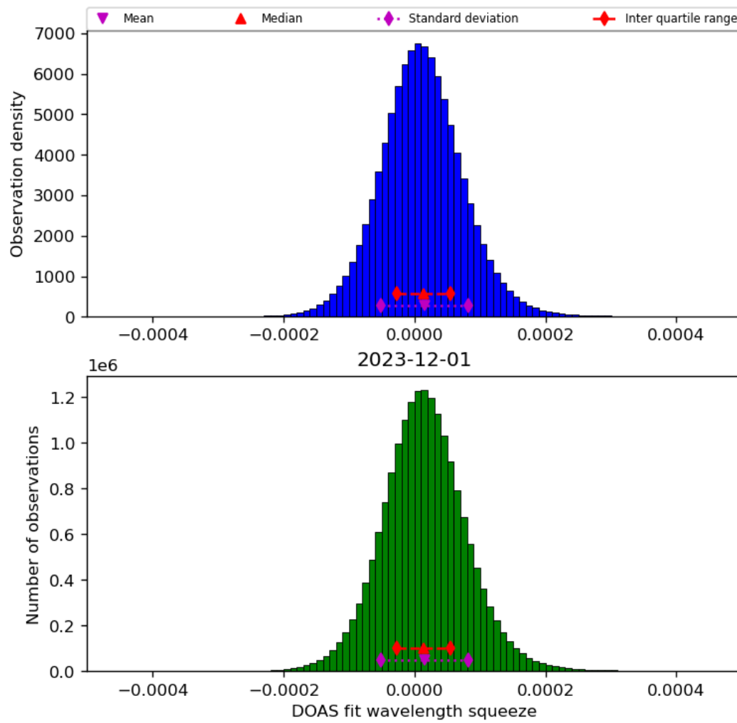
Figure 45: Histogram of “DOAS fit wavelength squeeze” for 2023-11-30 to 2023-12-02
