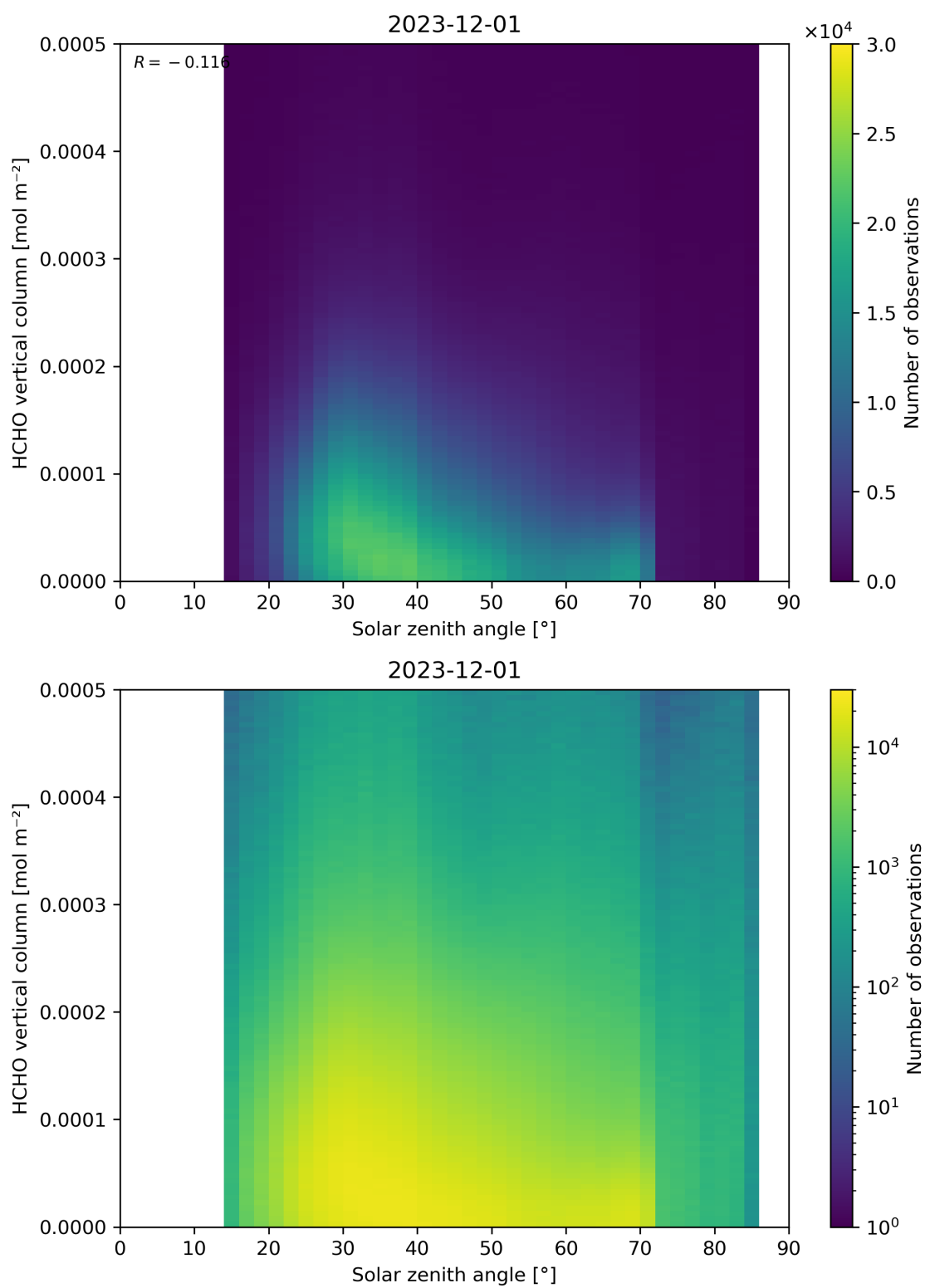
Figure 177: Scatter density plot of “Solar zenith angle” against “HCHO vertical column” for 2023-11-30 to 2023-12-02.
