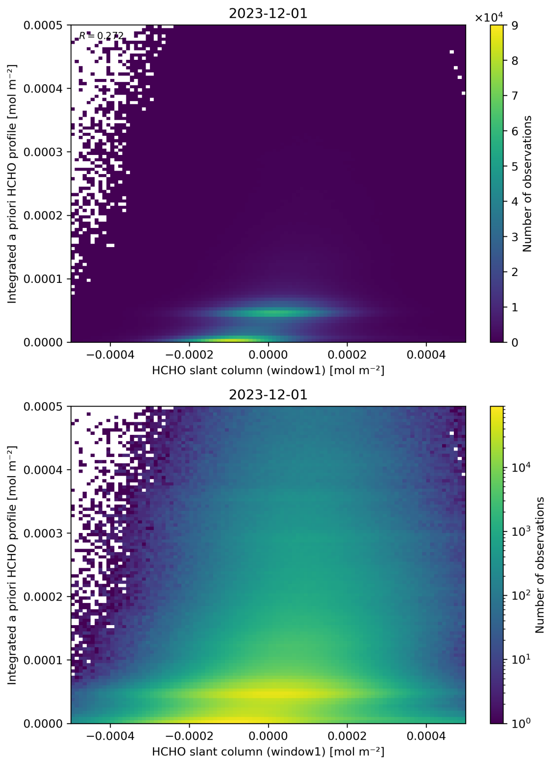
Figure 87: Scatter density plot of “HCHO slant column (window1)” against “Integrated a priori HCHO profile” for 2023-11-30 to 2023-12-02.
