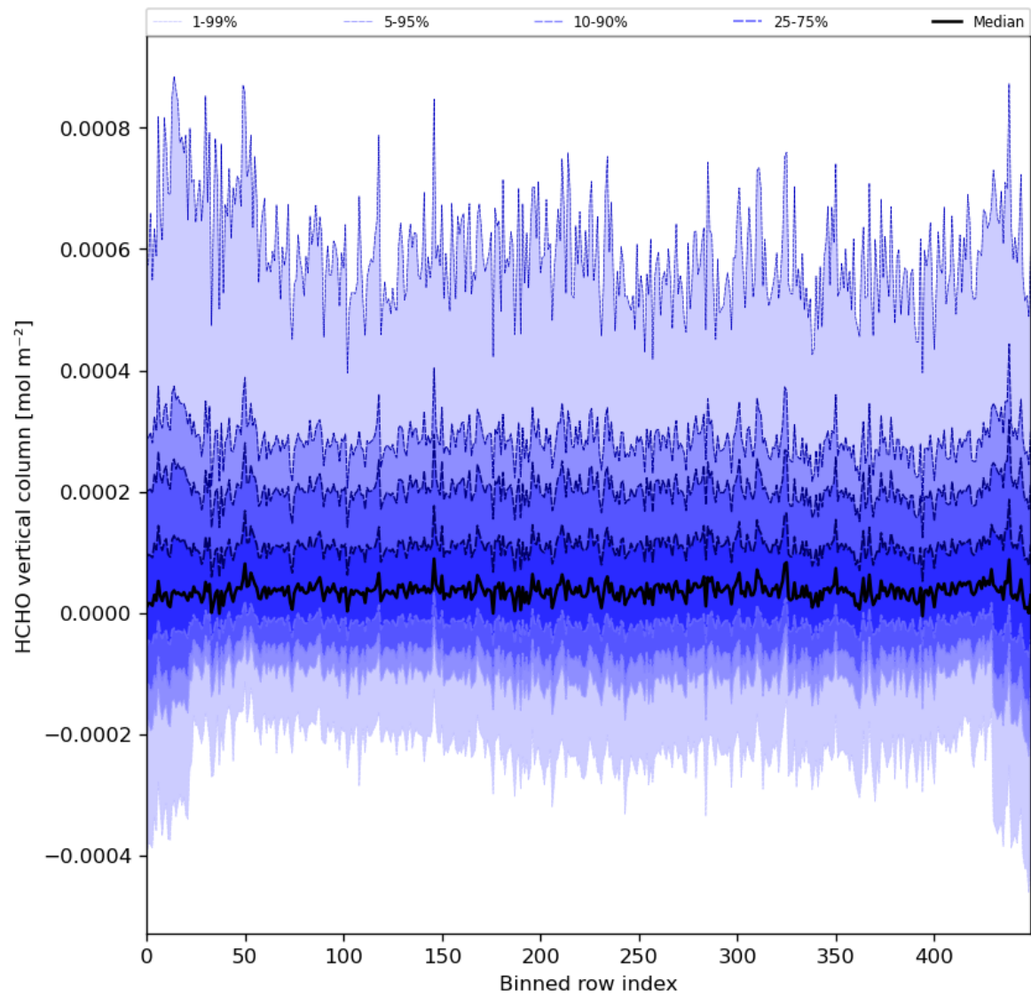
Figure 49: Along track statistics of “HCHO vertical column” for 2023-11-30 to 2023-12-02
