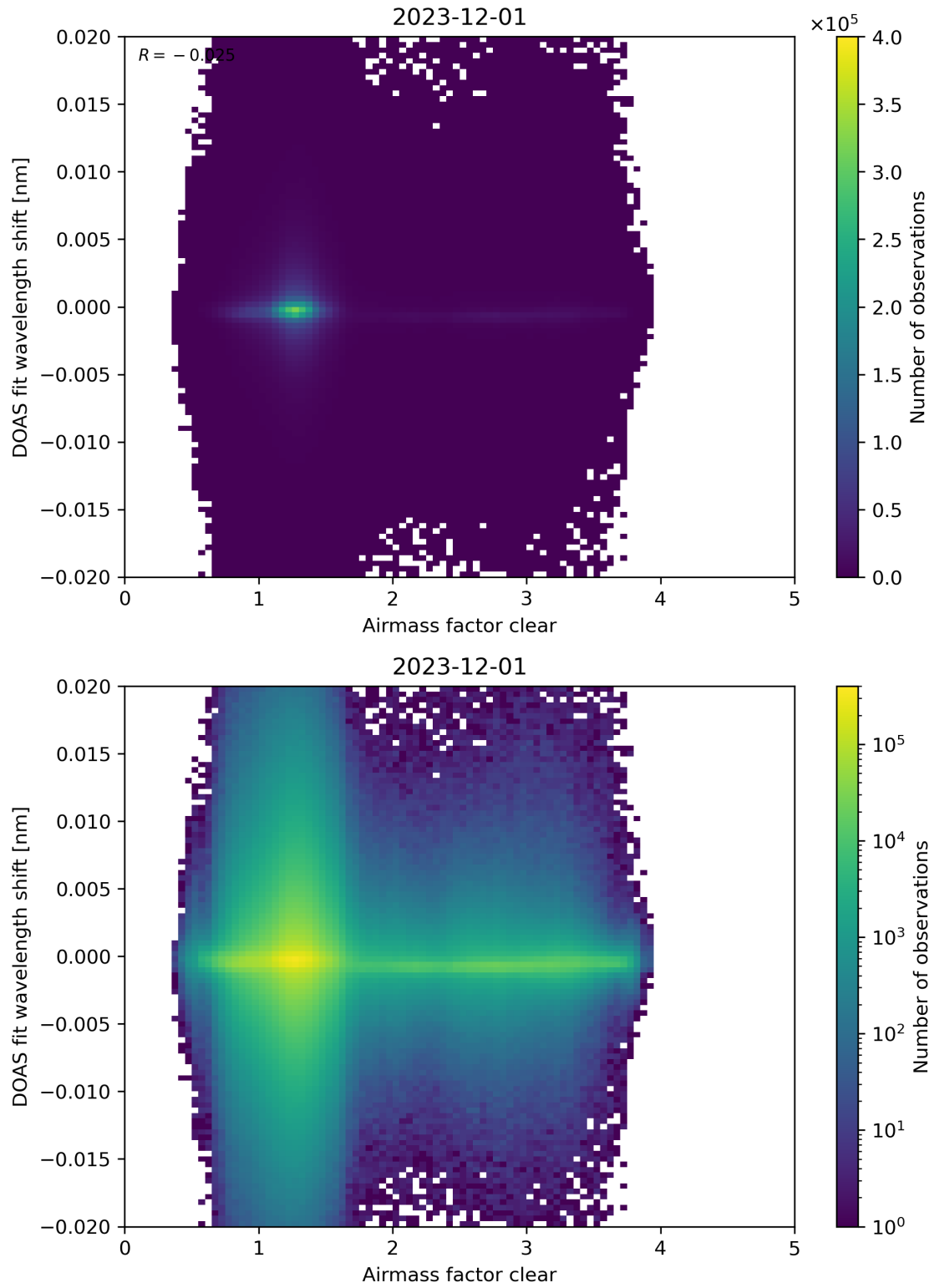
Figure 72: Scatter density plot of “Airmass factor clear” against “DOAS fit wavelength shift” for 2023-11-30 to 2023-12-02.
