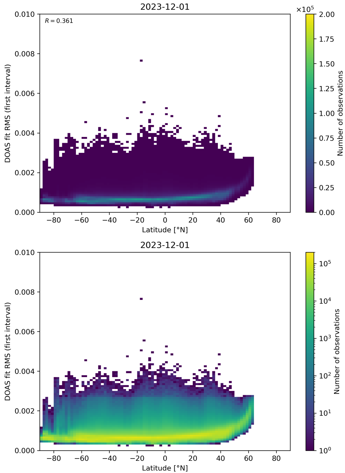
Figure 153: Scatter density plot of “Latitude” against “DOAS fit RMS (first interval)” for 2023-11-30 to 2023-12-02.
