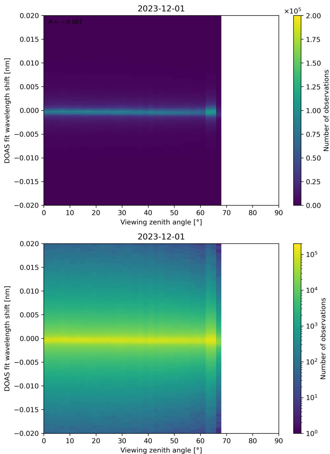
Figure 183: Scatter density plot of “Viewing zenith angle” against “DOAS fit wavelength shift” for 2023-11-30 to 2023-12-02.
