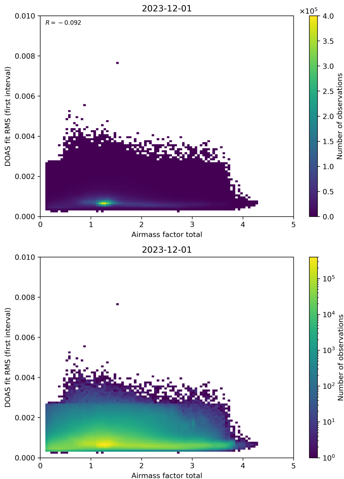
Figure 97: Scatter density plot of “Airmass factor total” against “DOAS fit RMS (first interval)” for 2023-11-30 to 2023-12-02.
