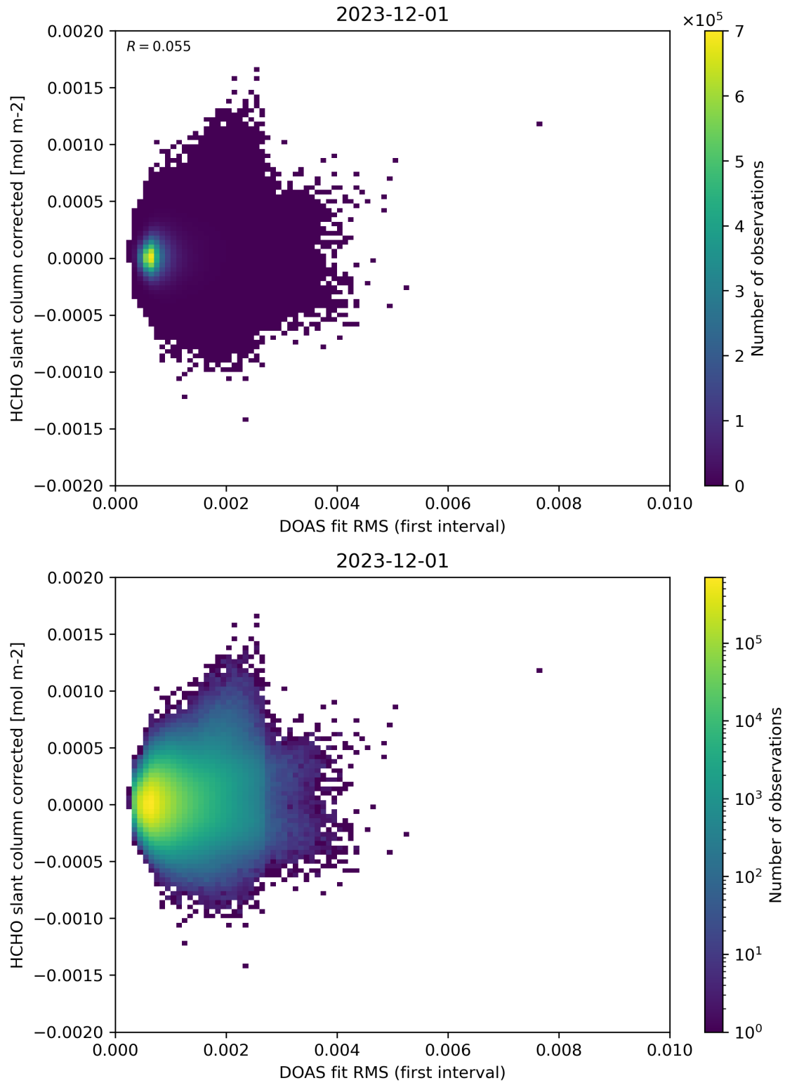
Figure 62: Scatter density plot of “DOAS fit RMS (first interval)” against “HCHO slant column corrected” for 2023-11-30 to 2023-12-02.
