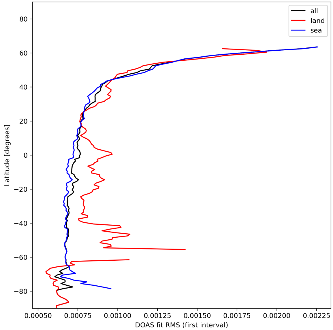
Figure 32: Zonal average of “DOAS fit RMS (first interval)” for 2023-11-30 to 2023-12-02.
