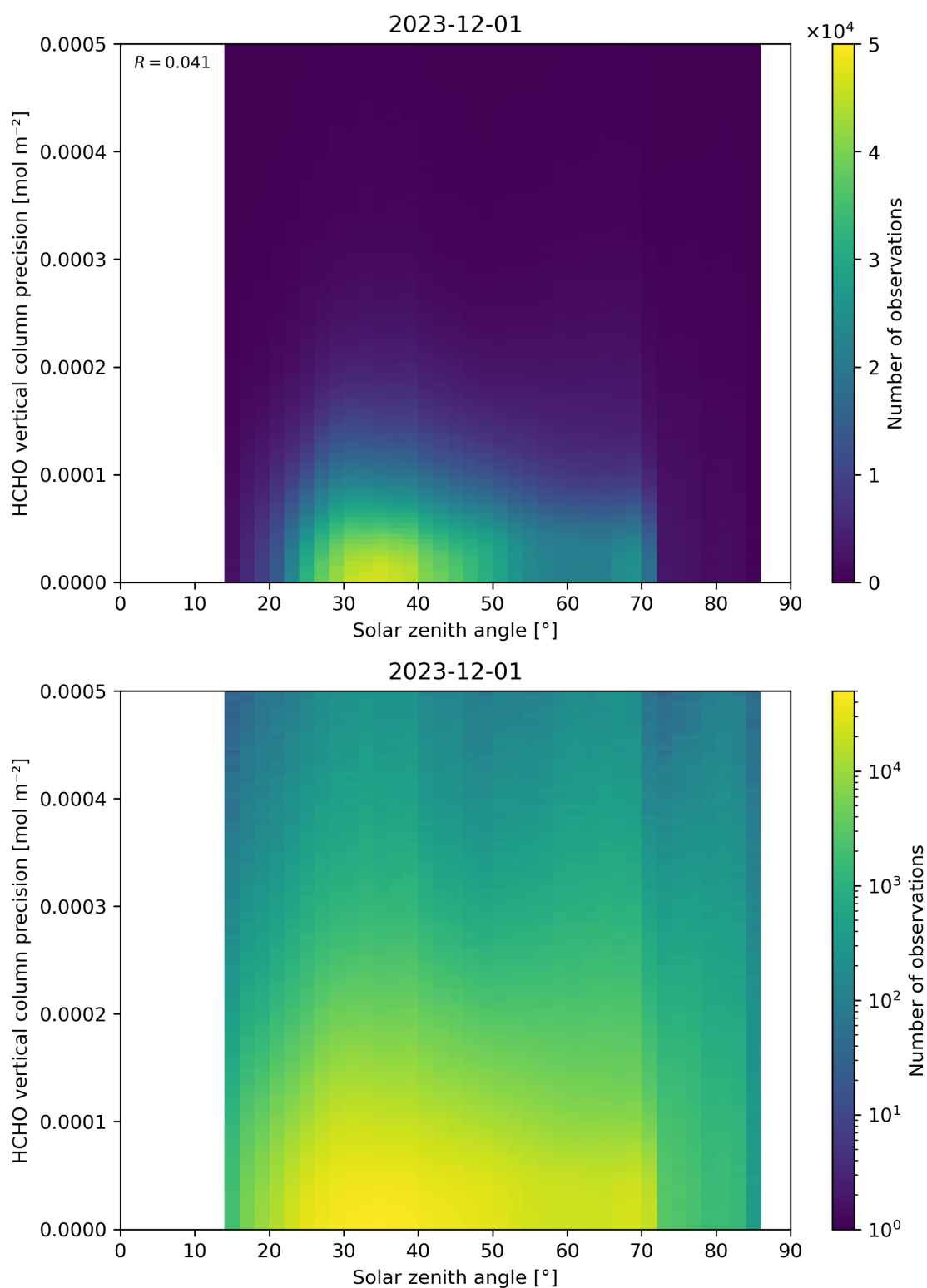
Figure 179: Scatter density plot of “Solar zenith angle” against “HCHO vertical column precision” for 2023-11-30 to 2023-12-02.
