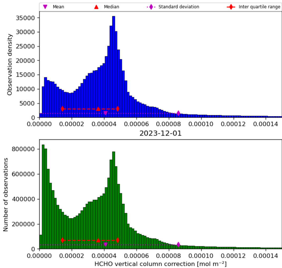
Figure 37: Histogram of “HCHO vertical column correction” for 2023-11-30 to 2023-12-02
