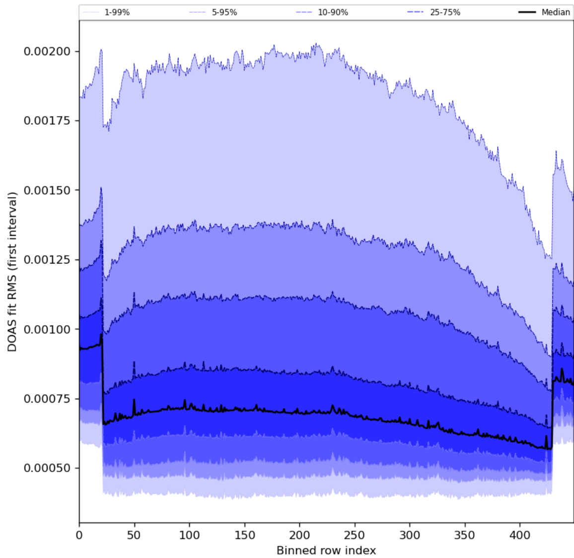
Figure 60: Along track statistics of “DOAS fit RMS (first interval)” for 2023-11-30 to 2023-12-02
