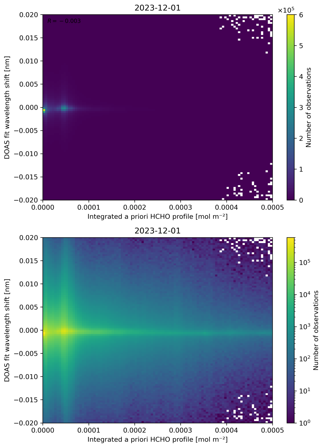
Figure 149: Scatter density plot of “Integrated a priori HCHO profile” against “DOAS fit wavelength shift” for 2023-11-30 to 2023-12-02.
