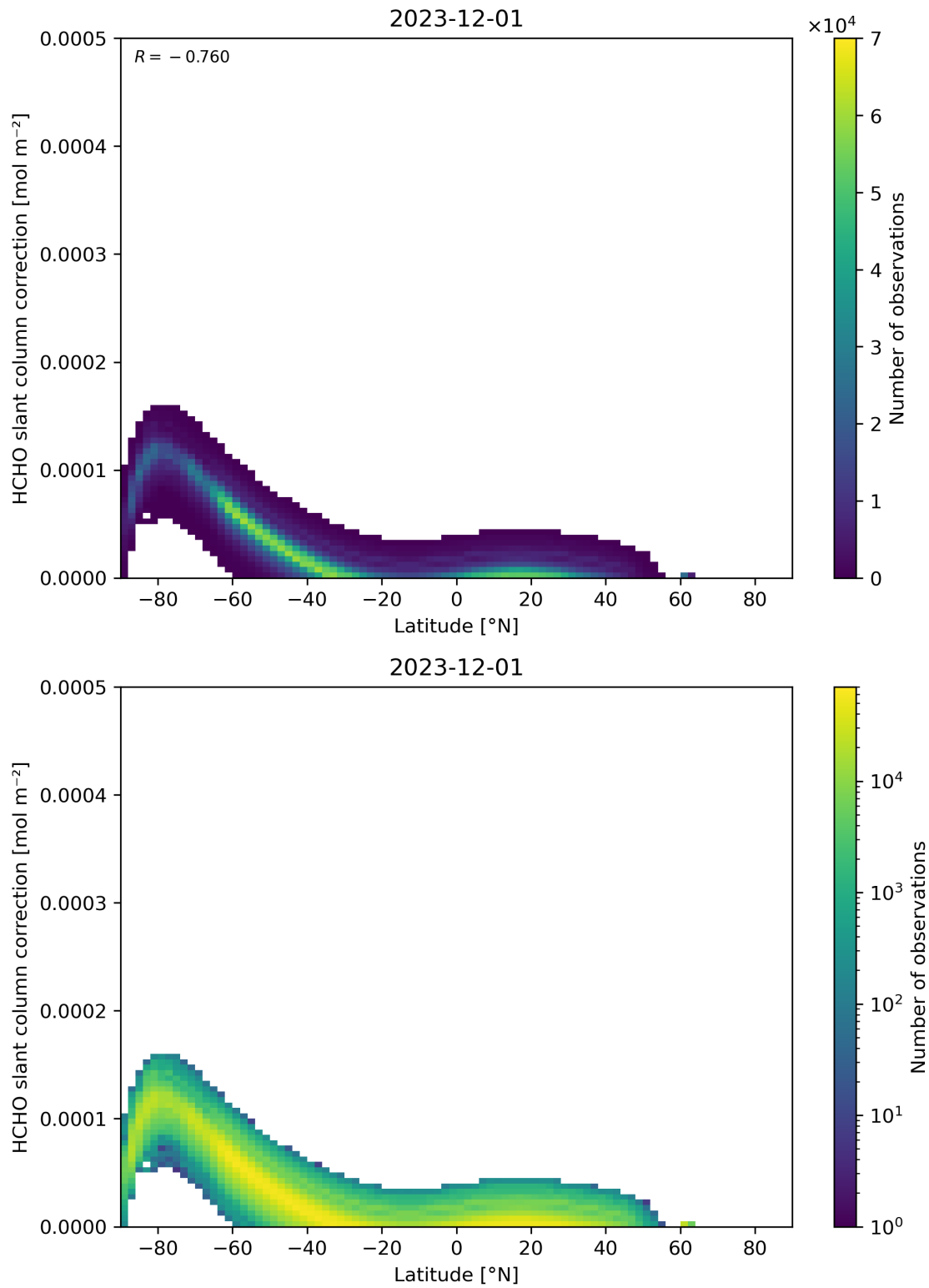
Figure 158: Scatter density plot of “Latitude” against “HCHO slant column correction” for 2023-11-30 to 2023-12-02.
