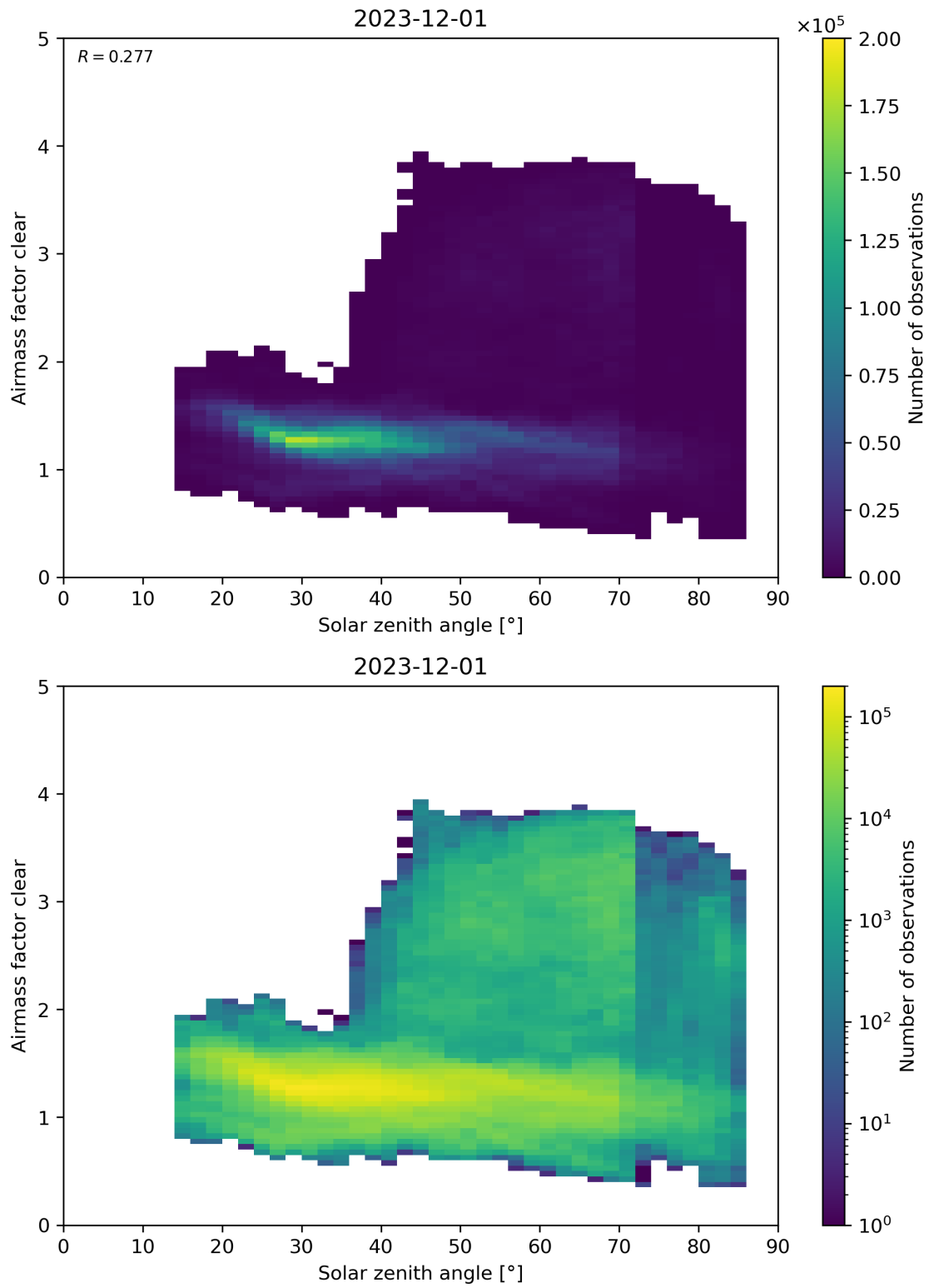
Figure 170: Scatter density plot of “Solar zenith angle” against “Airmass factor clear” for 2023-11-30 to 2023-12-02.
