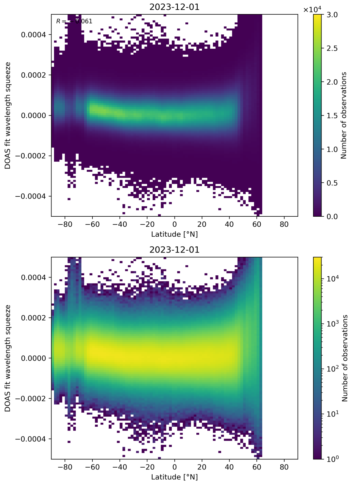
Figure 155: Scatter density plot of “Latitude” against “DOAS fit wavelength squeeze” for 2023-11-30 to 2023-12-02.
