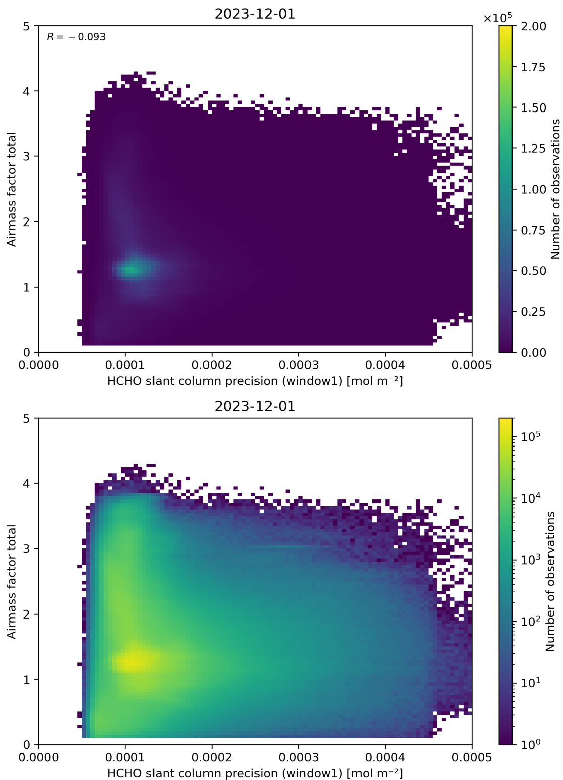
Figure 94: Scatter density plot of “HCHO slant column precision (window1)” against “Airmass factor total” for 2023-11-30 to 2023-12-02.
