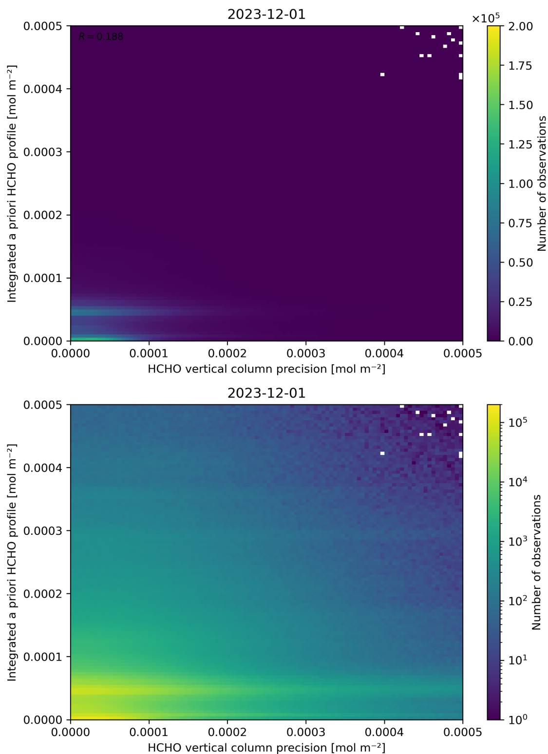
Figure 147: Scatter density plot of “HCHO vertical column precision” against “Integrated a priori HCHO profile” for 2023-11-30 to 2023-12-02.
