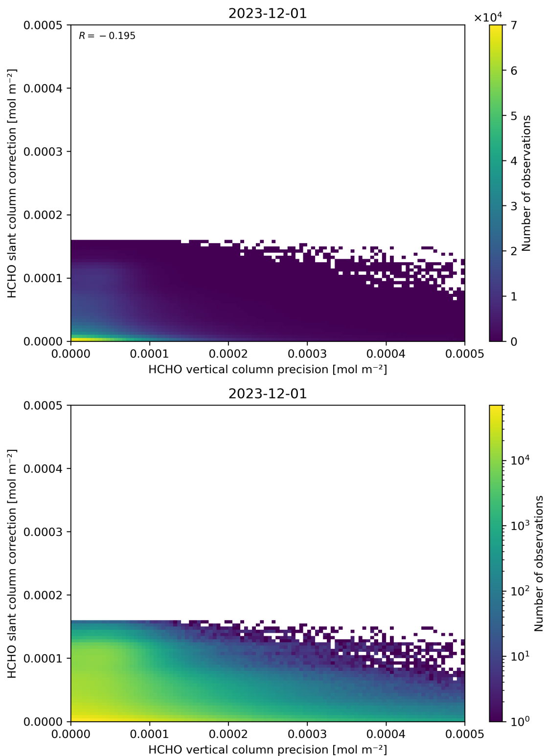
Figure 141: Scatter density plot of “HCHO vertical column precision” against “HCHO slant column correction” for 2023-11-30 to 2023-12-02.
