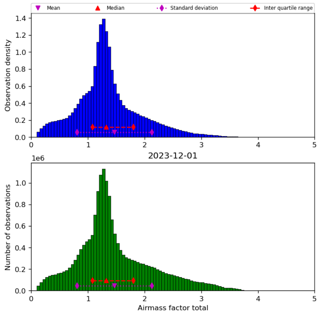
Figure 40: Histogram of “Airmass factor total” for 2023-11-30 to 2023-12-02
