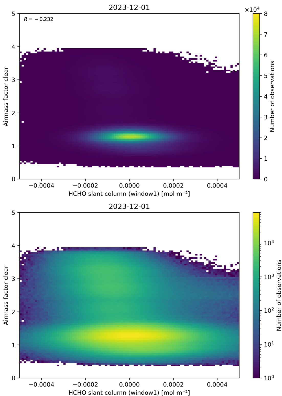
Figure 81: Scatter density plot of “HCHO slant column (window1)” against “Airmass factor clear” for 2023-11-30 to 2023-12-02.
