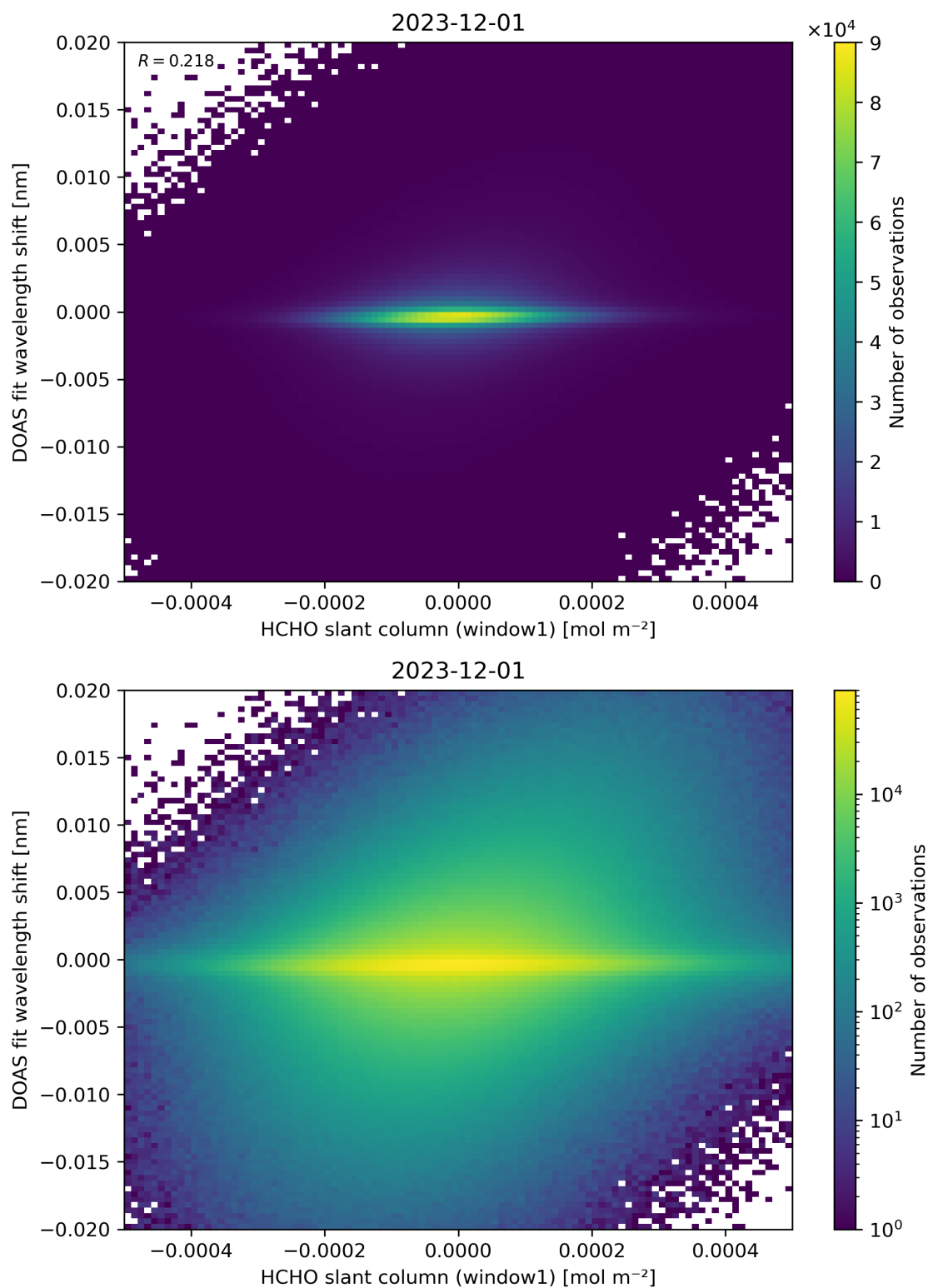
Figure 79: Scatter density plot of “HCHO slant column (window1)” against “DOAS fit wavelength shift” for 2023-11-30 to 2023-12-02.
