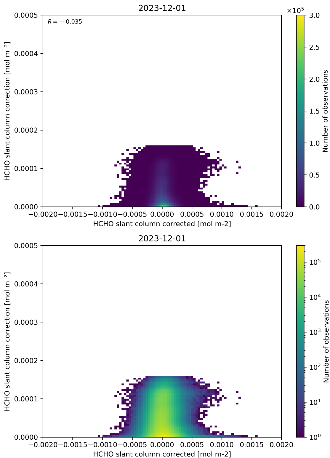
Figure 77: Scatter density plot of “HCHO slant column corrected” against “HCHO slant column correction” for 2023-11-30 to 2023-12-02.
