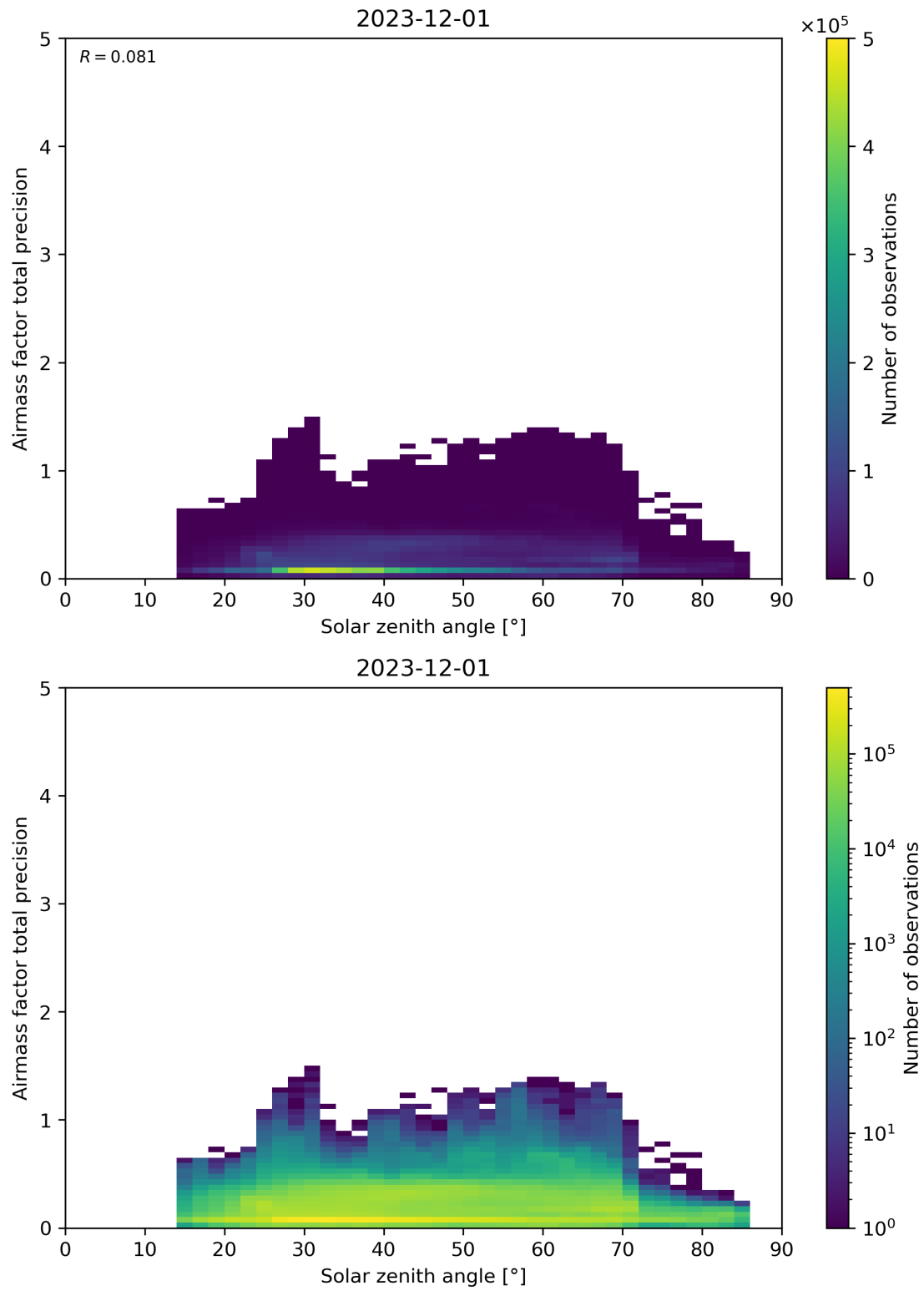
Figure 176: Scatter density plot of “Solar zenith angle” against “Airmass factor total precision” for 2023-11-30 to 2023-12-02.
