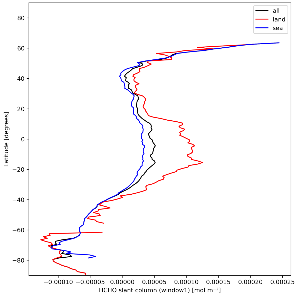
Figure 24: Zonal average of “HCHO slant column (window1)” for 2023-11-30 to 2023-12-02.
