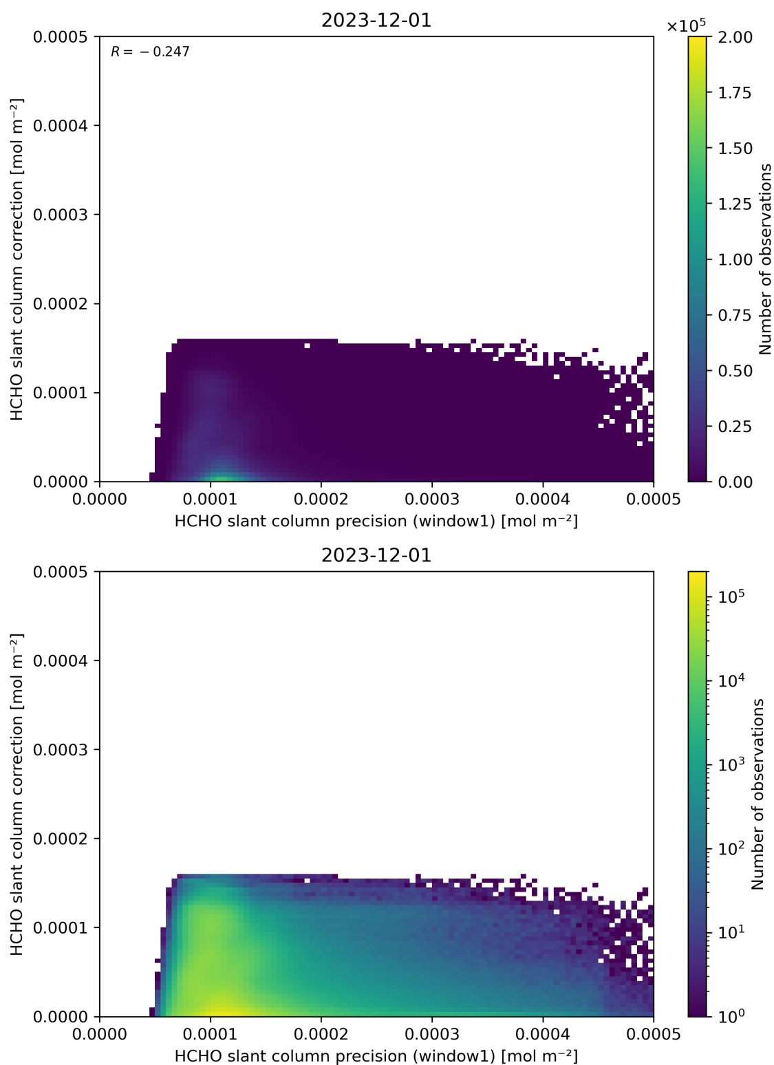
Figure 93: Scatter density plot of “HCHO slant column precision (window1)” against “HCHO slant column correction” for 2023-11-30 to 2023-12-02.
