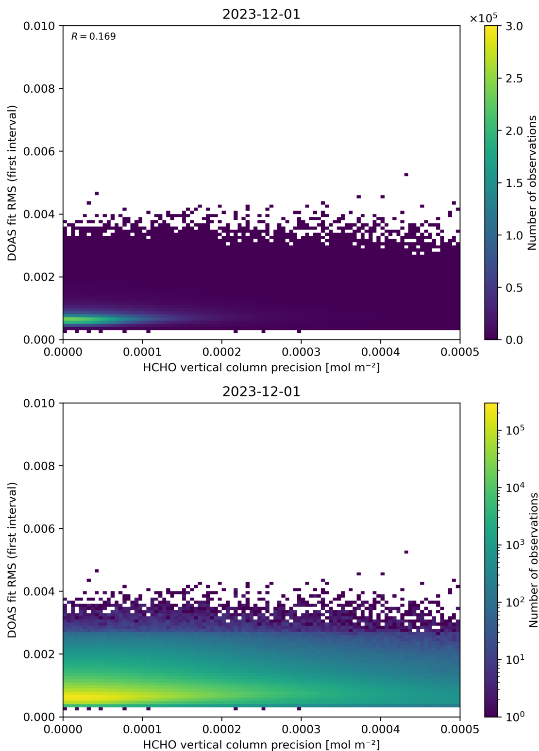
Figure 136: Scatter density plot of “HCHO vertical column precision” against “DOAS fit RMS (first interval)” for 2023-11-30 to 2023-12-02.
