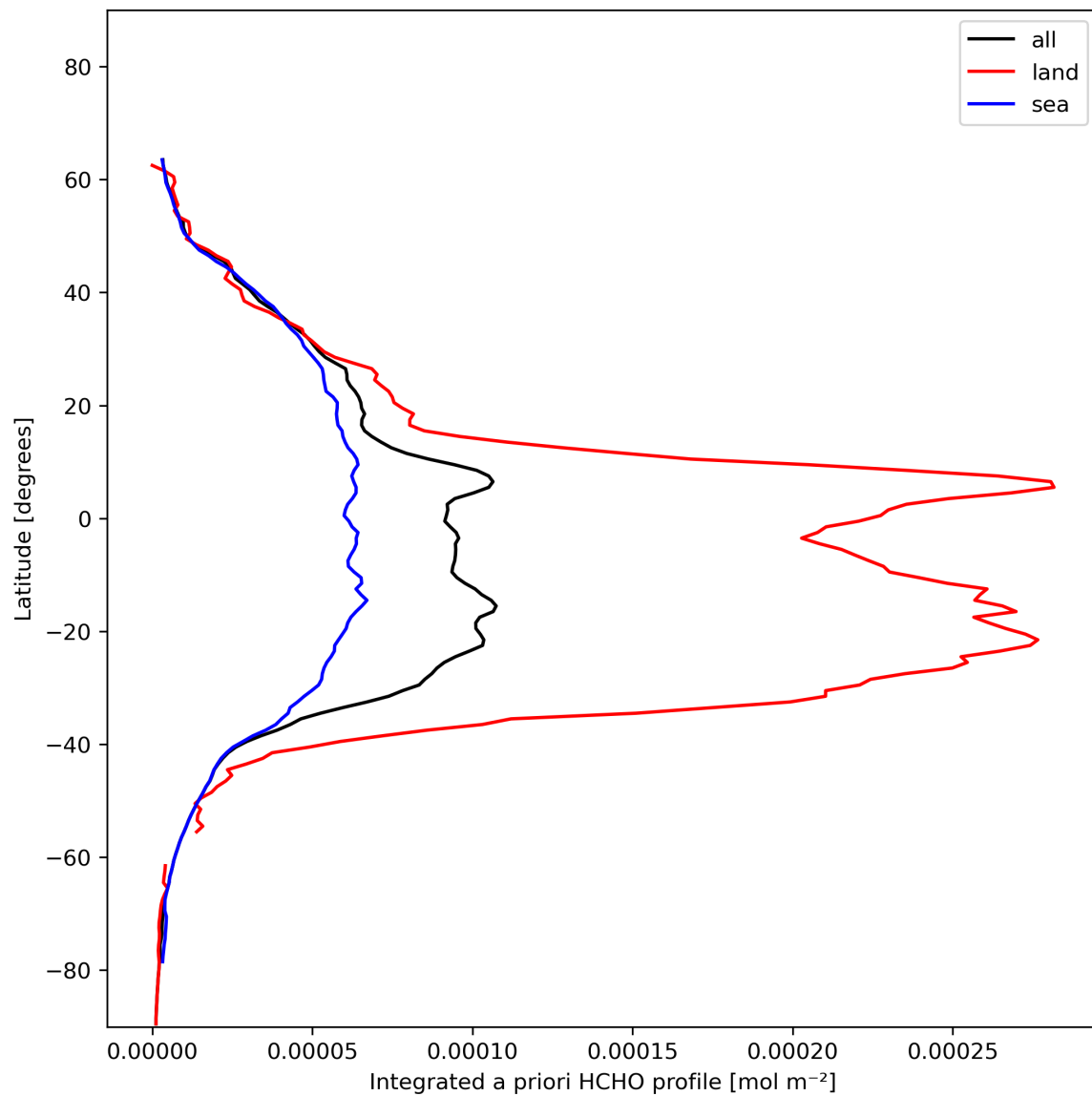
Figure 29: Zonal average of “Integrated a priori HCHO profile” for 2023-11-30 to 2023-12-02.
