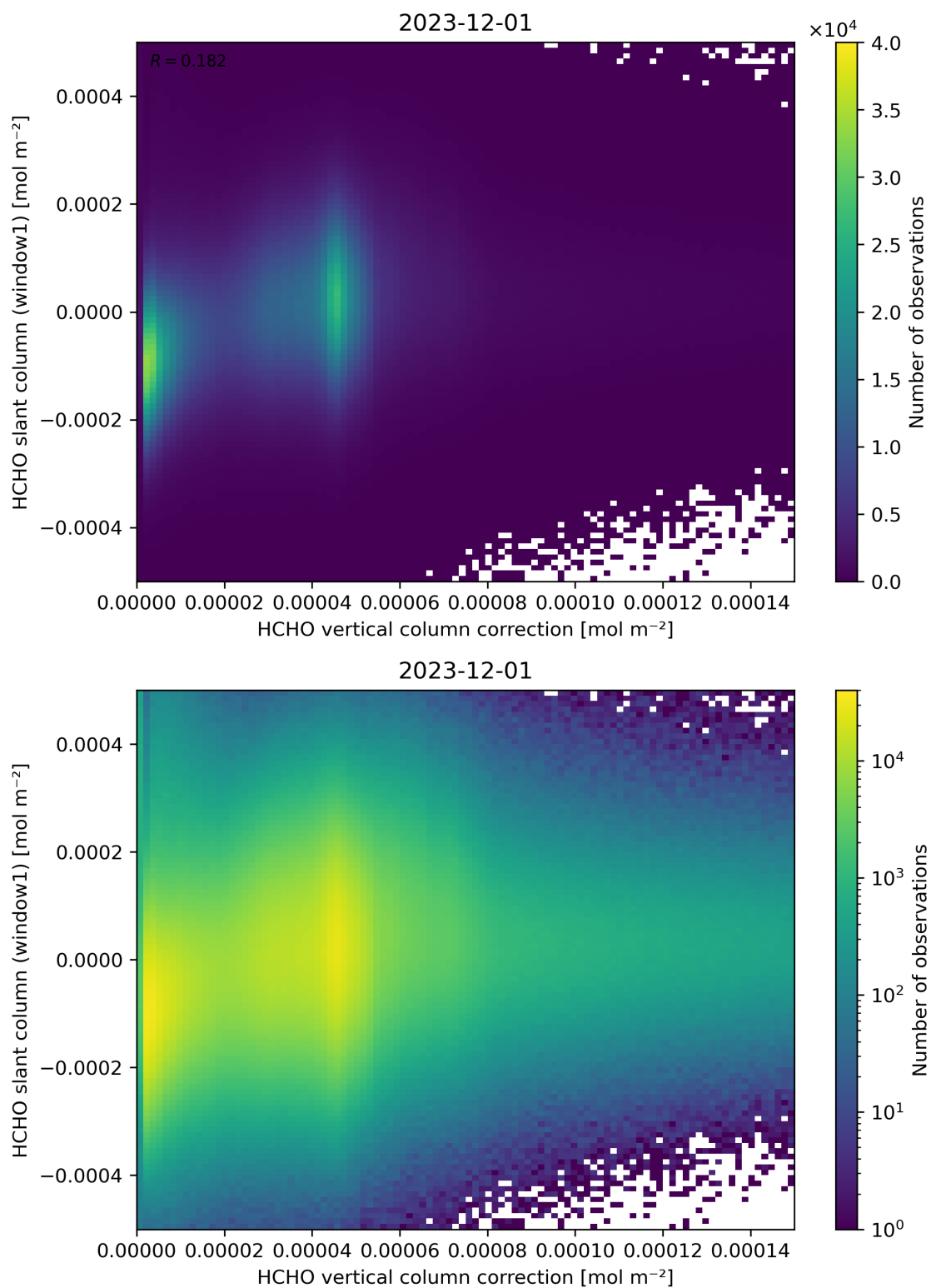
Figure 118: Scatter density plot of “HCHO vertical column correction” against “HCHO slant column (window1)” for 2023-11-30 to 2023-12-02.
