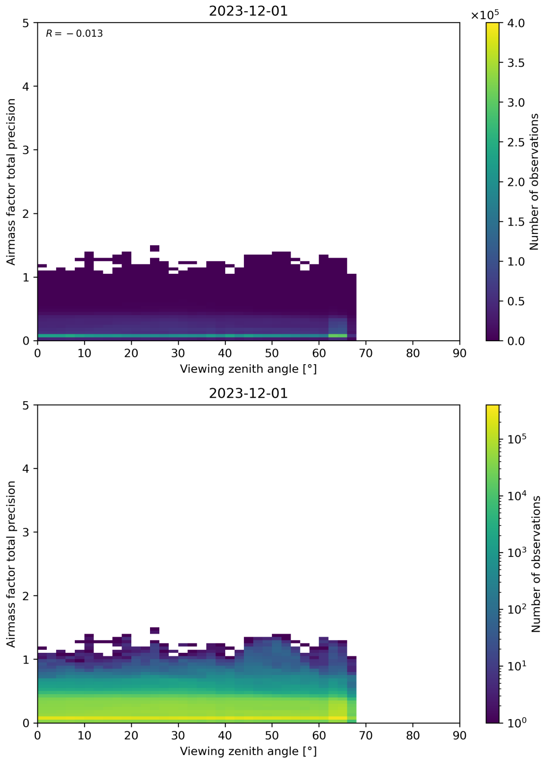
Figure 191: Scatter density plot of “Viewing zenith angle” against “Airmass factor total precision” for 2023-11-30 to 2023-12-02.
