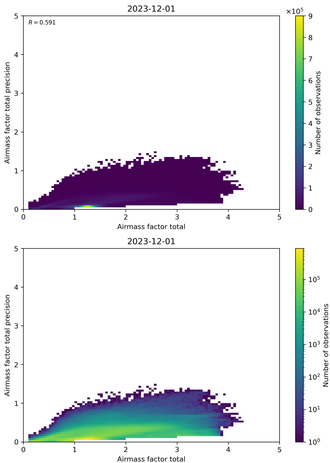
Figure 103: Scatter density plot of “Airmass factor total” against “Airmass factor total precision” for 2023-11-30 to 2023-12-02.
