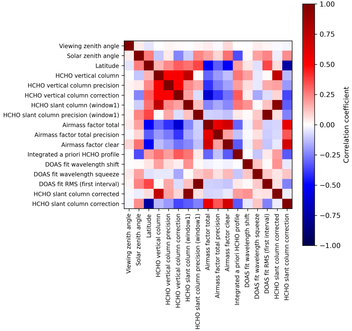
Figure 2: Map of correlation matrix for 2023-11-30 to 2023-12-02.
