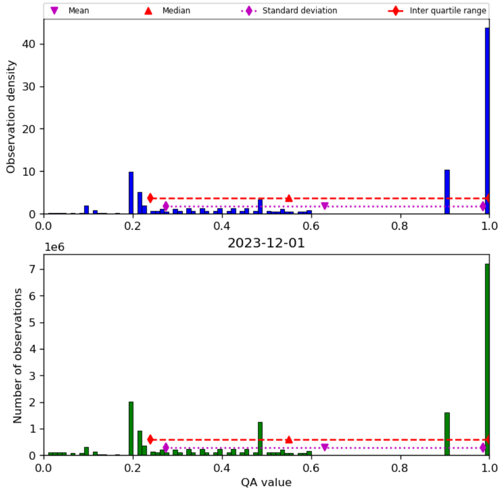
Figure 34: Histogram of “QA value” for 2023-11-30 to 2023-12-02
