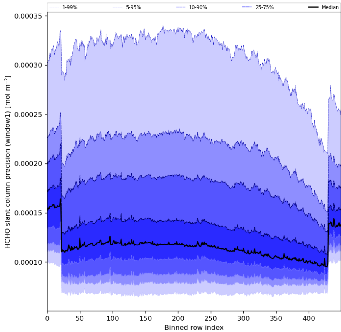
Figure 53: Along track statistics of “HCHO slant column precision (window1)” for 2023-11-30 to 2023-12-02
