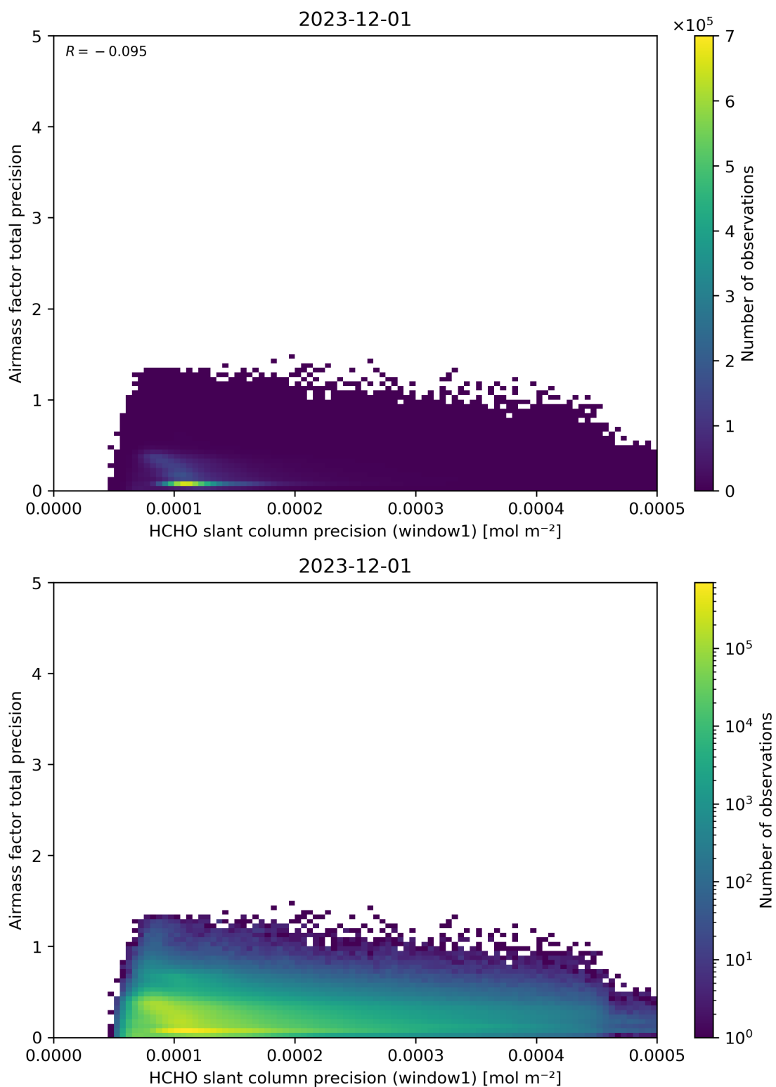
Figure 95: Scatter density plot of “HCHO slant column precision (window1)” against “Airmass factor total precision” for 2023-11-30 to 2023-12-02.
