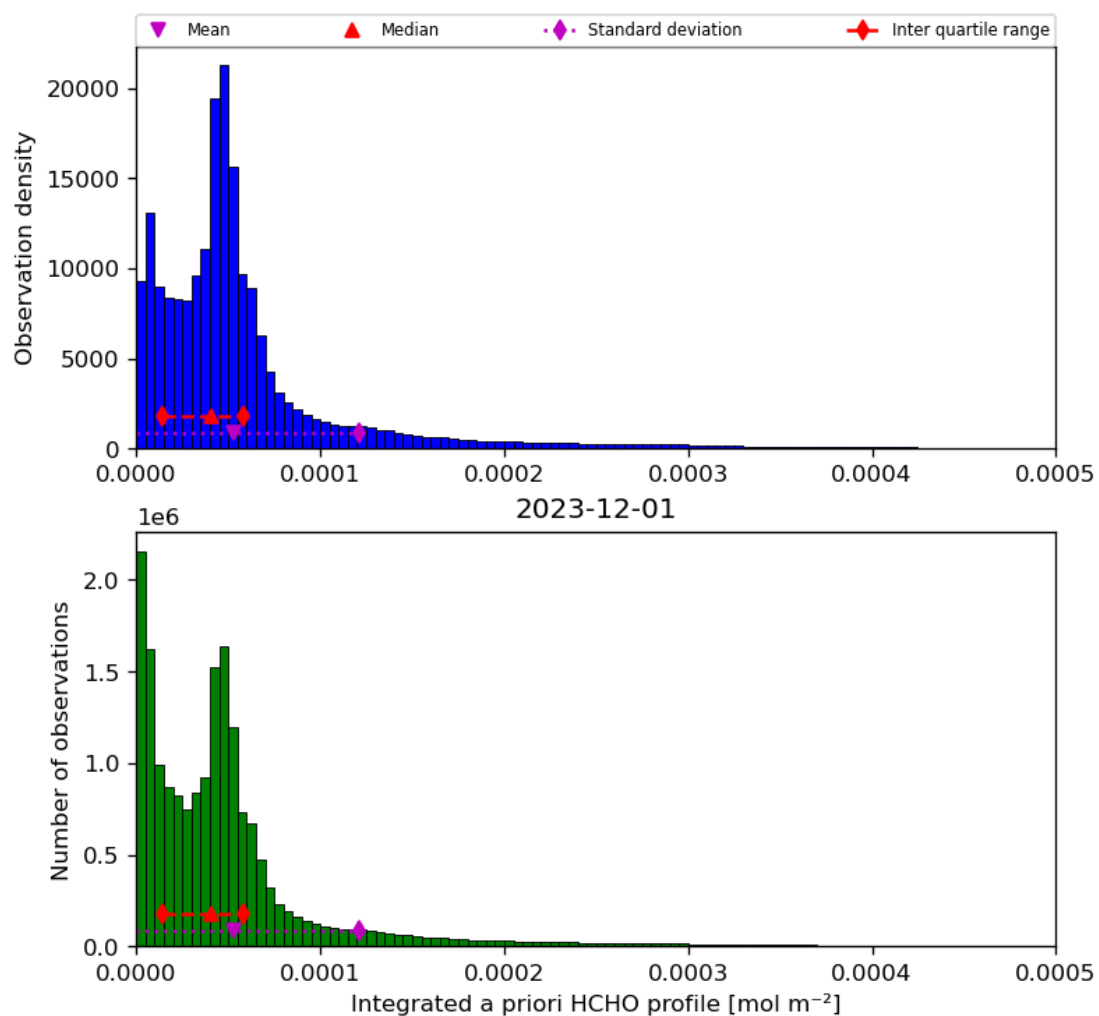
Figure 43: Histogram of “Integrated a priori HCHO profile” for 2023-11-30 to 2023-12-02
