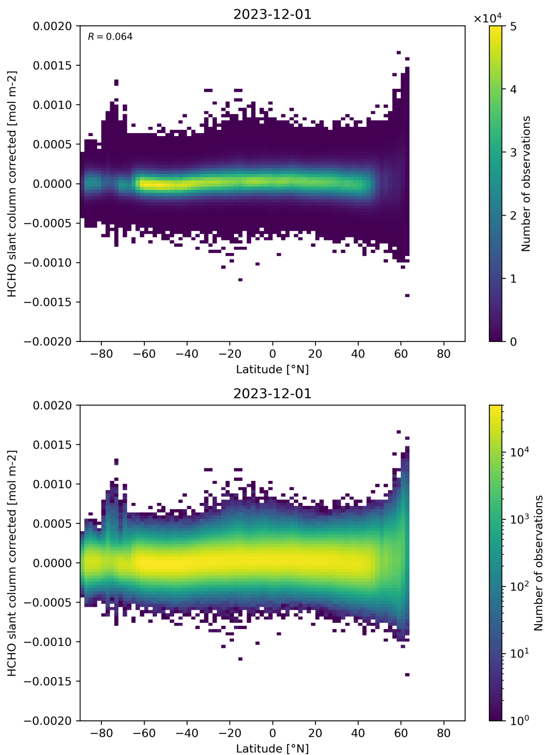
Figure 157: Scatter density plot of “Latitude” against “HCHO slant column corrected” for 2023-11-30 to 2023-12-02.
