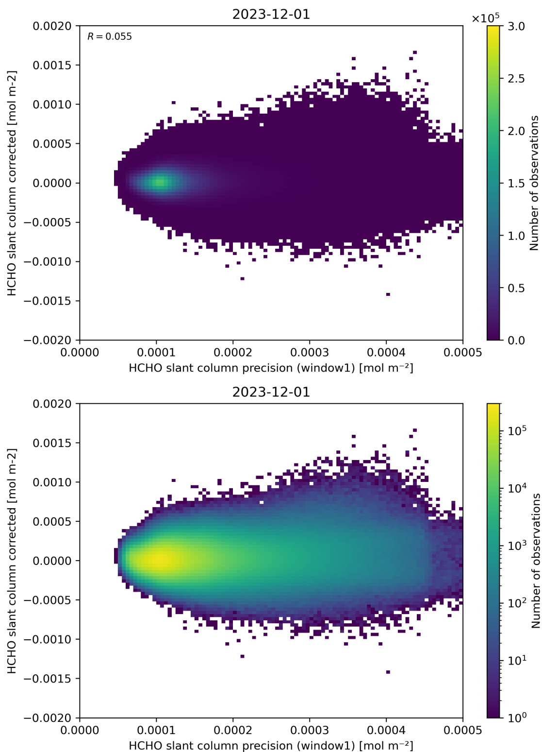
Figure 92: Scatter density plot of “HCHO slant column precision (window1)” against “HCHO slant column corrected” for 2023-11-30 to 2023-12-02.
