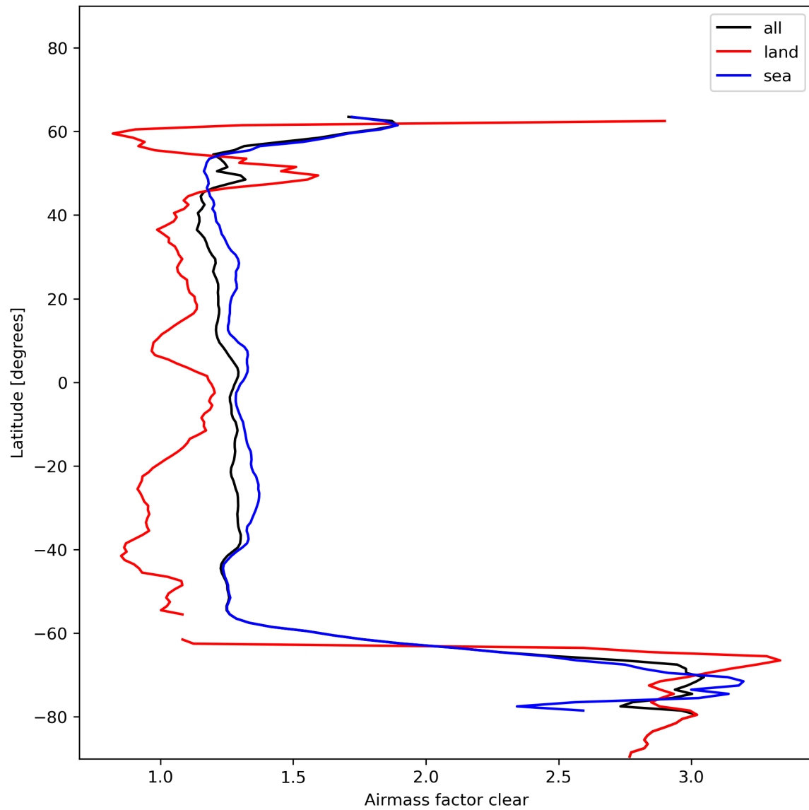
Figure 28: Zonal average of “Airmass factor clear” for 2023-11-30 to 2023-12-02.
