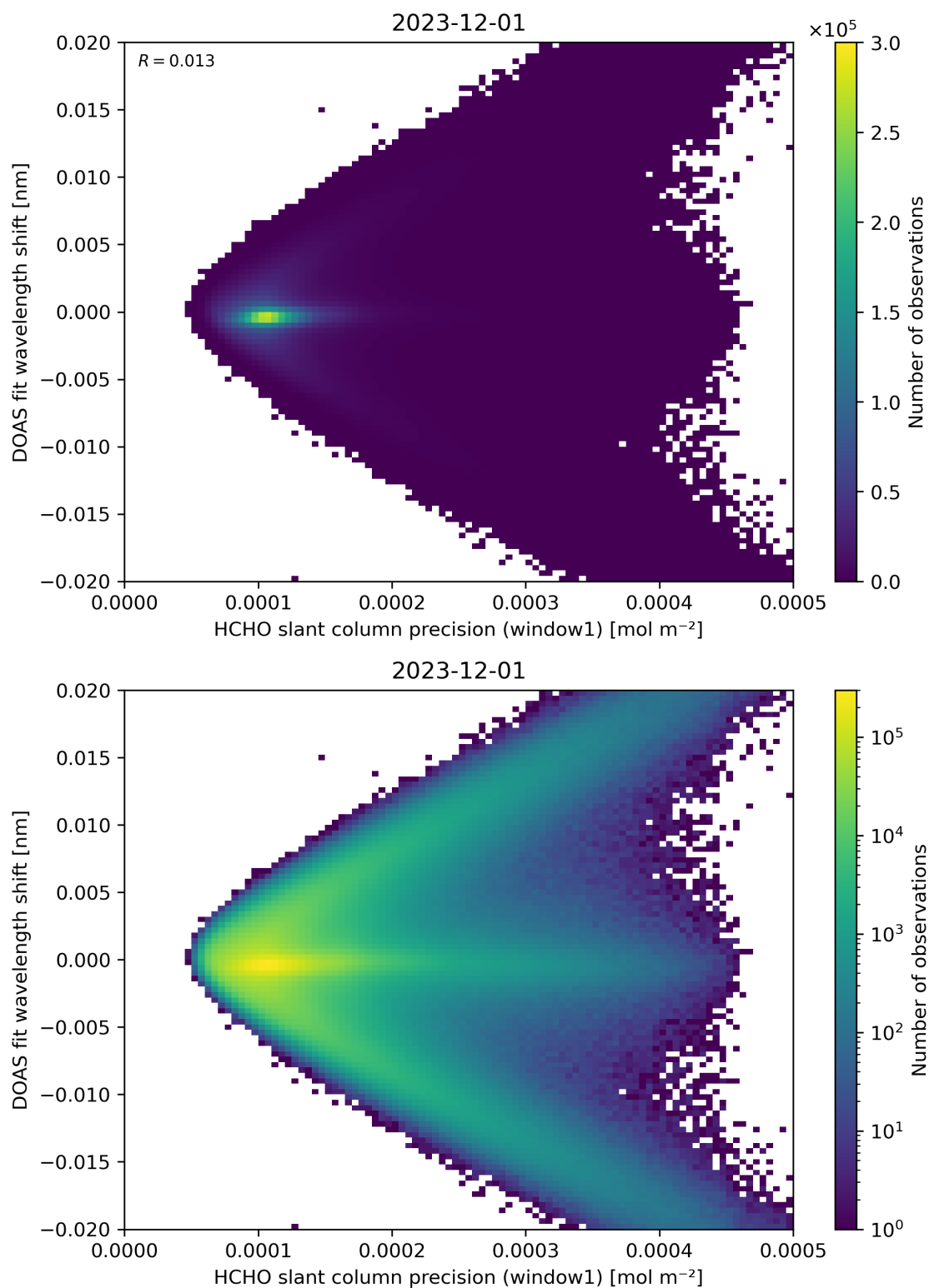
Figure 89: Scatter density plot of “HCHO slant column precision (window1)” against “DOAS fit wavelength shift” for 2023-11-30 to 2023-12-02.
