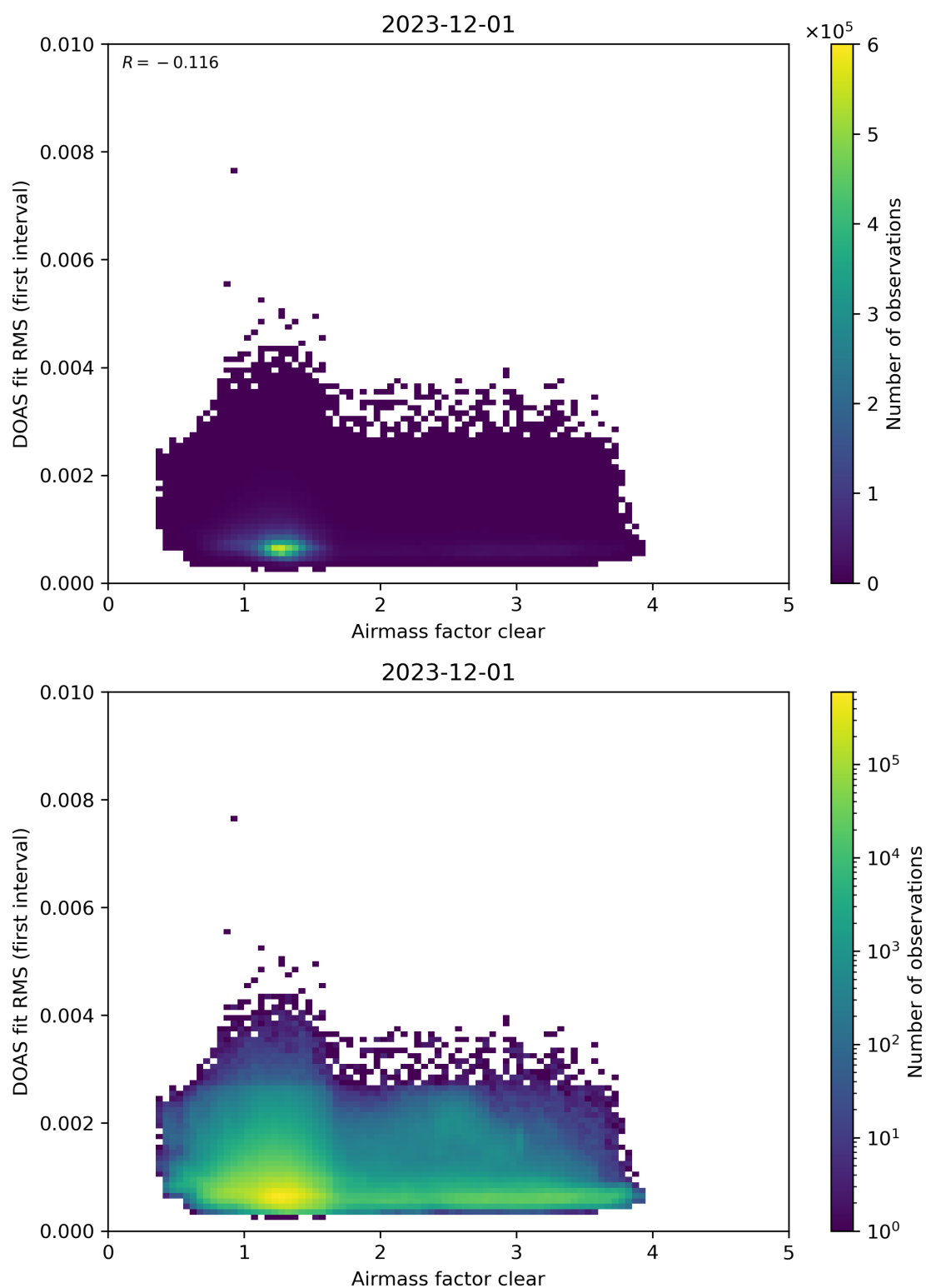
Figure 71: Scatter density plot of “Airmass factor clear” against “DOAS fit RMS (first interval)” for 2023-11-30 to 2023-12-02.
