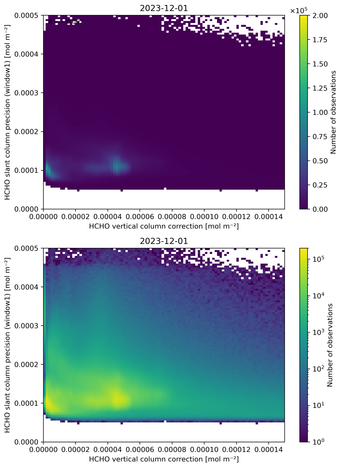
Figure 119: Scatter density plot of “HCHO vertical column correction” against “HCHO slant column precision (window1)” for 2023-11-30 to 2023-12-02.
