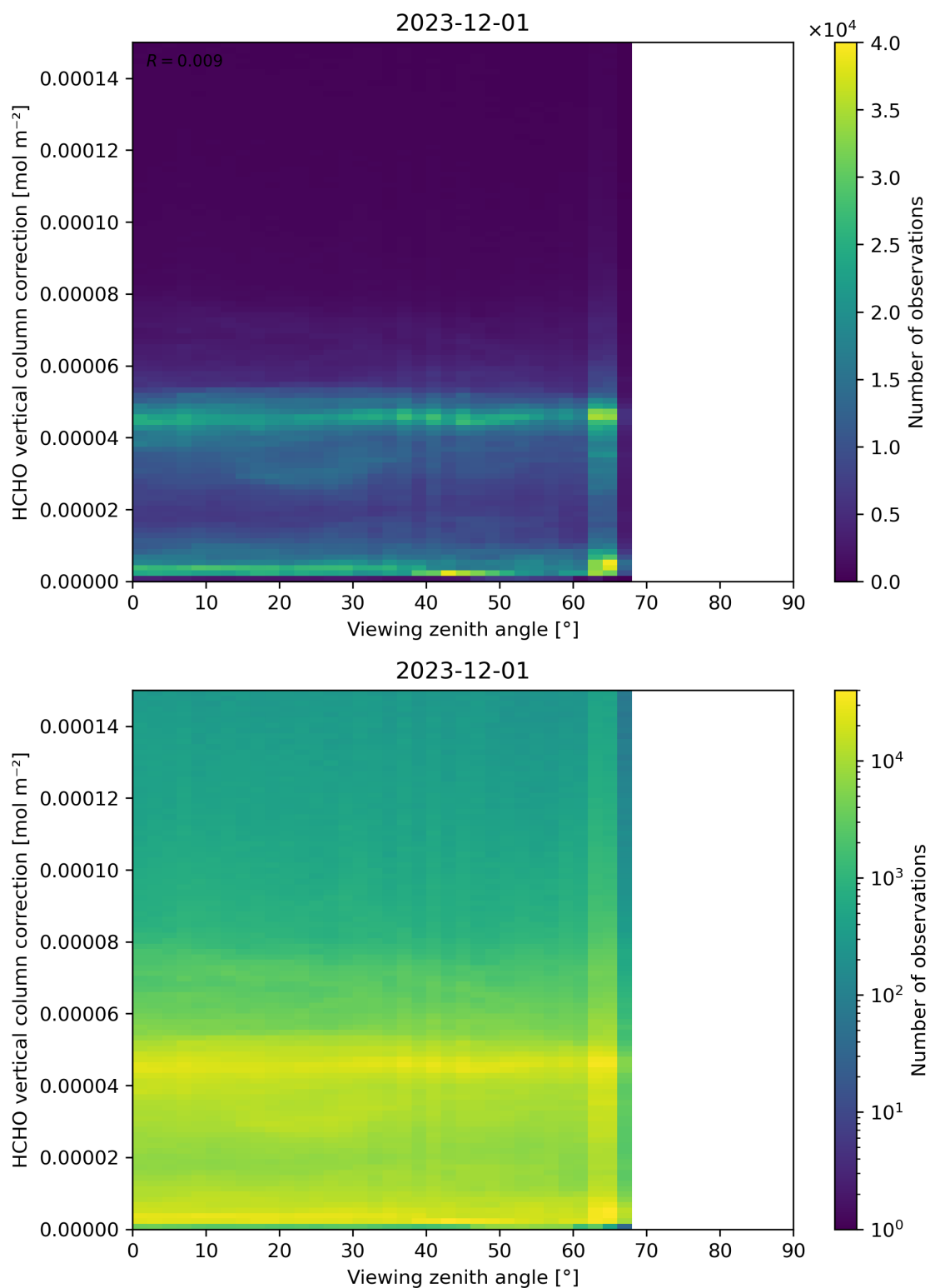
Figure 193: Scatter density plot of “Viewing zenith angle” against “HCHO vertical column correction” for 2023-11-30 to 2023-12-02.
