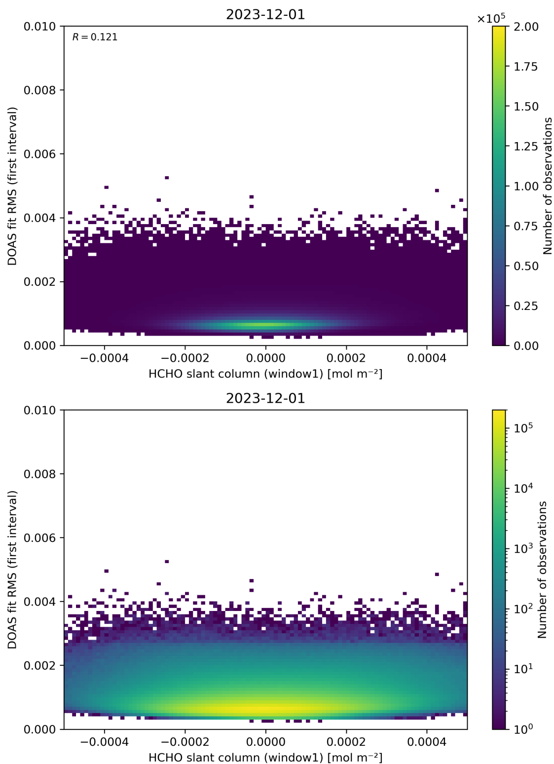
Figure 78: Scatter density plot of “HCHO slant column (window1)” against “DOAS fit RMS (first interval)” for 2023-11-30 to 2023-12-02.
