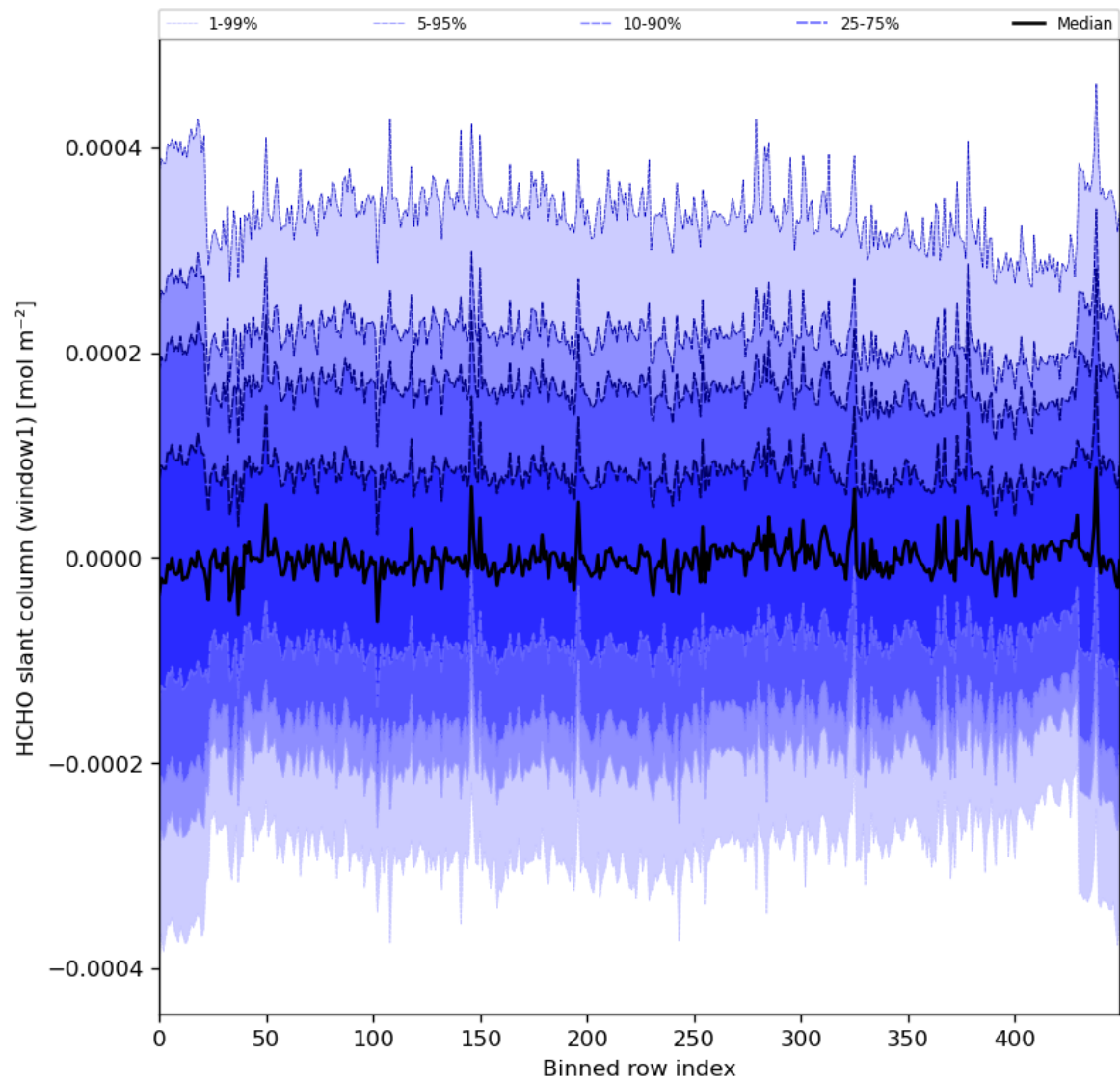
Figure 52: Along track statistics of “HCHO slant column (window1)” for 2023-11-30 to 2023-12-02
