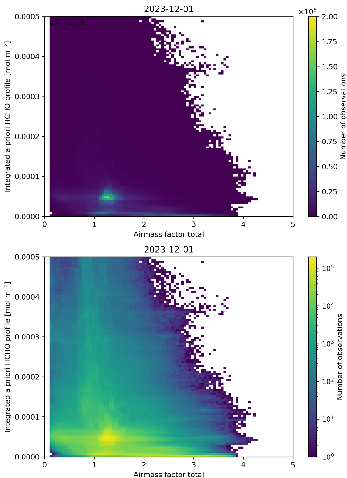
Figure 104: Scatter density plot of “Airmass factor total” against “Integrated a priori HCHO profile” for 2023-11-30 to 2023-12-02.
