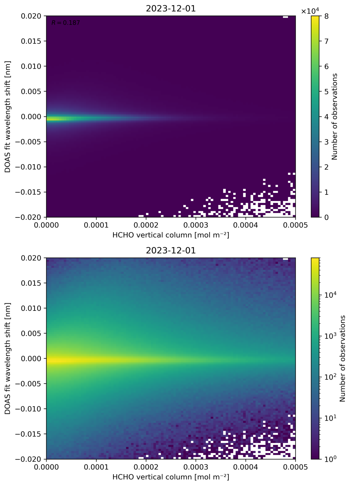
Figure 124: Scatter density plot of “HCHO vertical column” against “DOAS fit wavelength shift” for 2023-11-30 to 2023-12-02.
