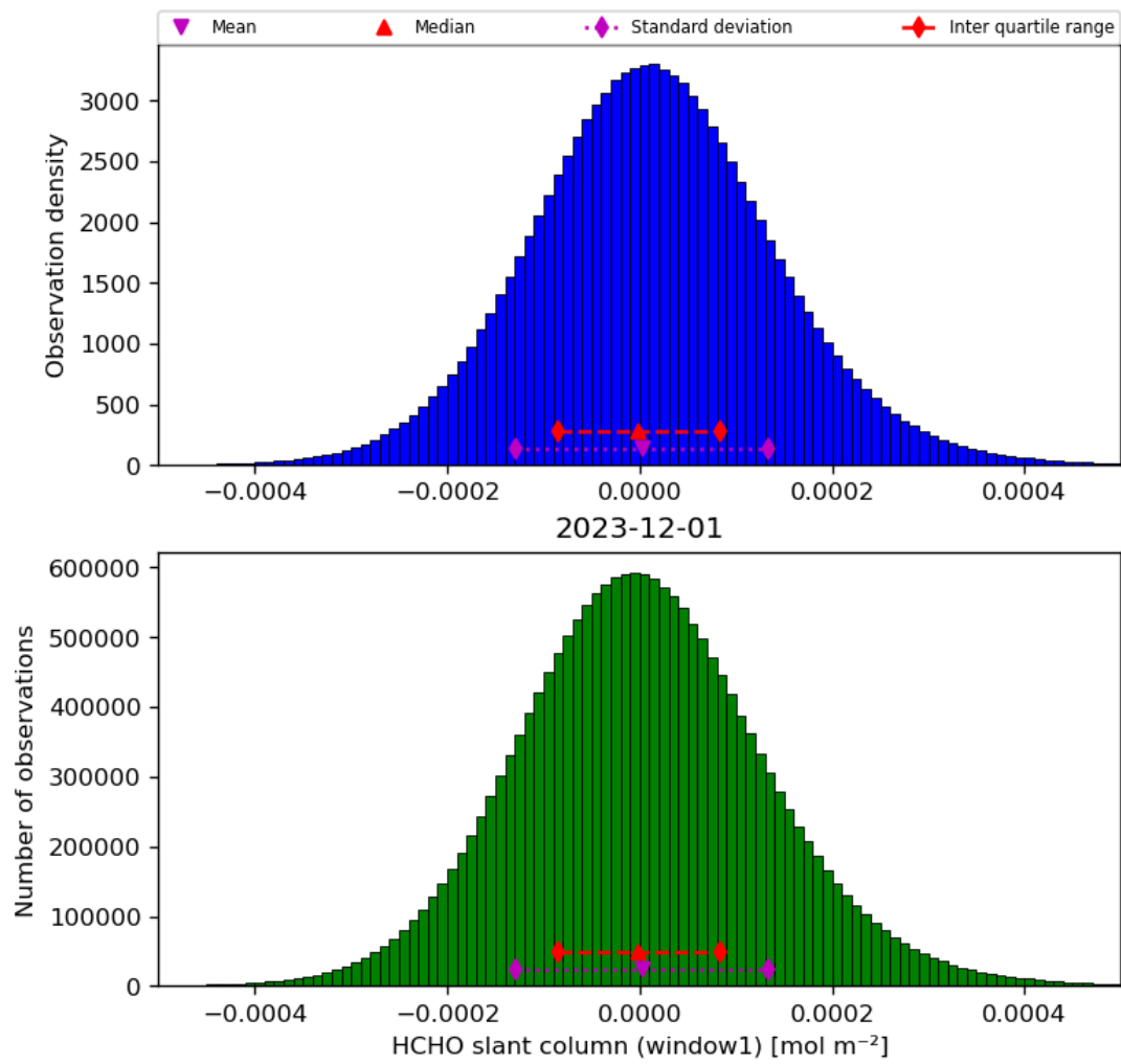
Figure 38: Histogram of “HCHO slant column (window1)” for 2023-11-30 to 2023-12-02
