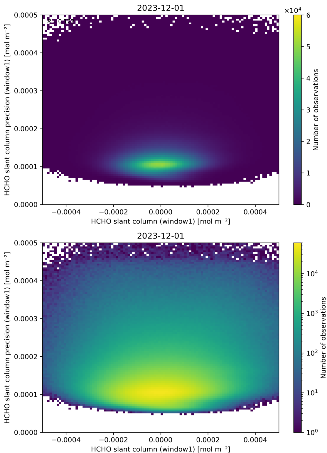
Figure 84: Scatter density plot of “HCHO slant column (window1)” against “HCHO slant column precision (window1)” for 2023-11-30 to 2023-12-02.
