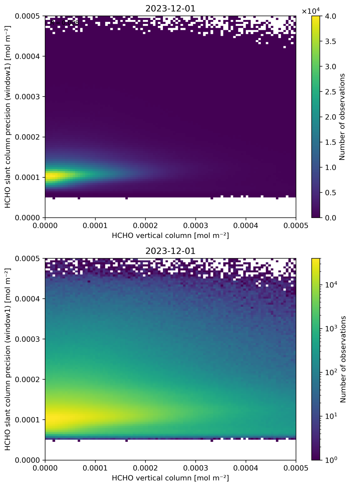
Figure 130: Scatter density plot of “HCHO vertical column” against “HCHO slant column precision (window1)” for 2023-11-30 to 2023-12-02.
