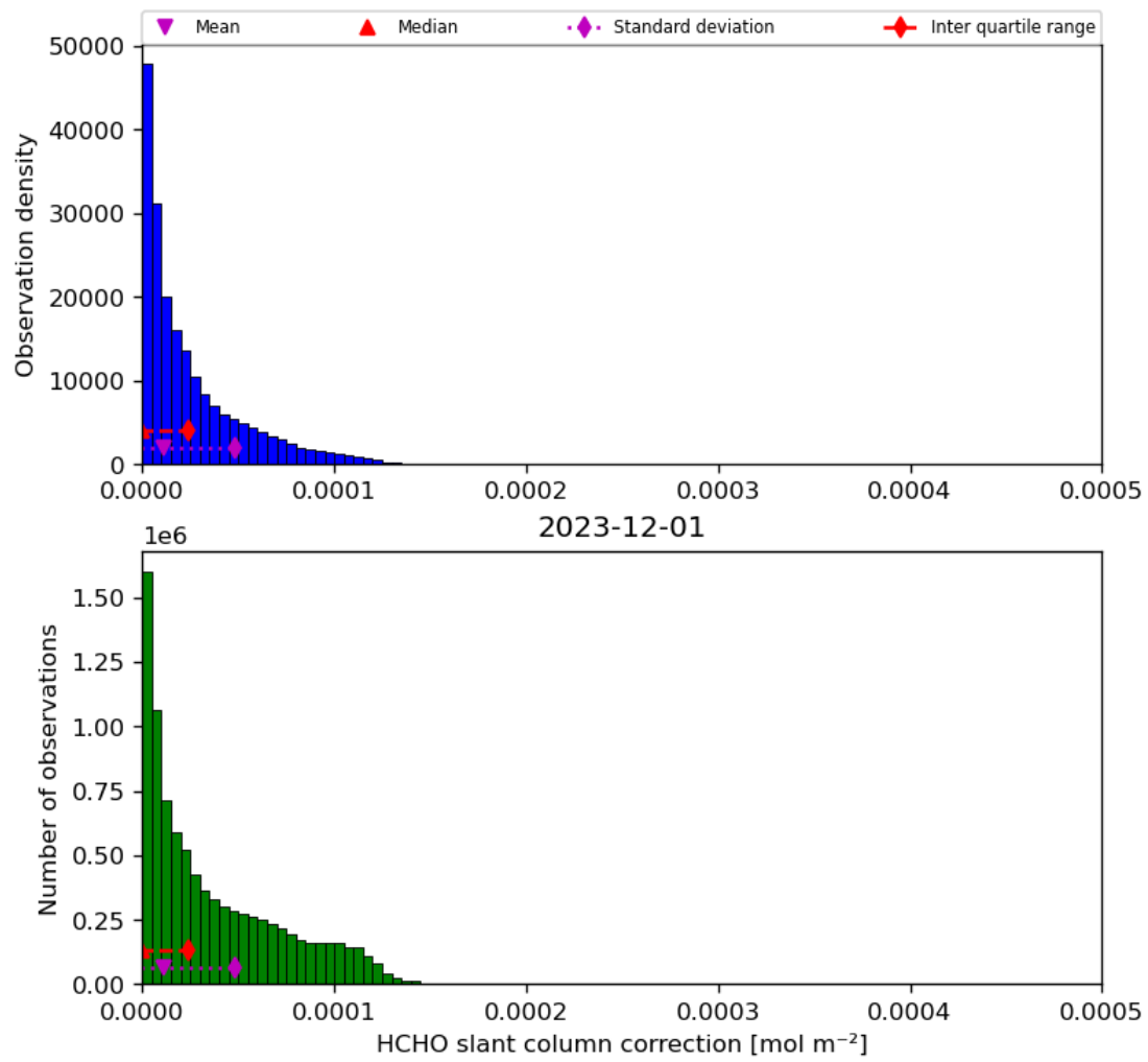
Figure 47: Histogram of “HCHO slant column correction” for 2023-11-30 to 2023-12-02
