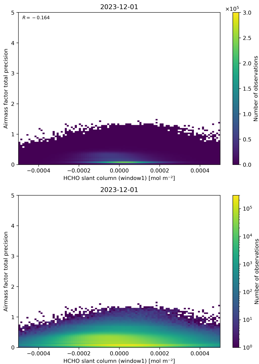
Figure 86: Scatter density plot of “HCHO slant column (window1)” against “Airmass factor total precision” for 2023-11-30 to 2023-12-02.
