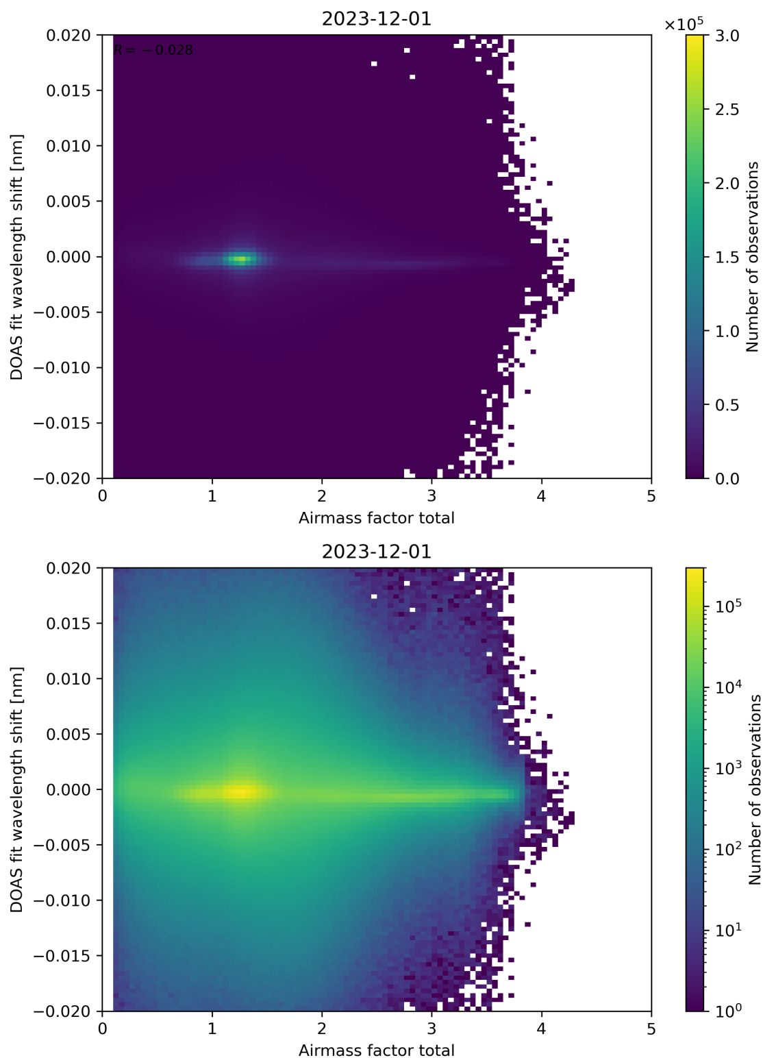
Figure 98: Scatter density plot of “Airmass factor total” against “DOAS fit wavelength shift” for 2023-11-30 to 2023-12-02.
