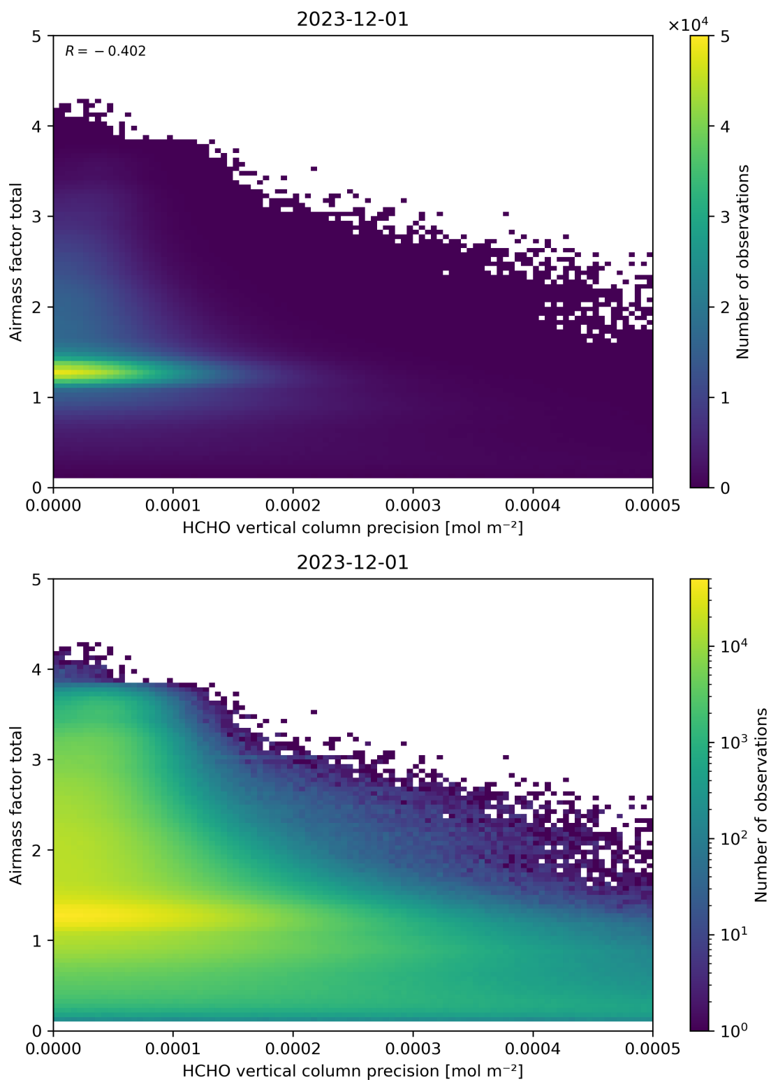
Figure 144: Scatter density plot of “HCHO vertical column precision” against “Airmass factor total” for 2023-11-30 to 2023-12-02.
