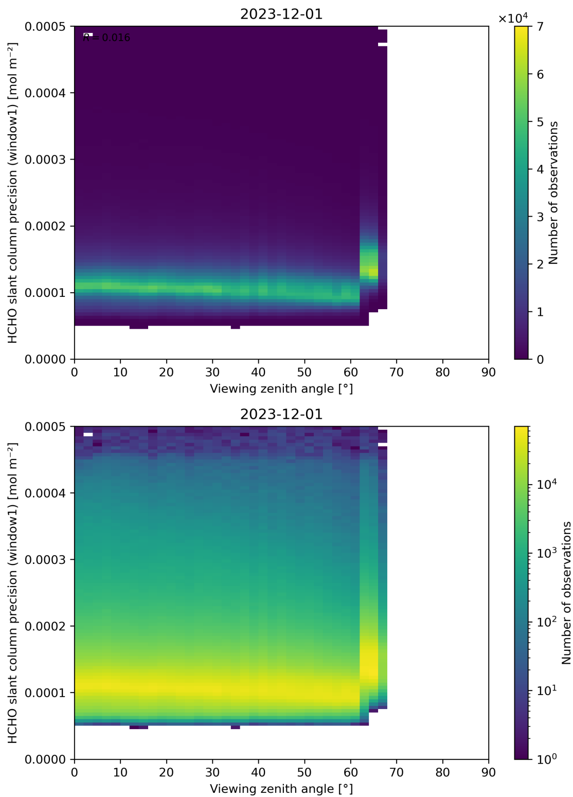
Figure 189: Scatter density plot of “Viewing zenith angle” against “HCHO slant column precision (window1)” for 2023-11-30 to 2023-12-02.
