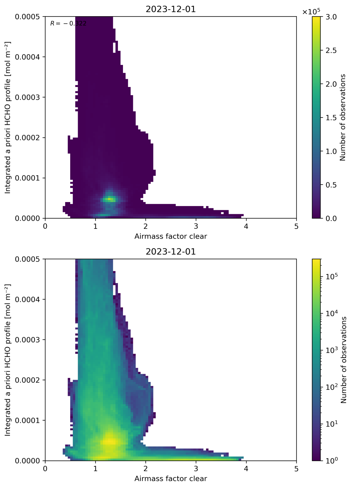
Figure 76: Scatter density plot of “Airmass factor clear” against “Integrated a priori HCHO profile” for 2023-11-30 to 2023-12-02.
