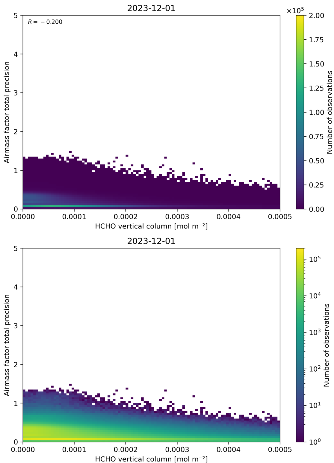
Figure 132: Scatter density plot of “HCHO vertical column” against “Airmass factor total precision” for 2023-11-30 to 2023-12-02.
