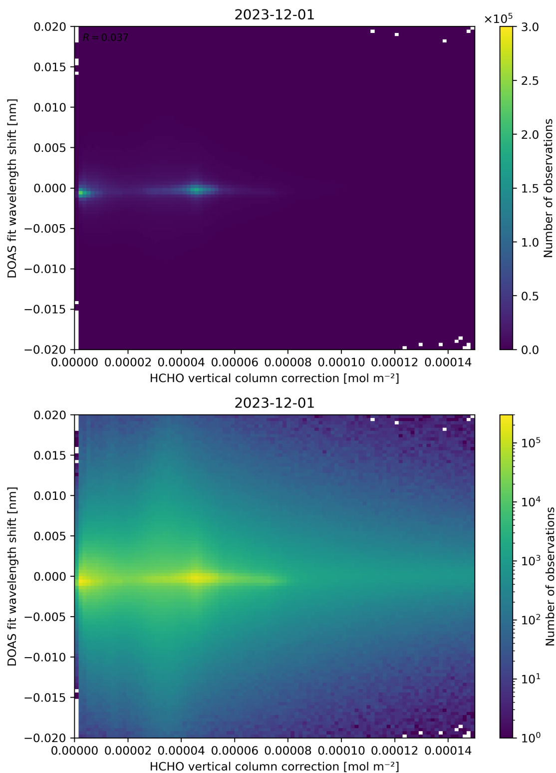
Figure 113: Scatter density plot of “HCHO vertical column correction” against “DOAS fit wavelength shift” for 2023-11-30 to 2023-12-02.
