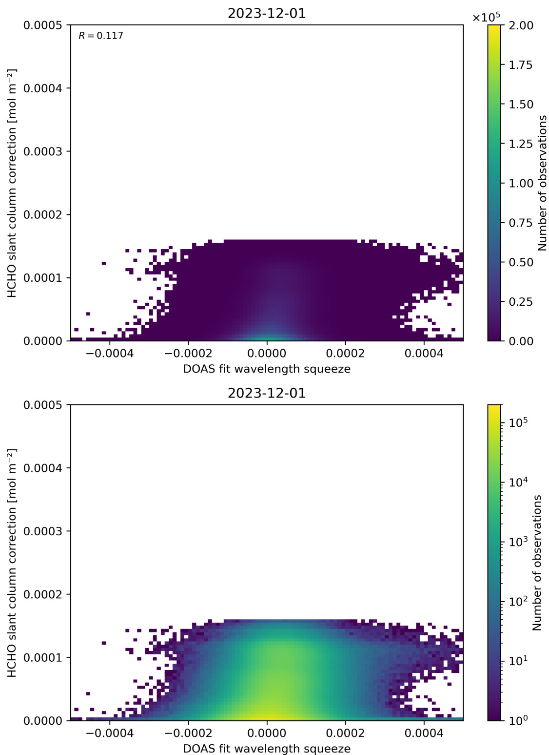
Figure 70: Scatter density plot of “DOAS fit wavelength squeeze” against “HCHO slant column correction” for 2023-11-30 to 2023-12-02.
