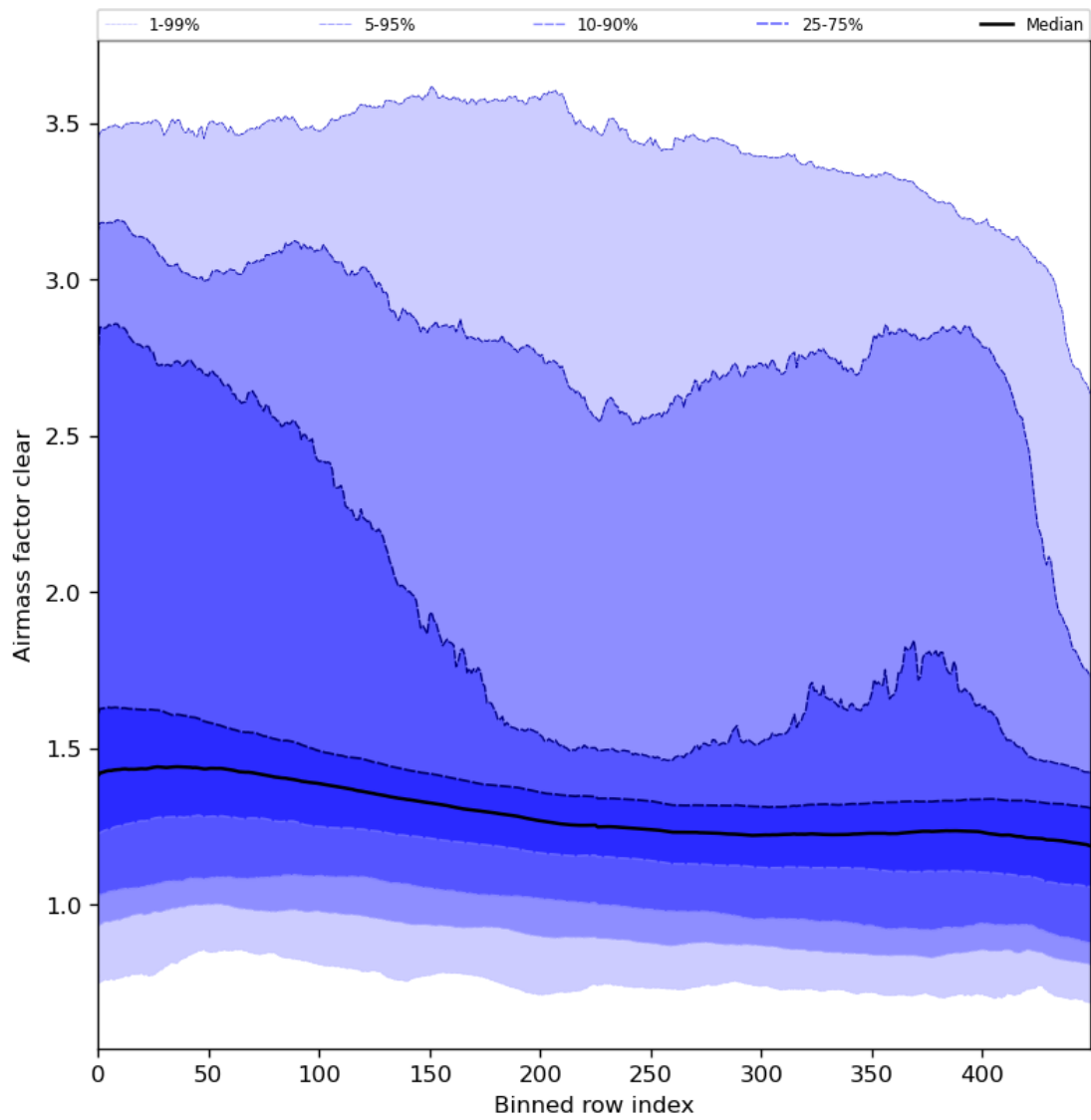
Figure 56: Along track statistics of “Airmass factor clear” for 2023-11-30 to 2023-12-02
