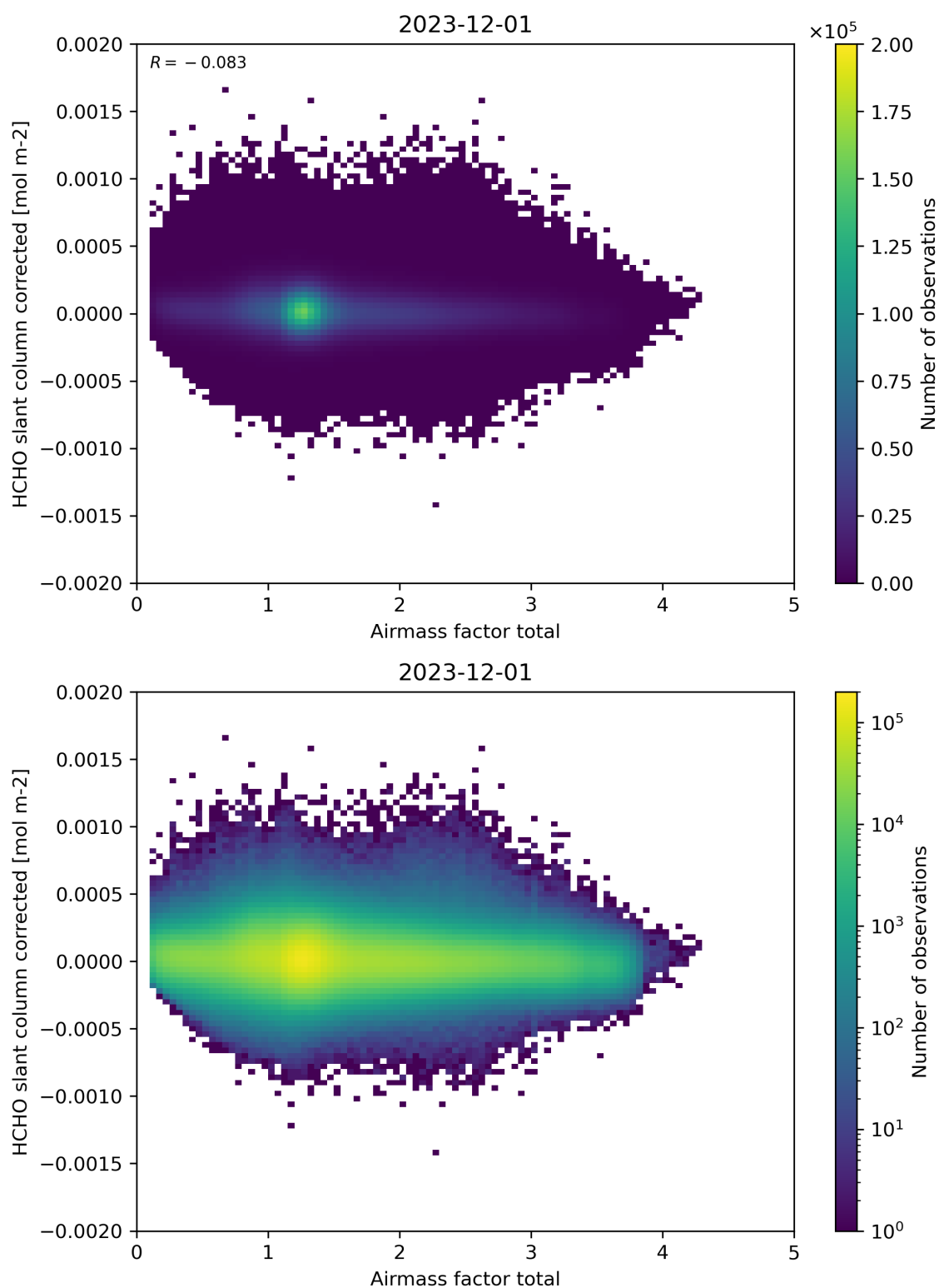
Figure 101: Scatter density plot of “Airmass factor total” against “HCHO slant column corrected” for 2023-11-30 to 2023-12-02.
