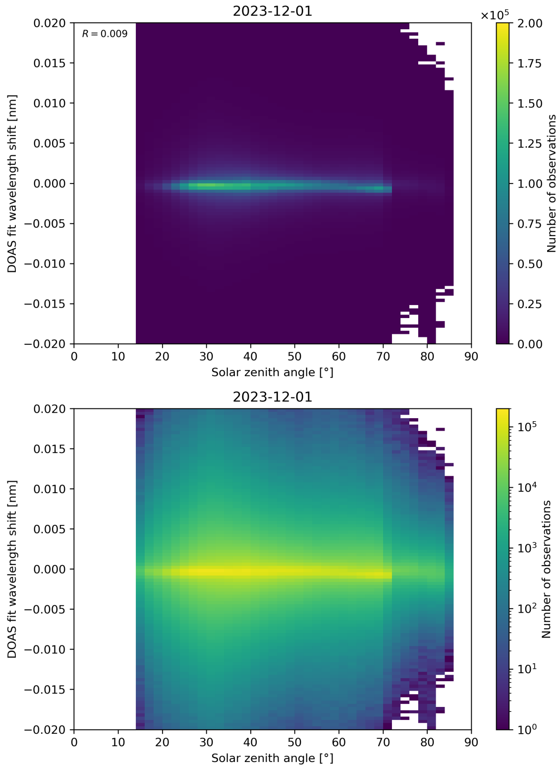
Figure 168: Scatter density plot of “Solar zenith angle” against “DOAS fit wavelength shift” for 2023-11-30 to 2023-12-02.
