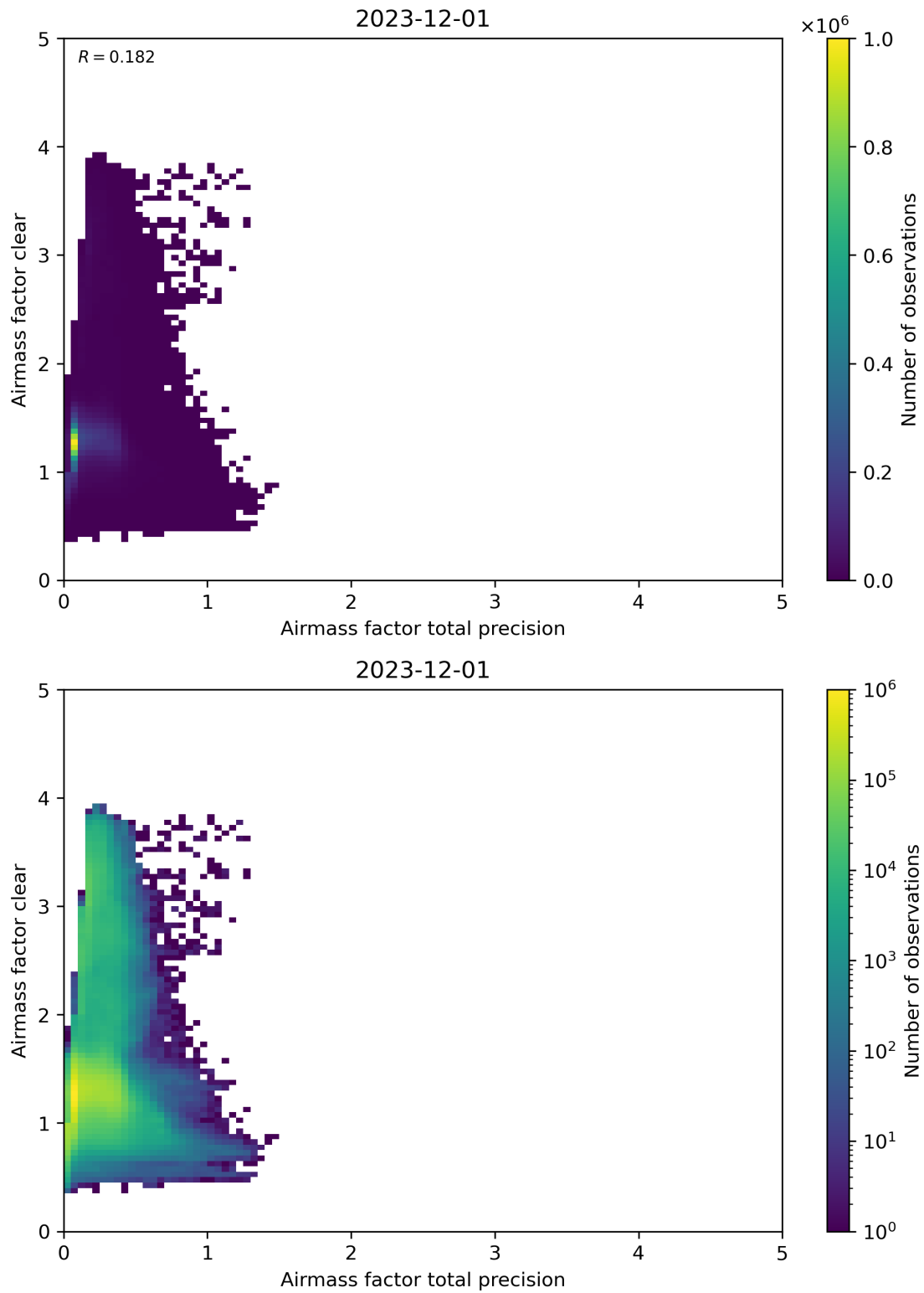
Figure 108: Scatter density plot of “Airmass factor total precision” against “Airmass factor clear” for 2023-11-30 to 2023-12-02.
