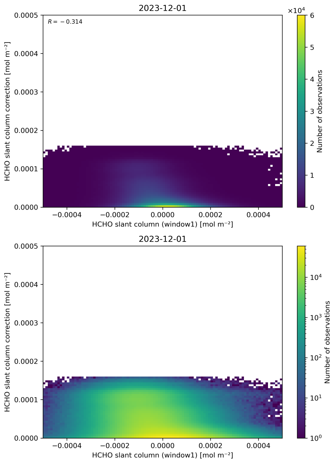
Figure 83: Scatter density plot of “HCHO slant column (window1)” against “HCHO slant column correction” for 2023-11-30 to 2023-12-02.
