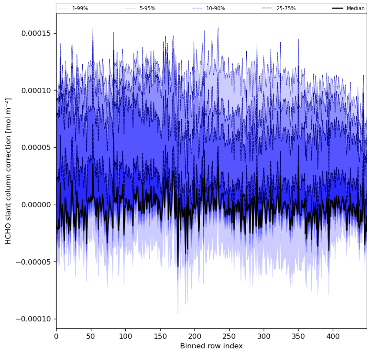
Figure 61: Along track statistics of “HCHO slant column correction” for 2023-11-30 to 2023-12-02
