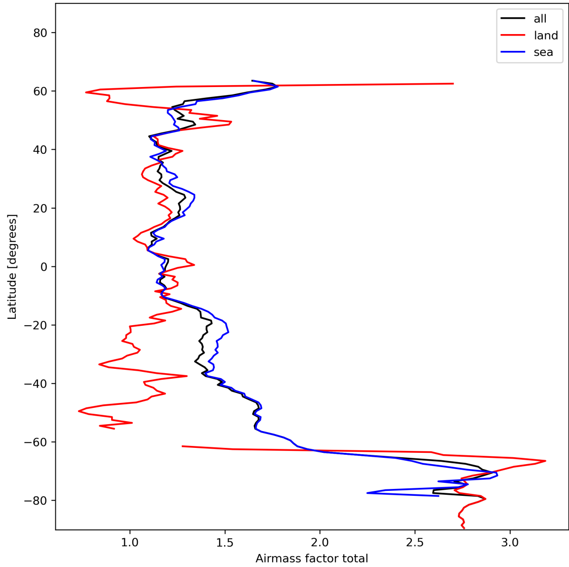
Figure 26: Zonal average of “Airmass factor total” for 2023-11-30 to 2023-12-02.
