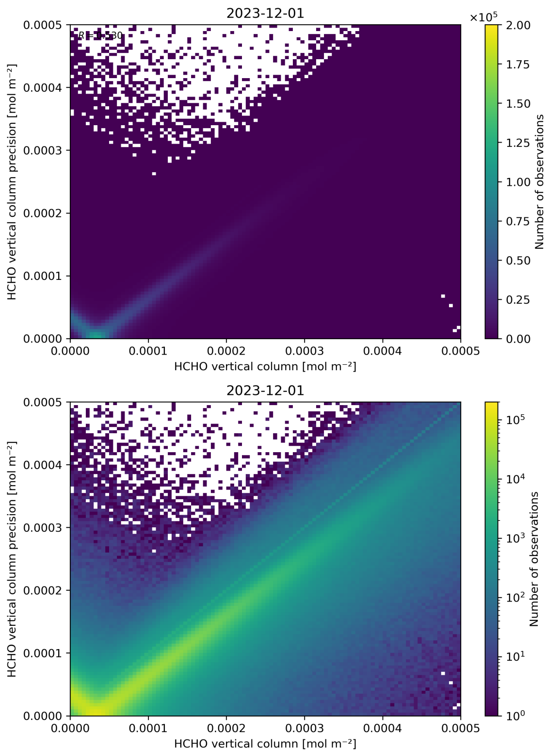
Figure 134: Scatter density plot of “HCHO vertical column” against “HCHO vertical column precision” for 2023-11-30 to 2023-12-02.
