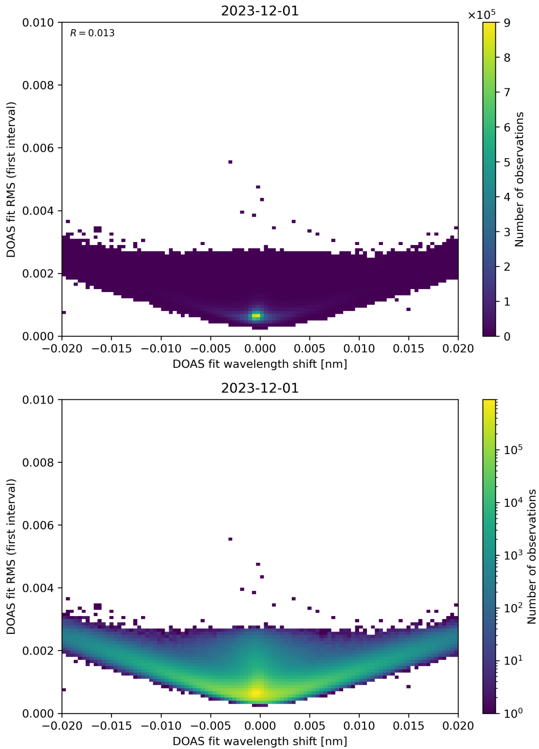
Figure 64: Scatter density plot of “DOAS fit wavelength shift” against “DOAS fit RMS (first interval)” for 2023-11-30 to 2023-12-02.
