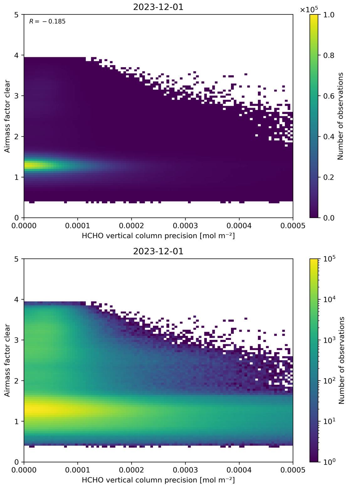
Figure 139: Scatter density plot of “HCHO vertical column precision” against “Airmass factor clear” for 2023-11-30 to 2023-12-02.
