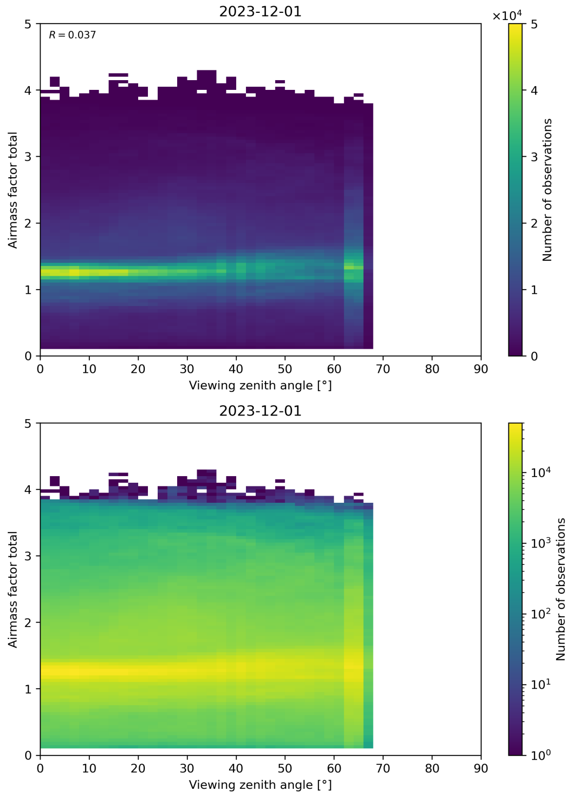
Figure 190: Scatter density plot of “Viewing zenith angle” against “Airmass factor total” for 2023-11-30 to 2023-12-02.
