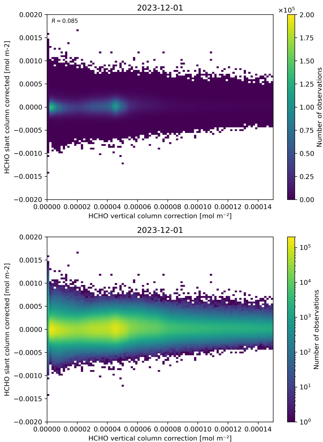
Figure 116: Scatter density plot of “HCHO vertical column correction” against “HCHO slant column corrected” for 2023-11-30 to 2023-12-02.
