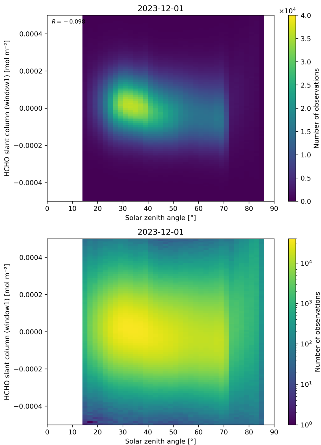
Figure 173: Scatter density plot of “Solar zenith angle” against “HCHO slant column (window1)” for 2023-11-30 to 2023-12-02.
