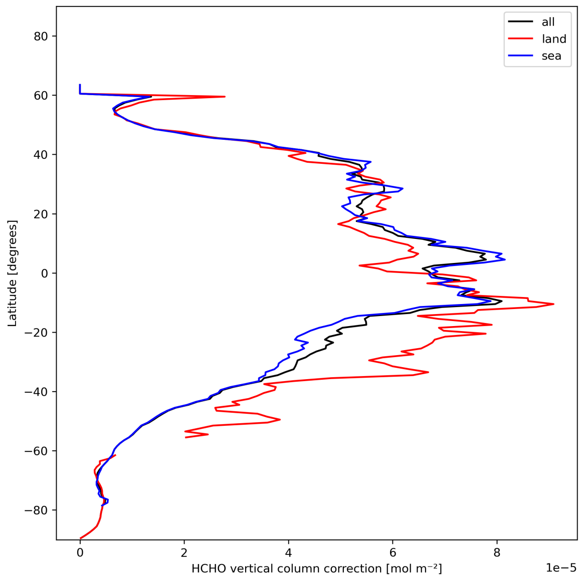
Figure 23: Zonal average of “HCHO vertical column correction” for 2023-11-30 to 2023-12-02.
