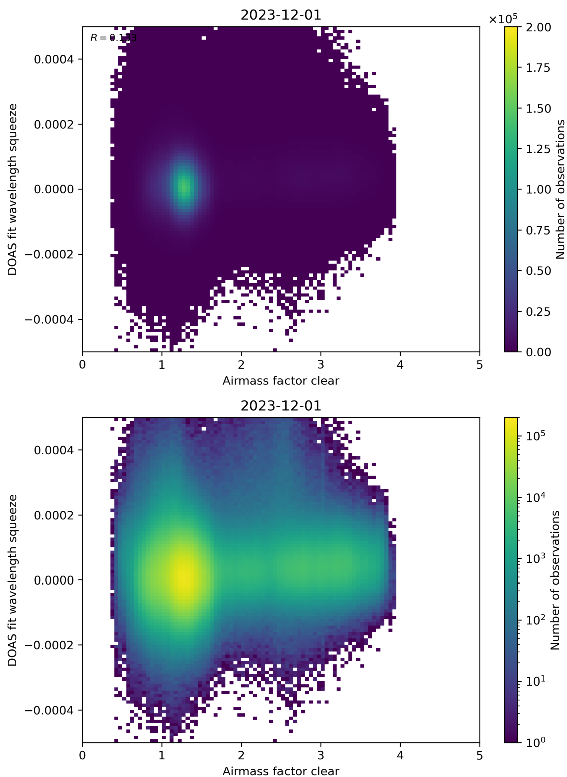
Figure 73: Scatter density plot of “Airmass factor clear” against “DOAS fit wavelength squeeze” for 2023-11-30 to 2023-12-02.
