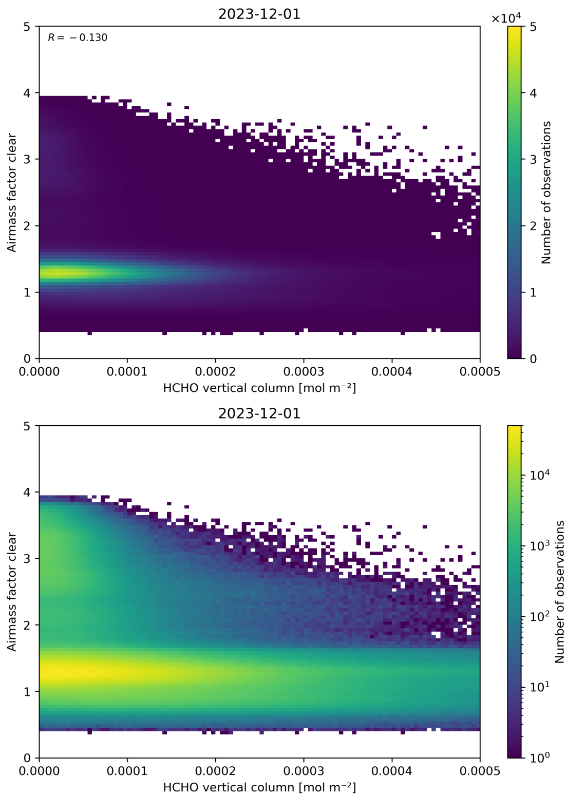
Figure 126: Scatter density plot of “HCHO vertical column” against “Airmass factor clear” for 2023-11-30 to 2023-12-02.
