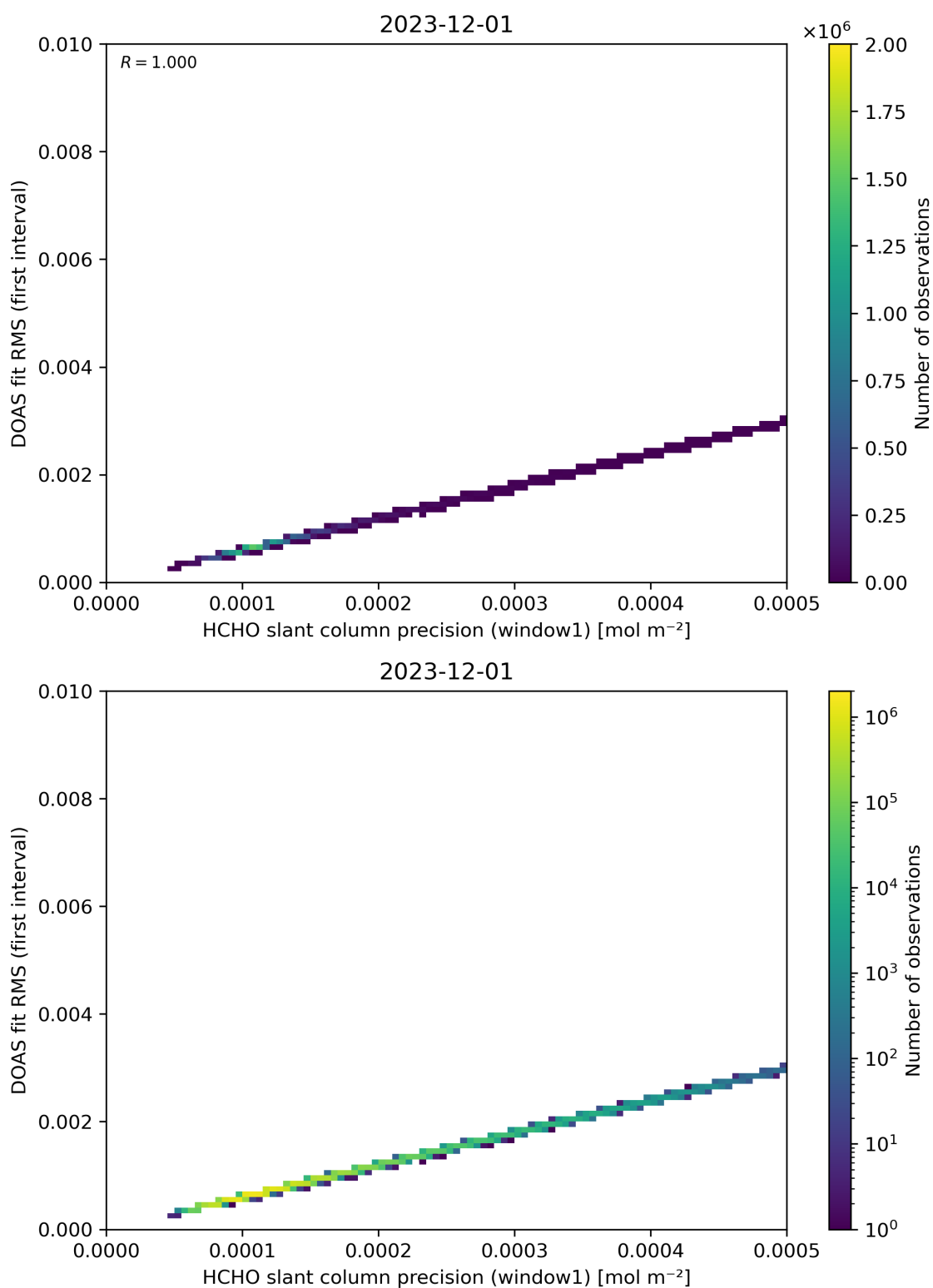
Figure 88: Scatter density plot of “HCHO slant column precision (window1)” against “DOAS fit RMS (first interval)” for 2023-11-30 to 2023-12-02.
