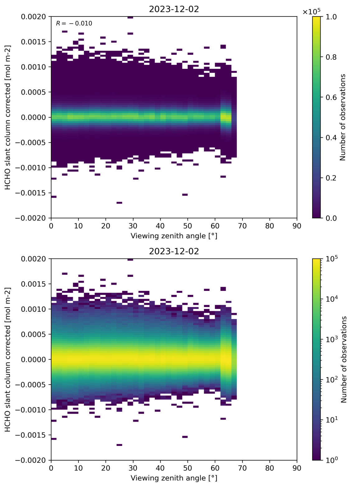
Figure 186: Scatter density plot of “Viewing zenith angle” against “HCHO slant column corrected” for 2023-12-01 to 2023-12-03.
