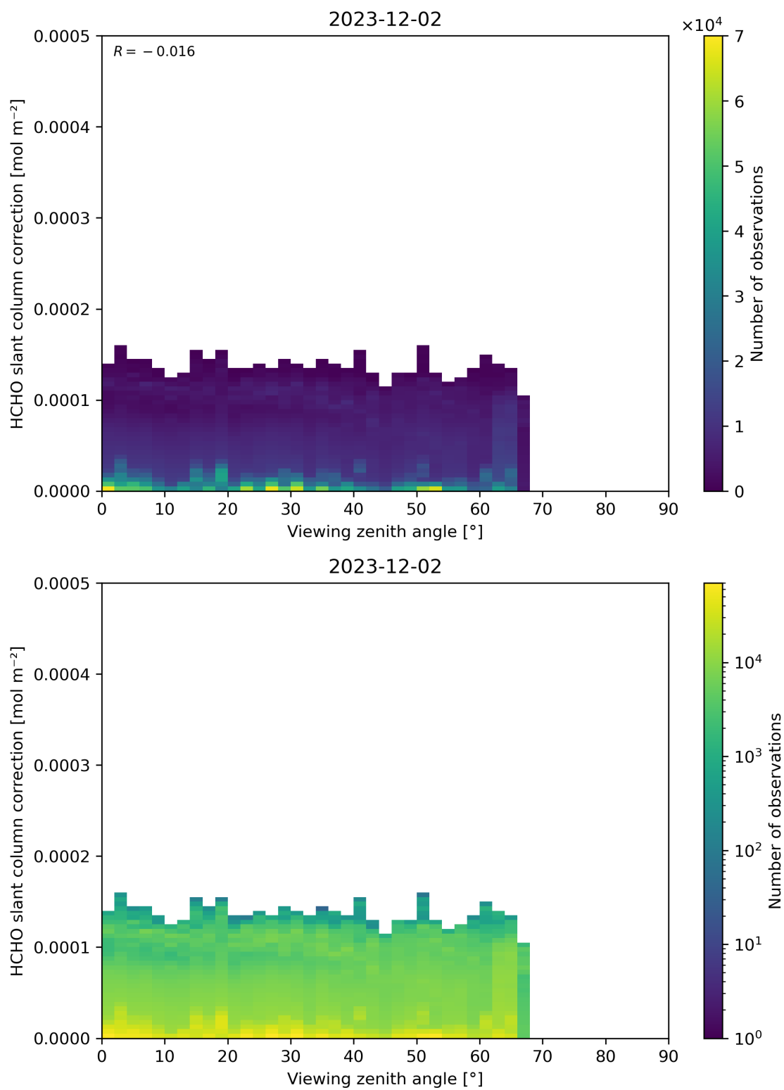
Figure 187: Scatter density plot of “Viewing zenith angle” against “HCHO slant column correction” for 2023-12-01 to 2023-12-03.
