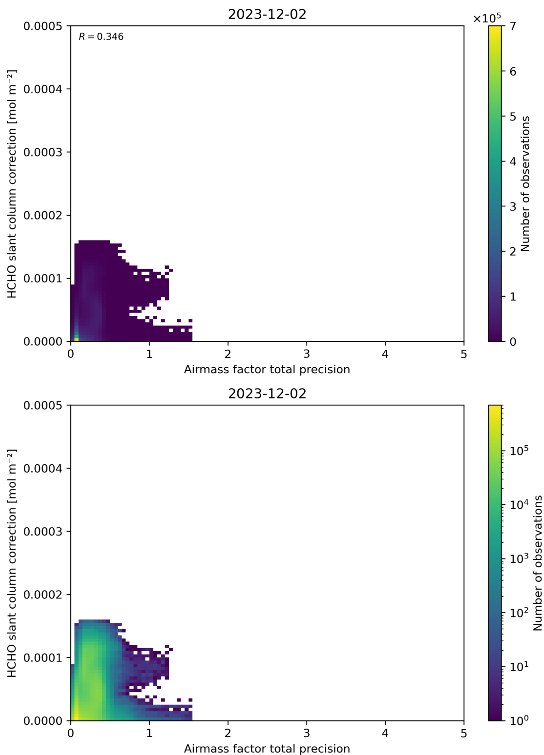
Figure 110: Scatter density plot of “Airmass factor total precision” against “HCHO slant column correction” for 2023-12-01 to 2023-12-03.
