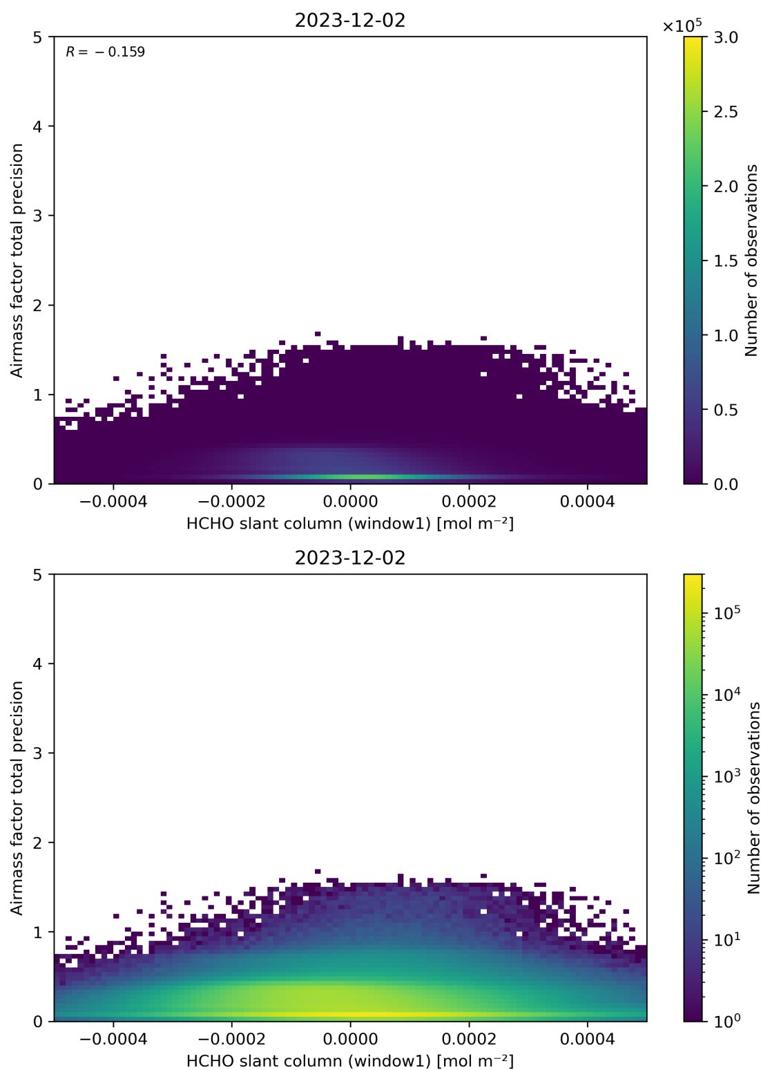
Figure 86: Scatter density plot of “HCHO slant column (window1)” against “Airmass factor total precision” for 2023-12-01 to 2023-12-03.
