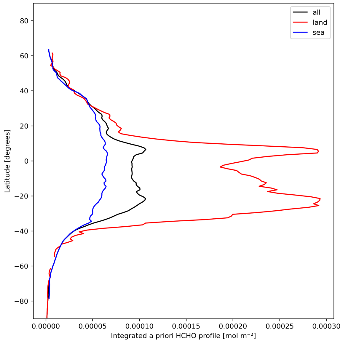
Figure 29: Zonal average of “Integrated a priori HCHO profile” for 2023-12-01 to 2023-12-03.
