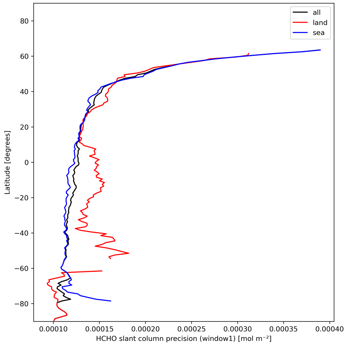
Figure 25: Zonal average of “HCHO slant column precision (window1)” for 2023-12-01 to 2023-12-03.
