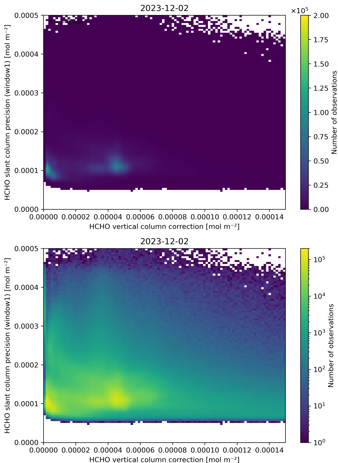
Figure 119: Scatter density plot of “HCHO vertical column correction” against “HCHO slant column precision (window1)” for 2023-12-01 to 2023-12-03.
