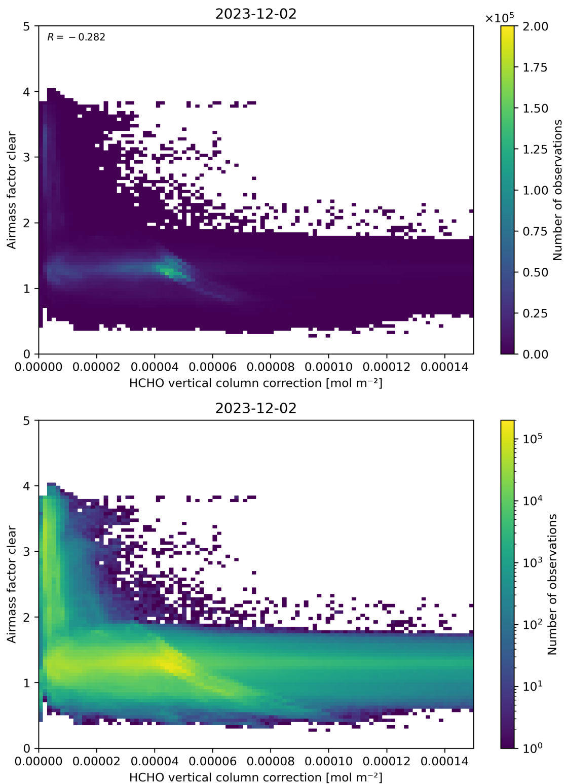
Figure 115: Scatter density plot of “HCHO vertical column correction” against “Airmass factor clear” for 2023-12-01 to 2023-12-03.
