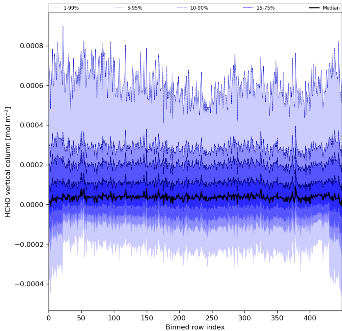
Figure 49: Along track statistics of "HCHO vertical column" for 2023-12-01 to 2023-12-03
