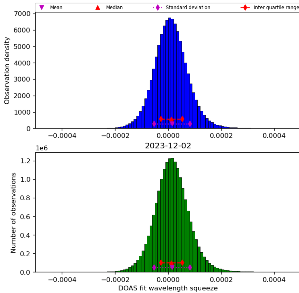
Figure 45: Histogram of “DOAS fit wavelength squeeze” for 2023-12-01 to 2023-12-03
