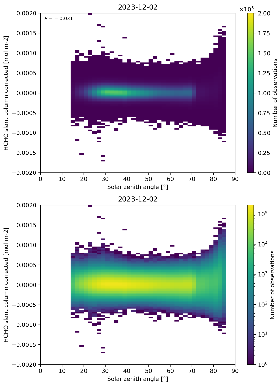
Figure 171: Scatter density plot of “Solar zenith angle” against “HCHO slant column corrected” for 2023-12-01 to 2023-12-03.
