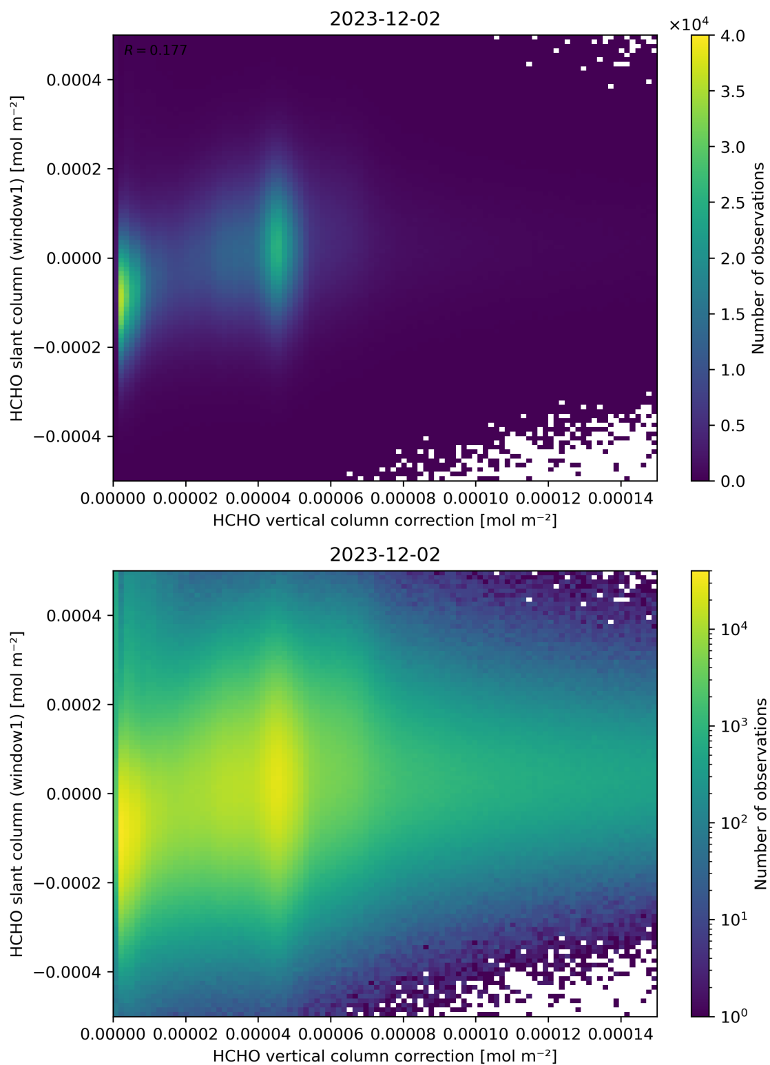
Figure 118: Scatter density plot of “HCHO vertical column correction” against “HCHO slant column (window1)” for 2023-12-01 to 2023-12-03.
