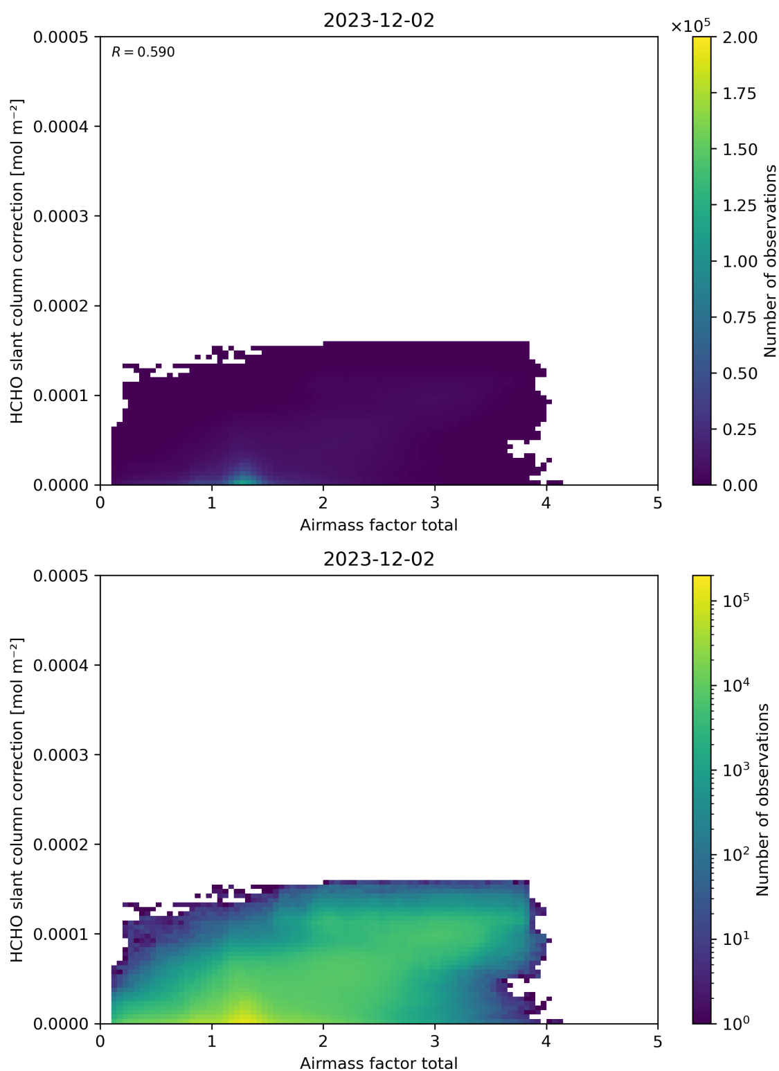
Figure 102: Scatter density plot of “Airmass factor total” against “HCHO slant column correction” for 2023-12-01 to 2023-12-03.
