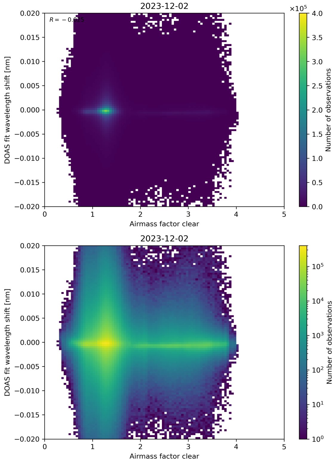
Figure 72: Scatter density plot of “Airmass factor clear” against “DOAS fit wavelength shift” for 2023-12-01 to 2023-12-03.
