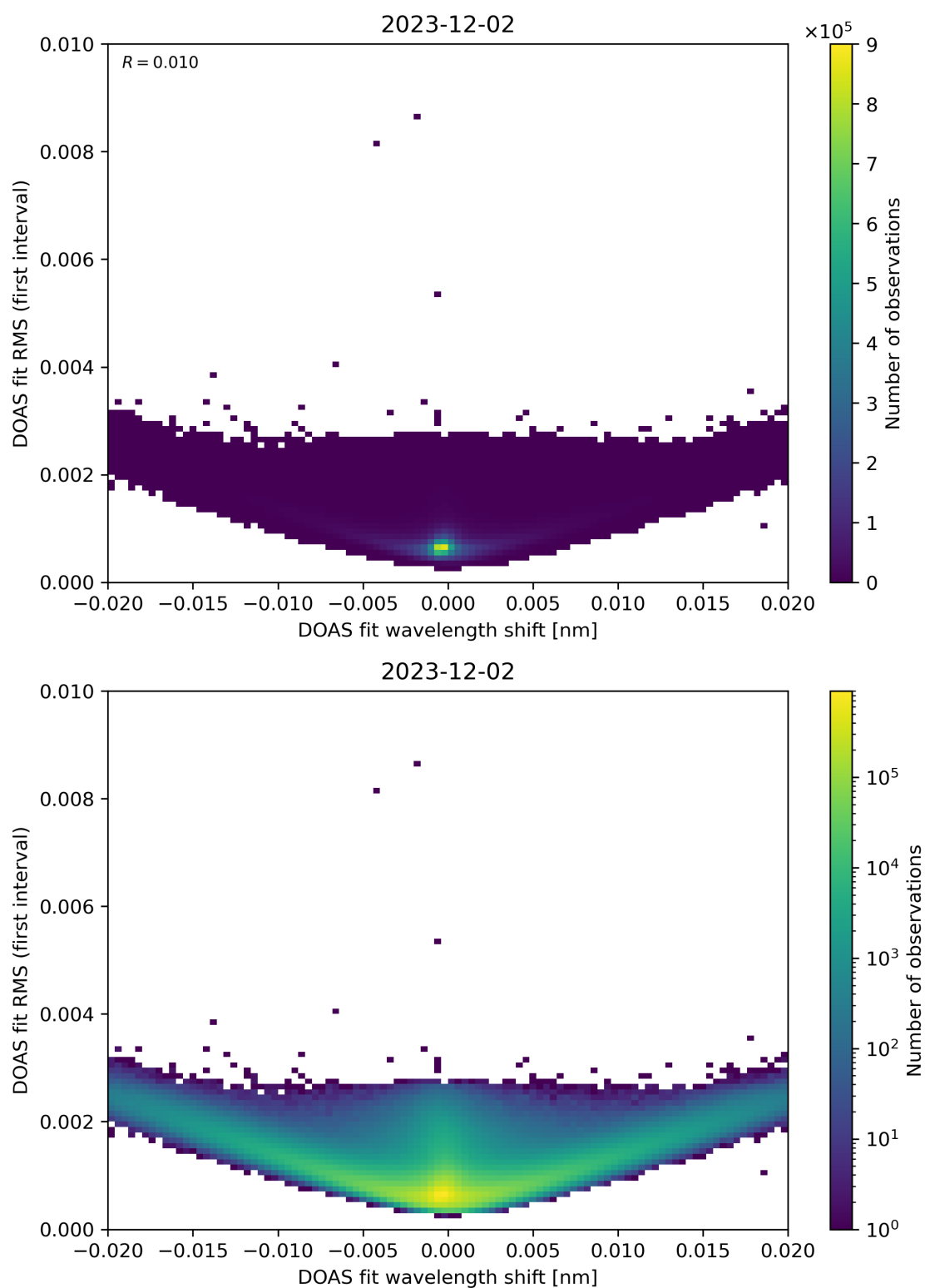
Figure 64: Scatter density plot of “DOAS fit wavelength shift” against “DOAS fit RMS (first interval)” for 2023-12-01 to 2023-12-03.
