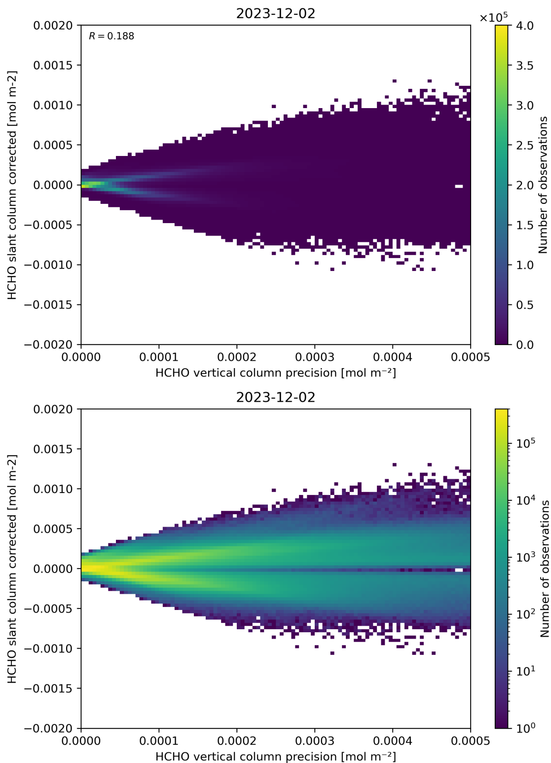
Figure 140: Scatter density plot of “HCHO vertical column precision” against “HCHO slant column corrected” for 2023-12-01 to 2023-12-03.
