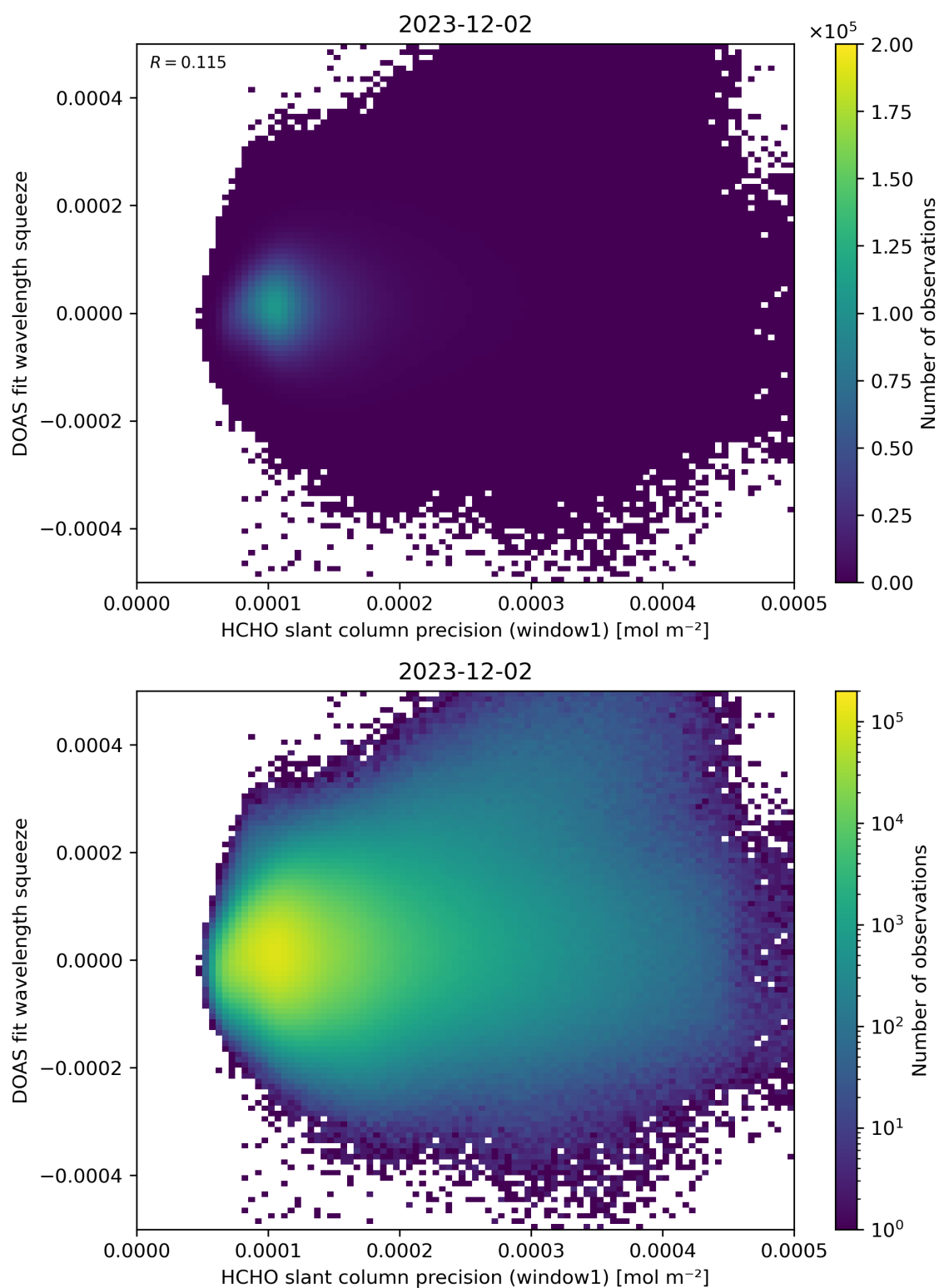
Figure 90: Scatter density plot of “HCHO slant column precision (window1)” against “DOAS fit wavelength squeeze” for 2023-12-01 to 2023-12-03.
