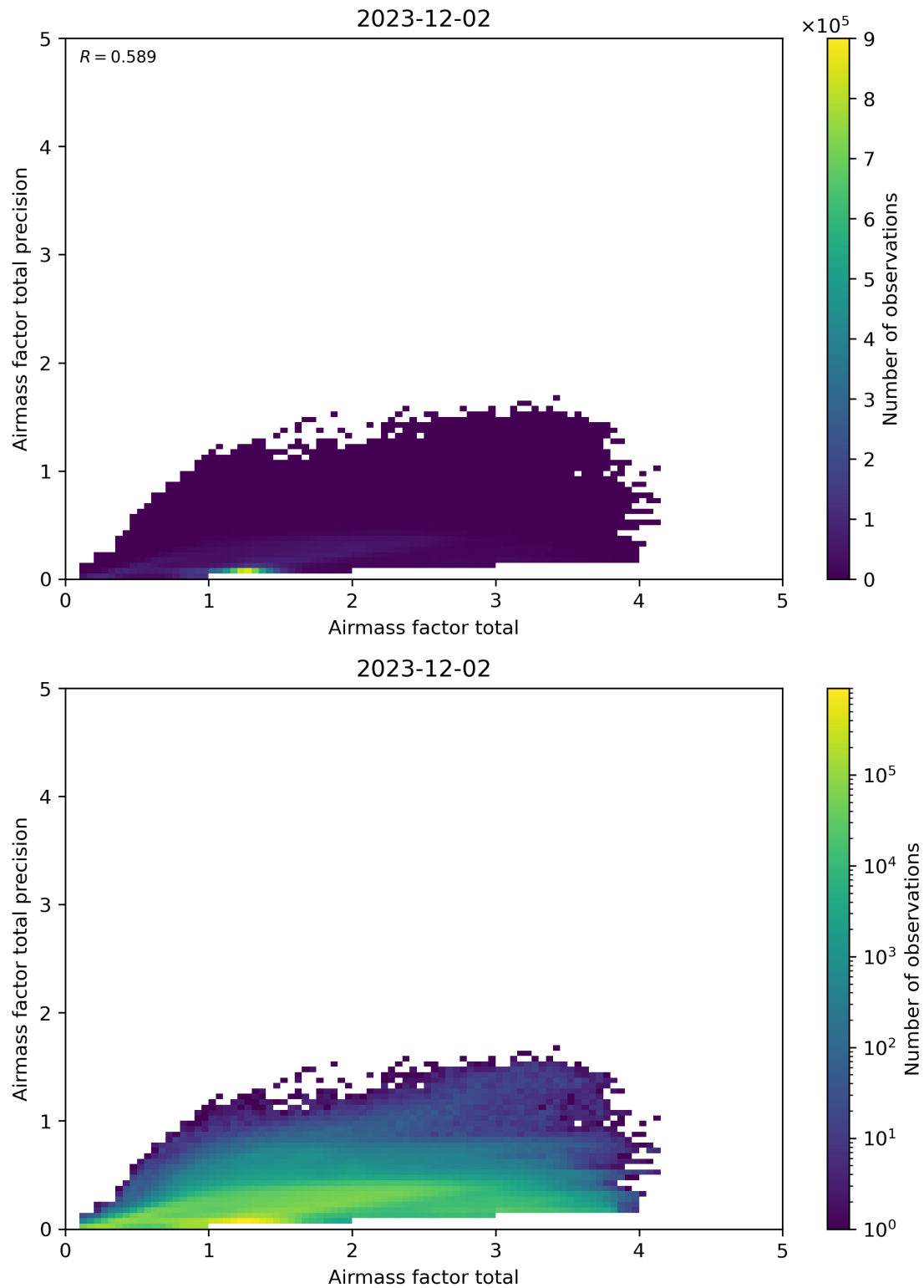
Figure 103: Scatter density plot of “Airmass factor total” against “Airmass factor total precision” for 2023-12-01 to 2023-12-03.
