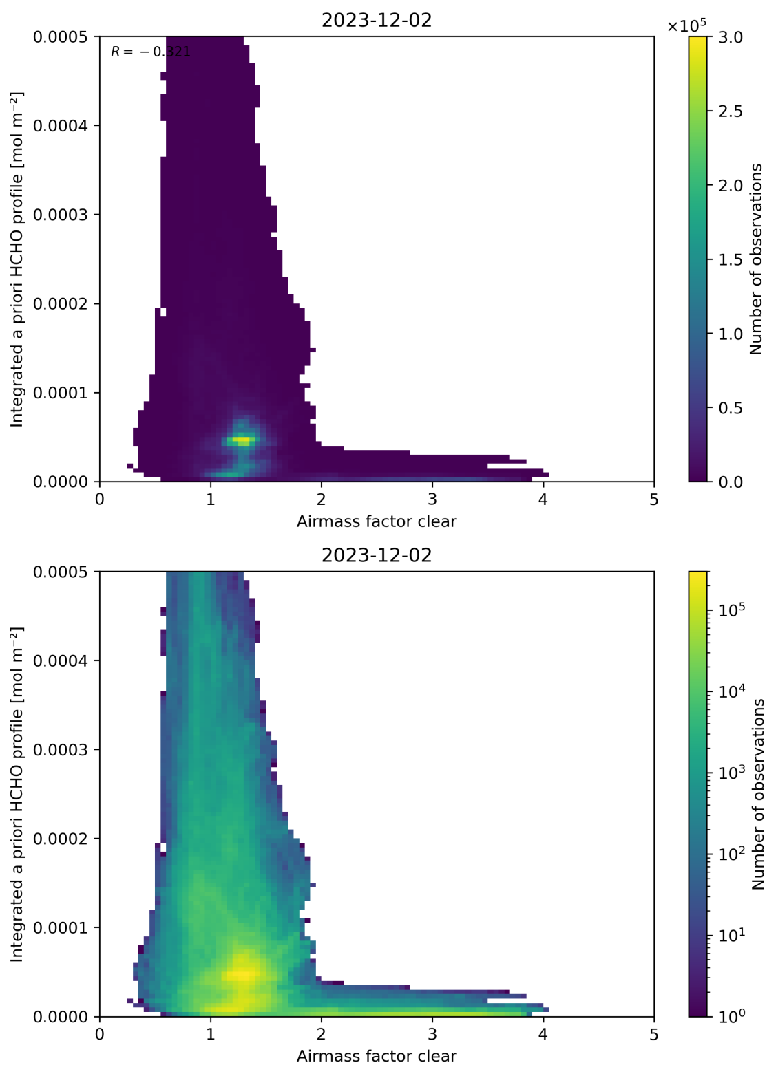
Figure 76: Scatter density plot of “Airmass factor clear” against “Integrated a priori HCHO profile” for 2023-12-01 to 2023-12-03.
