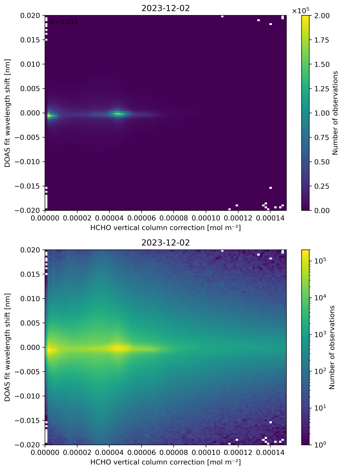
Figure 113: Scatter density plot of “HCHO vertical column correction” against “DOAS fit wavelength shift” for 2023-12-01 to 2023-12-03.
