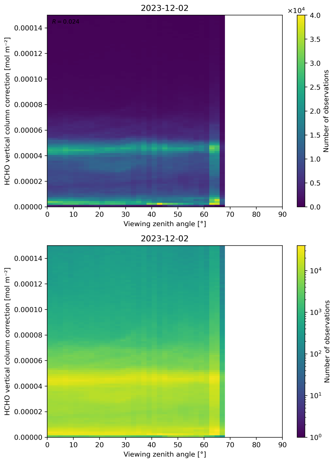
Figure 193: Scatter density plot of “Viewing zenith angle” against “HCHO vertical column correction” for 2023-12-01 to 2023-12-03.
