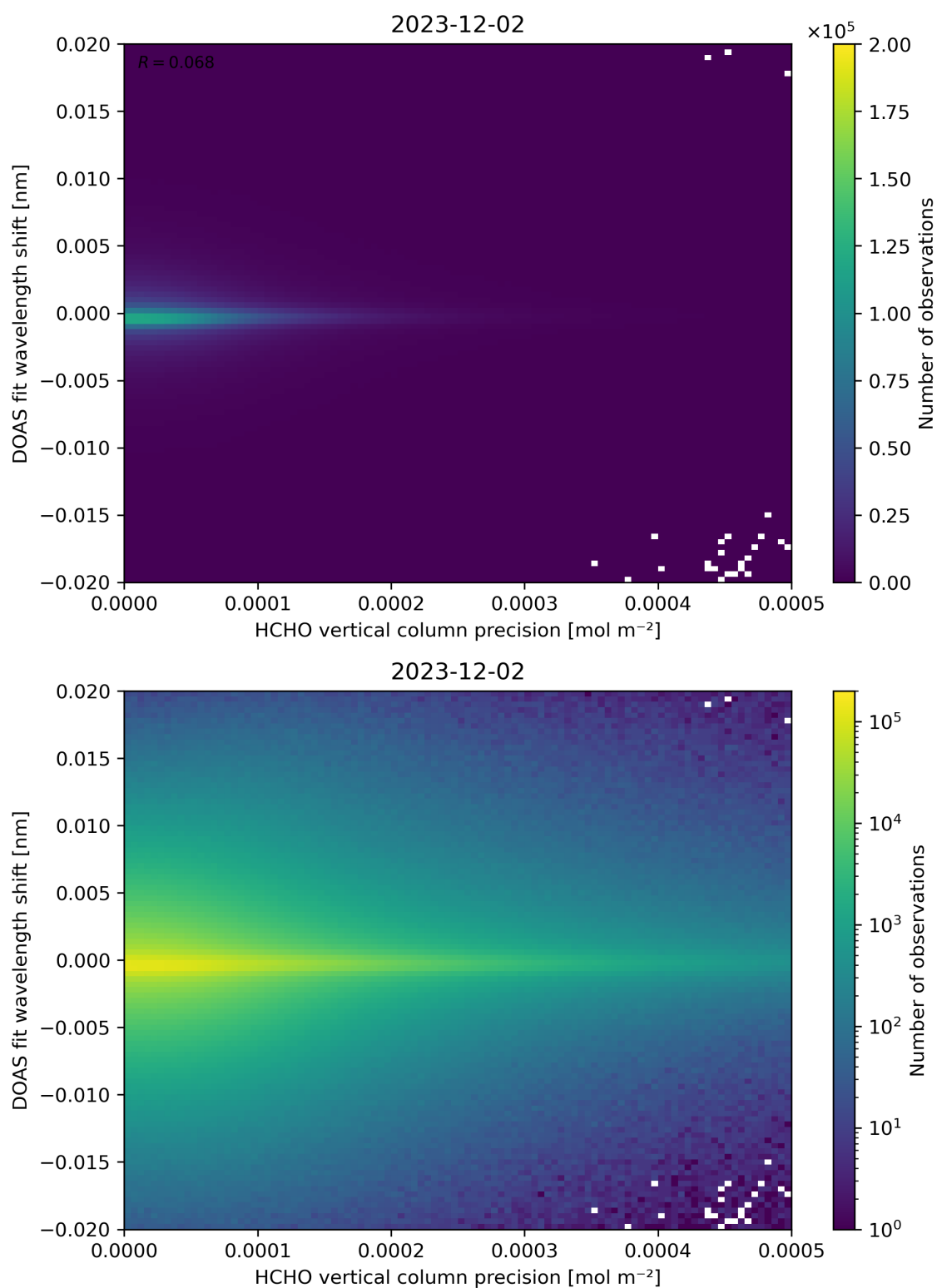
Figure 137: Scatter density plot of “HCHO vertical column precision” against “DOAS fit wavelength shift” for 2023-12-01 to 2023-12-03.
