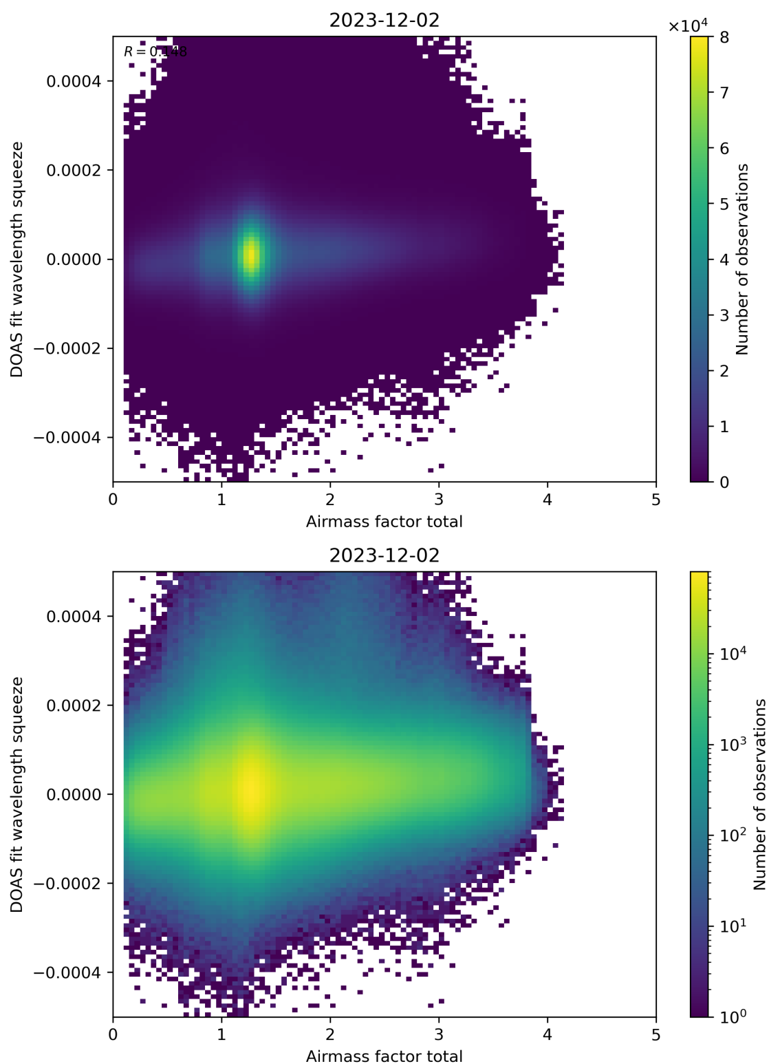
Figure 99: Scatter density plot of “Airmass factor total” against “DOAS fit wavelength squeeze” for 2023-12-01 to 2023-12-03.
