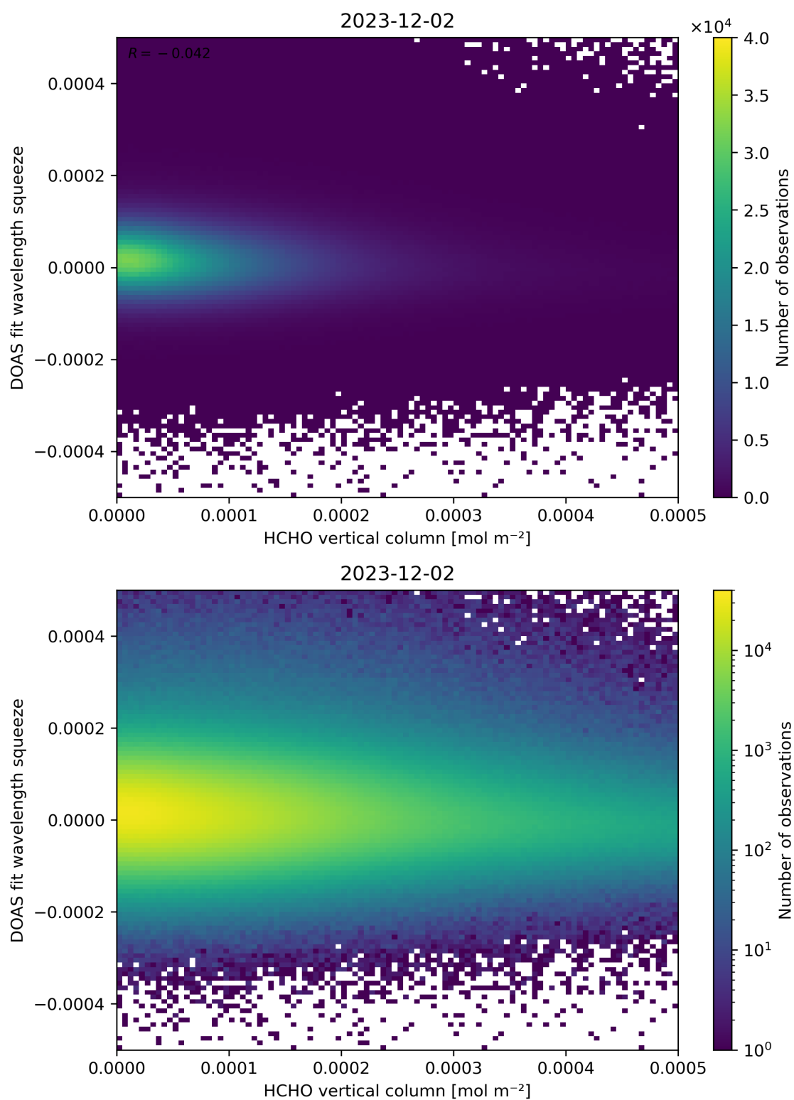
Figure 125: Scatter density plot of “HCHO vertical column” against “DOAS fit wavelength squeeze” for 2023-12-01 to 2023-12-03.
