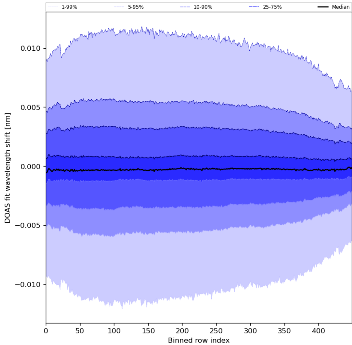
Figure 58: Along track statistics of “DOAS fit wavelength shift” for 2023-12-01 to 2023-12-03
