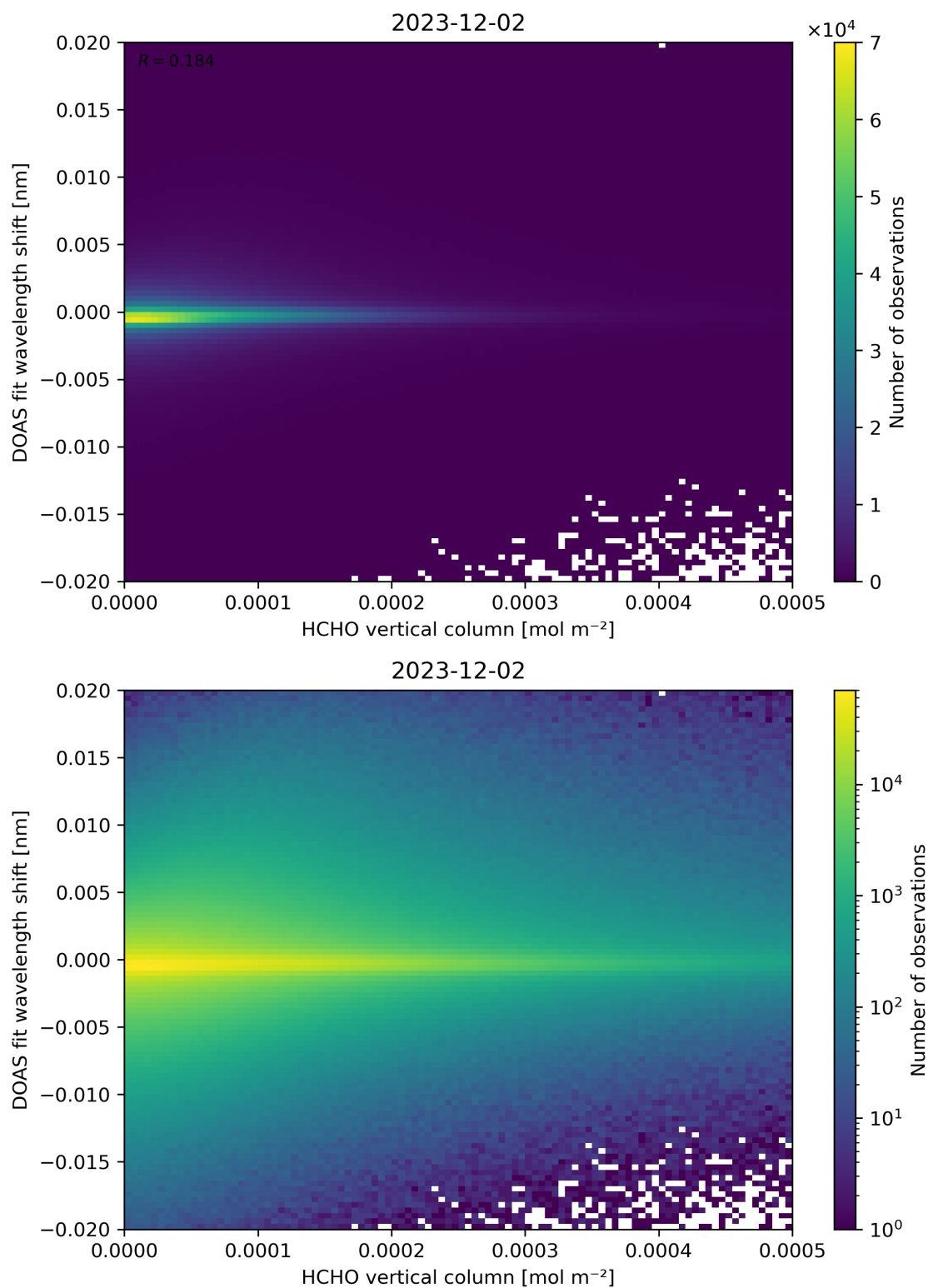
Figure 124: Scatter density plot of “HCHO vertical column” against “DOAS fit wavelength shift” for 2023-12-01 to 2023-12-03.
