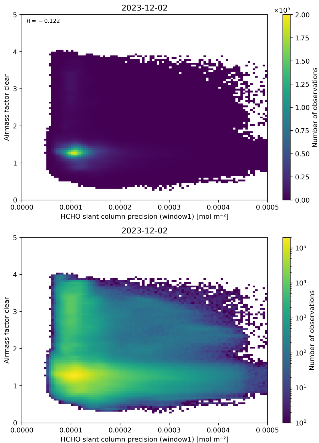
Figure 91: Scatter density plot of “HCHO slant column precision (window1)” against “Airmass factor clear” for 2023-12-01 to 2023-12-03.
