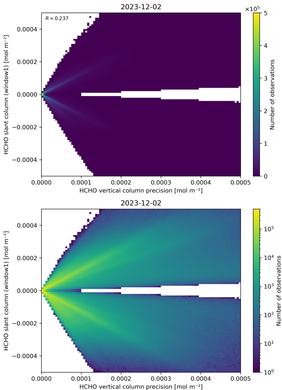
Figure 142: Scatter density plot of “HCHO vertical column precision” against “HCHO slant column (window1)” for 2023-12-01 to 2023-12-03.
