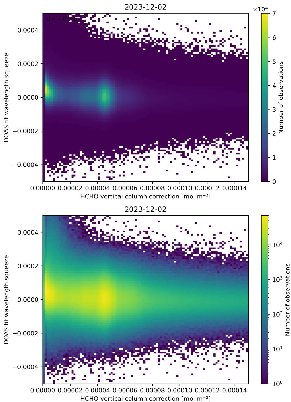
Figure 114: Scatter density plot of “HCHO vertical column correction” against “DOAS fit wavelength squeeze” for 2023-12-01 to 2023-12-03.
