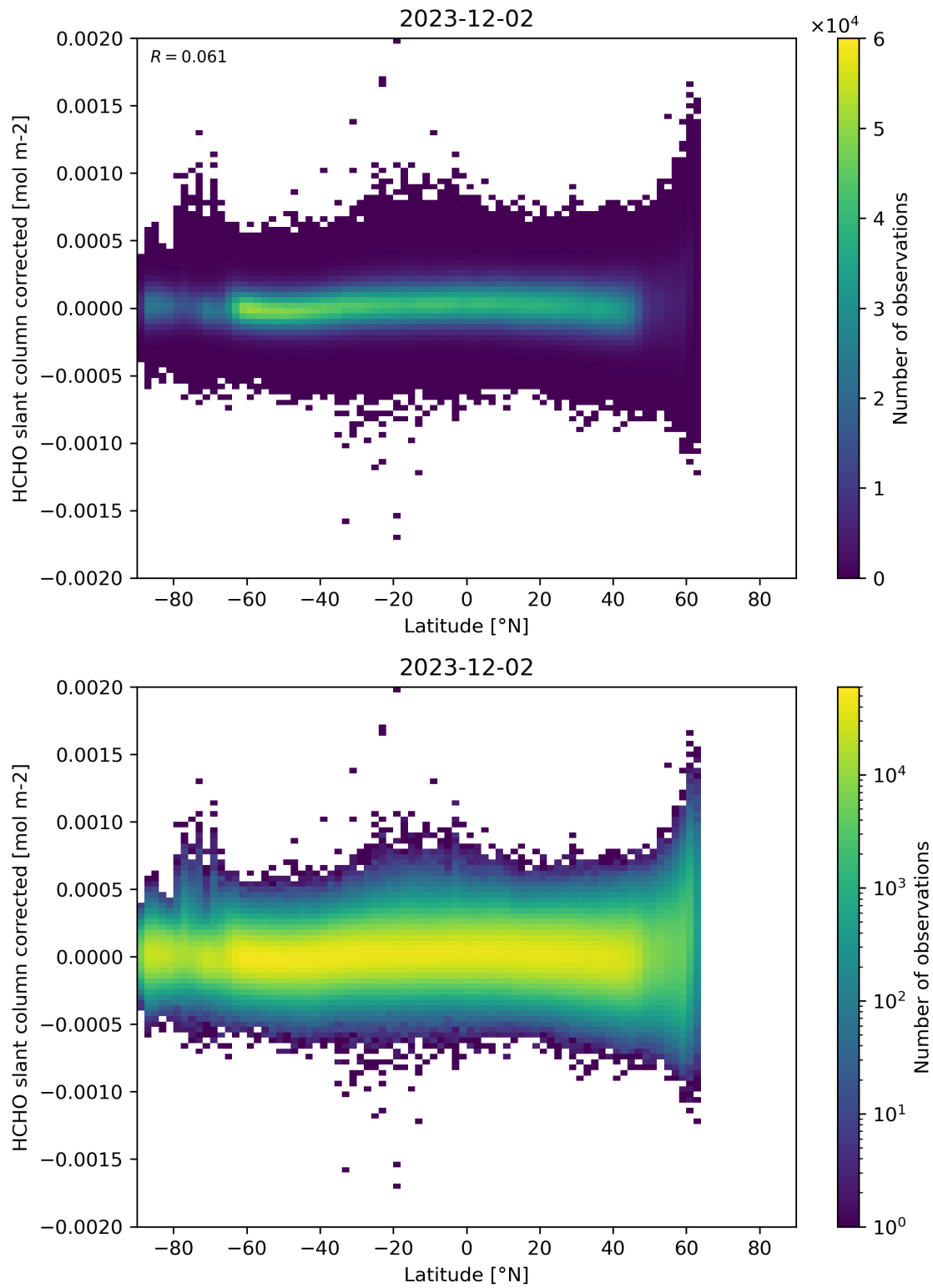
Figure 157: Scatter density plot of “Latitude” against “HCHO slant column corrected” for 2023-12-01 to 2023-12-03.
