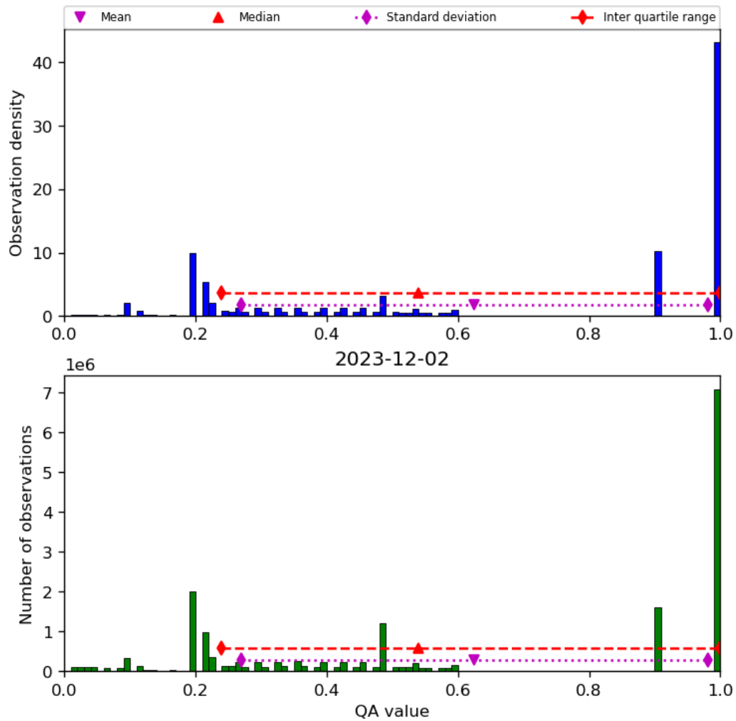
Figure 34: Histogram of “QA value” for 2023-12-01 to 2023-12-03
