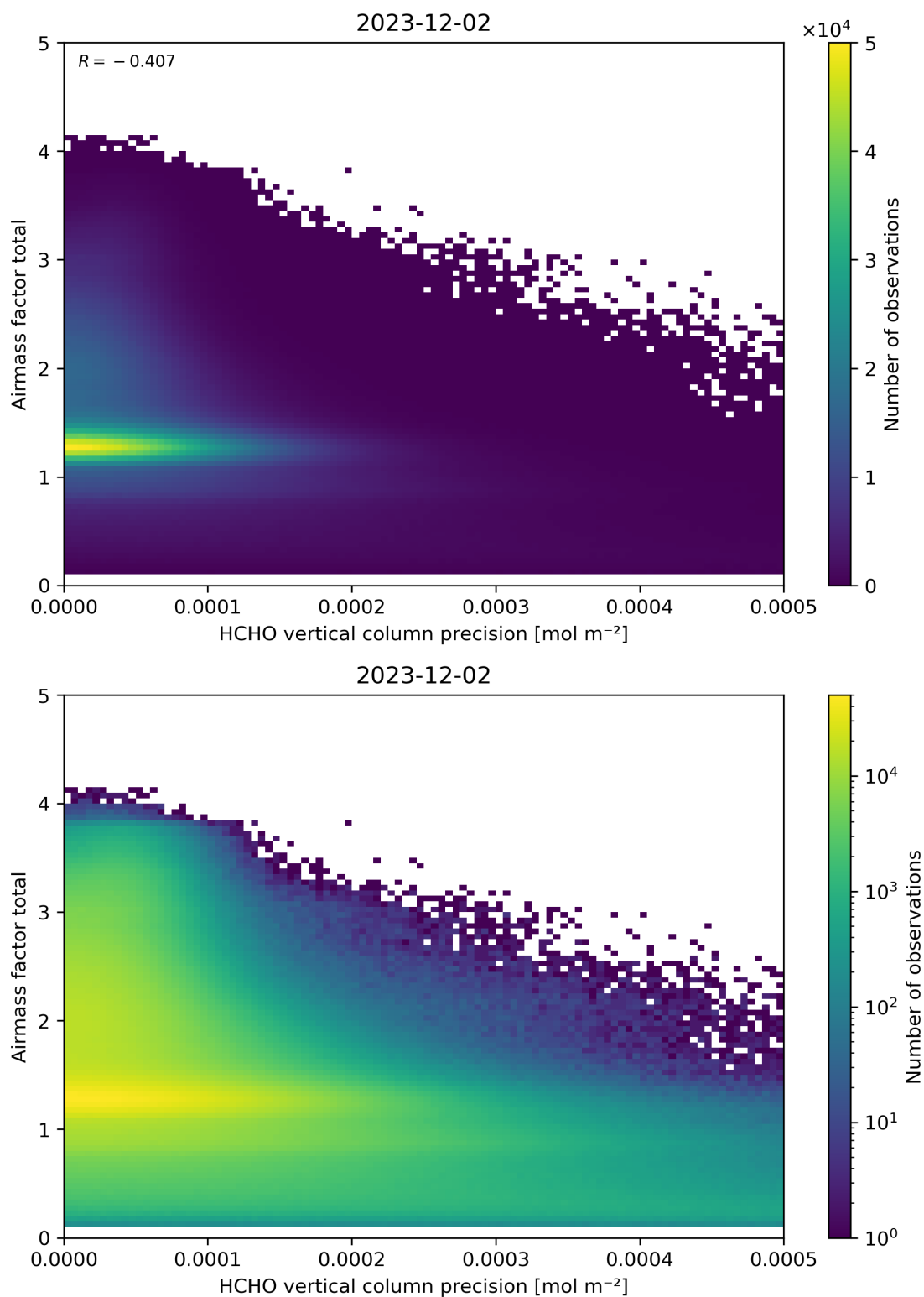
Figure 144: Scatter density plot of “HCHO vertical column precision” against “Airmass factor total” for 2023-12-01 to 2023-12-03.
