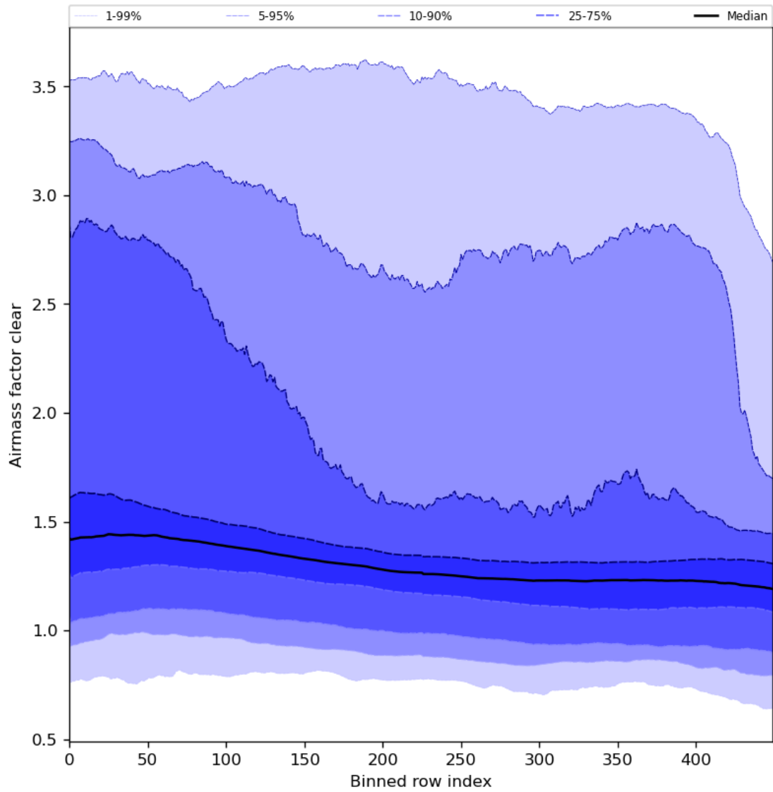
Figure 56: Along track statistics of “Airmass factor clear” for 2023-12-01 to 2023-12-03
