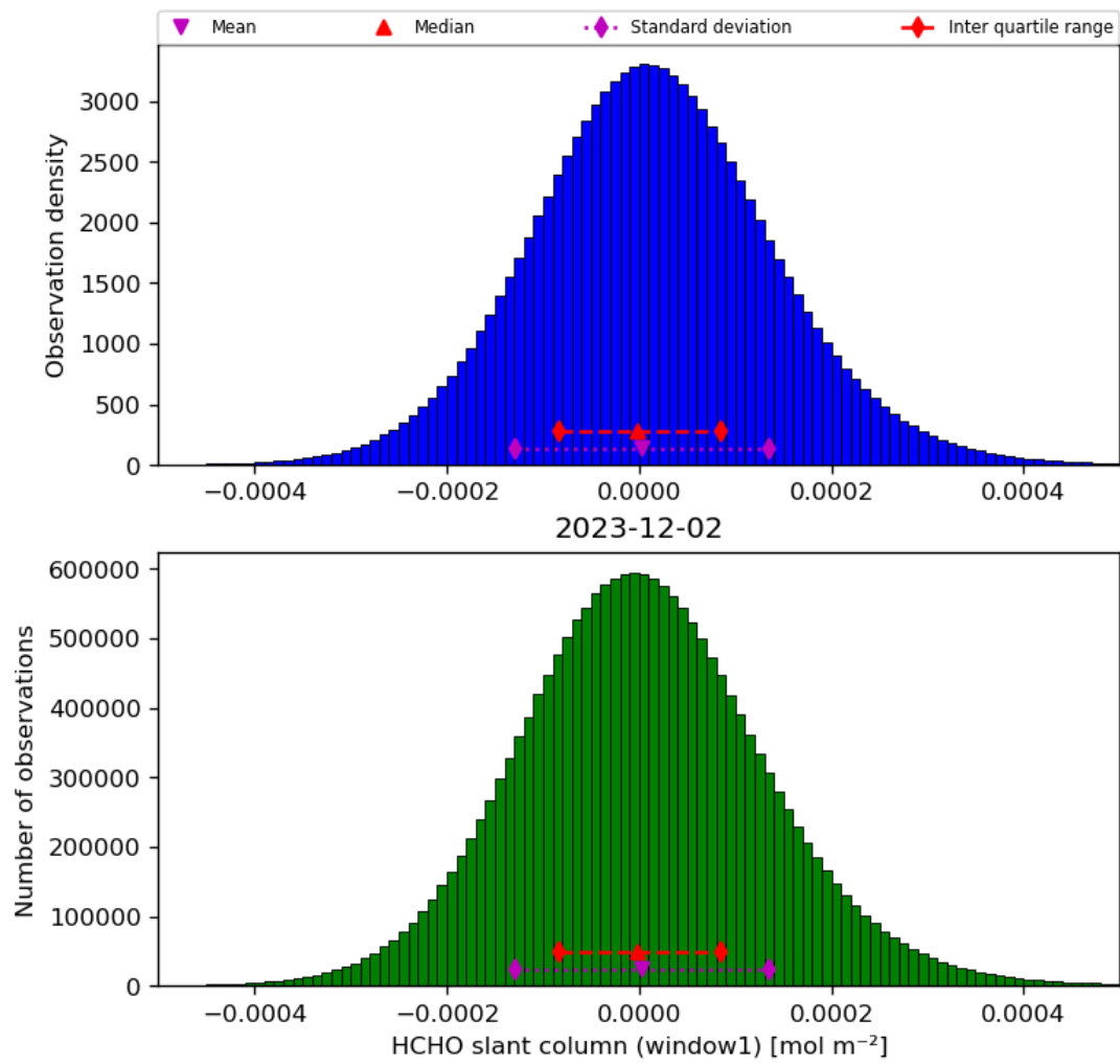
Figure 38: Histogram of “HCHO slant column (window1)” for 2023-12-01 to 2023-12-03
