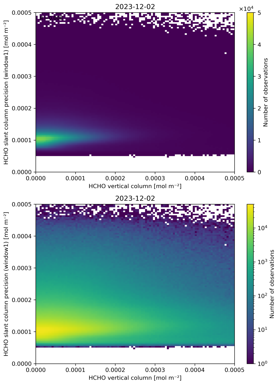
Figure 130: Scatter density plot of “HCHO vertical column” against “HCHO slant column precision (window1)” for 2023-12-01 to 2023-12-03.
