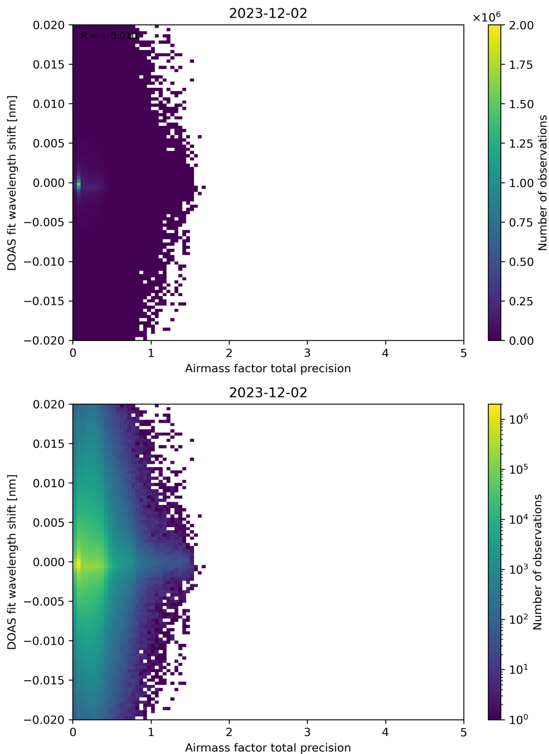
Figure 106: Scatter density plot of “Airmass factor total precision” against “DOAS fit wavelength shift” for 2023-12-01 to 2023-12-03.
