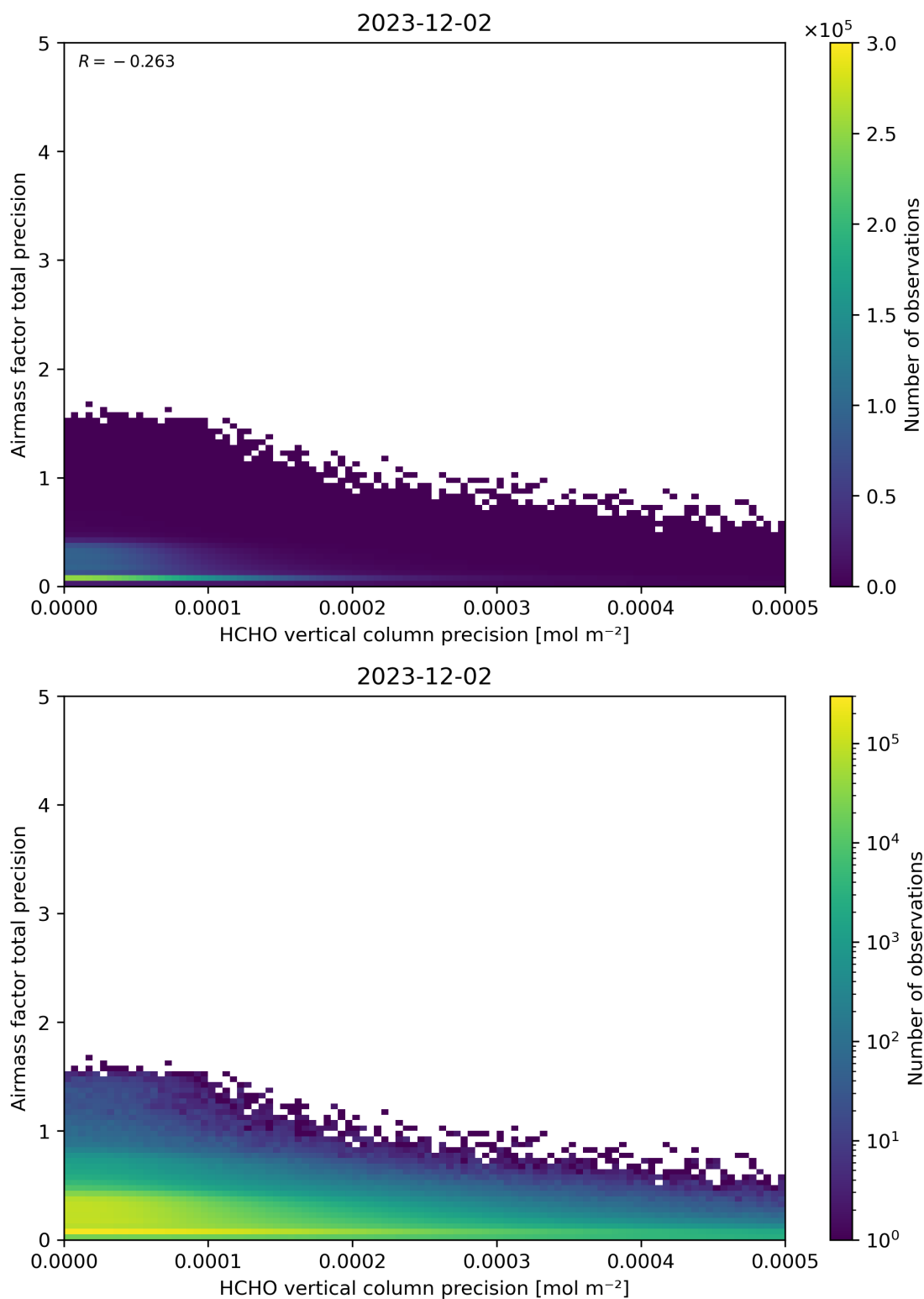
Figure 145: Scatter density plot of “HCHO vertical column precision” against “Airmass factor total precision” for 2023-12-01 to 2023-12-03.
