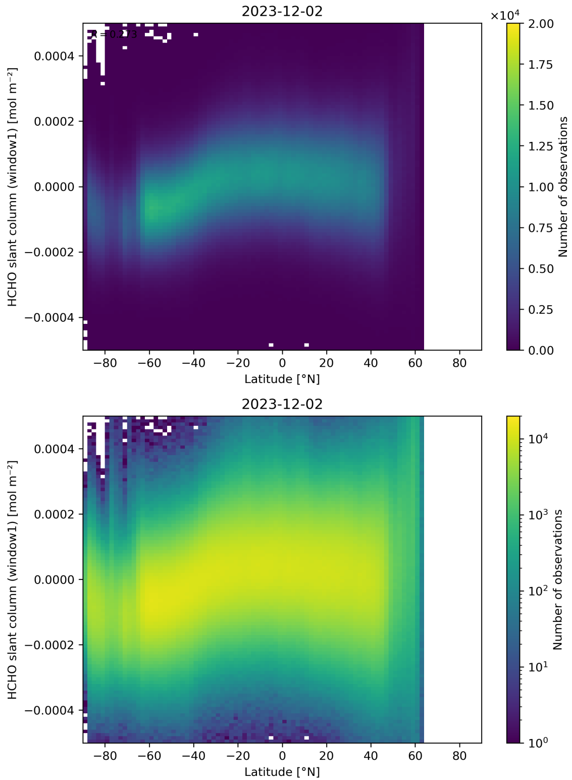
Figure 159: Scatter density plot of “Latitude” against “HCHO slant column (window1)” for 2023-12-01 to 2023-12-03.
