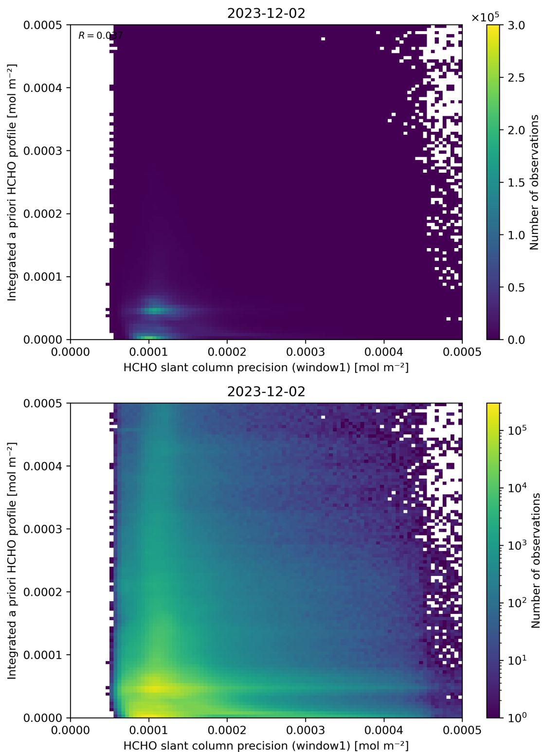
Figure 96: Scatter density plot of “HCHO slant column precision (window1)” against “Integrated a priori HCHO profile” for 2023-12-01 to 2023-12-03.
