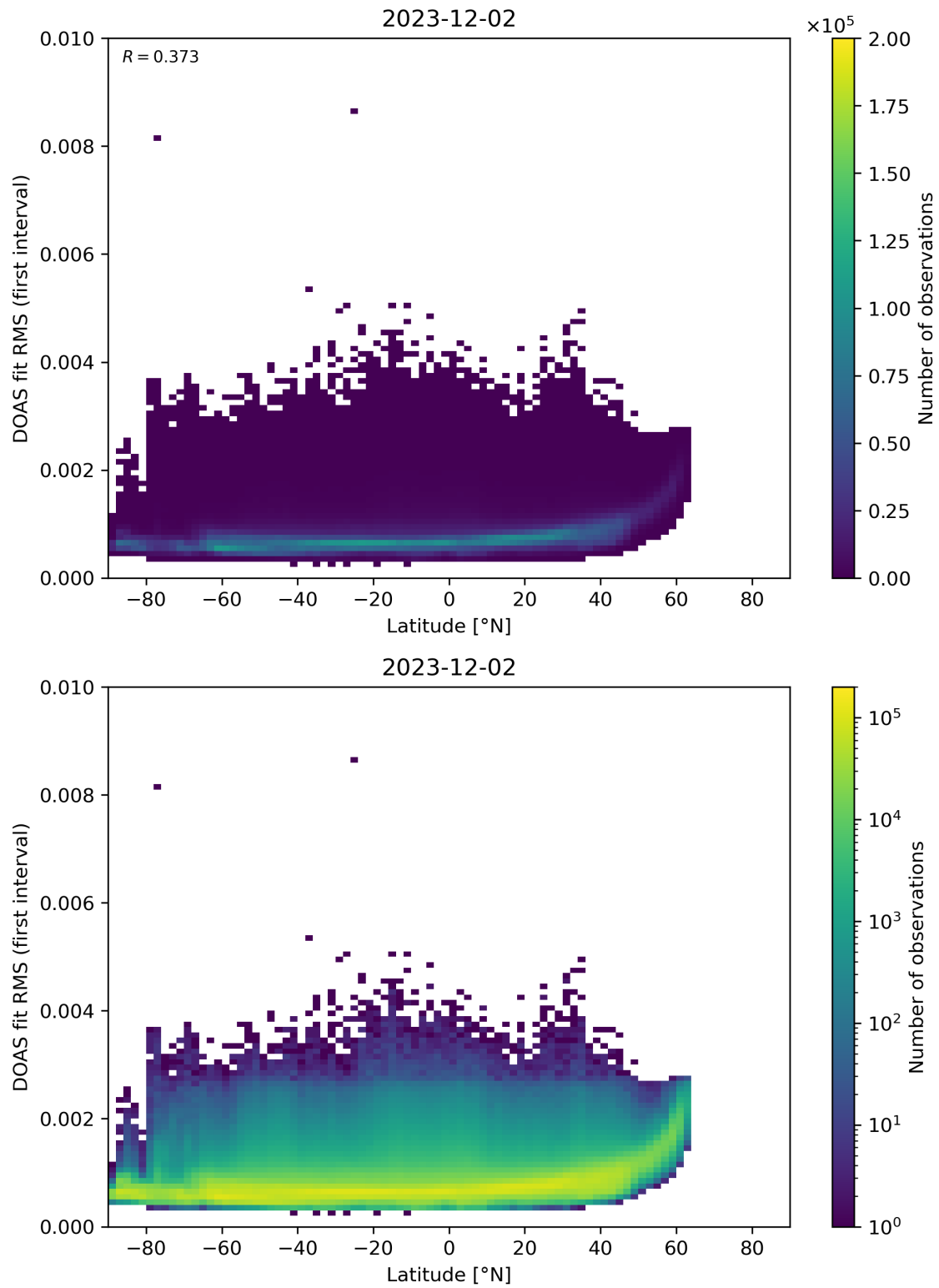
Figure 153: Scatter density plot of “Latitude” against “DOAS fit RMS (first interval)” for 2023-12-01 to 2023-12-03.
