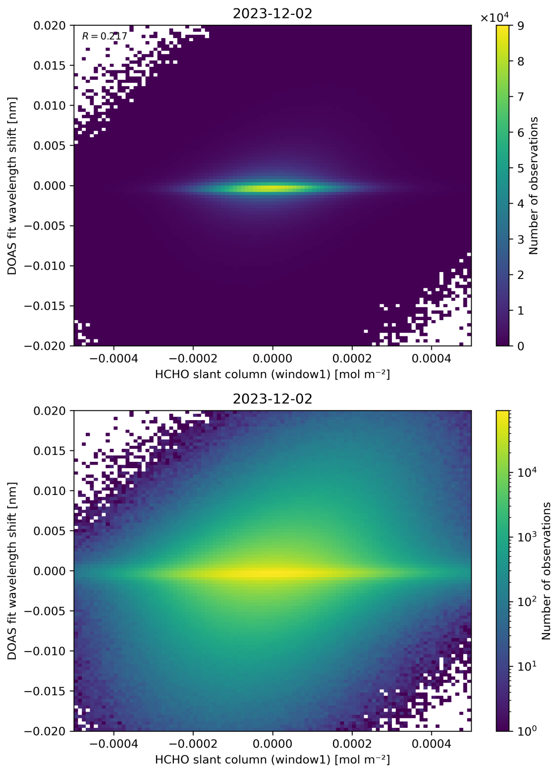
Figure 79: Scatter density plot of “HCHO slant column (window1)” against “DOAS fit wavelength shift” for 2023-12-01 to 2023-12-03.
