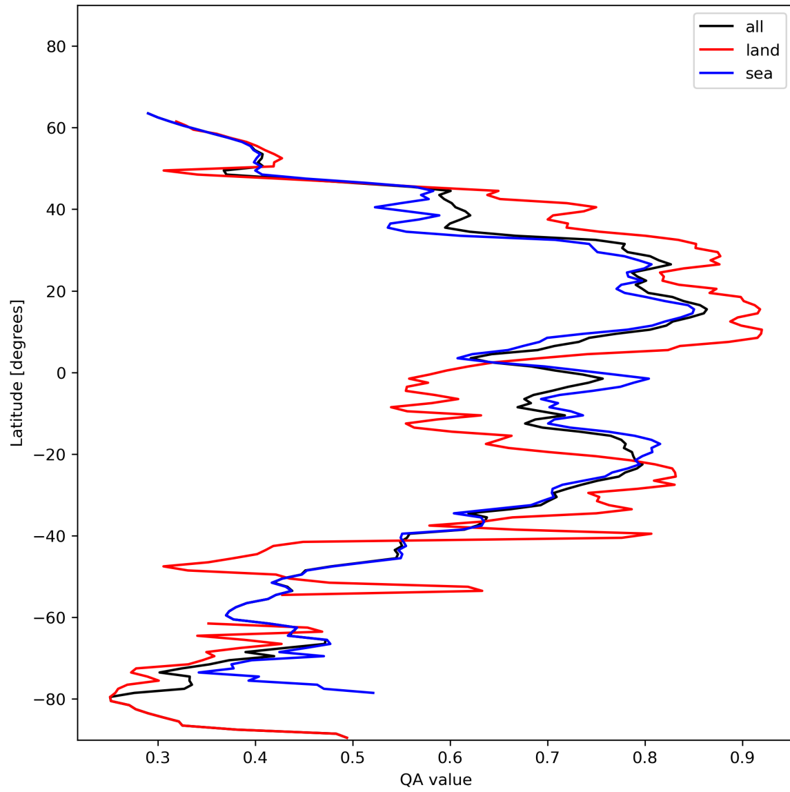
Figure 20: Zonal average of “QA value” for 2023-12-01 to 2023-12-03.
