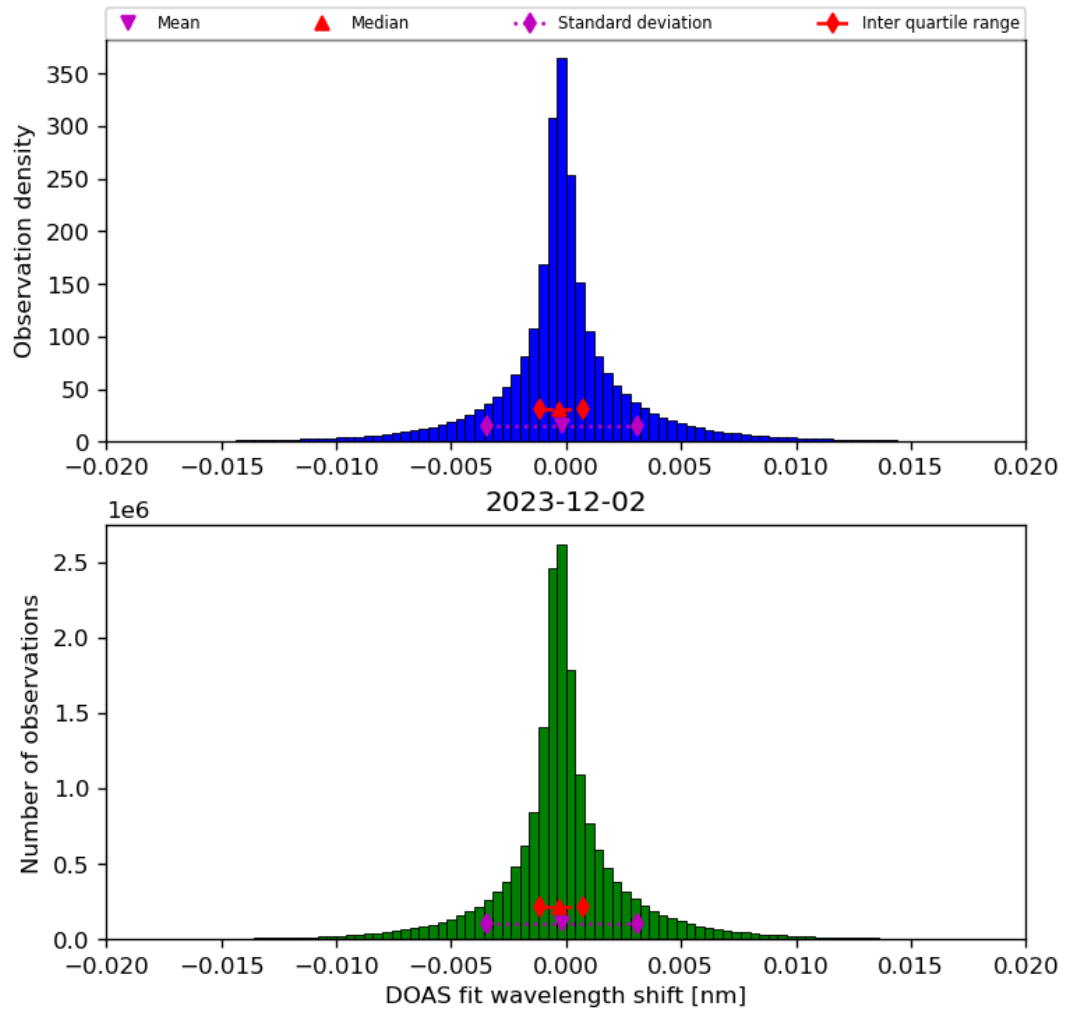
Figure 44: Histogram of “DOAS fit wavelength shift” for 2023-12-01 to 2023-12-03
