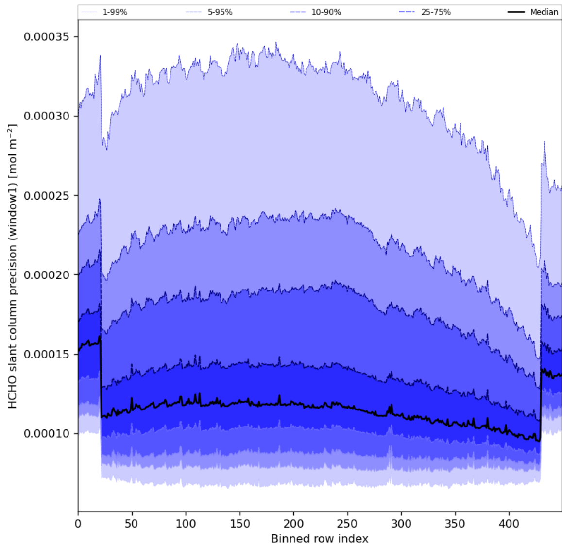
Figure 53: Along track statistics of “HCHO slant column precision (window1)” for 2023-12-01 to 2023-12-03
