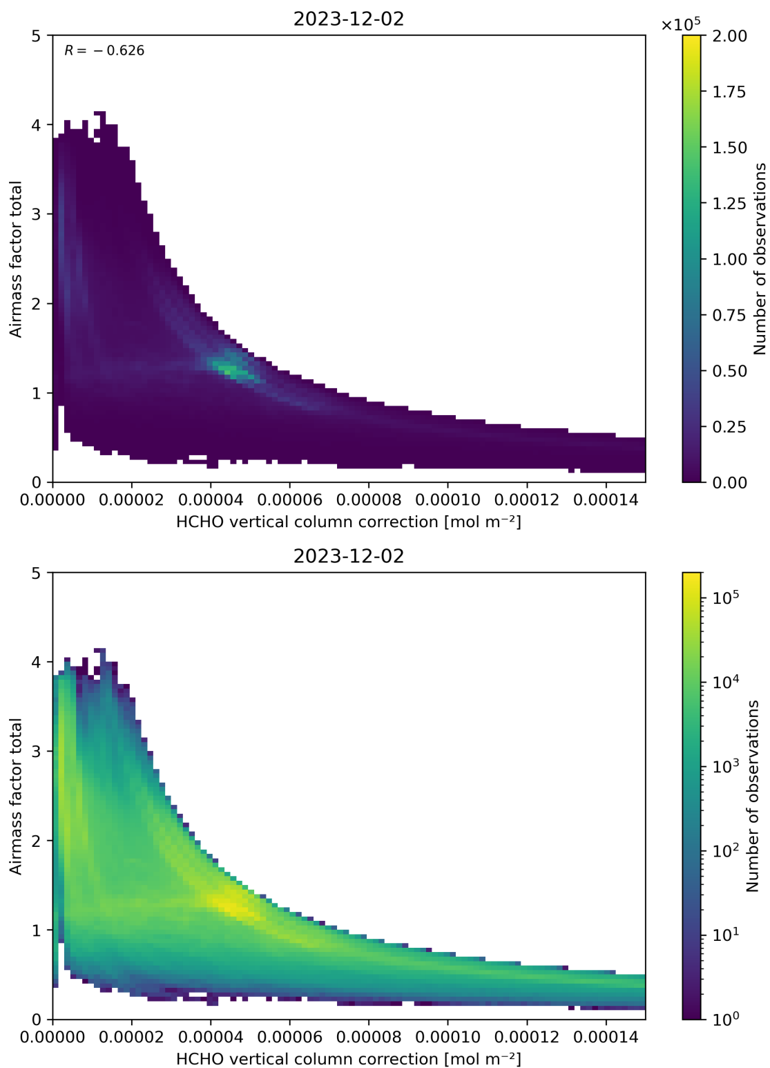
Figure 120: Scatter density plot of “HCHO vertical column correction” against “Airmass factor total” for 2023-12-01 to 2023-12-03.
