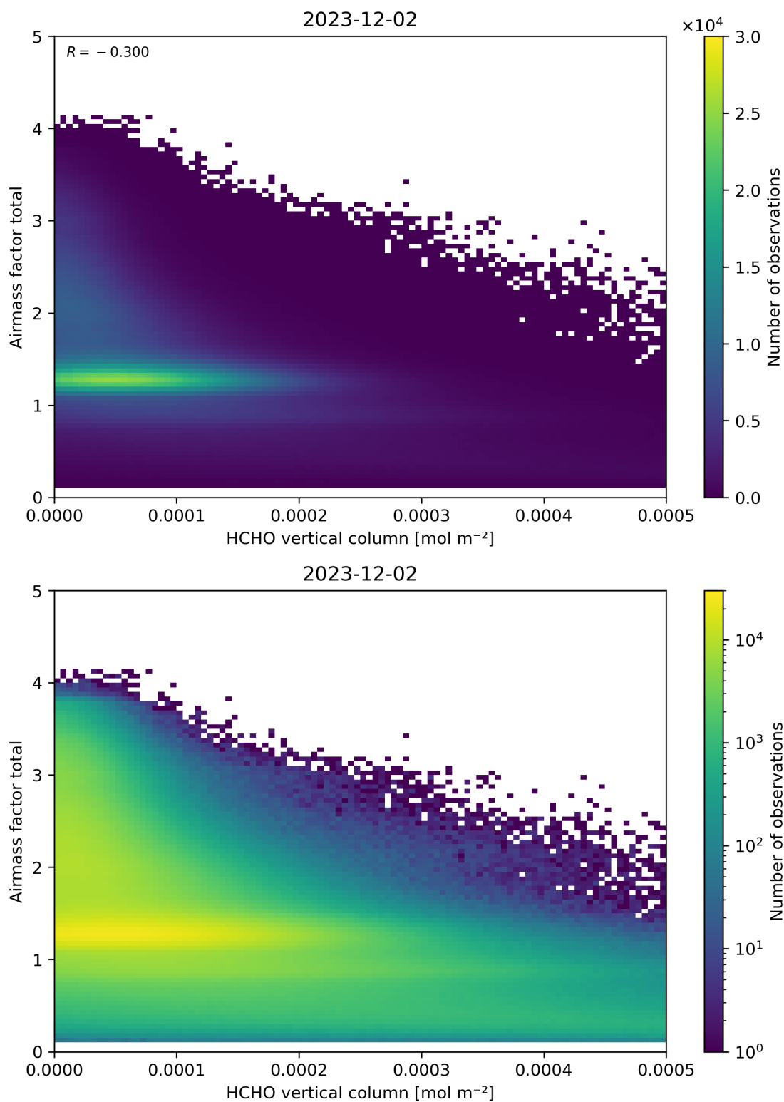
Figure 131: Scatter density plot of “HCHO vertical column” against “Airmass factor total” for 2023-12-01 to 2023-12-03.
