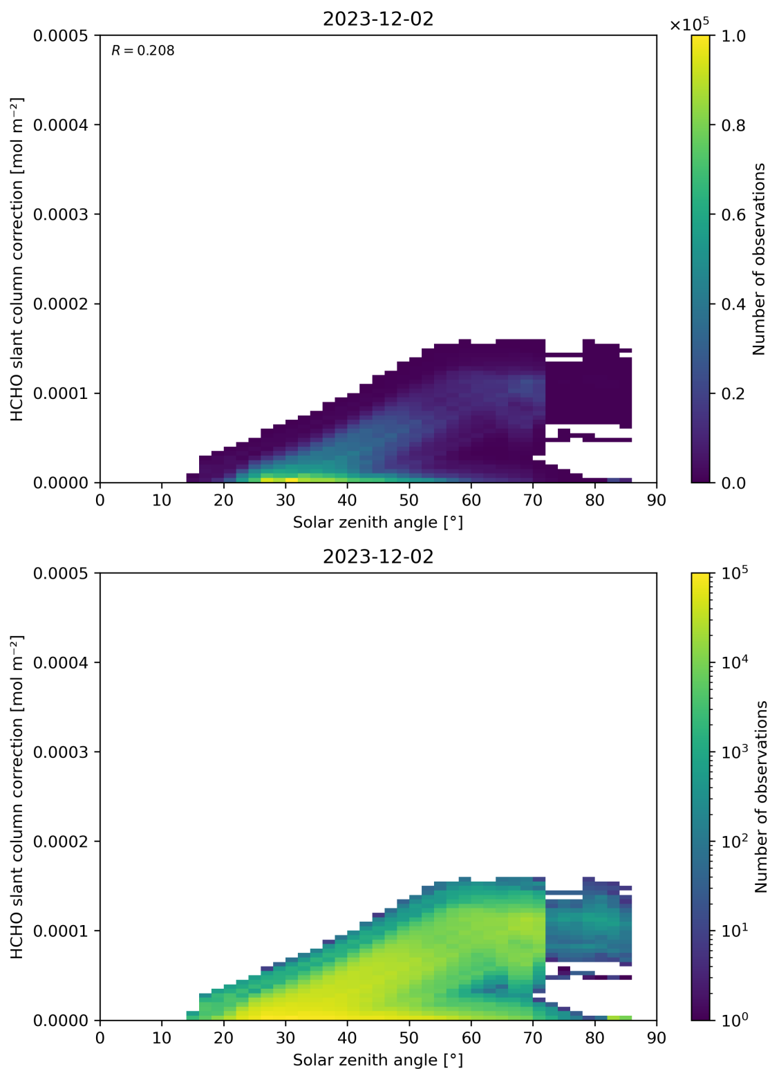
Figure 172: Scatter density plot of “Solar zenith angle” against “HCHO slant column correction” for 2023-12-01 to 2023-12-03.
