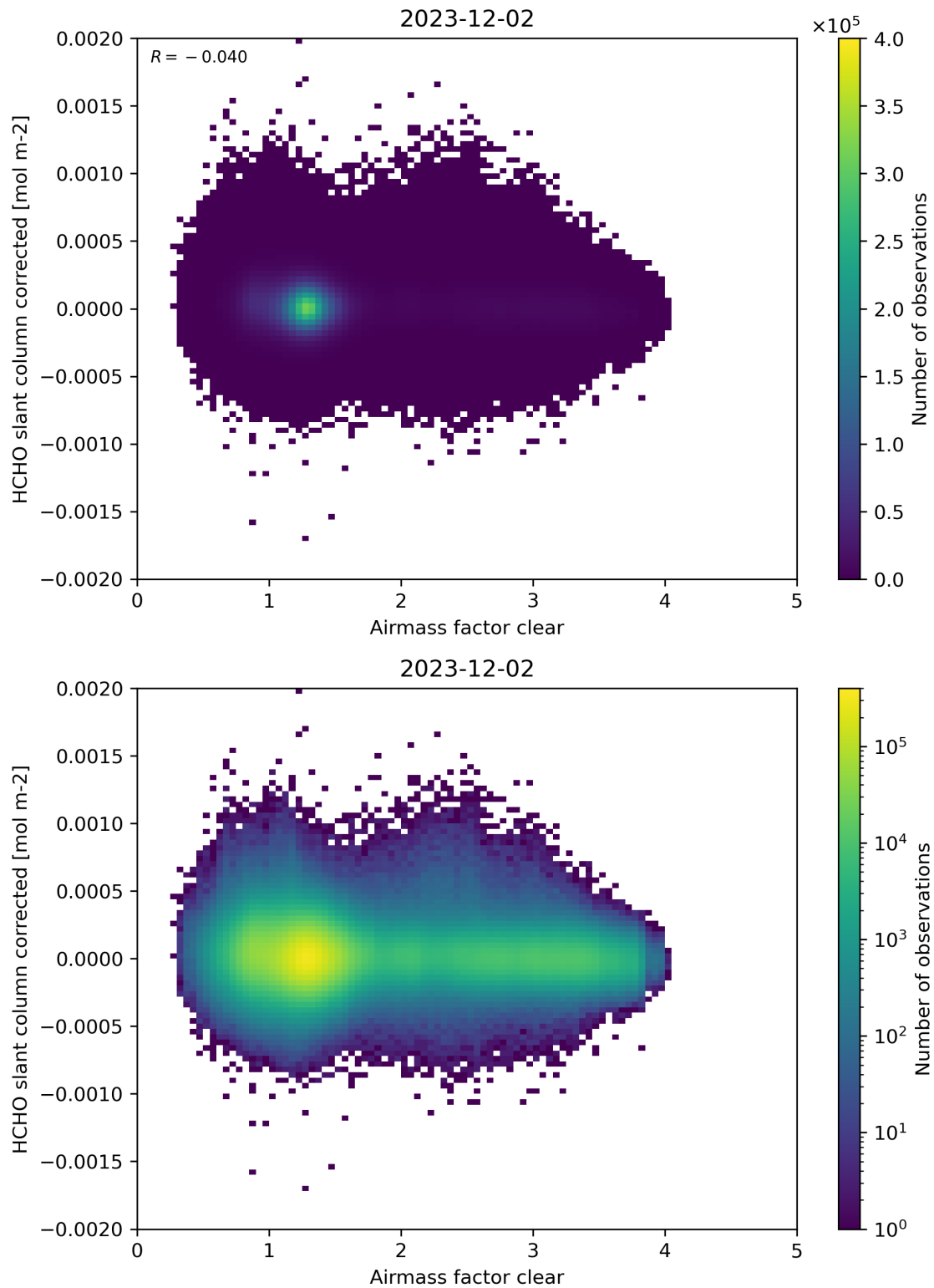
Figure 74: Scatter density plot of “Airmass factor clear” against “HCHO slant column corrected” for 2023-12-01 to 2023-12-03.
