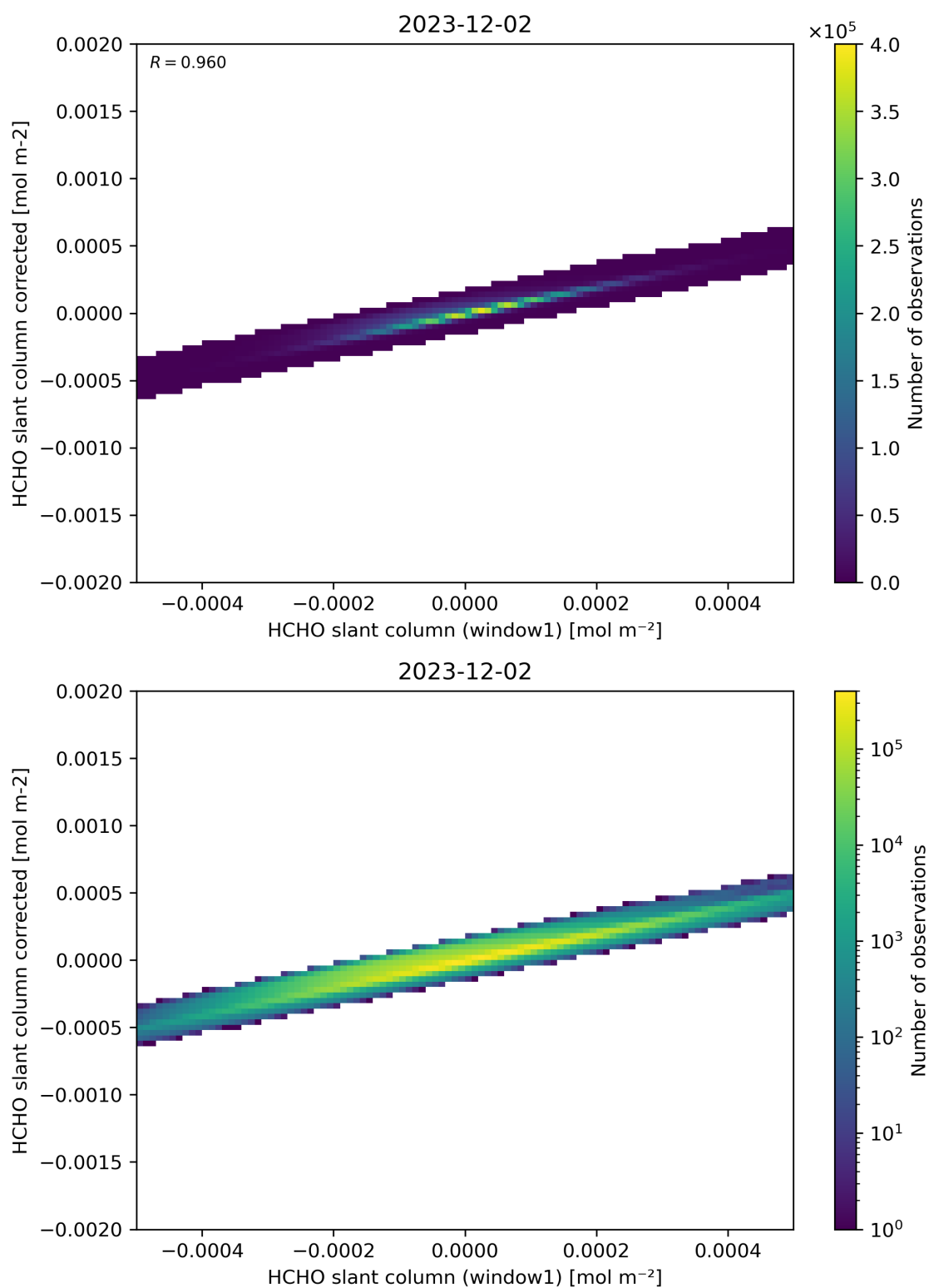
Figure 82: Scatter density plot of “HCHO slant column (window1)” against “HCHO slant column corrected” for 2023-12-01 to 2023-12-03.
