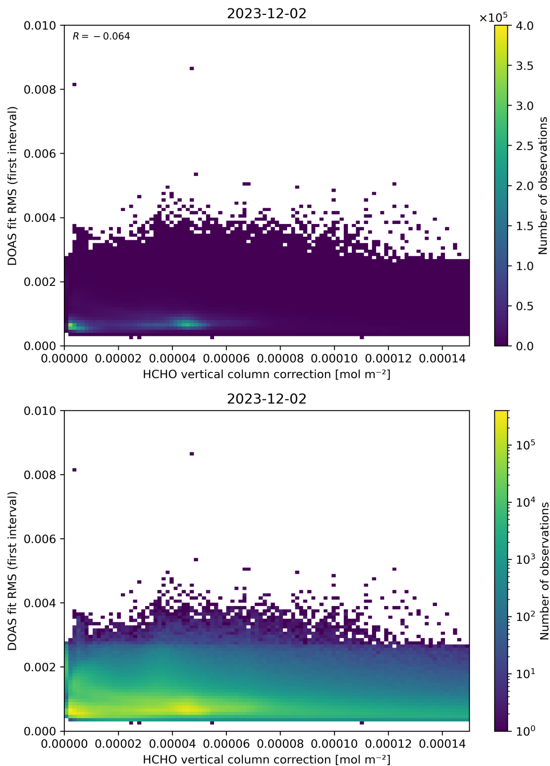
Figure 112: Scatter density plot of “HCHO vertical column correction” against “DOAS fit RMS (first interval)” for 2023-12-01 to 2023-12-03.
