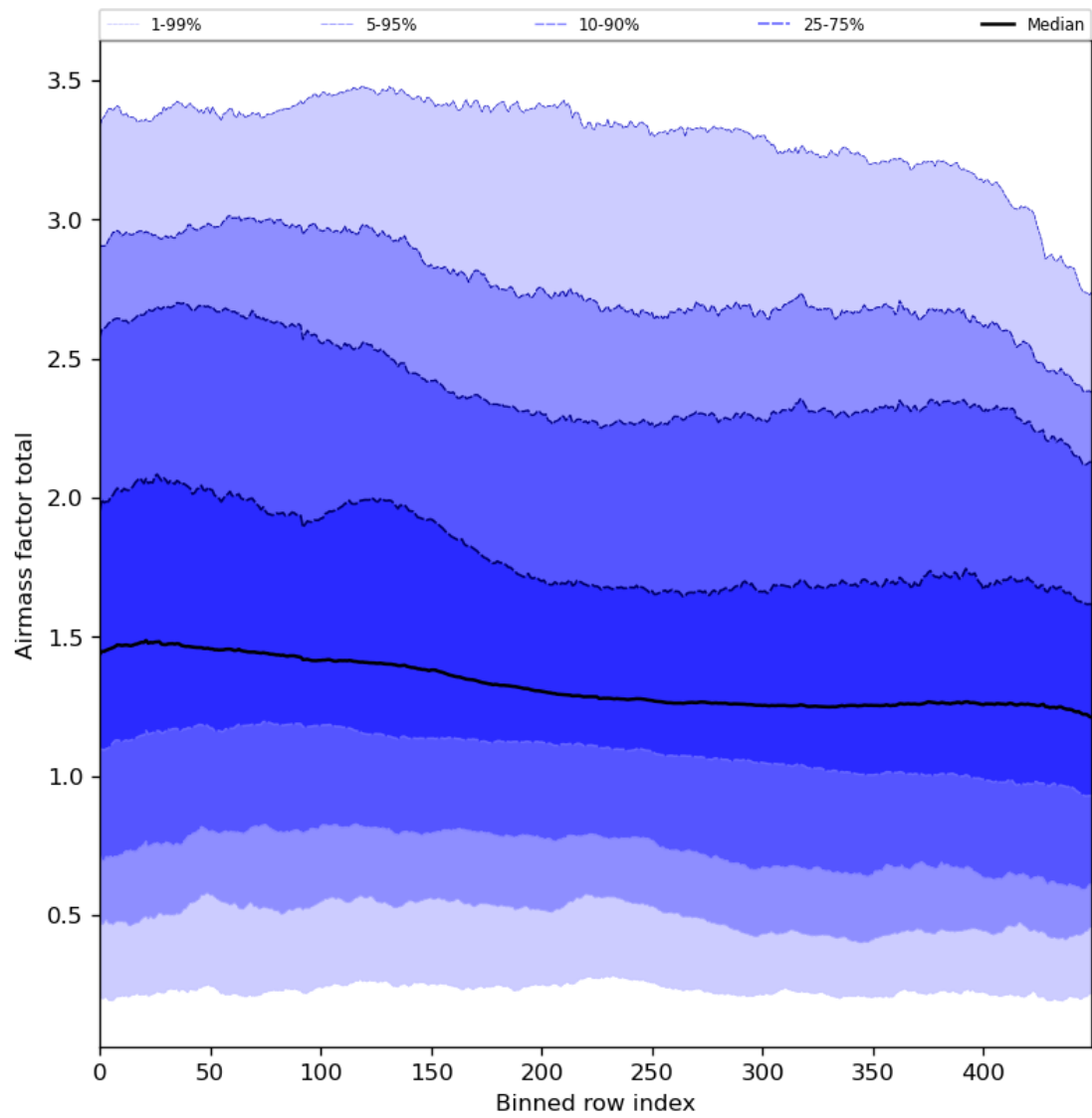
Figure 54: Along track statistics of “Airmass factor total” for 2023-12-01 to 2023-12-03
