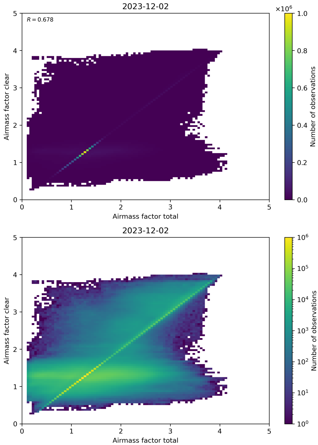
Figure 100: Scatter density plot of “Airmass factor total” against “Airmass factor clear” for 2023-12-01 to 2023-12-03.
