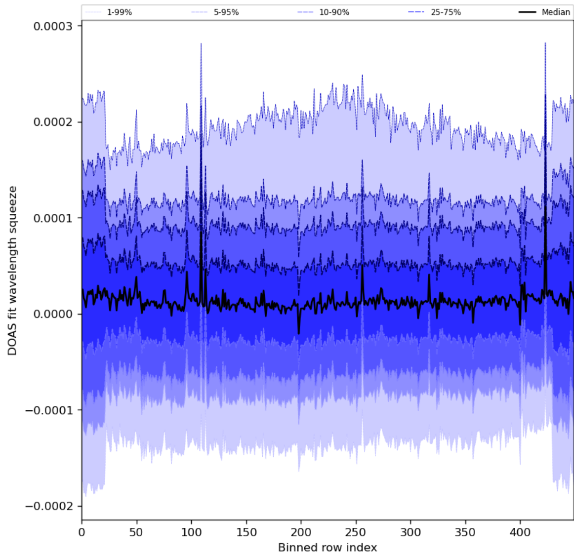
Figure 59: Along track statistics of “DOAS fit wavelength squeeze” for 2023-12-01 to 2023-12-03
