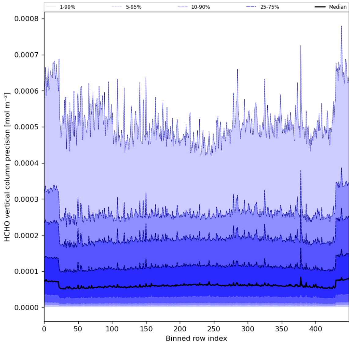
Figure 50: Along track statistics of “HCHO vertical column precision” for 2023-12-01 to 2023-12-03
