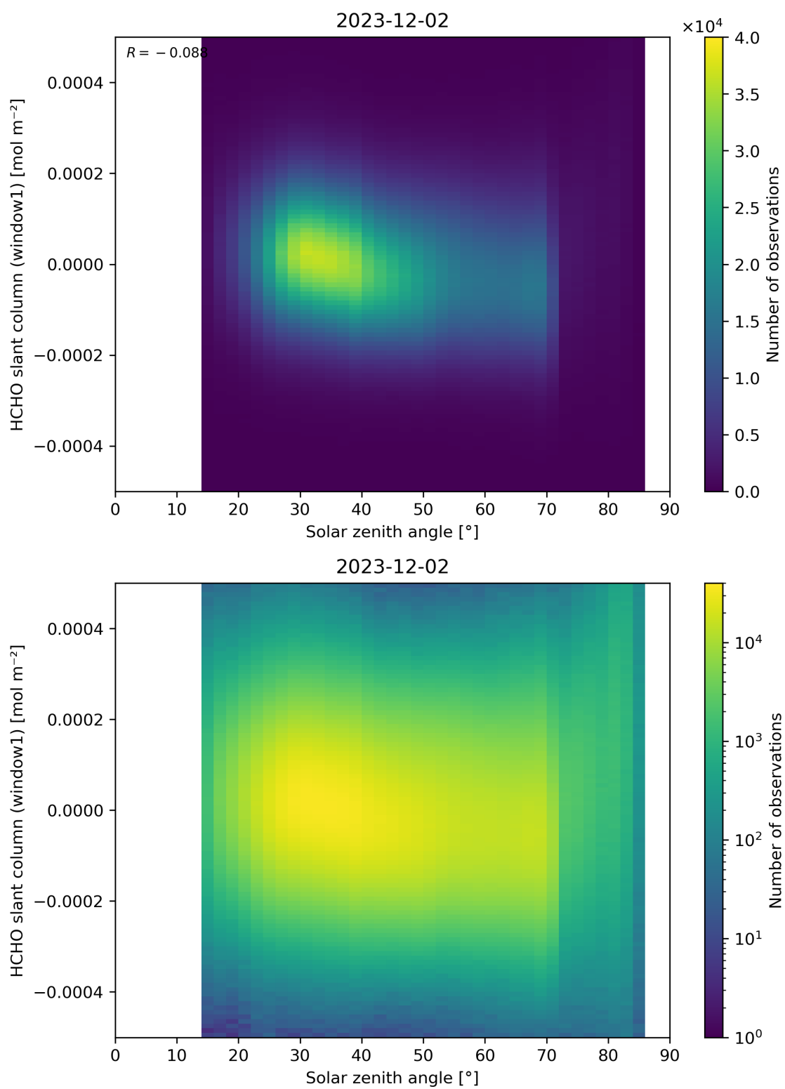
Figure 173: Scatter density plot of “Solar zenith angle” against “HCHO slant column (window1)” for 2023-12-01 to 2023-12-03.
