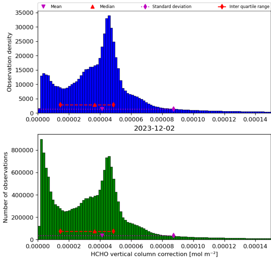
Figure 37: Histogram of “HCHO vertical column correction” for 2023-12-01 to 2023-12-03
