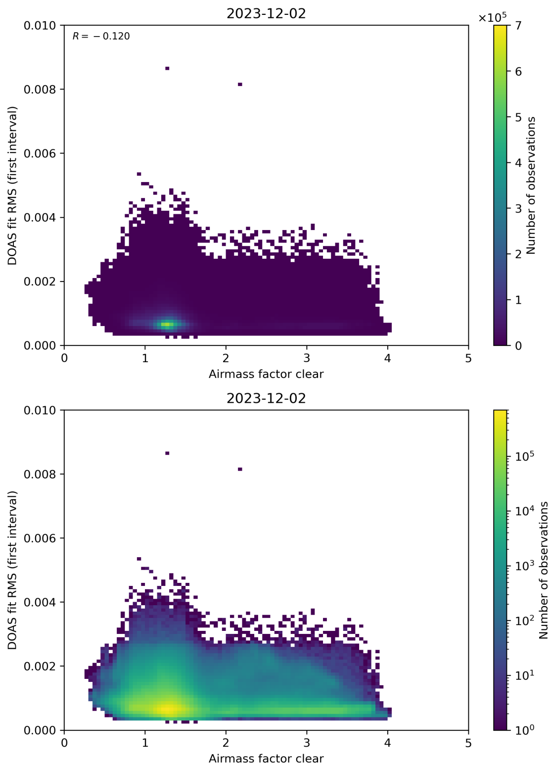
Figure 71: Scatter density plot of “Airmass factor clear” against “DOAS fit RMS (first interval)” for 2023-12-01 to 2023-12-03.
