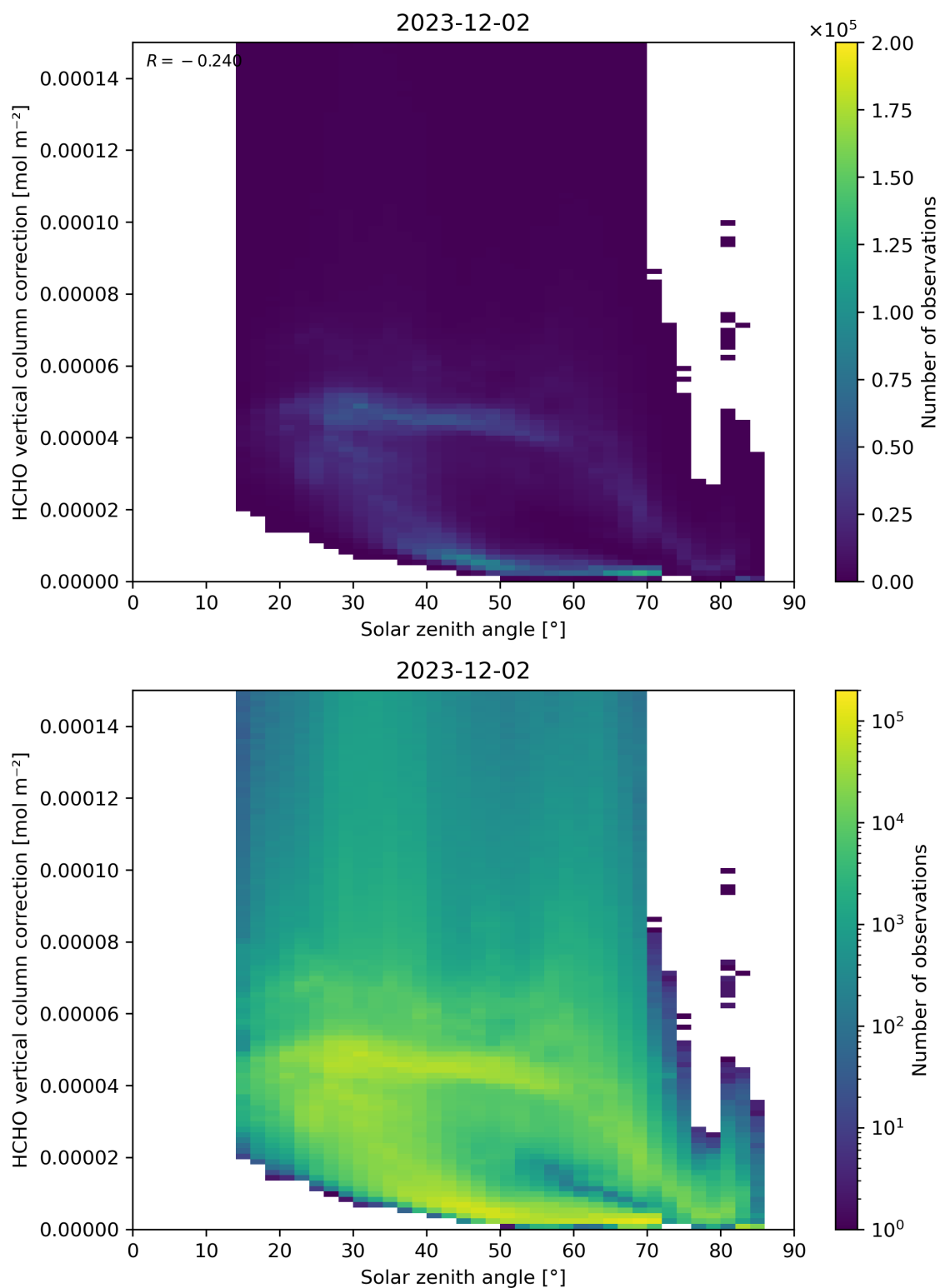
Figure 178: Scatter density plot of “Solar zenith angle” against “HCHO vertical column correction” for 2023-12-01 to 2023-12-03.
