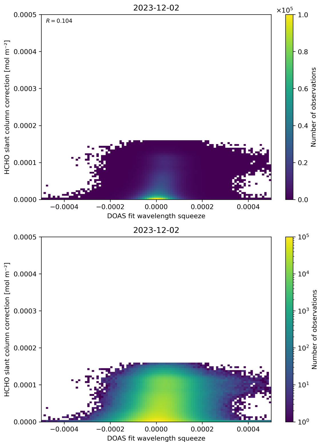
Figure 70: Scatter density plot of “DOAS fit wavelength squeeze” against “HCHO slant column correction” for 2023-12-01 to 2023-12-03.
