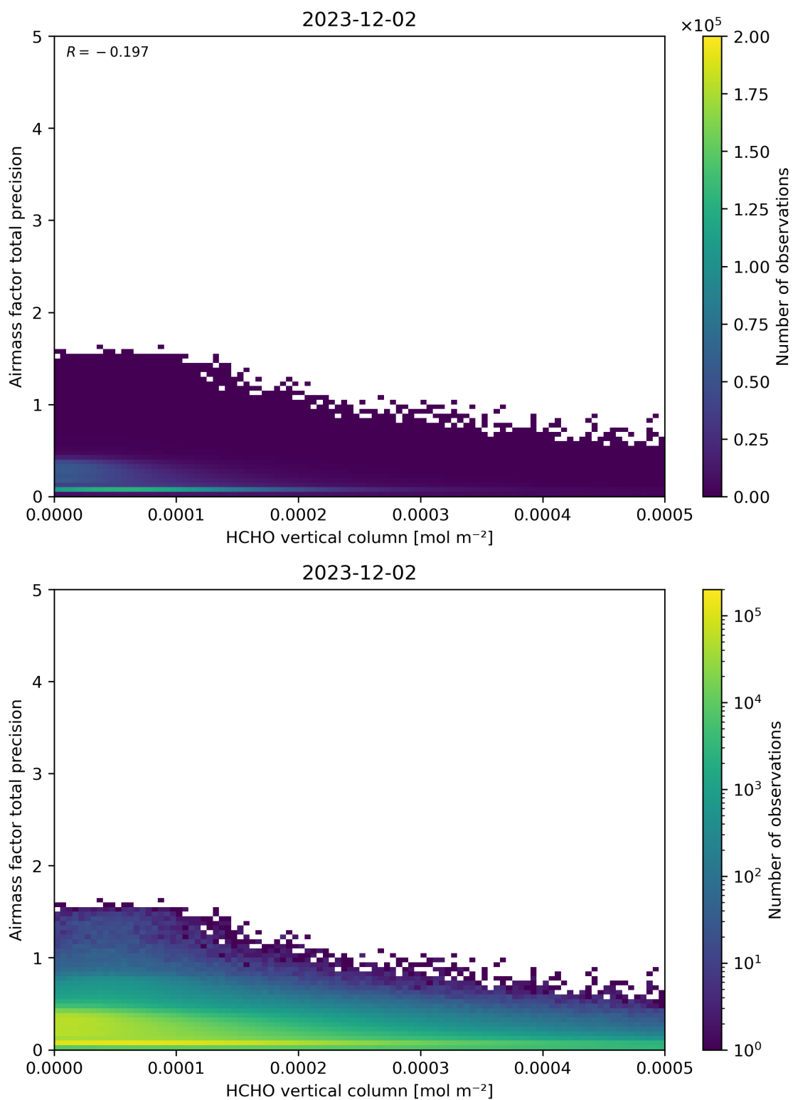
Figure 132: Scatter density plot of “HCHO vertical column” against “Airmass factor total precision” for 2023-12-01 to 2023-12-03.
