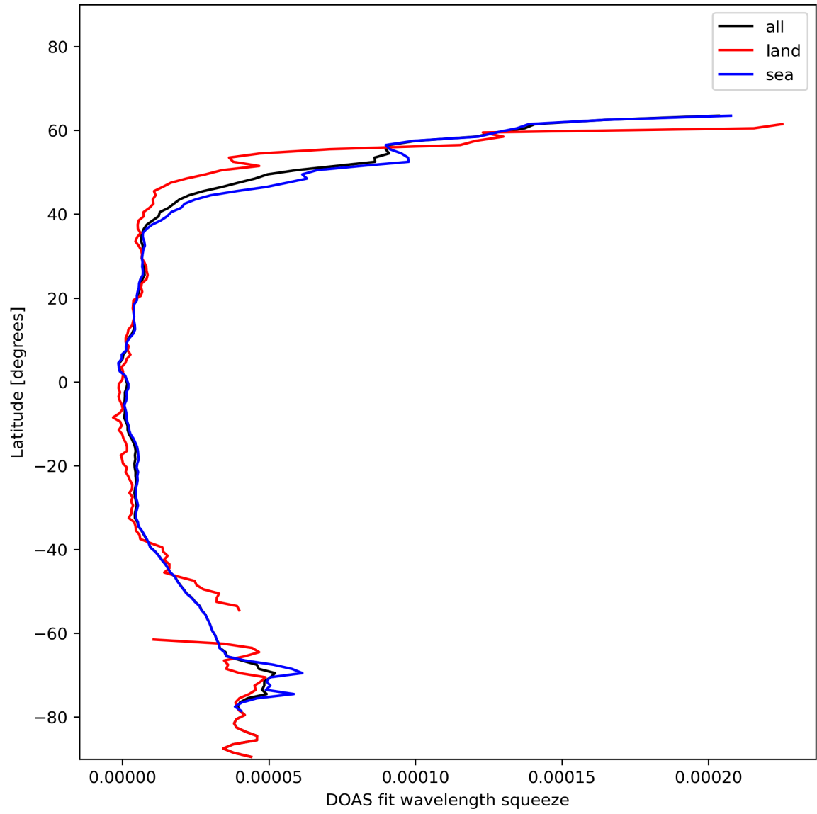
Figure 31: Zonal average of “DOAS fit wavelength squeeze” for 2023-12-01 to 2023-12-03.
