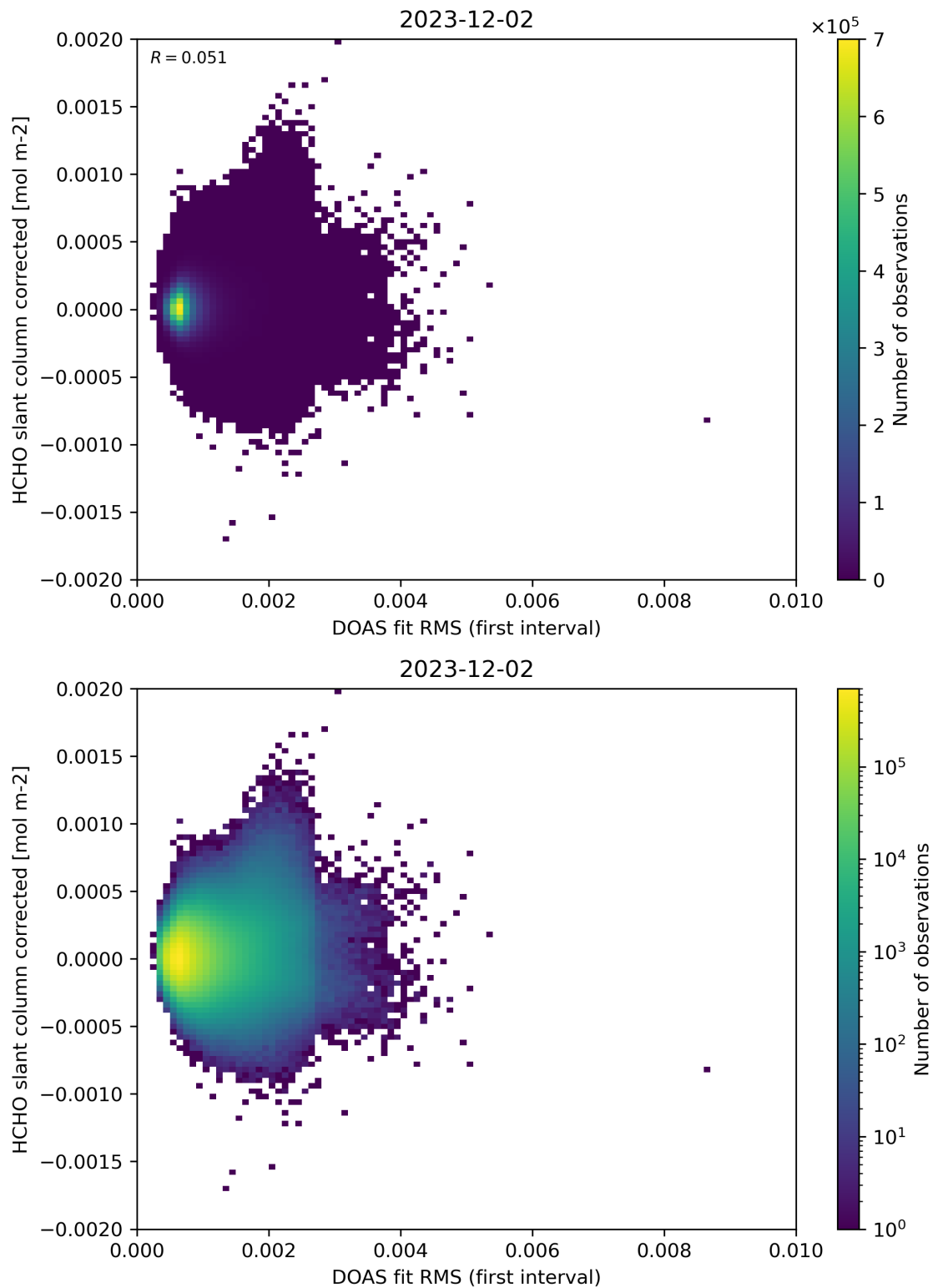
Figure 62: Scatter density plot of “DOAS fit RMS (first interval)” against “HCHO slant column corrected” for 2023-12-01 to 2023-12-03.
