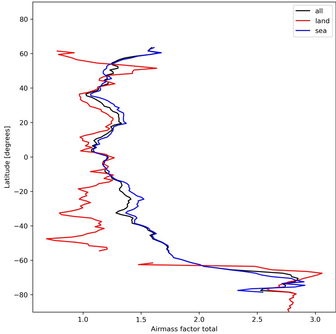
Figure 26: Zonal average of “Airmass factor total” for 2023-12-01 to 2023-12-03.
