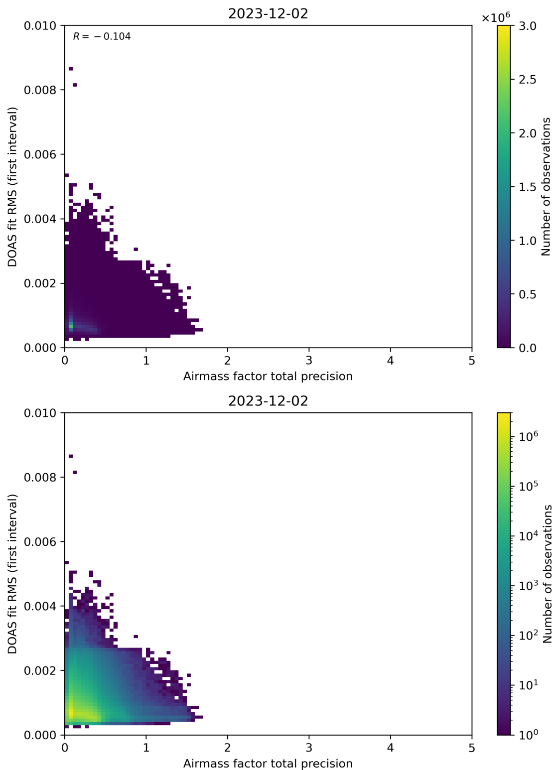
Figure 105: Scatter density plot of “Airmass factor total precision” against “DOAS fit RMS (first interval)” for 2023-12-01 to 2023-12-03.
