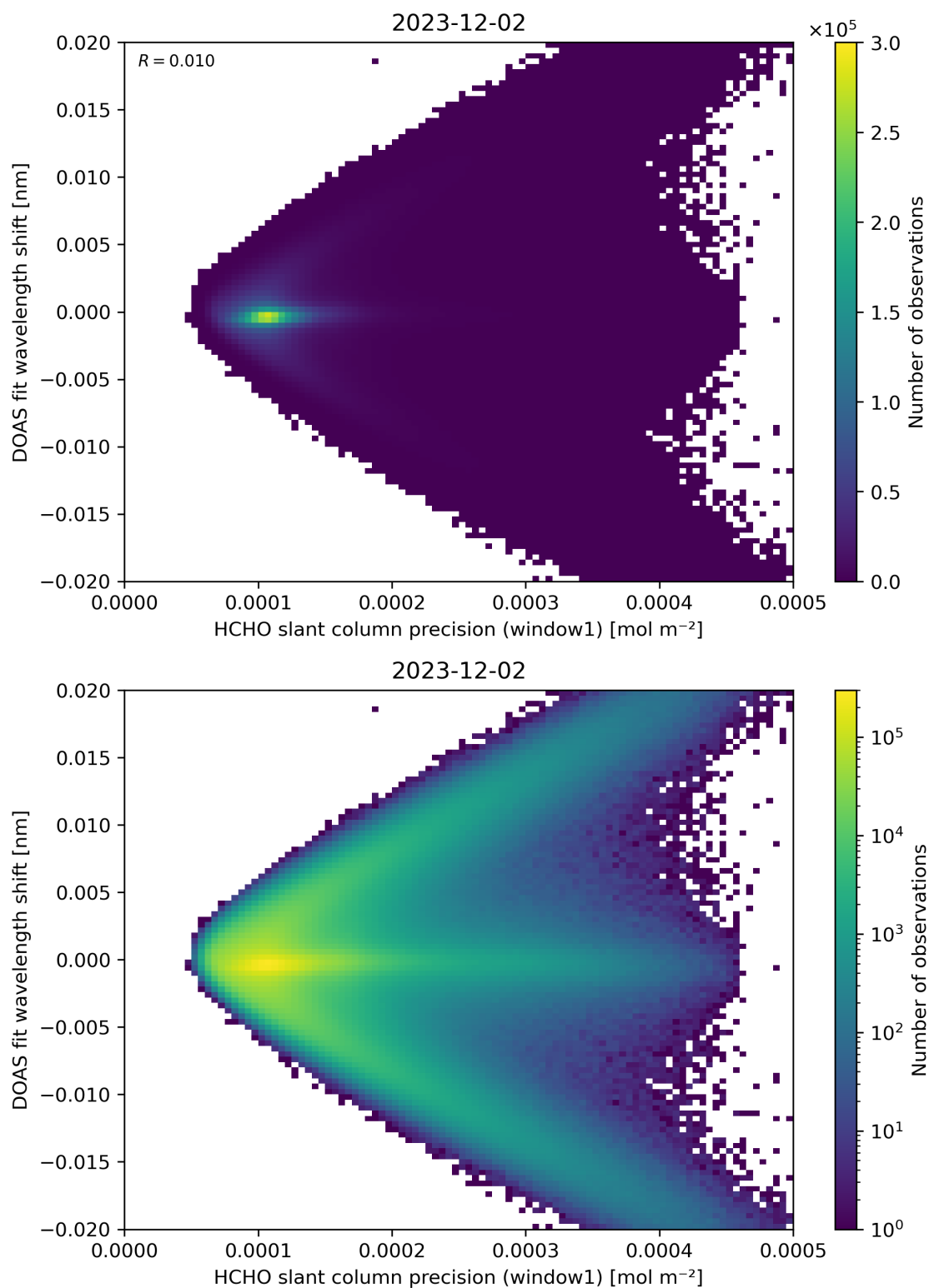
Figure 89: Scatter density plot of “HCHO slant column precision (window1)” against “DOAS fit wavelength shift” for 2023-12-01 to 2023-12-03.
