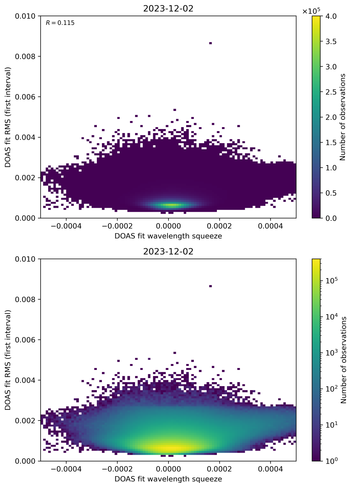
Figure 68: Scatter density plot of “DOAS fit wavelength squeeze” against “DOAS fit RMS (first interval)” for 2023-12-01 to 2023-12-03.
