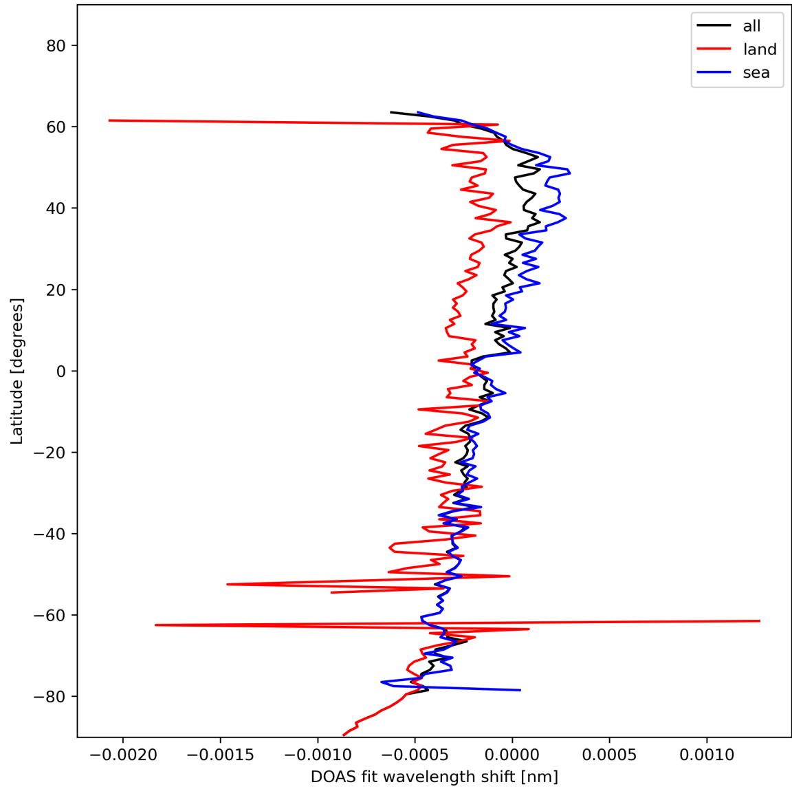
Figure 30: Zonal average of “DOAS fit wavelength shift” for 2023-12-01 to 2023-12-03.
