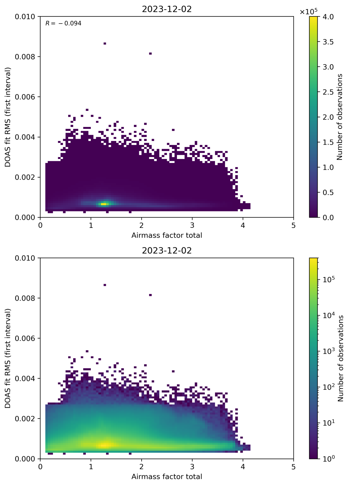
Figure 97: Scatter density plot of “Airmass factor total” against “DOAS fit RMS (first interval)” for 2023-12-01 to 2023-12-03.
