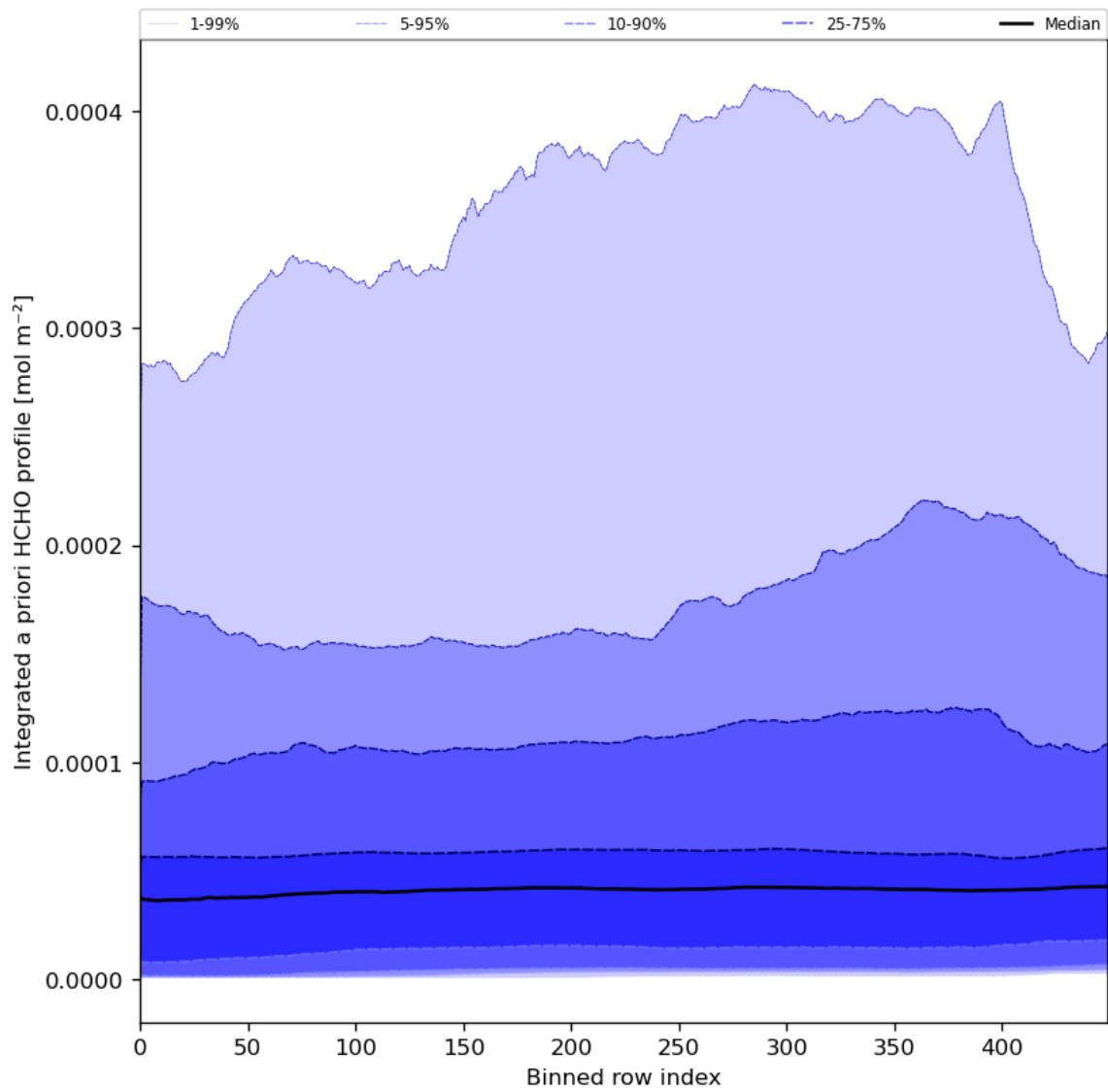
Figure 57: Along track statistics of “Integrated a priori HCHO profile” for 2023-12-01 to 2023-12-03
