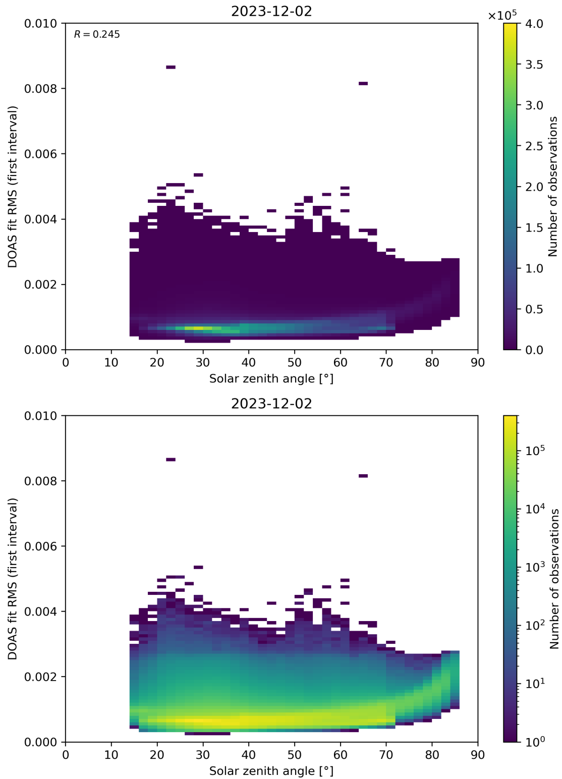
Figure 167: Scatter density plot of “Solar zenith angle” against “DOAS fit RMS (first interval)” for 2023-12-01 to 2023-12-03.
