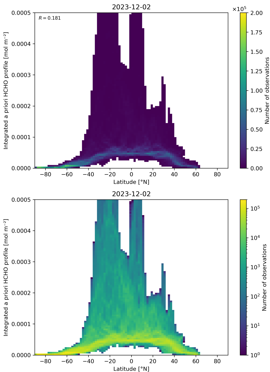
Figure 166: Scatter density plot of “Latitude” against “Integrated a priori HCHO profile” for 2023-12-01 to 2023-12-03.
