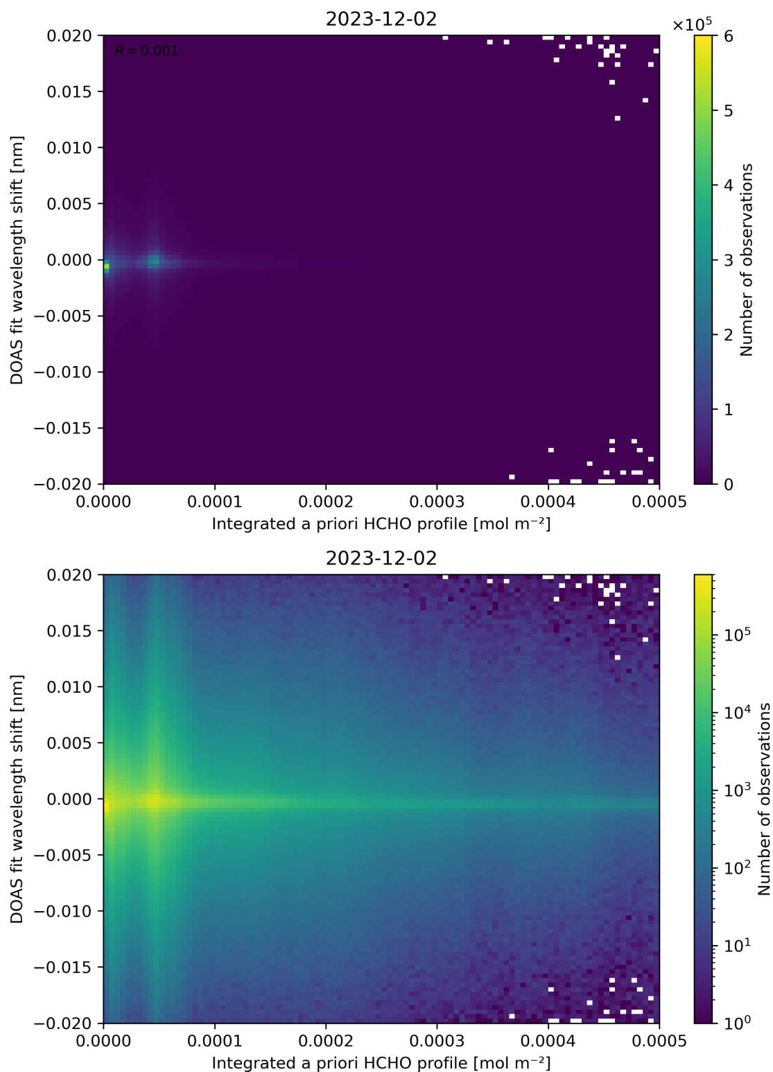
Figure 149: Scatter density plot of “Integrated a priori HCHO profile” against “DOAS fit wavelength shift” for 2023-12-01 to 2023-12-03.
