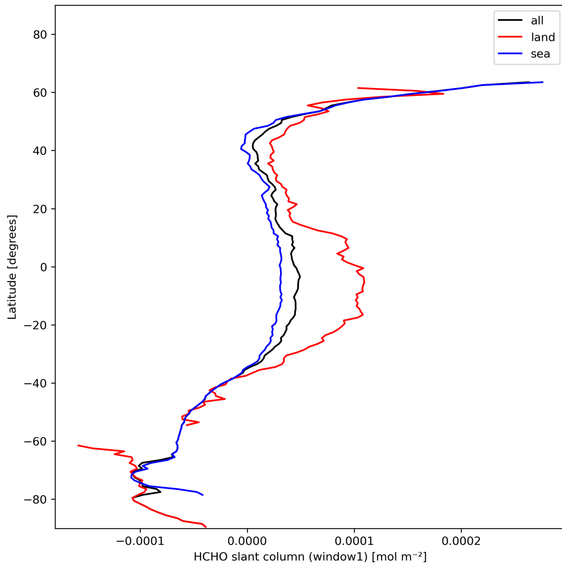
Figure 24: Zonal average of “HCHO slant column (window1)” for 2023-12-01 to 2023-12-03.
