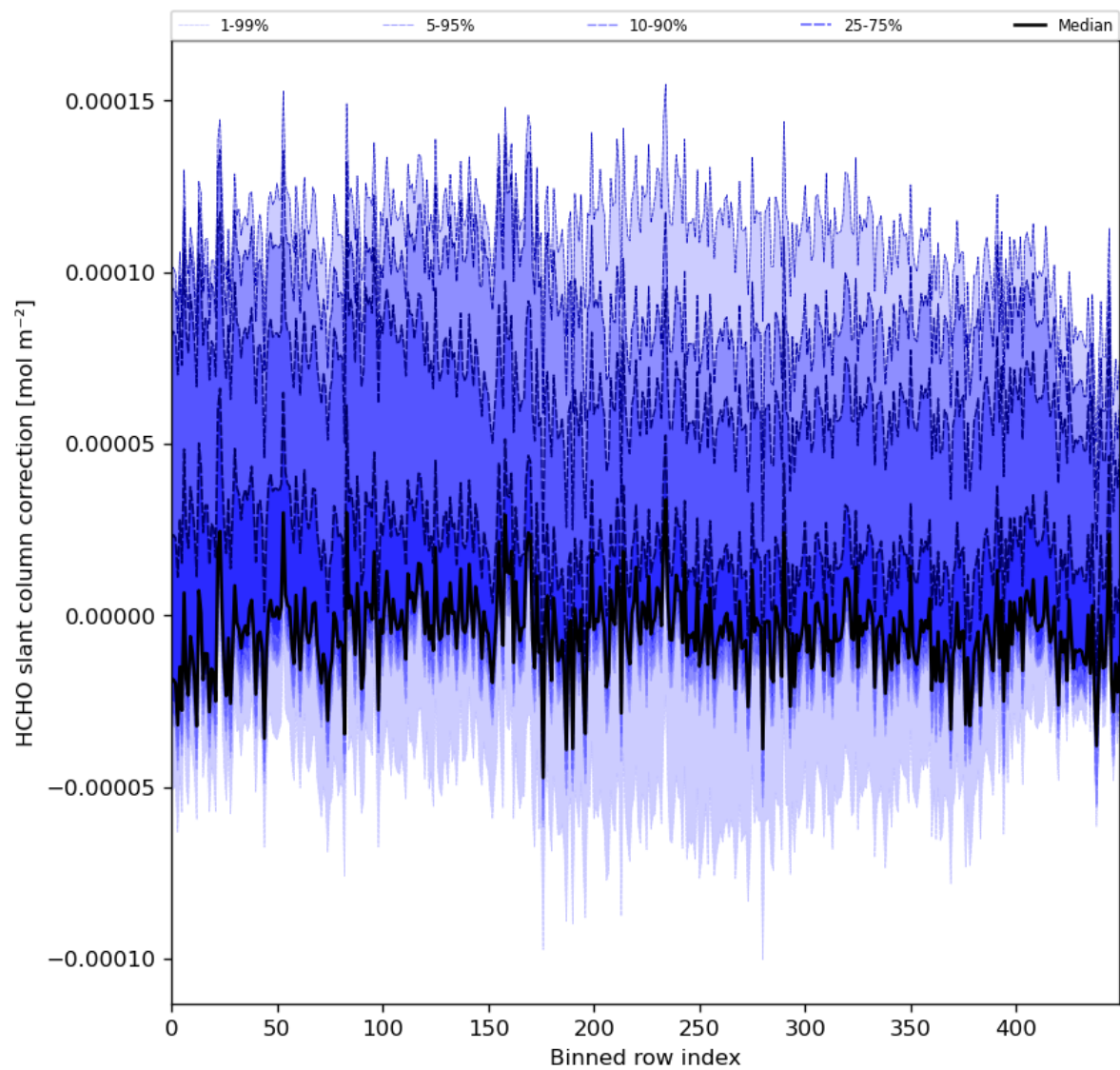
Figure 61: Along track statistics of “HCHO slant column correction” for 2023-12-01 to 2023-12-03
