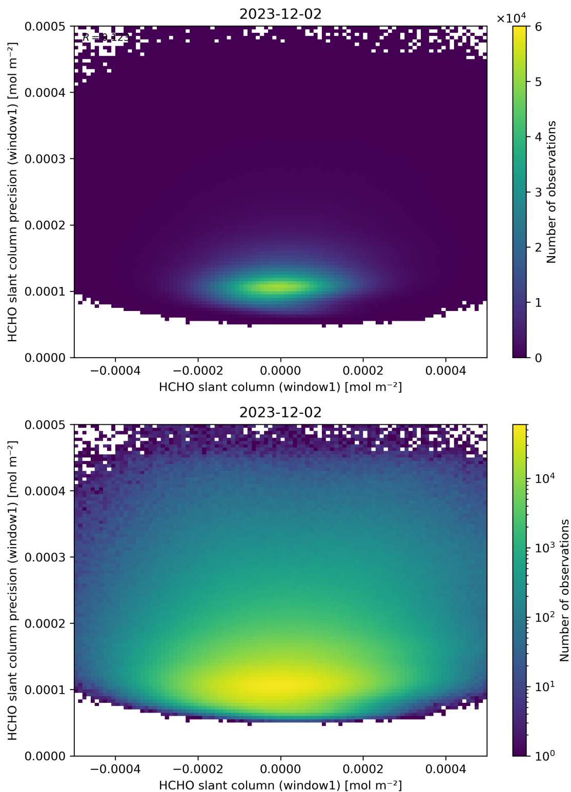
Figure 84: Scatter density plot of “HCHO slant column (window1)” against “HCHO slant column precision (window1)” for 2023-12-01 to 2023-12-03.
