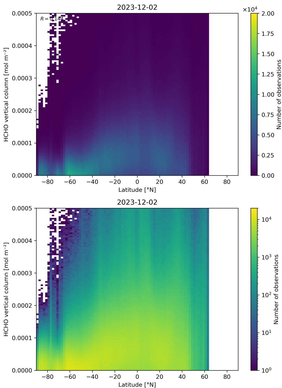
Figure 163: Scatter density plot of “Latitude” against “HCHO vertical column” for 2023-12-01 to 2023-12-03.
