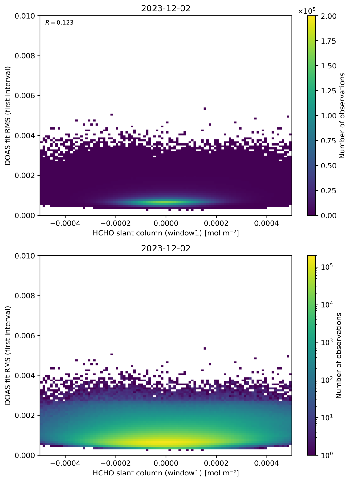
Figure 78: Scatter density plot of “HCHO slant column (window1)” against “DOAS fit RMS (first interval)” for 2023-12-01 to 2023-12-03.
