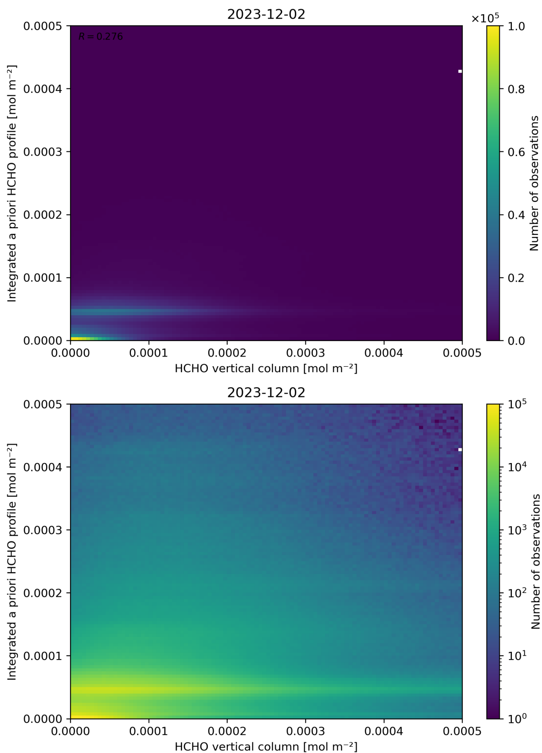
Figure 135: Scatter density plot of “HCHO vertical column” against “Integrated a priori HCHO profile” for 2023-12-01 to 2023-12-03.
