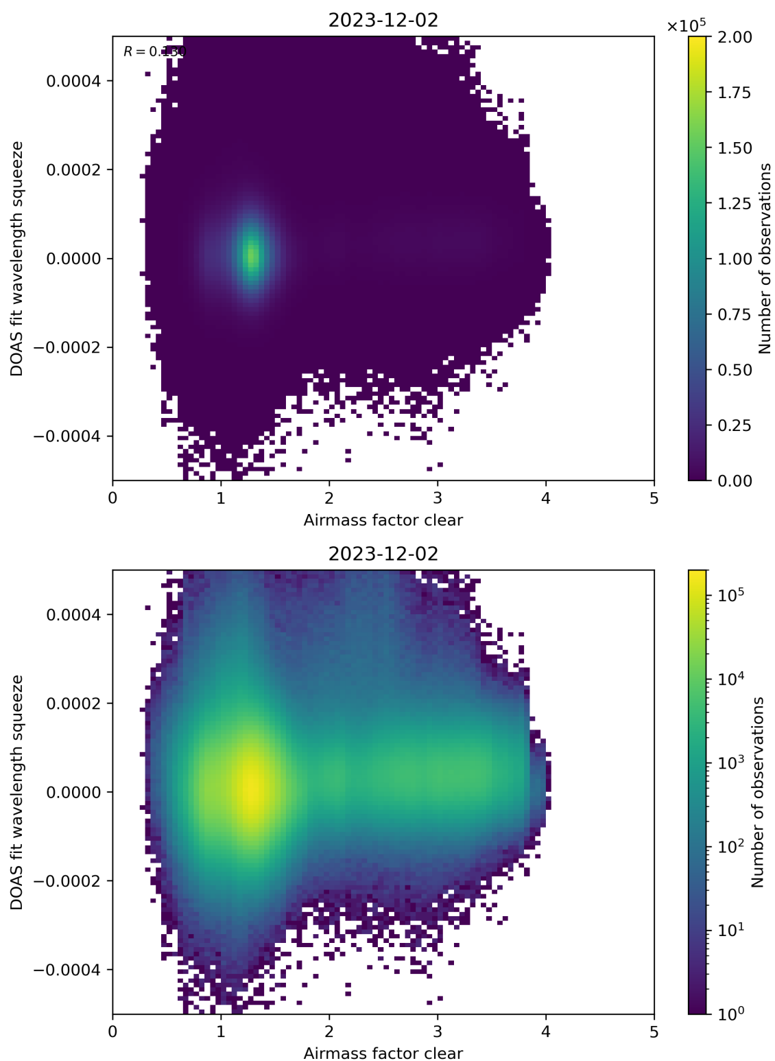
Figure 73: Scatter density plot of “Airmass factor clear” against “DOAS fit wavelength squeeze” for 2023-12-01 to 2023-12-03.
