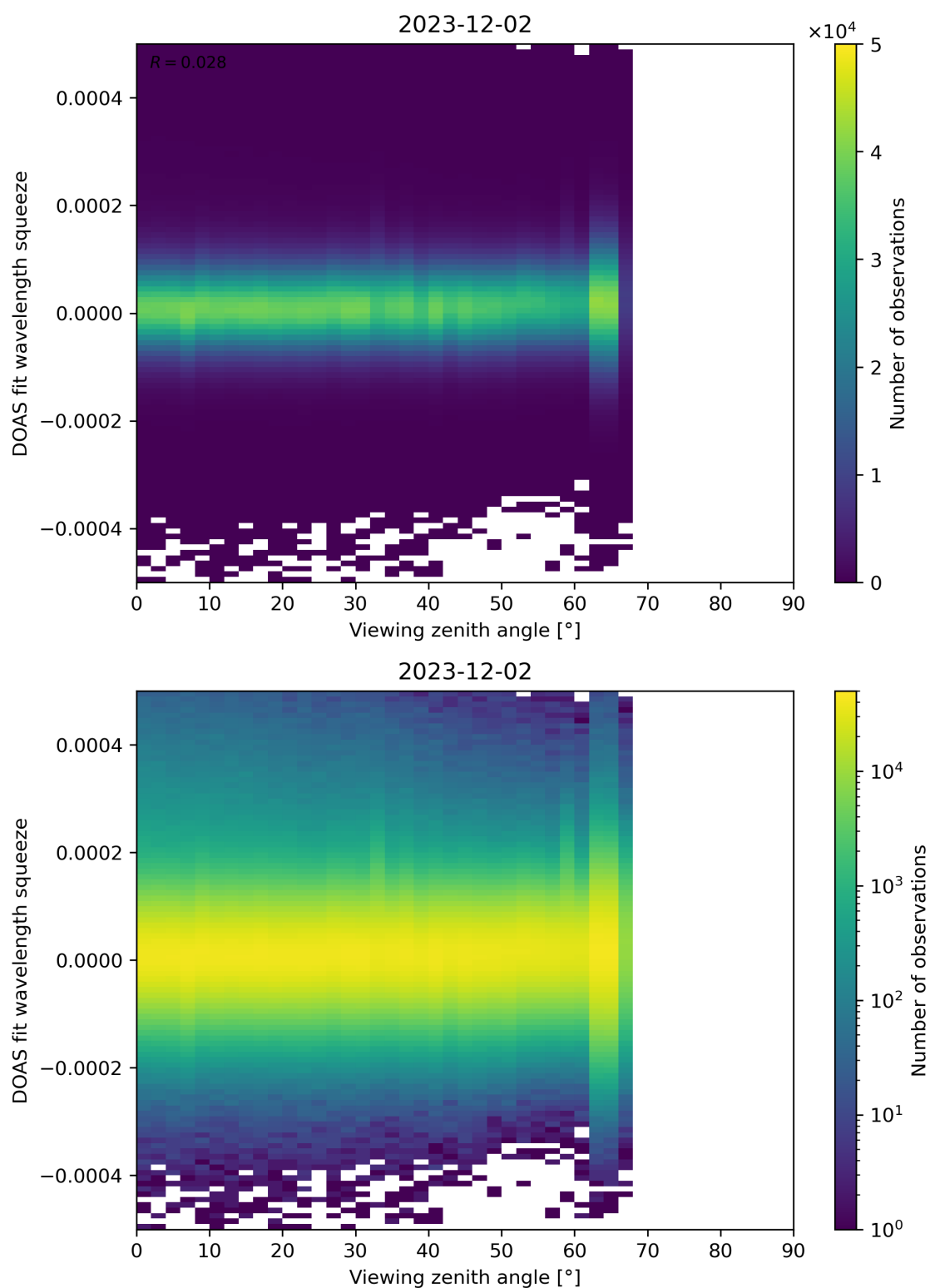
Figure 184: Scatter density plot of “Viewing zenith angle” against “DOAS fit wavelength squeeze” for 2023-12-01 to 2023-12-03.
