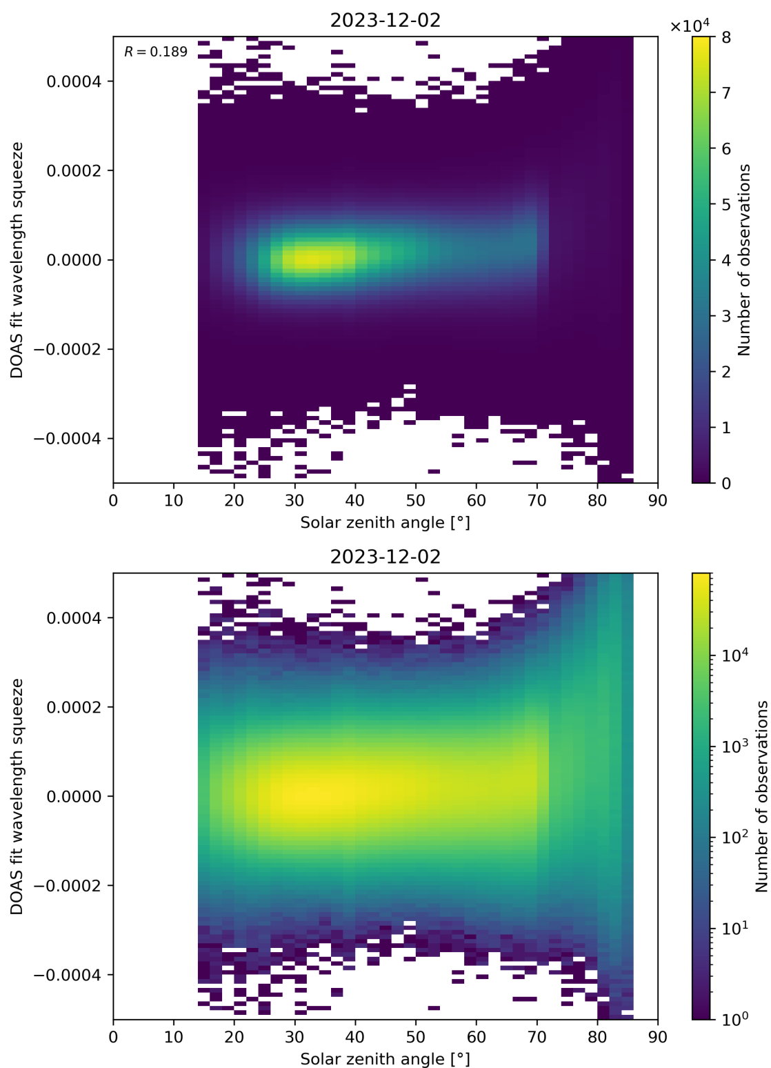
Figure 169: Scatter density plot of “Solar zenith angle” against “DOAS fit wavelength squeeze” for 2023-12-01 to 2023-12-03.
