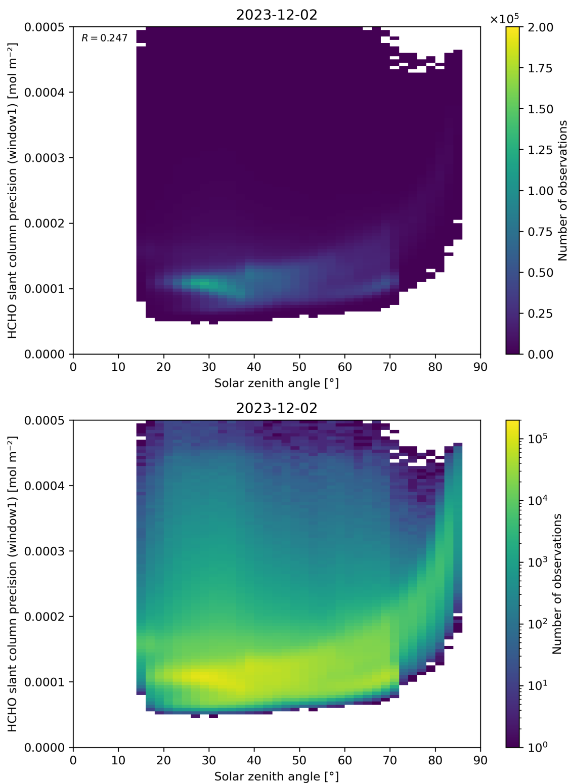
Figure 174: Scatter density plot of “Solar zenith angle” against “HCHO slant column precision (window1)” for 2023-12-01 to 2023-12-03.
