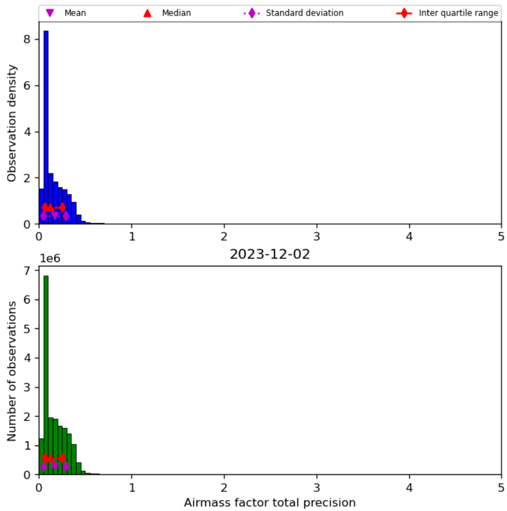
Figure 41: Histogram of “Airmass factor total precision” for 2023-12-01 to 2023-12-03
