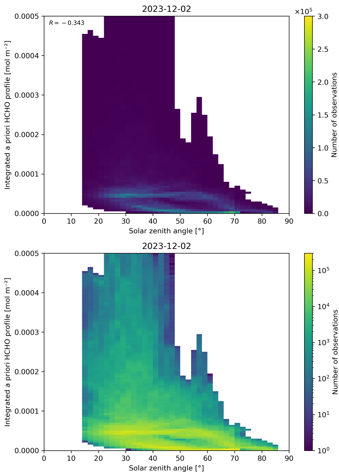
Figure 180: Scatter density plot of “Solar zenith angle” against “Integrated a priori HCHO profile” for 2023-12-01 to 2023-12-03.
