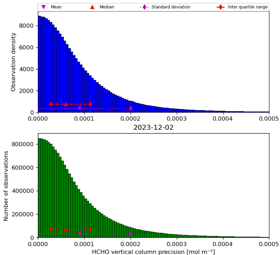
Figure 36: Histogram of “HCHO vertical column precision” for 2023-12-01 to 2023-12-03
