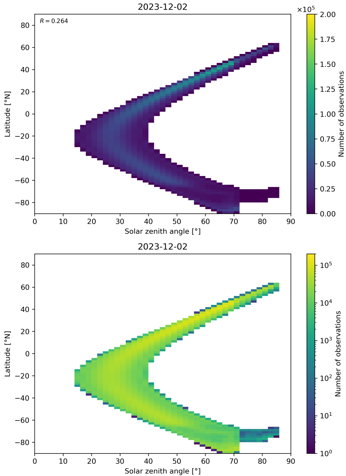
Figure 181: Scatter density plot of “Solar zenith angle” against “Latitude” for 2023-12-01 to 2023-12-03.
