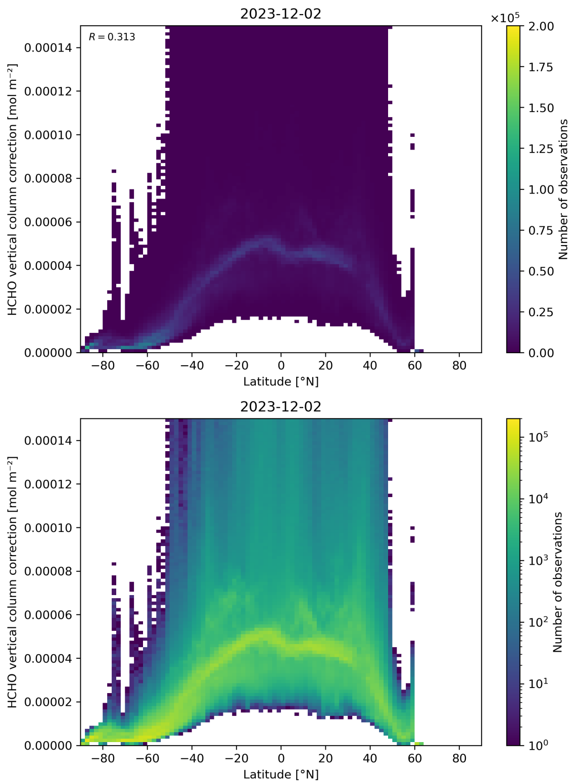
Figure 164: Scatter density plot of “Latitude” against “HCHO vertical column correction” for 2023-12-01 to 2023-12-03.
