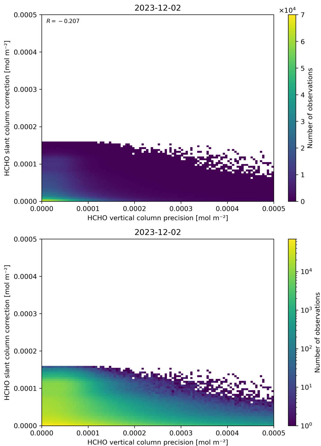
Figure 141: Scatter density plot of “HCHO vertical column precision” against “HCHO slant column correction” for 2023-12-01 to 2023-12-03.
