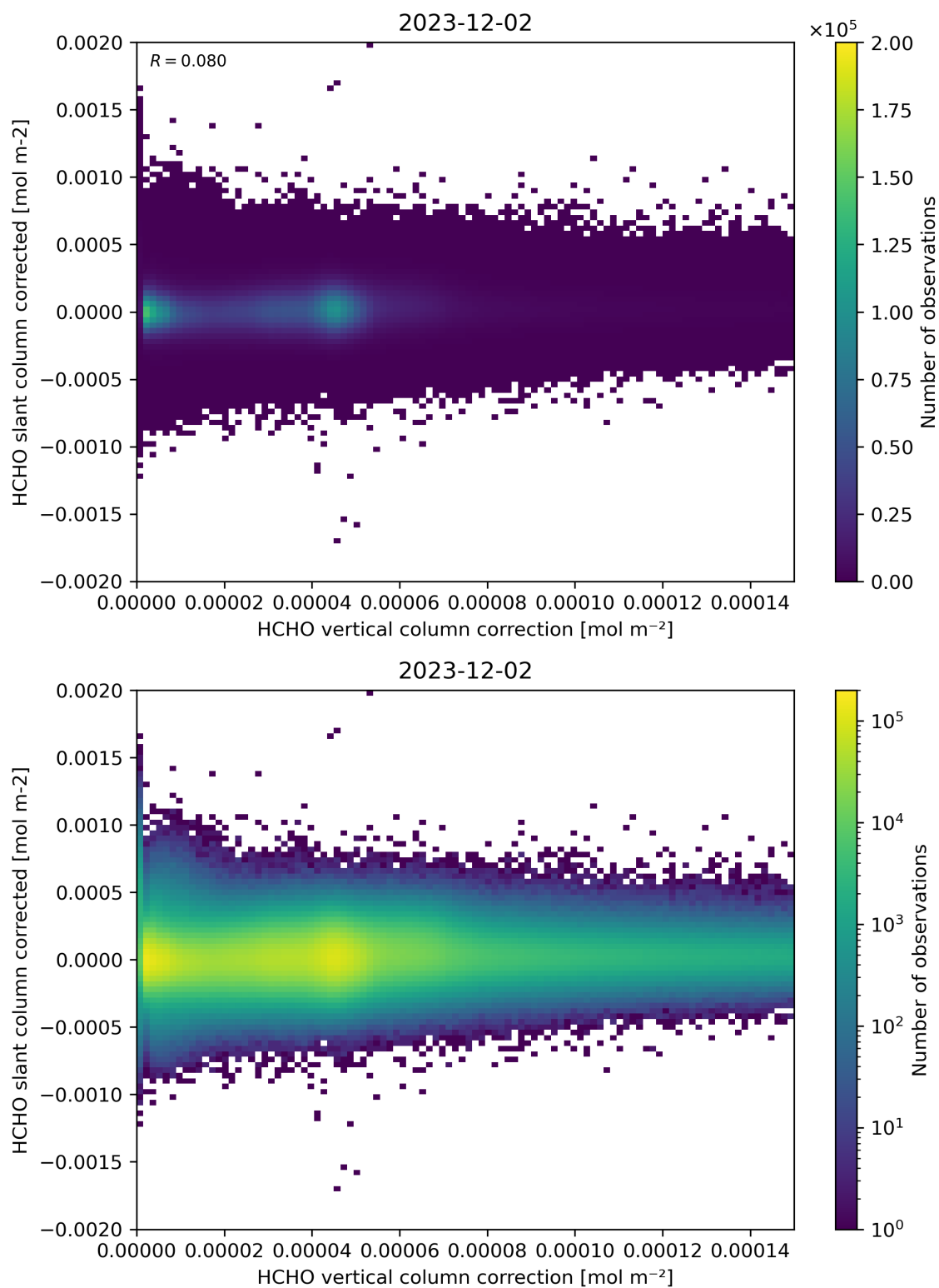
Figure 116: Scatter density plot of “HCHO vertical column correction” against “HCHO slant column corrected” for 2023-12-01 to 2023-12-03.
