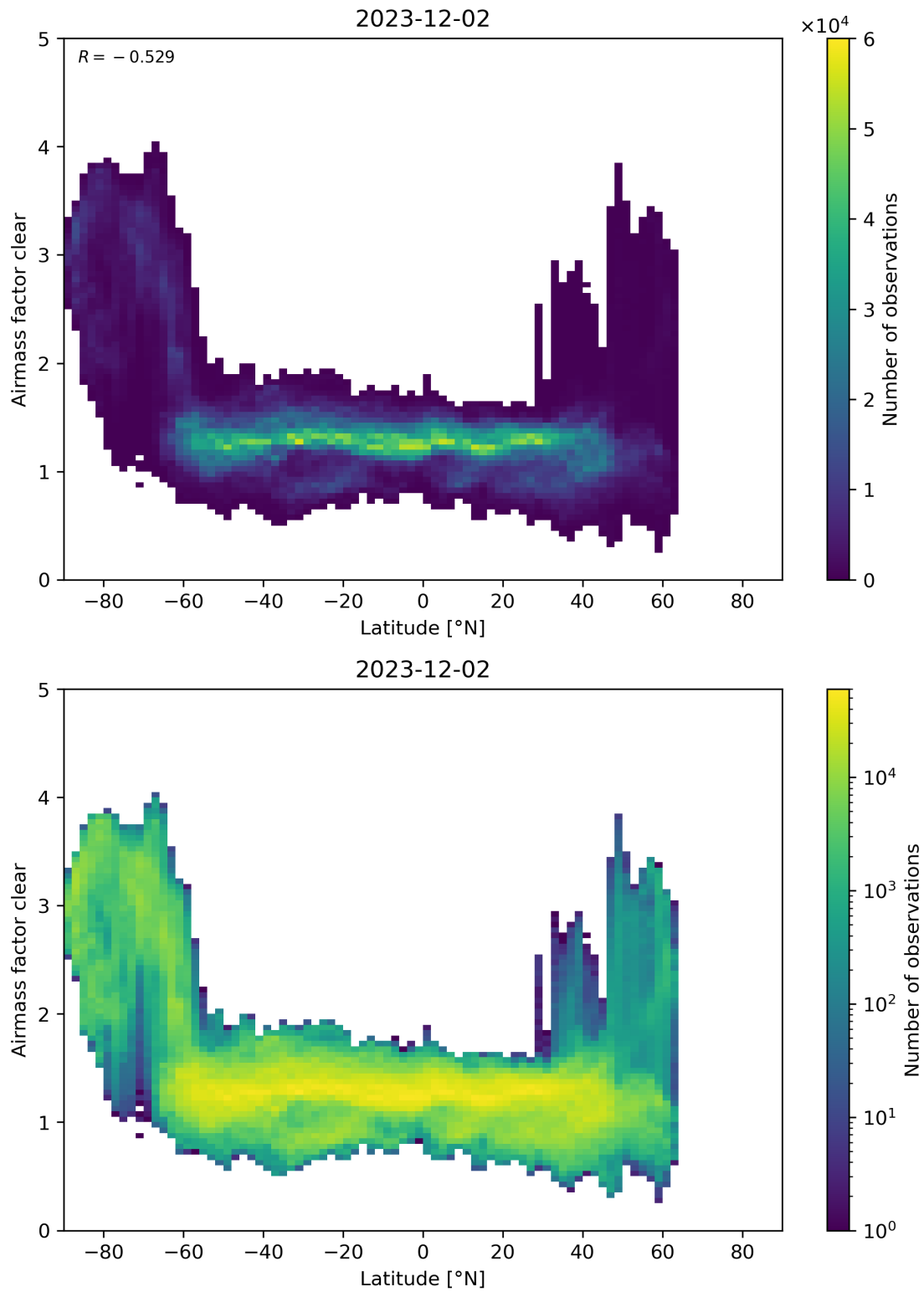
Figure 156: Scatter density plot of “Latitude” against “Airmass factor clear” for 2023-12-01 to 2023-12-03.
