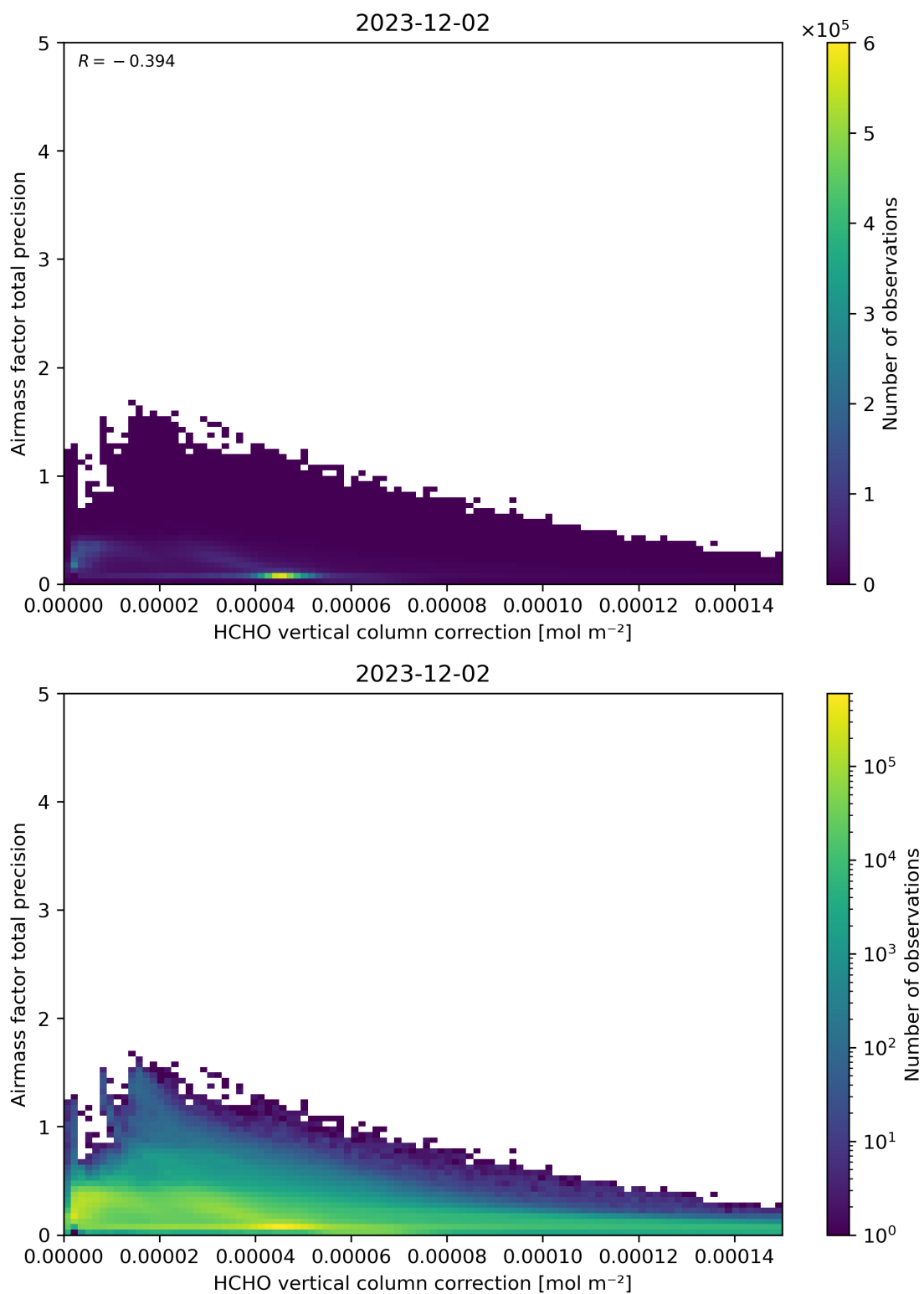
Figure 121: Scatter density plot of “HCHO vertical column correction” against “Airmass factor total precision” for 2023-12-01 to 2023-12-03.
