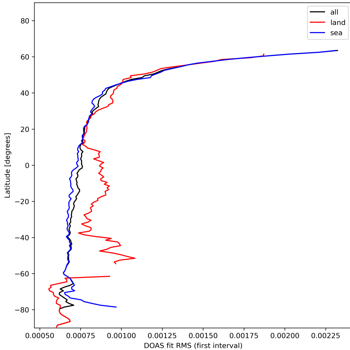
Figure 32: Zonal average of “DOAS fit RMS (first interval)” for 2023-12-01 to 2023-12-03.
