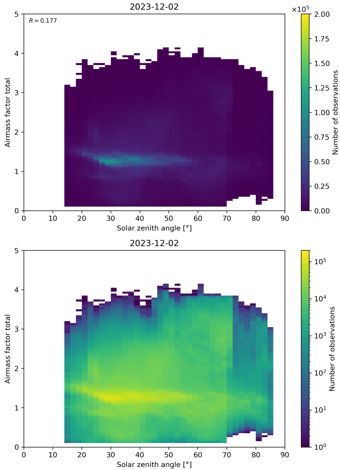
Figure 175: Scatter density plot of “Solar zenith angle” against “Airmass factor total” for 2023-12-01 to 2023-12-03.
