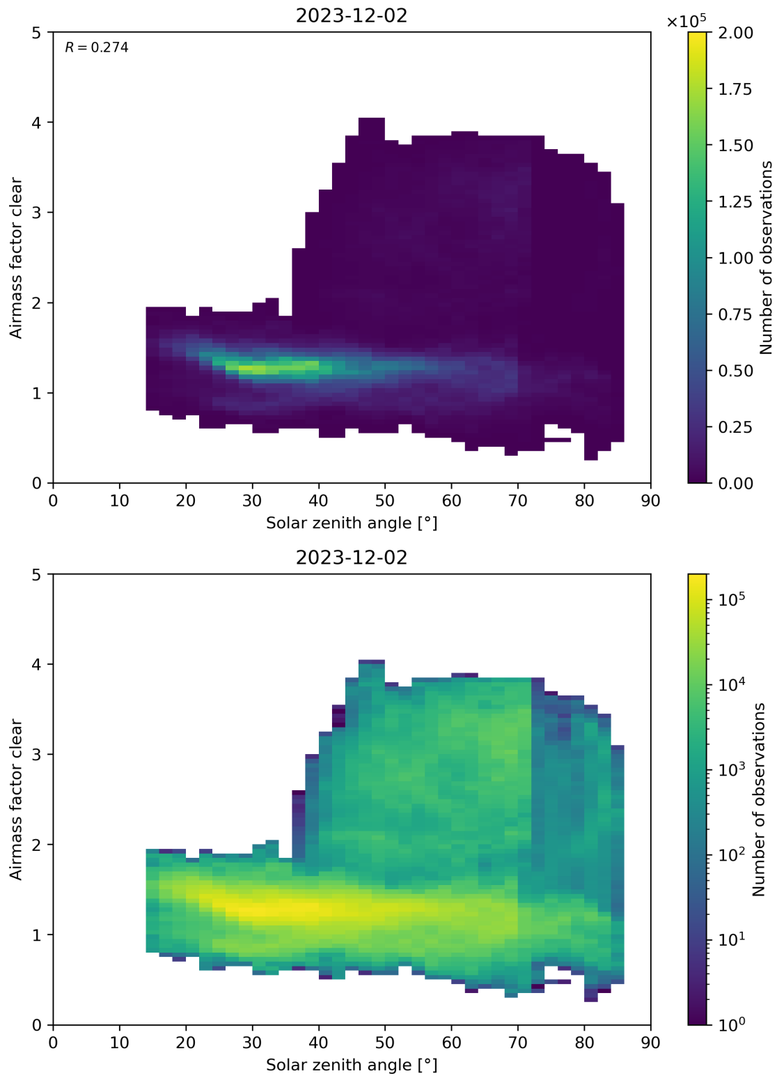
Figure 170: Scatter density plot of “Solar zenith angle” against “Airmass factor clear” for 2023-12-01 to 2023-12-03.
