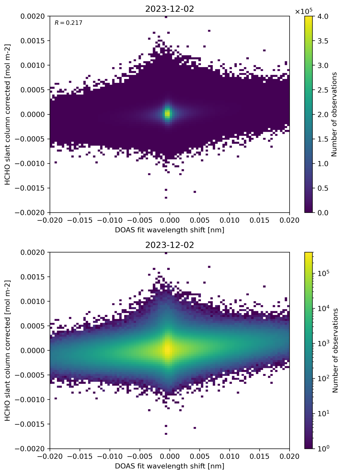
Figure 66: Scatter density plot of “DOAS fit wavelength shift” against “HCHO slant column corrected” for 2023-12-01 to 2023-12-03.
