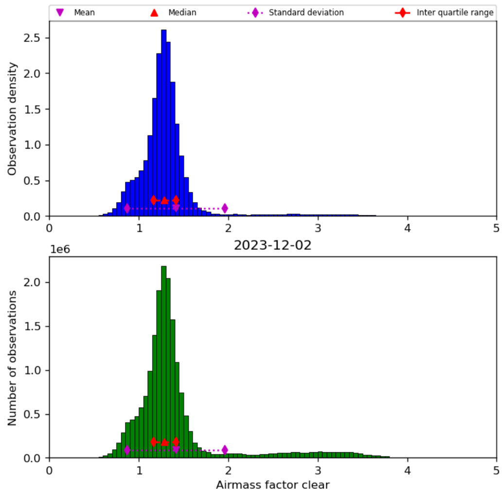
Figure 42: Histogram of “Airmass factor clear” for 2023-12-01 to 2023-12-03
