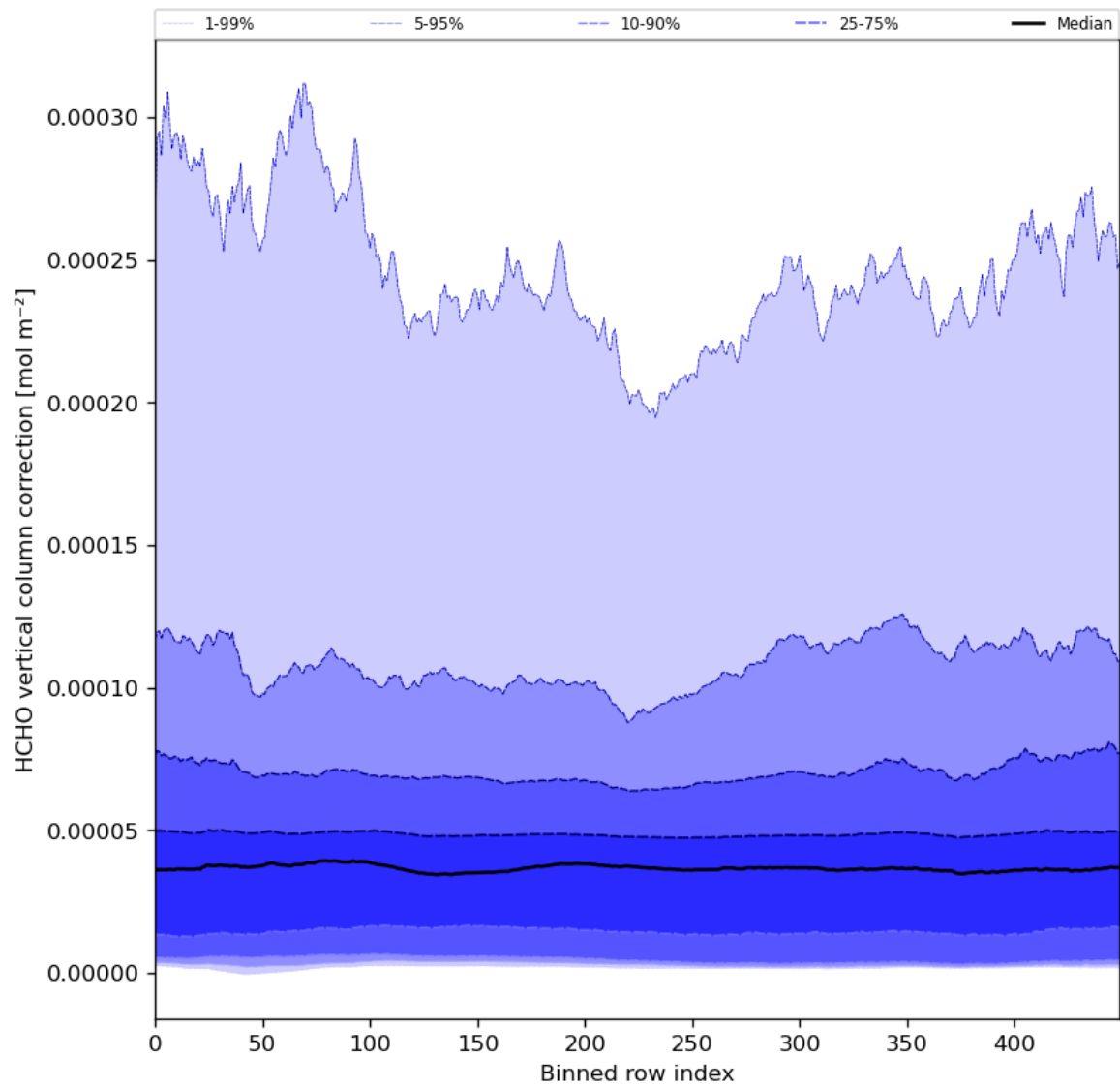
Figure 51: Along track statistics of “HCHO vertical column correction” for 2023-12-01 to 2023-12-03
