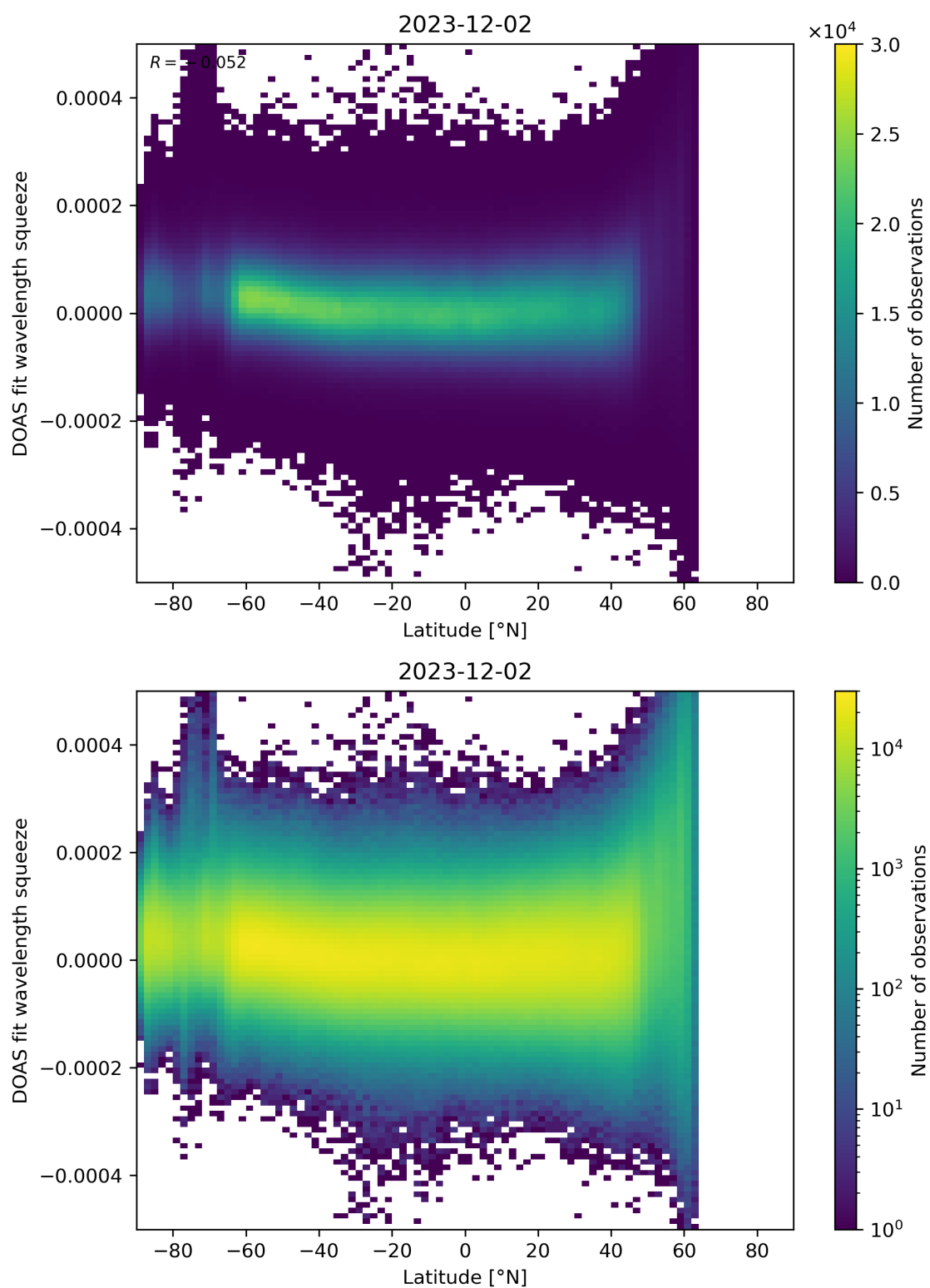
Figure 155: Scatter density plot of “Latitude” against “DOAS fit wavelength squeeze” for 2023-12-01 to 2023-12-03.
