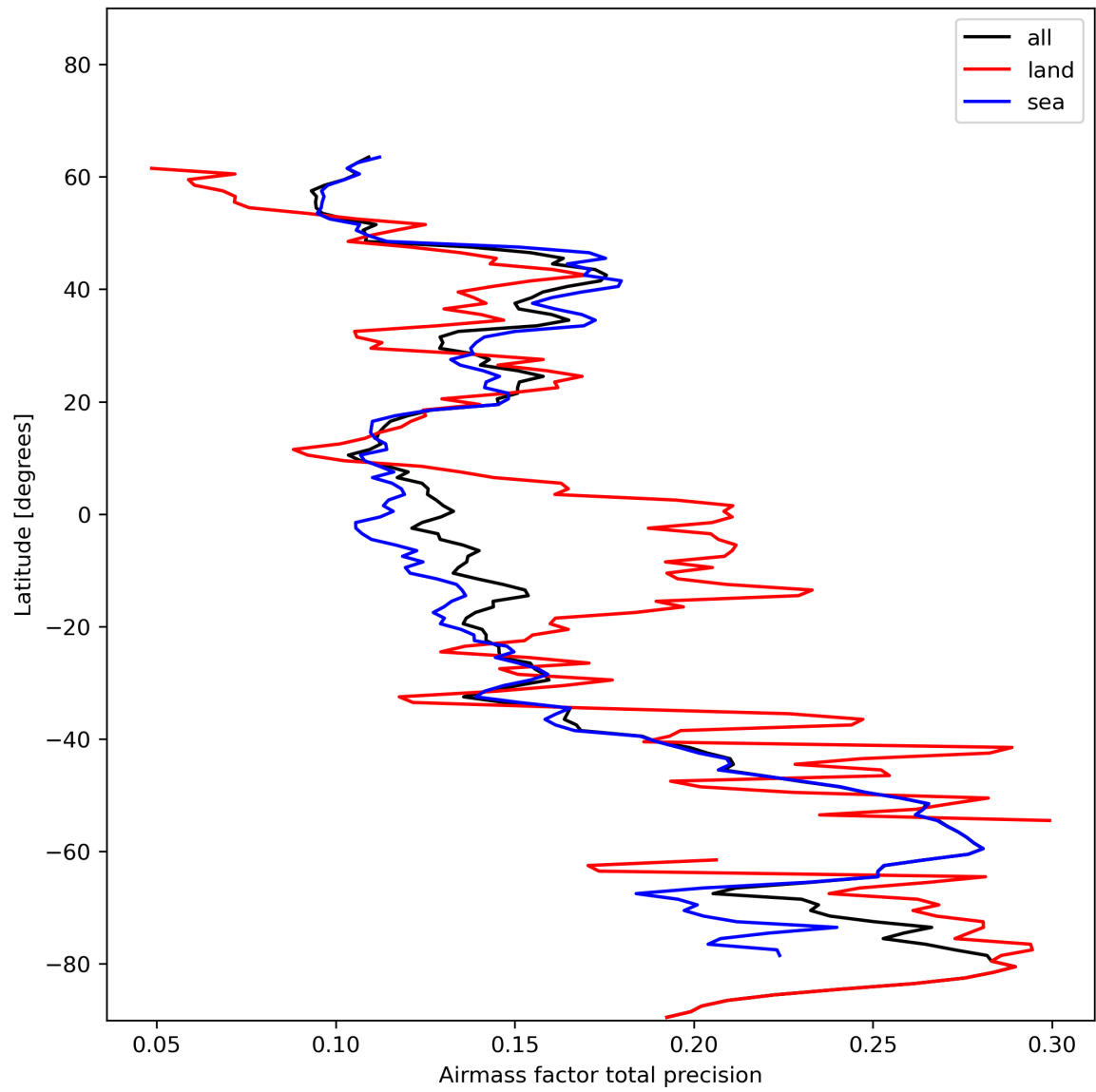
Figure 27: Zonal average of “Airmass factor total precision” for 2023-12-01 to 2023-12-03.
