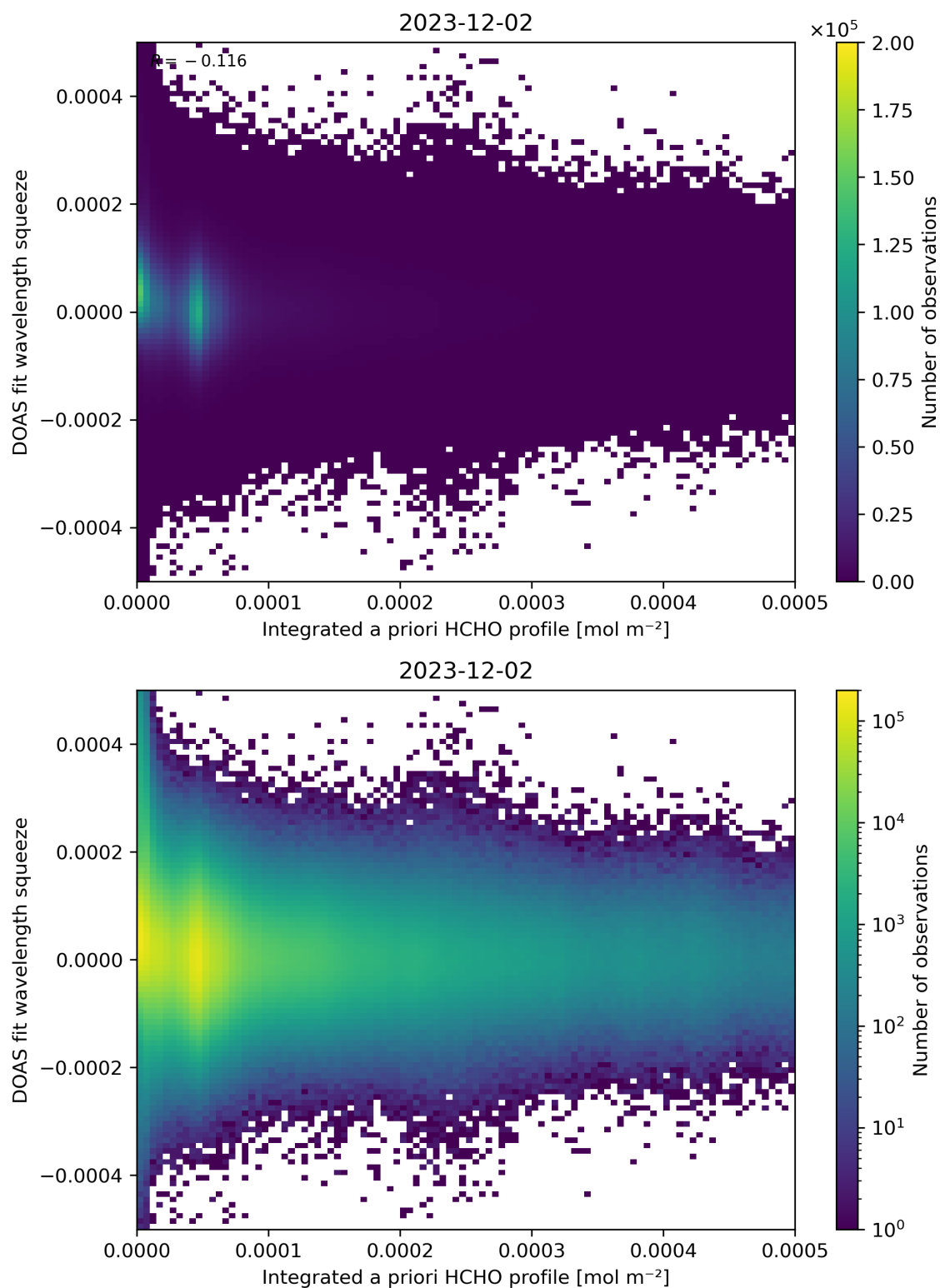
Figure 150: Scatter density plot of “Integrated a priori HCHO profile” against “DOAS fit wavelength squeeze” for 2023-12-01 to 2023-12-03.
