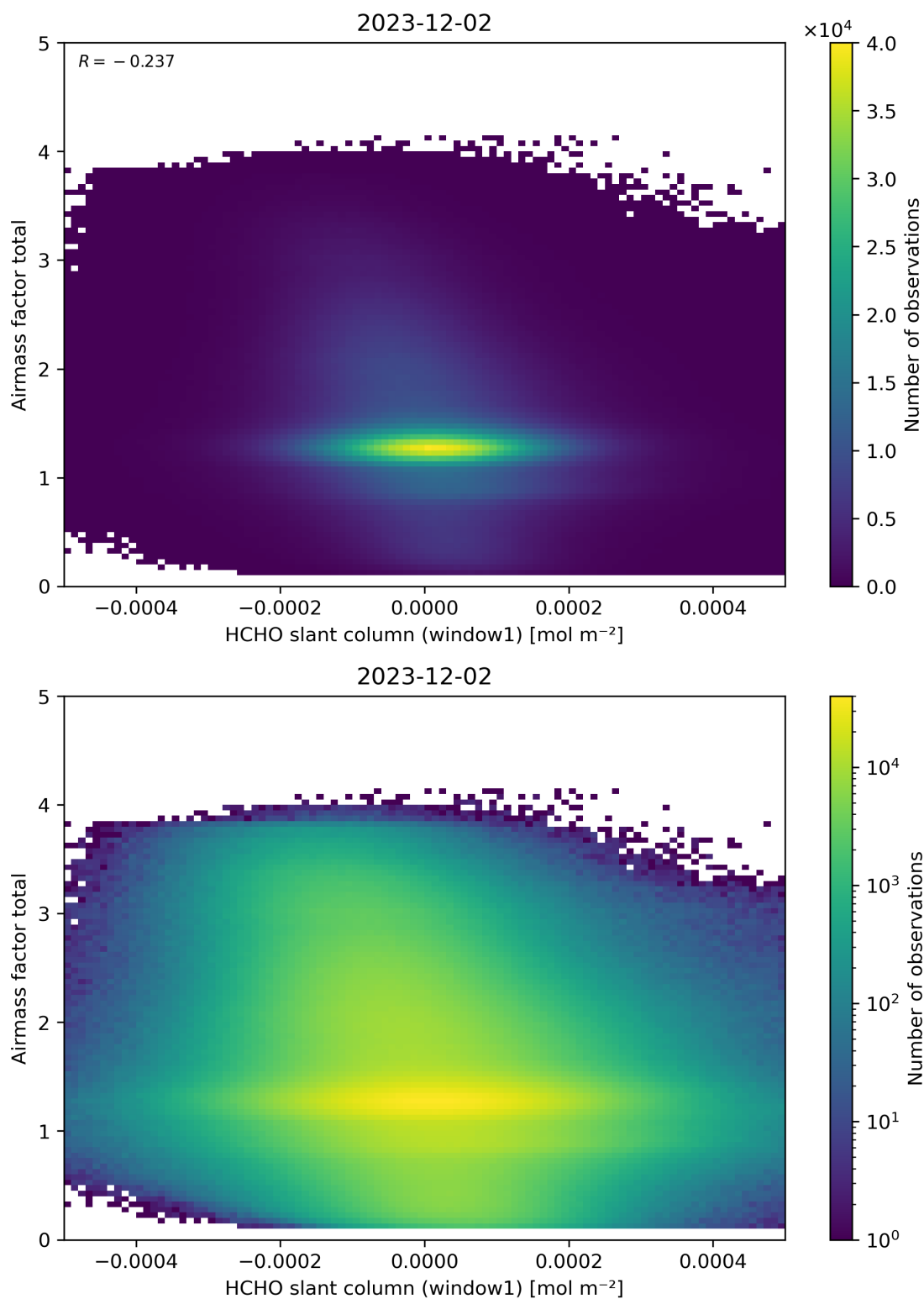
Figure 85: Scatter density plot of “HCHO slant column (window1)” against “Airmass factor total” for 2023-12-01 to 2023-12-03.
