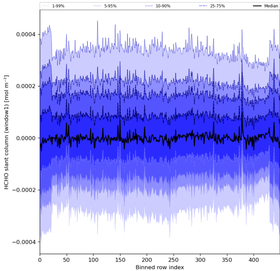
Figure 52: Along track statistics of “HCHO slant column (window1)” for 2023-12-01 to 2023-12-03
