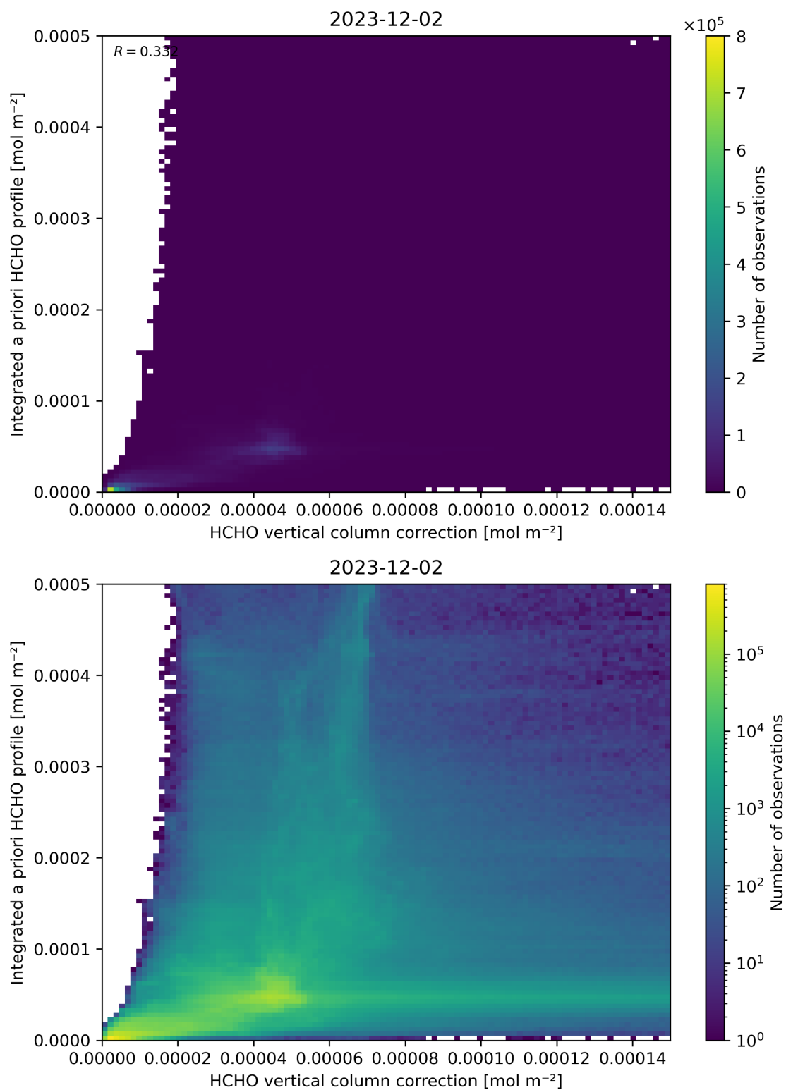
Figure 122: Scatter density plot of “HCHO vertical column correction” against “Integrated a priori HCHO profile” for 2023-12-01 to 2023-12-03.
