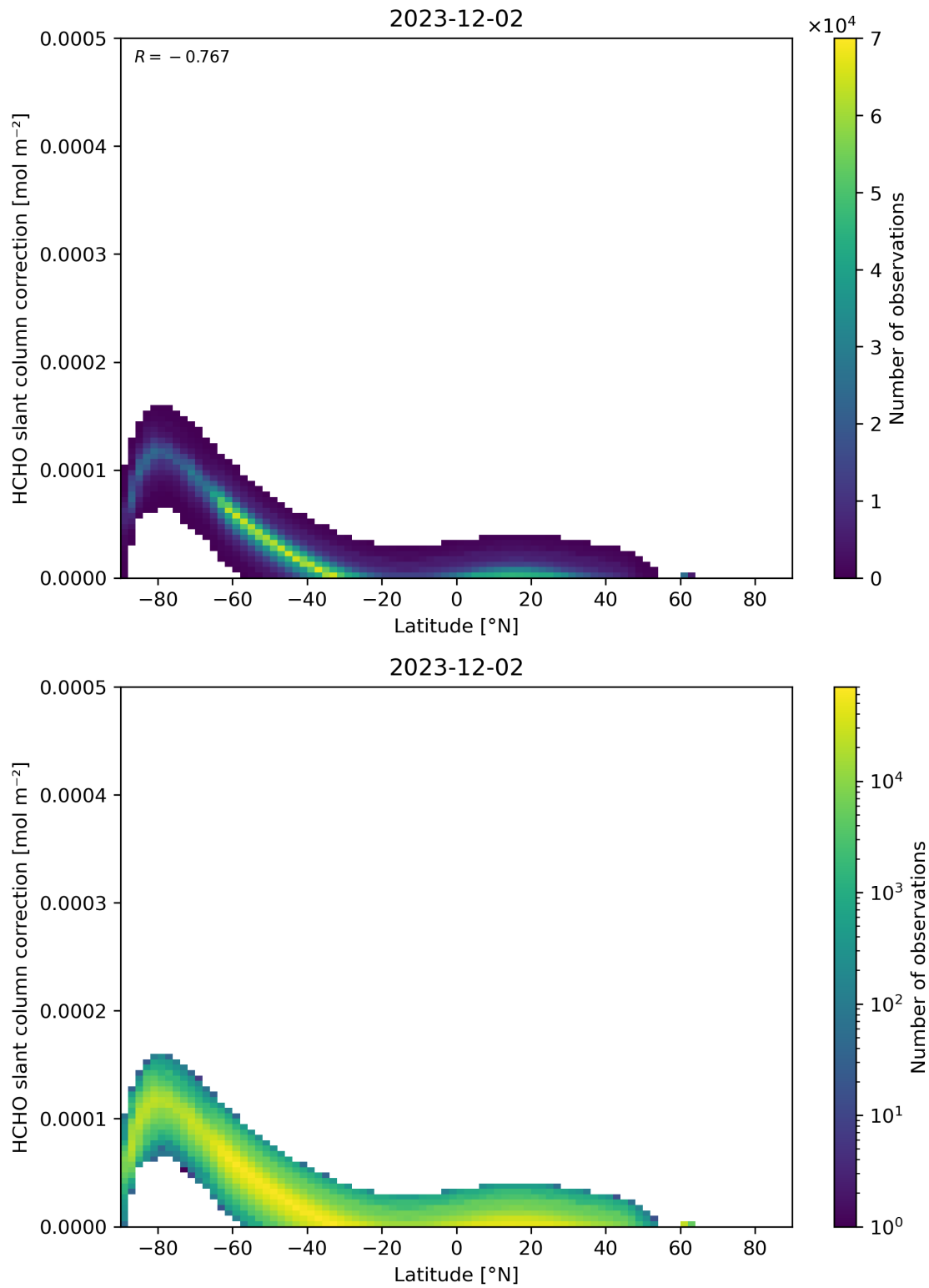
Figure 158: Scatter density plot of “Latitude” against “HCHO slant column correction” for 2023-12-01 to 2023-12-03.
