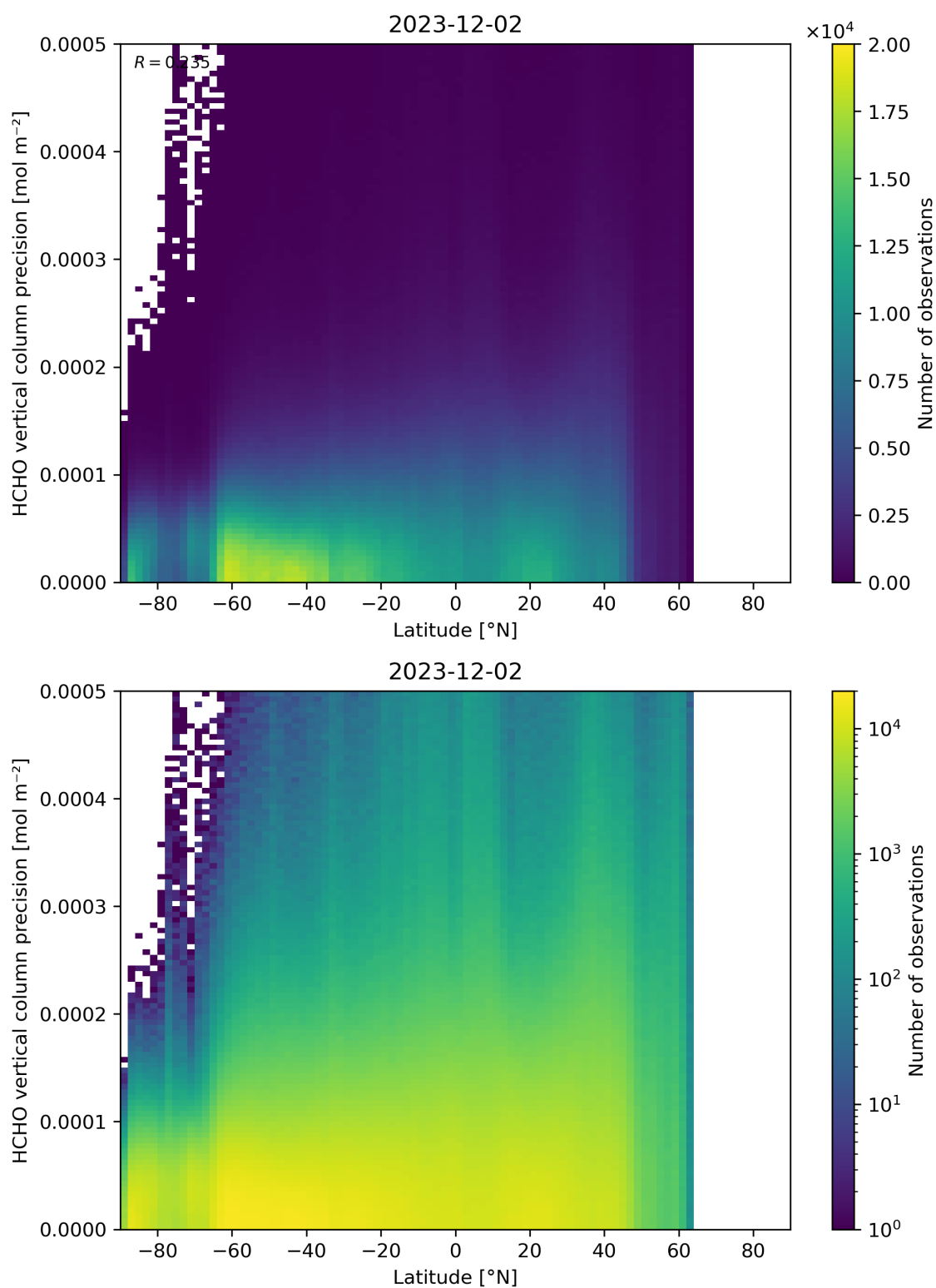
Figure 165: Scatter density plot of “Latitude” against “HCHO vertical column precision” for 2023-12-01 to 2023-12-03.
