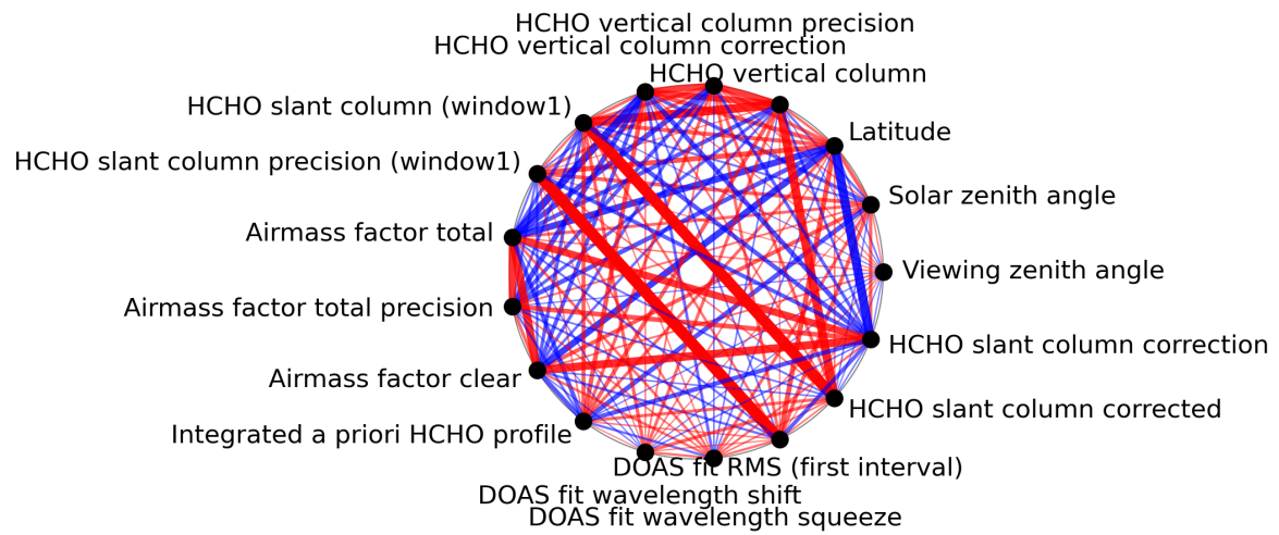
Figure 1: Map of correlation graph for 2023-12-01 to 2023-12-03.
