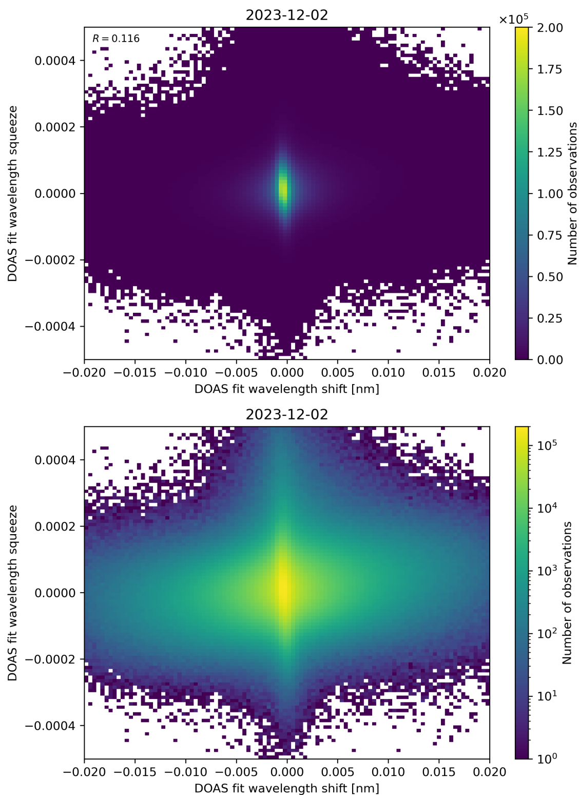
Figure 65: Scatter density plot of “DOAS fit wavelength shift” against “DOAS fit wavelength squeeze” for 2023-12-01 to 2023-12-03.
