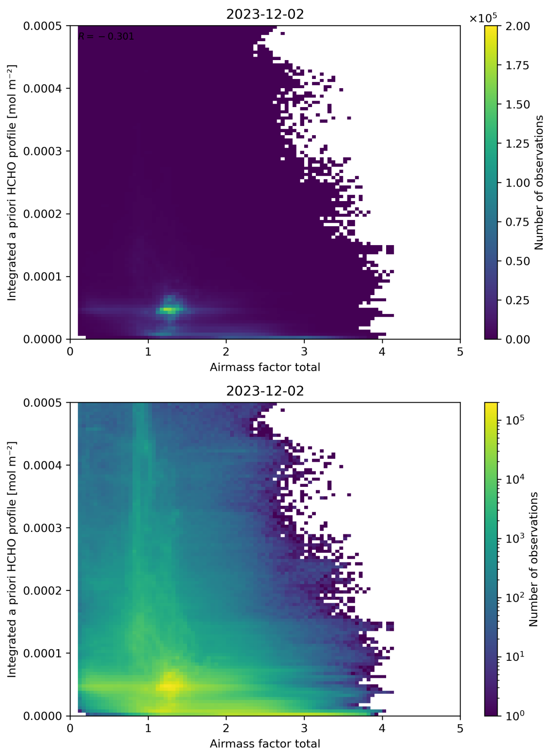
Figure 104: Scatter density plot of “Airmass factor total” against “Integrated a priori HCHO profile” for 2023-12-01 to 2023-12-03.
