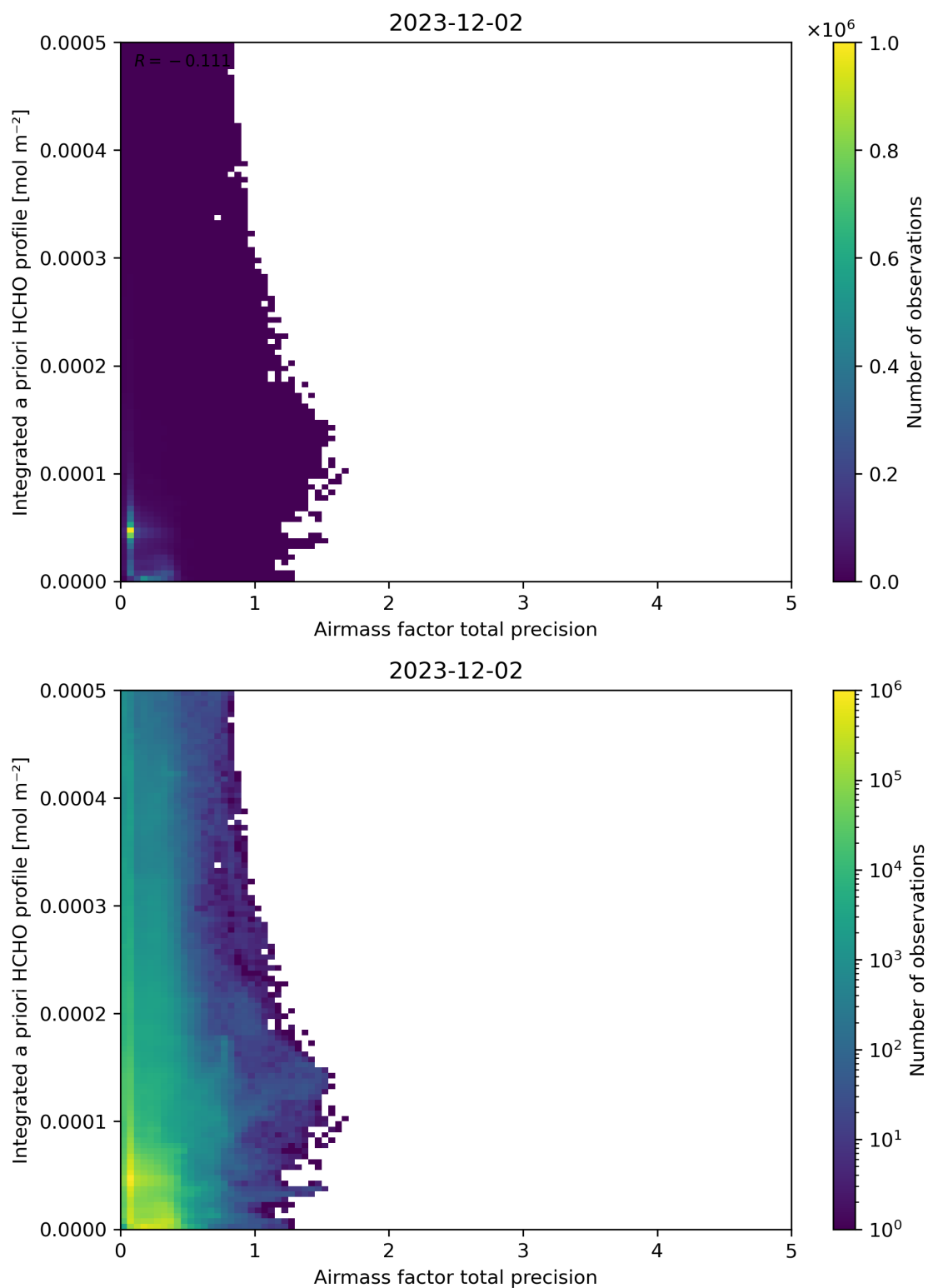
Figure 111: Scatter density plot of “Airmass factor total precision” against “Integrated a priori HCHO profile” for 2023-12-01 to 2023-12-03.
