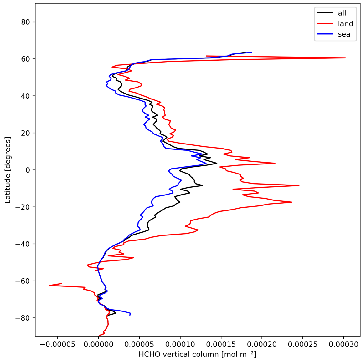
Figure 21: Zonal average of “HCHO vertical column” for 2023-12-01 to 2023-12-03.
