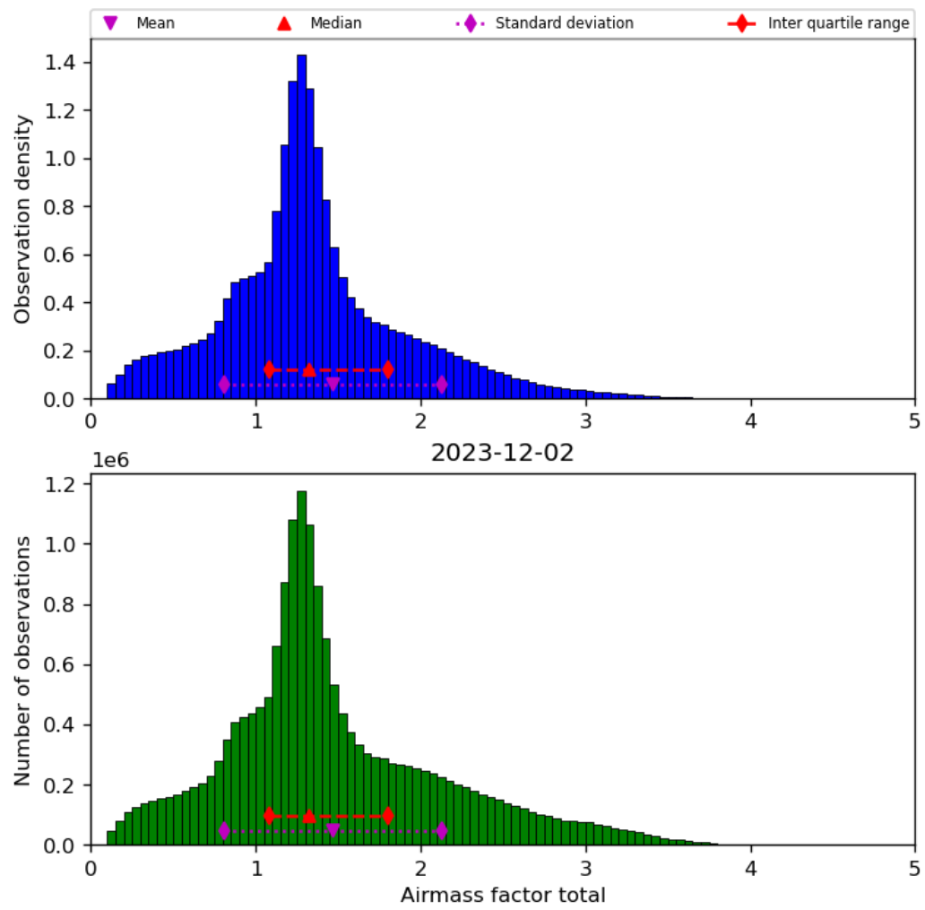
Figure 40: Histogram of “Airmass factor total” for 2023-12-01 to 2023-12-03
