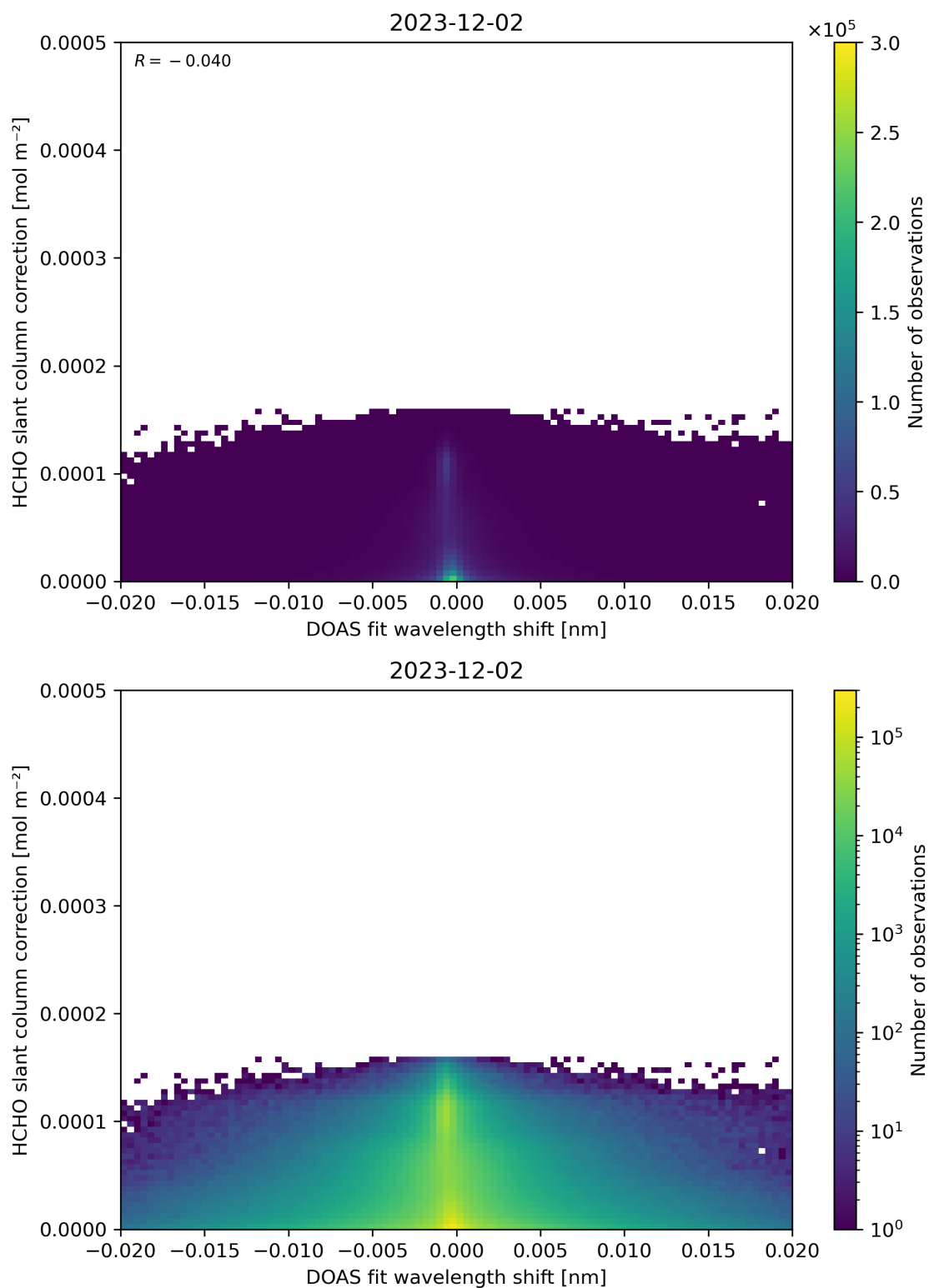
Figure 67: Scatter density plot of “DOAS fit wavelength shift” against “HCHO slant column correction” for 2023-12-01 to 2023-12-03.
