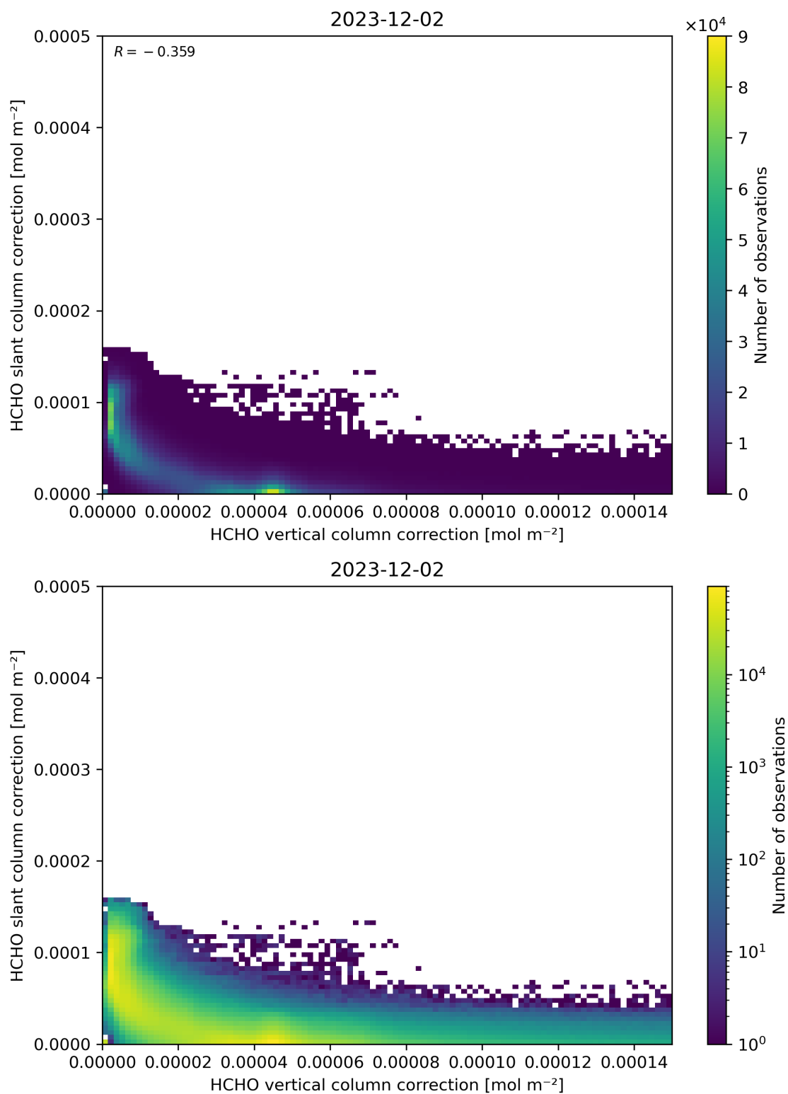
Figure 117: Scatter density plot of “HCHO vertical column correction” against “HCHO slant column correction” for 2023-12-01 to 2023-12-03.
