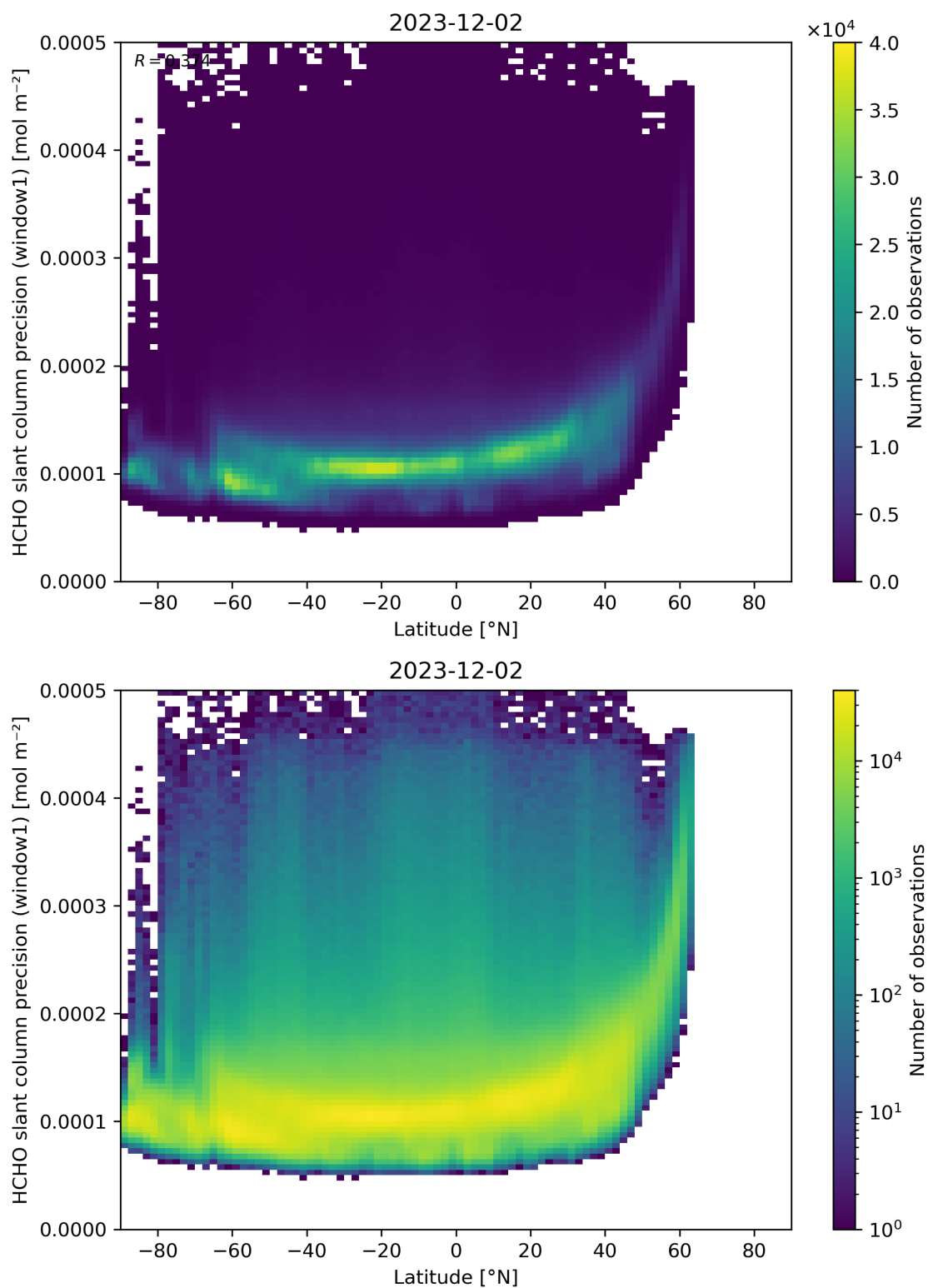
Figure 160: Scatter density plot of “Latitude” against “HCHO slant column precision (window1)” for 2023-12-01 to 2023-12-03.
