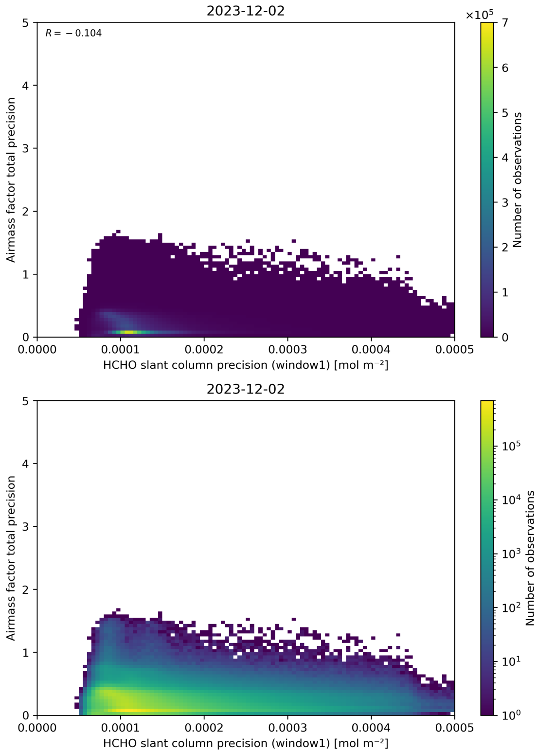
Figure 95: Scatter density plot of “HCHO slant column precision (window1)” against “Airmass factor total precision” for 2023-12-01 to 2023-12-03.
