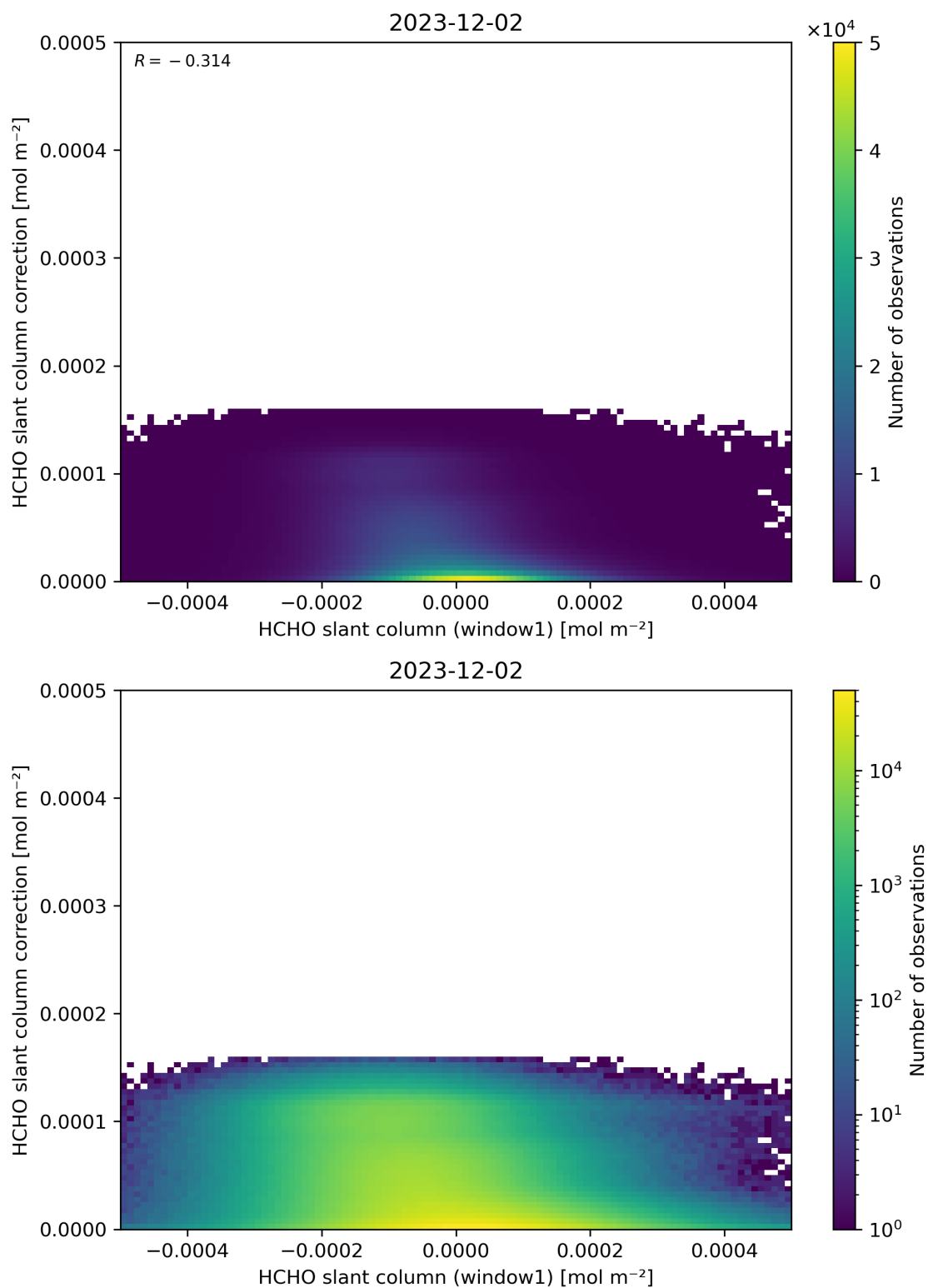
Figure 83: Scatter density plot of “HCHO slant column (window1)” against “HCHO slant column correction” for 2023-12-01 to 2023-12-03.
