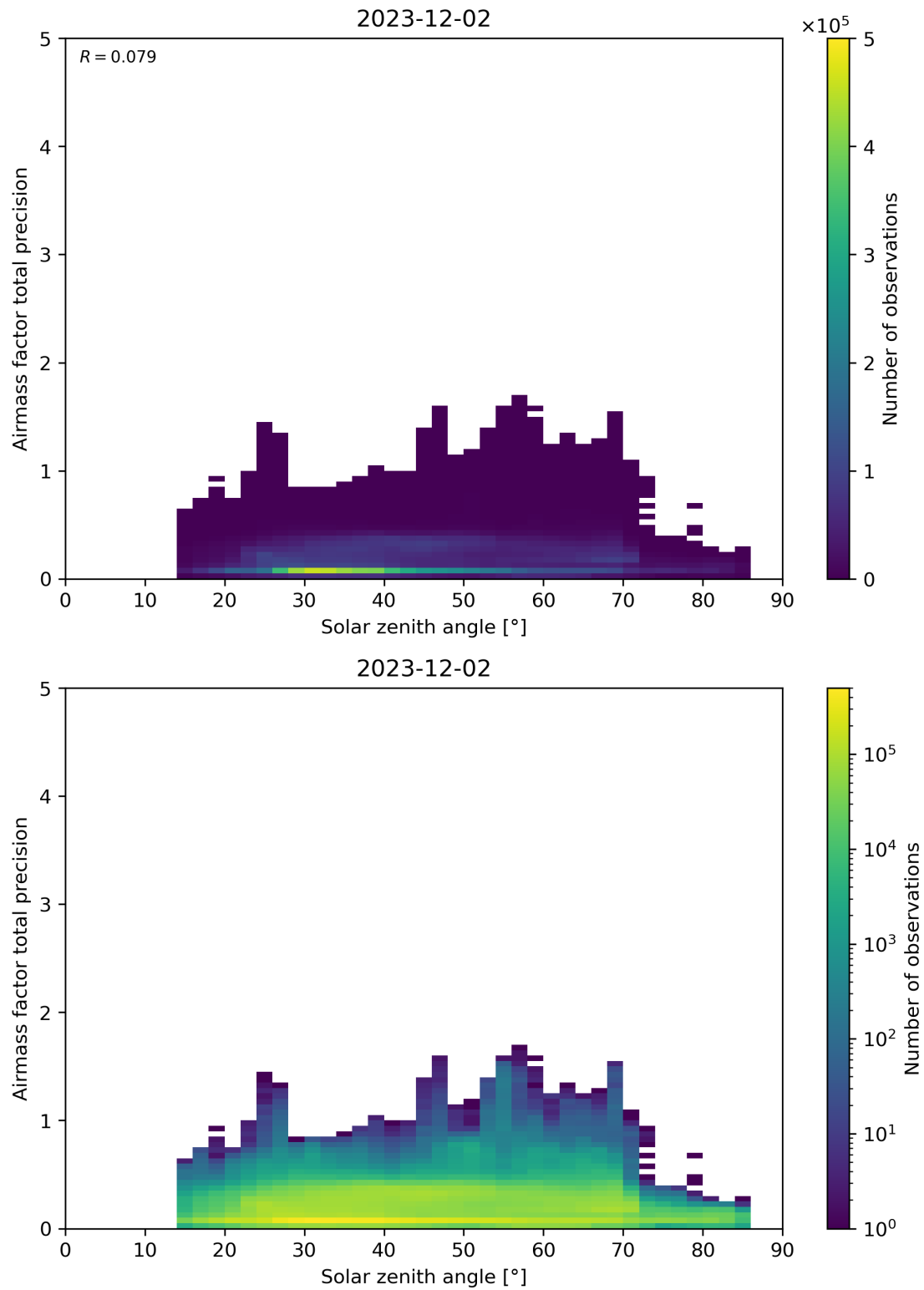
Figure 176: Scatter density plot of “Solar zenith angle” against “Airmass factor total precision” for 2023-12-01 to 2023-12-03.
