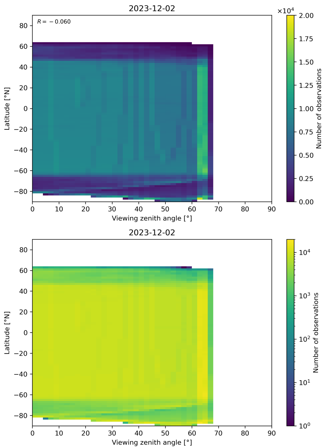
Figure 196: Scatter density plot of “Viewing zenith angle” against “Latitude” for 2023-12-01 to 2023-12-03.
