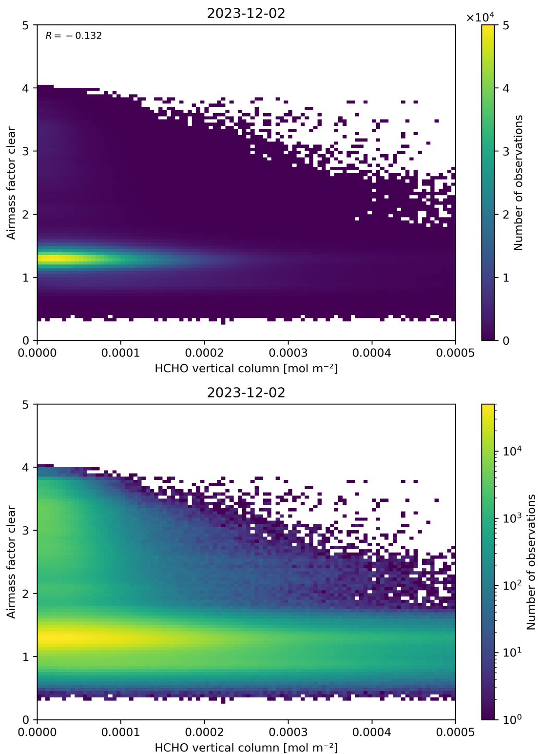
Figure 126: Scatter density plot of “HCHO vertical column” against “Airmass factor clear” for 2023-12-01 to 2023-12-03.
