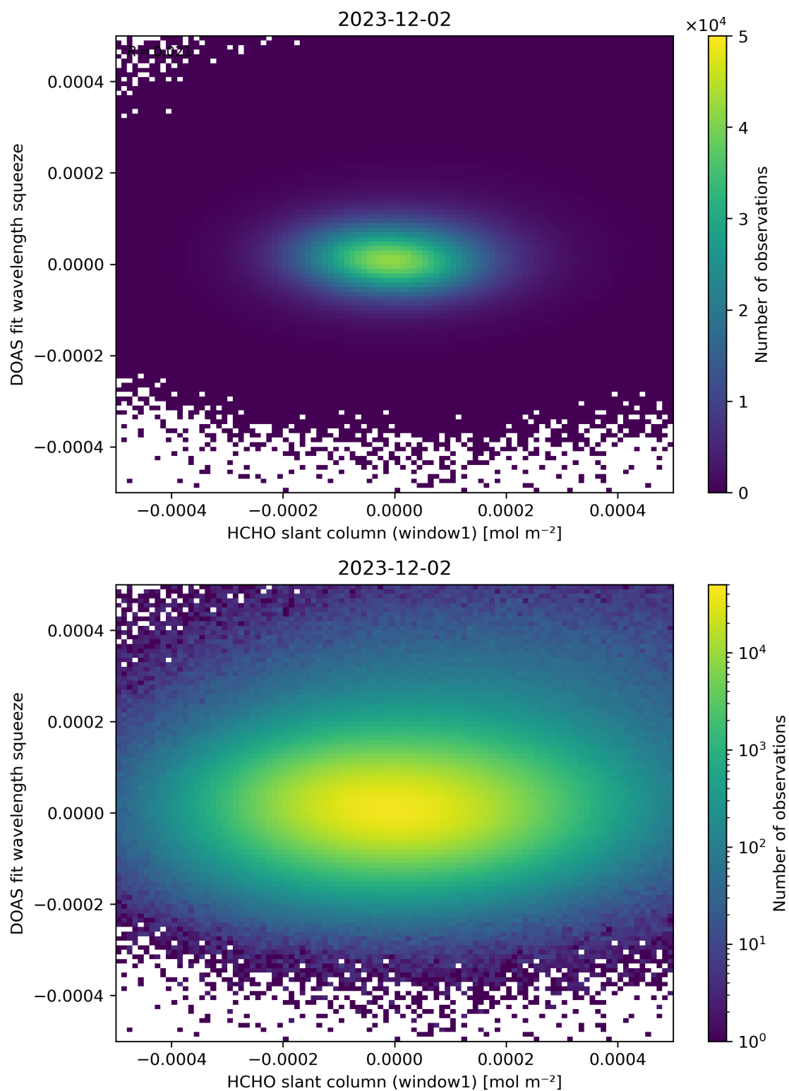
Figure 80: Scatter density plot of “HCHO slant column (window1)” against “DOAS fit wavelength squeeze” for 2023-12-01 to 2023-12-03.
