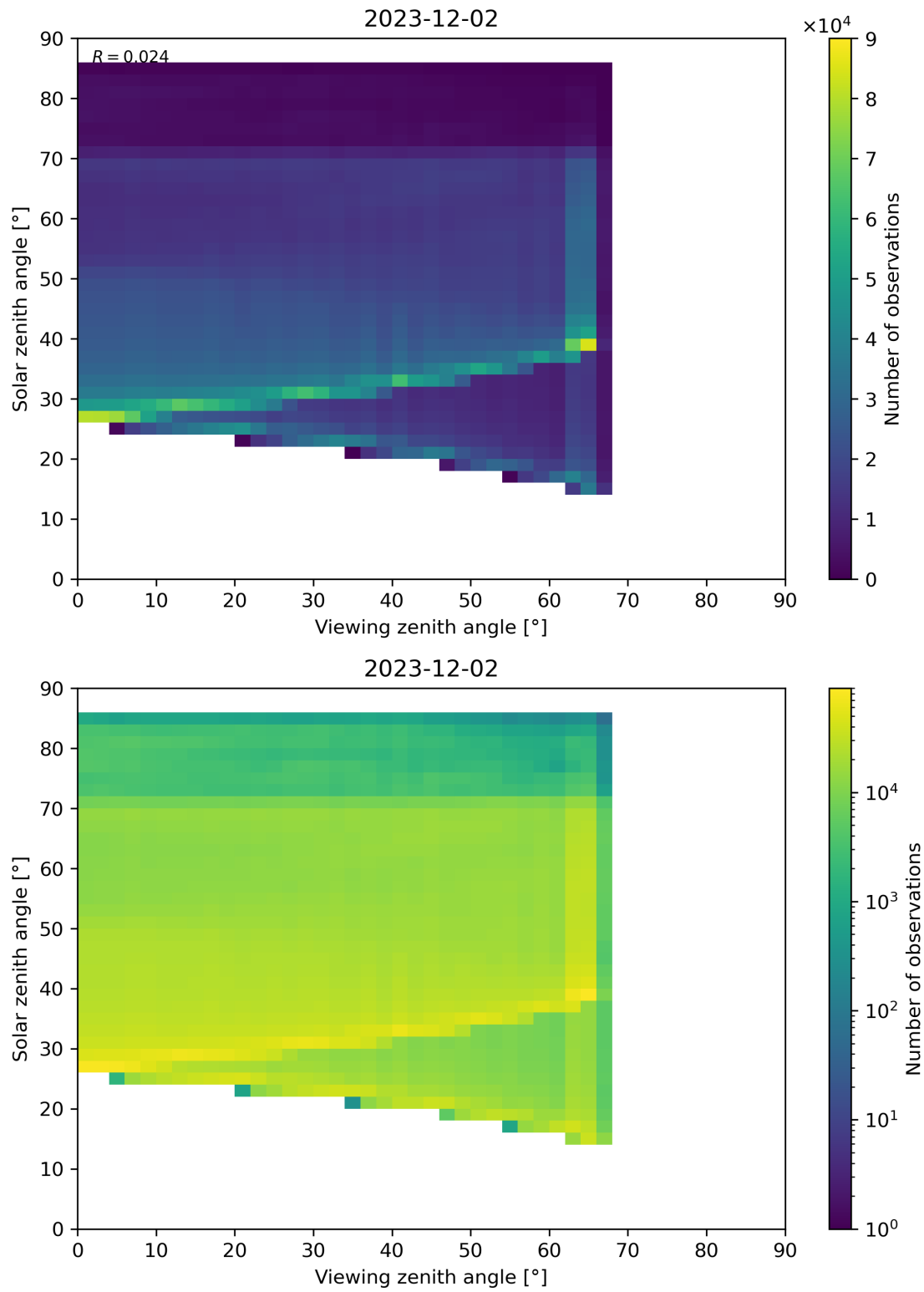
Figure 197: Scatter density plot of “Viewing zenith angle” against “Solar zenith angle” for 2023-12-01 to 2023-12-03.
