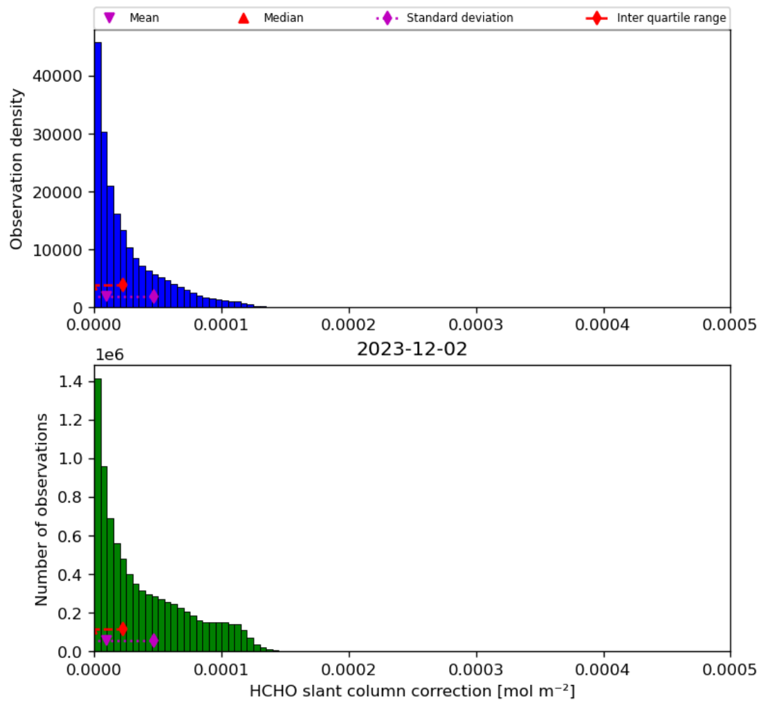
Figure 47: Histogram of “HCHO slant column correction” for 2023-12-01 to 2023-12-03
