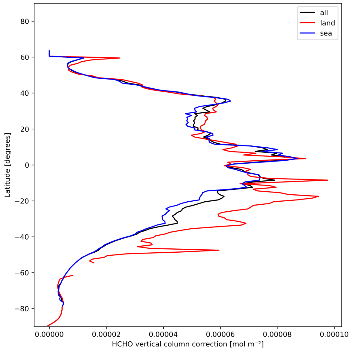
Figure 23: Zonal average of “HCHO vertical column correction” for 2023-12-01 to 2023-12-03.
