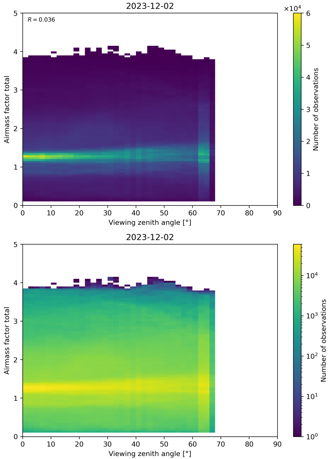
Figure 190: Scatter density plot of “Viewing zenith angle” against “Airmass factor total” for 2023-12-01 to 2023-12-03.
