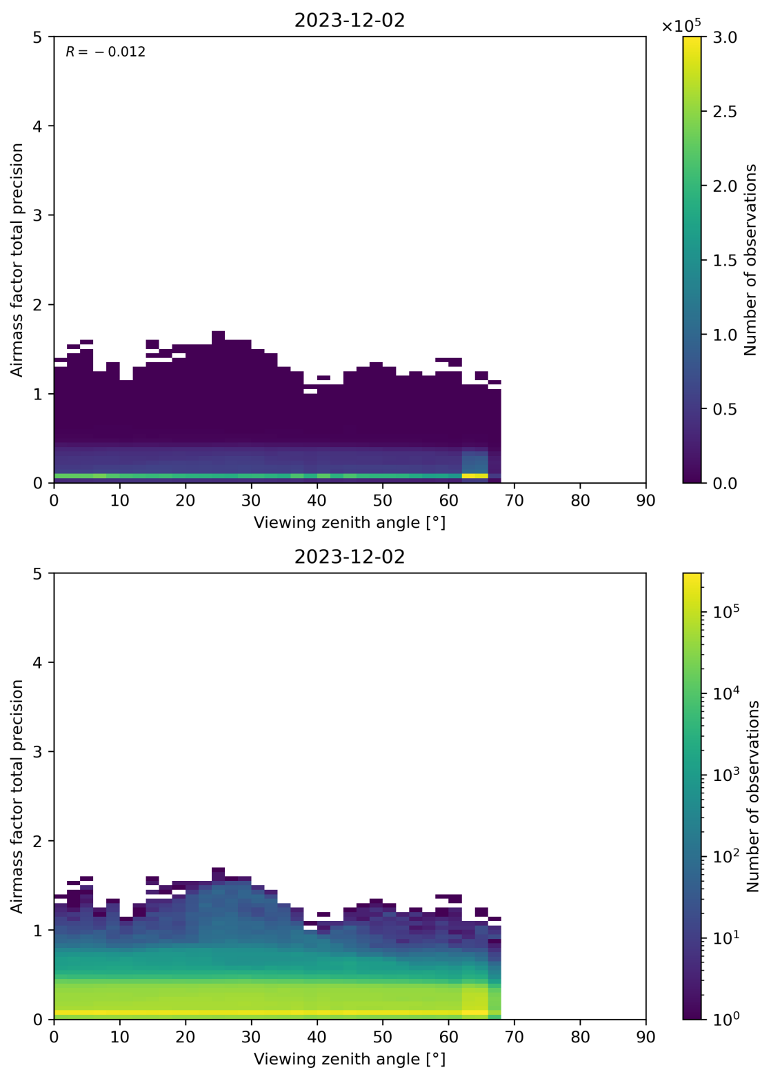
Figure 191: Scatter density plot of “Viewing zenith angle” against “Airmass factor total precision” for 2023-12-01 to 2023-12-03.
