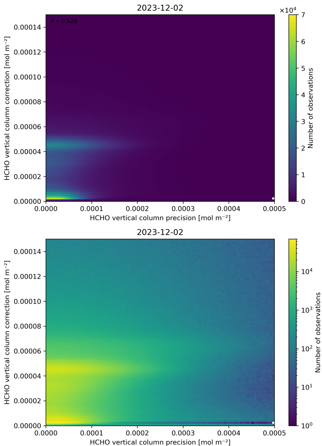
Figure 146: Scatter density plot of “HCHO vertical column precision” against “HCHO vertical column correction” for 2023-12-01 to 2023-12-03.
