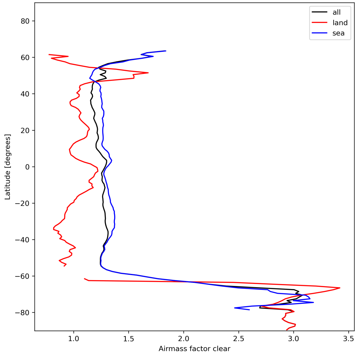
Figure 28: Zonal average of “Airmass factor clear” for 2023-12-01 to 2023-12-03.
