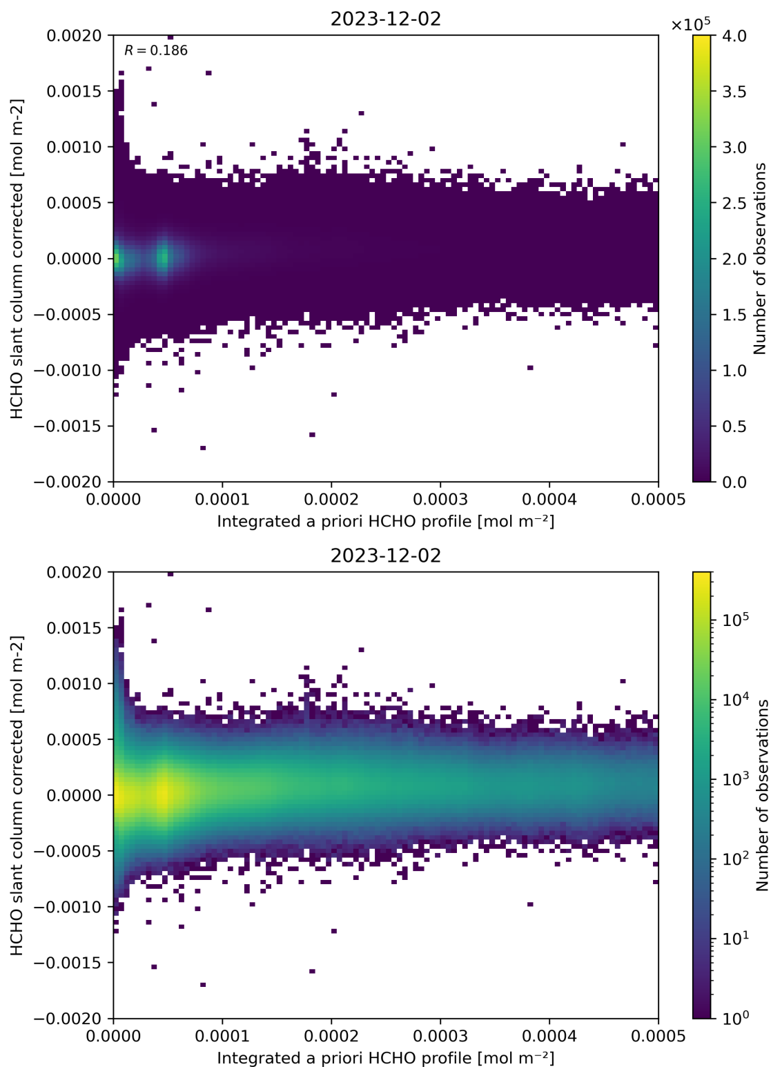
Figure 151: Scatter density plot of “Integrated a priori HCHO profile” against “HCHO slant column corrected” for 2023-12-01 to 2023-12-03.
