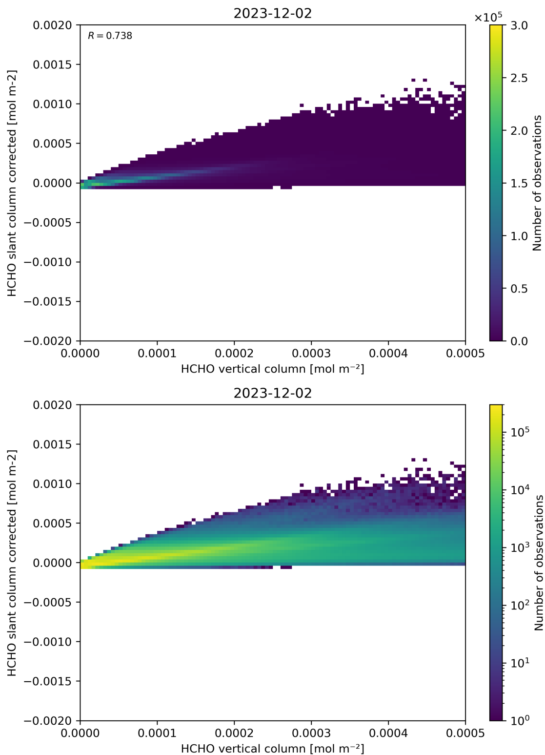
Figure 127: Scatter density plot of “HCHO vertical column” against “HCHO slant column corrected” for 2023-12-01 to 2023-12-03.
