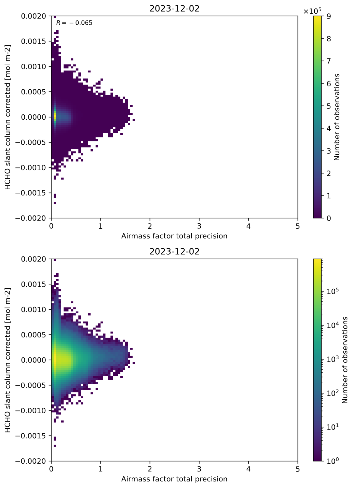
Figure 109: Scatter density plot of “Airmass factor total precision” against “HCHO slant column corrected” for 2023-12-01 to 2023-12-03.
