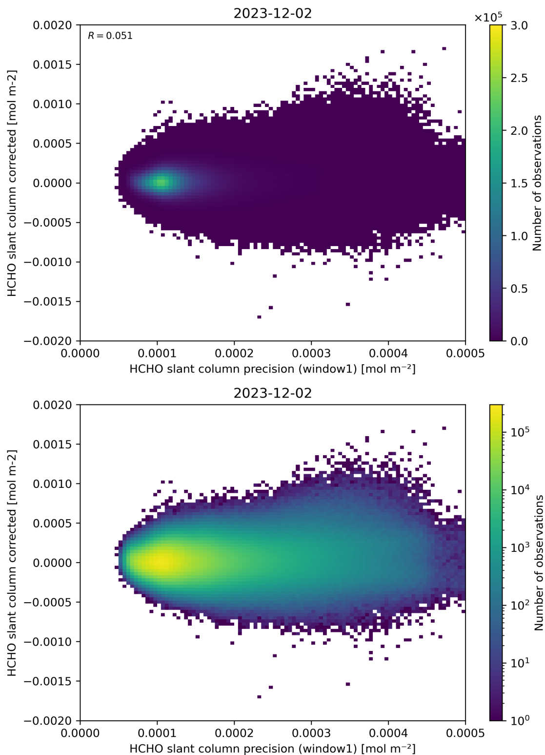
Figure 92: Scatter density plot of “HCHO slant column precision (window1)” against “HCHO slant column corrected” for 2023-12-01 to 2023-12-03.
