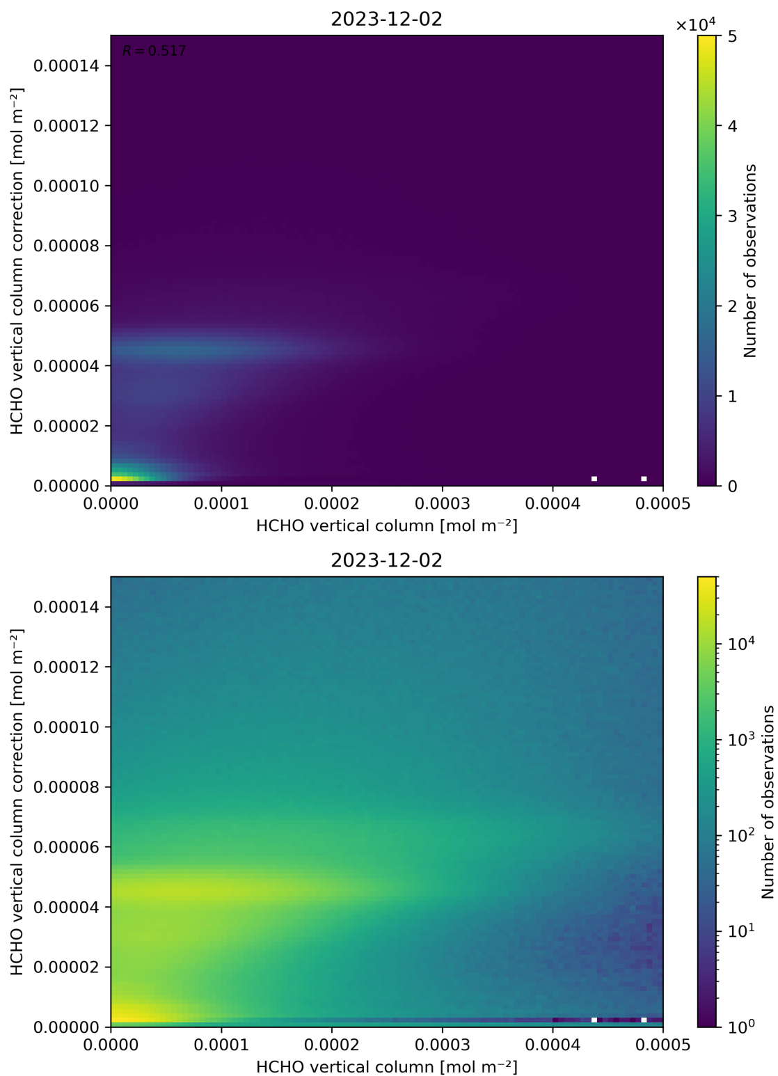
Figure 133: Scatter density plot of “HCHO vertical column” against “HCHO vertical column correction” for 2023-12-01 to 2023-12-03.
