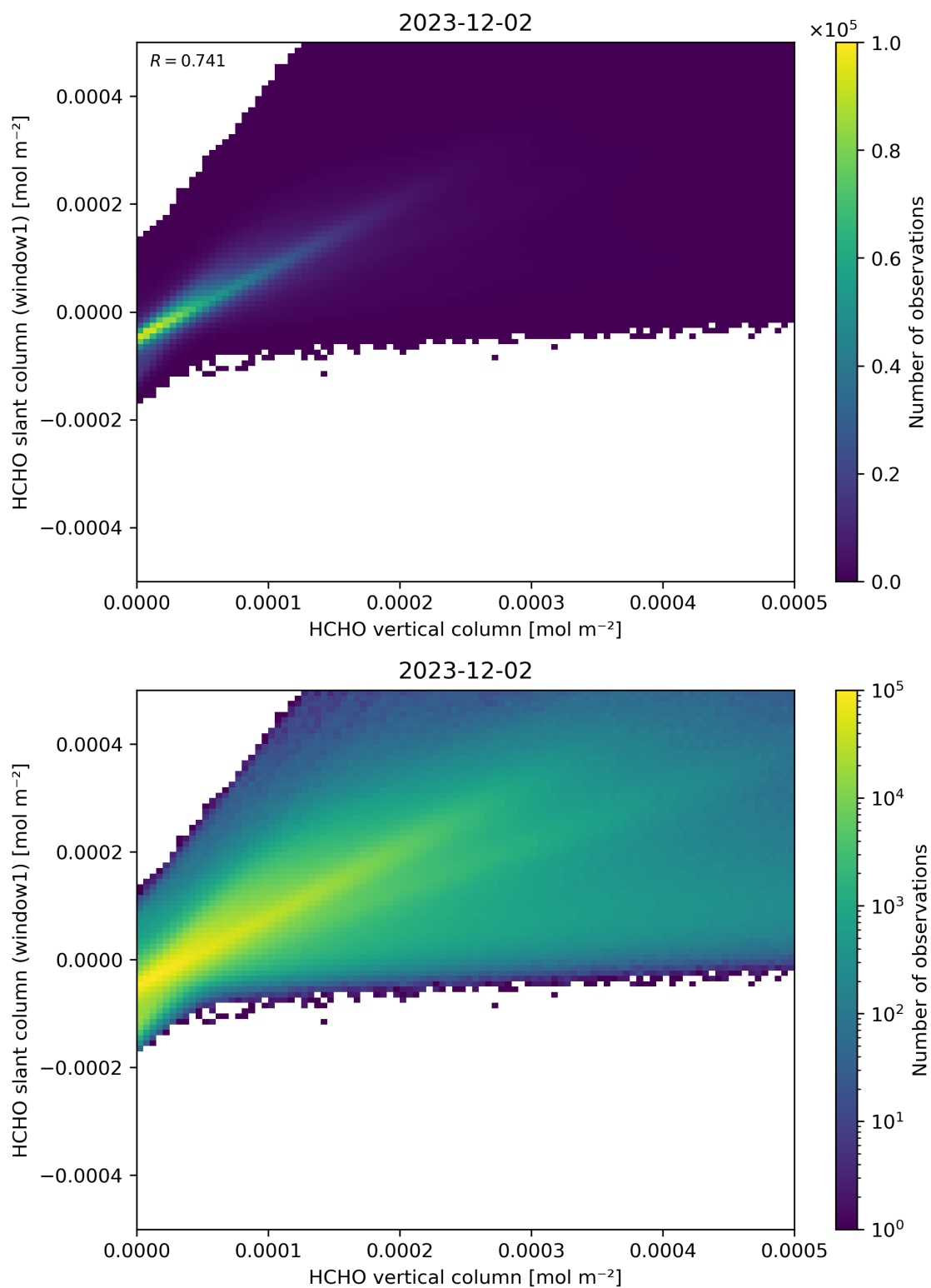
Figure 129: Scatter density plot of “HCHO vertical column” against “HCHO slant column (window1)” for 2023-12-01 to 2023-12-03.
