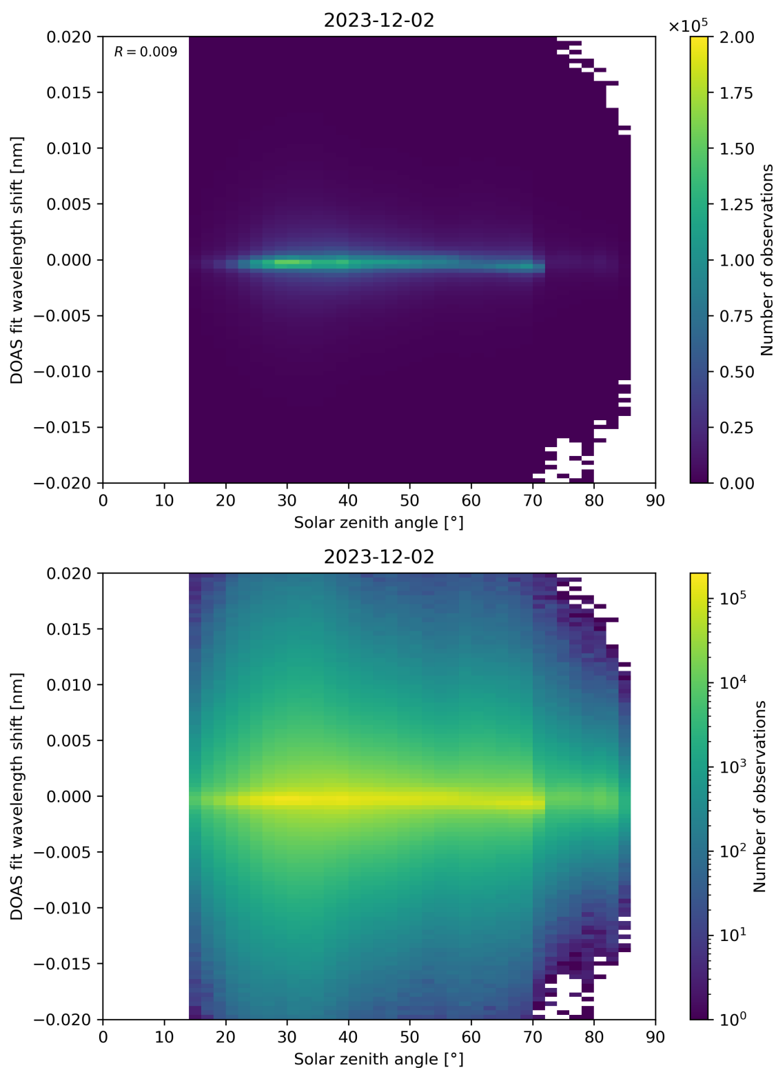
Figure 168: Scatter density plot of “Solar zenith angle” against “DOAS fit wavelength shift” for 2023-12-01 to 2023-12-03.
