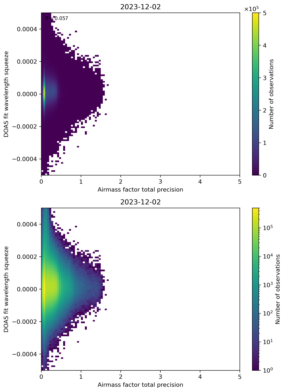
Figure 107: Scatter density plot of “Airmass factor total precision” against “DOAS fit wavelength squeeze” for 2023-12-01 to 2023-12-03.
