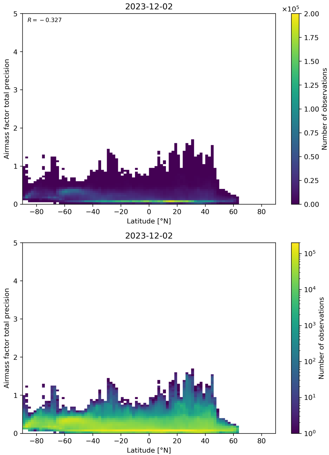
Figure 162: Scatter density plot of “Latitude” against “Airmass factor total precision” for 2023-12-01 to 2023-12-03.
