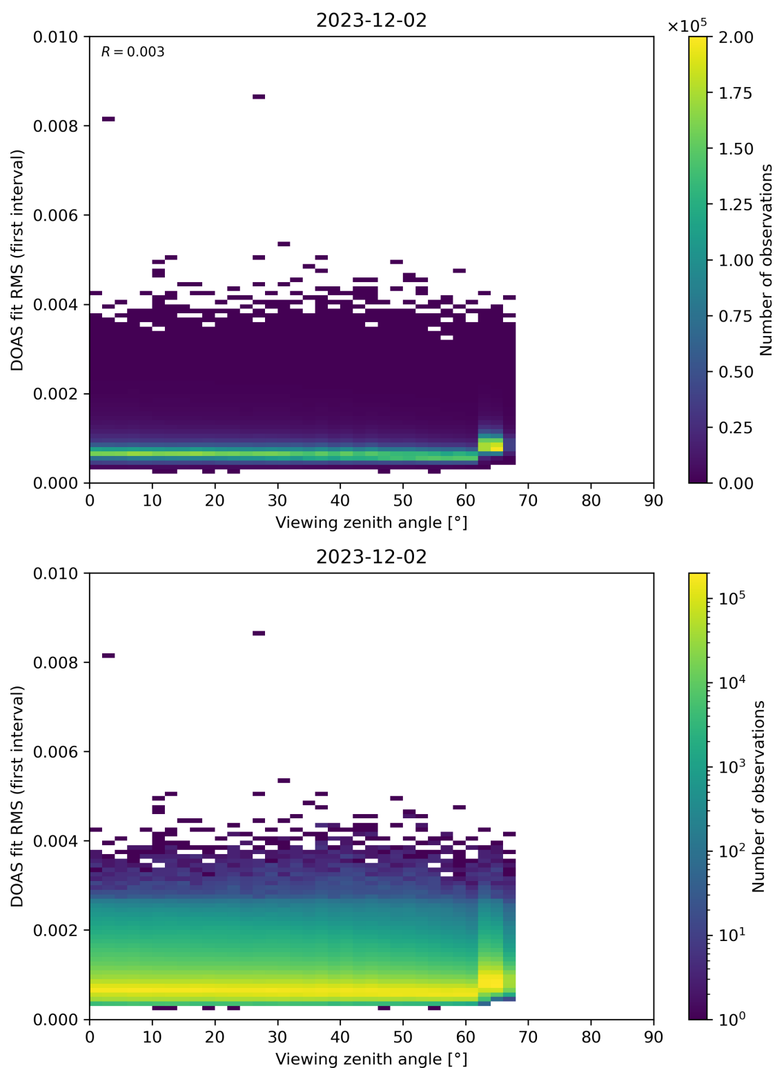
Figure 182: Scatter density plot of “Viewing zenith angle” against “DOAS fit RMS (first interval)” for 2023-12-01 to 2023-12-03.
