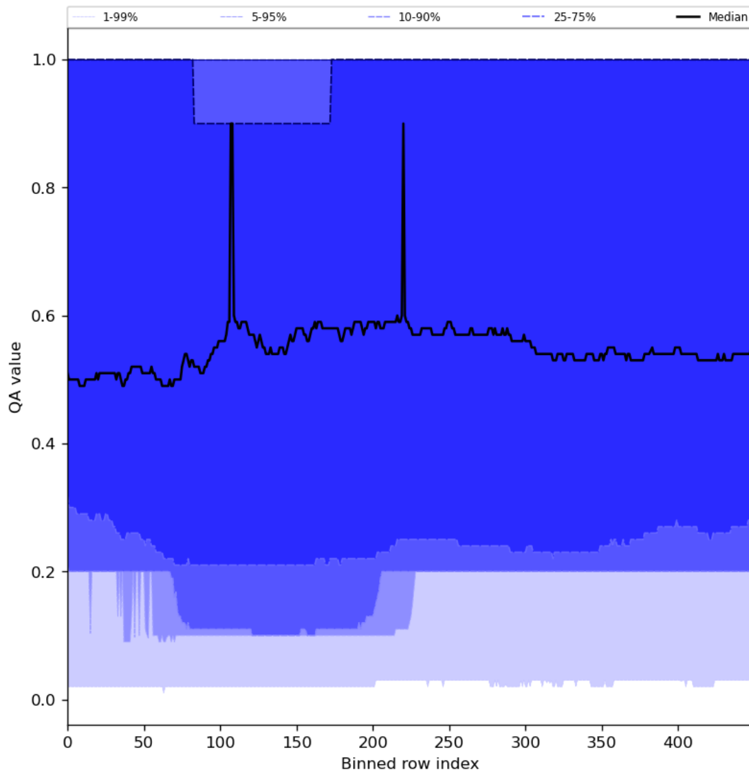
Figure 48: Along track statistics of “QA value” for 2023-12-01 to 2023-12-03
