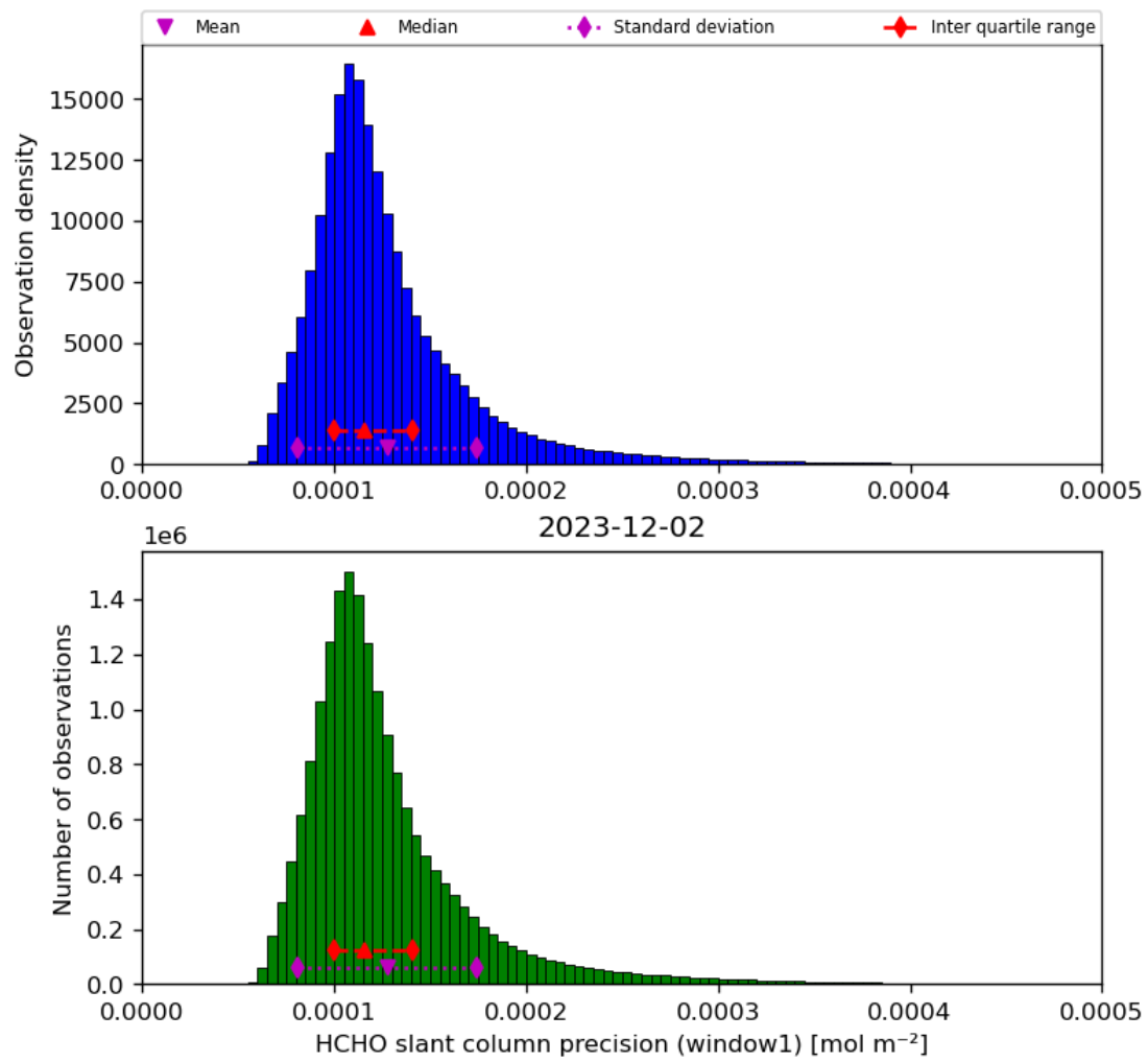
Figure 39: Histogram of “HCHO slant column precision (window1)” for 2023-12-01 to 2023-12-03
