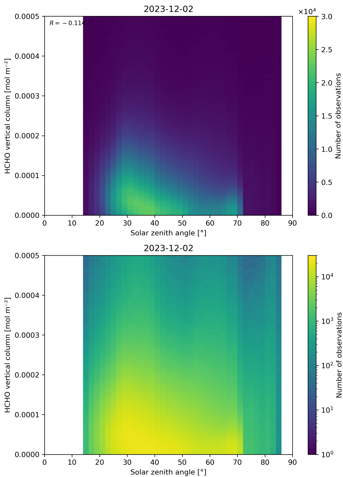
Figure 177: Scatter density plot of “Solar zenith angle” against “HCHO vertical column” for 2023-12-01 to 2023-12-03.
