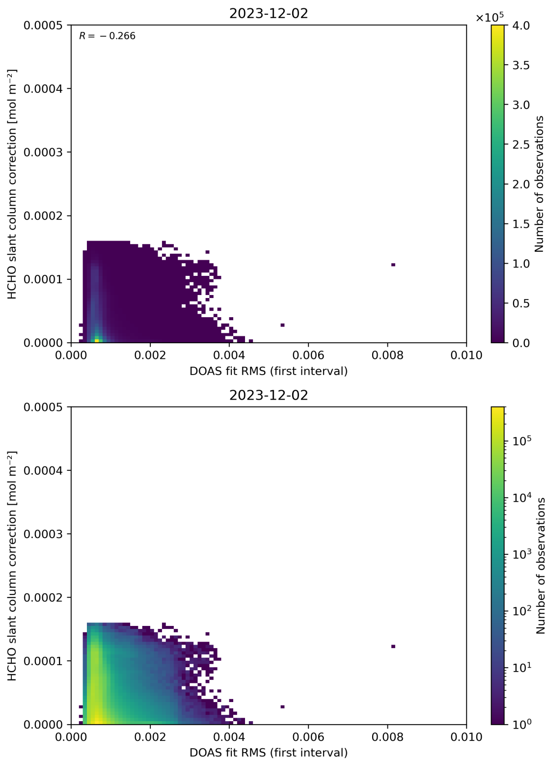
Figure 63: Scatter density plot of “DOAS fit RMS (first interval)” against “HCHO slant column correction” for 2023-12-01 to 2023-12-03.
