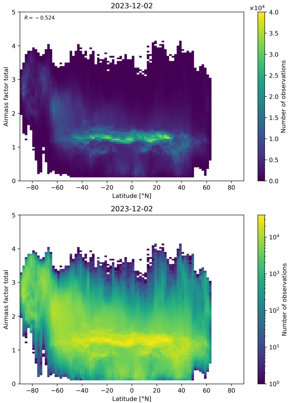
Figure 161: Scatter density plot of “Latitude” against “Airmass factor total” for 2023-12-01 to 2023-12-03.
