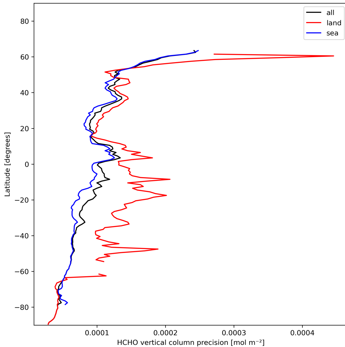
Figure 22: Zonal average of “HCHO vertical column precision” for 2023-12-01 to 2023-12-03.
