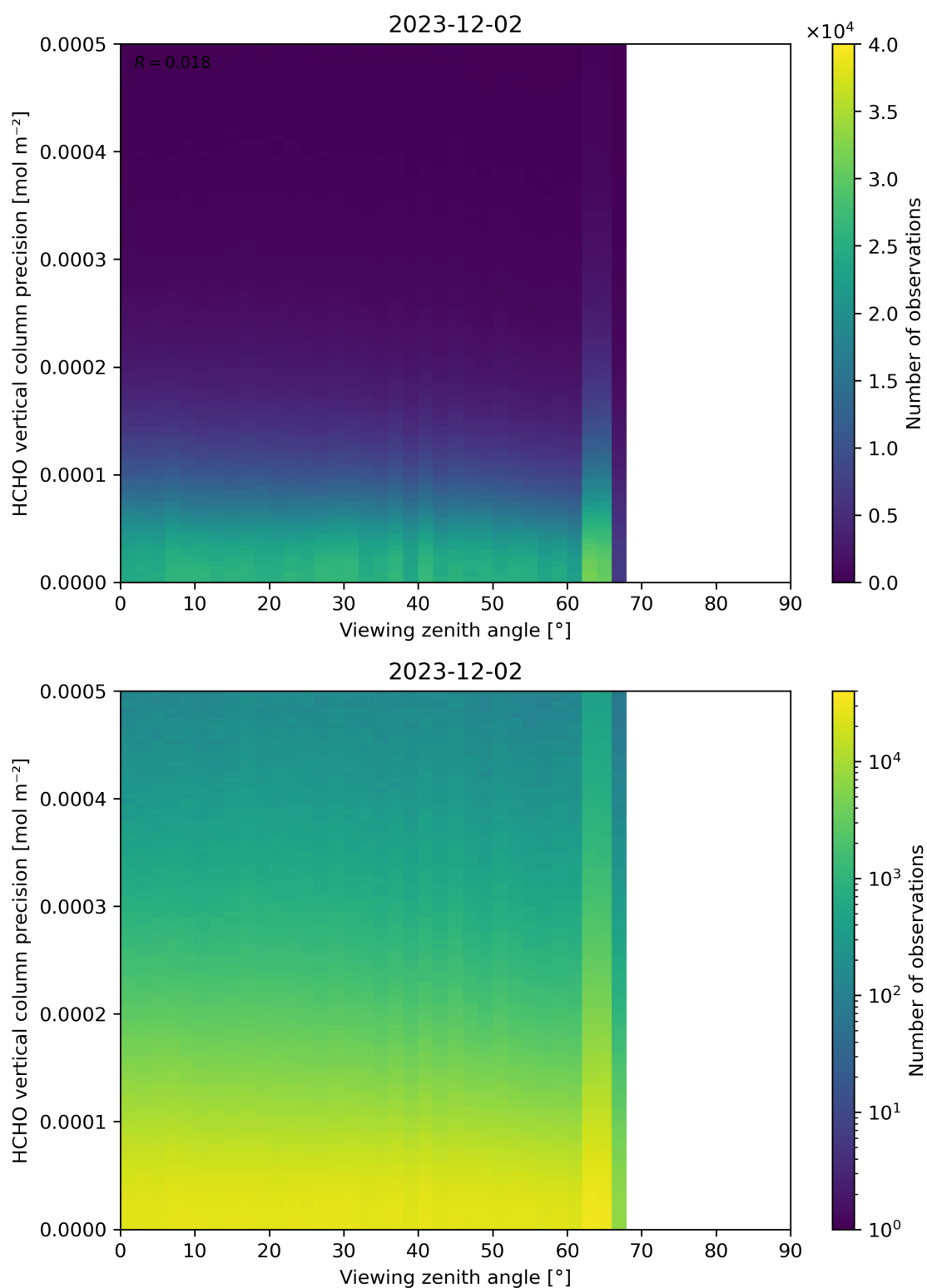
Figure 194: Scatter density plot of “Viewing zenith angle” against “HCHO vertical column precision” for 2023-12-01 to 2023-12-03.
