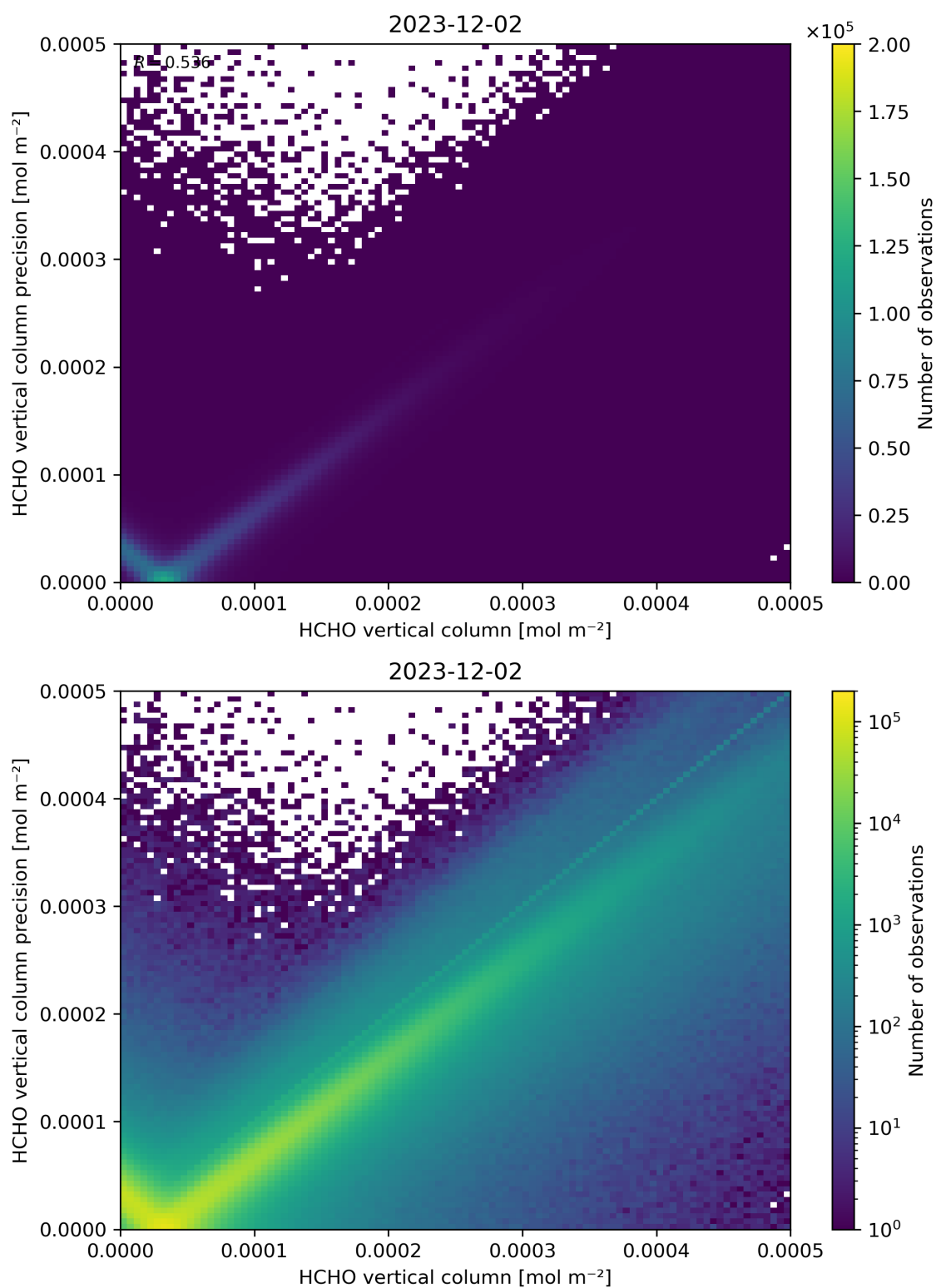
Figure 134: Scatter density plot of “HCHO vertical column” against “HCHO vertical column precision” for 2023-12-01 to 2023-12-03.
