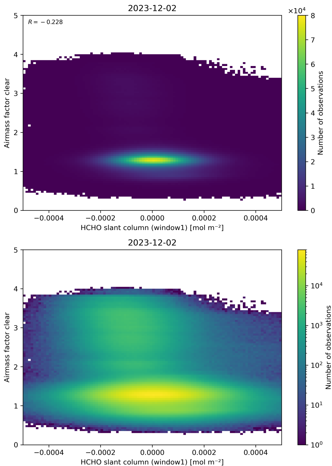
Figure 81: Scatter density plot of “HCHO slant column (window1)” against “Airmass factor clear” for 2023-12-01 to 2023-12-03.
