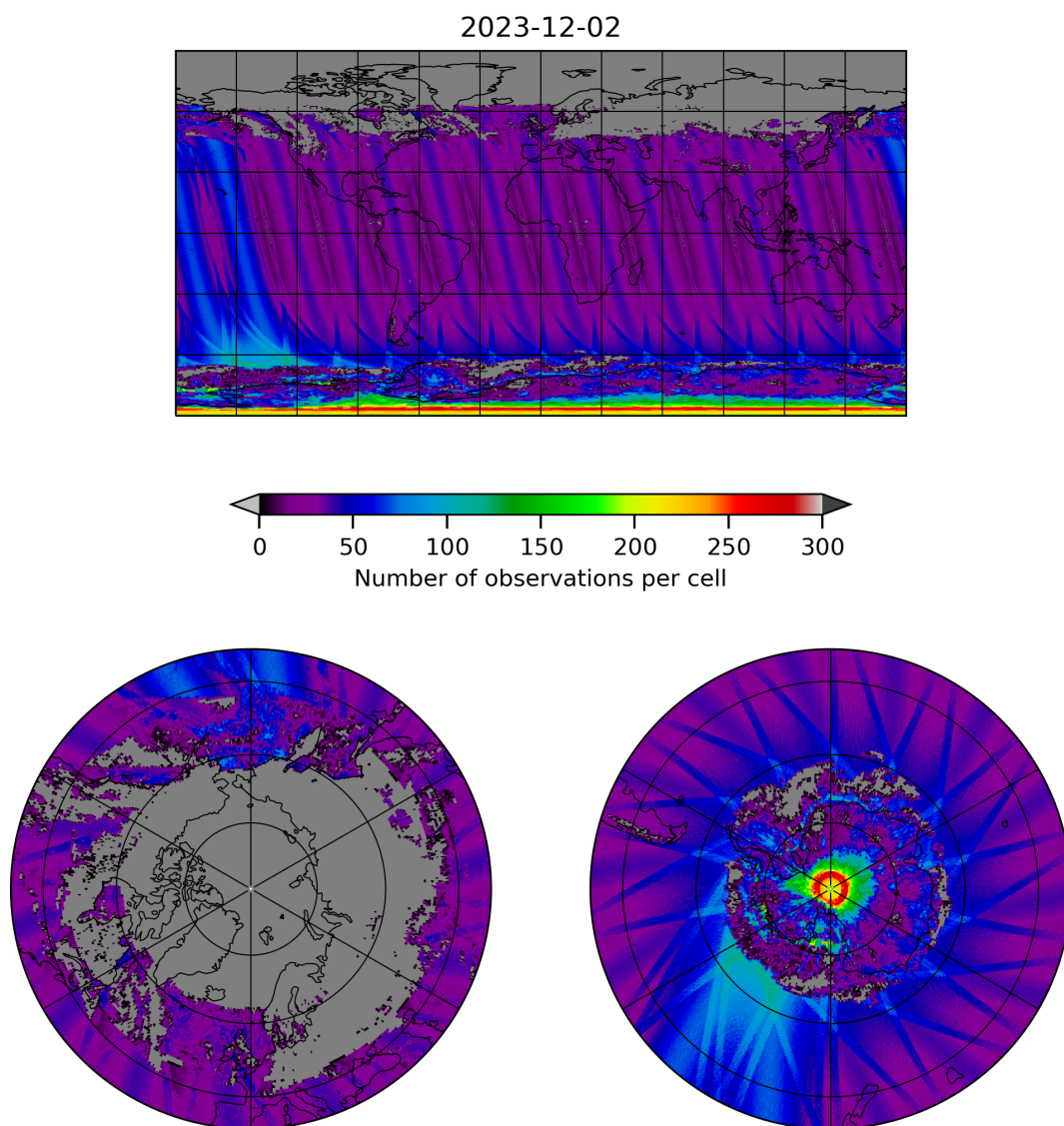
Figure 19: Map of the number of observations for 2023-12-01 to 2023-12-03
