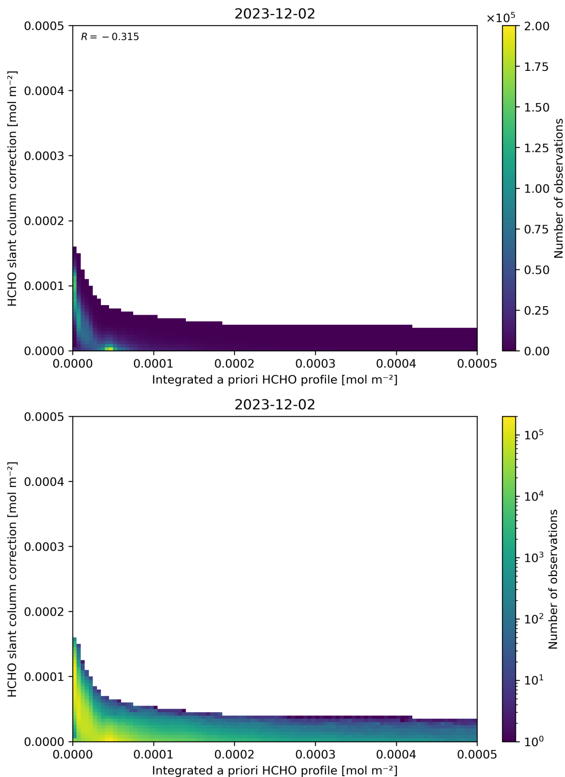
Figure 152: Scatter density plot of “Integrated a priori HCHO profile” against “HCHO slant column correction” for 2023-12-01 to 2023-12-03.
