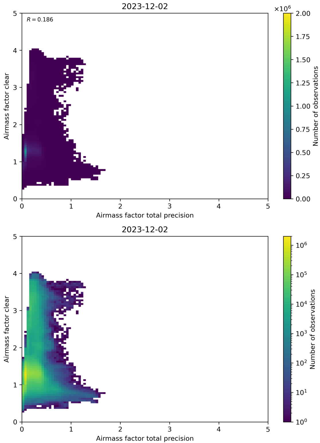
Figure 108: Scatter density plot of “Airmass factor total precision” against “Airmass factor clear” for 2023-12-01 to 2023-12-03.
