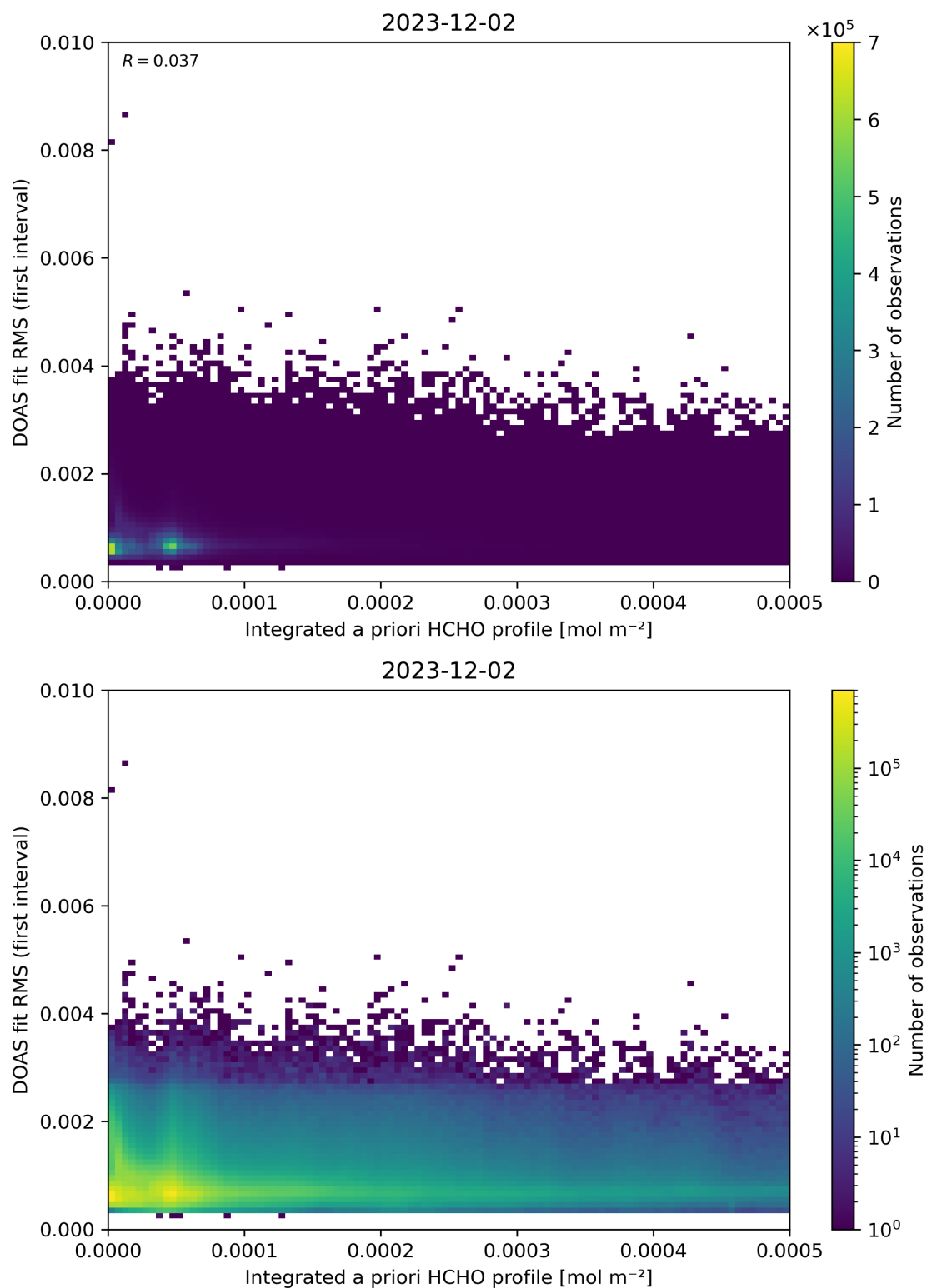
Figure 148: Scatter density plot of “Integrated a priori HCHO profile” against “DOAS fit RMS (first interval)” for 2023-12-01 to 2023-12-03.
