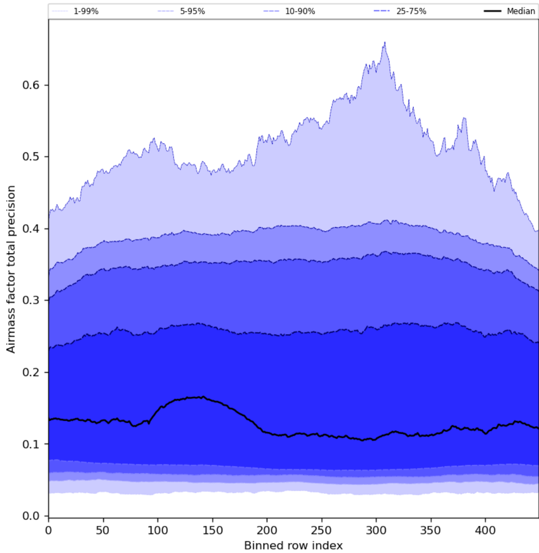
Figure 55: Along track statistics of “Airmass factor total precision” for 2023-12-01 to 2023-12-03
