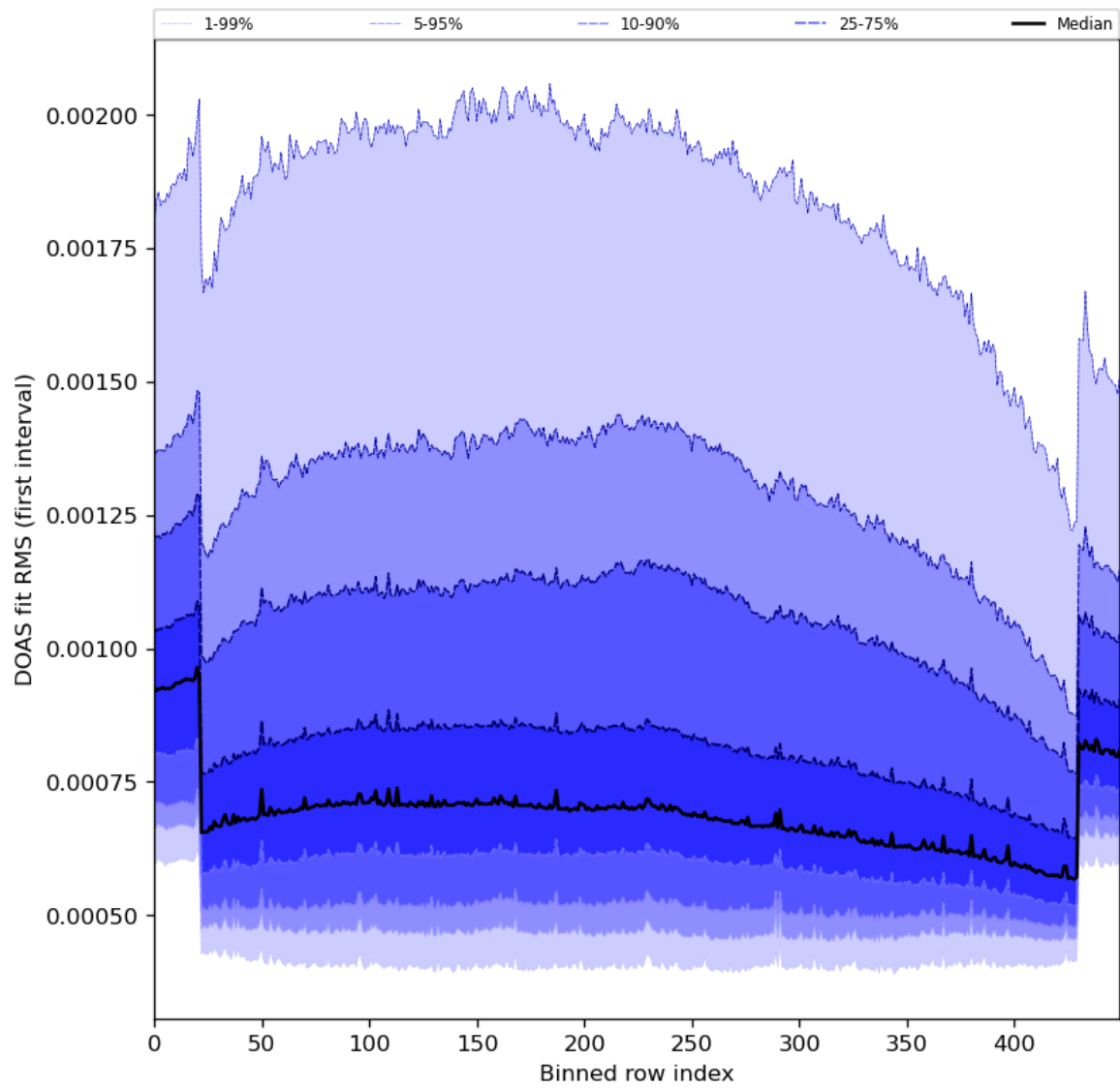
Figure 60: Along track statistics of “DOAS fit RMS (first interval)” for 2023-12-01 to 2023-12-03
