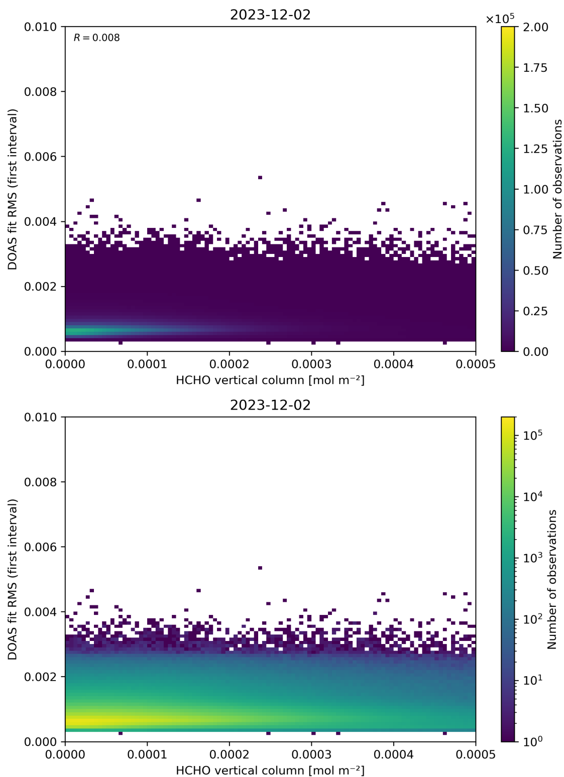
Figure 123: Scatter density plot of “HCHO vertical column” against “DOAS fit RMS (first interval)” for 2023-12-01 to 2023-12-03.
