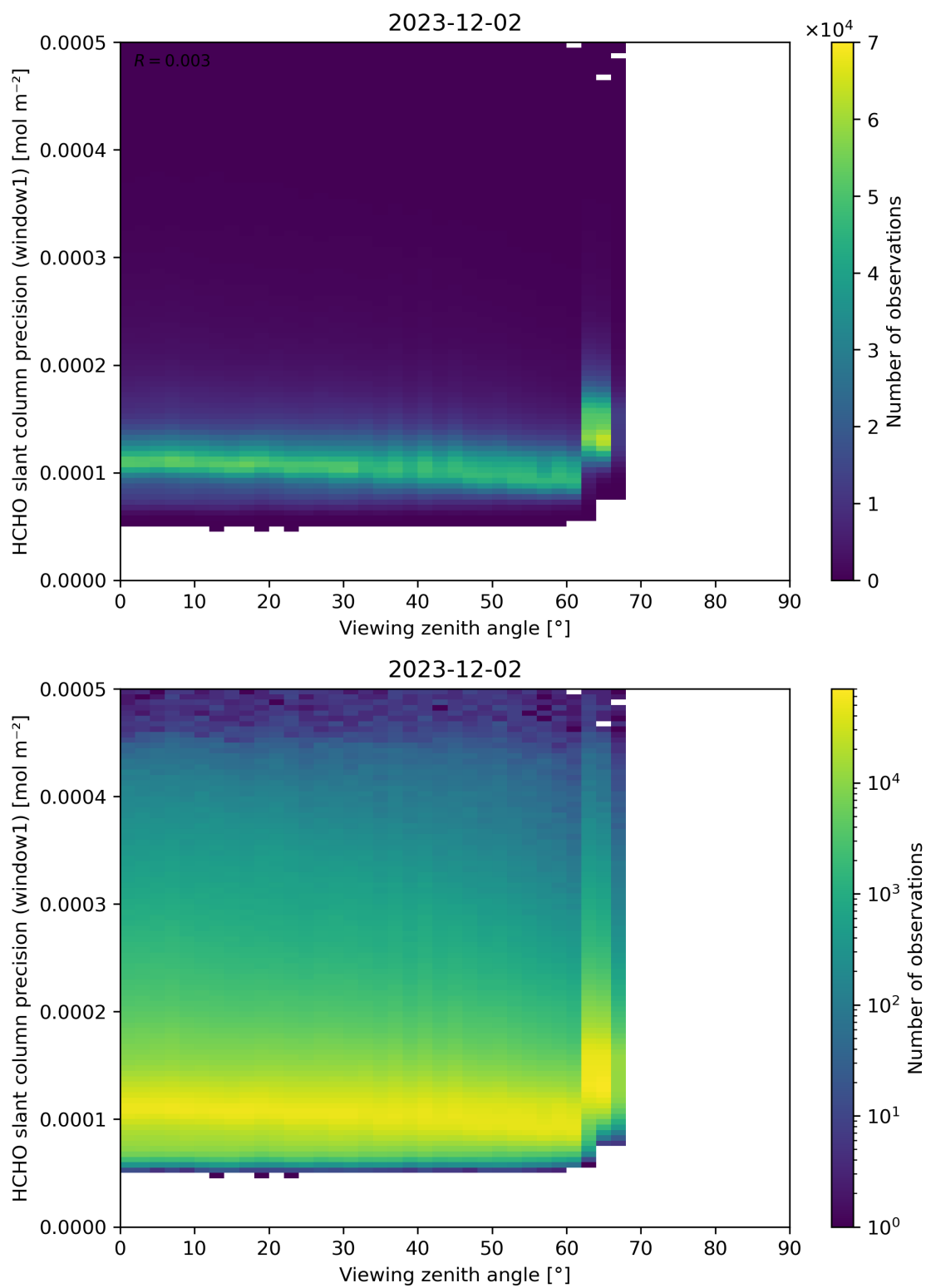
Figure 189: Scatter density plot of “Viewing zenith angle” against “HCHO slant column precision (window1)” for 2023-12-01 to 2023-12-03.
