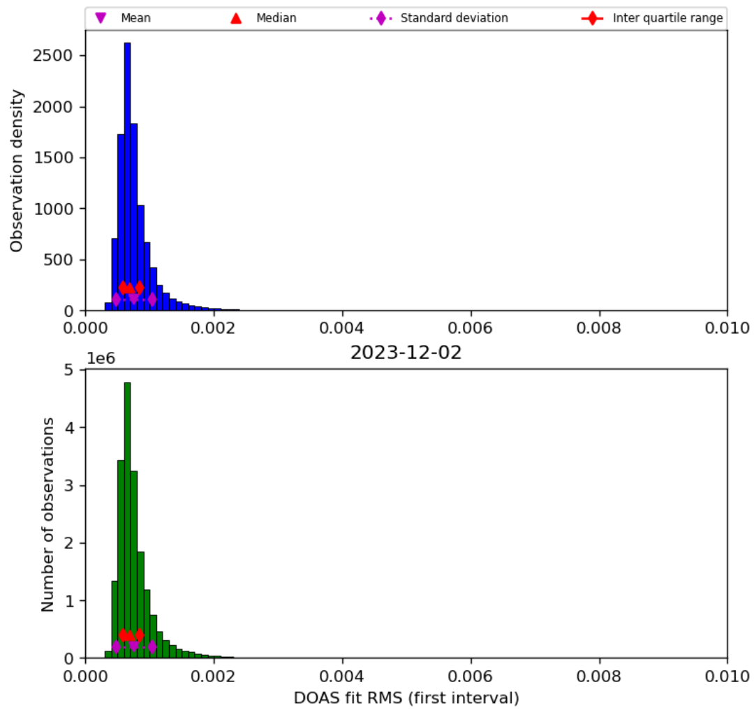
Figure 46: Histogram of “DOAS fit RMS (first interval)” for 2023-12-01 to 2023-12-03
