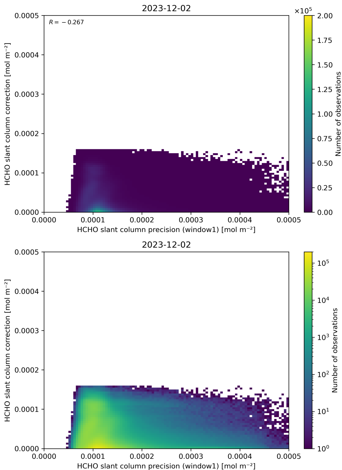
Figure 93: Scatter density plot of “HCHO slant column precision (window1)” against “HCHO slant column correction” for 2023-12-01 to 2023-12-03.
