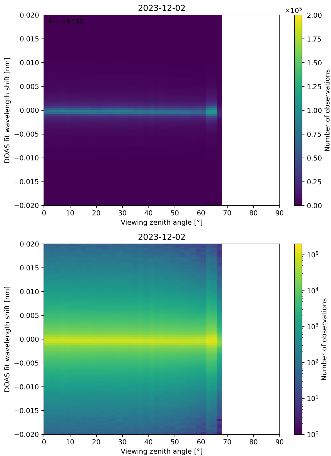
Figure 183: Scatter density plot of “Viewing zenith angle” against “DOAS fit wavelength shift” for 2023-12-01 to 2023-12-03.
