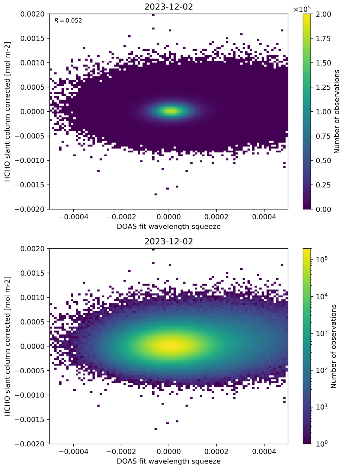
Figure 69: Scatter density plot of “DOAS fit wavelength squeeze” against “HCHO slant column corrected” for 2023-12-01 to 2023-12-03.
