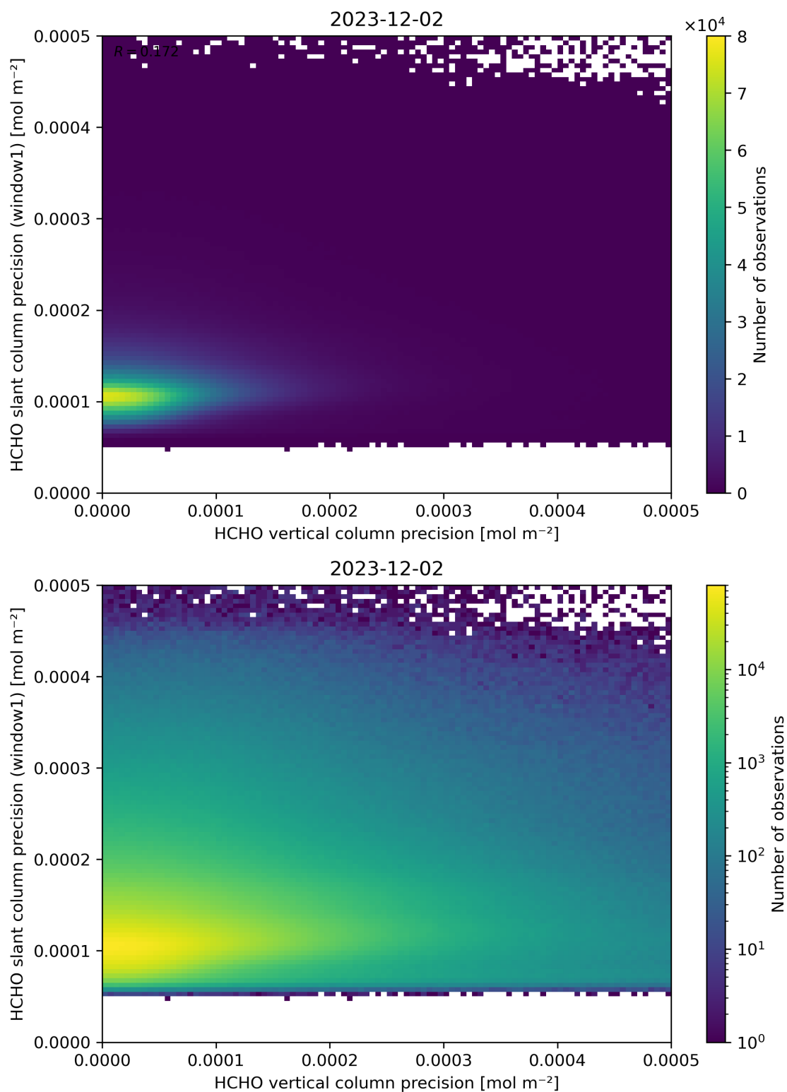
Figure 143: Scatter density plot of “HCHO vertical column precision” against “HCHO slant column precision (window1)” for 2023-12-01 to 2023-12-03.
