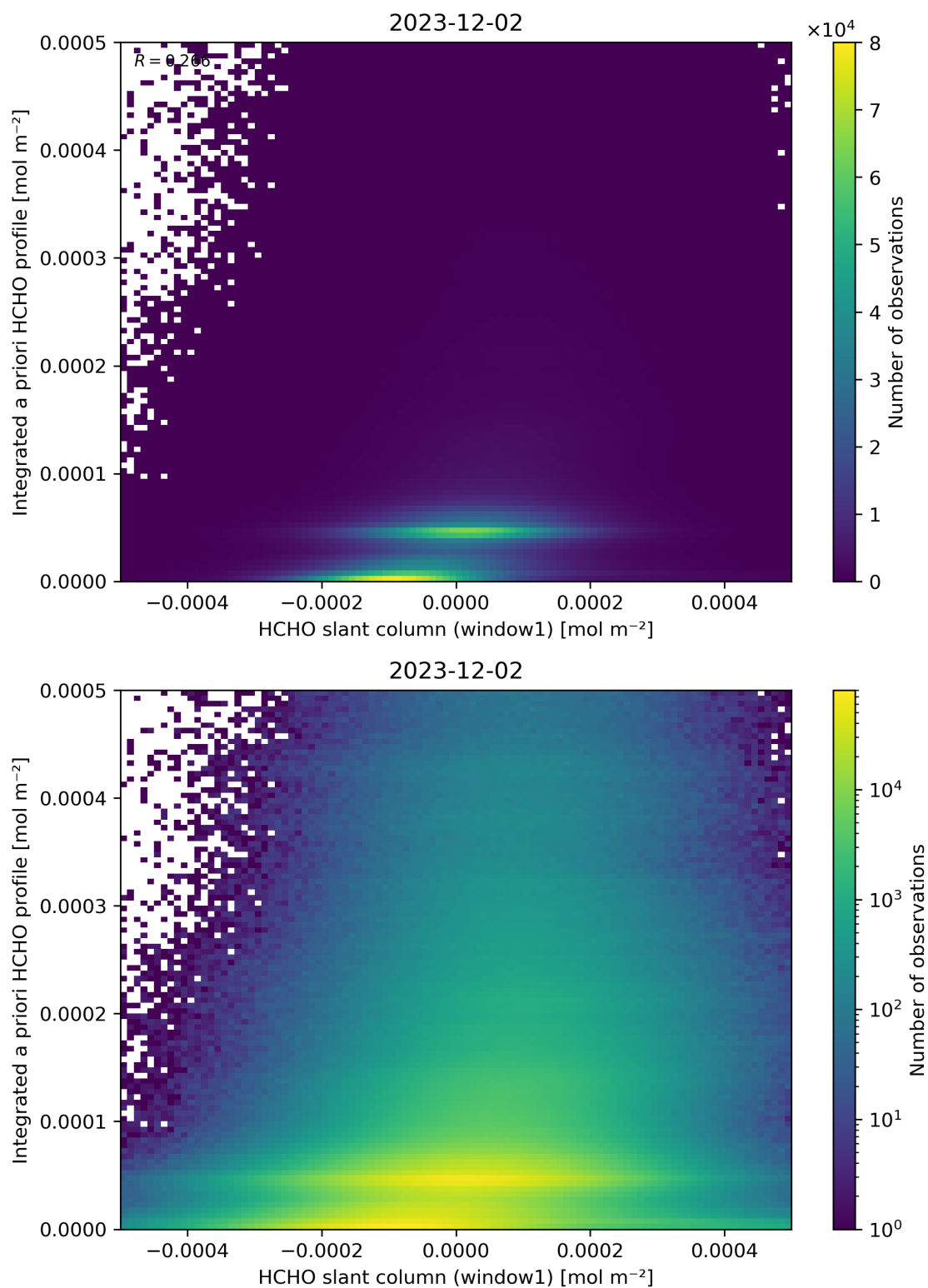
Figure 87: Scatter density plot of “HCHO slant column (window1)” against “Integrated a priori HCHO profile” for 2023-12-01 to 2023-12-03.
