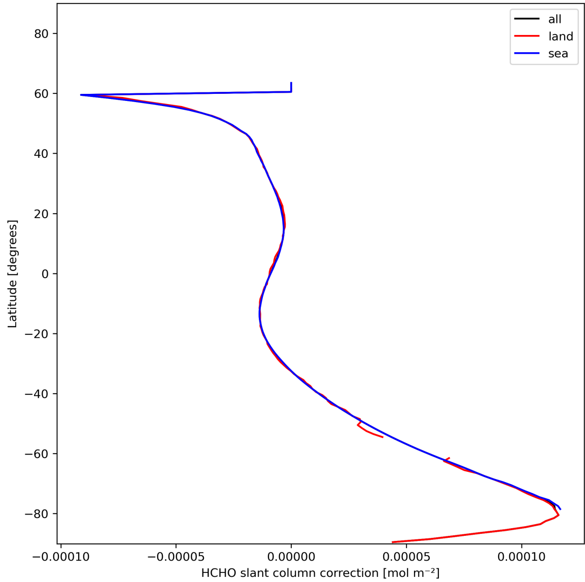
Figure 33: Zonal average of “HCHO slant column correction” for 2023-12-01 to 2023-12-03.
