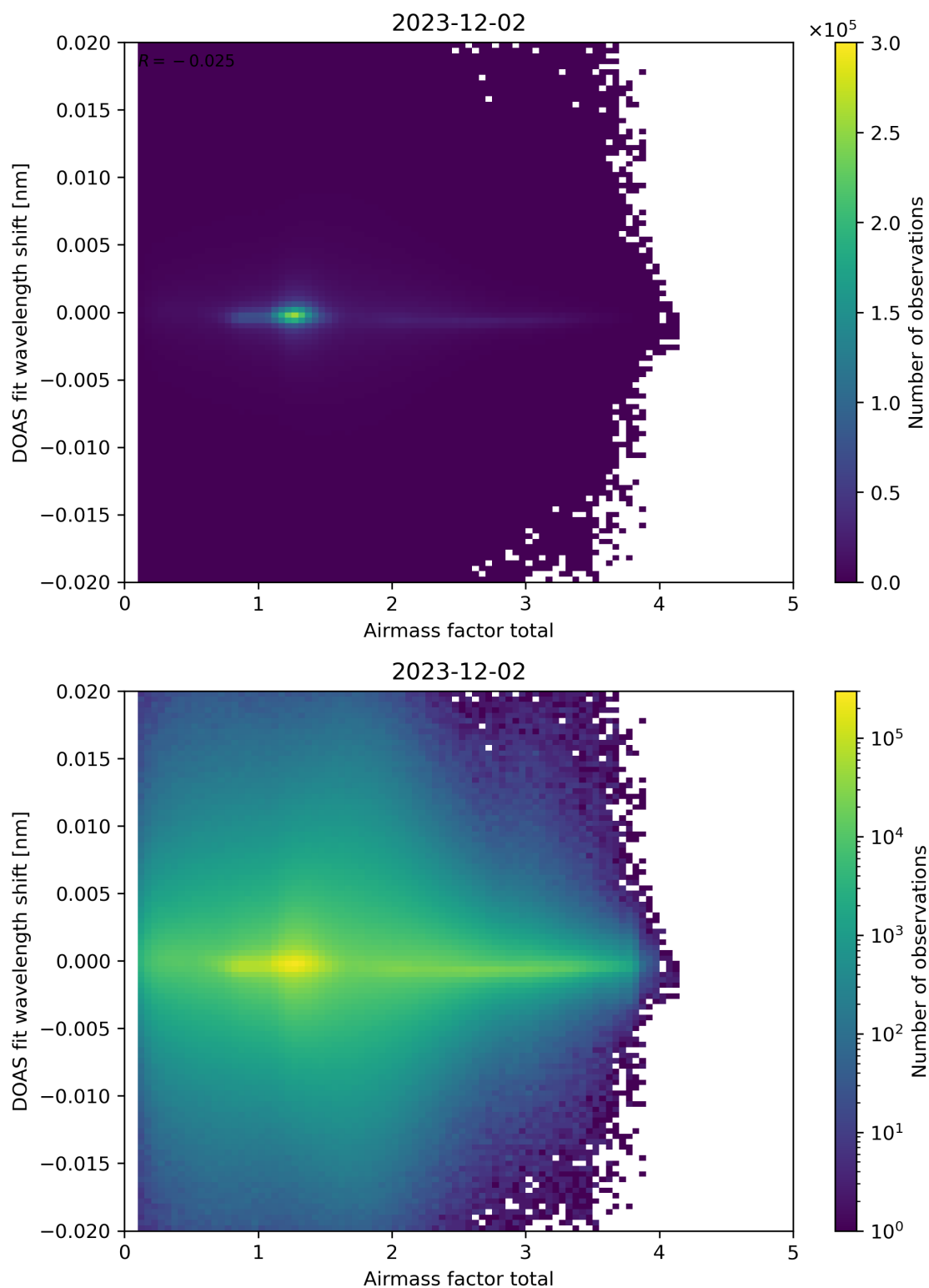
Figure 98: Scatter density plot of “Airmass factor total” against “DOAS fit wavelength shift” for 2023-12-01 to 2023-12-03.
