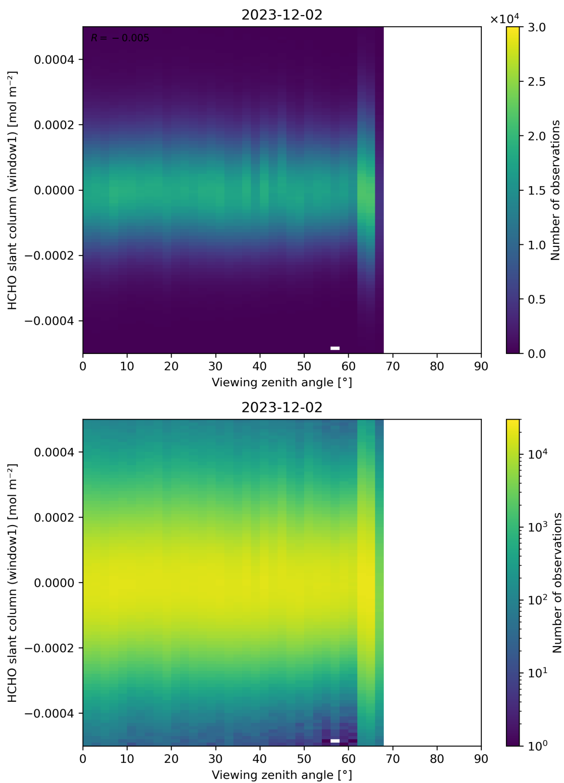
Figure 188: Scatter density plot of “Viewing zenith angle” against “HCHO slant column (window1)” for 2023-12-01 to 2023-12-03.
