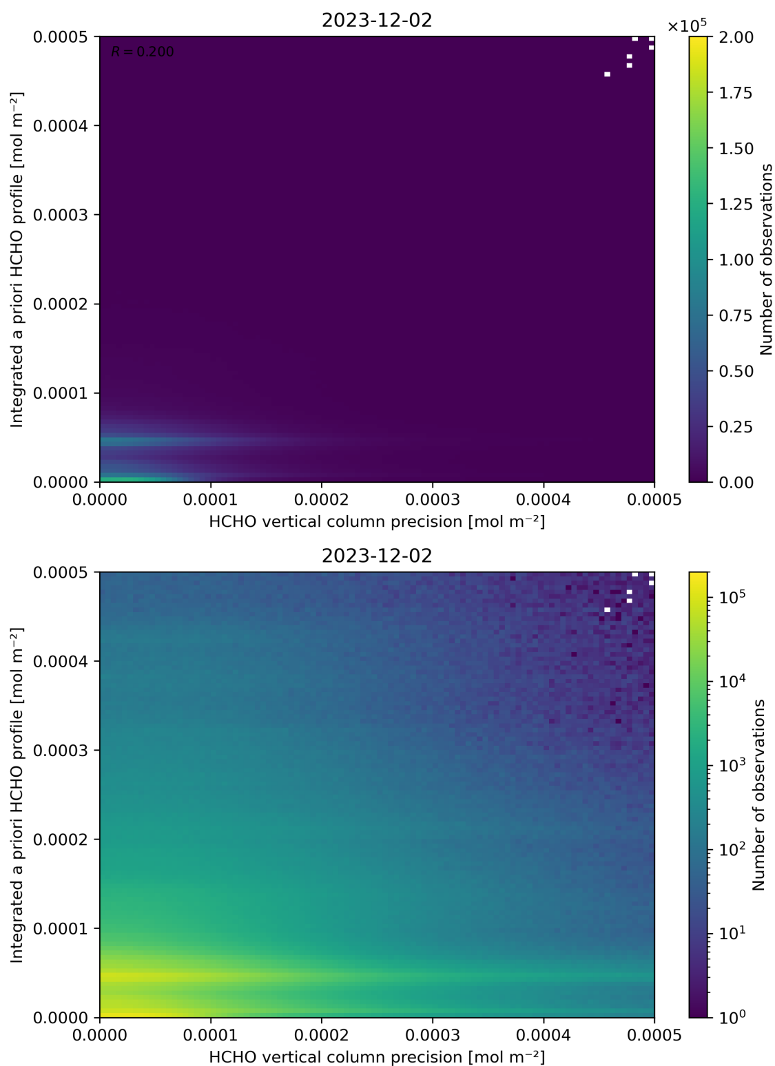
Figure 147: Scatter density plot of “HCHO vertical column precision” against “Integrated a priori HCHO profile” for 2023-12-01 to 2023-12-03.
