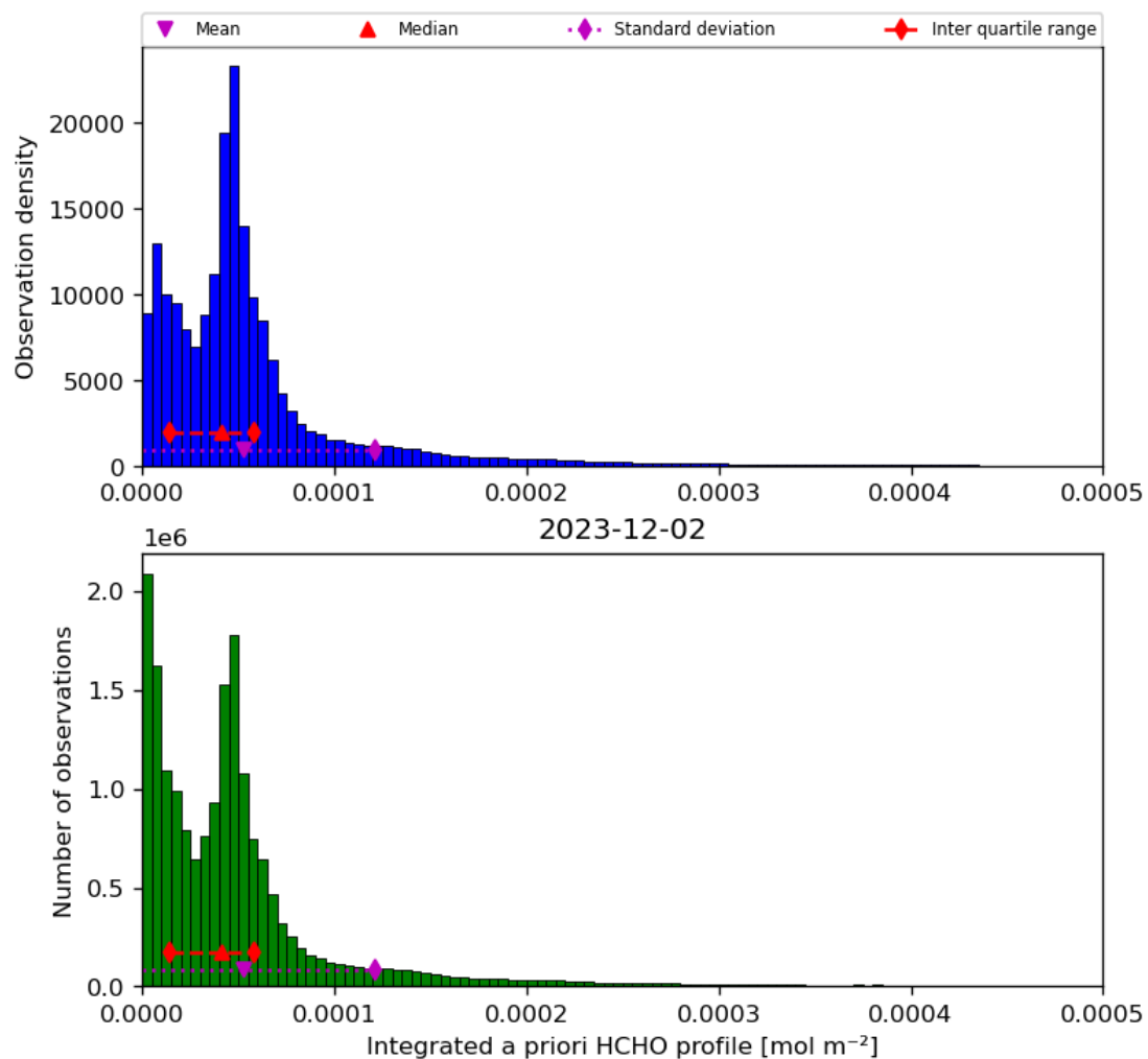
Figure 43: Histogram of “Integrated a priori HCHO profile” for 2023-12-01 to 2023-12-03
