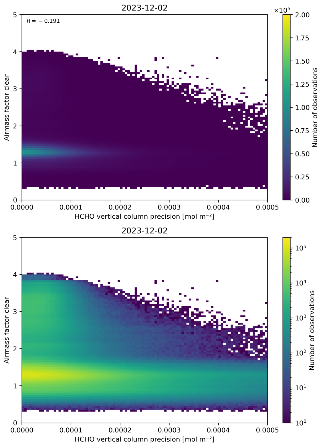
Figure 139: Scatter density plot of “HCHO vertical column precision” against “Airmass factor clear” for 2023-12-01 to 2023-12-03.
