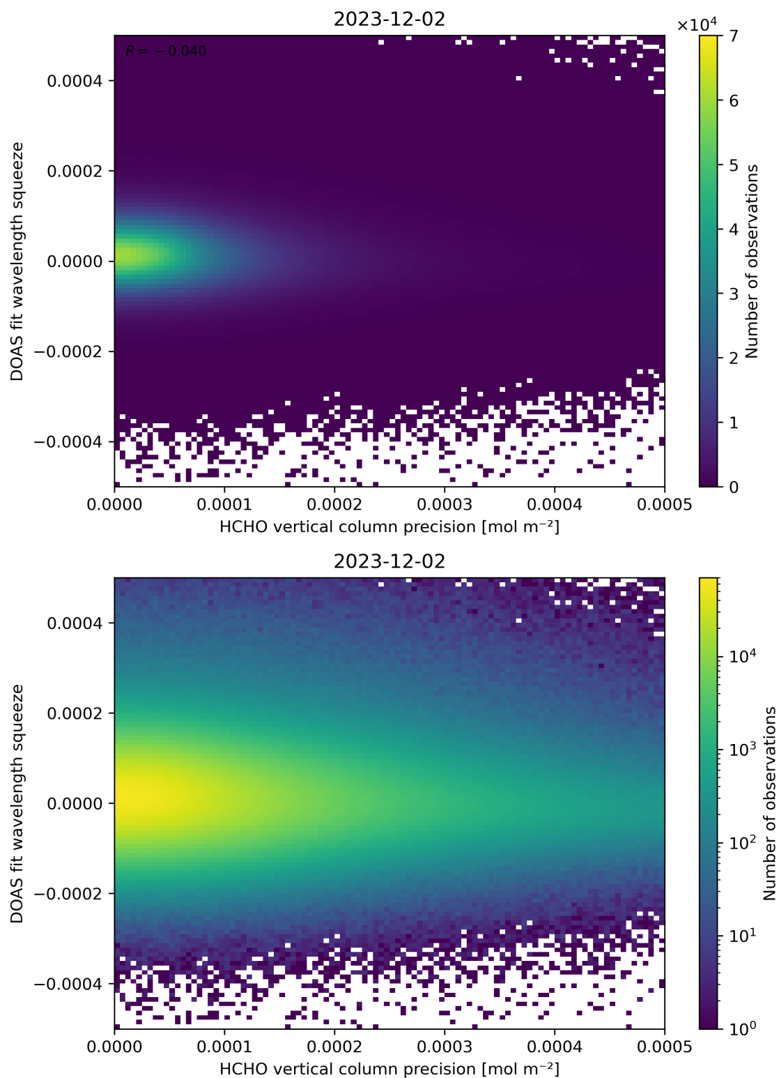
Figure 138: Scatter density plot of “HCHO vertical column precision” against “DOAS fit wavelength squeeze” for 2023-12-01 to 2023-12-03.
