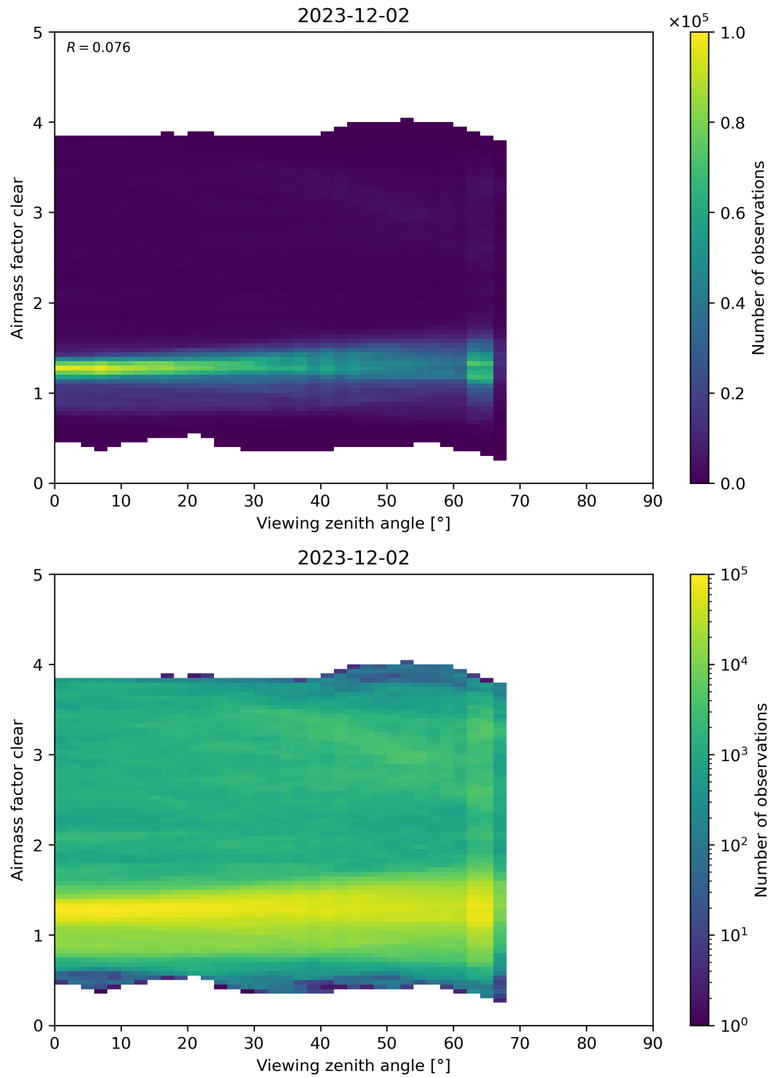
Figure 185: Scatter density plot of “Viewing zenith angle” against “Airmass factor clear” for 2023-12-01 to 2023-12-03.
