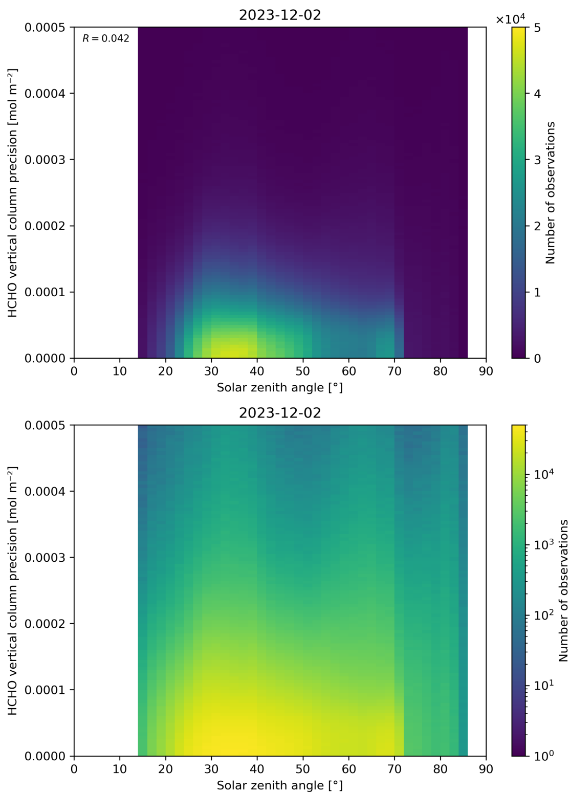
Figure 179: Scatter density plot of “Solar zenith angle” against “HCHO vertical column precision” for 2023-12-01 to 2023-12-03.
