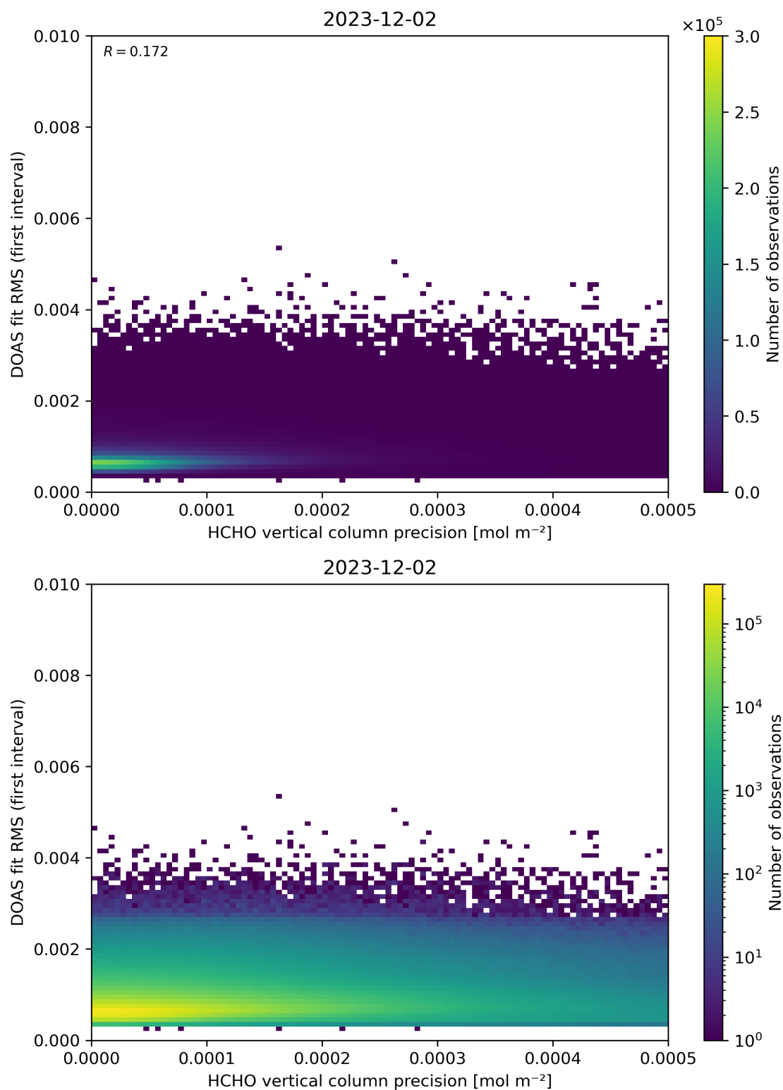
Figure 136: Scatter density plot of “HCHO vertical column precision” against “DOAS fit RMS (first interval)” for 2023-12-01 to 2023-12-03.
