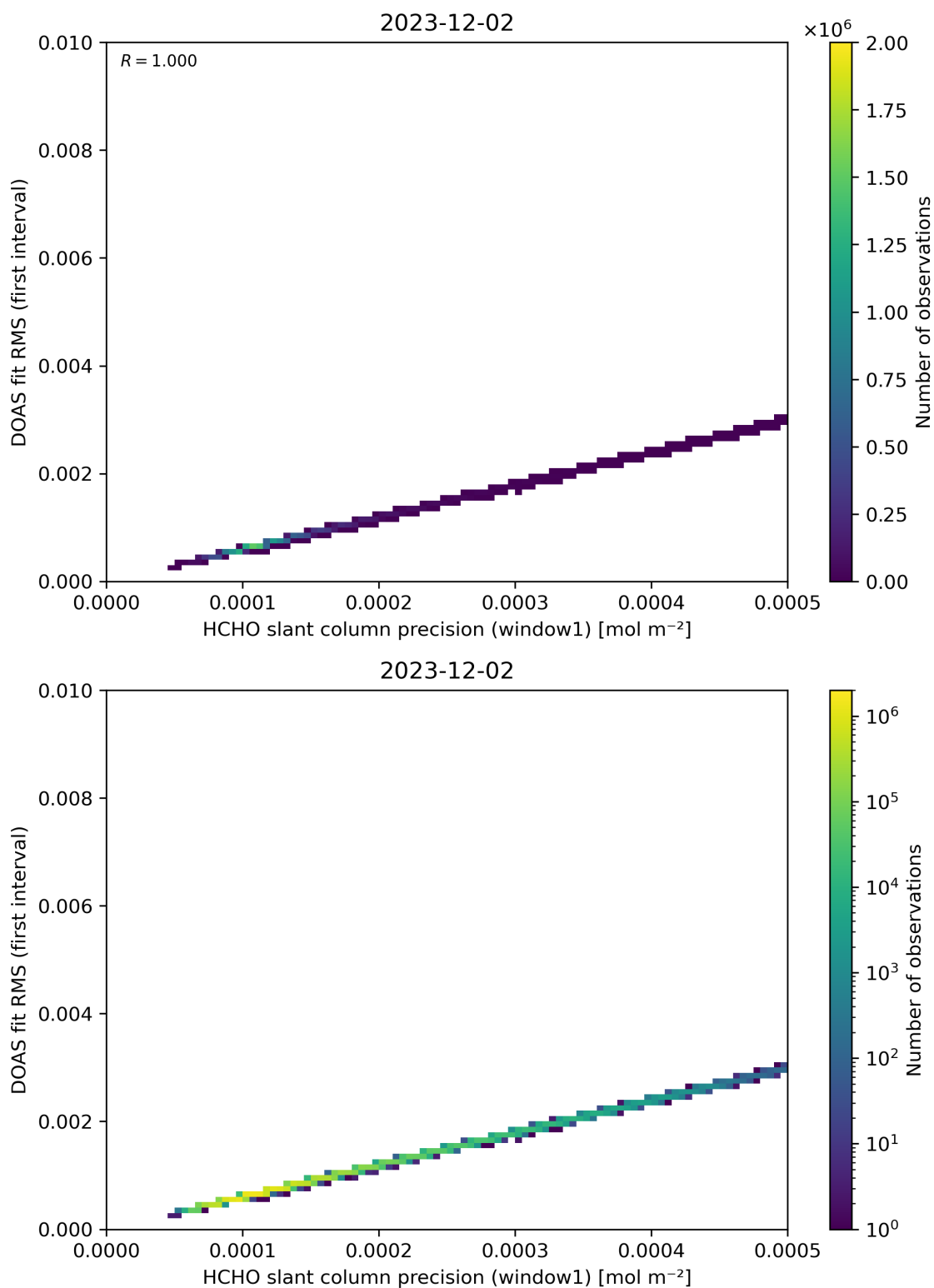
Figure 88: Scatter density plot of “HCHO slant column precision (window1)” against “DOAS fit RMS (first interval)” for 2023-12-01 to 2023-12-03.
