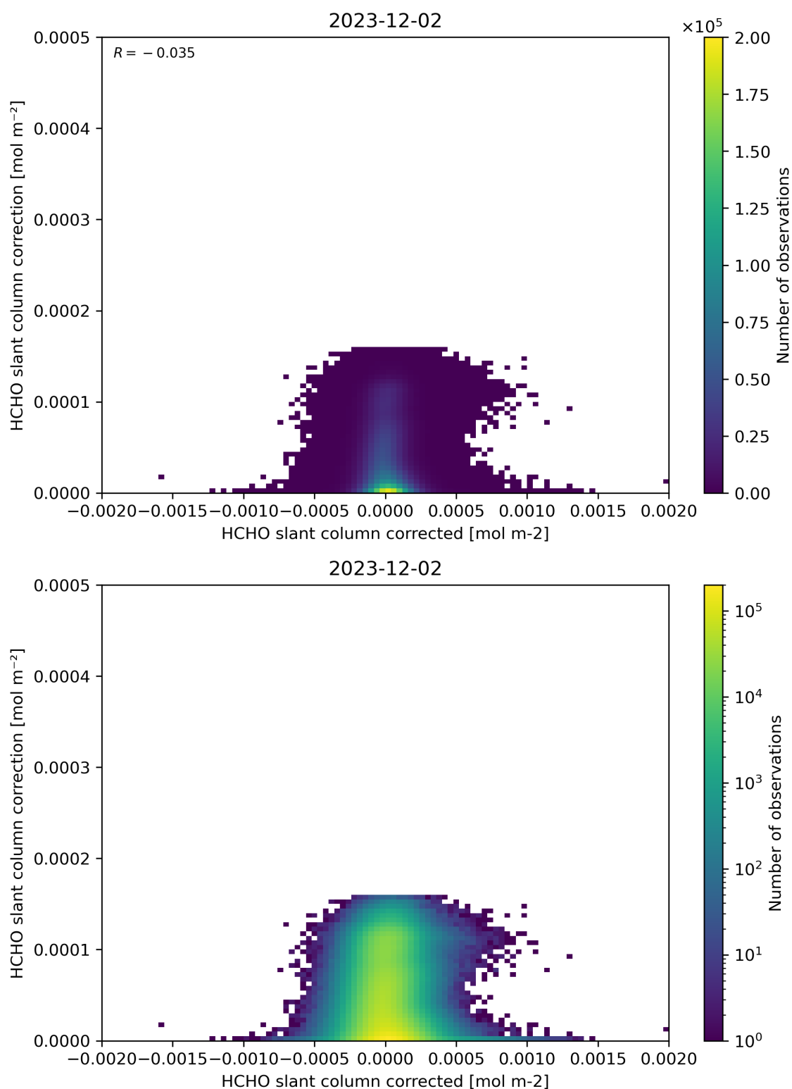
Figure 77: Scatter density plot of “HCHO slant column corrected” against “HCHO slant column correction” for 2023-12-01 to 2023-12-03.
