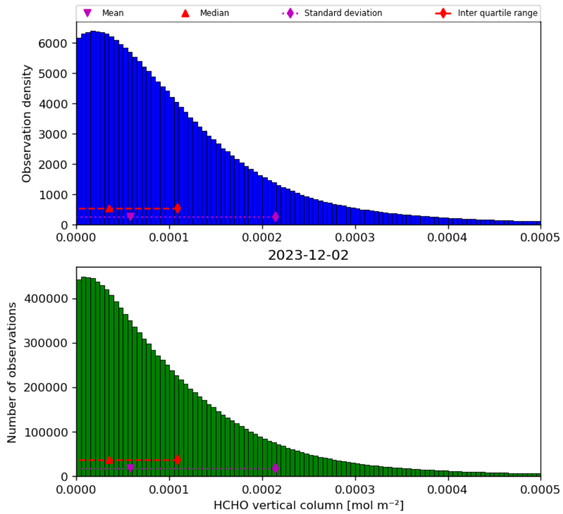
Figure 35: Histogram of “HCHO vertical column” for 2023-12-01 to 2023-12-03
