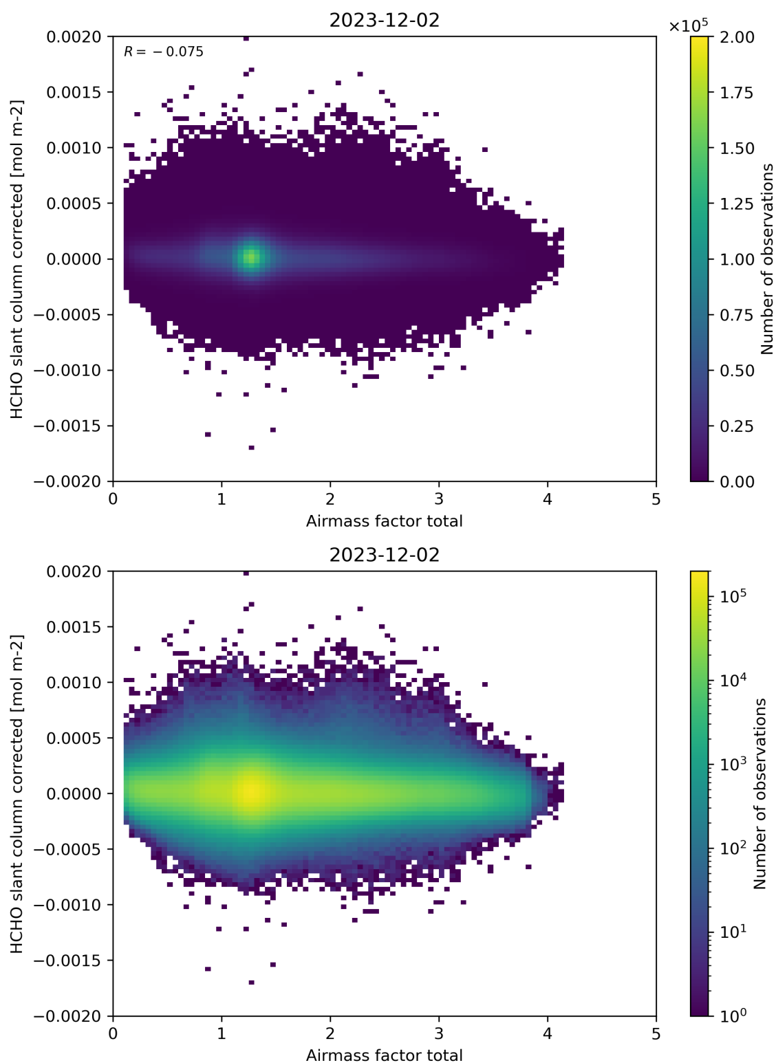
Figure 101: Scatter density plot of “Airmass factor total” against “HCHO slant column corrected” for 2023-12-01 to 2023-12-03.
