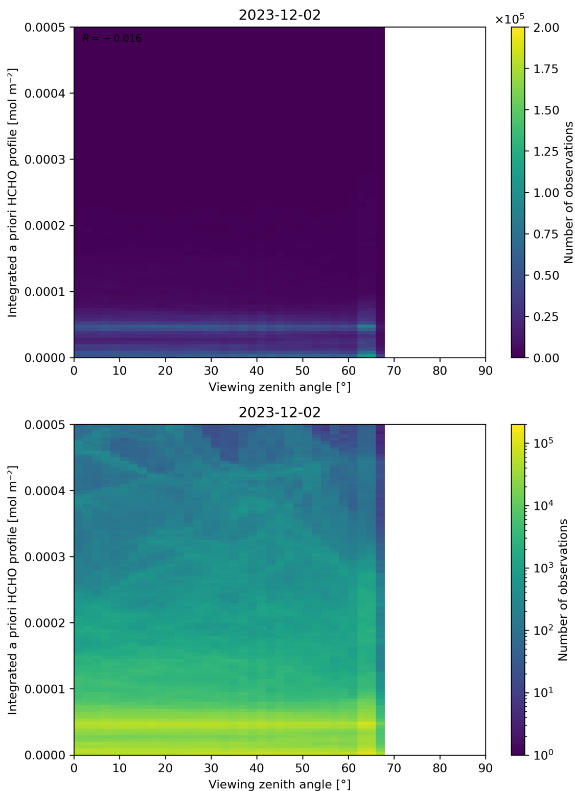
Figure 195: Scatter density plot of “Viewing zenith angle” against “Integrated a priori HCHO profile” for 2023-12-01 to 2023-12-03.
