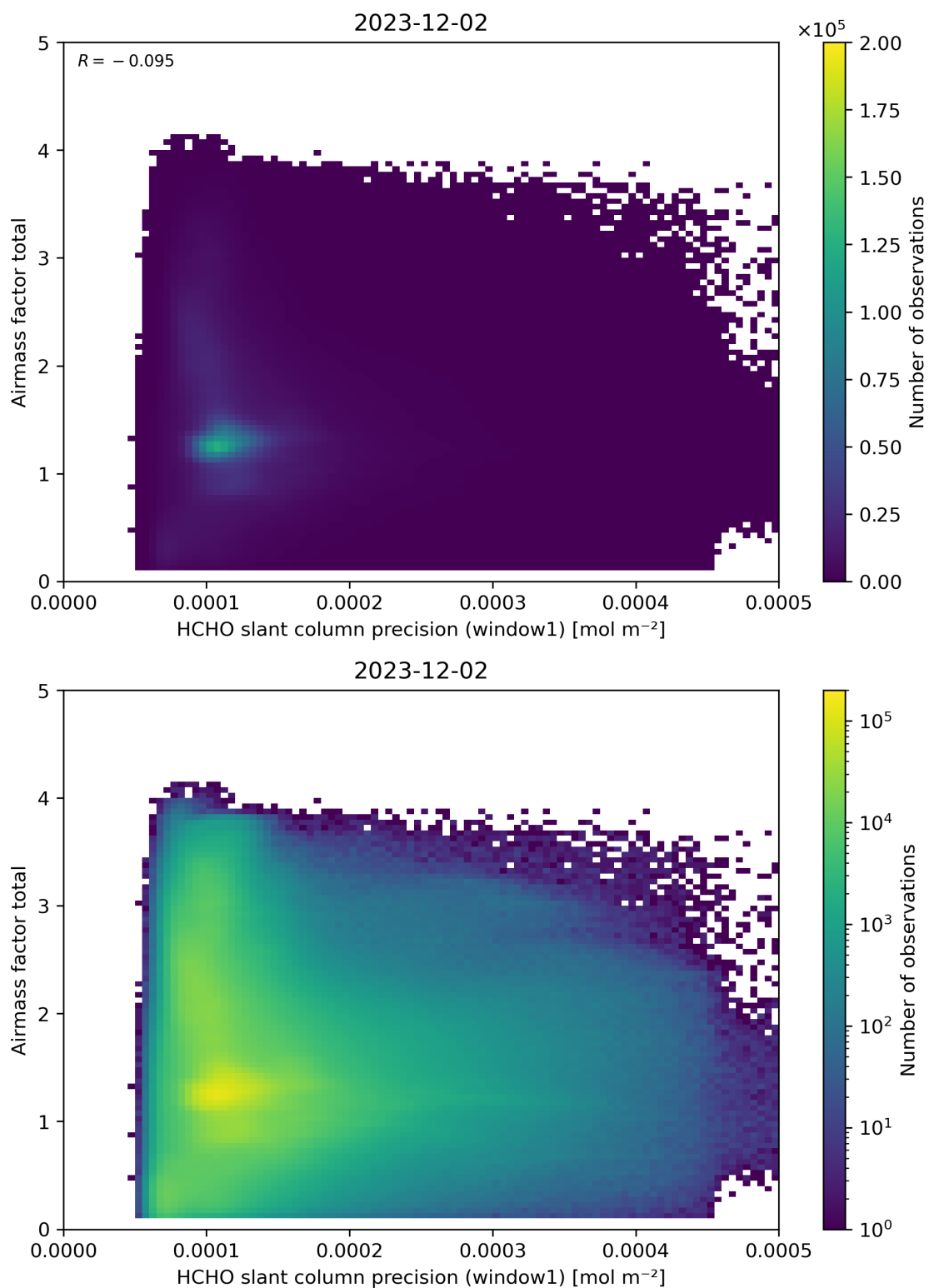
Figure 94: Scatter density plot of “HCHO slant column precision (window1)” against “Airmass factor total” for 2023-12-01 to 2023-12-03.
