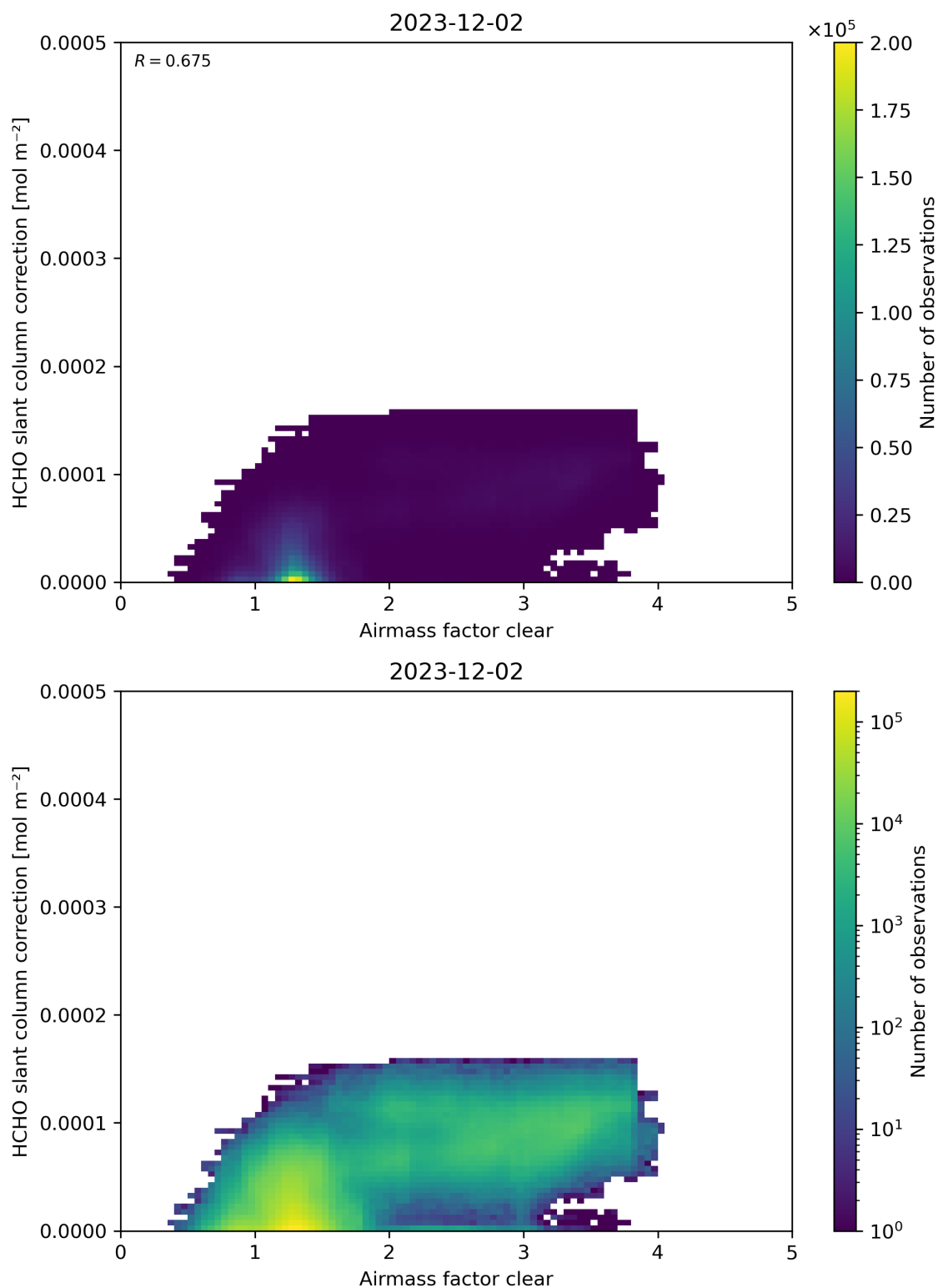
Figure 75: Scatter density plot of “Airmass factor clear” against “HCHO slant column correction” for 2023-12-01 to 2023-12-03.
