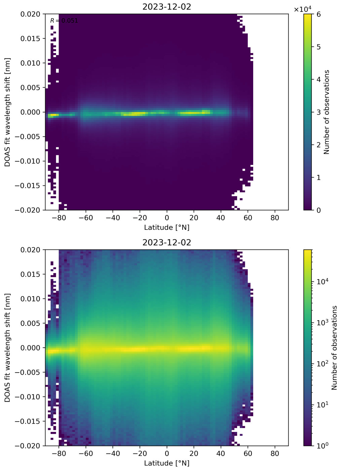
Figure 154: Scatter density plot of “Latitude” against “DOAS fit wavelength shift” for 2023-12-01 to 2023-12-03.
