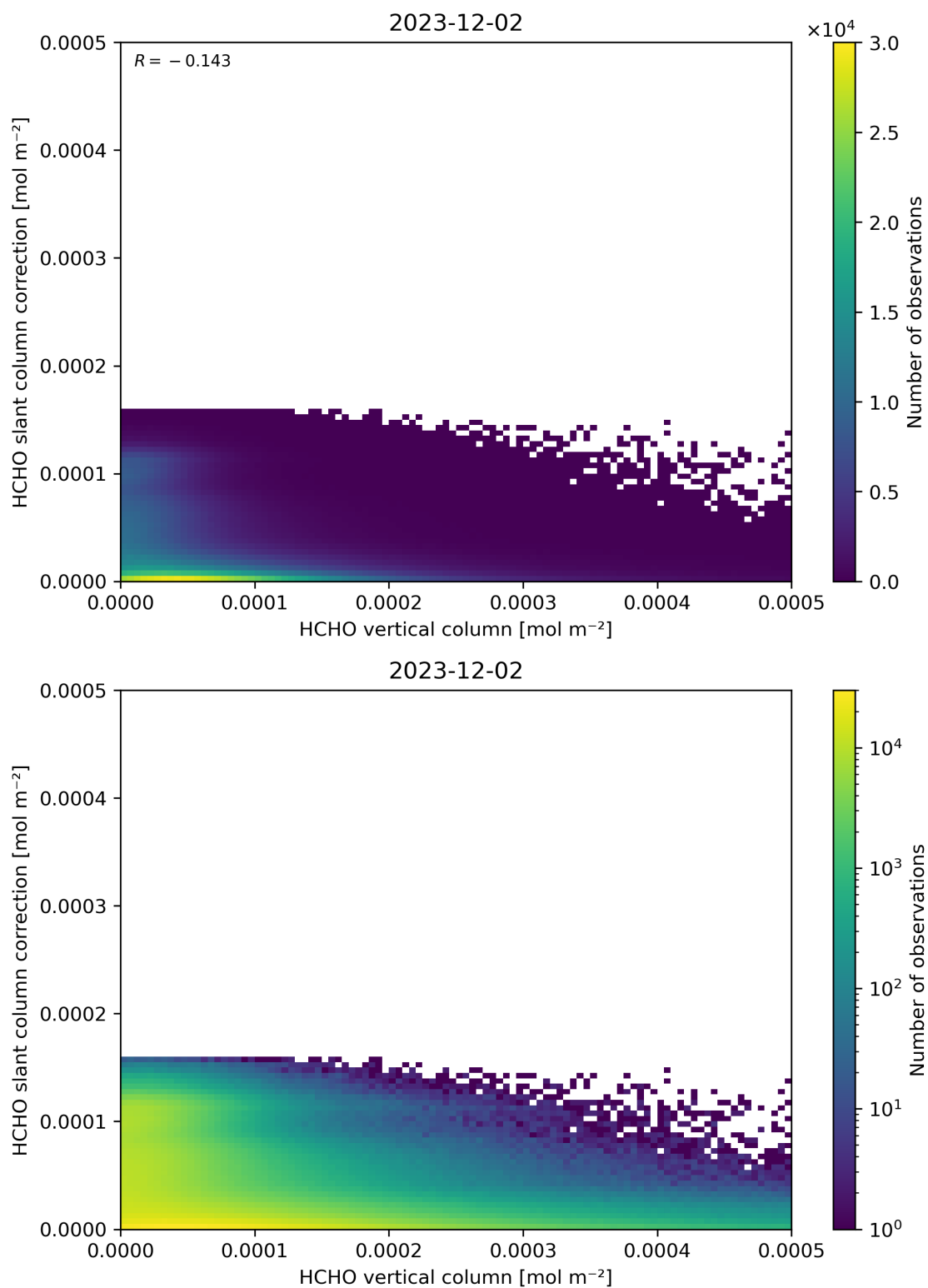
Figure 128: Scatter density plot of “HCHO vertical column” against “HCHO slant column correction” for 2023-12-01 to 2023-12-03.
