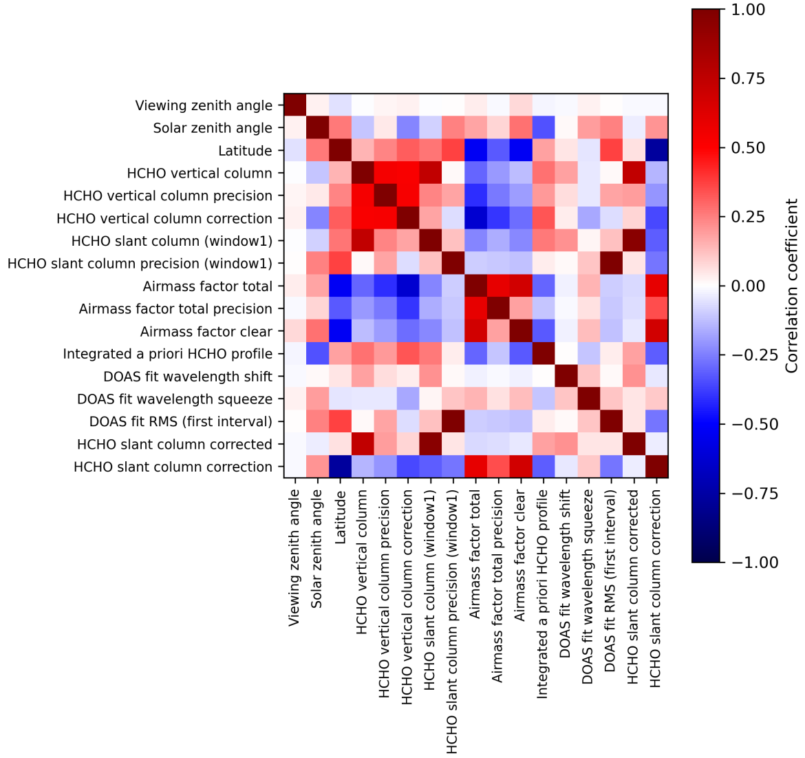
Figure 2: Map of correlation matrix for 2023-12-01 to 2023-12-03.
