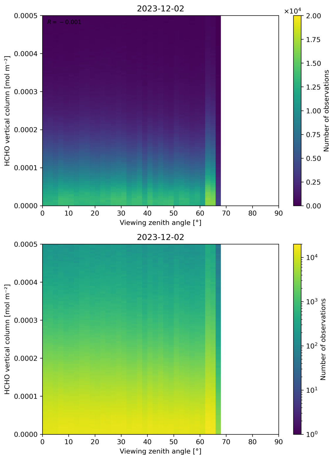
Figure 192: Scatter density plot of “Viewing zenith angle” against “HCHO vertical column” for 2023-12-01 to 2023-12-03.
