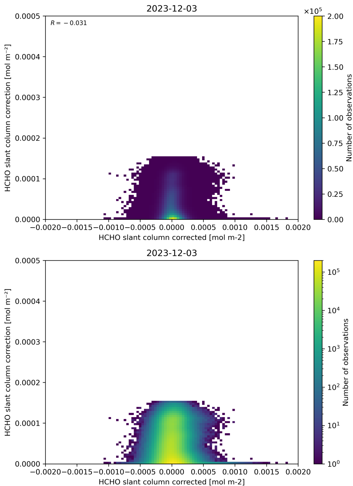
Figure 77: Scatter density plot of “HCHO slant column corrected” against “HCHO slant column correction” for 2023-12-02 to 2023-12-04.
