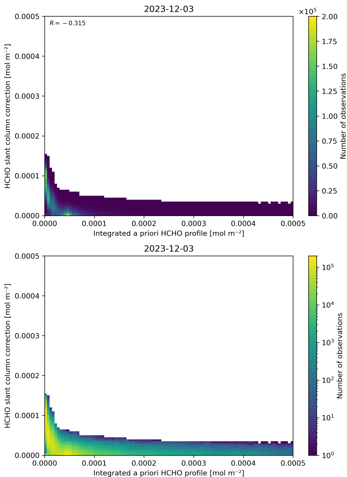
Figure 152: Scatter density plot of “Integrated a priori HCHO profile” against “HCHO slant column correction” for 2023-12-02 to 2023-12-04.
