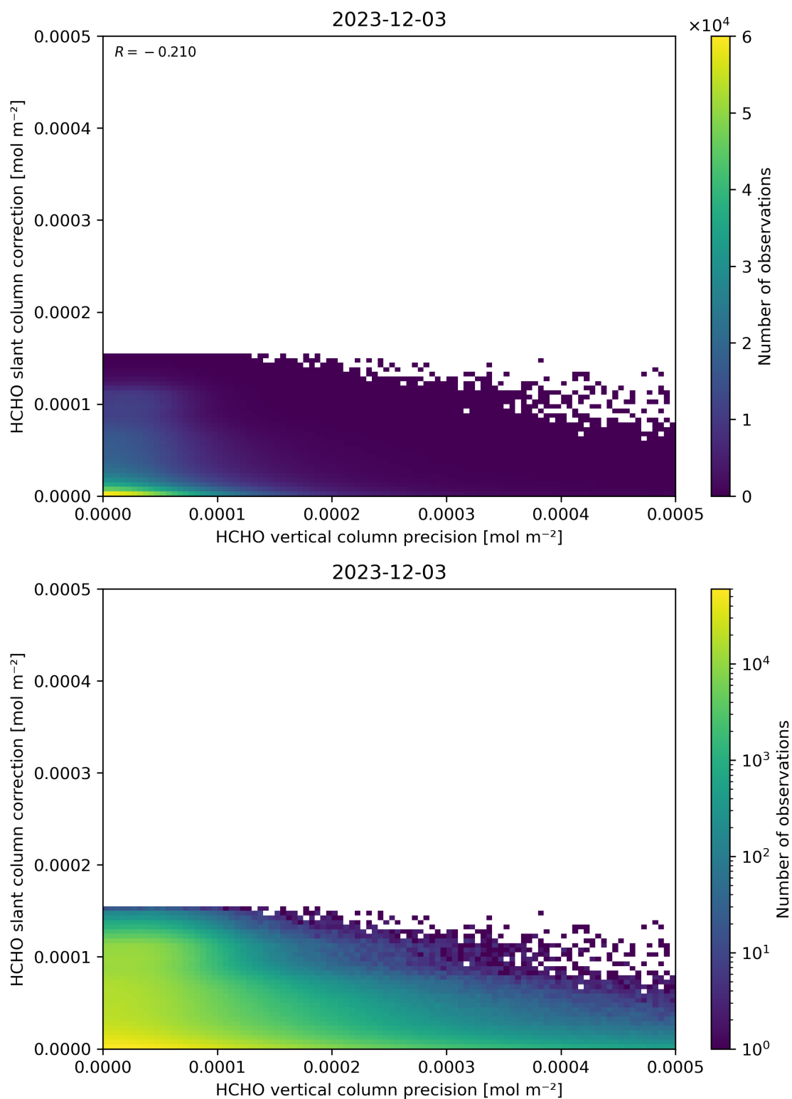
Figure 141: Scatter density plot of “HCHO vertical column precision” against “HCHO slant column correction” for 2023-12-02 to 2023-12-04.
