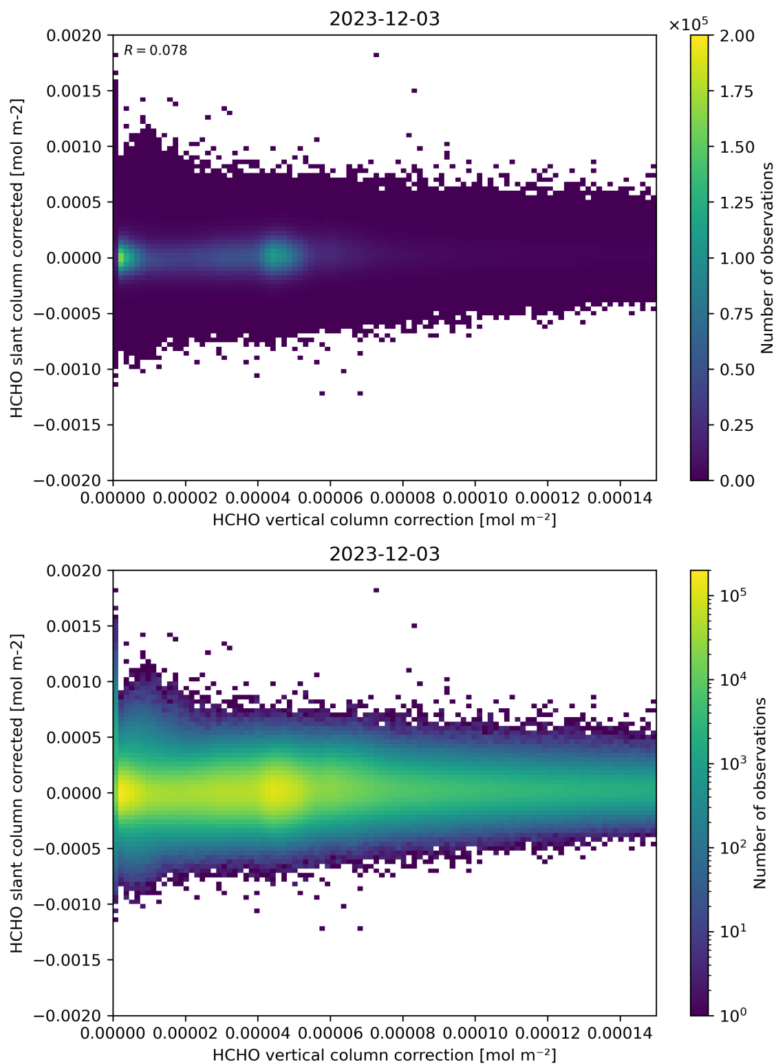
Figure 116: Scatter density plot of “HCHO vertical column correction” against “HCHO slant column corrected” for 2023-12-02 to 2023-12-04.
