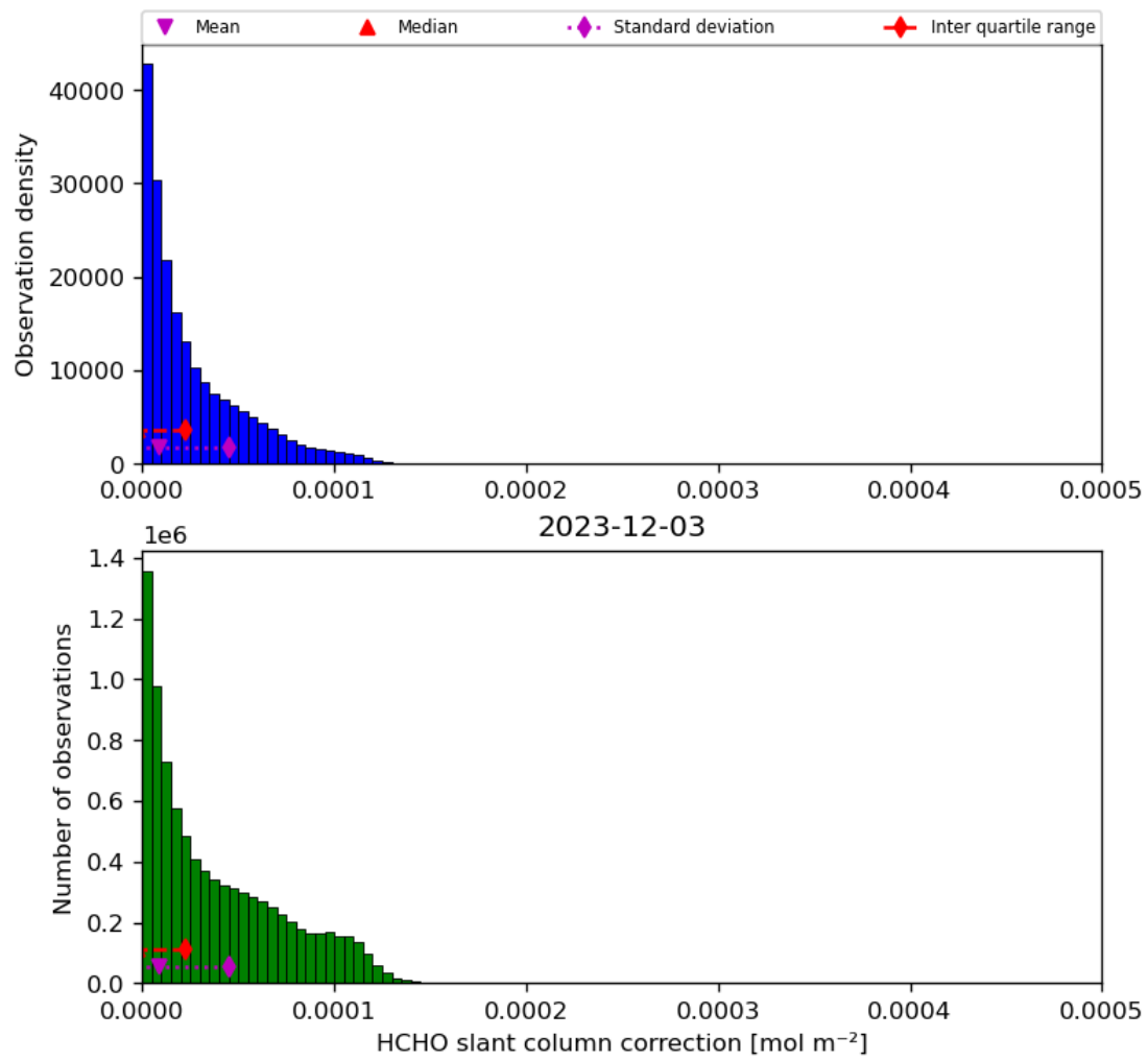
Figure 47: Histogram of “HCHO slant column correction” for 2023-12-02 to 2023-12-04
