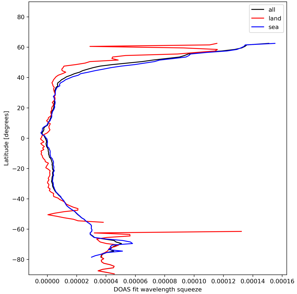
Figure 31: Zonal average of “DOAS fit wavelength squeeze” for 2023-12-02 to 2023-12-04.
