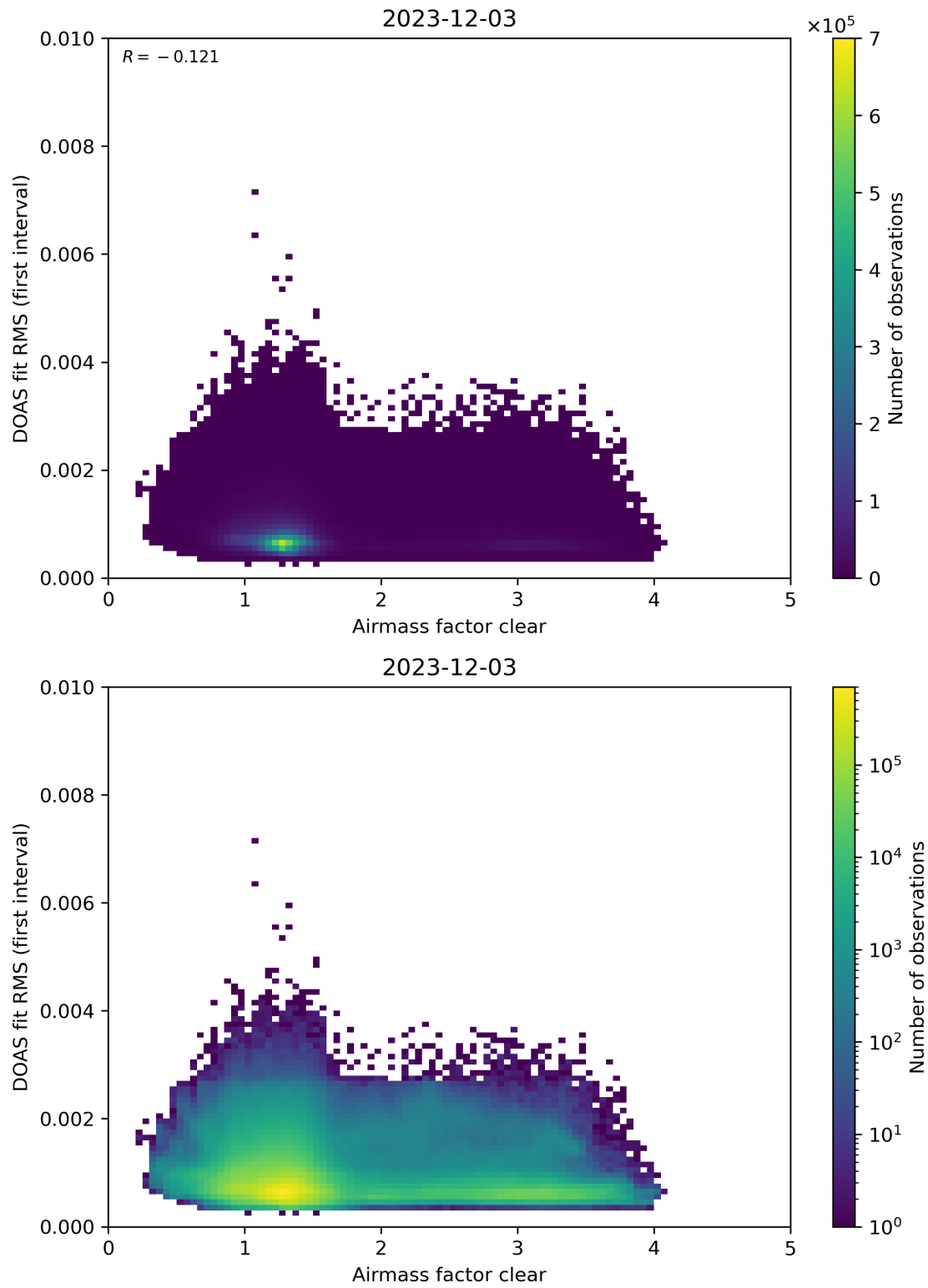
Figure 71: Scatter density plot of “Airmass factor clear” against “DOAS fit RMS (first interval)” for 2023-12-02 to 2023-12-04.
