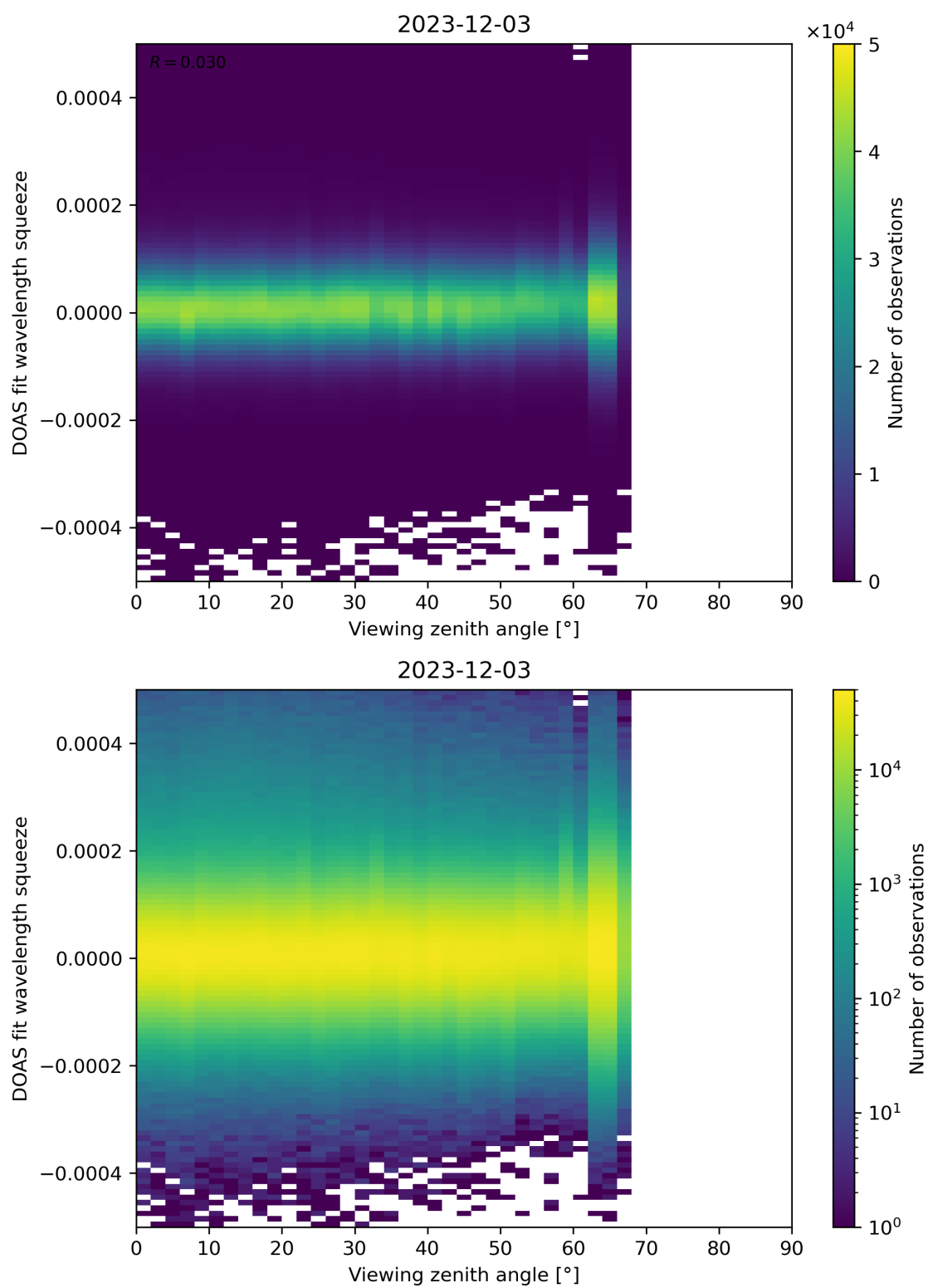
Figure 184: Scatter density plot of “Viewing zenith angle” against “DOAS fit wavelength squeeze” for 2023-12-02 to 2023-12-04.
