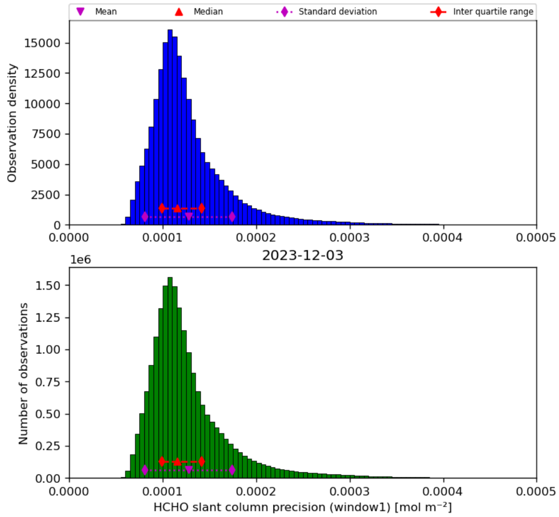
Figure 39: Histogram of “HCHO slant column precision (window1)” for 2023-12-02 to 2023-12-04
