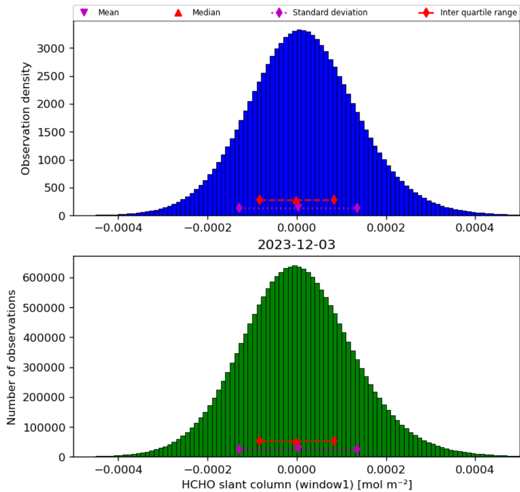
Figure 38: Histogram of “HCHO slant column (window1)” for 2023-12-02 to 2023-12-04
