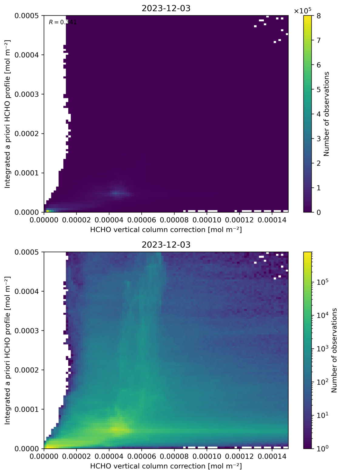
Figure 122: Scatter density plot of “HCHO vertical column correction” against “Integrated a priori HCHO profile” for 2023-12-02 to 2023-12-04.
