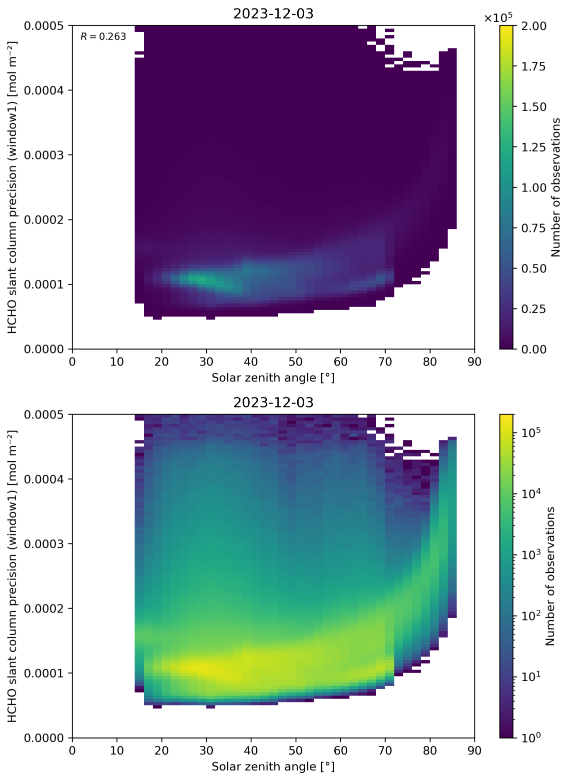
Figure 174: Scatter density plot of “Solar zenith angle” against “HCHO slant column precision (window1)” for 2023-12-02 to 2023-12-04.
