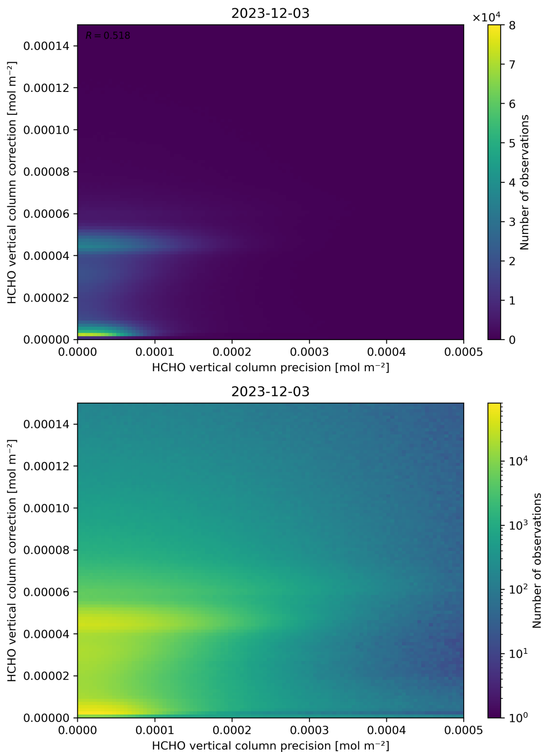
Figure 146: Scatter density plot of “HCHO vertical column precision” against “HCHO vertical column correction” for 2023-12-02 to 2023-12-04.
