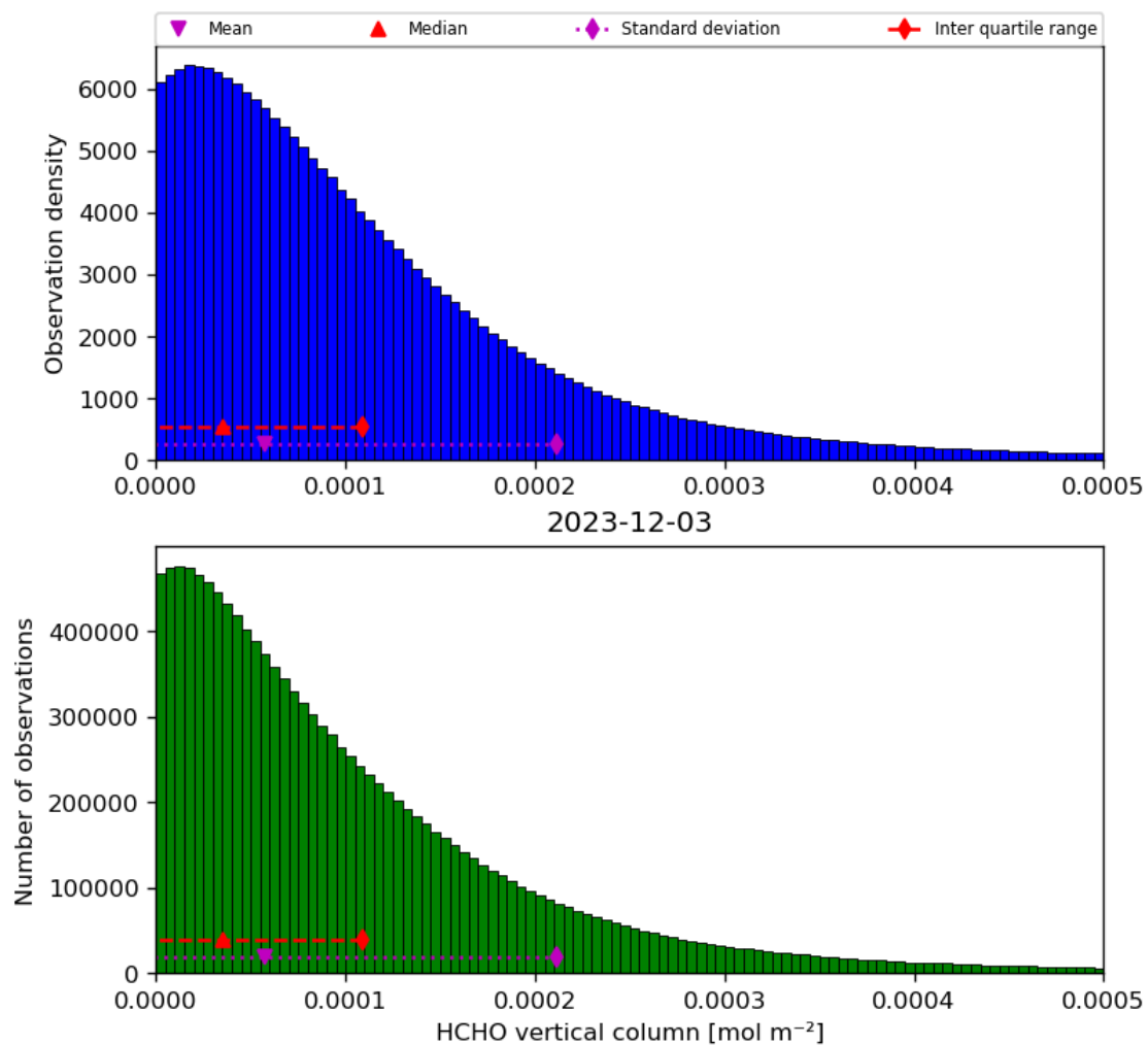
Figure 35: Histogram of “HCHO vertical column” for 2023-12-02 to 2023-12-04
