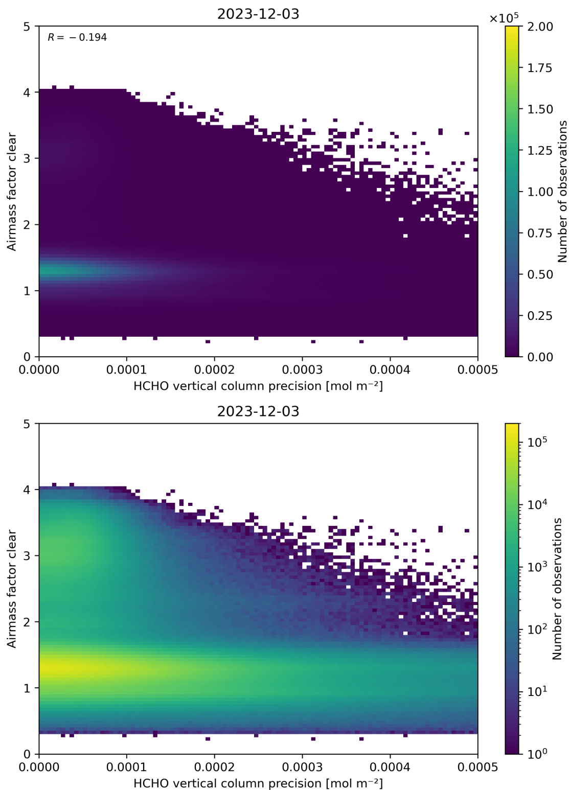
Figure 139: Scatter density plot of “HCHO vertical column precision” against “Airmass factor clear” for 2023-12-02 to 2023-12-04.
