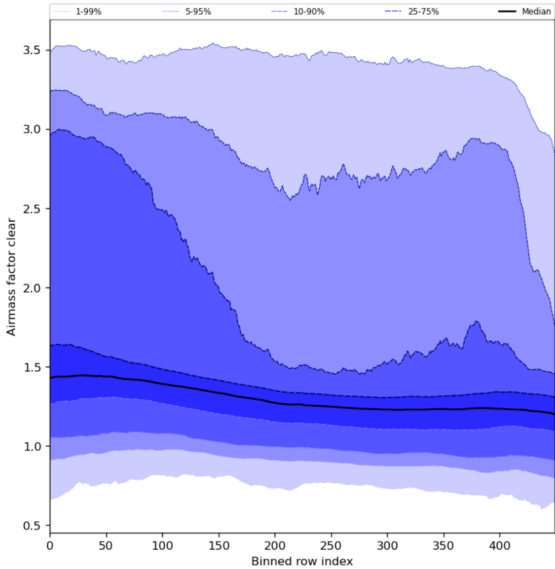
Figure 56: Along track statistics of “Airmass factor clear” for 2023-12-02 to 2023-12-04
