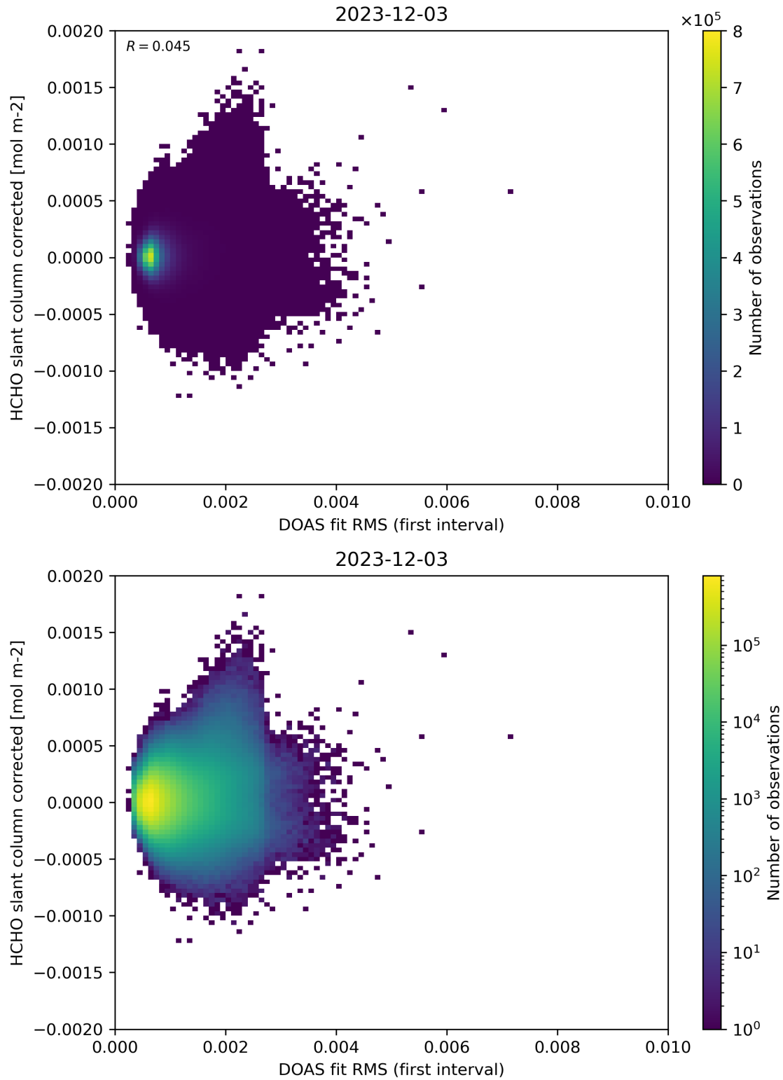
Figure 62: Scatter density plot of “DOAS fit RMS (first interval)” against “HCHO slant column corrected” for 2023-12-02 to 2023-12-04.
