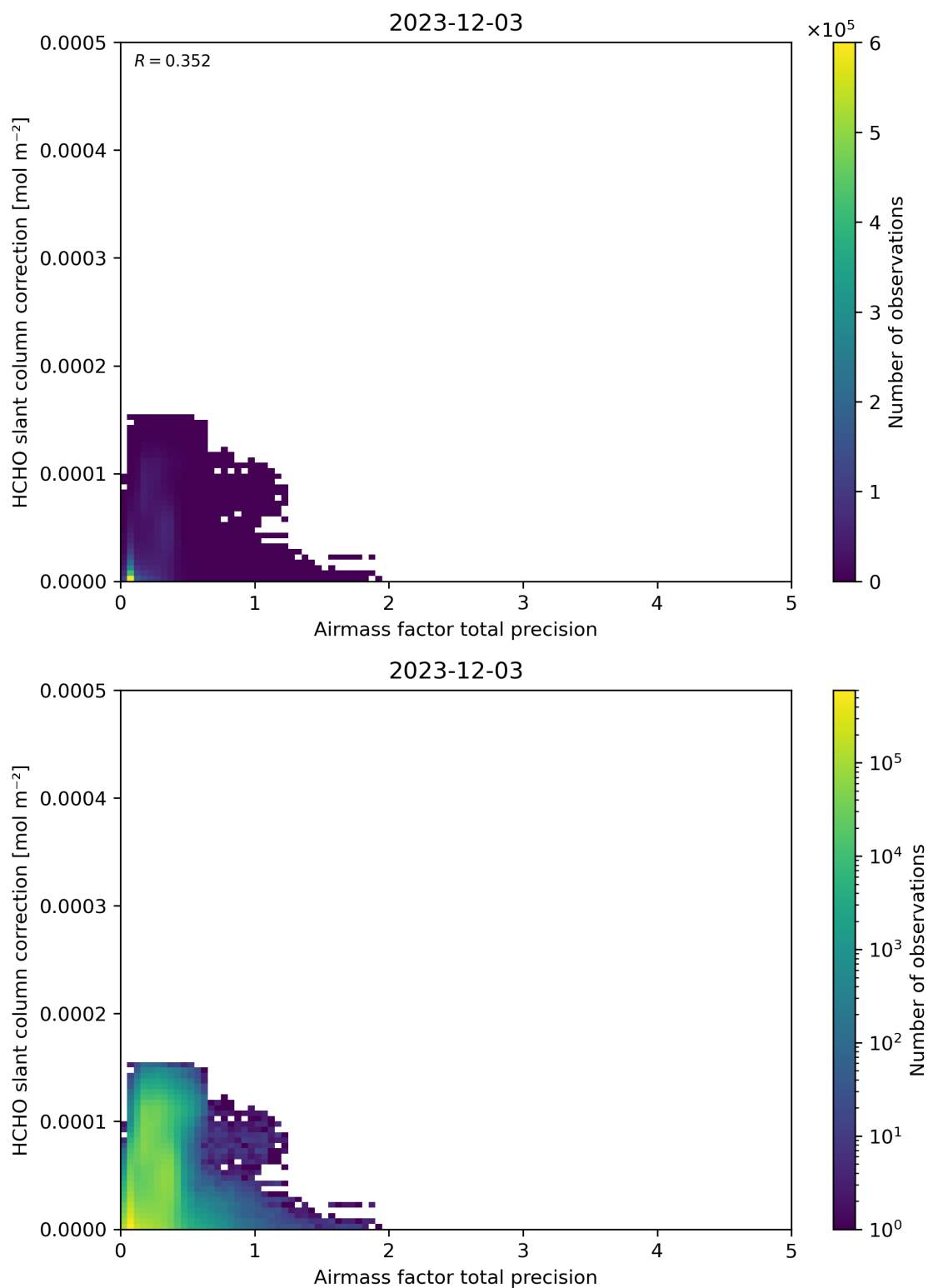
Figure 110: Scatter density plot of “Airmass factor total precision” against “HCHO slant column correction” for 2023-12-02 to 2023-12-04.
