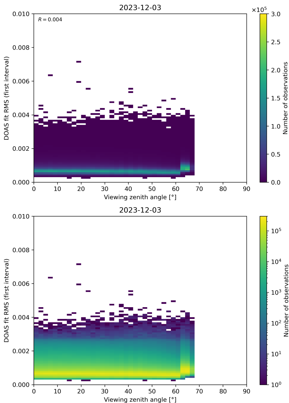
Figure 182: Scatter density plot of “Viewing zenith angle” against “DOAS fit RMS (first interval)” for 2023-12-02 to 2023-12-04.
