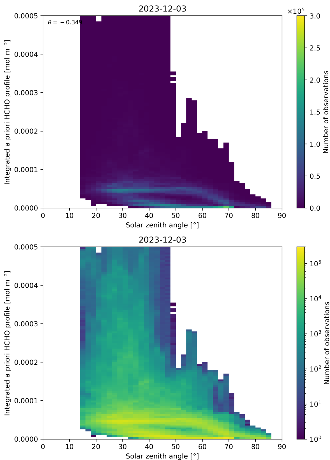
Figure 180: Scatter density plot of “Solar zenith angle” against “Integrated a priori HCHO profile” for 2023-12-02 to 2023-12-04.
