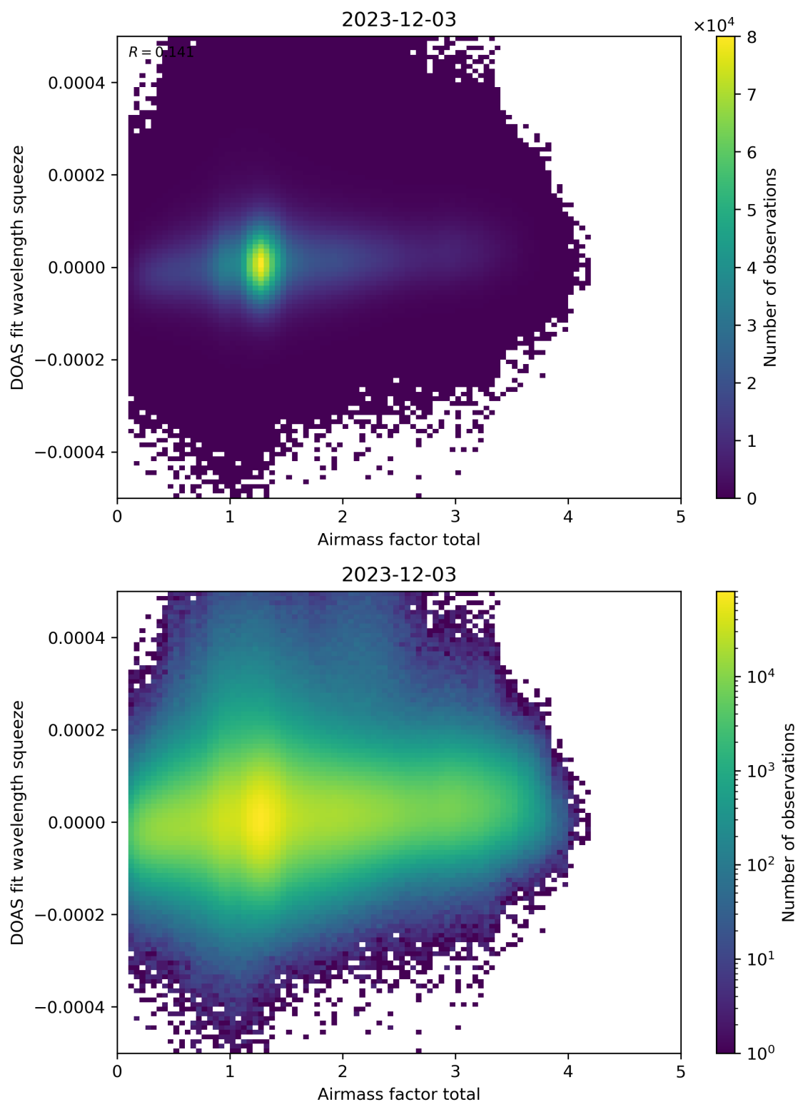
Figure 99: Scatter density plot of “Airmass factor total” against “DOAS fit wavelength squeeze” for 2023-12-02 to 2023-12-04.
