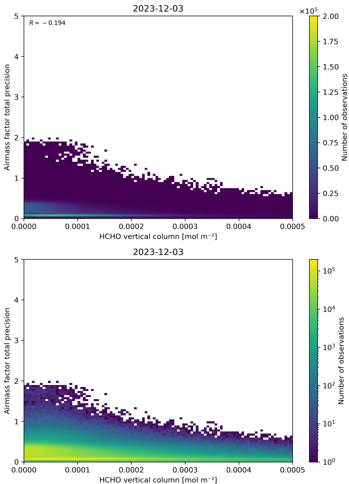
Figure 132: Scatter density plot of “HCHO vertical column” against “Airmass factor total precision” for 2023-12-02 to 2023-12-04.
