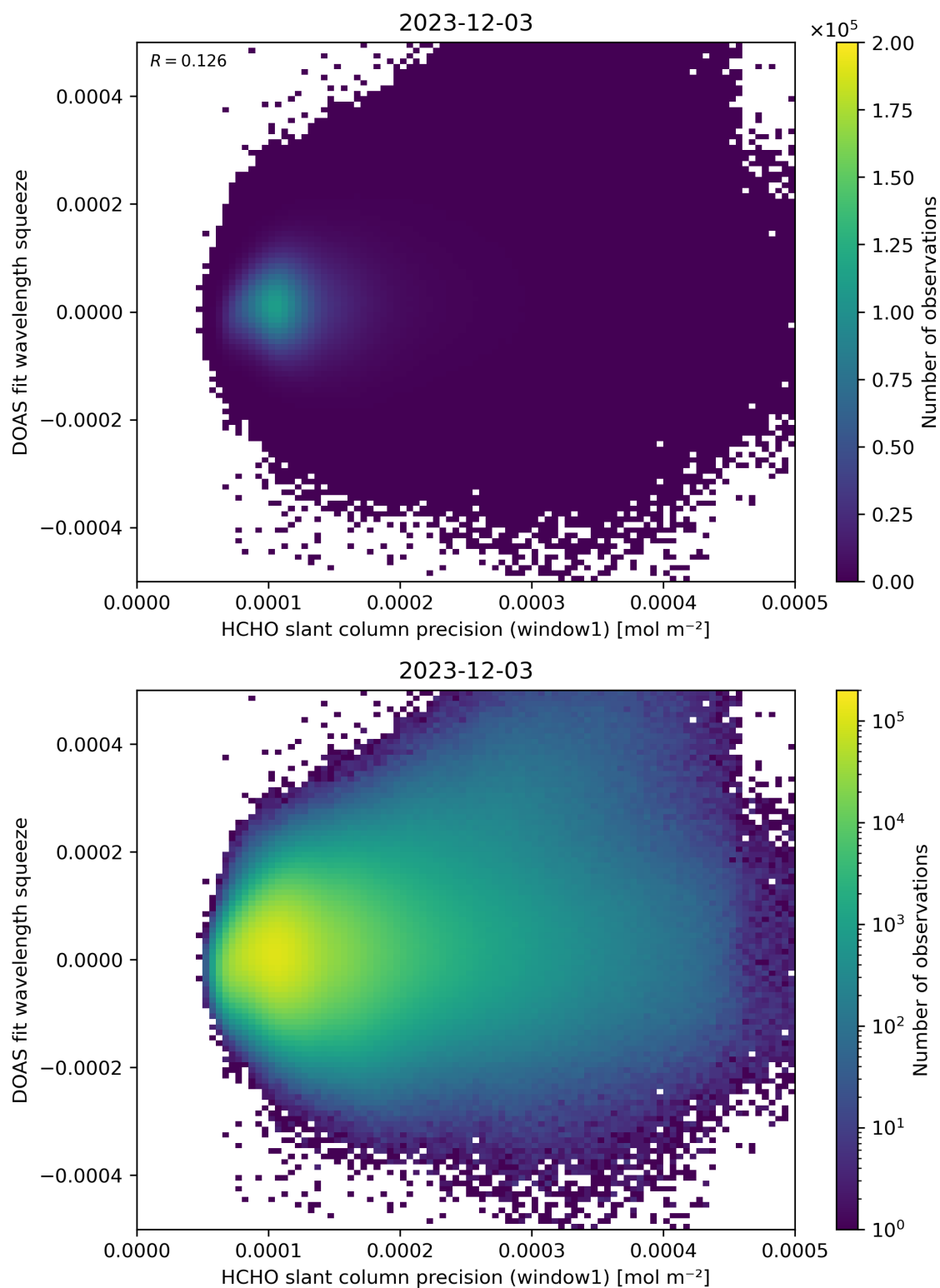
Figure 90: Scatter density plot of “HCHO slant column precision (window1)” against “DOAS fit wavelength squeeze” for 2023-12-02 to 2023-12-04.
