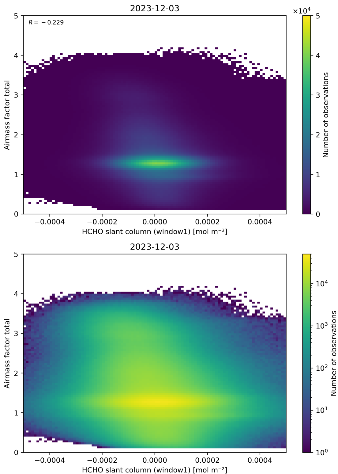
Figure 85: Scatter density plot of “HCHO slant column (window1)” against “Airmass factor total” for 2023-12-02 to 2023-12-04.
