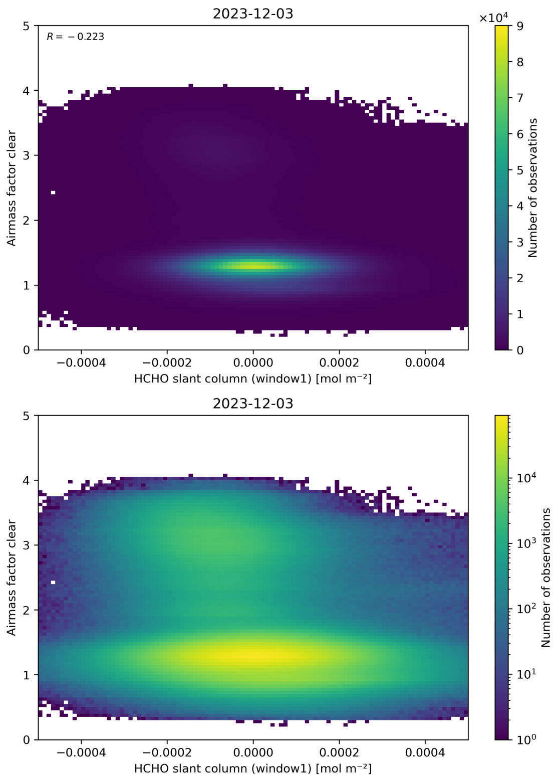
Figure 81: Scatter density plot of “HCHO slant column (window1)” against “Airmass factor clear” for 2023-12-02 to 2023-12-04.
