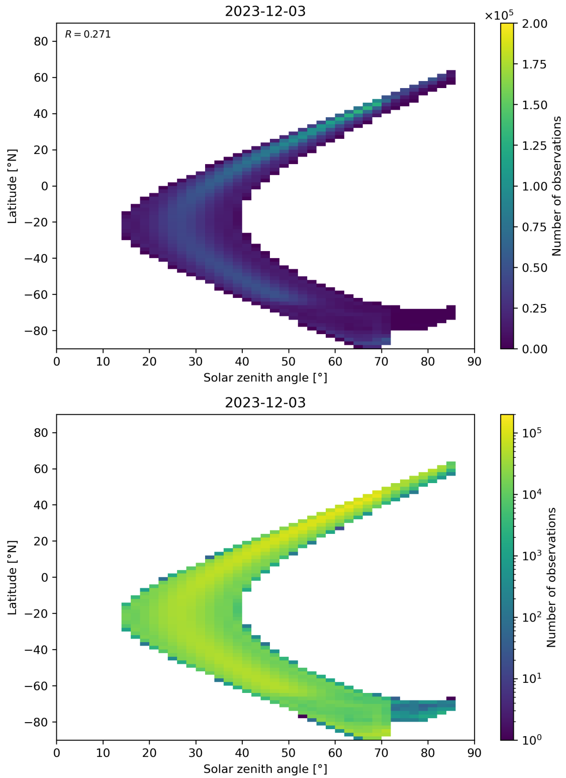
Figure 181: Scatter density plot of “Solar zenith angle” against “Latitude” for 2023-12-02 to 2023-12-04.
