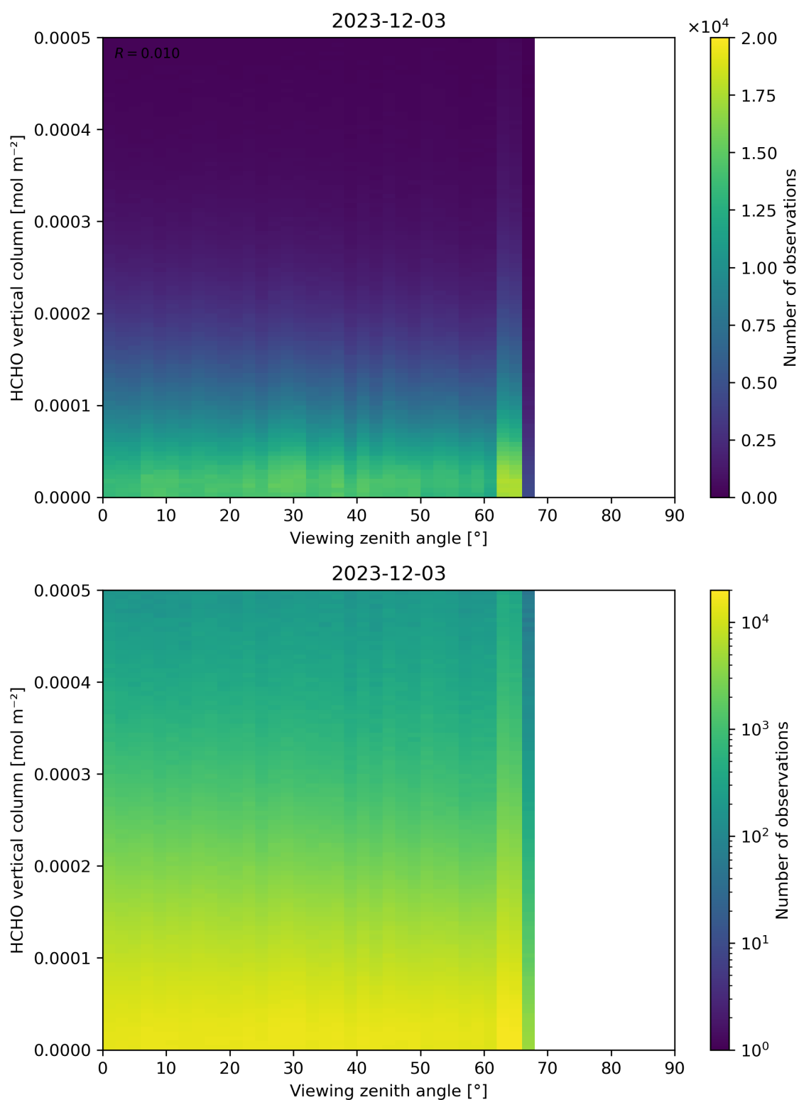
Figure 192: Scatter density plot of “Viewing zenith angle” against “HCHO vertical column” for 2023-12-02 to 2023-12-04.
