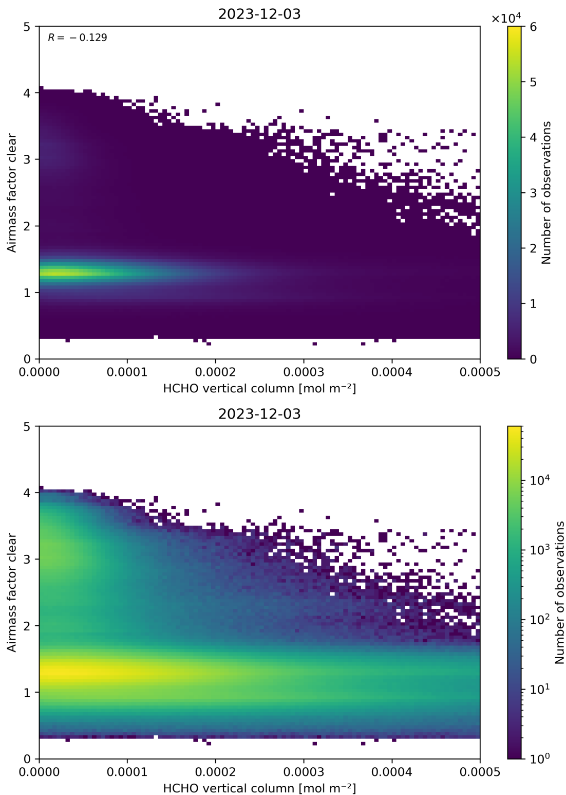
Figure 126: Scatter density plot of “HCHO vertical column” against “Airmass factor clear” for 2023-12-02 to 2023-12-04.
