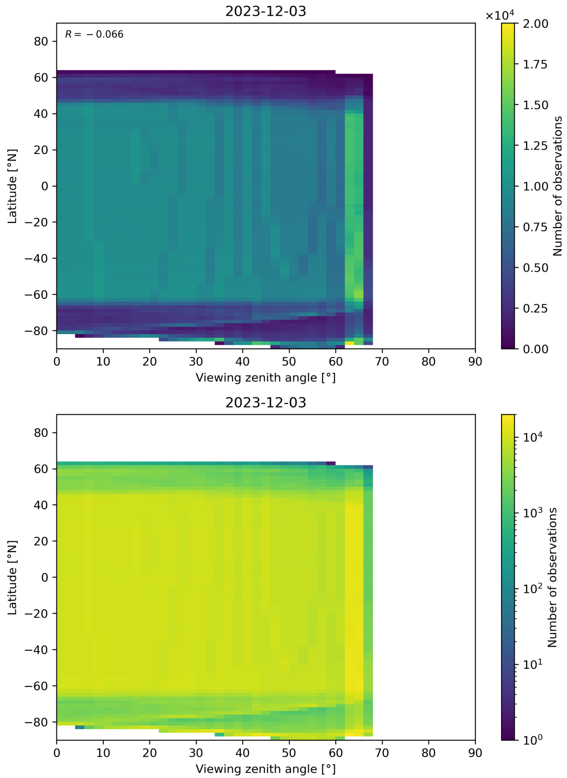
Figure 196: Scatter density plot of “Viewing zenith angle” against “Latitude” for 2023-12-02 to 2023-12-04.
