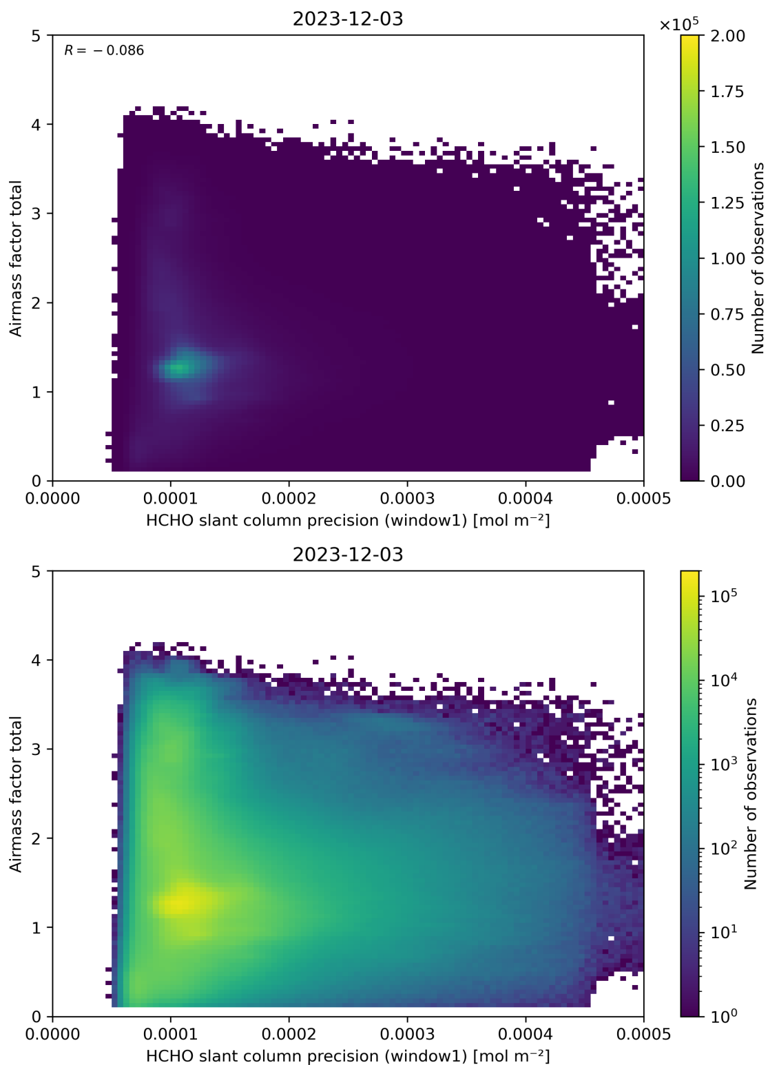
Figure 94: Scatter density plot of “HCHO slant column precision (window1)” against “Airmass factor total” for 2023-12-02 to 2023-12-04.
