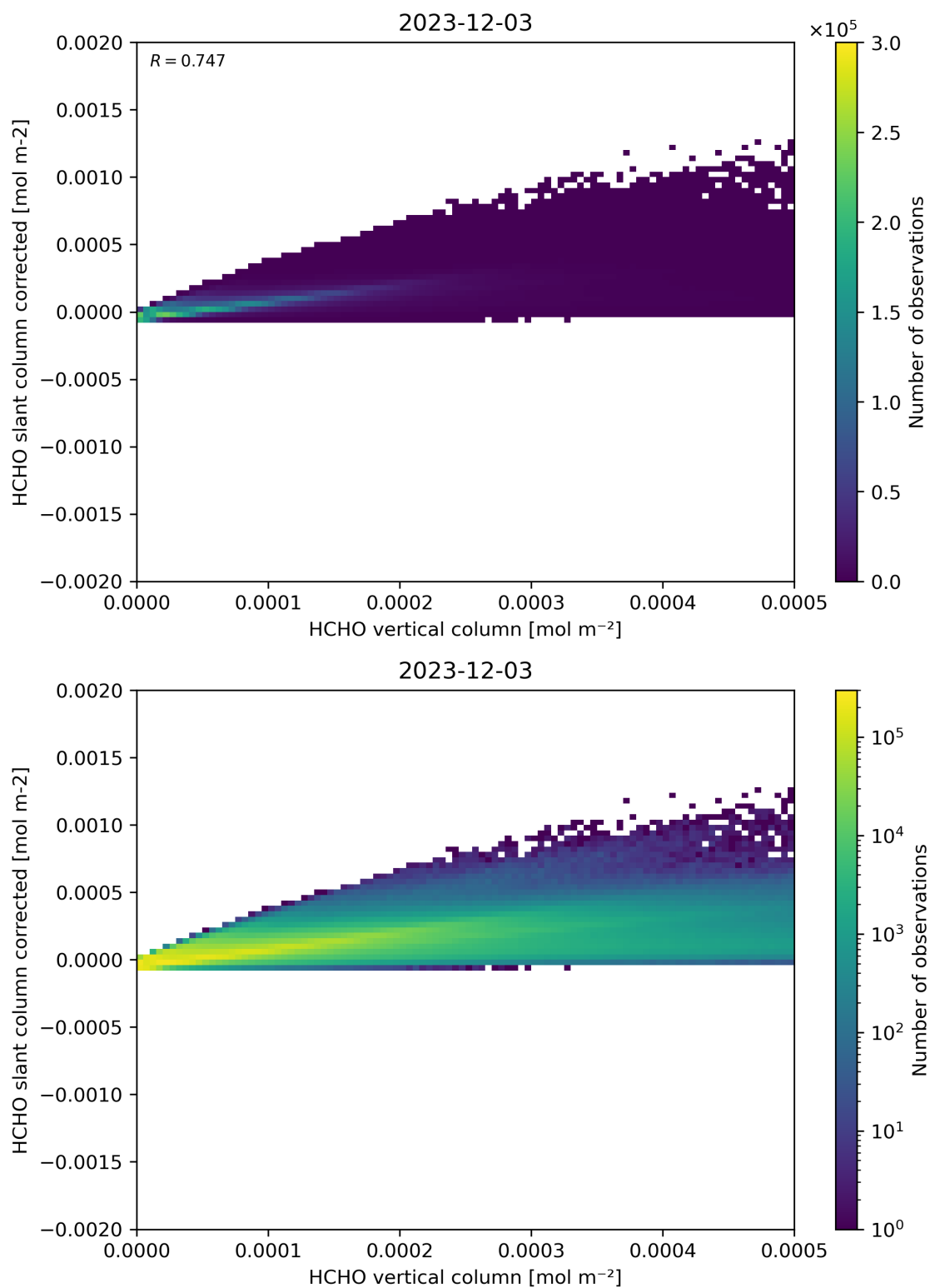
Figure 127: Scatter density plot of “HCHO vertical column” against “HCHO slant column corrected” for 2023-12-02 to 2023-12-04.
