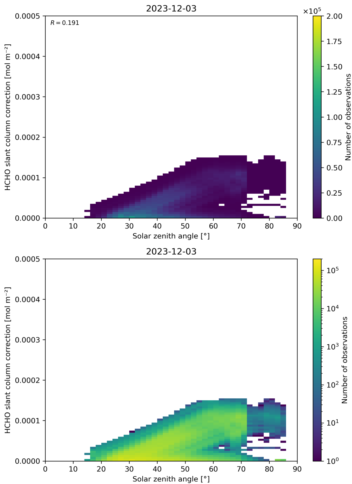
Figure 172: Scatter density plot of “Solar zenith angle” against “HCHO slant column correction” for 2023-12-02 to 2023-12-04.
