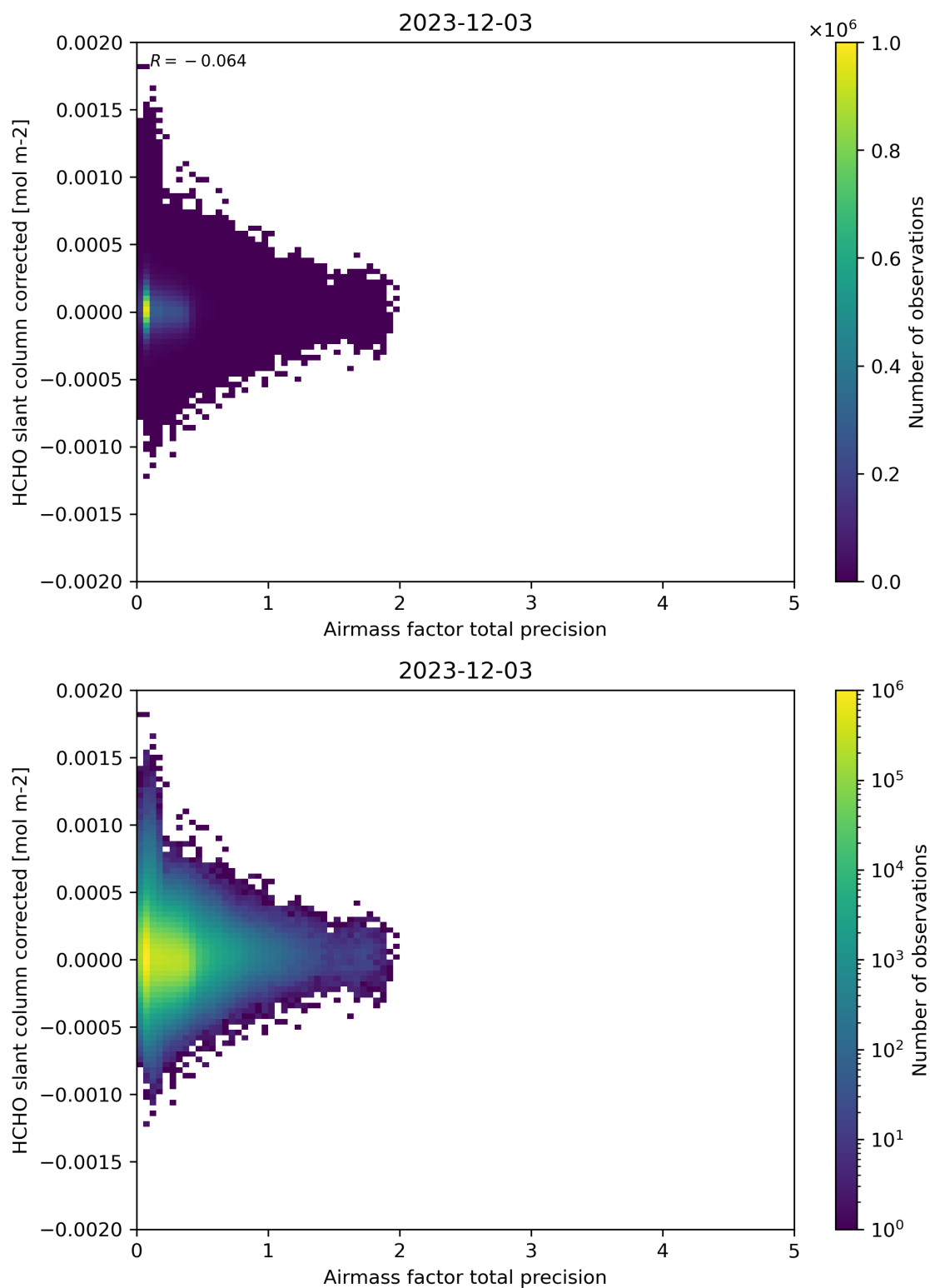
Figure 109: Scatter density plot of “Airmass factor total precision” against “HCHO slant column corrected” for 2023-12-02 to 2023-12-04.
