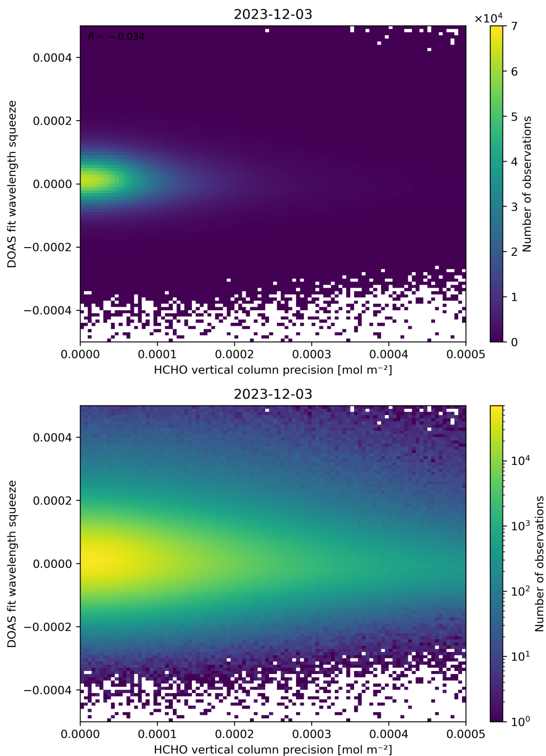
Figure 138: Scatter density plot of “HCHO vertical column precision” against “DOAS fit wavelength squeeze” for 2023-12-02 to 2023-12-04.
