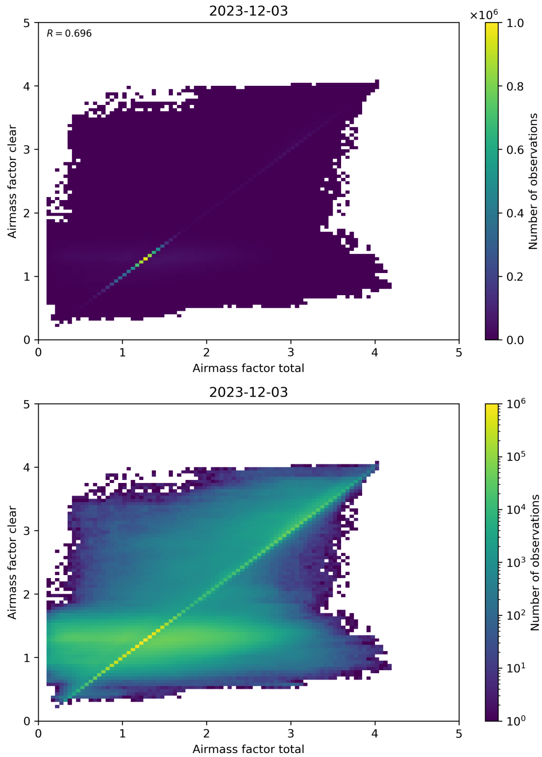
Figure 100: Scatter density plot of “Airmass factor total” against “Airmass factor clear” for 2023-12-02 to 2023-12-04.
