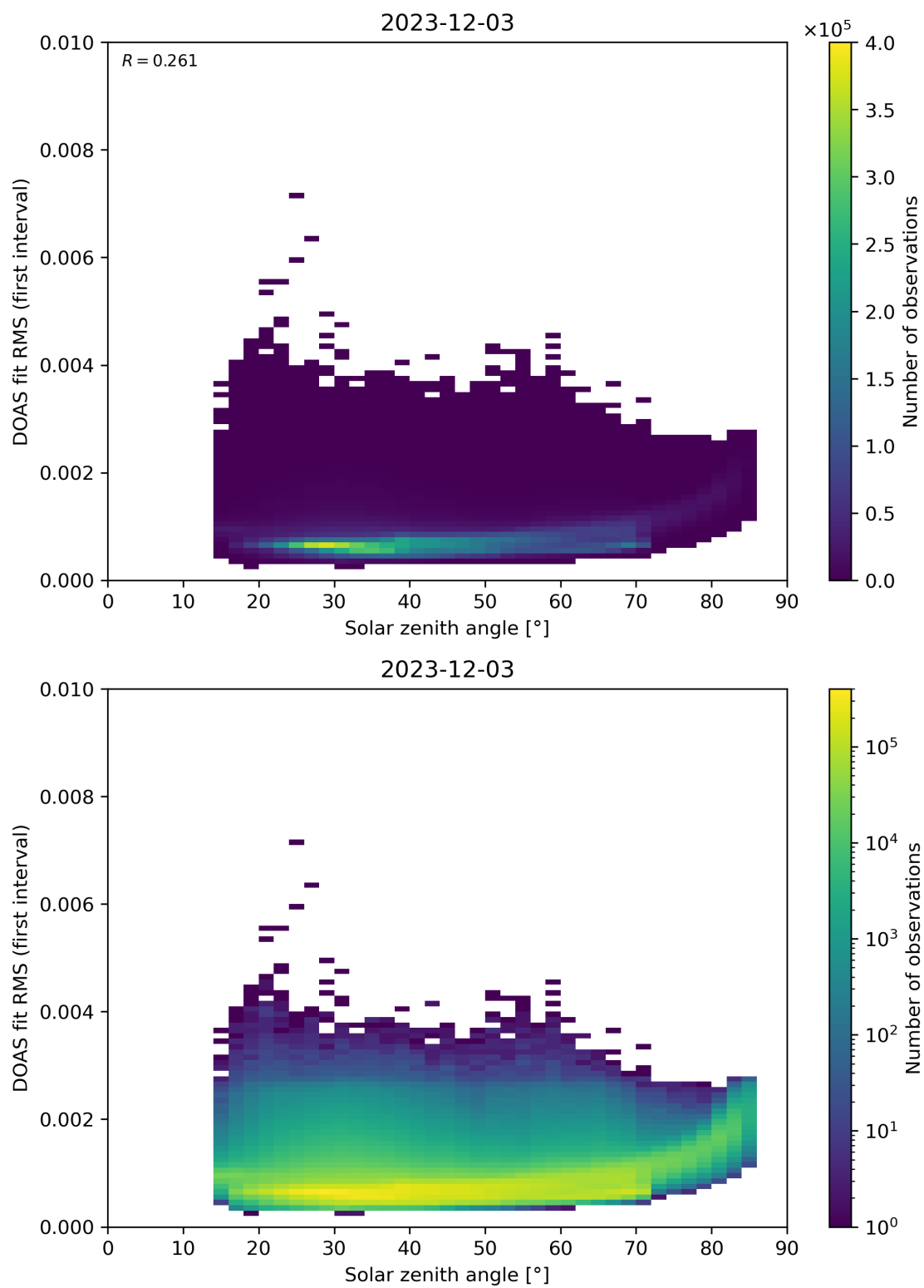
Figure 167: Scatter density plot of “Solar zenith angle” against “DOAS fit RMS (first interval)” for 2023-12-02 to 2023-12-04.
