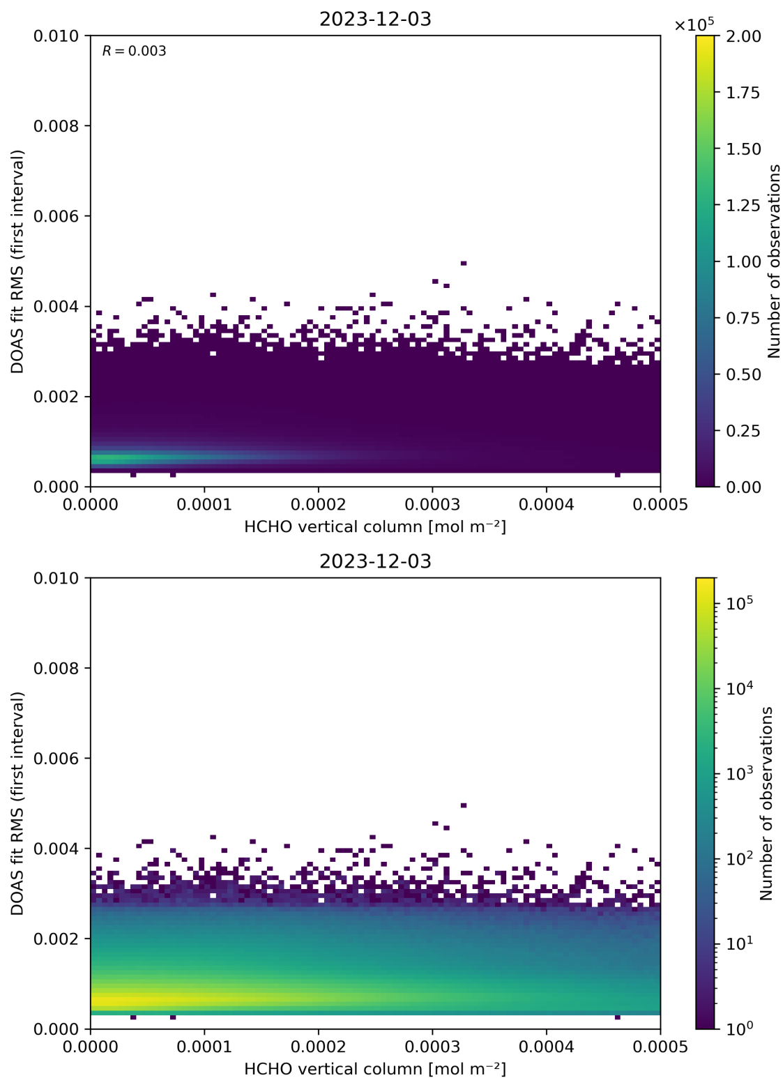
Figure 123: Scatter density plot of “HCHO vertical column” against “DOAS fit RMS (first interval)” for 2023-12-02 to 2023-12-04.
