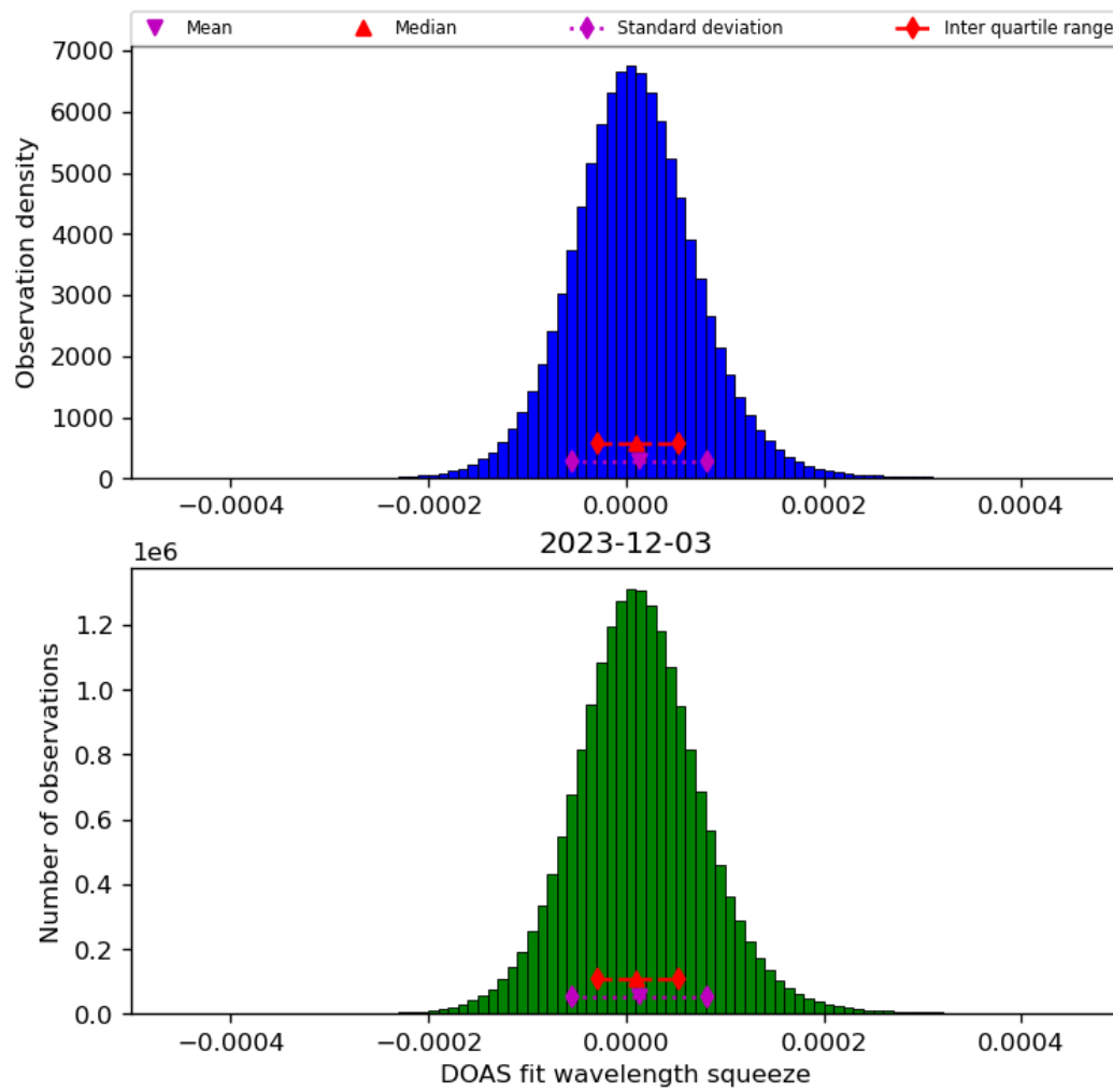
Figure 45: Histogram of “DOAS fit wavelength squeeze” for 2023-12-02 to 2023-12-04
