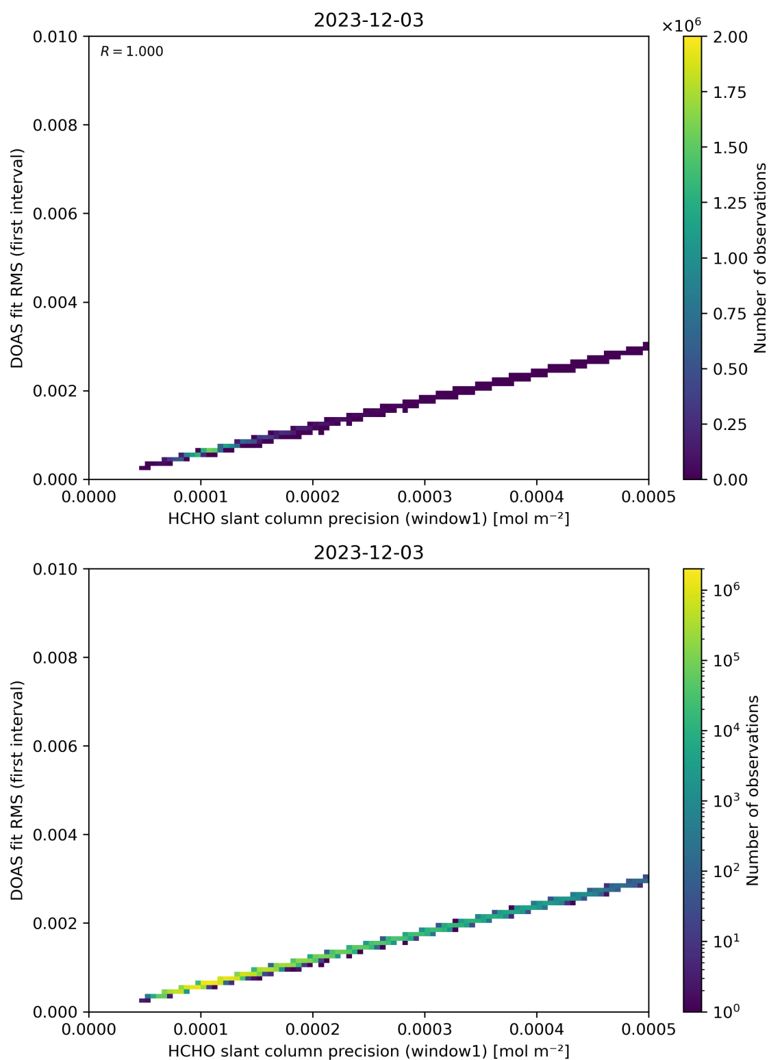
Figure 88: Scatter density plot of “HCHO slant column precision (window1)” against “DOAS fit RMS (first interval)” for 2023-12-02 to 2023-12-04.
