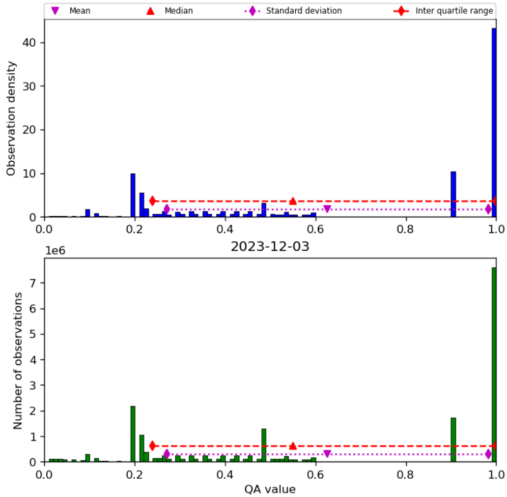
Figure 34: Histogram of “QA value” for 2023-12-02 to 2023-12-04
