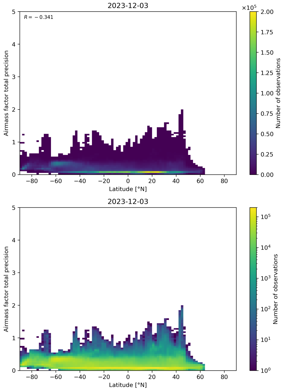
Figure 162: Scatter density plot of “Latitude” against “Airmass factor total precision” for 2023-12-02 to 2023-12-04.
