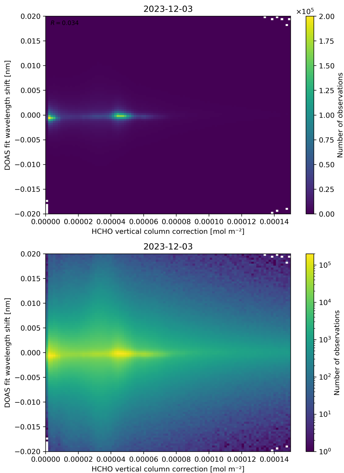
Figure 113: Scatter density plot of “HCHO vertical column correction” against “DOAS fit wavelength shift” for 2023-12-02 to 2023-12-04.
