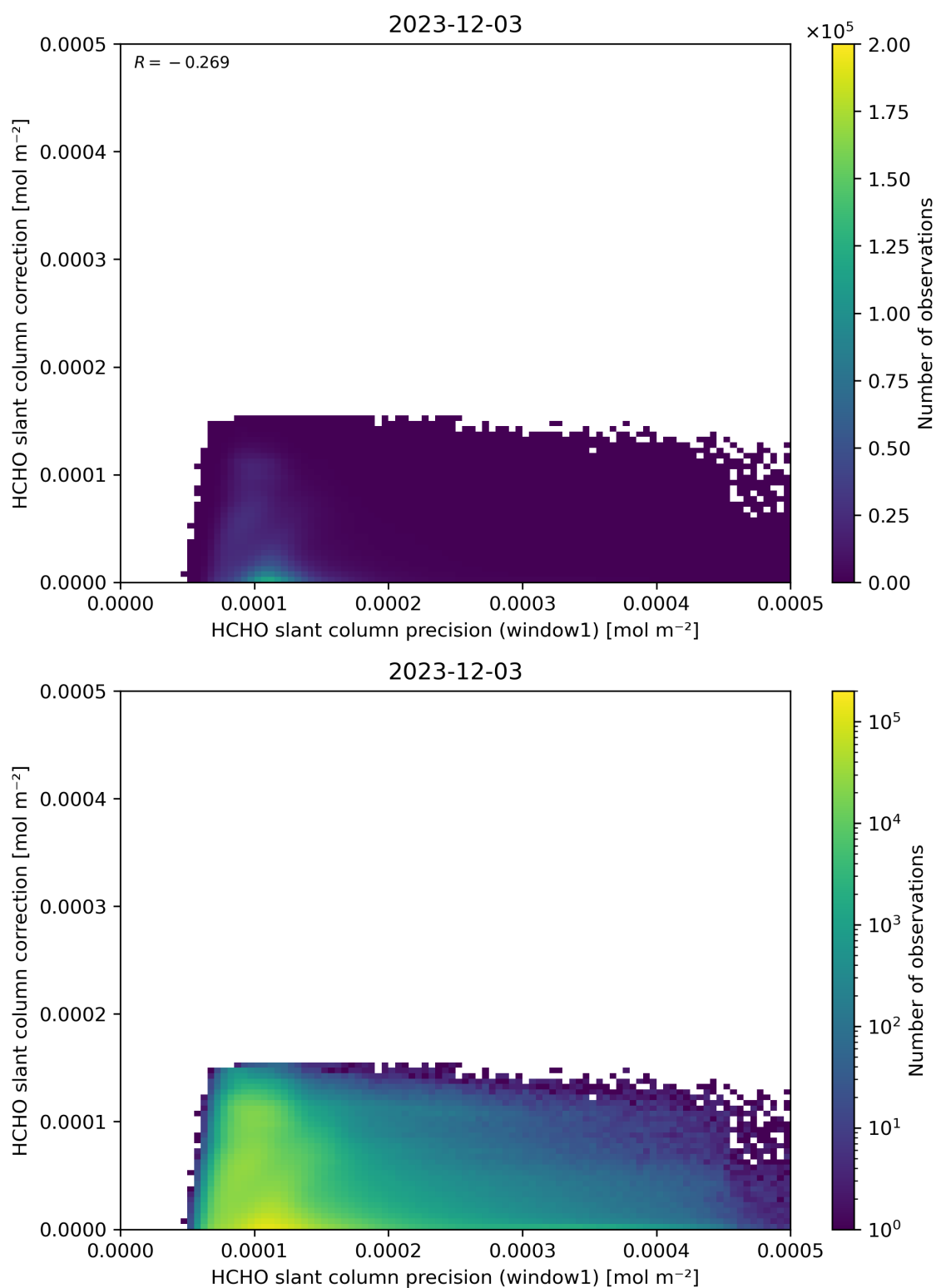
Figure 93: Scatter density plot of “HCHO slant column precision (window1)” against “HCHO slant column correction” for 2023-12-02 to 2023-12-04.
