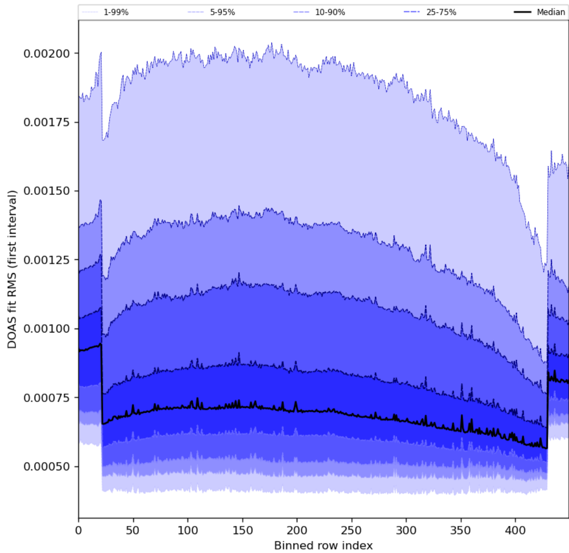
Figure 60: Along track statistics of “DOAS fit RMS (first interval)” for 2023-12-02 to 2023-12-04
