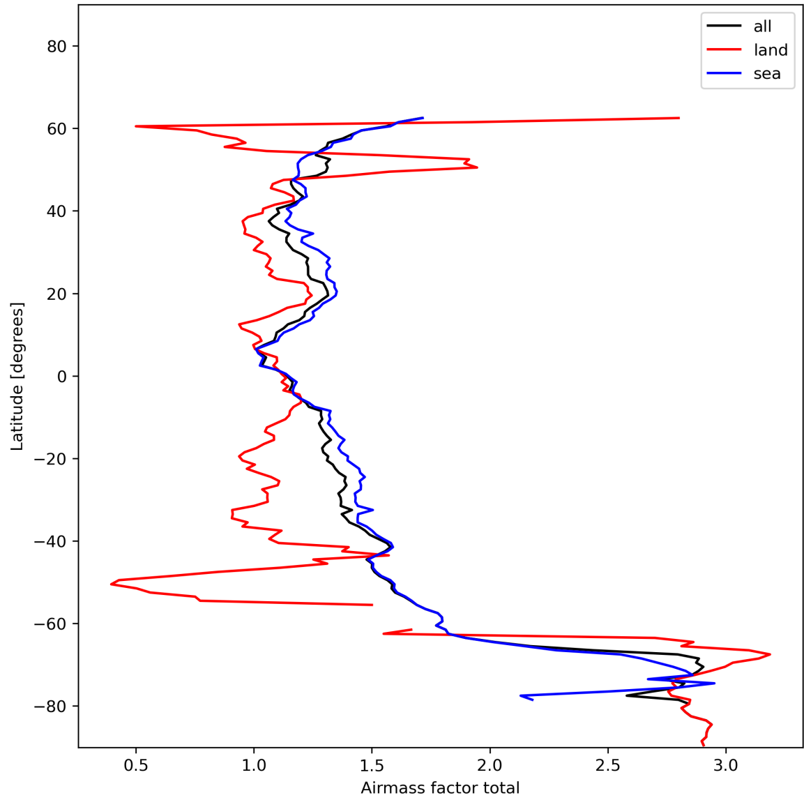
Figure 26: Zonal average of “Airmass factor total” for 2023-12-02 to 2023-12-04.
