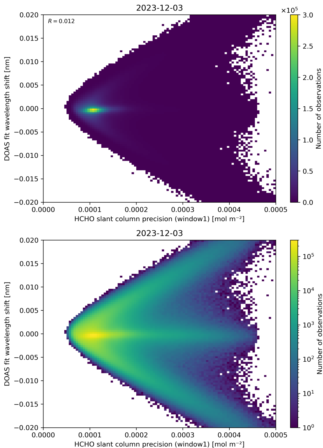
Figure 89: Scatter density plot of “HCHO slant column precision (window1)” against “DOAS fit wavelength shift” for 2023-12-02 to 2023-12-04.
