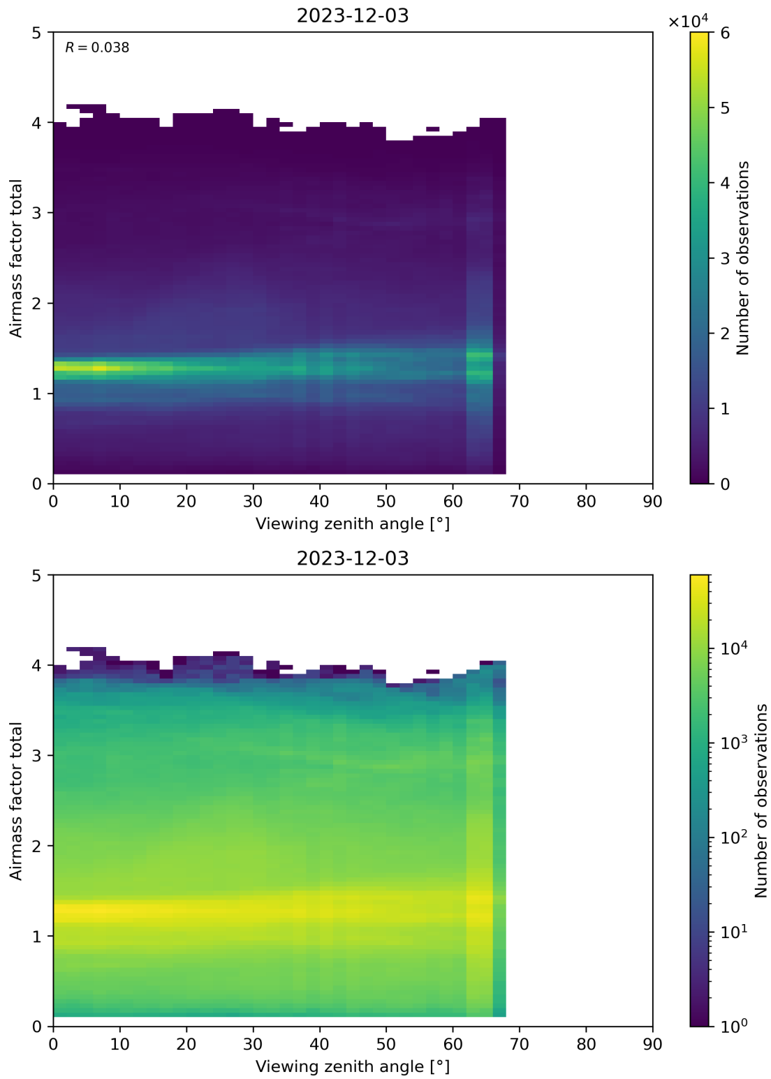
Figure 190: Scatter density plot of “Viewing zenith angle” against “Airmass factor total” for 2023-12-02 to 2023-12-04.
