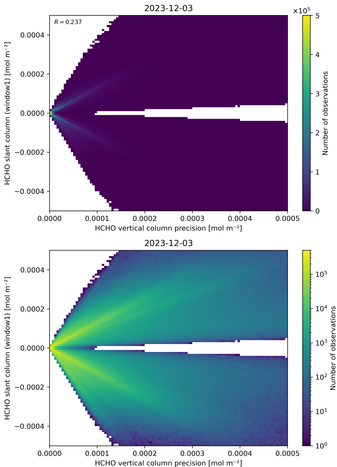
Figure 142: Scatter density plot of “HCHO vertical column precision” against “HCHO slant column (window1)” for 2023-12-02 to 2023-12-04.
