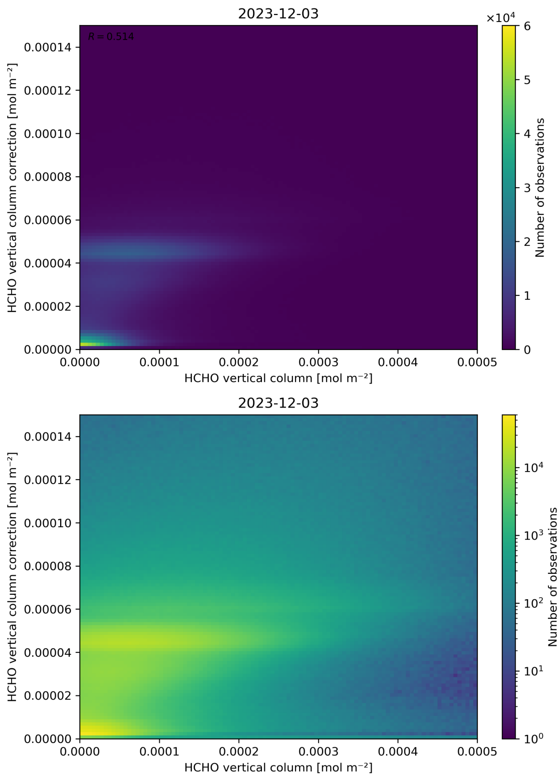
Figure 133: Scatter density plot of “HCHO vertical column” against “HCHO vertical column correction” for 2023-12-02 to 2023-12-04.
