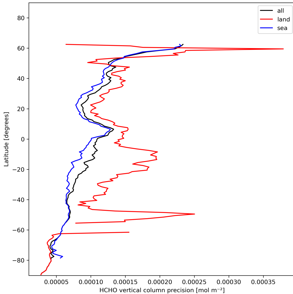
Figure 22: Zonal average of “HCHO vertical column precision” for 2023-12-02 to 2023-12-04.
