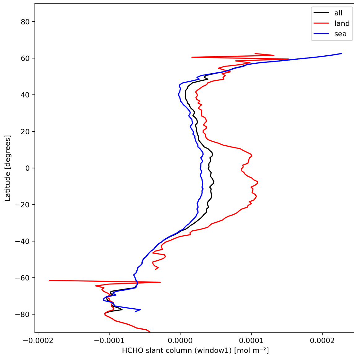
Figure 24: Zonal average of “HCHO slant column (window1)” for 2023-12-02 to 2023-12-04.
