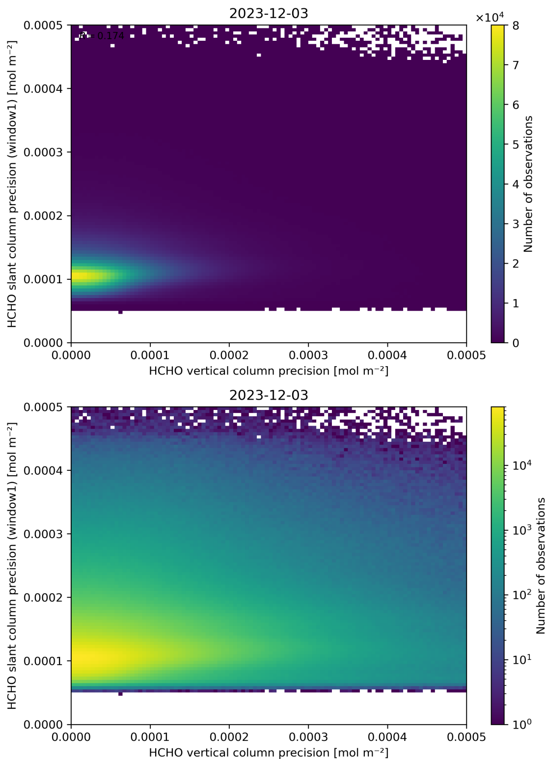
Figure 143: Scatter density plot of “HCHO vertical column precision” against “HCHO slant column precision (window1)” for 2023-12-02 to 2023-12-04.
