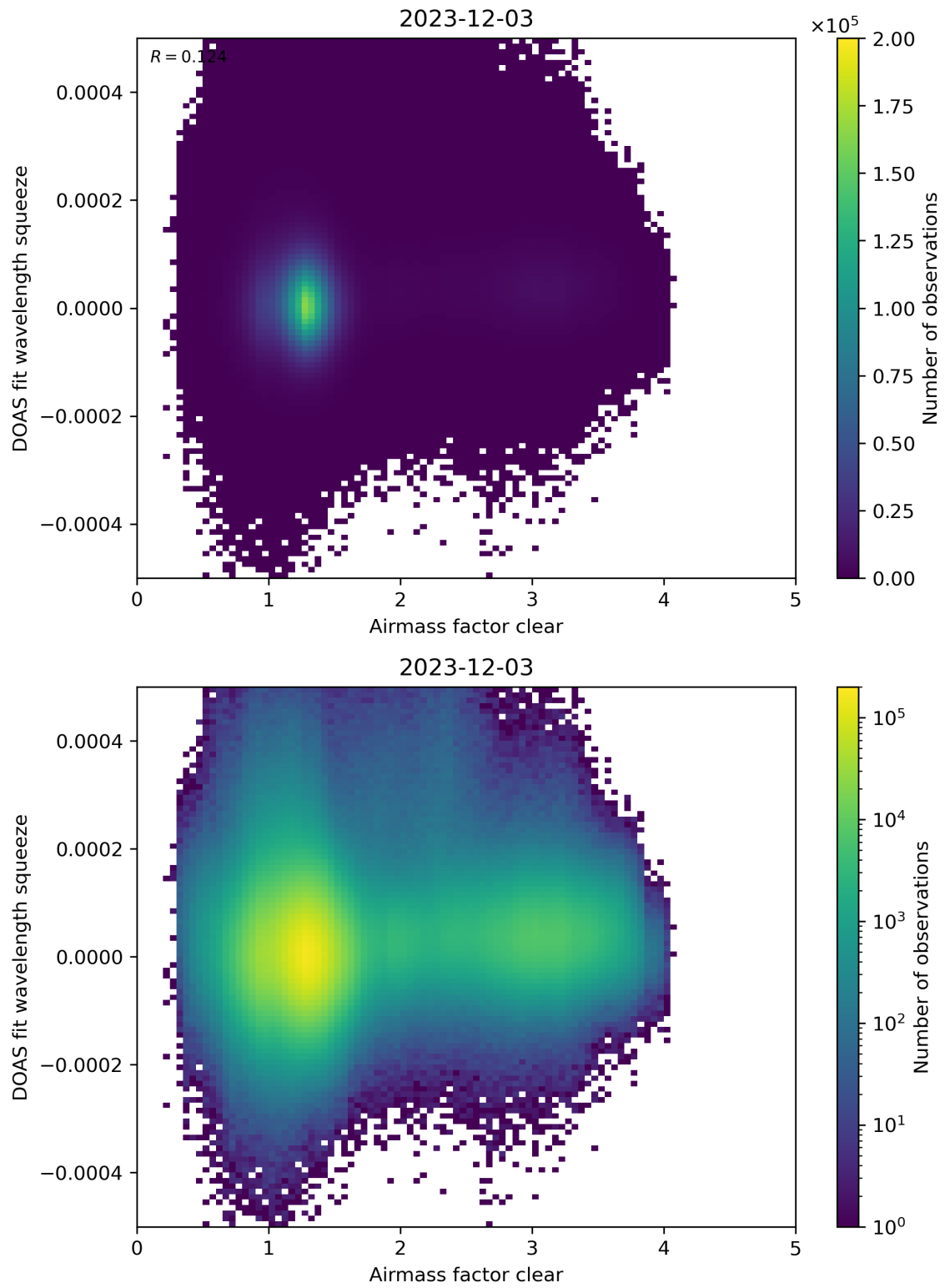
Figure 73: Scatter density plot of “Airmass factor clear” against “DOAS fit wavelength squeeze” for 2023-12-02 to 2023-12-04.
