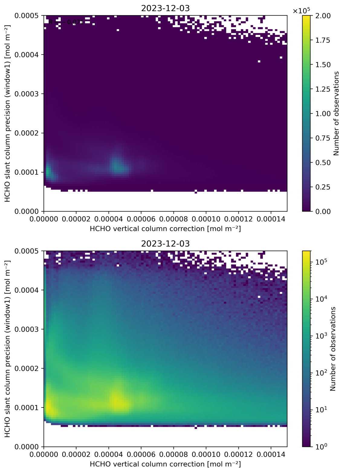
Figure 119: Scatter density plot of “HCHO vertical column correction” against “HCHO slant column precision (window1)” for 2023-12-02 to 2023-12-04.
