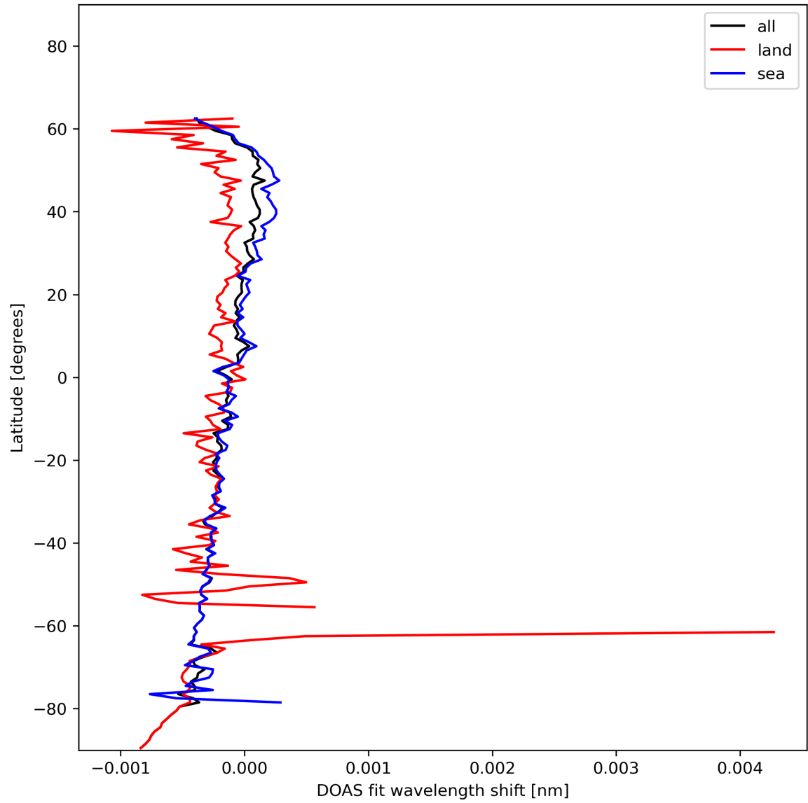
Figure 30: Zonal average of “DOAS fit wavelength shift” for 2023-12-02 to 2023-12-04.
