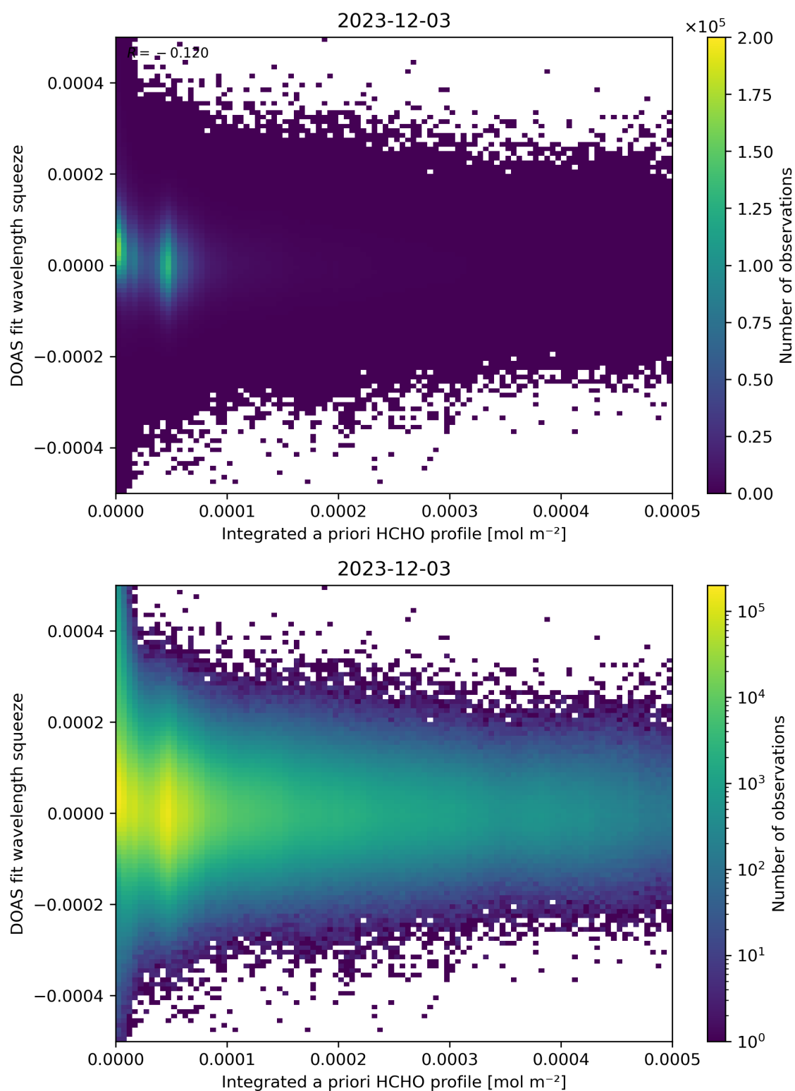
Figure 150: Scatter density plot of “Integrated a priori HCHO profile” against “DOAS fit wavelength squeeze” for 2023-12-02 to 2023-12-04.
