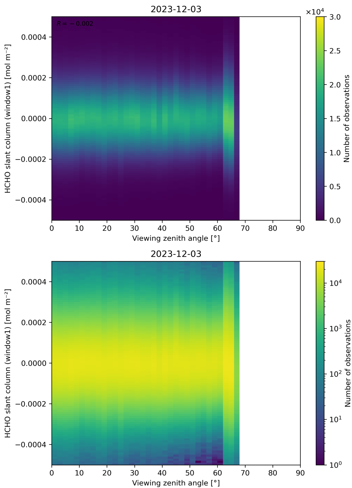
Figure 188: Scatter density plot of “Viewing zenith angle” against “HCHO slant column (window1)” for 2023-12-02 to 2023-12-04.
