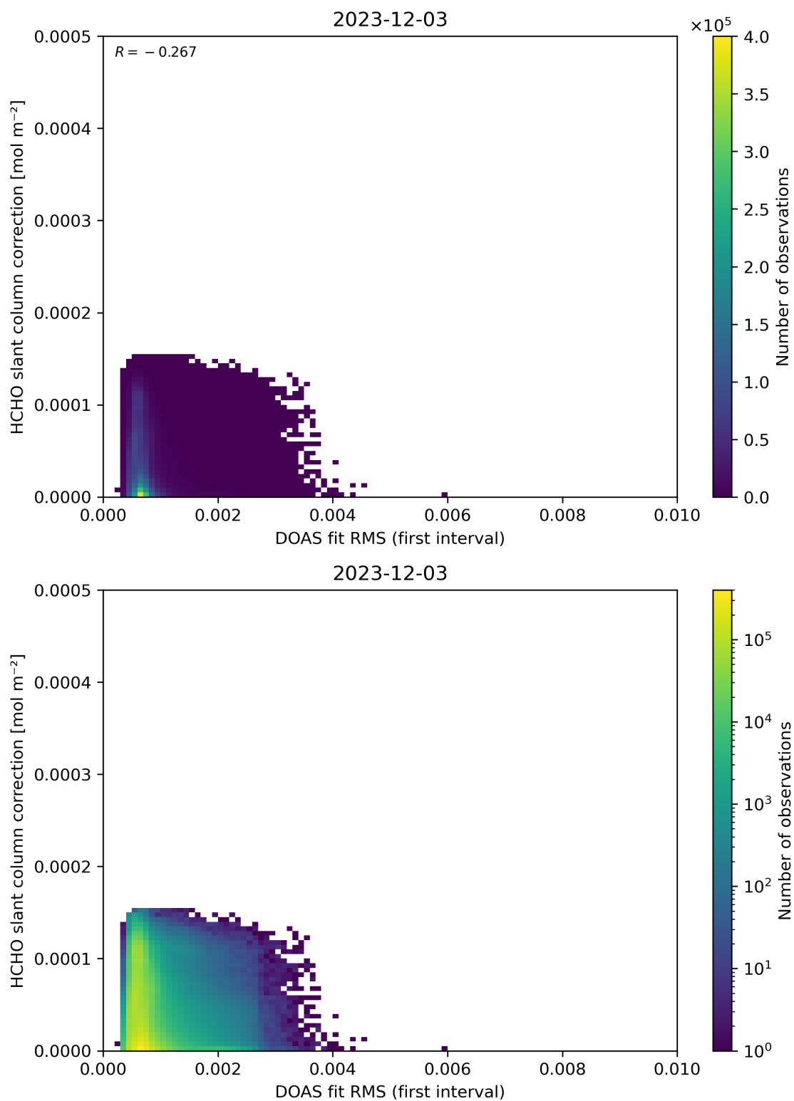
Figure 63: Scatter density plot of “DOAS fit RMS (first interval)” against “HCHO slant column correction” for 2023-12-02 to 2023-12-04.
