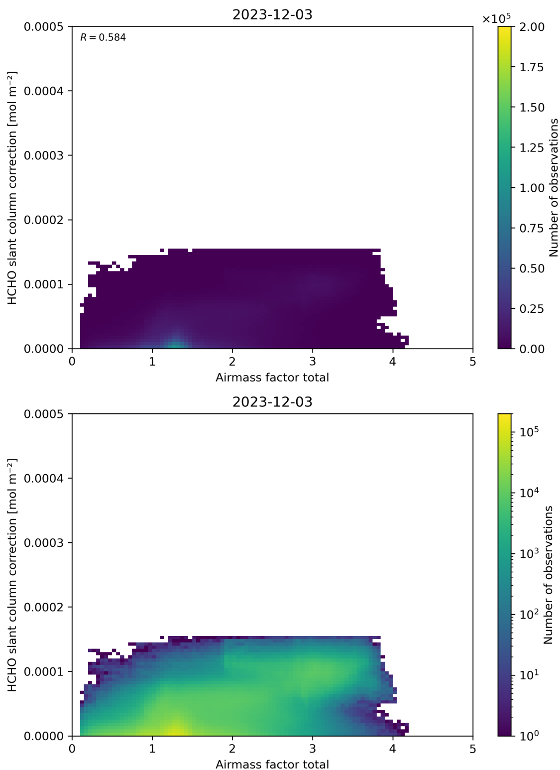
Figure 102: Scatter density plot of “Airmass factor total” against “HCHO slant column correction” for 2023-12-02 to 2023-12-04.
