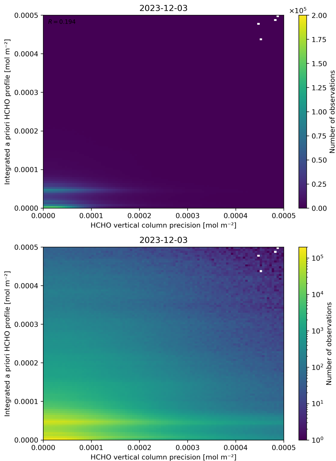
Figure 147: Scatter density plot of “HCHO vertical column precision” against “Integrated a priori HCHO profile” for 2023-12-02 to 2023-12-04.
