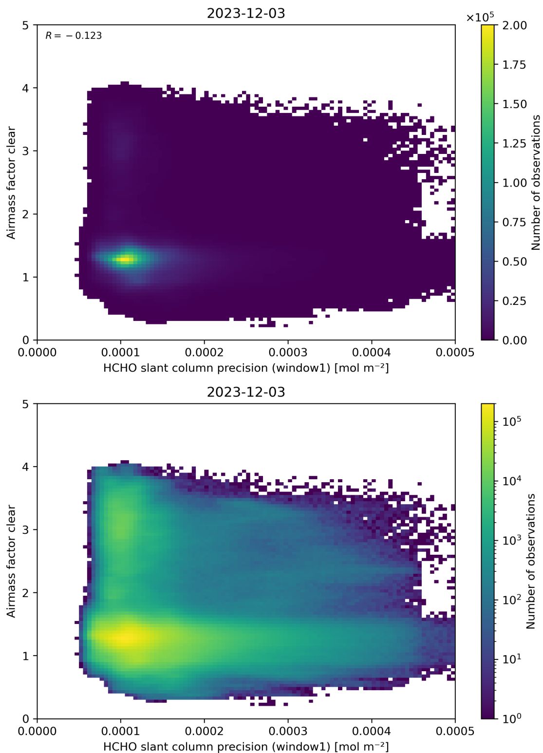
Figure 91: Scatter density plot of “HCHO slant column precision (window1)” against “Airmass factor clear” for 2023-12-02 to 2023-12-04.
