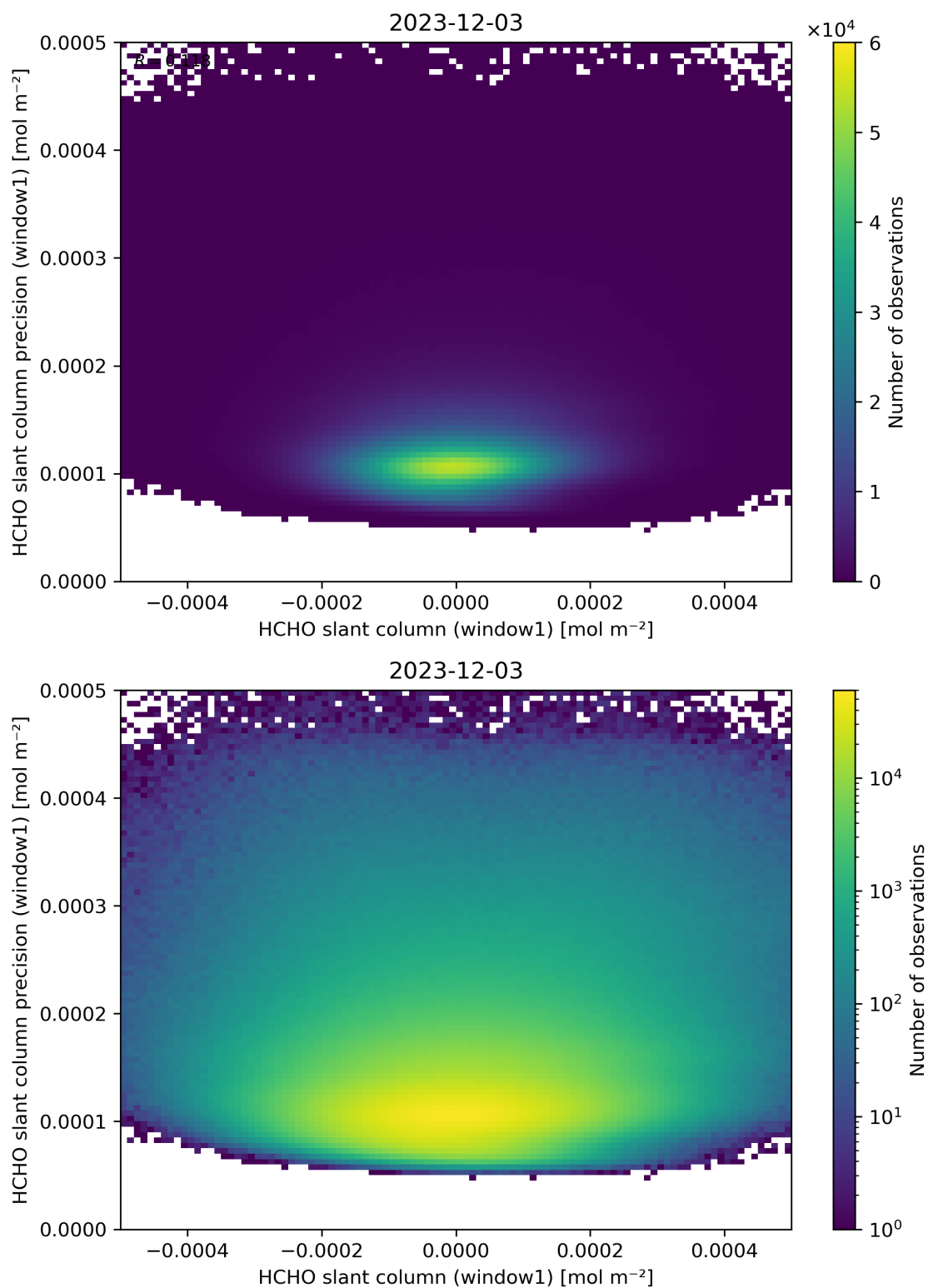
Figure 84: Scatter density plot of “HCHO slant column (window1)” against “HCHO slant column precision (window1)” for 2023-12-02 to 2023-12-04.
