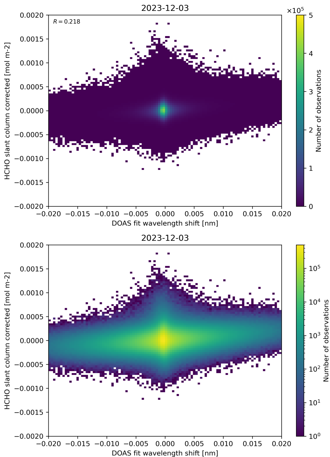
Figure 66: Scatter density plot of “DOAS fit wavelength shift” against “HCHO slant column corrected” for 2023-12-02 to 2023-12-04.
