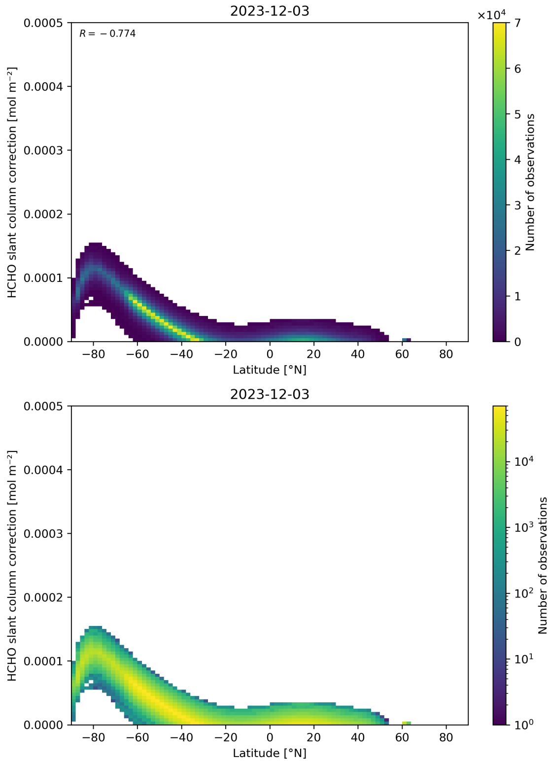
Figure 158: Scatter density plot of “Latitude” against “HCHO slant column correction” for 2023-12-02 to 2023-12-04.
