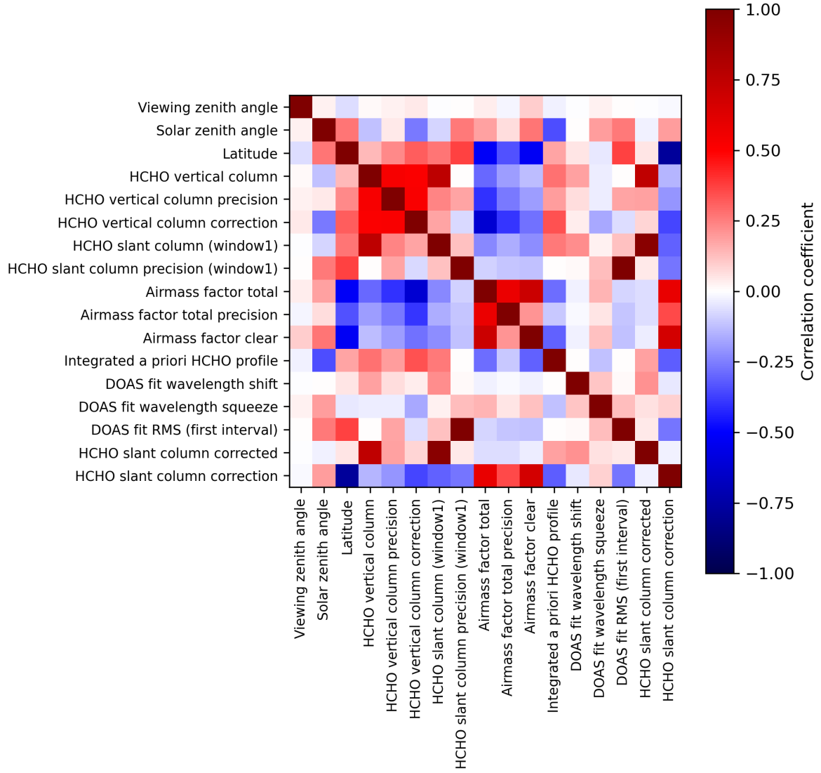
Figure 2: Map of correlation matrix for 2023-12-02 to 2023-12-04.
