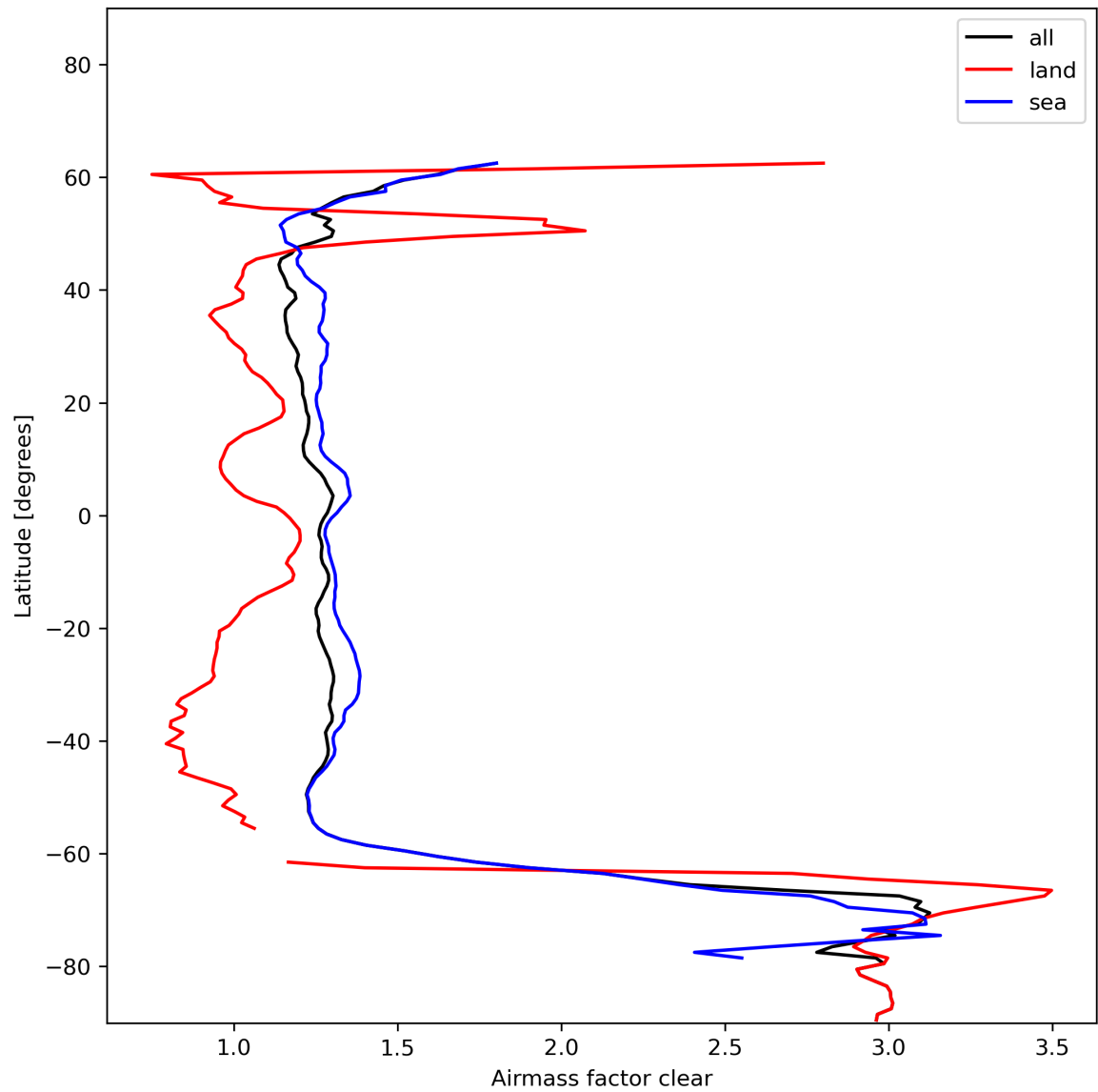
Figure 28: Zonal average of “Airmass factor clear” for 2023-12-02 to 2023-12-04.
