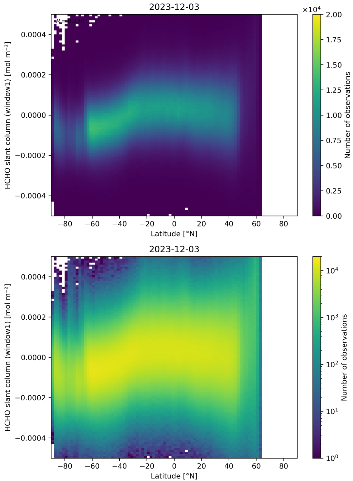
Figure 159: Scatter density plot of “Latitude” against “HCHO slant column (window1)” for 2023-12-02 to 2023-12-04.
