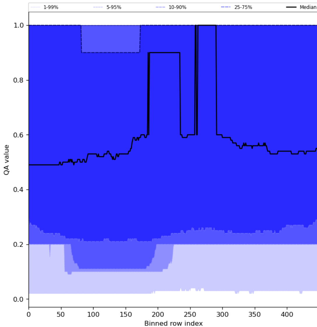
Figure 48: Along track statistics of “QA value” for 2023-12-02 to 2023-12-04
