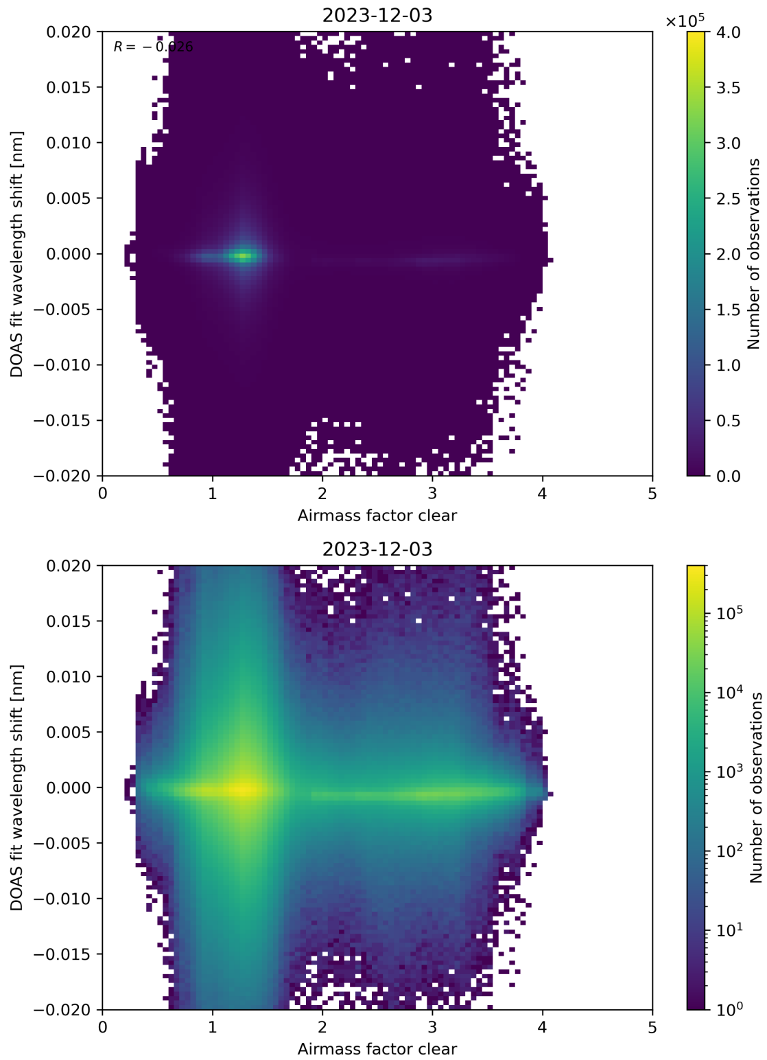
Figure 72: Scatter density plot of “Airmass factor clear” against “DOAS fit wavelength shift” for 2023-12-02 to 2023-12-04.
