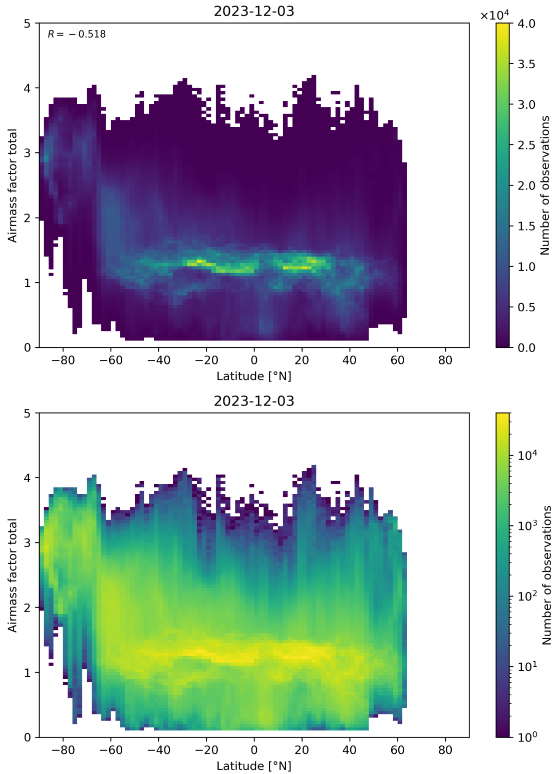
Figure 161: Scatter density plot of “Latitude” against “Airmass factor total” for 2023-12-02 to 2023-12-04.
