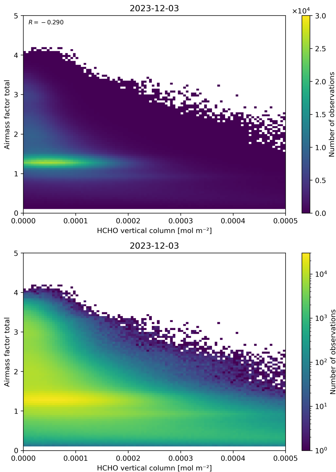
Figure 131: Scatter density plot of “HCHO vertical column” against “Airmass factor total” for 2023-12-02 to 2023-12-04.
