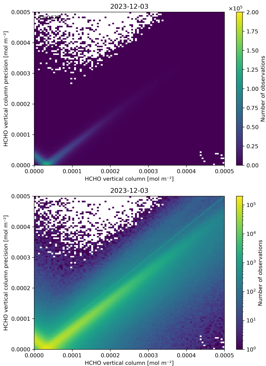
Figure 134: Scatter density plot of “HCHO vertical column” against “HCHO vertical column precision” for 2023-12-02 to 2023-12-04.
