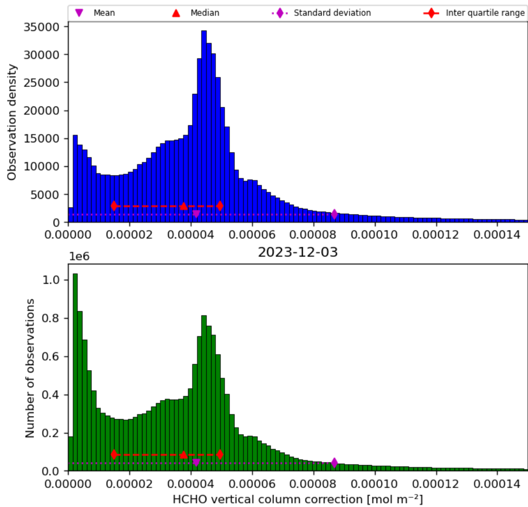
Figure 37: Histogram of “HCHO vertical column correction” for 2023-12-02 to 2023-12-04
