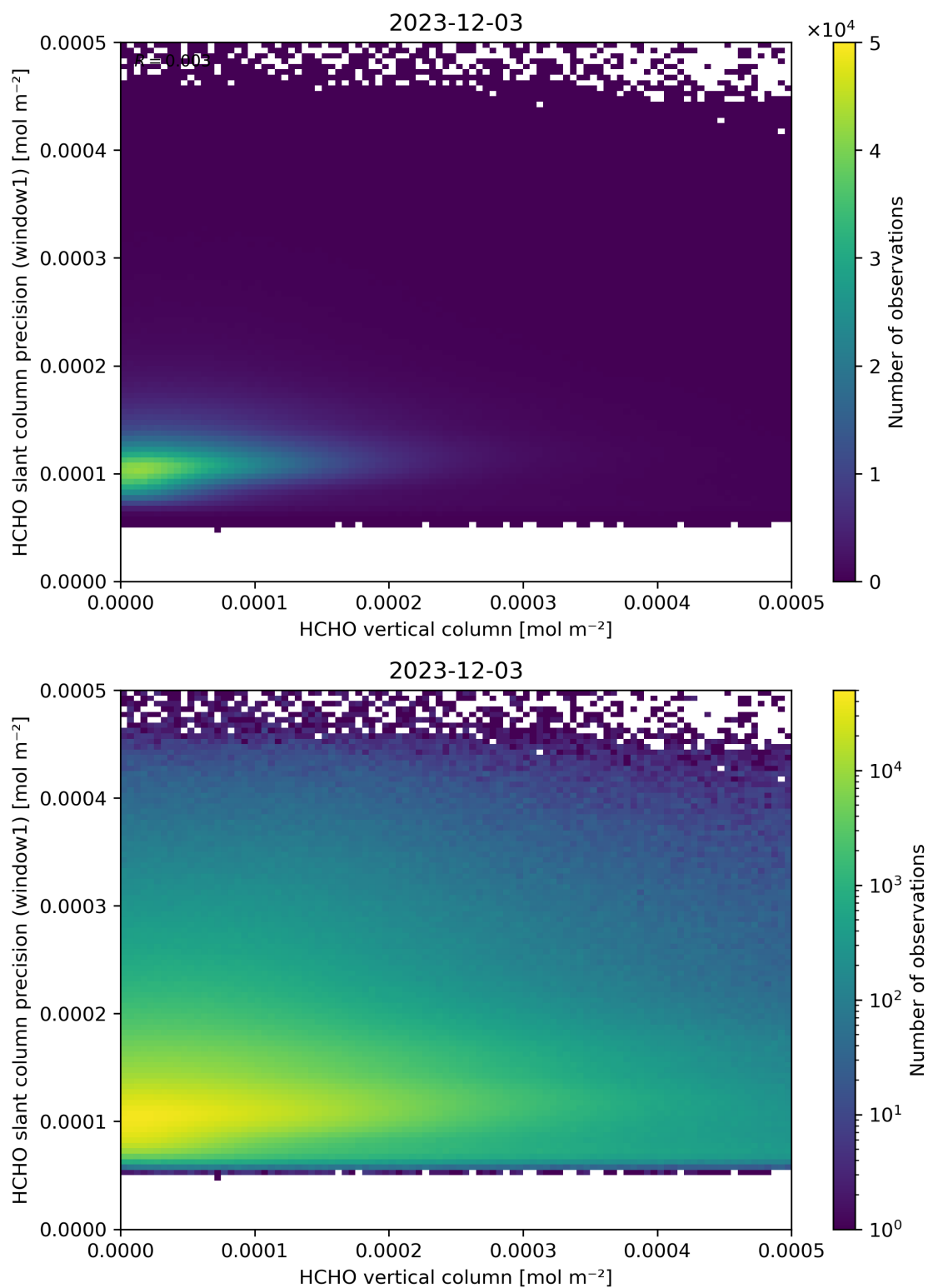
Figure 130: Scatter density plot of “HCHO vertical column” against “HCHO slant column precision (window1)” for 2023-12-02 to 2023-12-04.
