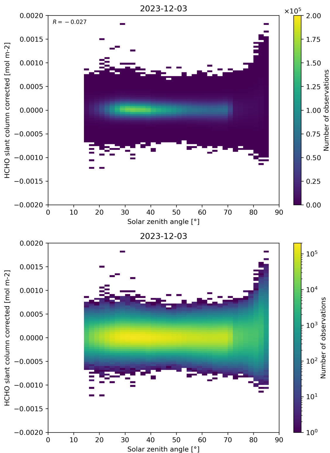
Figure 171: Scatter density plot of “Solar zenith angle” against “HCHO slant column corrected” for 2023-12-02 to 2023-12-04.
