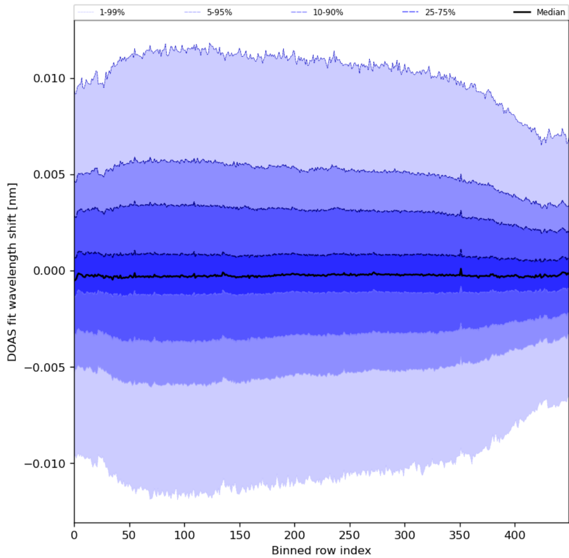
Figure 58: Along track statistics of “DOAS fit wavelength shift” for 2023-12-02 to 2023-12-04
