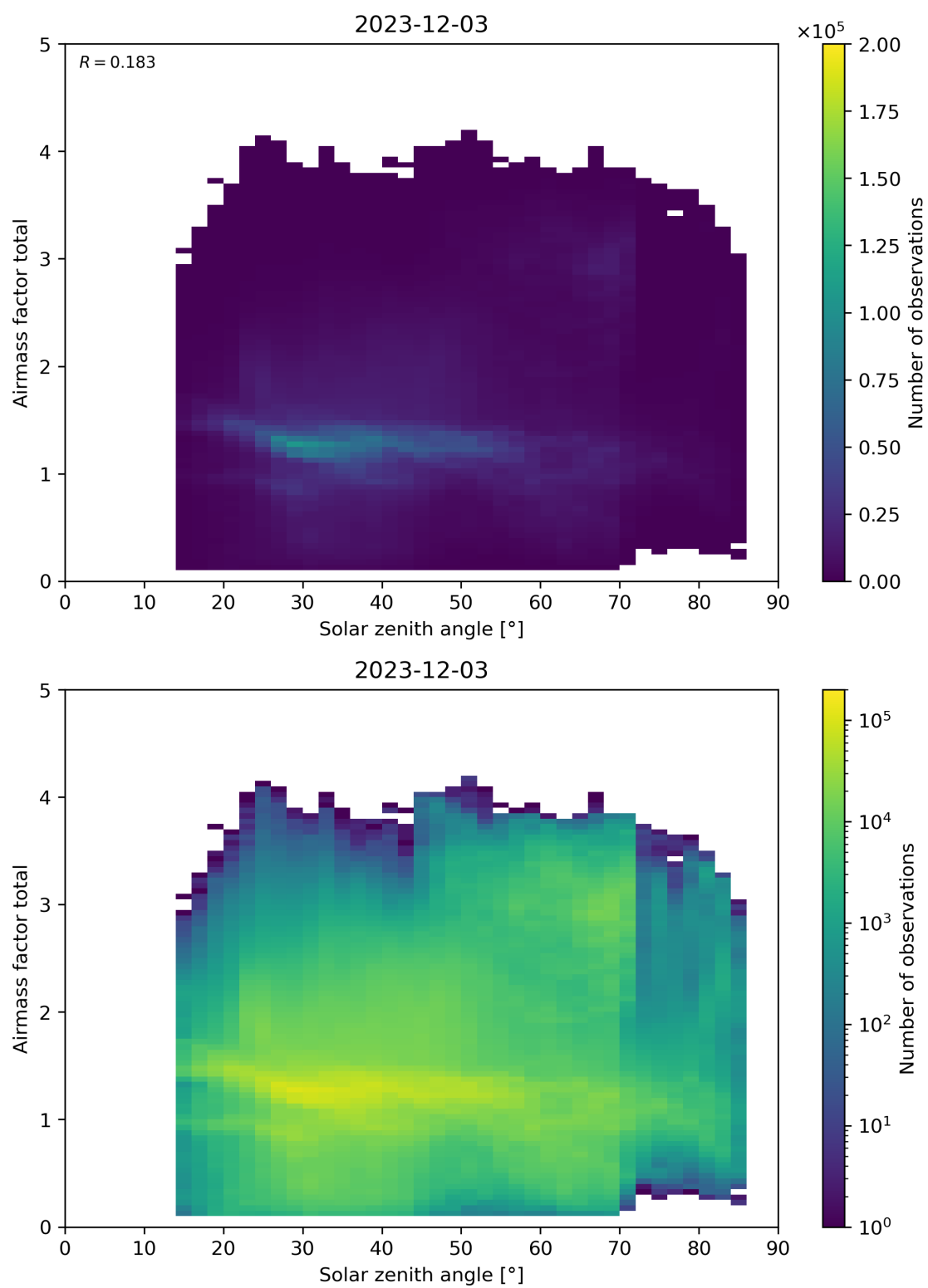
Figure 175: Scatter density plot of “Solar zenith angle” against “Airmass factor total” for 2023-12-02 to 2023-12-04.
