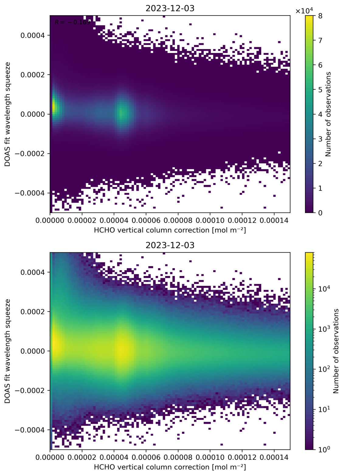
Figure 114: Scatter density plot of “HCHO vertical column correction” against “DOAS fit wavelength squeeze” for 2023-12-02 to 2023-12-04.
