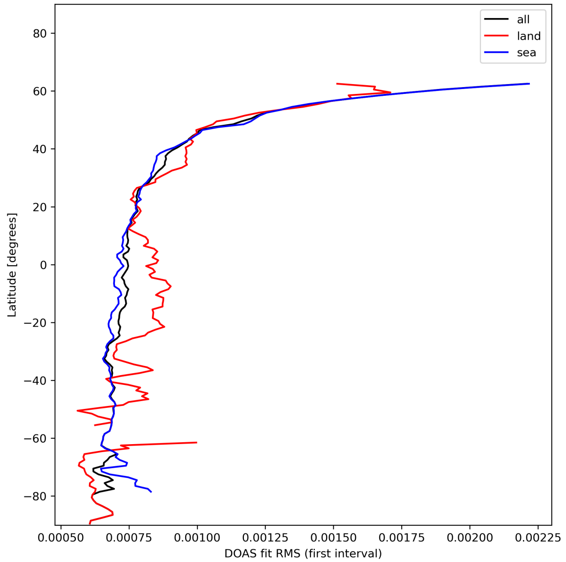
Figure 32: Zonal average of “DOAS fit RMS (first interval)” for 2023-12-02 to 2023-12-04.
