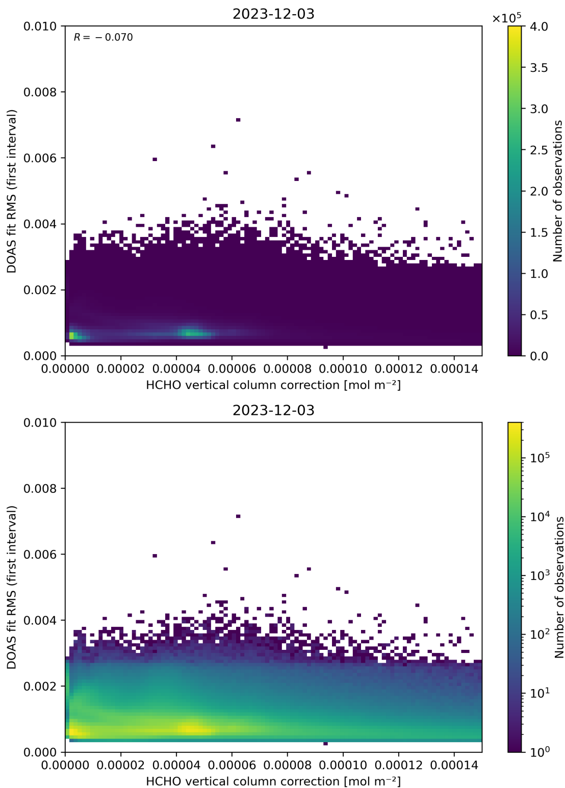
Figure 112: Scatter density plot of “HCHO vertical column correction” against “DOAS fit RMS (first interval)” for 2023-12-02 to 2023-12-04.
