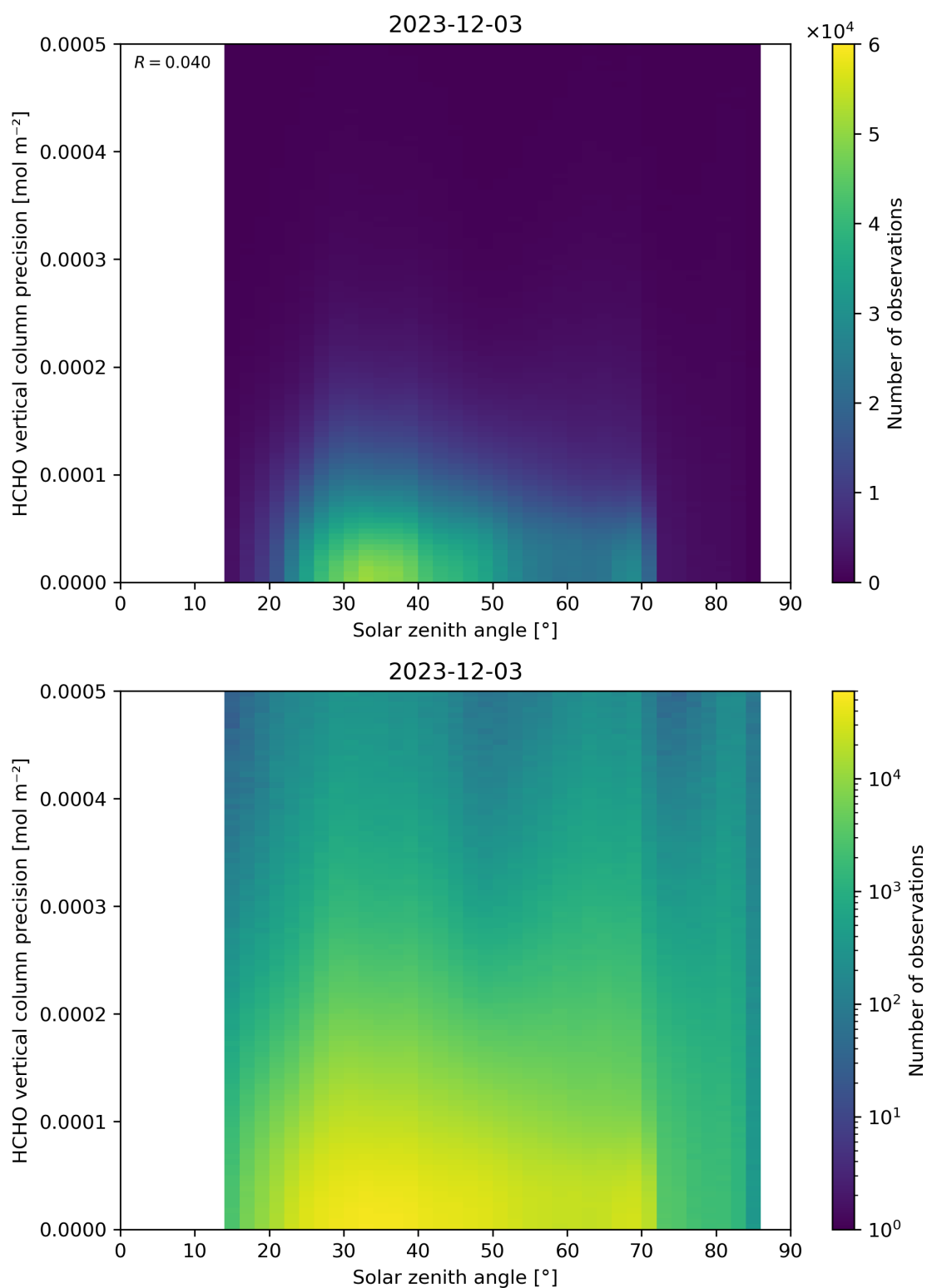
Figure 179: Scatter density plot of “Solar zenith angle” against “HCHO vertical column precision” for 2023-12-02 to 2023-12-04.
