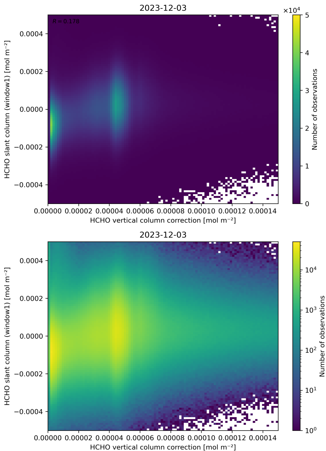
Figure 118: Scatter density plot of “HCHO vertical column correction” against “HCHO slant column (window1)” for 2023-12-02 to 2023-12-04.
