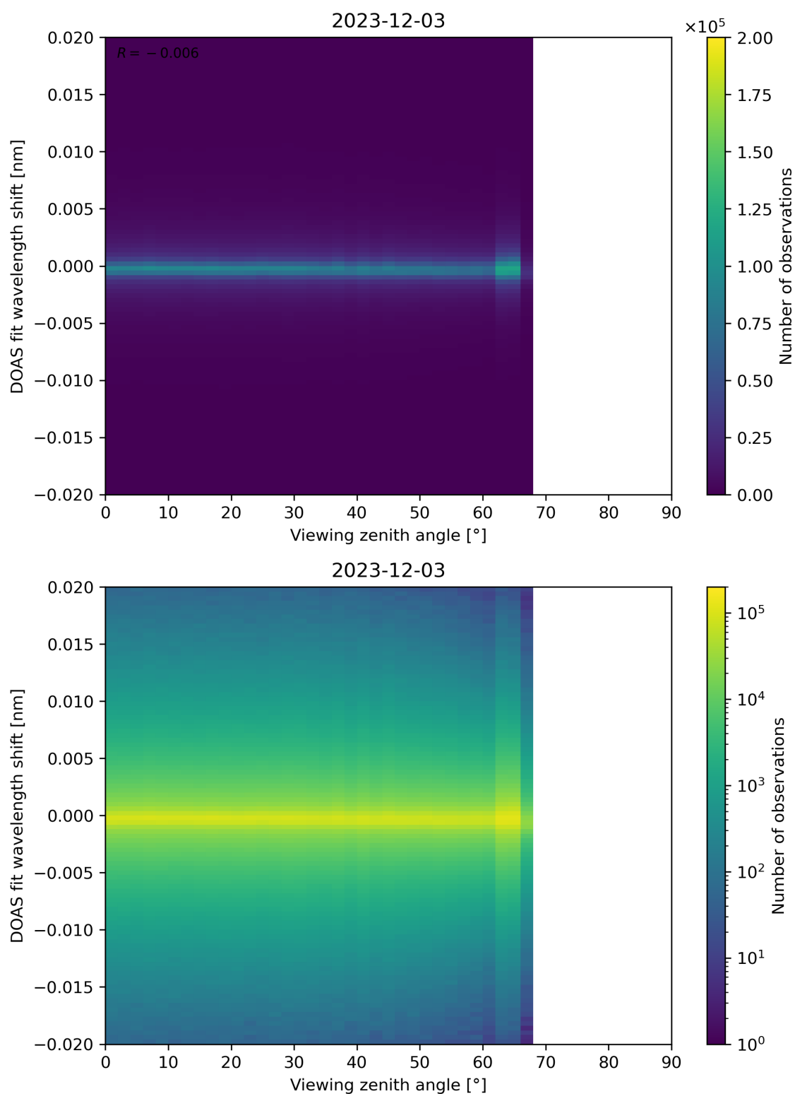
Figure 183: Scatter density plot of “Viewing zenith angle” against “DOAS fit wavelength shift” for 2023-12-02 to 2023-12-04.
