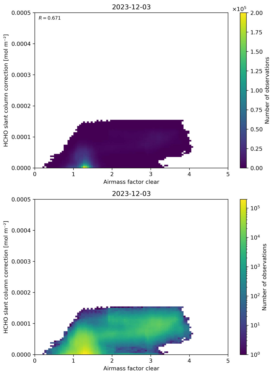
Figure 75: Scatter density plot of “Airmass factor clear” against “HCHO slant column correction” for 2023-12-02 to 2023-12-04.
