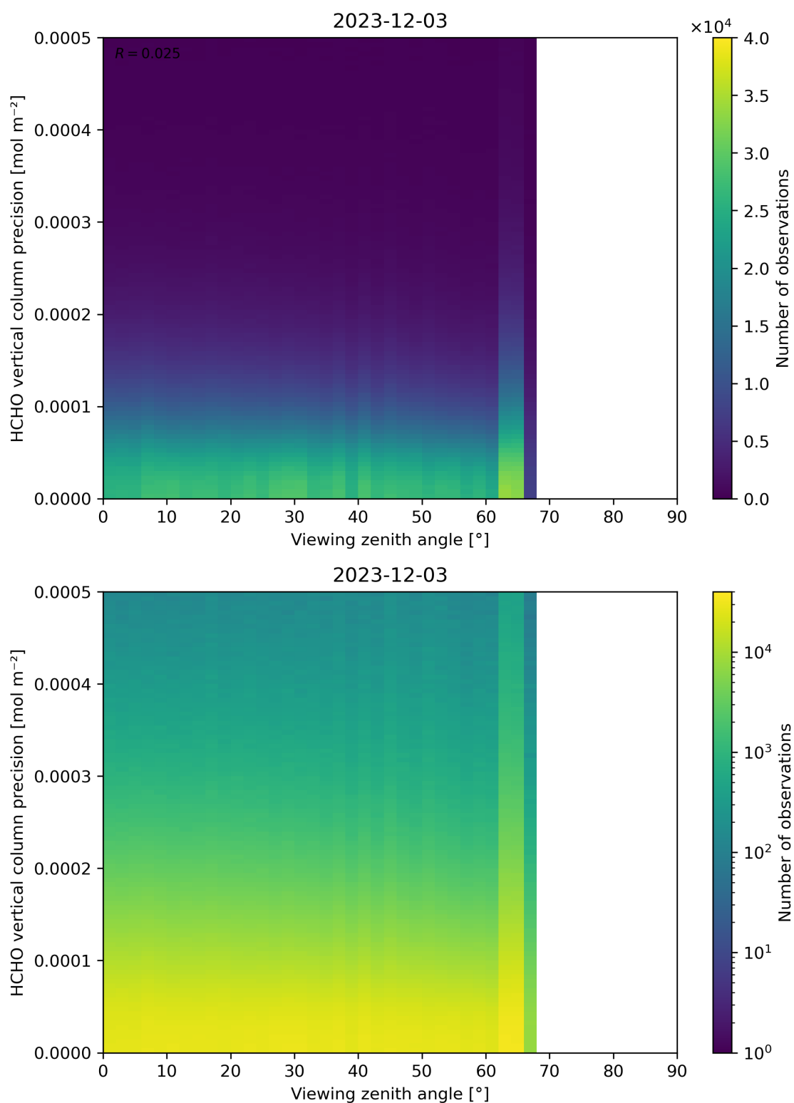
Figure 194: Scatter density plot of “Viewing zenith angle” against “HCHO vertical column precision” for 2023-12-02 to 2023-12-04.
