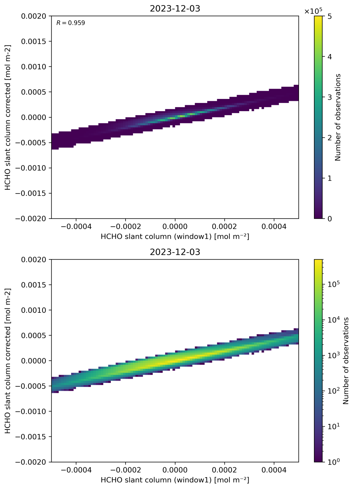
Figure 82: Scatter density plot of “HCHO slant column (window1)” against “HCHO slant column corrected” for 2023-12-02 to 2023-12-04.
