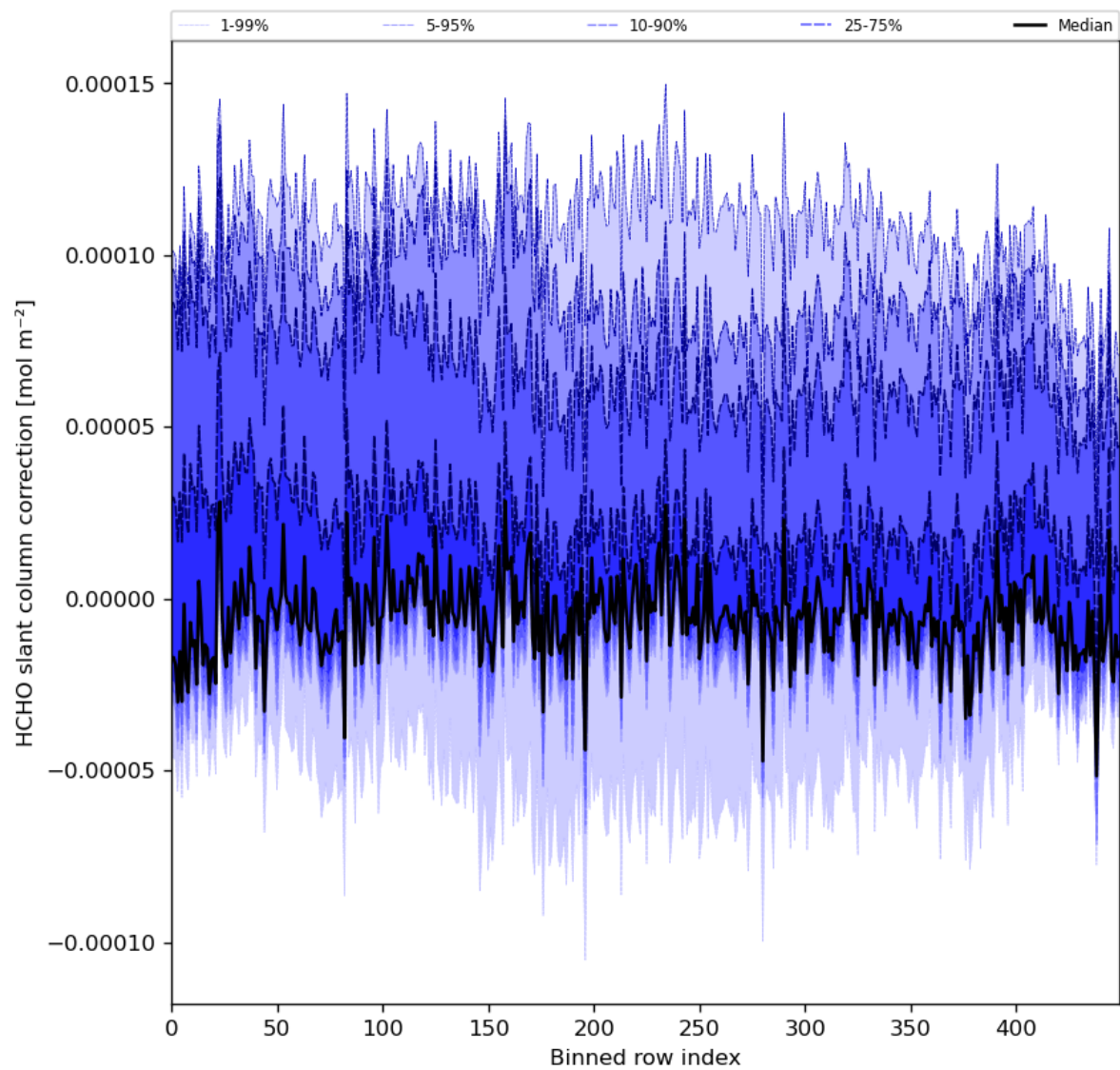
Figure 61: Along track statistics of “HCHO slant column correction” for 2023-12-02 to 2023-12-04
