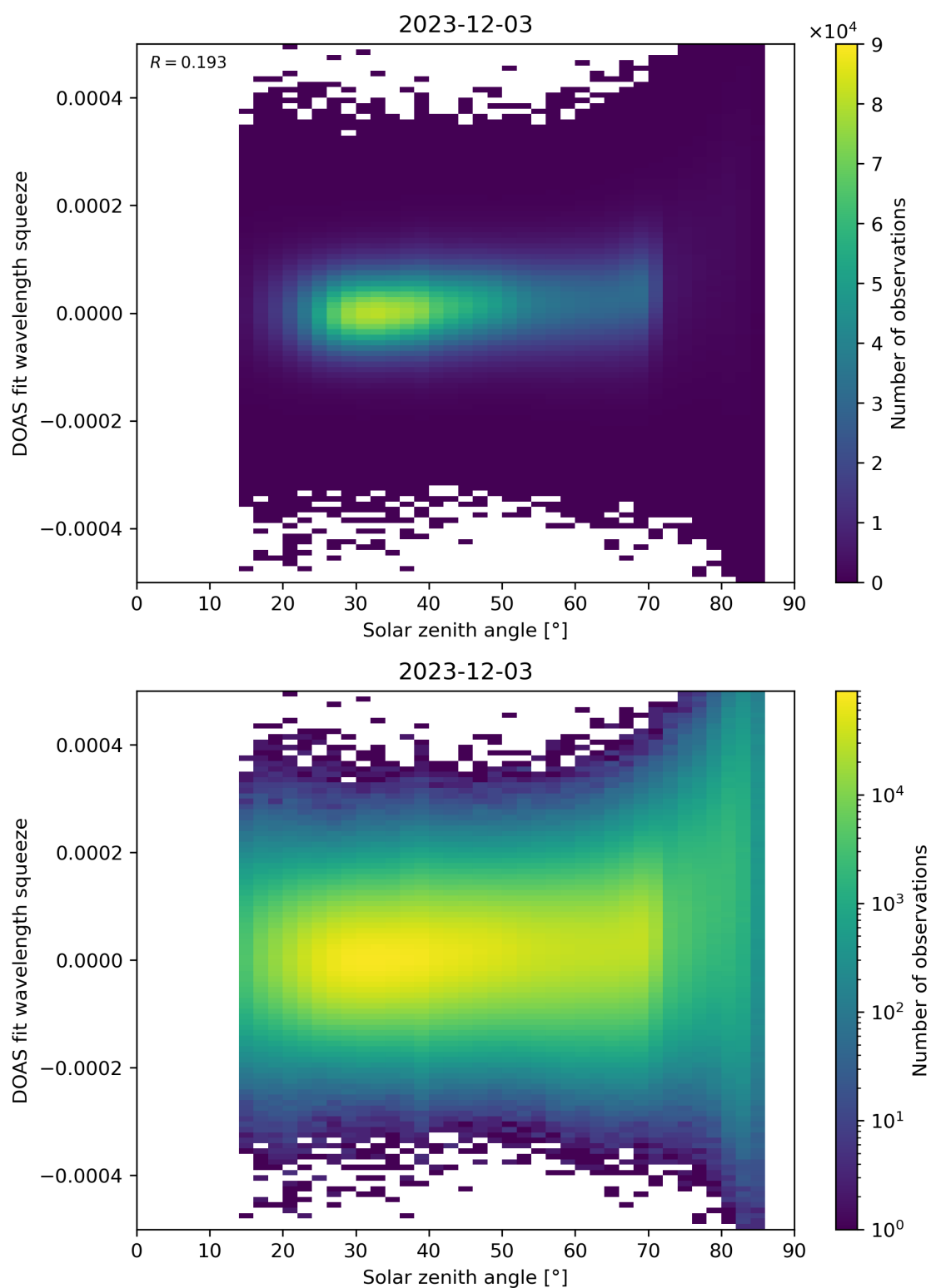
Figure 169: Scatter density plot of “Solar zenith angle” against “DOAS fit wavelength squeeze” for 2023-12-02 to 2023-12-04.
