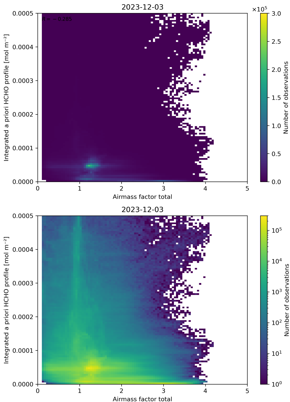
Figure 104: Scatter density plot of “Airmass factor total” against “Integrated a priori HCHO profile” for 2023-12-02 to 2023-12-04.
