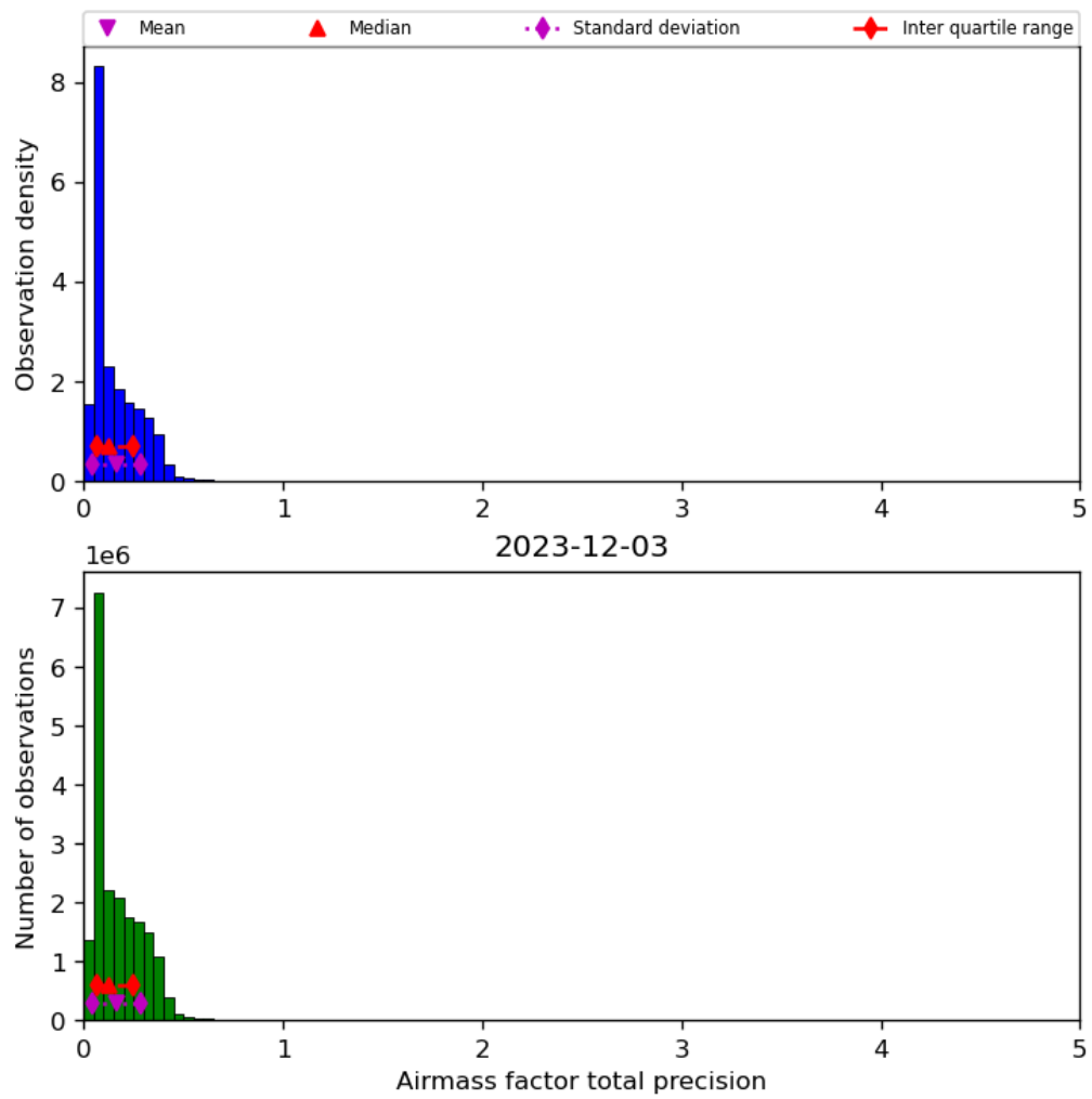
Figure 41: Histogram of “Airmass factor total precision” for 2023-12-02 to 2023-12-04
