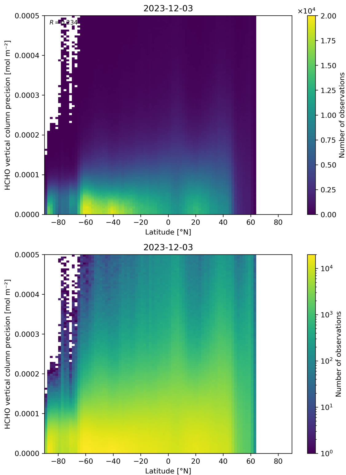
Figure 165: Scatter density plot of “Latitude” against “HCHO vertical column precision” for 2023-12-02 to 2023-12-04.
