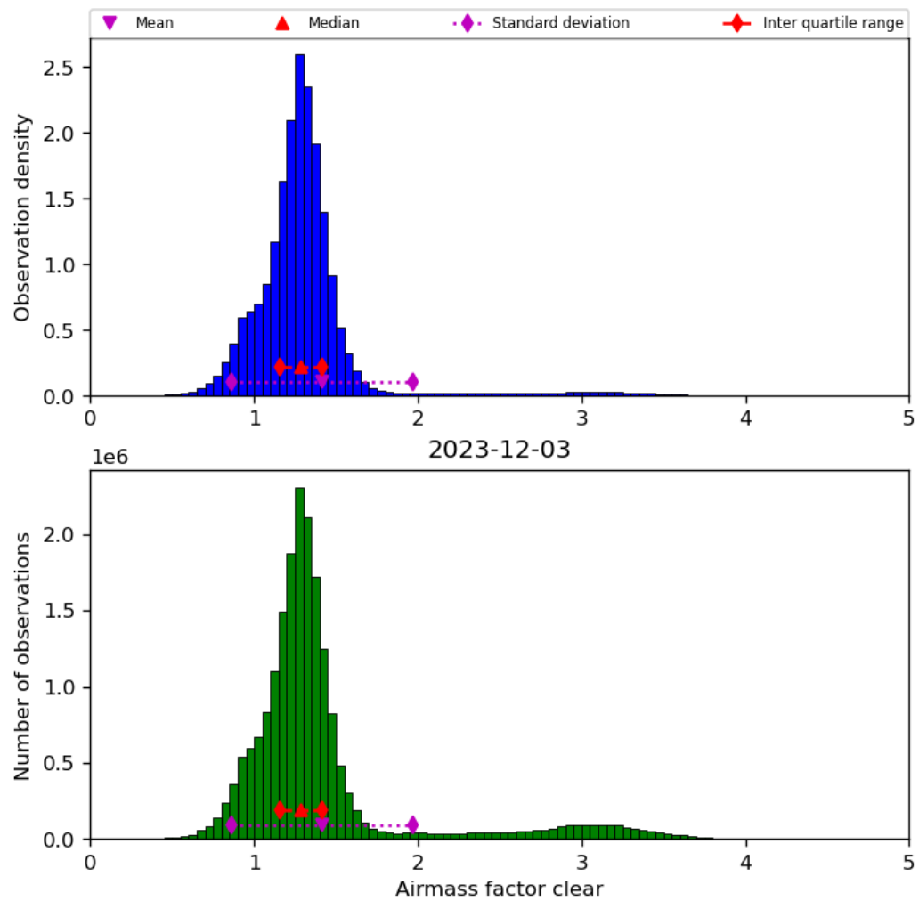
Figure 42: Histogram of “Airmass factor clear” for 2023-12-02 to 2023-12-04
