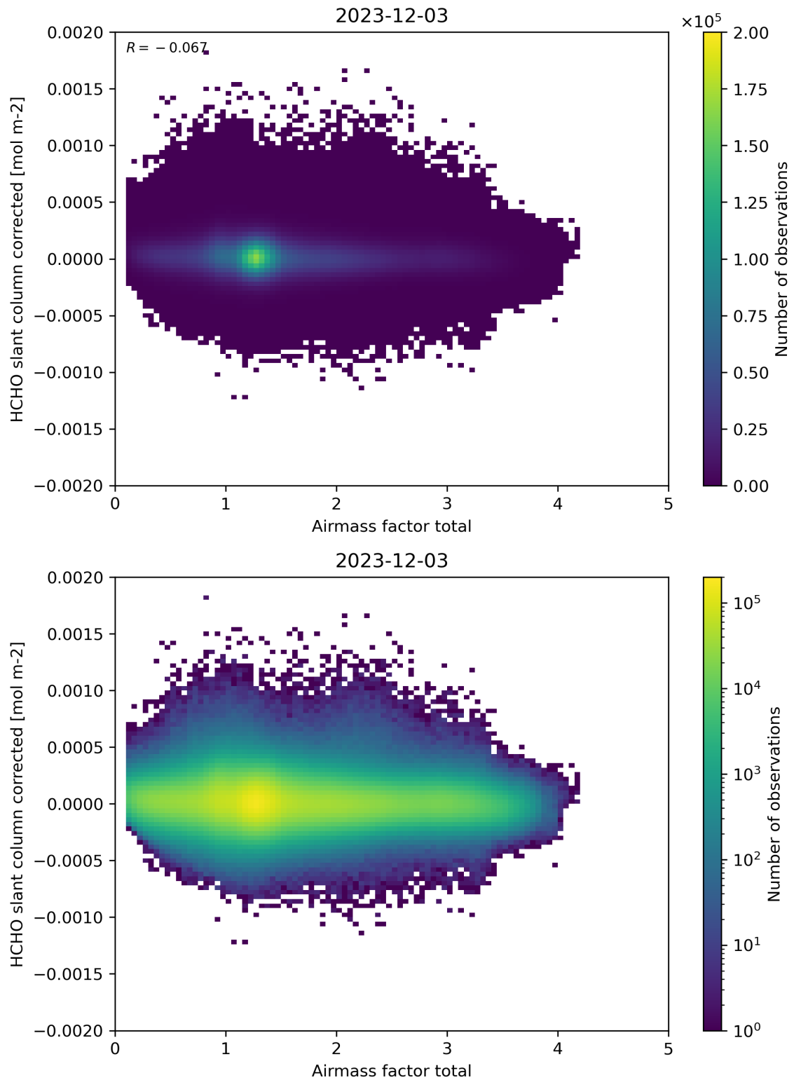
Figure 101: Scatter density plot of “Airmass factor total” against “HCHO slant column corrected” for 2023-12-02 to 2023-12-04.
