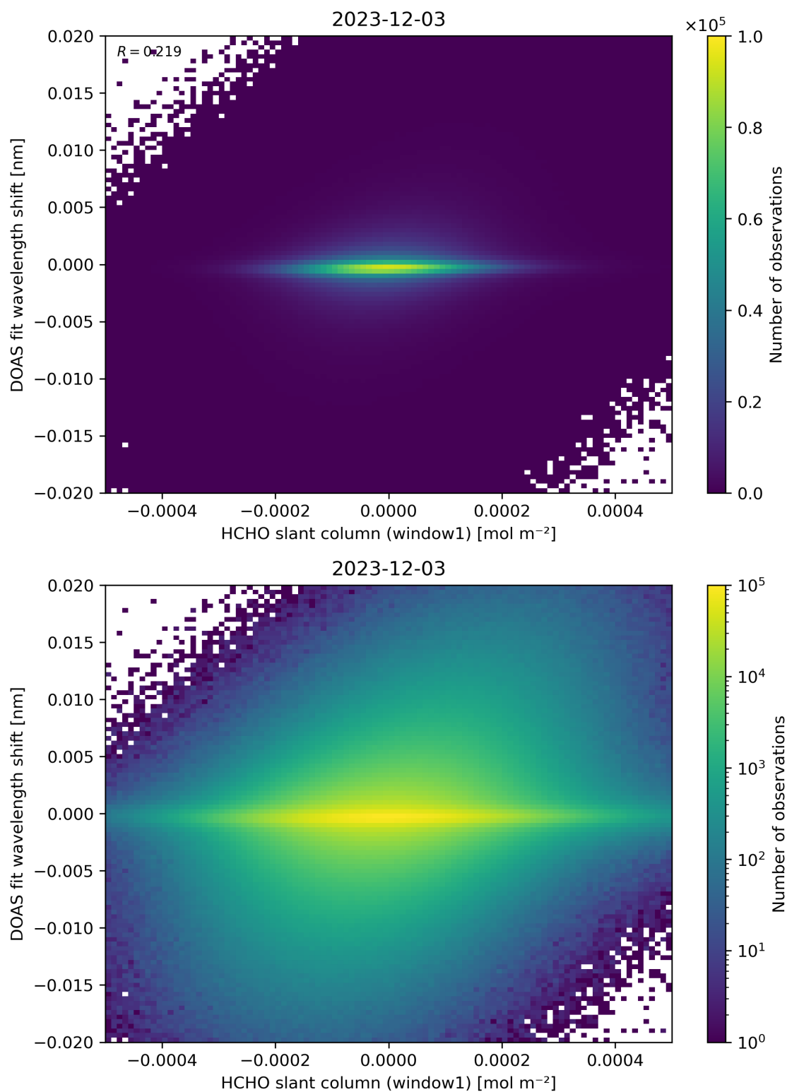
Figure 79: Scatter density plot of “HCHO slant column (window1)” against “DOAS fit wavelength shift” for 2023-12-02 to 2023-12-04.
