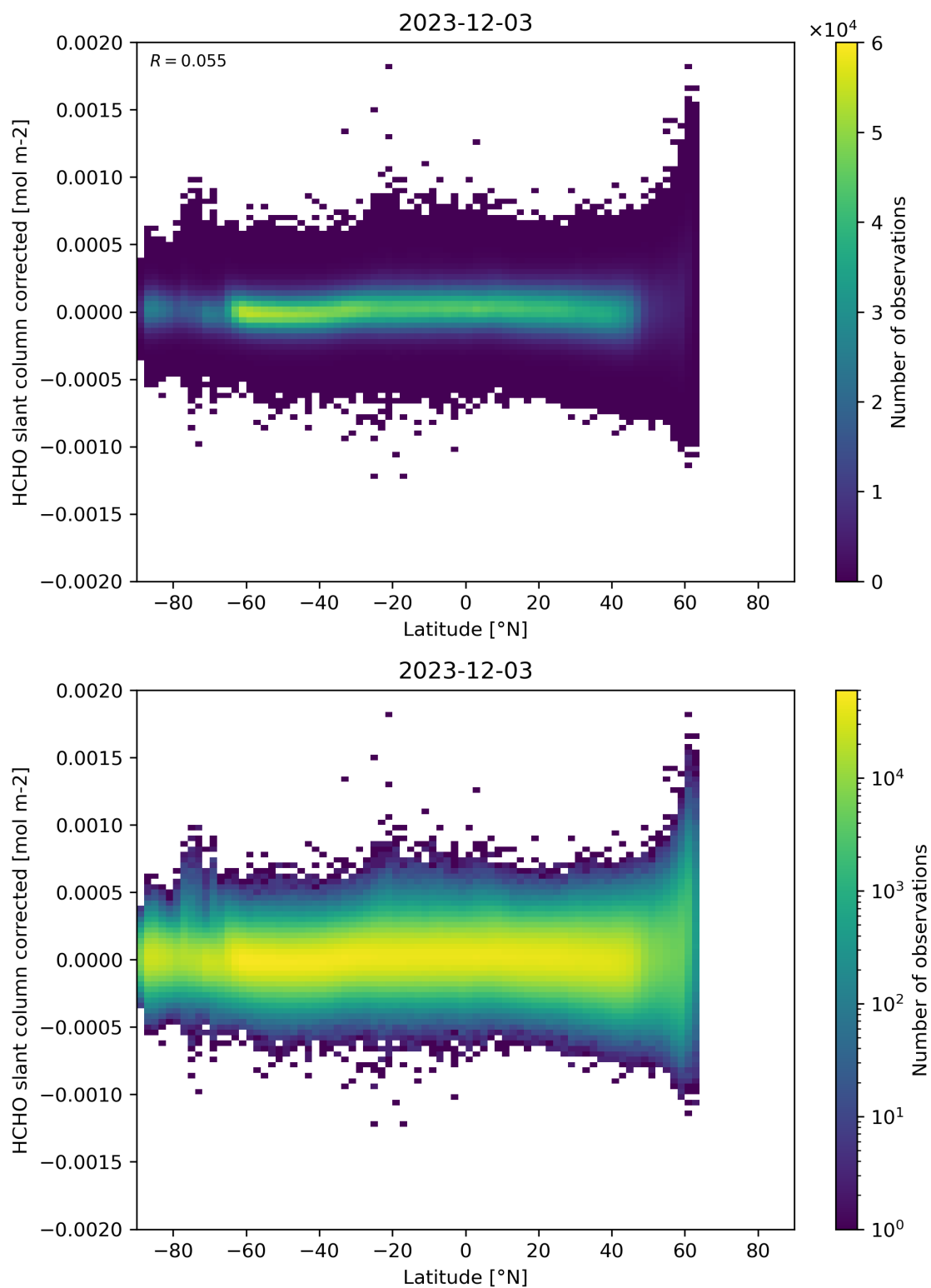
Figure 157: Scatter density plot of “Latitude” against “HCHO slant column corrected” for 2023-12-02 to 2023-12-04.
