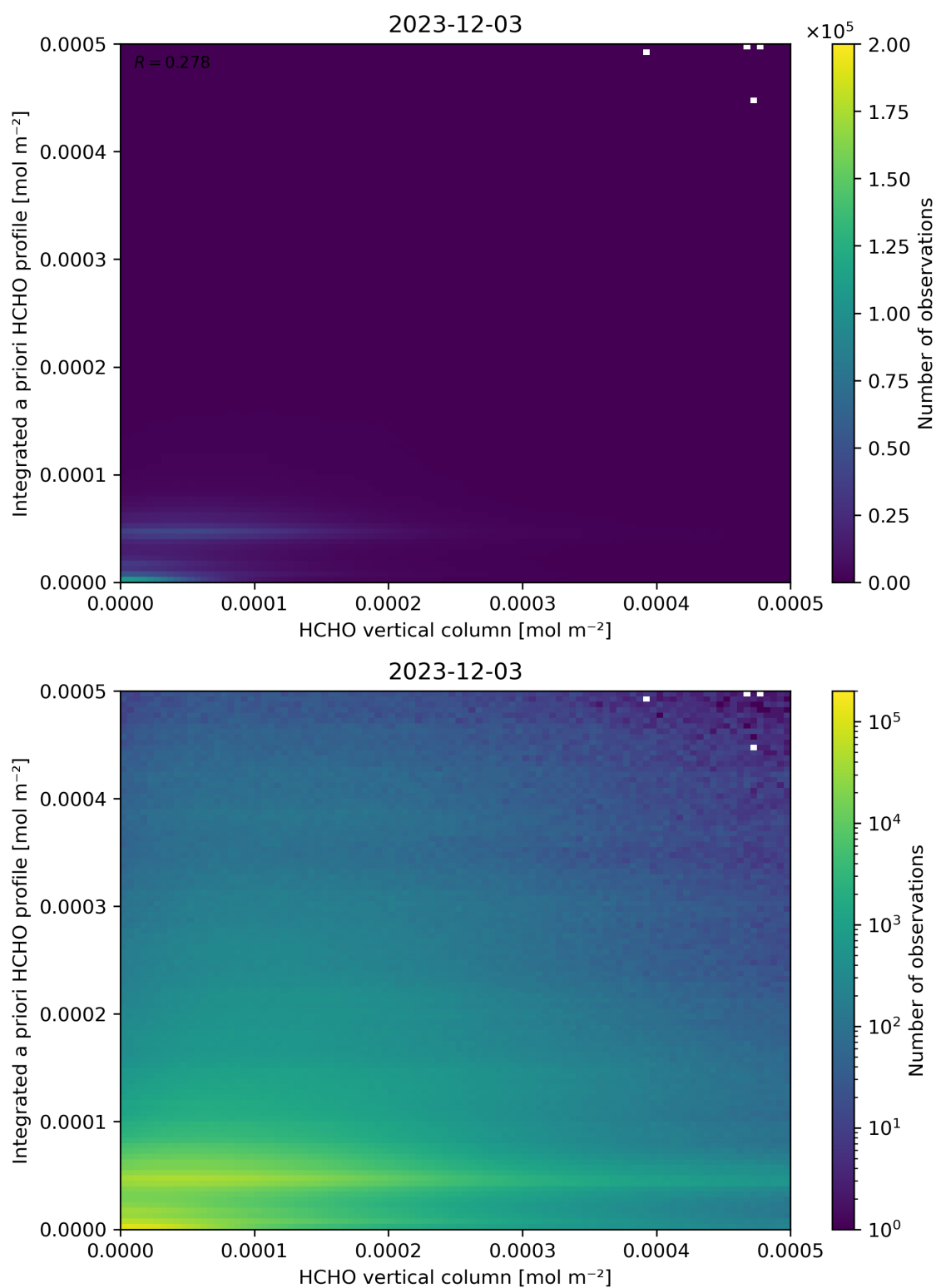
Figure 135: Scatter density plot of “HCHO vertical column” against “Integrated a priori HCHO profile” for 2023-12-02 to 2023-12-04.
