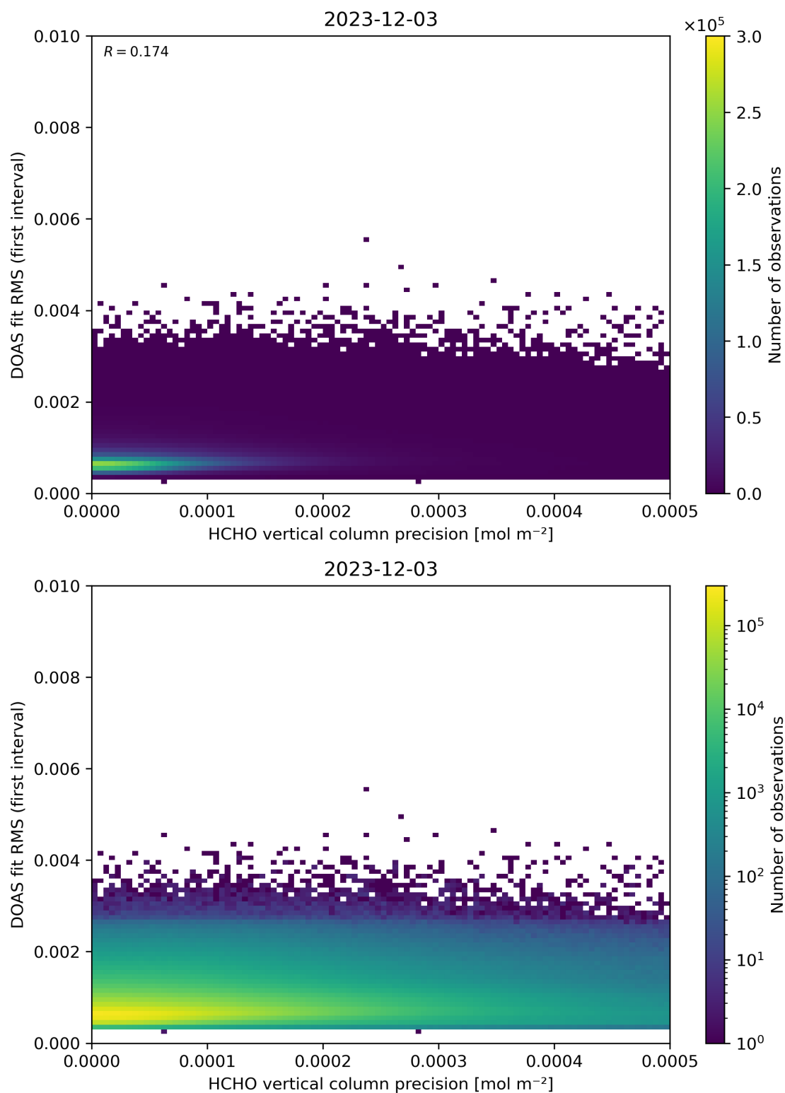
Figure 136: Scatter density plot of “HCHO vertical column precision” against “DOAS fit RMS (first interval)” for 2023-12-02 to 2023-12-04.
