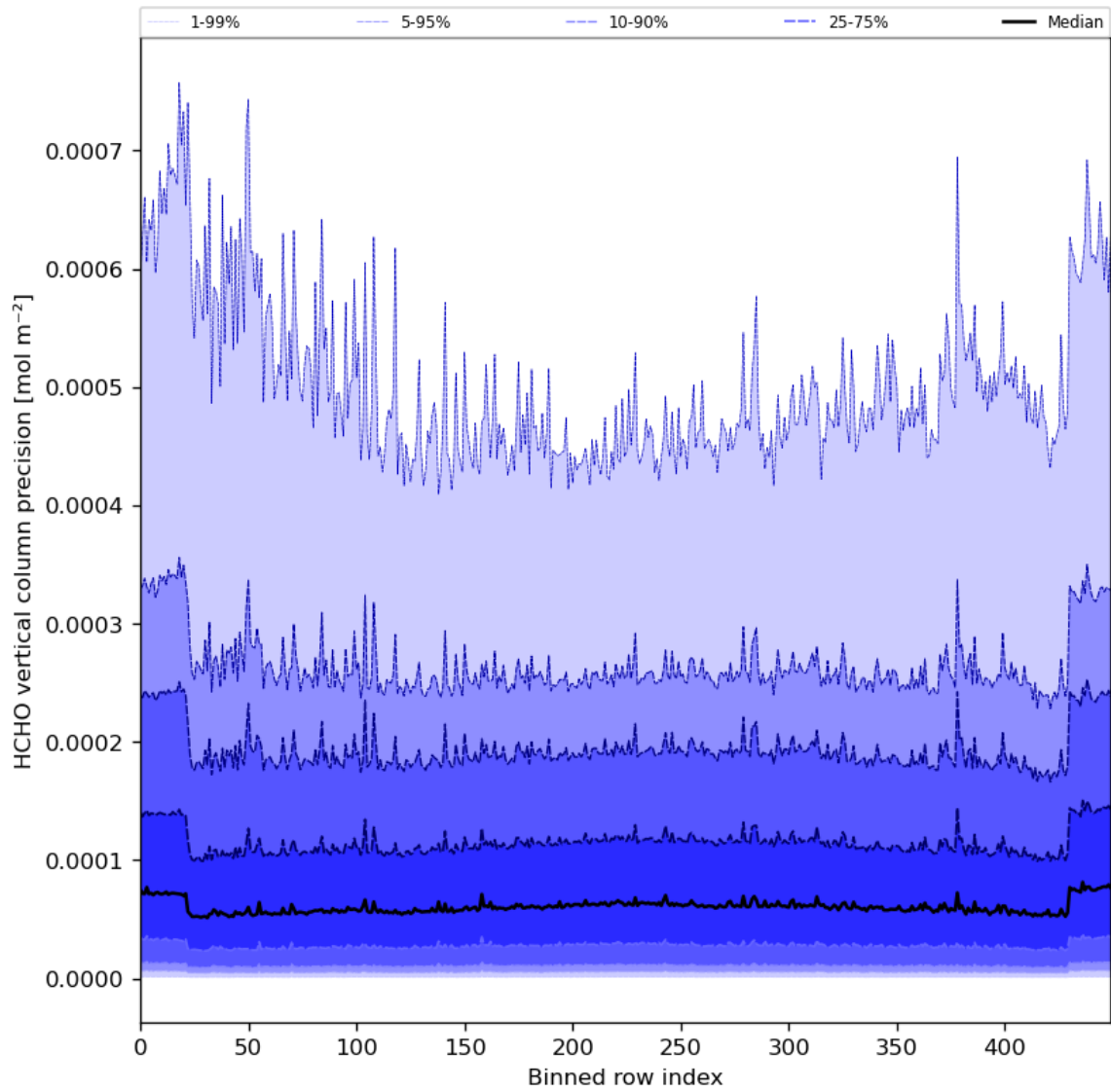
Figure 50: Along track statistics of “HCHO vertical column precision” for 2023-12-02 to 2023-12-04
