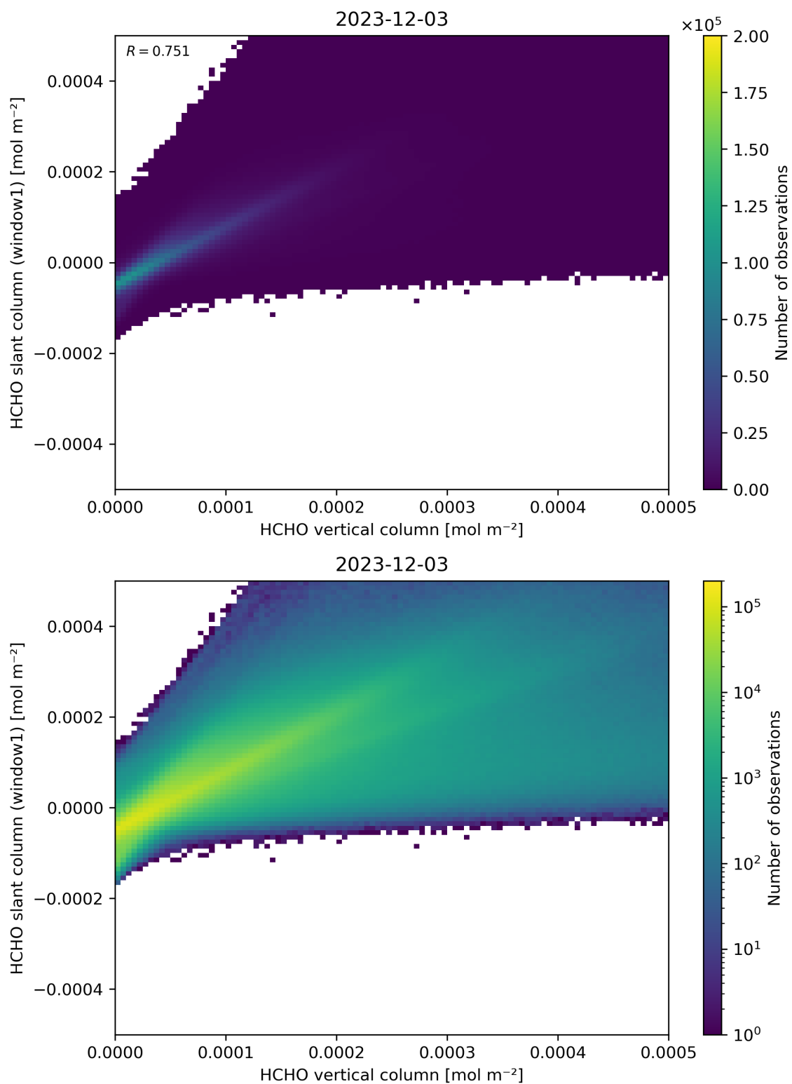
Figure 129: Scatter density plot of “HCHO vertical column” against “HCHO slant column (window1)” for 2023-12-02 to 2023-12-04.
