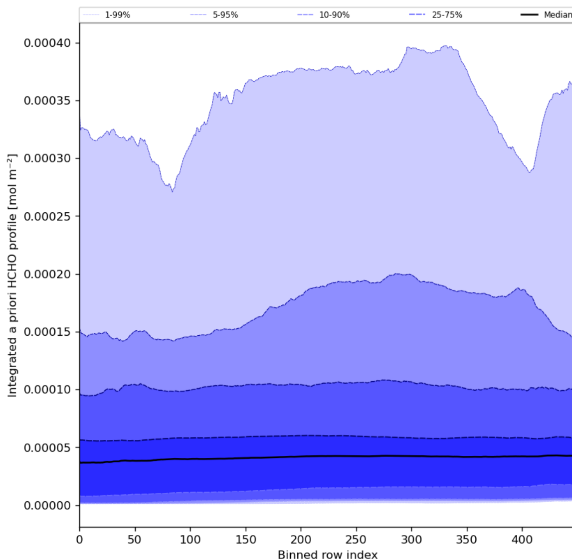
Figure 57: Along track statistics of “Integrated a priori HCHO profile” for 2023-12-02 to 2023-12-04
