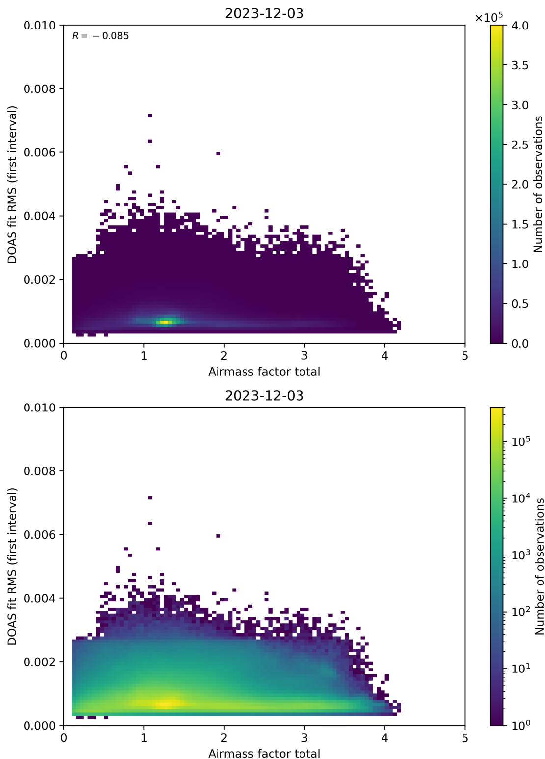
Figure 97: Scatter density plot of “Airmass factor total” against “DOAS fit RMS (first interval)” for 2023-12-02 to 2023-12-04.
