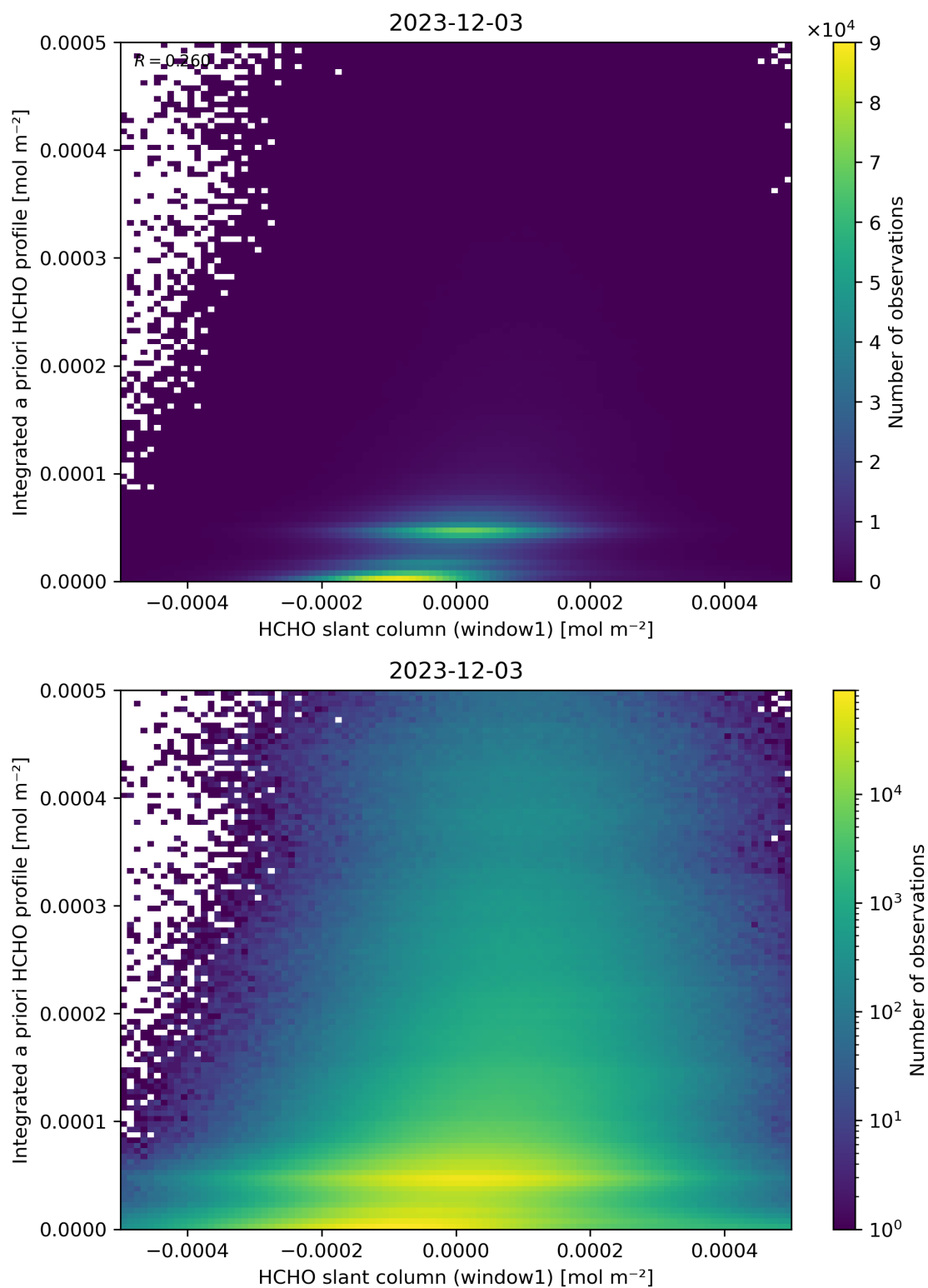
Figure 87: Scatter density plot of “HCHO slant column (window1)” against “Integrated a priori HCHO profile” for 2023-12-02 to 2023-12-04.
