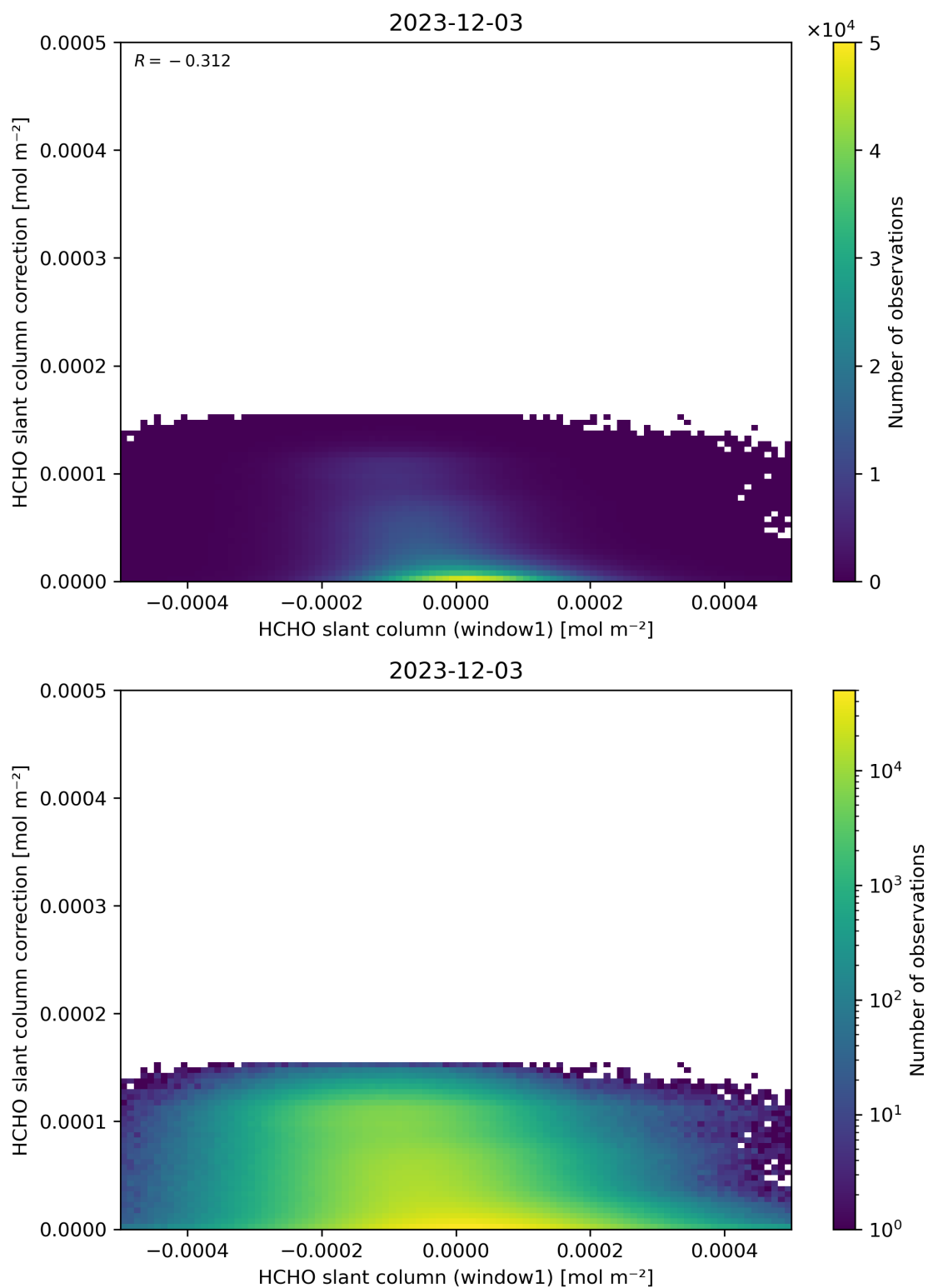
Figure 83: Scatter density plot of “HCHO slant column (window1)” against “HCHO slant column correction” for 2023-12-02 to 2023-12-04.
