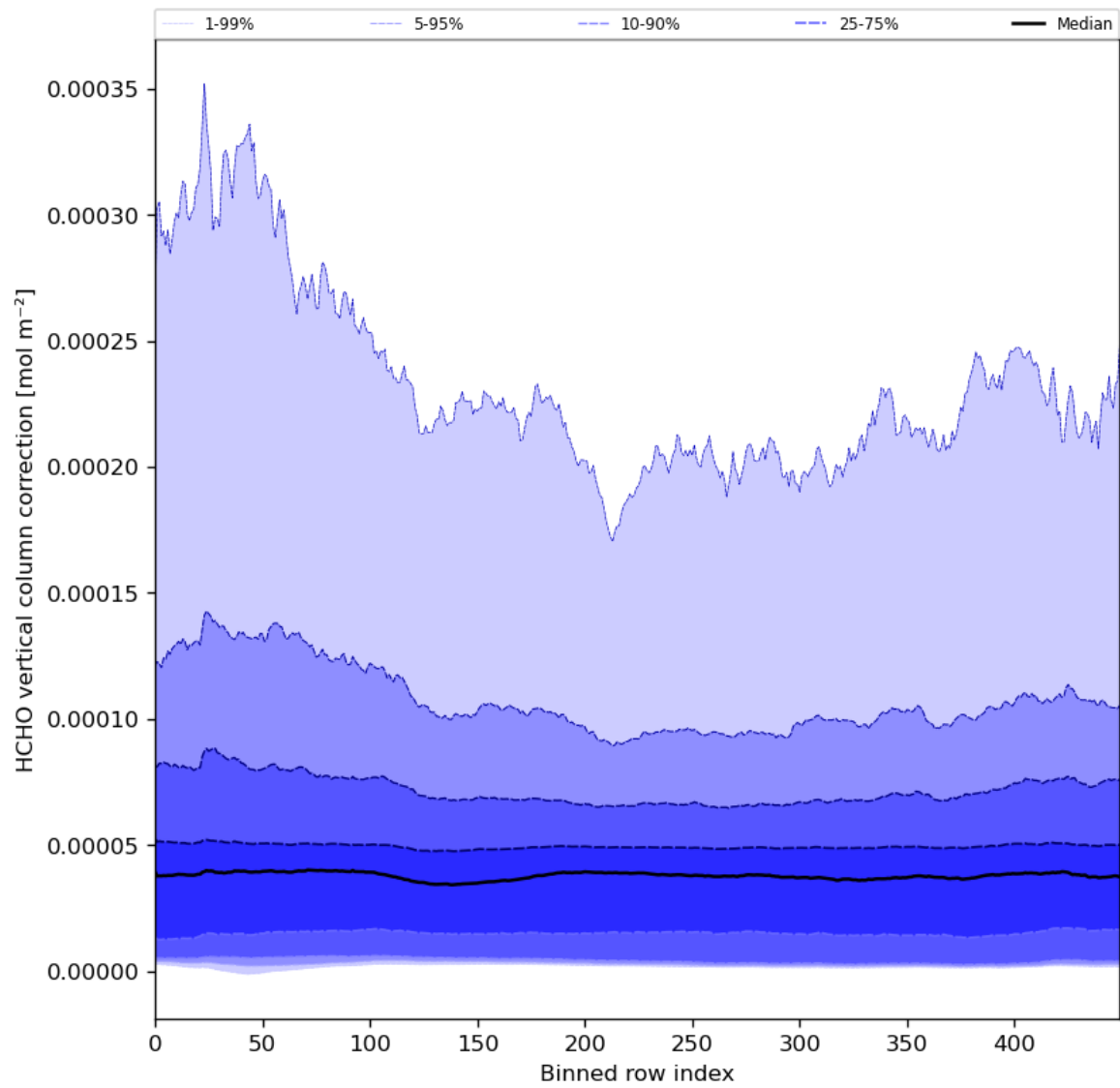
Figure 51: Along track statistics of “HCHO vertical column correction” for 2023-12-02 to 2023-12-04
