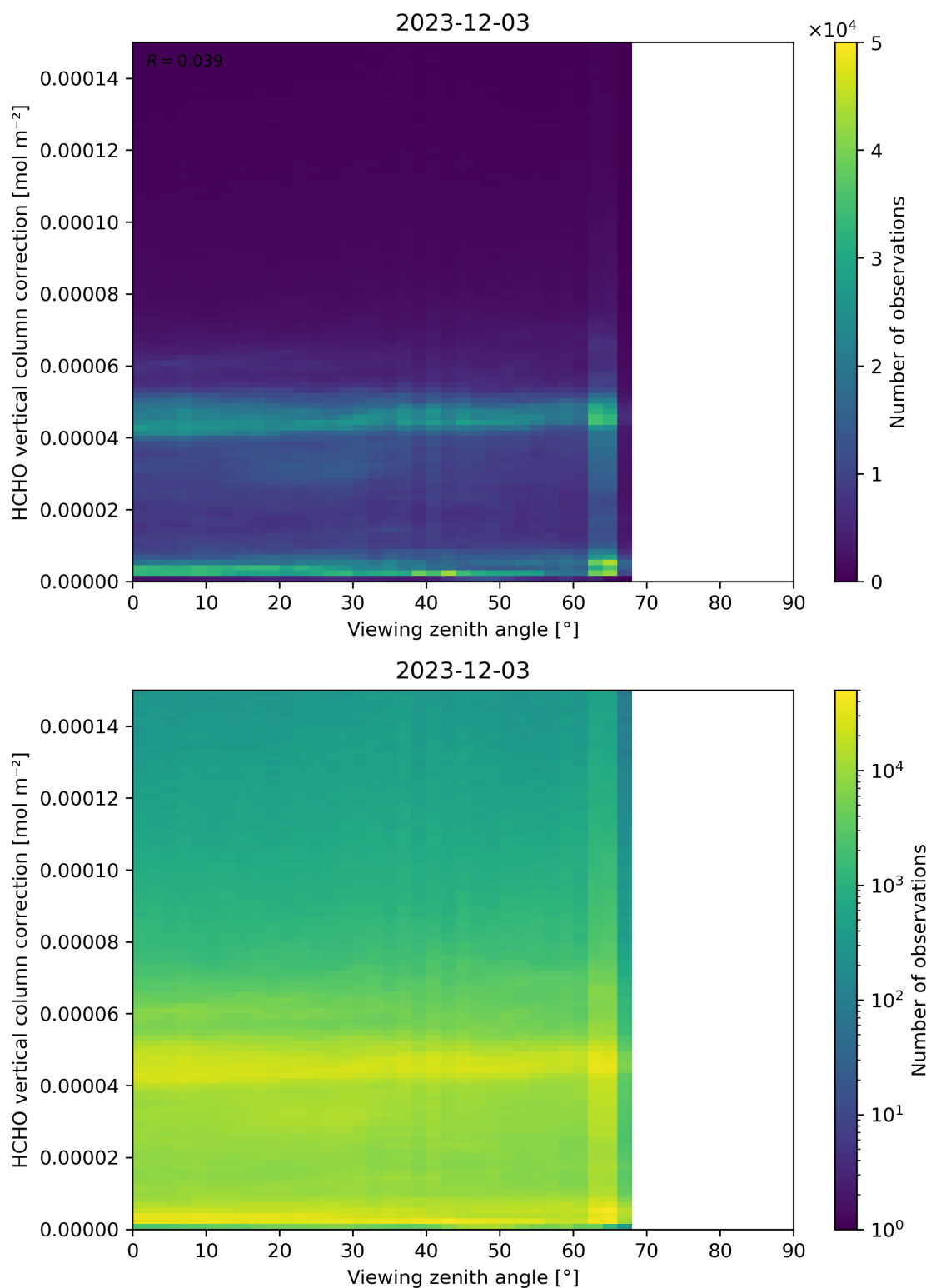
Figure 193: Scatter density plot of “Viewing zenith angle” against “HCHO vertical column correction” for 2023-12-02 to 2023-12-04.
