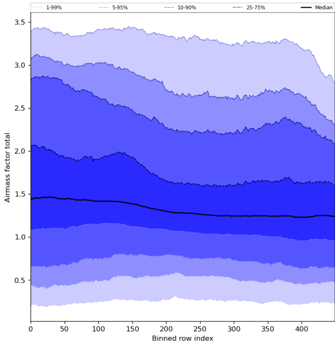
Figure 54: Along track statistics of “Airmass factor total” for 2023-12-02 to 2023-12-04
