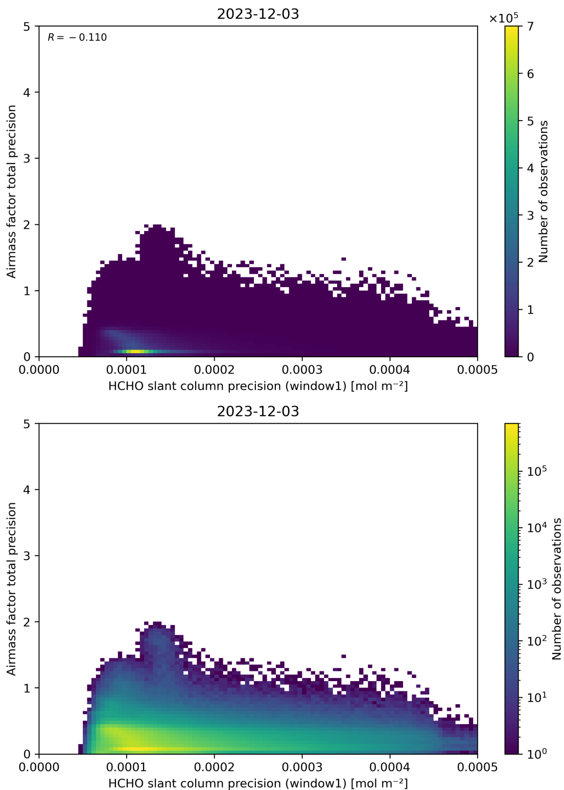
Figure 95: Scatter density plot of “HCHO slant column precision (window1)” against “Airmass factor total precision” for 2023-12-02 to 2023-12-04.
