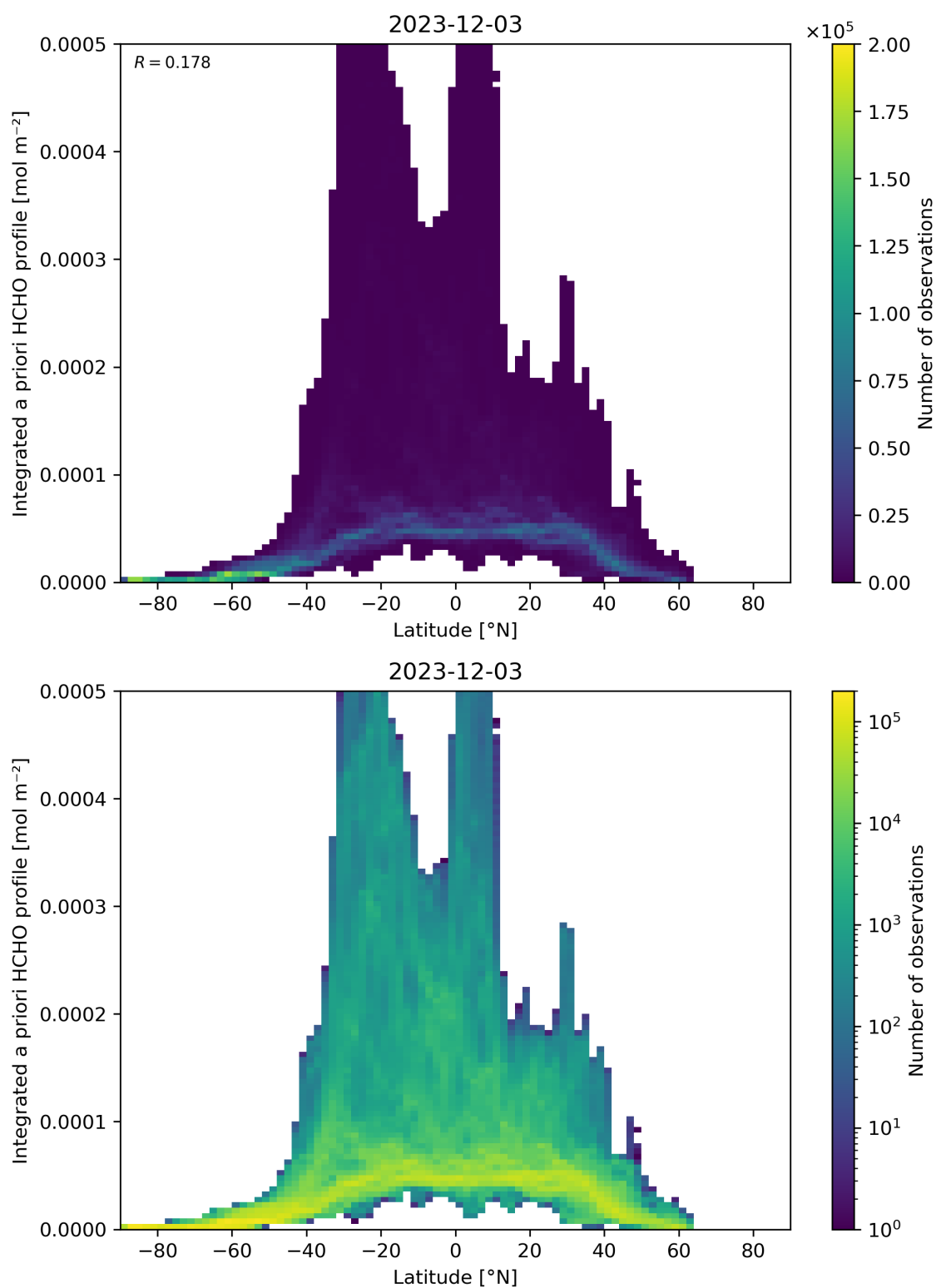
Figure 166: Scatter density plot of “Latitude” against “Integrated a priori HCHO profile” for 2023-12-02 to 2023-12-04.
