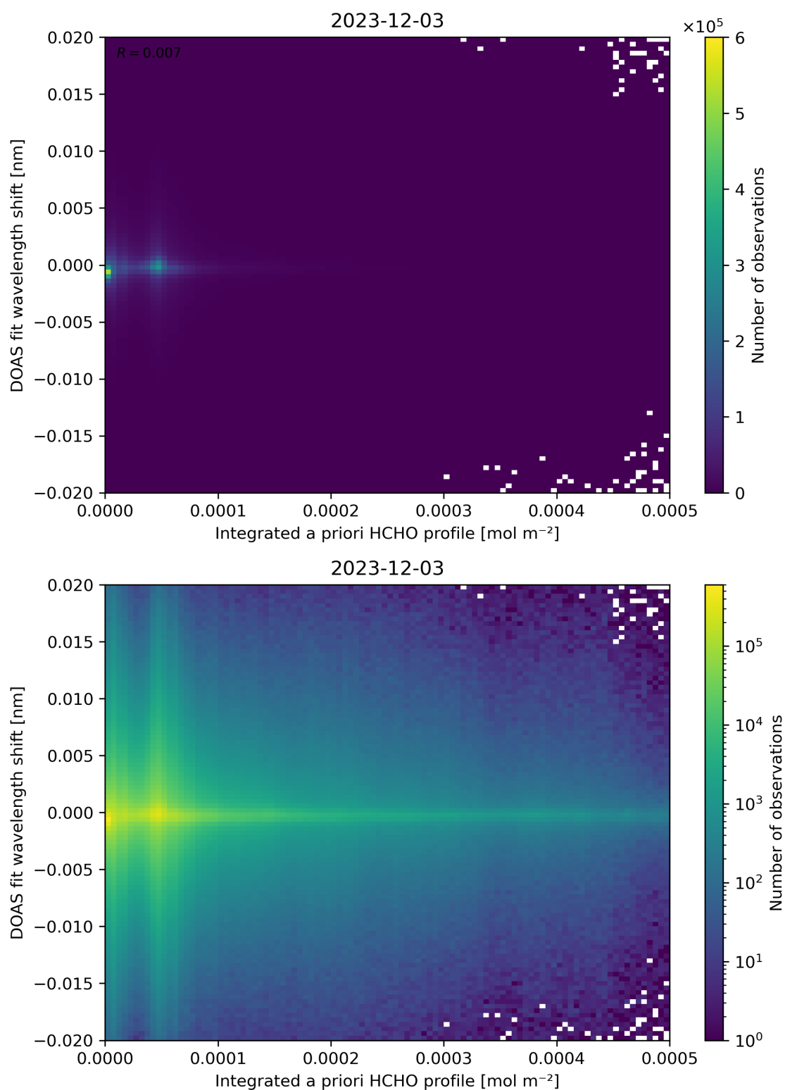
Figure 149: Scatter density plot of “Integrated a priori HCHO profile” against “DOAS fit wavelength shift” for 2023-12-02 to 2023-12-04.
