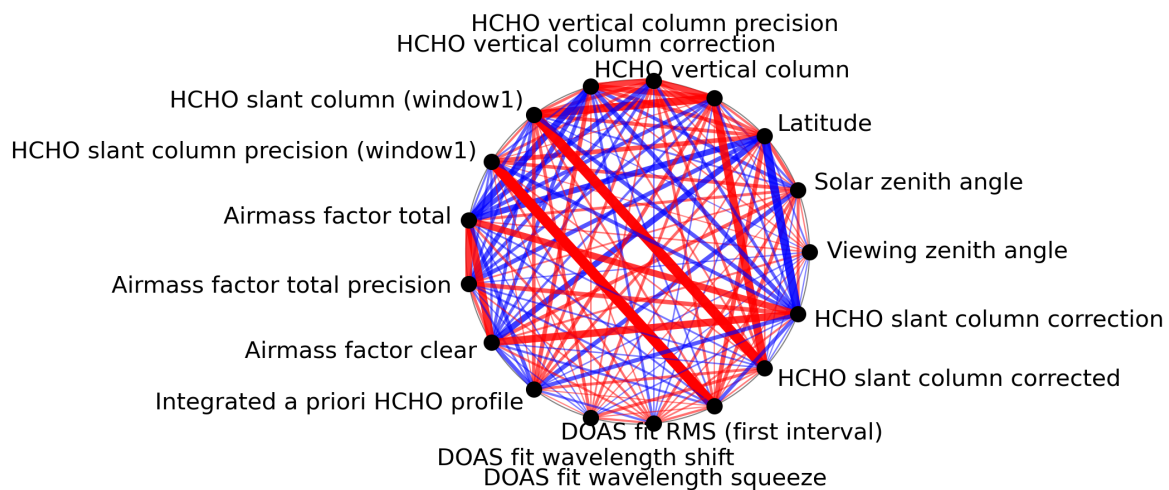
Figure 1: Map of correlation graph for 2023-12-02 to 2023-12-04.
