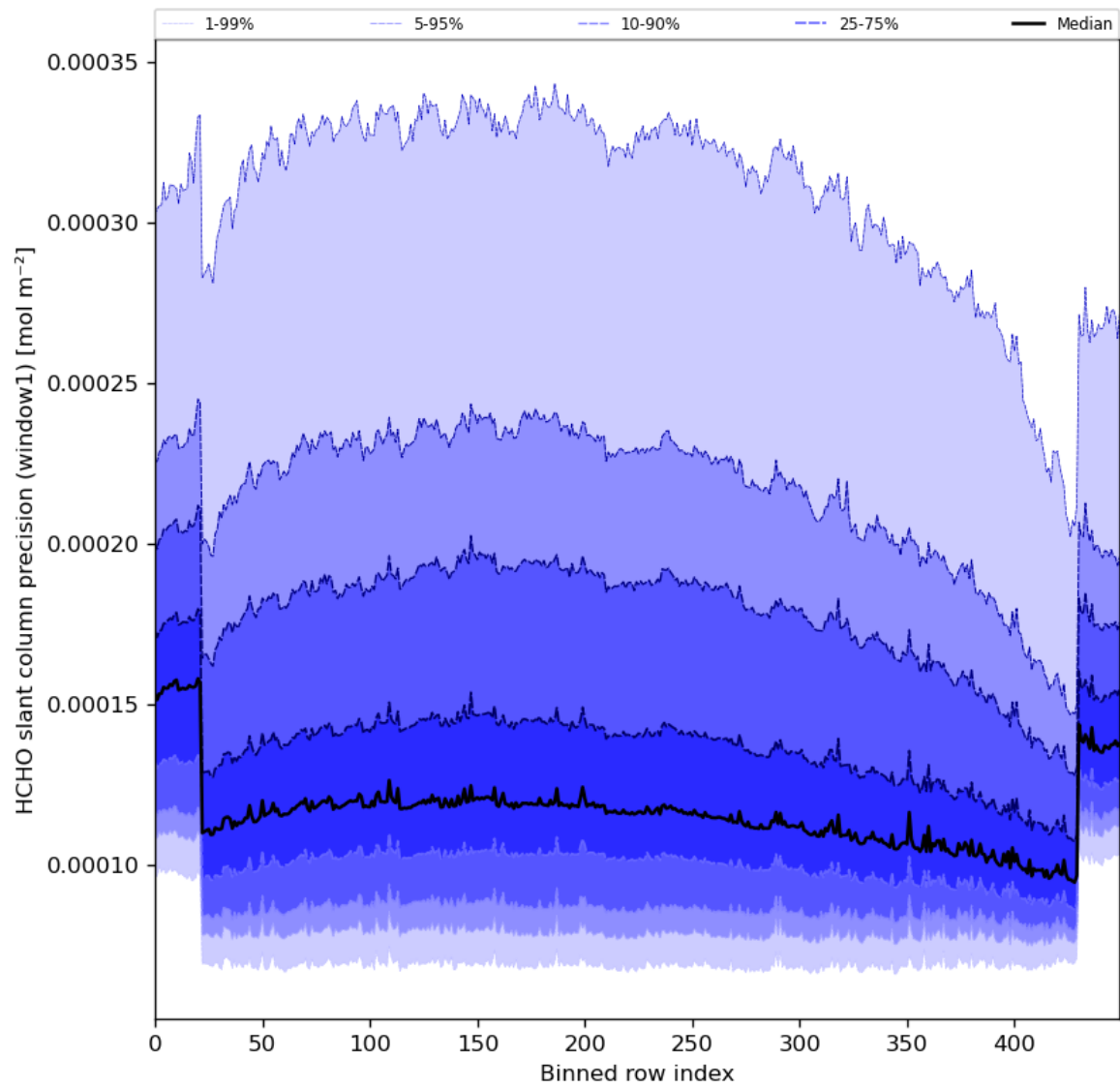
Figure 53: Along track statistics of “HCHO slant column precision (window1)” for 2023-12-02 to 2023-12-04
