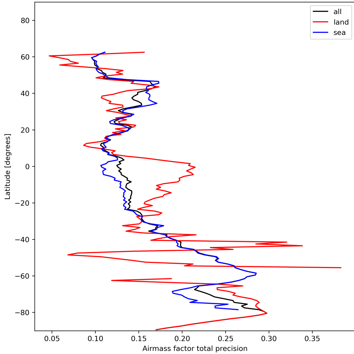
Figure 27: Zonal average of “Airmass factor total precision” for 2023-12-02 to 2023-12-04.
