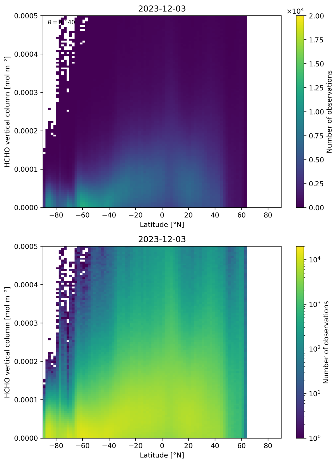
Figure 163: Scatter density plot of “Latitude” against “HCHO vertical column” for 2023-12-02 to 2023-12-04.
