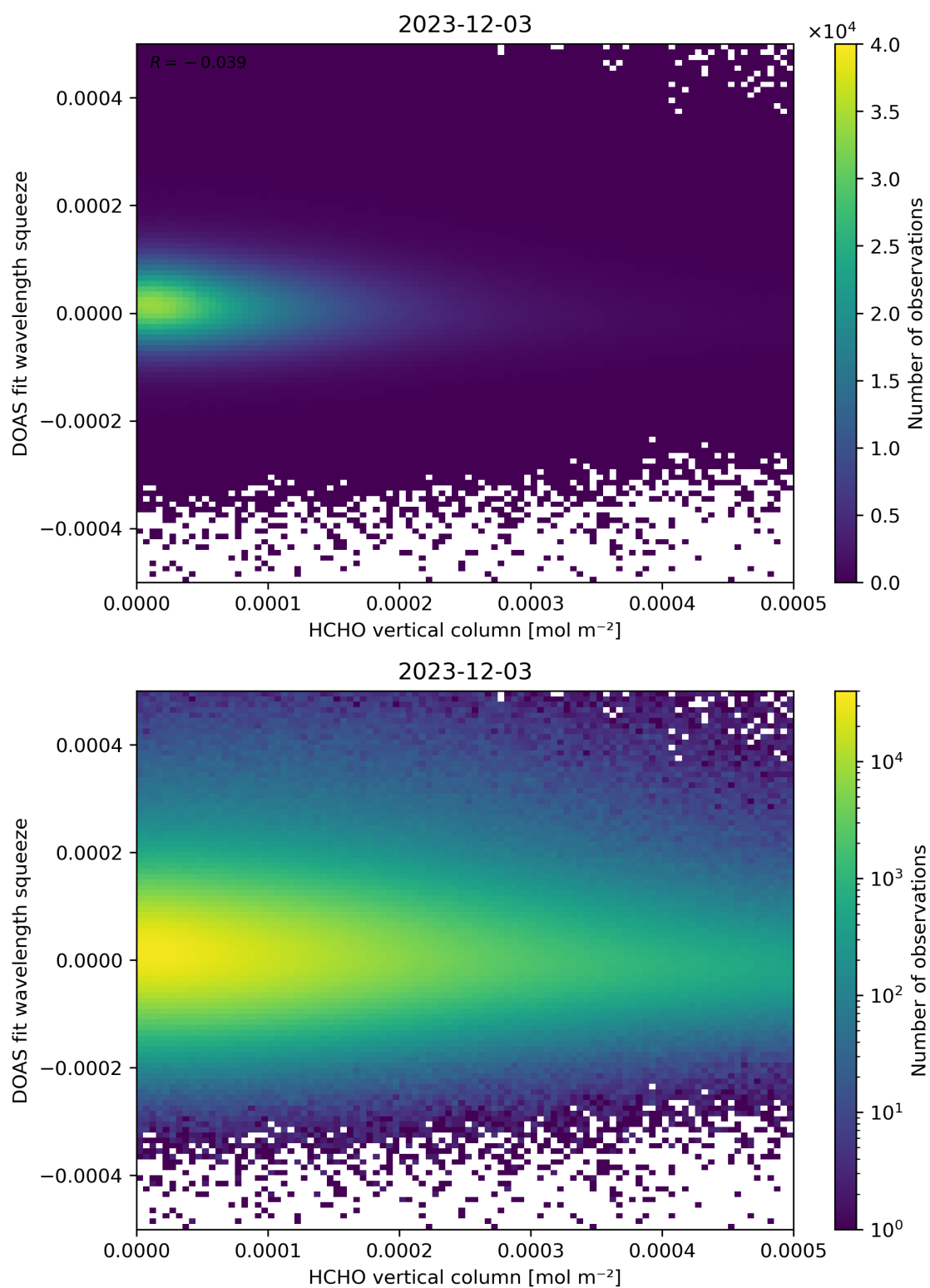
Figure 125: Scatter density plot of “HCHO vertical column” against “DOAS fit wavelength squeeze” for 2023-12-02 to 2023-12-04.
