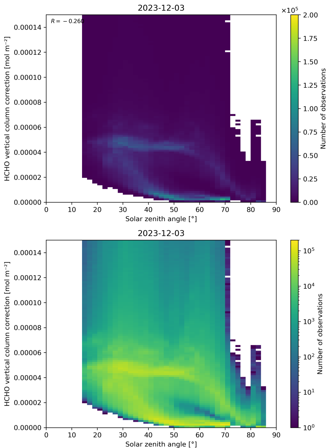
Figure 178: Scatter density plot of “Solar zenith angle” against “HCHO vertical column correction” for 2023-12-02 to 2023-12-04.
