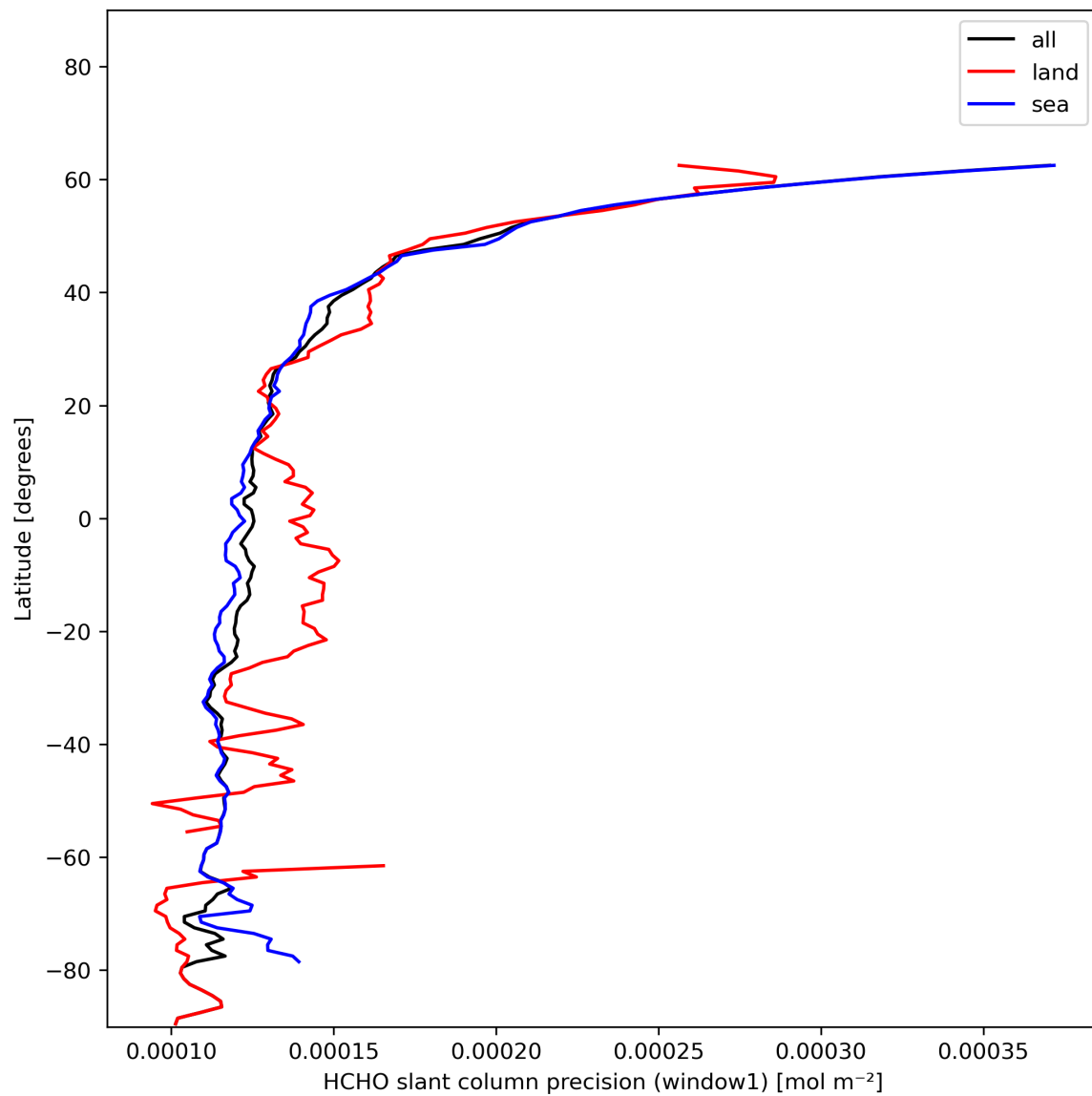
Figure 25: Zonal average of “HCHO slant column precision (window1)” for 2023-12-02 to 2023-12-04.
