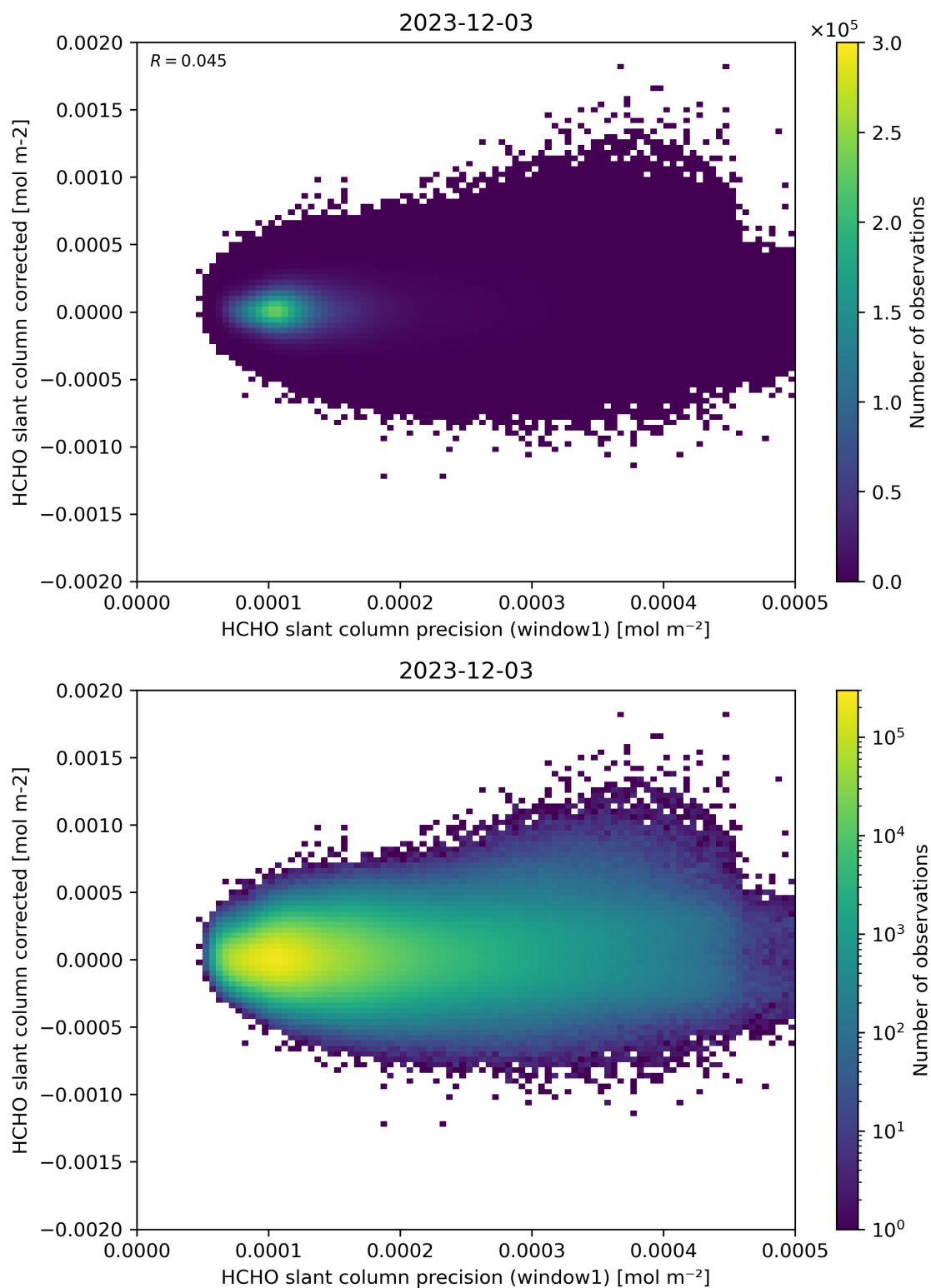
Figure 92: Scatter density plot of “HCHO slant column precision (window1)” against “HCHO slant column corrected” for 2023-12-02 to 2023-12-04.
