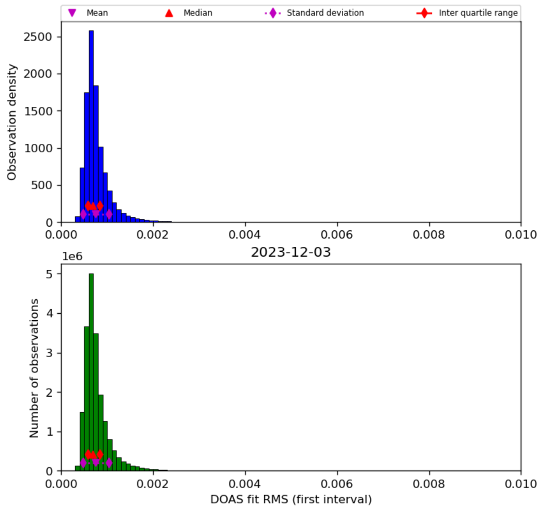
Figure 46: Histogram of “DOAS fit RMS (first interval)” for 2023-12-02 to 2023-12-04
