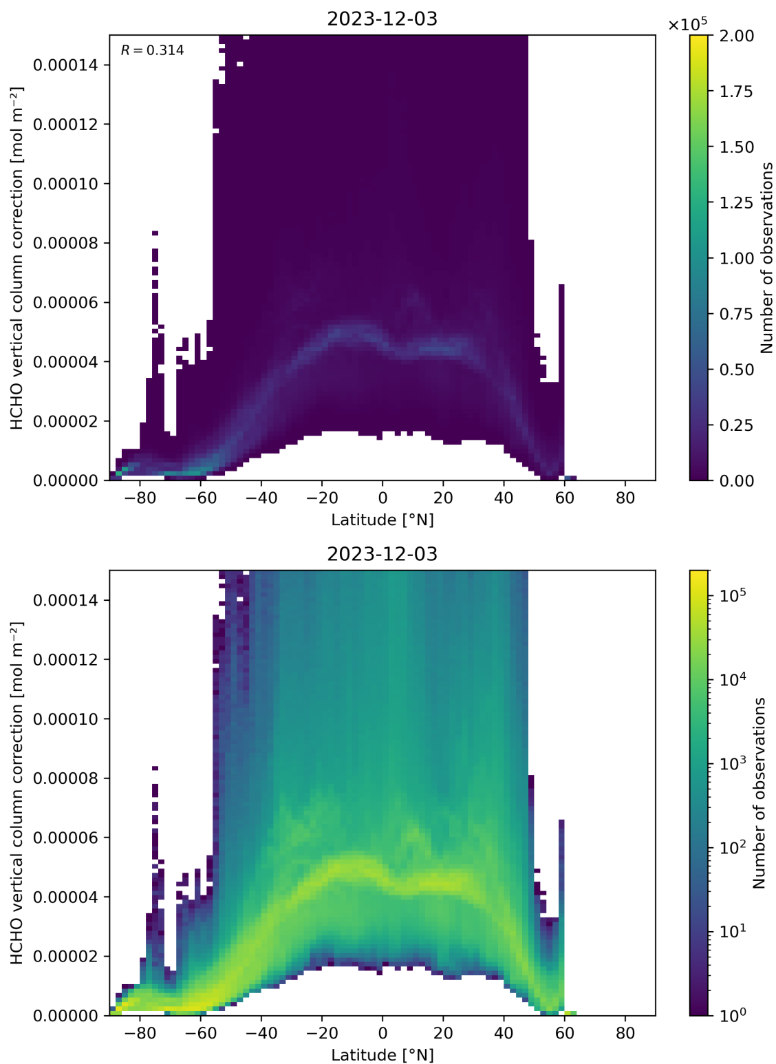
Figure 164: Scatter density plot of “Latitude” against “HCHO vertical column correction” for 2023-12-02 to 2023-12-04.
