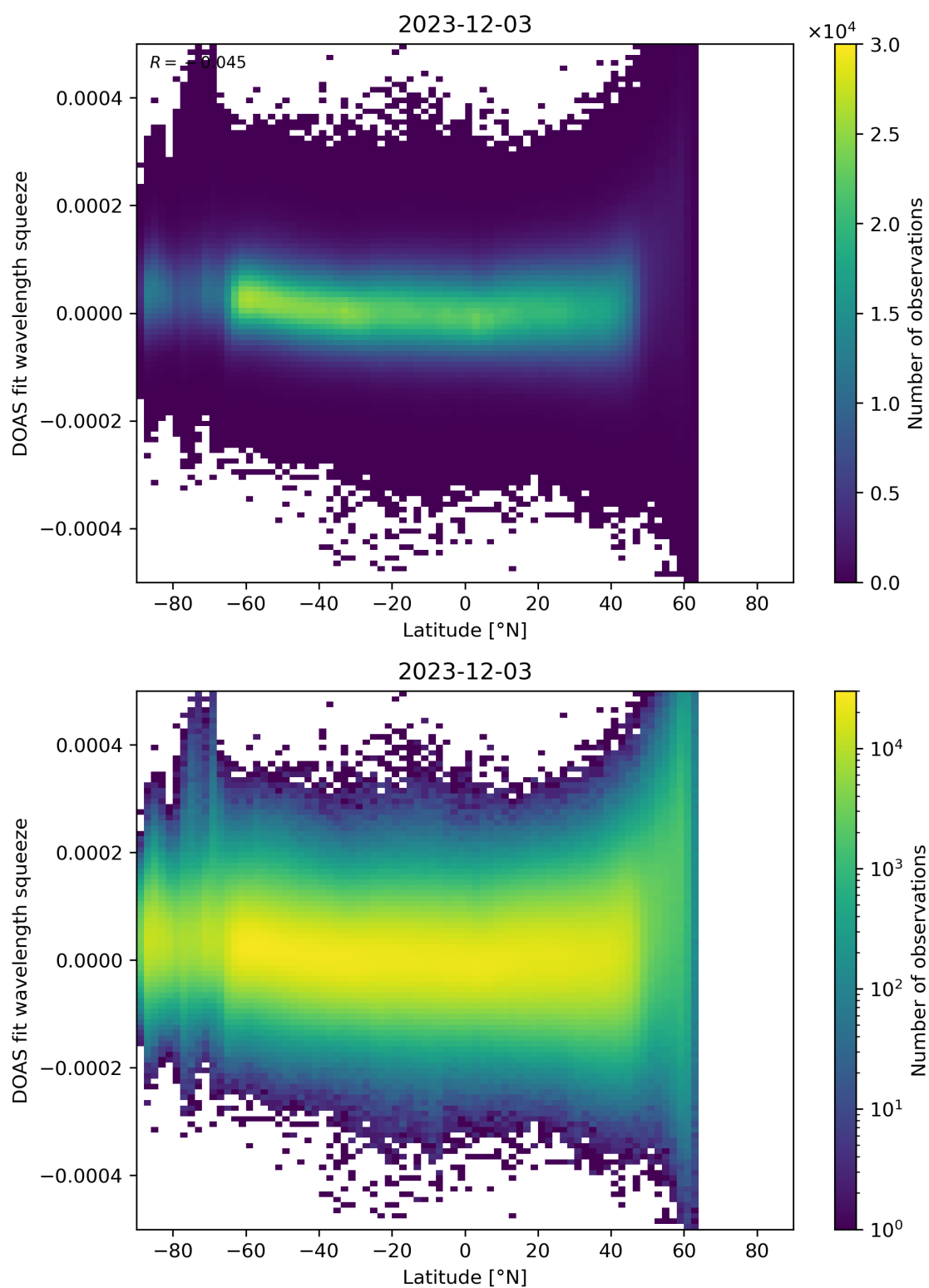
Figure 155: Scatter density plot of “Latitude” against “DOAS fit wavelength squeeze” for 2023-12-02 to 2023-12-04.
