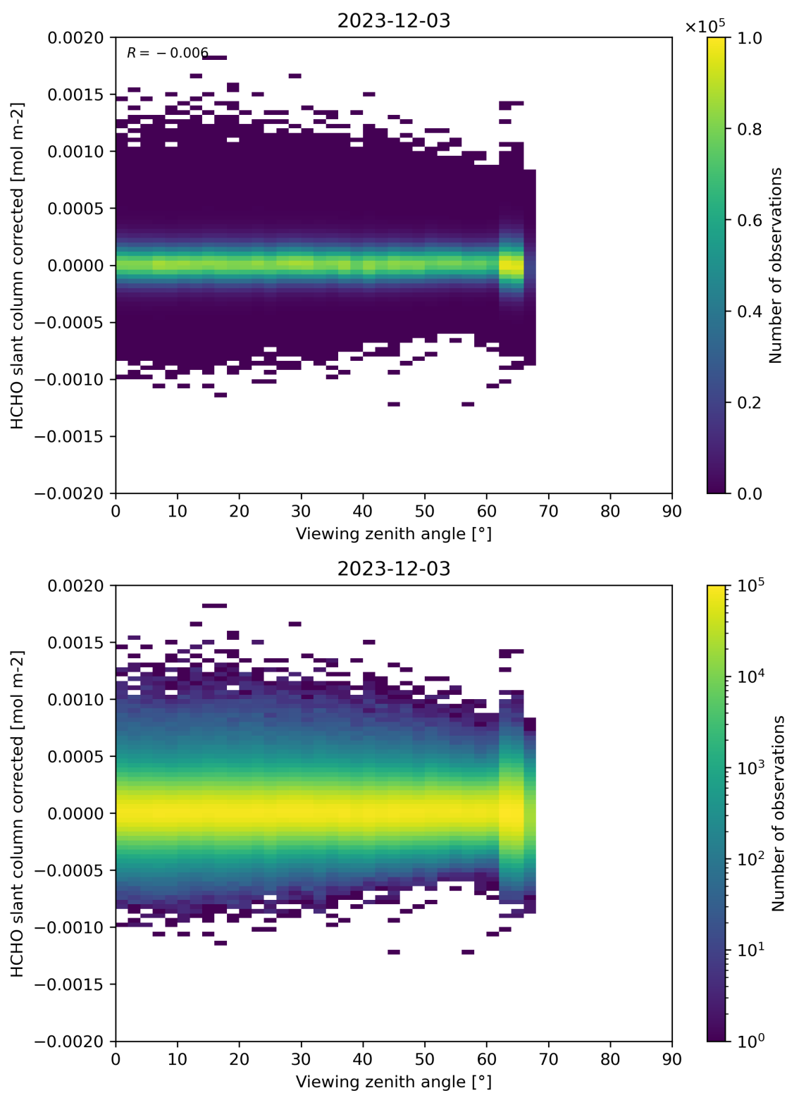
Figure 186: Scatter density plot of “Viewing zenith angle” against “HCHO slant column corrected” for 2023-12-02 to 2023-12-04.
