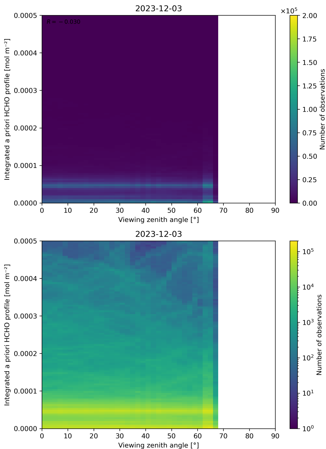
Figure 195: Scatter density plot of “Viewing zenith angle” against “Integrated a priori HCHO profile” for 2023-12-02 to 2023-12-04.
