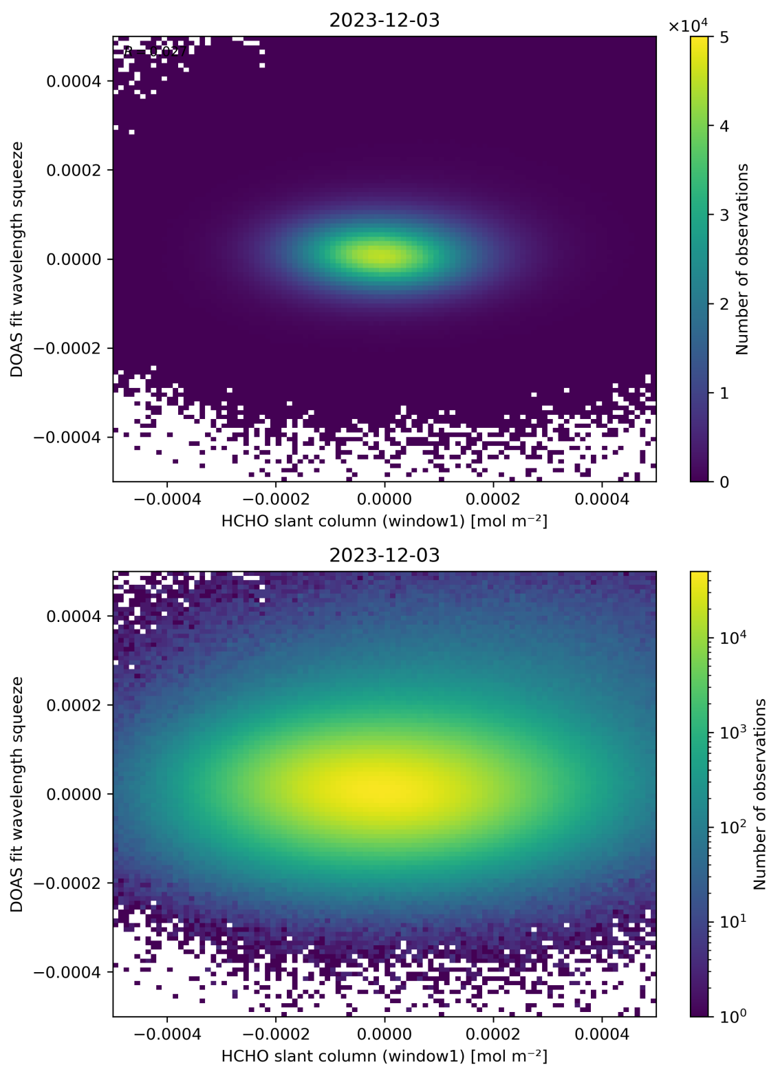
Figure 80: Scatter density plot of “HCHO slant column (window1)” against “DOAS fit wavelength squeeze” for 2023-12-02 to 2023-12-04.
