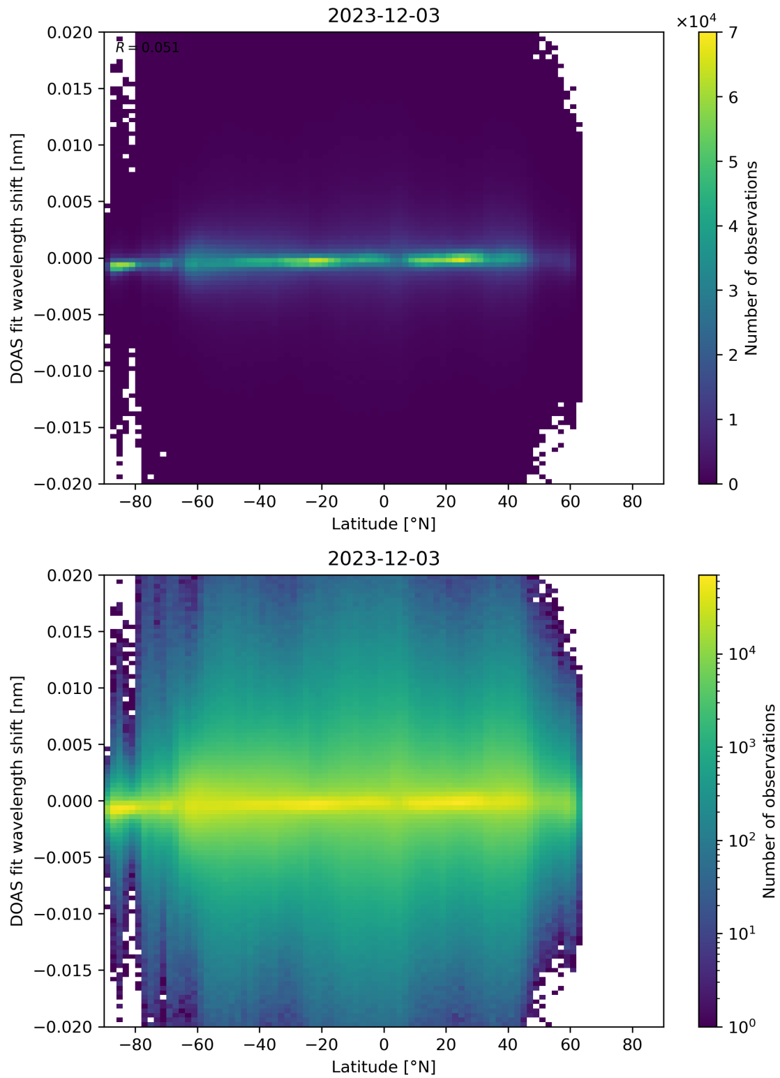
Figure 154: Scatter density plot of “Latitude” against “DOAS fit wavelength shift” for 2023-12-02 to 2023-12-04.
