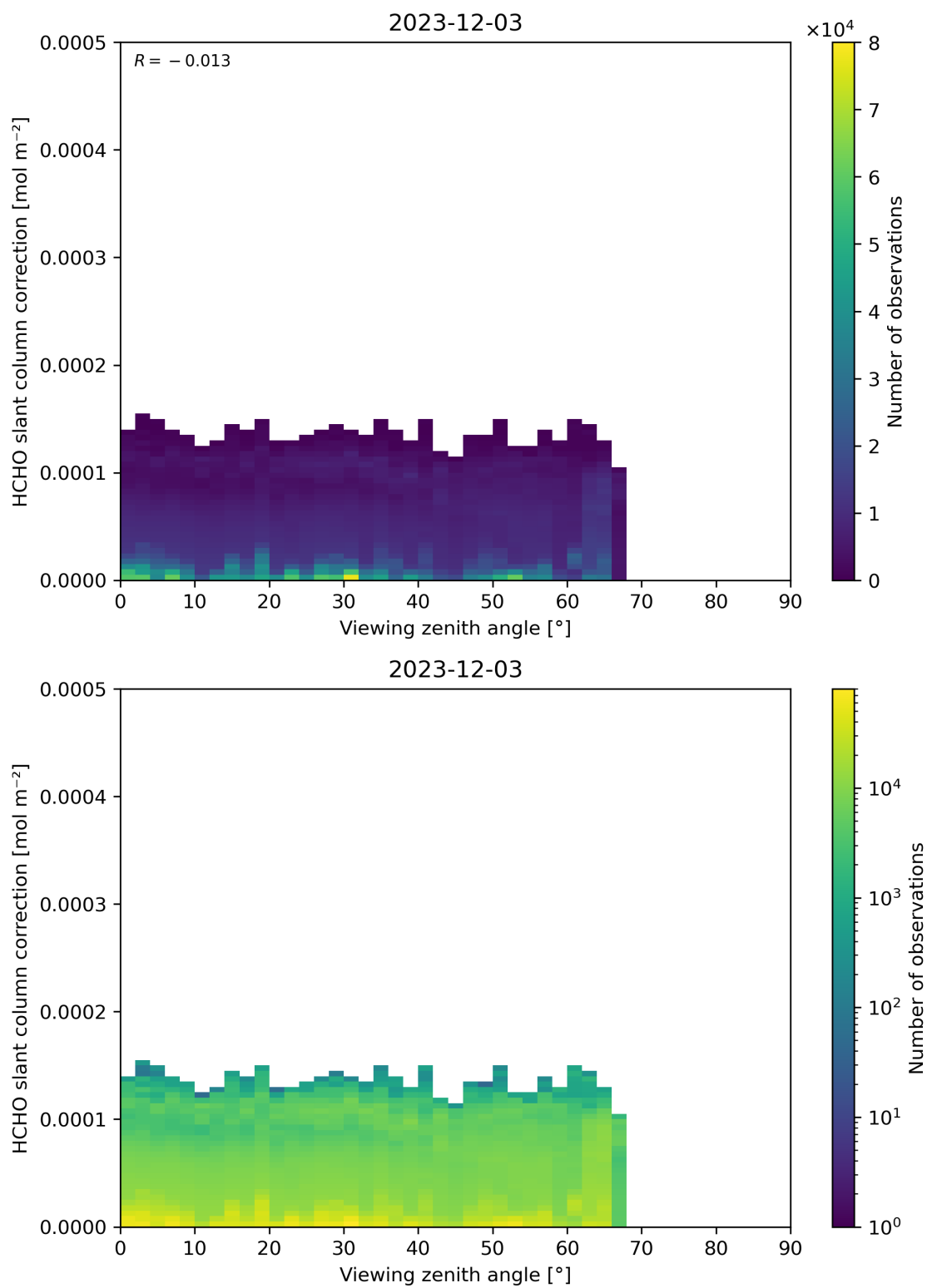
Figure 187: Scatter density plot of “Viewing zenith angle” against “HCHO slant column correction” for 2023-12-02 to 2023-12-04.
