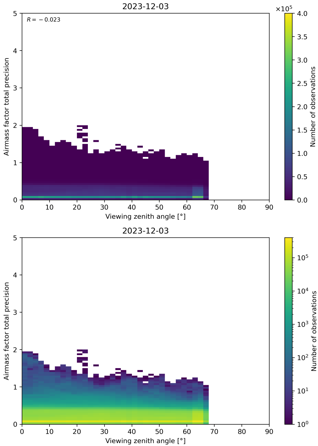
Figure 191: Scatter density plot of “Viewing zenith angle” against “Airmass factor total precision” for 2023-12-02 to 2023-12-04.
