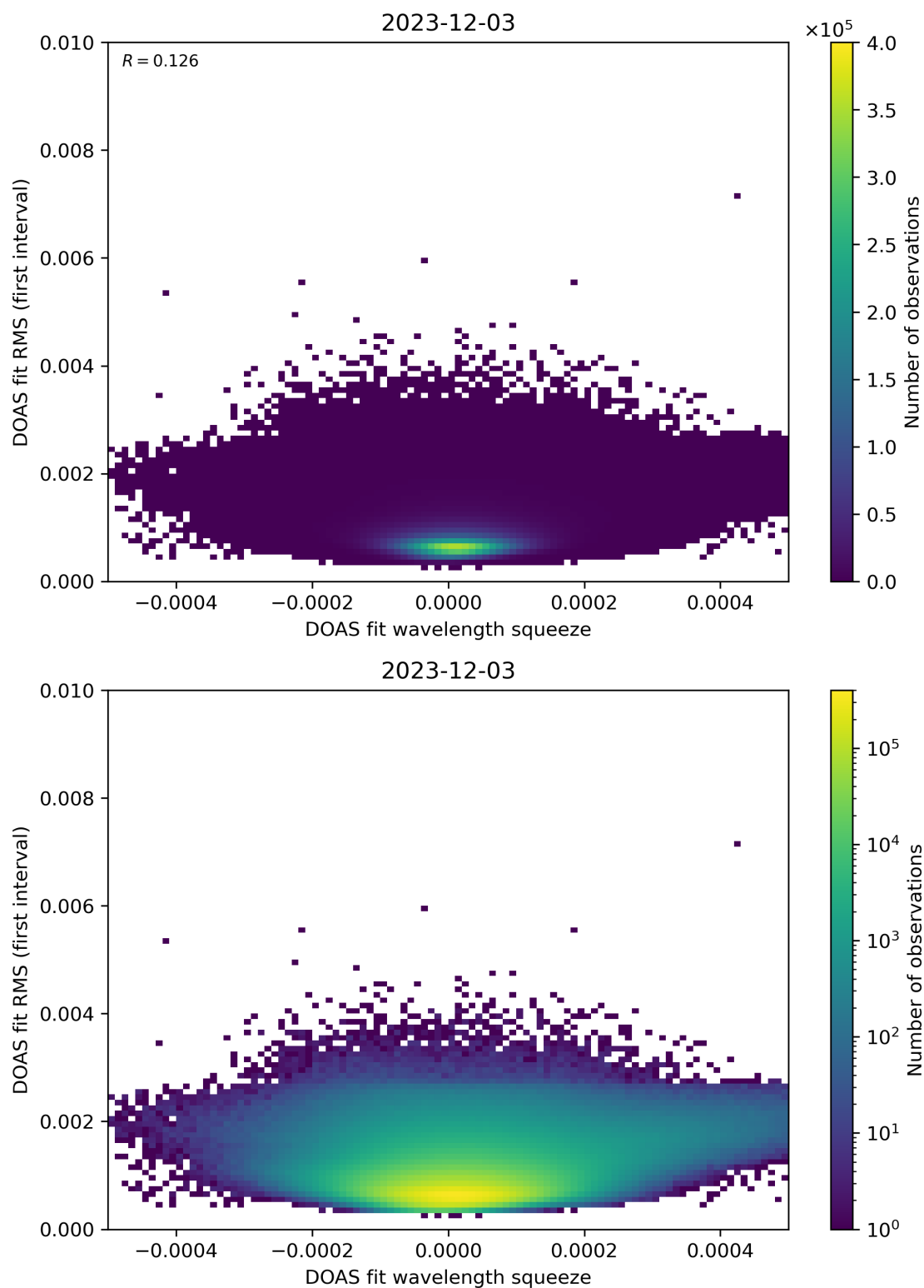
Figure 68: Scatter density plot of “DOAS fit wavelength squeeze” against “DOAS fit RMS (first interval)” for 2023-12-02 to 2023-12-04.
