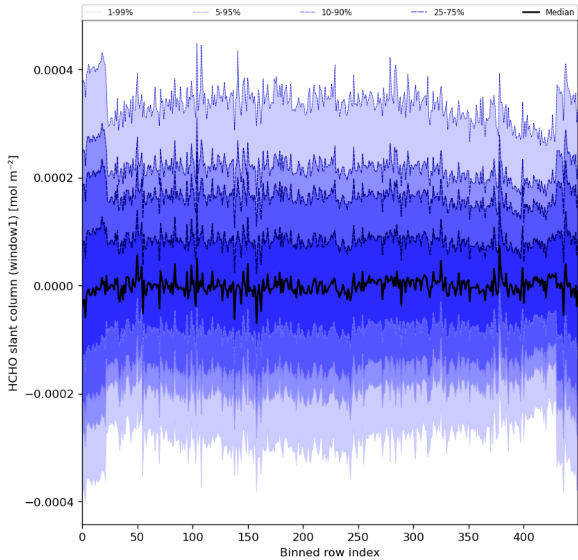
Figure 52: Along track statistics of “HCHO slant column (window1)” for 2023-12-02 to 2023-12-04
