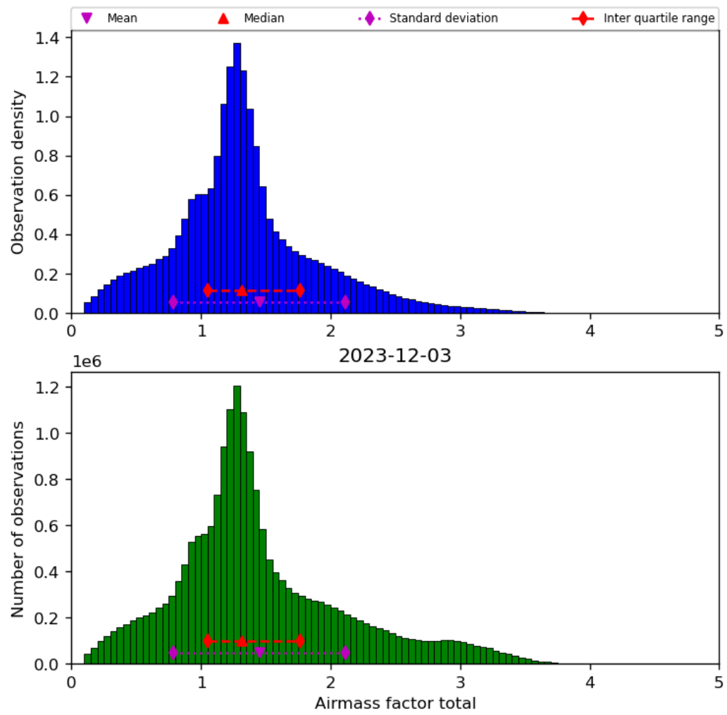
Figure 40: Histogram of “Airmass factor total” for 2023-12-02 to 2023-12-04
