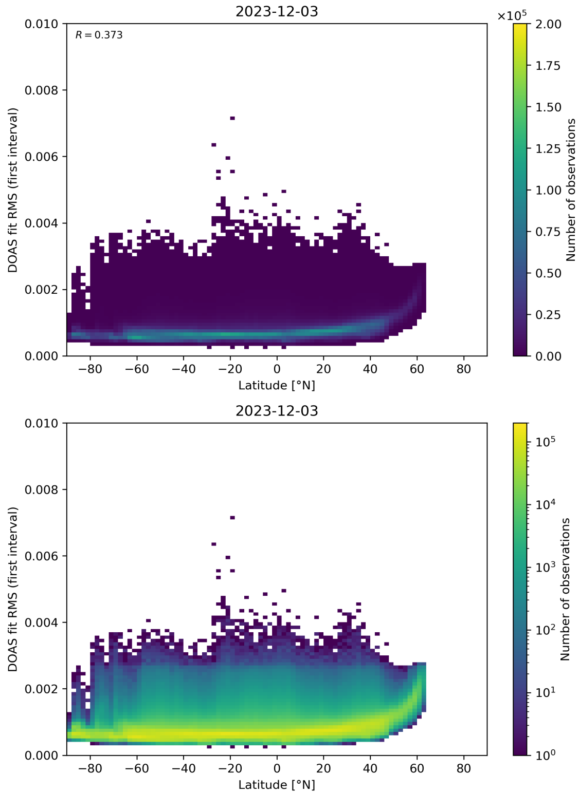
Figure 153: Scatter density plot of “Latitude” against “DOAS fit RMS (first interval)” for 2023-12-02 to 2023-12-04.
