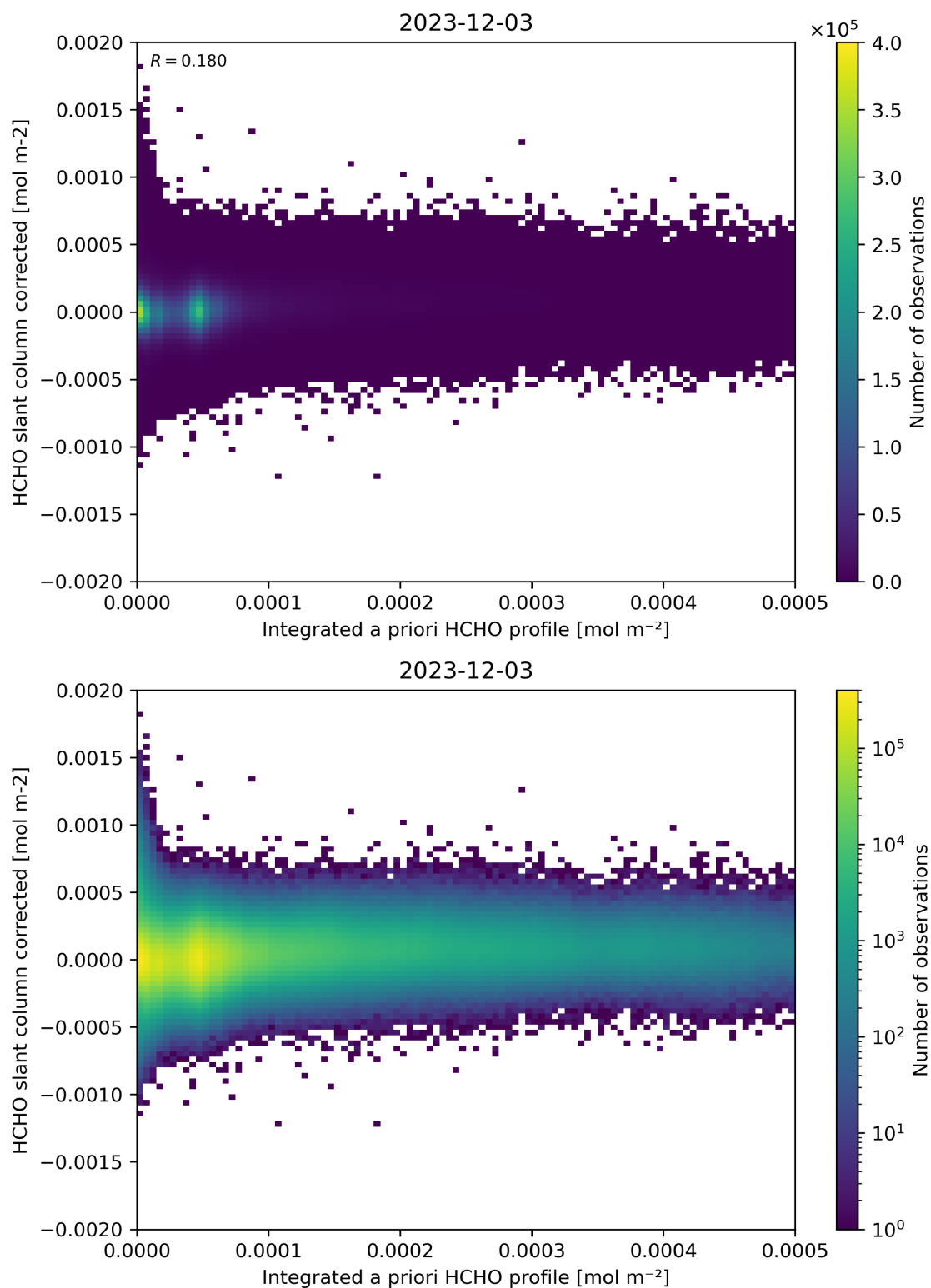
Figure 151: Scatter density plot of “Integrated a priori HCHO profile” against “HCHO slant column corrected” for 2023-12-02 to 2023-12-04.
