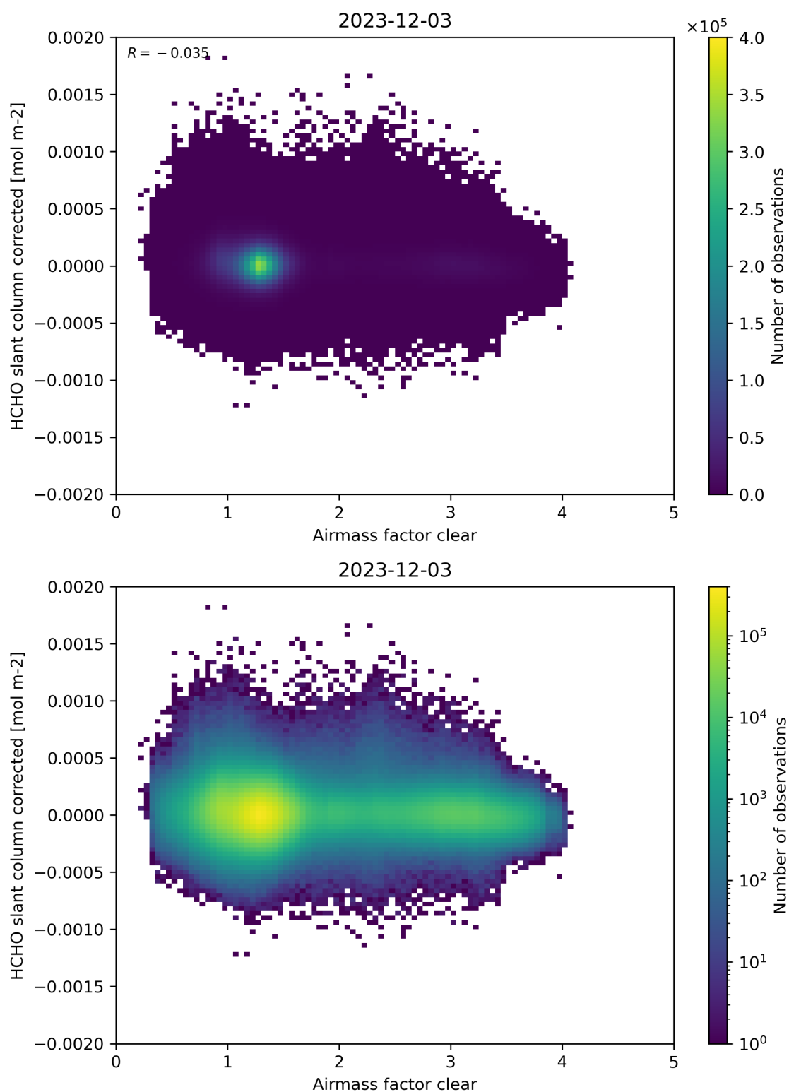
Figure 74: Scatter density plot of “Airmass factor clear” against “HCHO slant column corrected” for 2023-12-02 to 2023-12-04.
