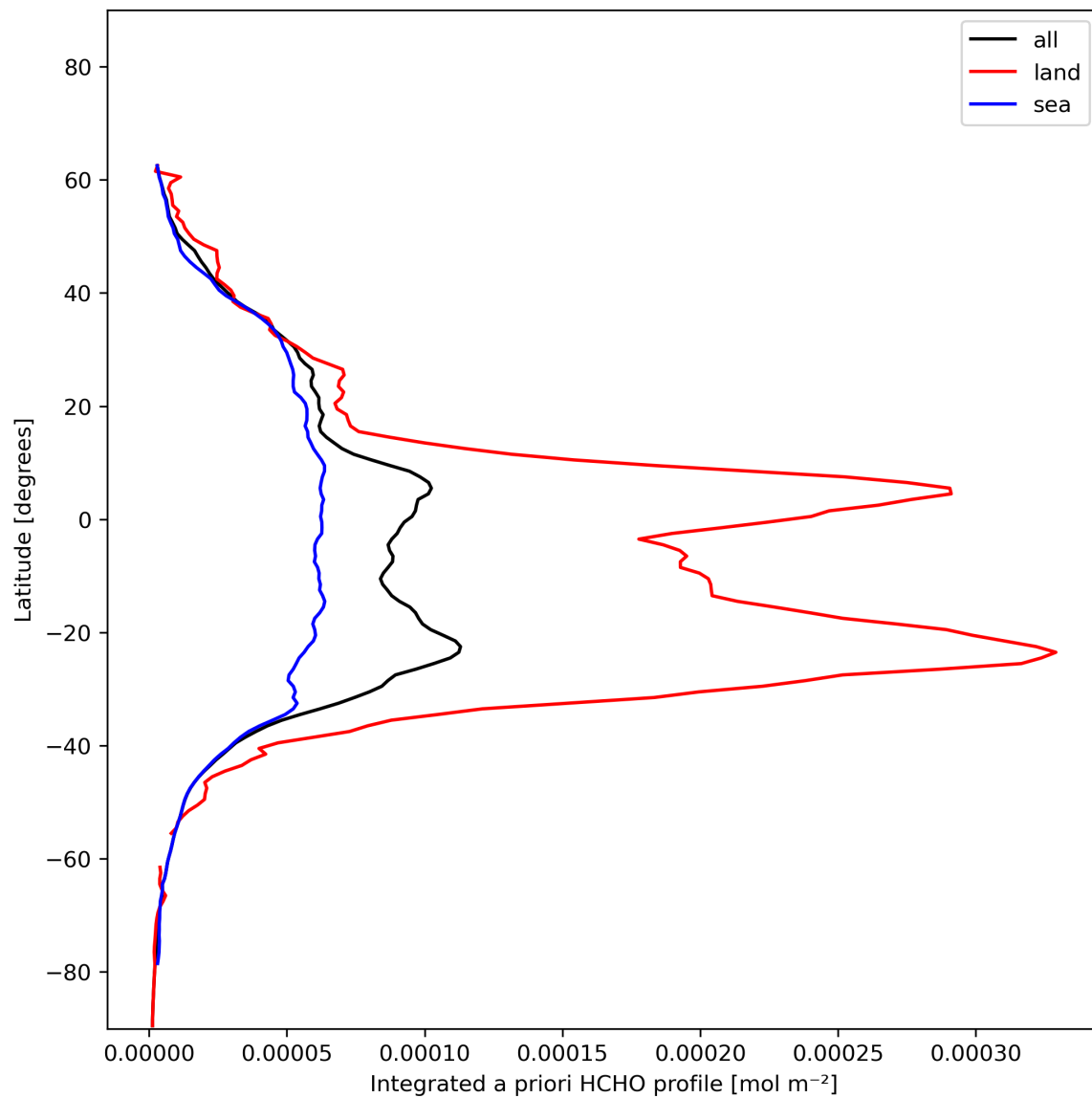
Figure 29: Zonal average of “Integrated a priori HCHO profile” for 2023-12-02 to 2023-12-04.
