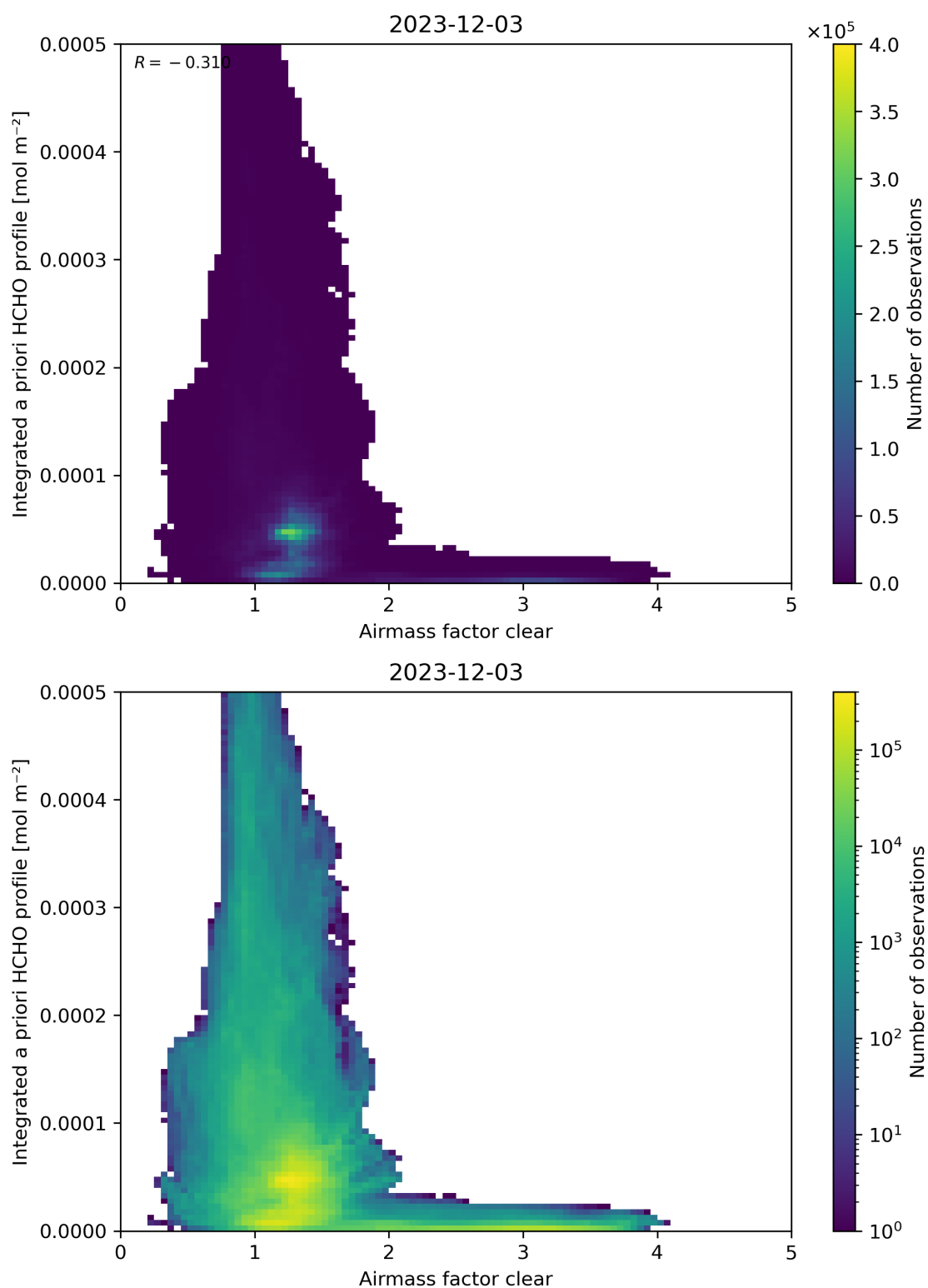
Figure 76: Scatter density plot of “Airmass factor clear” against “Integrated a priori HCHO profile” for 2023-12-02 to 2023-12-04.
