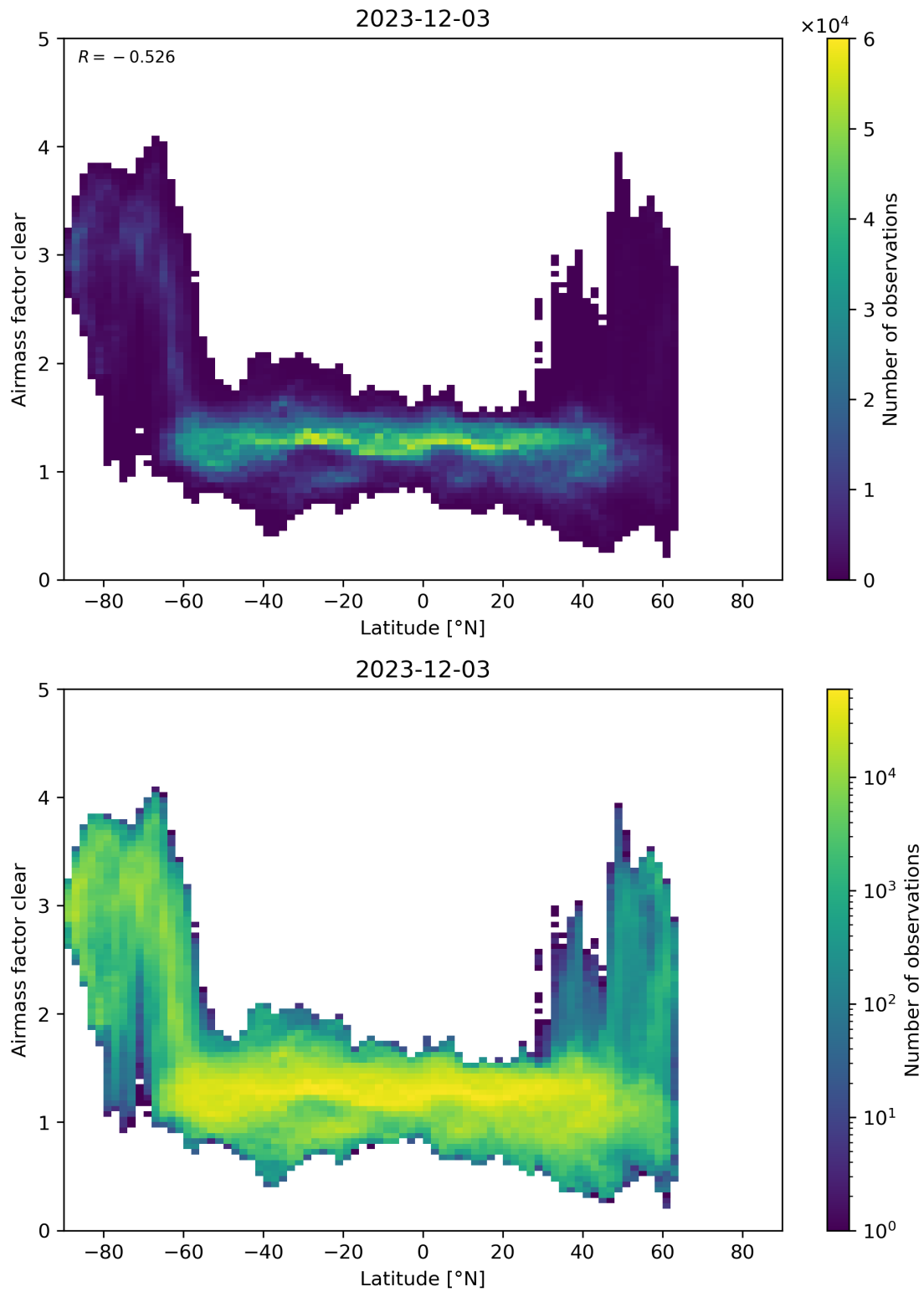
Figure 156: Scatter density plot of “Latitude” against “Airmass factor clear” for 2023-12-02 to 2023-12-04.
