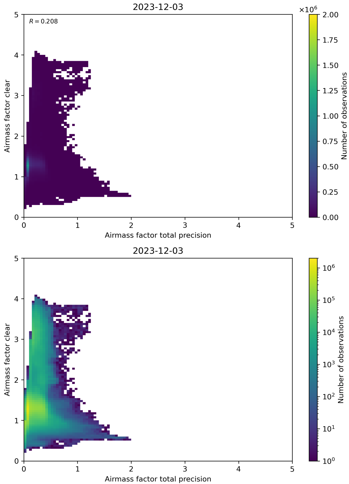
Figure 108: Scatter density plot of “Airmass factor total precision” against “Airmass factor clear” for 2023-12-02 to 2023-12-04.
