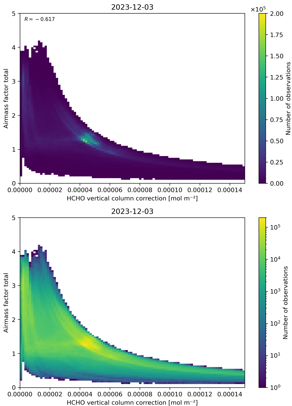
Figure 120: Scatter density plot of “HCHO vertical column correction” against “Airmass factor total” for 2023-12-02 to 2023-12-04.
