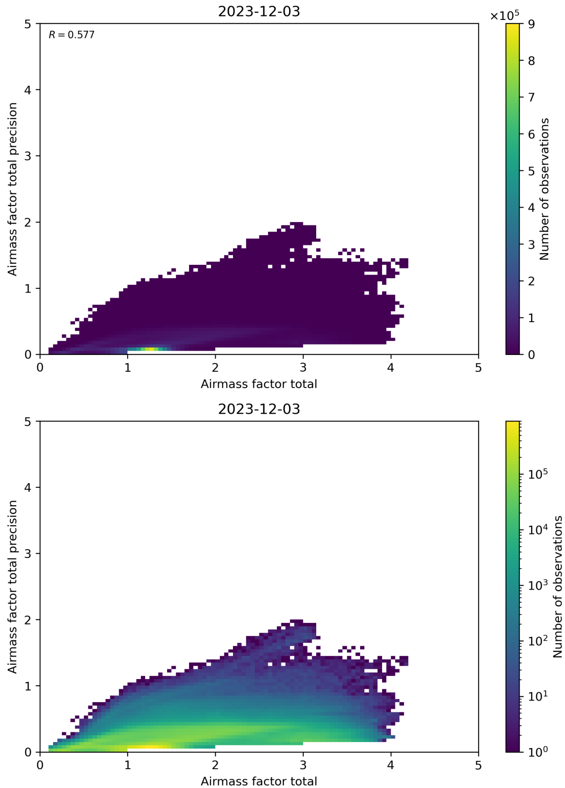
Figure 103: Scatter density plot of “Airmass factor total” against “Airmass factor total precision” for 2023-12-02 to 2023-12-04.
