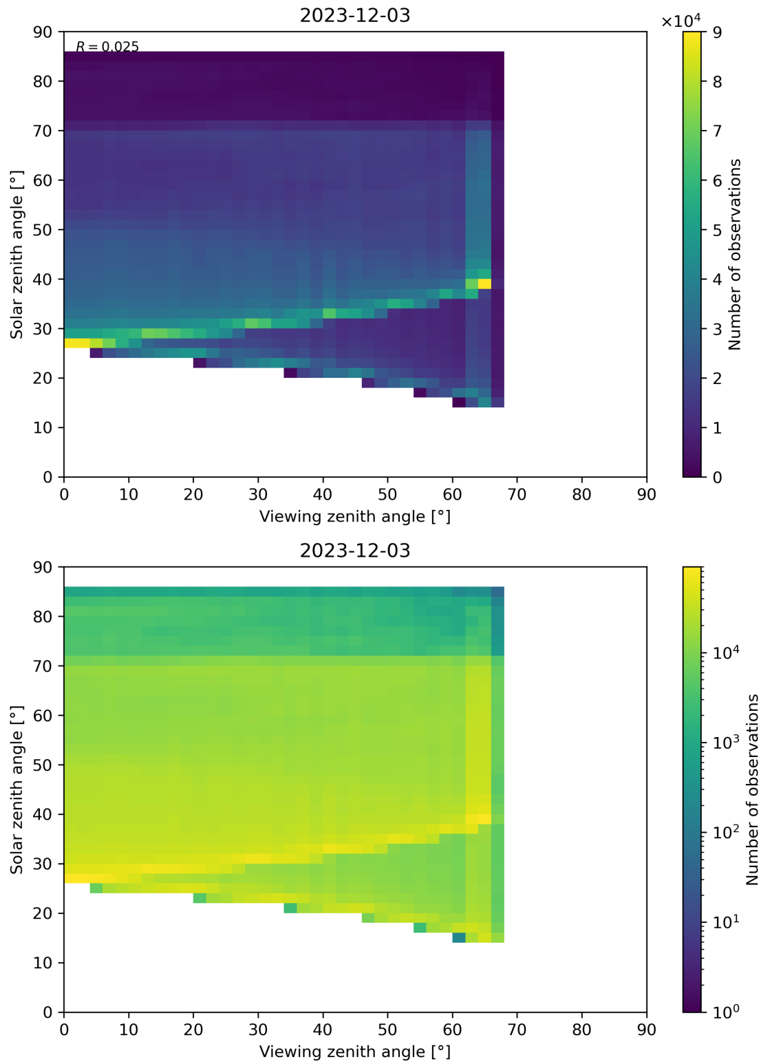
Figure 197: Scatter density plot of “Viewing zenith angle” against “Solar zenith angle” for 2023-12-02 to 2023-12-04.
