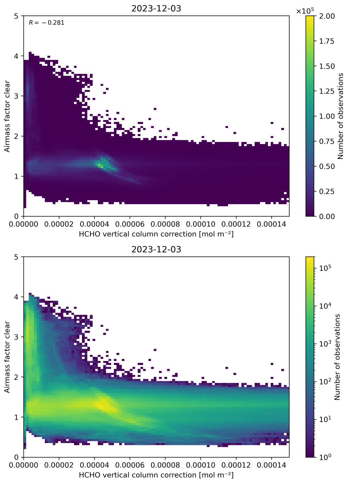
Figure 115: Scatter density plot of “HCHO vertical column correction” against “Airmass factor clear” for 2023-12-02 to 2023-12-04.
