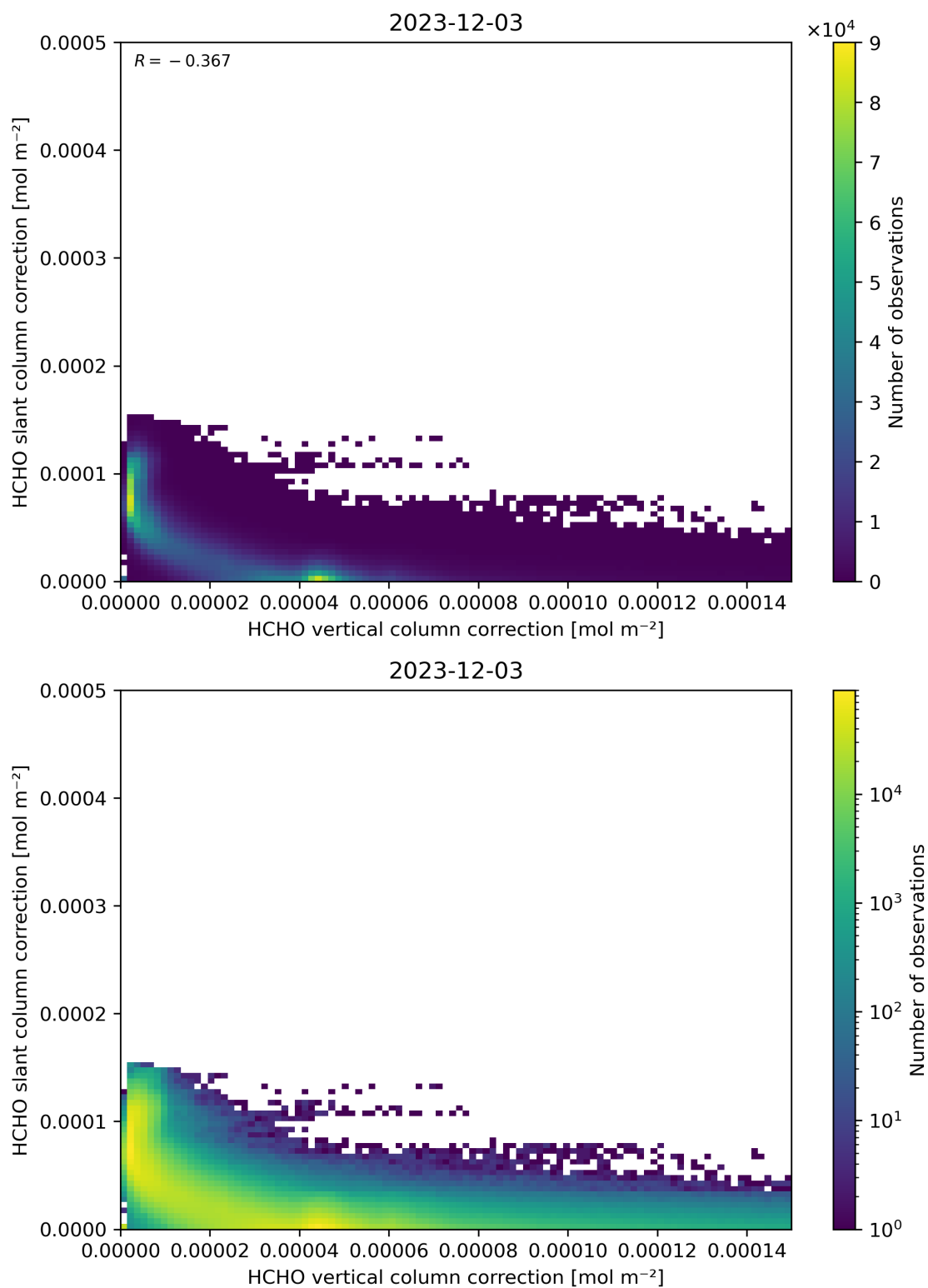
Figure 117: Scatter density plot of “HCHO vertical column correction” against “HCHO slant column correction” for 2023-12-02 to 2023-12-04.
