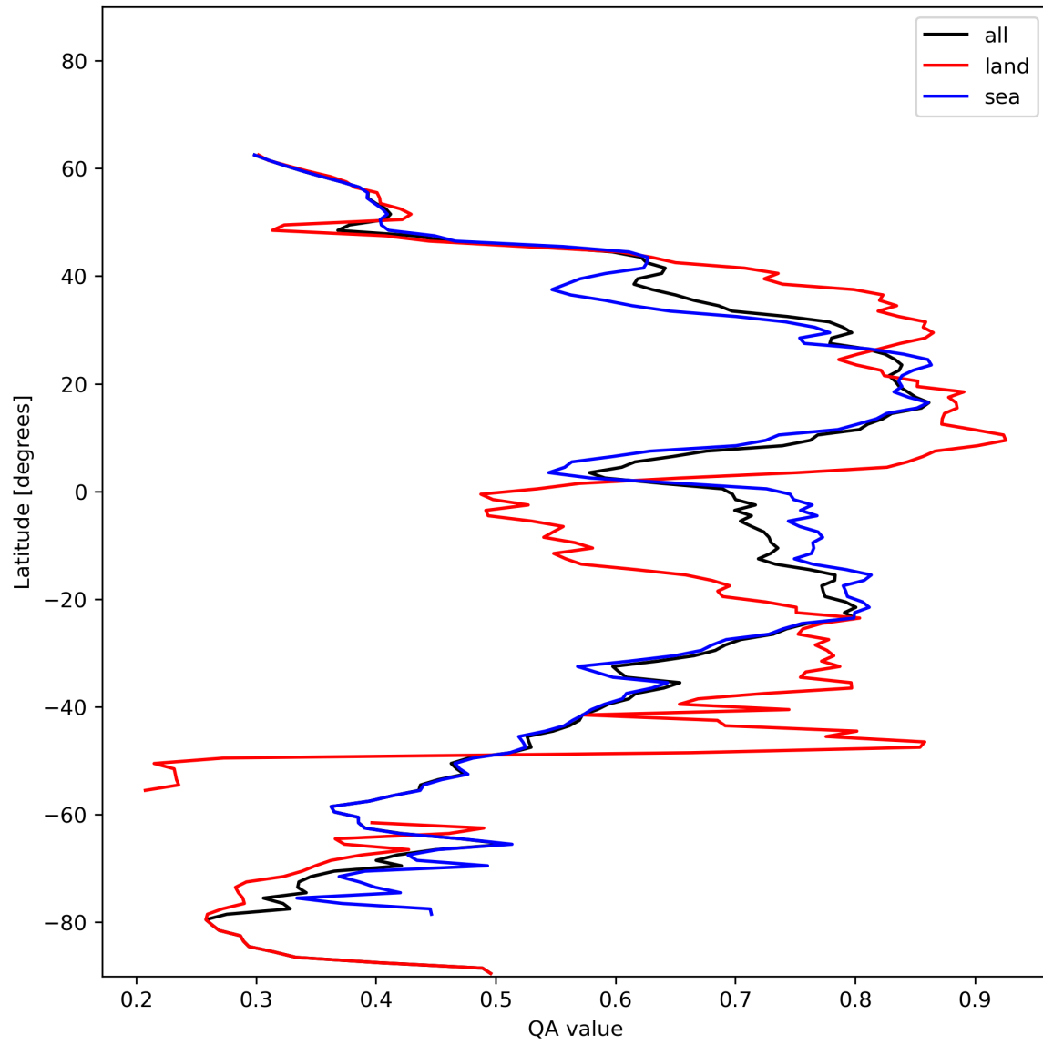
Figure 20: Zonal average of “QA value” for 2023-12-02 to 2023-12-04.
