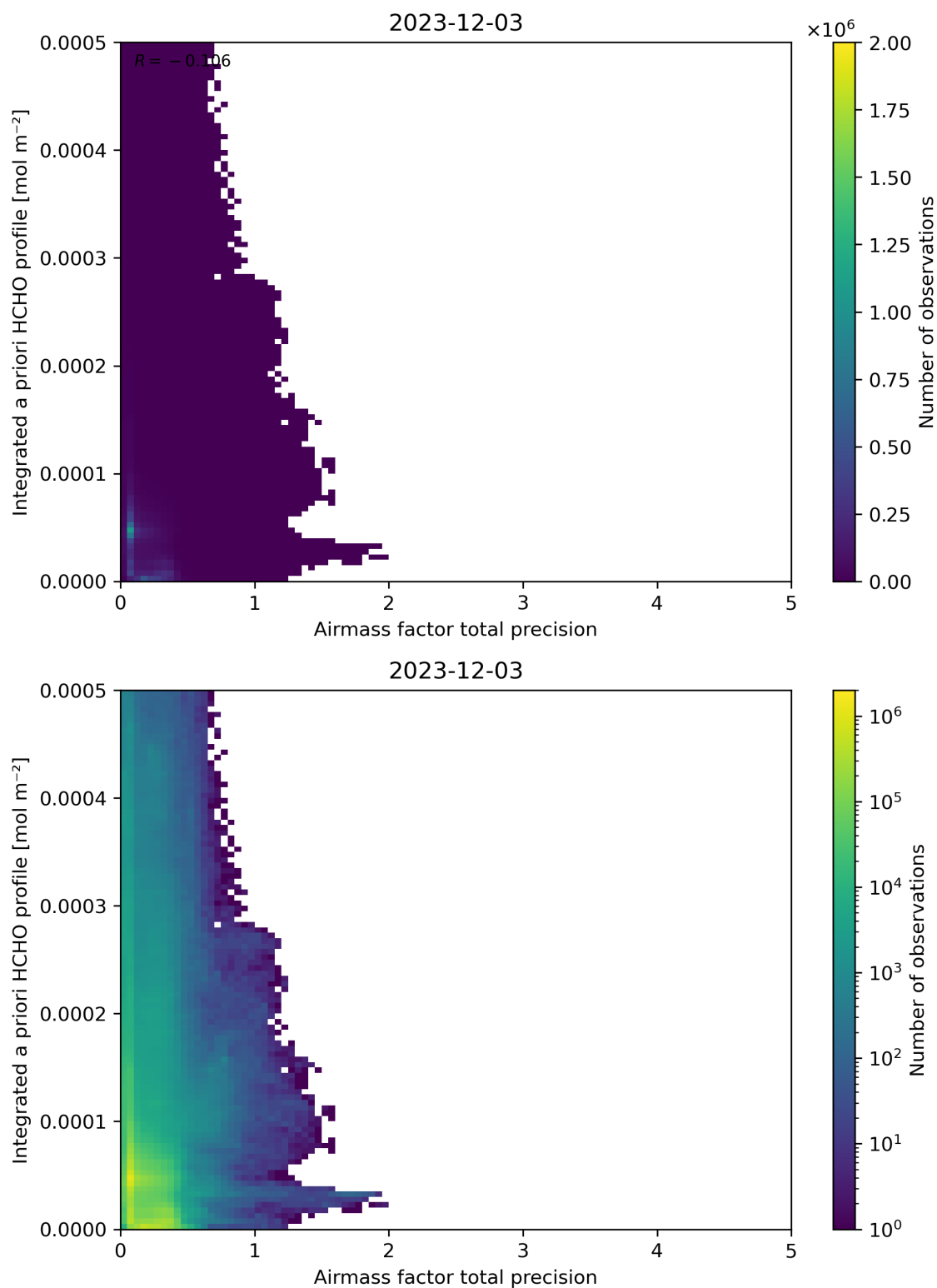
Figure 111: Scatter density plot of “Airmass factor total precision” against “Integrated a priori HCHO profile” for 2023-12-02 to 2023-12-04.
