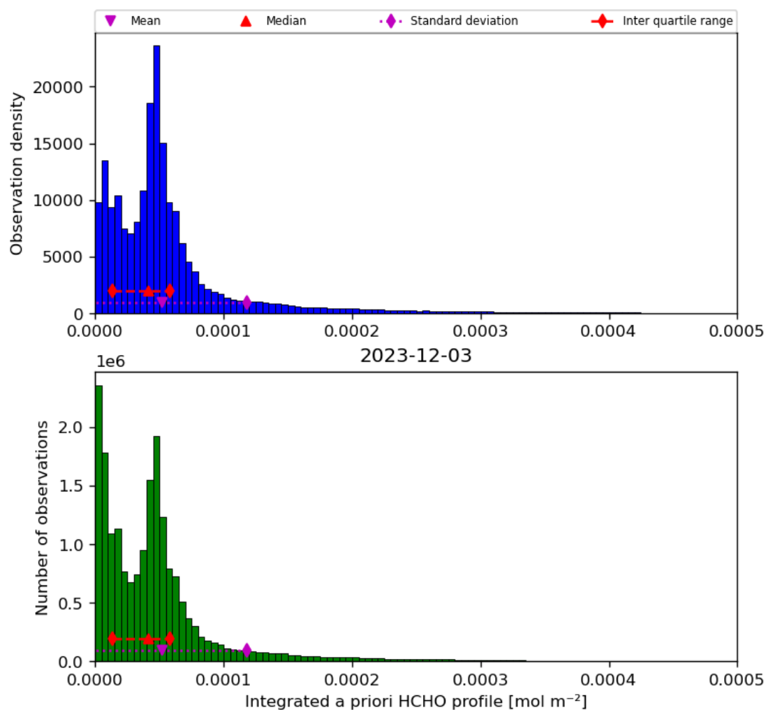
Figure 43: Histogram of “Integrated a priori HCHO profile” for 2023-12-02 to 2023-12-04
