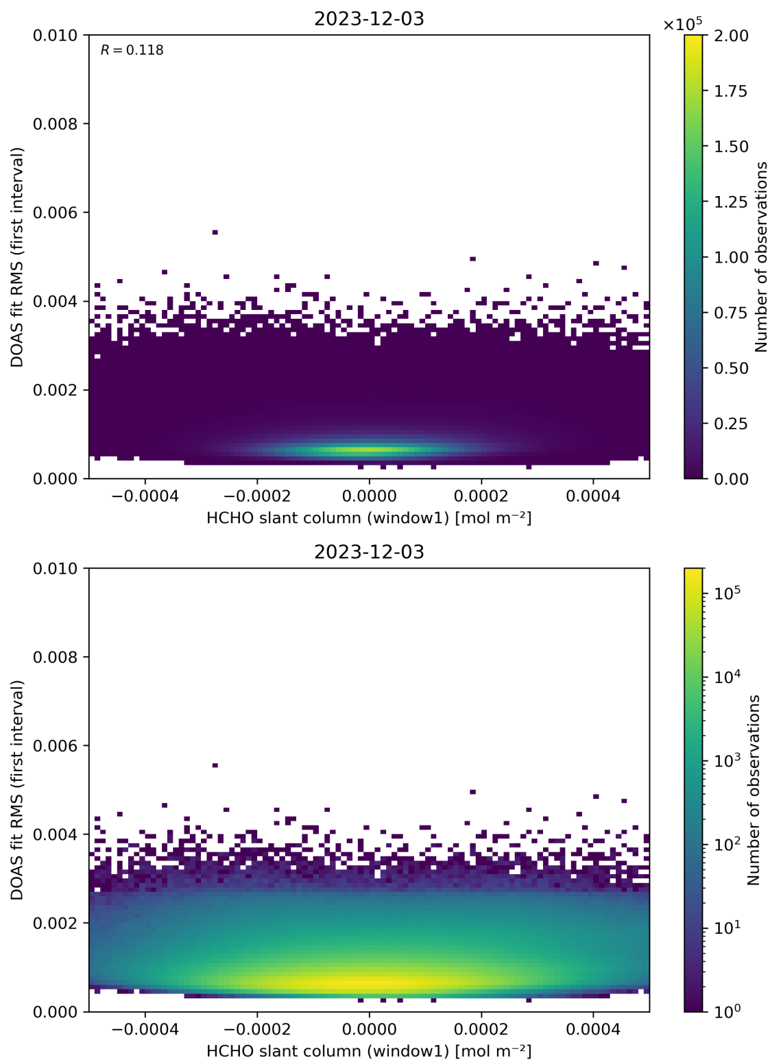
Figure 78: Scatter density plot of “HCHO slant column (window1)” against “DOAS fit RMS (first interval)” for 2023-12-02 to 2023-12-04.
