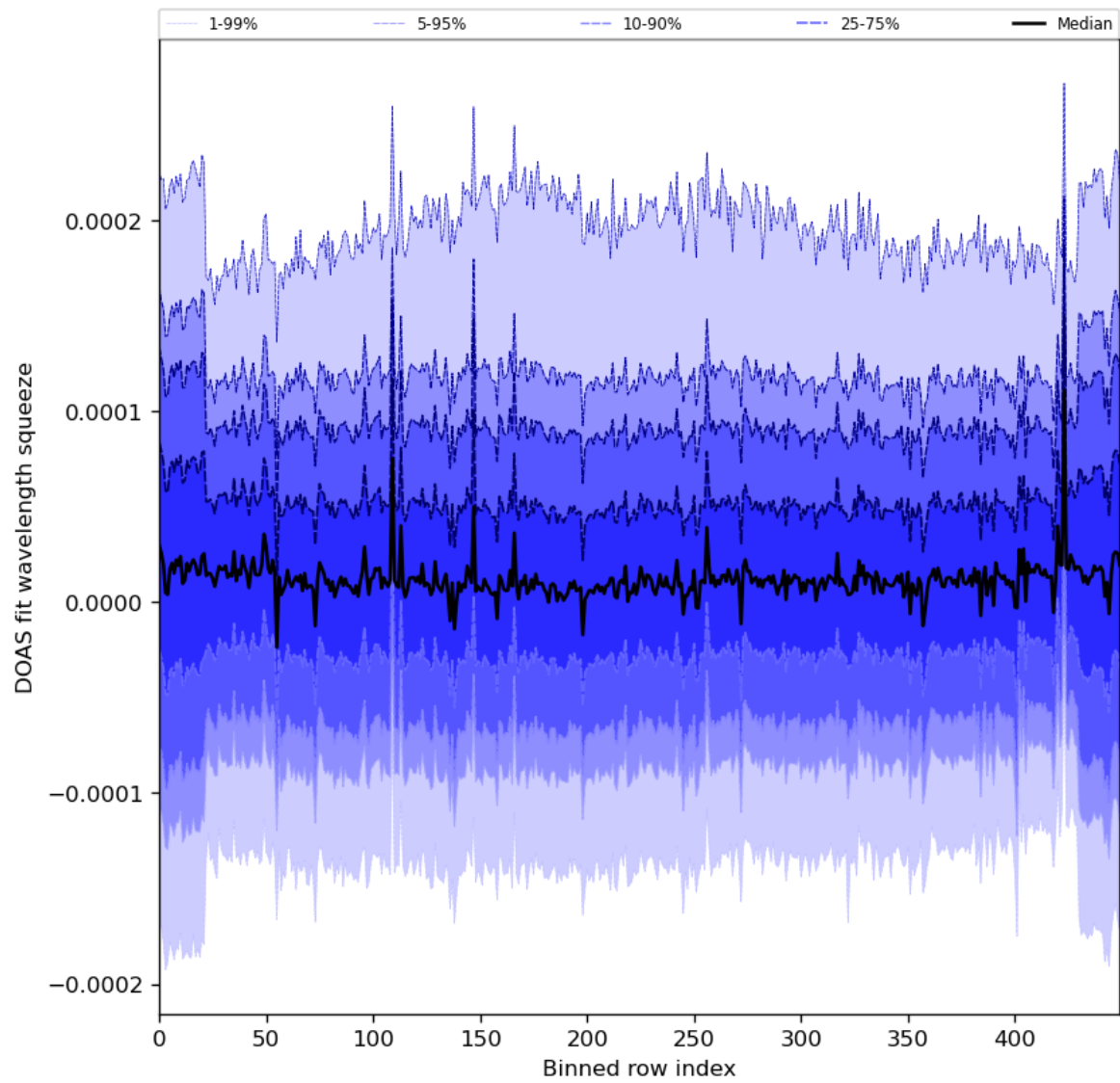
Figure 59: Along track statistics of “DOAS fit wavelength squeeze” for 2023-12-02 to 2023-12-04
