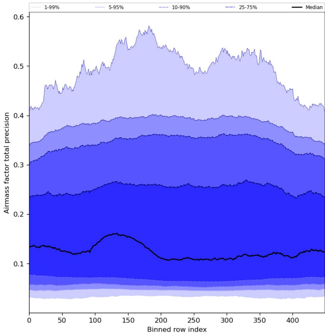
Figure 55: Along track statistics of “Airmass factor total precision” for 2023-12-02 to 2023-12-04
