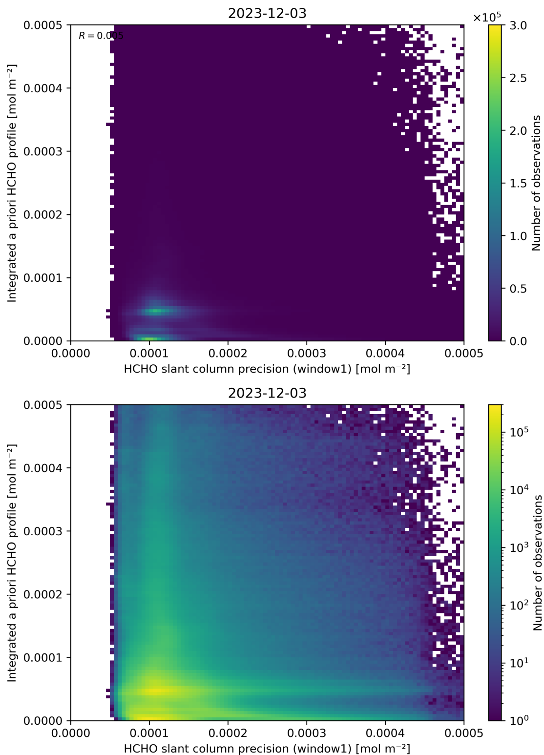
Figure 96: Scatter density plot of “HCHO slant column precision (window1)” against “Integrated a priori HCHO profile” for 2023-12-02 to 2023-12-04.
