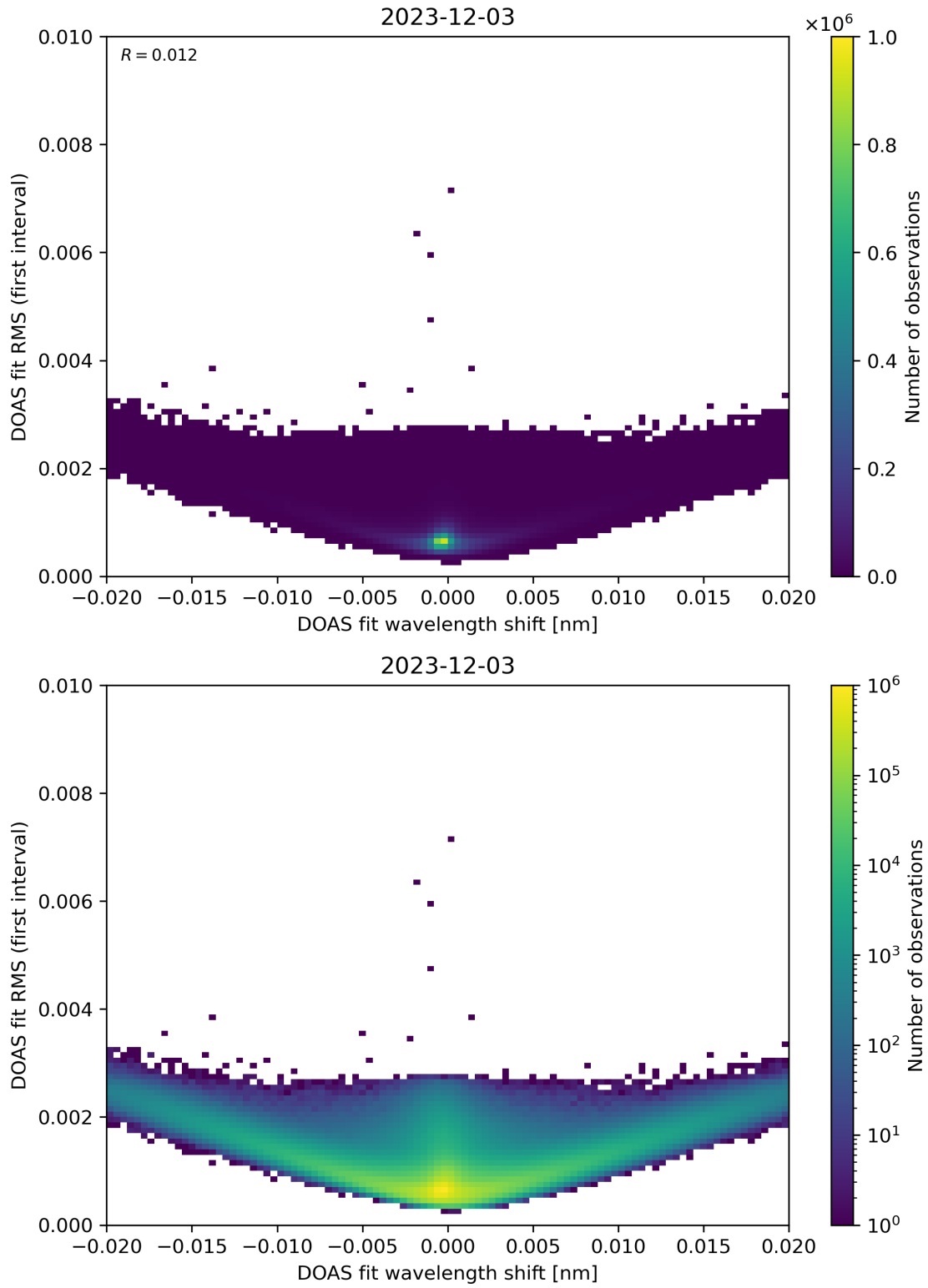
Figure 64: Scatter density plot of “DOAS fit wavelength shift” against “DOAS fit RMS (first interval)” for 2023-12-02 to 2023-12-04.
