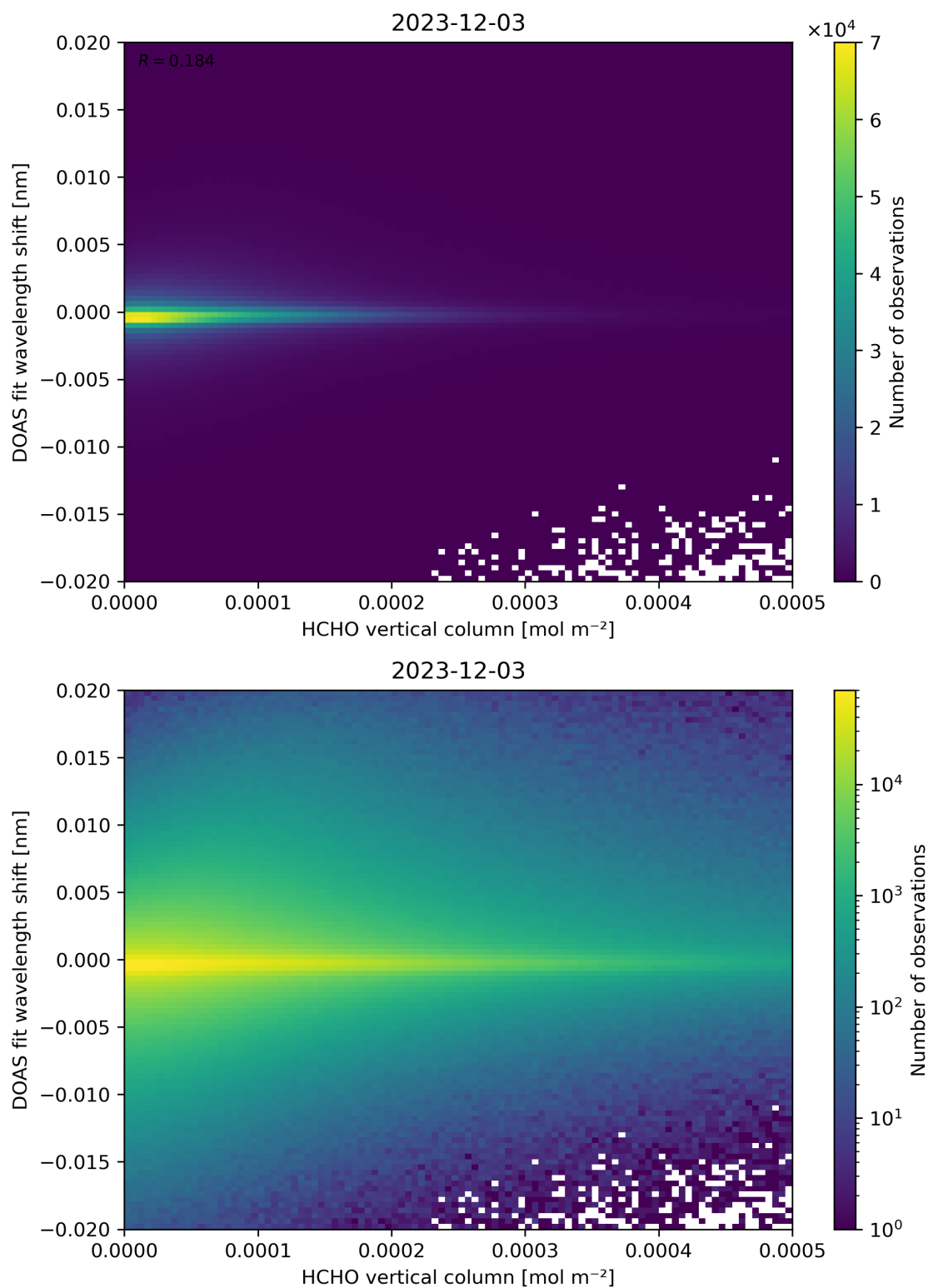
Figure 124: Scatter density plot of “HCHO vertical column” against “DOAS fit wavelength shift” for 2023-12-02 to 2023-12-04.
