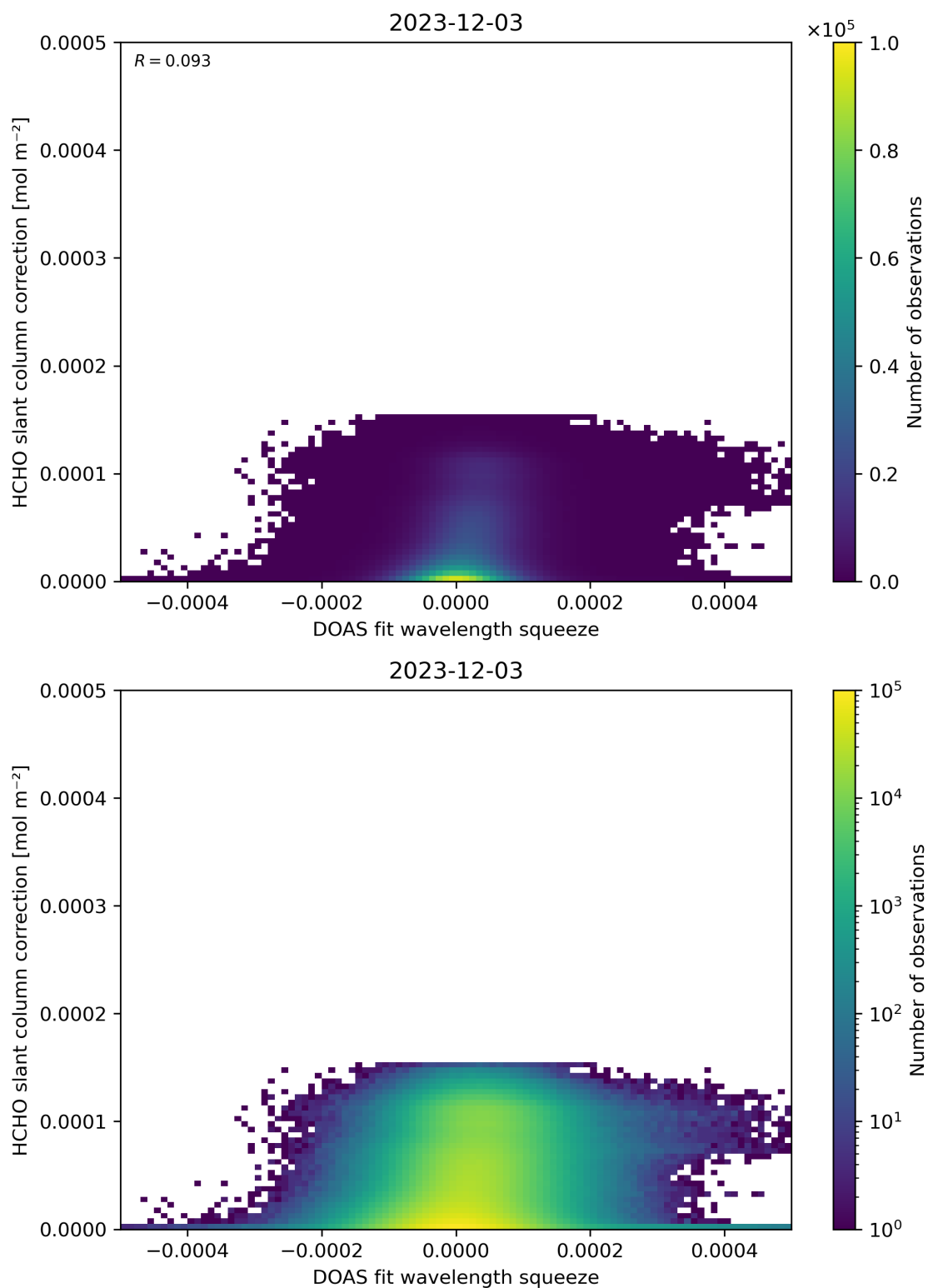
Figure 70: Scatter density plot of “DOAS fit wavelength squeeze” against “HCHO slant column correction” for 2023-12-02 to 2023-12-04.
