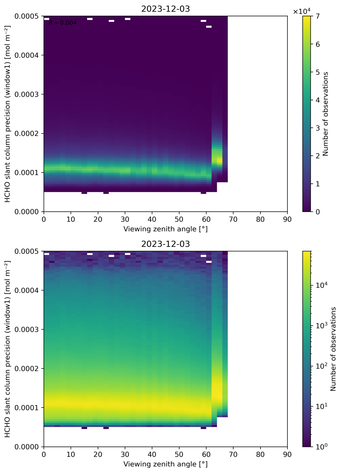
Figure 189: Scatter density plot of “Viewing zenith angle” against “HCHO slant column precision (window1)” for 2023-12-02 to 2023-12-04.
