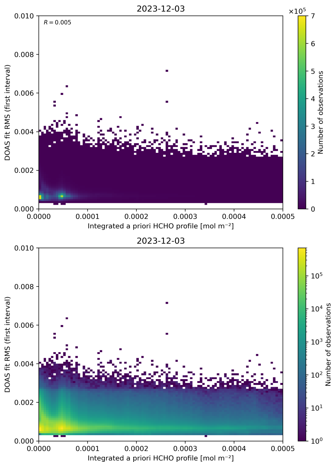
Figure 148: Scatter density plot of “Integrated a priori HCHO profile” against “DOAS fit RMS (first interval)” for 2023-12-02 to 2023-12-04.
