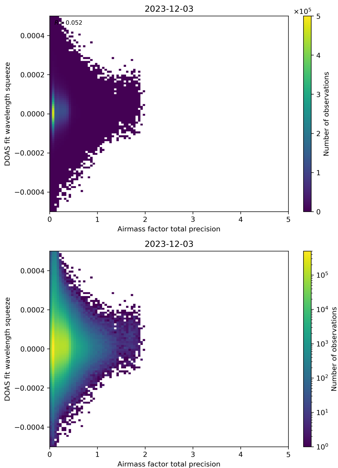
Figure 107: Scatter density plot of “Airmass factor total precision” against “DOAS fit wavelength squeeze” for 2023-12-02 to 2023-12-04.
