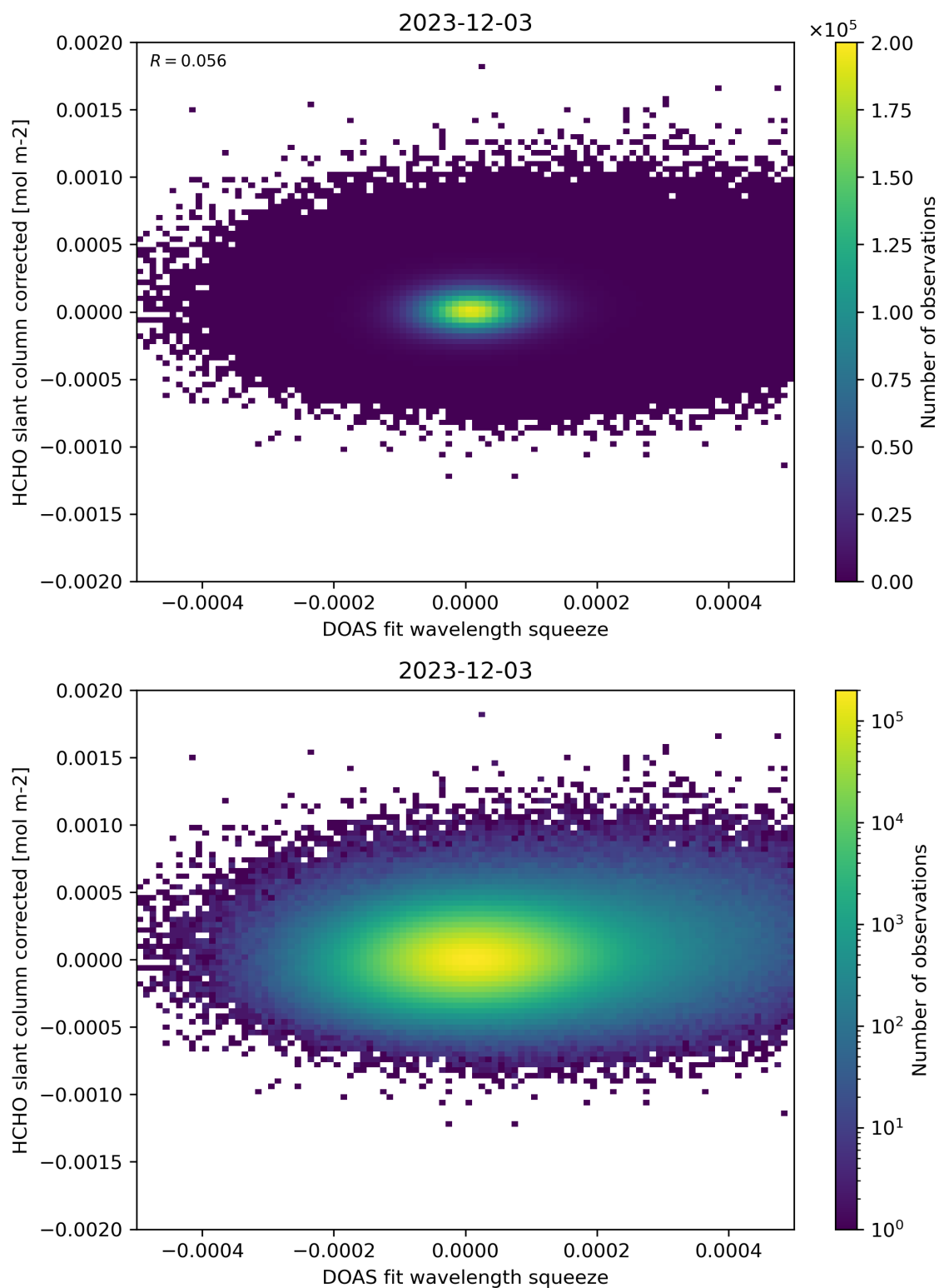
Figure 69: Scatter density plot of “DOAS fit wavelength squeeze” against “HCHO slant column corrected” for 2023-12-02 to 2023-12-04.
