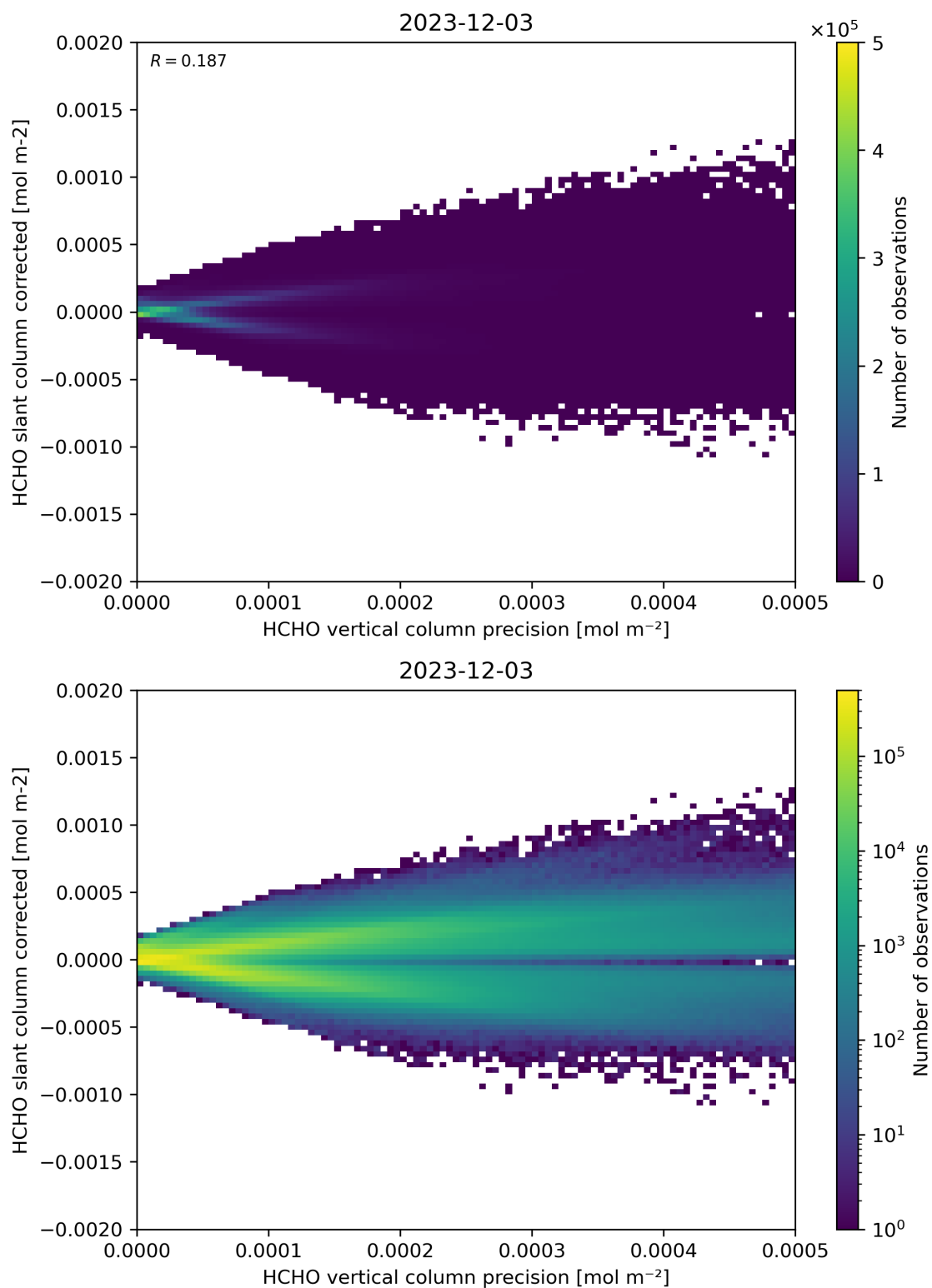
Figure 140: Scatter density plot of “HCHO vertical column precision” against “HCHO slant column corrected” for 2023-12-02 to 2023-12-04.
