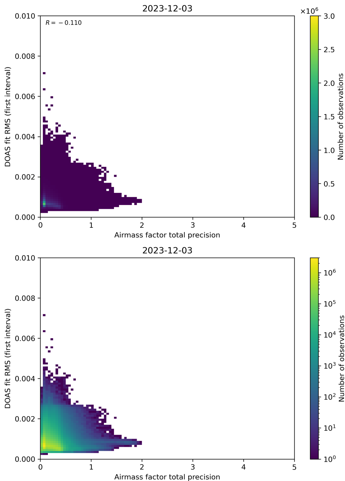
Figure 105: Scatter density plot of “Airmass factor total precision” against “DOAS fit RMS (first interval)” for 2023-12-02 to 2023-12-04.
