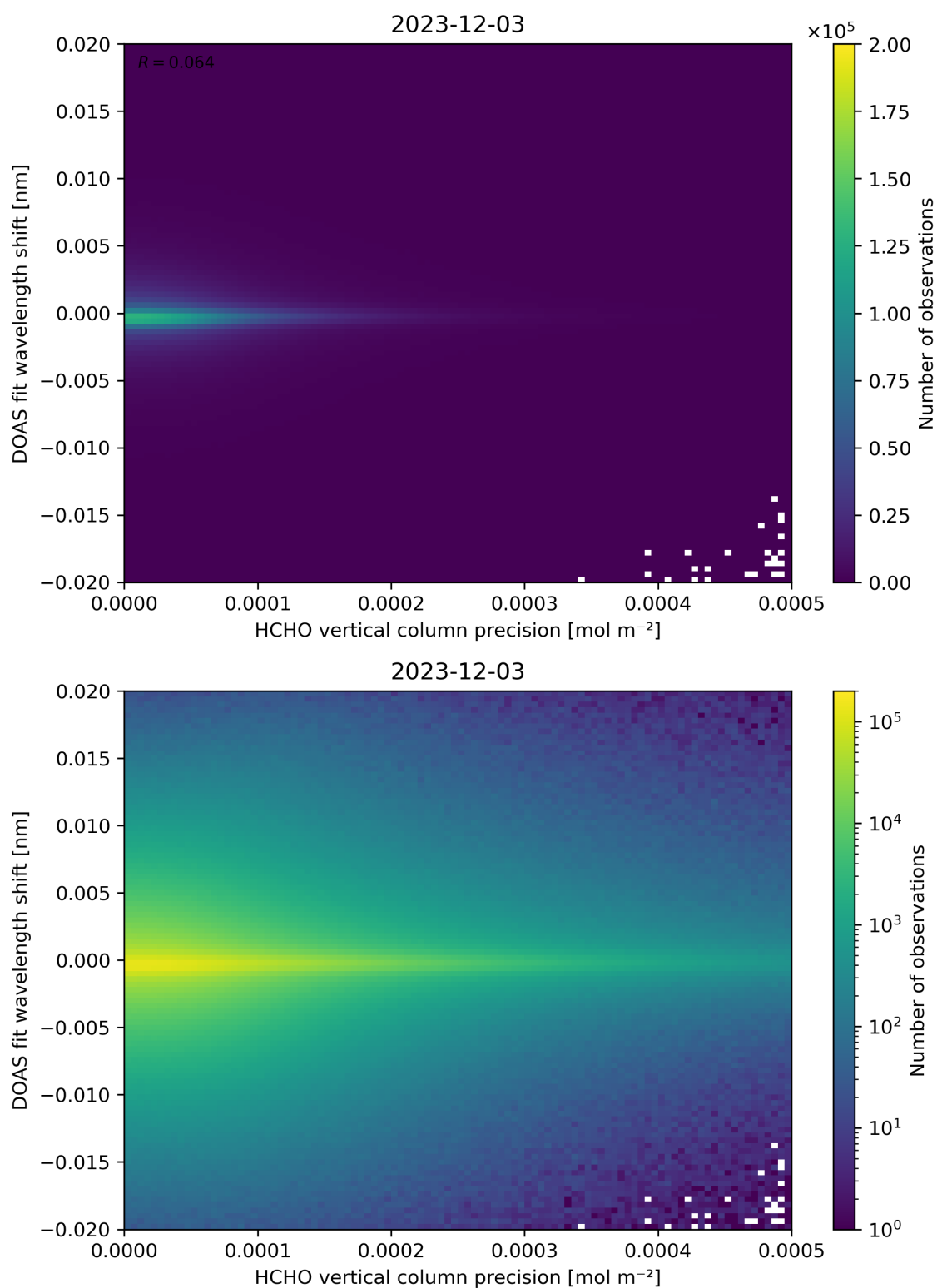
Figure 137: Scatter density plot of “HCHO vertical column precision” against “DOAS fit wavelength shift” for 2023-12-02 to 2023-12-04.
