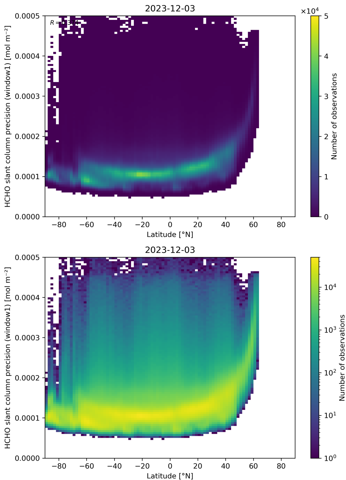
Figure 160: Scatter density plot of “Latitude” against “HCHO slant column precision (window1)” for 2023-12-02 to 2023-12-04.
