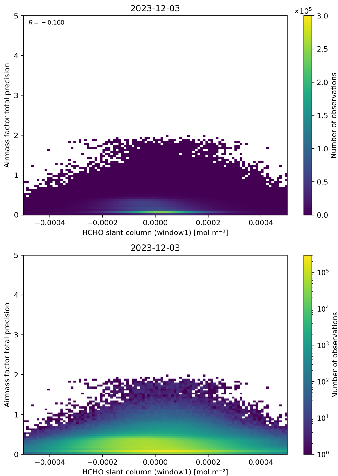
Figure 86: Scatter density plot of “HCHO slant column (window1)” against “Airmass factor total precision” for 2023-12-02 to 2023-12-04.
