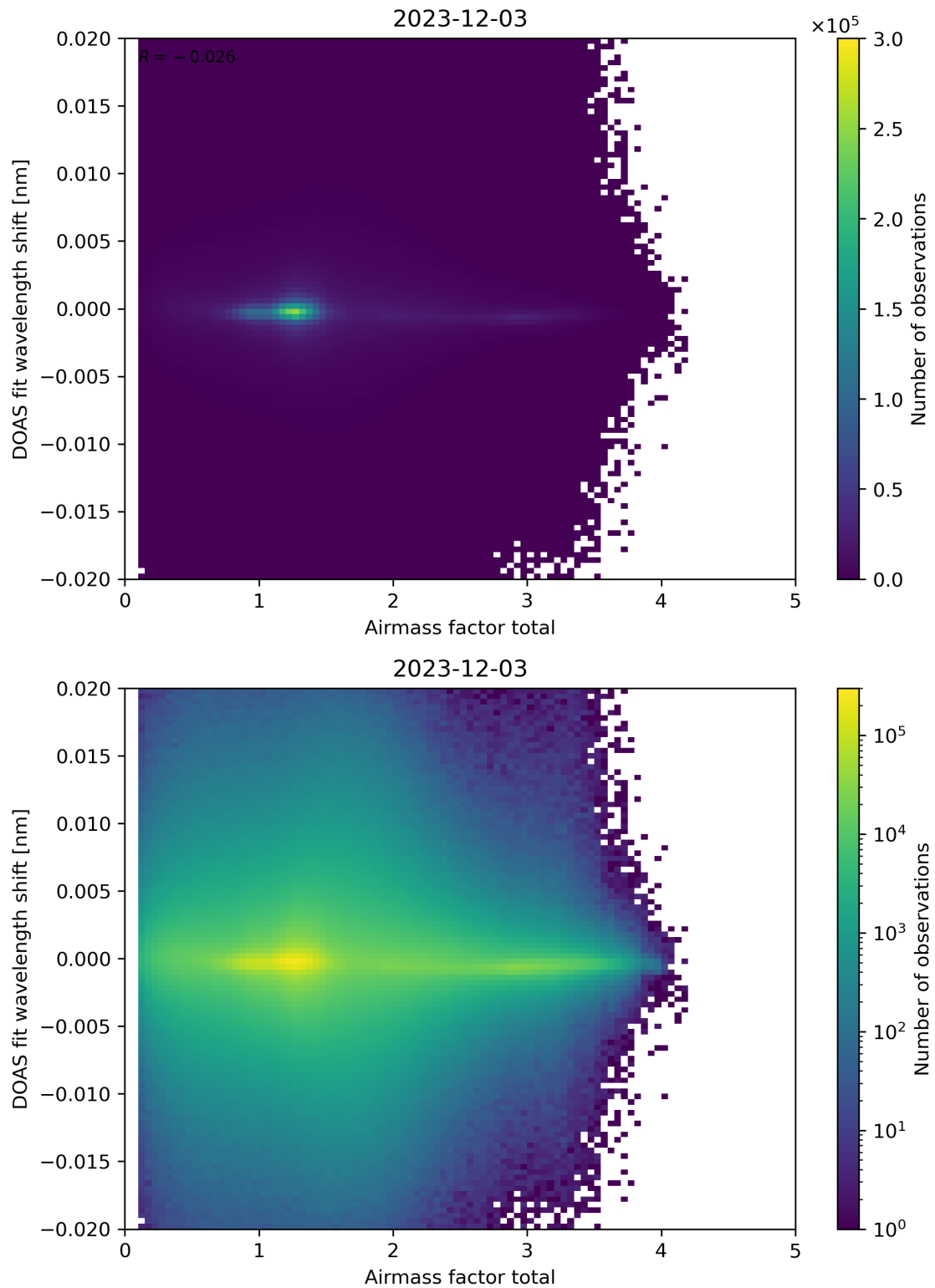
Figure 98: Scatter density plot of “Airmass factor total” against “DOAS fit wavelength shift” for 2023-12-02 to 2023-12-04.
