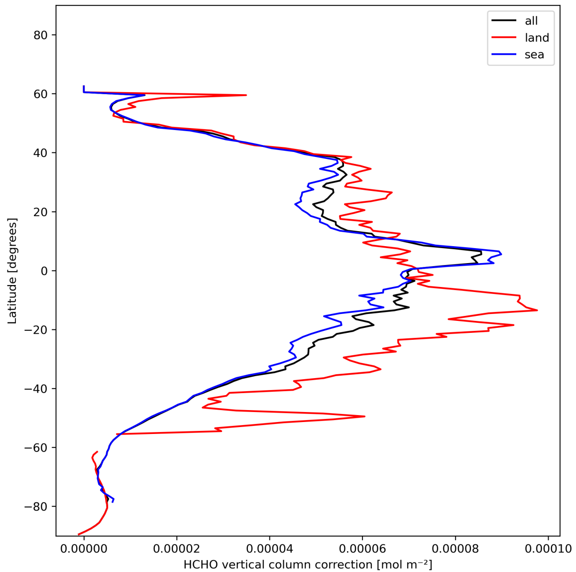
Figure 23: Zonal average of “HCHO vertical column correction” for 2023-12-02 to 2023-12-04.
