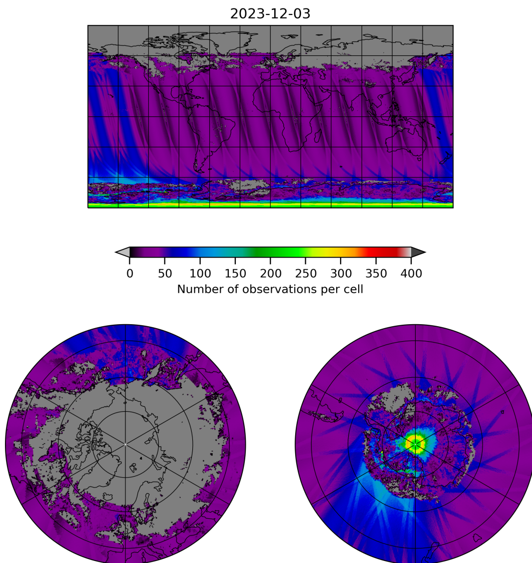
Figure 19: Map of the number of observations for 2023-12-02 to 2023-12-04
