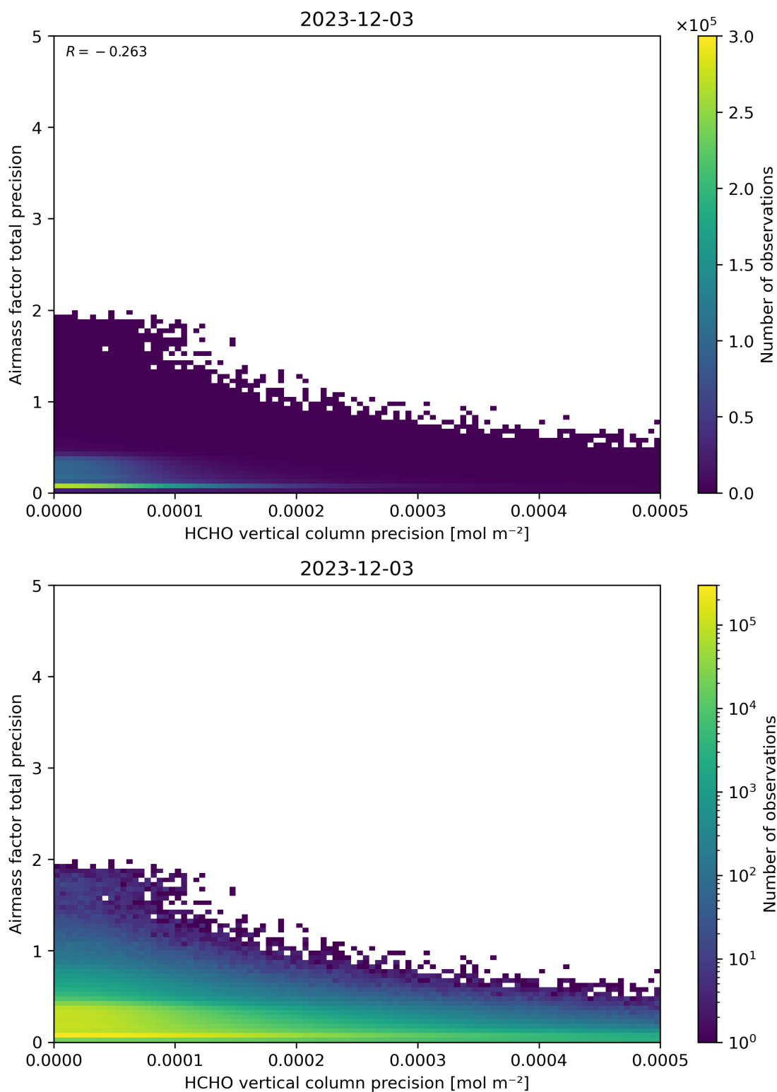
Figure 145: Scatter density plot of “HCHO vertical column precision” against “Airmass factor total precision” for 2023-12-02 to 2023-12-04.
