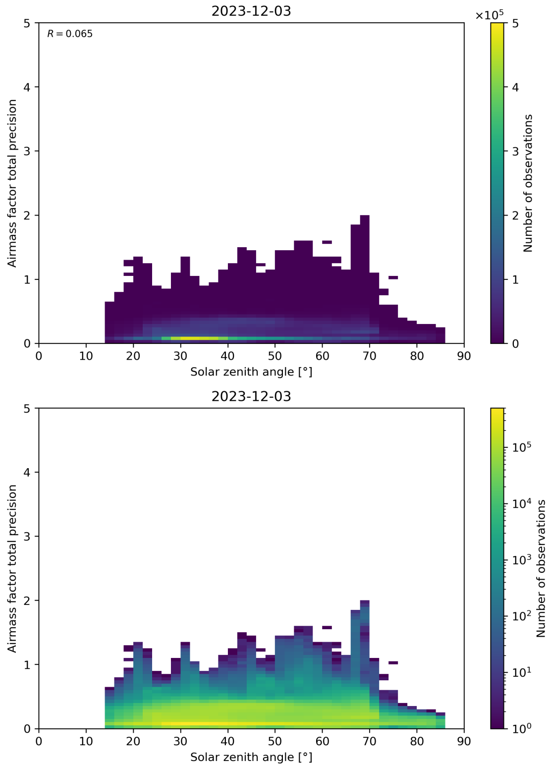
Figure 176: Scatter density plot of “Solar zenith angle” against “Airmass factor total precision” for 2023-12-02 to 2023-12-04.
