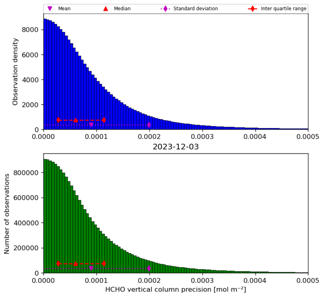
Figure 36: Histogram of “HCHO vertical column precision” for 2023-12-02 to 2023-12-04
