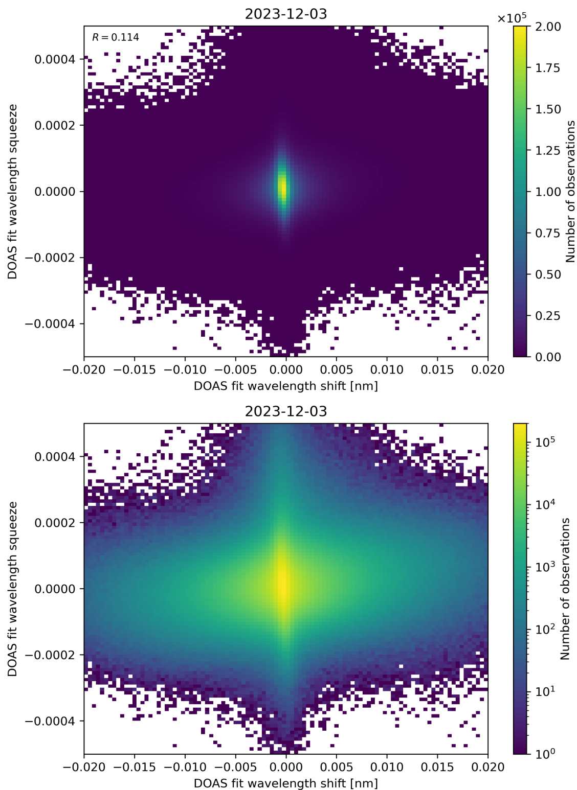
Figure 65: Scatter density plot of “DOAS fit wavelength shift” against “DOAS fit wavelength squeeze” for 2023-12-02 to 2023-12-04.
