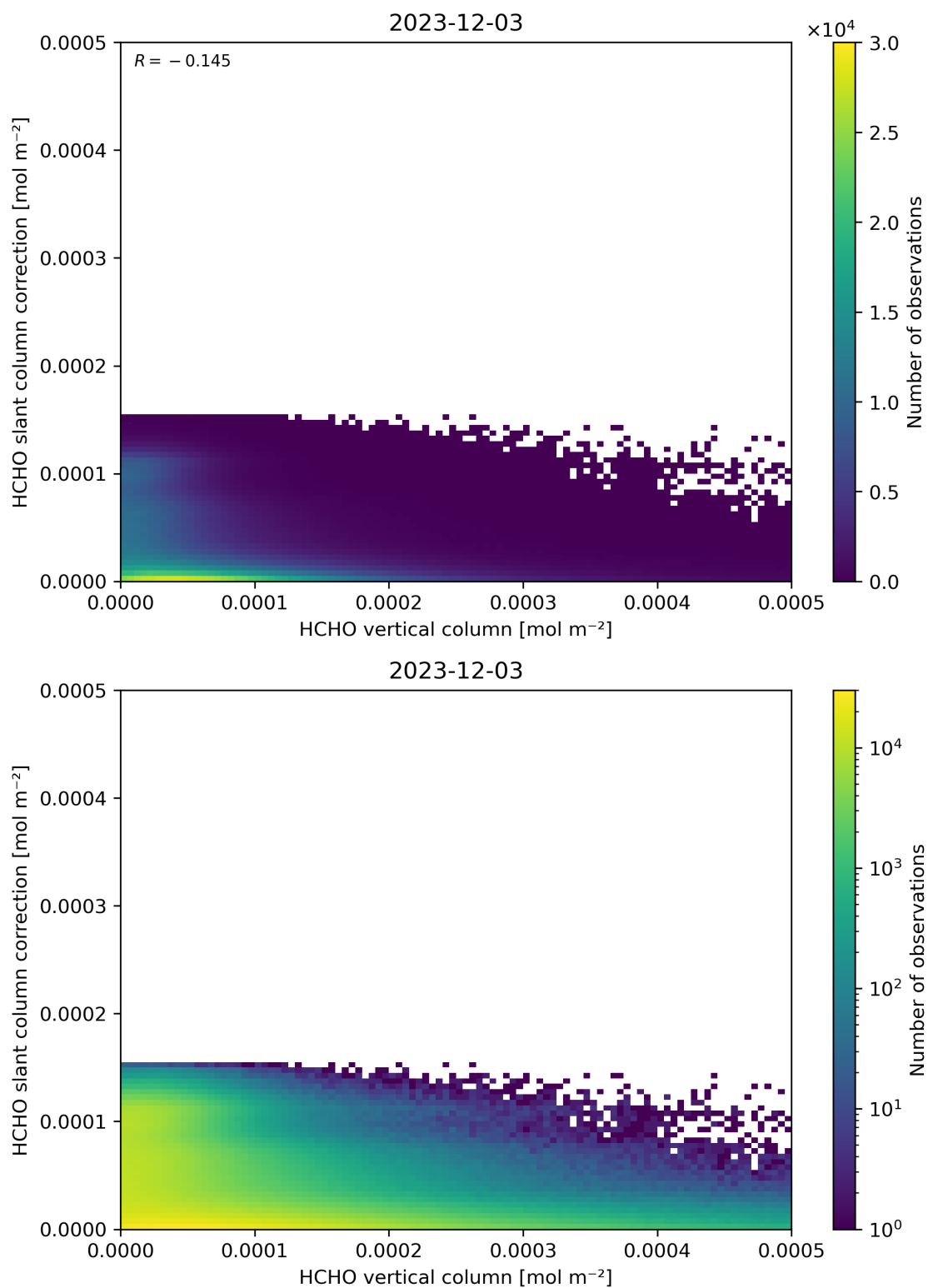
Figure 128: Scatter density plot of “HCHO vertical column” against “HCHO slant column correction” for 2023-12-02 to 2023-12-04.
