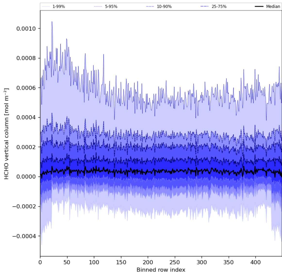
Figure 49: Along track statistics of “HCHO vertical column” for 2023-12-02 to 2023-12-04
