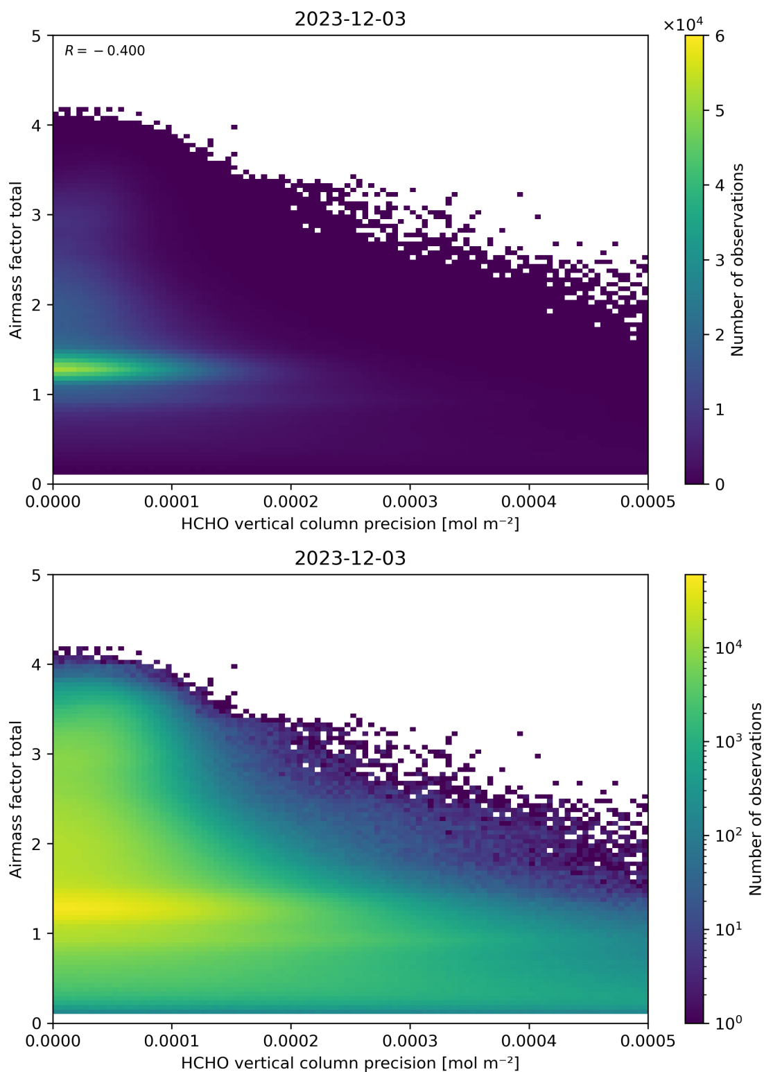
Figure 144: Scatter density plot of “HCHO vertical column precision” against “Airmass factor total” for 2023-12-02 to 2023-12-04.
