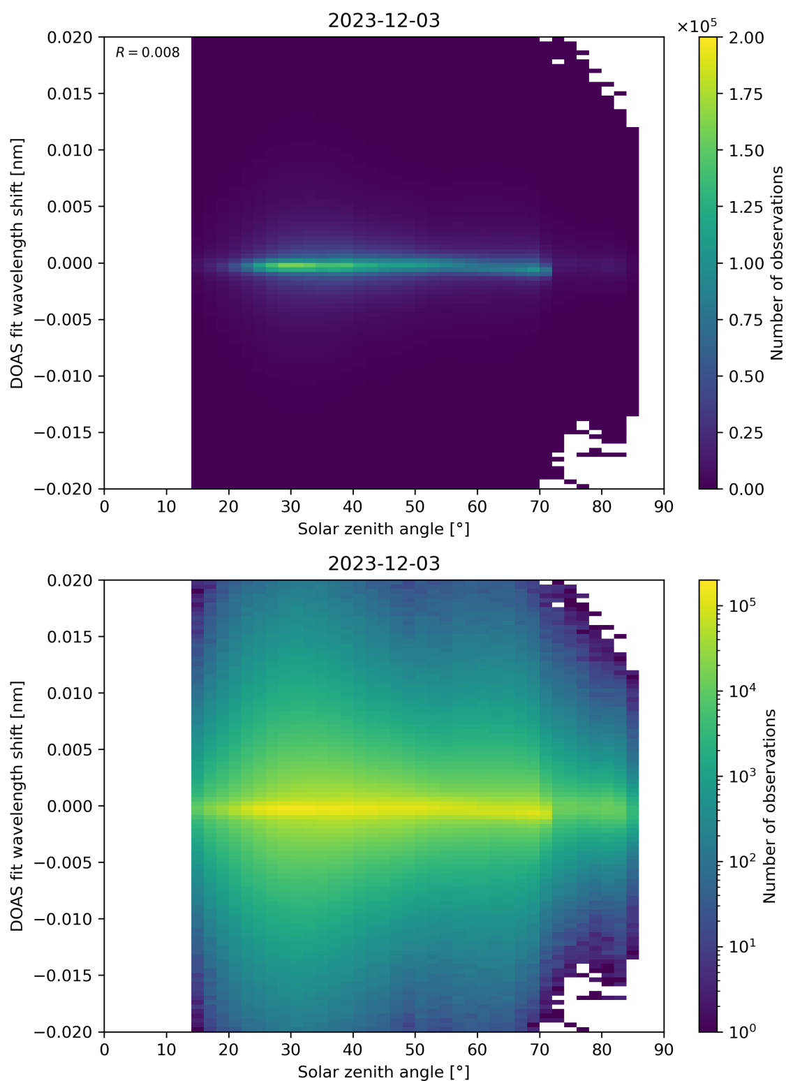
Figure 168: Scatter density plot of “Solar zenith angle” against “DOAS fit wavelength shift” for 2023-12-02 to 2023-12-04.
