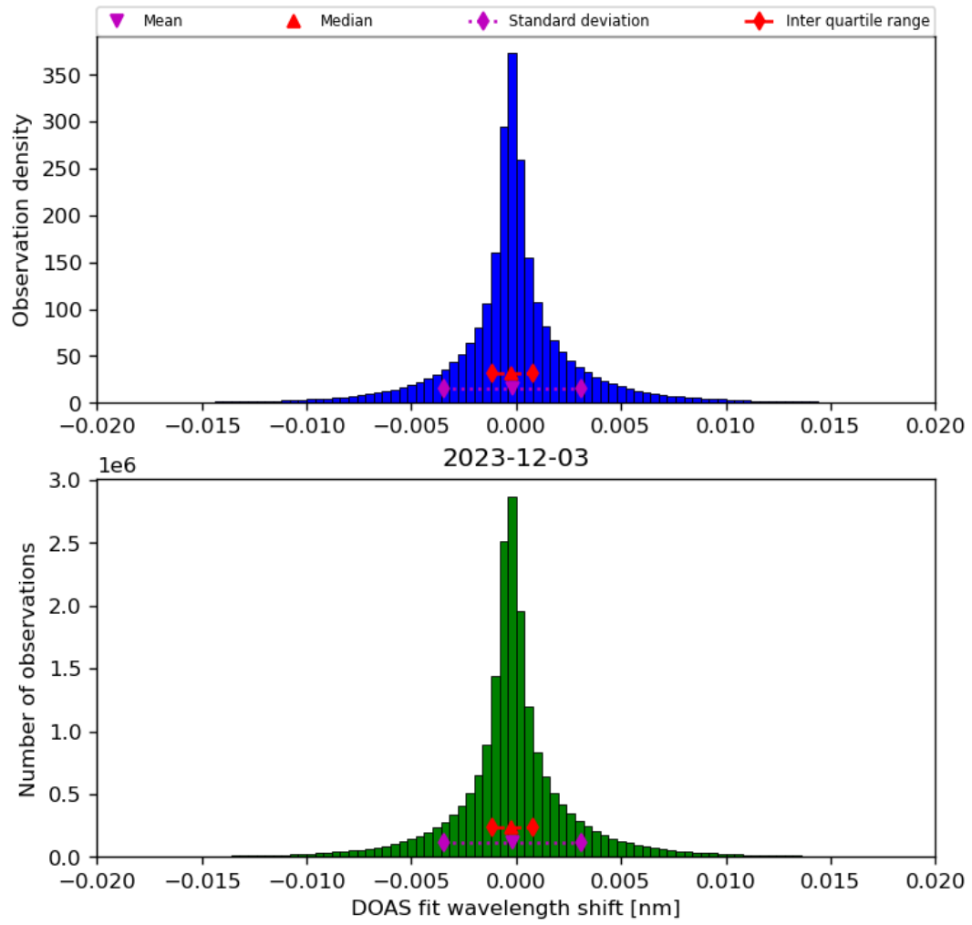
Figure 44: Histogram of “DOAS fit wavelength shift” for 2023-12-02 to 2023-12-04
