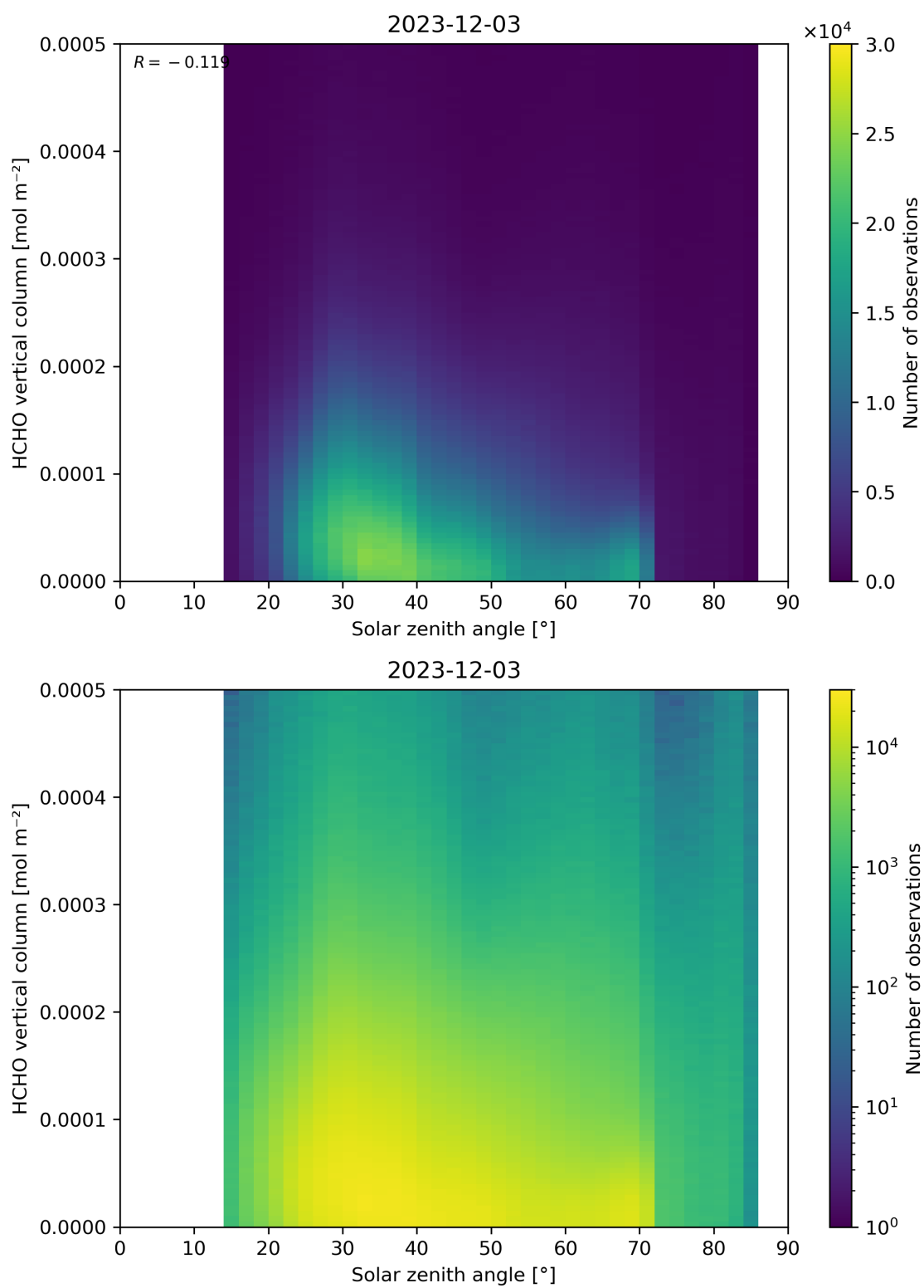
Figure 177: Scatter density plot of “Solar zenith angle” against “HCHO vertical column” for 2023-12-02 to 2023-12-04.
