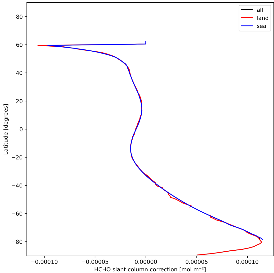
Figure 33: Zonal average of “HCHO slant column correction” for 2023-12-02 to 2023-12-04.
