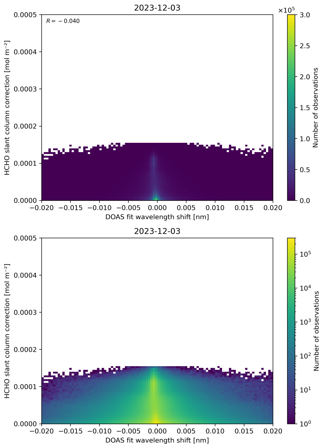
Figure 67: Scatter density plot of “DOAS fit wavelength shift” against “HCHO slant column correction” for 2023-12-02 to 2023-12-04.
