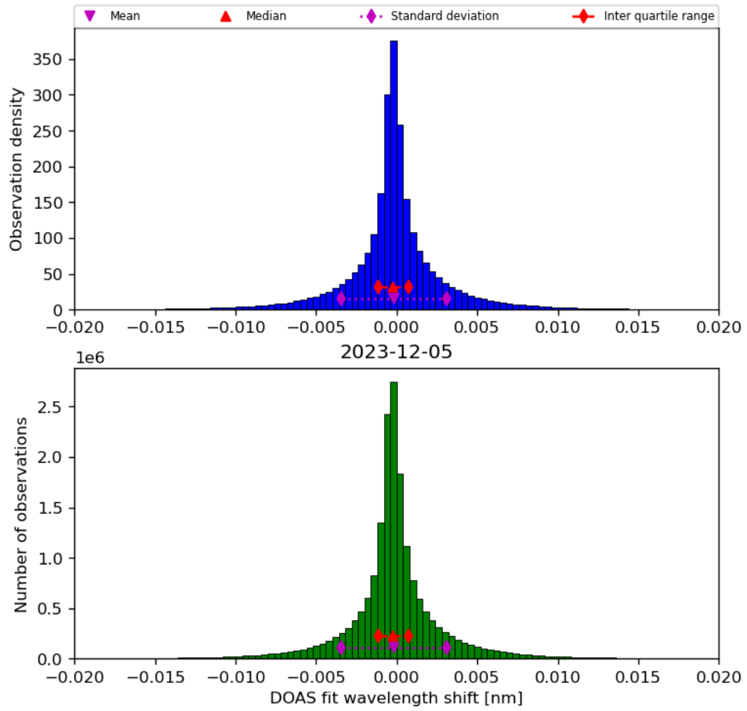
Figure 44: Histogram of “DOAS fit wavelength shift” for 2023-12-04 to 2023-12-06
