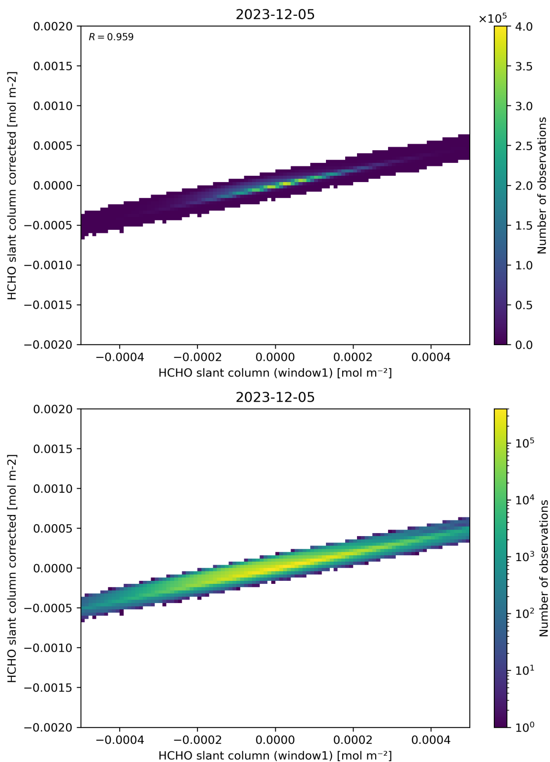
Figure 82: Scatter density plot of “HCHO slant column (window1)” against “HCHO slant column corrected” for 2023-12-04 to 2023-12-06.
