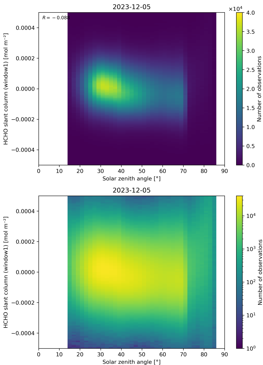
Figure 173: Scatter density plot of “Solar zenith angle” against “HCHO slant column (window1)” for 2023-12-04 to 2023-12-06.
