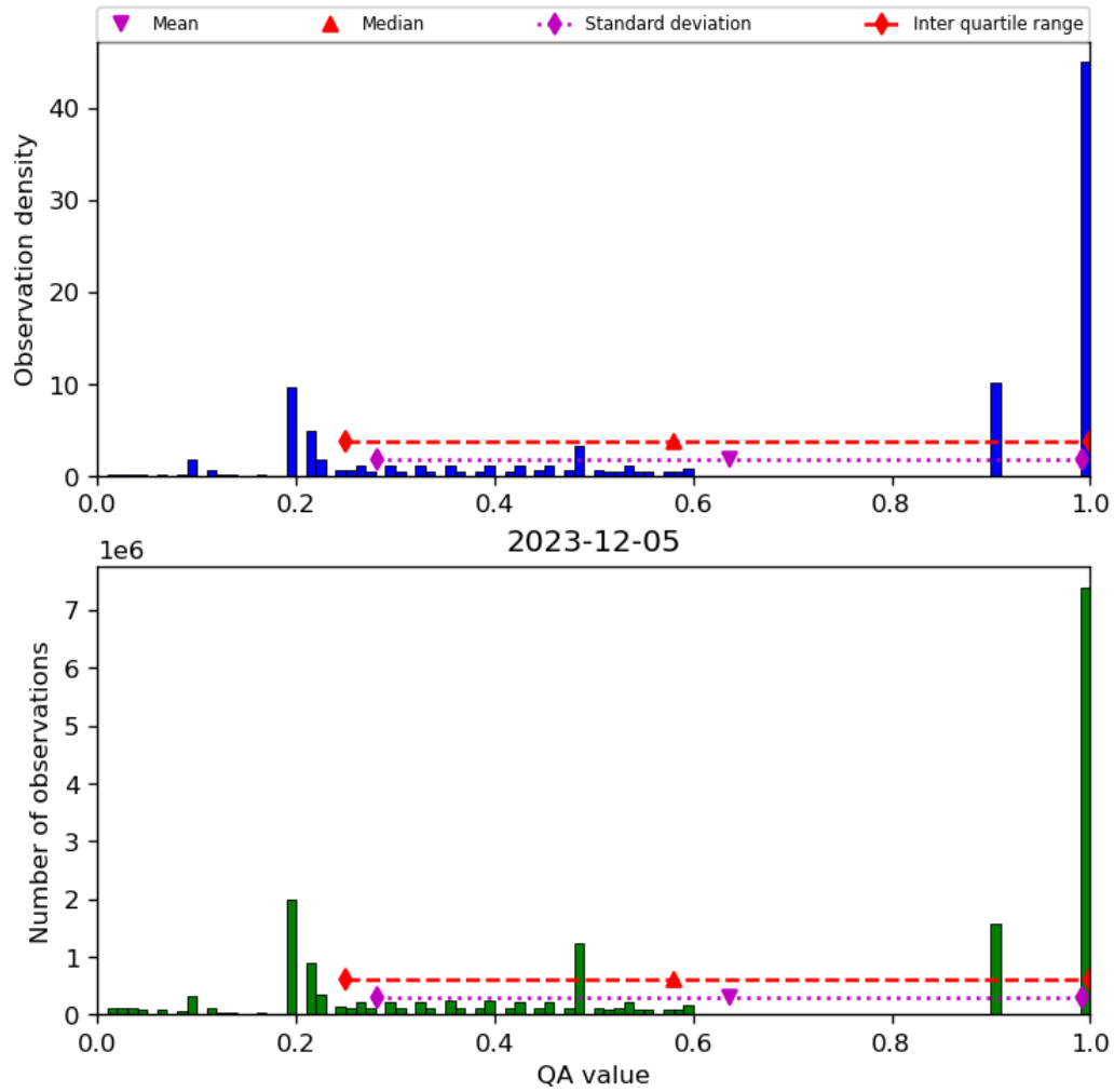
Figure 34: Histogram of “QA value” for 2023-12-04 to 2023-12-06
