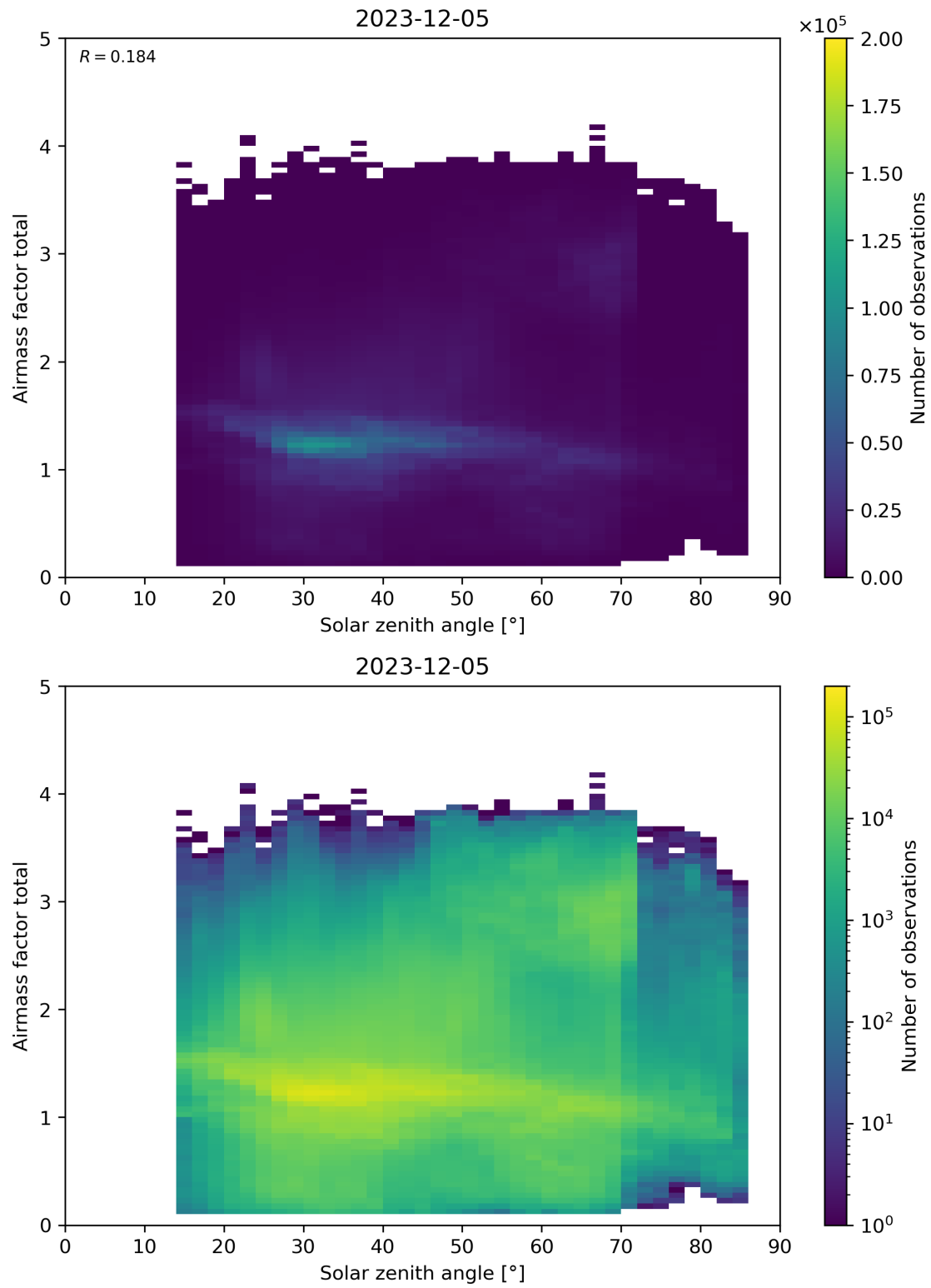
Figure 175: Scatter density plot of “Solar zenith angle” against “Airmass factor total” for 2023-12-04 to 2023-12-06.
