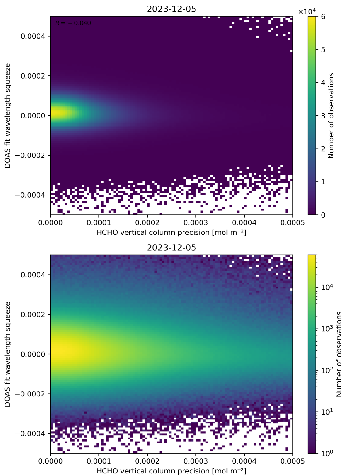
Figure 138: Scatter density plot of “HCHO vertical column precision” against “DOAS fit wavelength squeeze” for 2023-12-04 to 2023-12-06.
