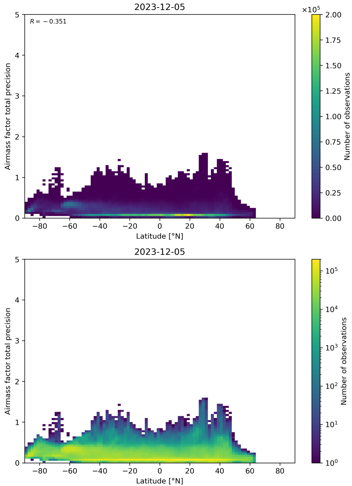
Figure 162: Scatter density plot of “Latitude” against “Airmass factor total precision” for 2023-12-04 to 2023-12-06.
