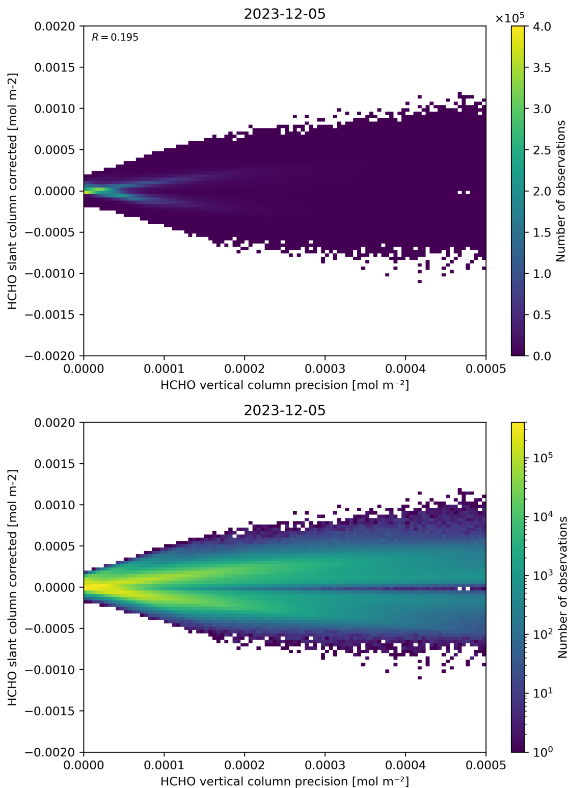
Figure 140: Scatter density plot of “HCHO vertical column precision” against “HCHO slant column corrected” for 2023-12-04 to 2023-12-06.
