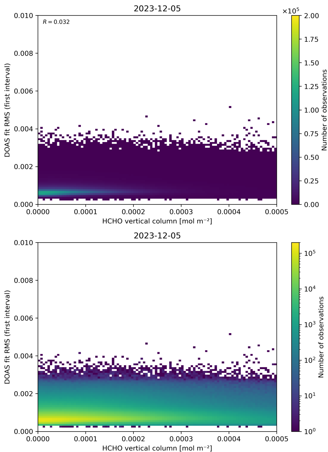
Figure 123: Scatter density plot of “HCHO vertical column” against “DOAS fit RMS (first interval)” for 2023-12-04 to 2023-12-06.
