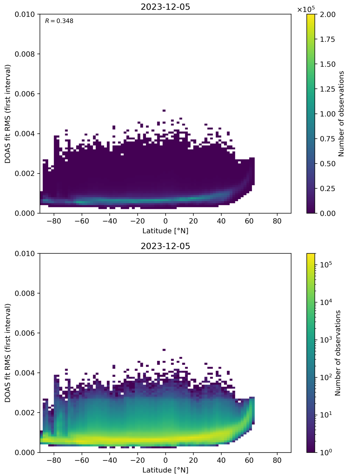
Figure 153: Scatter density plot of “Latitude” against “DOAS fit RMS (first interval)” for 2023-12-04 to 2023-12-06.
