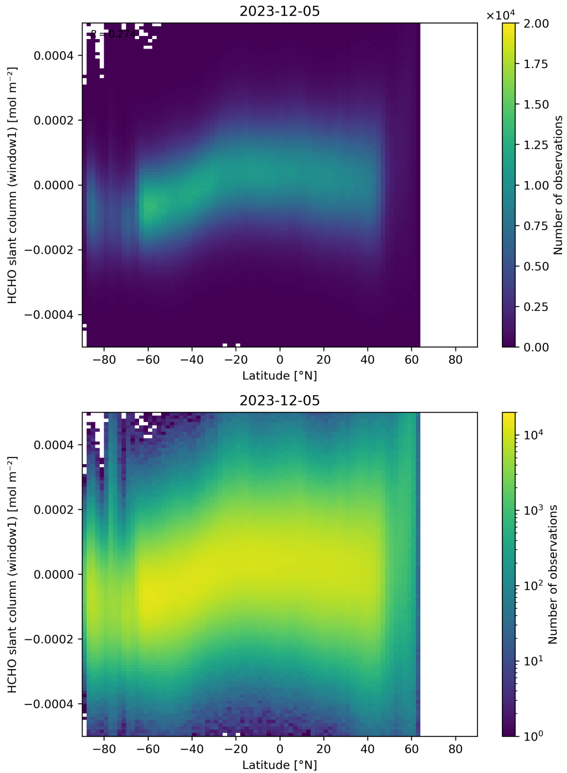
Figure 159: Scatter density plot of “Latitude” against “HCHO slant column (window1)” for 2023-12-04 to 2023-12-06.
