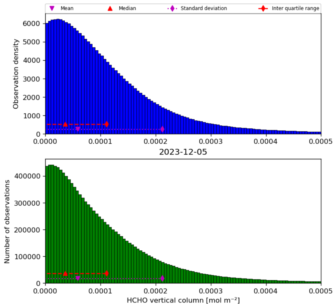
Figure 35: Histogram of “HCHO vertical column” for 2023-12-04 to 2023-12-06
