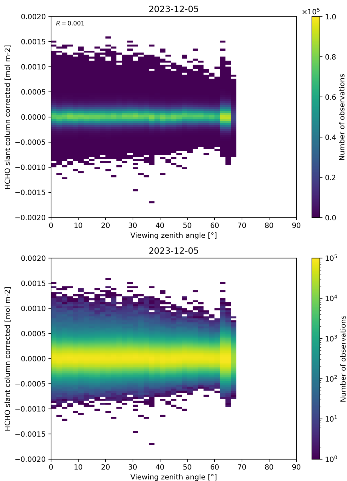
Figure 186: Scatter density plot of “Viewing zenith angle” against “HCHO slant column corrected” for 2023-12-04 to 2023-12-06.
