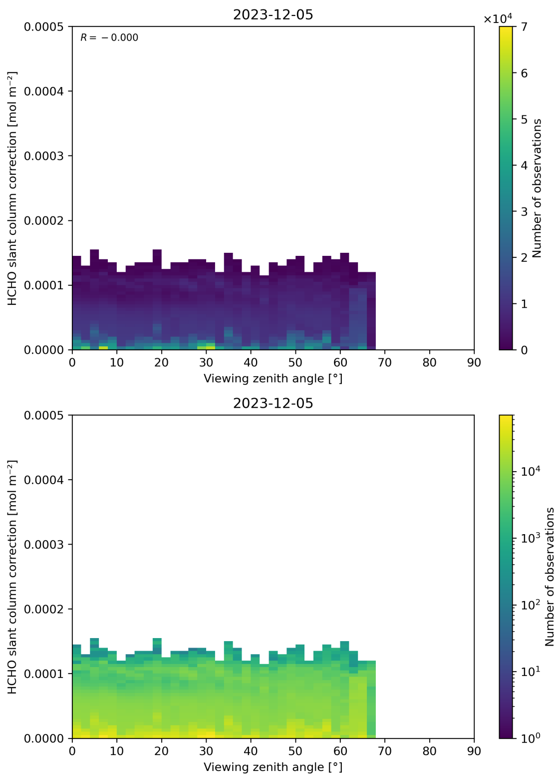
Figure 187: Scatter density plot of “Viewing zenith angle” against “HCHO slant column correction” for 2023-12-04 to 2023-12-06.
