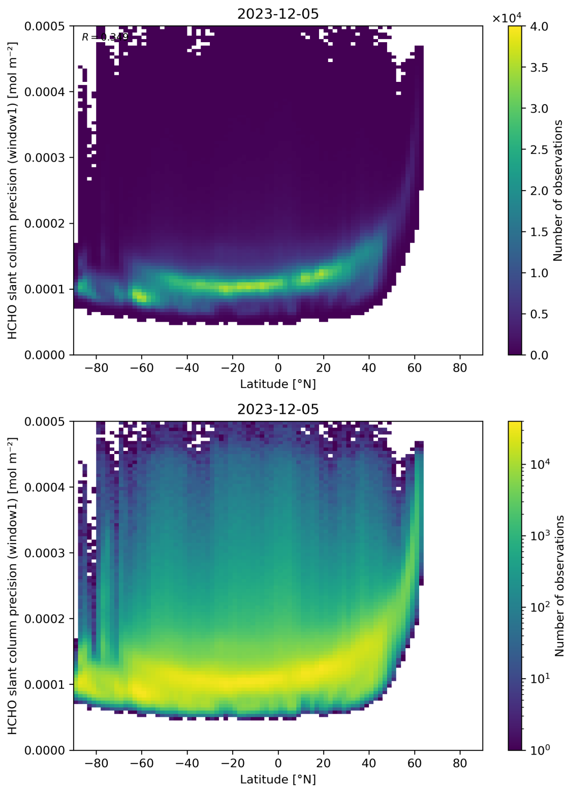
Figure 160: Scatter density plot of “Latitude” against “HCHO slant column precision (window1)” for 2023-12-04 to 2023-12-06.
