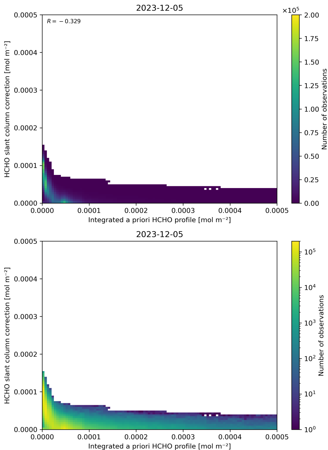
Figure 152: Scatter density plot of “Integrated a priori HCHO profile” against “HCHO slant column correction” for 2023-12-04 to 2023-12-06.
