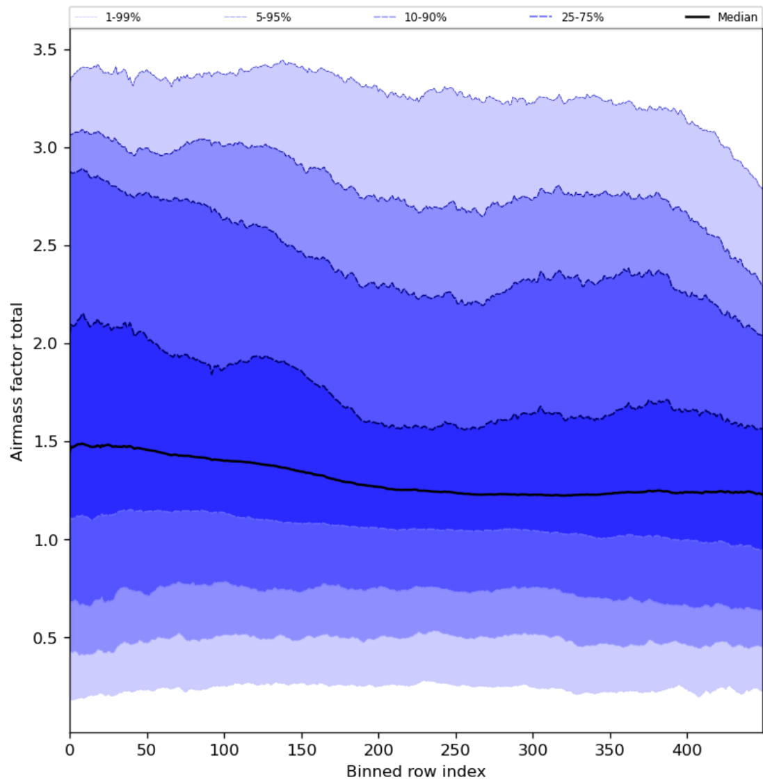
Figure 54: Along track statistics of “Airmass factor total” for 2023-12-04 to 2023-12-06
