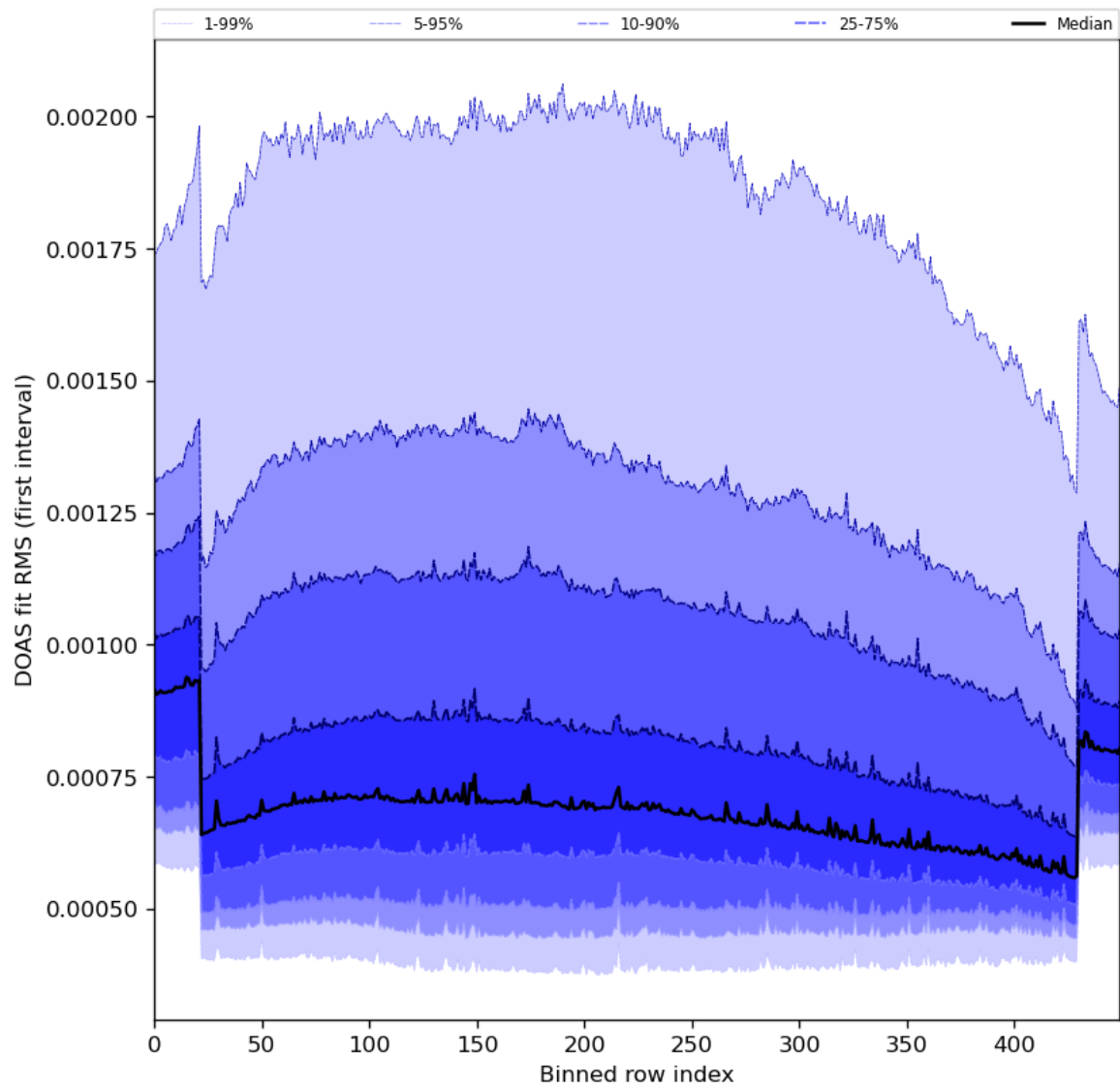
Figure 60: Along track statistics of “DOAS fit RMS (first interval)” for 2023-12-04 to 2023-12-06
