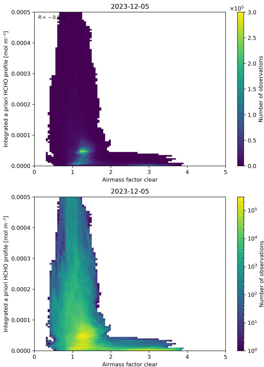
Figure 76: Scatter density plot of “Airmass factor clear” against “Integrated a priori HCHO profile” for 2023-12-04 to 2023-12-06.
