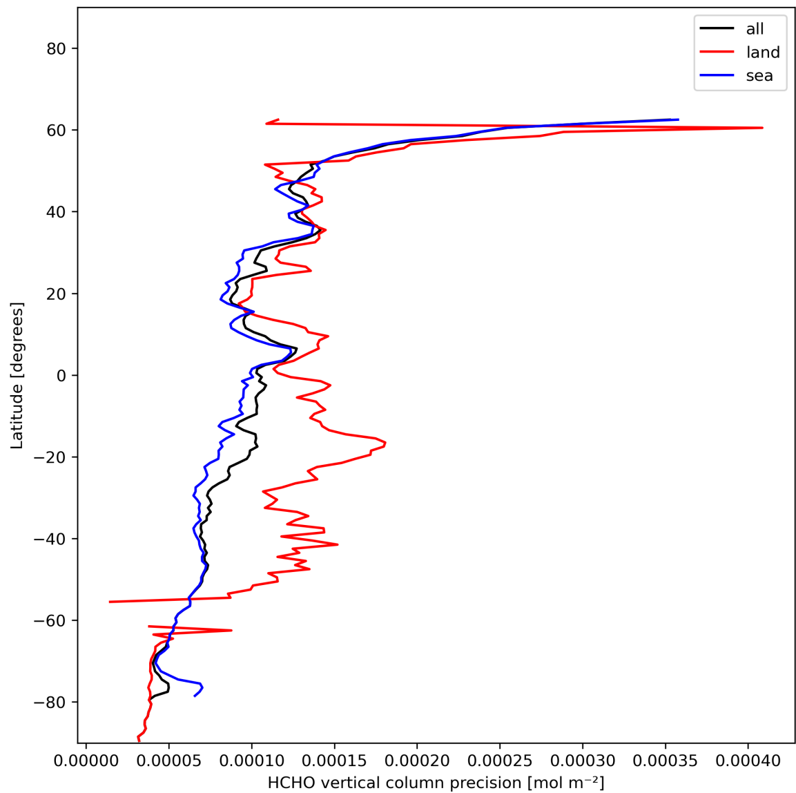
Figure 22: Zonal average of “HCHO vertical column precision” for 2023-12-04 to 2023-12-06.
