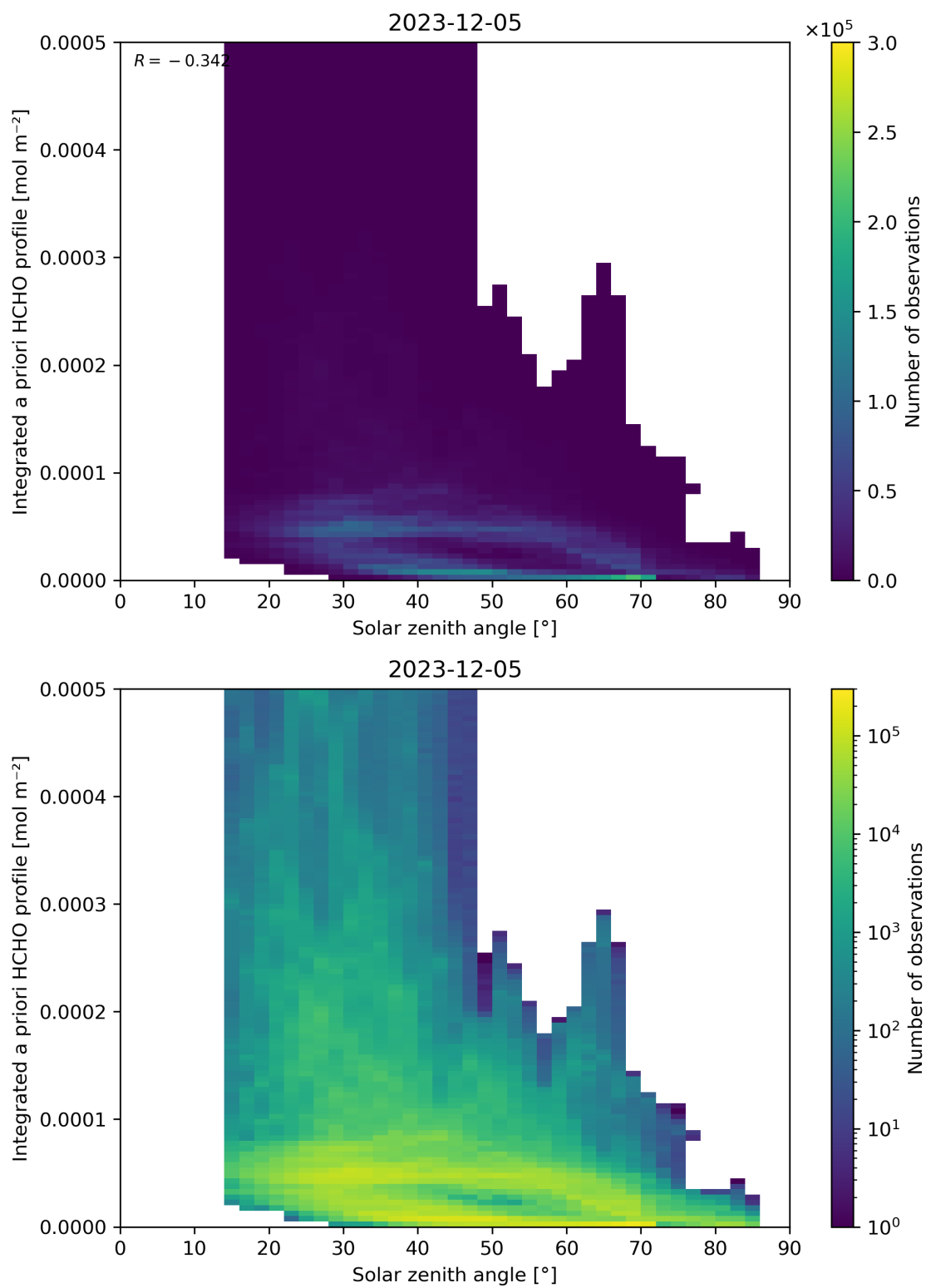
Figure 180: Scatter density plot of “Solar zenith angle” against “Integrated a priori HCHO profile” for 2023-12-04 to 2023-12-06.
