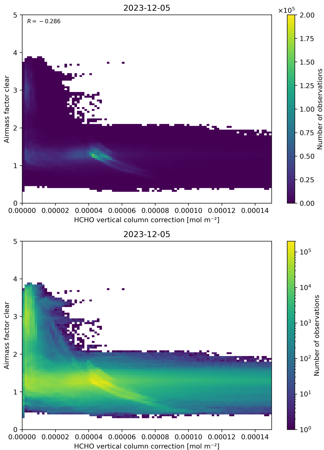
Figure 115: Scatter density plot of “HCHO vertical column correction” against “Airmass factor clear” for 2023-12-04 to 2023-12-06.
