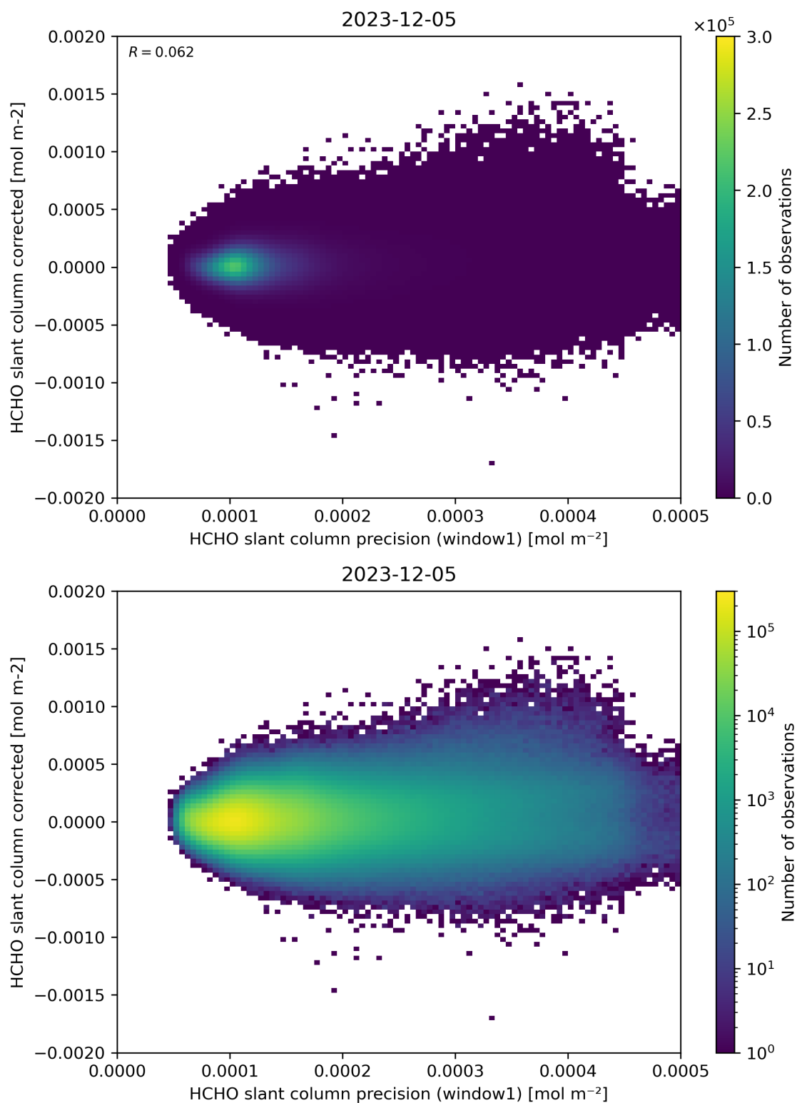
Figure 92: Scatter density plot of “HCHO slant column precision (window1)” against “HCHO slant column corrected” for 2023-12-04 to 2023-12-06.
