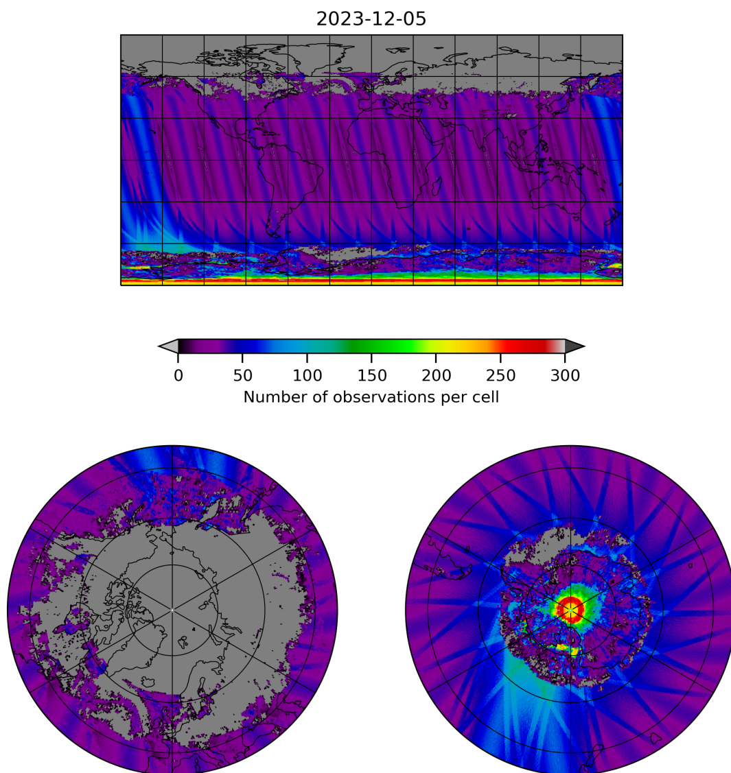
Figure 19: Map of the number of observations for 2023-12-04 to 2023-12-06
