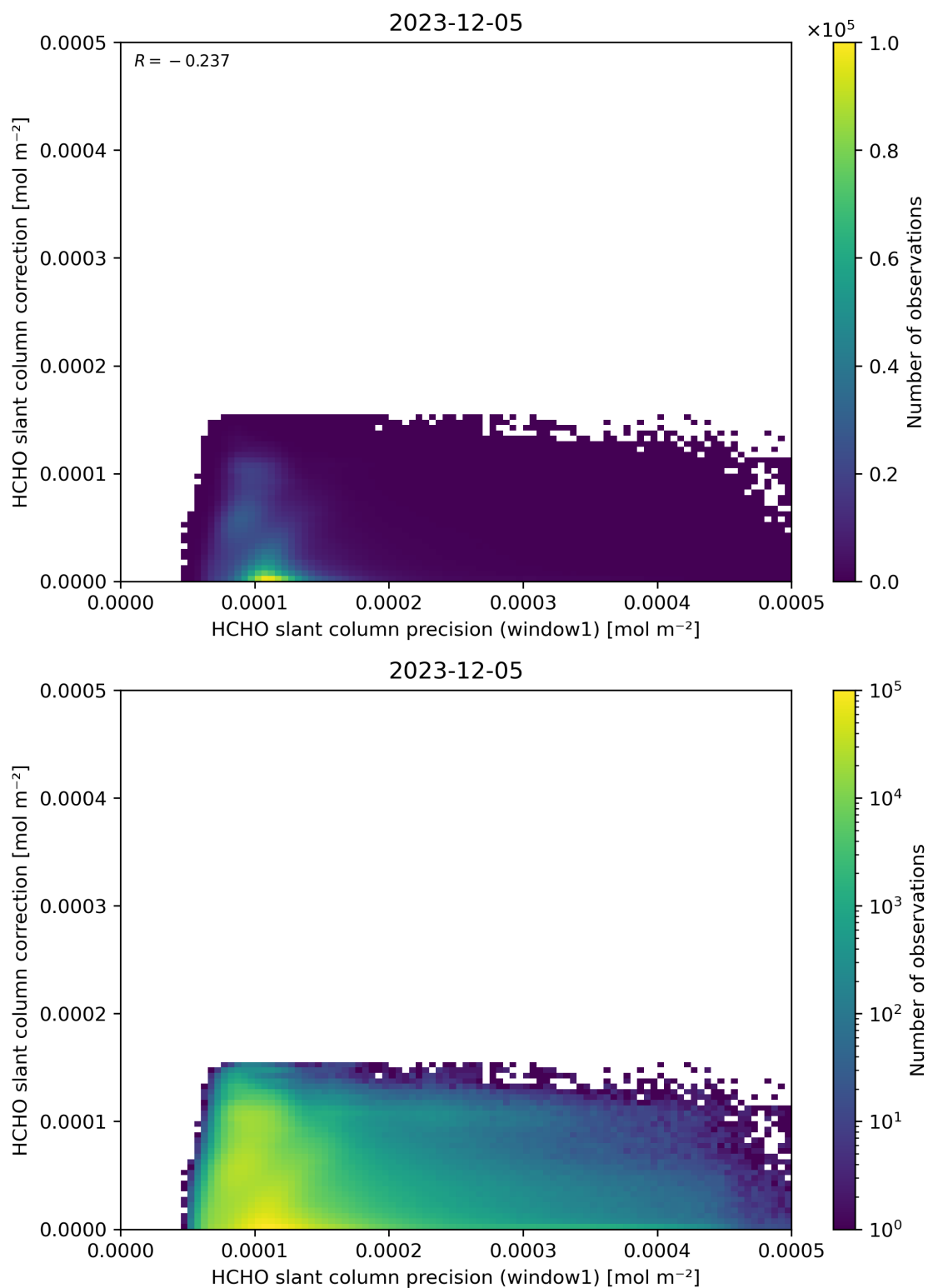
Figure 93: Scatter density plot of “HCHO slant column precision (window1)” against “HCHO slant column correction” for 2023-12-04 to 2023-12-06.
