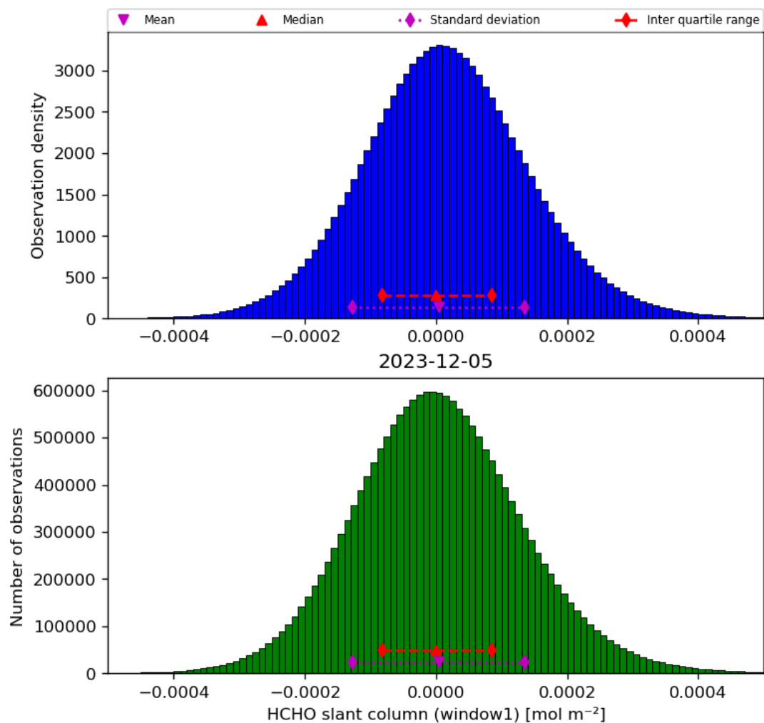
Figure 38: Histogram of “HCHO slant column (window1)” for 2023-12-04 to 2023-12-06
