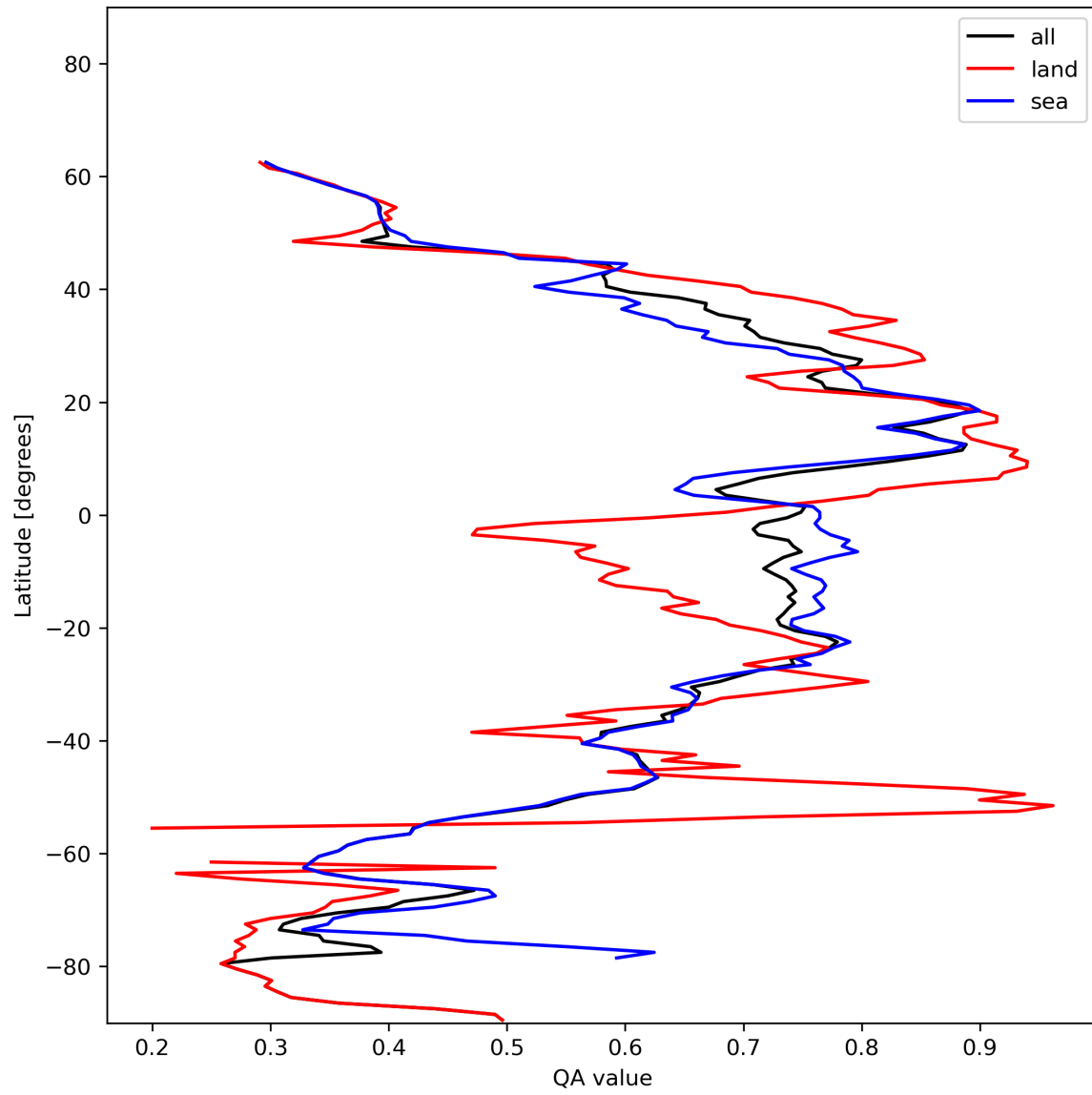
Figure 20: Zonal average of “QA value” for 2023-12-04 to 2023-12-06.
