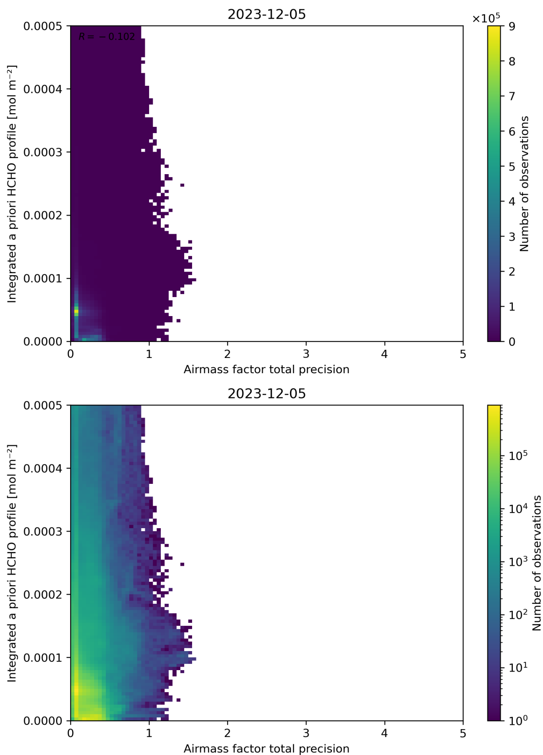
Figure 111: Scatter density plot of “Airmass factor total precision” against “Integrated a priori HCHO profile” for 2023-12-04 to 2023-12-06.
