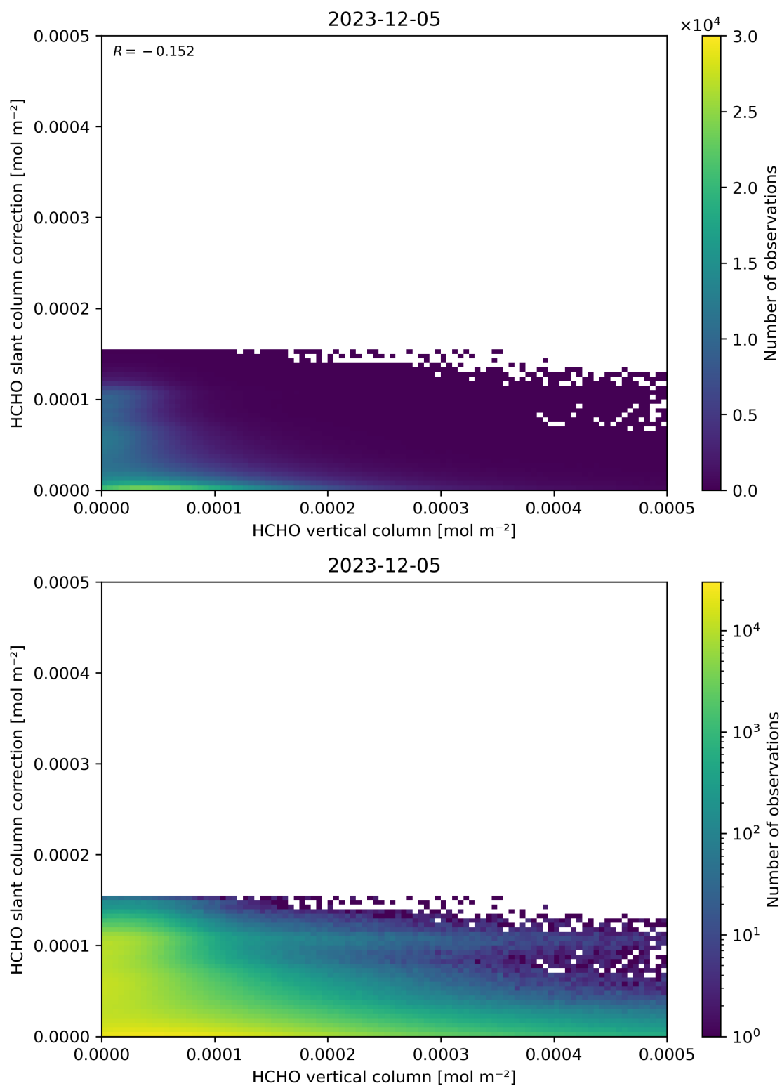
Figure 128: Scatter density plot of “HCHO vertical column” against “HCHO slant column correction” for 2023-12-04 to 2023-12-06.
