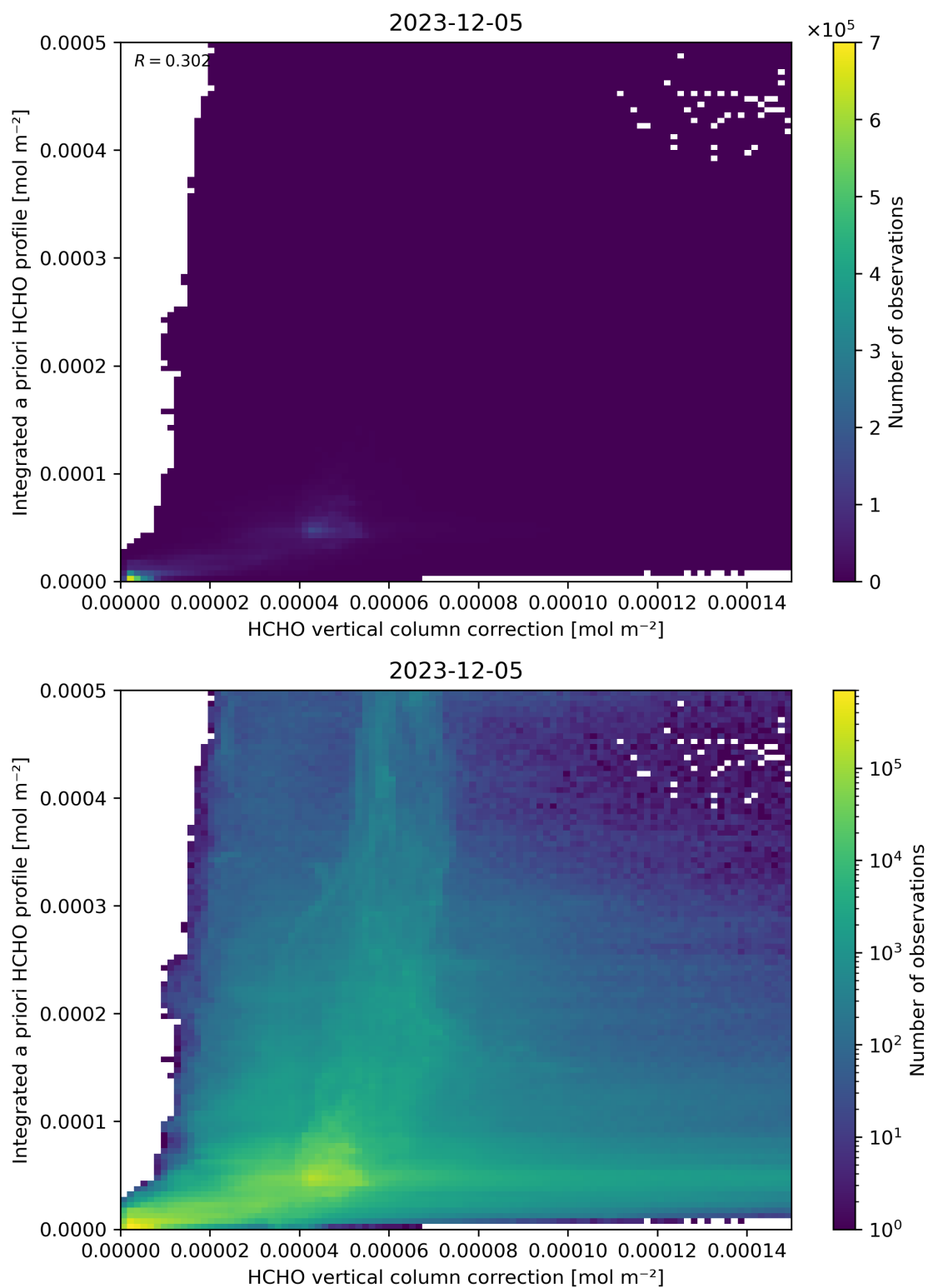
Figure 122: Scatter density plot of “HCHO vertical column correction” against “Integrated a priori HCHO profile” for 2023-12-04 to 2023-12-06.
