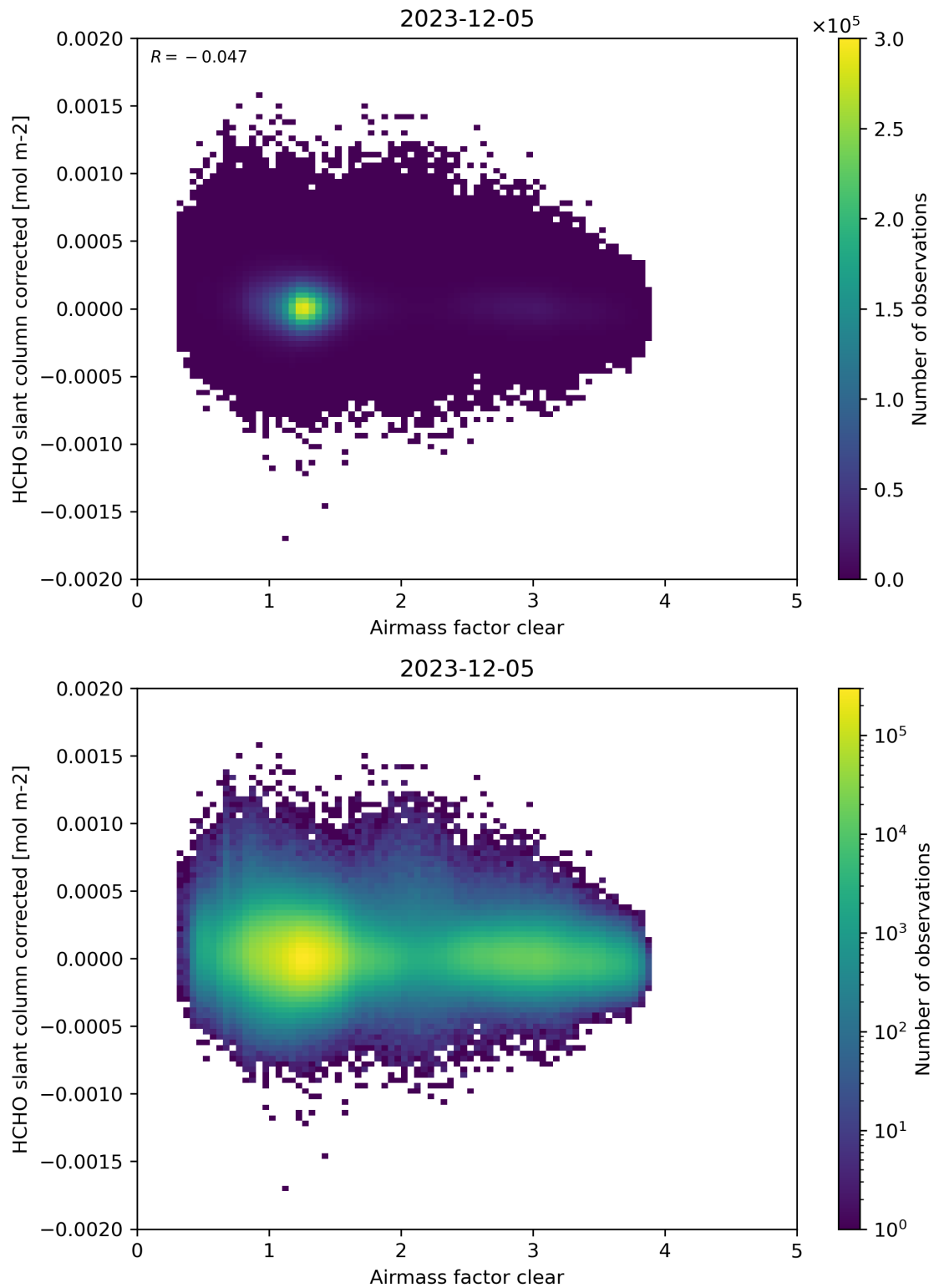
Figure 74: Scatter density plot of “Airmass factor clear” against “HCHO slant column corrected” for 2023-12-04 to 2023-12-06.
