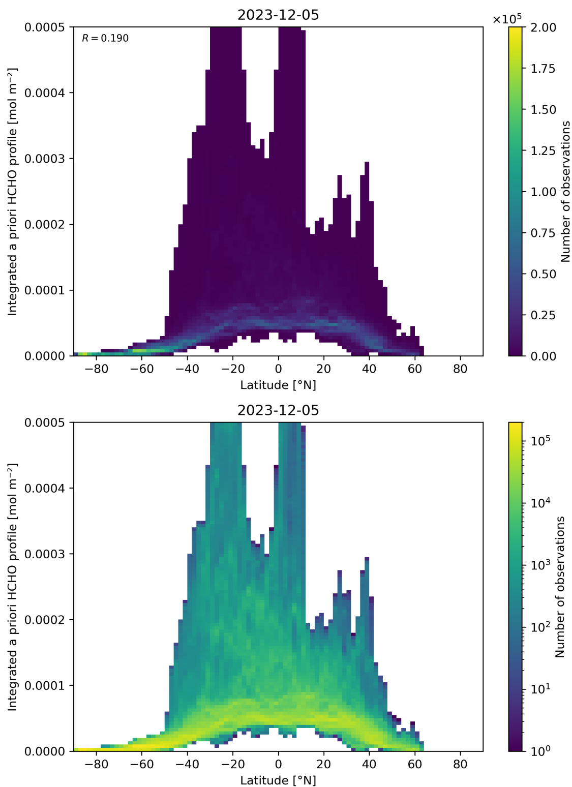
Figure 166: Scatter density plot of “Latitude” against “Integrated a priori HCHO profile” for 2023-12-04 to 2023-12-06.
