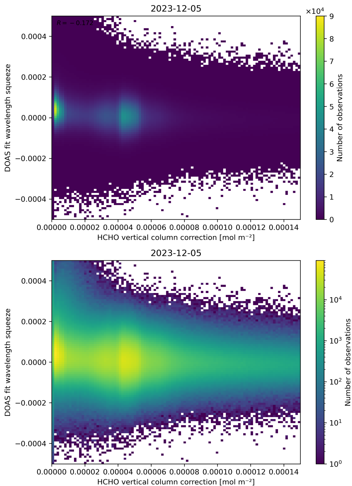
Figure 114: Scatter density plot of “HCHO vertical column correction” against “DOAS fit wavelength squeeze” for 2023-12-04 to 2023-12-06.
