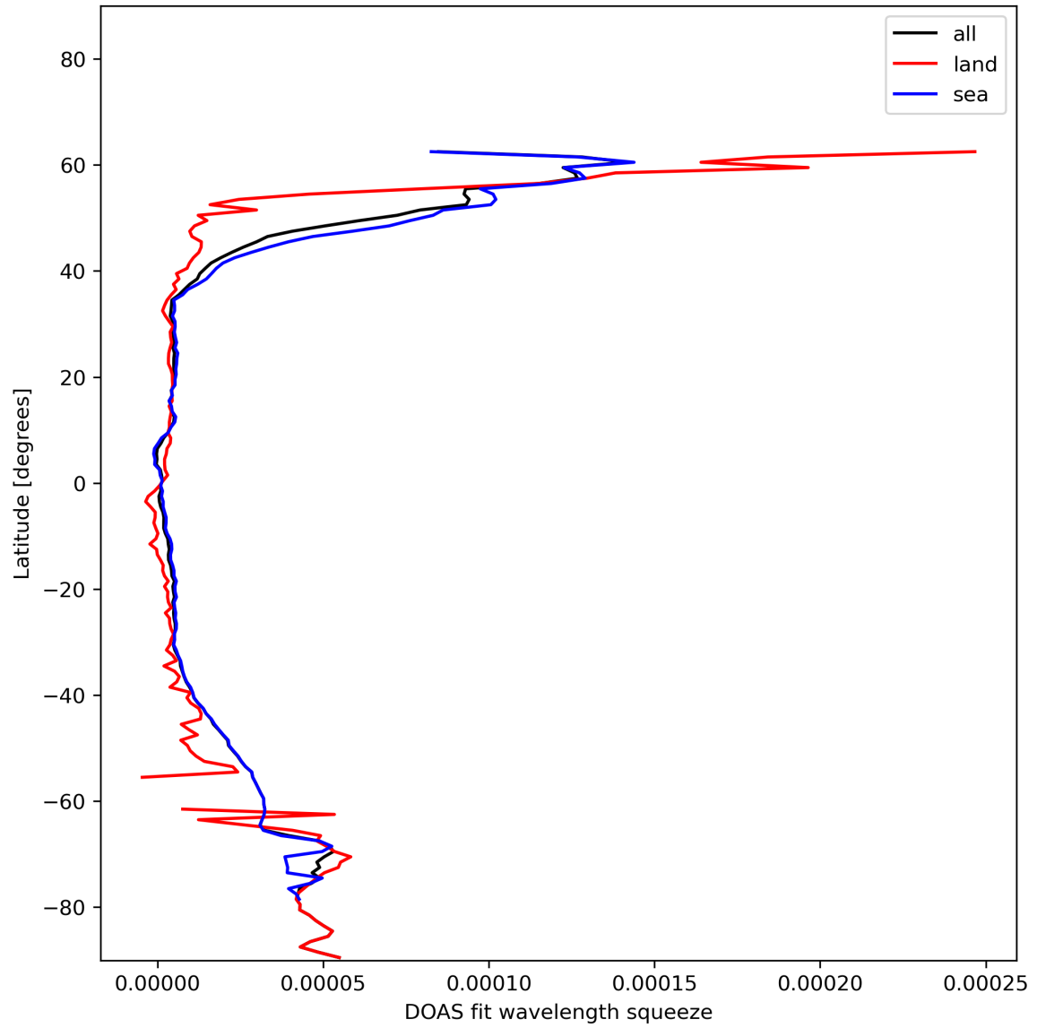
Figure 31: Zonal average of “DOAS fit wavelength squeeze” for 2023-12-04 to 2023-12-06.
