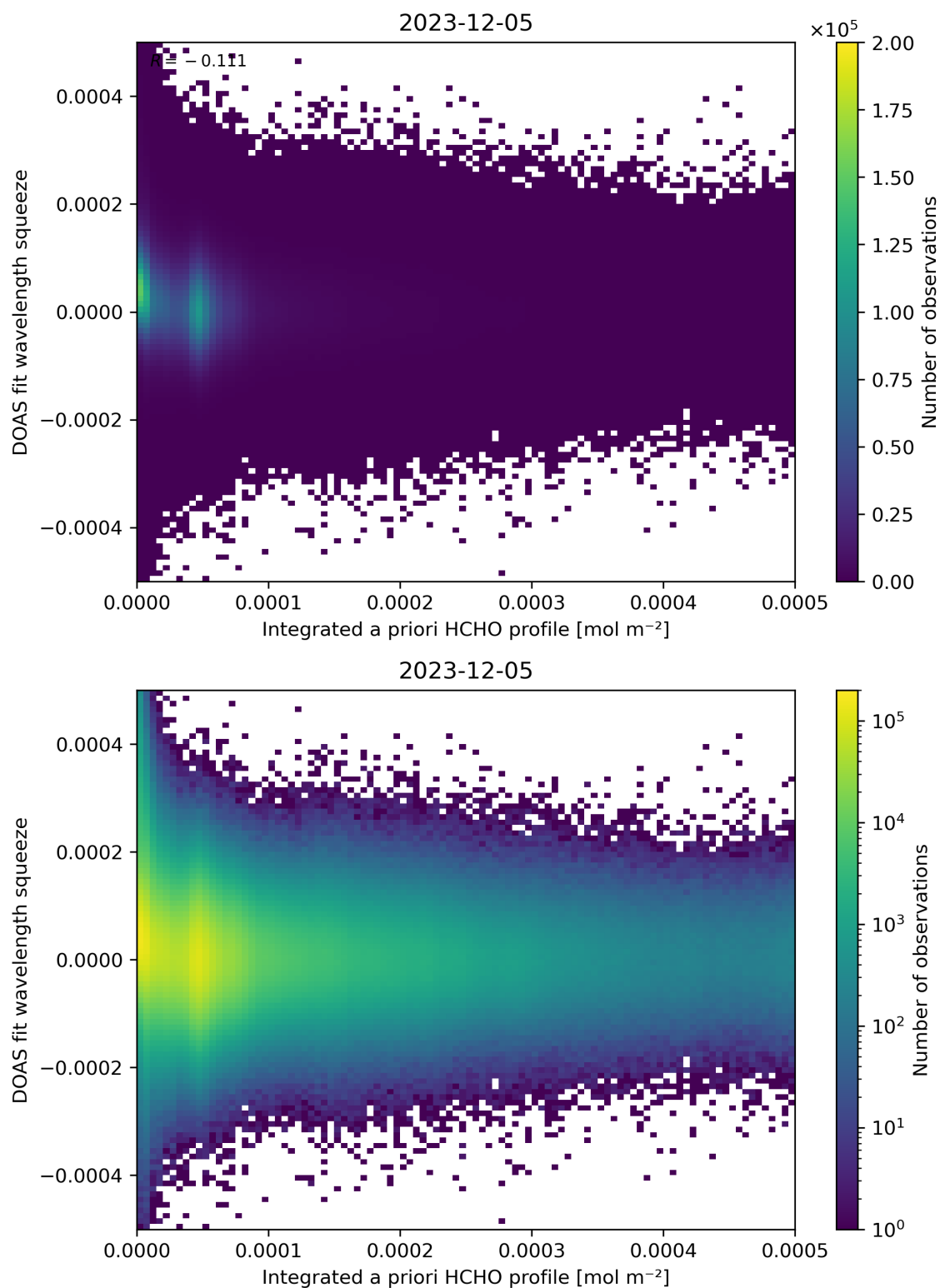
Figure 150: Scatter density plot of “Integrated a priori HCHO profile” against “DOAS fit wavelength squeeze” for 2023-12-04 to 2023-12-06.
