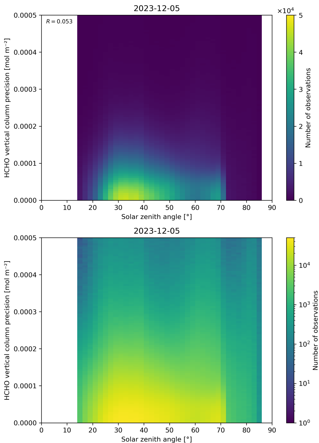
Figure 179: Scatter density plot of “Solar zenith angle” against “HCHO vertical column precision” for 2023-12-04 to 2023-12-06.
