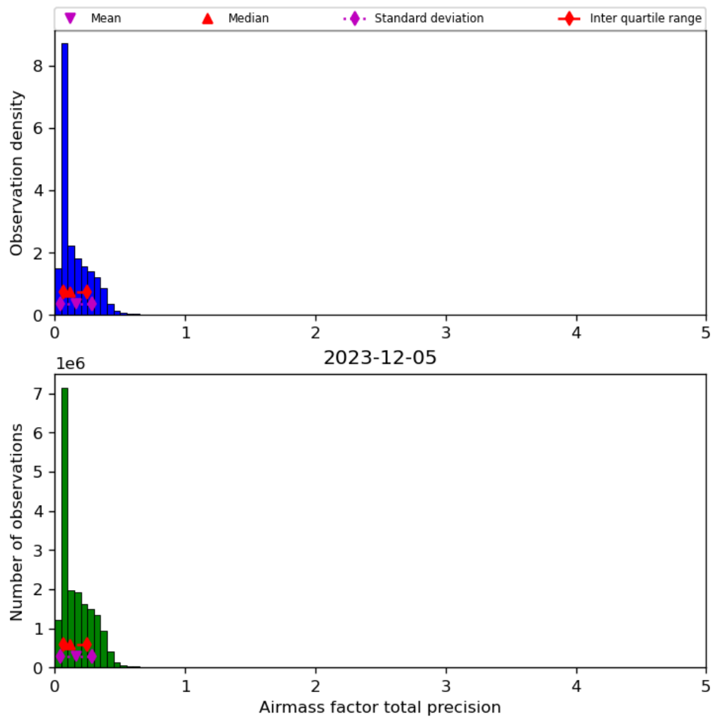
Figure 41: Histogram of “Airmass factor total precision” for 2023-12-04 to 2023-12-06
