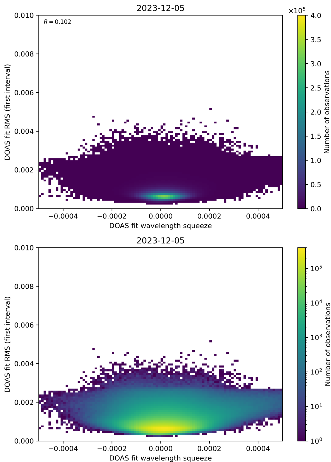
Figure 68: Scatter density plot of “DOAS fit wavelength squeeze” against “DOAS fit RMS (first interval)” for 2023-12-04 to 2023-12-06.
