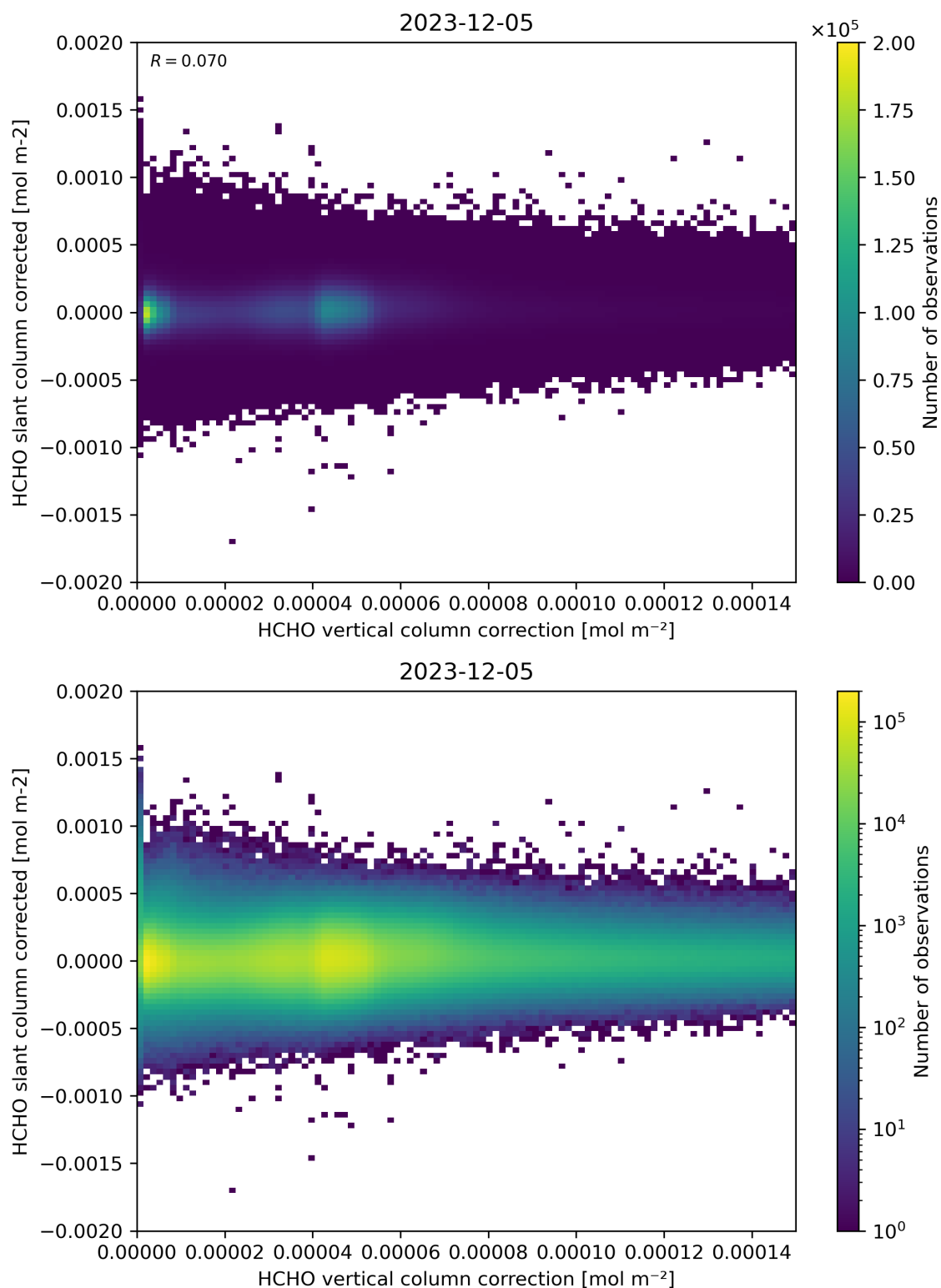
Figure 116: Scatter density plot of “HCHO vertical column correction” against “HCHO slant column corrected” for 2023-12-04 to 2023-12-06.
