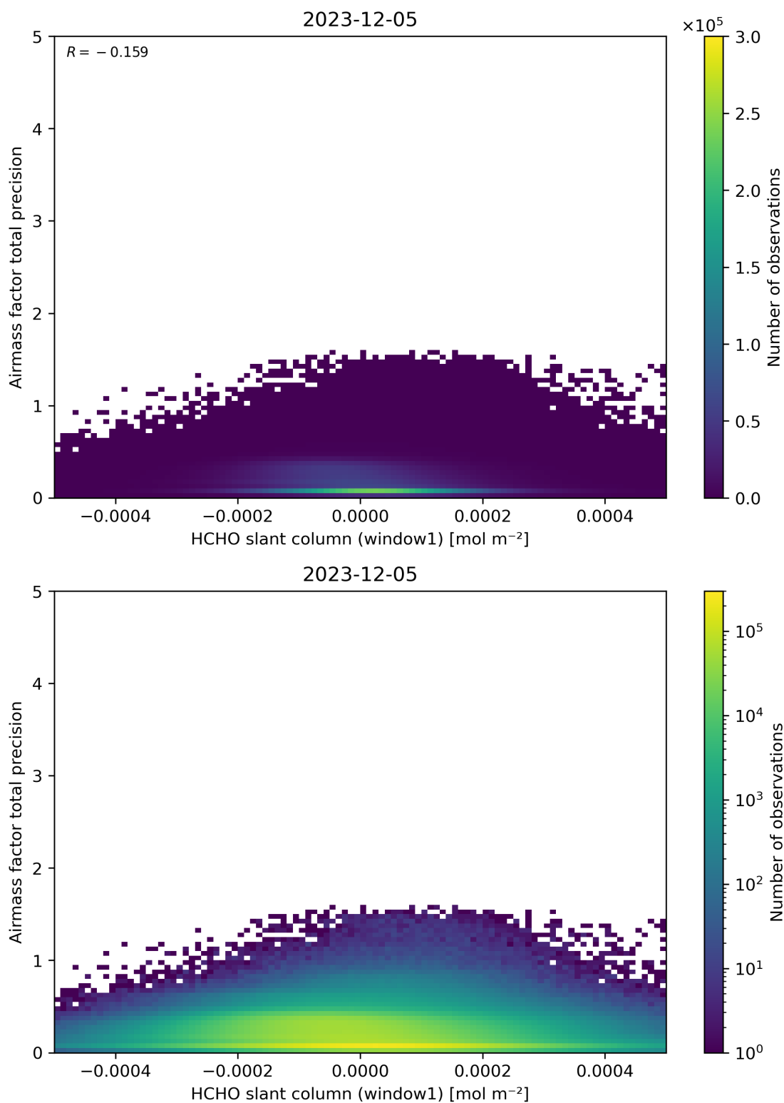
Figure 86: Scatter density plot of “HCHO slant column (window1)” against “Airmass factor total precision” for 2023-12-04 to 2023-12-06.
