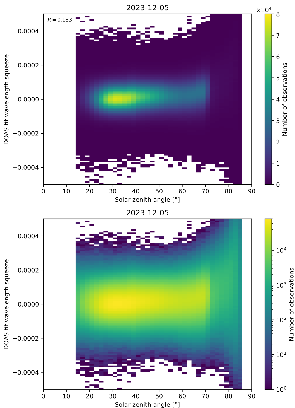
Figure 169: Scatter density plot of “Solar zenith angle” against “DOAS fit wavelength squeeze” for 2023-12-04 to 2023-12-06.
