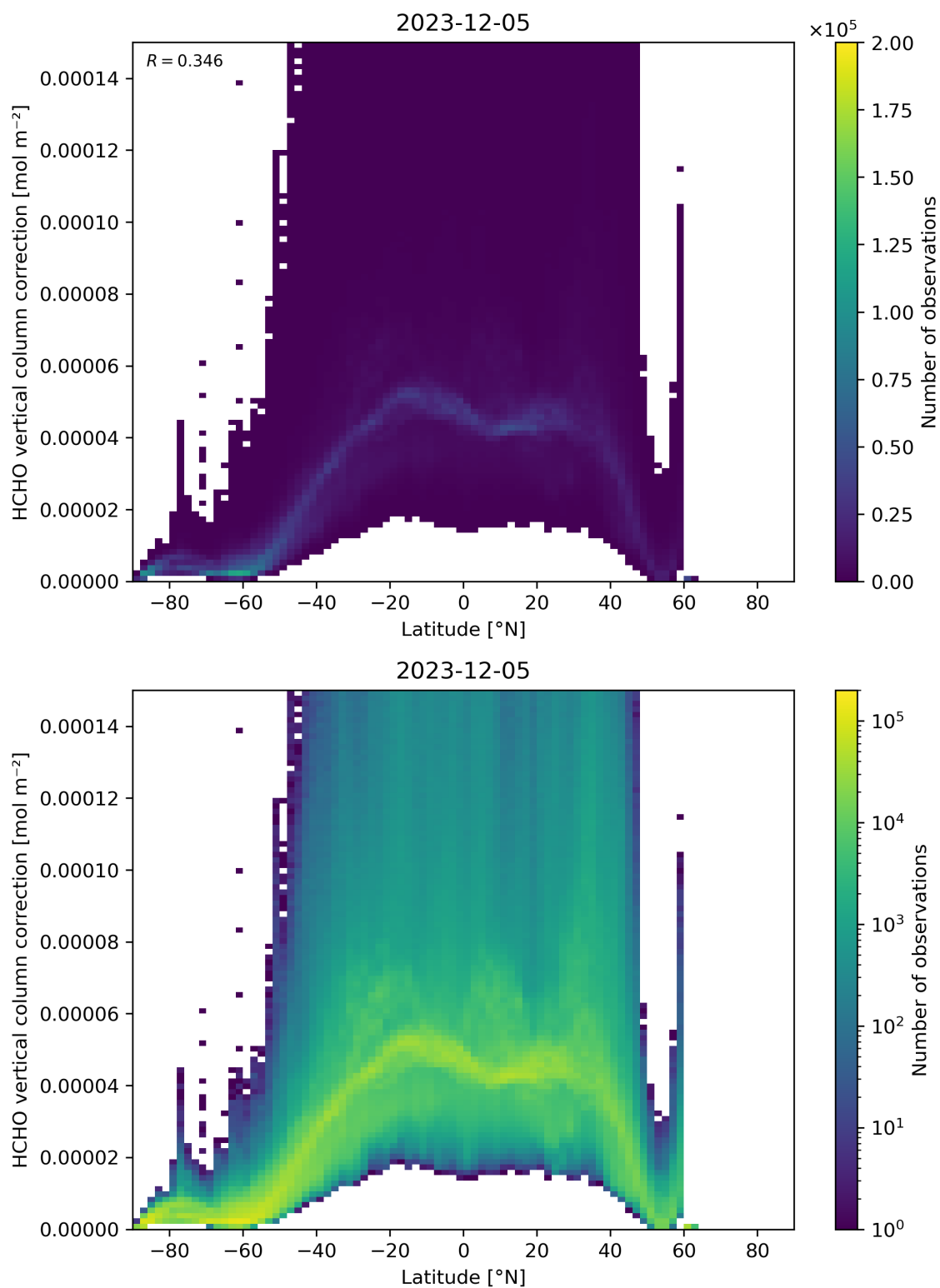
Figure 164: Scatter density plot of “Latitude” against “HCHO vertical column correction” for 2023-12-04 to 2023-12-06.
