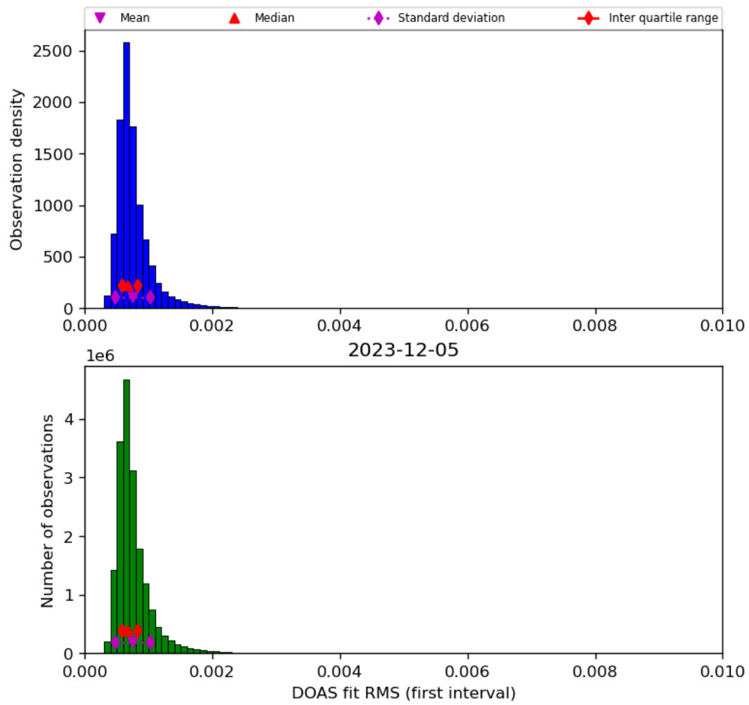
Figure 46: Histogram of “DOAS fit RMS (first interval)” for 2023-12-04 to 2023-12-06
