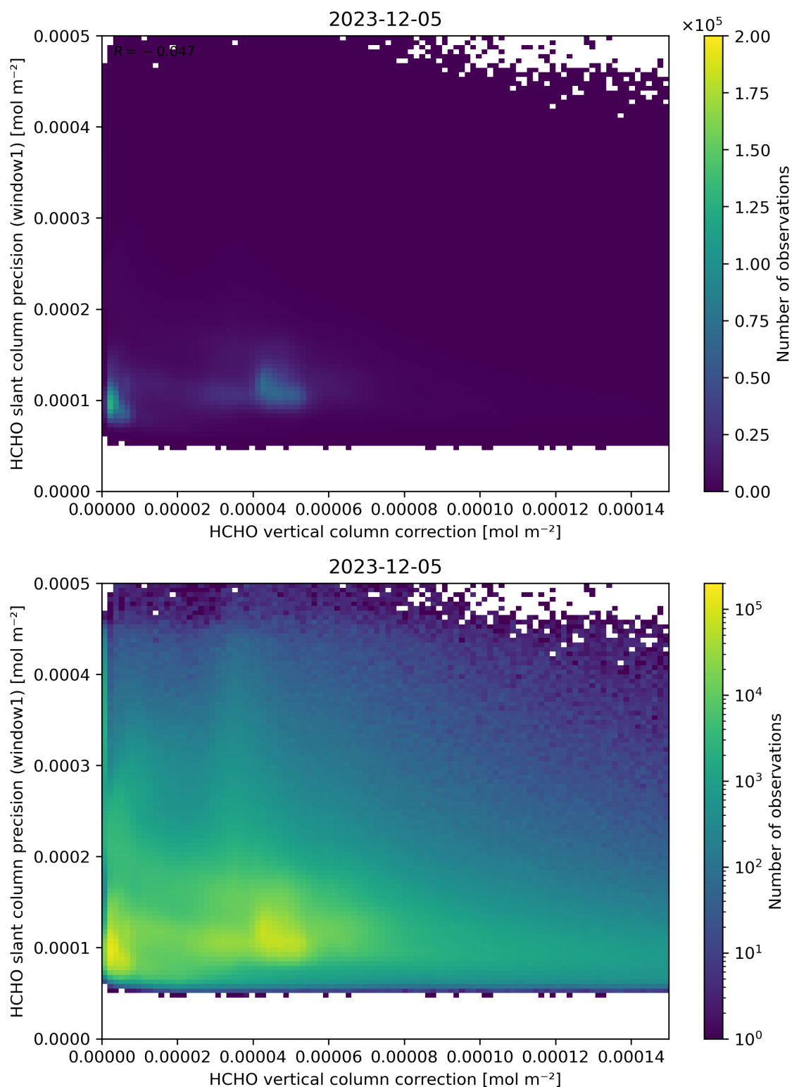
Figure 119: Scatter density plot of “HCHO vertical column correction” against “HCHO slant column precision (window1)” for 2023-12-04 to 2023-12-06.
