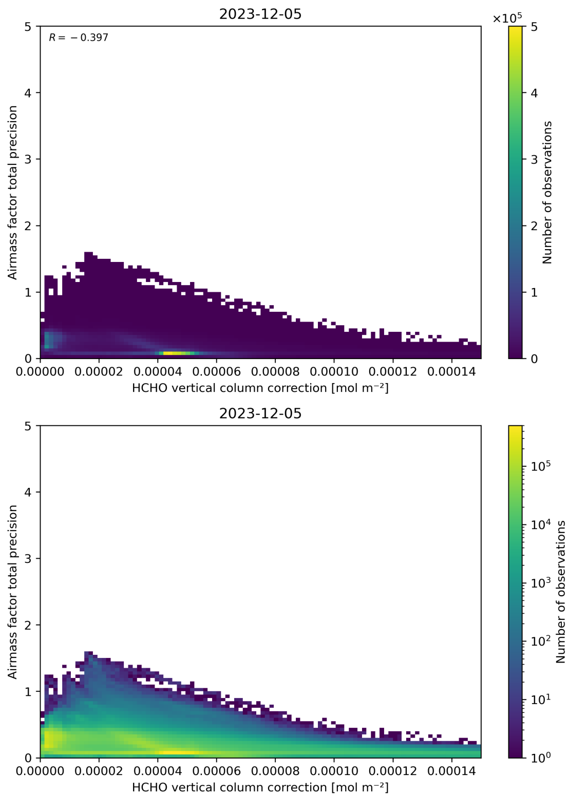
Figure 121: Scatter density plot of “HCHO vertical column correction” against “Airmass factor total precision” for 2023-12-04 to 2023-12-06.
