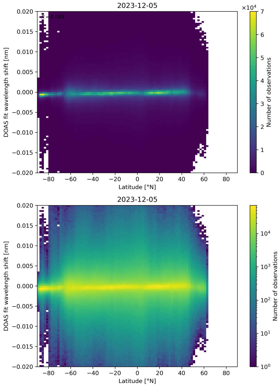
Figure 154: Scatter density plot of “Latitude” against “DOAS fit wavelength shift” for 2023-12-04 to 2023-12-06.
