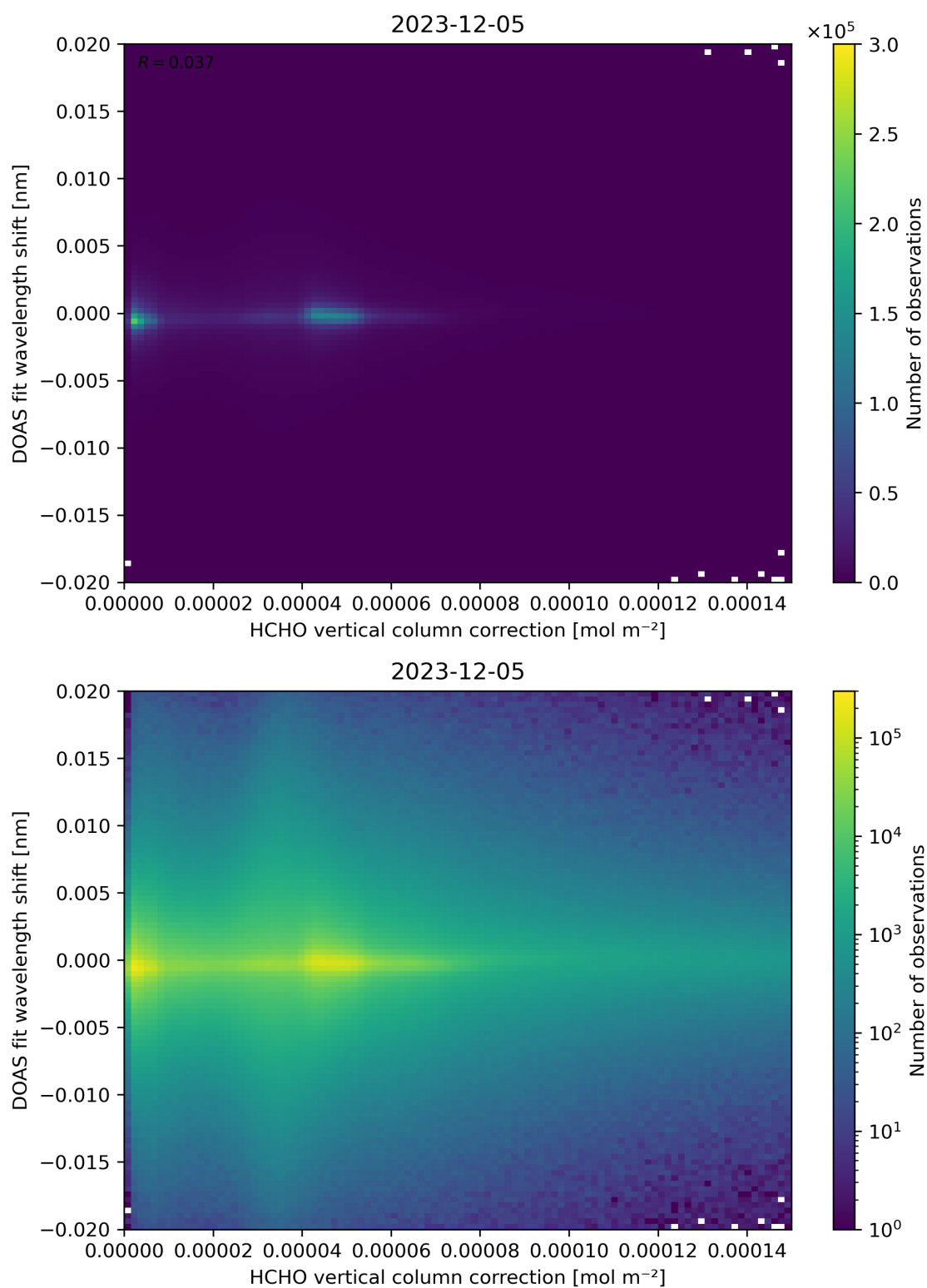
Figure 113: Scatter density plot of “HCHO vertical column correction” against “DOAS fit wavelength shift” for 2023-12-04 to 2023-12-06.
