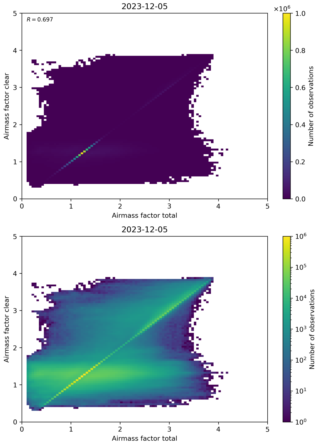
Figure 100: Scatter density plot of “Airmass factor total” against “Airmass factor clear” for 2023-12-04 to 2023-12-06.
