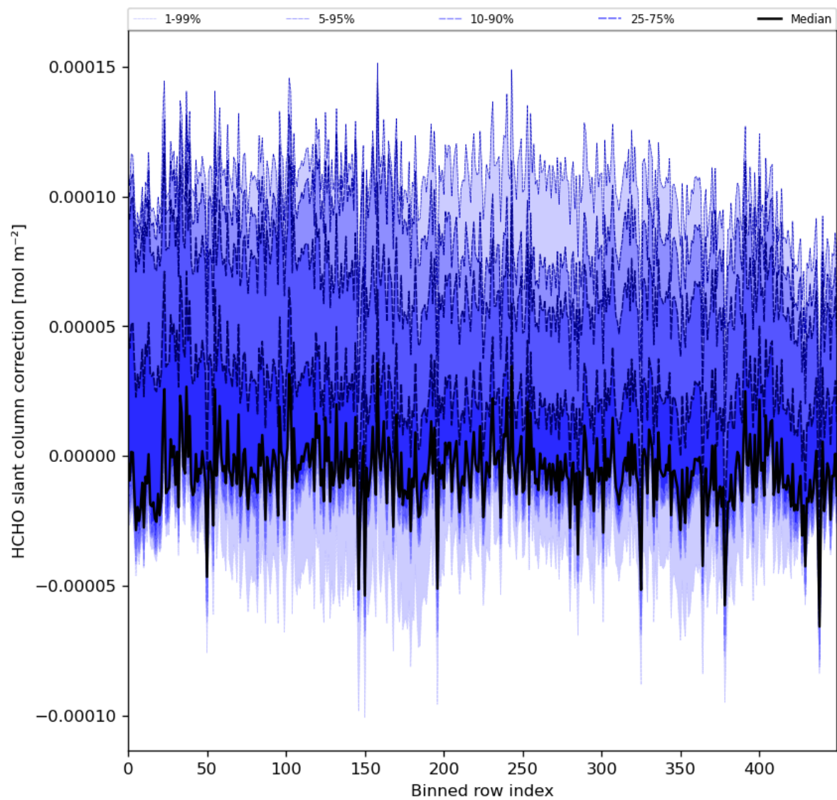
Figure 61: Along track statistics of “HCHO slant column correction” for 2023-12-04 to 2023-12-06
