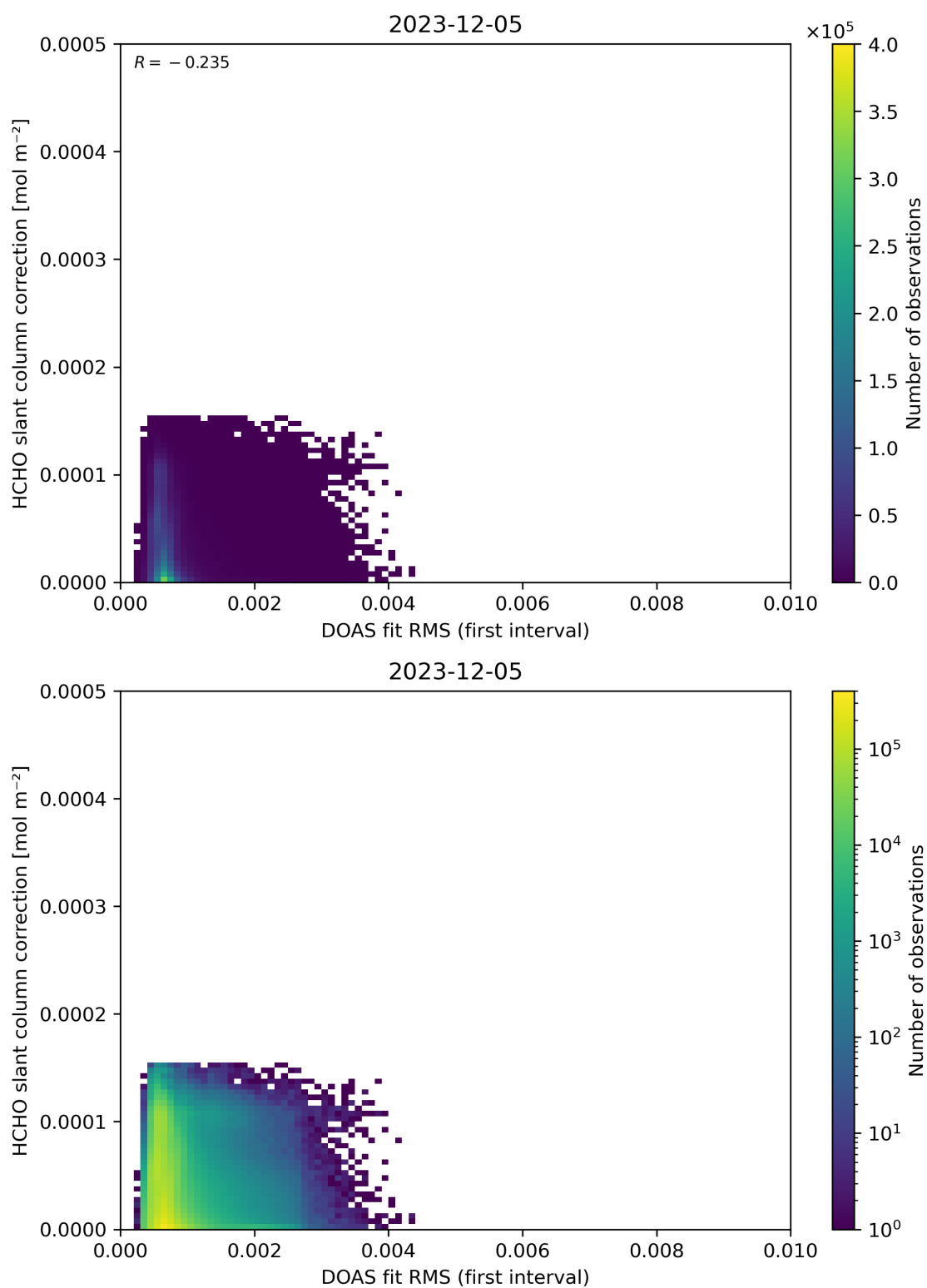
Figure 63: Scatter density plot of “DOAS fit RMS (first interval)” against “HCHO slant column correction” for 2023-12-04 to 2023-12-06.
