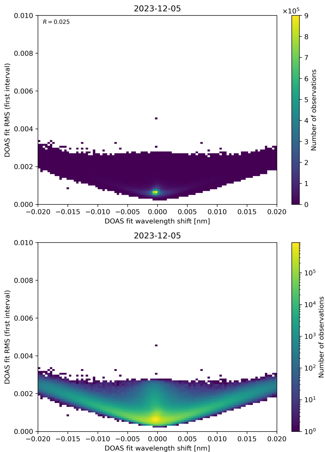
Figure 64: Scatter density plot of “DOAS fit wavelength shift” against “DOAS fit RMS (first interval)” for 2023-12-04 to 2023-12-06.
