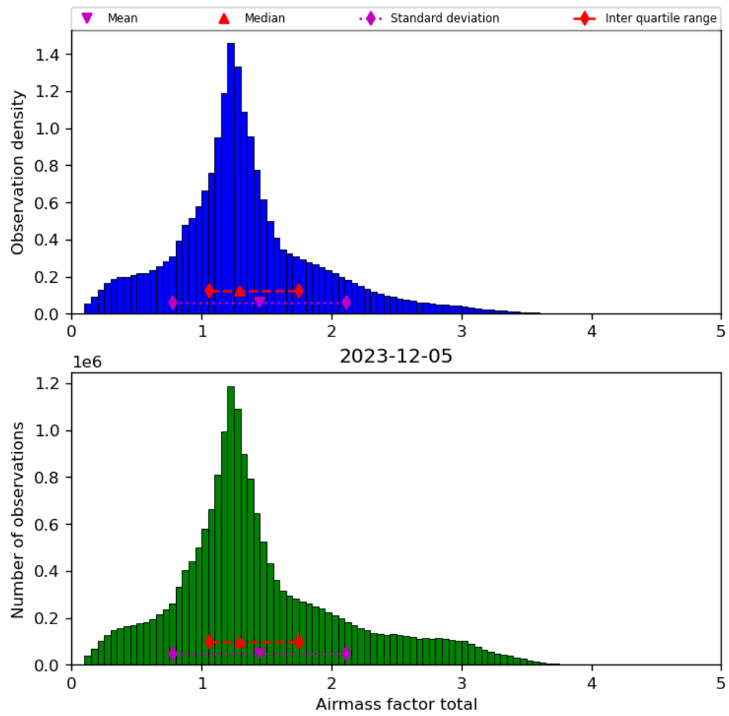
Figure 40: Histogram of “Airmass factor total” for 2023-12-04 to 2023-12-06
