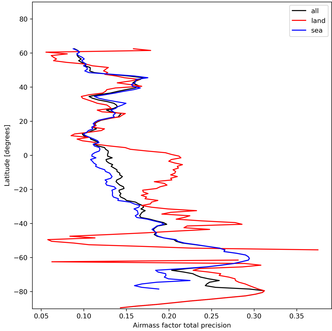
Figure 27: Zonal average of “Airmass factor total precision” for 2023-12-04 to 2023-12-06.
