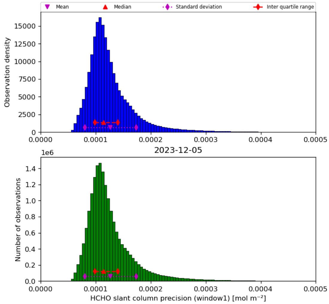
Figure 39: Histogram of “HCHO slant column precision (window1)” for 2023-12-04 to 2023-12-06
