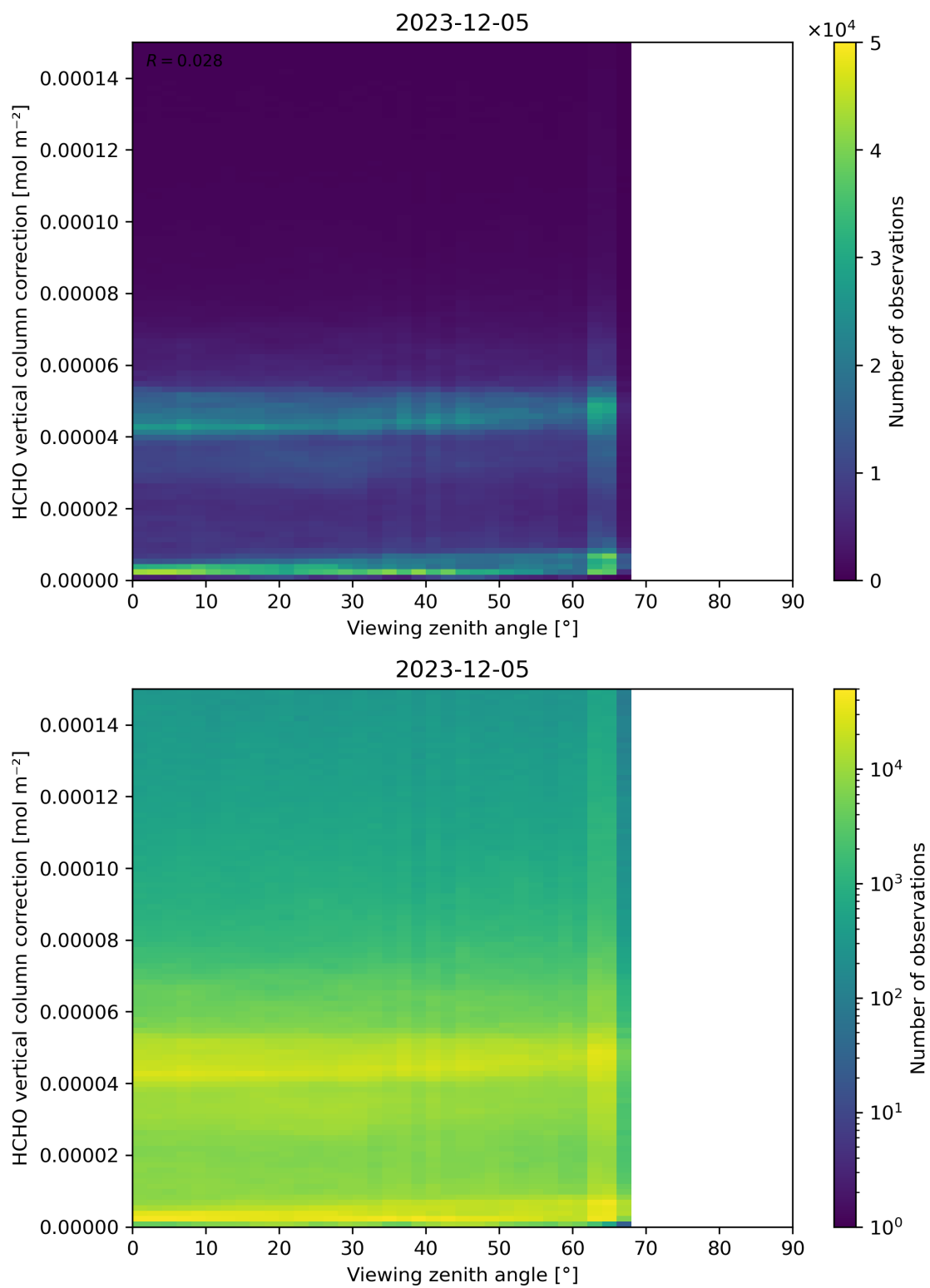
Figure 193: Scatter density plot of “Viewing zenith angle” against “HCHO vertical column correction” for 2023-12-04 to 2023-12-06.
