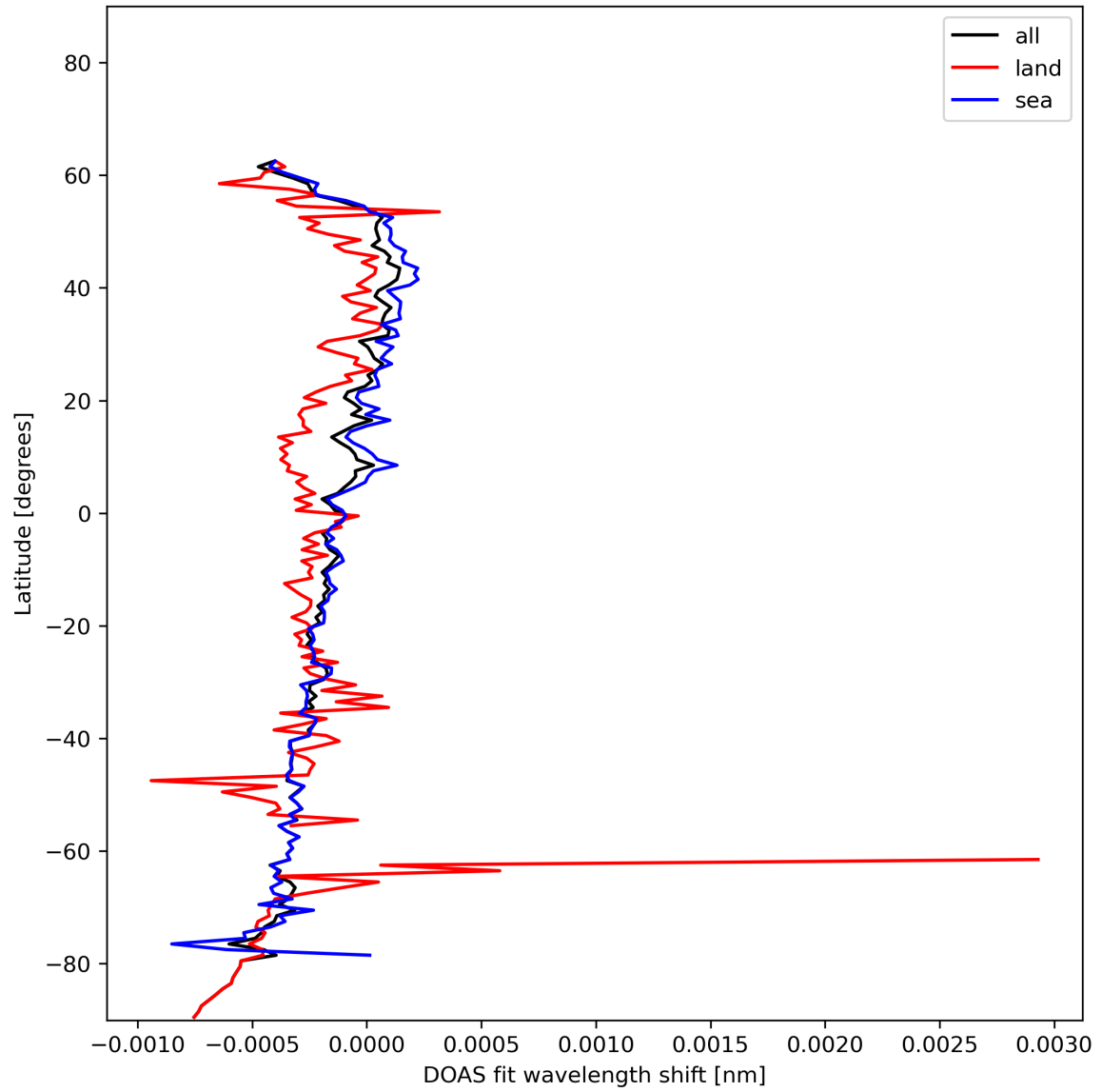
Figure 30: Zonal average of “DOAS fit wavelength shift” for 2023-12-04 to 2023-12-06.
