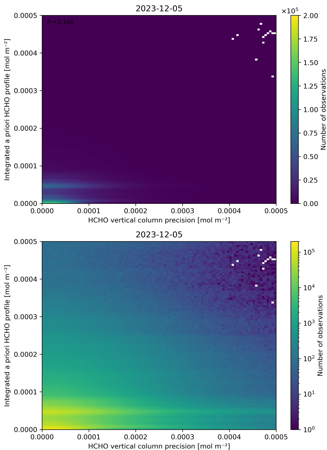
Figure 147: Scatter density plot of “HCHO vertical column precision” against “Integrated a priori HCHO profile” for 2023-12-04 to 2023-12-06.
