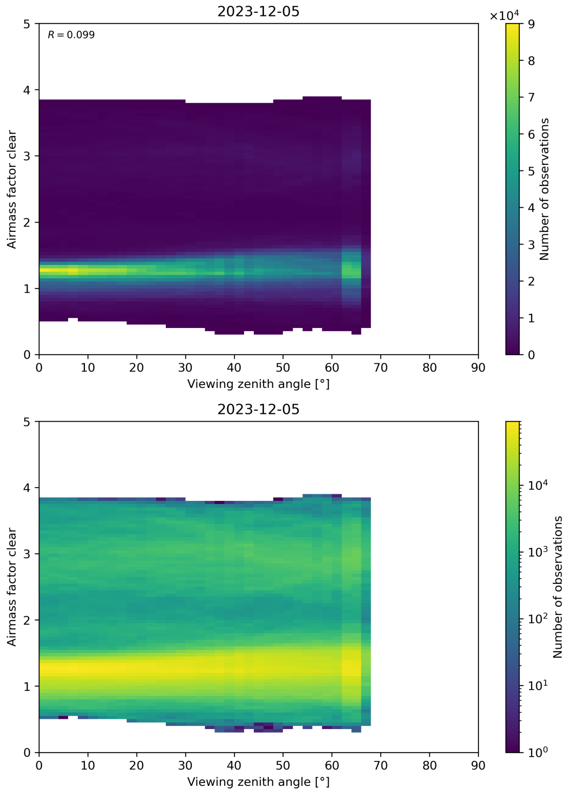
Figure 185: Scatter density plot of “Viewing zenith angle” against “Airmass factor clear” for 2023-12-04 to 2023-12-06.
