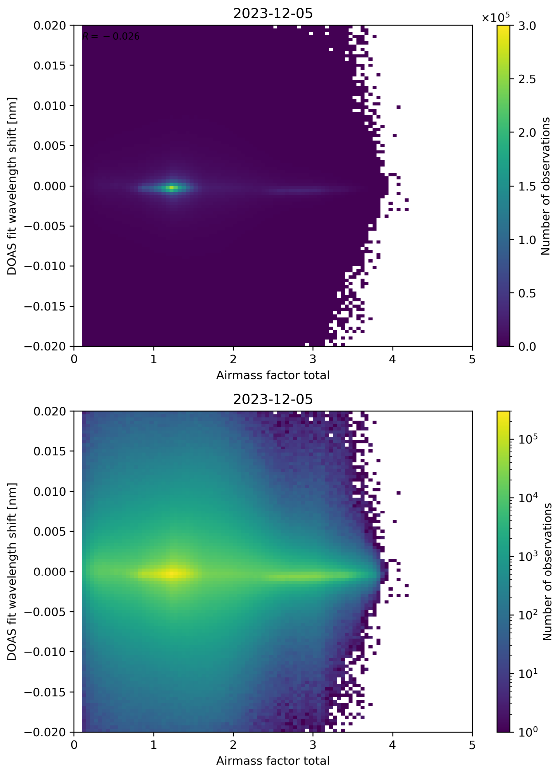
Figure 98: Scatter density plot of “Airmass factor total” against “DOAS fit wavelength shift” for 2023-12-04 to 2023-12-06.
