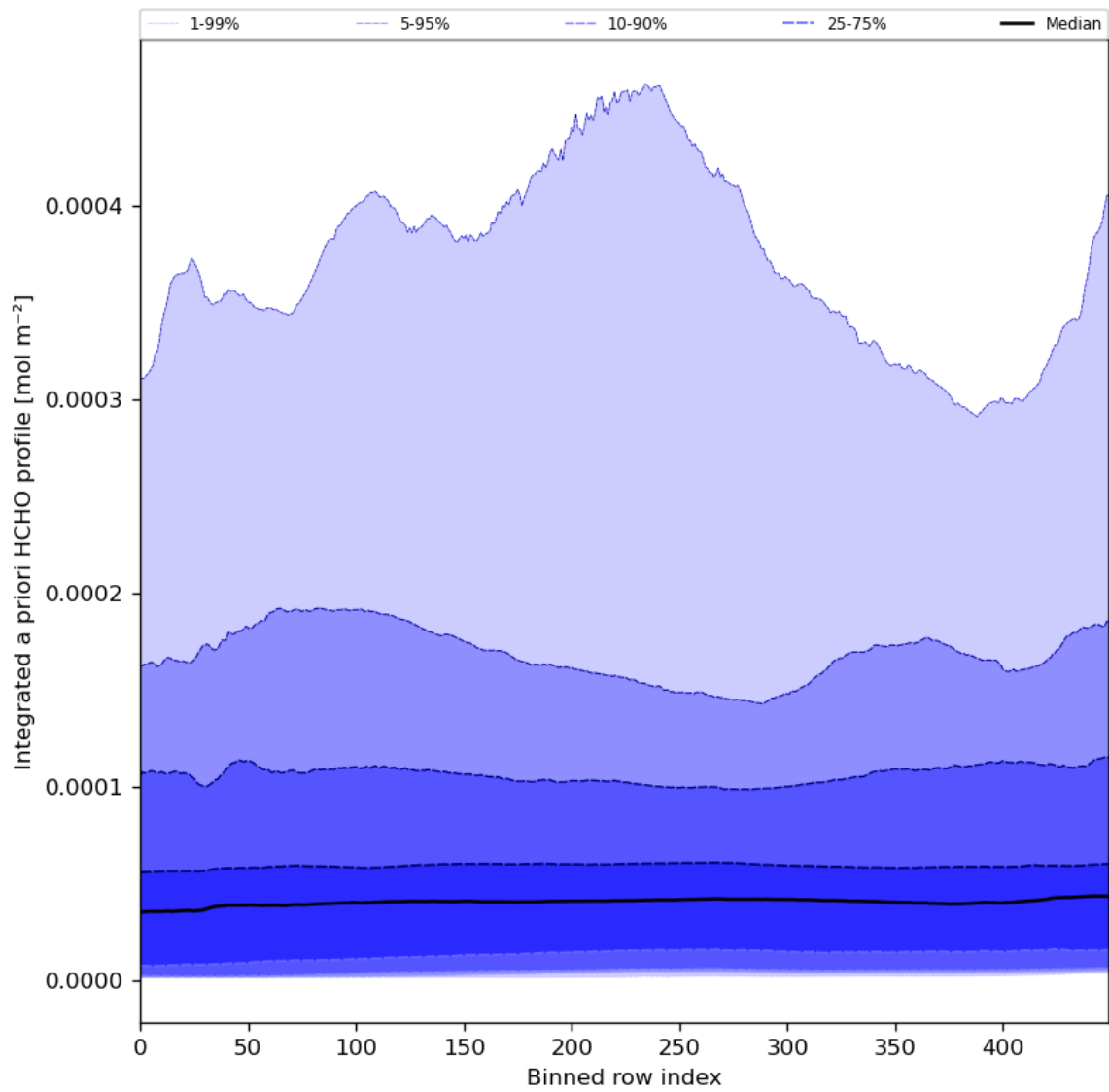
Figure 57: Along track statistics of "Integrated a priori HCHO profile" for 2023-12-04 to 2023-12-06
