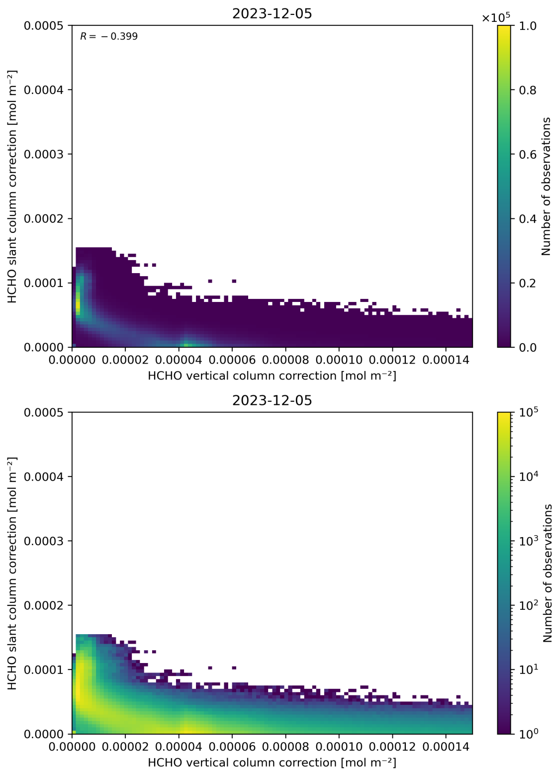
Figure 117: Scatter density plot of “HCHO vertical column correction” against “HCHO slant column correction” for 2023-12-04 to 2023-12-06.
