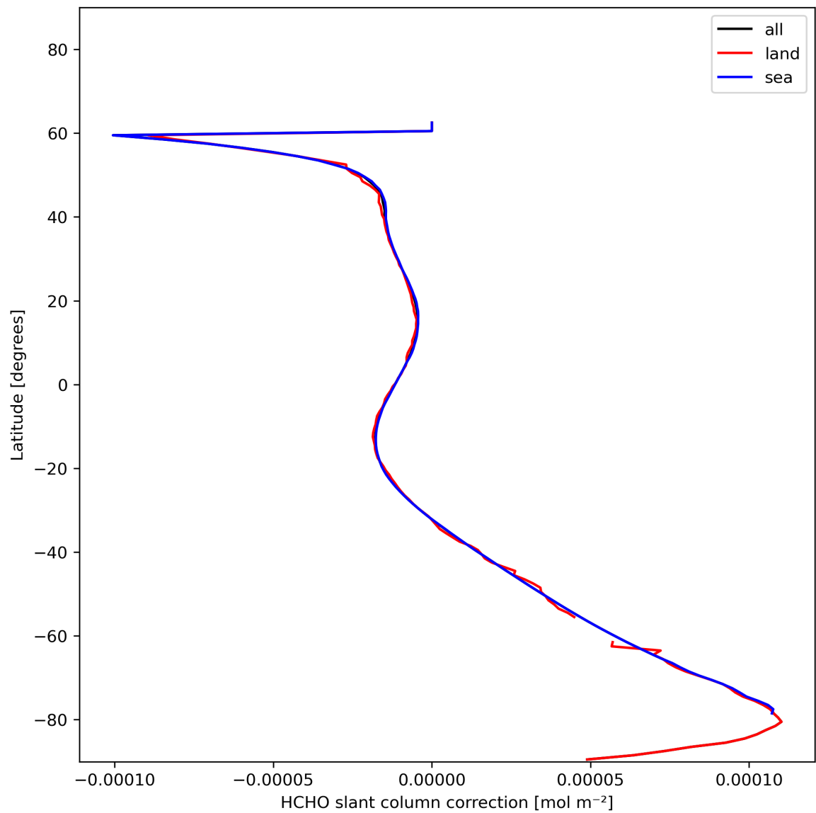
Figure 33: Zonal average of “HCHO slant column correction” for 2023-12-04 to 2023-12-06.
