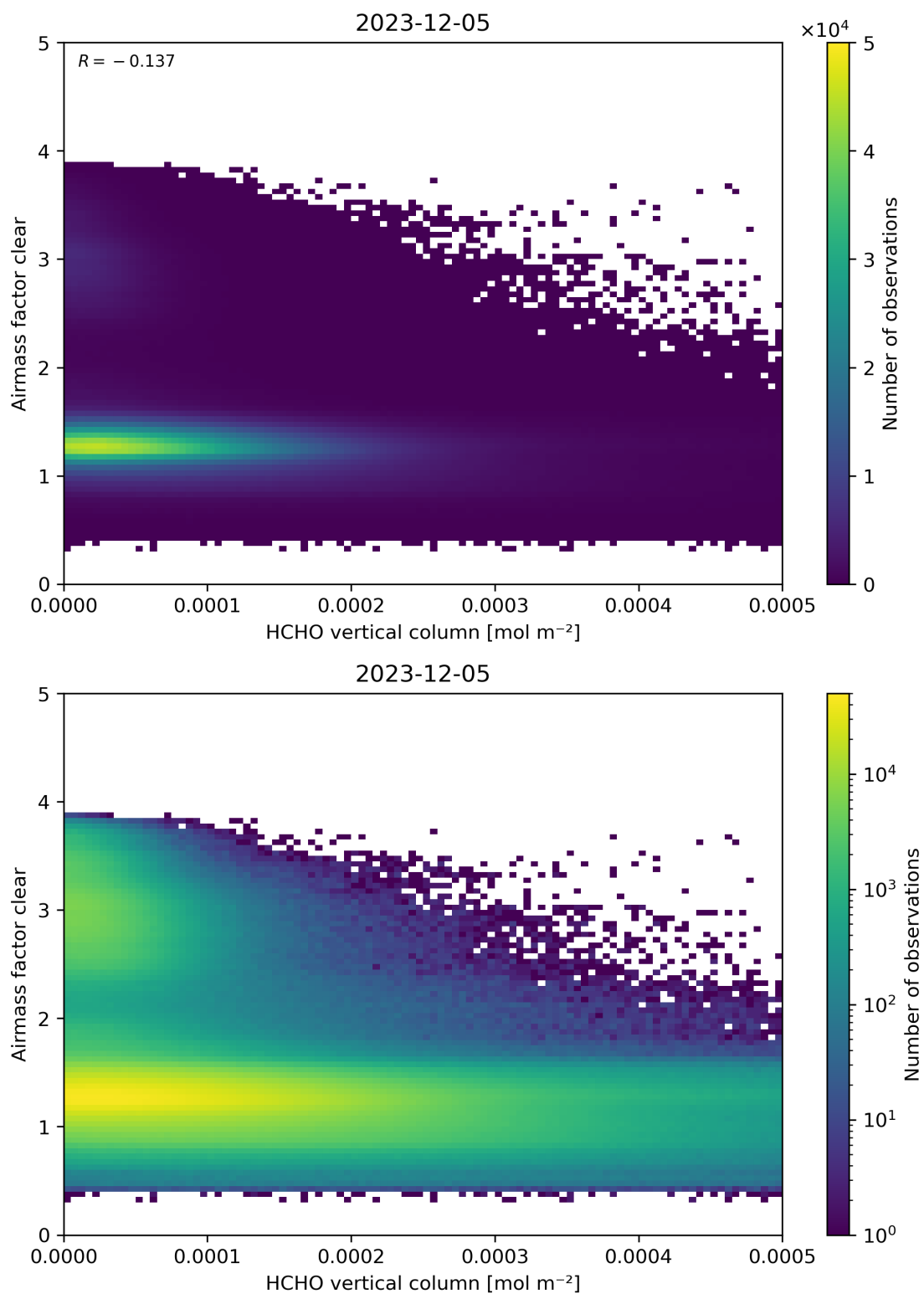
Figure 126: Scatter density plot of “HCHO vertical column” against “Airmass factor clear” for 2023-12-04 to 2023-12-06.
