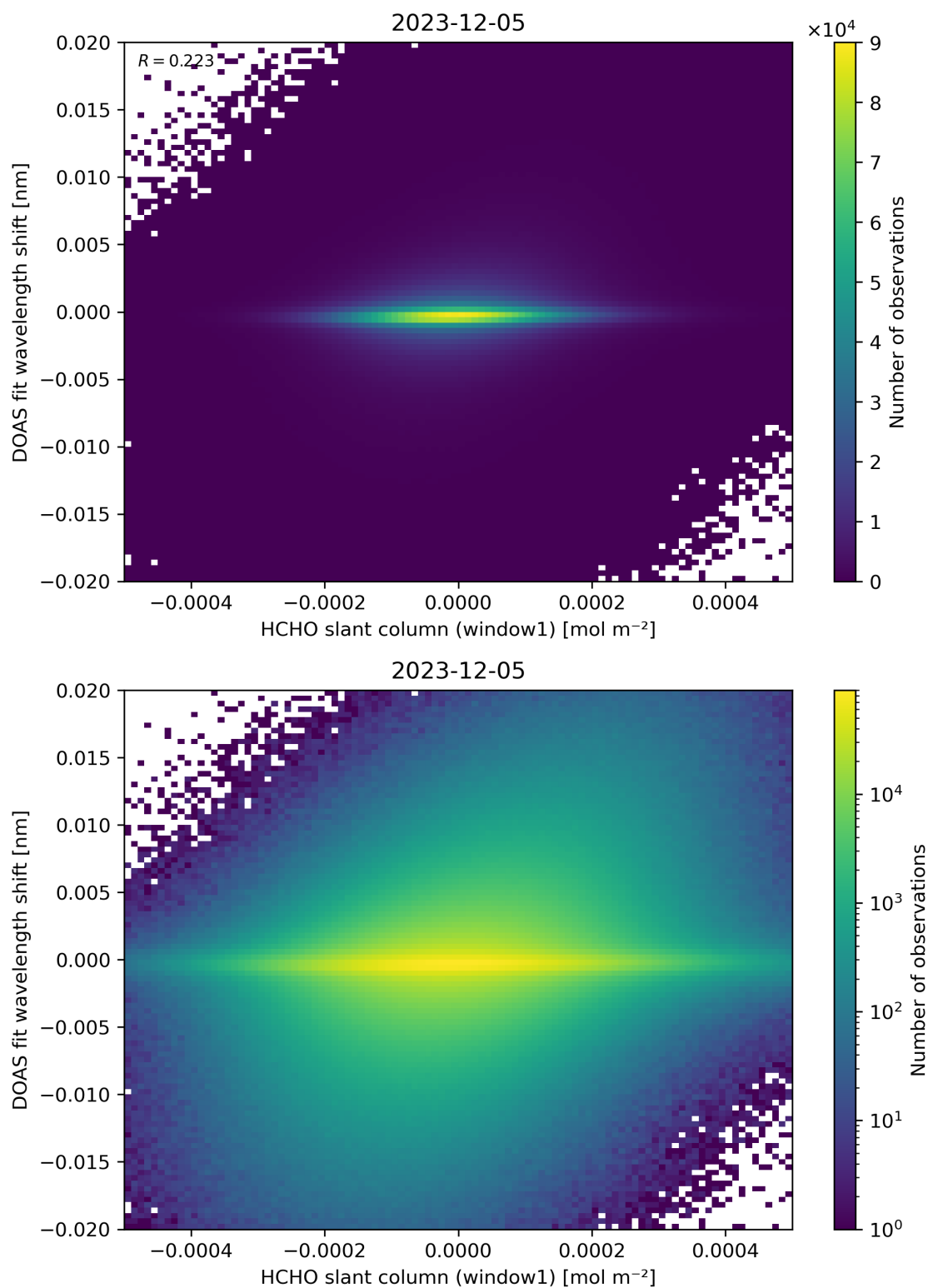
Figure 79: Scatter density plot of “HCHO slant column (window1)” against “DOAS fit wavelength shift” for 2023-12-04 to 2023-12-06.
