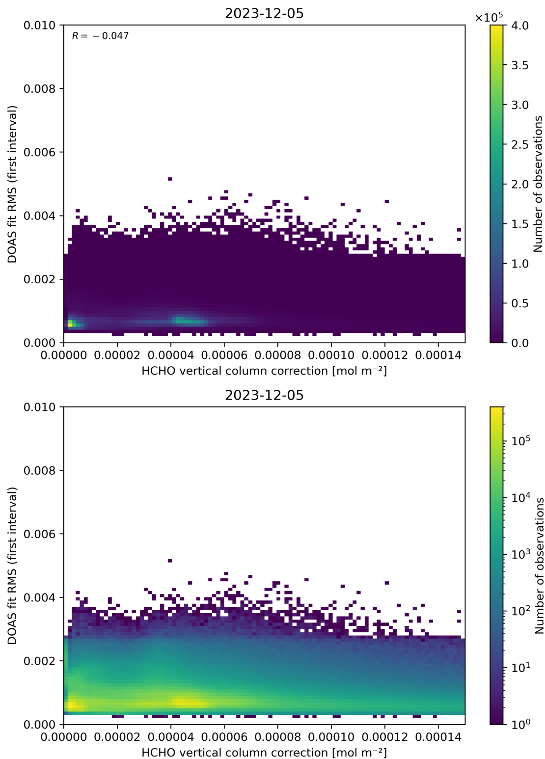
Figure 112: Scatter density plot of “HCHO vertical column correction” against “DOAS fit RMS (first interval)” for 2023-12-04 to 2023-12-06.
