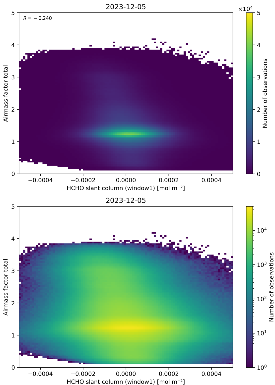
Figure 85: Scatter density plot of “HCHO slant column (window1)” against “Airmass factor total” for 2023-12-04 to 2023-12-06.
