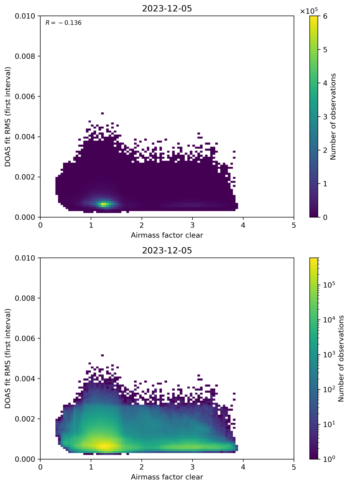
Figure 71: Scatter density plot of “Airmass factor clear” against “DOAS fit RMS (first interval)” for 2023-12-04 to 2023-12-06.
