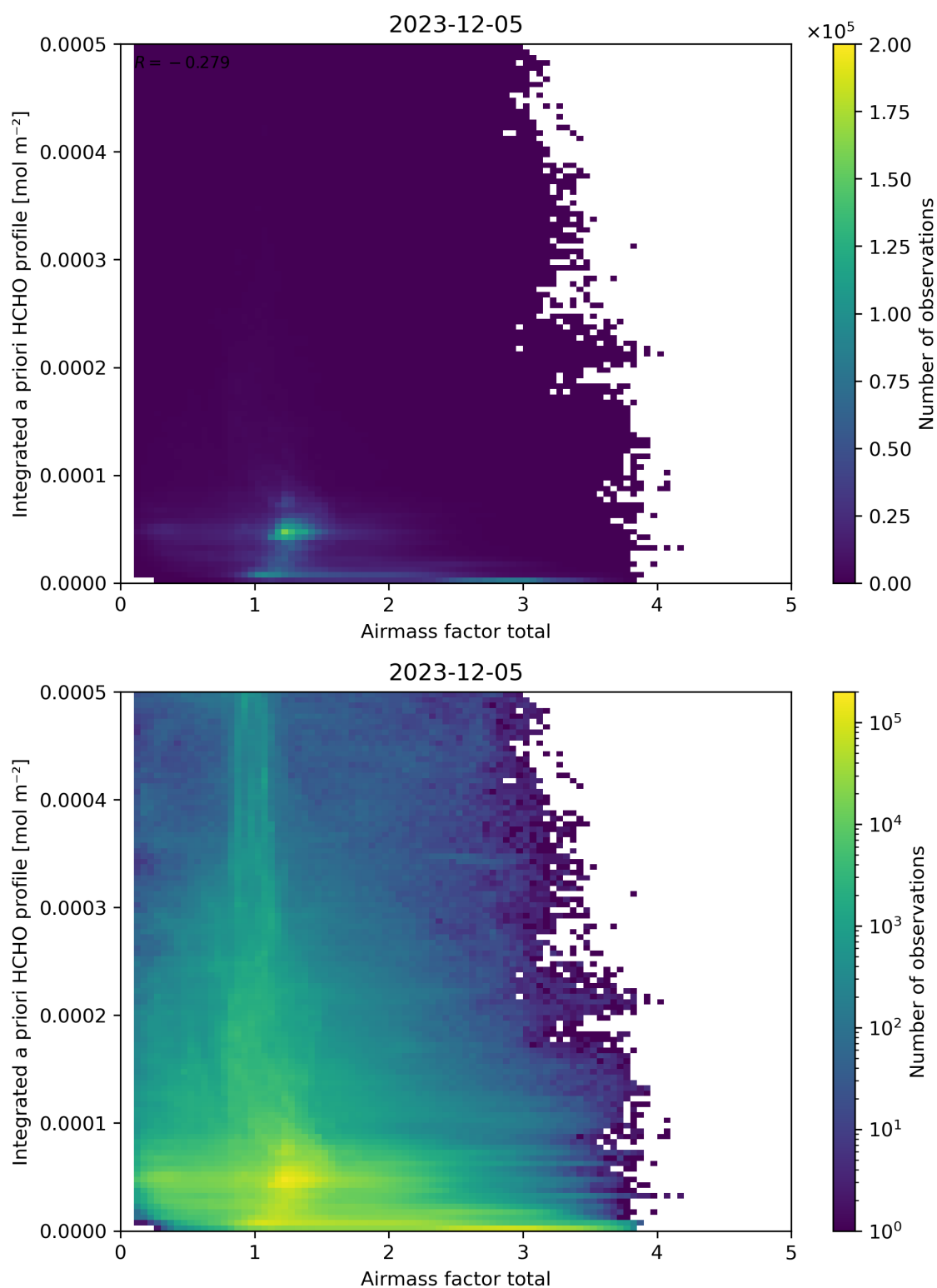
Figure 104: Scatter density plot of “Air mass factor total” against “Integrated a priori HCHO profile” for 2023-12-04 to 2023-12-06.
