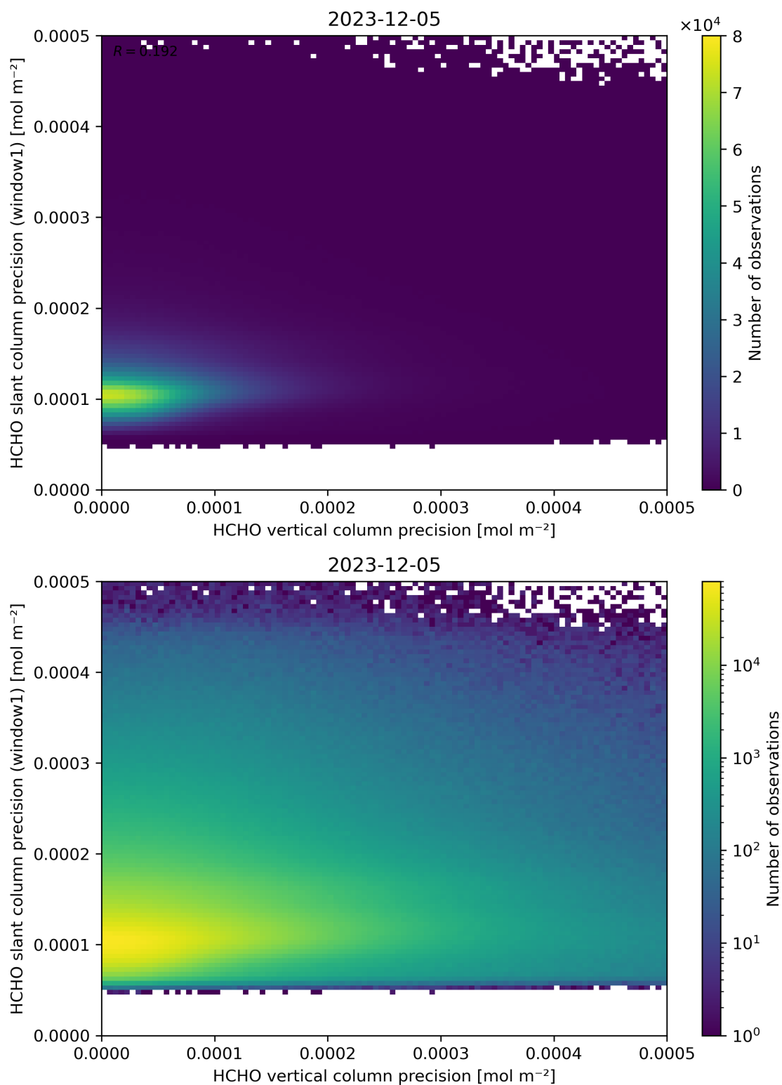
Figure 143: Scatter density plot of “HCHO vertical column precision” against “HCHO slant column precision (window1)” for 2023-12-04 to 2023-12-06.
