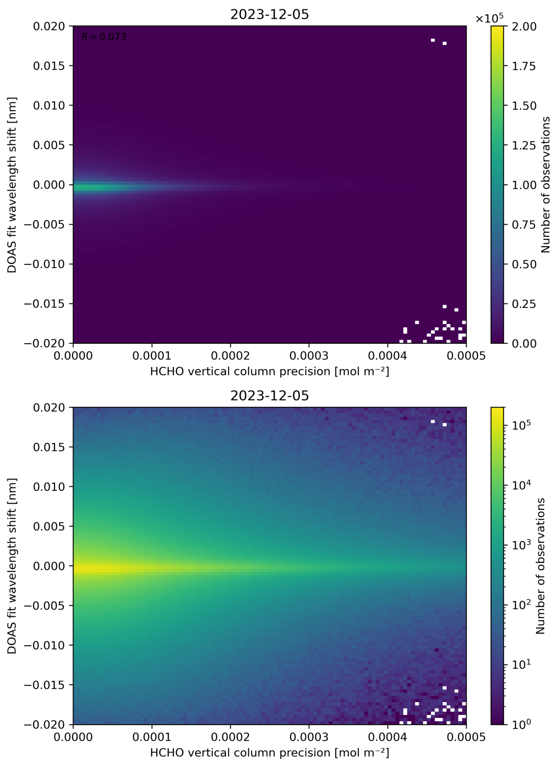
Figure 137: Scatter density plot of “HCHO vertical column precision” against “DOAS fit wavelength shift” for 2023-12-04 to 2023-12-06.
