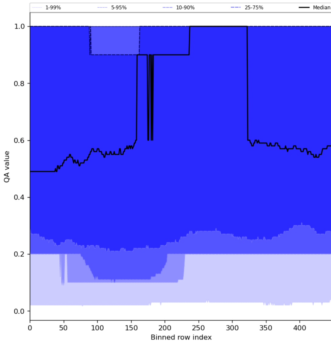
Figure 48: Along track statistics of “QA value” for 2023-12-04 to 2023-12-06
