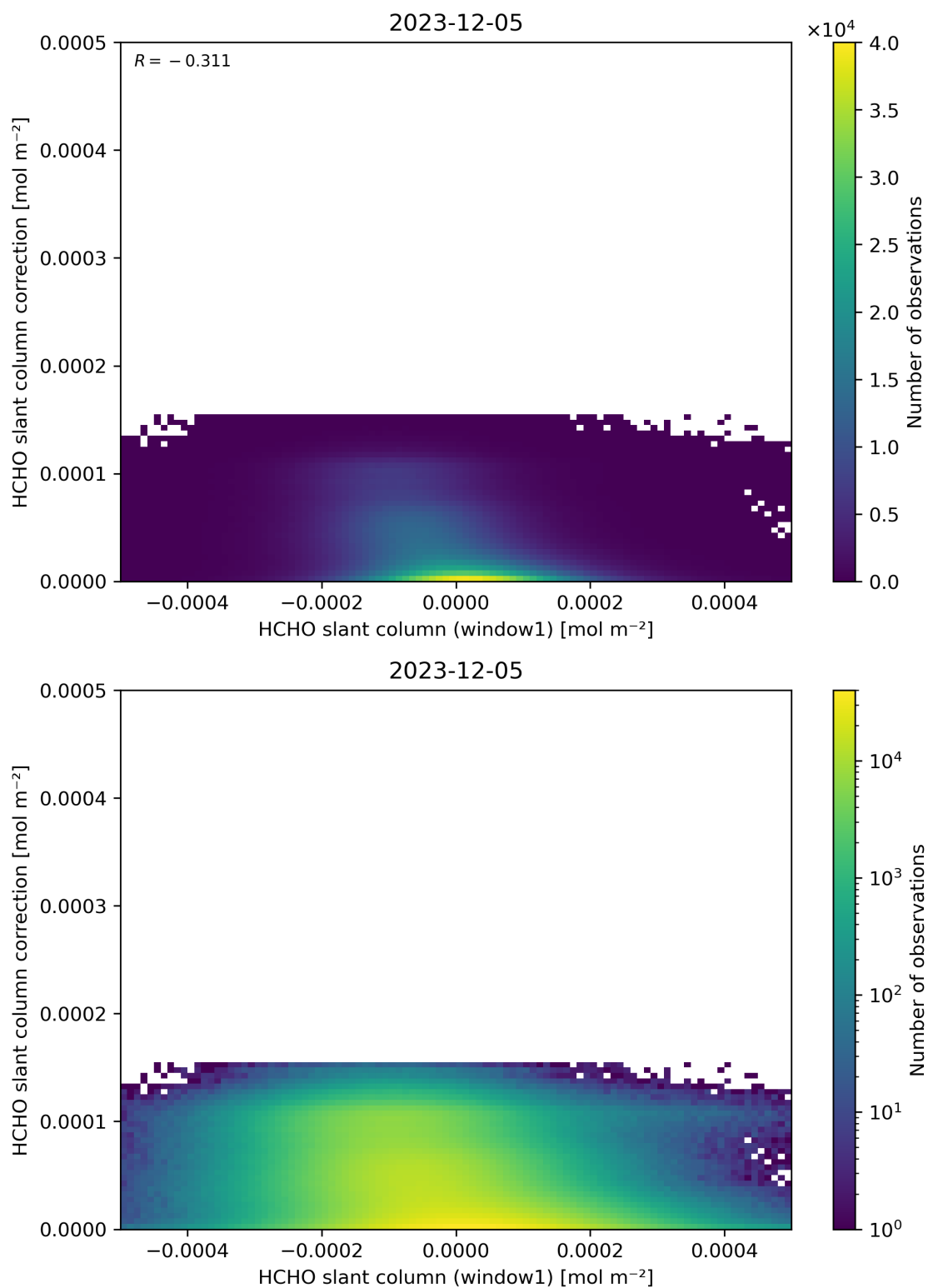
Figure 83: Scatter density plot of “HCHO slant column (window1)” against “HCHO slant column correction” for 2023-12-04 to 2023-12-06.
