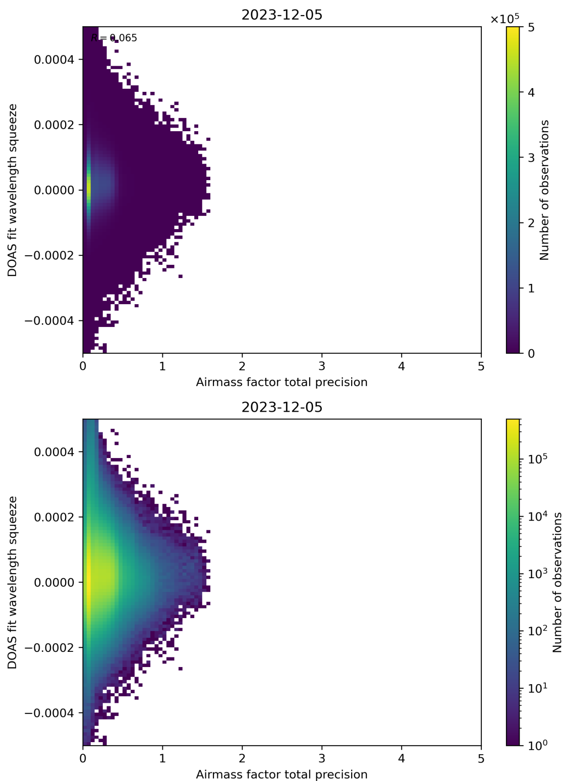
Figure 107: Scatter density plot of “Airmass factor total precision” against “DOAS fit wavelength squeeze” for 2023-12-04 to 2023-12-06.
