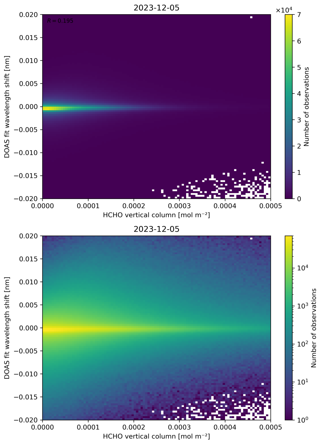
Figure 124: Scatter density plot of “HCHO vertical column” against “DOAS fit wavelength shift” for 2023-12-04 to 2023-12-06.
