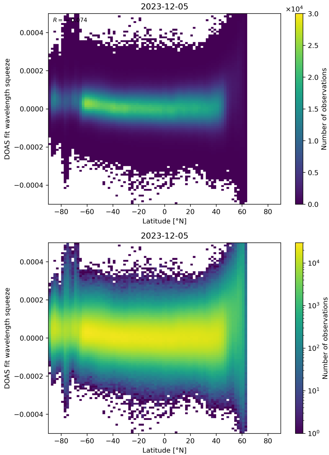
Figure 155: Scatter density plot of “Latitude” against “DOAS fit wavelength squeeze” for 2023-12-04 to 2023-12-06.
