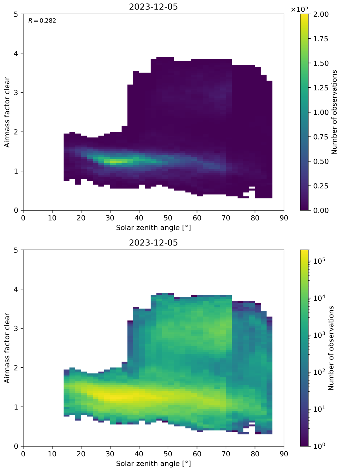
Figure 170: Scatter density plot of “Solar zenith angle” against “Airmass factor clear” for 2023-12-04 to 2023-12-06.
