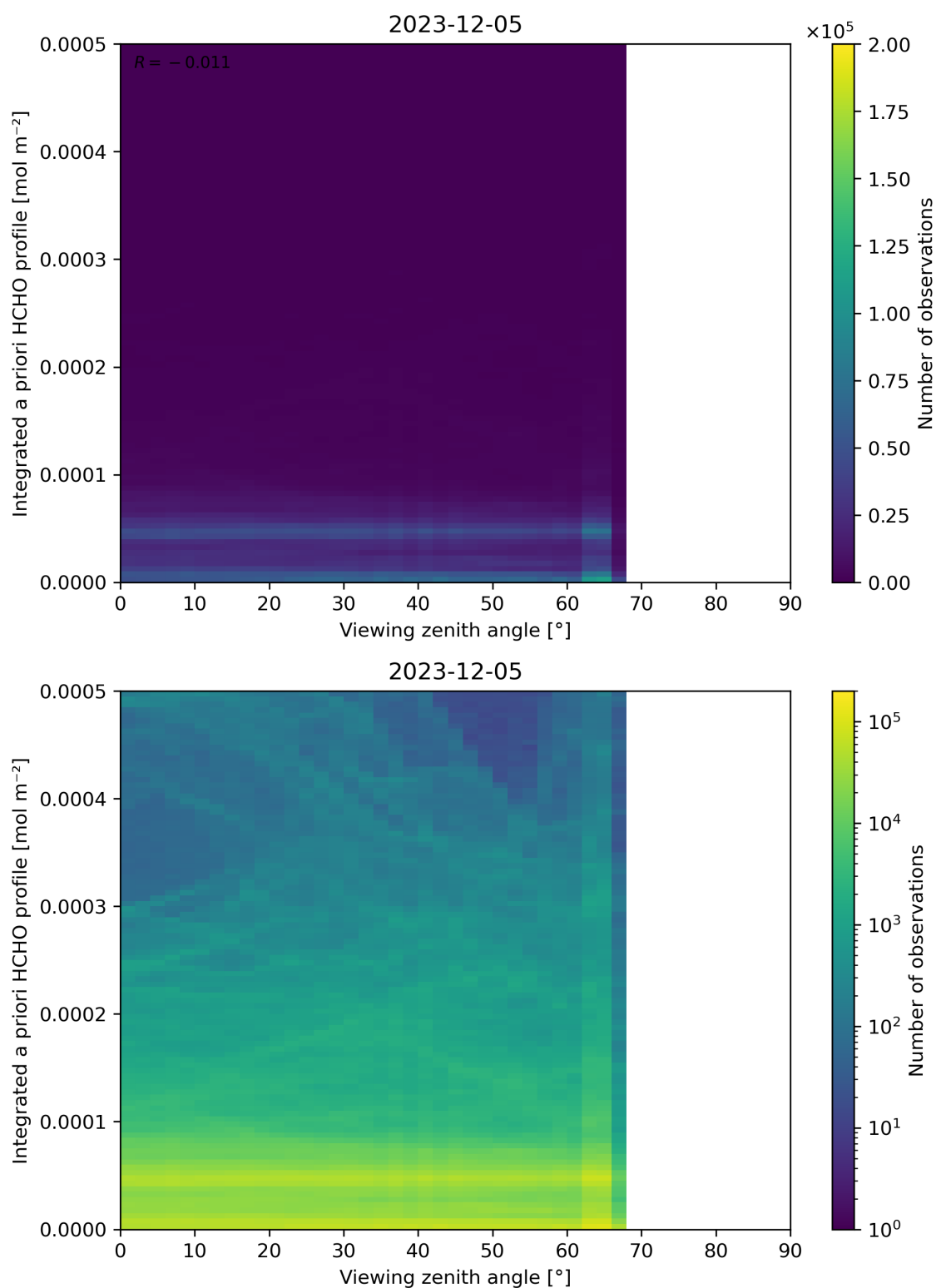
Figure 195: Scatter density plot of “Viewing zenith angle” against “Integrated a priori HCHO profile” for 2023-12-04 to 2023-12-06.
