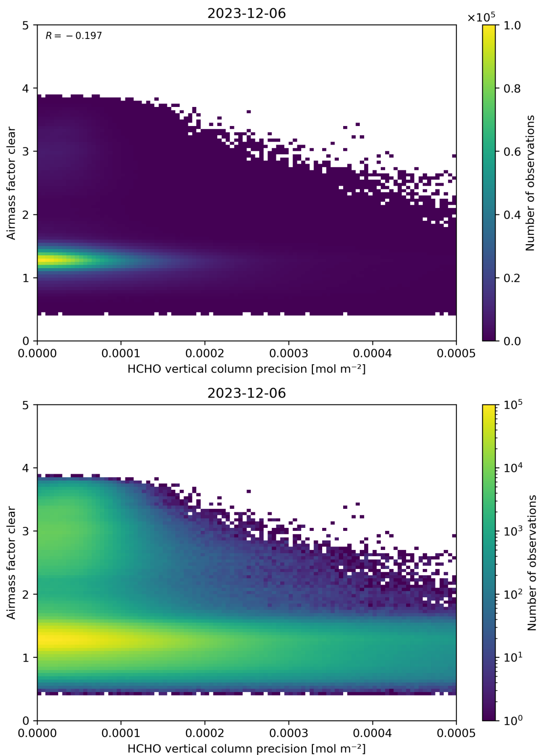
Figure 139: Scatter density plot of “HCHO vertical column precision” against “Airmass factor clear” for 2023-12-05 to 2023-12-07.
