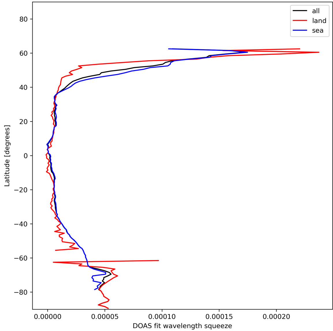
Figure 31: Zonal average of “DOAS fit wavelength squeeze” for 2023-12-05 to 2023-12-07.
