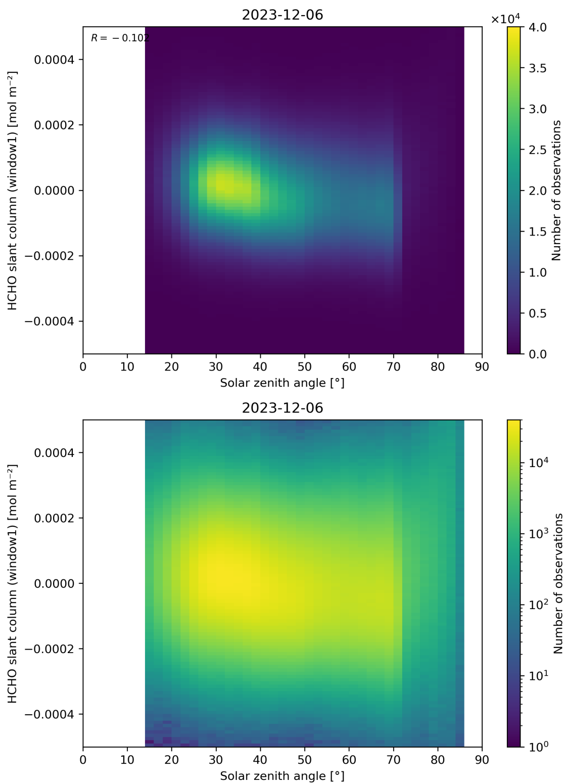
Figure 173: Scatter density plot of “Solar zenith angle” against “HCHO slant column (window1)” for 2023-12-05 to 2023-12-07.
