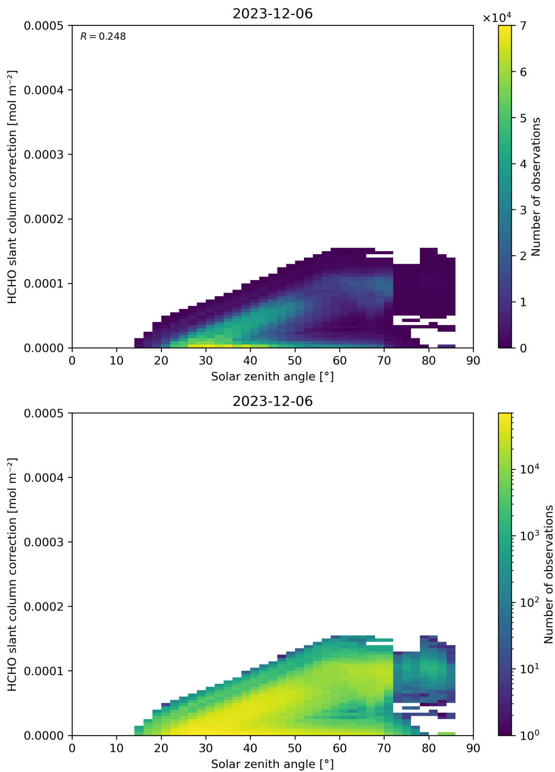
Figure 172: Scatter density plot of “Solar zenith angle” against “HCHO slant column correction” for 2023-12-05 to 2023-12-07.
