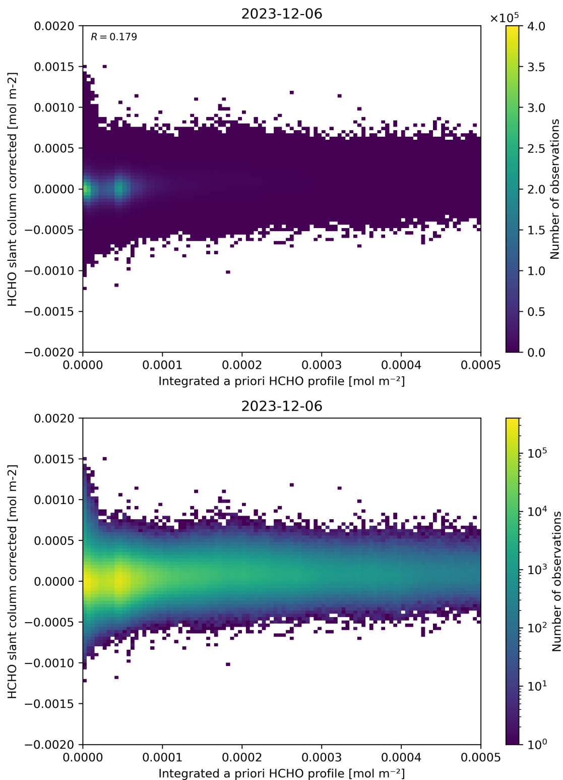
Figure 151: Scatter density plot of “Integrated a priori HCHO profile” against “HCHO slant column corrected” for 2023-12-05 to 2023-12-07.
