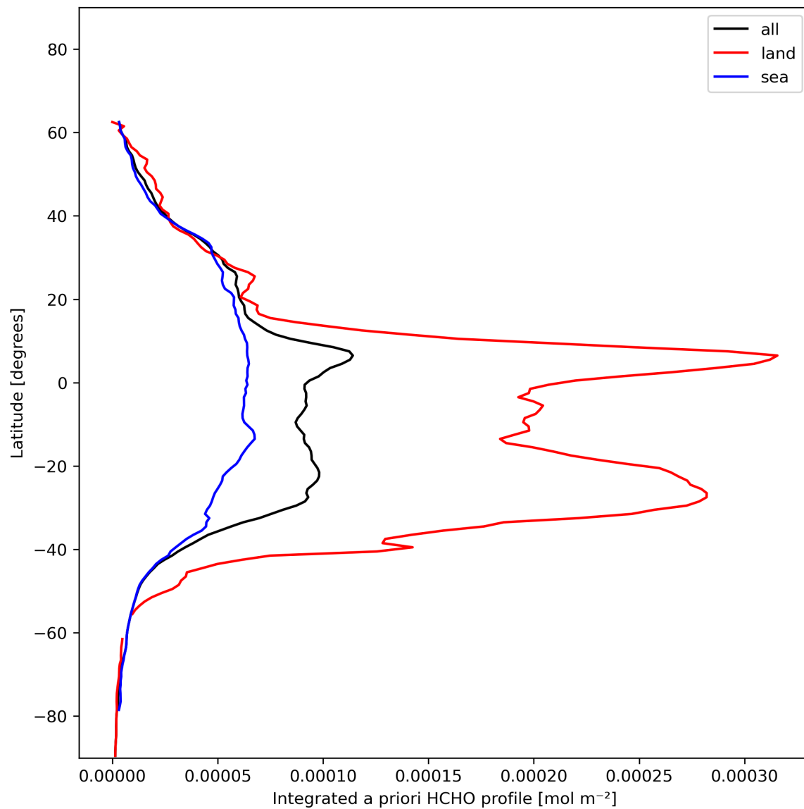
Figure 29: Zonal average of “Integrated a priori HCHO profile” for 2023-12-05 to 2023-12-07.
