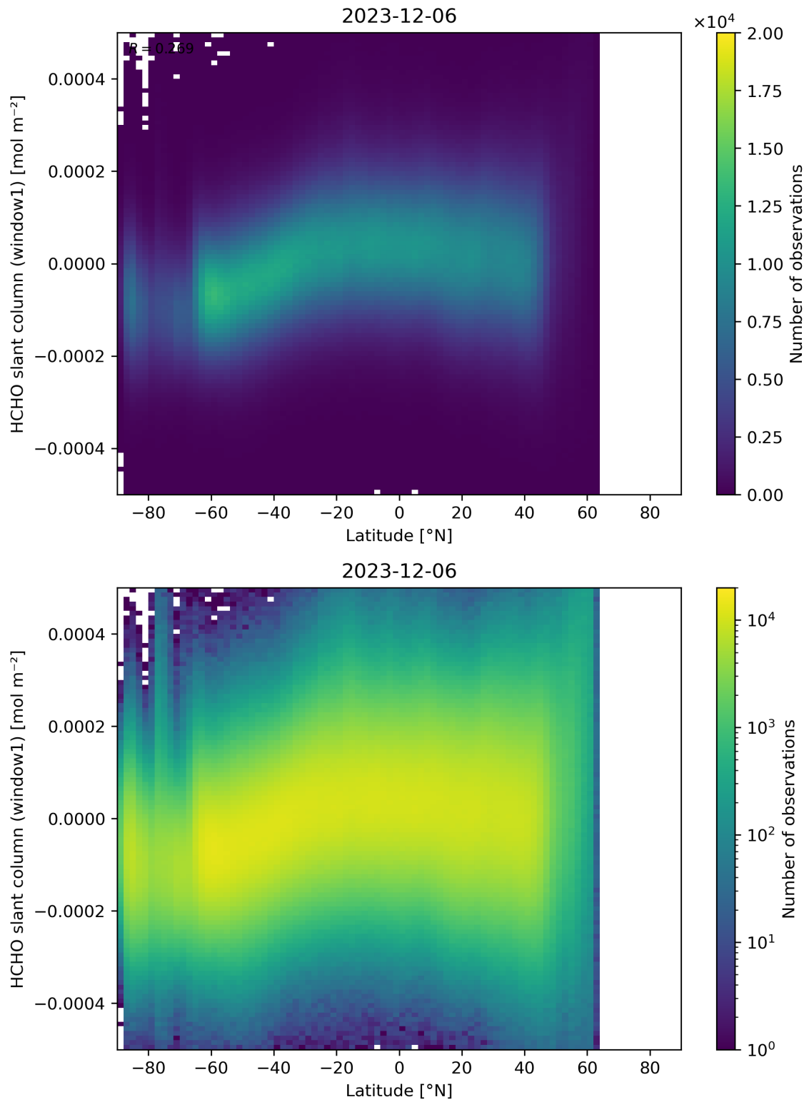
Figure 159: Scatter density plot of “Latitude” against “HCHO slant column (window1)” for 2023-12-05 to 2023-12-07.
