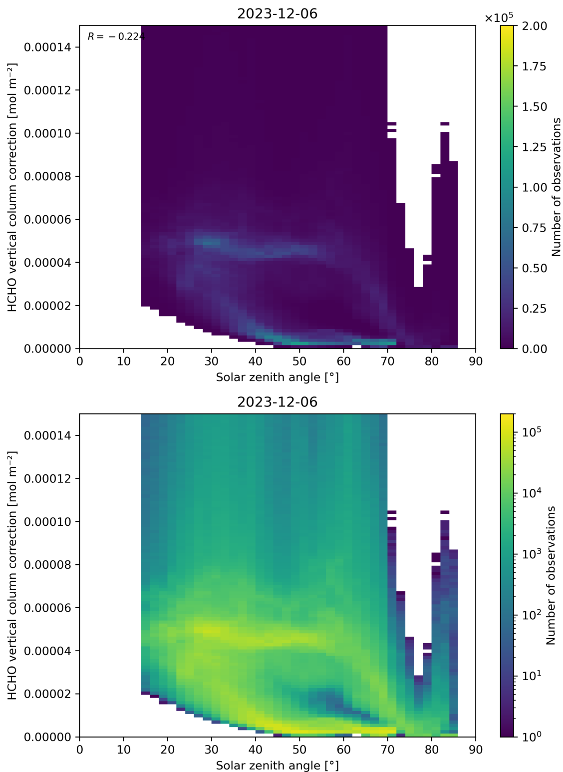
Figure 178: Scatter density plot of “Solar zenith angle” against “HCHO vertical column correction” for 2023-12-05 to 2023-12-07.
