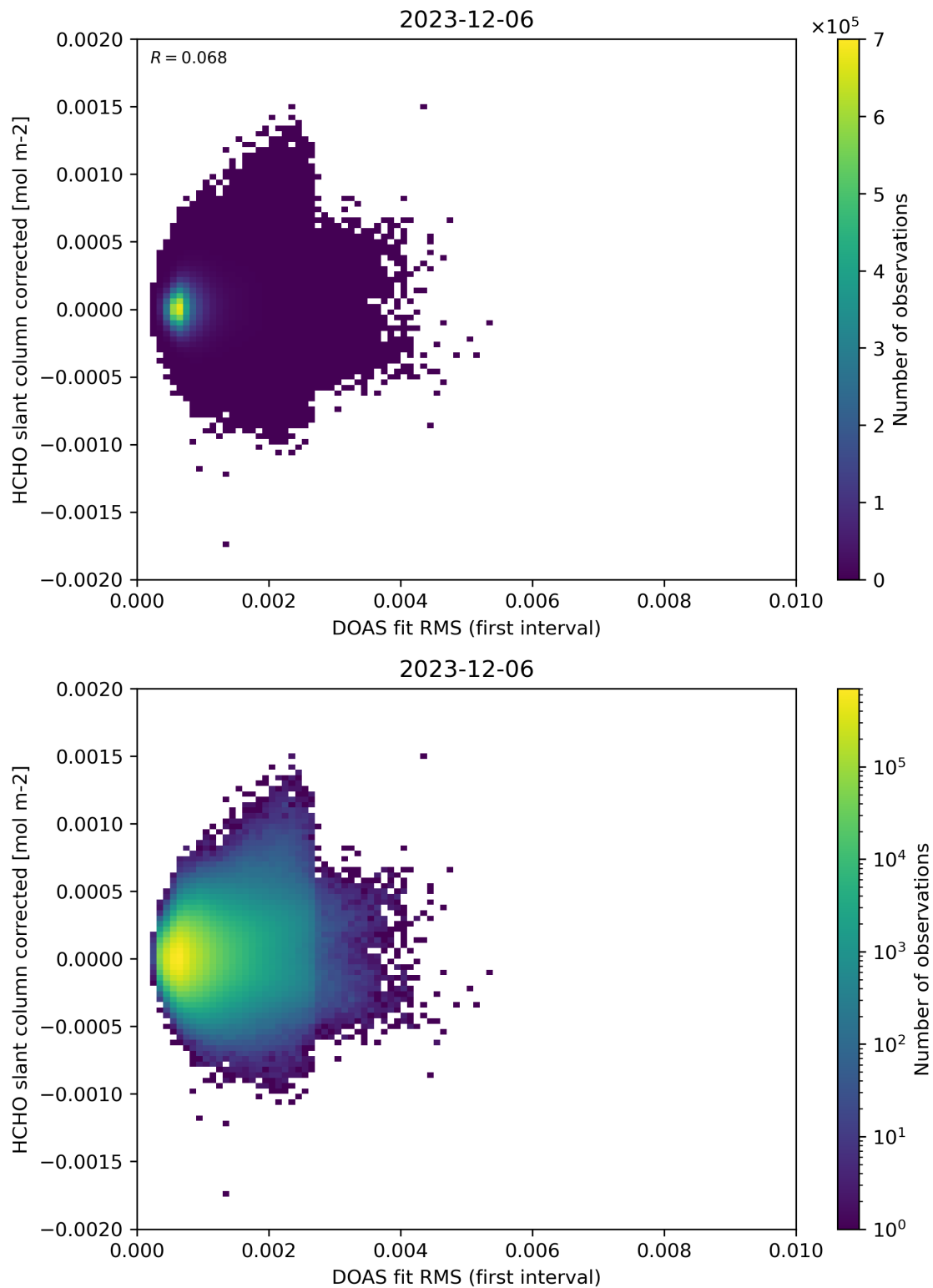
Figure 62: Scatter density plot of “DOAS fit RMS (first interval)” against “HCHO slant column corrected” for 2023-12-05 to 2023-12-07.
