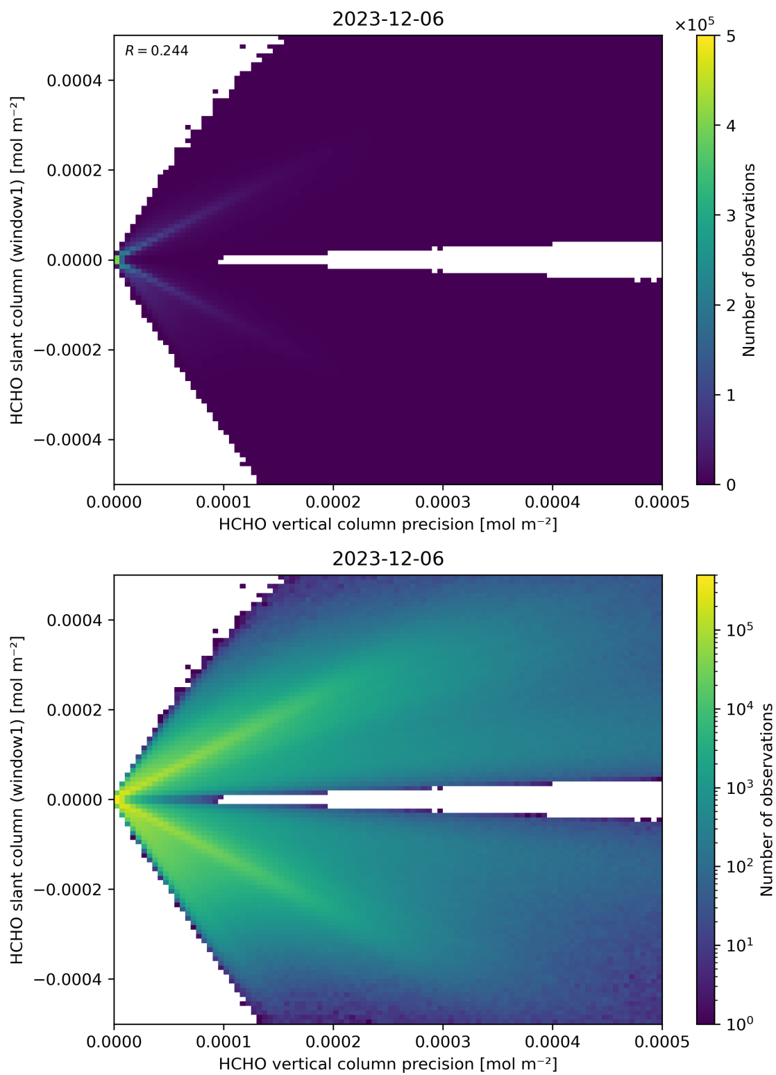
Figure 142: Scatter density plot of “HCHO vertical column precision” against “HCHO slant column (window1)” for 2023-12-05 to 2023-12-07.
