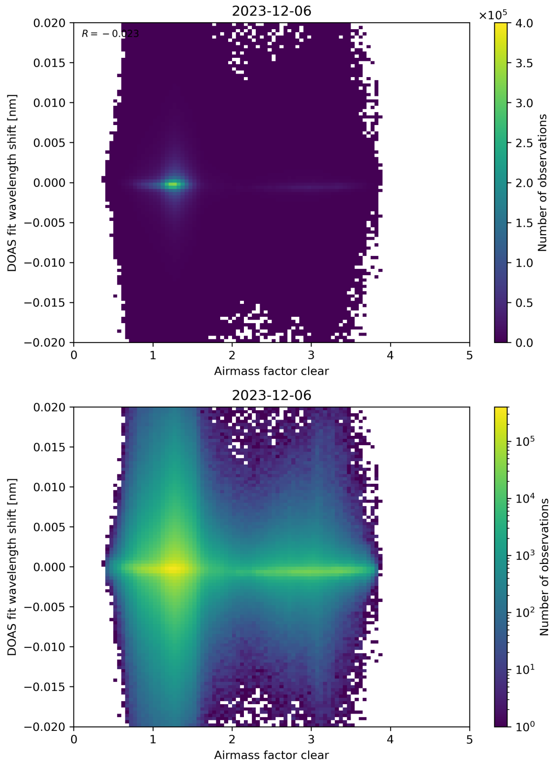
Figure 72: Scatter density plot of “Airmass factor clear” against “DOAS fit wavelength shift” for 2023-12-05 to 2023-12-07.
