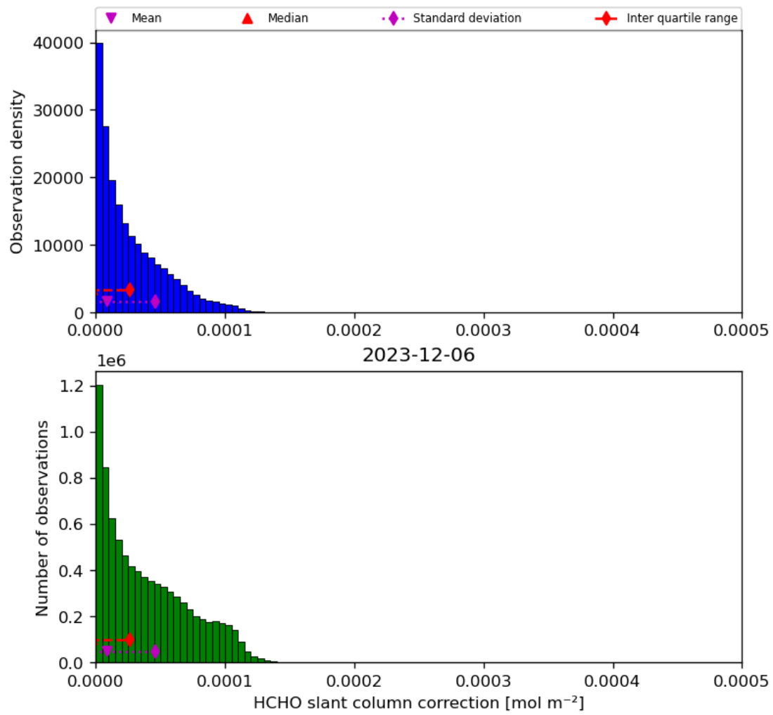
Figure 47: Histogram of “HCHO slant column correction” for 2023-12-05 to 2023-12-07
