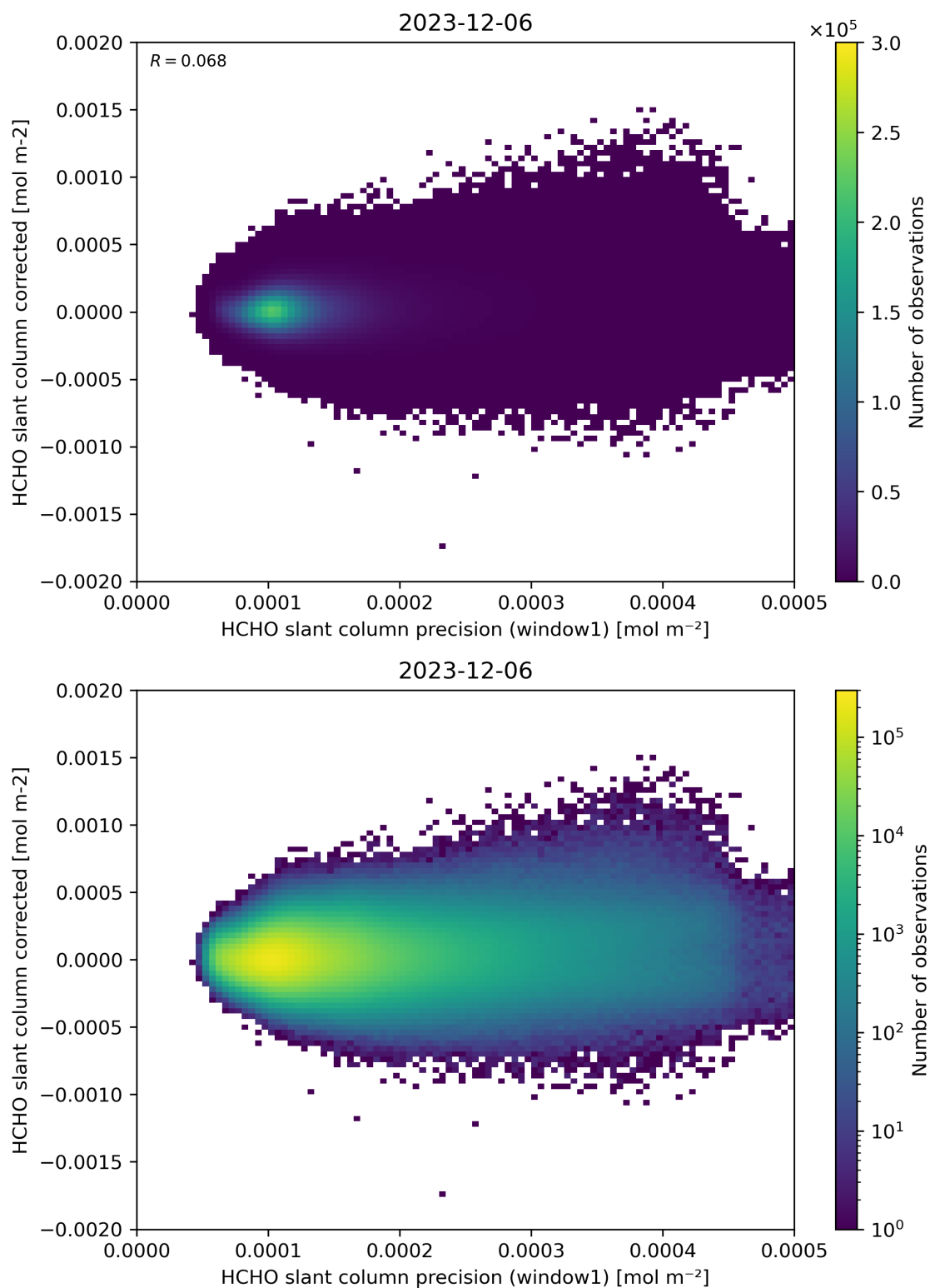
Figure 92: Scatter density plot of “HCHO slant column precision (window1)” against “HCHO slant column corrected” for 2023-12-05 to 2023-12-07.
