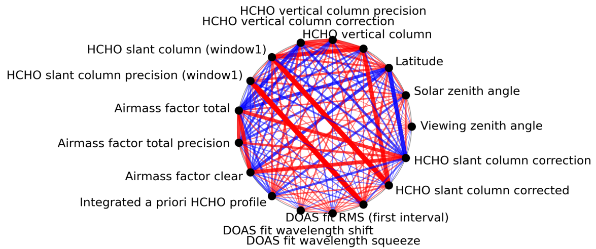
Figure 1: Map of correlation graph for 2023-12-05 to 2023-12-07.
