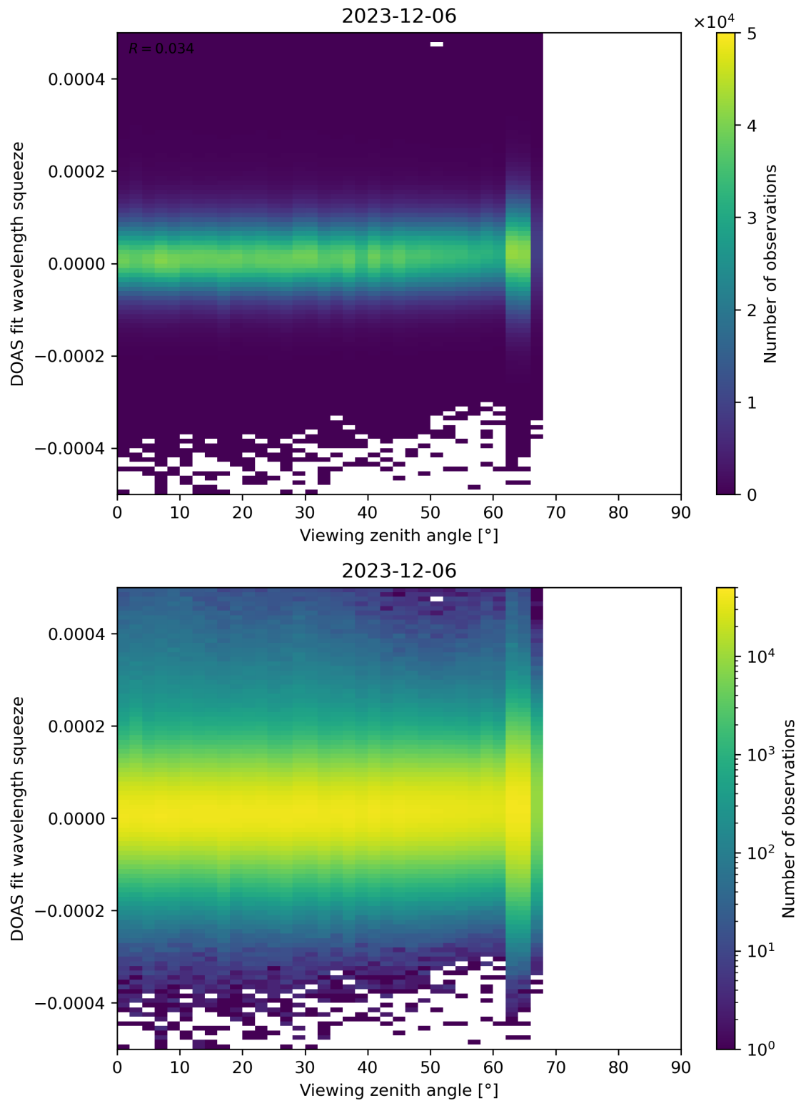
Figure 184: Scatter density plot of “Viewing zenith angle” against “DOAS fit wavelength squeeze” for 2023-12-05 to 2023-12-07.
