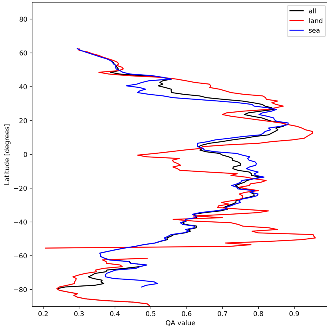
Figure 20: Zonal average of “QA value” for 2023-12-05 to 2023-12-07.
