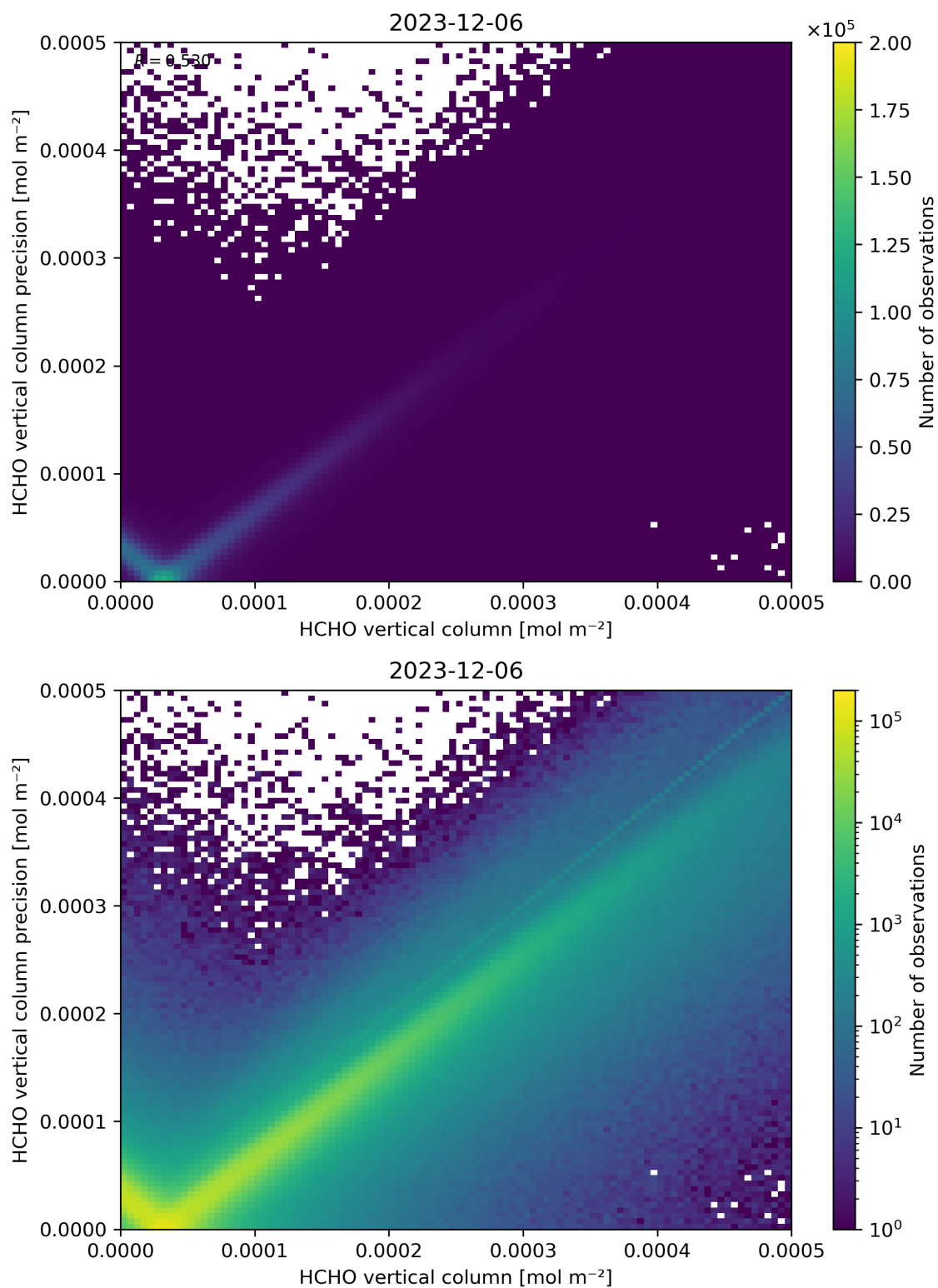
Figure 134: Scatter density plot of “HCHO vertical column” against “HCHO vertical column precision” for 2023-12-05 to 2023-12-07.
