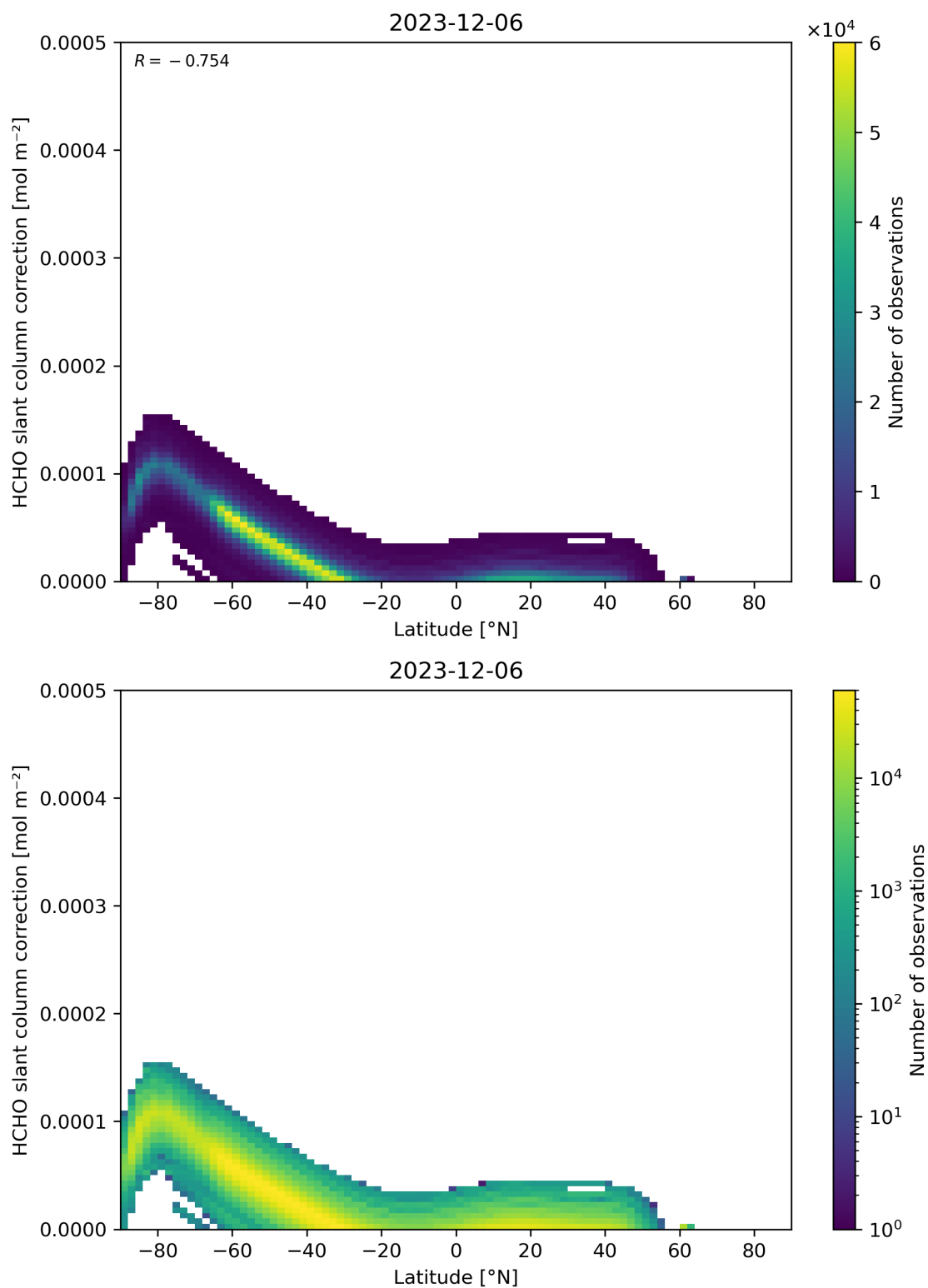
Figure 158: Scatter density plot of “Latitude” against “HCHO slant column correction” for 2023-12-05 to 2023-12-07.
