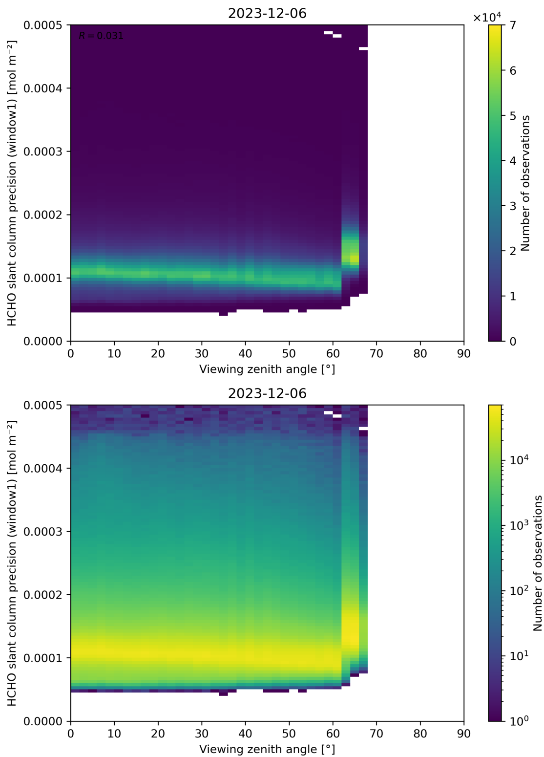
Figure 189: Scatter density plot of “Viewing zenith angle” against “HCHO slant column precision (window1)” for 2023-12-05 to 2023-12-07.
