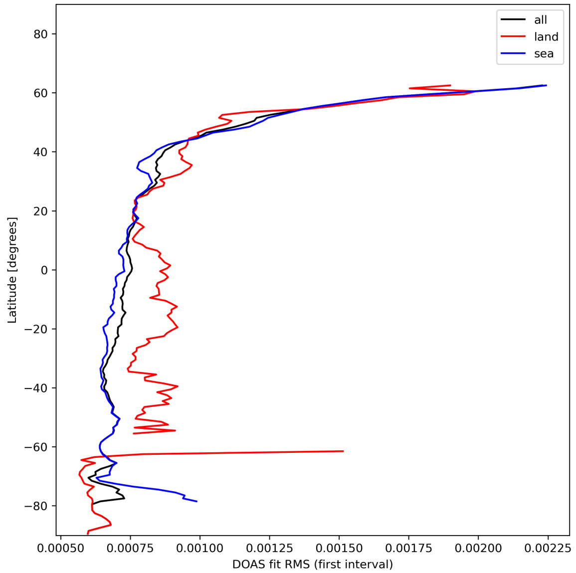
Figure 32: Zonal average of “DOAS fit RMS (first interval)” for 2023-12-05 to 2023-12-07.
