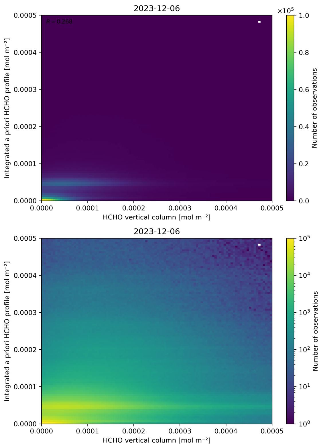
Figure 135: Scatter density plot of “HCHO vertical column” against “Integrated a priori HCHO profile” for 2023-12-05 to 2023-12-07.
