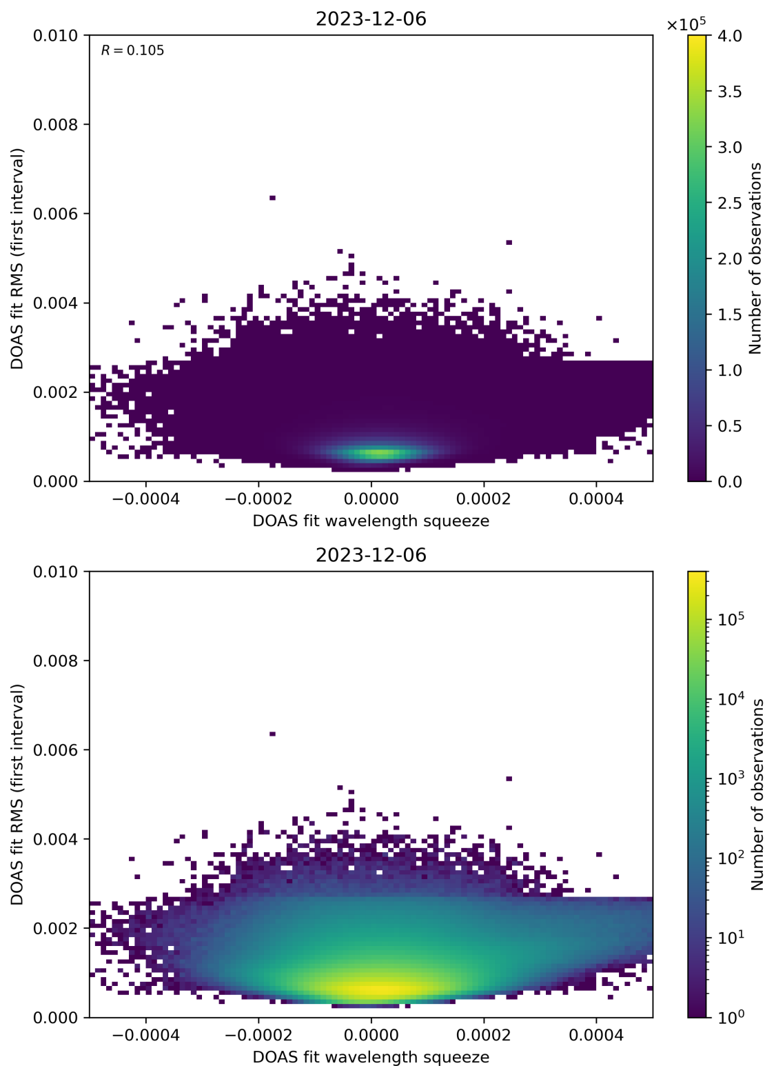
Figure 68: Scatter density plot of “DOAS fit wavelength squeeze” against “DOAS fit RMS (first interval)” for 2023-12-05 to 2023-12-07.
