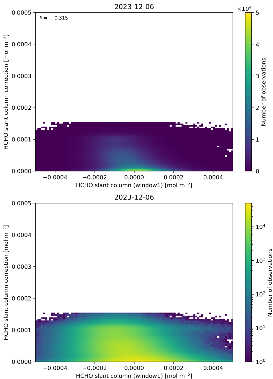
Figure 83: Scatter density plot of “HCHO slant column (window1)” against “HCHO slant column correction” for 2023-12-05 to 2023-12-07.
