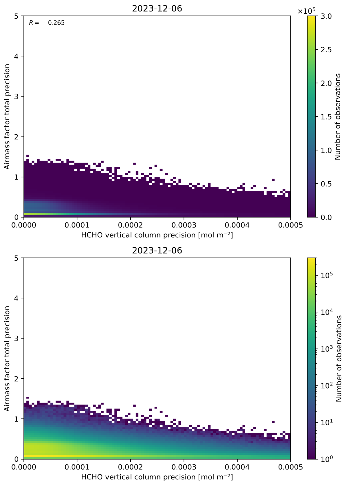
Figure 145: Scatter density plot of “HCHO vertical column precision” against “Airmass factor total precision” for 2023-12-05 to 2023-12-07.
