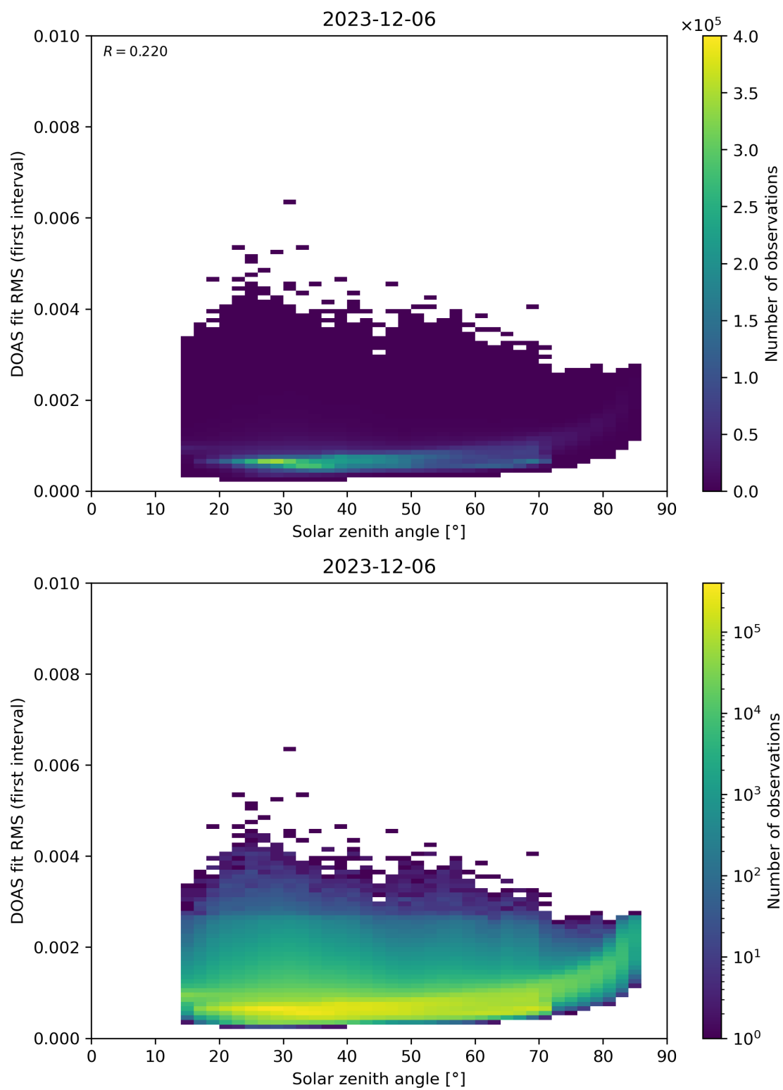
Figure 167: Scatter density plot of “Solar zenith angle” against “DOAS fit RMS (first interval)” for 2023-12-05 to 2023-12-07.
