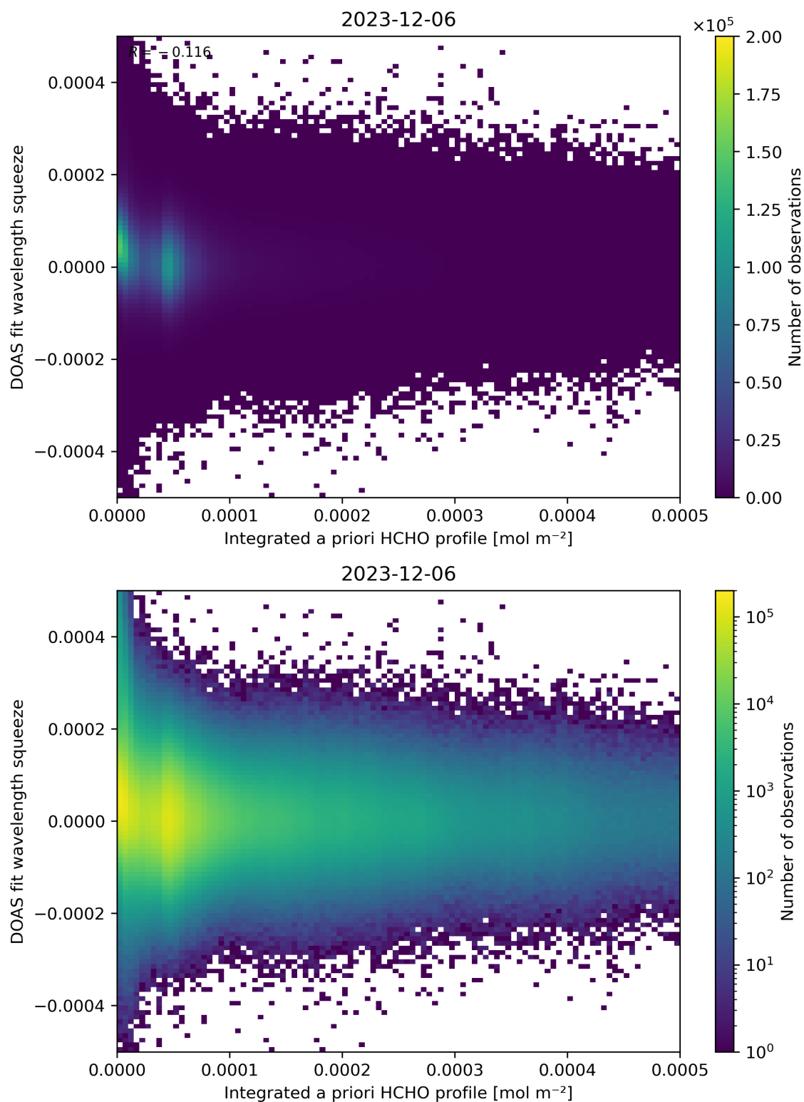
Figure 150: Scatter density plot of “Integrated a priori HCHO profile” against “DOAS fit wavelength squeeze” for 2023-12-05 to 2023-12-07.
