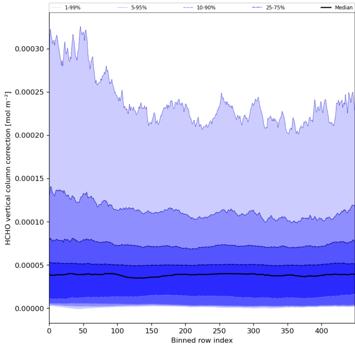
Figure 51: Along track statistics of “HCHO vertical column correction” for 2023-12-05 to 2023-12-07
