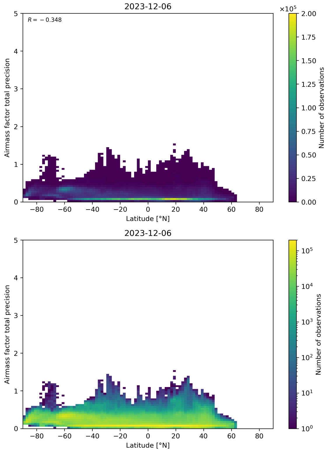
Figure 162: Scatter density plot of “Latitude” against “Airmass factor total precision” for 2023-12-05 to 2023-12-07.
