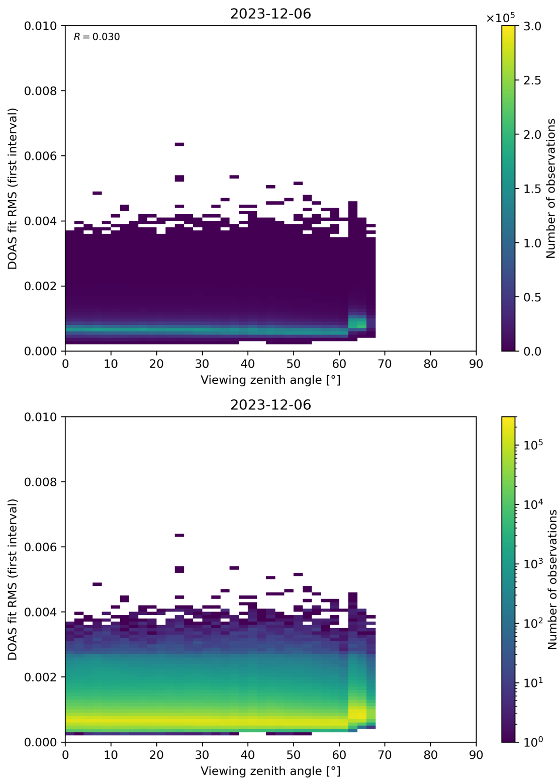
Figure 182: Scatter density plot of “Viewing zenith angle” against “DOAS fit RMS (first interval)” for 2023-12-05 to 2023-12-07.
