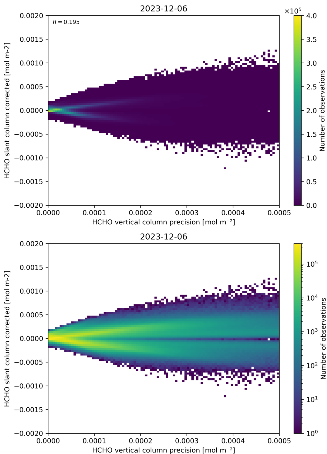
Figure 140: Scatter density plot of “HCHO vertical column precision” against “HCHO slant column corrected” for 2023-12-05 to 2023-12-07.
