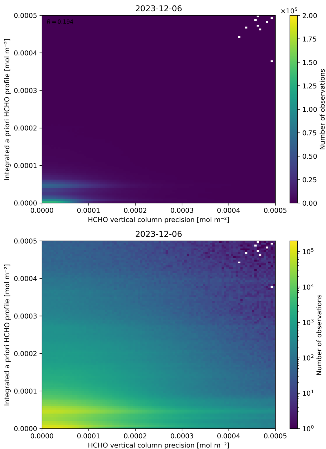
Figure 147: Scatter density plot of “HCHO vertical column precision” against “Integrated a priori HCHO profile” for 2023-12-05 to 2023-12-07.
