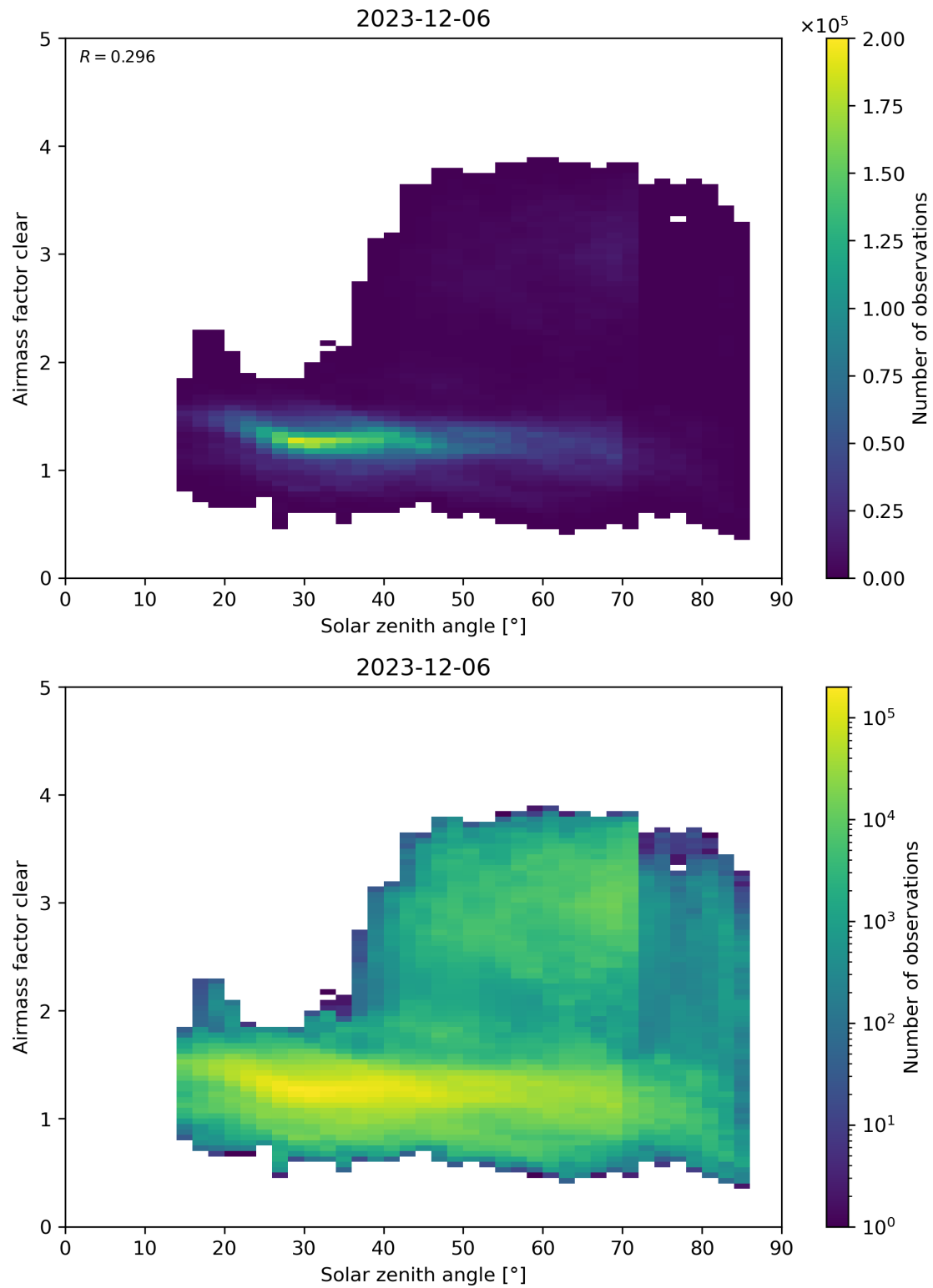
Figure 170: Scatter density plot of “Solar zenith angle” against “Airmass factor clear” for 2023-12-05 to 2023-12-07.
