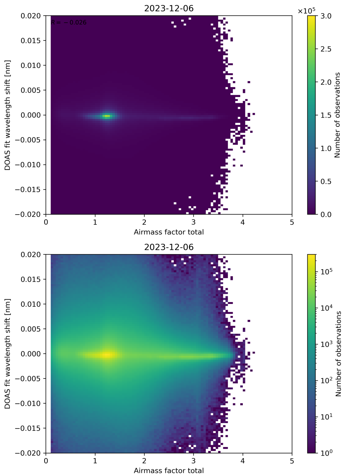
Figure 98: Scatter density plot of “Airmass factor total” against “DOAS fit wavelength shift” for 2023-12-05 to 2023-12-07.
