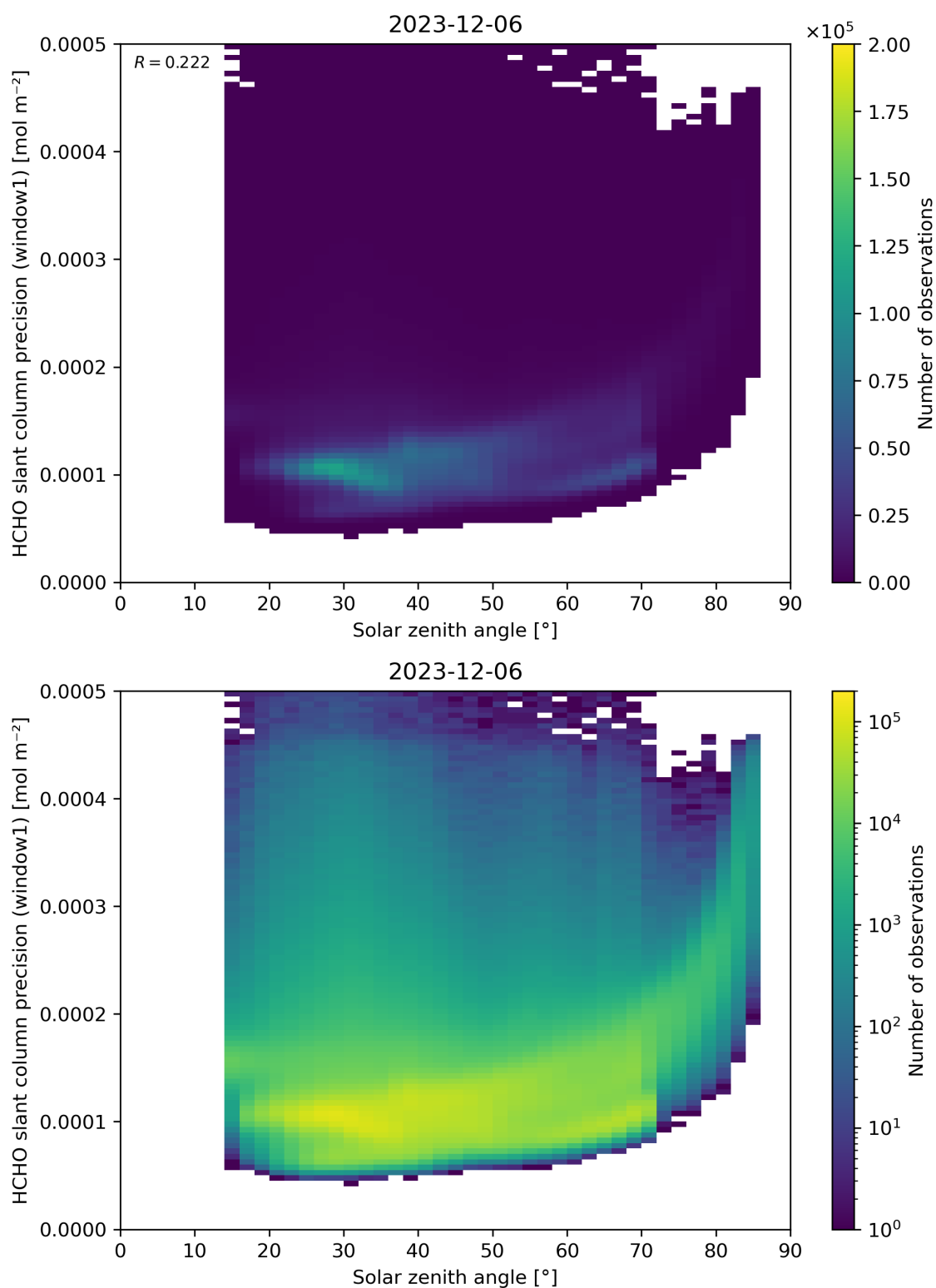
Figure 174: Scatter density plot of “Solar zenith angle” against “HCHO slant column precision (window1)” for 2023-12-05 to 2023-12-07.
