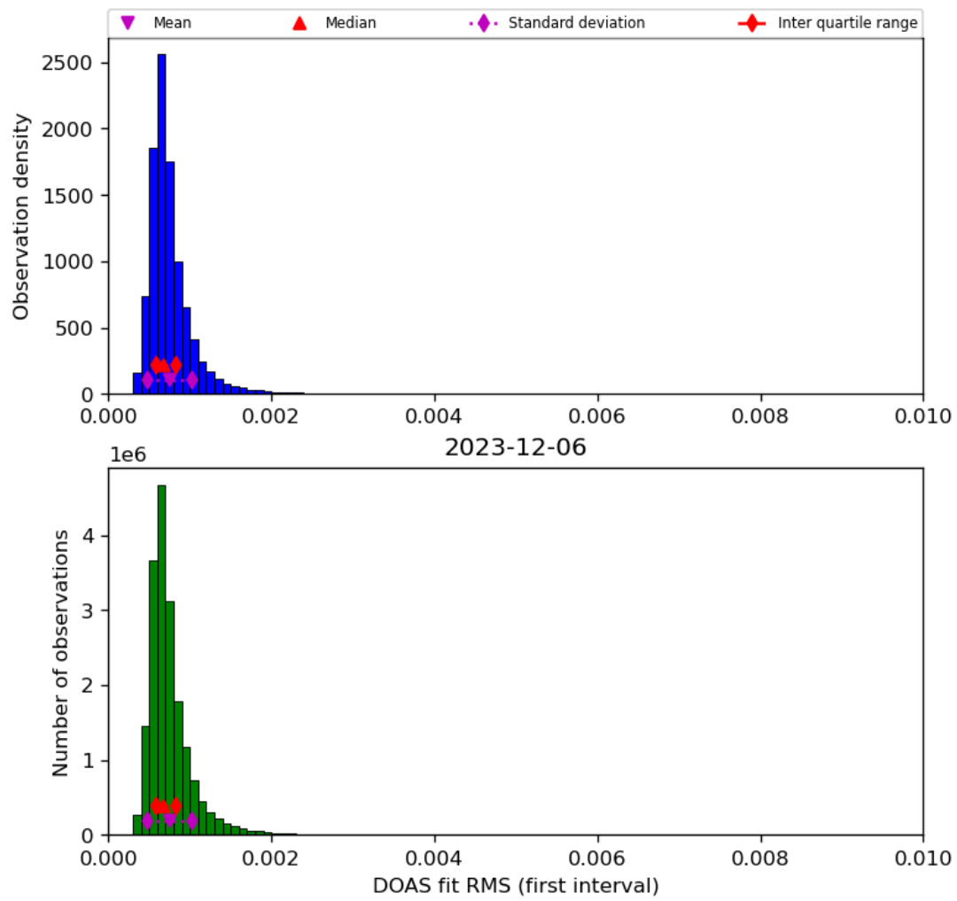
Figure 46: Histogram of “DOAS fit RMS (first interval)” for 2023-12-05 to 2023-12-07
