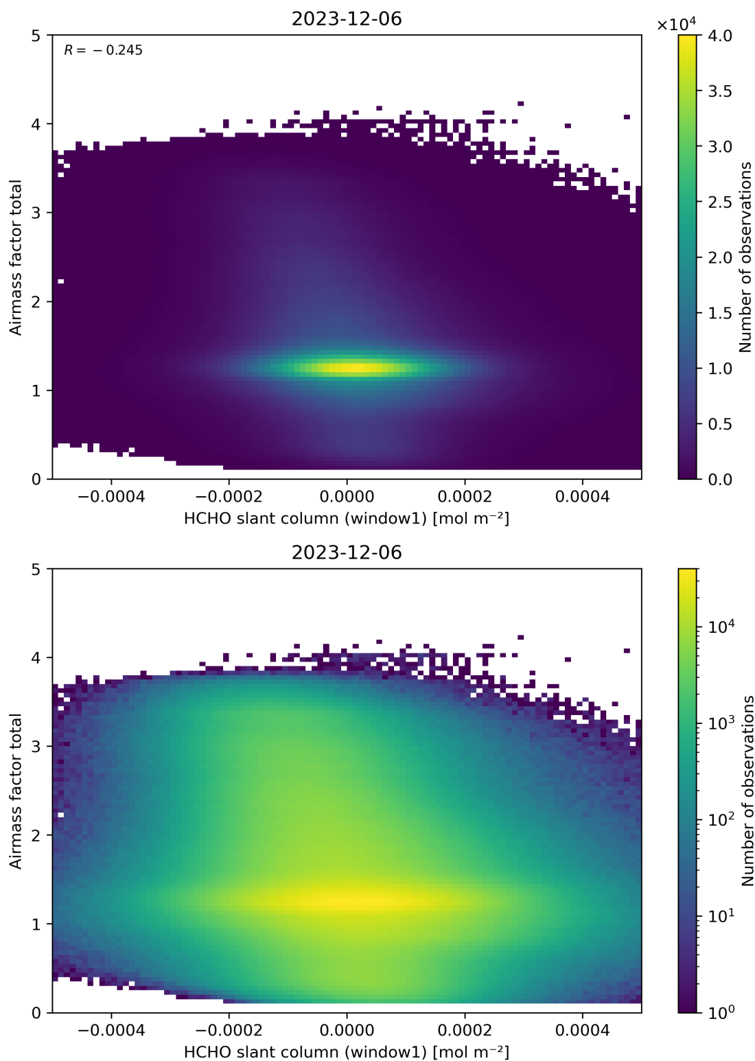
Figure 85: Scatter density plot of “HCHO slant column (window1)” against “Airmass factor total” for 2023-12-05 to 2023-12-07.
