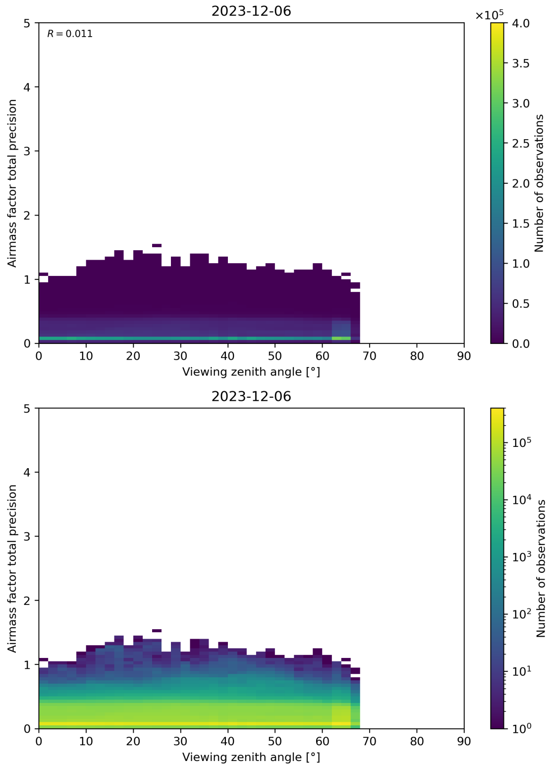
Figure 191: Scatter density plot of “Viewing zenith angle” against “Airmass factor total precision” for 2023-12-05 to 2023-12-07.
