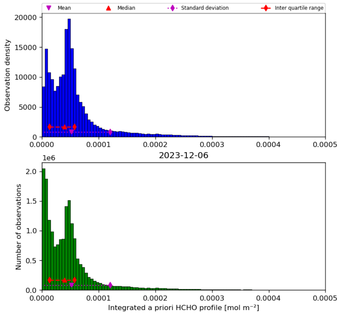
Figure 43: Histogram of “Integrated a priori HCHO profile” for 2023-12-05 to 2023-12-07
