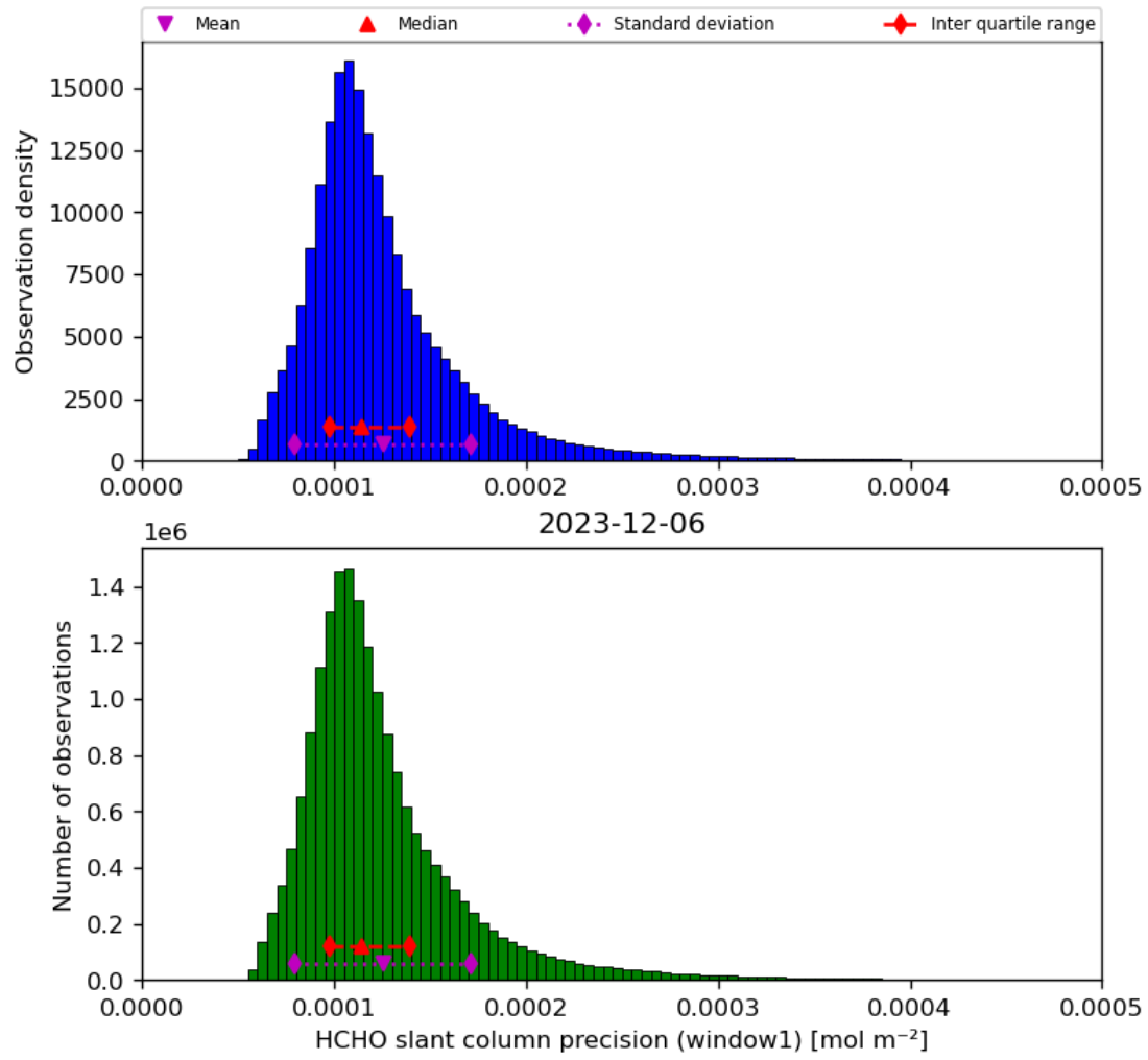
Figure 39: Histogram of “HCHO slant column precision (window1)” for 2023-12-05 to 2023-12-07
