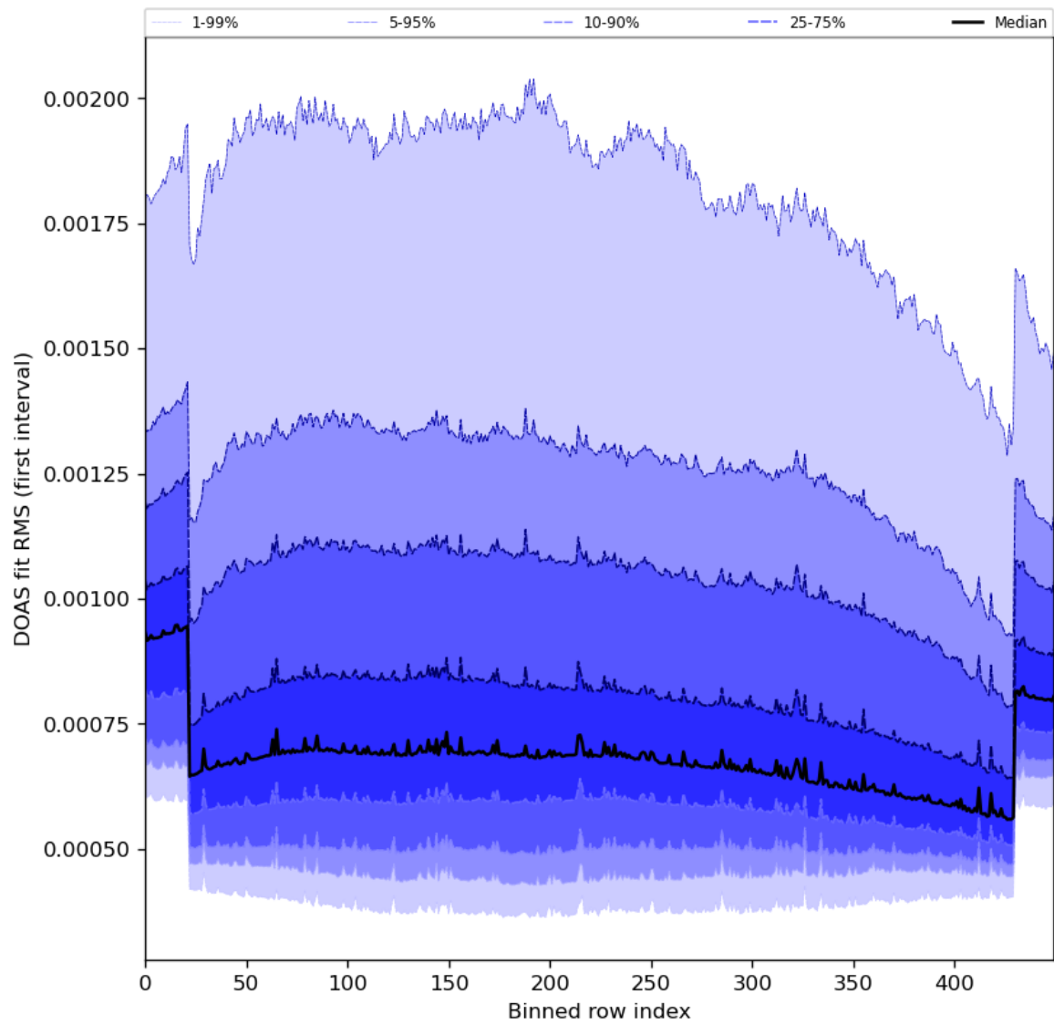
Figure 60: Along track statistics of “DOAS fit RMS (first interval)” for 2023-12-05 to 2023-12-07
