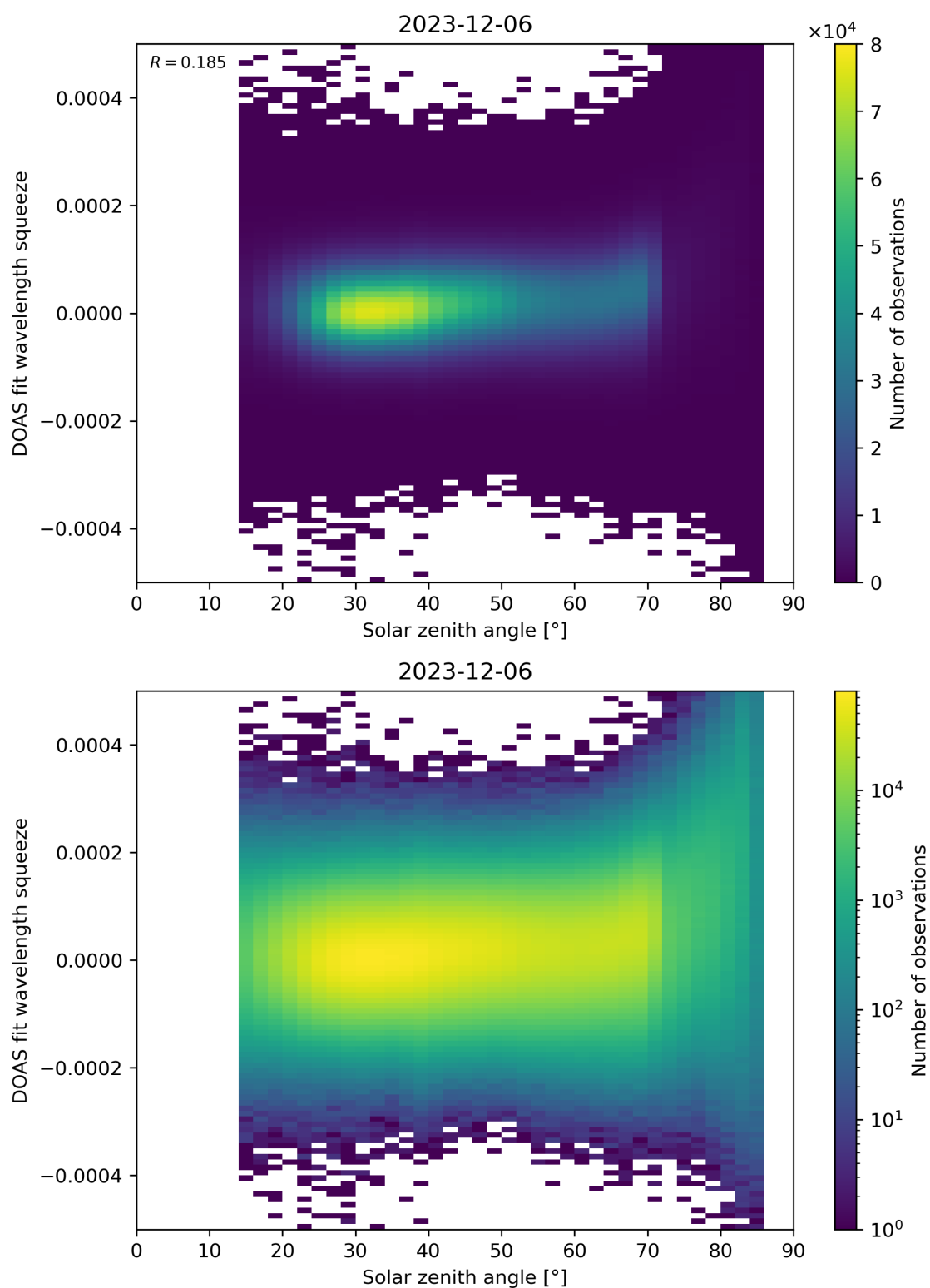
Figure 169: Scatter density plot of “Solar zenith angle” against “DOAS fit wavelength squeeze” for 2023-12-05 to 2023-12-07.
