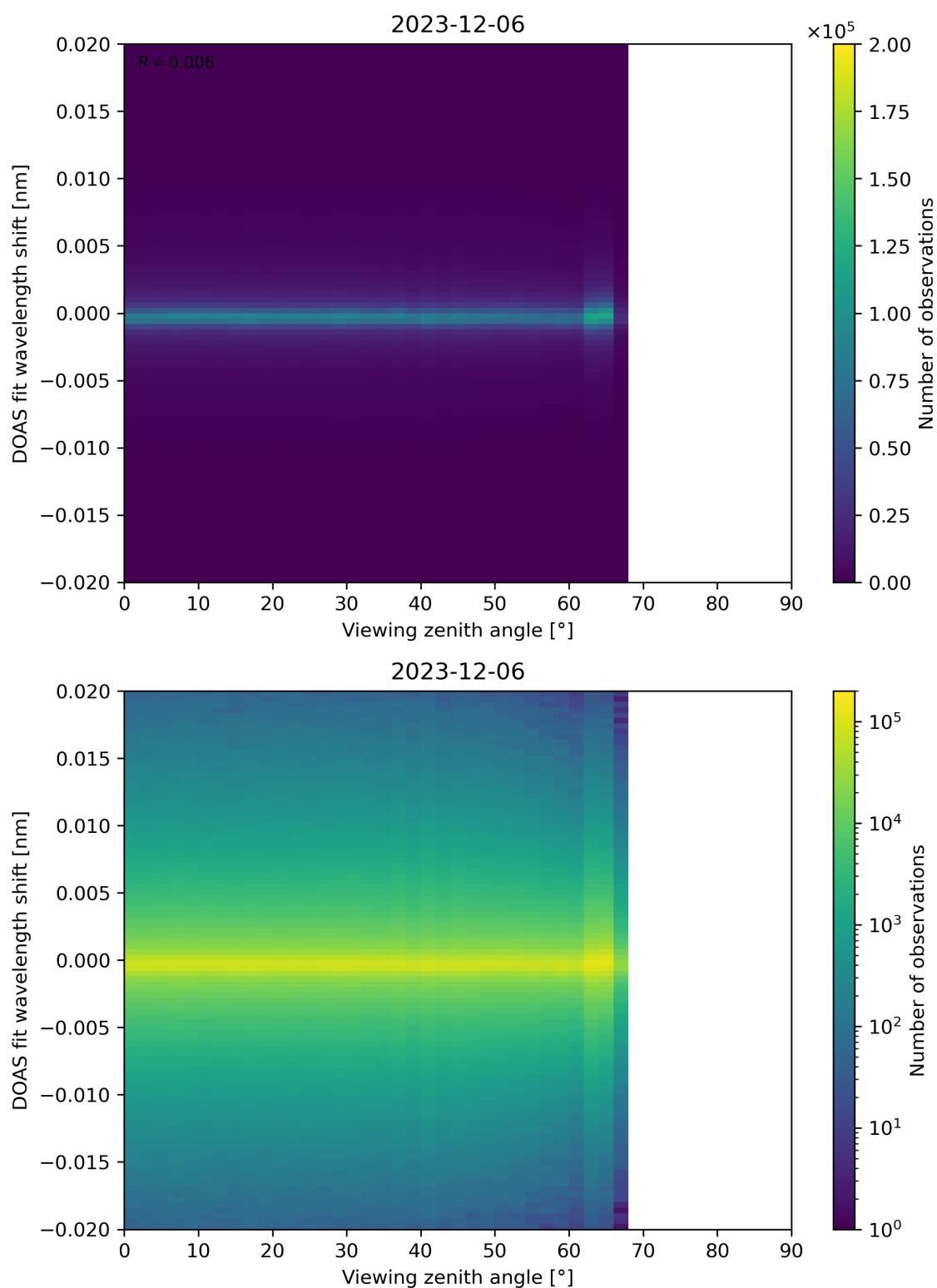
Figure 183: Scatter density plot of “Viewing zenith angle” against “DOAS fit wavelength shift” for 2023-12-05 to 2023-12-07.
