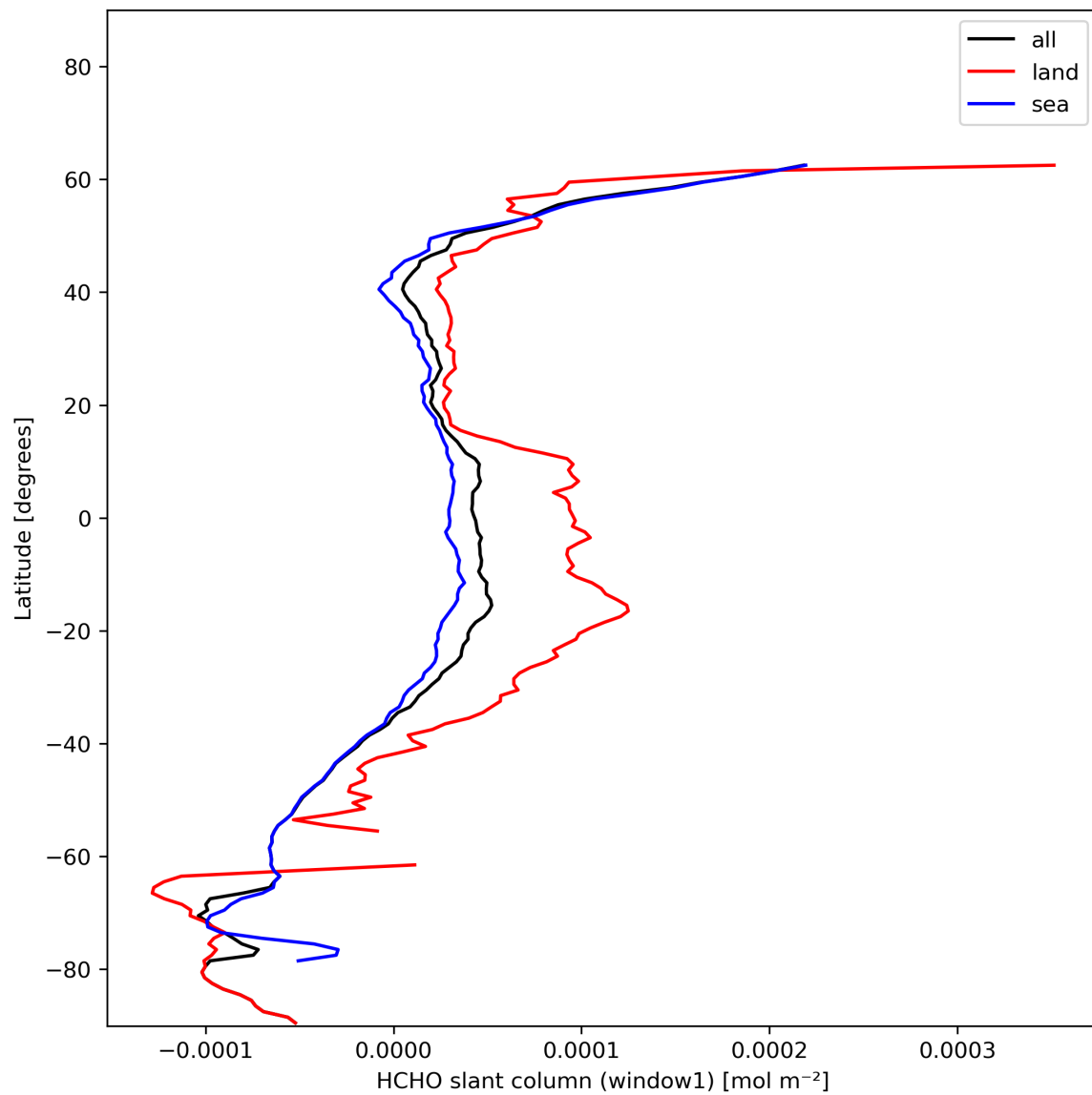
Figure 24: Zonal average of “HCHO slant column (window1)” for 2023-12-05 to 2023-12-07.
