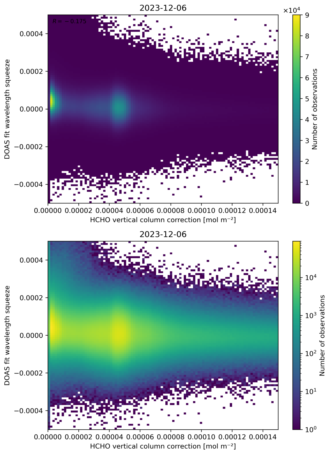
Figure 114: Scatter density plot of “HCHO vertical column correction” against “DOAS fit wavelength squeeze” for 2023-12-05 to 2023-12-07.
