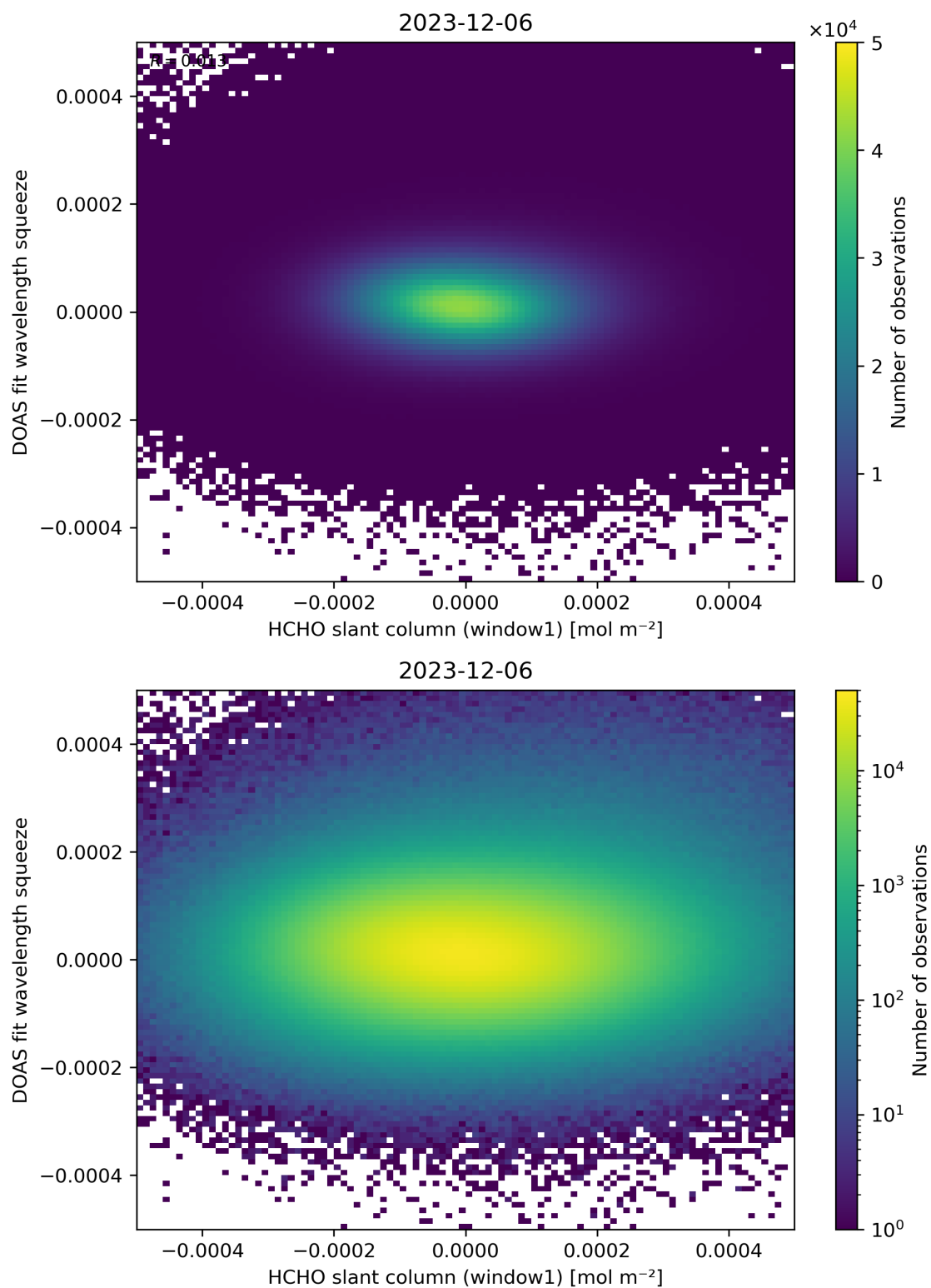
Figure 80: Scatter density plot of “HCHO slant column (window1)” against “DOAS fit wavelength squeeze” for 2023-12-05 to 2023-12-07.
