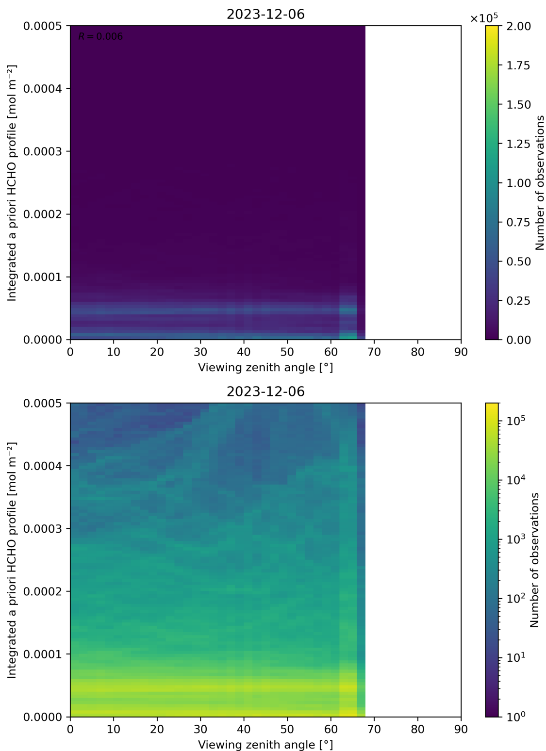
Figure 195: Scatter density plot of “Viewing zenith angle” against “Integrated a priori HCHO profile” for 2023-12-05 to 2023-12-07.
