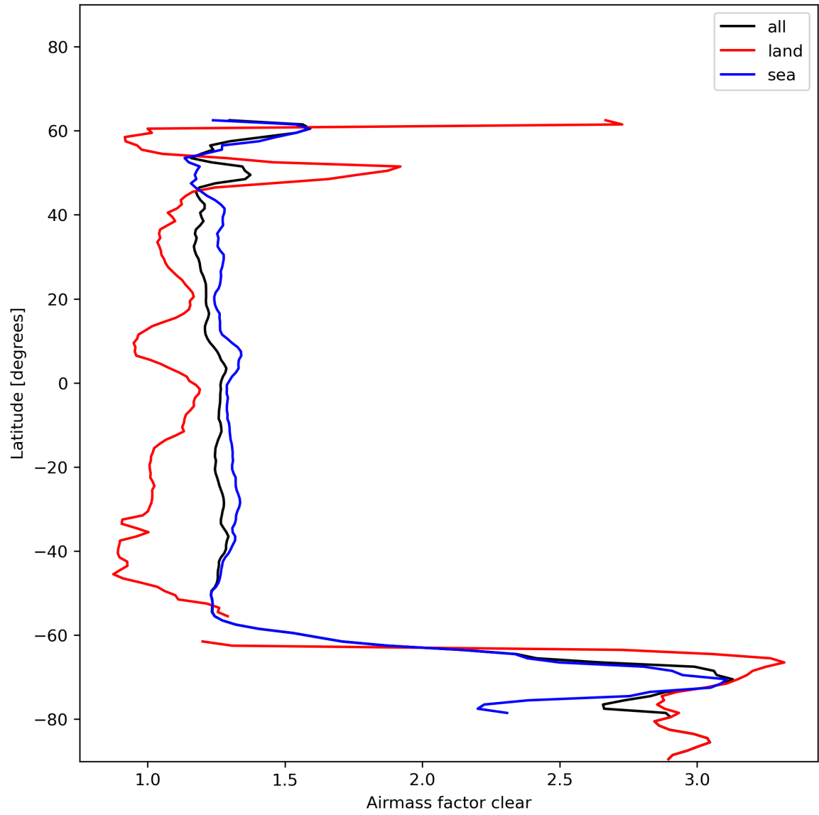
Figure 28: Zonal average of “Airmass factor clear” for 2023-12-05 to 2023-12-07.
