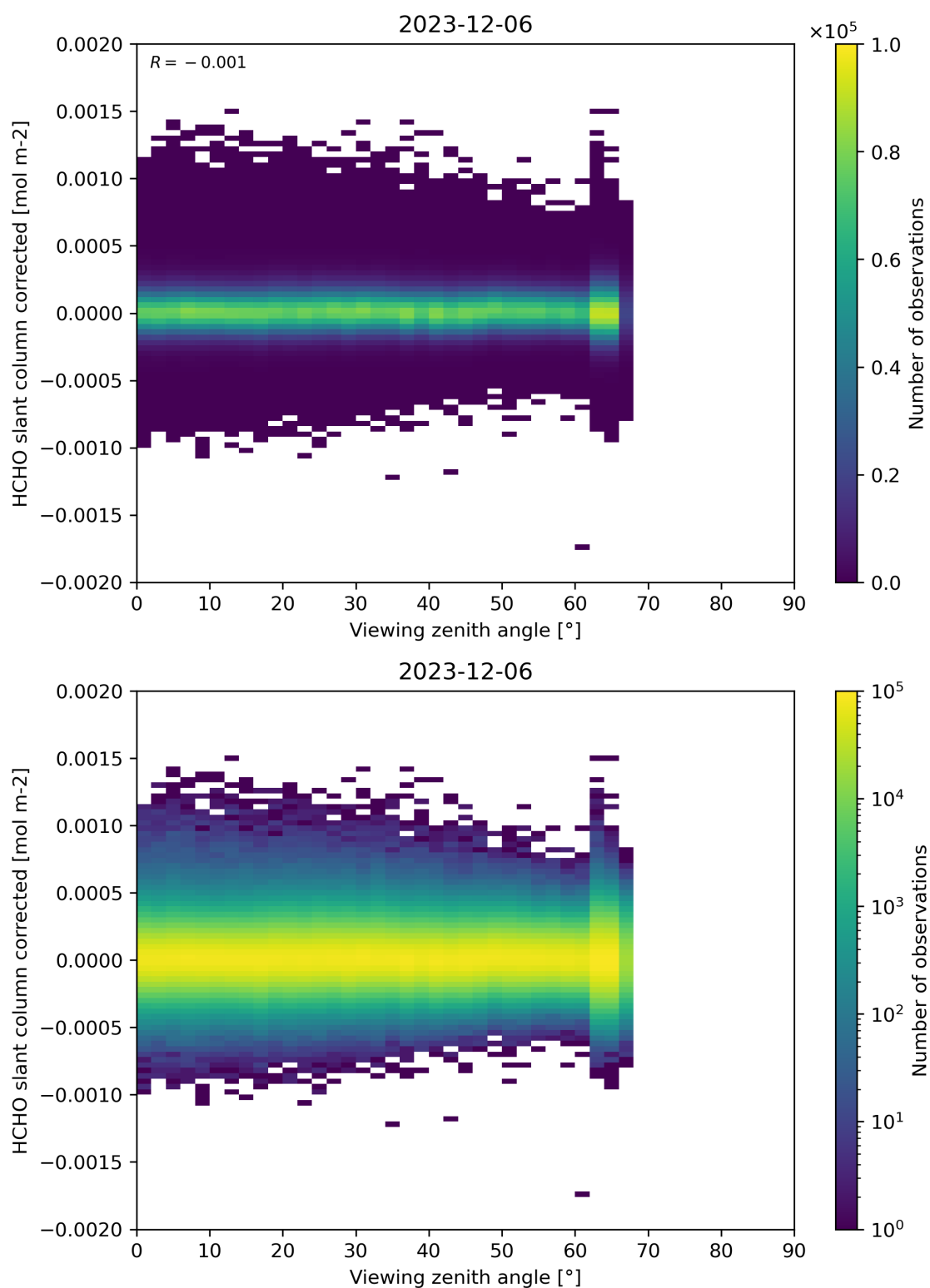
Figure 186: Scatter density plot of “Viewing zenith angle” against “HCHO slant column corrected” for 2023-12-05 to 2023-12-07.
