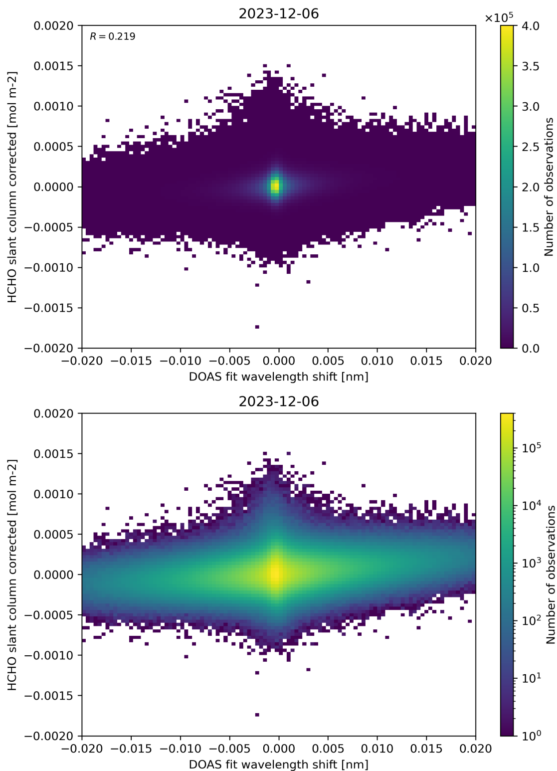
Figure 66: Scatter density plot of “DOAS fit wavelength shift” against “HCHO slant column corrected” for 2023-12-05 to 2023-12-07.
