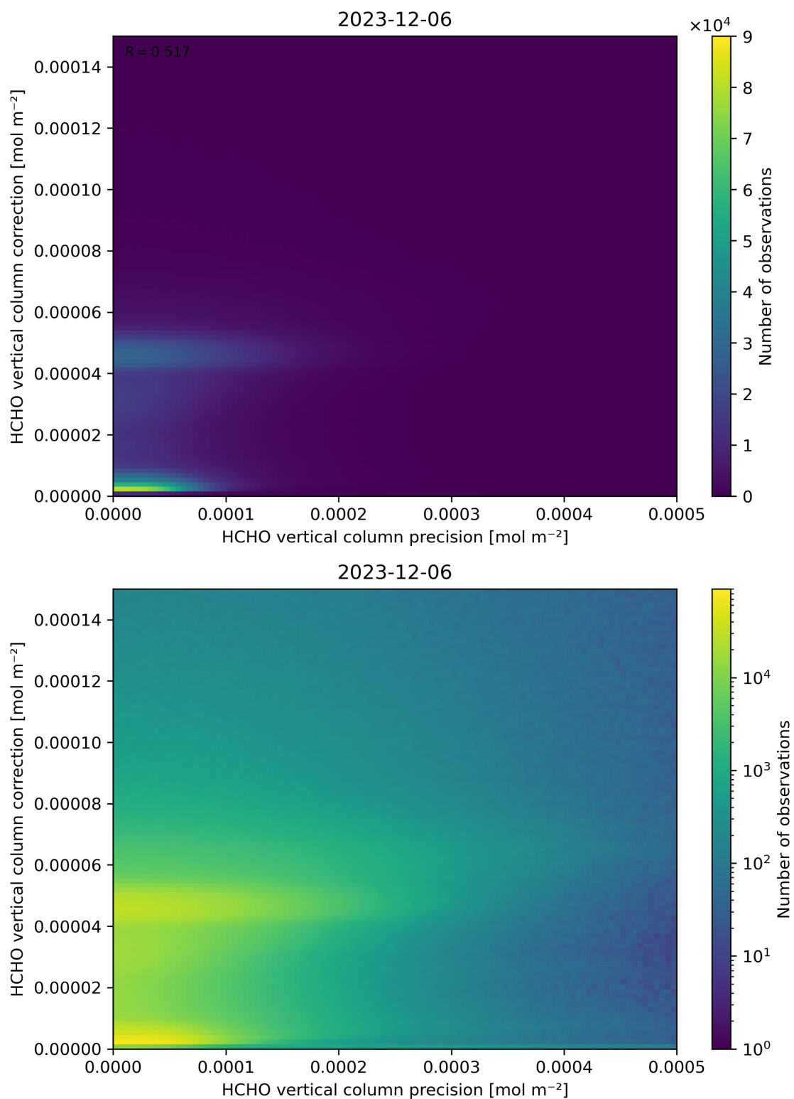
Figure 146: Scatter density plot of “HCHO vertical column precision” against “HCHO vertical column correction” for 2023-12-05 to 2023-12-07.
