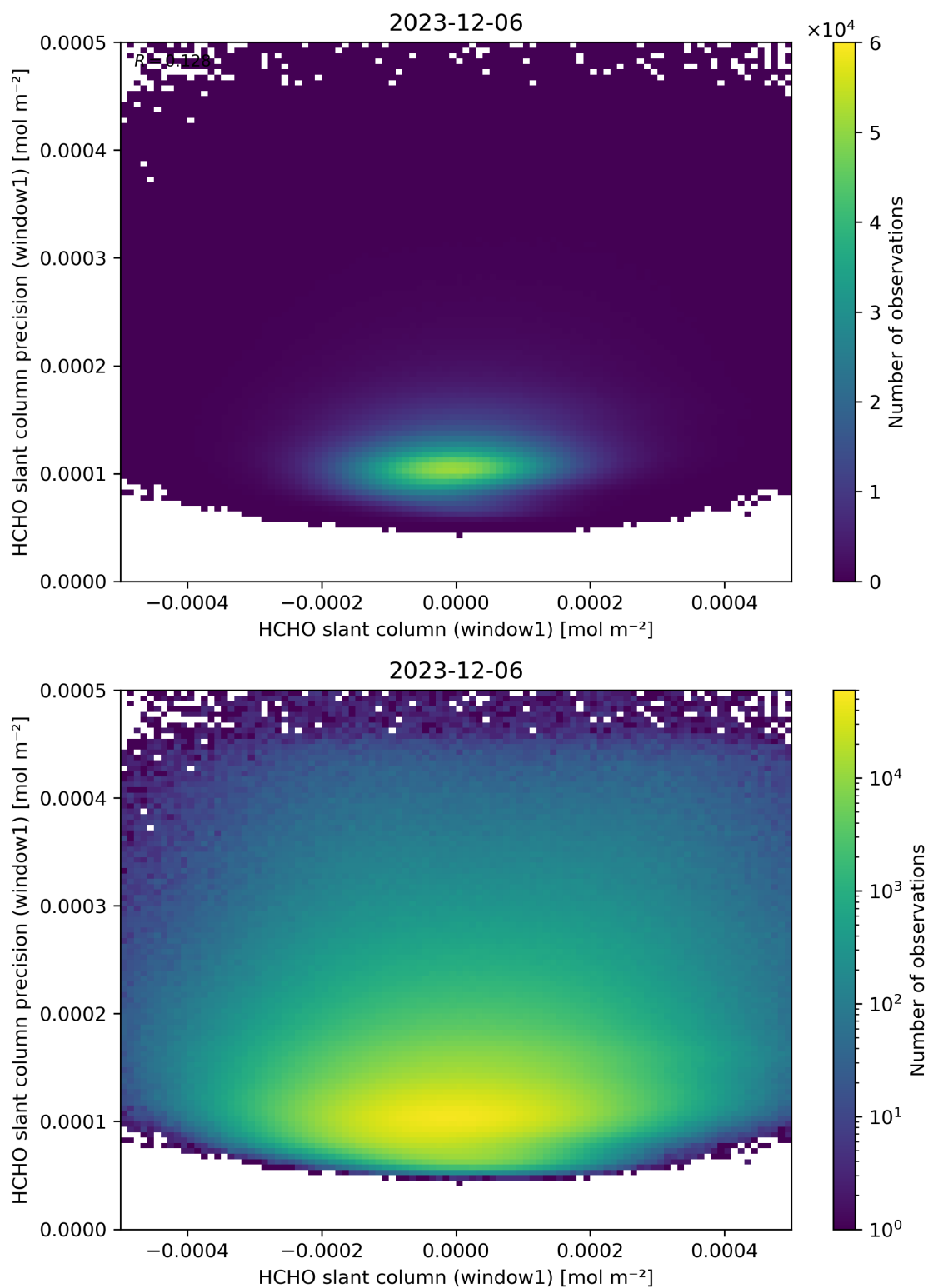
Figure 84: Scatter density plot of “HCHO slant column (window1)” against “HCHO slant column precision (window1)” for 2023-12-05 to 2023-12-07.
