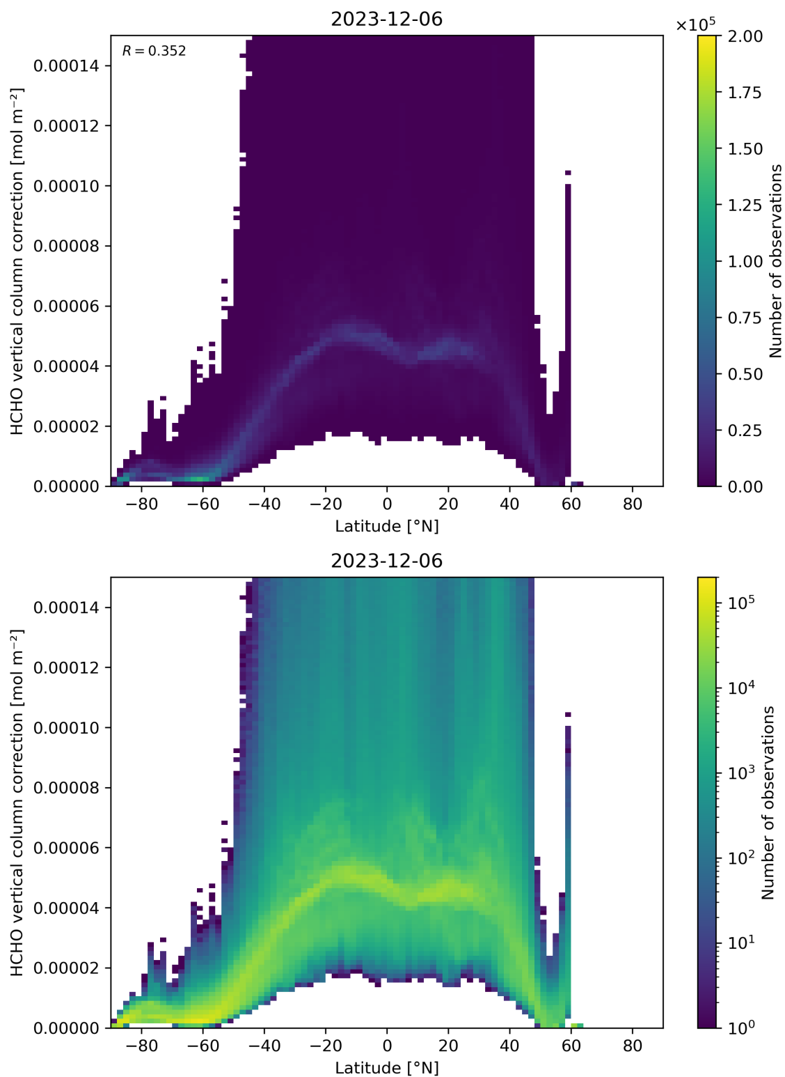
Figure 164: Scatter density plot of “Latitude” against “HCHO vertical column correction” for 2023-12-05 to 2023-12-07.
