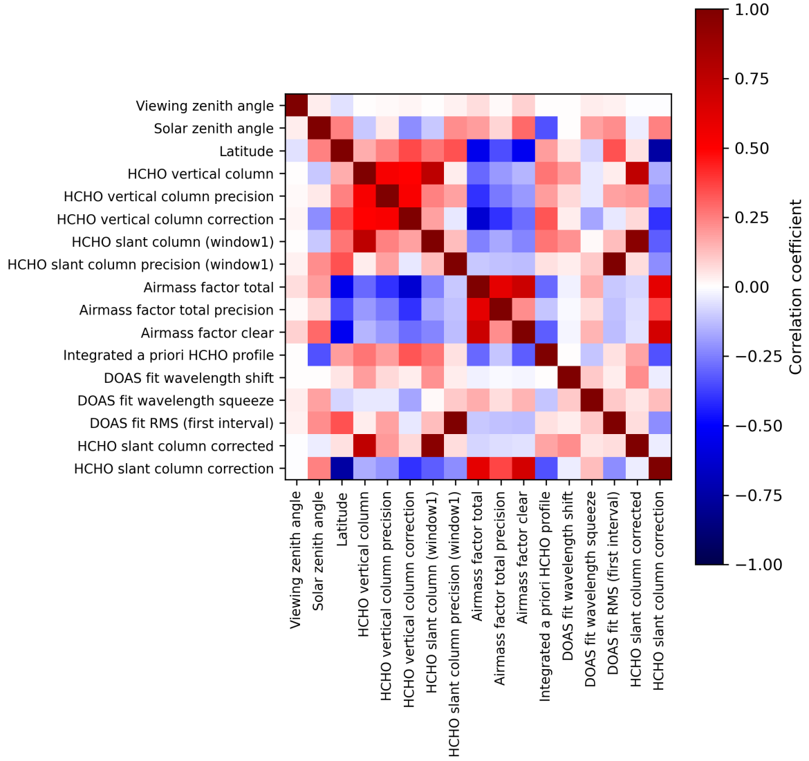
Figure 2: Map of correlation matrix for 2023-12-05 to 2023-12-07.
