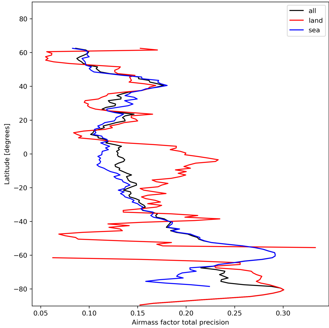
Figure 27: Zonal average of “Airmass factor total precision” for 2023-12-05 to 2023-12-07.
