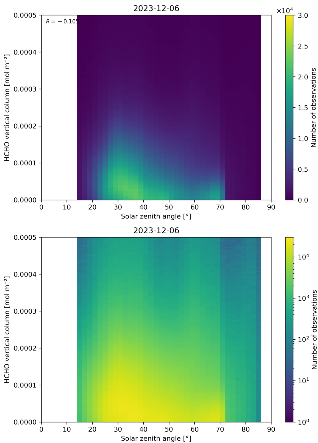
Figure 177: Scatter density plot of “Solar zenith angle” against “HCHO vertical column” for 2023-12-05 to 2023-12-07.
