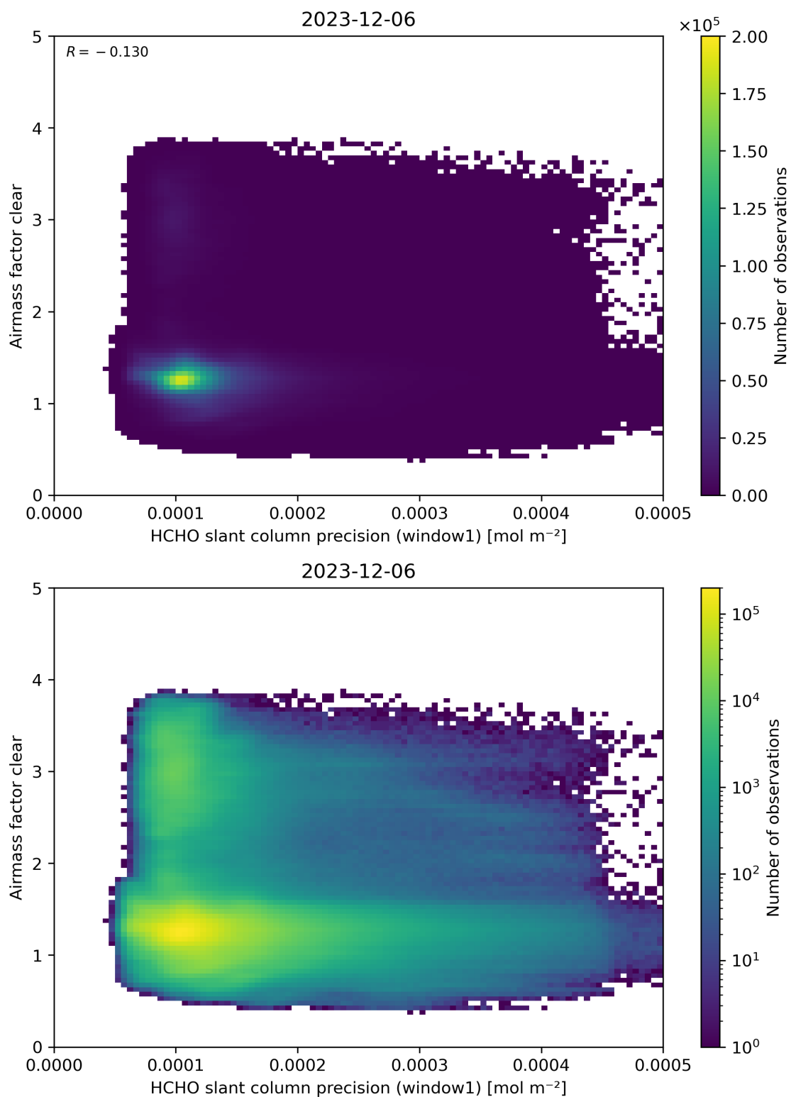
Figure 91: Scatter density plot of “HCHO slant column precision (window1)” against “Airmass factor clear” for 2023-12-05 to 2023-12-07.
