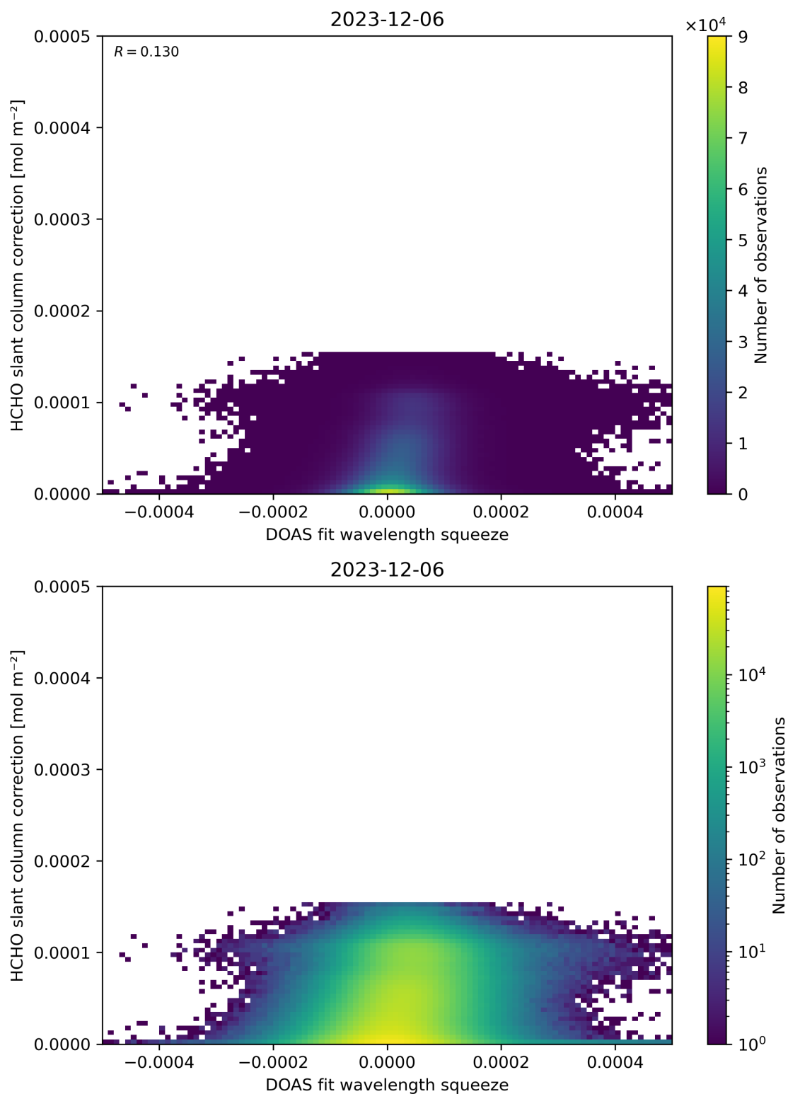
Figure 70: Scatter density plot of “DOAS fit wavelength squeeze” against “HCHO slant column correction” for 2023-12-05 to 2023-12-07.
