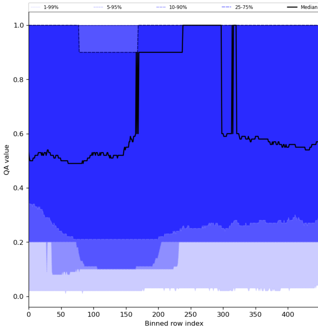
Figure 48: Along track statistics of “QA value” for 2023-12-05 to 2023-12-07
