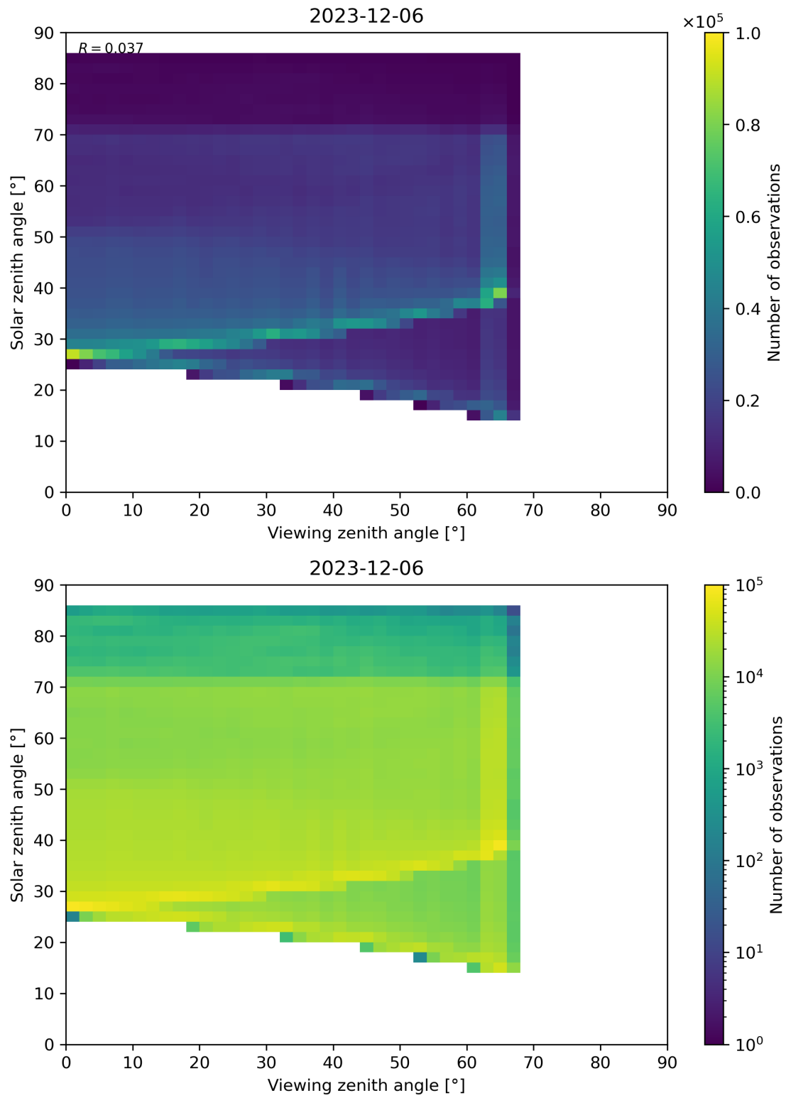
Figure 197: Scatter density plot of “Viewing zenith angle” against “Solar zenith angle” for 2023-12-05 to 2023-12-07.
