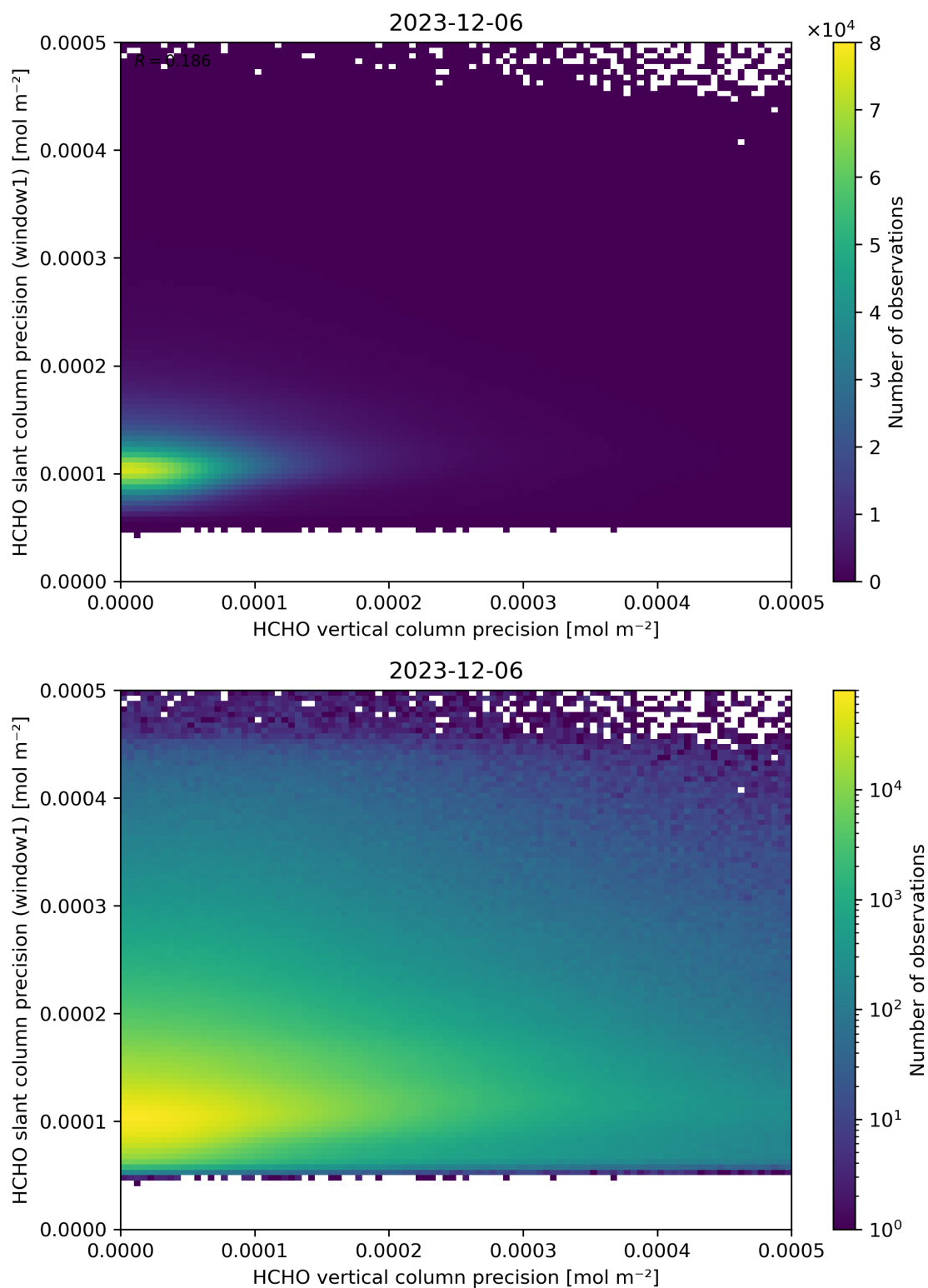
Figure 143: Scatter density plot of “HCHO vertical column precision” against “HCHO slant column precision (window1)” for 2023-12-05 to 2023-12-07.
