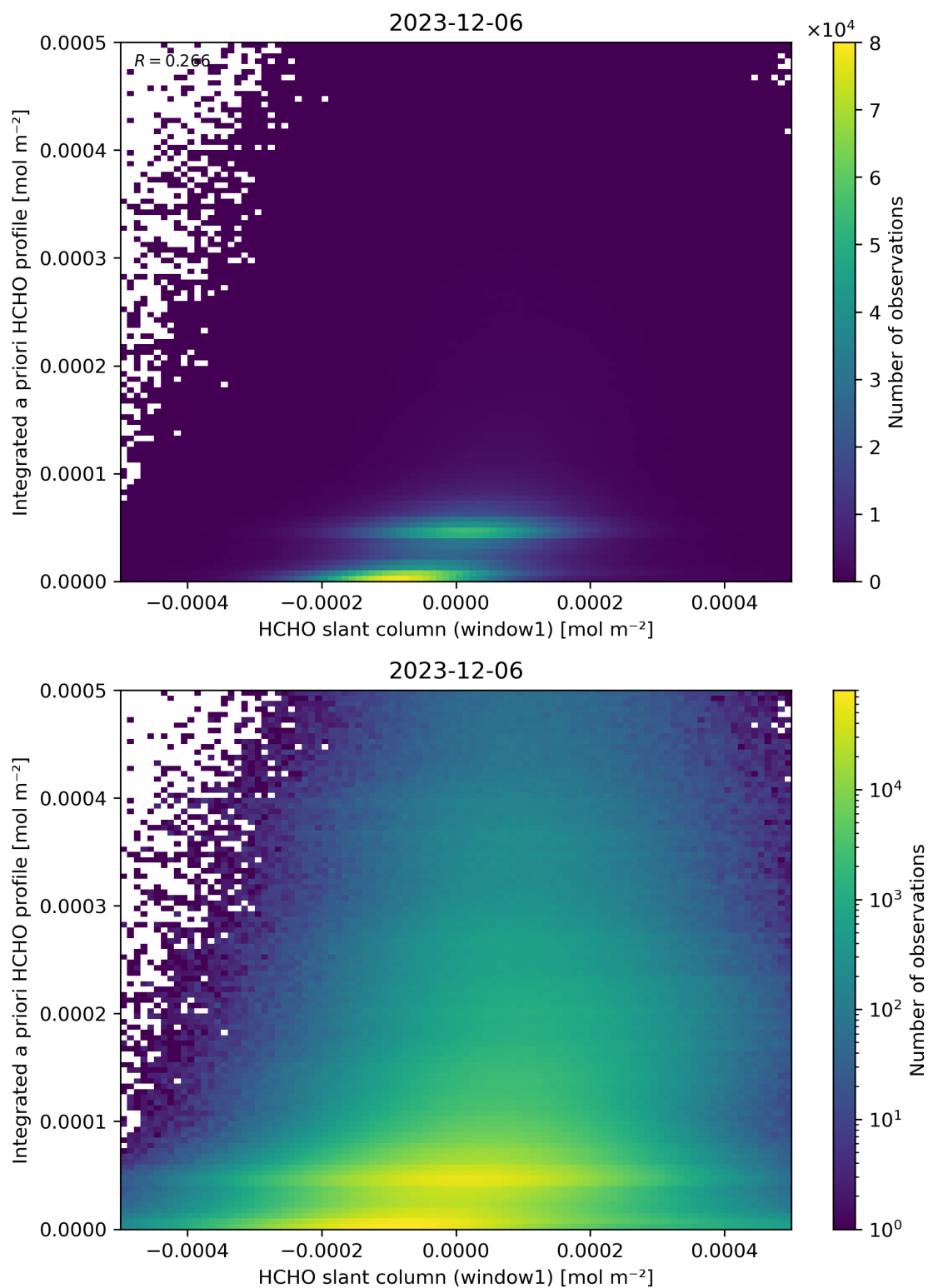
Figure 87: Scatter density plot of “HCHO slant column (window1)” against “Integrated a priori HCHO profile” for 2023-12-05 to 2023-12-07.
