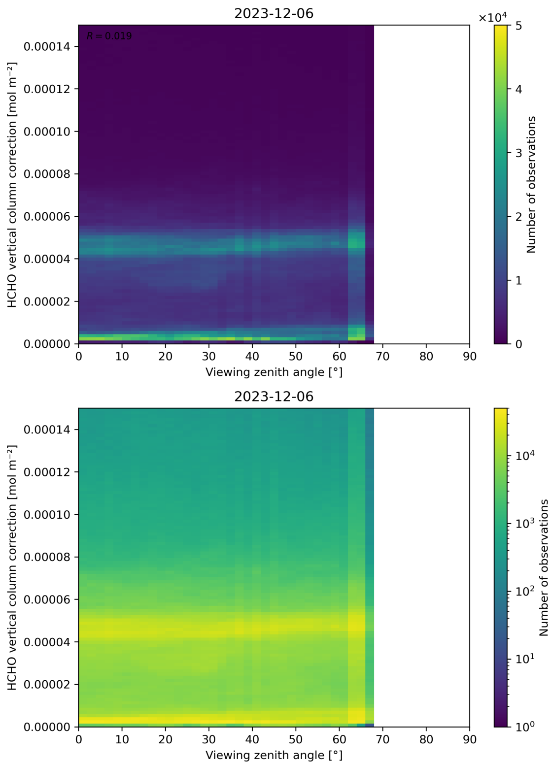
Figure 193: Scatter density plot of “Viewing zenith angle” against “HCHO vertical column correction” for 2023-12-05 to 2023-12-07.
