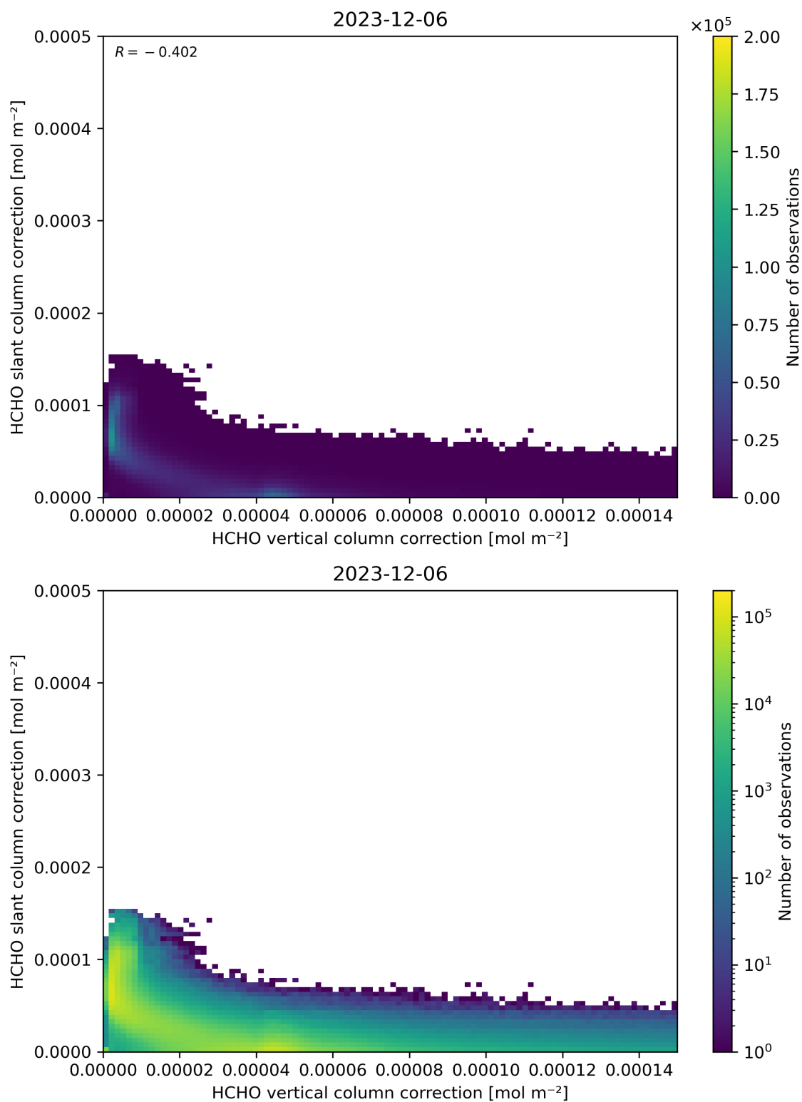
Figure 117: Scatter density plot of “HCHO vertical column correction” against “HCHO slant column correction” for 2023-12-05 to 2023-12-07.
