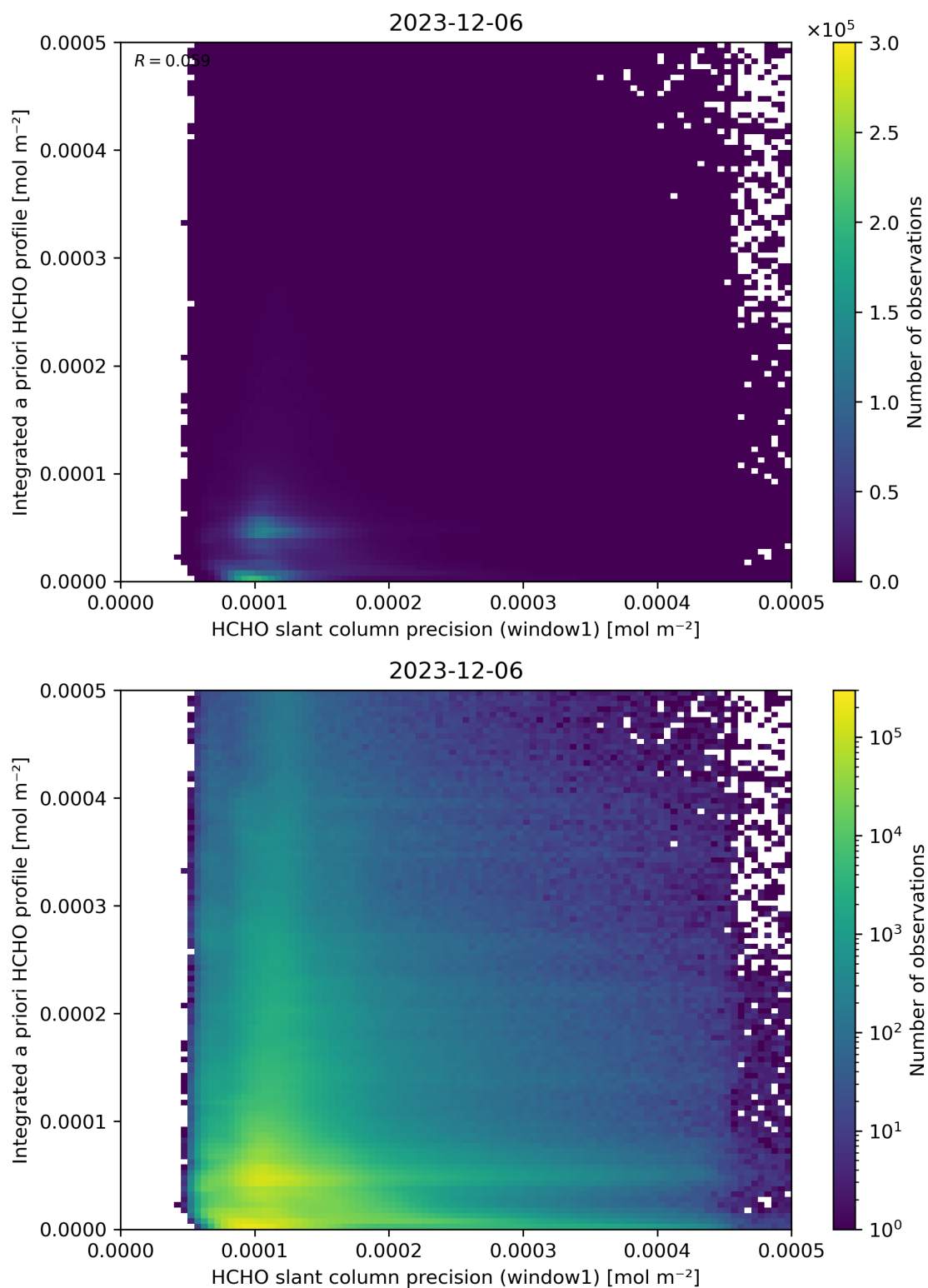
Figure 96: Scatter density plot of “HCHO slant column precision (window1)” against “Integrated a priori HCHO profile” for 2023-12-05 to 2023-12-07.
