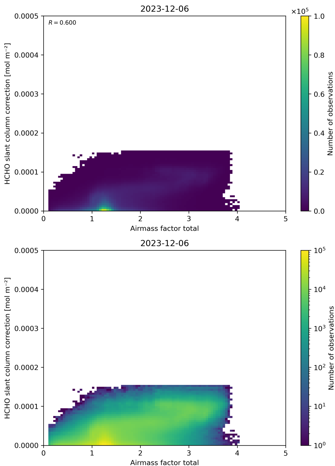
Figure 102: Scatter density plot of “Airmass factor total” against “HCHO slant column correction” for 2023-12-05 to 2023-12-07.
