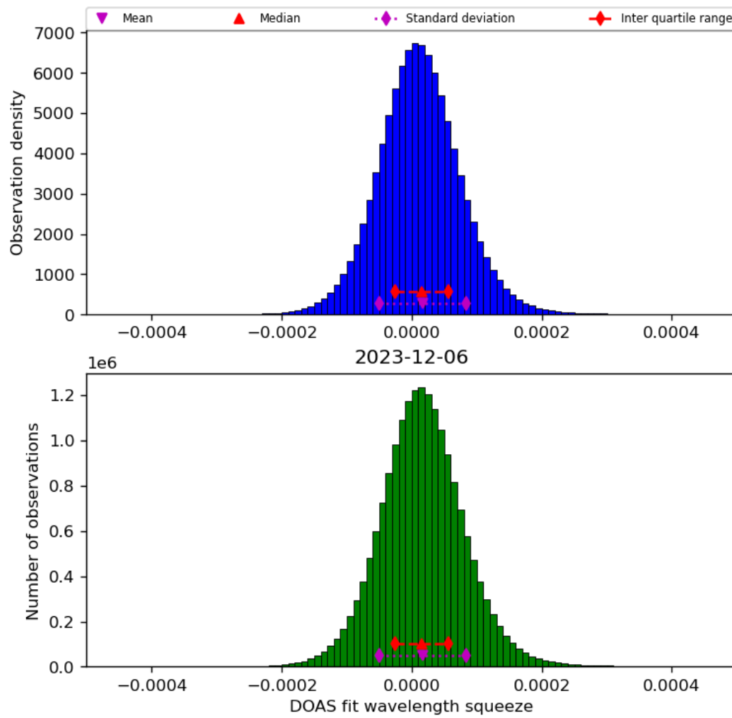
Figure 45: Histogram of “DOAS fit wavelength squeeze” for 2023-12-05 to 2023-12-07
