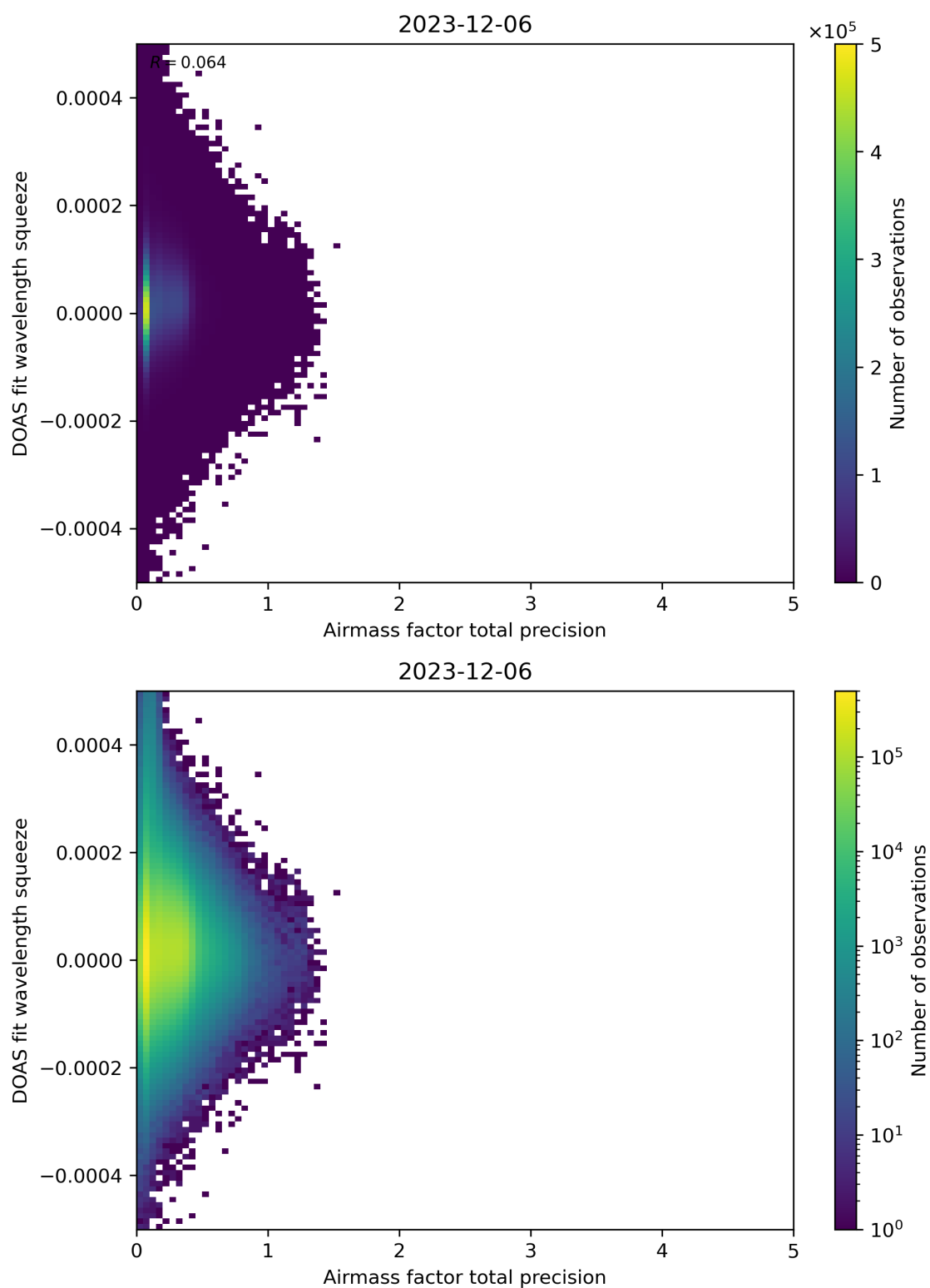
Figure 107: Scatter density plot of “Airmass factor total precision” against “DOAS fit wavelength squeeze” for 2023-12-05 to 2023-12-07.
