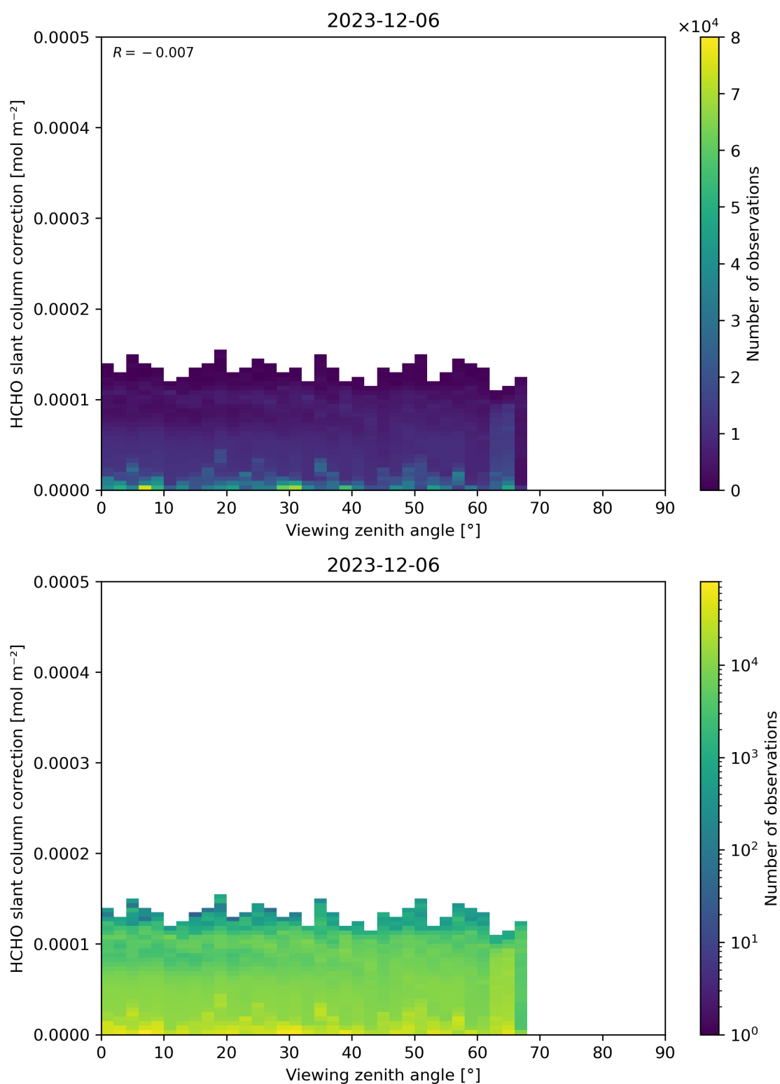
Figure 187: Scatter density plot of “Viewing zenith angle” against “HCHO slant column correction” for 2023-12-05 to 2023-12-07.
