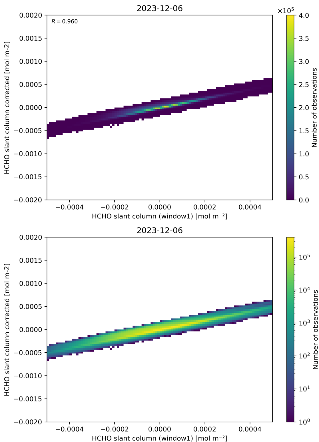
Figure 82: Scatter density plot of “HCHO slant column (window1)” against “HCHO slant column corrected” for 2023-12-05 to 2023-12-07.
