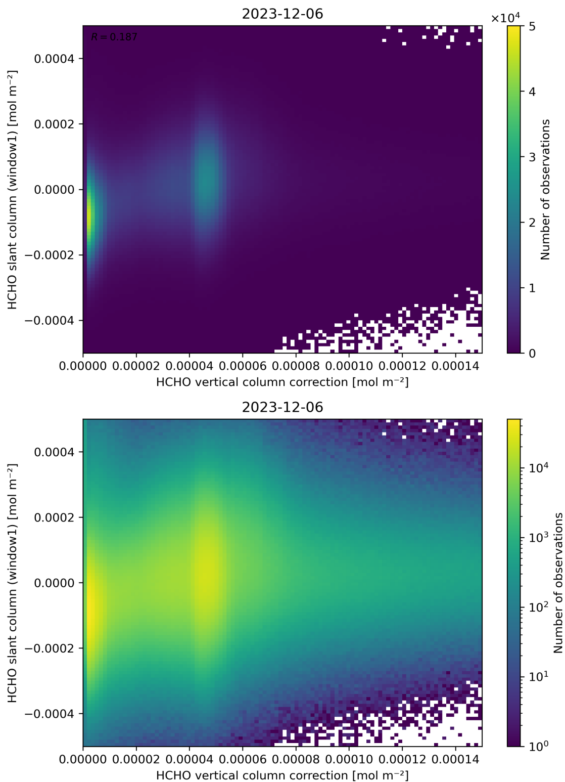
Figure 118: Scatter density plot of “HCHO vertical column correction” against “HCHO slant column (window1)” for 2023-12-05 to 2023-12-07.
