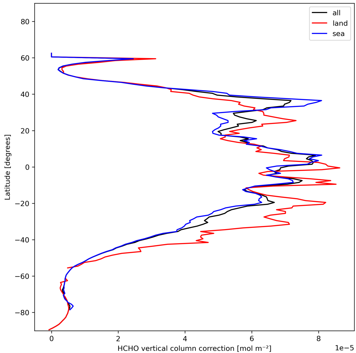
Figure 23: Zonal average of “HCHO vertical column correction” for 2023-12-05 to 2023-12-07.
