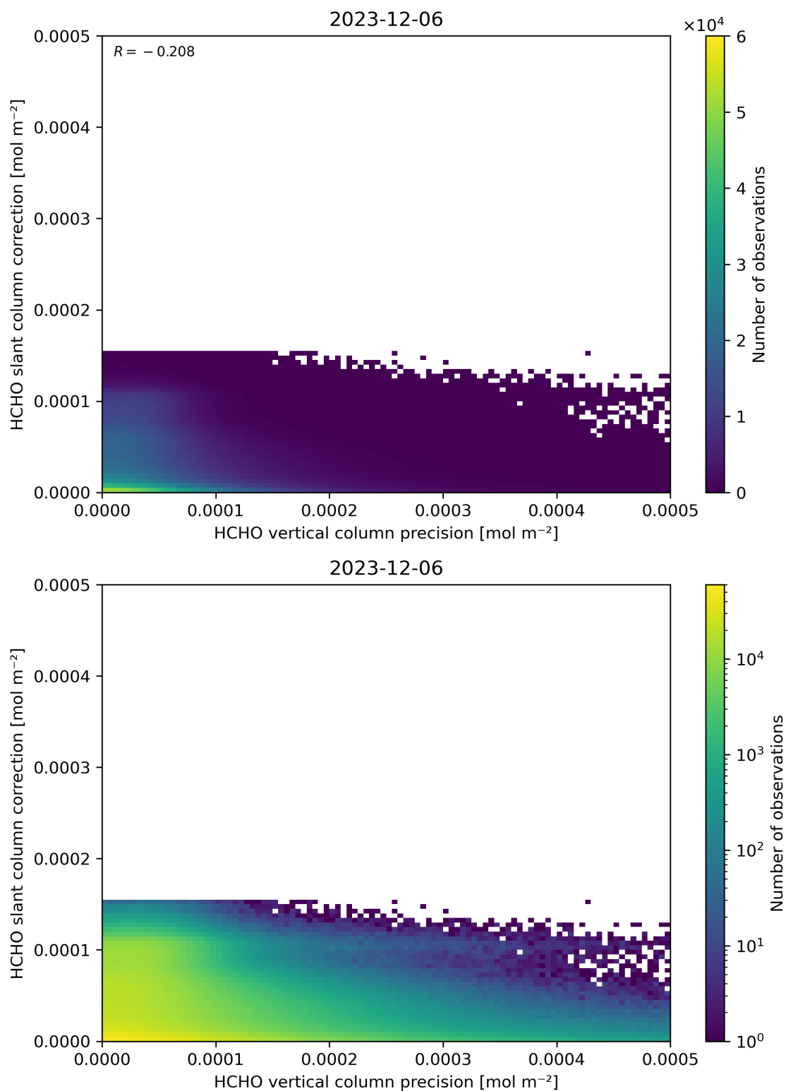
Figure 141: Scatter density plot of “HCHO vertical column precision” against “HCHO slant column correction” for 2023-12-05 to 2023-12-07.
