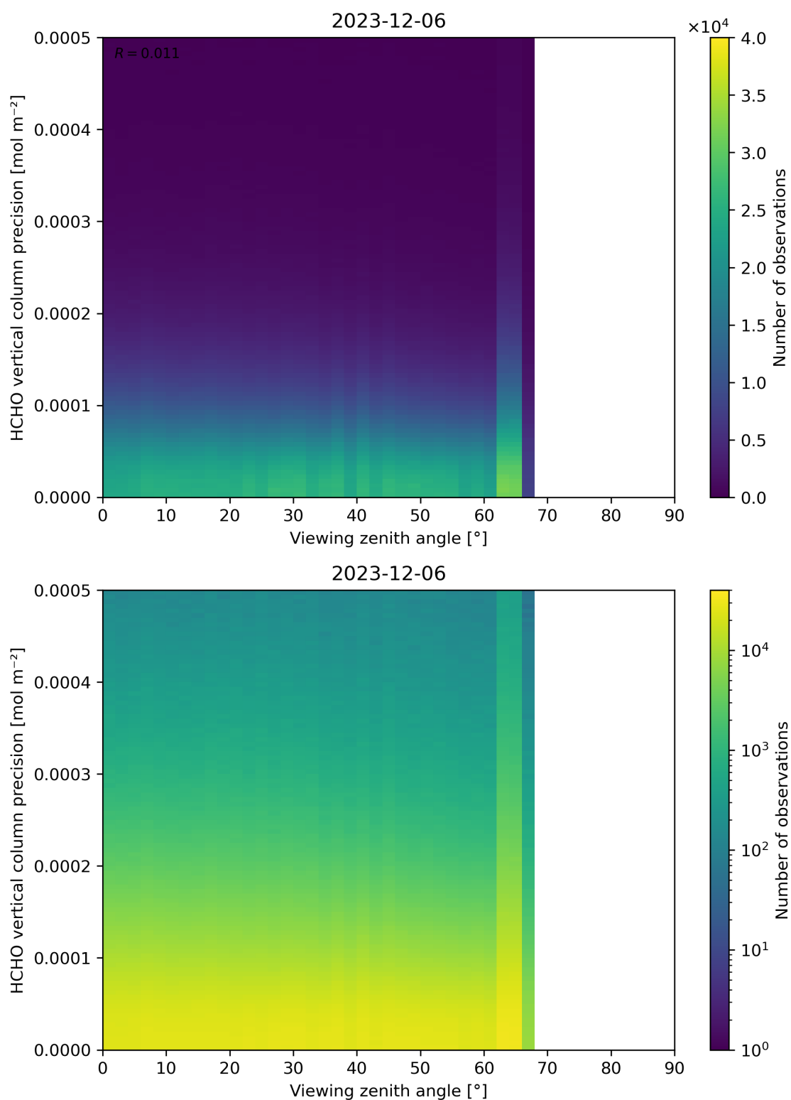
Figure 194: Scatter density plot of “Viewing zenith angle” against “HCHO vertical column precision” for 2023-12-05 to 2023-12-07.
