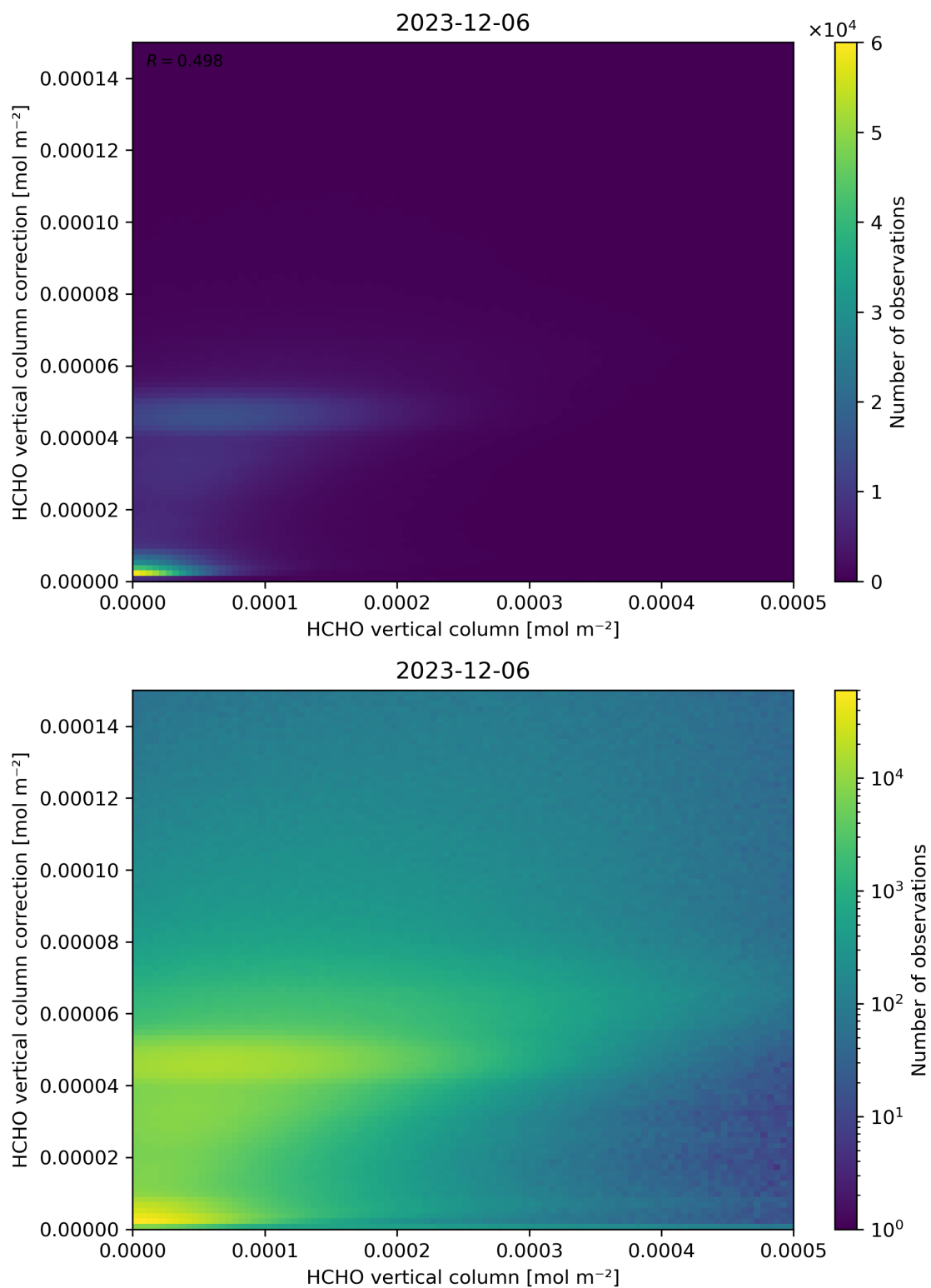
Figure 133: Scatter density plot of “HCHO vertical column” against “HCHO vertical column correction” for 2023-12-05 to 2023-12-07.
