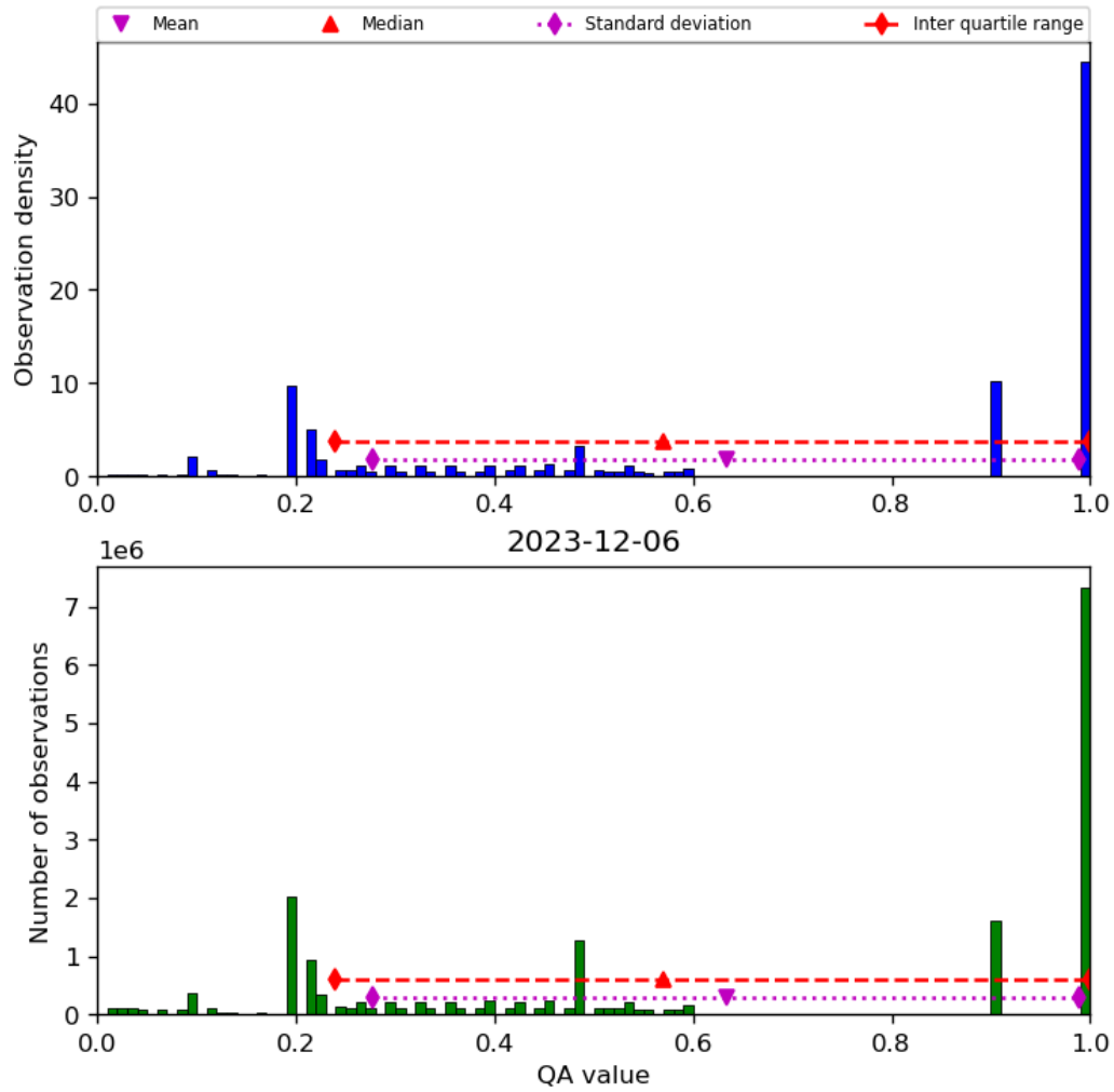
Figure 34: Histogram of “QA value” for 2023-12-05 to 2023-12-07
