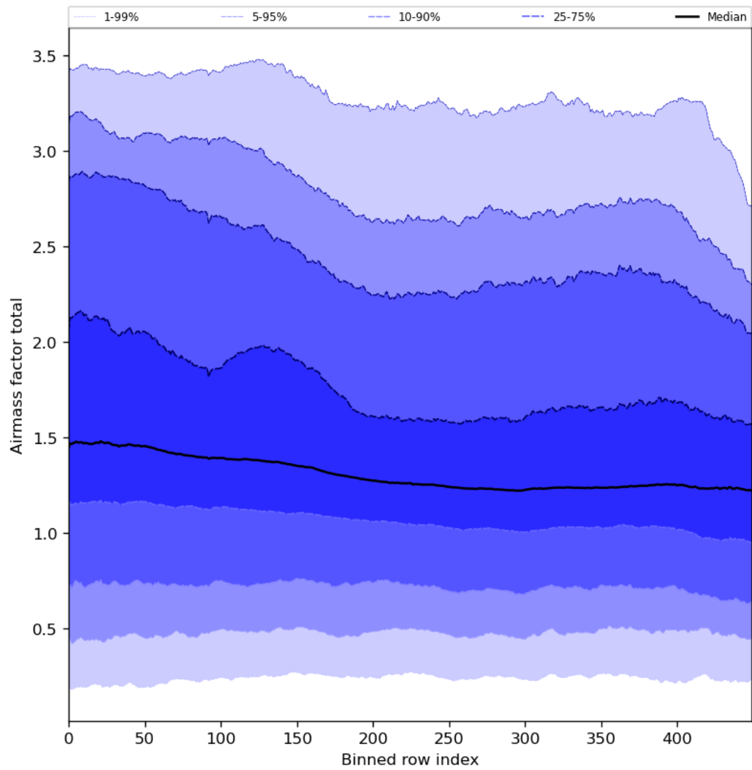
Figure 54: Along track statistics of “Airmass factor total” for 2023-12-05 to 2023-12-07
