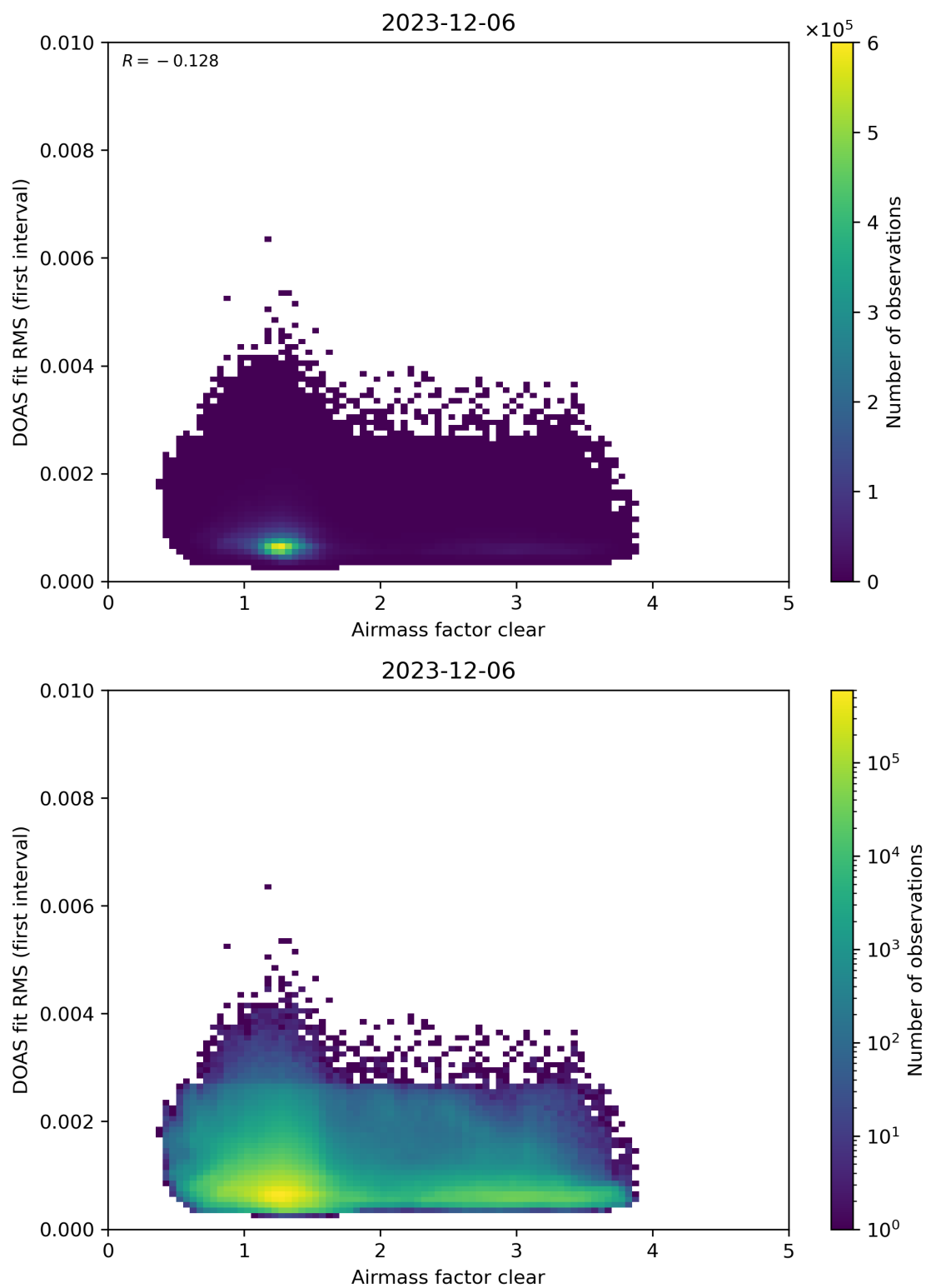
Figure 71: Scatter density plot of “Airmass factor clear” against “DOAS fit RMS (first interval)” for 2023-12-05 to 2023-12-07.
