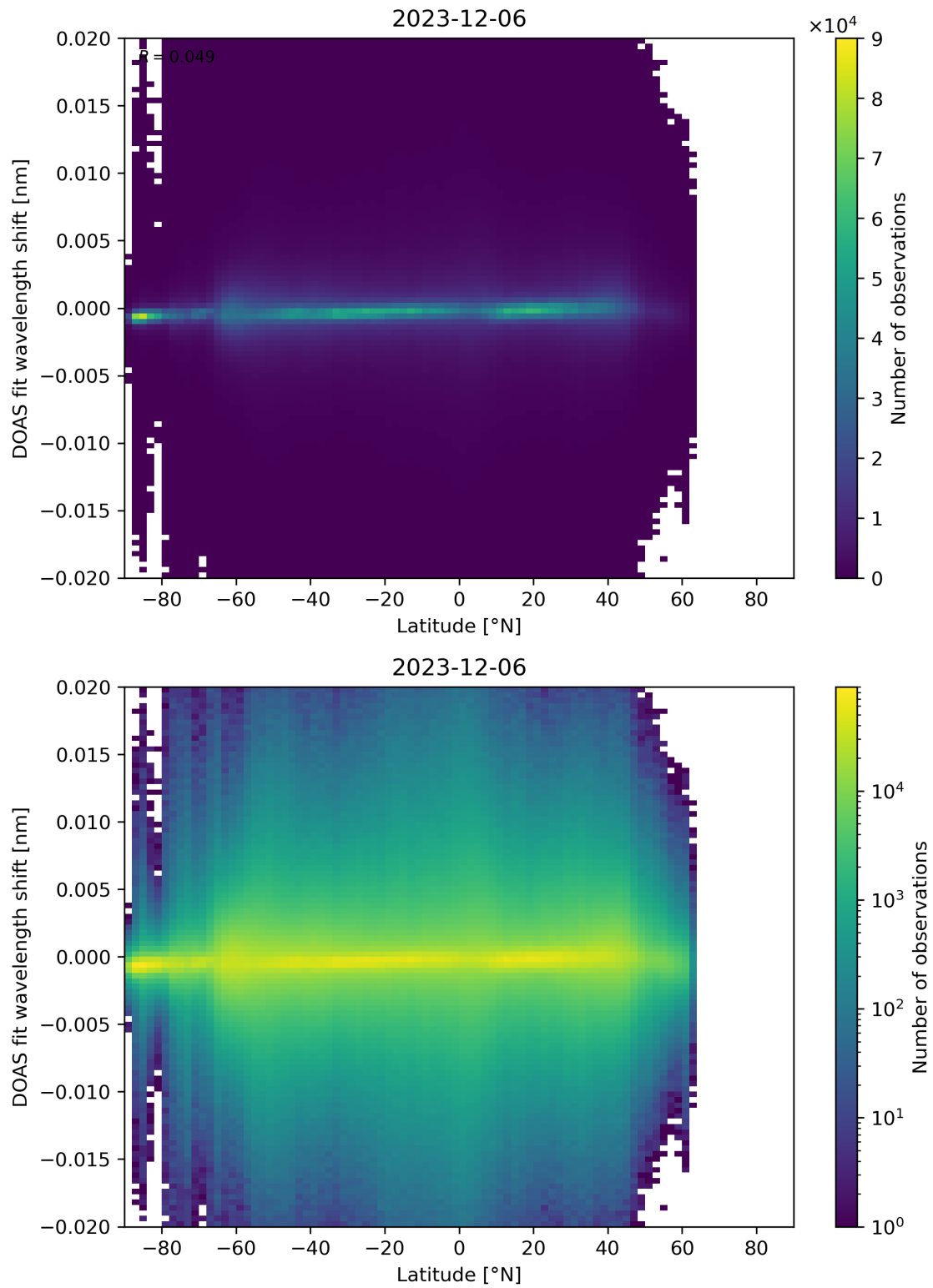
Figure 154: Scatter density plot of “Latitude” against “DOAS fit wavelength shift” for 2023-12-05 to 2023-12-07.
