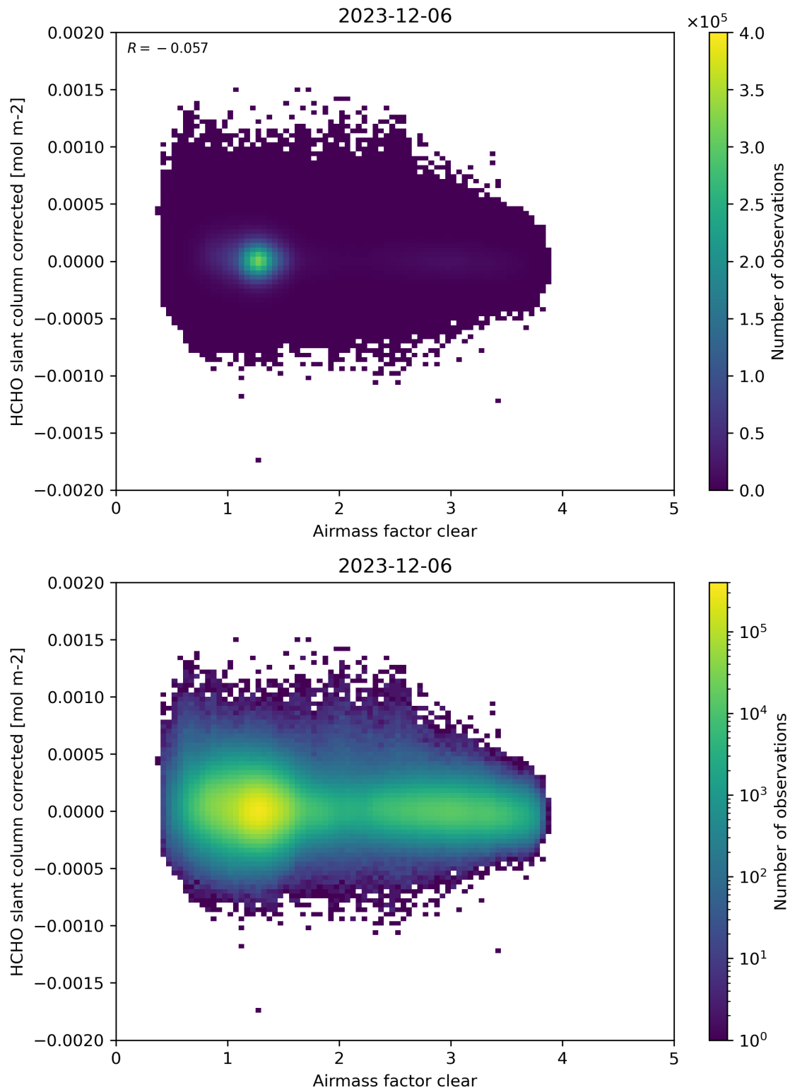
Figure 74: Scatter density plot of “Airmass factor clear” against “HCHO slant column corrected” for 2023-12-05 to 2023-12-07.
