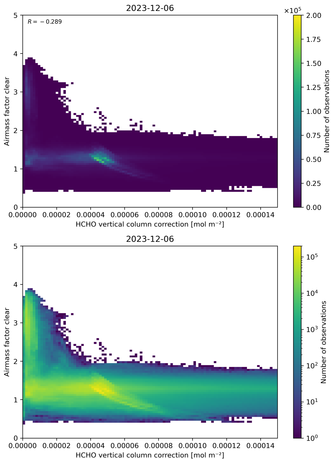
Figure 115: Scatter density plot of “HCHO vertical column correction” against “Airmass factor clear” for 2023-12-05 to 2023-12-07.
