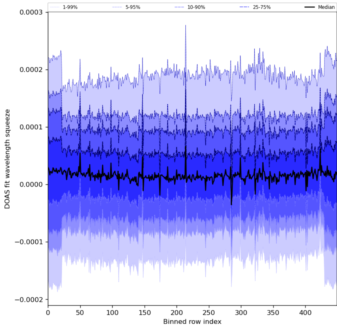
Figure 59: Along track statistics of “DOAS fit wavelength squeeze” for 2023-12-05 to 2023-12-07
