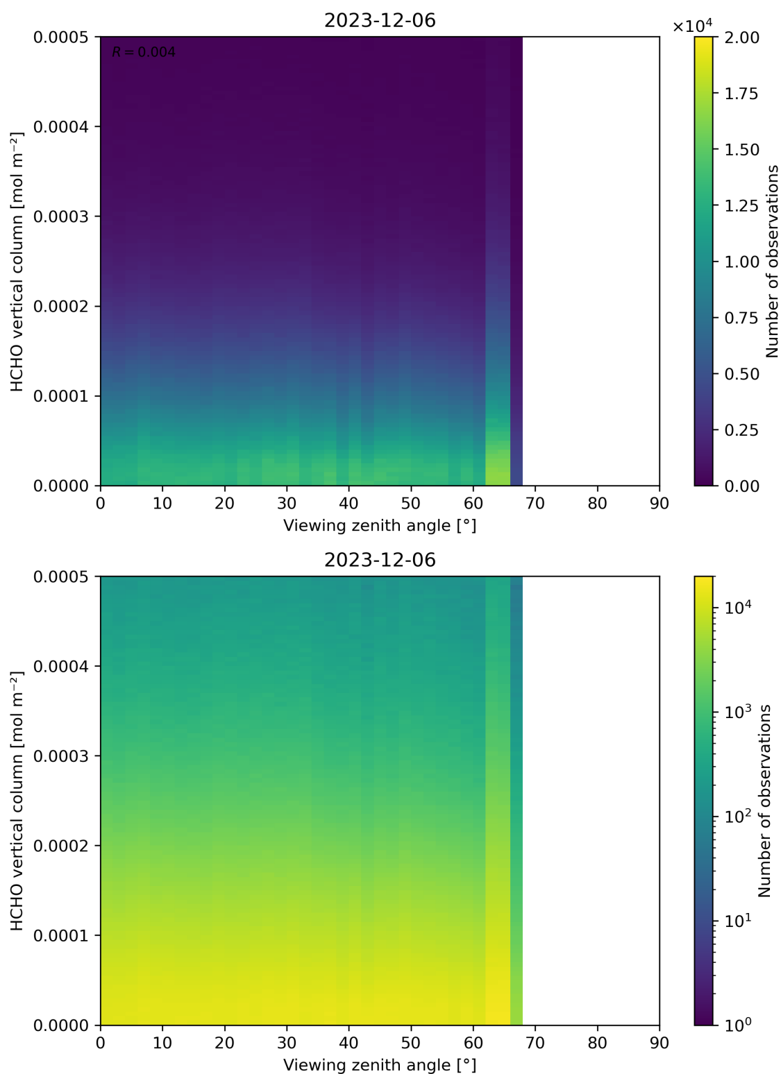
Figure 192: Scatter density plot of “Viewing zenith angle” against “HCHO vertical column” for 2023-12-05 to 2023-12-07.
