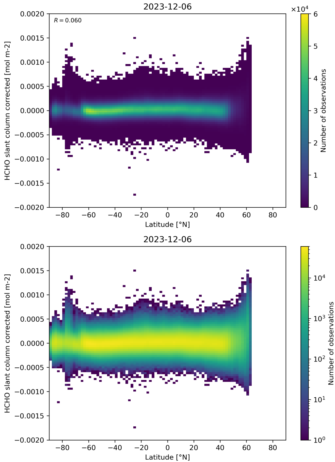
Figure 157: Scatter density plot of “Latitude” against “HCHO slant column corrected” for 2023-12-05 to 2023-12-07.
