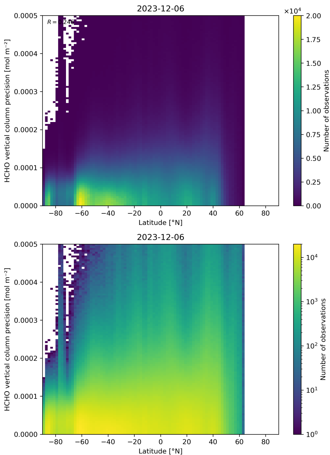
Figure 165: Scatter density plot of “Latitude” against “HCHO vertical column precision” for 2023-12-05 to 2023-12-07.
