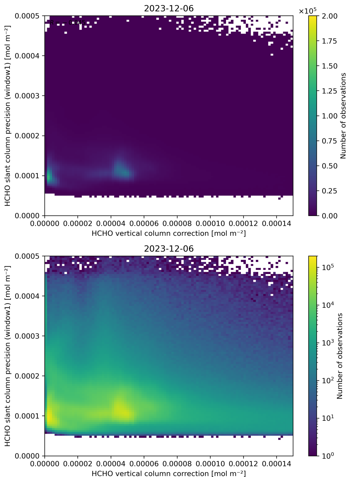
Figure 119: Scatter density plot of “HCHO vertical column correction” against “HCHO slant column precision (window1)” for 2023-12-05 to 2023-12-07.
