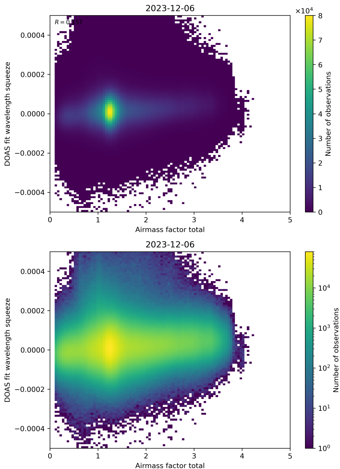
Figure 99: Scatter density plot of “Airmass factor total” against “DOAS fit wavelength squeeze” for 2023-12-05 to 2023-12-07.
