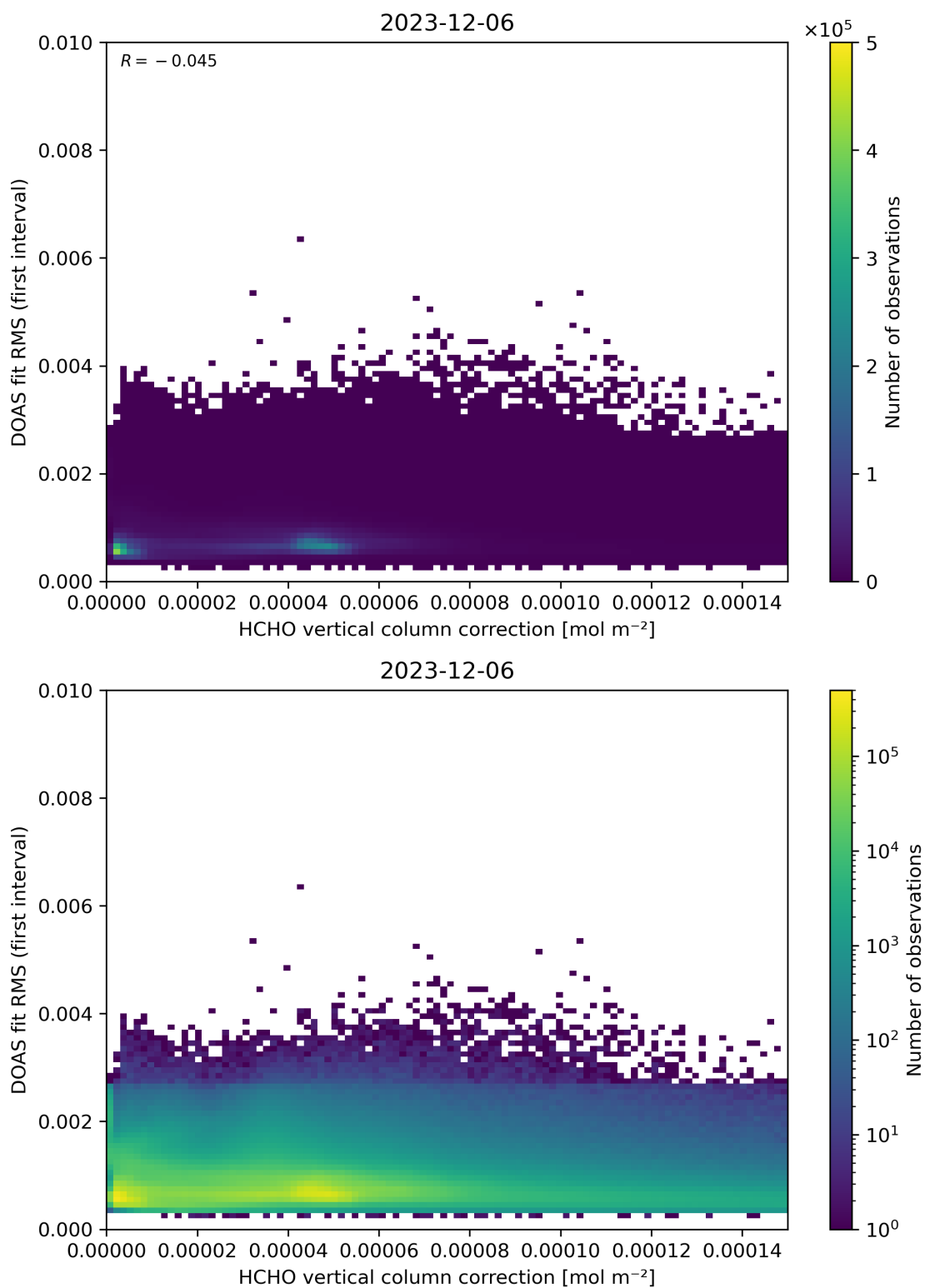
Figure 112: Scatter density plot of “HCHO vertical column correction” against “DOAS fit RMS (first interval)” for 2023-12-05 to 2023-12-07.
