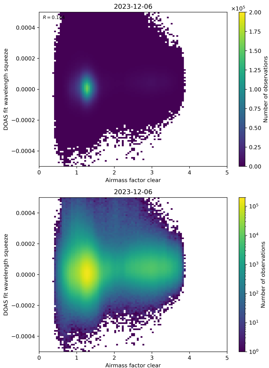
Figure 73: Scatter density plot of “Airmass factor clear” against “DOAS fit wavelength squeeze” for 2023-12-05 to 2023-12-07.
