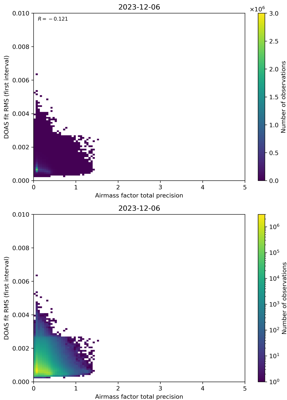
Figure 105: Scatter density plot of “Airmass factor total precision” against “DOAS fit RMS (first interval)” for 2023-12-05 to 2023-12-07.
