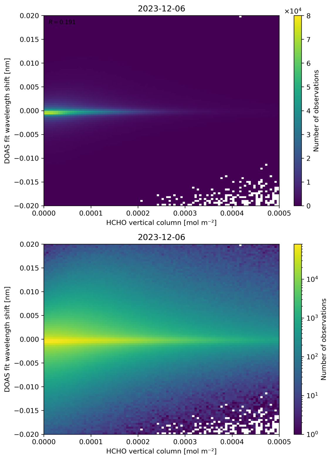
Figure 124: Scatter density plot of “HCHO vertical column” against “DOAS fit wavelength shift” for 2023-12-05 to 2023-12-07.
