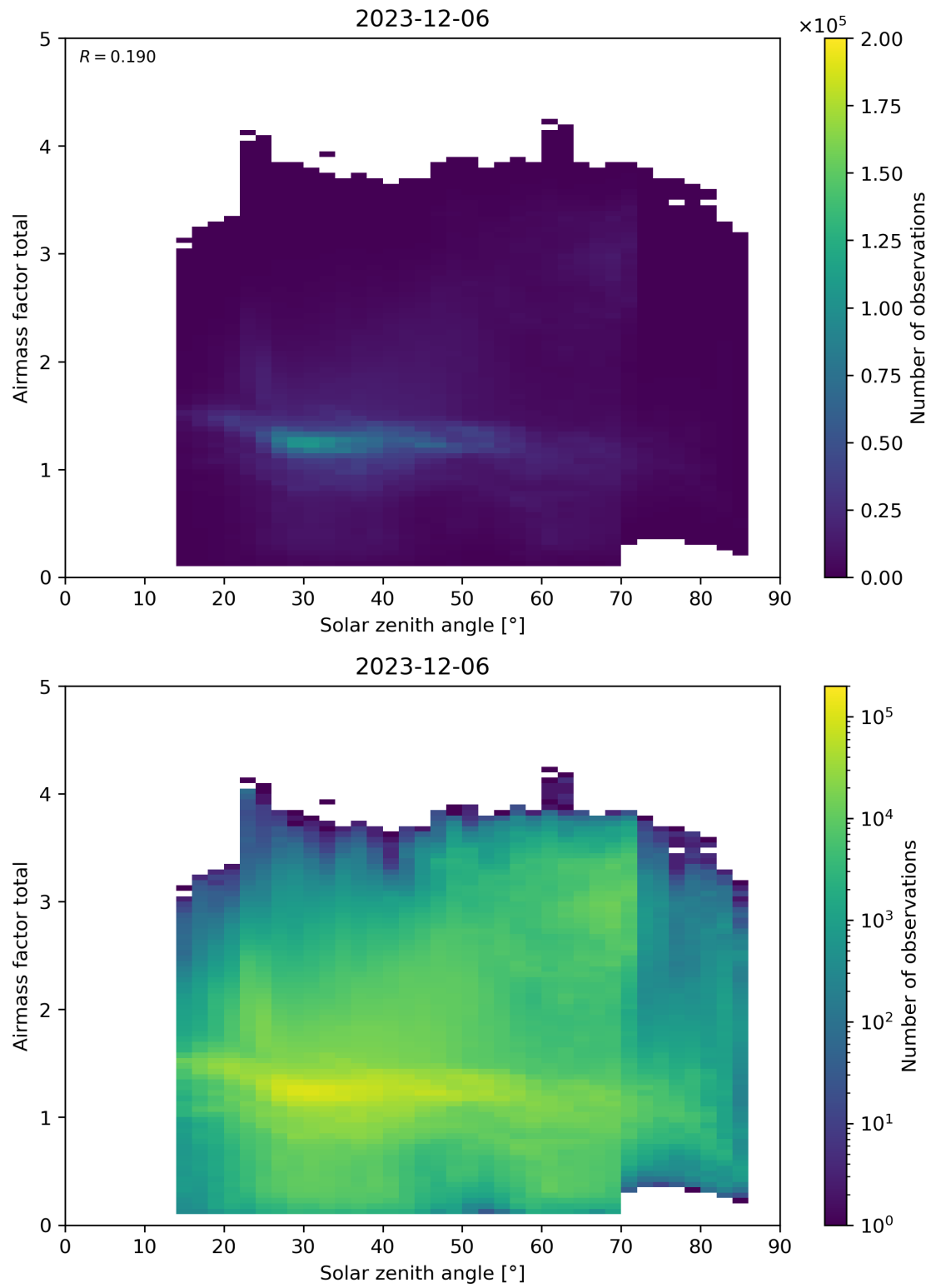
Figure 175: Scatter density plot of “Solar zenith angle” against “Airmass factor total” for 2023-12-05 to 2023-12-07.
