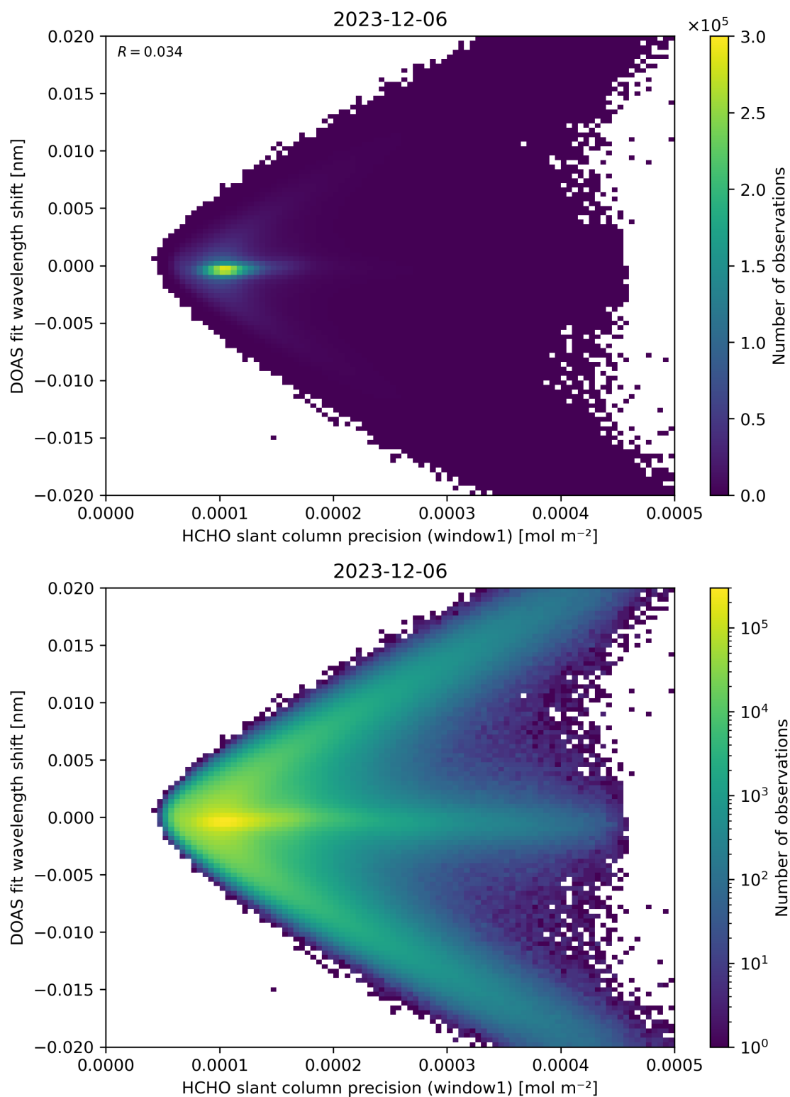
Figure 89: Scatter density plot of “HCHO slant column precision (window1)” against “DOAS fit wavelength shift” for 2023-12-05 to 2023-12-07.
