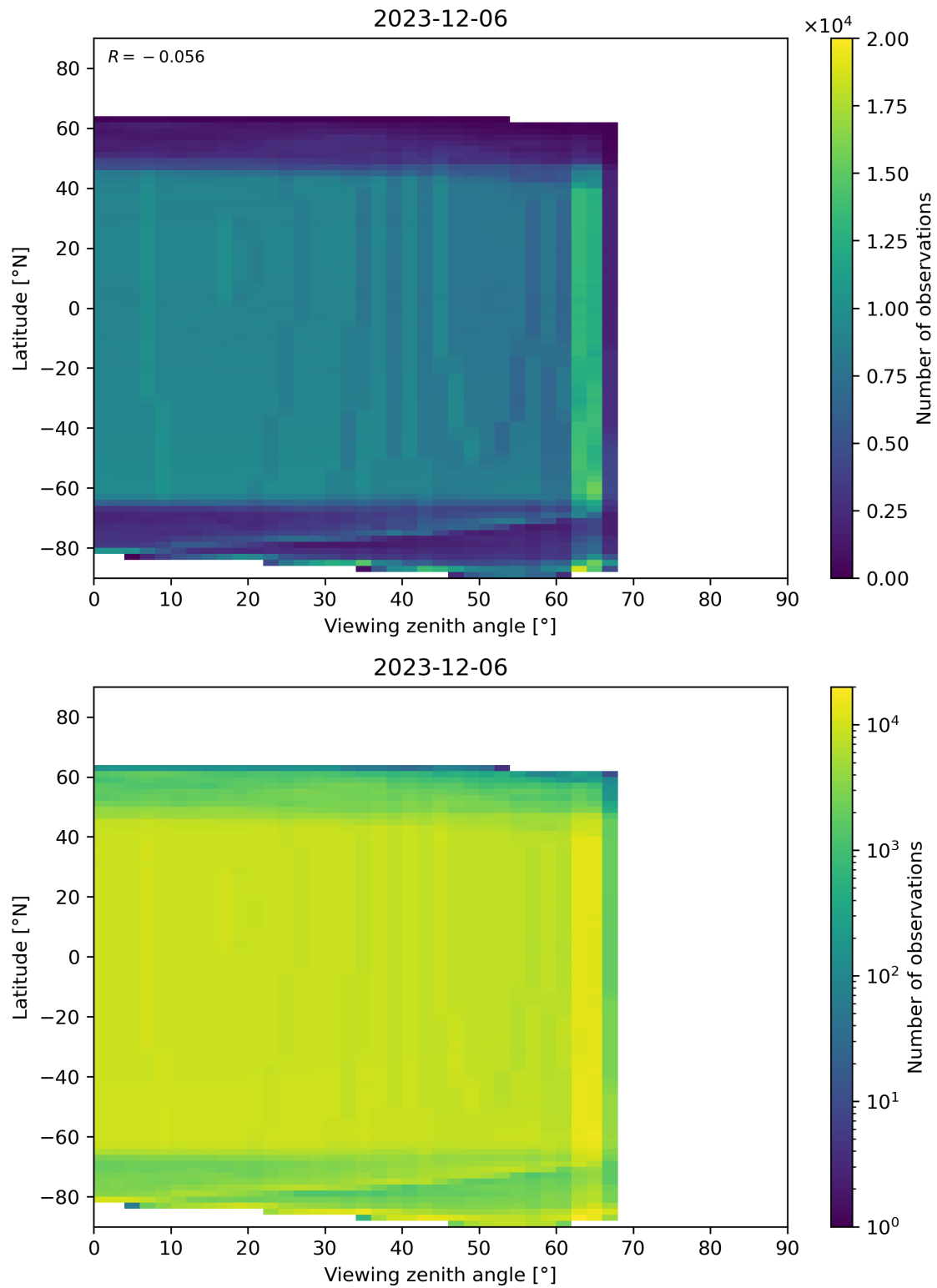
Figure 196: Scatter density plot of “Viewing zenith angle” against “Latitude” for 2023-12-05 to 2023-12-07.
