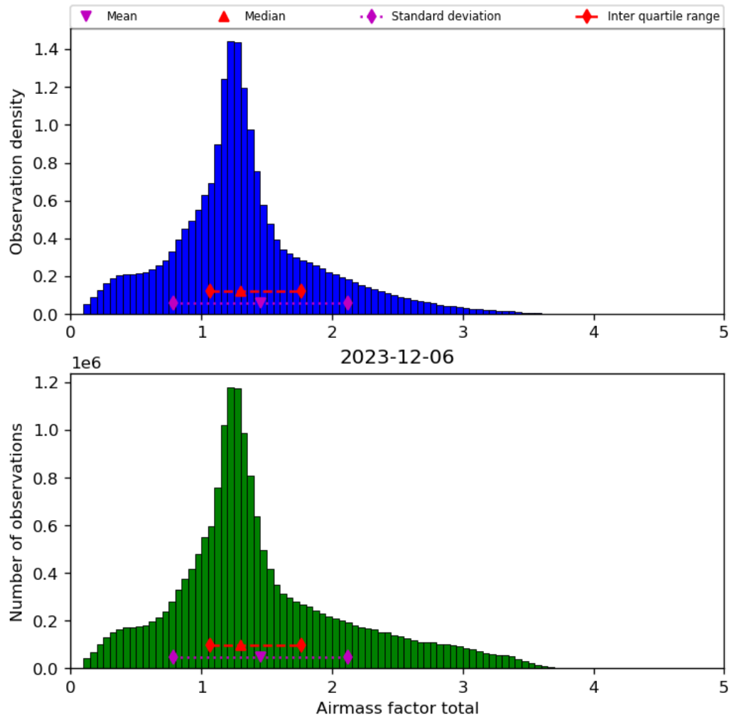
Figure 40: Histogram of “Airmass factor total” for 2023-12-05 to 2023-12-07
