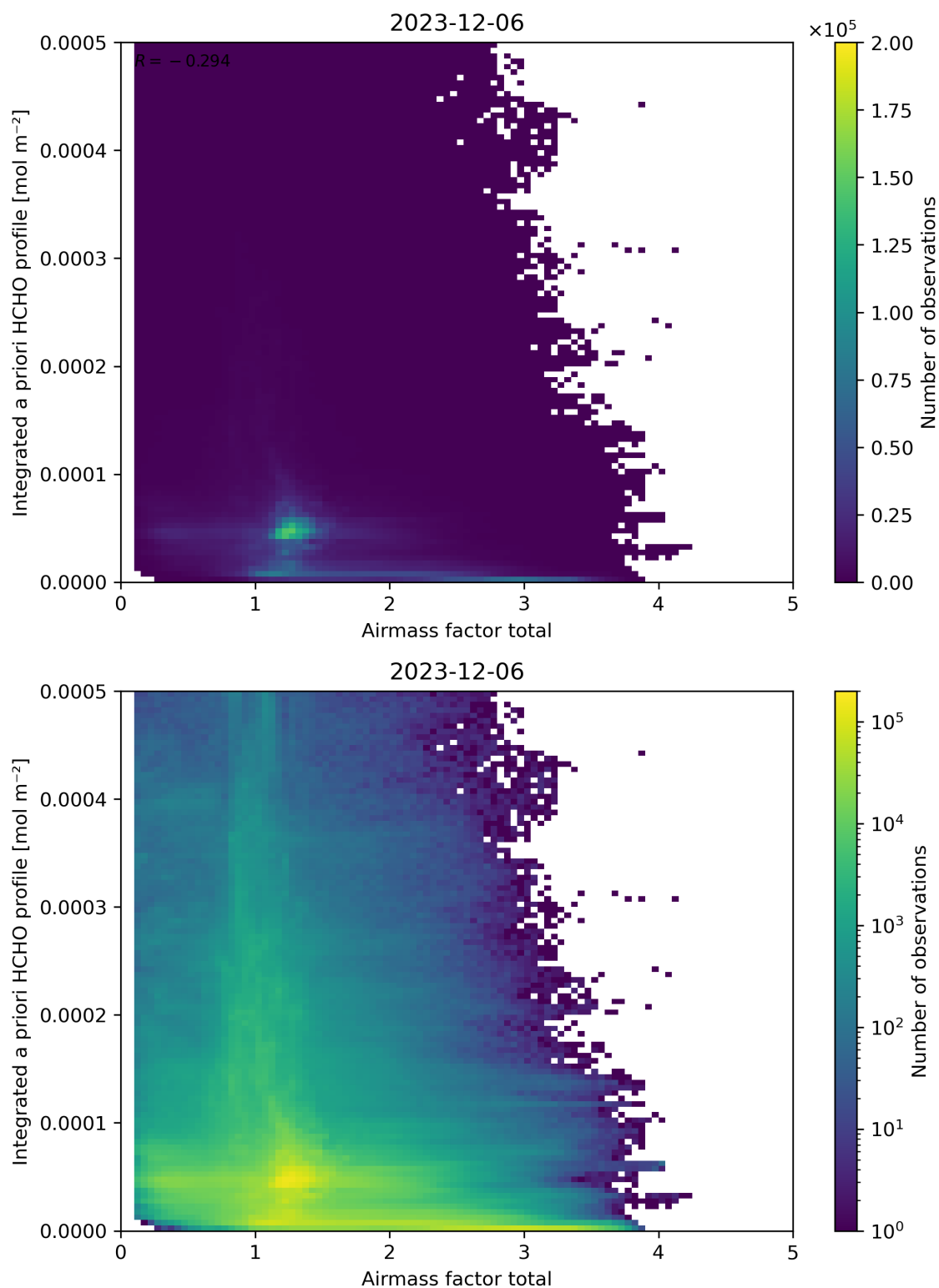
Figure 104: Scatter density plot of “Airmass factor total” against “Integrated a priori HCHO profile” for 2023-12-05 to 2023-12-07.
