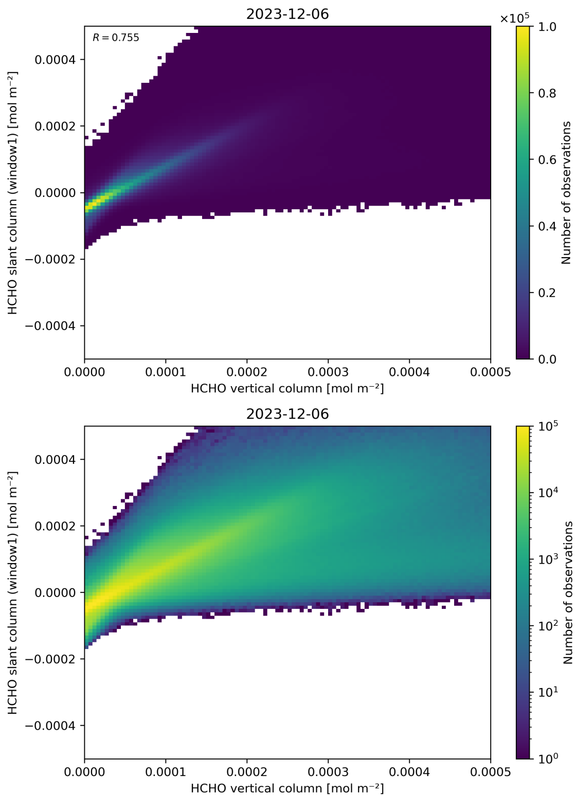
Figure 129: Scatter density plot of “HCHO vertical column” against “HCHO slant column (window1)” for 2023-12-05 to 2023-12-07.
