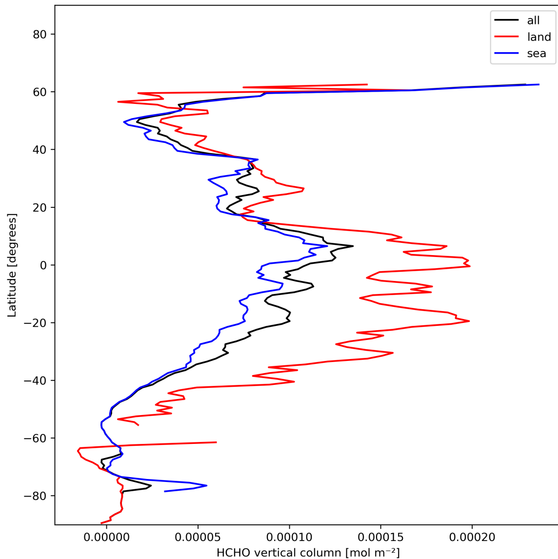
Figure 21: Zonal average of “HCHO vertical column” for 2023-12-05 to 2023-12-07.
