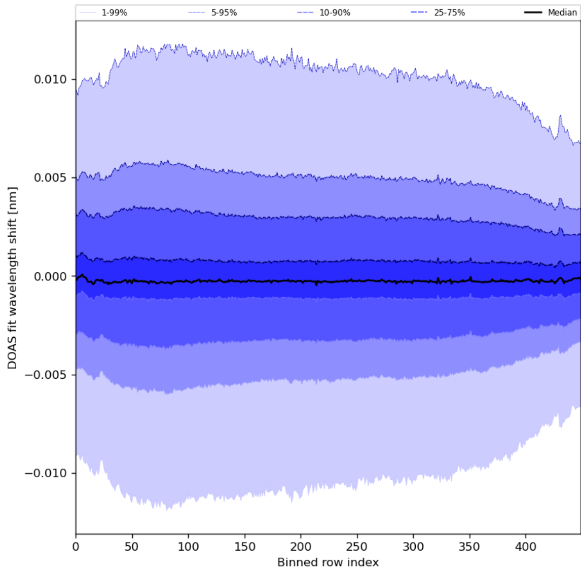
Figure 58: Along track statistics of “DOAS fit wavelength shift” for 2023-12-05 to 2023-12-07
