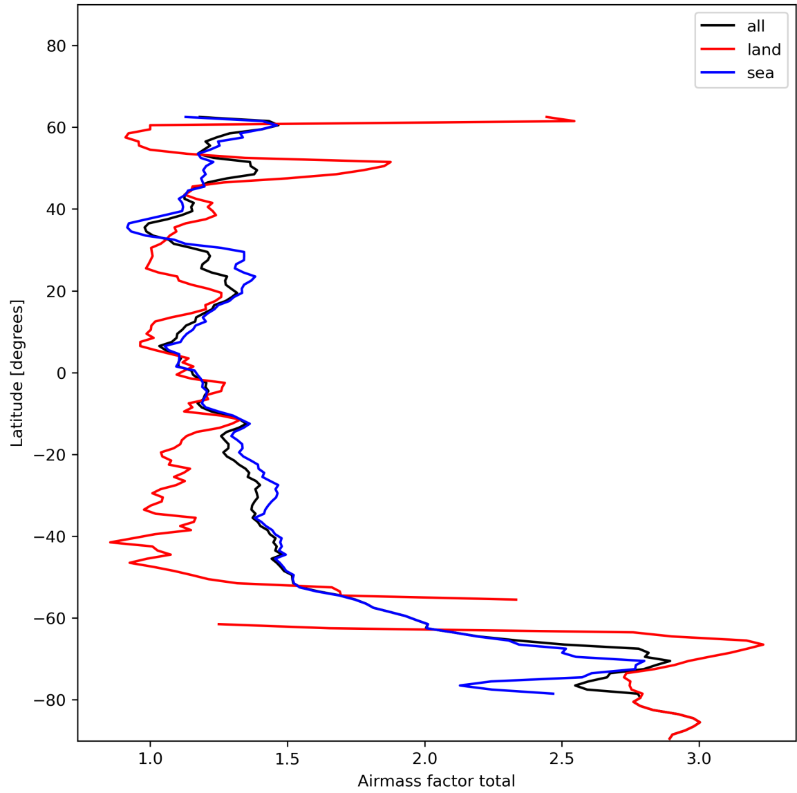
Figure 26: Zonal average of “Airmass factor total” for 2023-12-05 to 2023-12-07.
