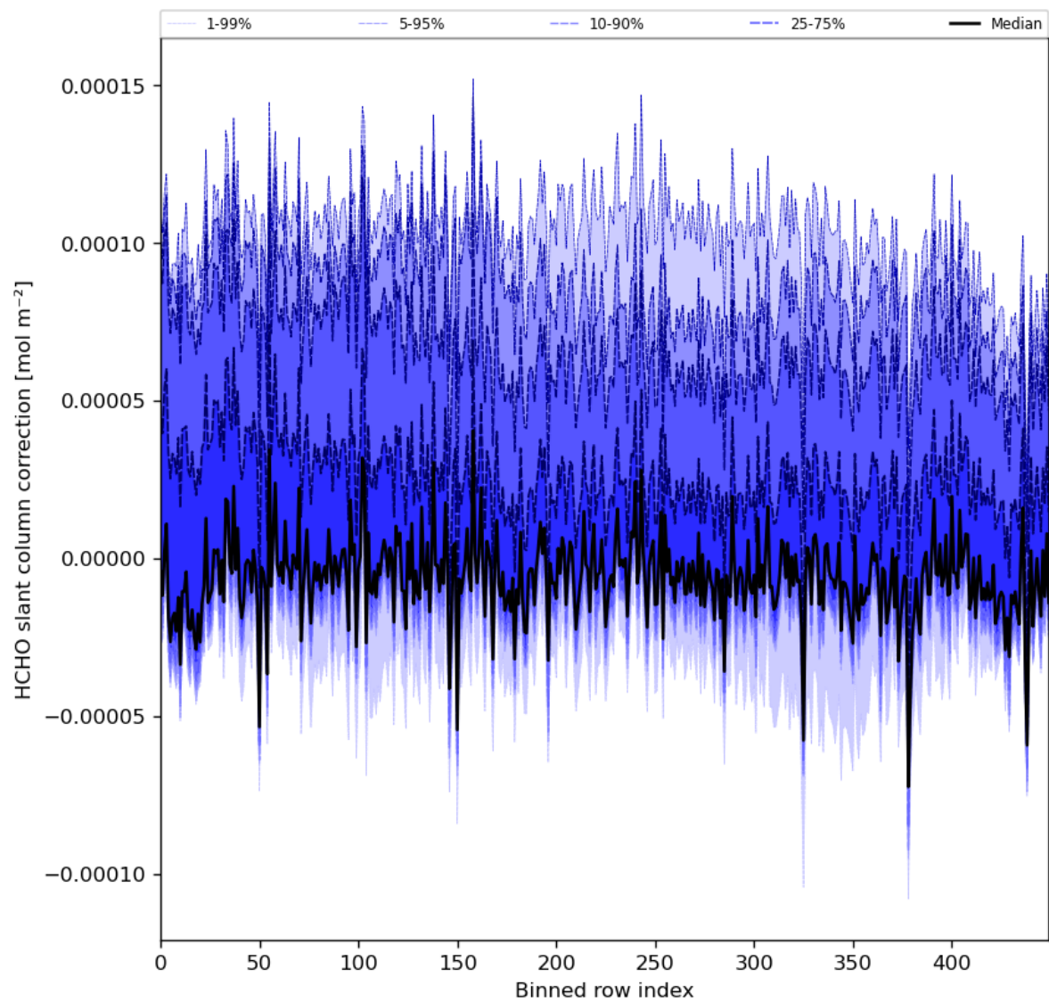
Figure 61: Along track statistics of “HCHO slant column correction” for 2023-12-05 to 2023-12-07
