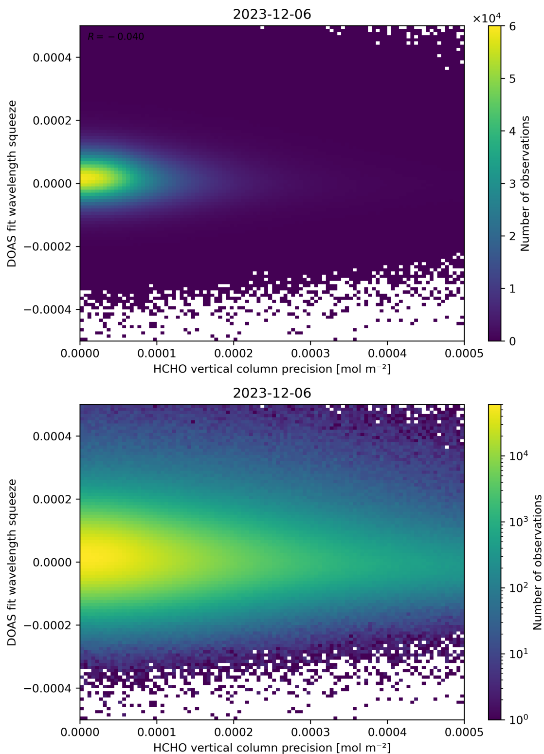
Figure 138: Scatter density plot of “HCHO vertical column precision” against “DOAS fit wavelength squeeze” for 2023-12-05 to 2023-12-07.
