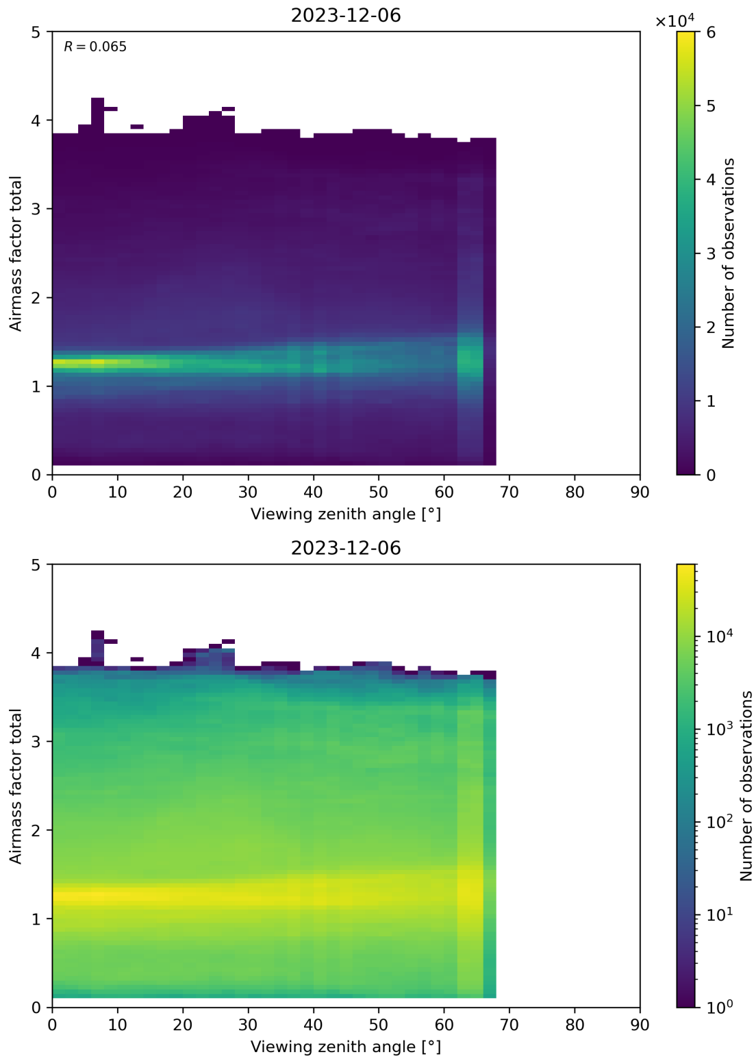
Figure 190: Scatter density plot of “Viewing zenith angle” against “Airmass factor total” for 2023-12-05 to 2023-12-07.
