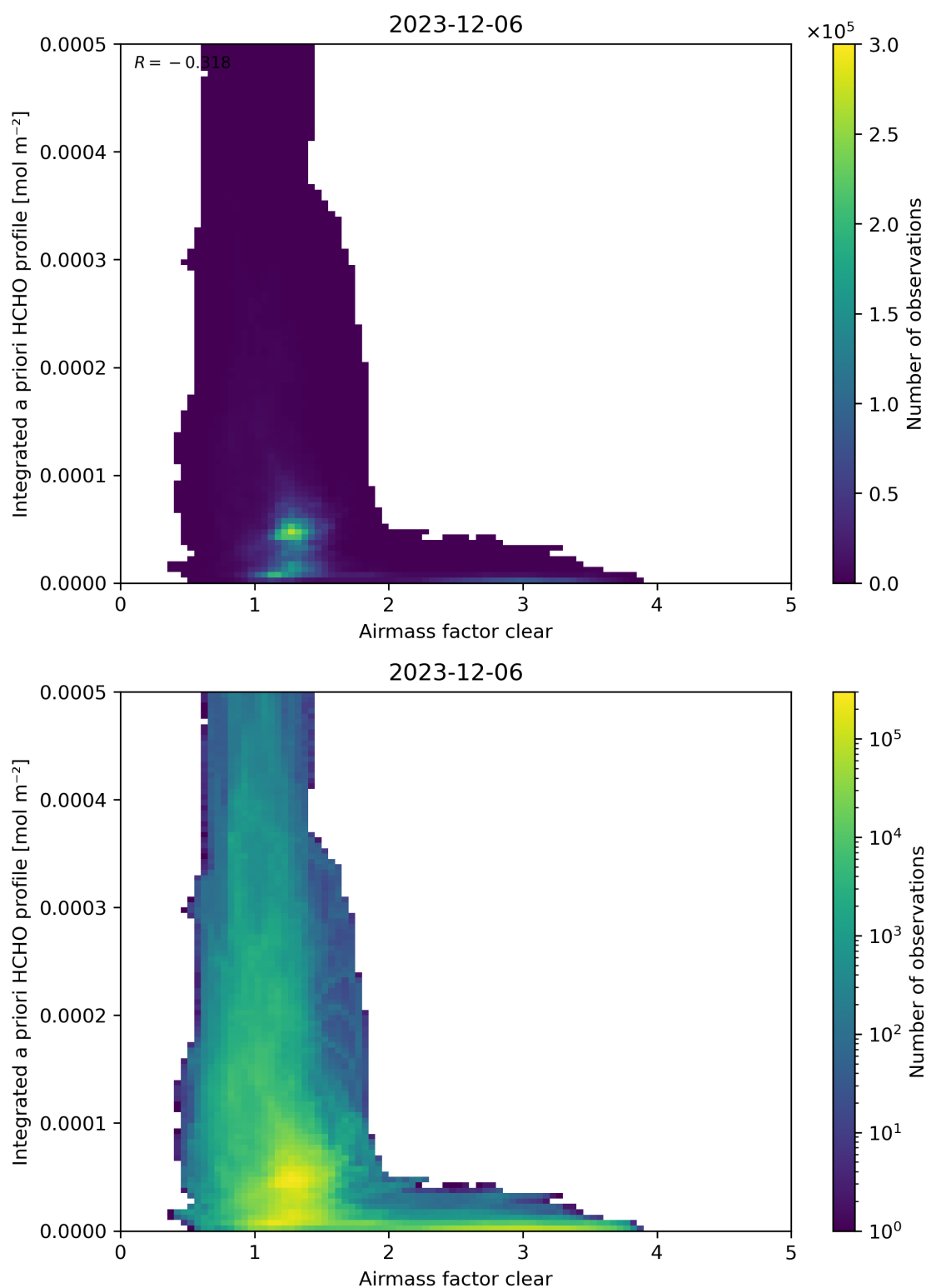
Figure 76: Scatter density plot of “Airmass factor clear” against “Integrated a priori HCHO profile” for 2023-12-05 to 2023-12-07.
