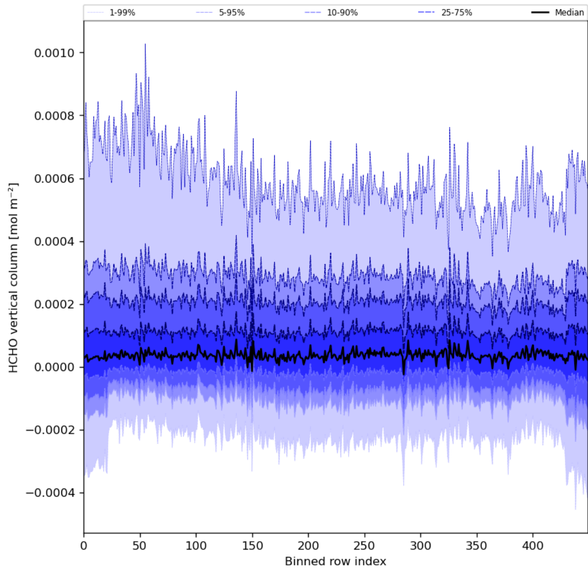
Figure 49: Along track statistics of “HCHO vertical column” for 2023-12-05 to 2023-12-07
