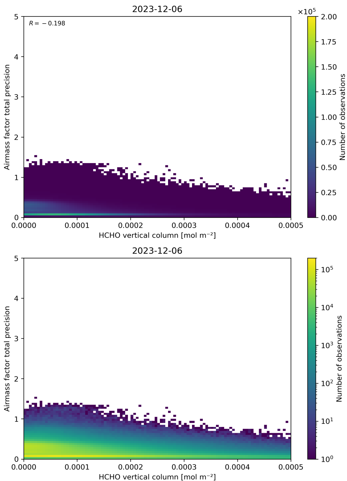
Figure 132: Scatter density plot of “HCHO vertical column” against “Airmass factor total precision” for 2023-12-05 to 2023-12-07.
