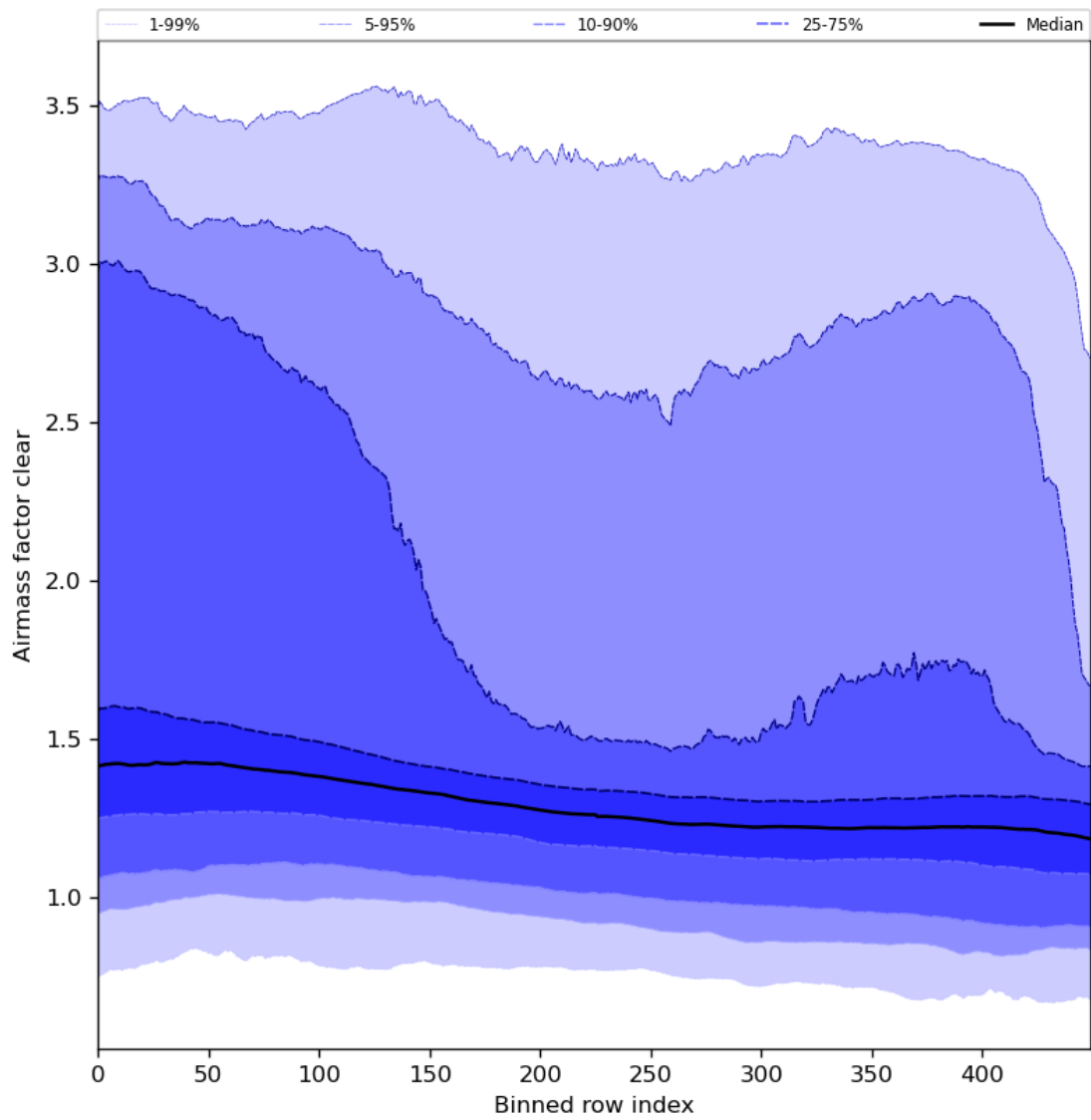
Figure 56: Along track statistics of “Airmass factor clear” for 2023-12-05 to 2023-12-07
