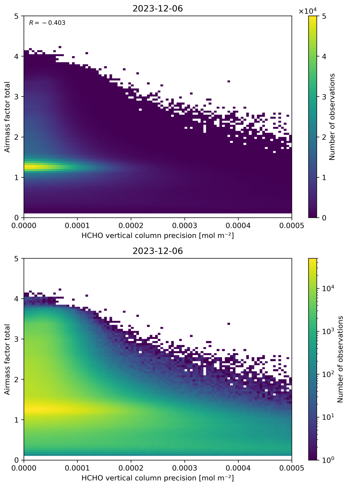
Figure 144: Scatter density plot of “HCHO vertical column precision” against “Airmass factor total” for 2023-12-05 to 2023-12-07.
