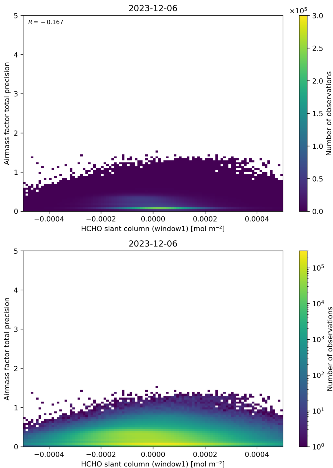
Figure 86: Scatter density plot of “HCHO slant column (window1)” against “Airmass factor total precision” for 2023-12-05 to 2023-12-07.
