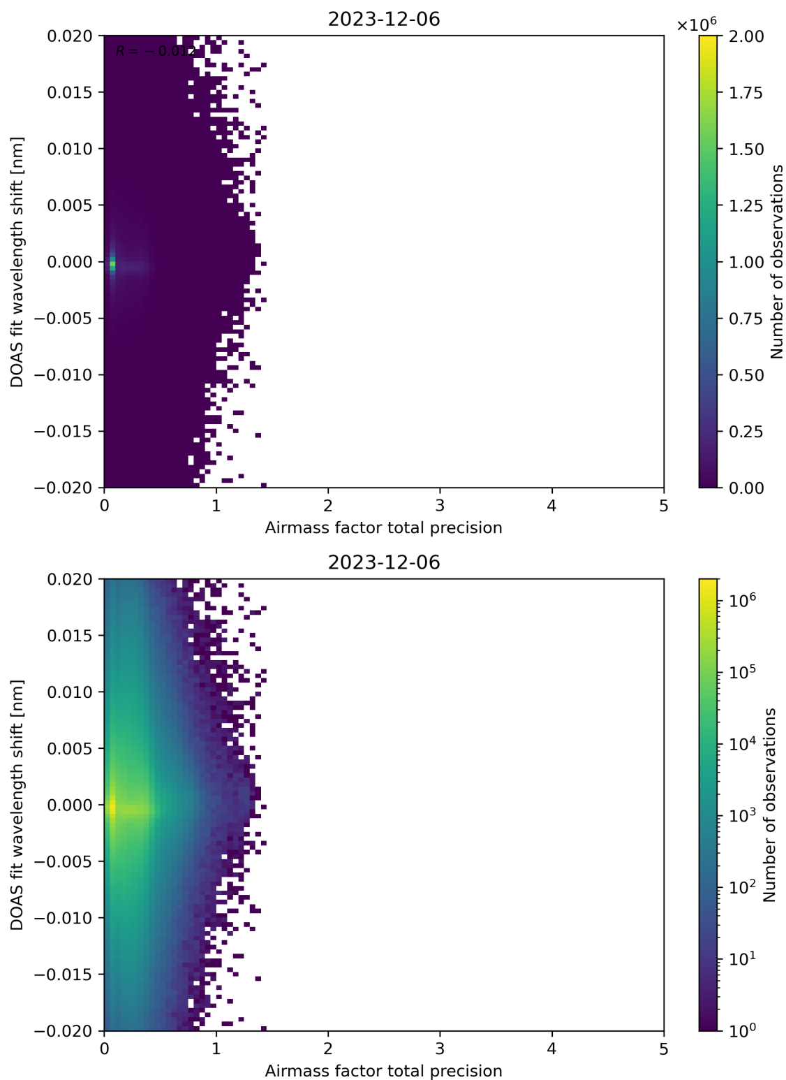
Figure 106: Scatter density plot of “Airmass factor total precision” against “DOAS fit wavelength shift” for 2023-12-05 to 2023-12-07.
