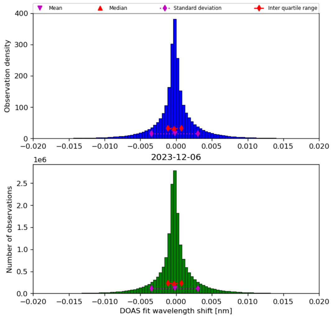
Figure 44: Histogram of “DOAS fit wavelength shift” for 2023-12-05 to 2023-12-07
