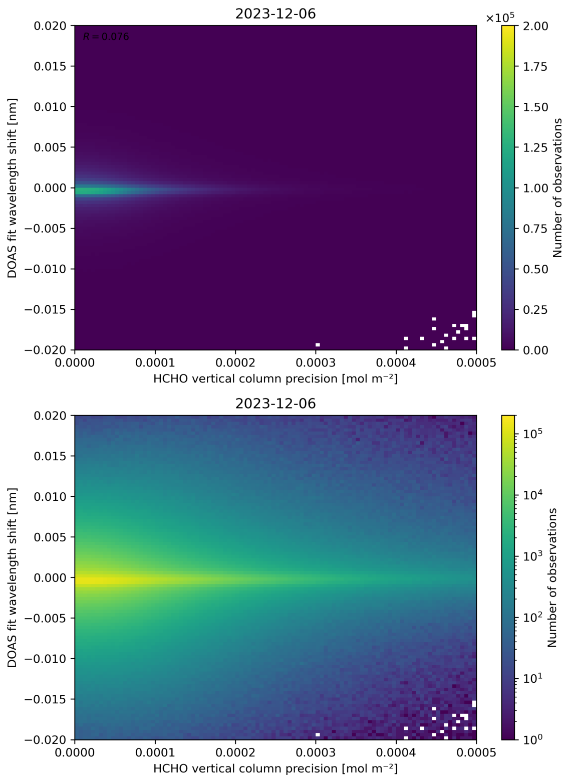
Figure 137: Scatter density plot of “HCHO vertical column precision” against “DOAS fit wavelength shift” for 2023-12-05 to 2023-12-07.
