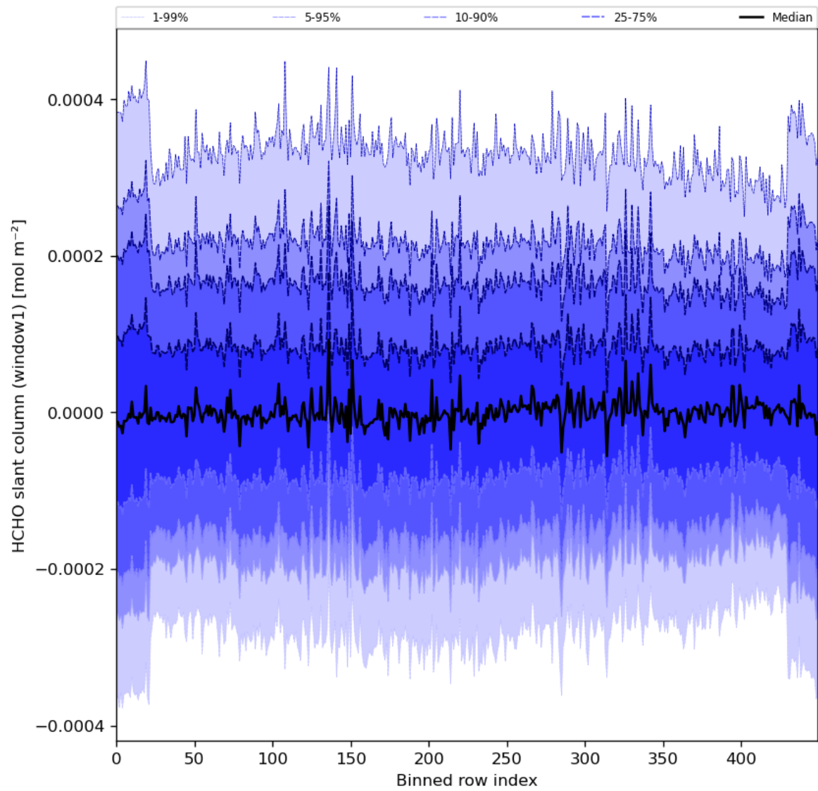
Figure 52: Along track statistics of “HCHO slant column (window1)” for 2023-12-05 to 2023-12-07
