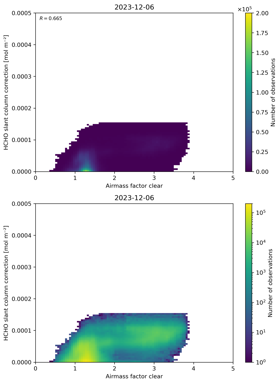
Figure 75: Scatter density plot of “Airmass factor clear” against “HCHO slant column correction” for 2023-12-05 to 2023-12-07.
