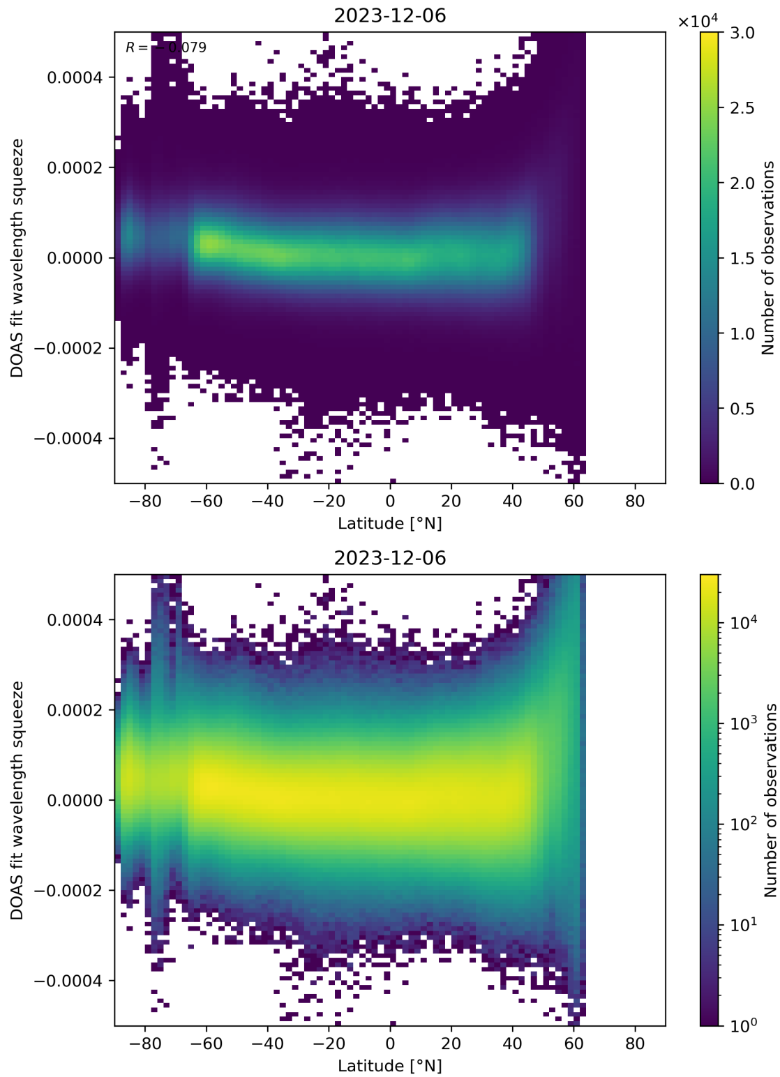
Figure 155: Scatter density plot of “Latitude” against “DOAS fit wavelength squeeze” for 2023-12-05 to 2023-12-07.
