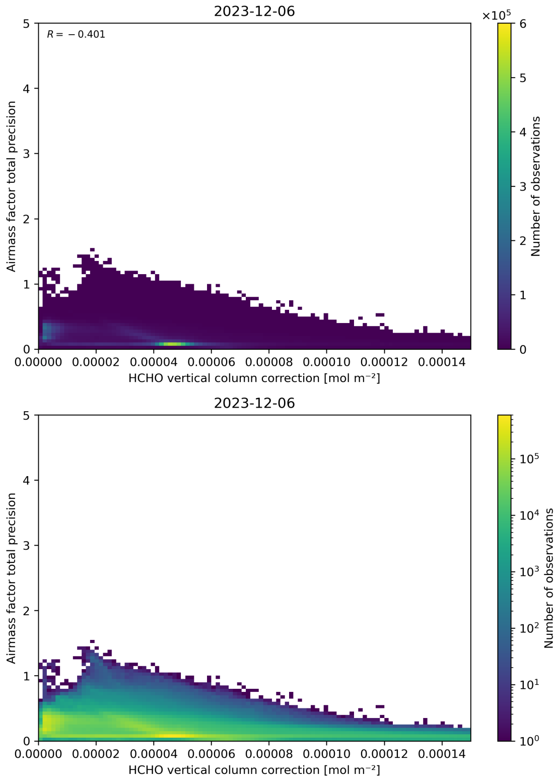
Figure 121: Scatter density plot of “HCHO vertical column correction” against “Airmass factor total precision” for 2023-12-05 to 2023-12-07.
