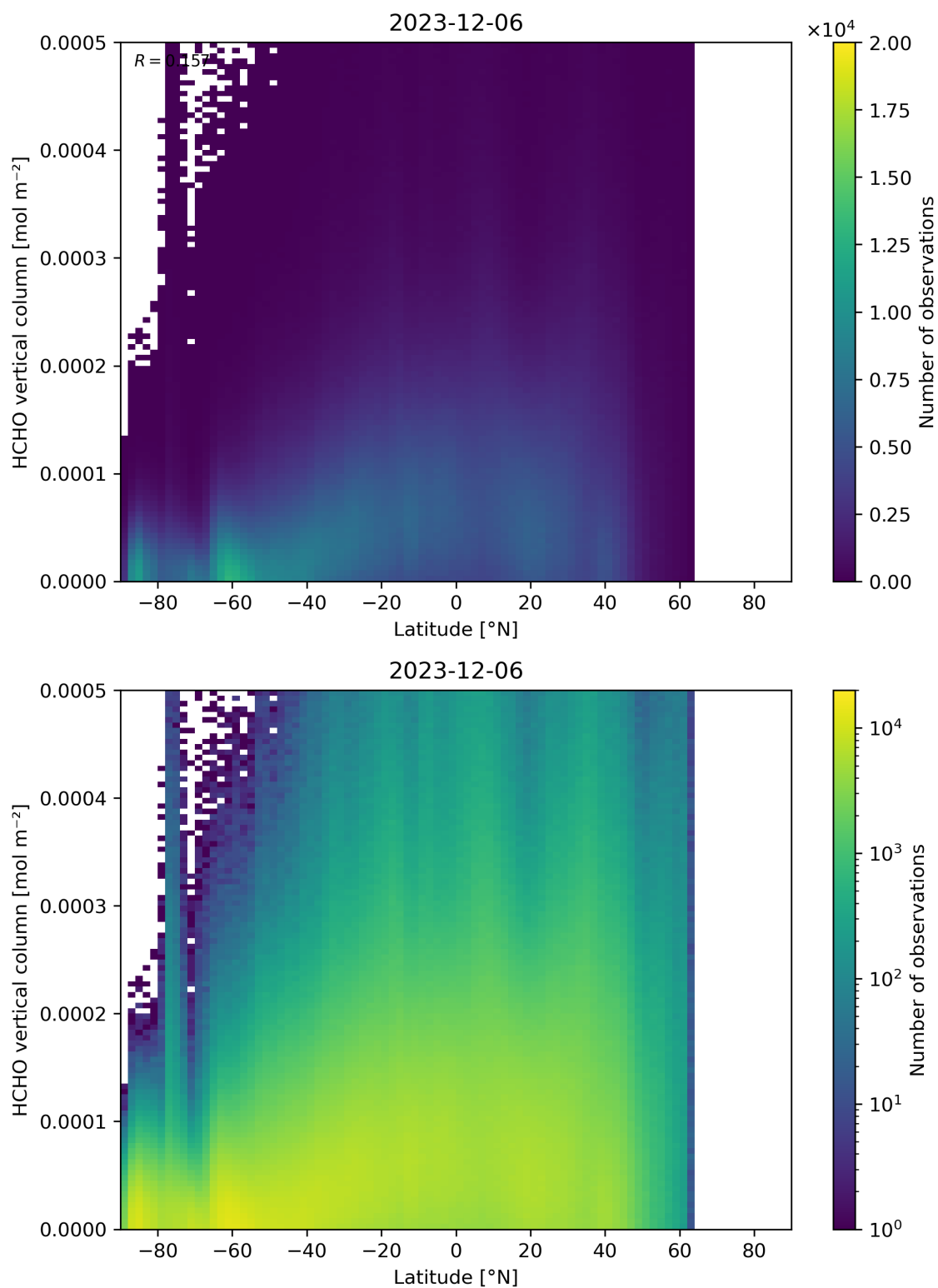
Figure 163: Scatter density plot of “Latitude” against “HCHO vertical column” for 2023-12-05 to 2023-12-07.
