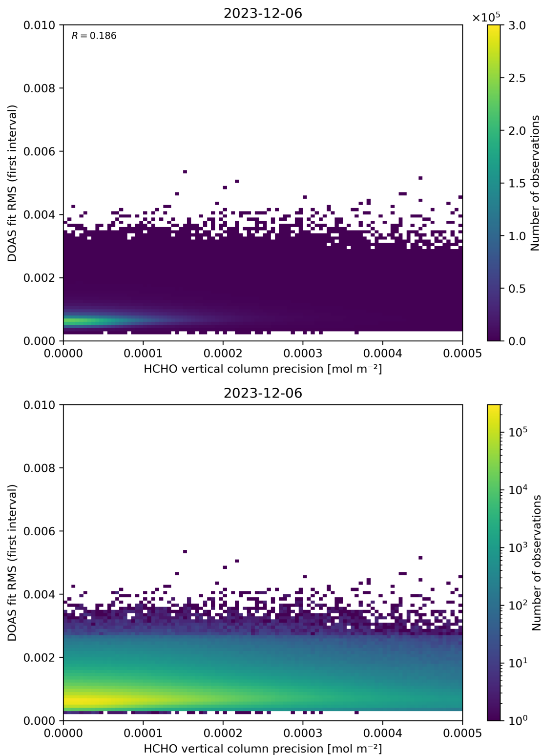
Figure 136: Scatter density plot of “HCHO vertical column precision” against “DOAS fit RMS (first interval)” for 2023-12-05 to 2023-12-07.
