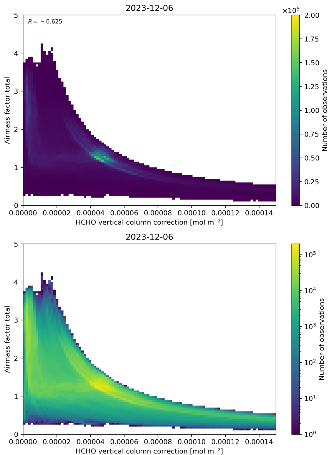
Figure 120: Scatter density plot of “HCHO vertical column correction” against “Airmass factor total” for 2023-12-05 to 2023-12-07.
