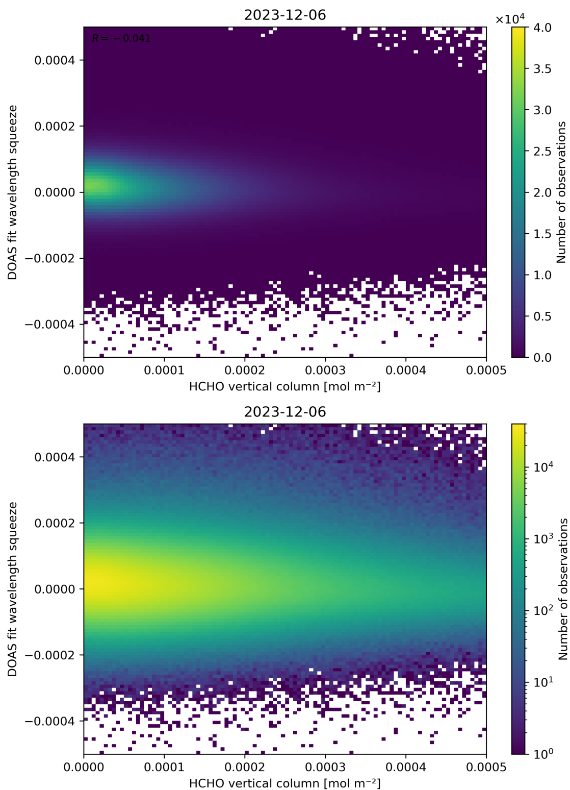
Figure 125: Scatter density plot of “HCHO vertical column” against “DOAS fit wavelength squeeze” for 2023-12-05 to 2023-12-07.
