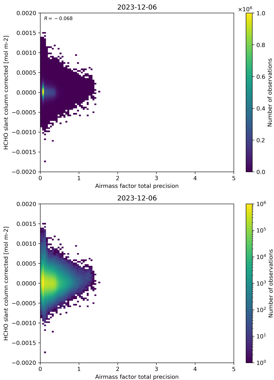
Figure 109: Scatter density plot of “Airmass factor total precision” against “HCHO slant column corrected” for 2023-12-05 to 2023-12-07.
