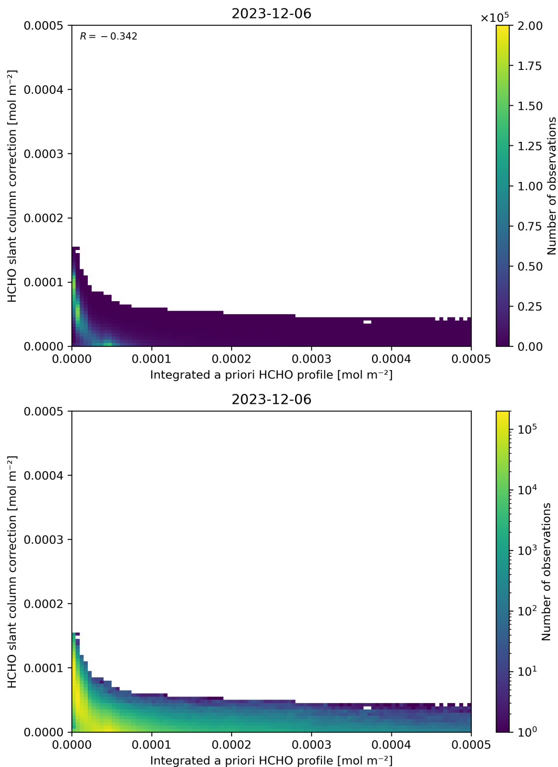
Figure 152: Scatter density plot of “Integrated a priori HCHO profile” against “HCHO slant column correction” for 2023-12-05 to 2023-12-07.
