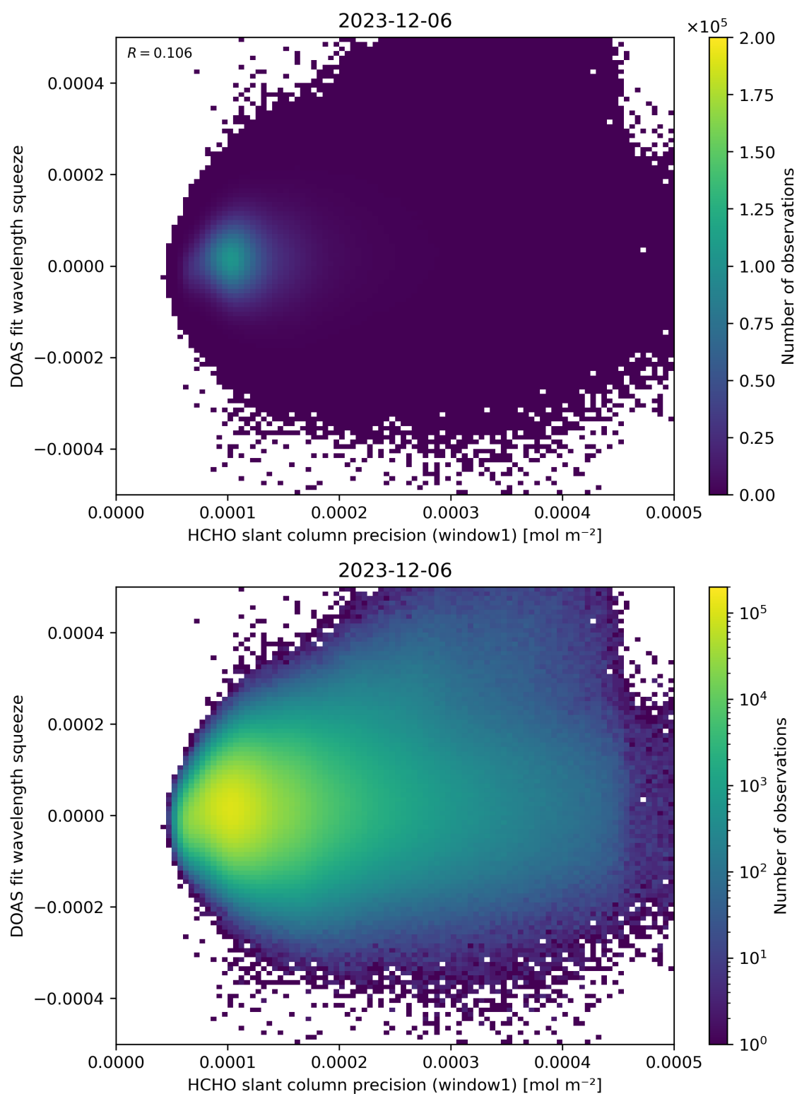
Figure 90: Scatter density plot of “HCHO slant column precision (window1)” against “DOAS fit wavelength squeeze” for 2023-12-05 to 2023-12-07.
