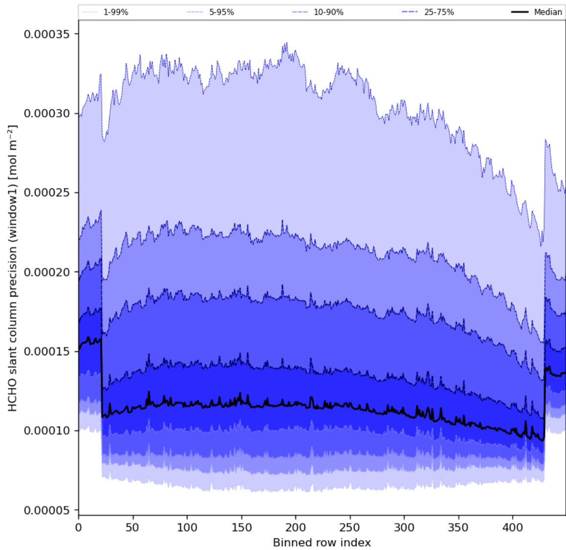
Figure 53: Along track statistics of “HCHO slant column precision (window1)” for 2023-12-05 to 2023-12-07
