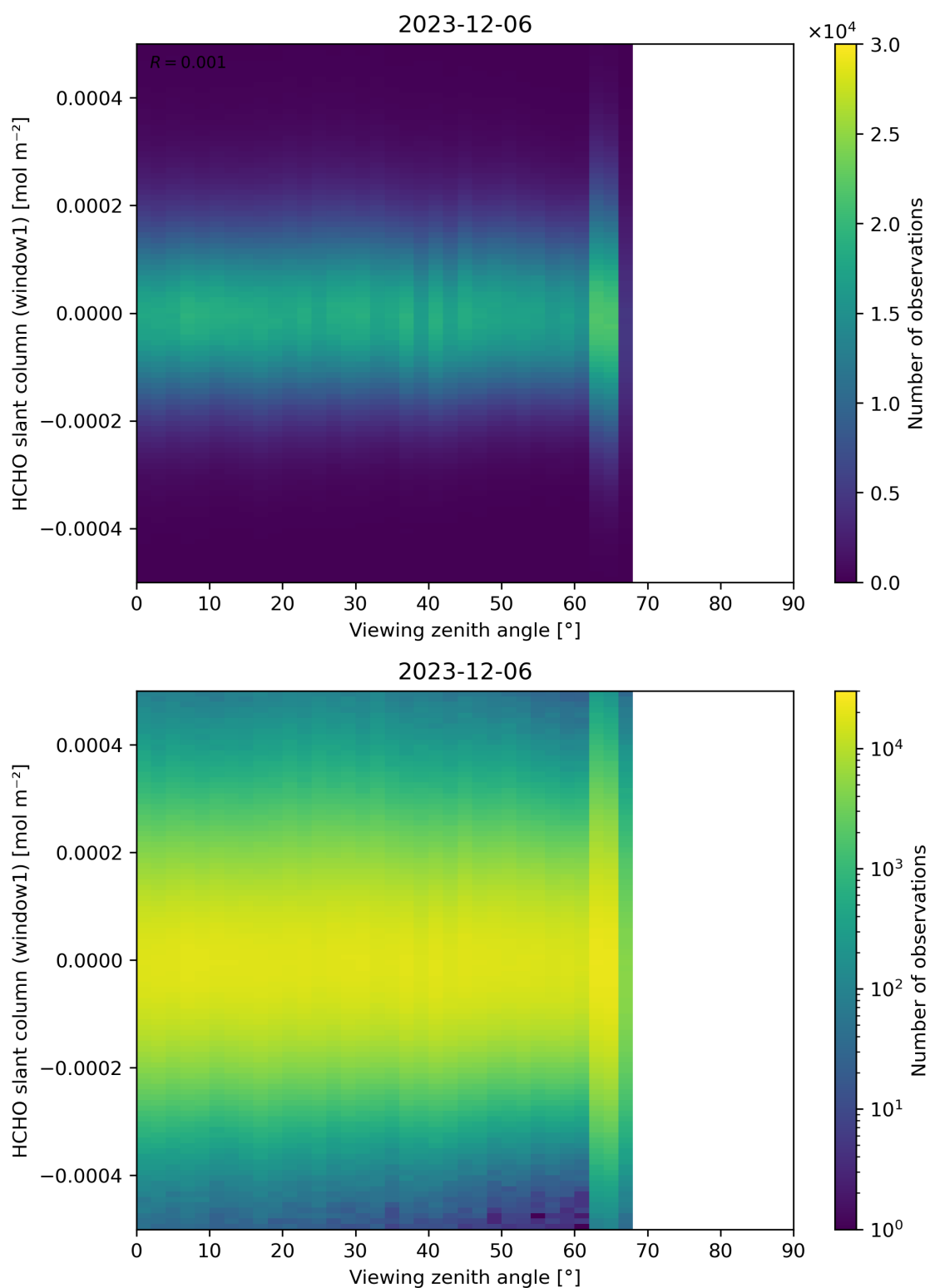
Figure 188: Scatter density plot of “Viewing zenith angle” against “HCHO slant column (window1)” for 2023-12-05 to 2023-12-07.
