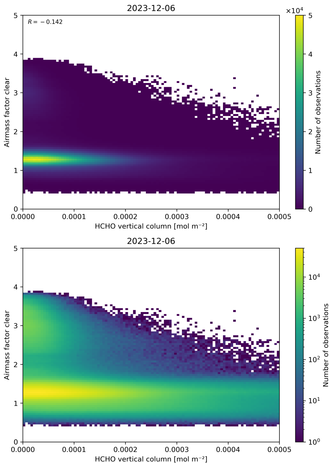
Figure 126: Scatter density plot of “HCHO vertical column” against “Airmass factor clear” for 2023-12-05 to 2023-12-07.
