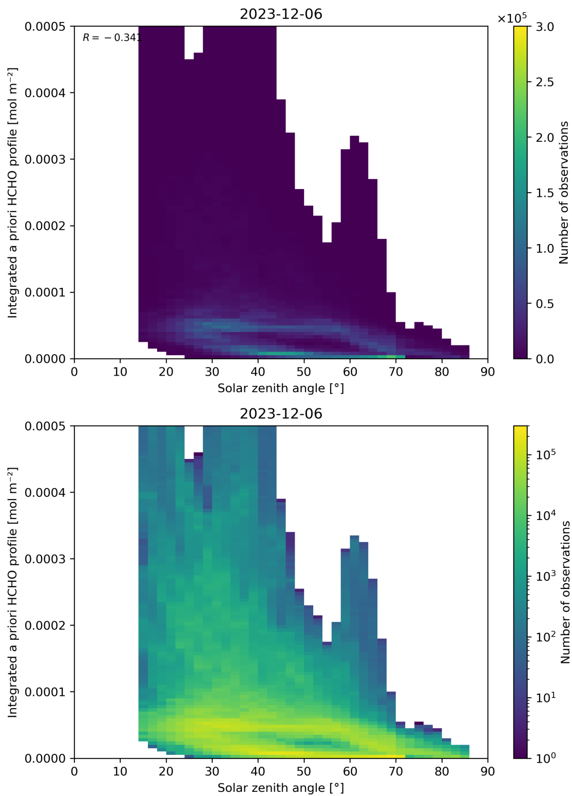
Figure 180: Scatter density plot of “Solar zenith angle” against “Integrated a priori HCHO profile” for 2023-12-05 to 2023-12-07.
