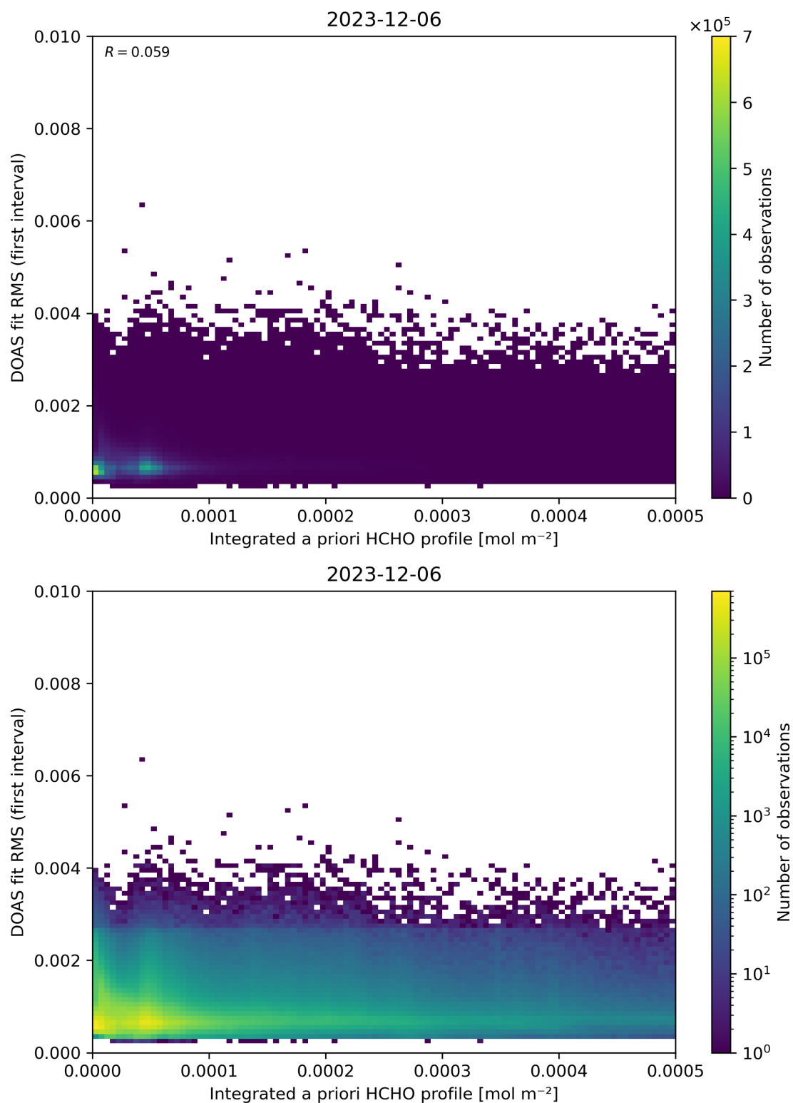
Figure 148: Scatter density plot of “Integrated a priori HCHO profile” against “DOAS fit RMS (first interval)” for 2023-12-05 to 2023-12-07.
