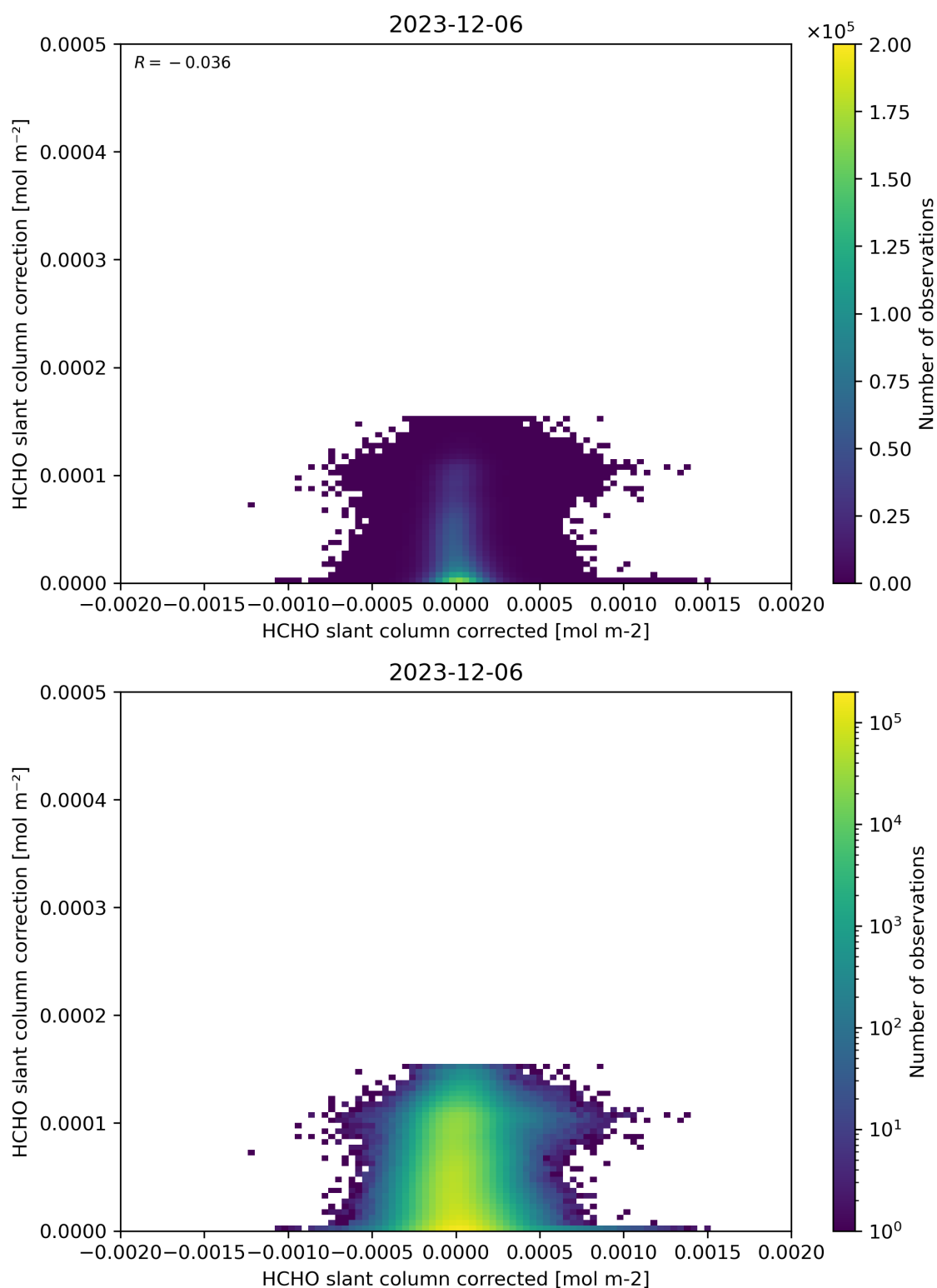
Figure 77: Scatter density plot of “HCHO slant column corrected” against “HCHO slant column correction” for 2023-12-05 to 2023-12-07.
