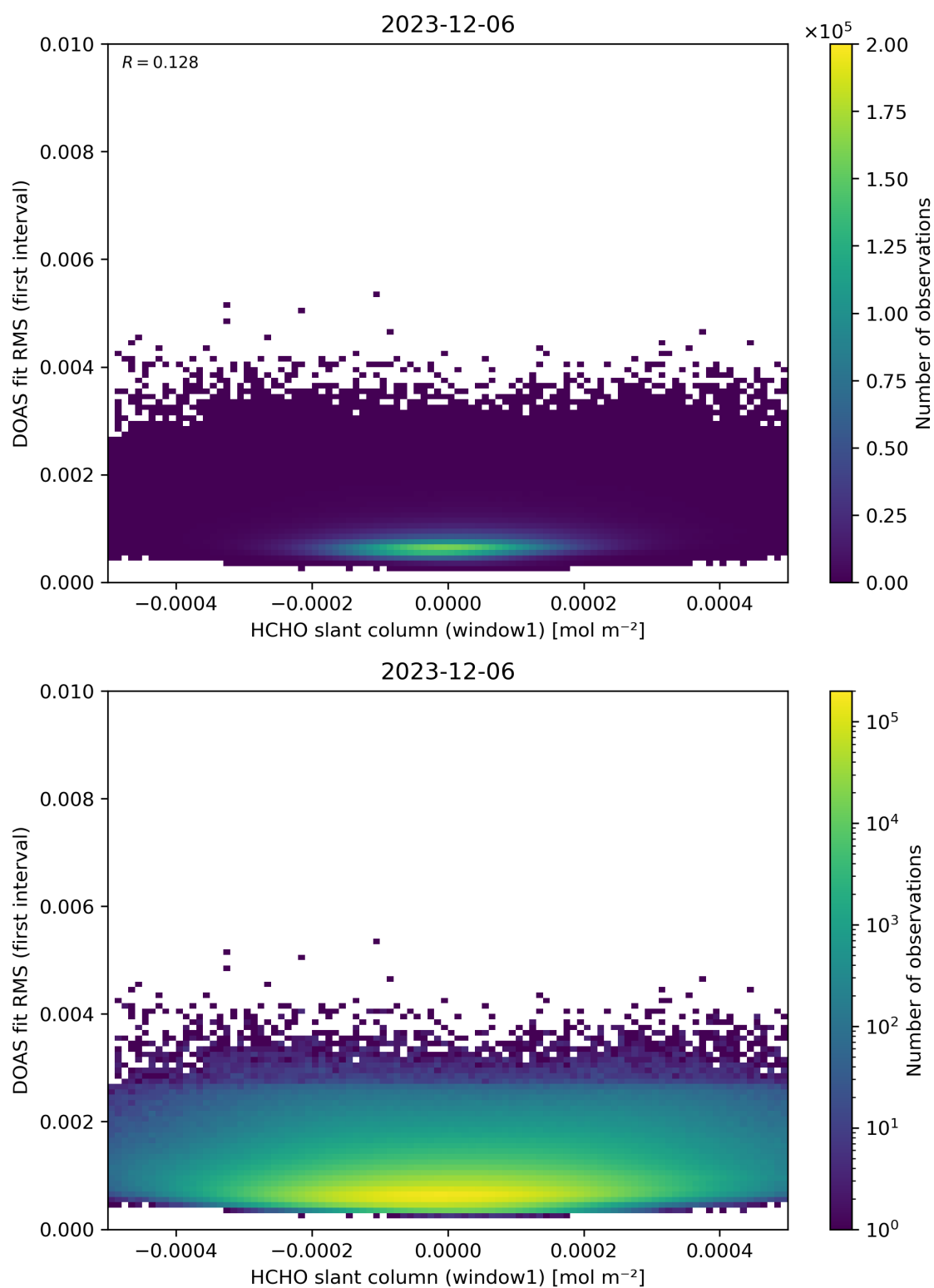
Figure 78: Scatter density plot of “HCHO slant column (window1)” against “DOAS fit RMS (first interval)” for 2023-12-05 to 2023-12-07.
