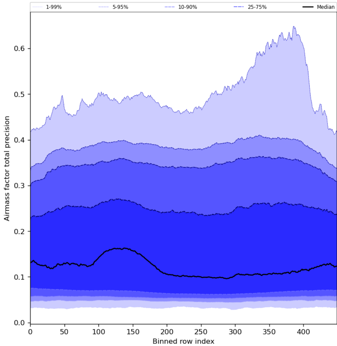
Figure 55: Along track statistics of “Airmass factor total precision” for 2023-12-05 to 2023-12-07
