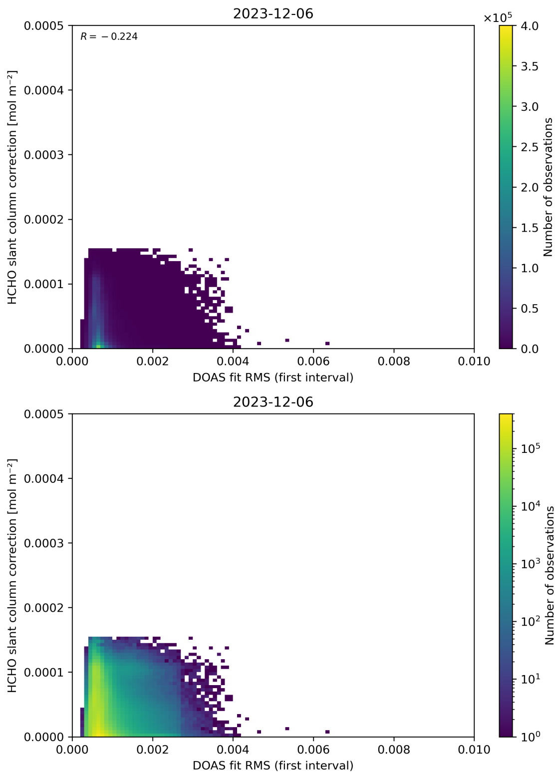
Figure 63: Scatter density plot of “DOAS fit RMS (first interval)” against “HCHO slant column correction” for 2023-12-05 to 2023-12-07.
