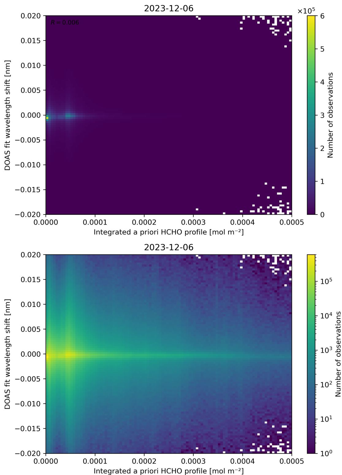
Figure 149: Scatter density plot of “Integrated a priori HCHO profile” against “DOAS fit wavelength shift” for 2023-12-05 to 2023-12-07.
