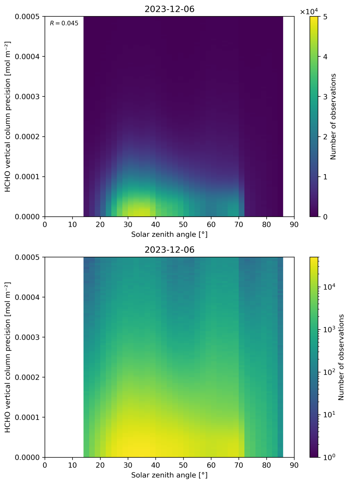
Figure 179: Scatter density plot of “Solar zenith angle” against “HCHO vertical column precision” for 2023-12-05 to 2023-12-07.
