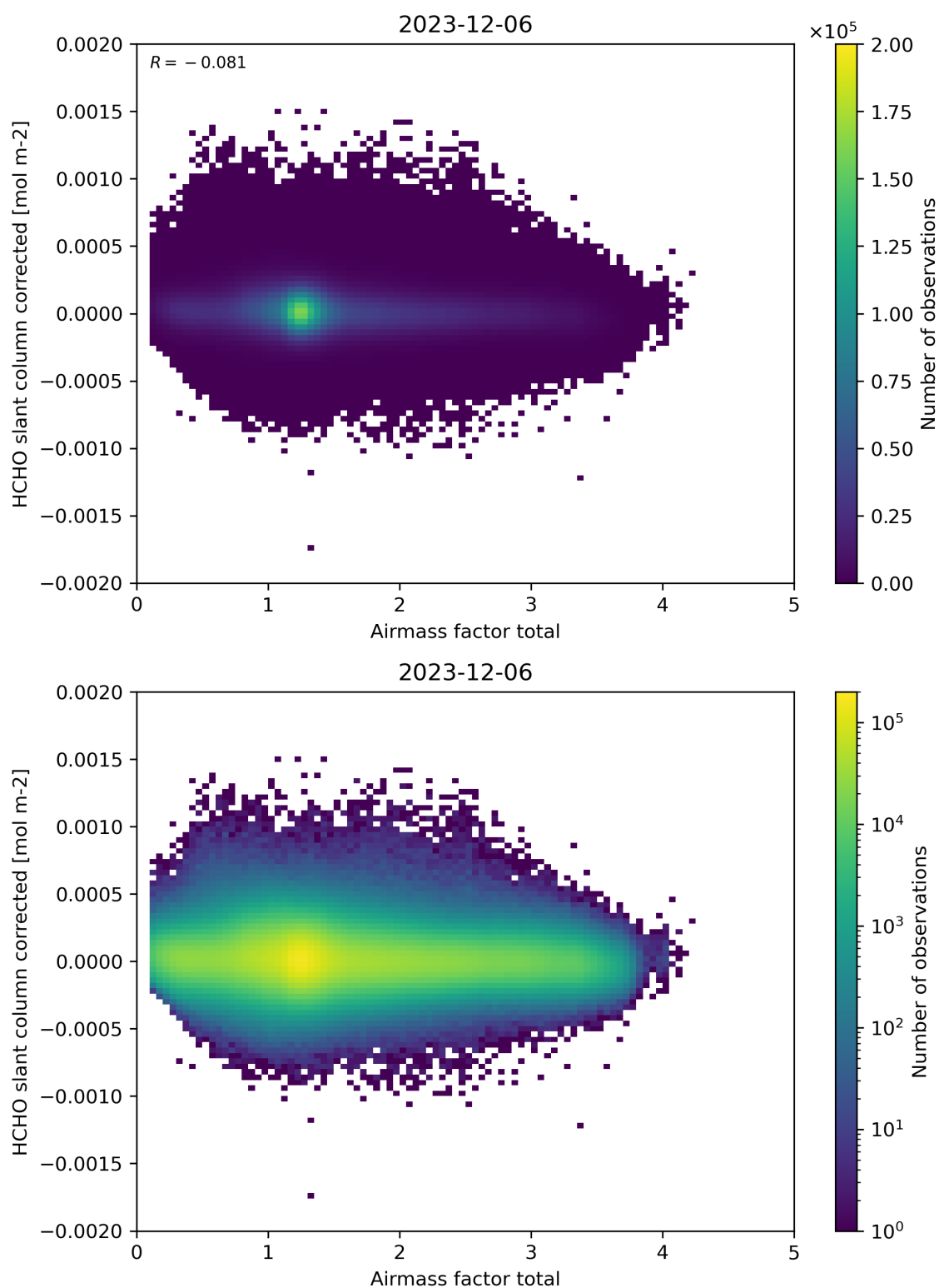
Figure 101: Scatter density plot of “Airmass factor total” against “HCHO slant column corrected” for 2023-12-05 to 2023-12-07.
