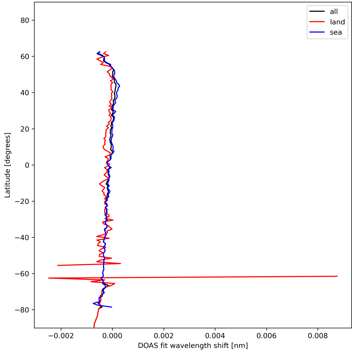
Figure 30: Zonal average of “DOAS fit wavelength shift” for 2023-12-05 to 2023-12-07.
