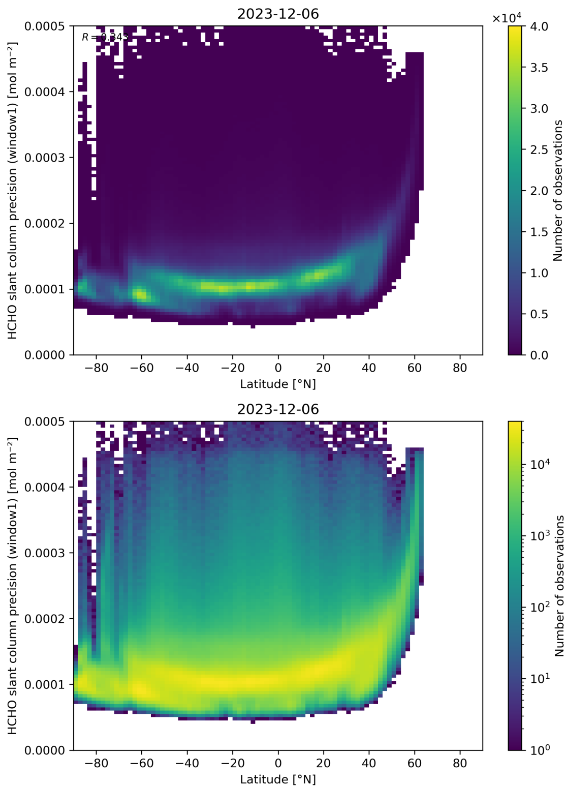
Figure 160: Scatter density plot of “Latitude” against “HCHO slant column precision (window1)” for 2023-12-05 to 2023-12-07.
