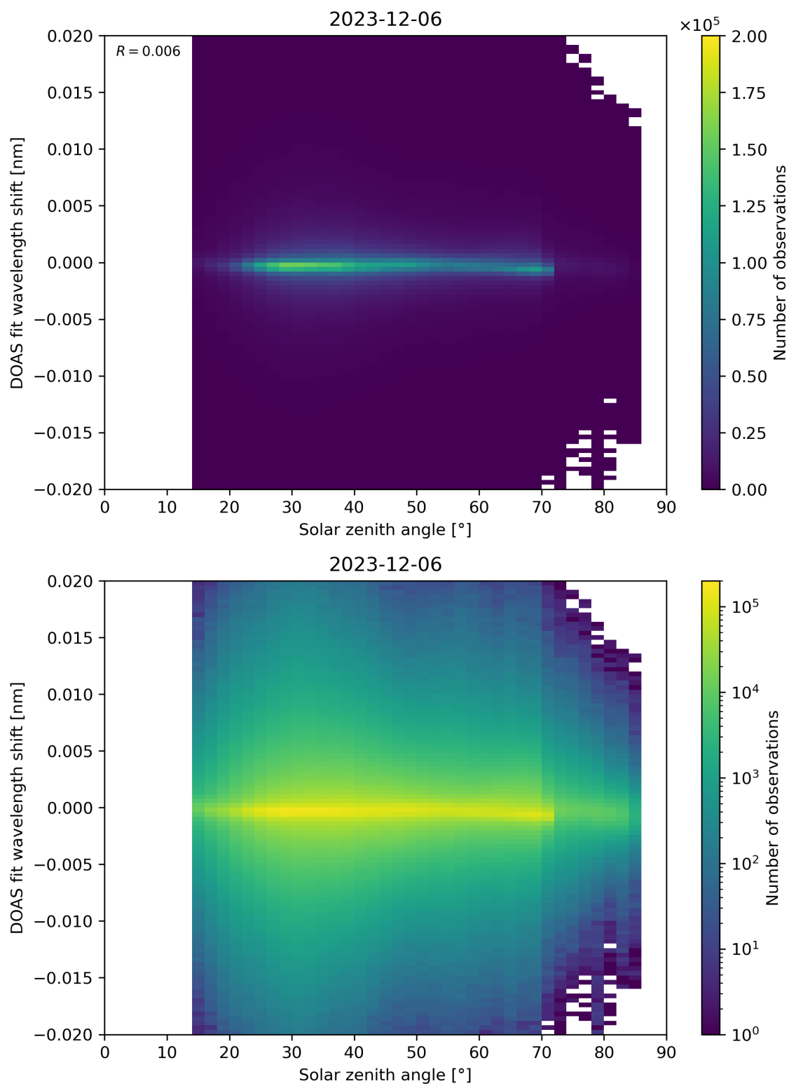
Figure 168: Scatter density plot of “Solar zenith angle” against “DOAS fit wavelength shift” for 2023-12-05 to 2023-12-07.
