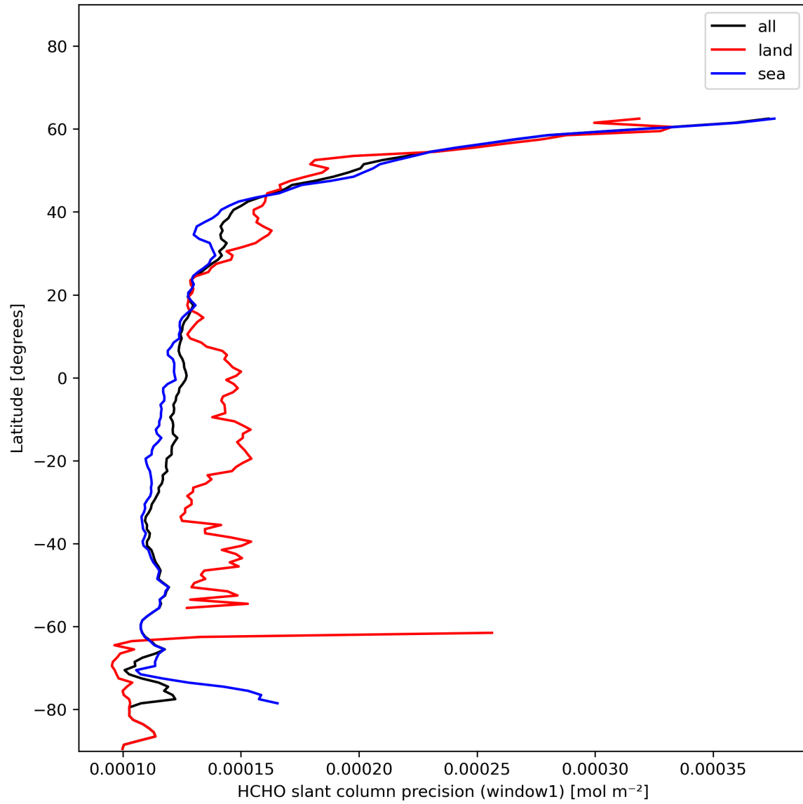
Figure 25: Zonal average of "HCHO slant column precision (window1)" for 2023-12-05 to 2023-12-07.
