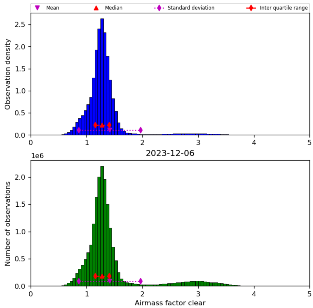
Figure 42: Histogram of “Airmass factor clear” for 2023-12-05 to 2023-12-07
