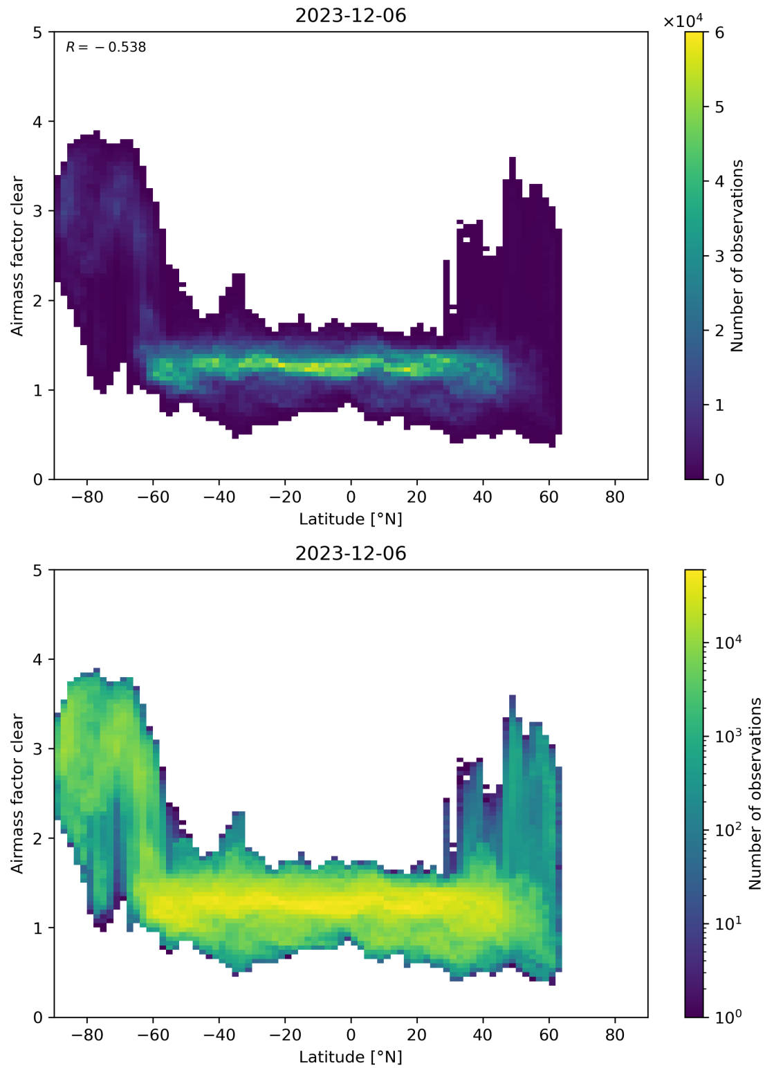
Figure 156: Scatter density plot of “Latitude” against “Airmass factor clear” for 2023-12-05 to 2023-12-07.
