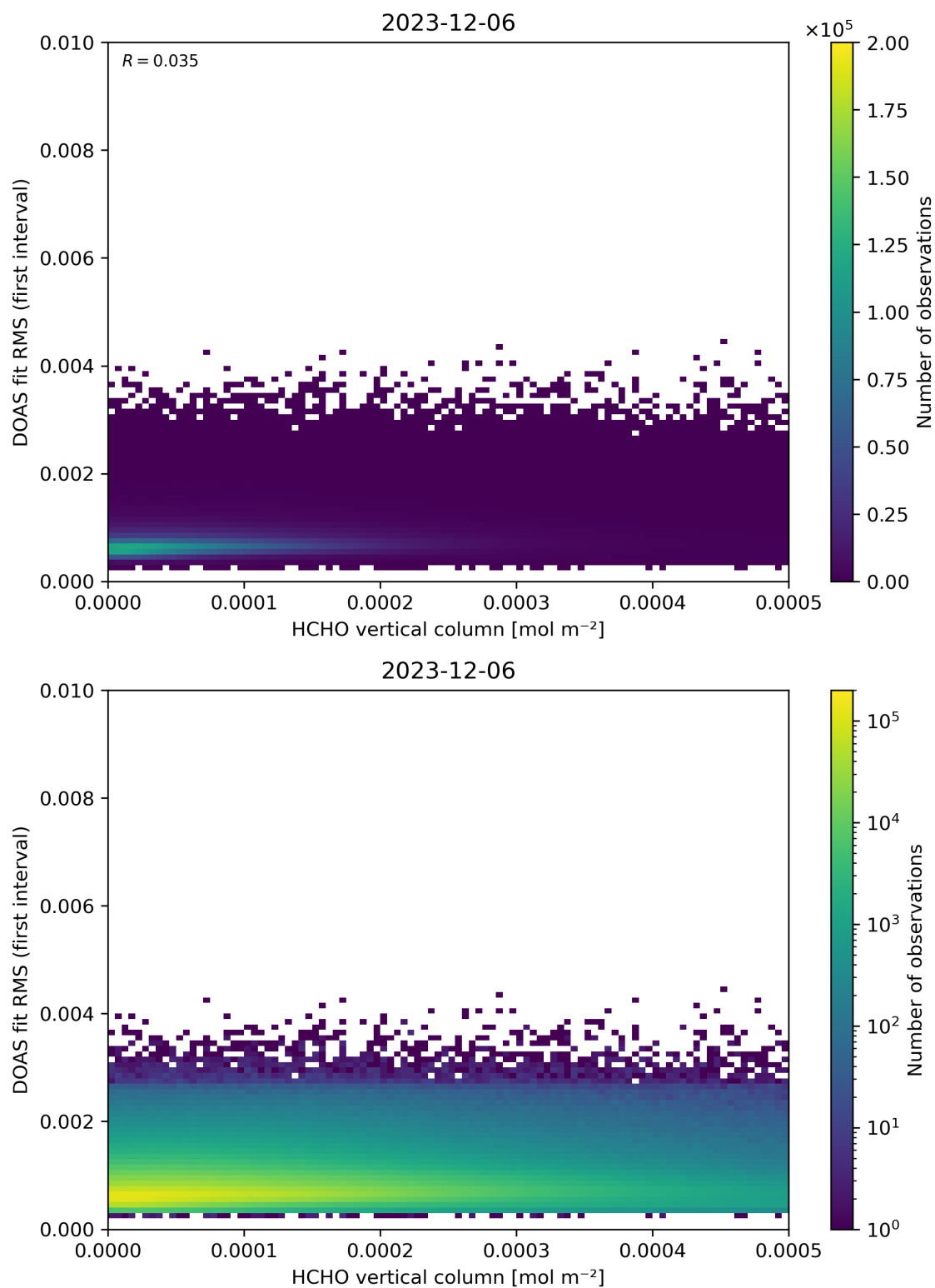
Figure 123: Scatter density plot of “HCHO vertical column” against “DOAS fit RMS (first interval)” for 2023-12-05 to 2023-12-07.
