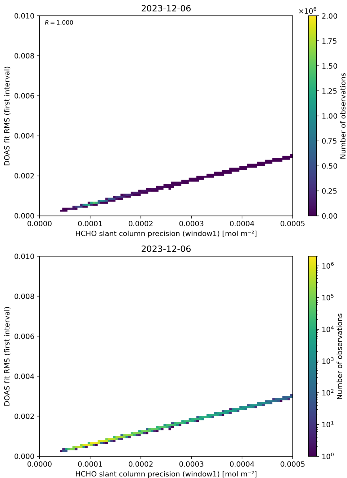
Figure 88: Scatter density plot of “HCHO slant column precision (window1)” against “DOAS fit RMS (first interval)” for 2023-12-05 to 2023-12-07.
