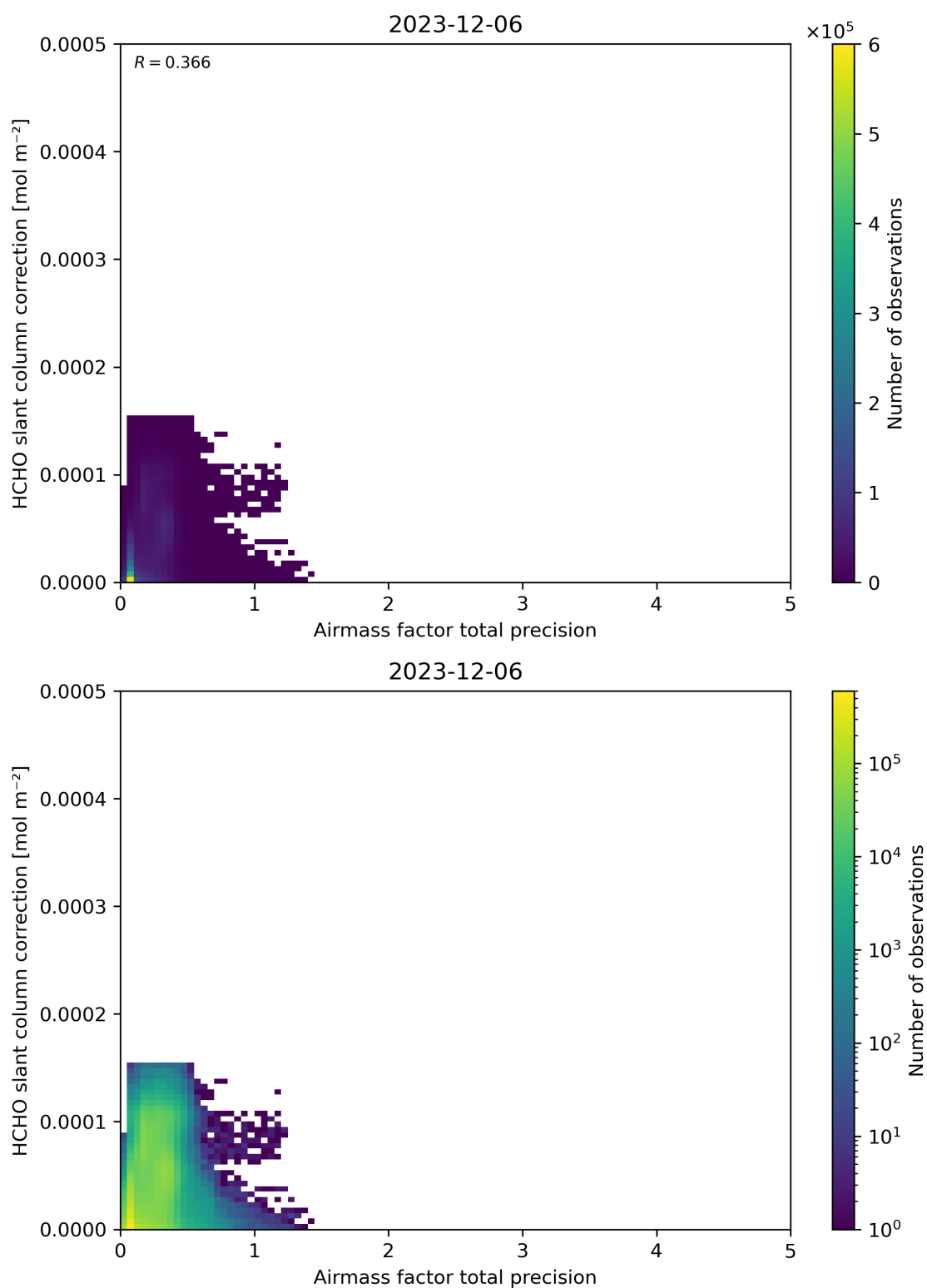
Figure 110: Scatter density plot of “Airmass factor total precision” against “HCHO slant column correction” for 2023-12-05 to 2023-12-07.
