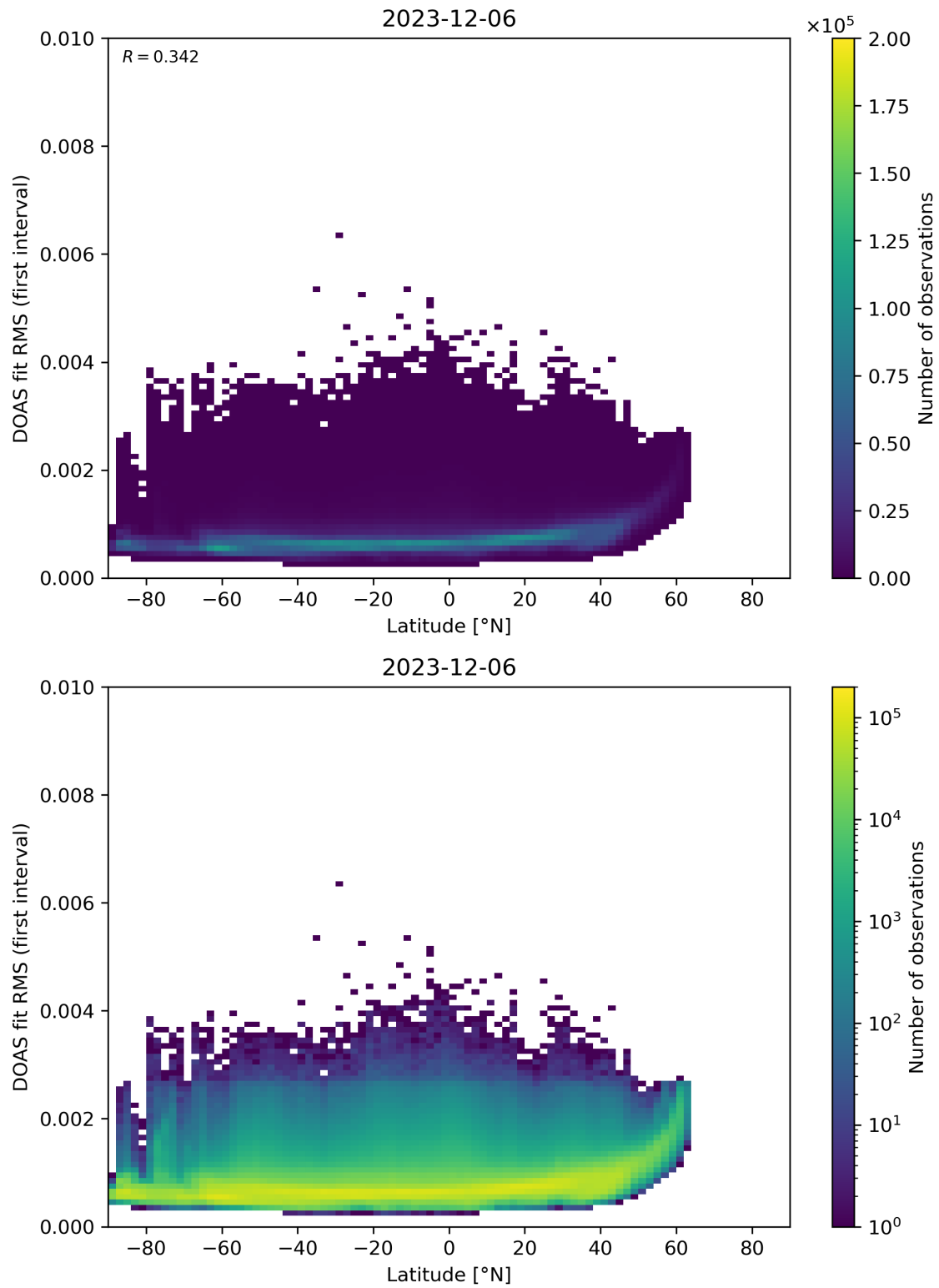
Figure 153: Scatter density plot of “Latitude” against “DOAS fit RMS (first interval)” for 2023-12-05 to 2023-12-07.
