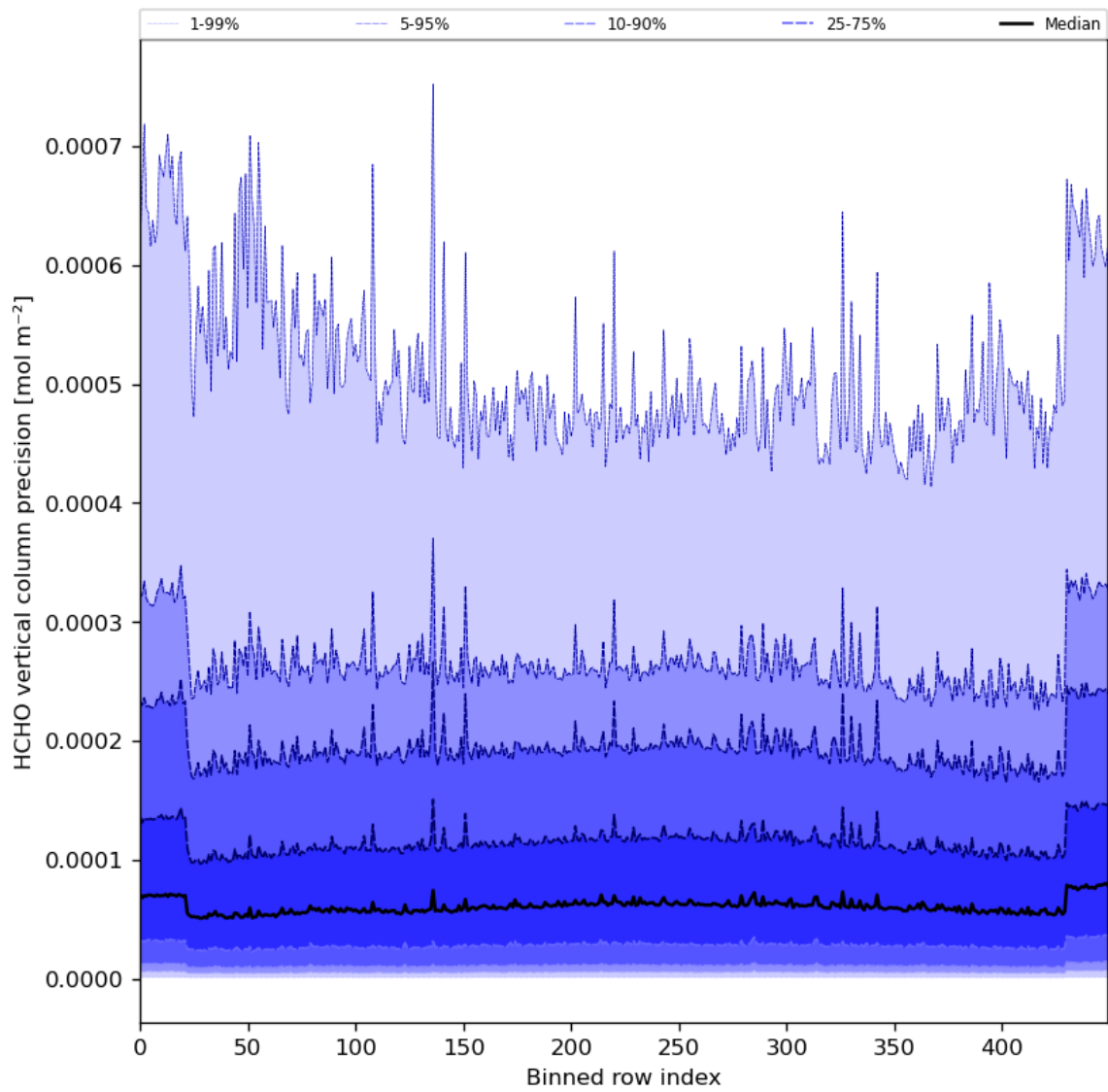
Figure 50: Along track statistics of “HCHO vertical column precision” for 2023-12-05 to 2023-12-07
