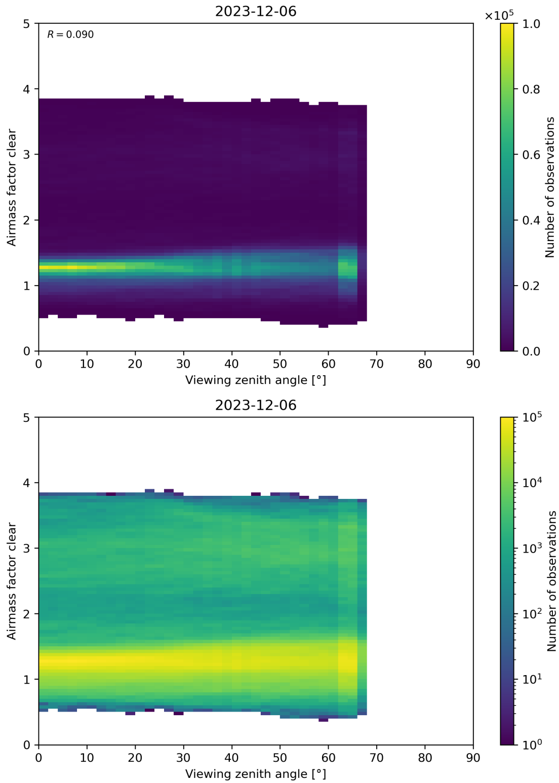
Figure 185: Scatter density plot of “Viewing zenith angle” against “Airmass factor clear” for 2023-12-05 to 2023-12-07.
