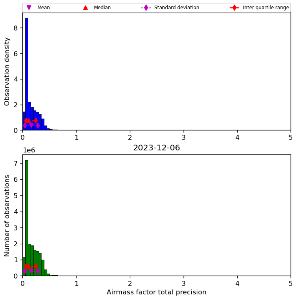
Figure 41: Histogram of “Airmass factor total precision” for 2023-12-05 to 2023-12-07
