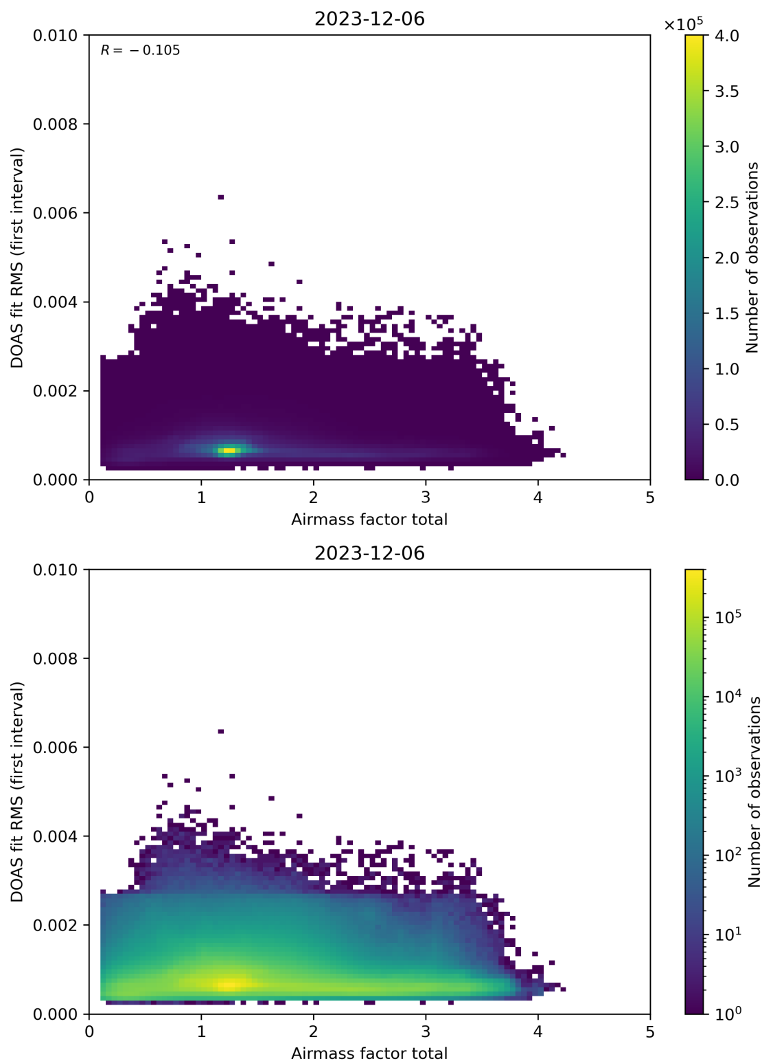
Figure 97: Scatter density plot of “Airmass factor total” against “DOAS fit RMS (first interval)” for 2023-12-05 to 2023-12-07.
