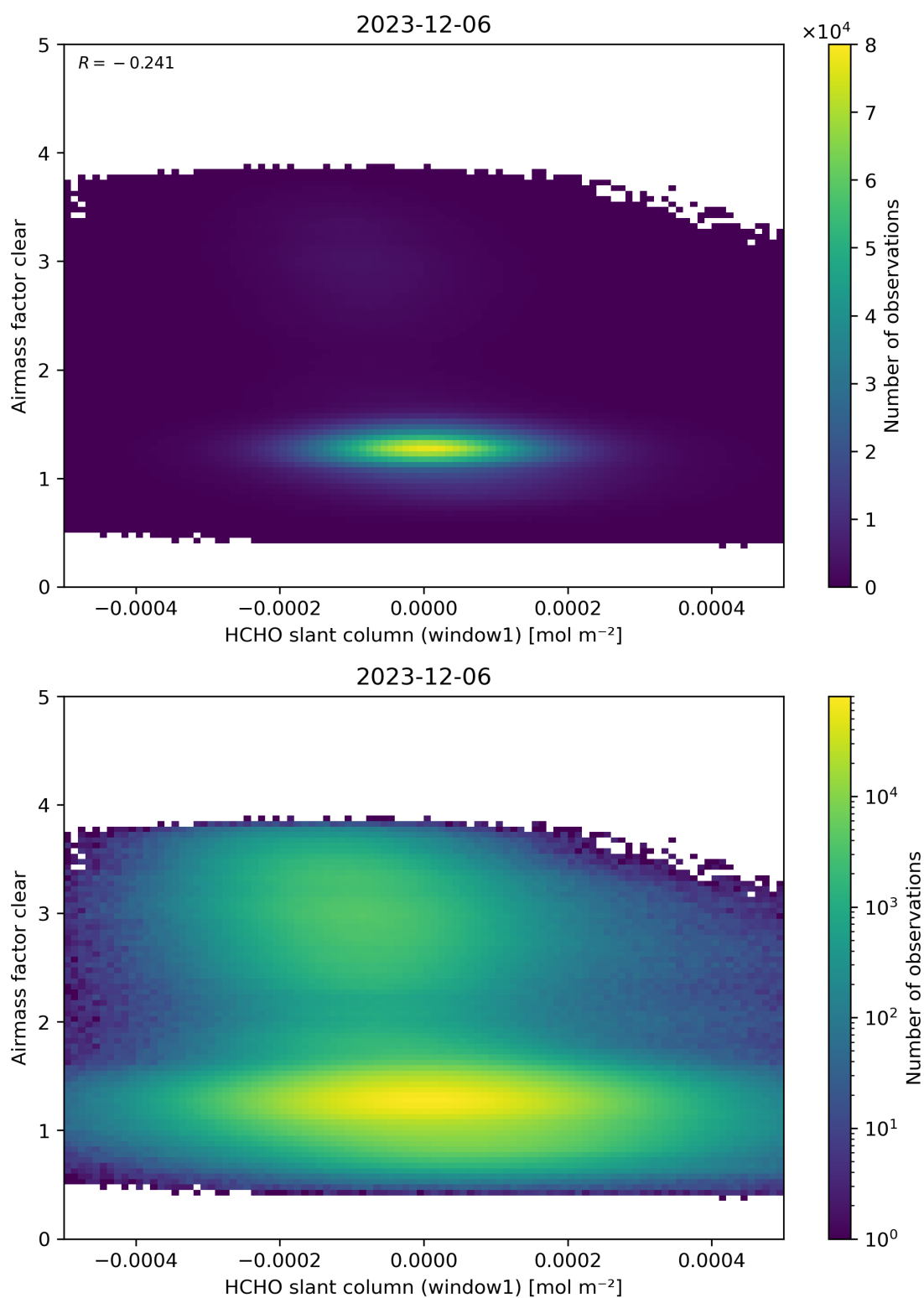
Figure 81: Scatter density plot of “HCHO slant column (window1)” against “Airmass factor clear” for 2023-12-05 to 2023-12-07.
