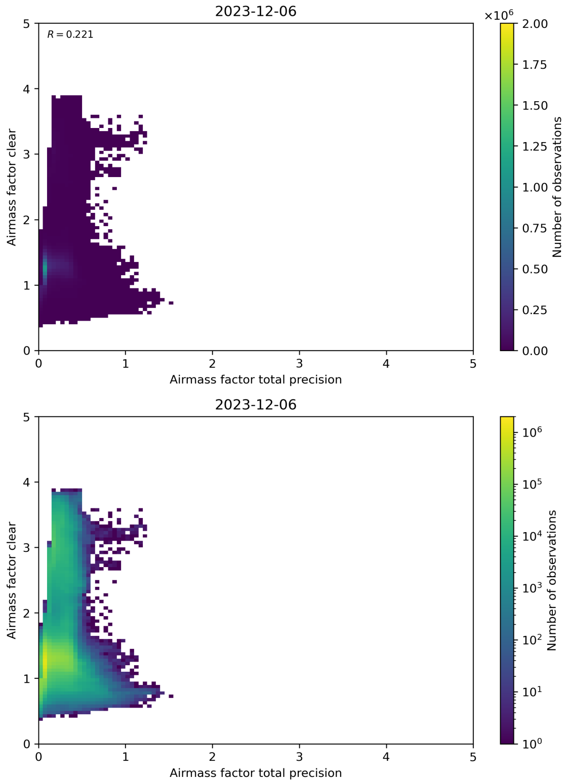
Figure 108: Scatter density plot of “Airmass factor total precision” against “Airmass factor clear” for 2023-12-05 to 2023-12-07.
