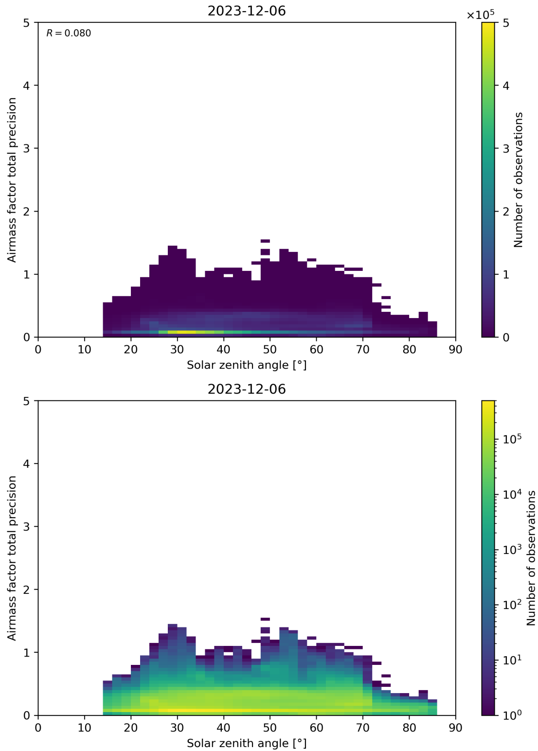
Figure 176: Scatter density plot of “Solar zenith angle” against “Airmass factor total precision” for 2023-12-05 to 2023-12-07.
