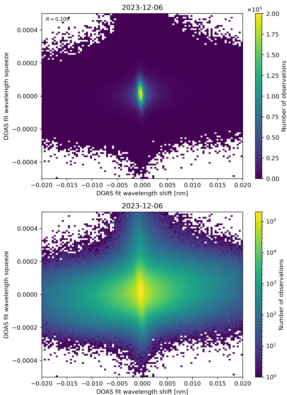
Figure 65: Scatter density plot of “DOAS fit wavelength shift” against “DOAS fit wavelength squeeze” for 2023-12-05 to 2023-12-07.
