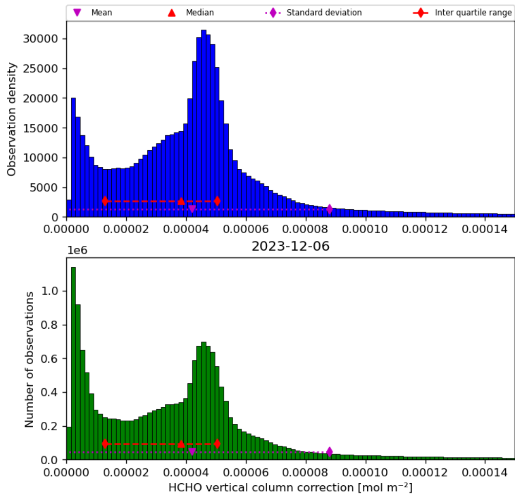
Figure 37: Histogram of “HCHO vertical column correction” for 2023-12-05 to 2023-12-07
