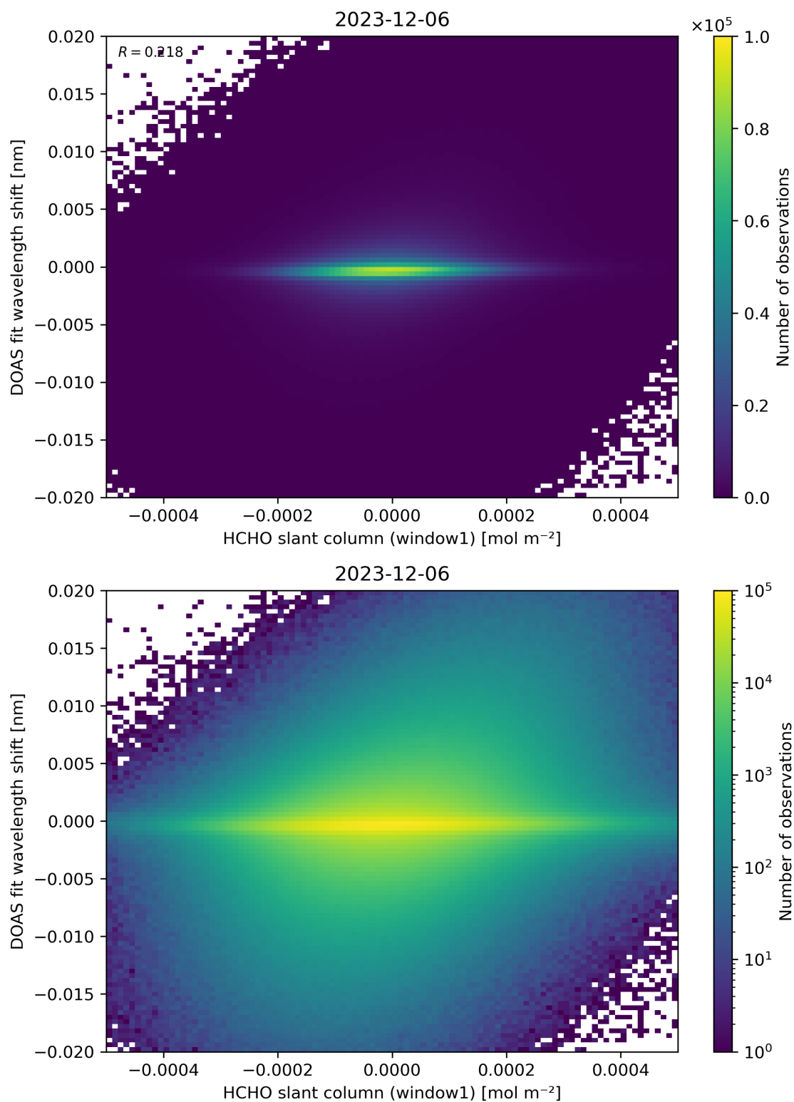
Figure 79: Scatter density plot of “HCHO slant column (window1)” against “DOAS fit wavelength shift” for 2023-12-05 to 2023-12-07.
