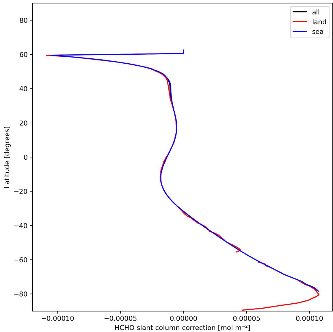
Figure 33: Zonal average of “HCHO slant column correction” for 2023-12-05 to 2023-12-07.
