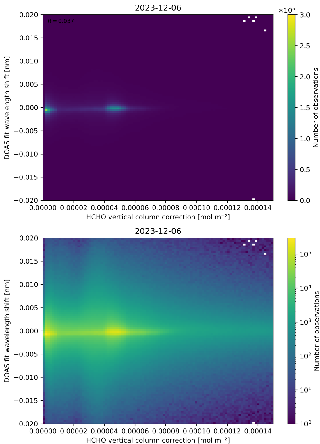
Figure 113: Scatter density plot of “HCHO vertical column correction” against “DOAS fit wavelength shift” for 2023-12-05 to 2023-12-07.
