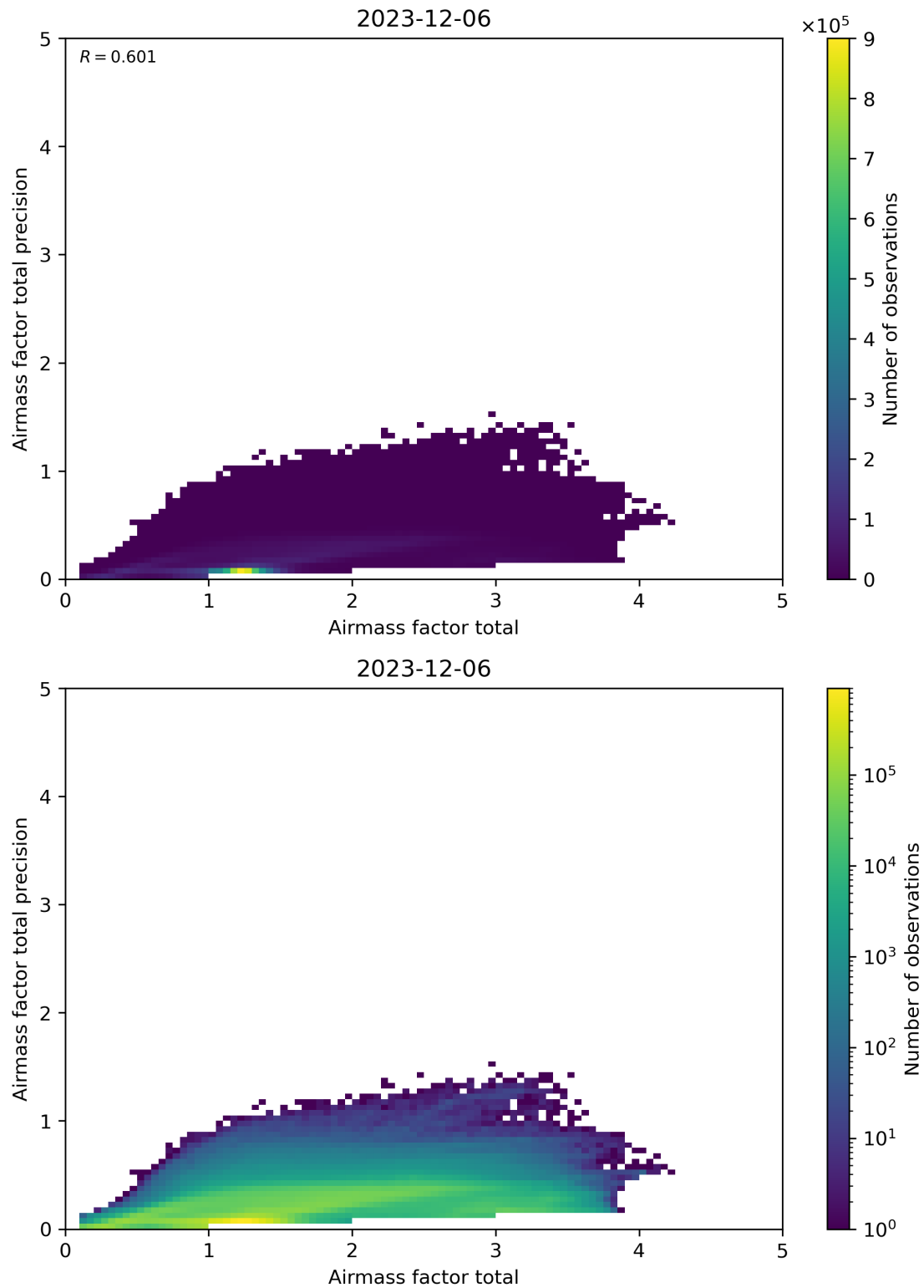
Figure 103: Scatter density plot of “Airmass factor total” against “Airmass factor total precision” for 2023-12-05 to 2023-12-07.
