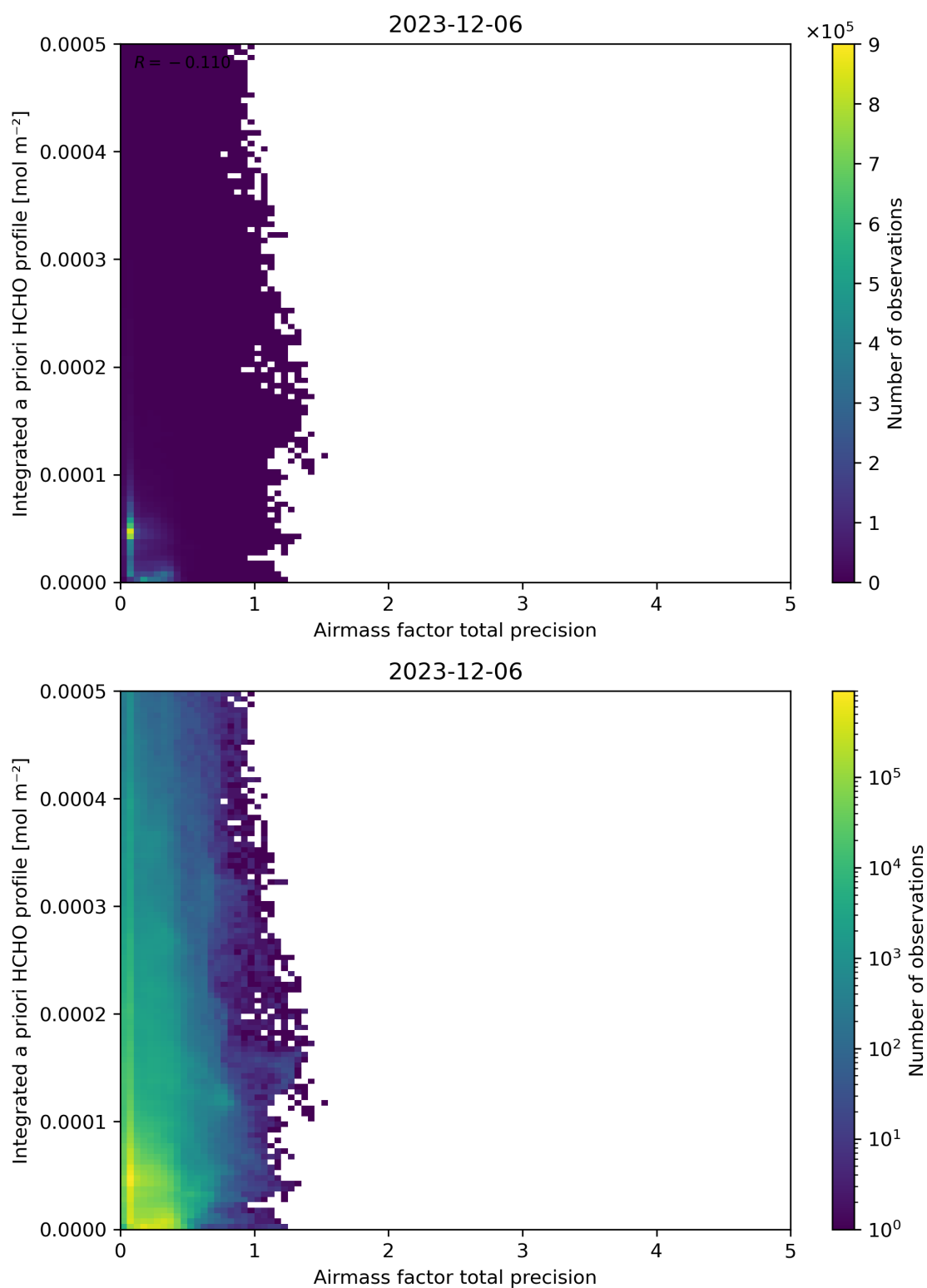
Figure 111: Scatter density plot of “Airmass factor total precision” against “Integrated a priori HCHO profile” for 2023-12-05 to 2023-12-07.
