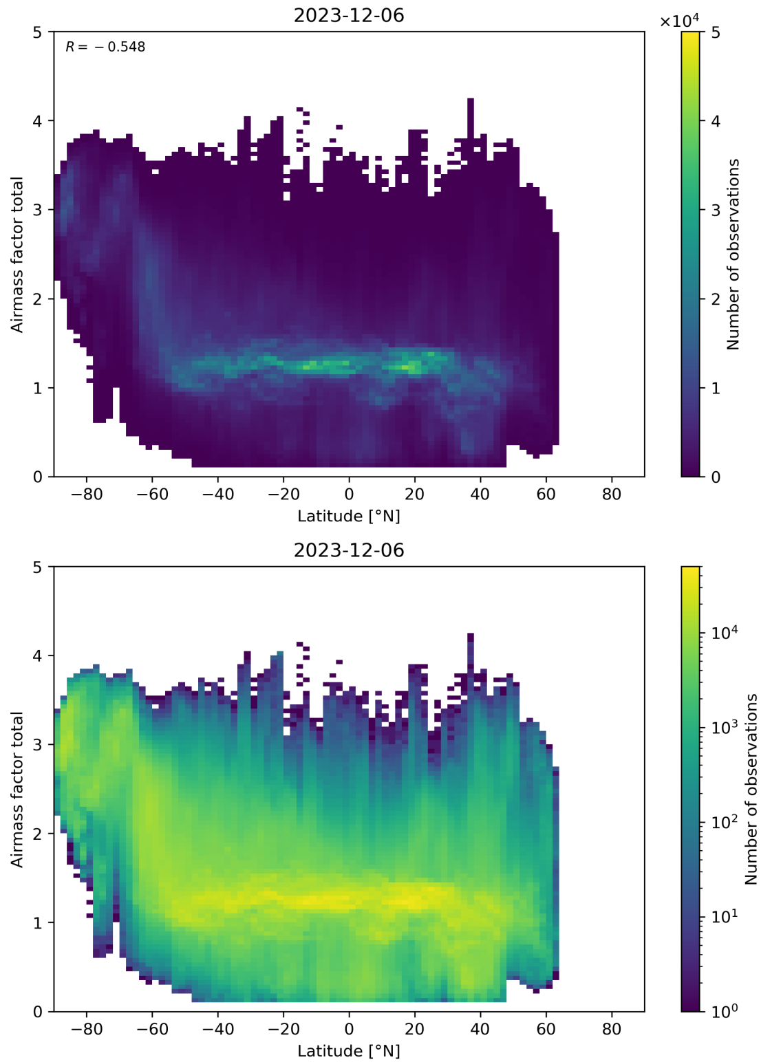
Figure 161: Scatter density plot of “Latitude” against “Airmass factor total” for 2023-12-05 to 2023-12-07.
