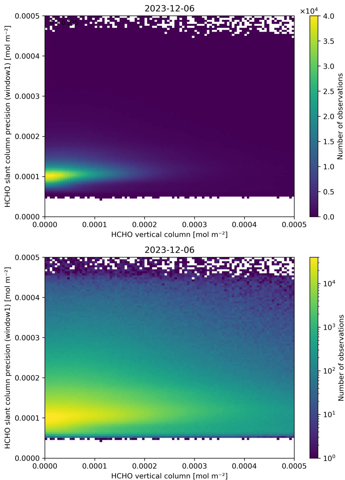
Figure 130: Scatter density plot of “HCHO vertical column” against “HCHO slant column precision (window1)” for 2023-12-05 to 2023-12-07.
