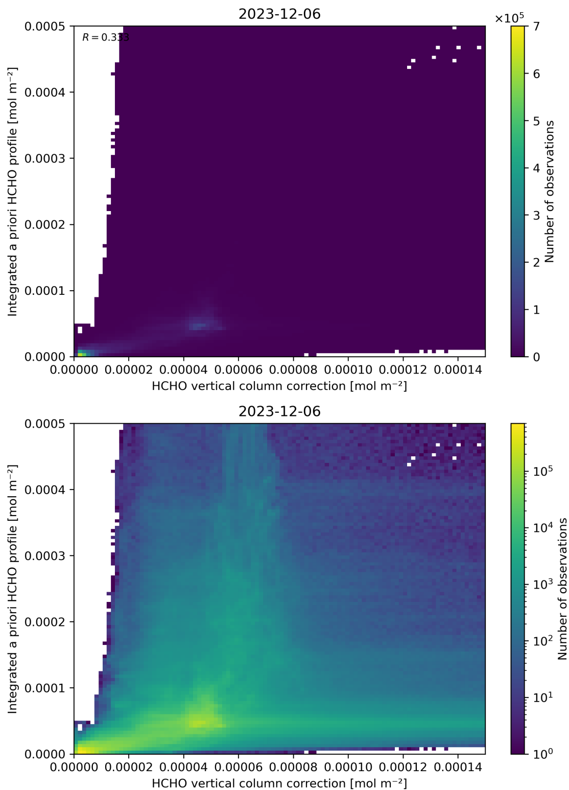
Figure 122: Scatter density plot of “HCHO vertical column correction” against “Integrated a priori HCHO profile” for 2023-12-05 to 2023-12-07.
