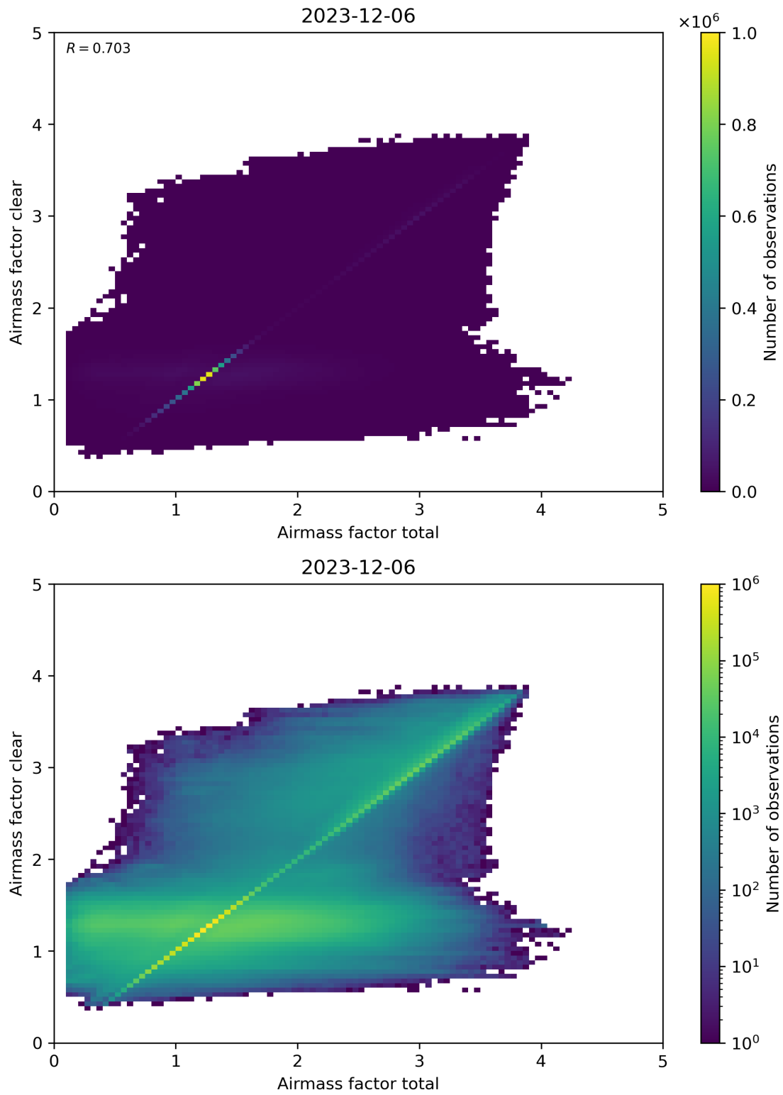
Figure 100: Scatter density plot of “Airmass factor total” against “Airmass factor clear” for 2023-12-05 to 2023-12-07.
