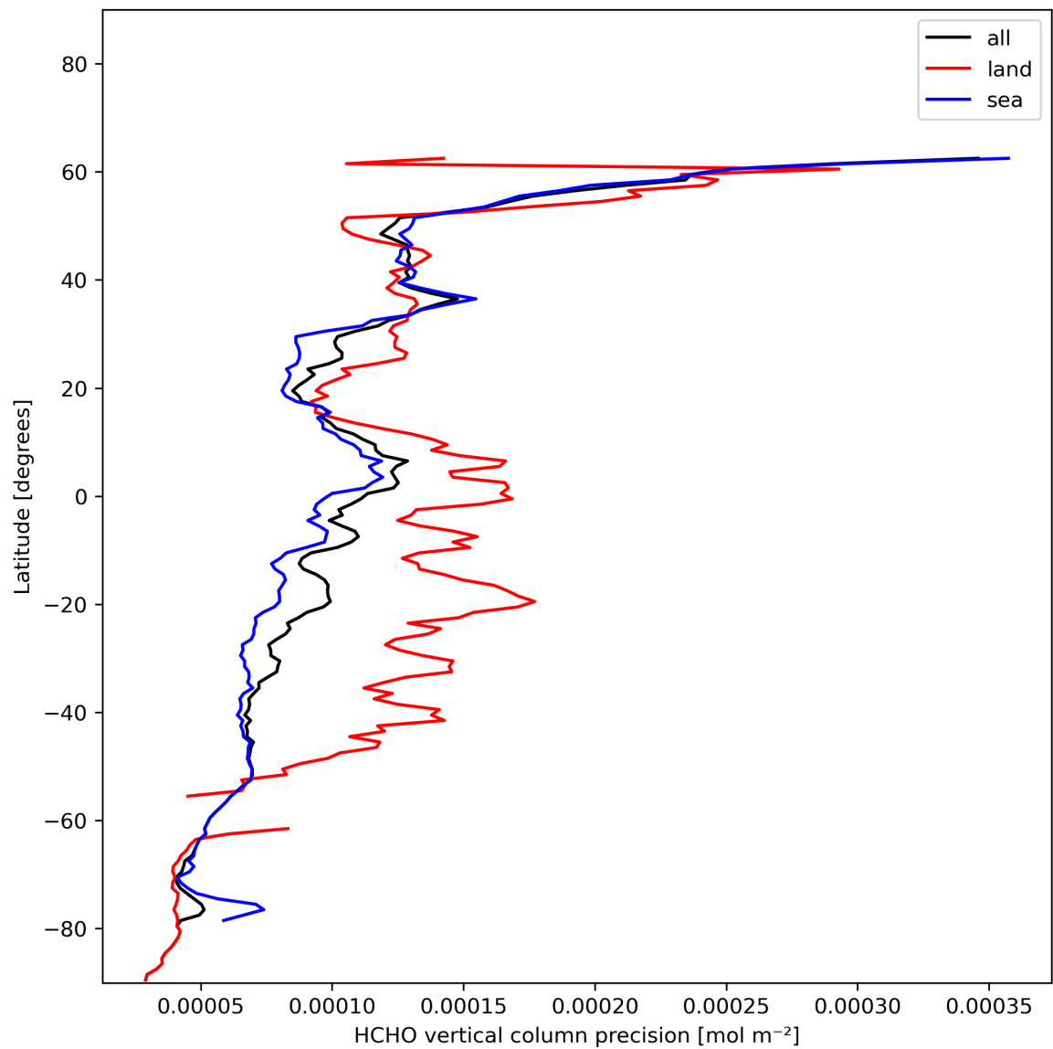
Figure 22: Zonal average of “HCHO vertical column precision” for 2023-12-05 to 2023-12-07.
