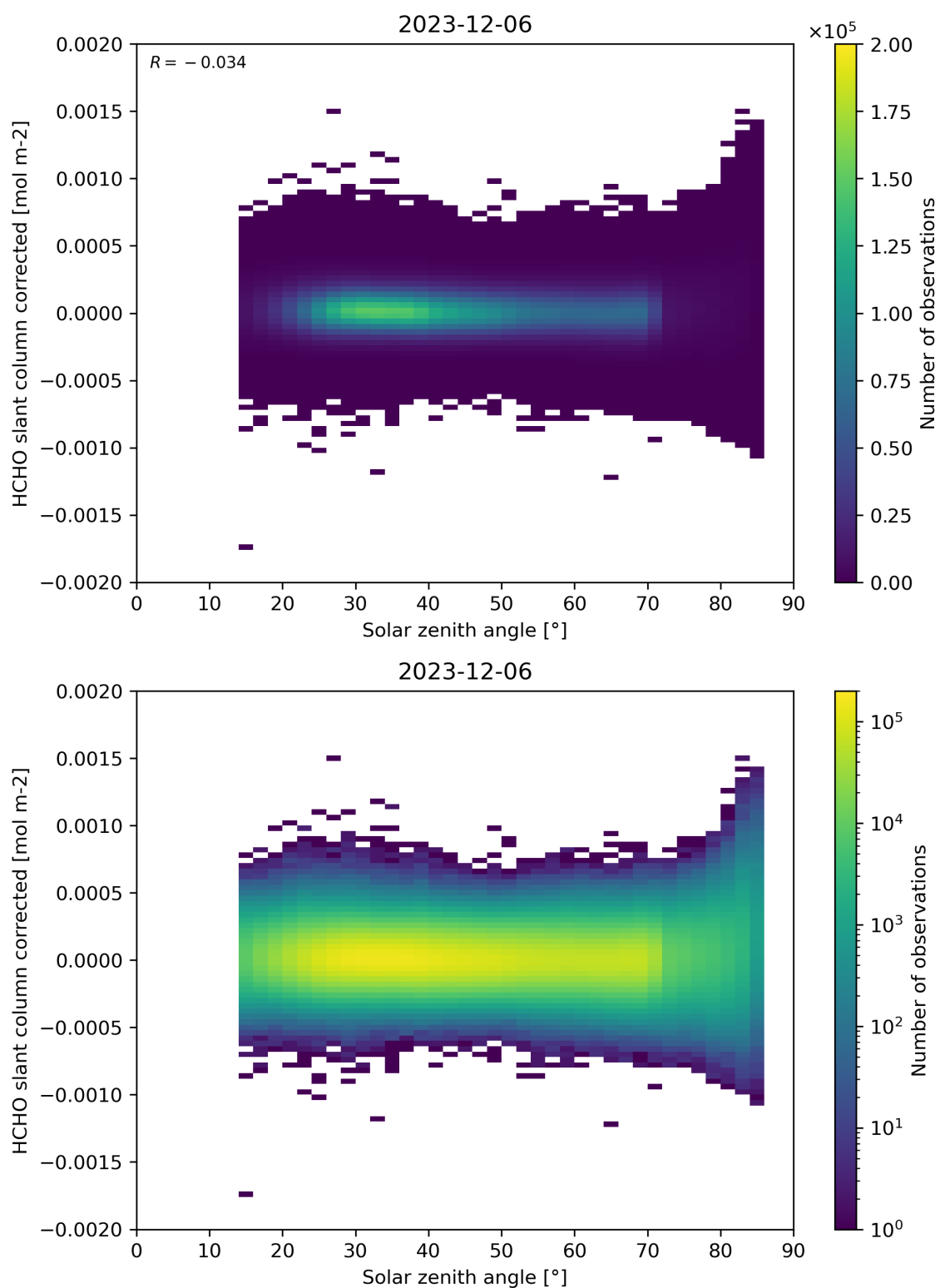
Figure 171: Scatter density plot of “Solar zenith angle” against “HCHO slant column corrected” for 2023-12-05 to 2023-12-07.
