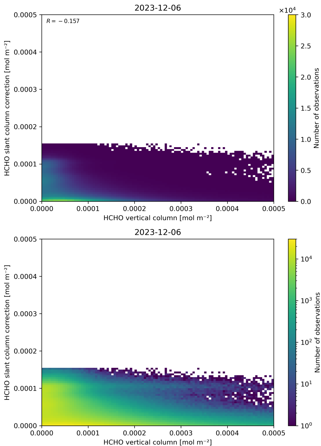
Figure 128: Scatter density plot of “HCHO vertical column” against “HCHO slant column correction” for 2023-12-05 to 2023-12-07.
