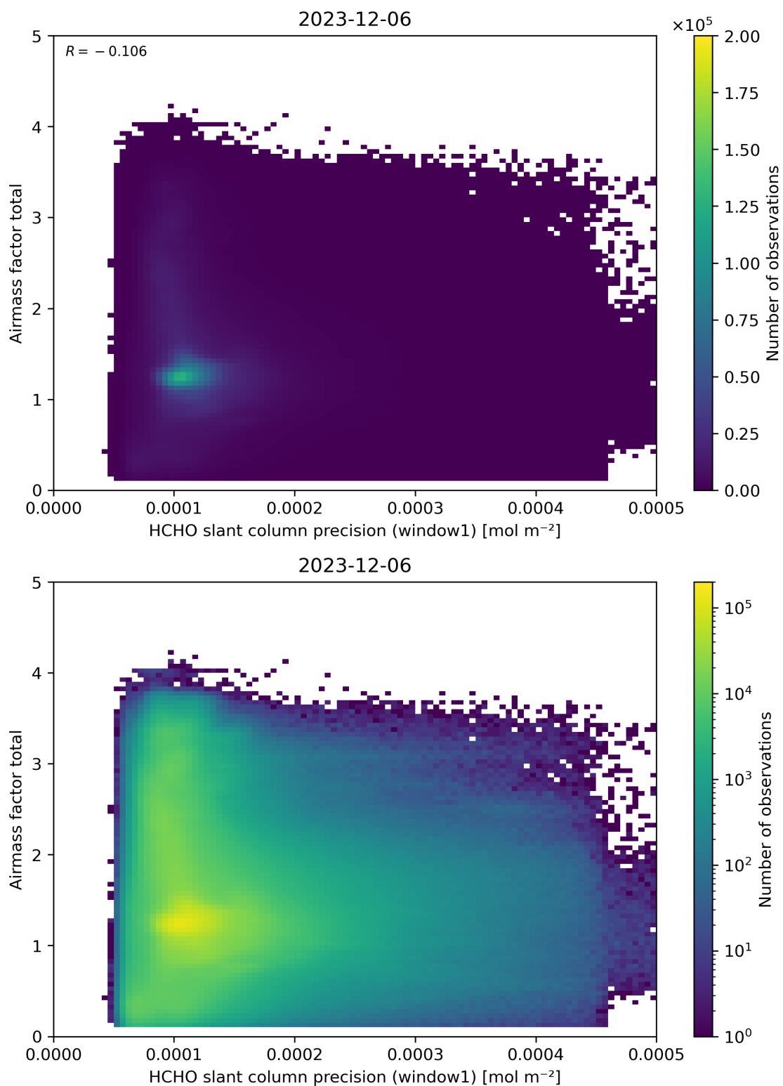
Figure 94: Scatter density plot of “HCHO slant column precision (window1)” against “Airmass factor total” for 2023-12-05 to 2023-12-07.
