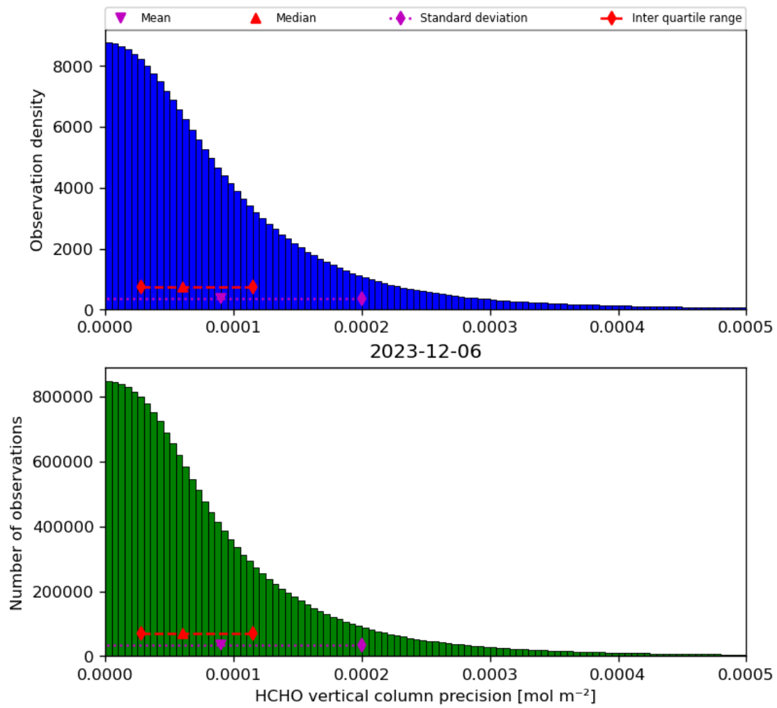
Figure 36: Histogram of “HCHO vertical column precision” for 2023-12-05 to 2023-12-07
