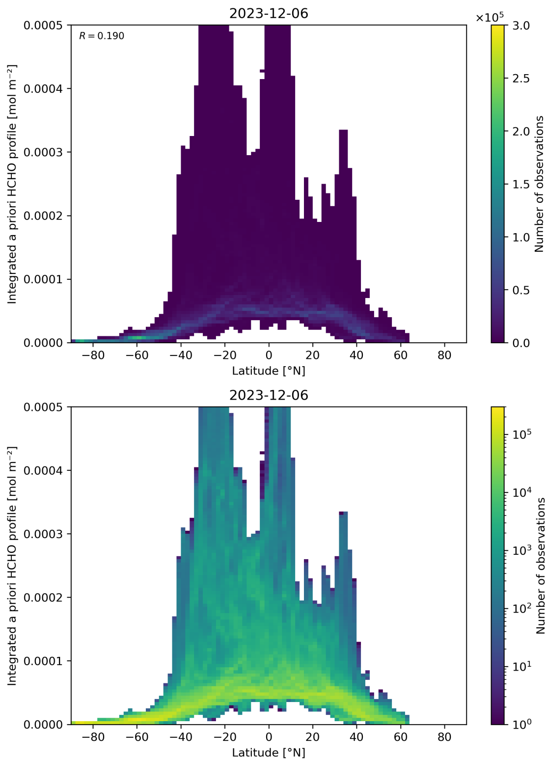
Figure 166: Scatter density plot of “Latitude” against “Integrated a priori HCHO profile” for 2023-12-05 to 2023-12-07.
