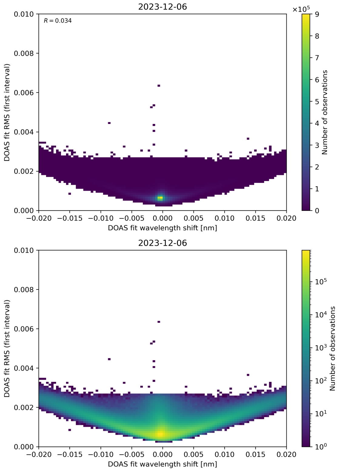
Figure 64: Scatter density plot of “DOAS fit wavelength shift” against “DOAS fit RMS (first interval)” for 2023-12-05 to 2023-12-07.
