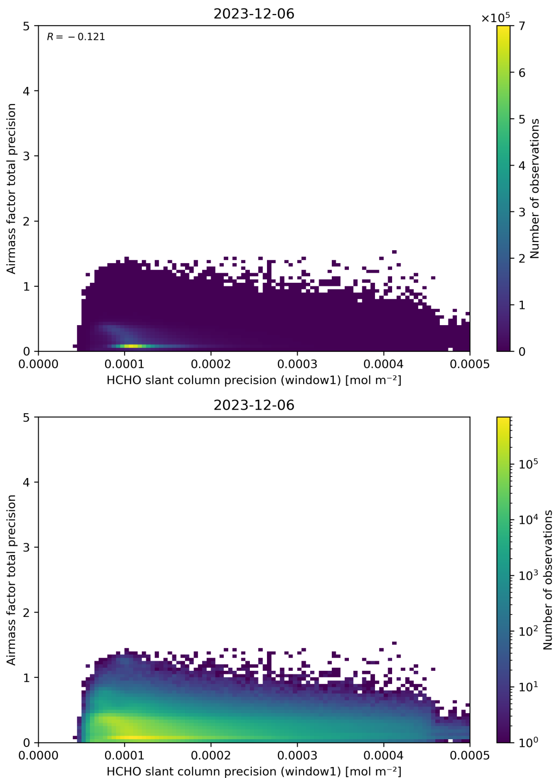
Figure 95: Scatter density plot of “HCHO slant column precision (window1)” against “Airmass factor total precision” for 2023-12-05 to 2023-12-07.
