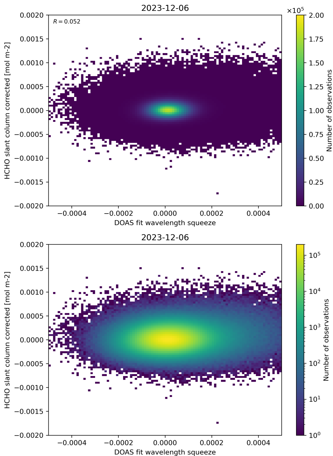
Figure 69: Scatter density plot of “DOAS fit wavelength squeeze” against “HCHO slant column corrected” for 2023-12-05 to 2023-12-07.
