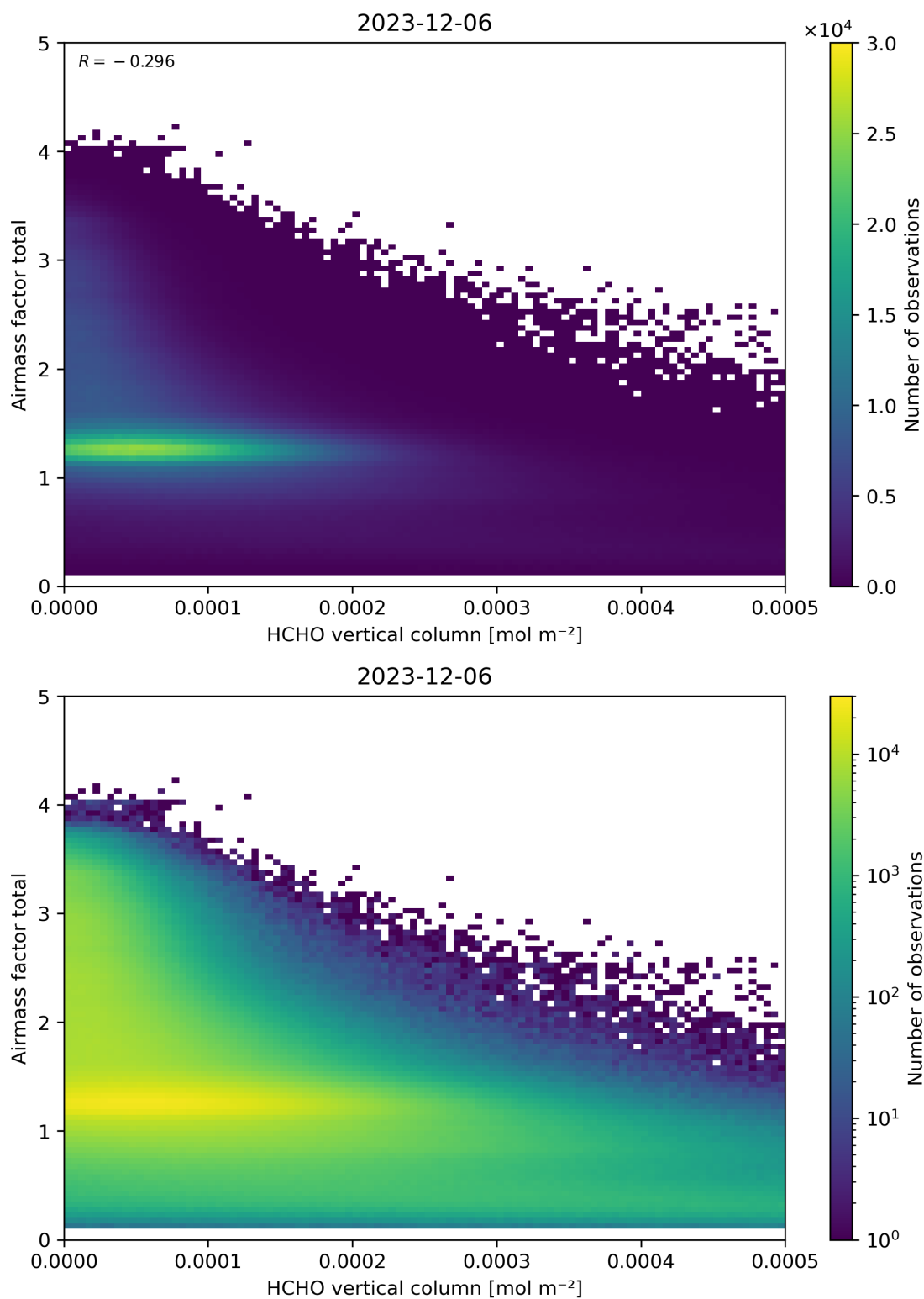
Figure 131: Scatter density plot of “HCHO vertical column” against “Airmass factor total” for 2023-12-05 to 2023-12-07.
