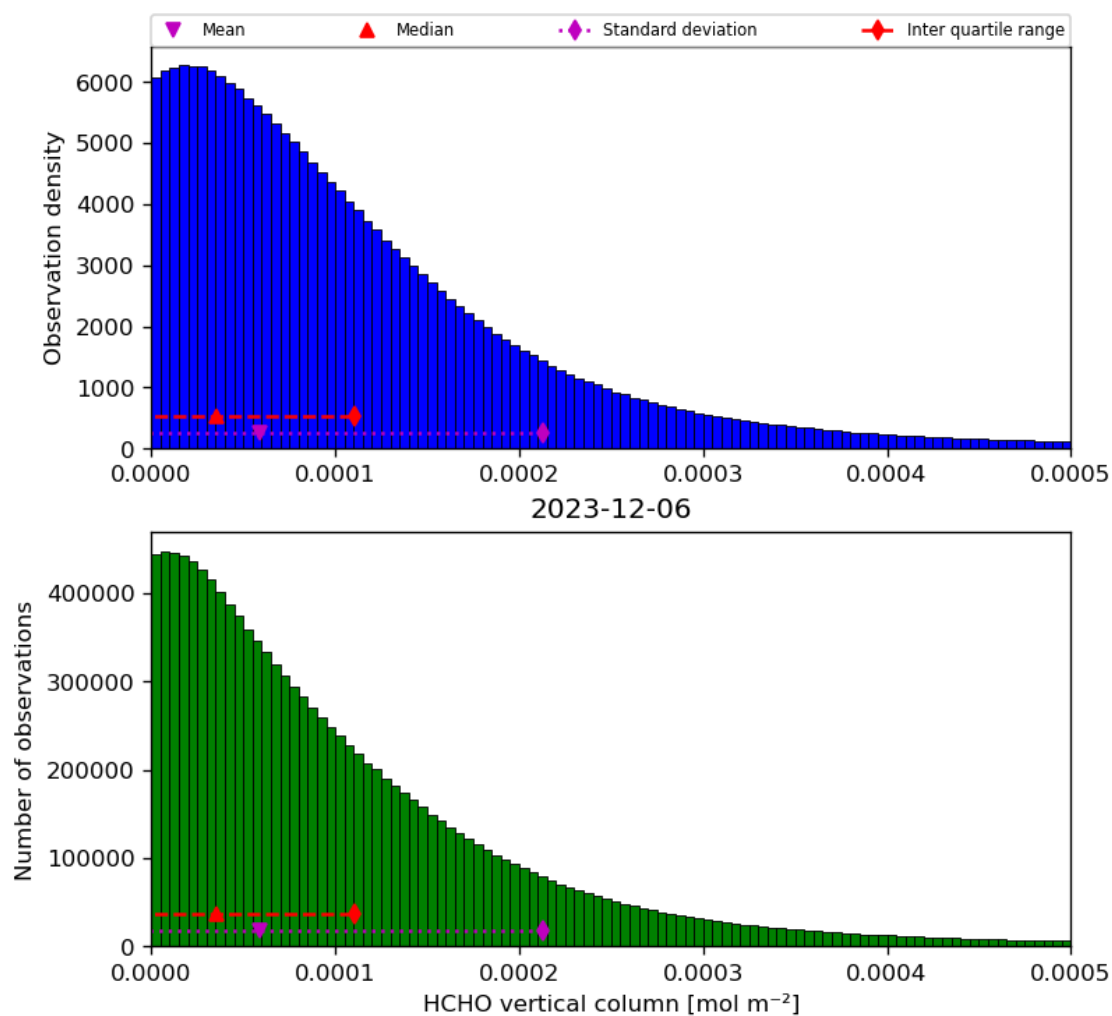
Figure 35: Histogram of “HCHO vertical column” for 2023-12-05 to 2023-12-07
