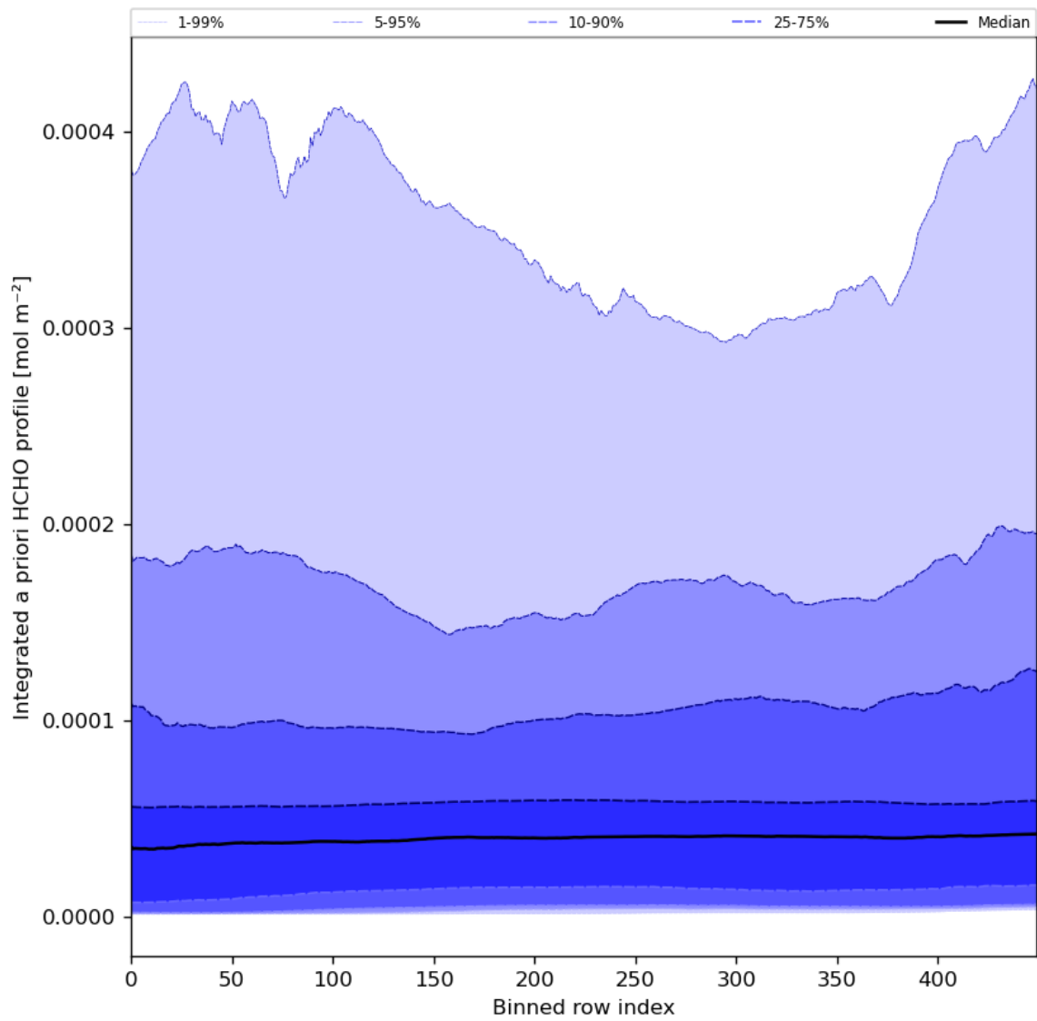
Figure 57: Along track statistics of “Integrated a priori HCHO profile” for 2023-12-05 to 2023-12-07
