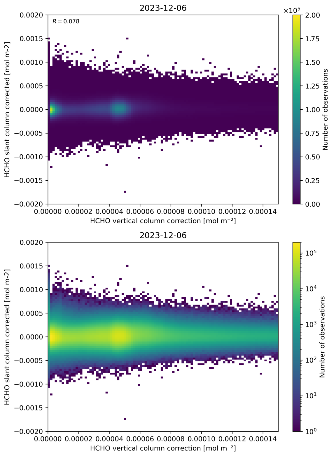
Figure 116: Scatter density plot of “HCHO vertical column correction” against “HCHO slant column corrected” for 2023-12-05 to 2023-12-07.
