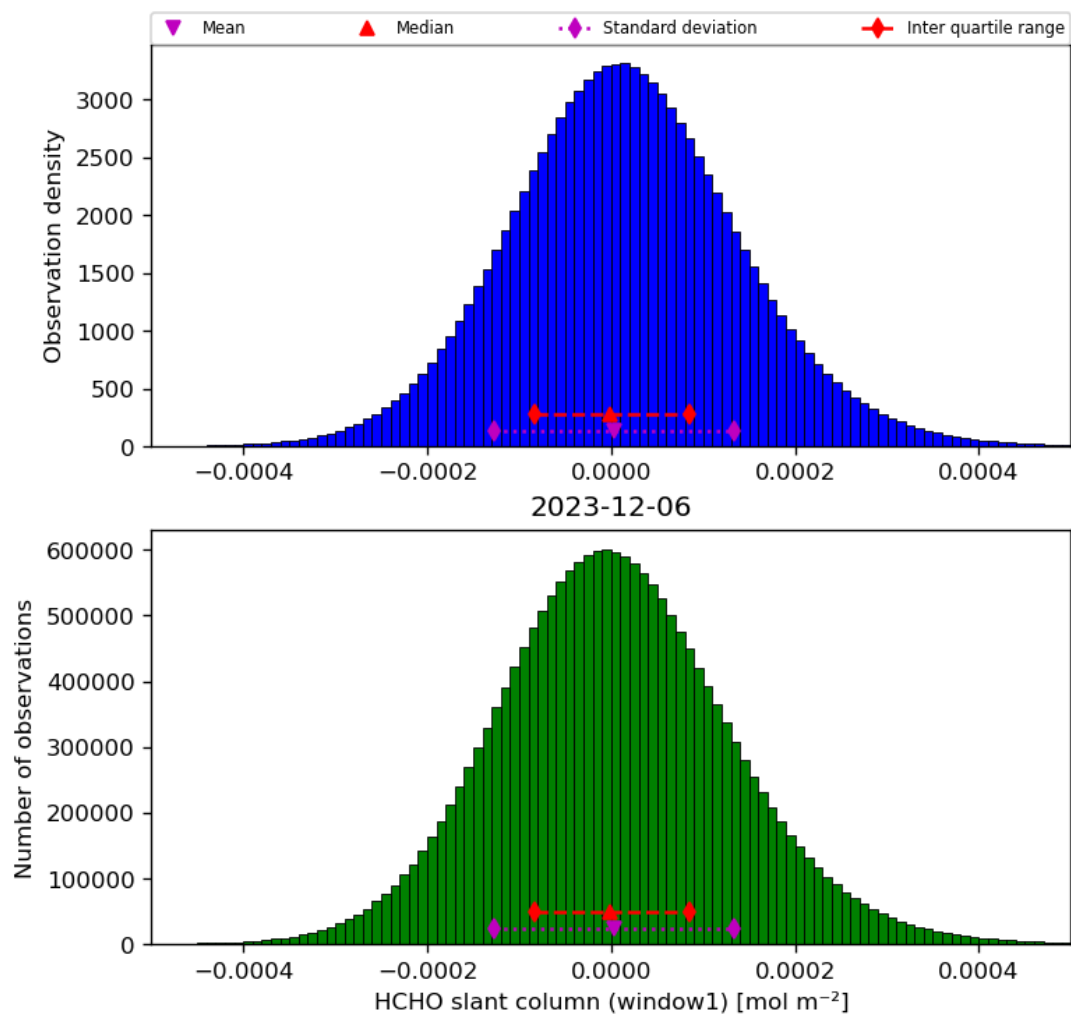
Figure 38: Histogram of “HCHO slant column (window1)” for 2023-12-05 to 2023-12-07
