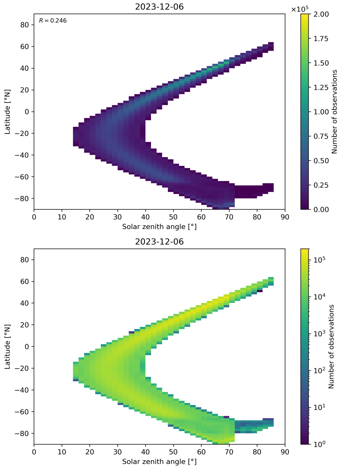
Figure 181: Scatter density plot of “Solar zenith angle” against “Latitude” for 2023-12-05 to 2023-12-07.
