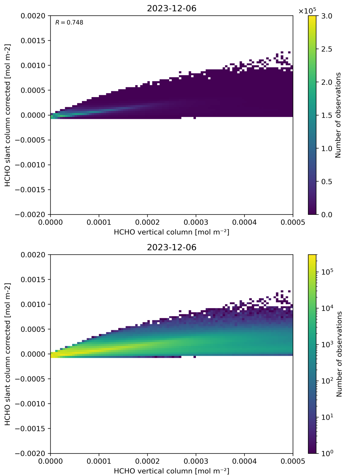
Figure 127: Scatter density plot of “HCHO vertical column” against “HCHO slant column corrected” for 2023-12-05 to 2023-12-07.
