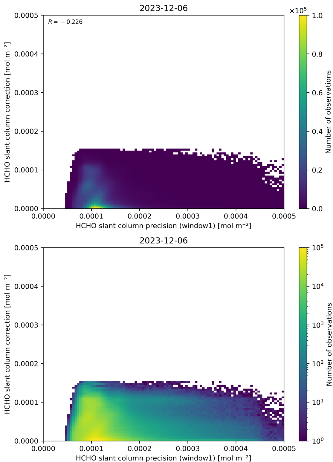
Figure 93: Scatter density plot of “HCHO slant column precision (window1)” against “HCHO slant column correction” for 2023-12-05 to 2023-12-07.
