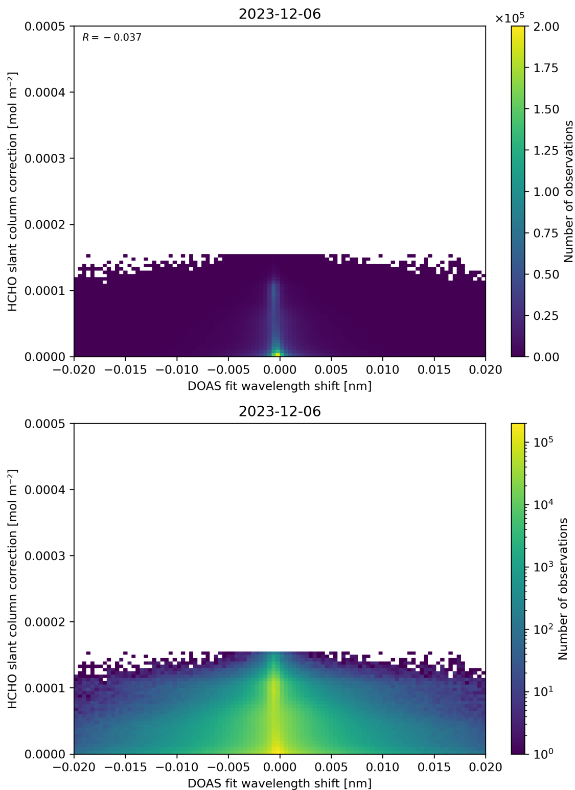
Figure 67: Scatter density plot of “DOAS fit wavelength shift” against “HCHO slant column correction” for 2023-12-05 to 2023-12-07.
