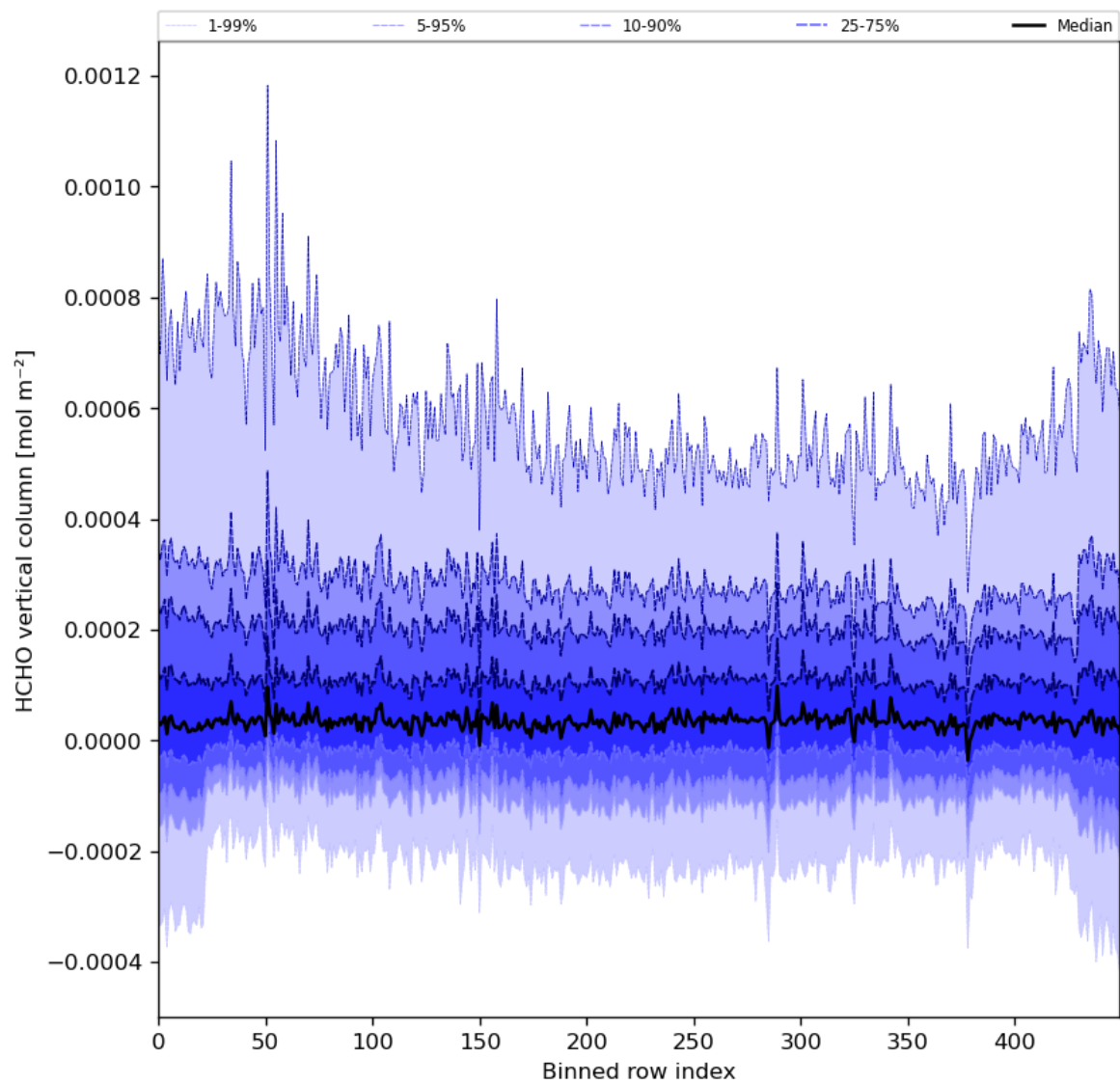
Figure 49: Along track statistics of “HCHO vertical column” for 2023-12-06 to 2023-12-08
