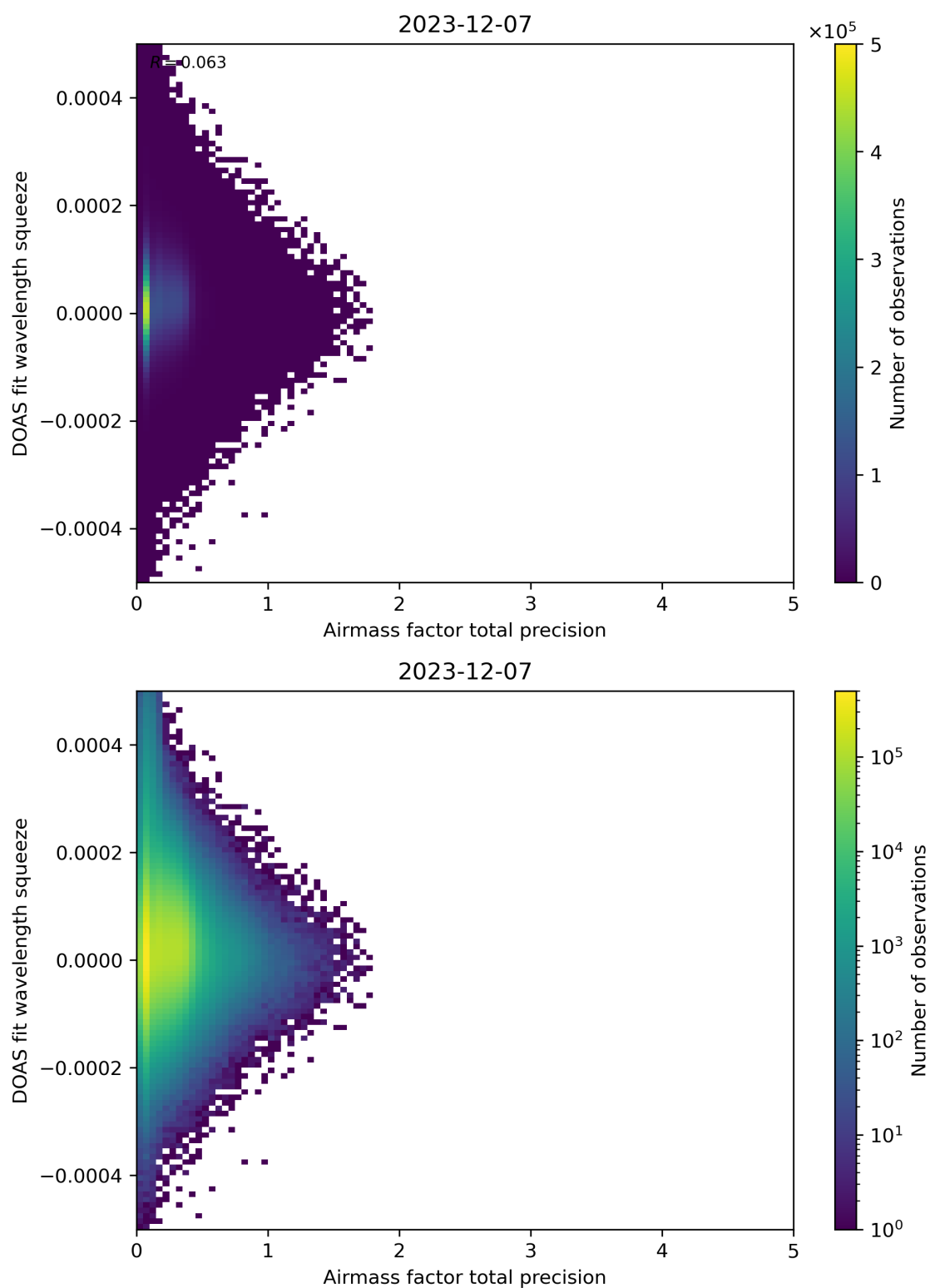
Figure 107: Scatter density plot of “Airmass factor total precision” against “DOAS fit wavelength squeeze” for 2023-12-06 to 2023-12-08.
