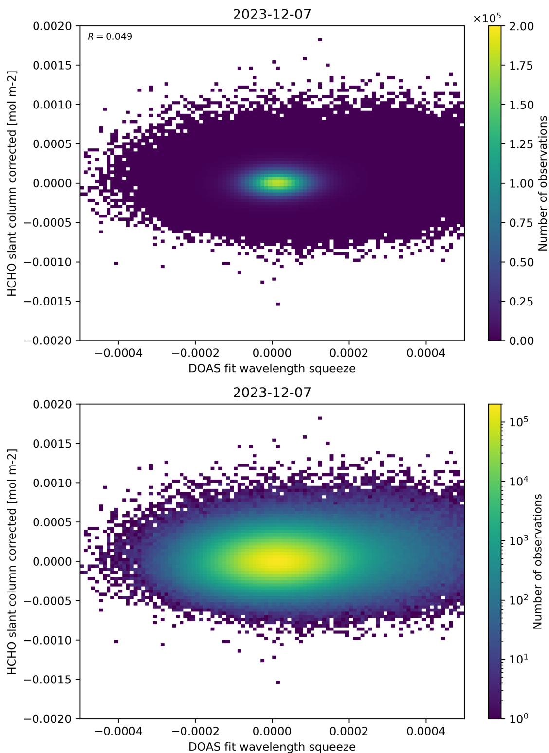
Figure 69: Scatter density plot of “DOAS fit wavelength squeeze” against “HCHO slant column corrected” for 2023-12-06 to 2023-12-08.
