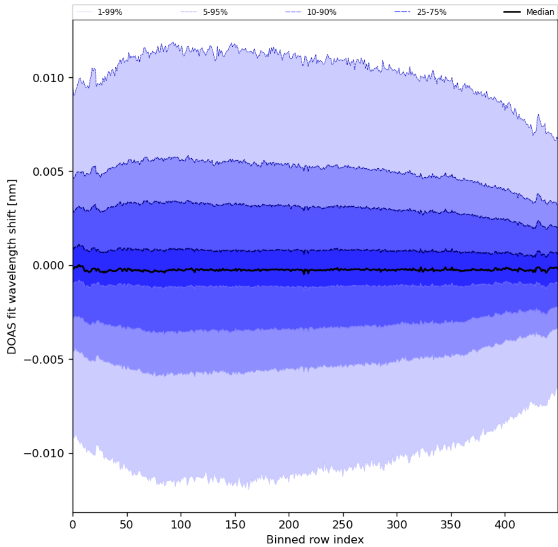
Figure 58: Along track statistics of “DOAS fit wavelength shift” for 2023-12-06 to 2023-12-08
