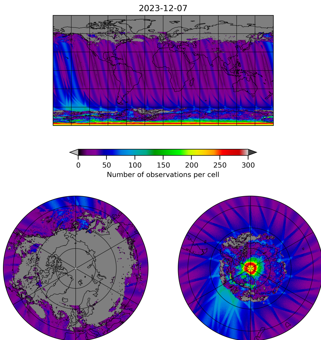
Figure 19: Map of the number of observations for 2023-12-06 to 2023-12-08
