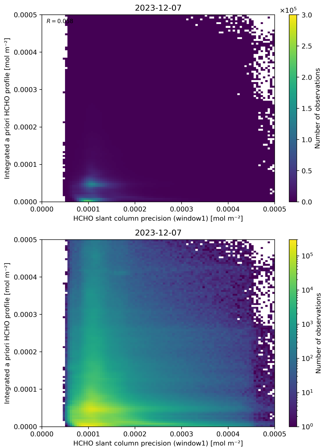
Figure 96: Scatter density plot of “HCHO slant column precision (window1)” against “Integrated a priori HCHO profile” for 2023-12-06 to 2023-12-08.
