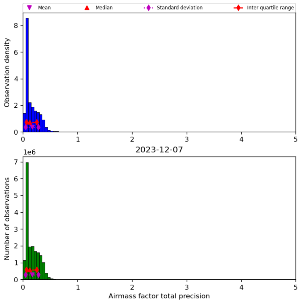
Figure 41: Histogram of “Airmass factor total precision” for 2023-12-06 to 2023-12-08
