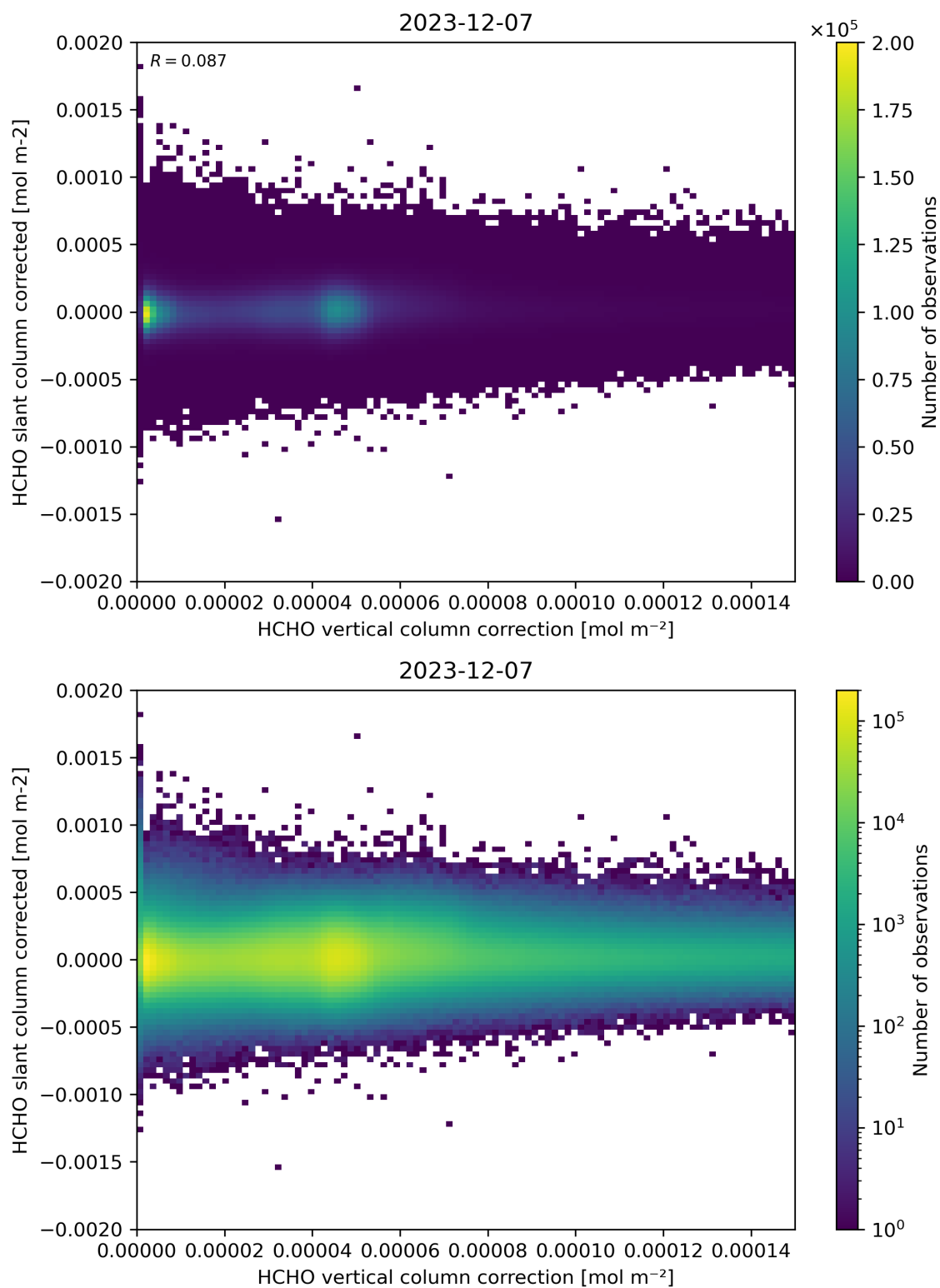
Figure 116: Scatter density plot of “HCHO vertical column correction” against “HCHO slant column corrected” for 2023-12-06 to 2023-12-08.
