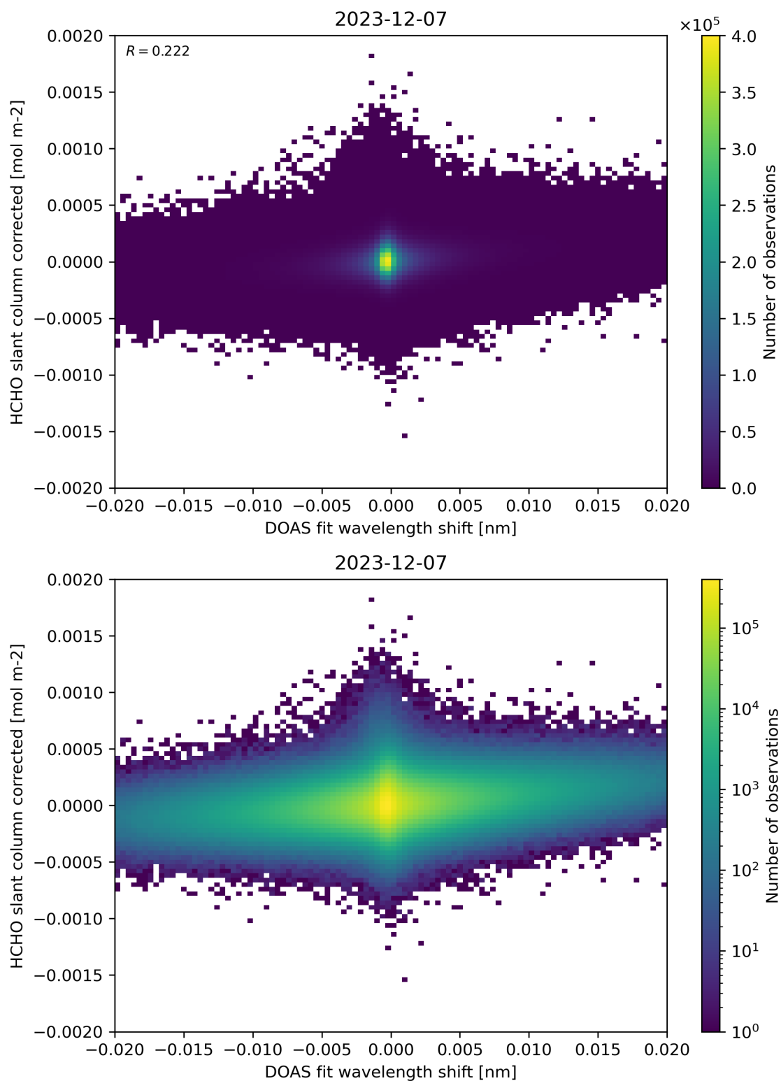
Figure 66: Scatter density plot of “DOAS fit wavelength shift” against “HCHO slant column corrected” for 2023-12-06 to 2023-12-08.
