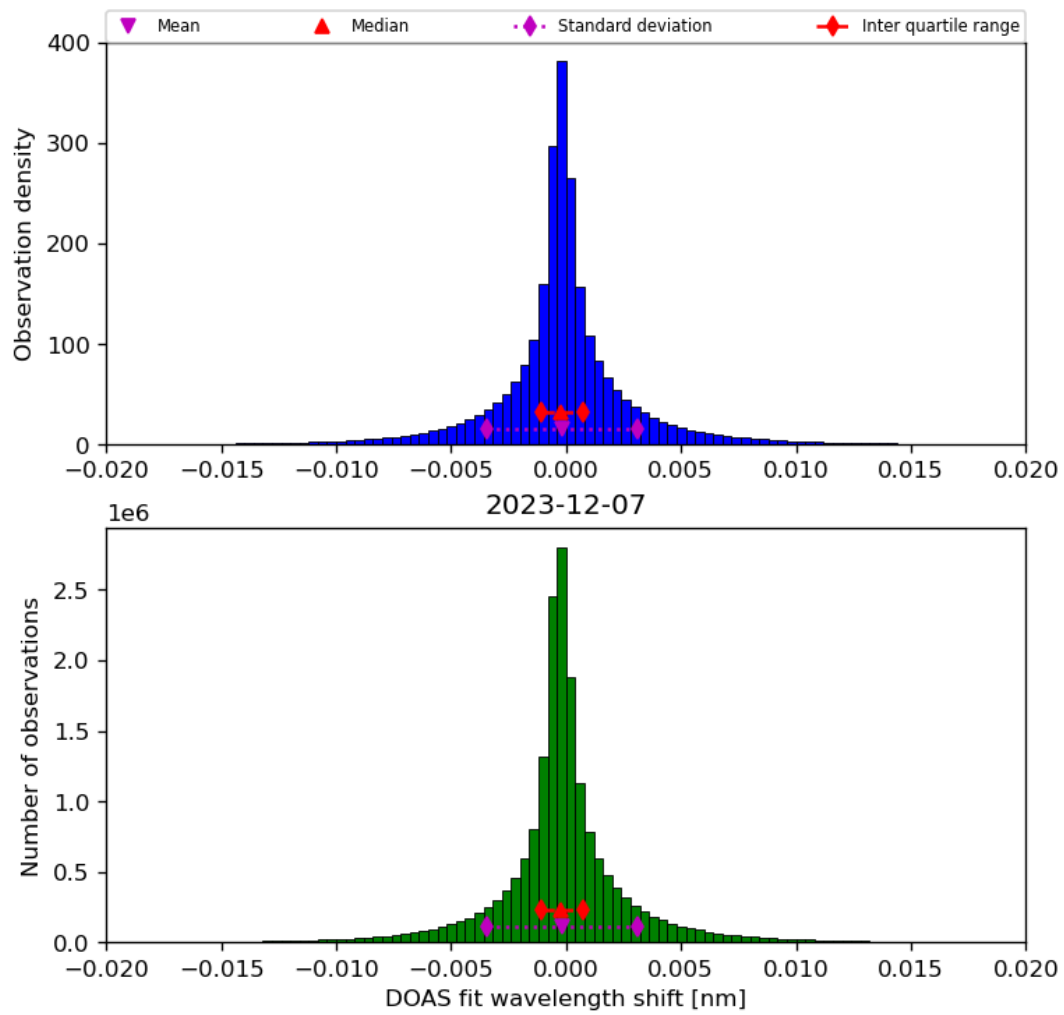
Figure 44: Histogram of “DOAS fit wavelength shift” for 2023-12-06 to 2023-12-08
