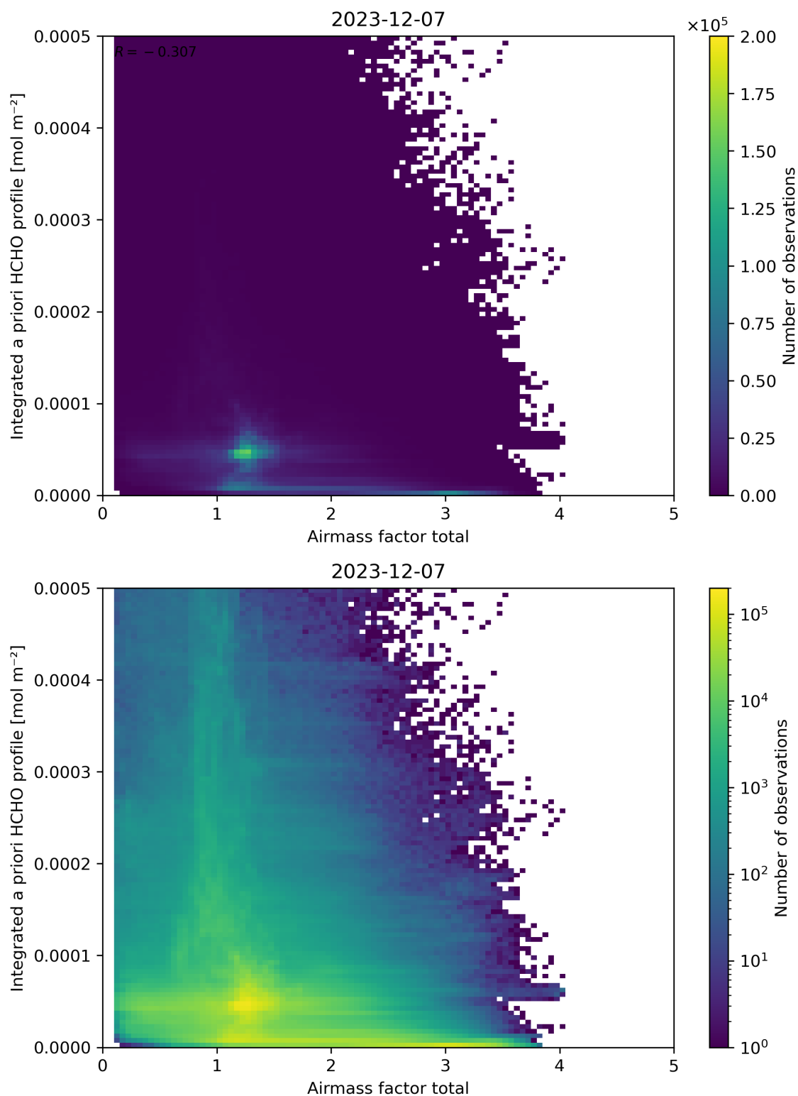
Figure 104: Scatter density plot of “Air mass factor total” against “Integrated a priori HCHO profile” for 2023-12-06 to 2023-12-08.
