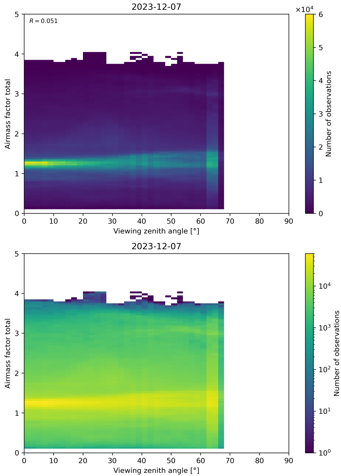
Figure 190: Scatter density plot of “Viewing zenith angle” against “Airmass factor total” for 2023-12-06 to 2023-12-08.
