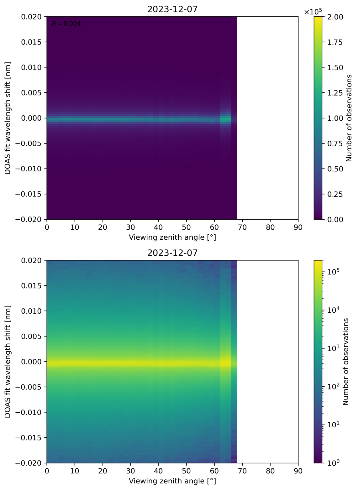
Figure 183: Scatter density plot of “Viewing zenith angle” against “DOAS fit wavelength shift” for 2023-12-06 to 2023-12-08.
