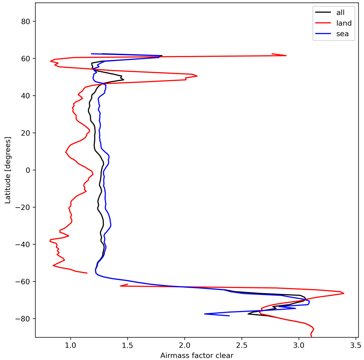
Figure 28: Zonal average of “Airmass factor clear” for 2023-12-06 to 2023-12-08.
