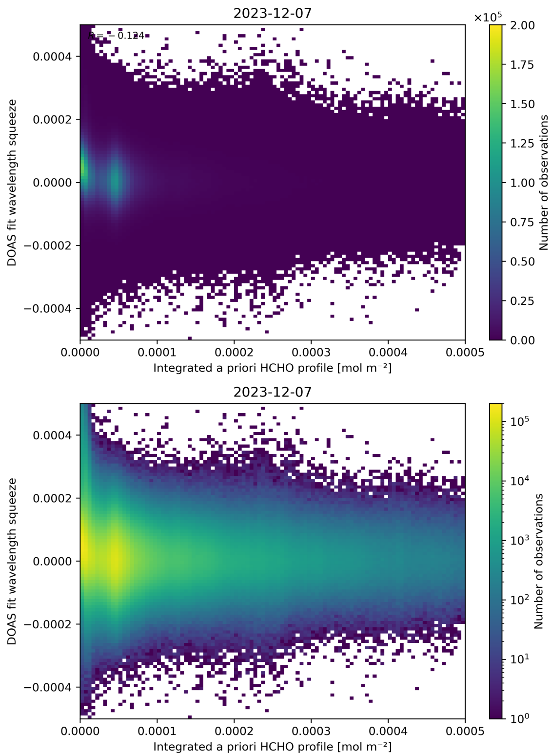
Figure 150: Scatter density plot of “Integrated a priori HCHO profile” against “DOAS fit wavelength squeeze” for 2023-12-06 to 2023-12-08.
