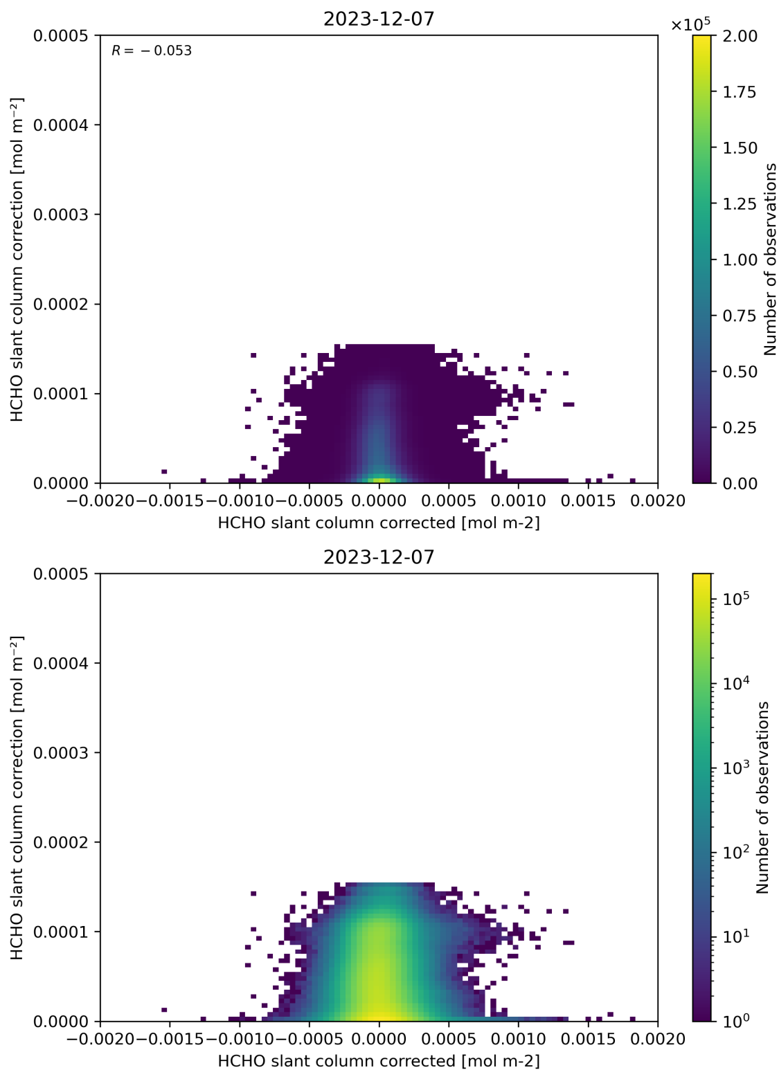
Figure 77: Scatter density plot of “HCHO slant column corrected” against “HCHO slant column correction” for 2023-12-06 to 2023-12-08.
