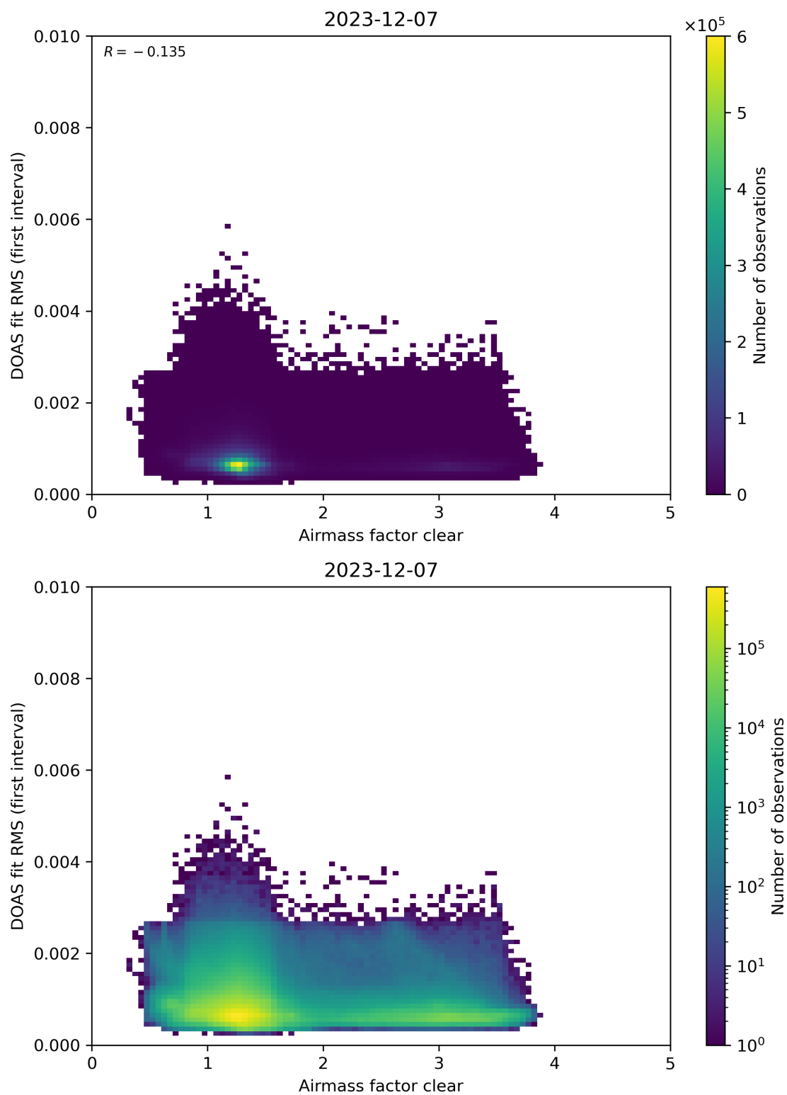
Figure 71: Scatter density plot of “Airmass factor clear” against “DOAS fit RMS (first interval)” for 2023-12-06 to 2023-12-08.
