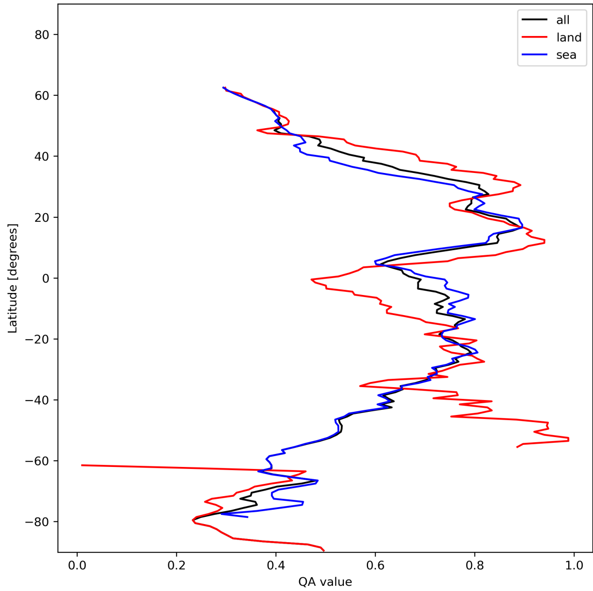
Figure 20: Zonal average of “QA value” for 2023-12-06 to 2023-12-08.
