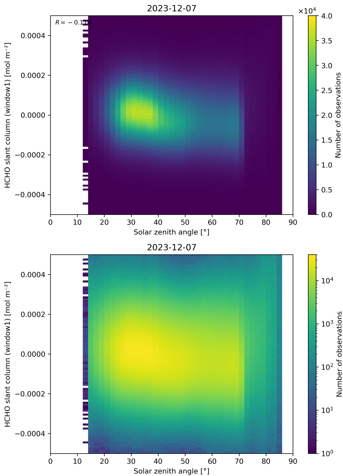
Figure 173: Scatter density plot of “Solar zenith angle” against “HCHO slant column (window1)” for 2023-12-06 to 2023-12-08.
