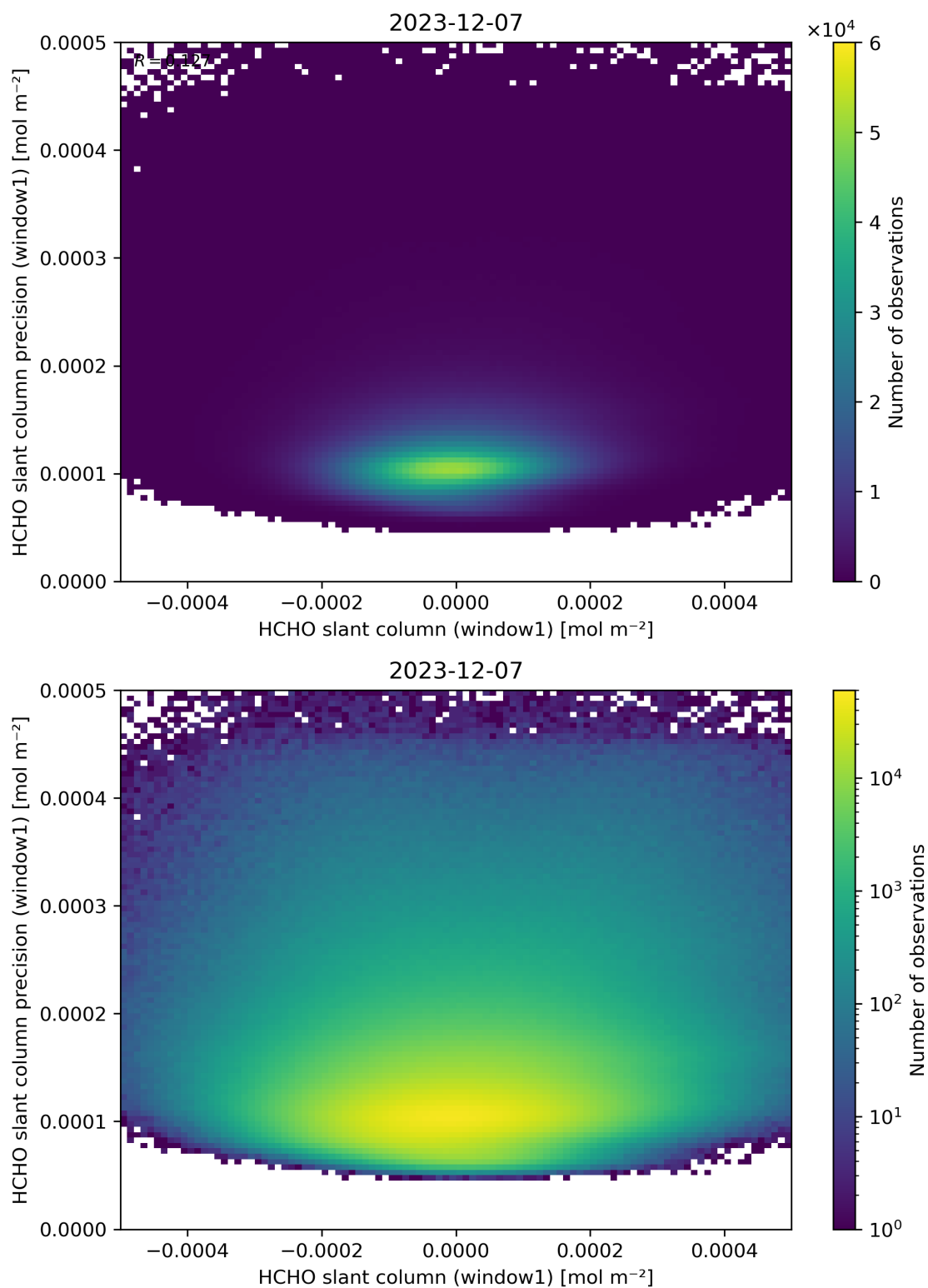
Figure 84: Scatter density plot of “HCHO slant column (window1)” against “HCHO slant column precision (window1)” for 2023-12-06 to 2023-12-08.
