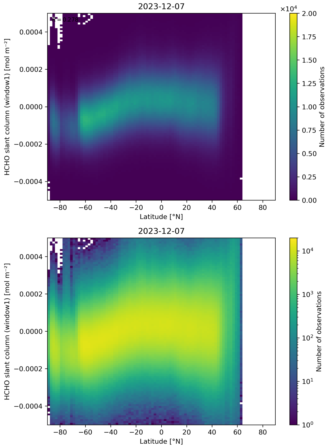
Figure 159: Scatter density plot of “Latitude” against “HCHO slant column (window1)” for 2023-12-06 to 2023-12-08.
