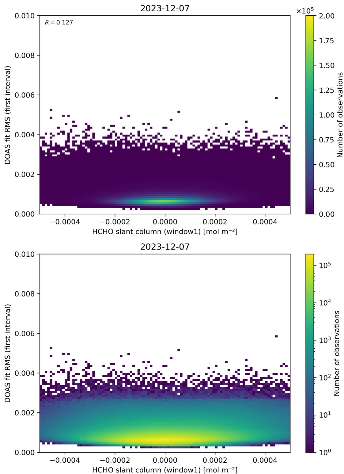
Figure 78: Scatter density plot of “HCHO slant column (window1)” against “DOAS fit RMS (first interval)” for 2023-12-06 to 2023-12-08.
