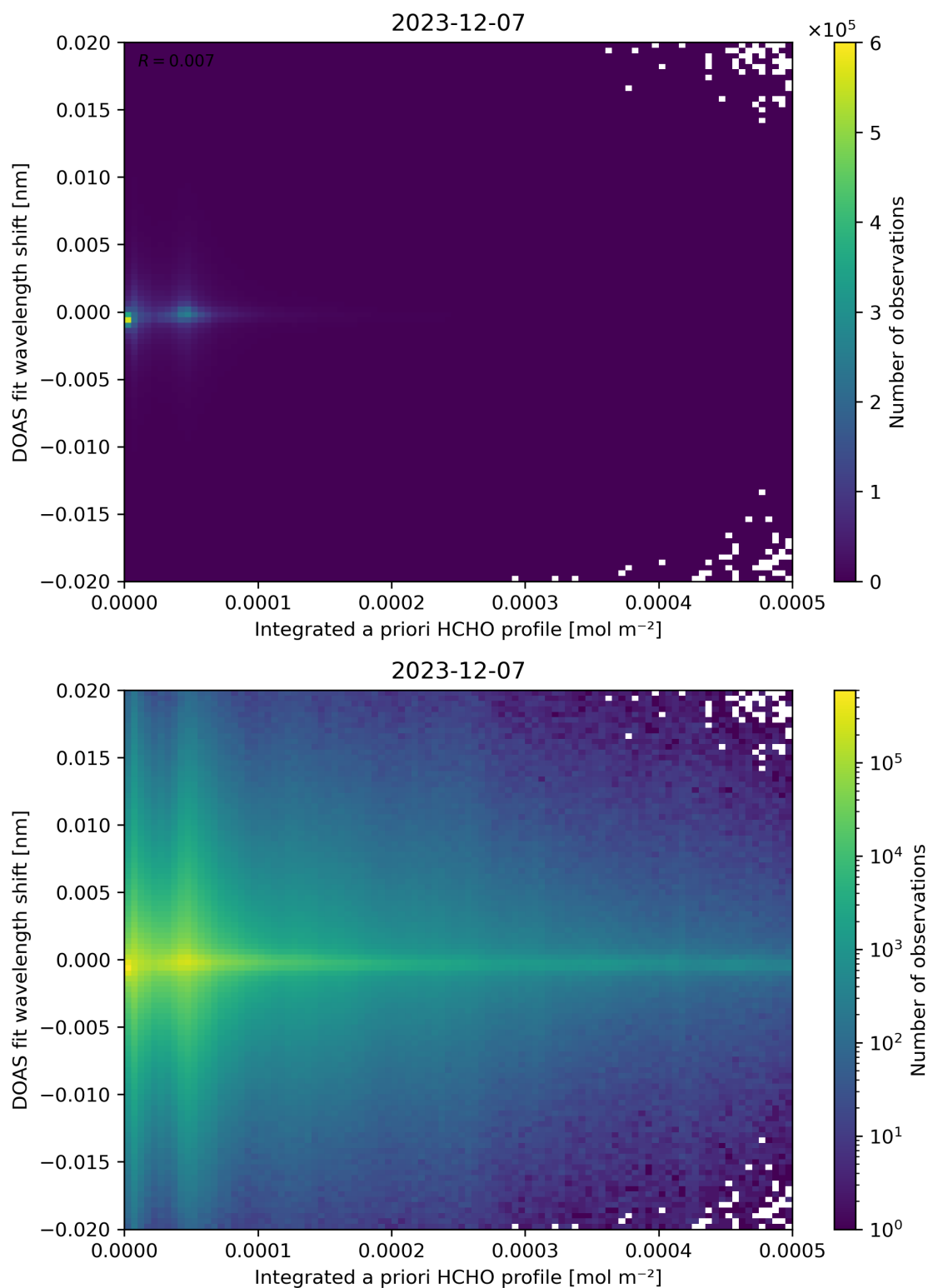
Figure 149: Scatter density plot of “Integrated a priori HCHO profile” against “DOAS fit wavelength shift” for 2023-12-06 to 2023-12-08.
