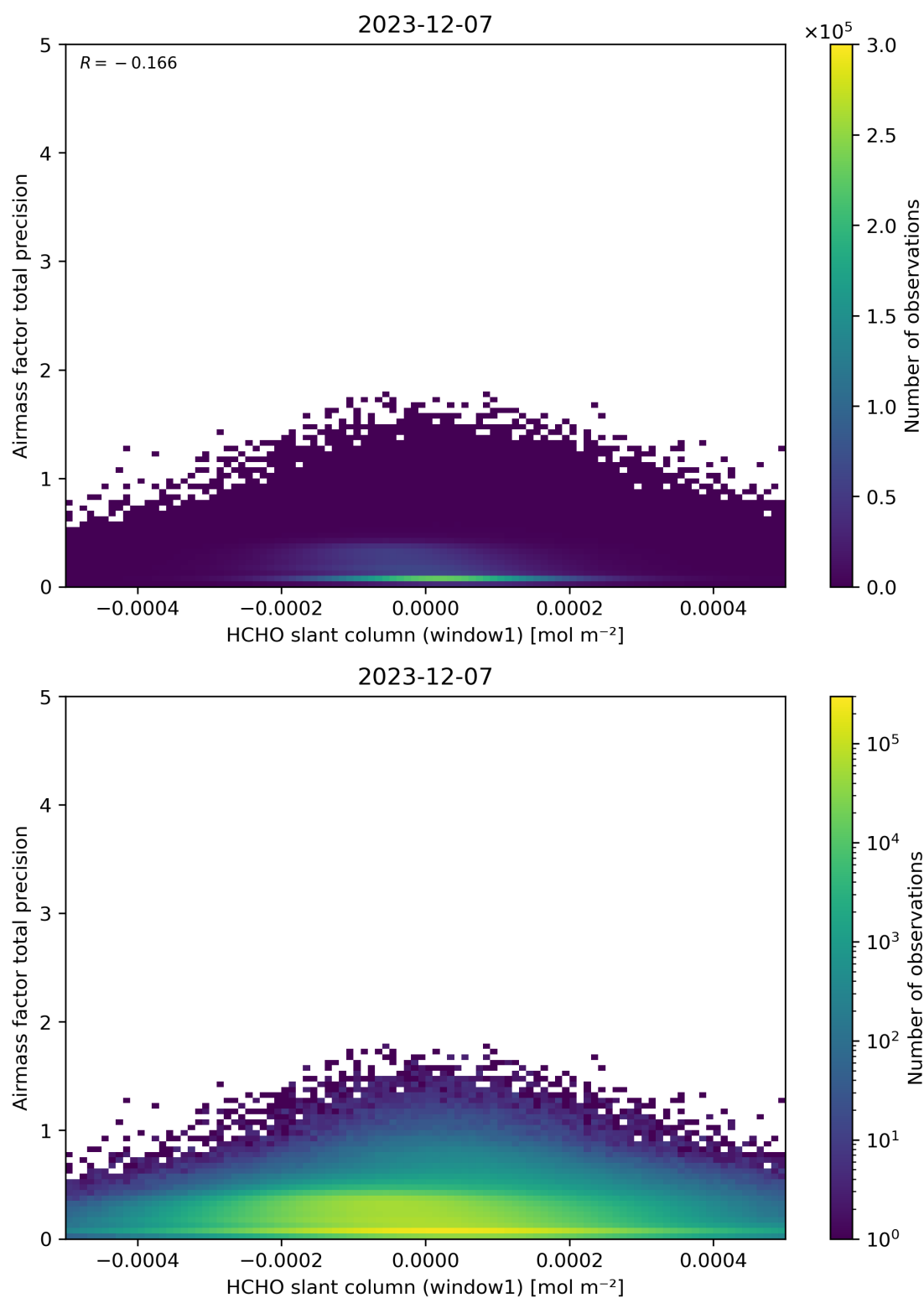
Figure 86: Scatter density plot of “HCHO slant column (window1)” against “Airmass factor total precision” for 2023-12-06 to 2023-12-08.
