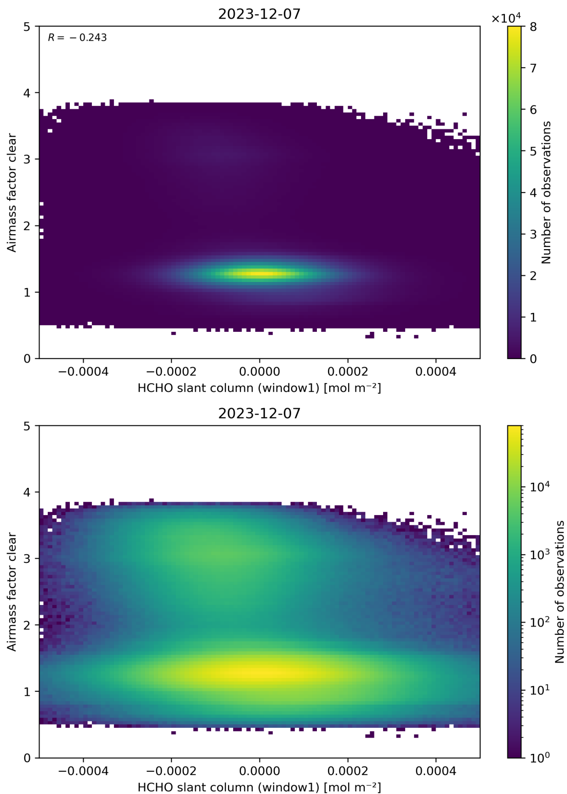
Figure 81: Scatter density plot of “HCHO slant column (window1)” against “Airmass factor clear” for 2023-12-06 to 2023-12-08.
