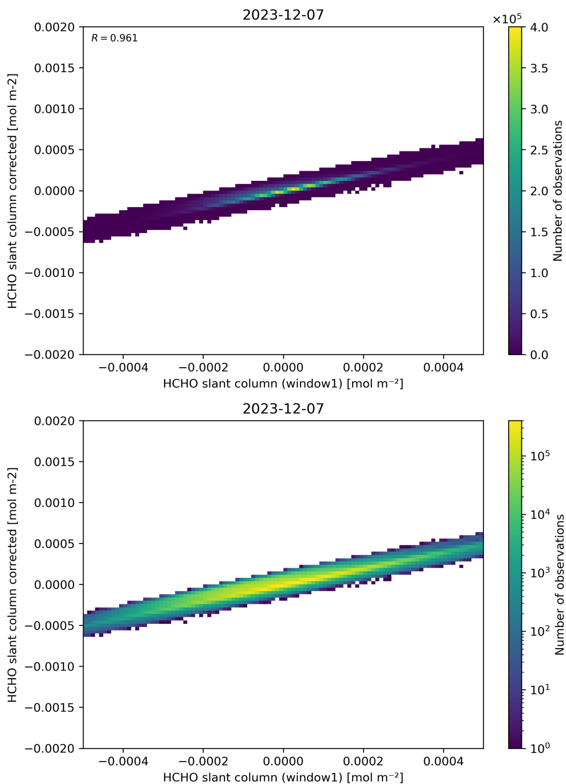
Figure 82: Scatter density plot of “HCHO slant column (window1)” against “HCHO slant column corrected” for 2023-12-06 to 2023-12-08.
