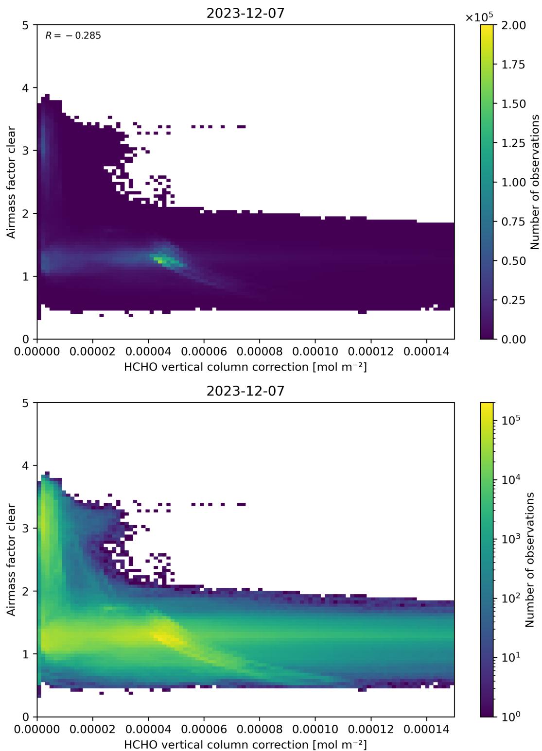
Figure 115: Scatter density plot of “HCHO vertical column correction” against “Airmass factor clear” for 2023-12-06 to 2023-12-08.
