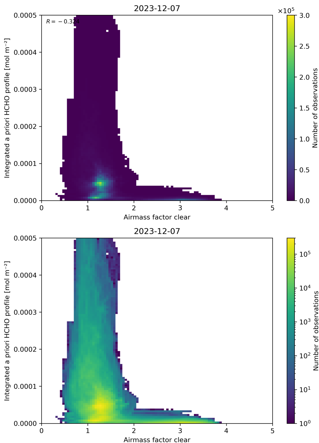
Figure 76: Scatter density plot of “Airmass factor clear” against “Integrated a priori HCHO profile” for 2023-12-06 to 2023-12-08.
