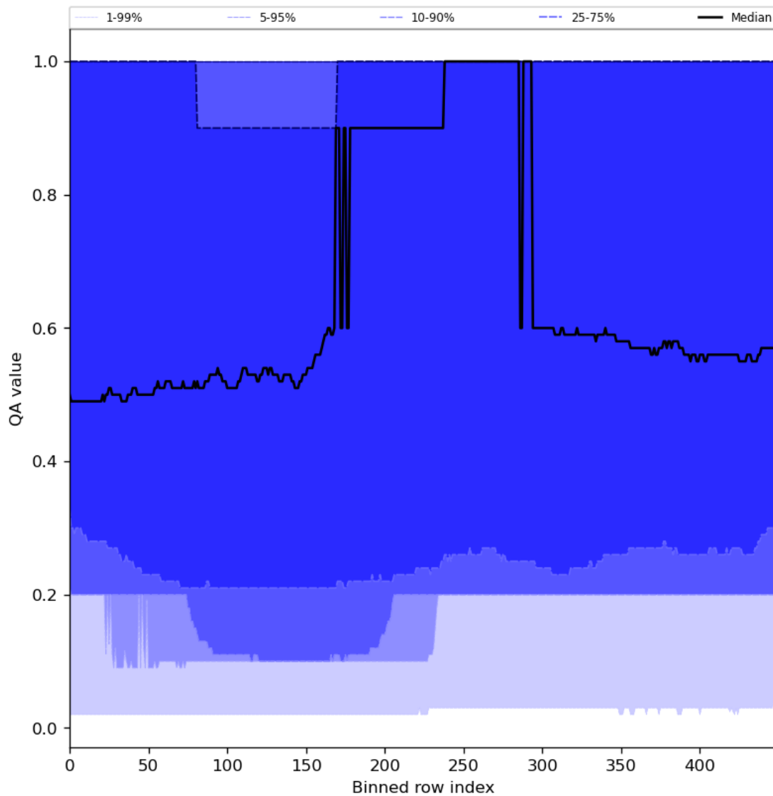
Figure 48: Along track statistics of “QA value” for 2023-12-06 to 2023-12-08
