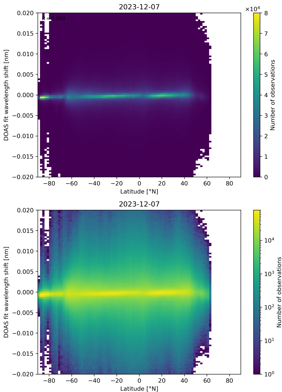
Figure 154: Scatter density plot of “Latitude” against “DOAS fit wavelength shift” for 2023-12-06 to 2023-12-08.
