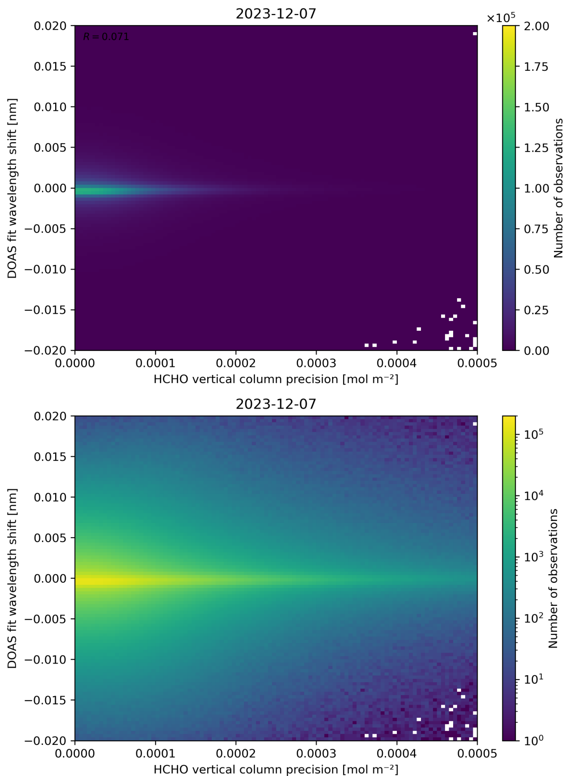
Figure 137: Scatter density plot of “HCHO vertical column precision” against “DOAS fit wavelength shift” for 2023-12-06 to 2023-12-08.
