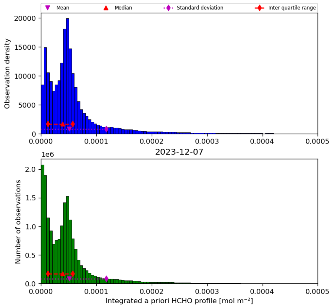
Figure 43: Histogram of “Integrated a priori HCHO profile” for 2023-12-06 to 2023-12-08
