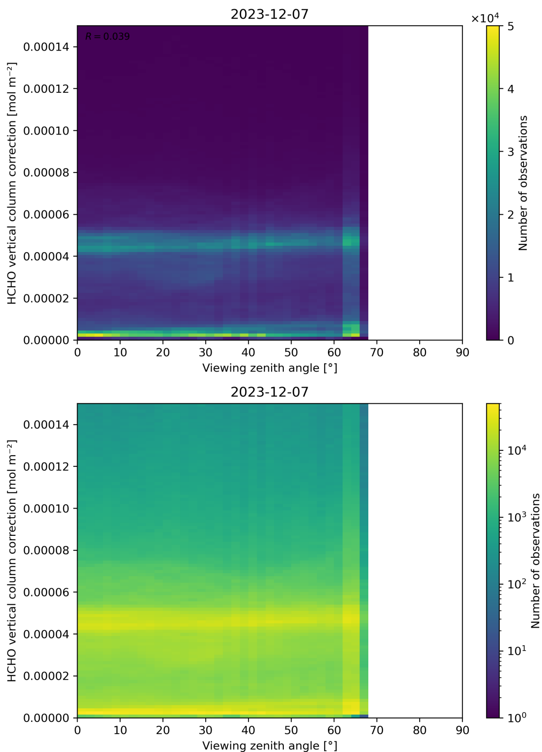
Figure 193: Scatter density plot of “Viewing zenith angle” against “HCHO vertical column correction” for 2023-12-06 to 2023-12-08.
