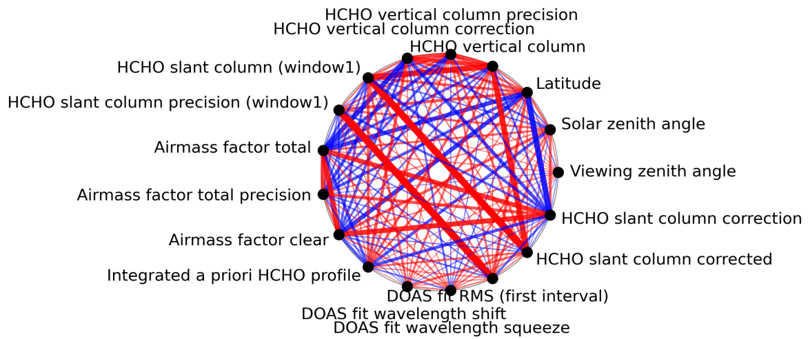
Figure 1: Map of correlation graph for 2023-12-06 to 2023-12-08.
