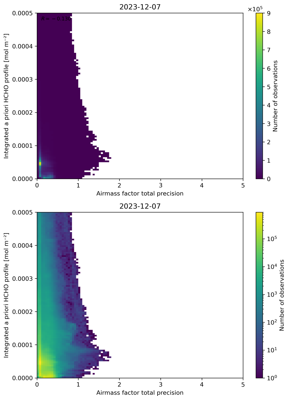
Figure 111: Scatter density plot of “Airmass factor total precision” against “Integrated a priori HCHO profile” for 2023-12-06 to 2023-12-08.
