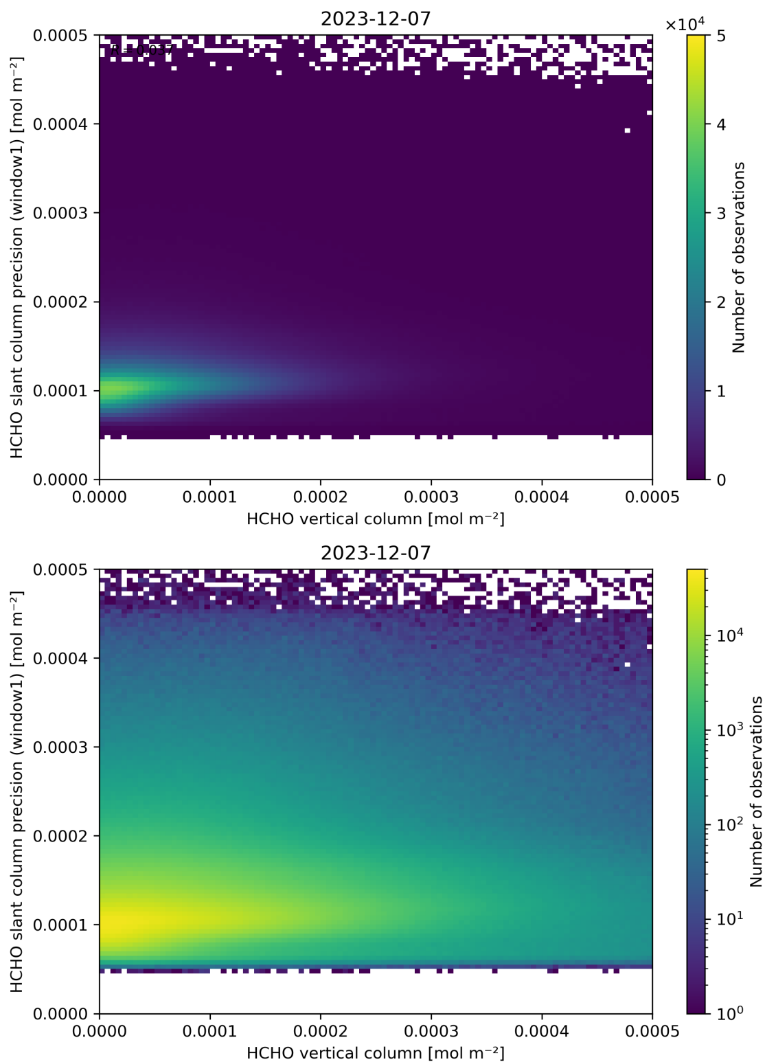
Figure 130: Scatter density plot of “HCHO vertical column” against “HCHO slant column precision (window1)” for 2023-12-06 to 2023-12-08.
