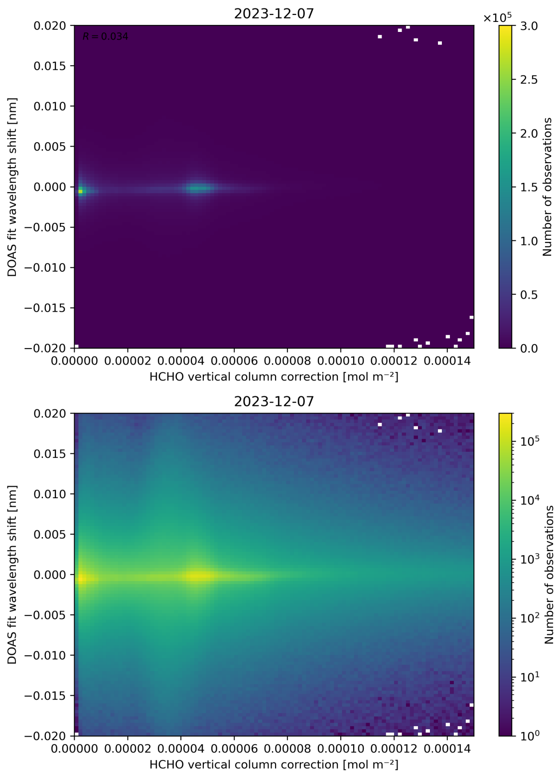
Figure 113: Scatter density plot of “HCHO vertical column correction” against “DOAS fit wavelength shift” for 2023-12-06 to 2023-12-08.
