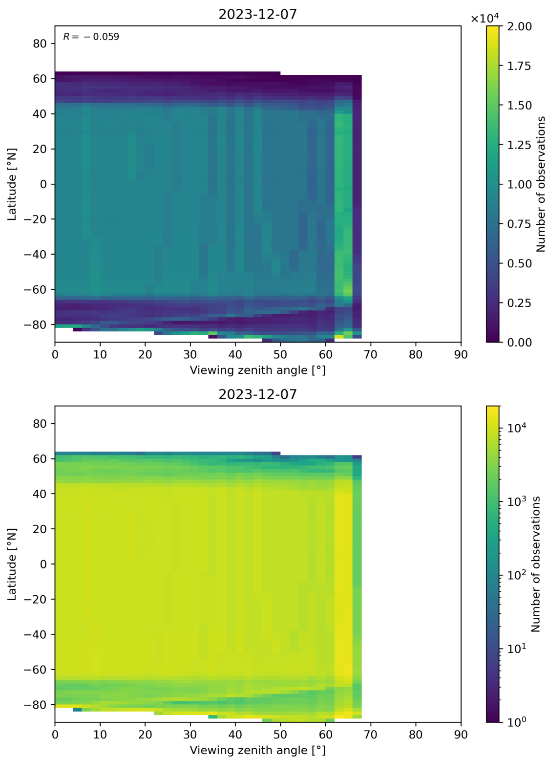
Figure 196: Scatter density plot of “Viewing zenith angle” against “Latitude” for 2023-12-06 to 2023-12-08.
