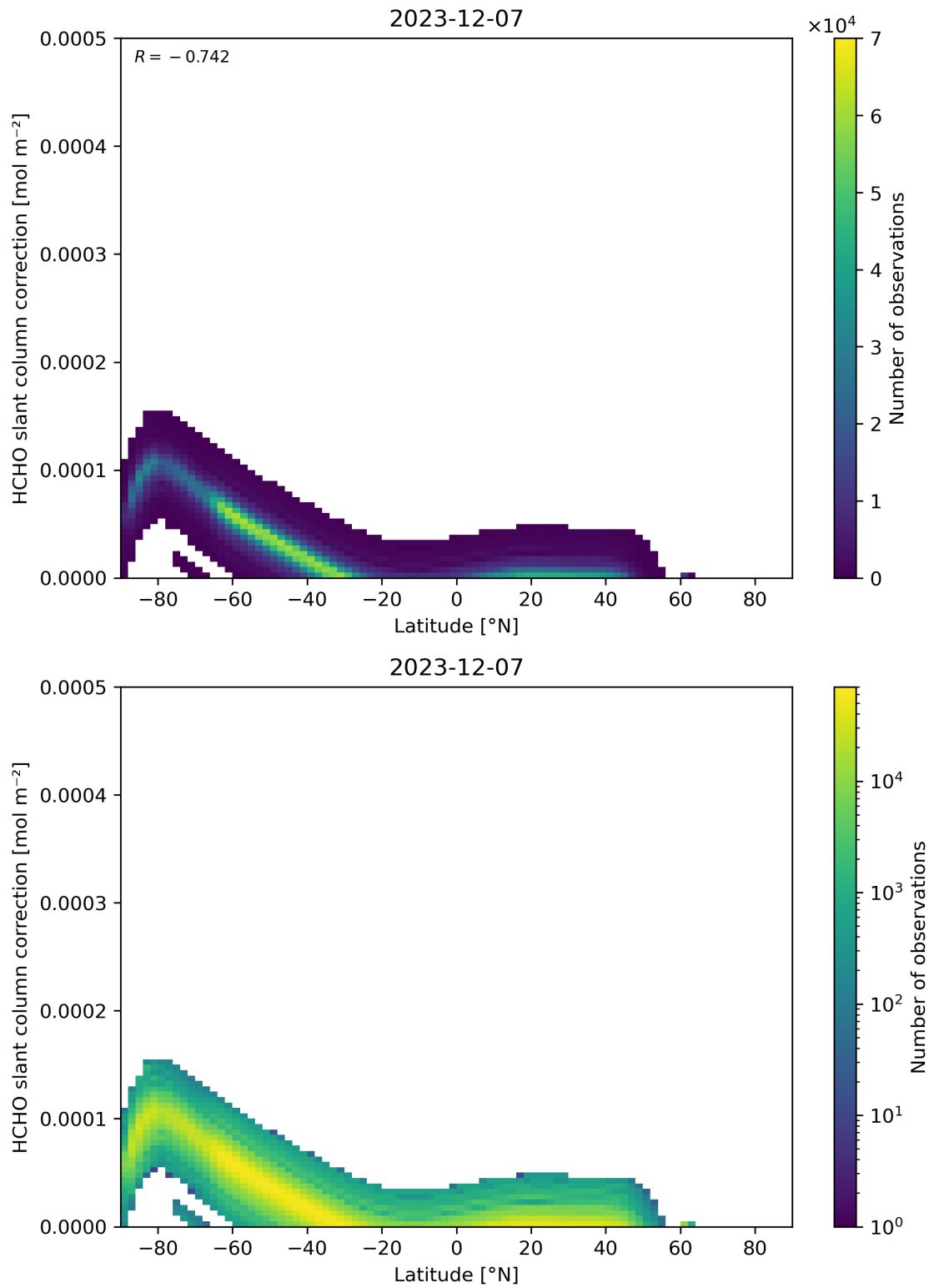
Figure 158: Scatter density plot of “Latitude” against “HCHO slant column correction” for 2023-12-06 to 2023-12-08.
