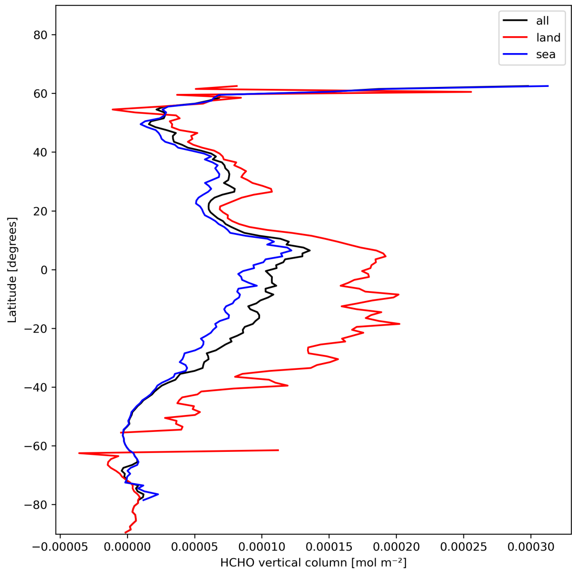
Figure 21: Zonal average of “HCHO vertical column” for 2023-12-06 to 2023-12-08.
