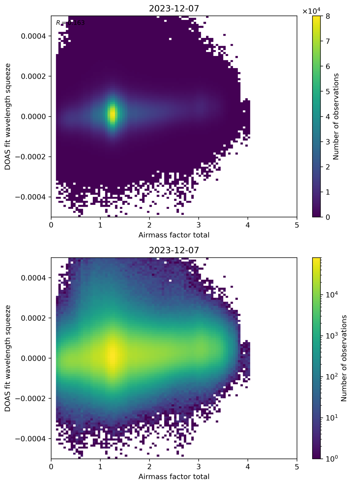
Figure 99: Scatter density plot of “Airmass factor total” against “DOAS fit wavelength squeeze” for 2023-12-06 to 2023-12-08.
