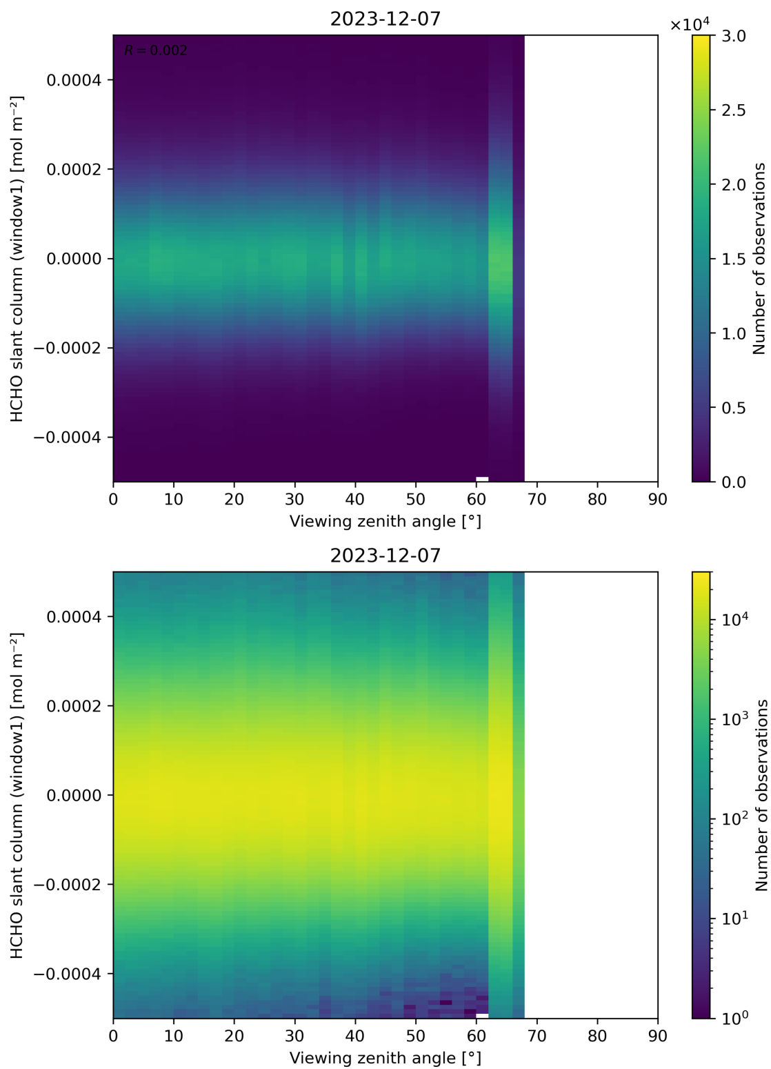
Figure 188: Scatter density plot of “Viewing zenith angle” against “HCHO slant column (window1)” for 2023-12-06 to 2023-12-08.
