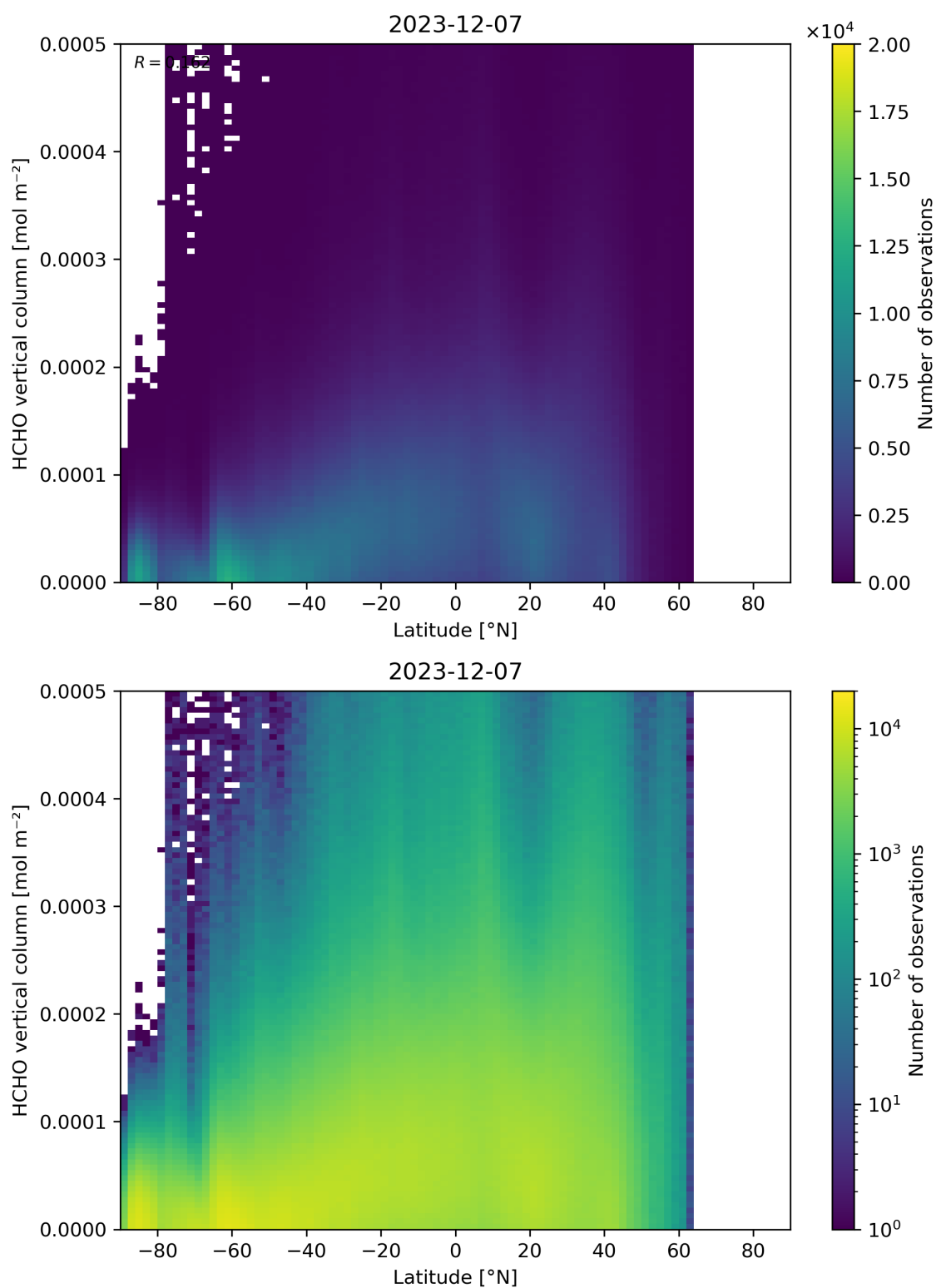
Figure 163: Scatter density plot of “Latitude” against “HCHO vertical column” for 2023-12-06 to 2023-12-08.
