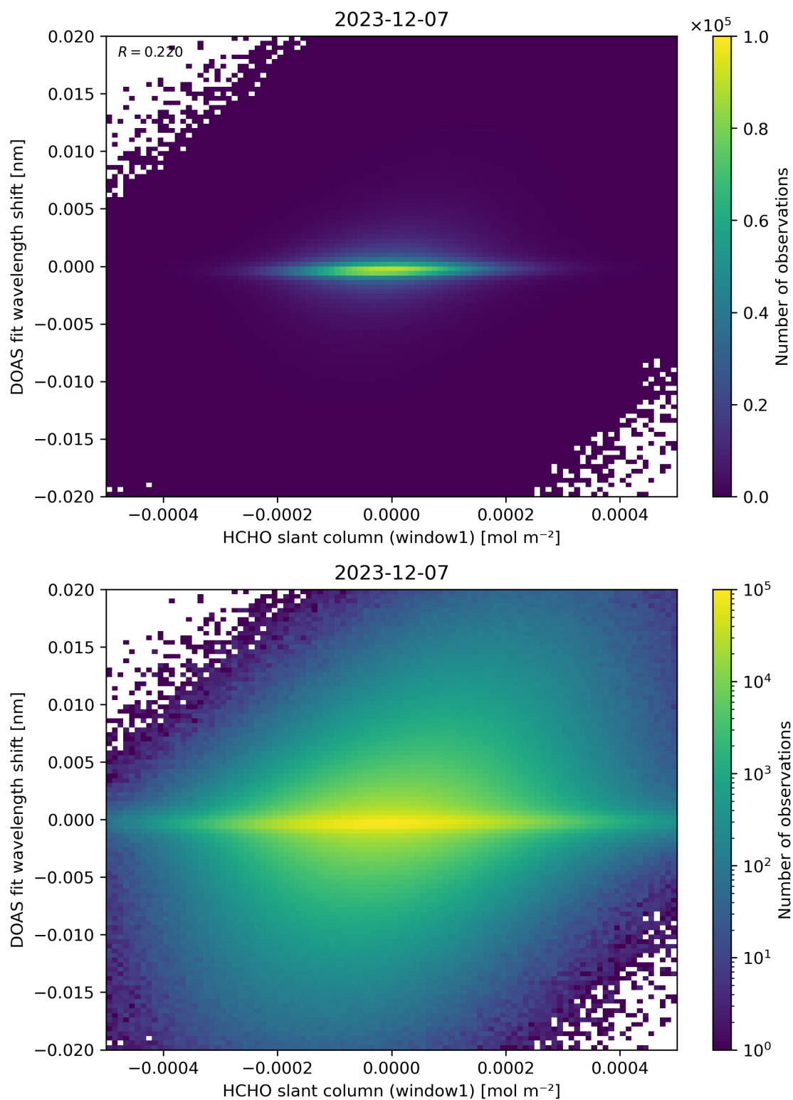
Figure 79: Scatter density plot of “HCHO slant column (window1)” against “DOAS fit wavelength shift” for 2023-12-06 to 2023-12-08.
