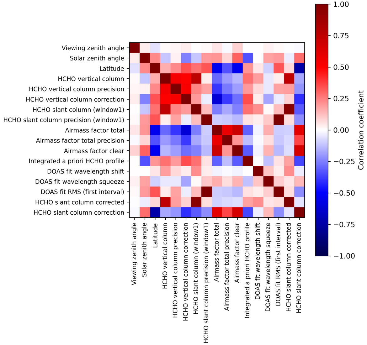
Figure 2: Map of correlation matrix for 2023-12-06 to 2023-12-08.
