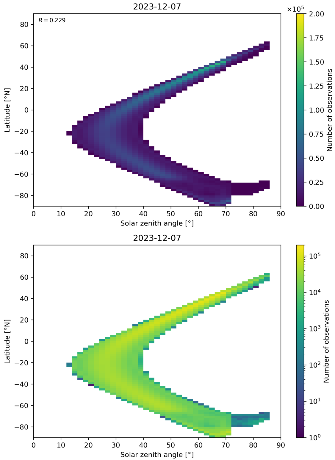
Figure 181: Scatter density plot of “Solar zenith angle” against “Latitude” for 2023-12-06 to 2023-12-08.
