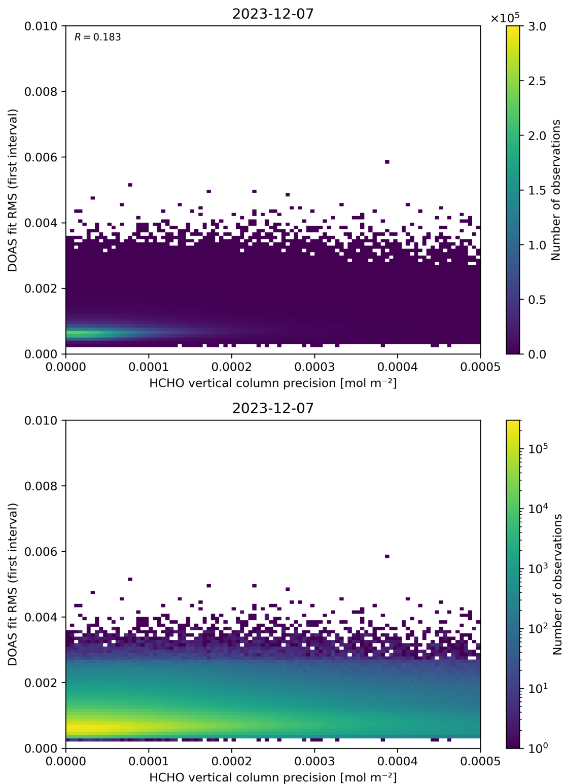
Figure 136: Scatter density plot of “HCHO vertical column precision” against “DOAS fit RMS (first interval)” for 2023-12-06 to 2023-12-08.
