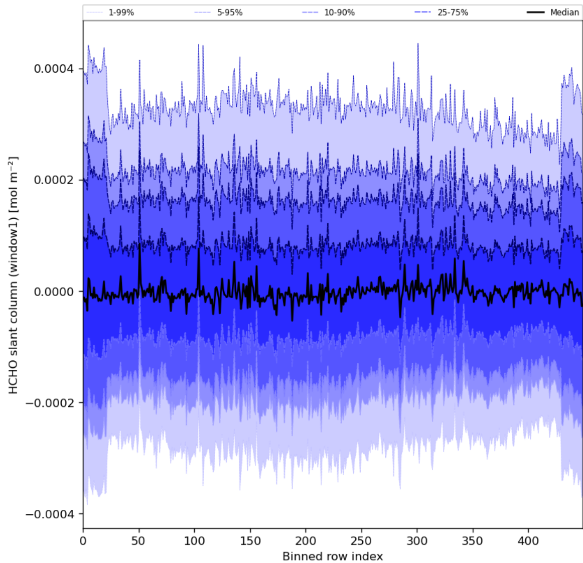
Figure 52: Along track statistics of “HCHO slant column (window1)” for 2023-12-06 to 2023-12-08
