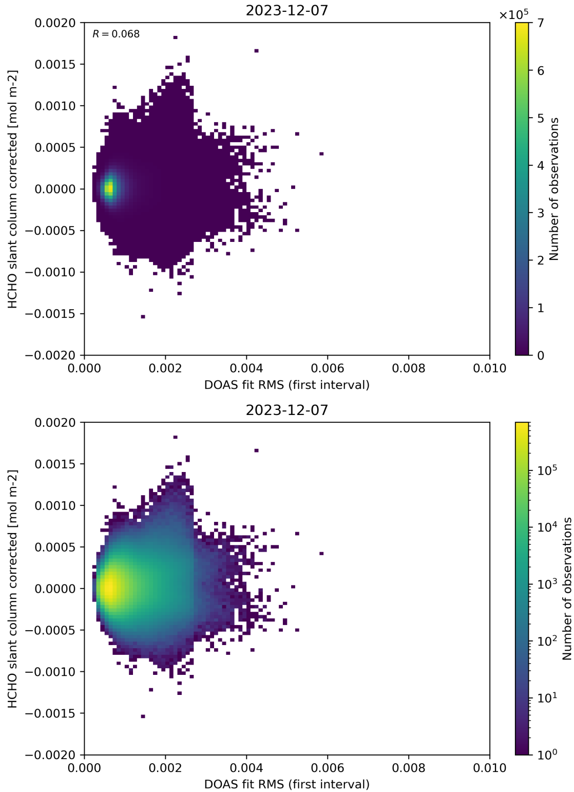
Figure 62: Scatter density plot of “DOAS fit RMS (first interval)” against “HCHO slant column corrected” for 2023-12-06 to 2023-12-08.
