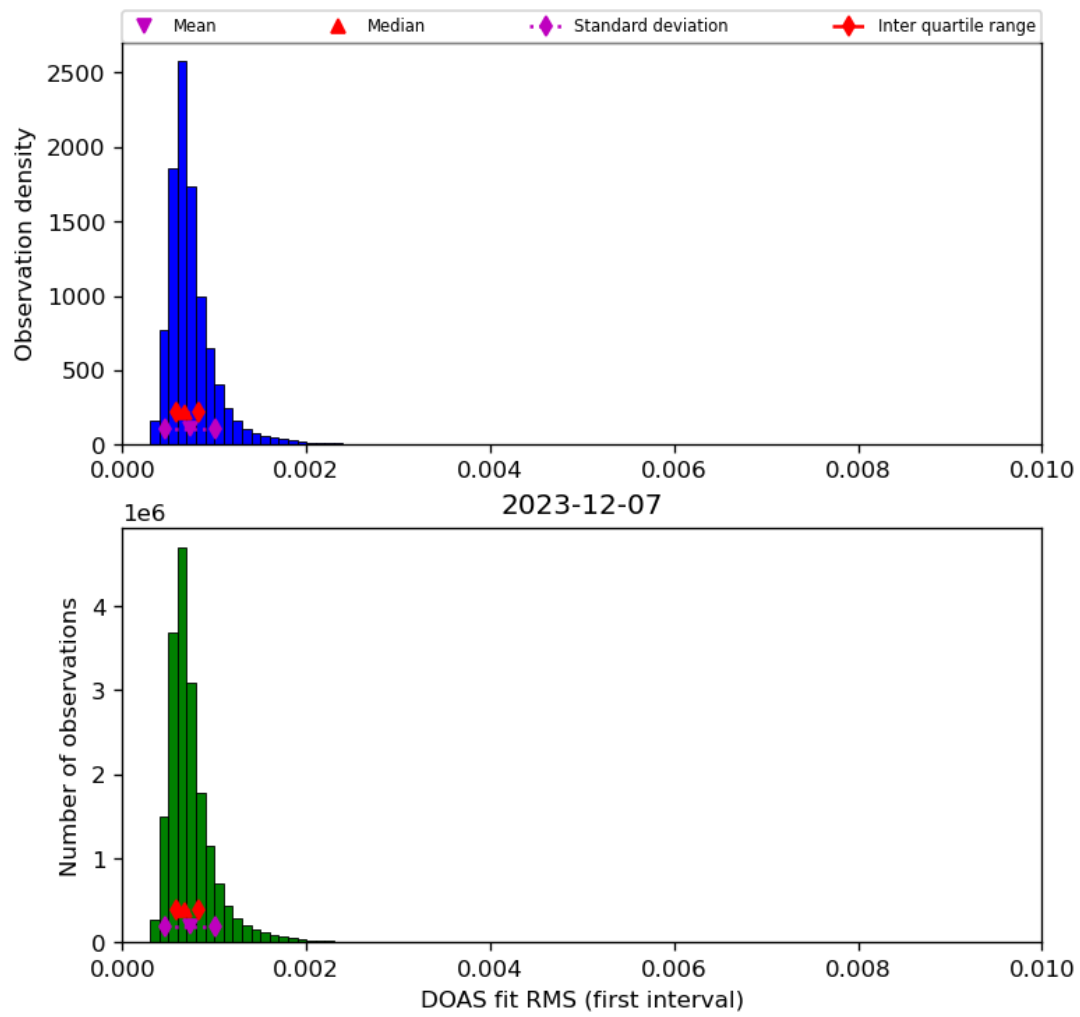
Figure 46: Histogram of “DOAS fit RMS (first interval)” for 2023-12-06 to 2023-12-08
