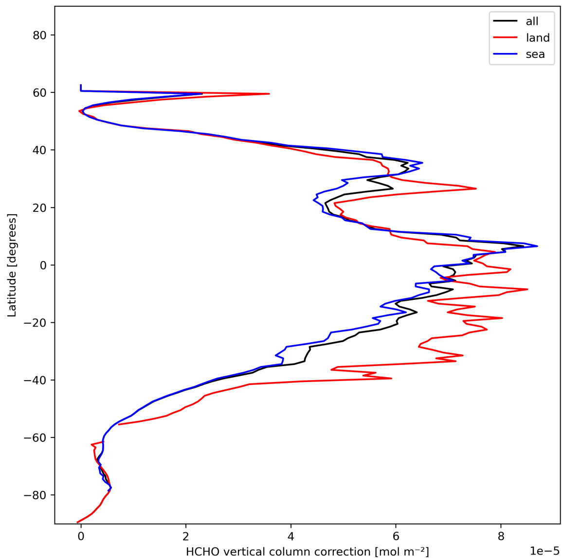
Figure 23: Zonal average of “HCHO vertical column correction” for 2023-12-06 to 2023-12-08.
