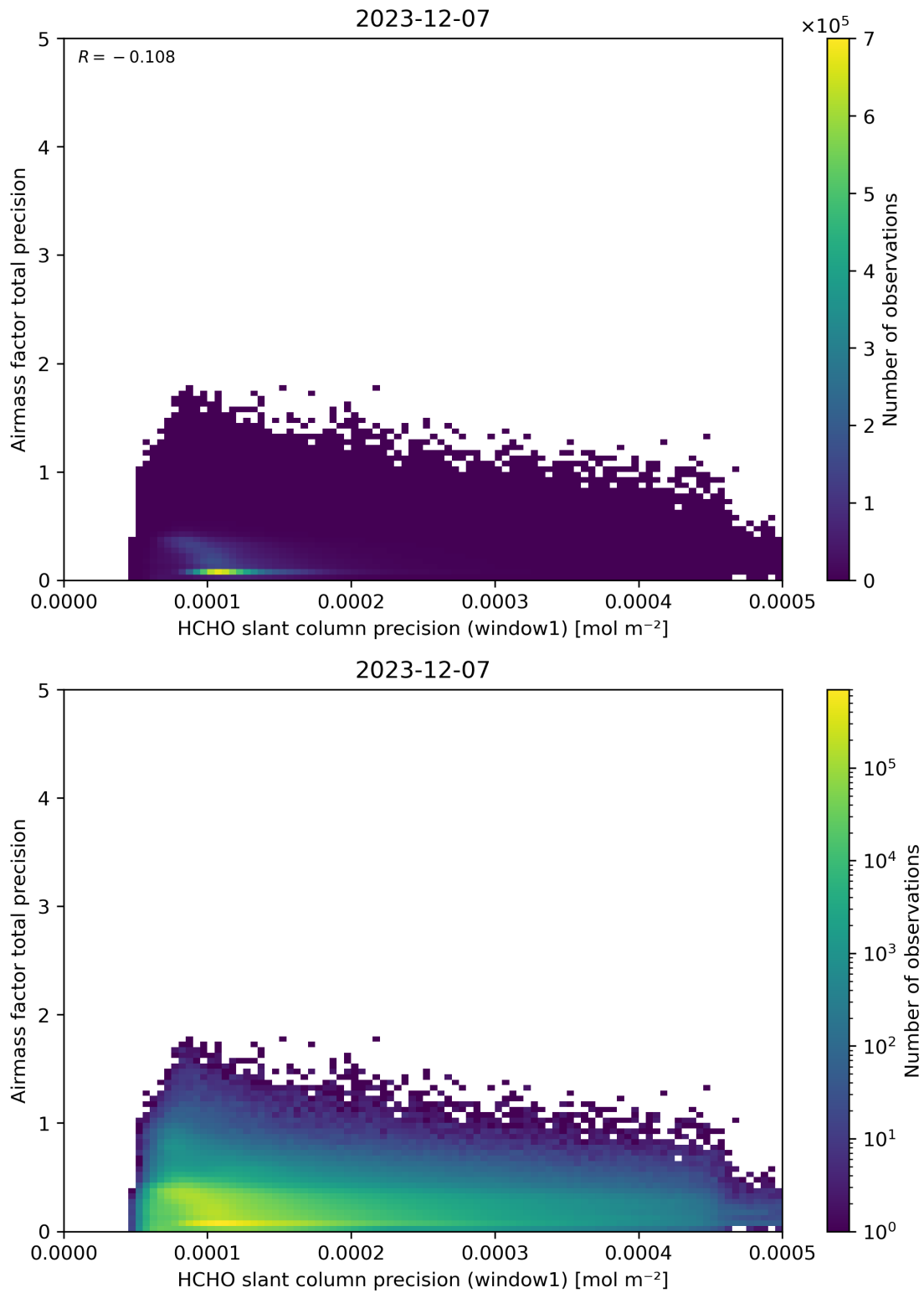
Figure 95: Scatter density plot of “HCHO slant column precision (window1)” against “Airmass factor total precision” for 2023-12-06 to 2023-12-08.
