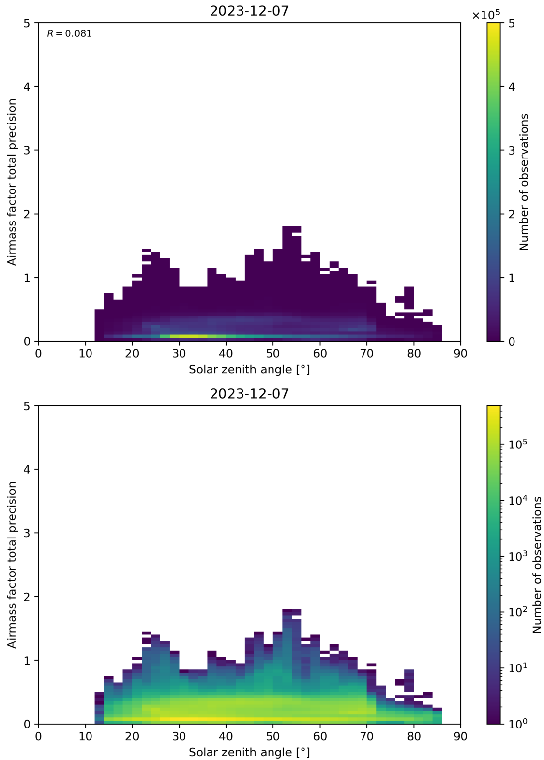
Figure 176: Scatter density plot of “Solar zenith angle” against “Airmass factor total precision” for 2023-12-06 to 2023-12-08.
