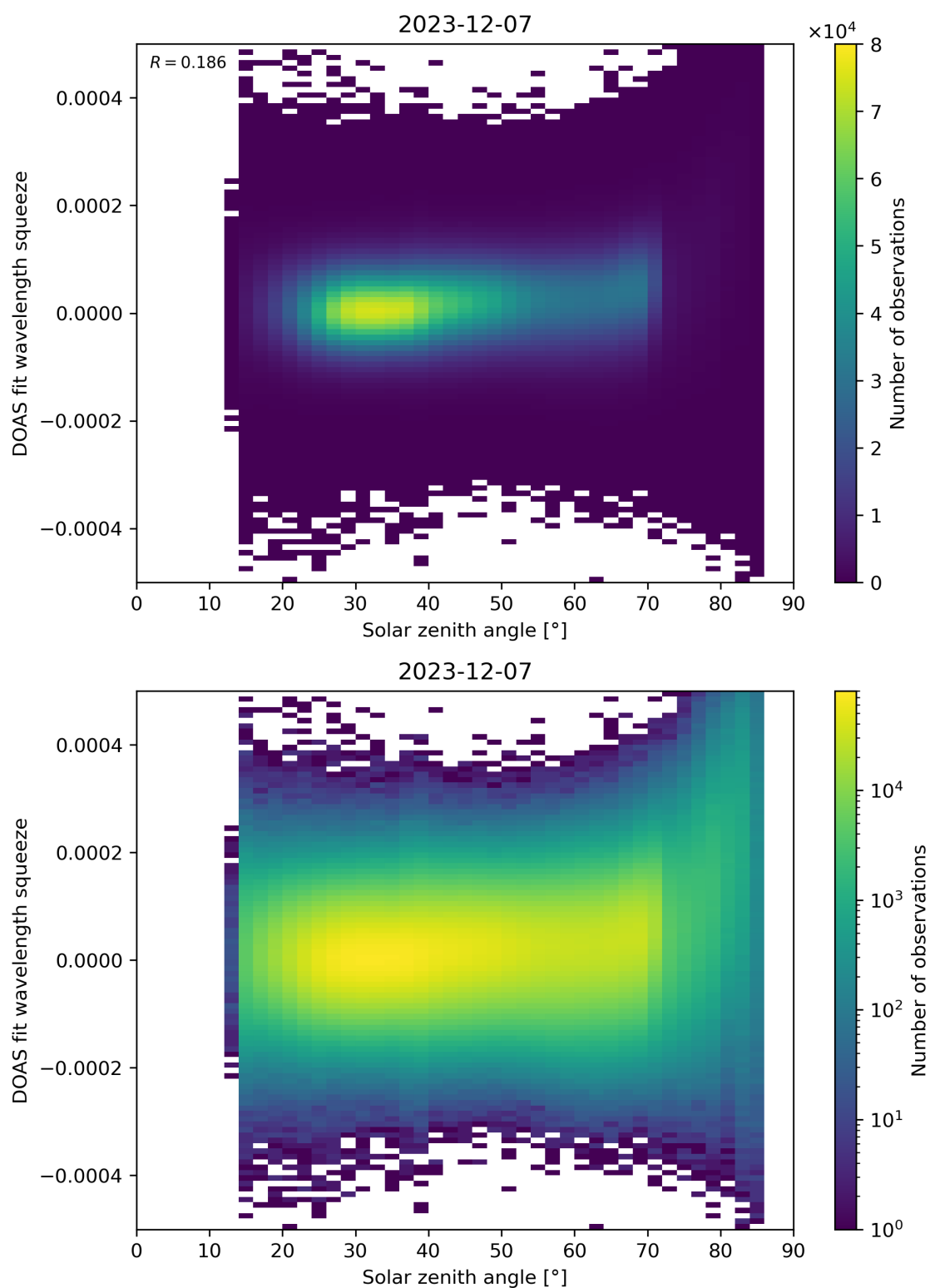
Figure 169: Scatter density plot of “Solar zenith angle” against “DOAS fit wavelength squeeze” for 2023-12-06 to 2023-12-08.
