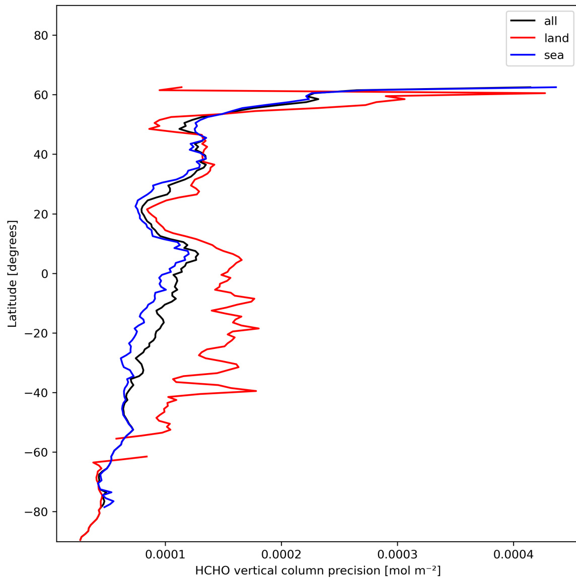
Figure 22: Zonal average of “HCHO vertical column precision” for 2023-12-06 to 2023-12-08.
