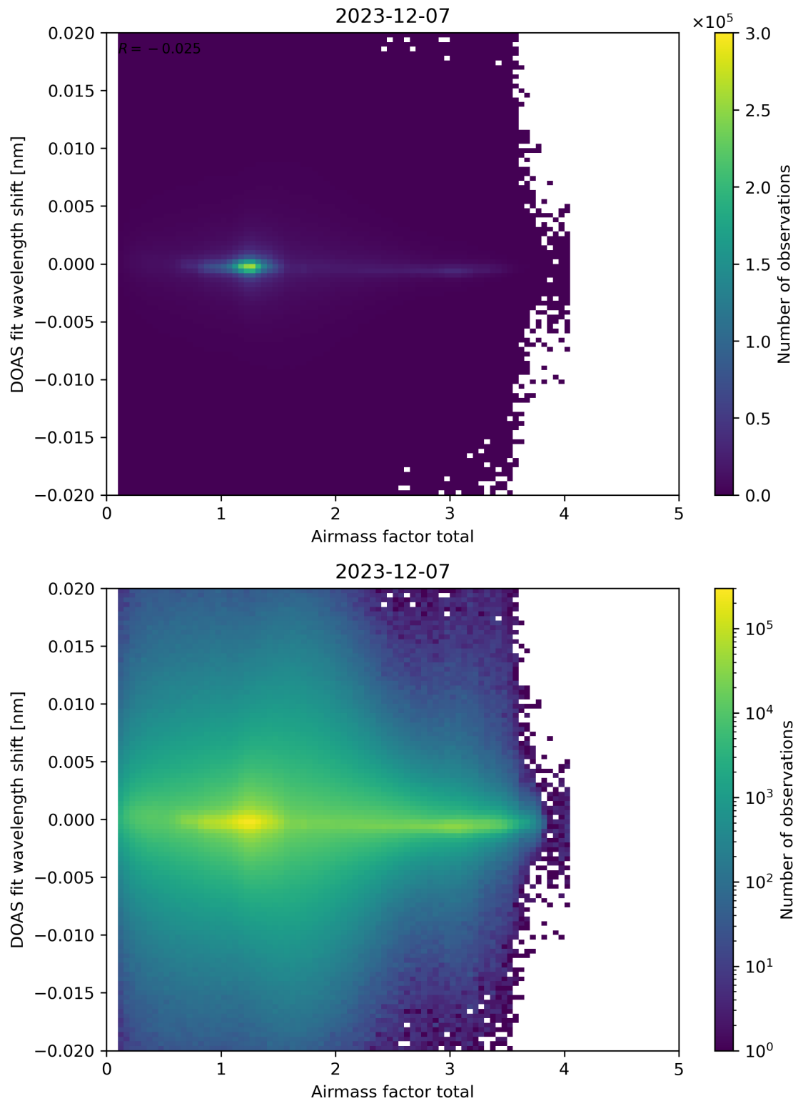
Figure 98: Scatter density plot of “Airmass factor total” against “DOAS fit wavelength shift” for 2023-12-06 to 2023-12-08.
