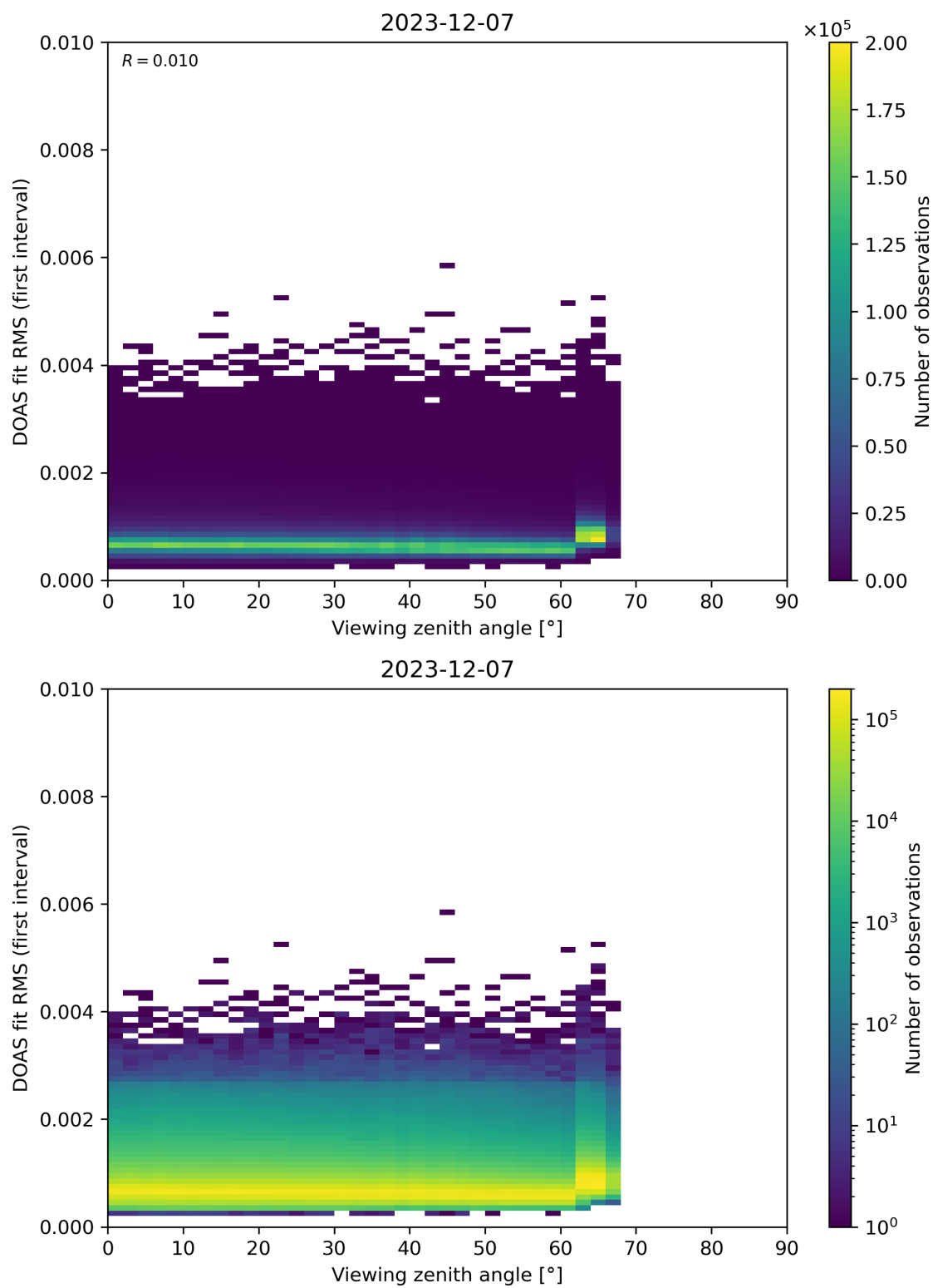
Figure 182: Scatter density plot of “Viewing zenith angle” against “DOAS fit RMS (first interval)” for 2023-12-06 to 2023-12-08.
