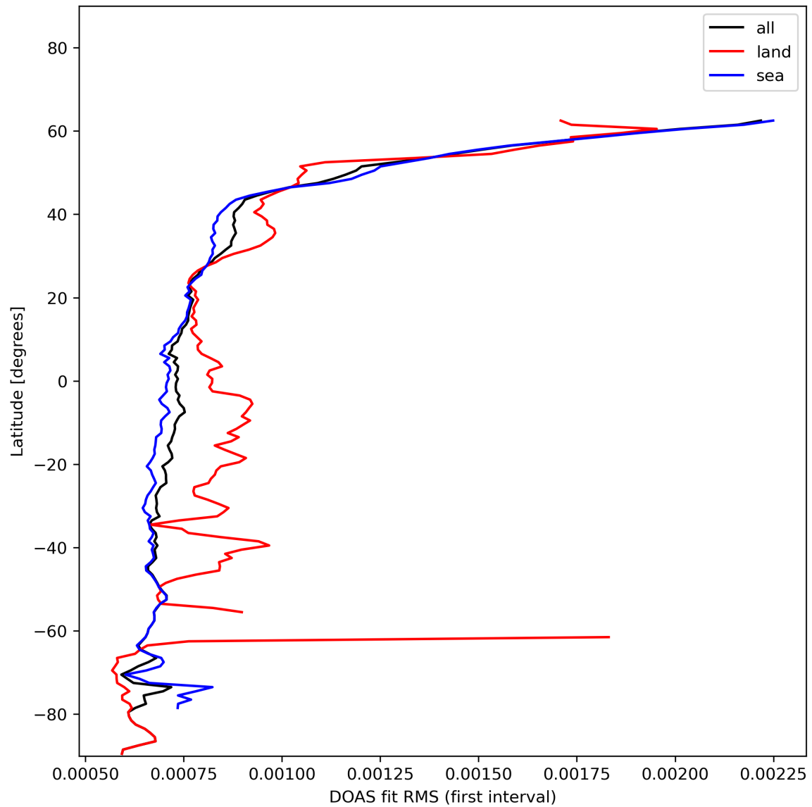
Figure 32: Zonal average of “DOAS fit RMS (first interval)” for 2023-12-06 to 2023-12-08.
