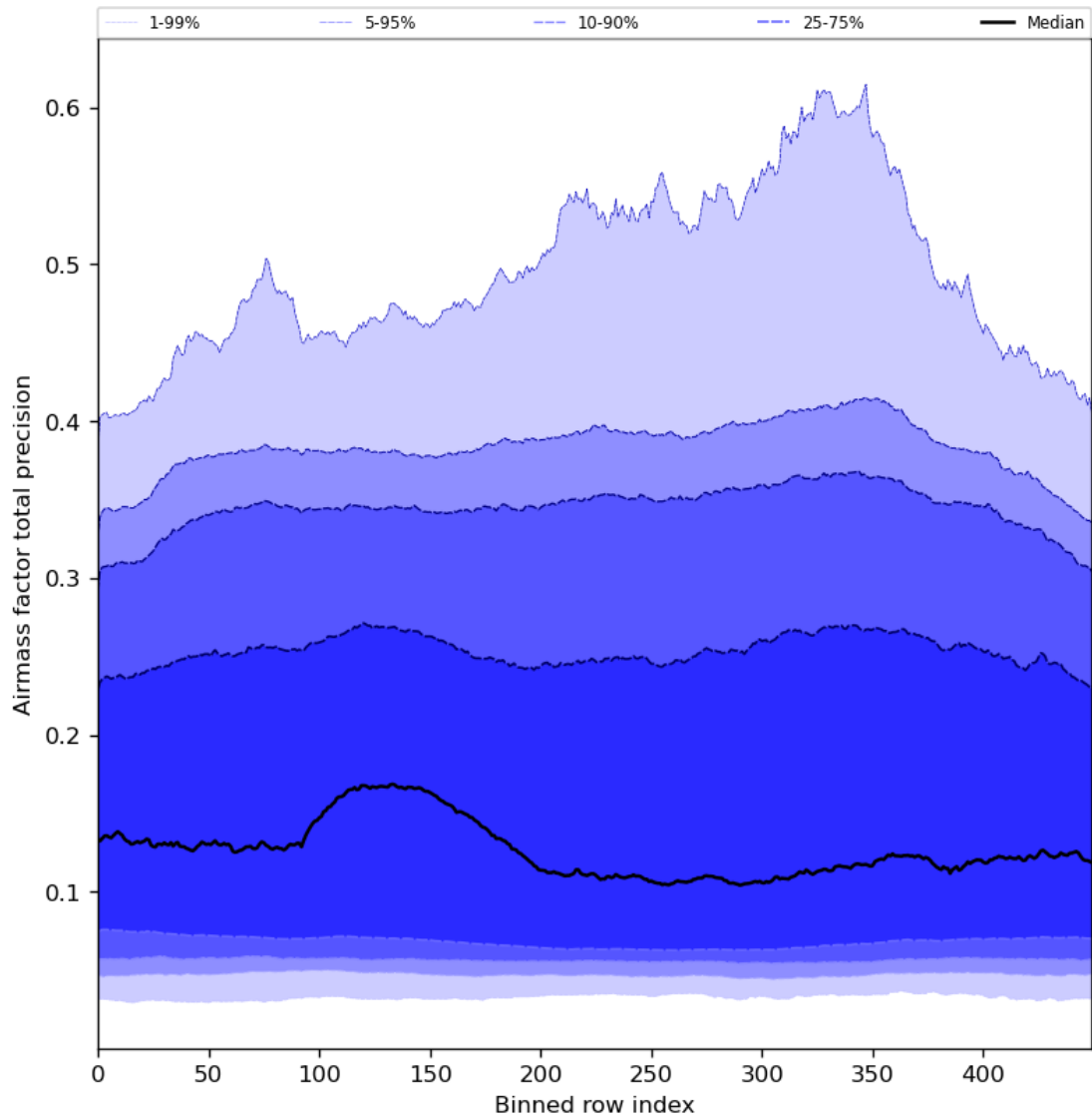
Figure 55: Along track statistics of “Airmass factor total precision” for 2023-12-06 to 2023-12-08
