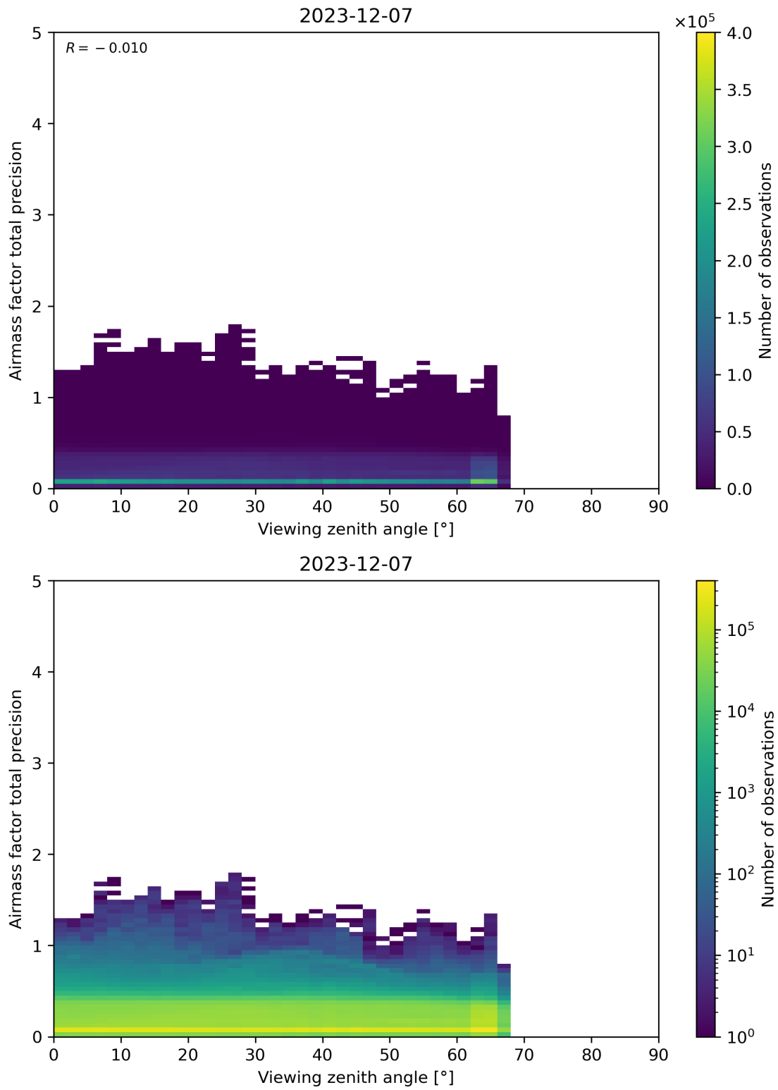
Figure 191: Scatter density plot of “Viewing zenith angle” against “Airmass factor total precision” for 2023-12-06 to 2023-12-08.
