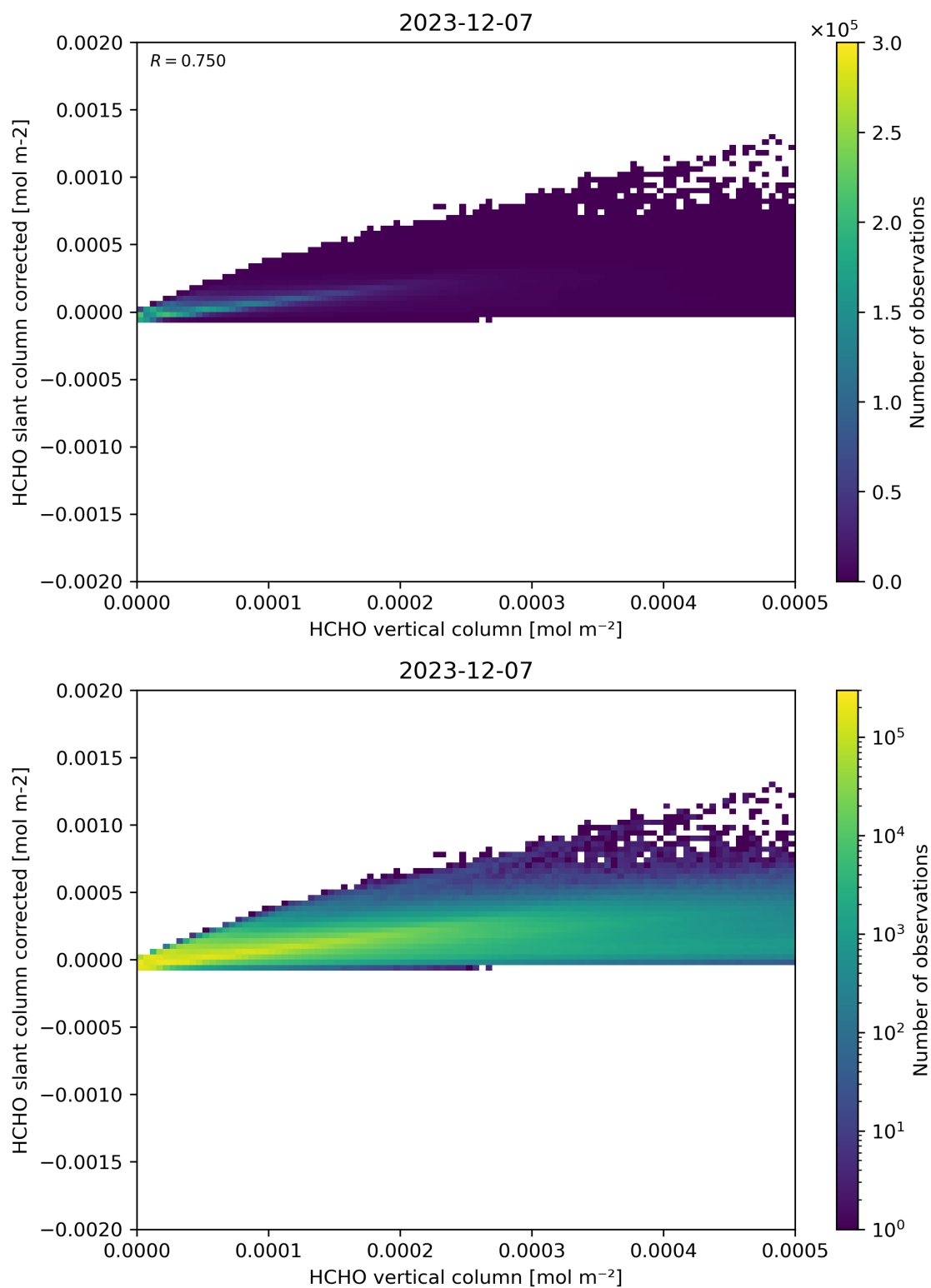
Figure 127: Scatter density plot of “HCHO vertical column” against “HCHO slant column corrected” for 2023-12-06 to 2023-12-08.
