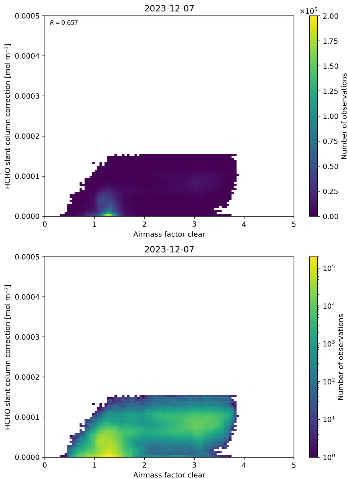
Figure 75: Scatter density plot of “Air mass factor clear” against “HCHO slant column correction” for 2023-12-06 to 2023-12-08.
