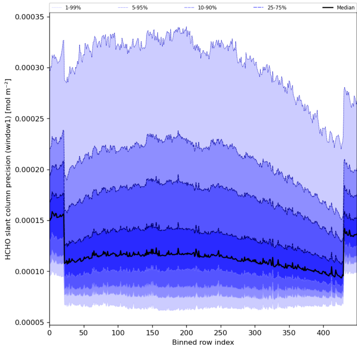
Figure 53: Along track statistics of “HCHO slant column precision (window1)” for 2023-12-06 to 2023-12-08
