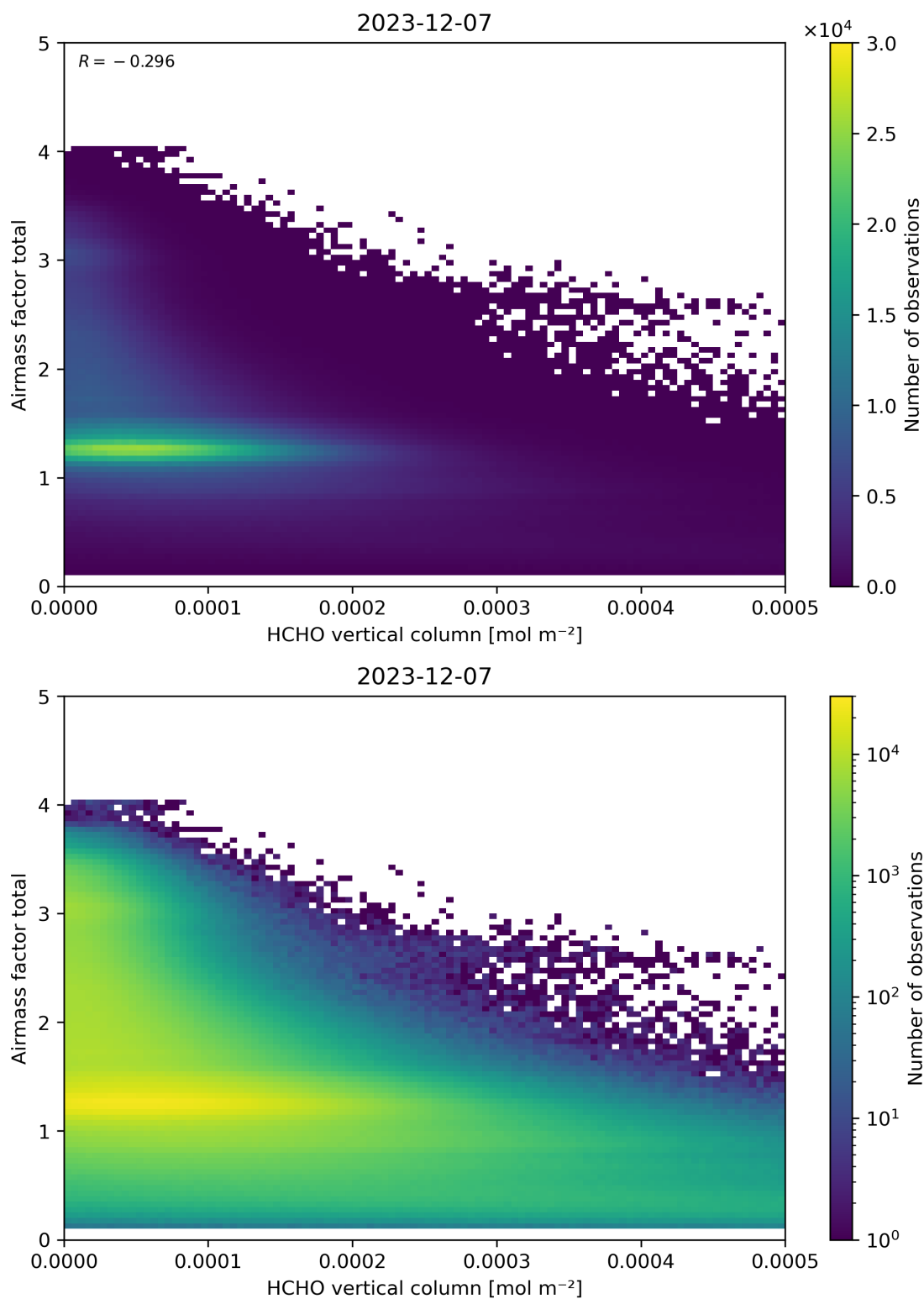
Figure 131: Scatter density plot of “HCHO vertical column” against “Airmass factor total” for 2023-12-06 to 2023-12-08.
