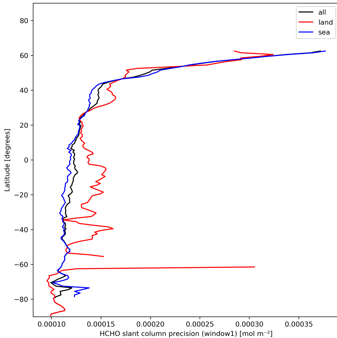
Figure 25: Zonal average of "HCHO slant column precision (window1)" for 2023-12-06 to 2023-12-08.
