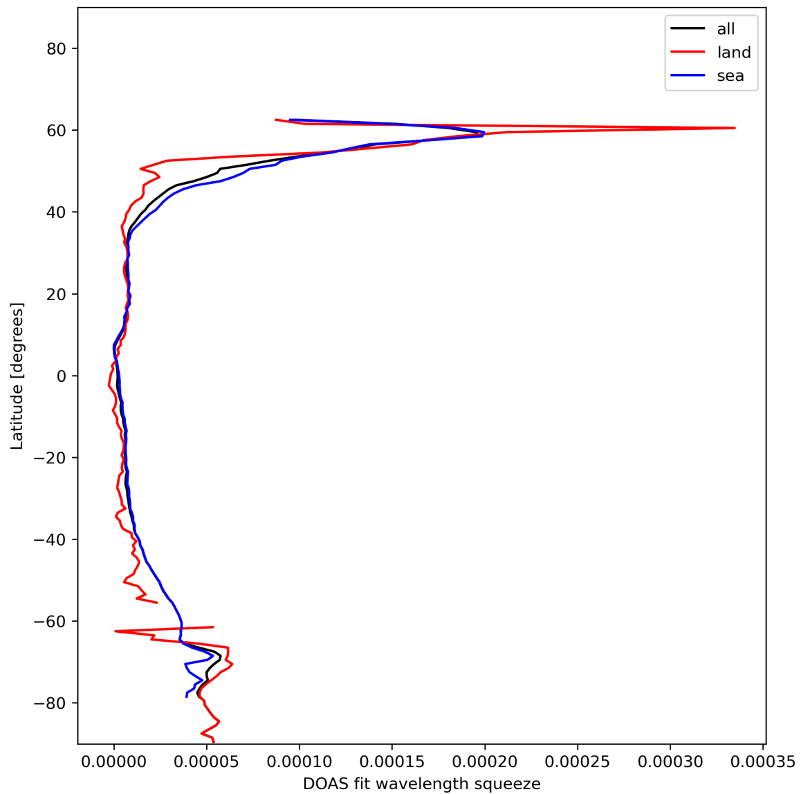
Figure 31: Zonal average of “DOAS fit wavelength squeeze” for 2023-12-06 to 2023-12-08.
