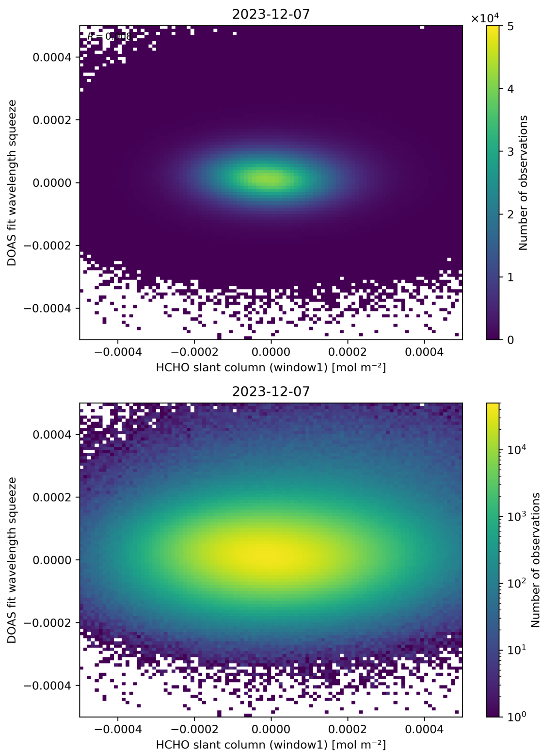
Figure 80: Scatter density plot of “HCHO slant column (window1)” against “DOAS fit wavelength squeeze” for 2023-12-06 to 2023-12-08.
