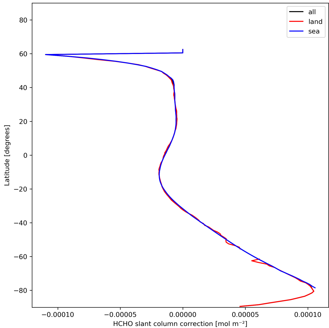
Figure 33: Zonal average of “HCHO slant column correction” for 2023-12-06 to 2023-12-08.
