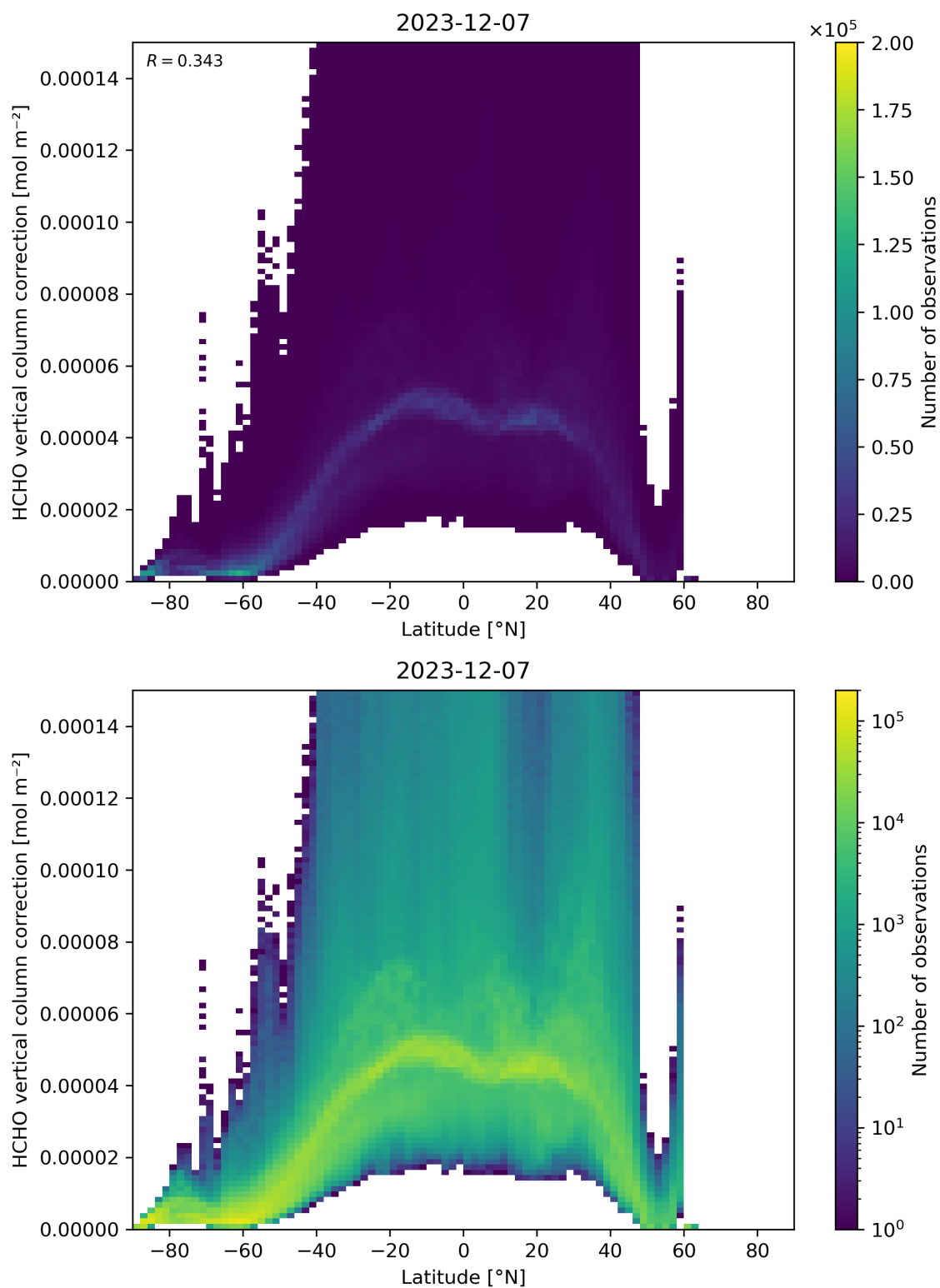
Figure 164: Scatter density plot of “Latitude” against “HCHO vertical column correction” for 2023-12-06 to 2023-12-08.
