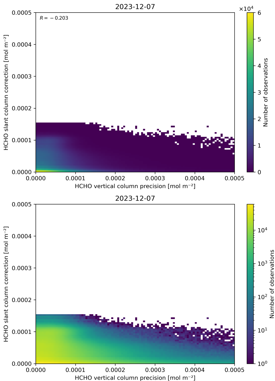
Figure 141: Scatter density plot of “HCHO vertical column precision” against “HCHO slant column correction” for 2023-12-06 to 2023-12-08.
