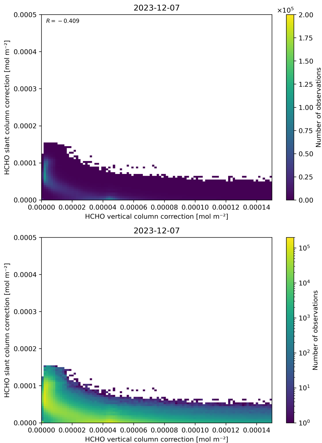
Figure 117: Scatter density plot of “HCHO vertical column correction” against “HCHO slant column correction” for 2023-12-06 to 2023-12-08.
