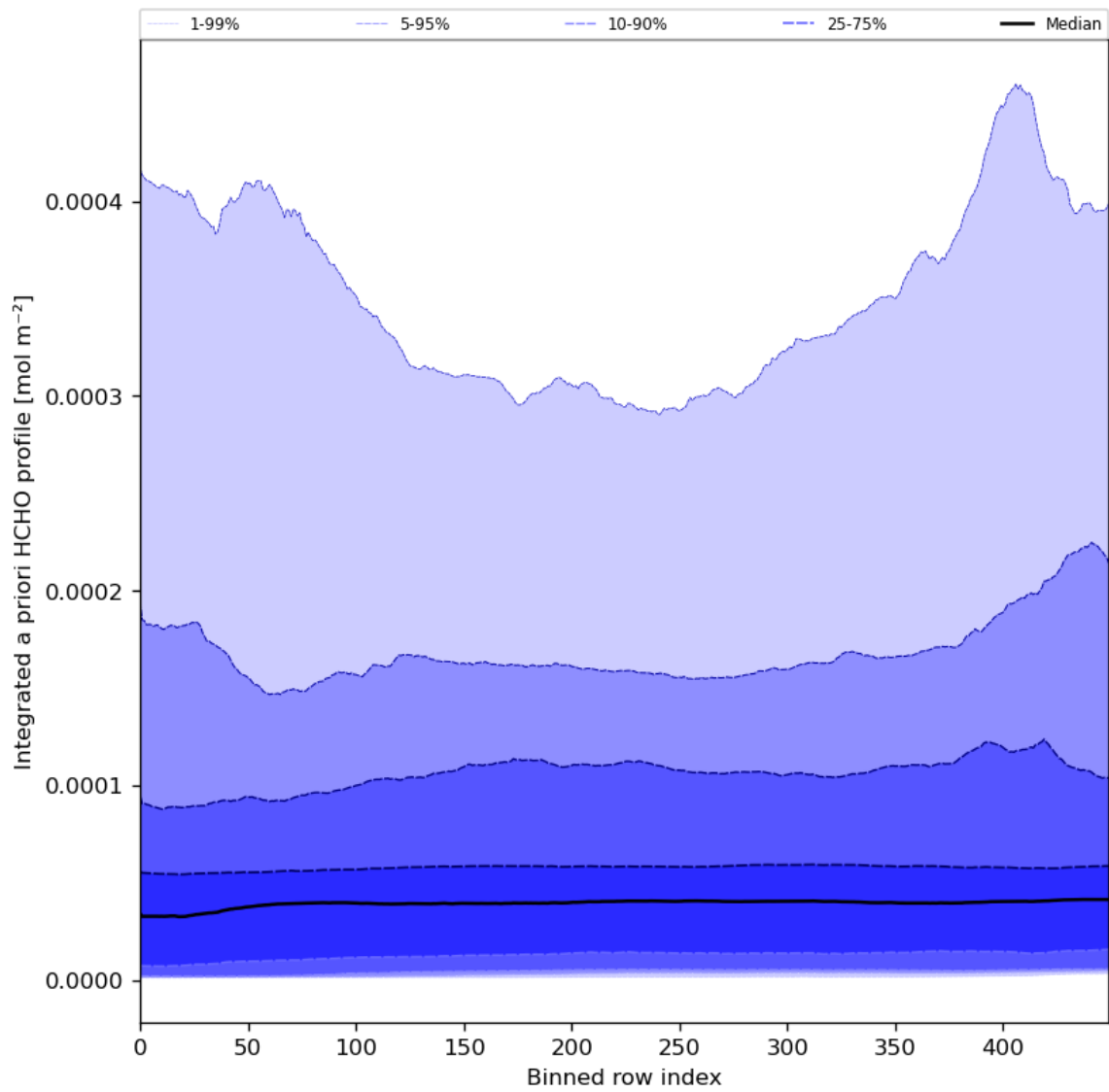
Figure 57: Along track statistics of “Integrated a priori HCHO profile” for 2023-12-06 to 2023-12-08
