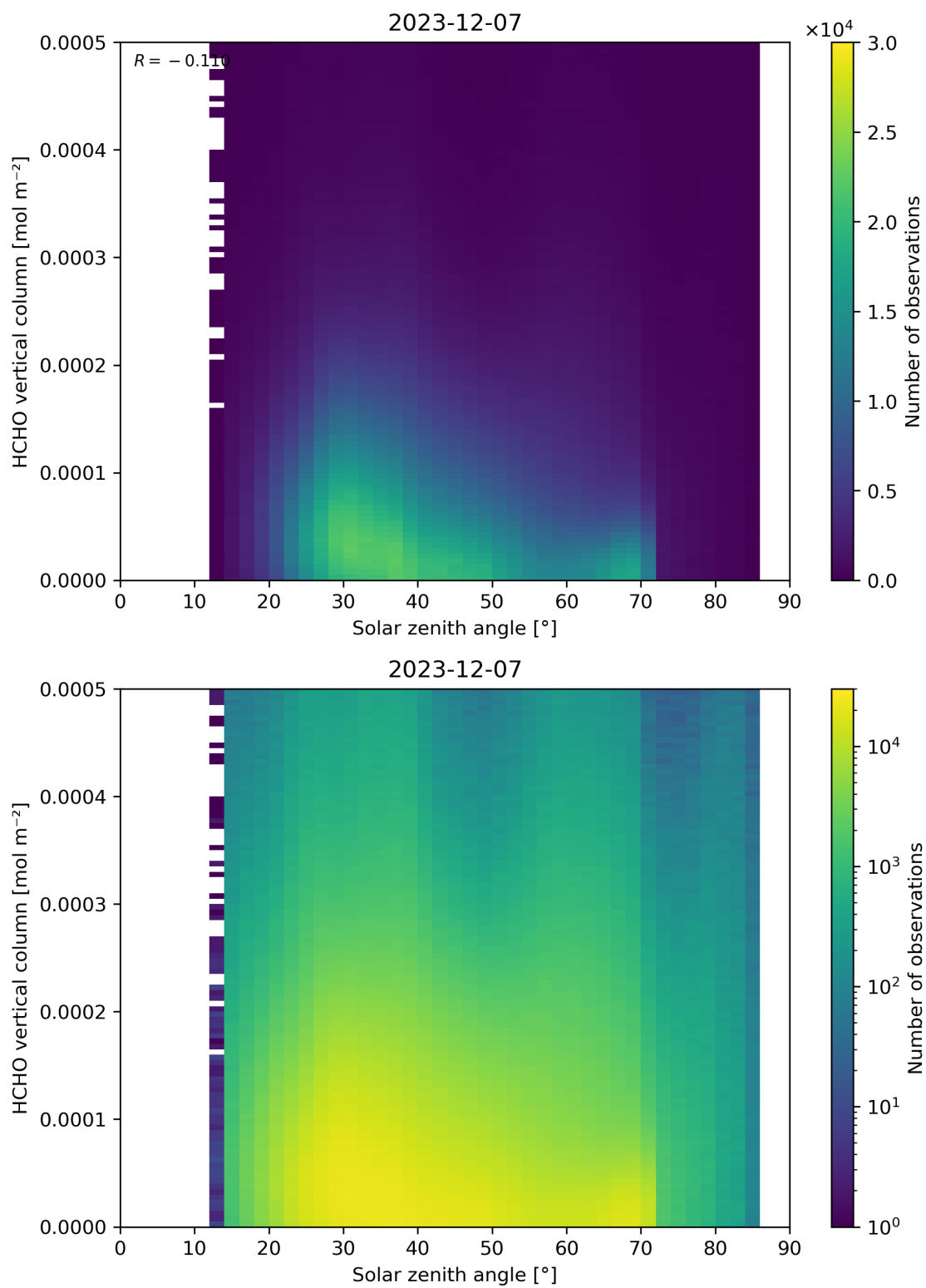
Figure 177: Scatter density plot of “Solar zenith angle” against “HCHO vertical column” for 2023-12-06 to 2023-12-08.
