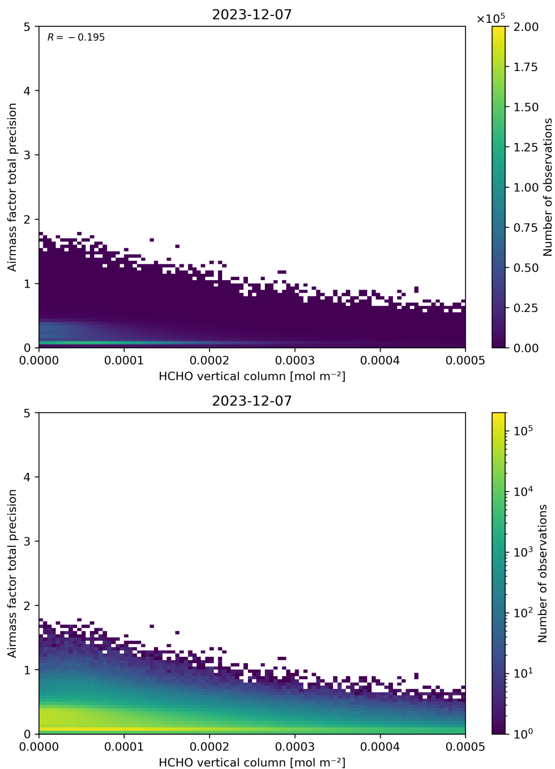
Figure 132: Scatter density plot of “HCHO vertical column” against “Airmass factor total precision” for 2023-12-06 to 2023-12-08.
