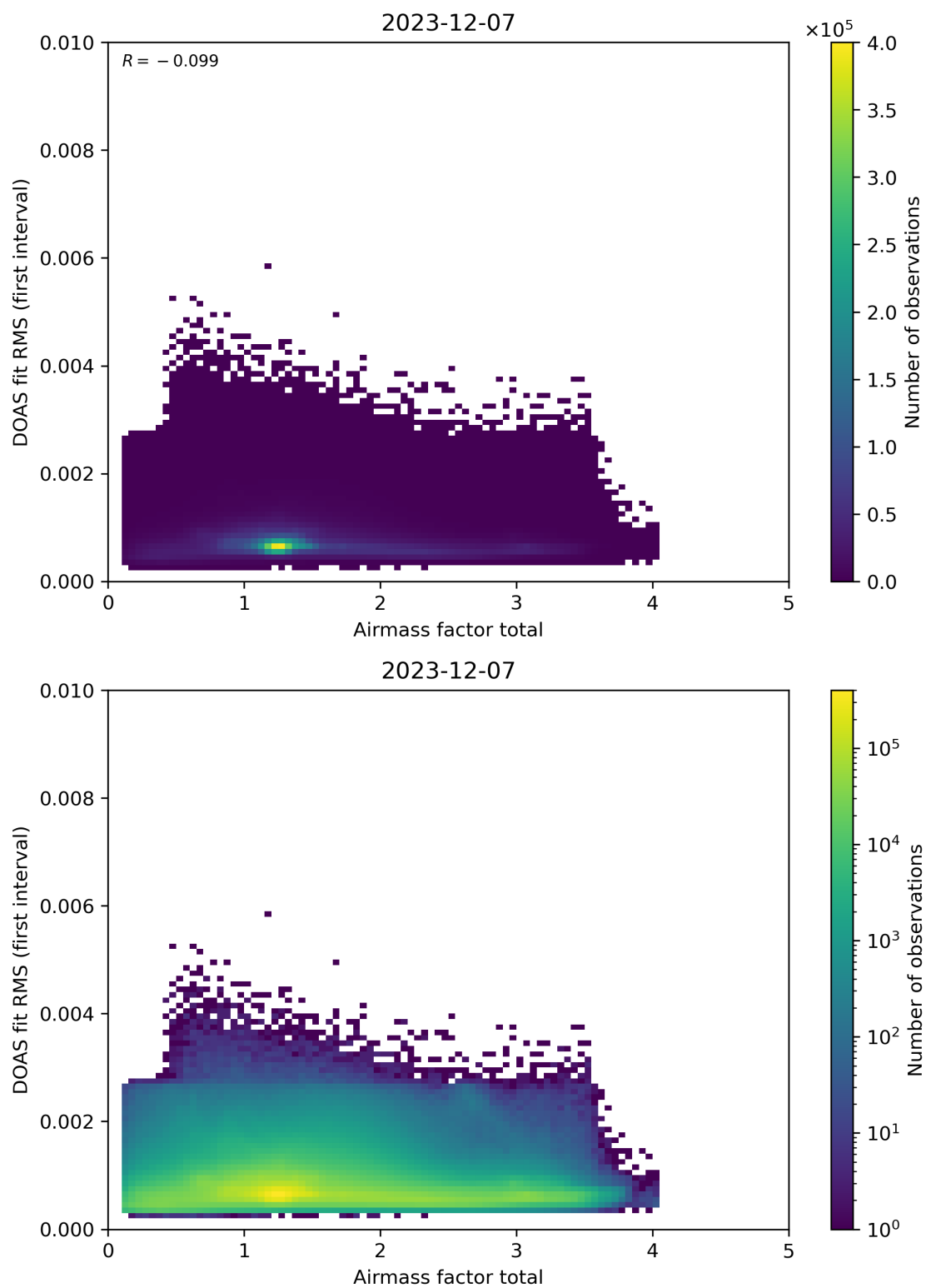
Figure 97: Scatter density plot of “Airmass factor total” against “DOAS fit RMS (first interval)” for 2023-12-06 to 2023-12-08.
