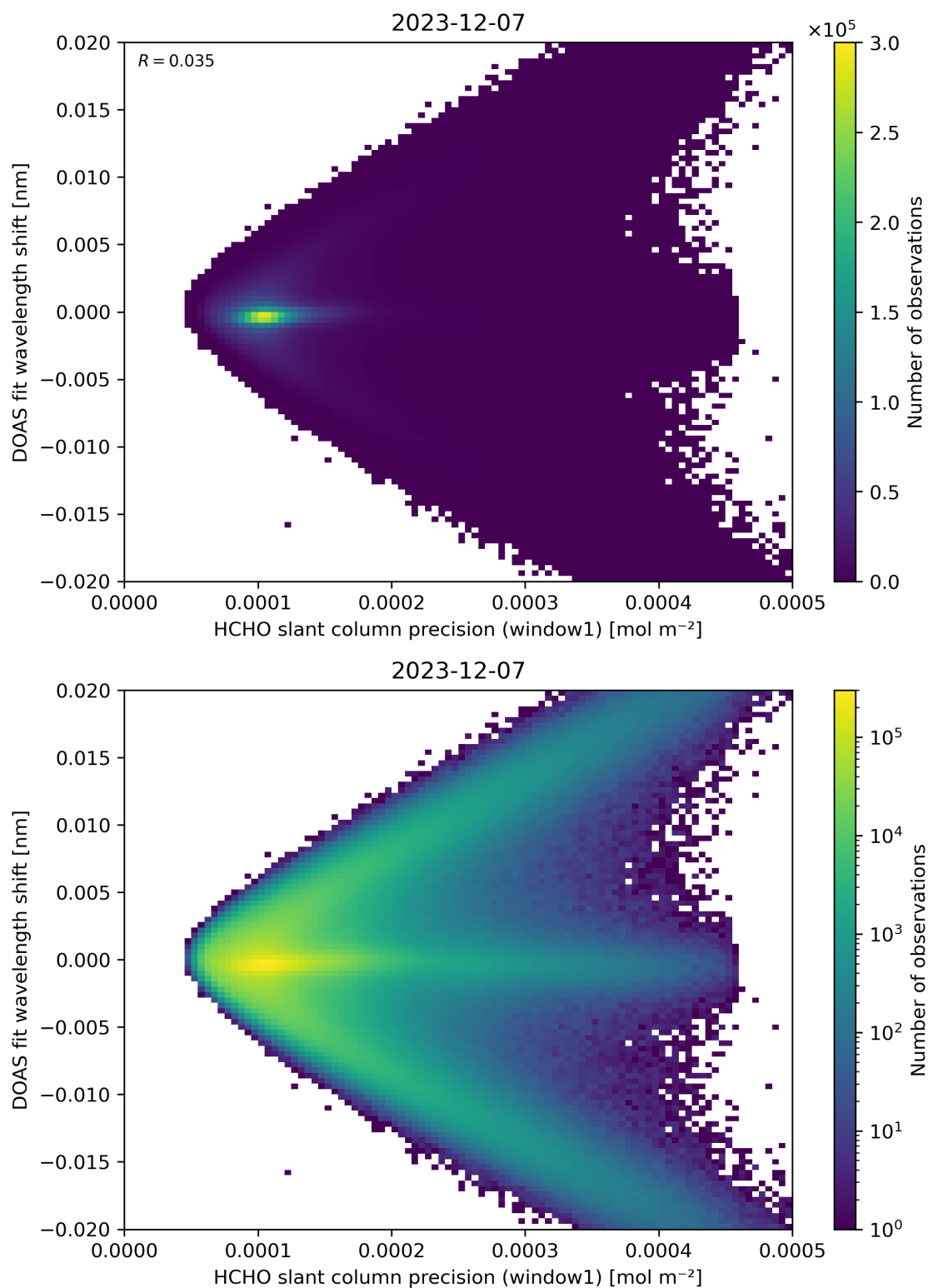
Figure 89: Scatter density plot of “HCHO slant column precision (window1)” against “DOAS fit wavelength shift” for 2023-12-06 to 2023-12-08.
