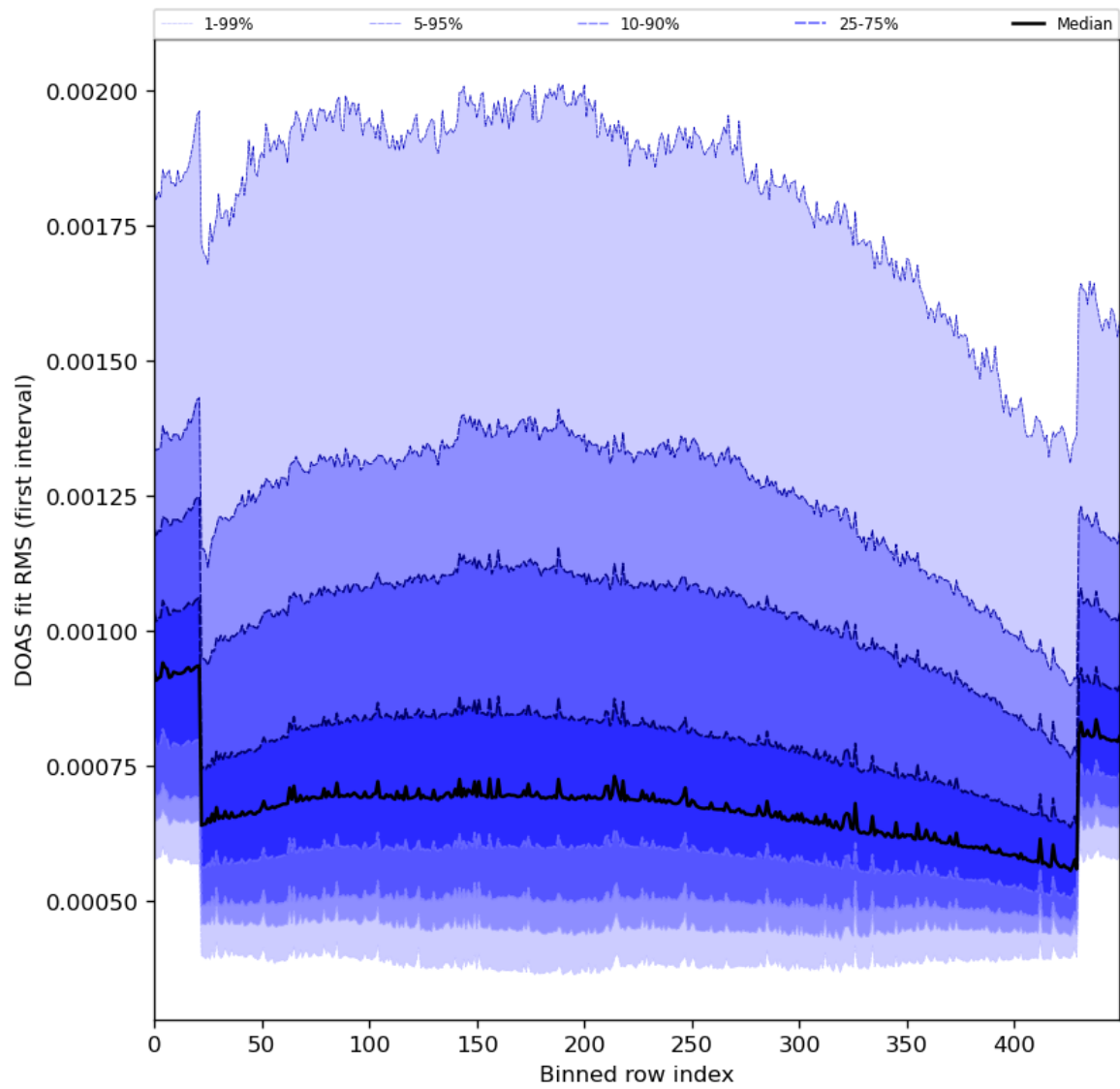
Figure 60: Along track statistics of “DOAS fit RMS (first interval)” for 2023-12-06 to 2023-12-08
