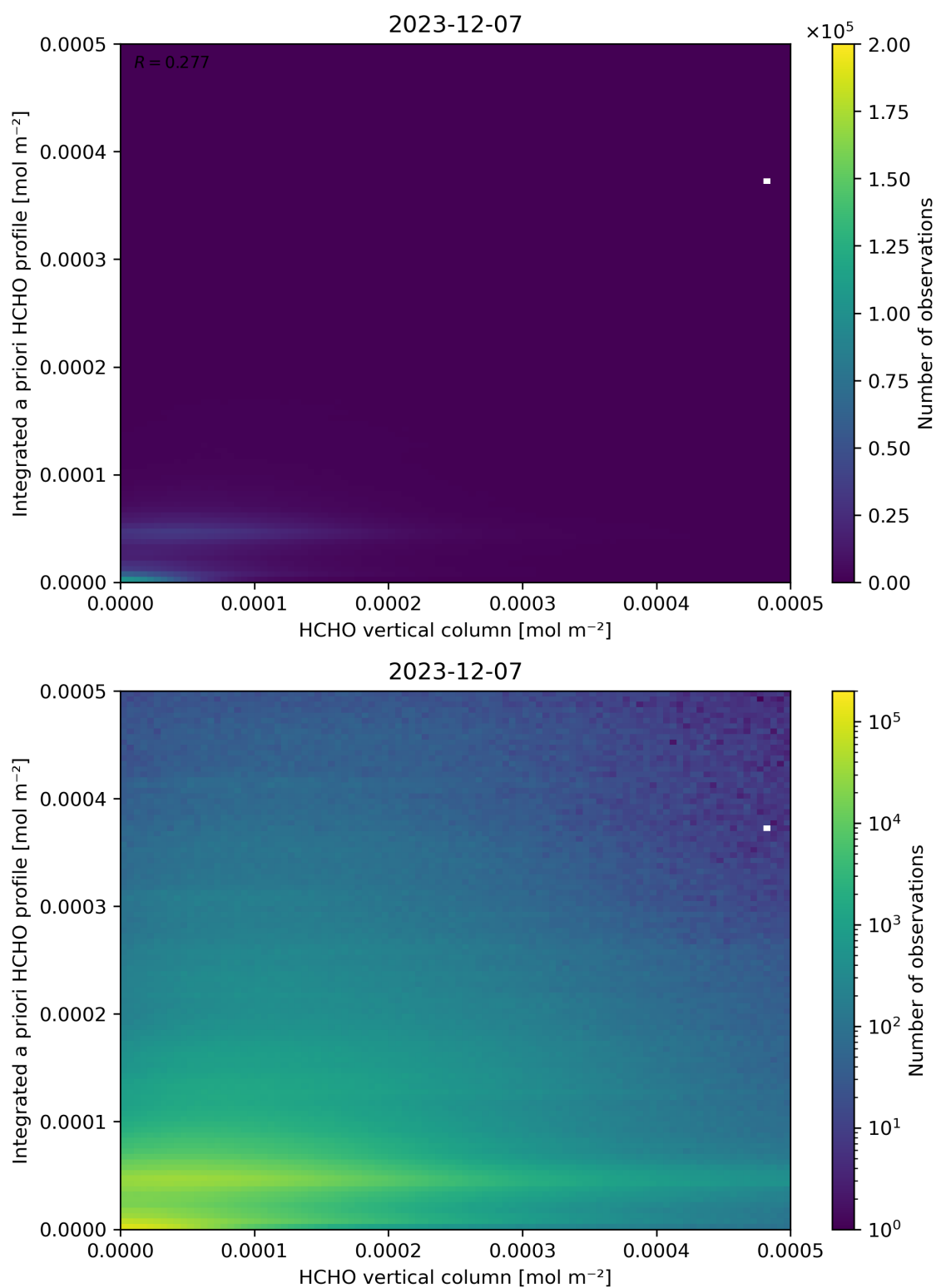
Figure 135: Scatter density plot of “HCHO vertical column” against “Integrated a priori HCHO profile” for 2023-12-06 to 2023-12-08.
