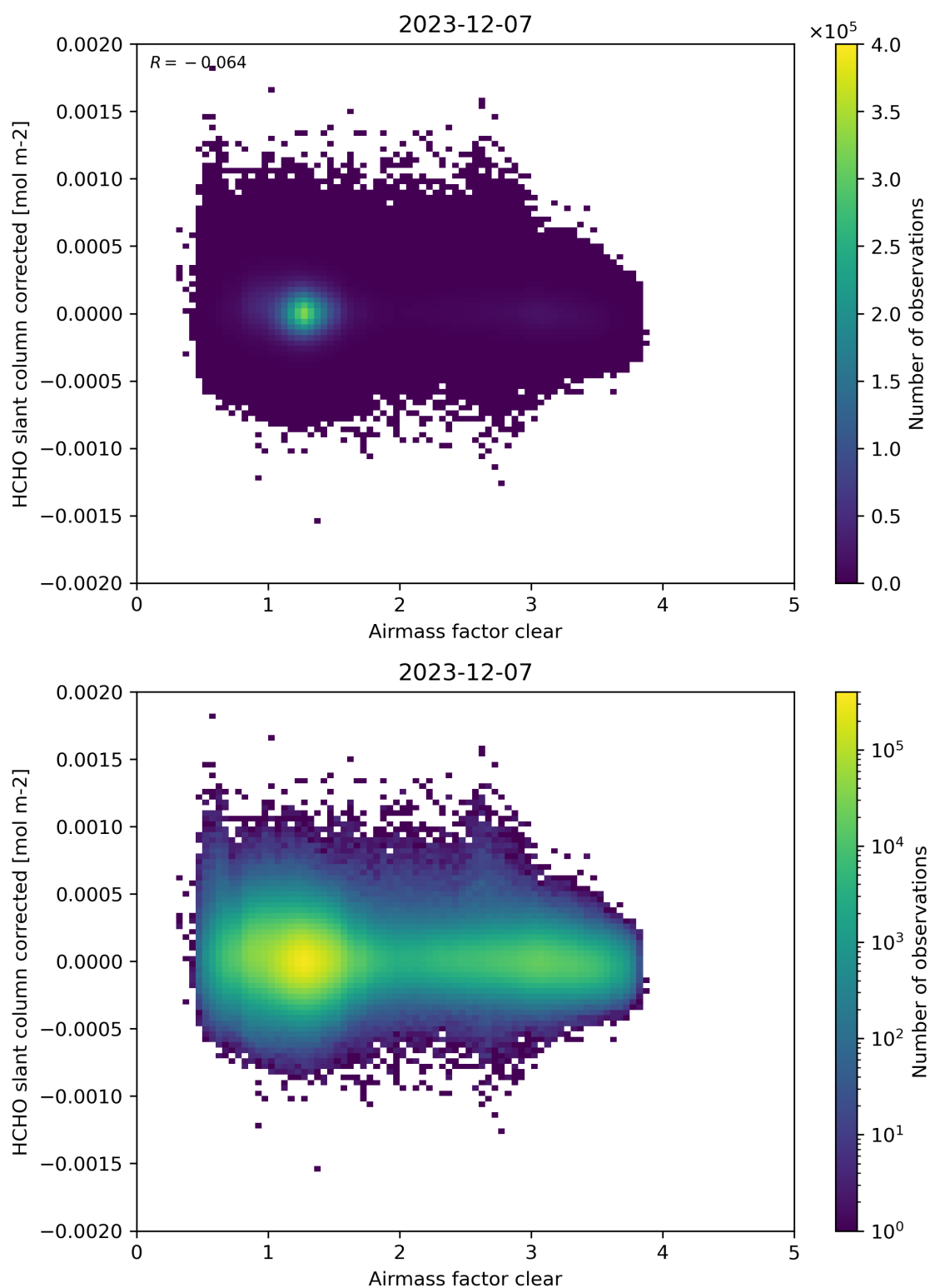
Figure 74: Scatter density plot of “Airmass factor clear” against “HCHO slant column corrected” for 2023-12-06 to 2023-12-08.
