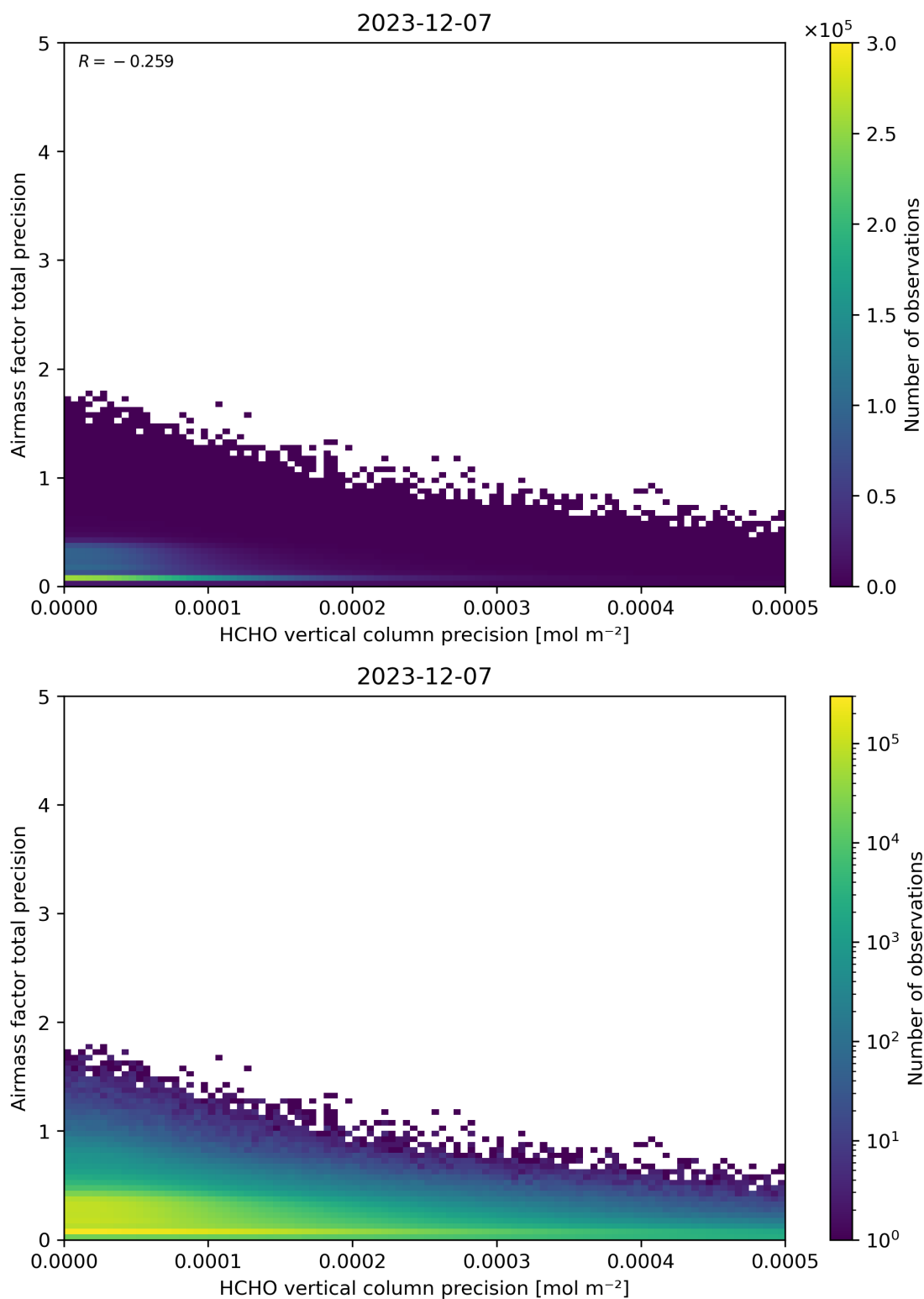
Figure 145: Scatter density plot of “HCHO vertical column precision” against “Airmass factor total precision” for 2023-12-06 to 2023-12-08.
