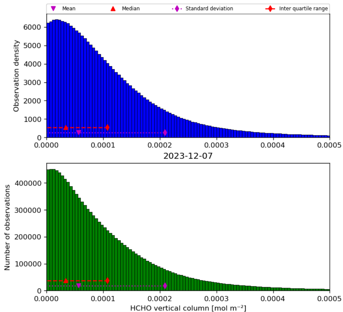
Figure 35: Histogram of “HCHO vertical column” for 2023-12-06 to 2023-12-08
