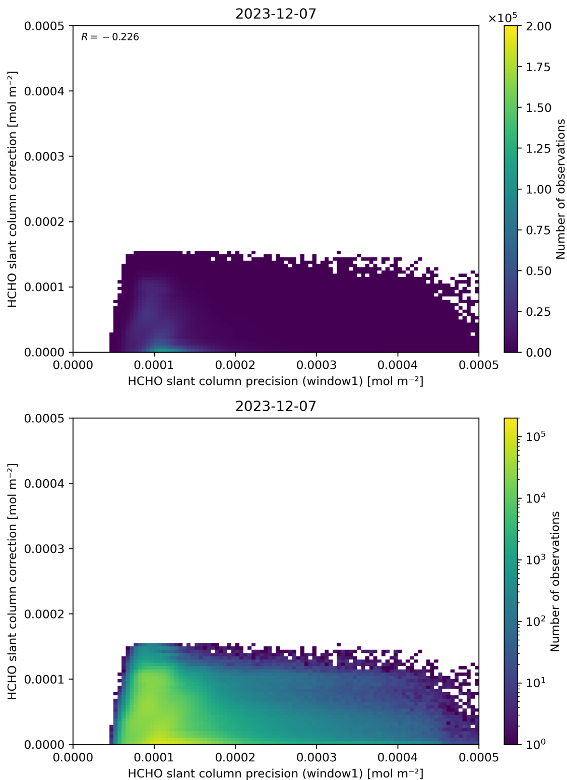
Figure 93: Scatter density plot of “HCHO slant column precision (window1)” against “HCHO slant column correction” for 2023-12-06 to 2023-12-08.
