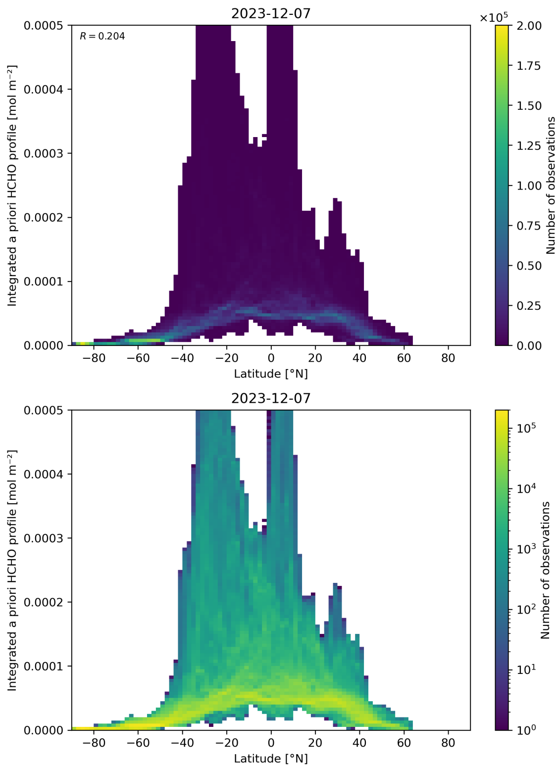
Figure 166: Scatter density plot of “Latitude” against “Integrated a priori HCHO profile” for 2023-12-06 to 2023-12-08.
