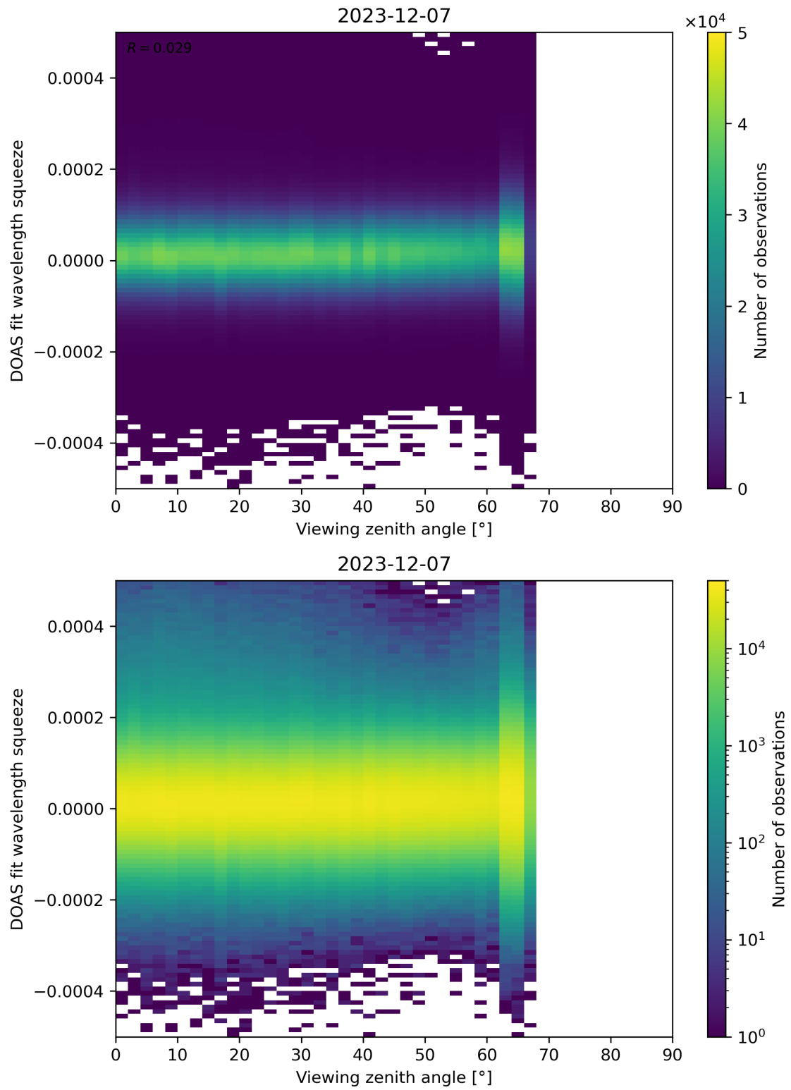
Figure 184: Scatter density plot of “Viewing zenith angle” against “DOAS fit wavelength squeeze” for 2023-12-06 to 2023-12-08.
