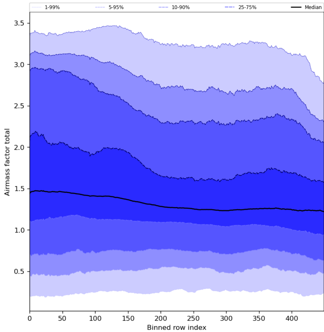
Figure 54: Along track statistics of “Airmass factor total” for 2023-12-06 to 2023-12-08
