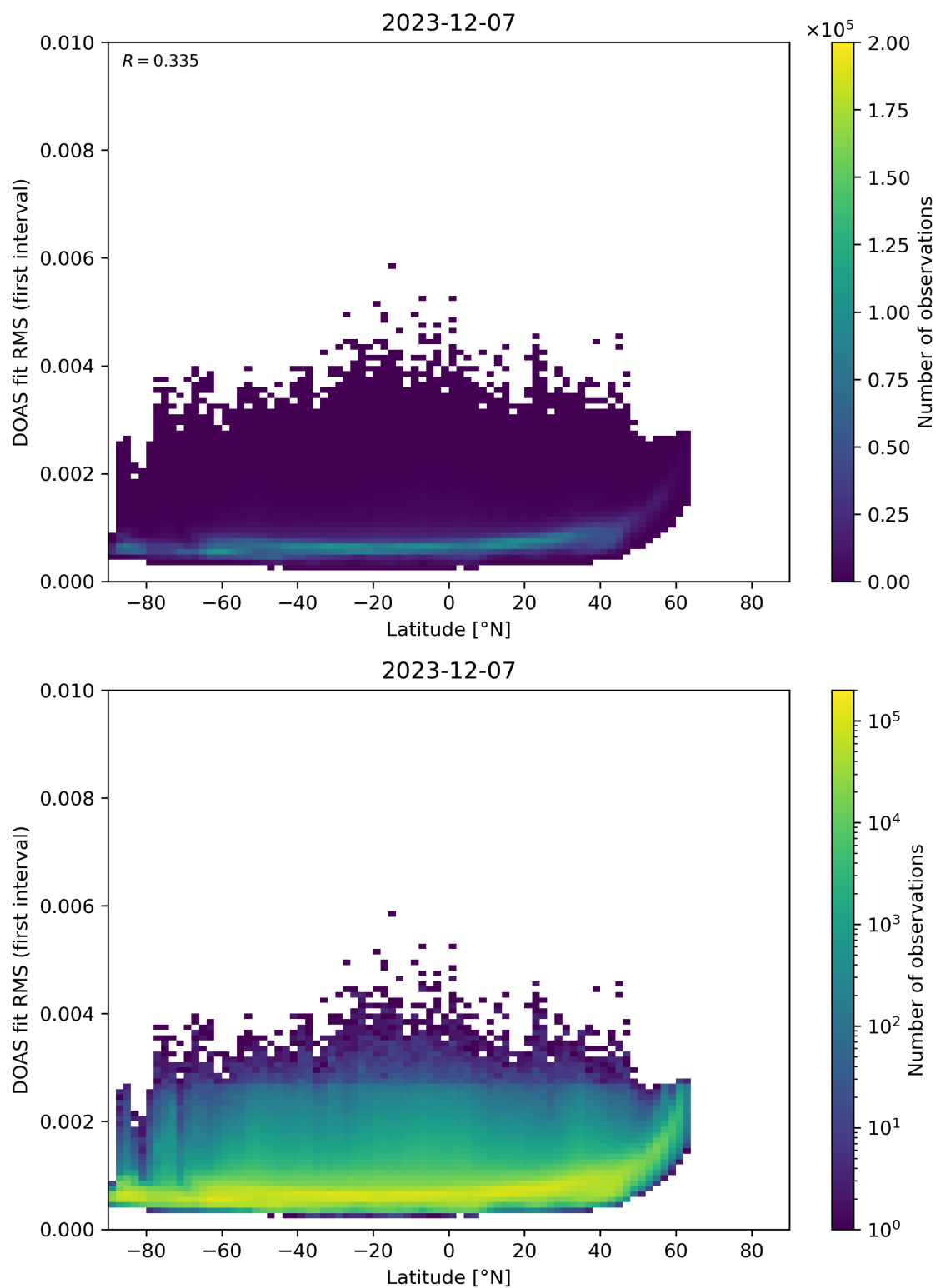
Figure 153: Scatter density plot of “Latitude” against “DOAS fit RMS (first interval)” for 2023-12-06 to 2023-12-08.
