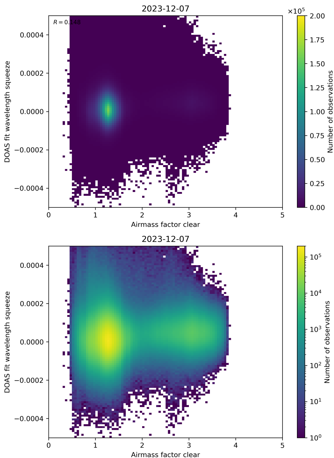
Figure 73: Scatter density plot of “Airmass factor clear” against “DOAS fit wavelength squeeze” for 2023-12-06 to 2023-12-08.
