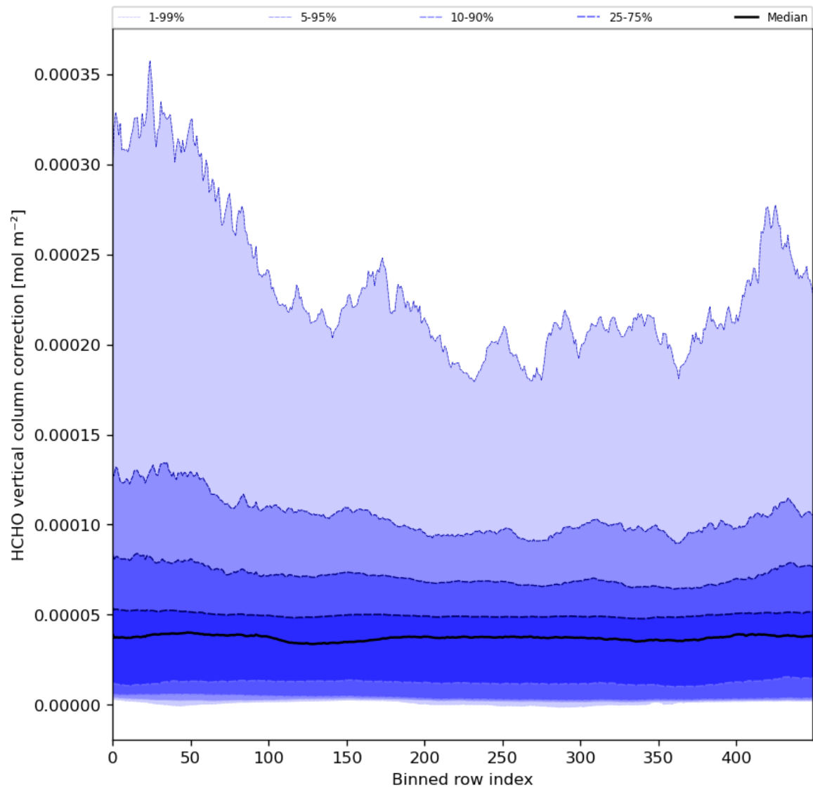
Figure 51: Along track statistics of “HCHO vertical column correction” for 2023-12-06 to 2023-12-08
