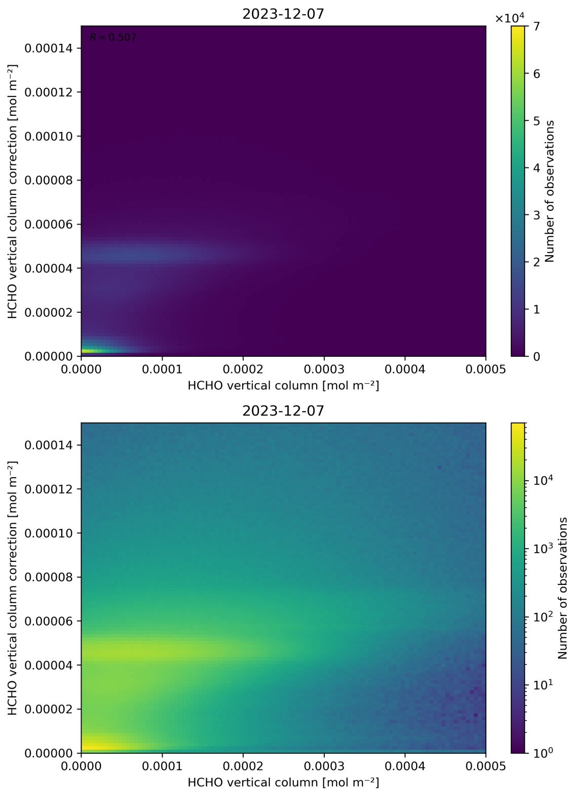
Figure 133: Scatter density plot of “HCHO vertical column” against “HCHO vertical column correction” for 2023-12-06 to 2023-12-08.
