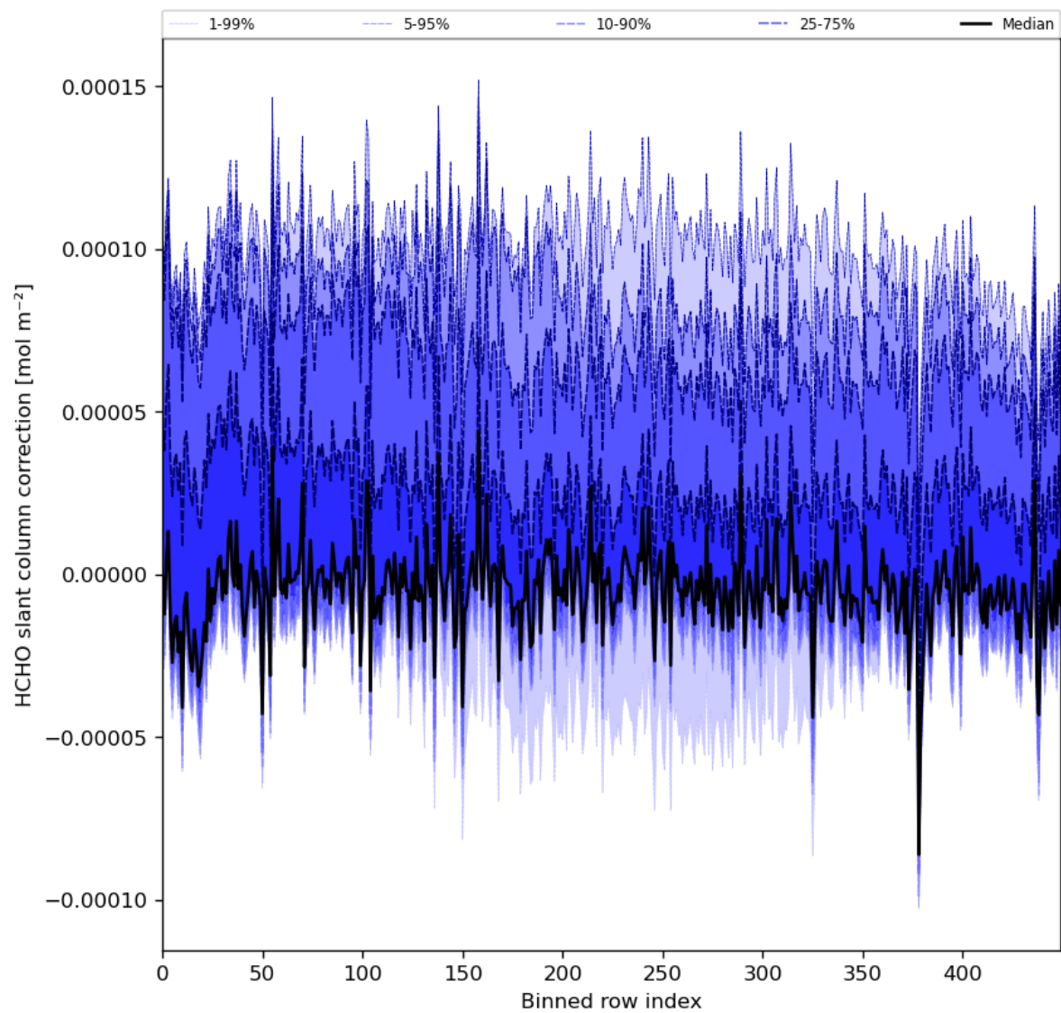
Figure 61: Along track statistics of “HCHO slant column correction” for 2023-12-06 to 2023-12-08
