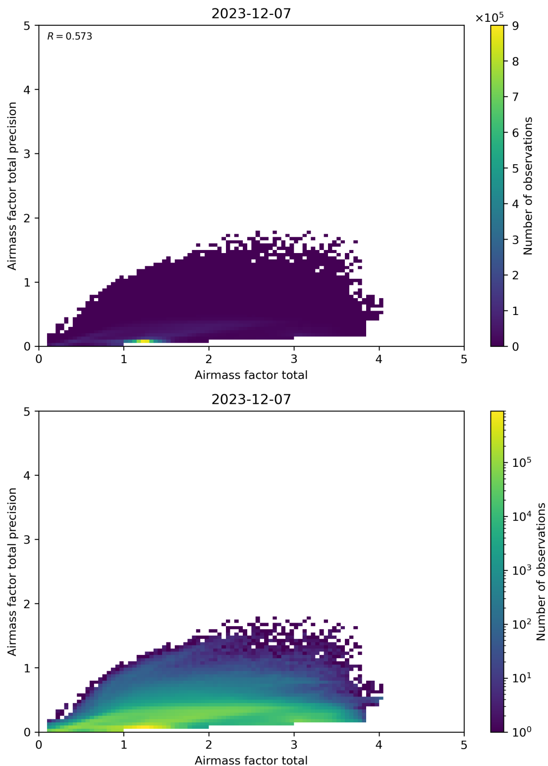
Figure 103: Scatter density plot of “Airmass factor total” against “Airmass factor total precision” for 2023-12-06 to 2023-12-08.
