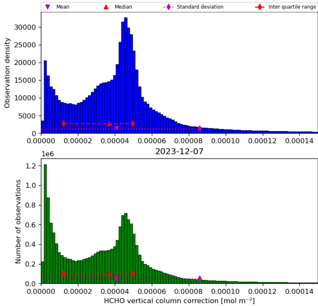
Figure 37: Histogram of “HCHO vertical column correction” for 2023-12-06 to 2023-12-08
