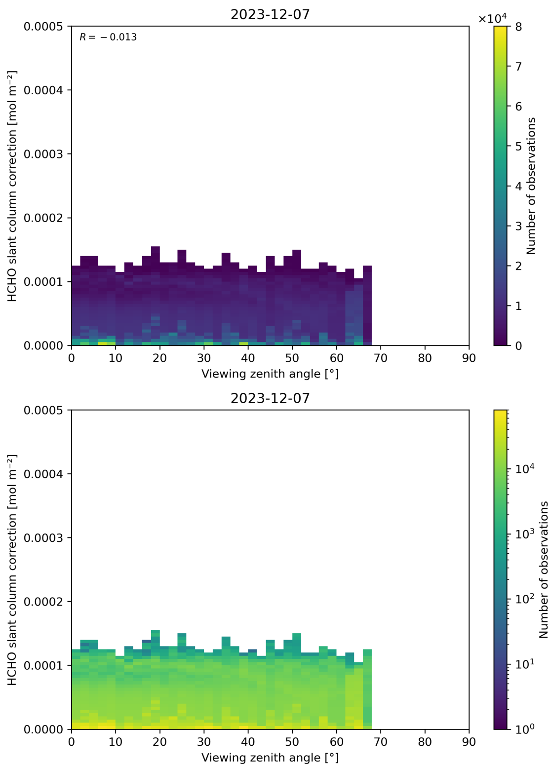
Figure 187: Scatter density plot of “Viewing zenith angle” against “HCHO slant column correction” for 2023-12-06 to 2023-12-08.
