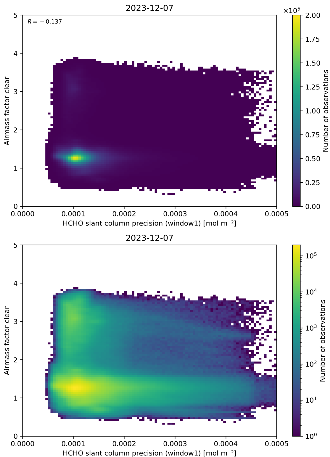
Figure 91: Scatter density plot of “HCHO slant column precision (window1)” against “Airmass factor clear” for 2023-12-06 to 2023-12-08.
