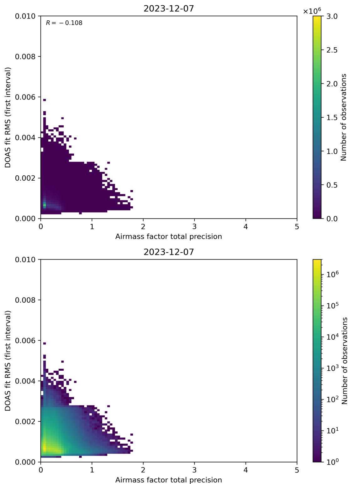
Figure 105: Scatter density plot of “Airmass factor total precision” against “DOAS fit RMS (first interval)” for 2023-12-06 to 2023-12-08.
