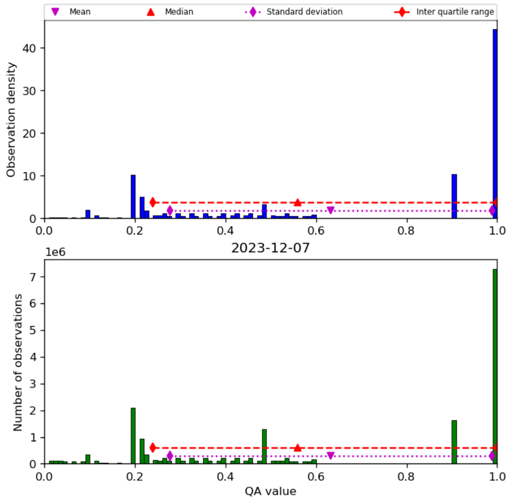
Figure 34: Histogram of “QA value” for 2023-12-06 to 2023-12-08
