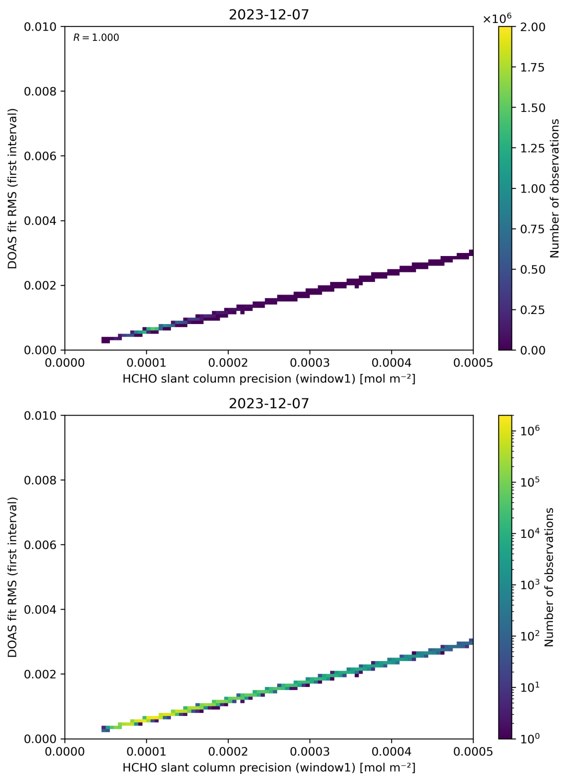
Figure 88: Scatter density plot of “HCHO slant column precision (window1)” against “DOAS fit RMS (first interval)” for 2023-12-06 to 2023-12-08.
