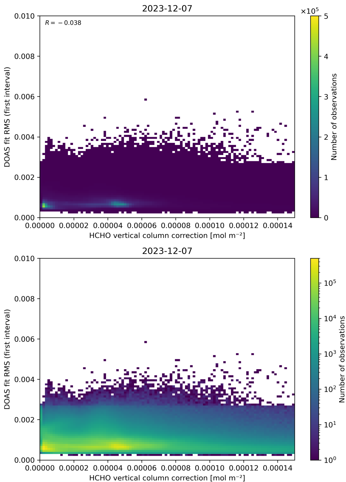
Figure 112: Scatter density plot of “HCHO vertical column correction” against “DOAS fit RMS (first interval)” for 2023-12-06 to 2023-12-08.
