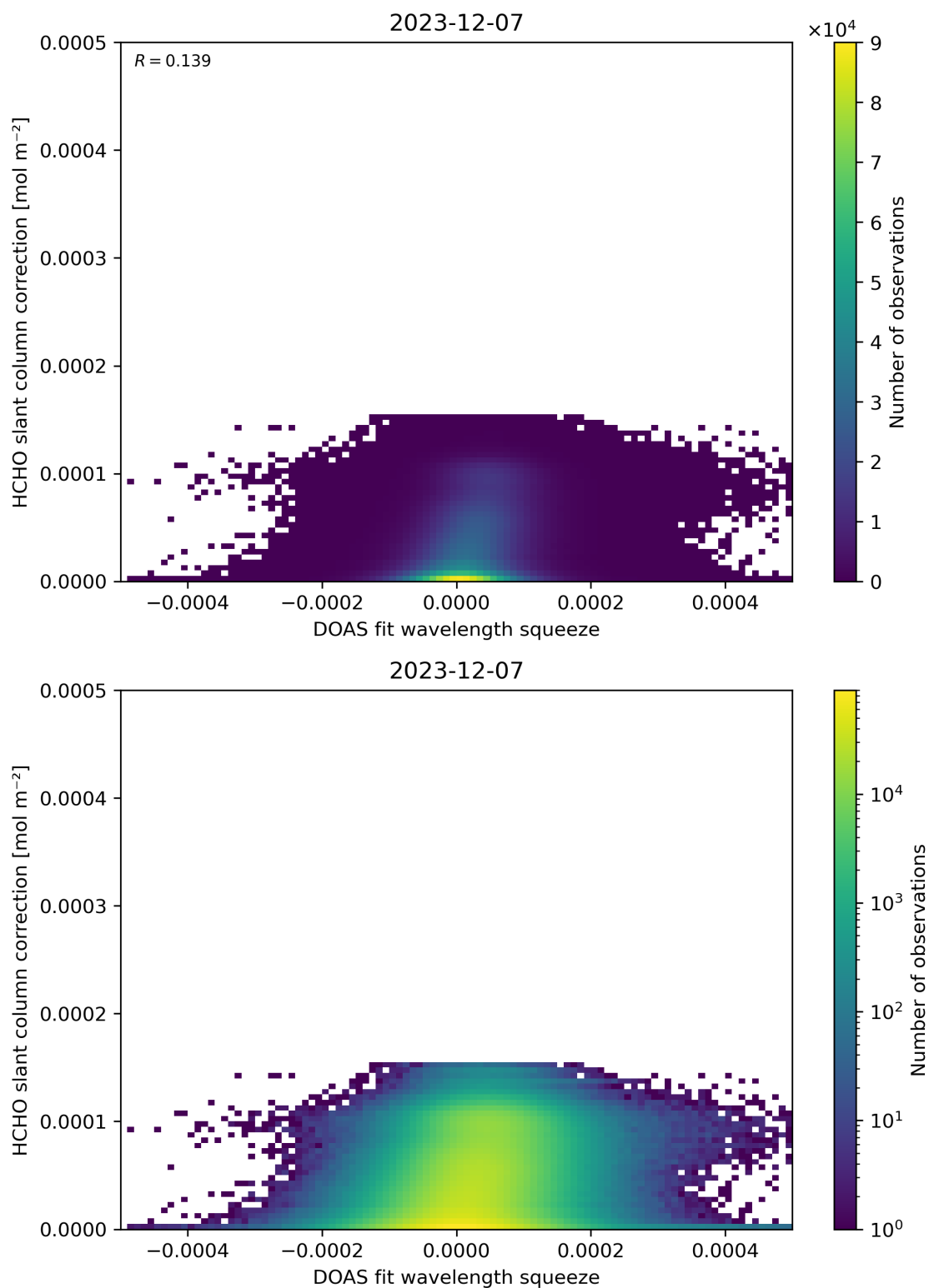
Figure 70: Scatter density plot of “DOAS fit wavelength squeeze” against “HCHO slant column correction” for 2023-12-06 to 2023-12-08.
