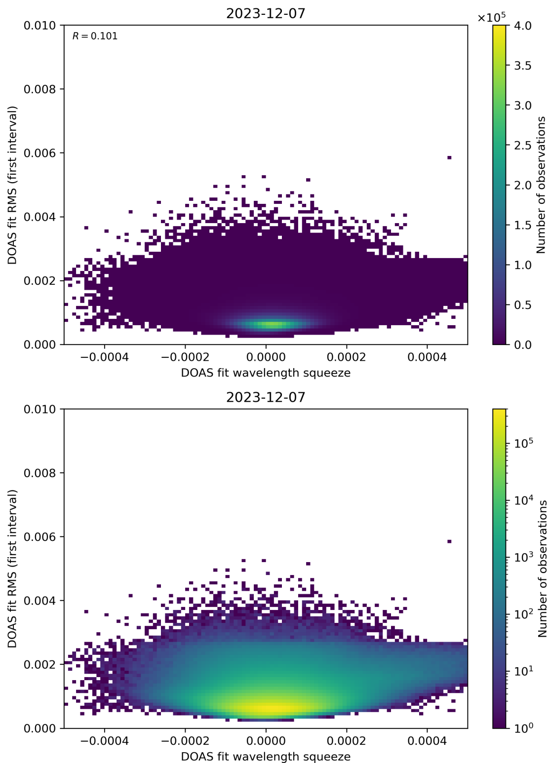
Figure 68: Scatter density plot of “DOAS fit wavelength squeeze” against “DOAS fit RMS (first interval)” for 2023-12-06 to 2023-12-08.
