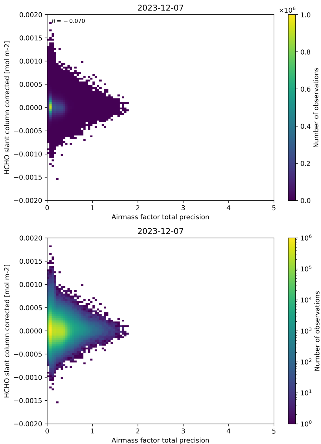
Figure 109: Scatter density plot of “Airmass factor total precision” against “HCHO slant column corrected” for 2023-12-06 to 2023-12-08.
