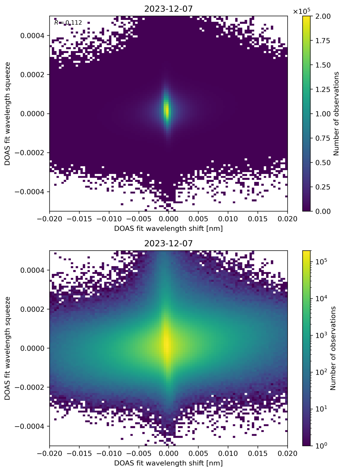
Figure 65: Scatter density plot of “DOAS fit wavelength shift” against “DOAS fit wavelength squeeze” for 2023-12-06 to 2023-12-08.
