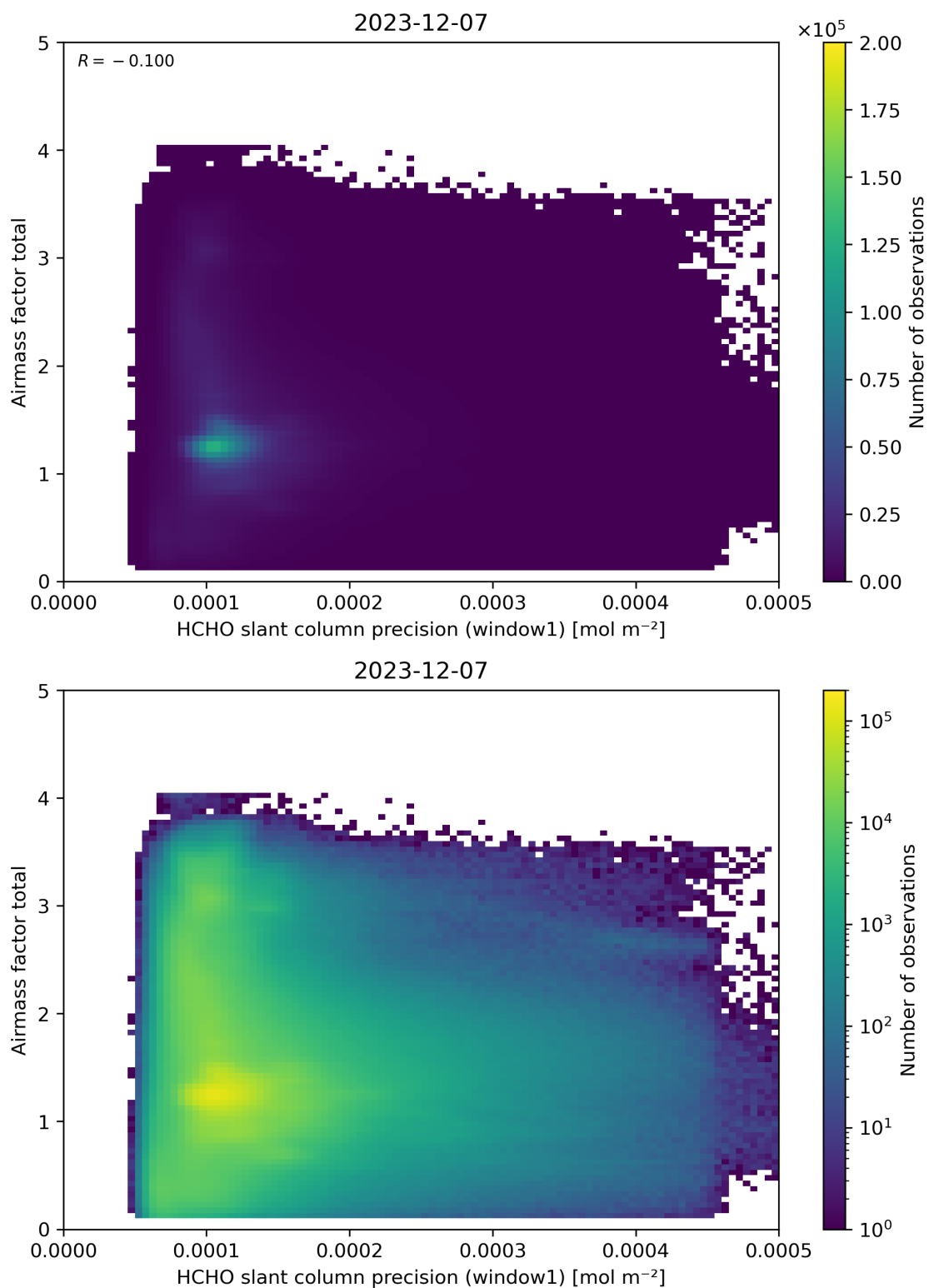
Figure 94: Scatter density plot of “HCHO slant column precision (window1)” against “Airmass factor total” for 2023-12-06 to 2023-12-08.
