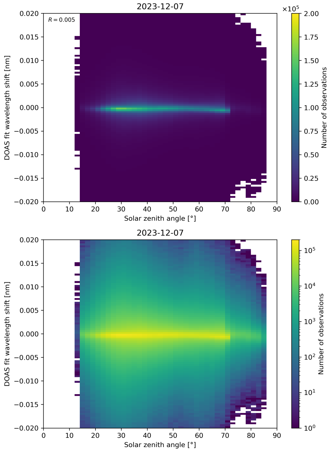
Figure 168: Scatter density plot of “Solar zenith angle” against “DOAS fit wavelength shift” for 2023-12-06 to 2023-12-08.
