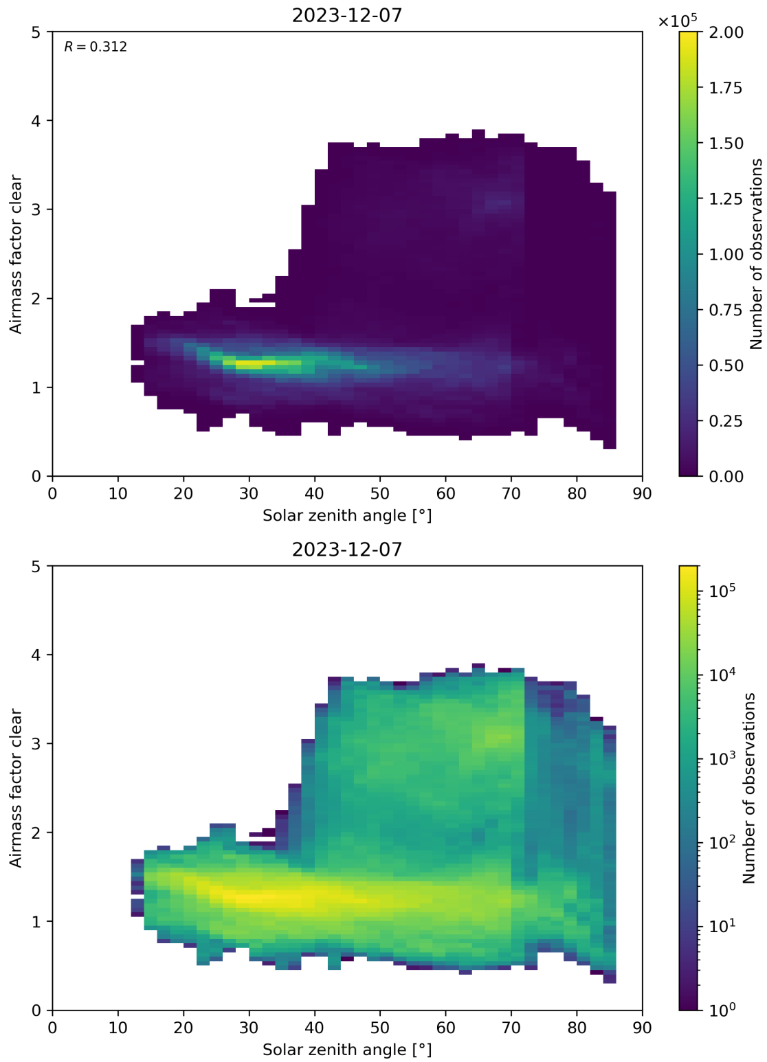
Figure 170: Scatter density plot of “Solar zenith angle” against “Airmass factor clear” for 2023-12-06 to 2023-12-08.
