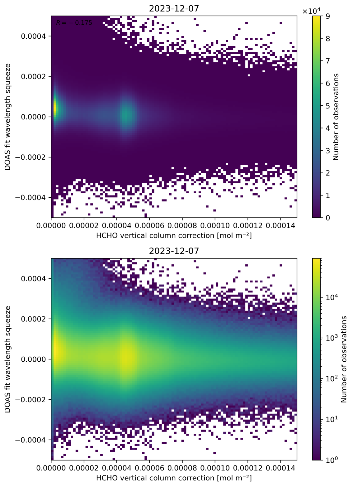
Figure 114: Scatter density plot of “HCHO vertical column correction” against “DOAS fit wavelength squeeze” for 2023-12-06 to 2023-12-08.
