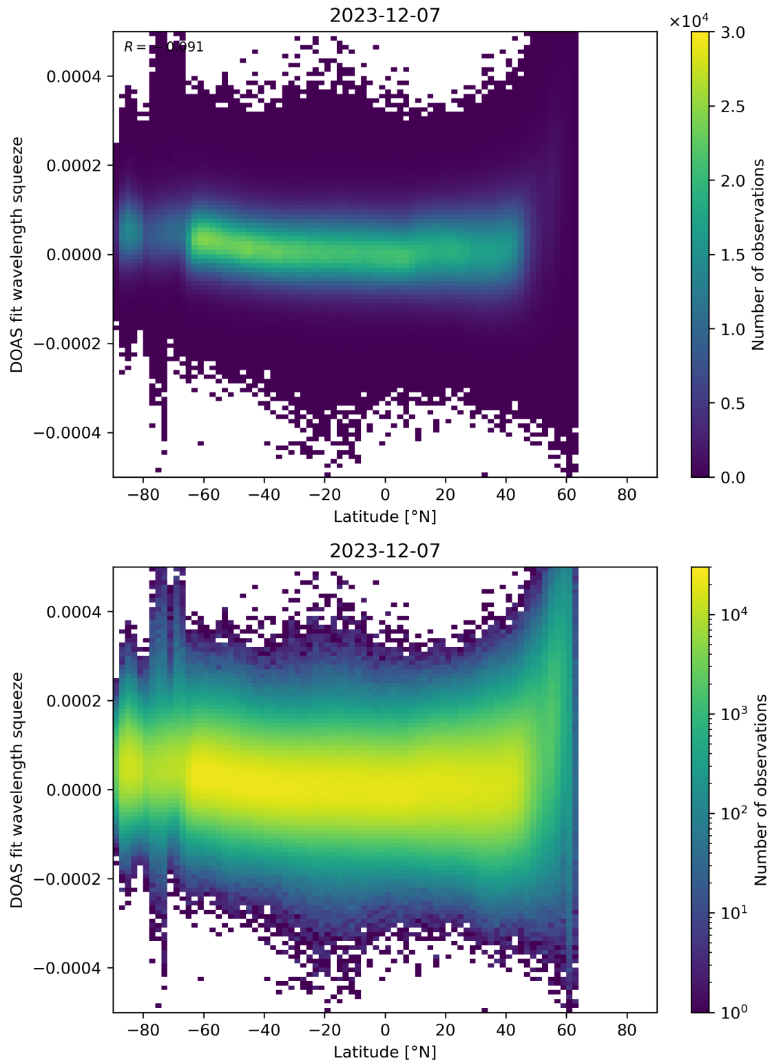
Figure 155: Scatter density plot of “Latitude” against “DOAS fit wavelength squeeze” for 2023-12-06 to 2023-12-08.
