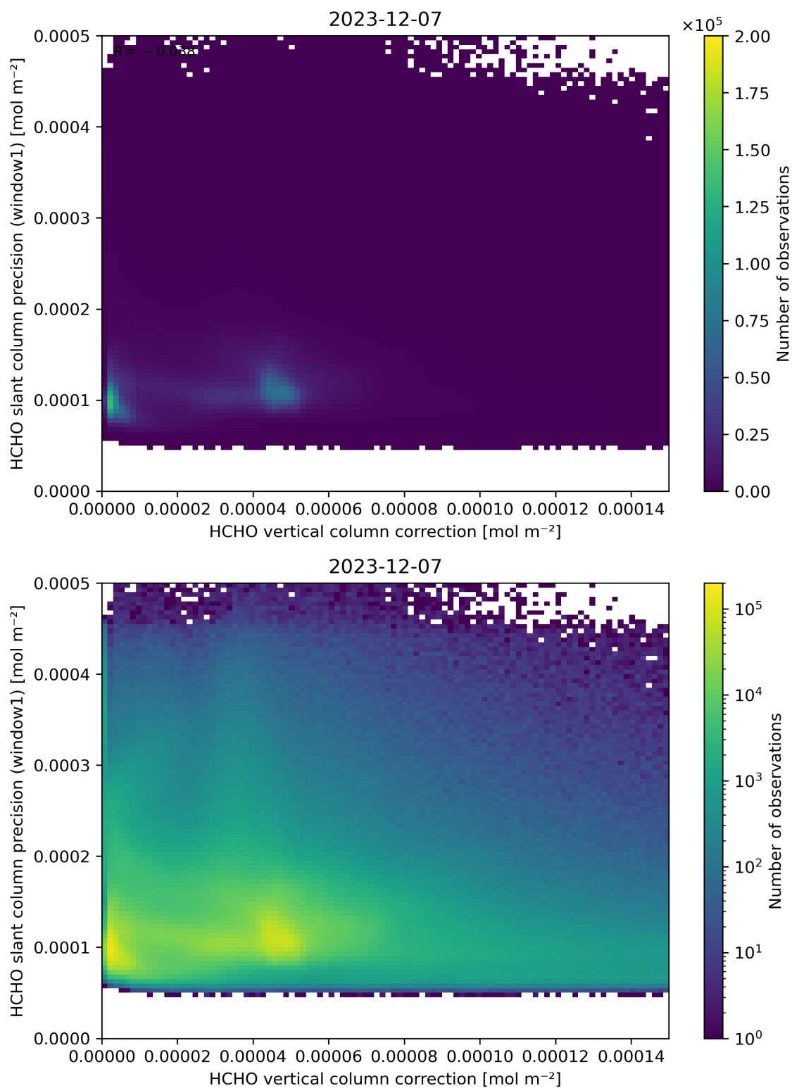
Figure 119: Scatter density plot of “HCHO vertical column correction” against “HCHO slant column precision (window1)” for 2023-12-06 to 2023-12-08.
