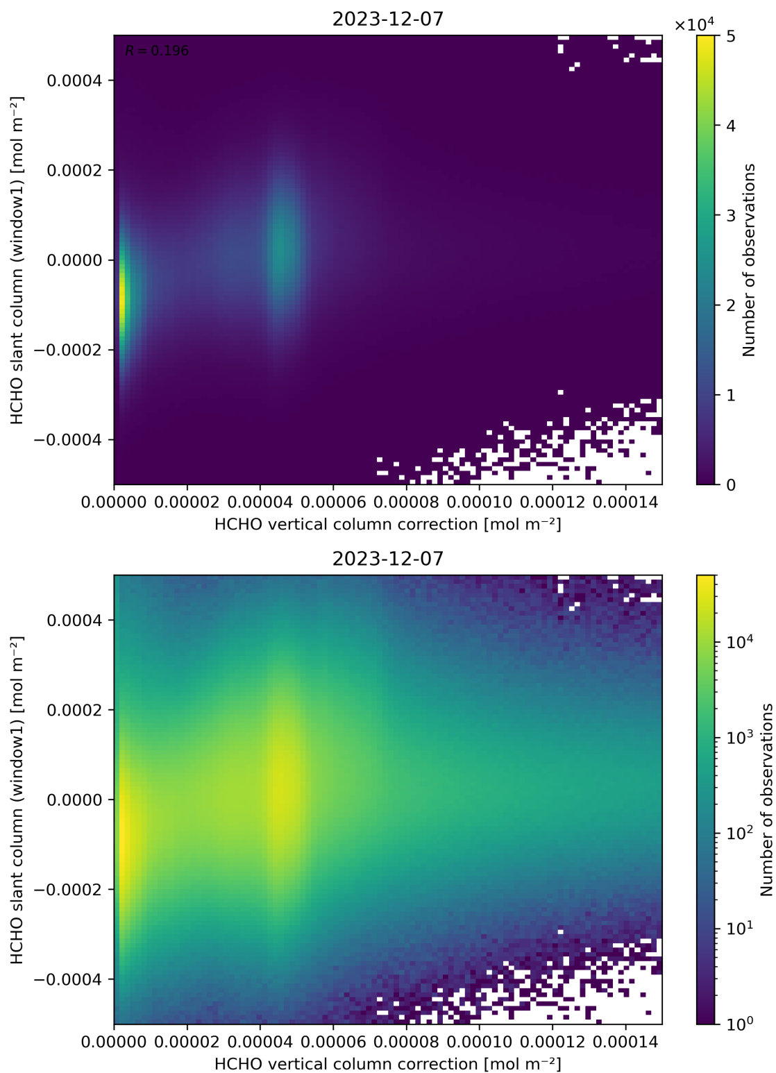
Figure 118: Scatter density plot of “HCHO vertical column correction” against “HCHO slant column (window1)” for 2023-12-06 to 2023-12-08.
