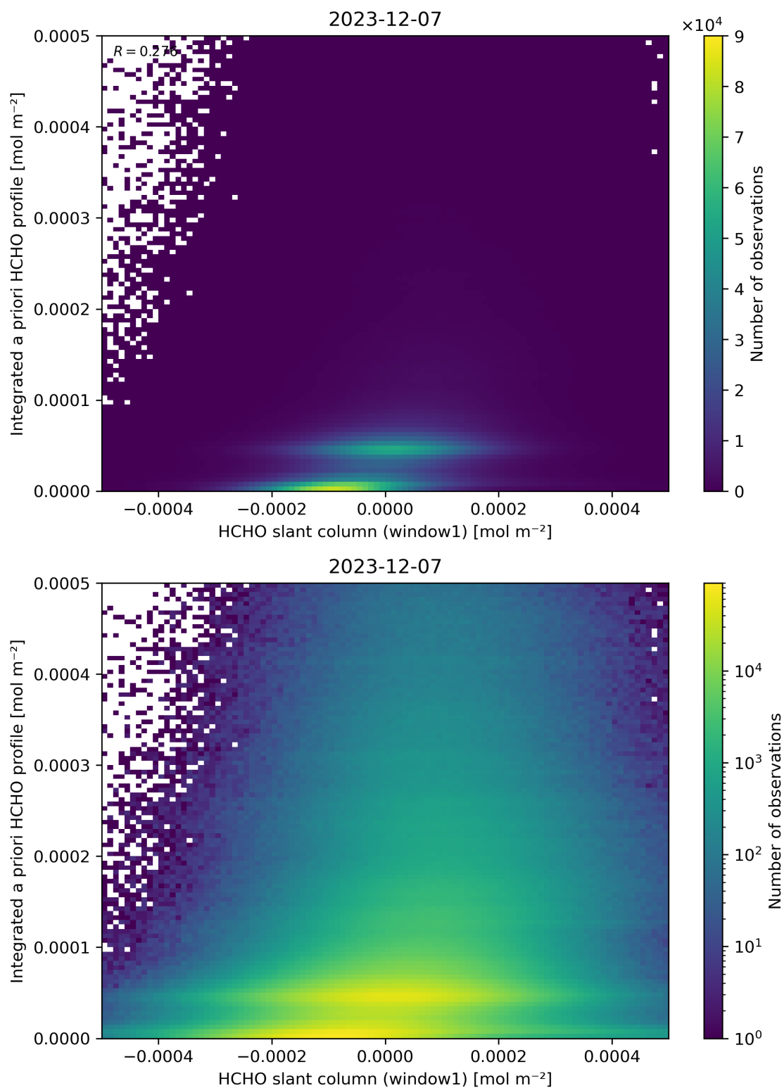
Figure 87: Scatter density plot of “HCHO slant column (window1)” against “Integrated a priori HCHO profile” for 2023-12-06 to 2023-12-08.
