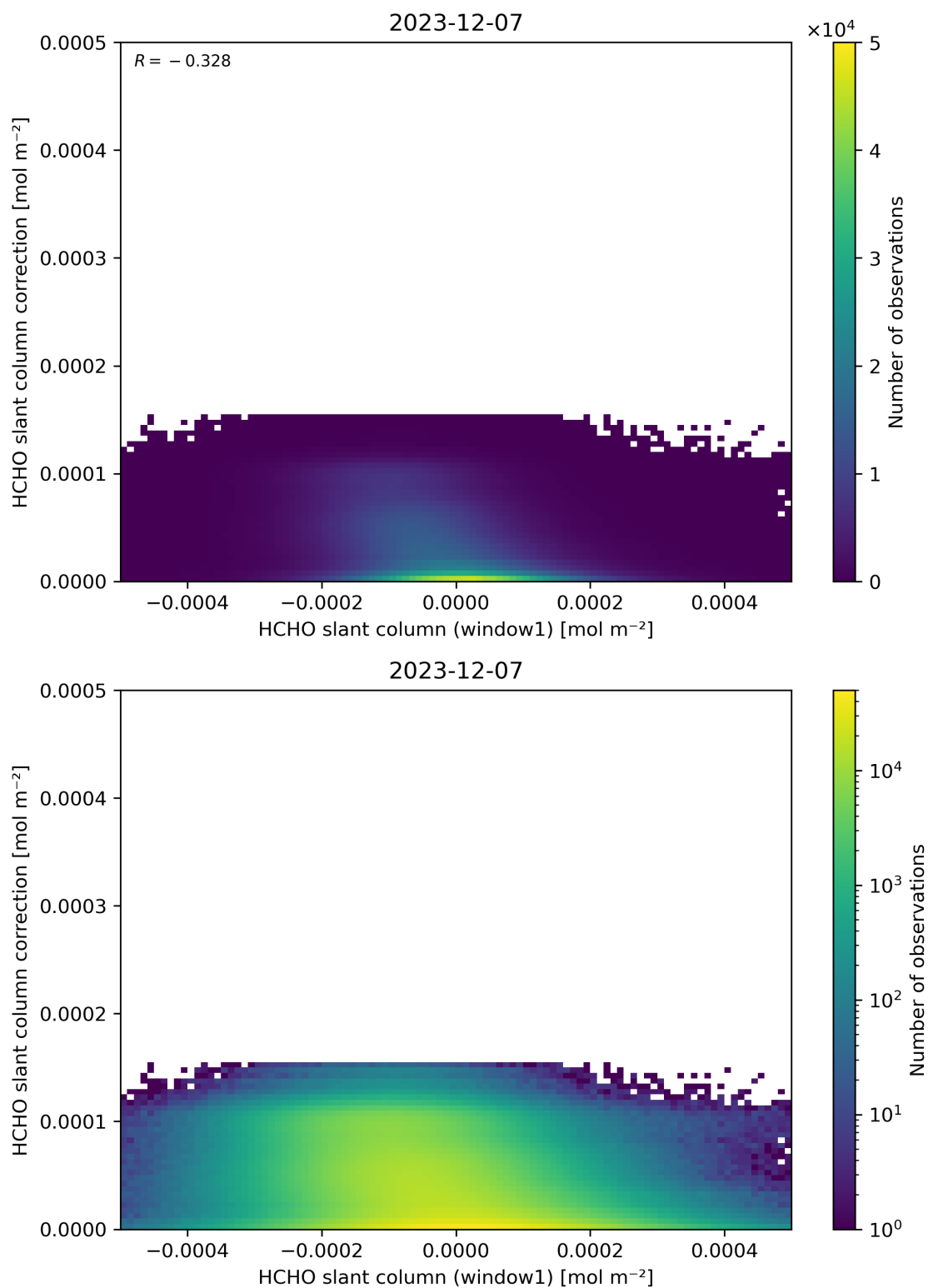
Figure 83: Scatter density plot of “HCHO slant column (window1)” against “HCHO slant column correction” for 2023-12-06 to 2023-12-08.
