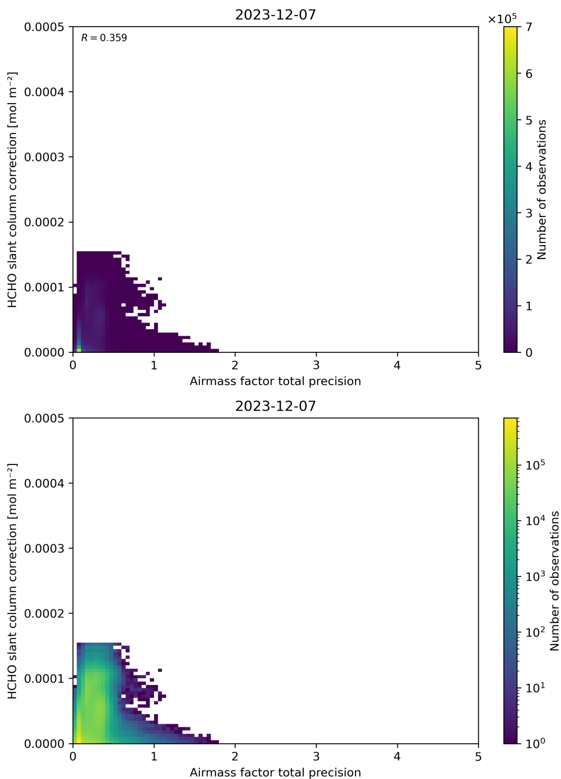
Figure 110: Scatter density plot of “Airmass factor total precision” against “HCHO slant column correction” for 2023-12-06 to 2023-12-08.
