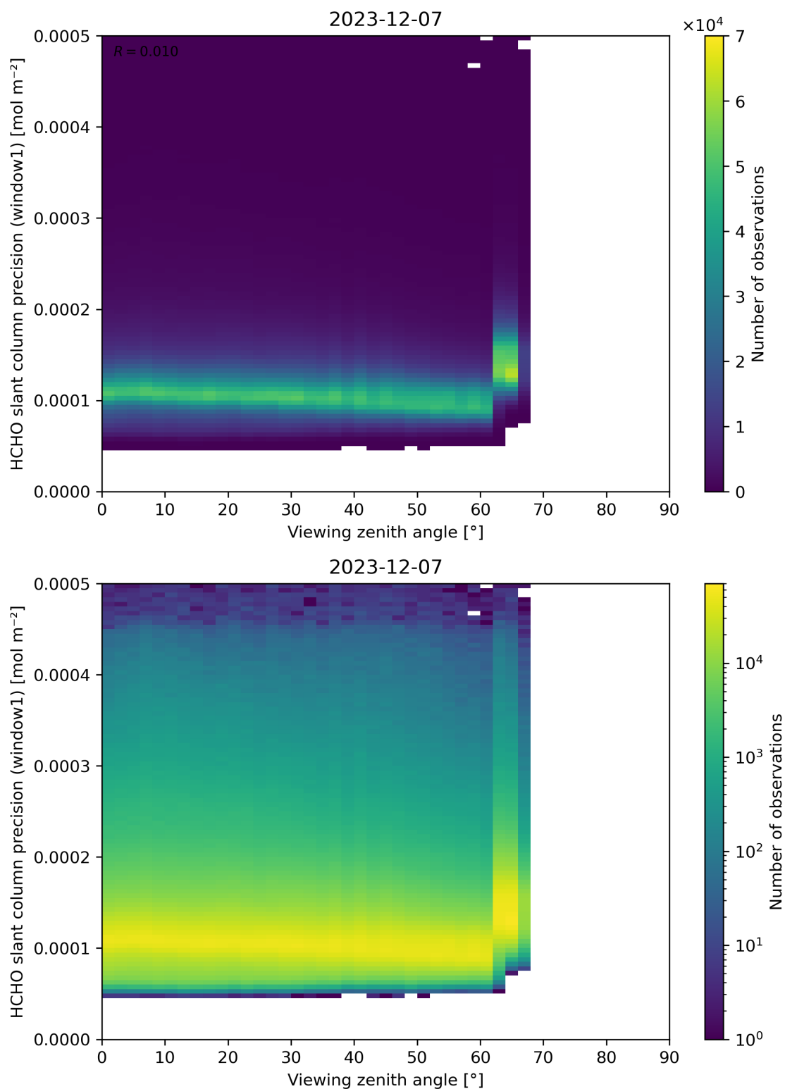
Figure 189: Scatter density plot of “Viewing zenith angle” against “HCHO slant column precision (window1)” for 2023-12-06 to 2023-12-08.
