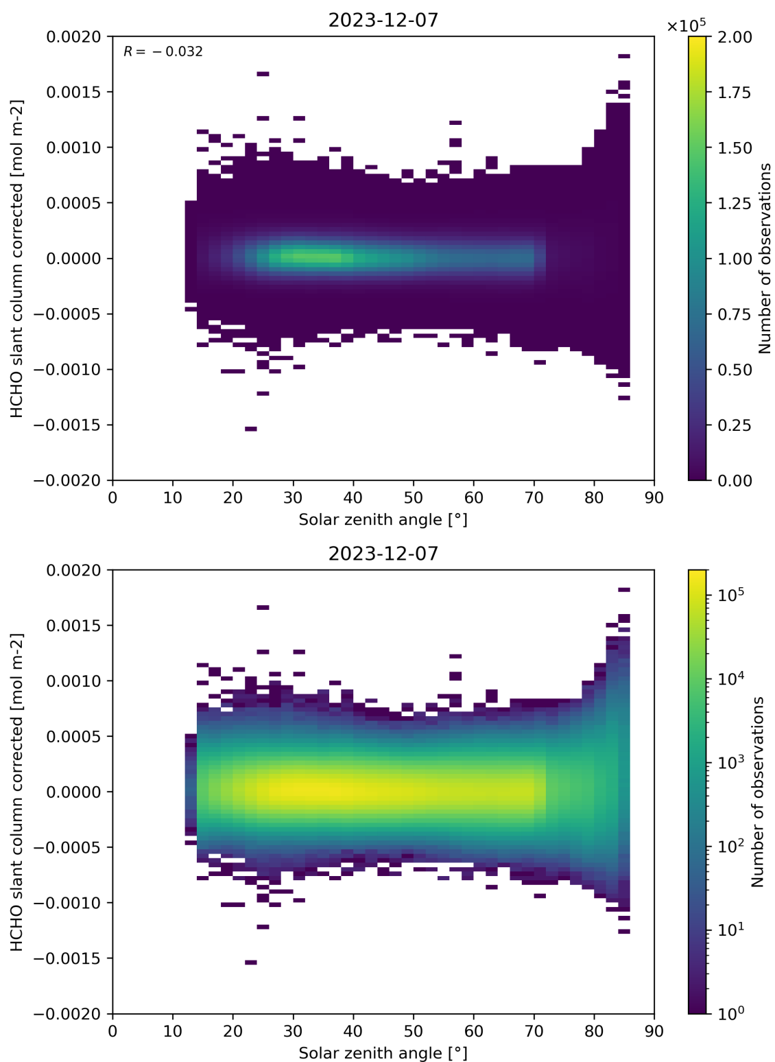
Figure 171: Scatter density plot of “Solar zenith angle” against “HCHO slant column corrected” for 2023-12-06 to 2023-12-08.
