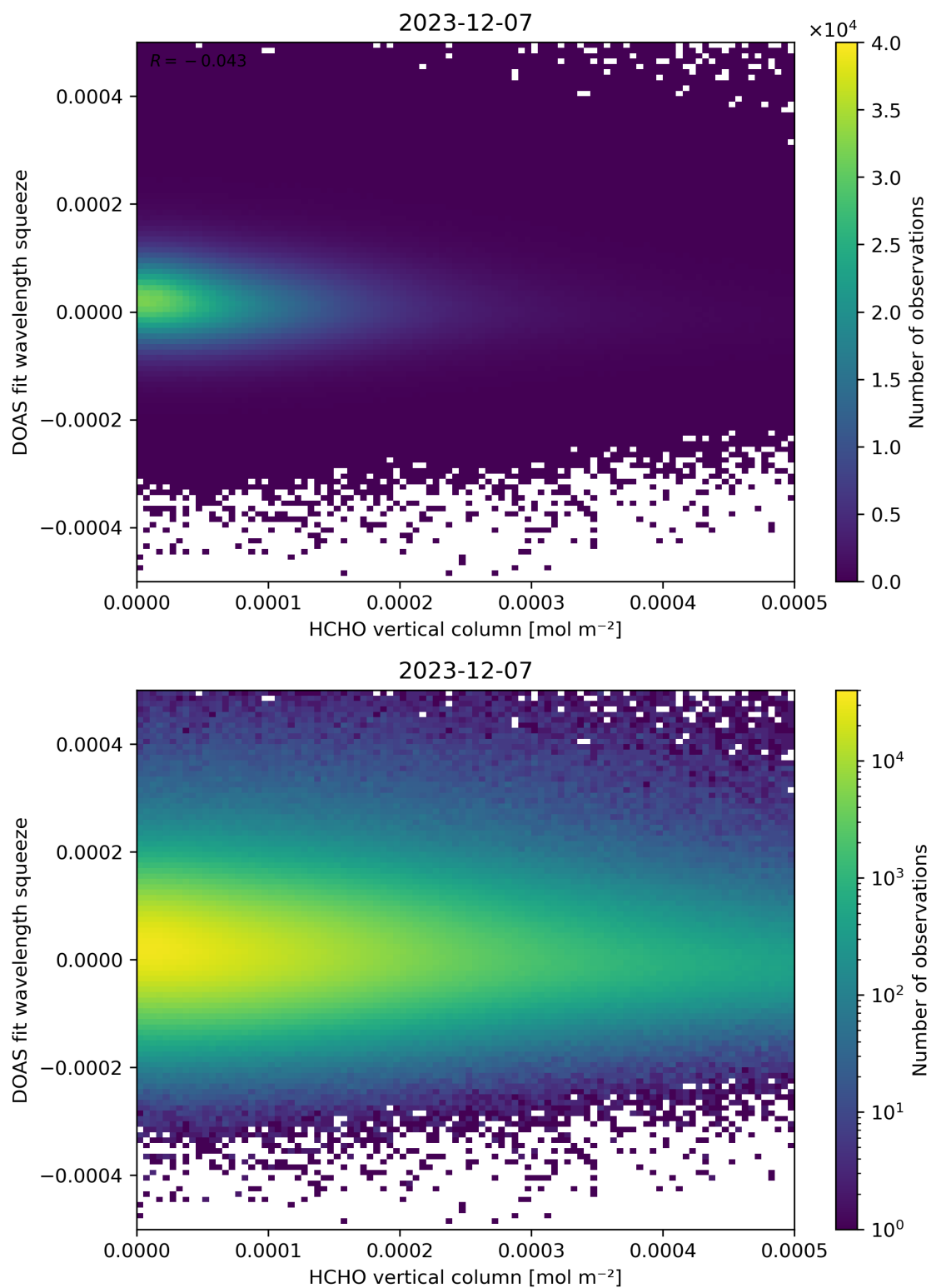
Figure 125: Scatter density plot of “HCHO vertical column” against “DOAS fit wavelength squeeze” for 2023-12-06 to 2023-12-08.
