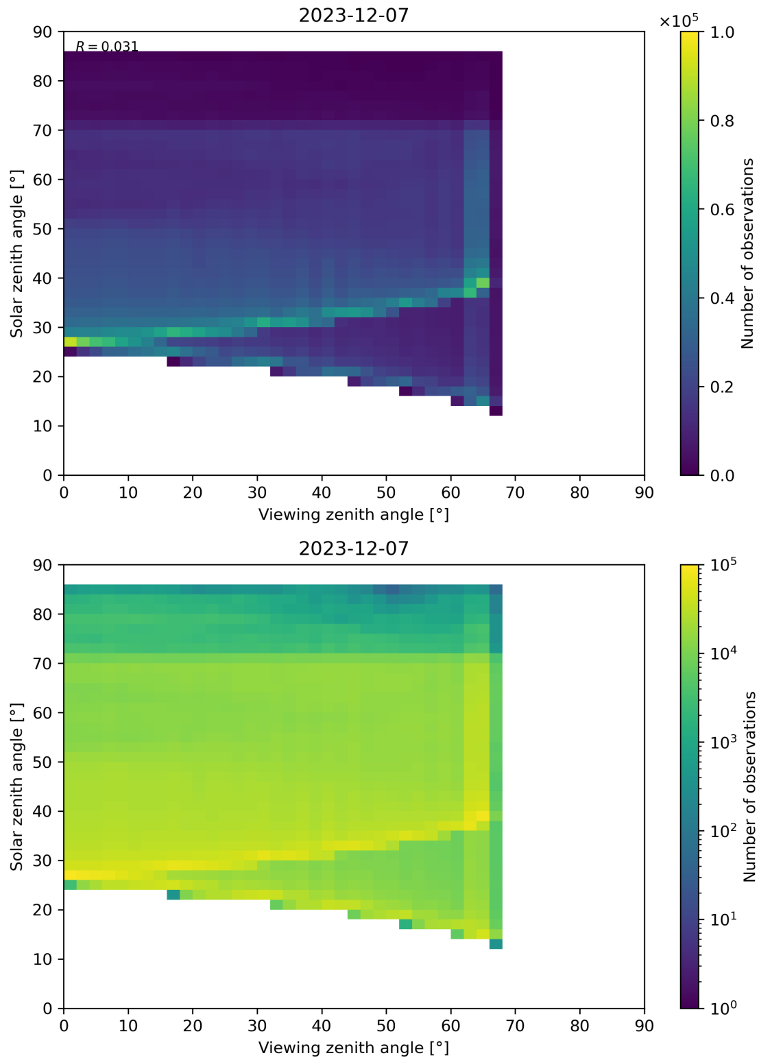
Figure 197: Scatter density plot of “Viewing zenith angle” against “Solar zenith angle” for 2023-12-06 to 2023-12-08.
