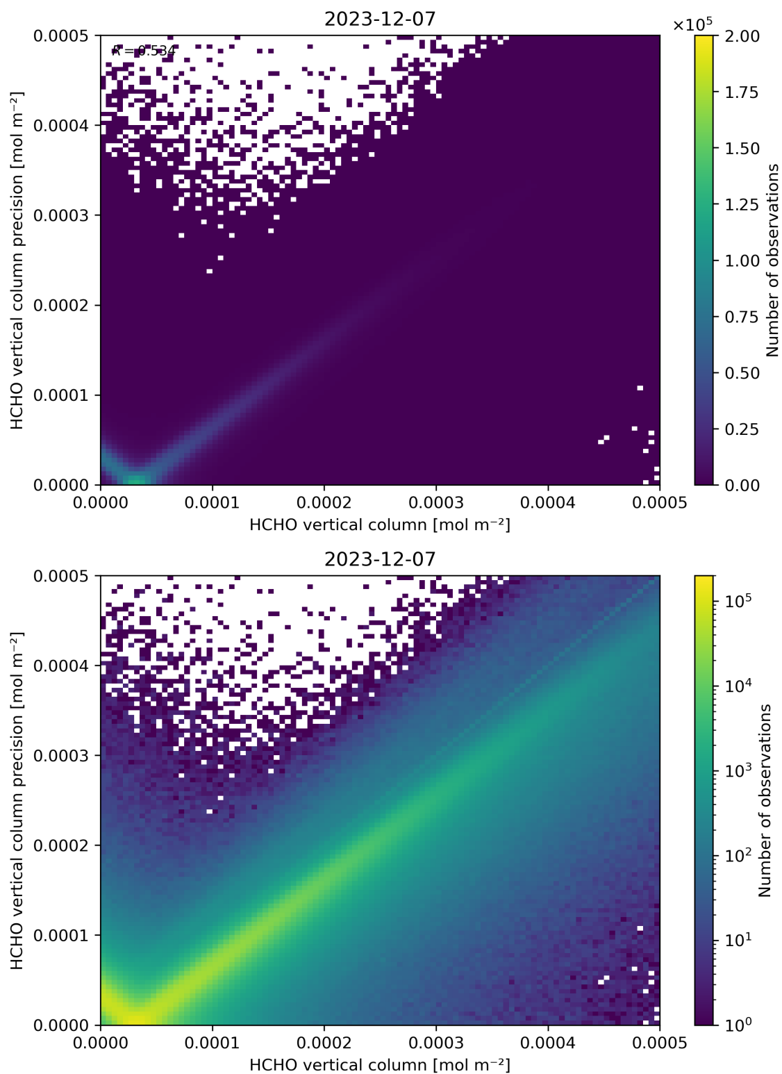
Figure 134: Scatter density plot of “HCHO vertical column” against “HCHO vertical column precision” for 2023-12-06 to 2023-12-08.
