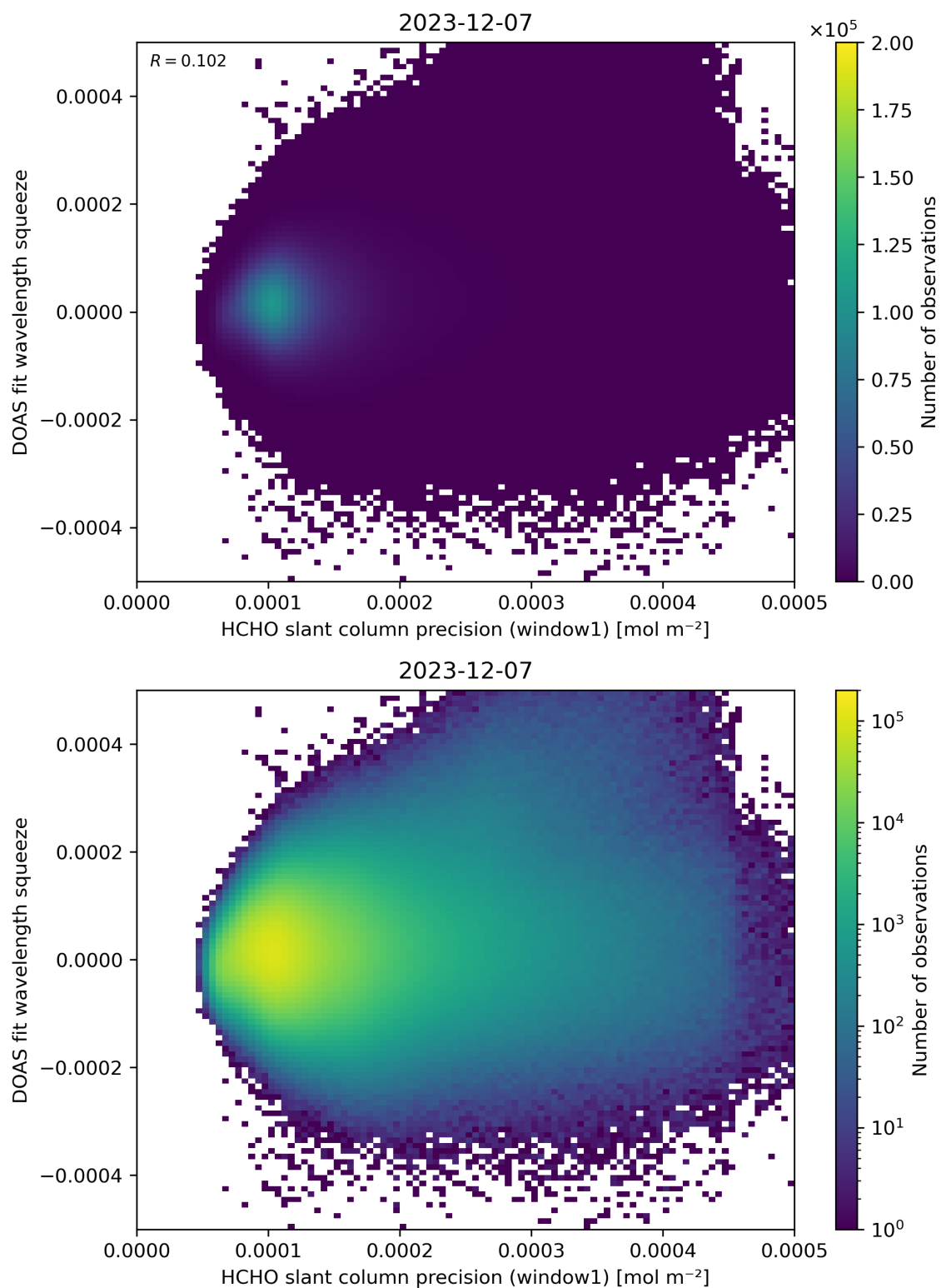
Figure 90: Scatter density plot of “HCHO slant column precision (window1)” against “DOAS fit wavelength squeeze” for 2023-12-06 to 2023-12-08.
