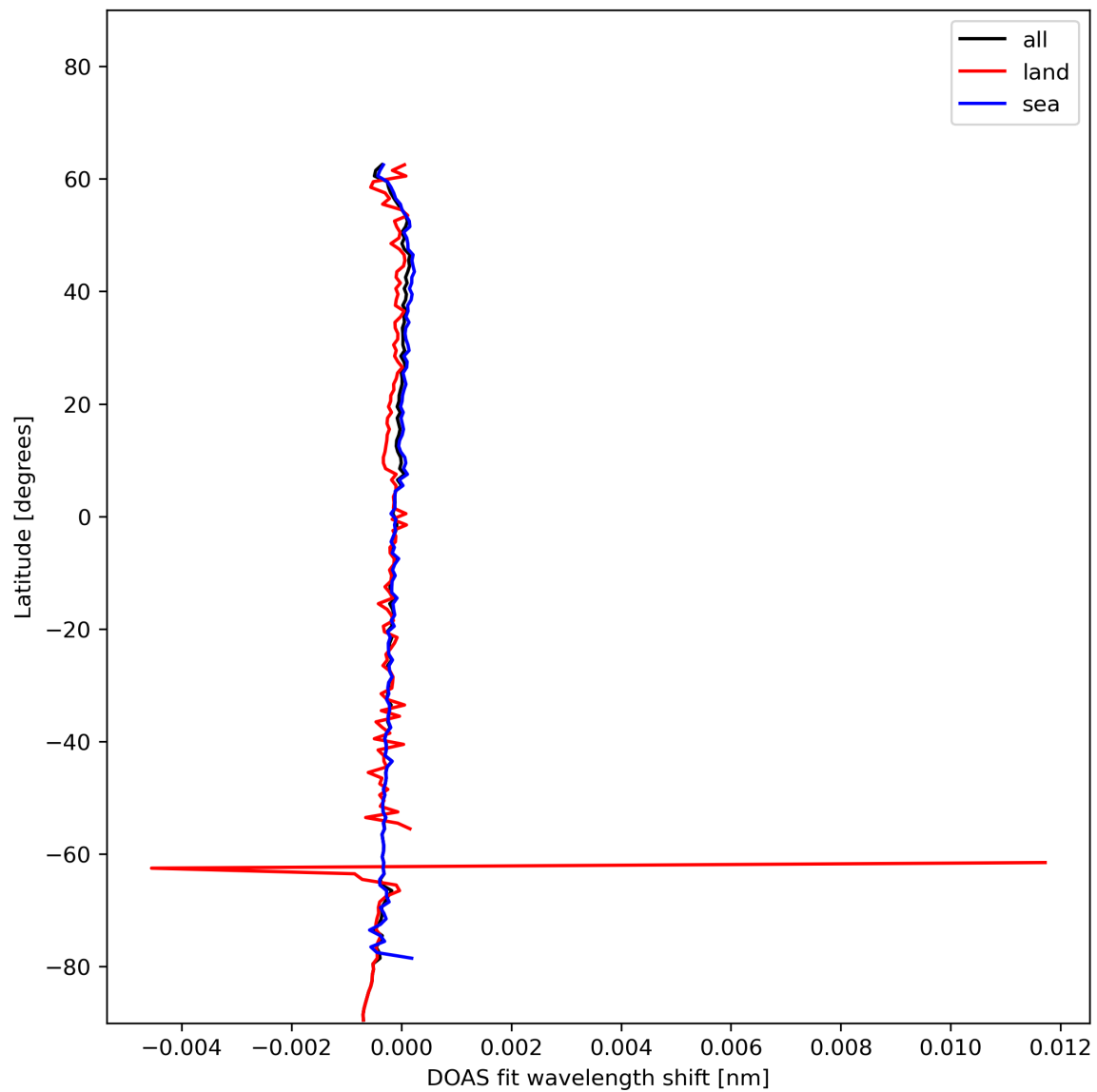
Figure 30: Zonal average of “DOAS fit wavelength shift” for 2023-12-06 to 2023-12-08.
