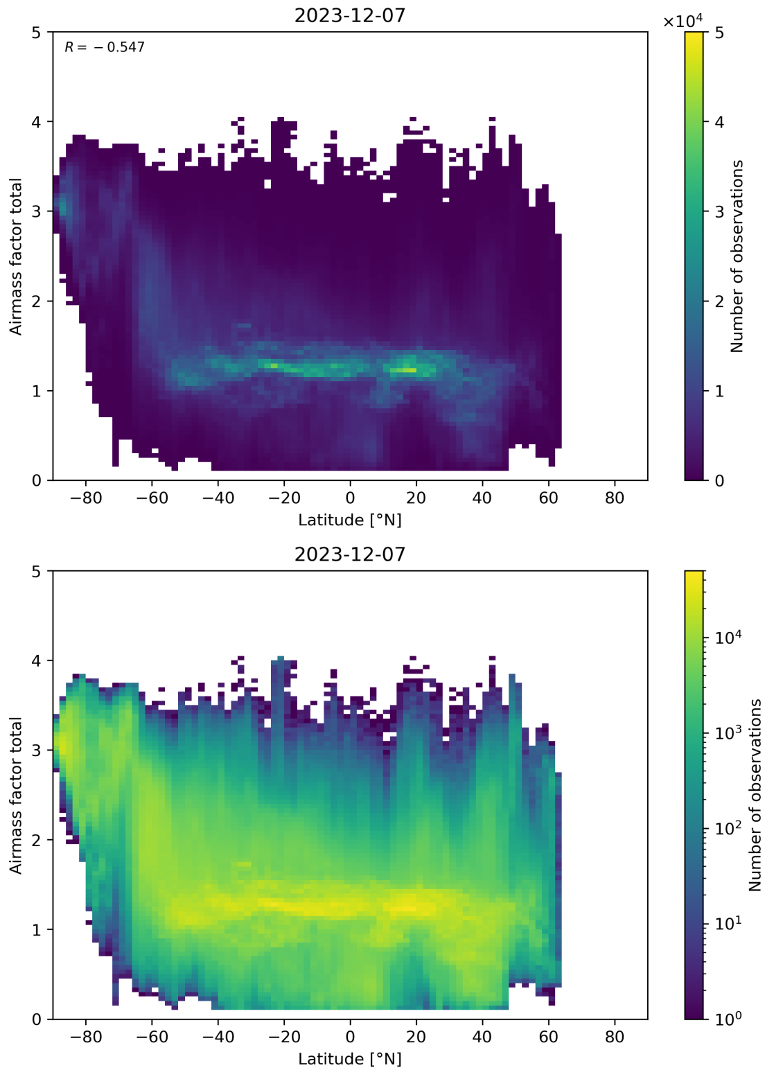
Figure 161: Scatter density plot of “Latitude” against “Airmass factor total” for 2023-12-06 to 2023-12-08.
