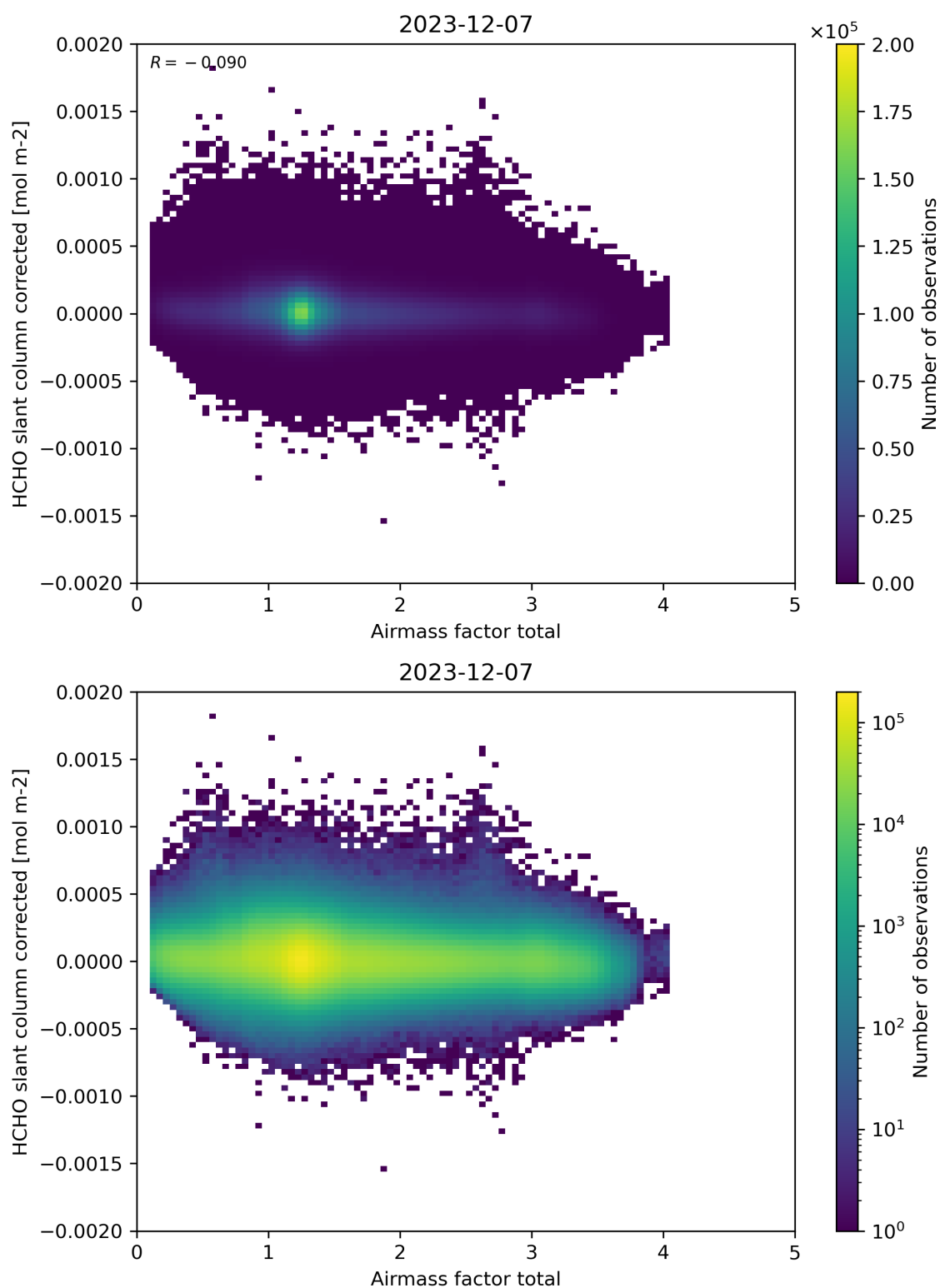
Figure 101: Scatter density plot of “Airmass factor total” against “HCHO slant column corrected” for 2023-12-06 to 2023-12-08.
