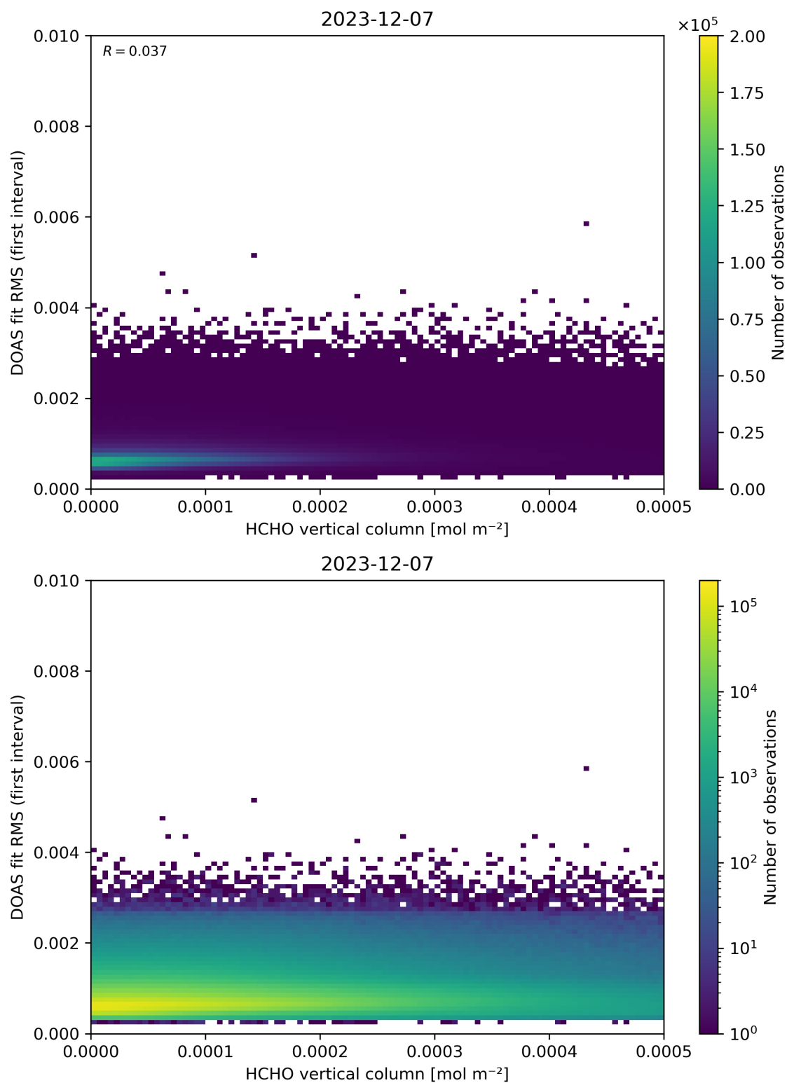
Figure 123: Scatter density plot of “HCHO vertical column” against “DOAS fit RMS (first interval)” for 2023-12-06 to 2023-12-08.
