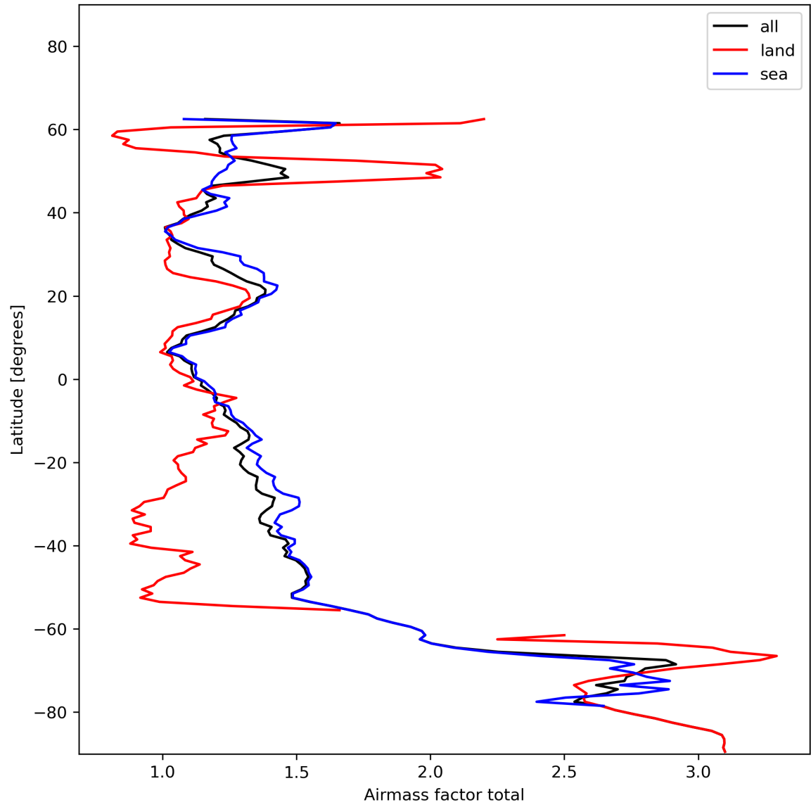
Figure 26: Zonal average of “Airmass factor total” for 2023-12-06 to 2023-12-08.
