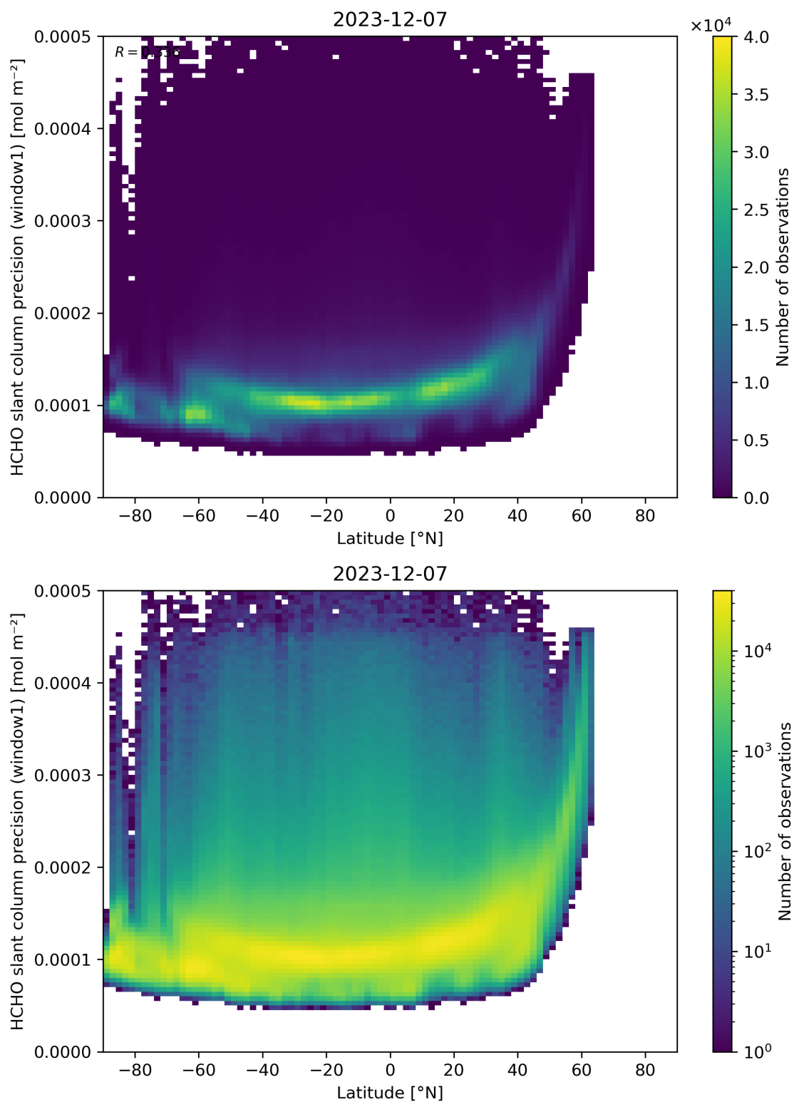
Figure 160: Scatter density plot of “Latitude” against “HCHO slant column precision (window1)” for 2023-12-06 to 2023-12-08.
