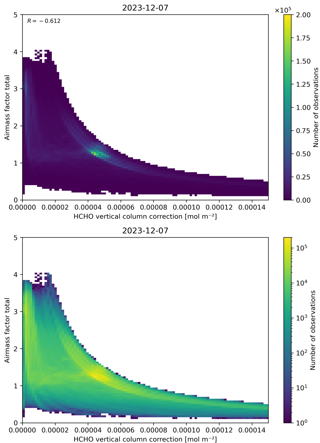
Figure 120: Scatter density plot of “HCHO vertical column correction” against “Airmass factor total” for 2023-12-06 to 2023-12-08.
