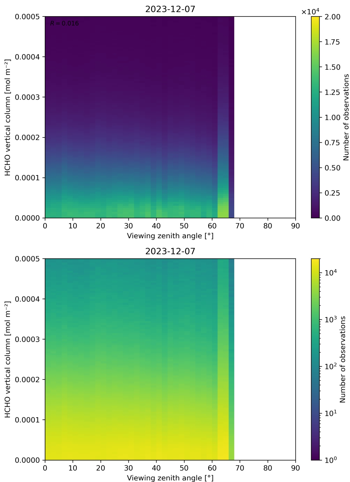
Figure 192: Scatter density plot of “Viewing zenith angle” against “HCHO vertical column” for 2023-12-06 to 2023-12-08.
