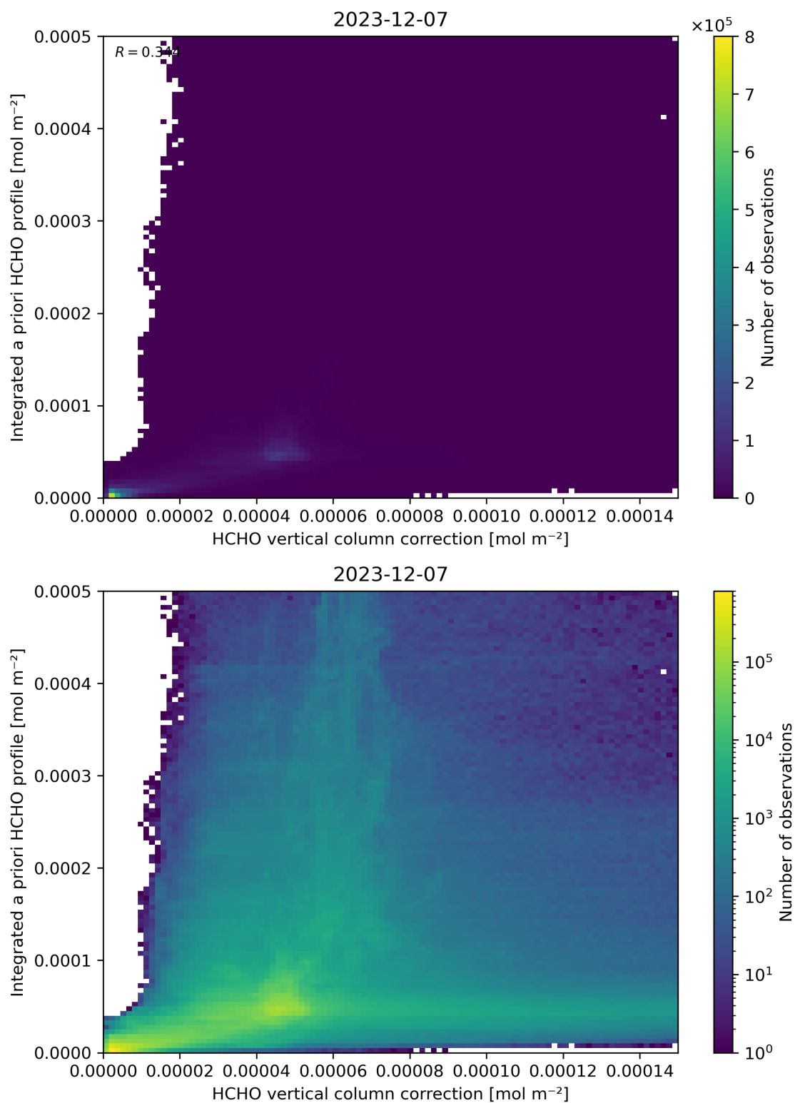
Figure 122: Scatter density plot of “HCHO vertical column correction” against “Integrated a priori HCHO profile” for 2023-12-06 to 2023-12-08.
