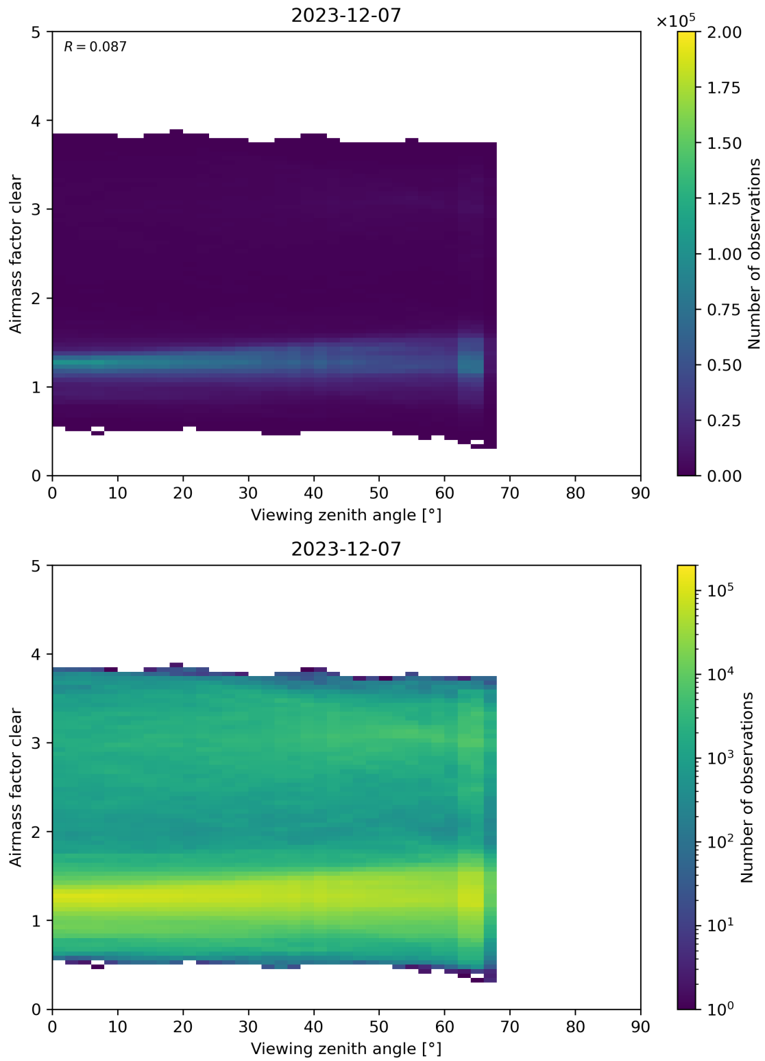
Figure 185: Scatter density plot of “Viewing zenith angle” against “Airmass factor clear” for 2023-12-06 to 2023-12-08.
