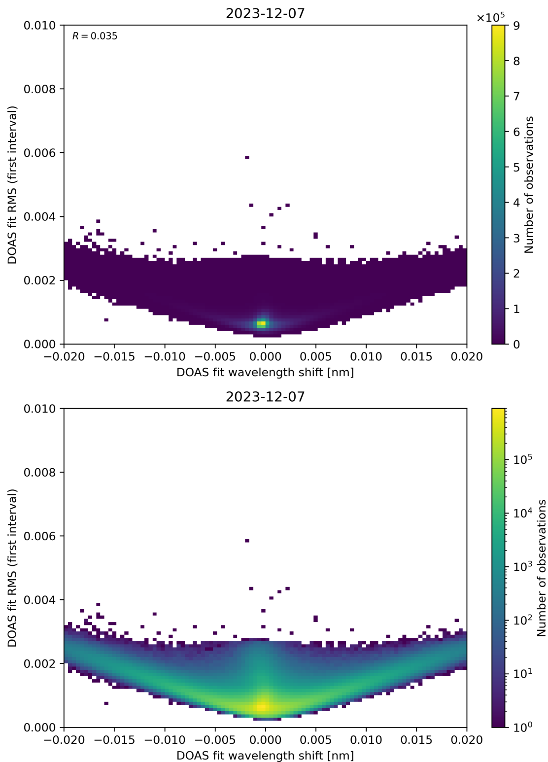
Figure 64: Scatter density plot of “DOAS fit wavelength shift” against “DOAS fit RMS (first interval)” for 2023-12-06 to 2023-12-08.
