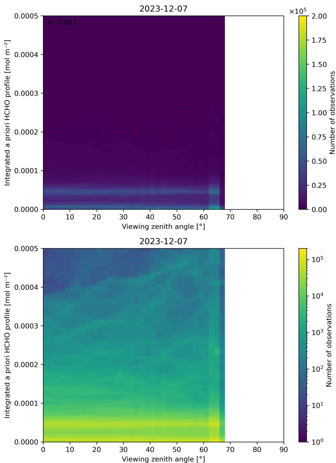
Figure 195: Scatter density plot of “Viewing zenith angle” against “Integrated a priori HCHO profile” for 2023-12-06 to 2023-12-08.
