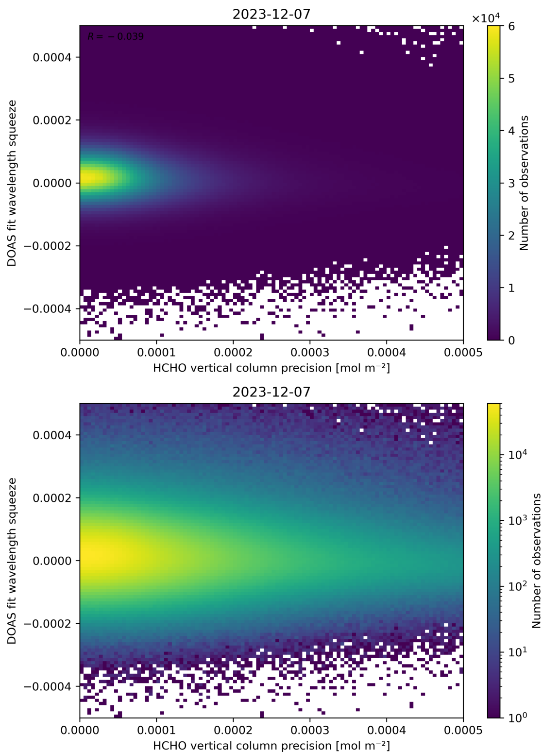
Figure 138: Scatter density plot of “HCHO vertical column precision” against “DOAS fit wavelength squeeze” for 2023-12-06 to 2023-12-08.
