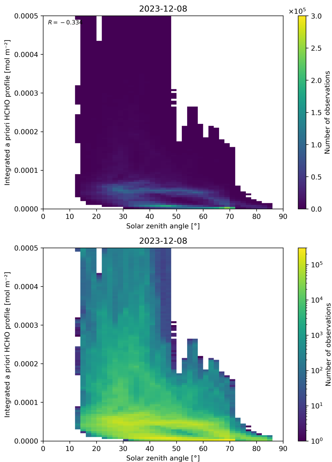
Figure 180: Scatter density plot of “Solar zenith angle” against “Integrated a priori HCHO profile” for 2023-12-07 to 2023-12-09.
