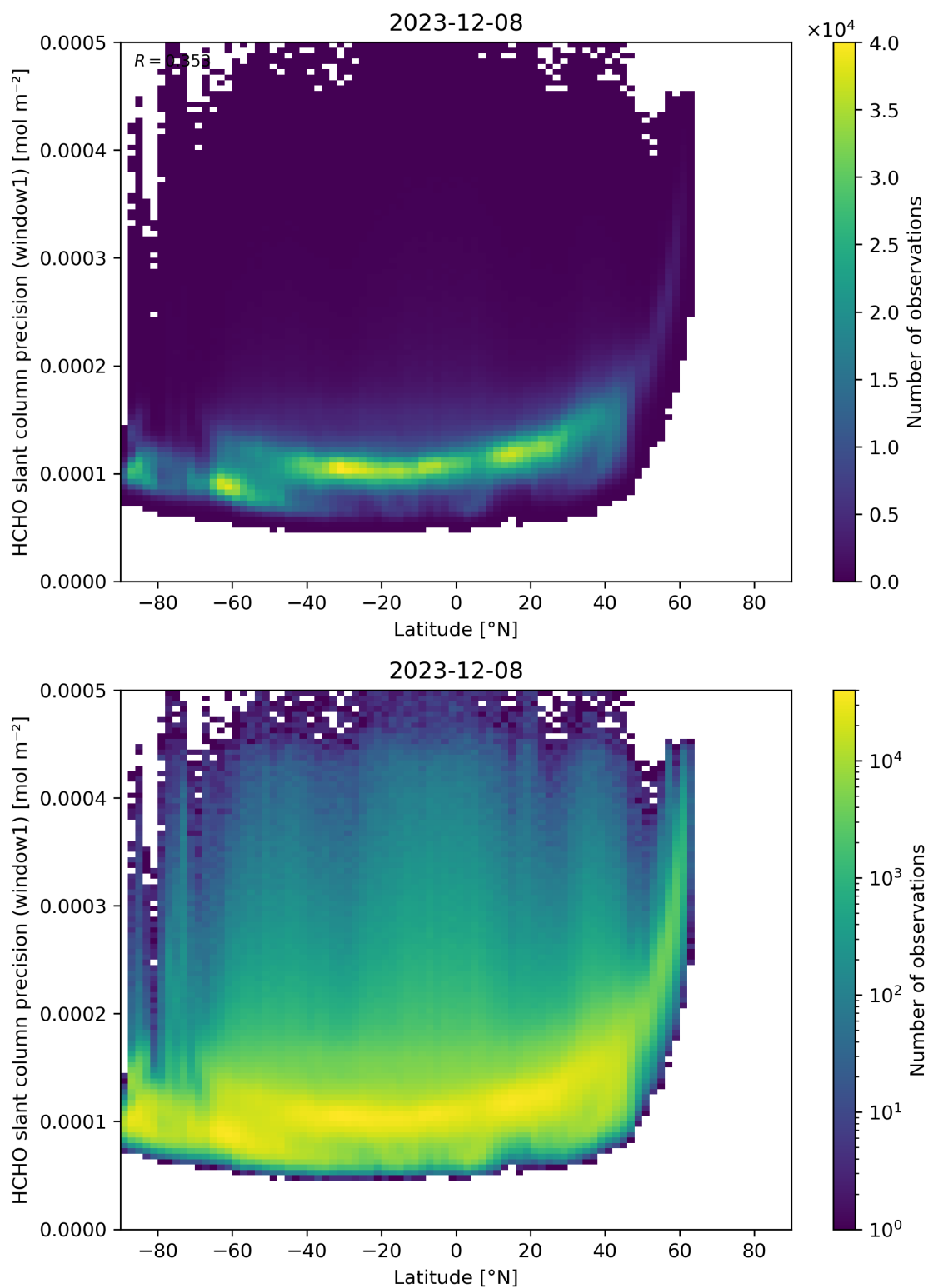
Figure 160: Scatter density plot of “Latitude” against “HCHO slant column precision (window1)” for 2023-12-07 to 2023-12-09.
