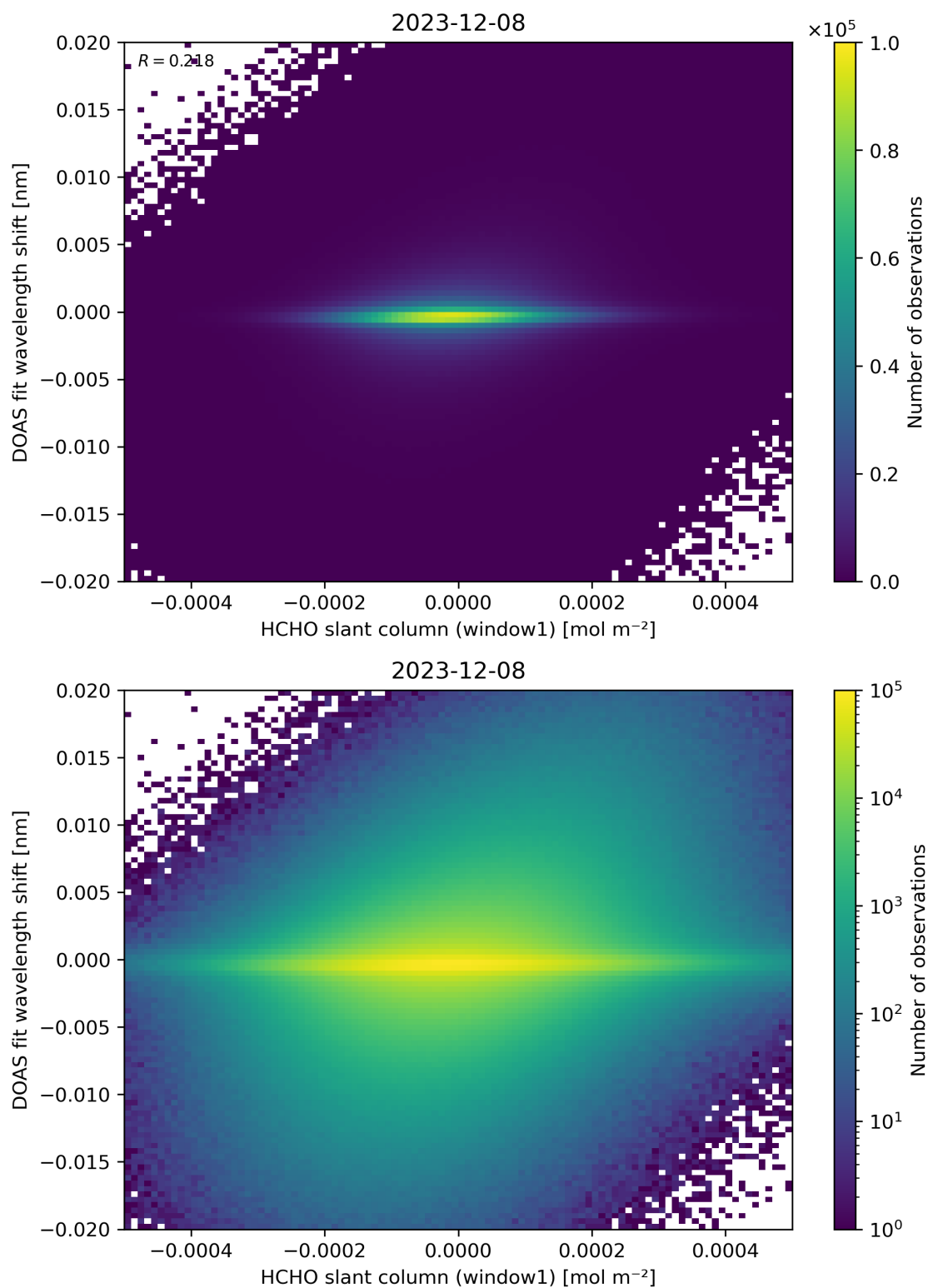
Figure 79: Scatter density plot of “HCHO slant column (window1)” against “DOAS fit wavelength shift” for 2023-12-07 to 2023-12-09.
