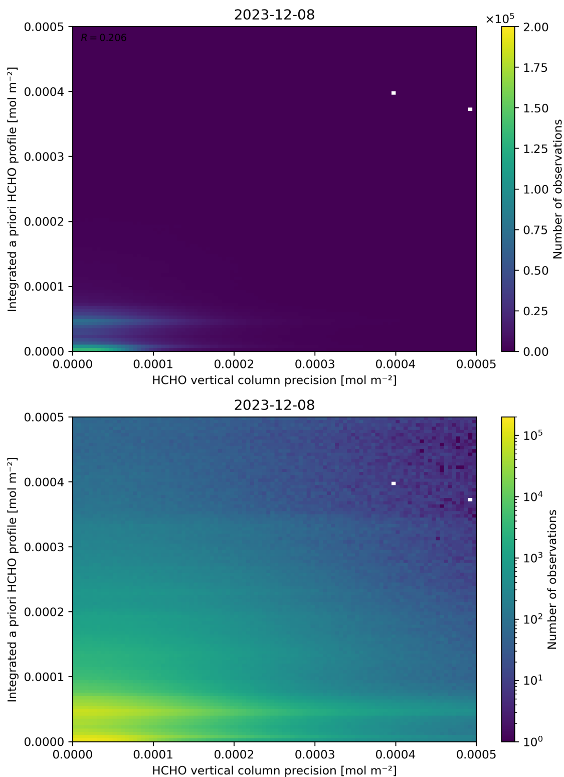
Figure 147: Scatter density plot of “HCHO vertical column precision” against “Integrated a priori HCHO profile” for 2023-12-07 to 2023-12-09.
