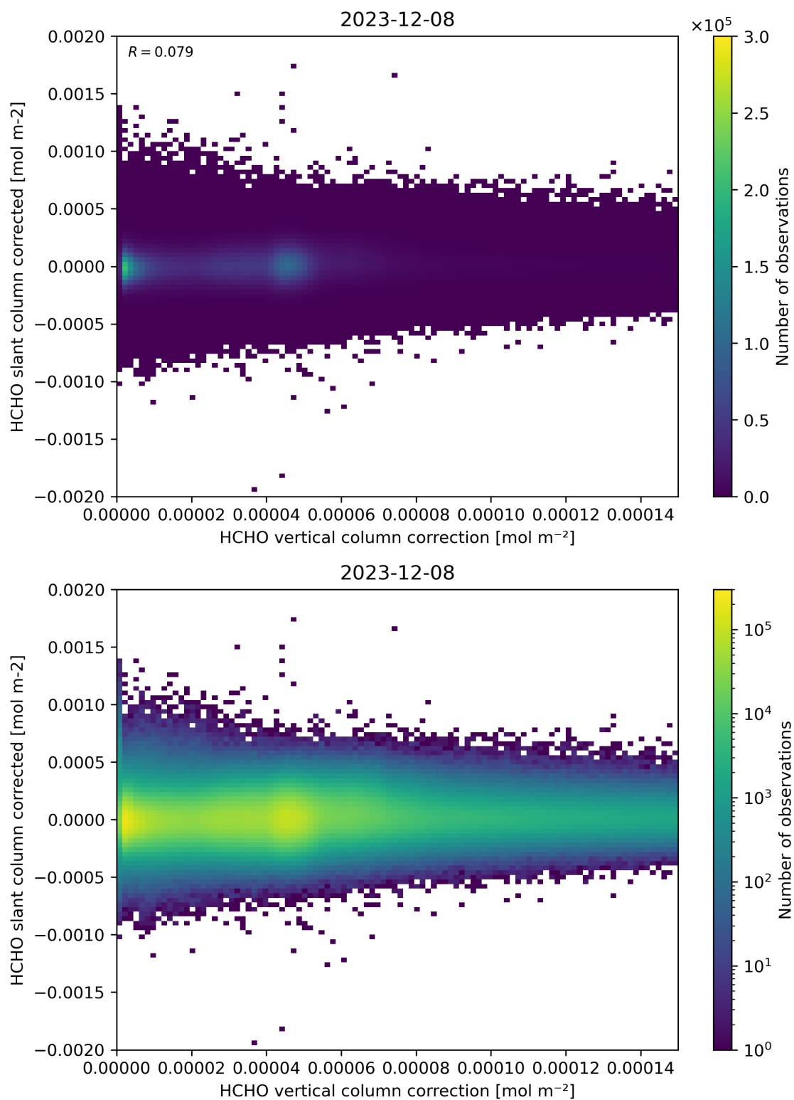
Figure 116: Scatter density plot of “HCHO vertical column correction” against “HCHO slant column corrected” for 2023-12-07 to 2023-12-09.
