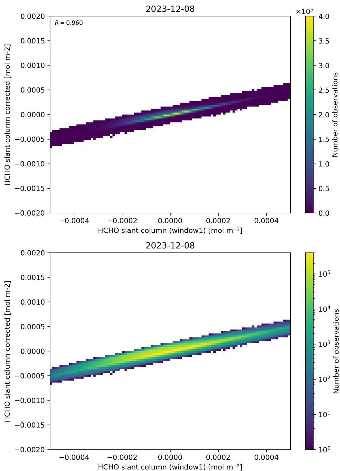
Figure 82: Scatter density plot of “HCHO slant column (window1)” against “HCHO slant column corrected” for 2023-12-07 to 2023-12-09.
