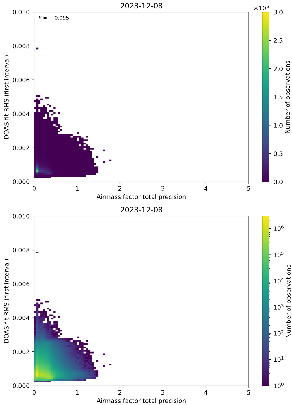
Figure 105: Scatter density plot of “Airmass factor total precision” against “DOAS fit RMS (first interval)” for 2023-12-07 to 2023-12-09.
