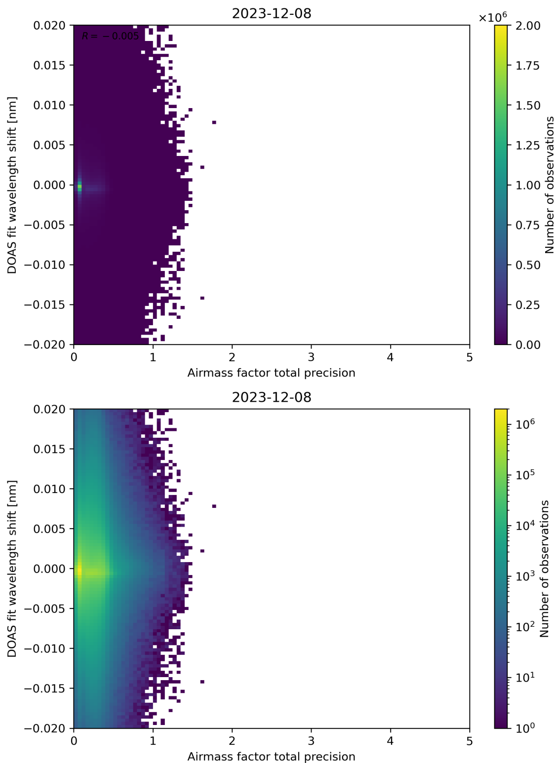
Figure 106: Scatter density plot of “Airmass factor total precision” against “DOAS fit wavelength shift” for 2023-12-07 to 2023-12-09.
