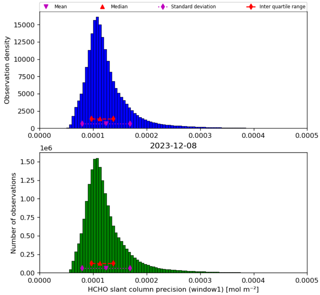
Figure 39: Histogram of “HCHO slant column precision (window1)” for 2023-12-07 to 2023-12-09
