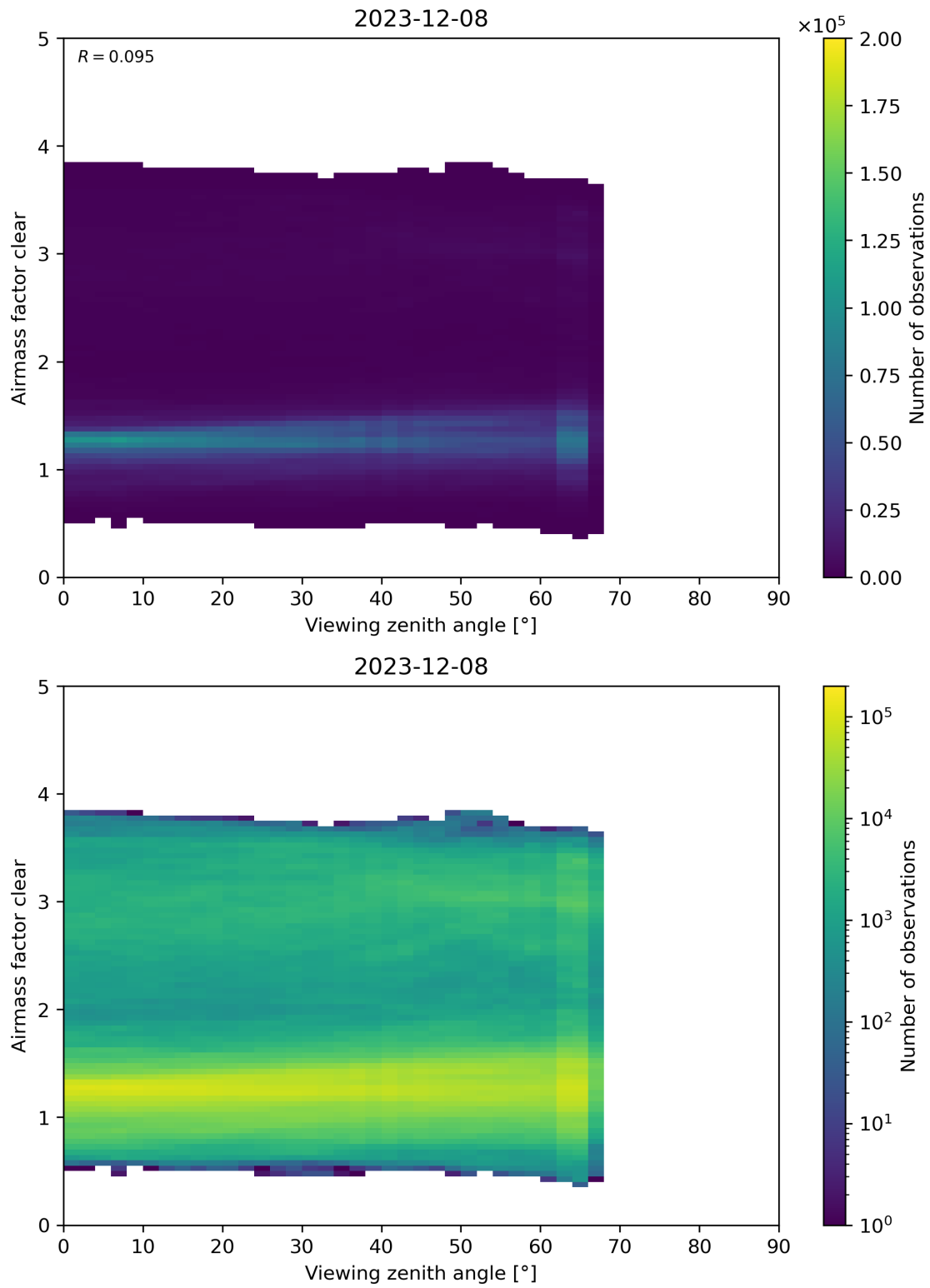
Figure 185: Scatter density plot of “Viewing zenith angle” against “Airmass factor clear” for 2023-12-07 to 2023-12-09.
