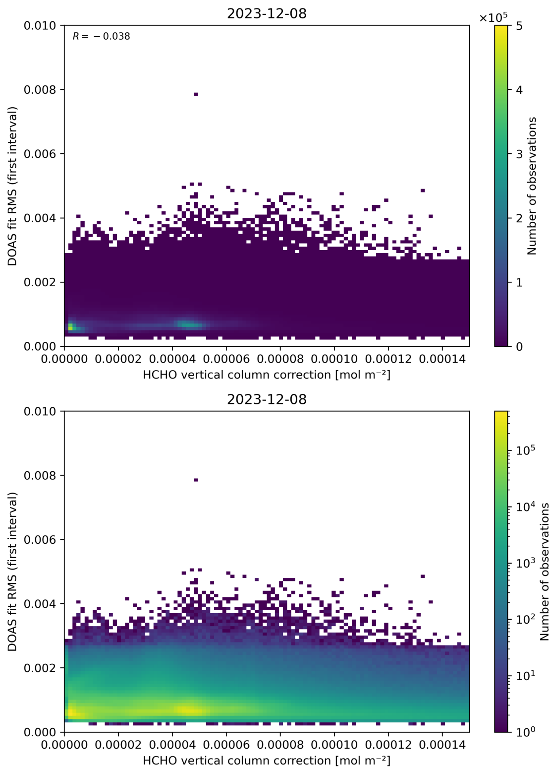
Figure 112: Scatter density plot of “HCHO vertical column correction” against “DOAS fit RMS (first interval)” for 2023-12-07 to 2023-12-09.
