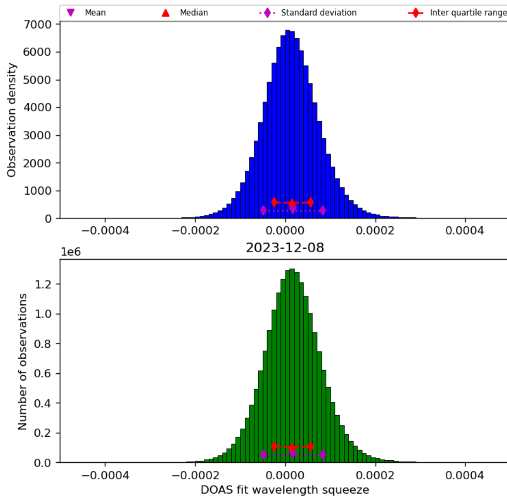
Figure 45: Histogram of “DOAS fit wavelength squeeze” for 2023-12-07 to 2023-12-09
