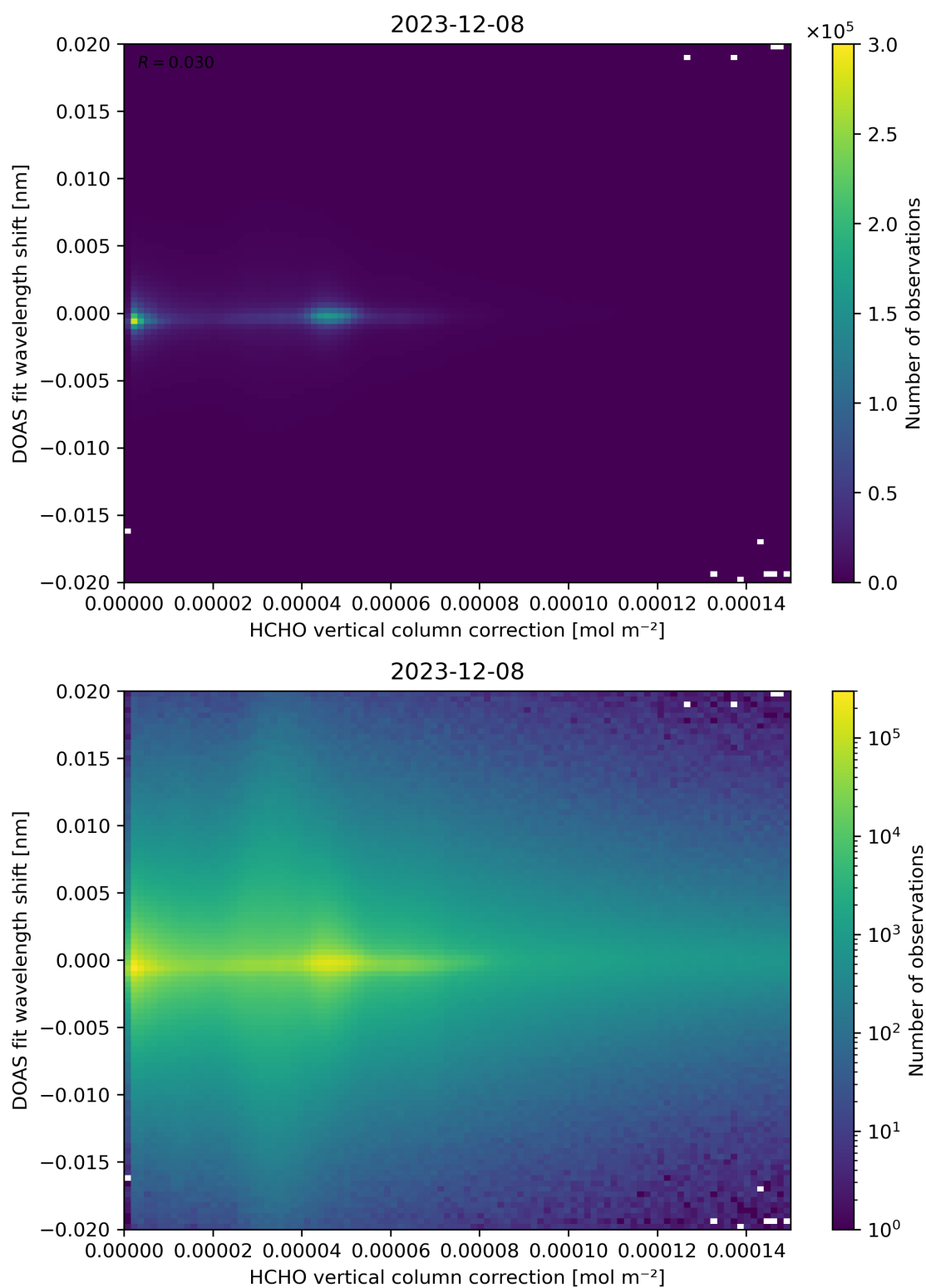
Figure 113: Scatter density plot of “HCHO vertical column correction” against “DOAS fit wavelength shift” for 2023-12-07 to 2023-12-09.
