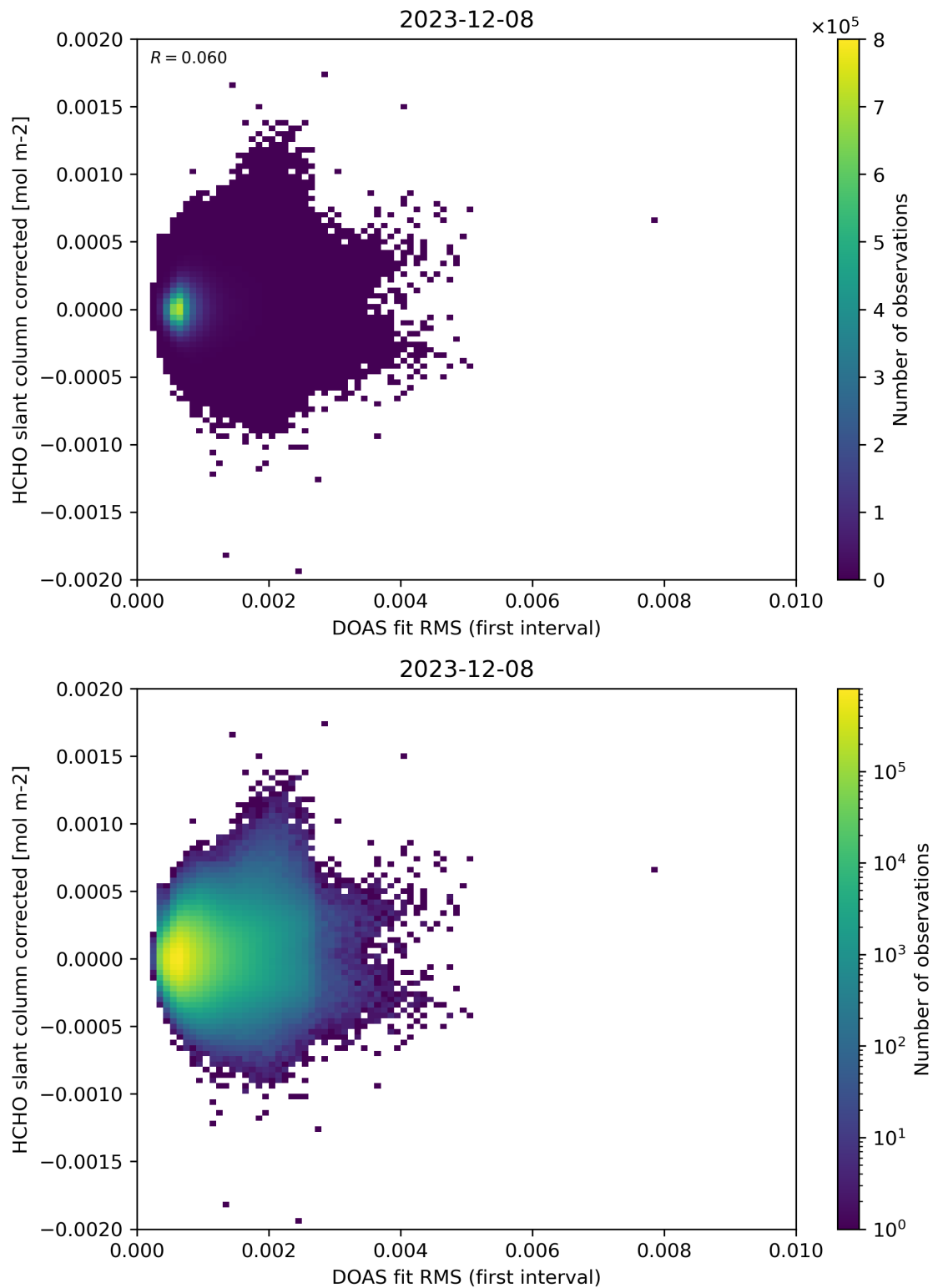
Figure 62: Scatter density plot of “DOAS fit RMS (first interval)” against “HCHO slant column corrected” for 2023-12-07 to 2023-12-09.
