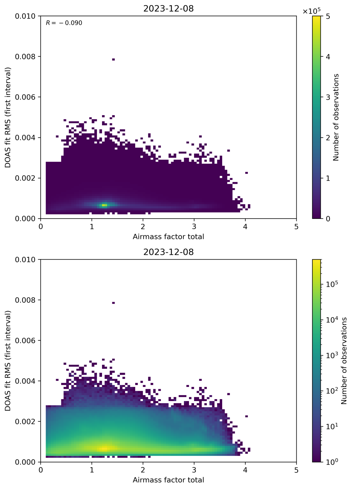
Figure 97: Scatter density plot of “Airmass factor total” against “DOAS fit RMS (first interval)” for 2023-12-07 to 2023-12-09.
