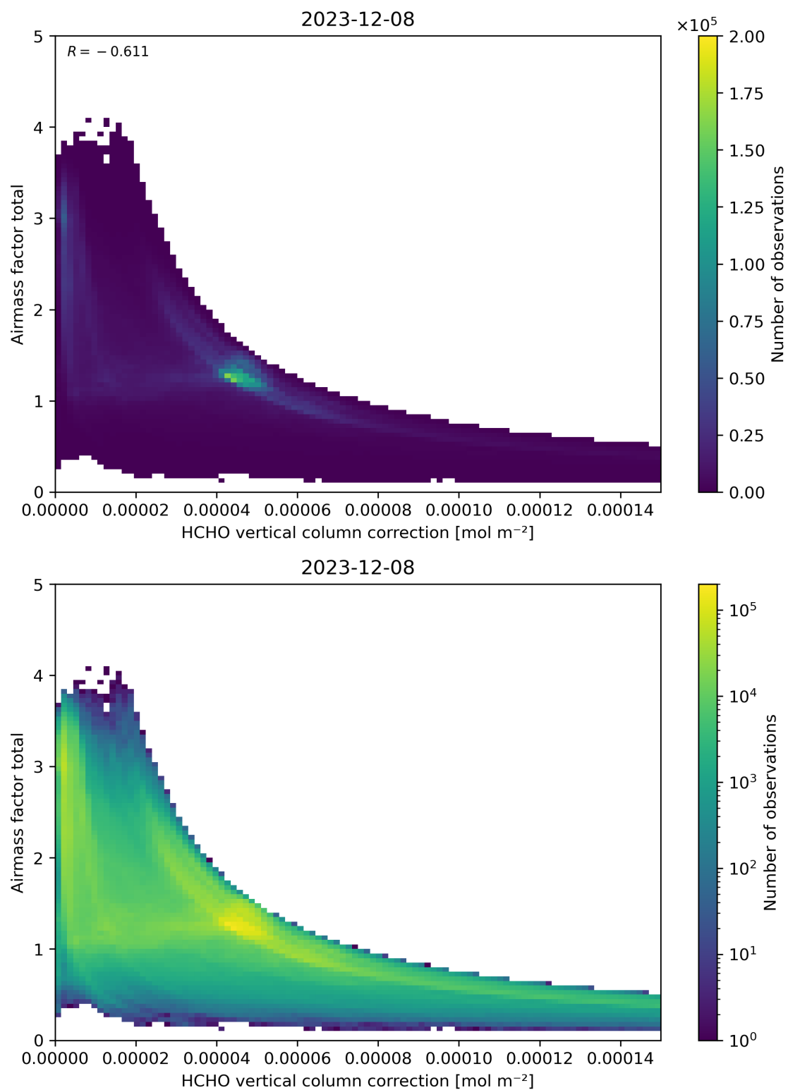
Figure 120: Scatter density plot of “HCHO vertical column correction” against “Airmass factor total” for 2023-12-07 to 2023-12-09.
