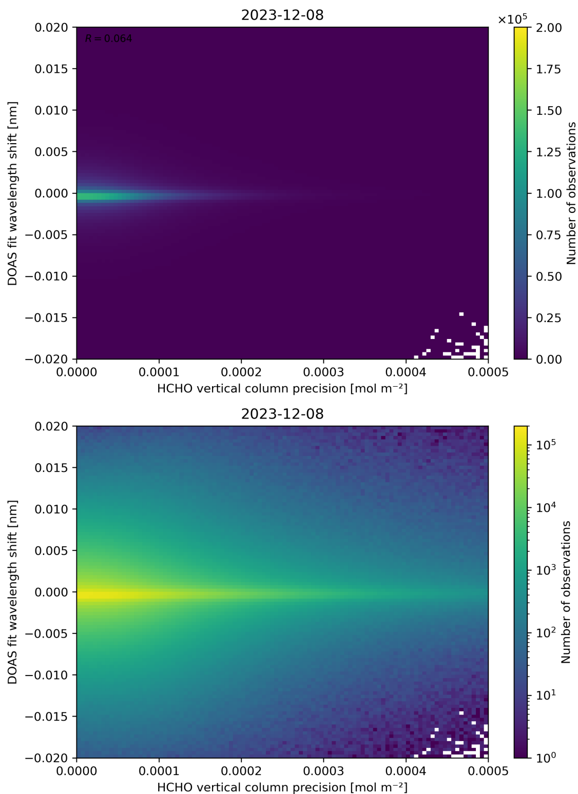
Figure 137: Scatter density plot of “HCHO vertical column precision” against “DOAS fit wavelength shift” for 2023-12-07 to 2023-12-09.
