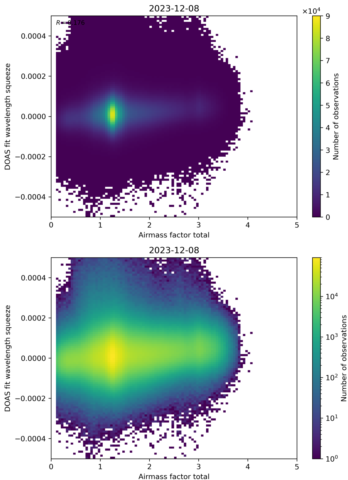
Figure 99: Scatter density plot of “Airmass factor total” against “DOAS fit wavelength squeeze” for 2023-12-07 to 2023-12-09.
