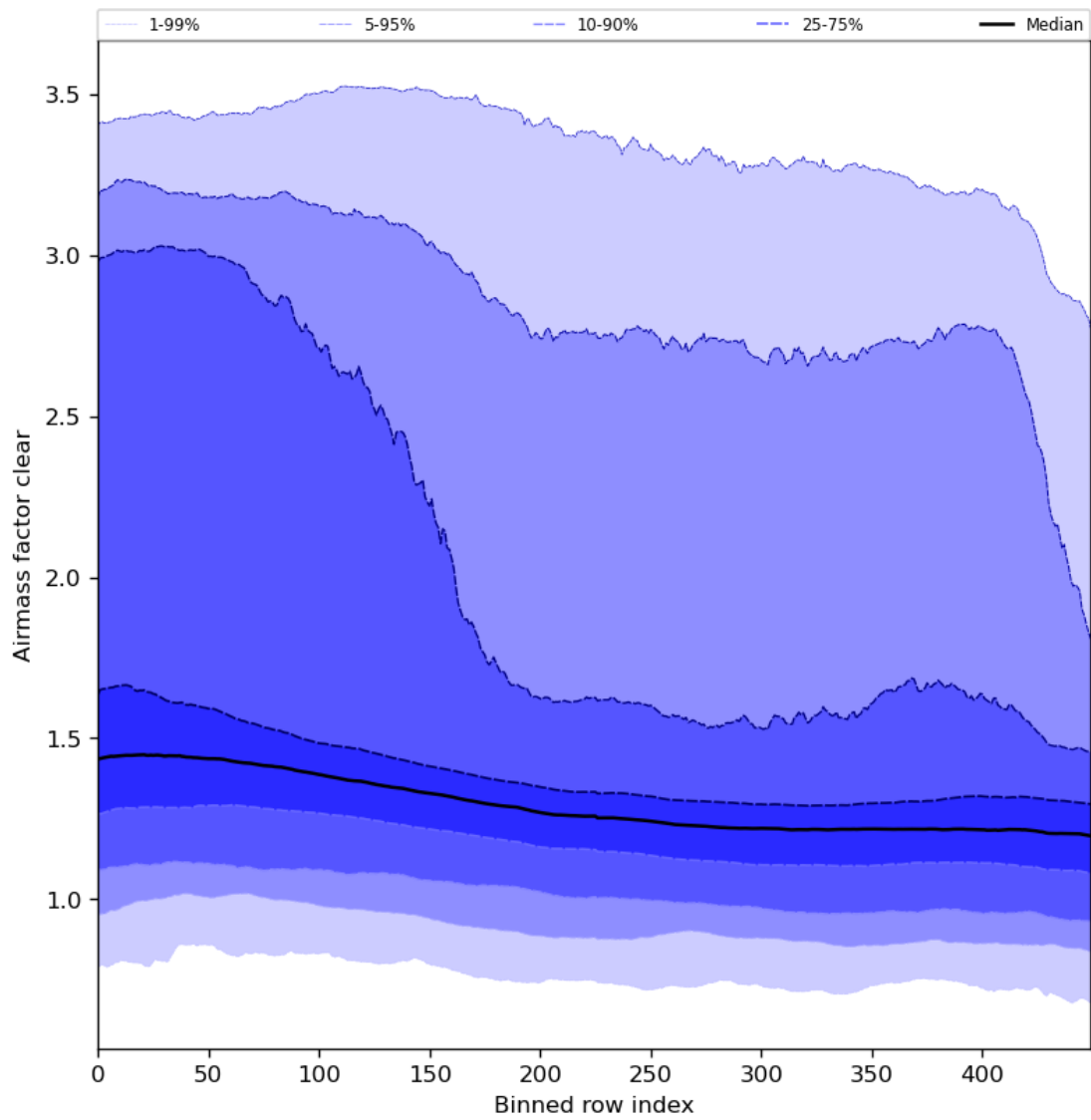
Figure 56: Along track statistics of “Airmass factor clear” for 2023-12-07 to 2023-12-09
