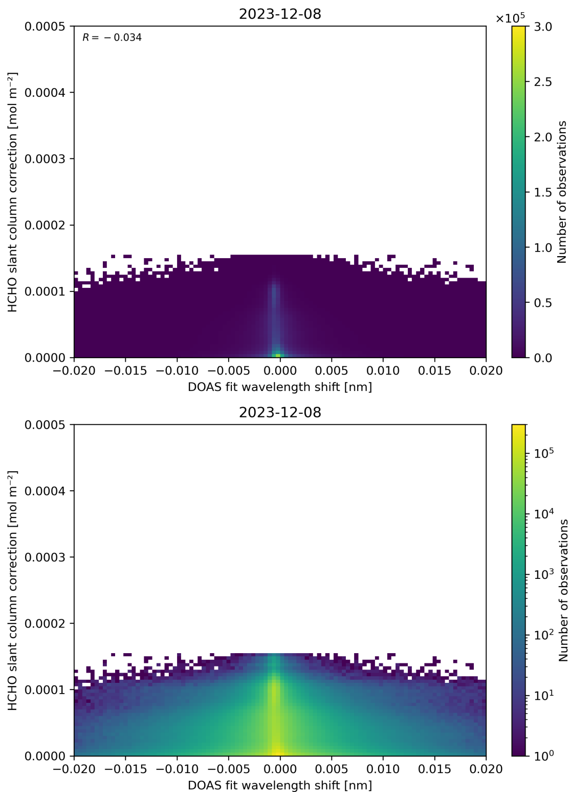
Figure 67: Scatter density plot of “DOAS fit wavelength shift” against “HCHO slant column correction” for 2023-12-07 to 2023-12-09.
