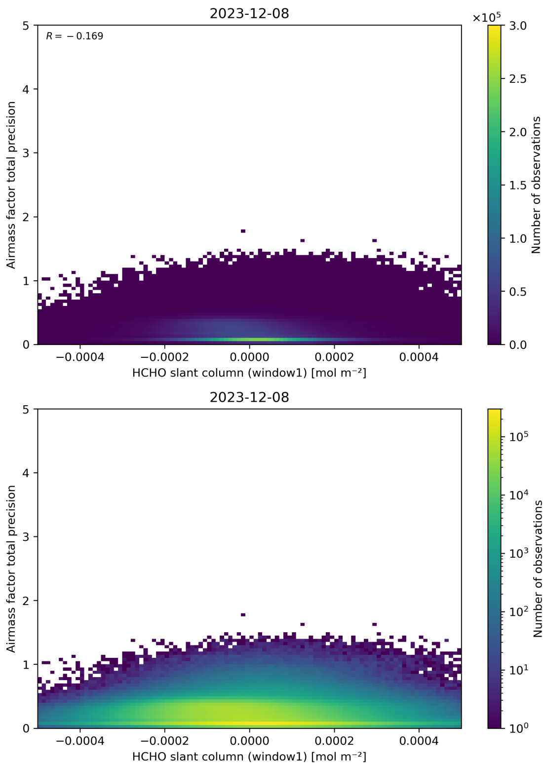
Figure 86: Scatter density plot of “HCHO slant column (window1)” against “Airmass factor total precision” for 2023-12-07 to 2023-12-09.
