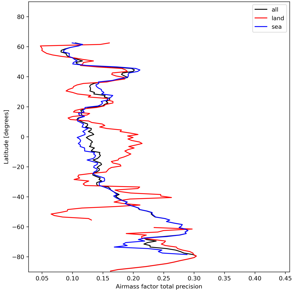
Figure 27: Zonal average of “Airmass factor total precision” for 2023-12-07 to 2023-12-09.
