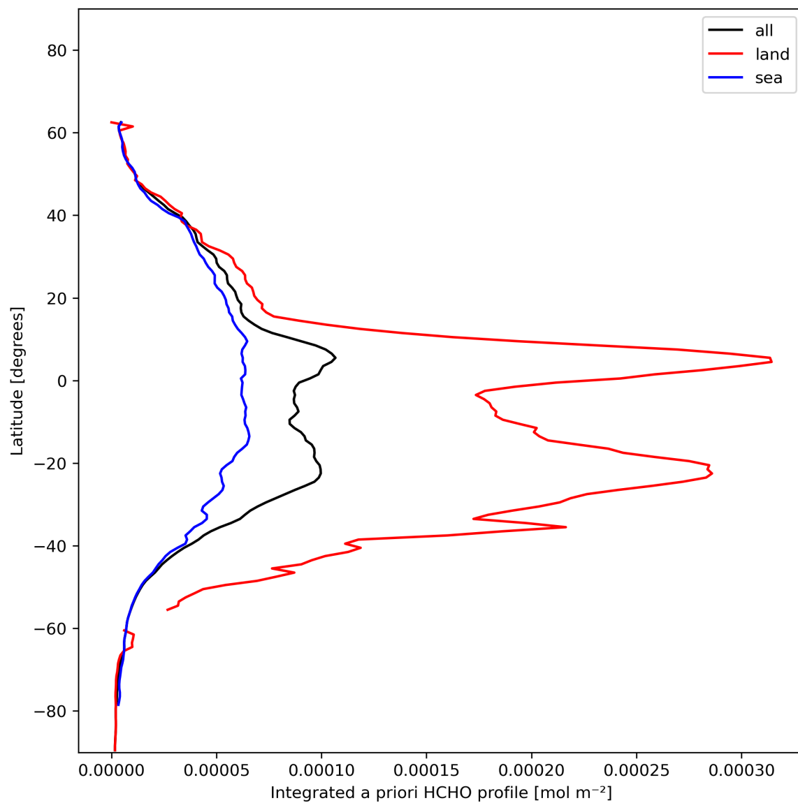
Figure 29: Zonal average of “Integrated a priori HCHO profile” for 2023-12-07 to 2023-12-09.
