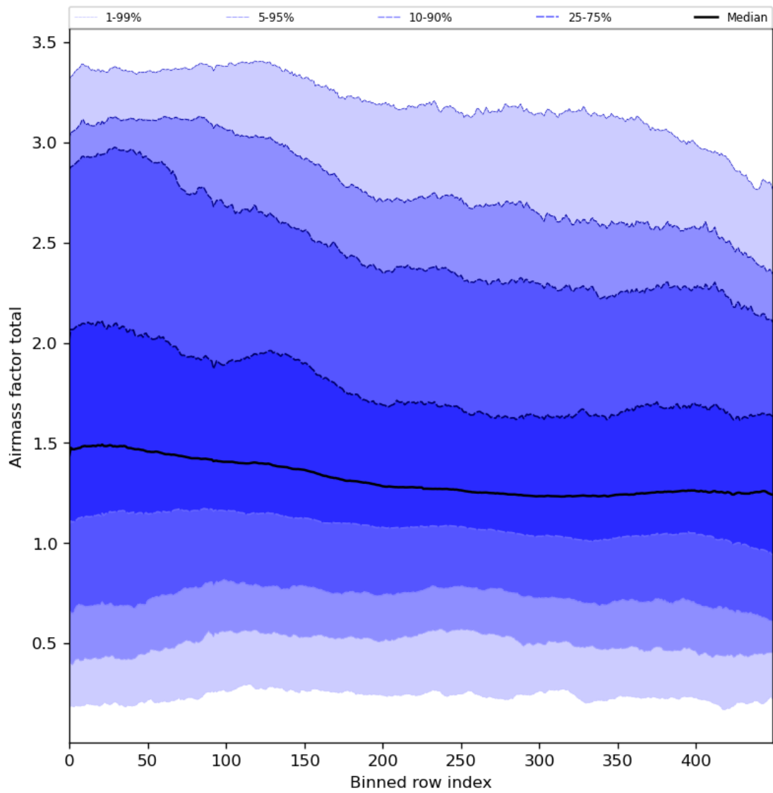
Figure 54: Along track statistics of “Airmass factor total” for 2023-12-07 to 2023-12-09
