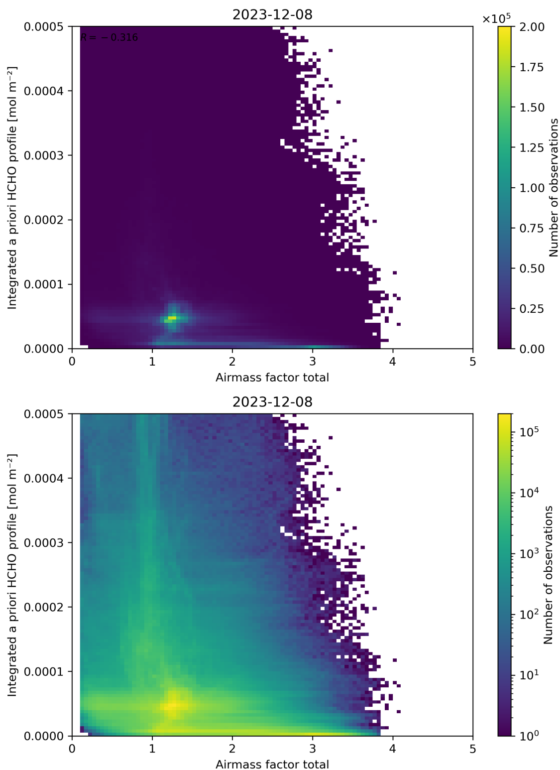
Figure 104: Scatter density plot of “Air mass factor total” against “Integrated a priori HCHO profile” for 2023-12-07 to 2023-12-09.
