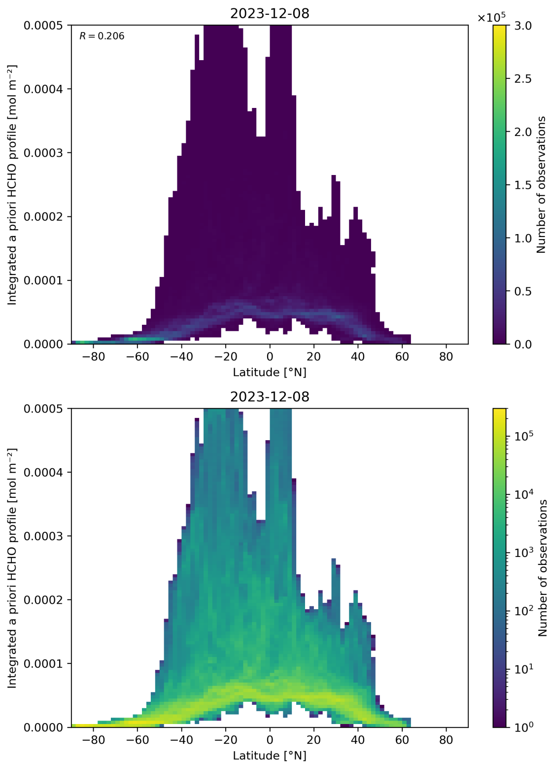
Figure 166: Scatter density plot of “Latitude” against “Integrated a priori HCHO profile” for 2023-12-07 to 2023-12-09.
