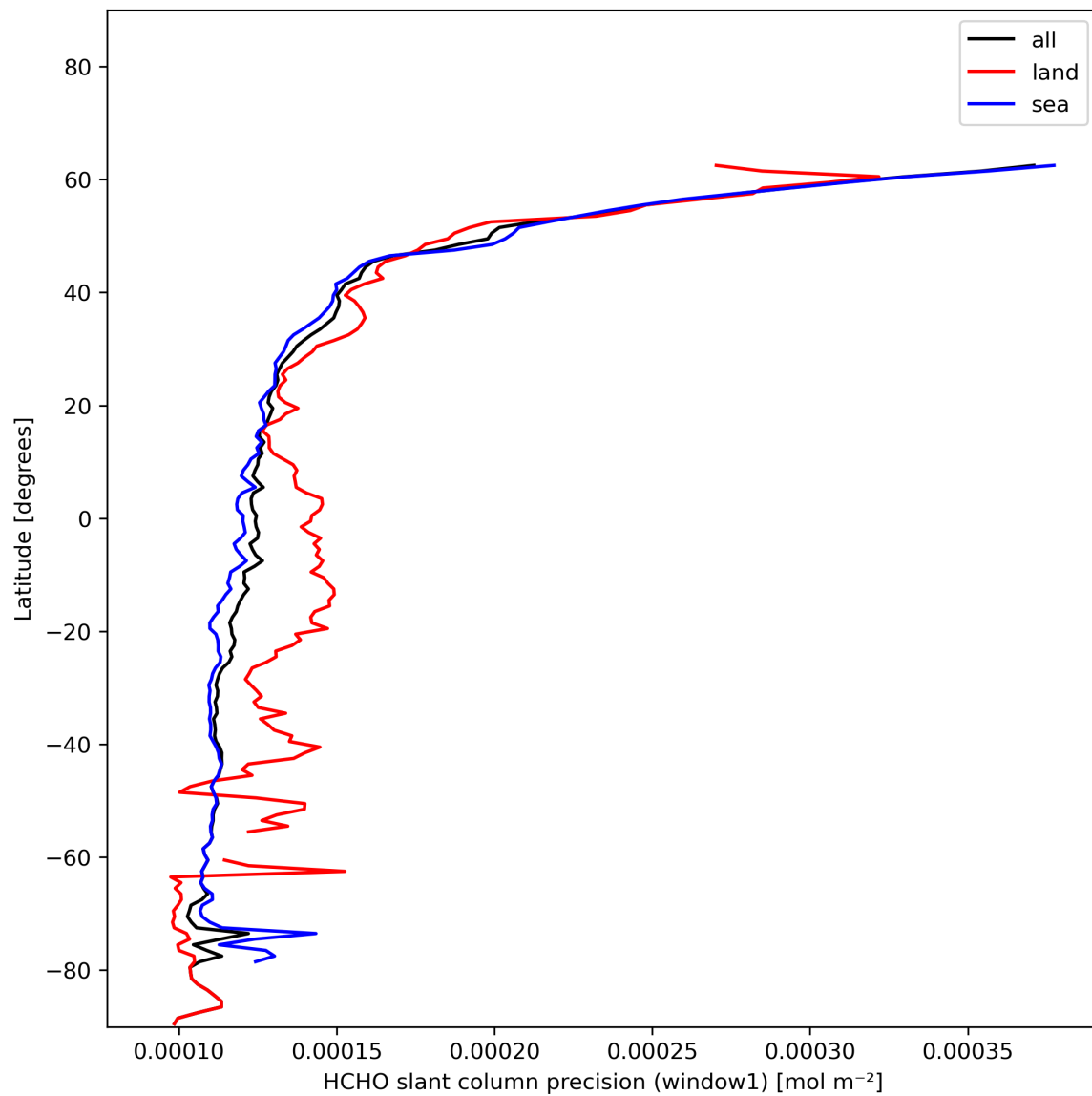
Figure 25: Zonal average of “HCHO slant column precision (window1)” for 2023-12-07 to 2023-12-09.
