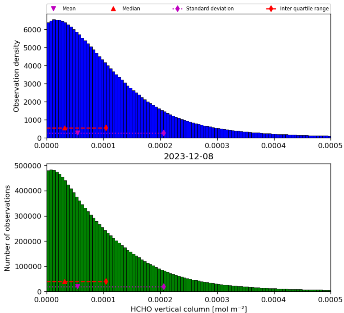
Figure 35: Histogram of “HCHO vertical column” for 2023-12-07 to 2023-12-09
