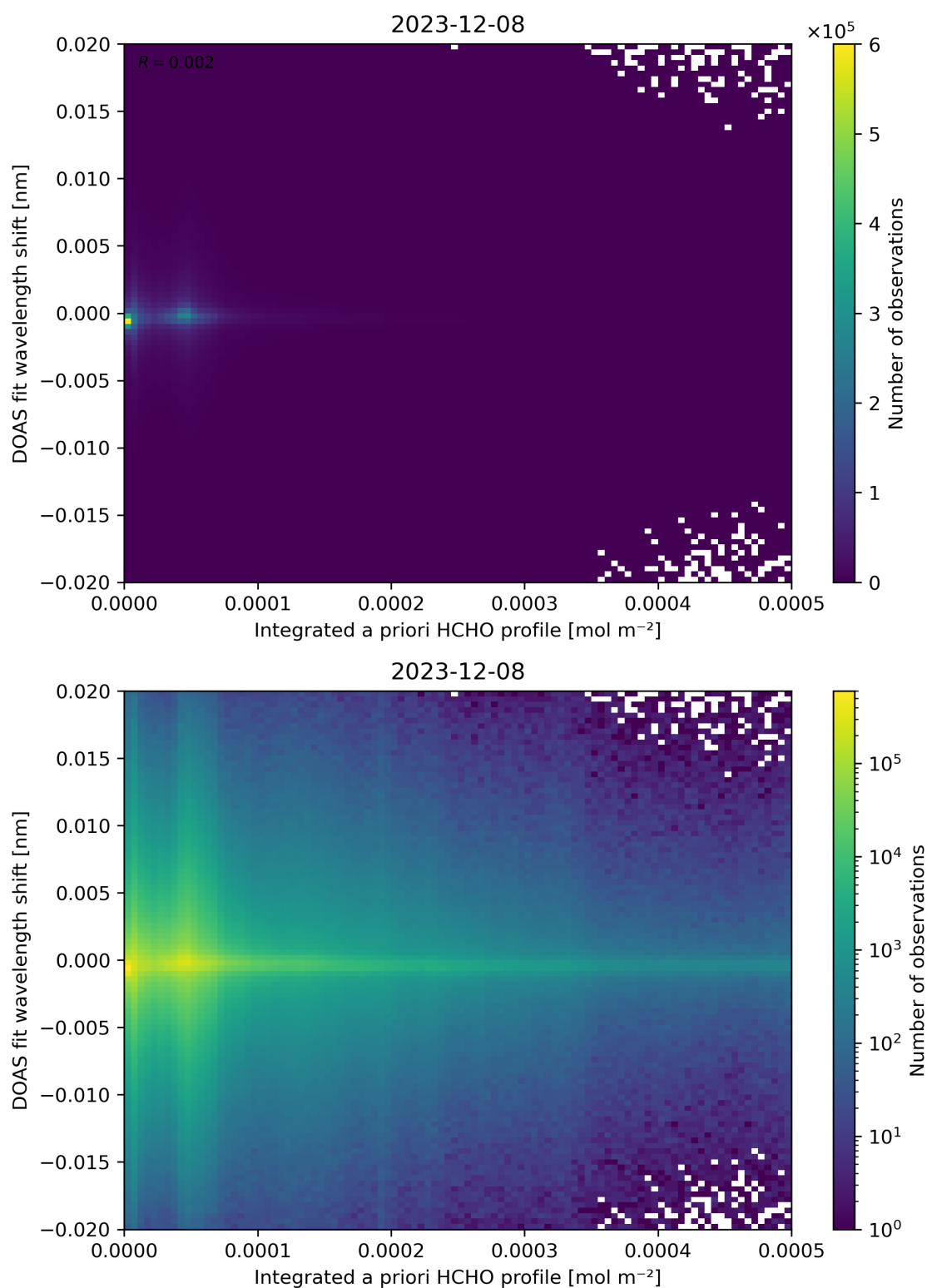
Figure 149: Scatter density plot of “Integrated a priori HCHO profile” against “DOAS fit wavelength shift” for 2023-12-07 to 2023-12-09.
