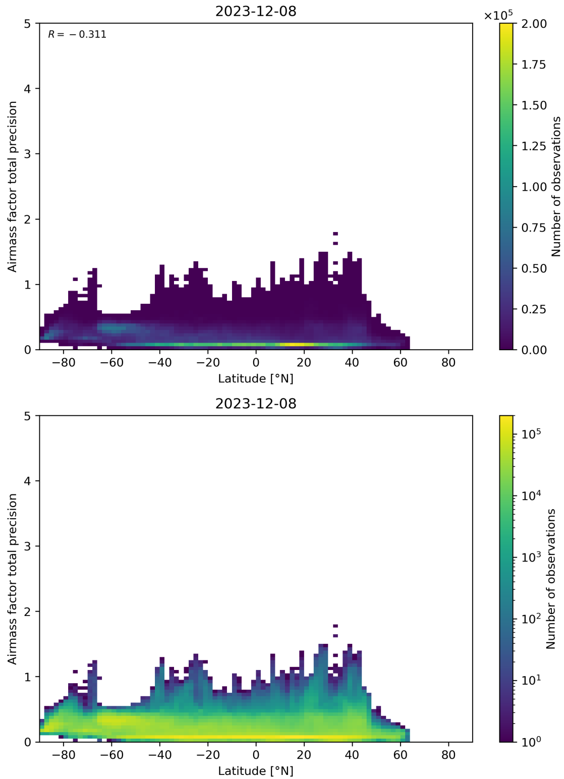
Figure 162: Scatter density plot of “Latitude” against “Airmass factor total precision” for 2023-12-07 to 2023-12-09.
