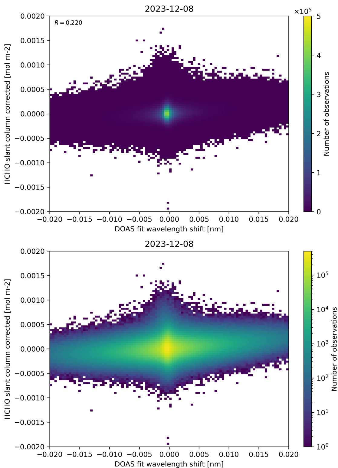
Figure 66: Scatter density plot of “DOAS fit wavelength shift” against “HCHO slant column corrected” for 2023-12-07 to 2023-12-09.
