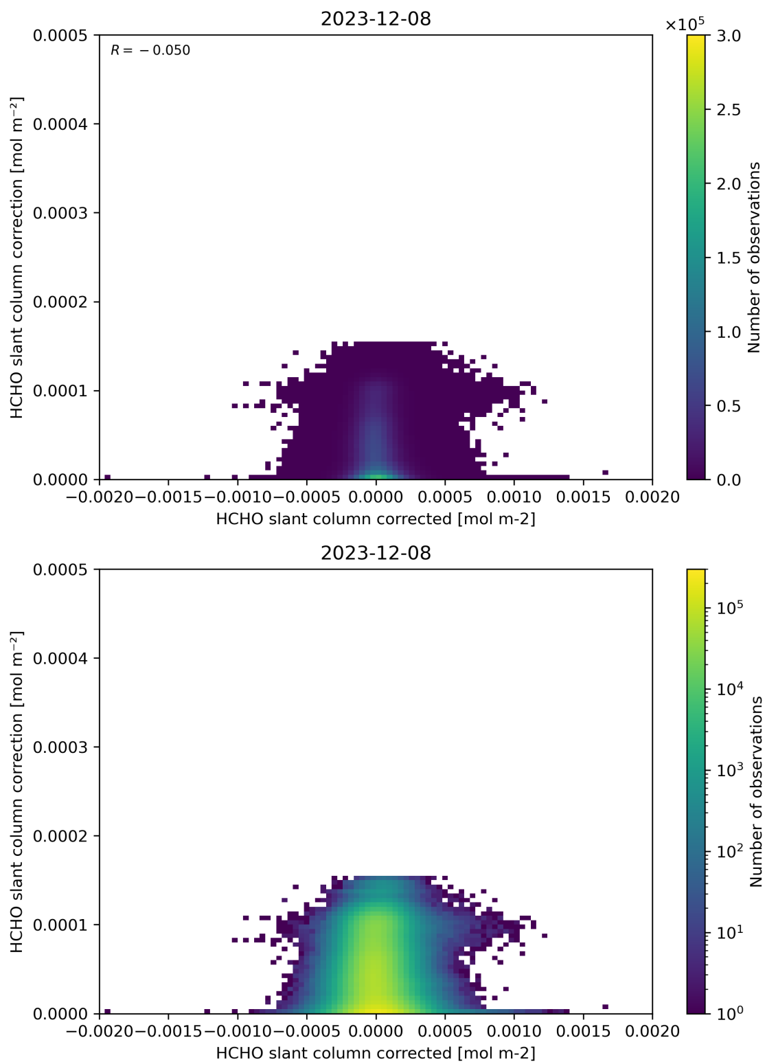
Figure 77: Scatter density plot of “HCHO slant column corrected” against “HCHO slant column correction” for 2023-12-07 to 2023-12-09.
