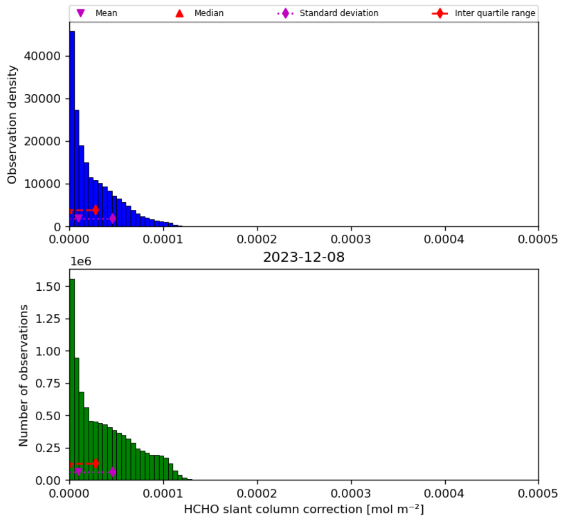
Figure 47: Histogram of “HCHO slant column correction” for 2023-12-07 to 2023-12-09
