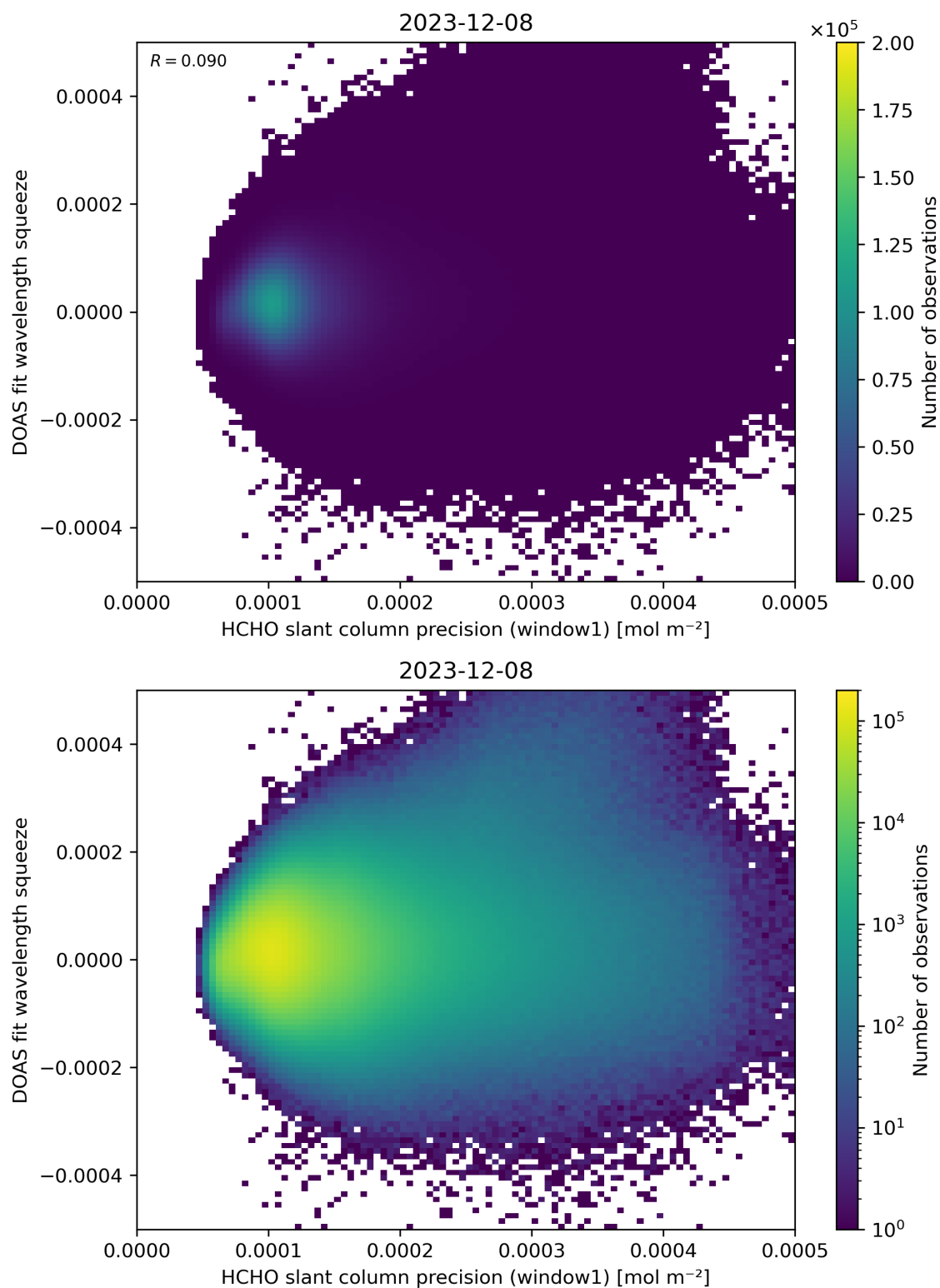
Figure 90: Scatter density plot of “HCHO slant column precision (window1)” against “DOAS fit wavelength squeeze” for 2023-12-07 to 2023-12-09.
