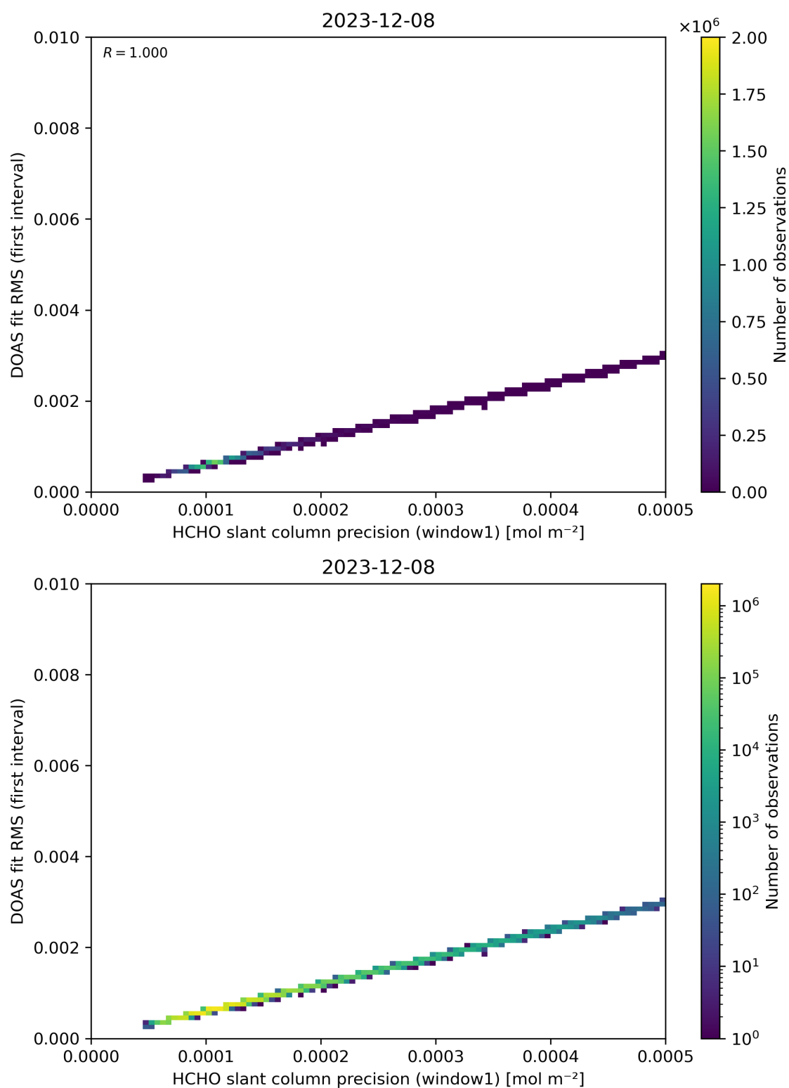
Figure 88: Scatter density plot of “HCHO slant column precision (window1)” against “DOAS fit RMS (first interval)” for 2023-12-07 to 2023-12-09.
