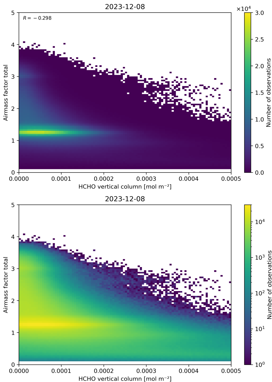
Figure 131: Scatter density plot of “HCHO vertical column” against “Airmass factor total” for 2023-12-07 to 2023-12-09.
