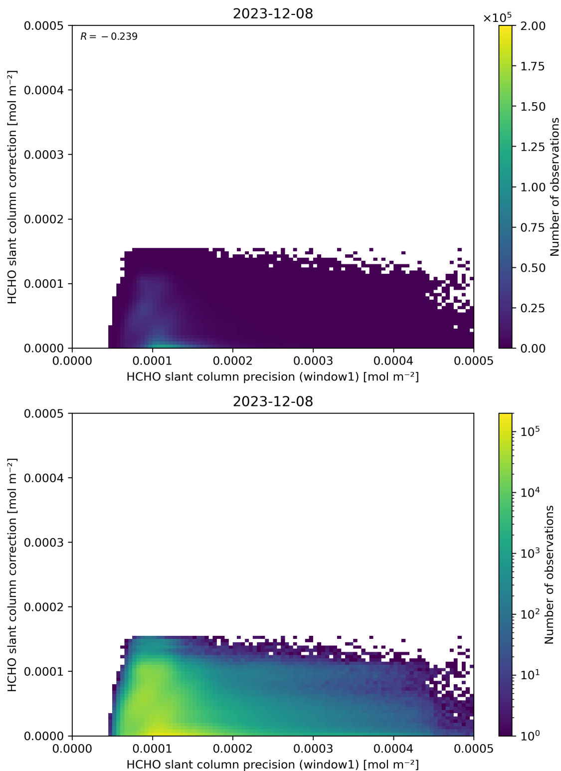
Figure 93: Scatter density plot of “HCHO slant column precision (window1)” against “HCHO slant column correction” for 2023-12-07 to 2023-12-09.
