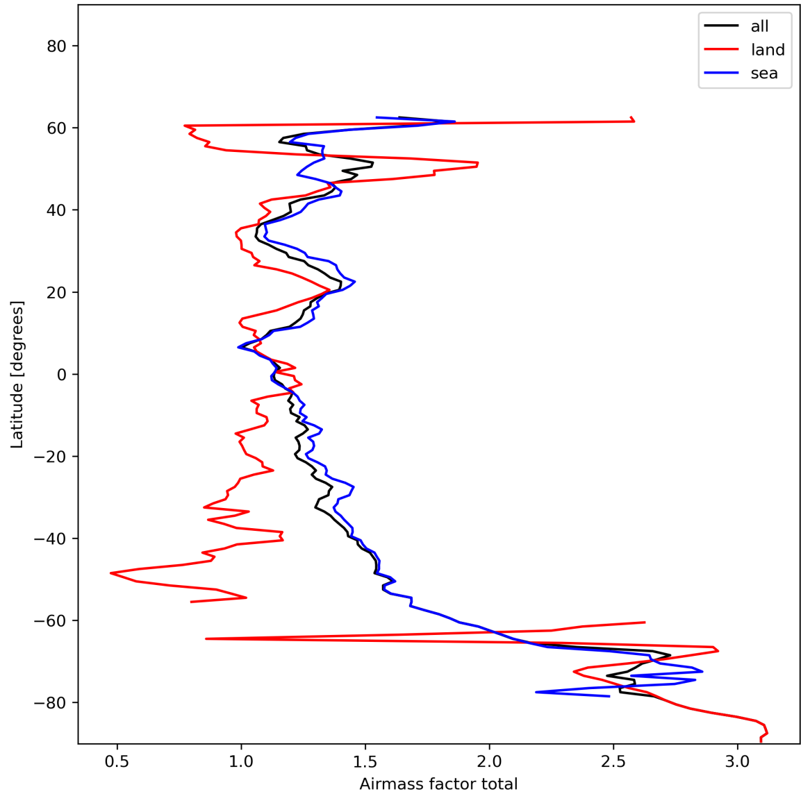
Figure 26: Zonal average of “Airmass factor total” for 2023-12-07 to 2023-12-09.
