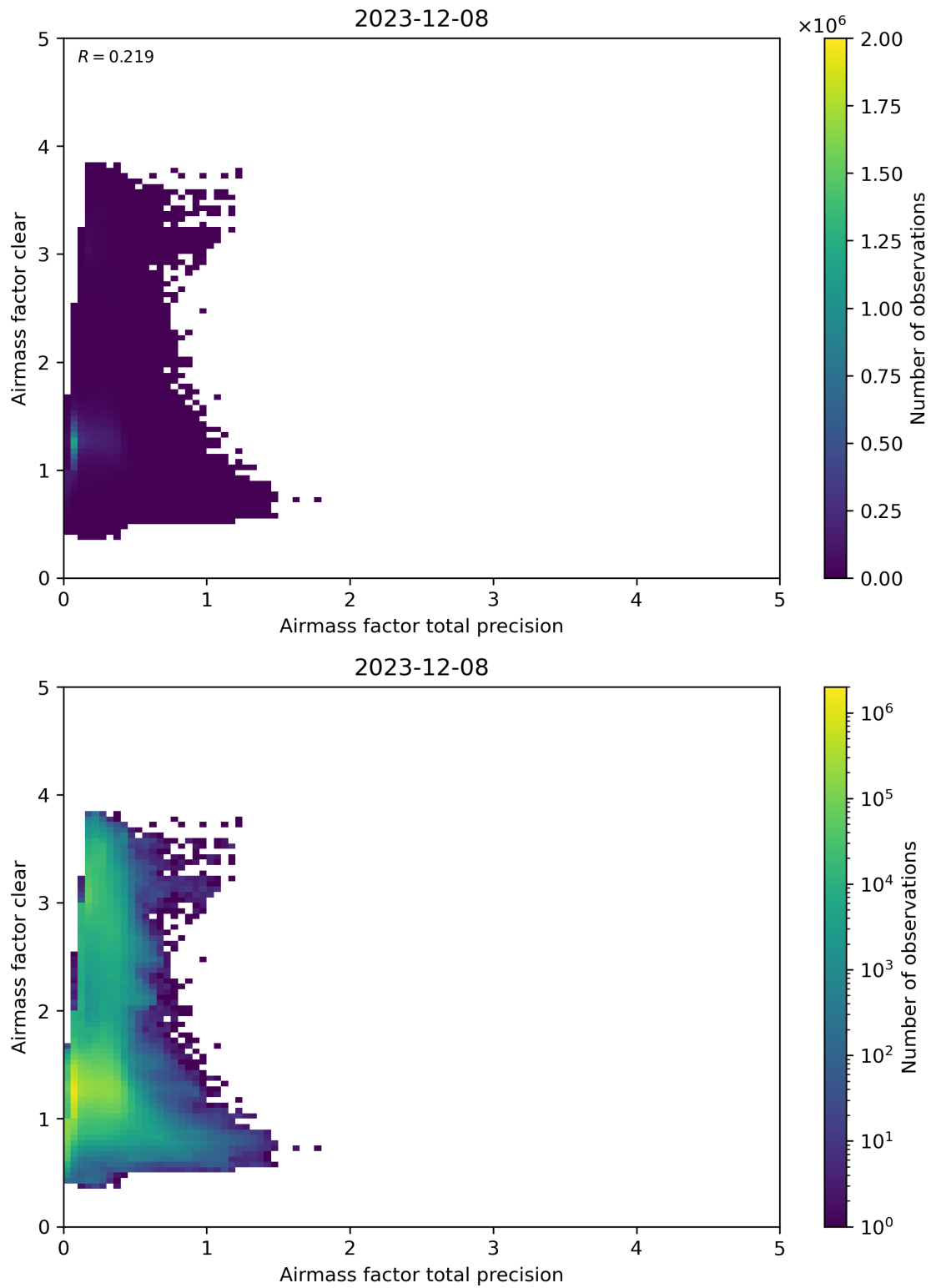
Figure 108: Scatter density plot of “Airmass factor total precision” against “Airmass factor clear” for 2023-12-07 to 2023-12-09.
