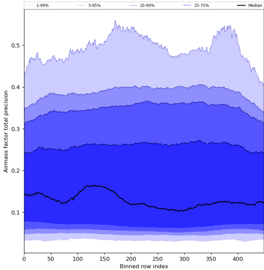
Figure 55: Along track statistics of “Airmass factor total precision” for 2023-12-07 to 2023-12-09
