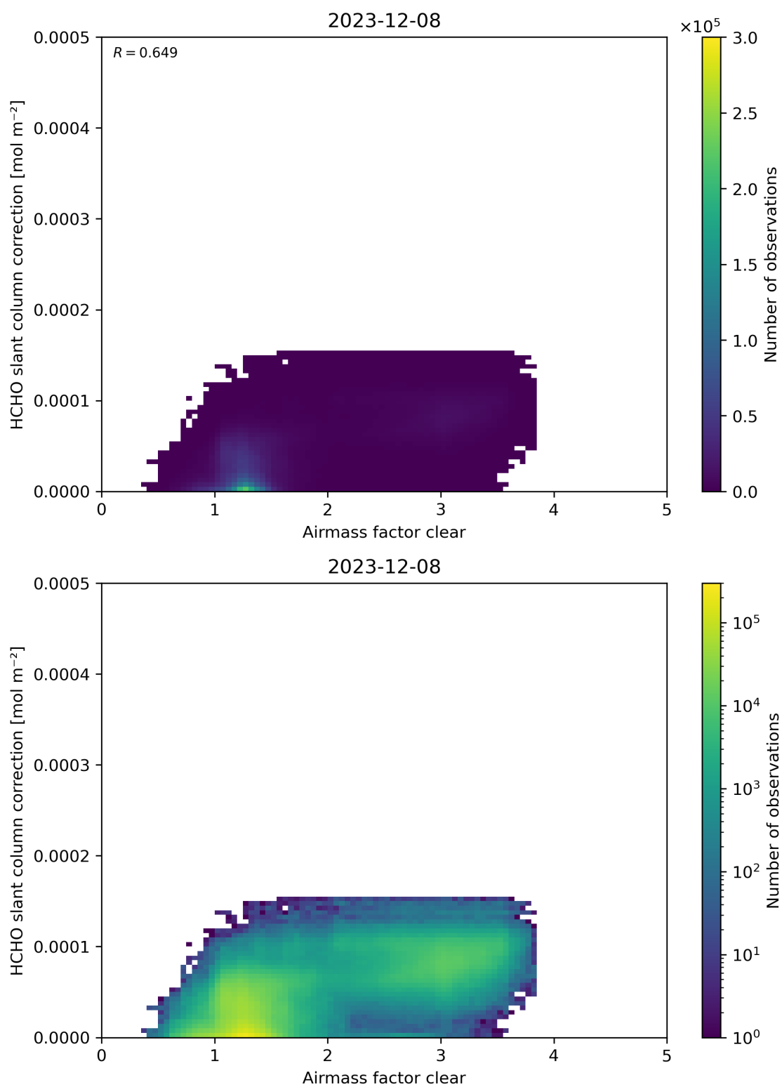
Figure 75: Scatter density plot of “Air mass factor clear” against “HCHO slant column correction” for 2023-12-07 to 2023-12-09.
