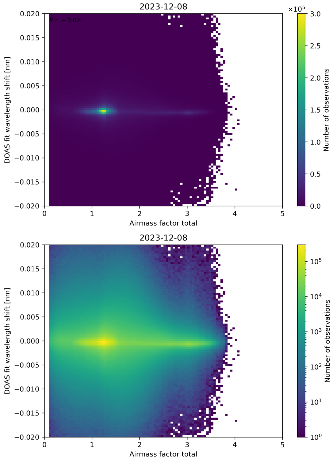
Figure 98: Scatter density plot of “Airmass factor total” against “DOAS fit wavelength shift” for 2023-12-07 to 2023-12-09.
