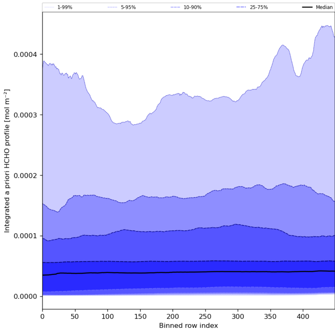
Figure 57: Along track statistics of “Integrated a priori HCHO profile” for 2023-12-07 to 2023-12-09
