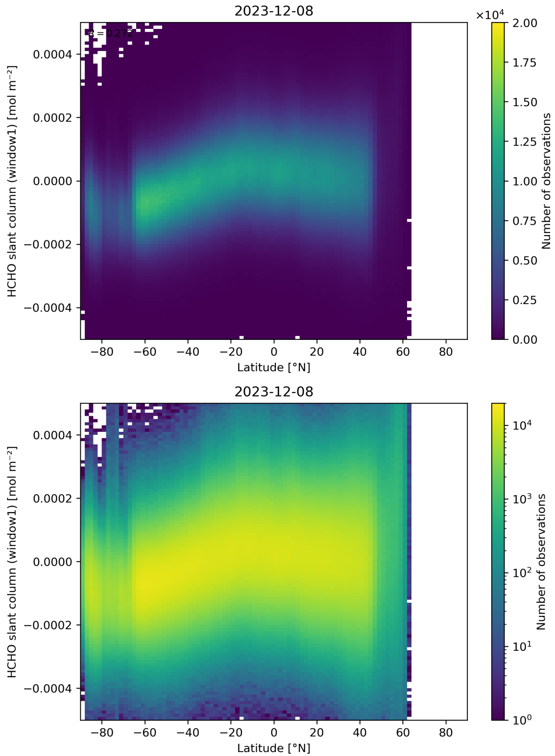
Figure 159: Scatter density plot of “Latitude” against “HCHO slant column (window1)” for 2023-12-07 to 2023-12-09.
