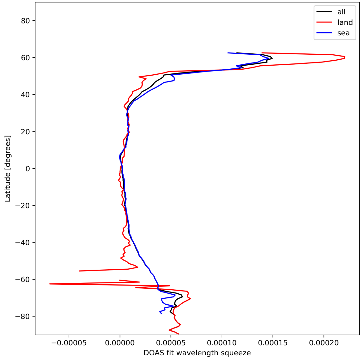
Figure 31: Zonal average of “DOAS fit wavelength squeeze” for 2023-12-07 to 2023-12-09.
