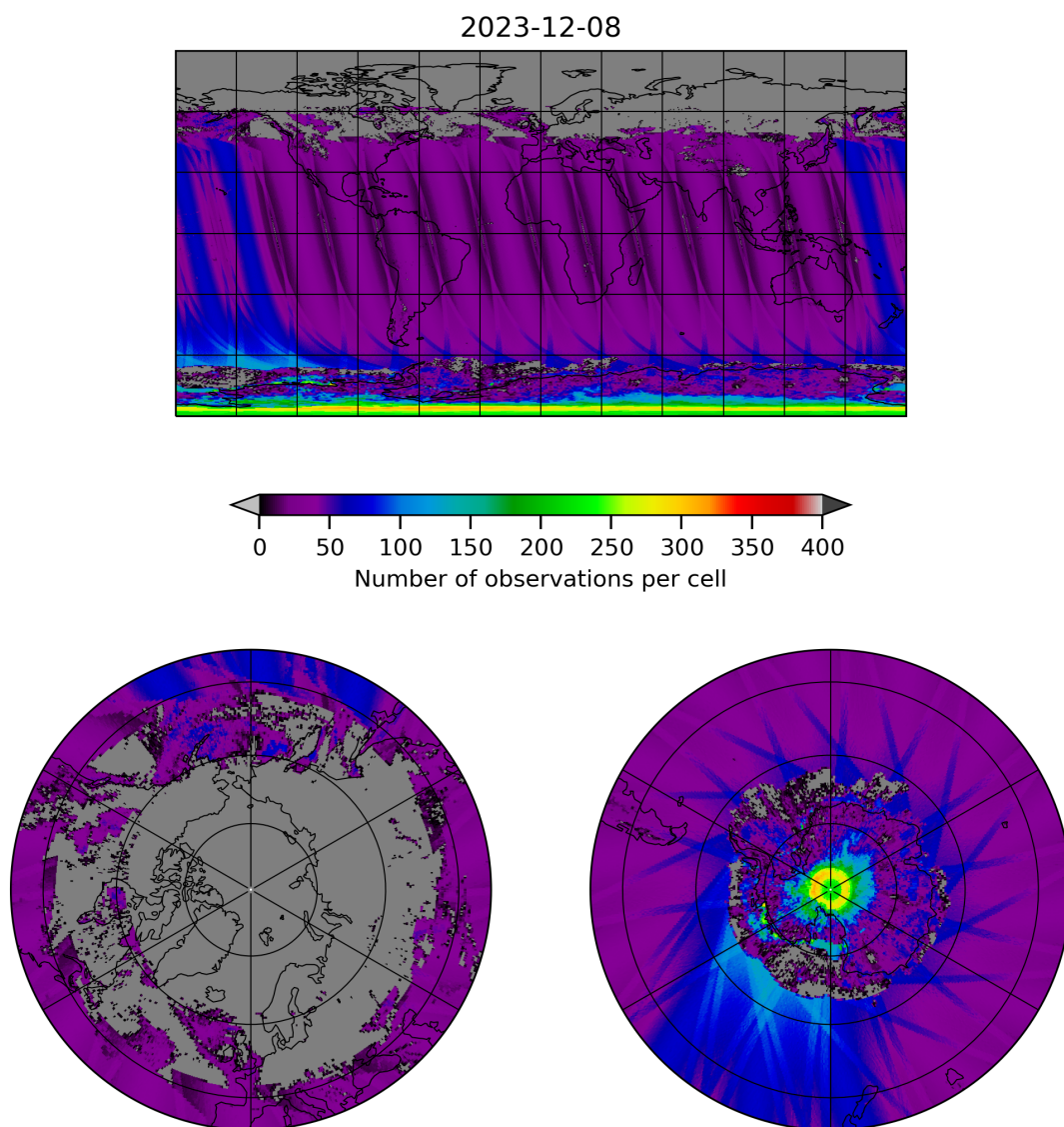
Figure 19: Map of the number of observations for 2023-12-07 to 2023-12-09
