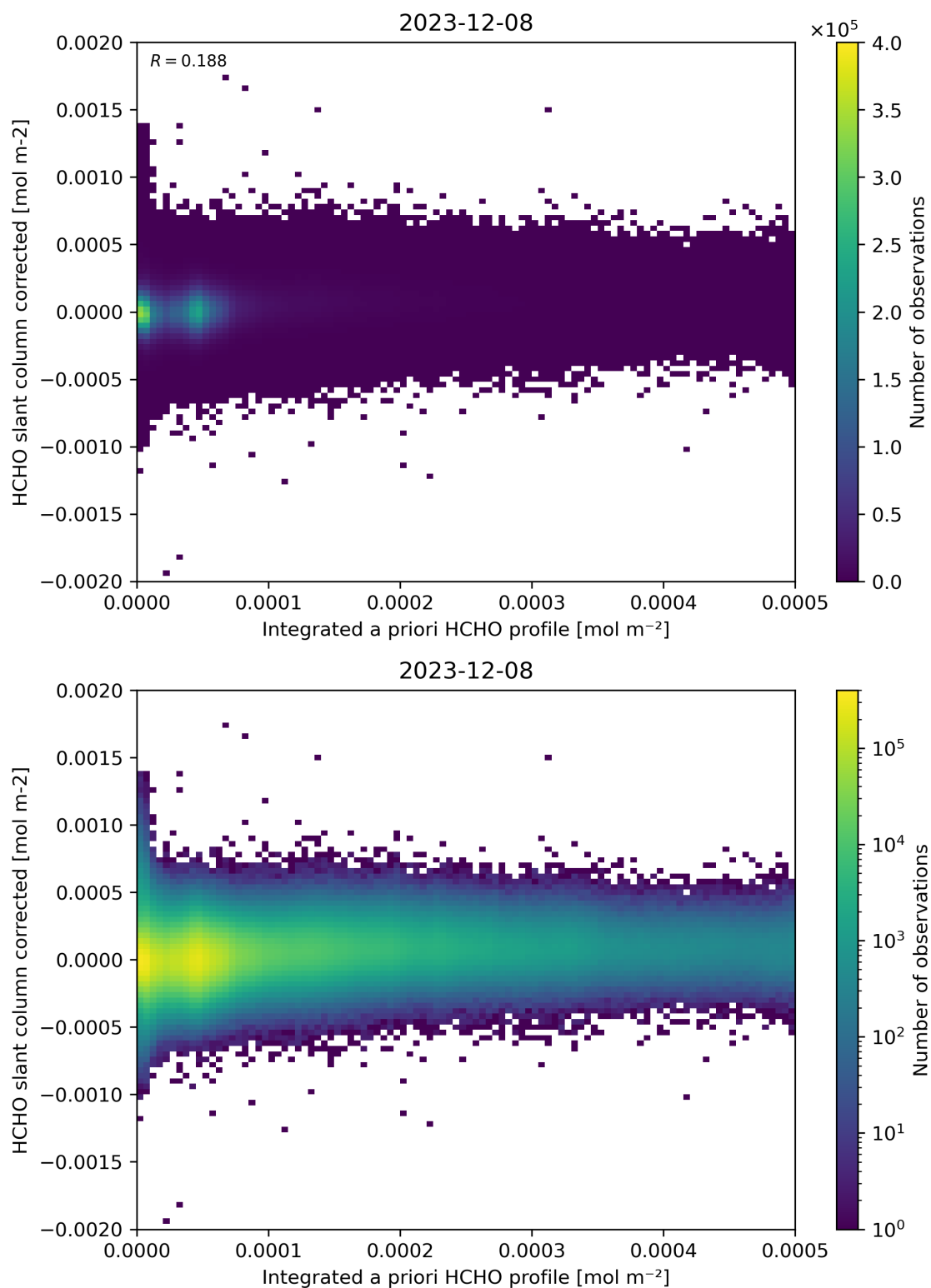
Figure 151: Scatter density plot of “Integrated a priori HCHO profile” against “HCHO slant column corrected” for 2023-12-07 to 2023-12-09.
