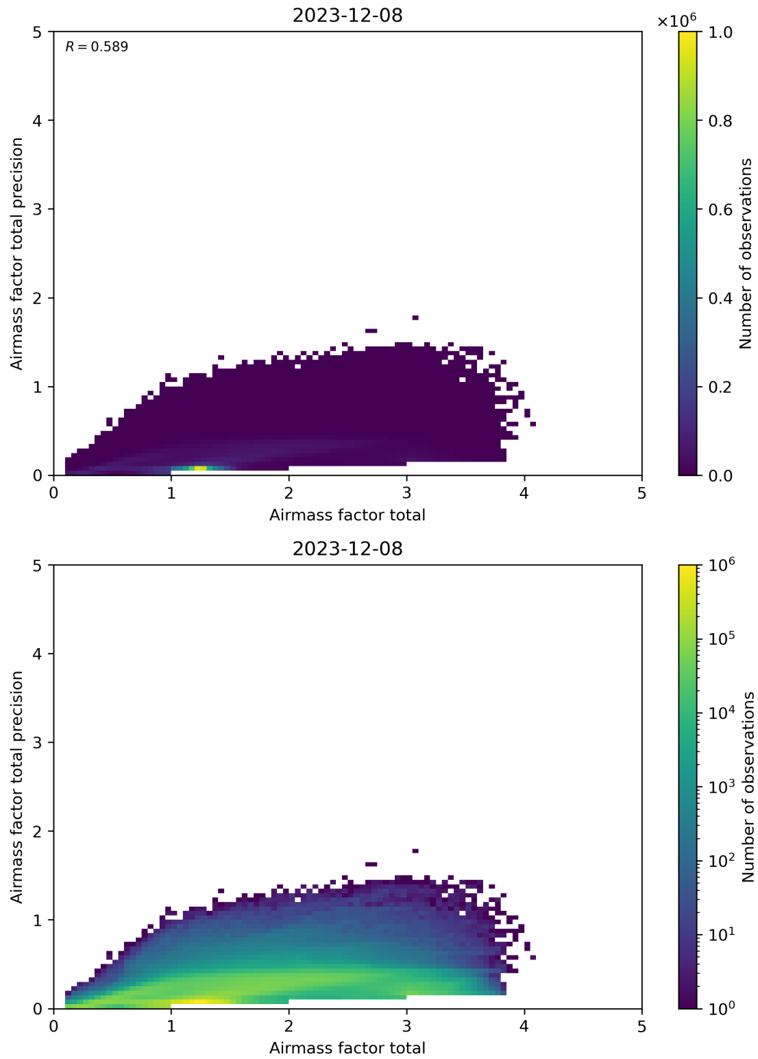
Figure 103: Scatter density plot of “Airmass factor total” against “Airmass factor total precision” for 2023-12-07 to 2023-12-09.
