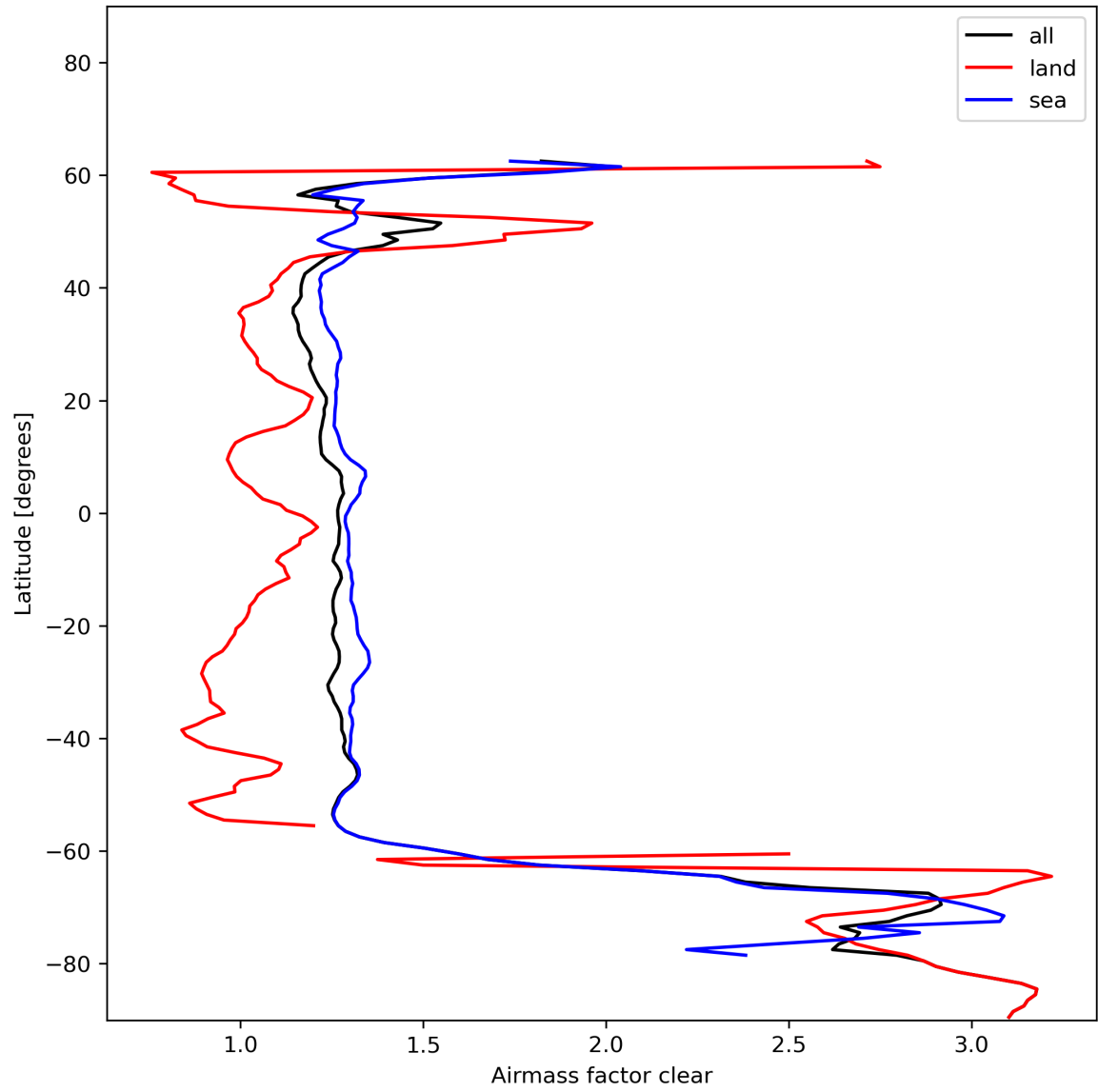
Figure 28: Zonal average of “Airmass factor clear” for 2023-12-07 to 2023-12-09.
