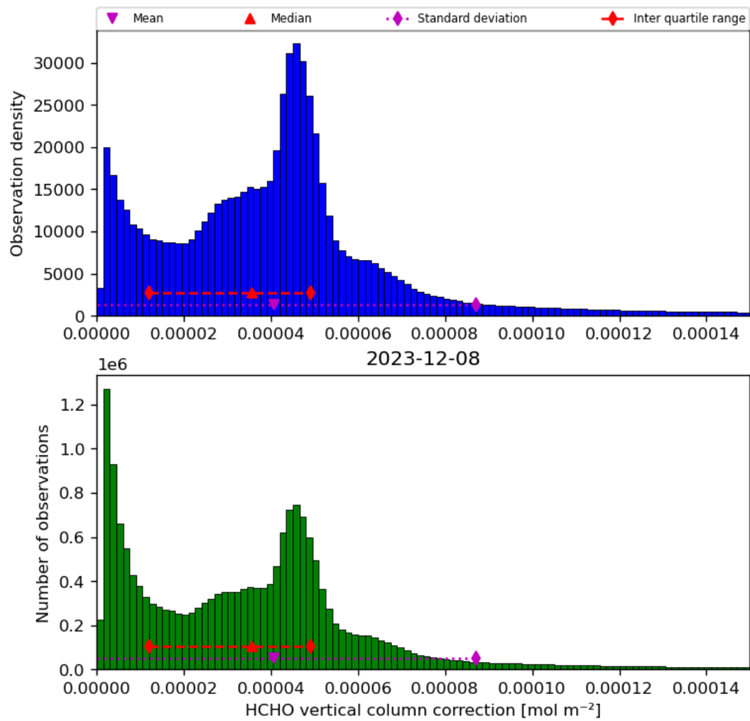
Figure 37: Histogram of “HCHO vertical column correction” for 2023-12-07 to 2023-12-09
