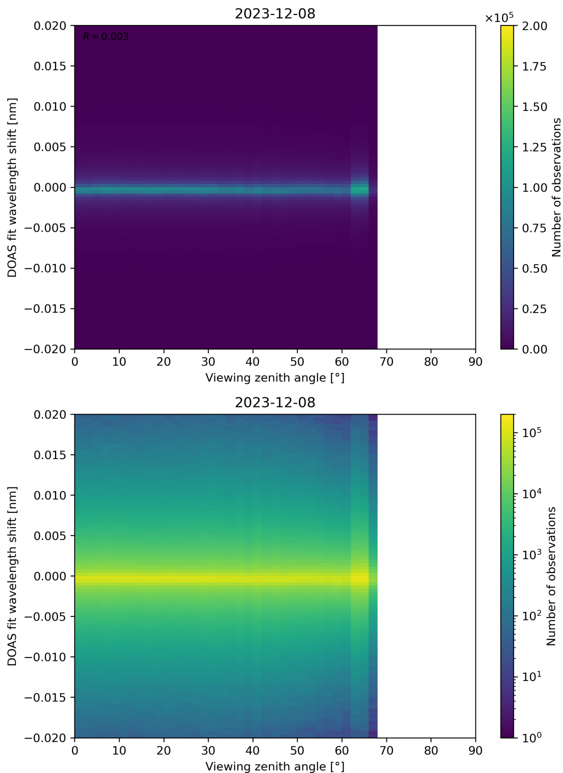
Figure 183: Scatter density plot of “Viewing zenith angle” against “DOAS fit wavelength shift” for 2023-12-07 to 2023-12-09.
