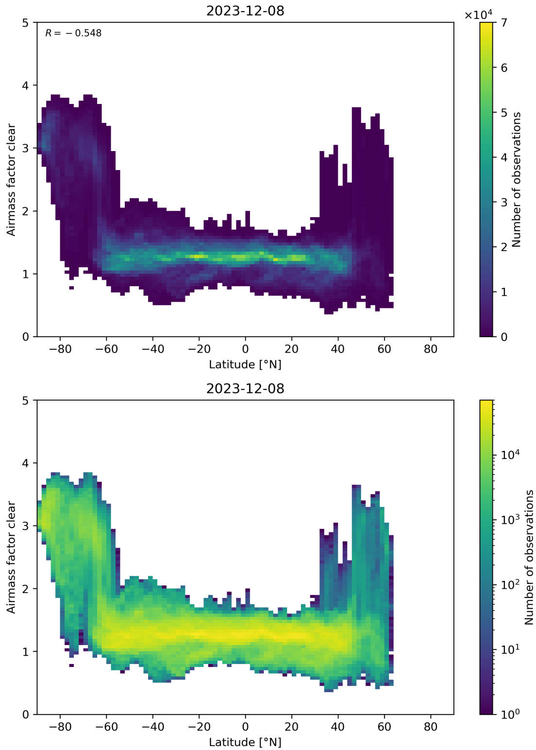
Figure 156: Scatter density plot of “Latitude” against “Airmass factor clear” for 2023-12-07 to 2023-12-09.
