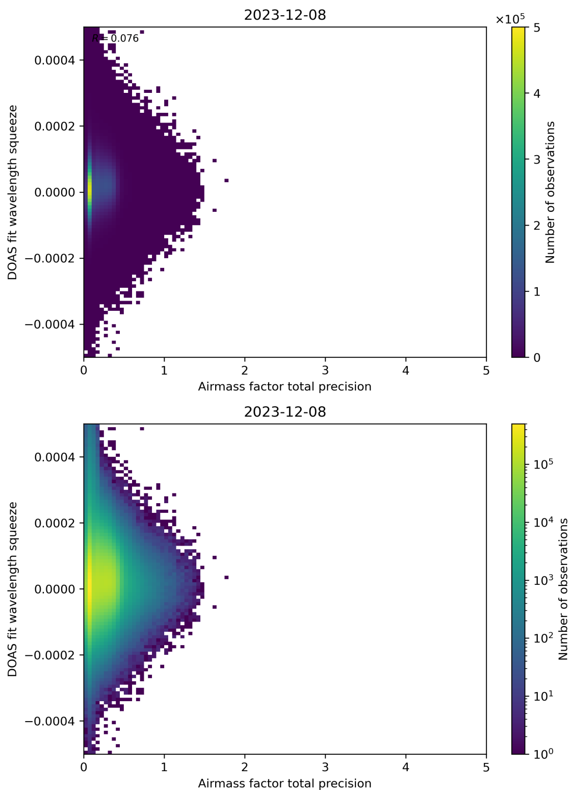
Figure 107: Scatter density plot of “Airmass factor total precision” against “DOAS fit wavelength squeeze” for 2023-12-07 to 2023-12-09.
