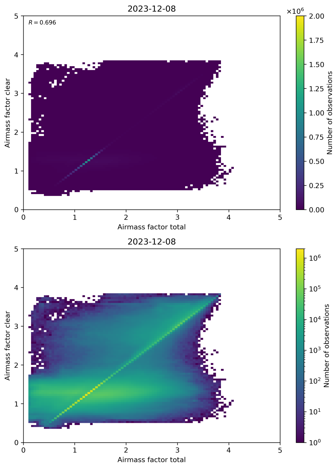
Figure 100: Scatter density plot of “Airmass factor total” against “Airmass factor clear” for 2023-12-07 to 2023-12-09.
