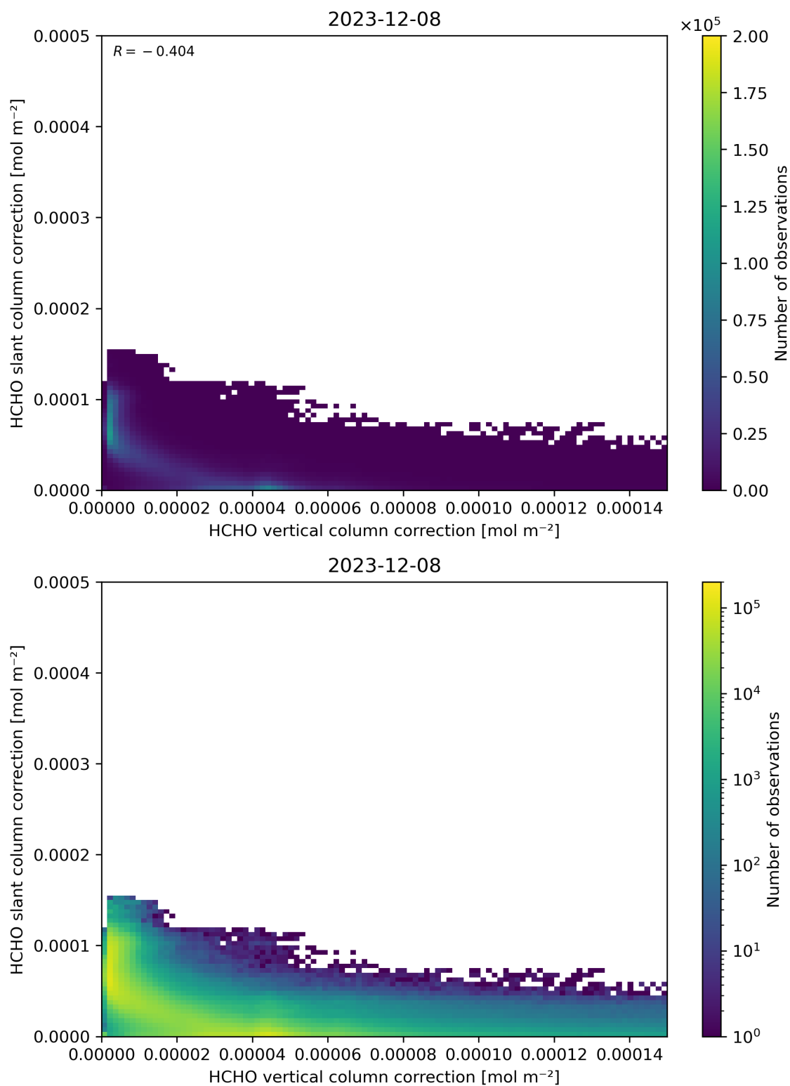
Figure 117: Scatter density plot of “HCHO vertical column correction” against “HCHO slant column correction” for 2023-12-07 to 2023-12-09.
