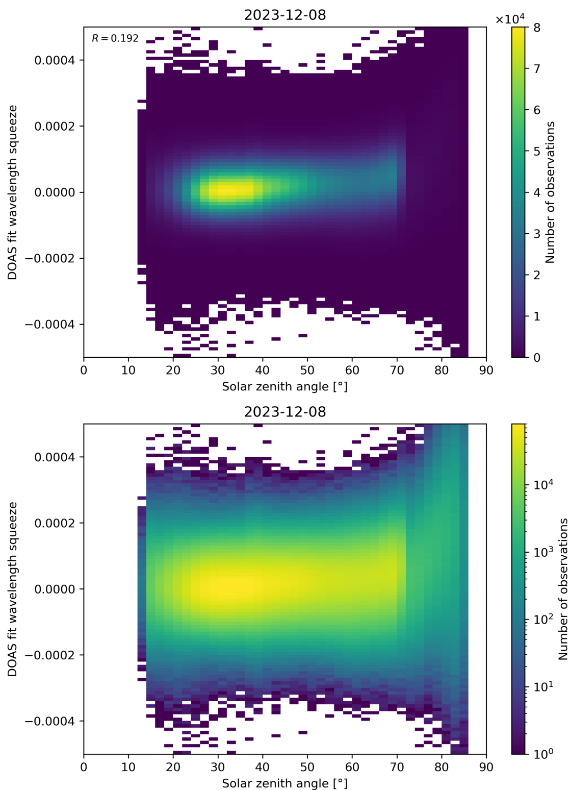
Figure 169: Scatter density plot of “Solar zenith angle” against “DOAS fit wavelength squeeze” for 2023-12-07 to 2023-12-09.
