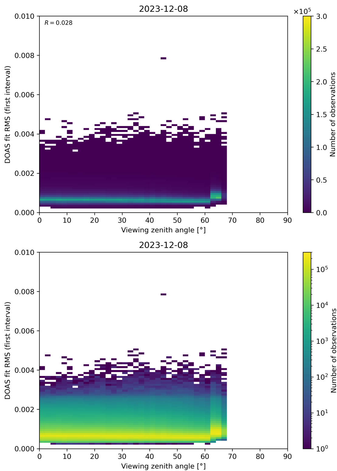
Figure 182: Scatter density plot of “Viewing zenith angle” against “DOAS fit RMS (first interval)” for 2023-12-07 to 2023-12-09.
