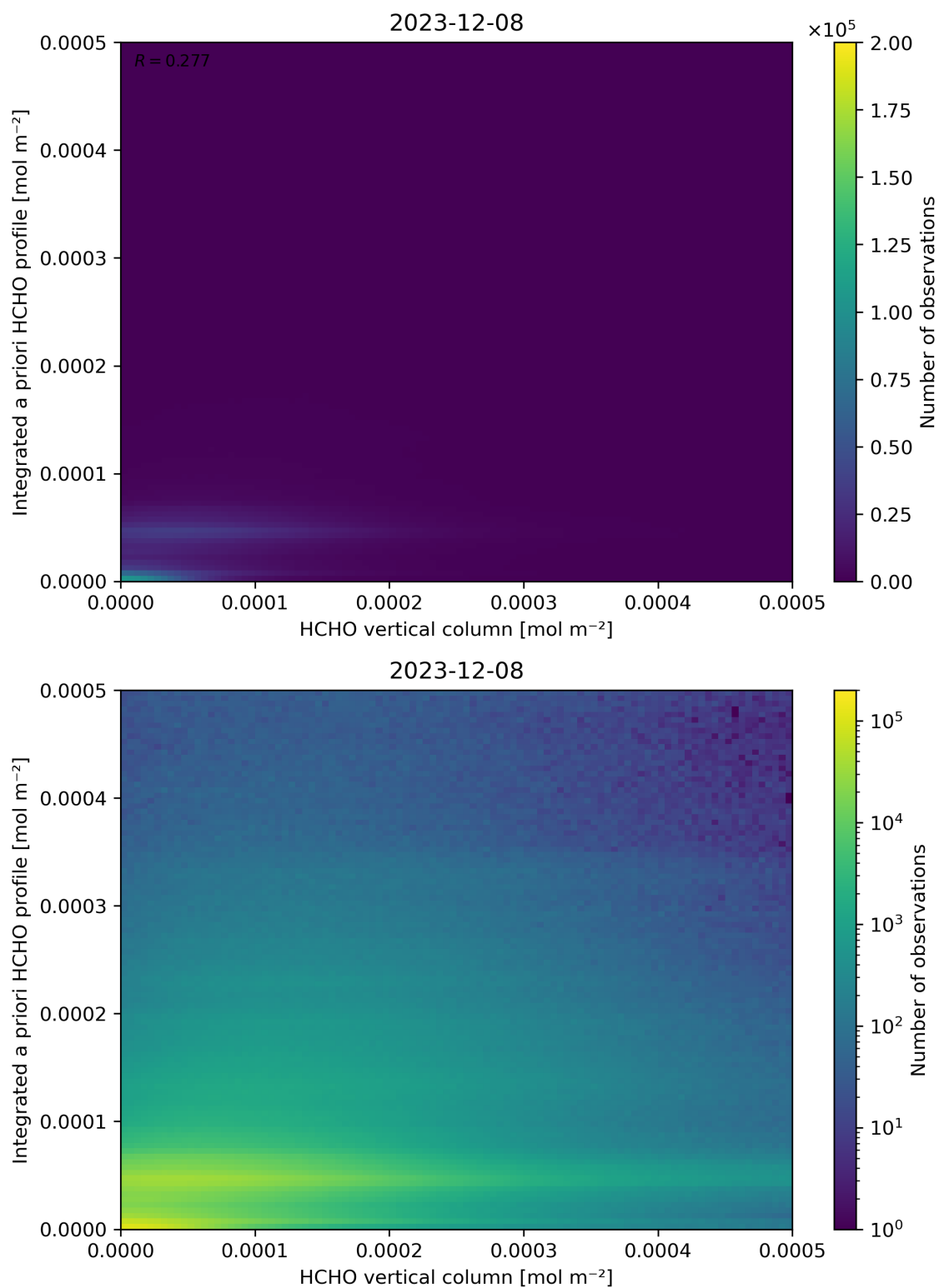
Figure 135: Scatter density plot of “HCHO vertical column” against “Integrated a priori HCHO profile” for 2023-12-07 to 2023-12-09.
