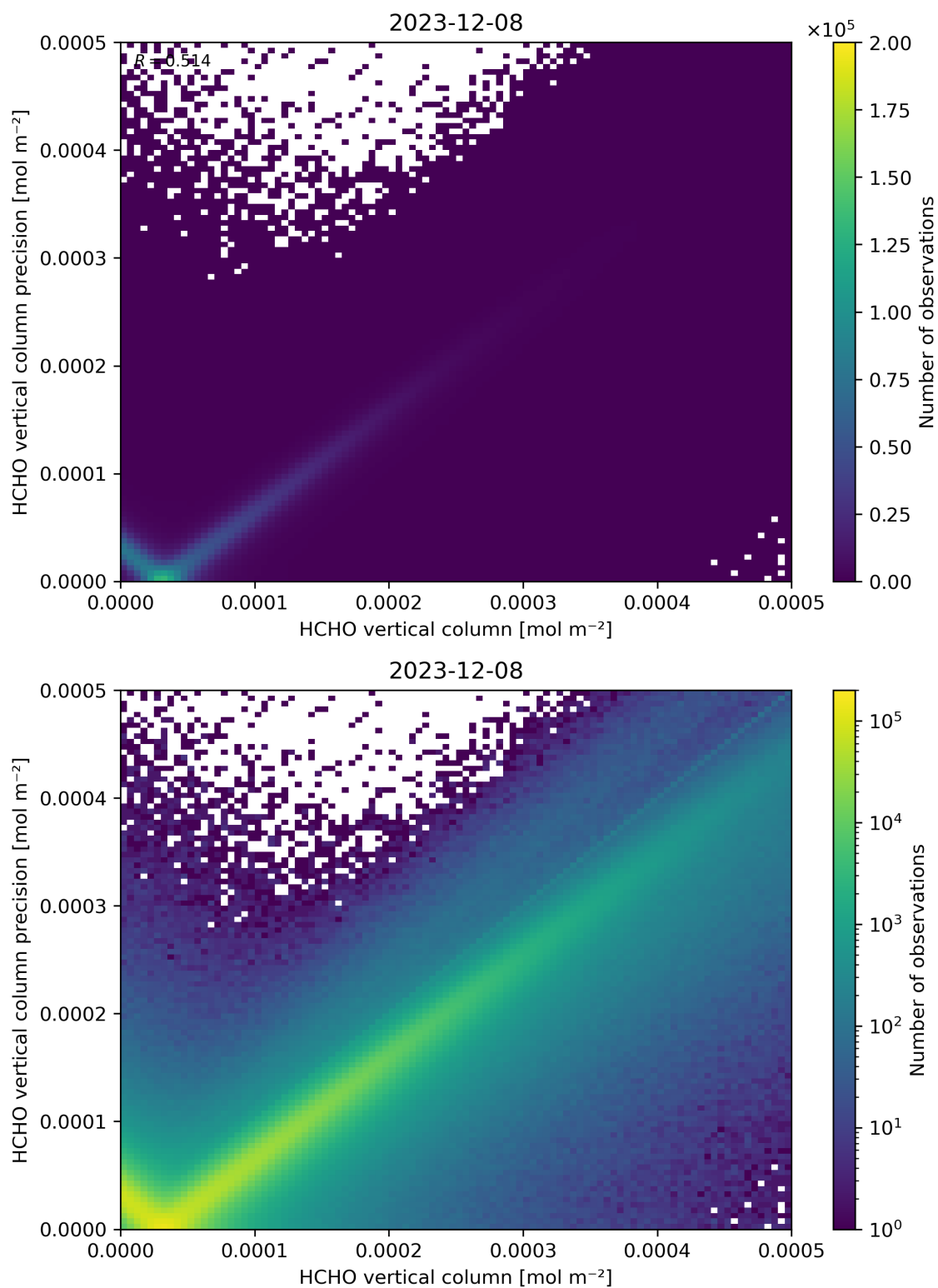
Figure 134: Scatter density plot of “HCHO vertical column” against “HCHO vertical column precision” for 2023-12-07 to 2023-12-09.
