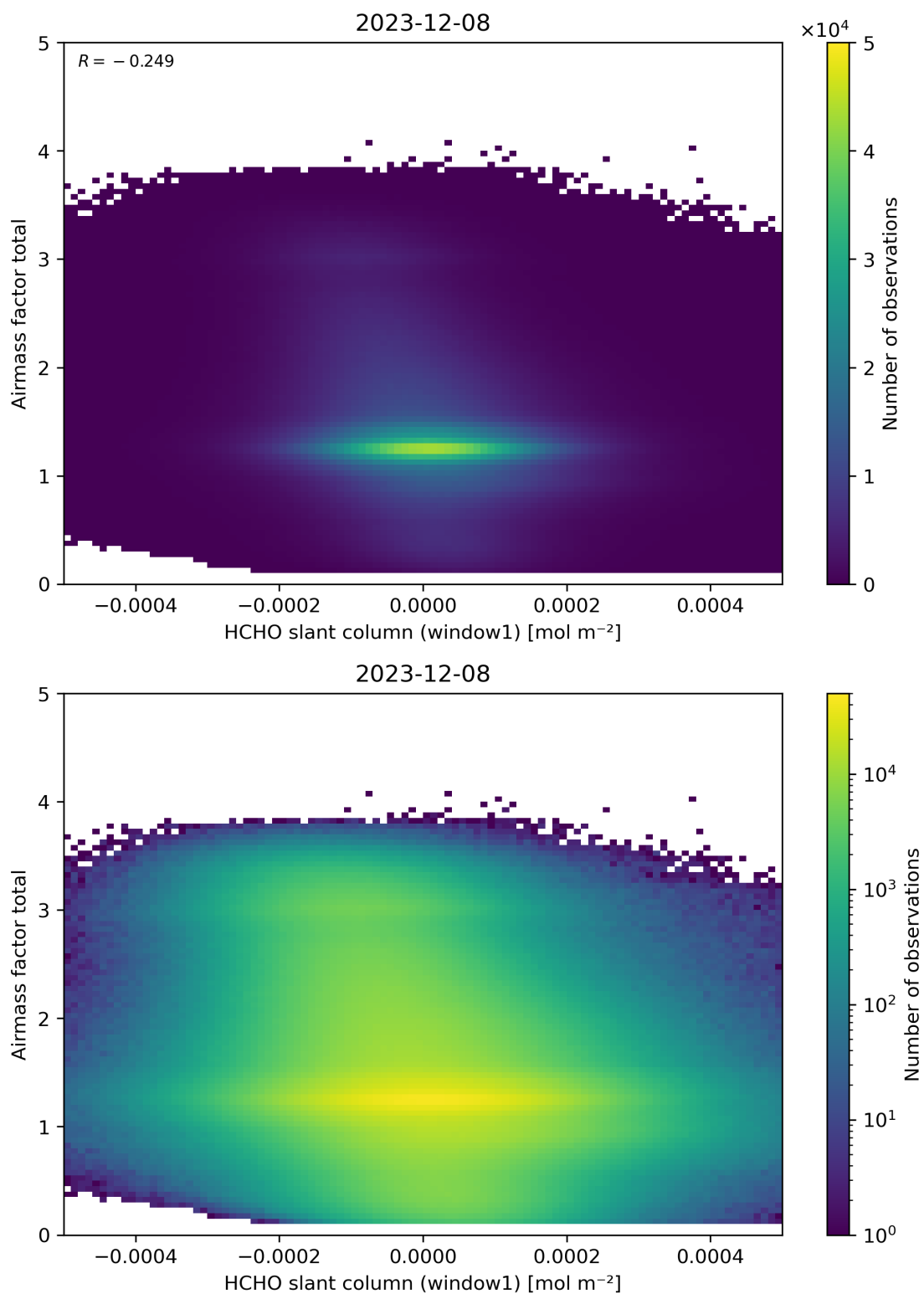
Figure 85: Scatter density plot of “HCHO slant column (window1)” against “Airmass factor total” for 2023-12-07 to 2023-12-09.
