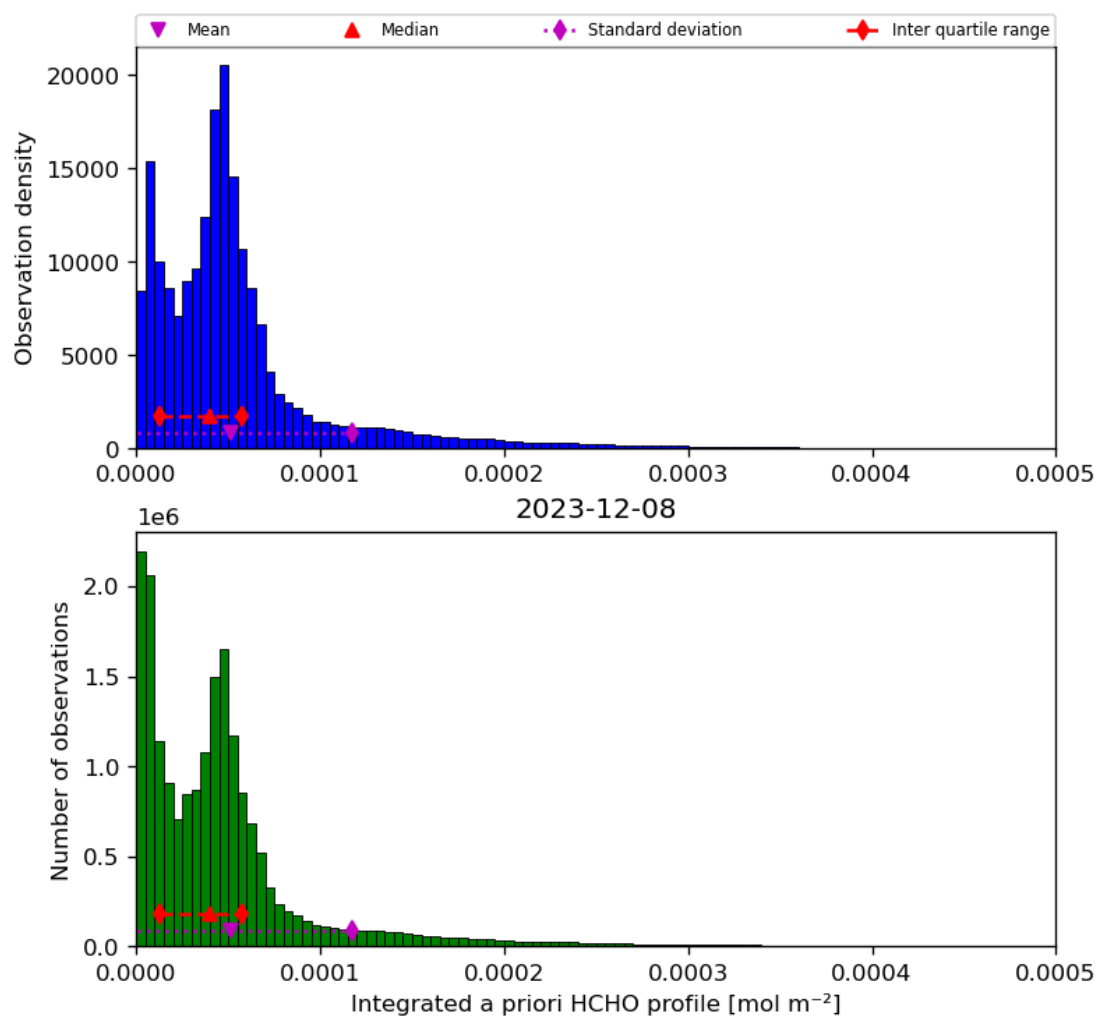
Figure 43: Histogram of “Integrated a priori HCHO profile” for 2023-12-07 to 2023-12-09
