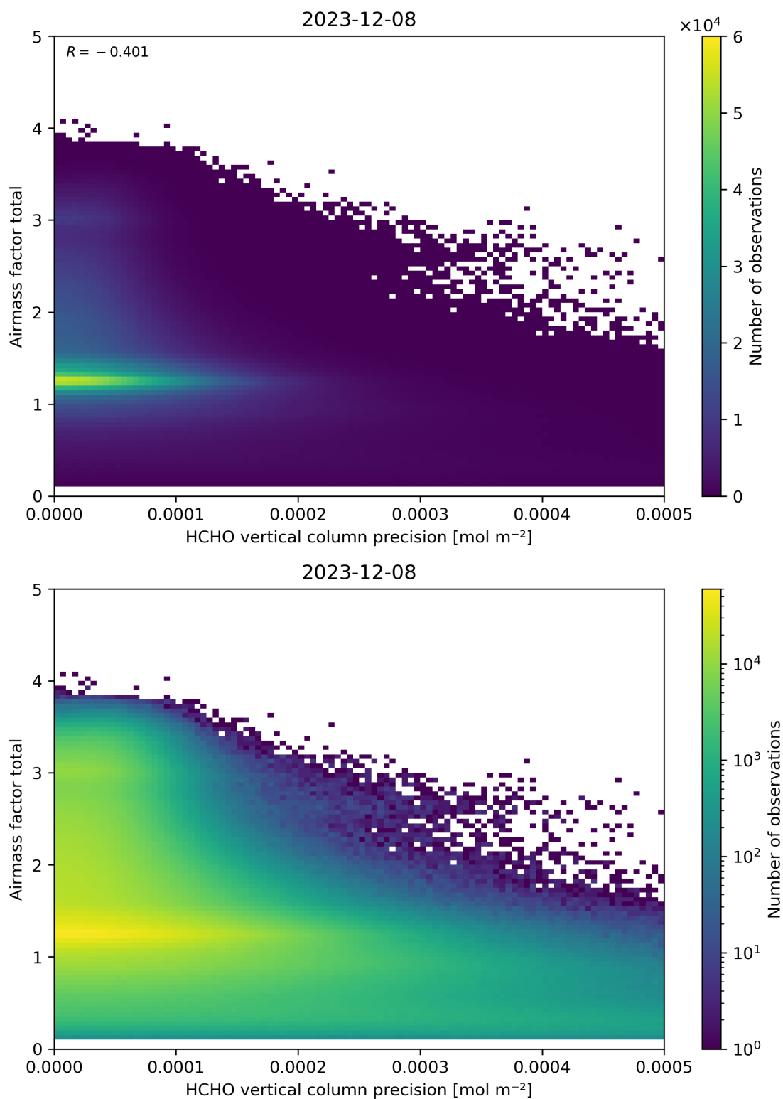
Figure 144: Scatter density plot of “HCHO vertical column precision” against “Airmass factor total” for 2023-12-07 to 2023-12-09.
