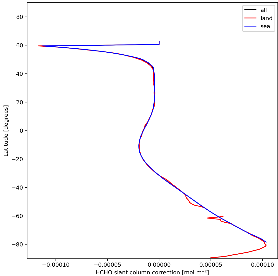
Figure 33: Zonal average of “HCHO slant column correction” for 2023-12-07 to 2023-12-09.
