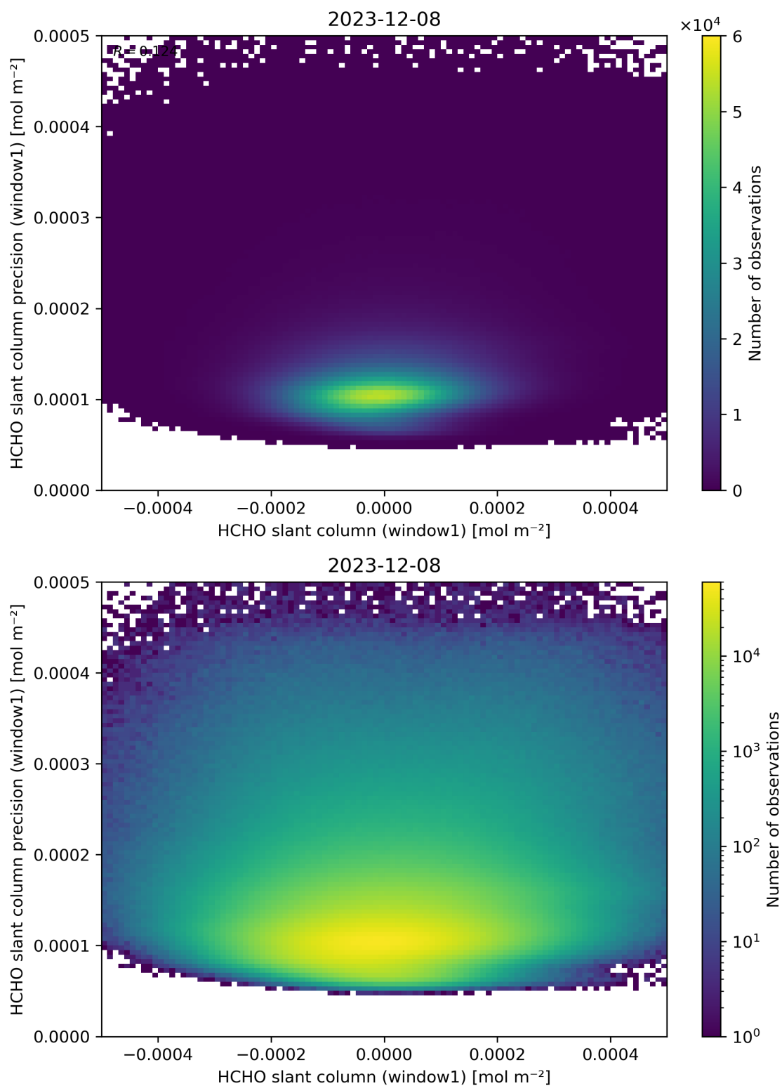
Figure 84: Scatter density plot of “HCHO slant column (window1)” against “HCHO slant column precision (window1)” for 2023-12-07 to 2023-12-09.
