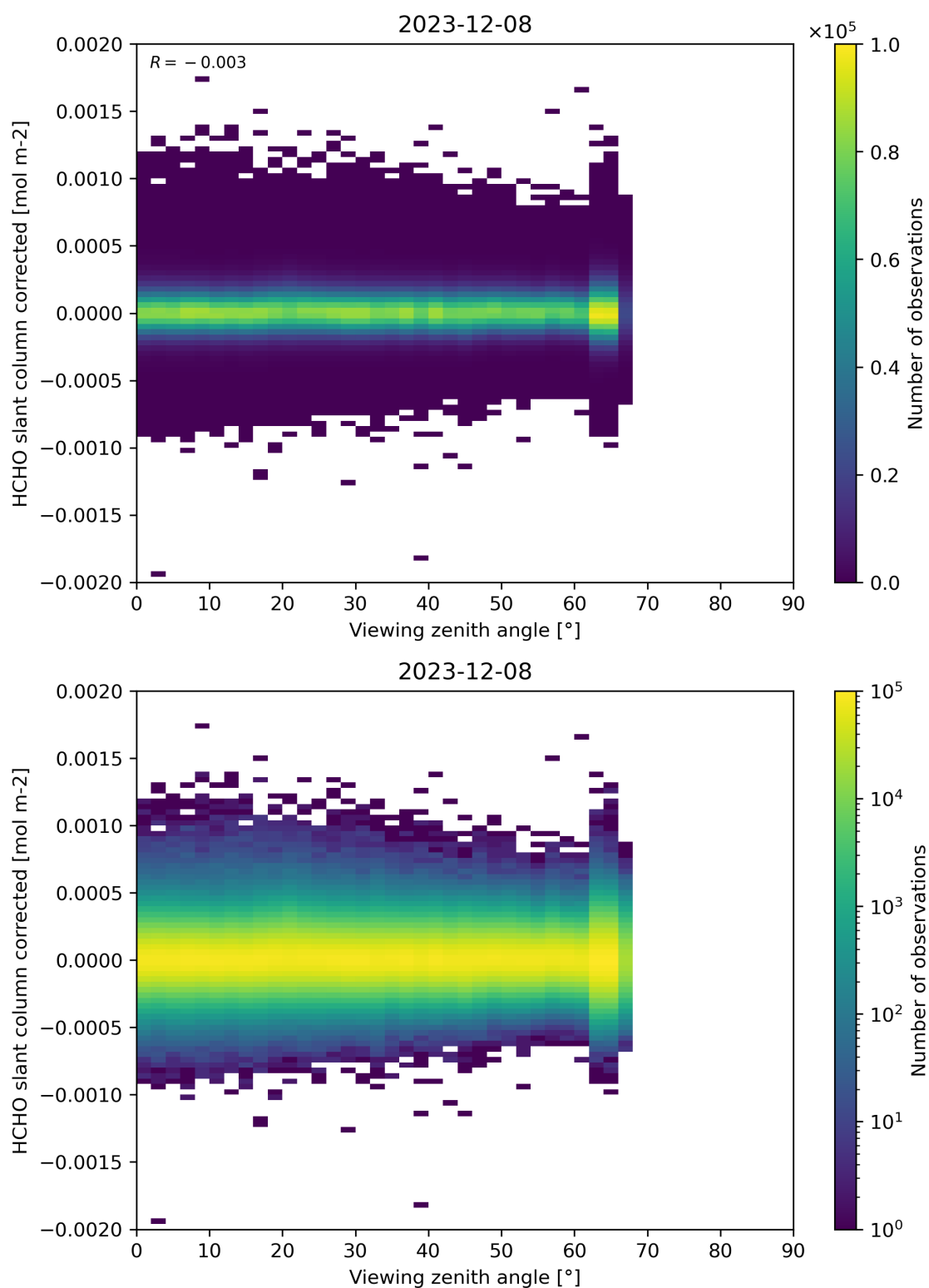
Figure 186: Scatter density plot of “Viewing zenith angle” against “HCHO slant column corrected” for 2023-12-07 to 2023-12-09.
