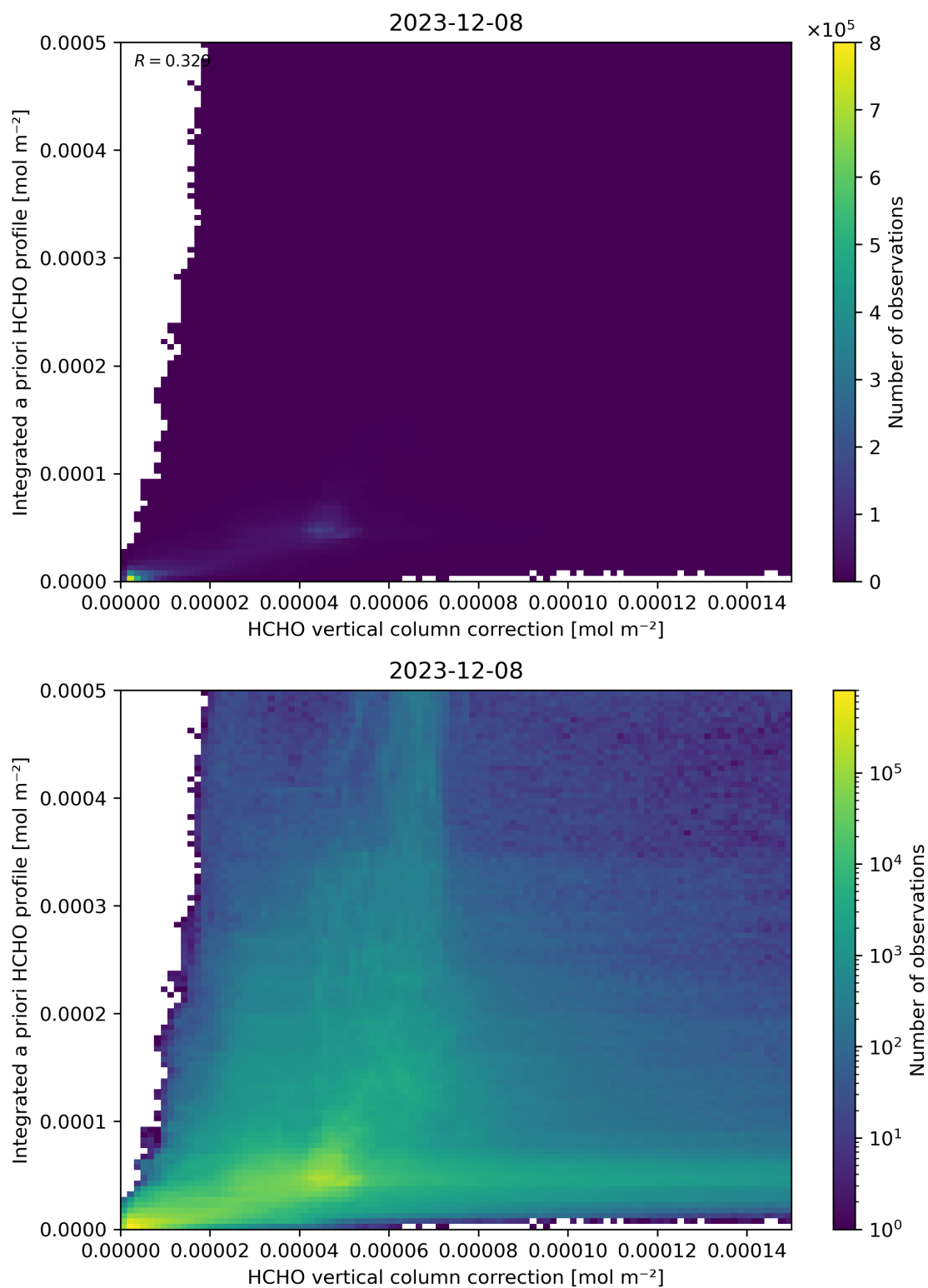
Figure 122: Scatter density plot of “HCHO vertical column correction” against “Integrated a priori HCHO profile” for 2023-12-07 to 2023-12-09.
