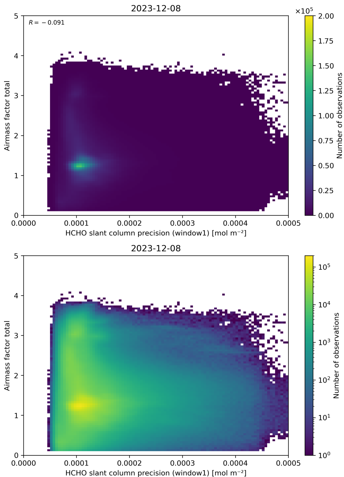
Figure 94: Scatter density plot of “HCHO slant column precision (window1)” against “Airmass factor total” for 2023-12-07 to 2023-12-09.
