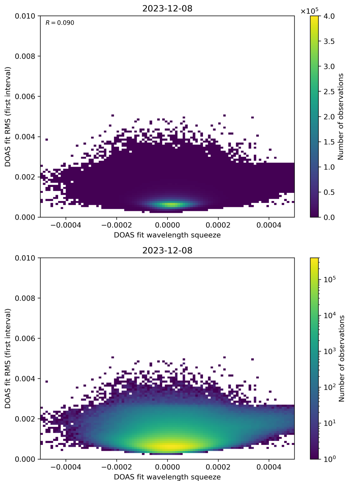
Figure 68: Scatter density plot of “DOAS fit wavelength squeeze” against “DOAS fit RMS (first interval)” for 2023-12-07 to 2023-12-09.
