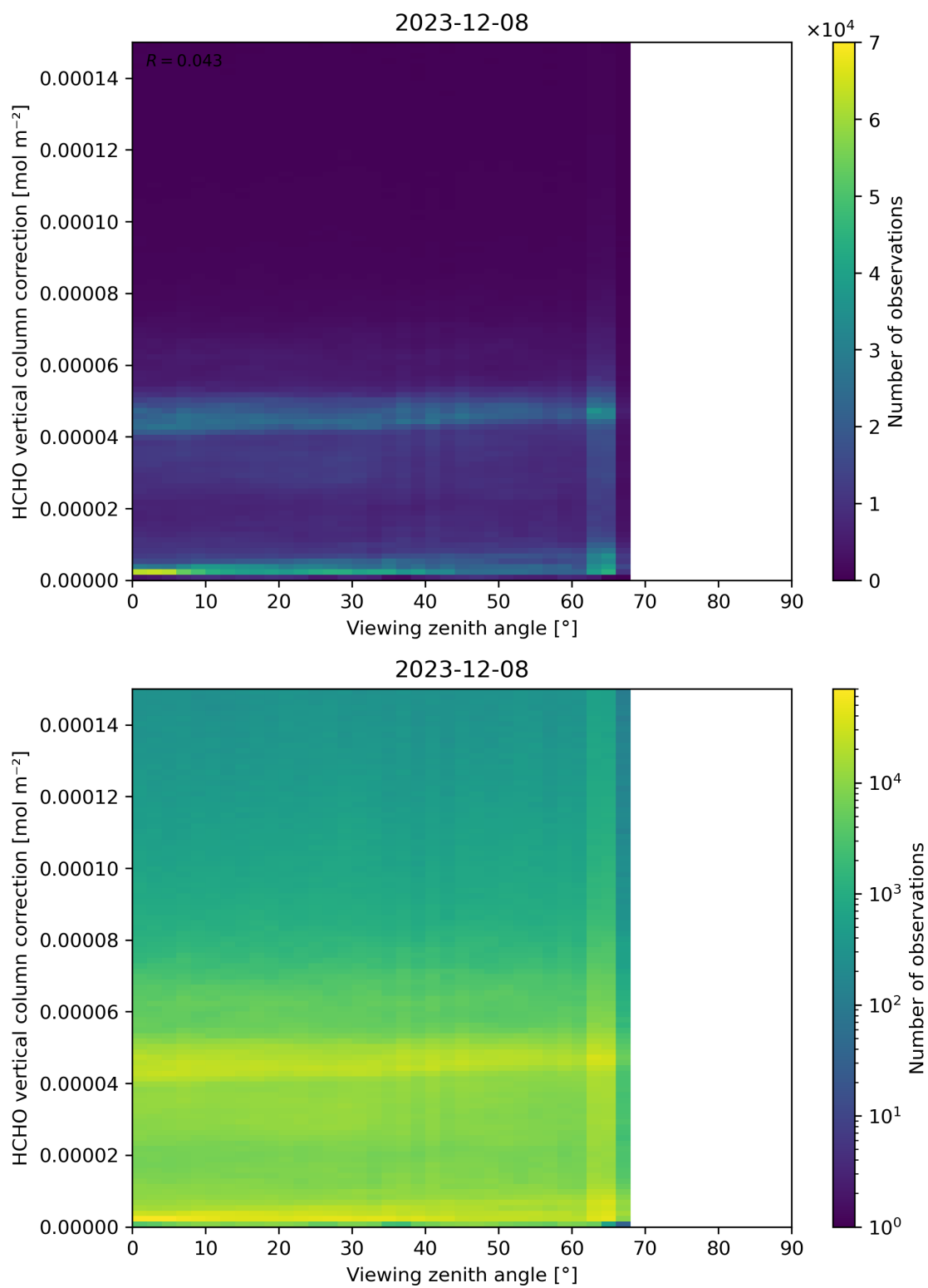
Figure 193: Scatter density plot of “Viewing zenith angle” against “HCHO vertical column correction” for 2023-12-07 to 2023-12-09.
