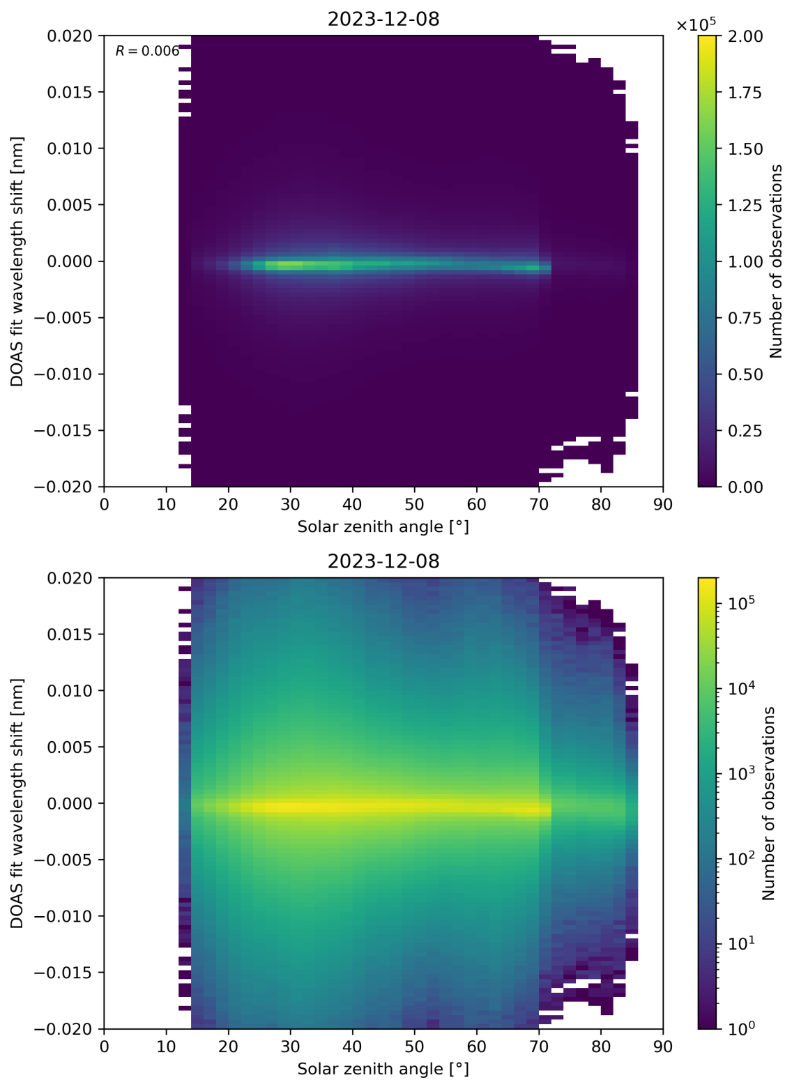
Figure 168: Scatter density plot of “Solar zenith angle” against “DOAS fit wavelength shift” for 2023-12-07 to 2023-12-09.
