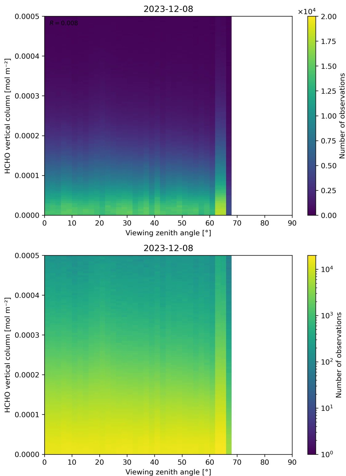
Figure 192: Scatter density plot of “Viewing zenith angle” against “HCHO vertical column” for 2023-12-07 to 2023-12-09.
