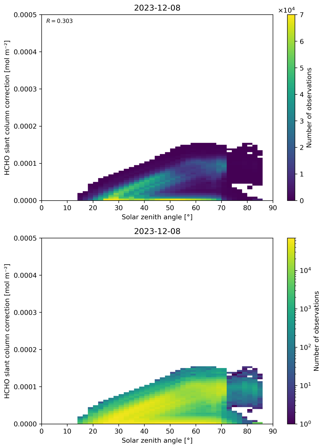
Figure 172: Scatter density plot of “Solar zenith angle” against “HCHO slant column correction” for 2023-12-07 to 2023-12-09.
