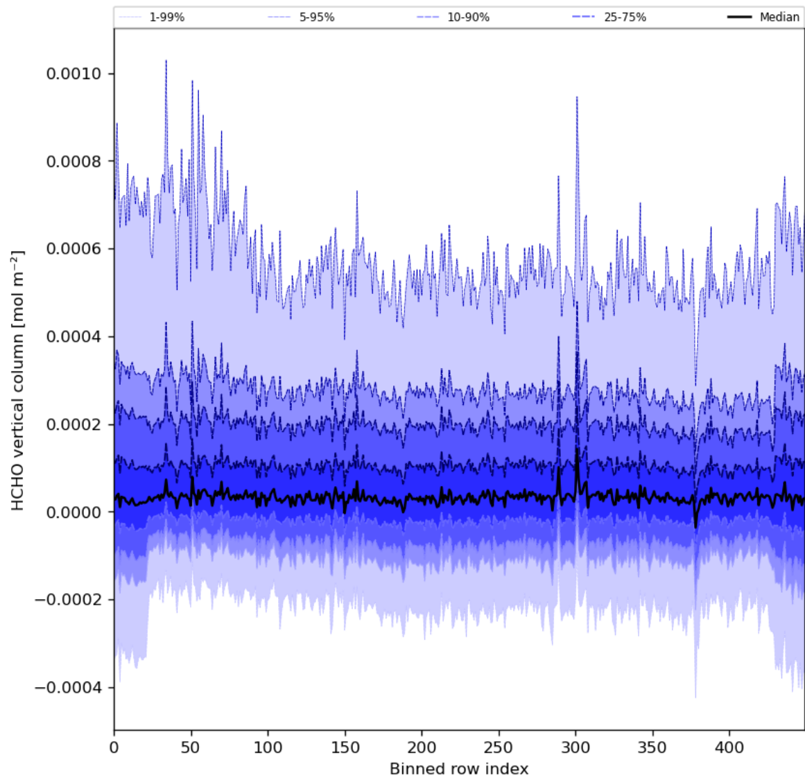
Figure 49: Along track statistics of “HCHO vertical column” for 2023-12-07 to 2023-12-09
