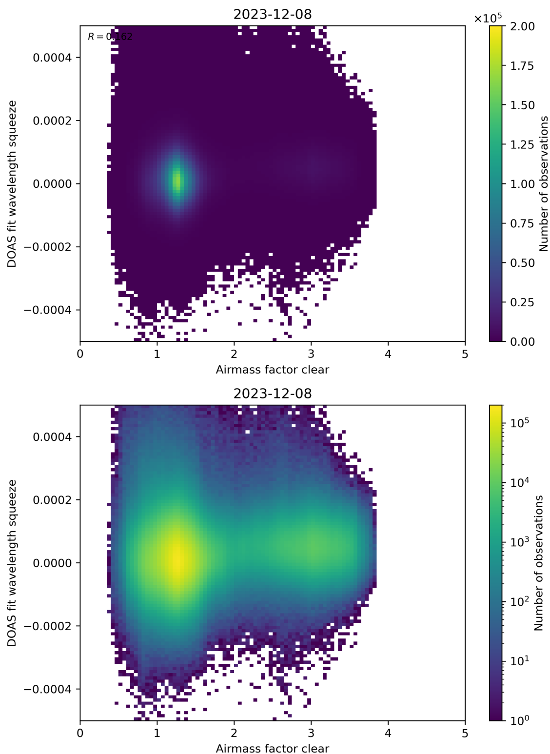
Figure 73: Scatter density plot of “Airmass factor clear” against “DOAS fit wavelength squeeze” for 2023-12-07 to 2023-12-09.
