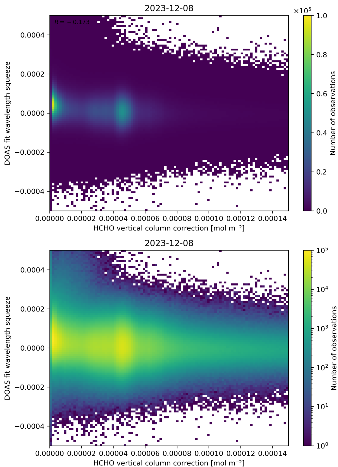
Figure 114: Scatter density plot of “HCHO vertical column correction” against “DOAS fit wavelength squeeze” for 2023-12-07 to 2023-12-09.
