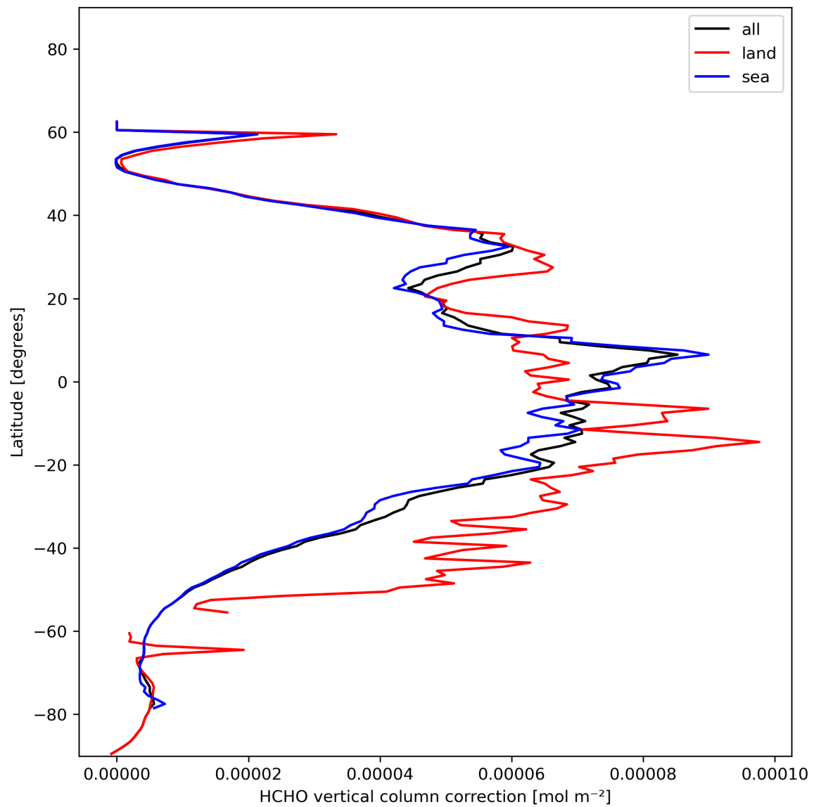
Figure 23: Zonal average of “HCHO vertical column correction” for 2023-12-07 to 2023-12-09.
