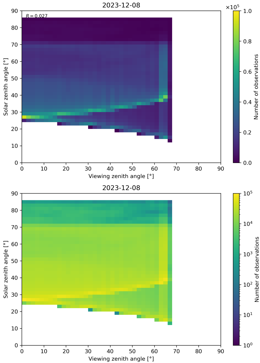
Figure 197: Scatter density plot of “Viewing zenith angle” against “Solar zenith angle” for 2023-12-07 to 2023-12-09.
