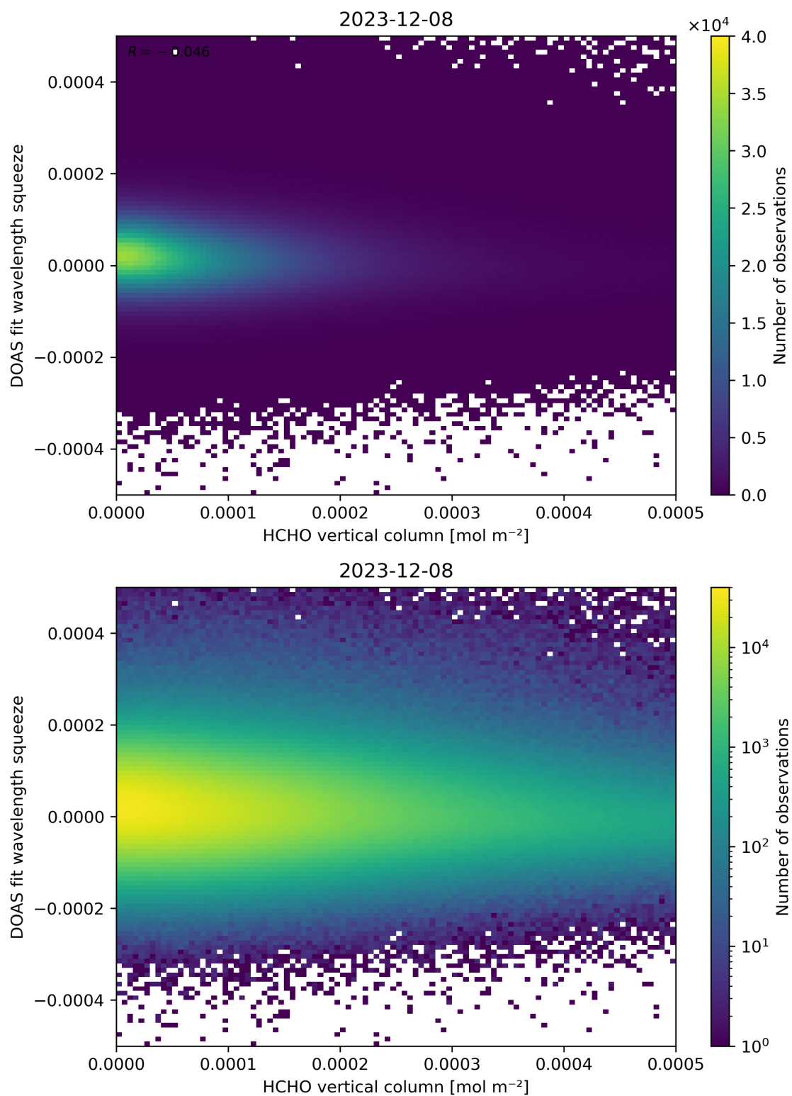
Figure 125: Scatter density plot of “HCHO vertical column” against “DOAS fit wavelength squeeze” for 2023-12-07 to 2023-12-09.
