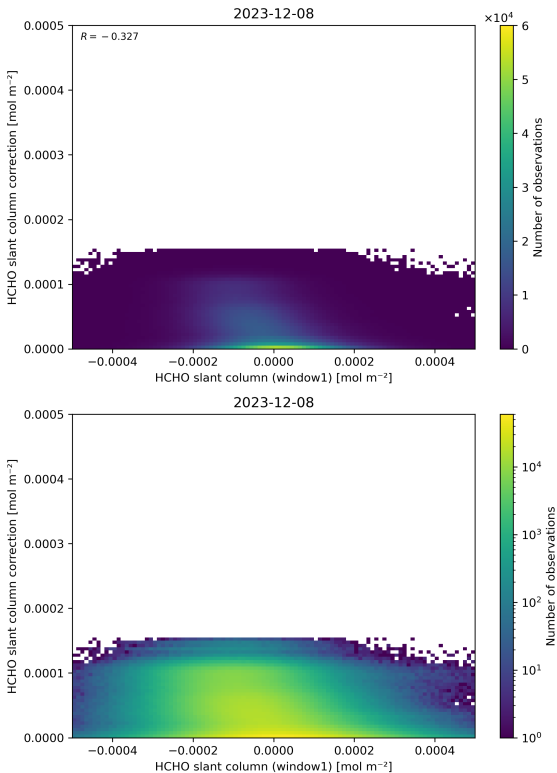
Figure 83: Scatter density plot of “HCHO slant column (window1)” against “HCHO slant column correction” for 2023-12-07 to 2023-12-09.
