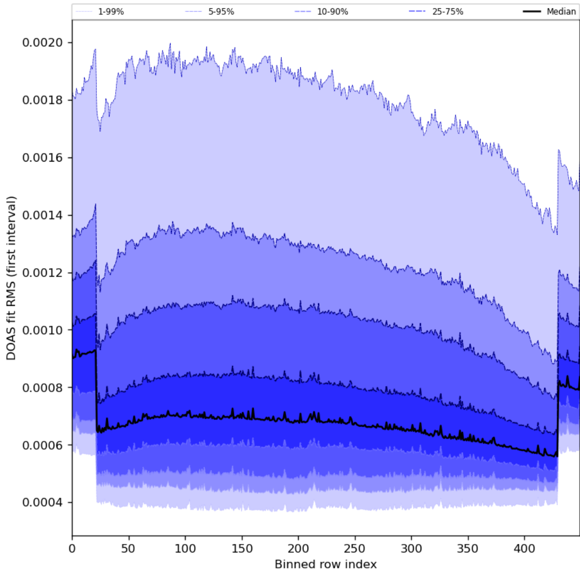
Figure 60: Along track statistics of “DOAS fit RMS (first interval)” for 2023-12-07 to 2023-12-09
