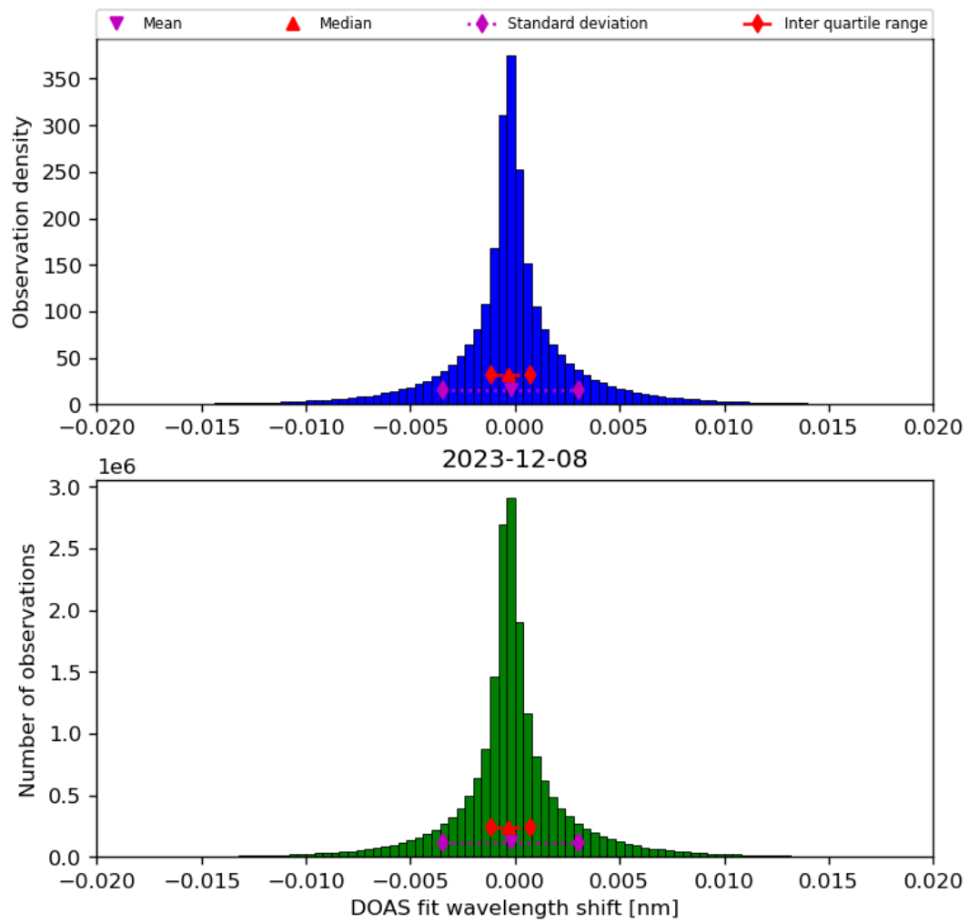
Figure 44: Histogram of “DOAS fit wavelength shift” for 2023-12-07 to 2023-12-09
