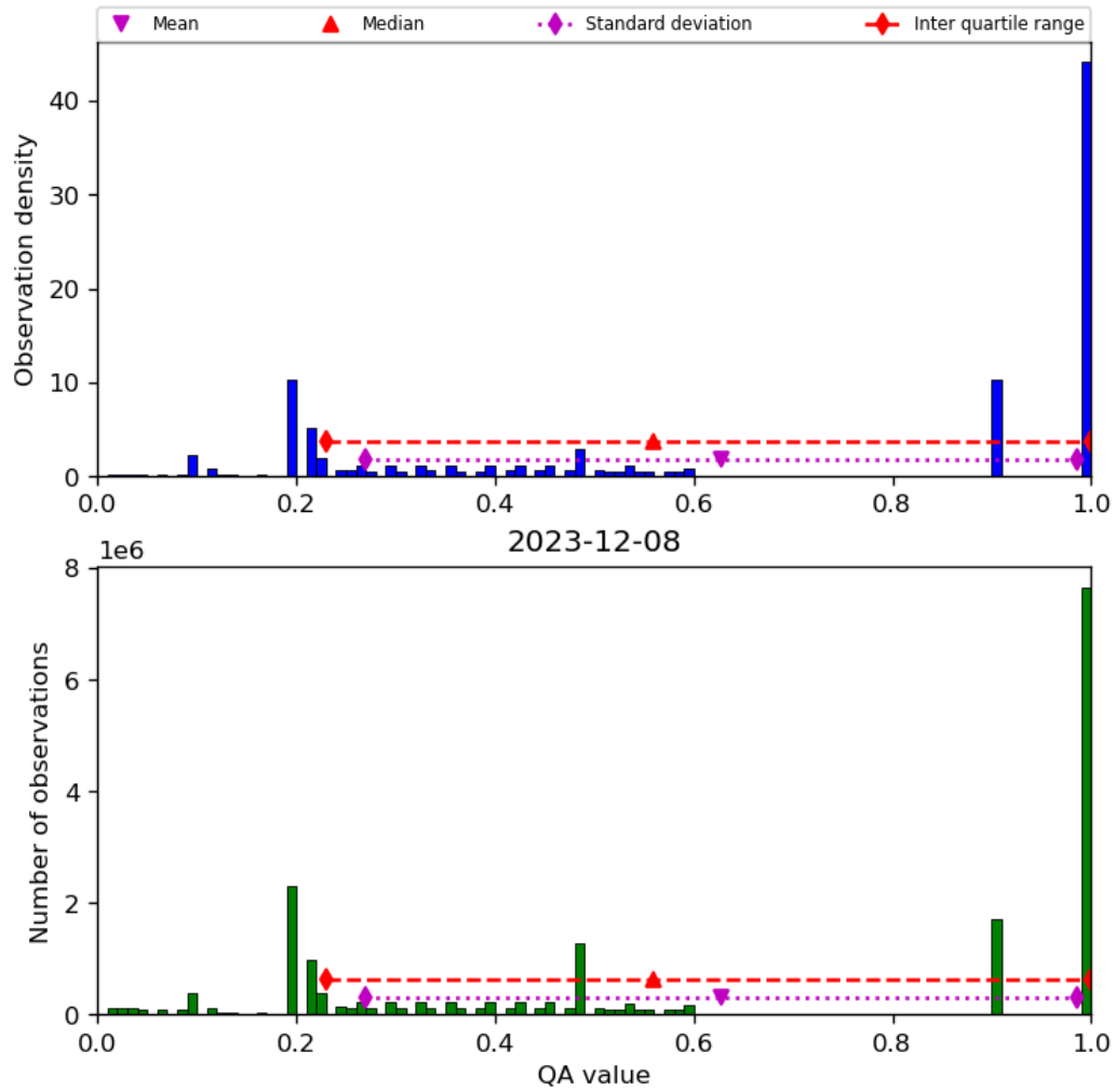
Figure 34: Histogram of “QA value” for 2023-12-07 to 2023-12-09
