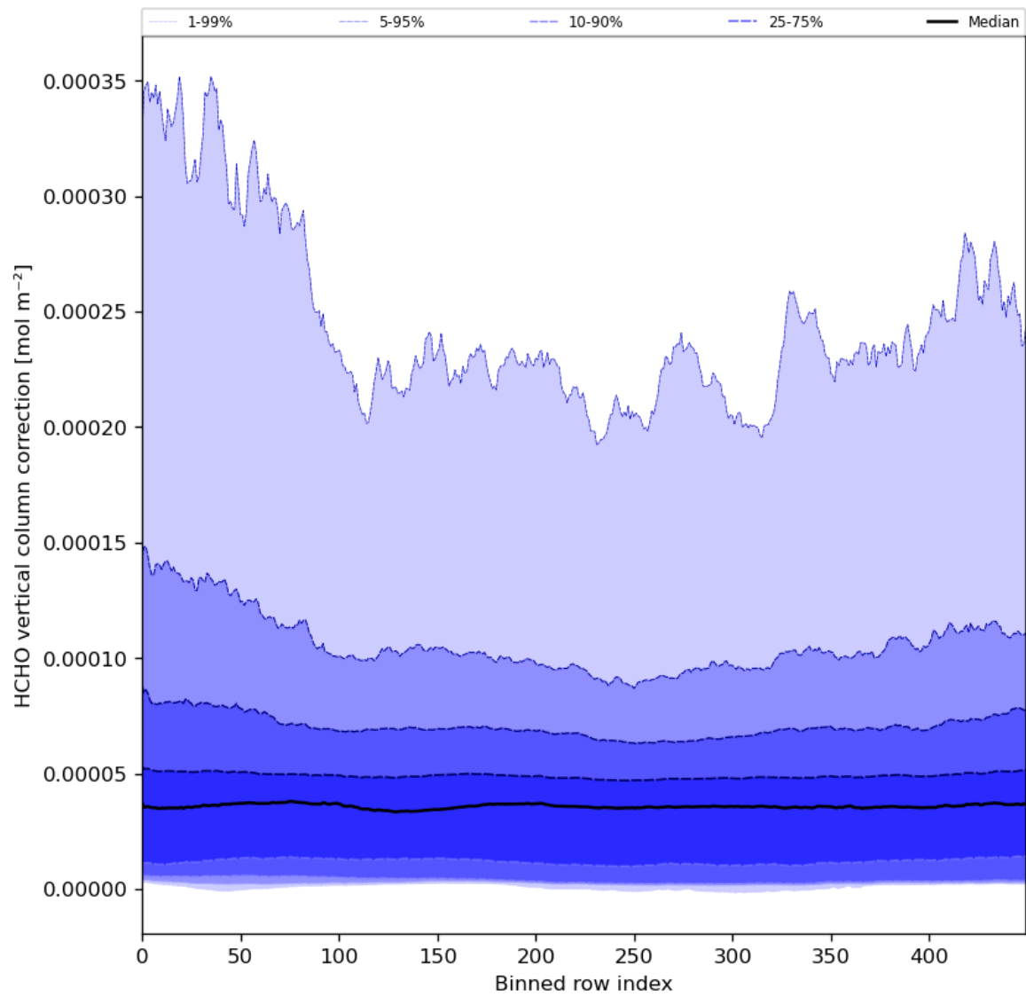
Figure 51: Along track statistics of “HCHO vertical column correction” for 2023-12-07 to 2023-12-09
