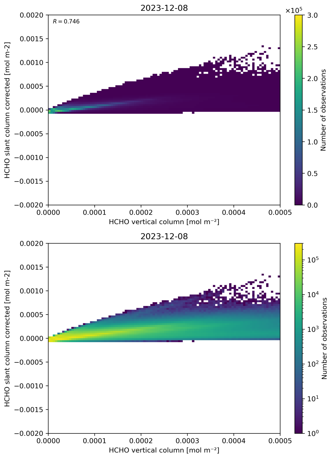
Figure 127: Scatter density plot of “HCHO vertical column” against “HCHO slant column corrected” for 2023-12-07 to 2023-12-09.
