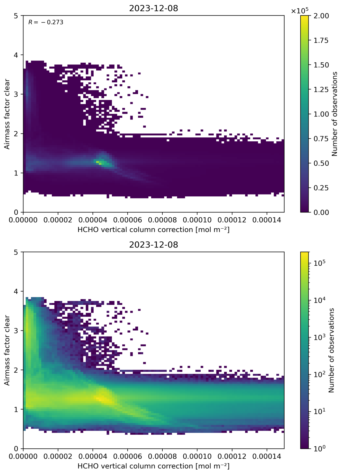
Figure 115: Scatter density plot of “HCHO vertical column correction” against “Airmass factor clear” for 2023-12-07 to 2023-12-09.
