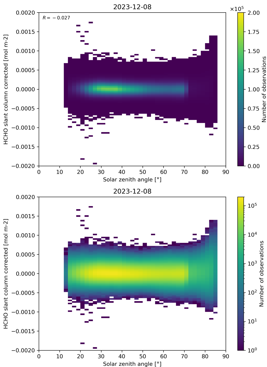
Figure 171: Scatter density plot of “Solar zenith angle” against “HCHO slant column corrected” for 2023-12-07 to 2023-12-09.
