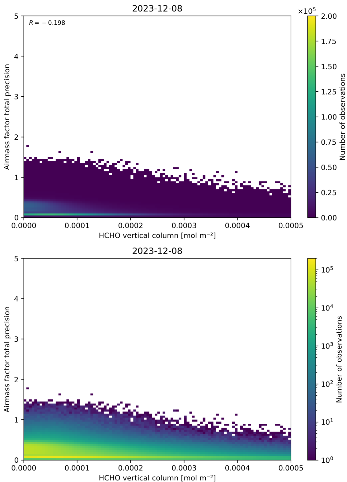
Figure 132: Scatter density plot of “HCHO vertical column” against “Airmass factor total precision” for 2023-12-07 to 2023-12-09.
