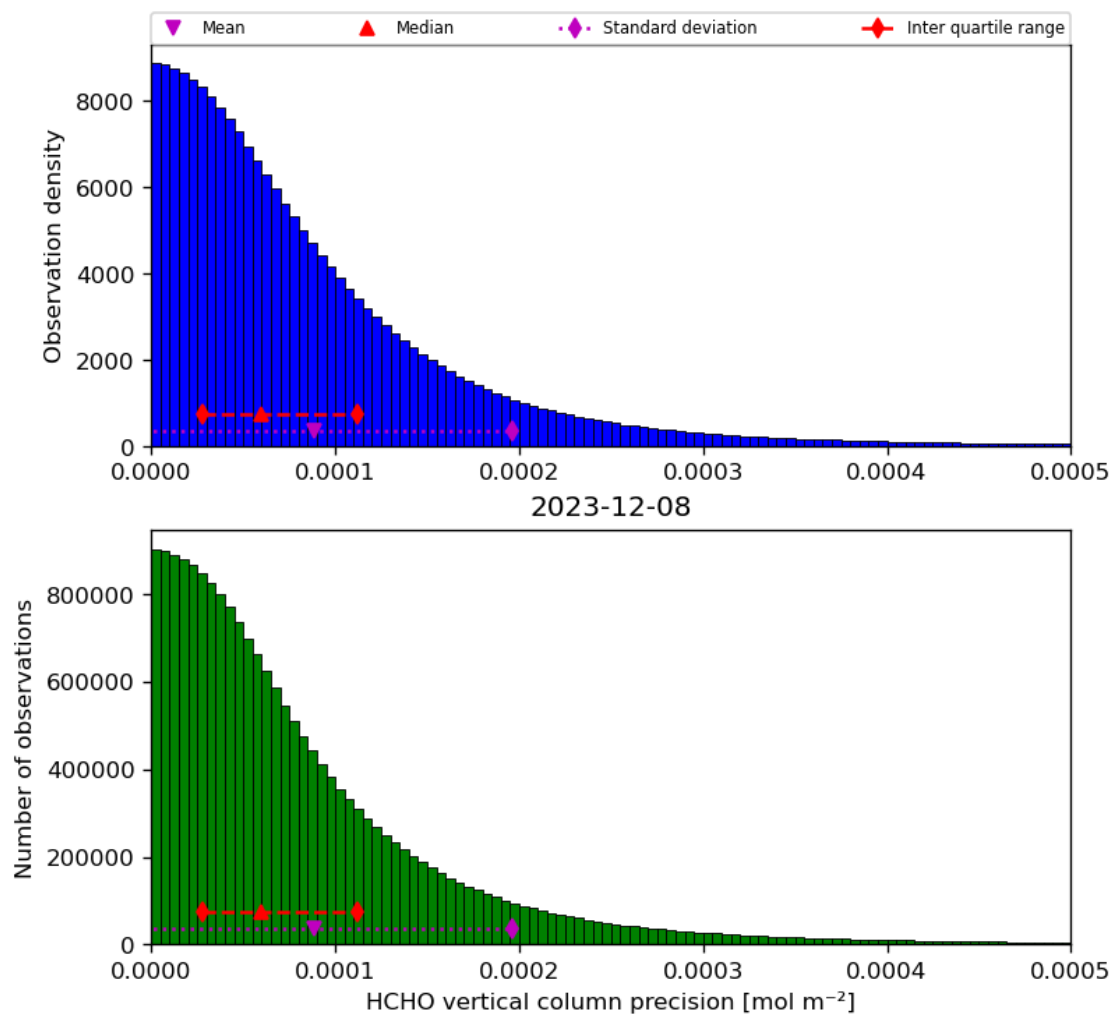
Figure 36: Histogram of “HCHO vertical column precision” for 2023-12-07 to 2023-12-09
