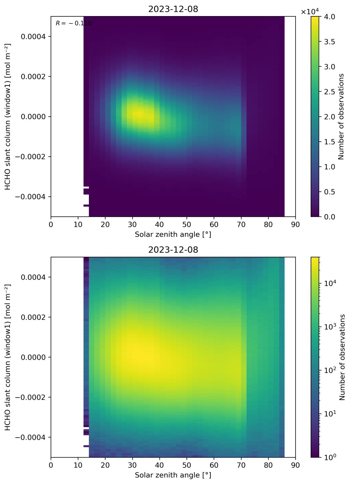
Figure 173: Scatter density plot of “Solar zenith angle” against “HCHO slant column (window1)” for 2023-12-07 to 2023-12-09.
