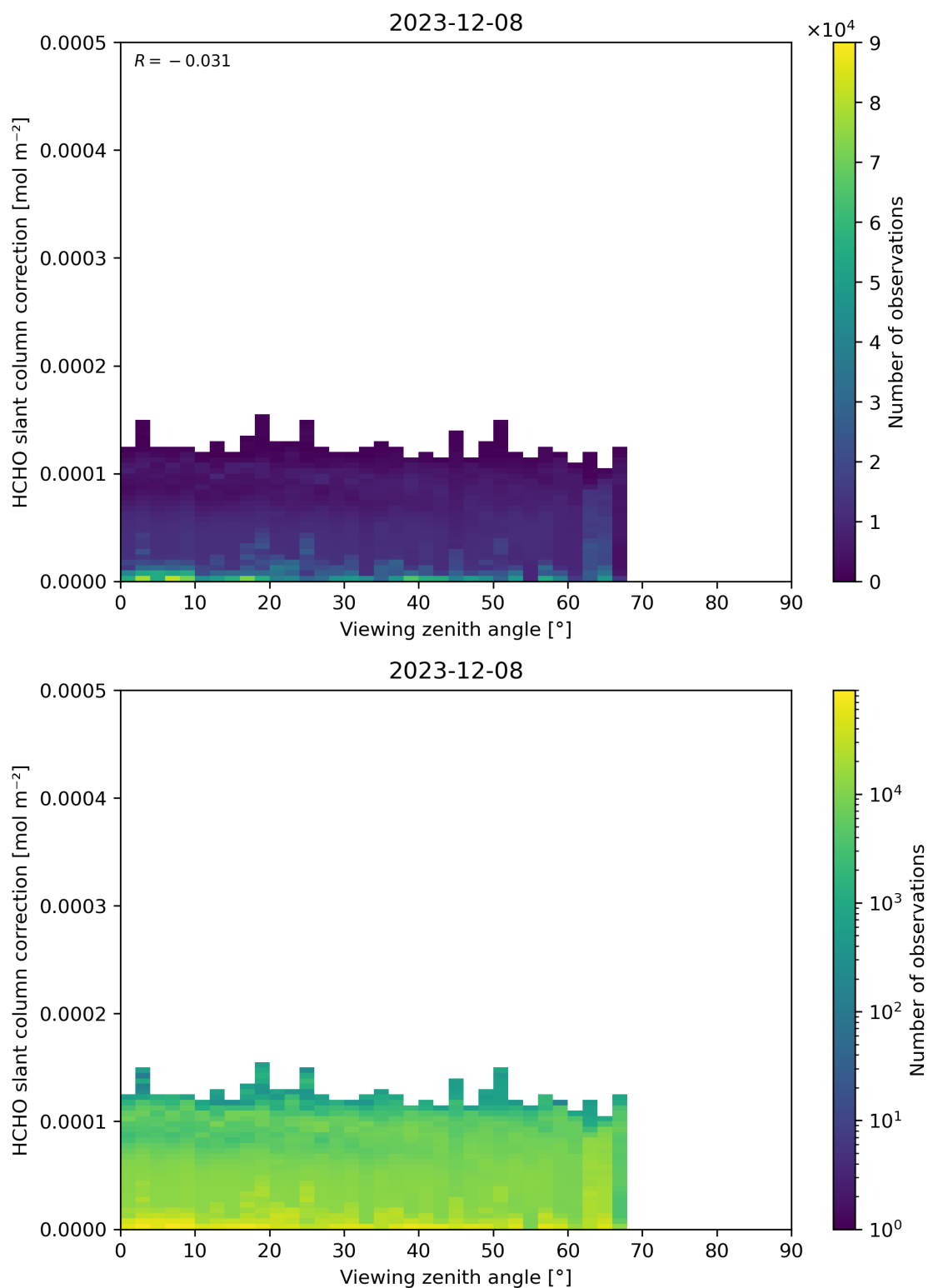
Figure 187: Scatter density plot of “Viewing zenith angle” against “HCHO slant column correction” for 2023-12-07 to 2023-12-09.
