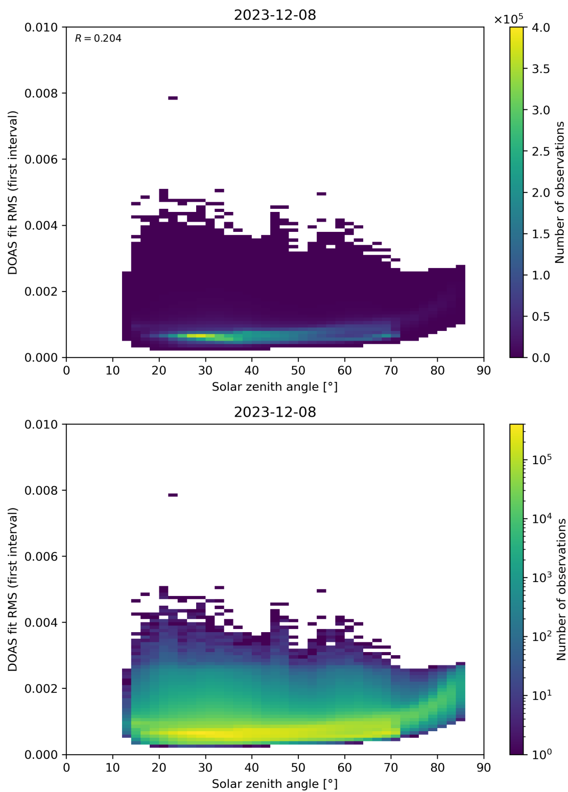
Figure 167: Scatter density plot of “Solar zenith angle” against “DOAS fit RMS (first interval)” for 2023-12-07 to 2023-12-09.
