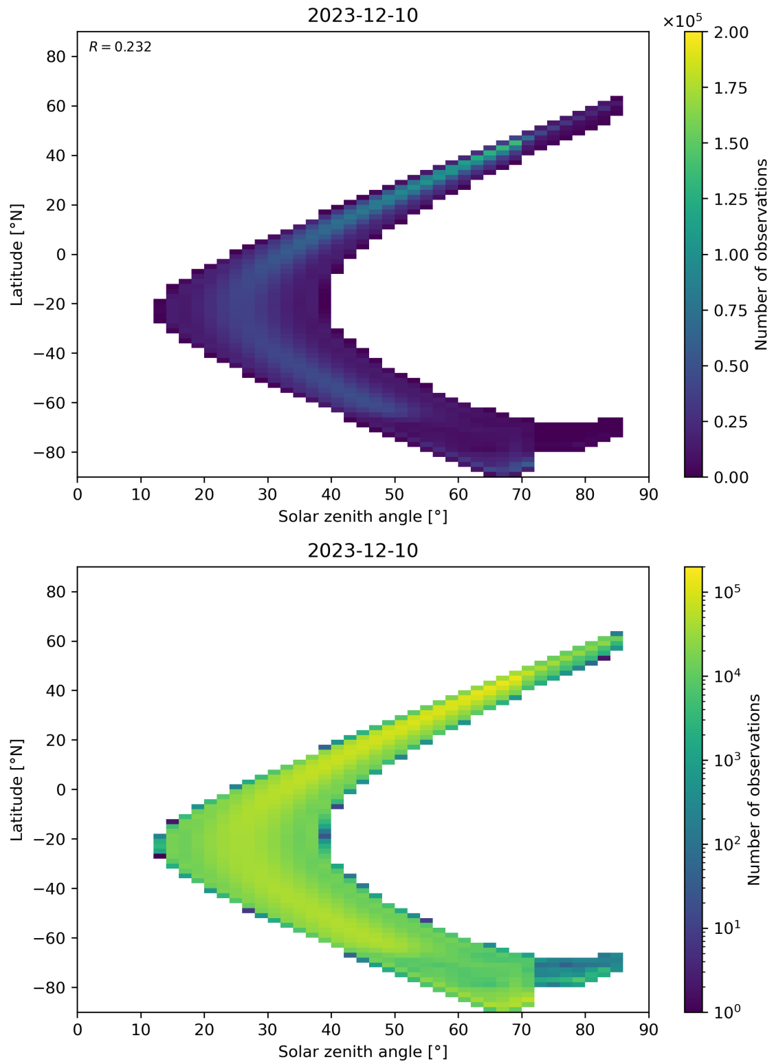
Figure 181: Scatter density plot of “Solar zenith angle” against “Latitude” for 2023-12-09 to 2023-12-11.
