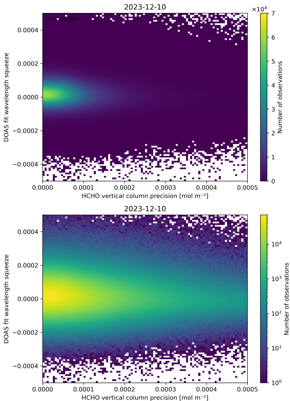
Figure 138: Scatter density plot of “HCHO vertical column precision” against “DOAS fit wavelength squeeze” for 2023-12-09 to 2023-12-11.
