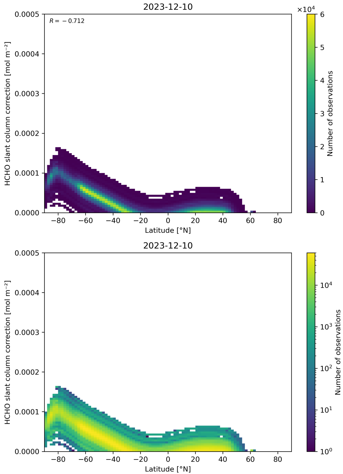
Figure 158: Scatter density plot of “Latitude” against “HCHO slant column correction” for 2023-12-09 to 2023-12-11.
