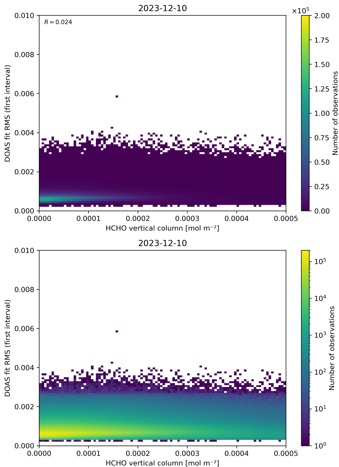
Figure 123: Scatter density plot of “HCHO vertical column” against “DOAS fit RMS (first interval)” for 2023-12-09 to 2023-12-11.
