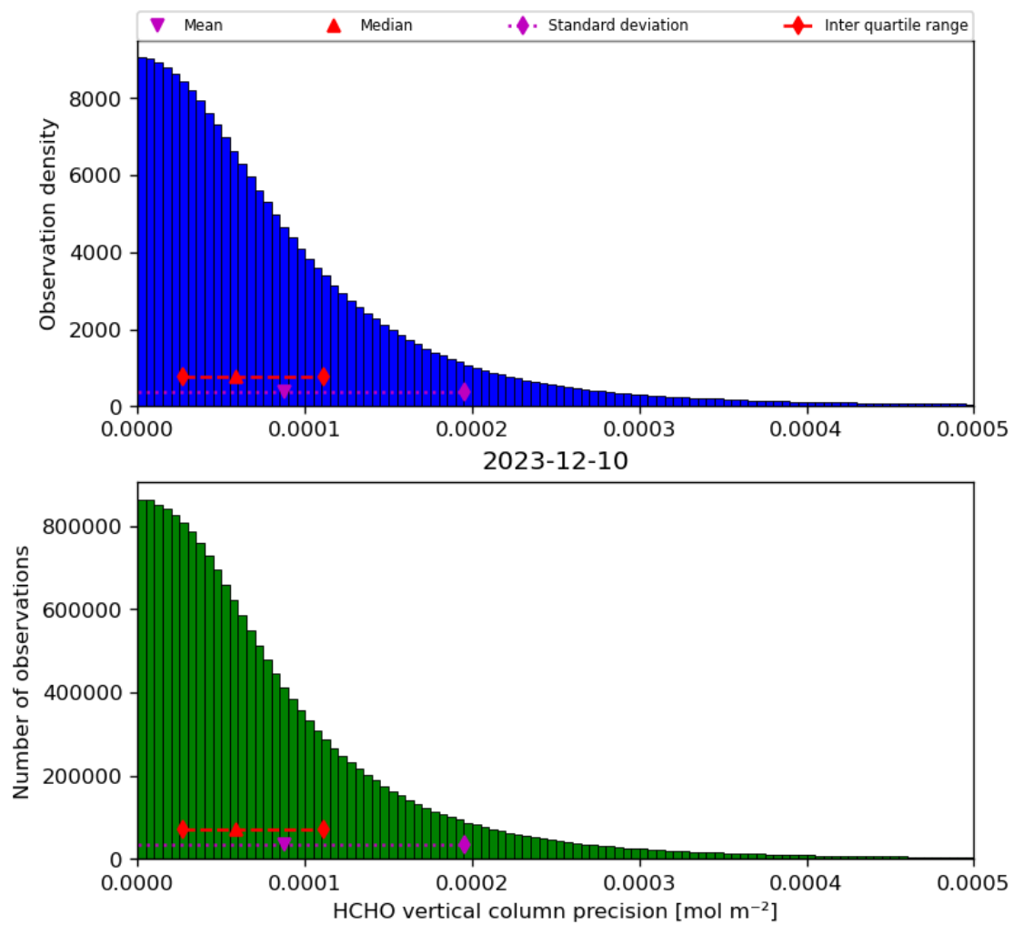
Figure 36: Histogram of “HCHO vertical column precision” for 2023-12-09 to 2023-12-11
