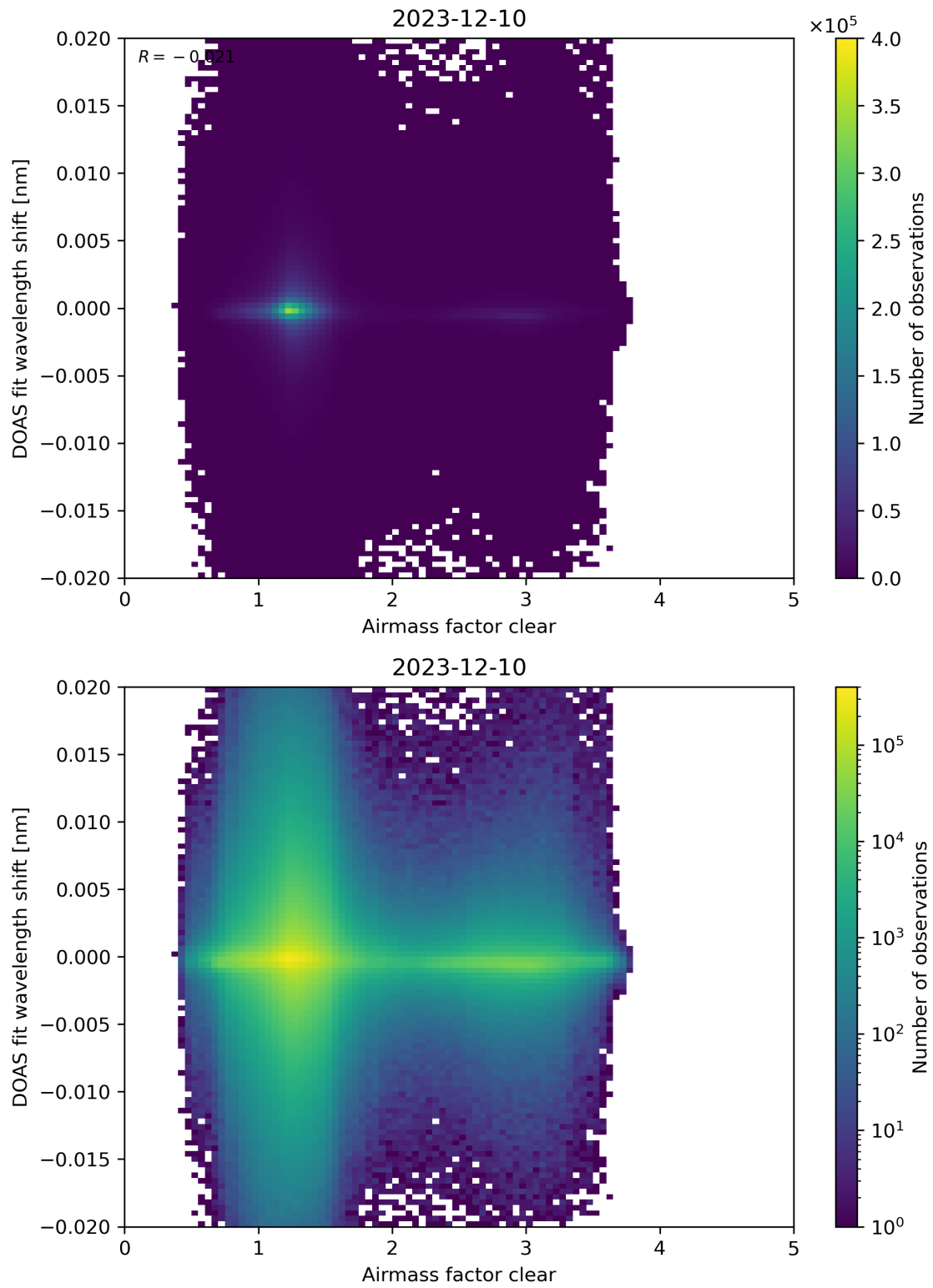
Figure 72: Scatter density plot of “Airmass factor clear” against “DOAS fit wavelength shift” for 2023-12-09 to 2023-12-11.
