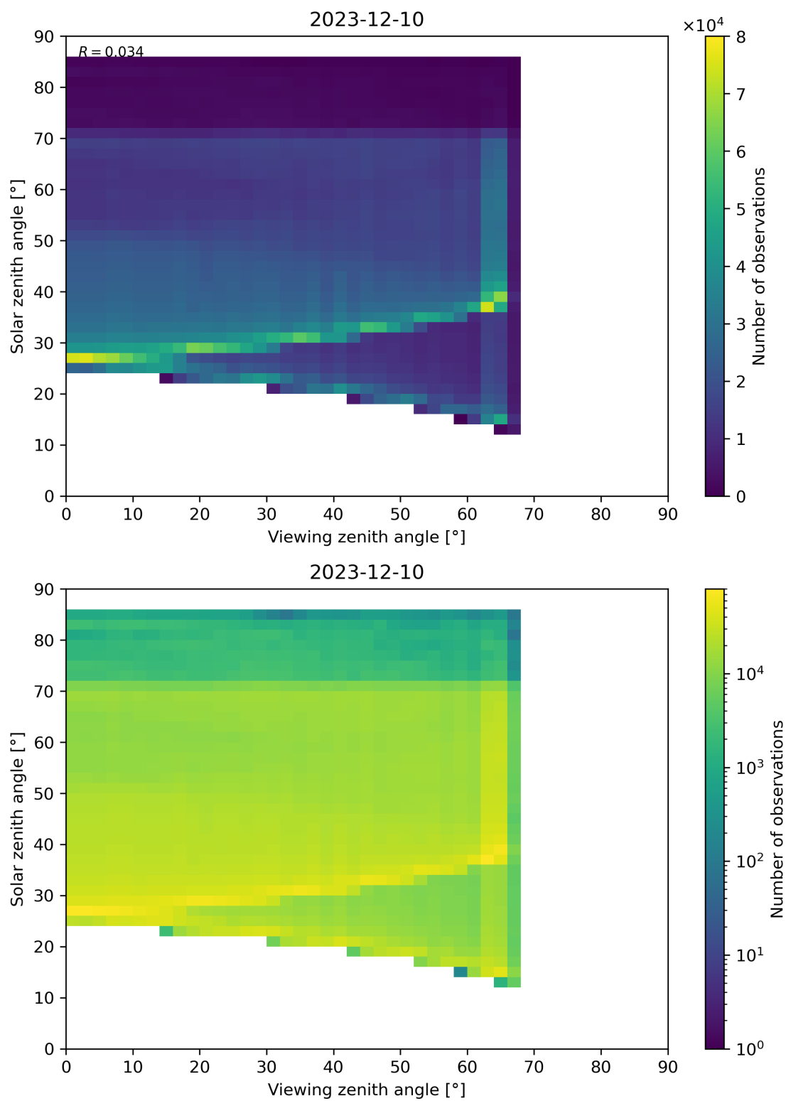
Figure 197: Scatter density plot of “Viewing zenith angle” against “Solar zenith angle” for 2023-12-09 to 2023-12-11.
