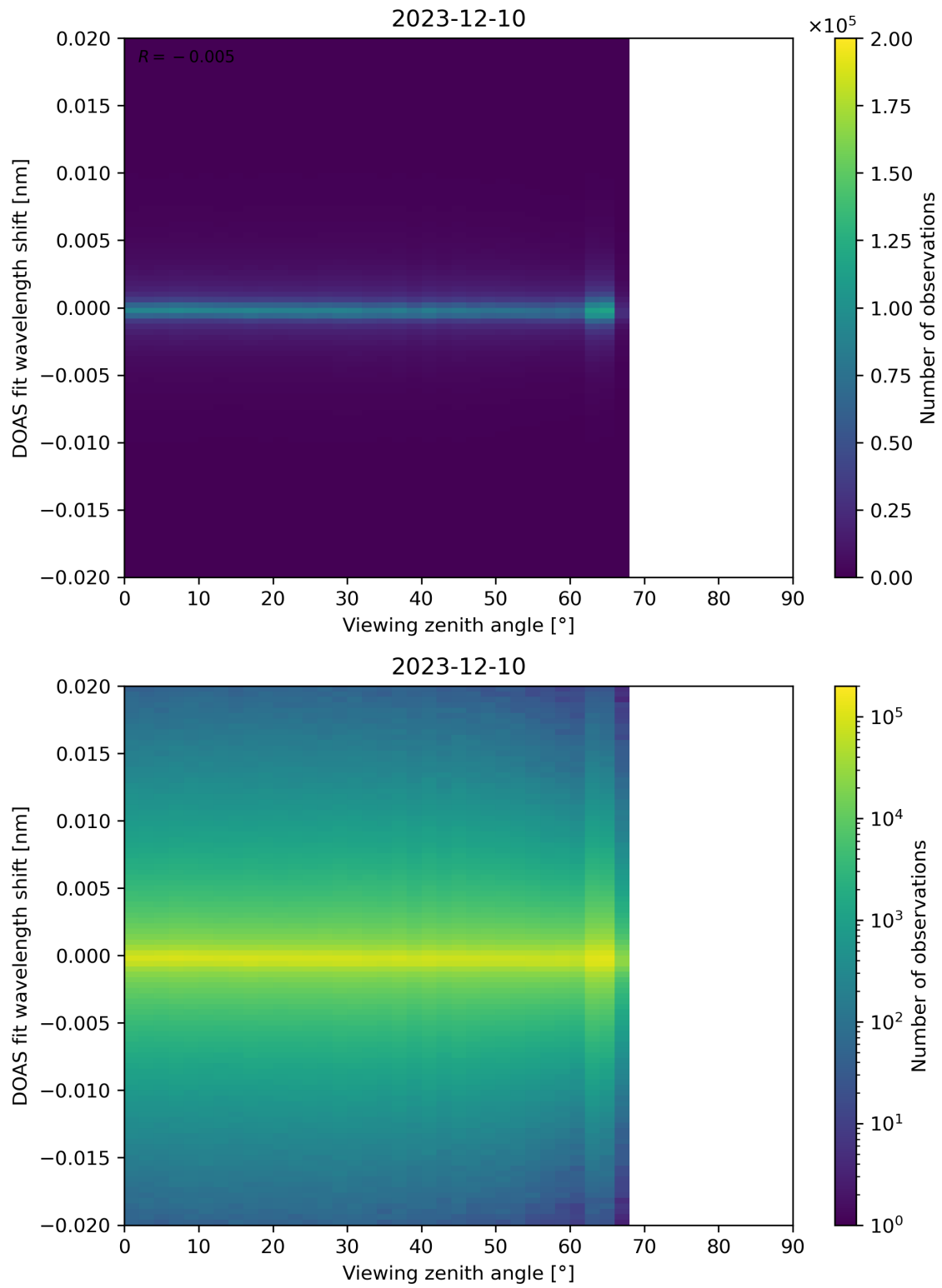
Figure 183: Scatter density plot of “Viewing zenith angle” against “DOAS fit wavelength shift” for 2023-12-09 to 2023-12-11.
