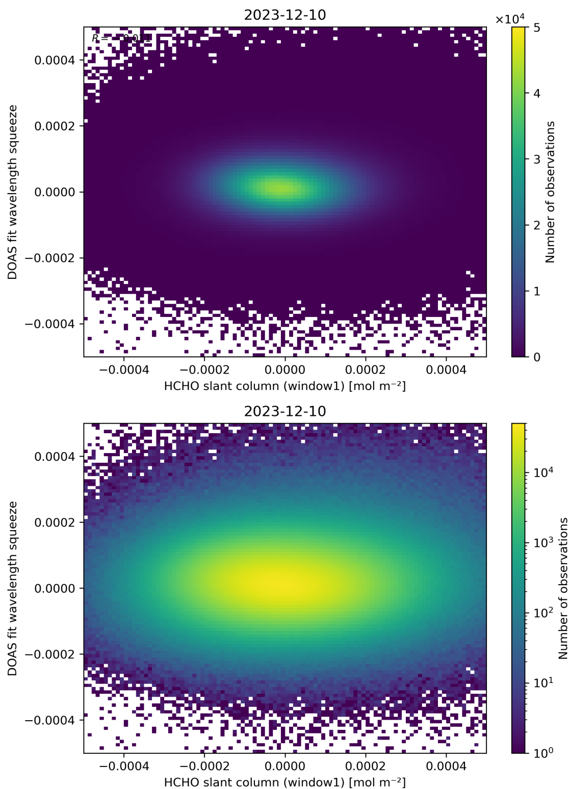
Figure 80: Scatter density plot of “HCHO slant column (window1)” against “DOAS fit wavelength squeeze” for 2023-12-09 to 2023-12-11.
