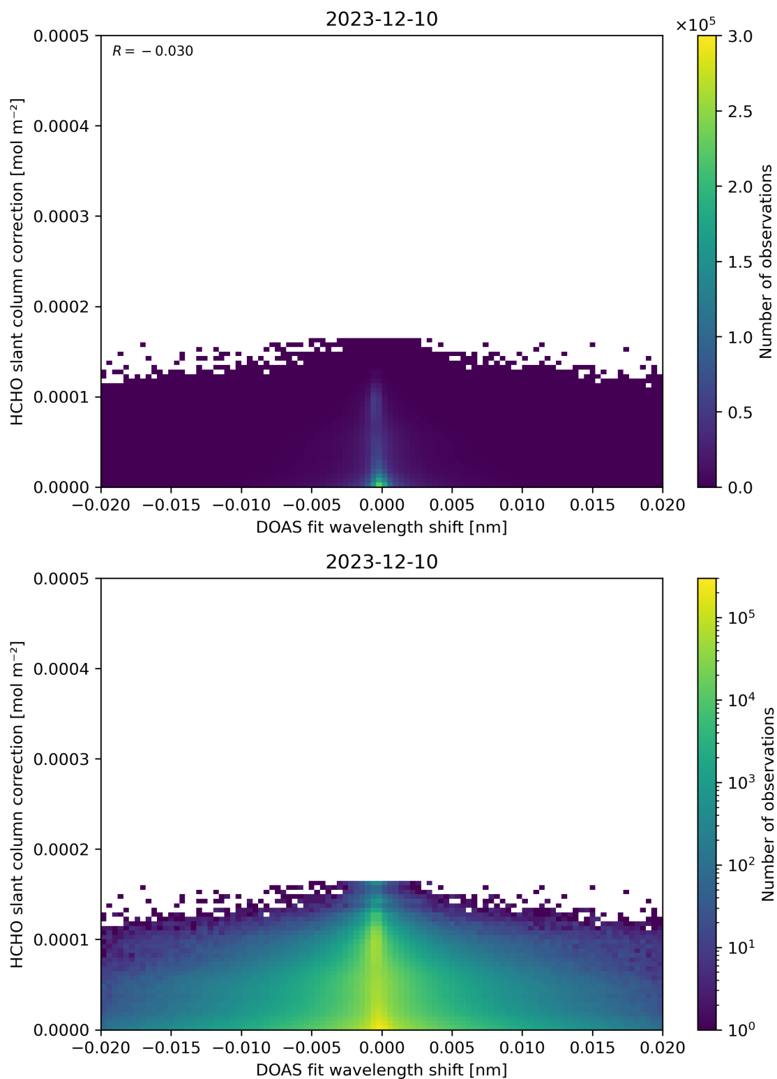
Figure 67: Scatter density plot of “DOAS fit wavelength shift” against “HCHO slant column correction” for 2023-12-09 to 2023-12-11.
