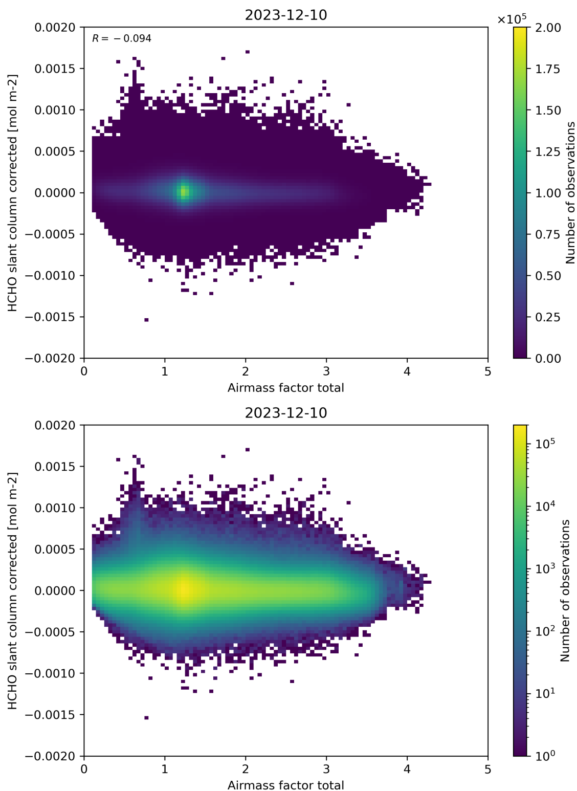
Figure 101: Scatter density plot of “Airmass factor total” against “HCHO slant column corrected” for 2023-12-09 to 2023-12-11.
