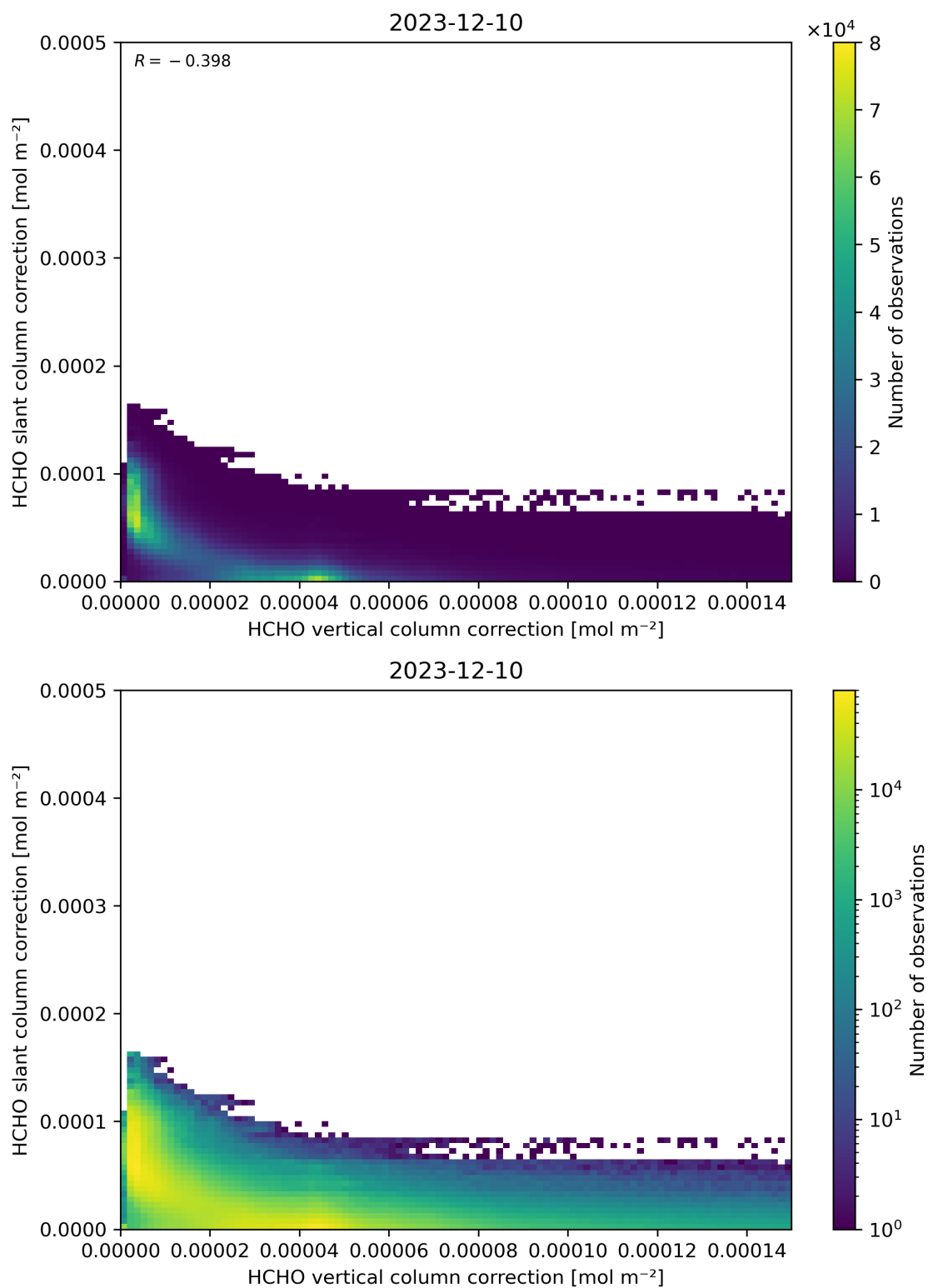
Figure 117: Scatter density plot of “HCHO vertical column correction” against “HCHO slant column correction” for 2023-12-09 to 2023-12-11.
