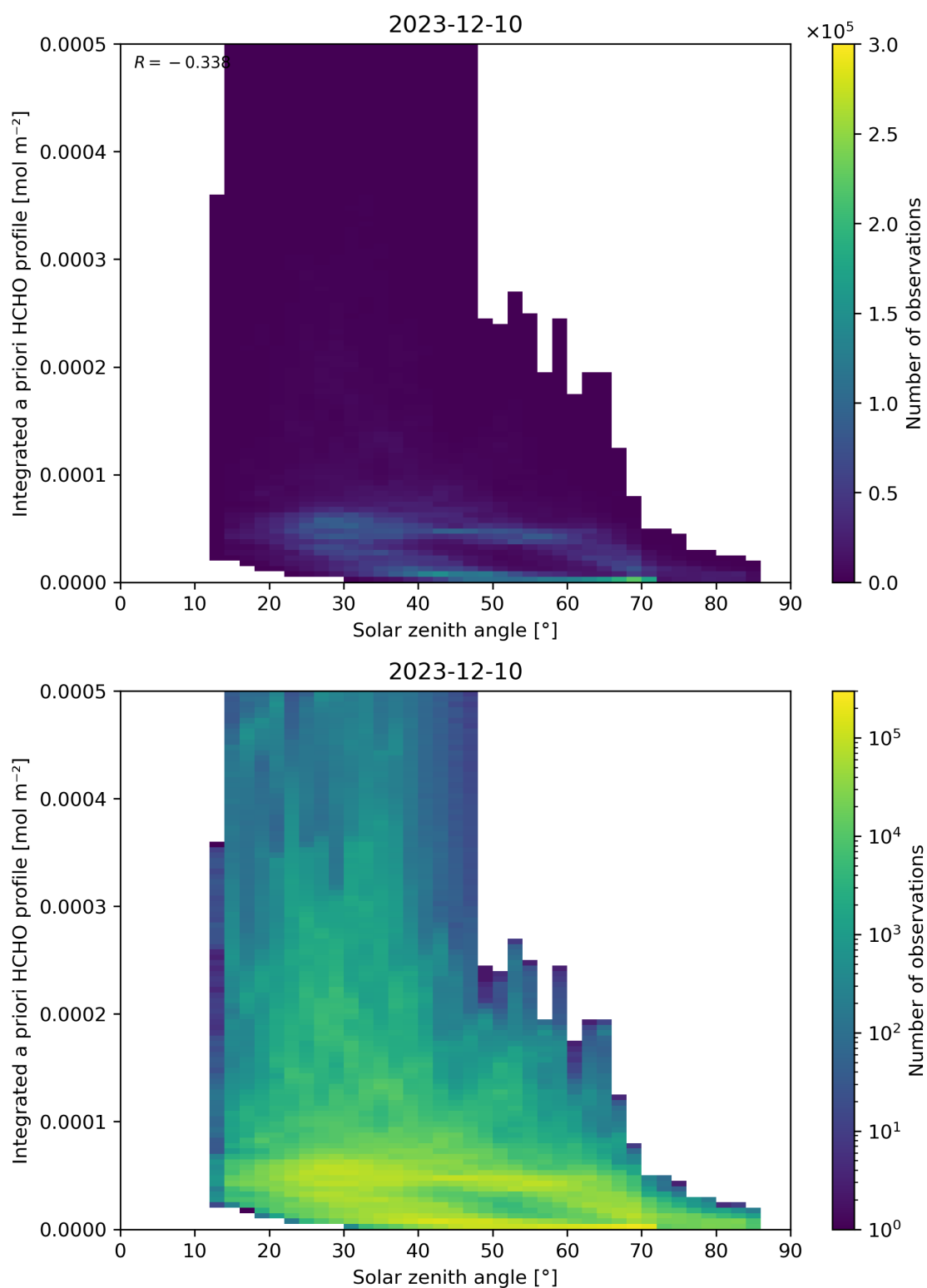
Figure 180: Scatter density plot of “Solar zenith angle” against “Integrated a priori HCHO profile” for 2023-12-09 to 2023-12-11.
