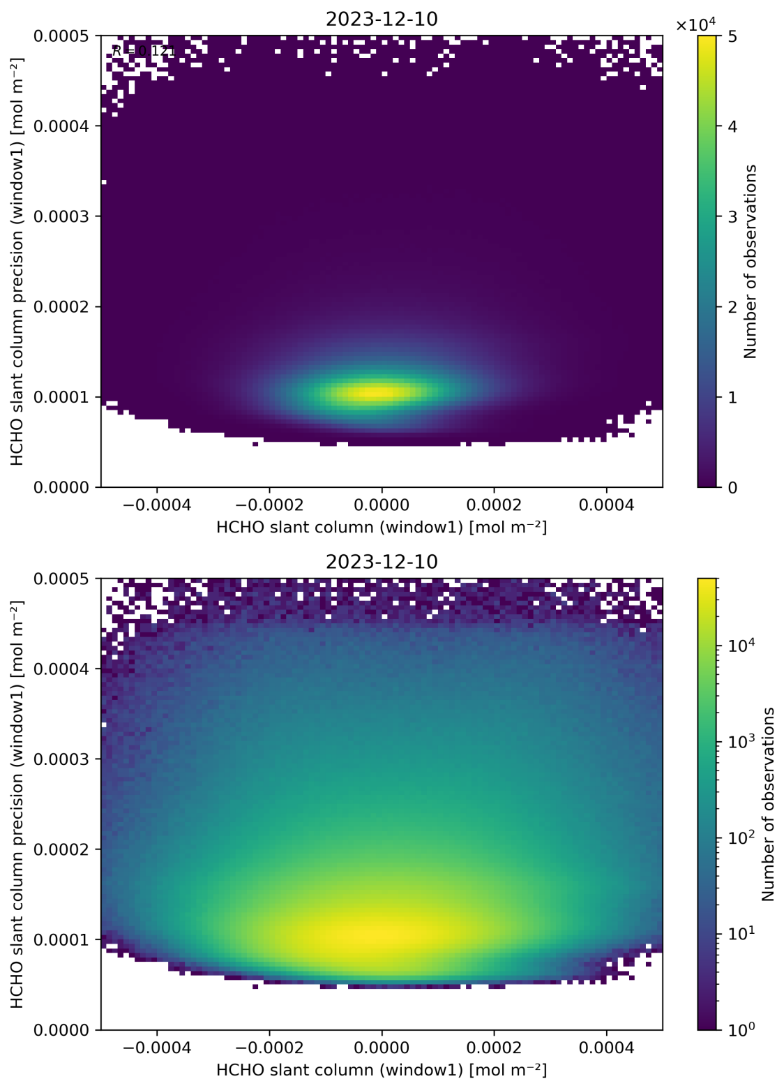
Figure 84: Scatter density plot of “HCHO slant column (window1)” against “HCHO slant column precision (window1)” for 2023-12-09 to 2023-12-11.
