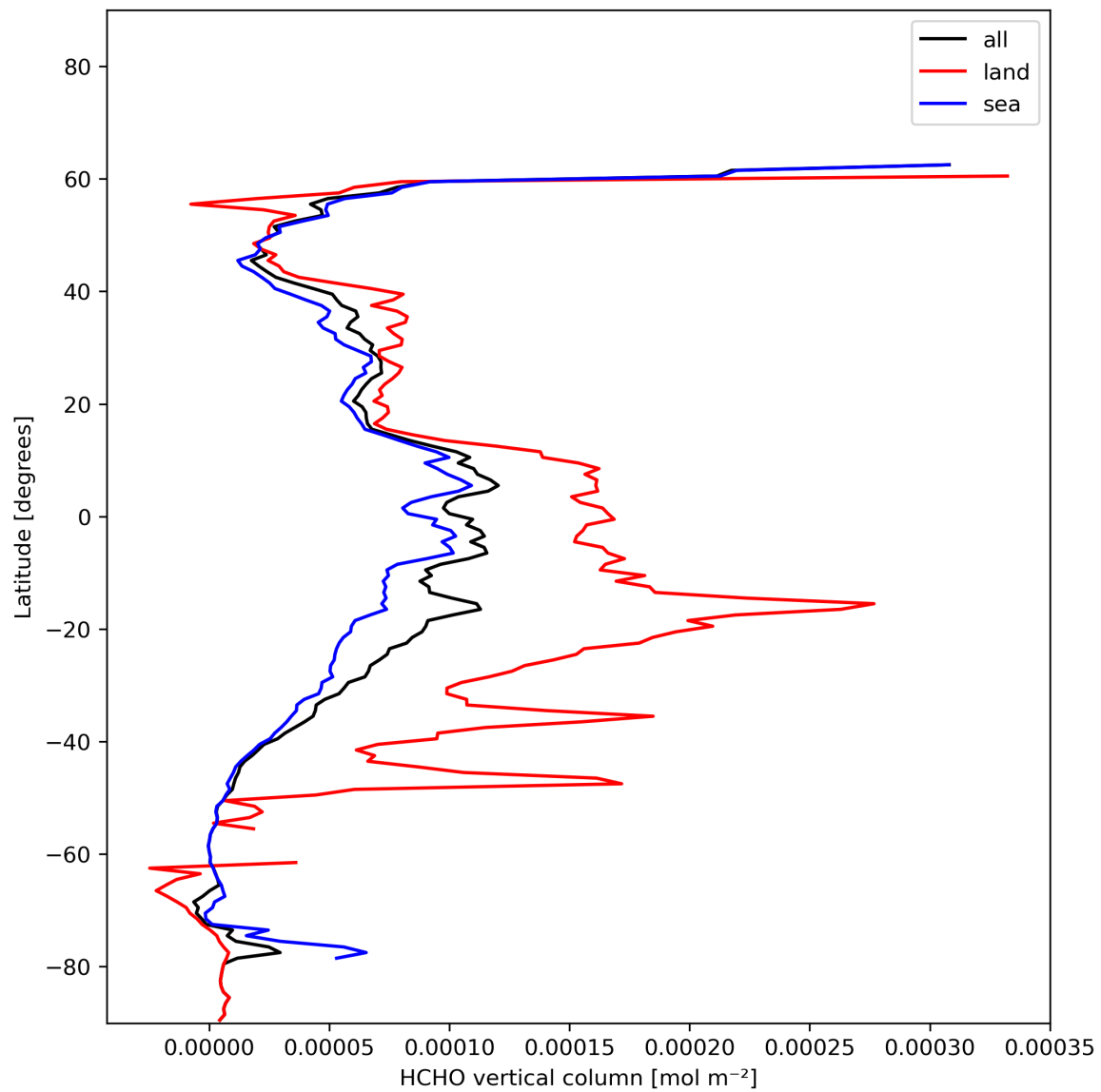
Figure 21: Zonal average of “HCHO vertical column” for 2023-12-09 to 2023-12-11.
