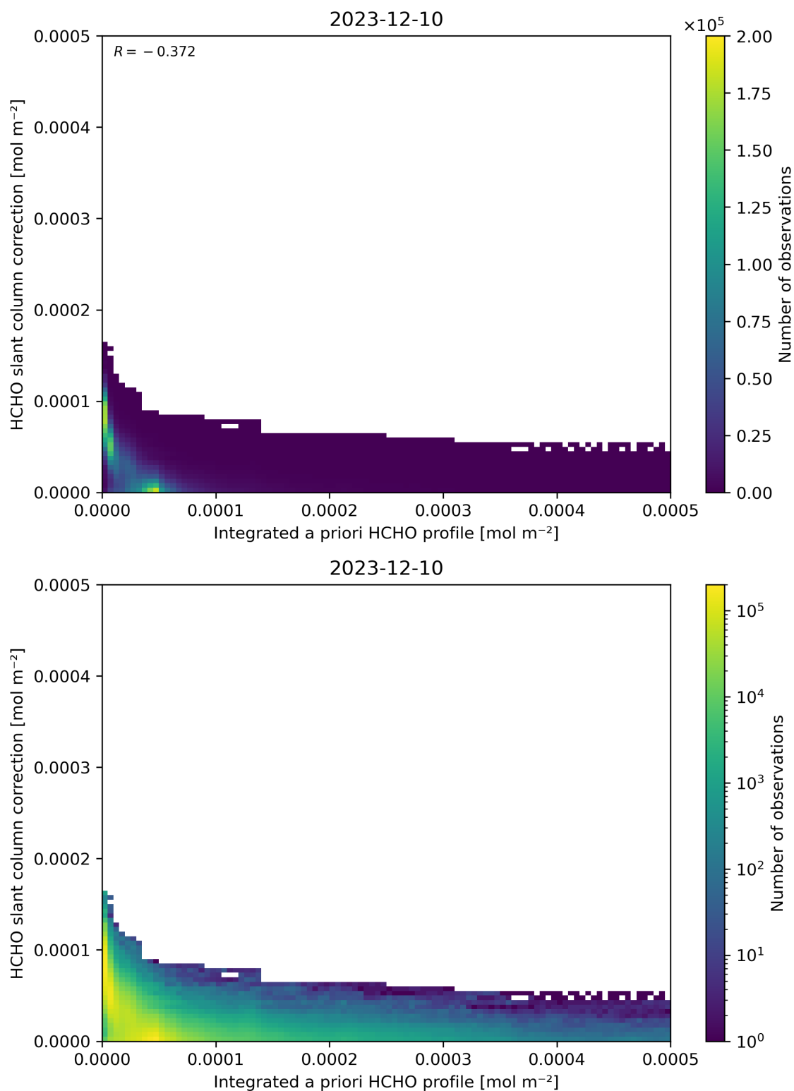
Figure 152: Scatter density plot of “Integrated a priori HCHO profile” against “HCHO slant column correction” for 2023-12-09 to 2023-12-11.
