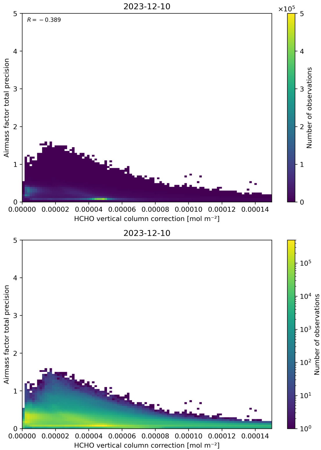
Figure 121: Scatter density plot of “HCHO vertical column correction” against “Airmass factor total precision” for 2023-12-09 to 2023-12-11.
