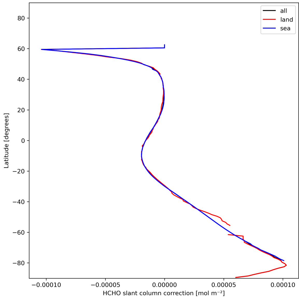
Figure 33: Zonal average of “HCHO slant column correction” for 2023-12-09 to 2023-12-11.
