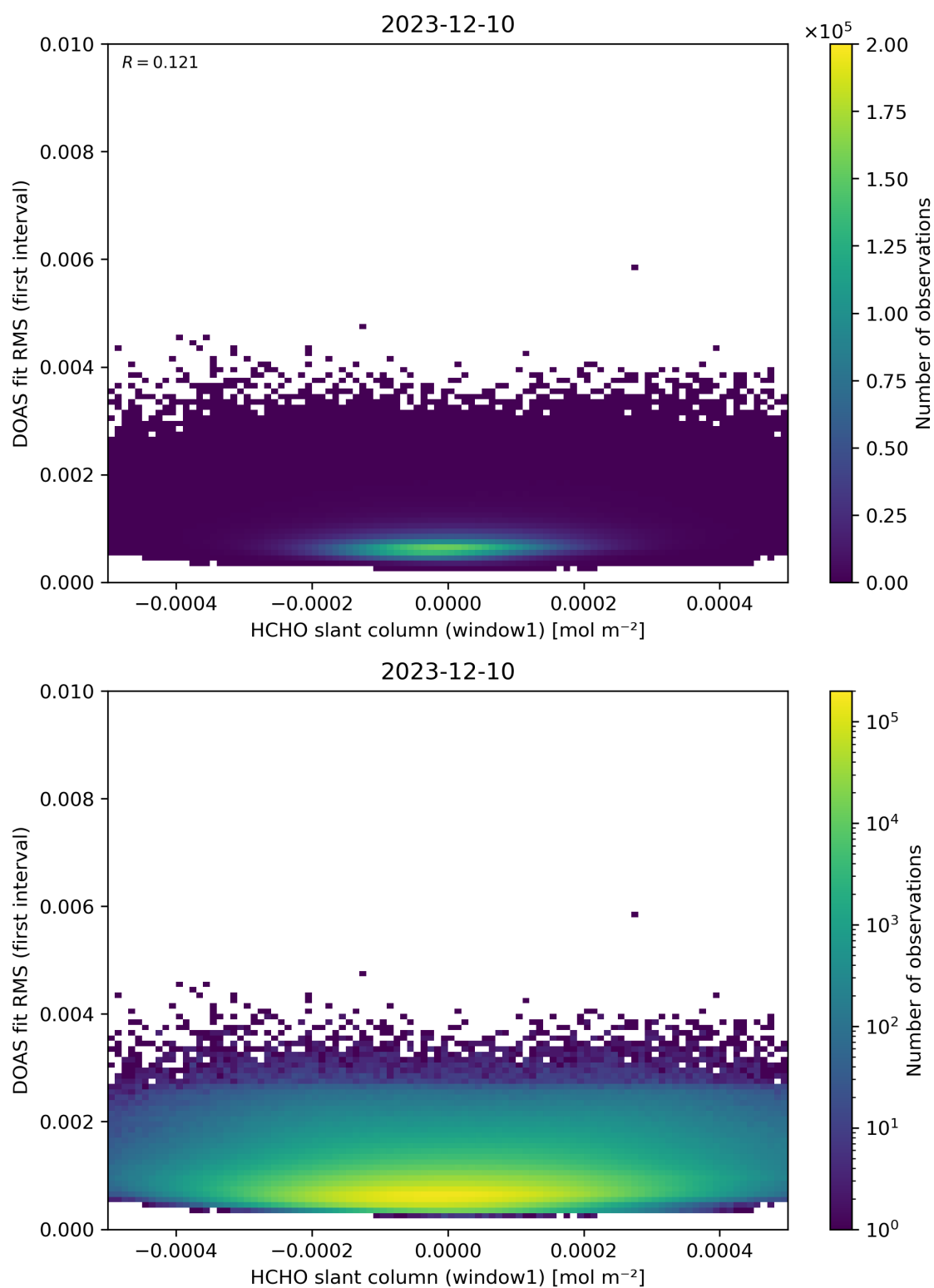
Figure 78: Scatter density plot of “HCHO slant column (window1)” against “DOAS fit RMS (first interval)” for 2023-12-09 to 2023-12-11.
