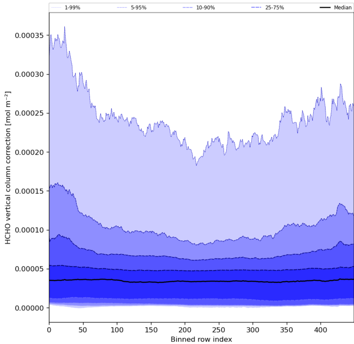
Figure 51: Along track statistics of “HCHO vertical column correction” for 2023-12-09 to 2023-12-11
