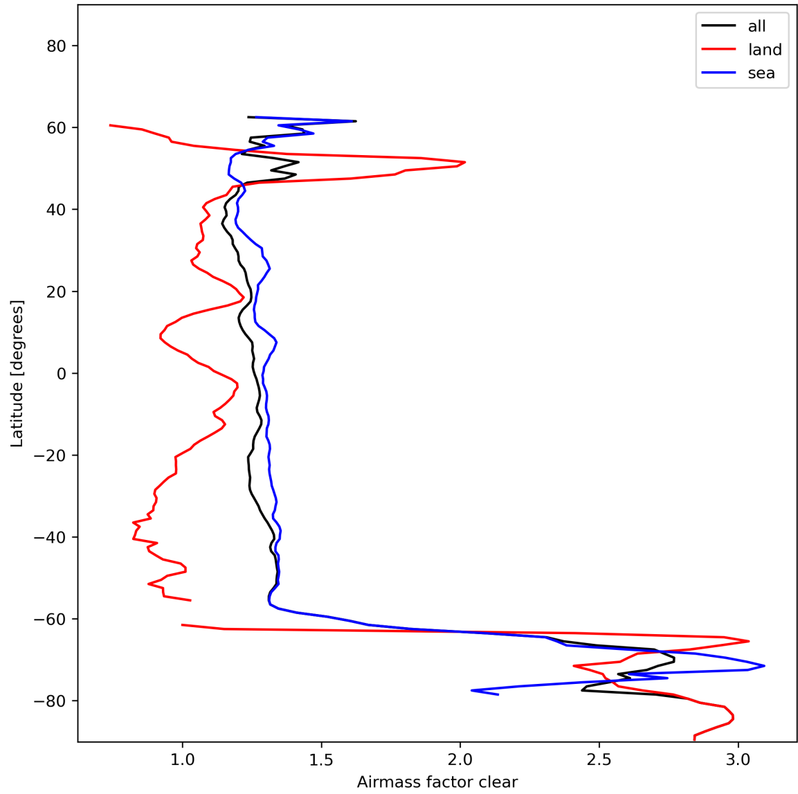
Figure 28: Zonal average of “Airmass factor clear” for 2023-12-09 to 2023-12-11.
