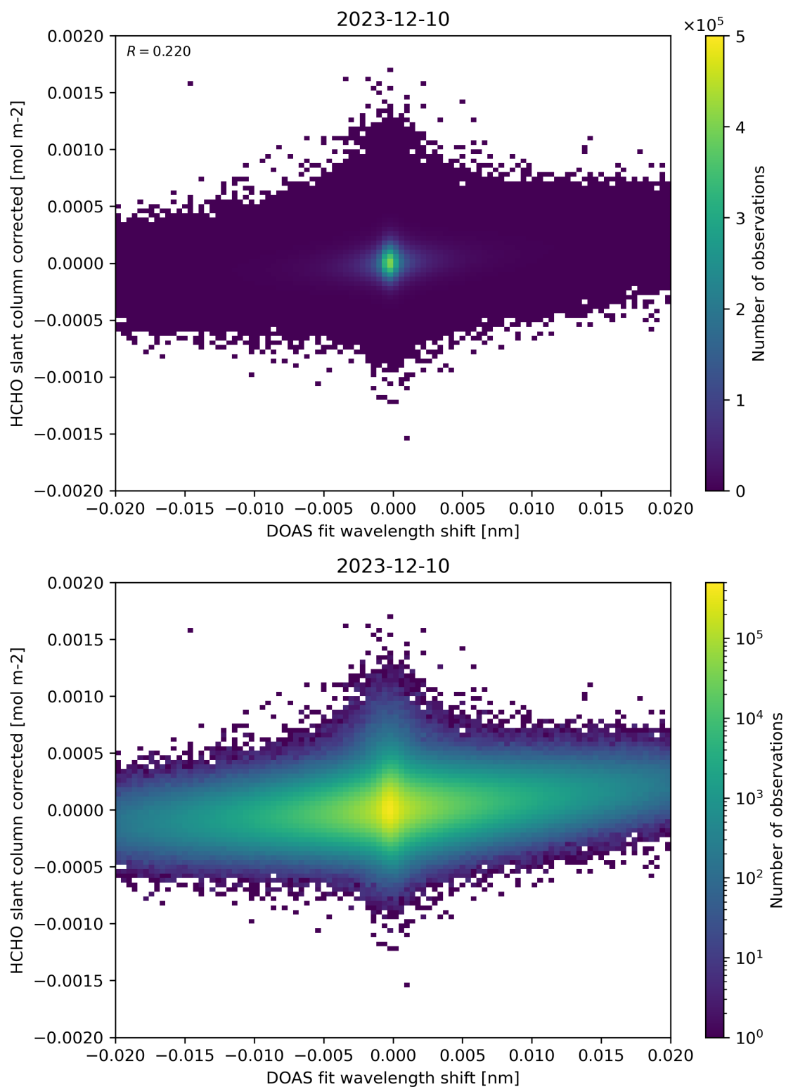
Figure 66: Scatter density plot of “DOAS fit wavelength shift” against “HCHO slant column corrected” for 2023-12-09 to 2023-12-11.
