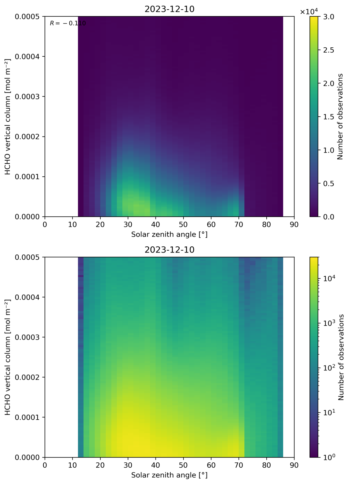
Figure 177: Scatter density plot of “Solar zenith angle” against “HCHO vertical column” for 2023-12-09 to 2023-12-11.
