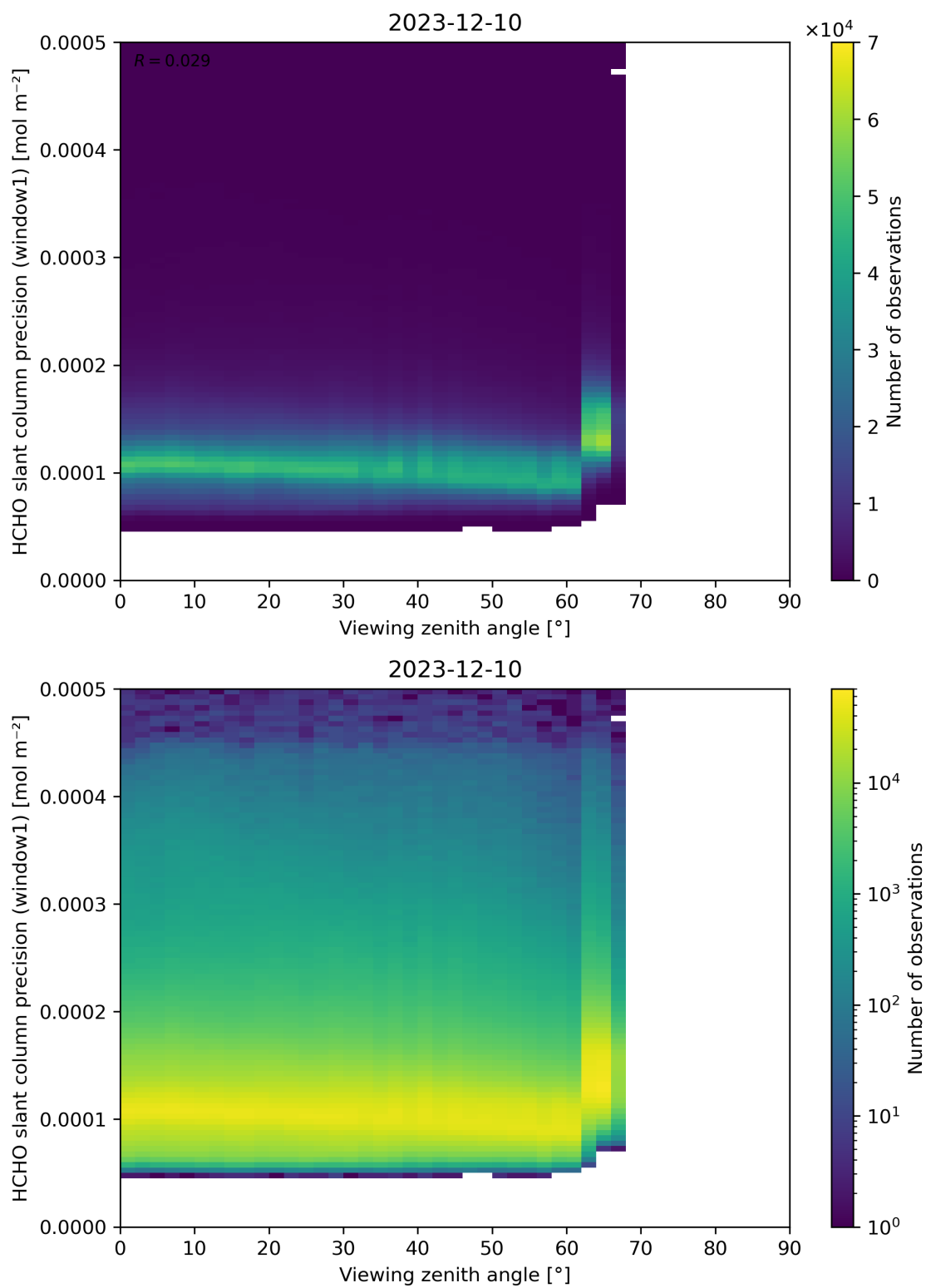
Figure 189: Scatter density plot of “Viewing zenith angle” against “HCHO slant column precision (window1)” for 2023-12-09 to 2023-12-11.
