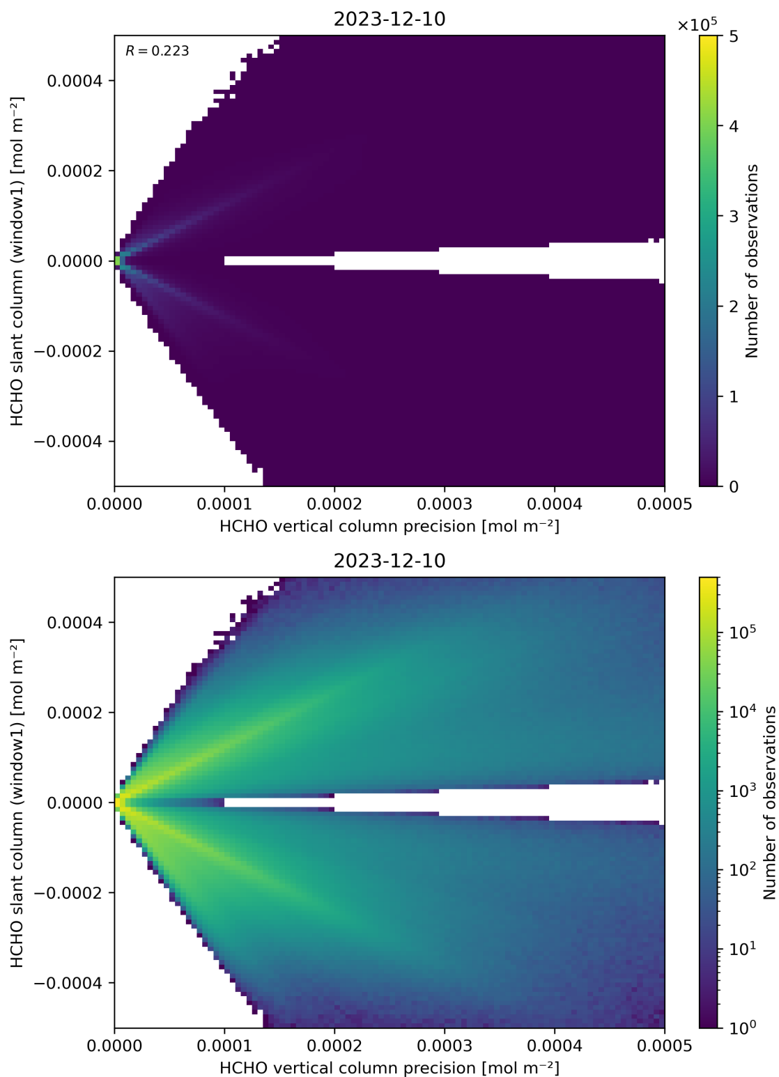
Figure 142: Scatter density plot of “HCHO vertical column precision” against “HCHO slant column (window1)” for 2023-12-09 to 2023-12-11.
