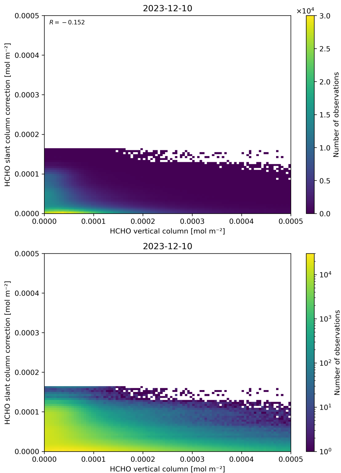
Figure 128: Scatter density plot of “HCHO vertical column” against “HCHO slant column correction” for 2023-12-09 to 2023-12-11.
