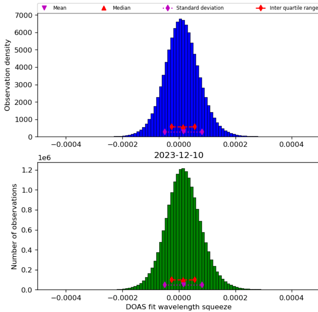
Figure 45: Histogram of “DOAS fit wavelength squeeze” for 2023-12-09 to 2023-12-11
