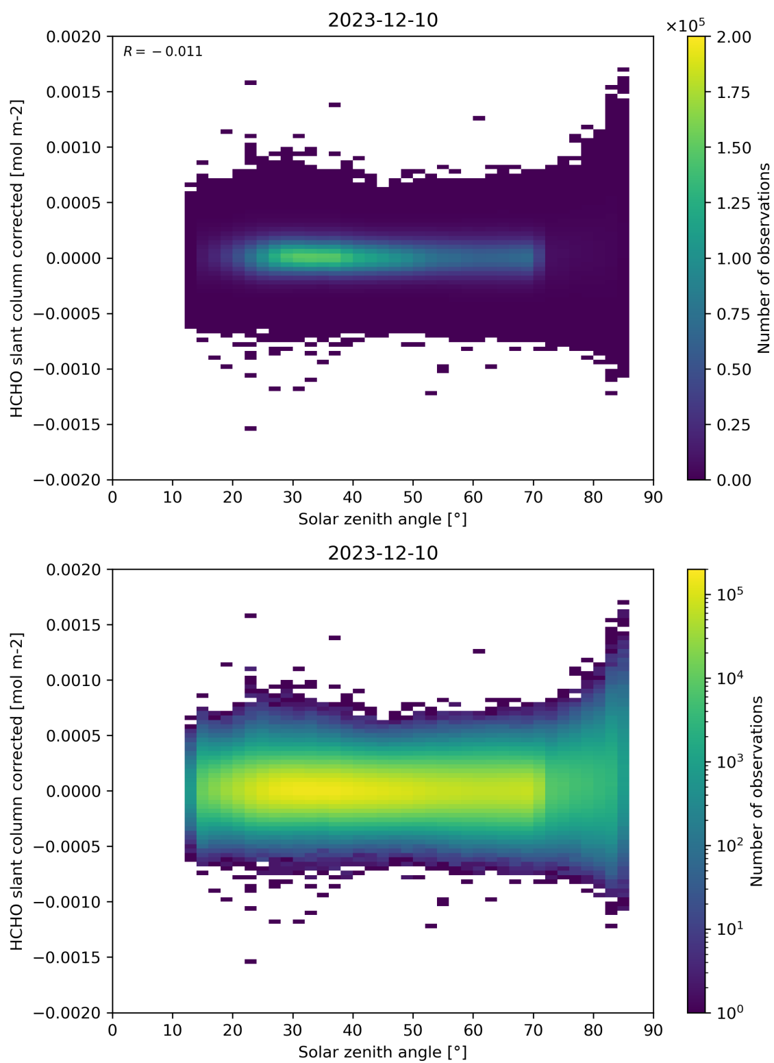
Figure 171: Scatter density plot of “Solar zenith angle” against “HCHO slant column corrected” for 2023-12-09 to 2023-12-11.
