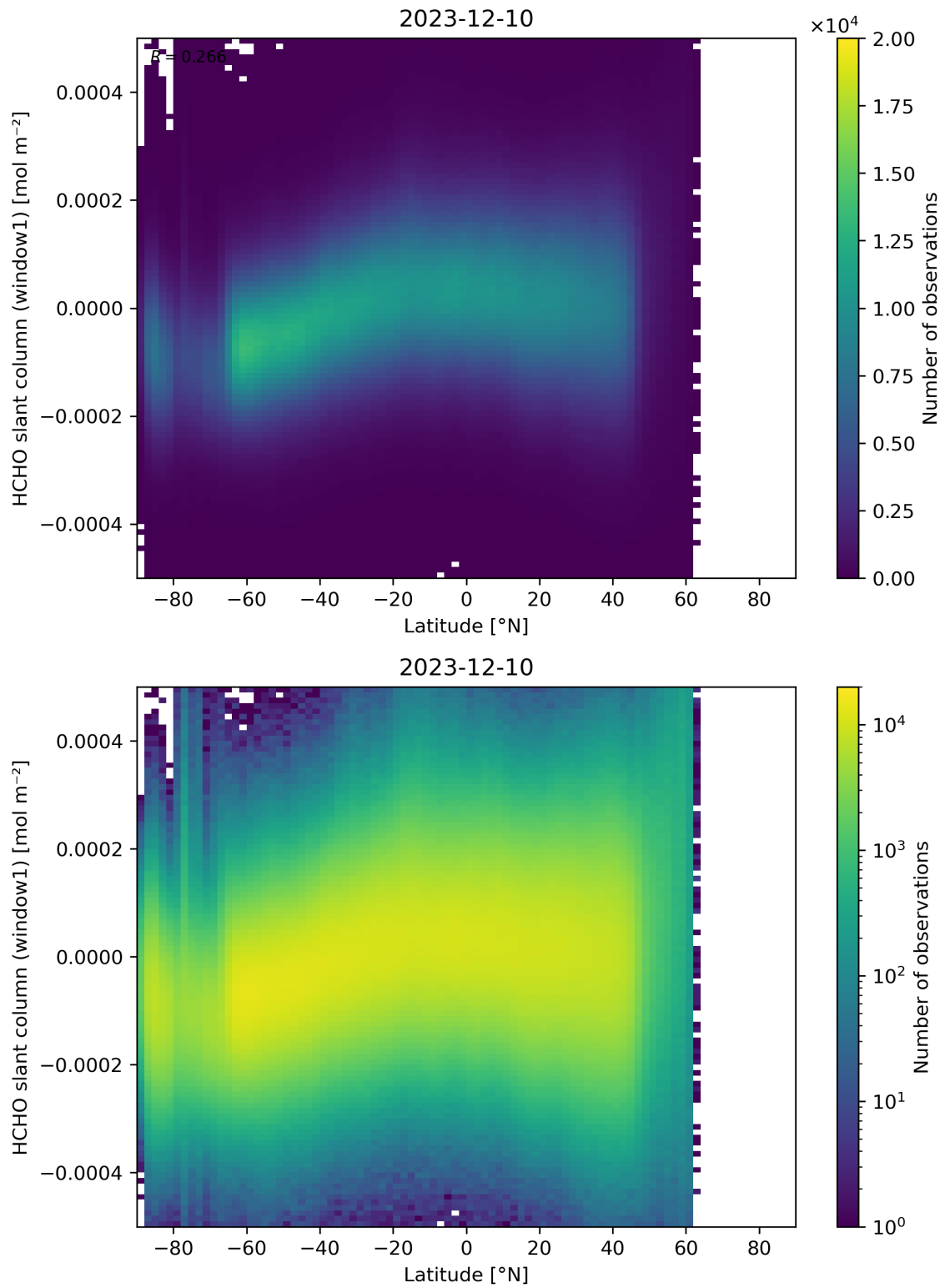
Figure 159: Scatter density plot of “Latitude” against “HCHO slant column (window1)” for 2023-12-09 to 2023-12-11.
