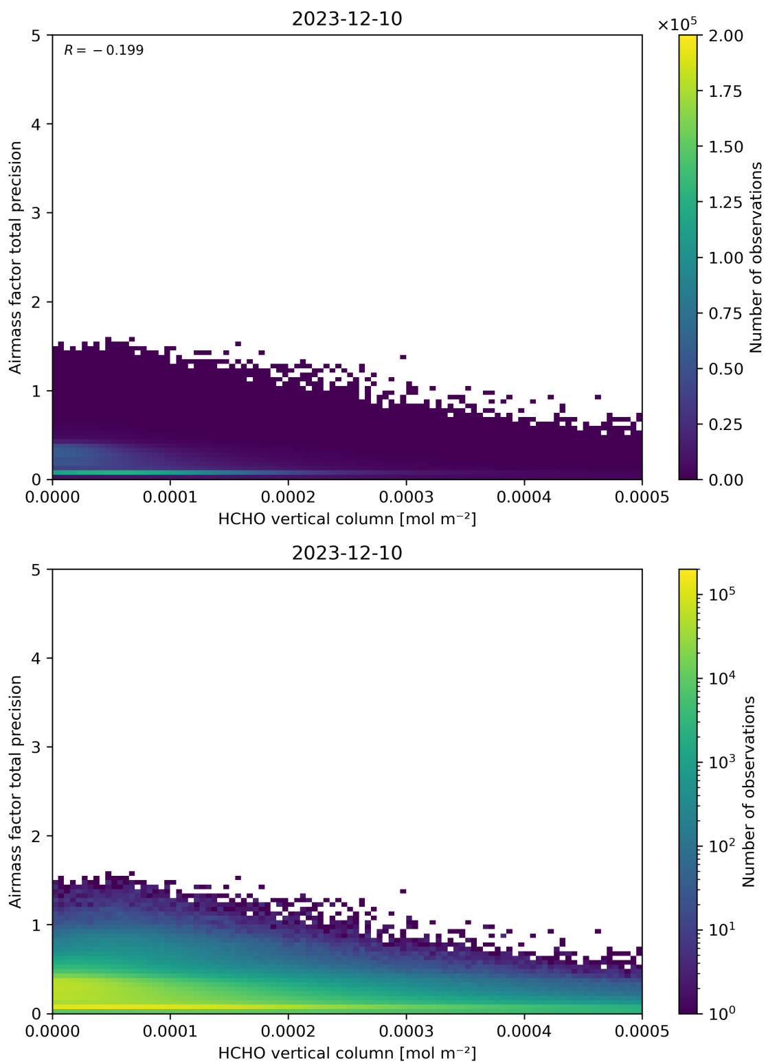
Figure 132: Scatter density plot of “HCHO vertical column” against “Airmass factor total precision” for 2023-12-09 to 2023-12-11.
