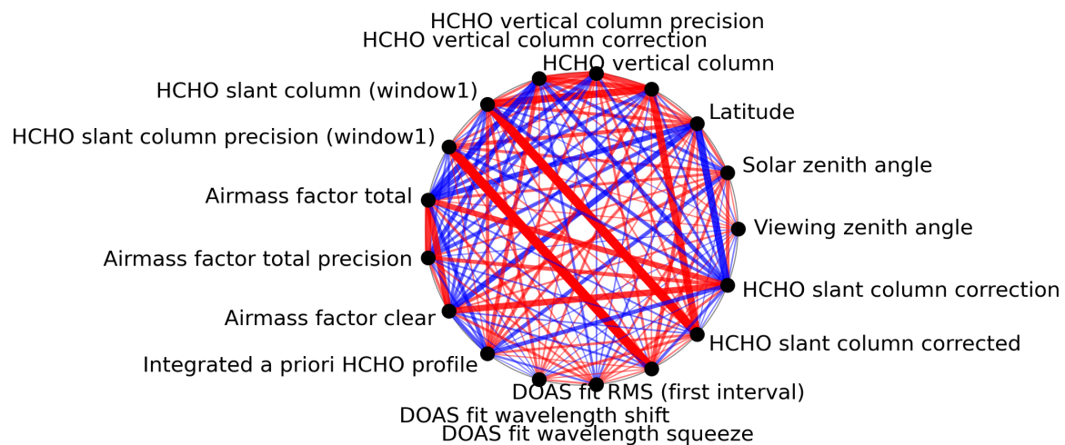
Figure 1: Map of correlation graph for 2023-12-09 to 2023-12-11.
