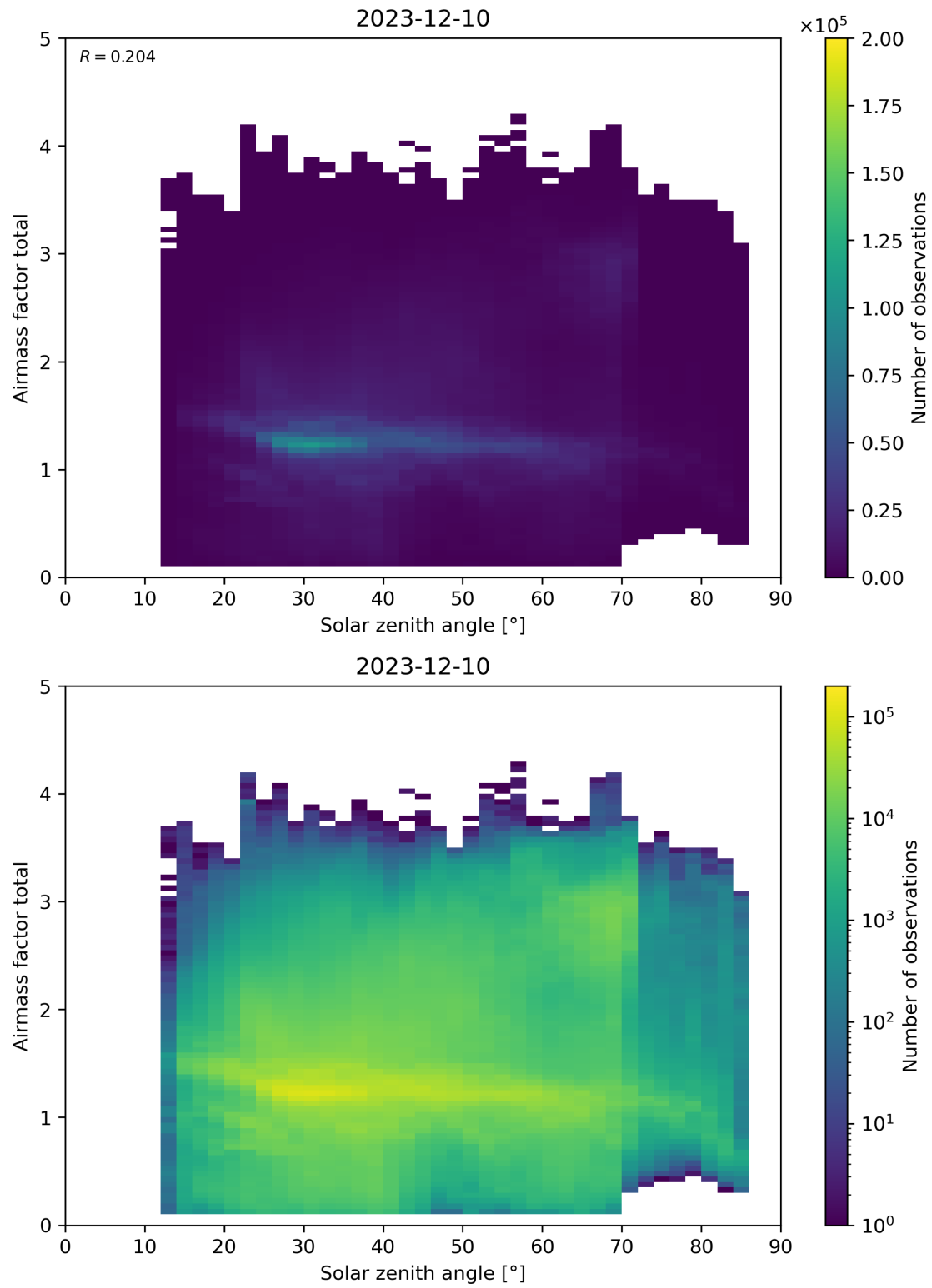
Figure 175: Scatter density plot of “Solar zenith angle” against “Airmass factor total” for 2023-12-09 to 2023-12-11.
