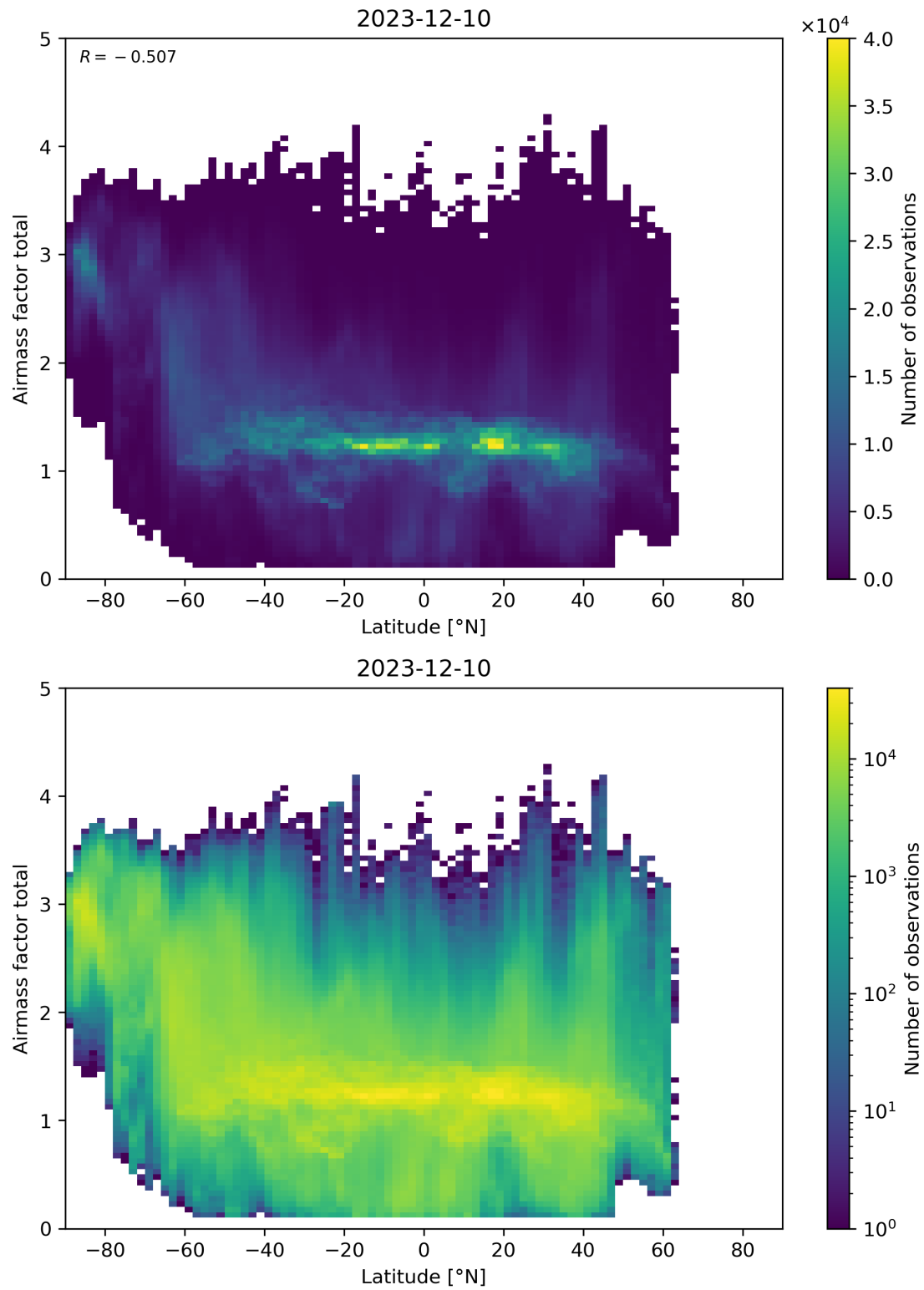
Figure 161: Scatter density plot of “Latitude” against “Airmass factor total” for 2023-12-09 to 2023-12-11.
