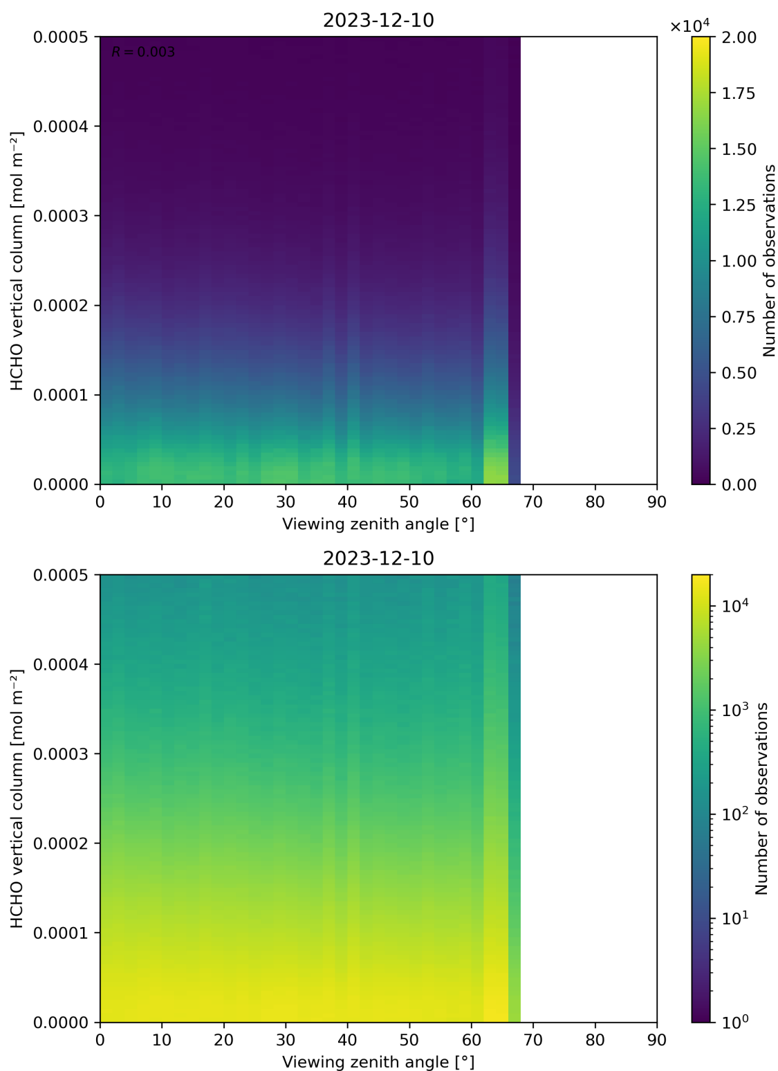
Figure 192: Scatter density plot of “Viewing zenith angle” against “HCHO vertical column” for 2023-12-09 to 2023-12-11.
