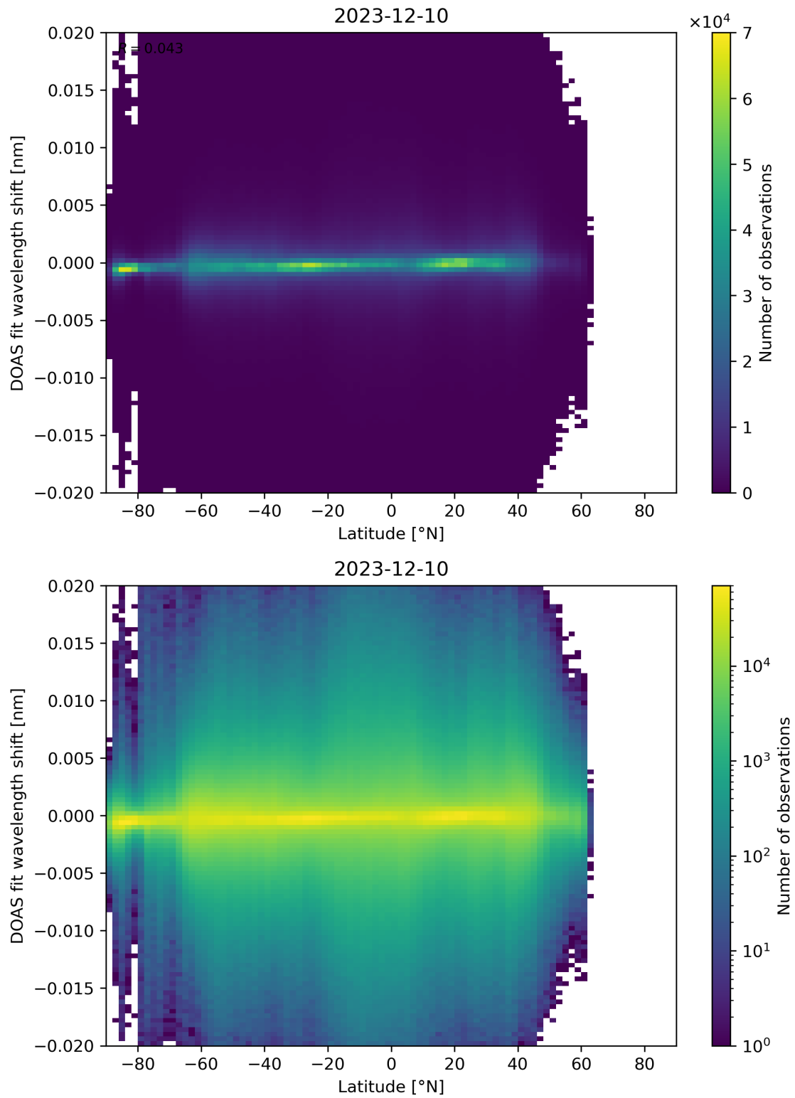
Figure 154: Scatter density plot of “Latitude” against “DOAS fit wavelength shift” for 2023-12-09 to 2023-12-11.
