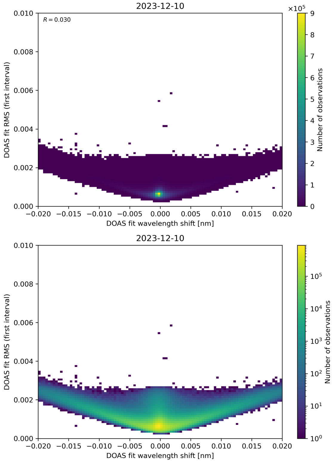
Figure 64: Scatter density plot of “DOAS fit wavelength shift” against “DOAS fit RMS (first interval)” for 2023-12-09 to 2023-12-11.
