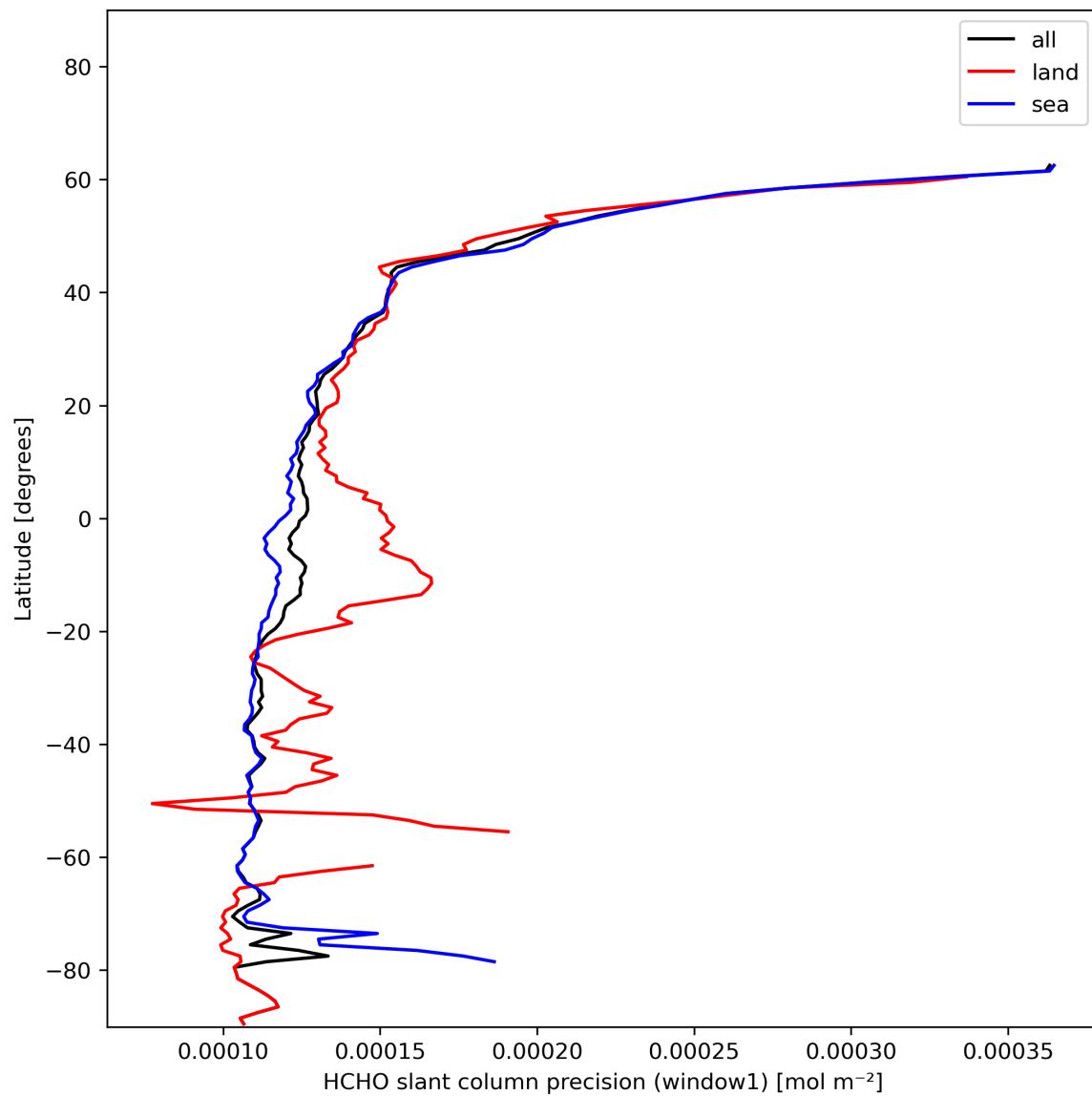
Figure 25: Zonal average of “HCHO slant column precision (window1)” for 2023-12-09 to 2023-12-11.
