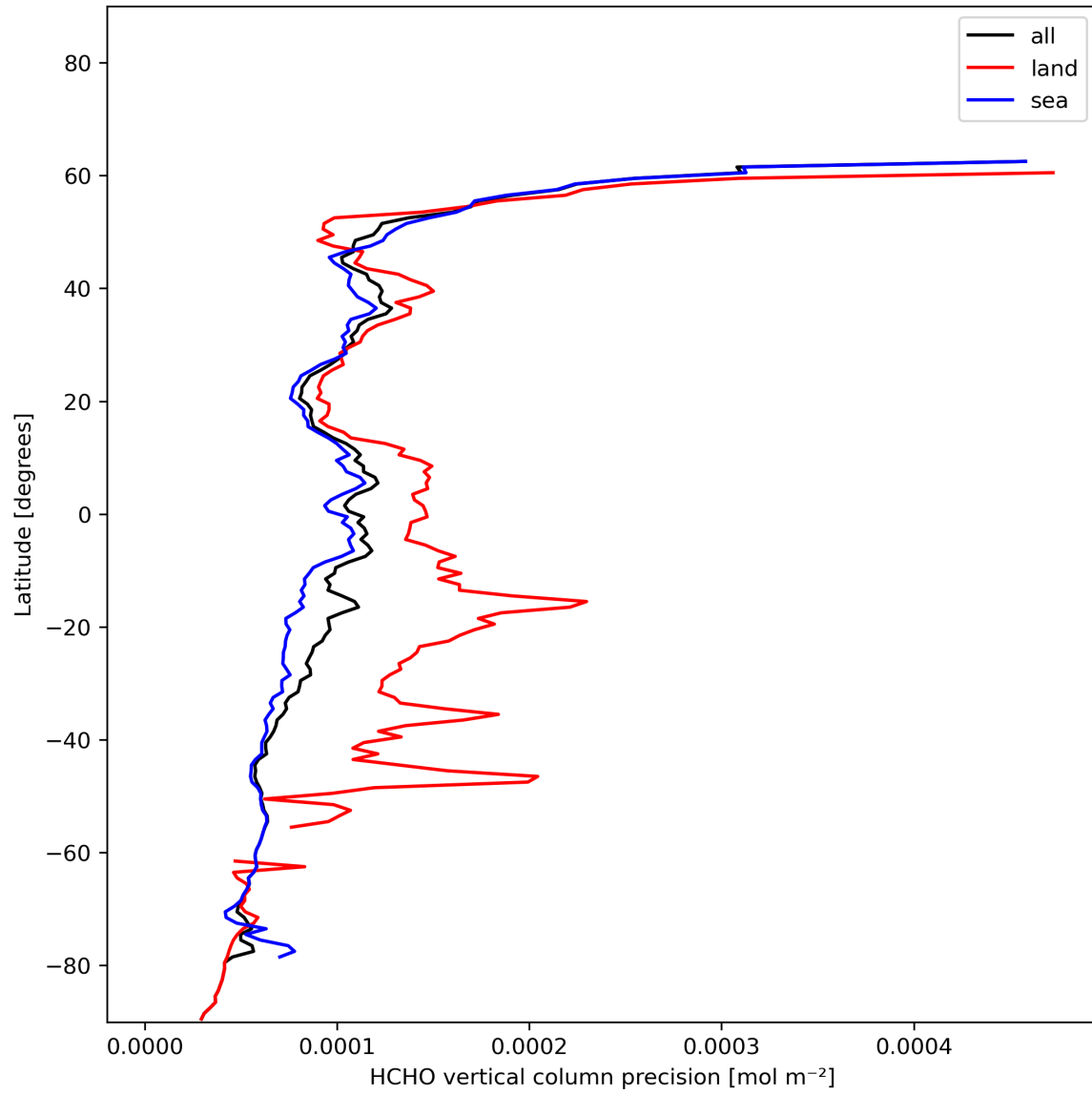
Figure 22: Zonal average of “HCHO vertical column precision” for 2023-12-09 to 2023-12-11.
