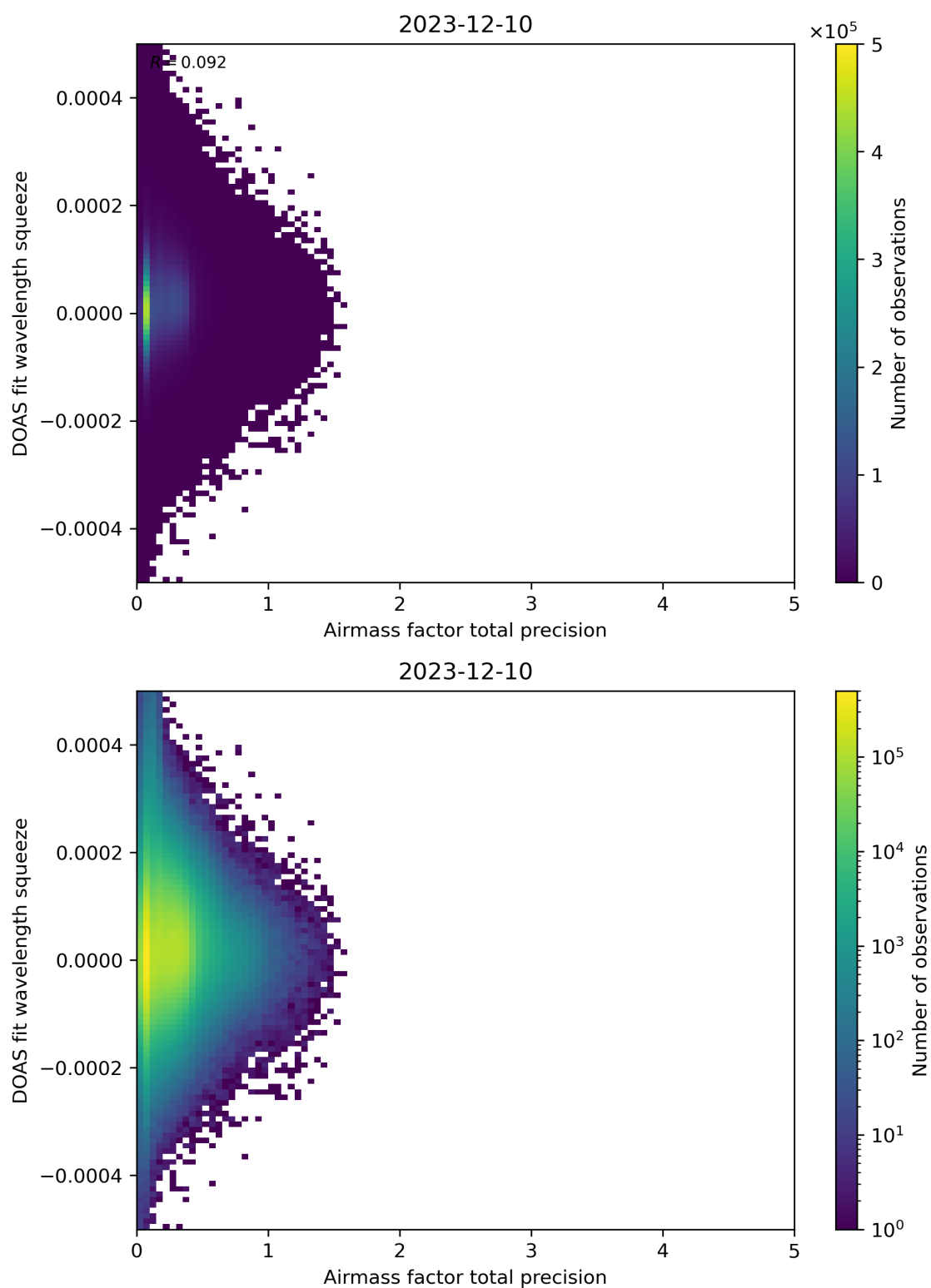
Figure 107: Scatter density plot of “Airmass factor total precision” against “DOAS fit wavelength squeeze” for 2023-12-09 to 2023-12-11.
