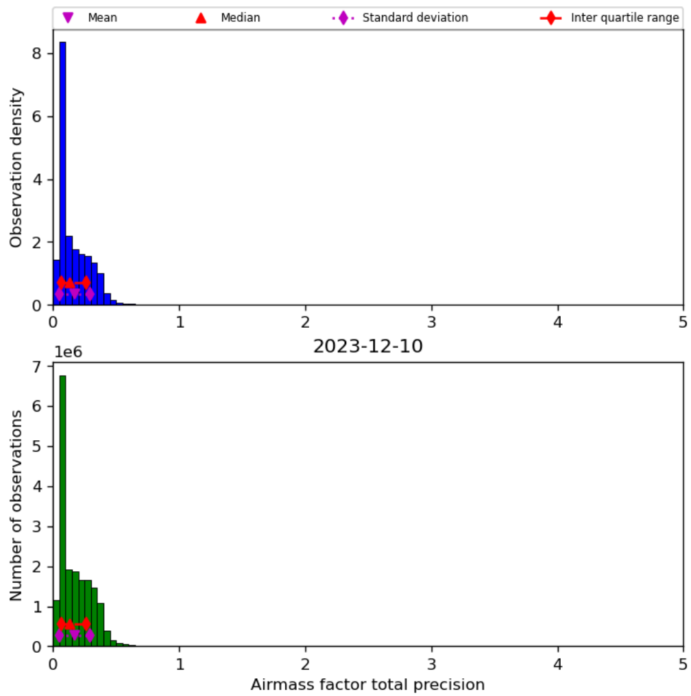
Figure 41: Histogram of “Airmass factor total precision” for 2023-12-09 to 2023-12-11
