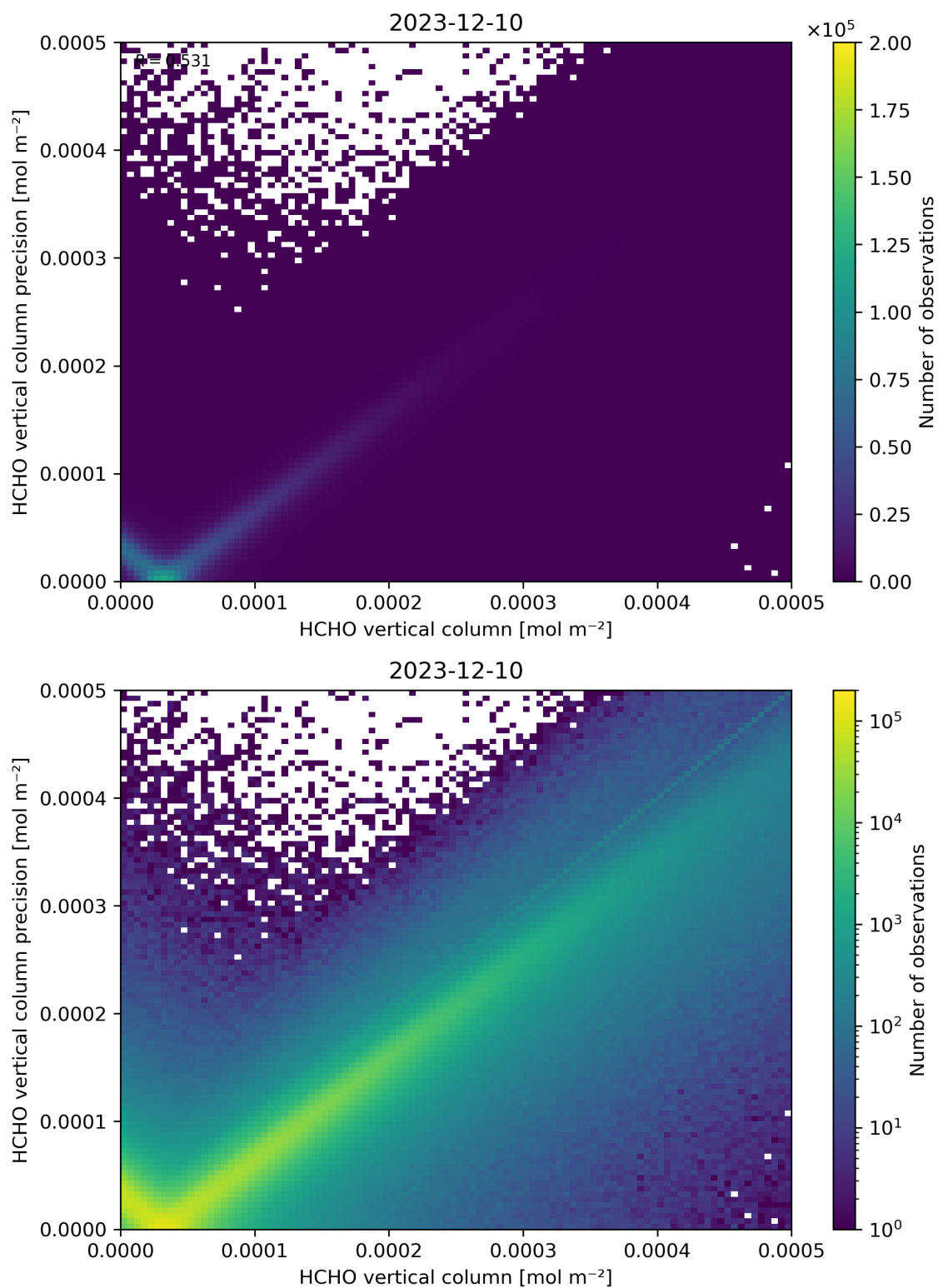
Figure 134: Scatter density plot of “HCHO vertical column” against “HCHO vertical column precision” for 2023-12-09 to 2023-12-11.
