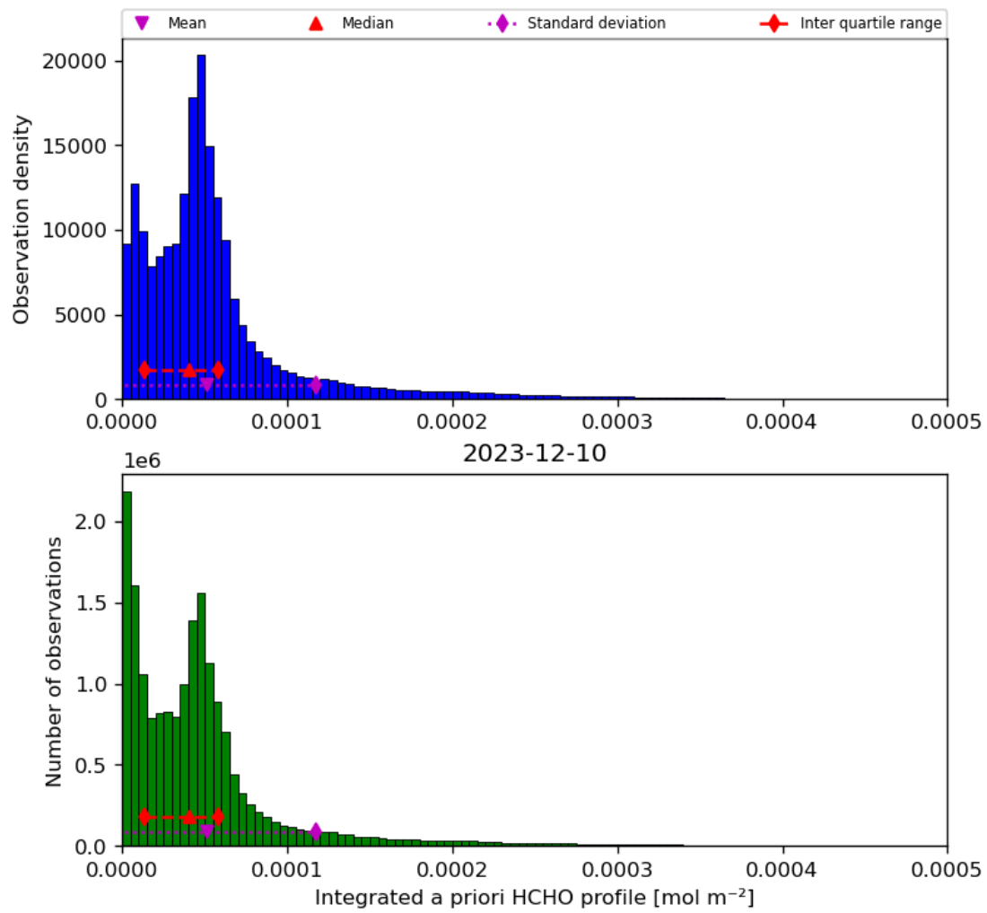
Figure 43: Histogram of “Integrated a priori HCHO profile” for 2023-12-09 to 2023-12-11
