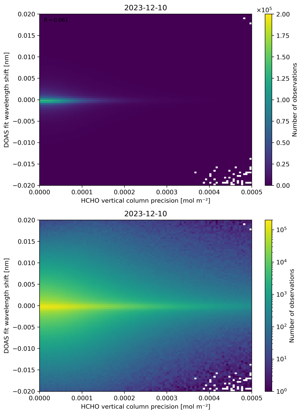
Figure 137: Scatter density plot of “HCHO vertical column precision” against “DOAS fit wavelength shift” for 2023-12-09 to 2023-12-11.
