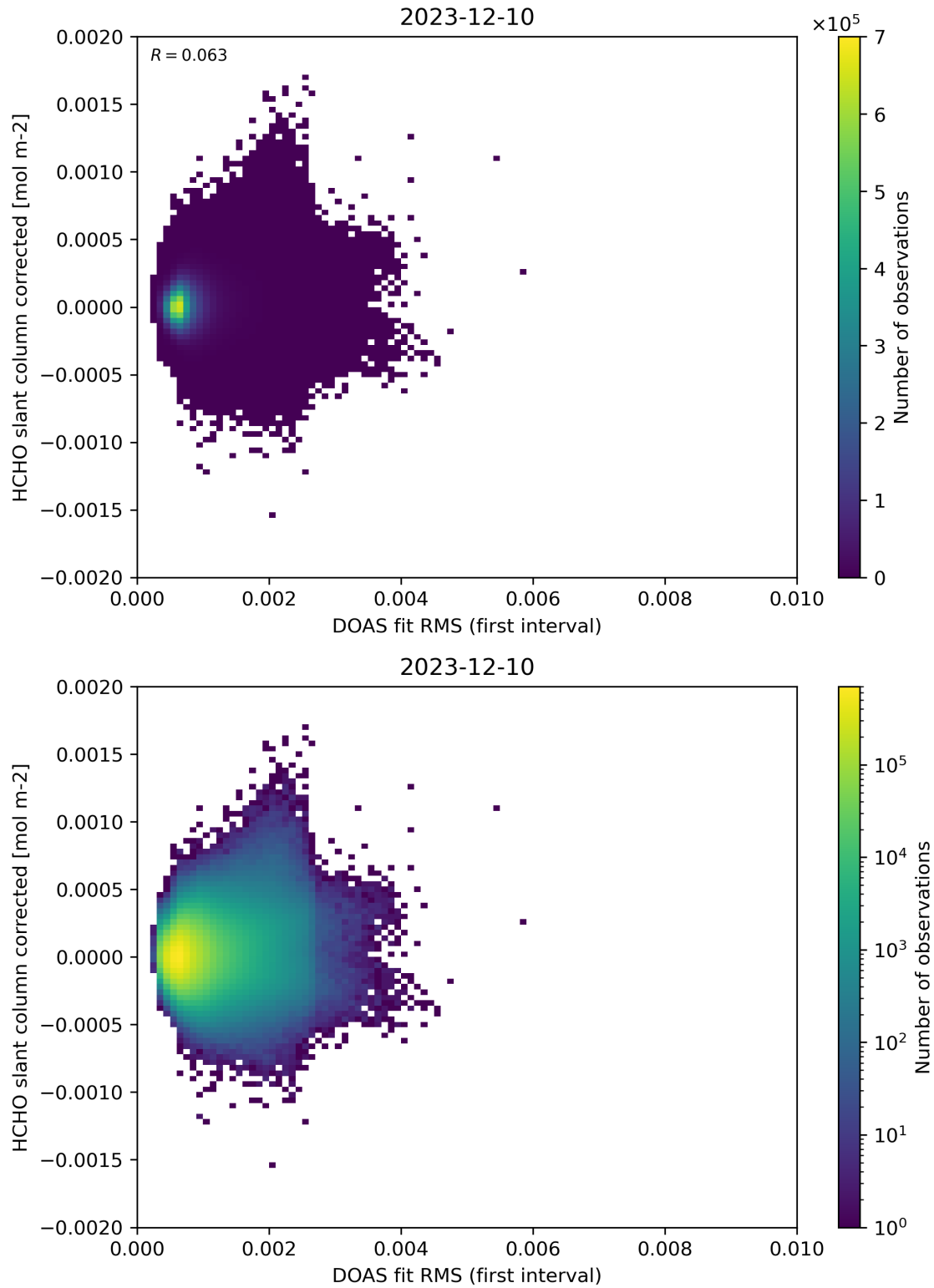
Figure 62: Scatter density plot of “DOAS fit RMS (first interval)” against “HCHO slant column corrected” for 2023-12-09 to 2023-12-11.
