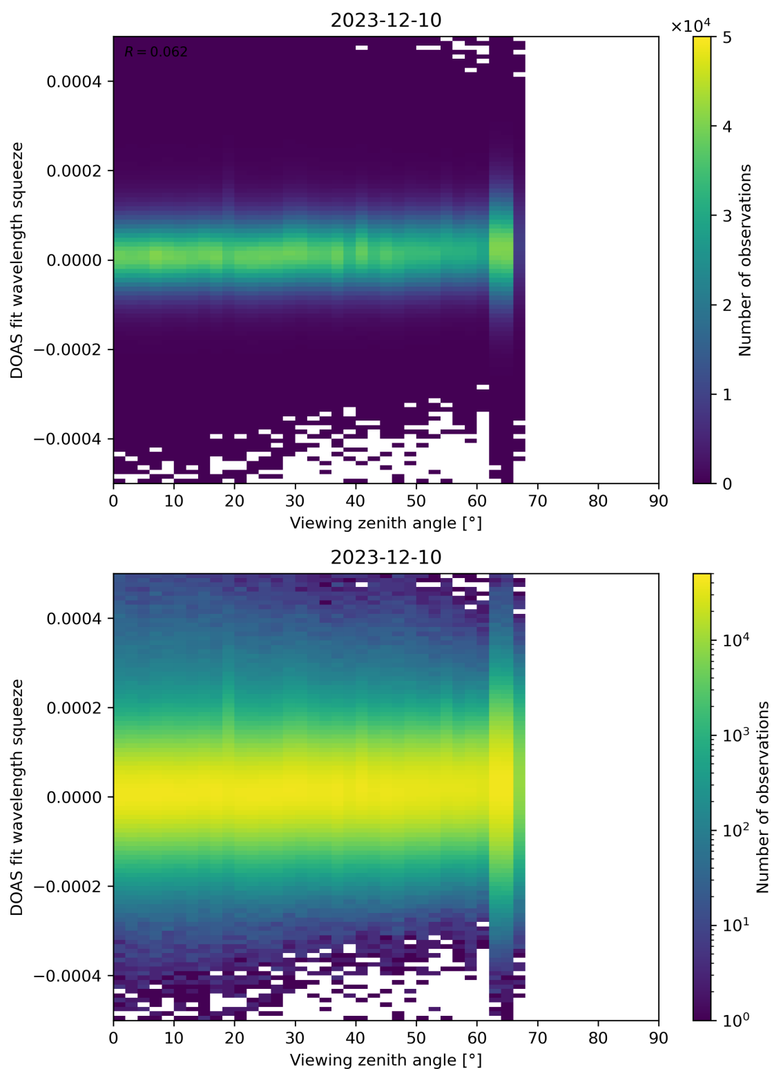
Figure 184: Scatter density plot of “Viewing zenith angle” against “DOAS fit wavelength squeeze” for 2023-12-09 to 2023-12-11.
