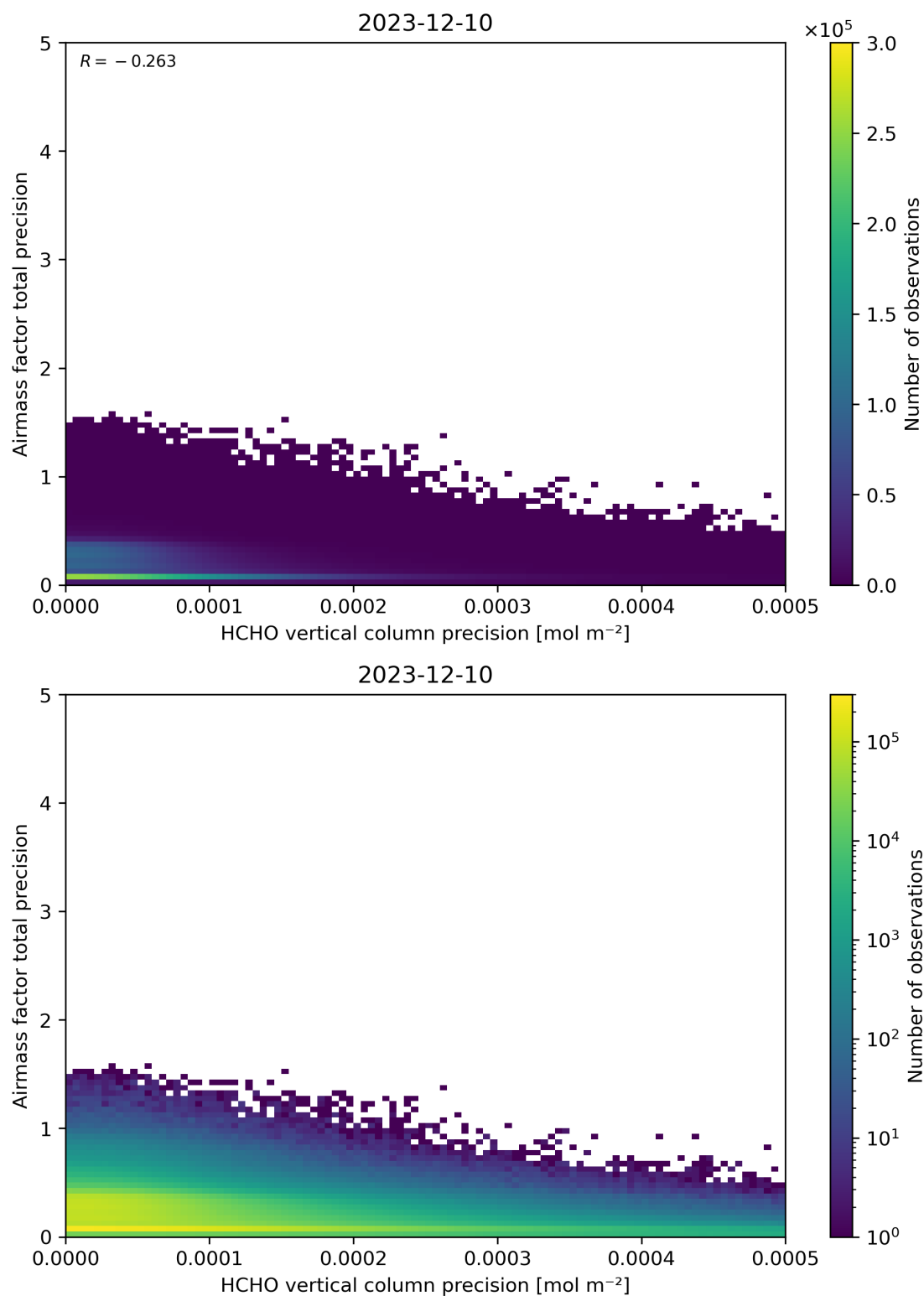
Figure 145: Scatter density plot of “HCHO vertical column precision” against “Airmass factor total precision” for 2023-12-09 to 2023-12-11.
