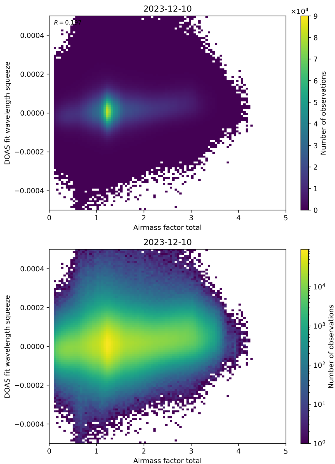
Figure 99: Scatter density plot of “Airmass factor total” against “DOAS fit wavelength squeeze” for 2023-12-09 to 2023-12-11.
