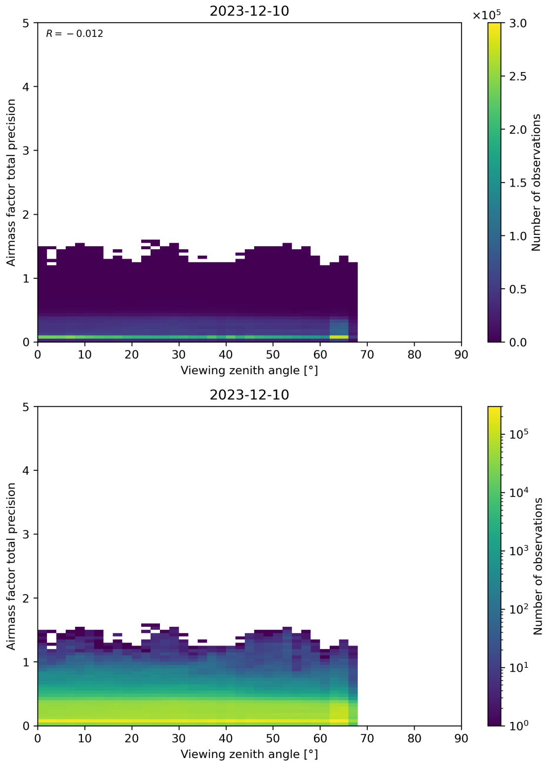
Figure 191: Scatter density plot of “Viewing zenith angle” against “Airmass factor total precision” for 2023-12-09 to 2023-12-11.
