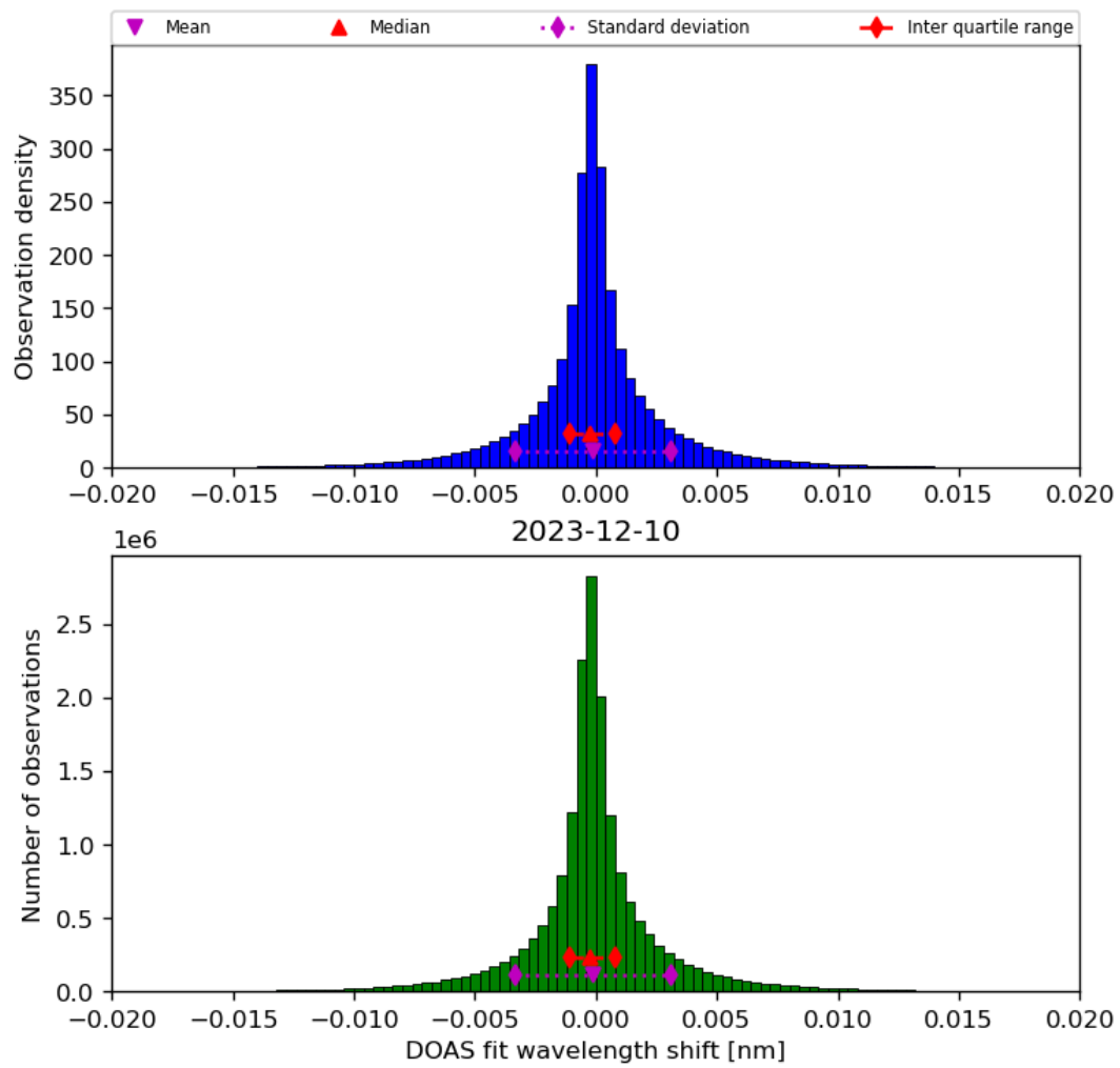
Figure 44: Histogram of “DOAS fit wavelength shift” for 2023-12-09 to 2023-12-11
