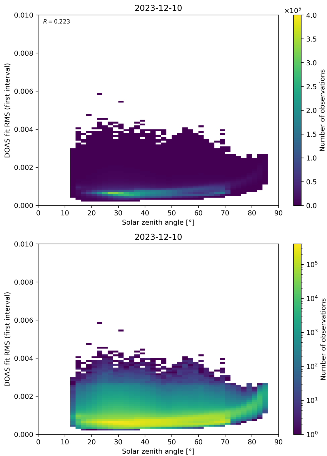
Figure 167: Scatter density plot of “Solar zenith angle” against “DOAS fit RMS (first interval)” for 2023-12-09 to 2023-12-11.
