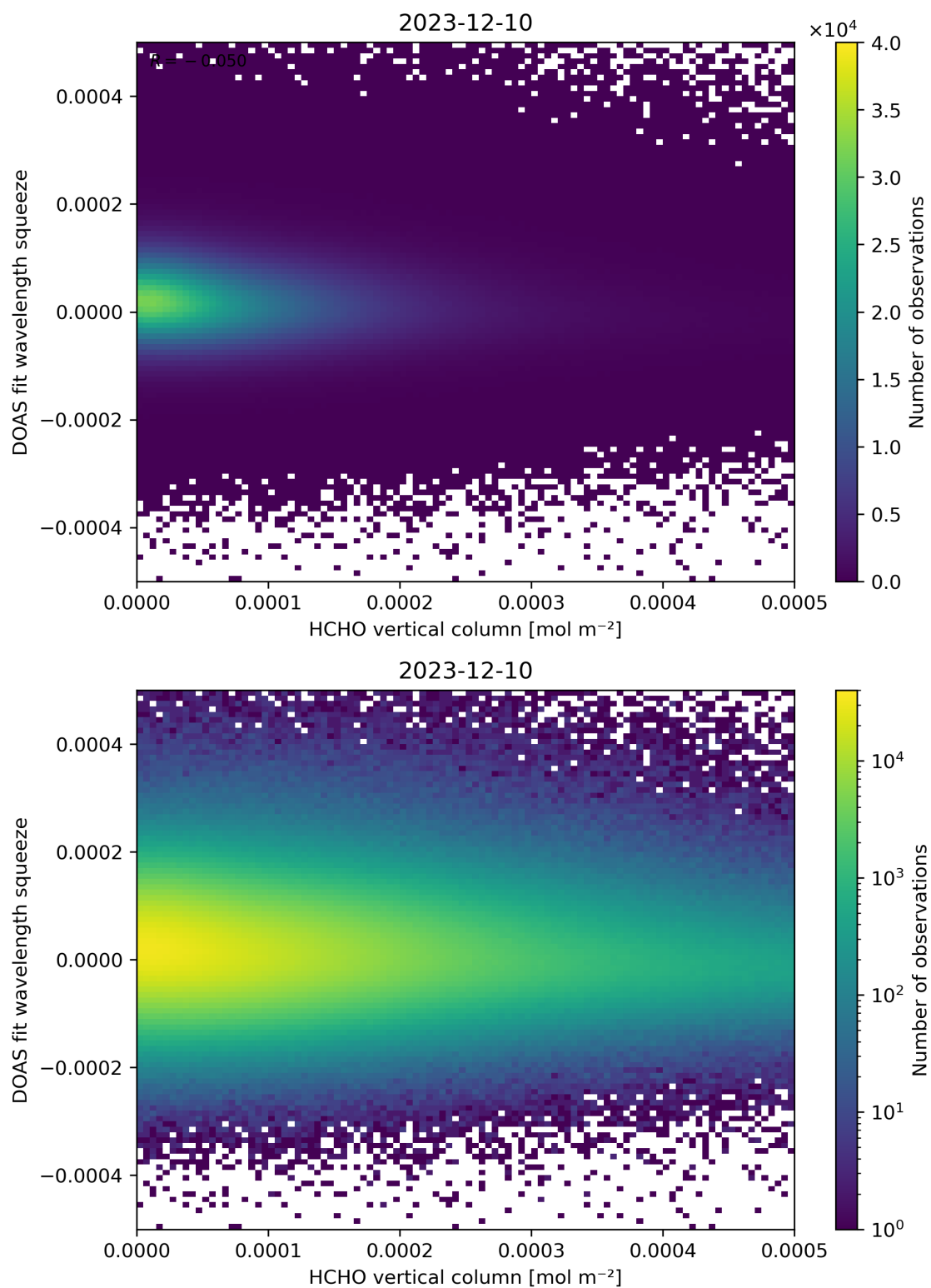
Figure 125: Scatter density plot of “HCHO vertical column” against “DOAS fit wavelength squeeze” for 2023-12-09 to 2023-12-11.
