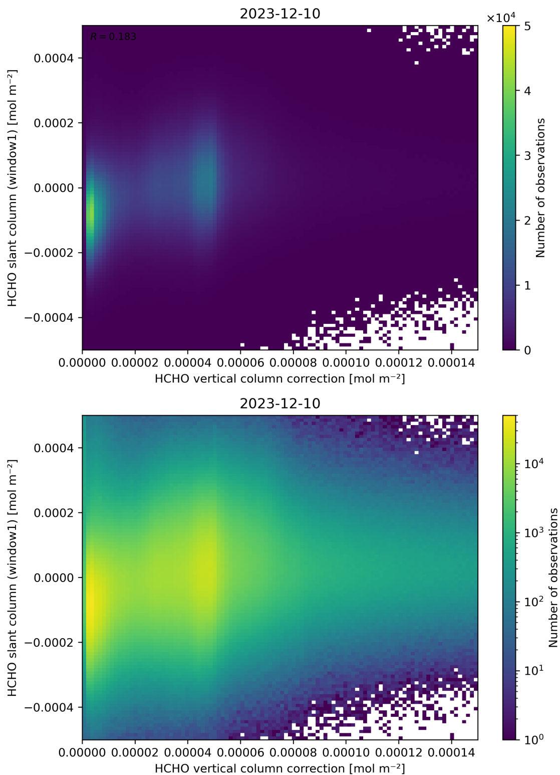
Figure 118: Scatter density plot of “HCHO vertical column correction” against “HCHO slant column (window1)” for 2023-12-09 to 2023-12-11.
