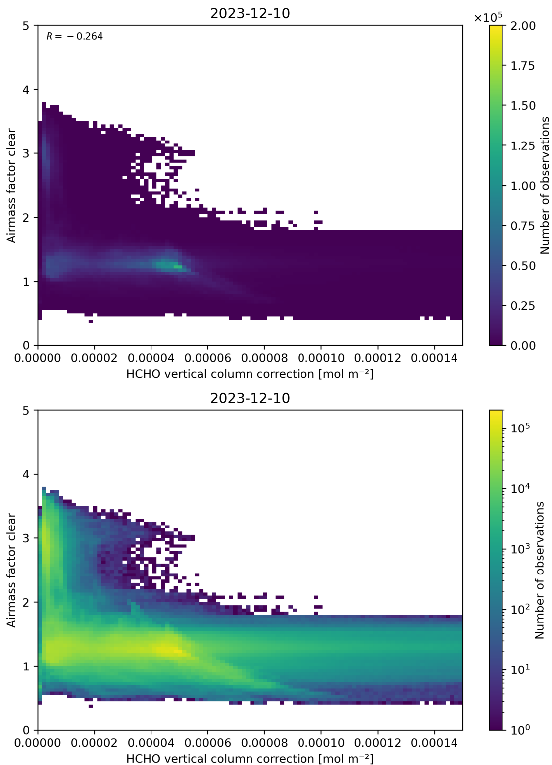
Figure 115: Scatter density plot of “HCHO vertical column correction” against “Airmass factor clear” for 2023-12-09 to 2023-12-11.
