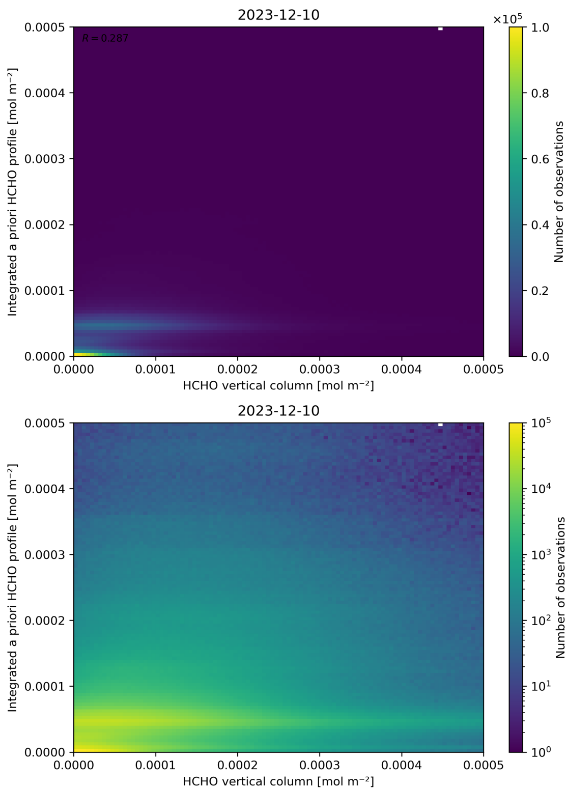
Figure 135: Scatter density plot of “HCHO vertical column” against “Integrated a priori HCHO profile” for 2023-12-09 to 2023-12-11.
