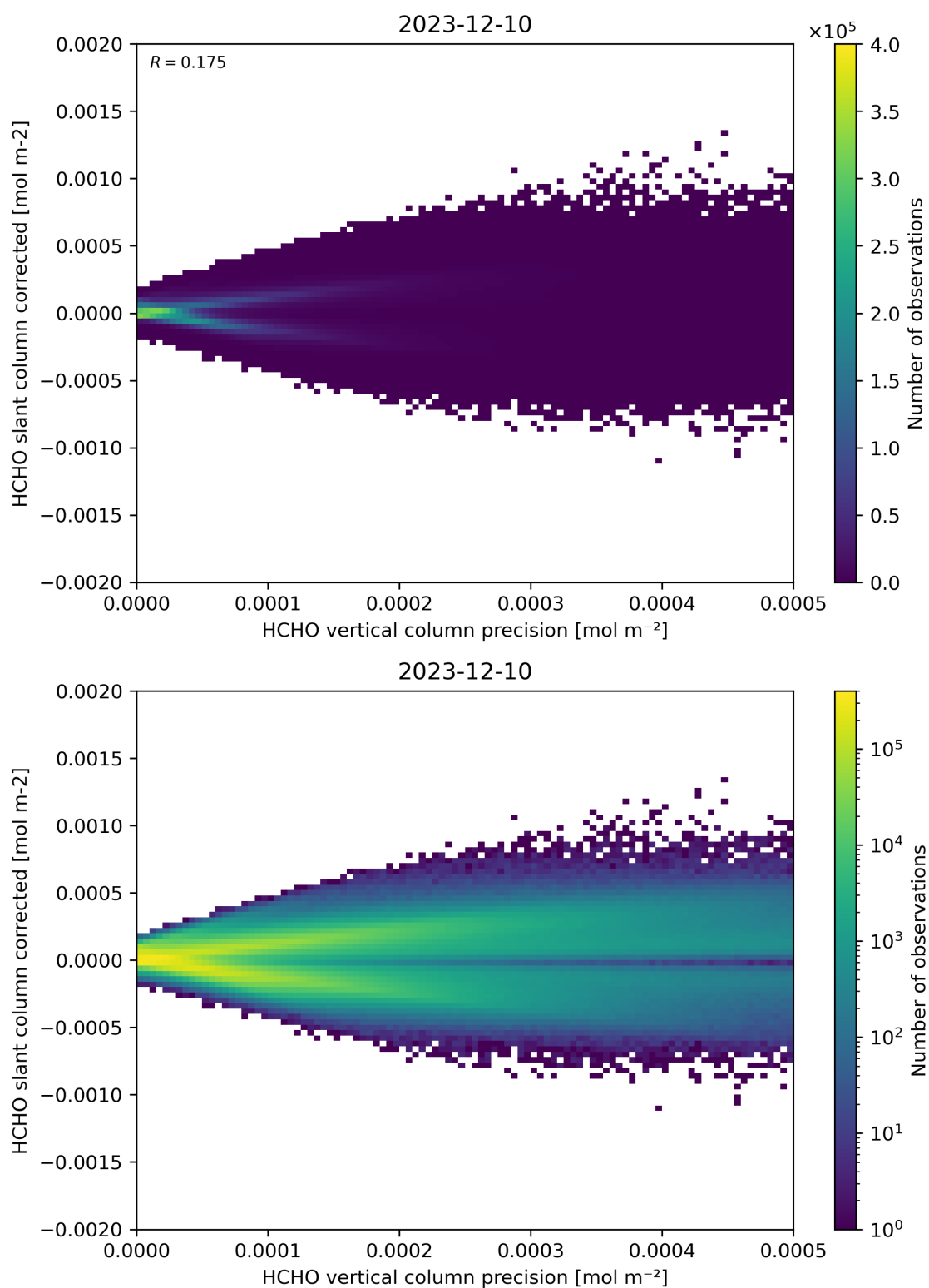
Figure 140: Scatter density plot of “HCHO vertical column precision” against “HCHO slant column corrected” for 2023-12-09 to 2023-12-11.
