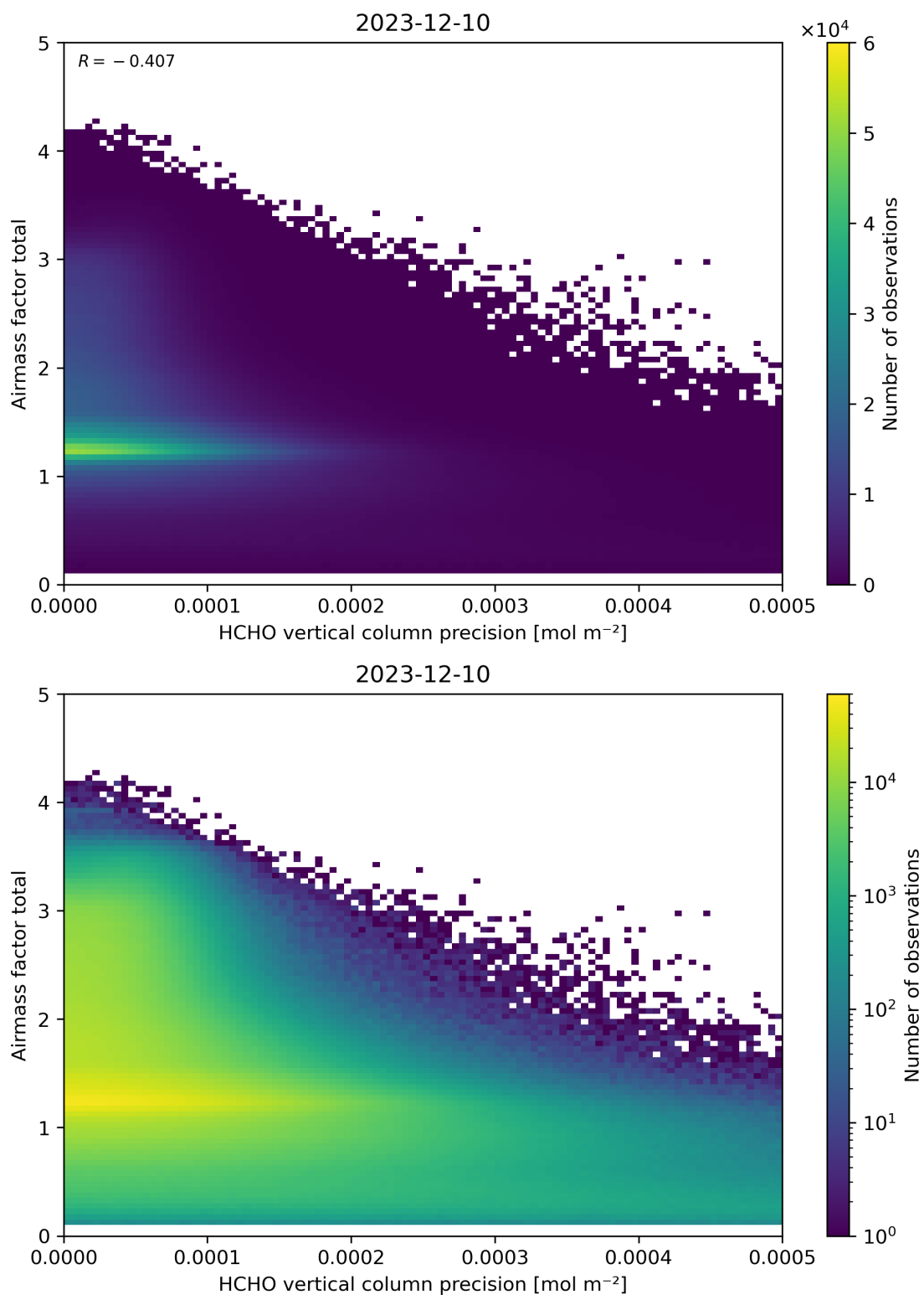
Figure 144: Scatter density plot of “HCHO vertical column precision” against “Airmass factor total” for 2023-12-09 to 2023-12-11.
