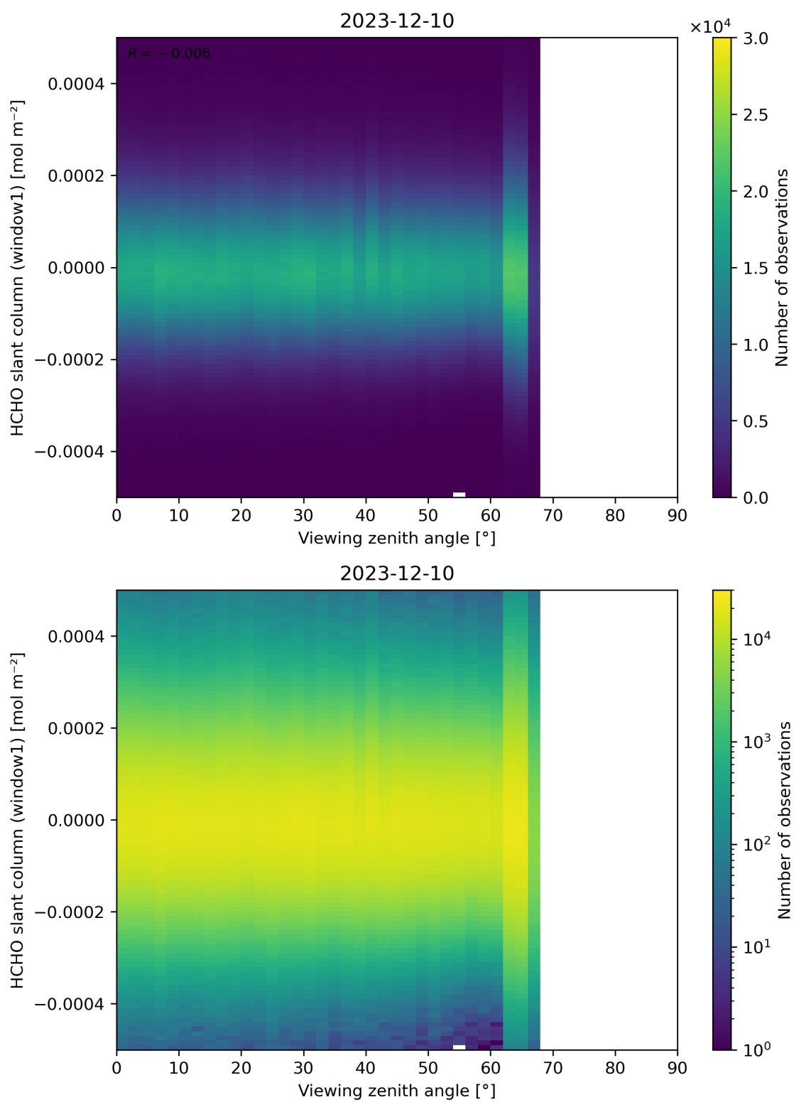
Figure 188: Scatter density plot of “Viewing zenith angle” against “HCHO slant column (window1)” for 2023-12-09 to 2023-12-11.
