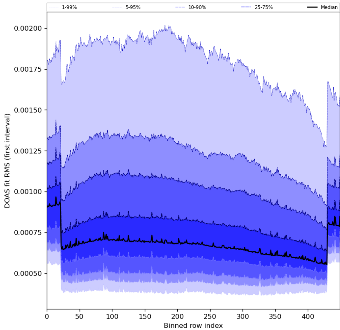
Figure 60: Along track statistics of “DOAS fit RMS (first interval)” for 2023-12-09 to 2023-12-11
