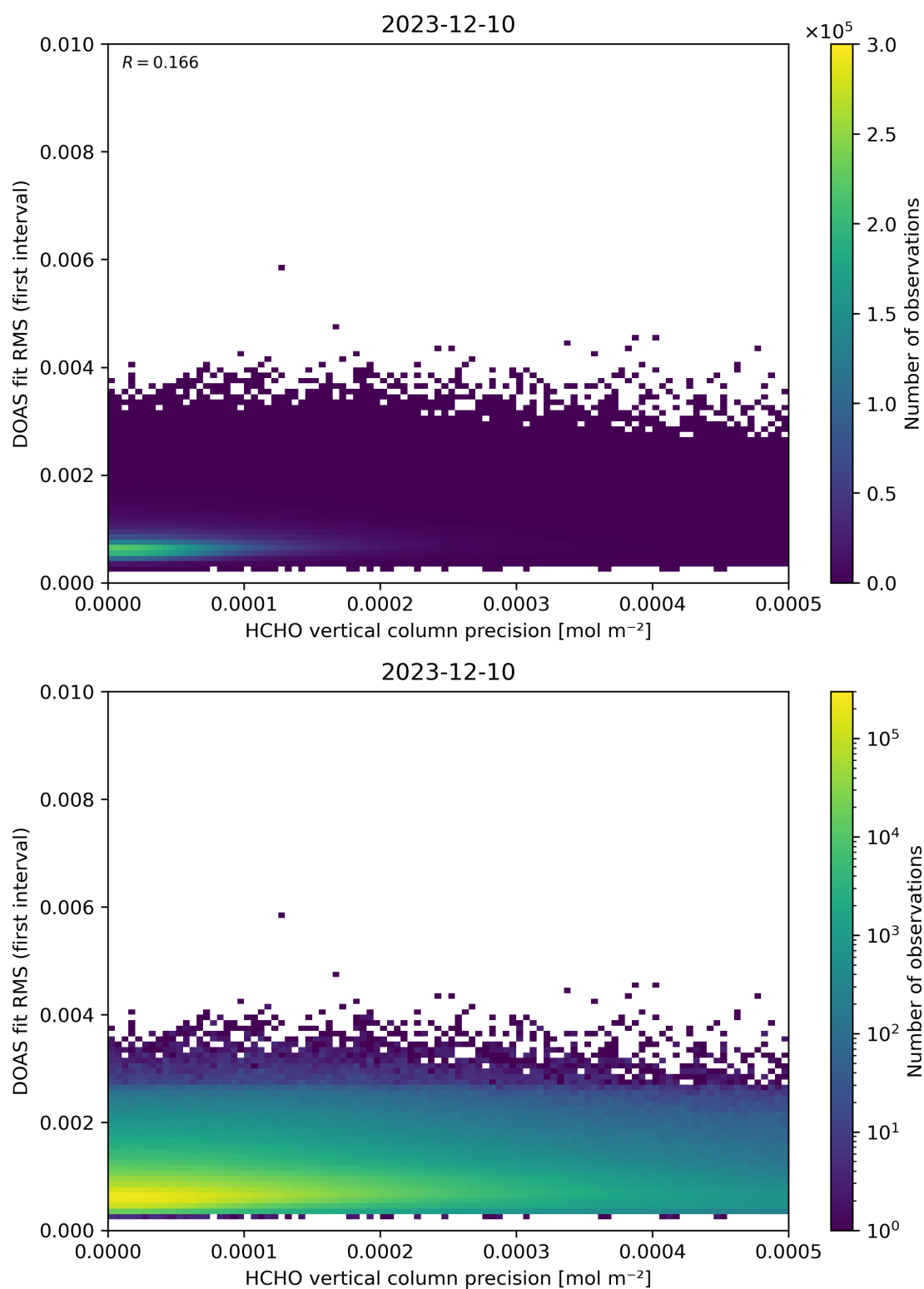
Figure 136: Scatter density plot of “HCHO vertical column precision” against “DOAS fit RMS (first interval)” for 2023-12-09 to 2023-12-11.
