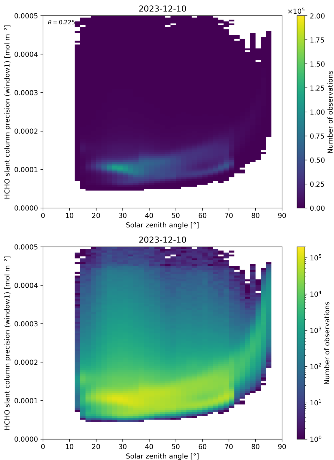
Figure 174: Scatter density plot of “Solar zenith angle” against “HCHO slant column precision (window1)” for 2023-12-09 to 2023-12-11.
