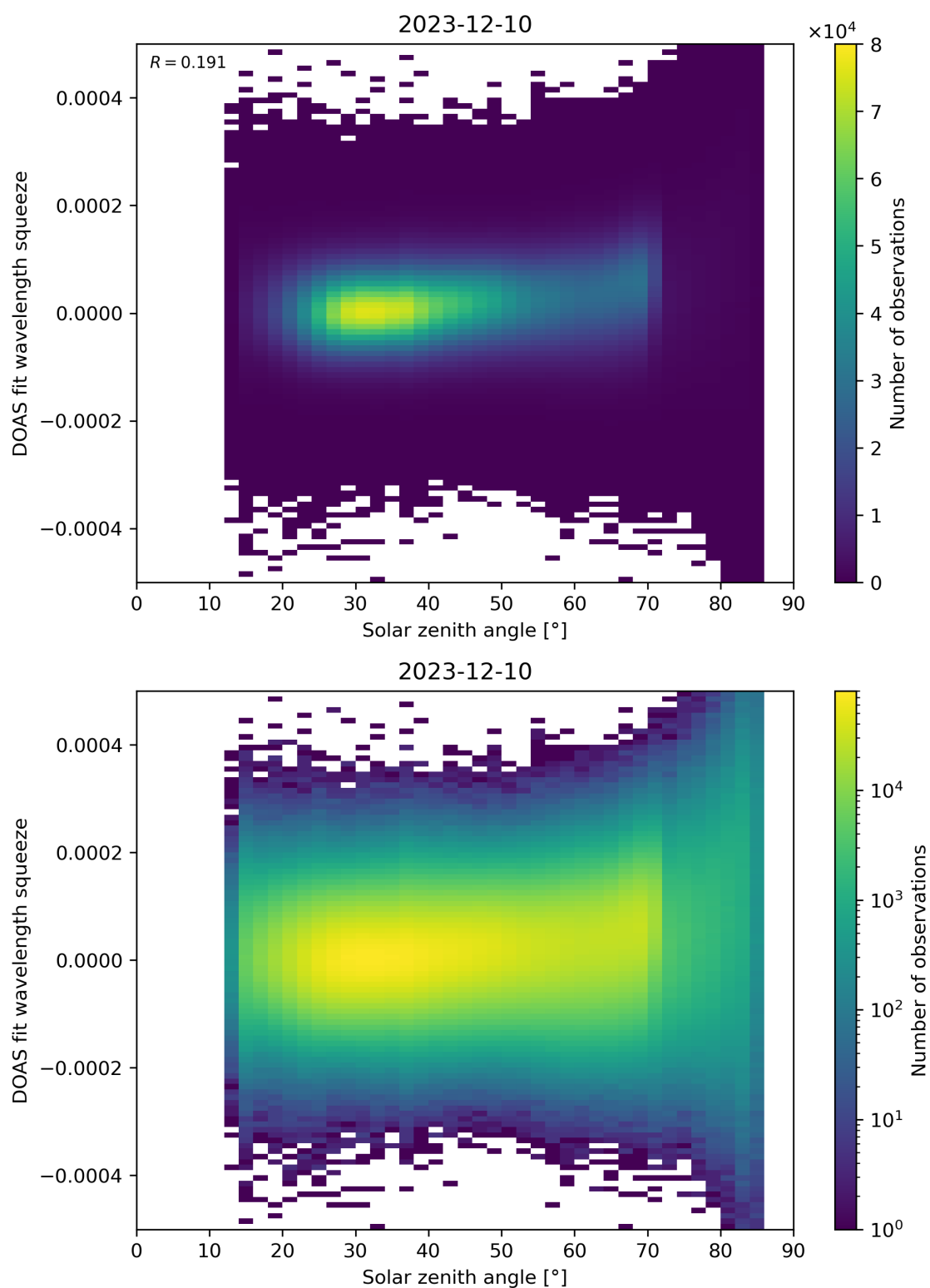
Figure 169: Scatter density plot of “Solar zenith angle” against “DOAS fit wavelength squeeze” for 2023-12-09 to 2023-12-11.
