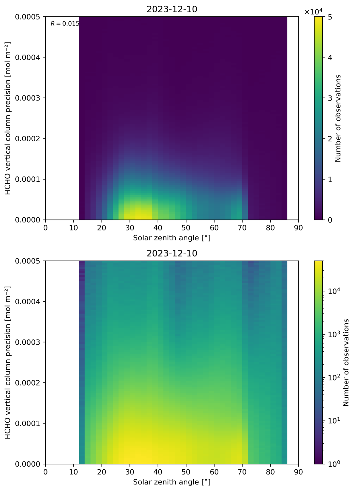
Figure 179: Scatter density plot of “Solar zenith angle” against “HCHO vertical column precision” for 2023-12-09 to 2023-12-11.
