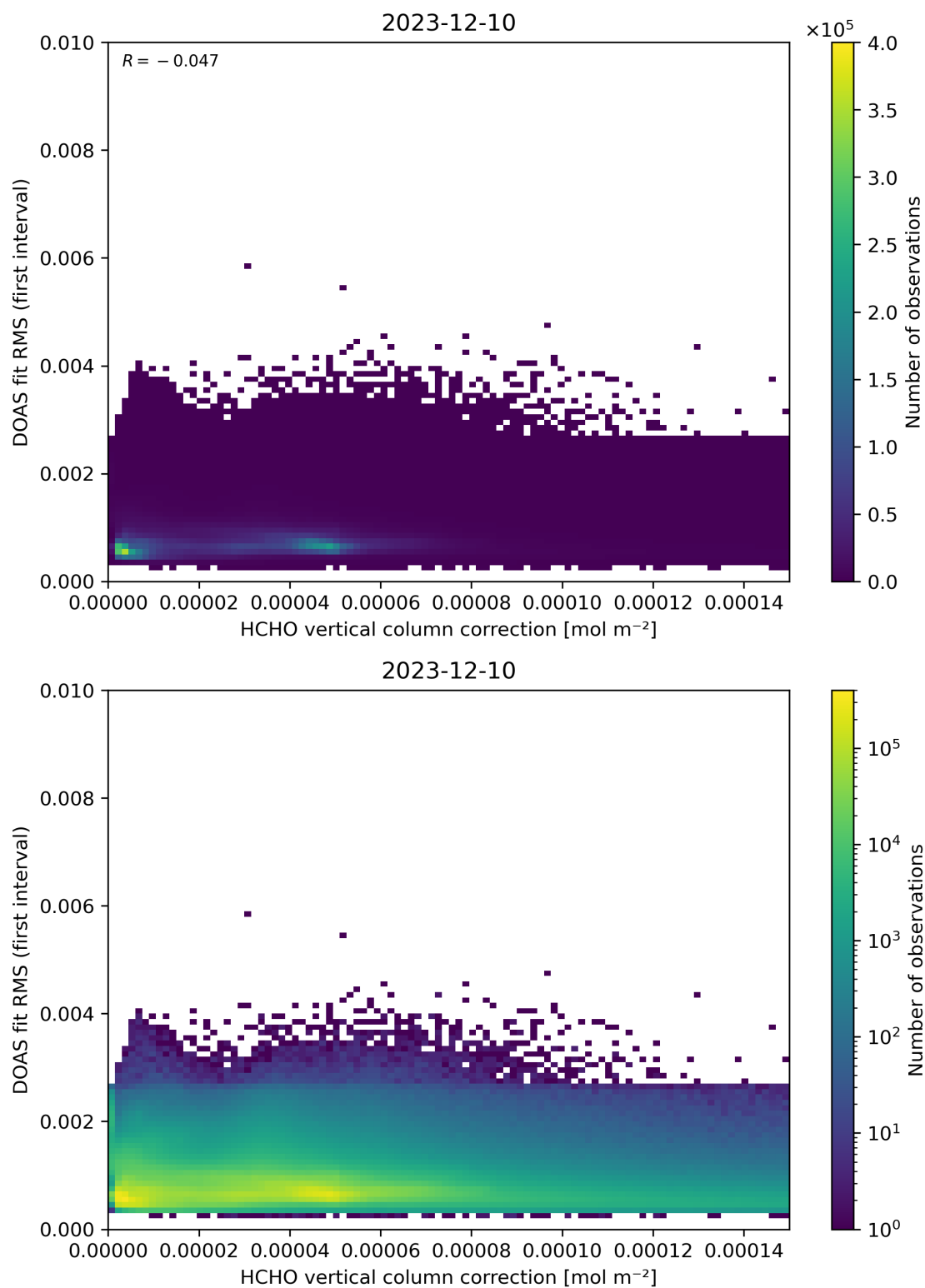
Figure 112: Scatter density plot of “HCHO vertical column correction” against “DOAS fit RMS (first interval)” for 2023-12-09 to 2023-12-11.
