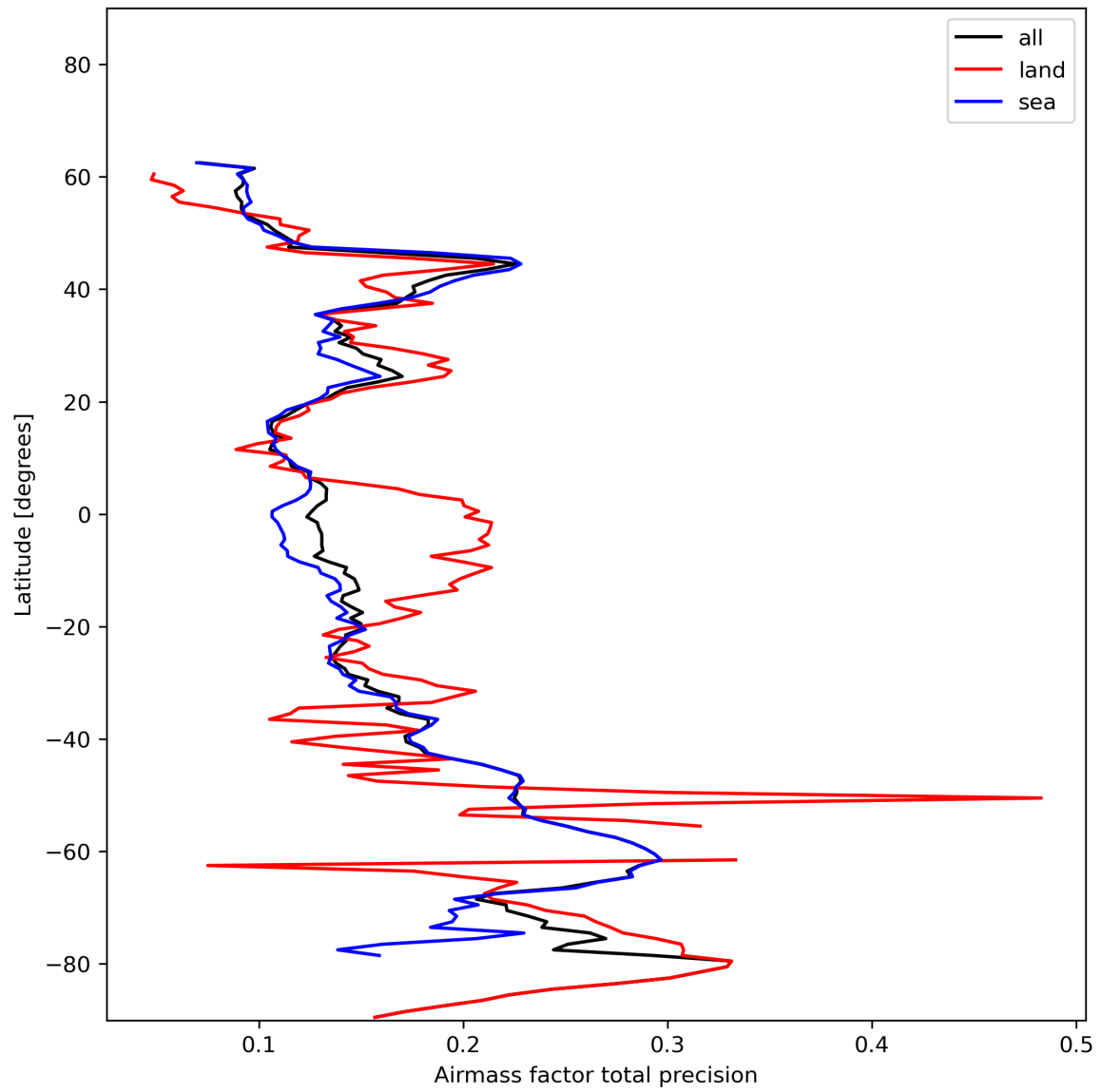
Figure 27: Zonal average of “Airmass factor total precision” for 2023-12-09 to 2023-12-11.
