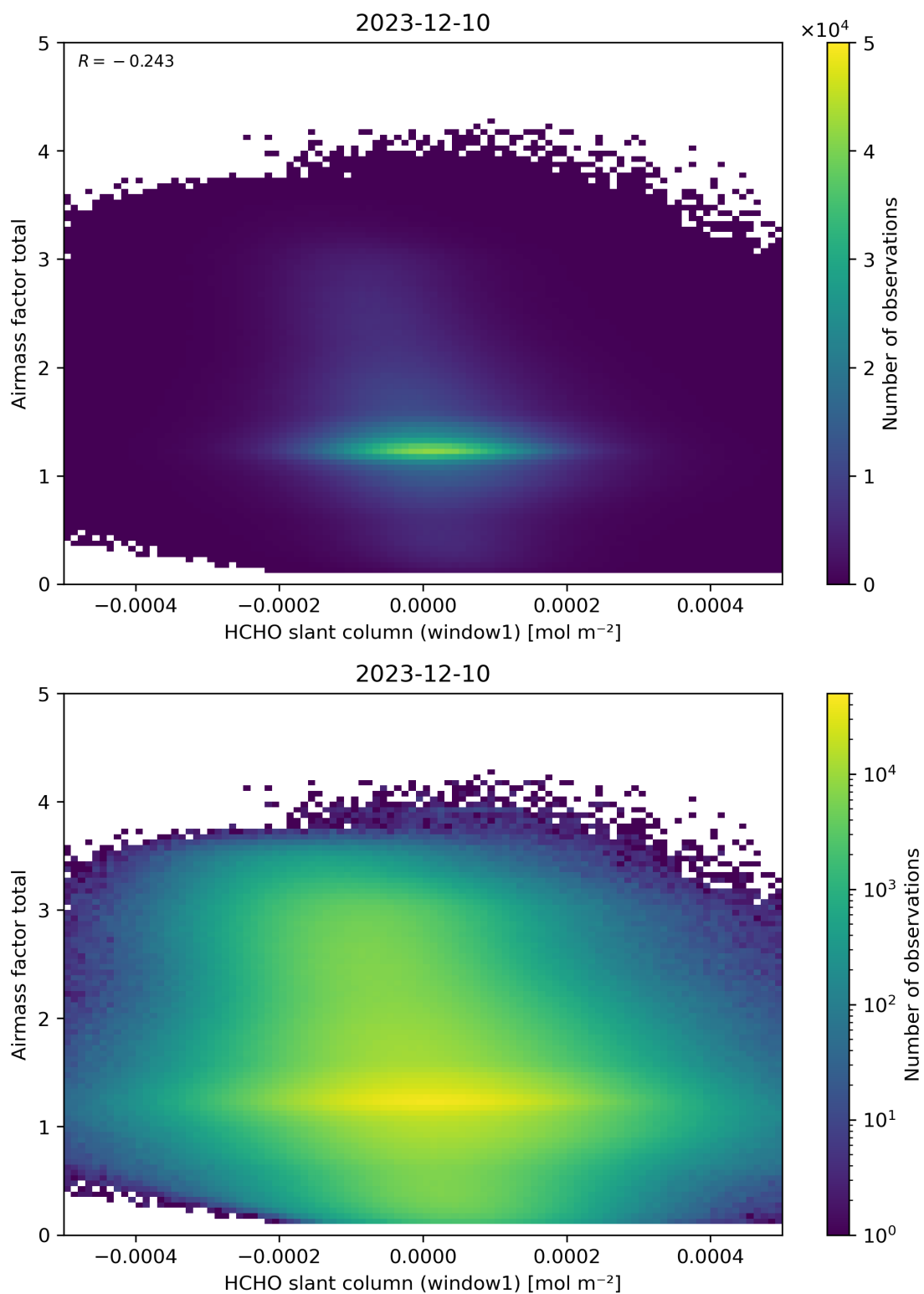
Figure 85: Scatter density plot of “HCHO slant column (window1)” against “Airmass factor total” for 2023-12-09 to 2023-12-11.
