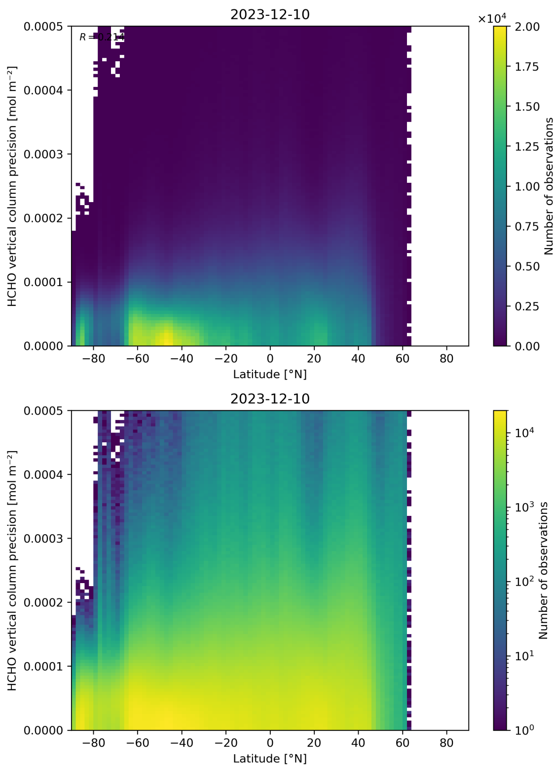
Figure 165: Scatter density plot of “Latitude” against “HCHO vertical column precision” for 2023-12-09 to 2023-12-11.
