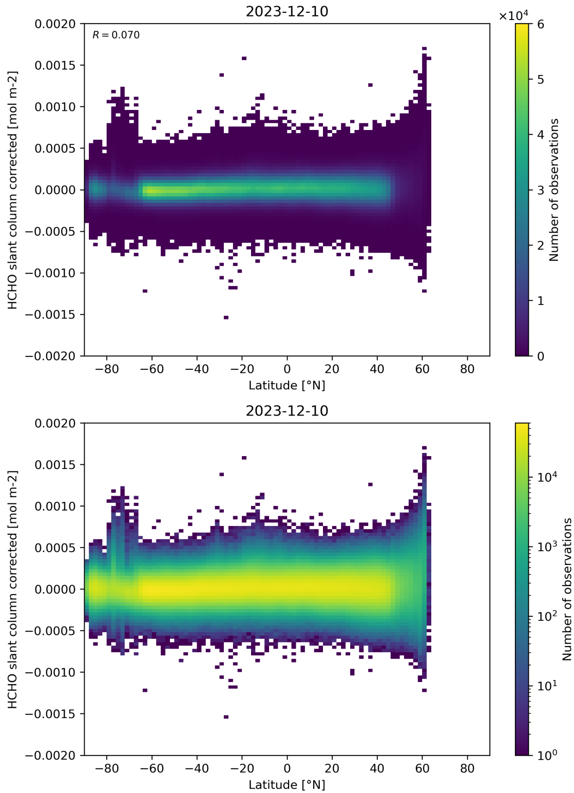
Figure 157: Scatter density plot of “Latitude” against “HCHO slant column corrected” for 2023-12-09 to 2023-12-11.
