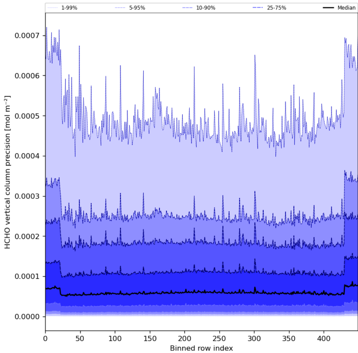
Figure 50: Along track statistics of “HCHO vertical column precision” for 2023-12-09 to 2023-12-11
