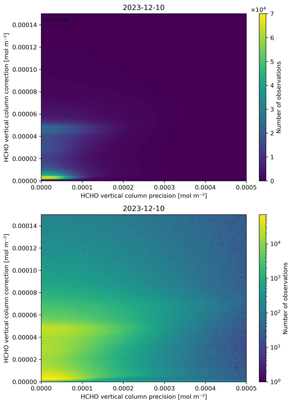
Figure 146: Scatter density plot of “HCHO vertical column precision” against “HCHO vertical column correction” for 2023-12-09 to 2023-12-11.
