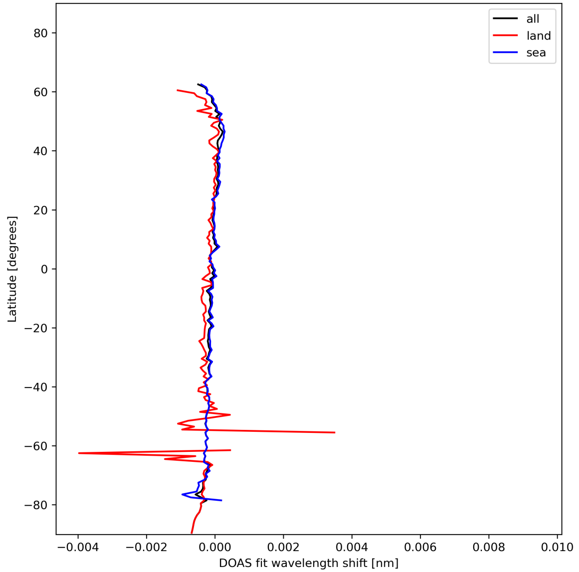
Figure 30: Zonal average of “DOAS fit wavelength shift” for 2023-12-09 to 2023-12-11.
