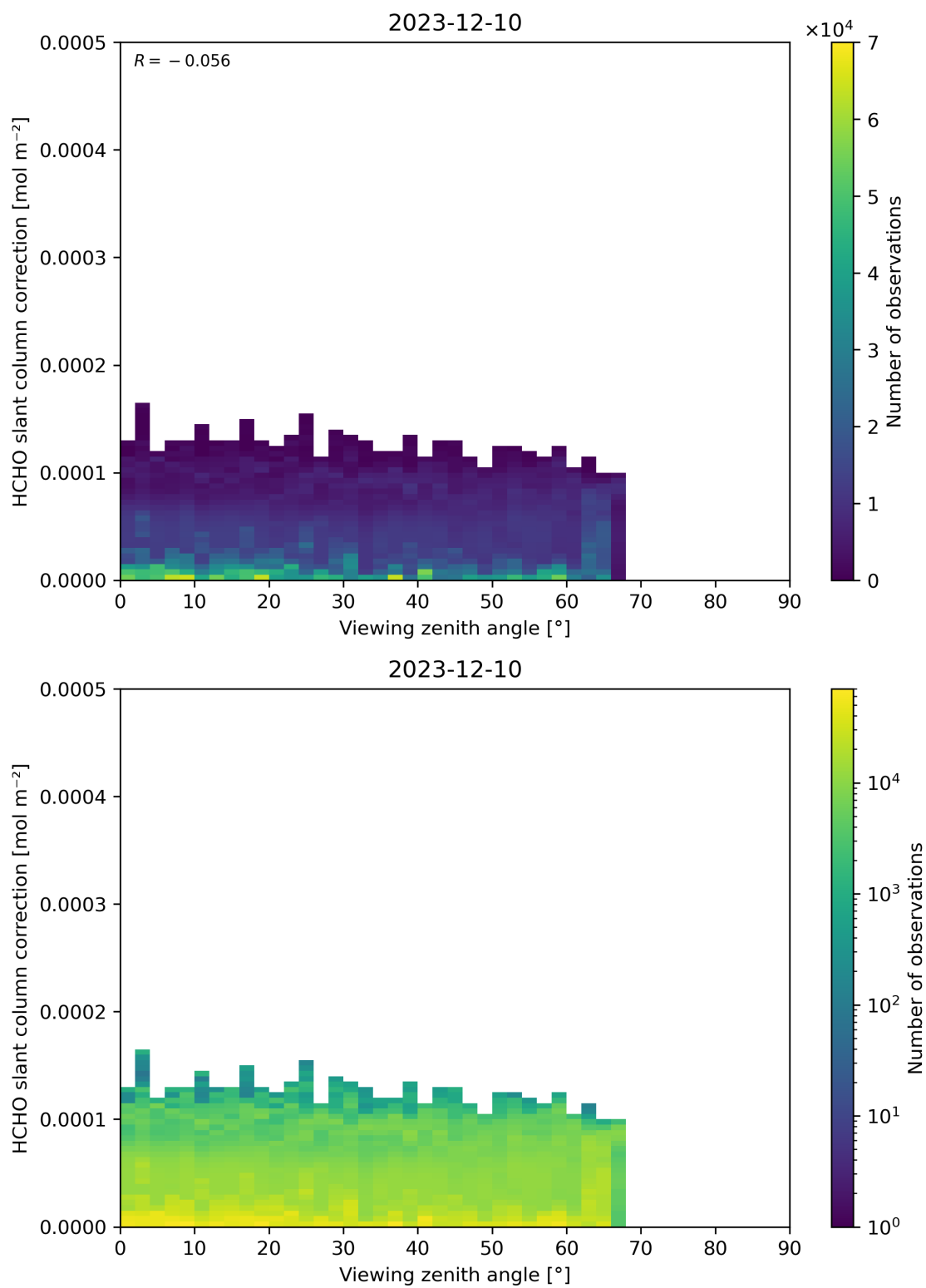
Figure 187: Scatter density plot of “Viewing zenith angle” against “HCHO slant column correction” for 2023-12-09 to 2023-12-11.
