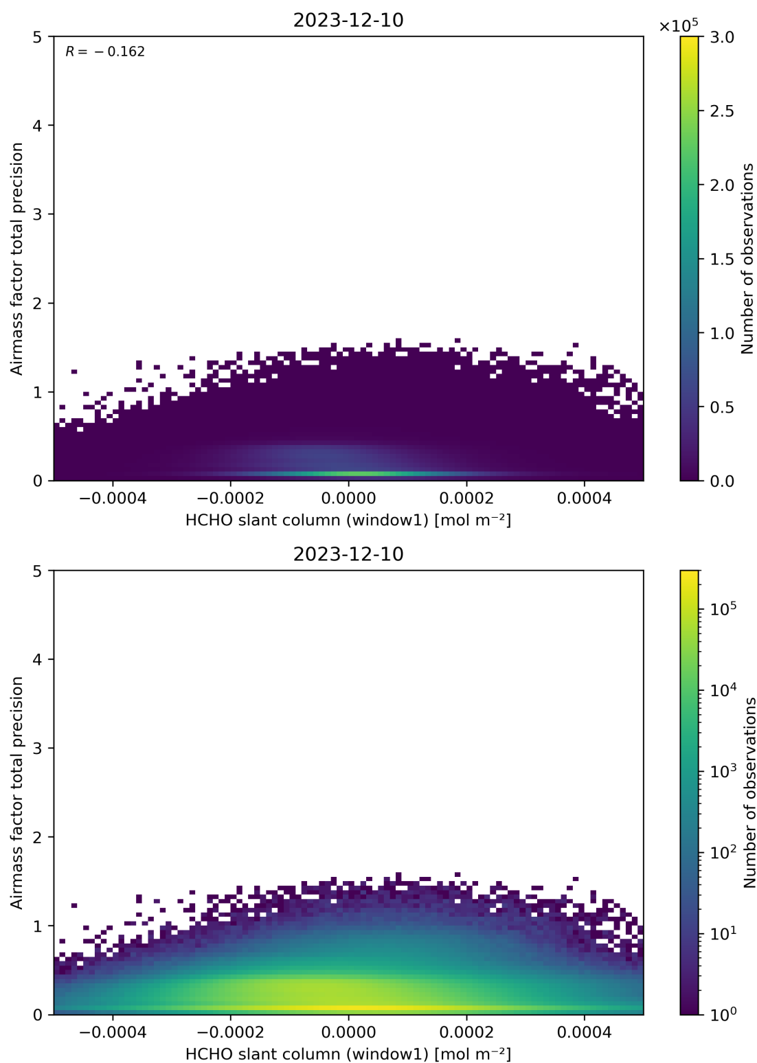
Figure 86: Scatter density plot of “HCHO slant column (window1)” against “Airmass factor total precision” for 2023-12-09 to 2023-12-11.
