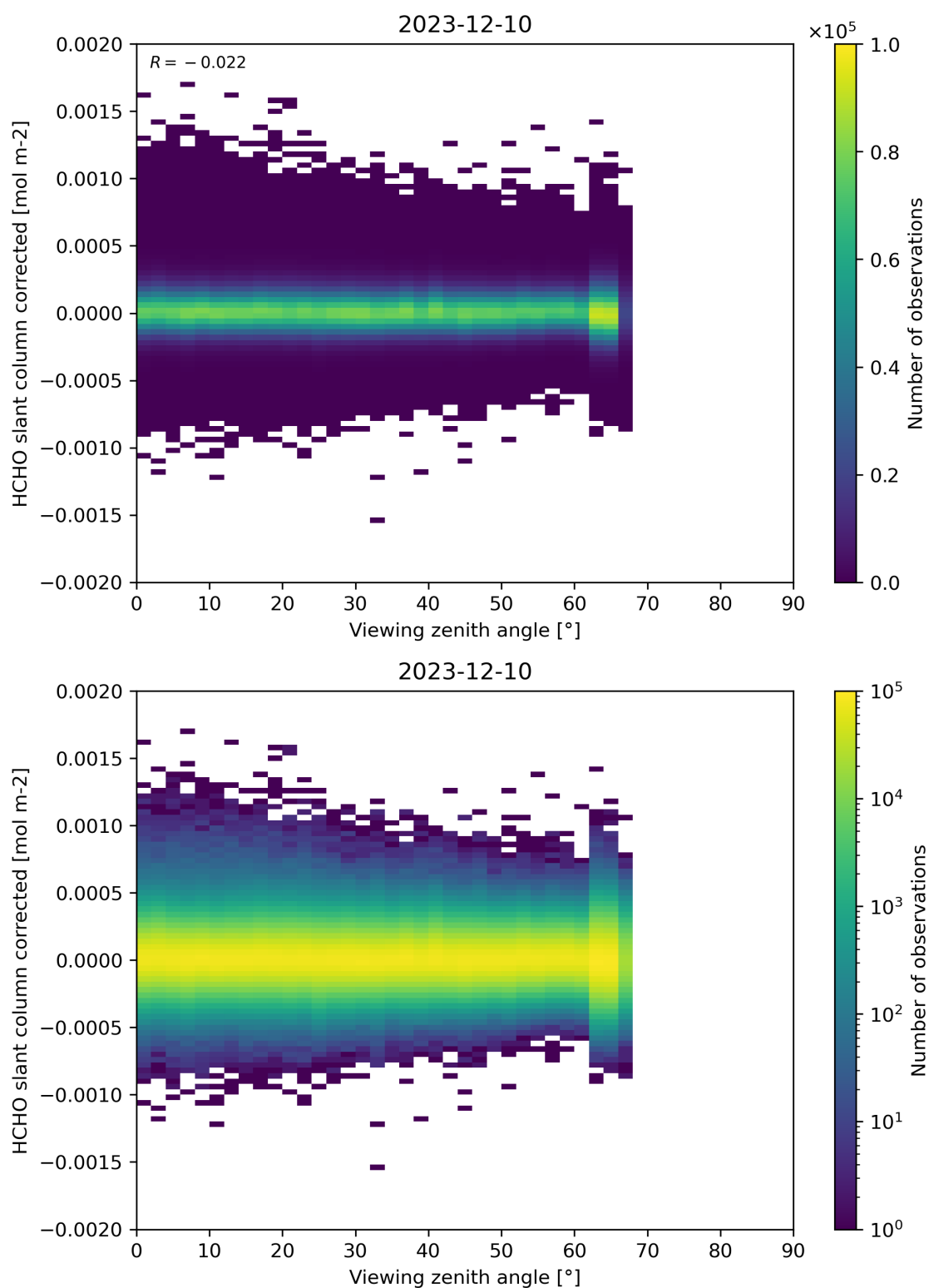
Figure 186: Scatter density plot of “Viewing zenith angle” against “HCHO slant column corrected” for 2023-12-09 to 2023-12-11.
