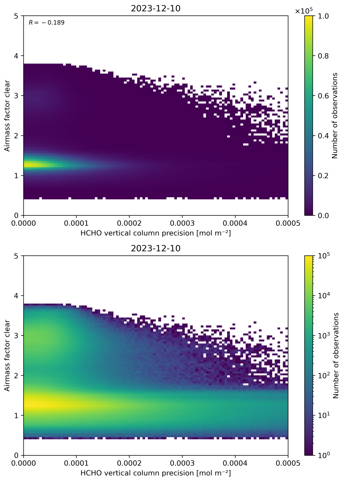
Figure 139: Scatter density plot of “HCHO vertical column precision” against “Airmass factor clear” for 2023-12-09 to 2023-12-11.
