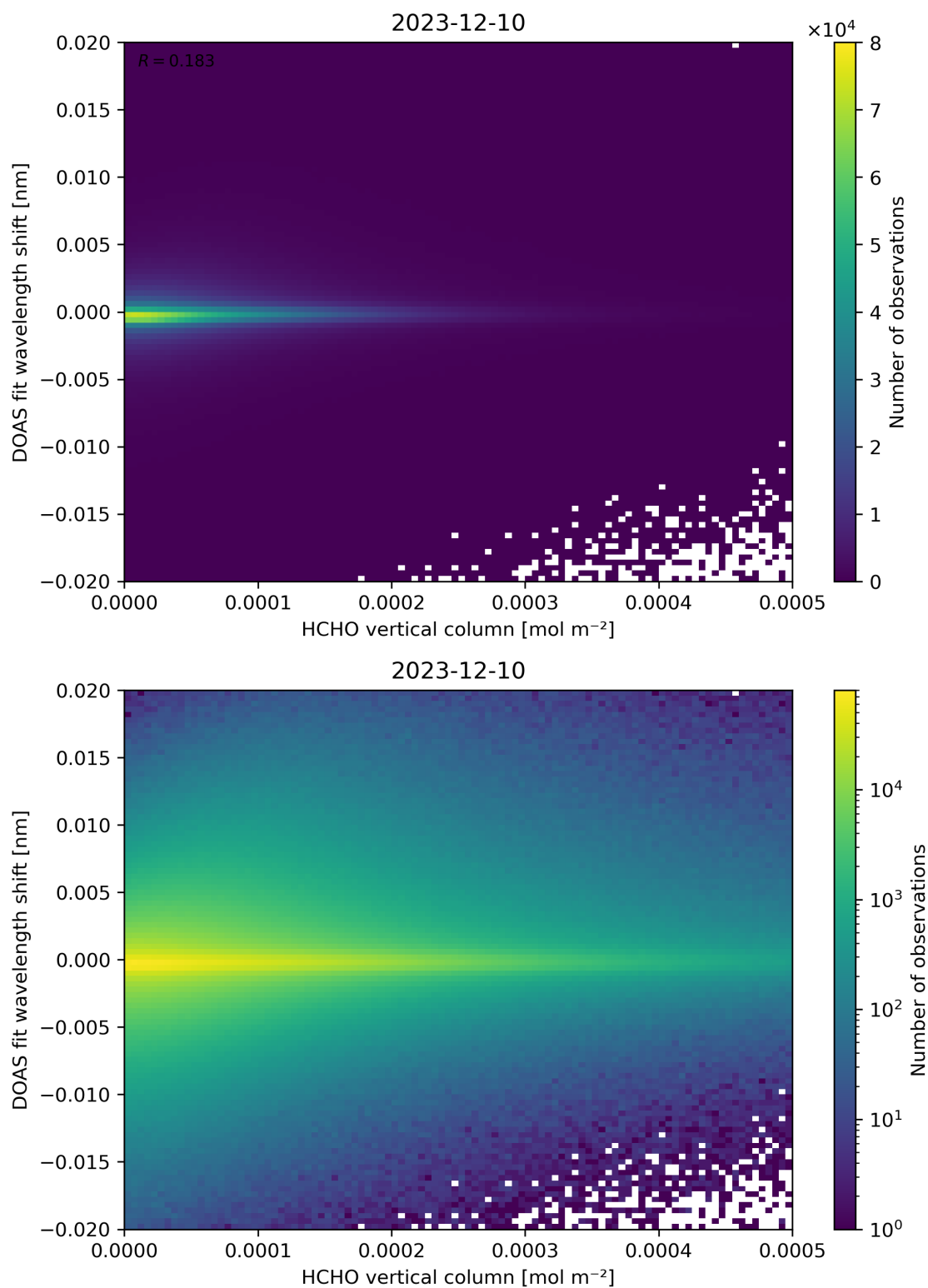
Figure 124: Scatter density plot of “HCHO vertical column” against “DOAS fit wavelength shift” for 2023-12-09 to 2023-12-11.
