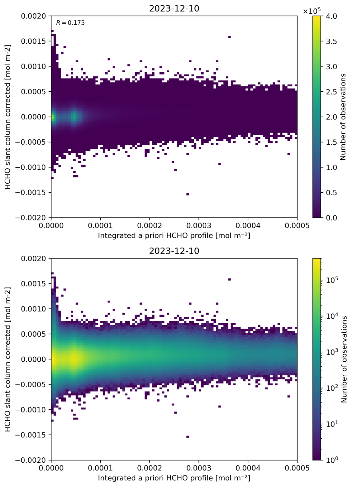
Figure 151: Scatter density plot of “Integrated a priori HCHO profile” against “HCHO slant column corrected” for 2023-12-09 to 2023-12-11.
