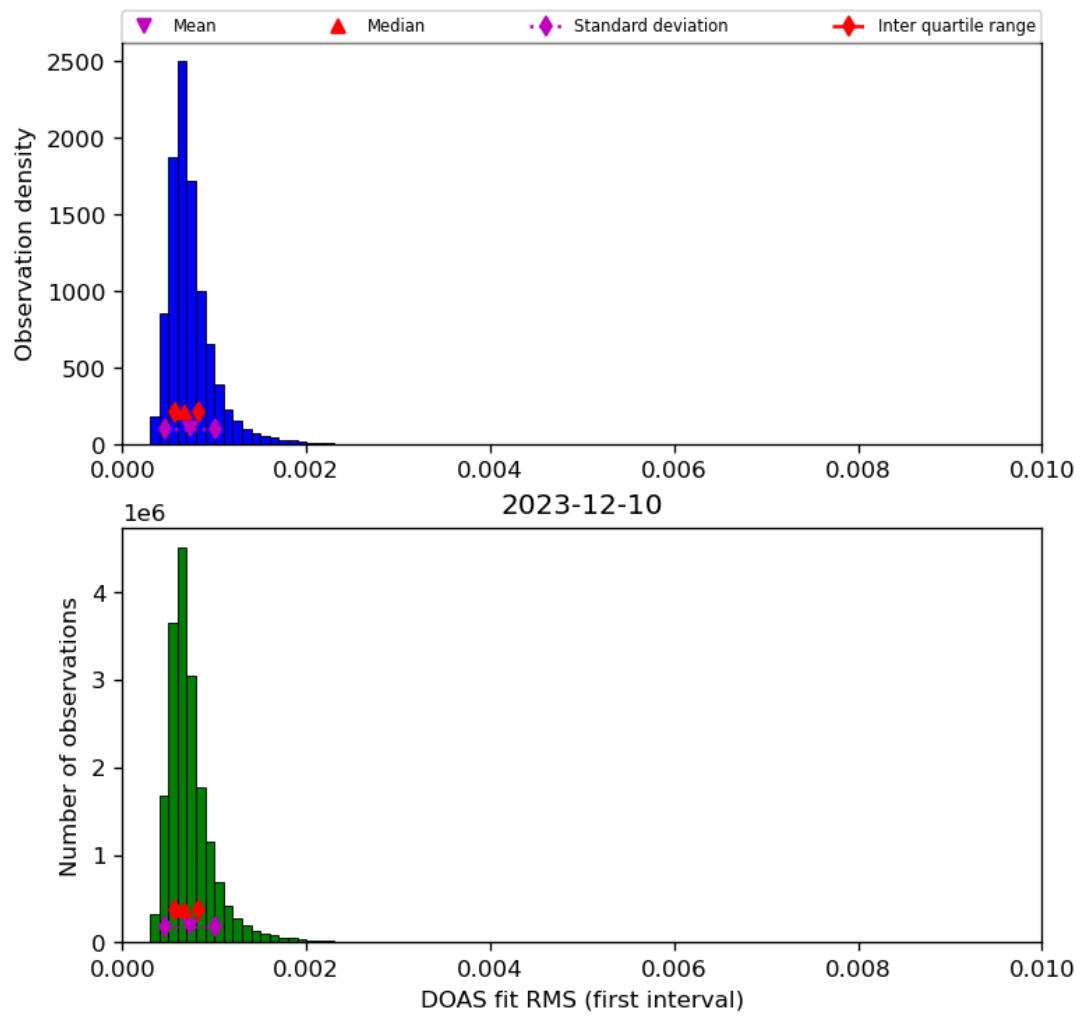
Figure 46: Histogram of “DOAS fit RMS (first interval)” for 2023-12-09 to 2023-12-11
