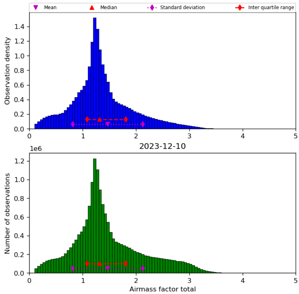
Figure 40: Histogram of “Airmass factor total” for 2023-12-09 to 2023-12-11
