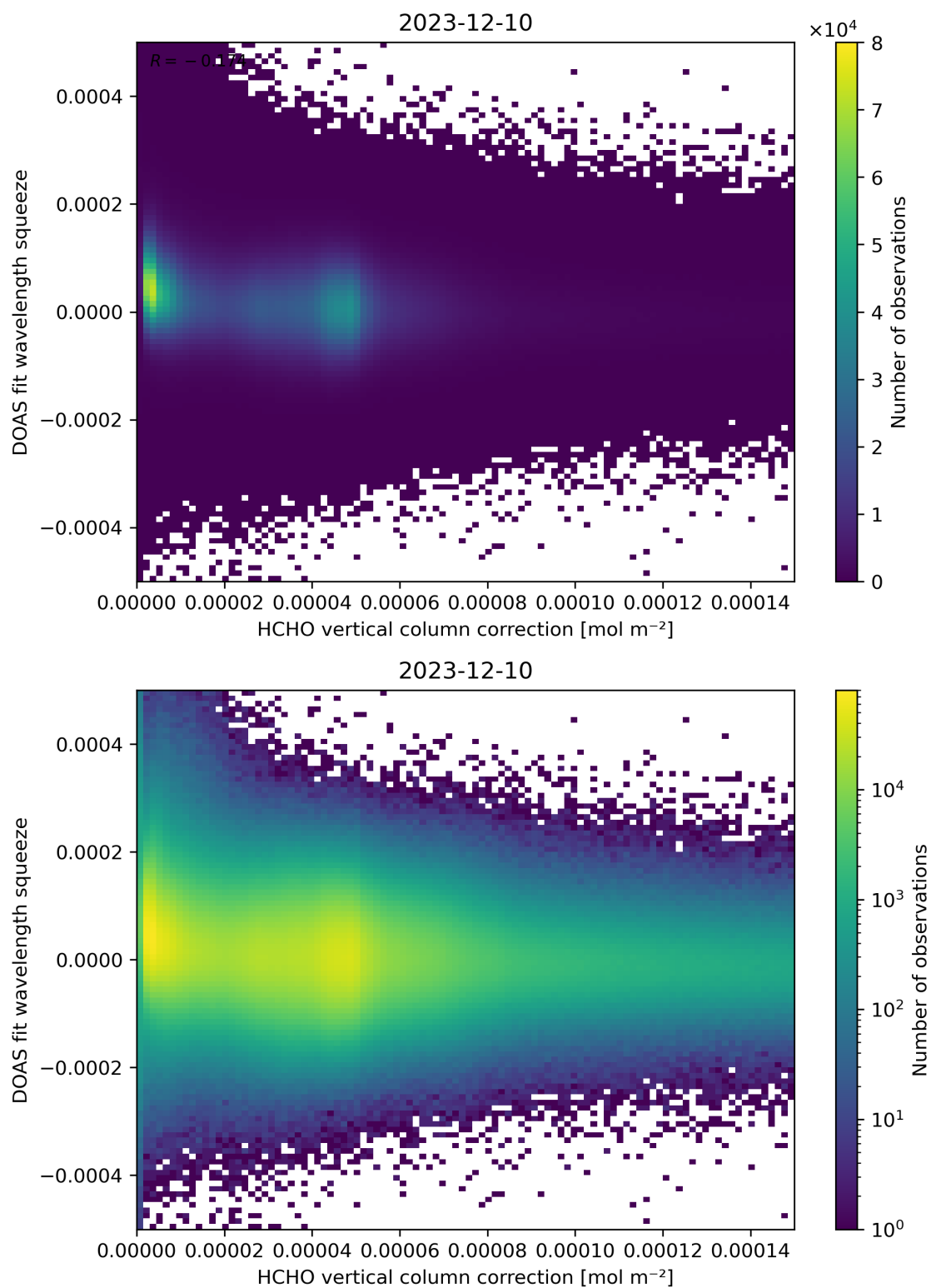
Figure 114: Scatter density plot of “HCHO vertical column correction” against “DOAS fit wavelength squeeze” for 2023-12-09 to 2023-12-11.
