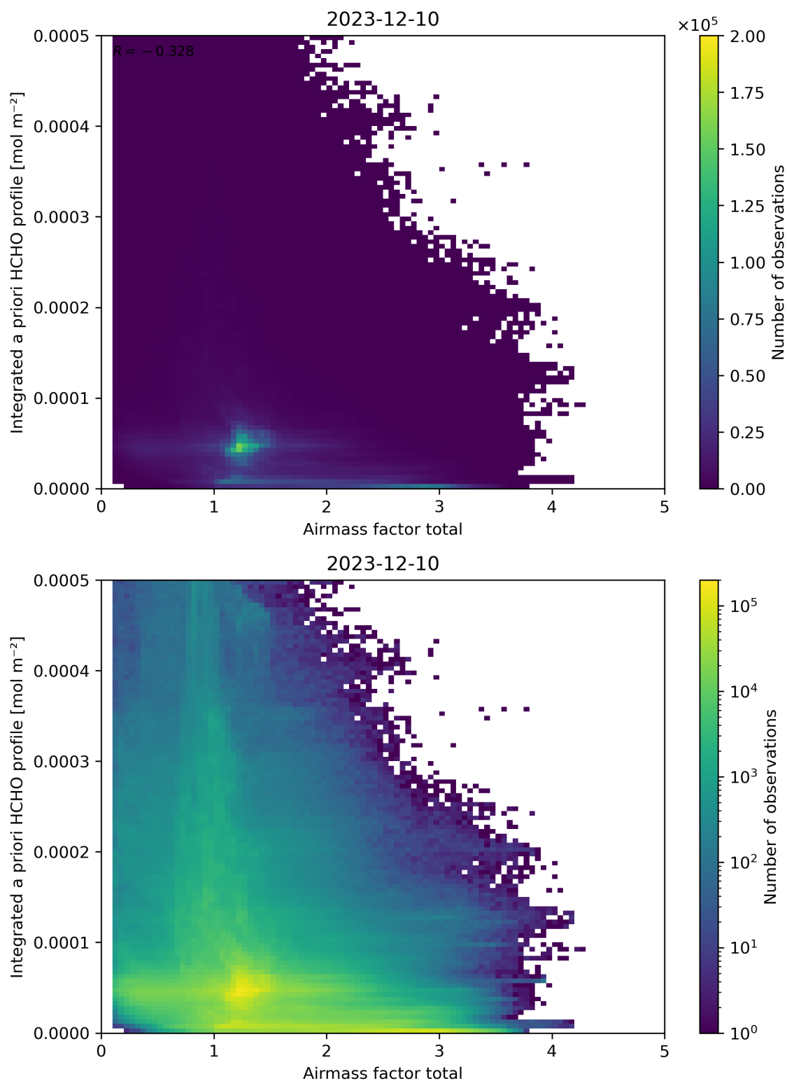
Figure 104: Scatter density plot of “Airmass factor total” against “Integrated a priori HCHO profile” for 2023-12-09 to 2023-12-11.
