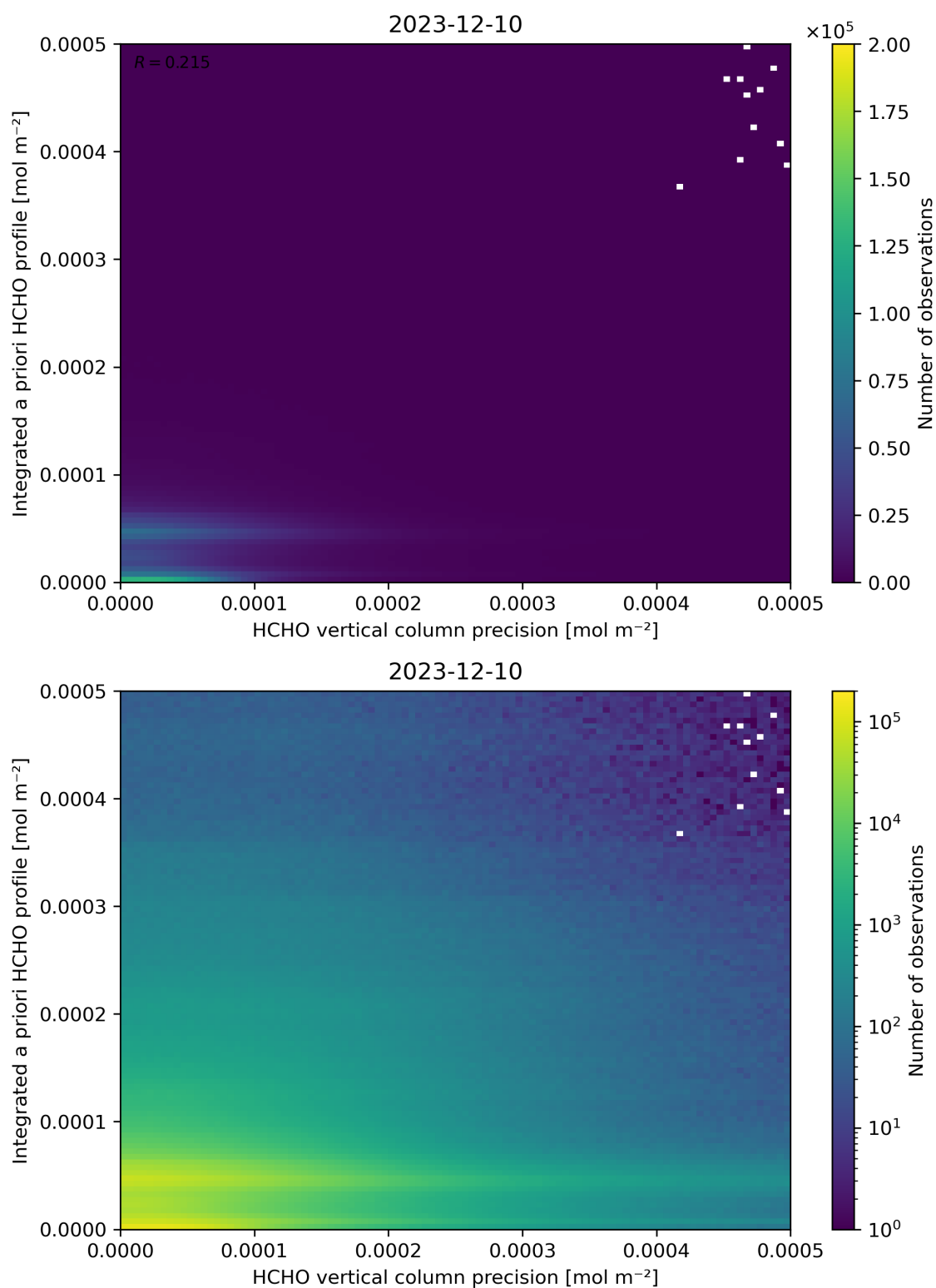
Figure 147: Scatter density plot of “HCHO vertical column precision” against “Integrated a priori HCHO profile” for 2023-12-09 to 2023-12-11.
