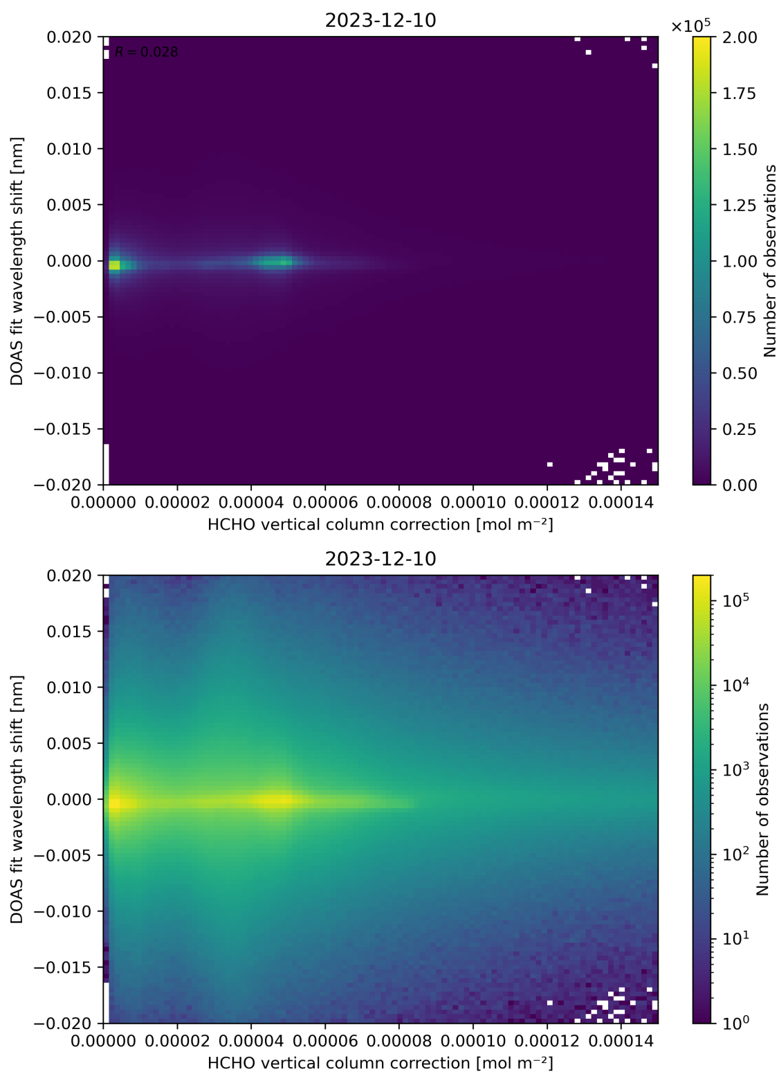
Figure 113: Scatter density plot of “HCHO vertical column correction” against “DOAS fit wavelength shift” for 2023-12-09 to 2023-12-11.
