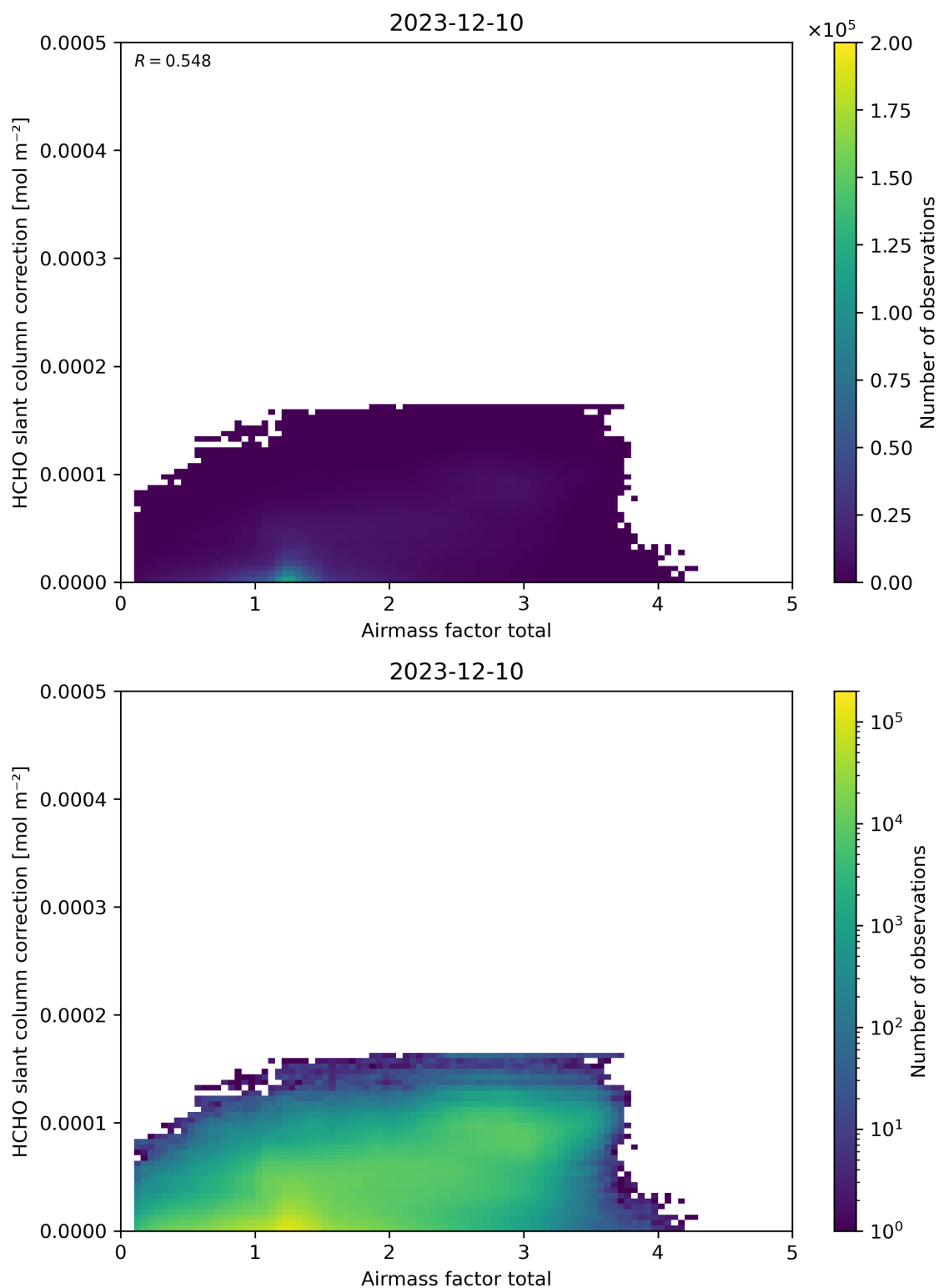
Figure 102: Scatter density plot of “Airmass factor total” against “HCHO slant column correction” for 2023-12-09 to 2023-12-11.
