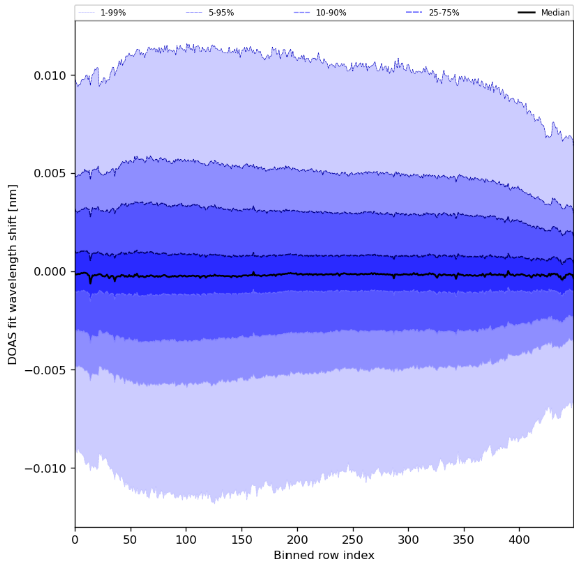
Figure 58: Along track statistics of “DOAS fit wavelength shift” for 2023-12-09 to 2023-12-11
