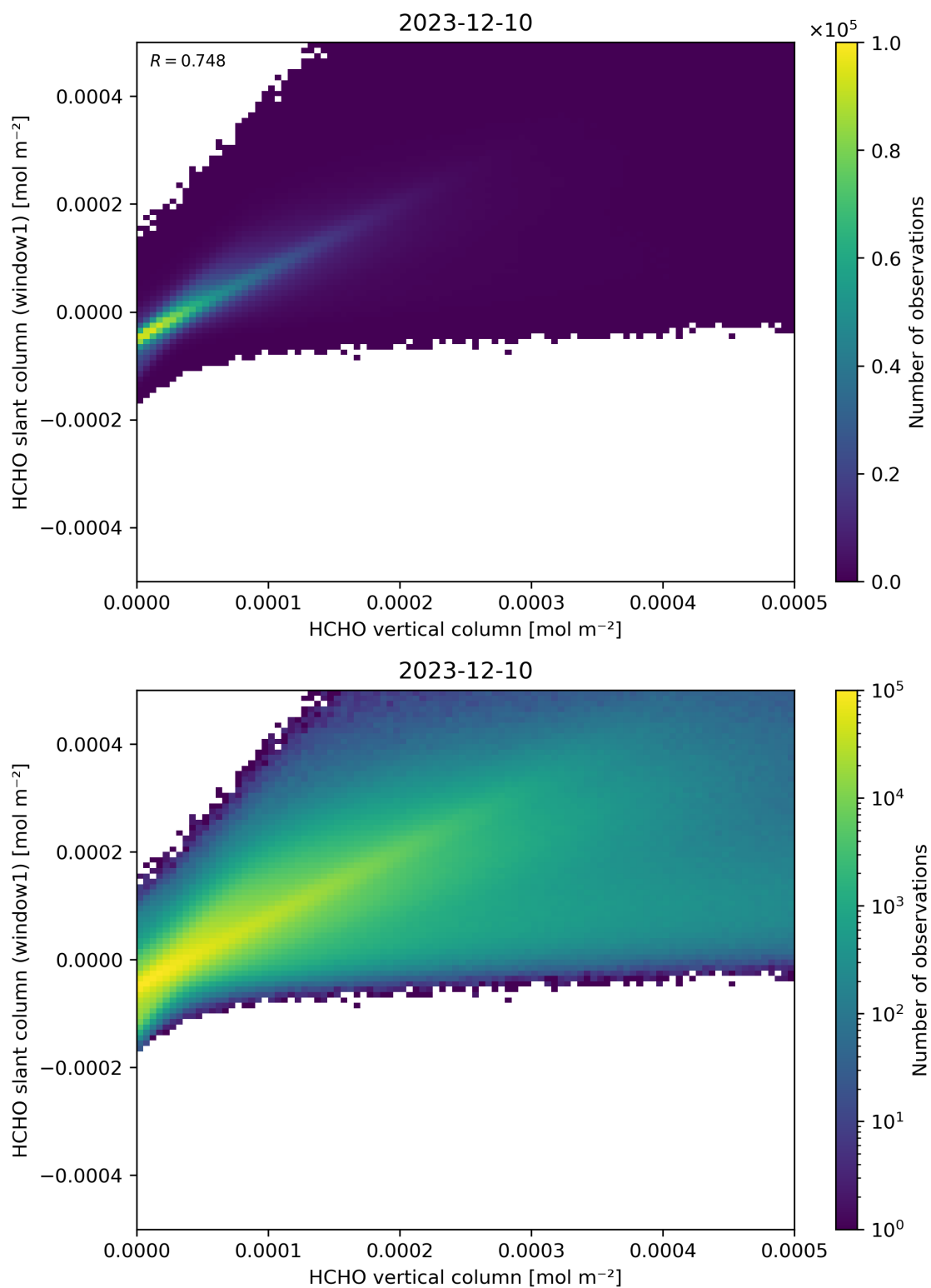
Figure 129: Scatter density plot of “HCHO vertical column” against “HCHO slant column (window1)” for 2023-12-09 to 2023-12-11.
