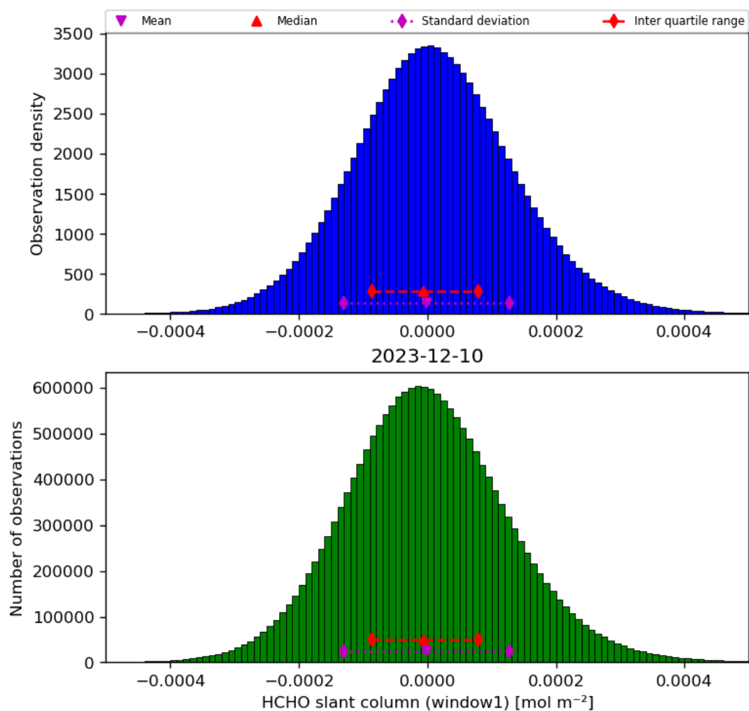
Figure 38: Histogram of “HCHO slant column (window1)” for 2023-12-09 to 2023-12-11
