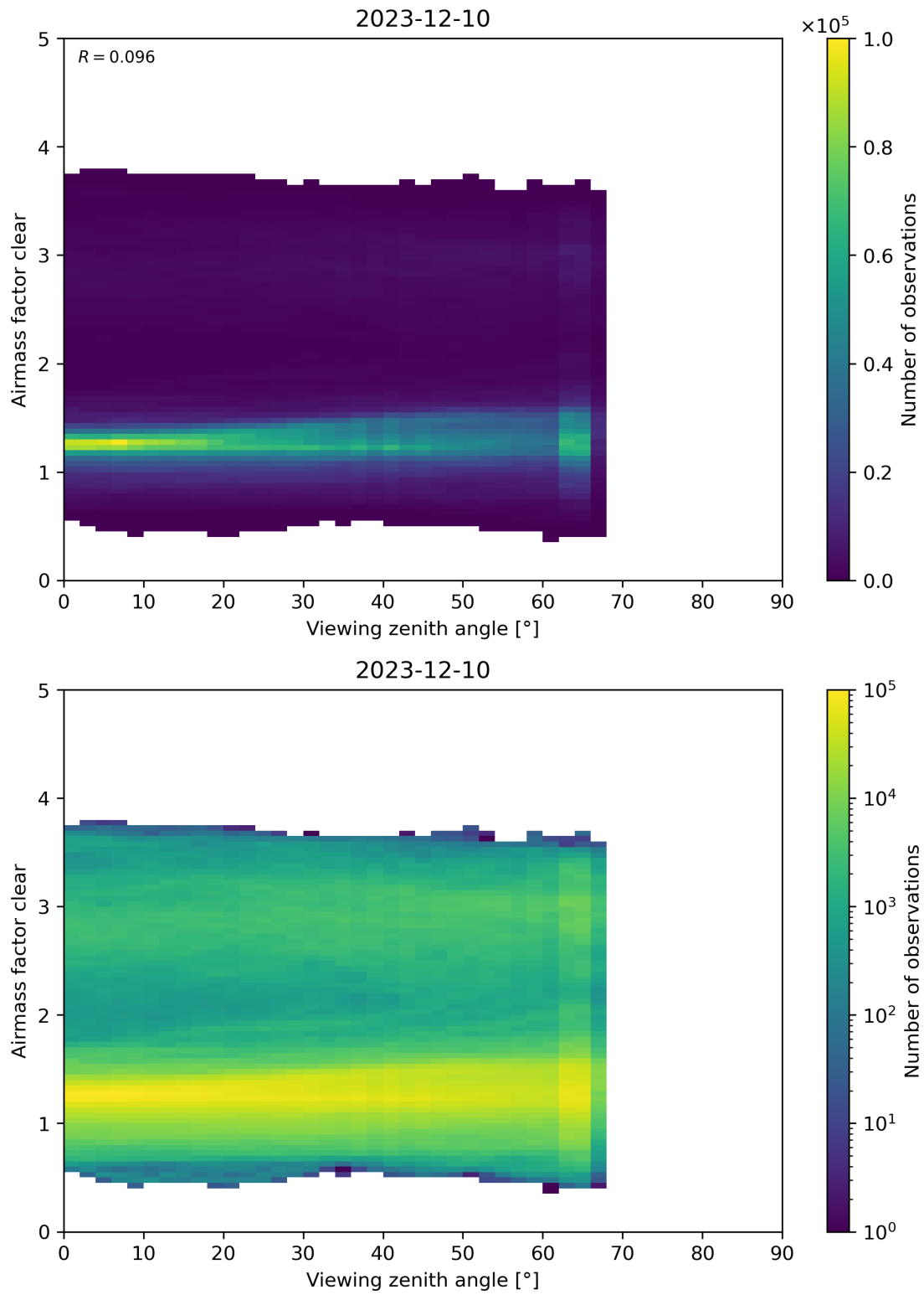
Figure 185: Scatter density plot of “Viewing zenith angle” against “Airmass factor clear” for 2023-12-09 to 2023-12-11.
