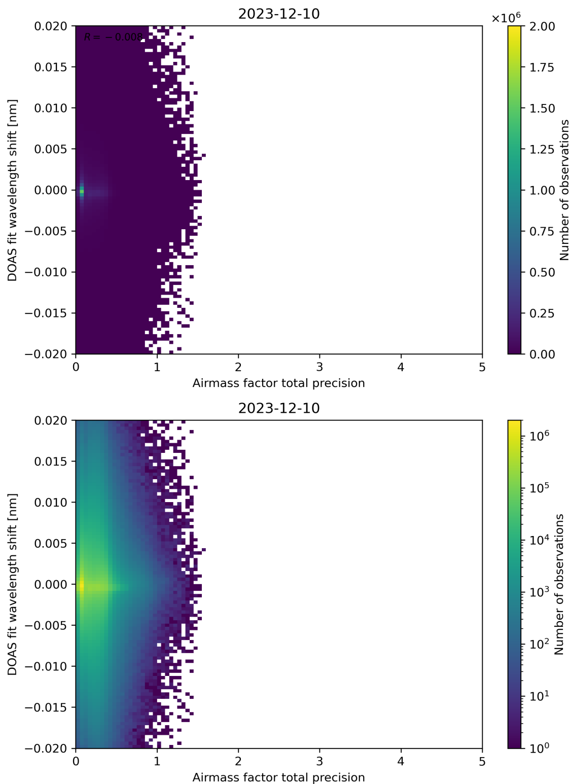
Figure 106: Scatter density plot of “Airmass factor total precision” against “DOAS fit wavelength shift” for 2023-12-09 to 2023-12-11.
