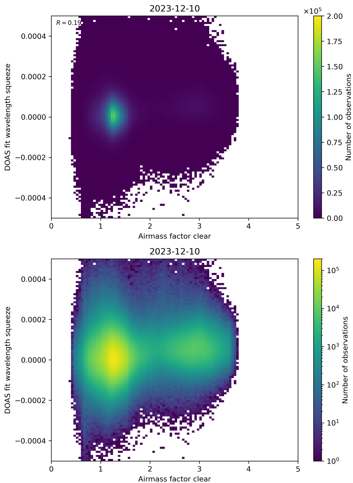
Figure 73: Scatter density plot of “Airmass factor clear” against “DOAS fit wavelength squeeze” for 2023-12-09 to 2023-12-11.
