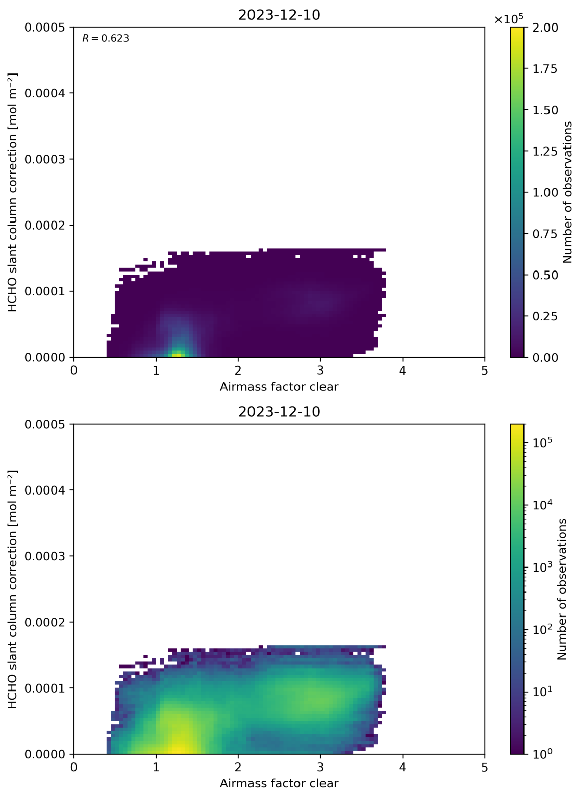
Figure 75: Scatter density plot of “Airmass factor clear” against “HCHO slant column correction” for 2023-12-09 to 2023-12-11.
