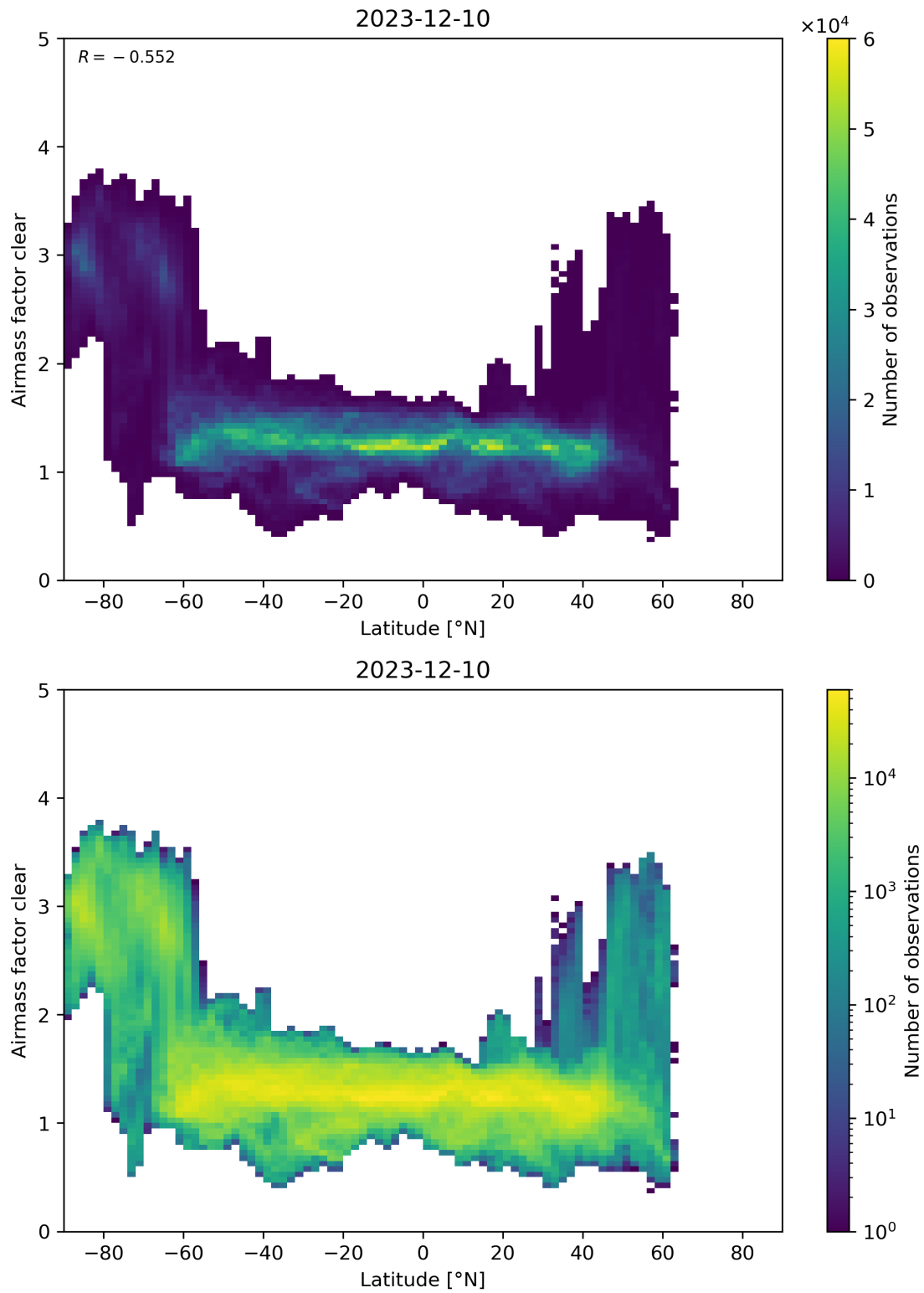
Figure 156: Scatter density plot of “Latitude” against “Airmass factor clear” for 2023-12-09 to 2023-12-11.
