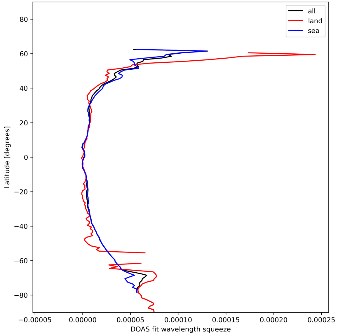
Figure 31: Zonal average of “DOAS fit wavelength squeeze” for 2023-12-09 to 2023-12-11.
