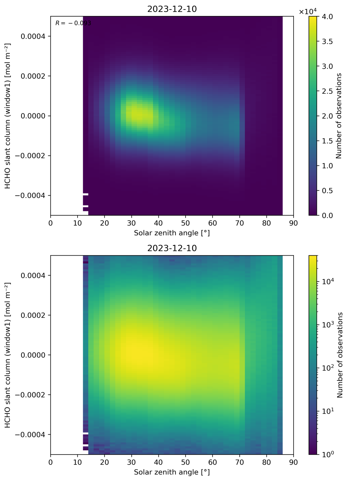
Figure 173: Scatter density plot of “Solar zenith angle” against “HCHO slant column (window1)” for 2023-12-09 to 2023-12-11.
