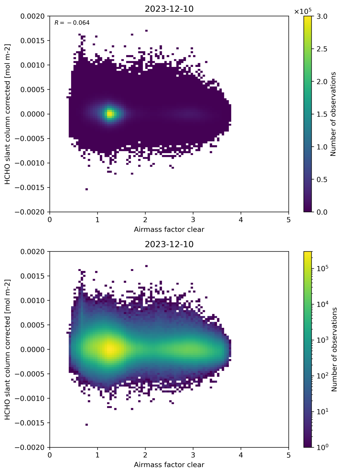
Figure 74: Scatter density plot of “Airmass factor clear” against “HCHO slant column corrected” for 2023-12-09 to 2023-12-11.
