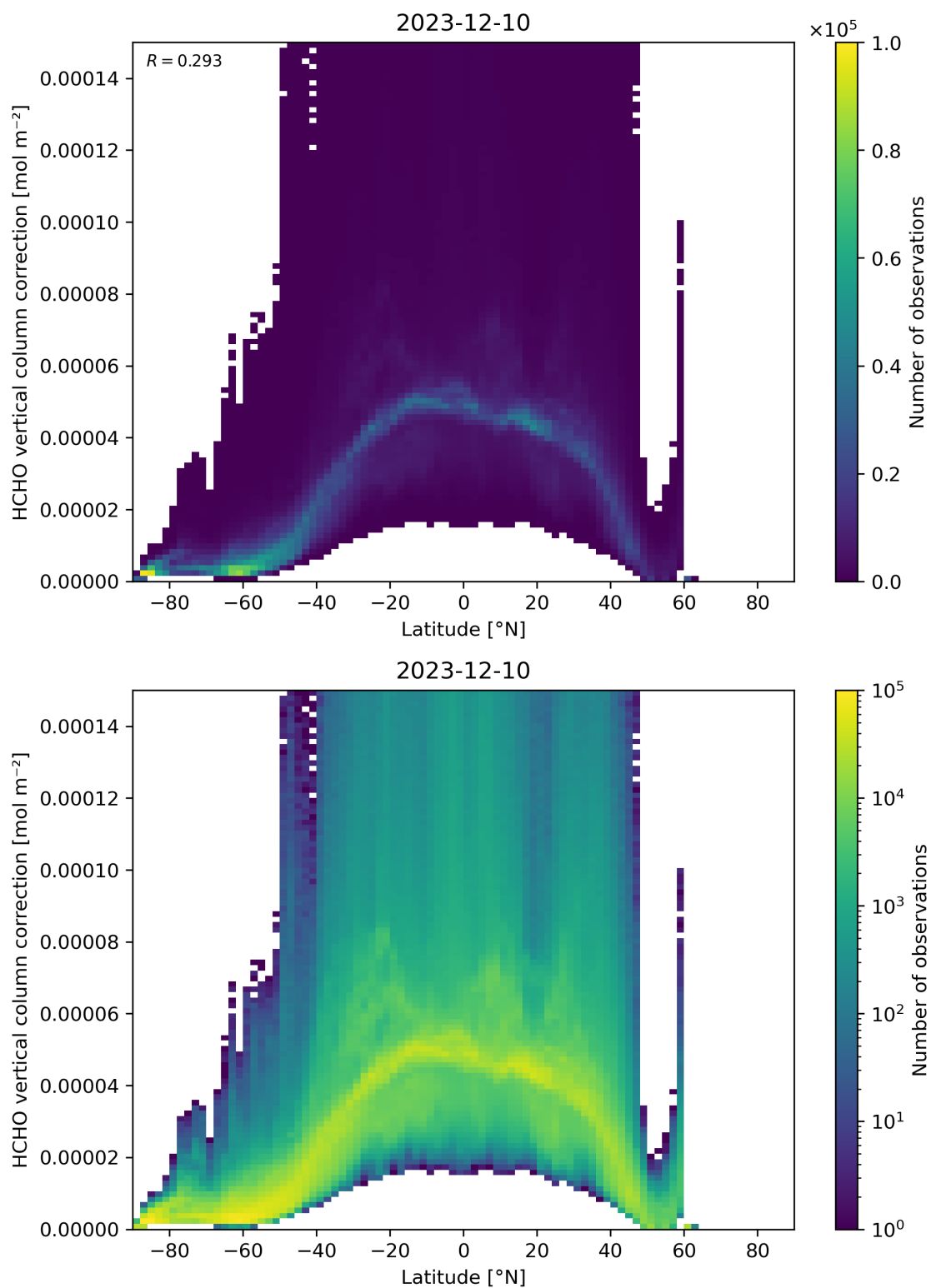
Figure 164: Scatter density plot of “Latitude” against “HCHO vertical column correction” for 2023-12-09 to 2023-12-11.
