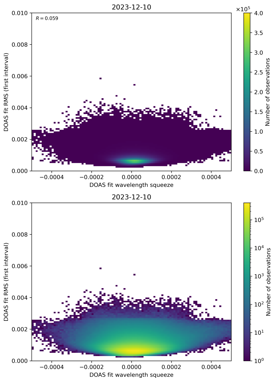
Figure 68: Scatter density plot of “DOAS fit wavelength squeeze” against “DOAS fit RMS (first interval)” for 2023-12-09 to 2023-12-11.
