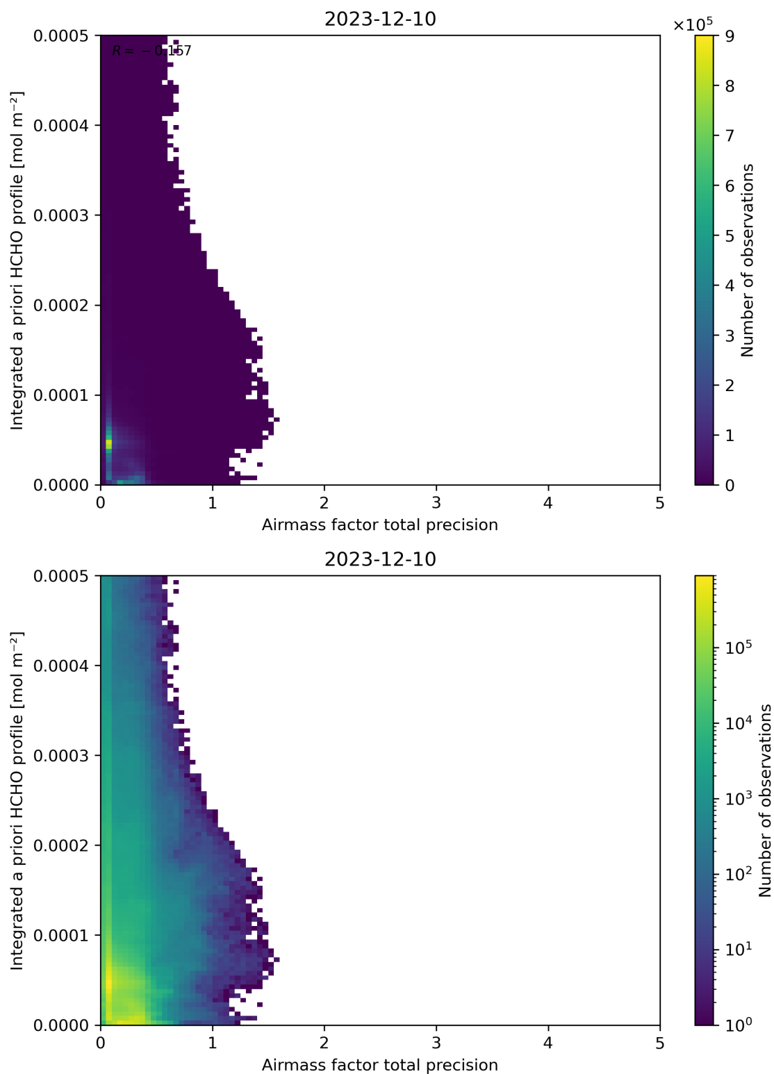
Figure 111: Scatter density plot of “Airmass factor total precision” against “Integrated a priori HCHO profile” for 2023-12-09 to 2023-12-11.
