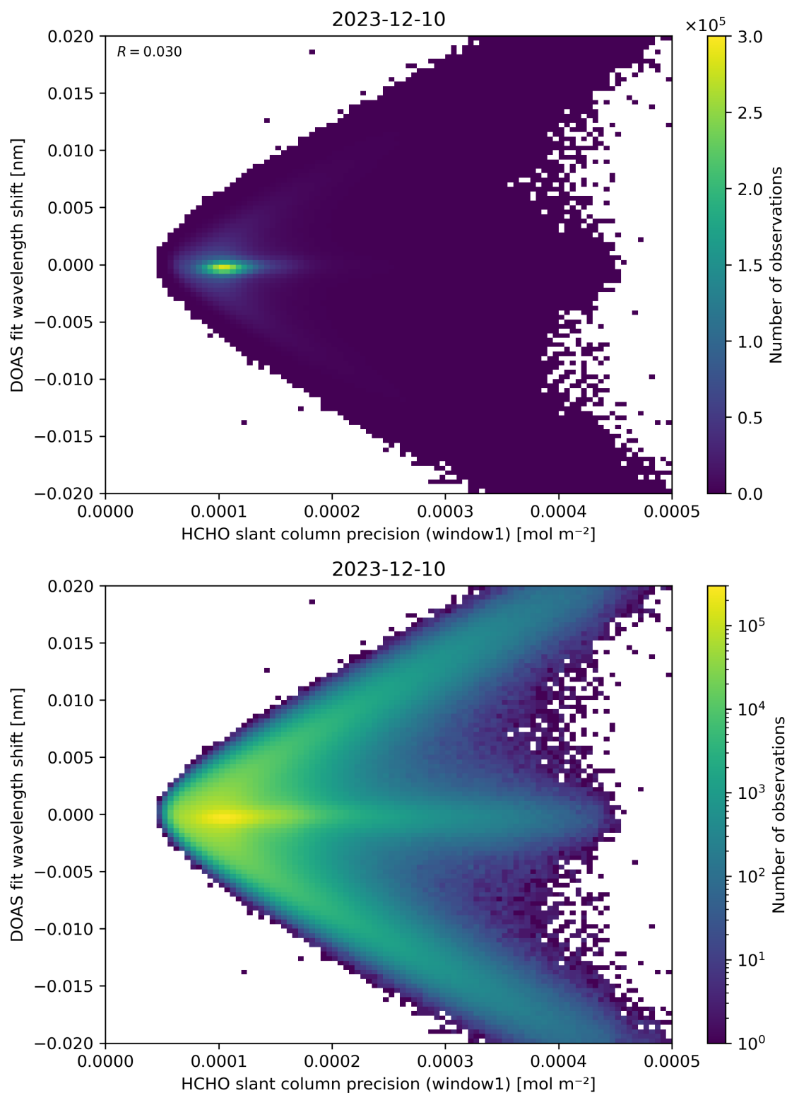
Figure 89: Scatter density plot of “HCHO slant column precision (window1)” against “DOAS fit wavelength shift” for 2023-12-09 to 2023-12-11.
