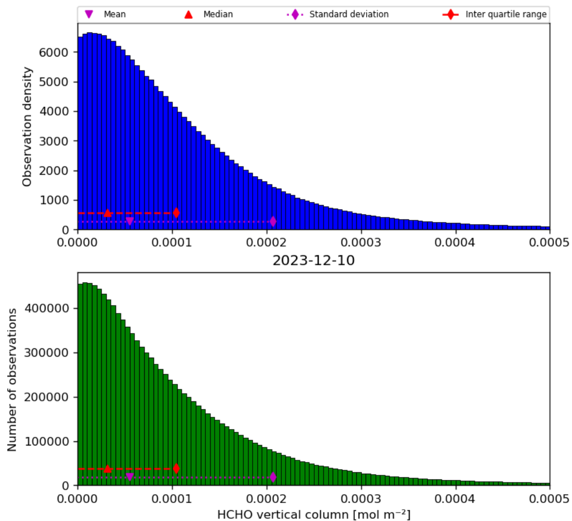
Figure 35: Histogram of “HCHO vertical column” for 2023-12-09 to 2023-12-11
