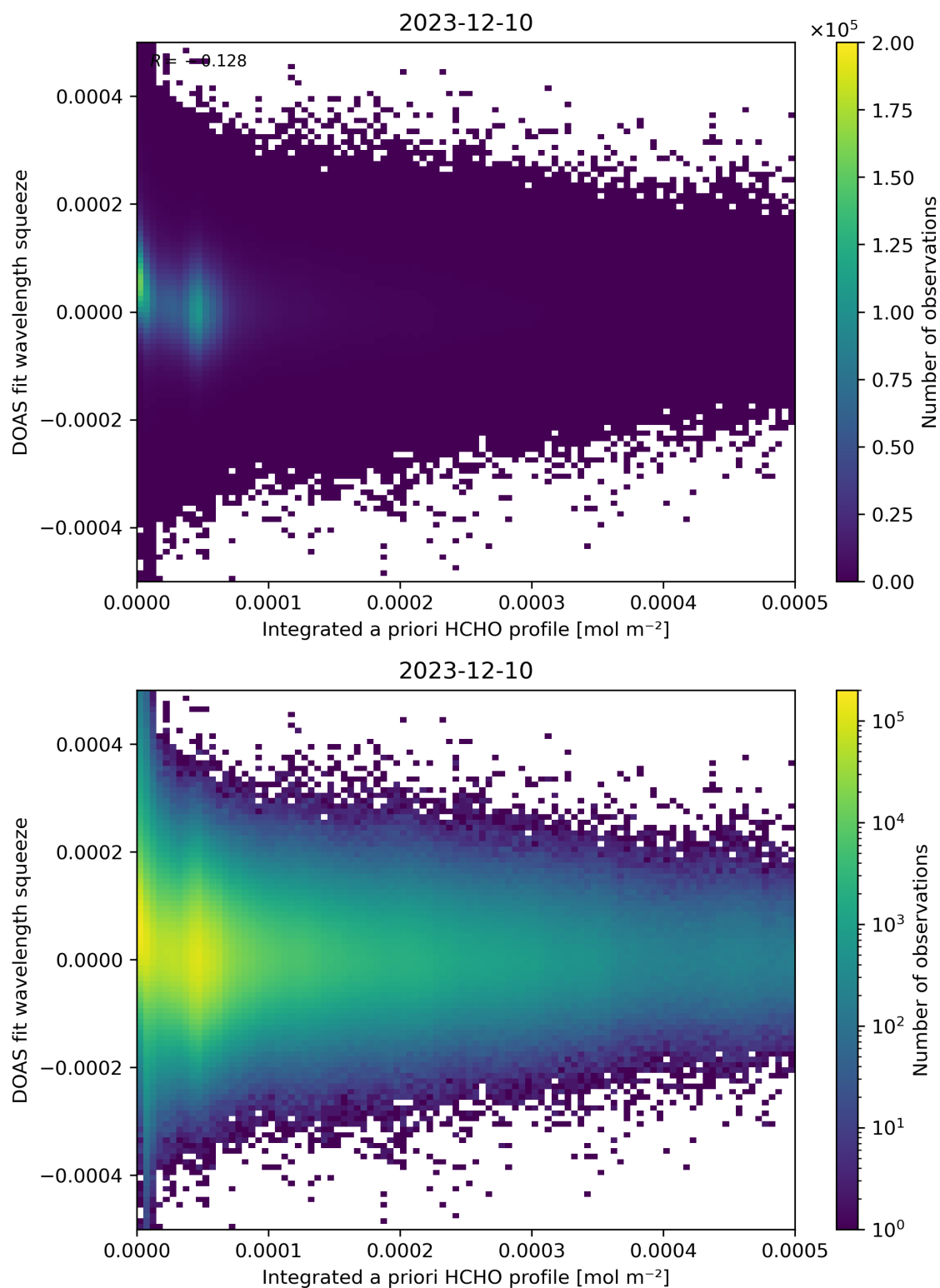
Figure 150: Scatter density plot of “Integrated a priori HCHO profile” against “DOAS fit wavelength squeeze” for 2023-12-09 to 2023-12-11.
