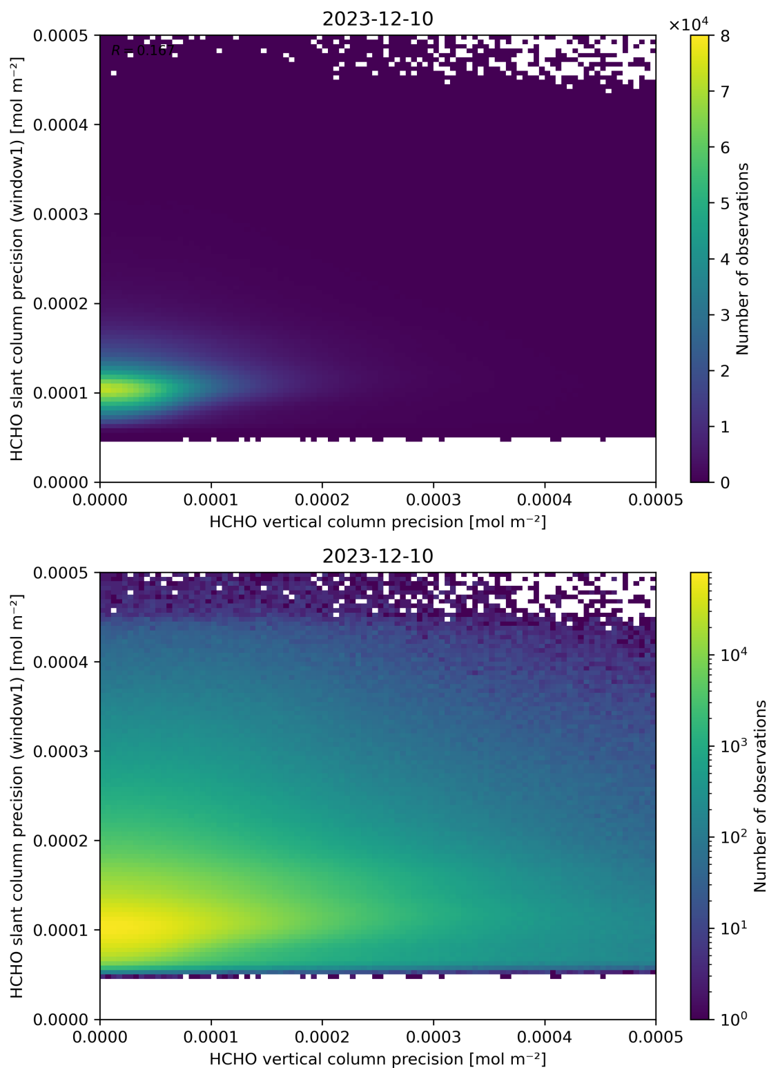
Figure 143: Scatter density plot of “HCHO vertical column precision” against “HCHO slant column precision (window1)” for 2023-12-09 to 2023-12-11.
