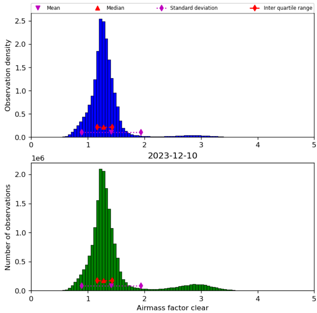
Figure 42: Histogram of “Airmass factor clear” for 2023-12-09 to 2023-12-11
