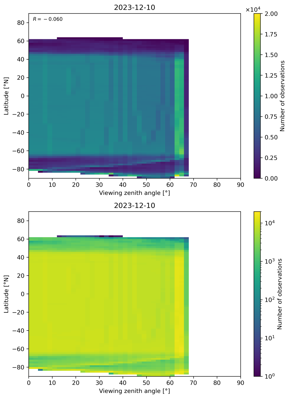
Figure 196: Scatter density plot of “Viewing zenith angle” against “Latitude” for 2023-12-09 to 2023-12-11.
