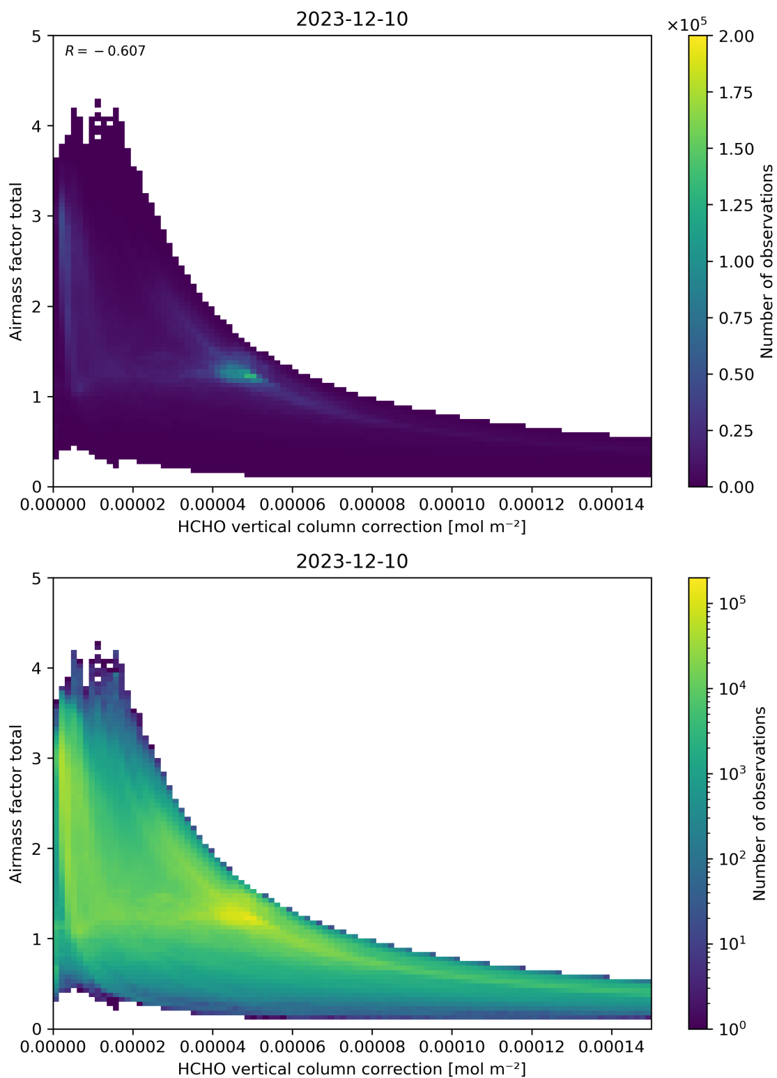
Figure 120: Scatter density plot of “HCHO vertical column correction” against “Airmass factor total” for 2023-12-09 to 2023-12-11.
