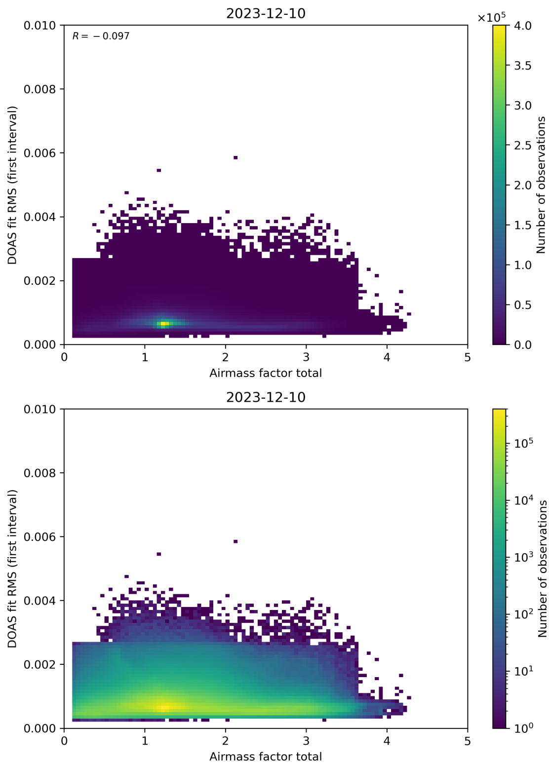
Figure 97: Scatter density plot of “Airmass factor total” against “DOAS fit RMS (first interval)” for 2023-12-09 to 2023-12-11.
