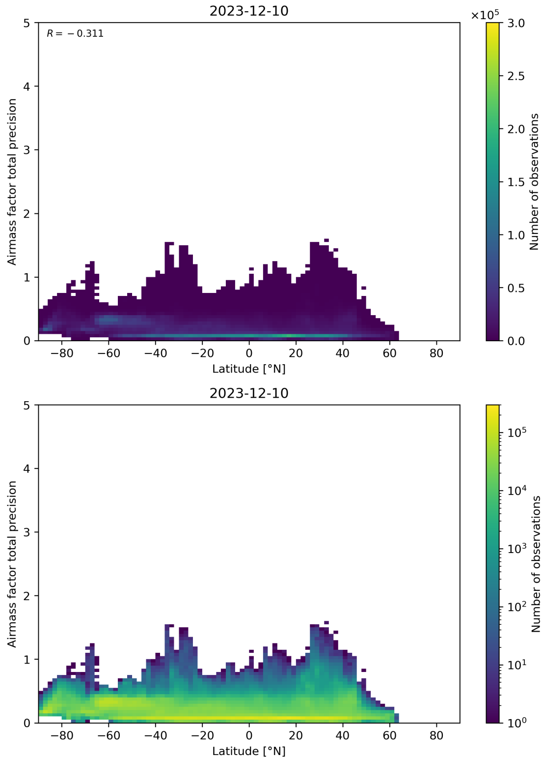
Figure 162: Scatter density plot of “Latitude” against “Airmass factor total precision” for 2023-12-09 to 2023-12-11.
