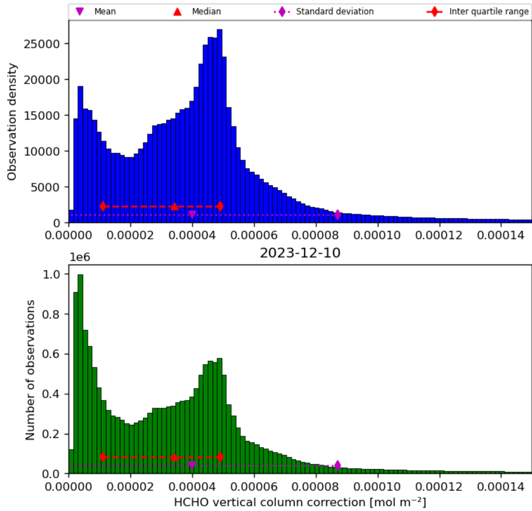
Figure 37: Histogram of “HCHO vertical column correction” for 2023-12-09 to 2023-12-11
