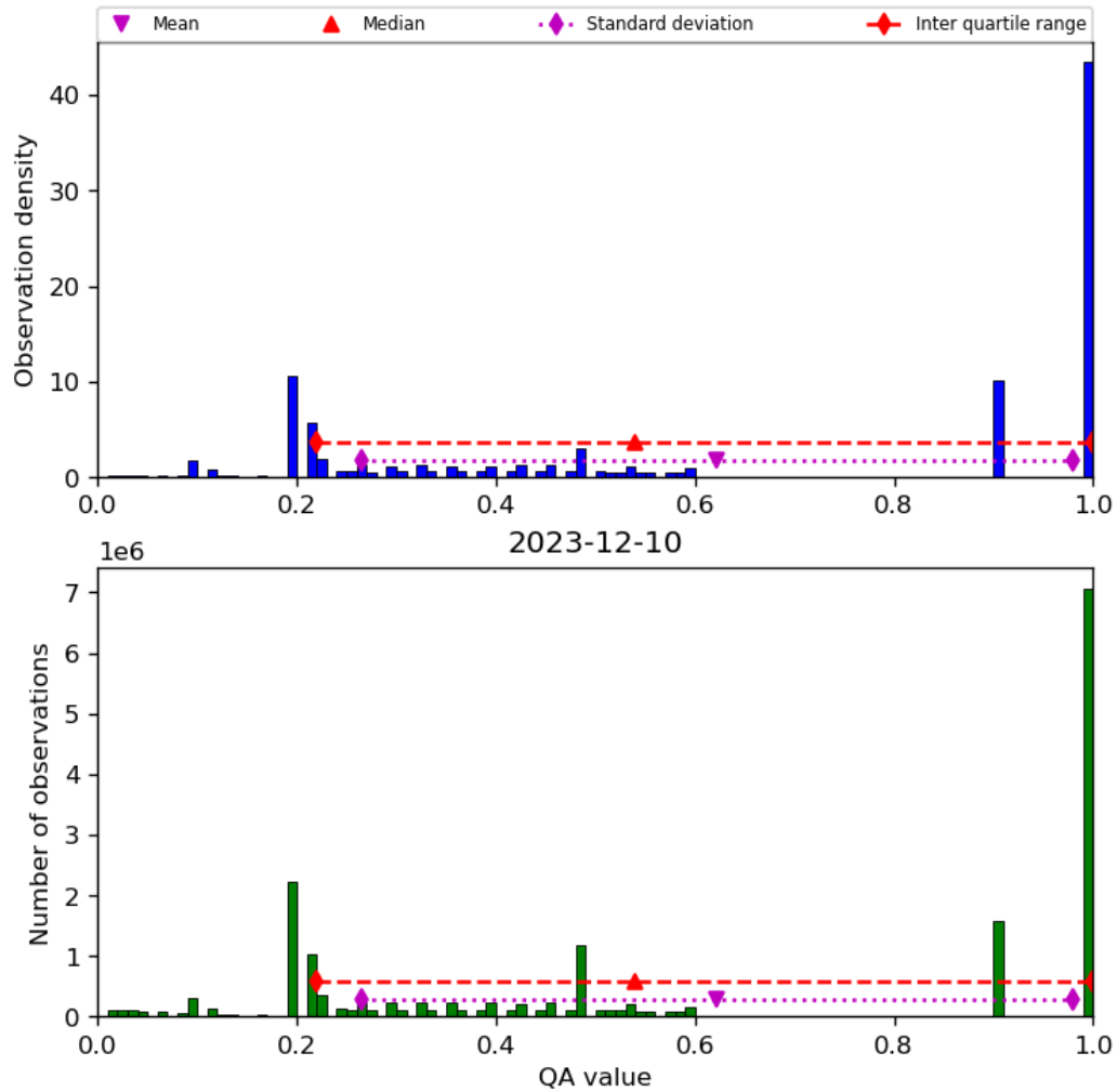
Figure 34: Histogram of “QA value” for 2023-12-09 to 2023-12-11
