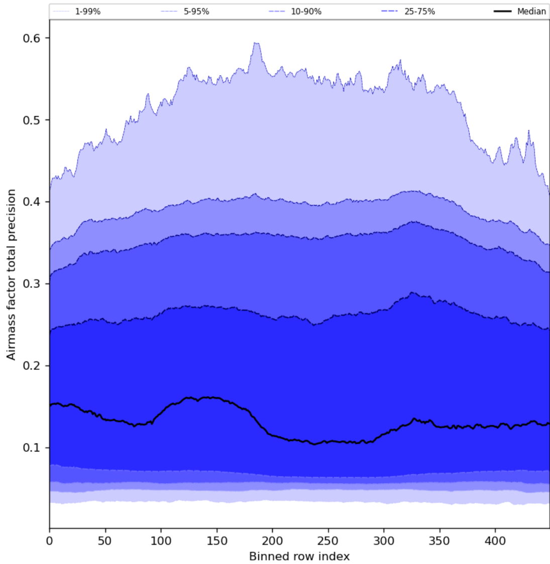
Figure 55: Along track statistics of “Airmass factor total precision” for 2023-12-09 to 2023-12-11
