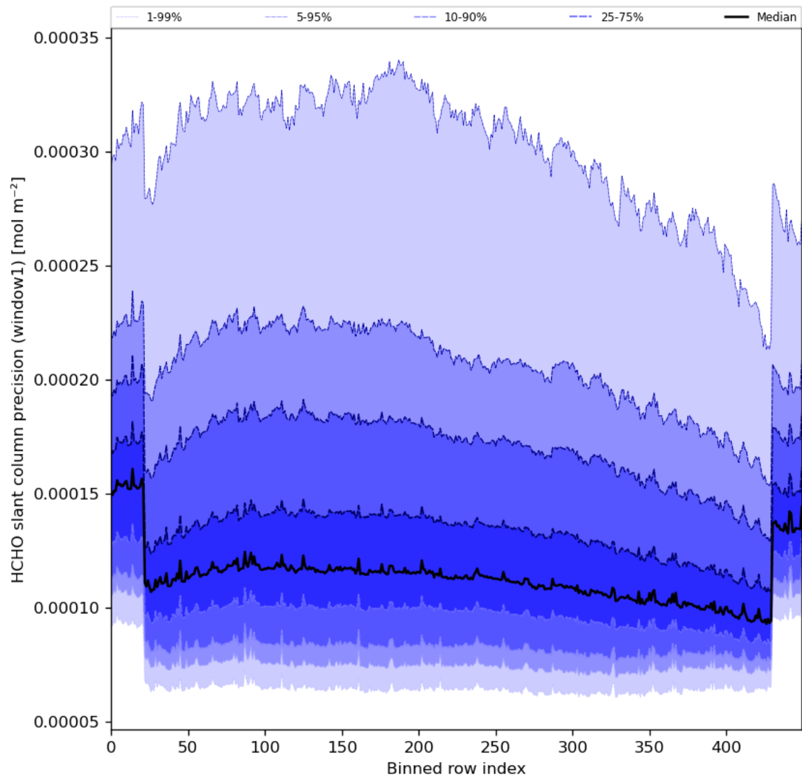
Figure 53: Along track statistics of “HCHO slant column precision (window1)” for 2023-12-09 to 2023-12-11
