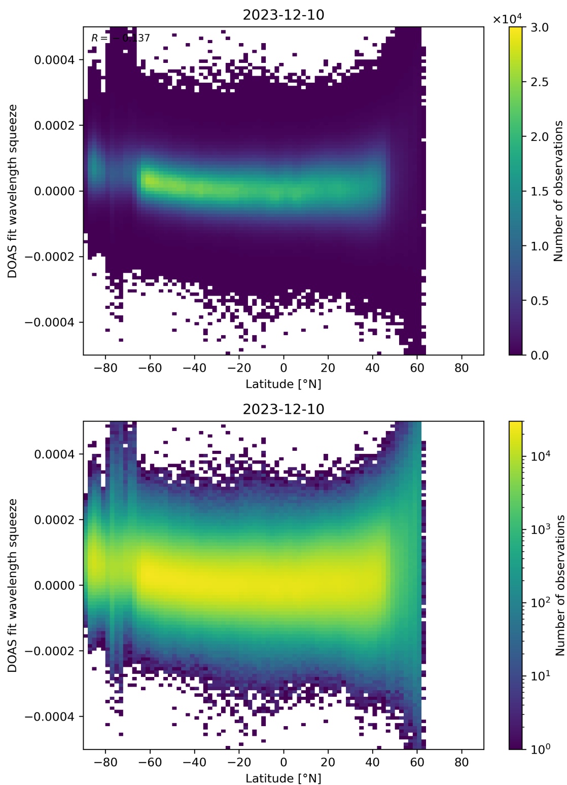
Figure 155: Scatter density plot of “Latitude” against “DOAS fit wavelength squeeze” for 2023-12-09 to 2023-12-11.
