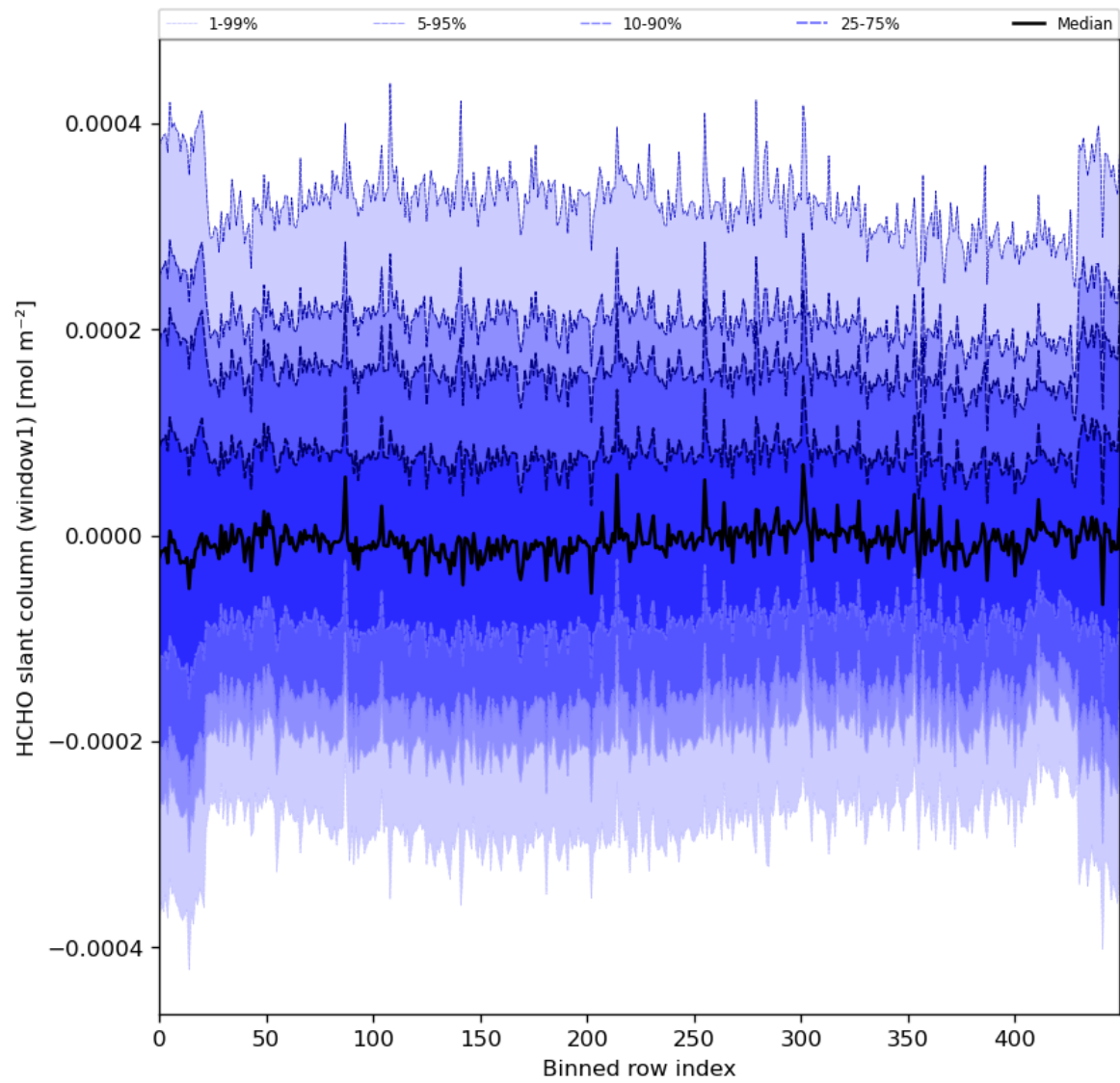
Figure 52: Along track statistics of “HCHO slant column (window1)” for 2023-12-09 to 2023-12-11
