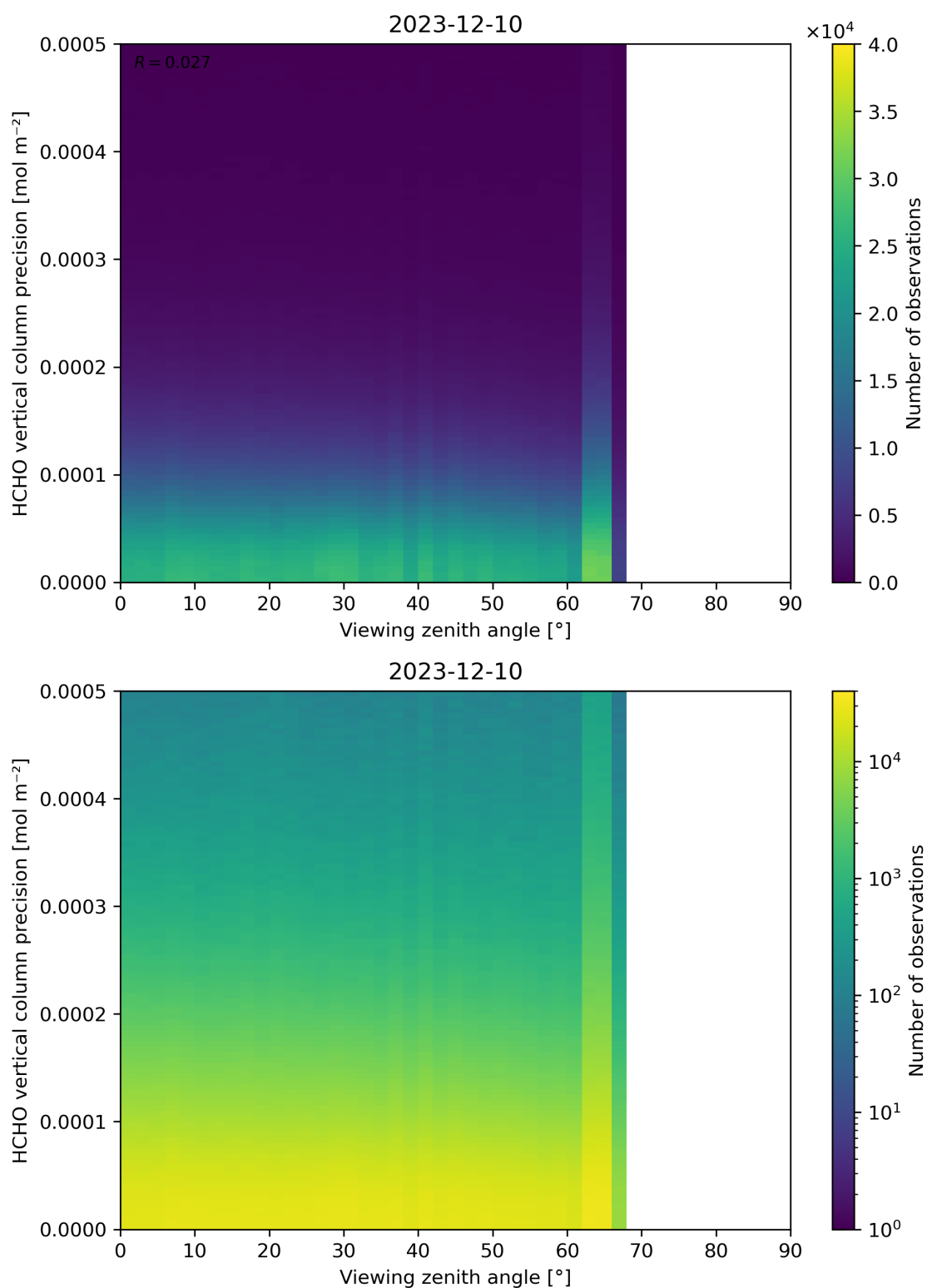
Figure 194: Scatter density plot of “Viewing zenith angle” against “HCHO vertical column precision” for 2023-12-09 to 2023-12-11.
