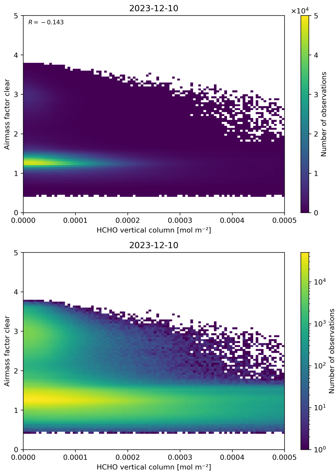
Figure 126: Scatter density plot of “HCHO vertical column” against “Airmass factor clear” for 2023-12-09 to 2023-12-11.
