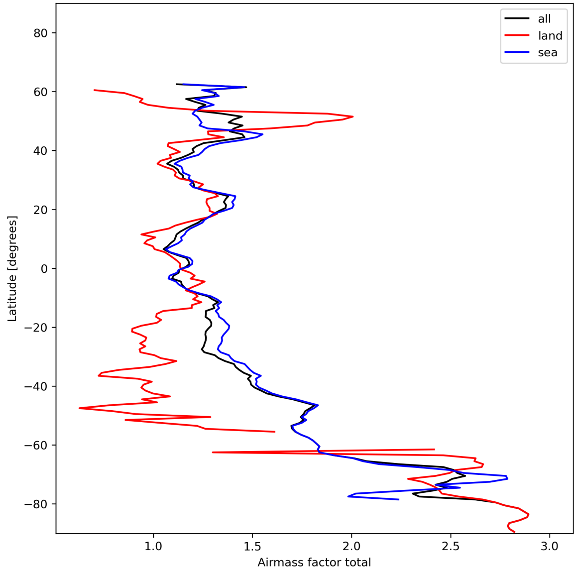
Figure 26: Zonal average of “Airmass factor total” for 2023-12-09 to 2023-12-11.
