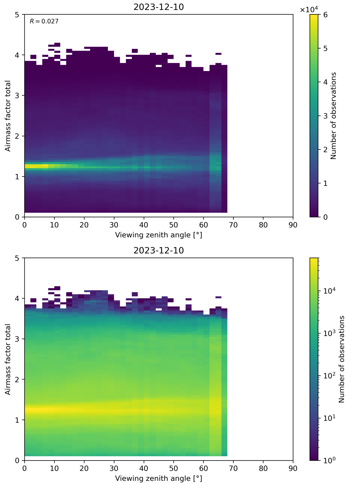
Figure 190: Scatter density plot of “Viewing zenith angle” against “Airmass factor total” for 2023-12-09 to 2023-12-11.
