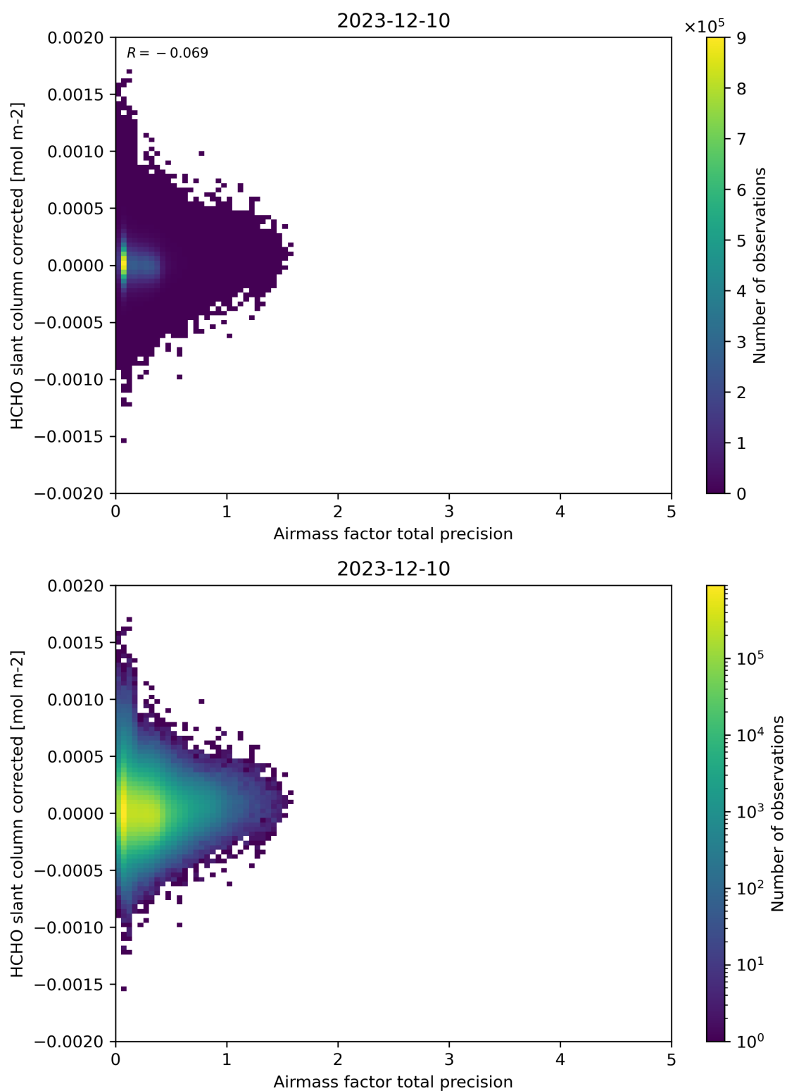
Figure 109: Scatter density plot of “Airmass factor total precision” against “HCHO slant column corrected” for 2023-12-09 to 2023-12-11.
