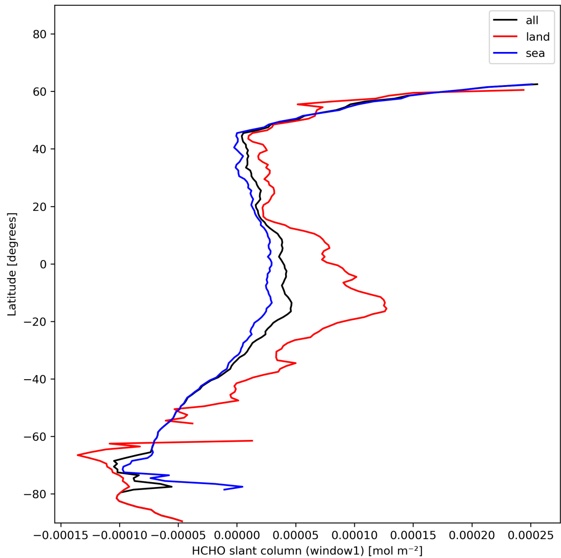
Figure 24: Zonal average of “HCHO slant column (window1)” for 2023-12-09 to 2023-12-11.
