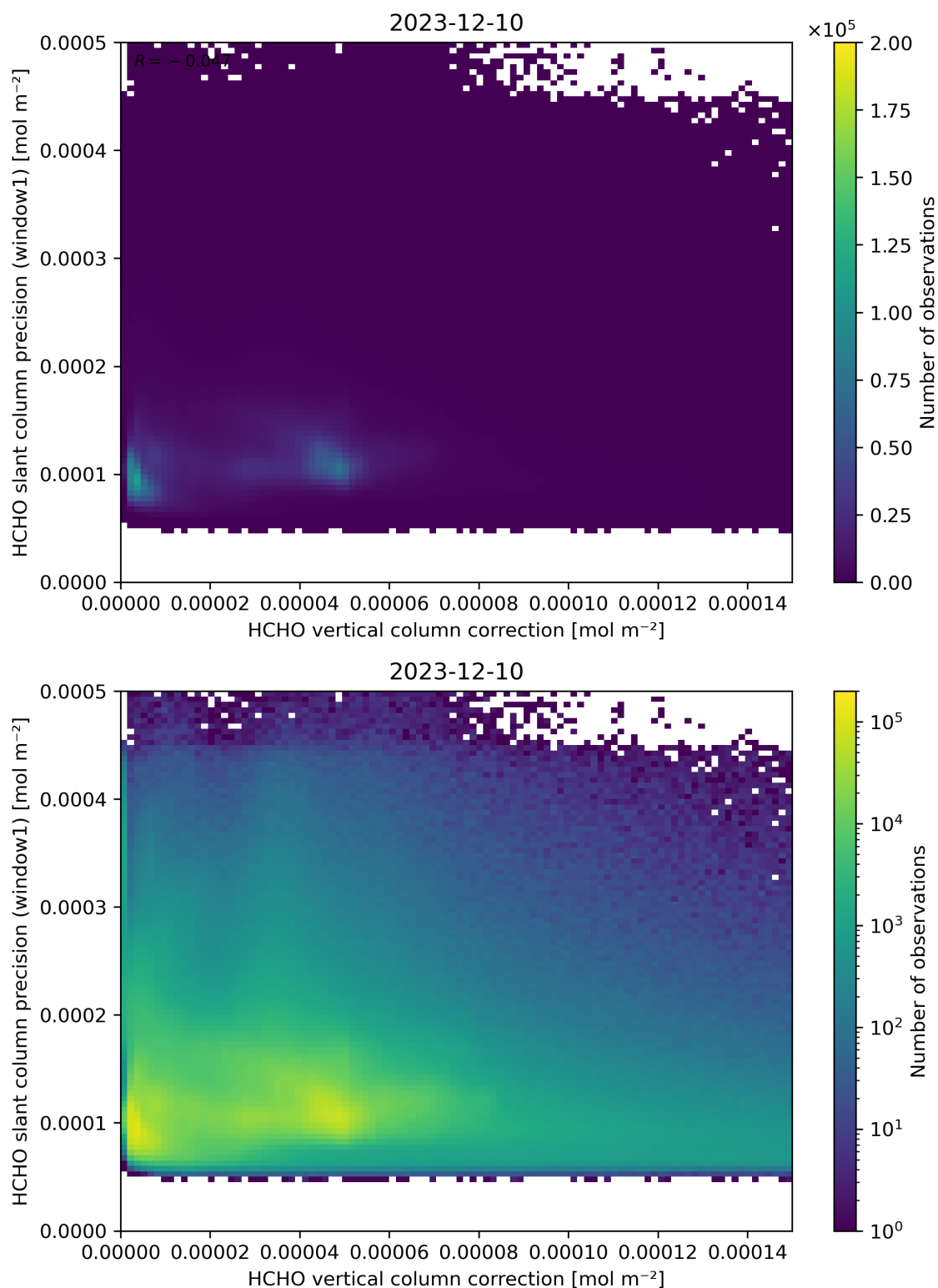
Figure 119: Scatter density plot of “HCHO vertical column correction” against “HCHO slant column precision (window1)” for 2023-12-09 to 2023-12-11.
