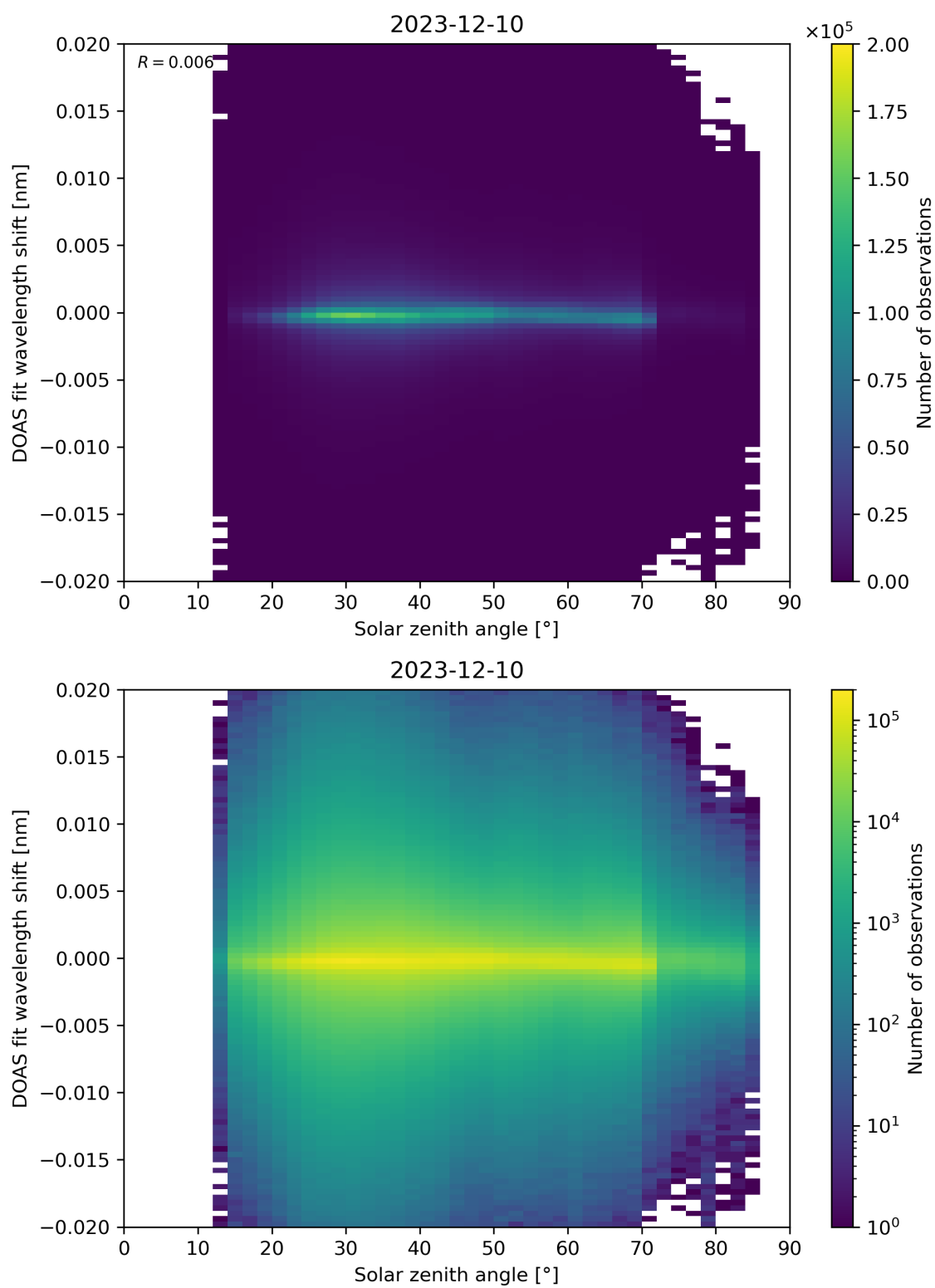
Figure 168: Scatter density plot of “Solar zenith angle” against “DOAS fit wavelength shift” for 2023-12-09 to 2023-12-11.
