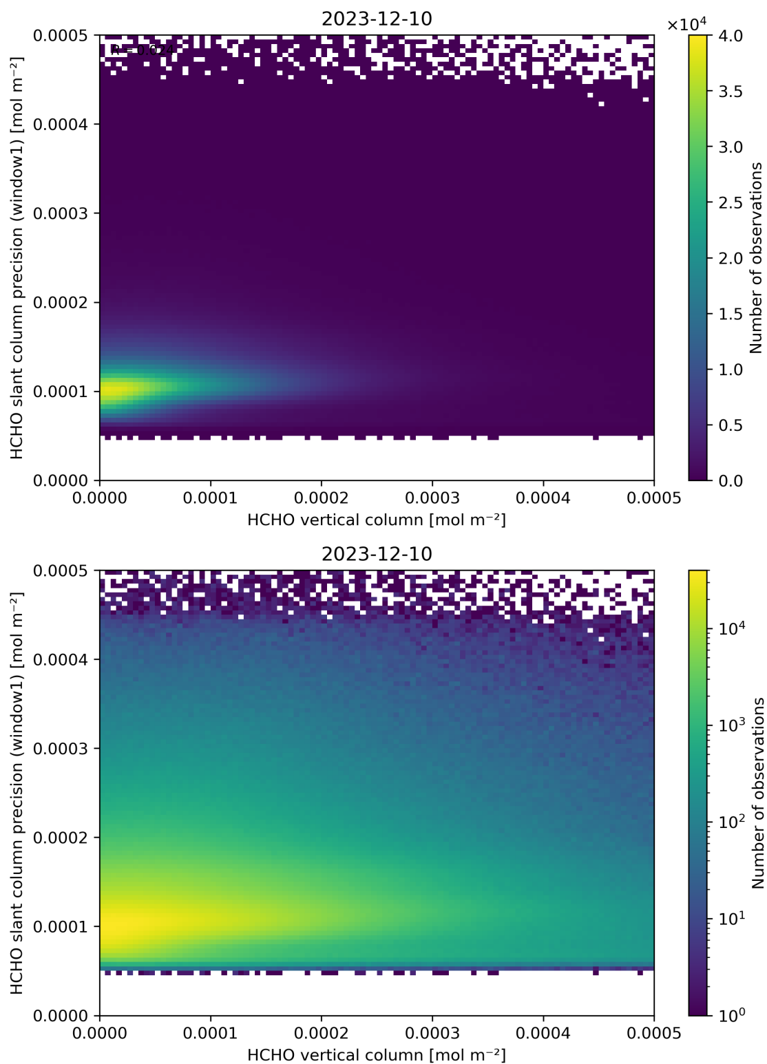
Figure 130: Scatter density plot of “HCHO vertical column” against “HCHO slant column precision (window1)” for 2023-12-09 to 2023-12-11.
