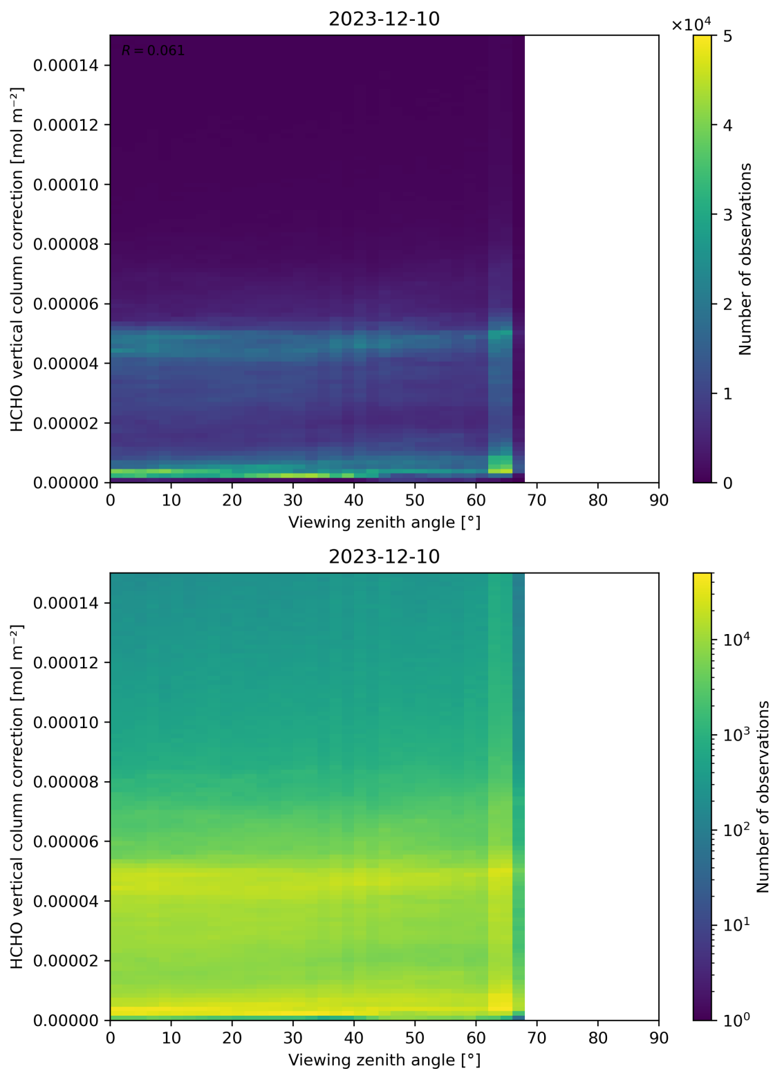
Figure 193: Scatter density plot of “Viewing zenith angle” against “HCHO vertical column correction” for 2023-12-09 to 2023-12-11.
