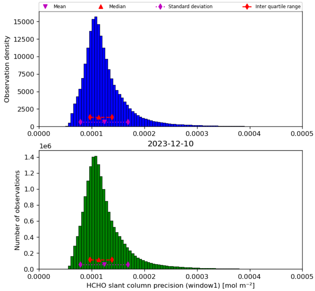
Figure 39: Histogram of “HCHO slant column precision (window1)” for 2023-12-09 to 2023-12-11
