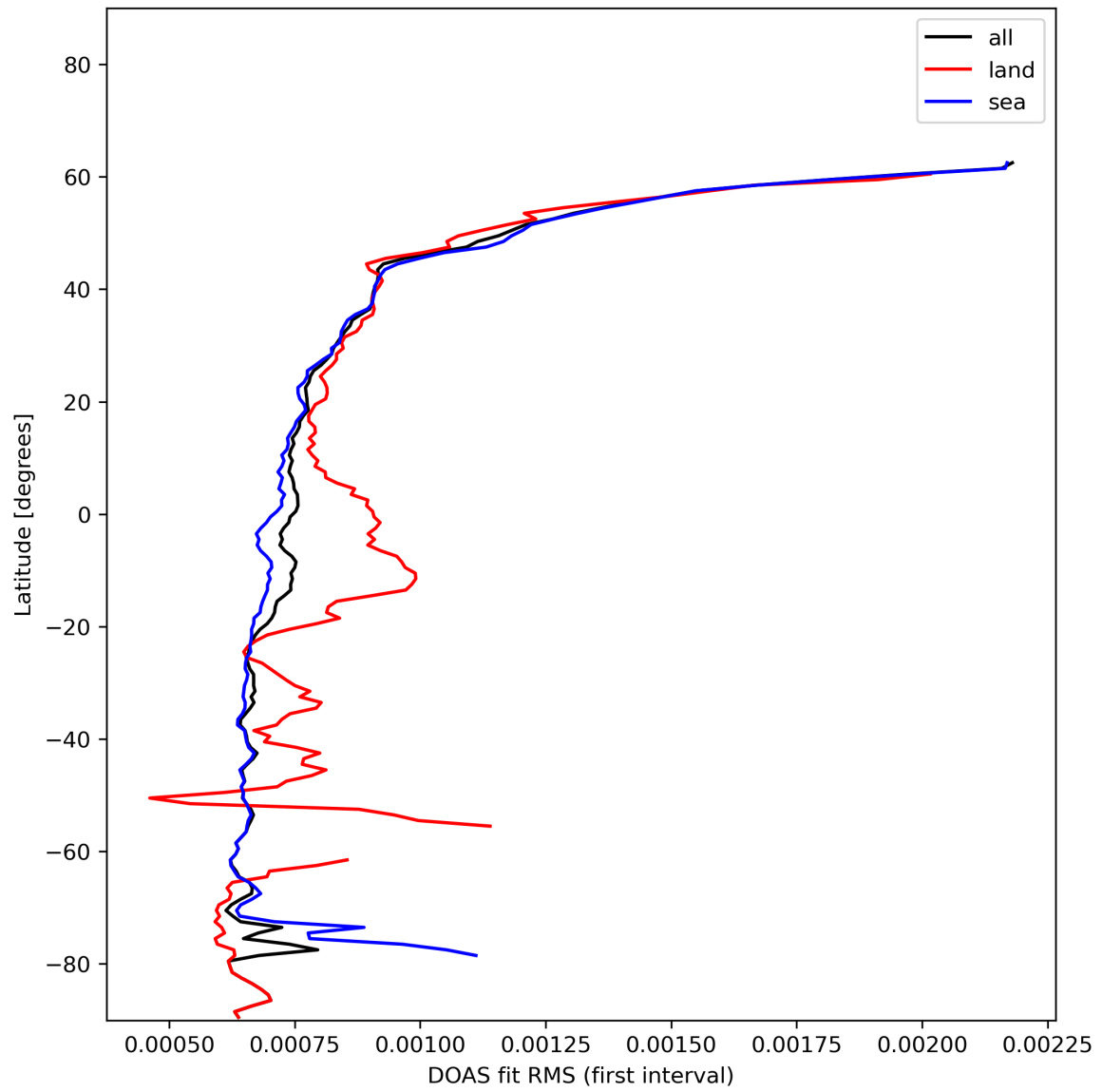
Figure 32: Zonal average of “DOAS fit RMS (first interval)” for 2023-12-09 to 2023-12-11.
