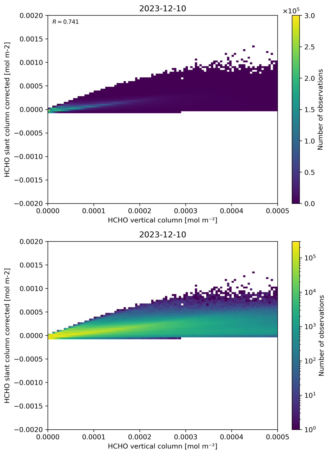
Figure 127: Scatter density plot of “HCHO vertical column” against “HCHO slant column corrected” for 2023-12-09 to 2023-12-11.
