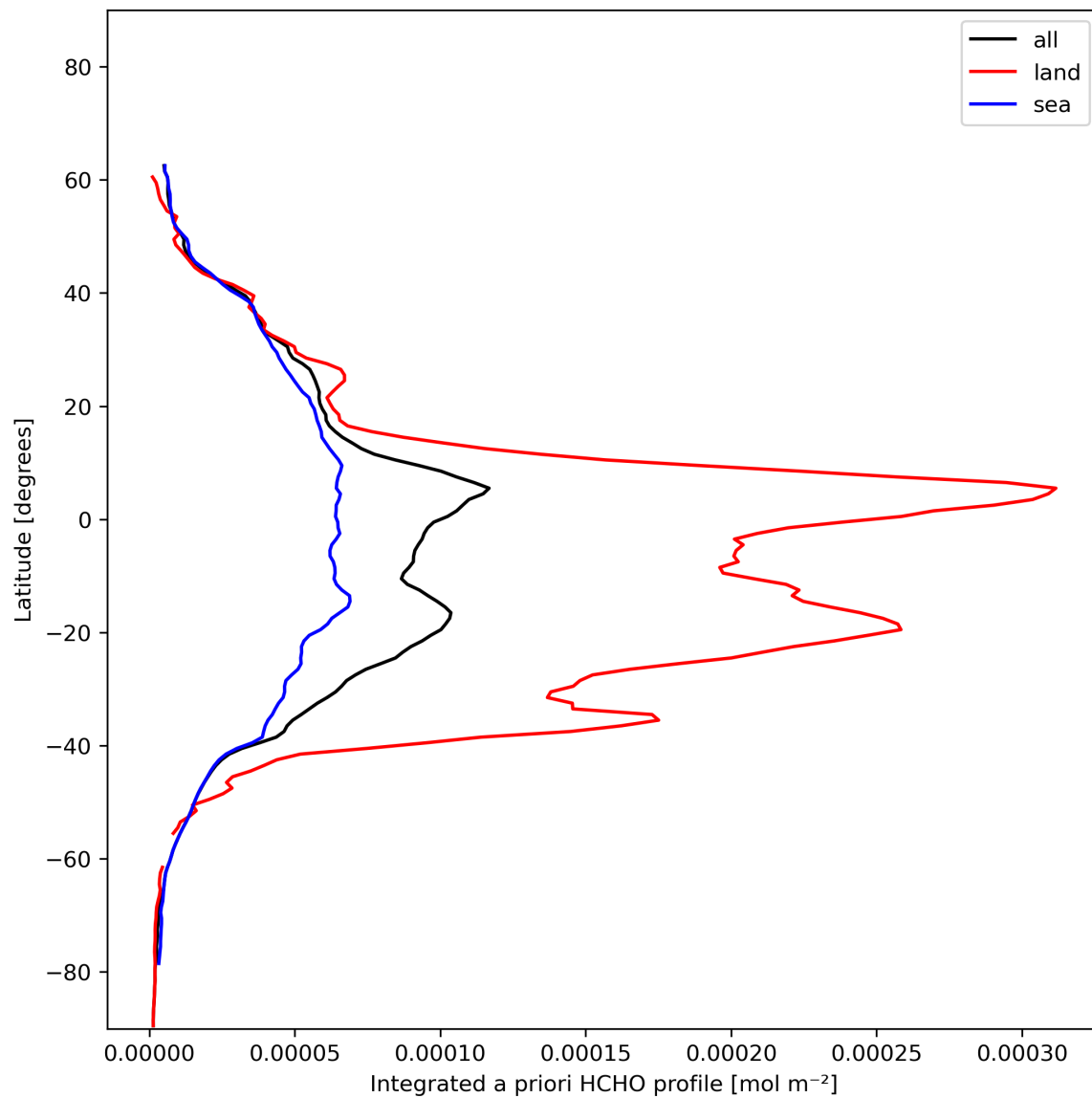
Figure 29: Zonal average of “Integrated a priori HCHO profile” for 2023-12-09 to 2023-12-11.
