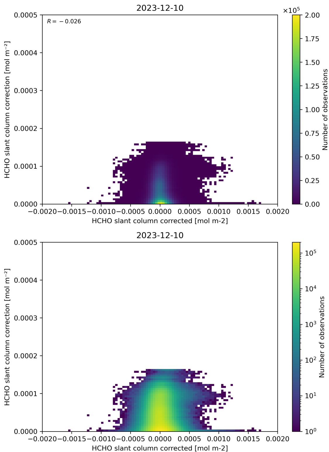
Figure 77: Scatter density plot of “HCHO slant column corrected” against “HCHO slant column correction” for 2023-12-09 to 2023-12-11.
