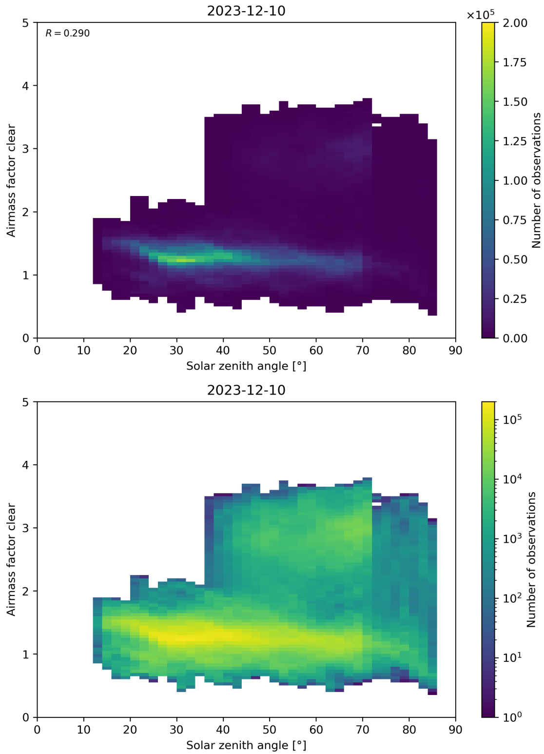
Figure 170: Scatter density plot of “Solar zenith angle” against “Airmass factor clear” for 2023-12-09 to 2023-12-11.
