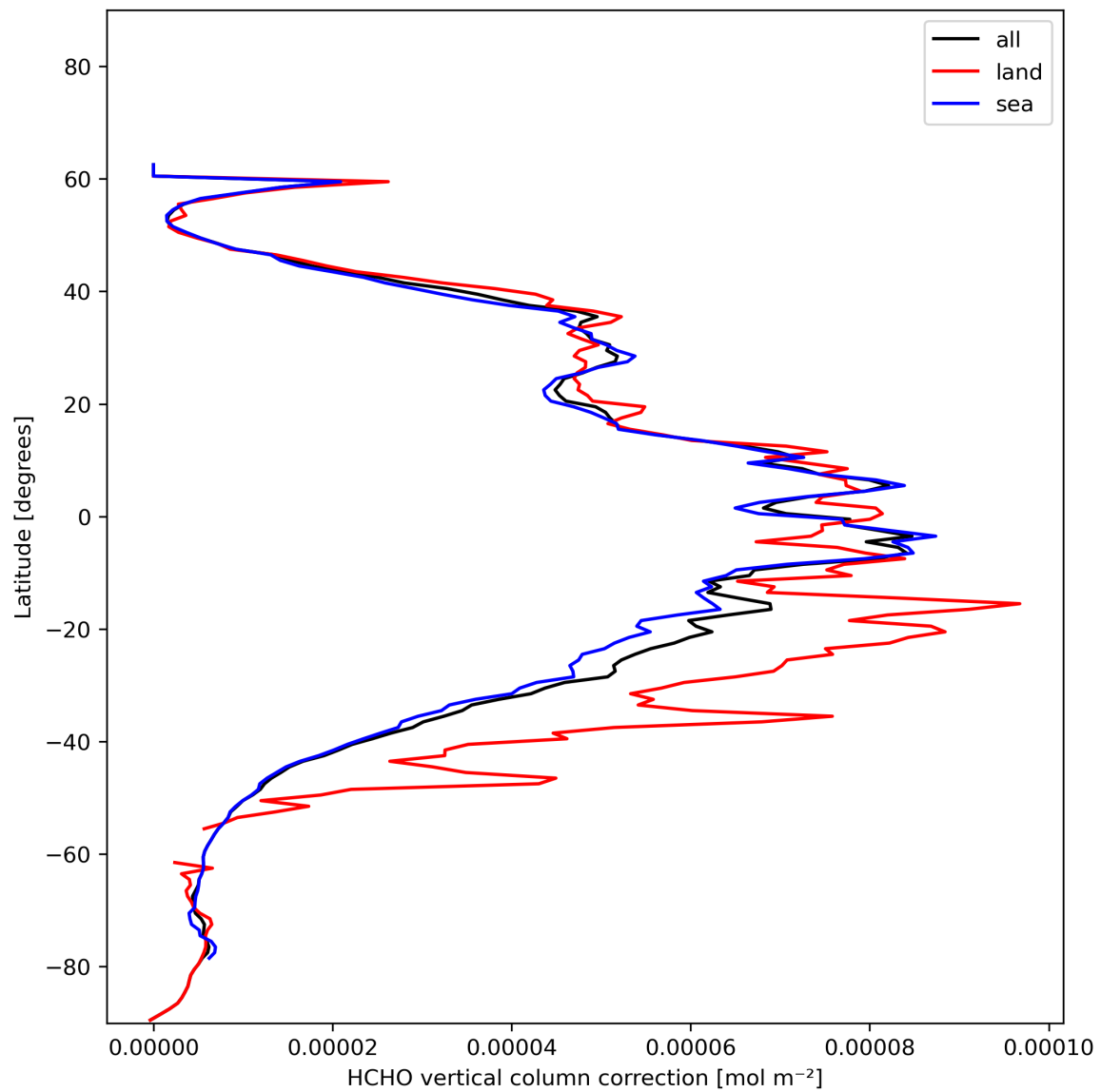
Figure 23: Zonal average of “HCHO vertical column correction” for 2023-12-09 to 2023-12-11.
