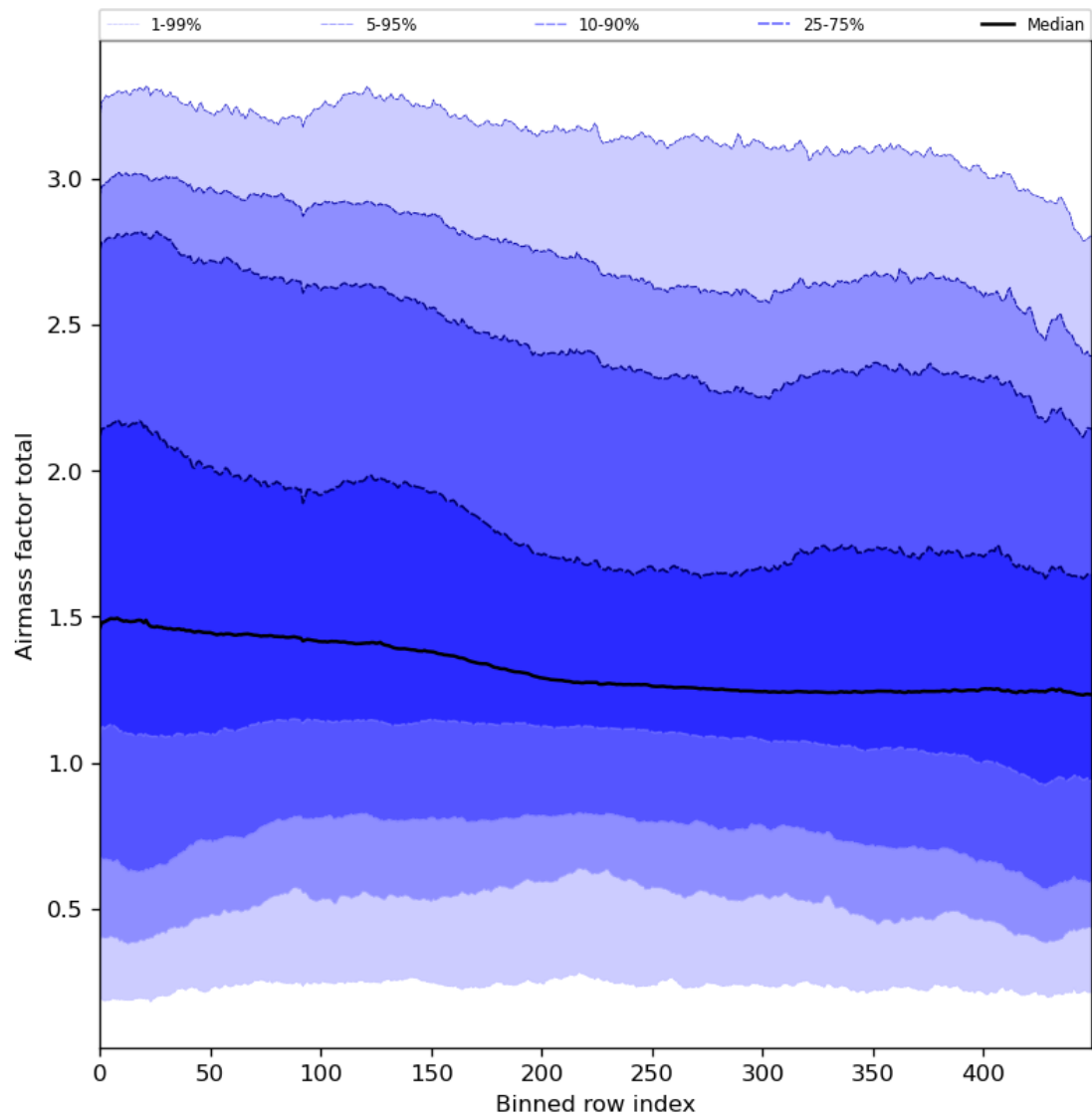
Figure 54: Along track statistics of “Airmass factor total” for 2023-12-09 to 2023-12-11
