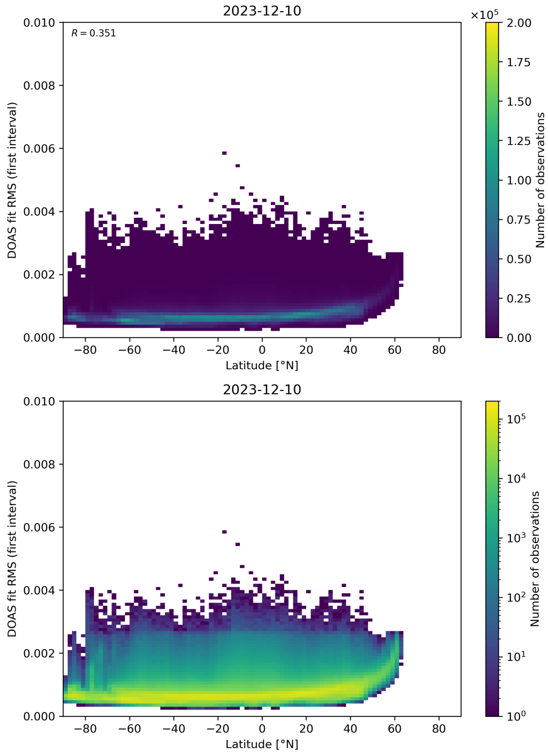
Figure 153: Scatter density plot of “Latitude” against “DOAS fit RMS (first interval)” for 2023-12-09 to 2023-12-11.
