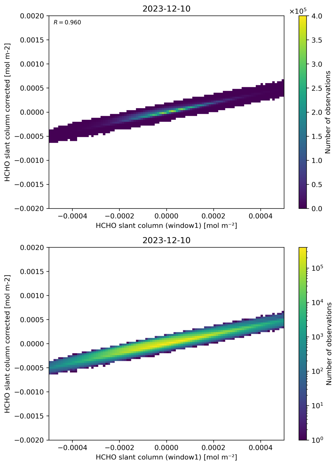
Figure 82: Scatter density plot of “HCHO slant column (window1)” against “HCHO slant column corrected” for 2023-12-09 to 2023-12-11.
