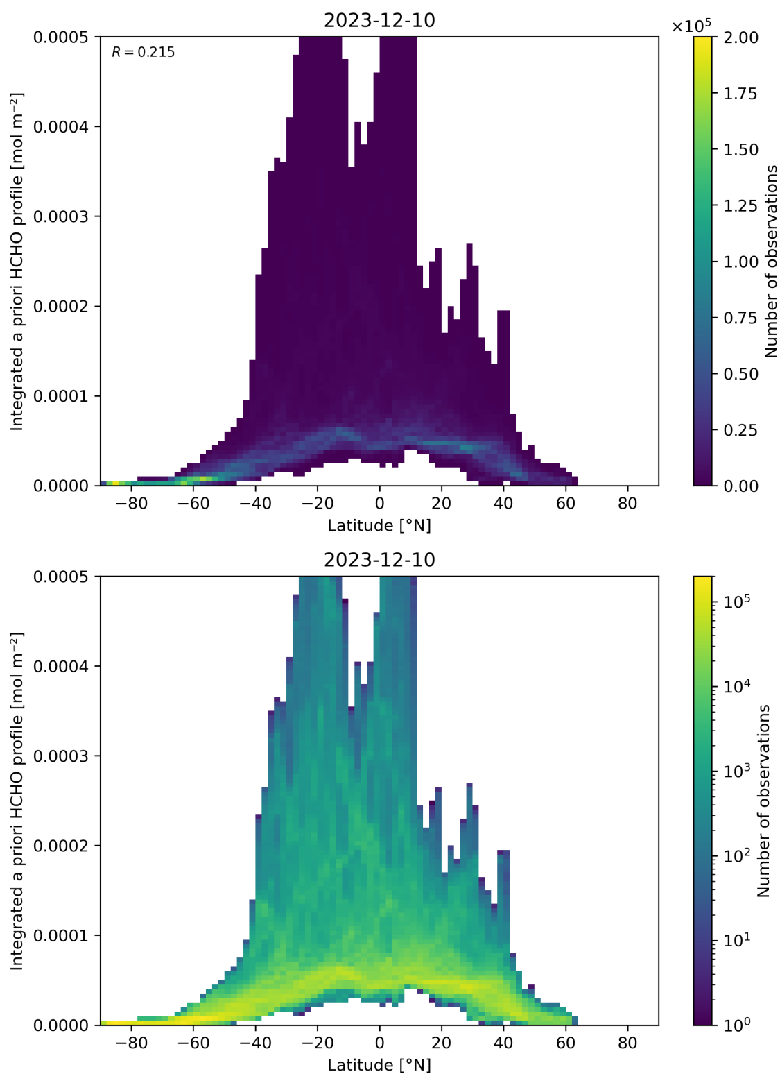
Figure 166: Scatter density plot of “Latitude” against “Integrated a priori HCHO profile” for 2023-12-09 to 2023-12-11.
