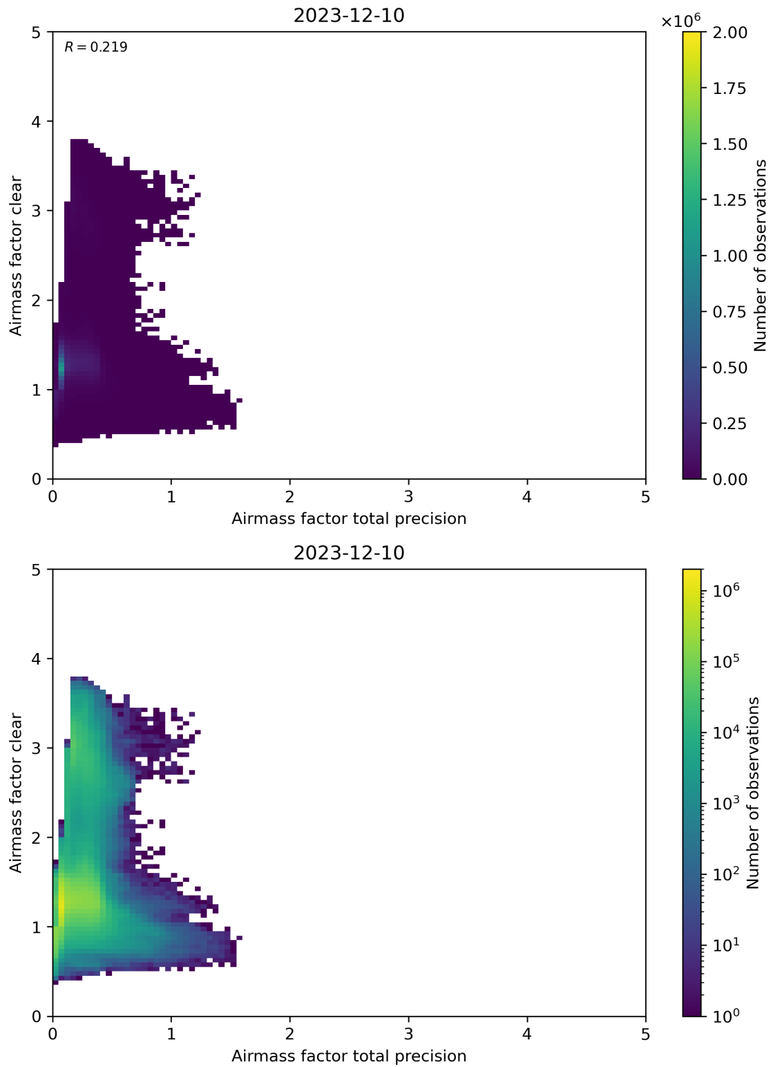
Figure 108: Scatter density plot of “Airmass factor total precision” against “Airmass factor clear” for 2023-12-09 to 2023-12-11.
