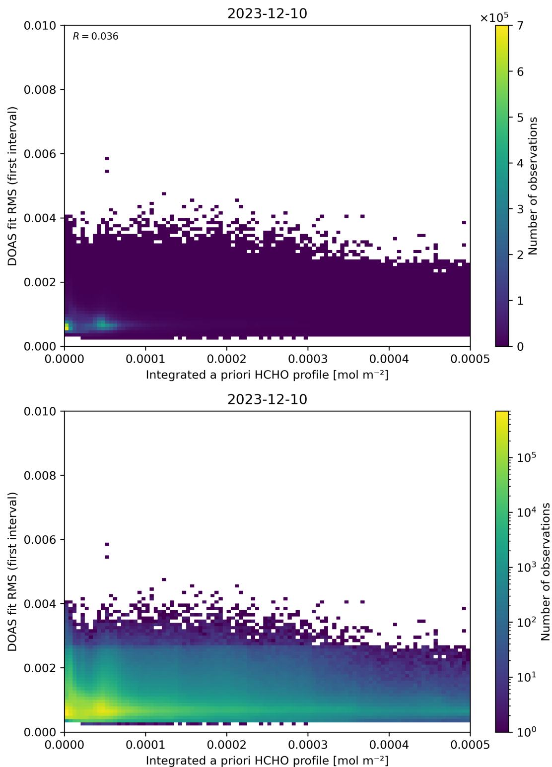
Figure 148: Scatter density plot of “Integrated a priori HCHO profile” against “DOAS fit RMS (first interval)” for 2023-12-09 to 2023-12-11.
