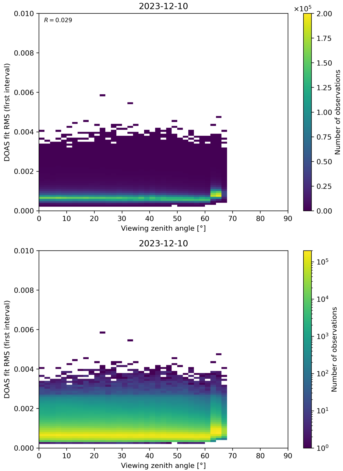
Figure 182: Scatter density plot of “Viewing zenith angle” against “DOAS fit RMS (first interval)” for 2023-12-09 to 2023-12-11.
