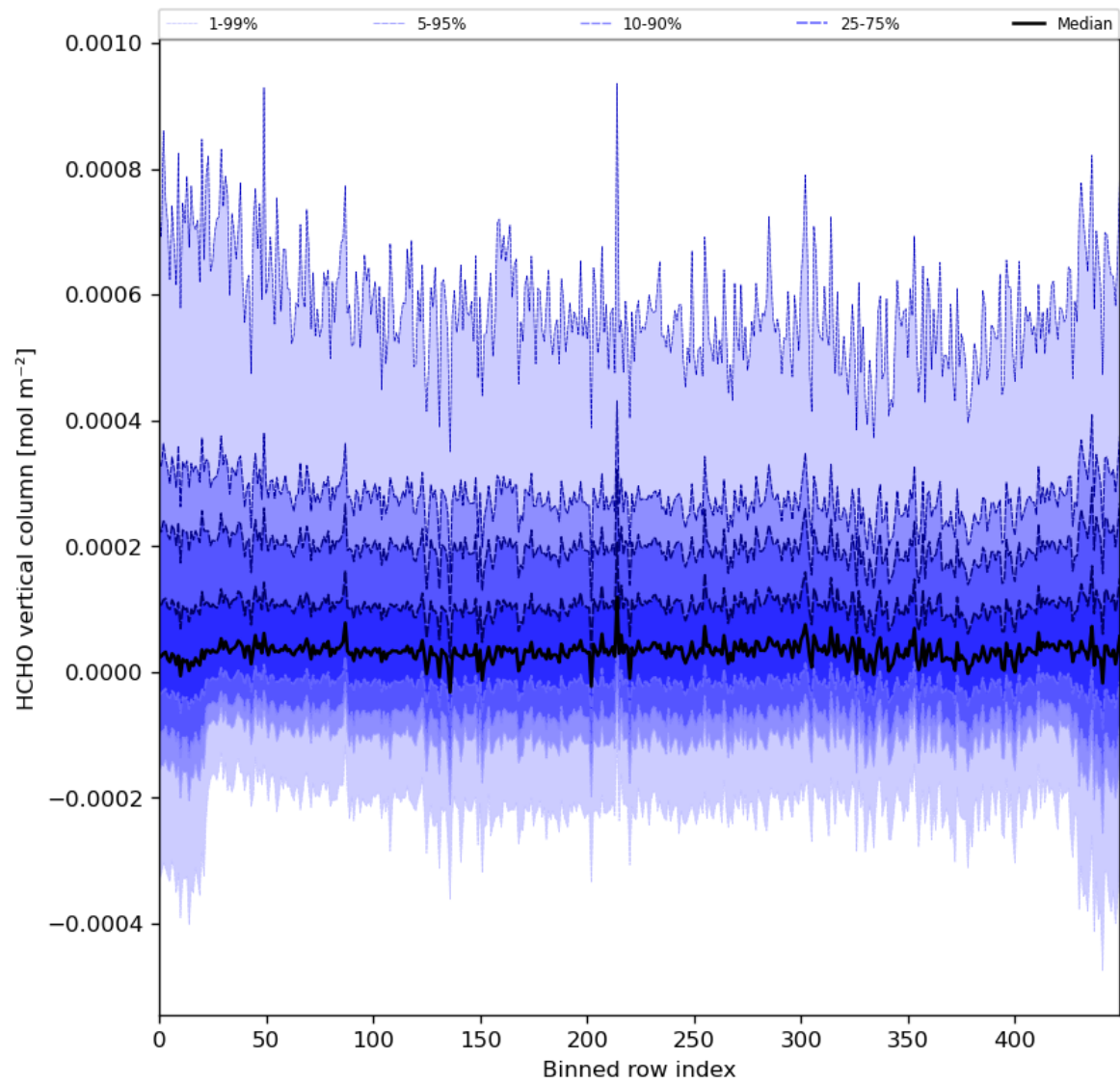
Figure 49: Along track statistics of “HCHO vertical column” for 2023-12-09 to 2023-12-11
