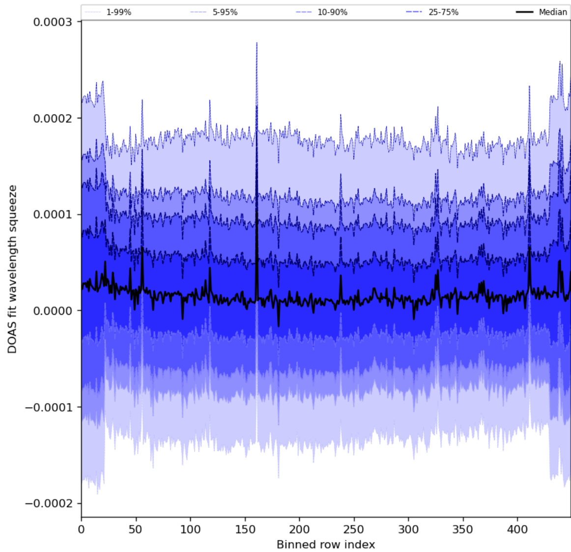
Figure 59: Along track statistics of “DOAS fit wavelength squeeze” for 2023-12-09 to 2023-12-11
