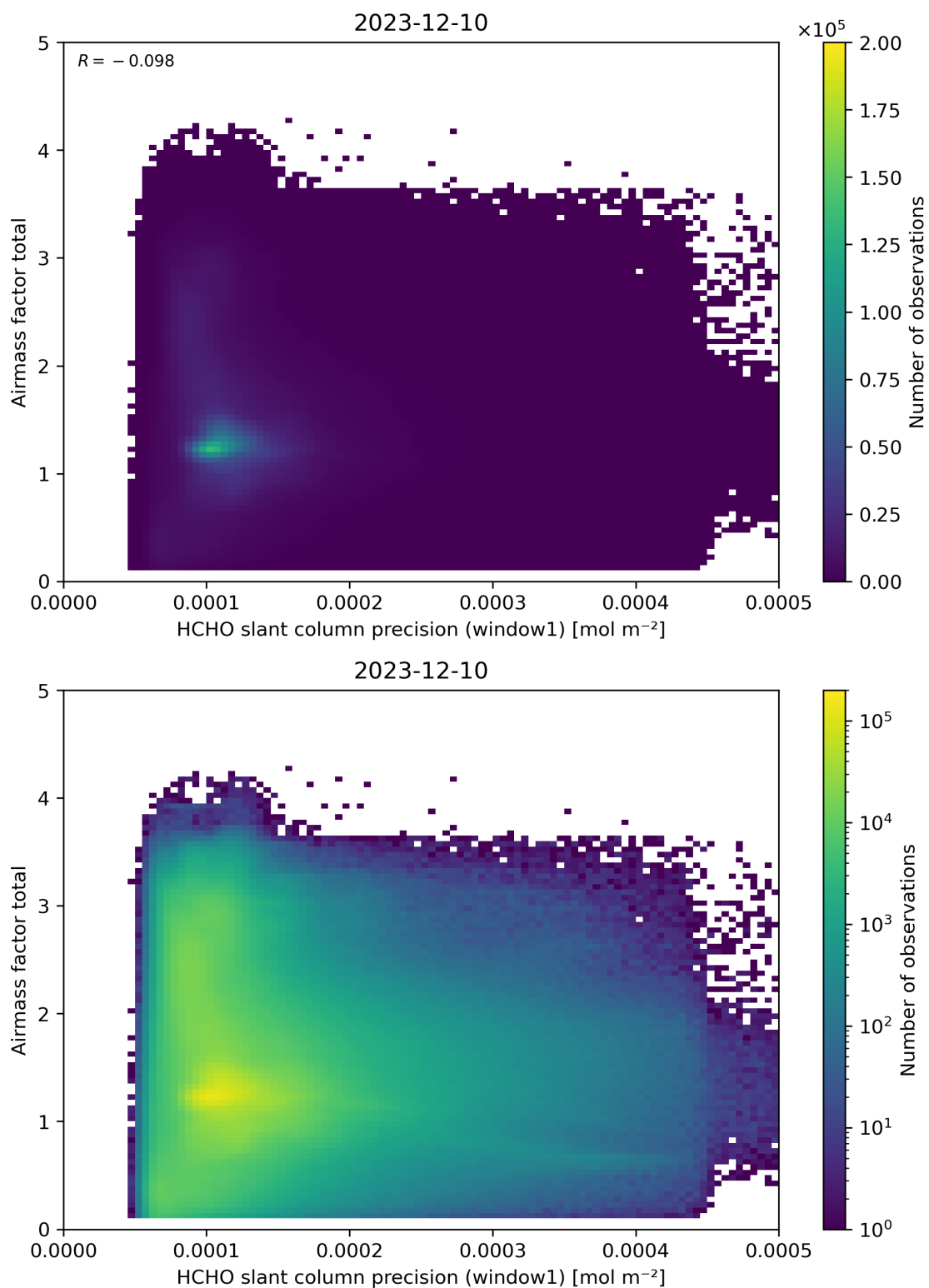
Figure 94: Scatter density plot of “HCHO slant column precision (window1)” against “Airmass factor total” for 2023-12-09 to 2023-12-11.
