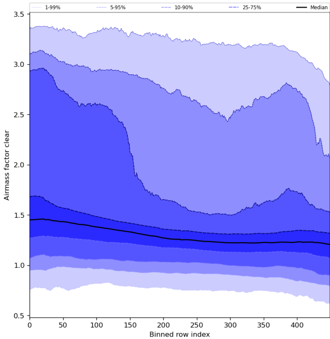
Figure 56: Along track statistics of “Airmass factor clear” for 2023-12-09 to 2023-12-11
