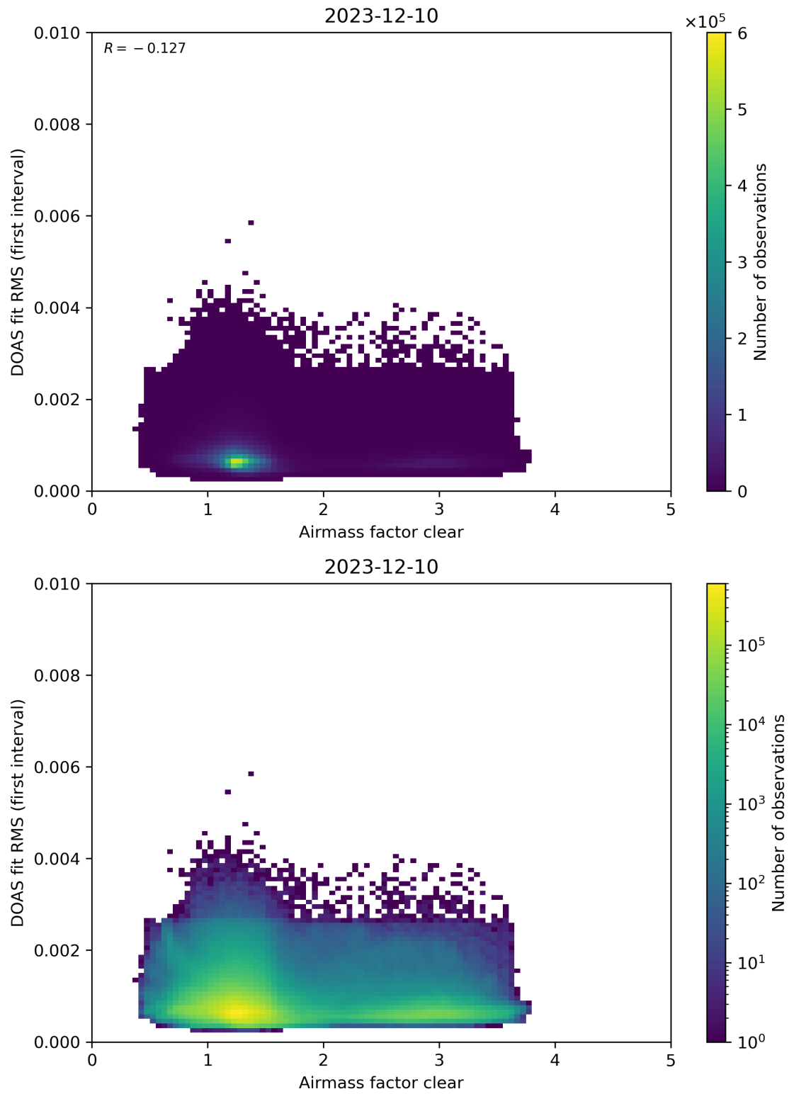
Figure 71: Scatter density plot of “Airmass factor clear” against “DOAS fit RMS (first interval)” for 2023-12-09 to 2023-12-11.
