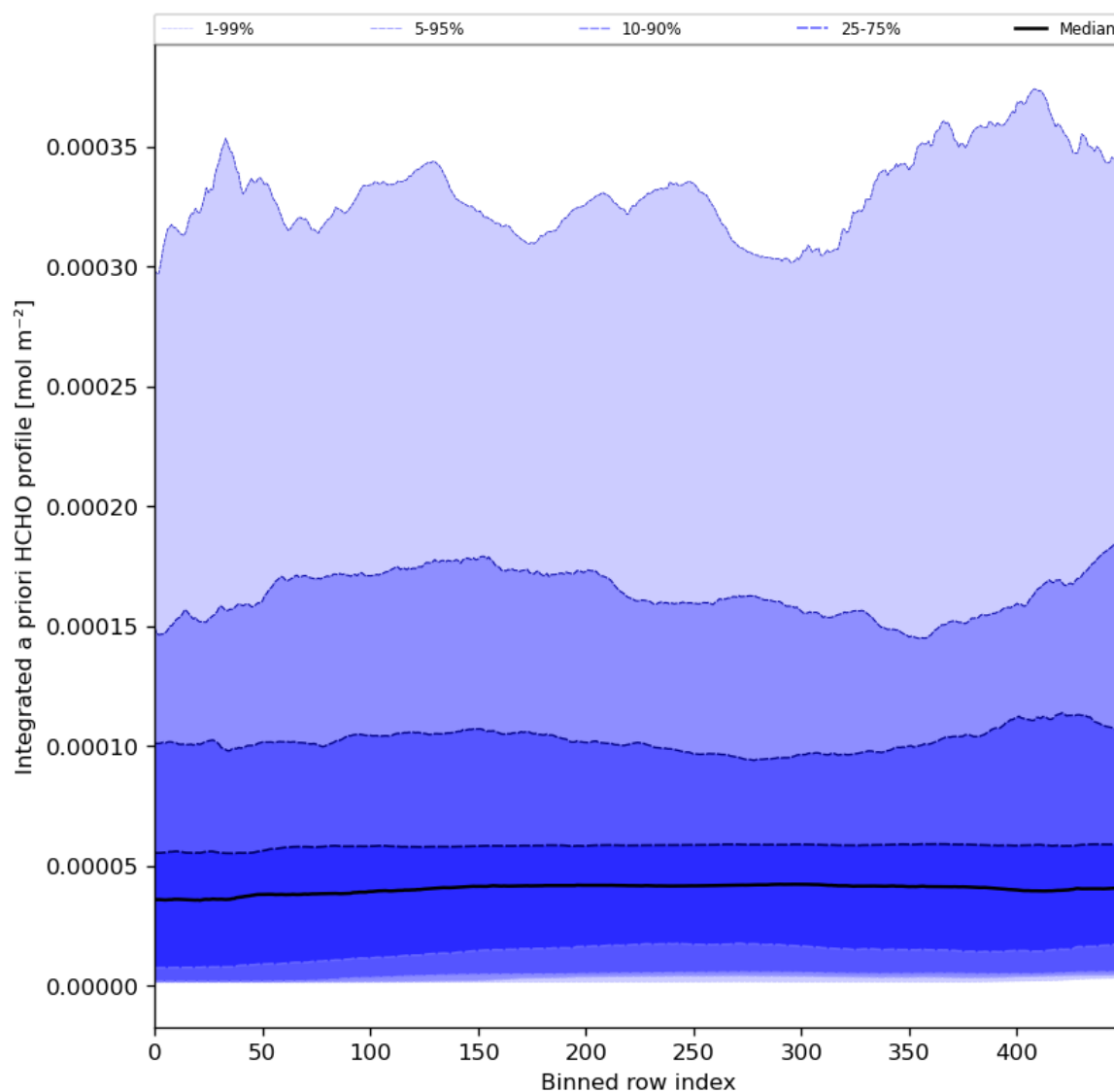
Figure 57: Along track statistics of “Integrated a priori HCHO profile” for 2023-12-09 to 2023-12-11
