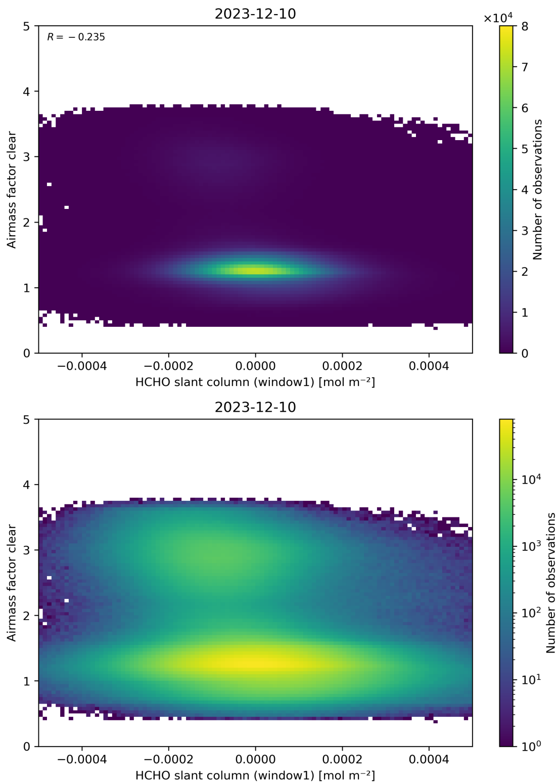
Figure 81: Scatter density plot of “HCHO slant column (window1)” against “Airmass factor clear” for 2023-12-09 to 2023-12-11.
