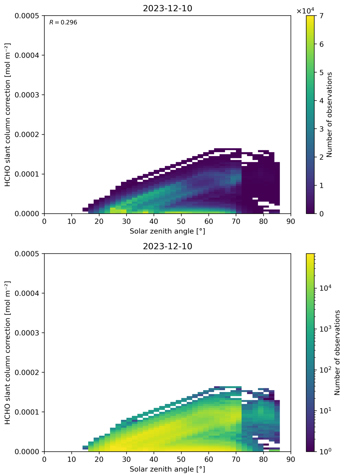
Figure 172: Scatter density plot of “Solar zenith angle” against “HCHO slant column correction” for 2023-12-09 to 2023-12-11.
