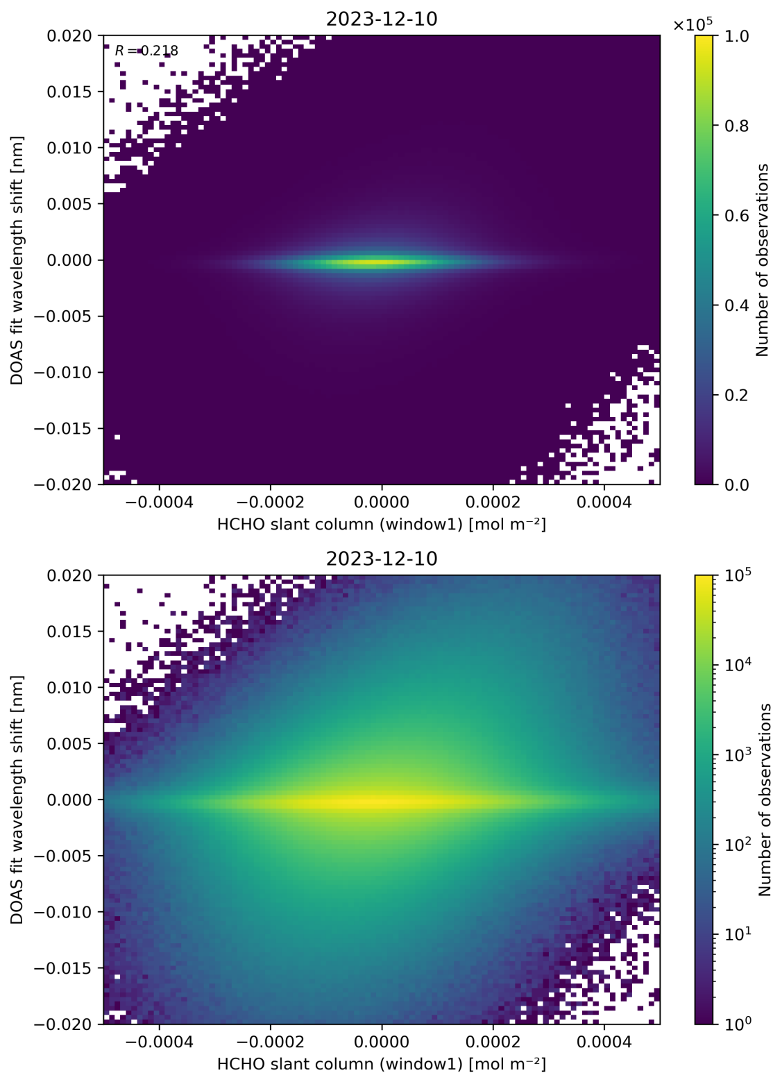
Figure 79: Scatter density plot of “HCHO slant column (window1)” against “DOAS fit wavelength shift” for 2023-12-09 to 2023-12-11.
