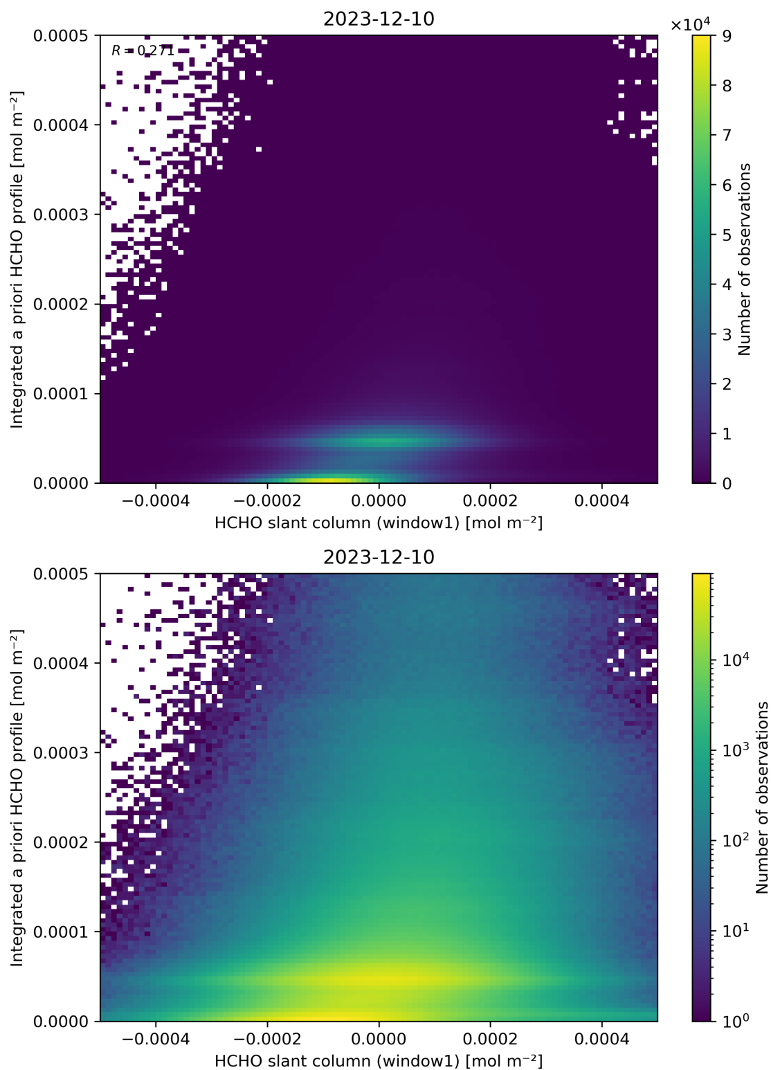
Figure 87: Scatter density plot of “HCHO slant column (window1)” against “Integrated a priori HCHO profile” for 2023-12-09 to 2023-12-11.
