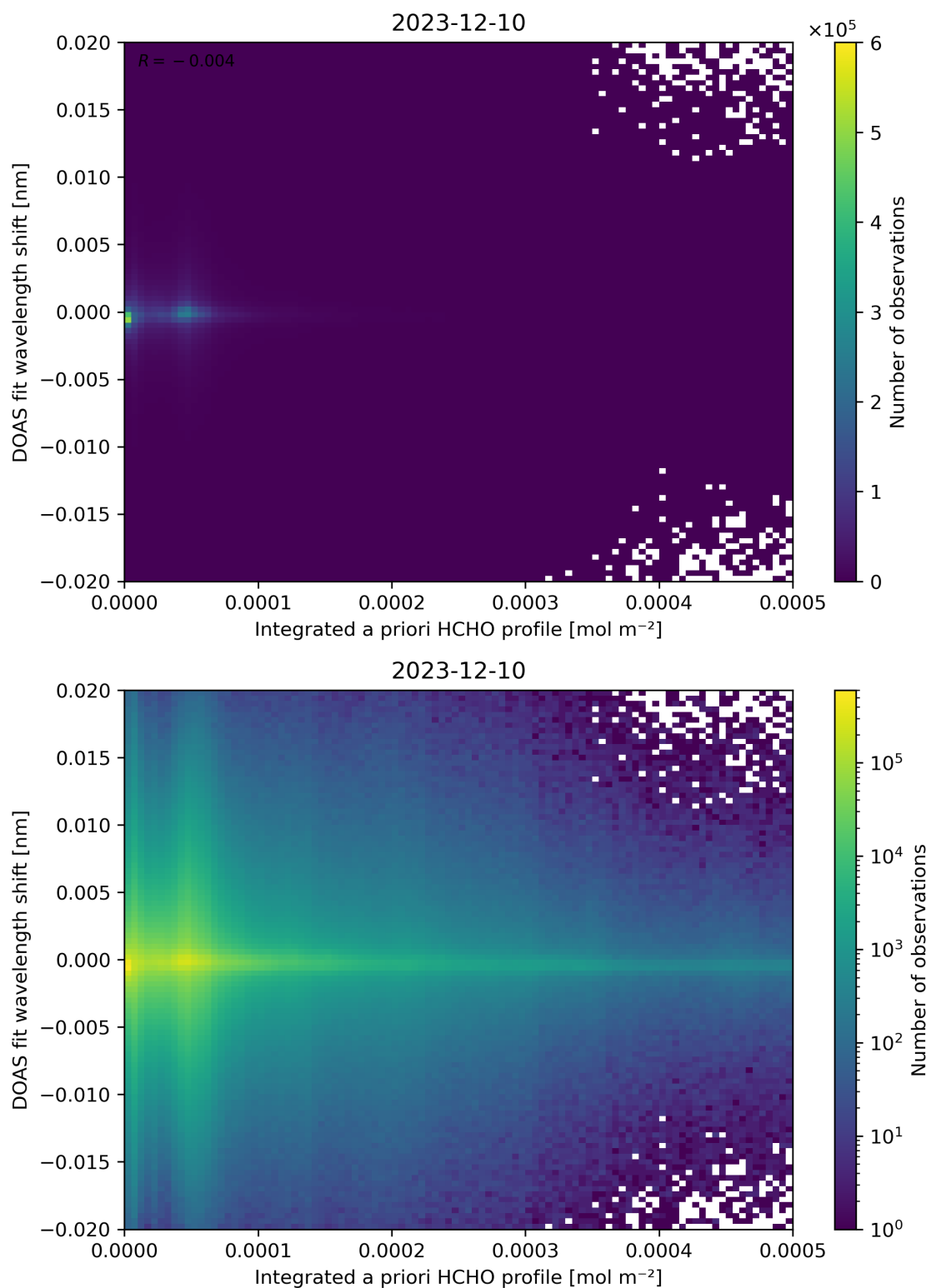
Figure 149: Scatter density plot of “Integrated a priori HCHO profile” against “DOAS fit wavelength shift” for 2023-12-09 to 2023-12-11.
