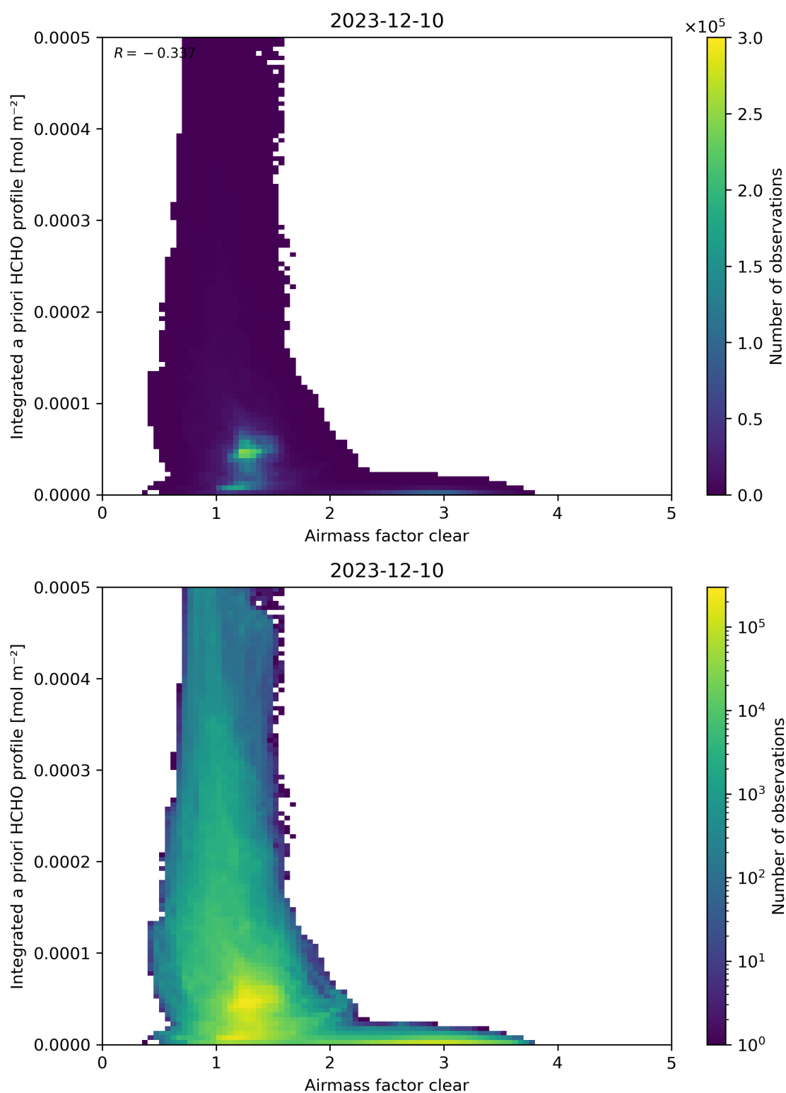
Figure 76: Scatter density plot of “Airmass factor clear” against “Integrated a priori HCHO profile” for 2023-12-09 to 2023-12-11.
