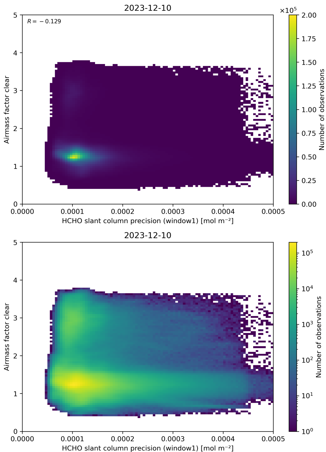
Figure 91: Scatter density plot of “HCHO slant column precision (window1)” against “Airmass factor clear” for 2023-12-09 to 2023-12-11.
