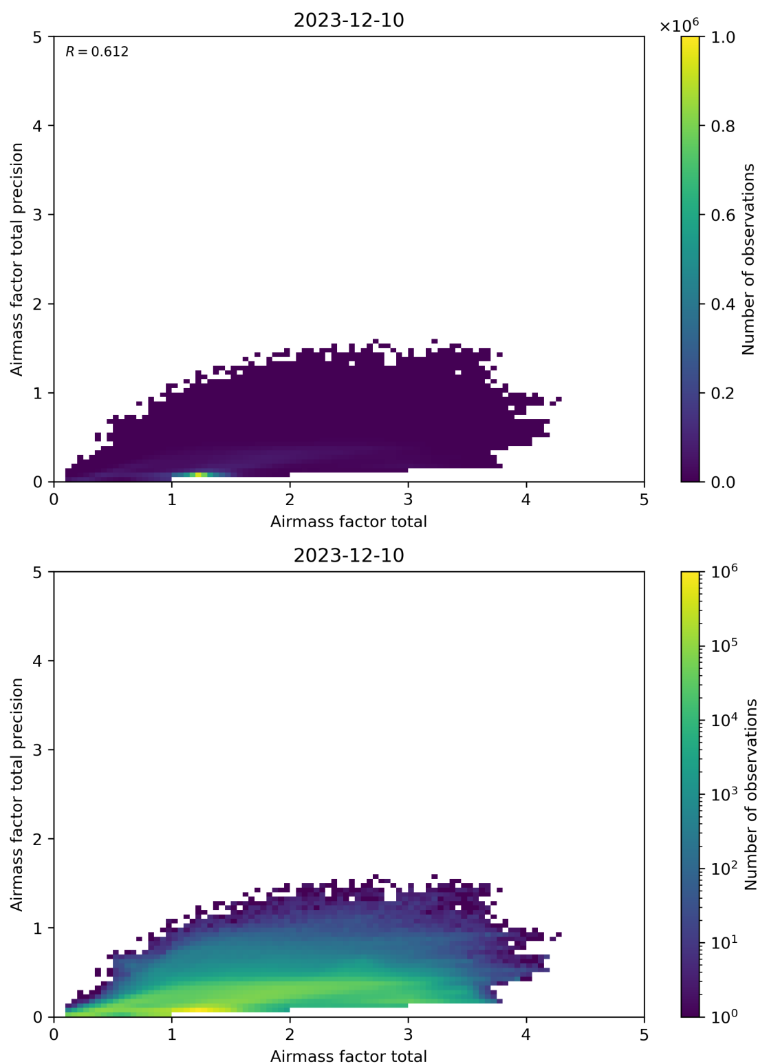
Figure 103: Scatter density plot of “Airmass factor total” against “Airmass factor total precision” for 2023-12-09 to 2023-12-11.
