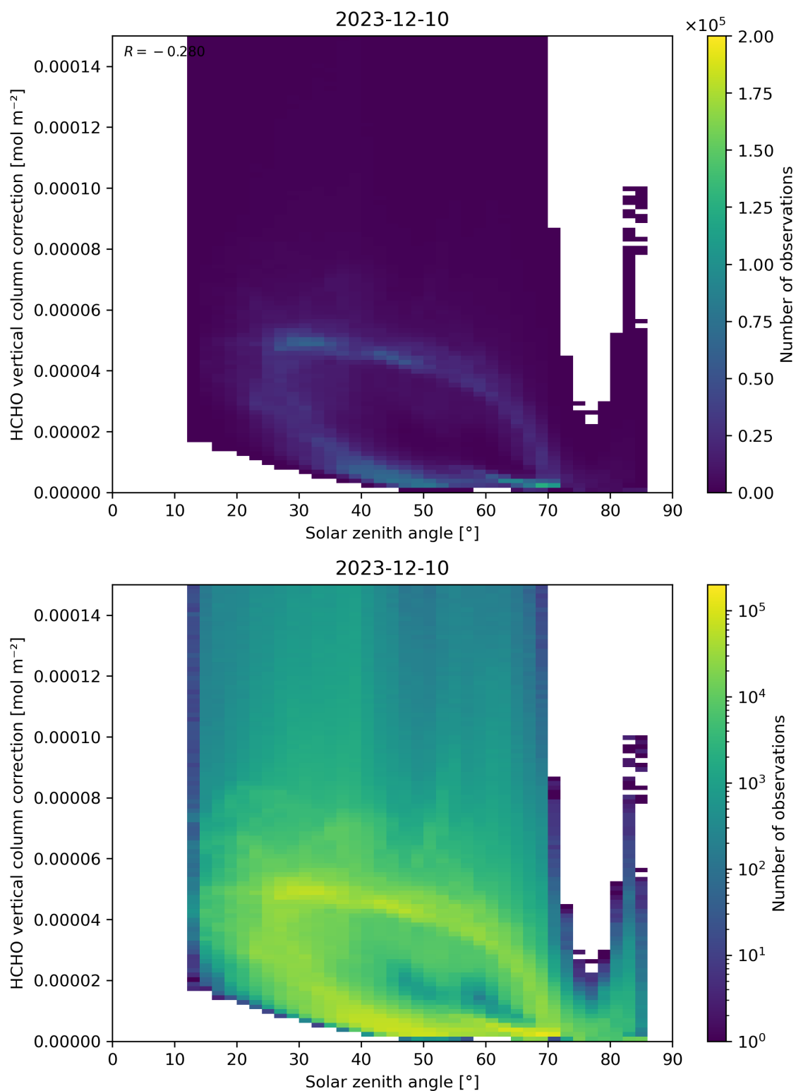
Figure 178: Scatter density plot of “Solar zenith angle” against “HCHO vertical column correction” for 2023-12-09 to 2023-12-11.
