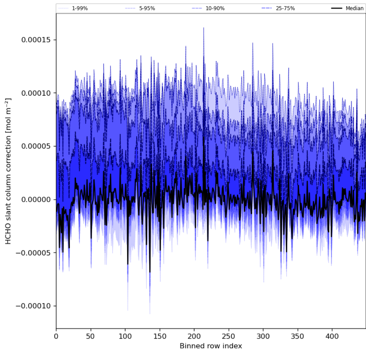
Figure 61: Along track statistics of “HCHO slant column correction” for 2023-12-09 to 2023-12-11
