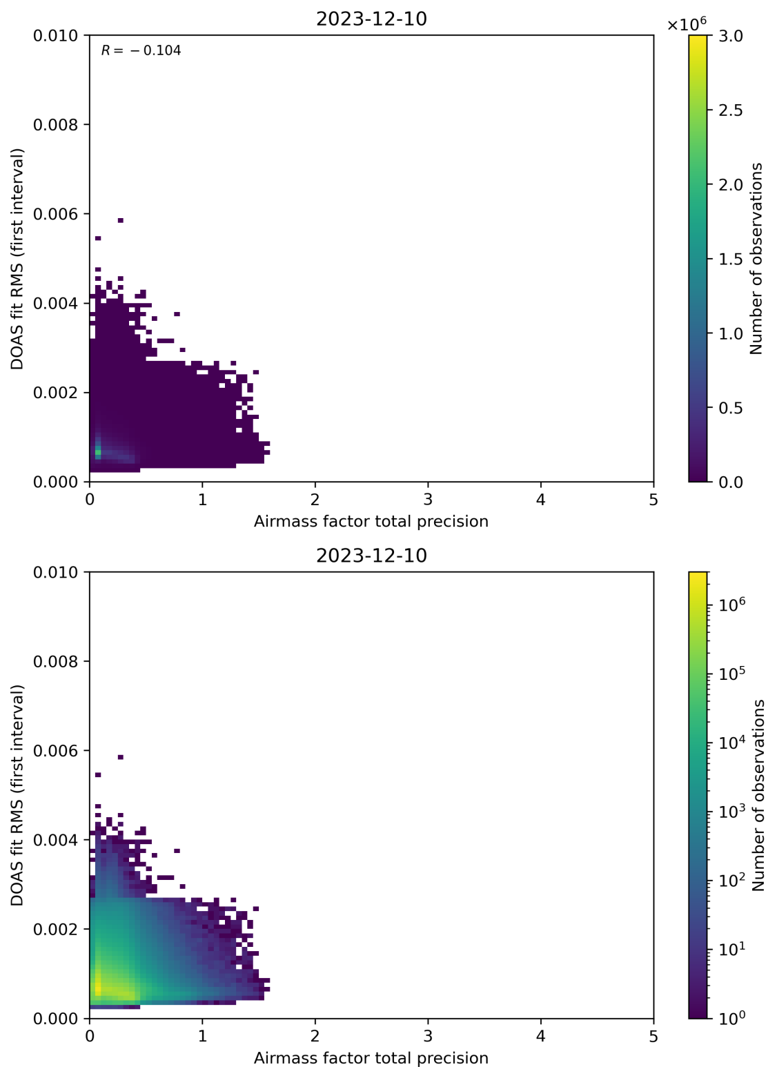
Figure 105: Scatter density plot of “Airmass factor total precision” against “DOAS fit RMS (first interval)” for 2023-12-09 to 2023-12-11.
