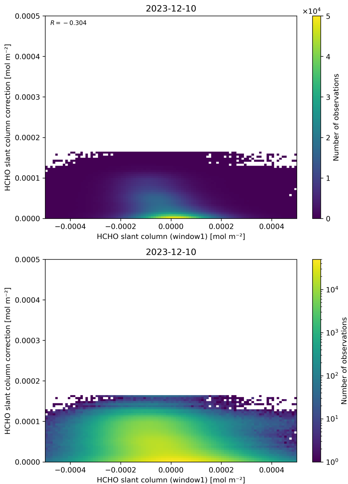
Figure 83: Scatter density plot of “HCHO slant column (window1)” against “HCHO slant column correction” for 2023-12-09 to 2023-12-11.
