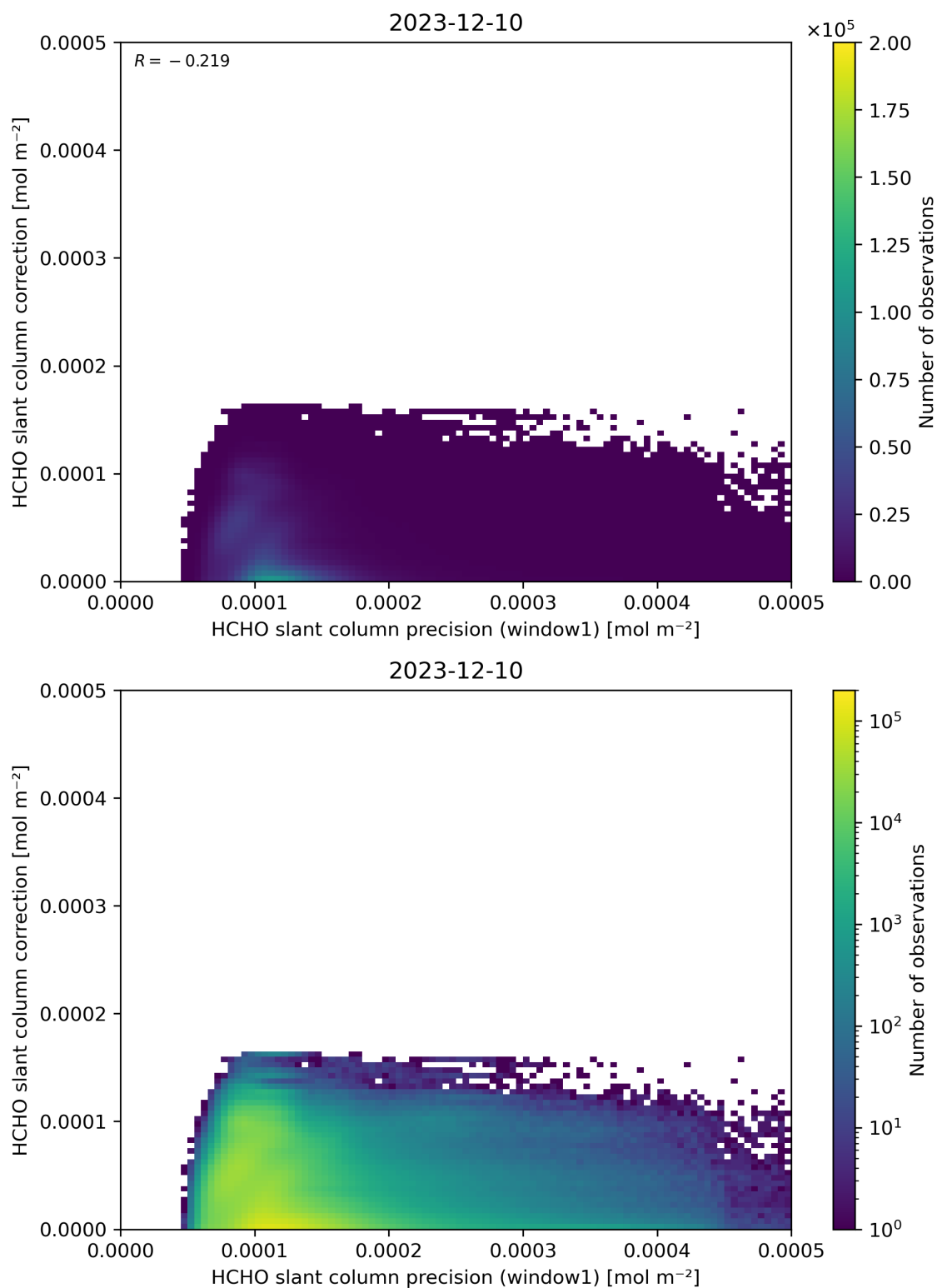
Figure 93: Scatter density plot of “HCHO slant column precision (window1)” against “HCHO slant column correction” for 2023-12-09 to 2023-12-11.
