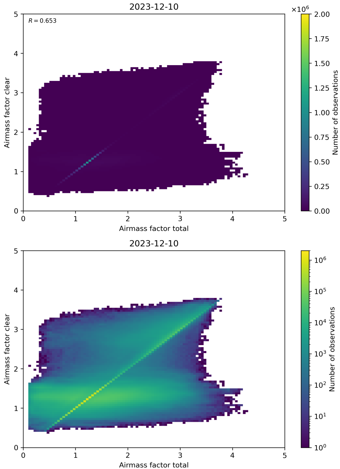
Figure 100: Scatter density plot of “Airmass factor total” against “Airmass factor clear” for 2023-12-09 to 2023-12-11.
