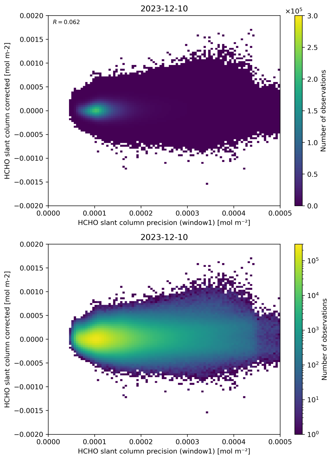
Figure 92: Scatter density plot of “HCHO slant column precision (window1)” against “HCHO slant column corrected” for 2023-12-09 to 2023-12-11.
