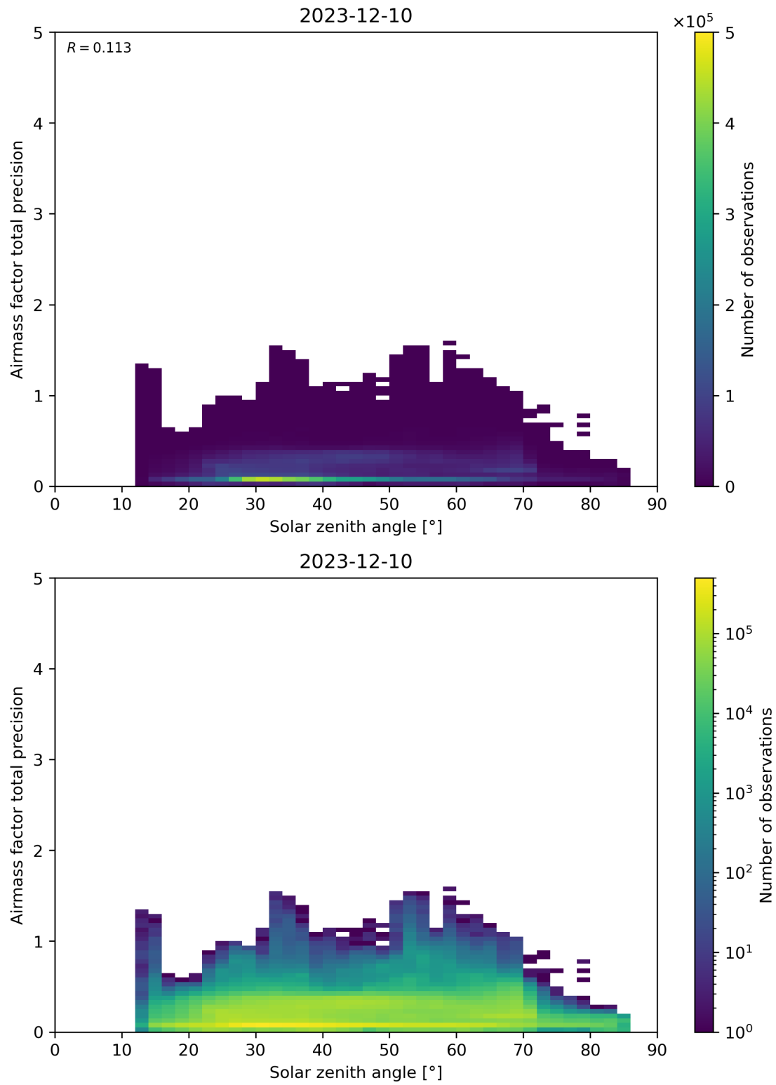
Figure 176: Scatter density plot of “Solar zenith angle” against “Airmass factor total precision” for 2023-12-09 to 2023-12-11.
