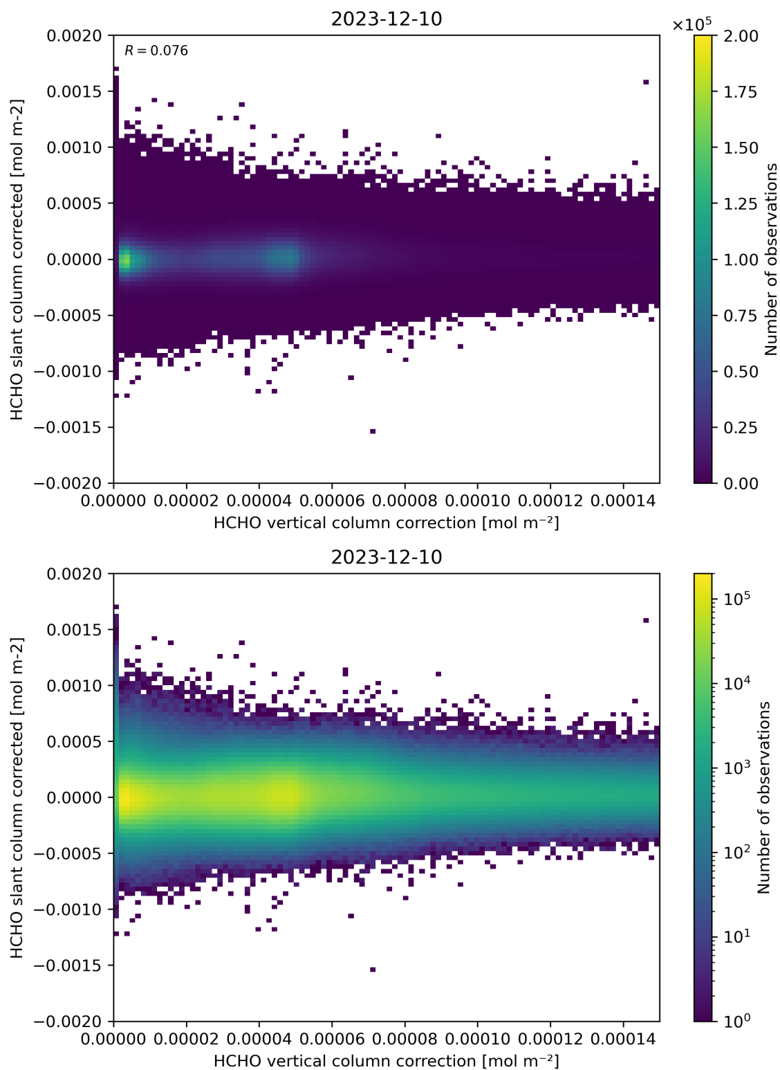
Figure 116: Scatter density plot of “HCHO vertical column correction” against “HCHO slant column corrected” for 2023-12-09 to 2023-12-11.
