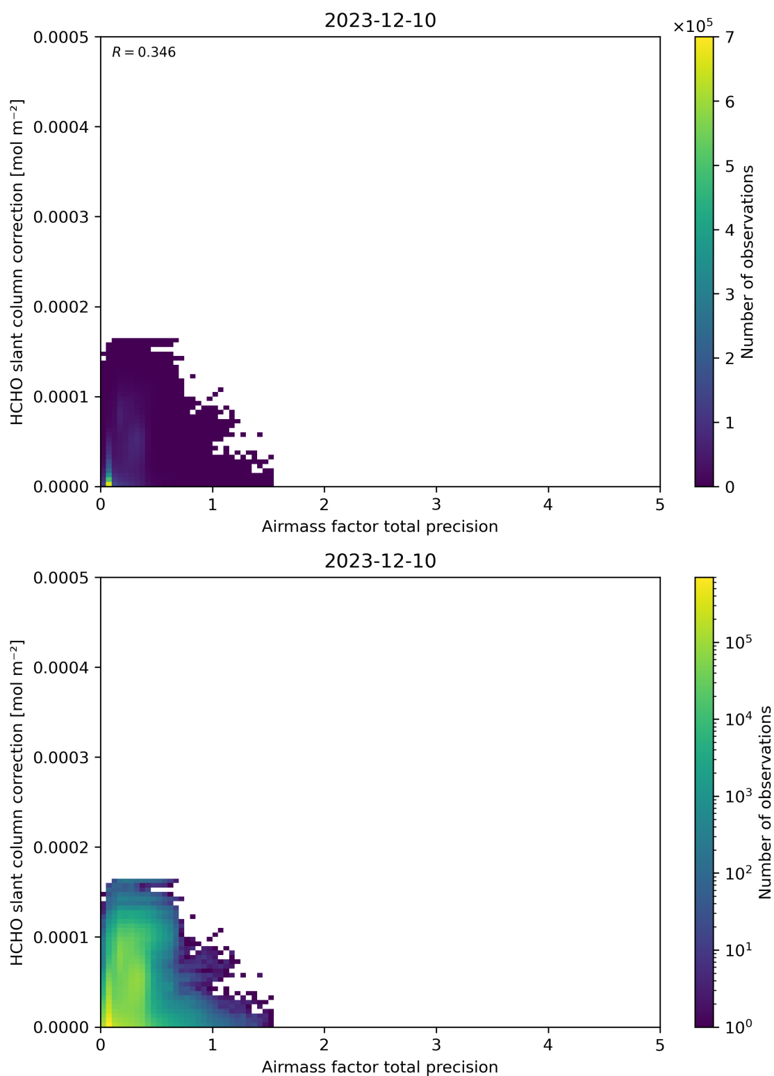
Figure 110: Scatter density plot of “Airmass factor total precision” against “HCHO slant column correction” for 2023-12-09 to 2023-12-11.
