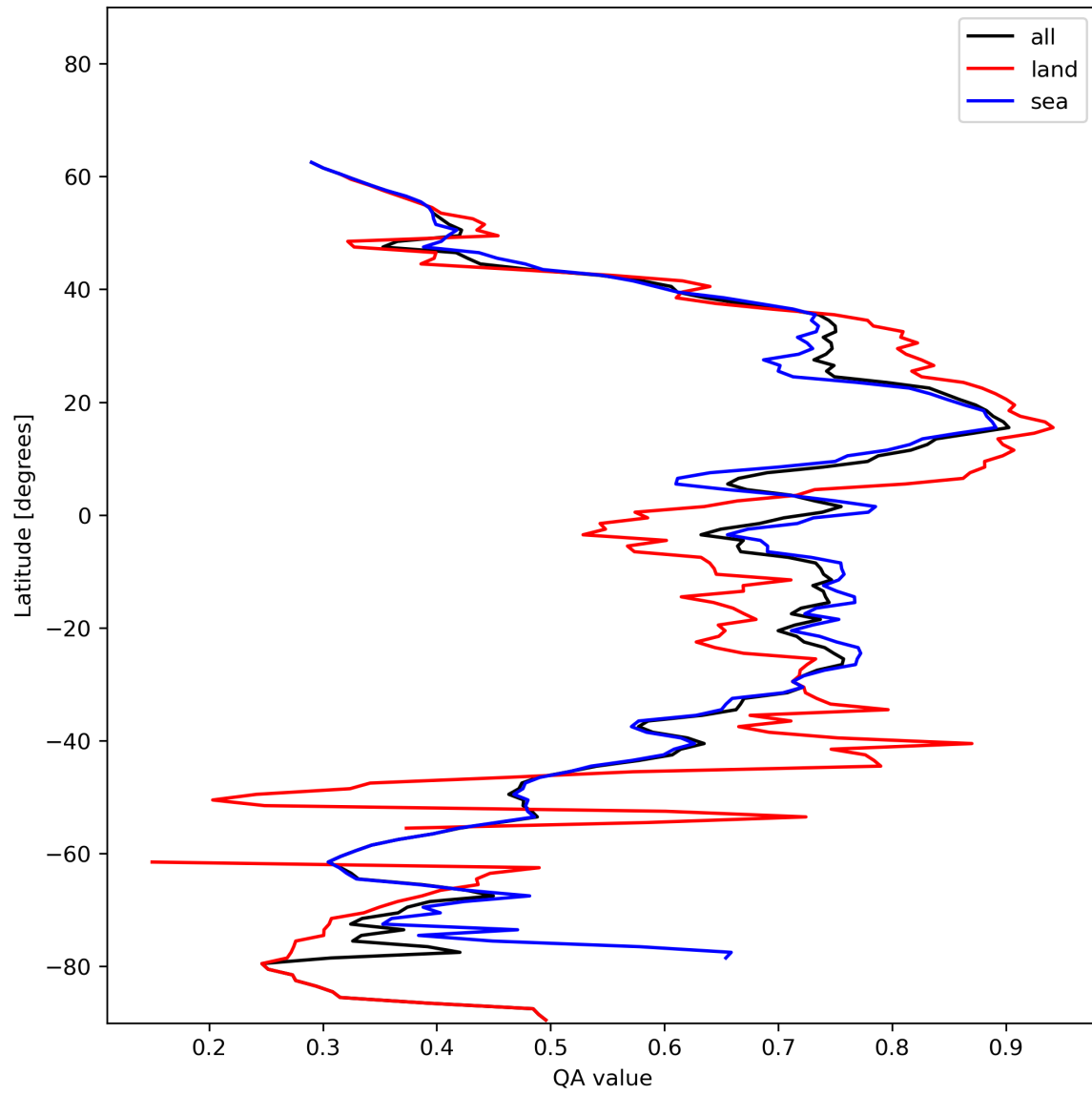
Figure 20: Zonal average of “QA value” for 2023-12-09 to 2023-12-11.
