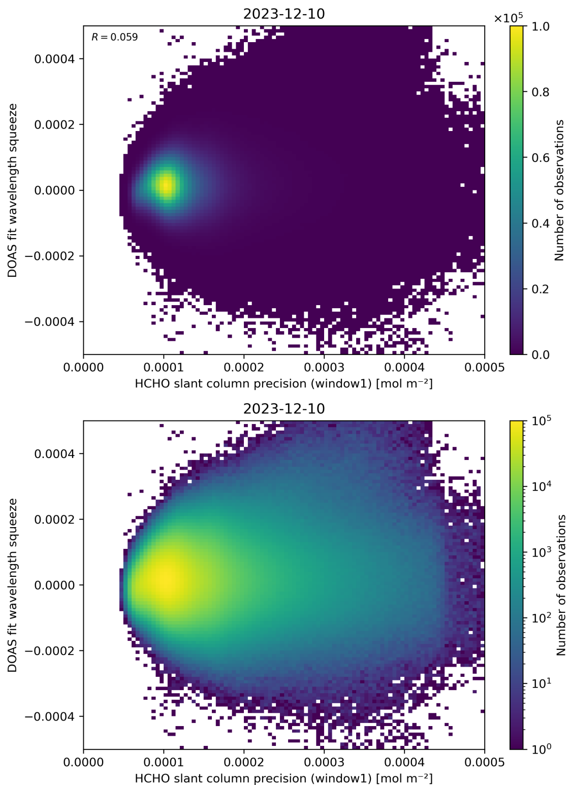
Figure 90: Scatter density plot of “HCHO slant column precision (window1)” against “DOAS fit wavelength squeeze” for 2023-12-09 to 2023-12-11.
