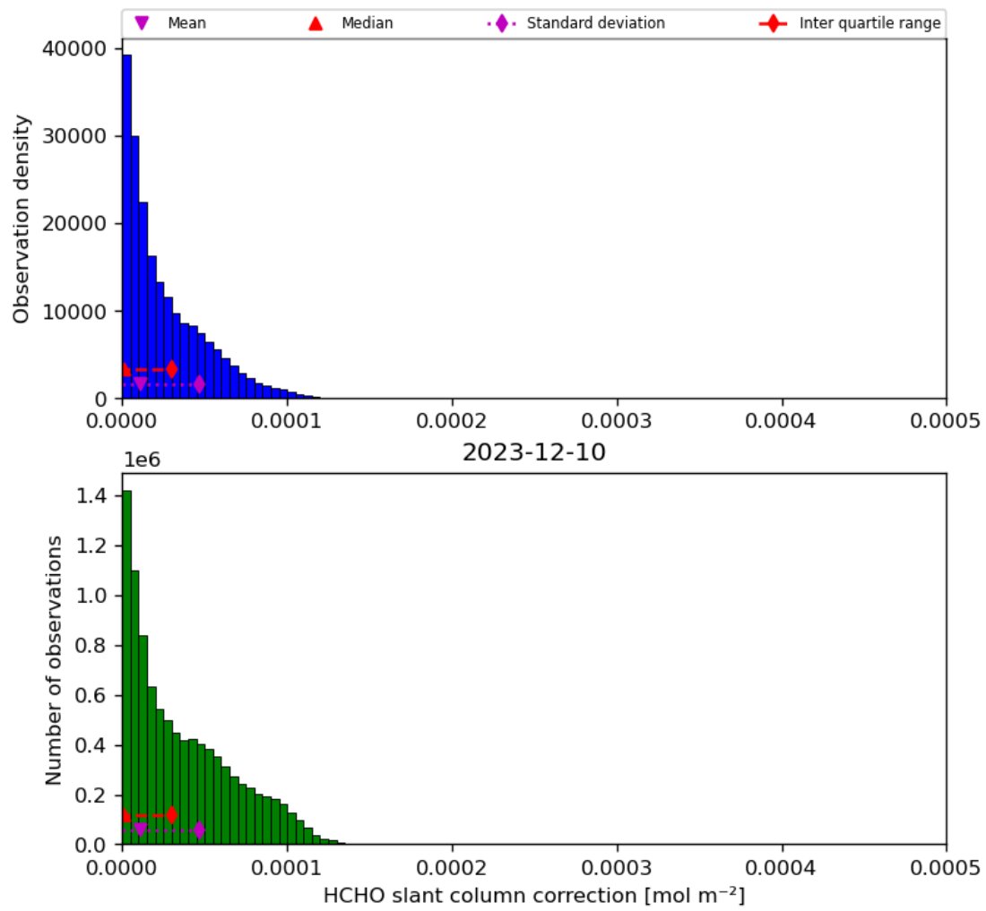
Figure 47: Histogram of “HCHO slant column correction” for 2023-12-09 to 2023-12-11
