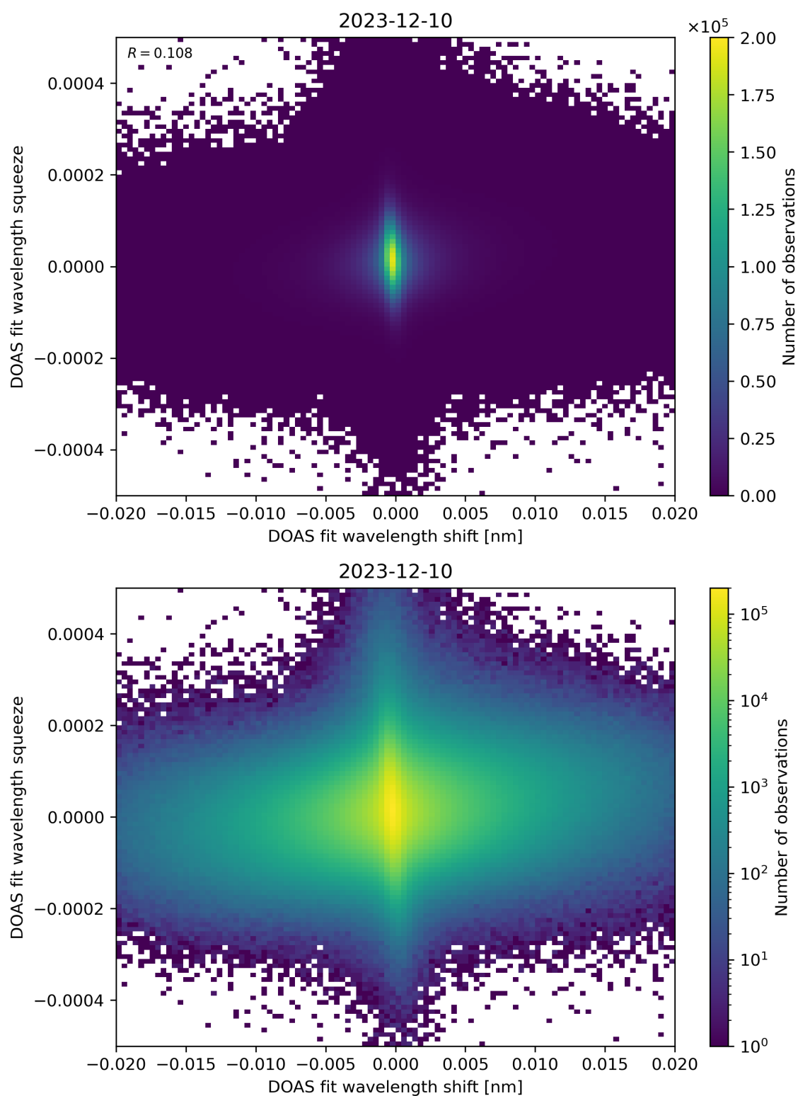
Figure 65: Scatter density plot of “DOAS fit wavelength shift” against “DOAS fit wavelength squeeze” for 2023-12-09 to 2023-12-11.
