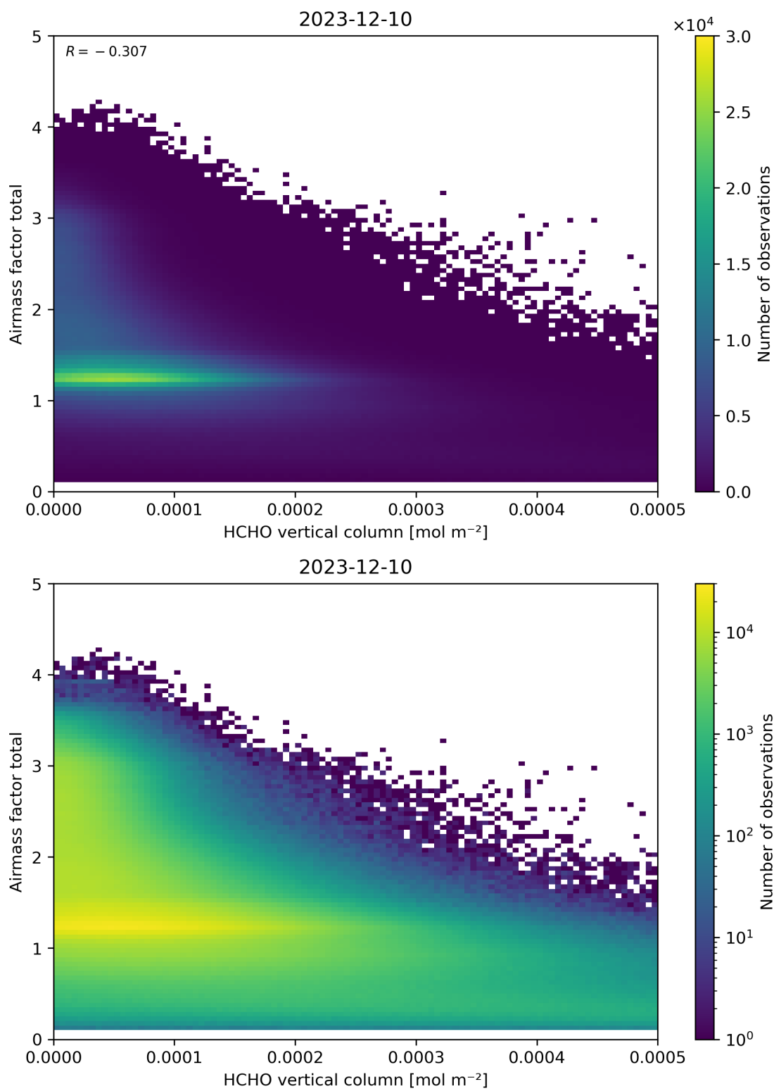
Figure 131: Scatter density plot of “HCHO vertical column” against “Airmass factor total” for 2023-12-09 to 2023-12-11.
