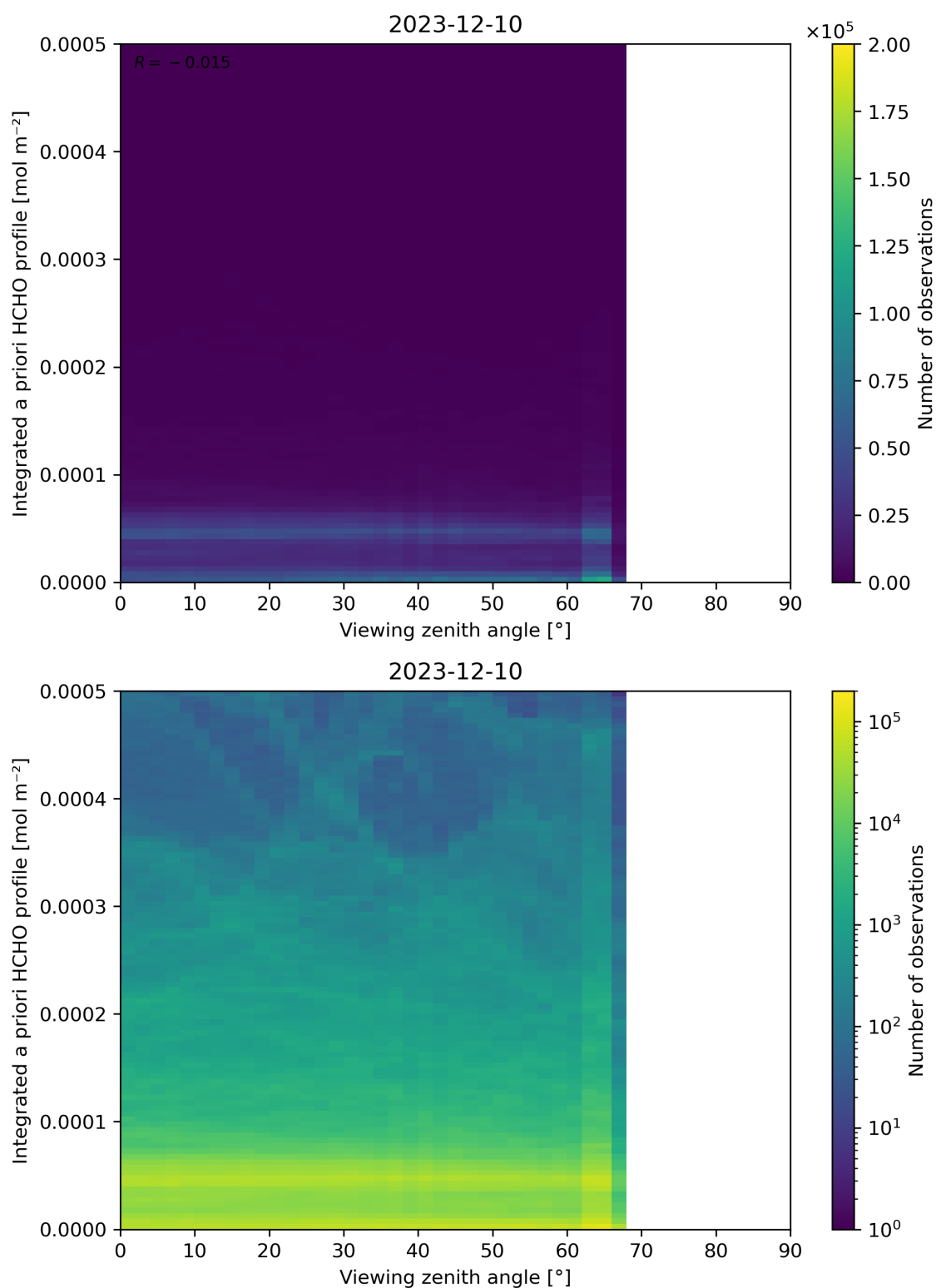
Figure 195: Scatter density plot of “Viewing zenith angle” against “Integrated a priori HCHO profile” for 2023-12-09 to 2023-12-11.
