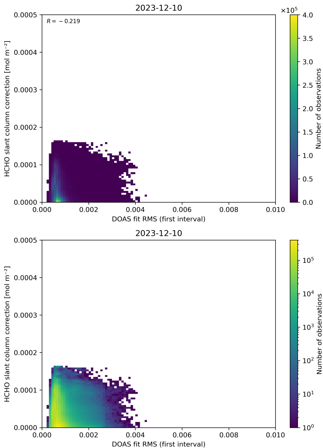
Figure 63: Scatter density plot of “DOAS fit RMS (first interval)” against “HCHO slant column correction” for 2023-12-09 to 2023-12-11.
