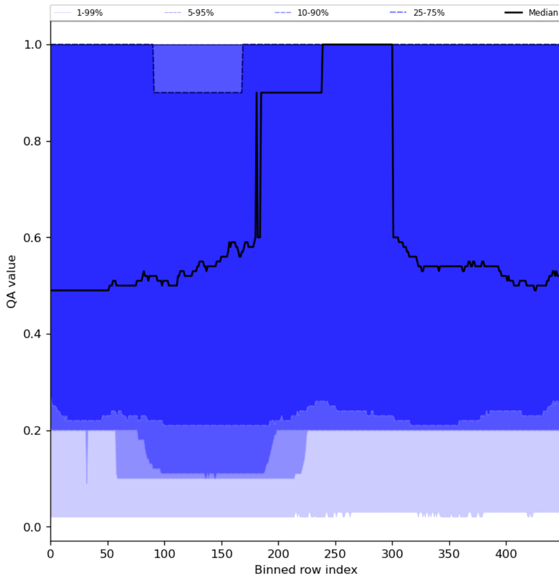
Figure 48: Along track statistics of “QA value” for 2023-12-09 to 2023-12-11
