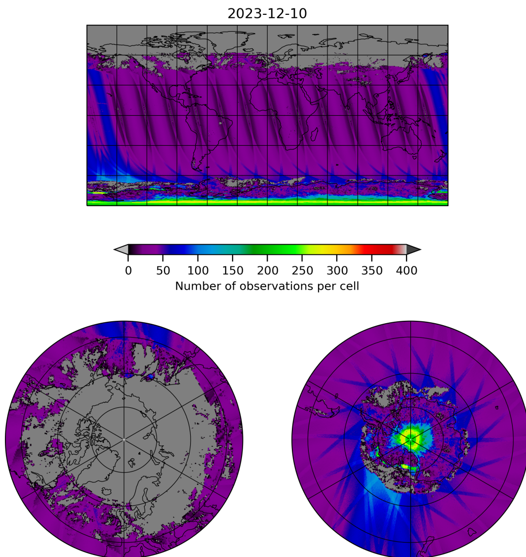
Figure 19: Map of the number of observations for 2023-12-09 to 2023-12-11
