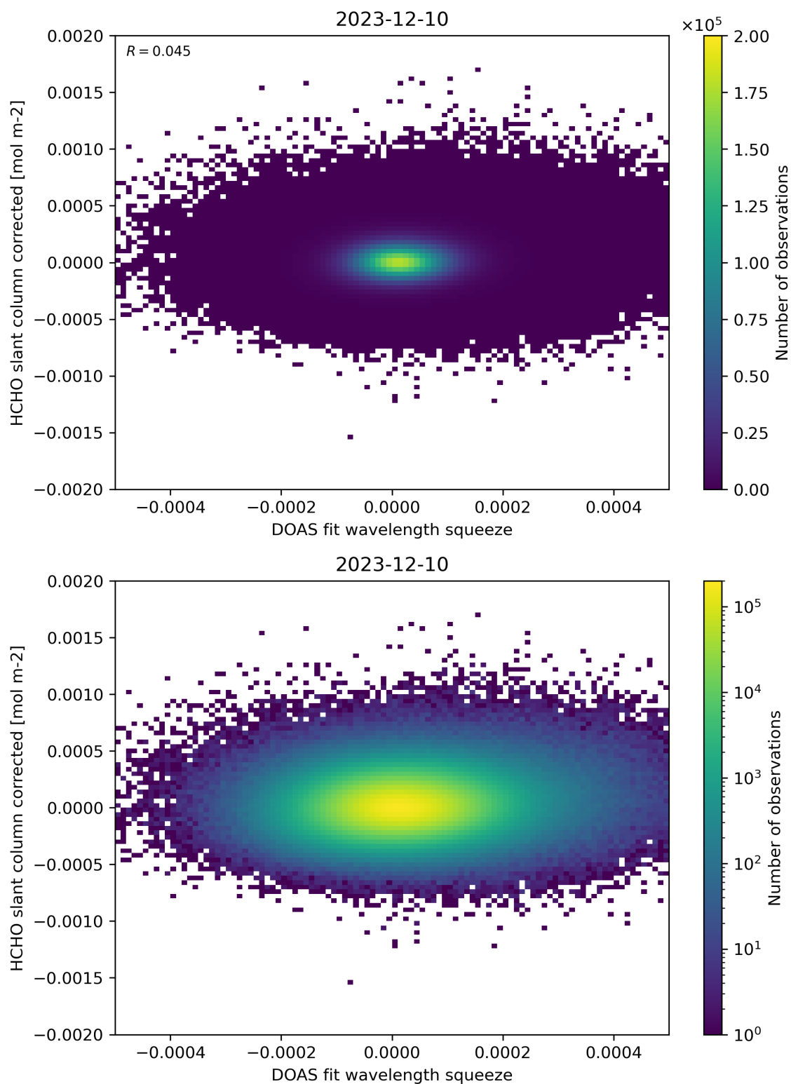
Figure 69: Scatter density plot of “DOAS fit wavelength squeeze” against “HCHO slant column corrected” for 2023-12-09 to 2023-12-11.
