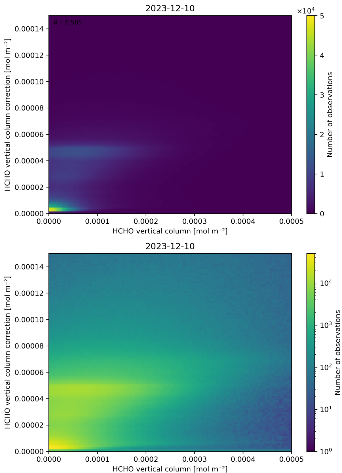
Figure 133: Scatter density plot of “HCHO vertical column” against “HCHO vertical column correction” for 2023-12-09 to 2023-12-11.
