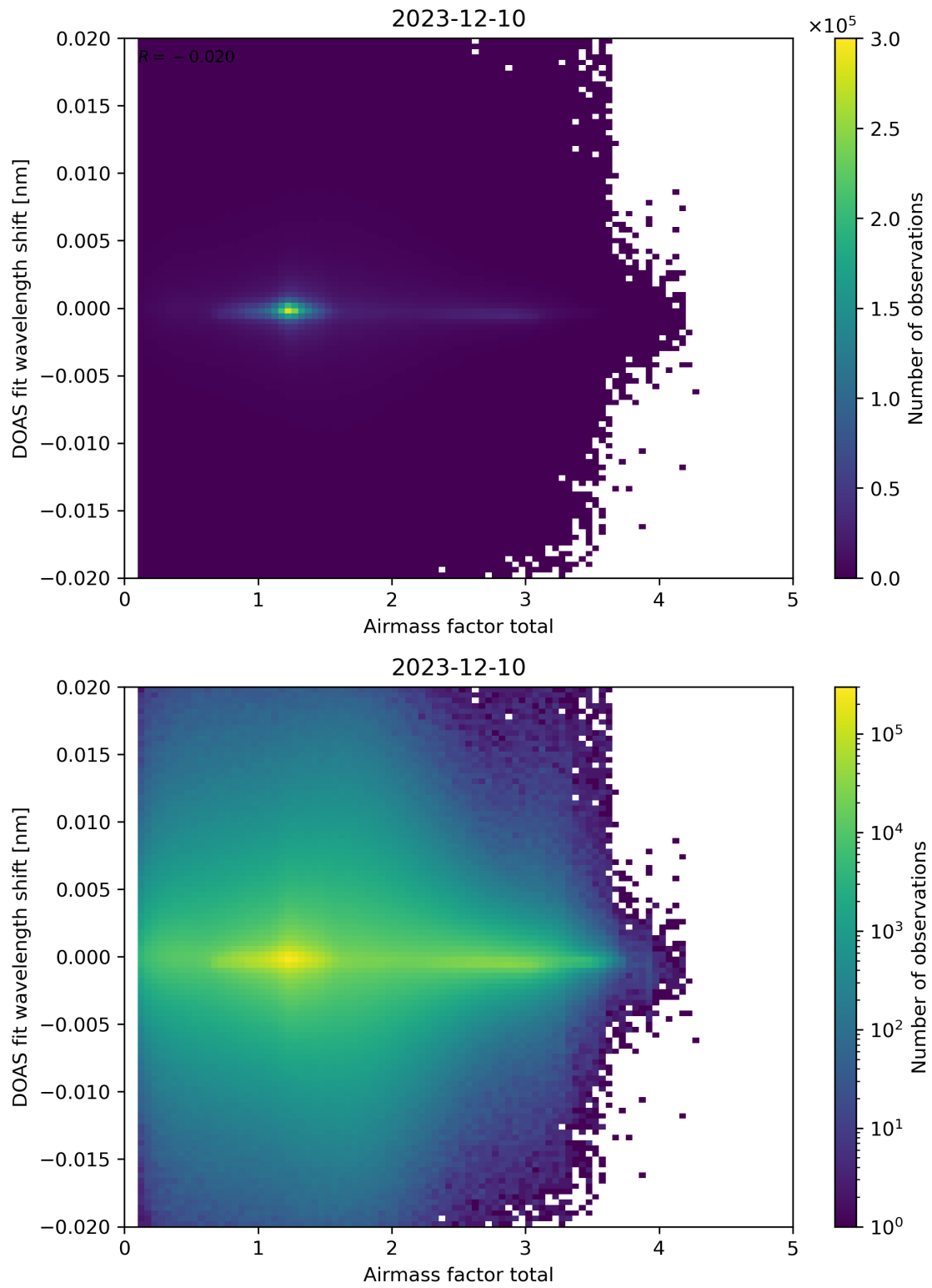
Figure 98: Scatter density plot of “Airmass factor total” against “DOAS fit wavelength shift” for 2023-12-09 to 2023-12-11.
