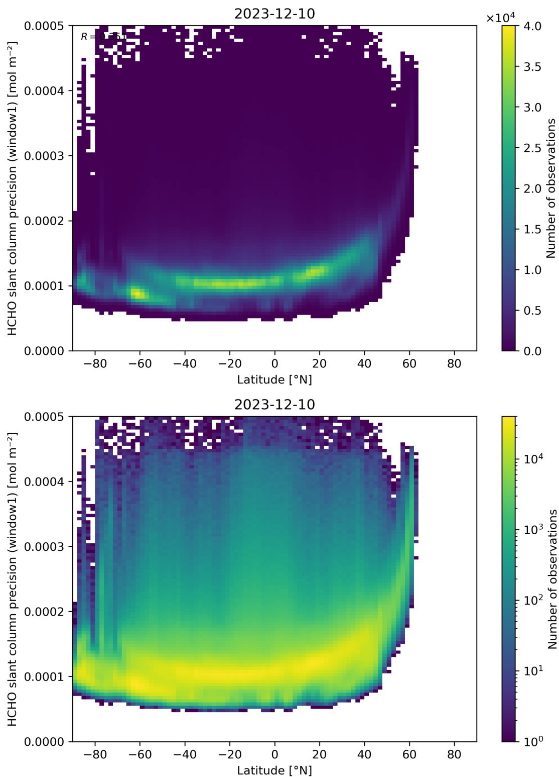
Figure 160: Scatter density plot of “Latitude” against “HCHO slant column precision (window1)” for 2023-12-09 to 2023-12-11.
