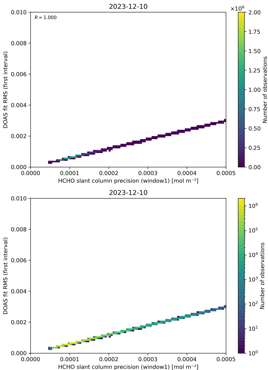
Figure 88: Scatter density plot of “HCHO slant column precision (window1)” against “DOAS fit RMS (first interval)” for 2023-12-09 to 2023-12-11.
