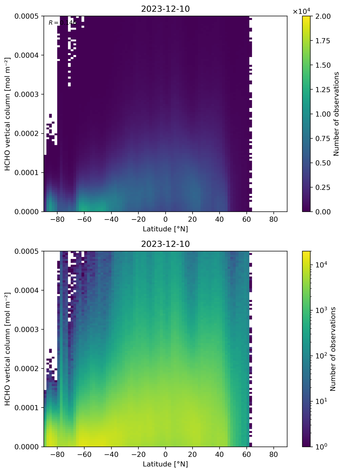
Figure 163: Scatter density plot of “Latitude” against “HCHO vertical column” for 2023-12-09 to 2023-12-11.
