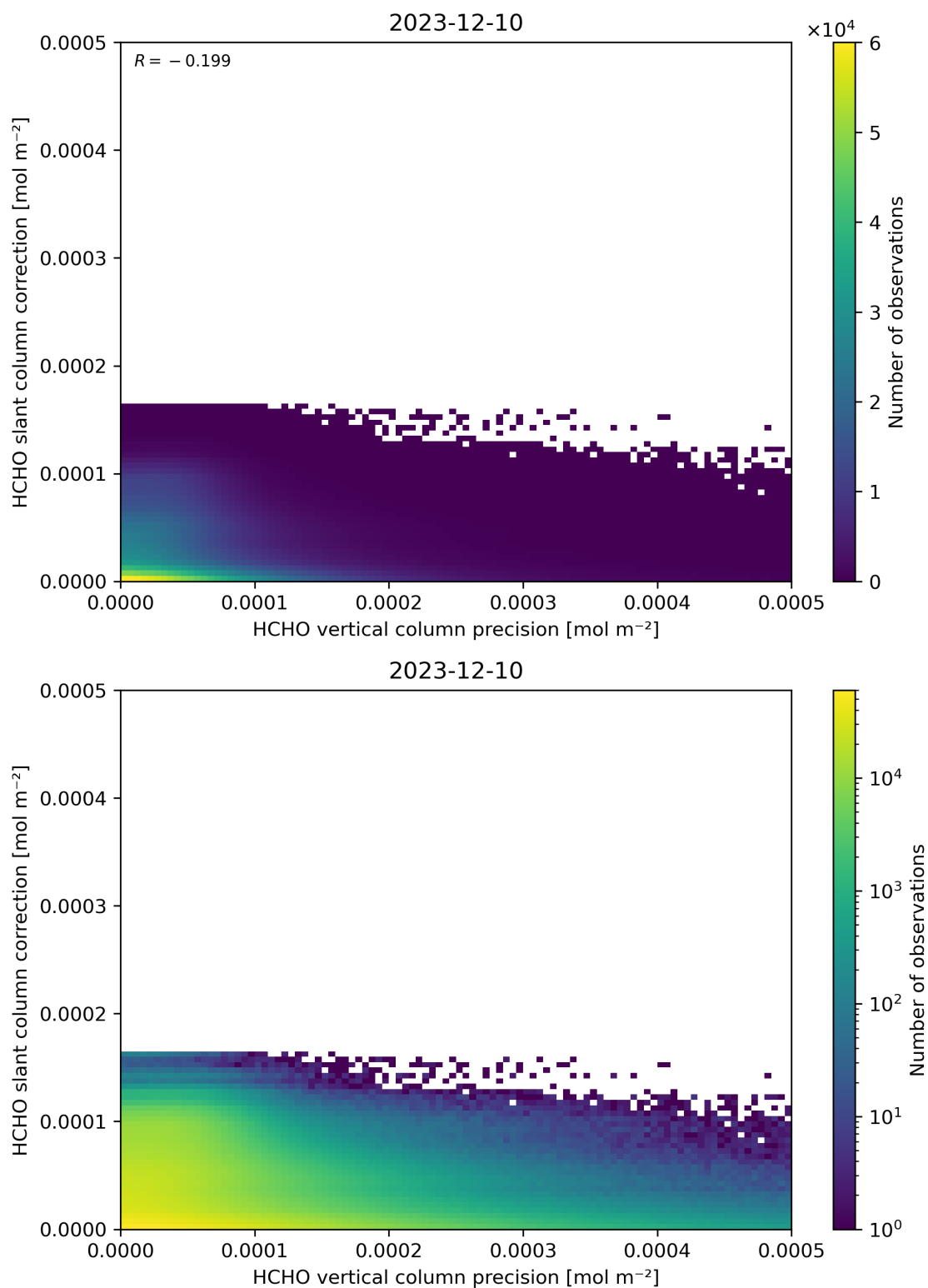
Figure 141: Scatter density plot of “HCHO vertical column precision” against “HCHO slant column correction” for 2023-12-09 to 2023-12-11.
