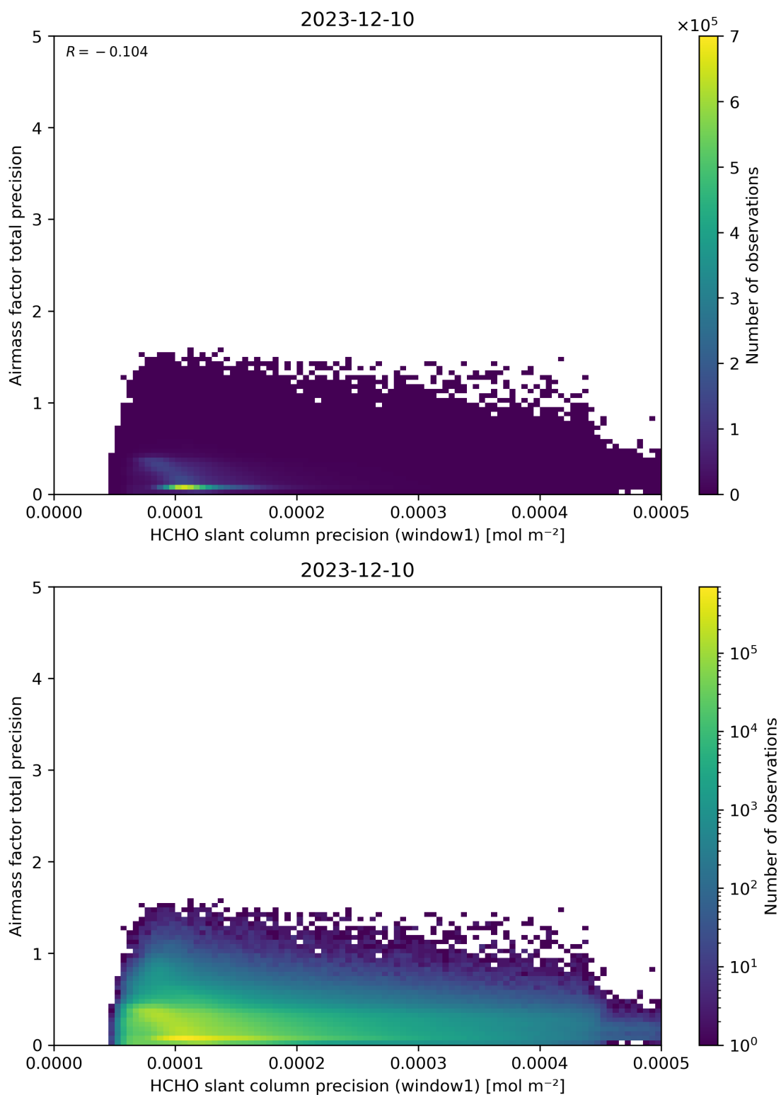
Figure 95: Scatter density plot of “HCHO slant column precision (window1)” against “Airmass factor total precision” for 2023-12-09 to 2023-12-11.
