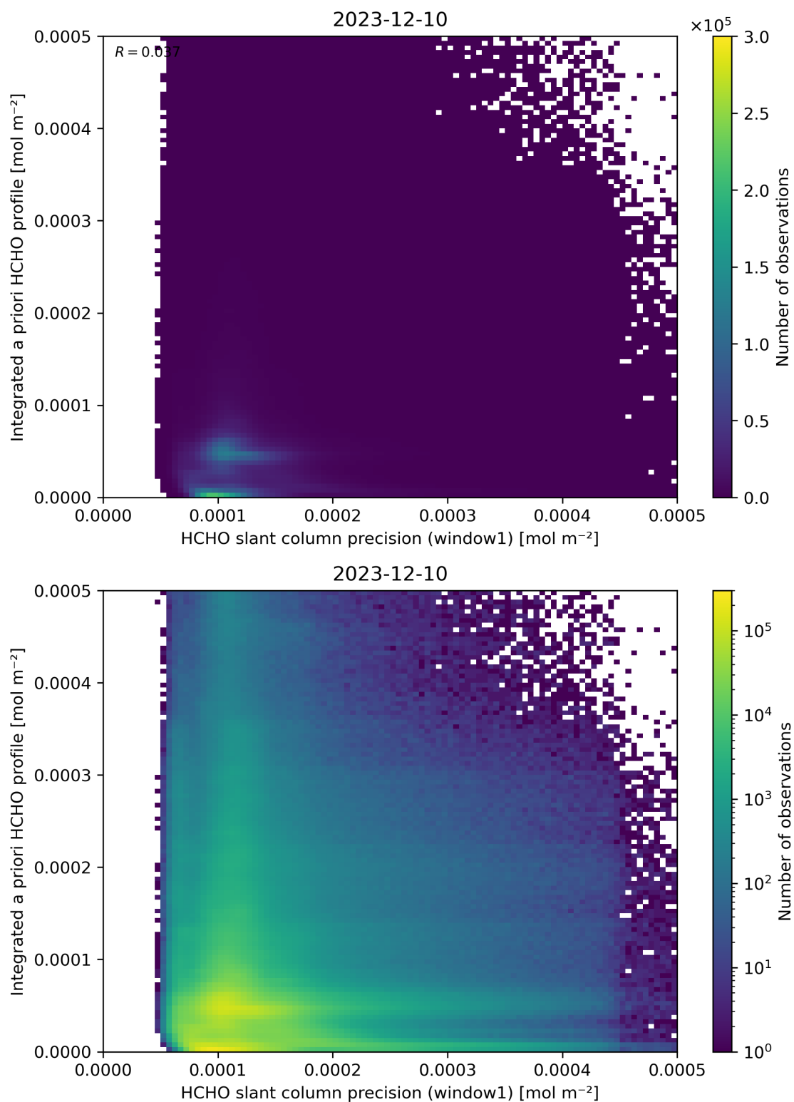
Figure 96: Scatter density plot of “HCHO slant column precision (window1)” against “Integrated a priori HCHO profile” for 2023-12-09 to 2023-12-11.
