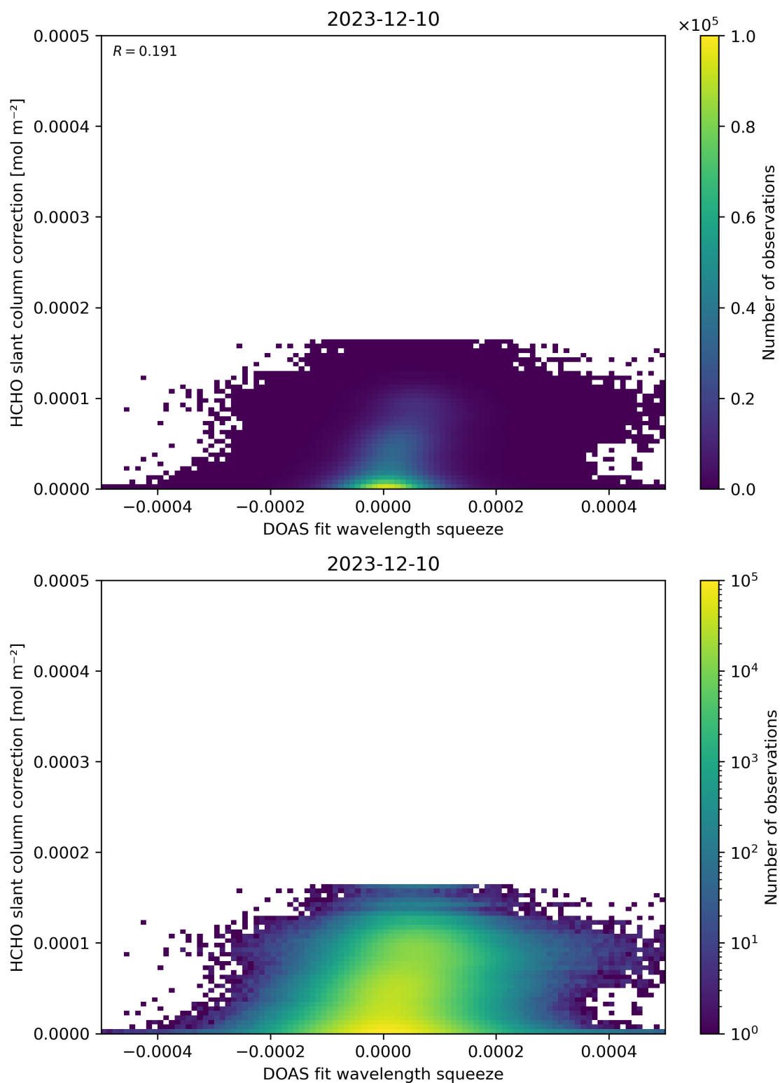
Figure 70: Scatter density plot of “DOAS fit wavelength squeeze” against “HCHO slant column correction” for 2023-12-09 to 2023-12-11.
