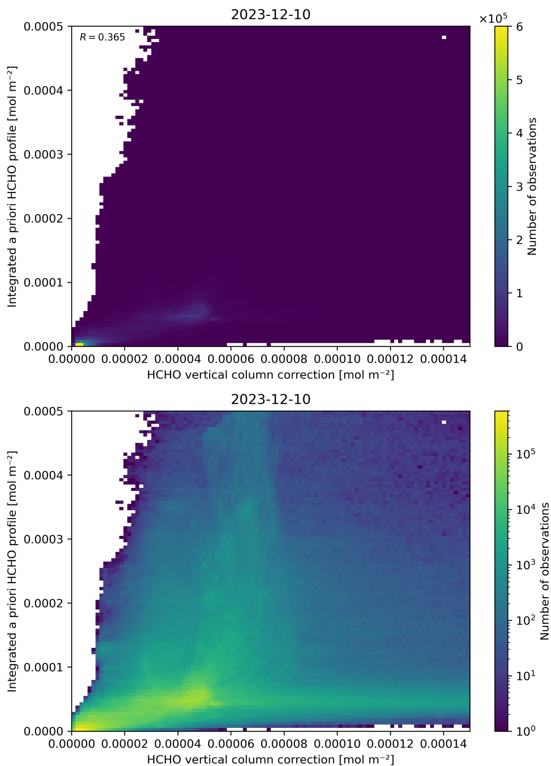
Figure 122: Scatter density plot of “HCHO vertical column correction” against “Integrated a priori HCHO profile” for 2023-12-09 to 2023-12-11.
