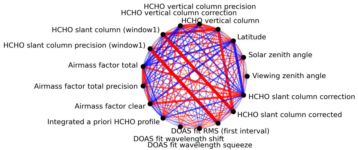
Figure 1: Map of correlation graph for 2023-12-10 to 2023-12-12.
