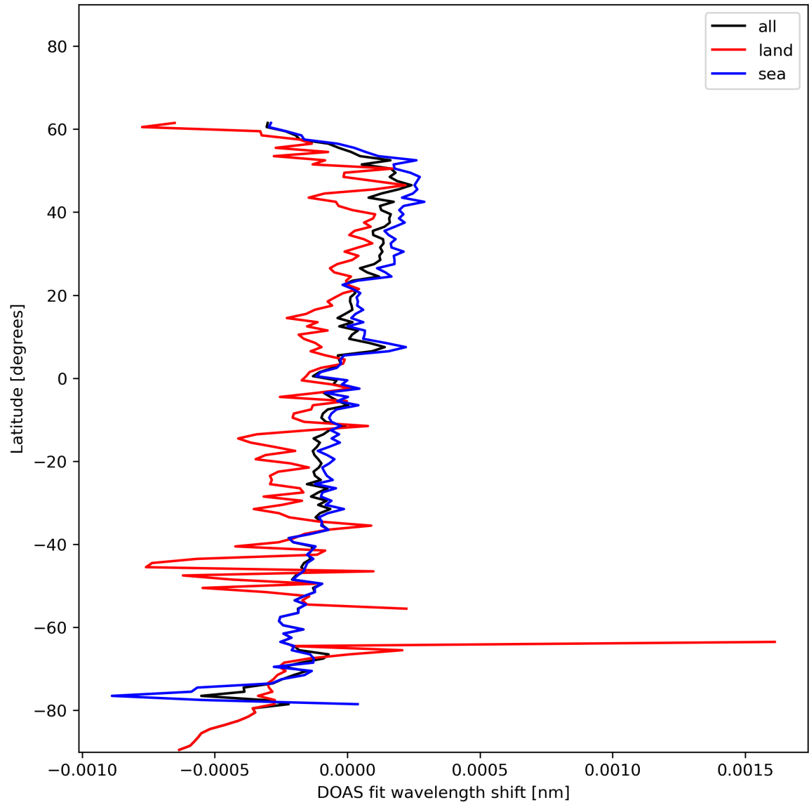
Figure 30: Zonal average of “DOAS fit wavelength shift” for 2023-12-10 to 2023-12-12.
