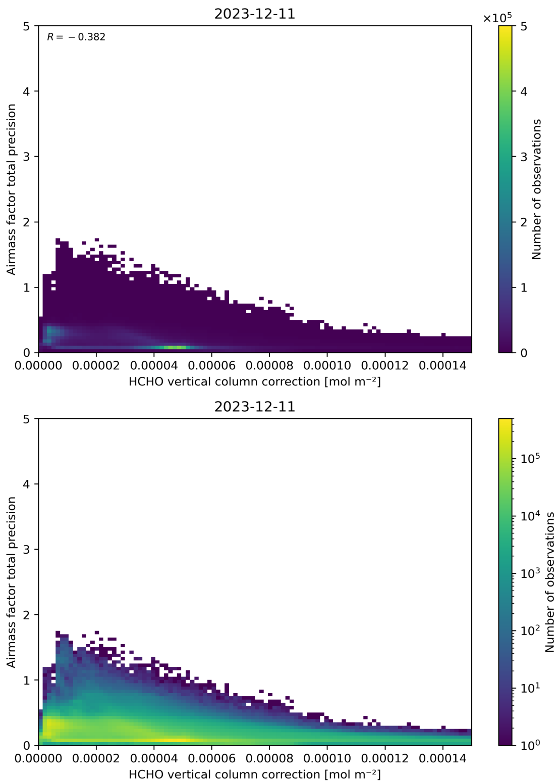
Figure 121: Scatter density plot of “HCHO vertical column correction” against “Airmass factor total precision” for 2023-12-10 to 2023-12-12.
