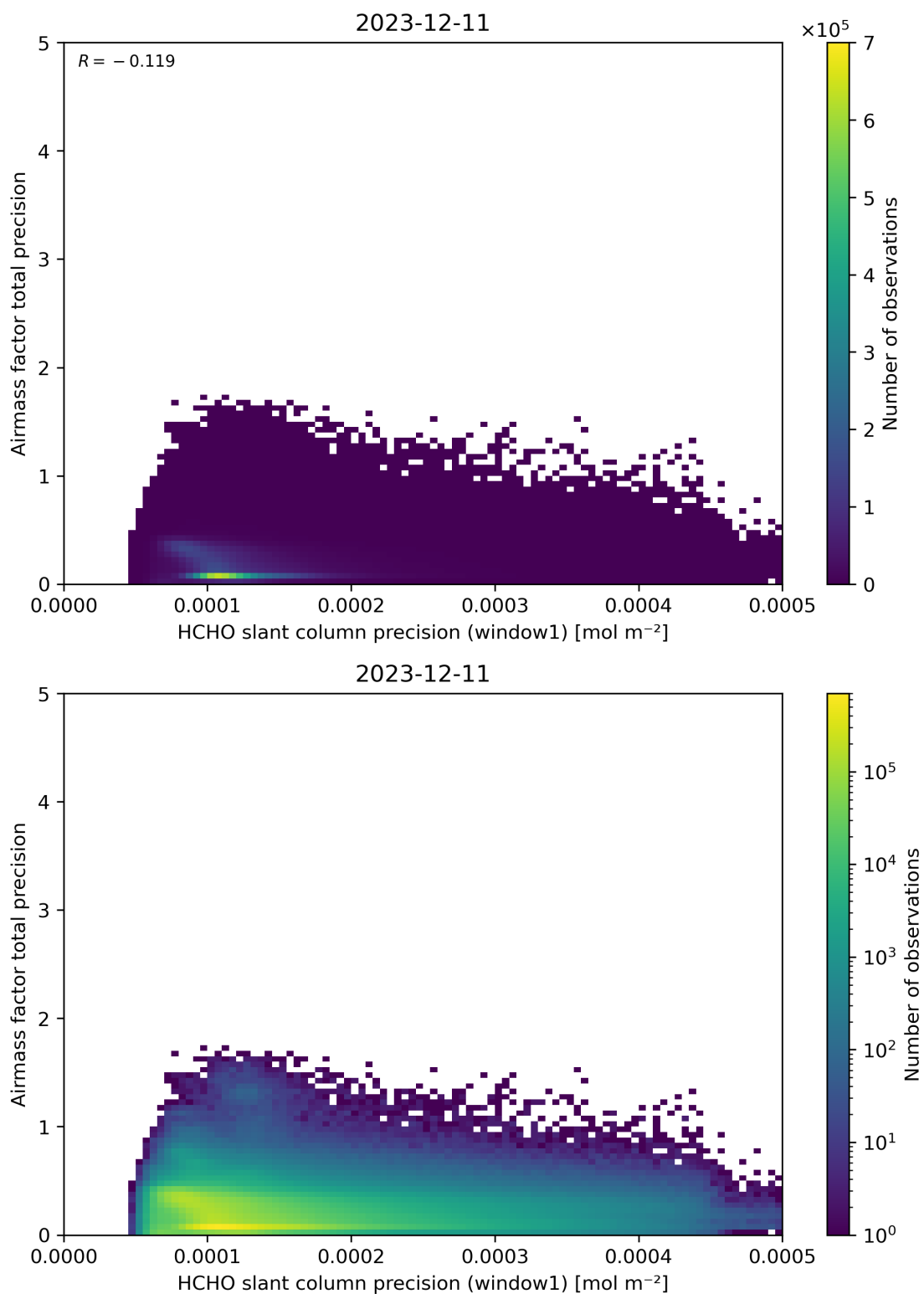
Figure 95: Scatter density plot of “HCHO slant column precision (window1)” against “Airmass factor total precision” for 2023-12-10 to 2023-12-12.
