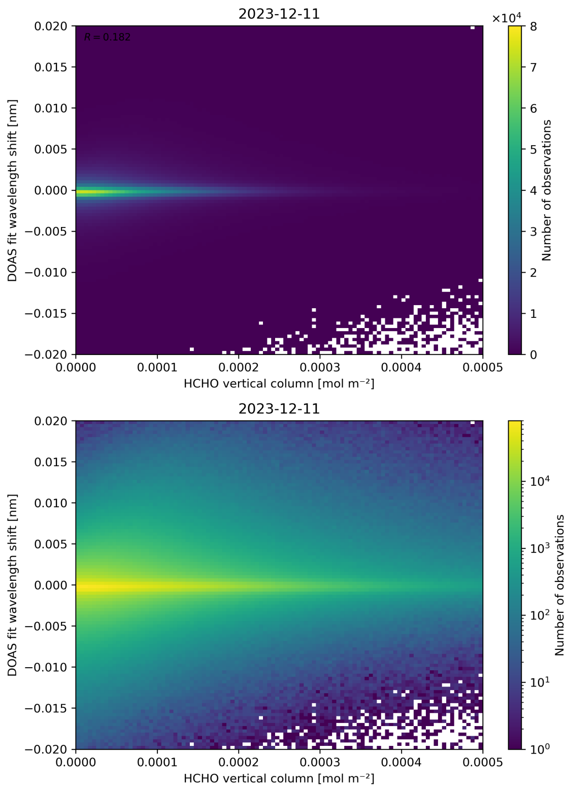
Figure 124: Scatter density plot of “HCHO vertical column” against “DOAS fit wavelength shift” for 2023-12-10 to 2023-12-12.
