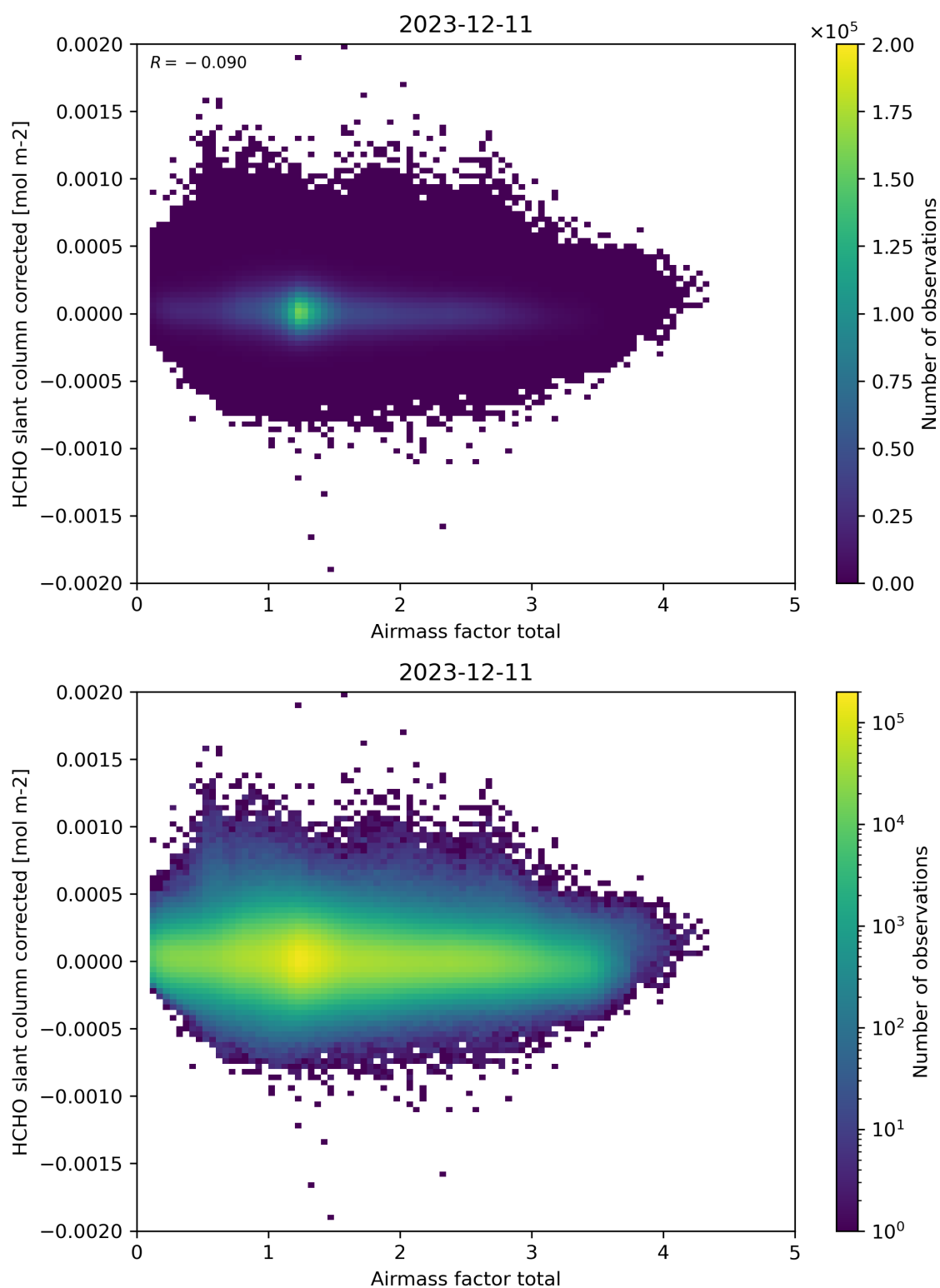
Figure 101: Scatter density plot of “Airmass factor total” against “HCHO slant column corrected” for 2023-12-10 to 2023-12-12.
