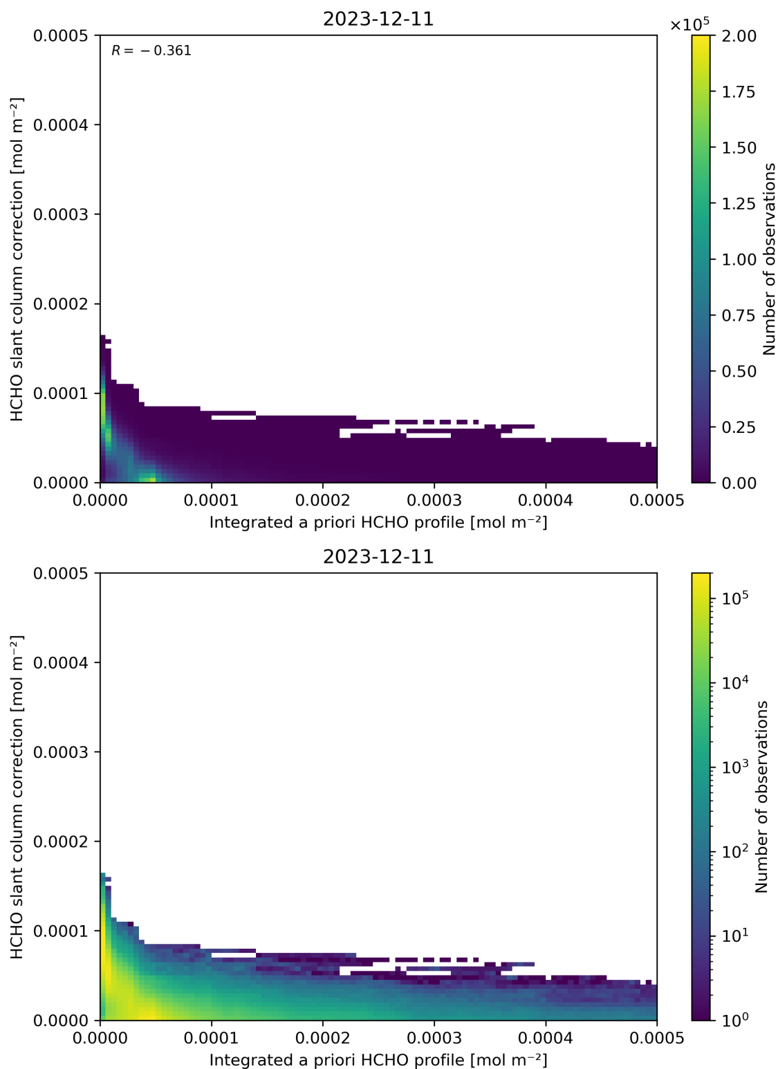
Figure 152: Scatter density plot of “Integrated a priori HCHO profile” against “HCHO slant column correction” for 2023-12-10 to 2023-12-12.
