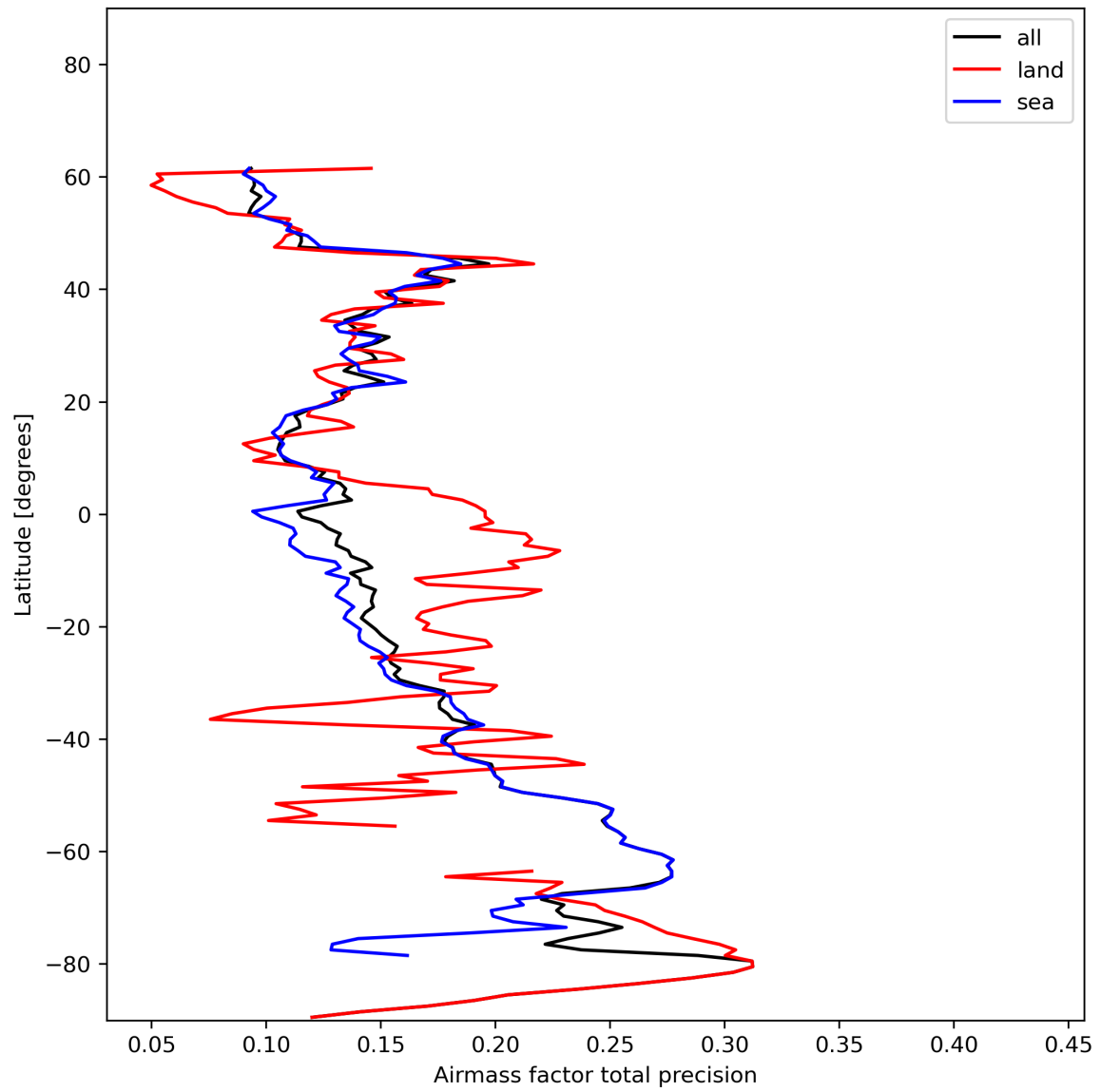
Figure 27: Zonal average of “Airmass factor total precision” for 2023-12-10 to 2023-12-12.
