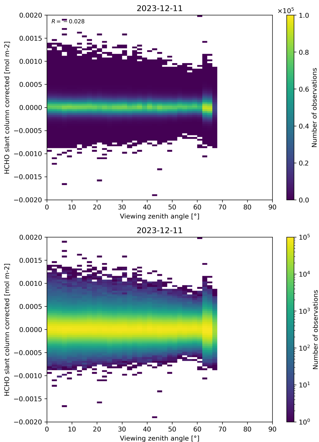
Figure 186: Scatter density plot of “Viewing zenith angle” against “HCHO slant column corrected” for 2023-12-10 to 2023-12-12.
