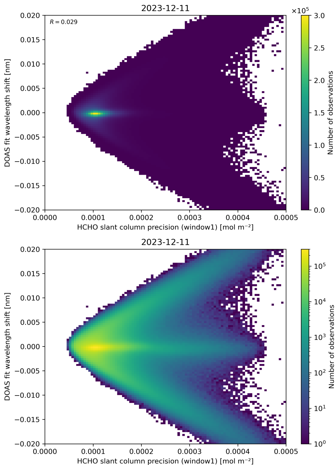
Figure 89: Scatter density plot of “HCHO slant column precision (window1)” against “DOAS fit wavelength shift” for 2023-12-10 to 2023-12-12.
