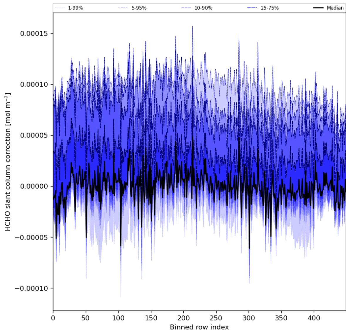
Figure 61: Along track statistics of “HCHO slant column correction” for 2023-12-10 to 2023-12-12
