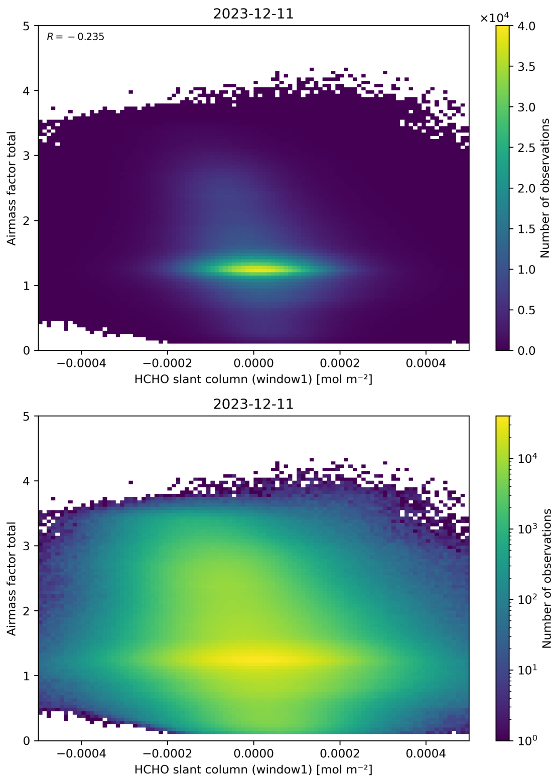
Figure 85: Scatter density plot of “HCHO slant column (window1)” against “Airmass factor total” for 2023-12-10 to 2023-12-12.
