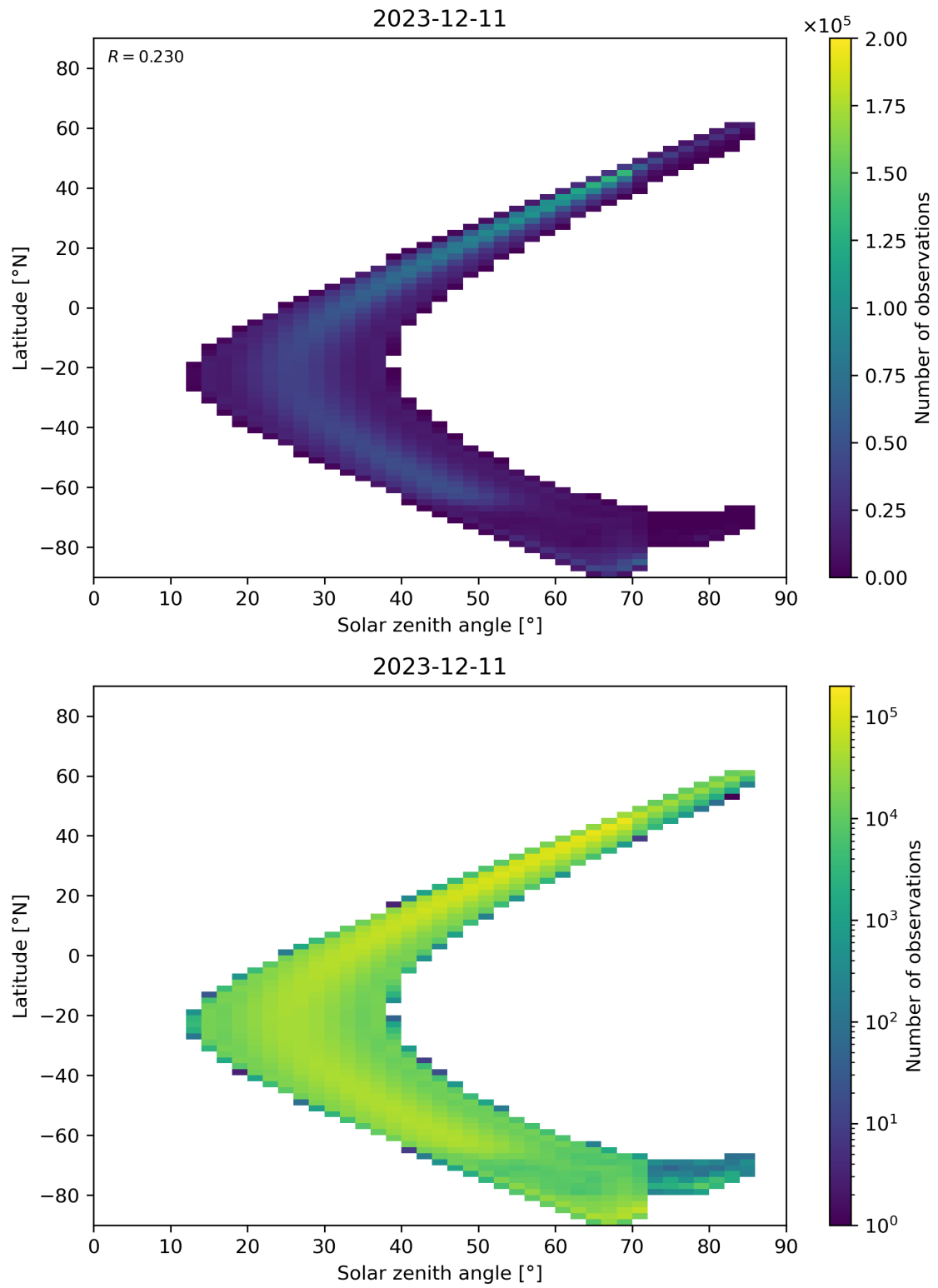
Figure 181: Scatter density plot of “Solar zenith angle” against “Latitude” for 2023-12-10 to 2023-12-12.
