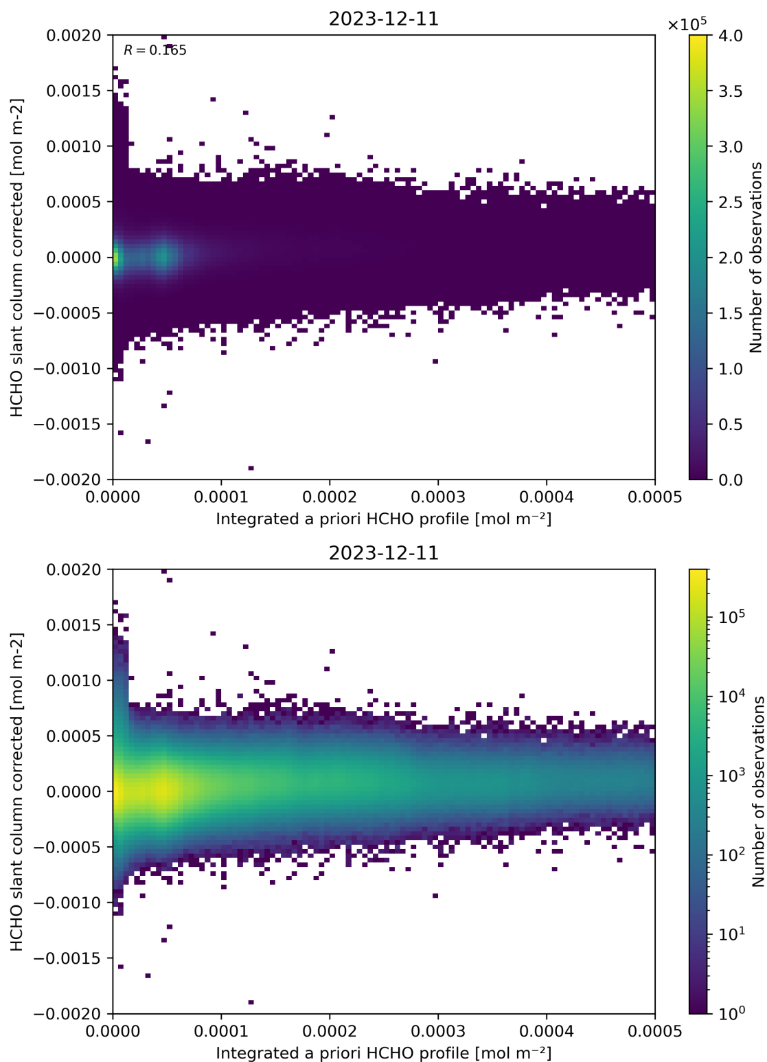
Figure 151: Scatter density plot of “Integrated a priori HCHO profile” against “HCHO slant column corrected” for 2023-12-10 to 2023-12-12.
