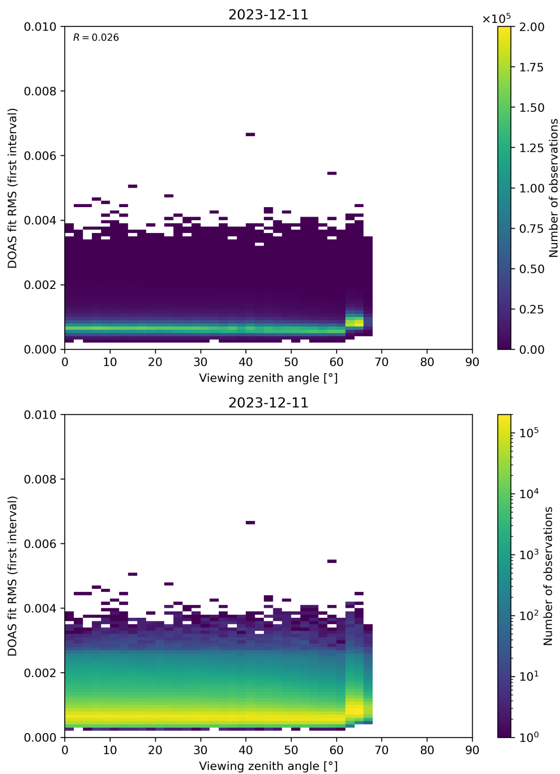
Figure 182: Scatter density plot of “Viewing zenith angle” against “DOAS fit RMS (first interval)” for 2023-12-10 to 2023-12-12.
