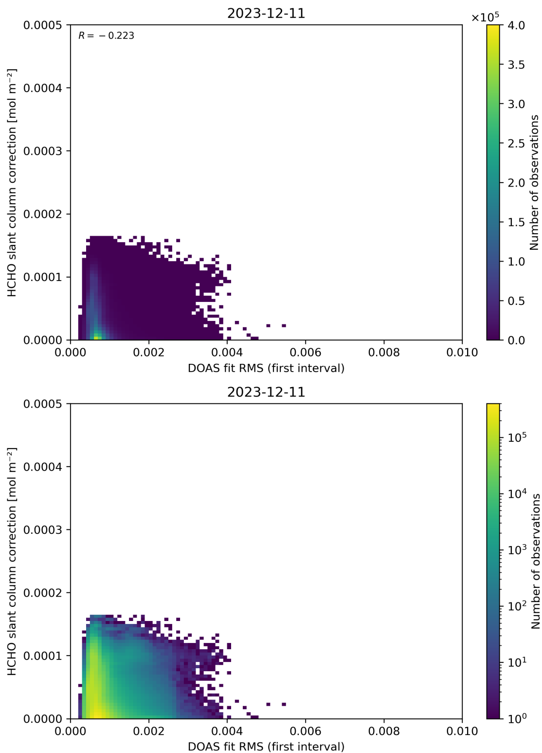
Figure 63: Scatter density plot of “DOAS fit RMS (first interval)” against “HCHO slant column correction” for 2023-12-10 to 2023-12-12.
