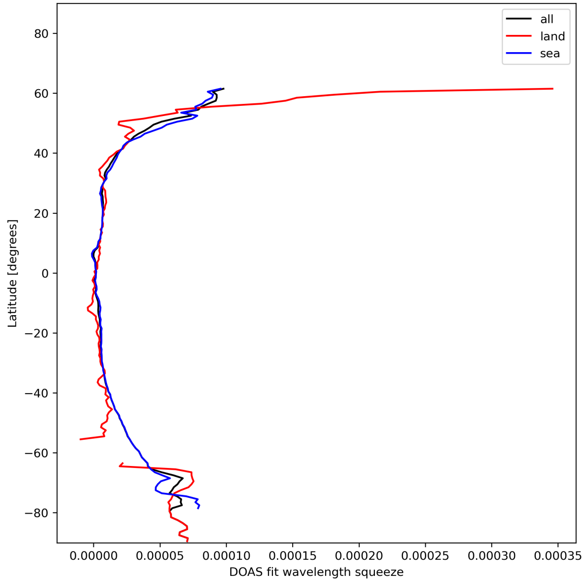
Figure 31: Zonal average of “DOAS fit wavelength squeeze” for 2023-12-10 to 2023-12-12.
