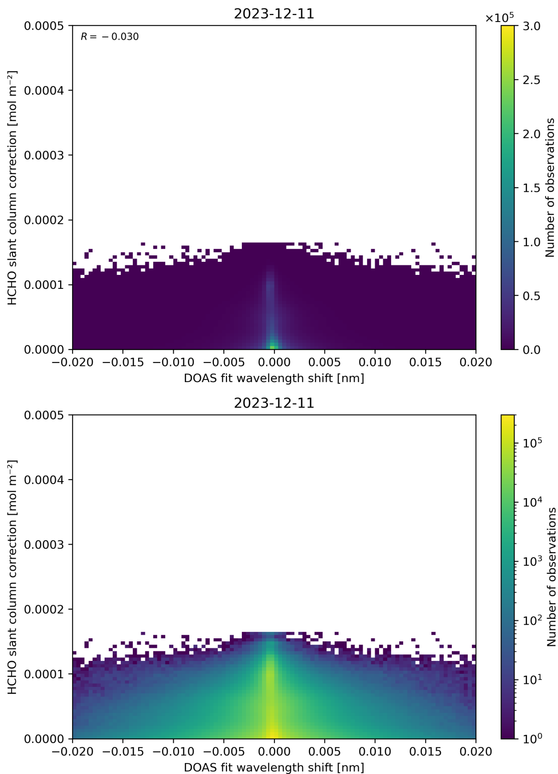
Figure 67: Scatter density plot of “DOAS fit wavelength shift” against “HCHO slant column correction” for 2023-12-10 to 2023-12-12.
