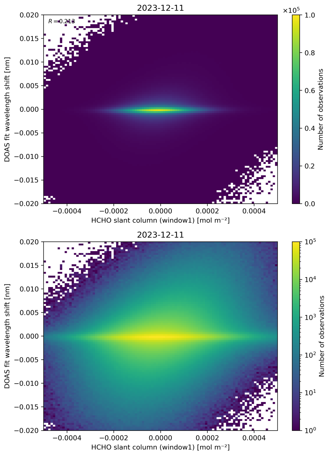
Figure 79: Scatter density plot of “HCHO slant column (window1)” against “DOAS fit wavelength shift” for 2023-12-10 to 2023-12-12.
