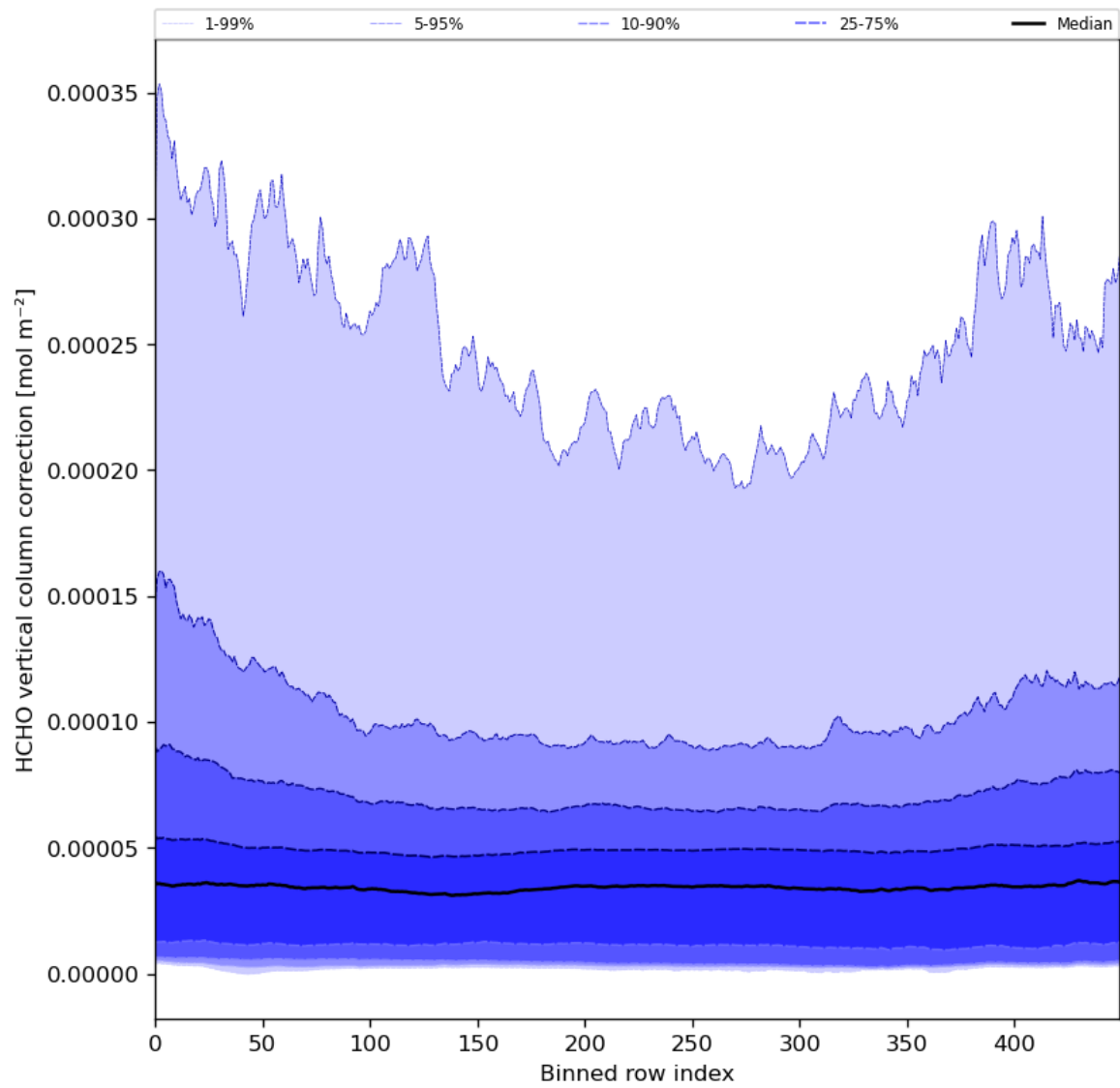
Figure 51: Along track statistics of “HCHO vertical column correction” for 2023-12-10 to 2023-12-12
