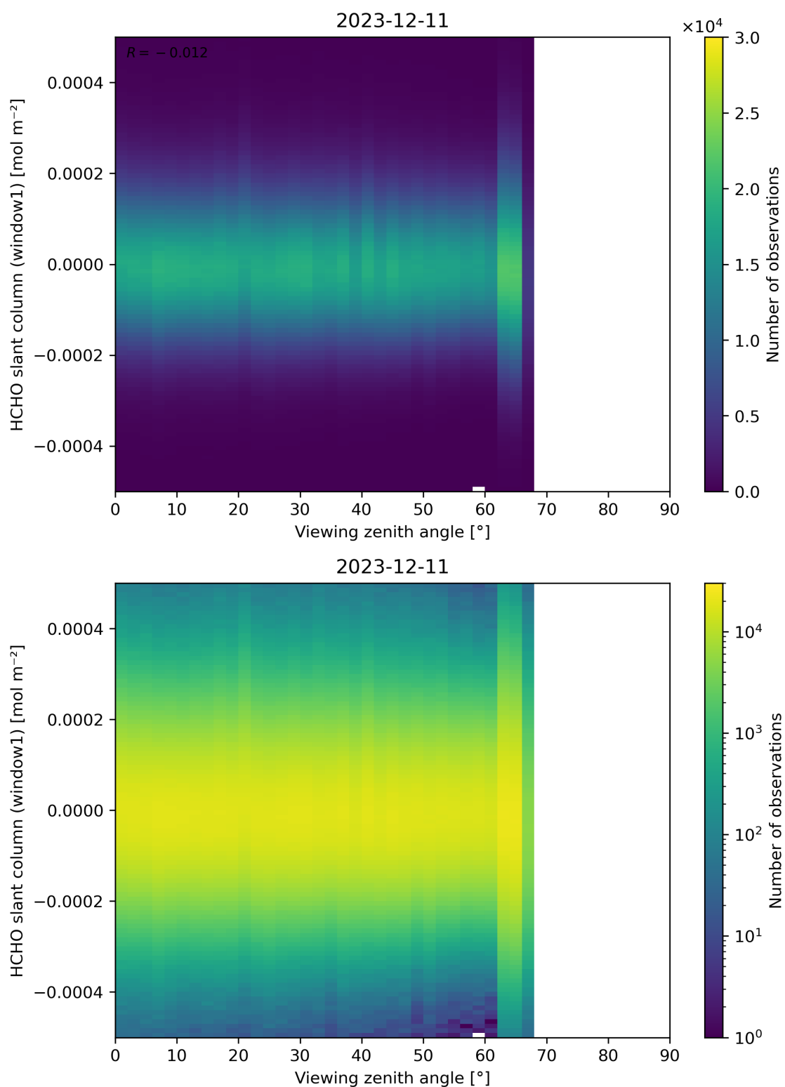
Figure 188: Scatter density plot of “Viewing zenith angle” against “HCHO slant column (window1)” for 2023-12-10 to 2023-12-12.
