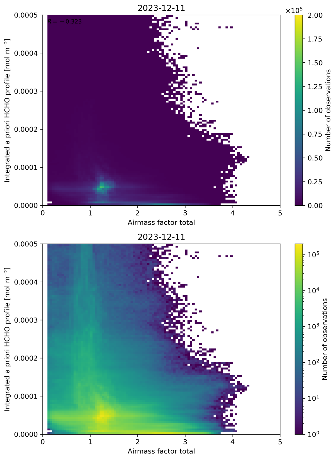
Figure 104: Scatter density plot of “Airmass factor total” against “Integrated a priori HCHO profile” for 2023-12-10 to 2023-12-12.
