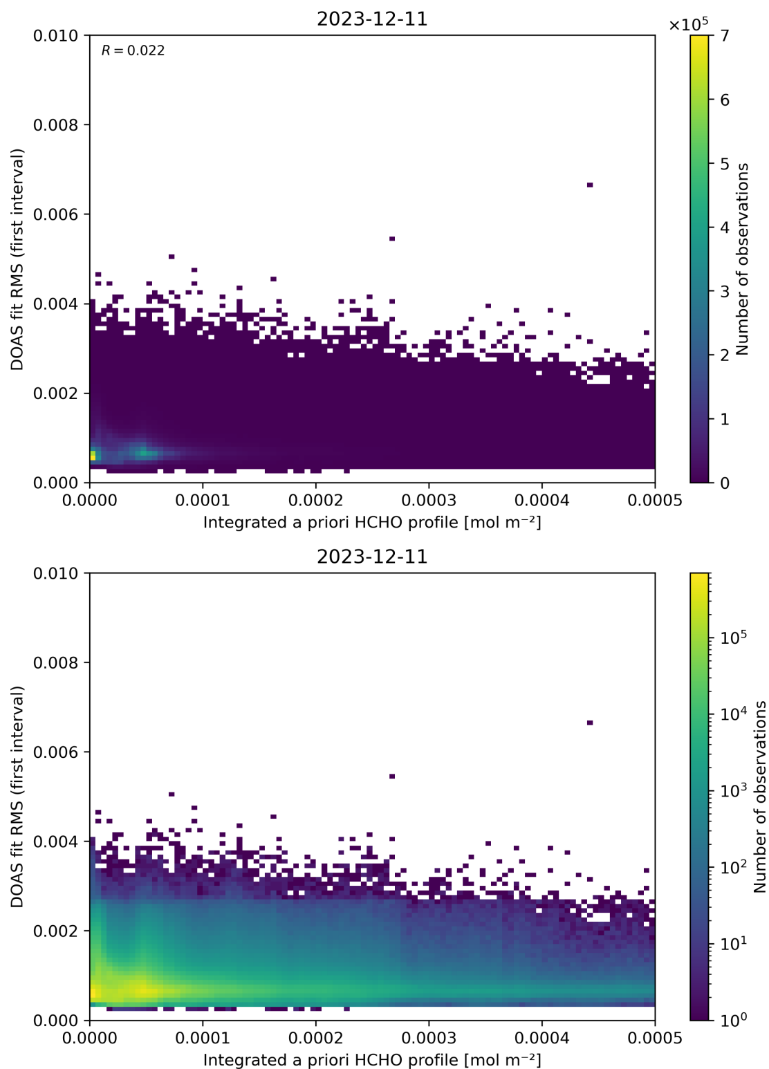
Figure 148: Scatter density plot of “Integrated a priori HCHO profile” against “DOAS fit RMS (first interval)” for 2023-12-10 to 2023-12-12.
