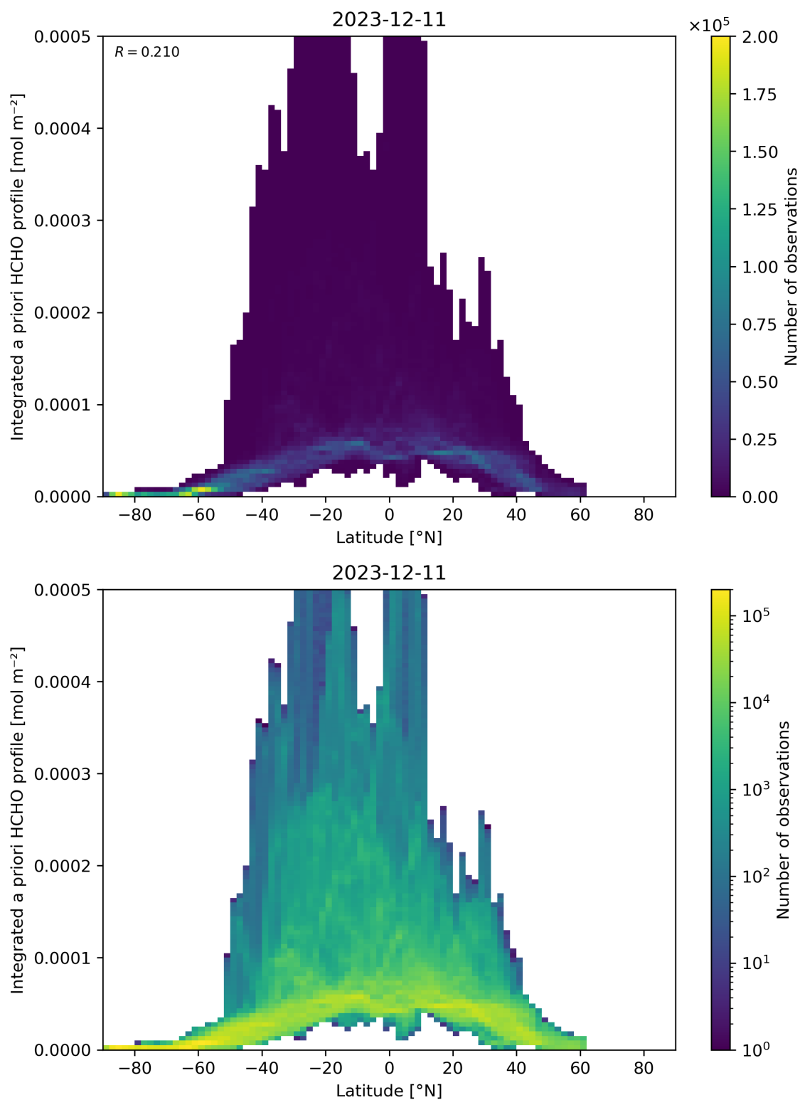
Figure 166: Scatter density plot of “Latitude” against “Integrated a priori HCHO profile” for 2023-12-10 to 2023-12-12.
