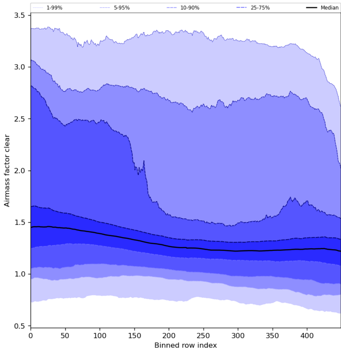
Figure 56: Along track statistics of “Airmass factor clear” for 2023-12-10 to 2023-12-12
