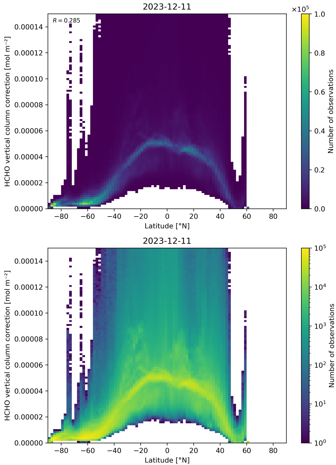
Figure 164: Scatter density plot of “Latitude” against “HCHO vertical column correction” for 2023-12-10 to 2023-12-12.
