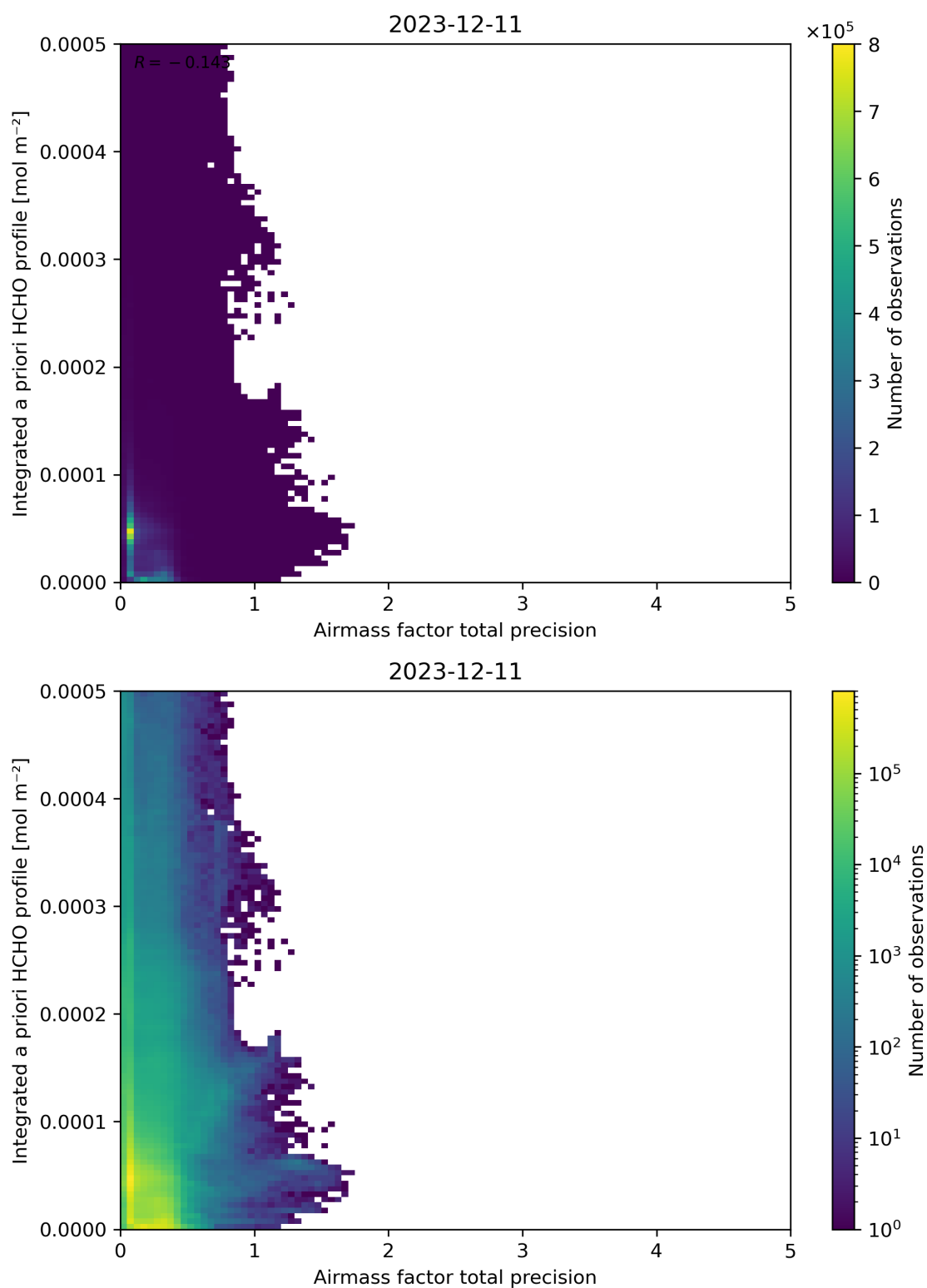
Figure 111: Scatter density plot of “Airmass factor total precision” against “Integrated a priori HCHO profile” for 2023-12-10 to 2023-12-12.
