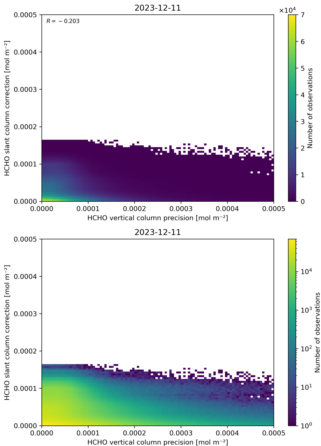
Figure 141: Scatter density plot of “HCHO vertical column precision” against “HCHO slant column correction” for 2023-12-10 to 2023-12-12.
