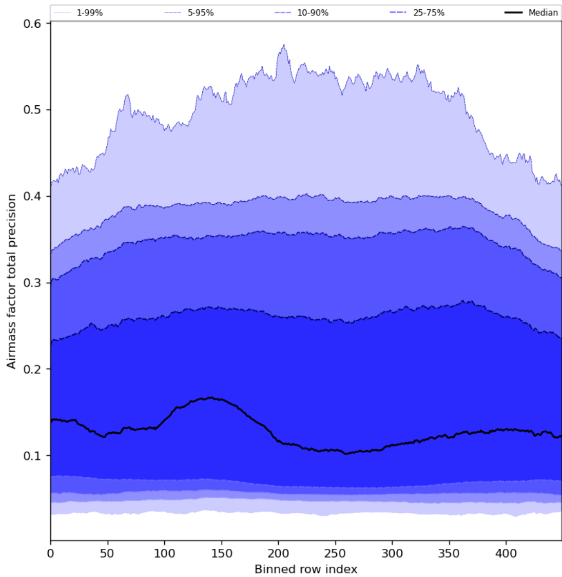
Figure 55: Along track statistics of “Airmass factor total precision” for 2023-12-10 to 2023-12-12
