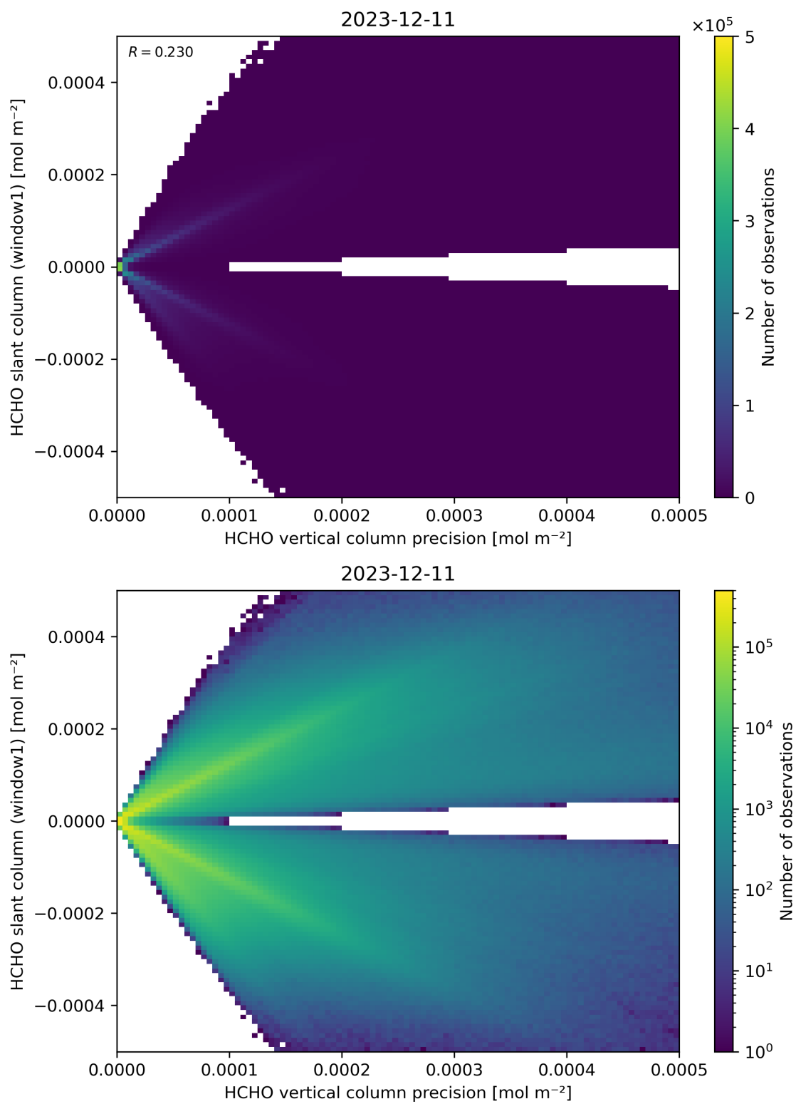
Figure 142: Scatter density plot of “HCHO vertical column precision” against “HCHO slant column (window1)” for 2023-12-10 to 2023-12-12.
