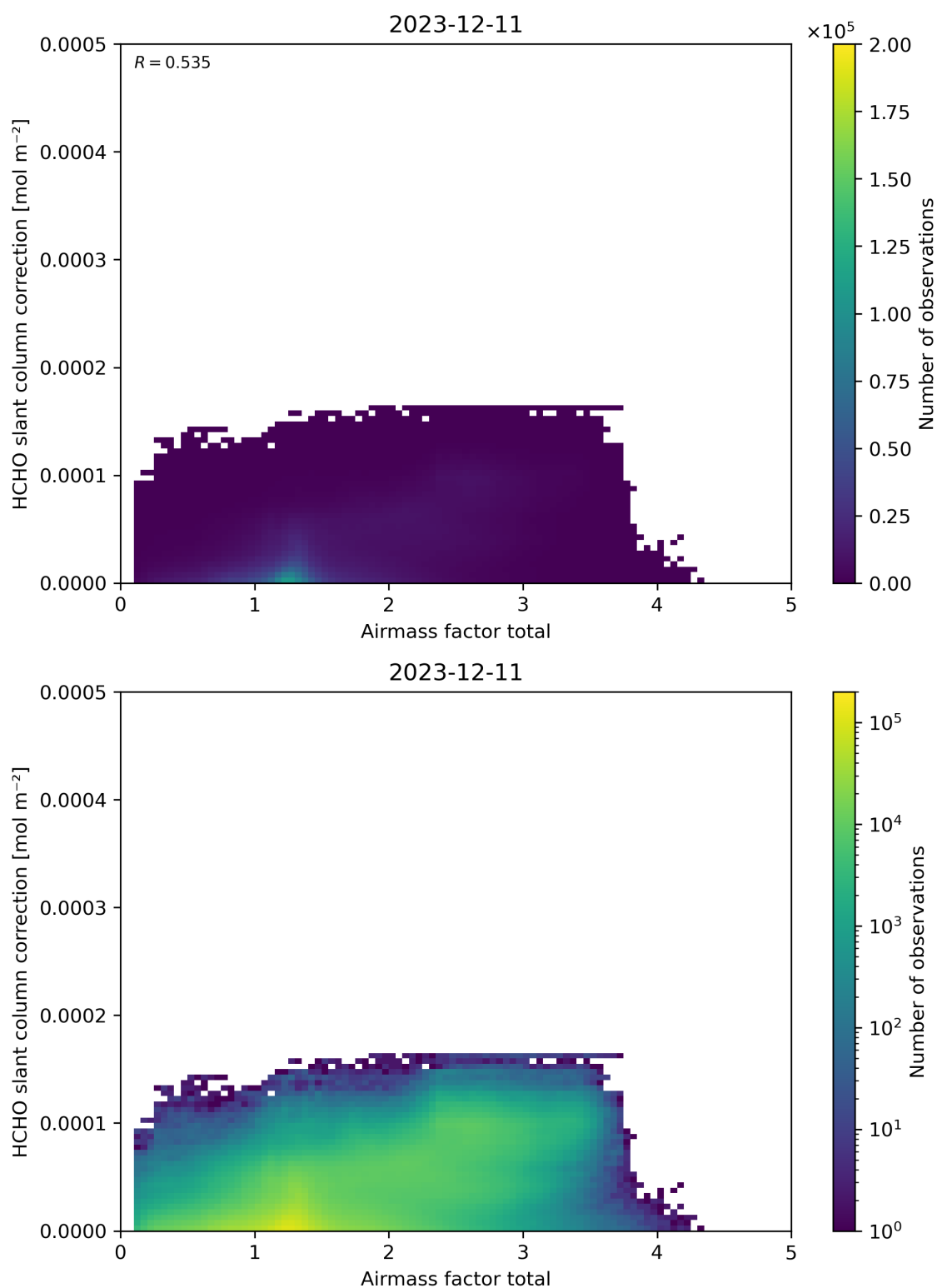
Figure 102: Scatter density plot of “Airmass factor total” against “HCHO slant column correction” for 2023-12-10 to 2023-12-12.
