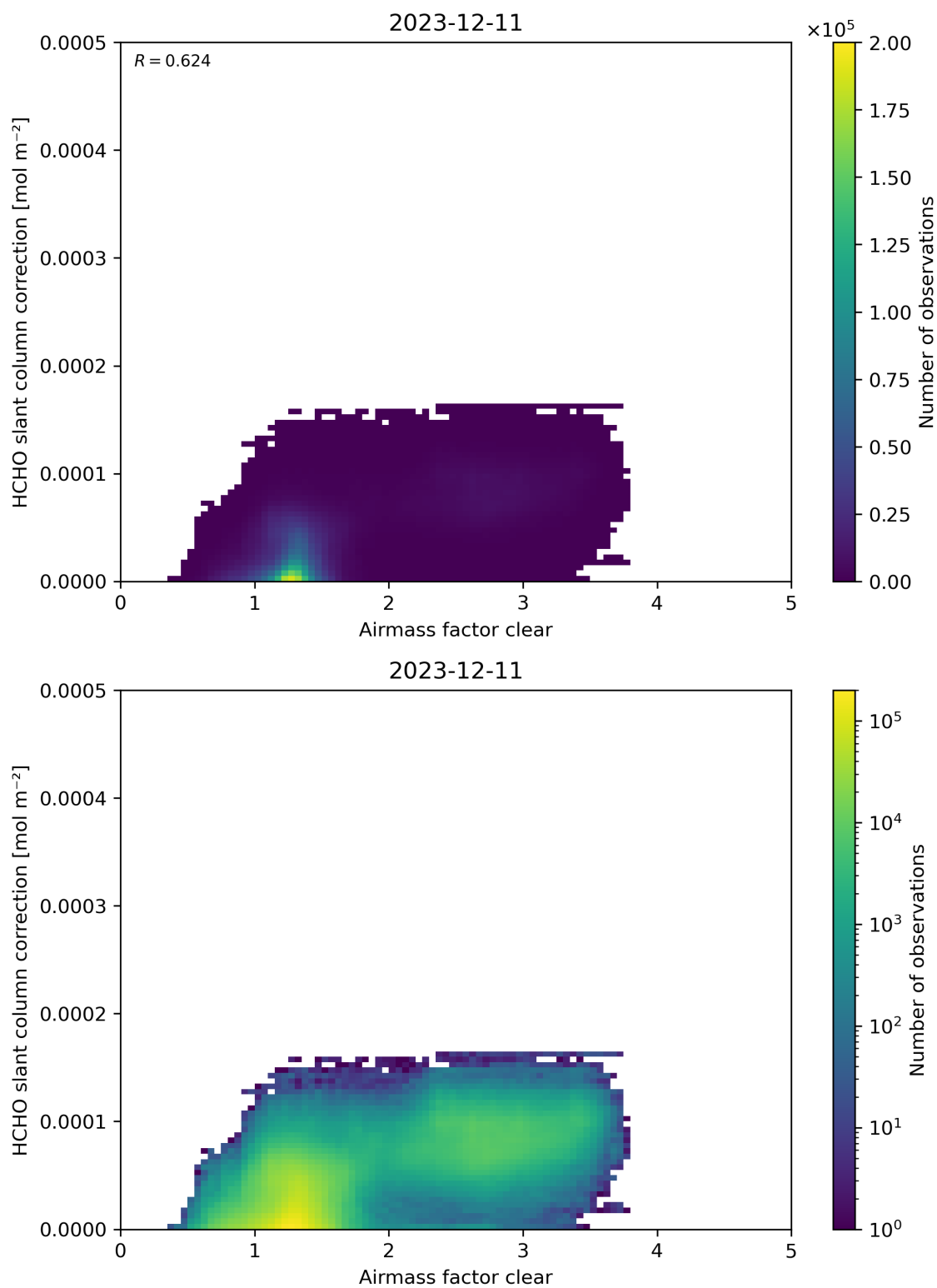
Figure 75: Scatter density plot of “Airmass factor clear” against “HCHO slant column correction” for 2023-12-10 to 2023-12-12.
