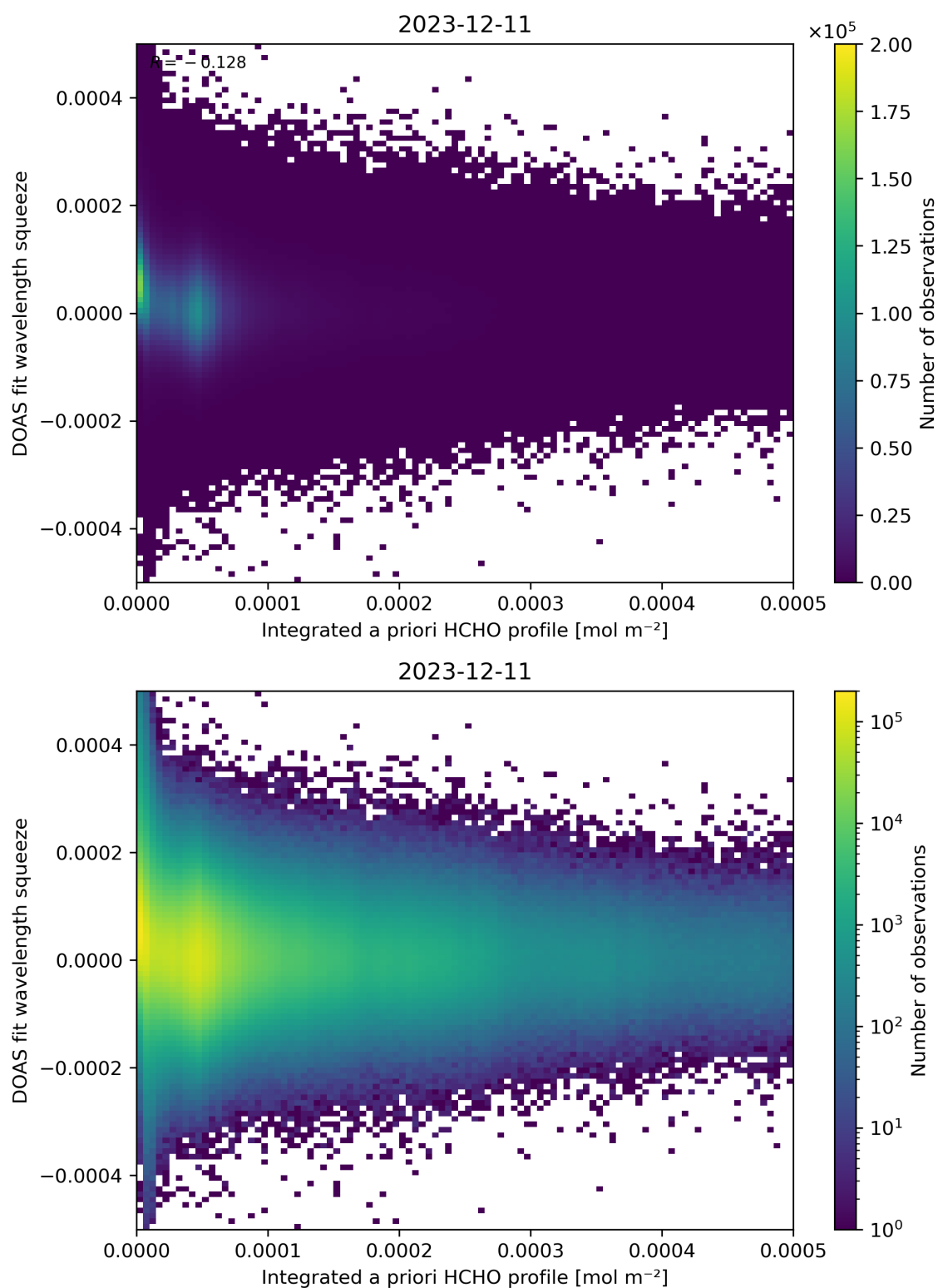
Figure 150: Scatter density plot of “Integrated a priori HCHO profile” against “DOAS fit wavelength squeeze” for 2023-12-10 to 2023-12-12.
