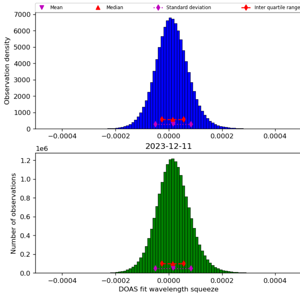
Figure 45: Histogram of “DOAS fit wavelength squeeze” for 2023-12-10 to 2023-12-12
