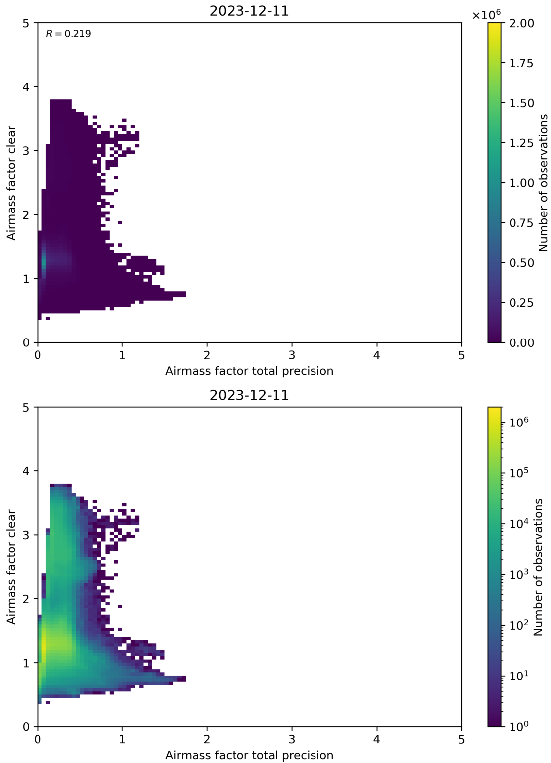
Figure 108: Scatter density plot of “Airmass factor total precision” against “Airmass factor clear” for 2023-12-10 to 2023-12-12.
