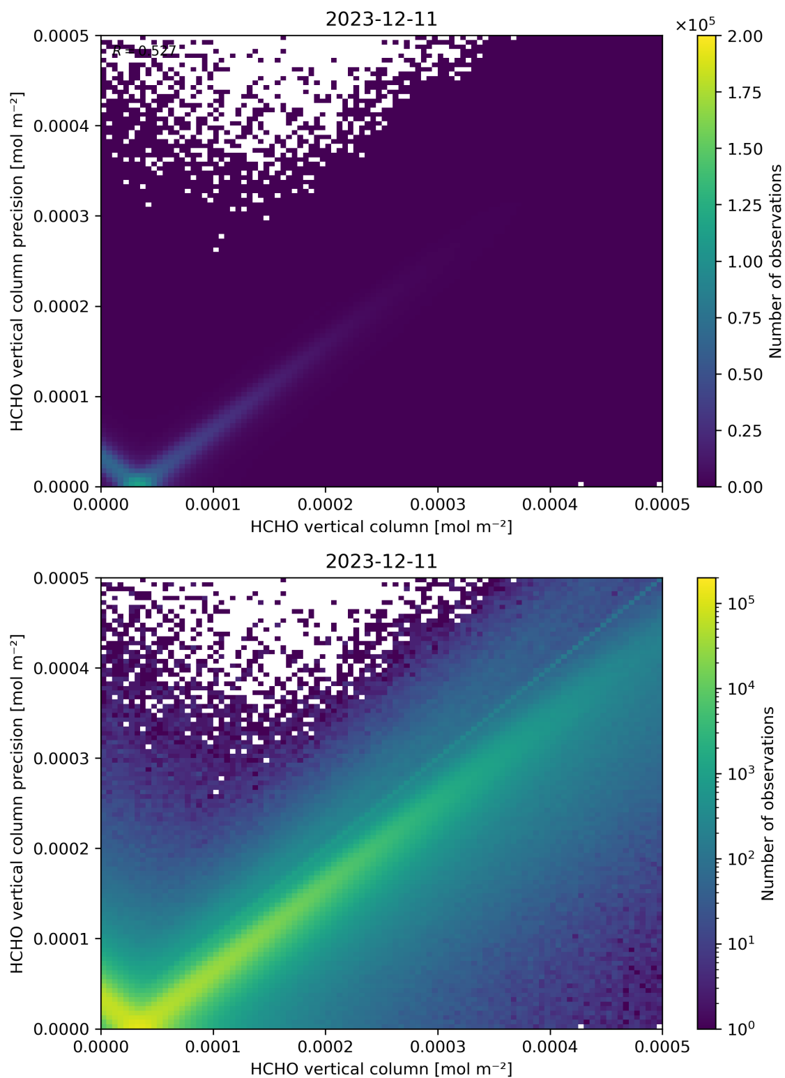
Figure 134: Scatter density plot of “HCHO vertical column” against “HCHO vertical column precision” for 2023-12-10 to 2023-12-12.
