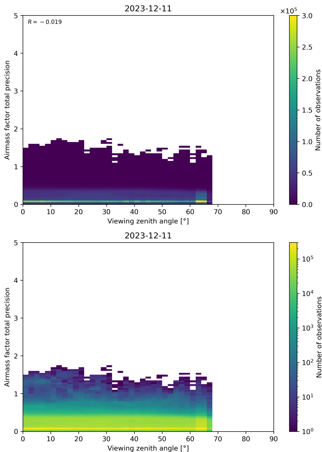
Figure 191: Scatter density plot of “Viewing zenith angle” against “Airmass factor total precision” for 2023-12-10 to 2023-12-12.
