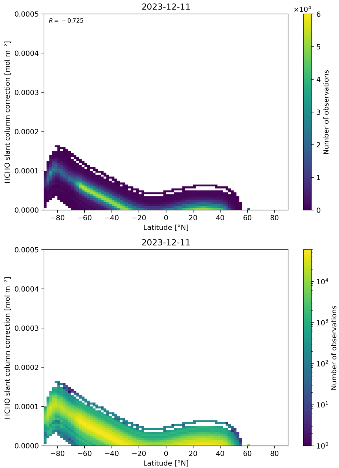
Figure 158: Scatter density plot of “Latitude” against “HCHO slant column correction” for 2023-12-10 to 2023-12-12.
