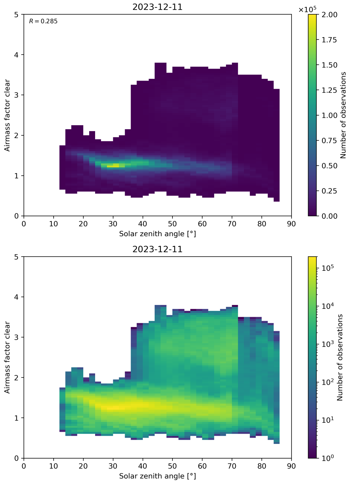
Figure 170: Scatter density plot of “Solar zenith angle” against “Airmass factor clear” for 2023-12-10 to 2023-12-12.
