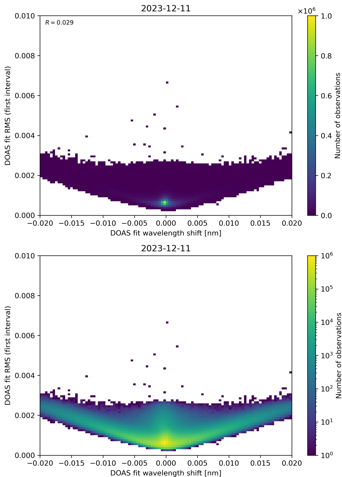
Figure 64: Scatter density plot of “DOAS fit wavelength shift” against “DOAS fit RMS (first interval)” for 2023-12-10 to 2023-12-12.
