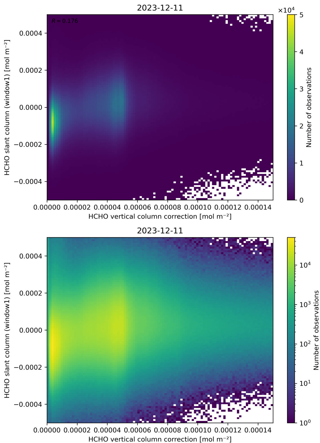
Figure 118: Scatter density plot of “HCHO vertical column correction” against “HCHO slant column (window1)” for 2023-12-10 to 2023-12-12.
