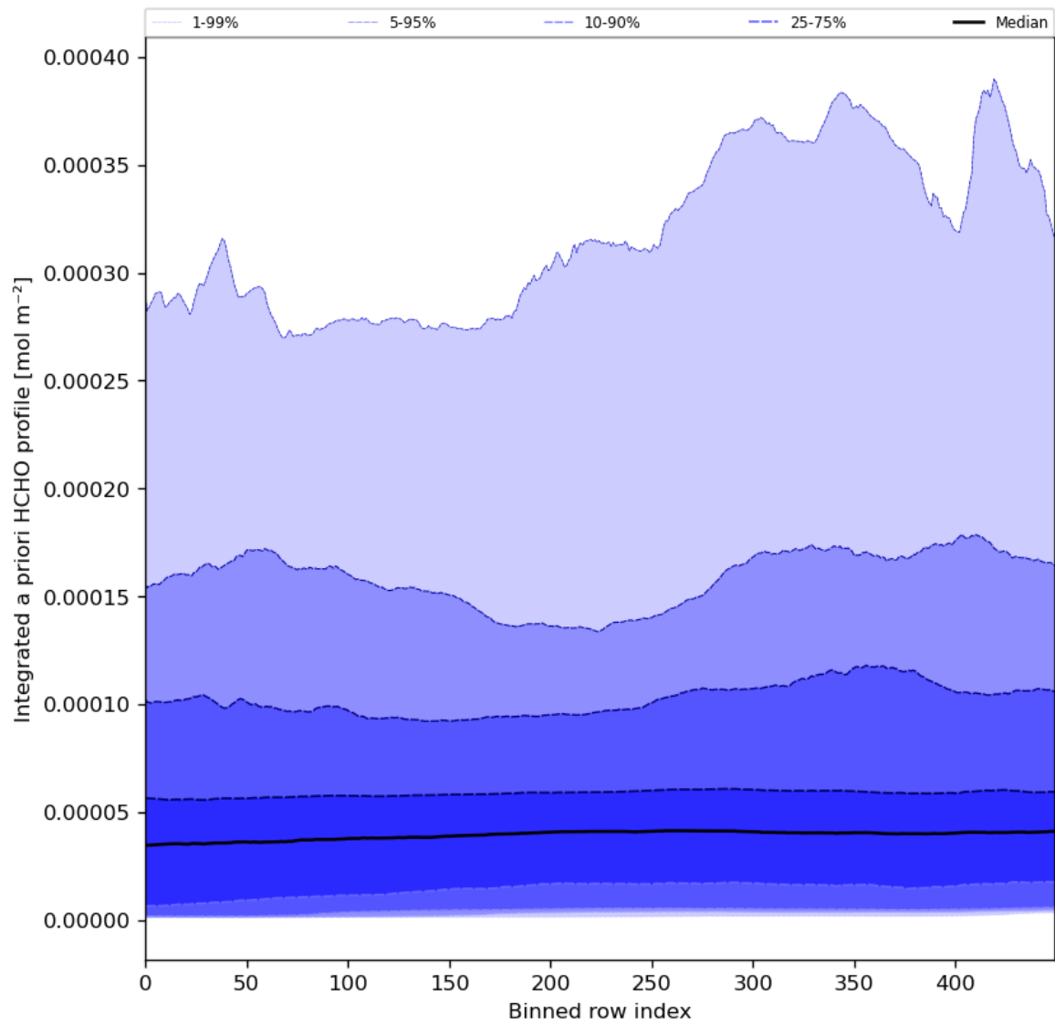
Figure 57: Along track statistics of “Integrated a priori HCHO profile” for 2023-12-10 to 2023-12-12
