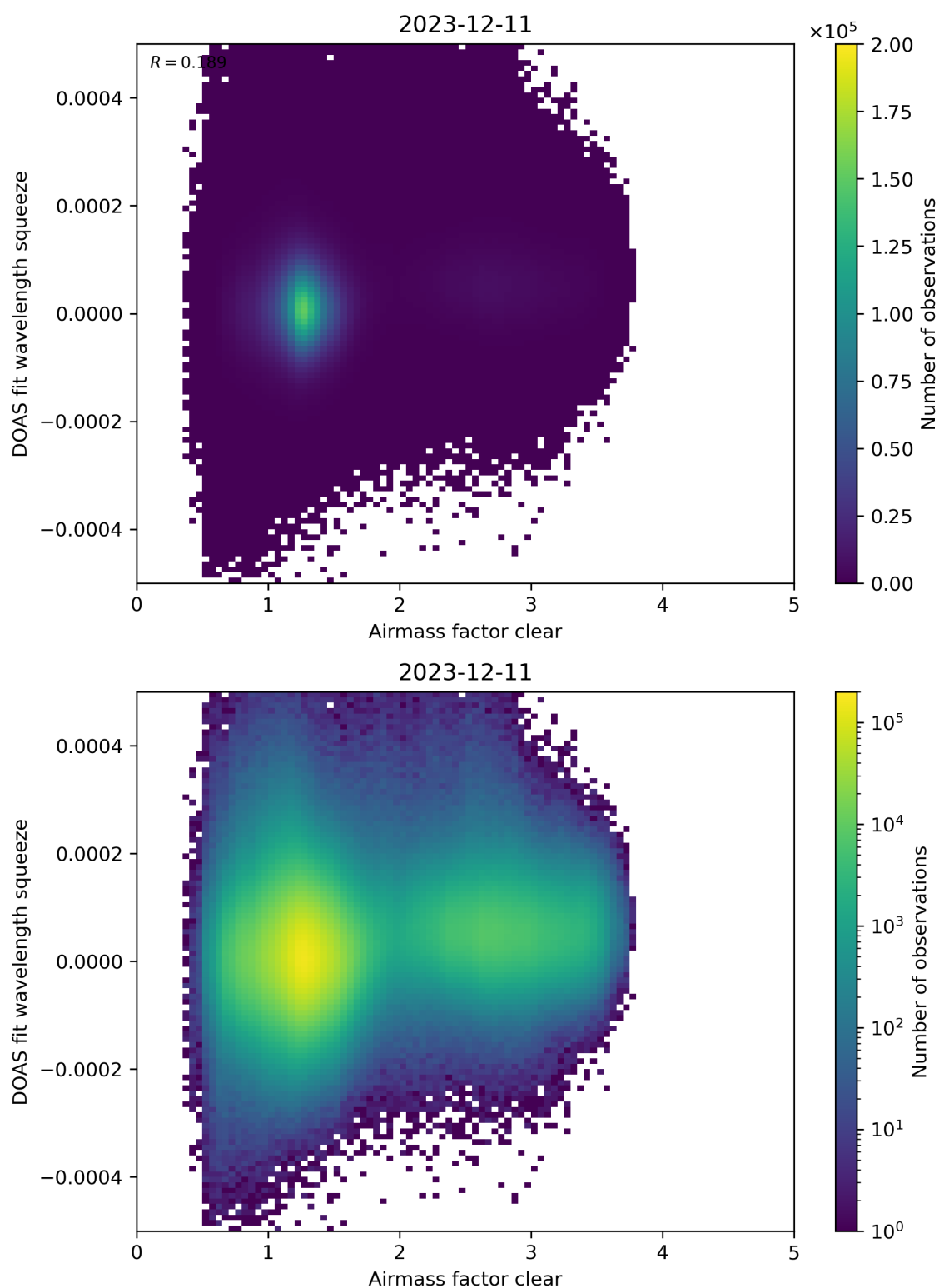
Figure 73: Scatter density plot of “Airmass factor clear” against “DOAS fit wavelength squeeze” for 2023-12-10 to 2023-12-12.
