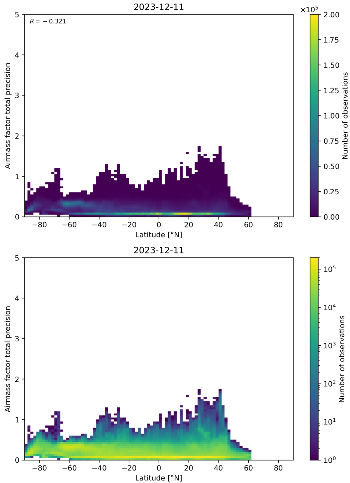
Figure 162: Scatter density plot of “Latitude” against “Airmass factor total precision” for 2023-12-10 to 2023-12-12.
