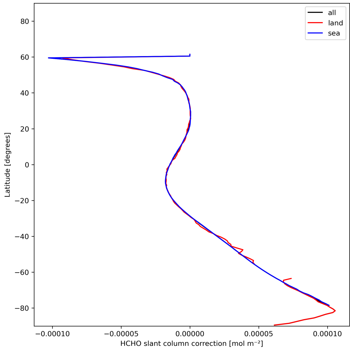
Figure 33: Zonal average of “HCHO slant column correction” for 2023-12-10 to 2023-12-12.
