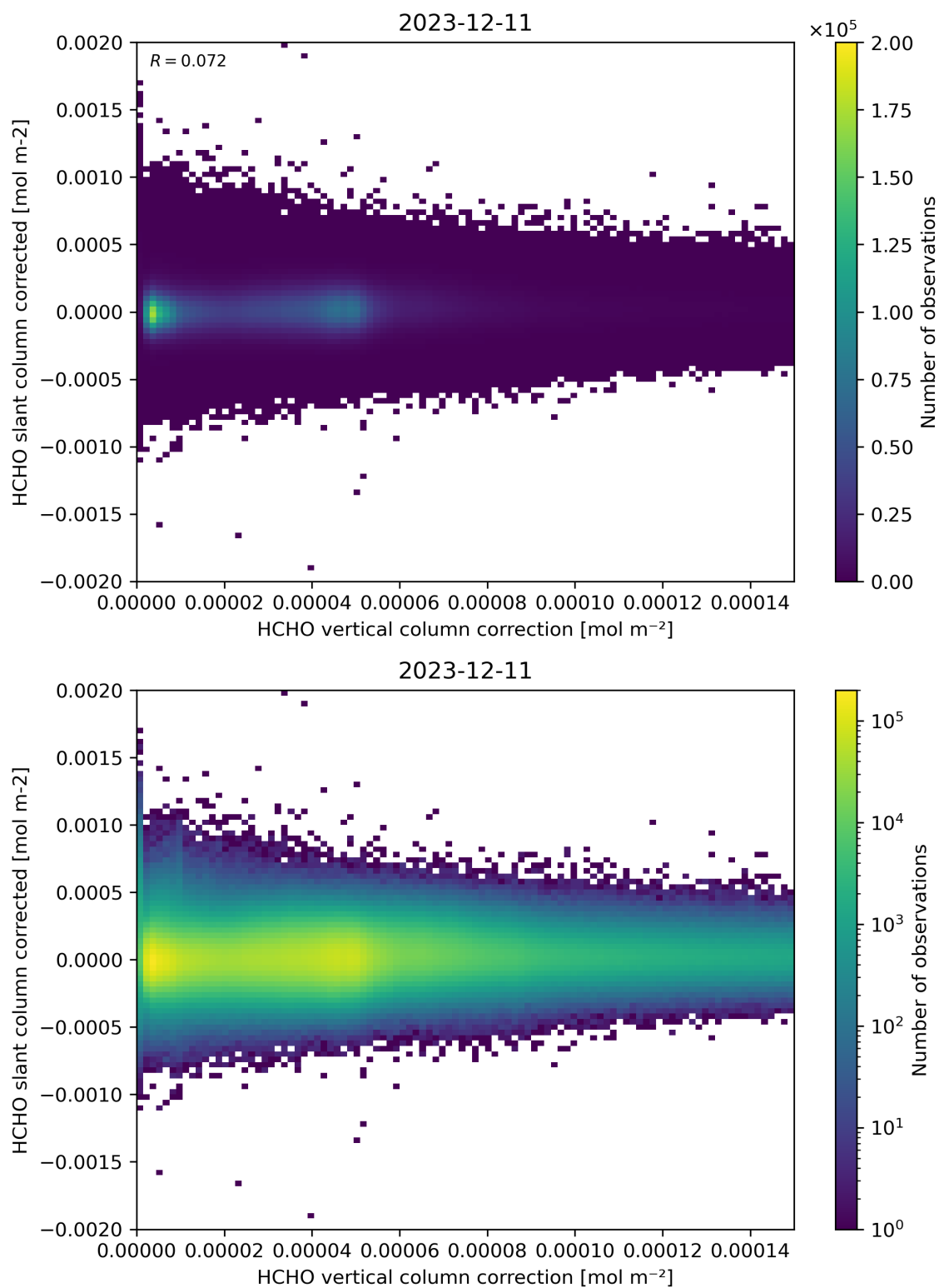
Figure 116: Scatter density plot of “HCHO vertical column correction” against “HCHO slant column corrected” for 2023-12-10 to 2023-12-12.
