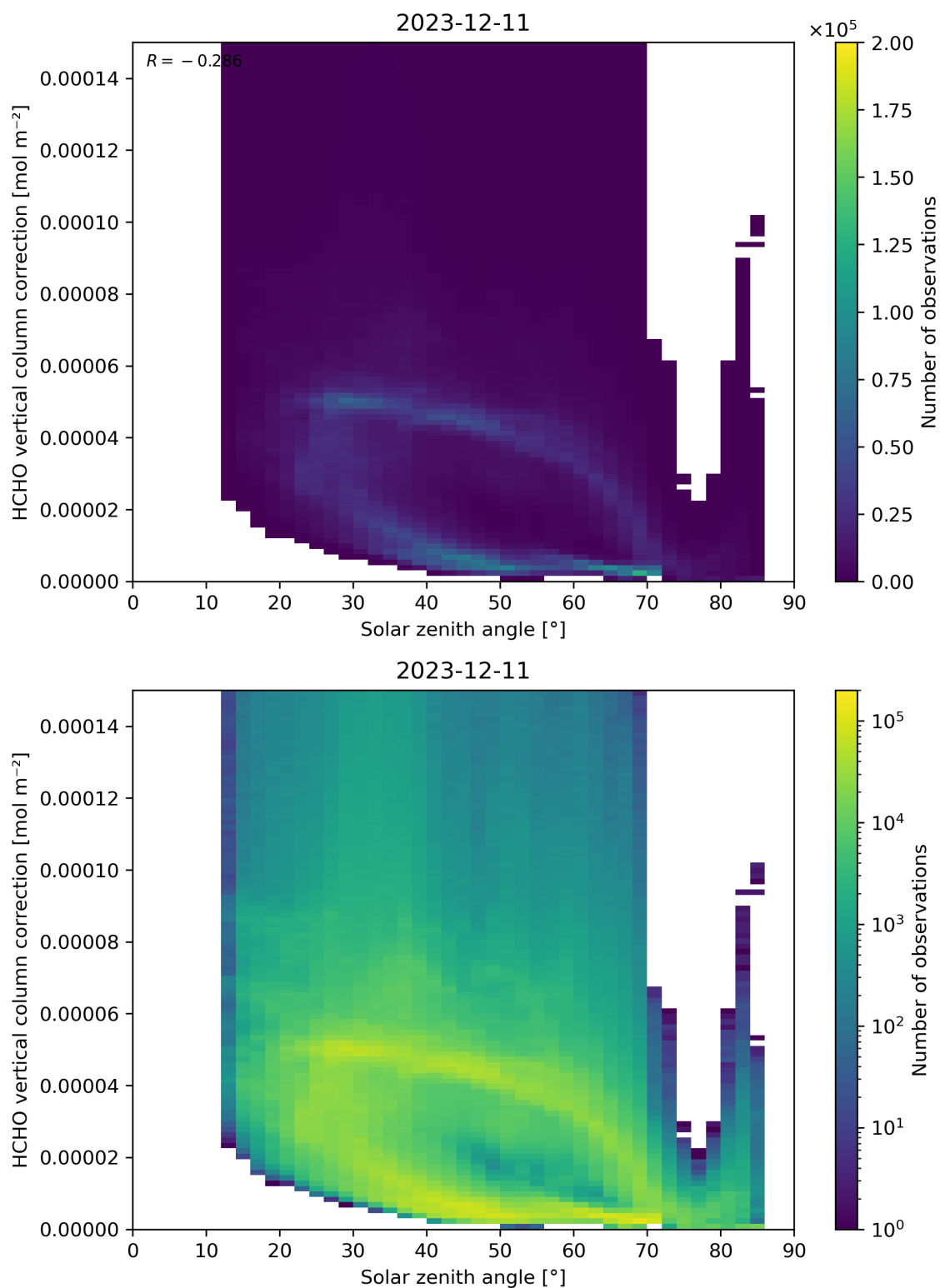
Figure 178: Scatter density plot of “Solar zenith angle” against “HCHO vertical column correction” for 2023-12-10 to 2023-12-12.
