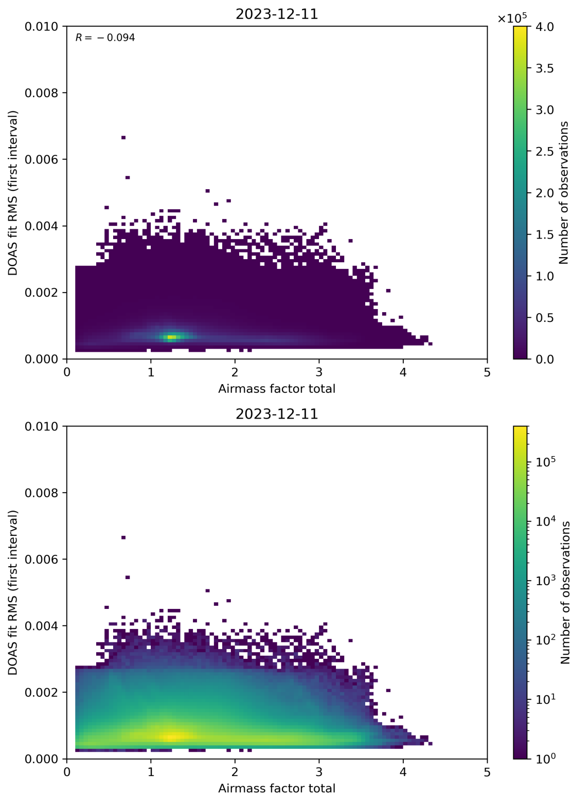
Figure 97: Scatter density plot of “Airmass factor total” against “DOAS fit RMS (first interval)” for 2023-12-10 to 2023-12-12.
