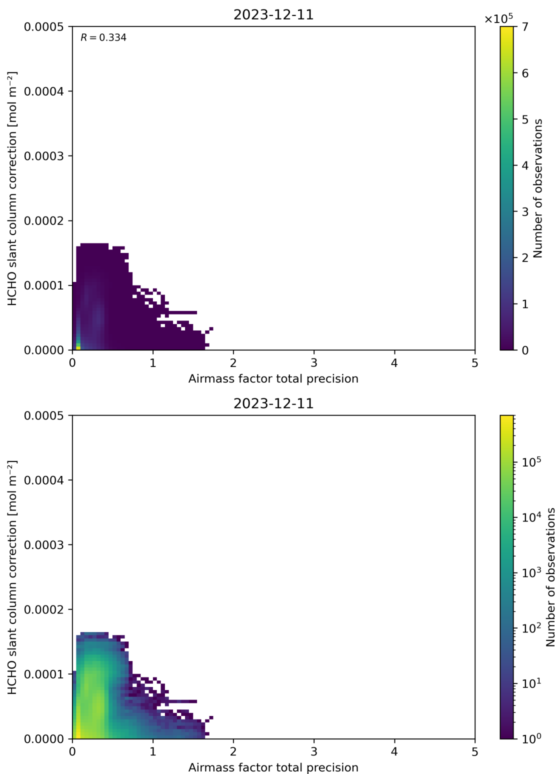
Figure 110: Scatter density plot of “Airmass factor total precision” against “HCHO slant column correction” for 2023-12-10 to 2023-12-12.
