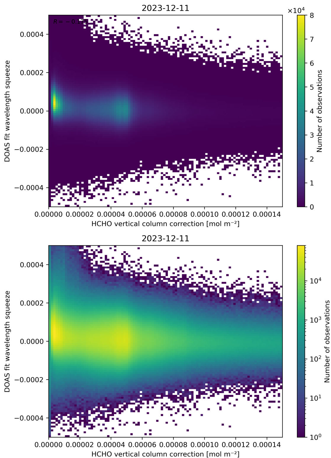
Figure 114: Scatter density plot of “HCHO vertical column correction” against “DOAS fit wavelength squeeze” for 2023-12-10 to 2023-12-12.
