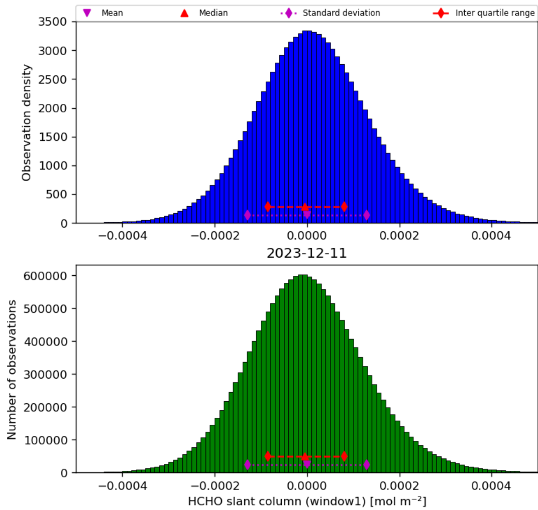
Figure 38: Histogram of “HCHO slant column (window1)” for 2023-12-10 to 2023-12-12
