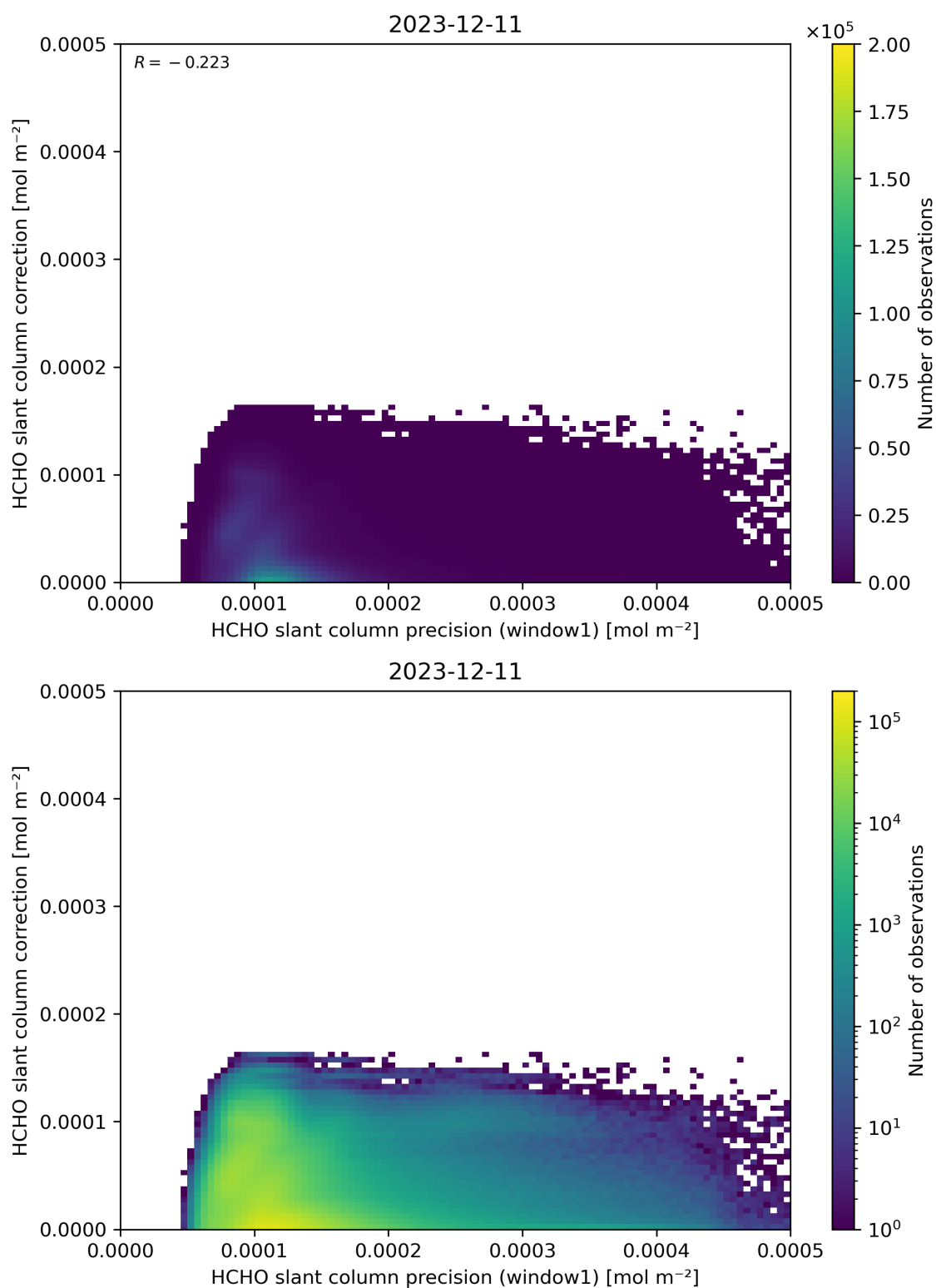
Figure 93: Scatter density plot of “HCHO slant column precision (window1)” against “HCHO slant column correction” for 2023-12-10 to 2023-12-12.
