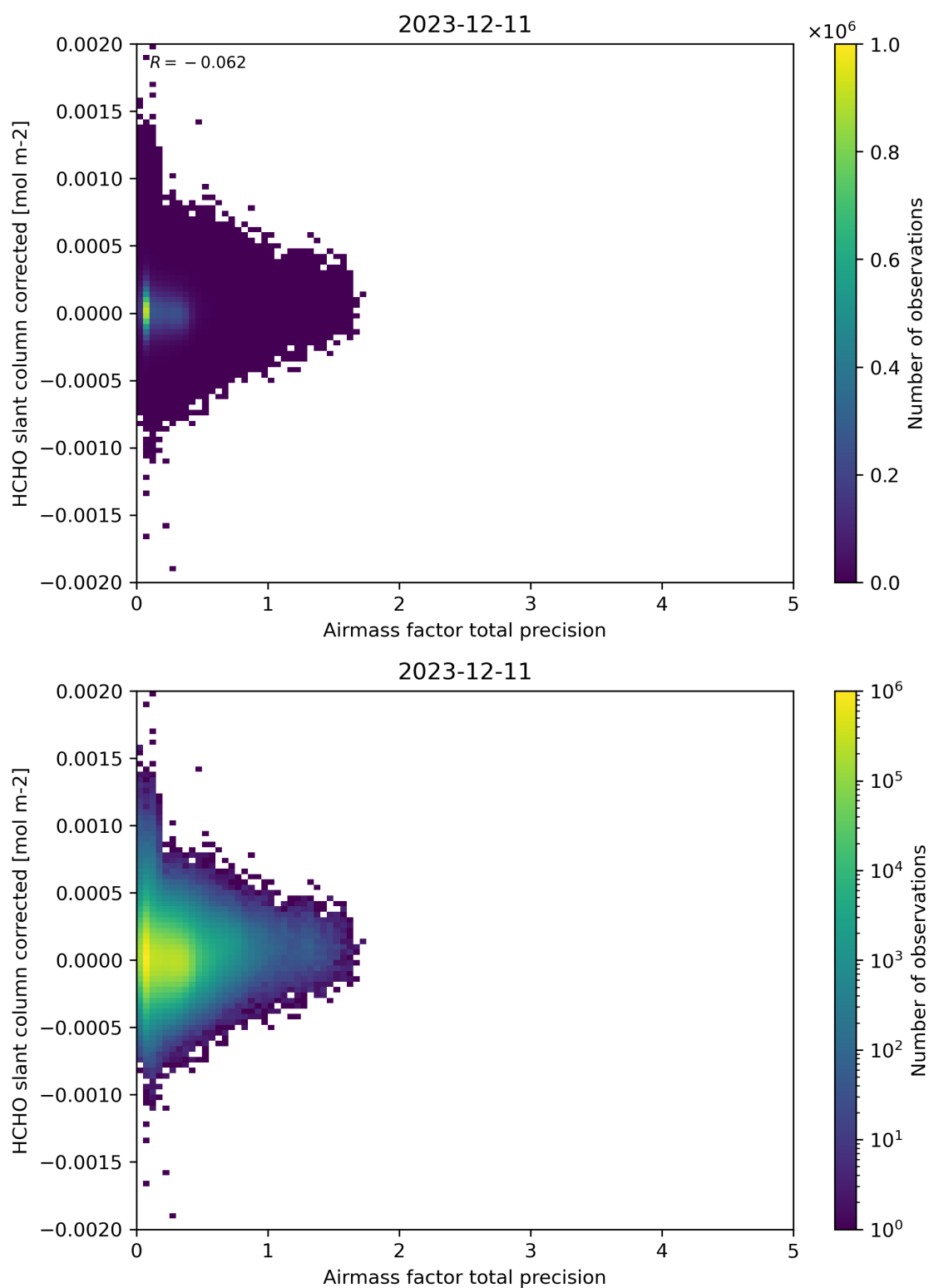
Figure 109: Scatter density plot of “Airmass factor total precision” against “HCHO slant column corrected” for 2023-12-10 to 2023-12-12.
