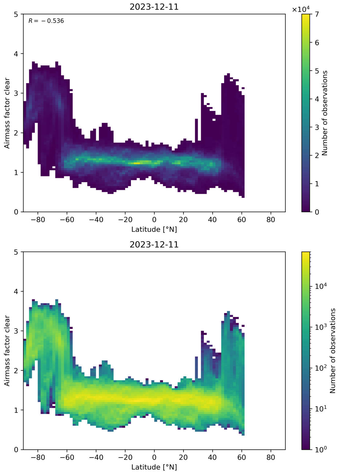
Figure 156: Scatter density plot of “Latitude” against “Airmass factor clear” for 2023-12-10 to 2023-12-12.
