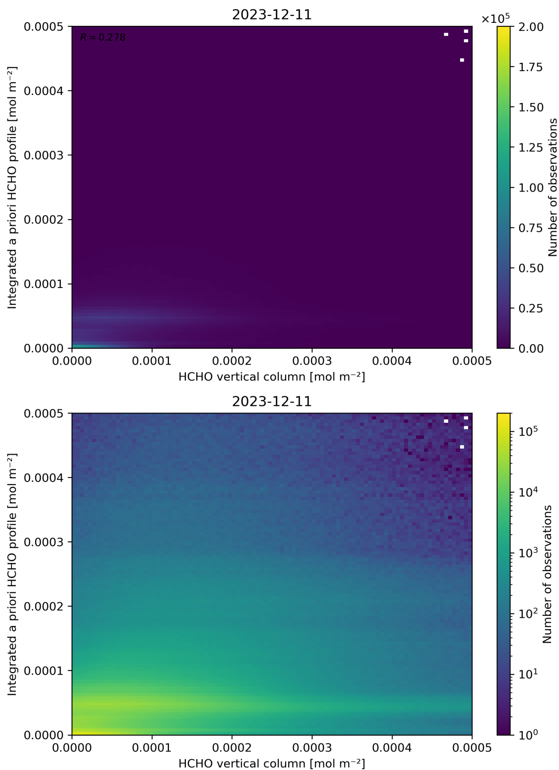
Figure 135: Scatter density plot of “HCHO vertical column” against “Integrated a priori HCHO profile” for 2023-12-10 to 2023-12-12.
