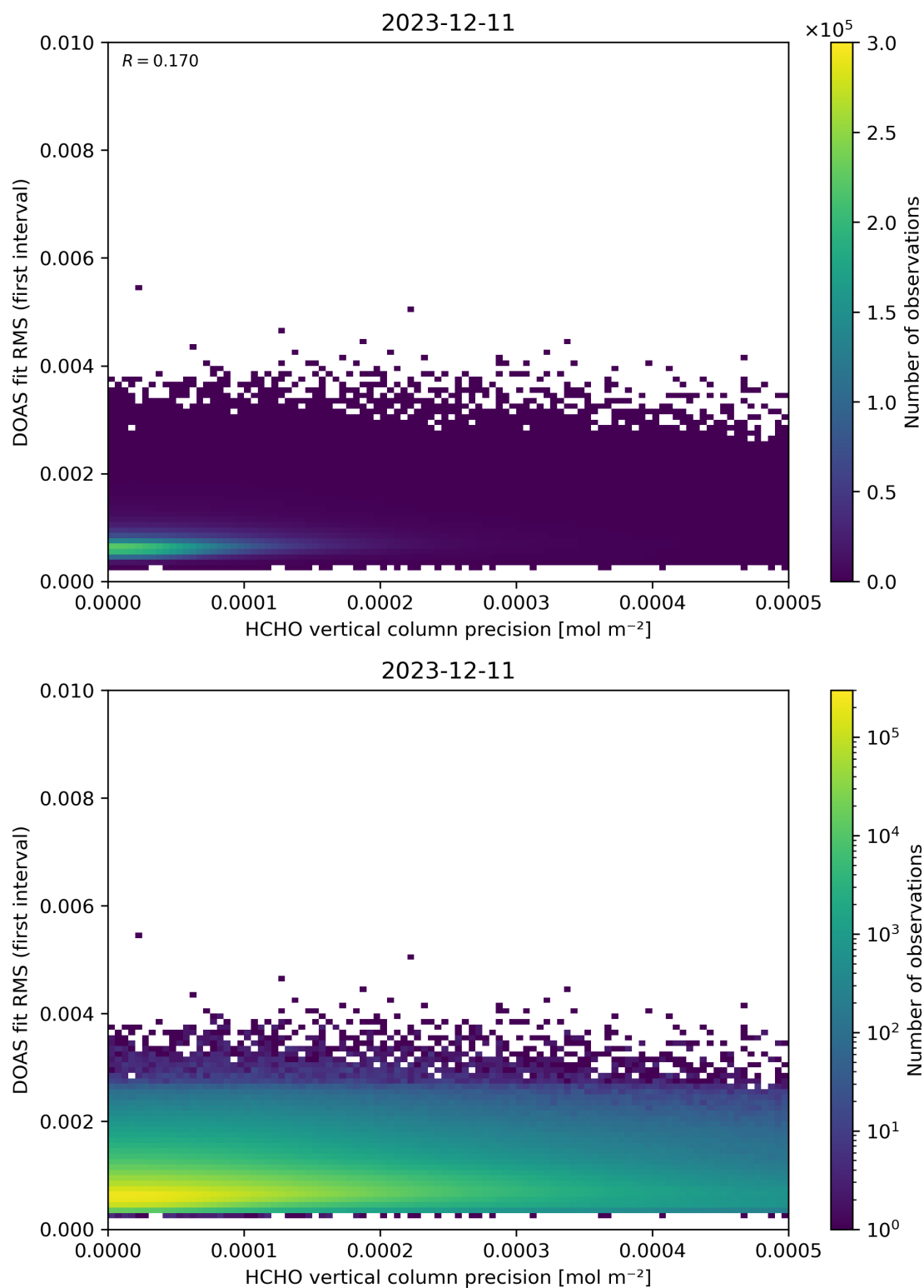
Figure 136: Scatter density plot of “HCHO vertical column precision” against “DOAS fit RMS (first interval)” for 2023-12-10 to 2023-12-12.
