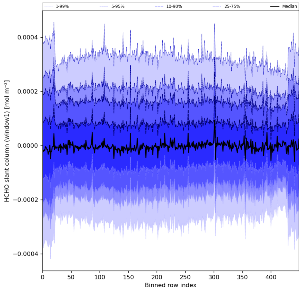
Figure 52: Along track statistics of “HCHO slant column (window1)” for 2023-12-10 to 2023-12-12
