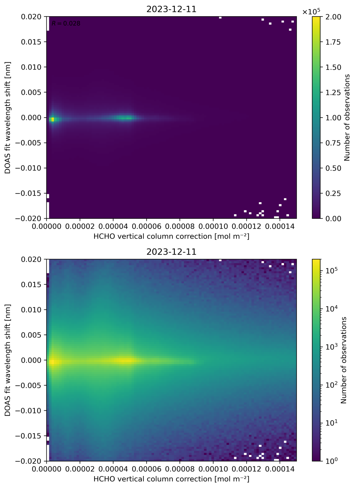
Figure 113: Scatter density plot of “HCHO vertical column correction” against “DOAS fit wavelength shift” for 2023-12-10 to 2023-12-12.
