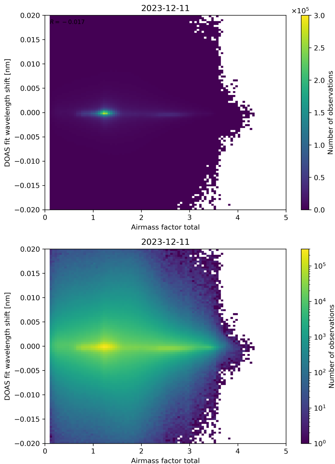
Figure 98: Scatter density plot of “Airmass factor total” against “DOAS fit wavelength shift” for 2023-12-10 to 2023-12-12.
