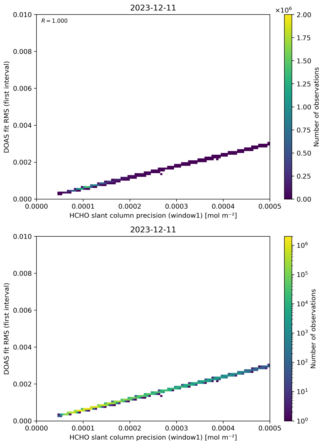
Figure 88: Scatter density plot of “HCHO slant column precision (window1)” against “DOAS fit RMS (first interval)” for 2023-12-10 to 2023-12-12.
