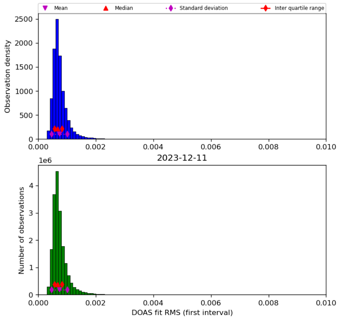
Figure 46: Histogram of “DOAS fit RMS (first interval)” for 2023-12-10 to 2023-12-12
