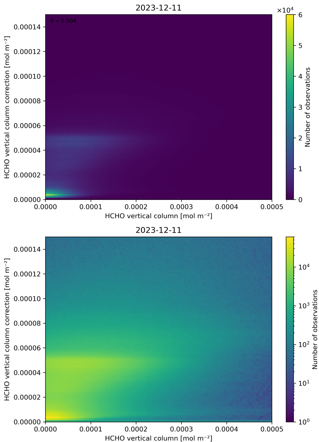
Figure 133: Scatter density plot of “HCHO vertical column” against “HCHO vertical column correction” for 2023-12-10 to 2023-12-12.
