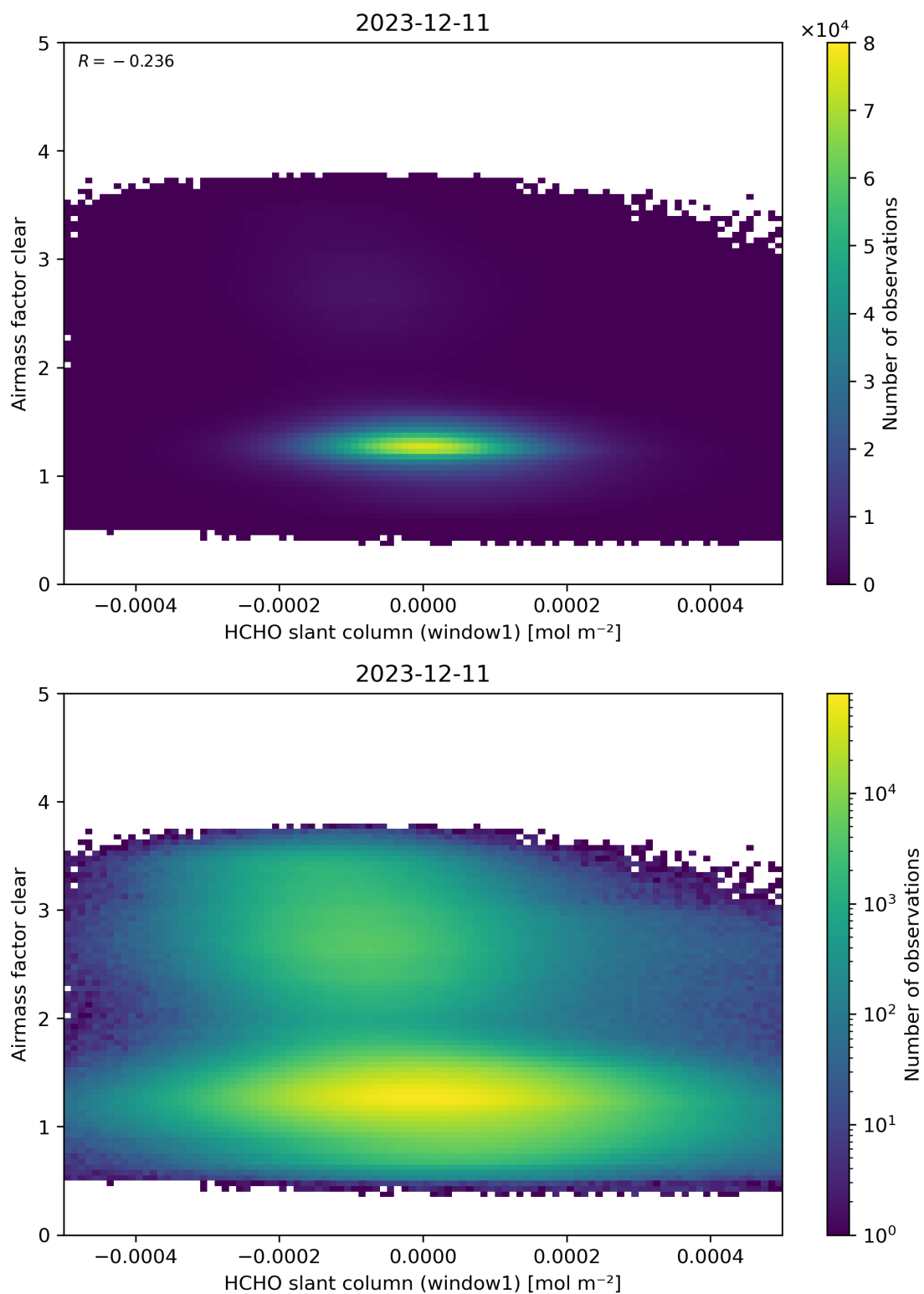
Figure 81: Scatter density plot of “HCHO slant column (window1)” against “Airmass factor clear” for 2023-12-10 to 2023-12-12.
