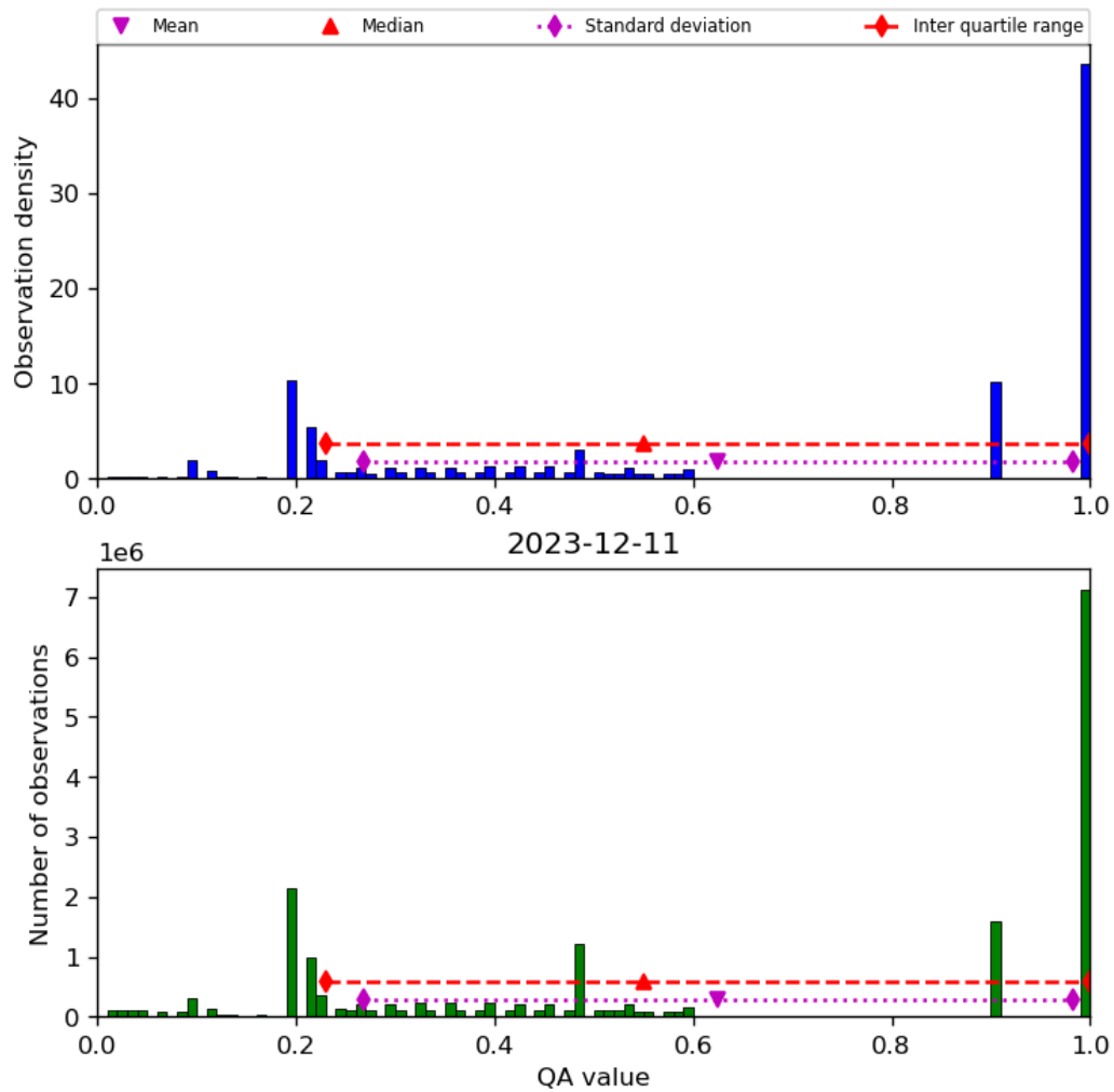
Figure 34: Histogram of “QA value” for 2023-12-10 to 2023-12-12
