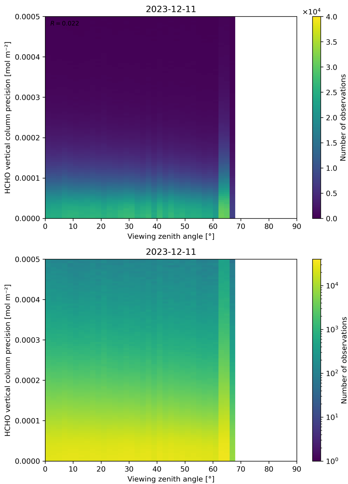
Figure 194: Scatter density plot of “Viewing zenith angle” against “HCHO vertical column precision” for 2023-12-10 to 2023-12-12.
