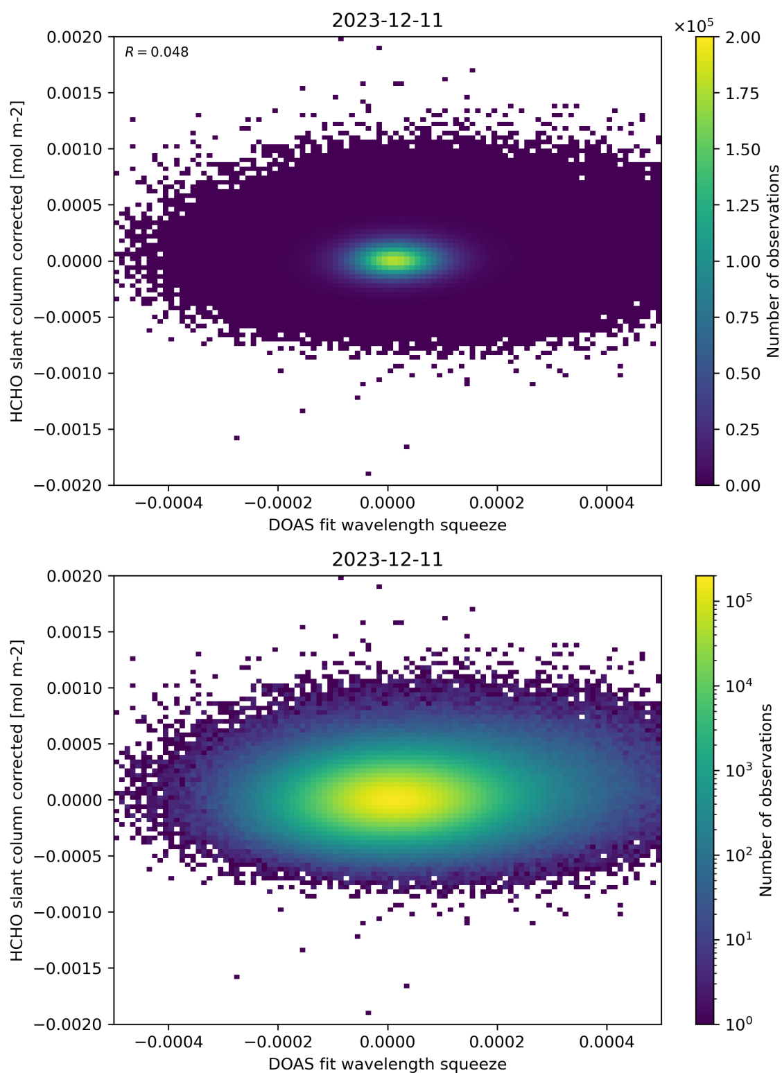
Figure 69: Scatter density plot of “DOAS fit wavelength squeeze” against “HCHO slant column corrected” for 2023-12-10 to 2023-12-12.
