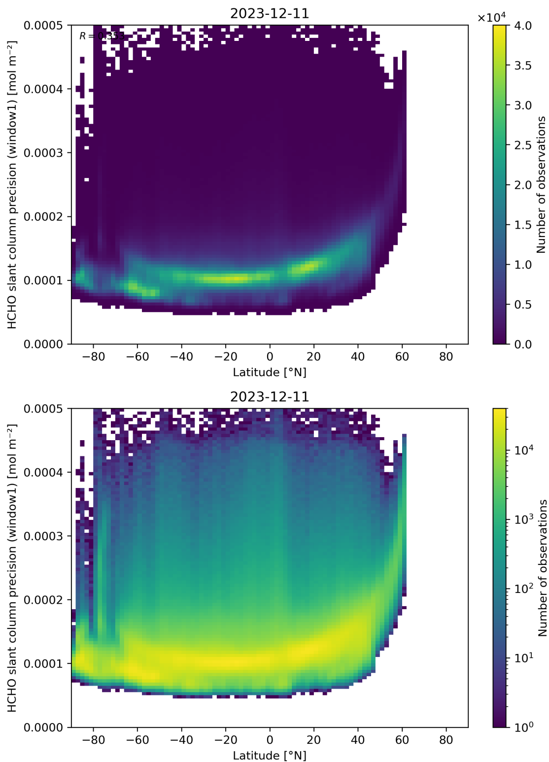
Figure 160: Scatter density plot of “Latitude” against “HCHO slant column precision (window1)” for 2023-12-10 to 2023-12-12.
