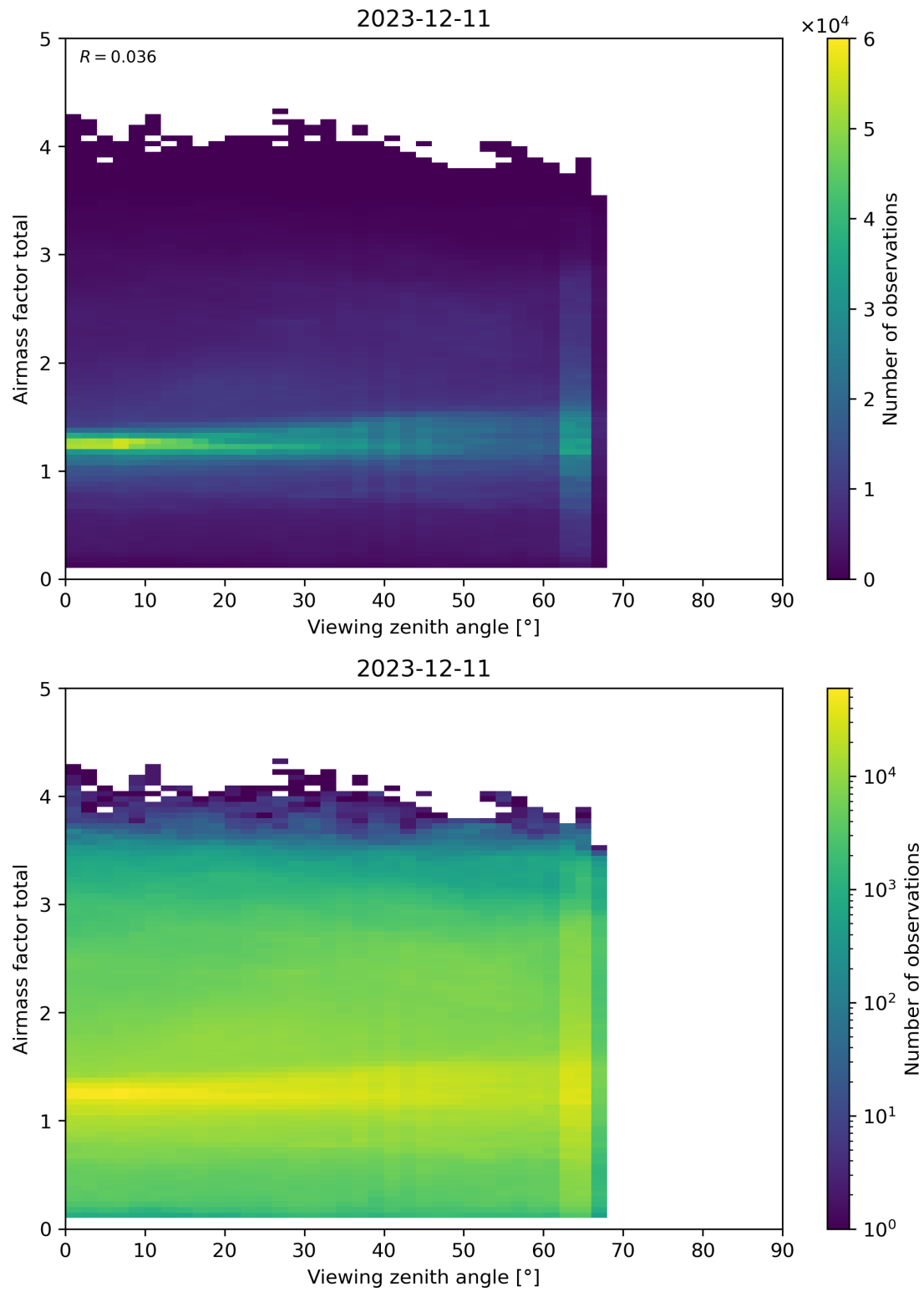
Figure 190: Scatter density plot of “Viewing zenith angle” against “Airmass factor total” for 2023-12-10 to 2023-12-12.
