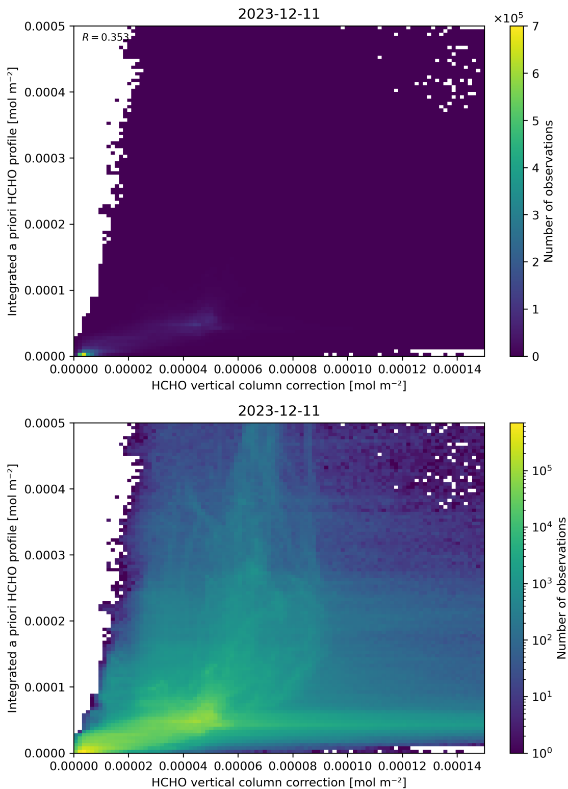
Figure 122: Scatter density plot of “HCHO vertical column correction” against “Integrated a priori HCHO profile” for 2023-12-10 to 2023-12-12.
