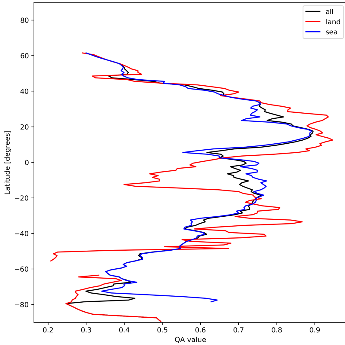
Figure 20: Zonal average of “QA value” for 2023-12-10 to 2023-12-12.
