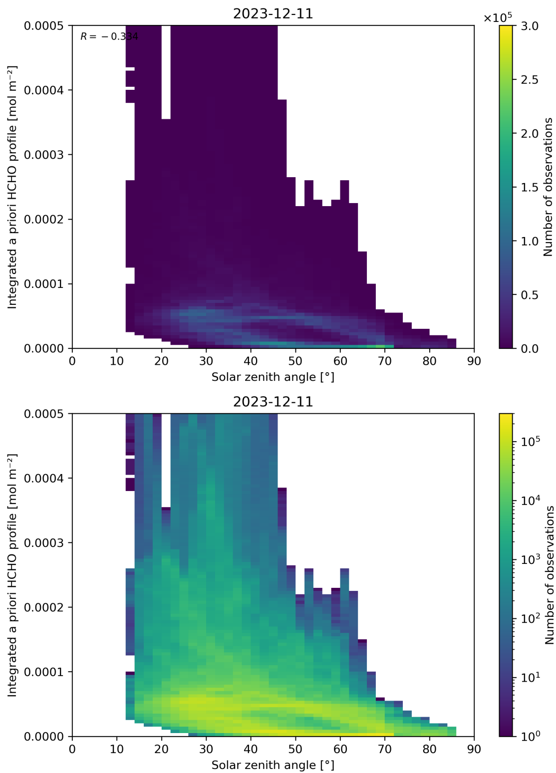
Figure 180: Scatter density plot of “Solar zenith angle” against “Integrated a priori HCHO profile” for 2023-12-10 to 2023-12-12.
