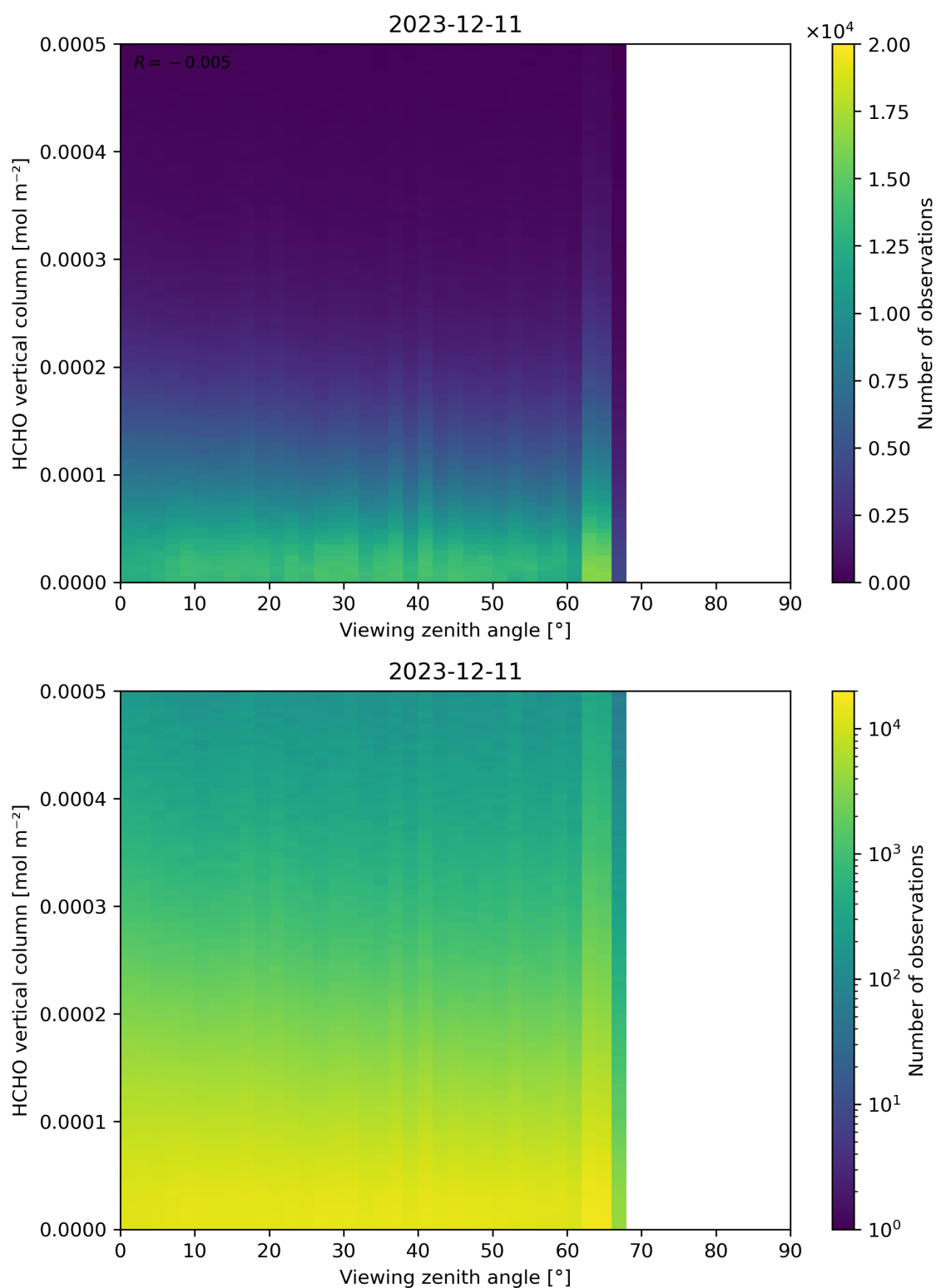
Figure 192: Scatter density plot of “Viewing zenith angle” against “HCHO vertical column” for 2023-12-10 to 2023-12-12.
