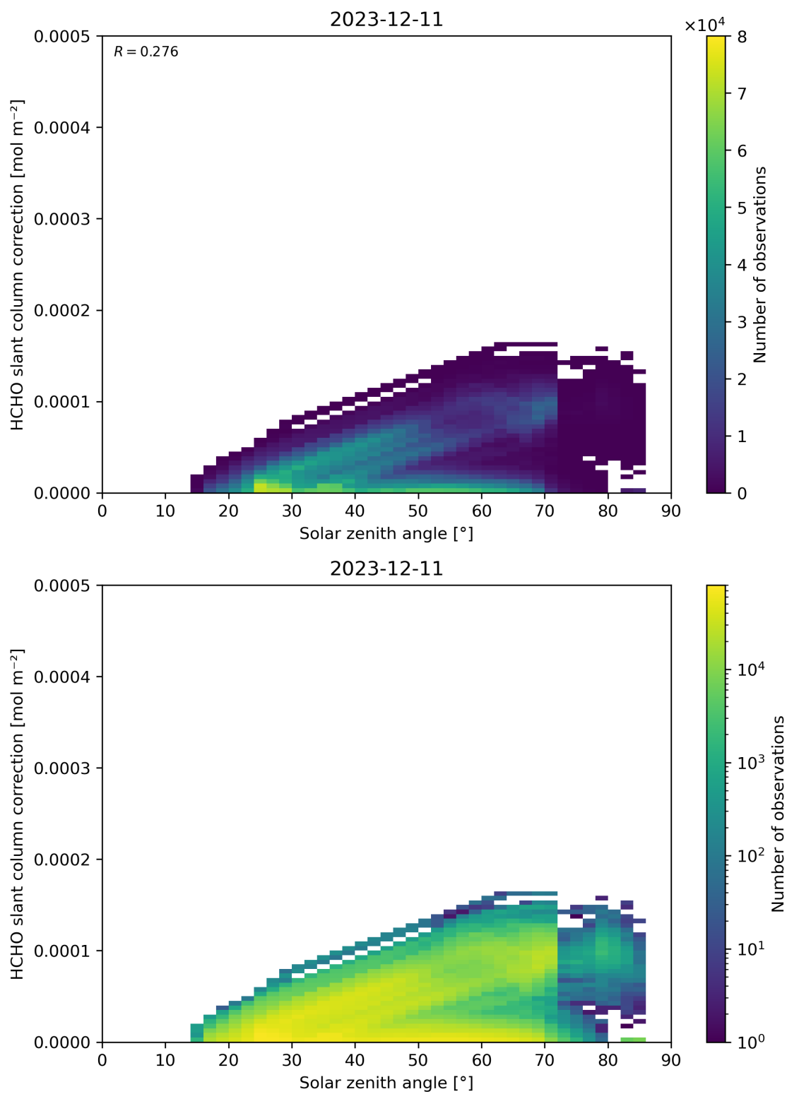
Figure 172: Scatter density plot of “Solar zenith angle” against “HCHO slant column correction” for 2023-12-10 to 2023-12-12.
