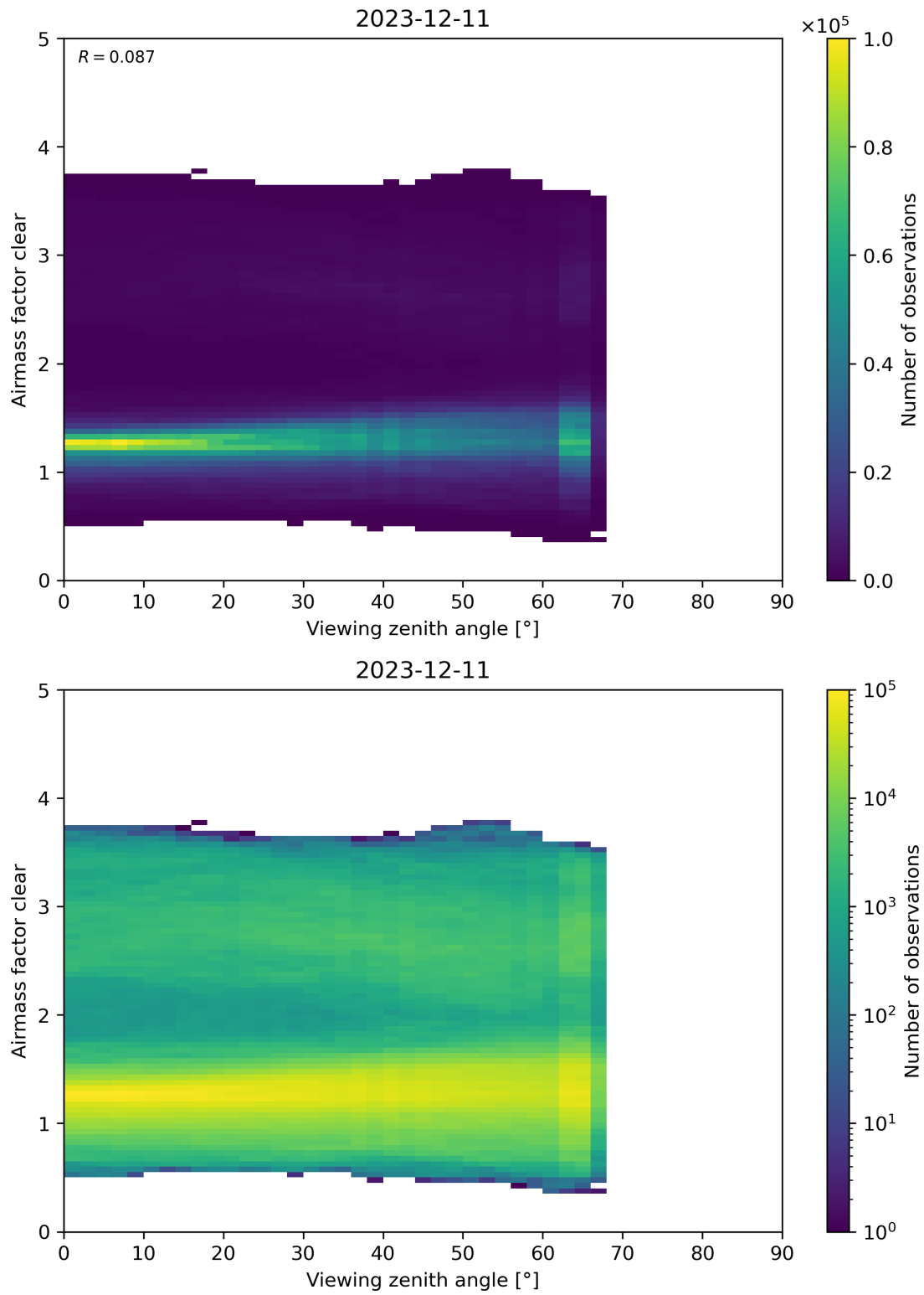
Figure 185: Scatter density plot of “Viewing zenith angle” against “Airmass factor clear” for 2023-12-10 to 2023-12-12.
