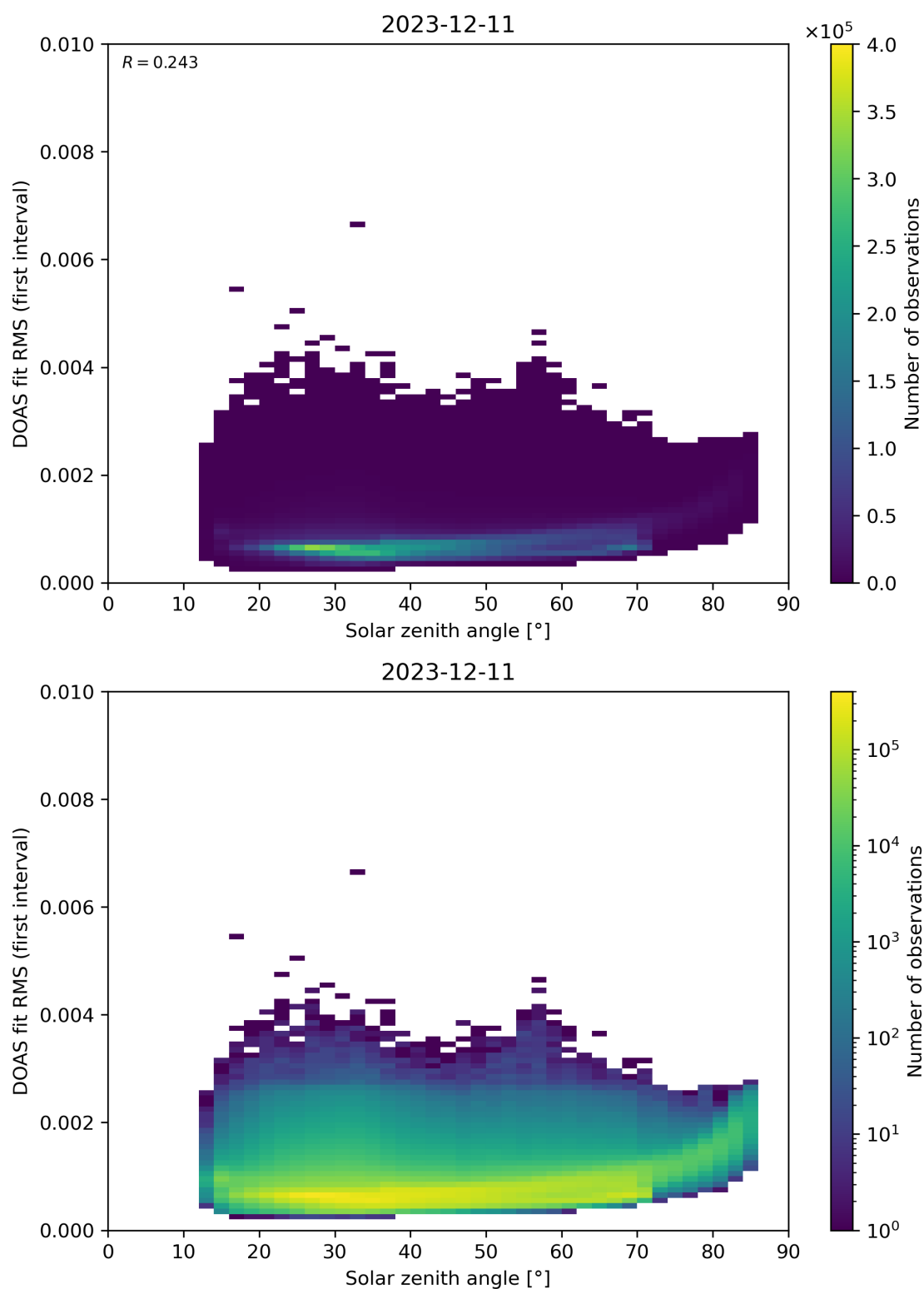
Figure 167: Scatter density plot of “Solar zenith angle” against “DOAS fit RMS (first interval)” for 2023-12-10 to 2023-12-12.
