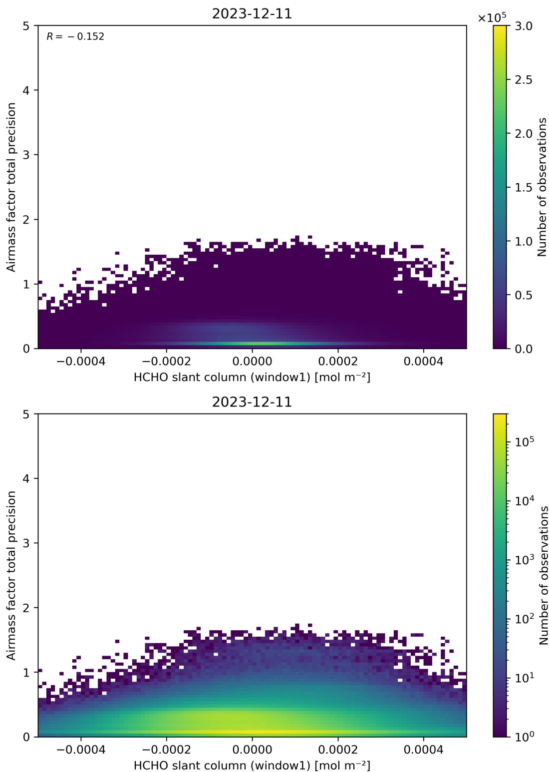
Figure 86: Scatter density plot of “HCHO slant column (window1)” against “Airmass factor total precision” for 2023-12-10 to 2023-12-12.
