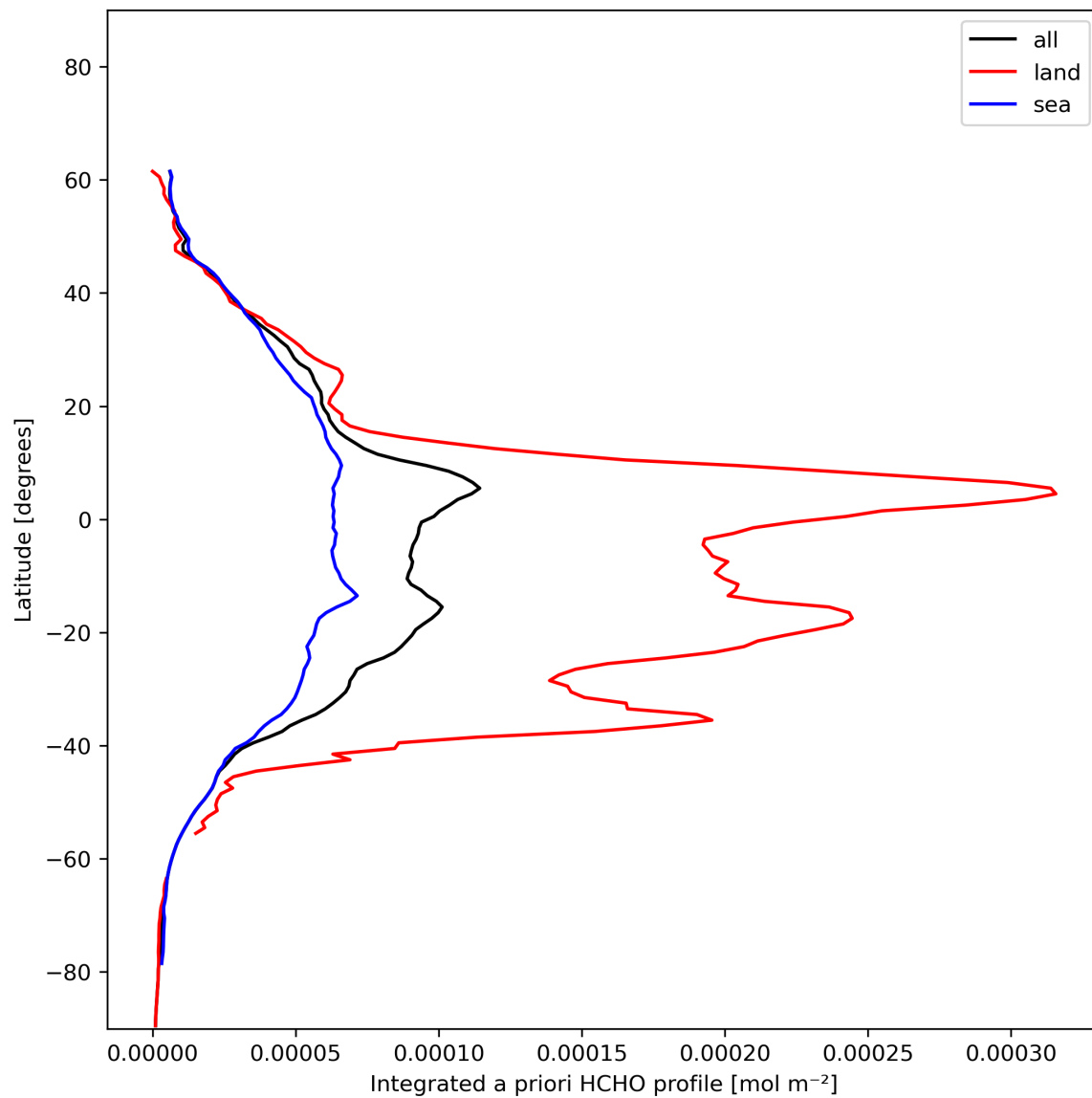
Figure 29: Zonal average of “Integrated a priori HCHO profile” for 2023-12-10 to 2023-12-12.
