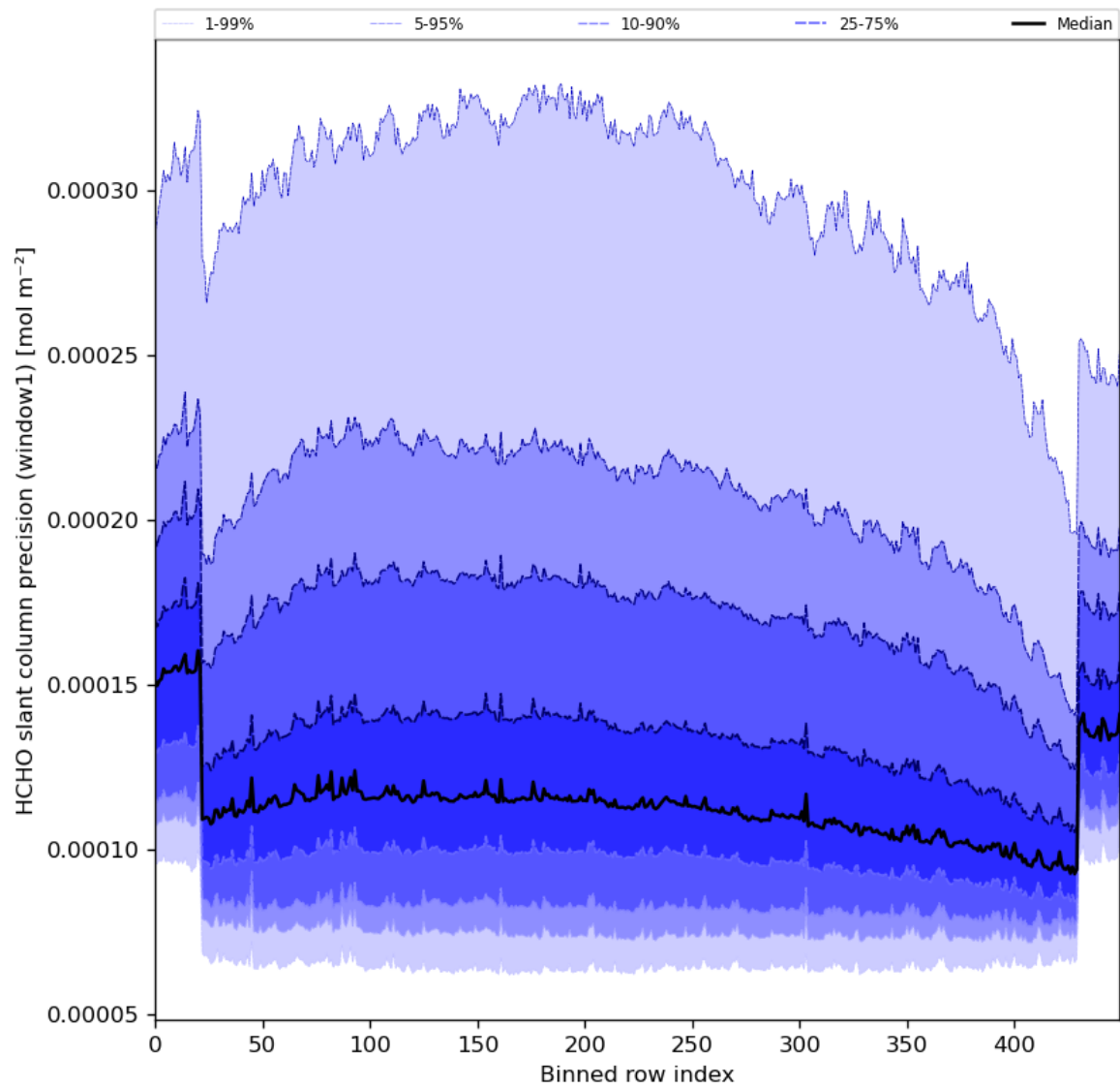
Figure 53: Along track statistics of “HCHO slant column precision (window1)” for 2023-12-10 to 2023-12-12
