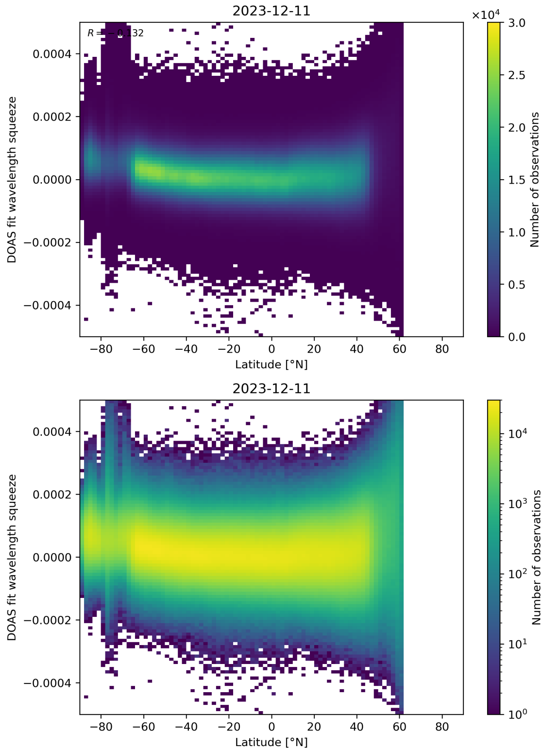
Figure 155: Scatter density plot of “Latitude” against “DOAS fit wavelength squeeze” for 2023-12-10 to 2023-12-12.
