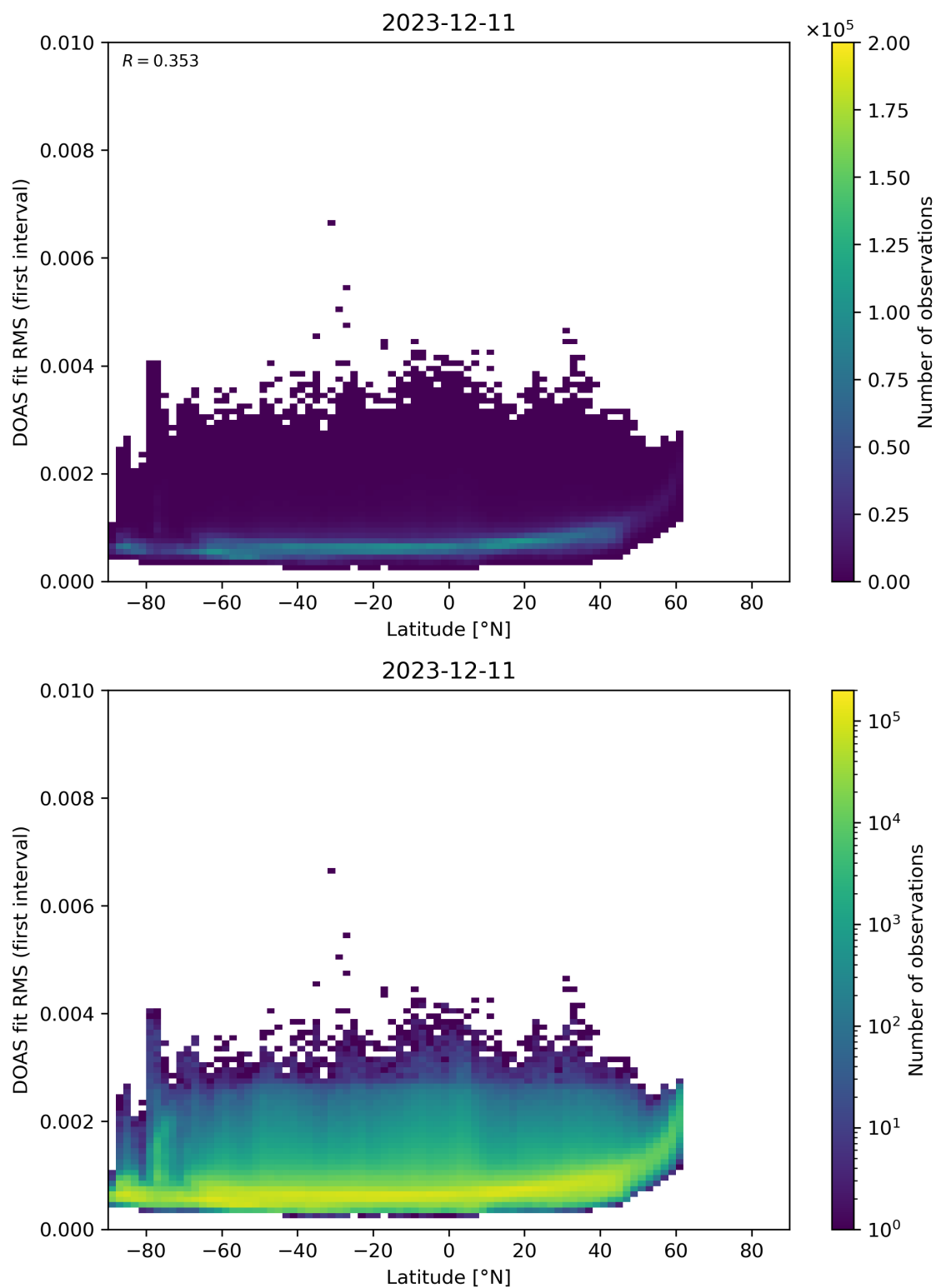
Figure 153: Scatter density plot of “Latitude” against “DOAS fit RMS (first interval)” for 2023-12-10 to 2023-12-12.
