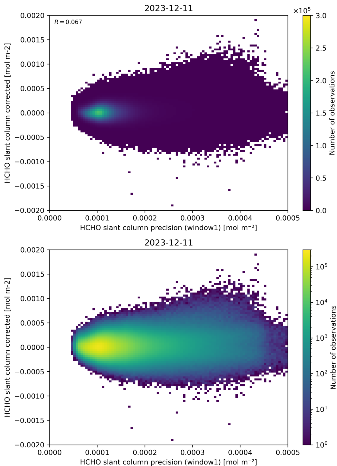
Figure 92: Scatter density plot of “HCHO slant column precision (window1)” against “HCHO slant column corrected” for 2023-12-10 to 2023-12-12.
