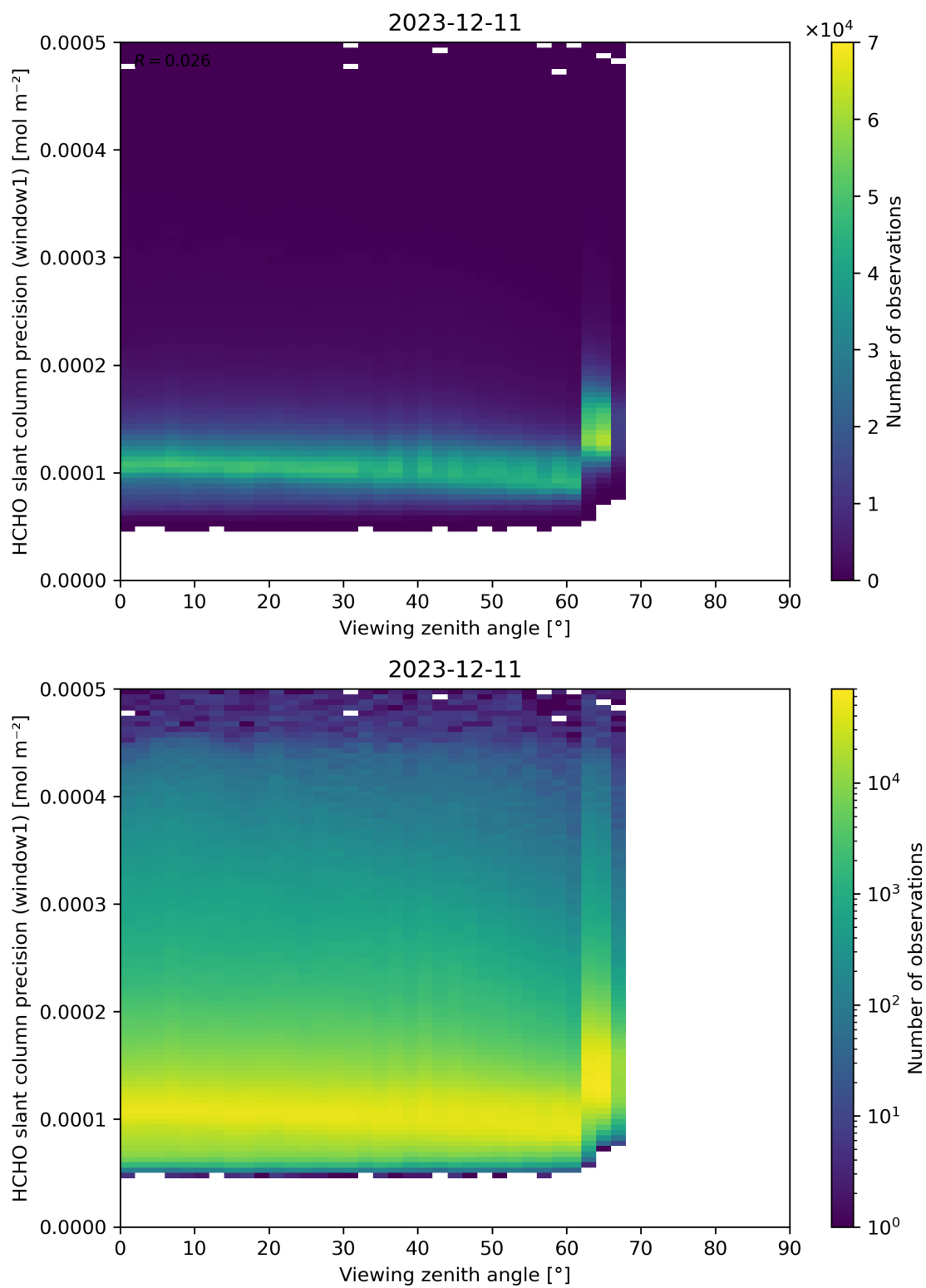
Figure 189: Scatter density plot of “Viewing zenith angle” against “HCHO slant column precision (window1)” for 2023-12-10 to 2023-12-12.
