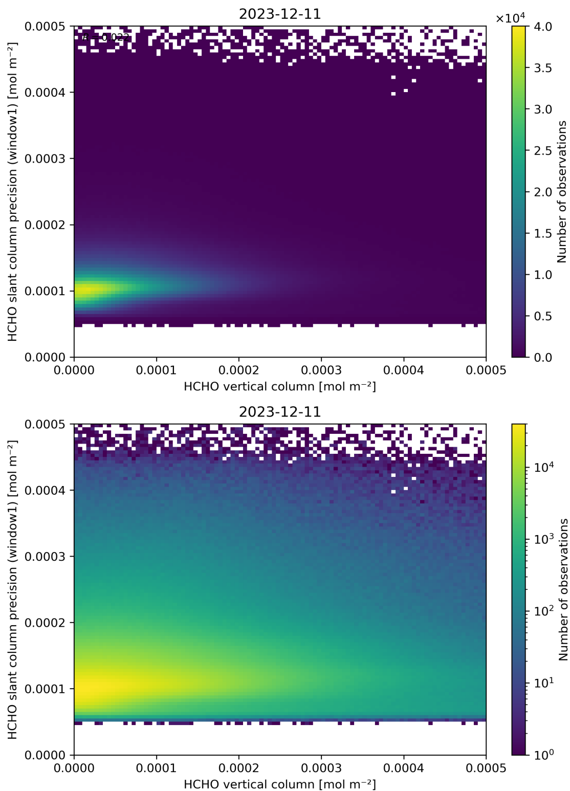
Figure 130: Scatter density plot of “HCHO vertical column” against “HCHO slant column precision (window1)” for 2023-12-10 to 2023-12-12.
