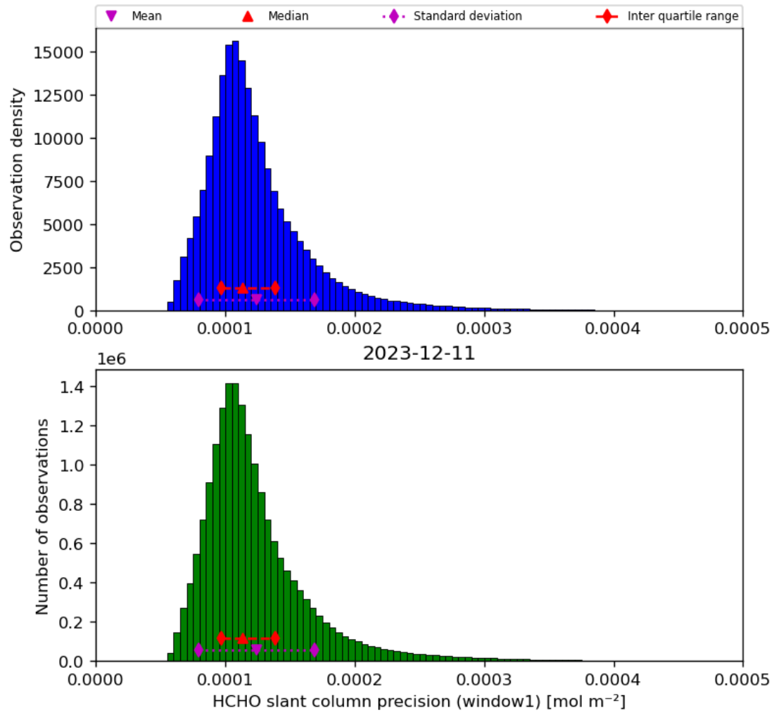
Figure 39: Histogram of “HCHO slant column precision (window1)” for 2023-12-10 to 2023-12-12
