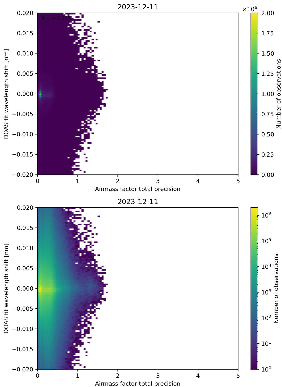
Figure 106: Scatter density plot of “Airmass factor total precision” against “DOAS fit wavelength shift” for 2023-12-10 to 2023-12-12.
