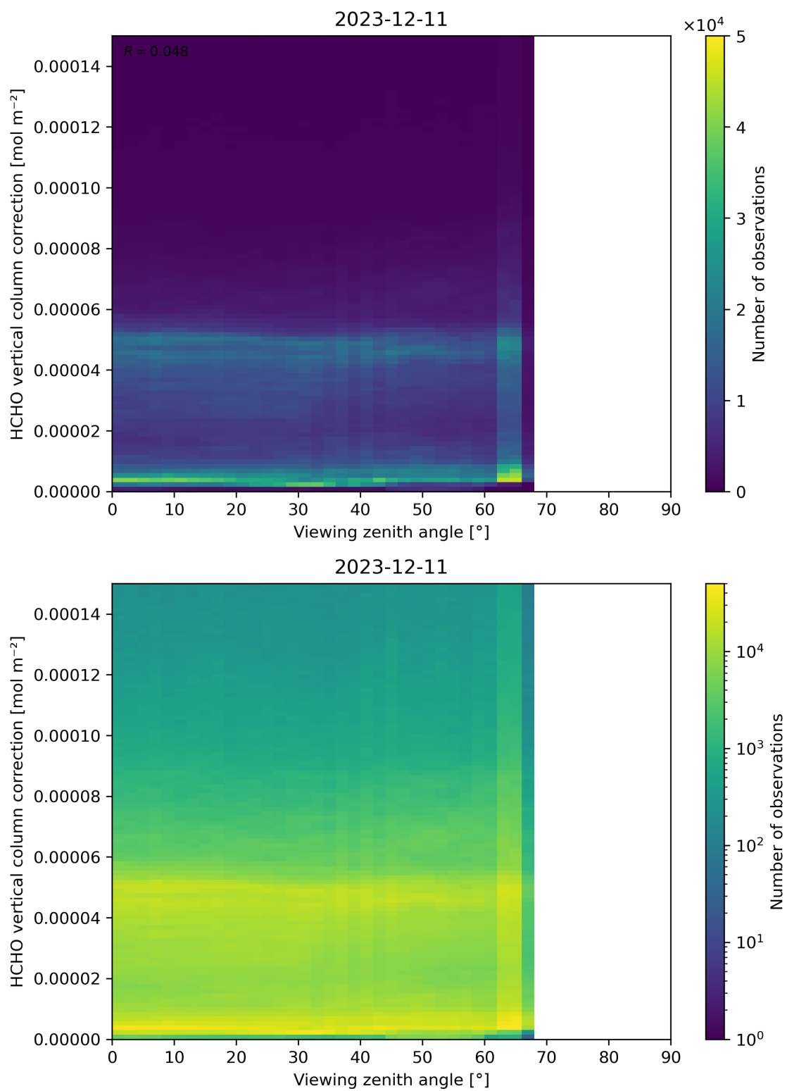
Figure 193: Scatter density plot of “Viewing zenith angle” against “HCHO vertical column correction” for 2023-12-10 to 2023-12-12.
