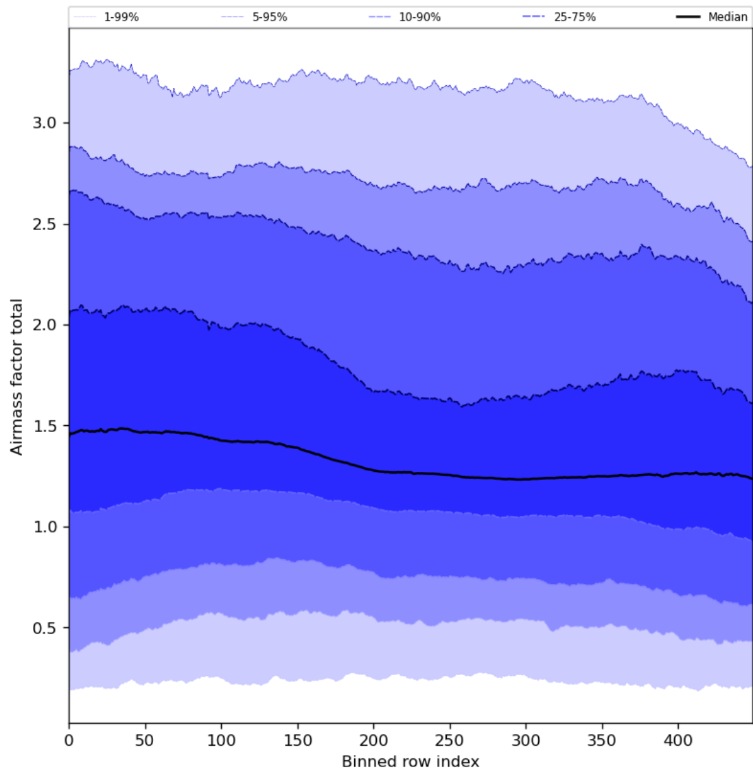
Figure 54: Along track statistics of “Airmass factor total” for 2023-12-10 to 2023-12-12
