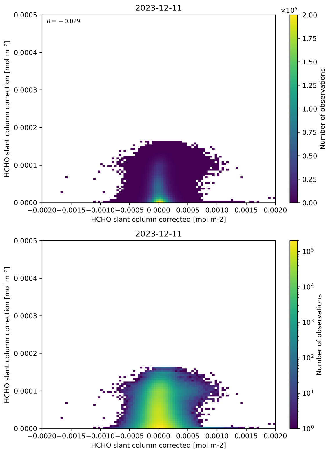
Figure 77: Scatter density plot of “HCHO slant column corrected” against “HCHO slant column correction” for 2023-12-10 to 2023-12-12.
