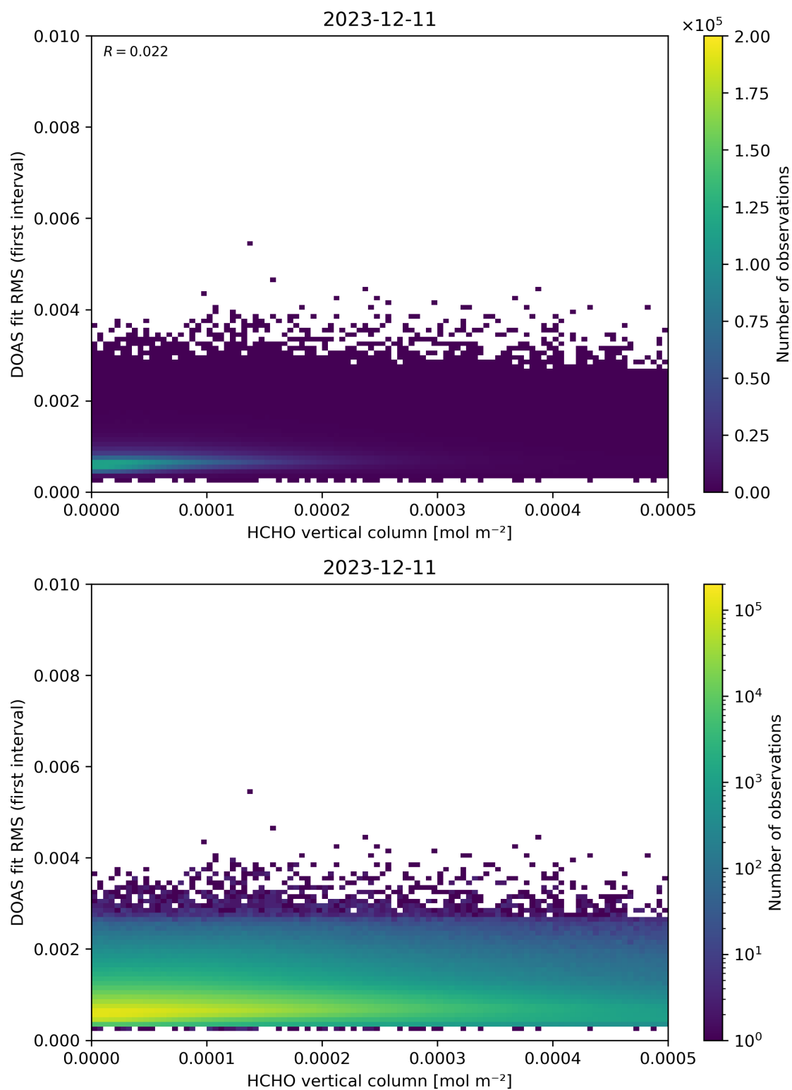
Figure 123: Scatter density plot of “HCHO vertical column” against “DOAS fit RMS (first interval)” for 2023-12-10 to 2023-12-12.
