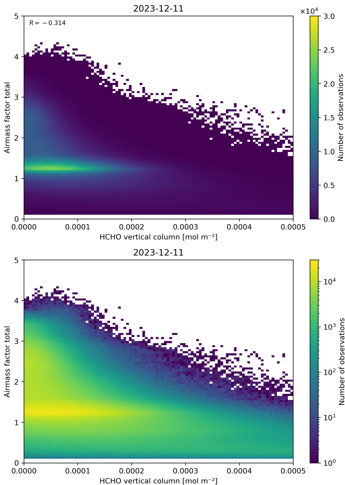
Figure 131: Scatter density plot of “HCHO vertical column” against “Airmass factor total” for 2023-12-10 to 2023-12-12.
