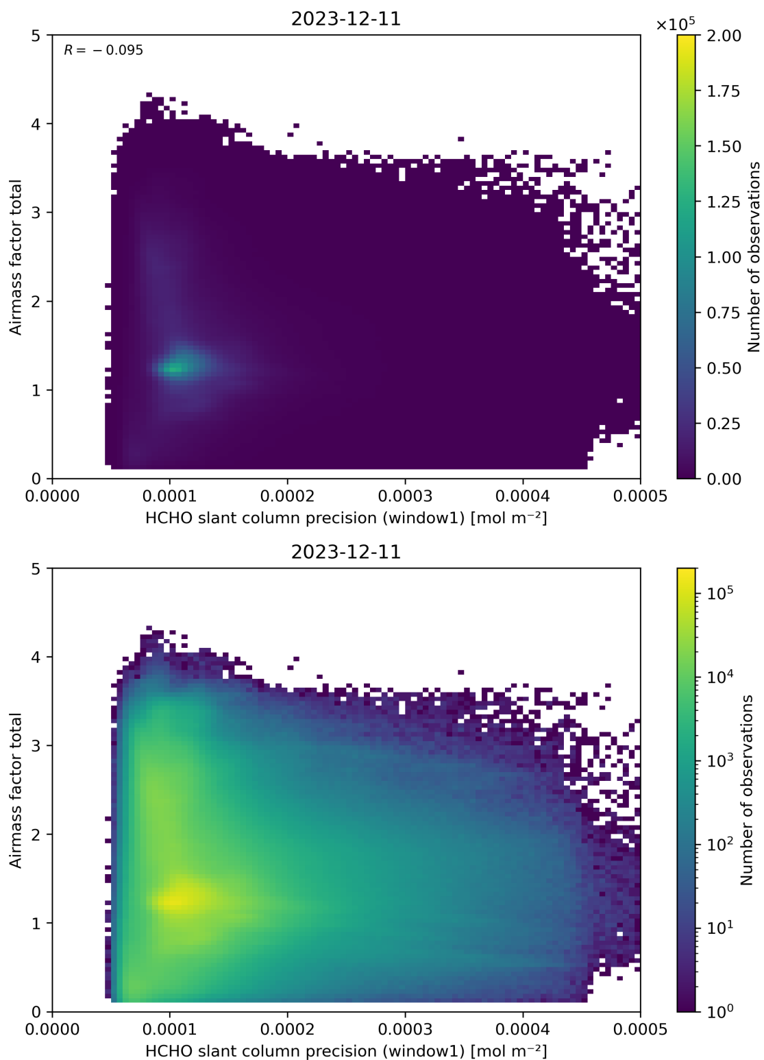
Figure 94: Scatter density plot of “HCHO slant column precision (window1)” against “Airmass factor total” for 2023-12-10 to 2023-12-12.
