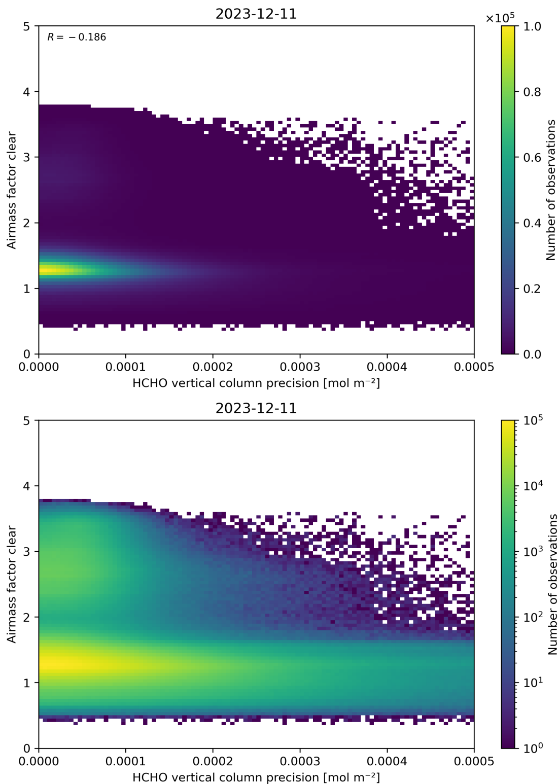
Figure 139: Scatter density plot of “HCHO vertical column precision” against “Airmass factor clear” for 2023-12-10 to 2023-12-12.
