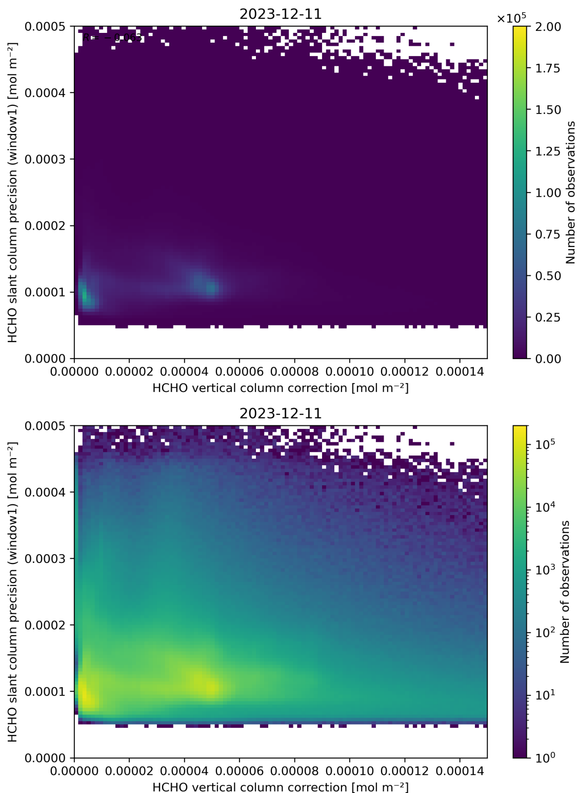
Figure 119: Scatter density plot of “HCHO vertical column correction” against “HCHO slant column precision (window1)” for 2023-12-10 to 2023-12-12.
