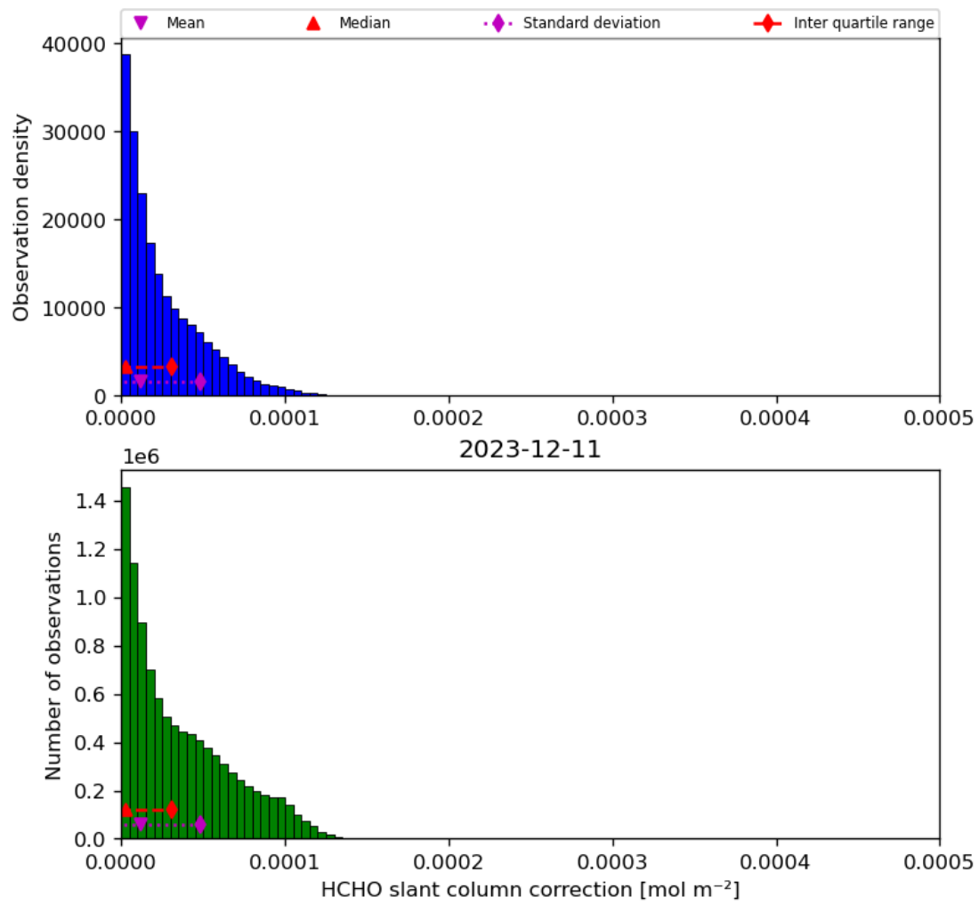
Figure 47: Histogram of “HCHO slant column correction” for 2023-12-10 to 2023-12-12
