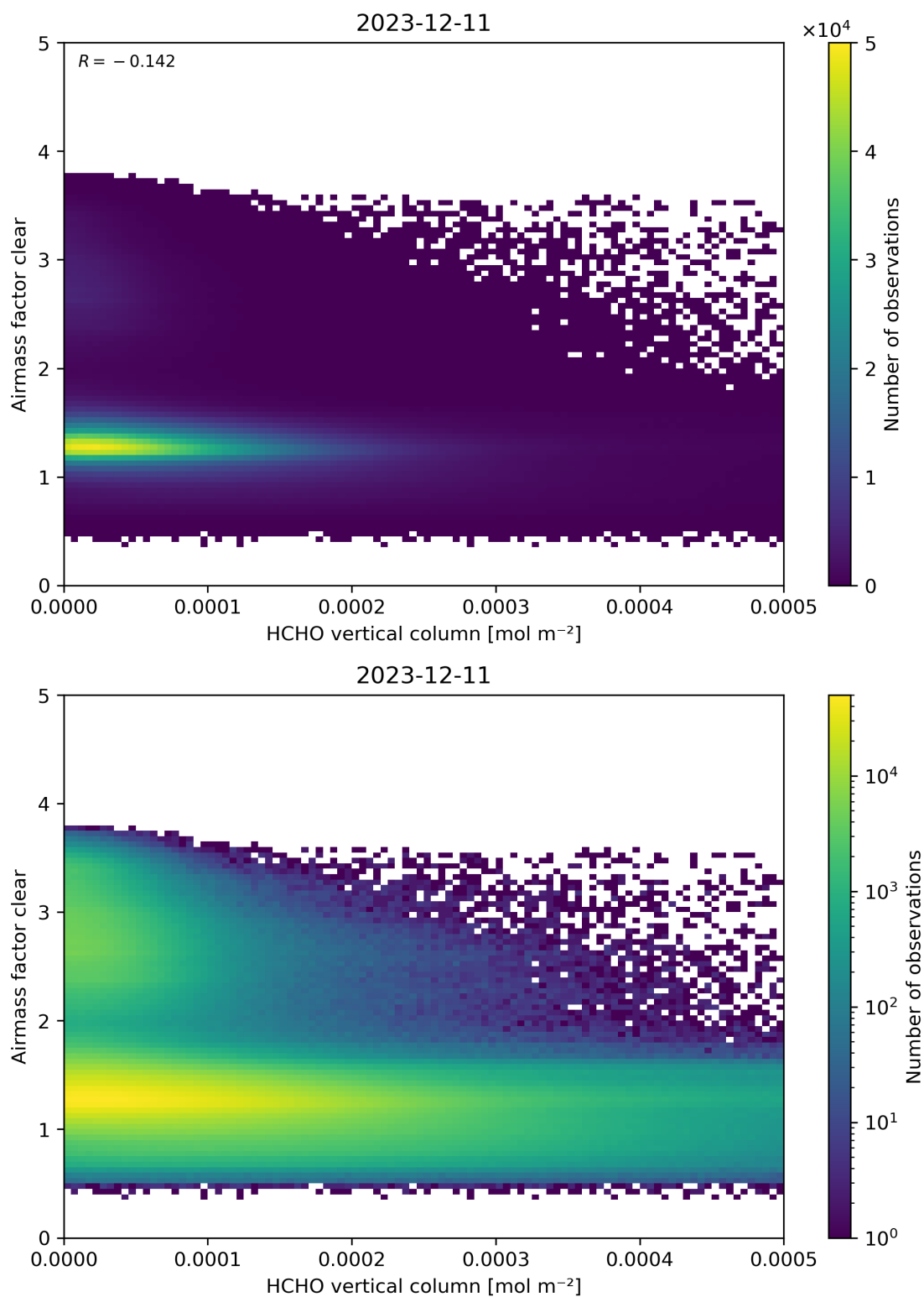
Figure 126: Scatter density plot of “HCHO vertical column” against “Airmass factor clear” for 2023-12-10 to 2023-12-12.
