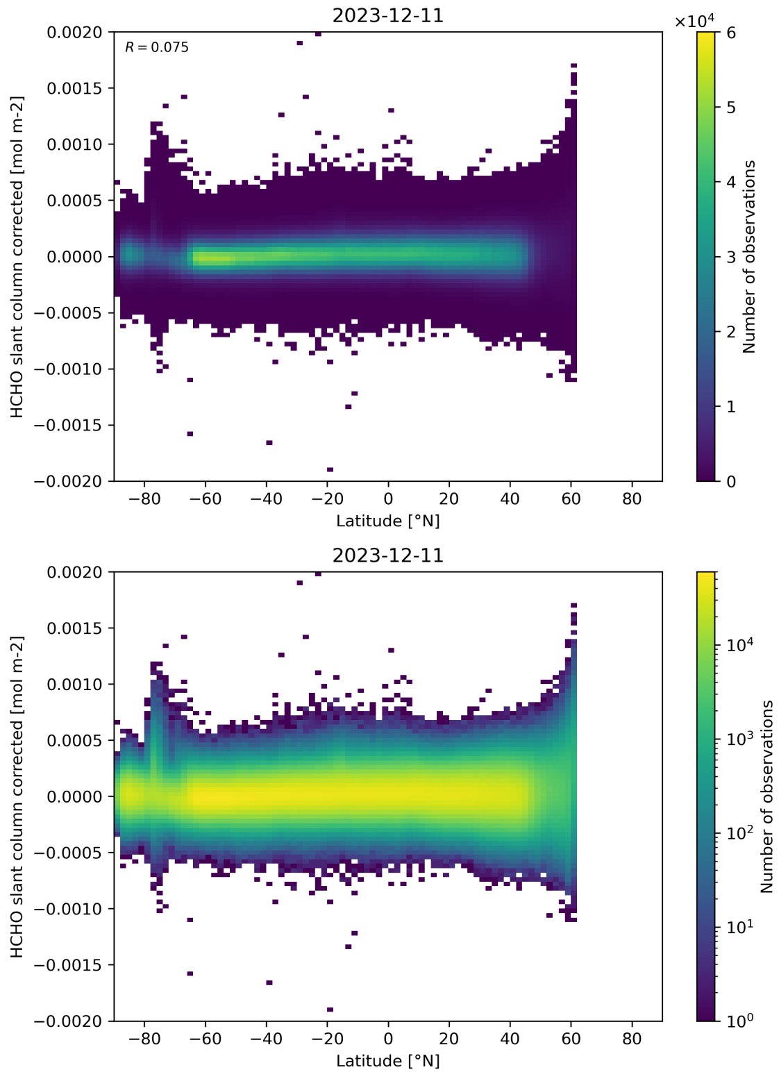
Figure 157: Scatter density plot of “Latitude” against “HCHO slant column corrected” for 2023-12-10 to 2023-12-12.
