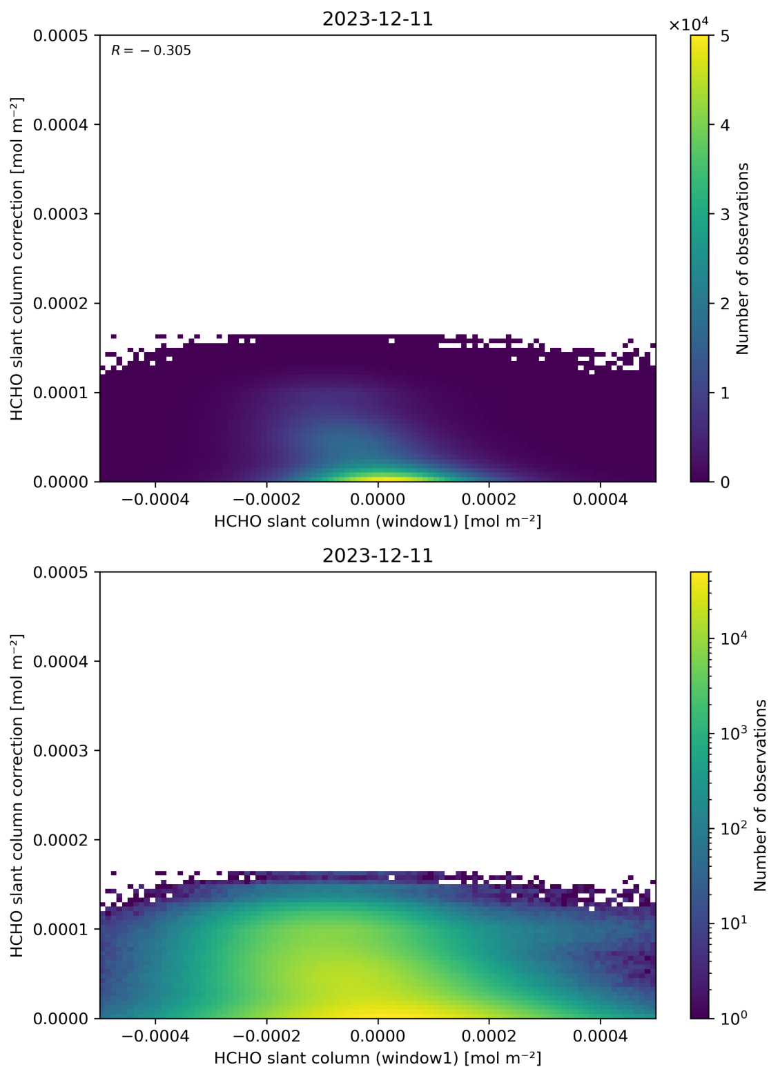
Figure 83: Scatter density plot of “HCHO slant column (window1)” against “HCHO slant column correction” for 2023-12-10 to 2023-12-12.
