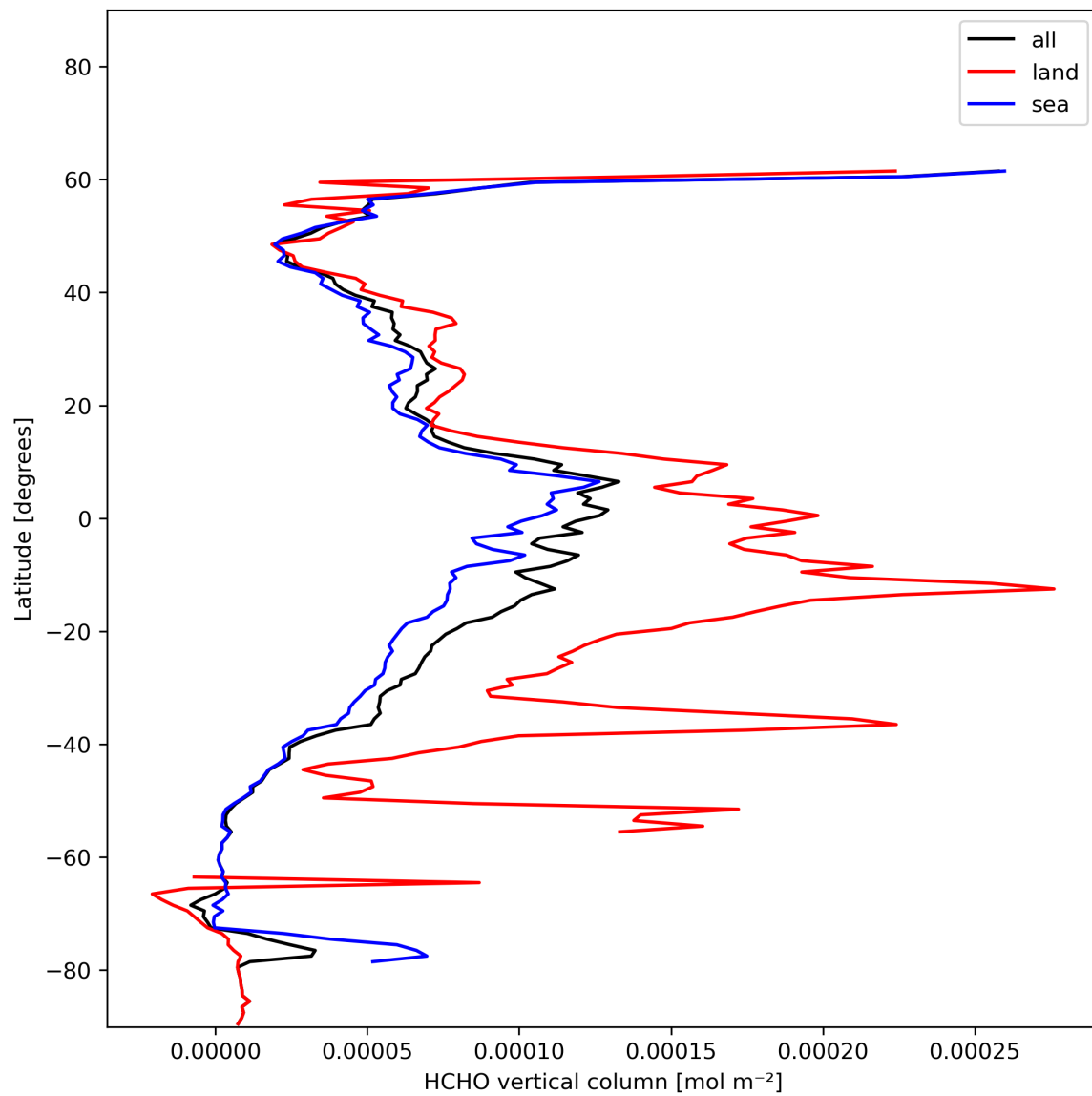
Figure 21: Zonal average of “HCHO vertical column” for 2023-12-10 to 2023-12-12.
