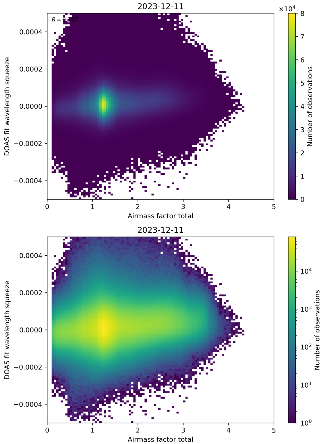
Figure 99: Scatter density plot of “Airmass factor total” against “DOAS fit wavelength squeeze” for 2023-12-10 to 2023-12-12.
