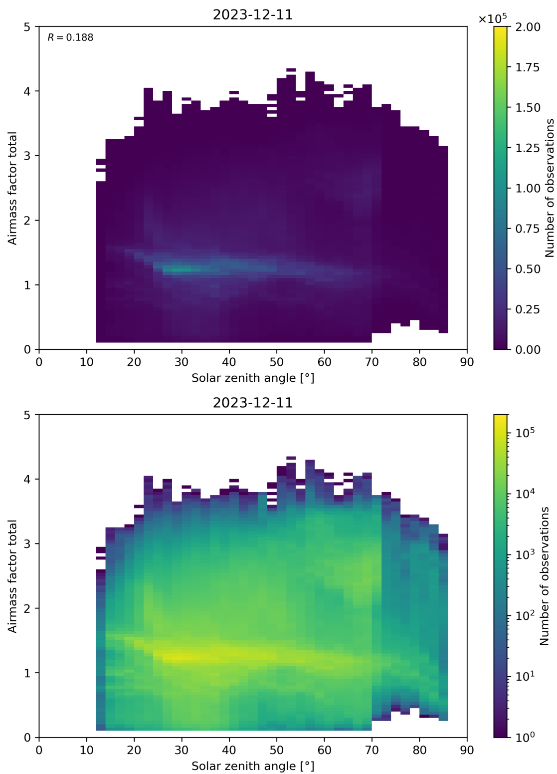
Figure 175: Scatter density plot of “Solar zenith angle” against “Airmass factor total” for 2023-12-10 to 2023-12-12.
