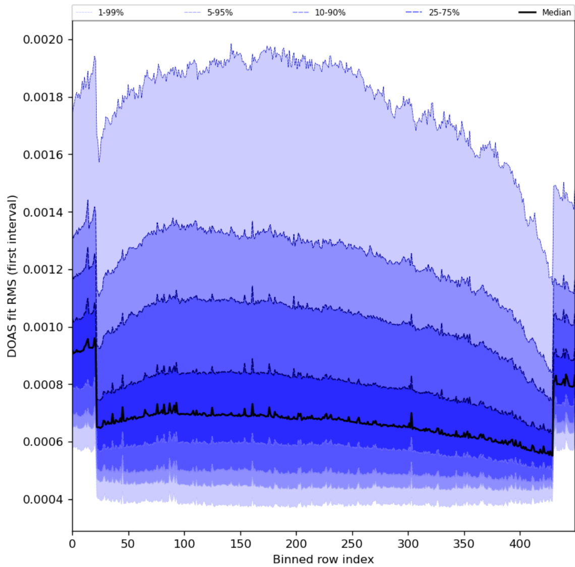
Figure 60: Along track statistics of “DOAS fit RMS (first interval)” for 2023-12-10 to 2023-12-12
