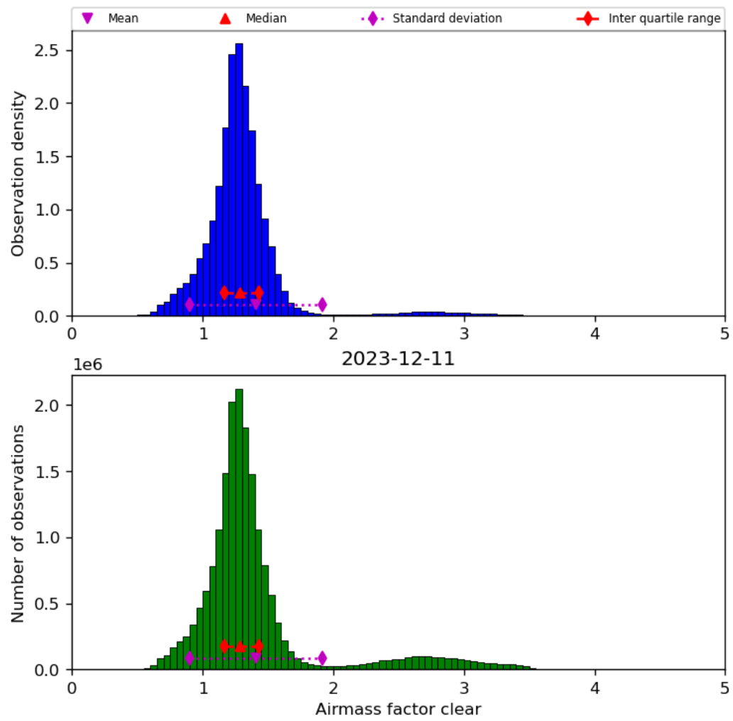
Figure 42: Histogram of “Airmass factor clear” for 2023-12-10 to 2023-12-12
