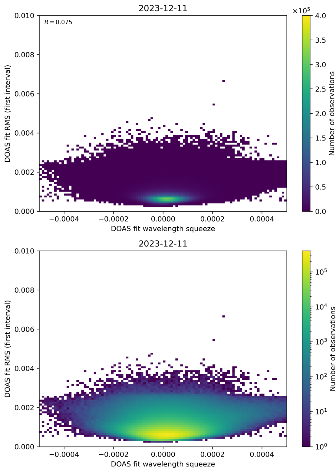
Figure 68: Scatter density plot of “DOAS fit wavelength squeeze” against “DOAS fit RMS (first interval)” for 2023-12-10 to 2023-12-12.
