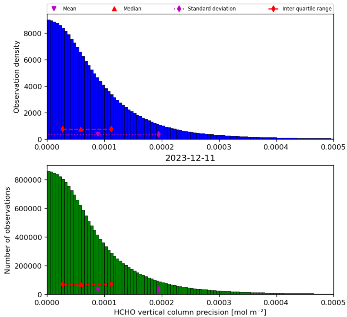
Figure 36: Histogram of “HCHO vertical column precision” for 2023-12-10 to 2023-12-12
