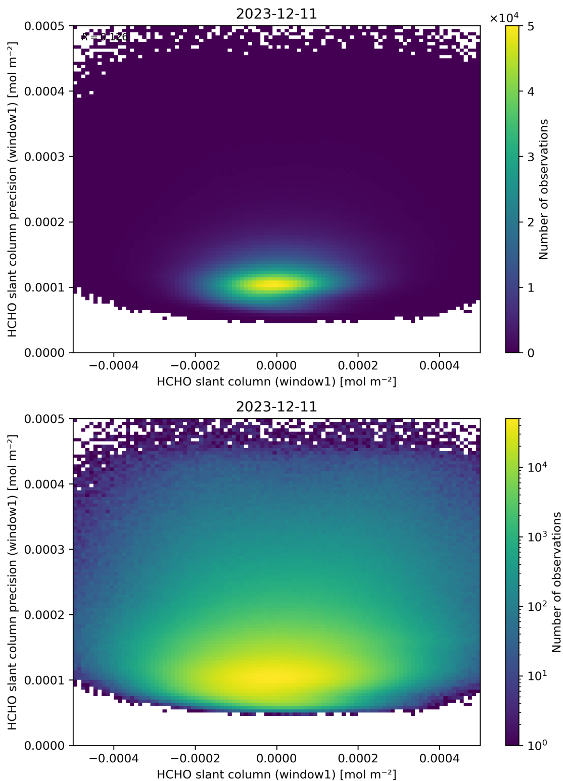
Figure 84: Scatter density plot of “HCHO slant column (window1)” against “HCHO slant column precision (window1)” for 2023-12-10 to 2023-12-12.
