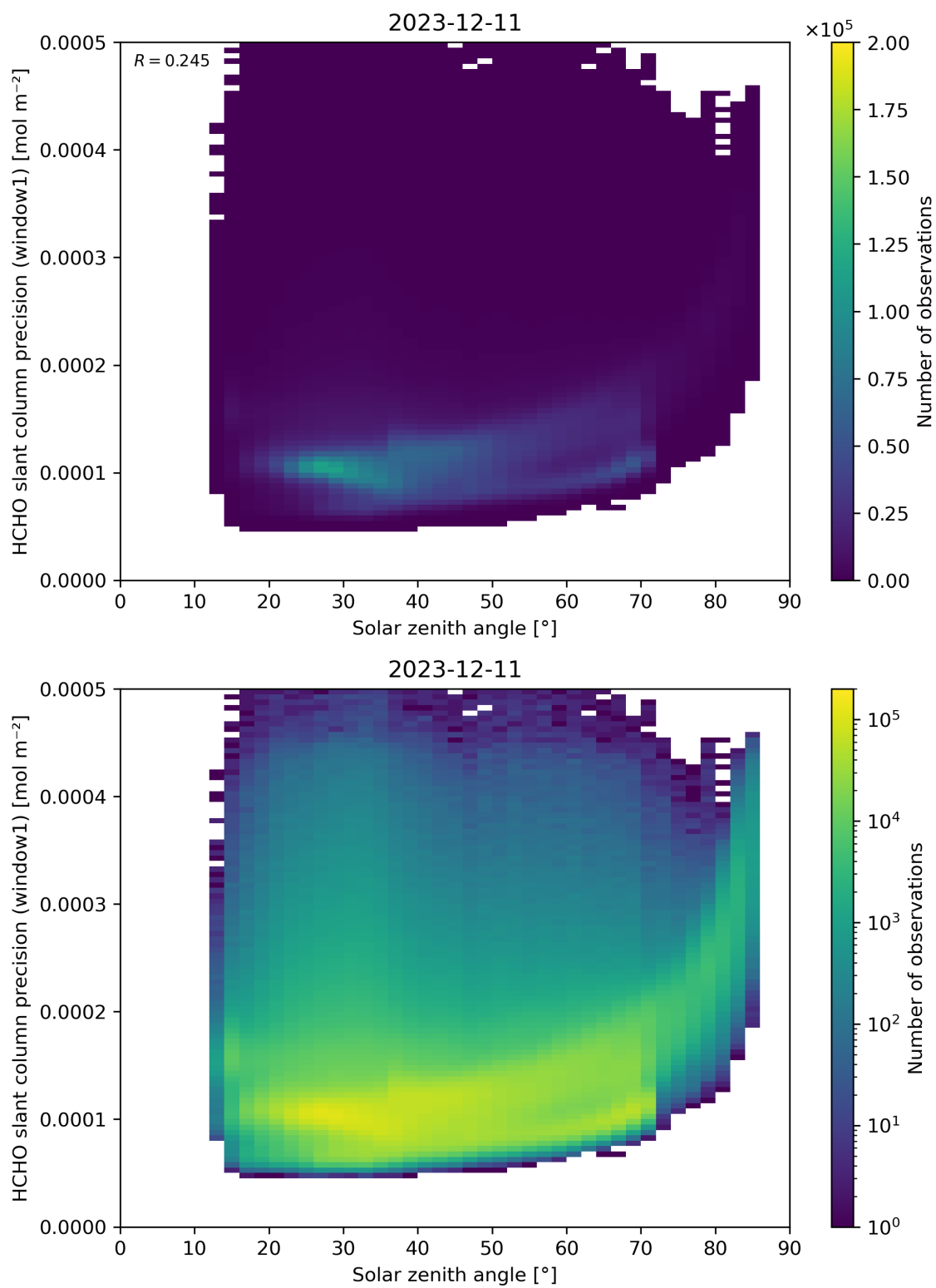
Figure 174: Scatter density plot of “Solar zenith angle” against “HCHO slant column precision (window1)” for 2023-12-10 to 2023-12-12.
