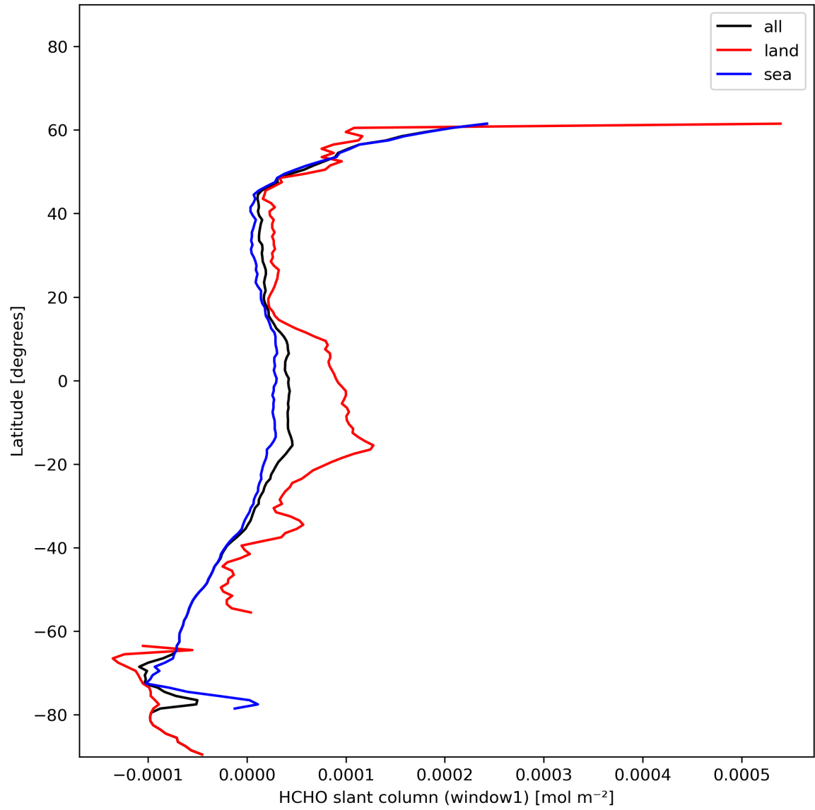
Figure 24: Zonal average of “HCHO slant column (window1)” for 2023-12-10 to 2023-12-12.
