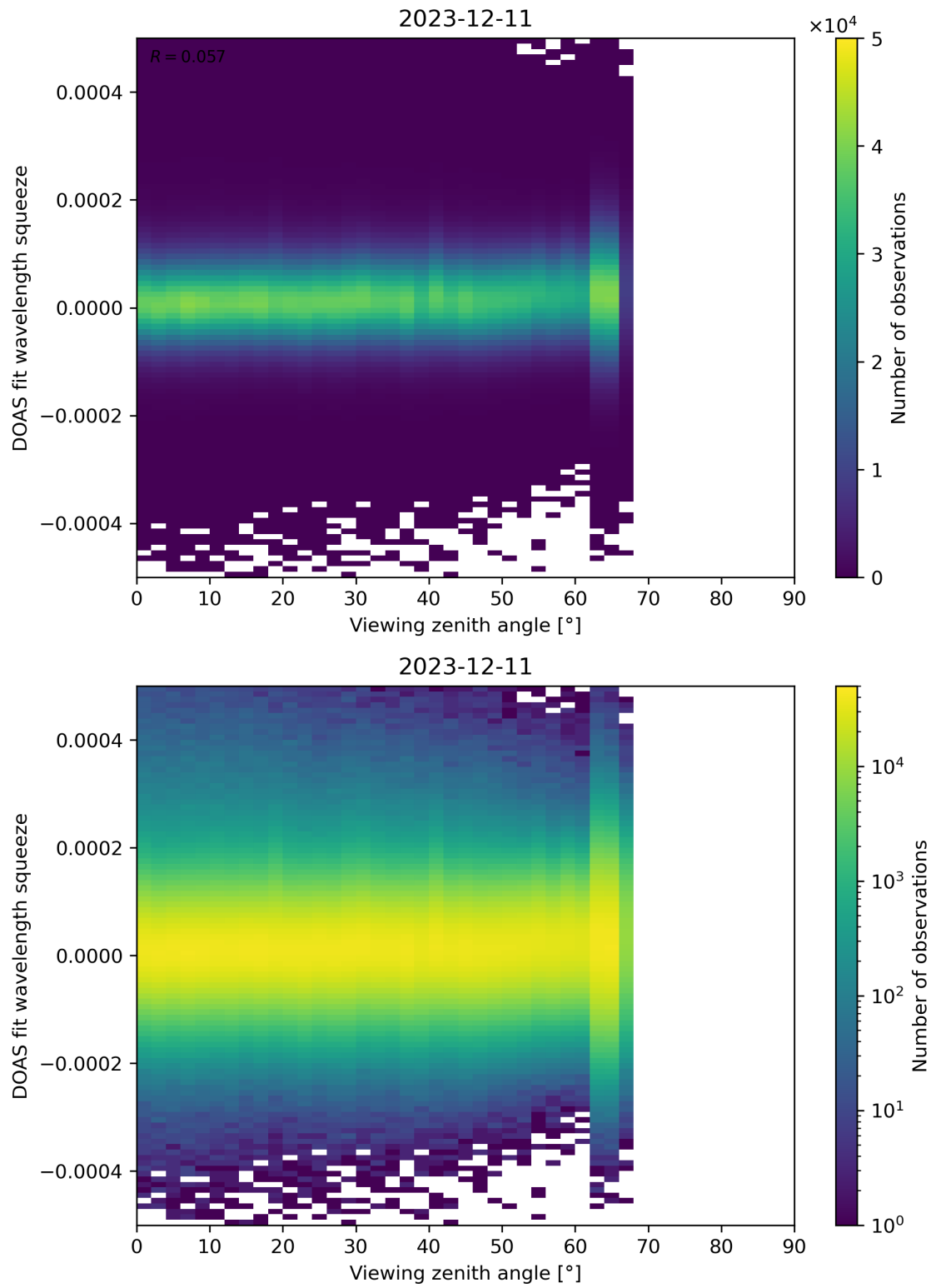
Figure 184: Scatter density plot of “Viewing zenith angle” against “DOAS fit wavelength squeeze” for 2023-12-10 to 2023-12-12.
