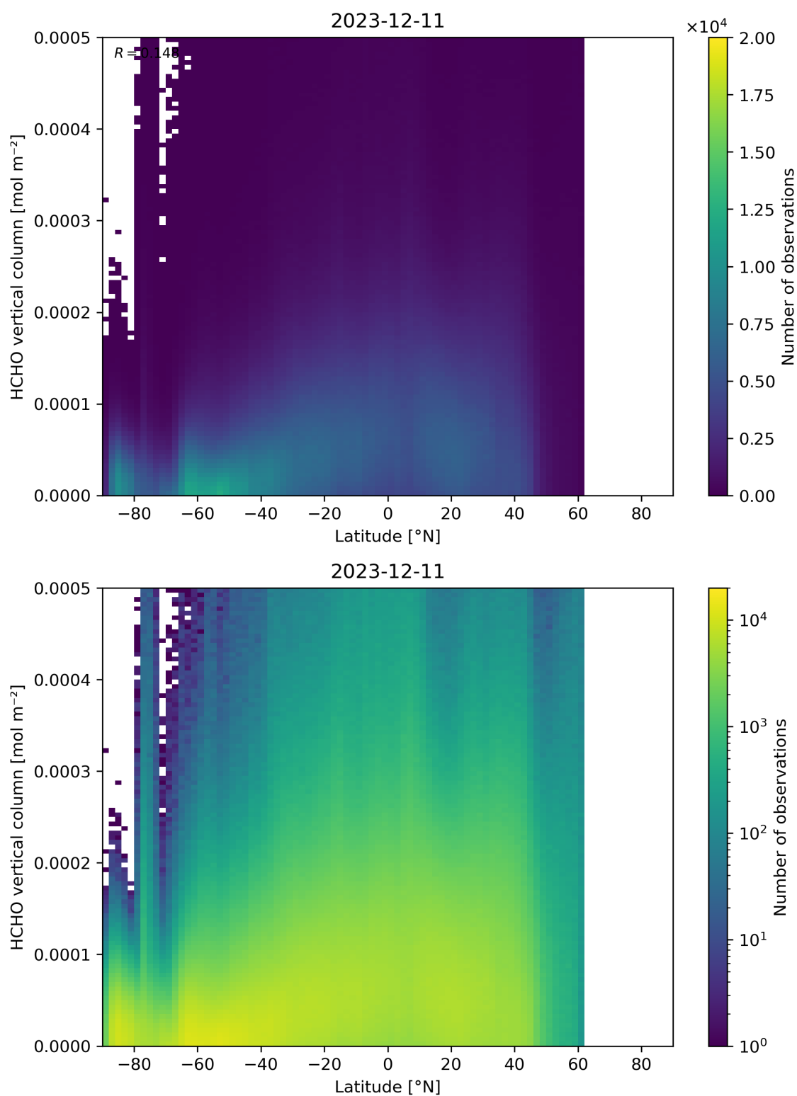
Figure 163: Scatter density plot of “Latitude” against “HCHO vertical column” for 2023-12-10 to 2023-12-12.
