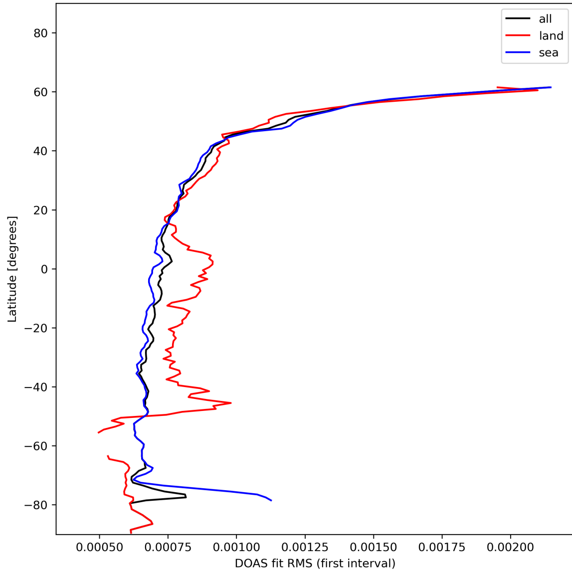
Figure 32: Zonal average of “DOAS fit RMS (first interval)” for 2023-12-10 to 2023-12-12.
