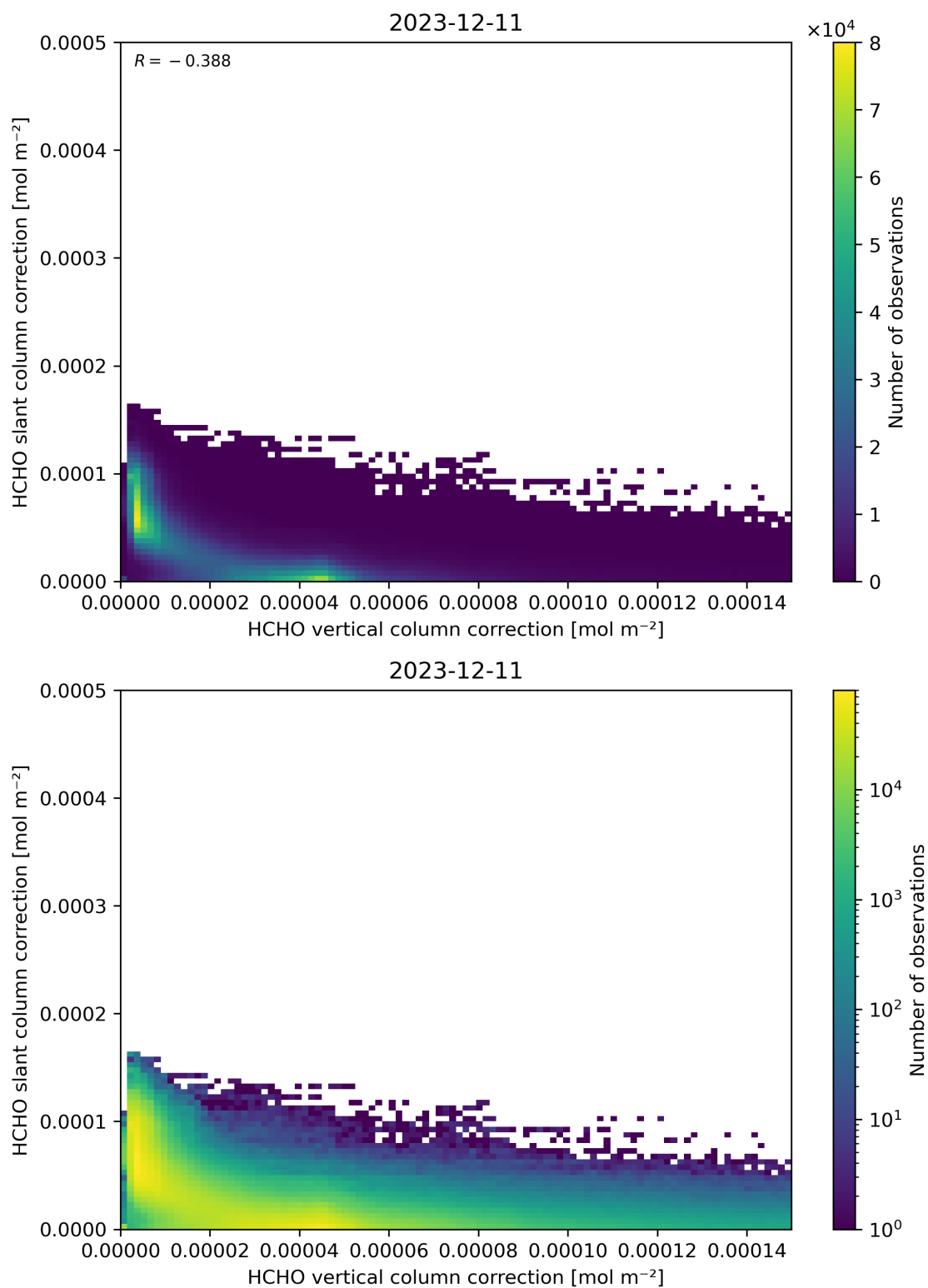
Figure 117: Scatter density plot of “HCHO vertical column correction” against “HCHO slant column correction” for 2023-12-10 to 2023-12-12.
