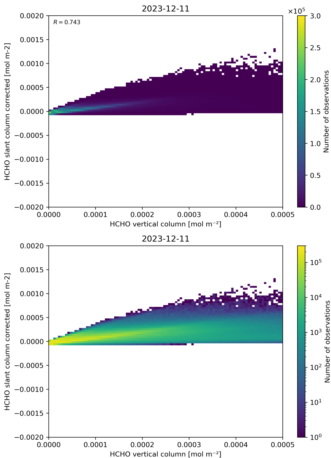
Figure 127: Scatter density plot of “HCHO vertical column” against “HCHO slant column corrected” for 2023-12-10 to 2023-12-12.
