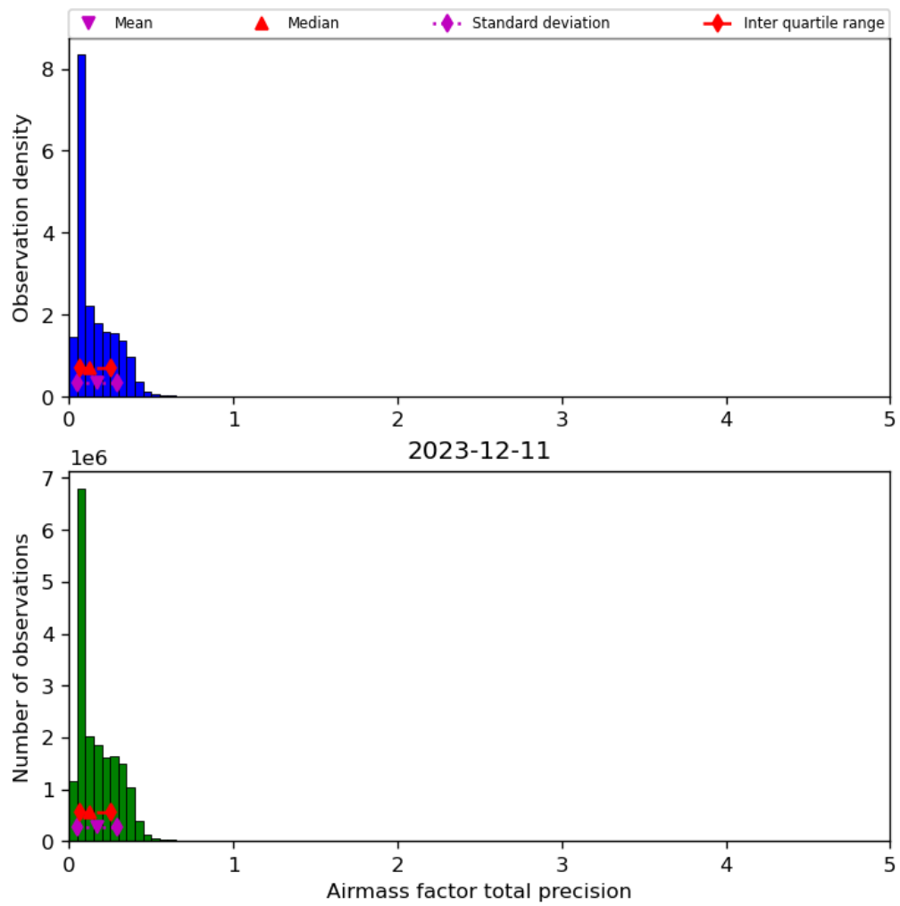
Figure 41: Histogram of “Airmass factor total precision” for 2023-12-10 to 2023-12-12
