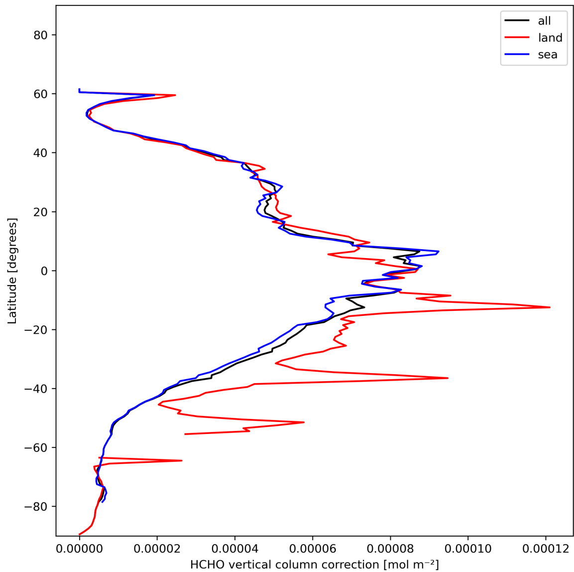
Figure 23: Zonal average of “HCHO vertical column correction” for 2023-12-10 to 2023-12-12.
