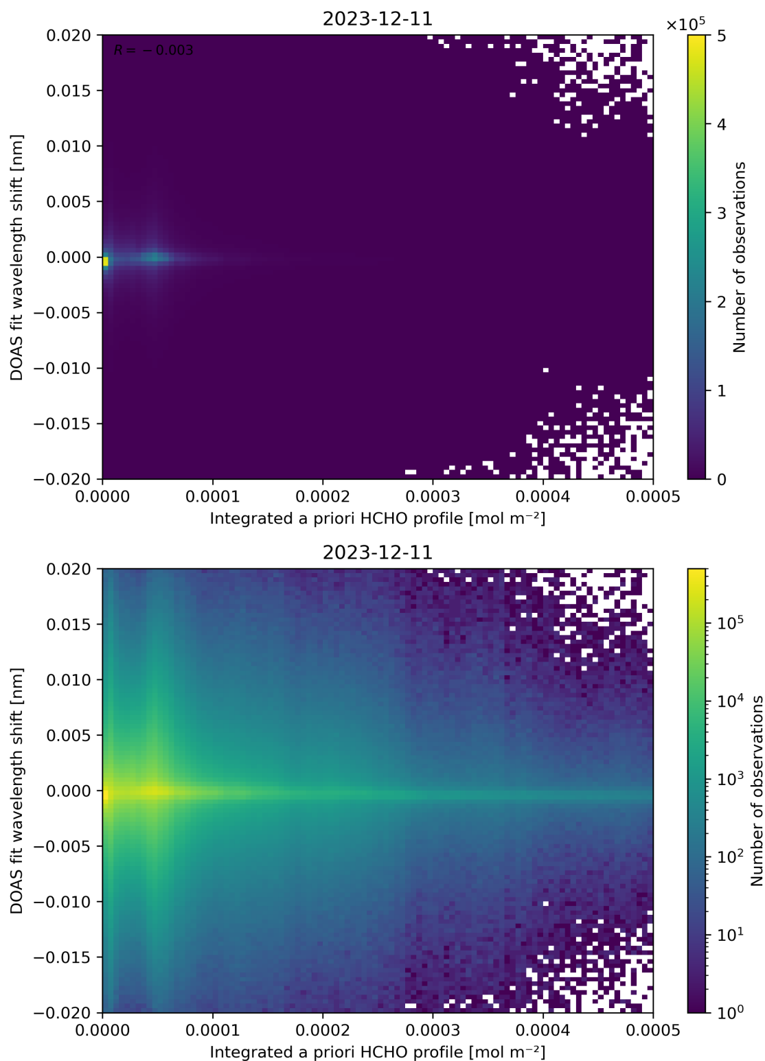
Figure 149: Scatter density plot of “Integrated a priori HCHO profile” against “DOAS fit wavelength shift” for 2023-12-10 to 2023-12-12.
