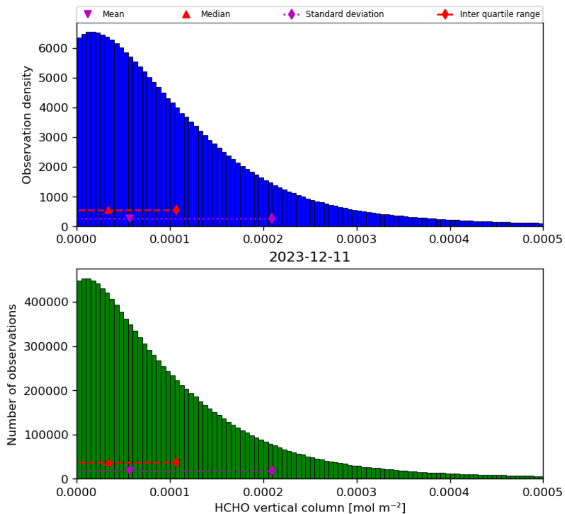
Figure 35: Histogram of “HCHO vertical column” for 2023-12-10 to 2023-12-12
