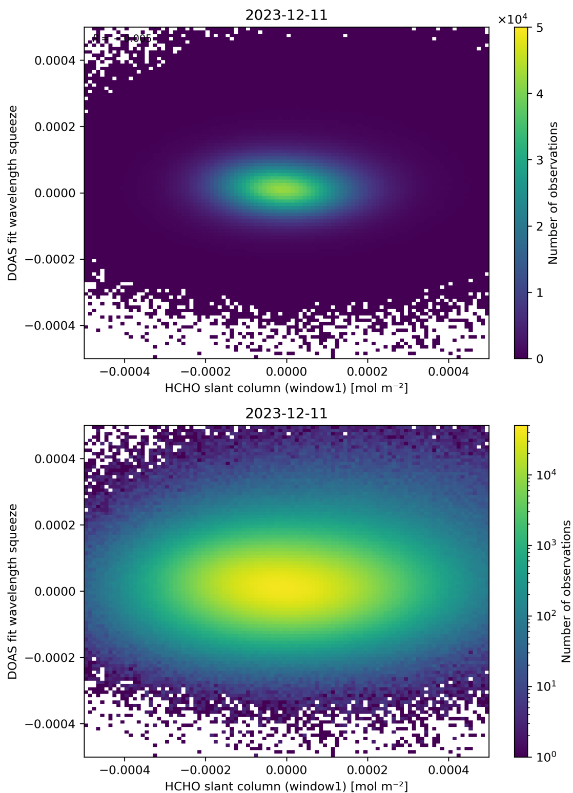
Figure 80: Scatter density plot of “HCHO slant column (window1)” against “DOAS fit wavelength squeeze” for 2023-12-10 to 2023-12-12.
