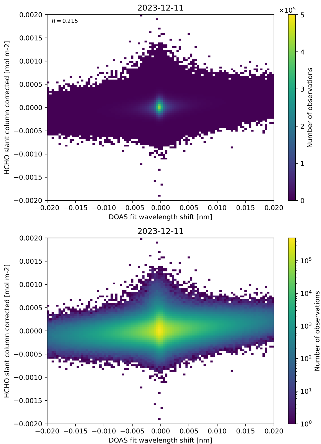
Figure 66: Scatter density plot of “DOAS fit wavelength shift” against “HCHO slant column corrected” for 2023-12-10 to 2023-12-12.
