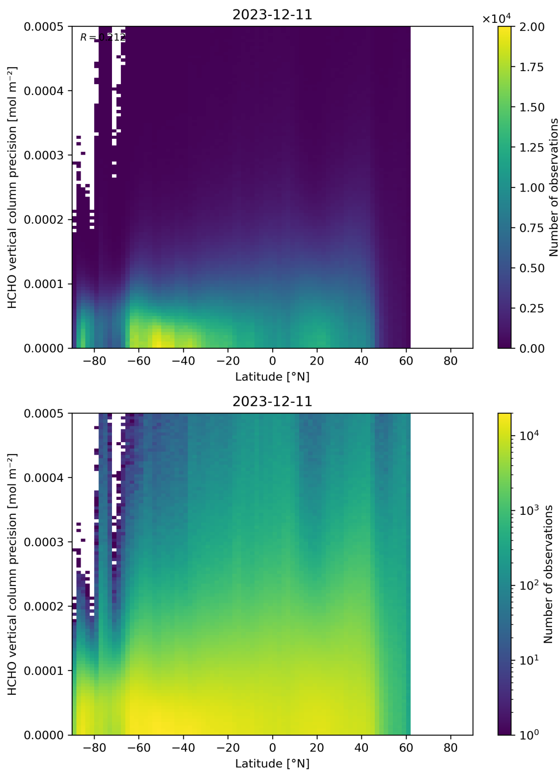
Figure 165: Scatter density plot of “Latitude” against “HCHO vertical column precision” for 2023-12-10 to 2023-12-12.
