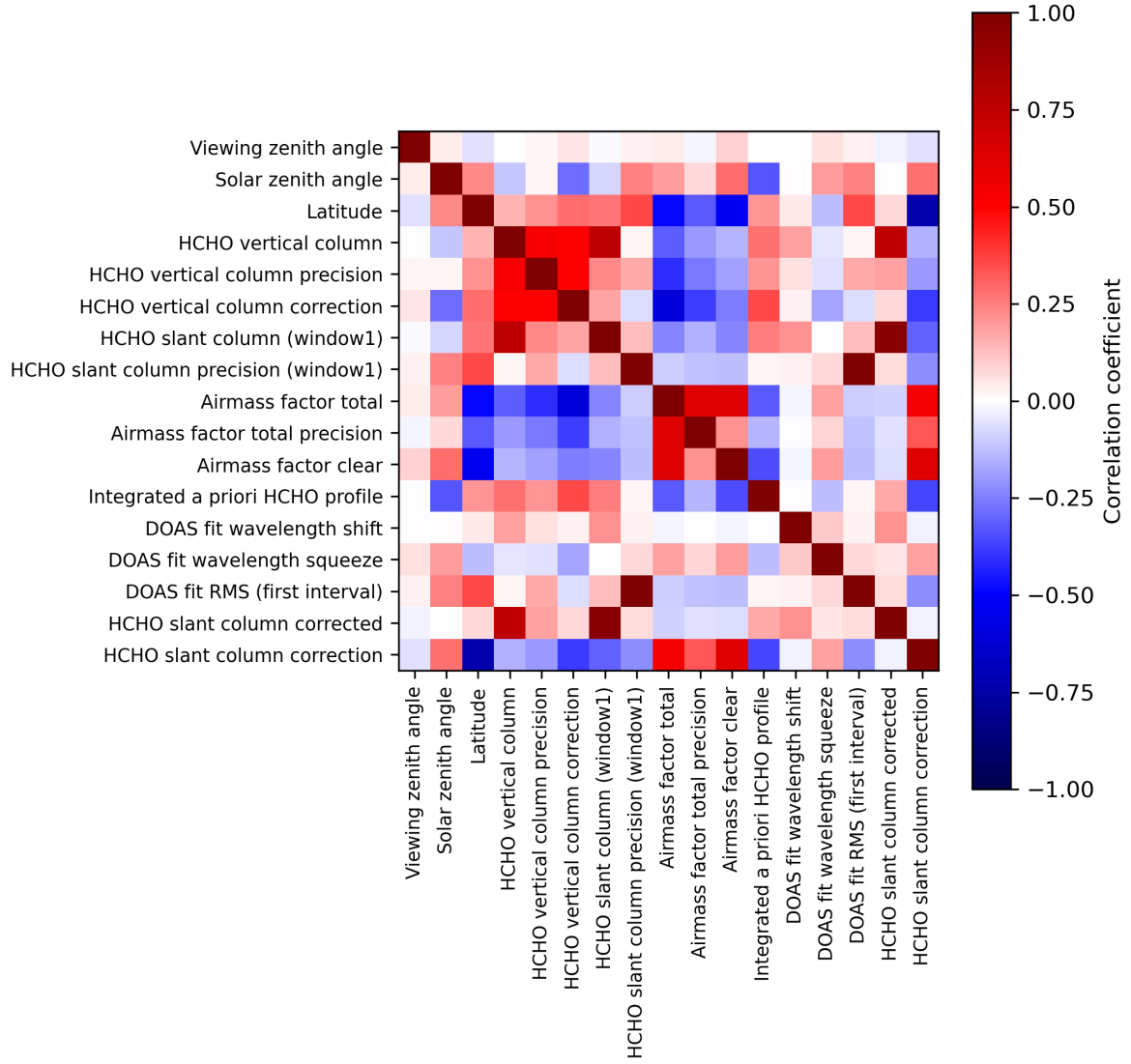
Figure 2: Map of correlation matrix for 2023-12-10 to 2023-12-12.
