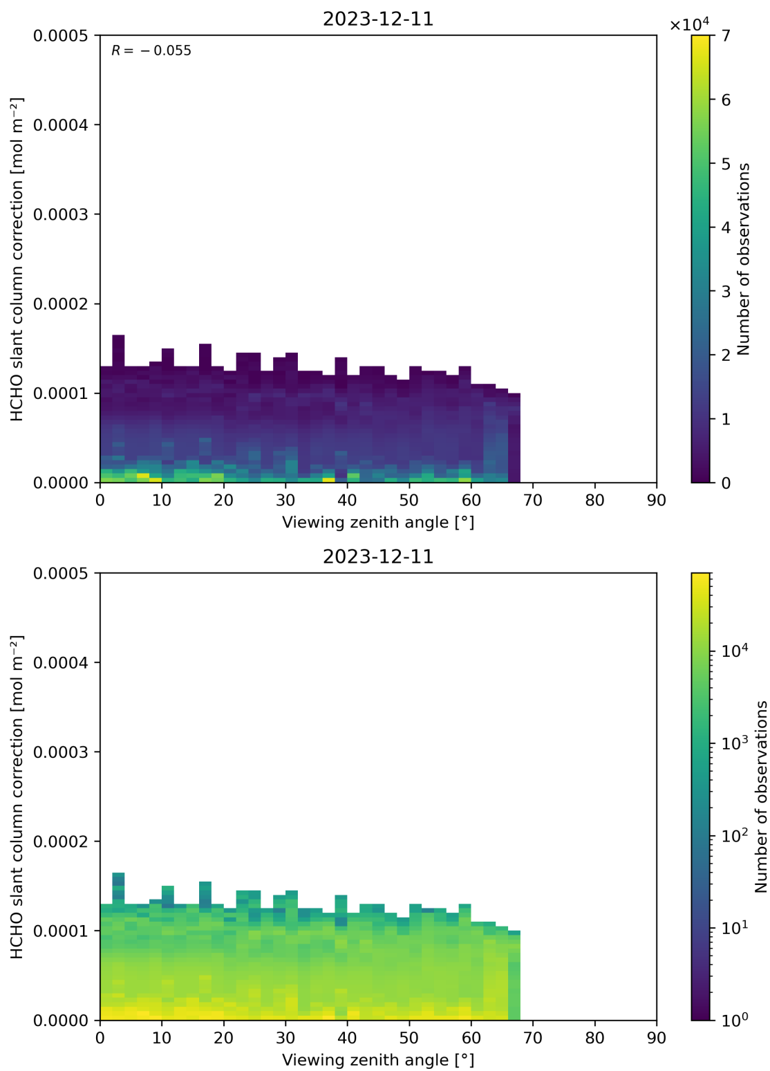
Figure 187: Scatter density plot of “Viewing zenith angle” against “HCHO slant column correction” for 2023-12-10 to 2023-12-12.
