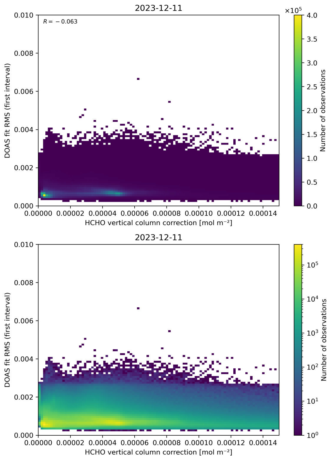
Figure 112: Scatter density plot of “HCHO vertical column correction” against “DOAS fit RMS (first interval)” for 2023-12-10 to 2023-12-12.
