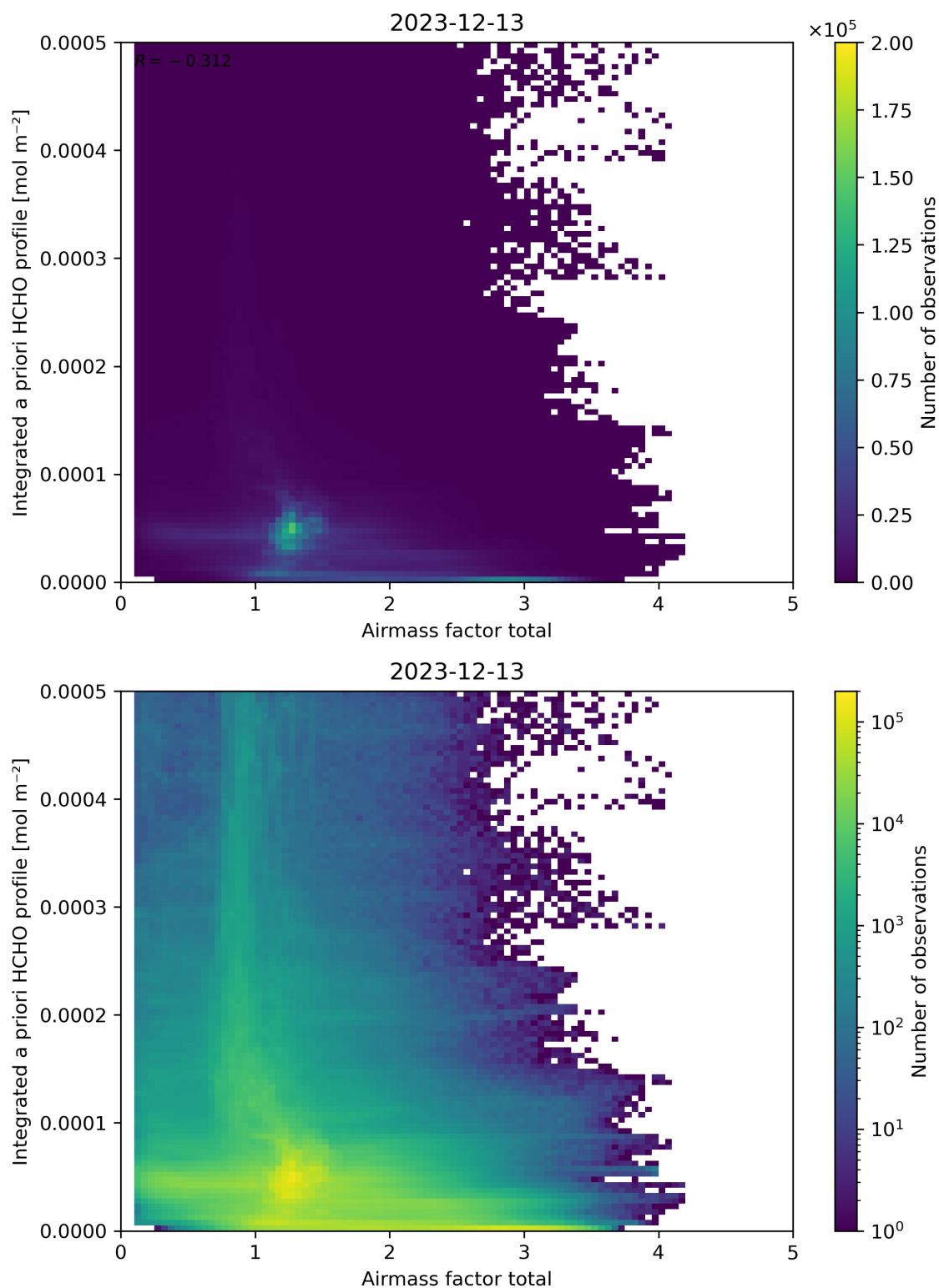
Figure 104: Scatter density plot of “Airmass factor total” against “Integrated a priori HCHO profile” for 2023-12-12 to 2023-12-14.
