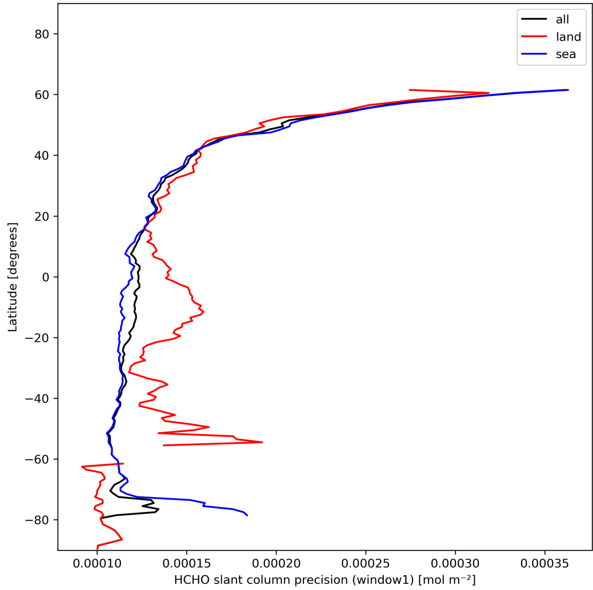
Figure 25: Zonal average of “HCHO slant column precision (window1)” for 2023-12-12 to 2023-12-14.
