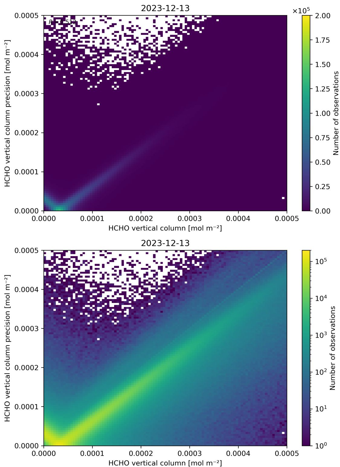
Figure 134: Scatter density plot of “HCHO vertical column” against “HCHO vertical column precision” for 2023-12-12 to 2023-12-14.
