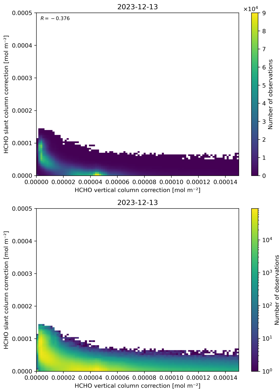
Figure 117: Scatter density plot of “HCHO vertical column correction” against “HCHO slant column correction” for 2023-12-12 to 2023-12-14.
