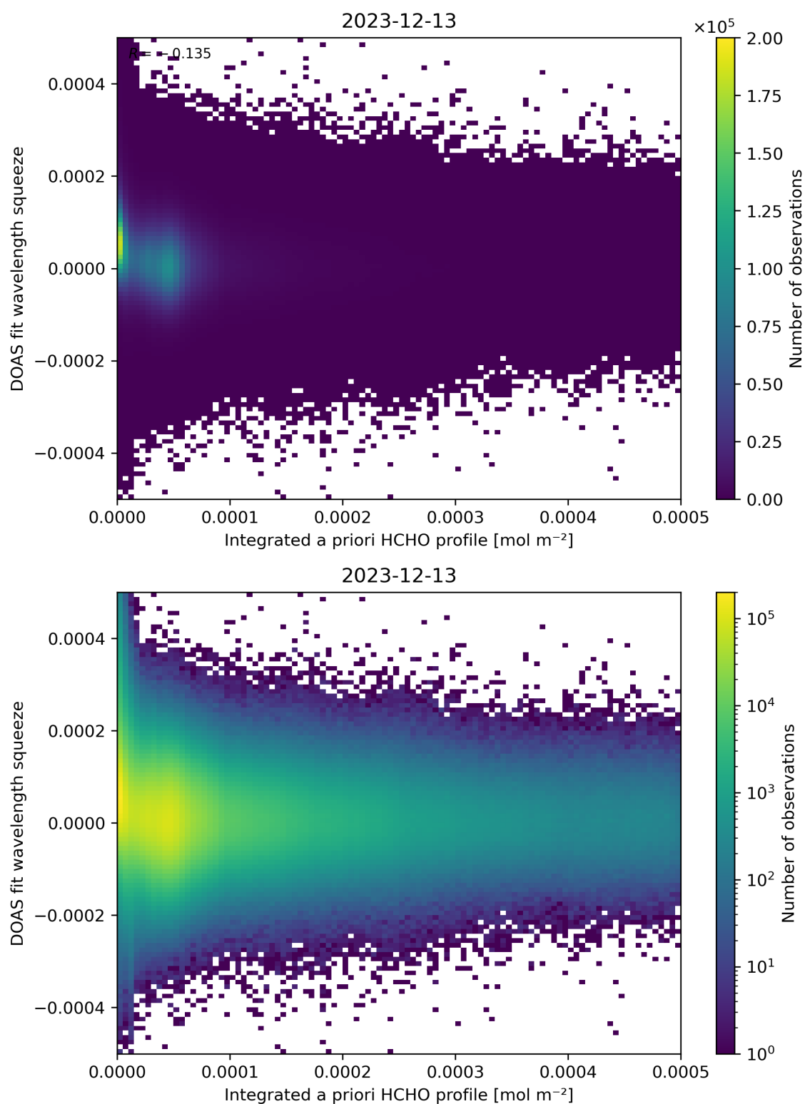
Figure 150: Scatter density plot of “Integrated a priori HCHO profile” against “DOAS fit wavelength squeeze” for 2023-12-12 to 2023-12-14.
