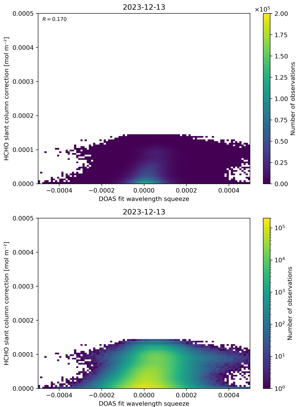
Figure 70: Scatter density plot of “DOAS fit wavelength squeeze” against “HCHO slant column correction” for 2023-12-12 to 2023-12-14.
