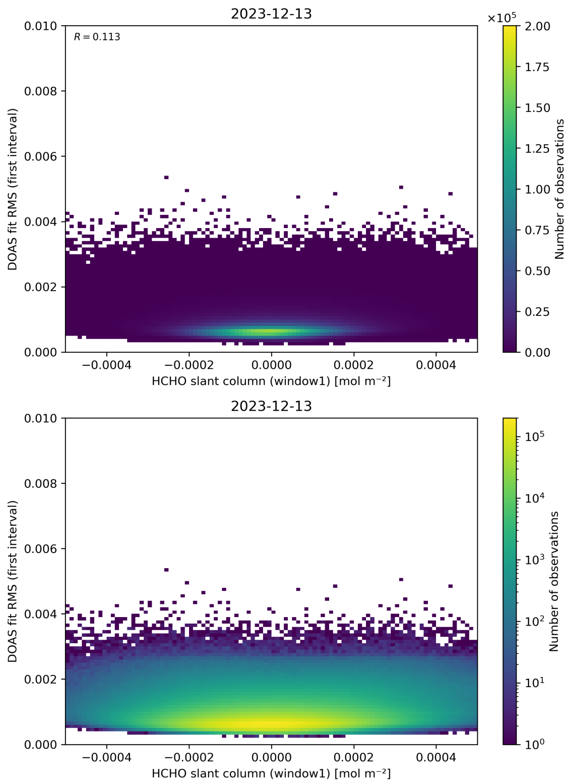
Figure 78: Scatter density plot of “HCHO slant column (window1)” against “DOAS fit RMS (first interval)” for 2023-12-12 to 2023-12-14.
