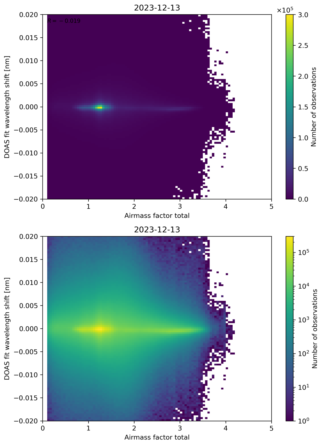
Figure 98: Scatter density plot of “Airmass factor total” against “DOAS fit wavelength shift” for 2023-12-12 to 2023-12-14.
