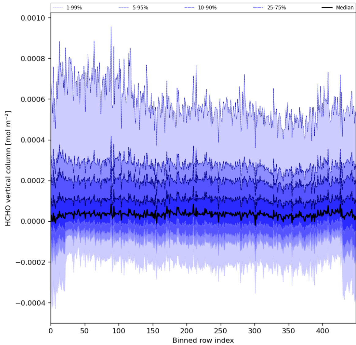
Figure 49: Along track statistics of “HCHO vertical column” for 2023-12-12 to 2023-12-14
