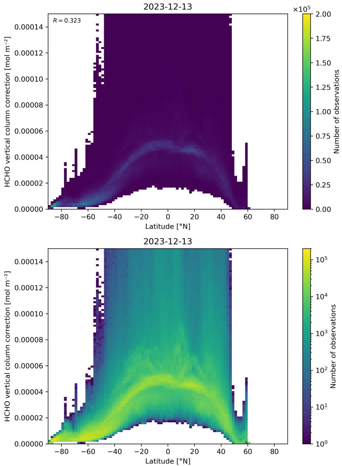
Figure 164: Scatter density plot of “Latitude” against “HCHO vertical column correction” for 2023-12-12 to 2023-12-14.
