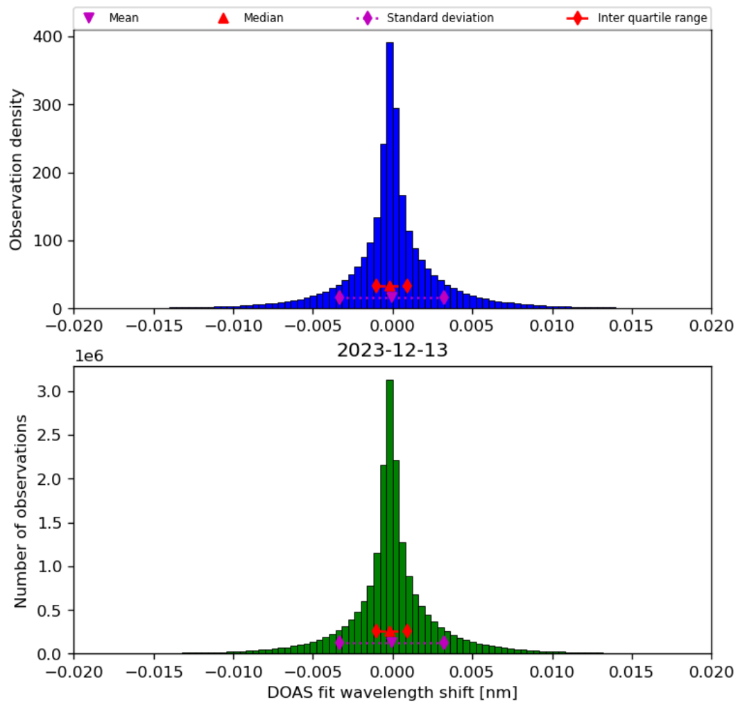
Figure 44: Histogram of “DOAS fit wavelength shift” for 2023-12-12 to 2023-12-14
