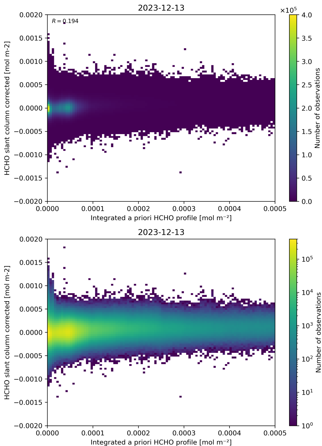
Figure 151: Scatter density plot of “Integrated a priori HCHO profile” against “HCHO slant column corrected” for 2023-12-12 to 2023-12-14.
