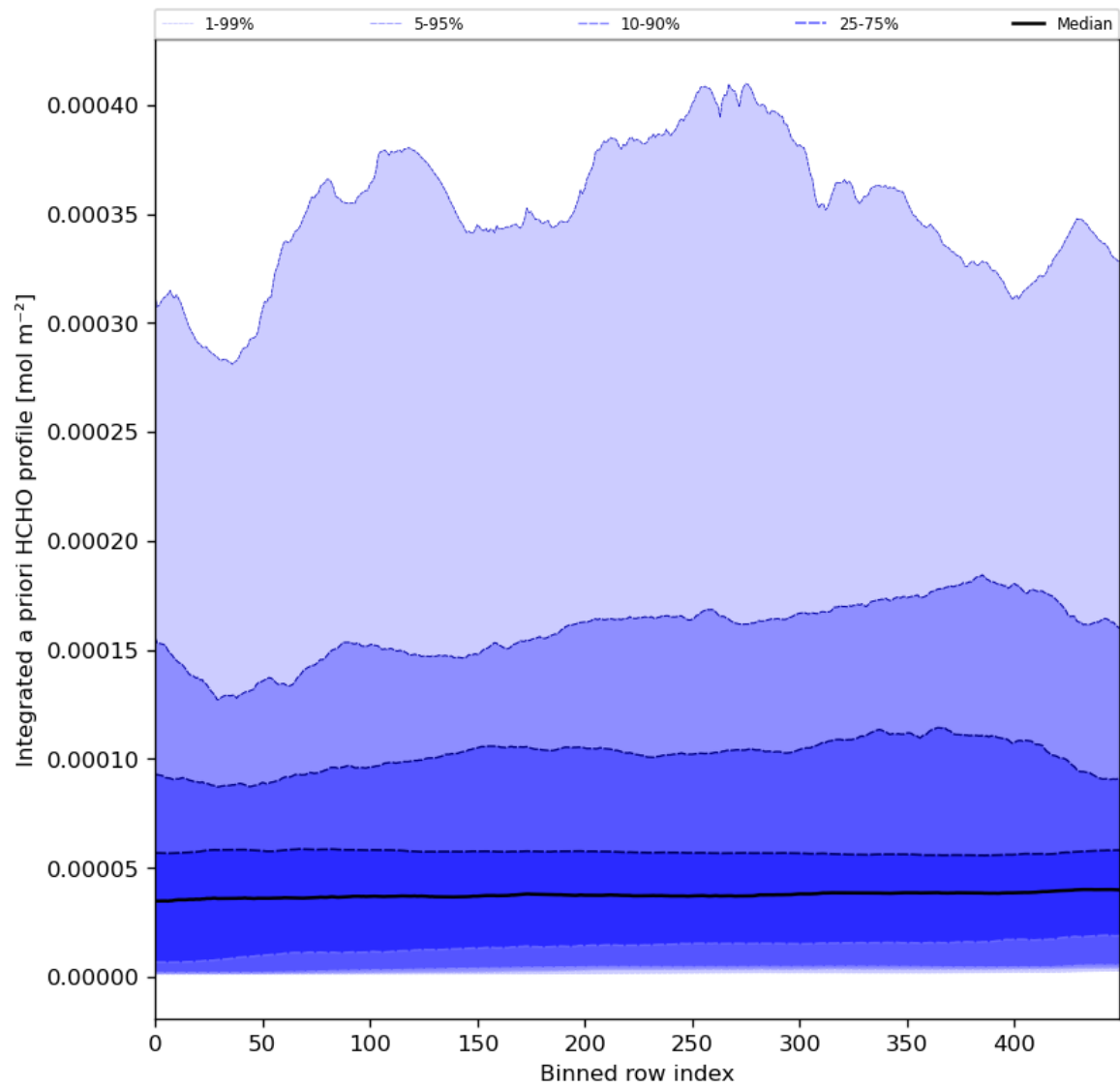
Figure 57: Along track statistics of “Integrated a priori HCHO profile” for 2023-12-12 to 2023-12-14
