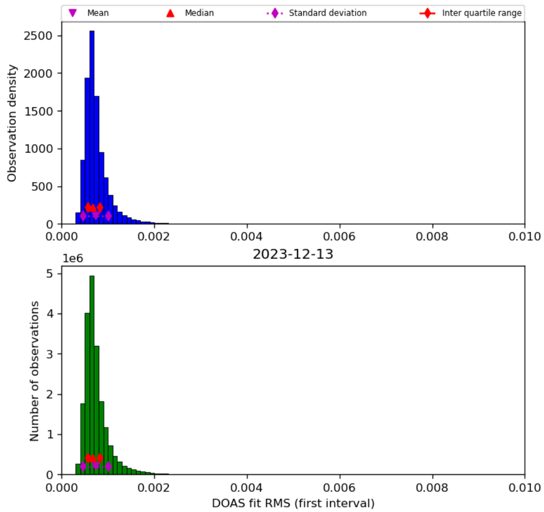
Figure 46: Histogram of “DOAS fit RMS (first interval)” for 2023-12-12 to 2023-12-14
