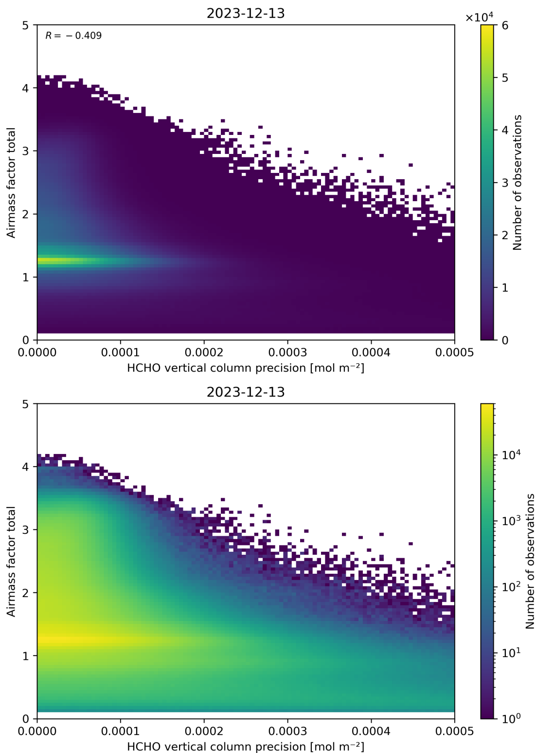
Figure 144: Scatter density plot of “HCHO vertical column precision” against “Airmass factor total” for 2023-12-12 to 2023-12-14.
