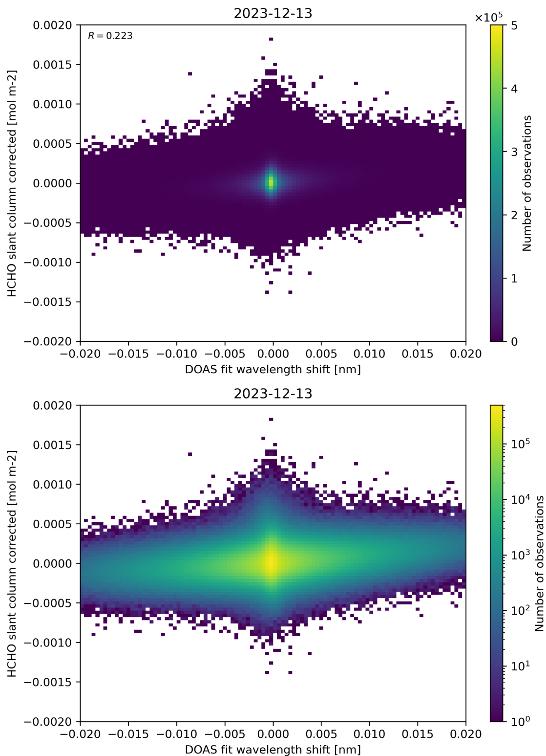
Figure 66: Scatter density plot of “DOAS fit wavelength shift” against “HCHO slant column corrected” for 2023-12-12 to 2023-12-14.
