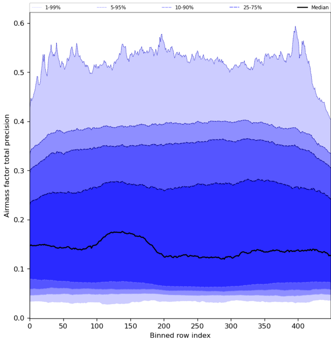
Figure 55: Along track statistics of “Airmass factor total precision” for 2023-12-12 to 2023-12-14
