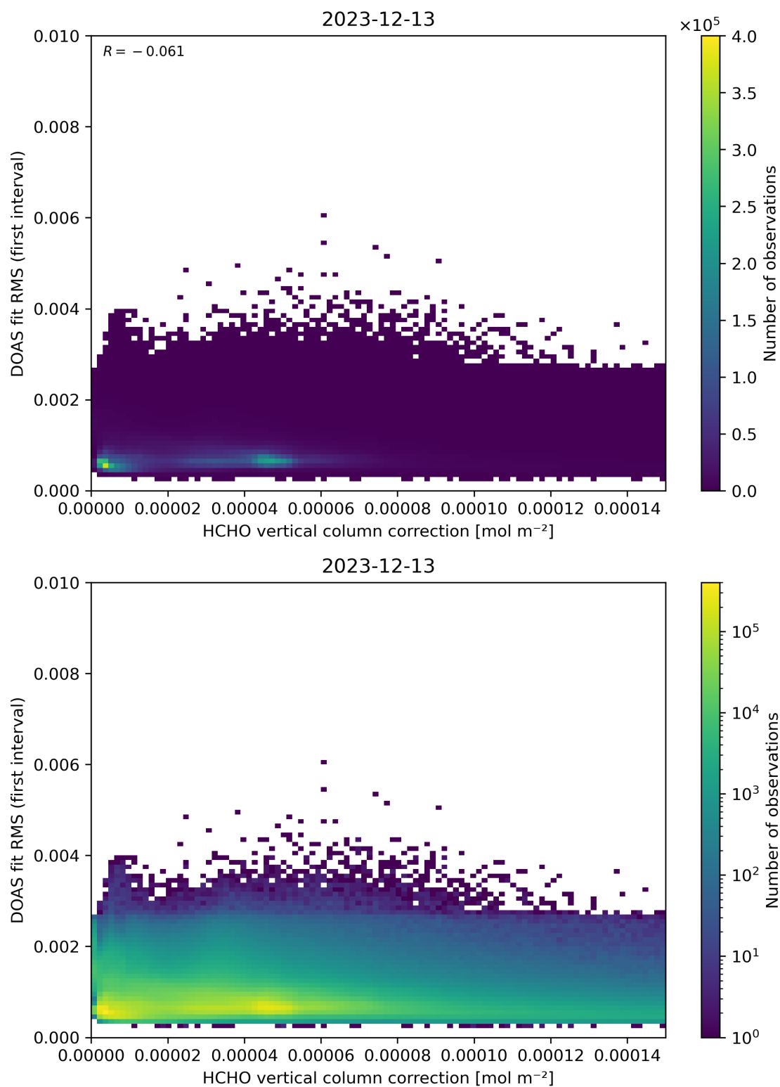
Figure 112: Scatter density plot of “HCHO vertical column correction” against “DOAS fit RMS (first interval)” for 2023-12-12 to 2023-12-14.
