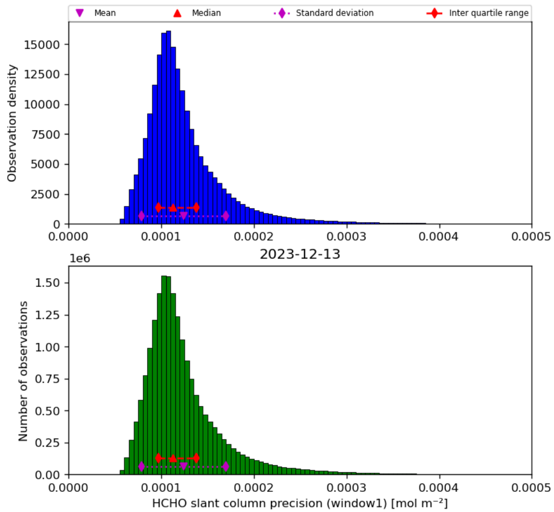
Figure 39: Histogram of “HCHO slant column precision (window1)” for 2023-12-12 to 2023-12-14
