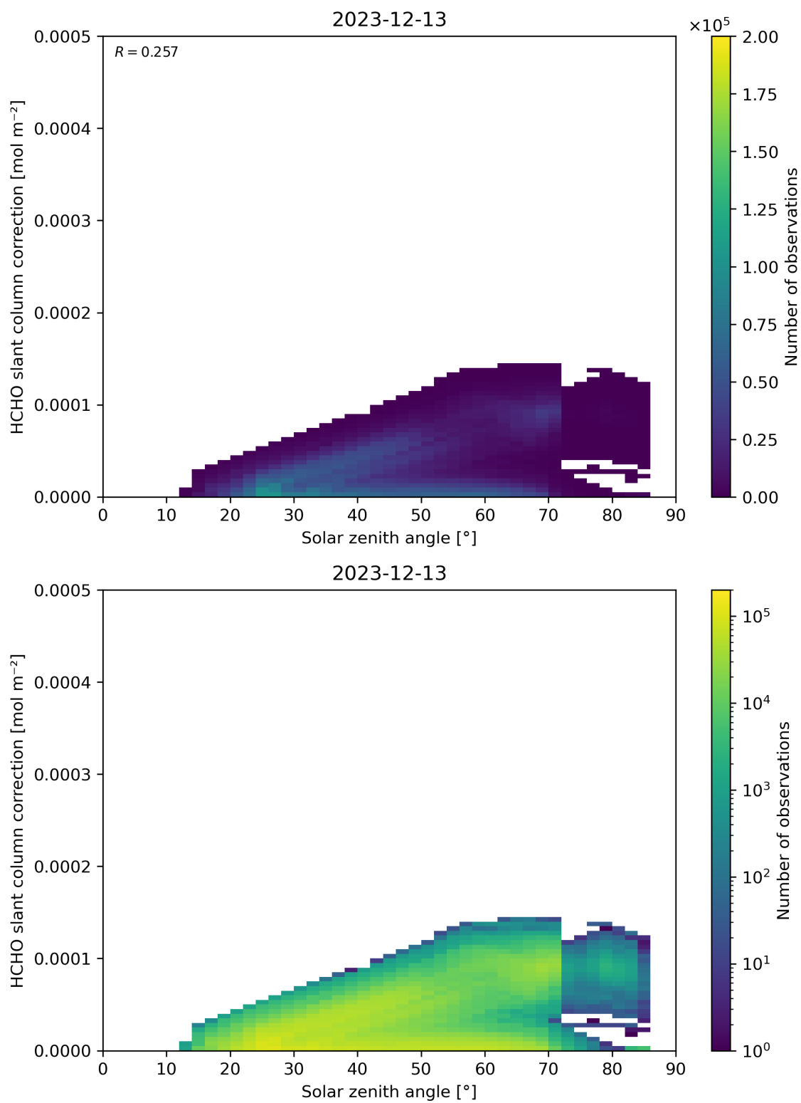
Figure 172: Scatter density plot of “Solar zenith angle” against “HCHO slant column correction” for 2023-12-12 to 2023-12-14.
