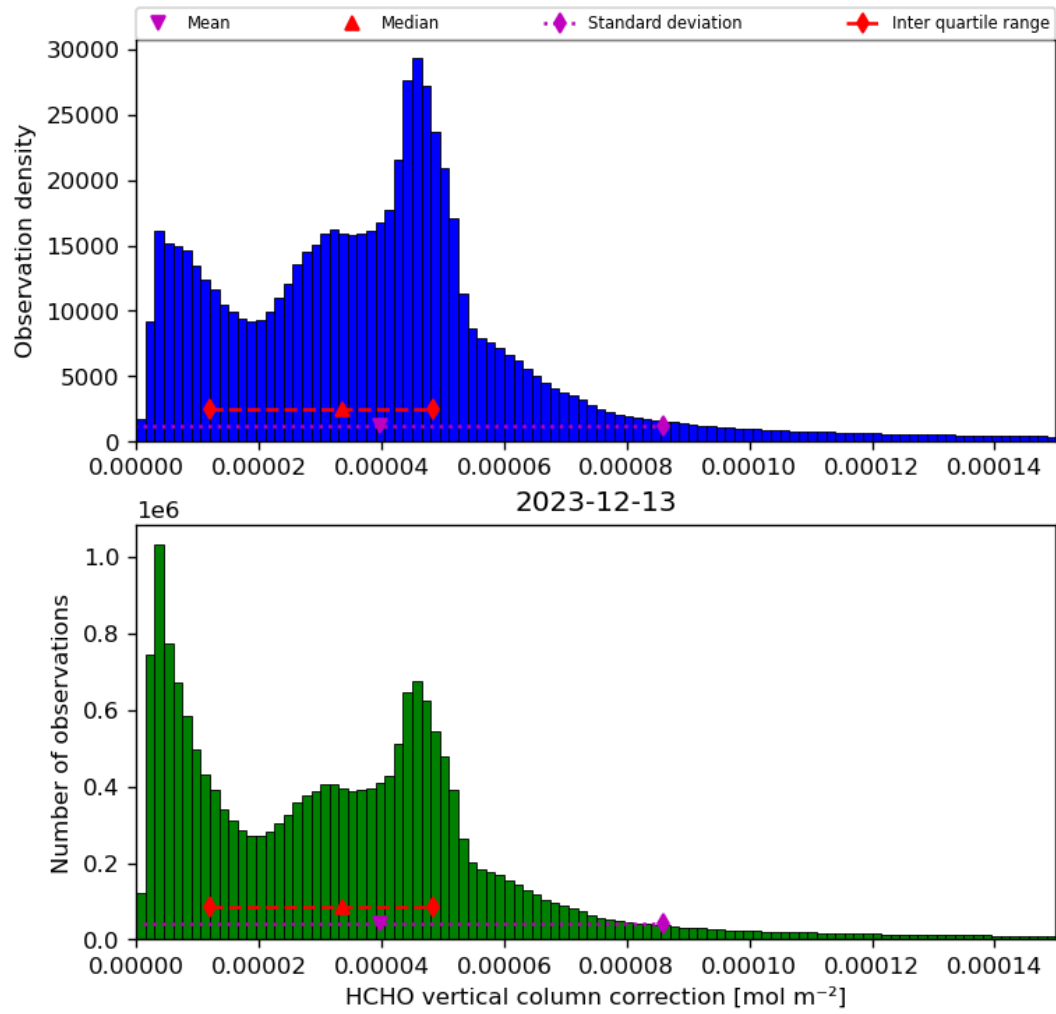
Figure 37: Histogram of “HCHO vertical column correction” for 2023-12-12 to 2023-12-14
