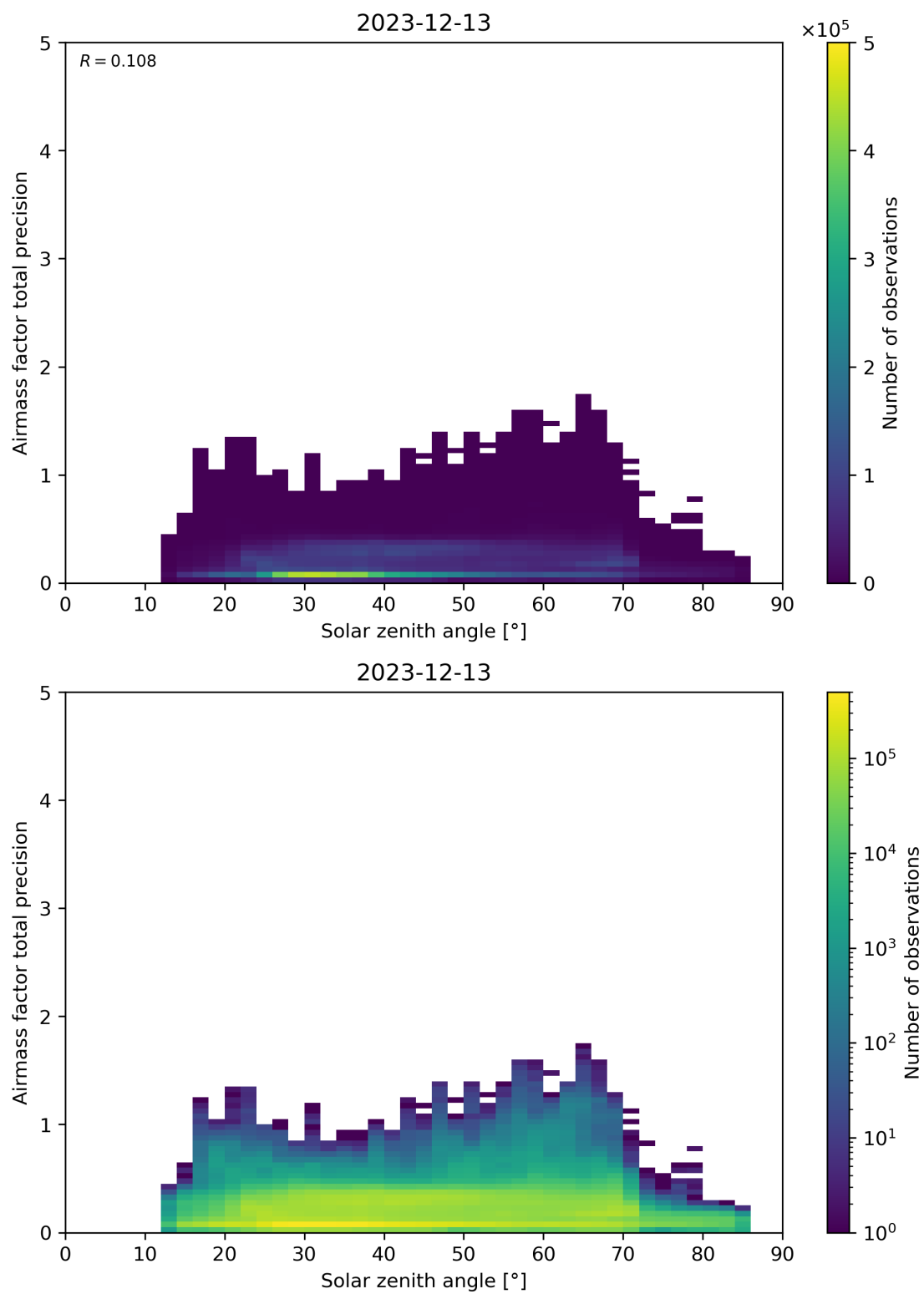
Figure 176: Scatter density plot of “Solar zenith angle” against “Airmass factor total precision” for 2023-12-12 to 2023-12-14.
