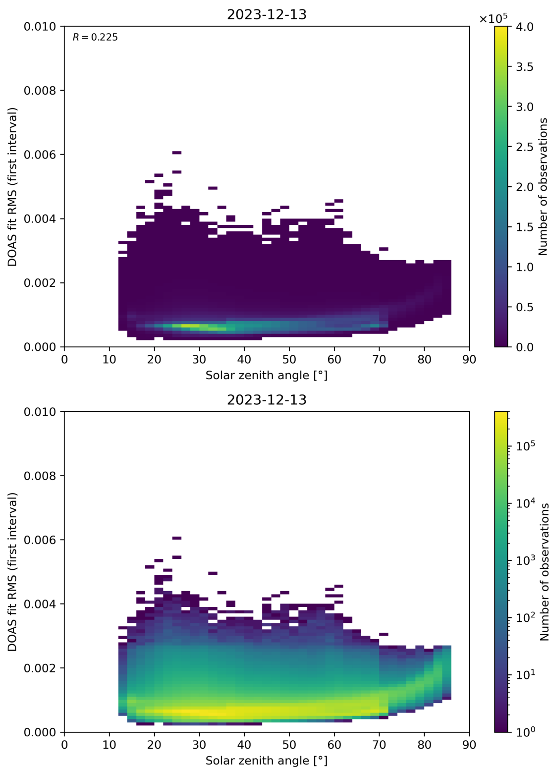
Figure 167: Scatter density plot of “Solar zenith angle” against “DOAS fit RMS (first interval)” for 2023-12-12 to 2023-12-14.
