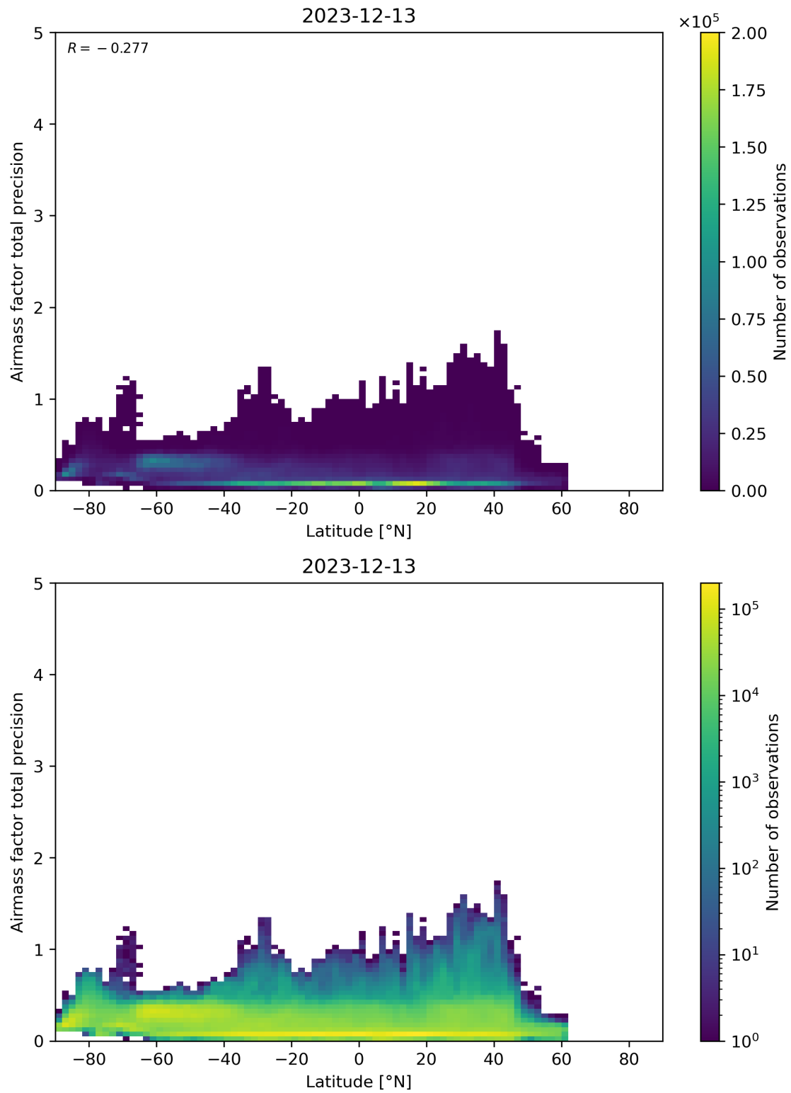
Figure 162: Scatter density plot of “Latitude” against “Airmass factor total precision” for 2023-12-12 to 2023-12-14.
