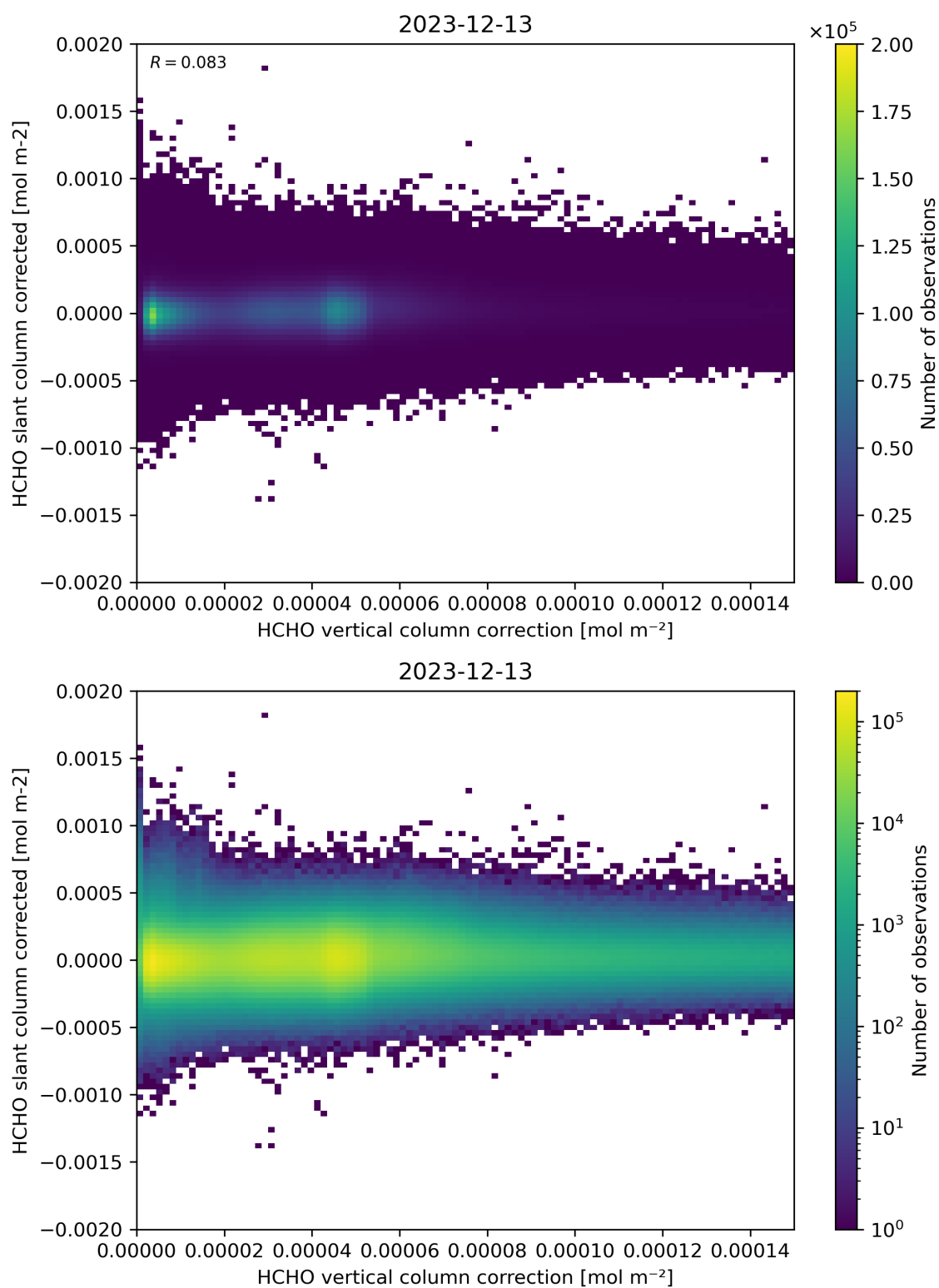
Figure 116: Scatter density plot of “HCHO vertical column correction” against “HCHO slant column corrected” for 2023-12-12 to 2023-12-14.
