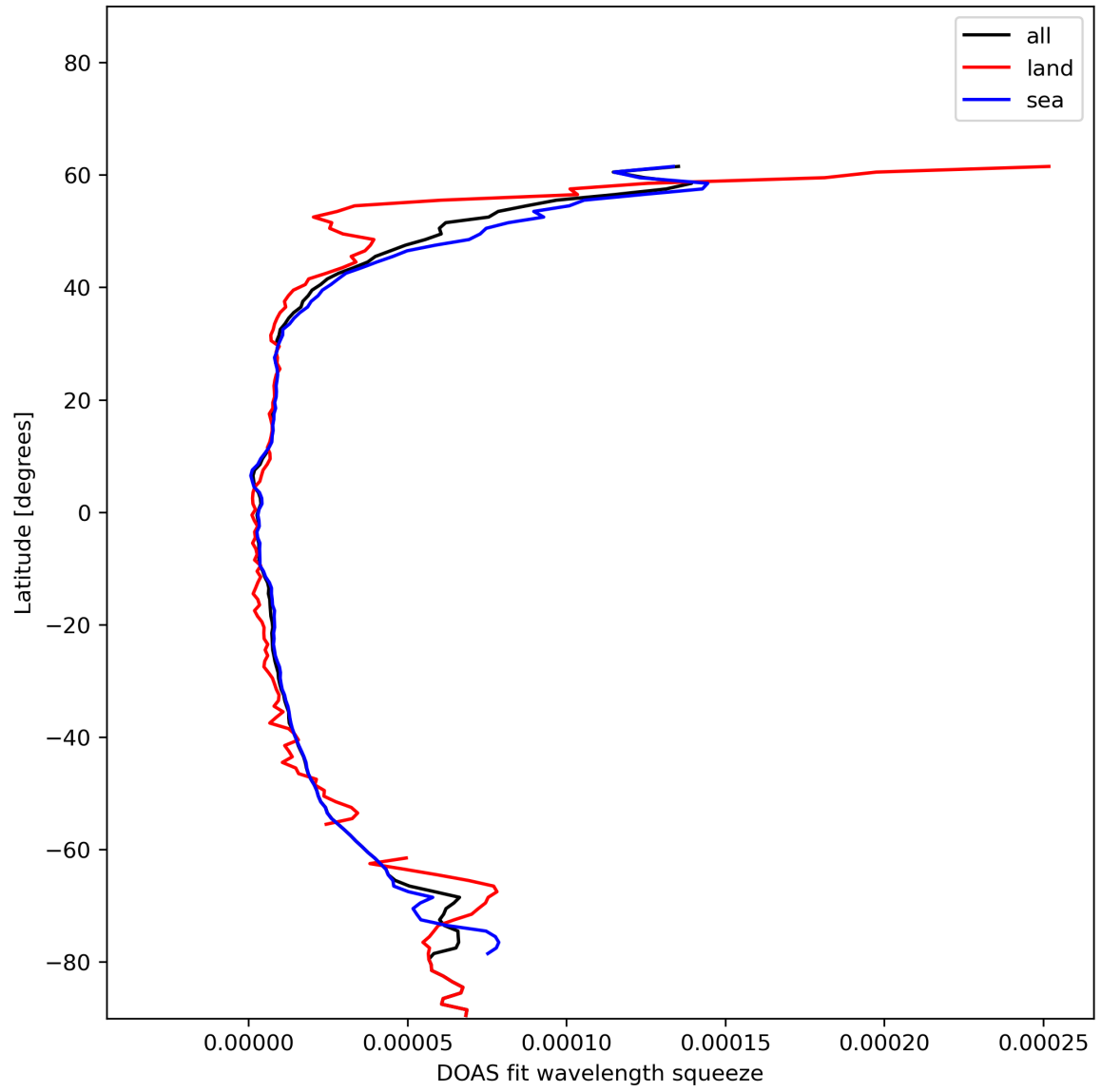
Figure 31: Zonal average of “DOAS fit wavelength squeeze” for 2023-12-12 to 2023-12-14.
