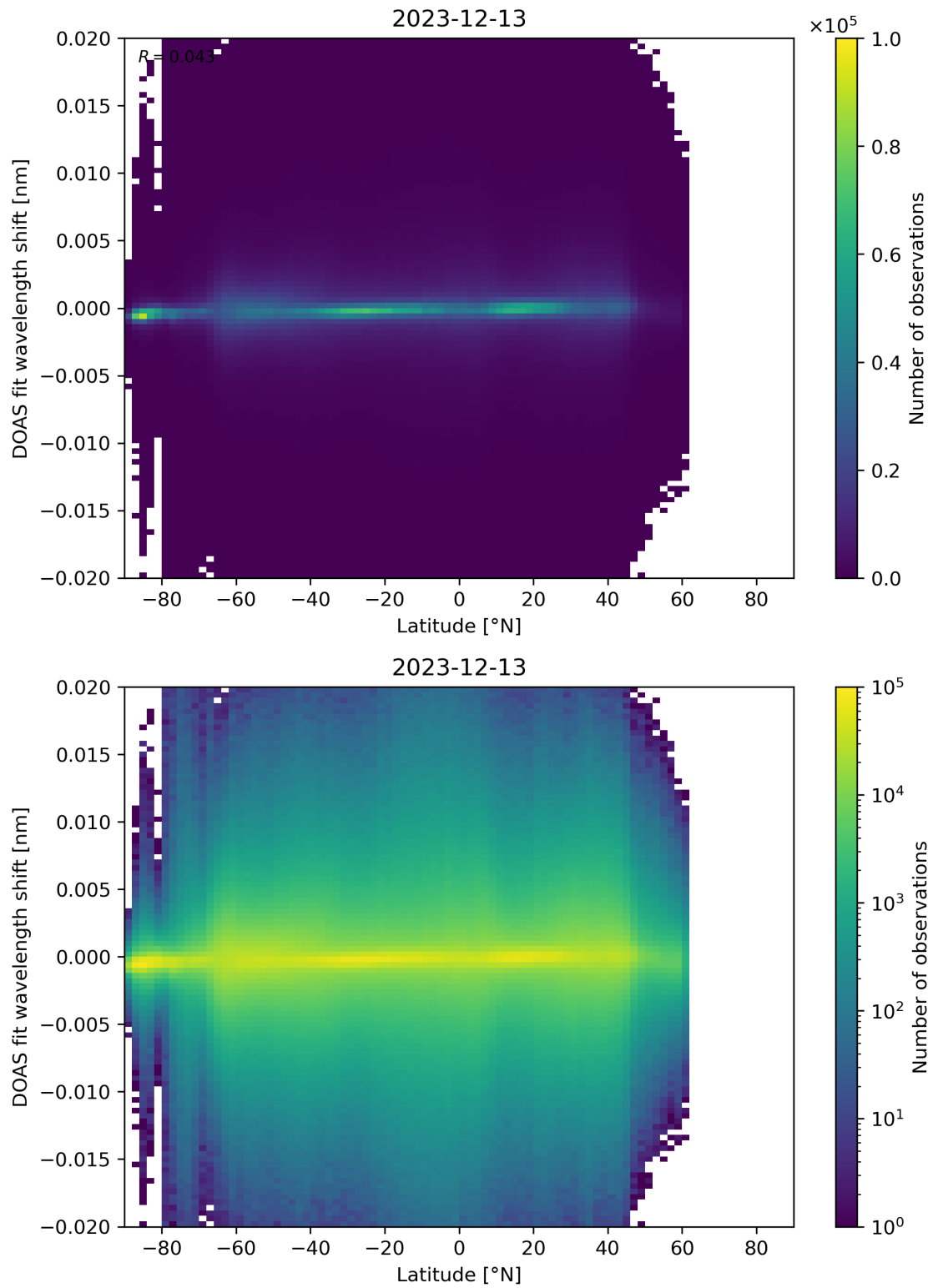
Figure 154: Scatter density plot of “Latitude” against “DOAS fit wavelength shift” for 2023-12-12 to 2023-12-14.
