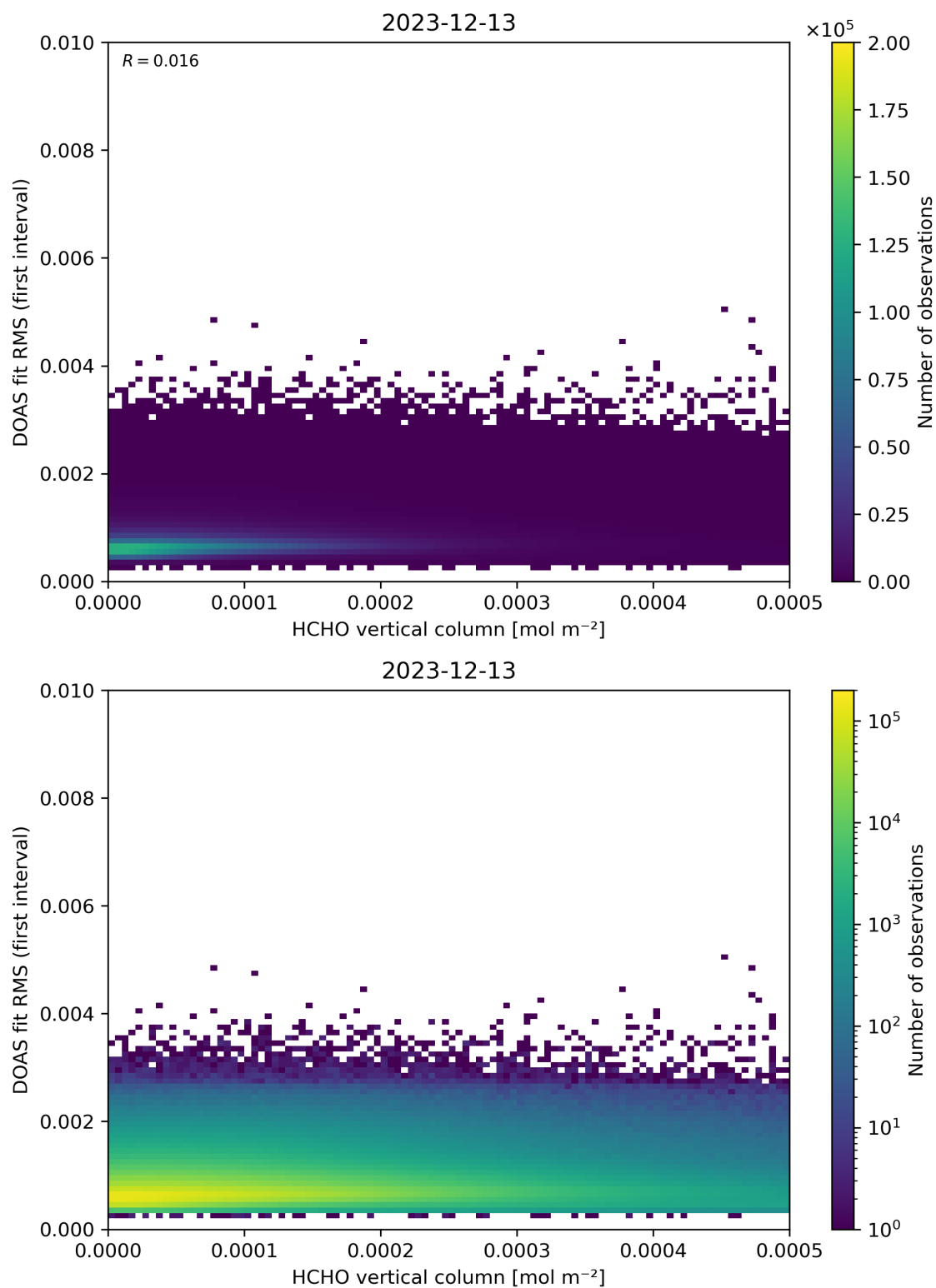
Figure 123: Scatter density plot of “HCHO vertical column” against “DOAS fit RMS (first interval)” for 2023-12-12 to 2023-12-14.
