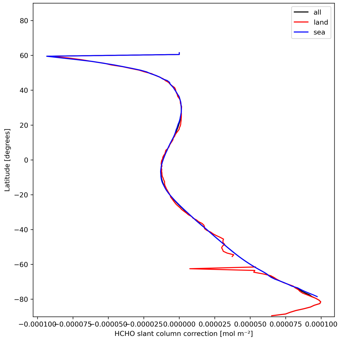
Figure 33: Zonal average of “HCHO slant column correction” for 2023-12-12 to 2023-12-14.
