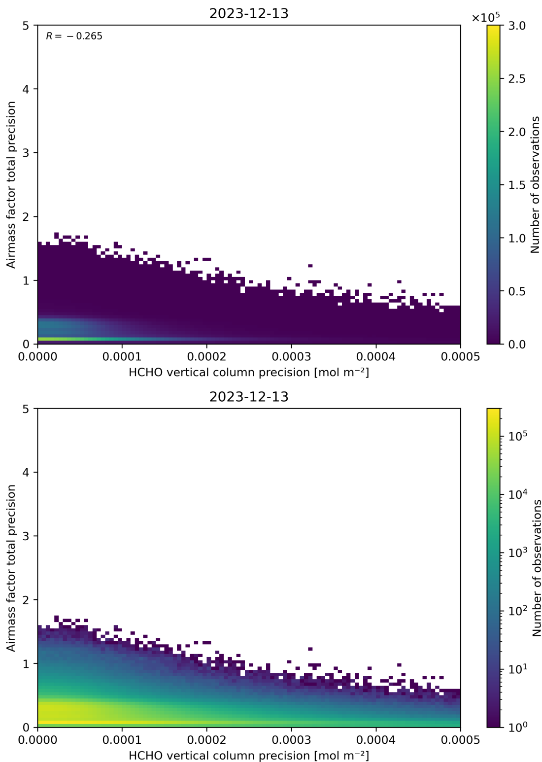
Figure 145: Scatter density plot of “HCHO vertical column precision” against “Airmass factor total precision” for 2023-12-12 to 2023-12-14.
