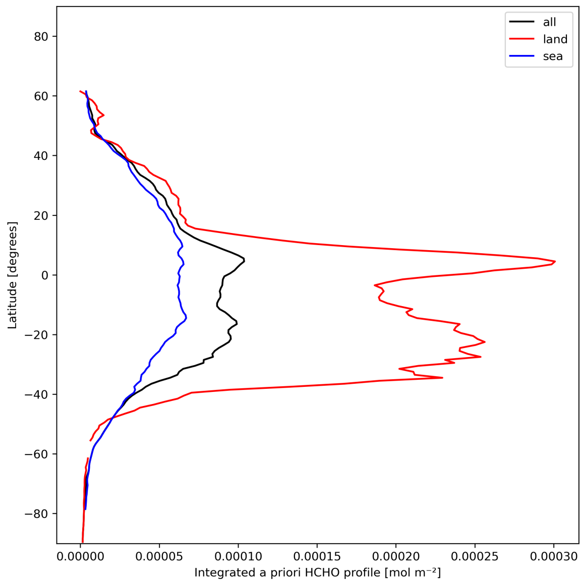
Figure 29: Zonal average of “Integrated a priori HCHO profile” for 2023-12-12 to 2023-12-14.
