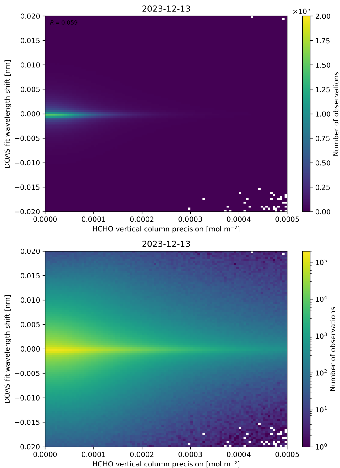
Figure 137: Scatter density plot of “HCHO vertical column precision” against “DOAS fit wavelength shift” for 2023-12-12 to 2023-12-14.
