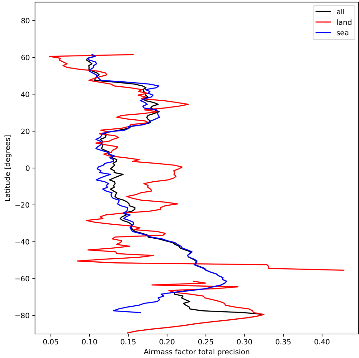
Figure 27: Zonal average of “Airmass factor total precision” for 2023-12-12 to 2023-12-14.
