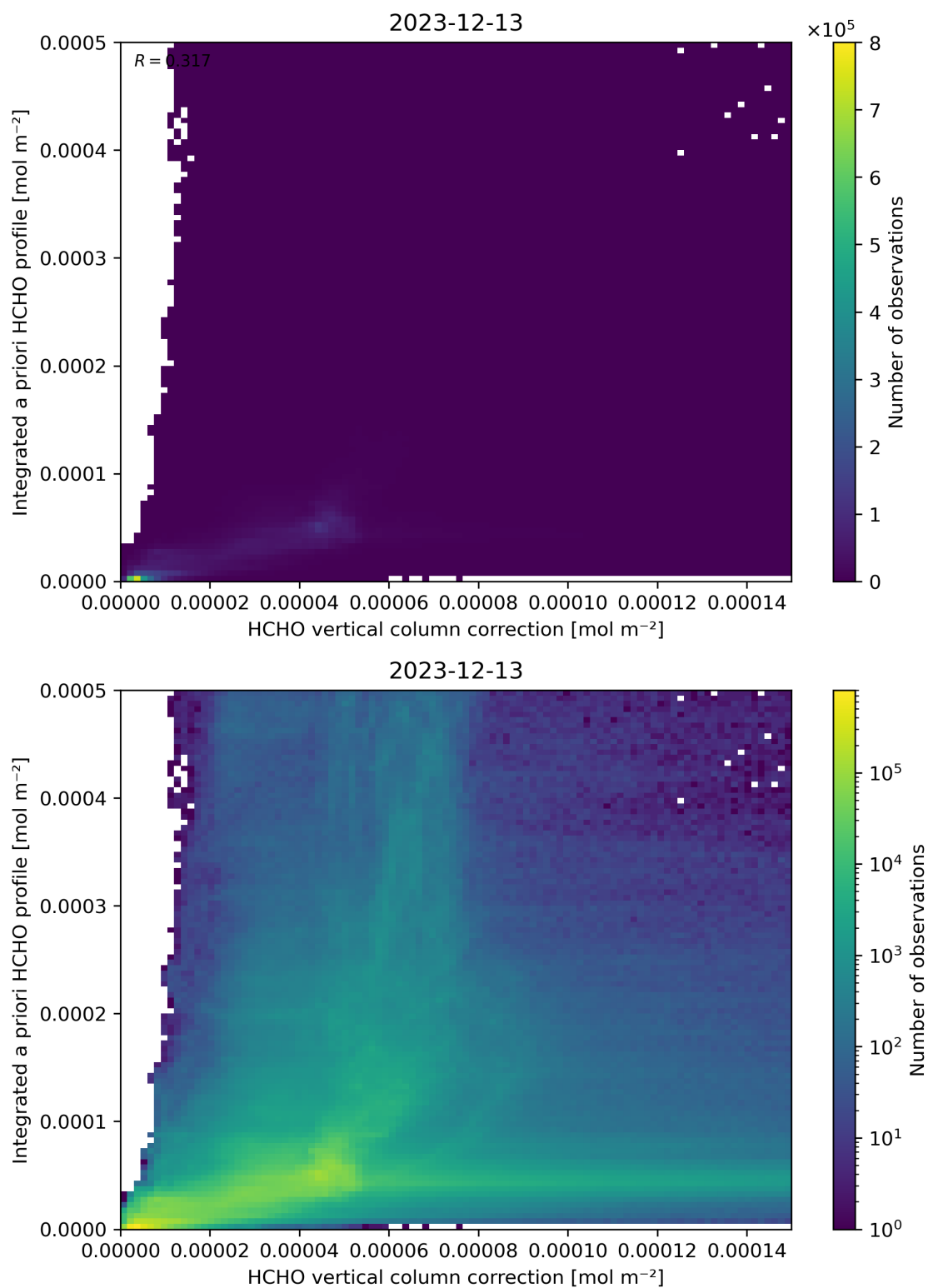
Figure 122: Scatter density plot of “HCHO vertical column correction” against “Integrated a priori HCHO profile” for 2023-12-12 to 2023-12-14.
