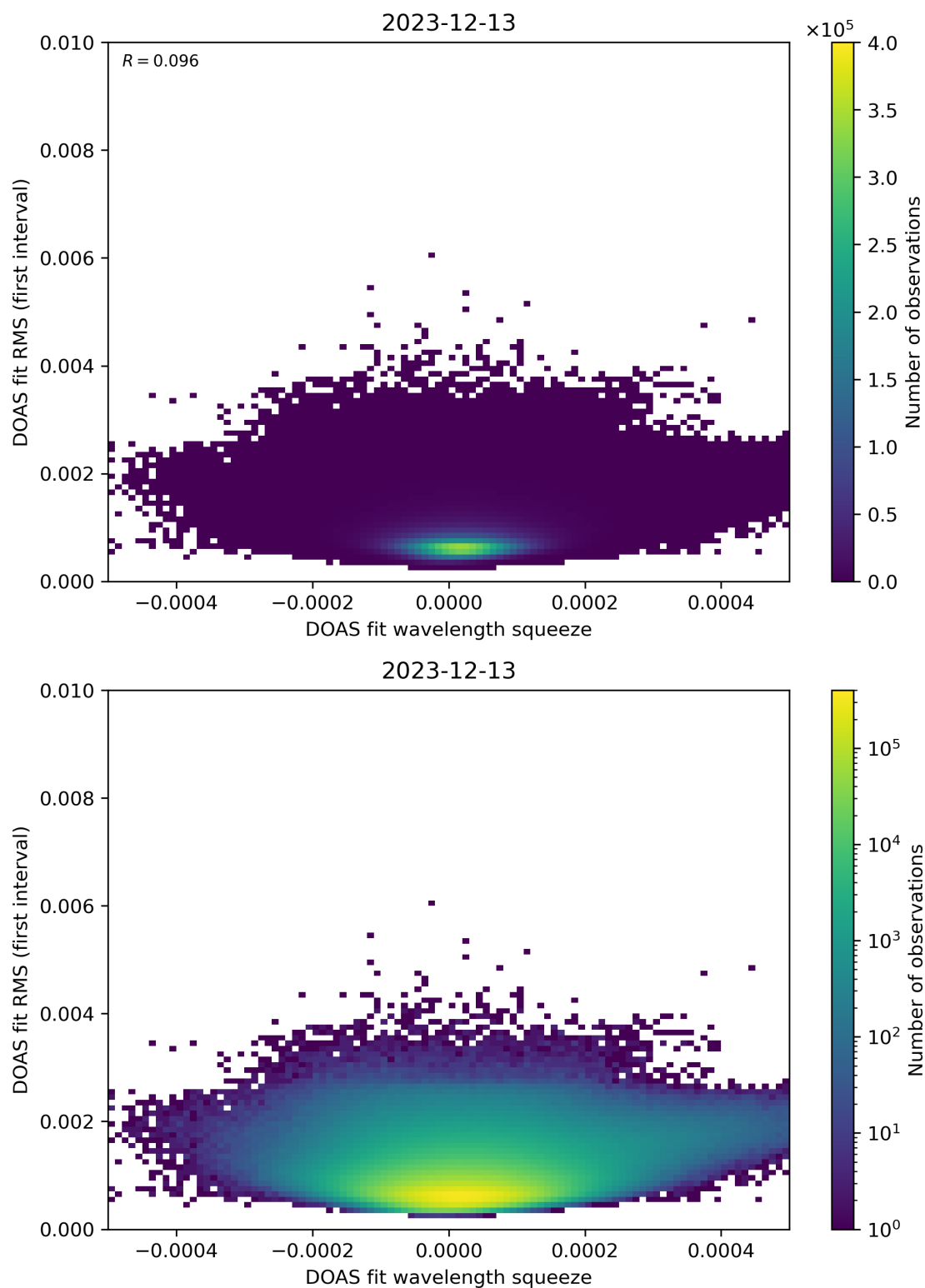
Figure 68: Scatter density plot of “DOAS fit wavelength squeeze” against “DOAS fit RMS (first interval)” for 2023-12-12 to 2023-12-14.
