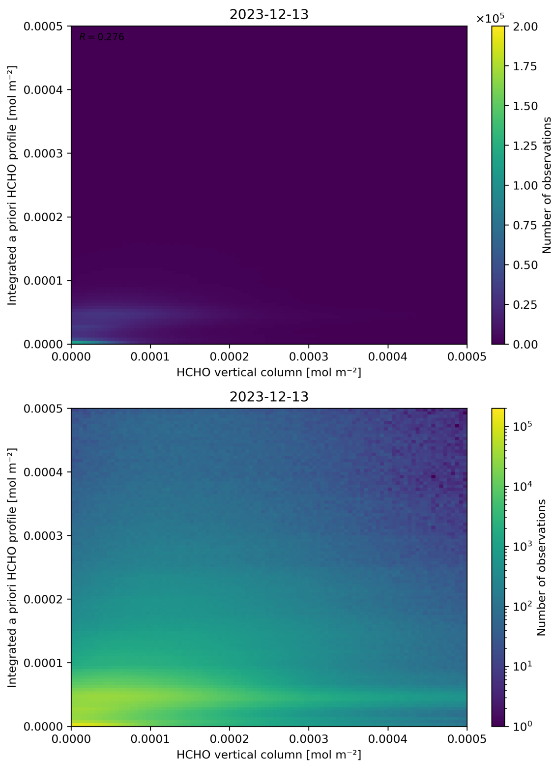
Figure 135: Scatter density plot of “HCHO vertical column” against “Integrated a priori HCHO profile” for 2023-12-12 to 2023-12-14.
