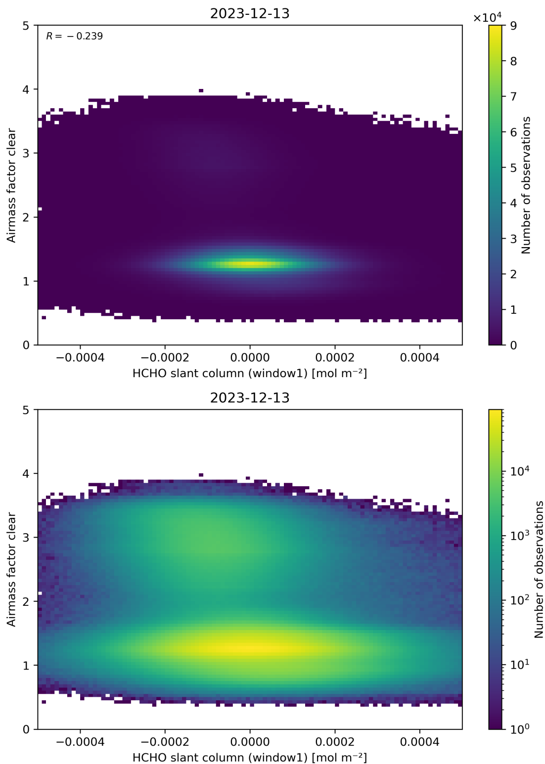
Figure 81: Scatter density plot of “HCHO slant column (window1)” against “Airmass factor clear” for 2023-12-12 to 2023-12-14.
