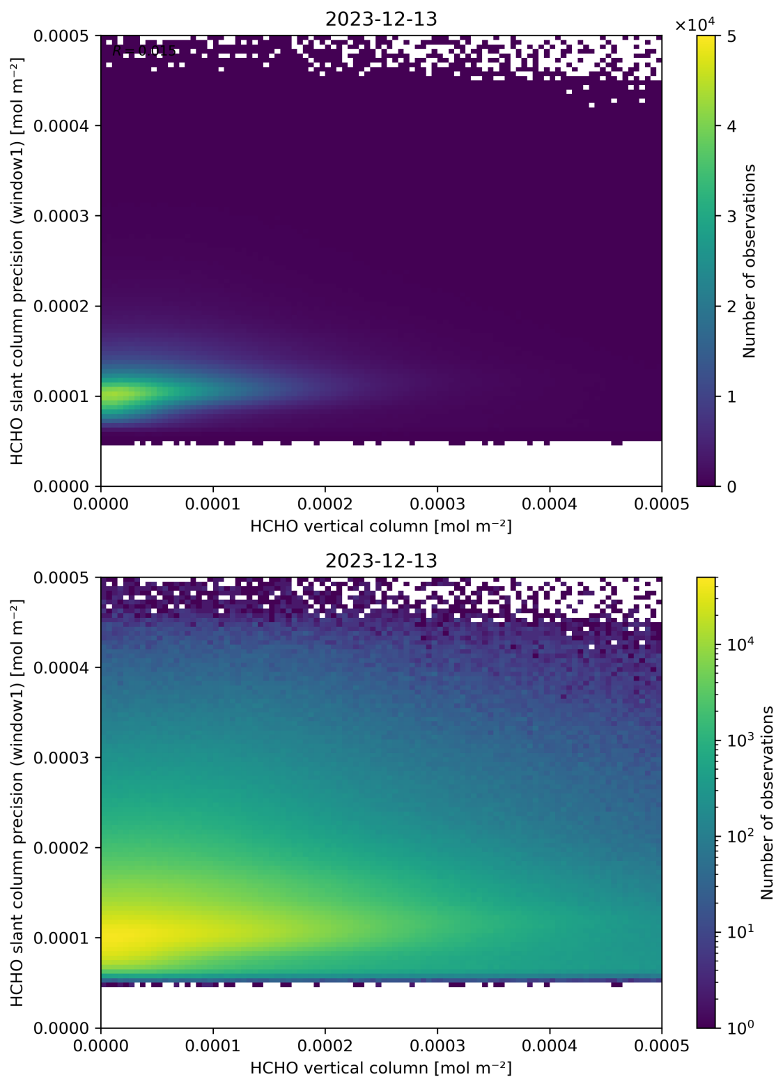
Figure 130: Scatter density plot of “HCHO vertical column” against “HCHO slant column precision (window1)” for 2023-12-12 to 2023-12-14.
