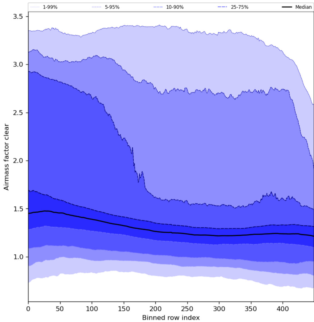
Figure 56: Along track statistics of “Airmass factor clear” for 2023-12-12 to 2023-12-14
