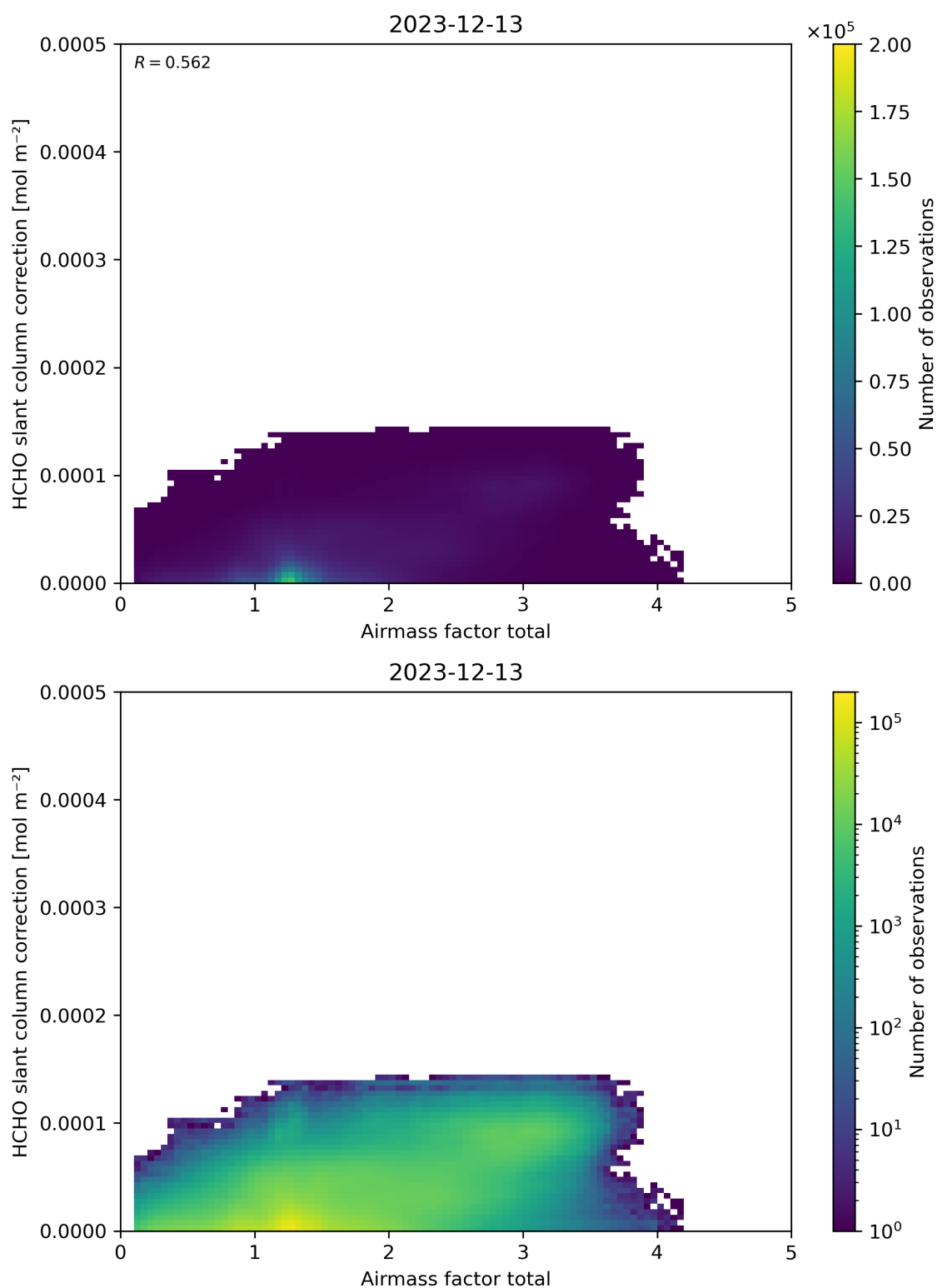
Figure 102: Scatter density plot of “Airmass factor total” against “HCHO slant column correction” for 2023-12-12 to 2023-12-14.
