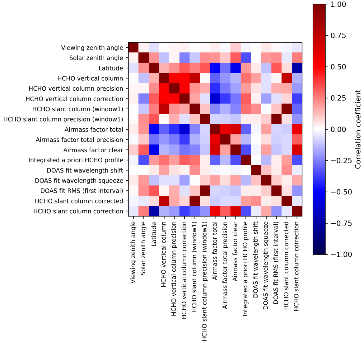
Figure 2: Map of correlation matrix for 2023-12-12 to 2023-12-14.
