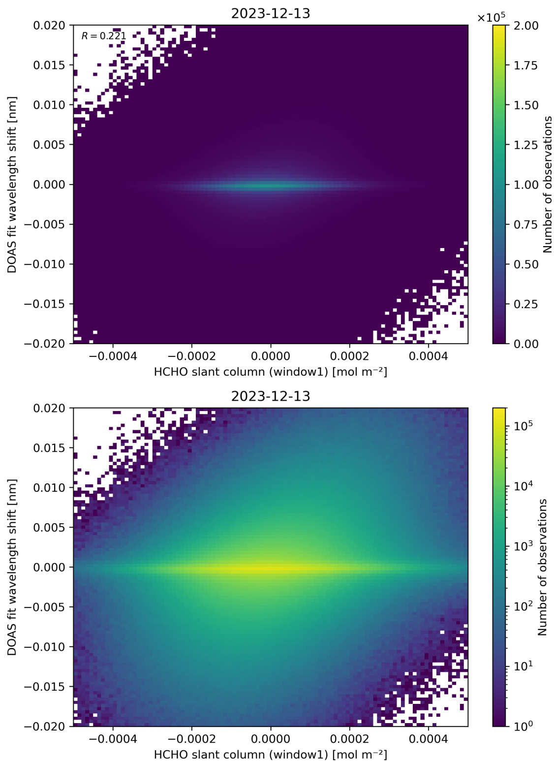
Figure 79: Scatter density plot of “HCHO slant column (window1)” against “DOAS fit wavelength shift” for 2023-12-12 to 2023-12-14.
