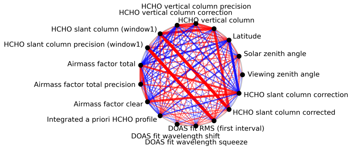
Figure 1: Map of correlation graph for 2023-12-12 to 2023-12-14.
