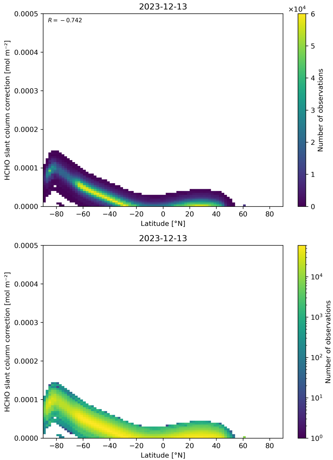
Figure 158: Scatter density plot of “Latitude” against “HCHO slant column correction” for 2023-12-12 to 2023-12-14.
