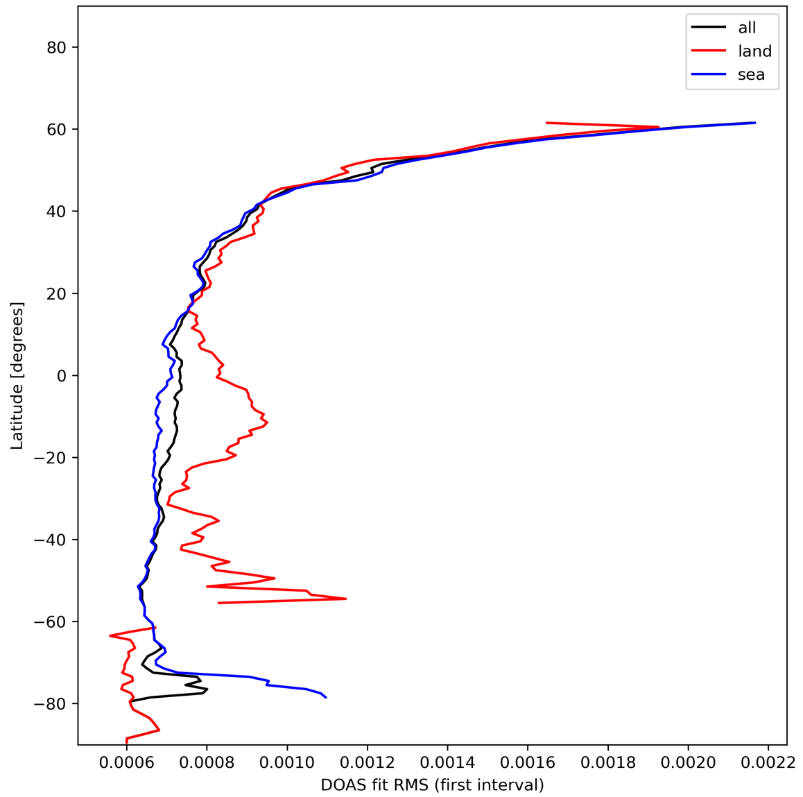
Figure 32: Zonal average of “DOAS fit RMS (first interval)” for 2023-12-12 to 2023-12-14.
