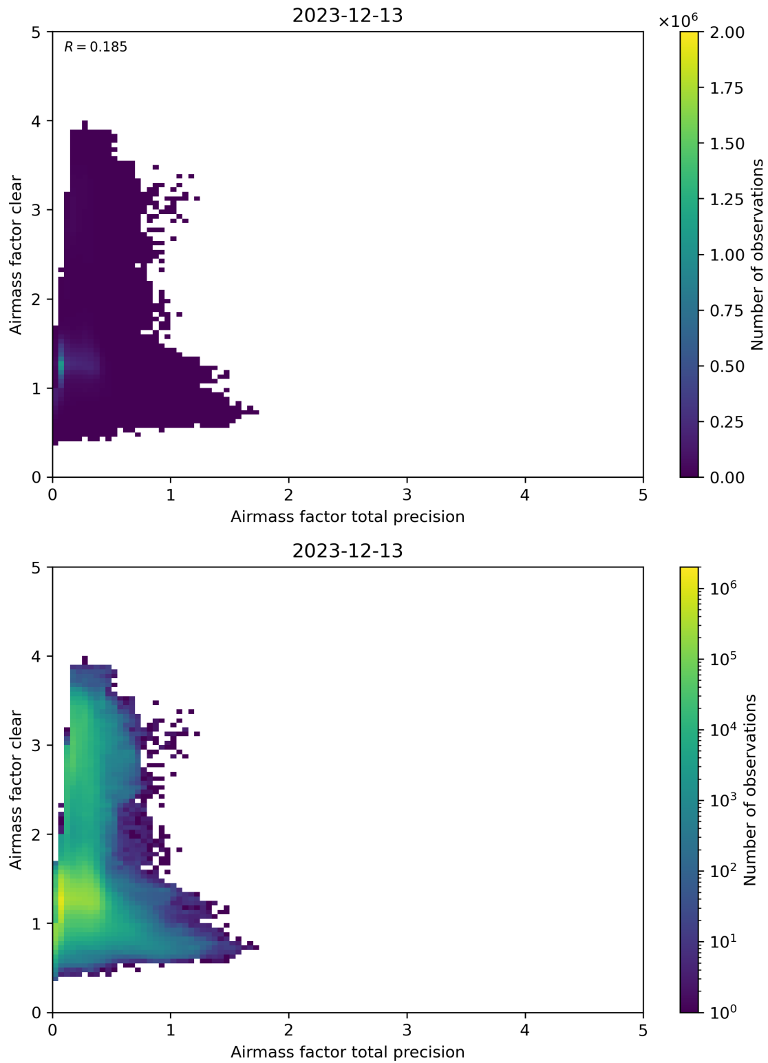
Figure 108: Scatter density plot of “Airmass factor total precision” against “Airmass factor clear” for 2023-12-12 to 2023-12-14.
