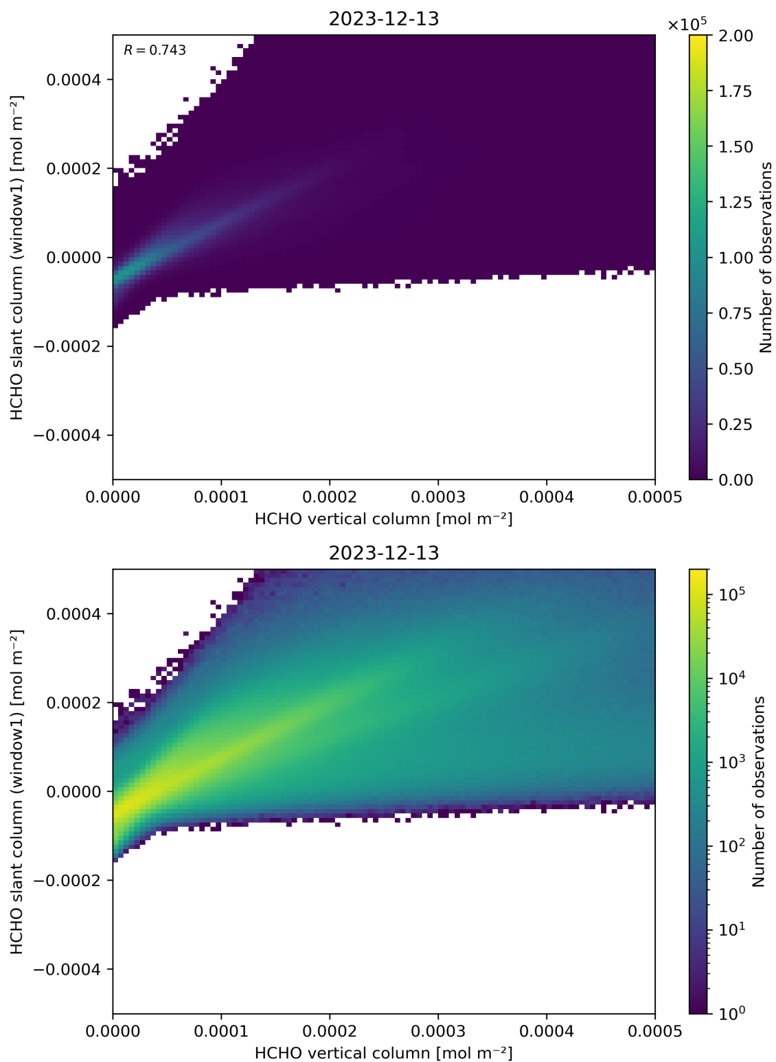
Figure 129: Scatter density plot of “HCHO vertical column” against “HCHO slant column (window1)” for 2023-12-12 to 2023-12-14.
