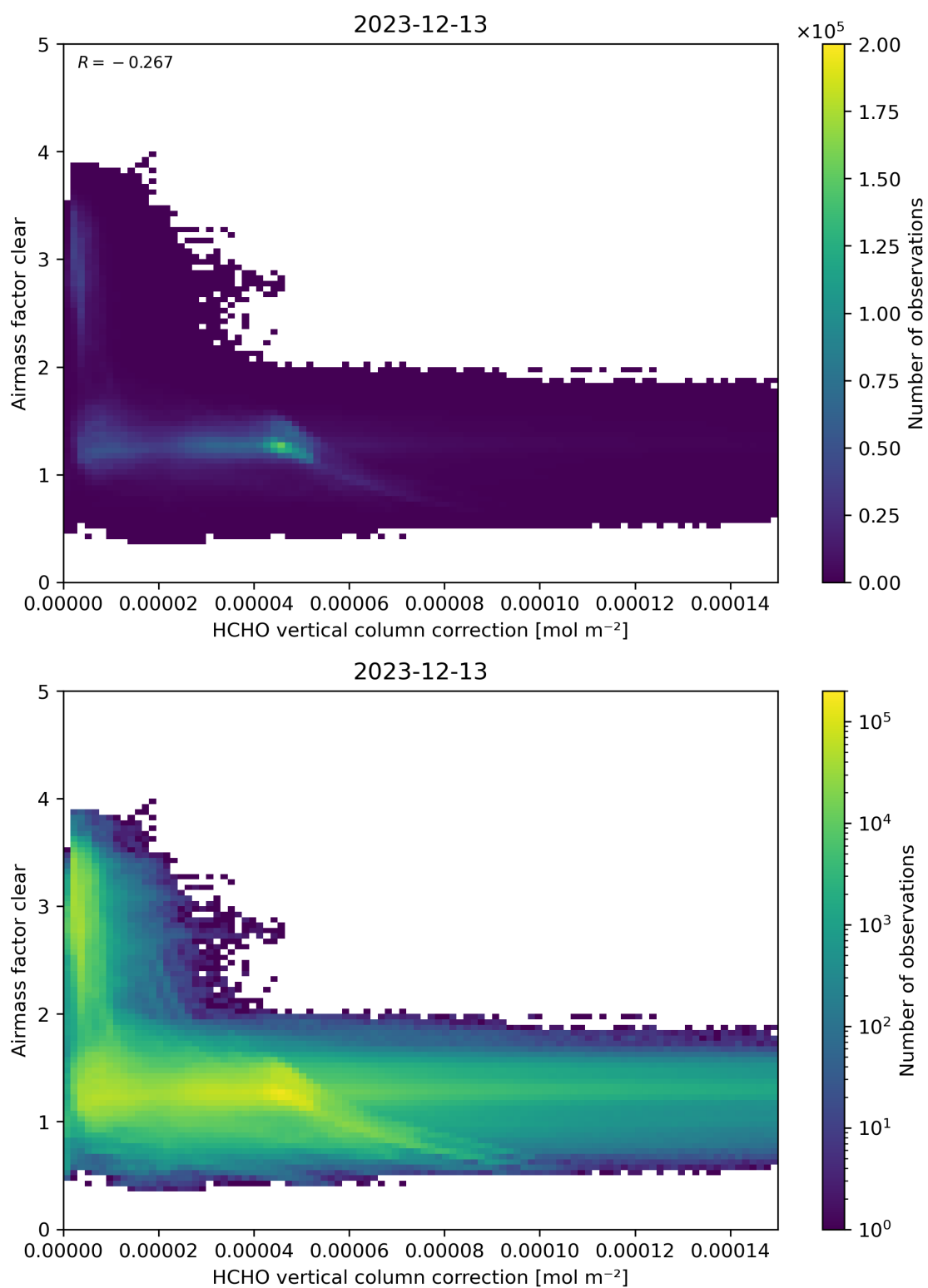
Figure 115: Scatter density plot of “HCHO vertical column correction” against “Airmass factor clear” for 2023-12-12 to 2023-12-14.
