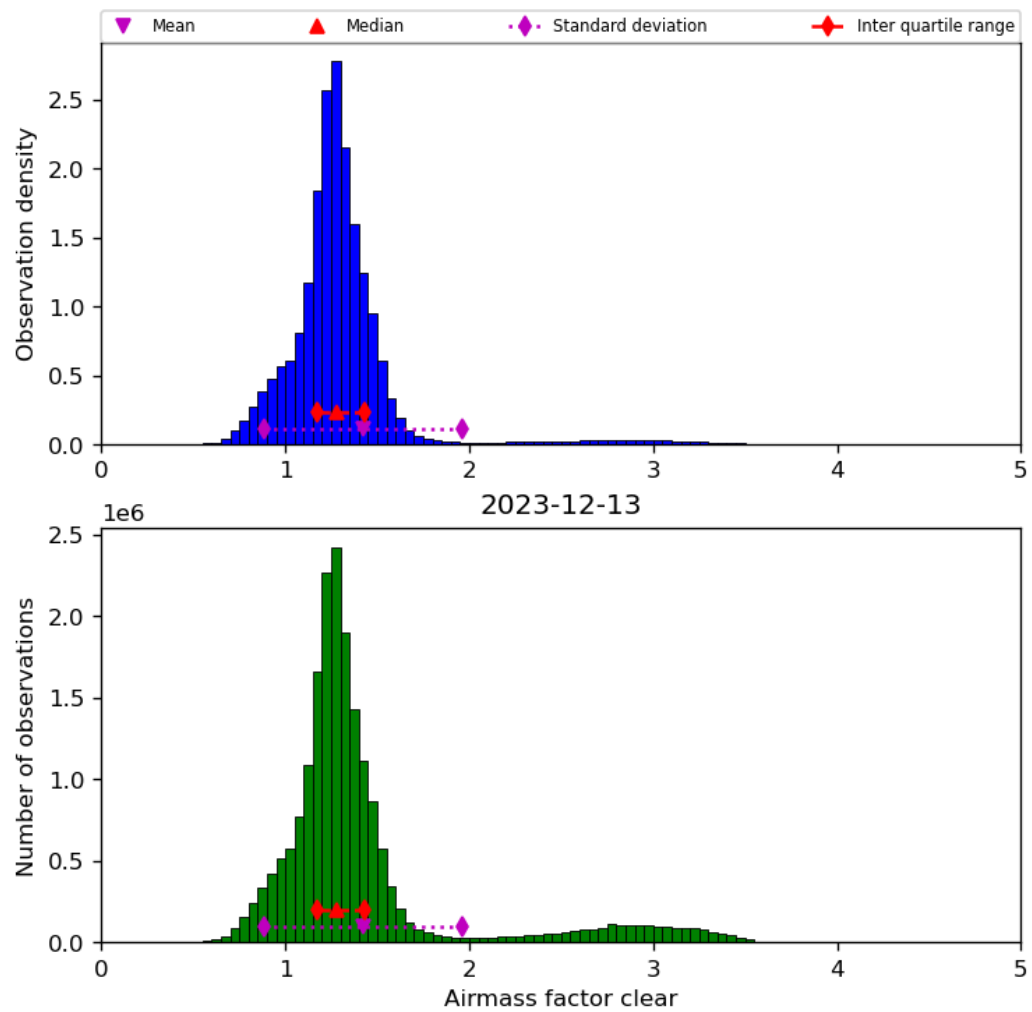
Figure 42: Histogram of “Airmass factor clear” for 2023-12-12 to 2023-12-14
