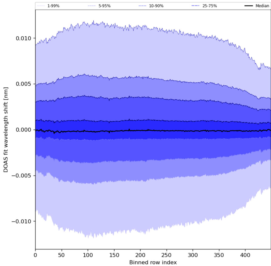
Figure 58: Along track statistics of “DOAS fit wavelength shift” for 2023-12-12 to 2023-12-14
