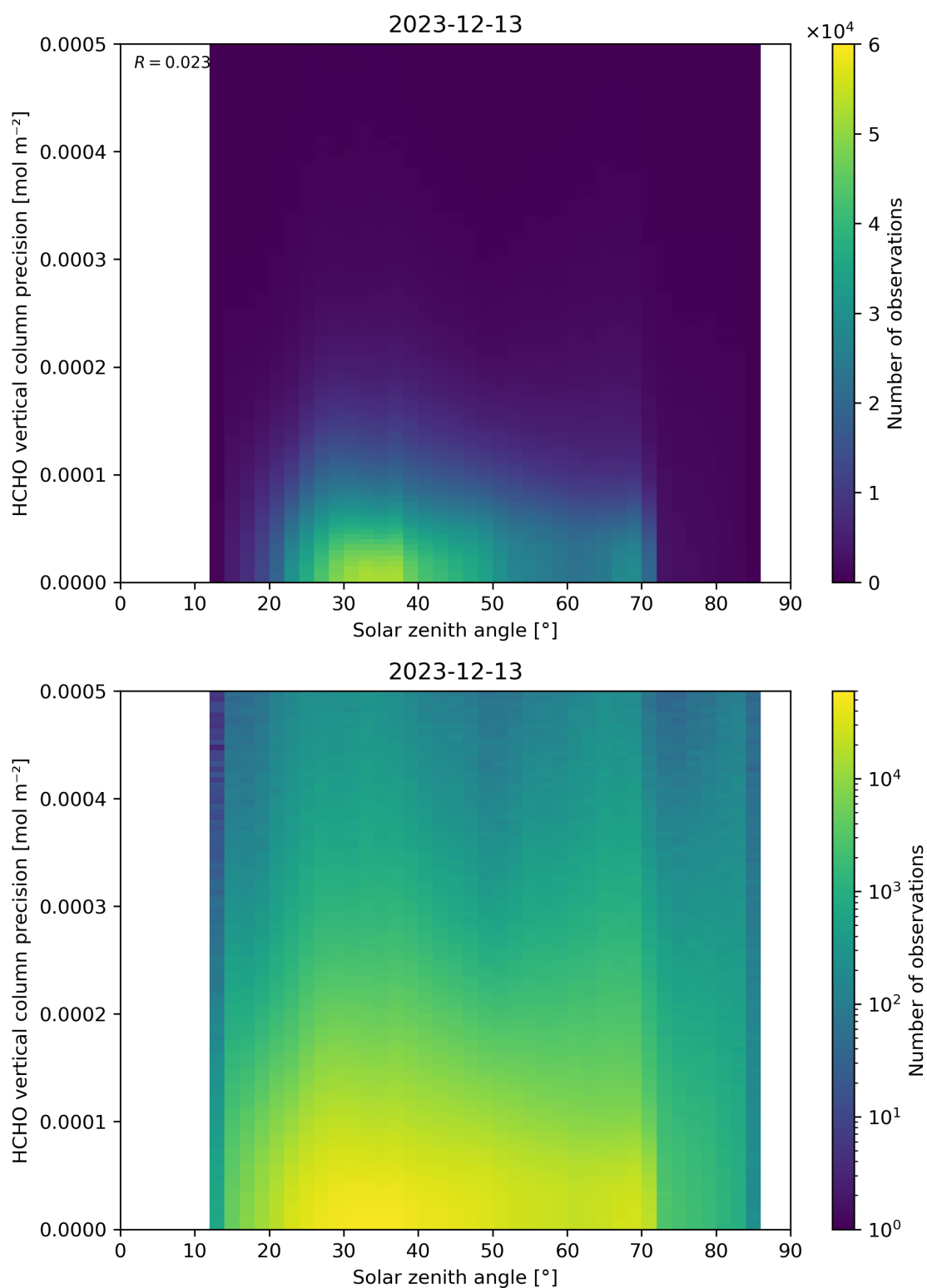
Figure 179: Scatter density plot of “Solar zenith angle” against “HCHO vertical column precision” for 2023-12-12 to 2023-12-14.
