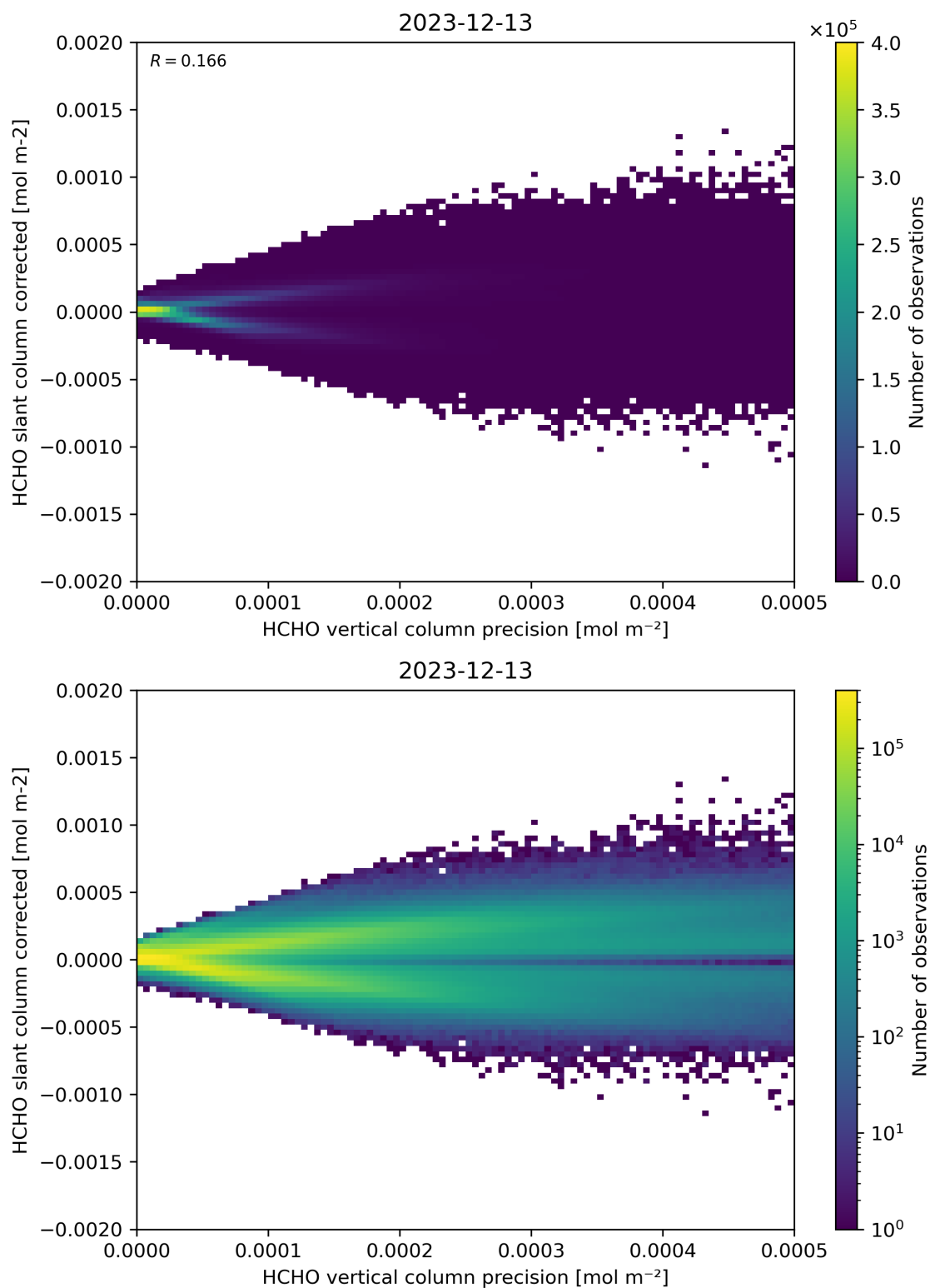
Figure 140: Scatter density plot of “HCHO vertical column precision” against “HCHO slant column corrected” for 2023-12-12 to 2023-12-14.
