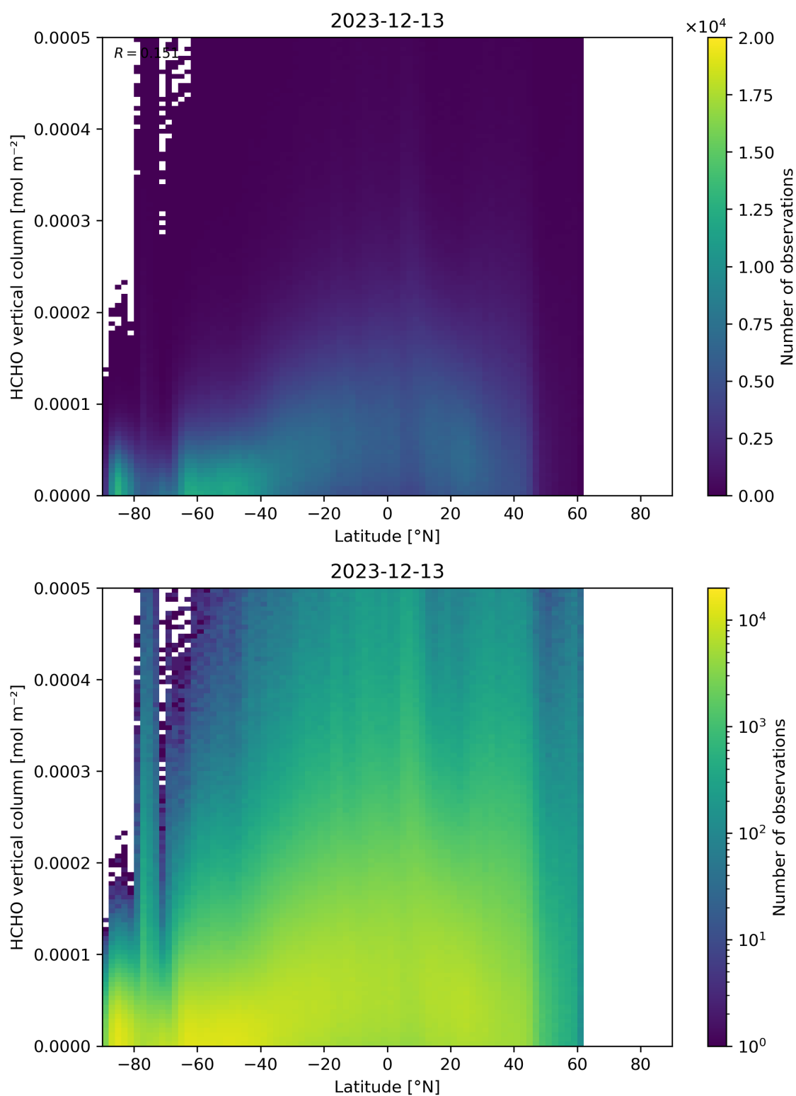
Figure 163: Scatter density plot of “Latitude” against “HCHO vertical column” for 2023-12-12 to 2023-12-14.
