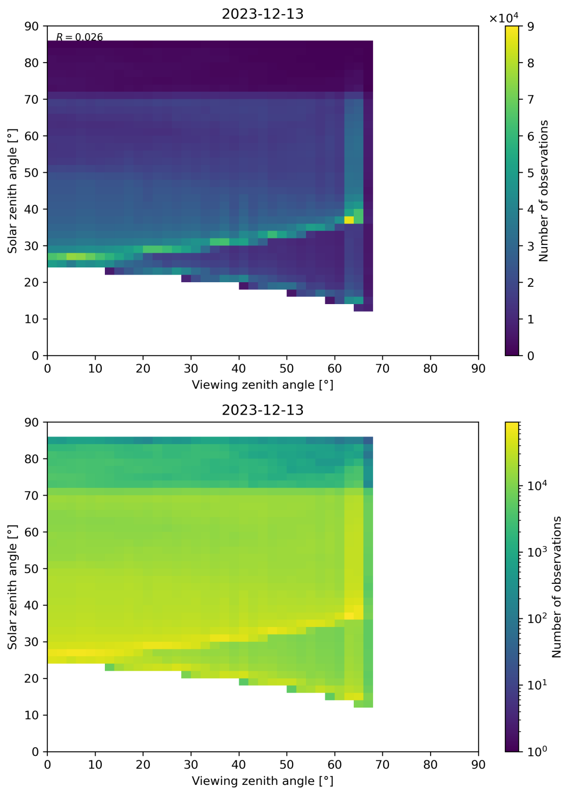
Figure 197: Scatter density plot of “Viewing zenith angle” against “Solar zenith angle” for 2023-12-12 to 2023-12-14.
