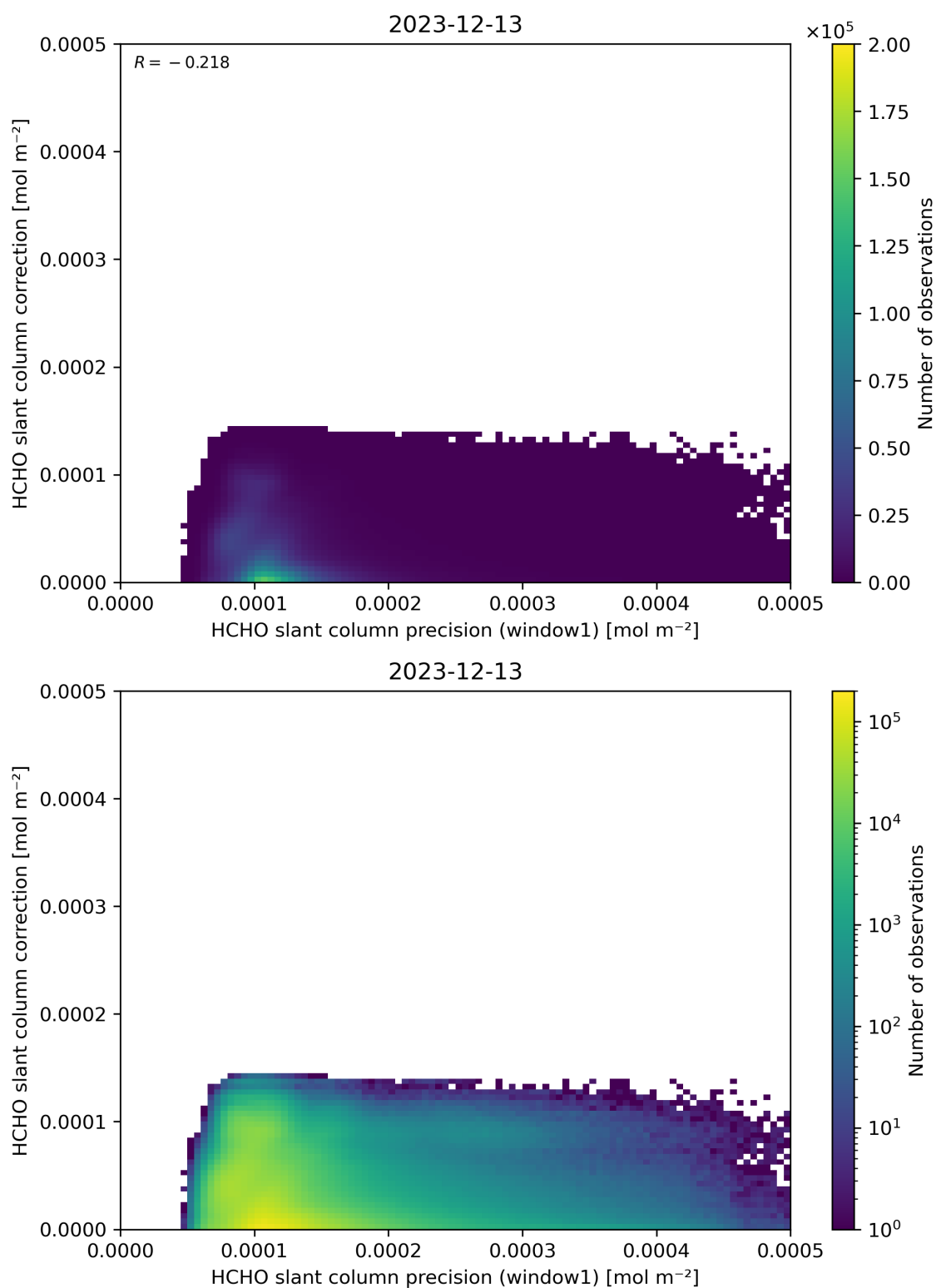
Figure 93: Scatter density plot of “HCHO slant column precision (window1)” against “HCHO slant column correction” for 2023-12-12 to 2023-12-14.
