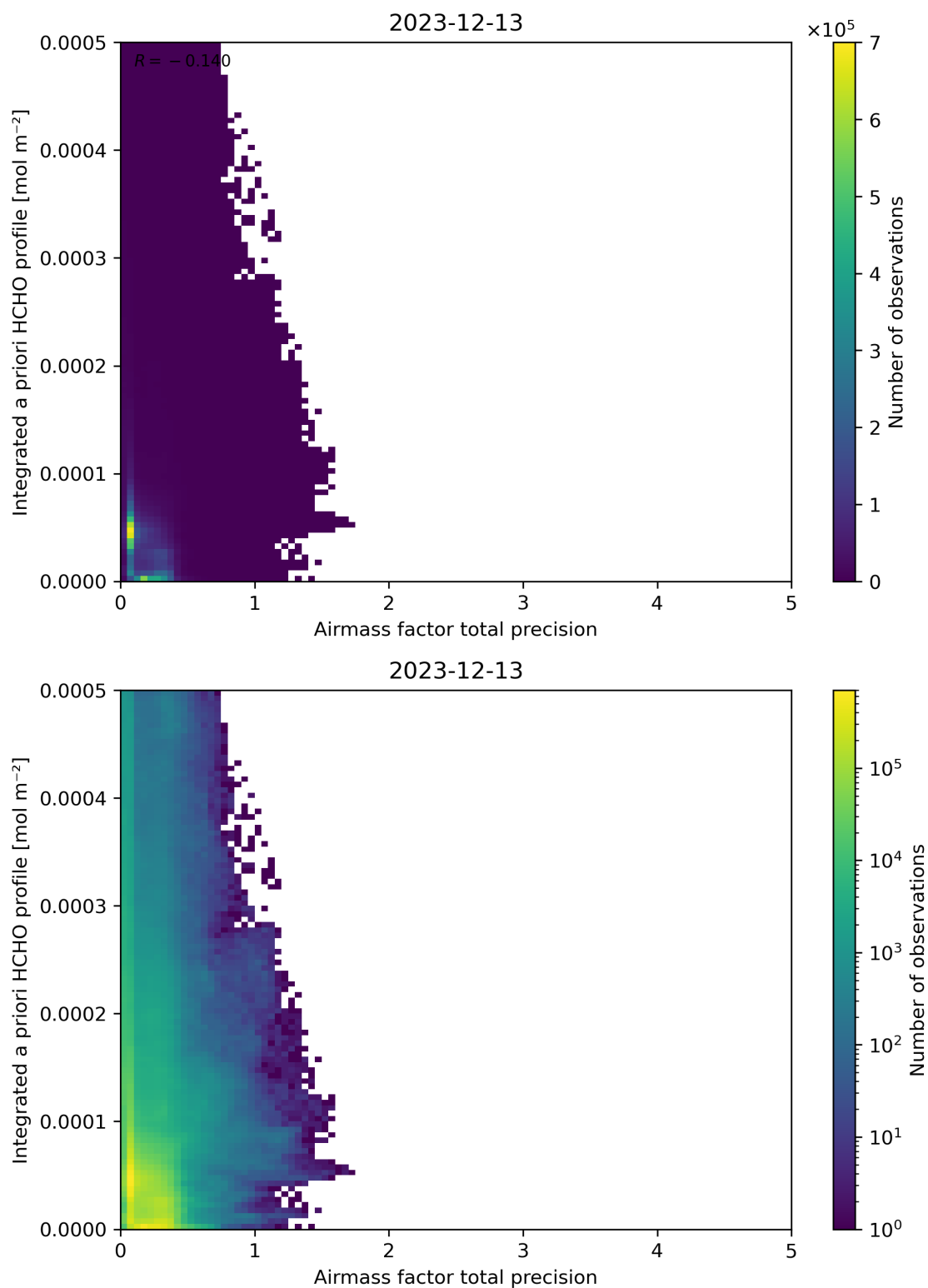
Figure 111: Scatter density plot of “Airmass factor total precision” against “Integrated a priori HCHO profile” for 2023-12-12 to 2023-12-14.
