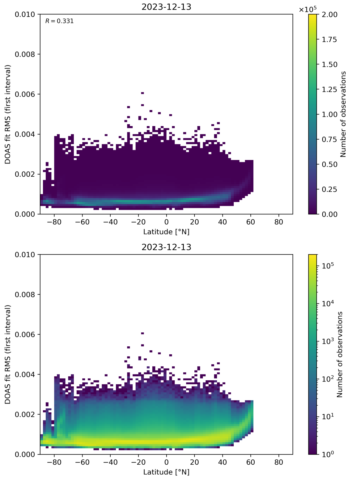
Figure 153: Scatter density plot of “Latitude” against “DOAS fit RMS (first interval)” for 2023-12-12 to 2023-12-14.
