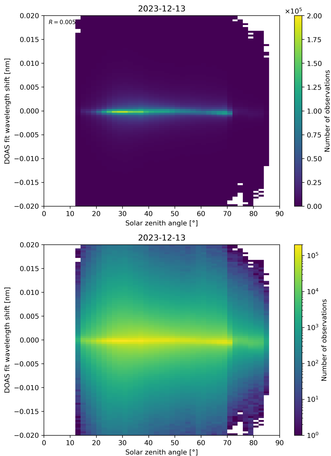
Figure 168: Scatter density plot of “Solar zenith angle” against “DOAS fit wavelength shift” for 2023-12-12 to 2023-12-14.
