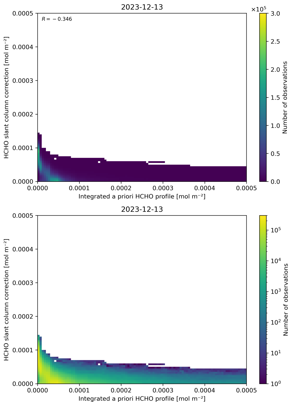
Figure 152: Scatter density plot of “Integrated a priori HCHO profile” against “HCHO slant column correction” for 2023-12-12 to 2023-12-14.
