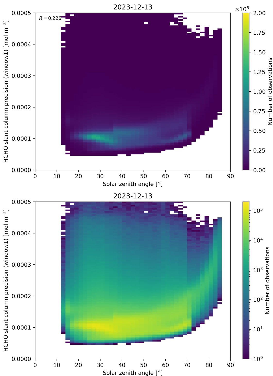
Figure 174: Scatter density plot of “Solar zenith angle” against “HCHO slant column precision (window1)” for 2023-12-12 to 2023-12-14.
