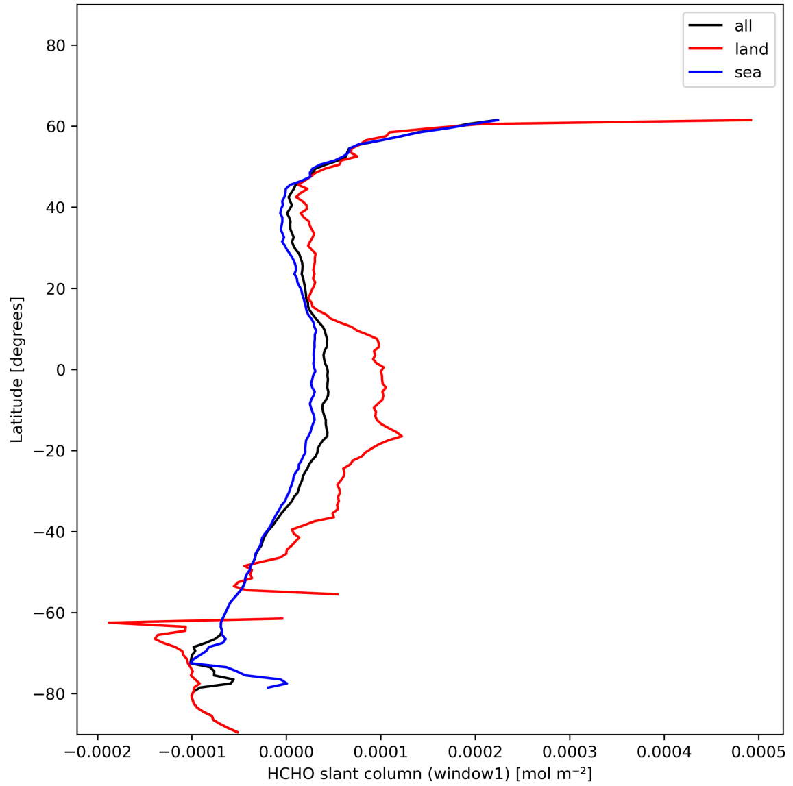
Figure 24: Zonal average of “HCHO slant column (window1)” for 2023-12-12 to 2023-12-14.
