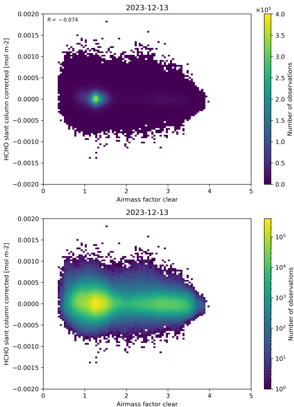
Figure 74: Scatter density plot of “Airmass factor clear” against “HCHO slant column corrected” for 2023-12-12 to 2023-12-14.
