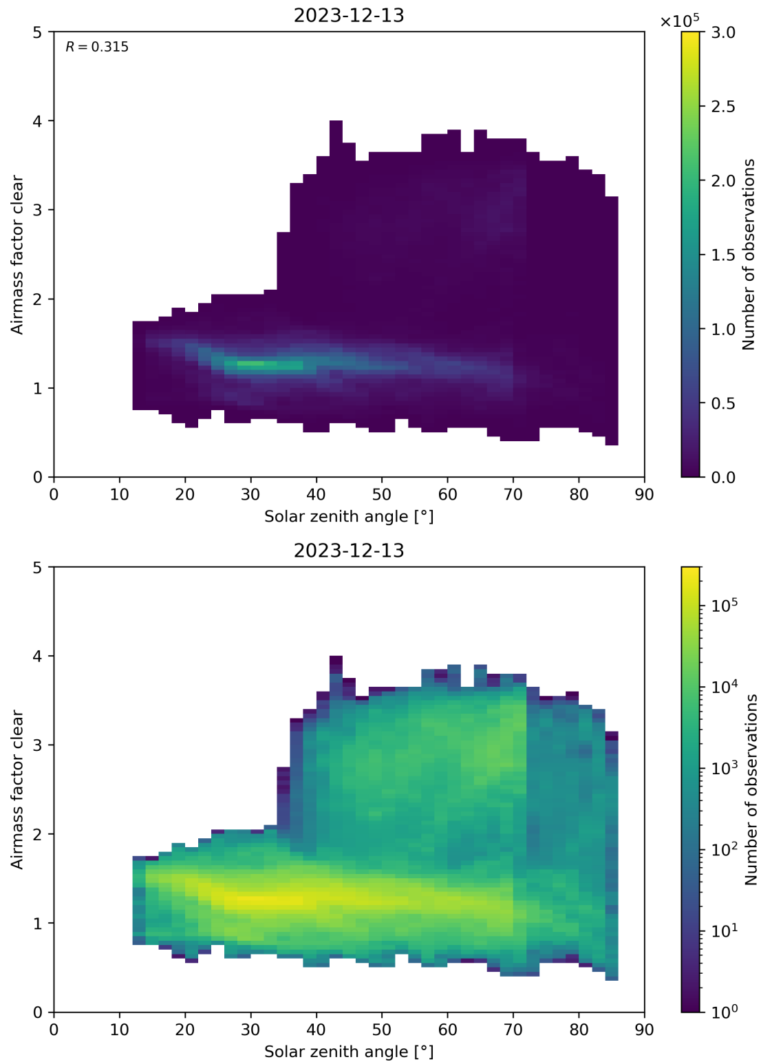
Figure 170: Scatter density plot of “Solar zenith angle” against “Airmass factor clear” for 2023-12-12 to 2023-12-14.
