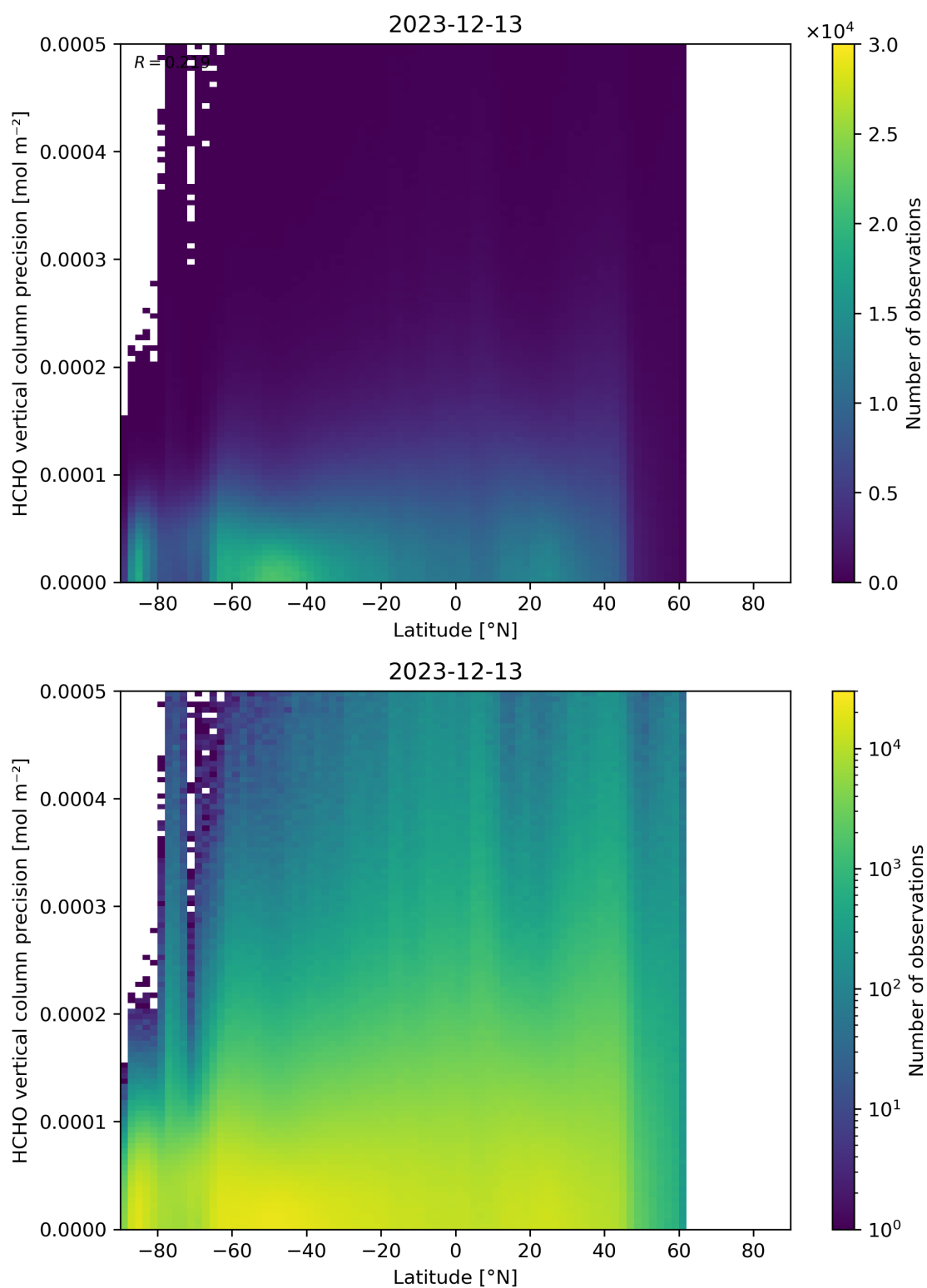
Figure 165: Scatter density plot of “Latitude” against “HCHO vertical column precision” for 2023-12-12 to 2023-12-14.
