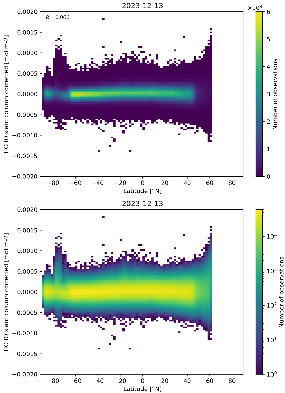
Figure 157: Scatter density plot of “Latitude” against “HCHO slant column corrected” for 2023-12-12 to 2023-12-14.
