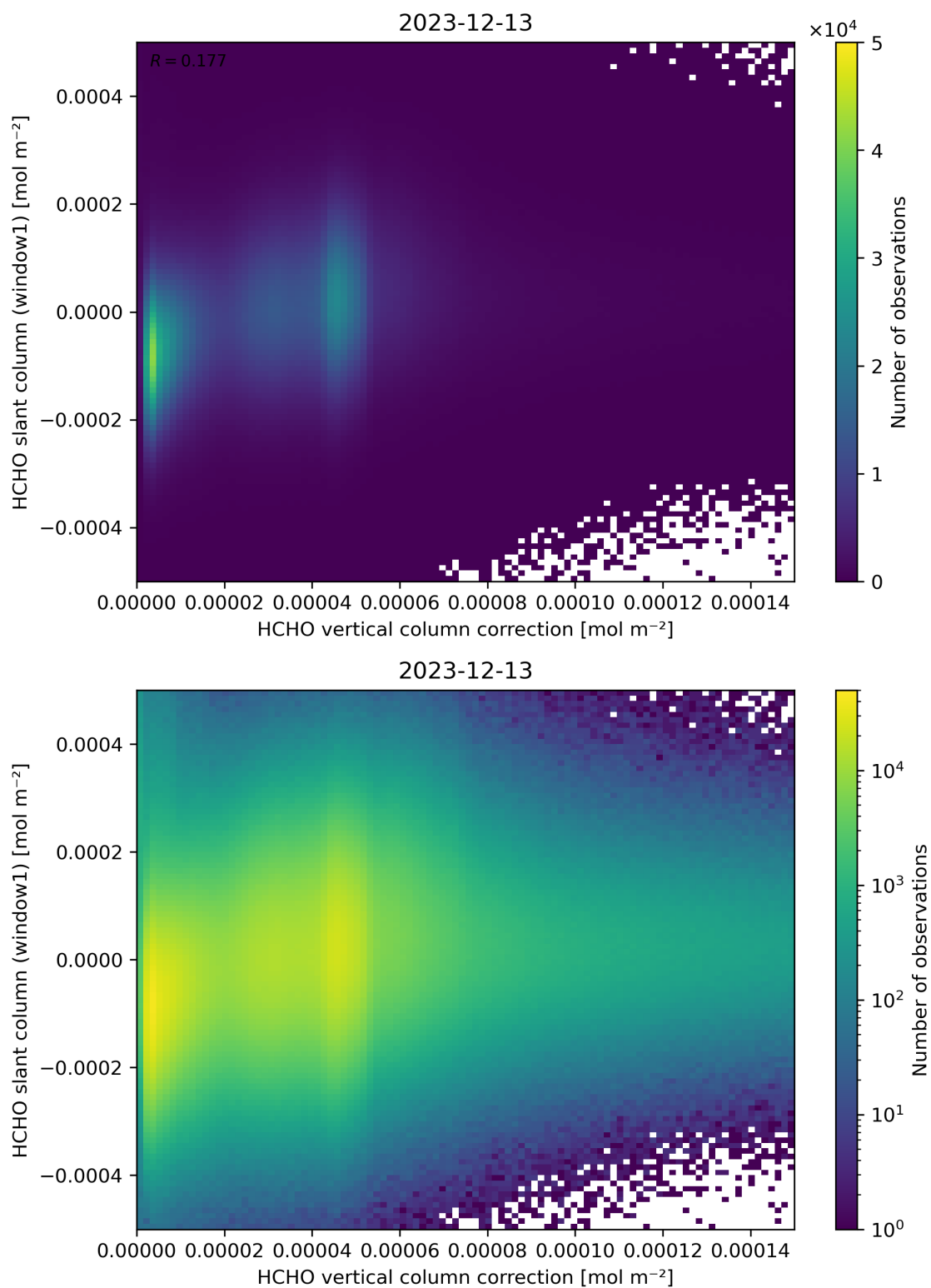
Figure 118: Scatter density plot of “HCHO vertical column correction” against “HCHO slant column (window1)” for 2023-12-12 to 2023-12-14.
