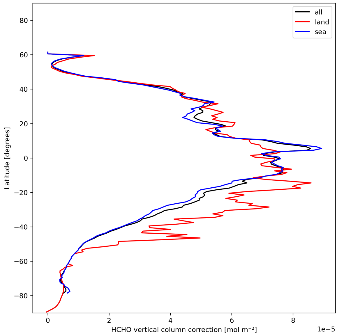
Figure 23: Zonal average of “HCHO vertical column correction” for 2023-12-12 to 2023-12-14.
