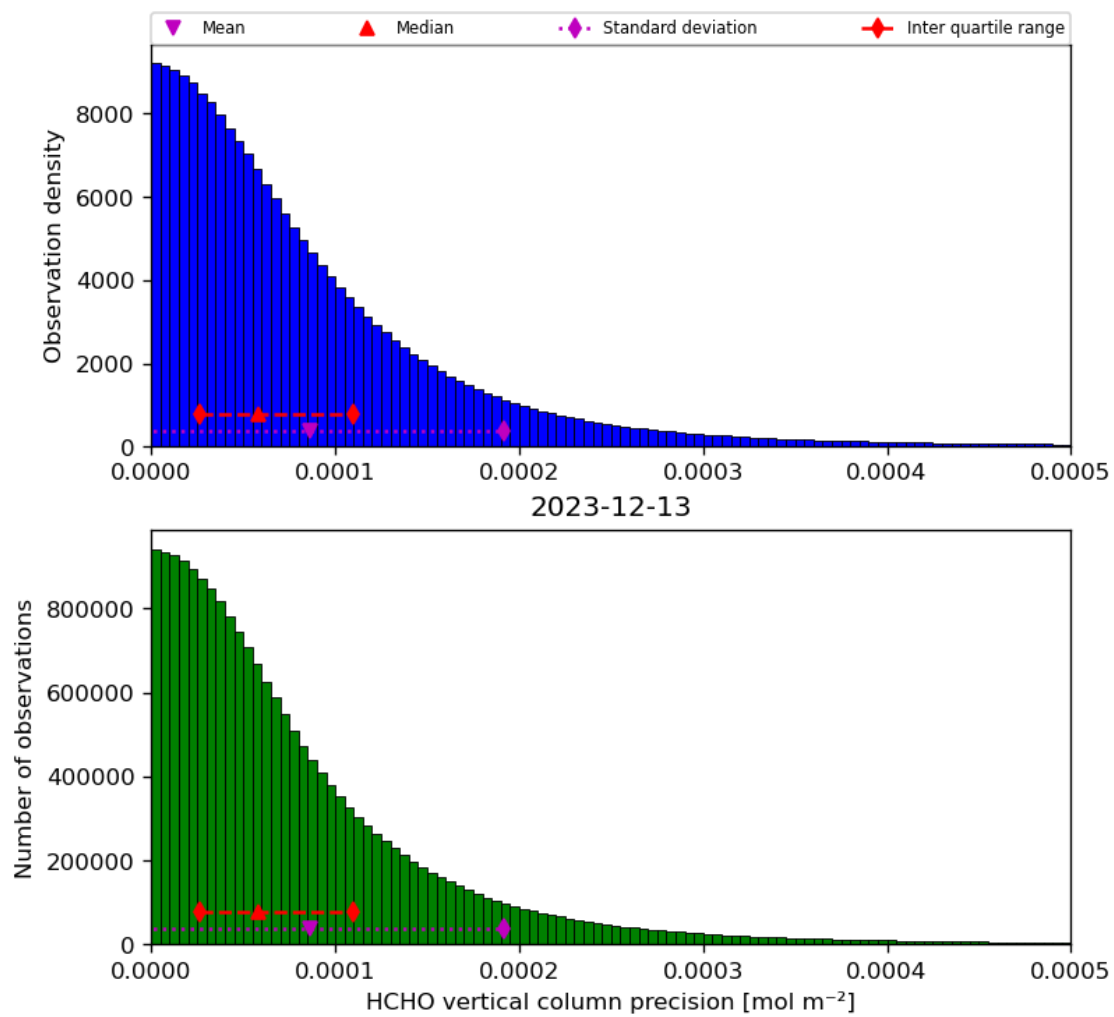
Figure 36: Histogram of “HCHO vertical column precision” for 2023-12-12 to 2023-12-14
