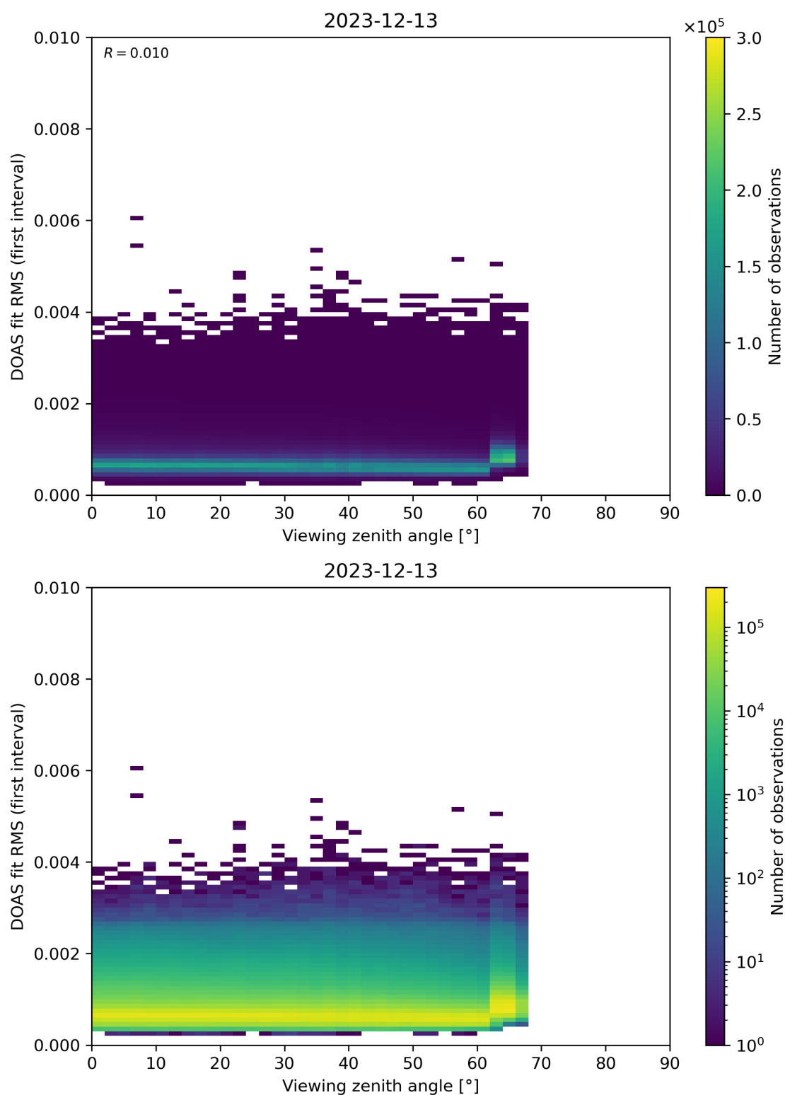
Figure 182: Scatter density plot of “Viewing zenith angle” against “DOAS fit RMS (first interval)” for 2023-12-12 to 2023-12-14.
