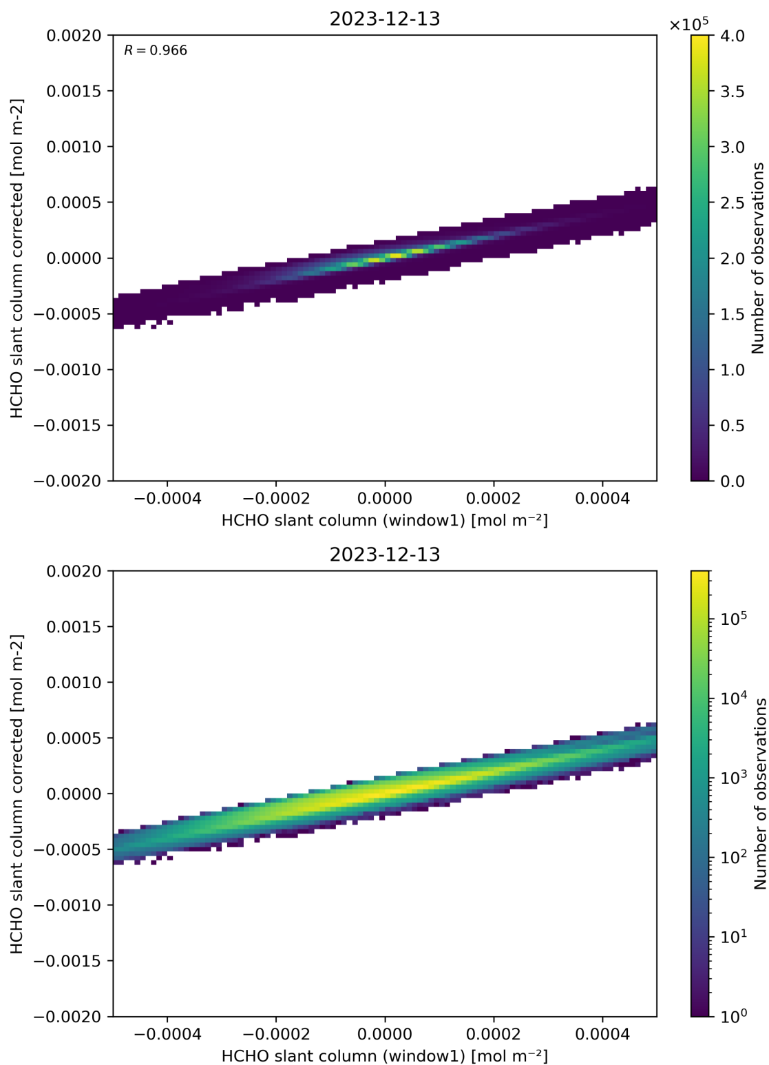
Figure 82: Scatter density plot of “HCHO slant column (window1)” against “HCHO slant column corrected” for 2023-12-12 to 2023-12-14.
