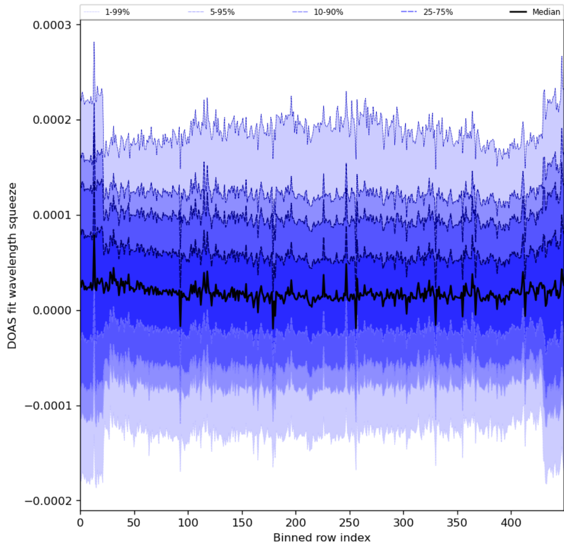
Figure 59: Along track statistics of “DOAS fit wavelength squeeze” for 2023-12-12 to 2023-12-14
