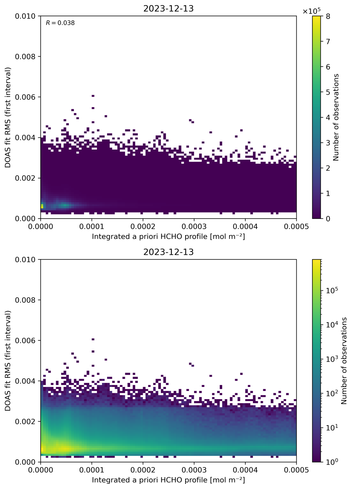
Figure 148: Scatter density plot of “Integrated a priori HCHO profile” against “DOAS fit RMS (first interval)” for 2023-12-12 to 2023-12-14.
