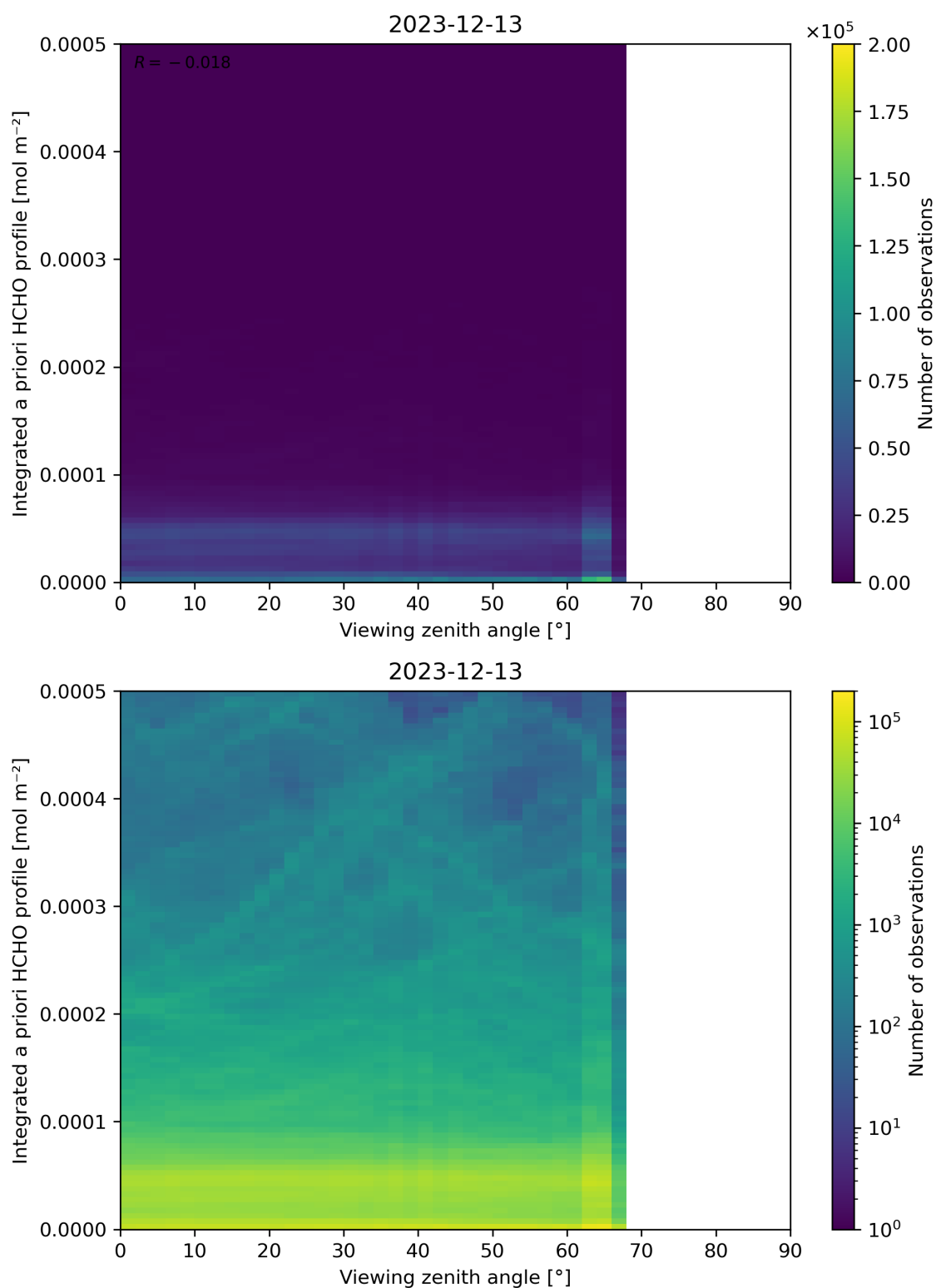
Figure 195: Scatter density plot of “Viewing zenith angle” against “Integrated a priori HCHO profile” for 2023-12-12 to 2023-12-14.
