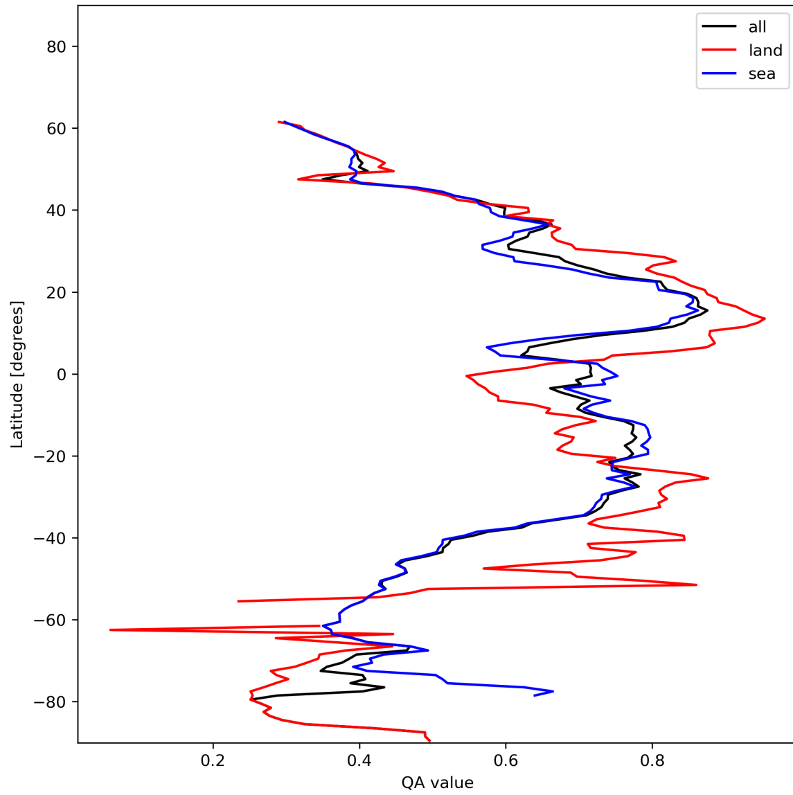
Figure 20: Zonal average of “QA value” for 2023-12-12 to 2023-12-14.
