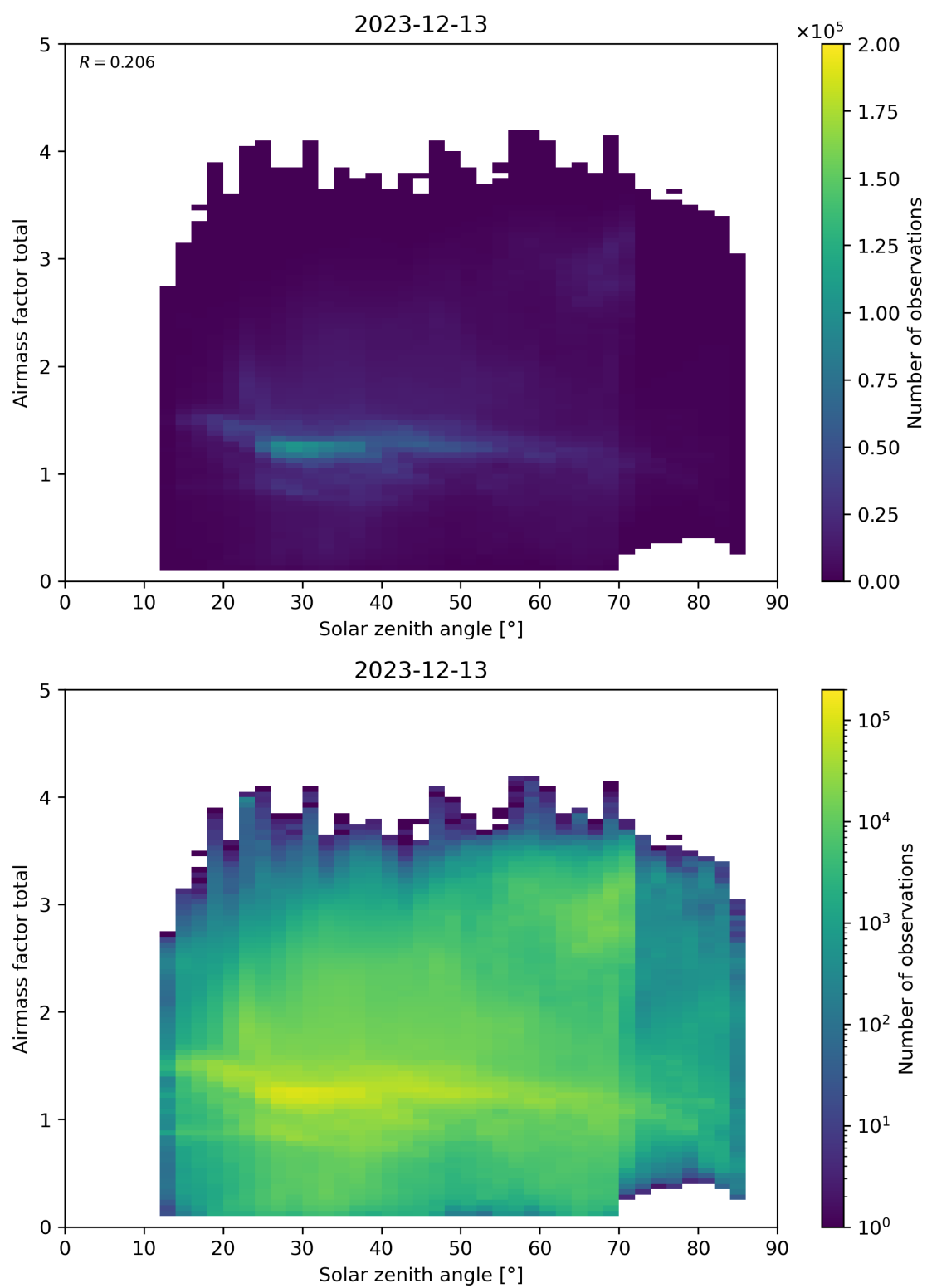
Figure 175: Scatter density plot of “Solar zenith angle” against “Airmass factor total” for 2023-12-12 to 2023-12-14.
