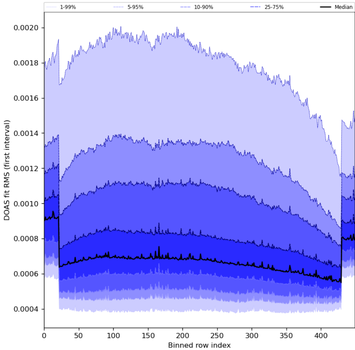
Figure 60: Along track statistics of “DOAS fit RMS (first interval)” for 2023-12-12 to 2023-12-14
