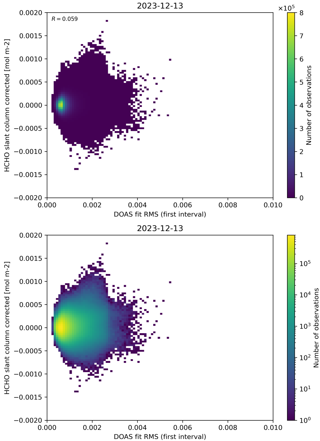
Figure 62: Scatter density plot of “DOAS fit RMS (first interval)” against “HCHO slant column corrected” for 2023-12-12 to 2023-12-14.
