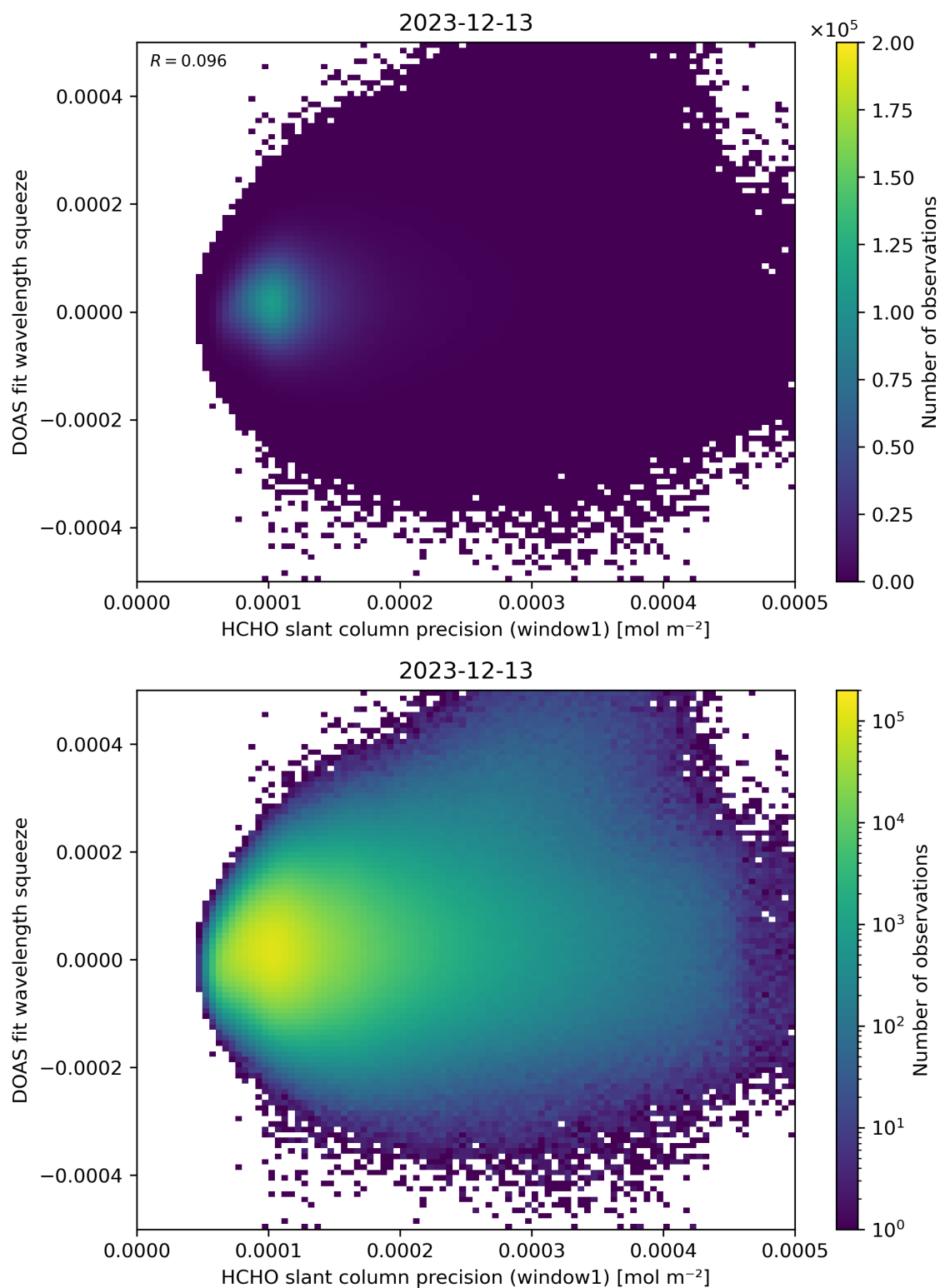
Figure 90: Scatter density plot of “HCHO slant column precision (window1)” against “DOAS fit wavelength squeeze” for 2023-12-12 to 2023-12-14.
