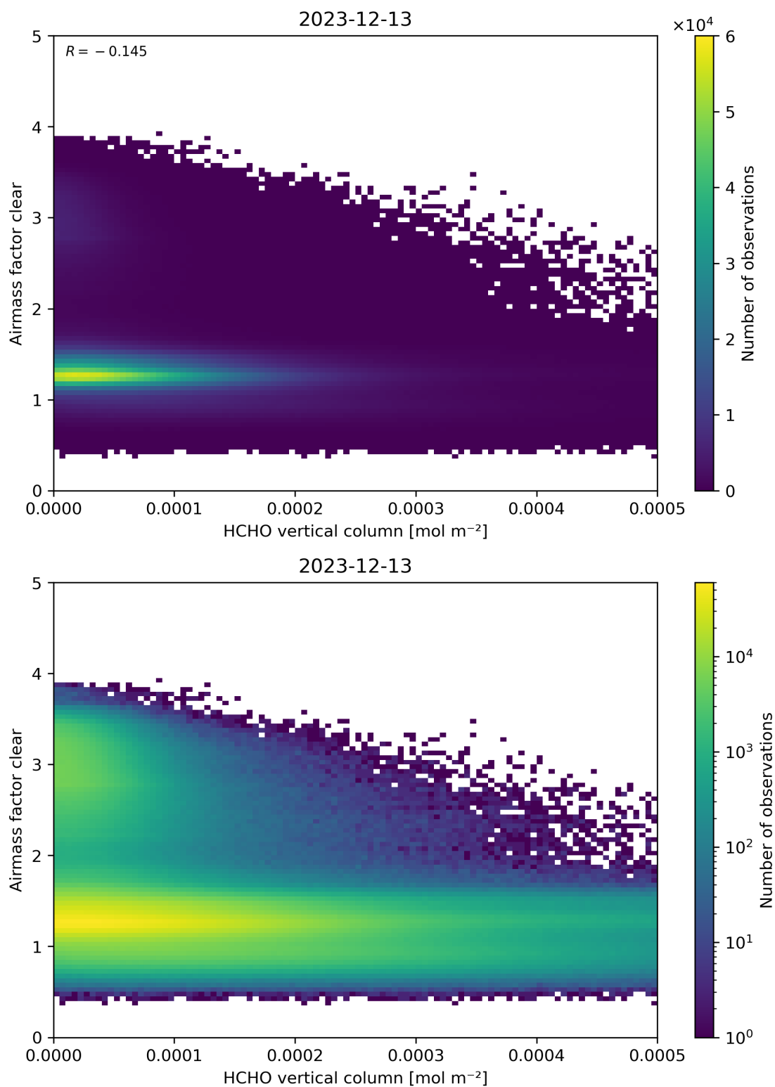
Figure 126: Scatter density plot of “HCHO vertical column” against “Airmass factor clear” for 2023-12-12 to 2023-12-14.
