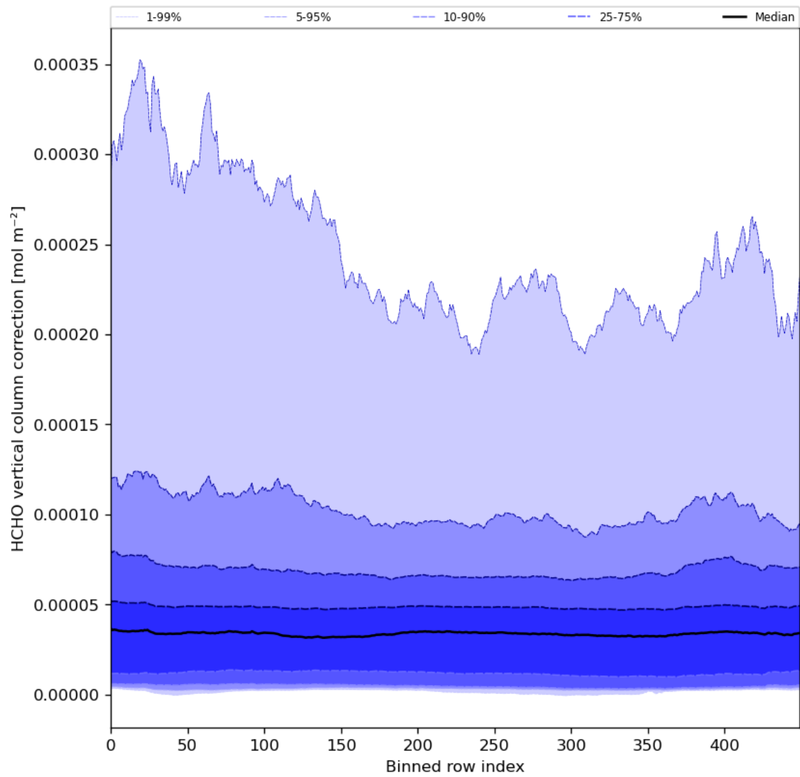
Figure 51: Along track statistics of “HCHO vertical column correction” for 2023-12-12 to 2023-12-14
