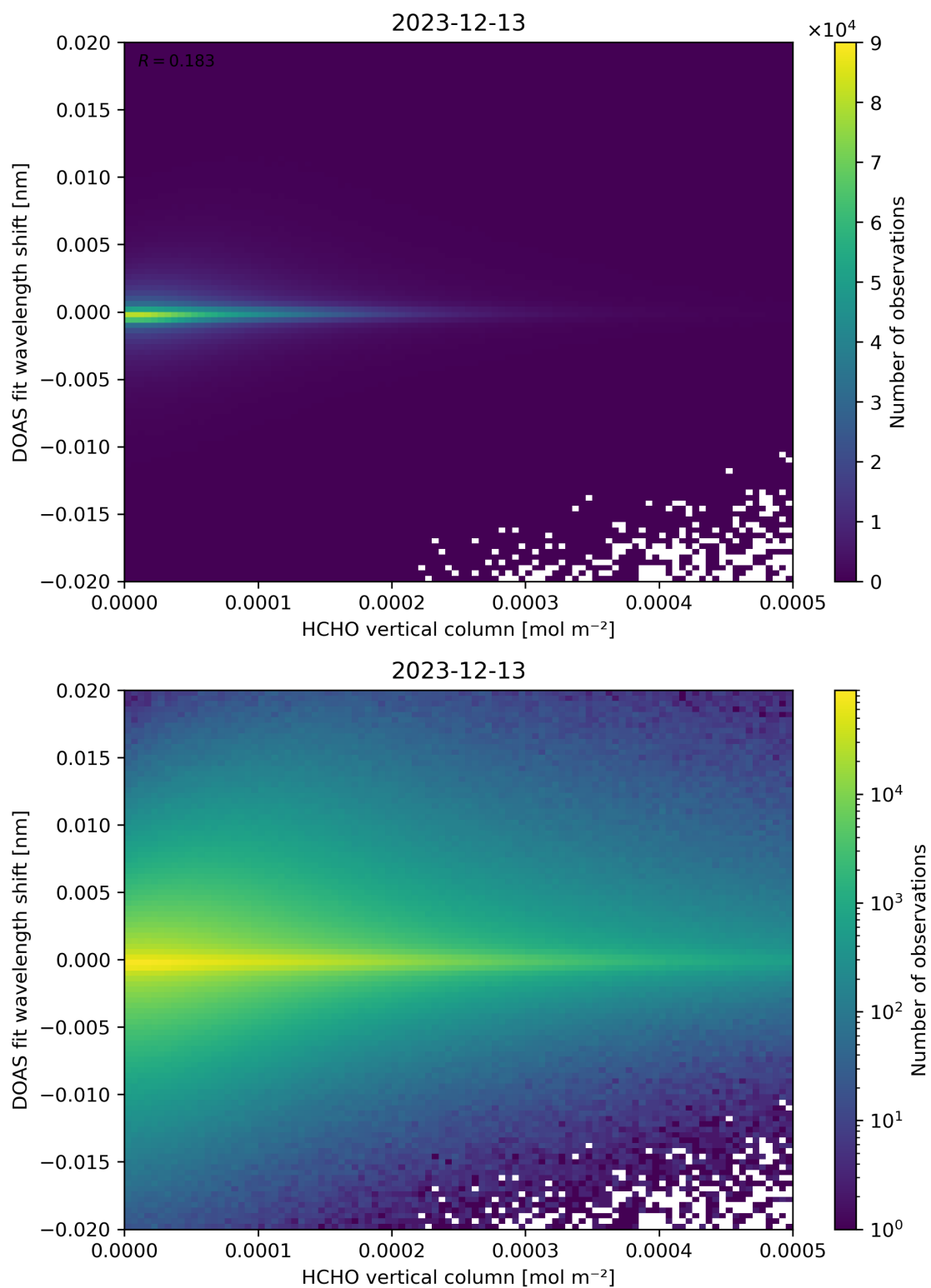
Figure 124: Scatter density plot of “HCHO vertical column” against “DOAS fit wavelength shift” for 2023-12-12 to 2023-12-14.
