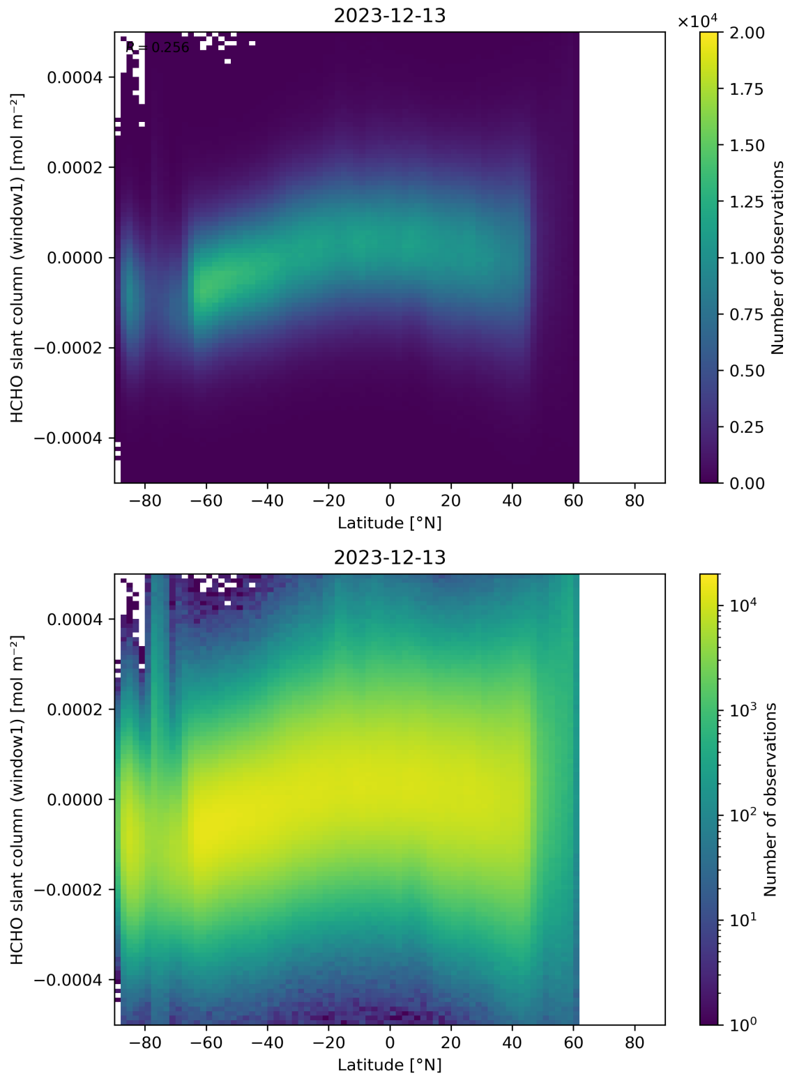
Figure 159: Scatter density plot of “Latitude” against “HCHO slant column (window1)” for 2023-12-12 to 2023-12-14.
