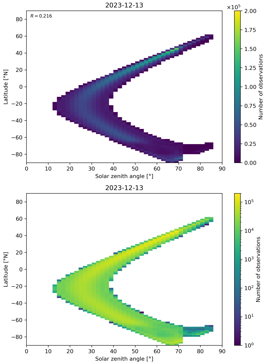
Figure 181: Scatter density plot of “Solar zenith angle” against “Latitude” for 2023-12-12 to 2023-12-14.
