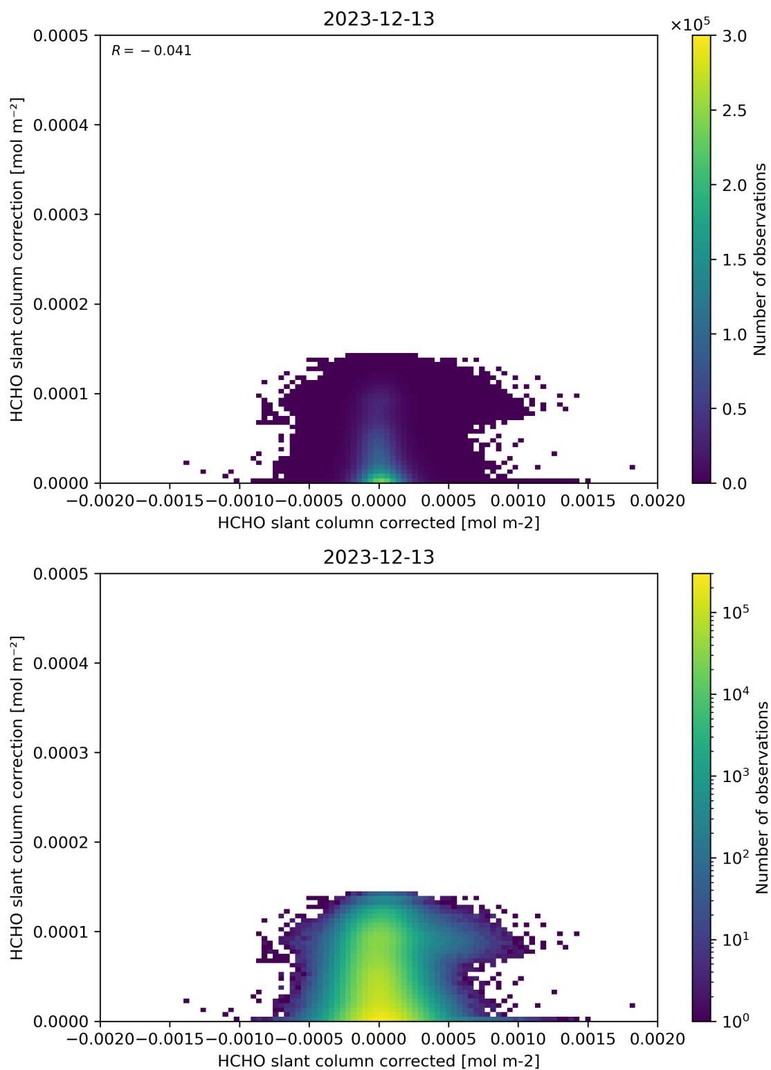
Figure 77: Scatter density plot of “HCHO slant column corrected” against “HCHO slant column correction” for 2023-12-12 to 2023-12-14.
