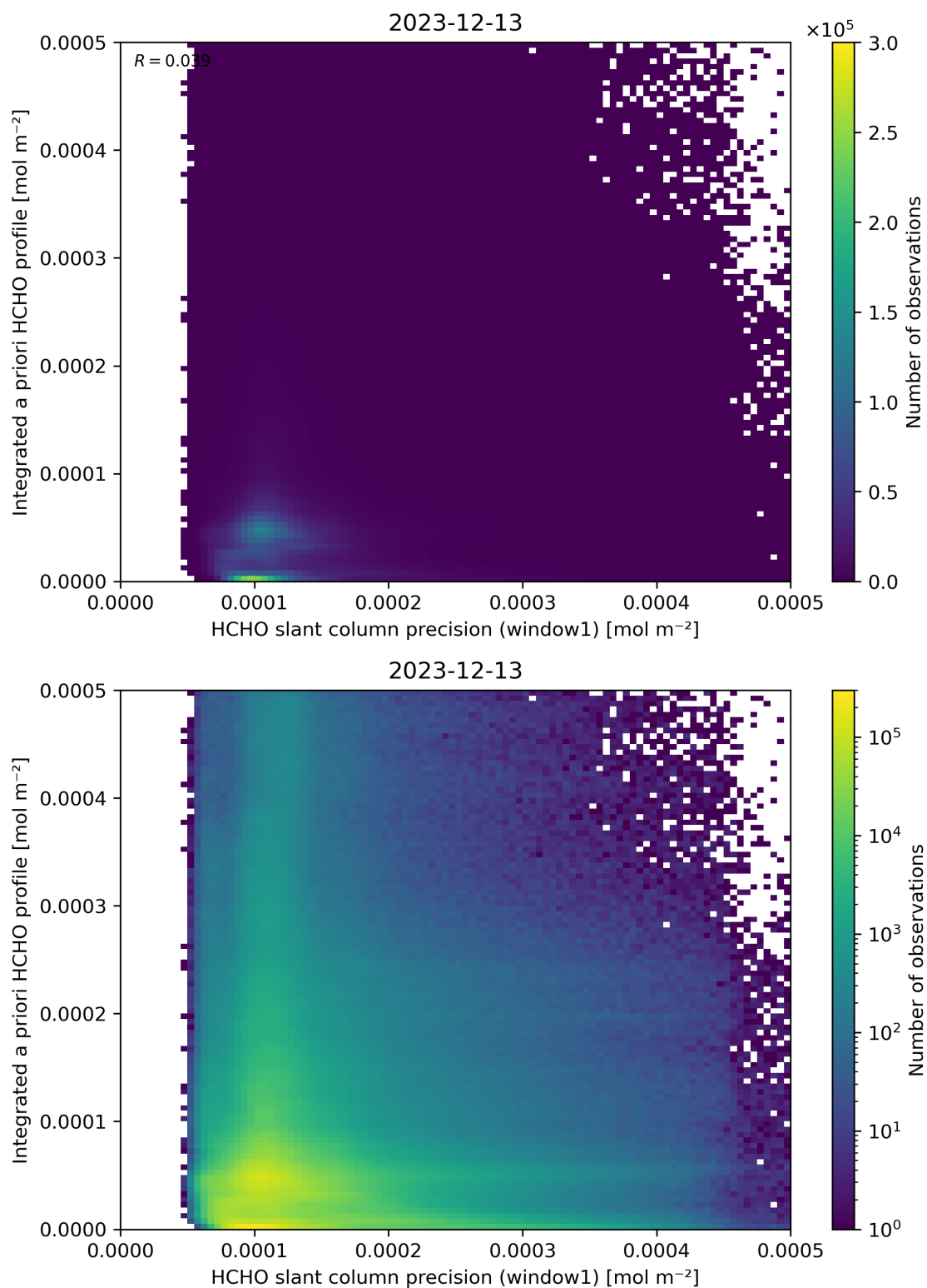
Figure 96: Scatter density plot of “HCHO slant column precision (window1)” against “Integrated a priori HCHO profile” for 2023-12-12 to 2023-12-14.
