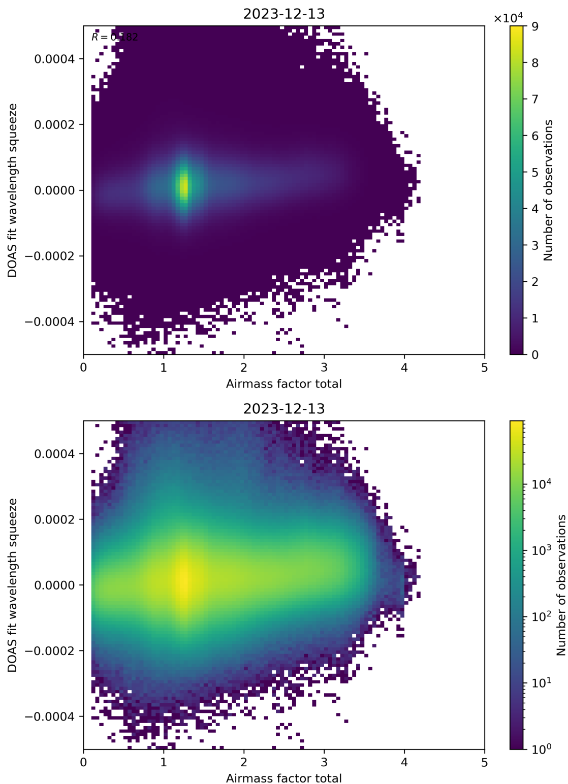
Figure 99: Scatter density plot of “Airmass factor total” against “DOAS fit wavelength squeeze” for 2023-12-12 to 2023-12-14.
