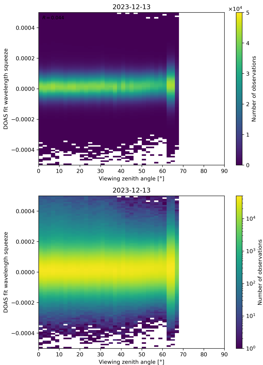
Figure 184: Scatter density plot of “Viewing zenith angle” against “DOAS fit wavelength squeeze” for 2023-12-12 to 2023-12-14.
