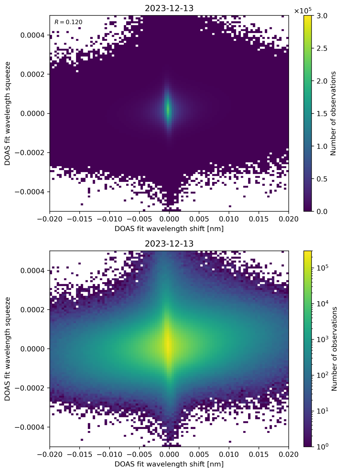
Figure 65: Scatter density plot of “DOAS fit wavelength shift” against “DOAS fit wavelength squeeze” for 2023-12-12 to 2023-12-14.
