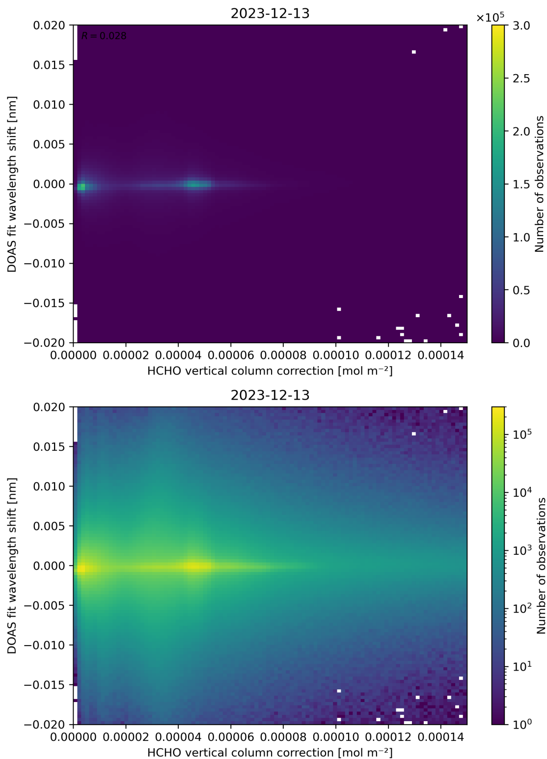
Figure 113: Scatter density plot of “HCHO vertical column correction” against “DOAS fit wavelength shift” for 2023-12-12 to 2023-12-14.
