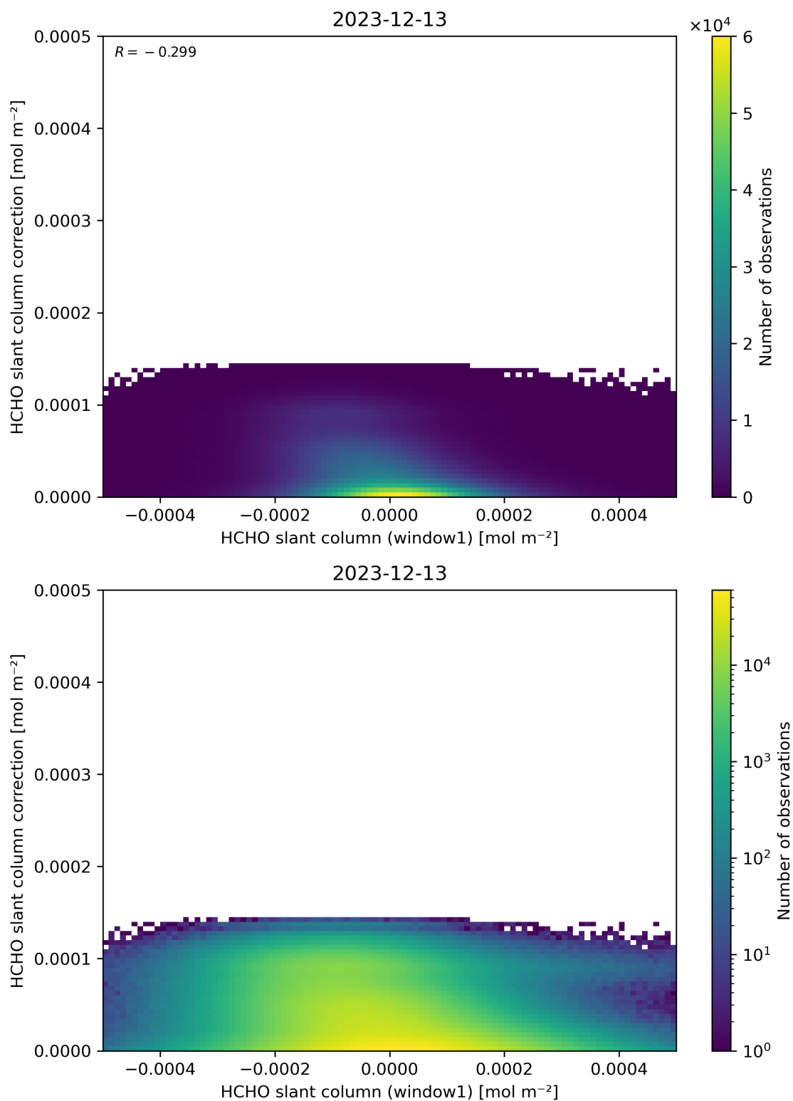
Figure 83: Scatter density plot of “HCHO slant column (window1)” against “HCHO slant column correction” for 2023-12-12 to 2023-12-14.
