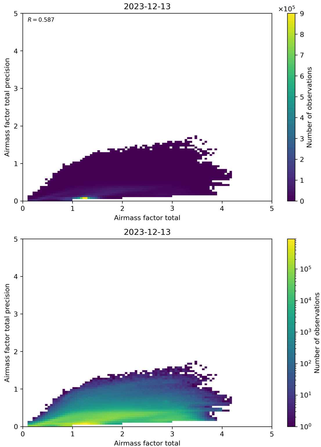
Figure 103: Scatter density plot of “Airmass factor total” against “Airmass factor total precision” for 2023-12-12 to 2023-12-14.
