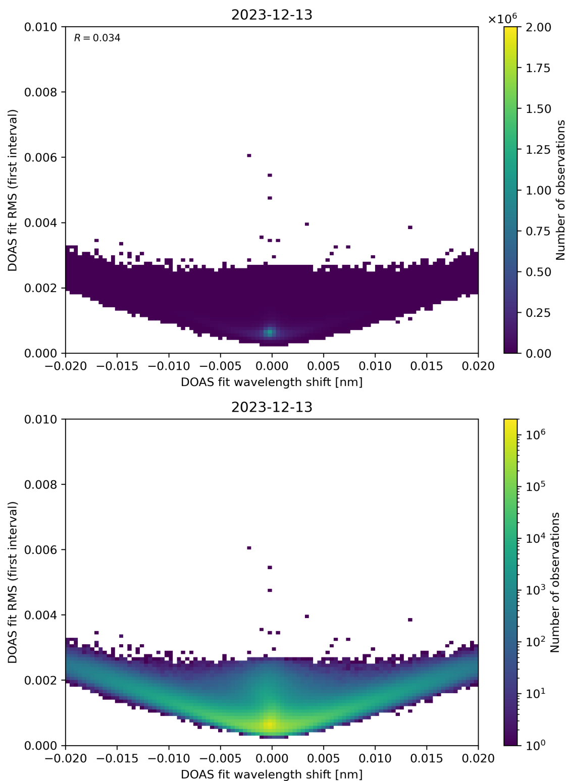
Figure 64: Scatter density plot of “DOAS fit wavelength shift” against “DOAS fit RMS (first interval)” for 2023-12-12 to 2023-12-14.
