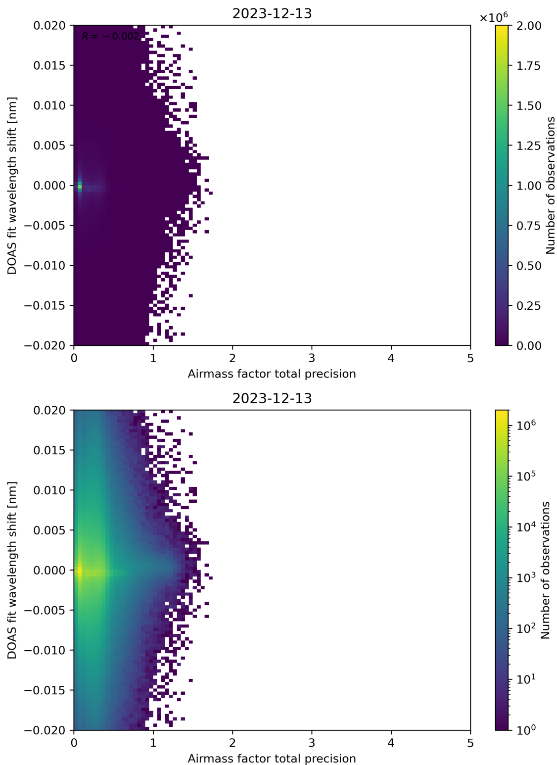
Figure 106: Scatter density plot of “Airmass factor total precision” against “DOAS fit wavelength shift” for 2023-12-12 to 2023-12-14.
