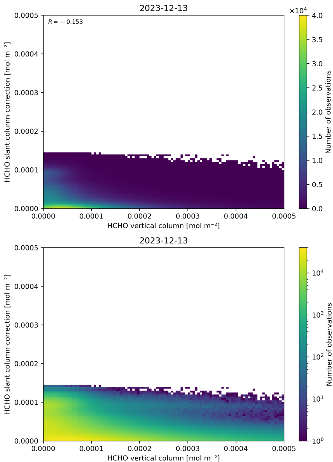
Figure 128: Scatter density plot of “HCHO vertical column” against “HCHO slant column correction” for 2023-12-12 to 2023-12-14.
