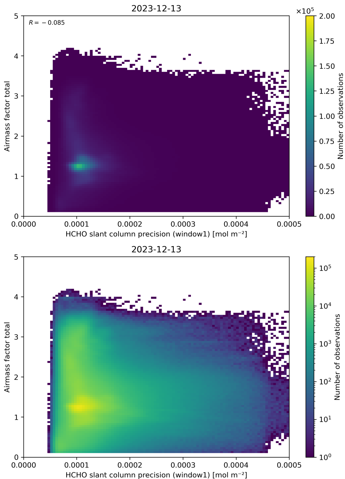
Figure 94: Scatter density plot of “HCHO slant column precision (window1)” against “Airmass factor total” for 2023-12-12 to 2023-12-14.
