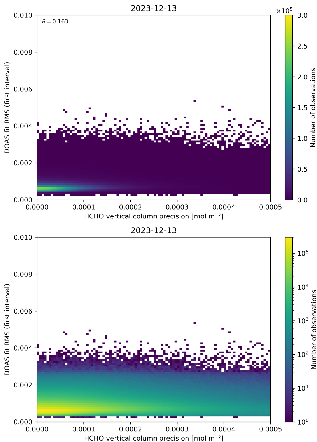
Figure 136: Scatter density plot of “HCHO vertical column precision” against “DOAS fit RMS (first interval)” for 2023-12-12 to 2023-12-14.
