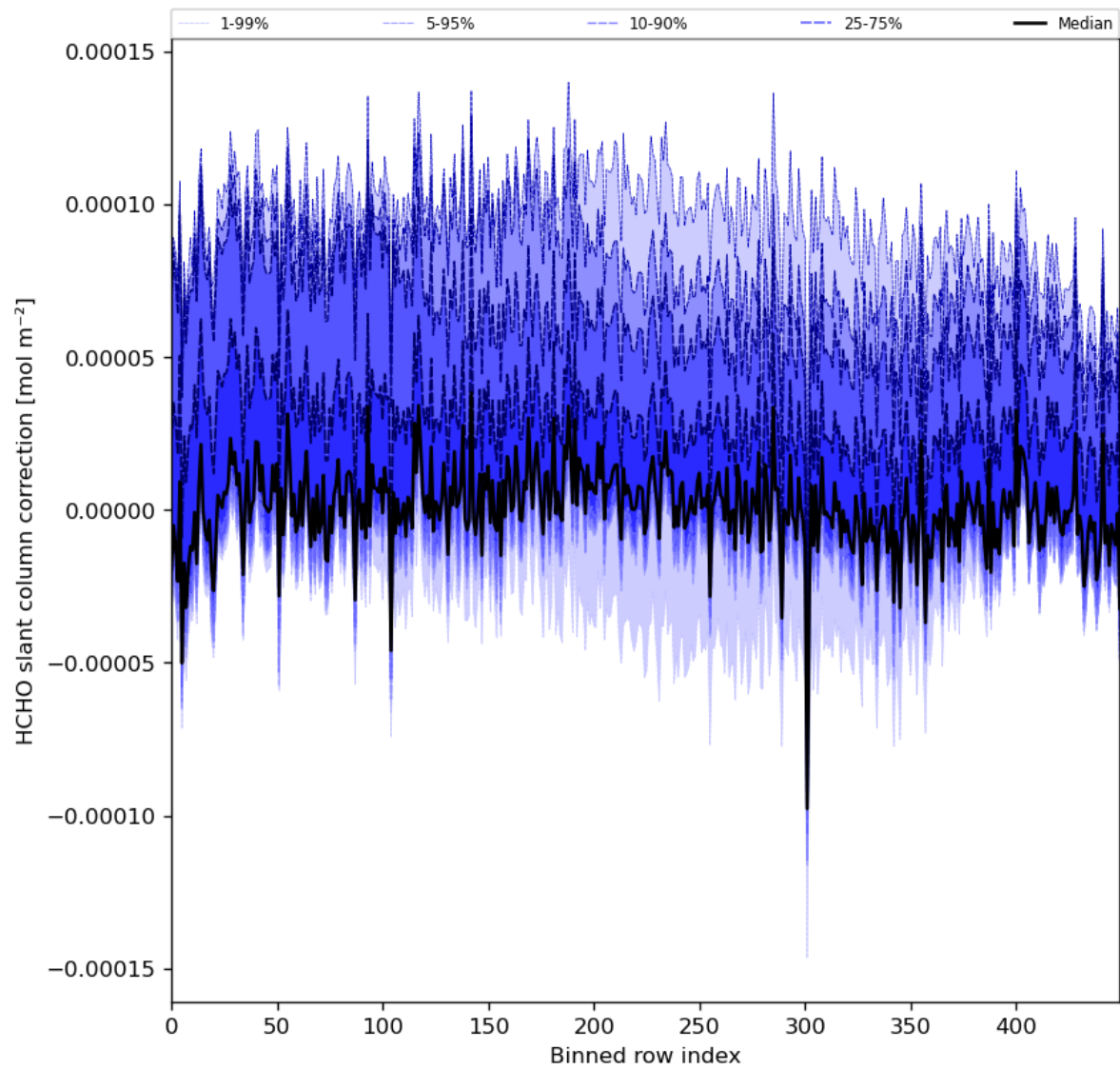
Figure 61: Along track statistics of “HCHO slant column correction” for 2023-12-12 to 2023-12-14
