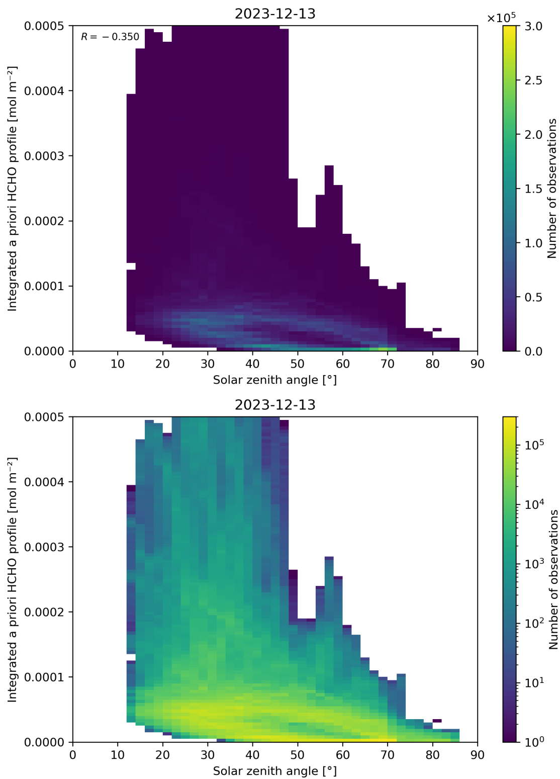
Figure 180: Scatter density plot of “Solar zenith angle” against “Integrated a priori HCHO profile” for 2023-12-12 to 2023-12-14.
