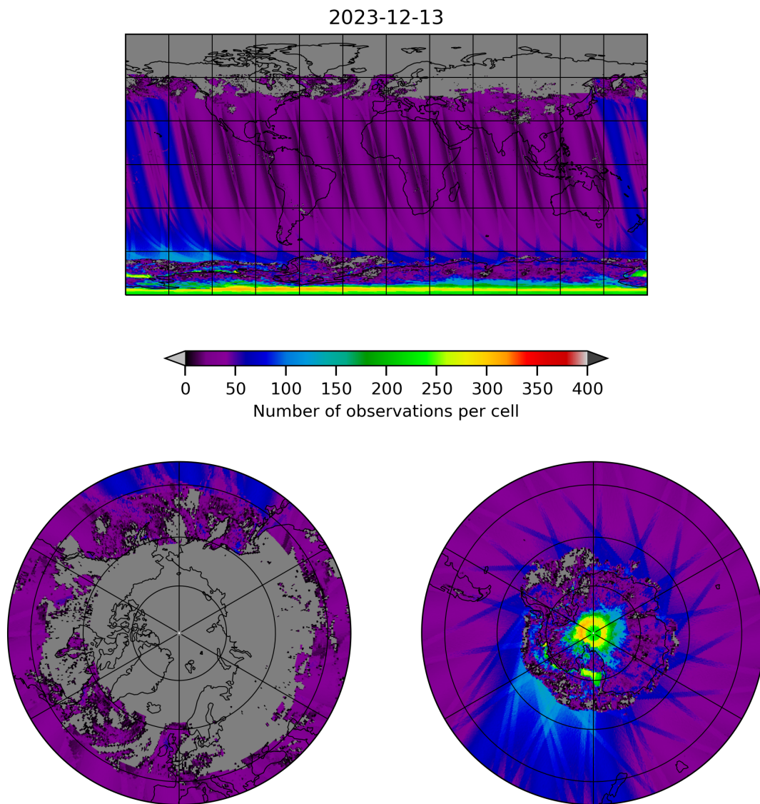
Figure 19: Map of the number of observations for 2023-12-12 to 2023-12-14
