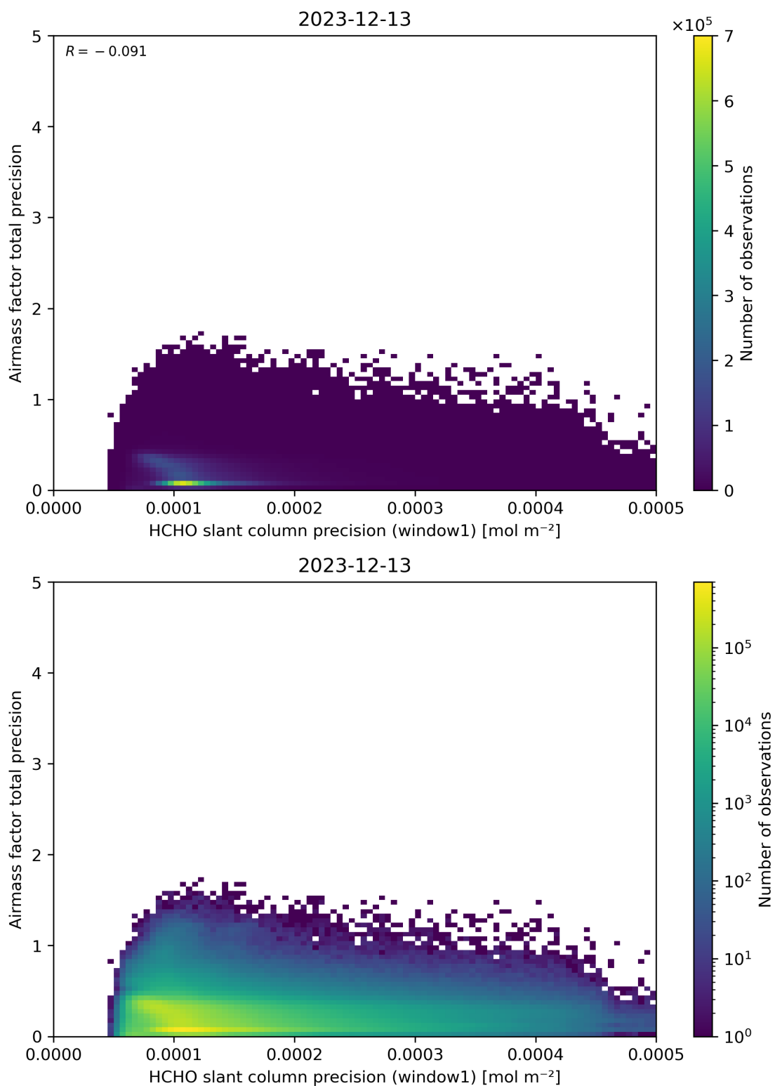
Figure 95: Scatter density plot of “HCHO slant column precision (window1)” against “Airmass factor total precision” for 2023-12-12 to 2023-12-14.
