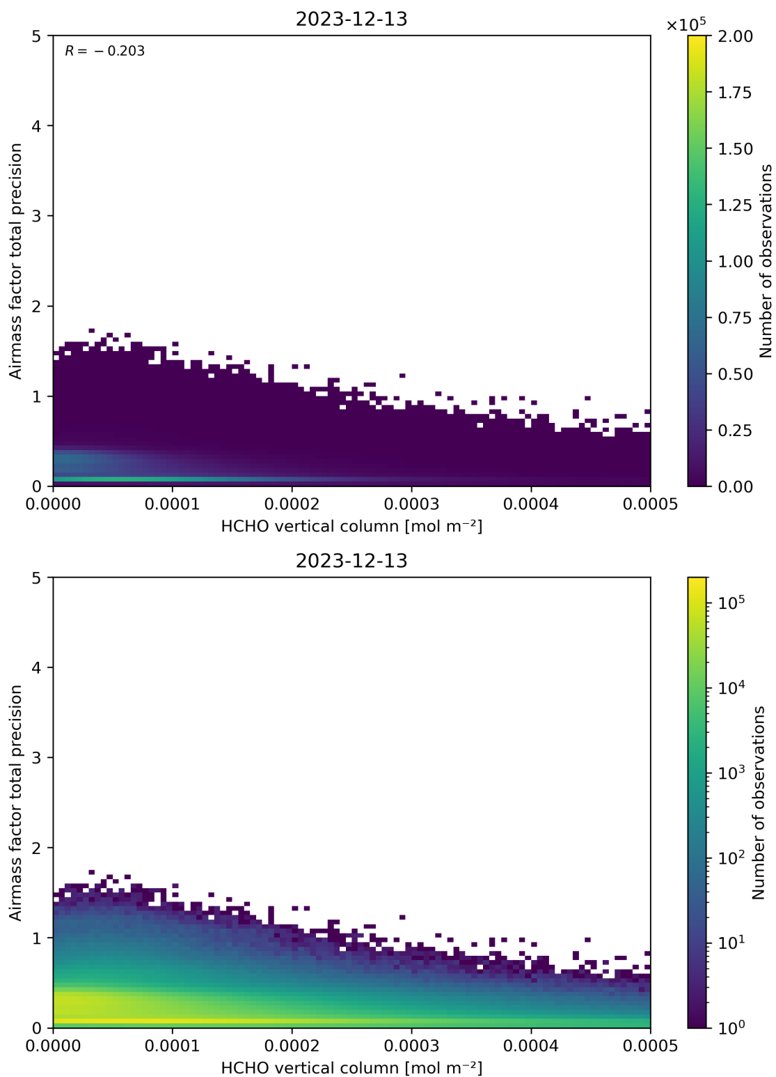
Figure 132: Scatter density plot of “HCHO vertical column” against “Airmass factor total precision” for 2023-12-12 to 2023-12-14.
