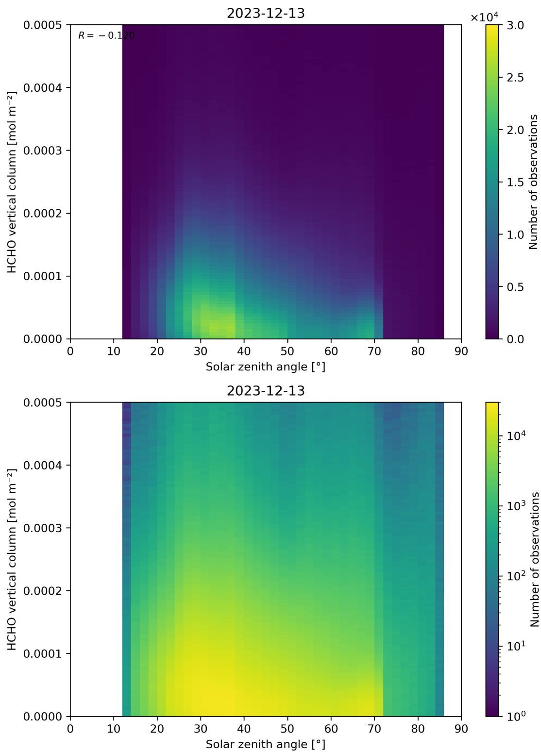
Figure 177: Scatter density plot of “Solar zenith angle” against “HCHO vertical column” for 2023-12-12 to 2023-12-14.
