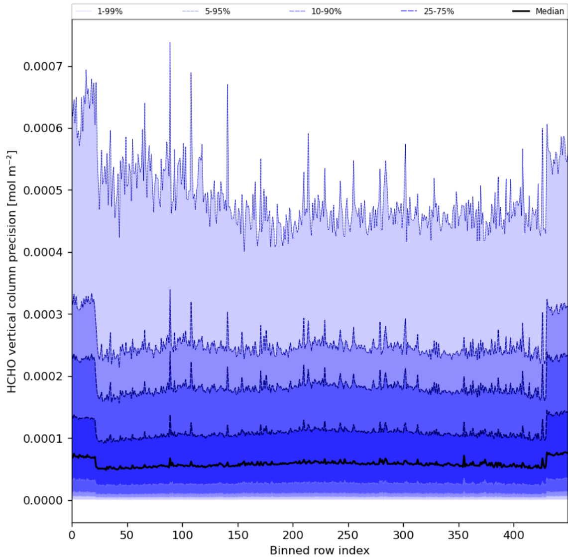
Figure 50: Along track statistics of “HCHO vertical column precision” for 2023-12-12 to 2023-12-14
