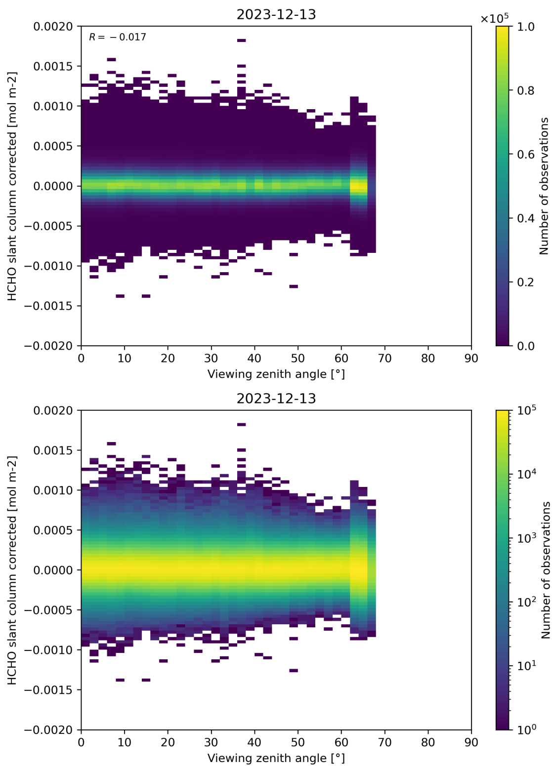
Figure 186: Scatter density plot of “Viewing zenith angle” against “HCHO slant column corrected” for 2023-12-12 to 2023-12-14.
