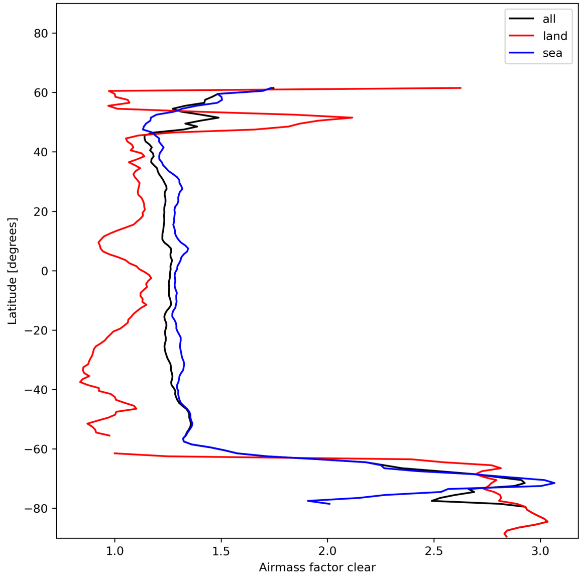
Figure 28: Zonal average of “Airmass factor clear” for 2023-12-12 to 2023-12-14.
