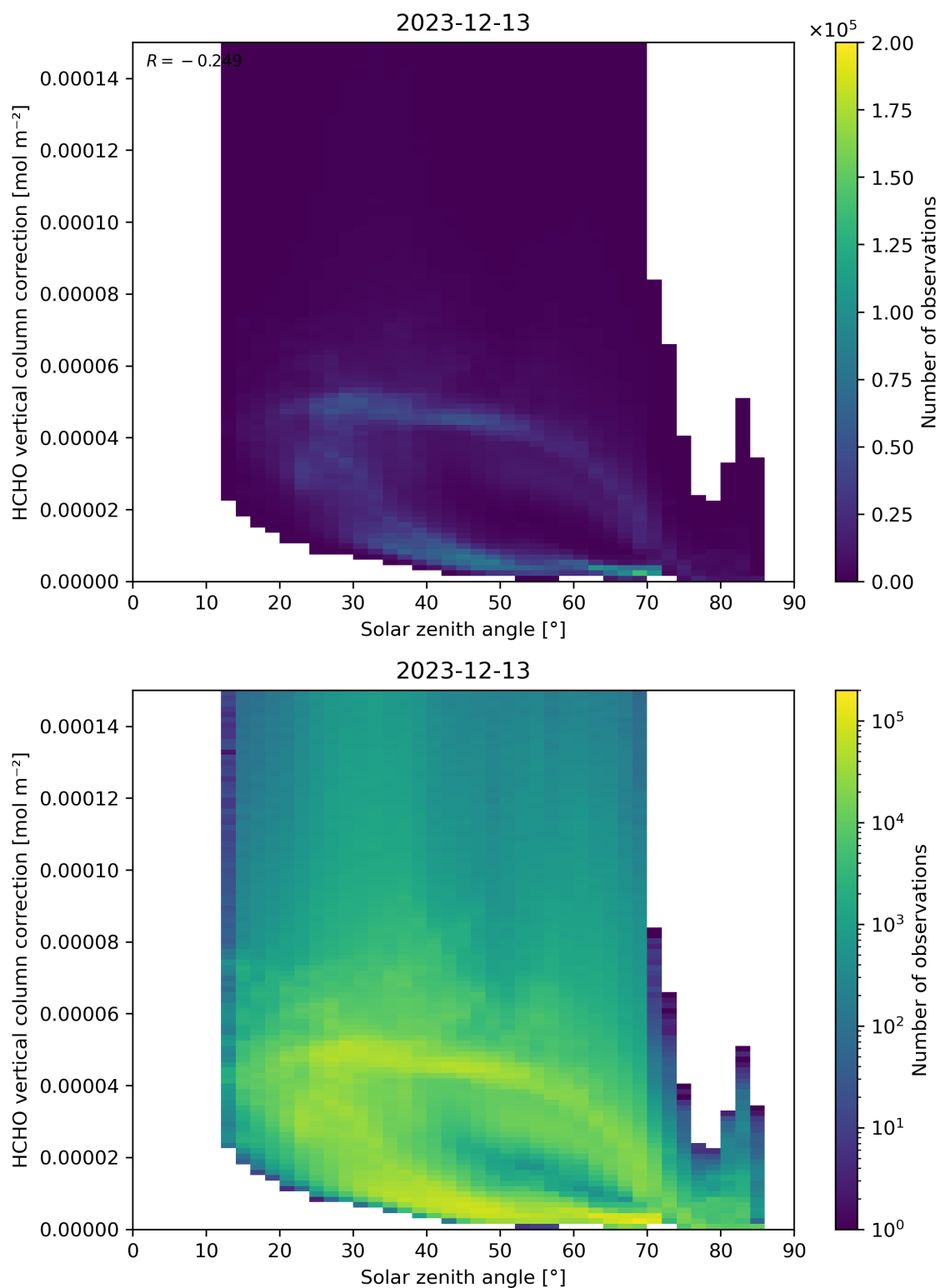
Figure 178: Scatter density plot of “Solar zenith angle” against “HCHO vertical column correction” for 2023-12-12 to 2023-12-14.
