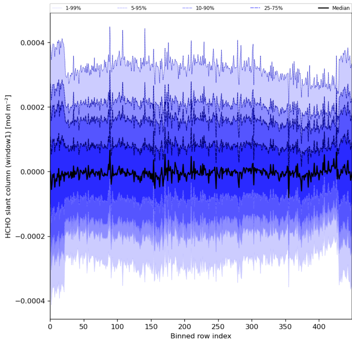
Figure 52: Along track statistics of “HCHO slant column (window1)” for 2023-12-12 to 2023-12-14
