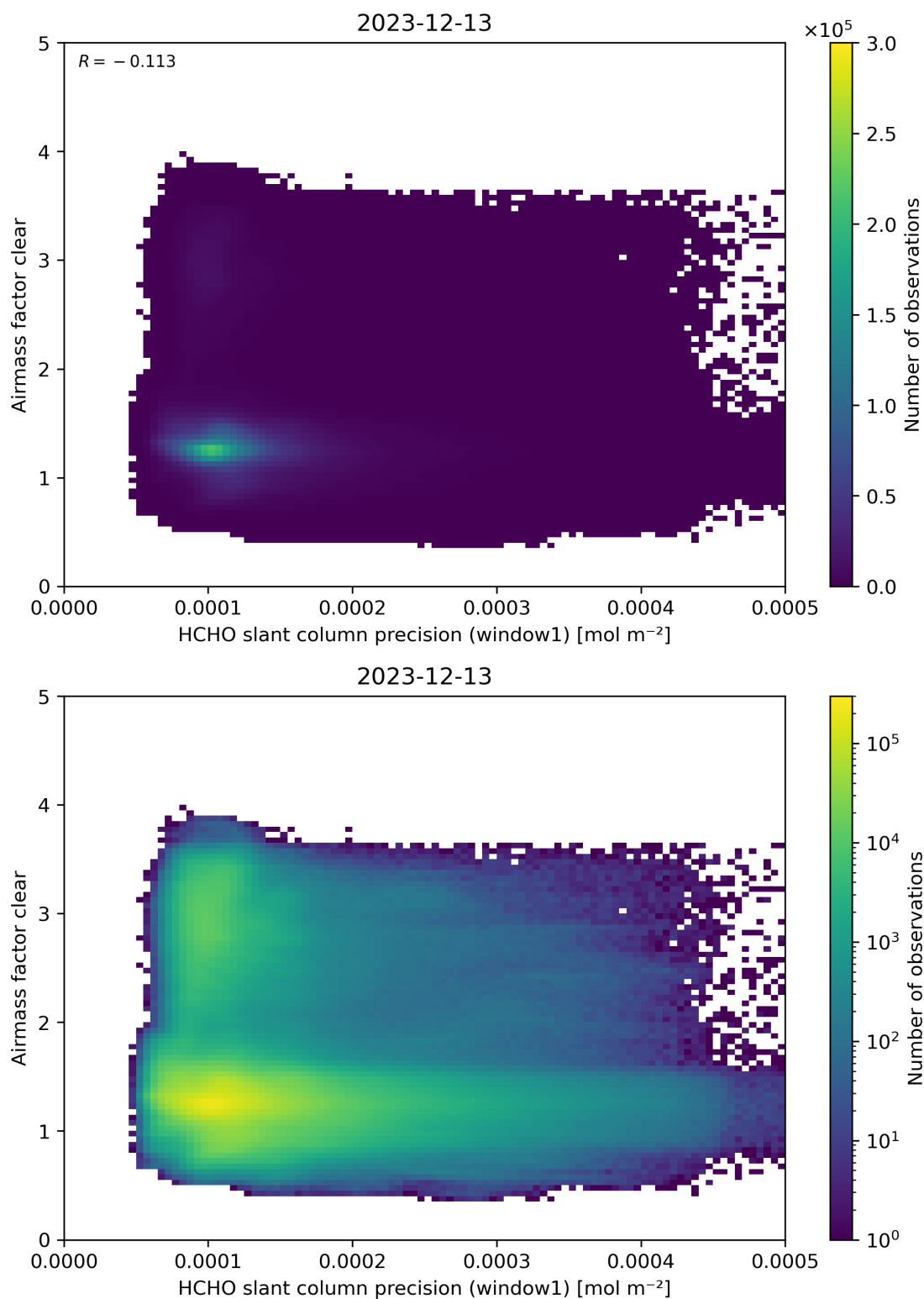
Figure 91: Scatter density plot of “HCHO slant column precision (window1)” against “Airmass factor clear” for 2023-12-12 to 2023-12-14.
