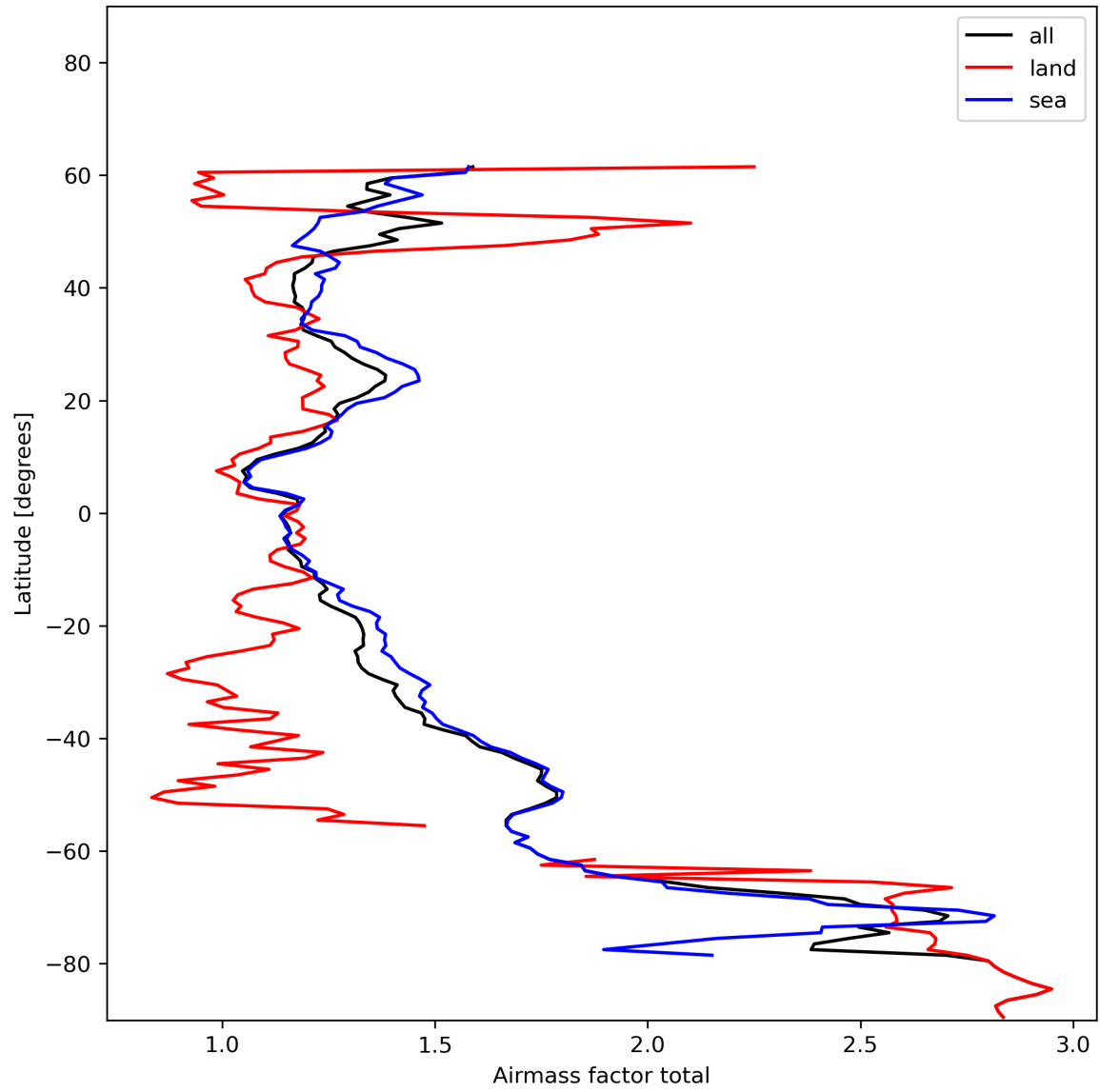
Figure 26: Zonal average of “Airmass factor total” for 2023-12-12 to 2023-12-14.
