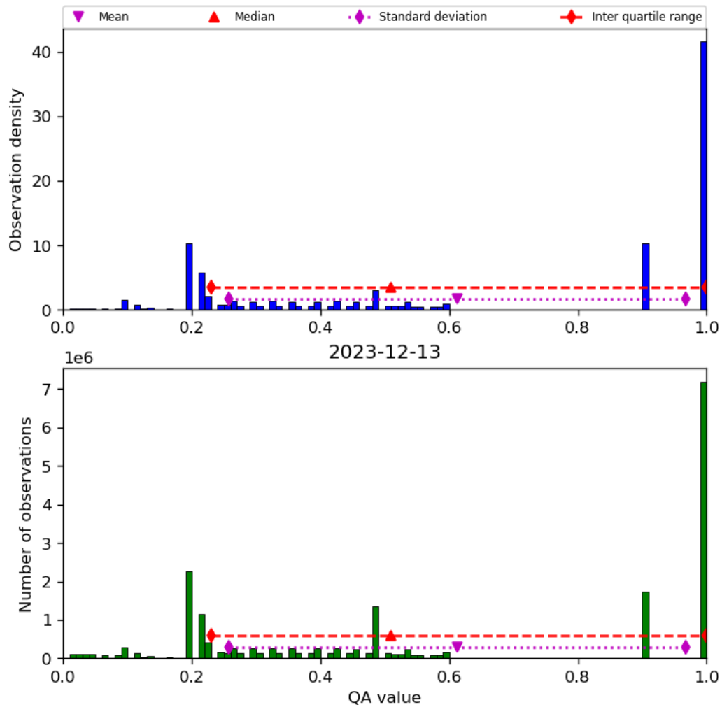
Figure 34: Histogram of “QA value” for 2023-12-12 to 2023-12-14
