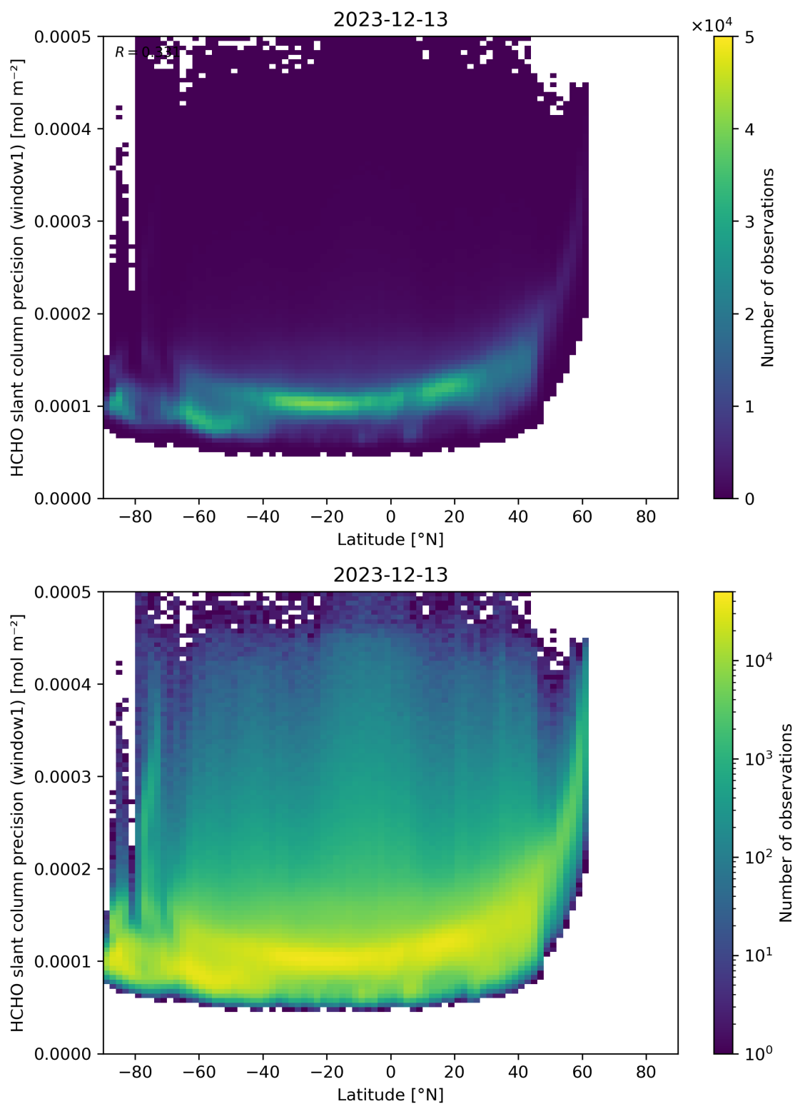
Figure 160: Scatter density plot of “Latitude” against “HCHO slant column precision (window1)” for 2023-12-12 to 2023-12-14.
