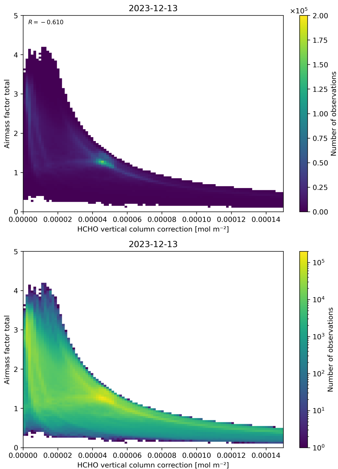
Figure 120: Scatter density plot of “HCHO vertical column correction” against “Airmass factor total” for 2023-12-12 to 2023-12-14.
