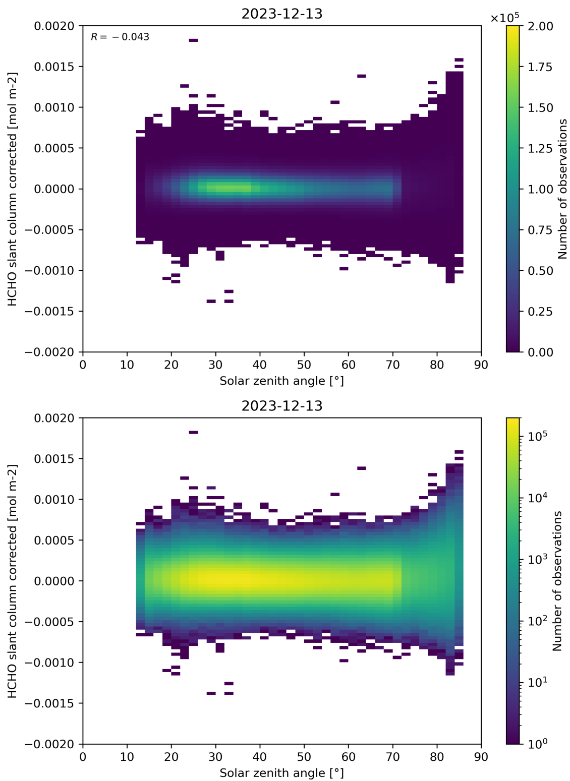
Figure 171: Scatter density plot of “Solar zenith angle” against “HCHO slant column corrected” for 2023-12-12 to 2023-12-14.
