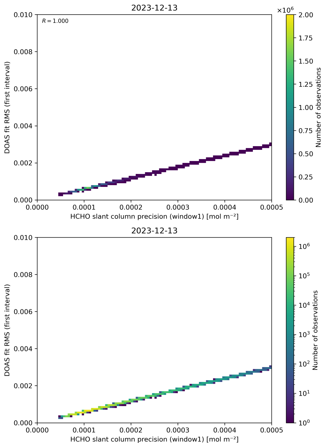
Figure 88: Scatter density plot of “HCHO slant column precision (window1)” against “DOAS fit RMS (first interval)” for 2023-12-12 to 2023-12-14.
