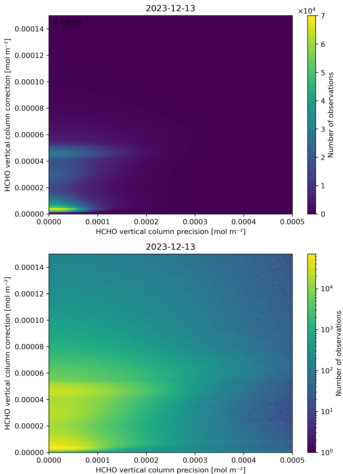
Figure 146: Scatter density plot of “HCHO vertical column precision” against “HCHO vertical column correction” for 2023-12-12 to 2023-12-14.
