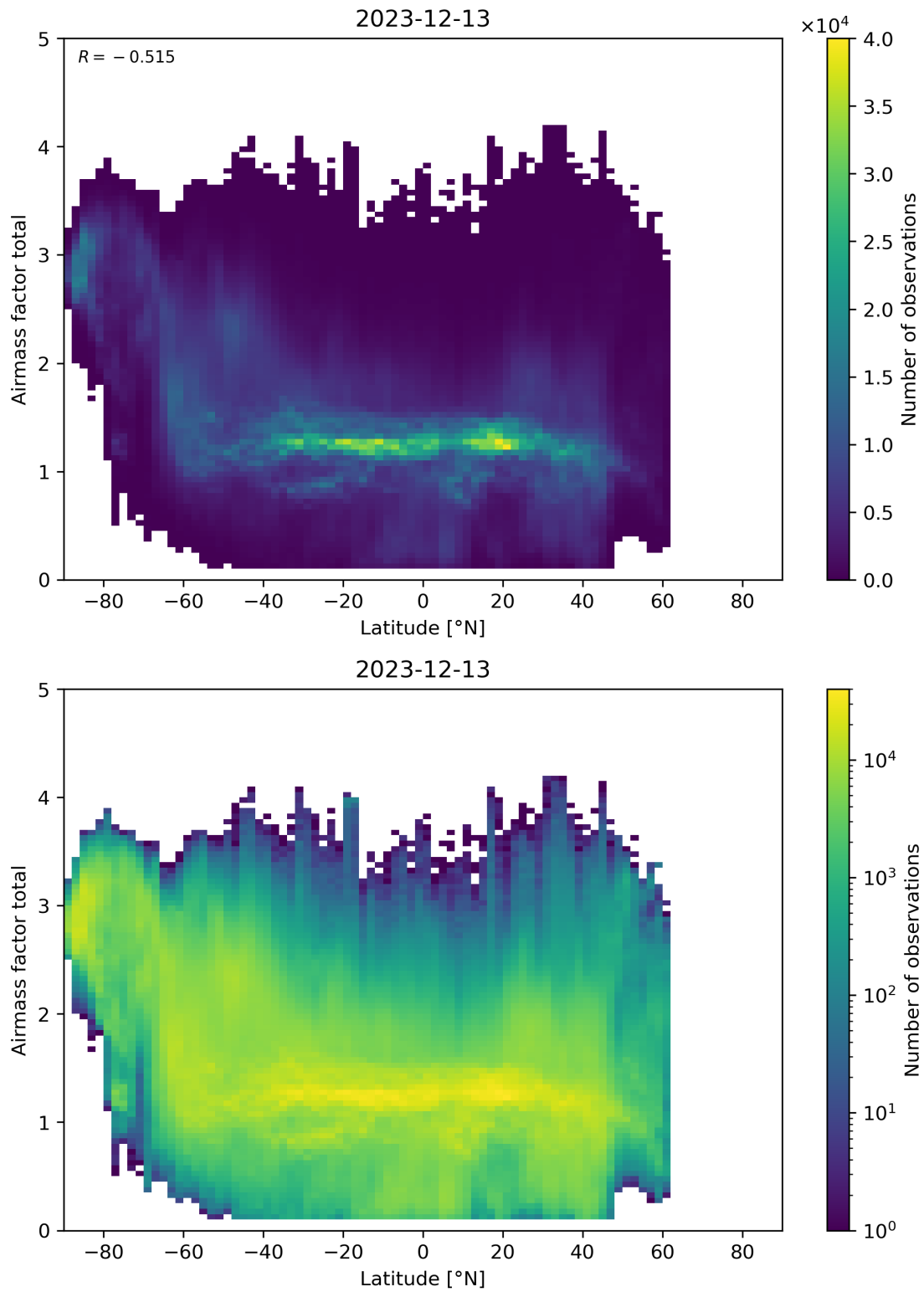
Figure 161: Scatter density plot of “Latitude” against “Airmass factor total” for 2023-12-12 to 2023-12-14.
