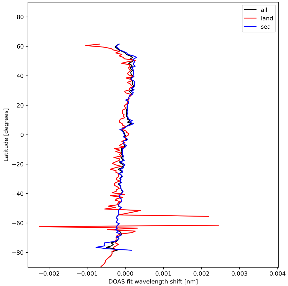
Figure 30: Zonal average of “DOAS fit wavelength shift” for 2023-12-12 to 2023-12-14.
