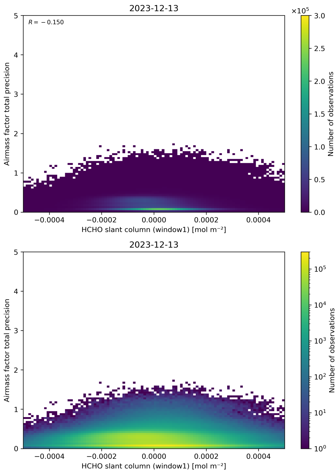
Figure 86: Scatter density plot of “HCHO slant column (window1)” against “Airmass factor total precision” for 2023-12-12 to 2023-12-14.
