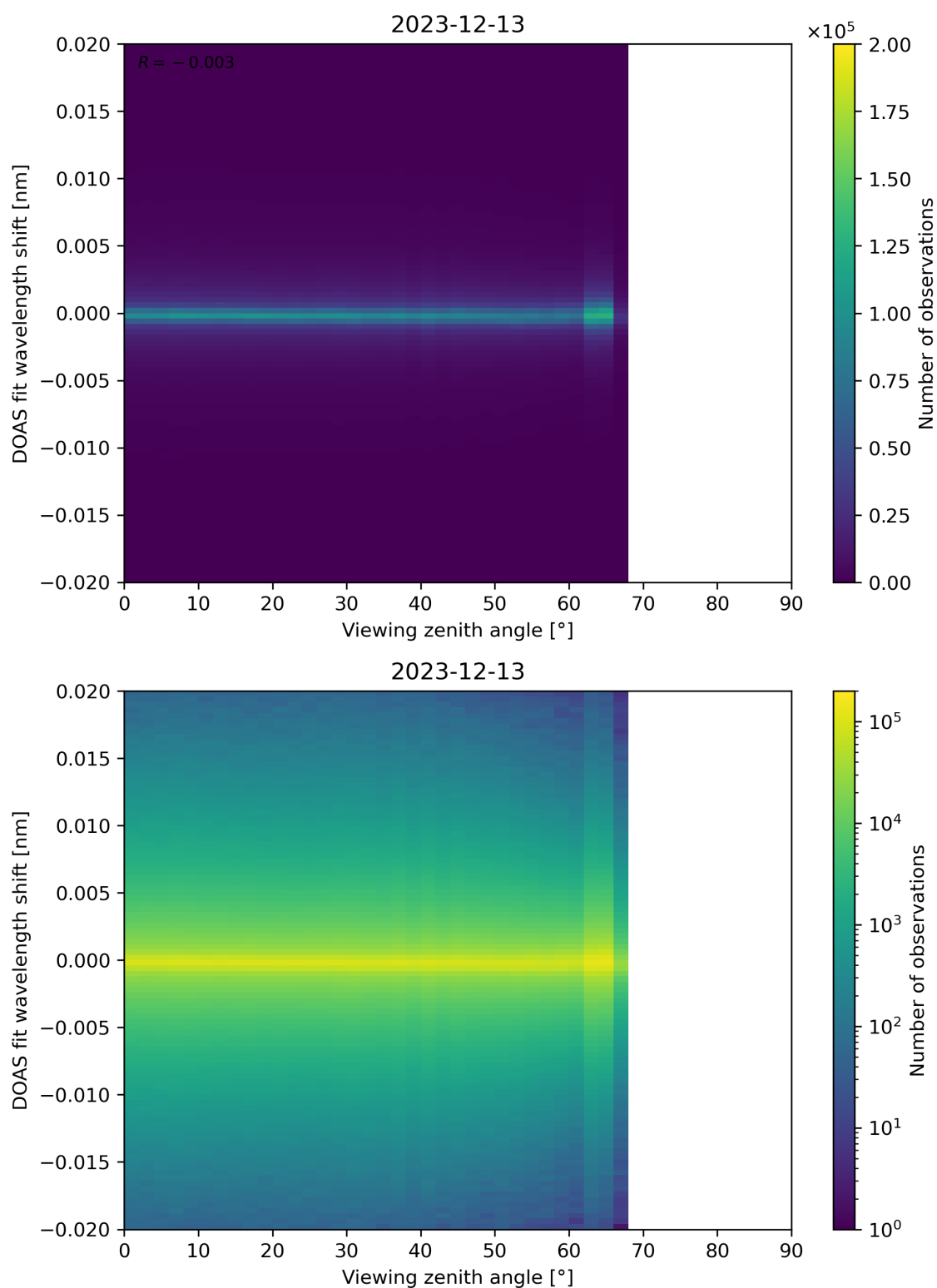
Figure 183: Scatter density plot of “Viewing zenith angle” against “DOAS fit wavelength shift” for 2023-12-12 to 2023-12-14.
