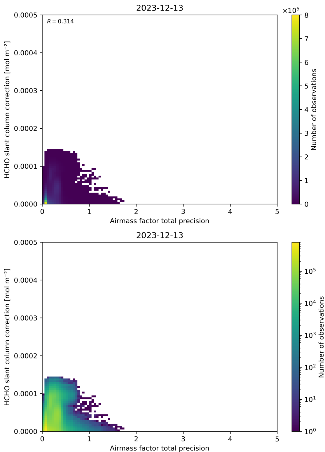
Figure 110: Scatter density plot of “Airmass factor total precision” against “HCHO slant column correction” for 2023-12-12 to 2023-12-14.
