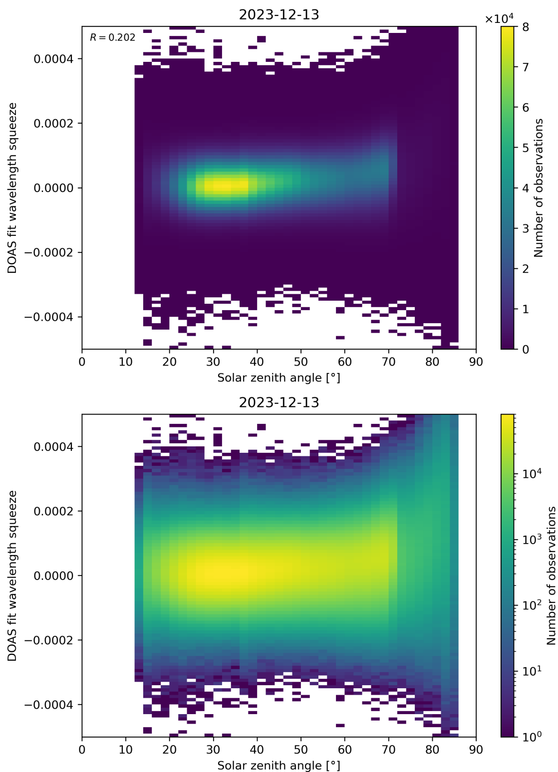
Figure 169: Scatter density plot of “Solar zenith angle” against “DOAS fit wavelength squeeze” for 2023-12-12 to 2023-12-14.
