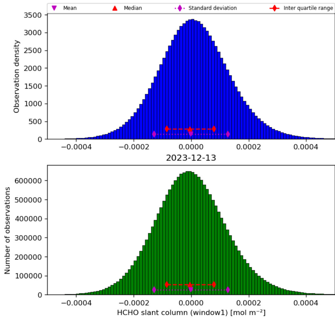
Figure 38: Histogram of “HCHO slant column (window1)” for 2023-12-12 to 2023-12-14
