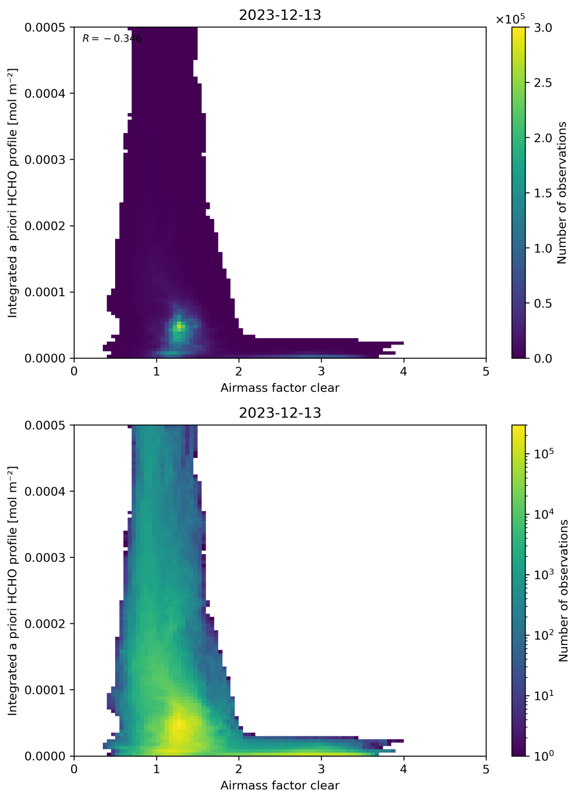
Figure 76: Scatter density plot of “Airmass factor clear” against “Integrated a priori HCHO profile” for 2023-12-12 to 2023-12-14.
