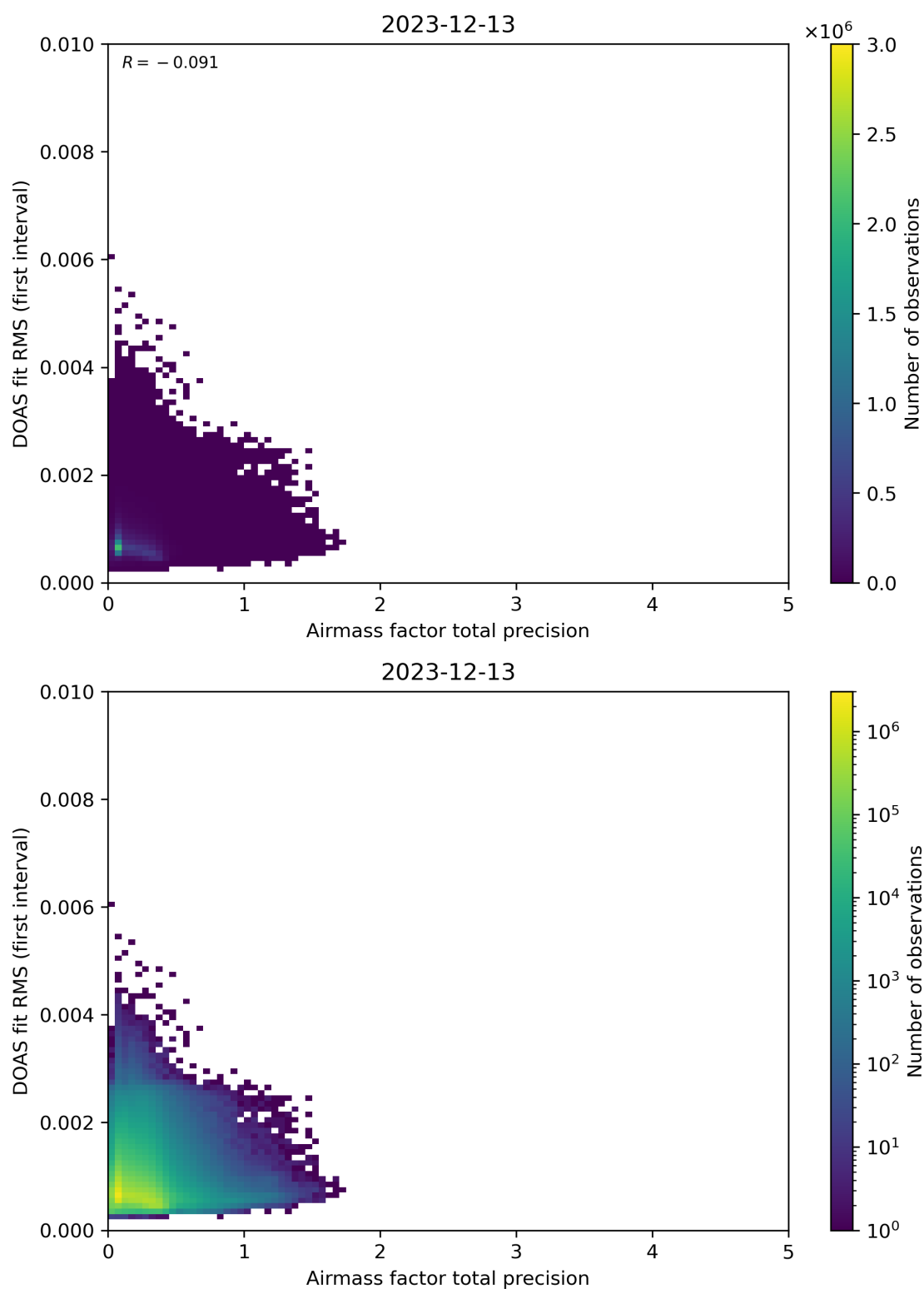
Figure 105: Scatter density plot of “Airmass factor total precision” against “DOAS fit RMS (first interval)” for 2023-12-12 to 2023-12-14.
