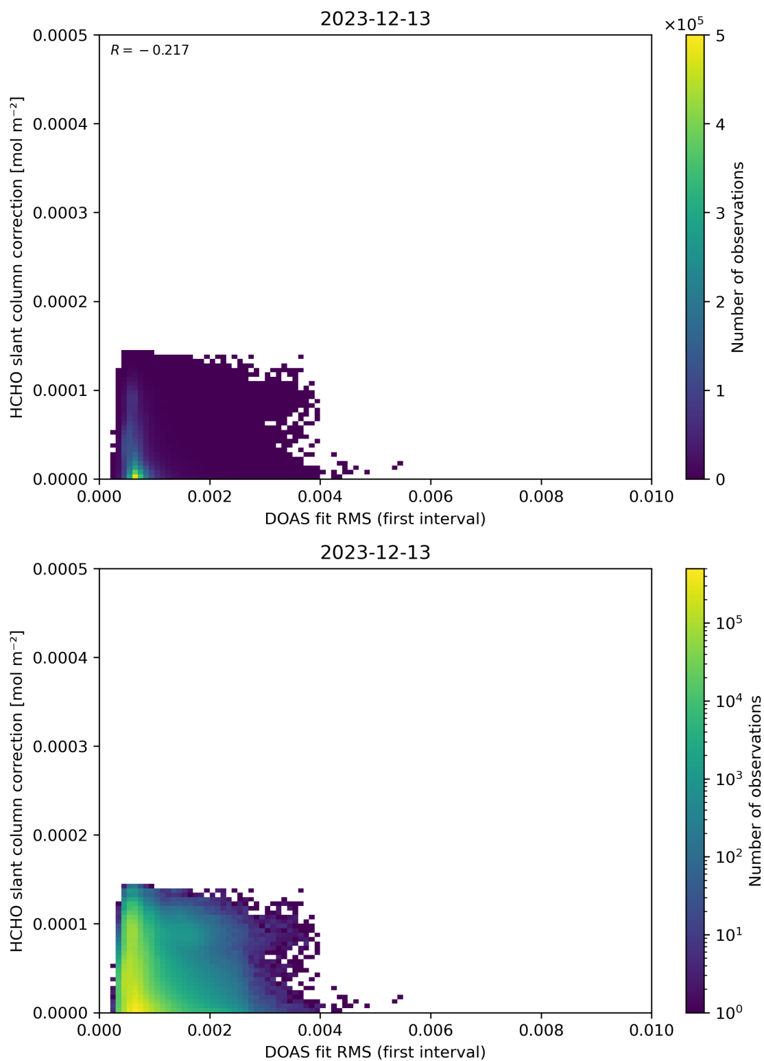
Figure 63: Scatter density plot of “DOAS fit RMS (first interval)” against “HCHO slant column correction” for 2023-12-12 to 2023-12-14.
