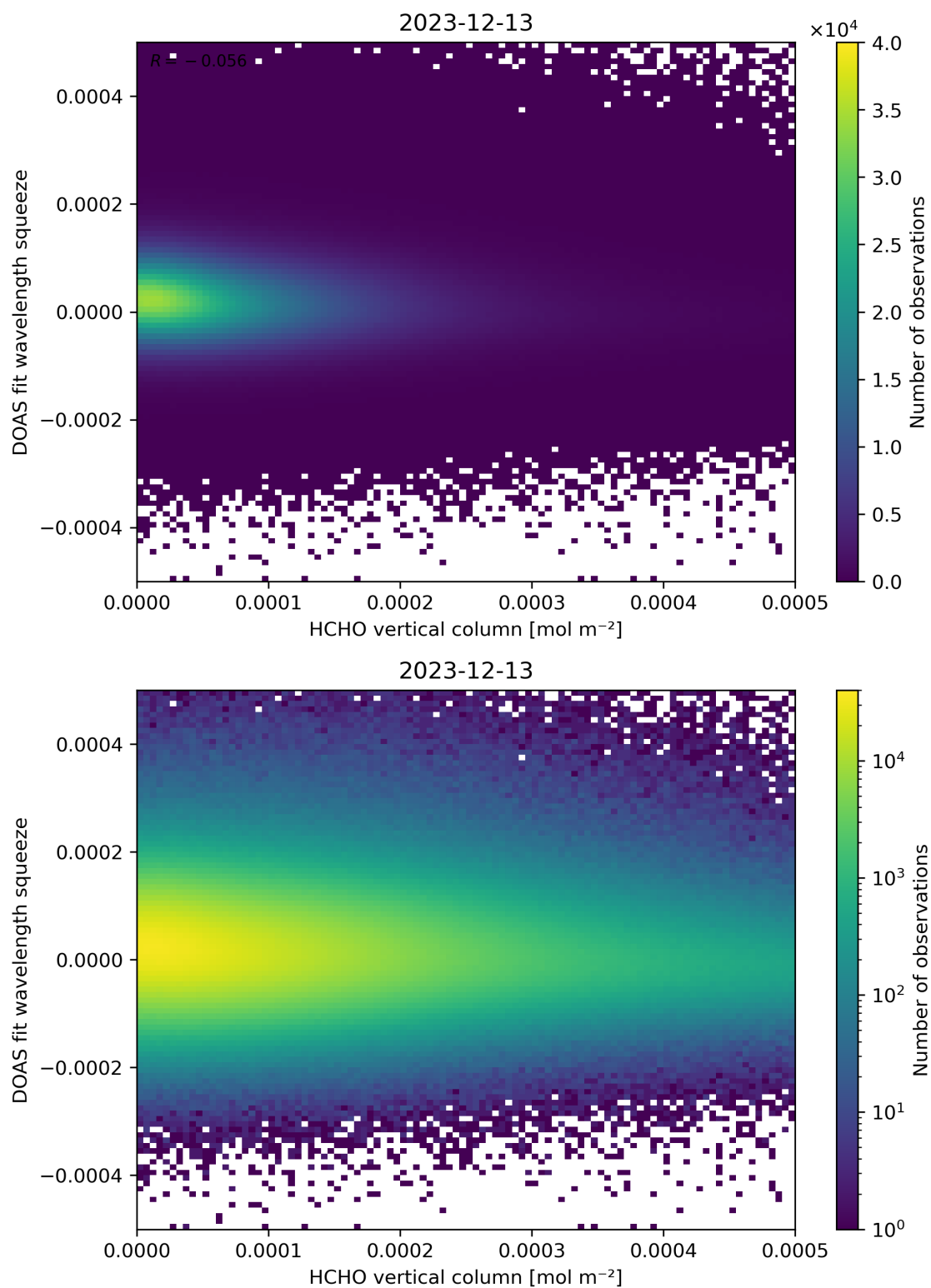
Figure 125: Scatter density plot of “HCHO vertical column” against “DOAS fit wavelength squeeze” for 2023-12-12 to 2023-12-14.
