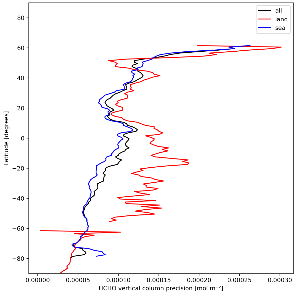
Figure 22: Zonal average of “HCHO vertical column precision” for 2023-12-12 to 2023-12-14.
