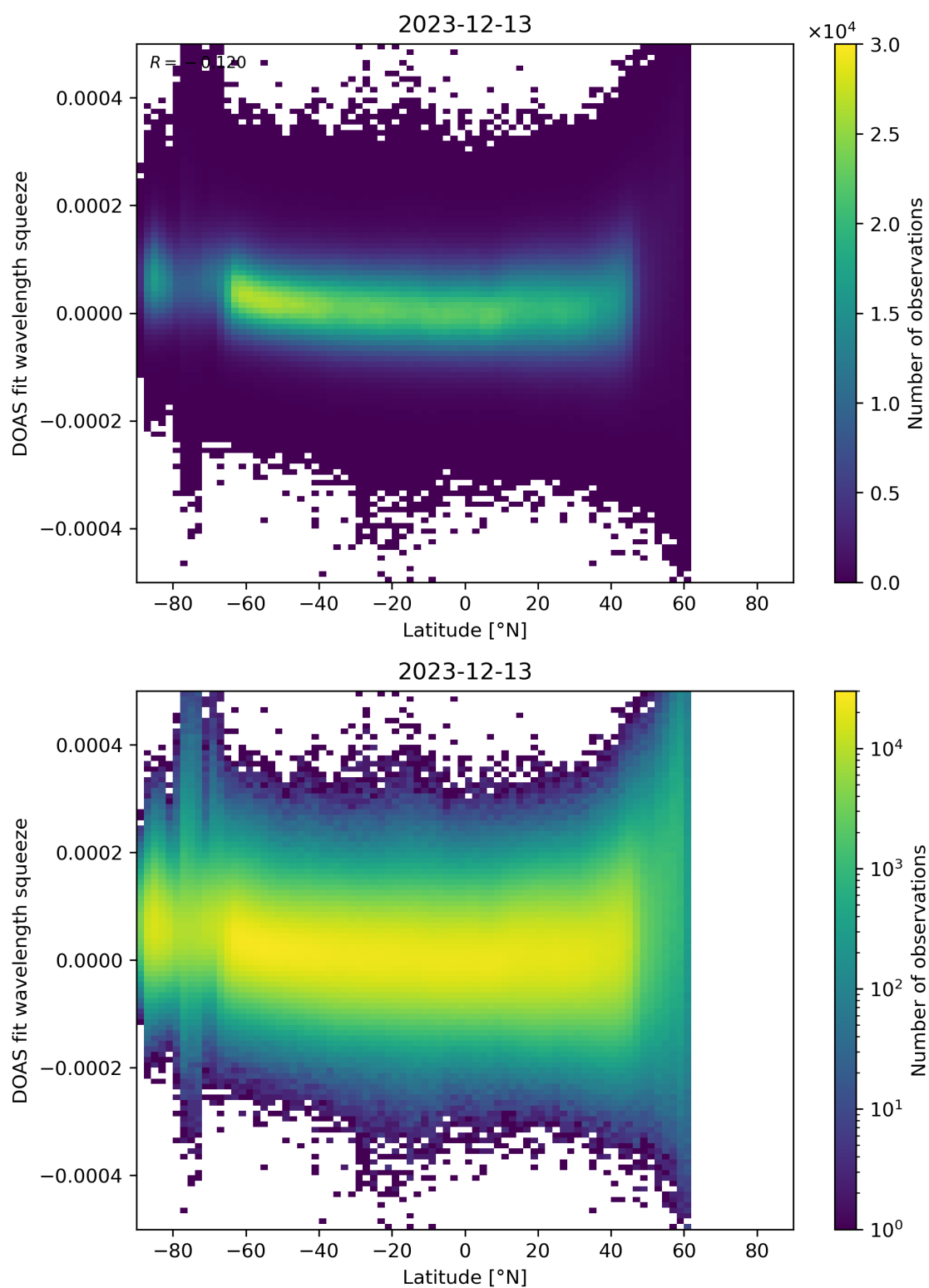
Figure 155: Scatter density plot of “Latitude” against “DOAS fit wavelength squeeze” for 2023-12-12 to 2023-12-14.
