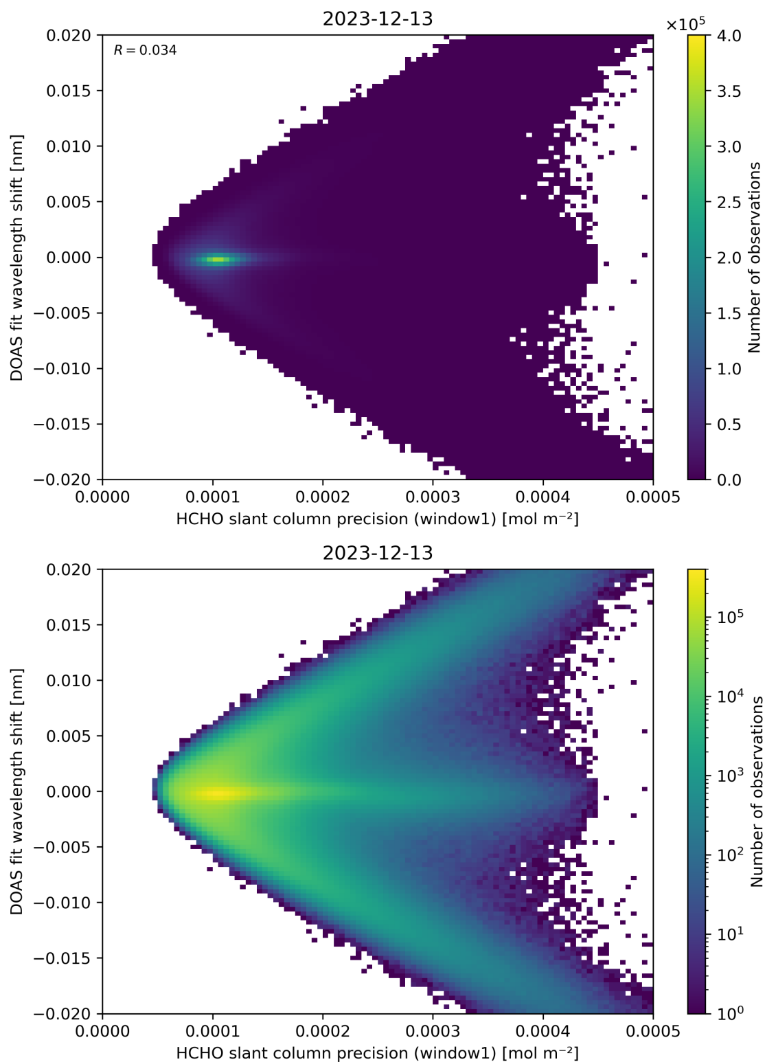
Figure 89: Scatter density plot of “HCHO slant column precision (window1)” against “DOAS fit wavelength shift” for 2023-12-12 to 2023-12-14.
