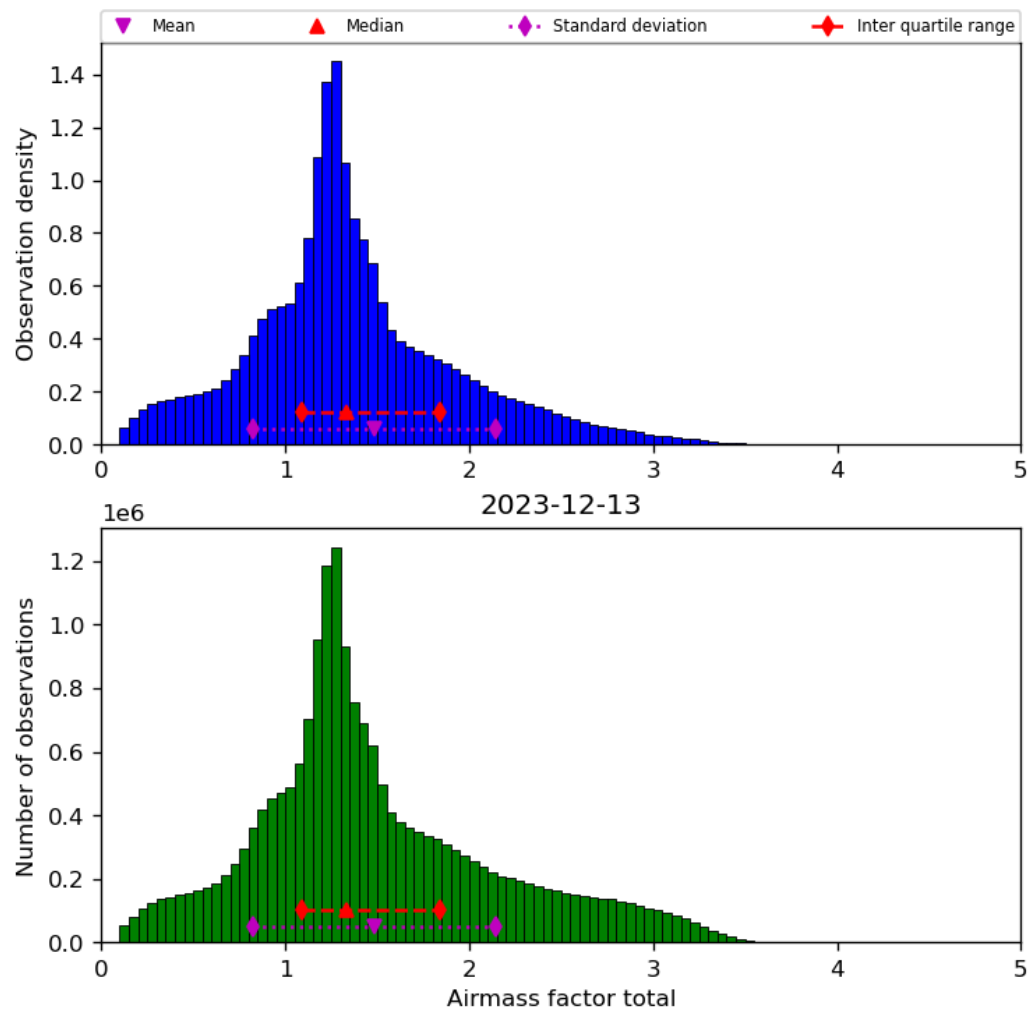
Figure 40: Histogram of “Airmass factor total” for 2023-12-12 to 2023-12-14
