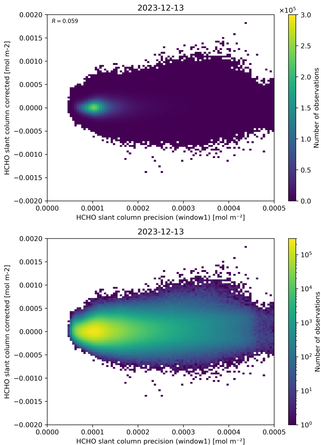
Figure 92: Scatter density plot of “HCHO slant column precision (window1)” against “HCHO slant column corrected” for 2023-12-12 to 2023-12-14.
