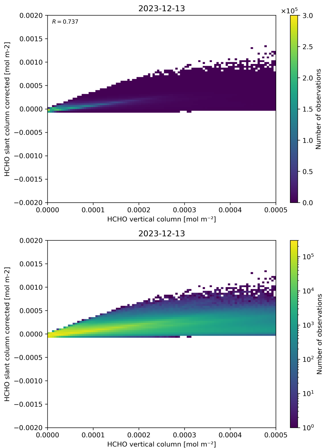
Figure 127: Scatter density plot of “HCHO vertical column” against “HCHO slant column corrected” for 2023-12-12 to 2023-12-14.
