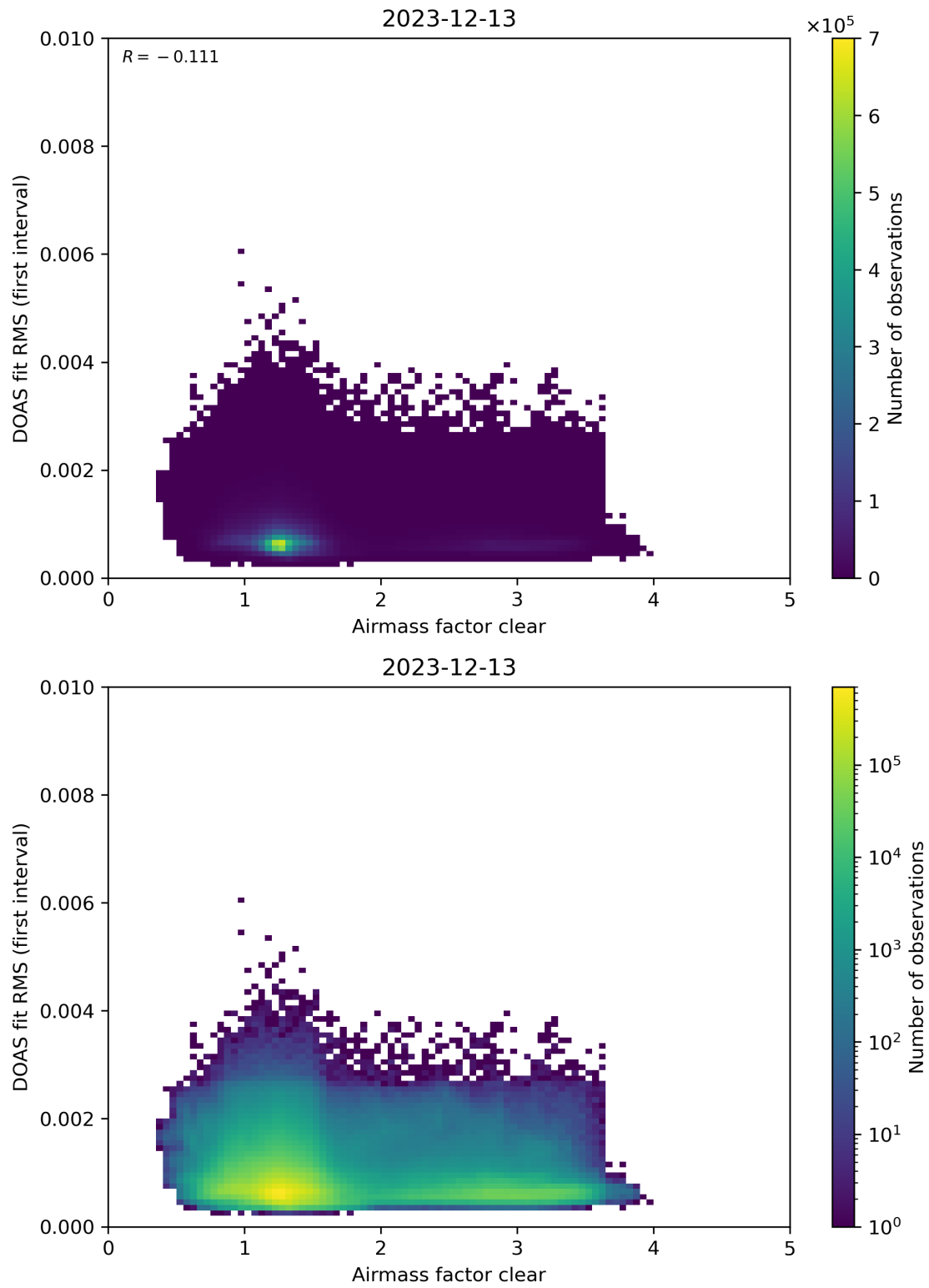
Figure 71: Scatter density plot of “Airmass factor clear” against “DOAS fit RMS (first interval)” for 2023-12-12 to 2023-12-14.
