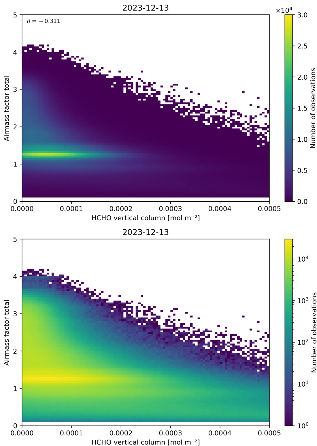
Figure 131: Scatter density plot of “HCHO vertical column” against “Airmass factor total” for 2023-12-12 to 2023-12-14.
