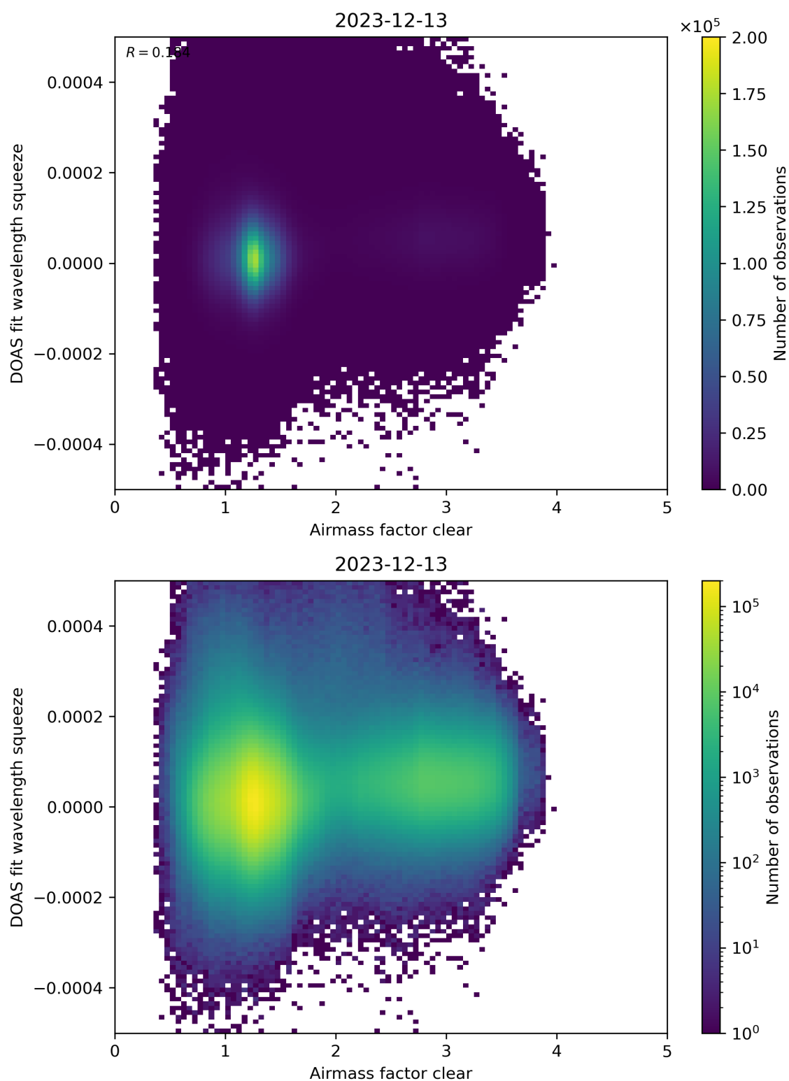
Figure 73: Scatter density plot of “Airmass factor clear” against “DOAS fit wavelength squeeze” for 2023-12-12 to 2023-12-14.
