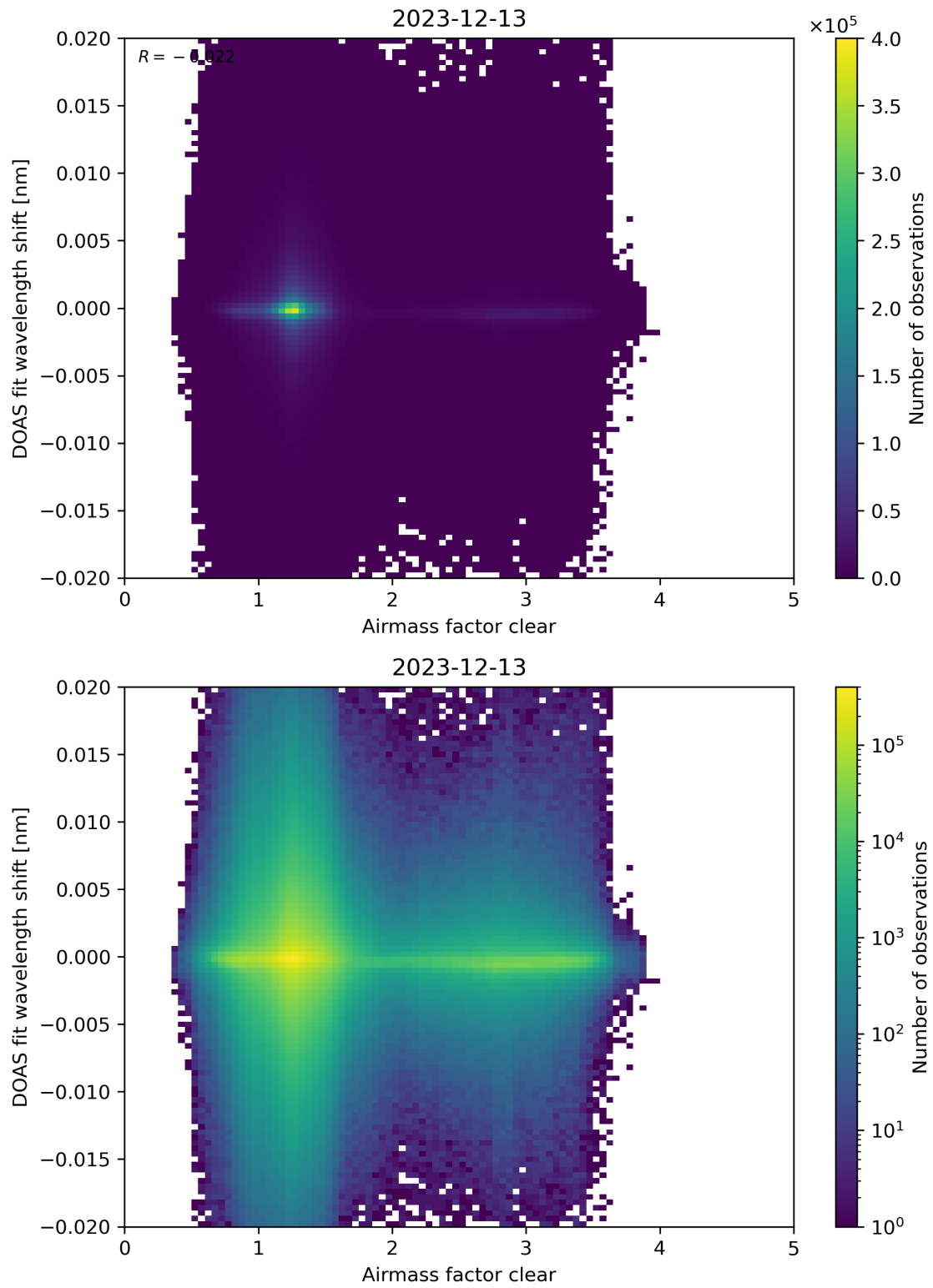
Figure 72: Scatter density plot of “Airmass factor clear” against “DOAS fit wavelength shift” for 2023-12-12 to 2023-12-14.
