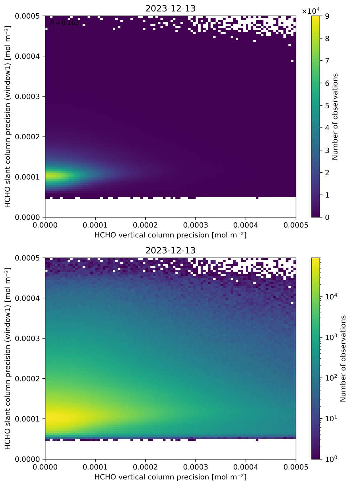
Figure 143: Scatter density plot of “HCHO vertical column precision” against “HCHO slant column precision (window1)” for 2023-12-12 to 2023-12-14.
