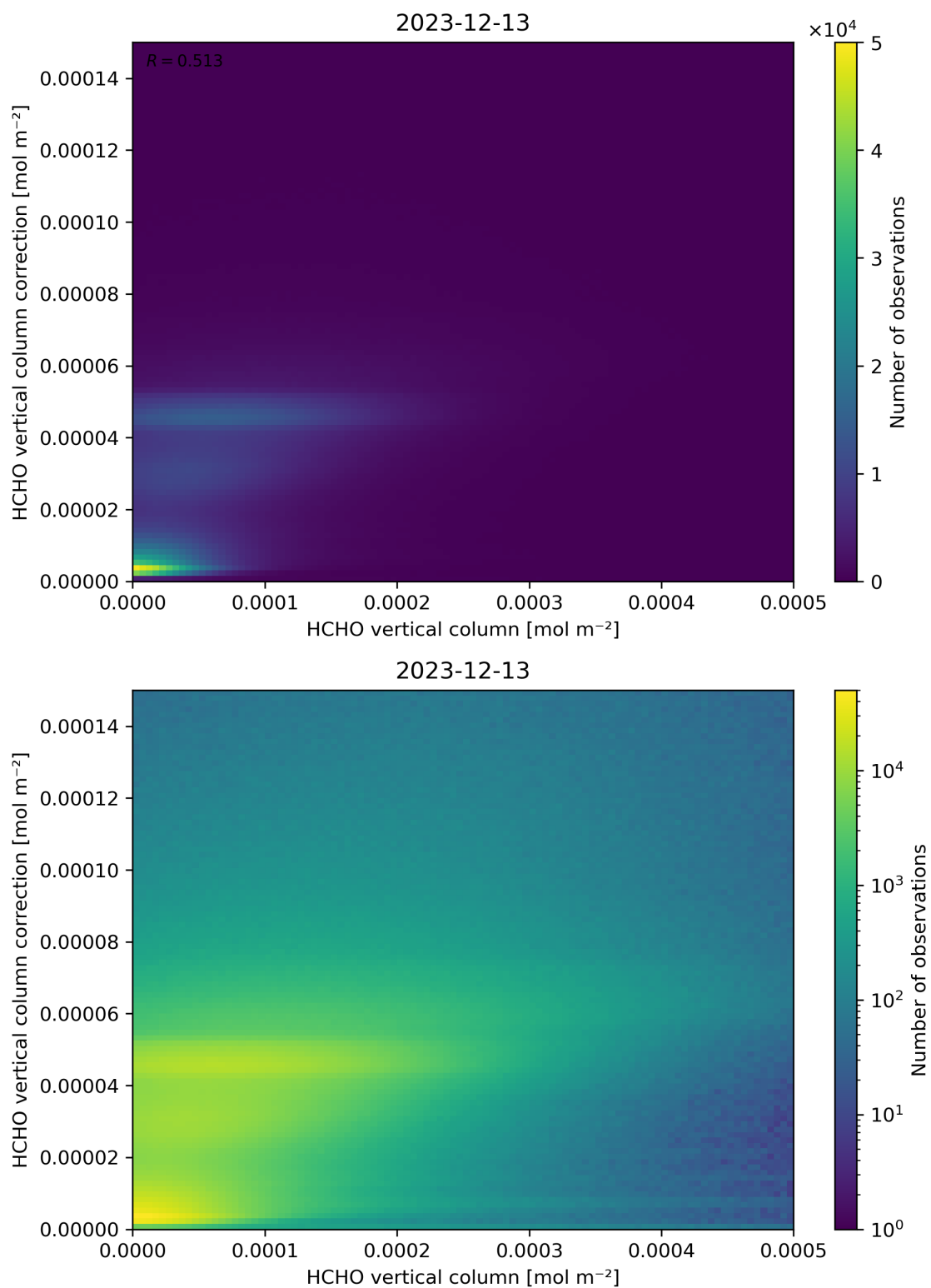
Figure 133: Scatter density plot of “HCHO vertical column” against “HCHO vertical column correction” for 2023-12-12 to 2023-12-14.
