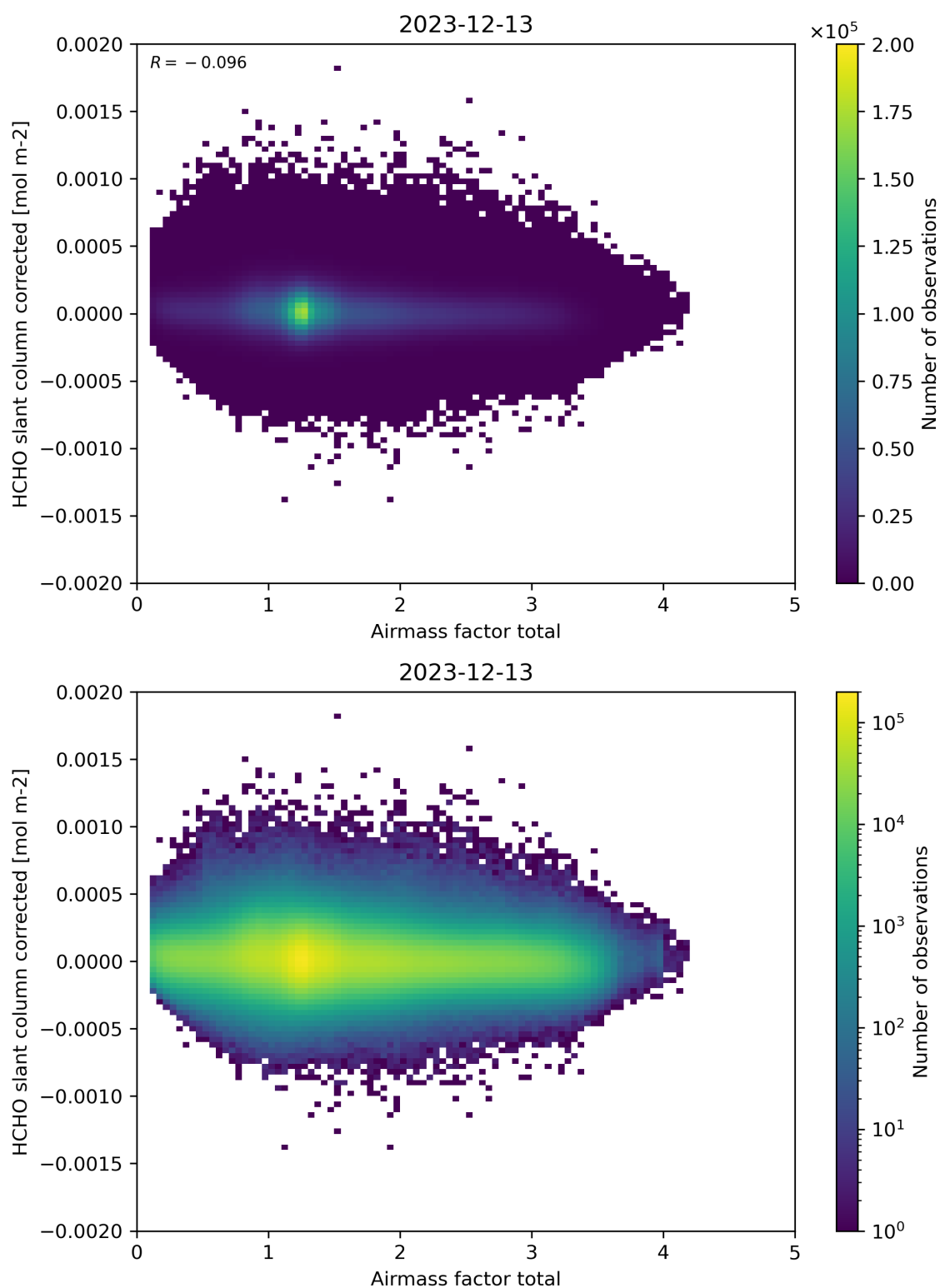
Figure 101: Scatter density plot of “Airmass factor total” against “HCHO slant column corrected” for 2023-12-12 to 2023-12-14.
