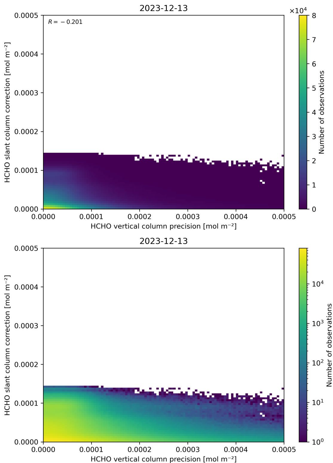
Figure 141: Scatter density plot of “HCHO vertical column precision” against “HCHO slant column correction” for 2023-12-12 to 2023-12-14.
