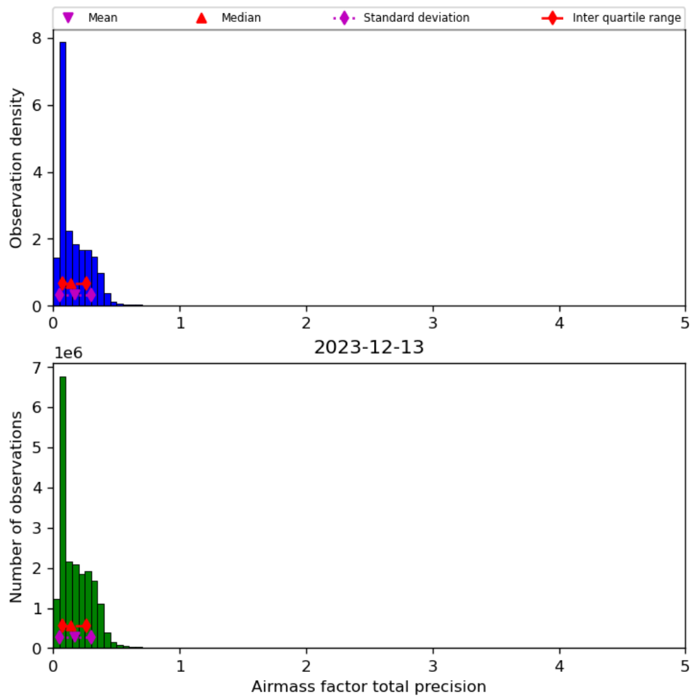
Figure 41: Histogram of “Airmass factor total precision” for 2023-12-12 to 2023-12-14
