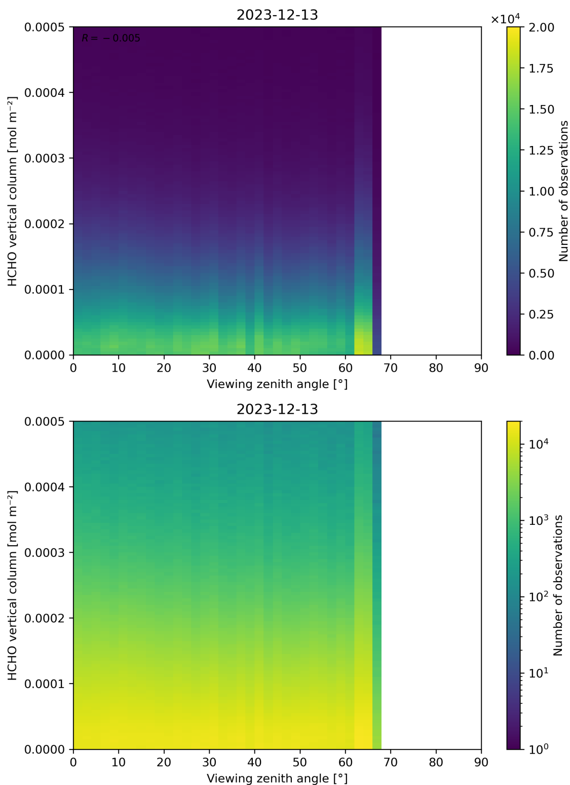
Figure 192: Scatter density plot of “Viewing zenith angle” against “HCHO vertical column” for 2023-12-12 to 2023-12-14.
