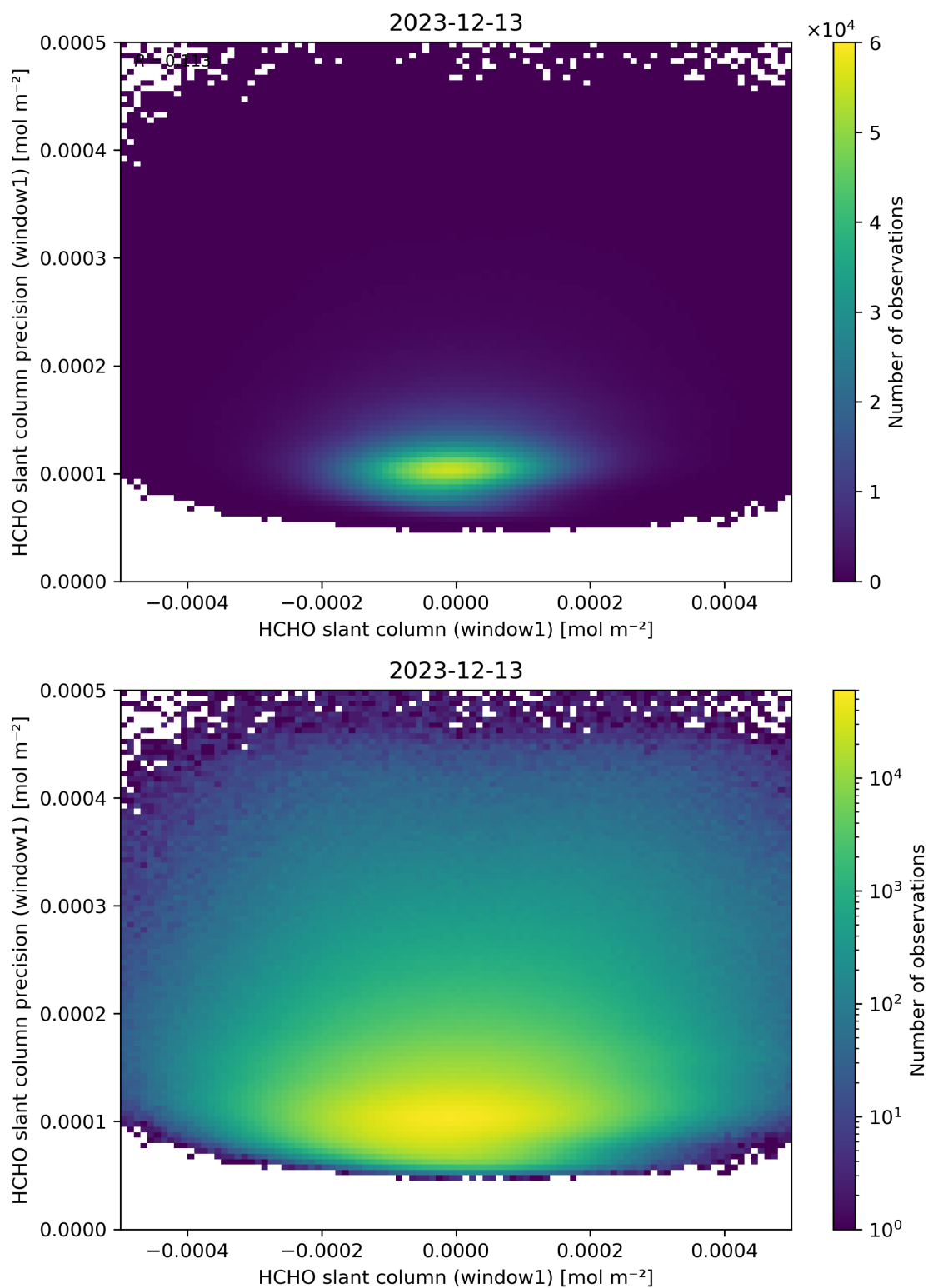
Figure 84: Scatter density plot of “HCHO slant column (window1)” against “HCHO slant column precision (window1)” for 2023-12-12 to 2023-12-14.
