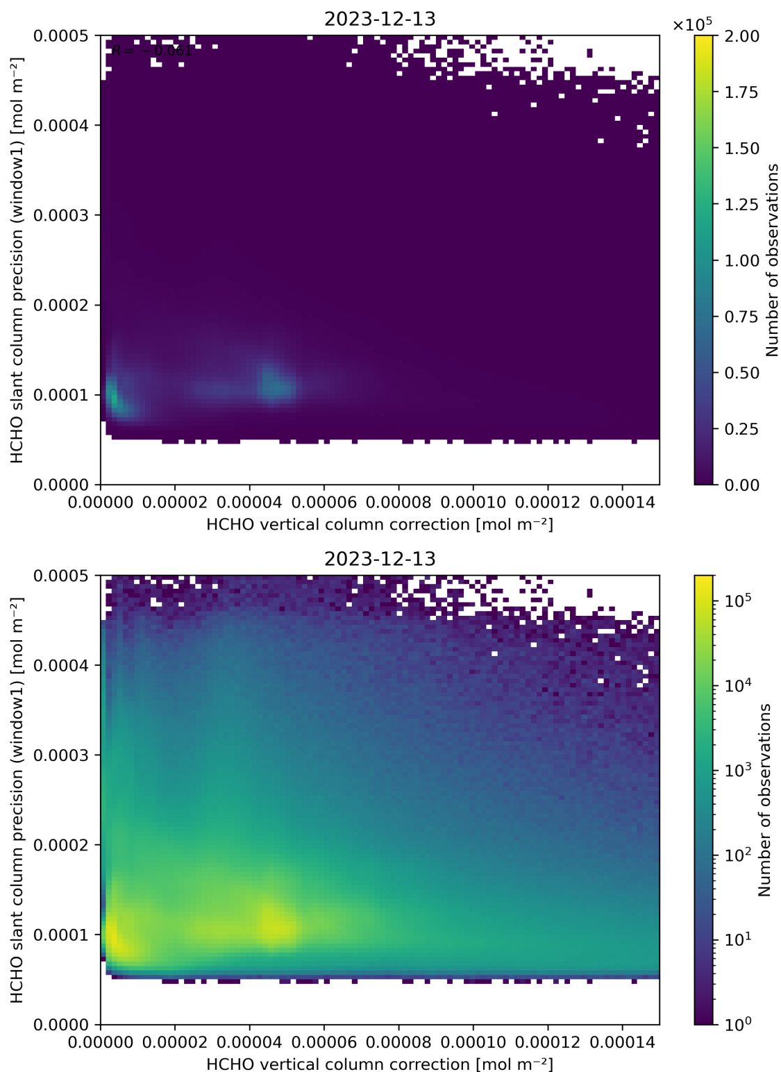
Figure 119: Scatter density plot of “HCHO vertical column correction” against “HCHO slant column precision (window1)” for 2023-12-12 to 2023-12-14.
