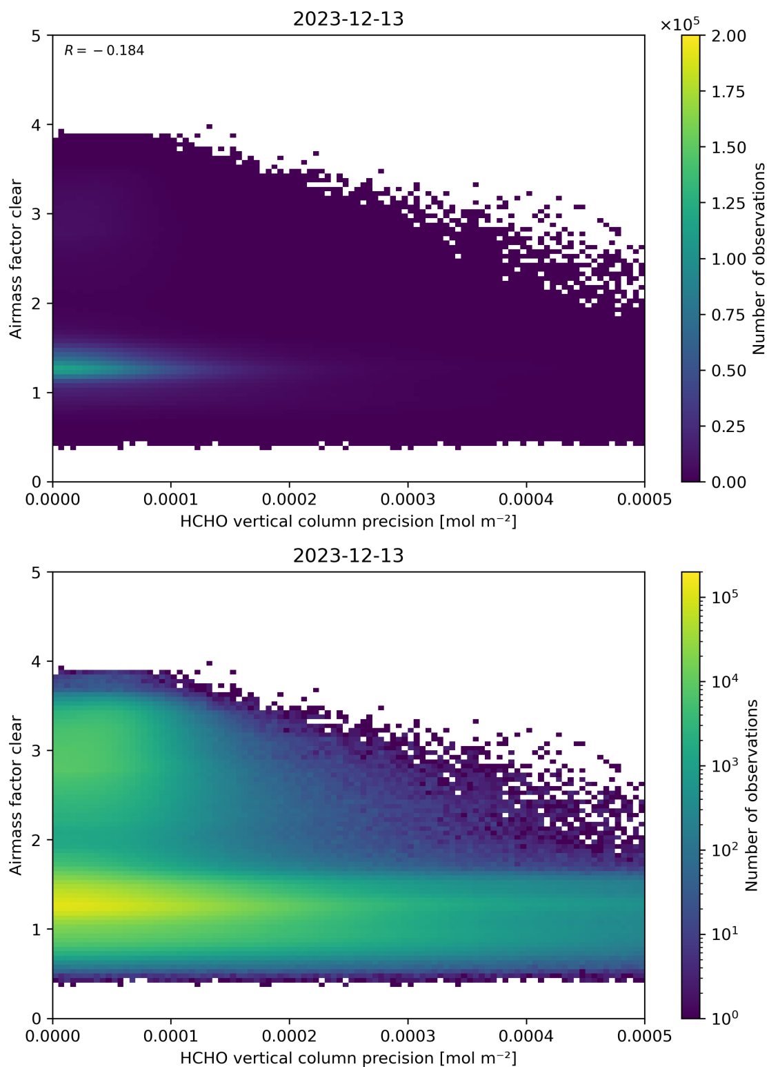
Figure 139: Scatter density plot of “HCHO vertical column precision” against “Airmass factor clear” for 2023-12-12 to 2023-12-14.
