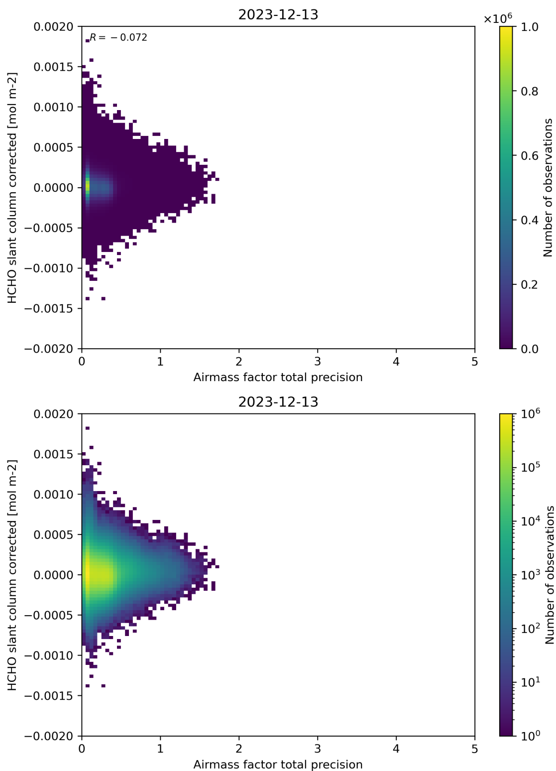
Figure 109: Scatter density plot of “Airmass factor total precision” against “HCHO slant column corrected” for 2023-12-12 to 2023-12-14.
