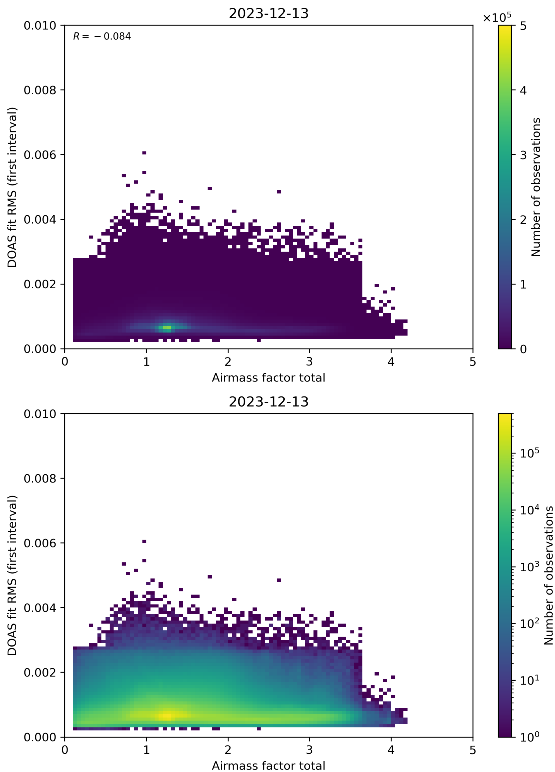
Figure 97: Scatter density plot of “Airmass factor total” against “DOAS fit RMS (first interval)” for 2023-12-12 to 2023-12-14.
