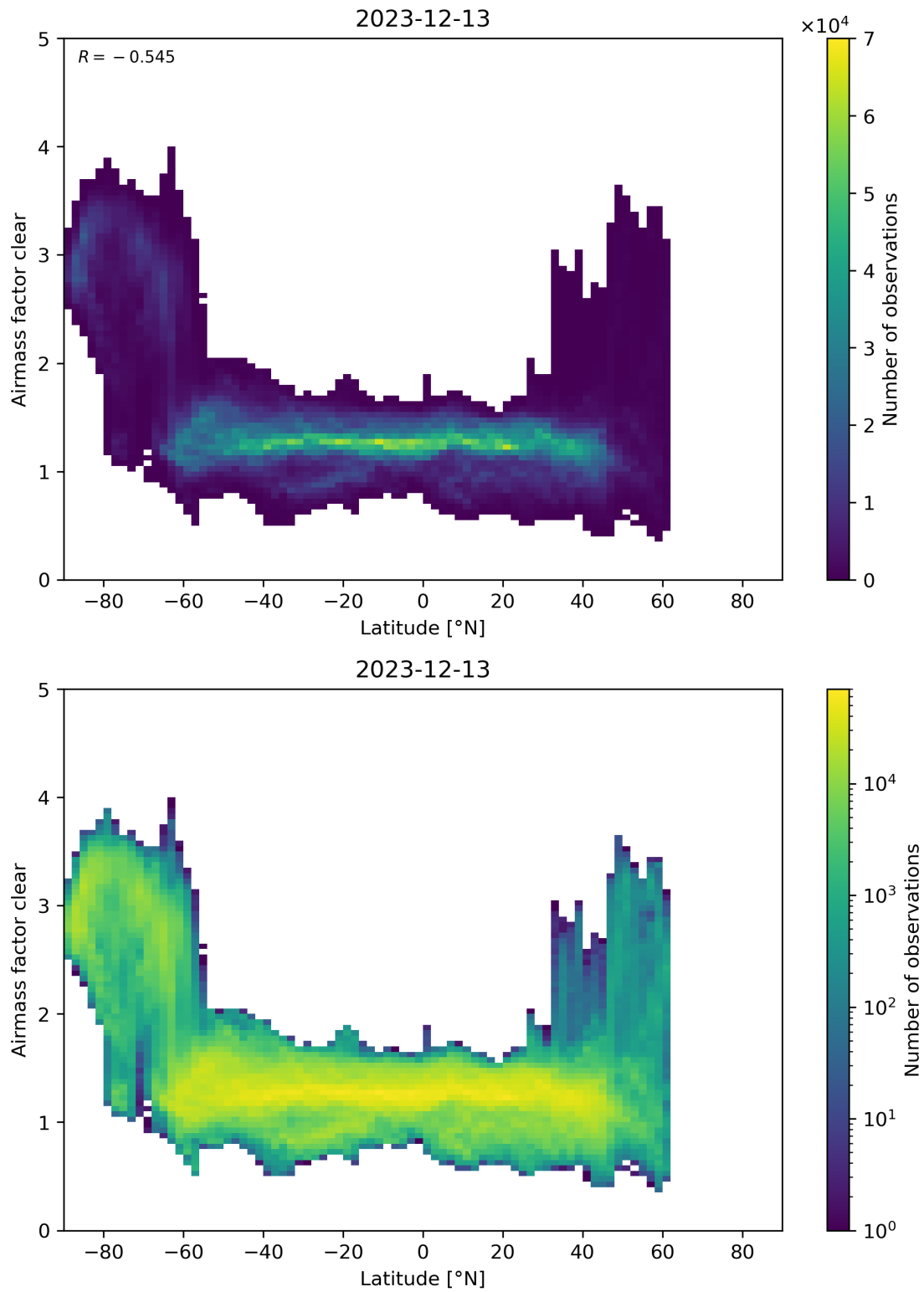
Figure 156: Scatter density plot of “Latitude” against “Airmass factor clear” for 2023-12-12 to 2023-12-14.
