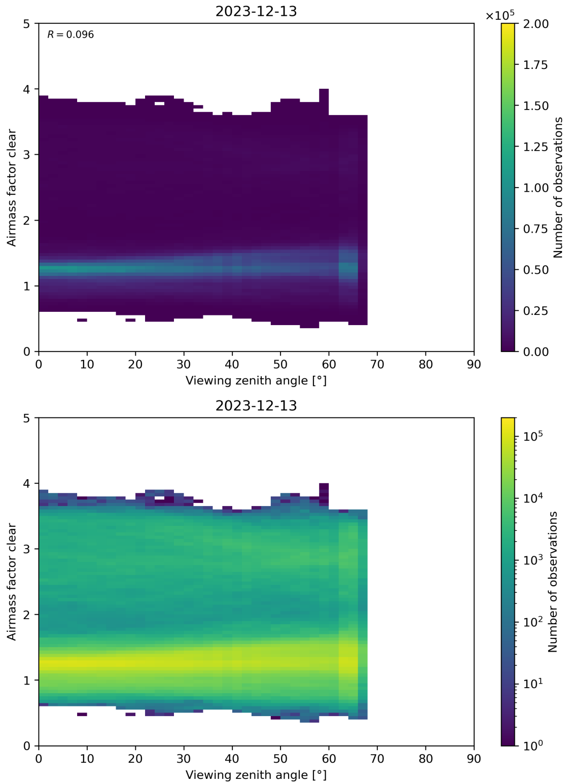
Figure 185: Scatter density plot of “Viewing zenith angle” against “Airmass factor clear” for 2023-12-12 to 2023-12-14.
