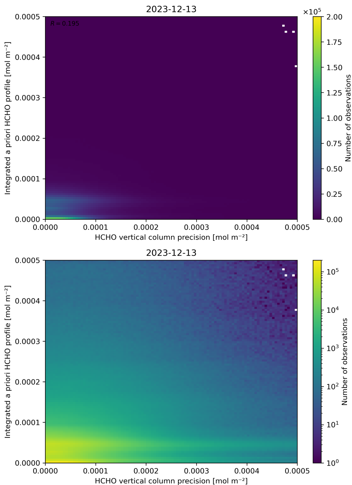
Figure 147: Scatter density plot of “HCHO vertical column precision” against “Integrated a priori HCHO profile” for 2023-12-12 to 2023-12-14.
