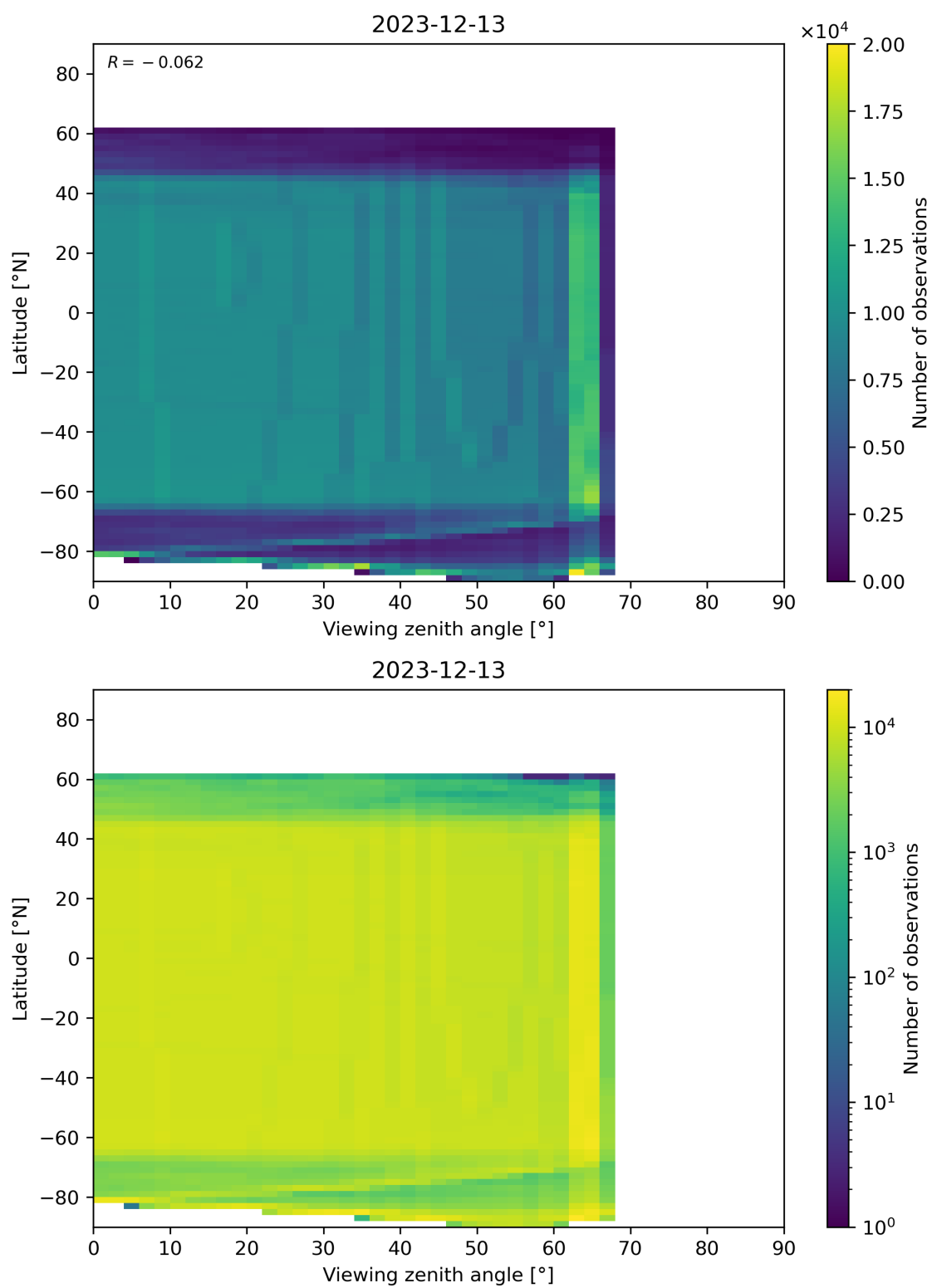
Figure 196: Scatter density plot of “Viewing zenith angle” against “Latitude” for 2023-12-12 to 2023-12-14.
