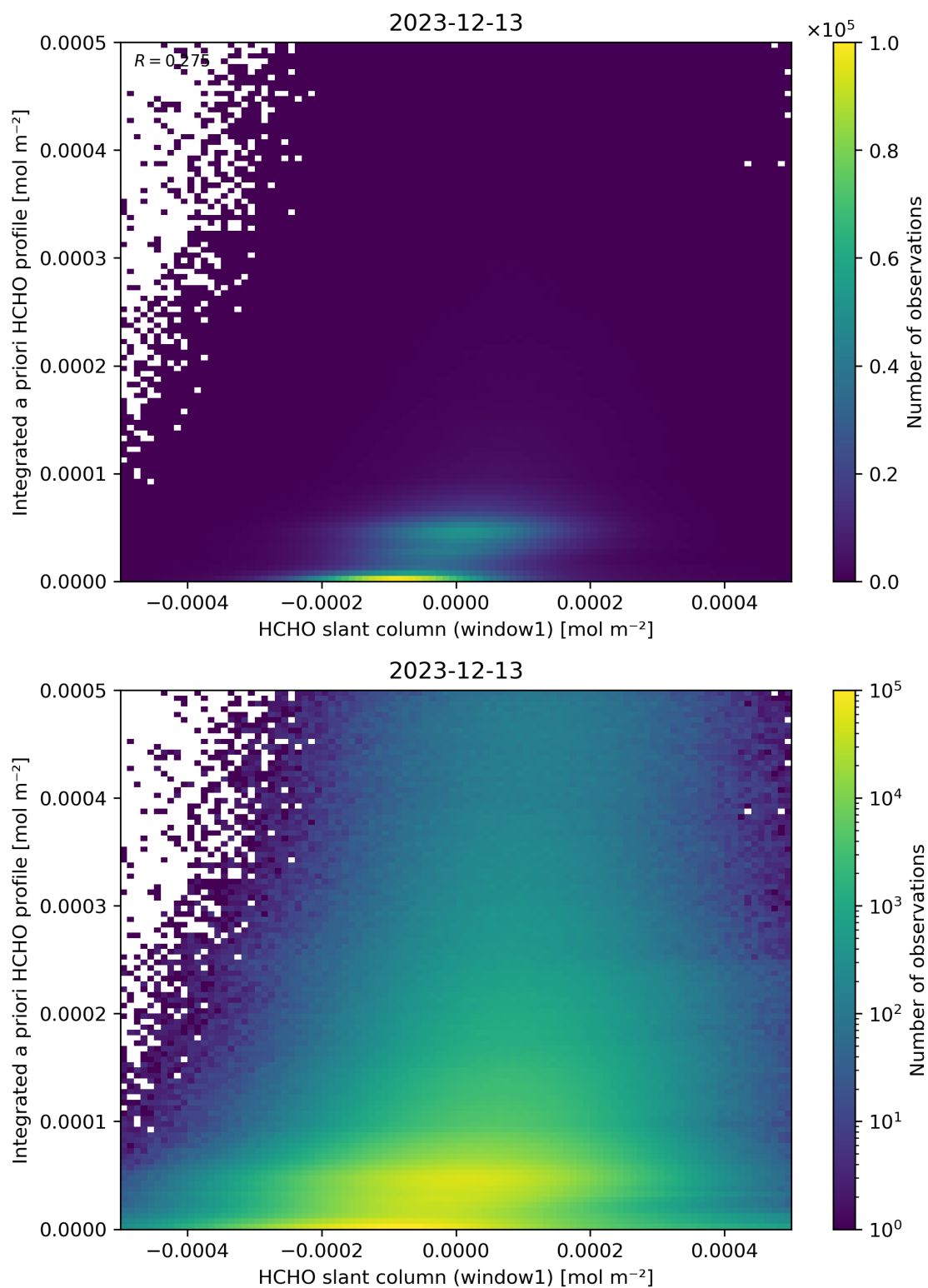
Figure 87: Scatter density plot of “HCHO slant column (window1)” against “Integrated a priori HCHO profile” for 2023-12-12 to 2023-12-14.
