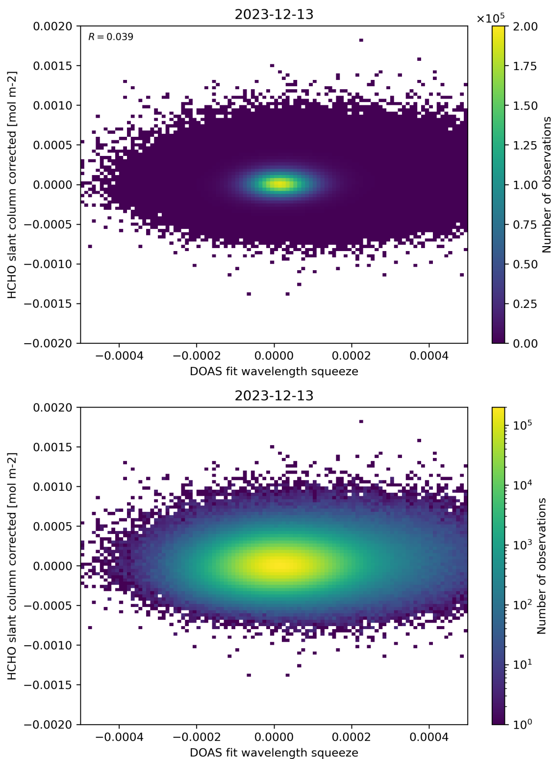
Figure 69: Scatter density plot of “DOAS fit wavelength squeeze” against “HCHO slant column corrected” for 2023-12-12 to 2023-12-14.
