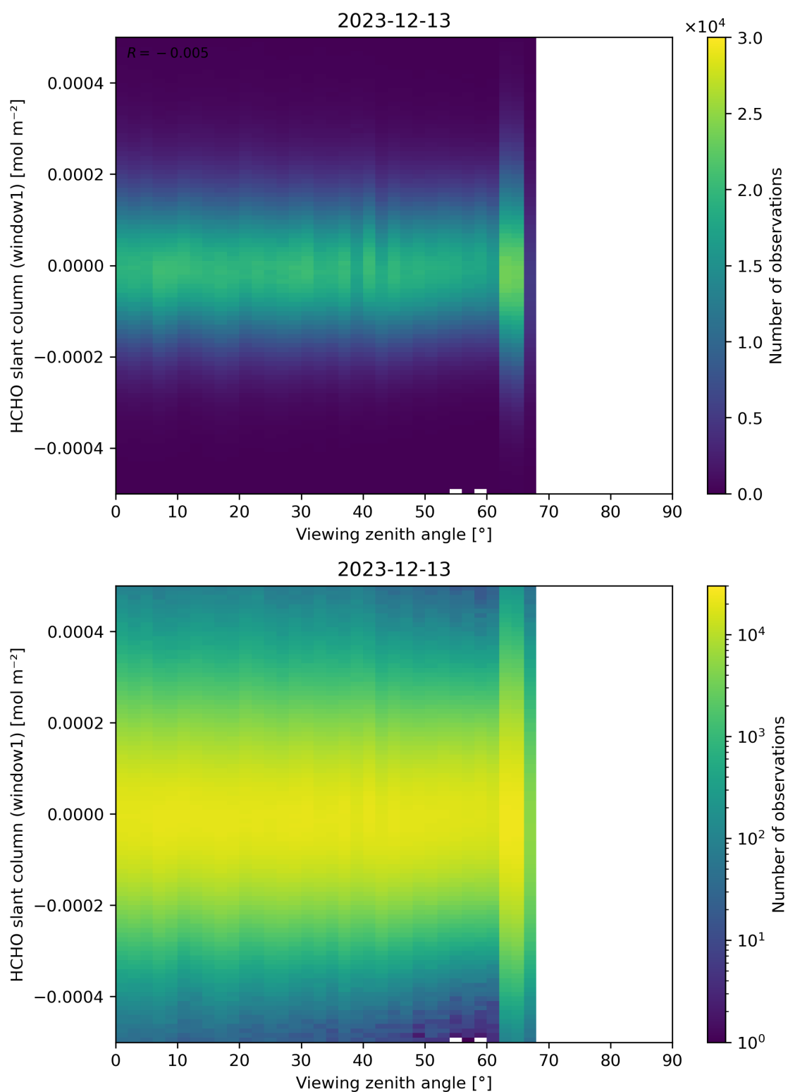
Figure 188: Scatter density plot of “Viewing zenith angle” against “HCHO slant column (window1)” for 2023-12-12 to 2023-12-14.
