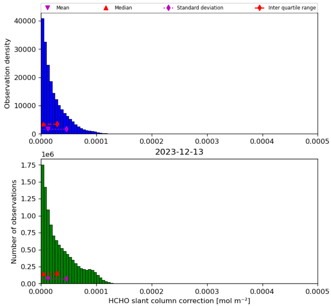
Figure 47: Histogram of “HCHO slant column correction” for 2023-12-12 to 2023-12-14
