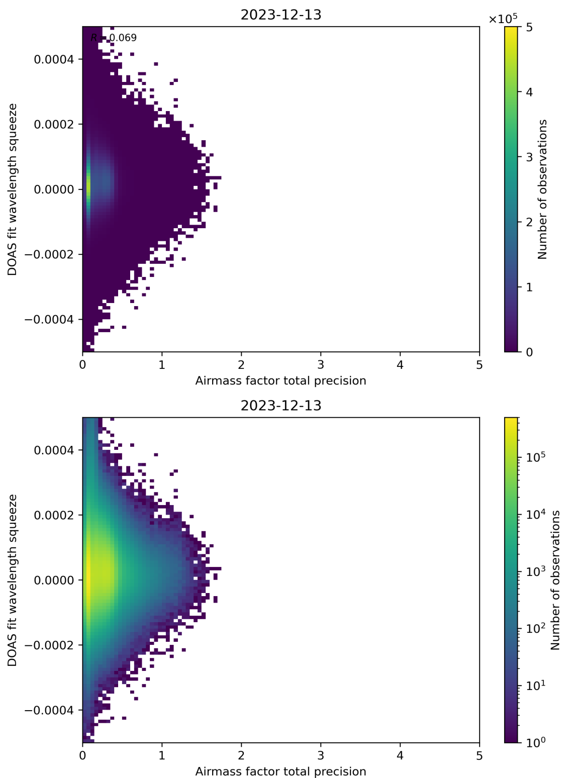
Figure 107: Scatter density plot of “Airmass factor total precision” against “DOAS fit wavelength squeeze” for 2023-12-12 to 2023-12-14.
