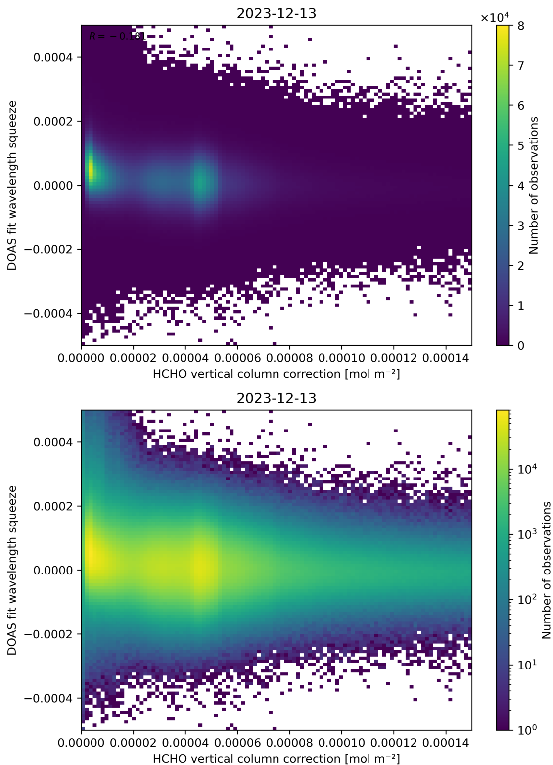
Figure 114: Scatter density plot of “HCHO vertical column correction” against “DOAS fit wavelength squeeze” for 2023-12-12 to 2023-12-14.
