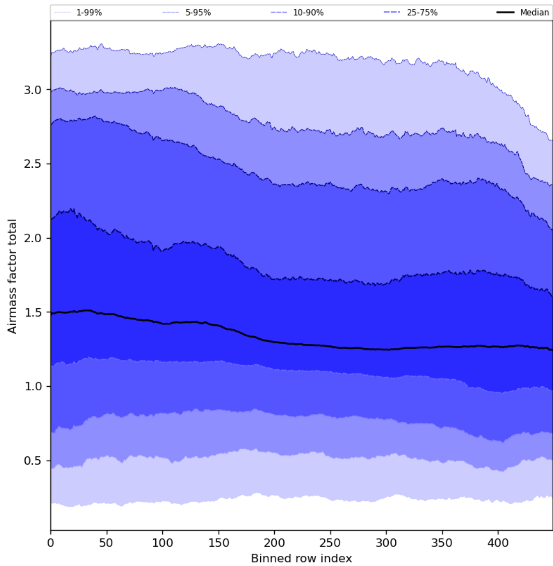
Figure 54: Along track statistics of “Airmass factor total” for 2023-12-12 to 2023-12-14
