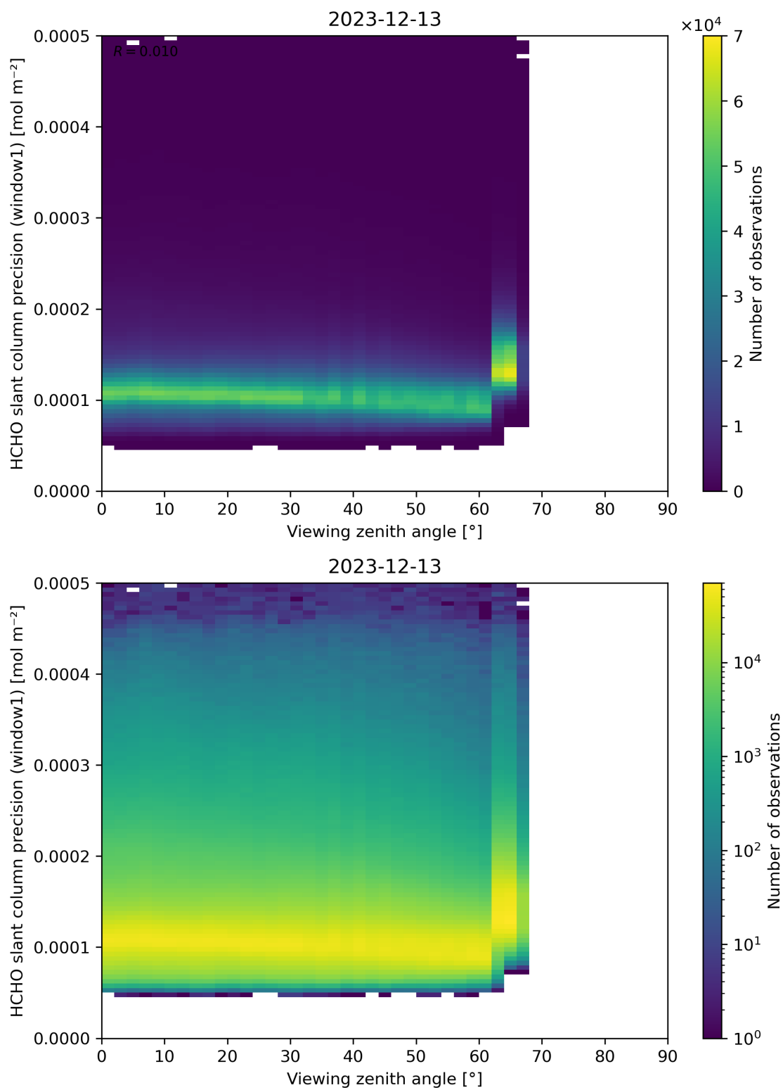
Figure 189: Scatter density plot of “Viewing zenith angle” against “HCHO slant column precision (window1)” for 2023-12-12 to 2023-12-14.
