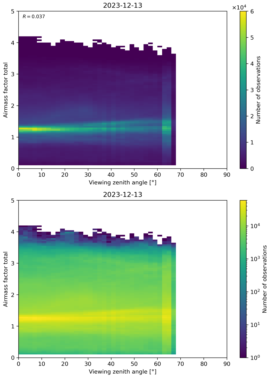
Figure 190: Scatter density plot of “Viewing zenith angle” against “Airmass factor total” for 2023-12-12 to 2023-12-14.
