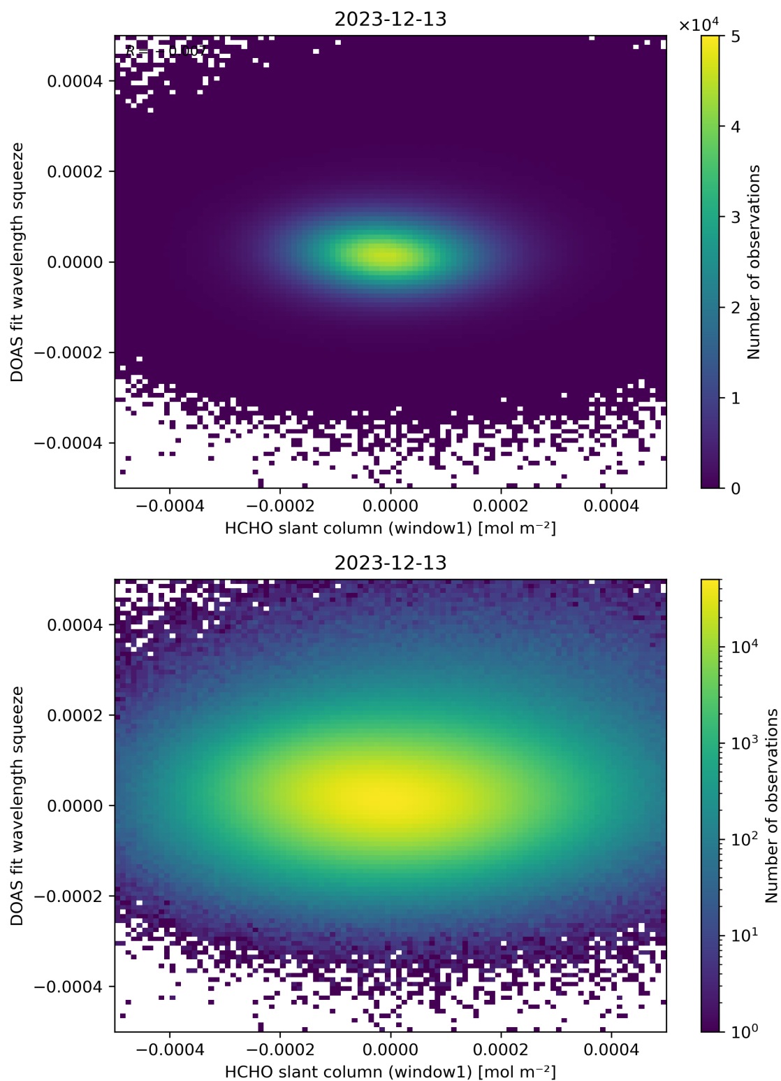
Figure 80: Scatter density plot of “HCHO slant column (window1)” against “DOAS fit wavelength squeeze” for 2023-12-12 to 2023-12-14.
