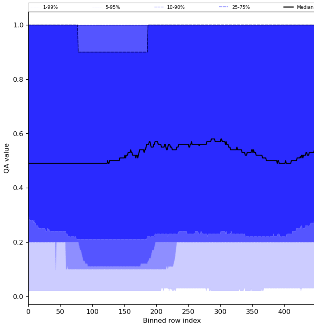
Figure 48: Along track statistics of “QA value” for 2023-12-12 to 2023-12-14
