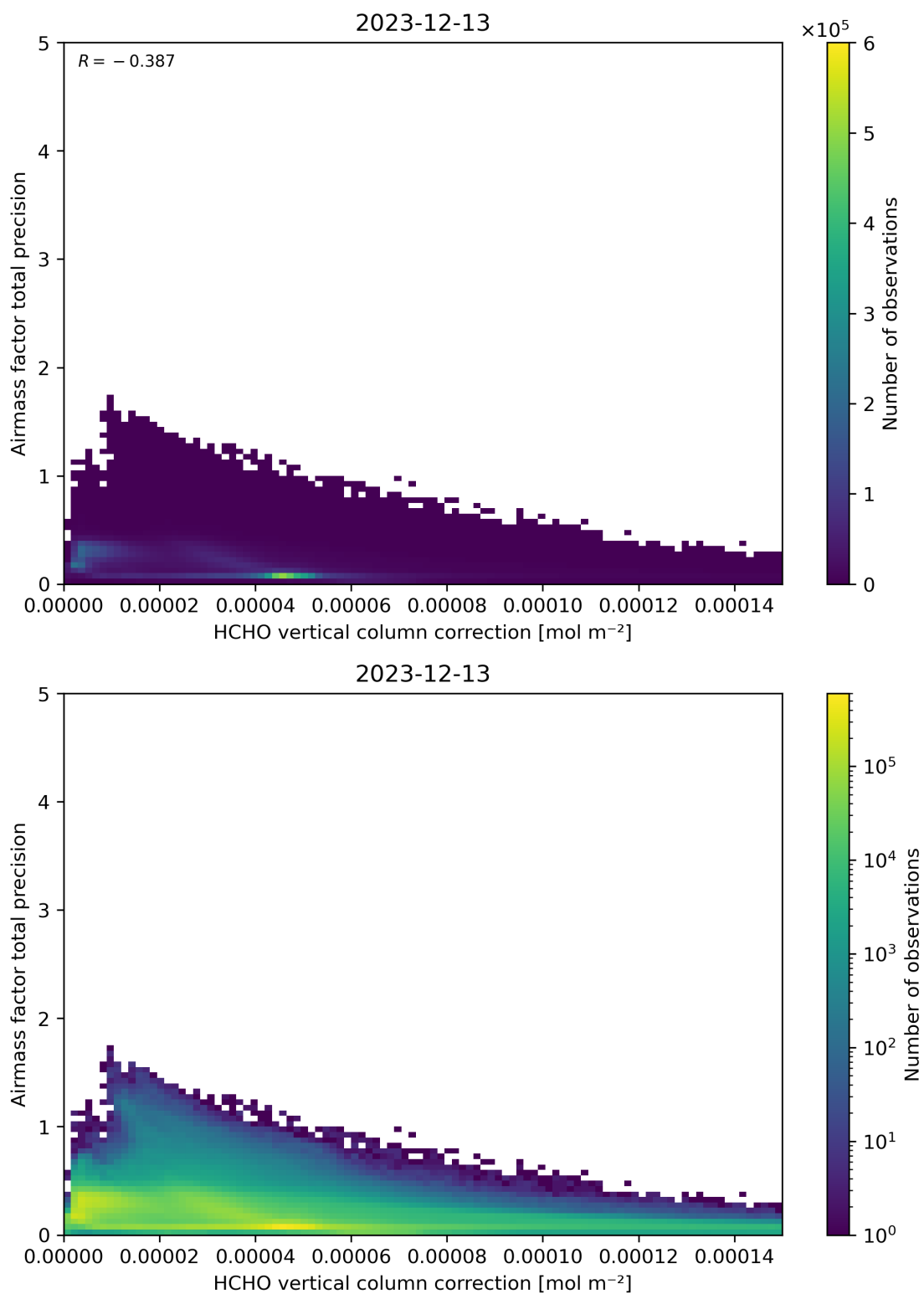
Figure 121: Scatter density plot of “HCHO vertical column correction” against “Airmass factor total precision” for 2023-12-12 to 2023-12-14.
