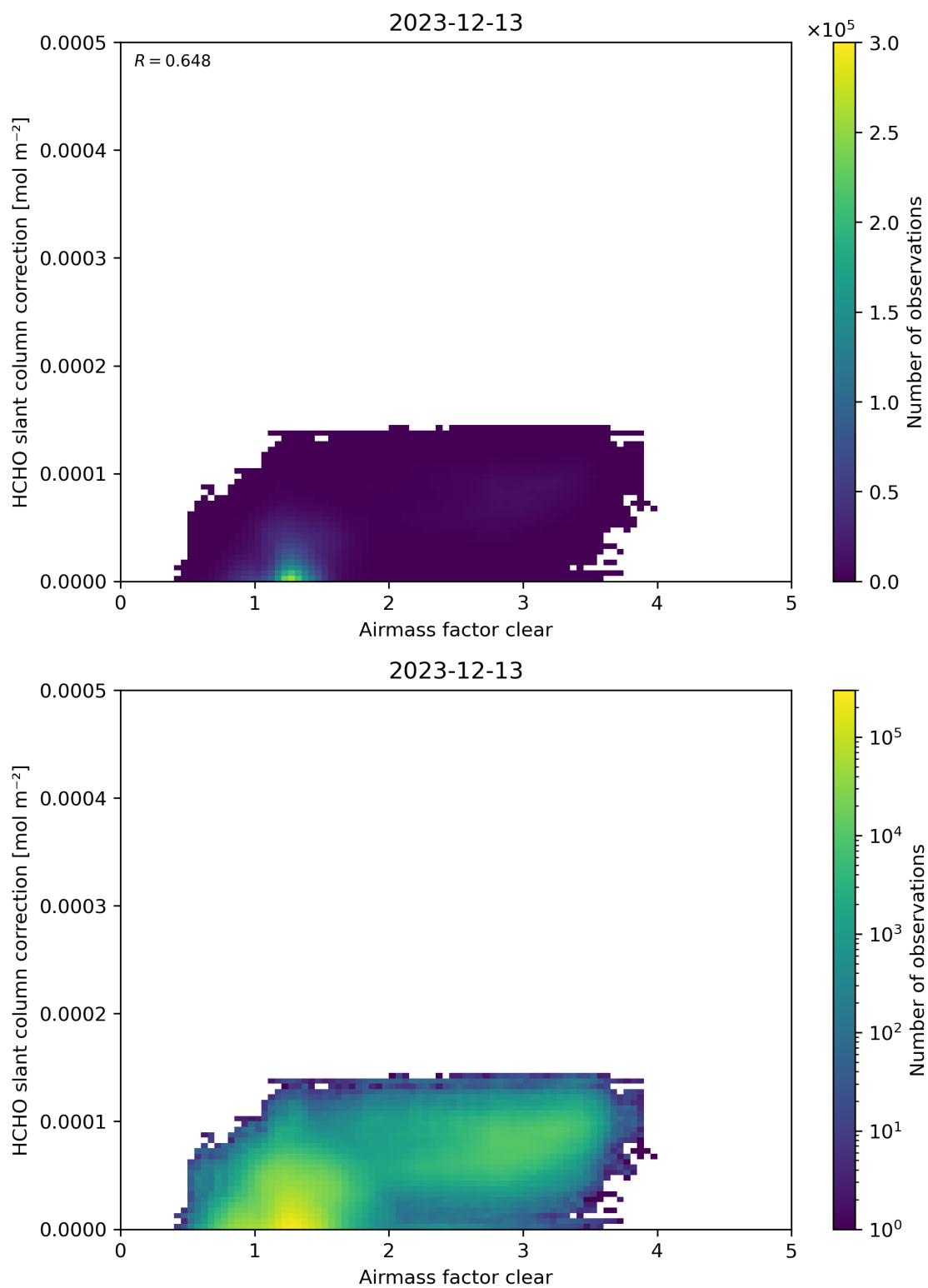
Figure 75: Scatter density plot of “Airmass factor clear” against “HCHO slant column correction” for 2023-12-12 to 2023-12-14.
