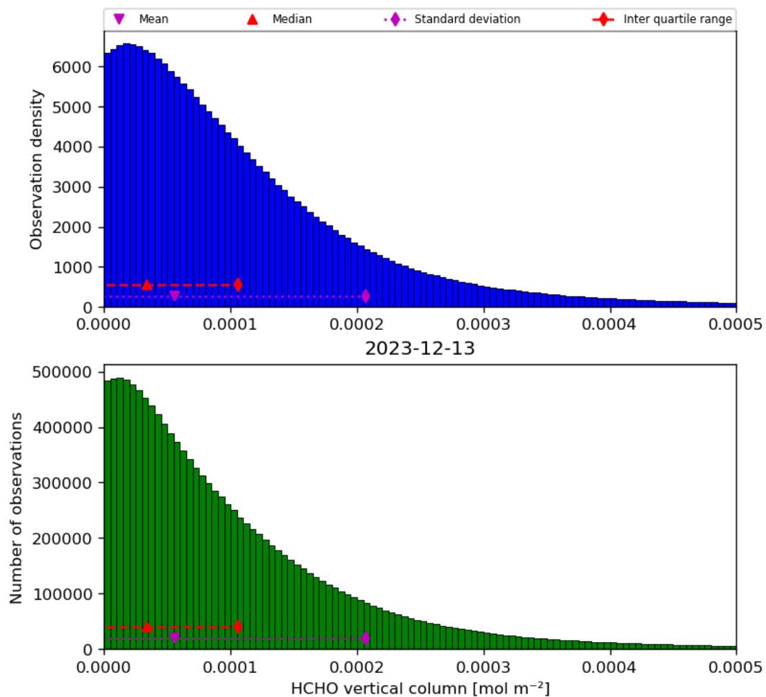
Figure 35: Histogram of “HCHO vertical column” for 2023-12-12 to 2023-12-14
