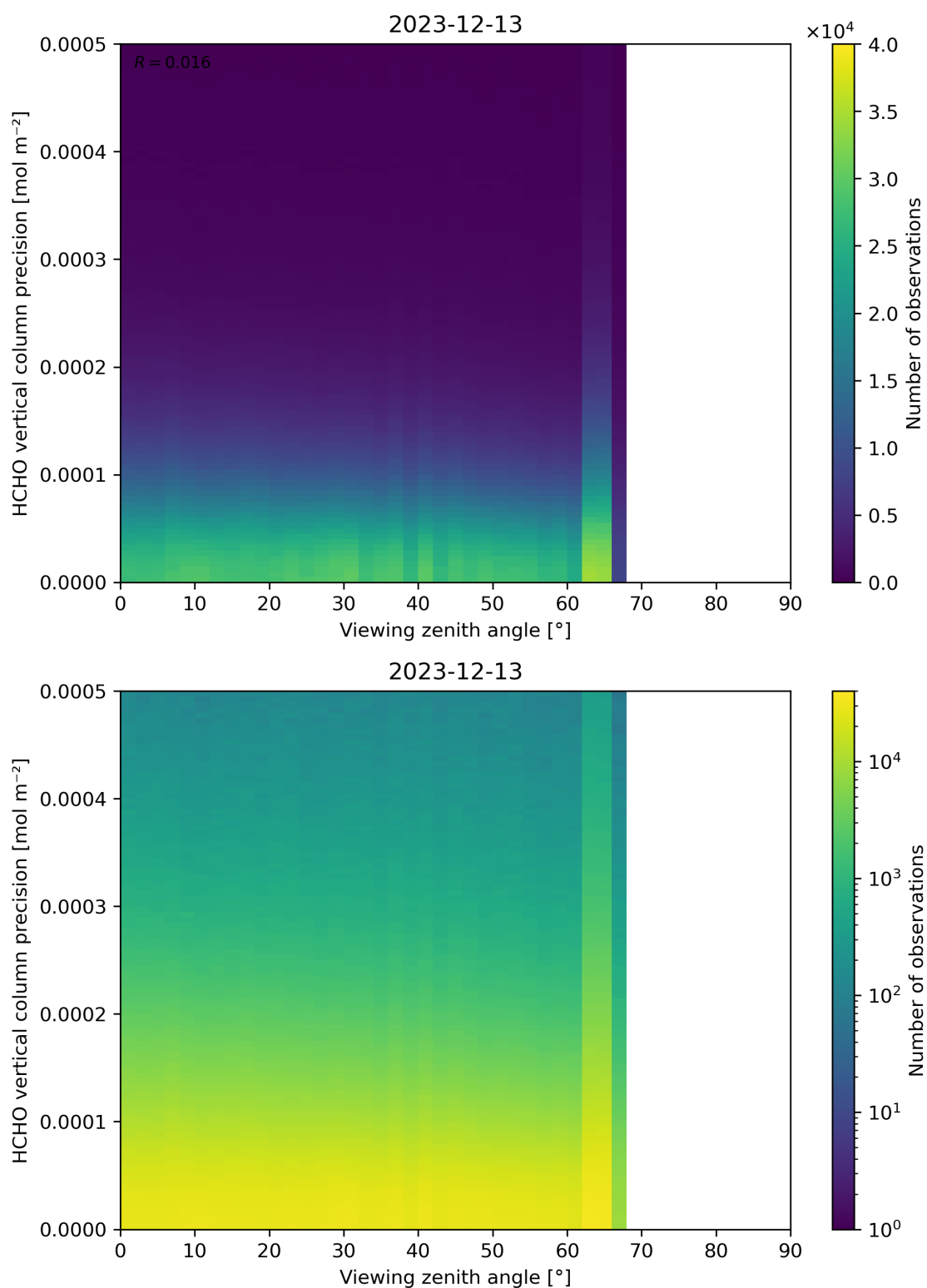
Figure 194: Scatter density plot of “Viewing zenith angle” against “HCHO vertical column precision” for 2023-12-12 to 2023-12-14.
