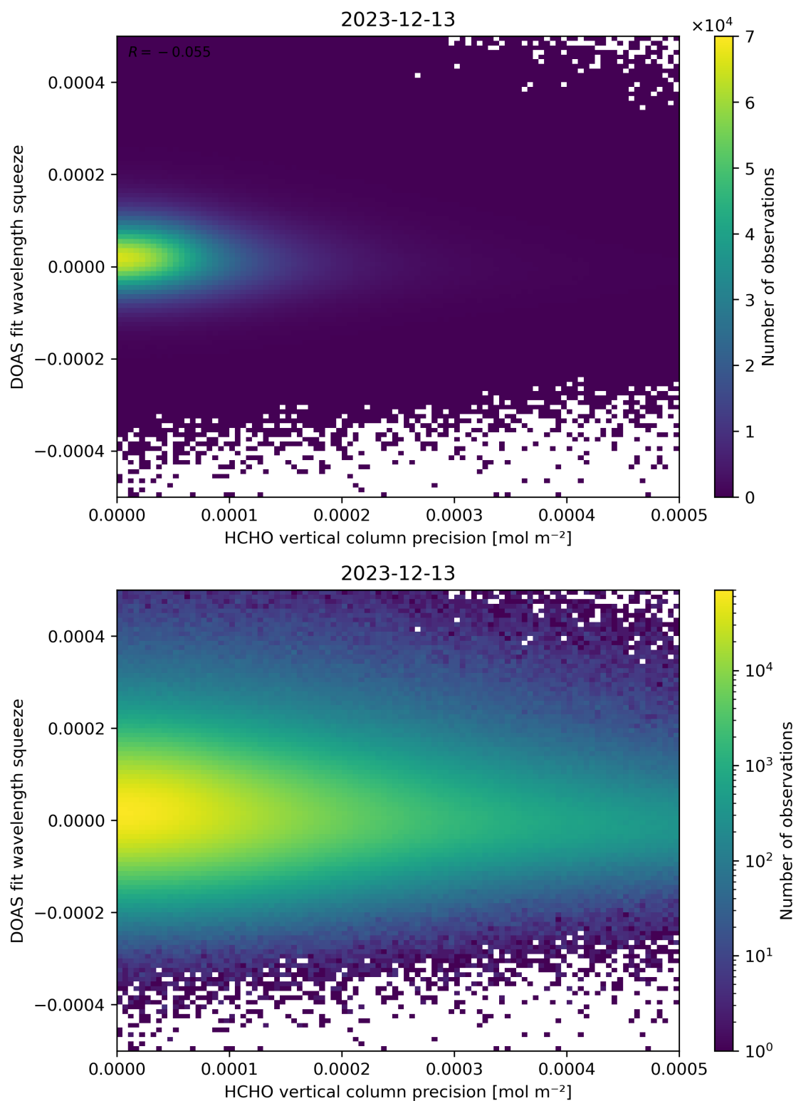
Figure 138: Scatter density plot of “HCHO vertical column precision” against “DOAS fit wavelength squeeze” for 2023-12-12 to 2023-12-14.
