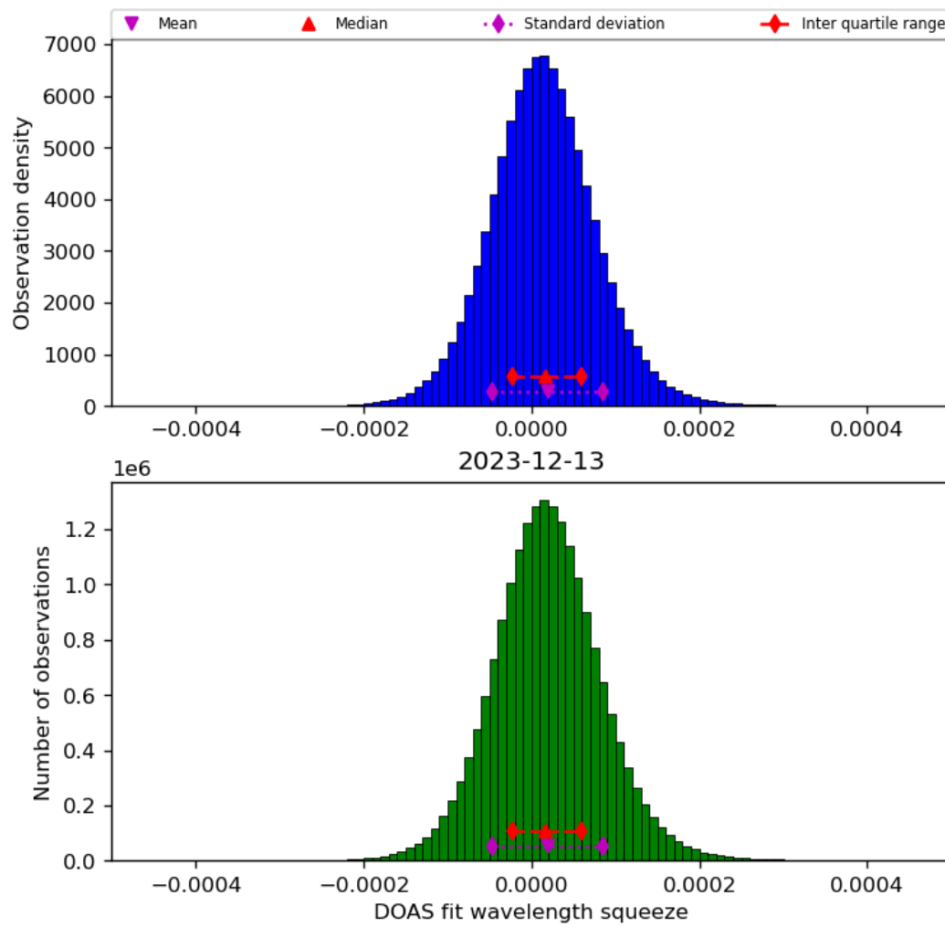
Figure 45: Histogram of “DOAS fit wavelength squeeze” for 2023-12-12 to 2023-12-14
