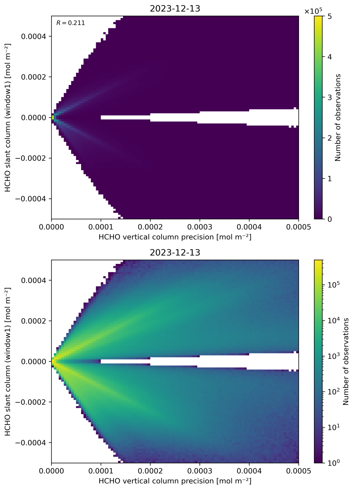
Figure 142: Scatter density plot of “HCHO vertical column precision” against “HCHO slant column (window1)” for 2023-12-12 to 2023-12-14.
