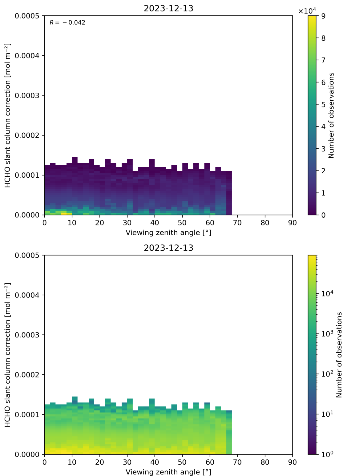
Figure 187: Scatter density plot of “Viewing zenith angle” against “HCHO slant column correction” for 2023-12-12 to 2023-12-14.
