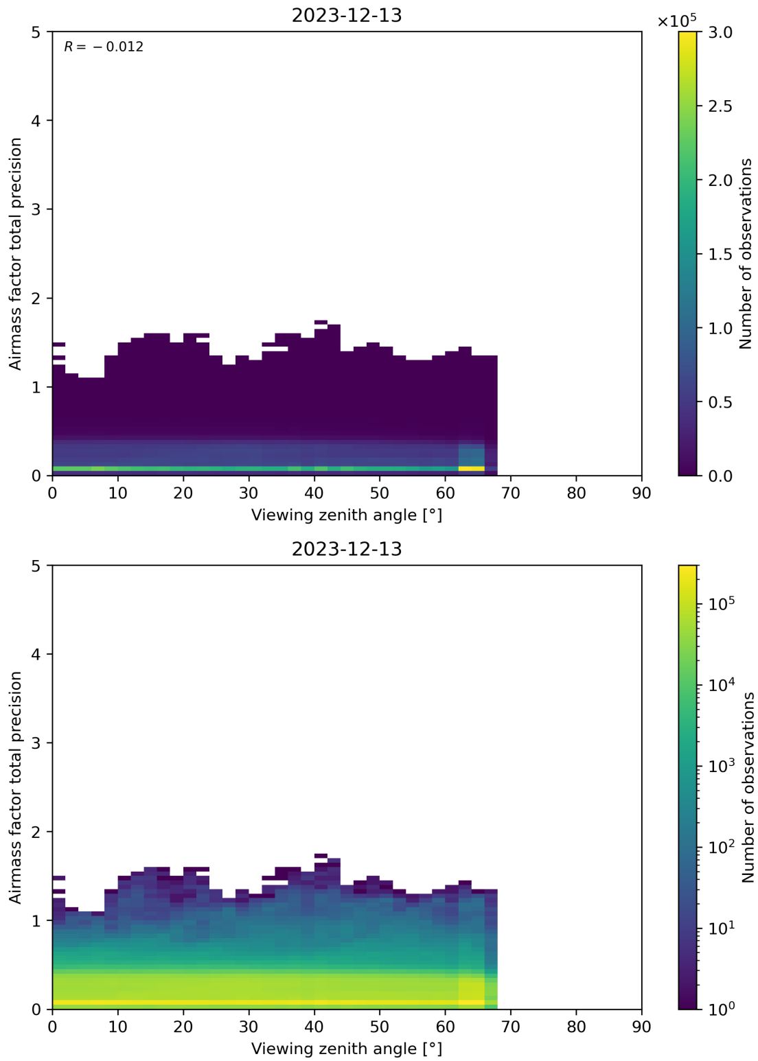
Figure 191: Scatter density plot of “Viewing zenith angle” against “Airmass factor total precision” for 2023-12-12 to 2023-12-14.
