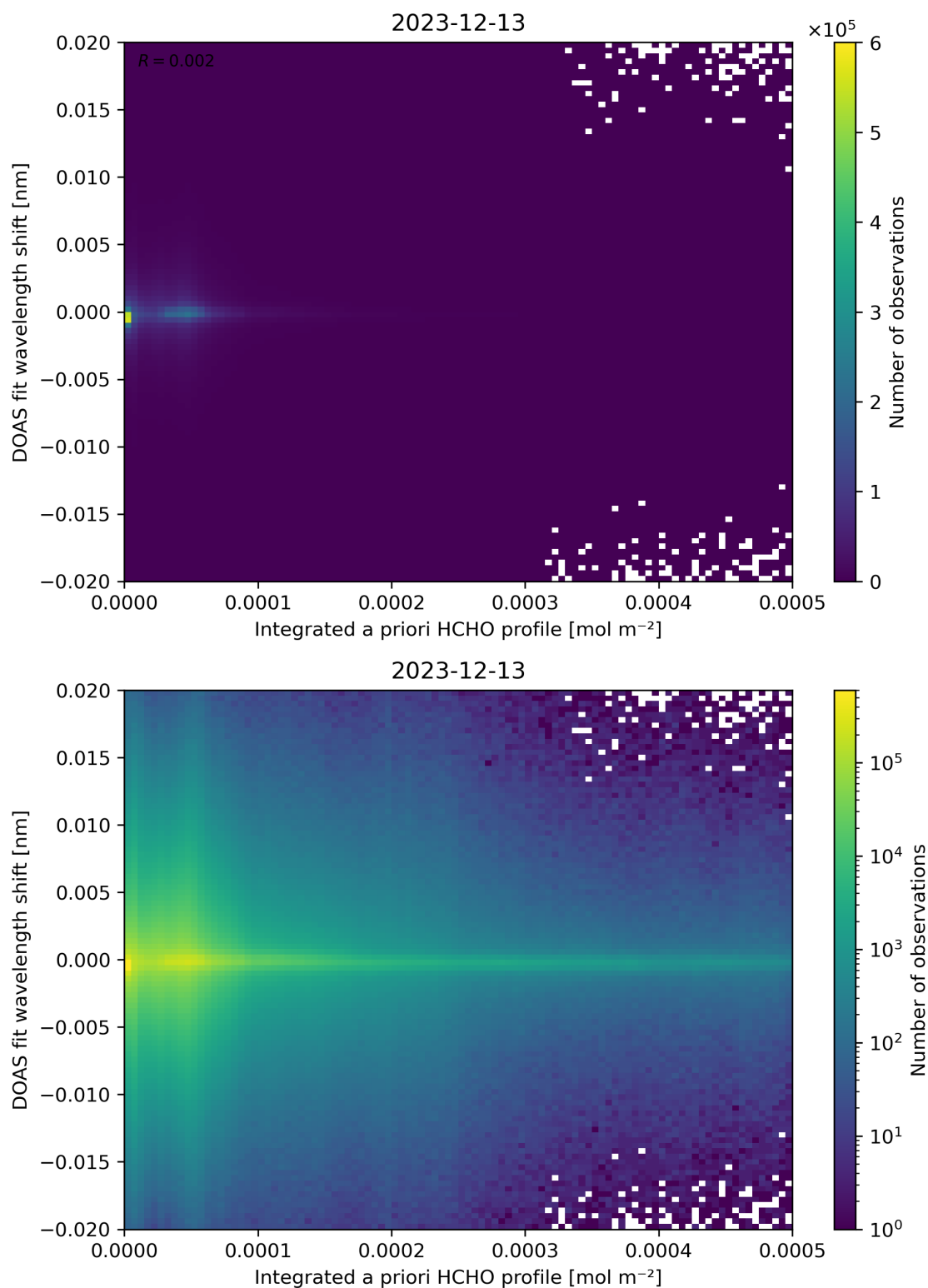
Figure 149: Scatter density plot of “Integrated a priori HCHO profile” against “DOAS fit wavelength shift” for 2023-12-12 to 2023-12-14.
