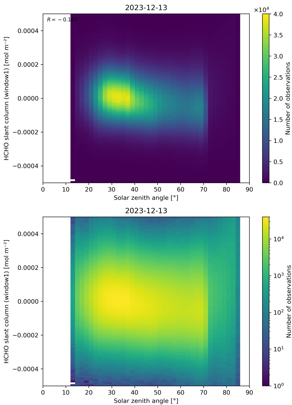
Figure 173: Scatter density plot of “Solar zenith angle” against “HCHO slant column (window1)” for 2023-12-12 to 2023-12-14.
