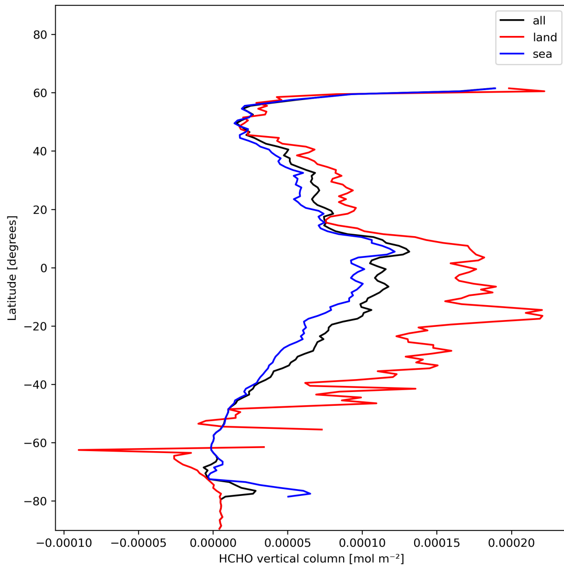
Figure 21: Zonal average of “HCHO vertical column” for 2023-12-12 to 2023-12-14.
