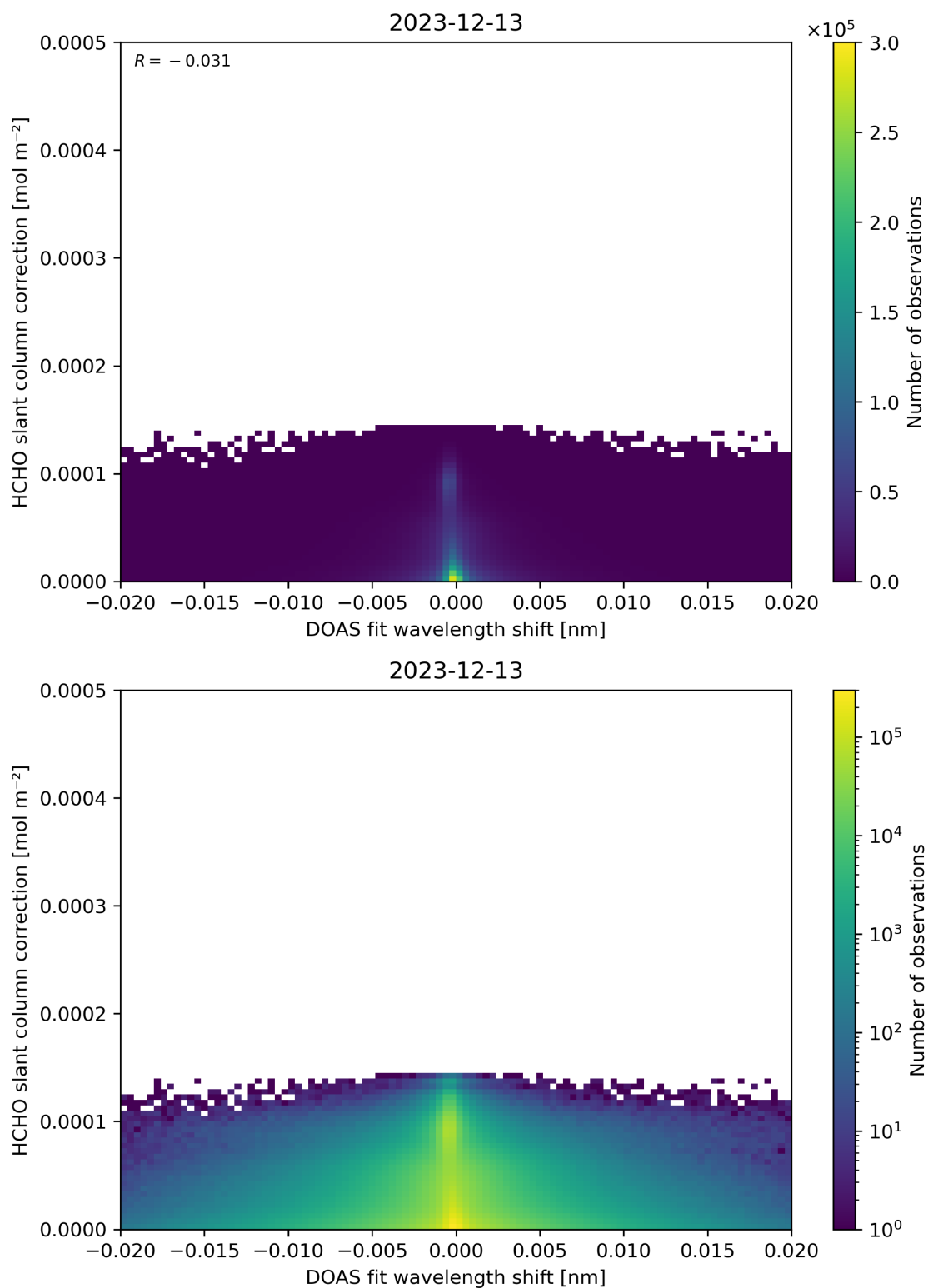
Figure 67: Scatter density plot of “DOAS fit wavelength shift” against “HCHO slant column correction” for 2023-12-12 to 2023-12-14.
