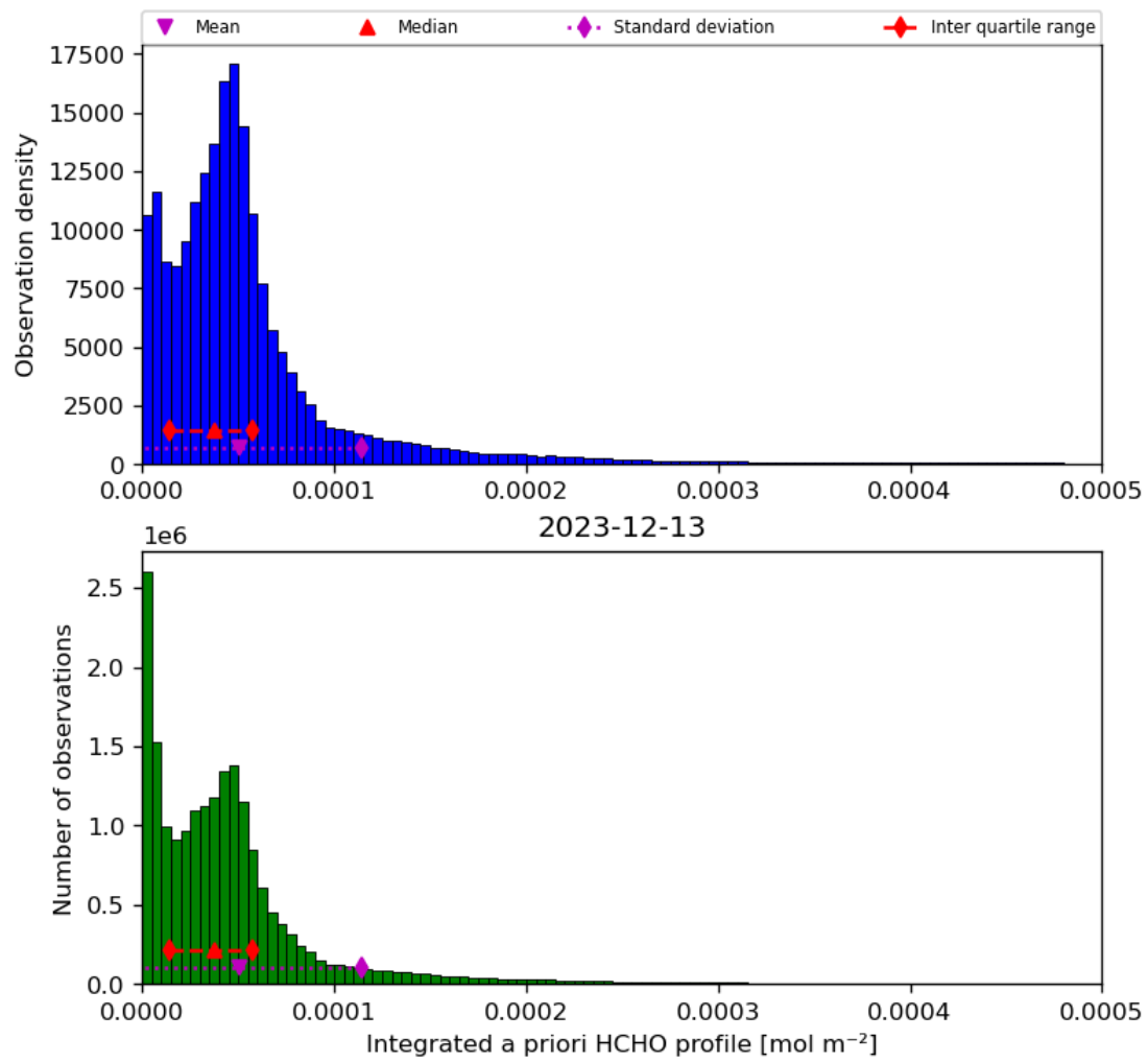
Figure 43: Histogram of “Integrated a priori HCHO profile” for 2023-12-12 to 2023-12-14
