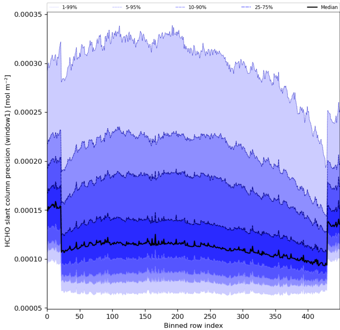
Figure 53: Along track statistics of “HCHO slant column precision (window1)” for 2023-12-12 to 2023-12-14
