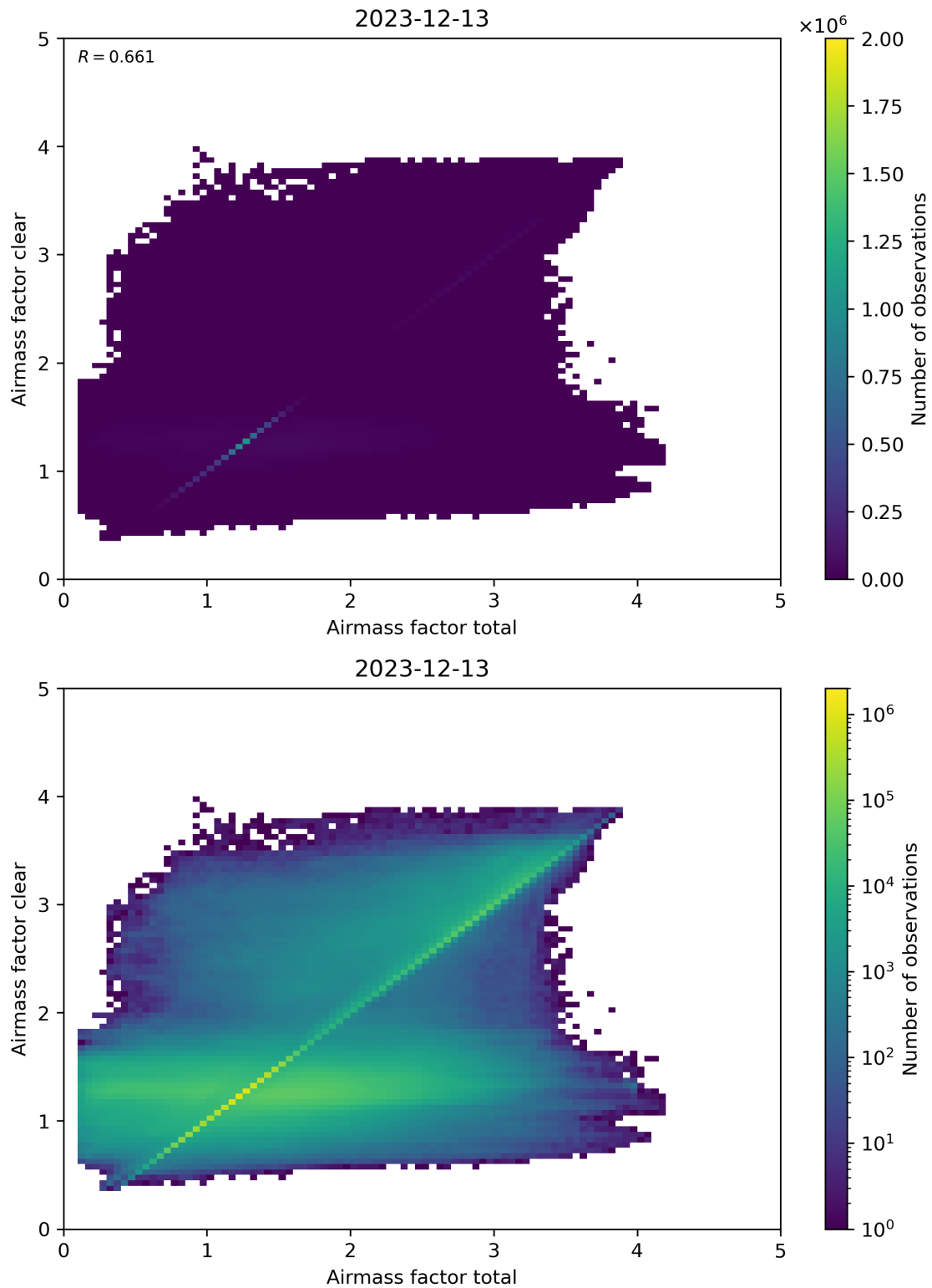
Figure 100: Scatter density plot of “Airmass factor total” against “Airmass factor clear” for 2023-12-12 to 2023-12-14.
