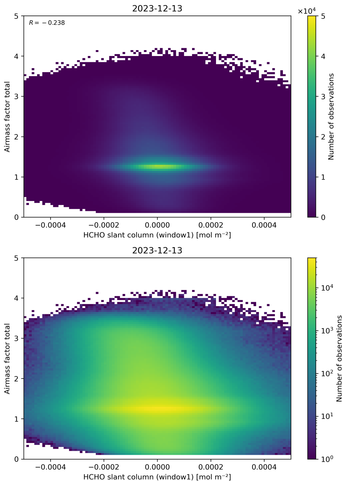
Figure 85: Scatter density plot of “HCHO slant column (window1)” against “Airmass factor total” for 2023-12-12 to 2023-12-14.
