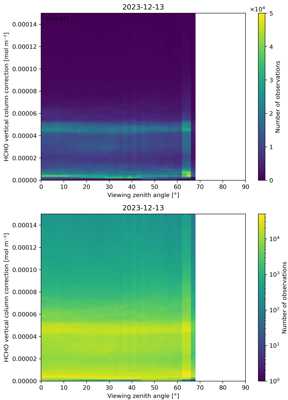
Figure 193: Scatter density plot of “Viewing zenith angle” against “HCHO vertical column correction” for 2023-12-12 to 2023-12-14.
