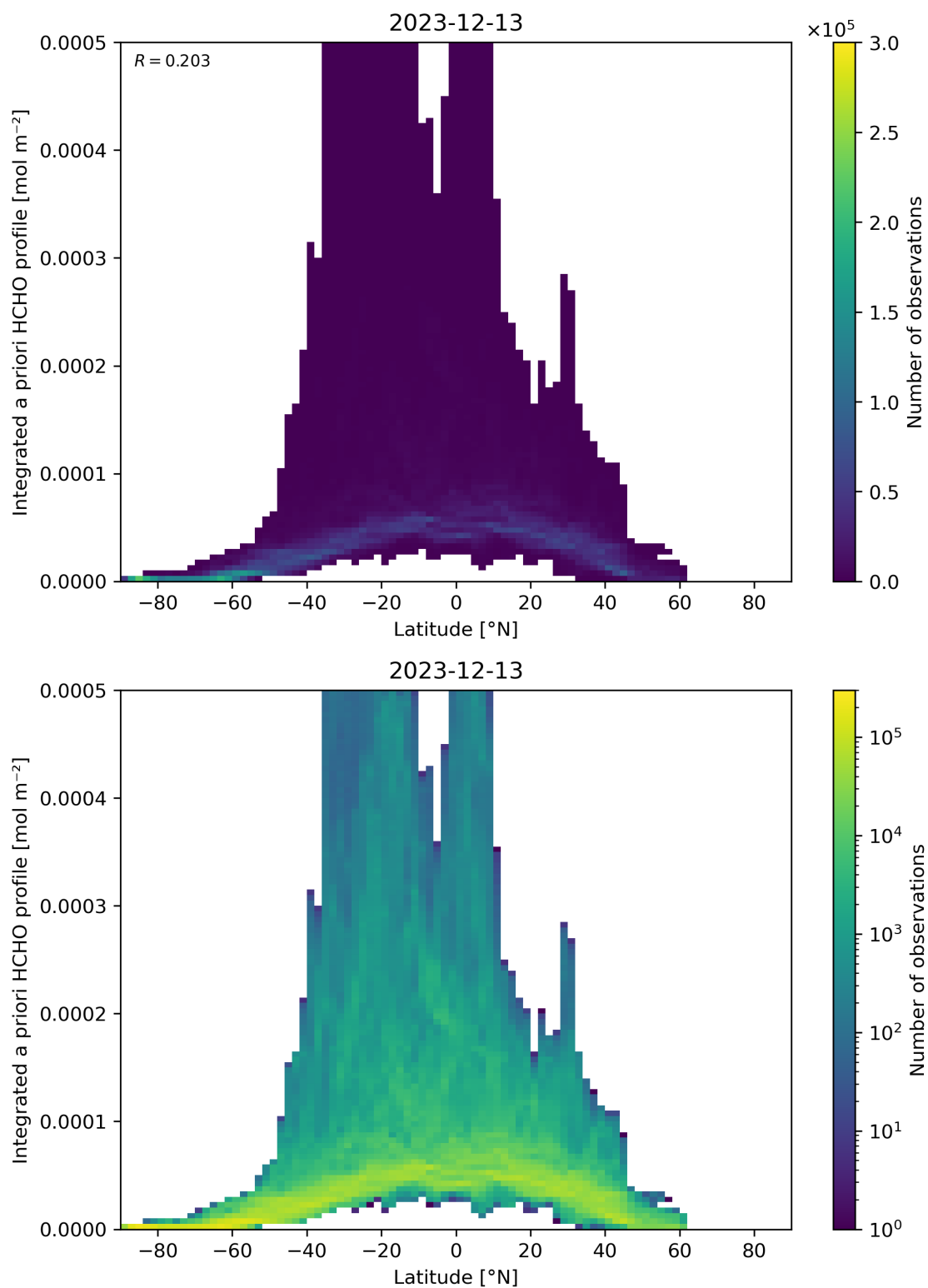
Figure 166: Scatter density plot of “Latitude” against “Integrated a priori HCHO profile” for 2023-12-12 to 2023-12-14.
